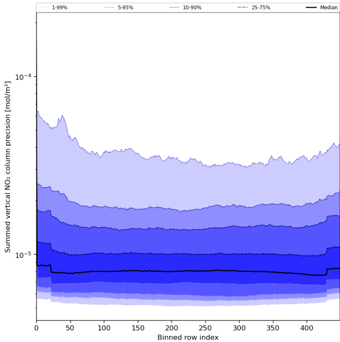
Figure 58: Along track statistics of “Summed vertical NO 2 column precision” for 2023-07-26 to 2023-07-28
