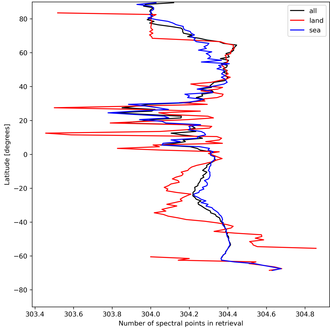
Figure 16: Zonal average of “Number of spectral points in retrieval” for 2023-07-26 to 2023-07-28.
