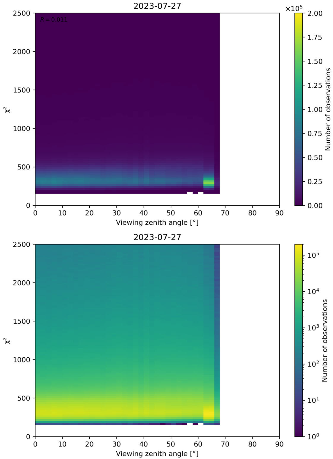
Figure 162: Scatter density plot of “Viewing zenith angle” against “ \chi^2 ” for 2023-07-26 to 2023-07-28.
