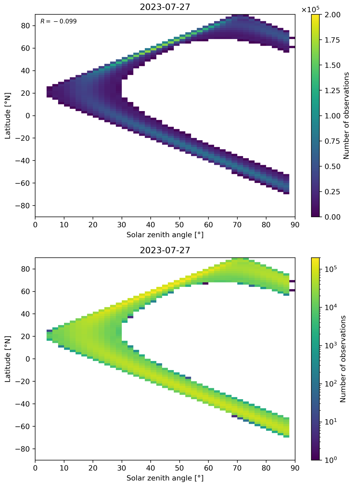
Figure 149: Scatter density plot of “Solar zenith angle” against “Latitude” for 2023-07-26 to 2023-07-28.
