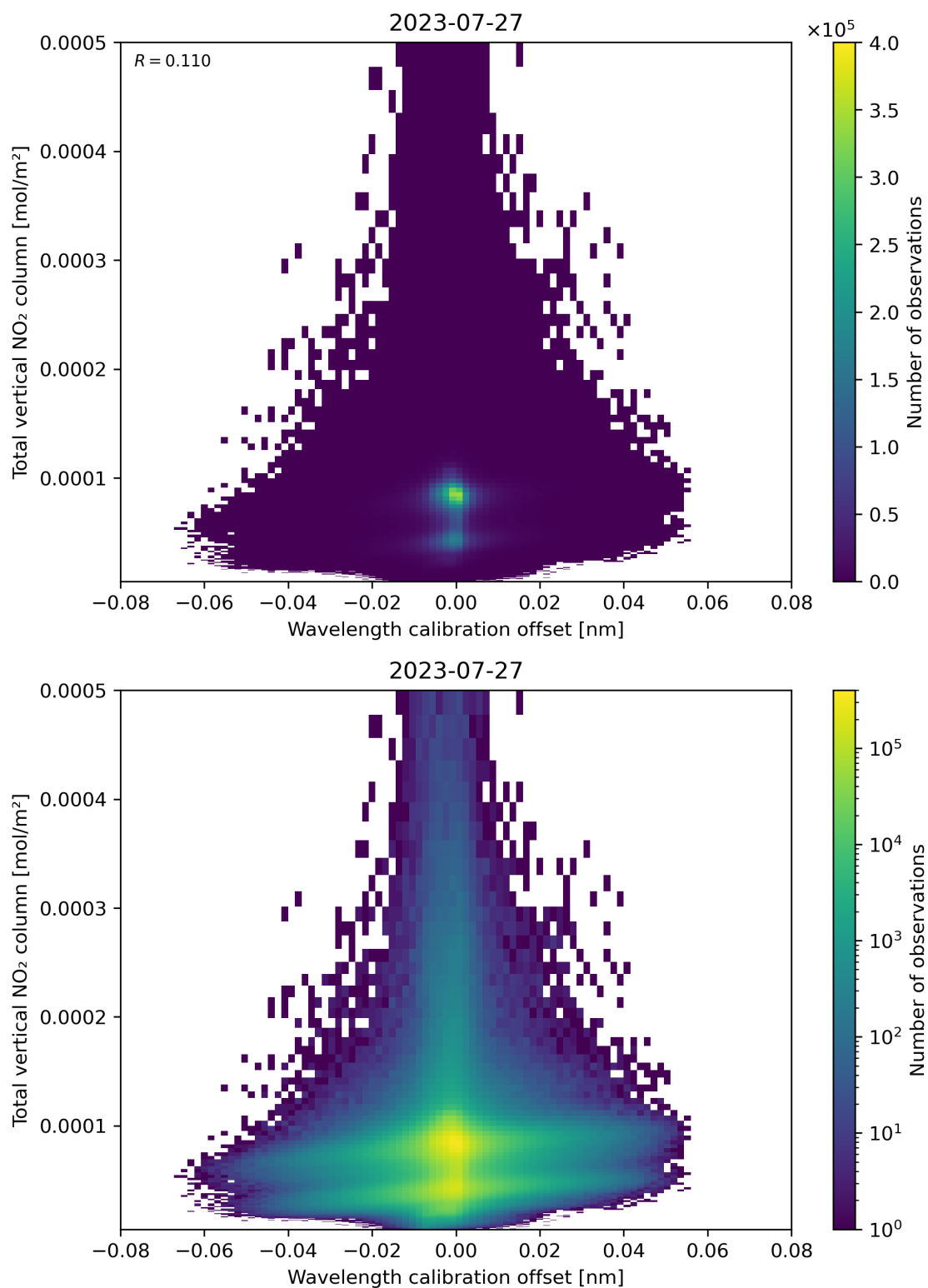
Figure 179: Scatter density plot of “Wavelength calibration offset” against “Total vertical NO 2 column” for 2023-07-26 to 2023-07-28.
