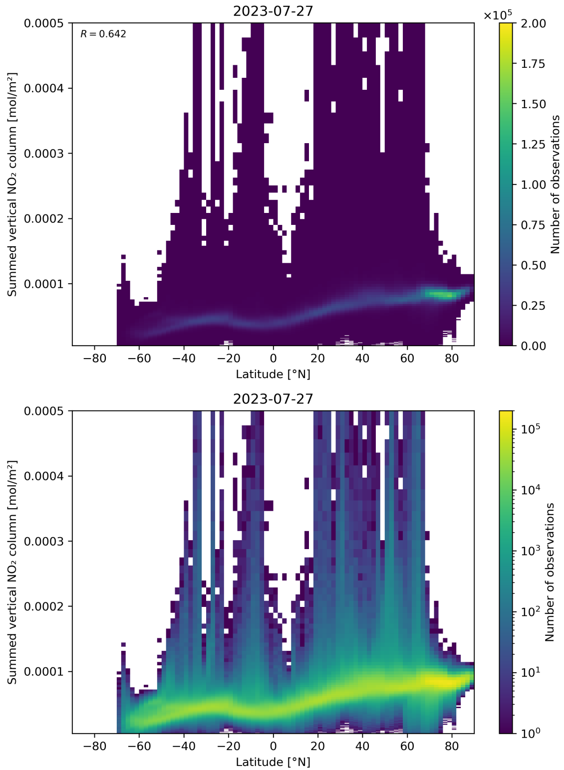
Figure 88: Scatter density plot of “Latitude” against “Summed vertical NO 2 column” for 2023-07-26 to 2023-07-28.
