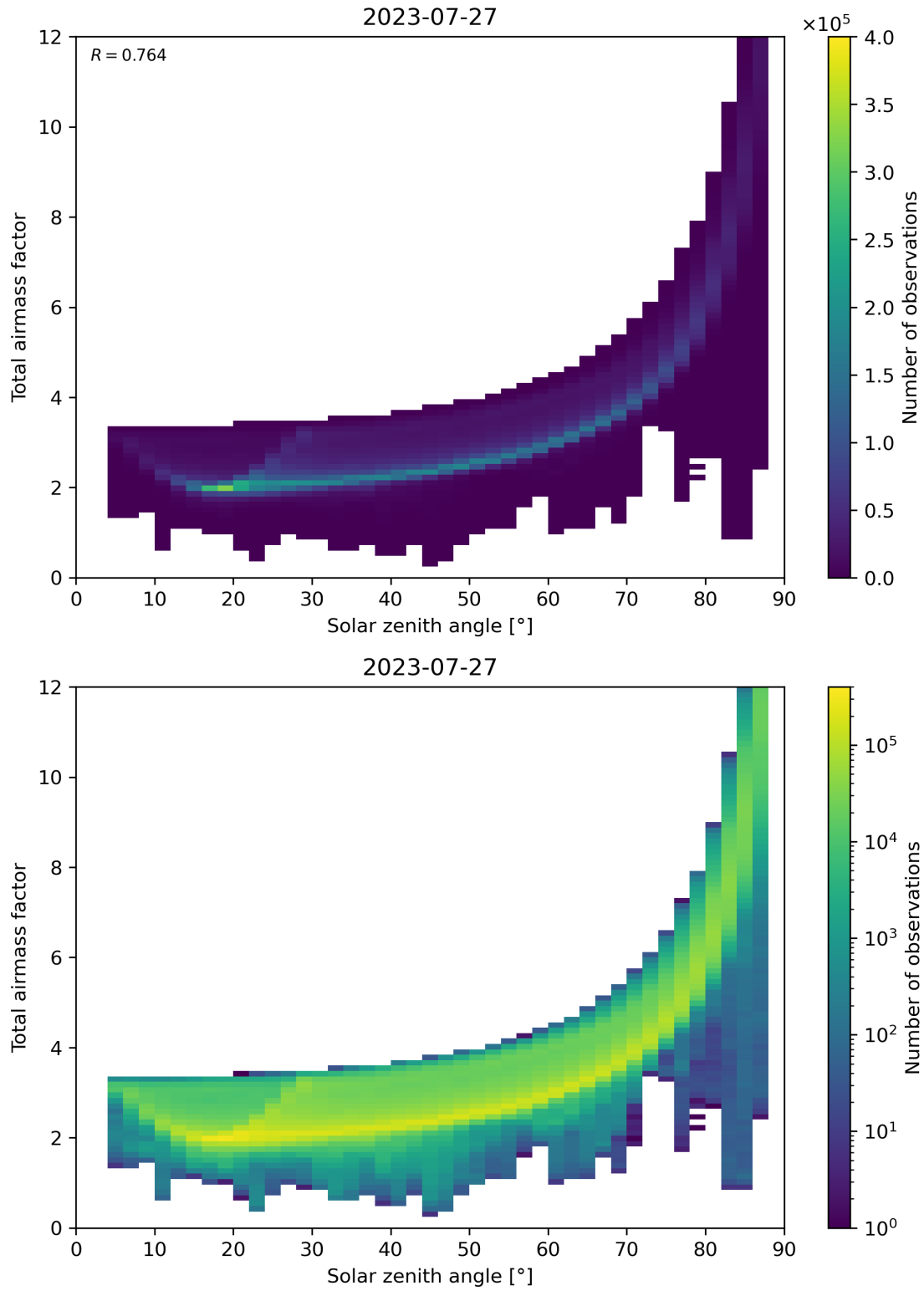
Figure 146: Scatter density plot of “Solar zenith angle” against “Total air mass factor” for 2023-07-26 to 2023-07-28.
