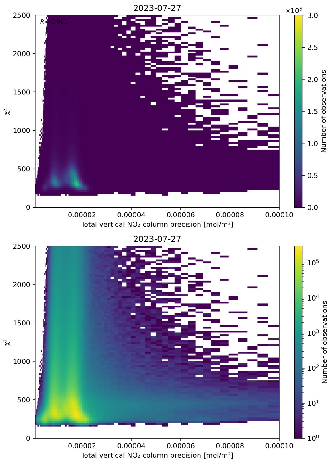
Figure 116: Scatter density plot of “Total vertical NO 2 column precision” against “ \chi^2 ” for 2023-07-26 to 2023-07-28.
