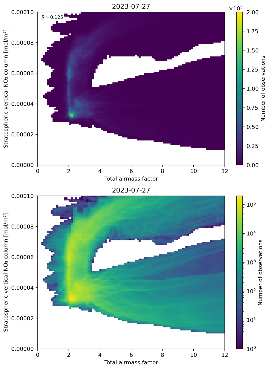
Figure 64: Scatter density plot of “Total airmass factor” against “Stratospheric vertical \text{NO}_2 column” for 2023-07-26 to 2023-07-28.
