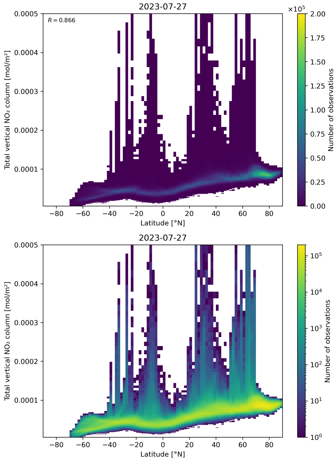
Figure 90: Scatter density plot of “Latitude” against “Total vertical NO 2 column” for 2023-07-26 to 2023-07-28.
