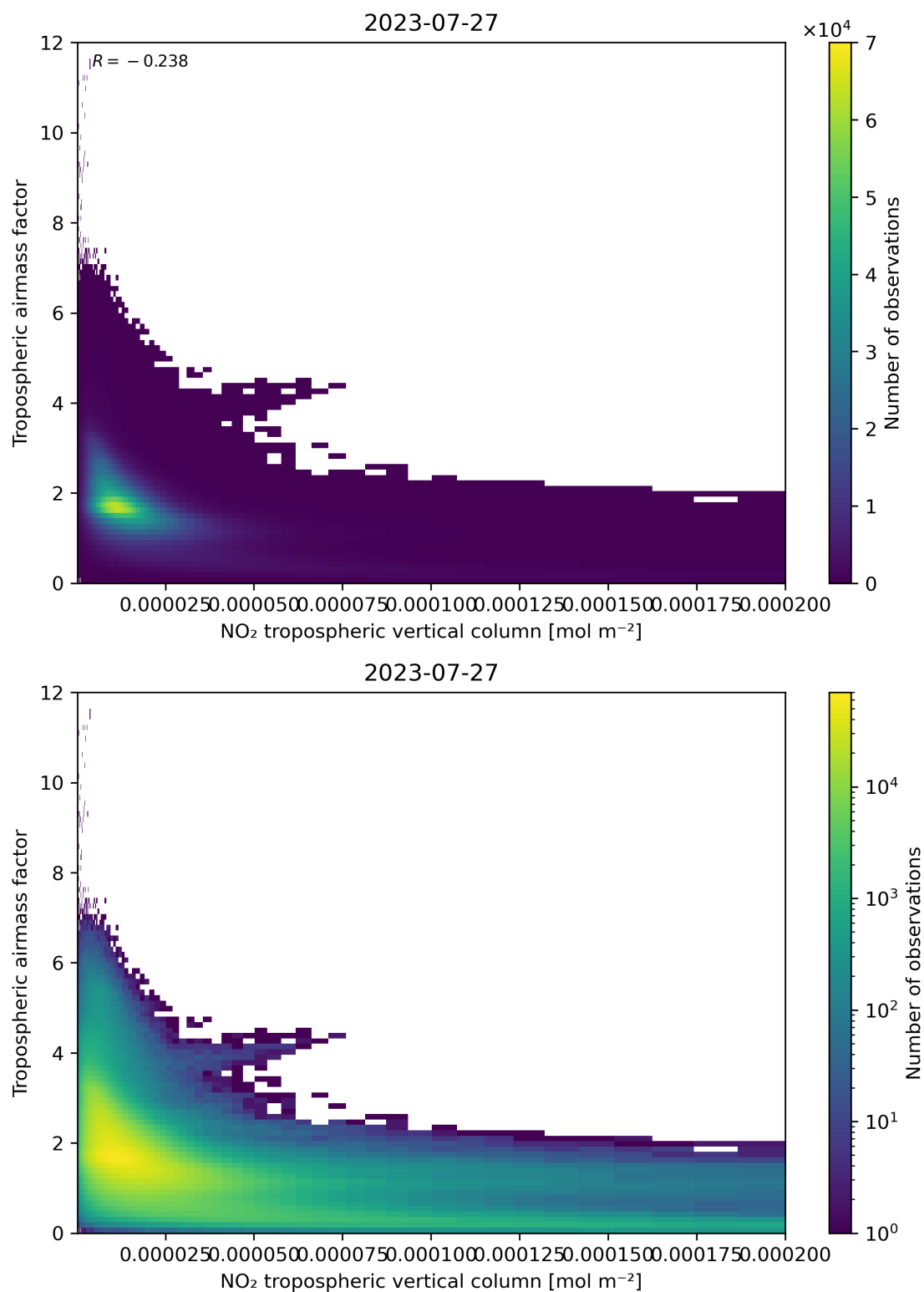
Figure 123: Scatter density plot of “NO 2 tropospheric vertical column” against “Tropospheric airmass factor” for 2023-07-26 to 2023-07-28.
