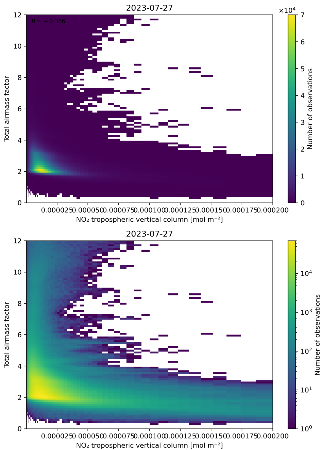
Figure 122: Scatter density plot of “NO 2 tropospheric vertical column” against “Total air mass factor” for 2023-07-26 to 2023-07-28.
