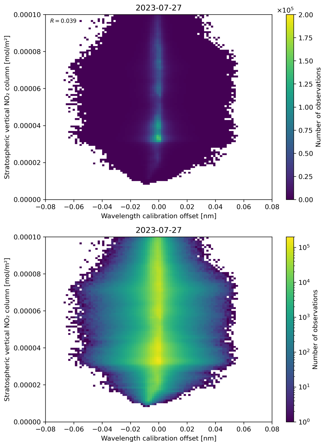
Figure 176: Scatter density plot of “Wavelength calibration offset” against “Stratospheric vertical NO 2 column” for 2023-07-26 to 2023-07-28.
