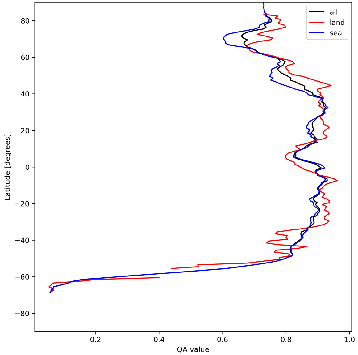
Figure 11: Zonal average of “QA value” for 2023-07-26 to 2023-07-28.
