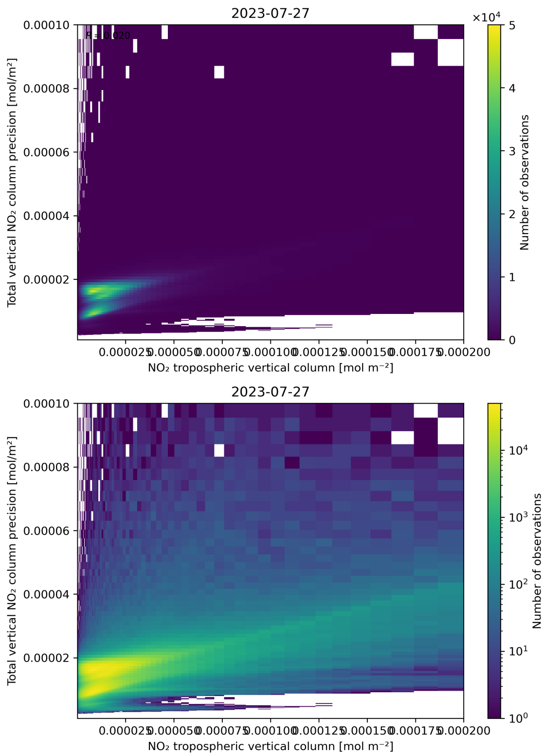
Figure 129: Scatter density plot of “NO 2 tropospheric vertical column” against “Total vertical NO 2 column precision” for 2023-07-26 to 2023-07-28.
