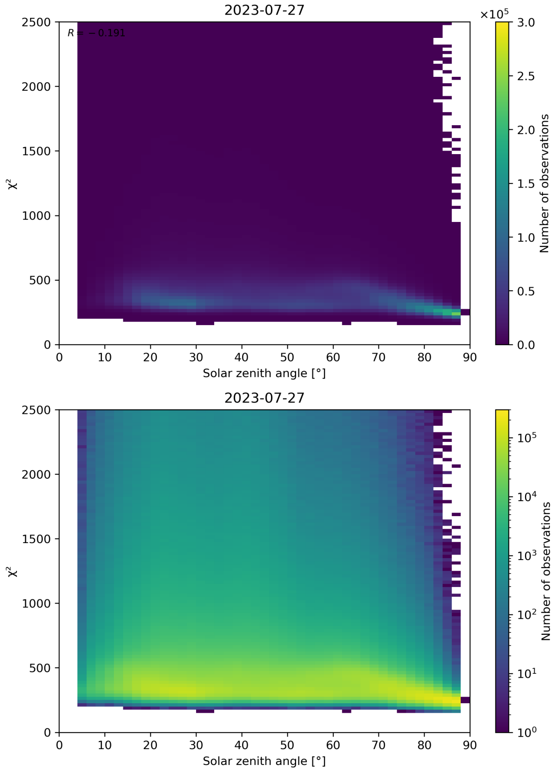
Figure 148: Scatter density plot of “Solar zenith angle” against “ \chi^2 ” for 2023-07-26 to 2023-07-28.
