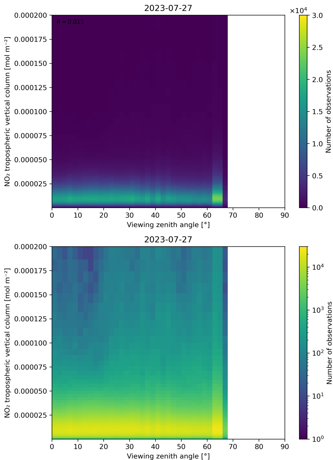
Figure 169: Scatter density plot of “Viewing zenith angle” against “NO 2 tropospheric vertical column” for 2023-07-26 to 2023-07-28.
