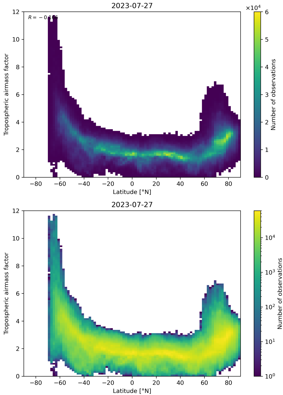
Figure 85: Scatter density plot of “Latitude” against “Tropospheric airmass factor” for 2023-07-26 to 2023-07-28.
