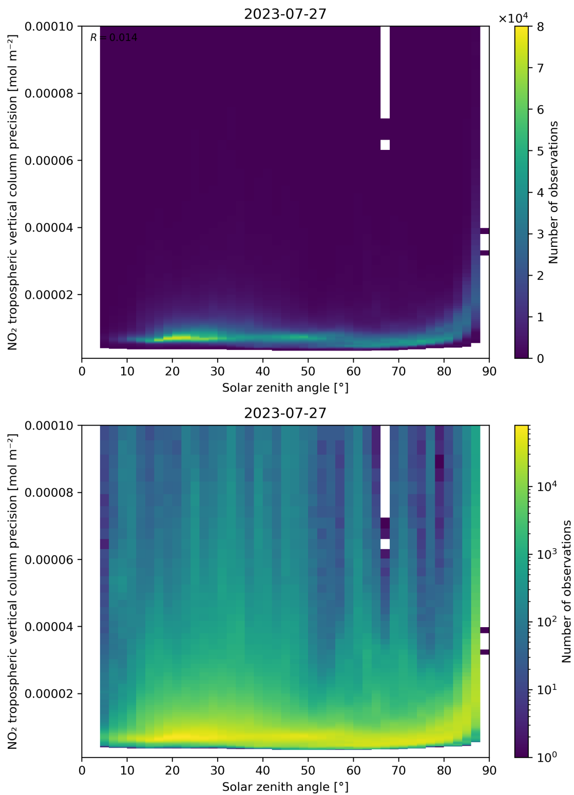
Figure 156: Scatter density plot of “Solar zenith angle” against “NO 2 tropospheric vertical column precision” for 2023-07-26 to 2023-07-28.
