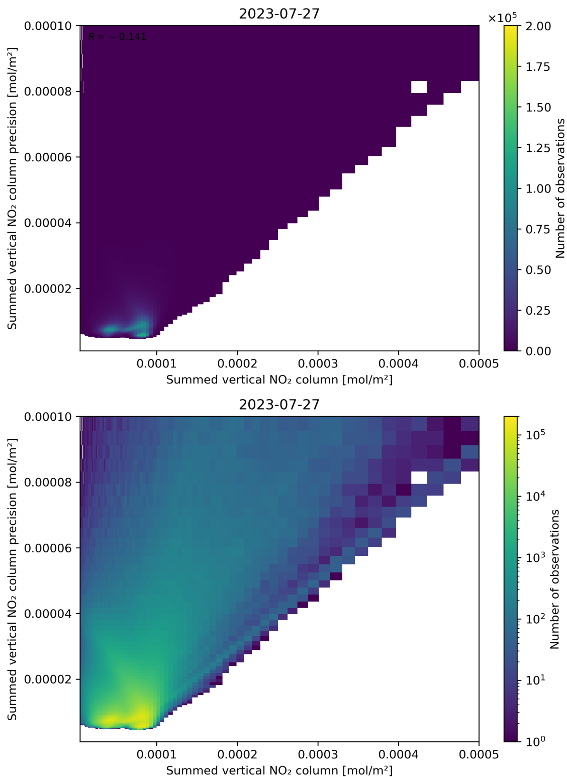
Figure 105: Scatter density plot of “Summed vertical NO 2 column” against “Summed vertical NO 2 column precision” for 2023-07-26 to 2023-07-28.
