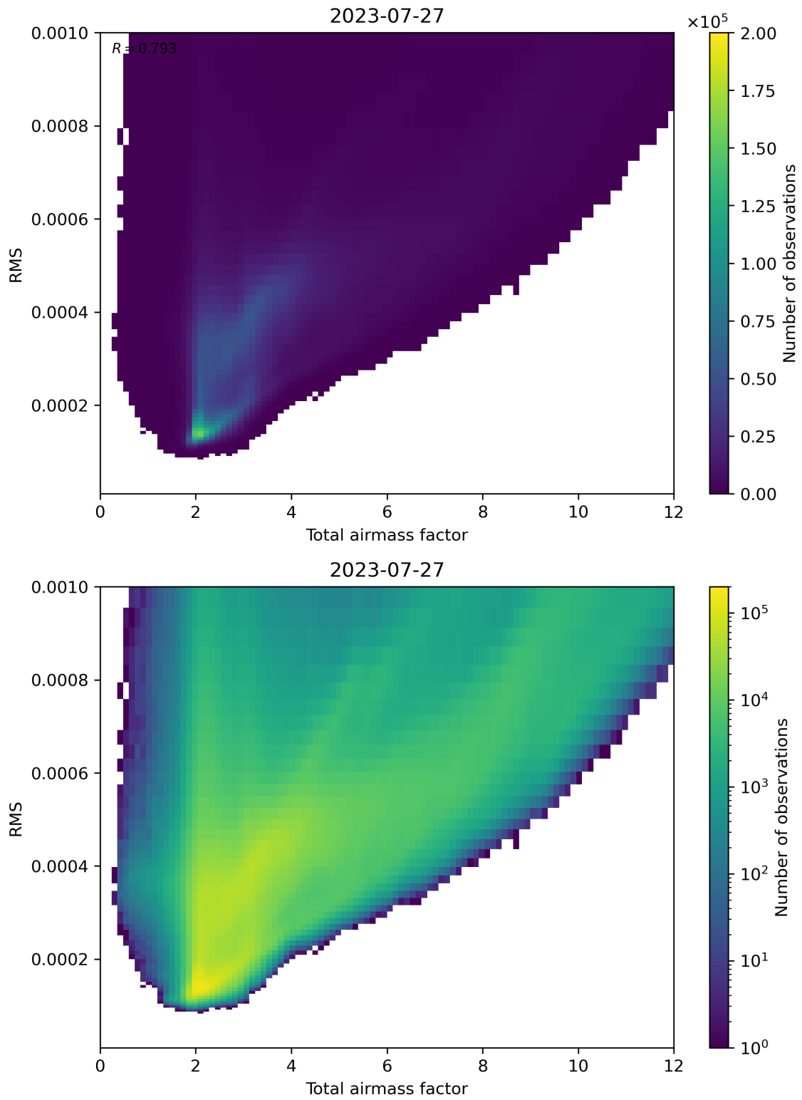
Figure 69: Scatter density plot of “Total airmass factor” against “RMS” for 2023-07-26 to 2023-07-28.
