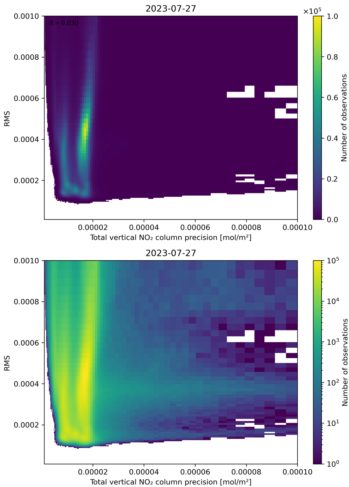
Figure 119: Scatter density plot of “Total vertical NO 2 column precision” against “RMS” for 2023-07-26 to 2023-07-28.
