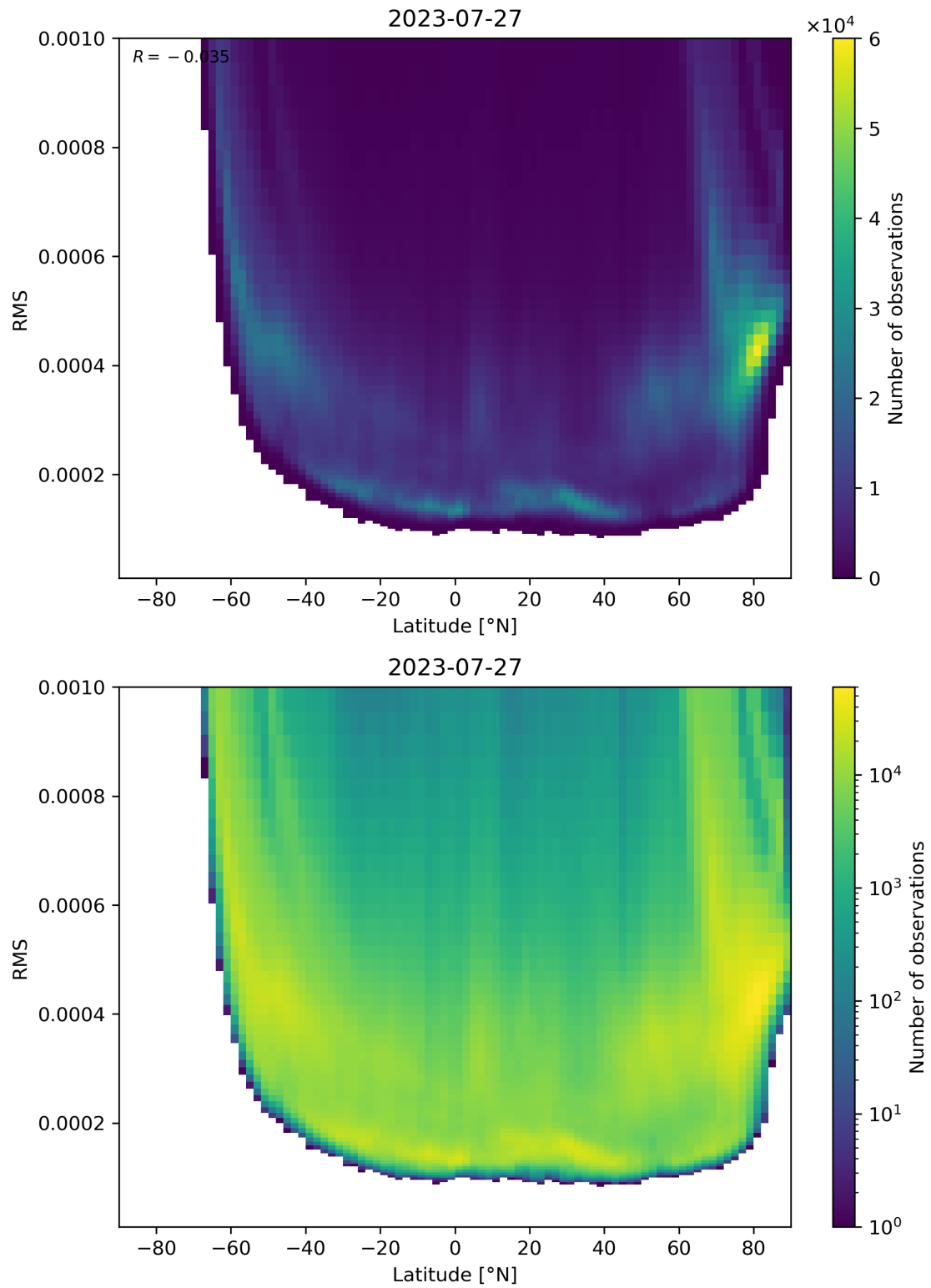
Figure 94: Scatter density plot of “Latitude” against “RMS” for 2023-07-26 to 2023-07-28.
