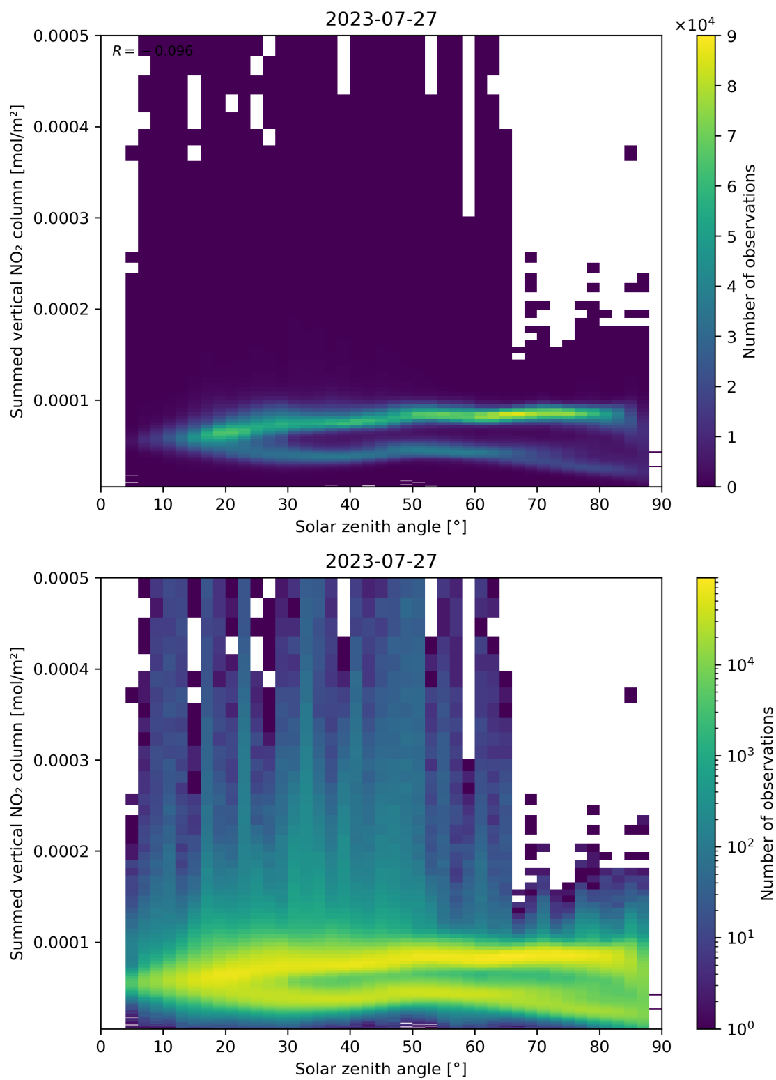
Figure 151: Scatter density plot of “Solar zenith angle” against “Summed vertical NO 2 column” for 2023-07-26 to 2023-07-28.
