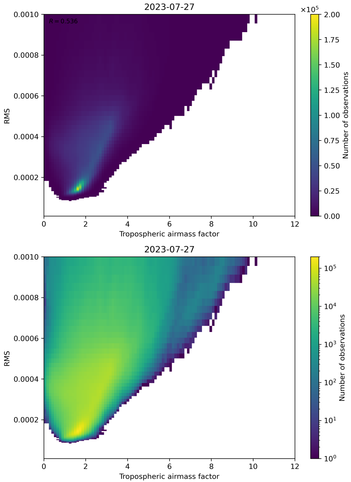
Figure 79: Scatter density plot of “Tropospheric airmass factor” against “RMS” for 2023-07-26 to 2023-07-28.
