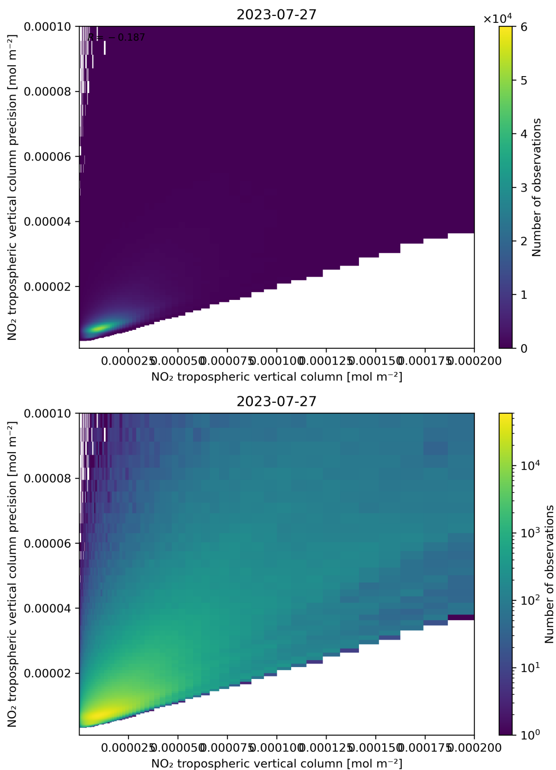
Figure 130: Scatter density plot of “NO 2 tropospheric vertical column” against “NO 2 tropospheric vertical column precision” for 2023-07-26 to 2023-07-28.
