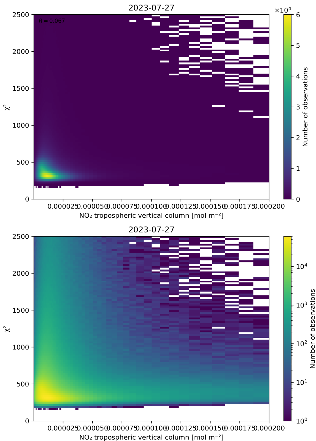
Figure 124: Scatter density plot of “NO 2 tropospheric vertical column” against “ \chi^2 ” for 2023-07-26 to 2023-07-28.
