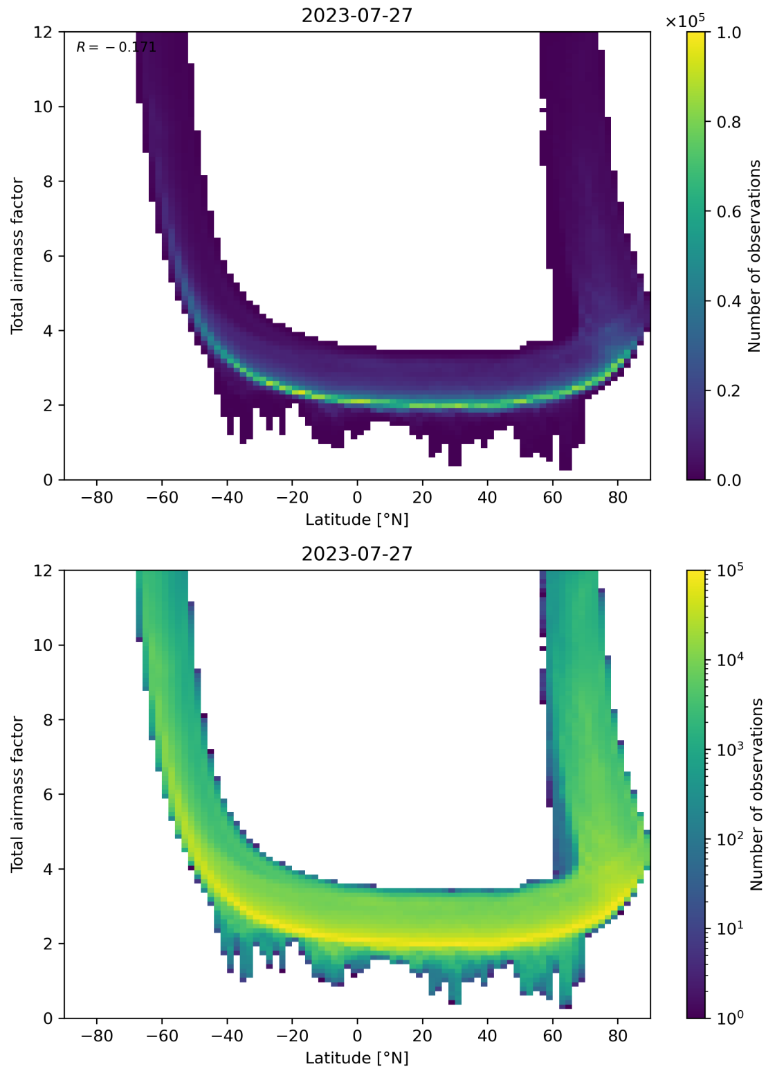
Figure 84: Scatter density plot of “Latitude” against “Total airmass factor” for 2023-07-26 to 2023-07-28.
