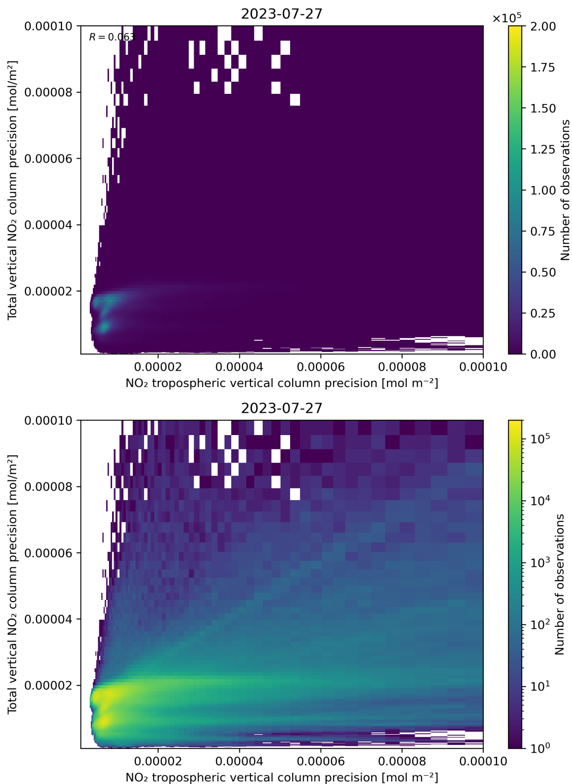
Figure 139: Scatter density plot of “NO 2 tropospheric vertical column precision” against “Total vertical NO 2 column precision” for 2023-07-26 to 2023-07-28.
