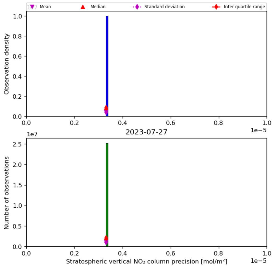
Figure 37: Histogram of “Stratospheric vertical NO 2 column precision” for 2023-07-26 to 2023-07-28
