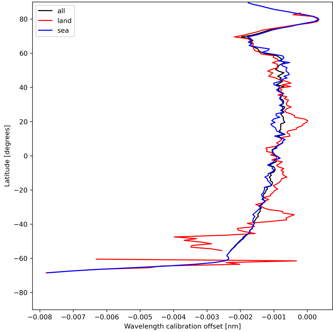
Figure 18: Zonal average of “Wavelength calibration offset” for 2023-07-26 to 2023-07-28.
