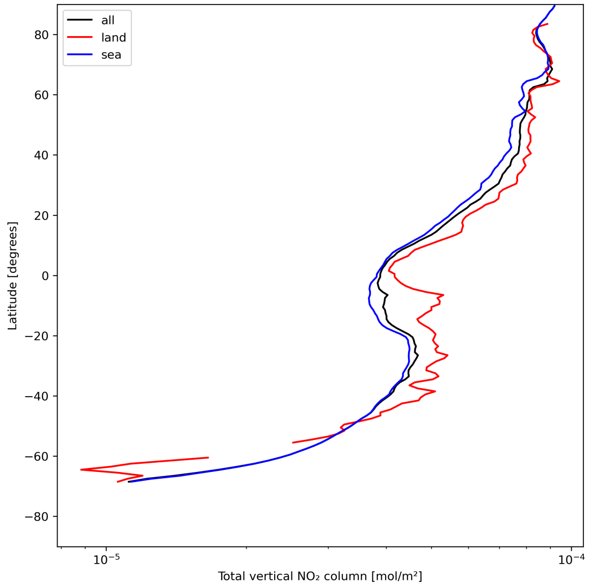
Figure 21: Zonal average of “Total vertical NO 2 column” for 2023-07-26 to 2023-07-28.
