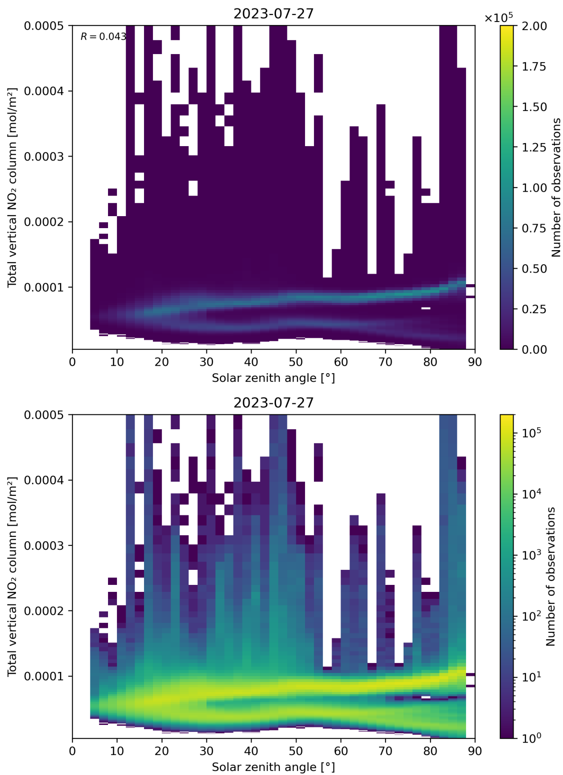
Figure 153: Scatter density plot of “Solar zenith angle” against “Total vertical NO 2 column” for 2023-07-26 to 2023-07-28.
