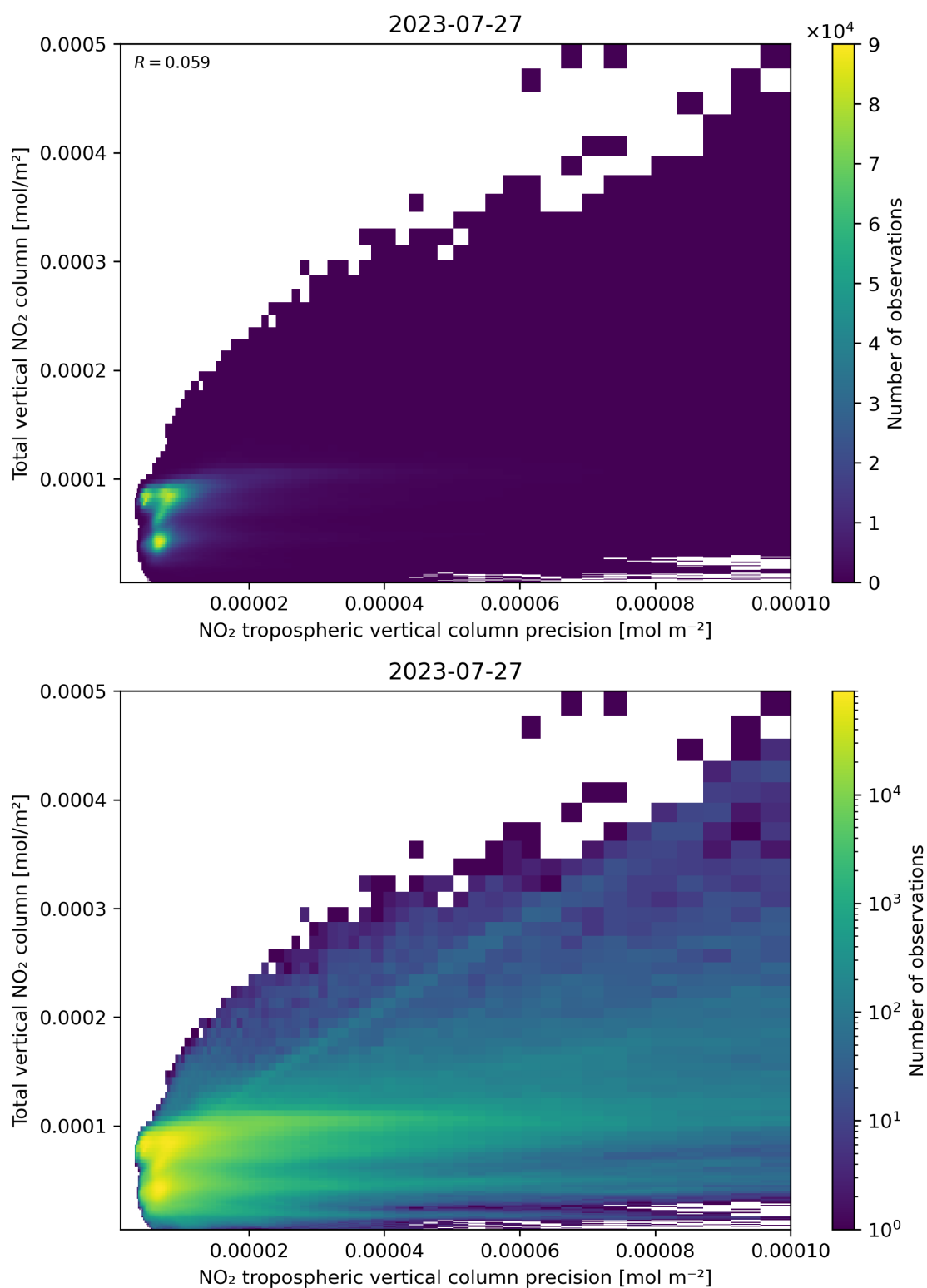
Figure 138: Scatter density plot of “NO 2 tropospheric vertical column precision” against “Total vertical NO 2 column” for 2023-07-26 to 2023-07-28.
