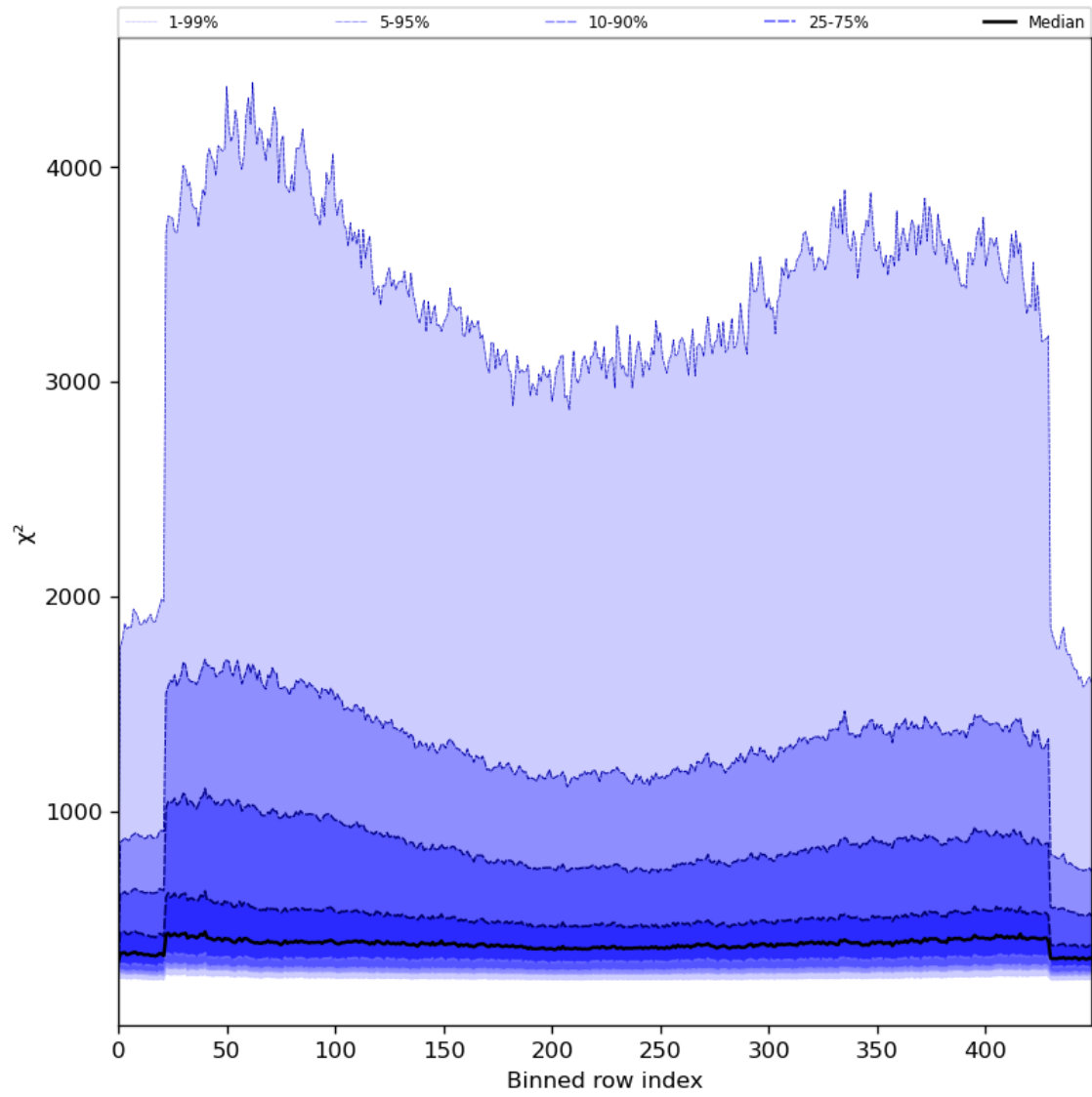
Figure 59: Along track statistics of “ \chi^2 ” for 2023-07-26 to 2023-07-28
