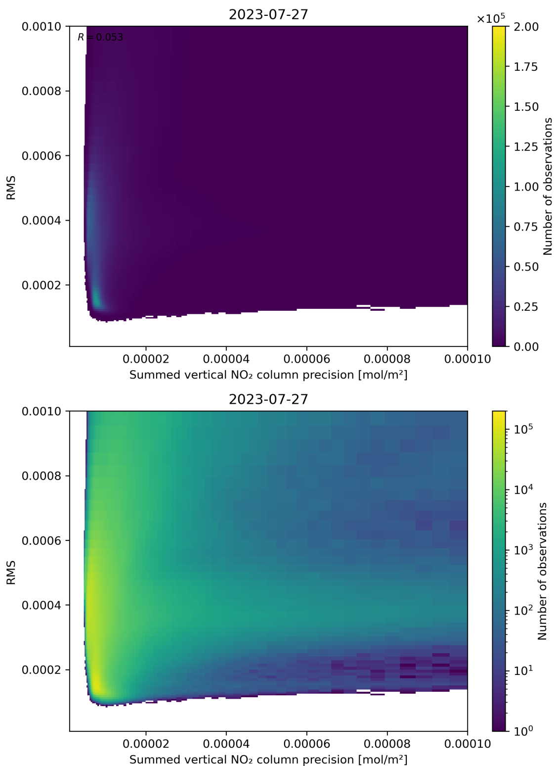
Figure 108: Scatter density plot of “Summed vertical NO 2 column precision” against “RMS” for 2023-07-26 to 2023-07-28.
