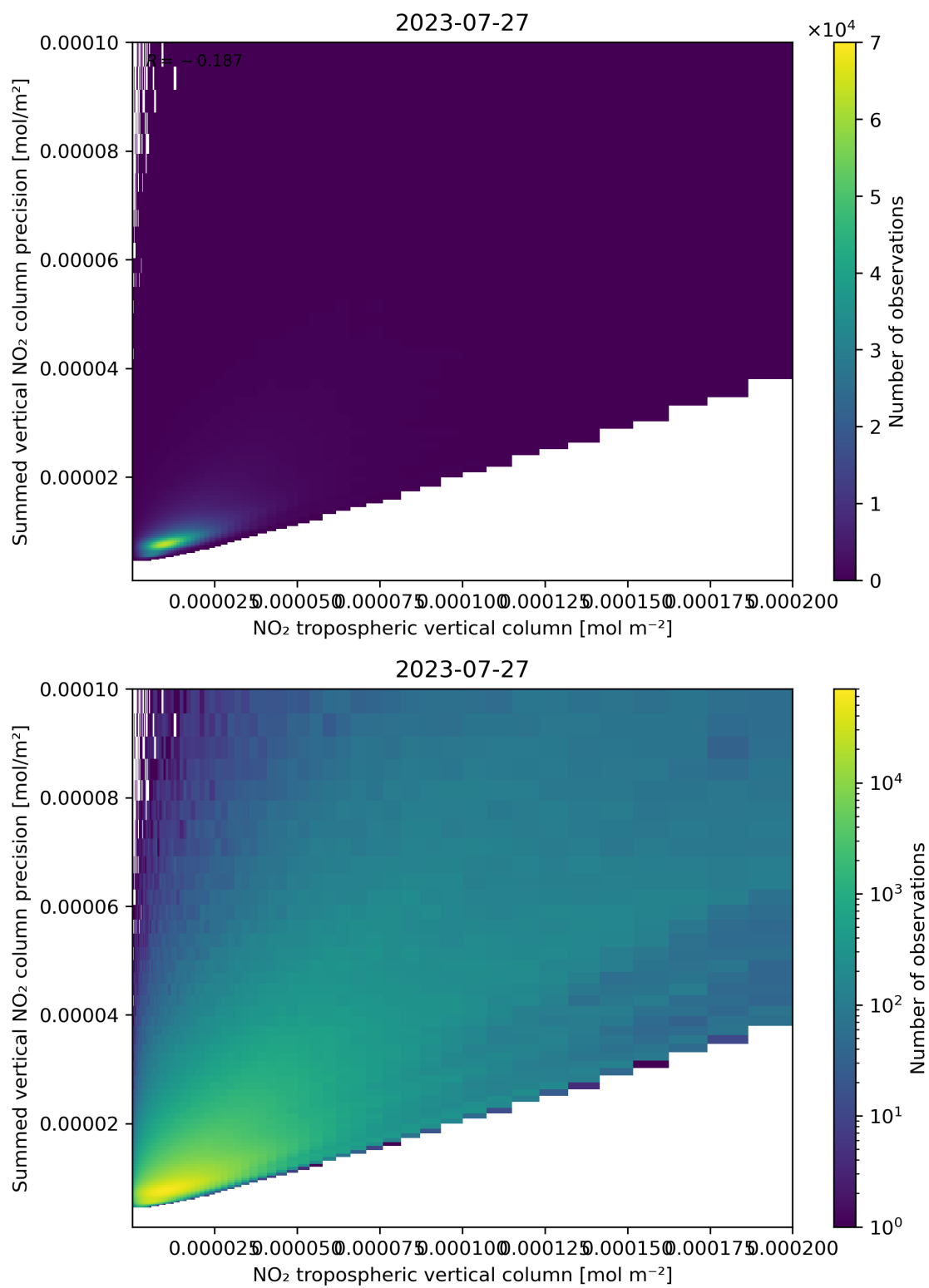
Figure 127: Scatter density plot of “NO 2 tropospheric vertical column” against “Summed vertical NO 2 column precision” for 2023-07-26 to 2023-07-28.
