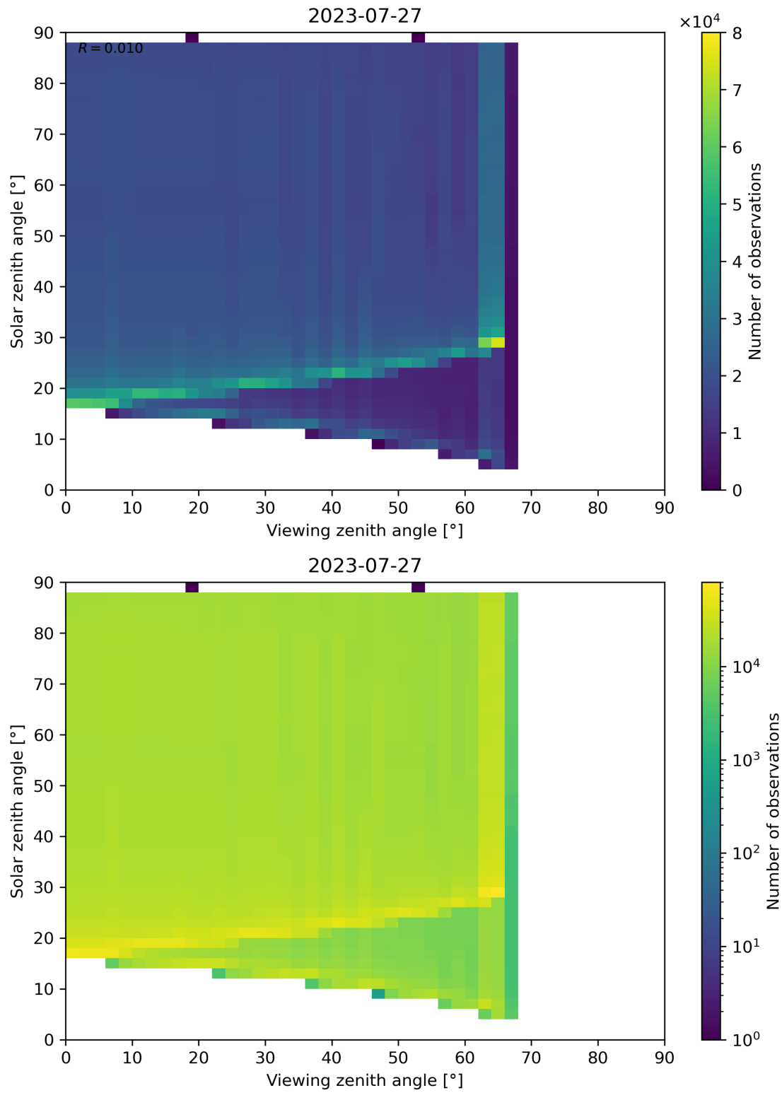
Figure 172: Scatter density plot of “Viewing zenith angle” against “Solar zenith angle” for 2023-07-26 to 2023-07-28.
