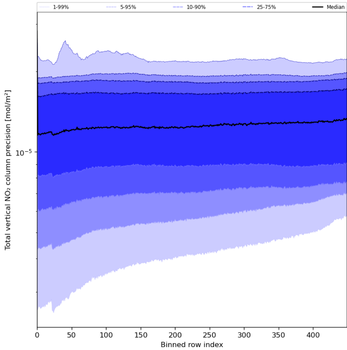
Figure 56: Along track statistics of “Total vertical NO 2 column precision” for 2023-07-26 to 2023-07-28
