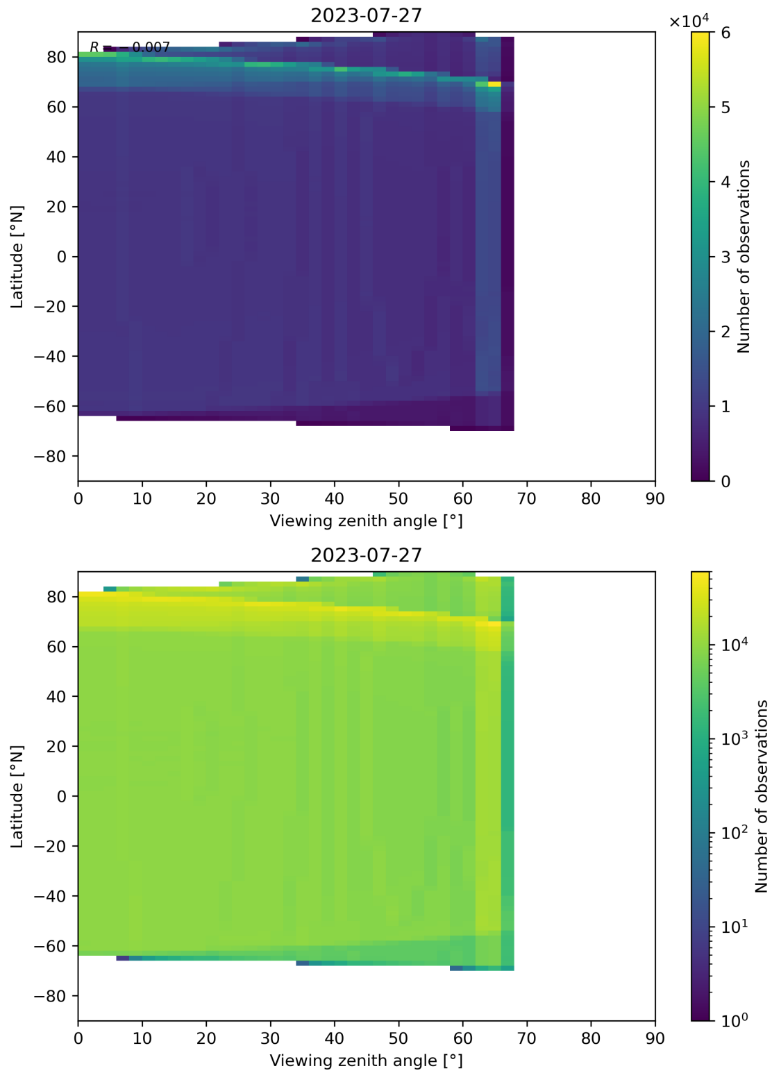
Figure 163: Scatter density plot of “Viewing zenith angle” against “Latitude” for 2023-07-26 to 2023-07-28.
