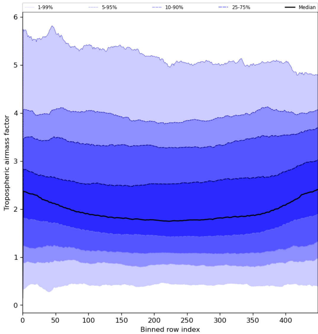
Figure 48: Along track statistics of “Tropospheric airmass factor” for 2023-07-26 to 2023-07-28
