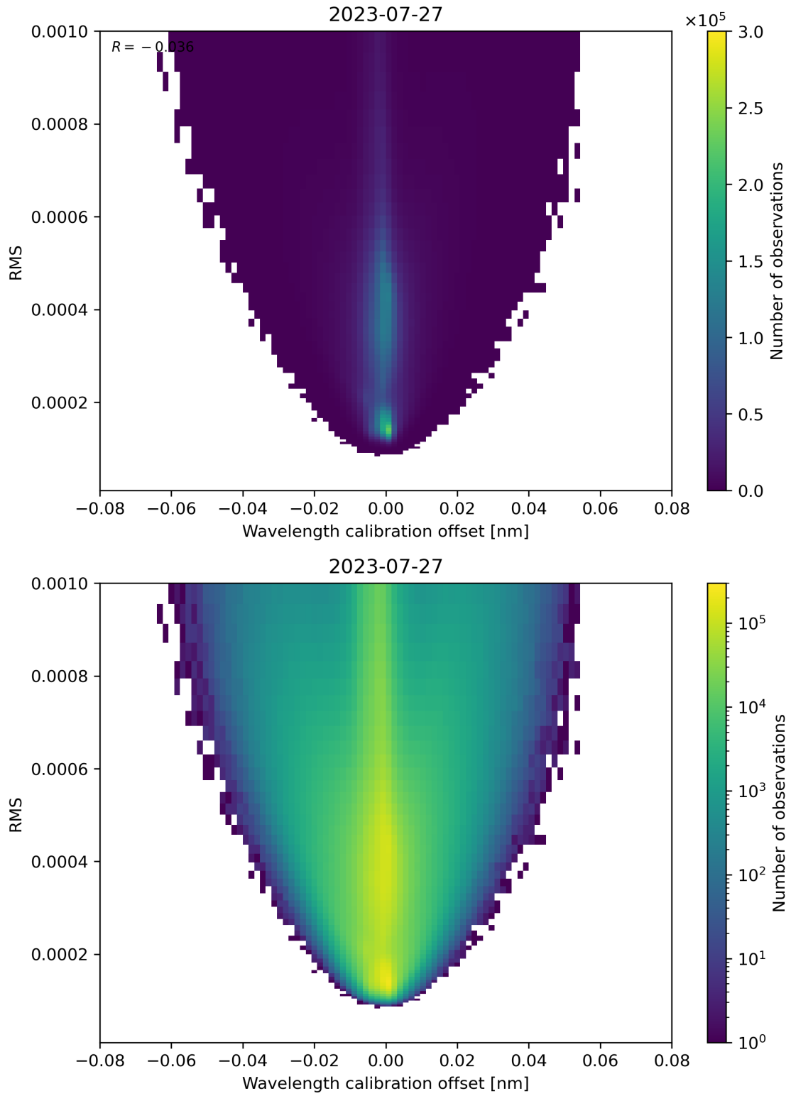
Figure 181: Scatter density plot of “Wavelength calibration offset” against “RMS” for 2023-07-26 to 2023-07-28.
