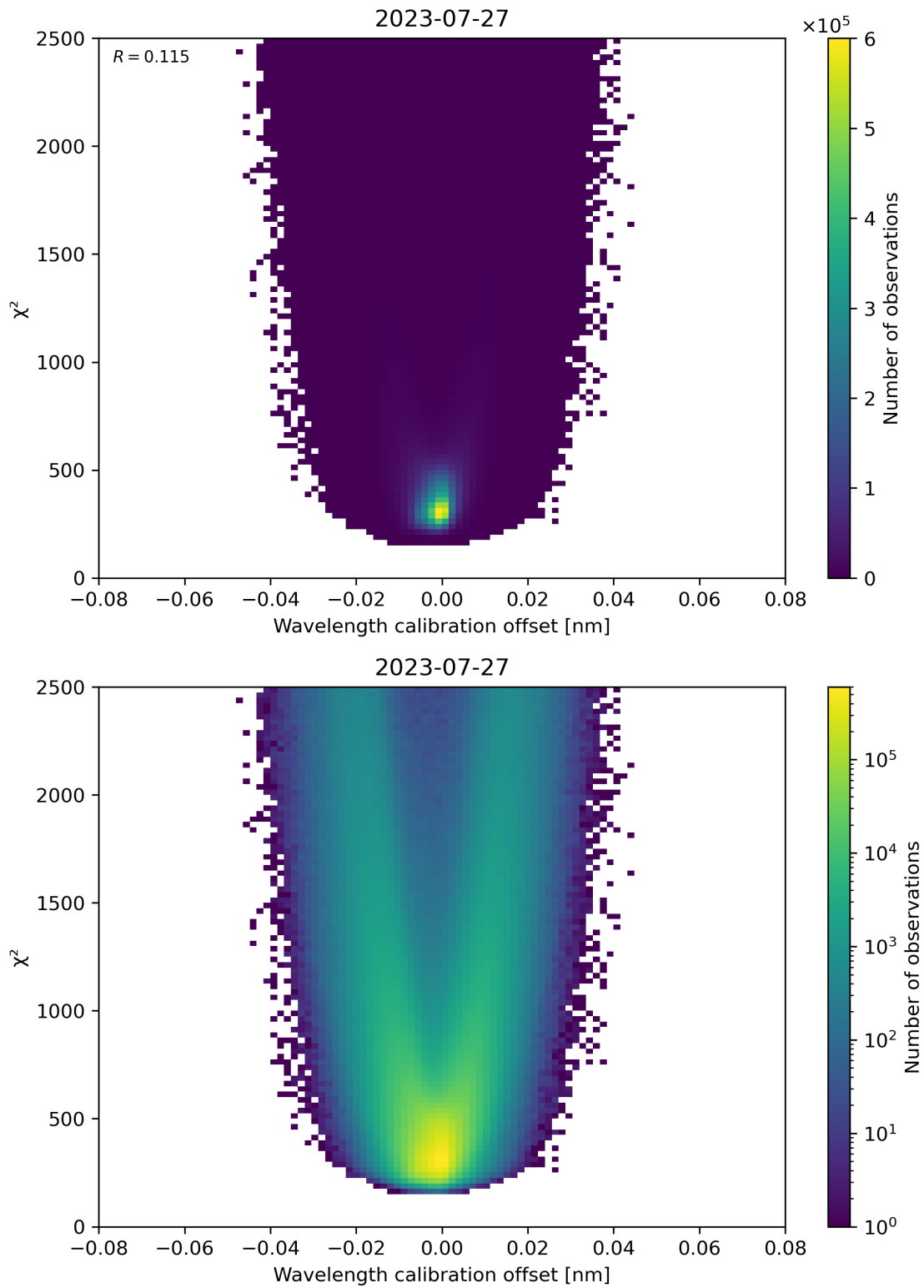
Figure 175: Scatter density plot of “Wavelength calibration offset” against “ \chi^2 ” for 2023-07-26 to 2023-07-28.
