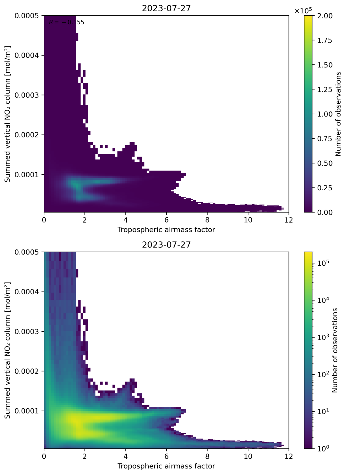
Figure 75: Scatter density plot of “Tropospheric airmass factor” against “Summed vertical NO 2 column” for 2023-07-26 to 2023-07-28.
