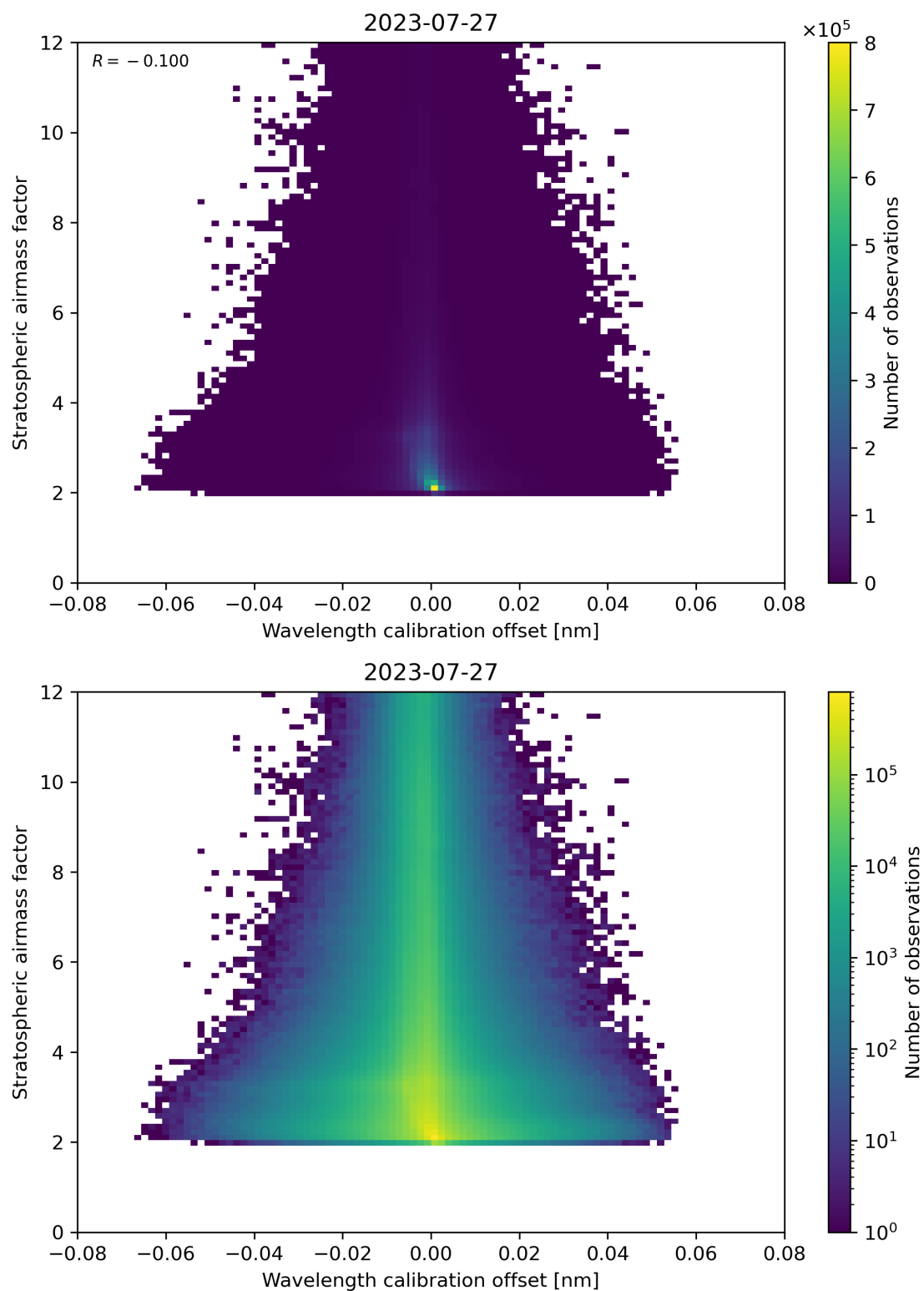
Figure 174: Scatter density plot of “Wavelength calibration offset” against “Stratospheric air mass factor” for 2023-07-26 to 2023-07-28.
