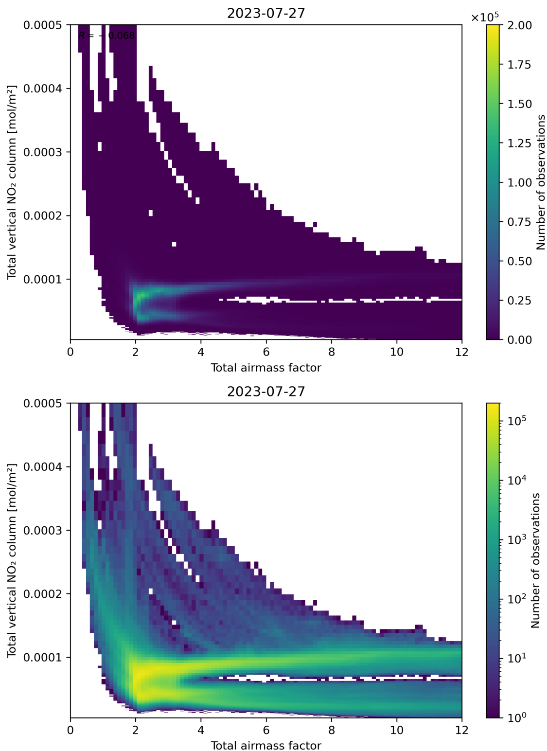
Figure 67: Scatter density plot of “Total airmass factor” against “Total vertical NO 2 column” for 2023-07-26 to 2023-07-28.
