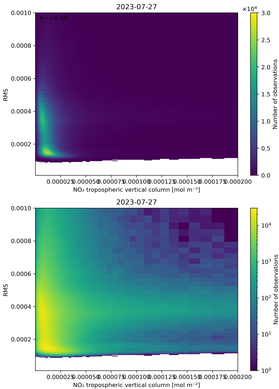
Figure 142: Scatter density plot of “NO 2 tropospheric vertical column” against “RMS” for 2023-07-26 to 2023-07-28.
