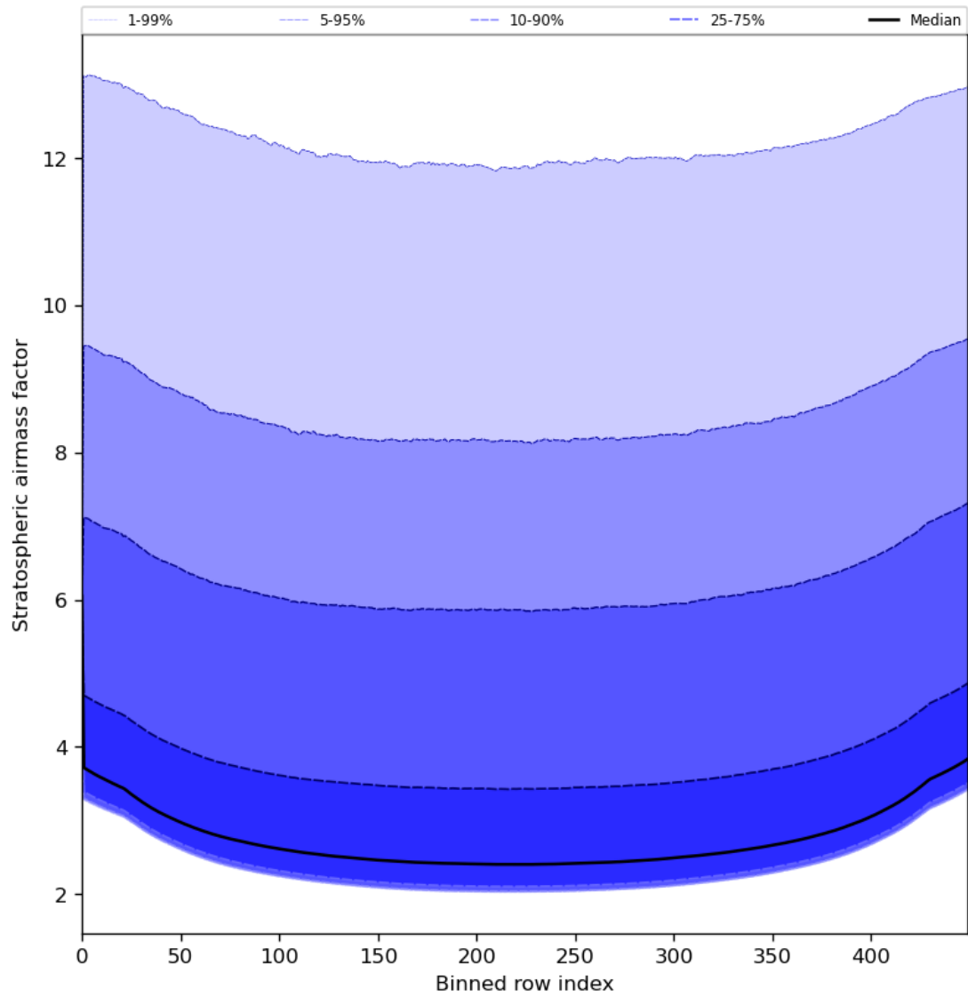
Figure 61: Along track statistics of “Stratospheric airmass factor” for 2023-07-26 to 2023-07-28
