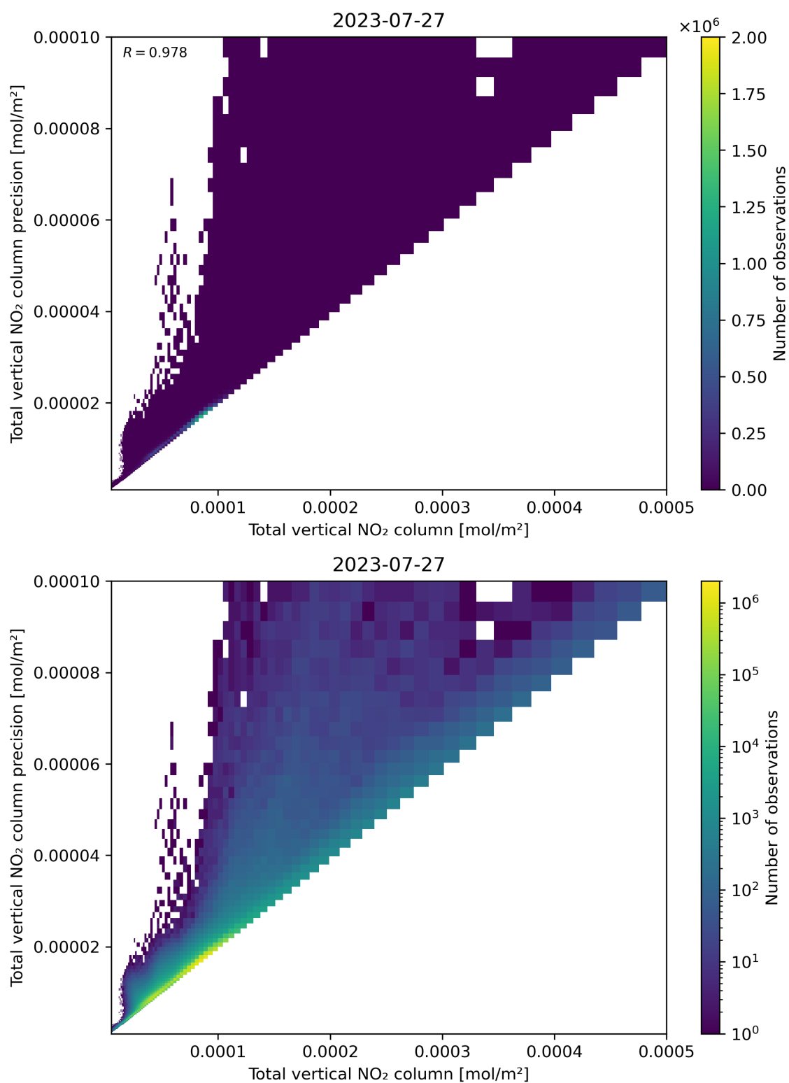
Figure 114: Scatter density plot of “Total vertical NO 2 column” against “Total vertical NO 2 column precision” for 2023-07-26 to 2023-07-28.
