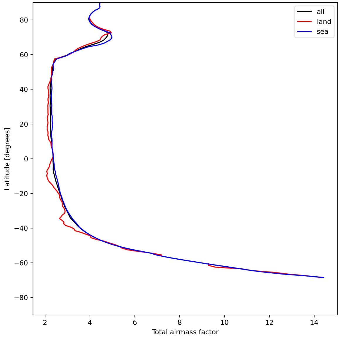
Figure 15: Zonal average of “Total airmass factor” for 2023-07-26 to 2023-07-28.
