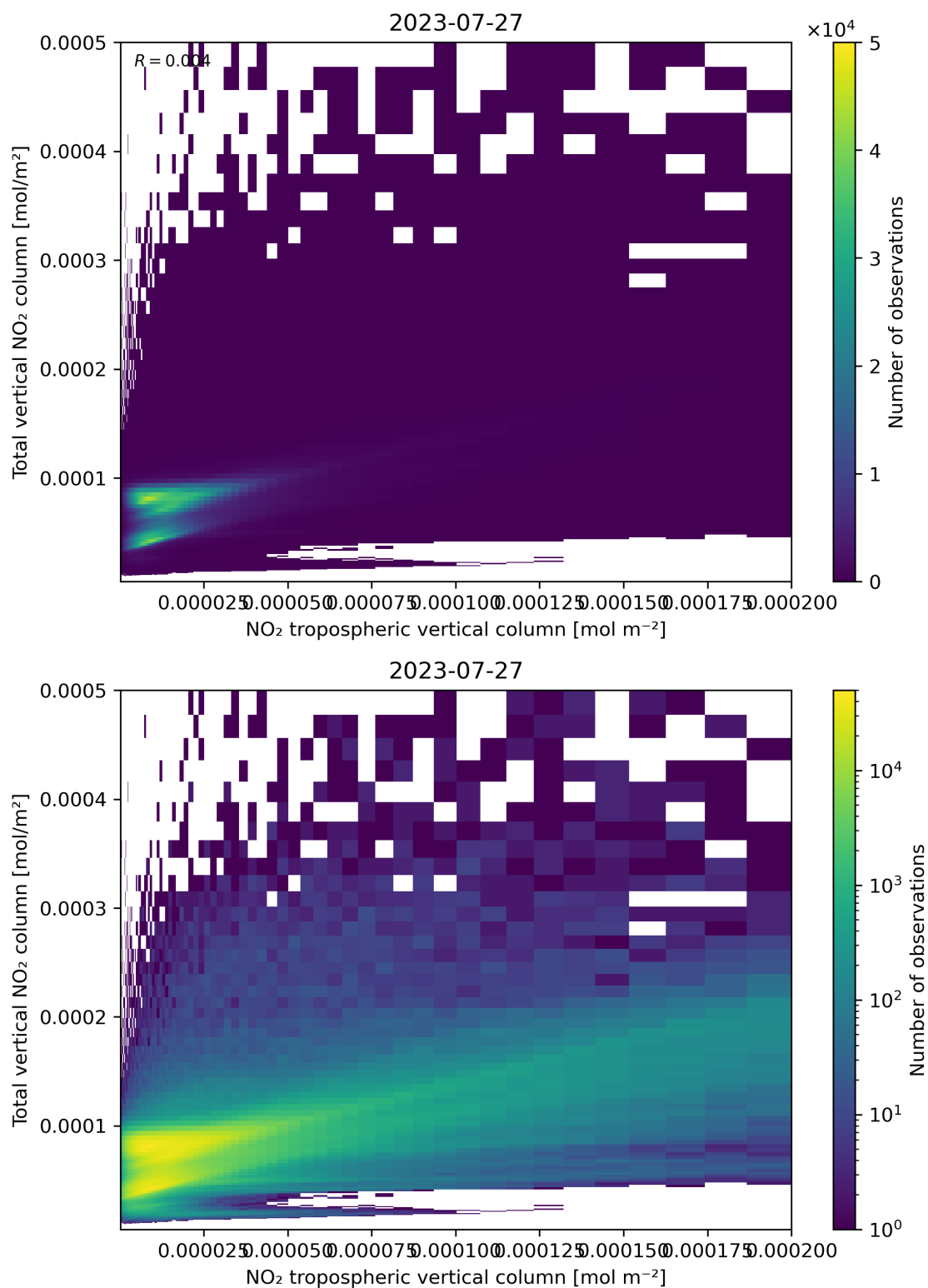
Figure 128: Scatter density plot of “NO 2 tropospheric vertical column” against “Total vertical NO 2 column” for 2023-07-26 to 2023-07-28.
