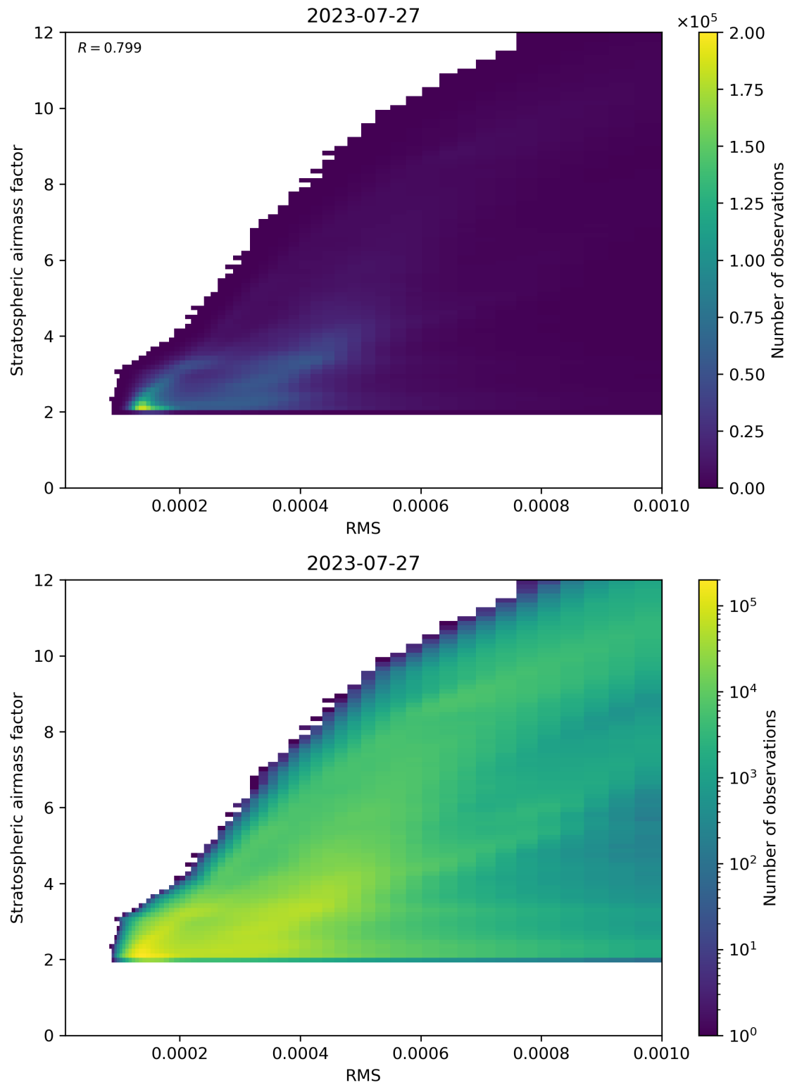
Figure 144: Scatter density plot of “RMS” against “Stratospheric airmass factor” for 2023-07-26 to 2023-07-28.
