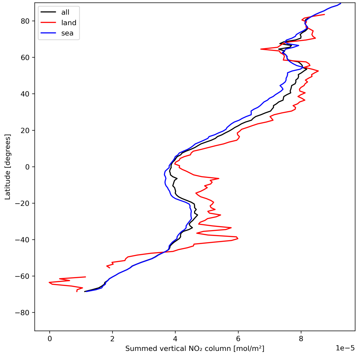
Figure 23: Zonal average of “Summed vertical NO 2 column” for 2023-07-26 to 2023-07-28.
