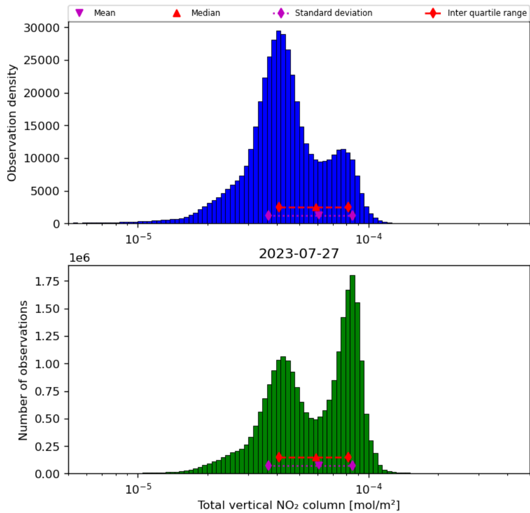
Figure 38: Histogram of “Total vertical NO 2 column” for 2023-07-26 to 2023-07-28
