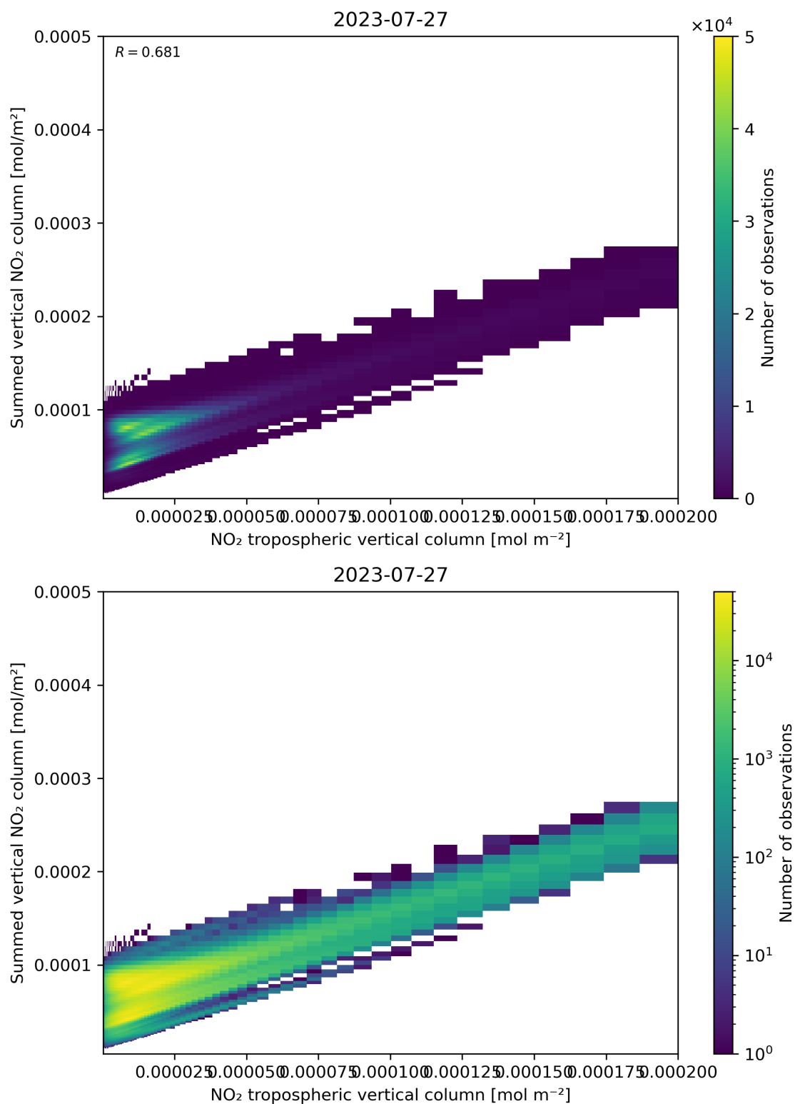
Figure 126: Scatter density plot of “NO 2 tropospheric vertical column” against “Summed vertical NO 2 column” for 2023-07-26 to 2023-07-28.
