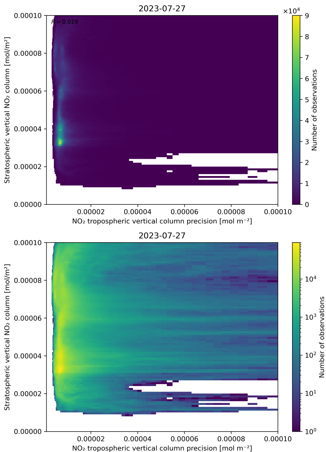
Figure 135: Scatter density plot of “NO 2 tropospheric vertical column precision” against “Stratospheric vertical NO 2 column” for 2023-07-26 to 2023-07-28.
