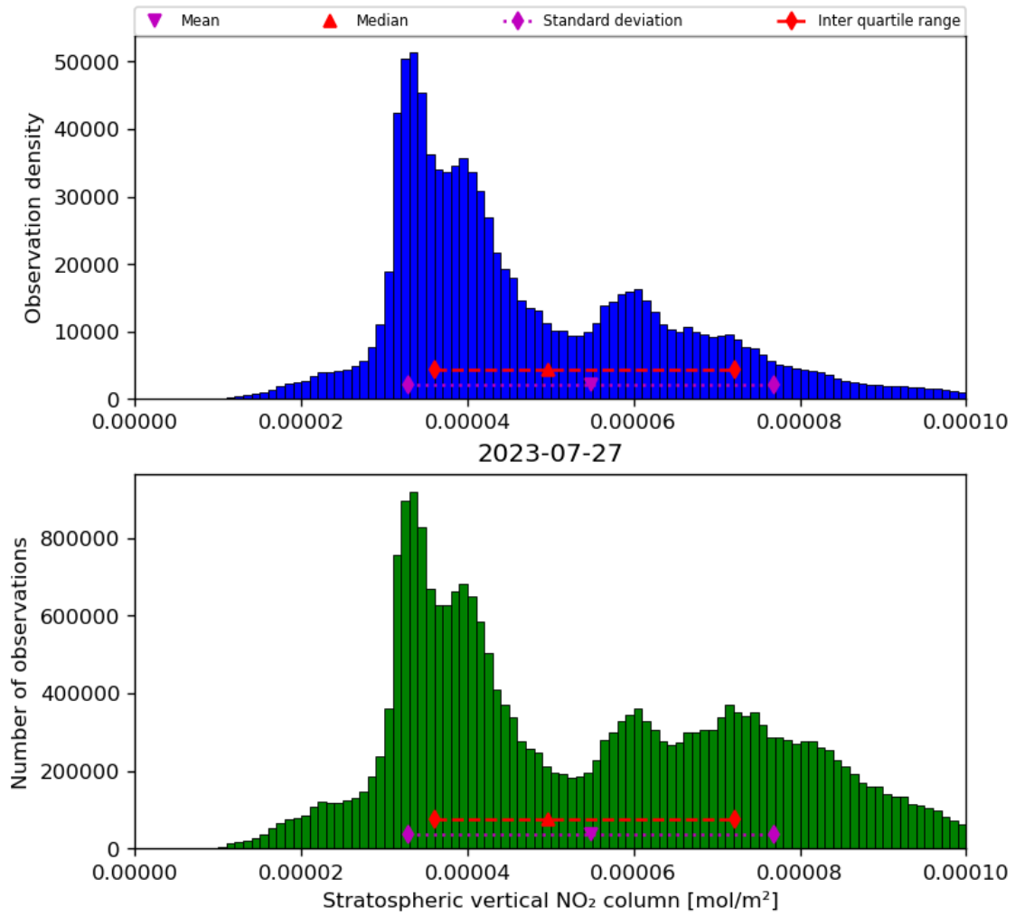
Figure 36: Histogram of “Stratospheric vertical NO 2 column” for 2023-07-26 to 2023-07-28
