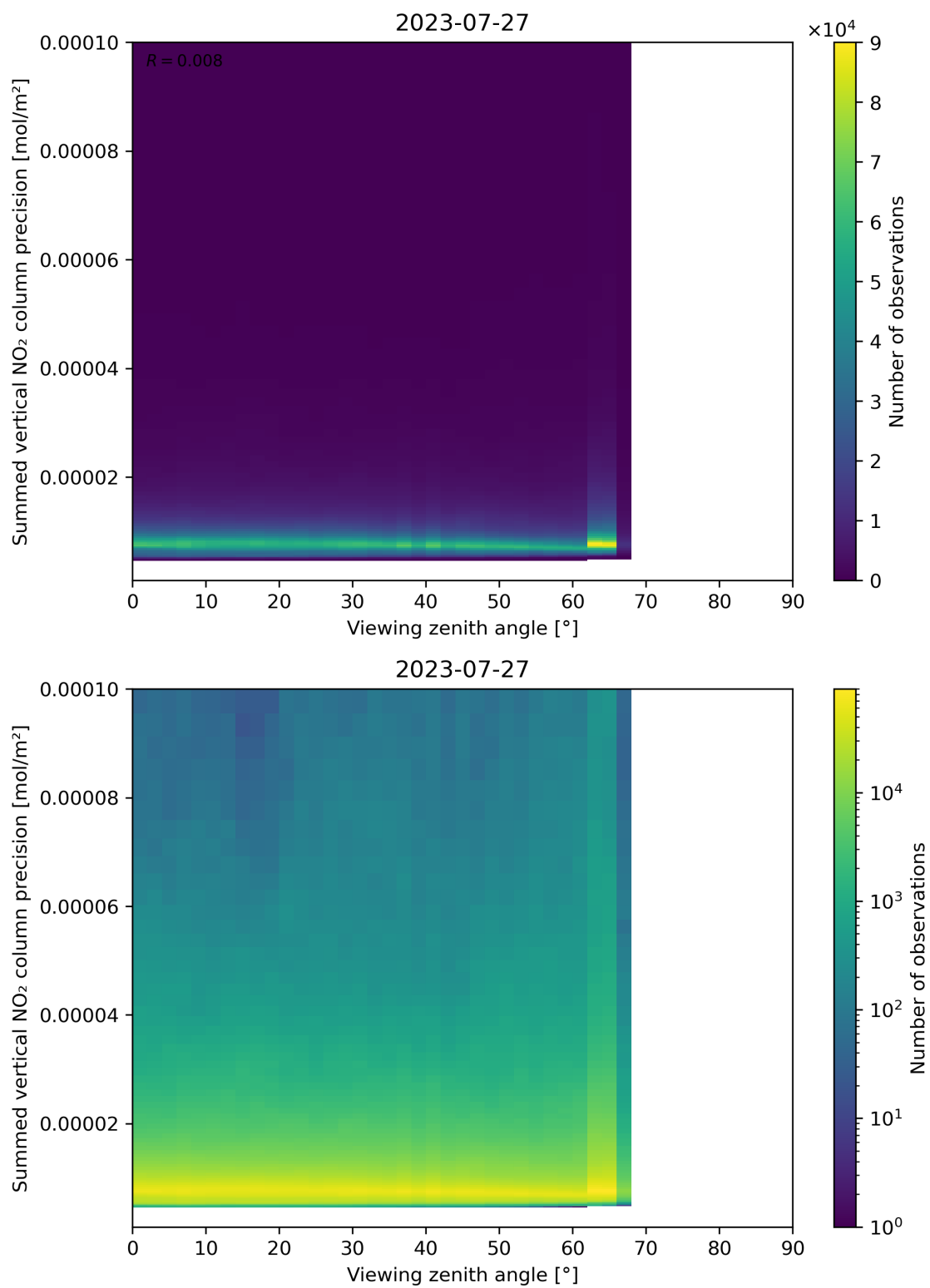
Figure 166: Scatter density plot of “Viewing zenith angle” against “Summed vertical NO 2 column precision” for 2023-07-26 to 2023-07-28.
