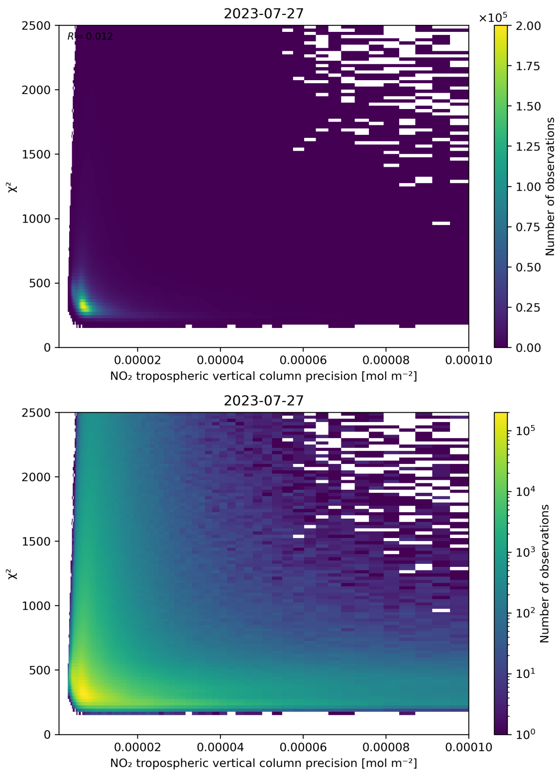
Figure 134: Scatter density plot of “NO 2 tropospheric vertical column precision” against “ \chi^2 ” for 2023-07-26 to 2023-07-28.
