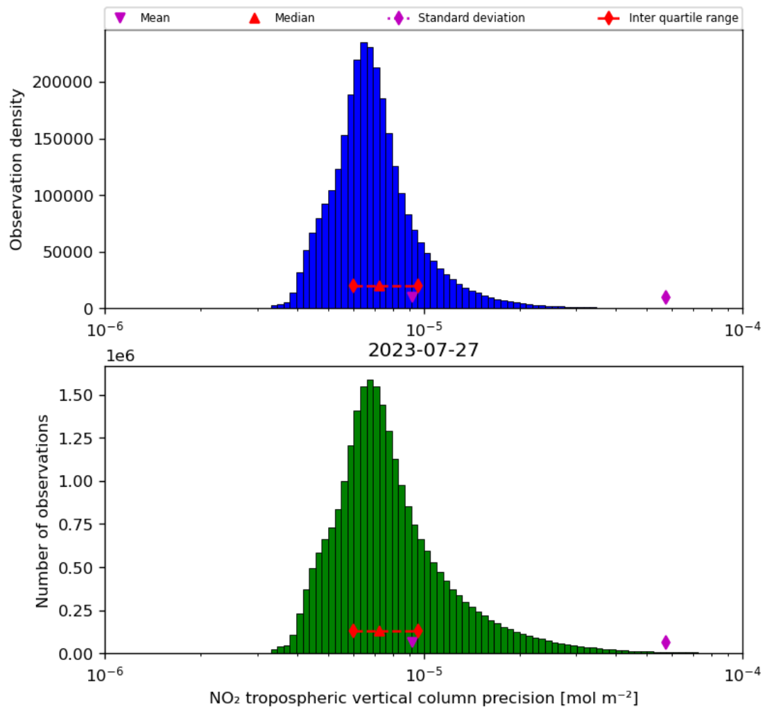
Figure 30: Histogram of “NO 2 tropospheric vertical column precision” for 2023-07-26 to 2023-07-28
