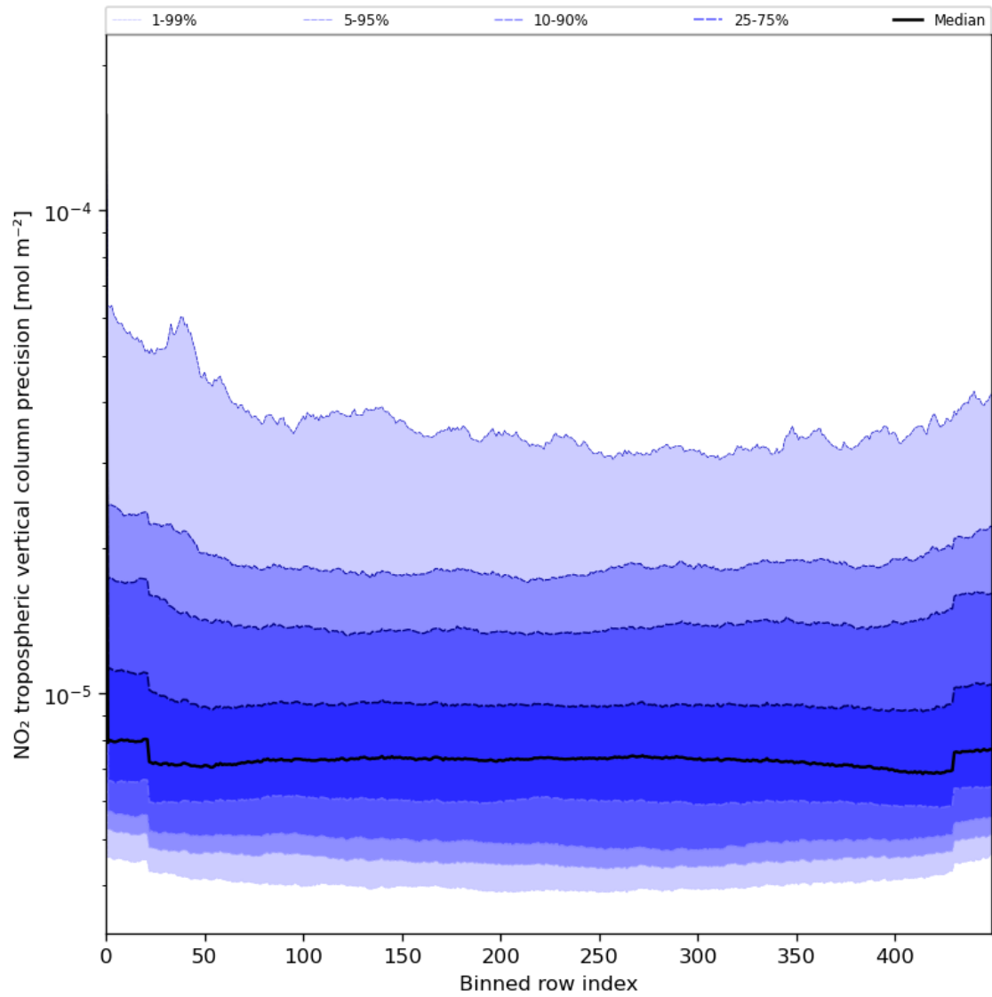
Figure 47: Along track statistics of “NO 2 tropospheric vertical column precision” for 2023-07-26 to 2023-07-28
