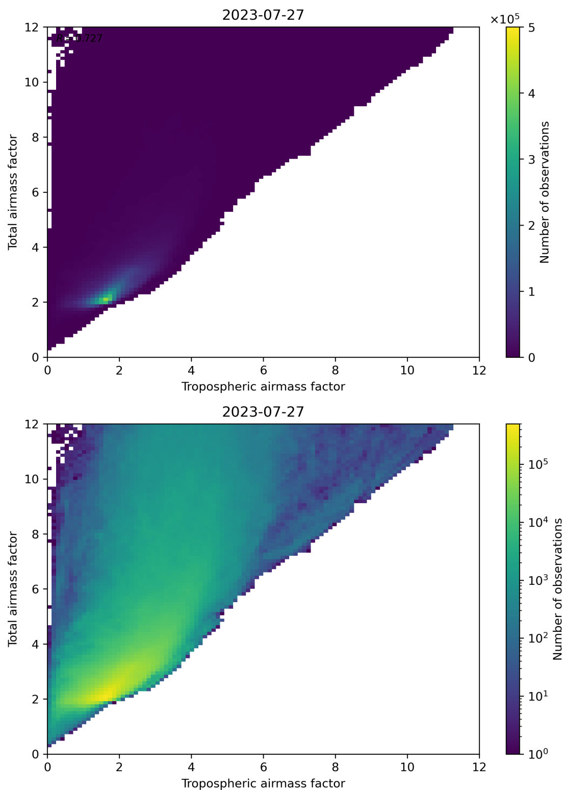
Figure 72: Scatter density plot of “Tropospheric airmass factor” against “Total airmass factor” for 2023-07-26 to 2023-07-28.
