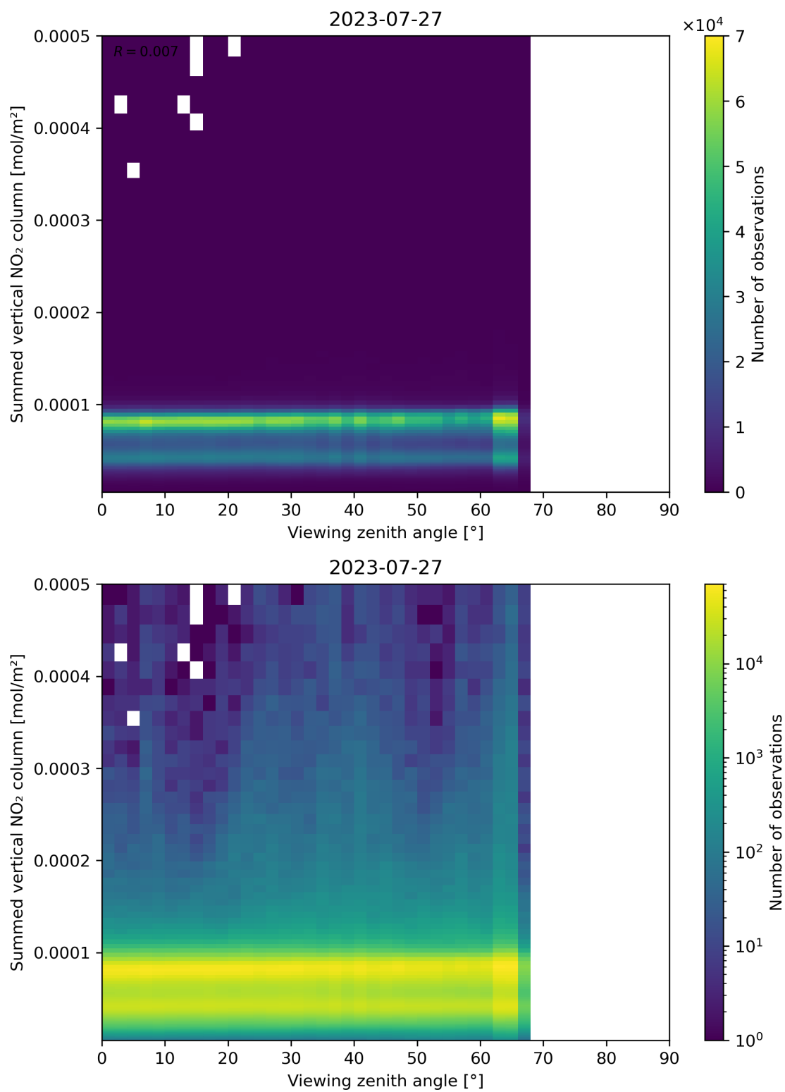
Figure 165: Scatter density plot of “Viewing zenith angle” against “Summed vertical NO 2 column” for 2023-07-26 to 2023-07-28.
