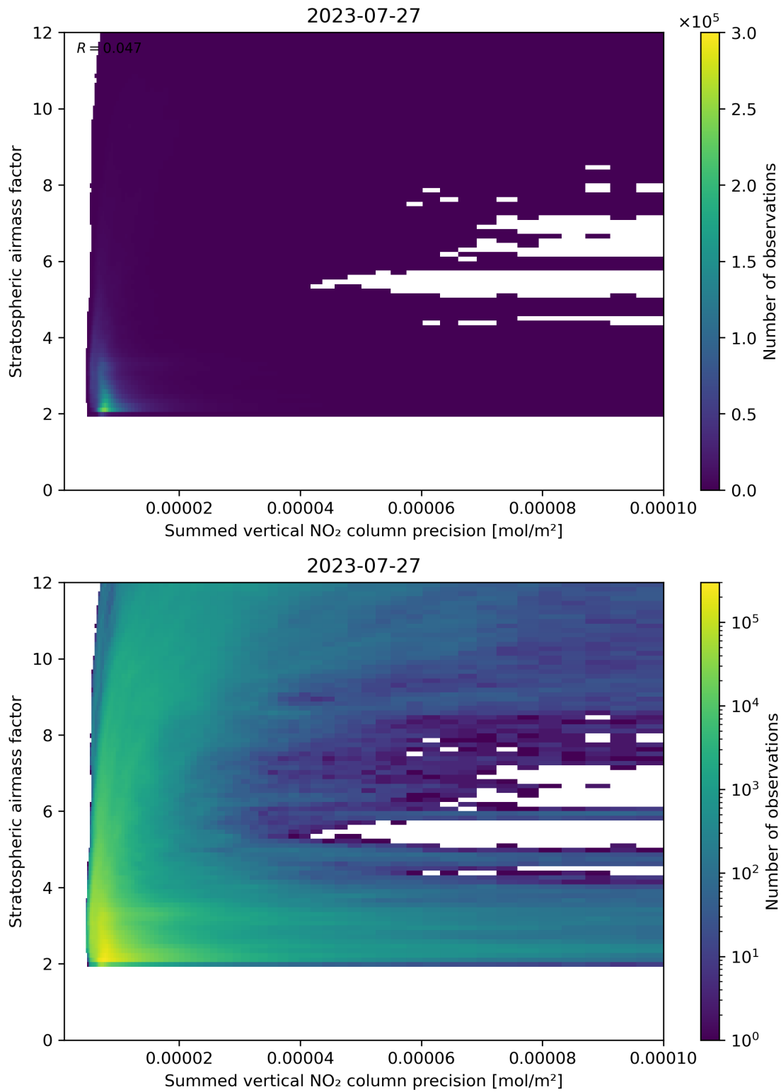
Figure 106: Scatter density plot of “Summed vertical NO 2 column precision” against “Stratospheric airmass factor” for 2023-07-26 to 2023-07-28.
