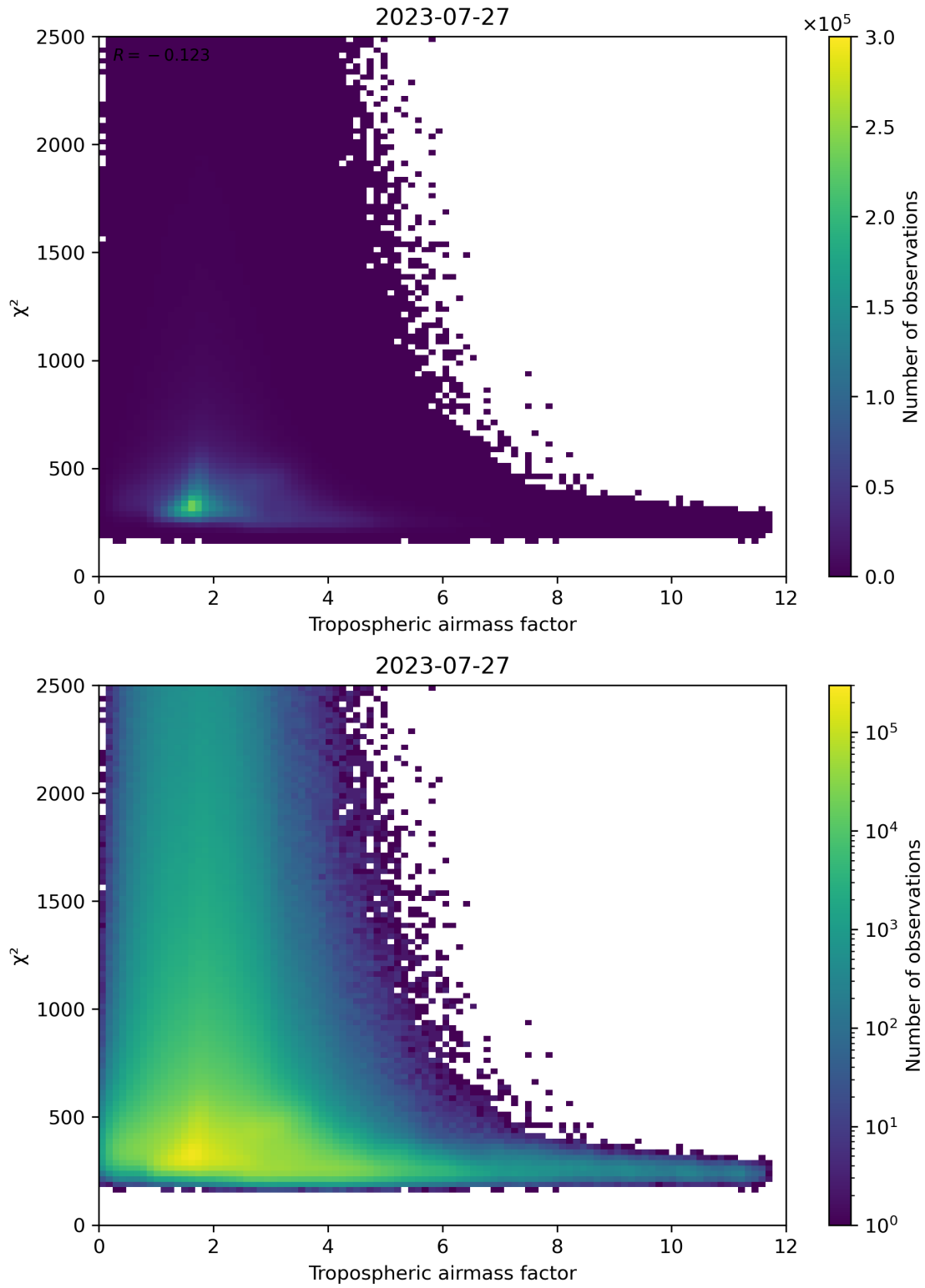
Figure 73: Scatter density plot of “Tropospheric airmass factor” against “ \chi^2 ” for 2023-07-26 to 2023-07-28.
