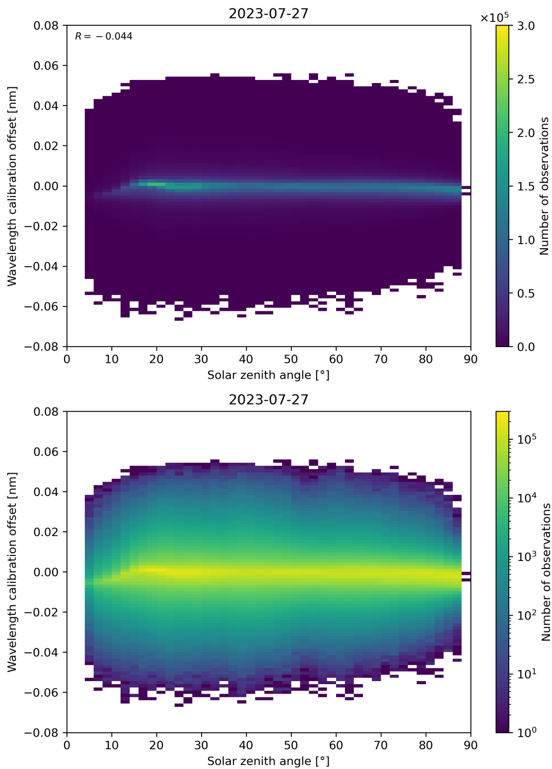
Figure 158: Scatter density plot of “Solar zenith angle” against “Wavelength calibration offset” for 2023-07-26 to 2023-07-28.
