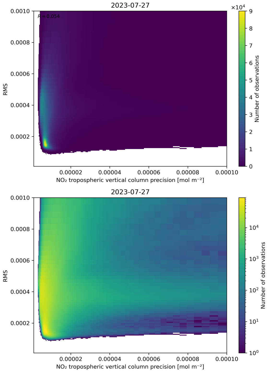
Figure 140: Scatter density plot of “NO 2 tropospheric vertical column precision” against “RMS” for 2023-07-26 to 2023-07-28.
