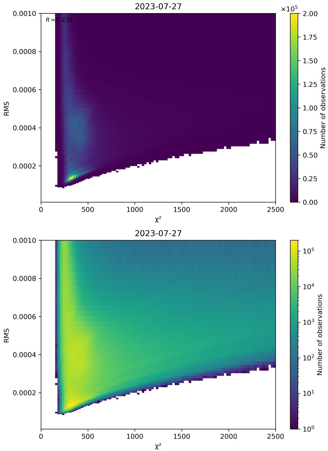
Figure 82: Scatter density plot of “ \chi^2 ” against “RMS” for 2023-07-26 to 2023-07-28.
