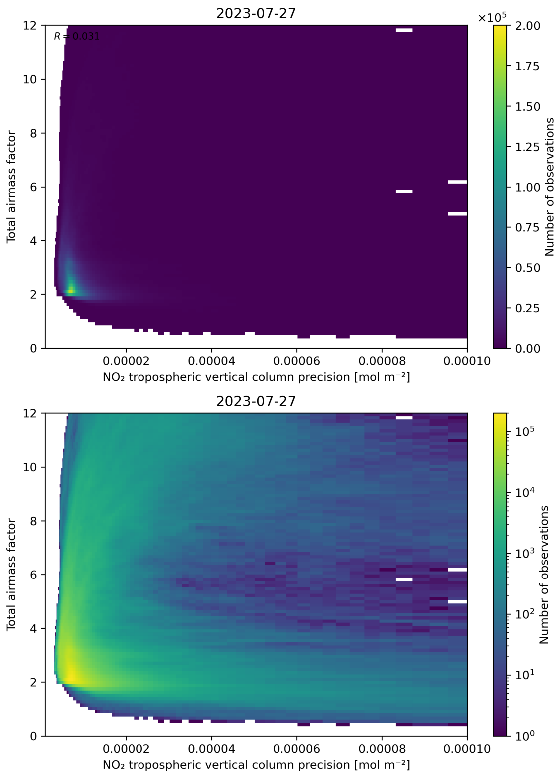
Figure 132: Scatter density plot of “NO 2 tropospheric vertical column precision” against “Total air mass factor” for 2023-07-26 to 2023-07-28.
