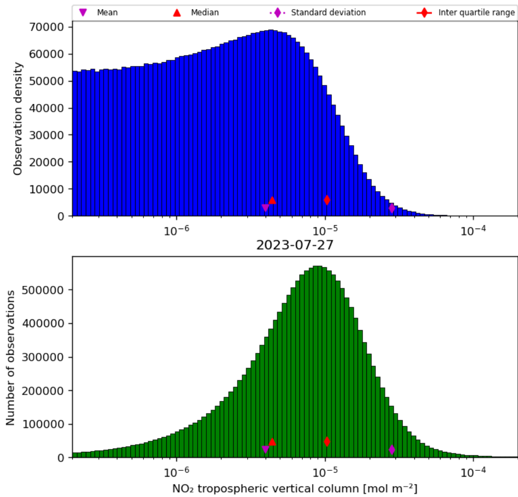
Figure 29: Histogram of “NO 2 tropospheric vertical column” for 2023-07-26 to 2023-07-28
