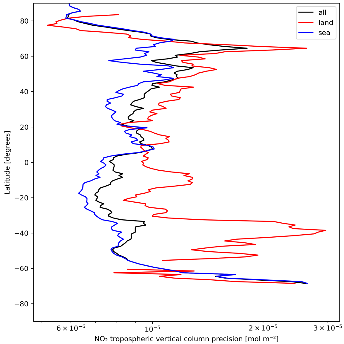
Figure 13: Zonal average of “NO 2 tropospheric vertical column precision” for 2023-07-26 to 2023-07-28.
