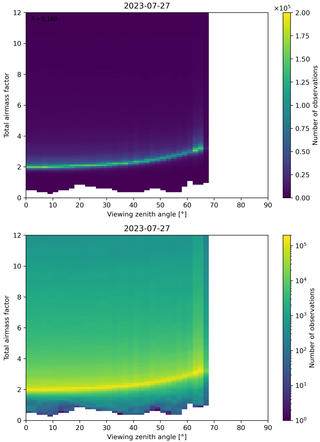
Figure 160: Scatter density plot of “Viewing zenith angle” against “Total airmass factor” for 2023-07-26 to 2023-07-28.
