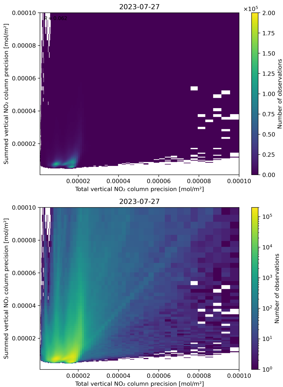
Figure 118: Scatter density plot of “Total vertical NO 2 column precision” against “Summed vertical NO 2 column precision” for 2023-07-26 to 2023-07-28.
