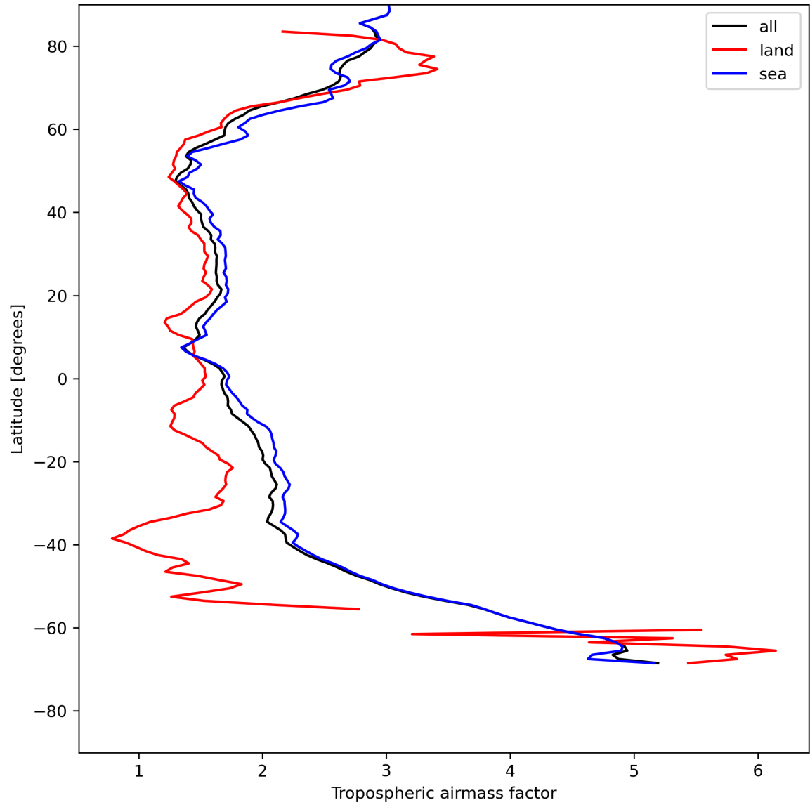
Figure 14: Zonal average of “Tropospheric airmass factor” for 2023-07-26 to 2023-07-28.
