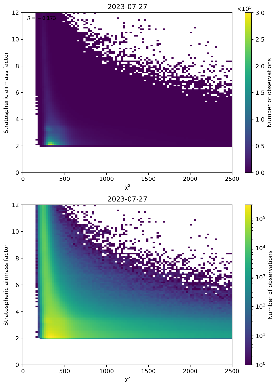
Figure 81: Scatter density plot of “ \chi^2 ” against “Stratospheric airmass factor” for 2023-07-26 to 2023-07-28.
