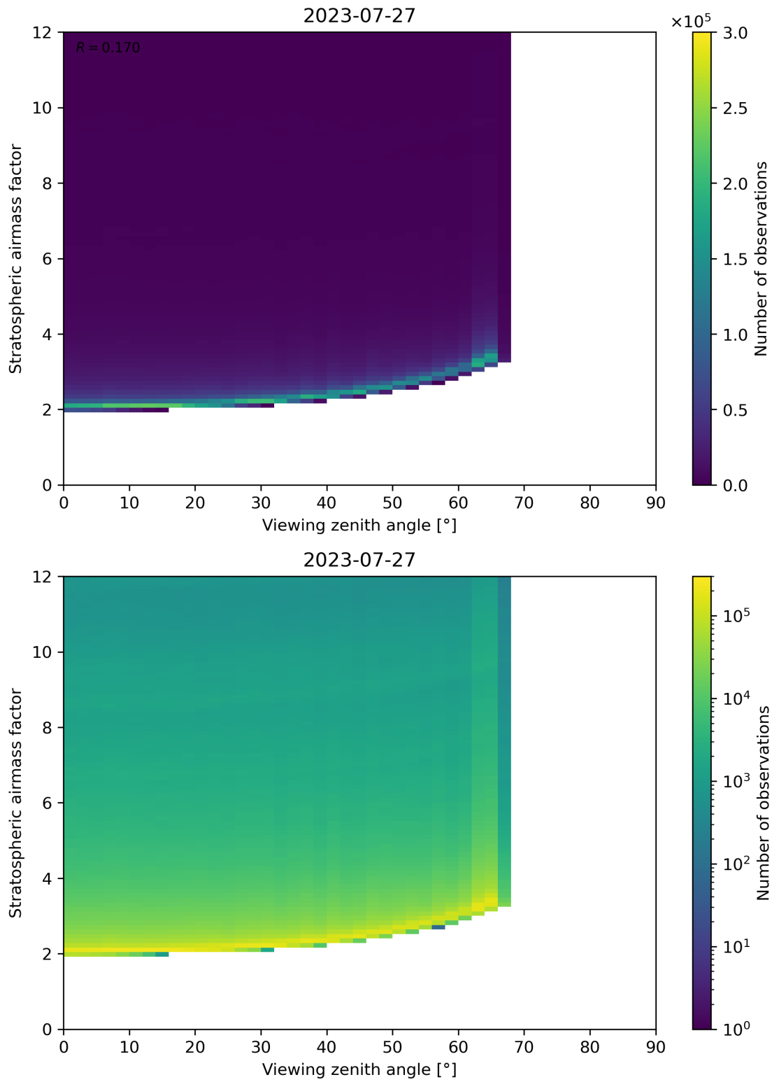
Figure 159: Scatter density plot of “Viewing zenith angle” against “Stratospheric airmass factor” for 2023-07-26 to 2023-07-28.
