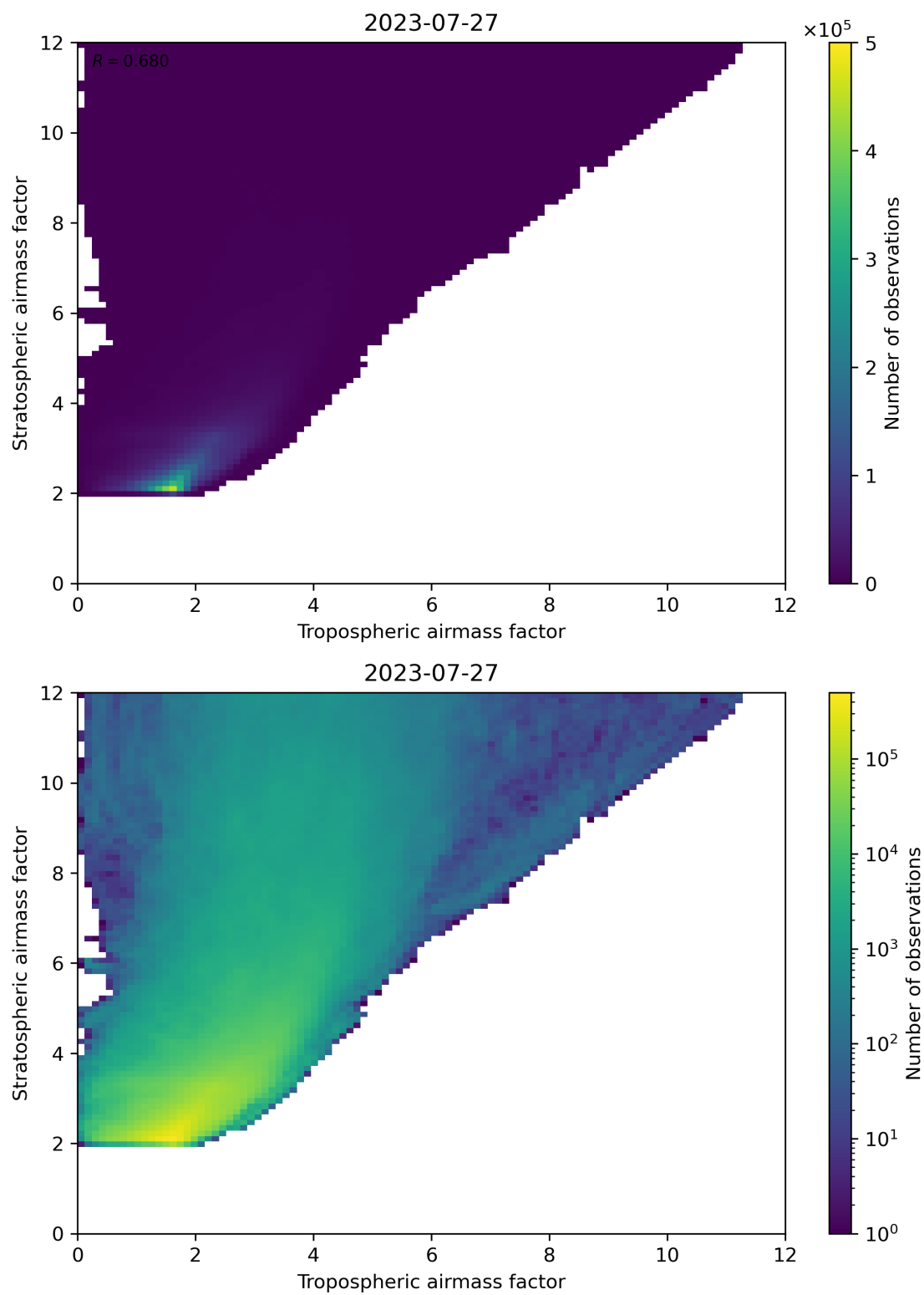
Figure 71: Scatter density plot of “Tropospheric airmass factor” against “Stratospheric airmass factor” for 2023-07-26 to 2023-07-28.
