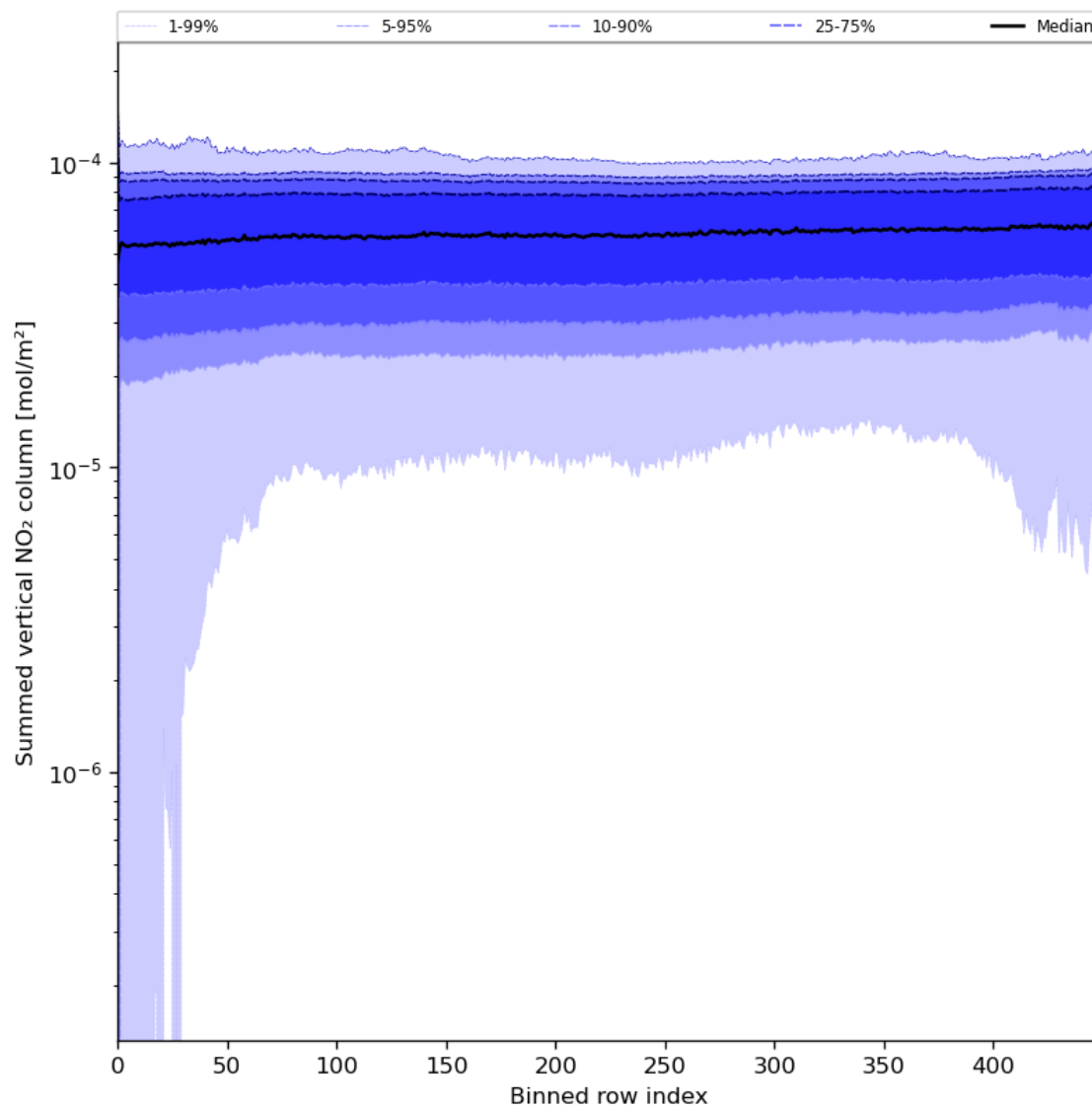
Figure 57: Along track statistics of “Summed vertical NO 2 column” for 2023-07-26 to 2023-07-28
