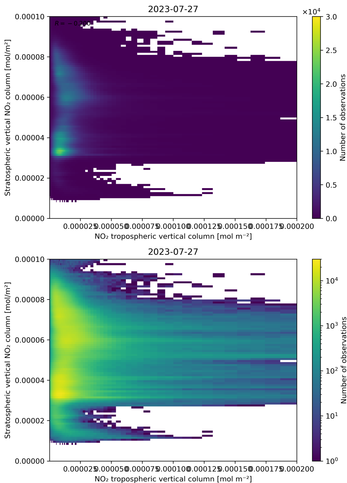
Figure 125: Scatter density plot of “NO 2 tropospheric vertical column” against “Stratospheric vertical NO 2 column” for 2023-07-26 to 2023-07-28.
