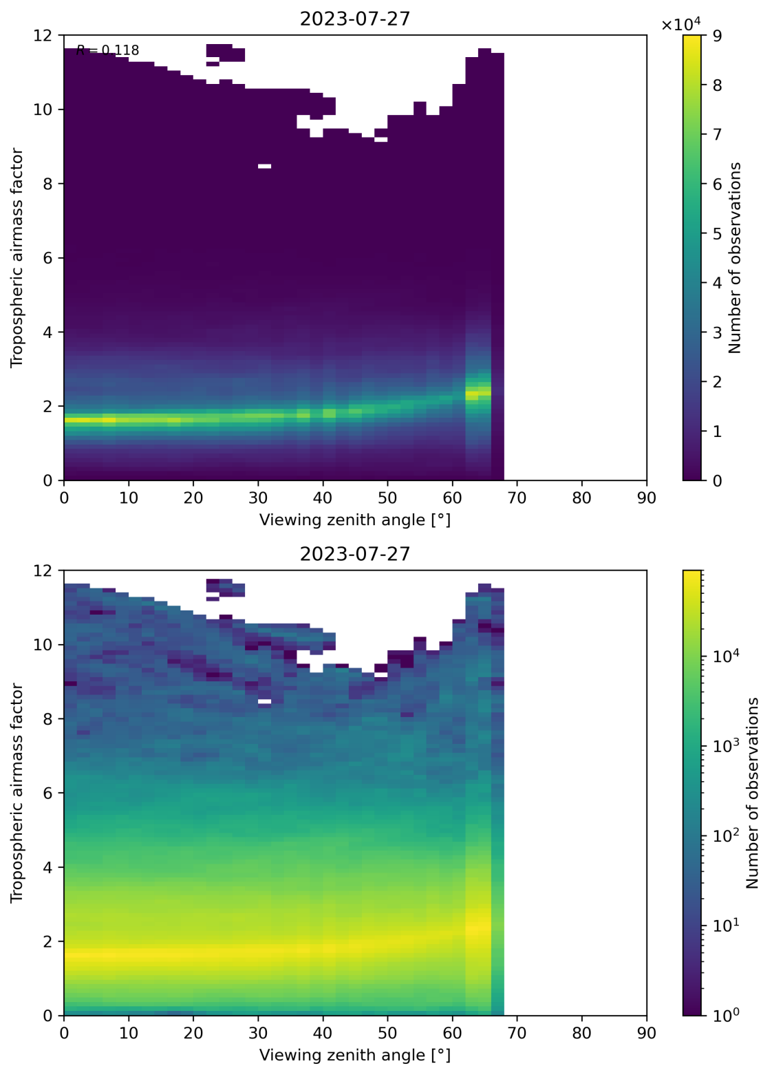
Figure 161: Scatter density plot of “Viewing zenith angle” against “Tropospheric airmass factor” for 2023-07-26 to 2023-07-28.
