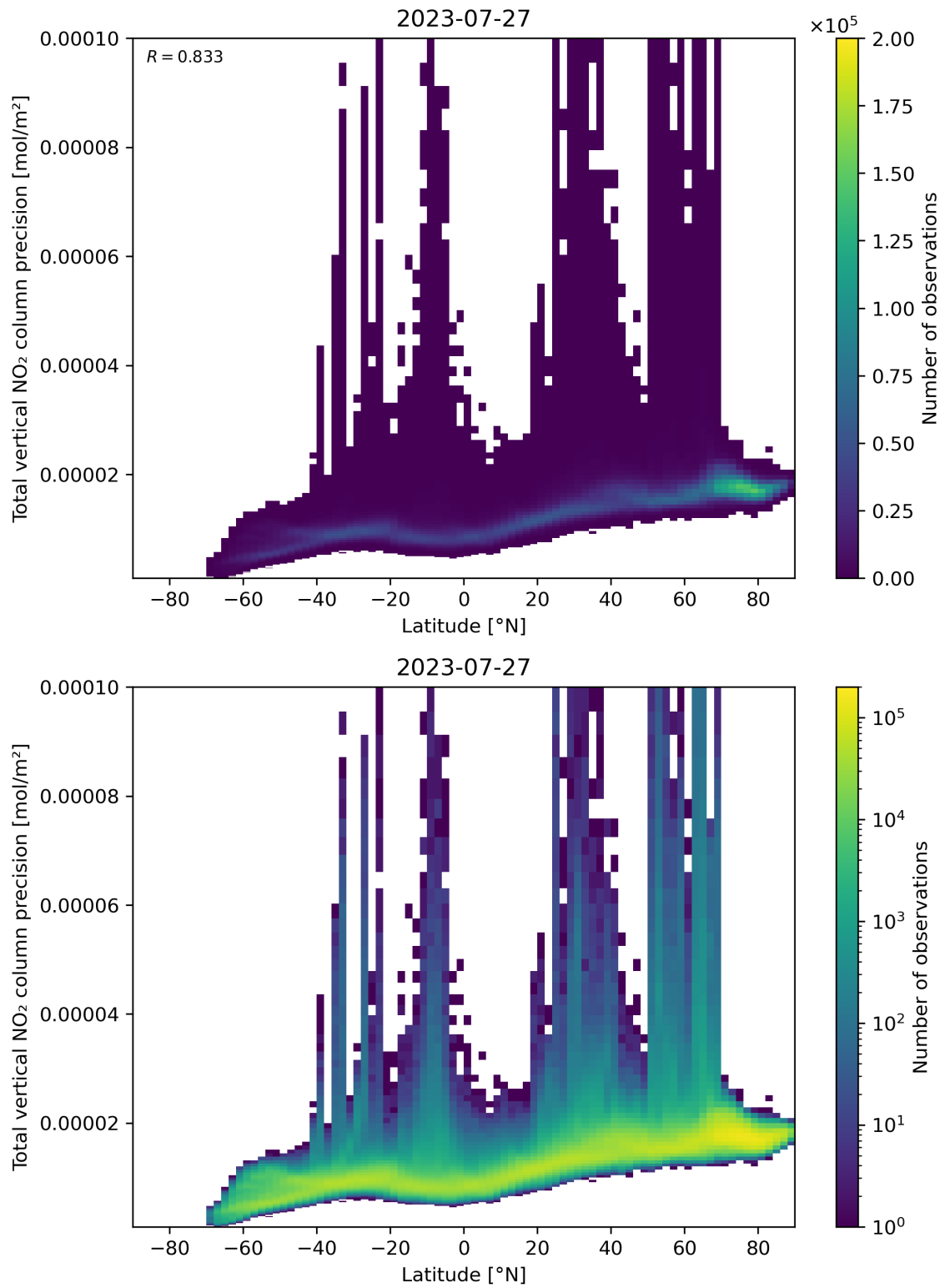
Figure 91: Scatter density plot of “Latitude” against “Total vertical NO 2 column precision” for 2023-07-26 to 2023-07-28.
