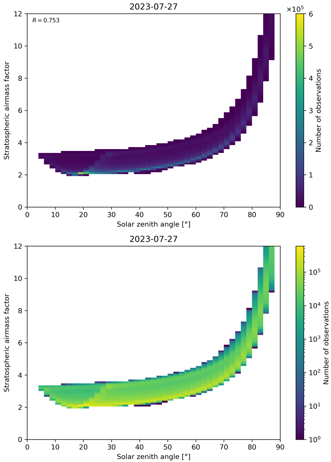
Figure 145: Scatter density plot of “Solar zenith angle” against “Stratospheric airmass factor” for 2023-07-26 to 2023-07-28.
