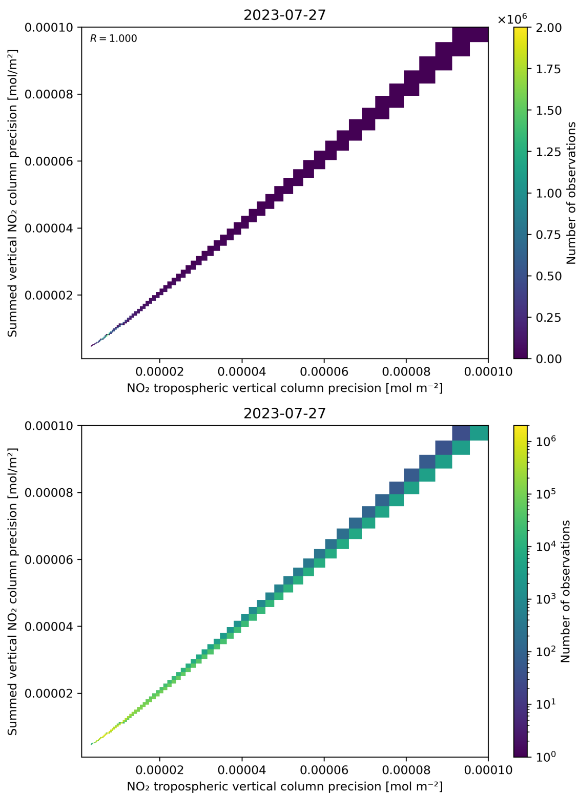
Figure 137: Scatter density plot of “NO 2 tropospheric vertical column precision” against “Summed vertical NO 2 column precision” for 2023-07-26 to 2023-07-28.
