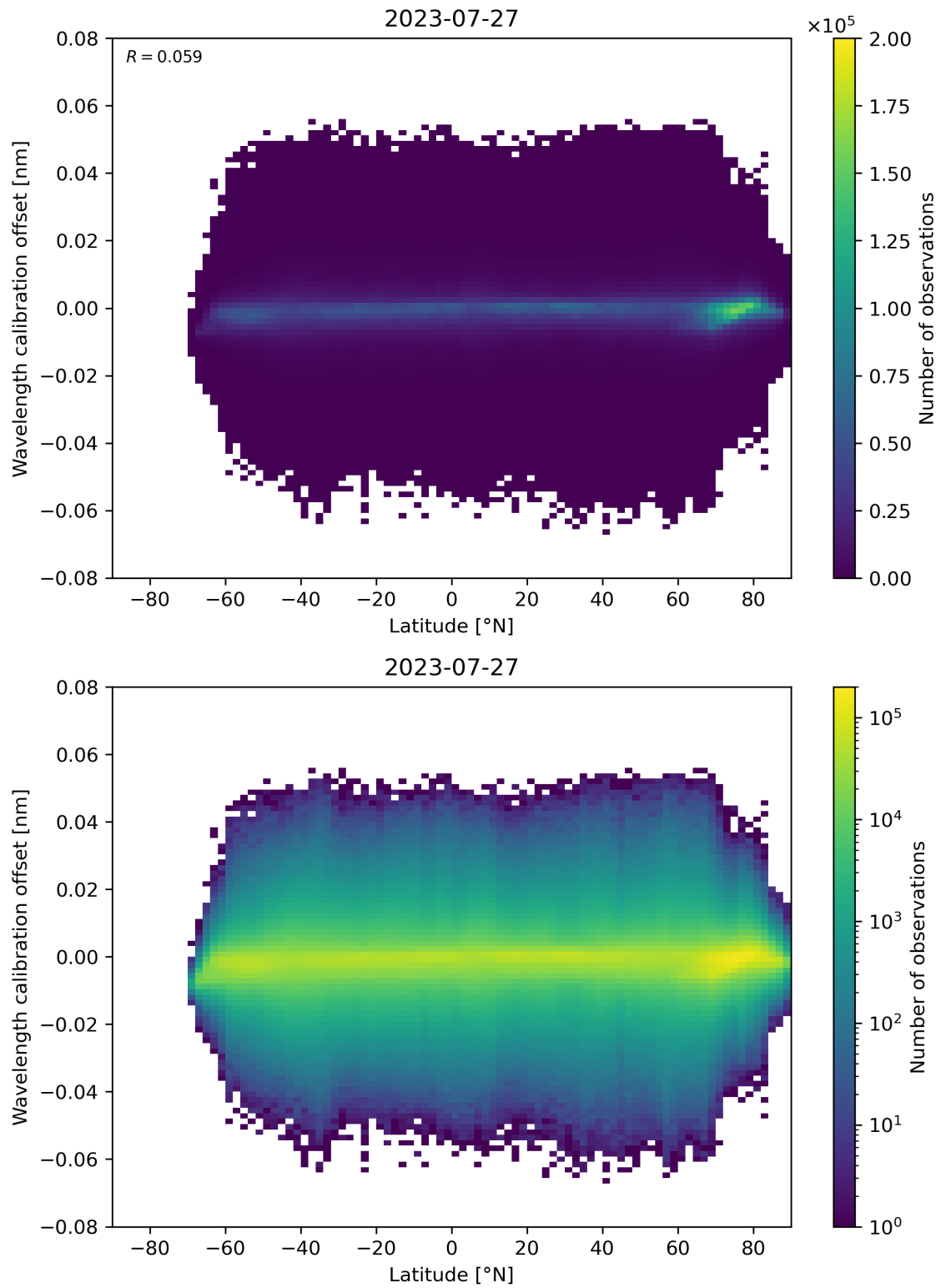
Figure 95: Scatter density plot of “Latitude” against “Wavelength calibration offset” for 2023-07-26 to 2023-07-28.
