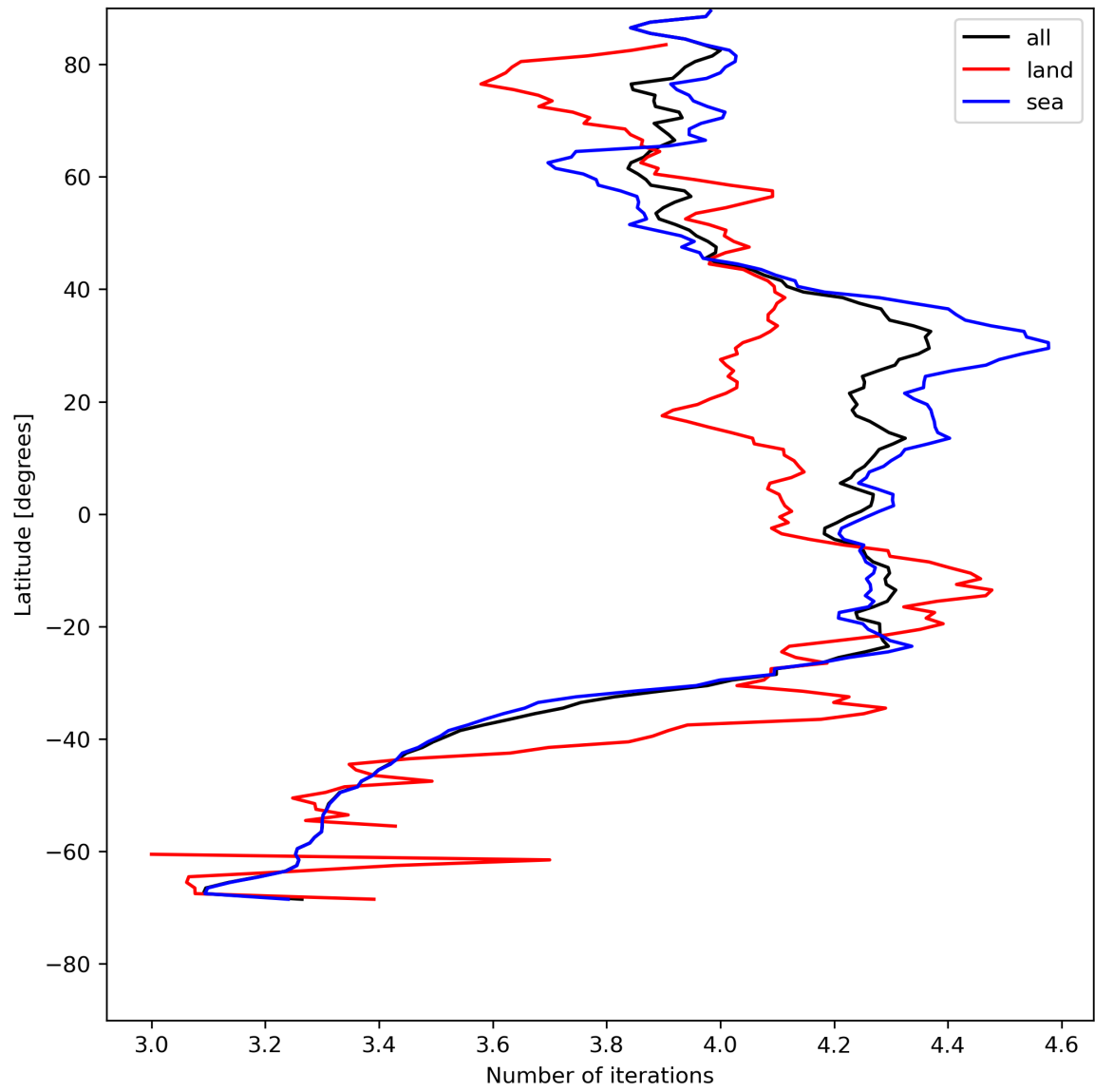
Figure 17: Zonal average of “Number of iterations” for 2023-07-26 to 2023-07-28.
