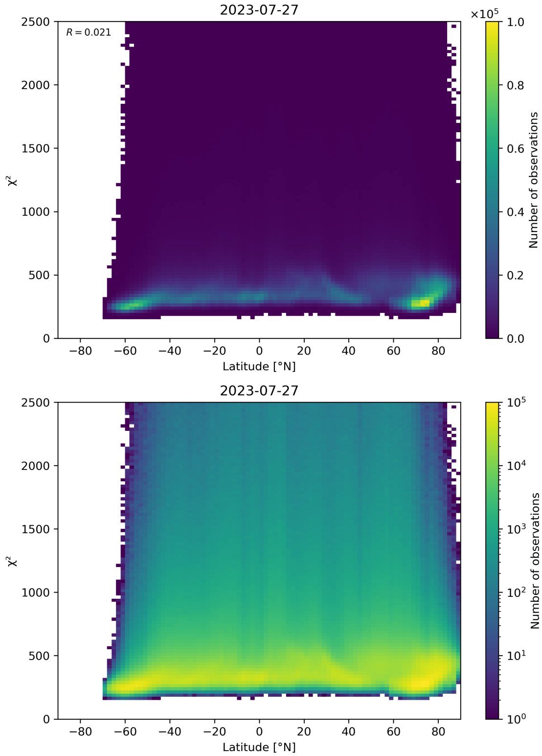
Figure 86: Scatter density plot of “Latitude” against “ \chi^2 ” for 2023-07-26 to 2023-07-28.
