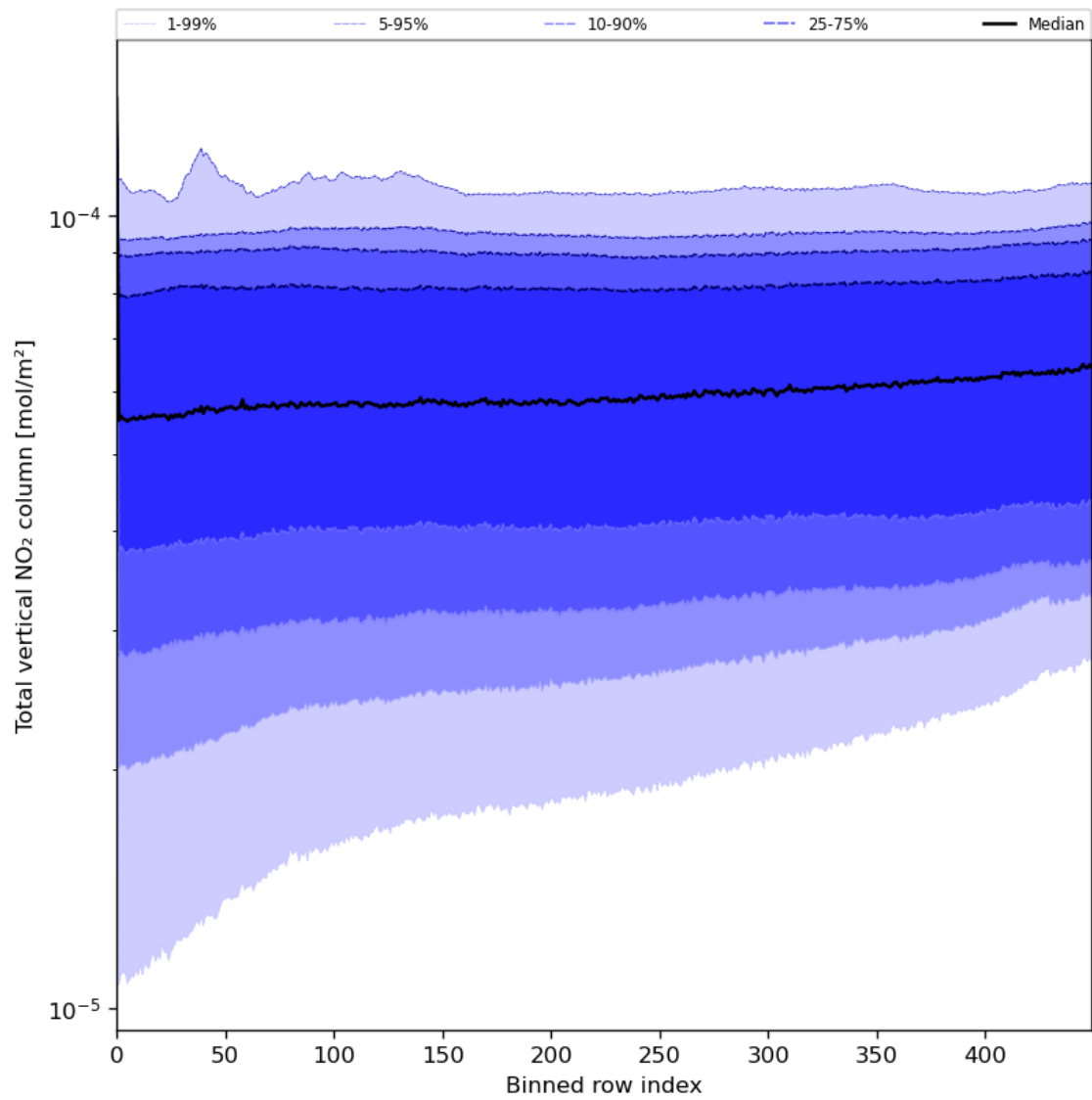
Figure 55: Along track statistics of “Total vertical NO 2 column” for 2023-07-26 to 2023-07-28
