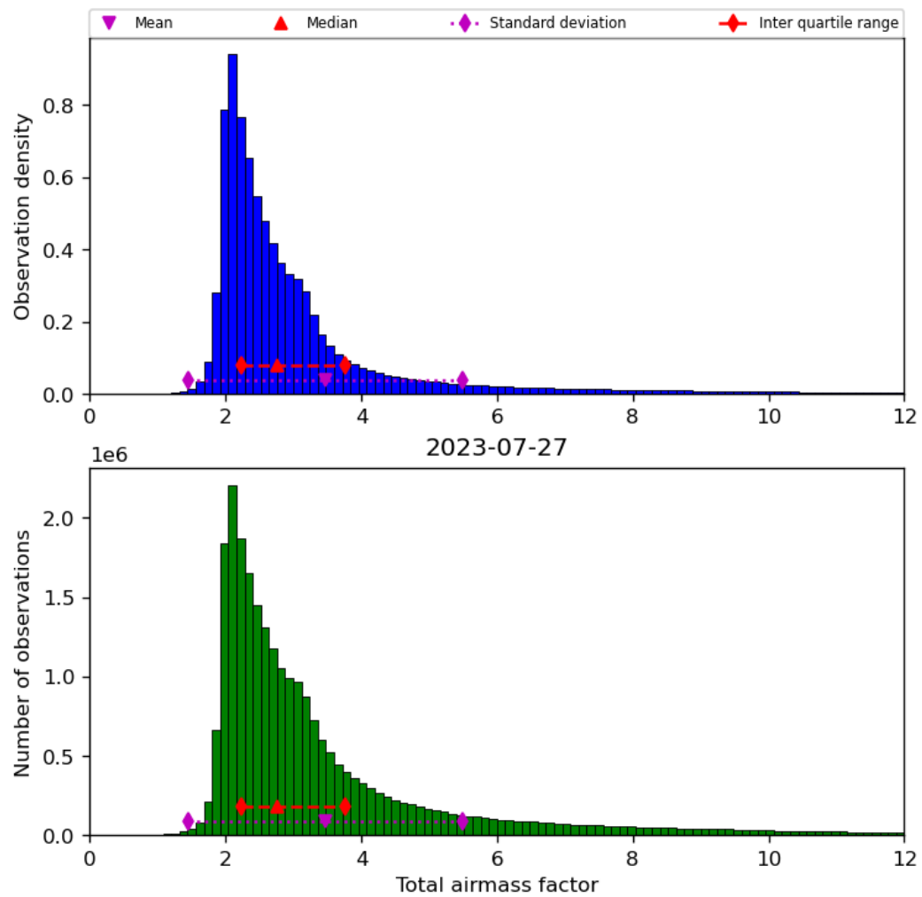
Figure 32: Histogram of “Total airmass factor” for 2023-07-26 to 2023-07-28
