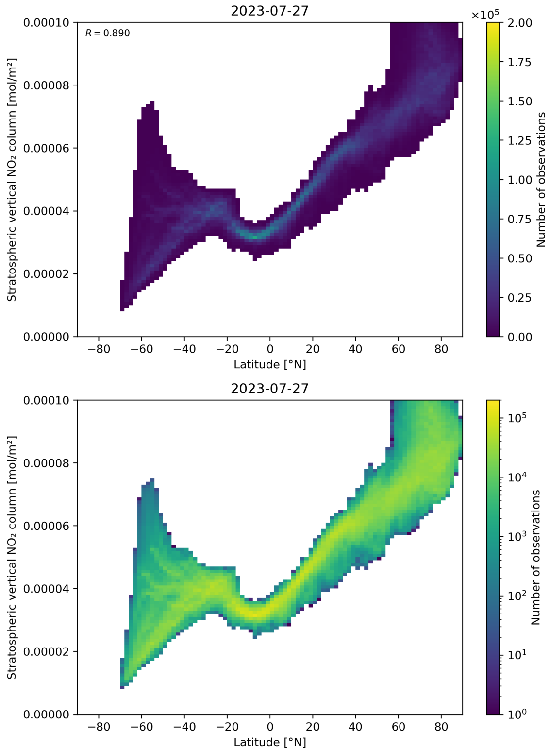
Figure 87: Scatter density plot of “Latitude” against “Stratospheric vertical \text{NO}_2 column” for 2023-07-26 to 2023-07-28.
