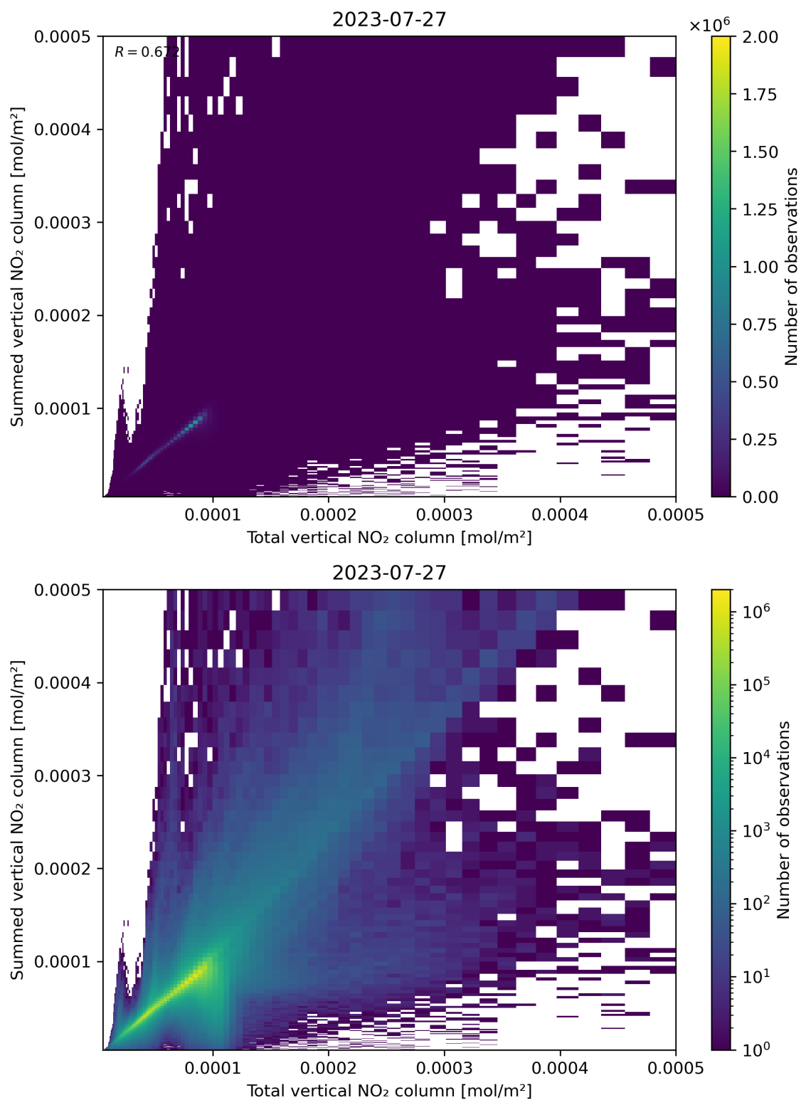
Figure 112: Scatter density plot of “Total vertical NO 2 column” against “Summed vertical NO 2 column” for 2023-07-26 to 2023-07-28.
