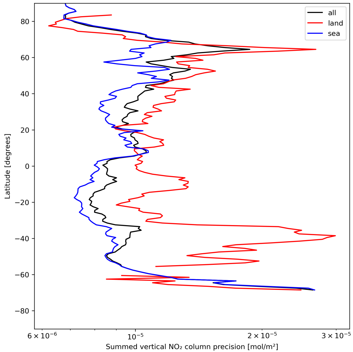
Figure 24: Zonal average of “Summed vertical NO 2 column precision” for 2023-07-26 to 2023-07-28.
