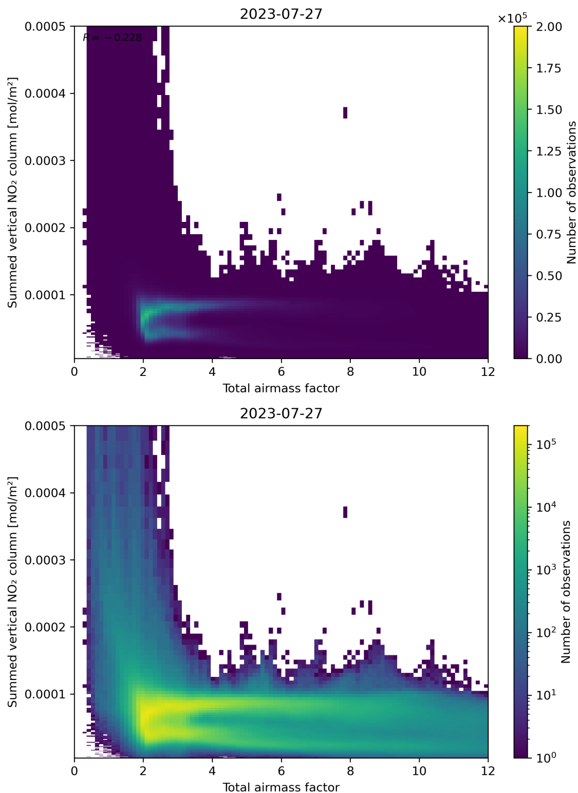
Figure 65: Scatter density plot of “Total airmass factor” against “Summed vertical NO 2 column” for 2023-07-26 to 2023-07-28.
