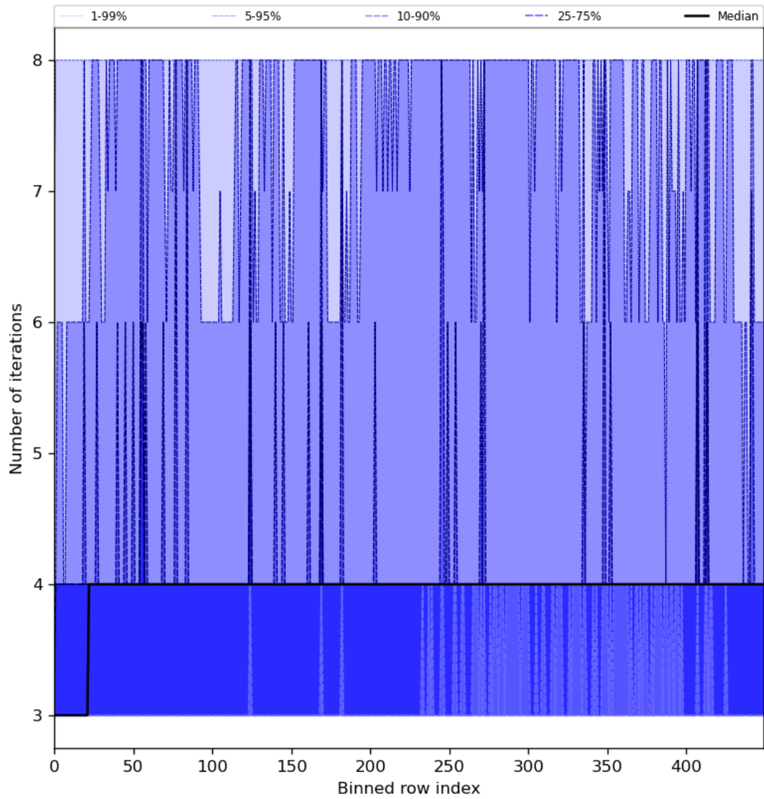
Figure 51: Along track statistics of “Number of iterations” for 2023-07-26 to 2023-07-28
