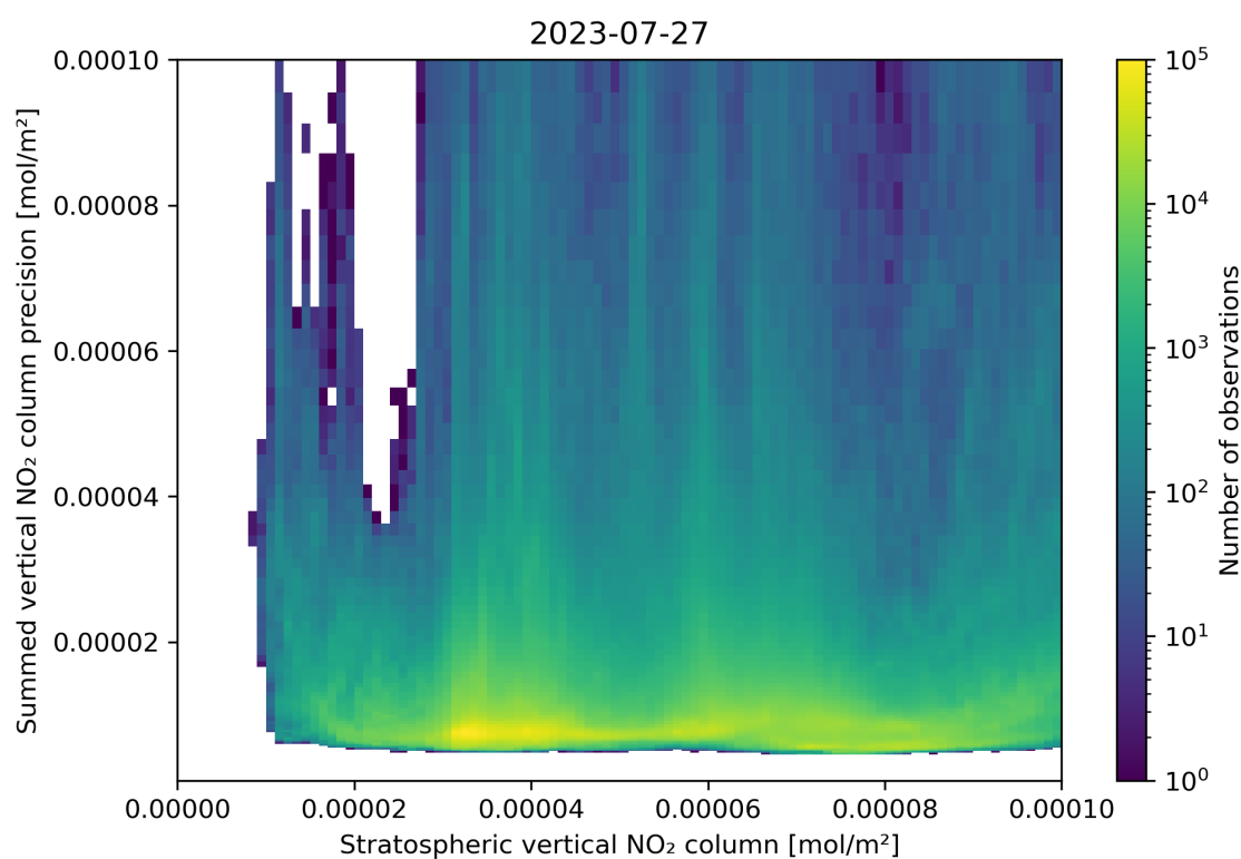
Figure 99: Scatter density plot of “Stratospheric vertical NO 2 column” against “Summed vertical NO 2 column precision” for 2023-07-26 to 2023-07-28.
