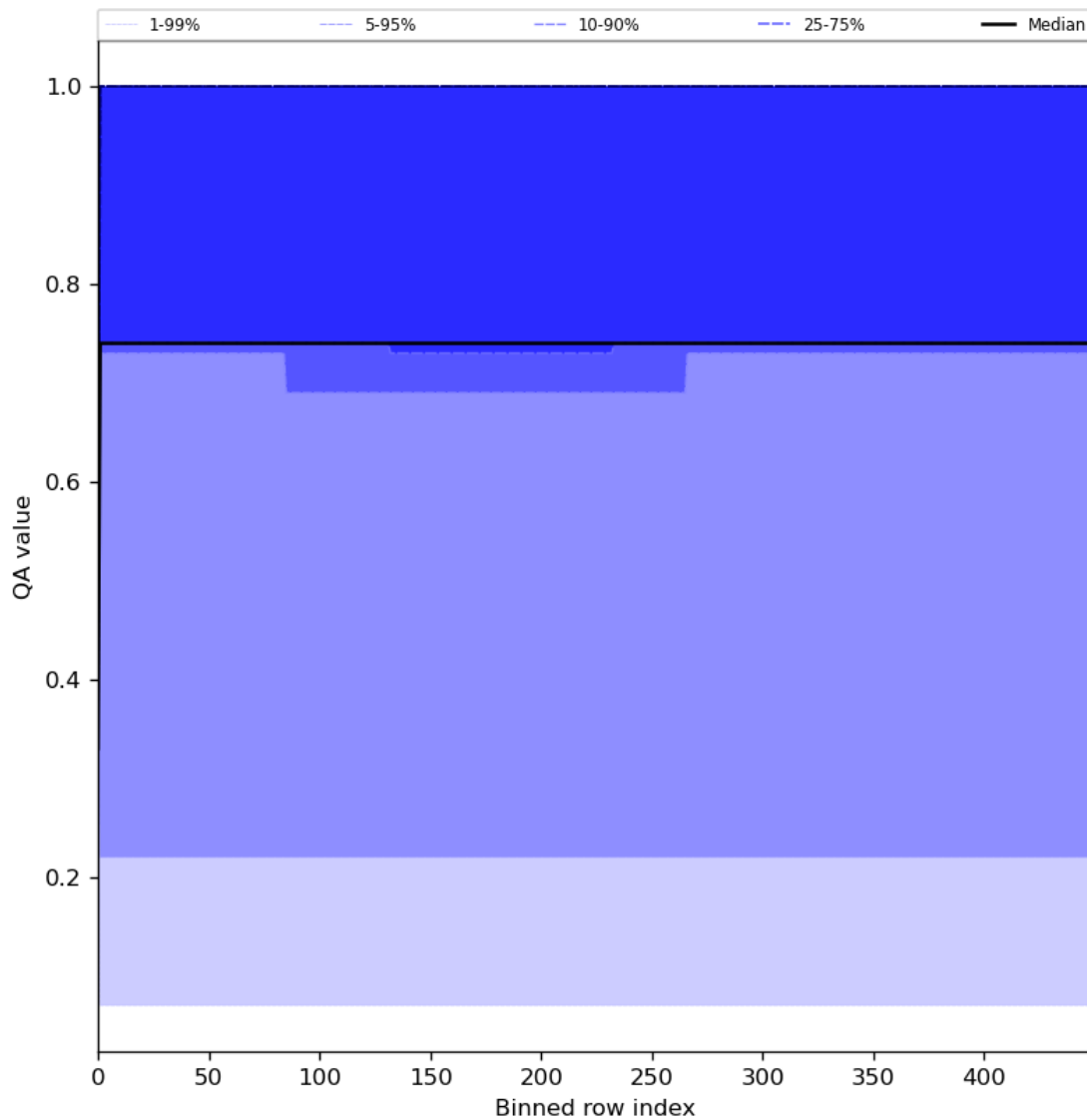
Figure 45: Along track statistics of “QA value” for 2023-07-26 to 2023-07-28
