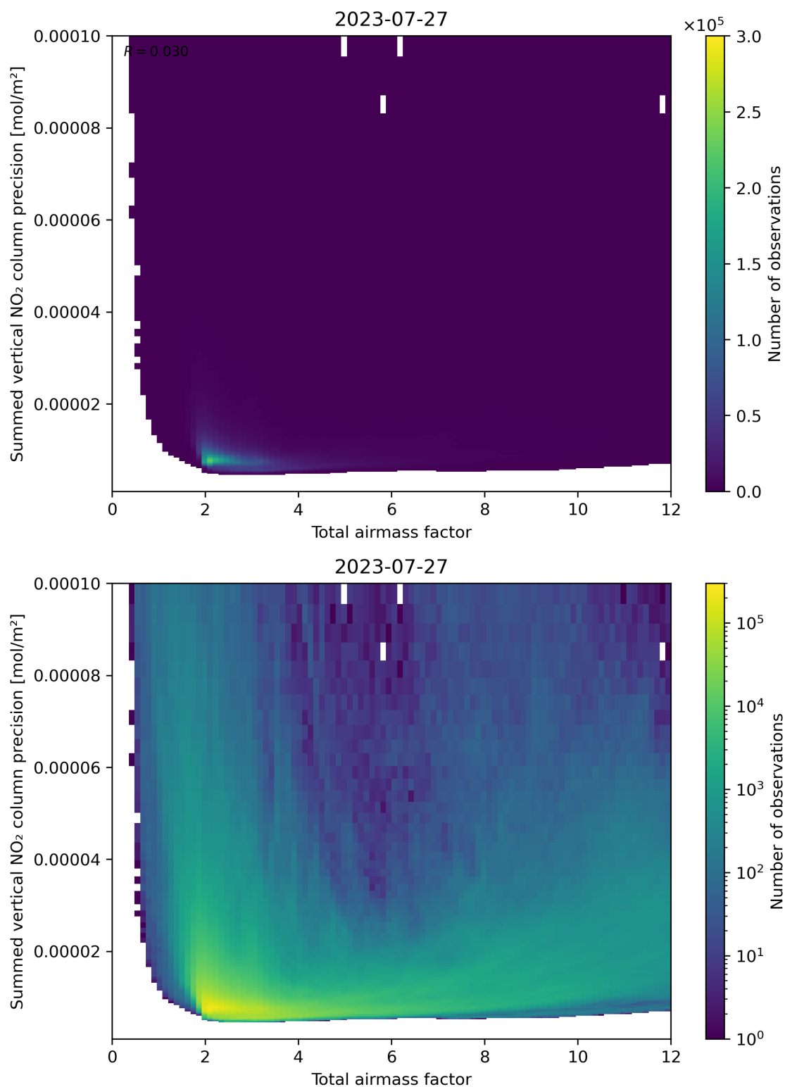
Figure 66: Scatter density plot of “Total airmass factor” against “Summed vertical NO 2 column precision” for 2023-07-26 to 2023-07-28.
