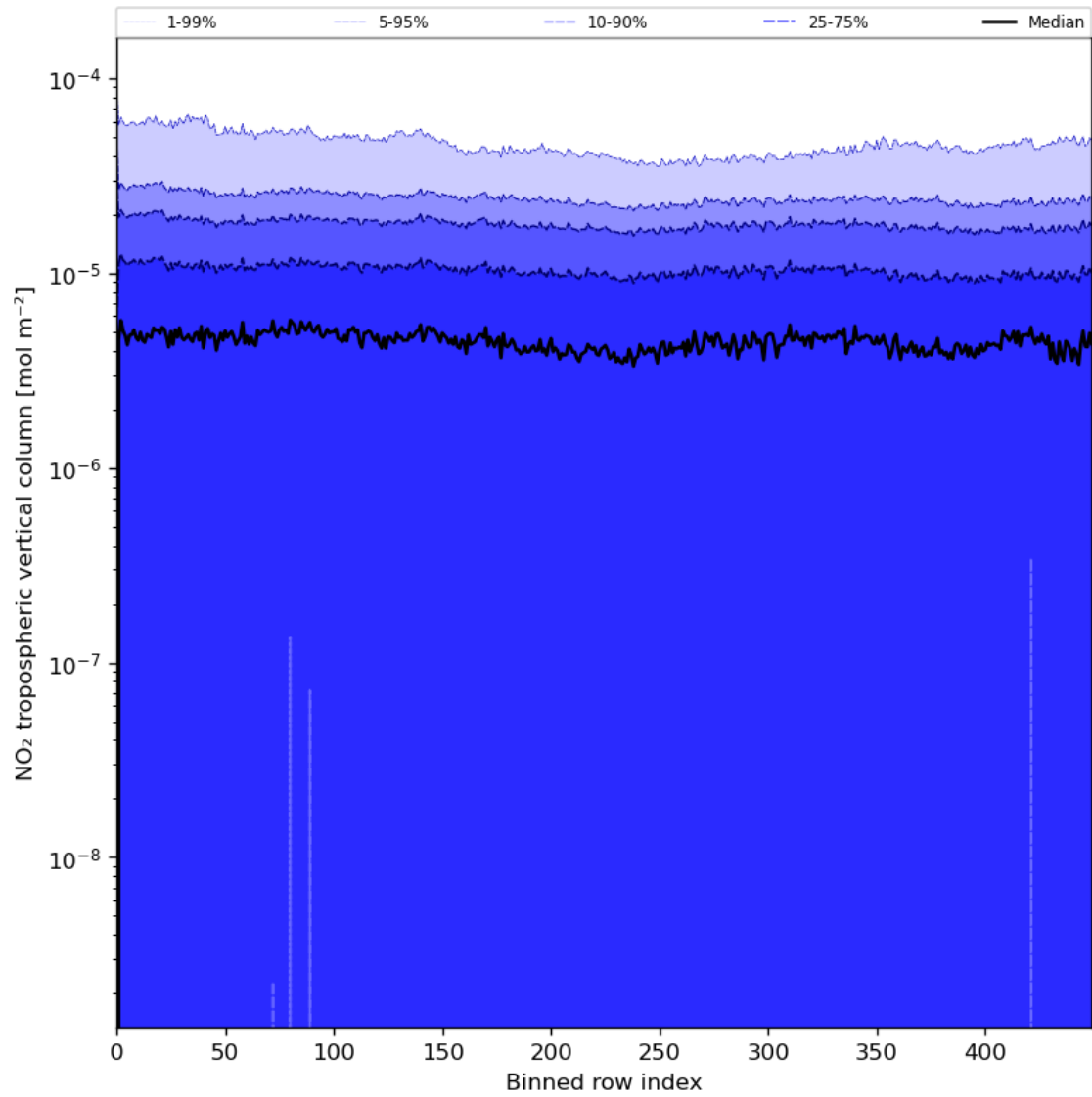
Figure 46: Along track statistics of “NO 2 tropospheric vertical column” for 2023-07-26 to 2023-07-28
