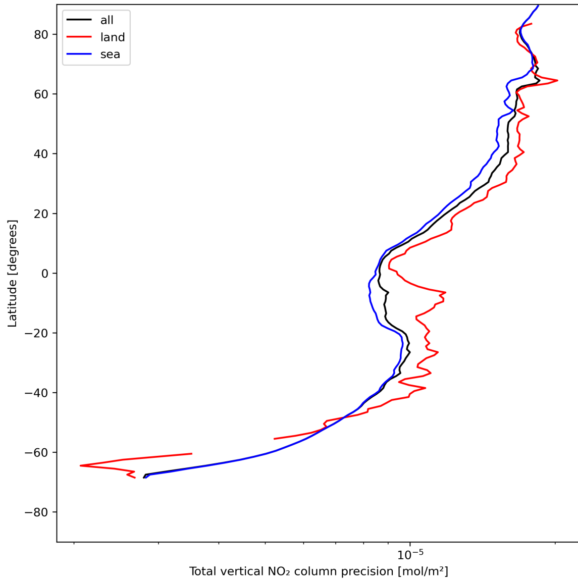
Figure 22: Zonal average of “Total vertical NO 2 column precision” for 2023-07-26 to 2023-07-28.
