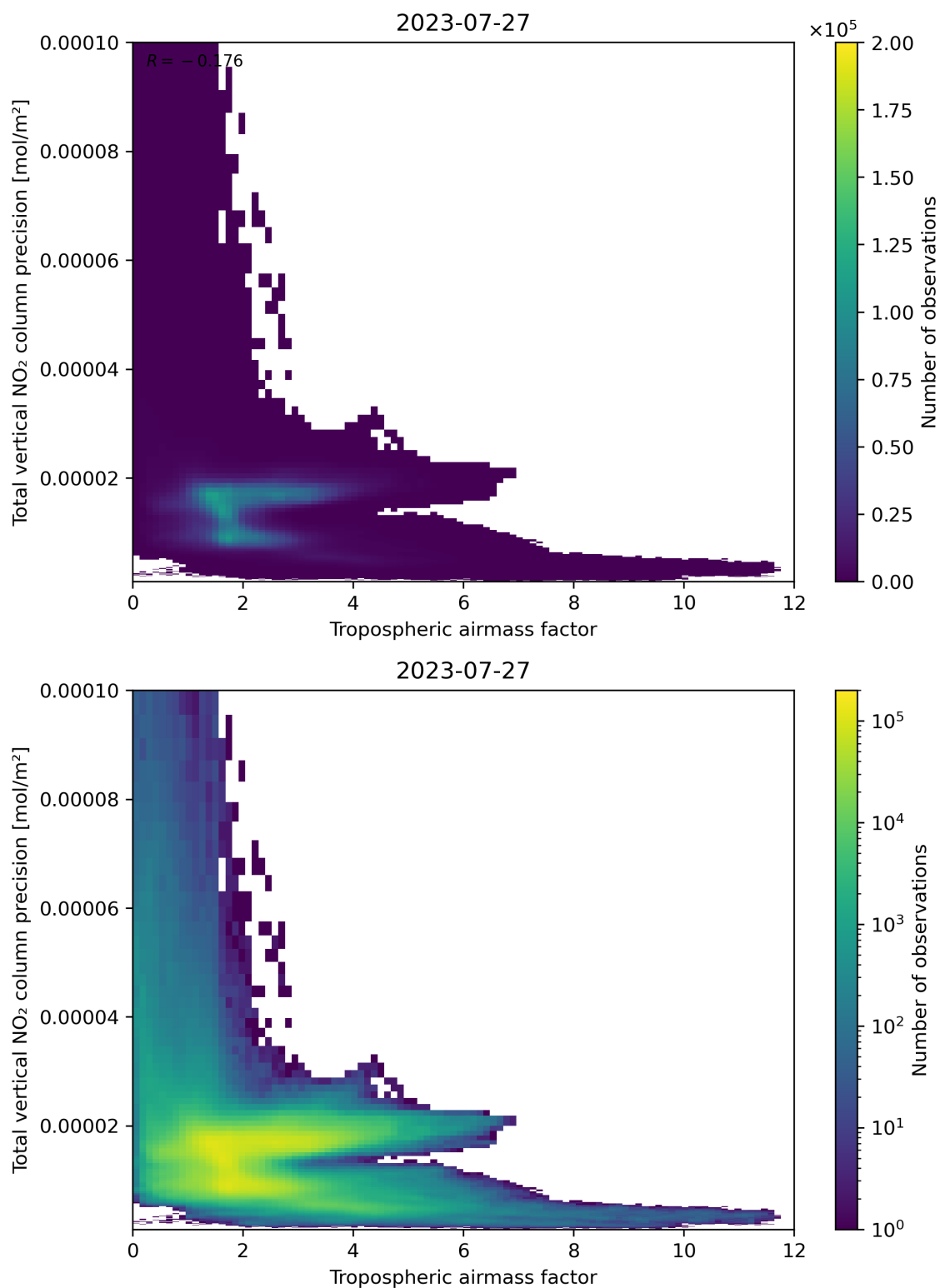
Figure 78: Scatter density plot of “Tropospheric airmass factor” against “Total vertical NO 2 column precision” for 2023-07-26 to 2023-07-28.
