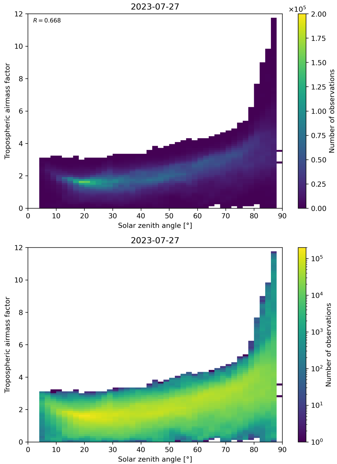
Figure 147: Scatter density plot of “Solar zenith angle” against “Tropospheric airmass factor” for 2023-07-26 to 2023-07-28.
