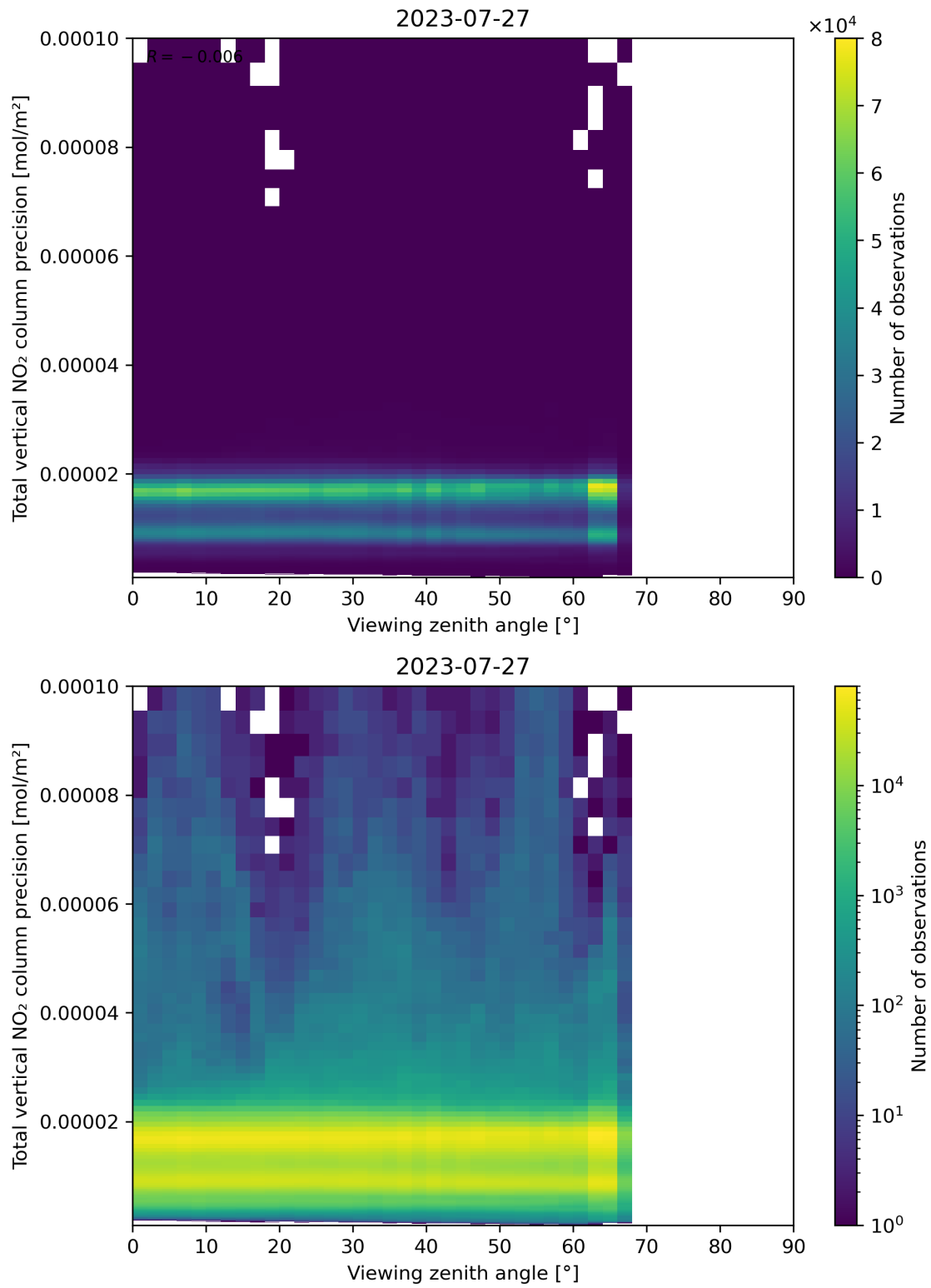
Figure 168: Scatter density plot of “Viewing zenith angle” against “Total vertical NO 2 column precision” for 2023-07-26 to 2023-07-28.
