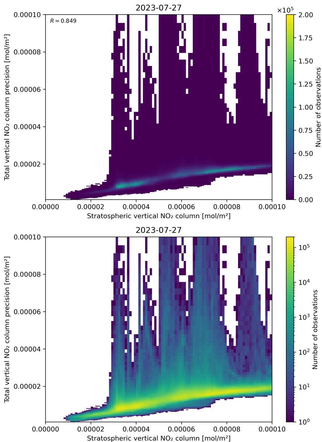
Figure 101: Scatter density plot of “Stratospheric vertical NO 2 column” against “Total vertical NO 2 column precision” for 2023-07-26 to 2023-07-28.
