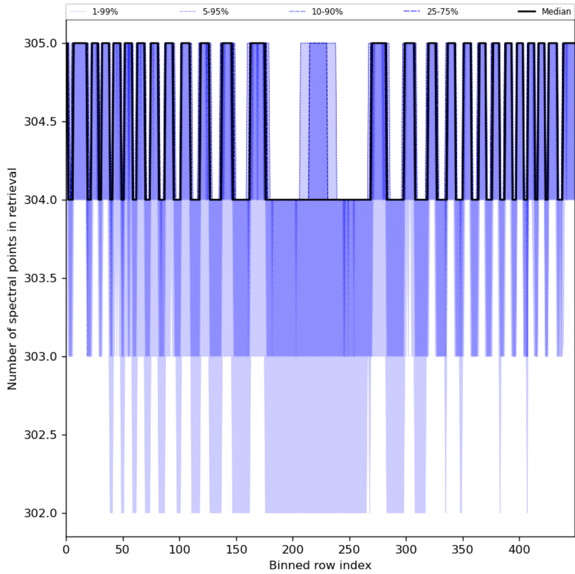
Figure 50: Along track statistics of “Number of spectral points in retrieval” for 2023-07-26 to 2023-07-28
