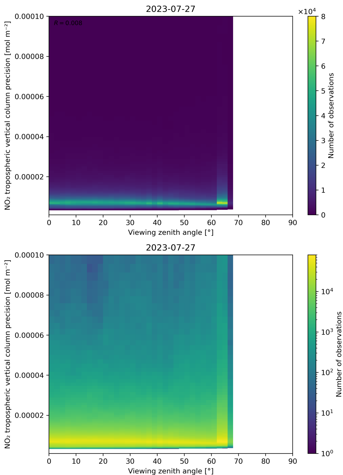
Figure 170: Scatter density plot of “Viewing zenith angle” against “NO 2 tropospheric vertical column precision” for 2023-07-26 to 2023-07-28.
