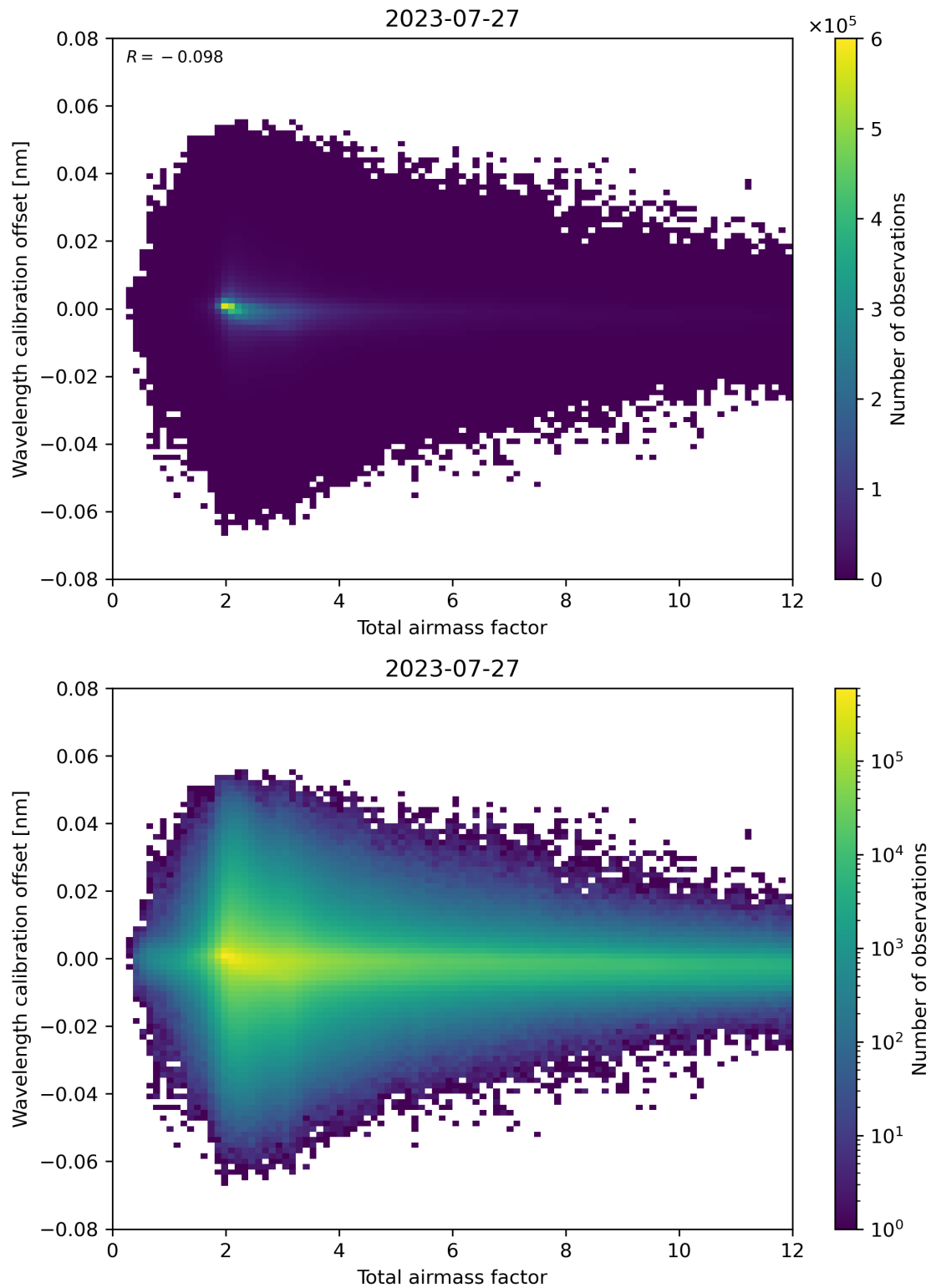
Figure 70: Scatter density plot of “Total airmass factor” against “Wavelength calibration offset” for 2023-07-26 to 2023-07-28.
