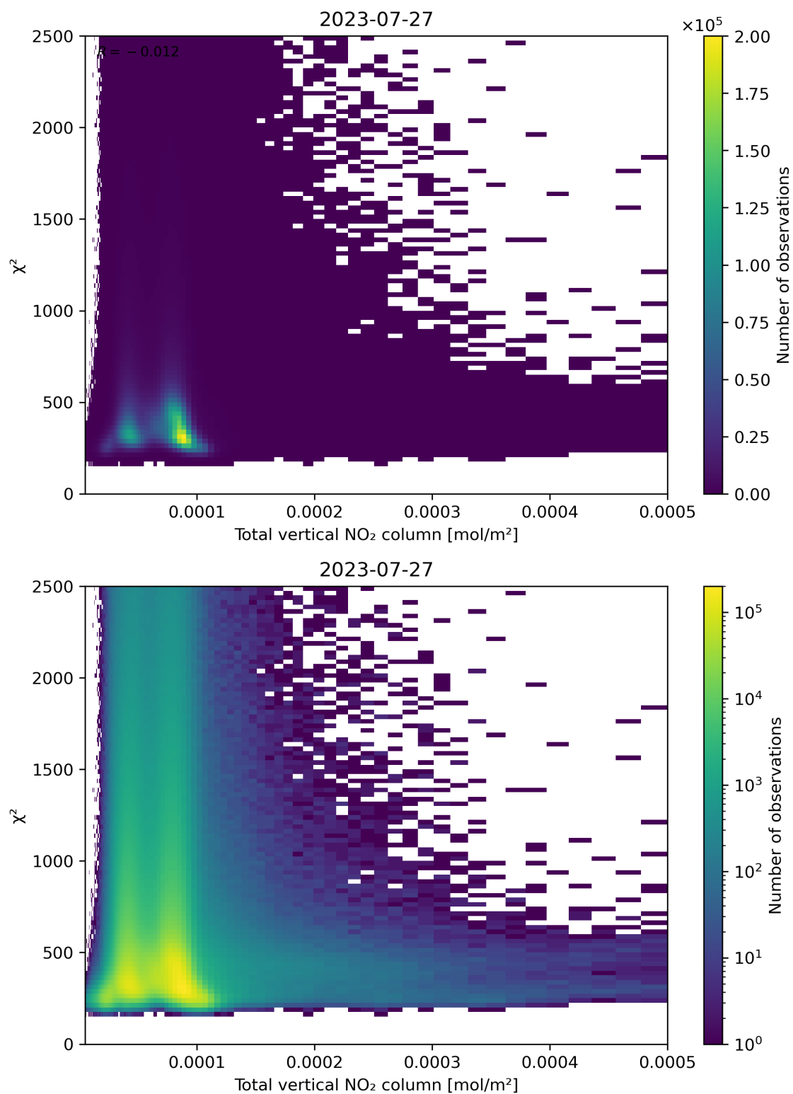
Figure 111: Scatter density plot of “Total vertical NO 2 column” against “ \chi^2 ” for 2023-07-26 to 2023-07-28.
