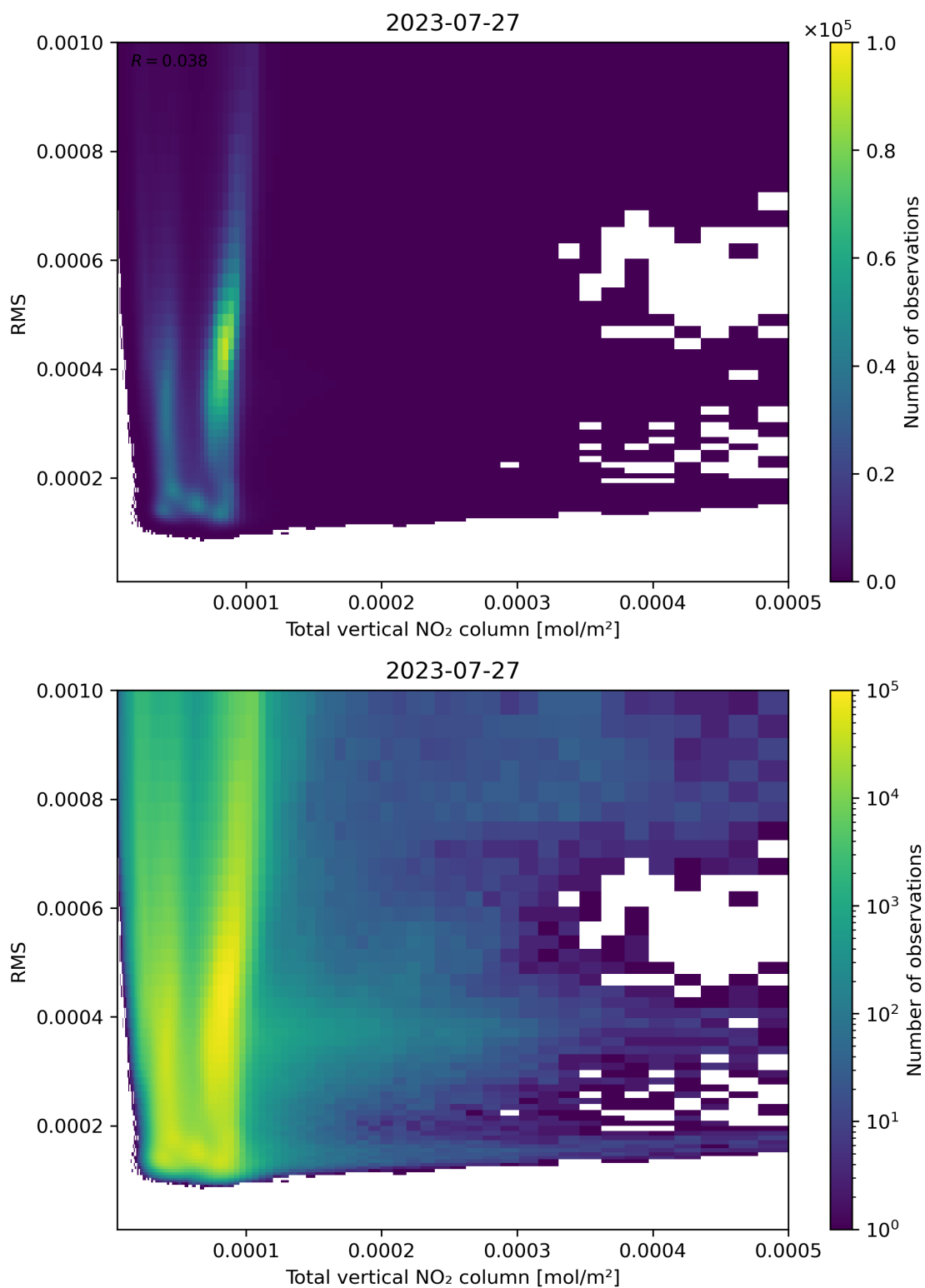
Figure 120: Scatter density plot of “Total vertical NO 2 column” against “RMS” for 2023-07-26 to 2023-07-28.
