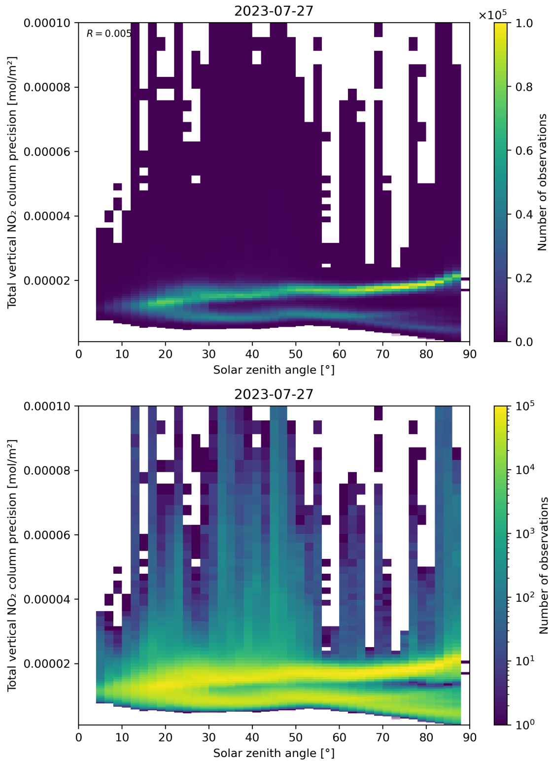
Figure 154: Scatter density plot of “Solar zenith angle” against “Total vertical NO 2 column precision” for 2023-07-26 to 2023-07-28.
