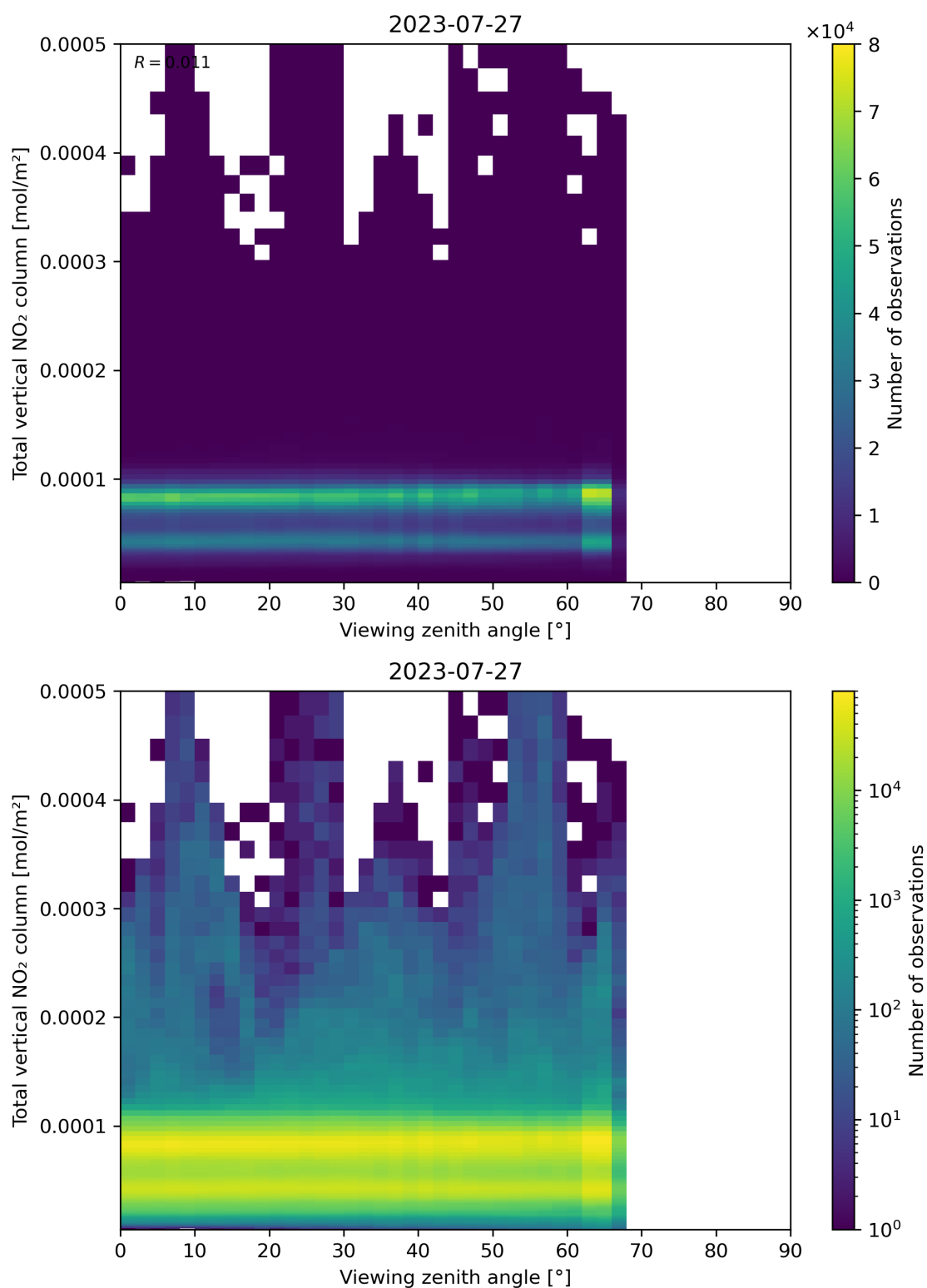
Figure 167: Scatter density plot of “Viewing zenith angle” against “Total vertical NO 2 column” for 2023-07-26 to 2023-07-28.
