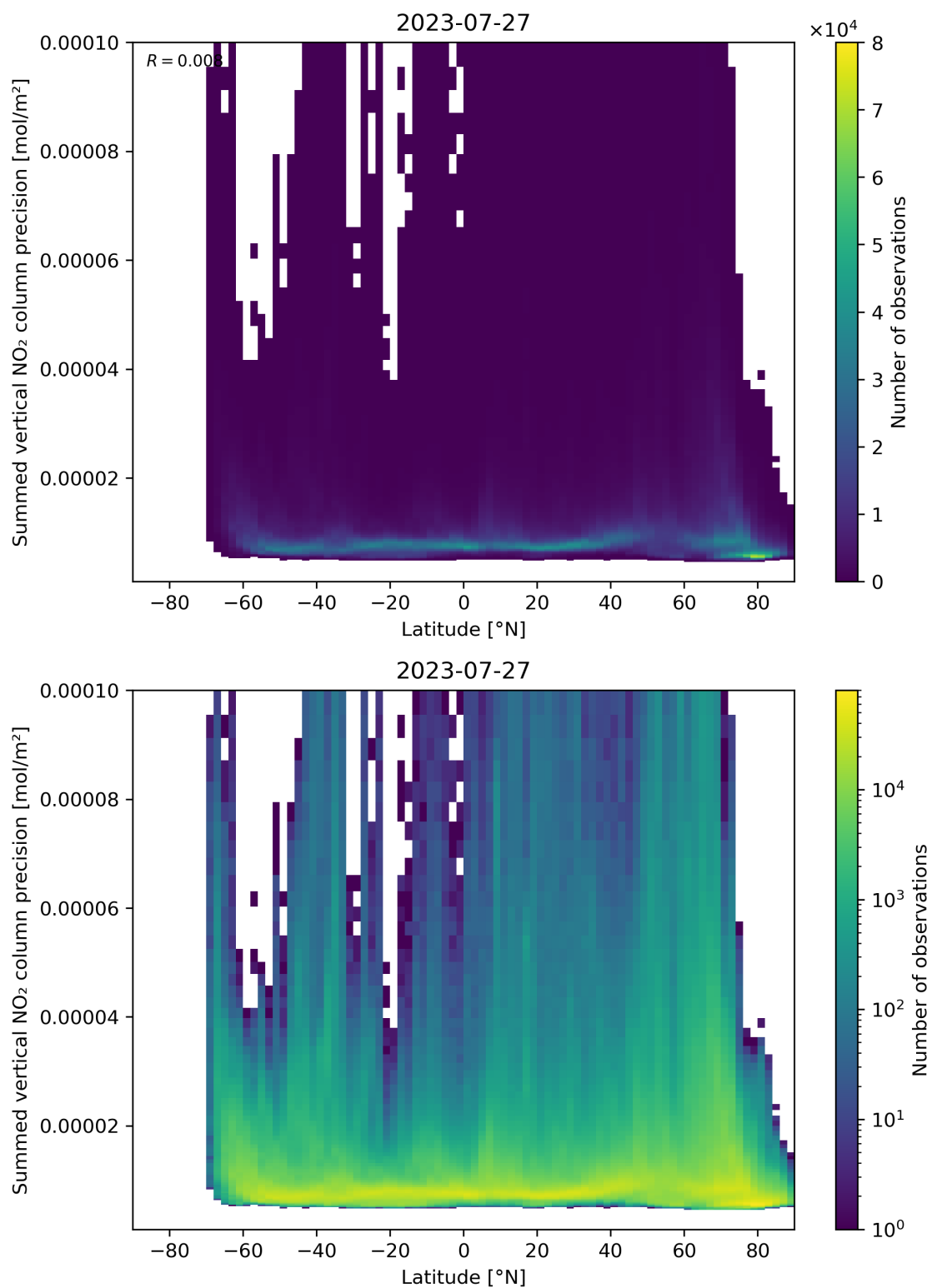
Figure 89: Scatter density plot of “Latitude” against “Summed vertical NO 2 column precision” for 2023-07-26 to 2023-07-28.
