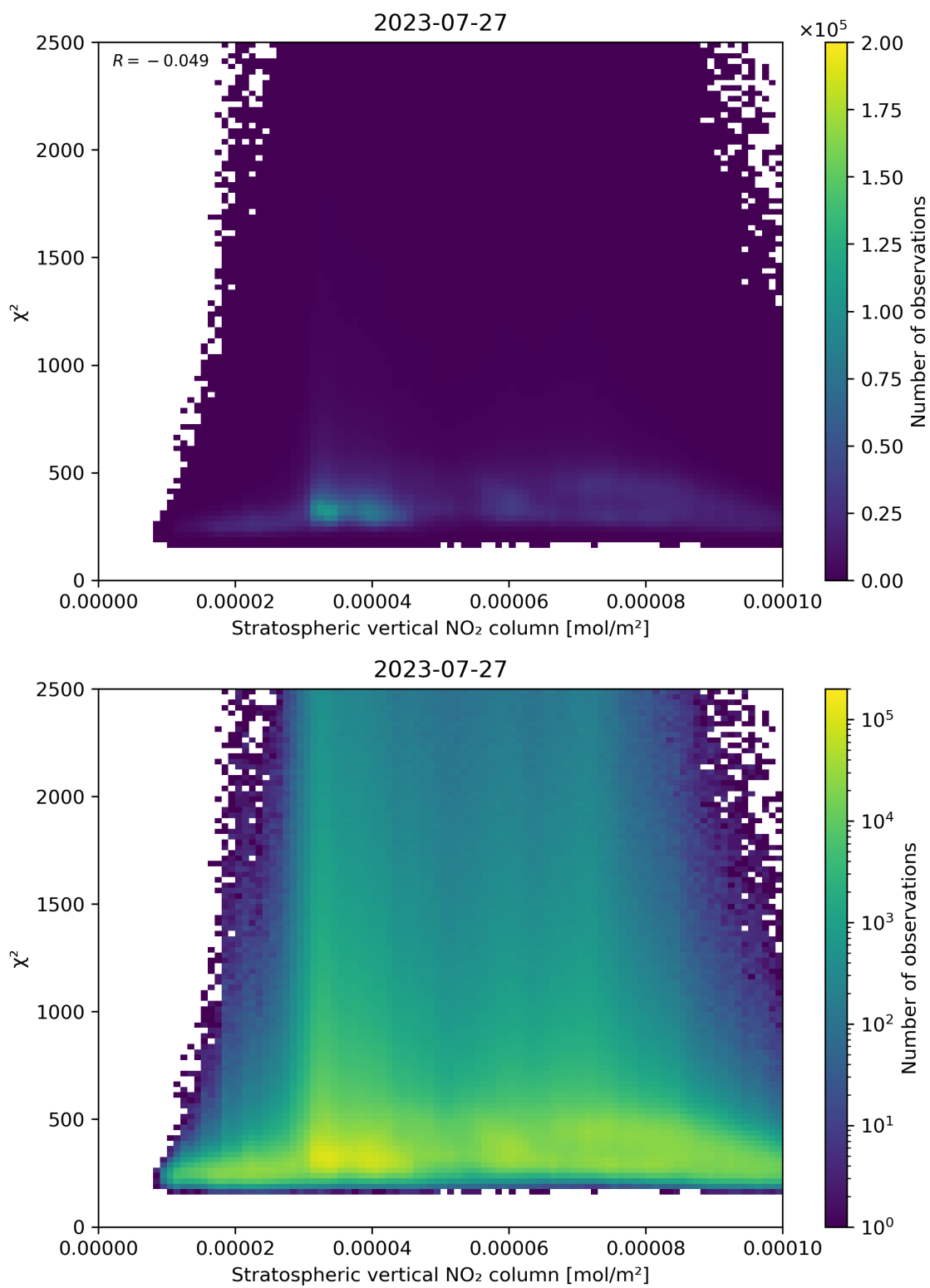
Figure 97: Scatter density plot of “Stratospheric vertical NO 2 column” against “ \chi^2 ” for 2023-07-26 to 2023-07-28.
