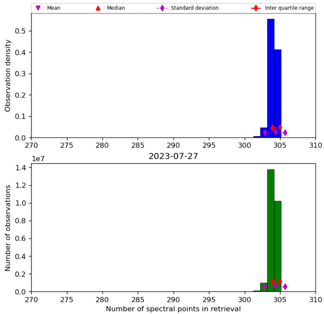
Figure 33: Histogram of “Number of spectral points in retrieval” for 2023-07-26 to 2023-07-28
