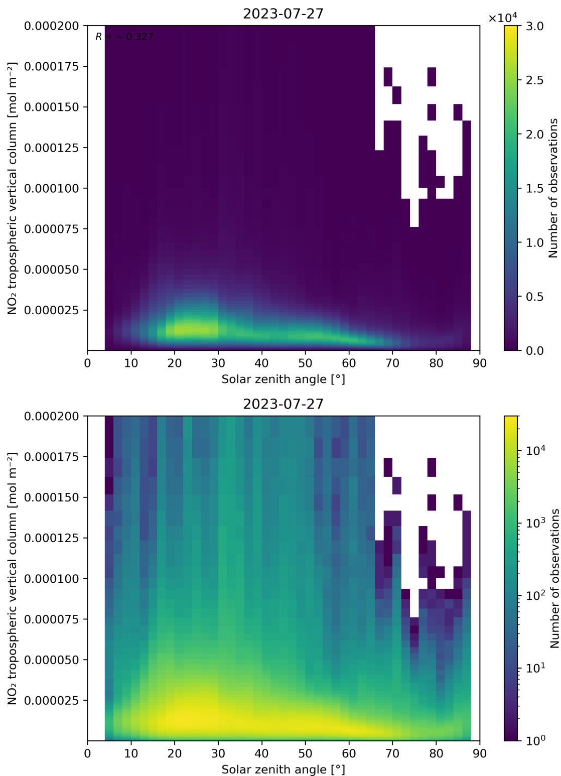
Figure 155: Scatter density plot of “Solar zenith angle” against “NO 2 tropospheric vertical column” for 2023-07-26 to 2023-07-28.
