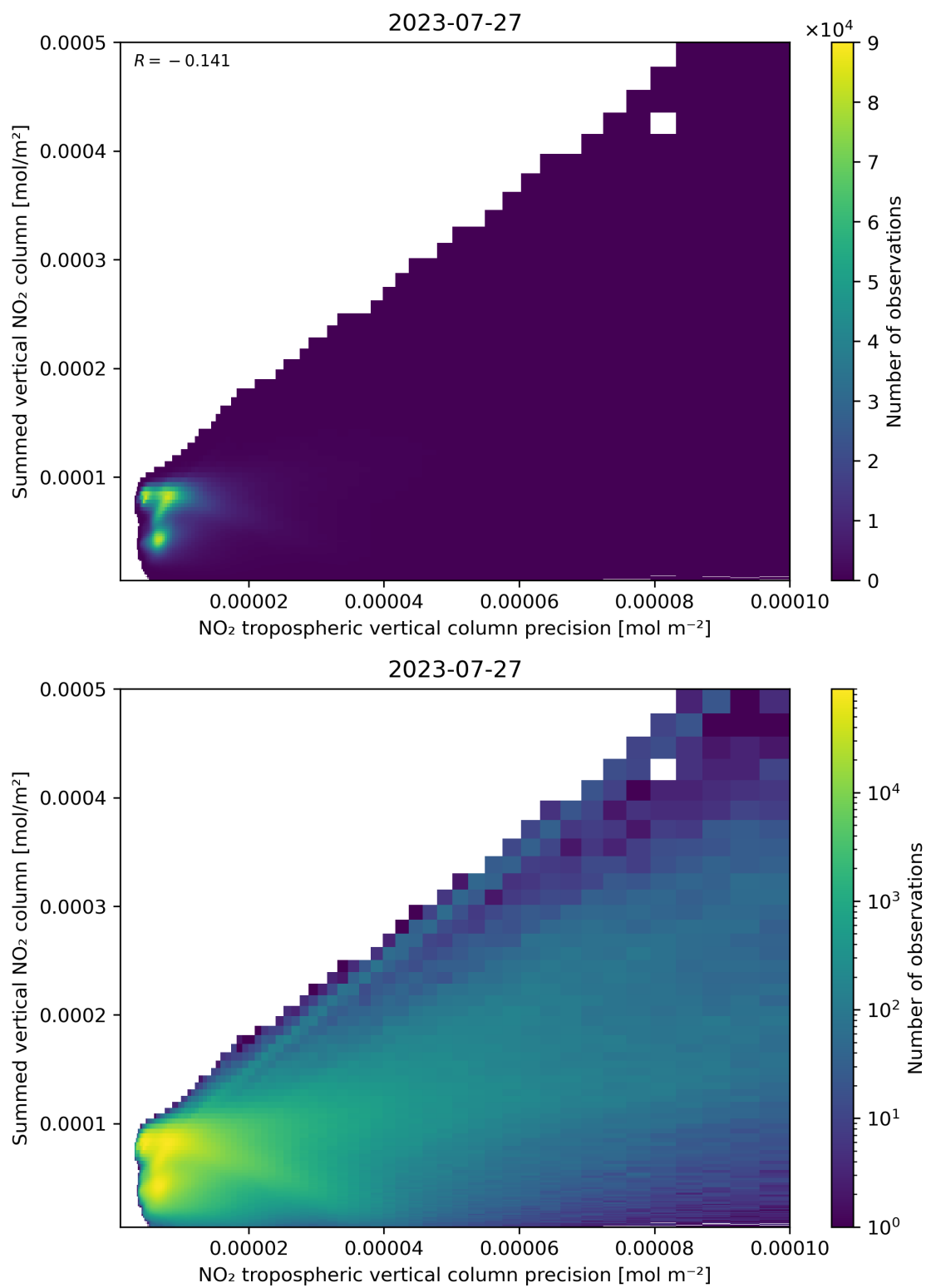
Figure 136: Scatter density plot of “NO 2 tropospheric vertical column precision” against “Summed vertical NO 2 column” for 2023-07-26 to 2023-07-28.
