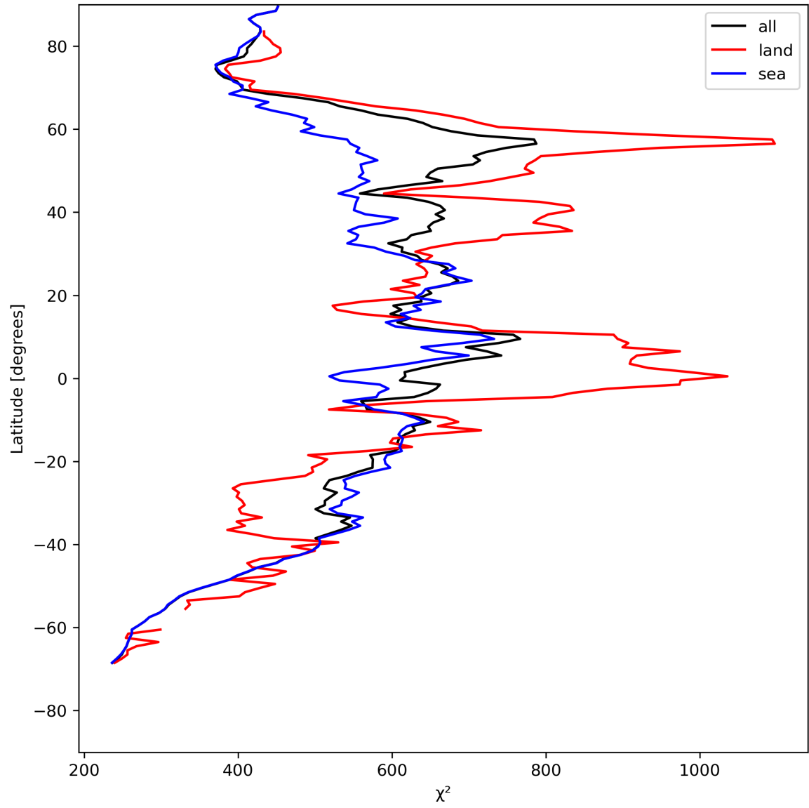
Figure 25: Zonal average of “ \chi^2 ” for 2023-07-26 to 2023-07-28.
