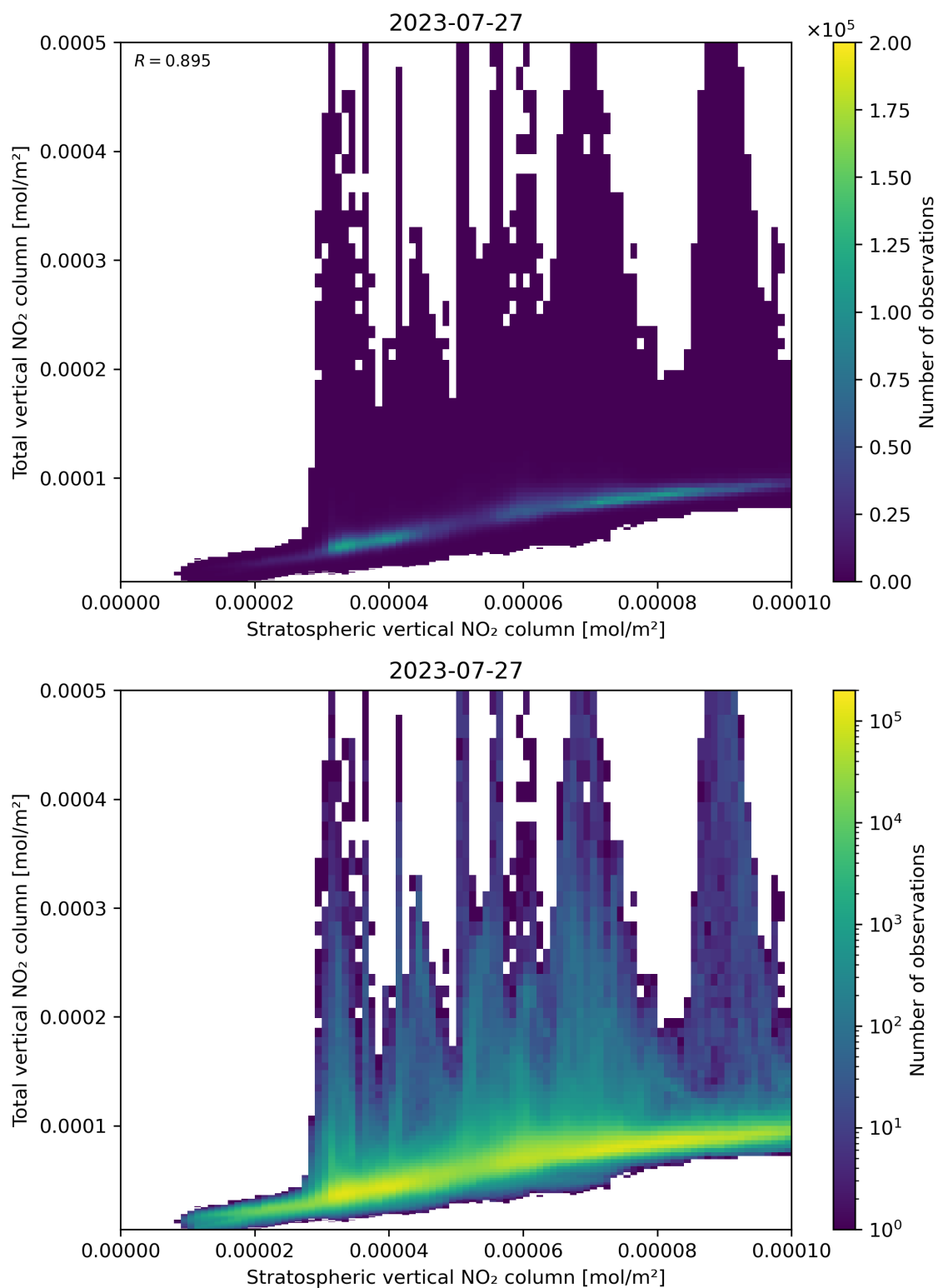
Figure 100: Scatter density plot of “Stratospheric vertical NO 2 column” against “Total vertical NO 2 column” for 2023-07-26 to 2023-07-28.
