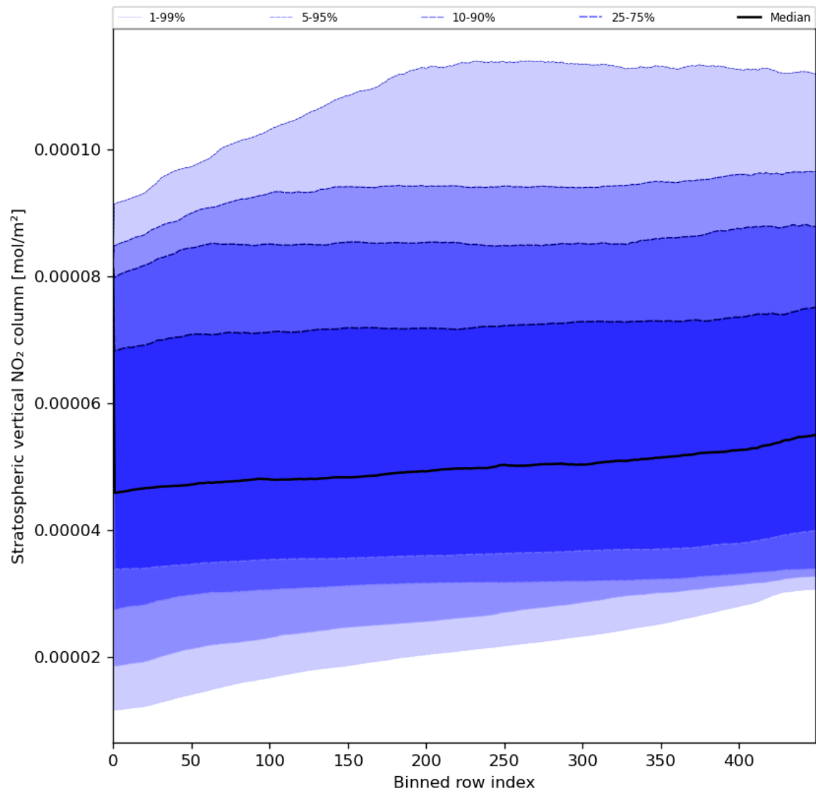
Figure 53: Along track statistics of “Stratospheric vertical NO 2 column” for 2023-07-26 to 2023-07-28
