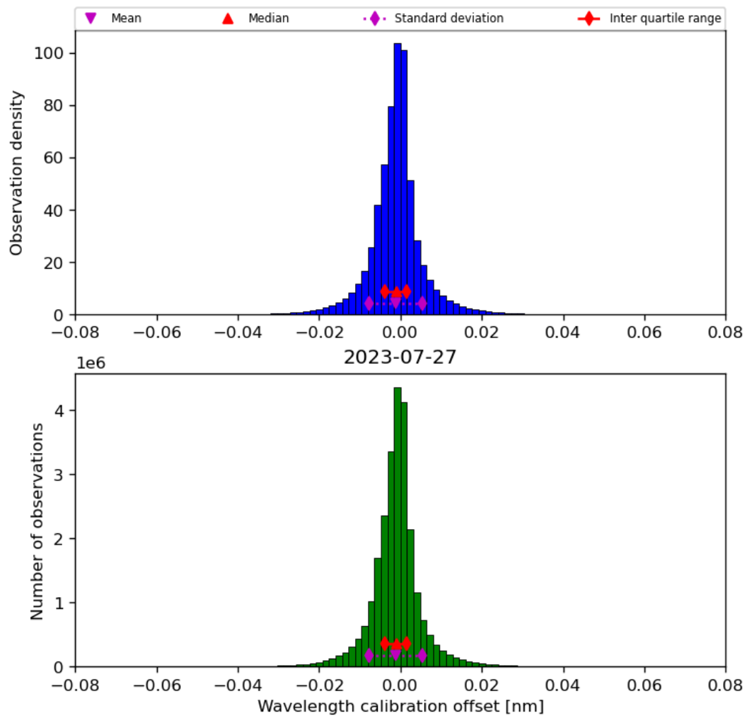
Figure 35: Histogram of “Wavelength calibration offset” for 2023-07-26 to 2023-07-28
