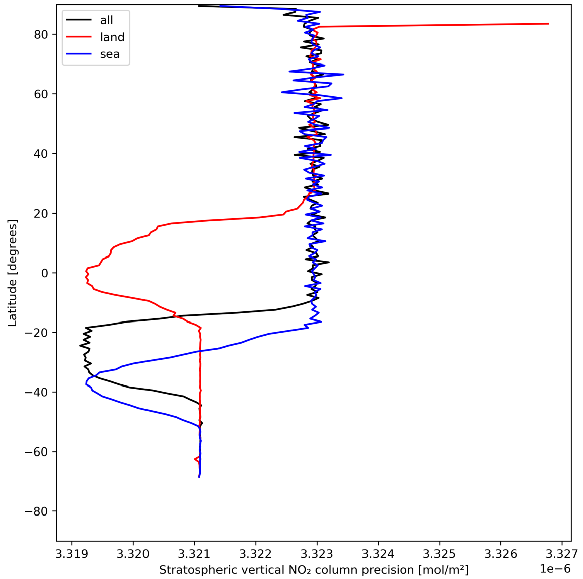
Figure 20: Zonal average of “Stratospheric vertical NO 2 column precision” for 2023-07-26 to 2023-07-28.
