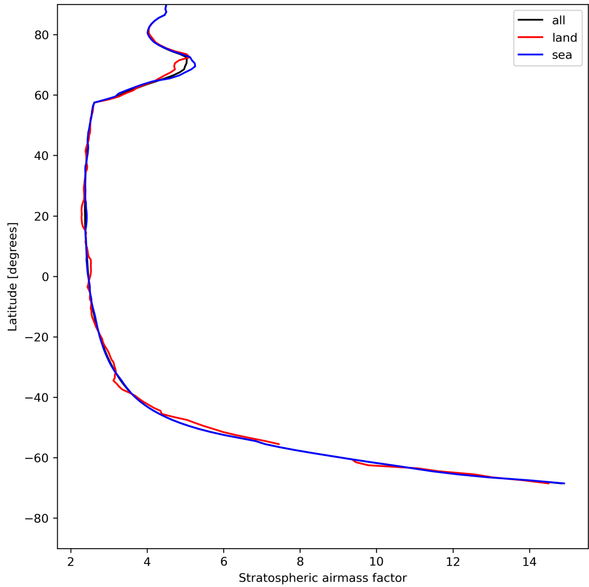
Figure 27: Zonal average of “Stratospheric air mass factor” for 2023-07-26 to 2023-07-28.
