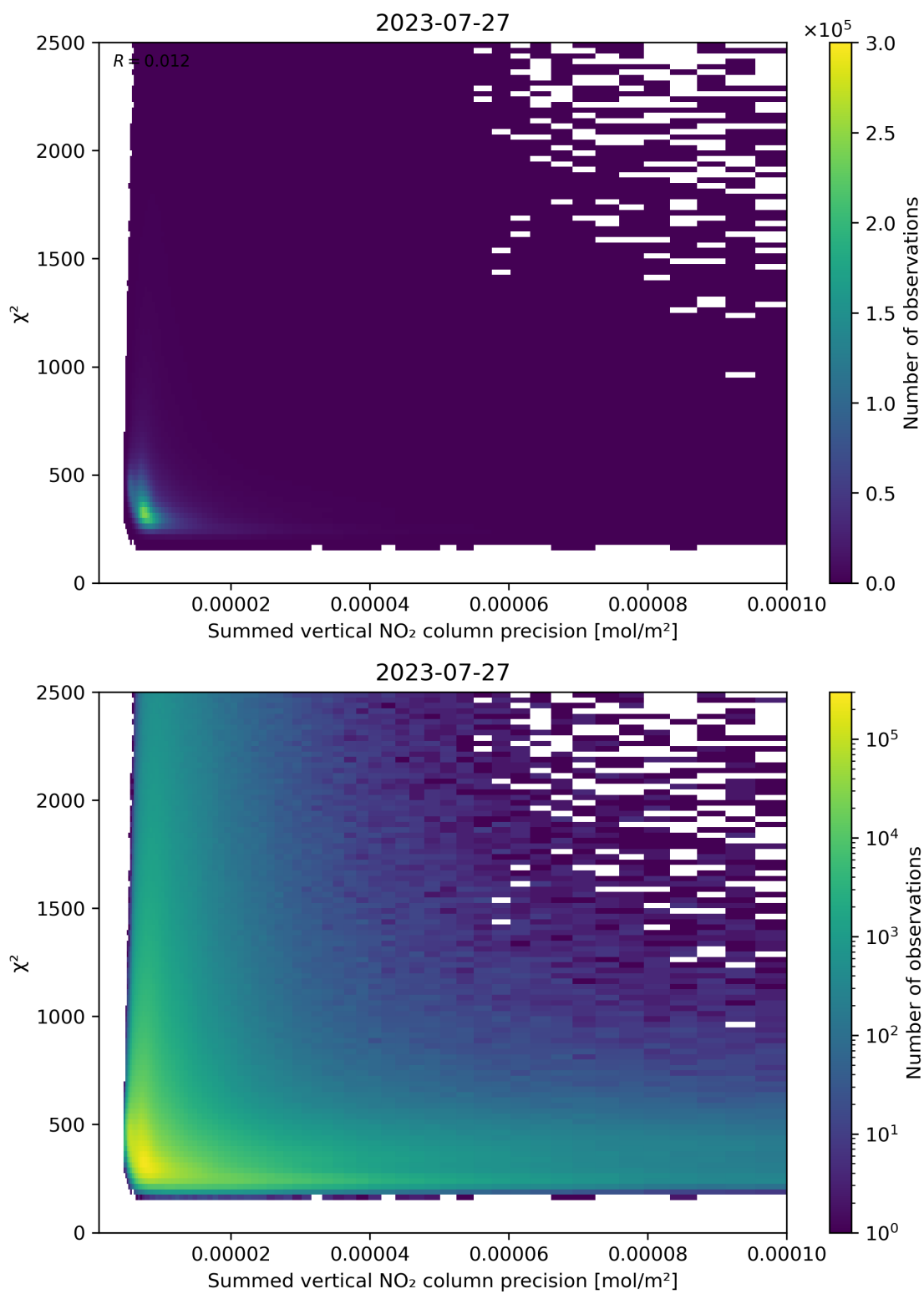
Figure 107: Scatter density plot of “Summed vertical NO 2 column precision” against “ \chi^2 ” for 2023-07-26 to 2023-07-28.
