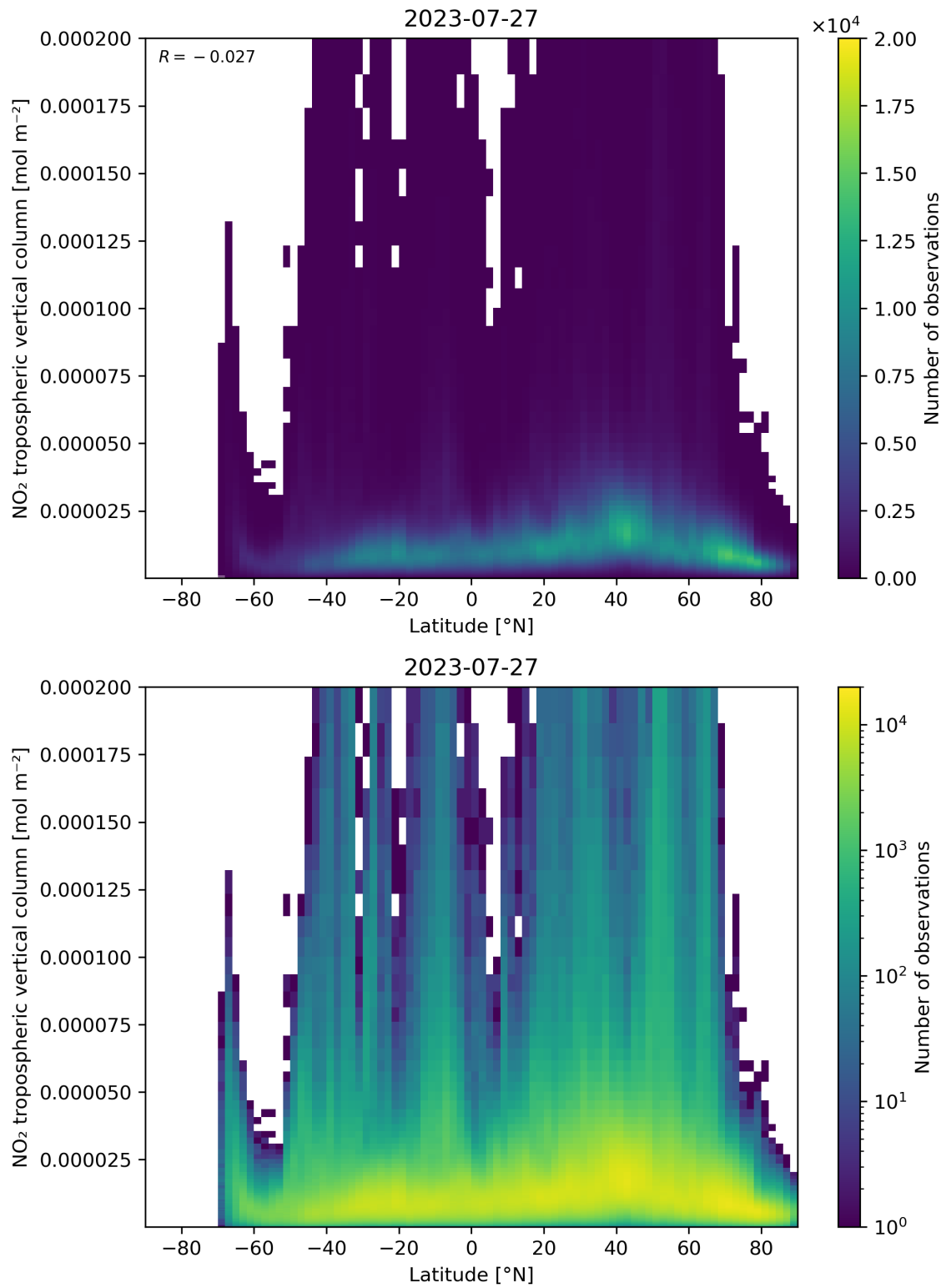
Figure 92: Scatter density plot of “Latitude” against “NO 2 tropospheric vertical column” for 2023-07-26 to 2023-07-28.
