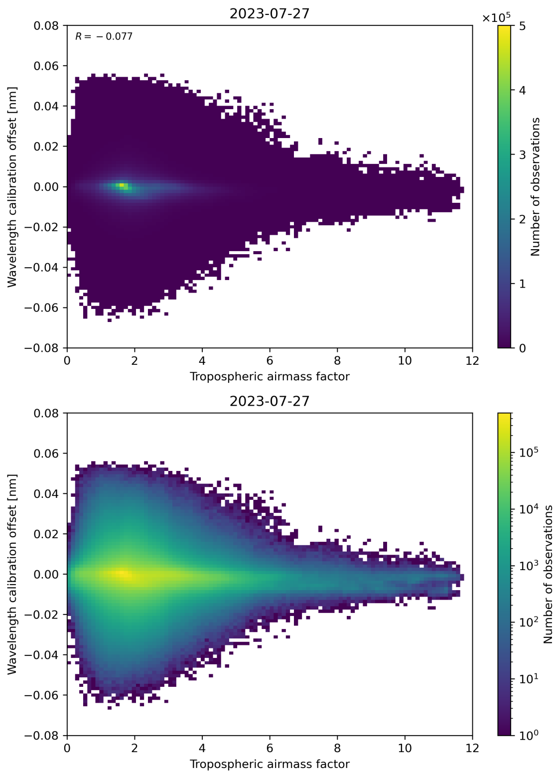
Figure 80: Scatter density plot of “Tropospheric air mass factor” against “Wavelength calibration offset” for 2023-07-26 to 2023-07-28.
