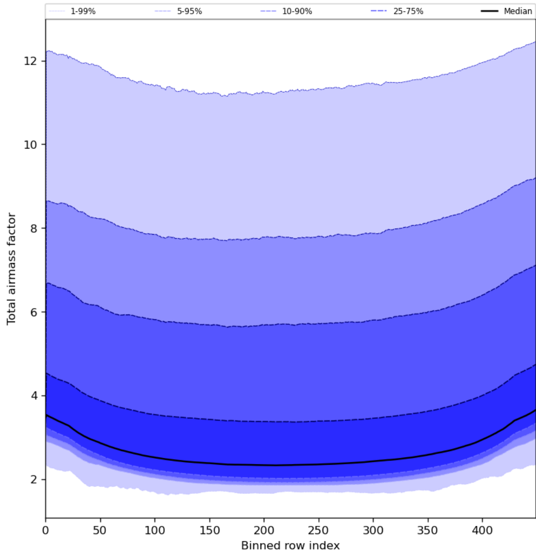
Figure 49: Along track statistics of “Total airmass factor” for 2023-07-26 to 2023-07-28
