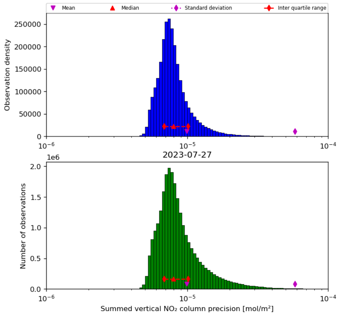
Figure 41: Histogram of “Summed vertical NO 2 column precision” for 2023-07-26 to 2023-07-28
