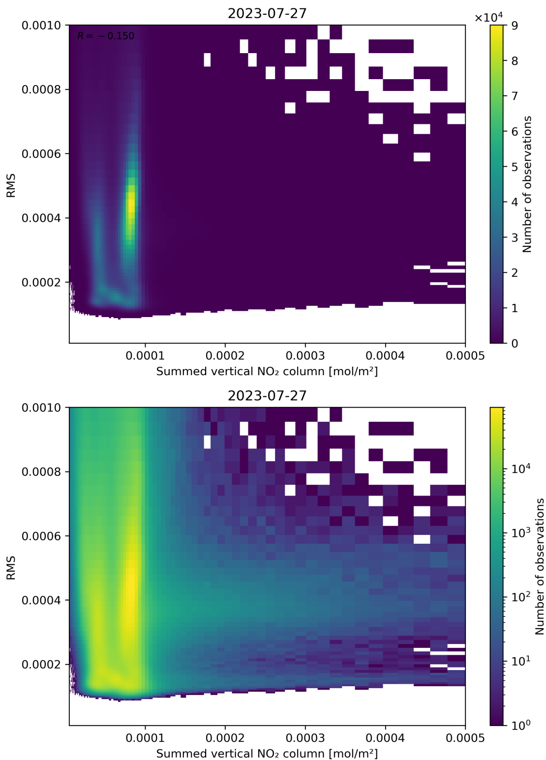
Figure 109: Scatter density plot of “Summed vertical NO 2 column” against “RMS” for 2023-07-26 to 2023-07-28.
