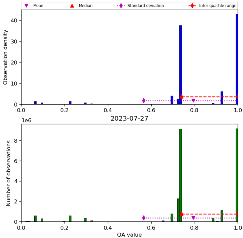
Figure 28: Histogram of “QA value” for 2023-07-26 to 2023-07-28
