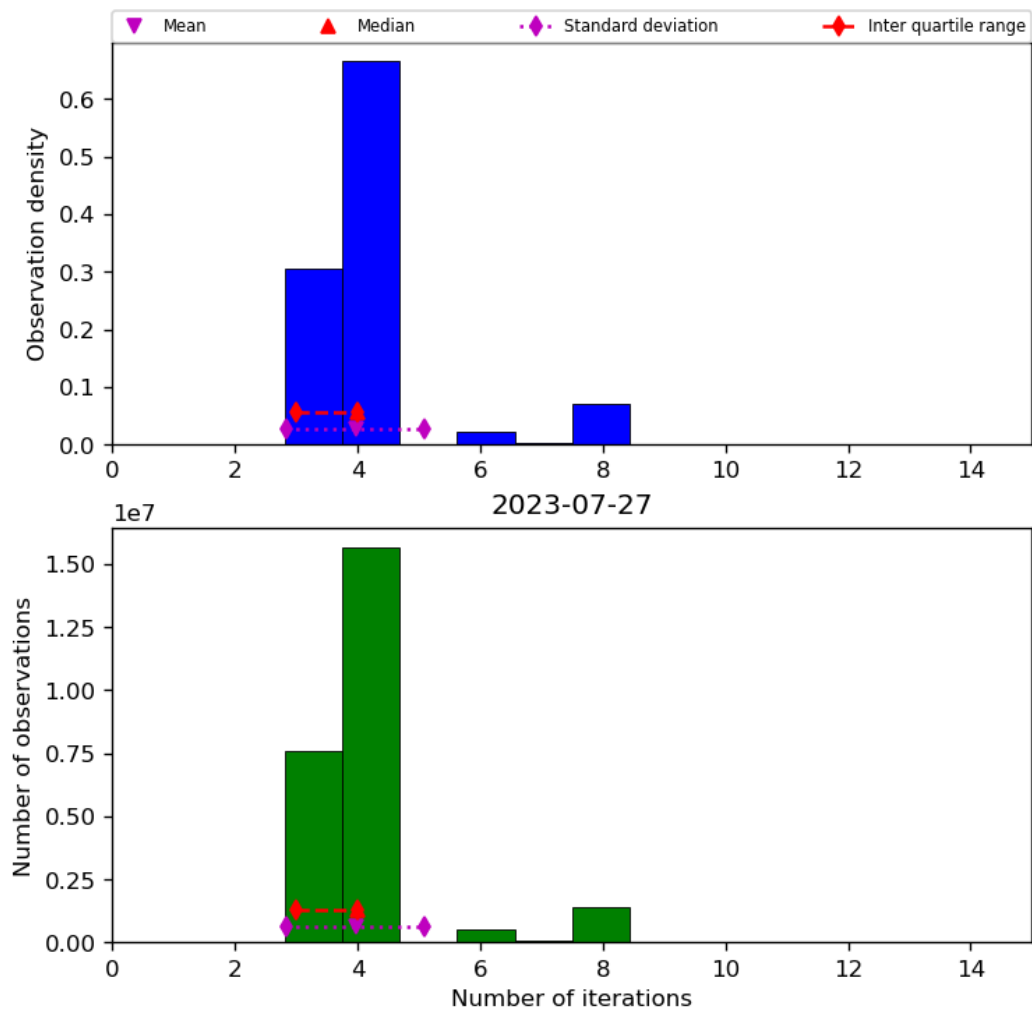
Figure 34: Histogram of “Number of iterations” for 2023-07-26 to 2023-07-28
