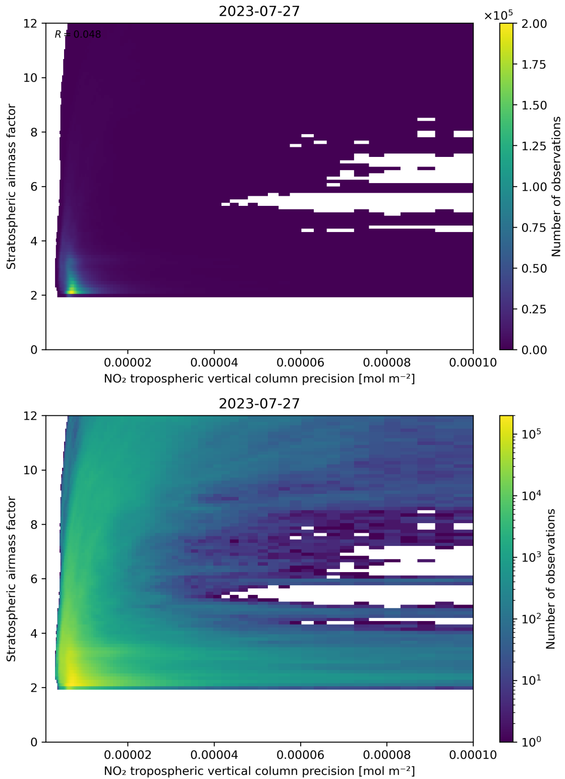
Figure 131: Scatter density plot of “NO 2 tropospheric vertical column precision” against “Stratospheric airmass factor” for 2023-07-26 to 2023-07-28.
