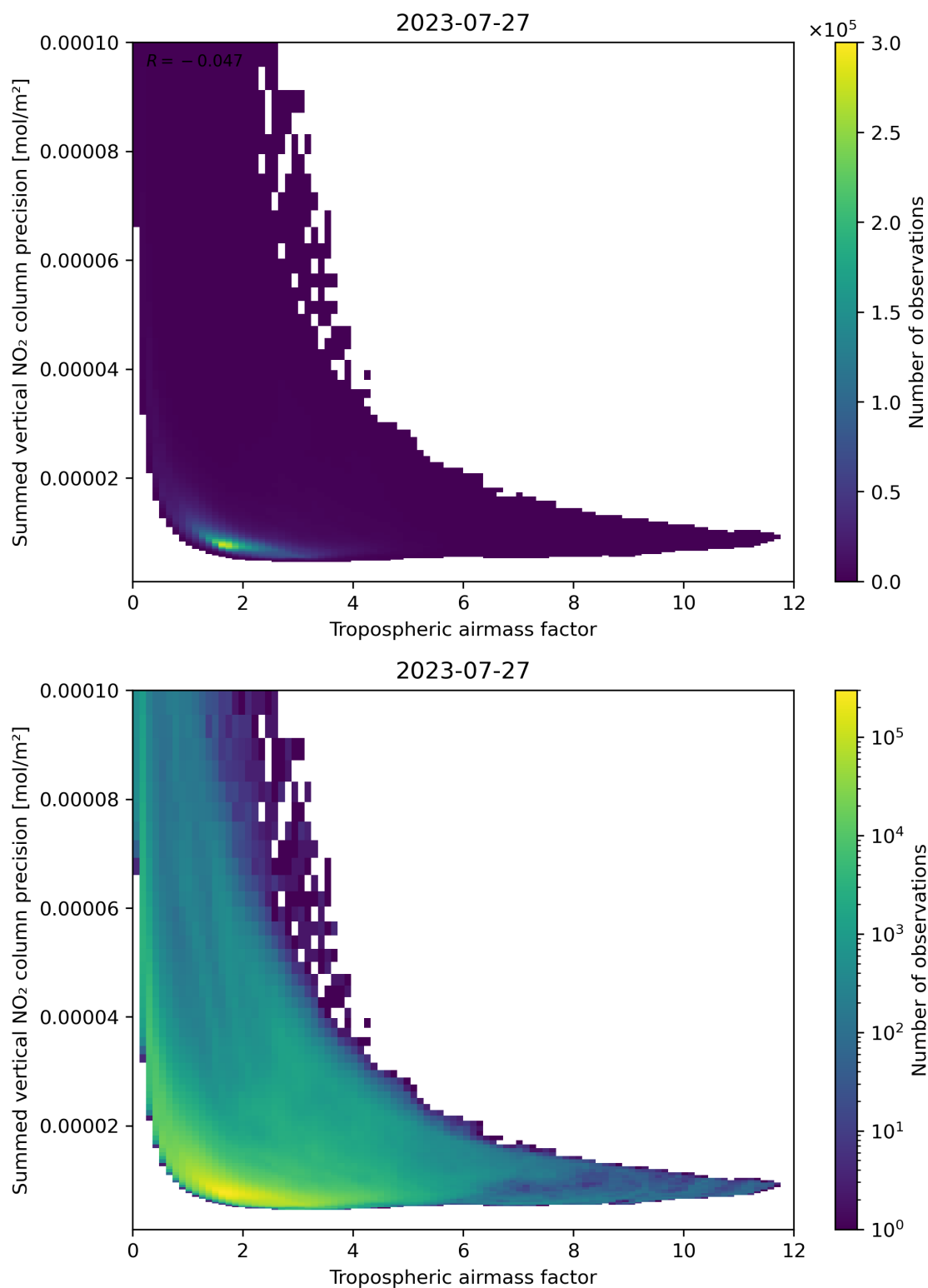
Figure 76: Scatter density plot of “Tropospheric air mass factor” against “Summed vertical NO 2 column precision” for 2023-07-26 to 2023-07-28.
