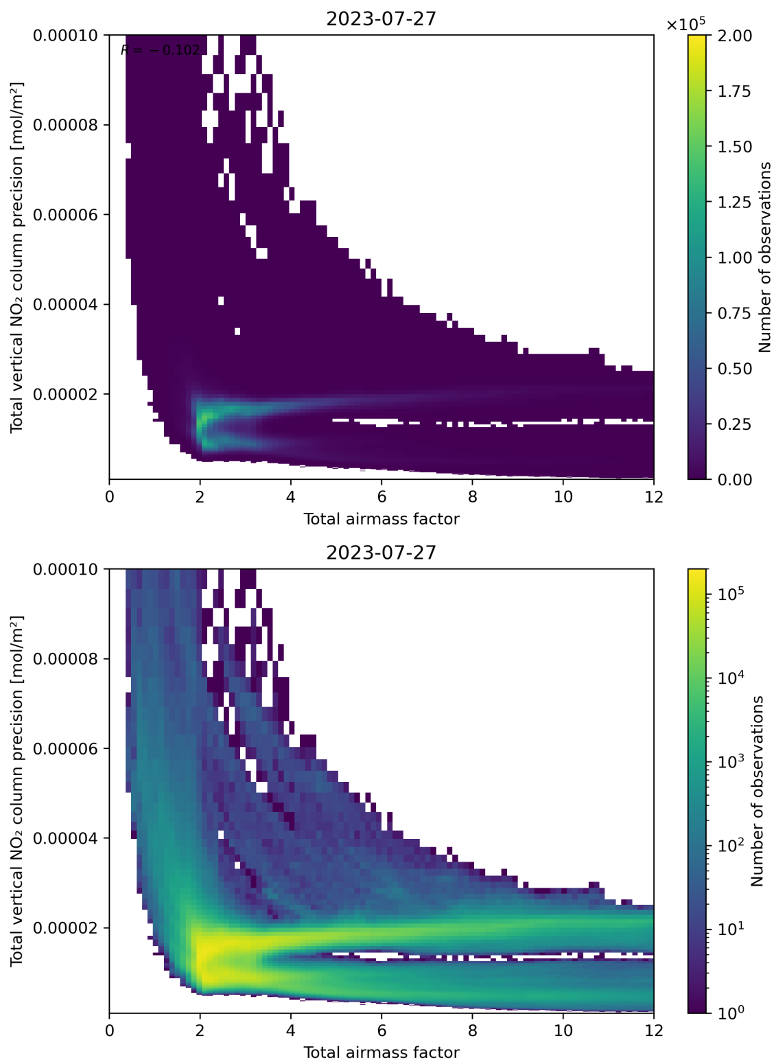
Figure 68: Scatter density plot of “Total airmass factor” against “Total vertical NO 2 column precision” for 2023-07-26 to 2023-07-28.
