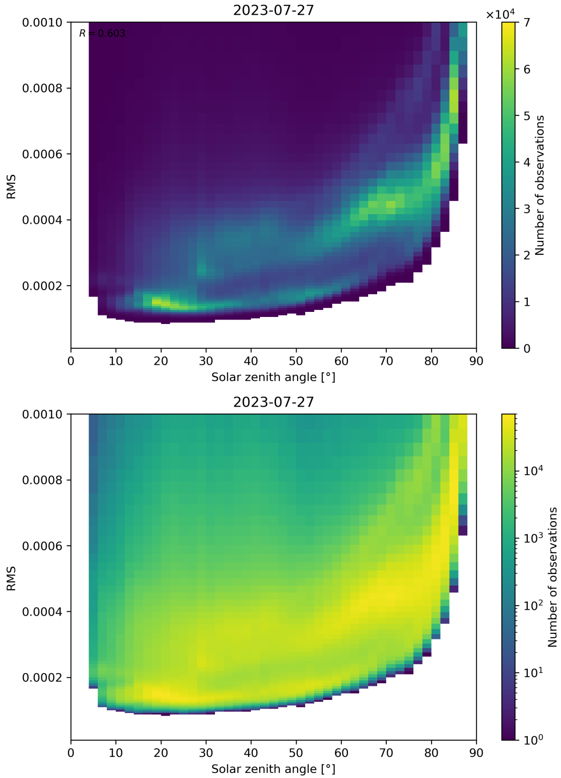
Figure 157: Scatter density plot of “Solar zenith angle” against “RMS” for 2023-07-26 to 2023-07-28.
