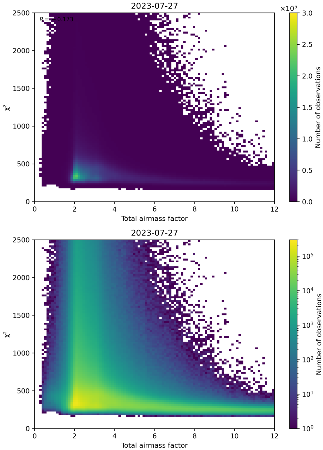
Figure 63: Scatter density plot of “Total airmass factor” against “ \chi^2 ” for 2023-07-26 to 2023-07-28.
