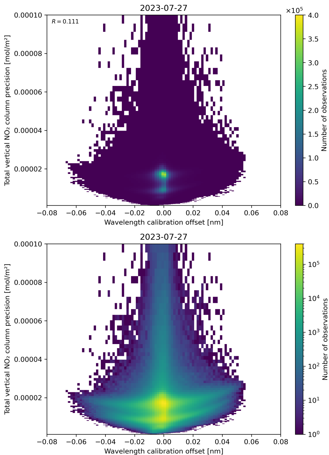
Figure 180: Scatter density plot of “Wavelength calibration offset” against “Total vertical NO 2 column precision” for 2023-07-26 to 2023-07-28.
