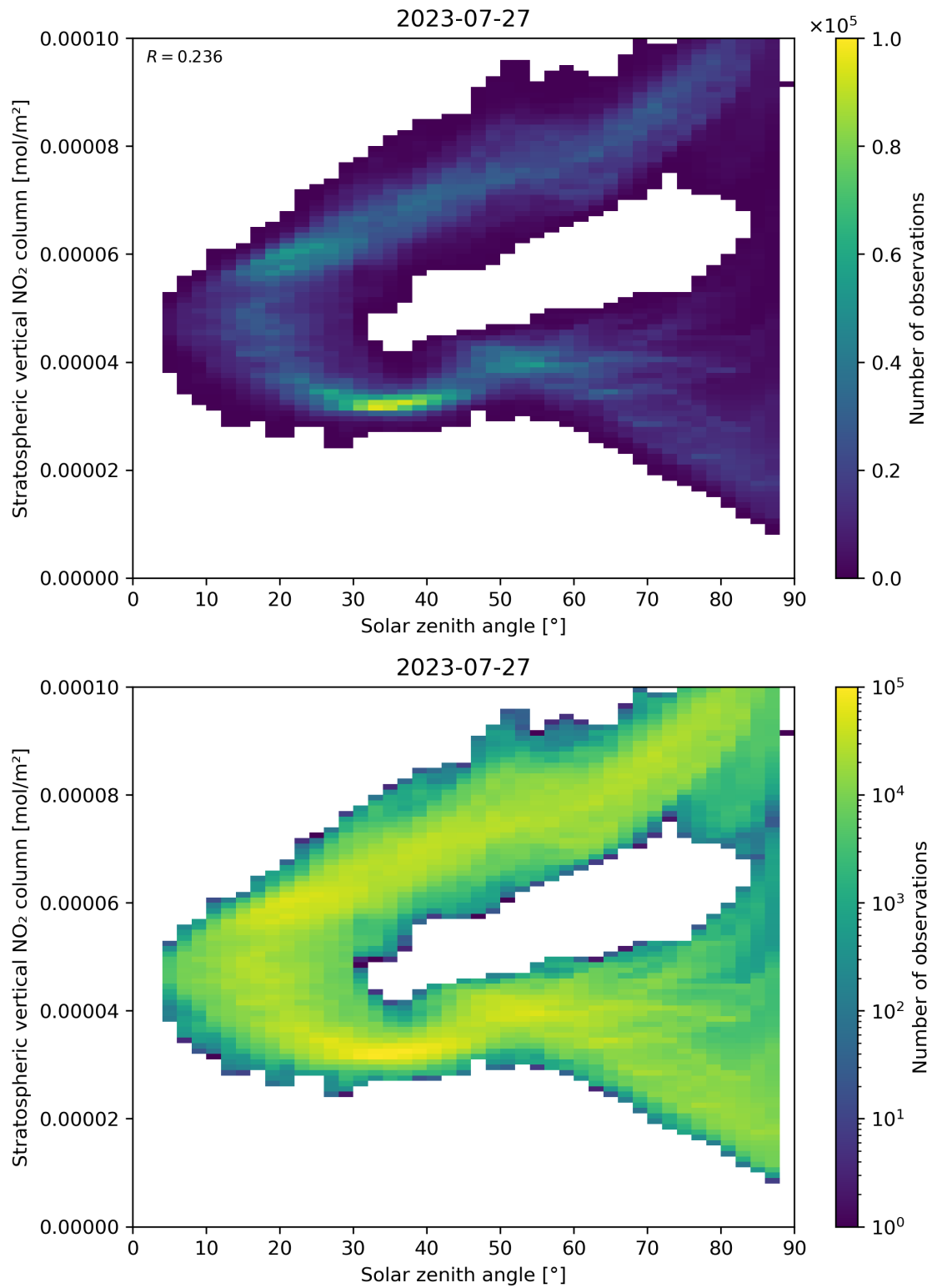
Figure 150: Scatter density plot of “Solar zenith angle” against “Stratospheric vertical NO 2 column” for 2023-07-26 to 2023-07-28.
