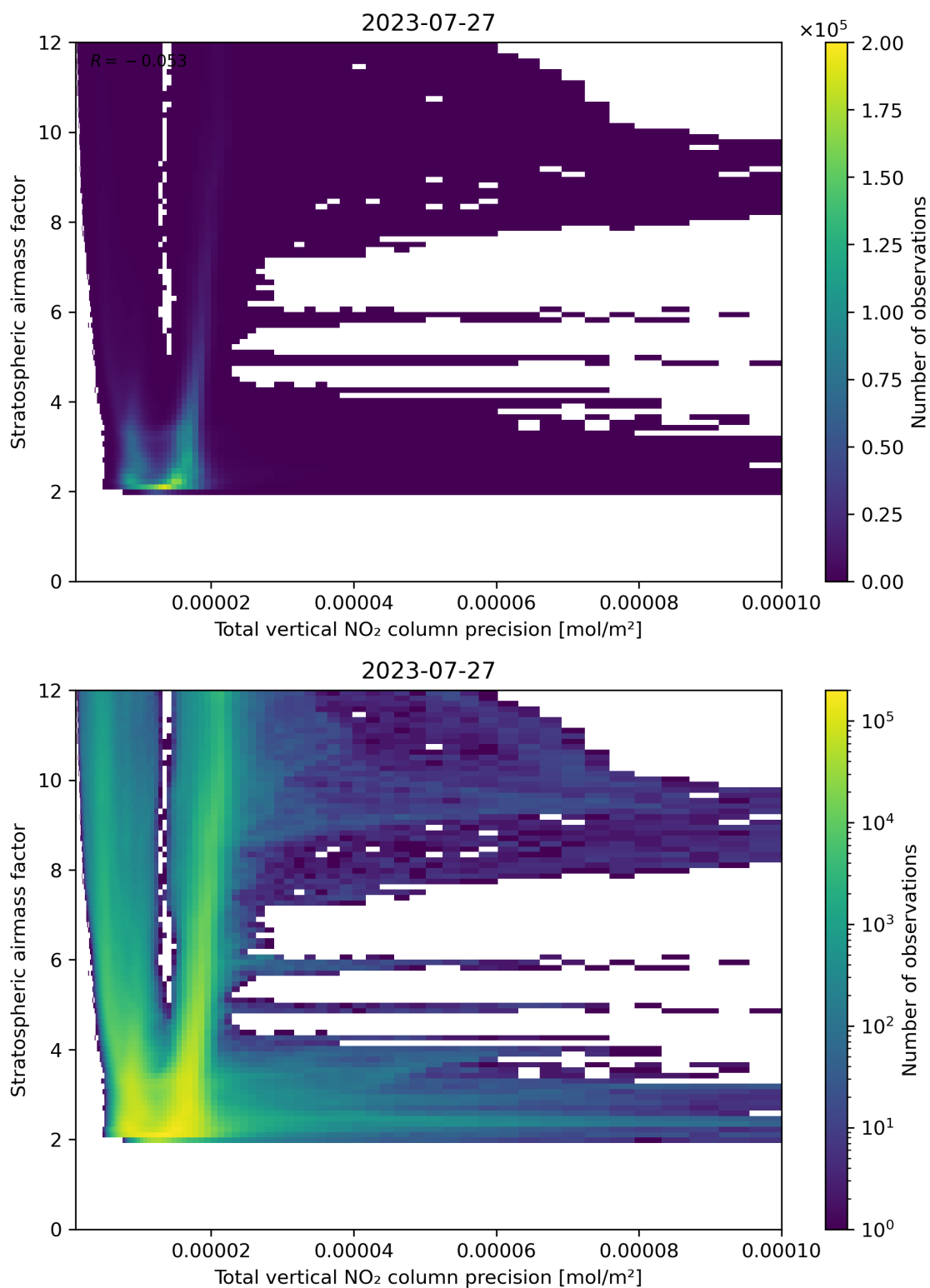
Figure 115: Scatter density plot of “Total vertical NO 2 column precision” against “Stratospheric air mass factor” for 2023-07-26 to 2023-07-28.
