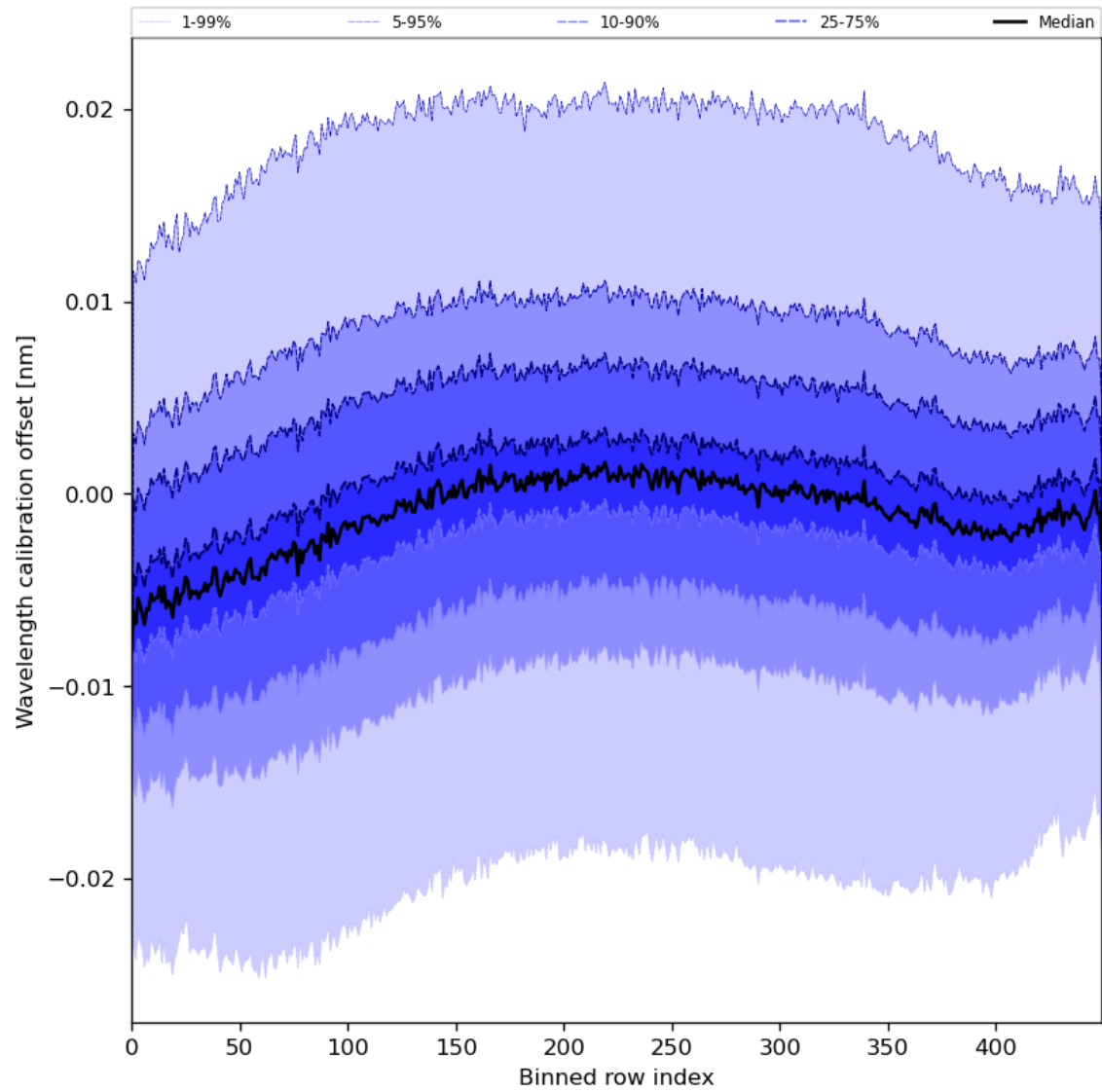
Figure 52: Along track statistics of “Wavelength calibration offset” for 2023-07-26 to 2023-07-28
