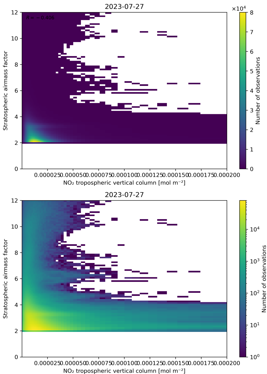
Figure 121: Scatter density plot of “NO 2 tropospheric vertical column” against “Stratospheric air mass factor” for 2023-07-26 to 2023-07-28.
