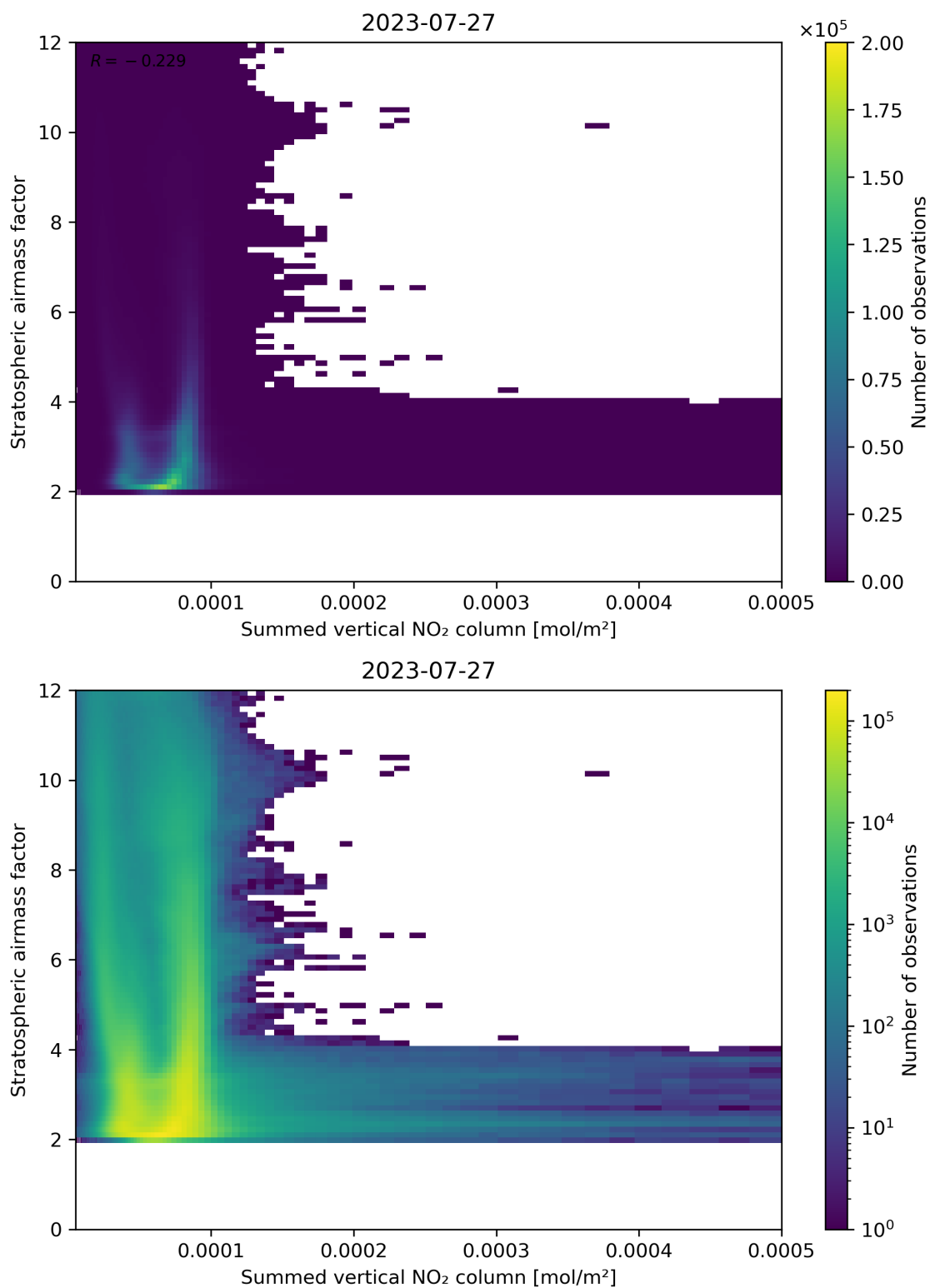
Figure 103: Scatter density plot of “Summed vertical NO 2 column” against “Stratospheric air mass factor” for 2023-07-26 to 2023-07-28.
