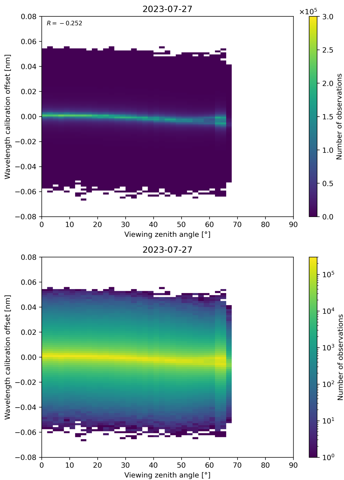
Figure 173: Scatter density plot of “Viewing zenith angle” against “Wavelength calibration offset” for 2023-07-26 to 2023-07-28.
