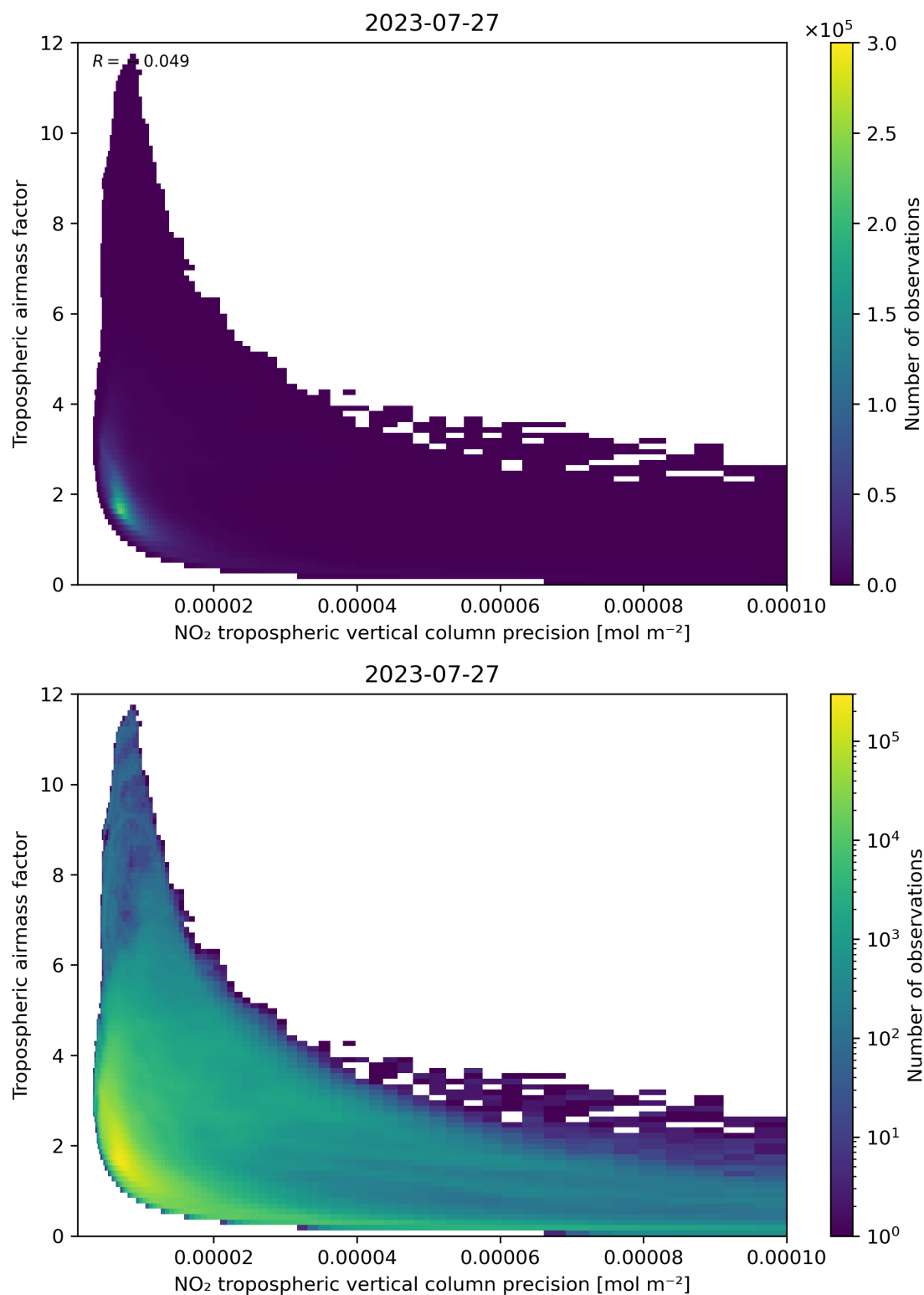
Figure 133: Scatter density plot of “NO 2 tropospheric vertical column precision” against “Tropospheric airmass factor” for 2023-07-26 to 2023-07-28.
