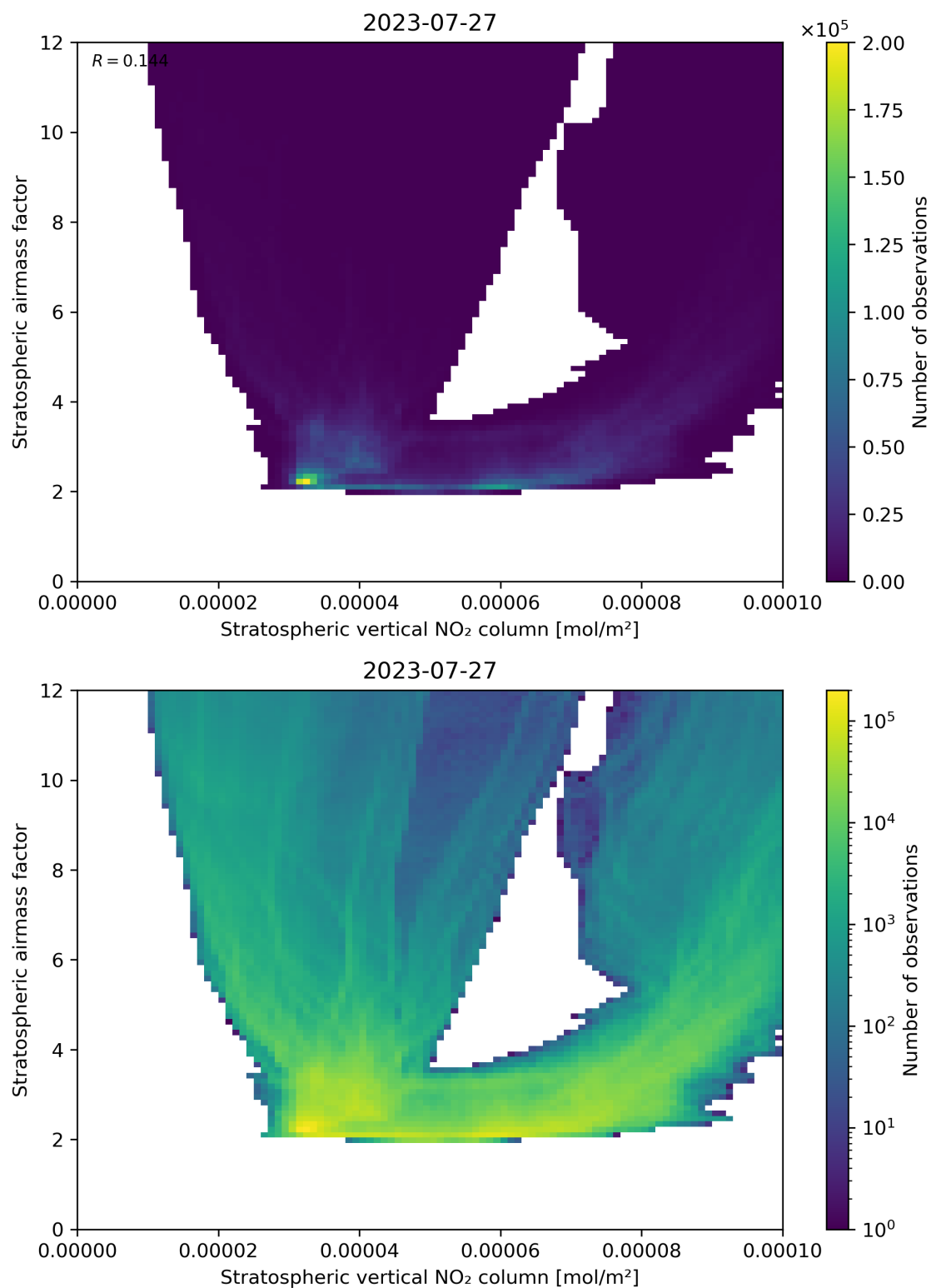
Figure 96: Scatter density plot of “Stratospheric vertical NO 2 column” against “Stratospheric airmass factor” for 2023-07-26 to 2023-07-28.
