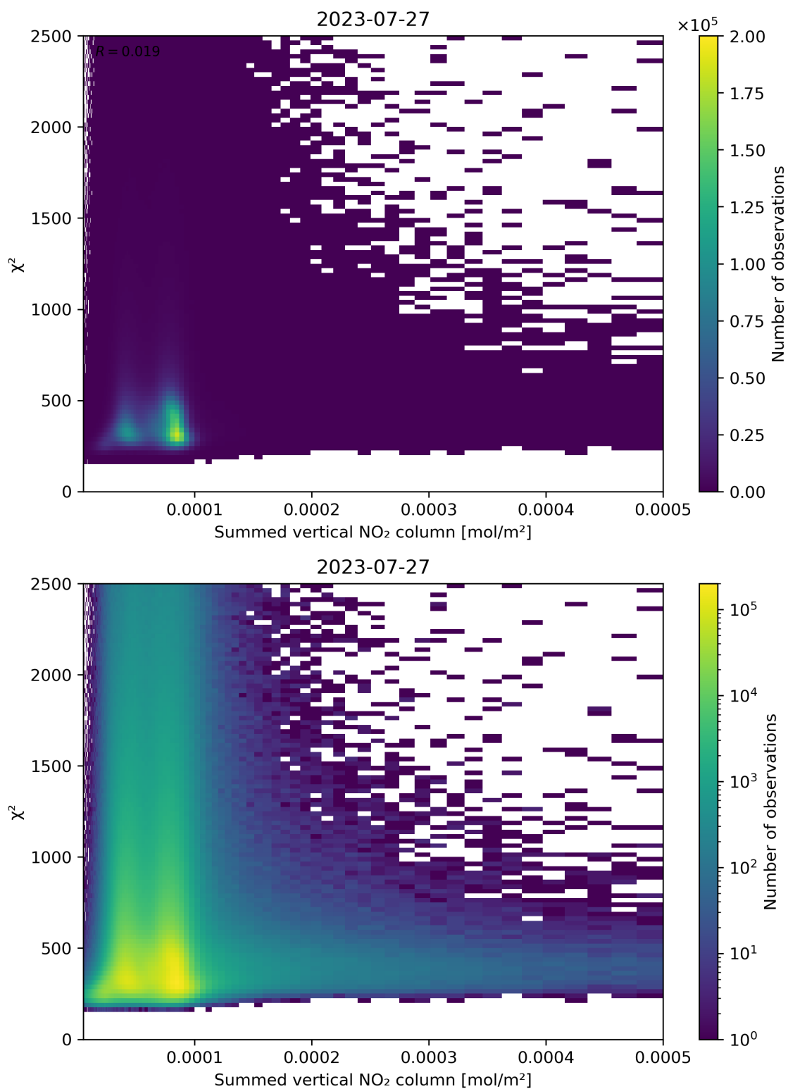
Figure 104: Scatter density plot of “Summed vertical NO 2 column” against “ \chi^2 ” for 2023-07-26 to 2023-07-28.
