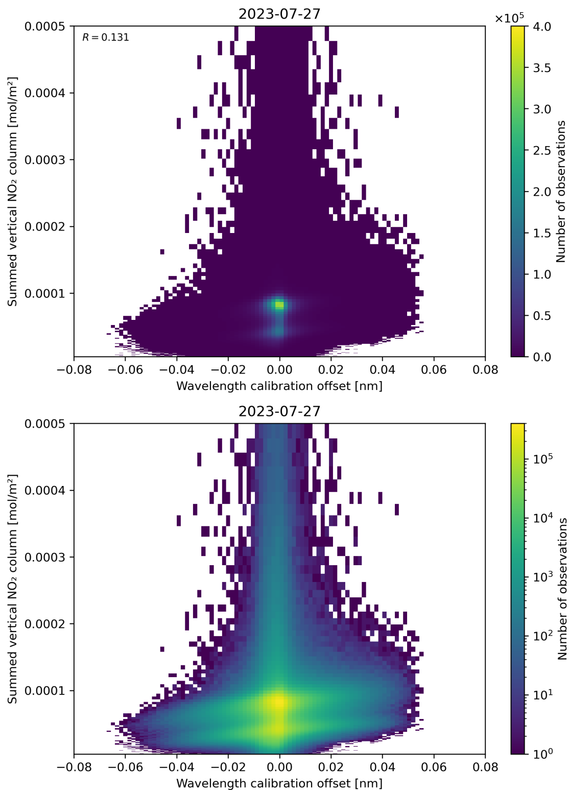
Figure 177: Scatter density plot of “Wavelength calibration offset” against “Summed vertical NO 2 column” for 2023-07-26 to 2023-07-28.
