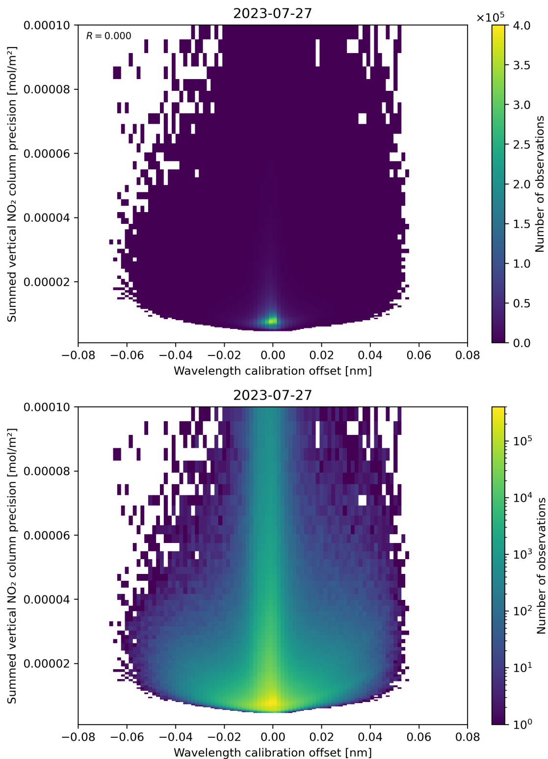
Figure 178: Scatter density plot of “Wavelength calibration offset” against “Summed vertical NO 2 column precision” for 2023-07-26 to 2023-07-28.
