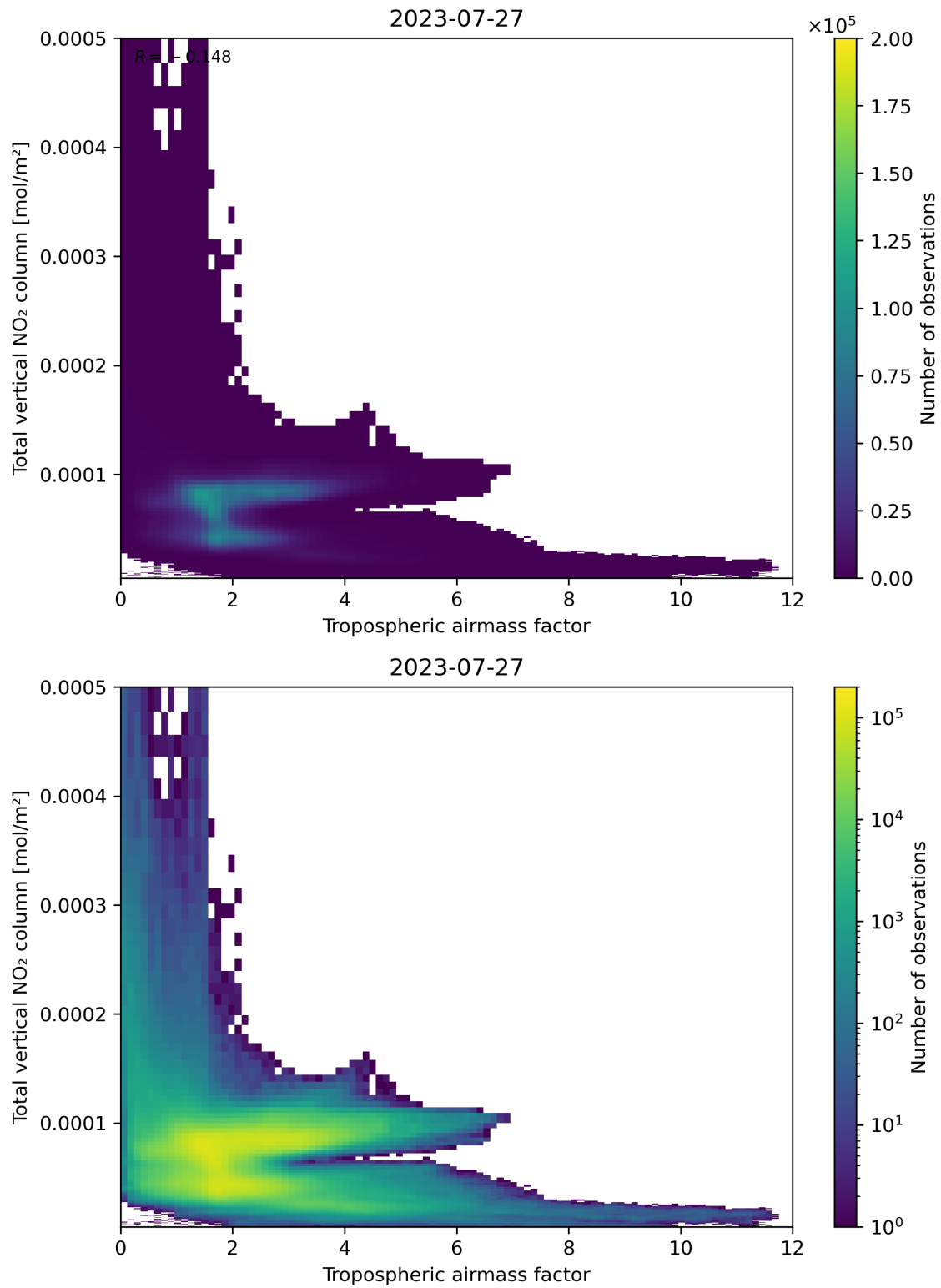
Figure 77: Scatter density plot of “Tropospheric airmass factor” against “Total vertical NO 2 column” for 2023-07-26 to 2023-07-28.
