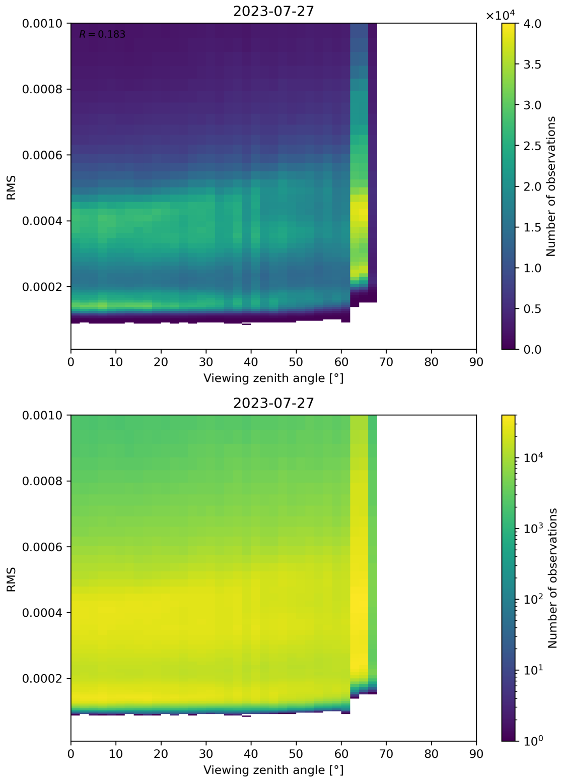
Figure 171: Scatter density plot of “Viewing zenith angle” against “RMS” for 2023-07-26 to 2023-07-28.
