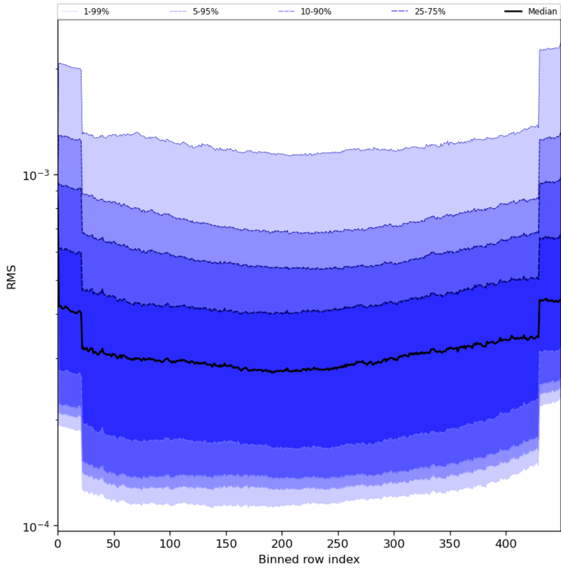
Figure 60: Along track statistics of “RMS” for 2023-07-26 to 2023-07-28
