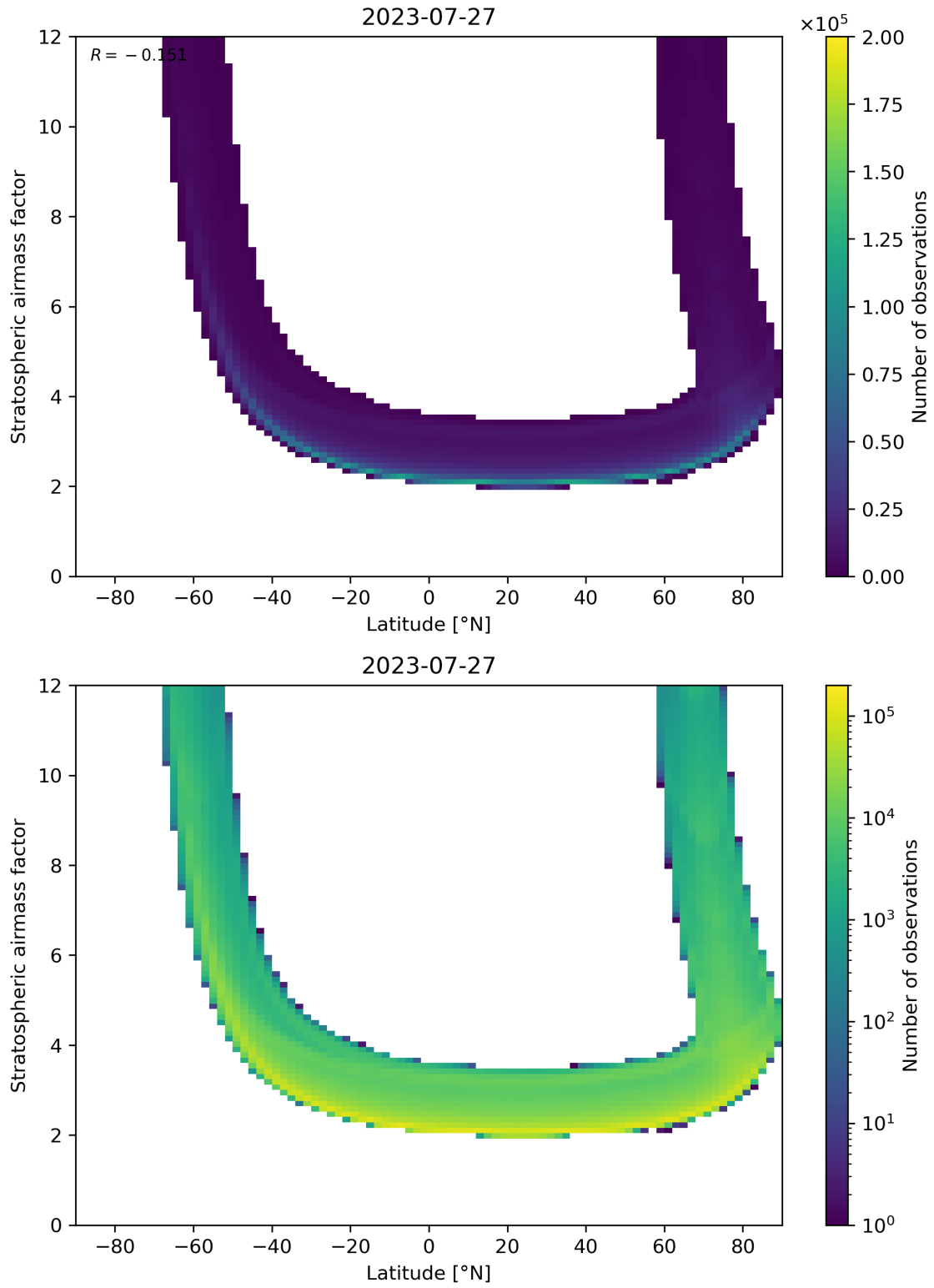
Figure 83: Scatter density plot of “Latitude” against “Stratospheric air mass factor” for 2023-07-26 to 2023-07-28.
