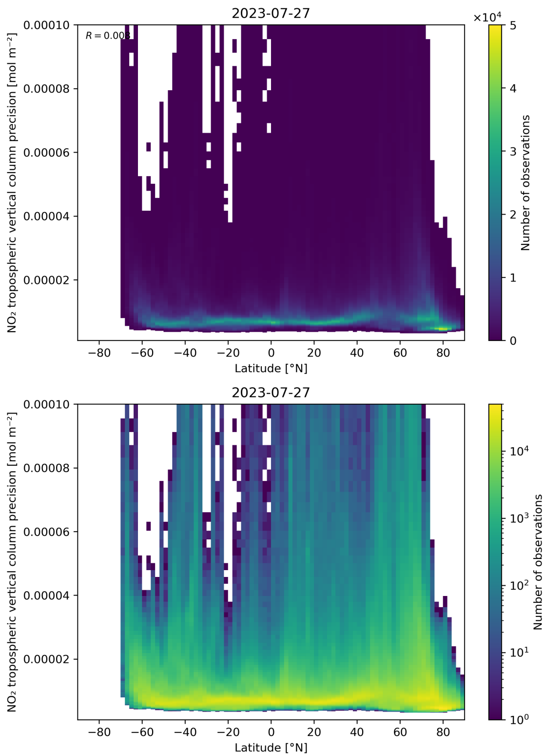
Figure 93: Scatter density plot of “Latitude” against “NO 2 tropospheric vertical column precision” for 2023-07-26 to 2023-07-28.
