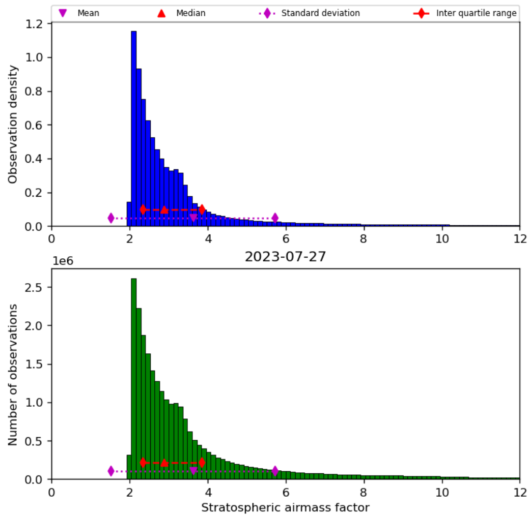
Figure 44: Histogram of “Stratospheric airmass factor” for 2023-07-26 to 2023-07-28
