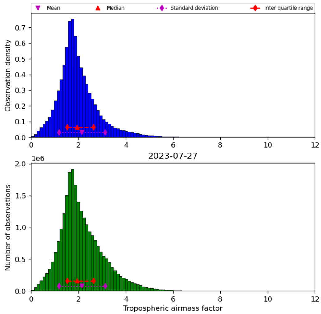
Figure 31: Histogram of “Tropospheric airmass factor” for 2023-07-26 to 2023-07-28
