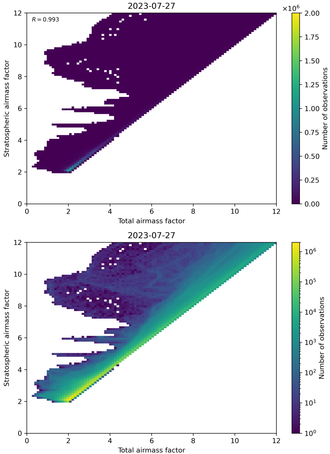
Figure 62: Scatter density plot of “Total air mass factor” against “Stratospheric air mass factor” for 2023-07-26 to 2023-07-28.
