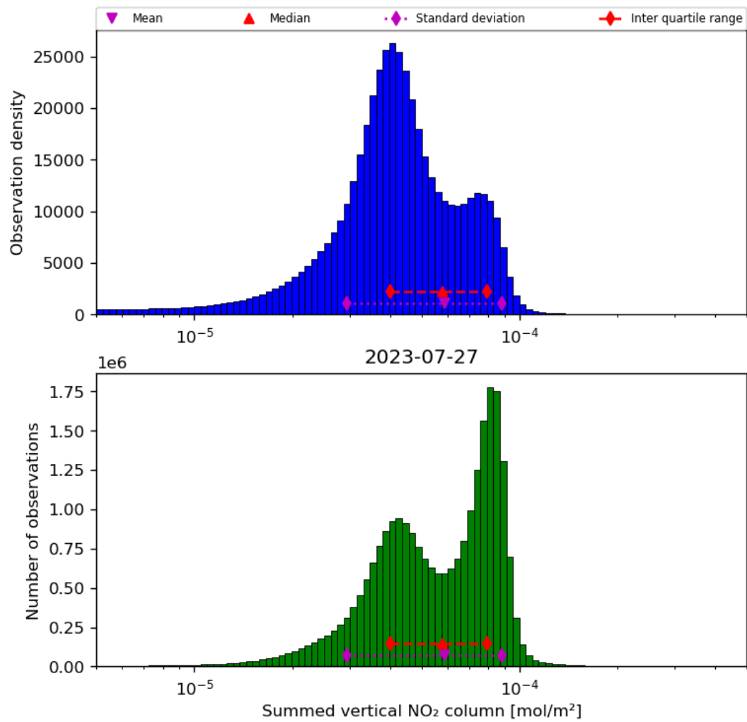
Figure 40: Histogram of “Summed vertical NO 2 column” for 2023-07-26 to 2023-07-28
