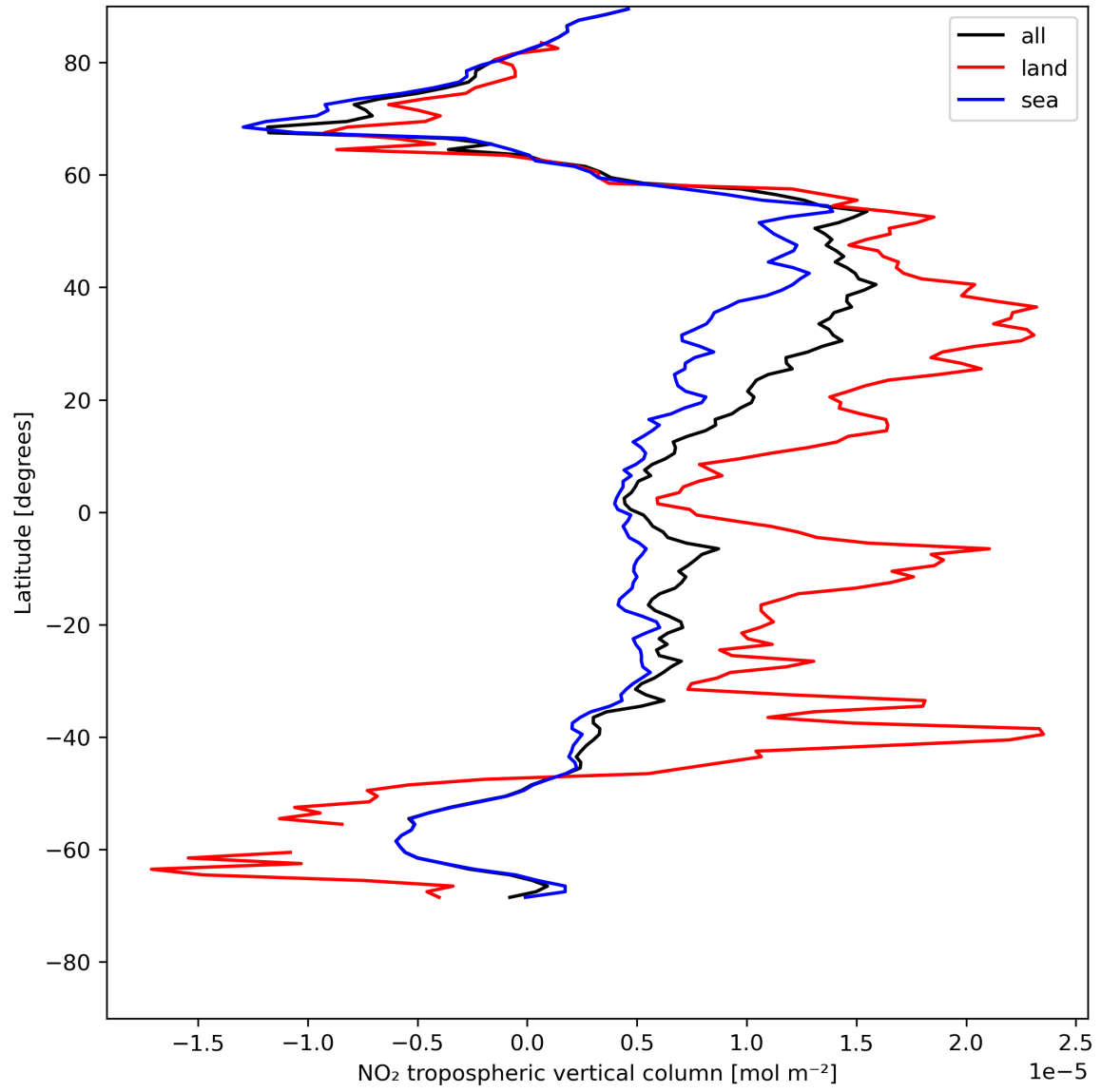
Figure 12: Zonal average of “NO 2 tropospheric vertical column” for 2023-07-26 to 2023-07-28.
