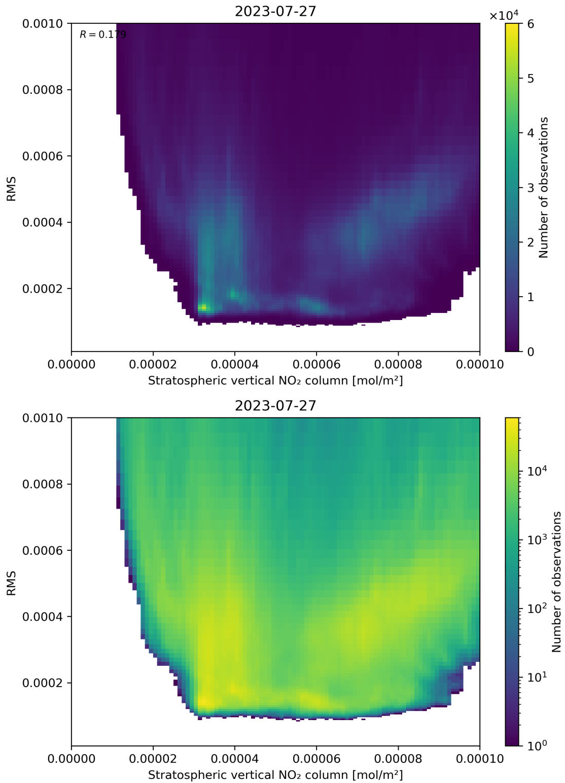
Figure 102: Scatter density plot of “Stratospheric vertical NO 2 column” against “RMS” for 2023-07-26 to 2023-07-28.
