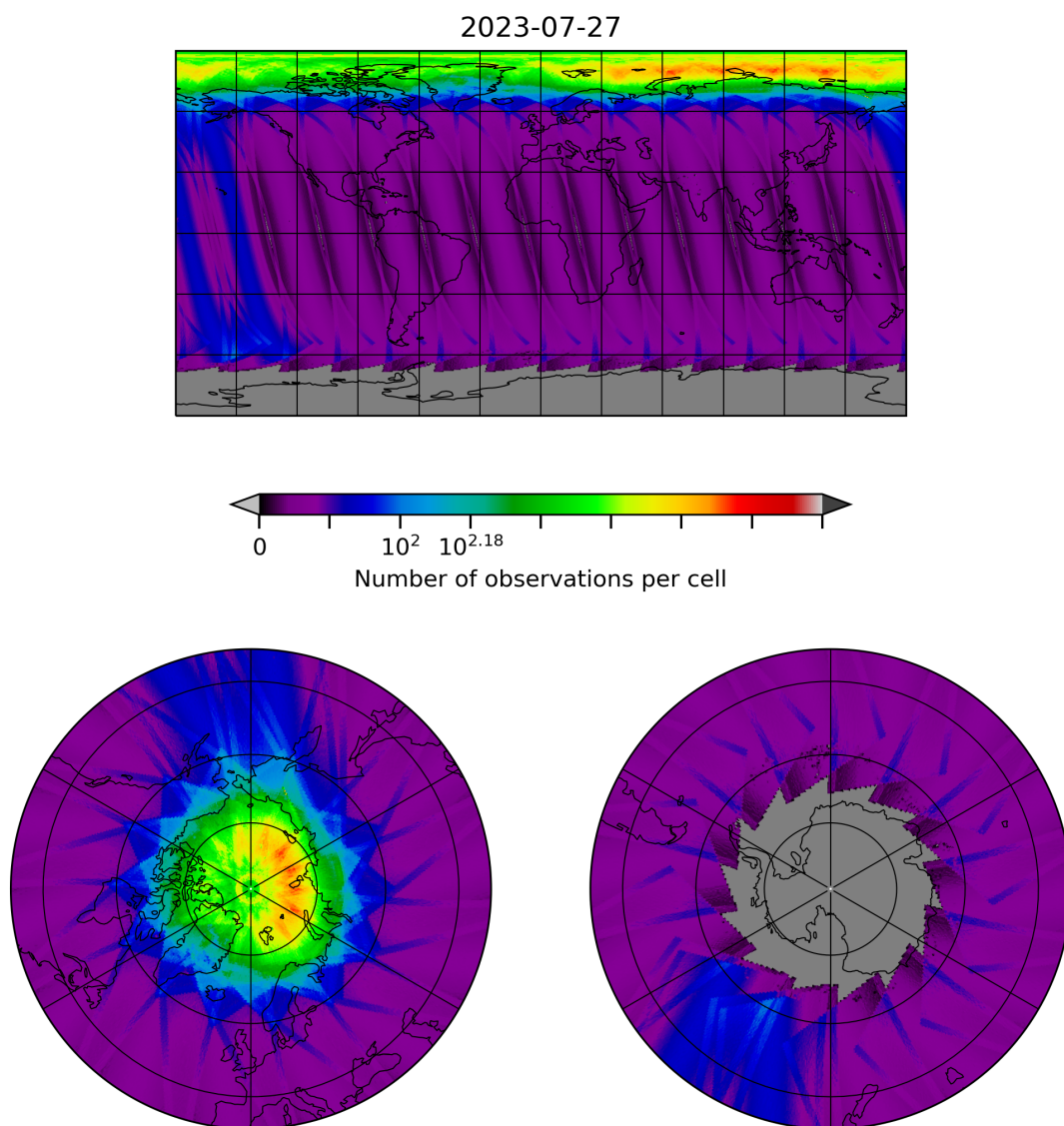
Figure 10: Map of the number of observations for 2023-07-26 to 2023-07-28
