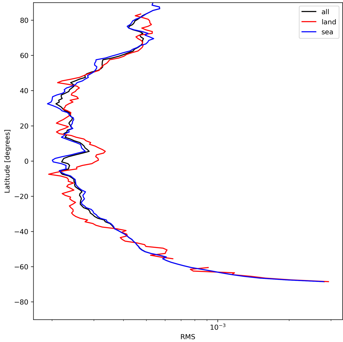
Figure 26: Zonal average of “RMS” for 2023-07-26 to 2023-07-28.
