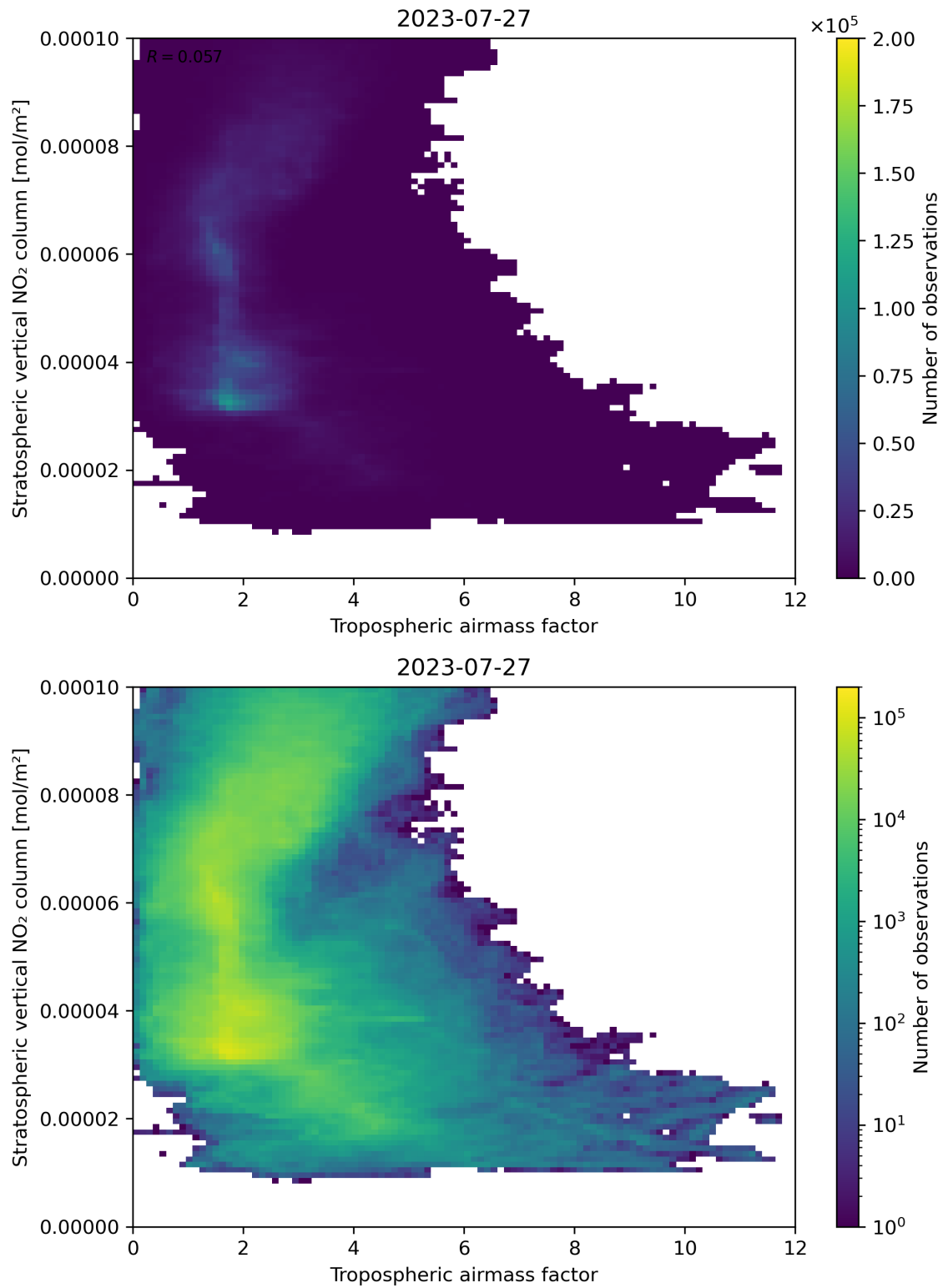
Figure 74: Scatter density plot of “Tropospheric air mass factor” against “Stratospheric vertical NO 2 column” for 2023-07-26 to 2023-07-28.
