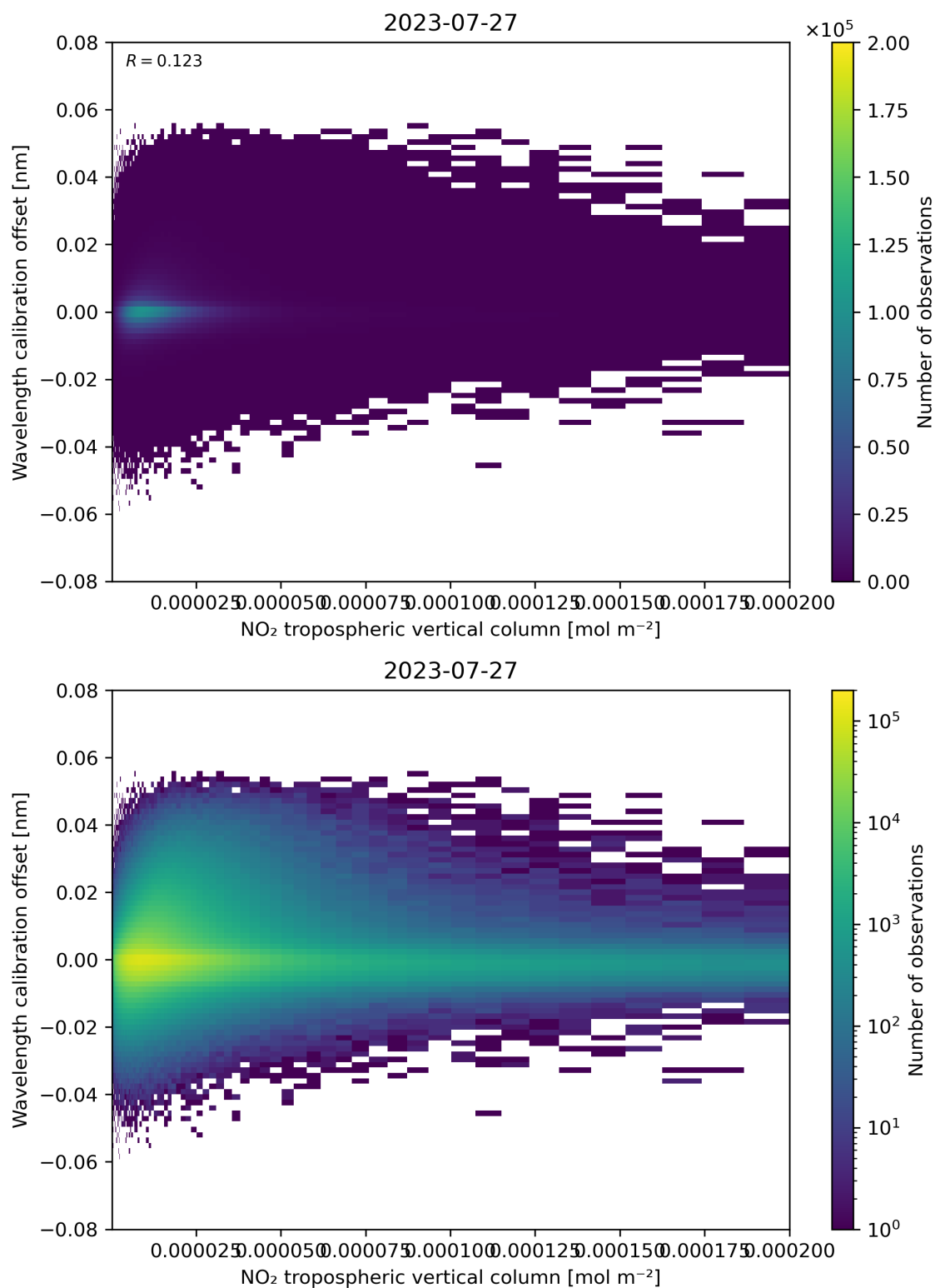
Figure 143: Scatter density plot of “NO 2 tropospheric vertical column” against “Wavelength calibration offset” for 2023-07-26 to 2023-07-28.
