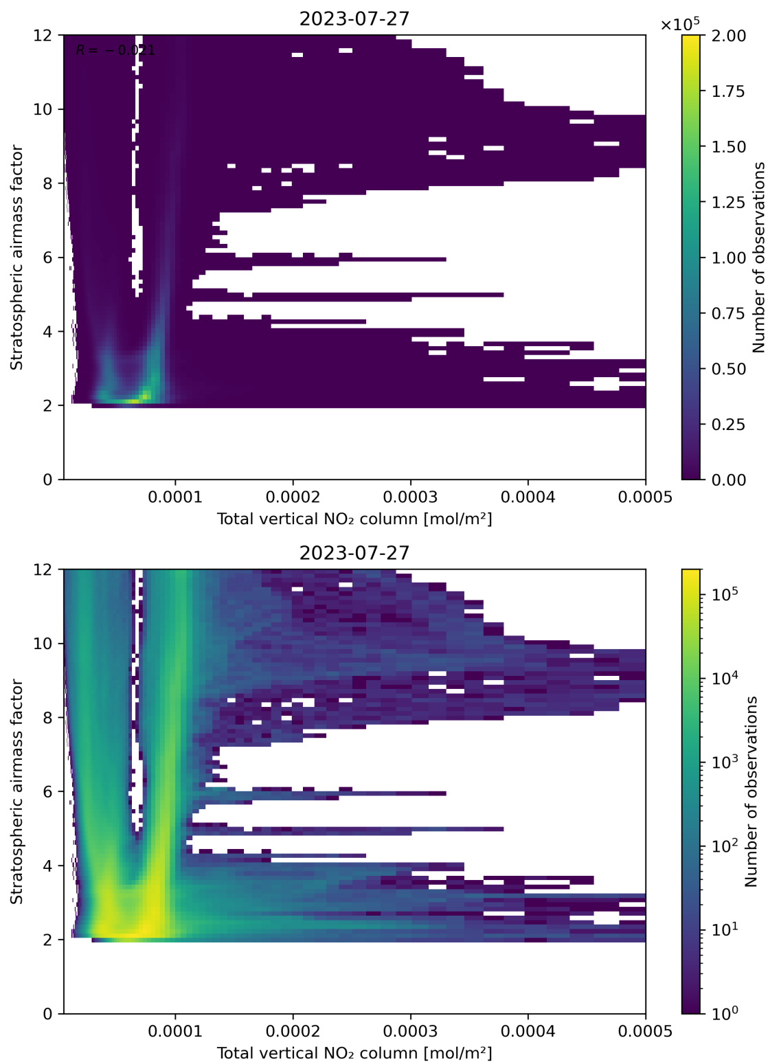
Figure 110: Scatter density plot of “Total vertical NO 2 column” against “Stratospheric airmass factor” for 2023-07-26 to 2023-07-28.
