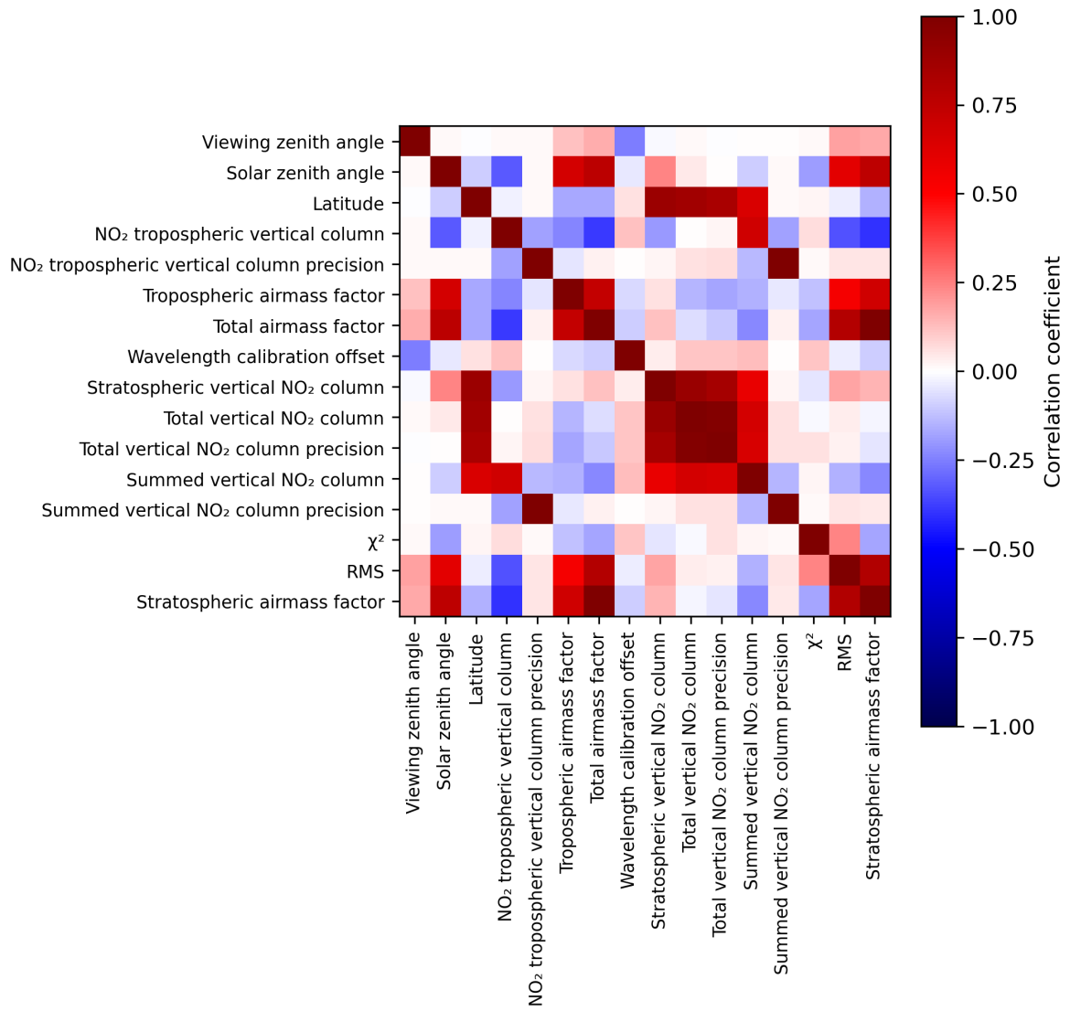
Figure 2: Map of correlation matrix for 2023-07-26 to 2023-07-28.
