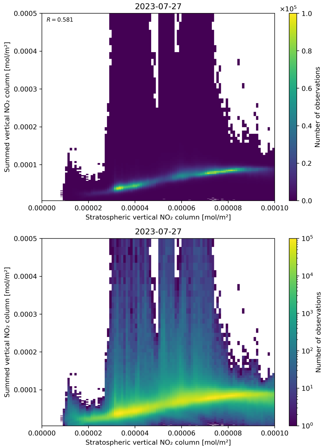
Figure 98: Scatter density plot of “Stratospheric vertical NO 2 column” against “Summed vertical NO 2 column” for 2023-07-26 to 2023-07-28.
