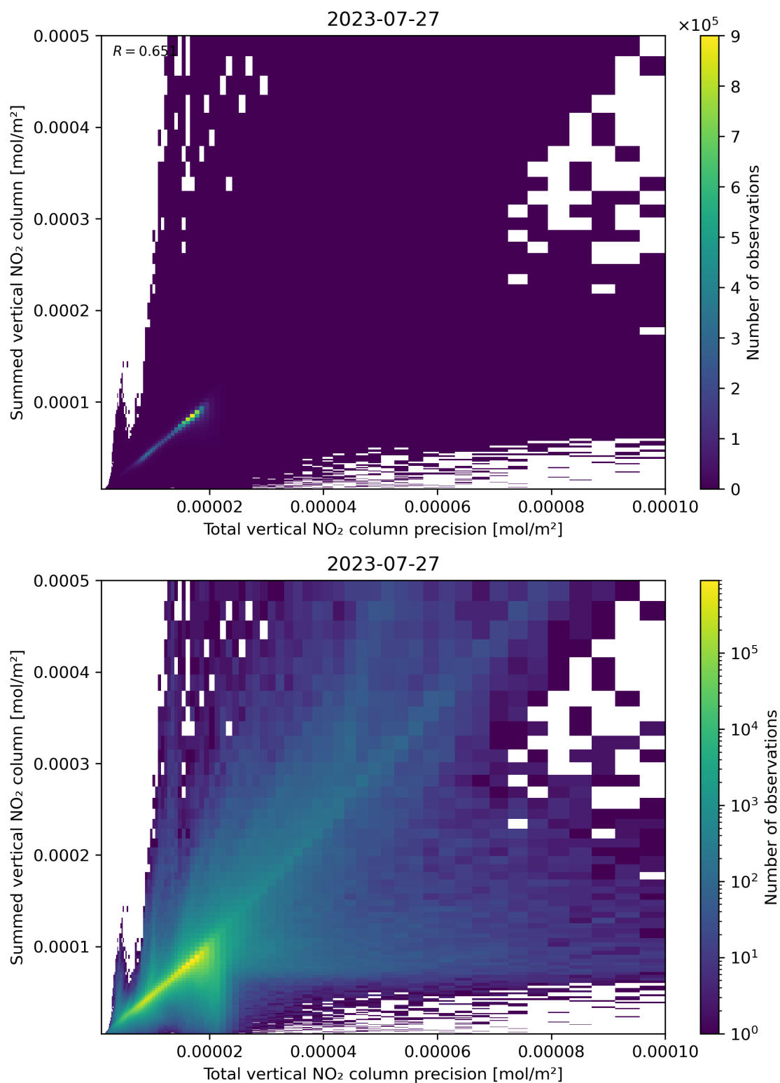
Figure 117: Scatter density plot of “Total vertical NO 2 column precision” against “Summed vertical NO 2 column” for 2023-07-26 to 2023-07-28.
