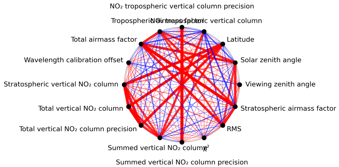
Figure 1: Map of correlation graph for 2023-07-26 to 2023-07-28.
