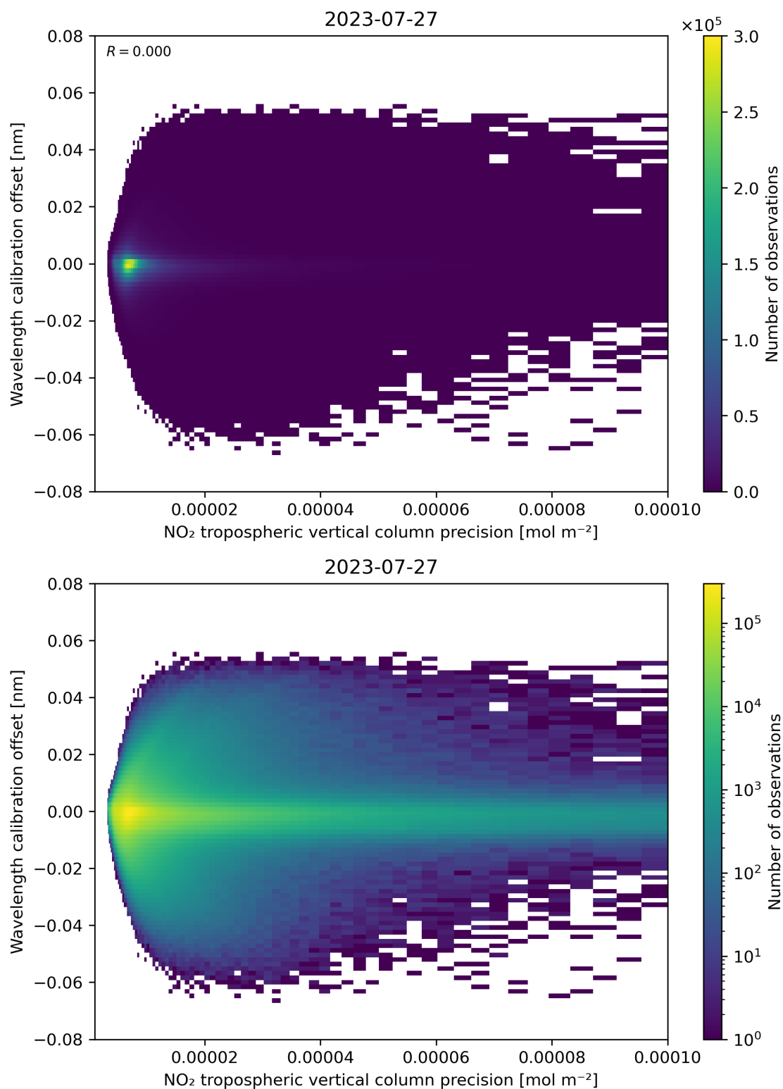
Figure 141: Scatter density plot of “NO 2 tropospheric vertical column precision” against “Wavelength calibration offset” for 2023-07-26 to 2023-07-28.
