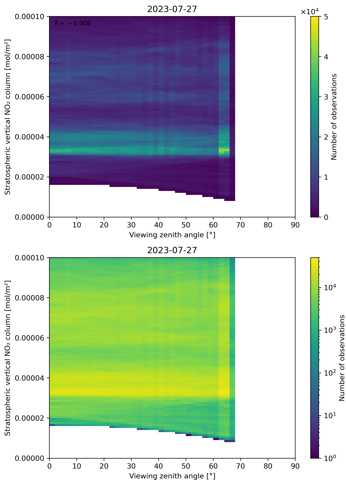
Figure 164: Scatter density plot of “Viewing zenith angle” against “Stratospheric vertical NO 2 column” for 2023-07-26 to 2023-07-28.
