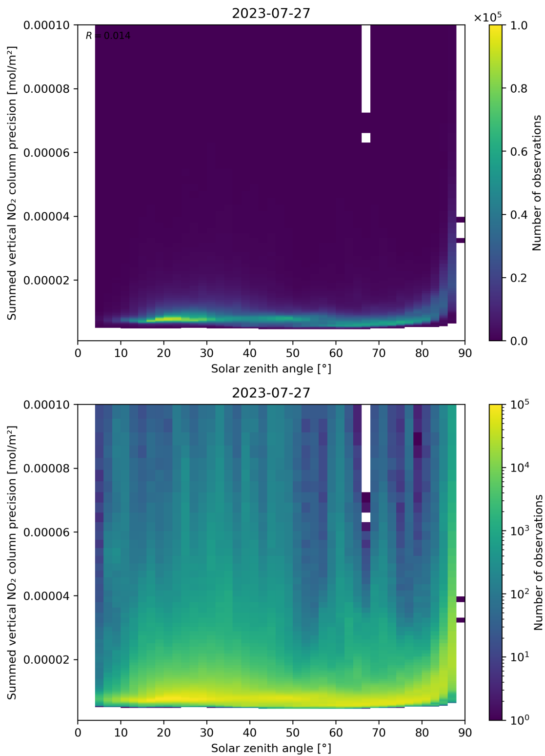
Figure 152: Scatter density plot of “Solar zenith angle” against “Summed vertical NO 2 column precision” for 2023-07-26 to 2023-07-28.
