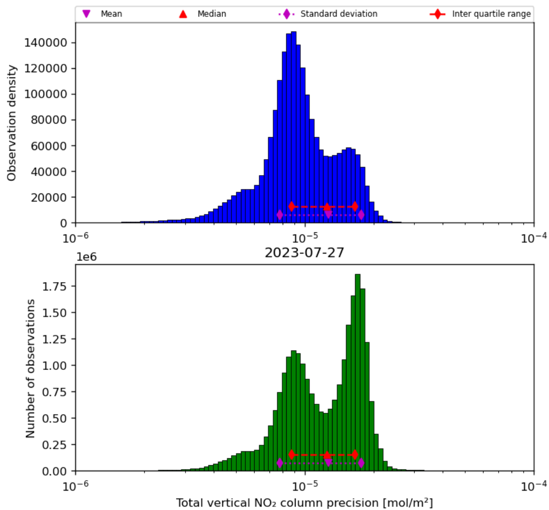
Figure 39: Histogram of "Total vertical NO 2 column precision" for 2023-07-26 to 2023-07-28
