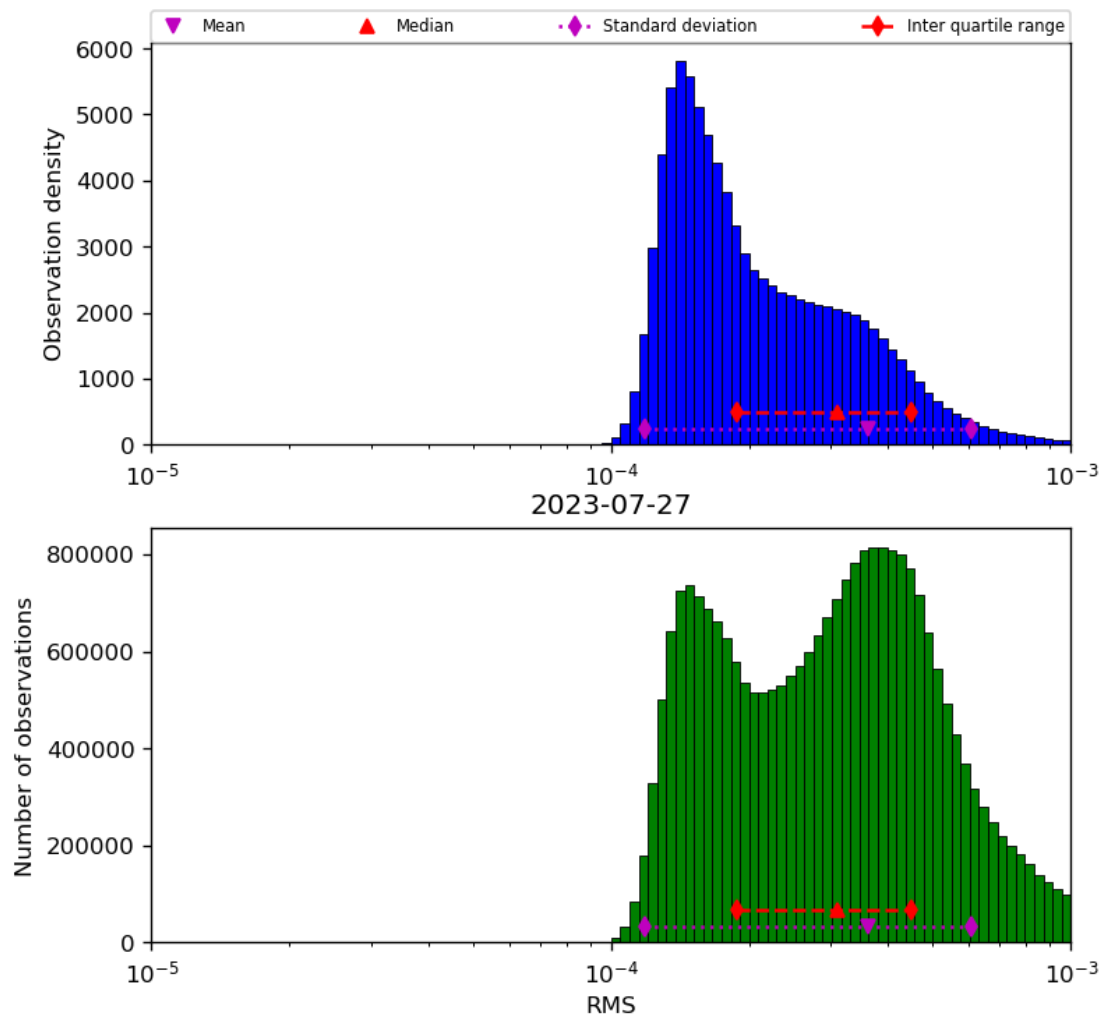
Figure 43: Histogram of “RMS” for 2023-07-26 to 2023-07-28
