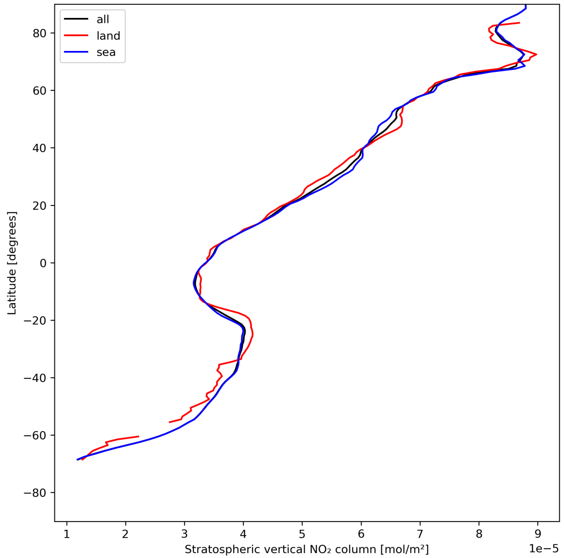
Figure 19: Zonal average of “Stratospheric vertical NO 2 column” for 2023-07-26 to 2023-07-28.
