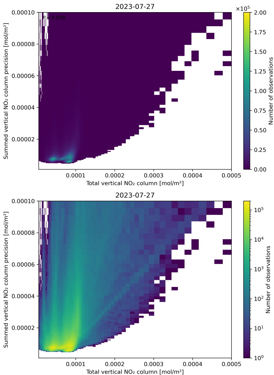
Figure 113: Scatter density plot of “Total vertical NO 2 column” against “Summed vertical NO 2 column precision” for 2023-07-26 to 2023-07-28.
