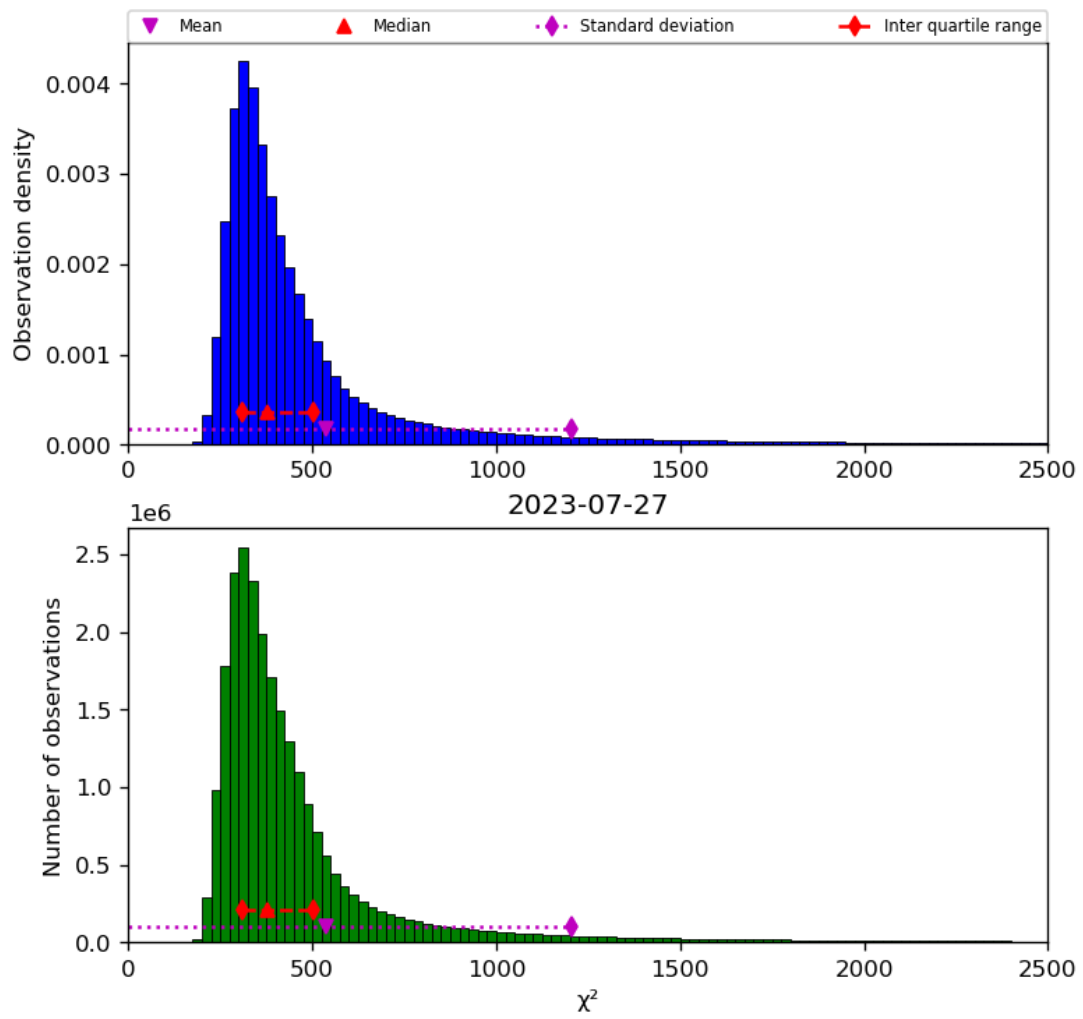
Figure 42: Histogram of “ \chi^2 ” for 2023-07-26 to 2023-07-28
