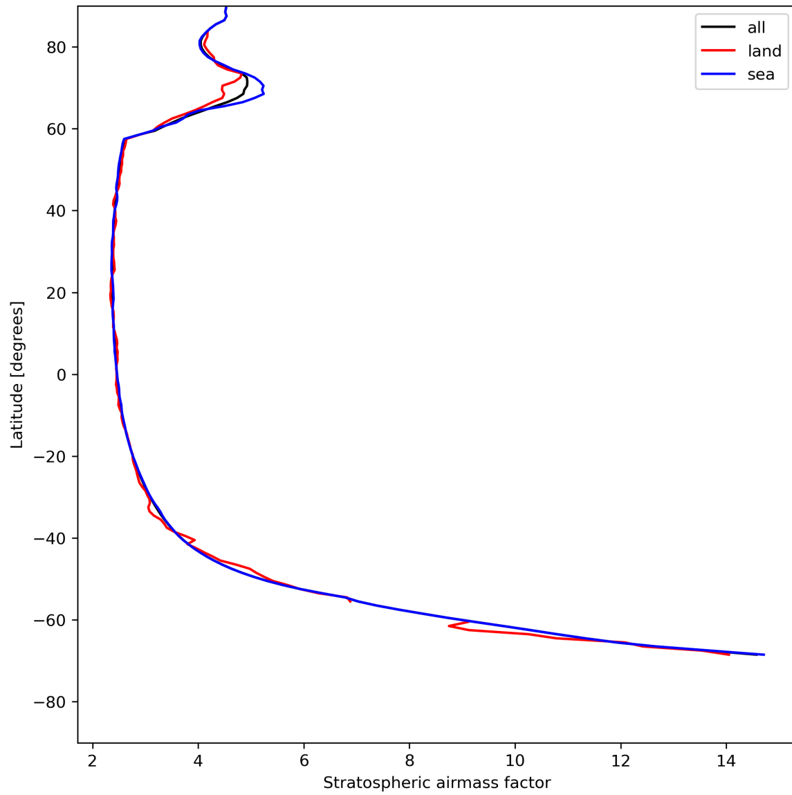
Figure 27: Zonal average of “Stratospheric air mass factor” for 2023-07-27 to 2023-07-29.
