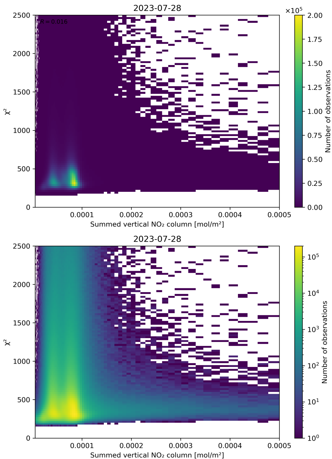
Figure 104: Scatter density plot of “Summed vertical NO 2 column” against “ \chi^2 ” for 2023-07-27 to 2023-07-29.
