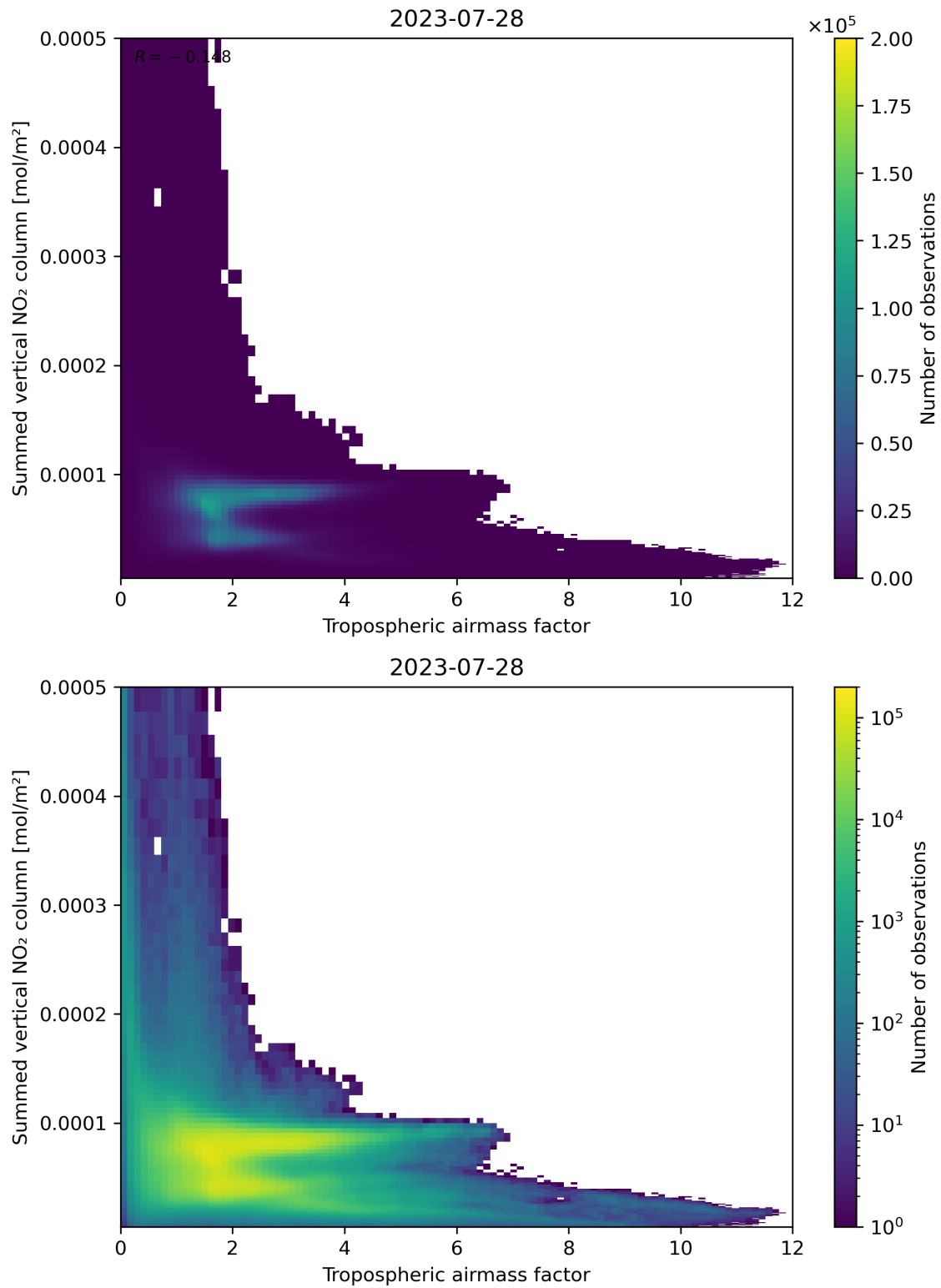
Figure 75: Scatter density plot of “Tropospheric airmass factor” against “Summed vertical NO 2 column” for 2023-07-27 to 2023-07-29.
