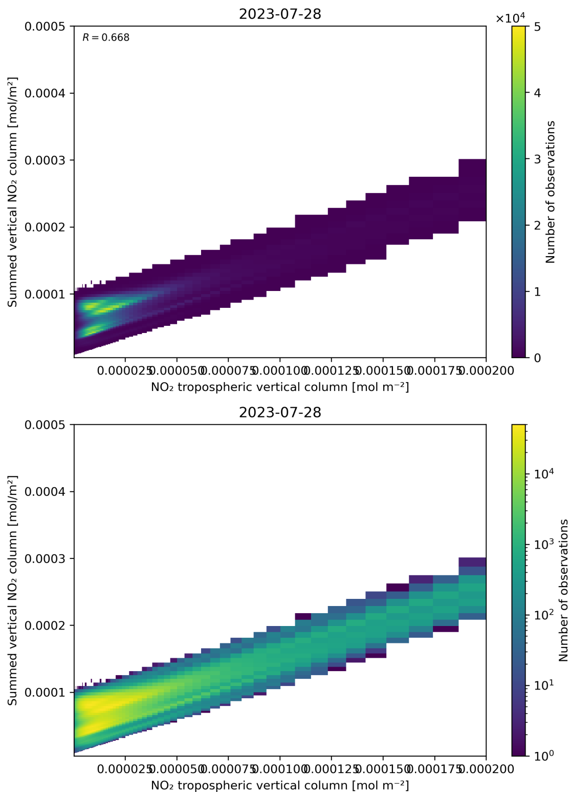
Figure 126: Scatter density plot of “NO 2 tropospheric vertical column” against “Summed vertical NO 2 column” for 2023-07-27 to 2023-07-29.
