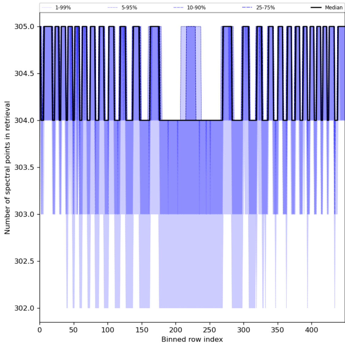
Figure 50: Along track statistics of “Number of spectral points in retrieval” for 2023-07-27 to 2023-07-29
