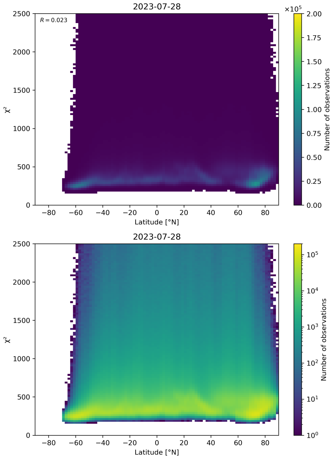
Figure 86: Scatter density plot of “Latitude” against “ \chi^2 ” for 2023-07-27 to 2023-07-29.
