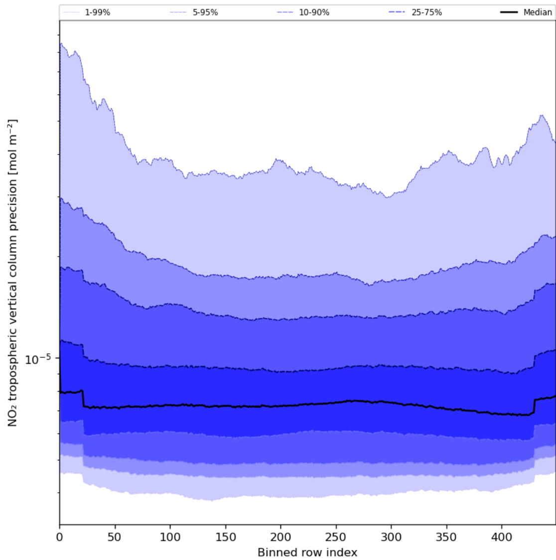
Figure 47: Along track statistics of “NO 2 tropospheric vertical column precision” for 2023-07-27 to 2023-07-29
