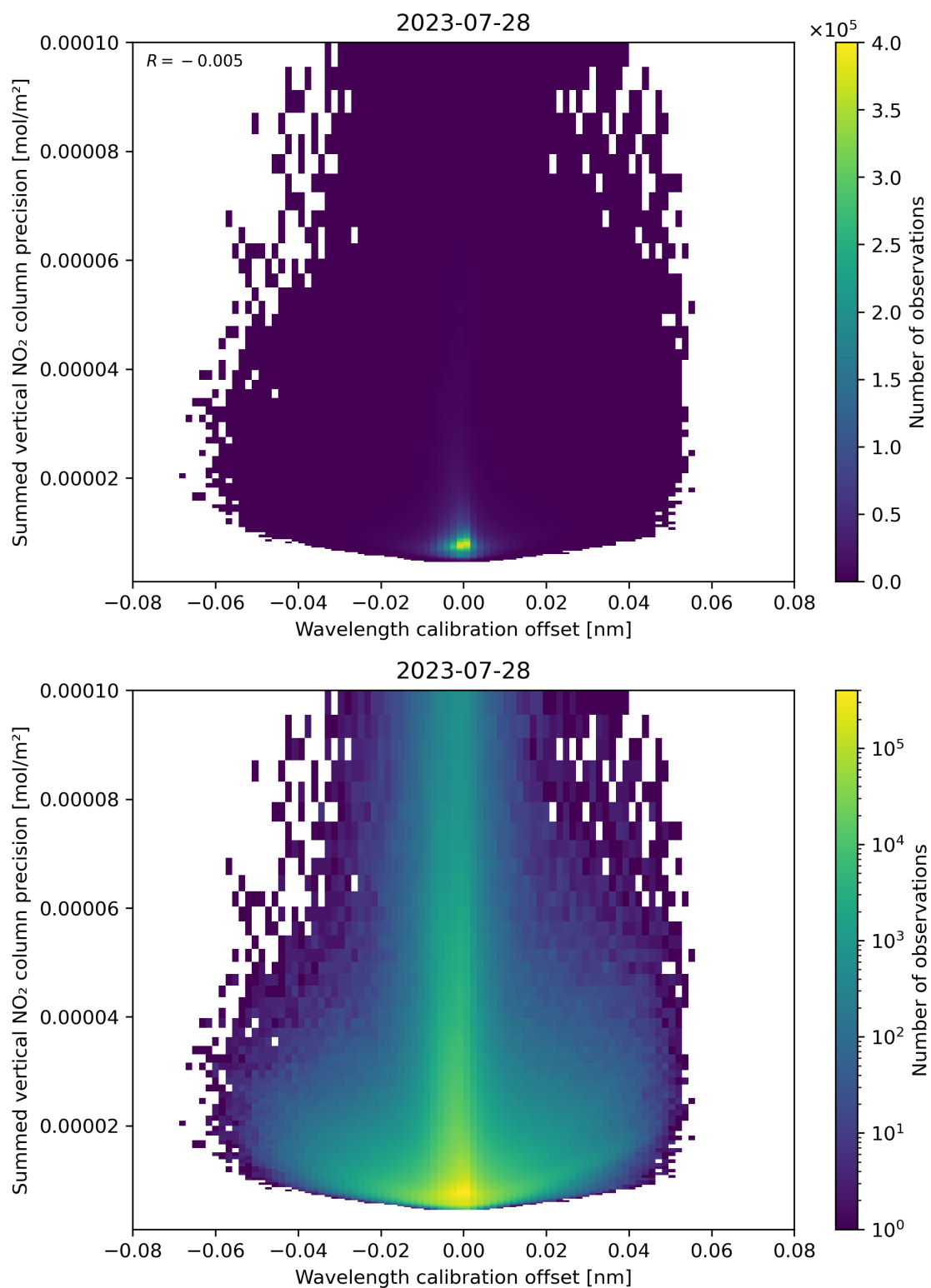
Figure 178: Scatter density plot of “Wavelength calibration offset” against “Summed vertical NO 2 column precision” for 2023-07-27 to 2023-07-29.
