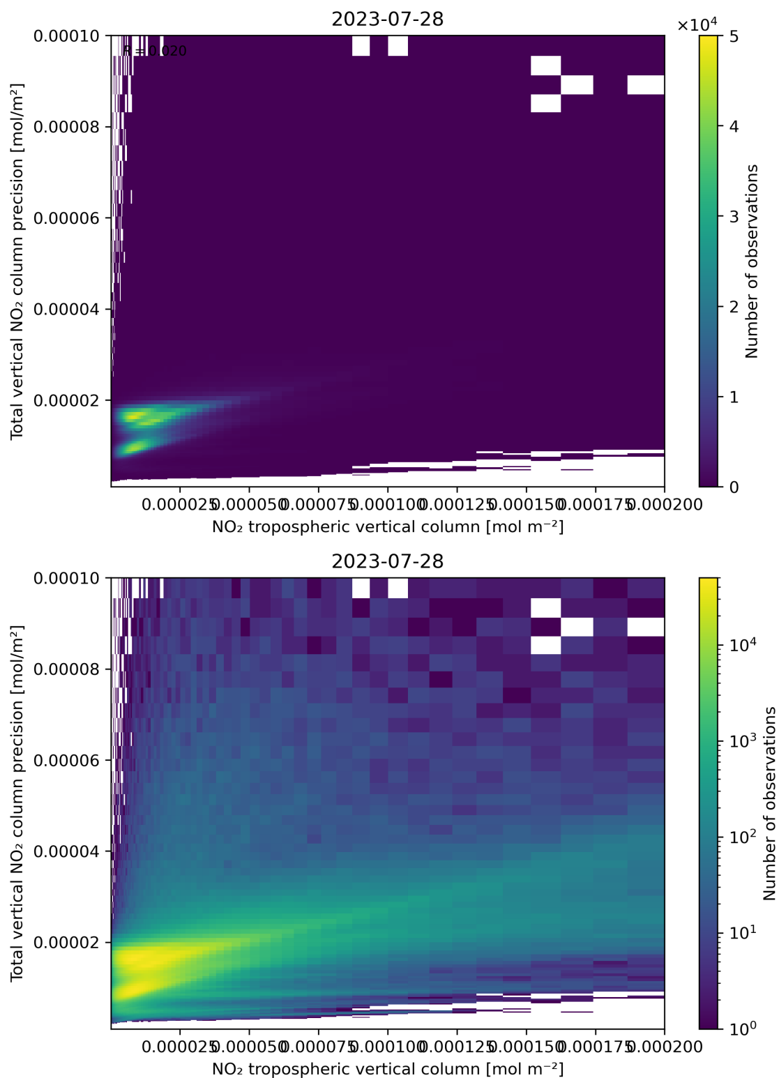
Figure 129: Scatter density plot of “NO 2 tropospheric vertical column” against “Total vertical NO 2 column precision” for 2023-07-27 to 2023-07-29.
