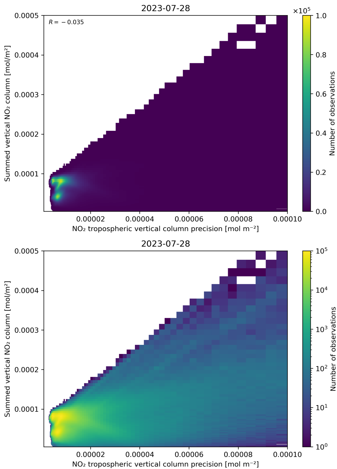
Figure 136: Scatter density plot of “NO 2 tropospheric vertical column precision” against “Summed vertical NO 2 column” for 2023-07-27 to 2023-07-29.
