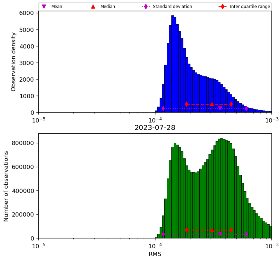
Figure 43: Histogram of “RMS” for 2023-07-27 to 2023-07-29
