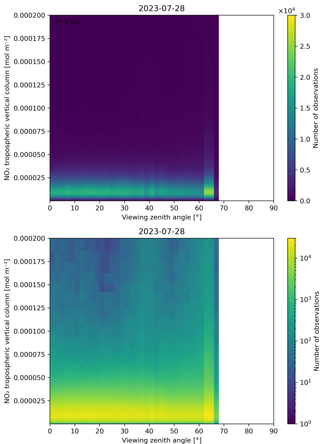
Figure 169: Scatter density plot of “Viewing zenith angle” against “NO 2 tropospheric vertical column” for 2023-07-27 to 2023-07-29.
