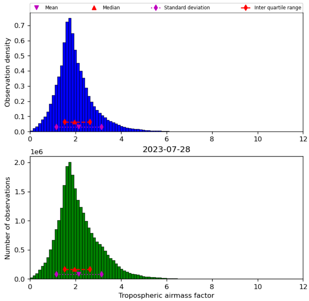
Figure 31: Histogram of “Tropospheric airmass factor” for 2023-07-27 to 2023-07-29
