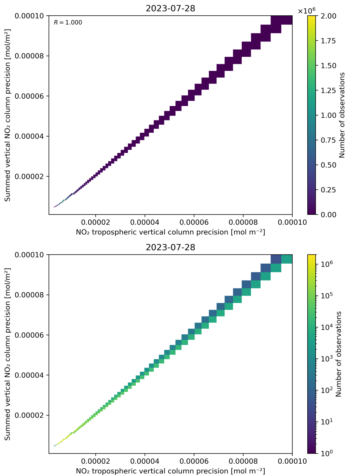
Figure 137: Scatter density plot of “NO 2 tropospheric vertical column precision” against “Summed vertical NO 2 column precision” for 2023-07-27 to 2023-07-29.
