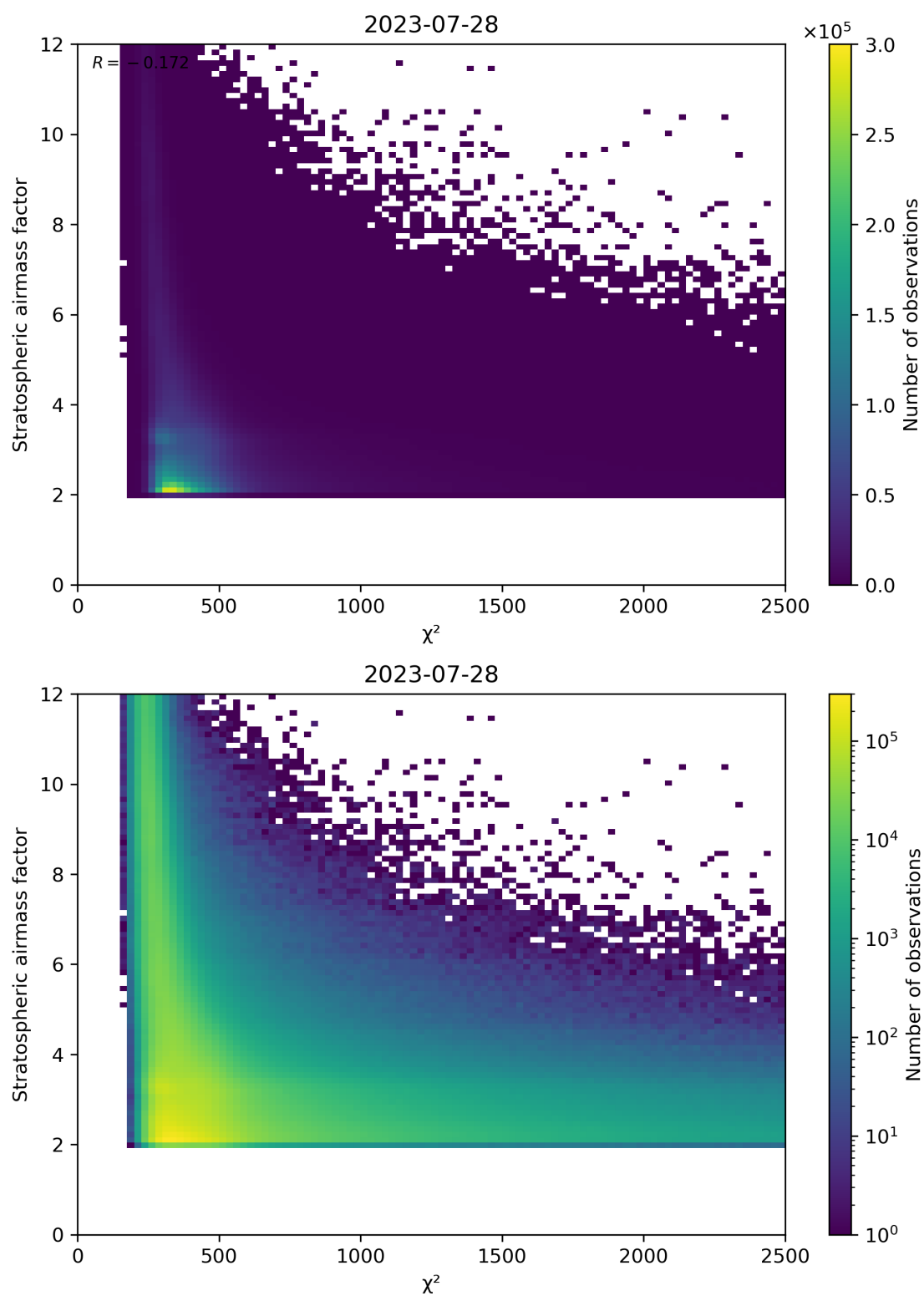
Figure 81: Scatter density plot of “ \chi^2 ” against “Stratospheric airmass factor” for 2023-07-27 to 2023-07-29.
