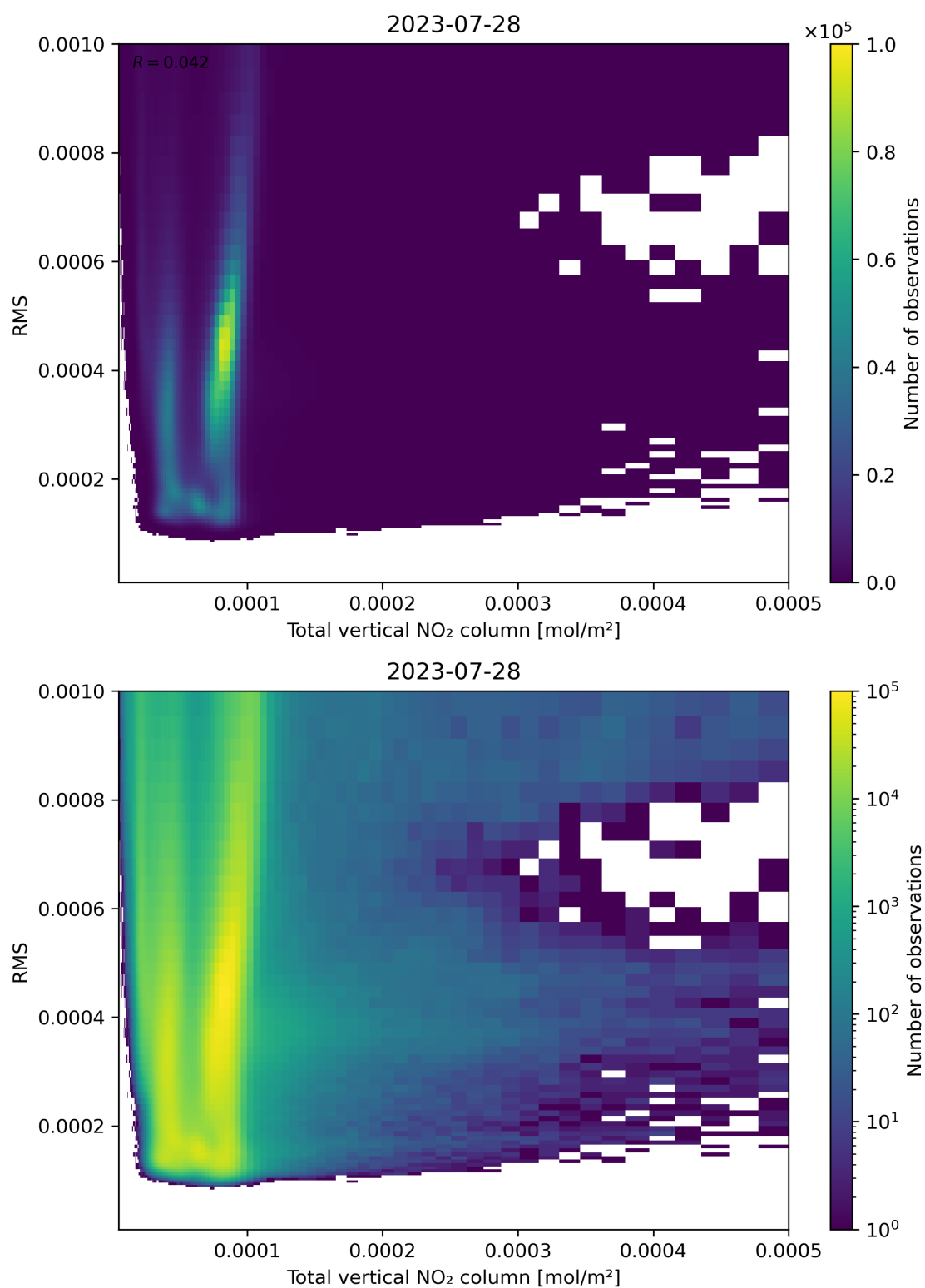
Figure 120: Scatter density plot of “Total vertical NO 2 column” against “RMS” for 2023-07-27 to 2023-07-29.
