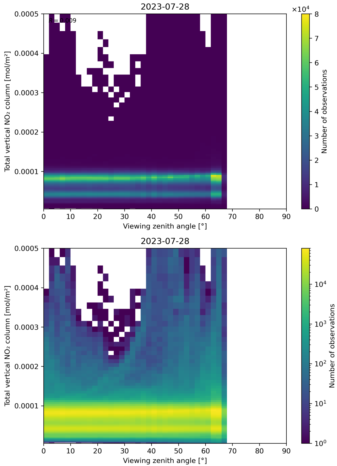
Figure 167: Scatter density plot of “Viewing zenith angle” against “Total vertical NO 2 column” for 2023-07-27 to 2023-07-29.
