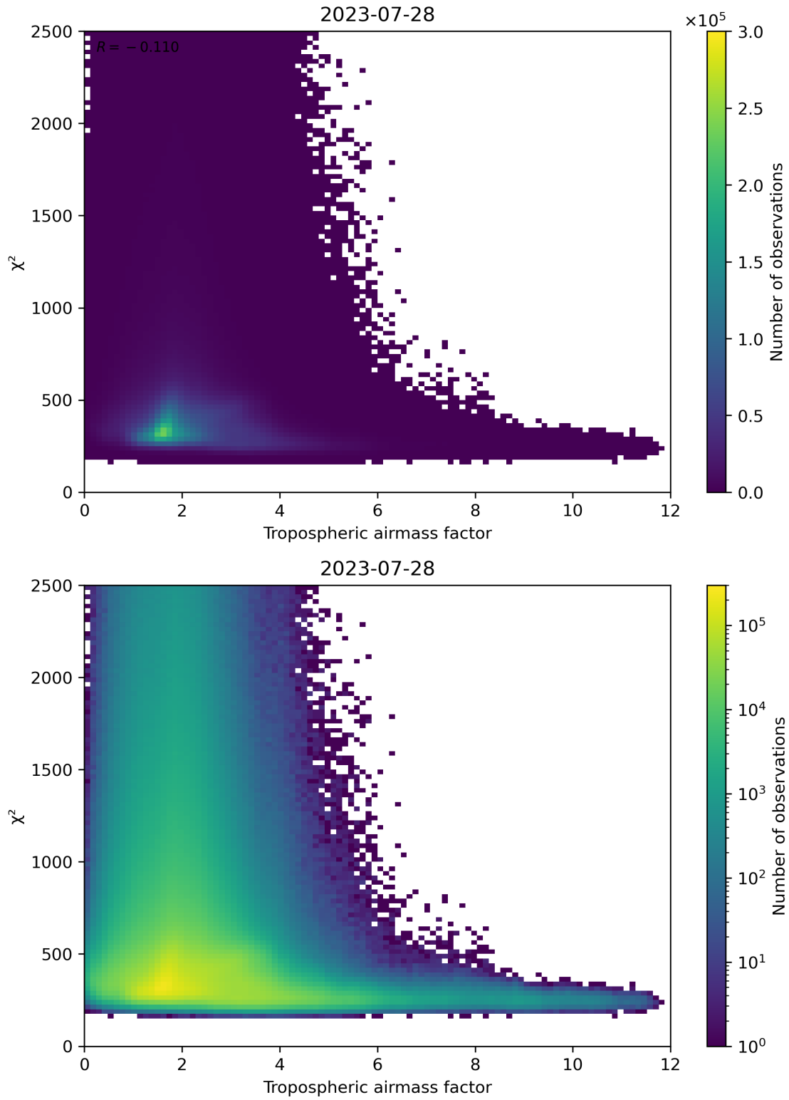
Figure 73: Scatter density plot of “Tropospheric airmass factor” against “ \chi^2 ” for 2023-07-27 to 2023-07-29.
