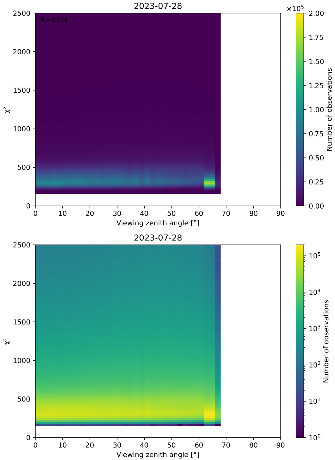
Figure 162: Scatter density plot of “Viewing zenith angle” against “ \chi^2 ” for 2023-07-27 to 2023-07-29.
