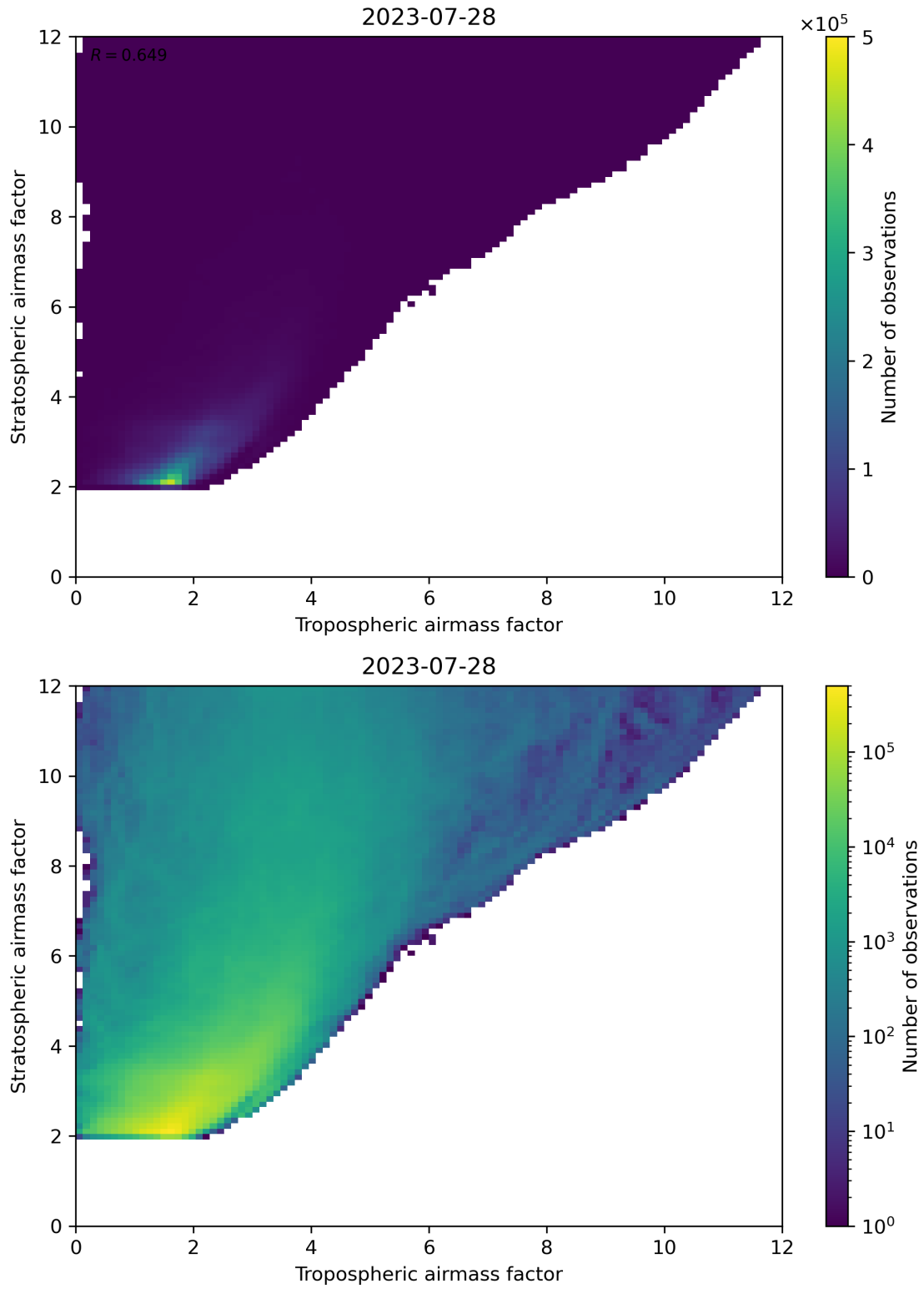
Figure 71: Scatter density plot of “Tropospheric airmass factor” against “Stratospheric airmass factor” for 2023-07-27 to 2023-07-29.
