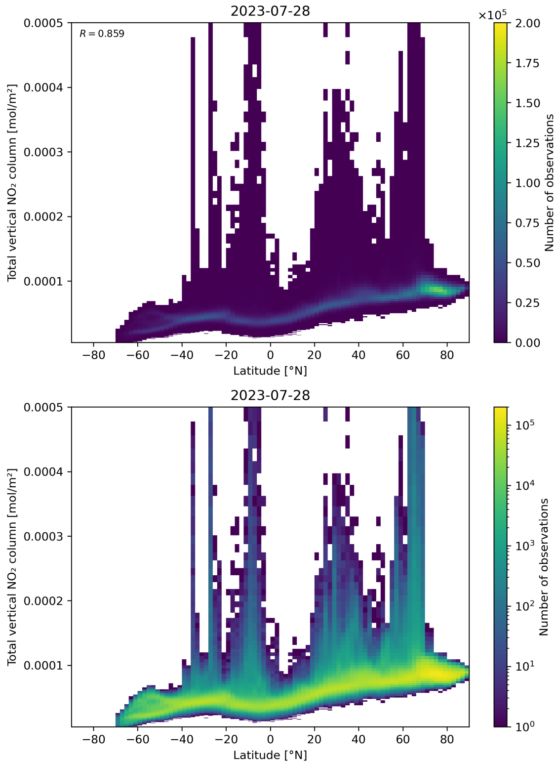
Figure 90: Scatter density plot of “Latitude” against “Total vertical NO 2 column” for 2023-07-27 to 2023-07-29.
