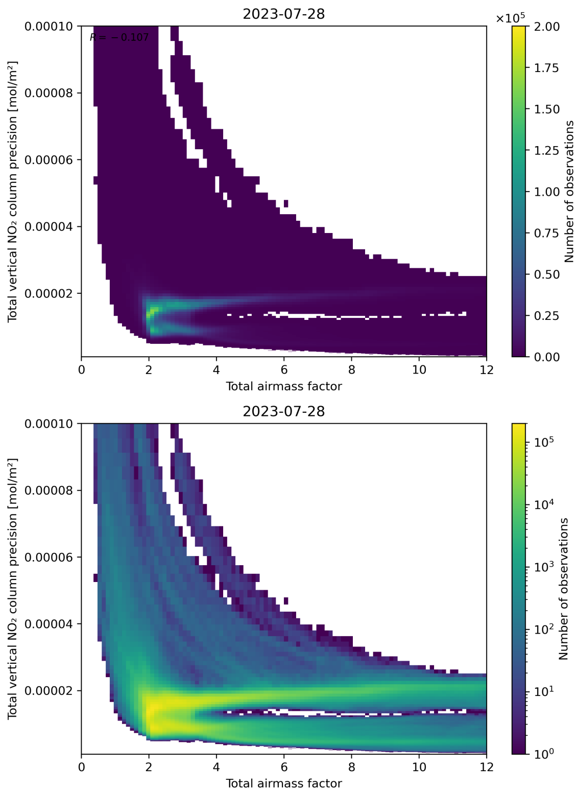
Figure 68: Scatter density plot of “Total airmass factor” against “Total vertical NO 2 column precision” for 2023-07-27 to 2023-07-29.
