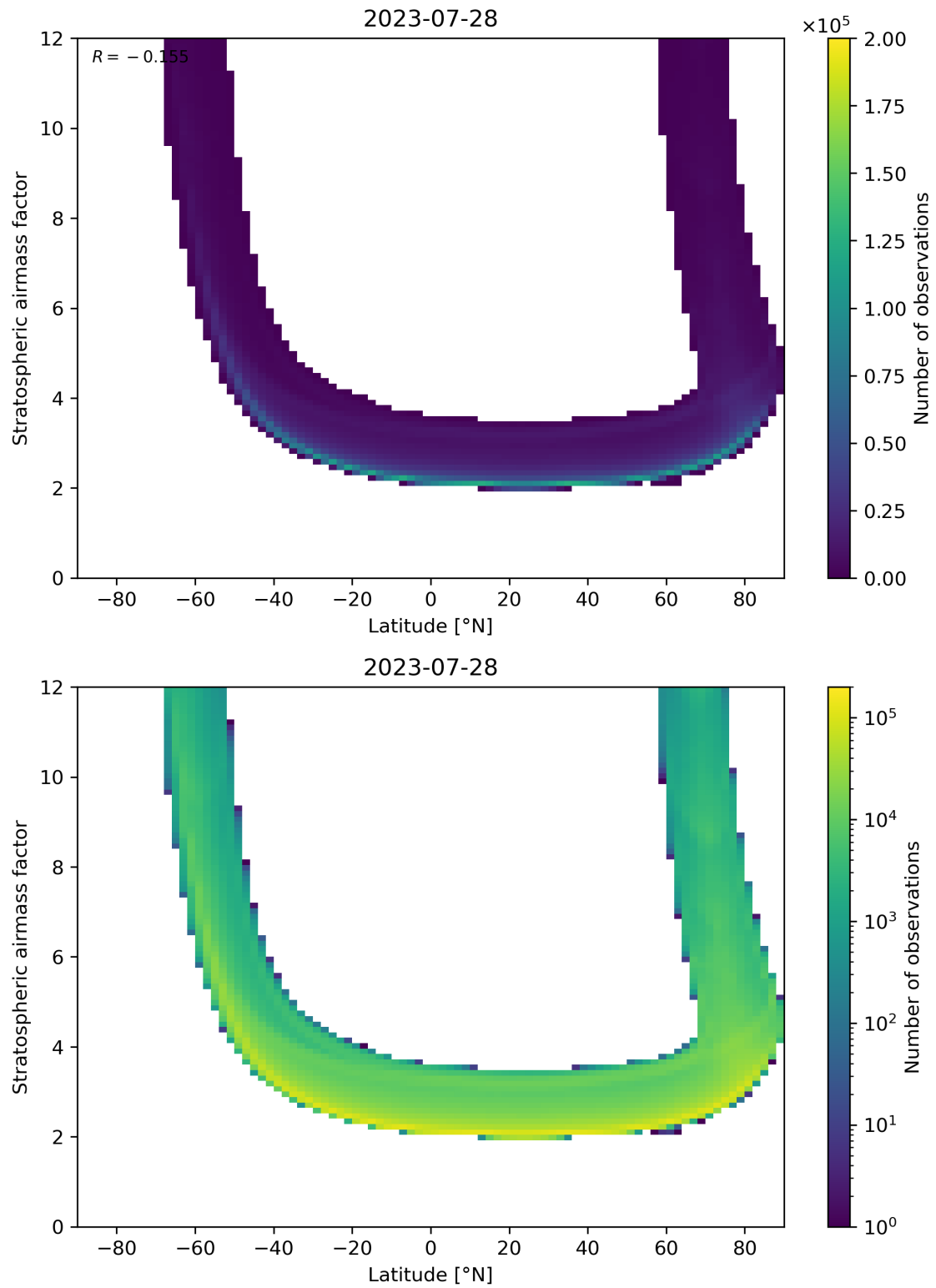
Figure 83: Scatter density plot of “Latitude” against “Stratospheric air mass factor” for 2023-07-27 to 2023-07-29.
