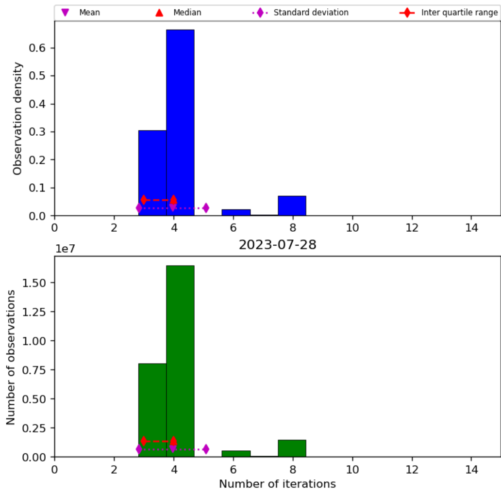
Figure 34: Histogram of “Number of iterations” for 2023-07-27 to 2023-07-29
