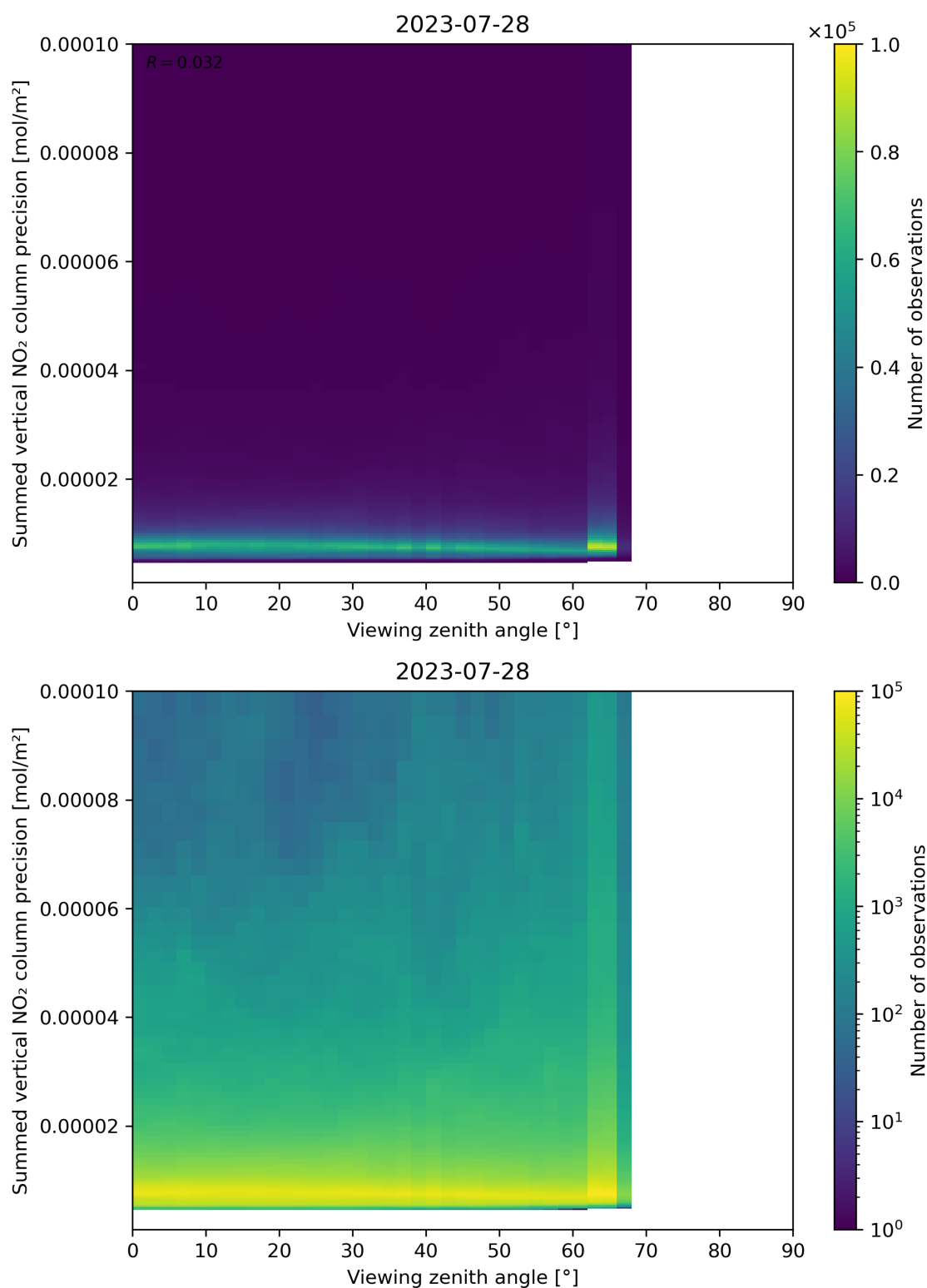
Figure 166: Scatter density plot of “Viewing zenith angle” against “Summed vertical NO 2 column precision” for 2023-07-27 to 2023-07-29.
