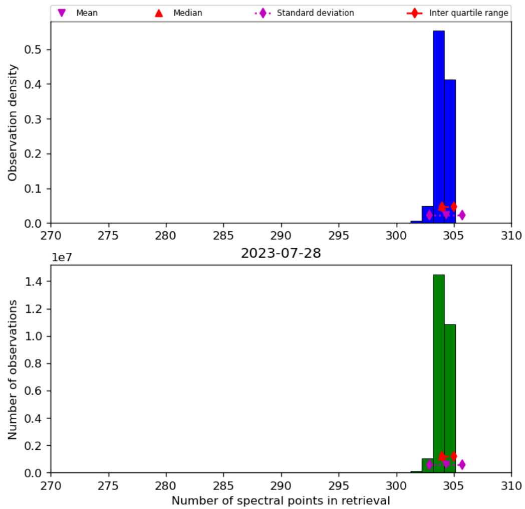
Figure 33: Histogram of “Number of spectral points in retrieval” for 2023-07-27 to 2023-07-29
