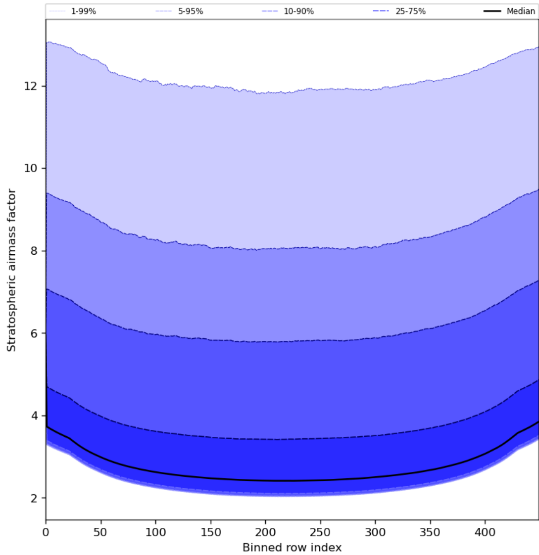
Figure 61: Along track statistics of “Stratospheric air mass factor” for 2023-07-27 to 2023-07-29
