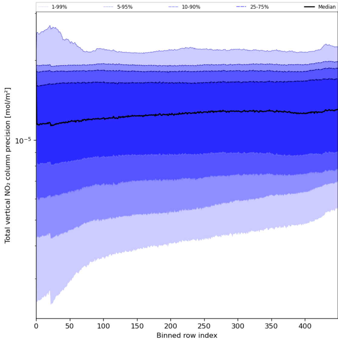
Figure 56: Along track statistics of “Total vertical NO 2 column precision” for 2023-07-27 to 2023-07-29
