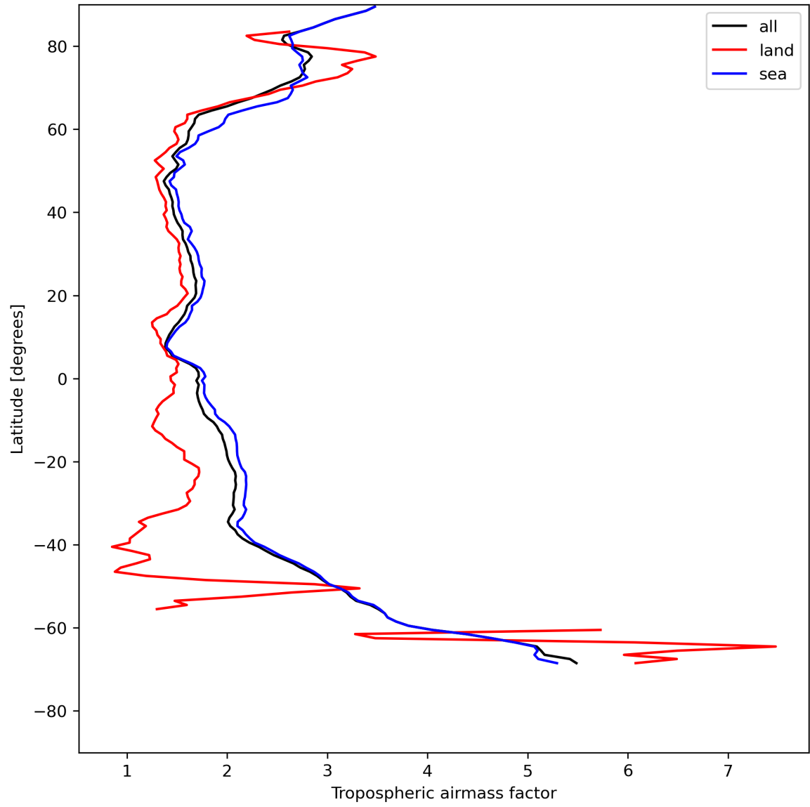
Figure 14: Zonal average of “Tropospheric air mass factor” for 2023-07-27 to 2023-07-29.
