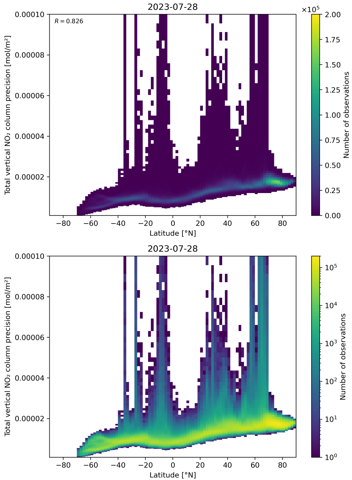
Figure 91: Scatter density plot of “Latitude” against “Total vertical NO 2 column precision” for 2023-07-27 to 2023-07-29.
