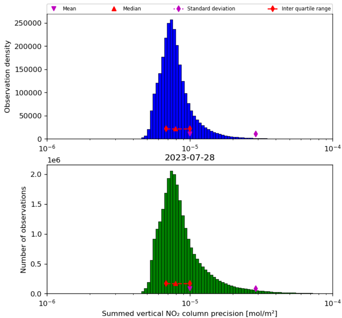
Figure 41: Histogram of “Summed vertical NO 2 column precision” for 2023-07-27 to 2023-07-29
