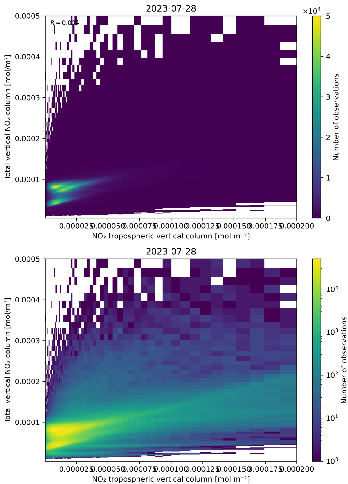
Figure 128: Scatter density plot of “NO 2 tropospheric vertical column” against “Total vertical NO 2 column” for 2023-07-27 to 2023-07-29.
