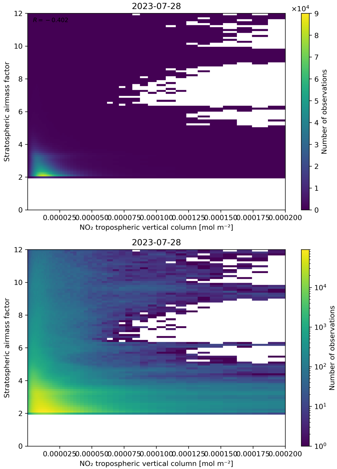
Figure 121: Scatter density plot of “NO 2 tropospheric vertical column” against “Stratospheric air mass factor” for 2023-07-27 to 2023-07-29.
