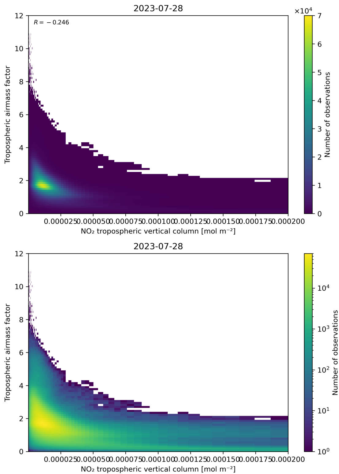
Figure 123: Scatter density plot of “NO 2 tropospheric vertical column” against “Tropospheric air mass factor” for 2023-07-27 to 2023-07-29.
