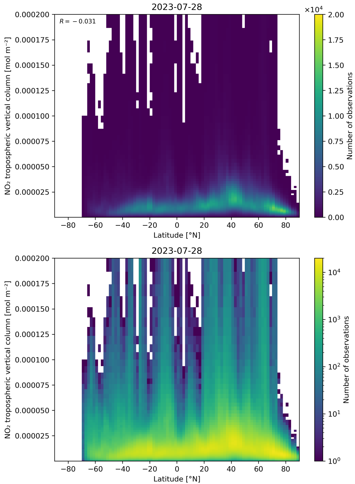
Figure 92: Scatter density plot of “Latitude” against “NO 2 tropospheric vertical column” for 2023-07-27 to 2023-07-29.
