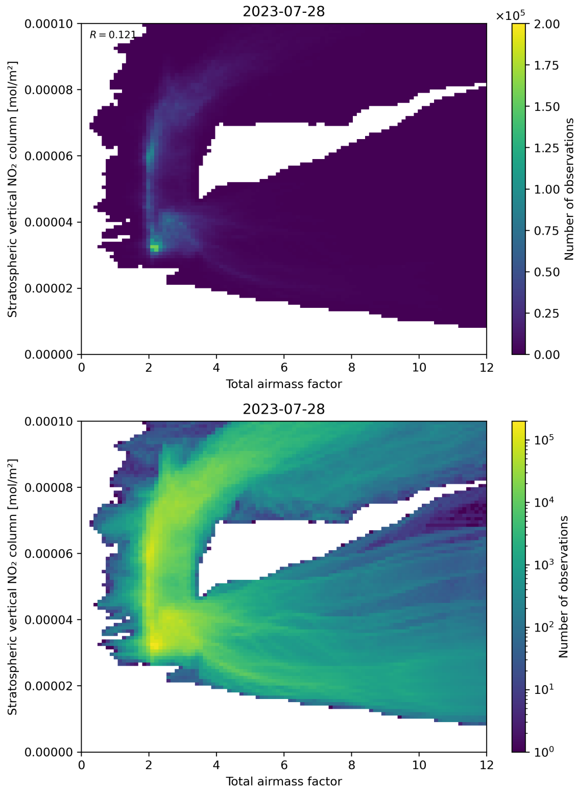
Figure 64: Scatter density plot of “Total airmass factor” against “Stratospheric vertical NO 2 column” for 2023-07-27 to 2023-07-29.
