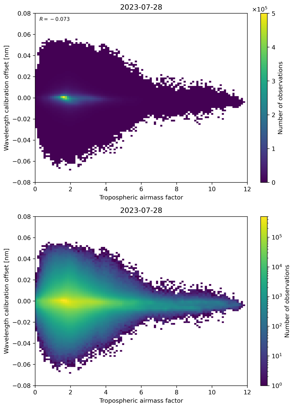
Figure 80: Scatter density plot of “Tropospheric airmass factor” against “Wavelength calibration offset” for 2023-07-27 to 2023-07-29.
