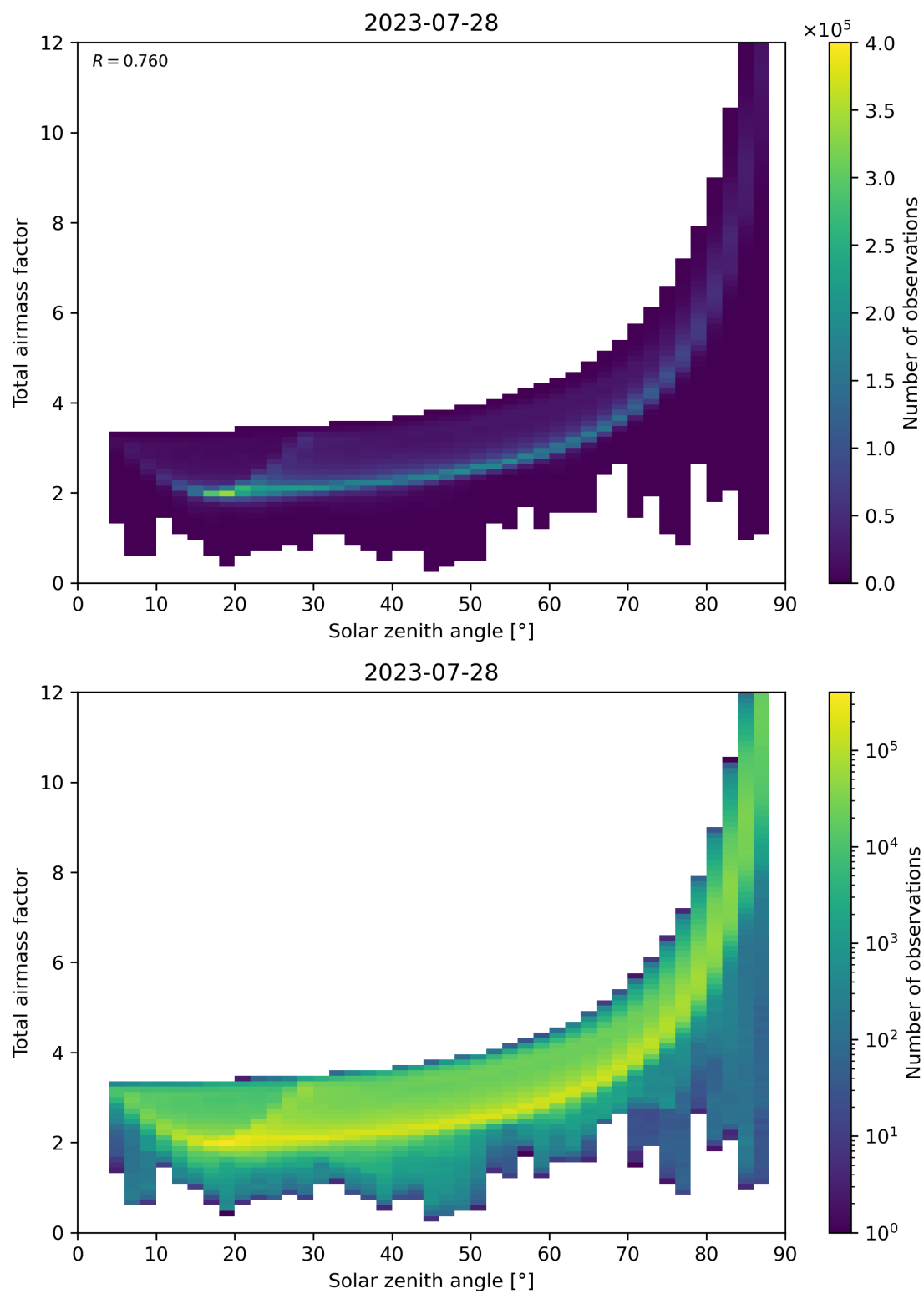
Figure 146: Scatter density plot of “Solar zenith angle” against “Total air mass factor” for 2023-07-27 to 2023-07-29.
