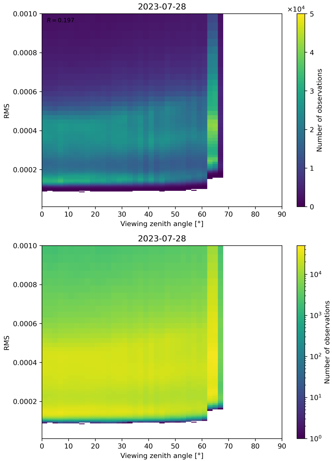
Figure 171: Scatter density plot of “Viewing zenith angle” against “RMS” for 2023-07-27 to 2023-07-29.
