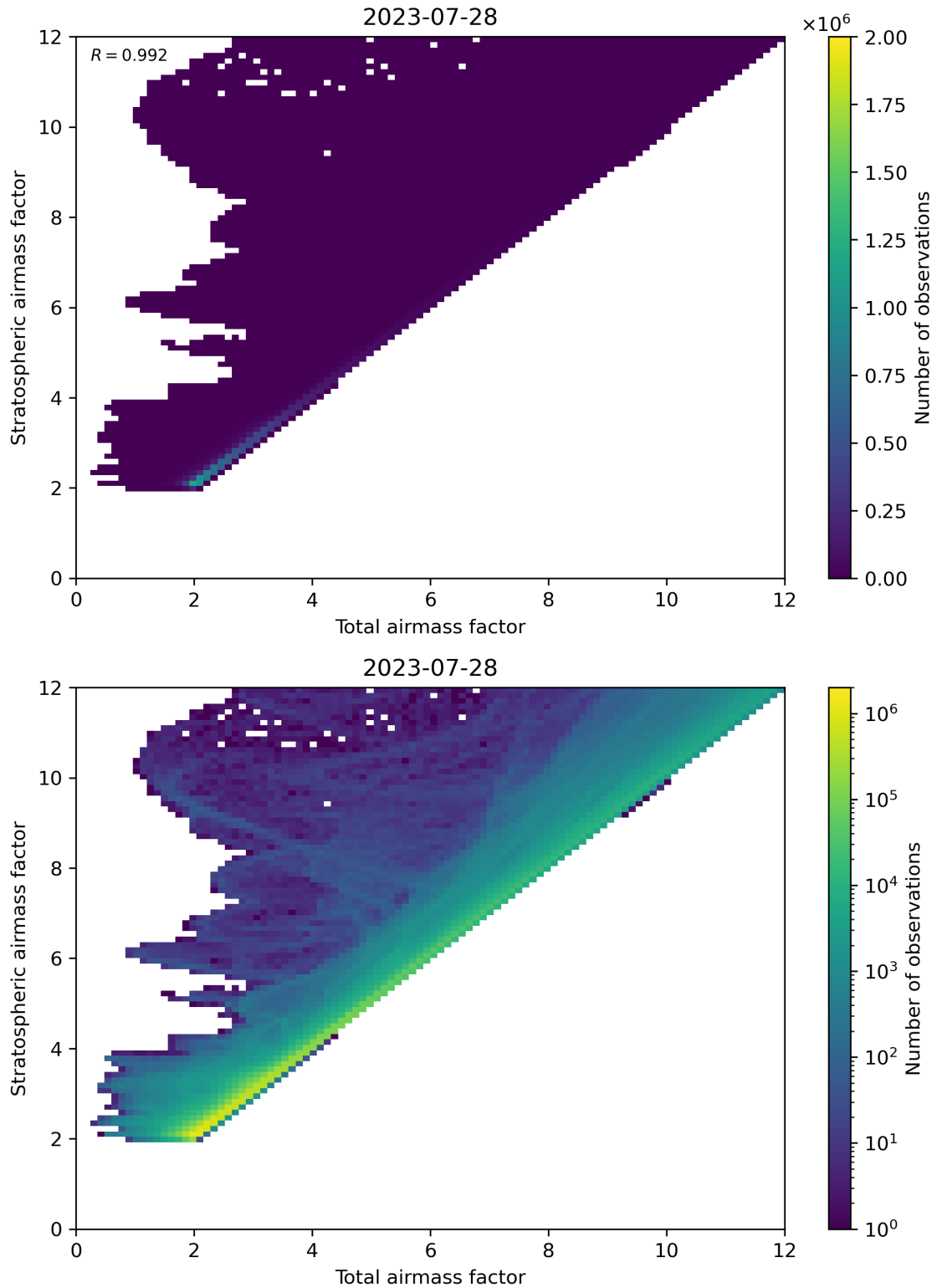
Figure 62: Scatter density plot of “Total airmass factor” against “Stratospheric airmass factor” for 2023-07-27 to 2023-07-29.
