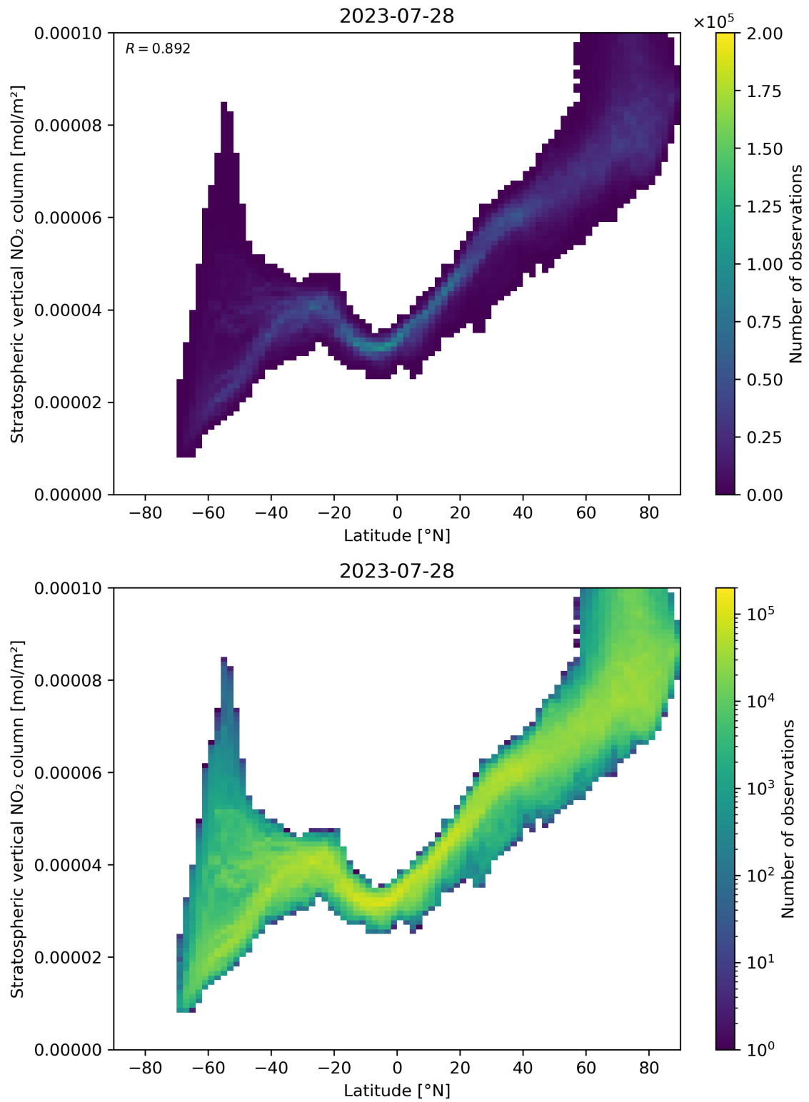
Figure 87: Scatter density plot of “Latitude” against “Stratospheric vertical NO 2 column” for 2023-07-27 to 2023-07-29.
