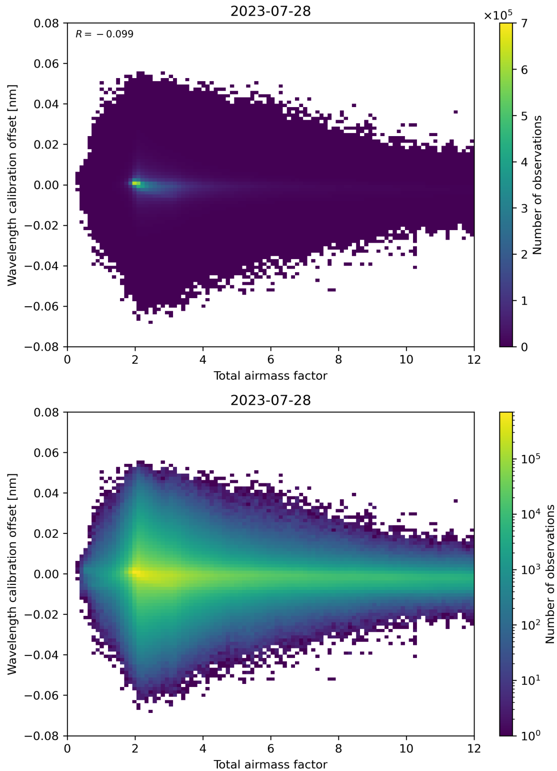
Figure 70: Scatter density plot of “Total airmass factor” against “Wavelength calibration offset” for 2023-07-27 to 2023-07-29.
