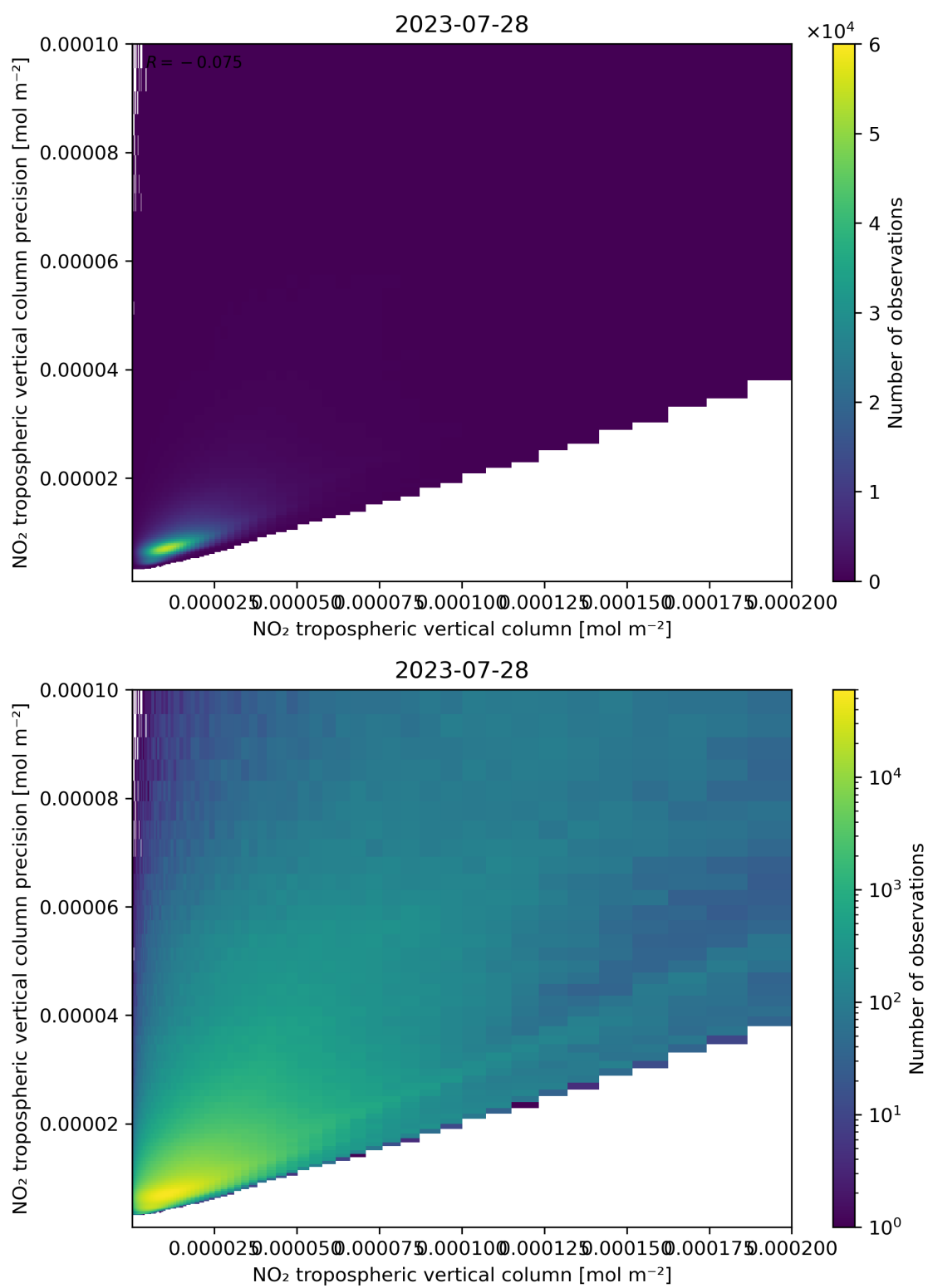
Figure 130: Scatter density plot of “NO 2 tropospheric vertical column” against “NO 2 tropospheric vertical column precision” for 2023-07-27 to 2023-07-29.
