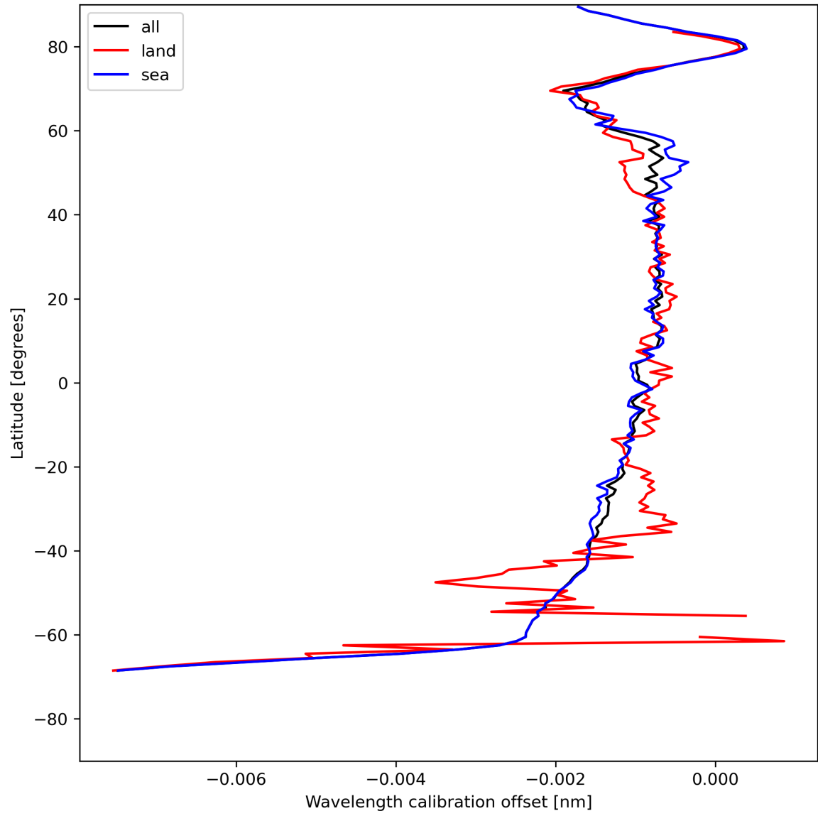
Figure 18: Zonal average of “Wavelength calibration offset” for 2023-07-27 to 2023-07-29.
