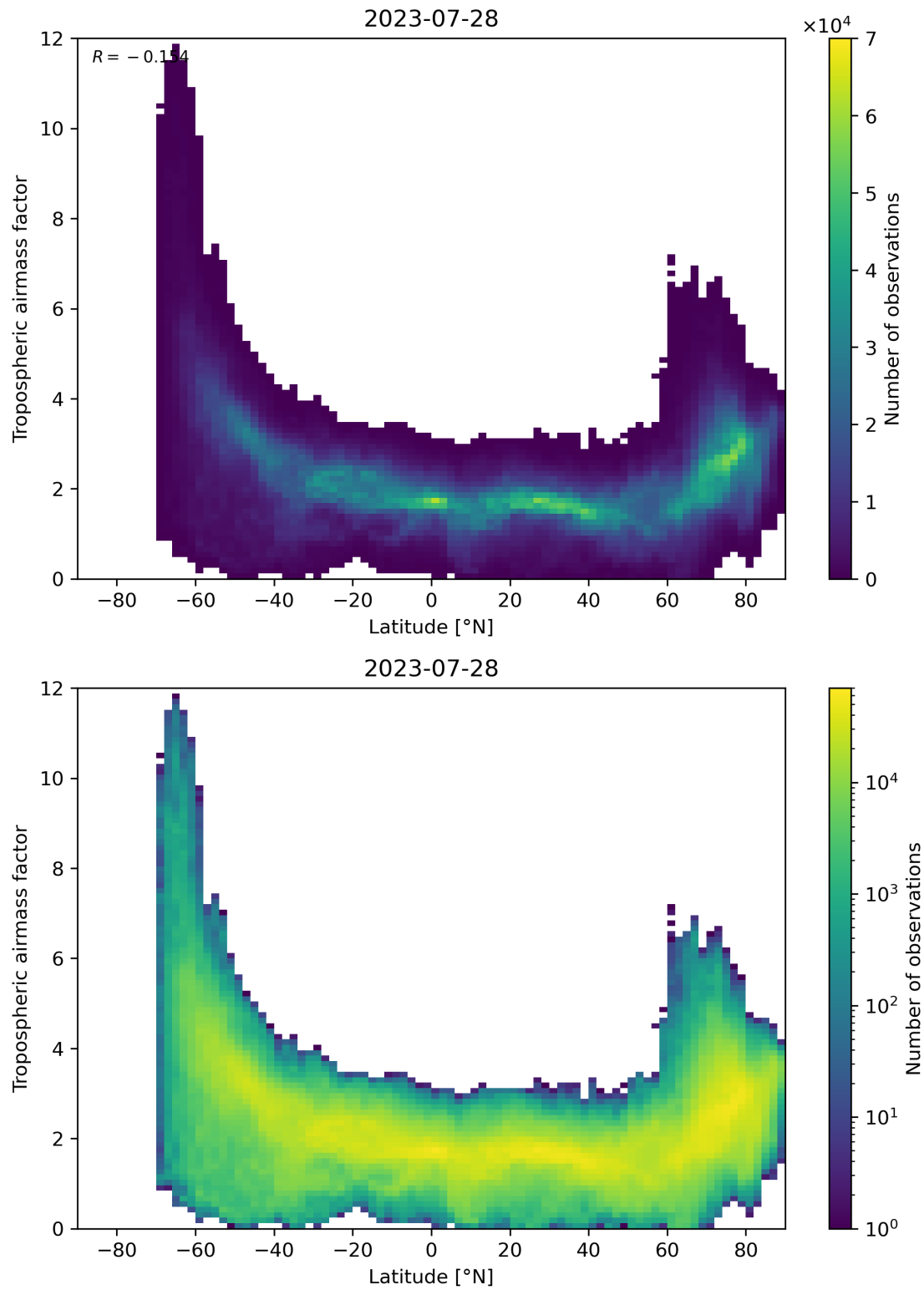
Figure 85: Scatter density plot of “Latitude” against “Tropospheric airmass factor” for 2023-07-27 to 2023-07-29.
