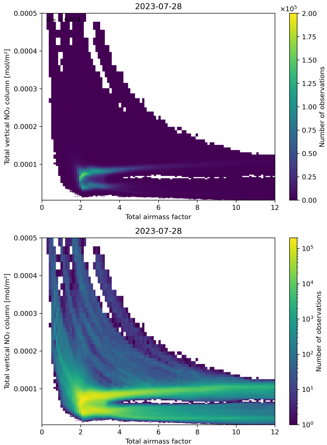
Figure 67: Scatter density plot of “Total airmass factor” against “Total vertical NO 2 column” for 2023-07-27 to 2023-07-29.
