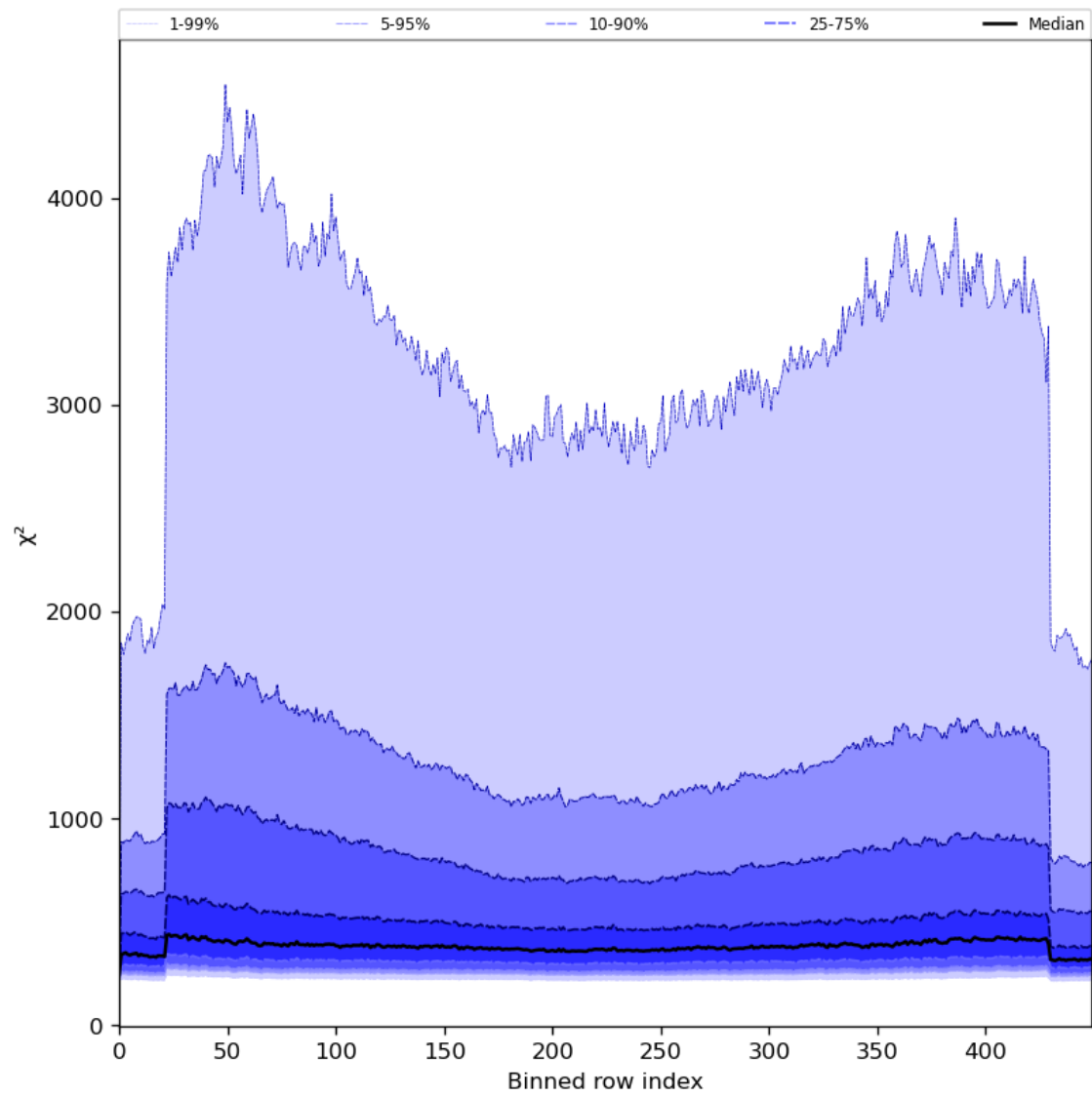
Figure 59: Along track statistics of “ \chi^2 ” for 2023-07-27 to 2023-07-29
