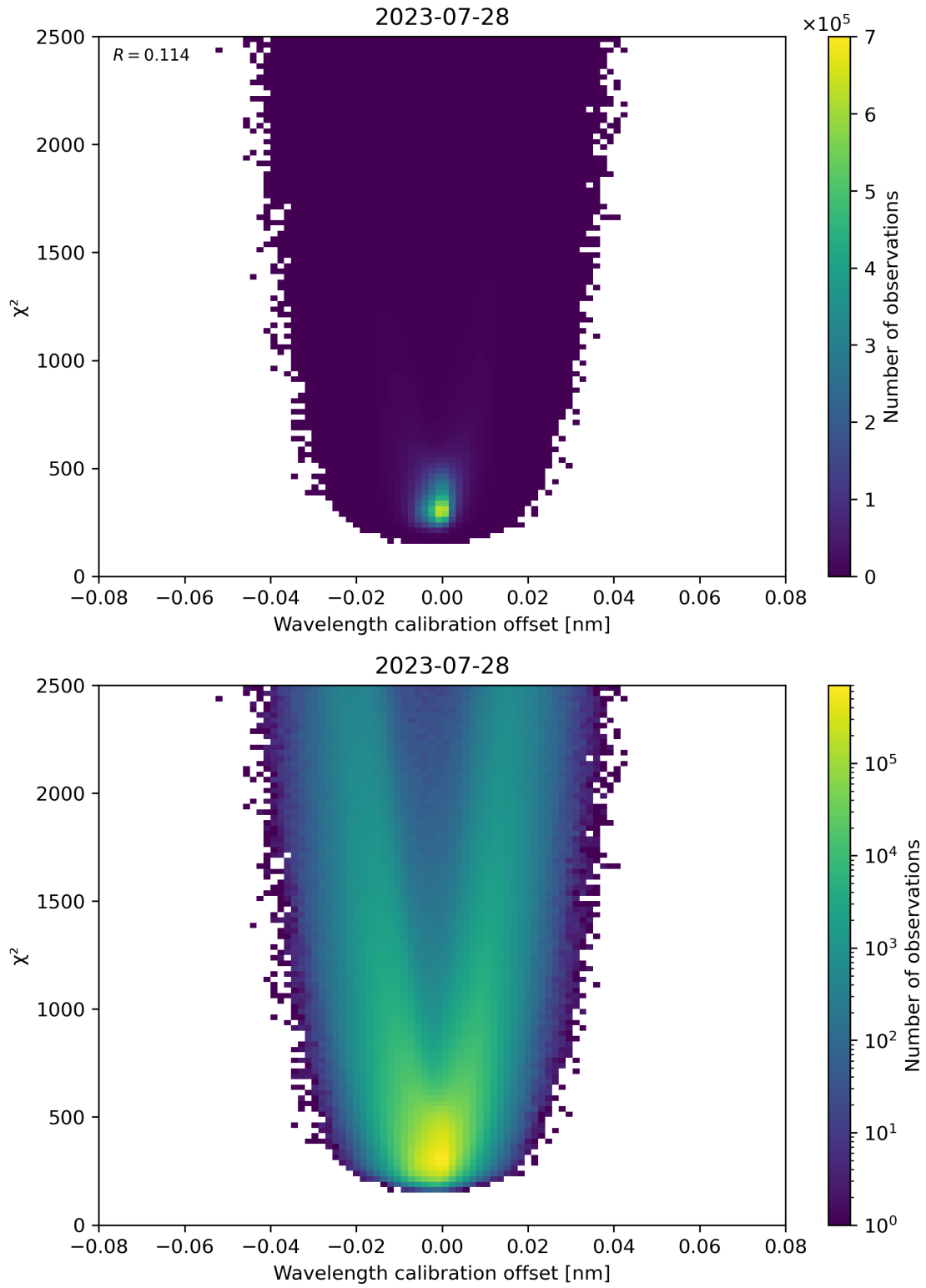
Figure 175: Scatter density plot of “Wavelength calibration offset” against “ \chi^2 ” for 2023-07-27 to 2023-07-29.
