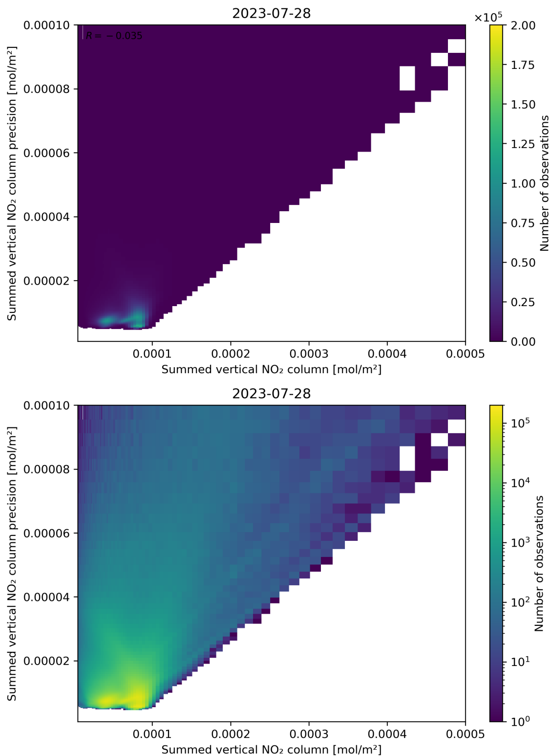
Figure 105: Scatter density plot of “Summed vertical NO 2 column” against “Summed vertical NO 2 column precision” for 2023-07-27 to 2023-07-29.
