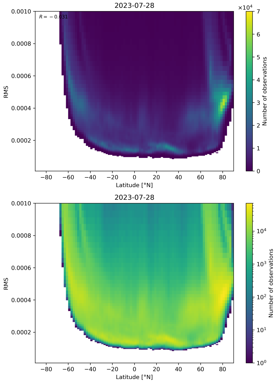
Figure 94: Scatter density plot of “Latitude” against “RMS” for 2023-07-27 to 2023-07-29.
