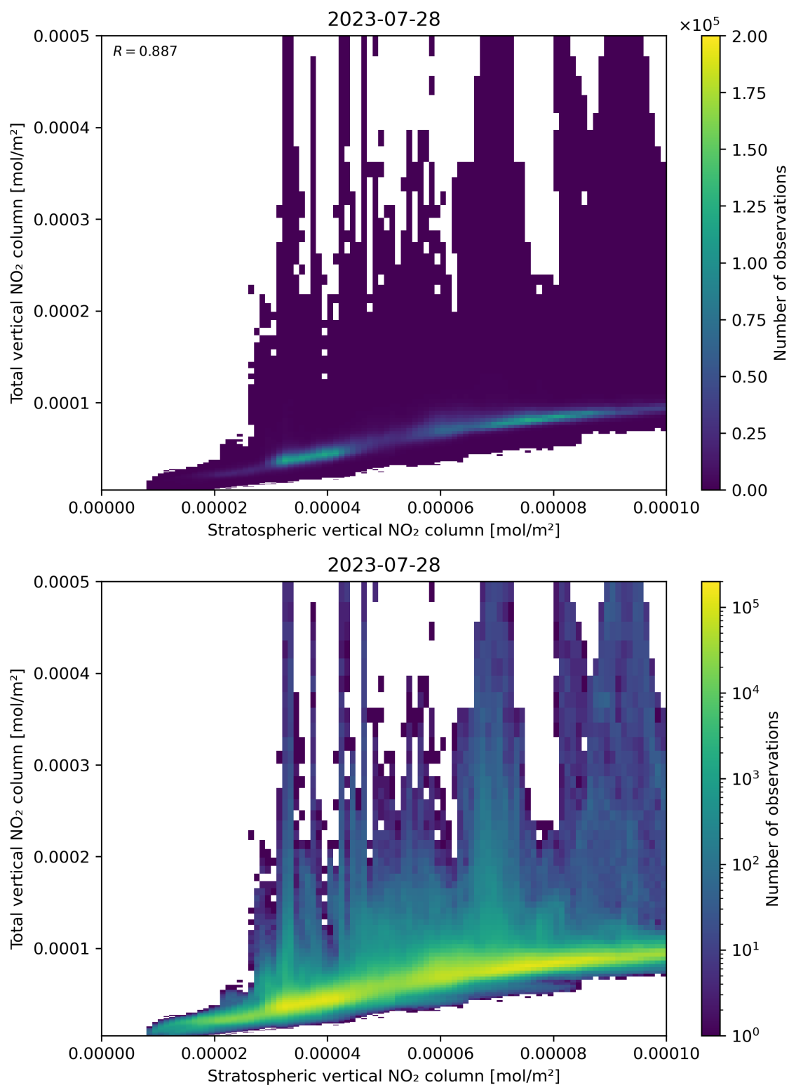
Figure 100: Scatter density plot of “Stratospheric vertical NO 2 column” against “Total vertical NO 2 column” for 2023-07-27 to 2023-07-29.
