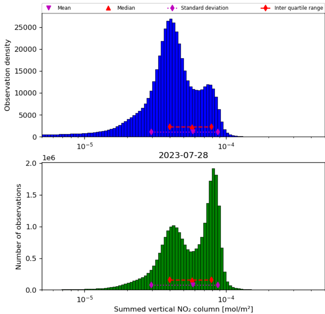
Figure 40: Histogram of "Summed vertical NO 2 column" for 2023-07-27 to 2023-07-29
