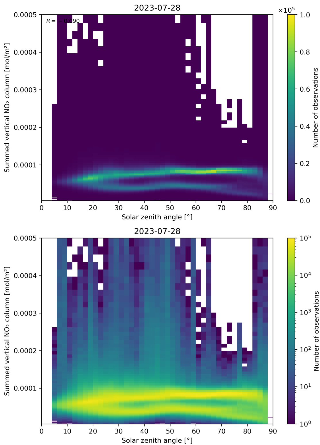
Figure 151: Scatter density plot of “Solar zenith angle” against “Summed vertical NO 2 column” for 2023-07-27 to 2023-07-29.
