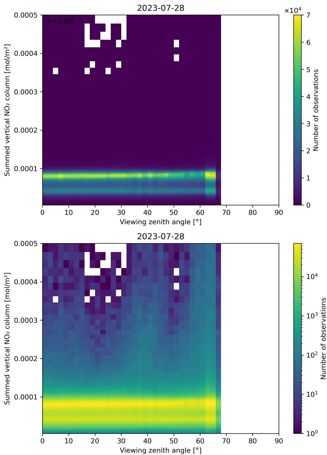
Figure 165: Scatter density plot of “Viewing zenith angle” against “Summed vertical NO 2 column” for 2023-07-27 to 2023-07-29.
