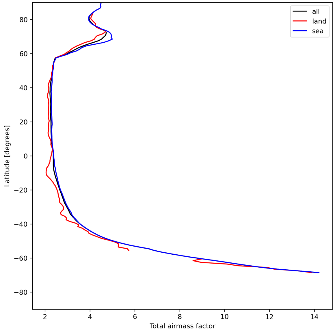
Figure 15: Zonal average of “Total airmass factor” for 2023-07-27 to 2023-07-29.
