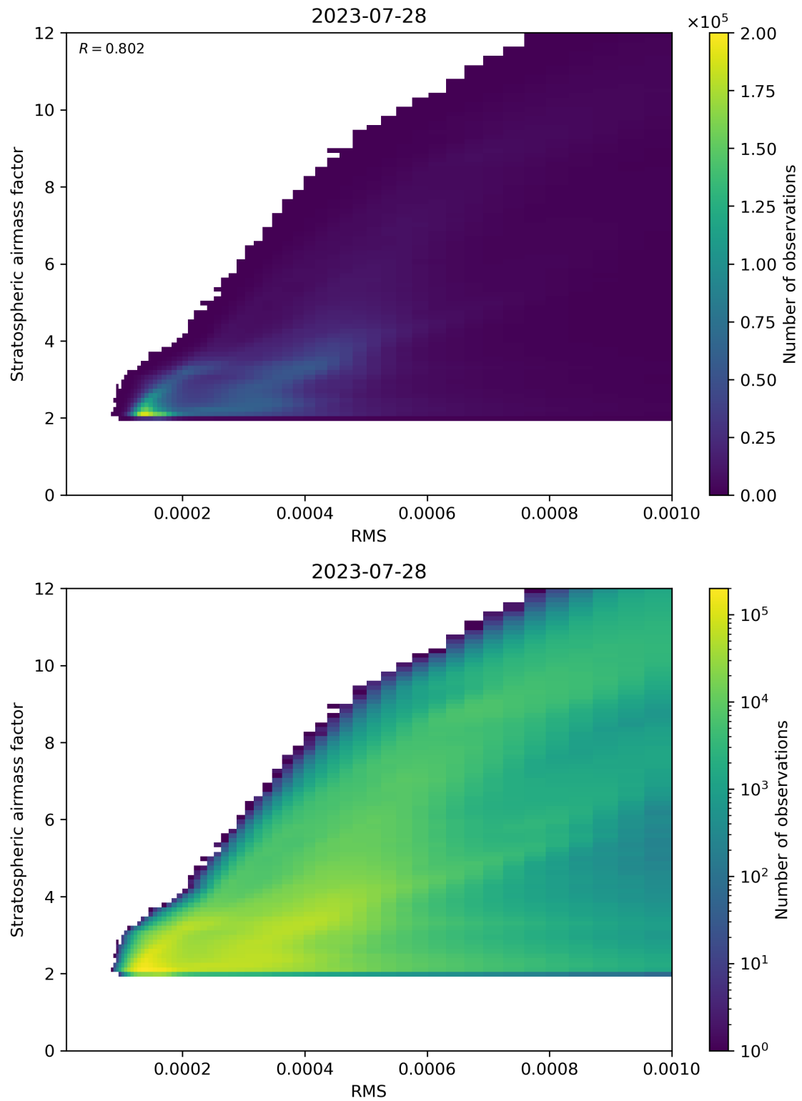
Figure 144: Scatter density plot of “RMS” against “Stratospheric airmass factor” for 2023-07-27 to 2023-07-29.
