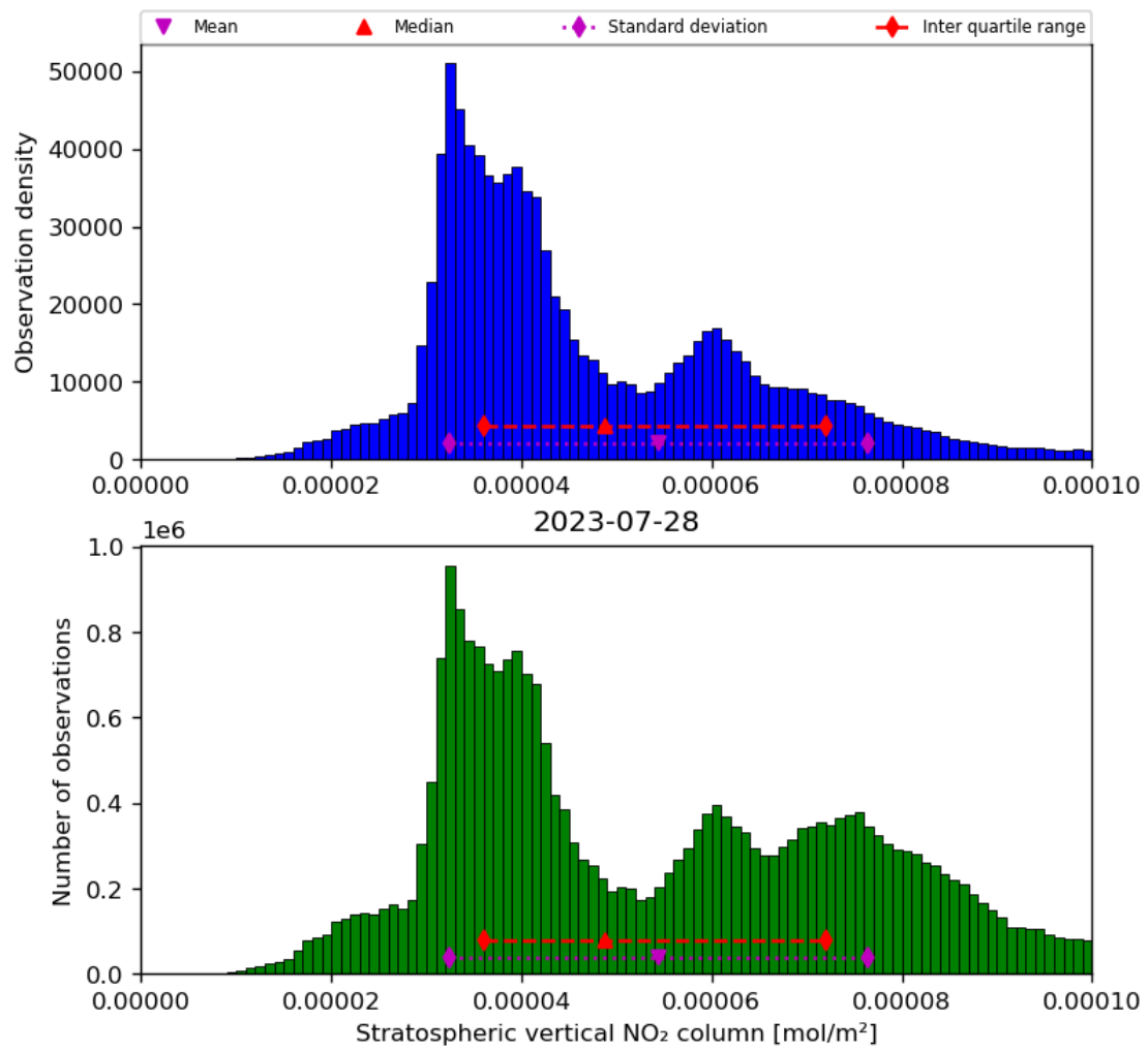
Figure 36: Histogram of “Stratospheric vertical NO 2 column” for 2023-07-27 to 2023-07-29
