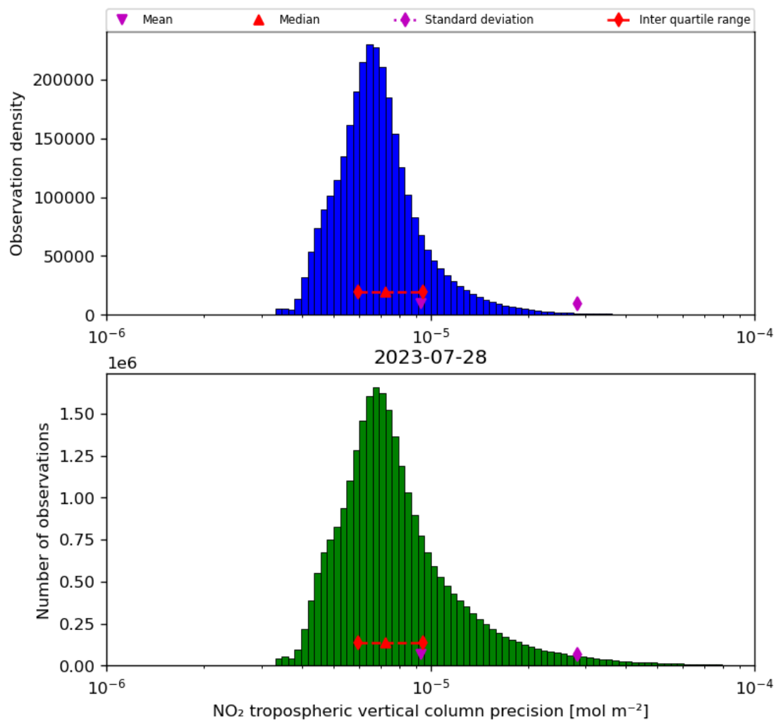
Figure 30: Histogram of “NO 2 tropospheric vertical column precision” for 2023-07-27 to 2023-07-29
