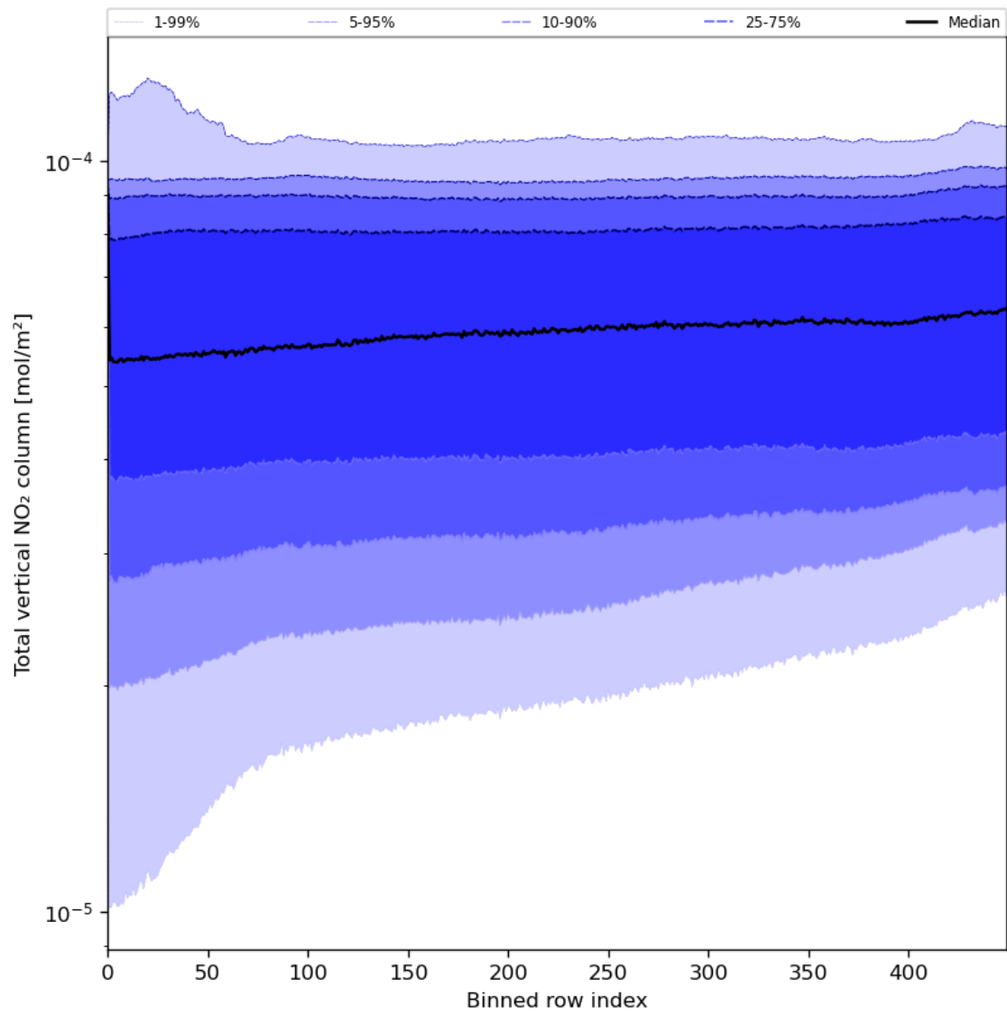
Figure 55: Along track statistics of “Total vertical NO 2 column” for 2023-07-27 to 2023-07-29
