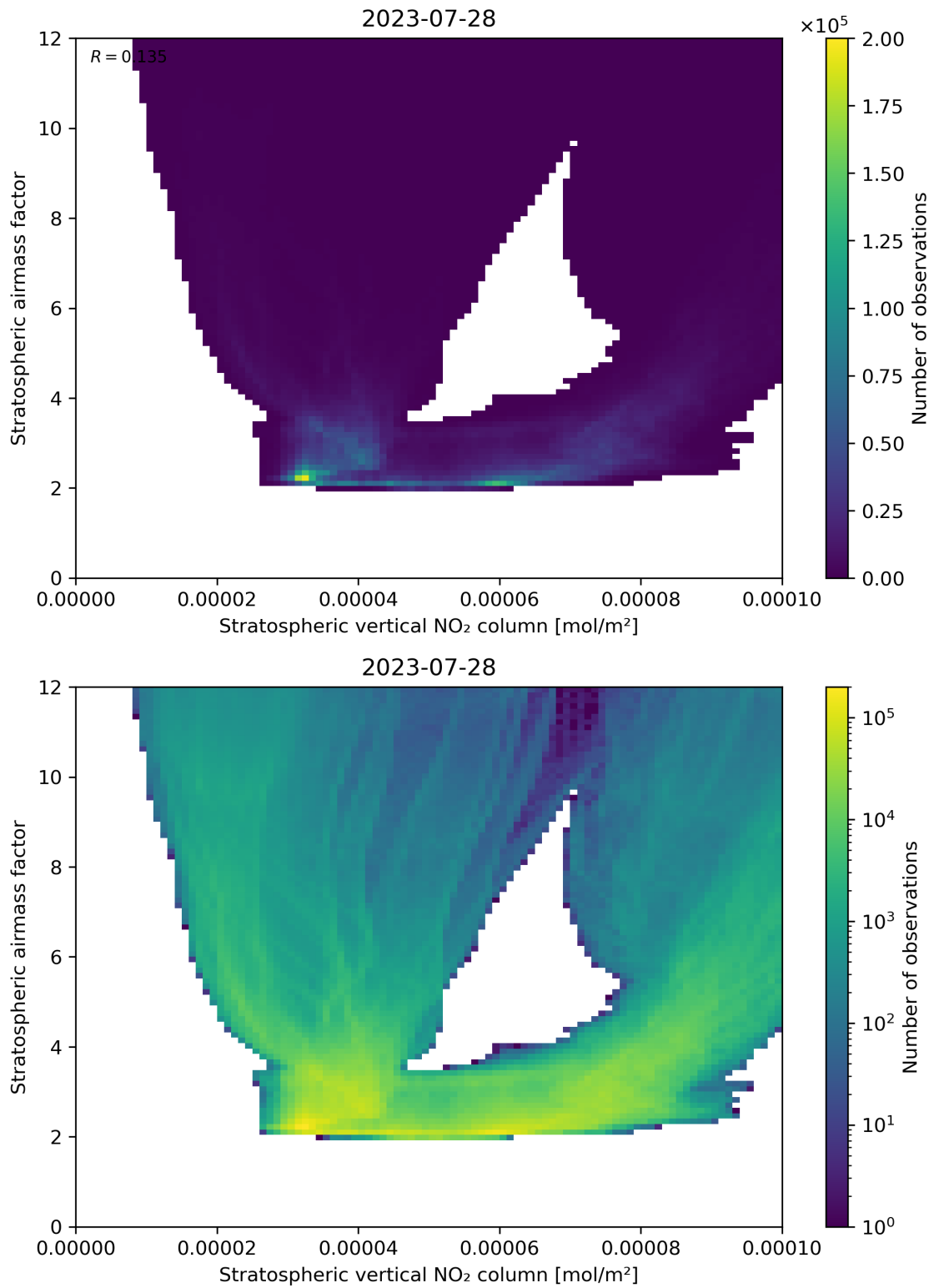
Figure 96: Scatter density plot of “Stratospheric vertical NO 2 column” against “Stratospheric airmass factor” for 2023-07-27 to 2023-07-29.
