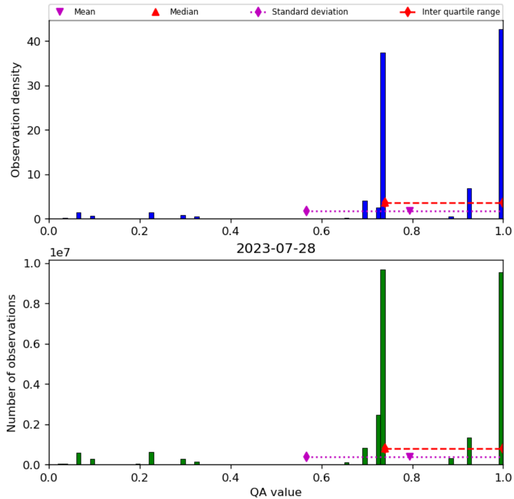
Figure 28: Histogram of “QA value” for 2023-07-27 to 2023-07-29
