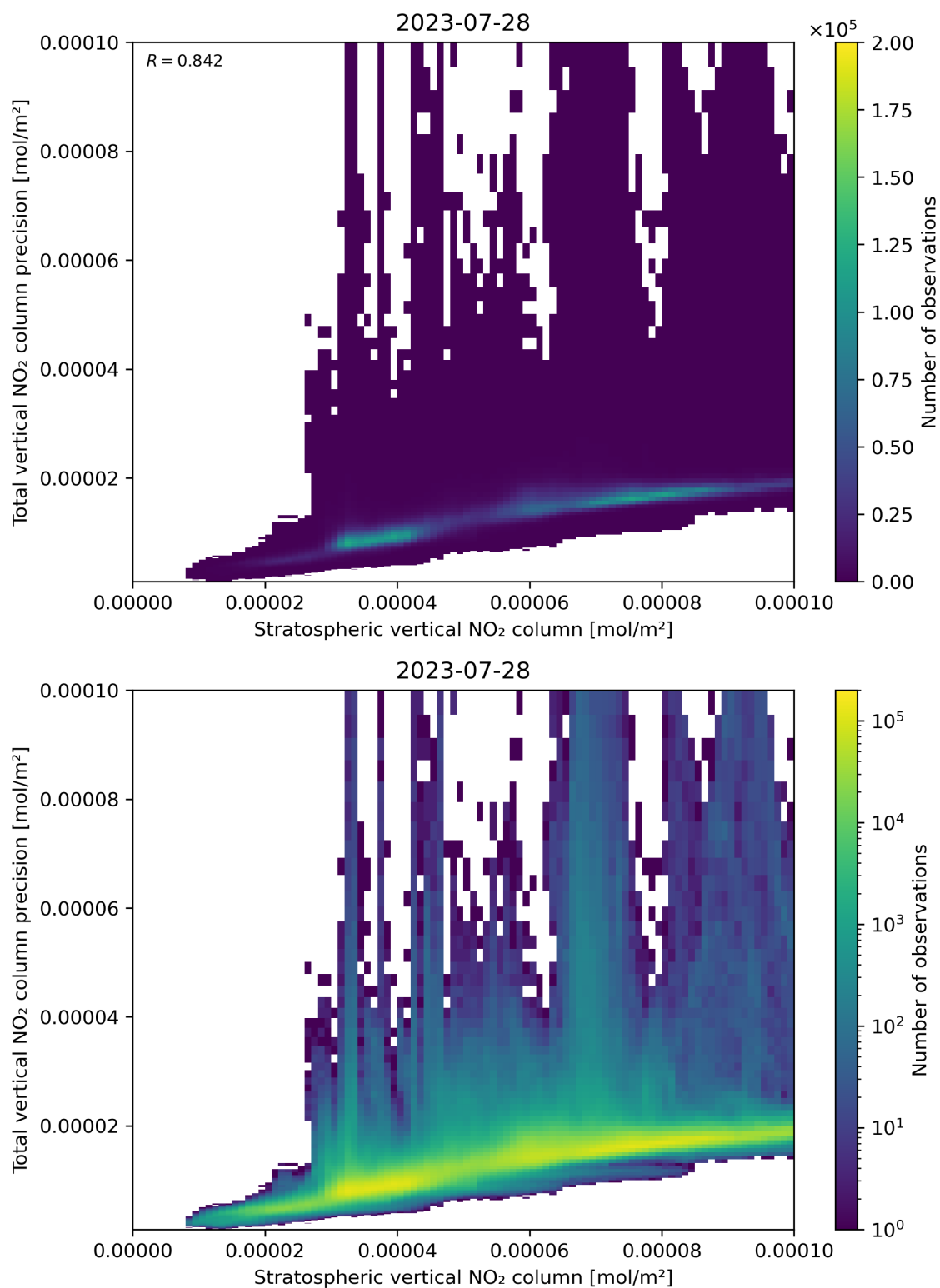
Figure 101: Scatter density plot of “Stratospheric vertical NO 2 column” against “Total vertical NO 2 column precision” for 2023-07-27 to 2023-07-29.
