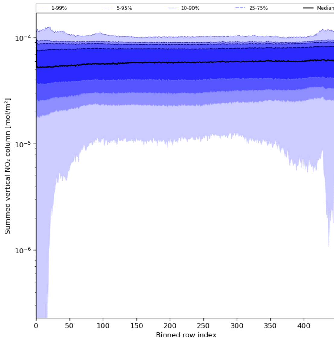
Figure 57: Along track statistics of “Summed vertical NO 2 column” for 2023-07-27 to 2023-07-29
