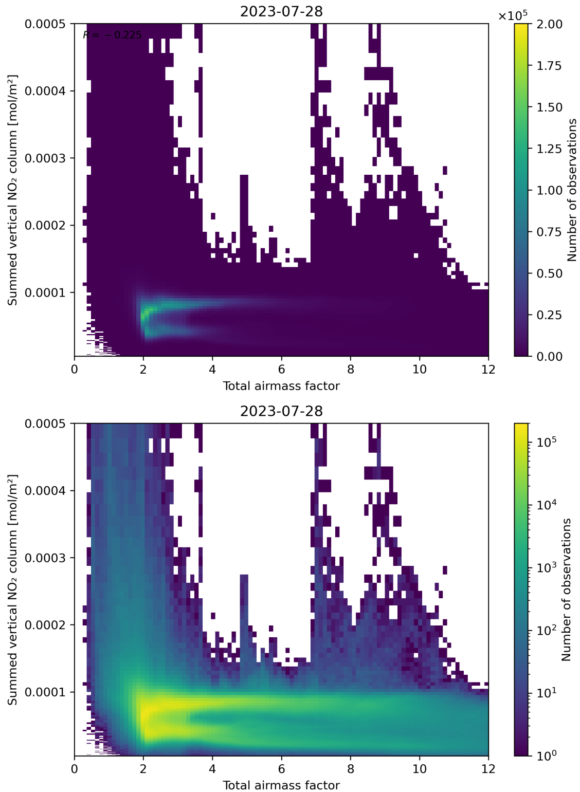
Figure 65: Scatter density plot of “Total airmass factor” against “Summed vertical NO 2 column” for 2023-07-27 to 2023-07-29.
