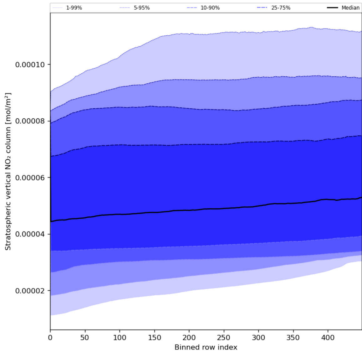
Figure 53: Along track statistics of “Stratospheric vertical NO 2 column” for 2023-07-27 to 2023-07-29
