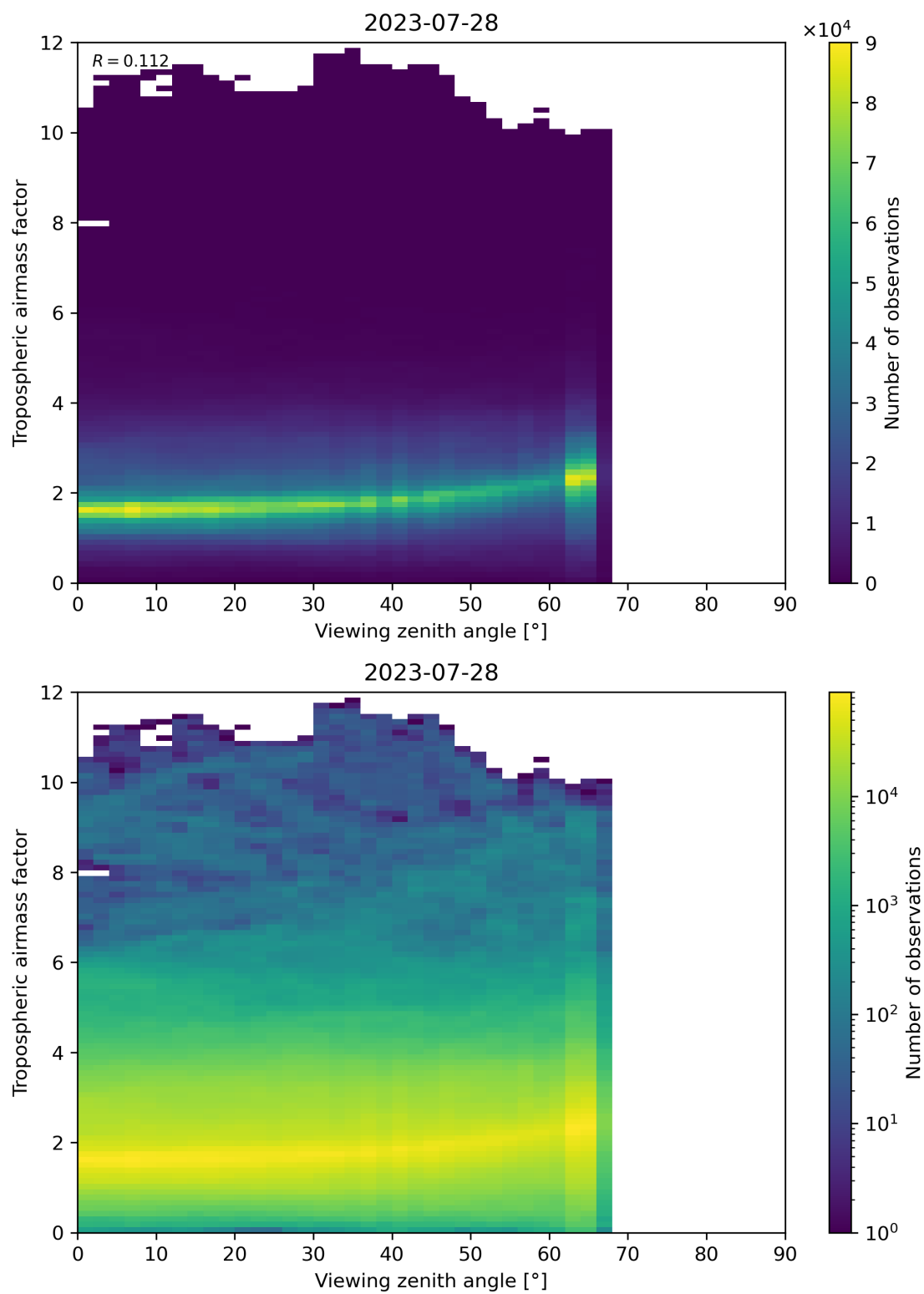
Figure 161: Scatter density plot of “Viewing zenith angle” against “Tropospheric airmass factor” for 2023-07-27 to 2023-07-29.
