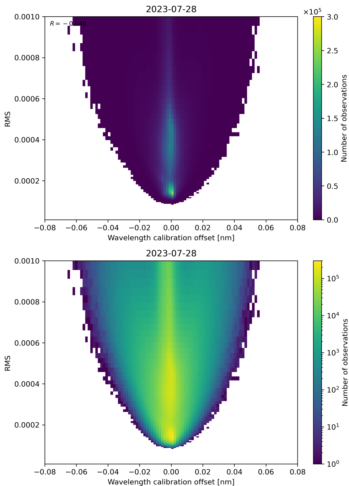
Figure 181: Scatter density plot of “Wavelength calibration offset” against “RMS” for 2023-07-27 to 2023-07-29.
