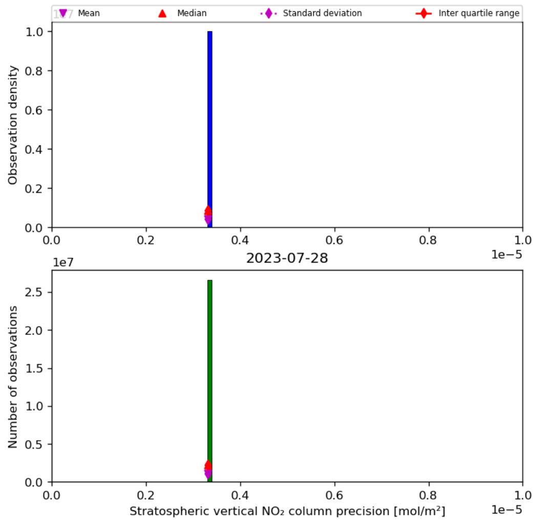
Figure 37: Histogram of “Stratospheric vertical NO 2 column precision” for 2023-07-27 to 2023-07-29
