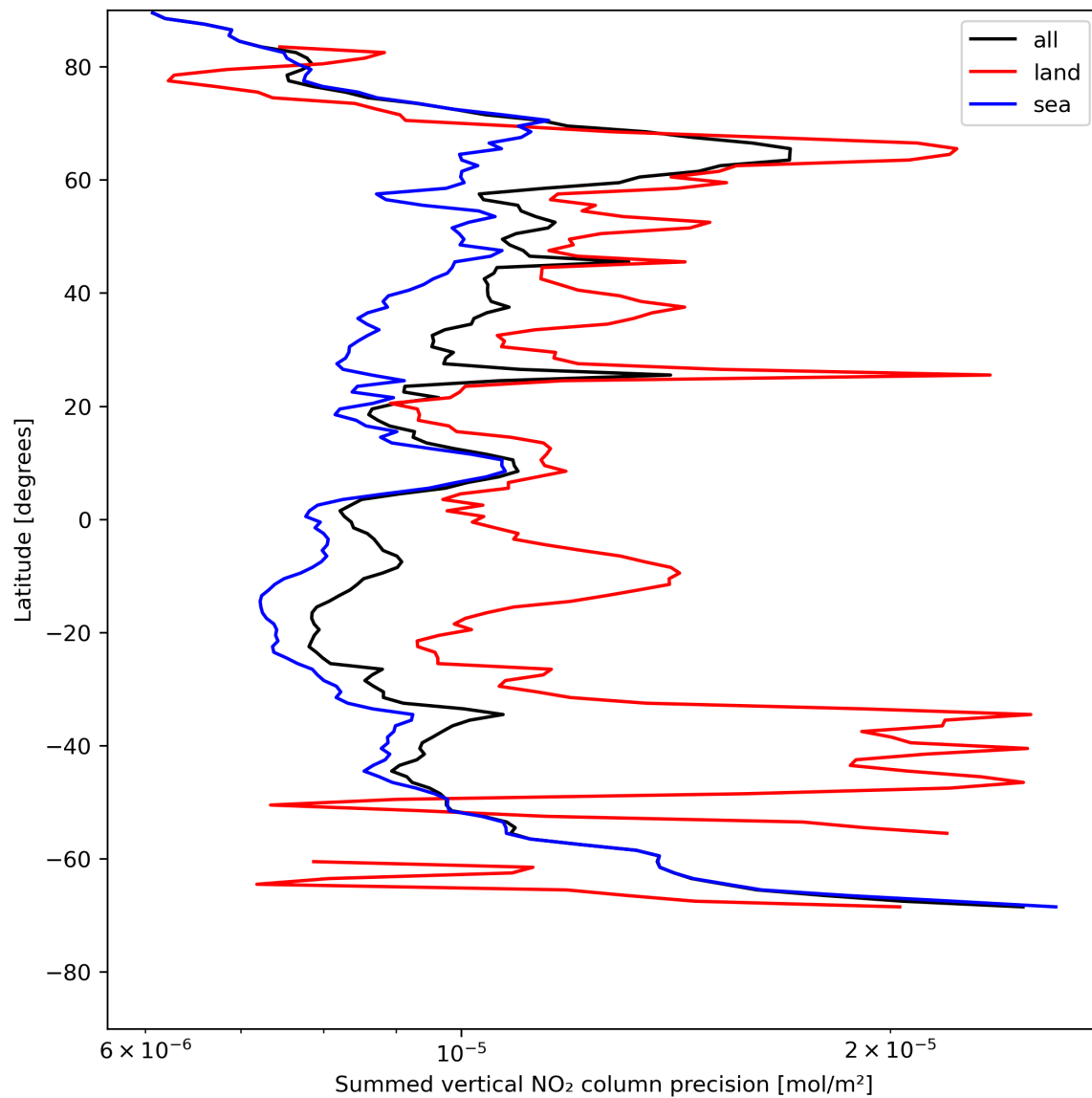
Figure 24: Zonal average of “Summed vertical NO 2 column precision” for 2023-07-27 to 2023-07-29.
