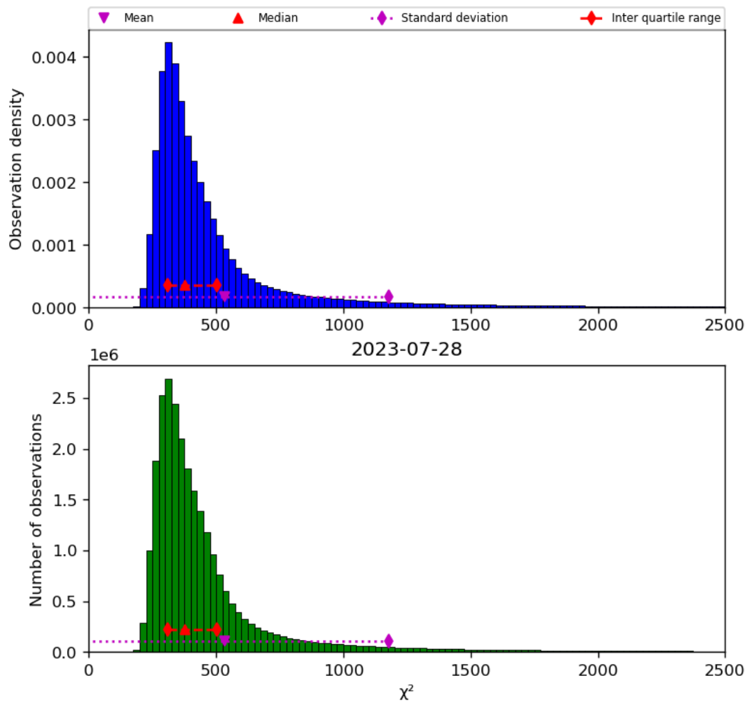
Figure 42: Histogram of “ \chi^2 ” for 2023-07-27 to 2023-07-29
