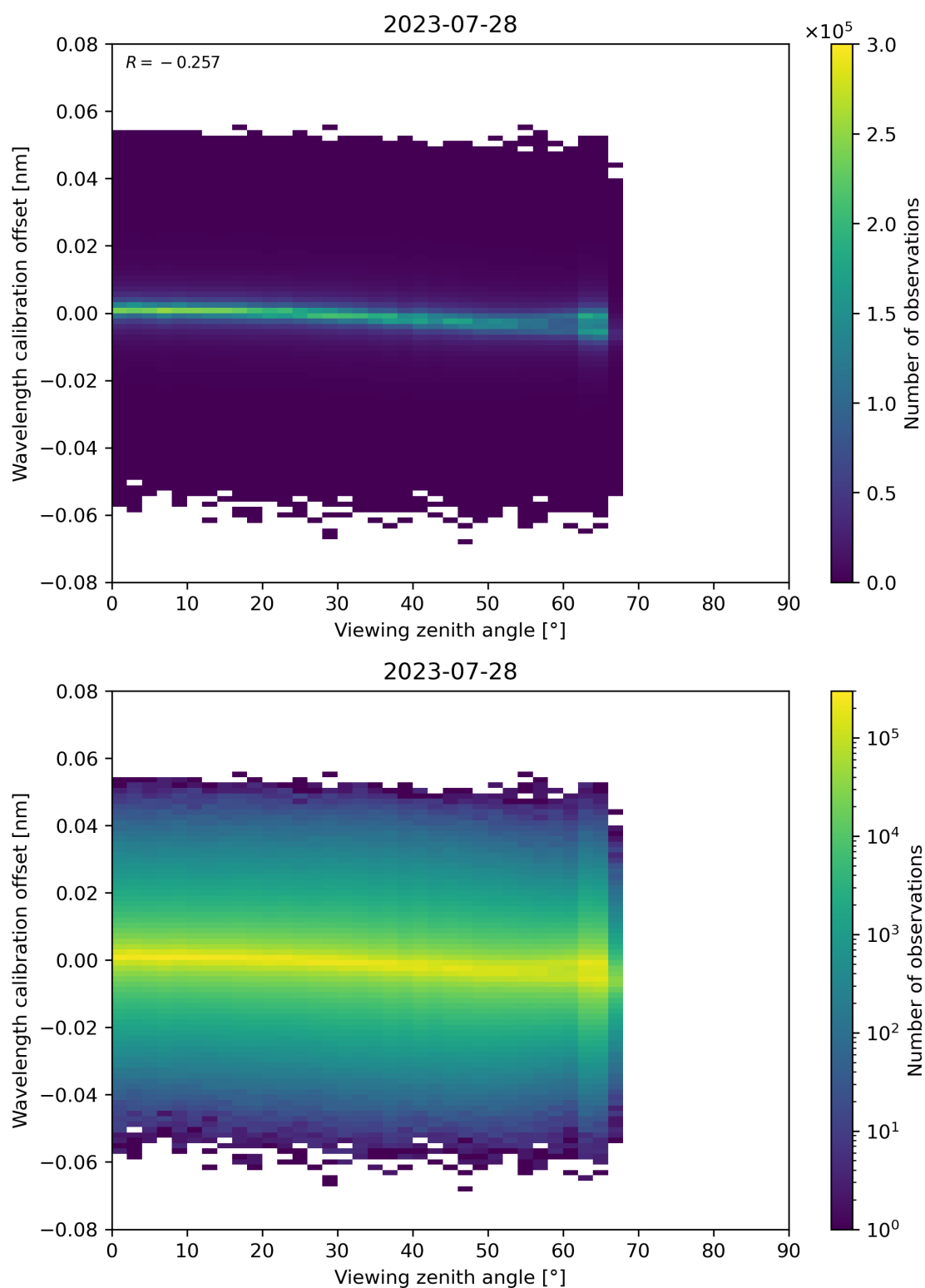
Figure 173: Scatter density plot of “Viewing zenith angle” against “Wavelength calibration offset” for 2023-07-27 to 2023-07-29.
