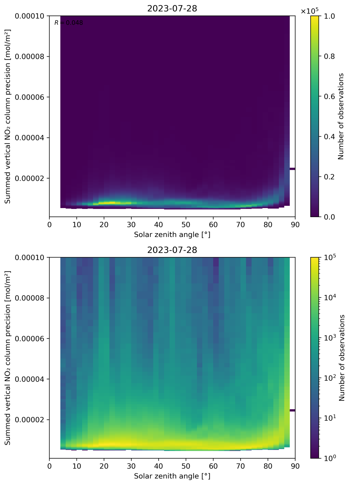
Figure 152: Scatter density plot of “Solar zenith angle” against “Summed vertical NO 2 column precision” for 2023-07-27 to 2023-07-29.
