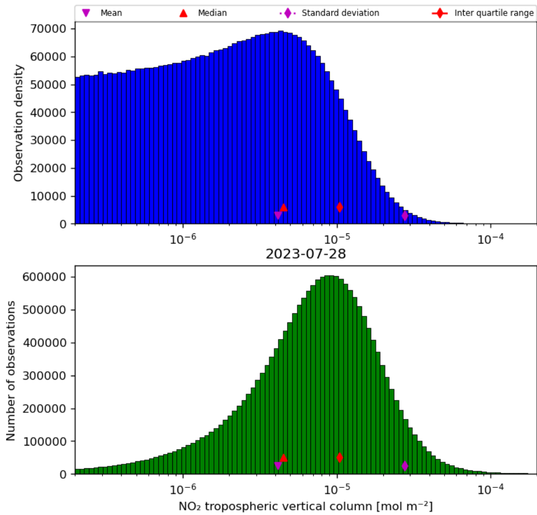
Figure 29: Histogram of “NO 2 tropospheric vertical column” for 2023-07-27 to 2023-07-29
