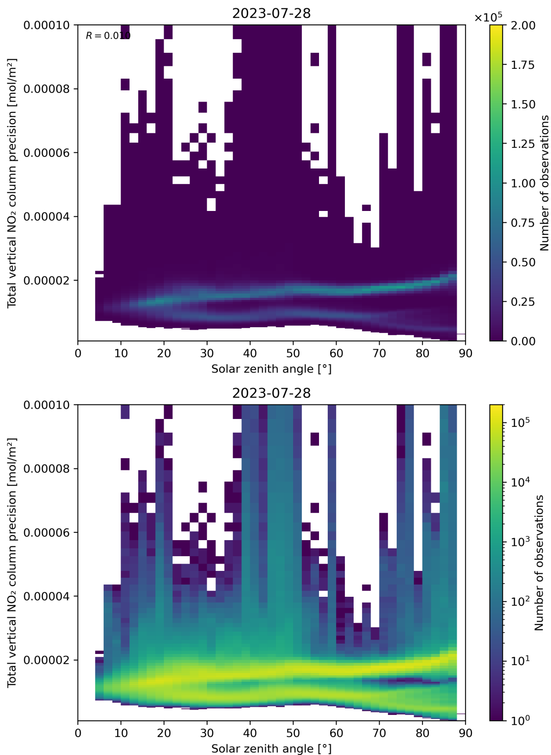
Figure 154: Scatter density plot of “Solar zenith angle” against “Total vertical NO 2 column precision” for 2023-07-27 to 2023-07-29.
