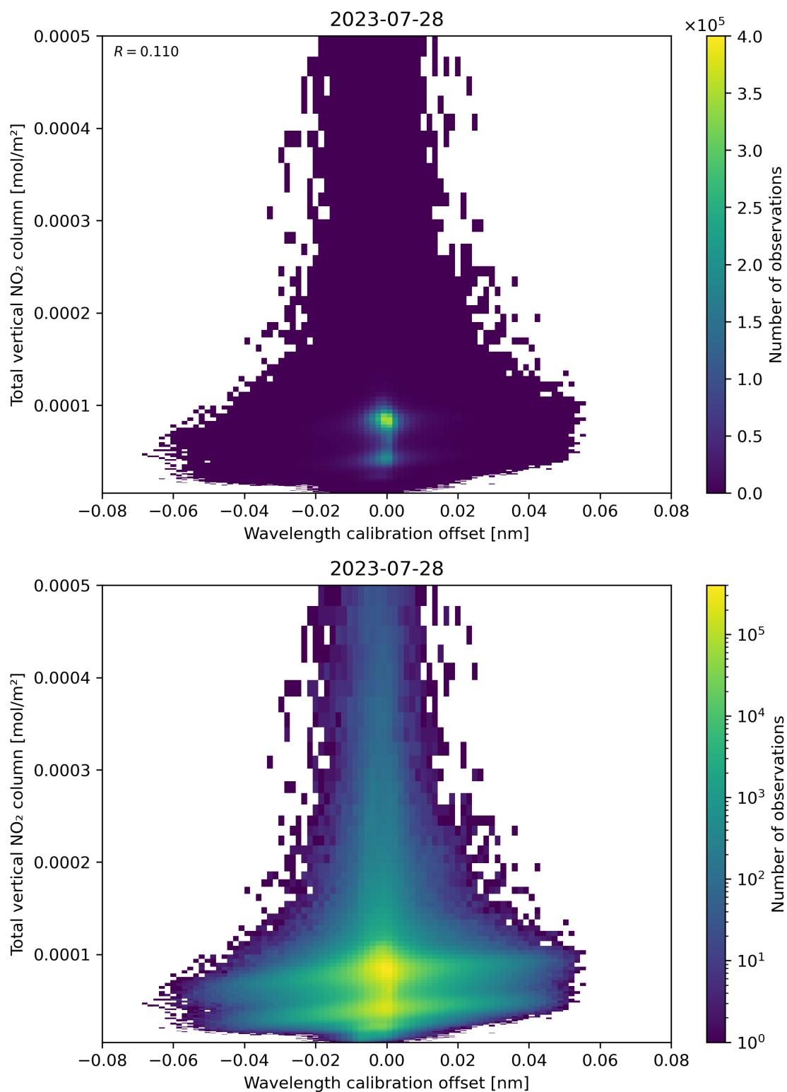
Figure 179: Scatter density plot of “Wavelength calibration offset” against “Total vertical NO 2 column” for 2023-07-27 to 2023-07-29.
