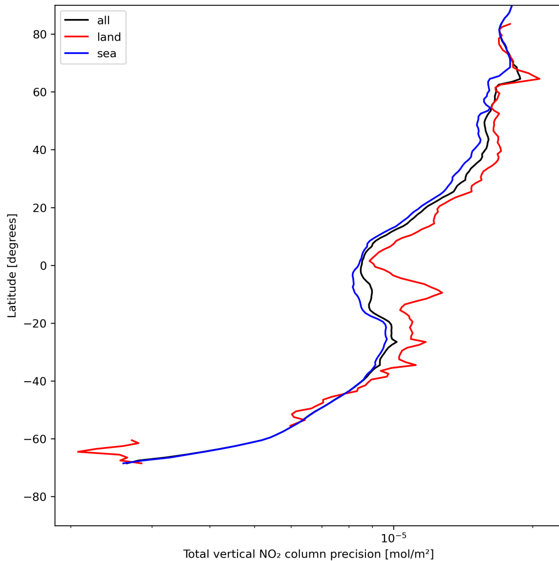
Figure 22: Zonal average of “Total vertical NO 2 column precision” for 2023-07-27 to 2023-07-29.
