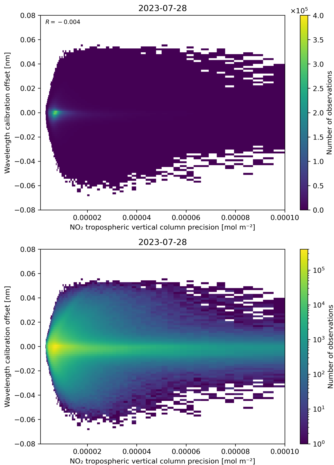
Figure 141: Scatter density plot of “NO 2 tropospheric vertical column precision” against “Wavelength calibration offset” for 2023-07-27 to 2023-07-29.
