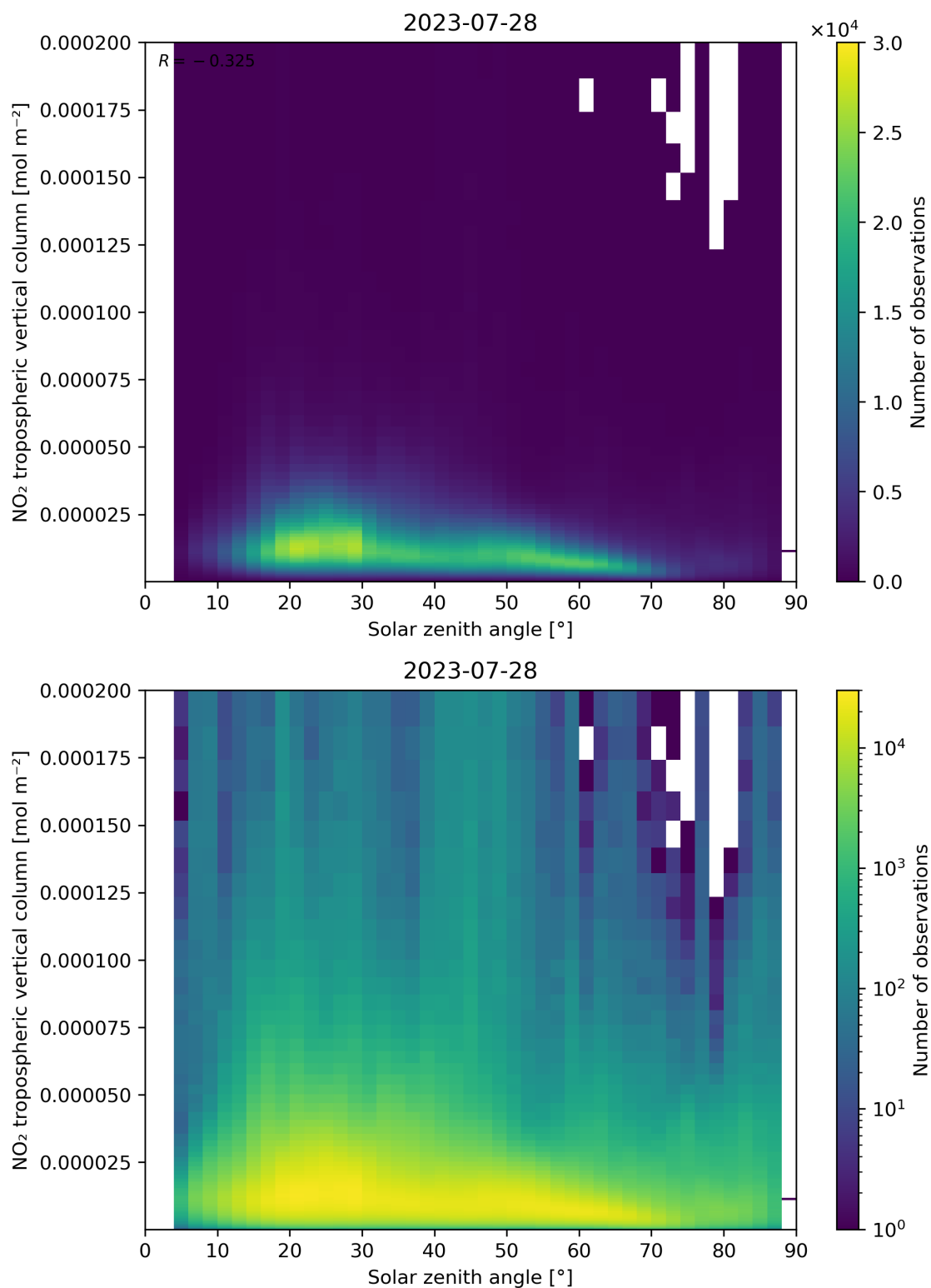
Figure 155: Scatter density plot of “Solar zenith angle” against “NO 2 tropospheric vertical column” for 2023-07-27 to 2023-07-29.
