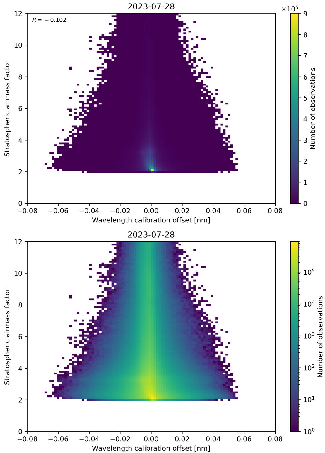
Figure 174: Scatter density plot of “Wavelength calibration offset” against “Stratospheric air mass factor” for 2023-07-27 to 2023-07-29.
