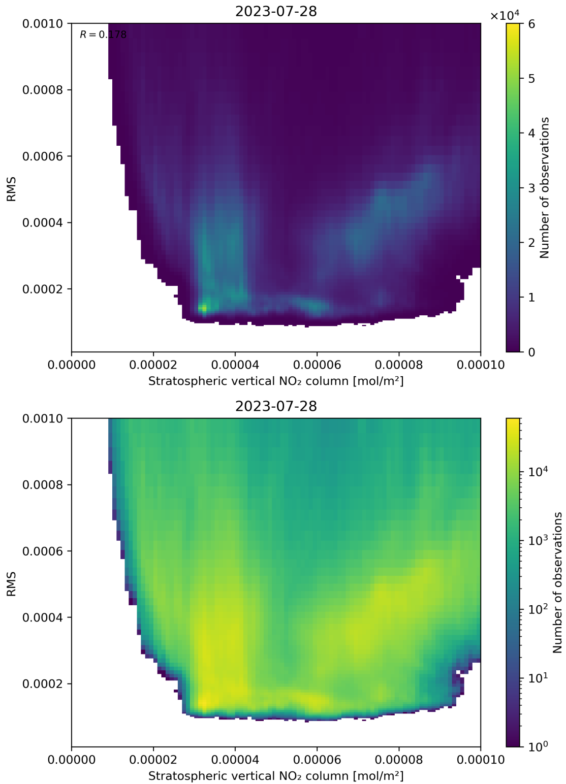
Figure 102: Scatter density plot of “Stratospheric vertical NO 2 column” against “RMS” for 2023-07-27 to 2023-07-29.
