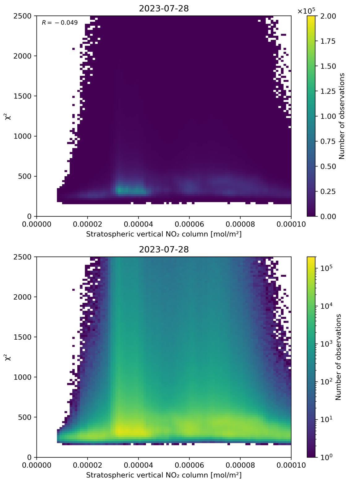
Figure 97: Scatter density plot of “Stratospheric vertical NO 2 column” against “ \chi^2 ” for 2023-07-27 to 2023-07-29.
