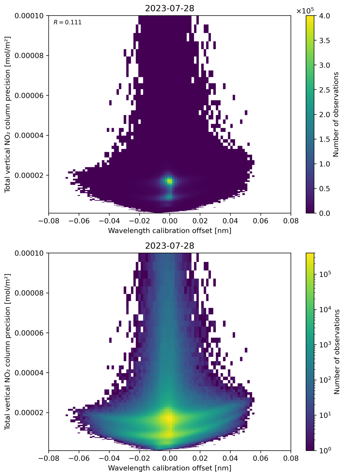
Figure 180: Scatter density plot of “Wavelength calibration offset” against “Total vertical NO 2 column precision” for 2023-07-27 to 2023-07-29.
