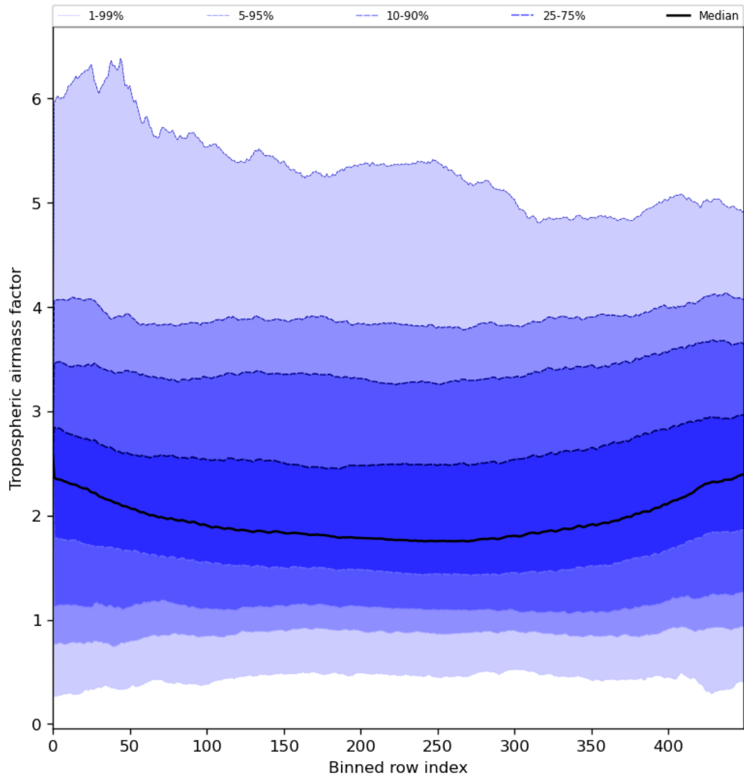
Figure 48: Along track statistics of “Tropospheric airmass factor” for 2023-07-27 to 2023-07-29
