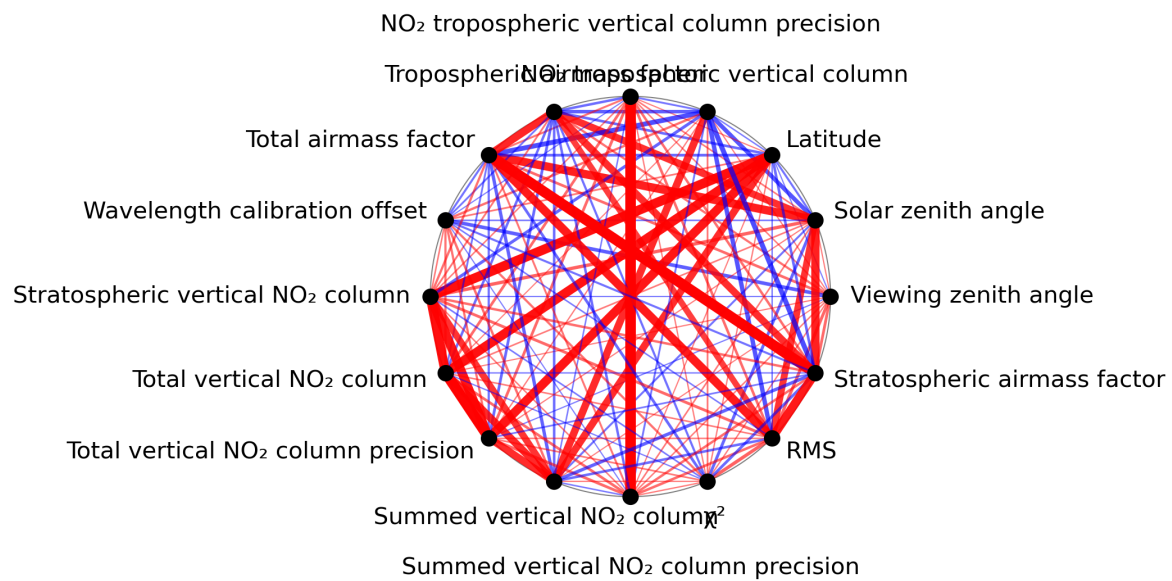
Figure 1: Map of correlation graph for 2023-07-27 to 2023-07-29.
