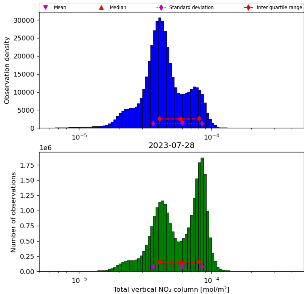
Figure 38: Histogram of “Total vertical NO 2 column” for 2023-07-27 to 2023-07-29
