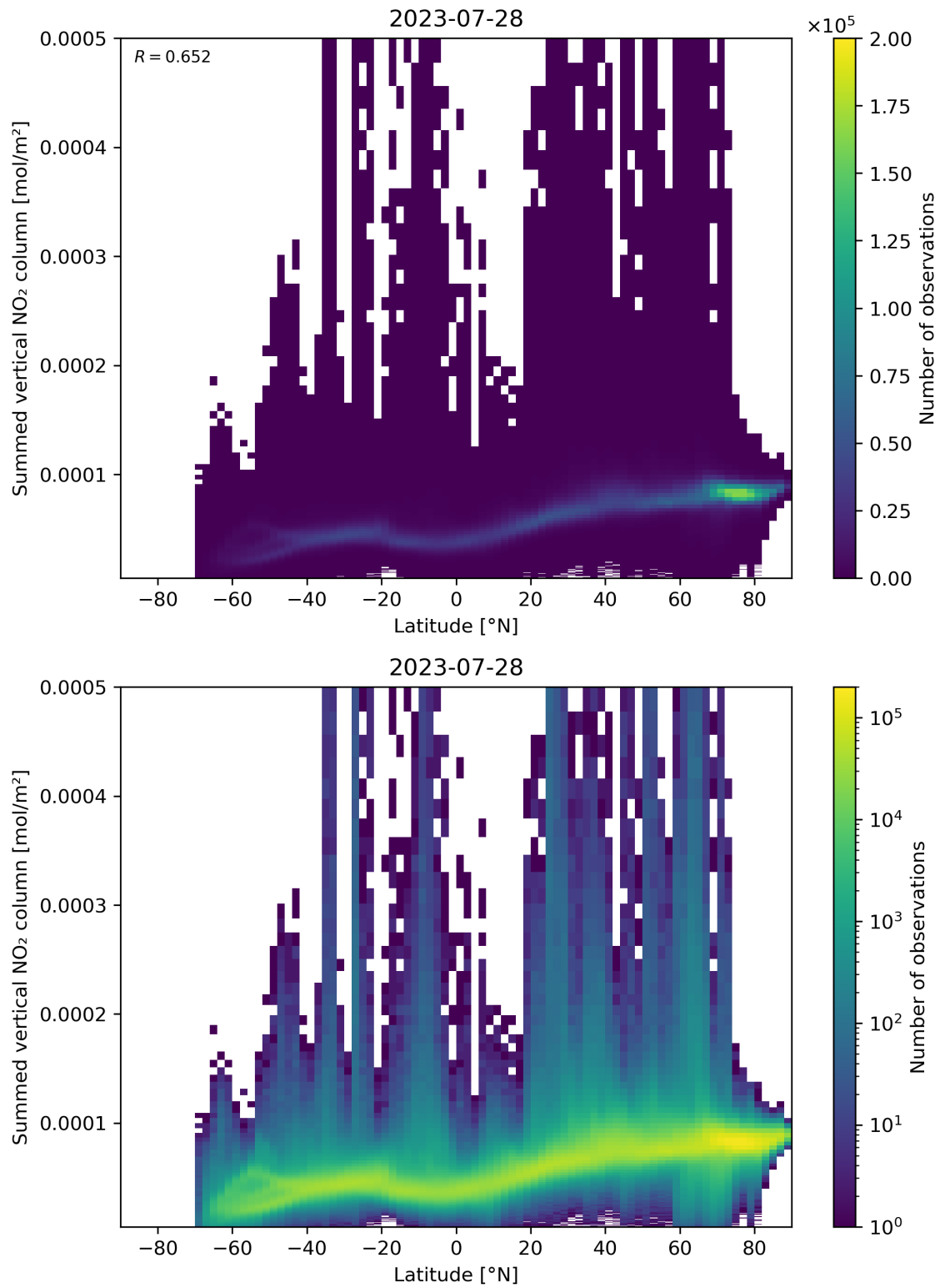
Figure 88: Scatter density plot of “Latitude” against “Summed vertical NO 2 column” for 2023-07-27 to 2023-07-29.
