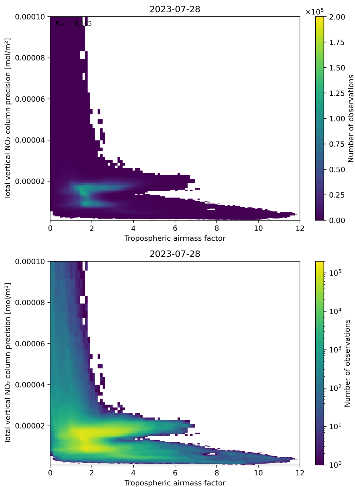
Figure 78: Scatter density plot of “Tropospheric air mass factor” against “Total vertical NO 2 column precision” for 2023-07-27 to 2023-07-29.
