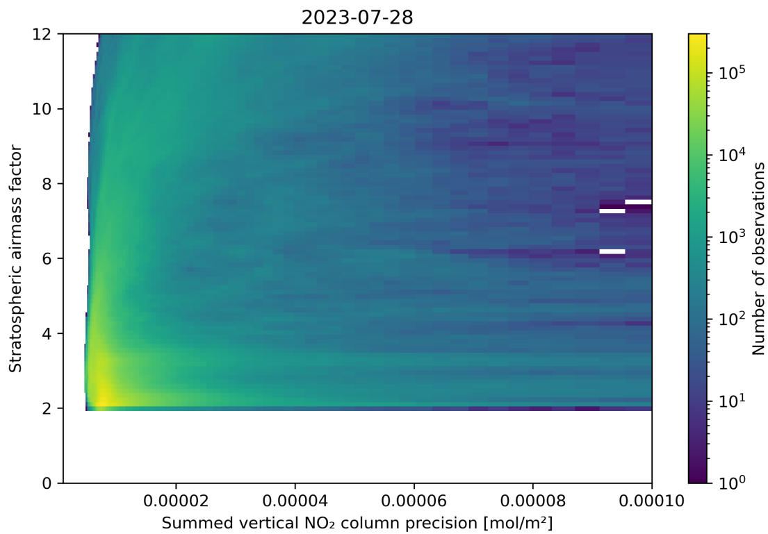
Figure 106: Scatter density plot of “Summed vertical NO 2 column precision” against “Stratospheric airmass factor” for 2023-07-27 to 2023-07-29.
