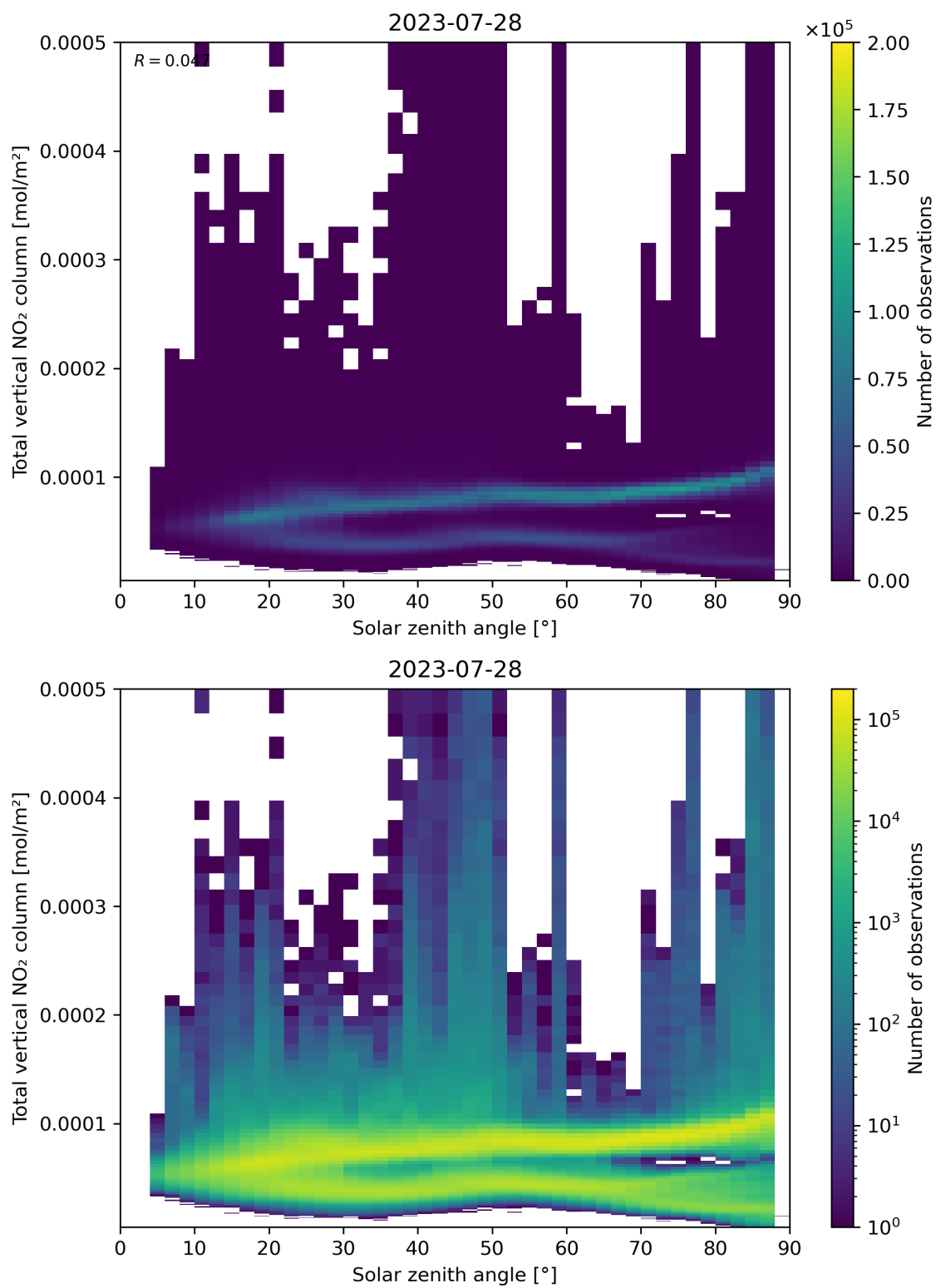
Figure 153: Scatter density plot of “Solar zenith angle” against “Total vertical NO 2 column” for 2023-07-27 to 2023-07-29.
