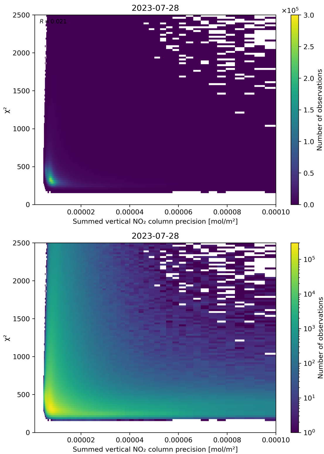
Figure 107: Scatter density plot of “Summed vertical NO 2 column precision” against “ \chi^2 ” for 2023-07-27 to 2023-07-29.
