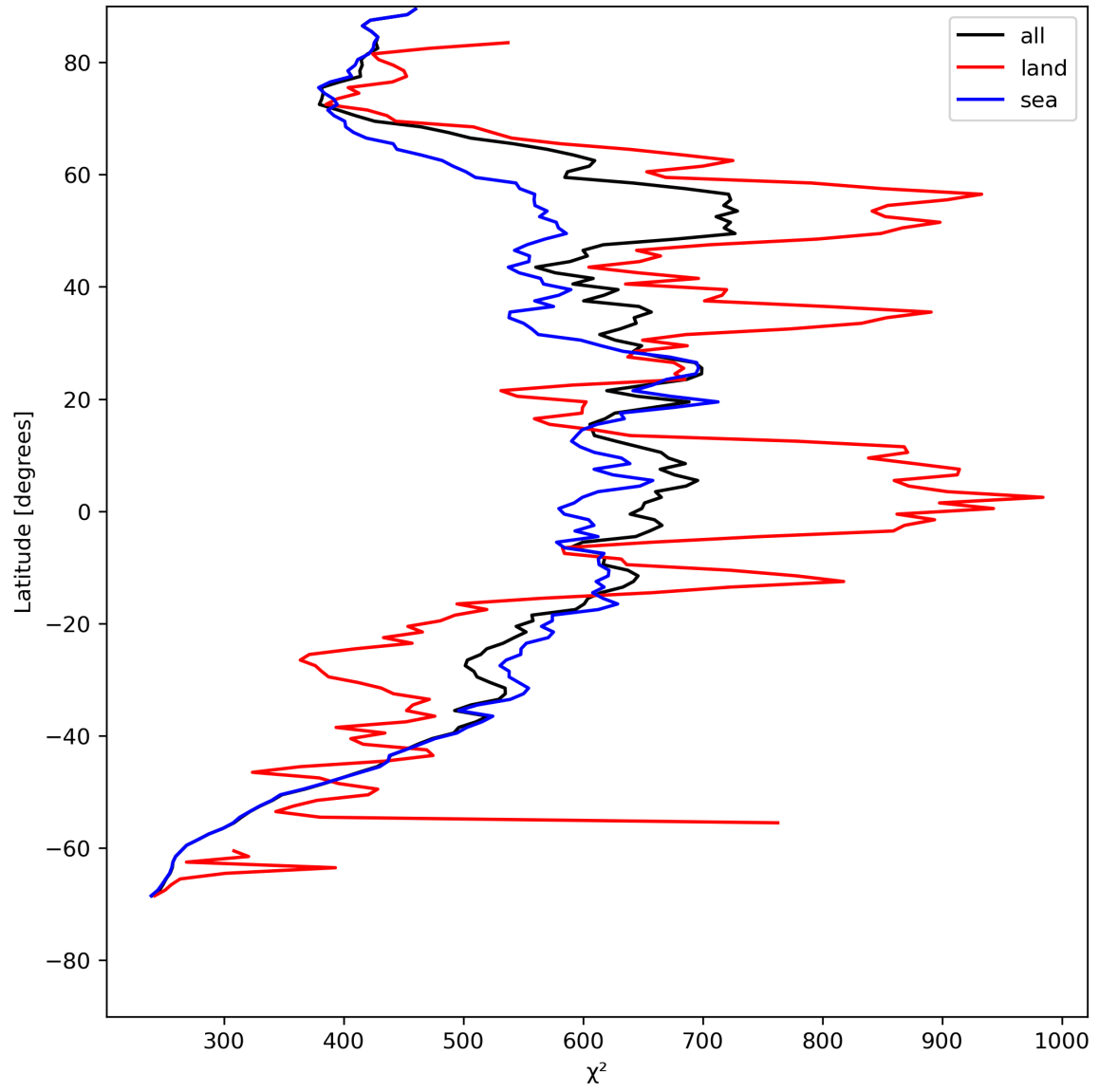
Figure 25: Zonal average of “ \chi^2 ” for 2023-07-27 to 2023-07-29.
