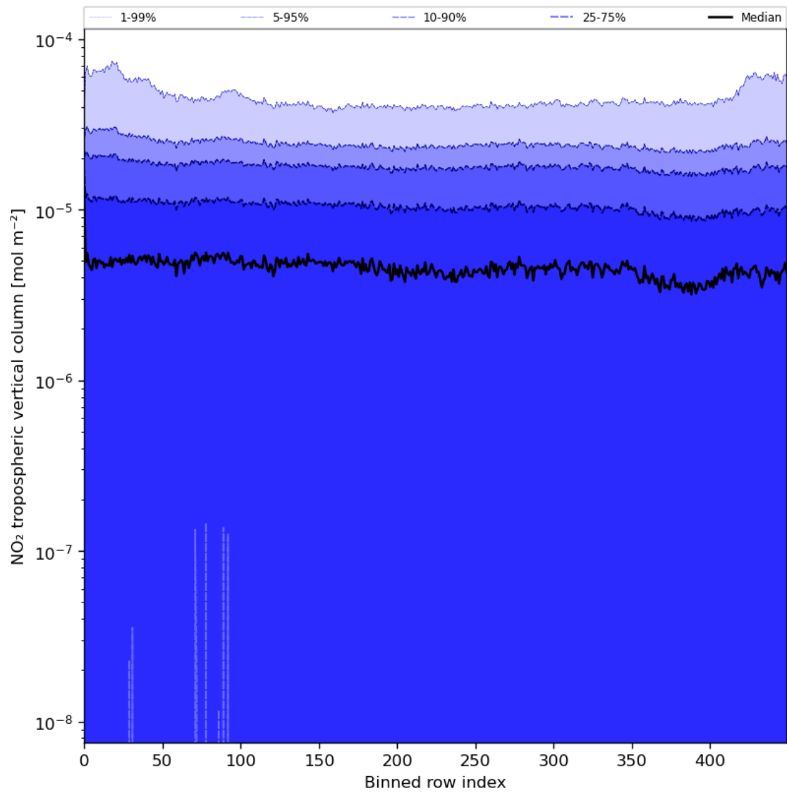
Figure 46: Along track statistics of “ \text{NO}_2 tropospheric vertical column” for 2023-07-27 to 2023-07-29
