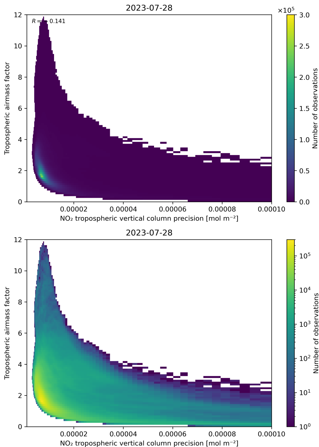
Figure 133: Scatter density plot of “NO 2 tropospheric vertical column precision” against “Tropospheric airmass factor” for 2023-07-27 to 2023-07-29.
