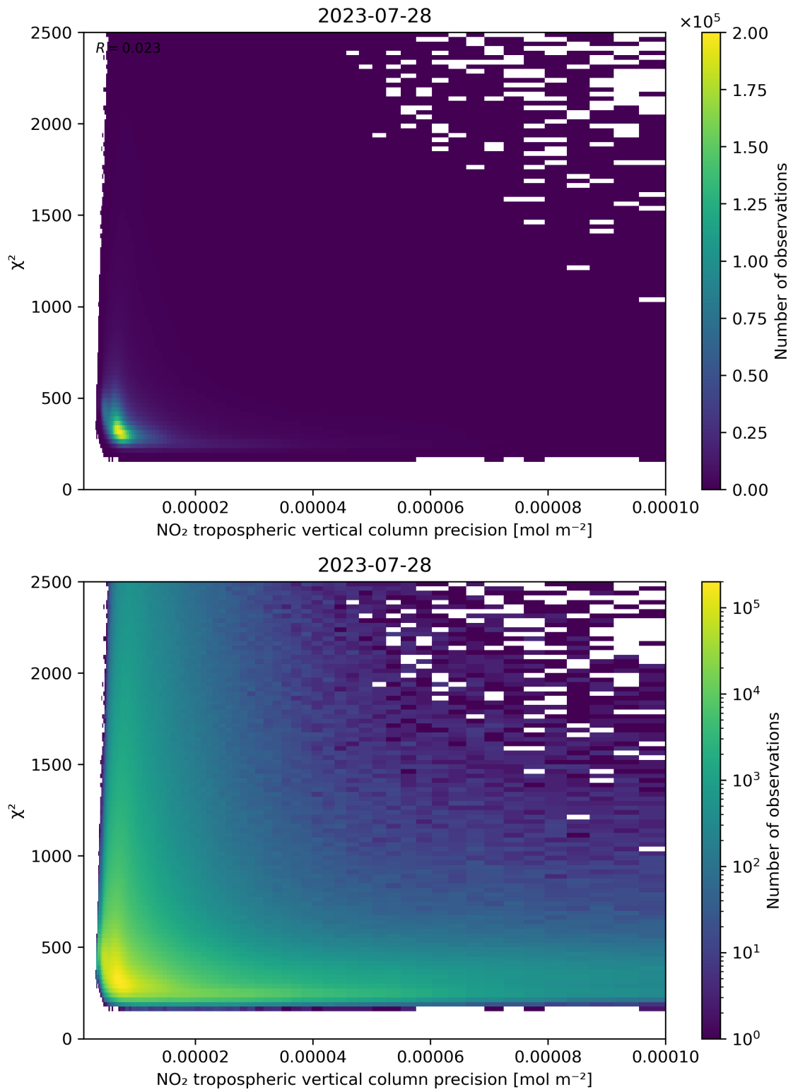
Figure 134: Scatter density plot of “NO 2 tropospheric vertical column precision” against “ \chi^2 ” for 2023-07-27 to 2023-07-29.
