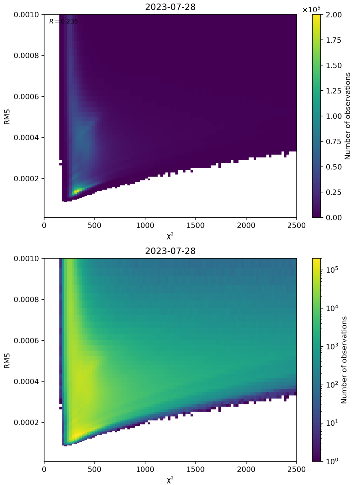
Figure 82: Scatter density plot of “ \chi^2 ” against “RMS” for 2023-07-27 to 2023-07-29.
