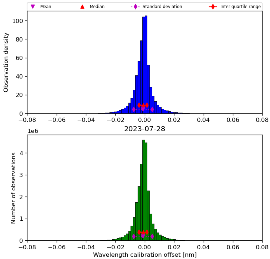
Figure 35: Histogram of “Wavelength calibration offset” for 2023-07-27 to 2023-07-29
