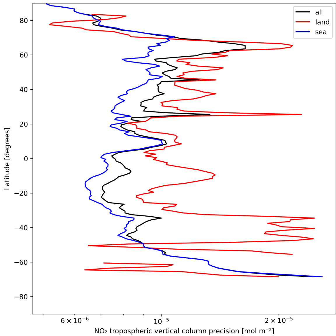
Figure 13: Zonal average of “NO 2 tropospheric vertical column precision” for 2023-07-27 to 2023-07-29.
