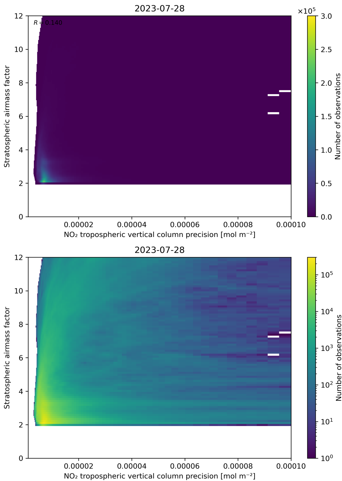
Figure 131: Scatter density plot of “NO 2 tropospheric vertical column precision” against “Stratospheric airmass factor” for 2023-07-27 to 2023-07-29.
