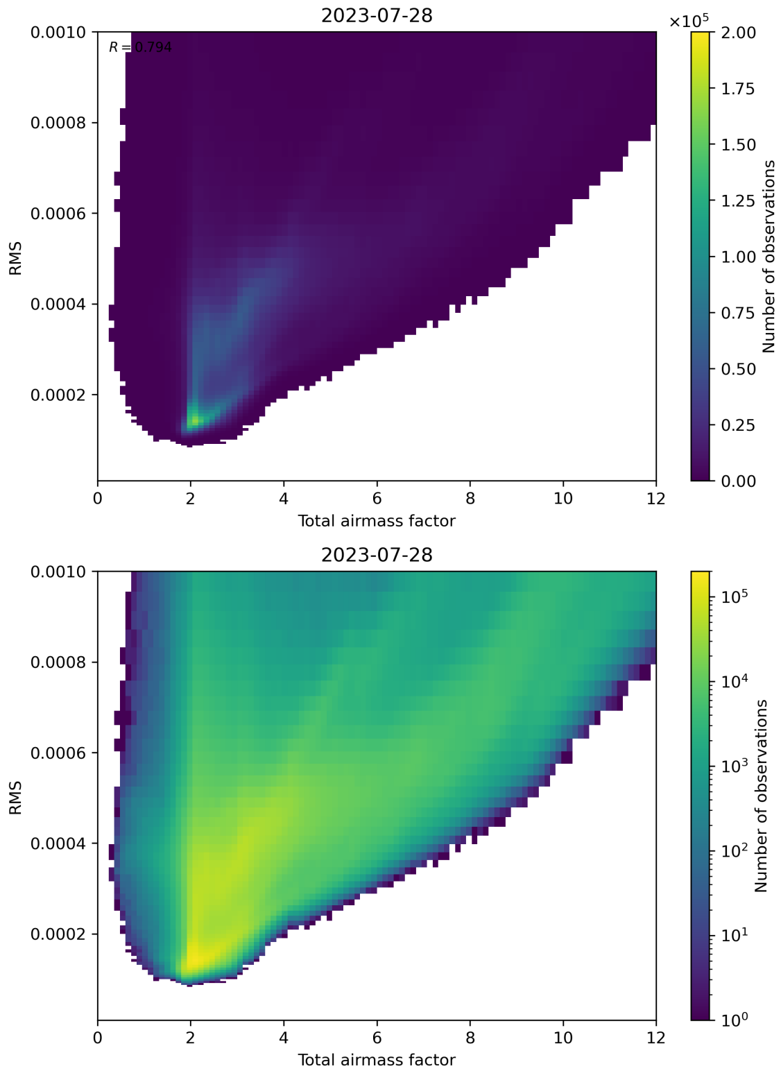
Figure 69: Scatter density plot of “Total airmass factor” against “RMS” for 2023-07-27 to 2023-07-29.
