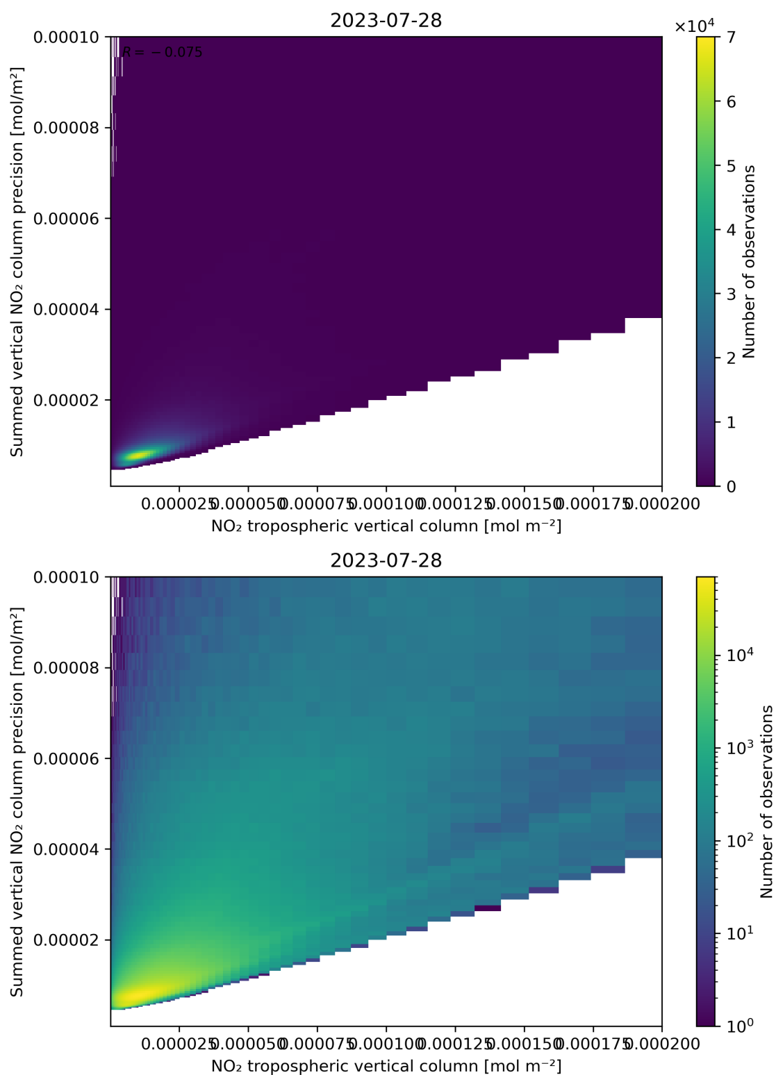
Figure 127: Scatter density plot of “NO 2 tropospheric vertical column” against “Summed vertical NO 2 column precision” for 2023-07-27 to 2023-07-29.
