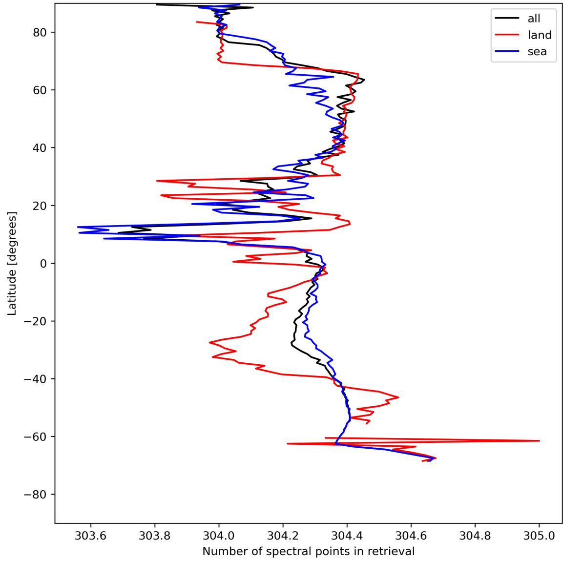
Figure 16: Zonal average of “Number of spectral points in retrieval” for 2023-07-27 to 2023-07-29.
