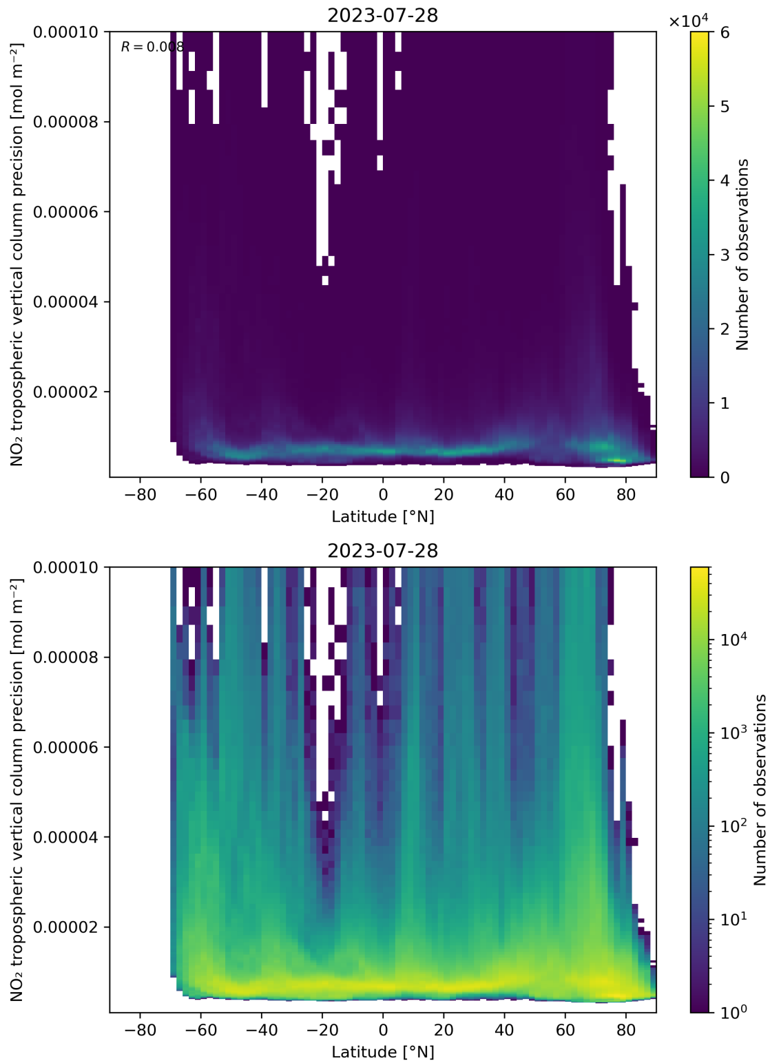
Figure 93: Scatter density plot of “Latitude” against “NO 2 tropospheric vertical column precision” for 2023-07-27 to 2023-07-29.
