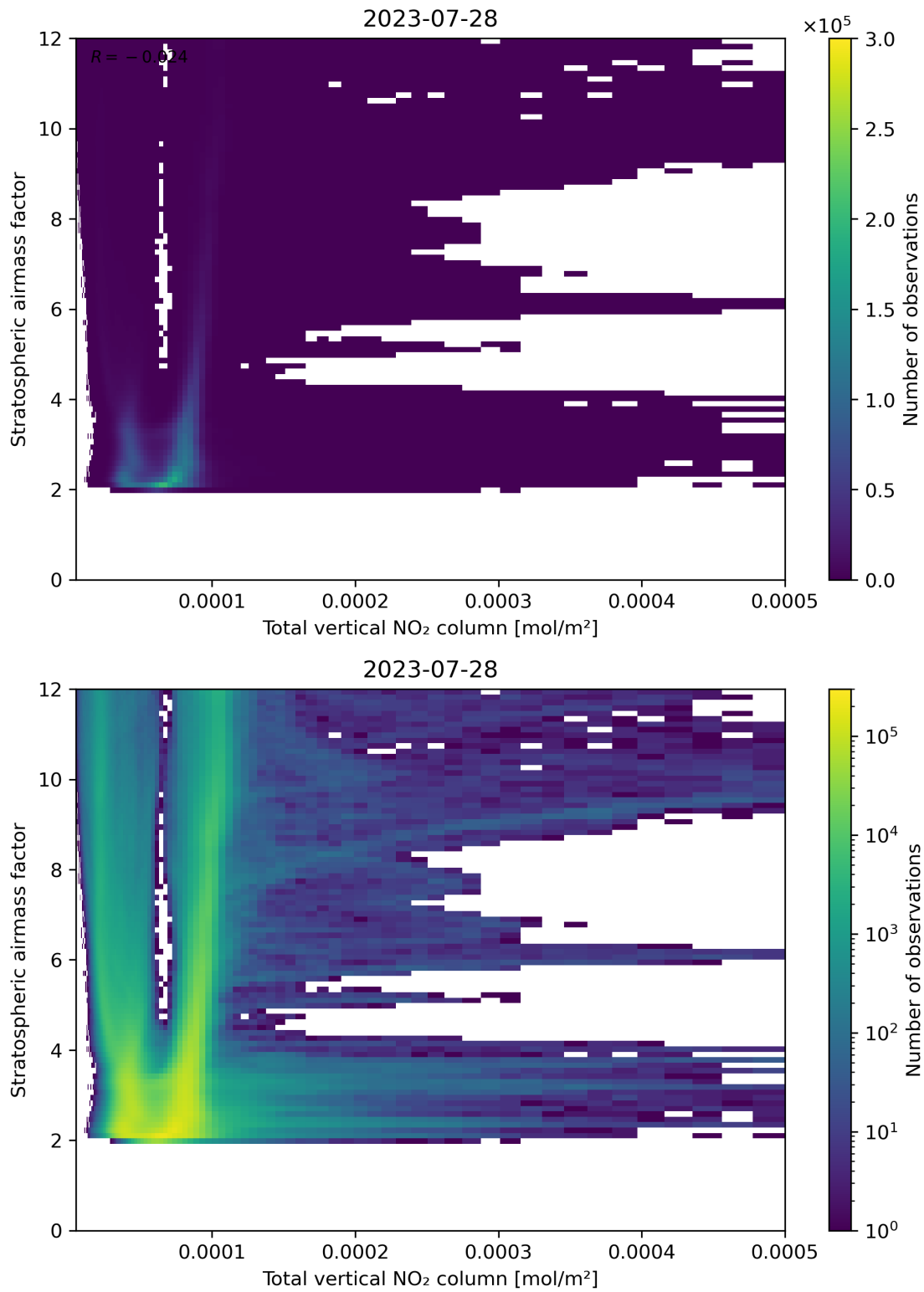
Figure 110: Scatter density plot of “Total vertical NO 2 column” against “Stratospheric airmass factor” for 2023-07-27 to 2023-07-29.
