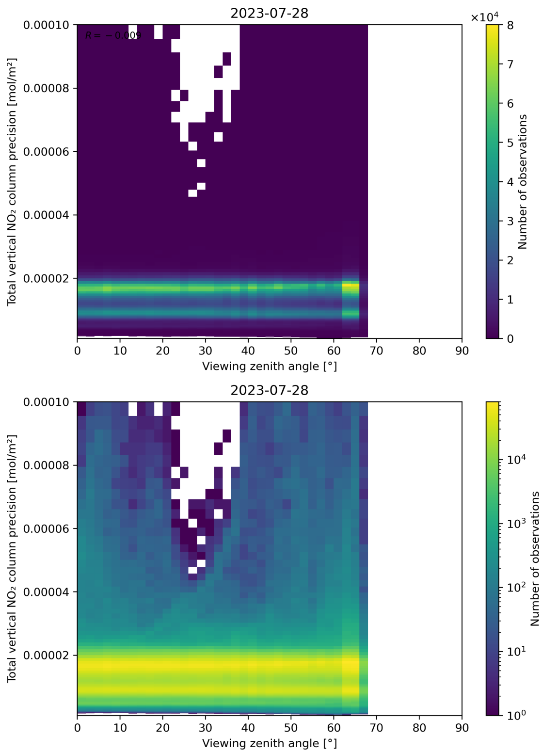
Figure 168: Scatter density plot of “Viewing zenith angle” against “Total vertical NO 2 column precision” for 2023-07-27 to 2023-07-29.
