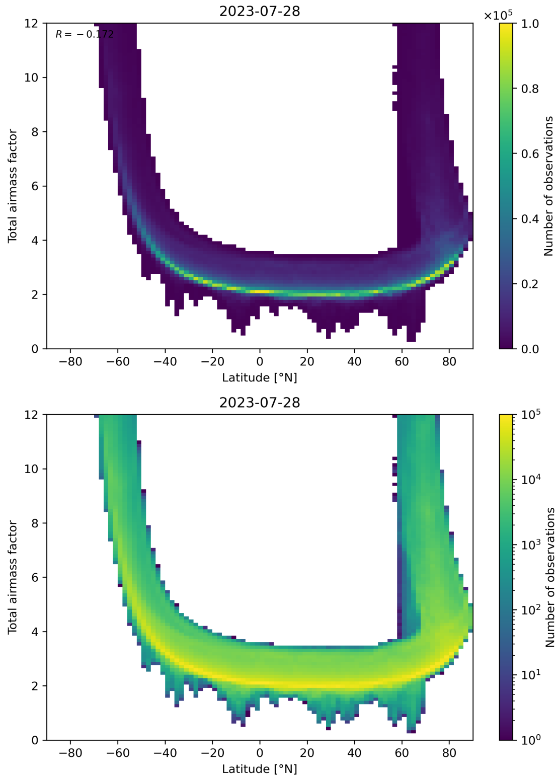
Figure 84: Scatter density plot of “Latitude” against “Total airmass factor” for 2023-07-27 to 2023-07-29.
