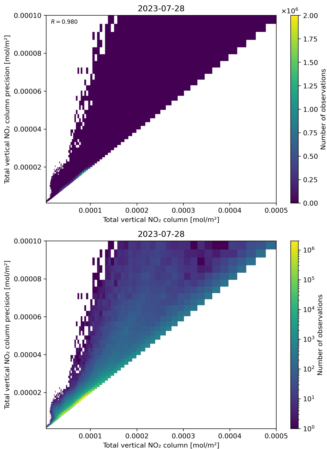
Figure 114: Scatter density plot of “Total vertical NO 2 column” against “Total vertical NO 2 column precision” for 2023-07-27 to 2023-07-29.
