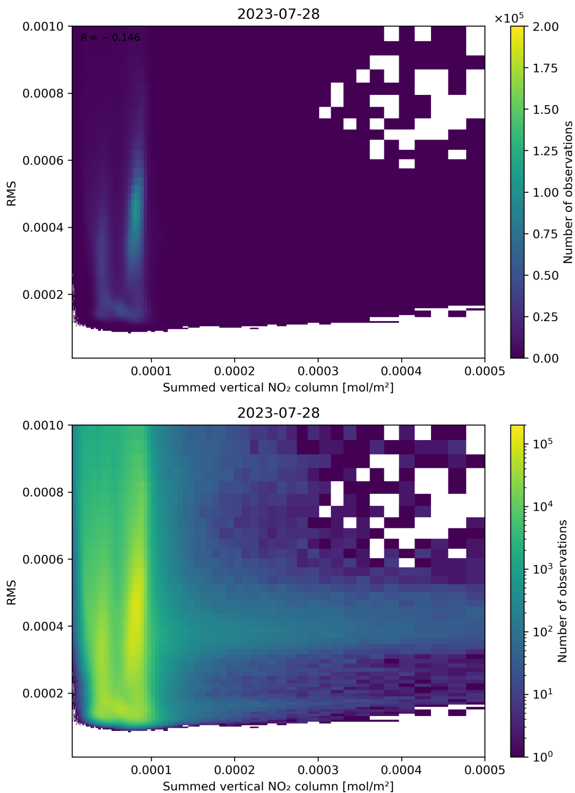
Figure 109: Scatter density plot of “Summed vertical NO 2 column” against “RMS” for 2023-07-27 to 2023-07-29.
