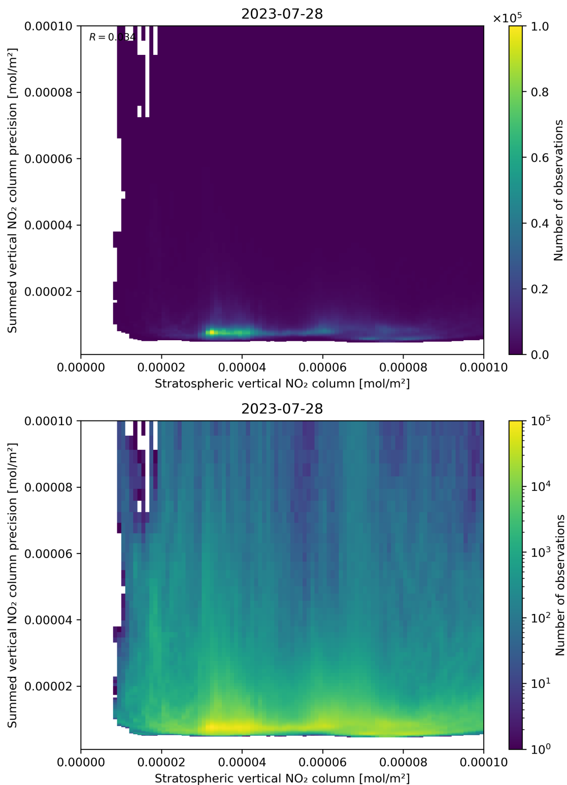
Figure 99: Scatter density plot of “Stratospheric vertical NO 2 column” against “Summed vertical NO 2 column precision” for 2023-07-27 to 2023-07-29.
