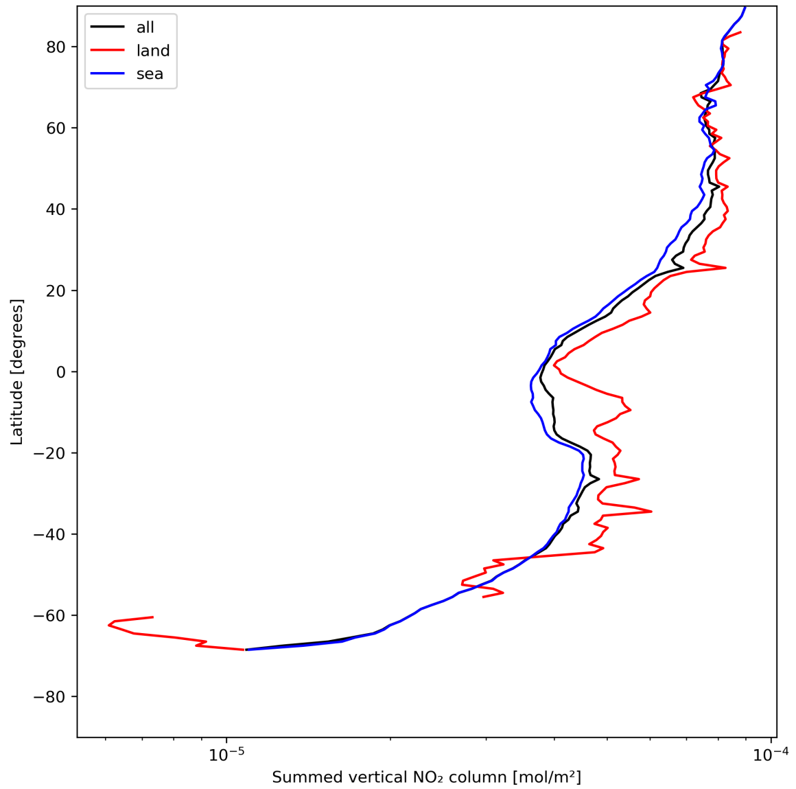
Figure 23: Zonal average of “Summed vertical NO 2 column” for 2023-07-27 to 2023-07-29.
