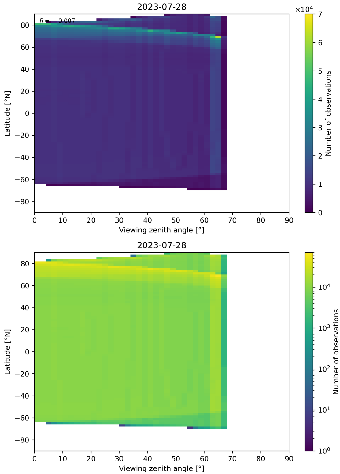
Figure 163: Scatter density plot of “Viewing zenith angle” against “Latitude” for 2023-07-27 to 2023-07-29.
