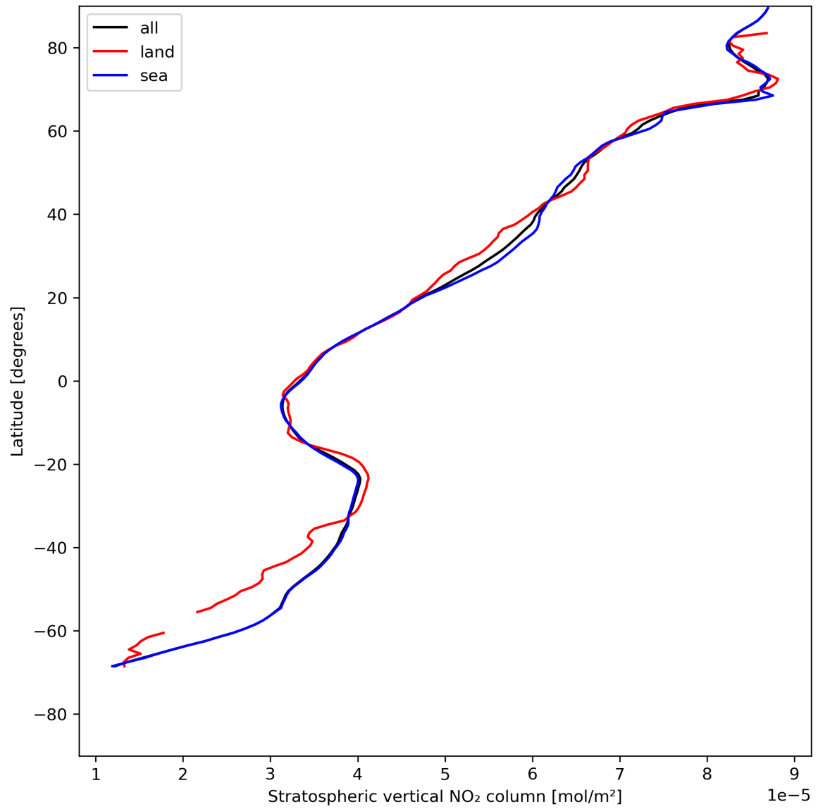
Figure 19: Zonal average of “Stratospheric vertical NO 2 column” for 2023-07-27 to 2023-07-29.
