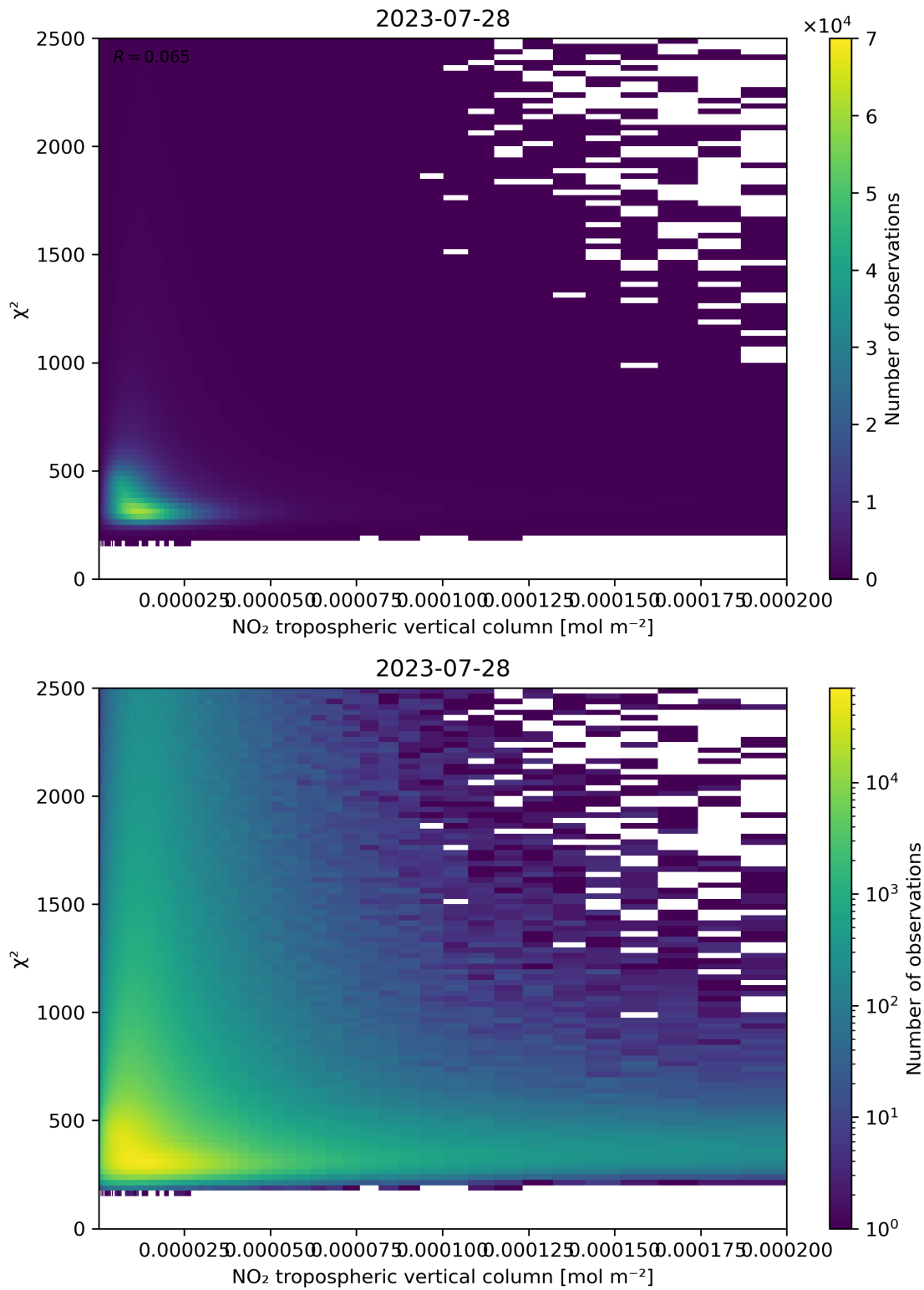
Figure 124: Scatter density plot of “NO 2 tropospheric vertical column” against “ \chi^2 ” for 2023-07-27 to 2023-07-29.
