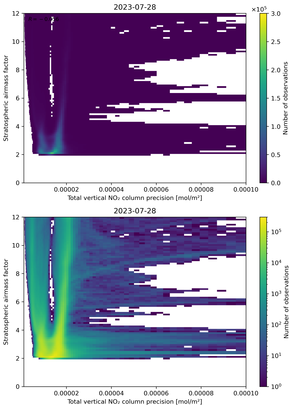
Figure 115: Scatter density plot of “Total vertical NO 2 column precision” against “Stratospheric air mass factor” for 2023-07-27 to 2023-07-29.
