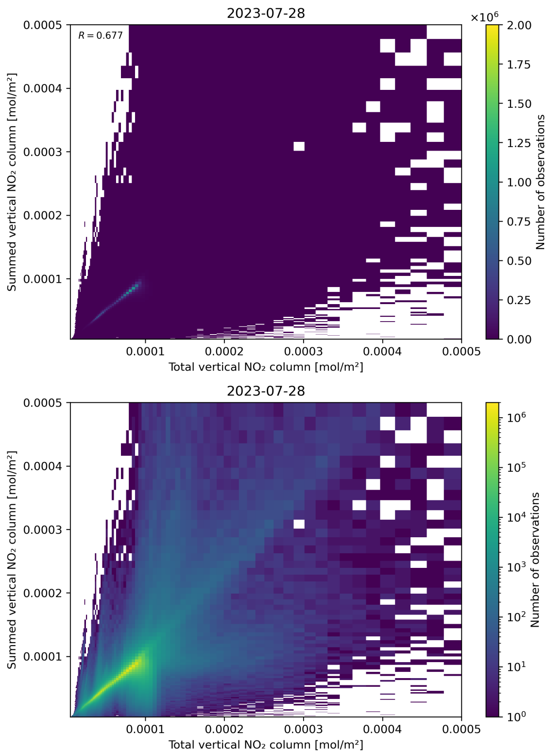
Figure 112: Scatter density plot of “Total vertical NO 2 column” against “Summed vertical NO 2 column” for 2023-07-27 to 2023-07-29.
