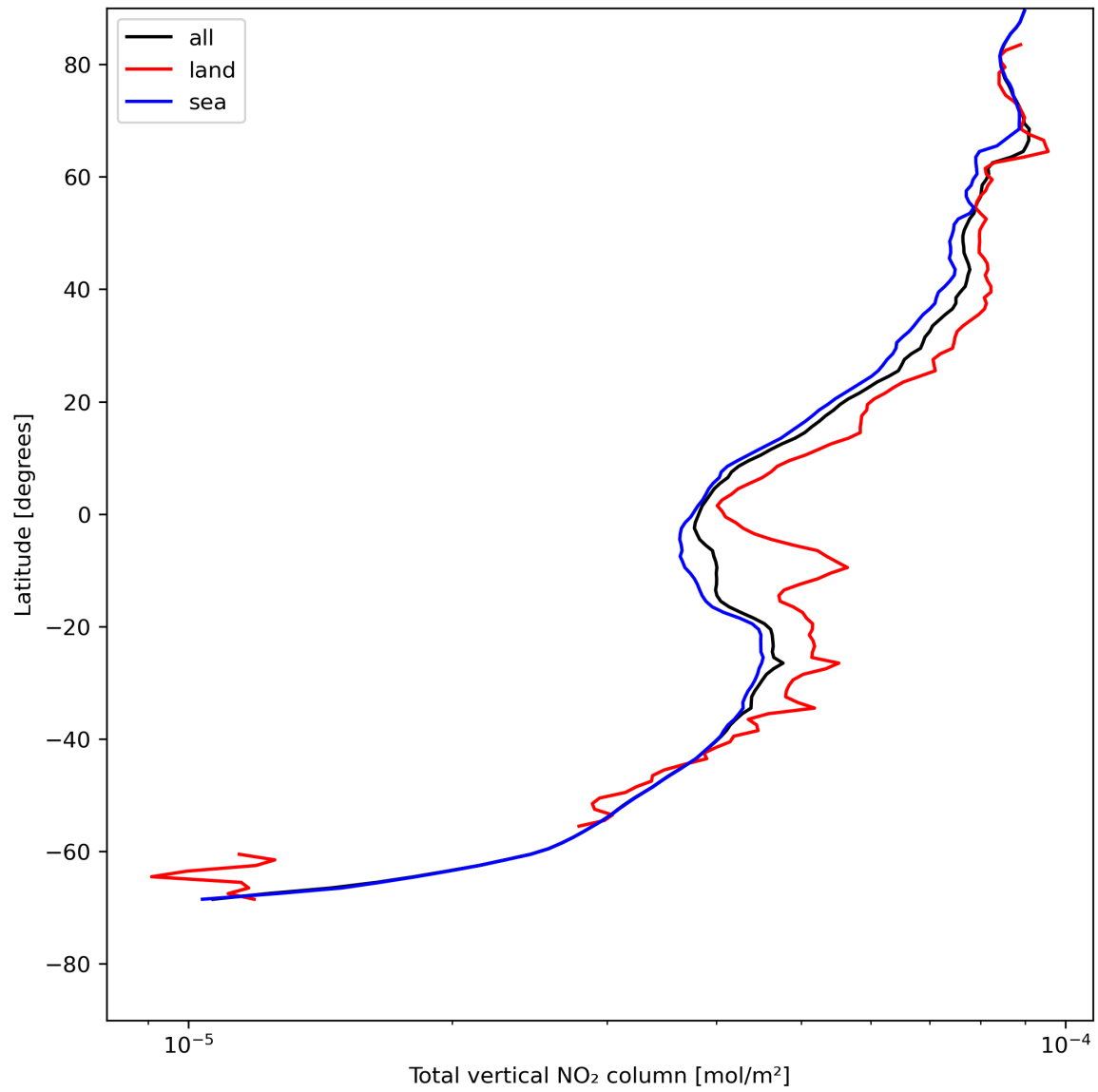
Figure 21: Zonal average of “Total vertical NO 2 column” for 2023-07-27 to 2023-07-29.
