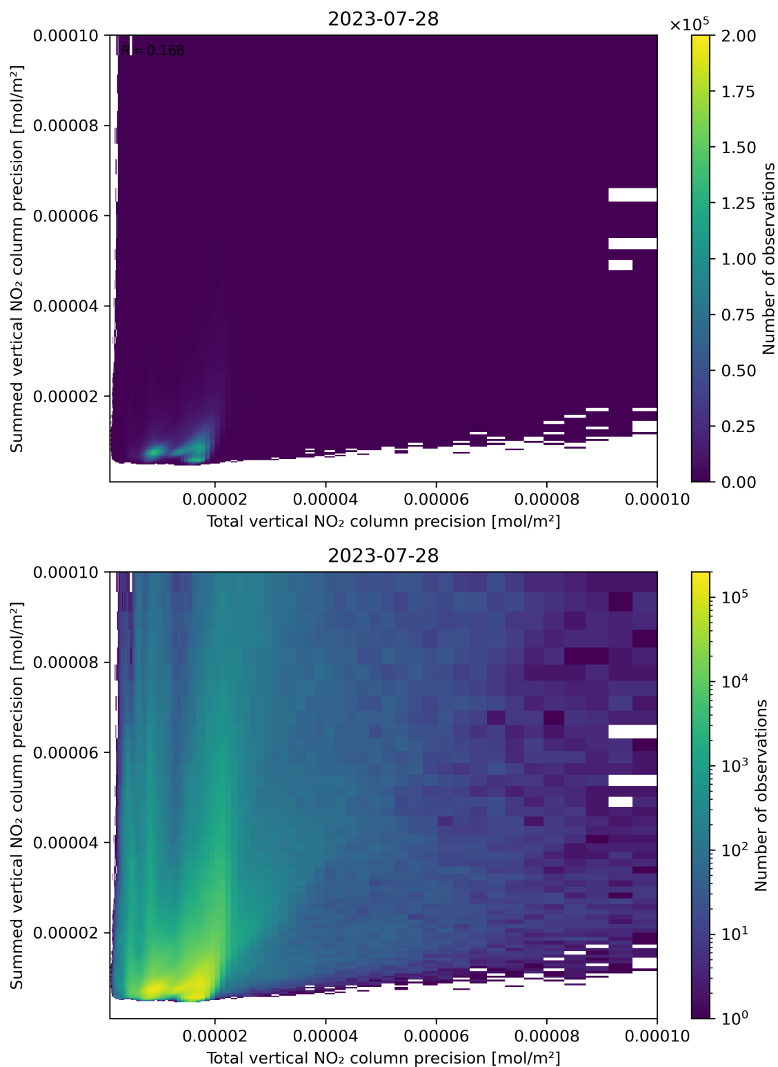
Figure 118: Scatter density plot of “Total vertical NO 2 column precision” against “Summed vertical NO 2 column precision” for 2023-07-27 to 2023-07-29.
