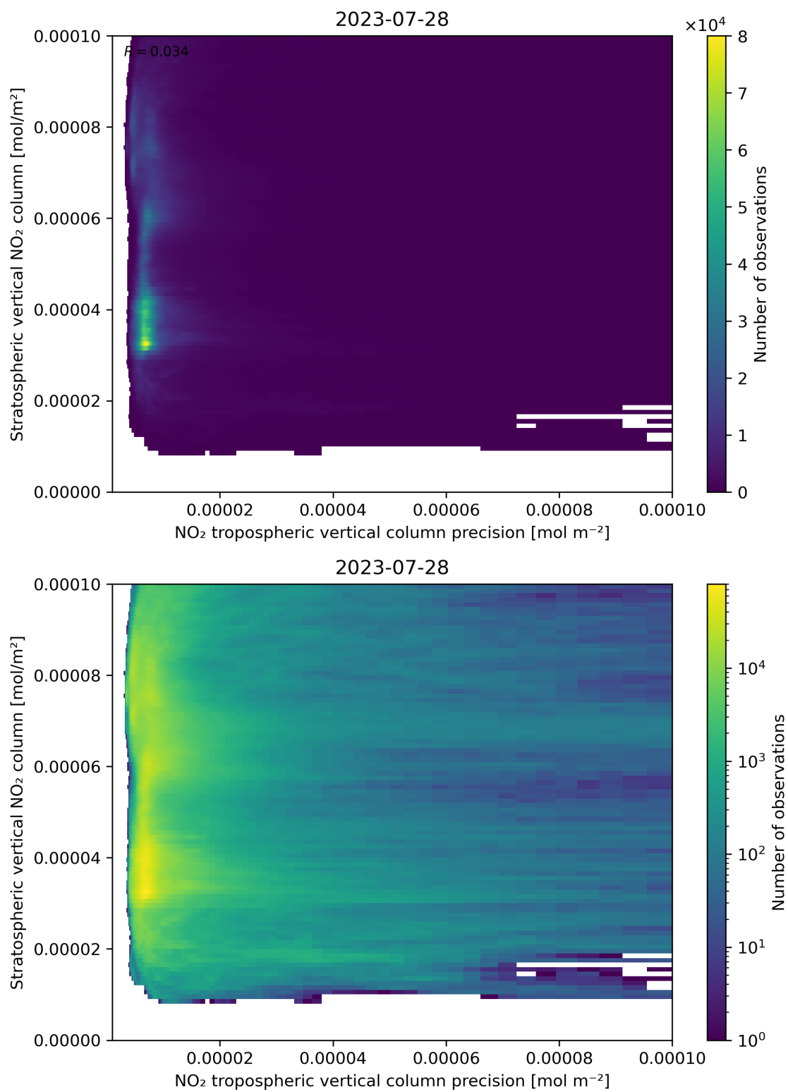
Figure 135: Scatter density plot of “NO 2 tropospheric vertical column precision” against “Stratospheric vertical NO 2 column” for 2023-07-27 to 2023-07-29.
