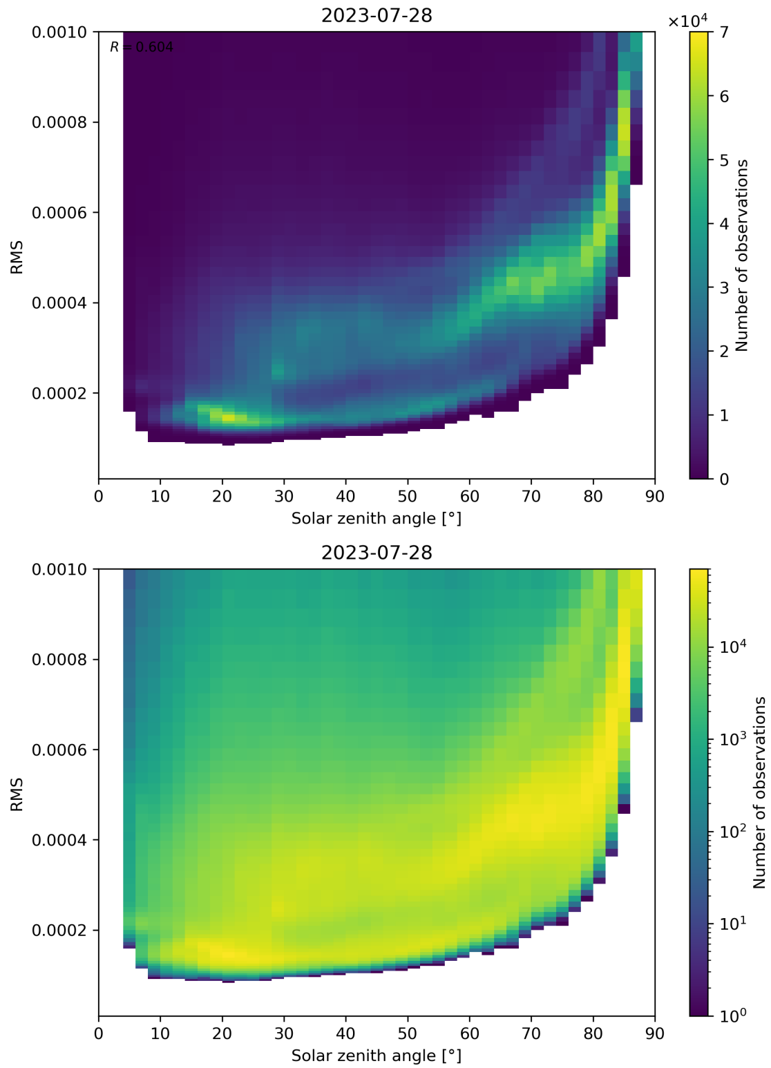
Figure 157: Scatter density plot of “Solar zenith angle” against “RMS” for 2023-07-27 to 2023-07-29.
