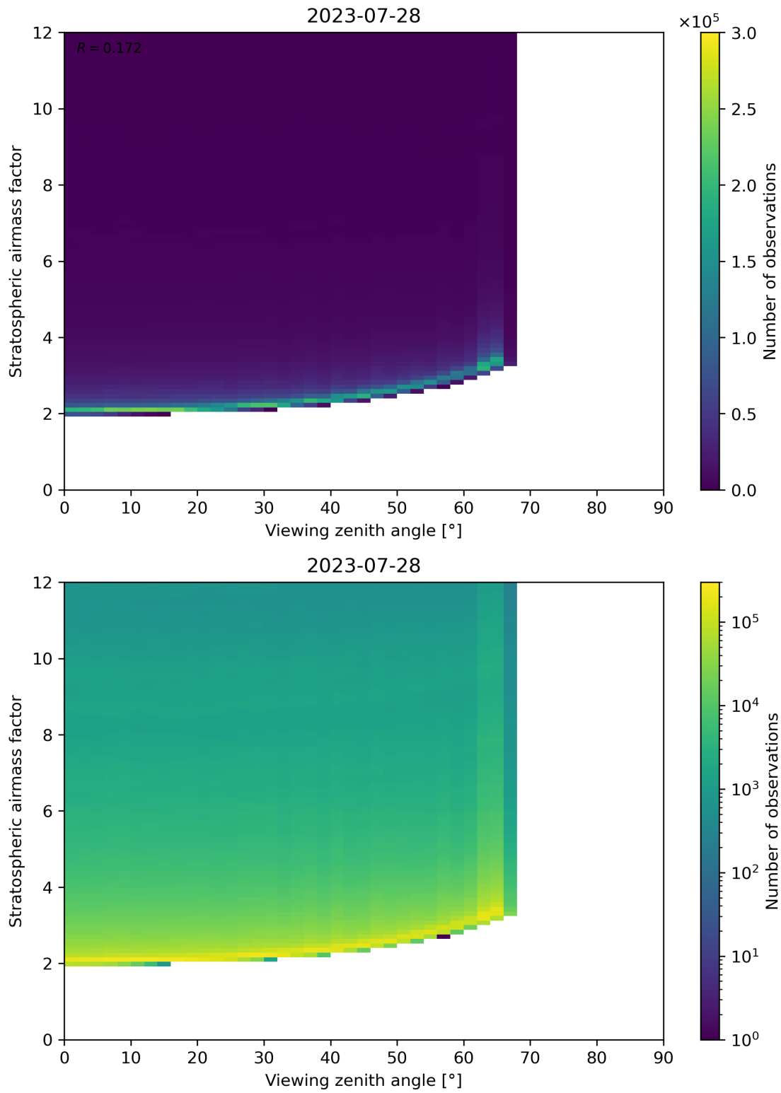
Figure 159: Scatter density plot of “Viewing zenith angle” against “Stratospheric airmass factor” for 2023-07-27 to 2023-07-29.
