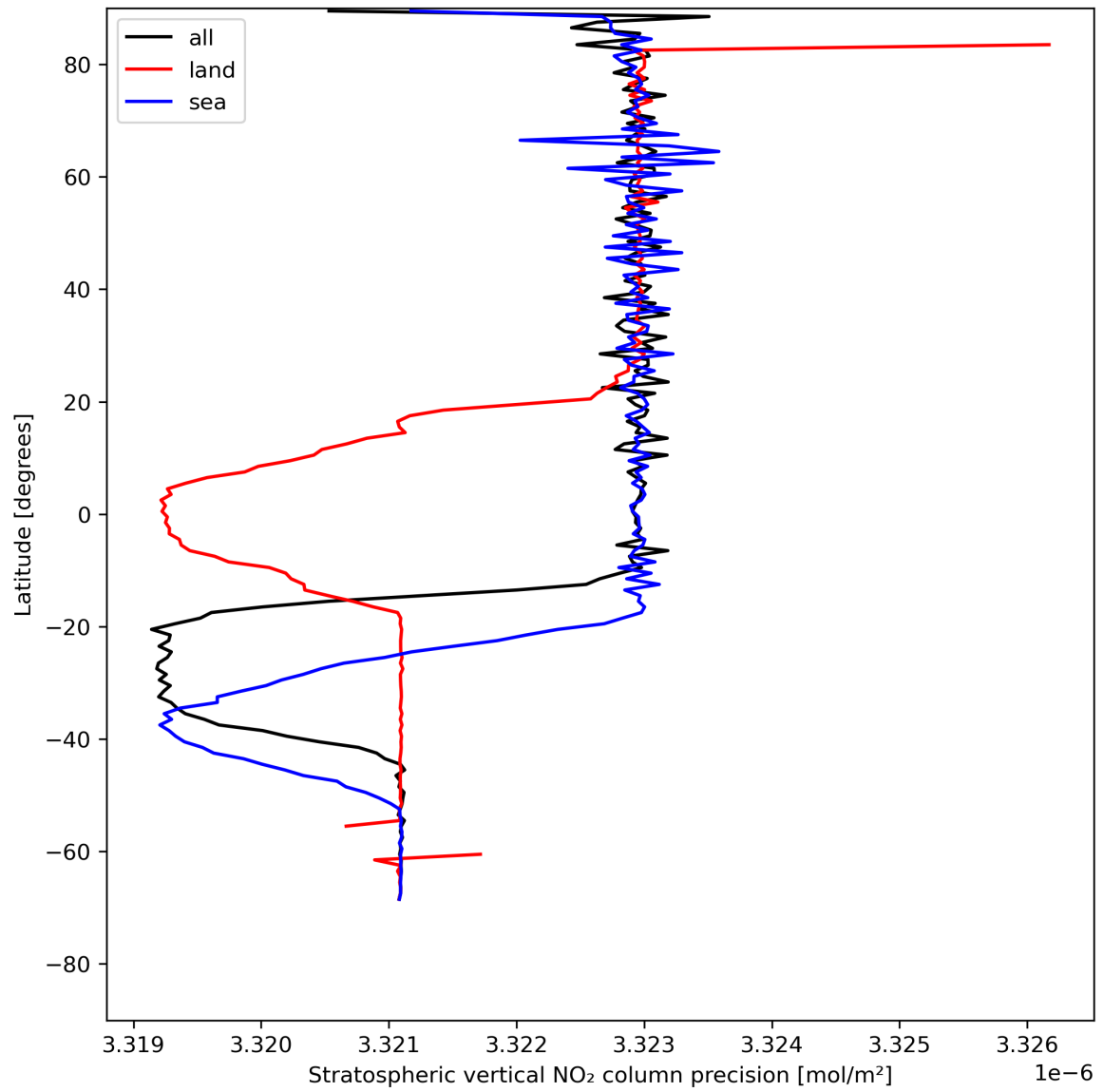
Figure 20: Zonal average of “Stratospheric vertical NO 2 column precision” for 2023-07-27 to 2023-07-29.
