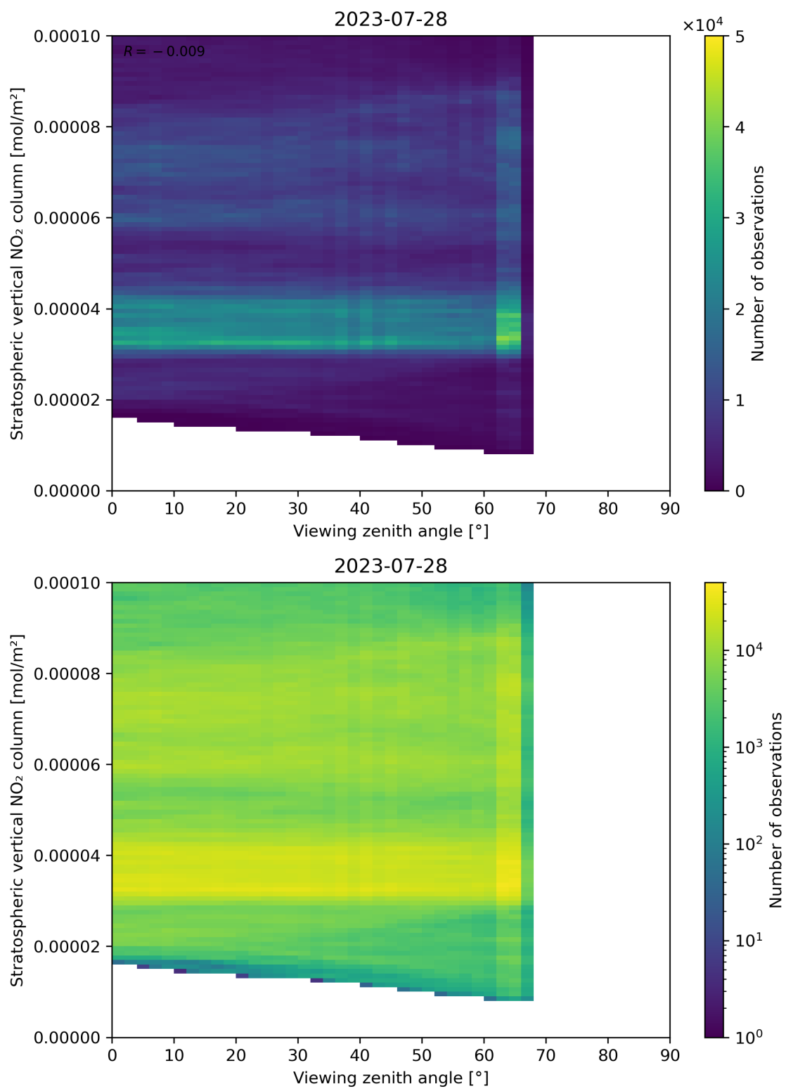
Figure 164: Scatter density plot of “Viewing zenith angle” against “Stratospheric vertical NO 2 column” for 2023-07-27 to 2023-07-29.
