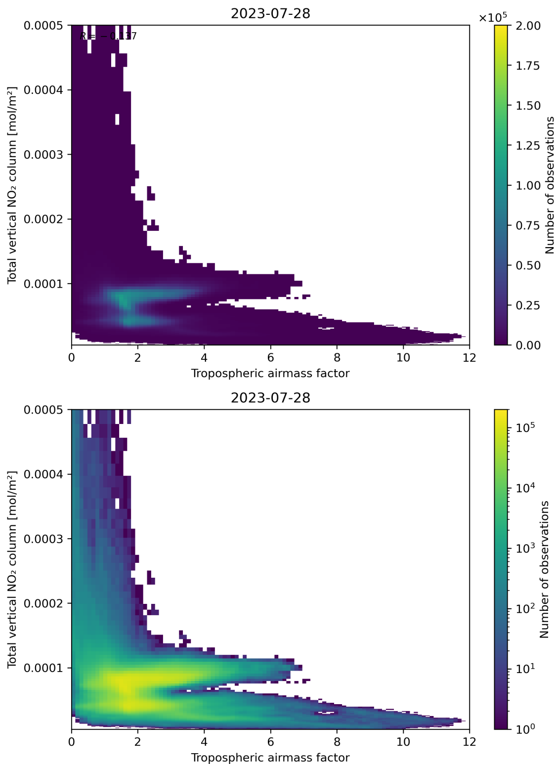
Figure 77: Scatter density plot of “Tropospheric airmass factor” against “Total vertical NO 2 column” for 2023-07-27 to 2023-07-29.
