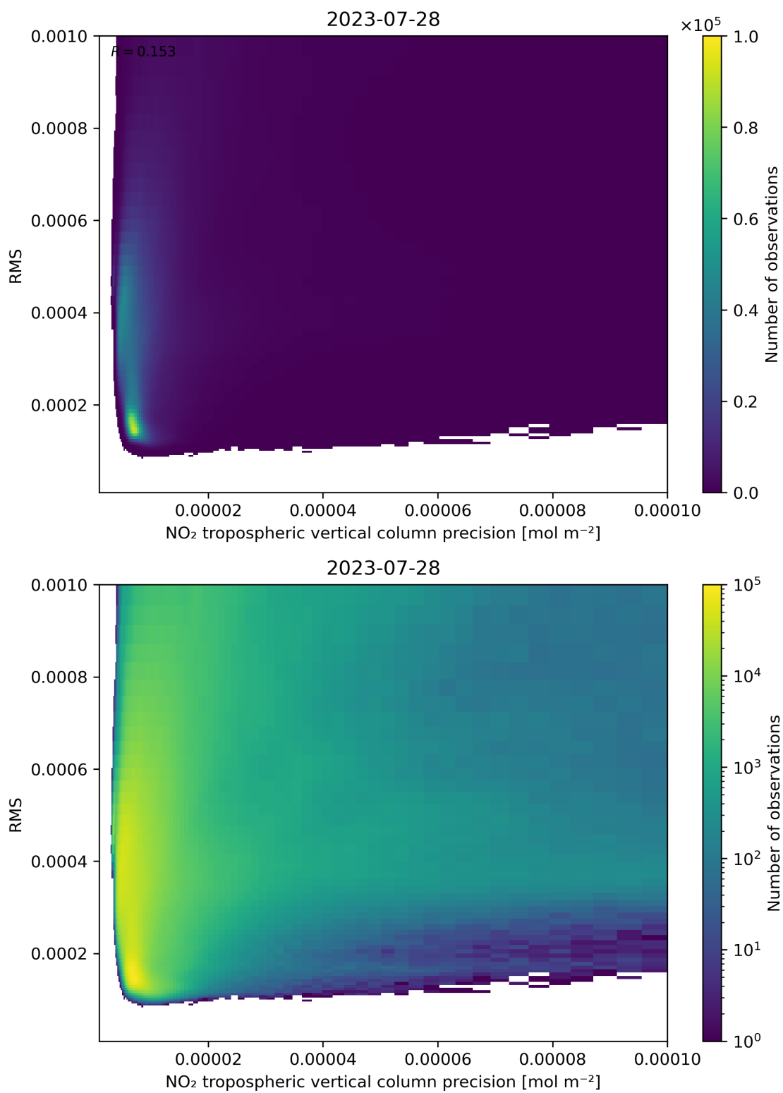
Figure 140: Scatter density plot of “NO 2 tropospheric vertical column precision” against “RMS” for 2023-07-27 to 2023-07-29.
