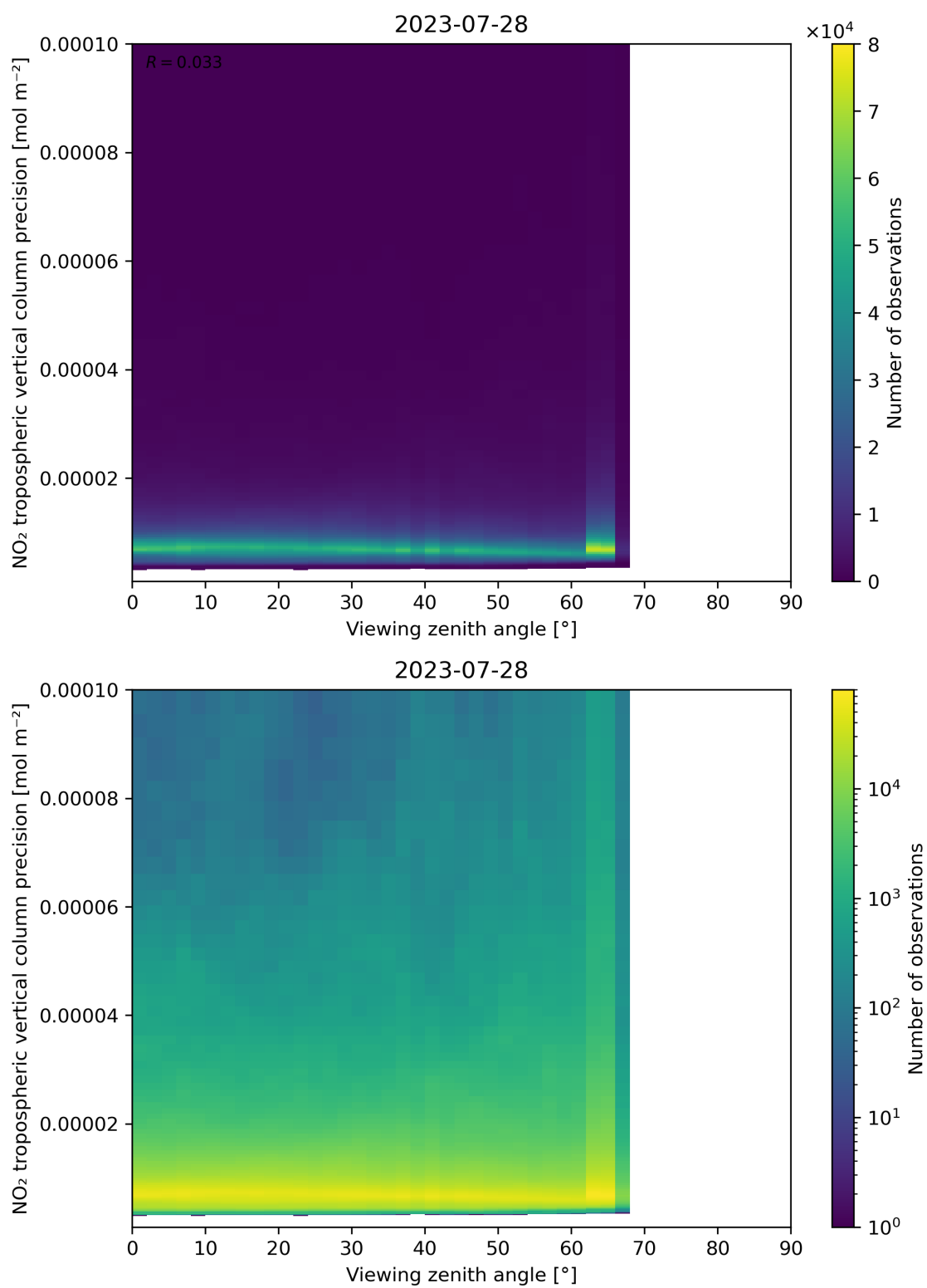
Figure 170: Scatter density plot of “Viewing zenith angle” against “NO 2 tropospheric vertical column precision” for 2023-07-27 to 2023-07-29.
