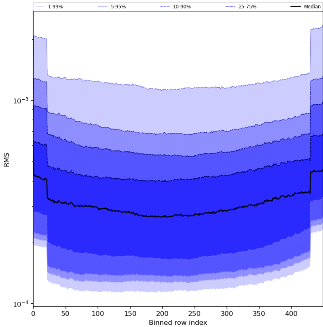
Figure 60: Along track statistics of “RMS” for 2023-07-27 to 2023-07-29
