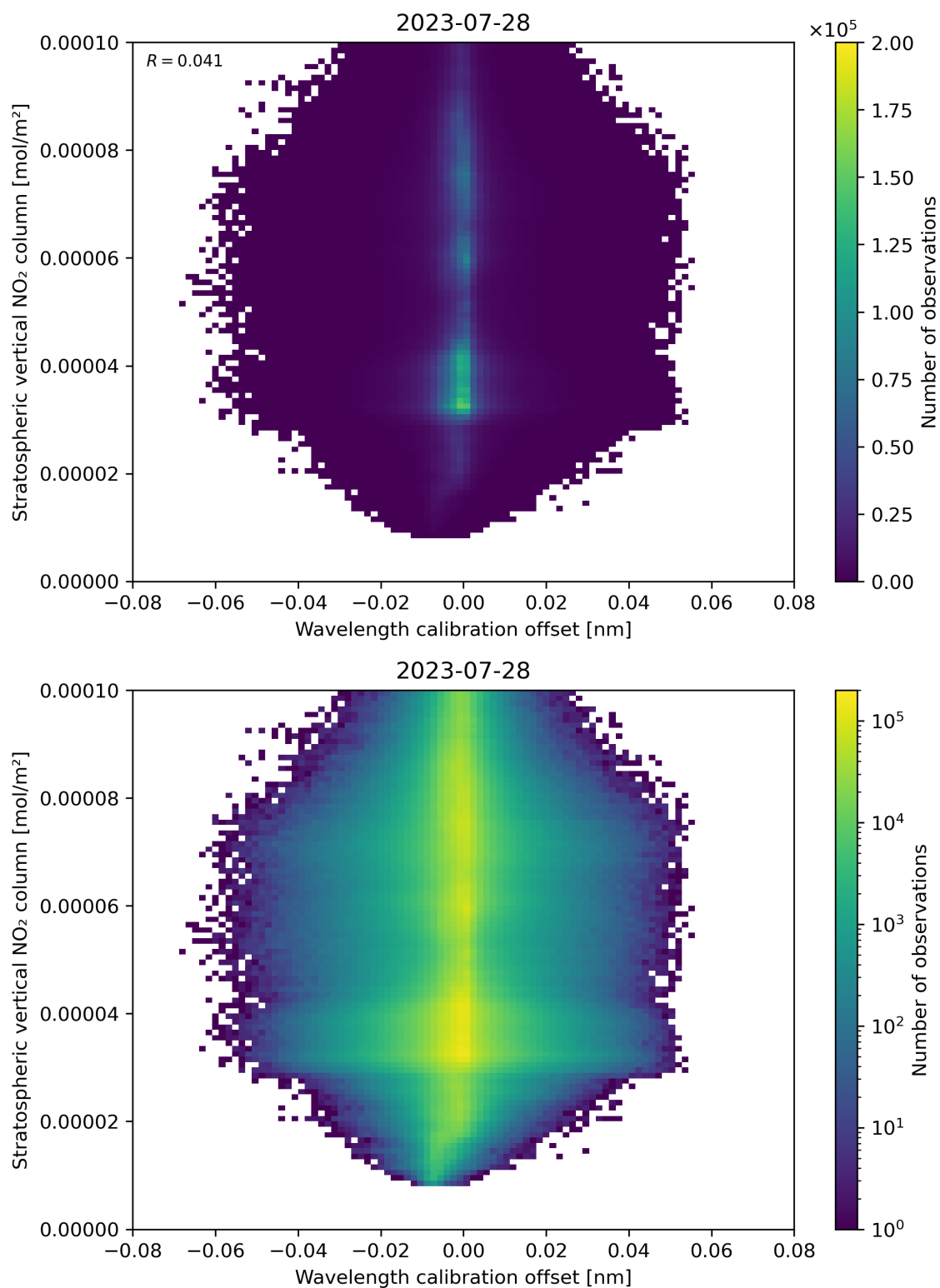
Figure 176: Scatter density plot of “Wavelength calibration offset” against “Stratospheric vertical NO 2 column” for 2023-07-27 to 2023-07-29.
