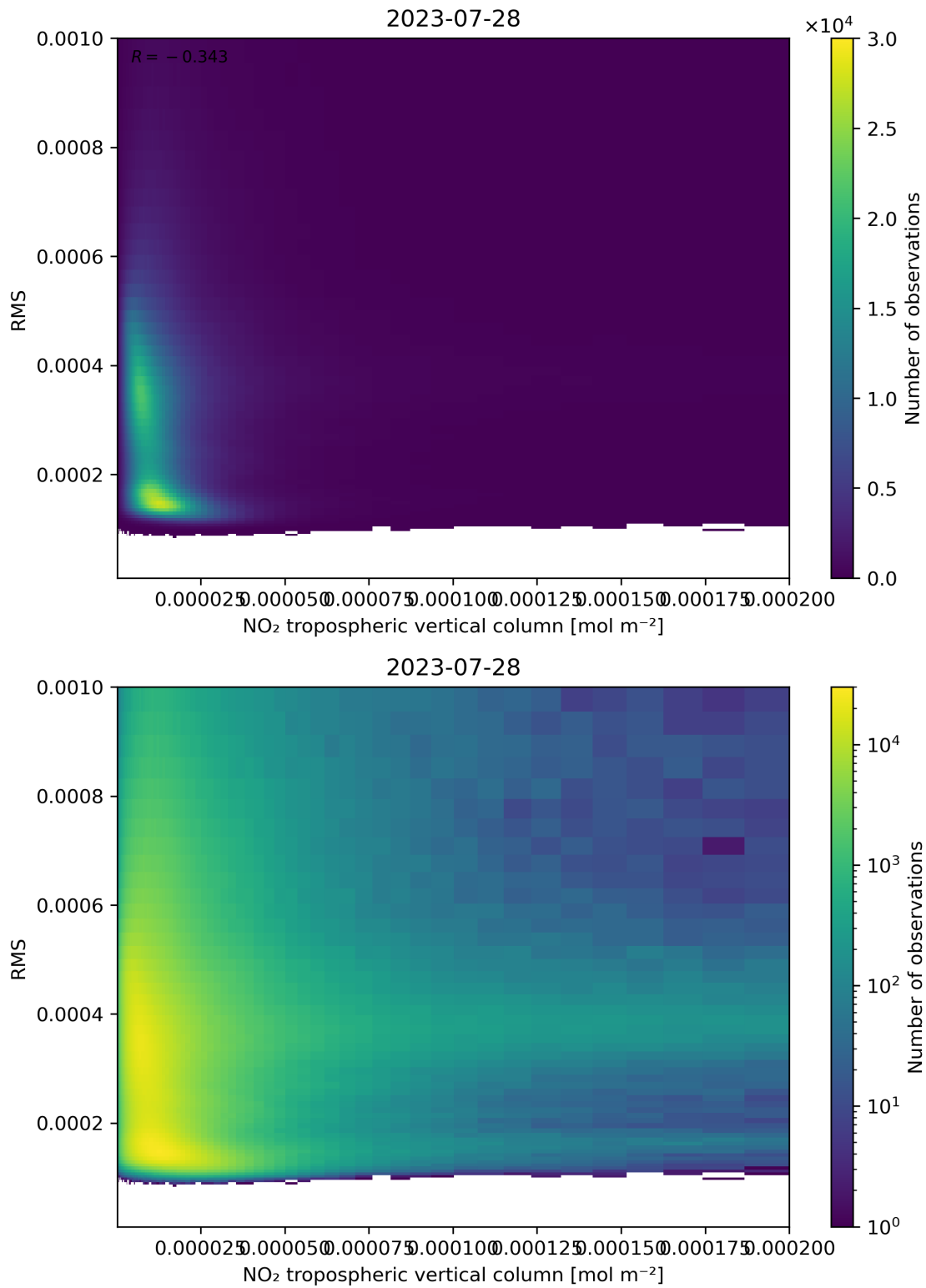
Figure 142: Scatter density plot of “NO 2 tropospheric vertical column” against “RMS” for 2023-07-27 to 2023-07-29.
