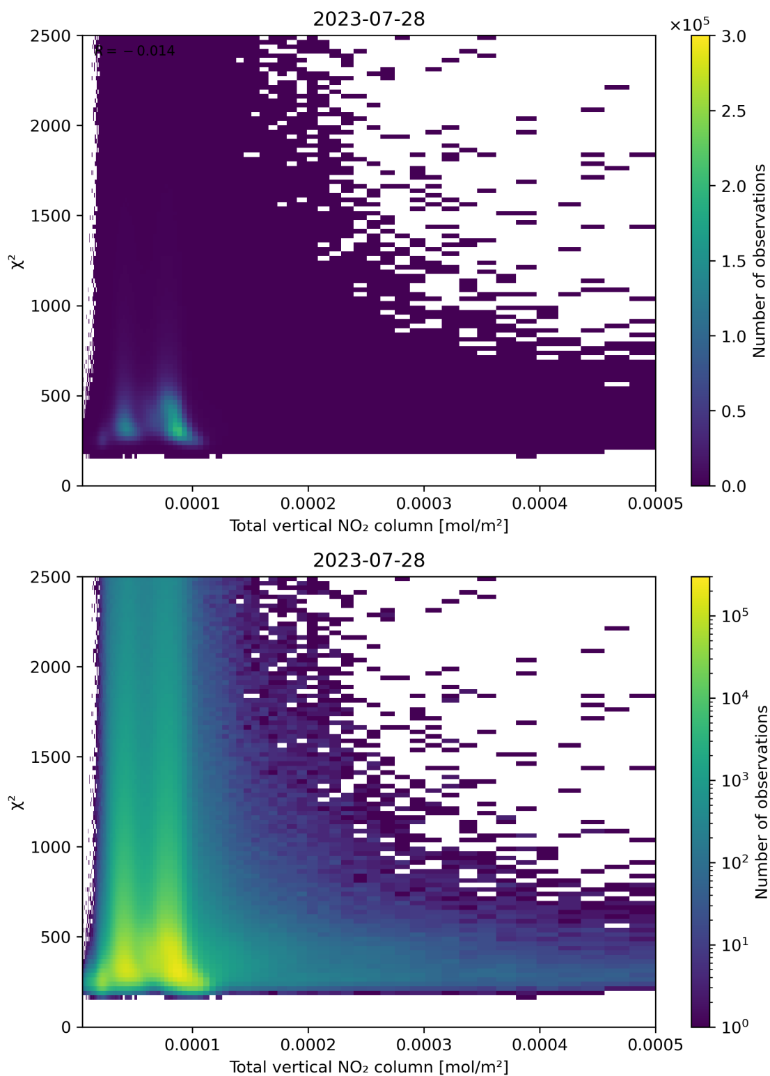
Figure 111: Scatter density plot of “Total vertical NO 2 column” against “ \chi^2 ” for 2023-07-27 to 2023-07-29.
