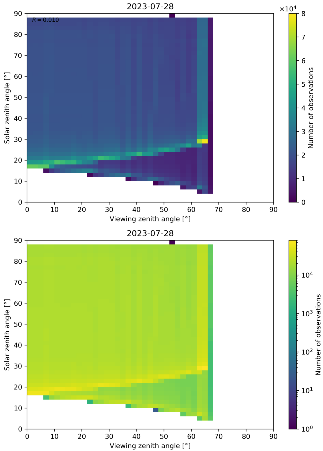
Figure 172: Scatter density plot of “Viewing zenith angle” against “Solar zenith angle” for 2023-07-27 to 2023-07-29.
