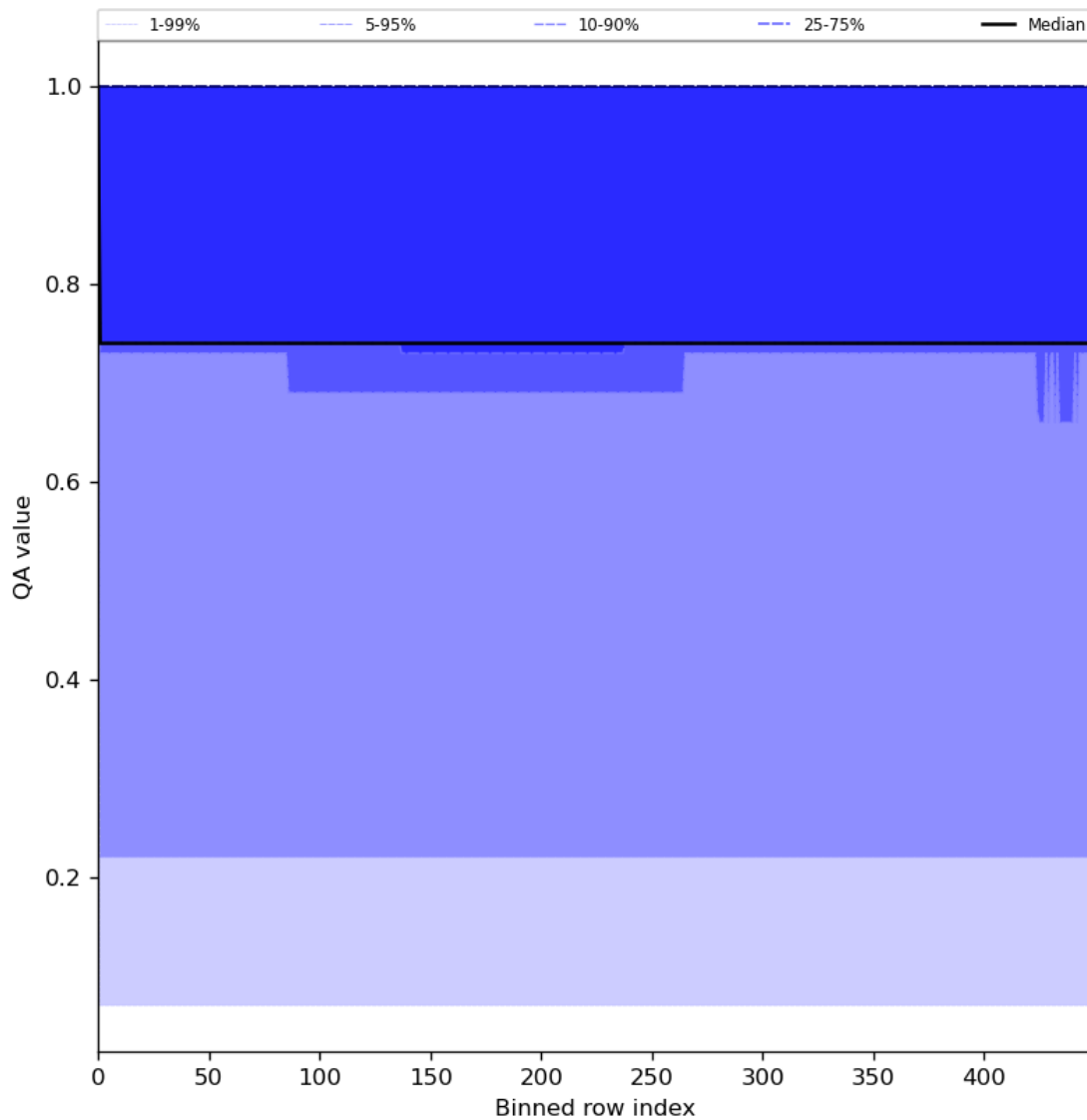
Figure 45: Along track statistics of “QA value” for 2023-07-27 to 2023-07-29
