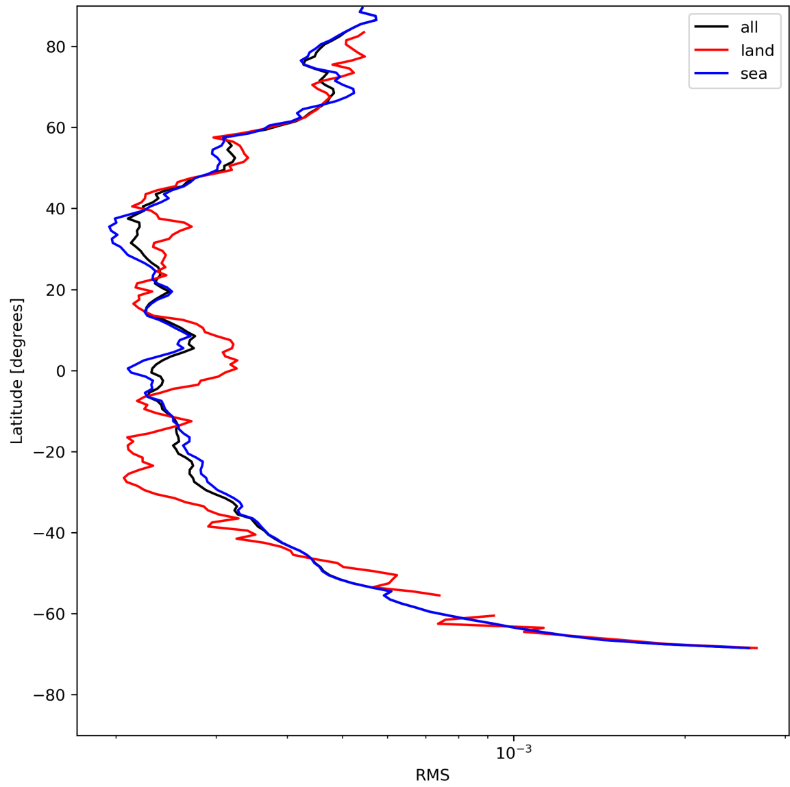
Figure 26: Zonal average of “RMS” for 2023-07-27 to 2023-07-29.
