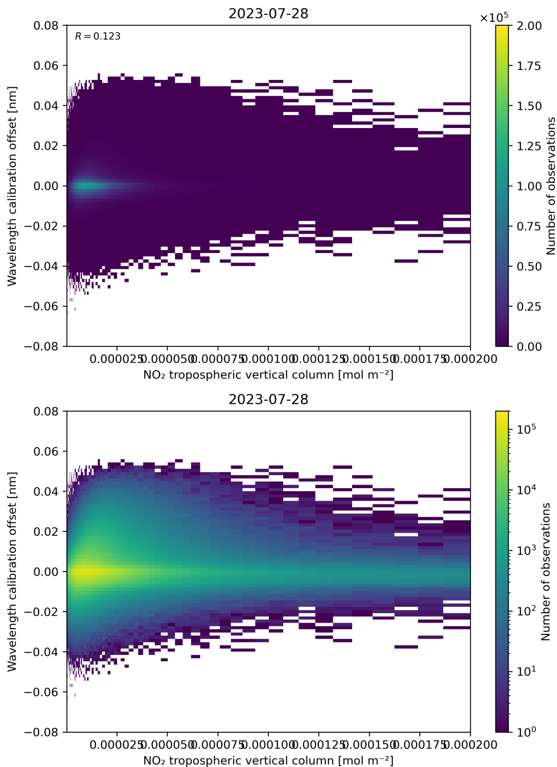
Figure 143: Scatter density plot of “NO 2 tropospheric vertical column” against “Wavelength calibration offset” for 2023-07-27 to 2023-07-29.
