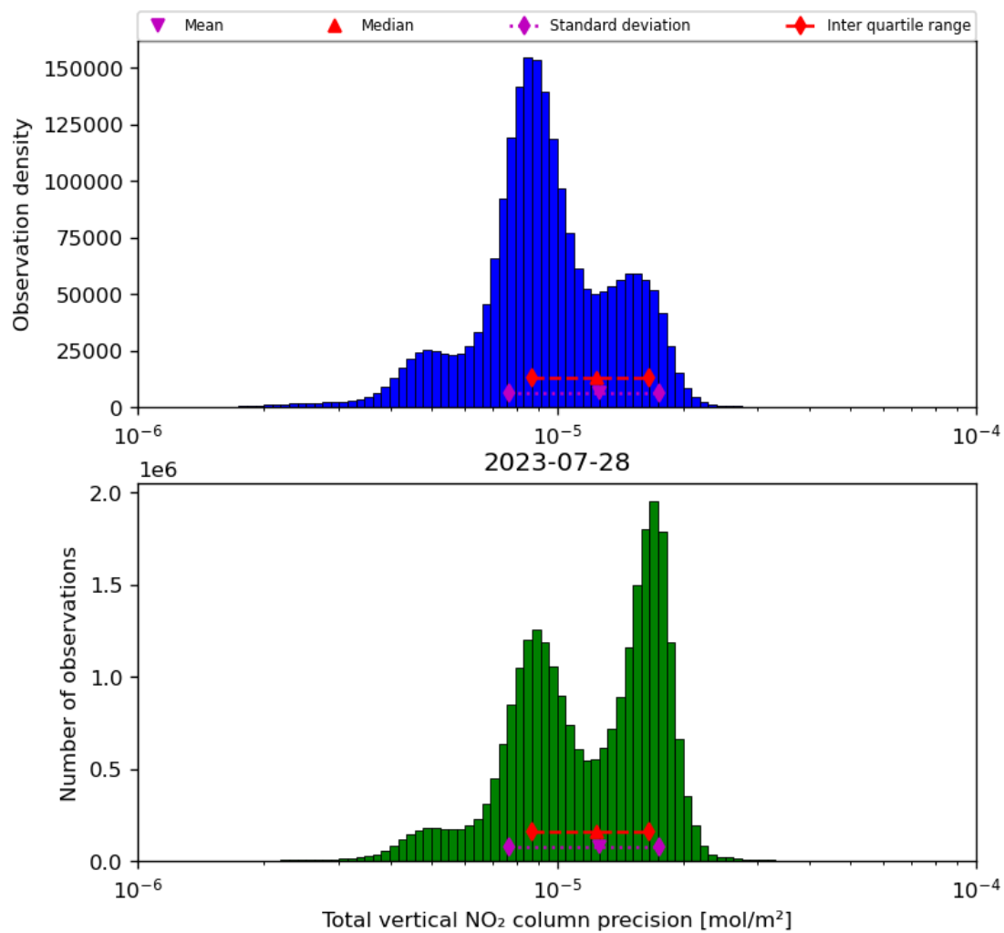
Figure 39: Histogram of "Total vertical NO 2 column precision" for 2023-07-27 to 2023-07-29
