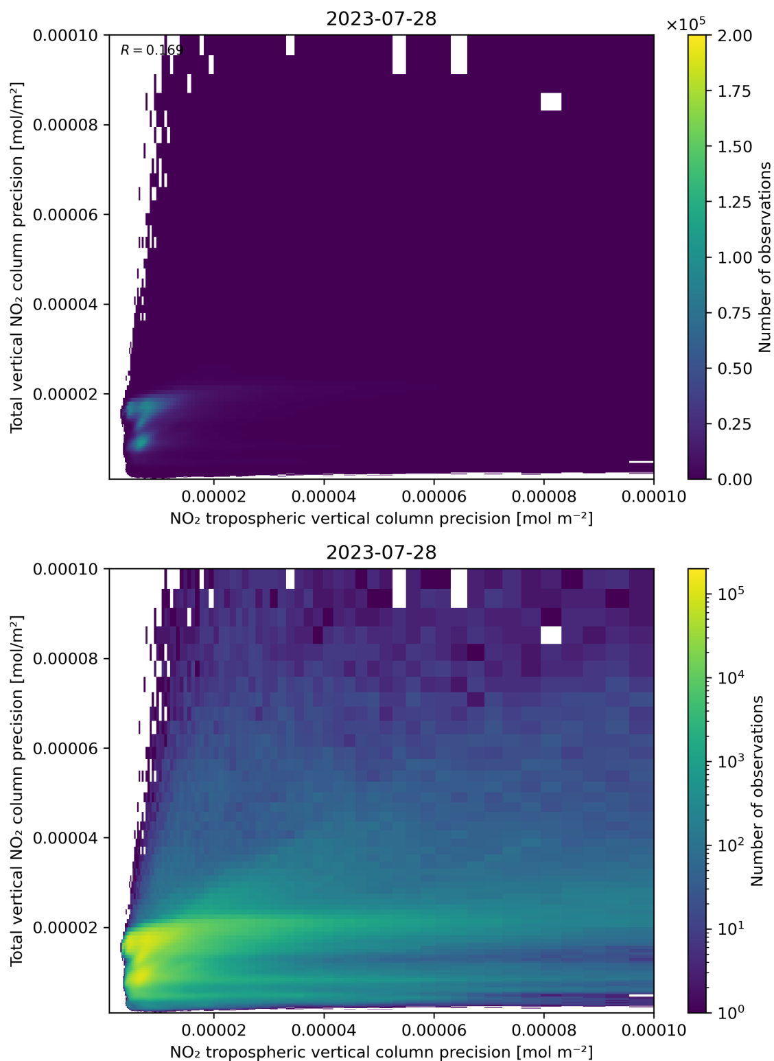
Figure 139: Scatter density plot of “NO 2 tropospheric vertical column precision” against “Total vertical NO 2 column precision” for 2023-07-27 to 2023-07-29.
