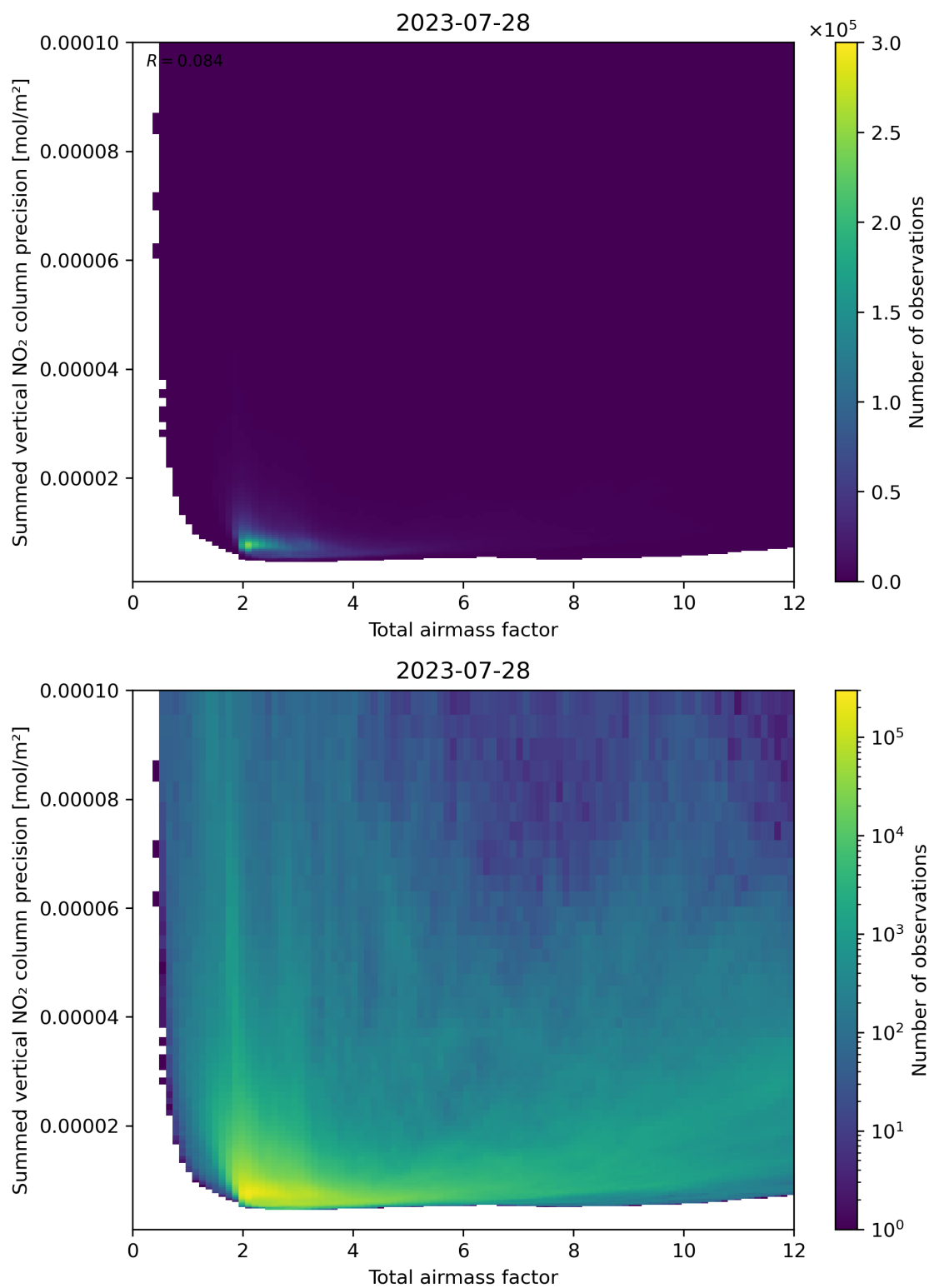
Figure 66: Scatter density plot of “Total airmass factor” against “Summed vertical NO 2 column precision” for 2023-07-27 to 2023-07-29.
