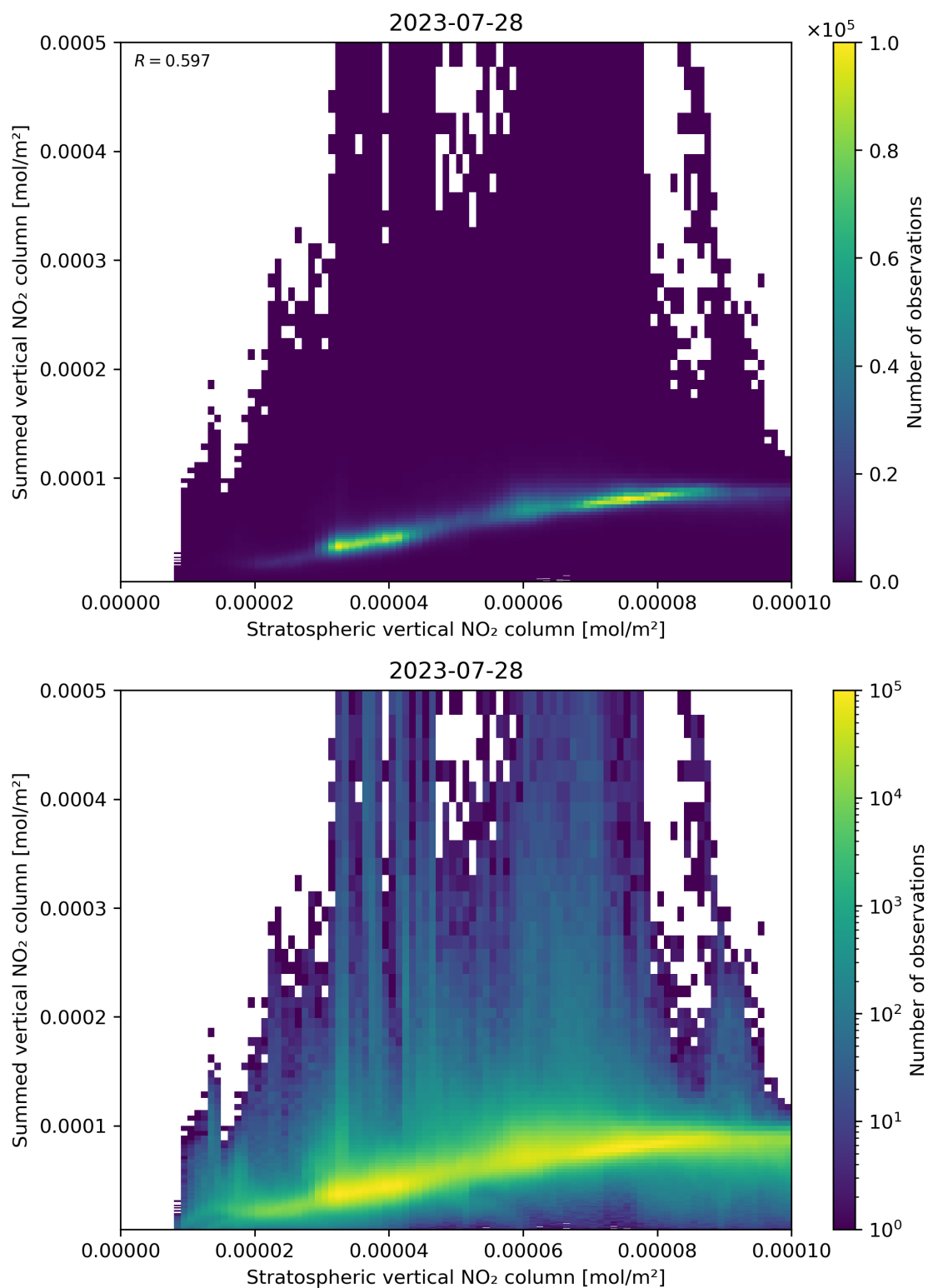
Figure 98: Scatter density plot of “Stratospheric vertical NO 2 column” against “Summed vertical NO 2 column” for 2023-07-27 to 2023-07-29.
