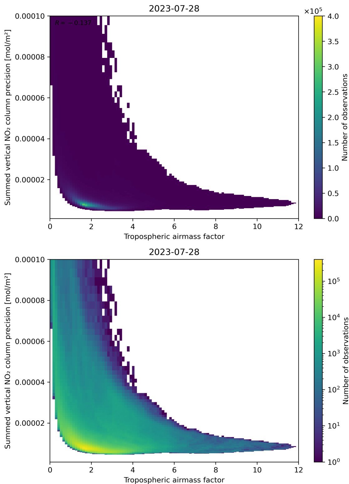
Figure 76: Scatter density plot of “Tropospheric air mass factor” against “Summed vertical NO 2 column precision” for 2023-07-27 to 2023-07-29.
