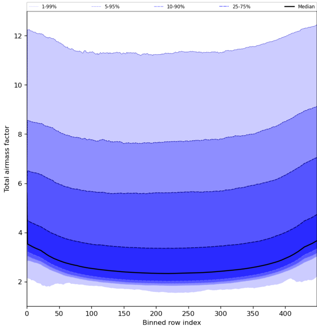
Figure 49: Along track statistics of “Total airmass factor” for 2023-07-27 to 2023-07-29
