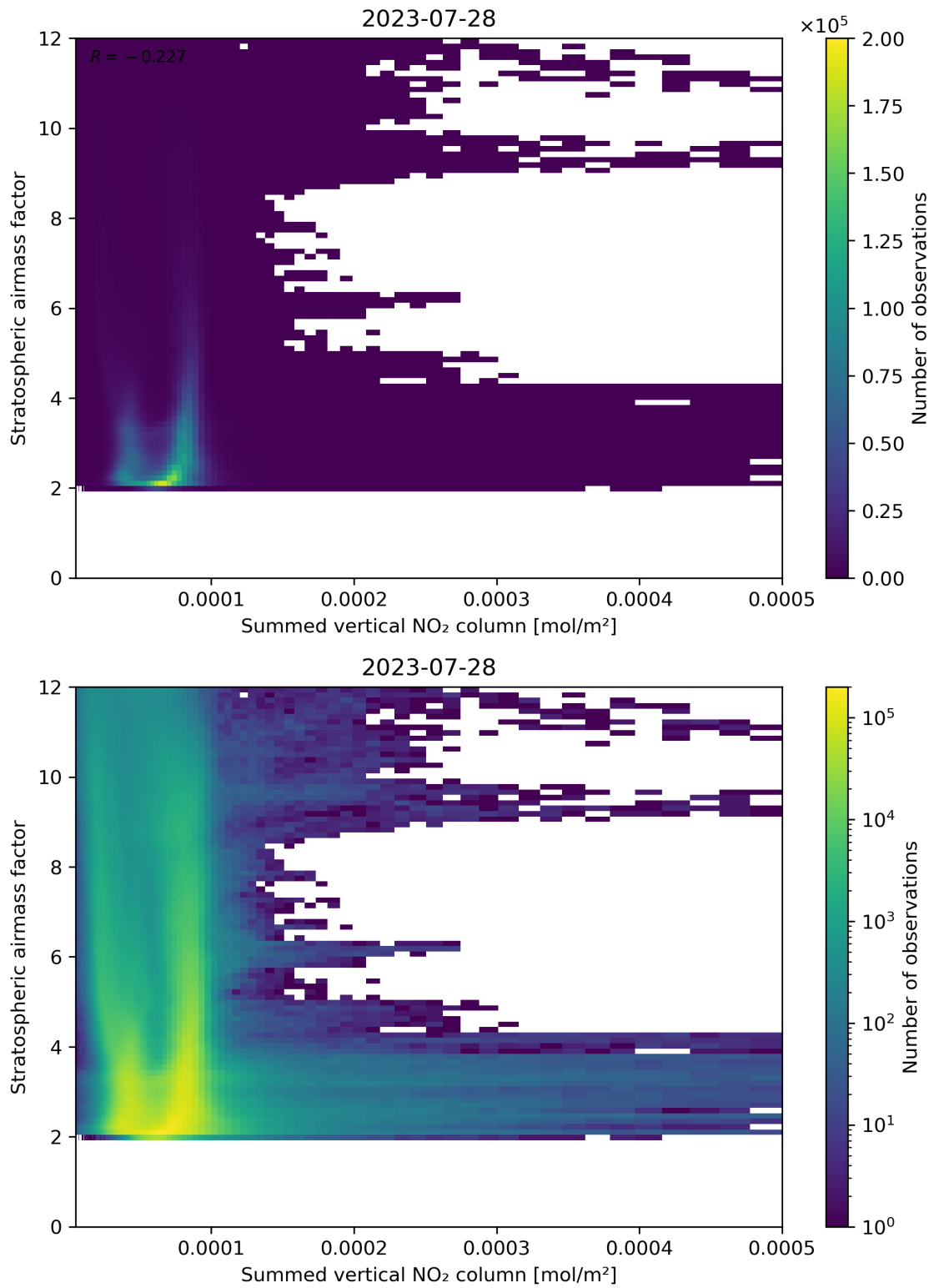
Figure 103: Scatter density plot of “Summed vertical NO 2 column” against “Stratospheric air mass factor” for 2023-07-27 to 2023-07-29.
