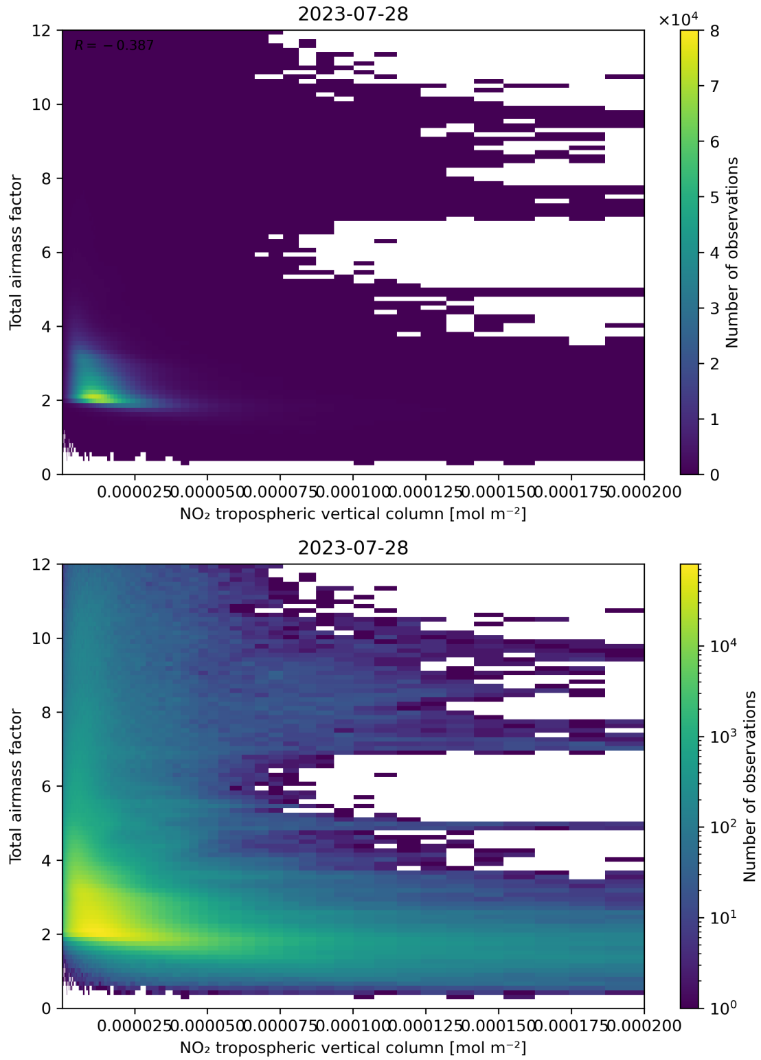
Figure 122: Scatter density plot of “NO 2 tropospheric vertical column” against “Total air mass factor” for 2023-07-27 to 2023-07-29.
