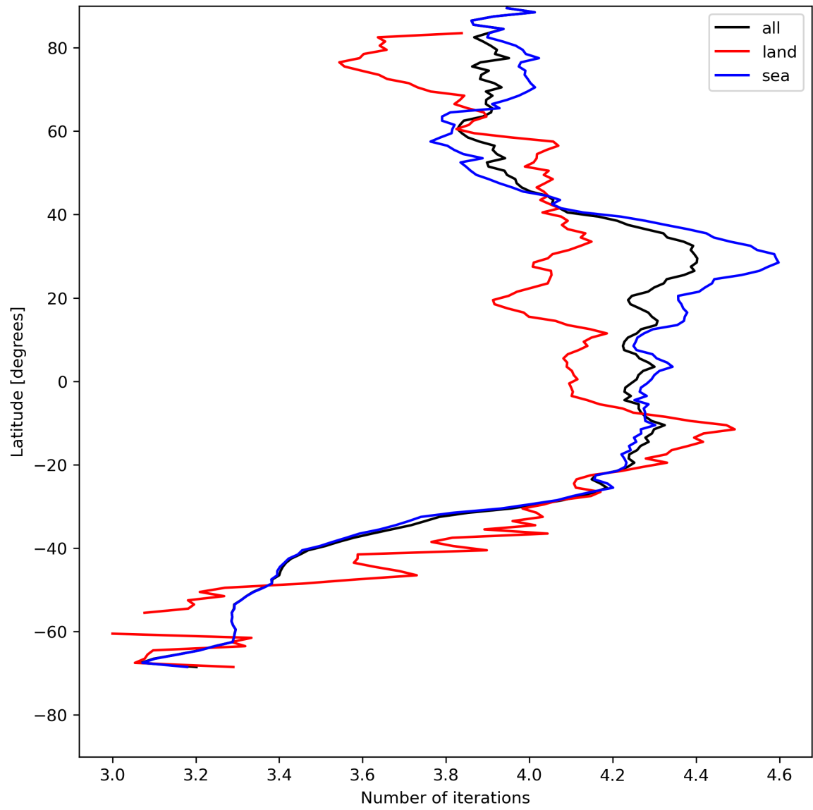
Figure 17: Zonal average of “Number of iterations” for 2023-07-27 to 2023-07-29.
