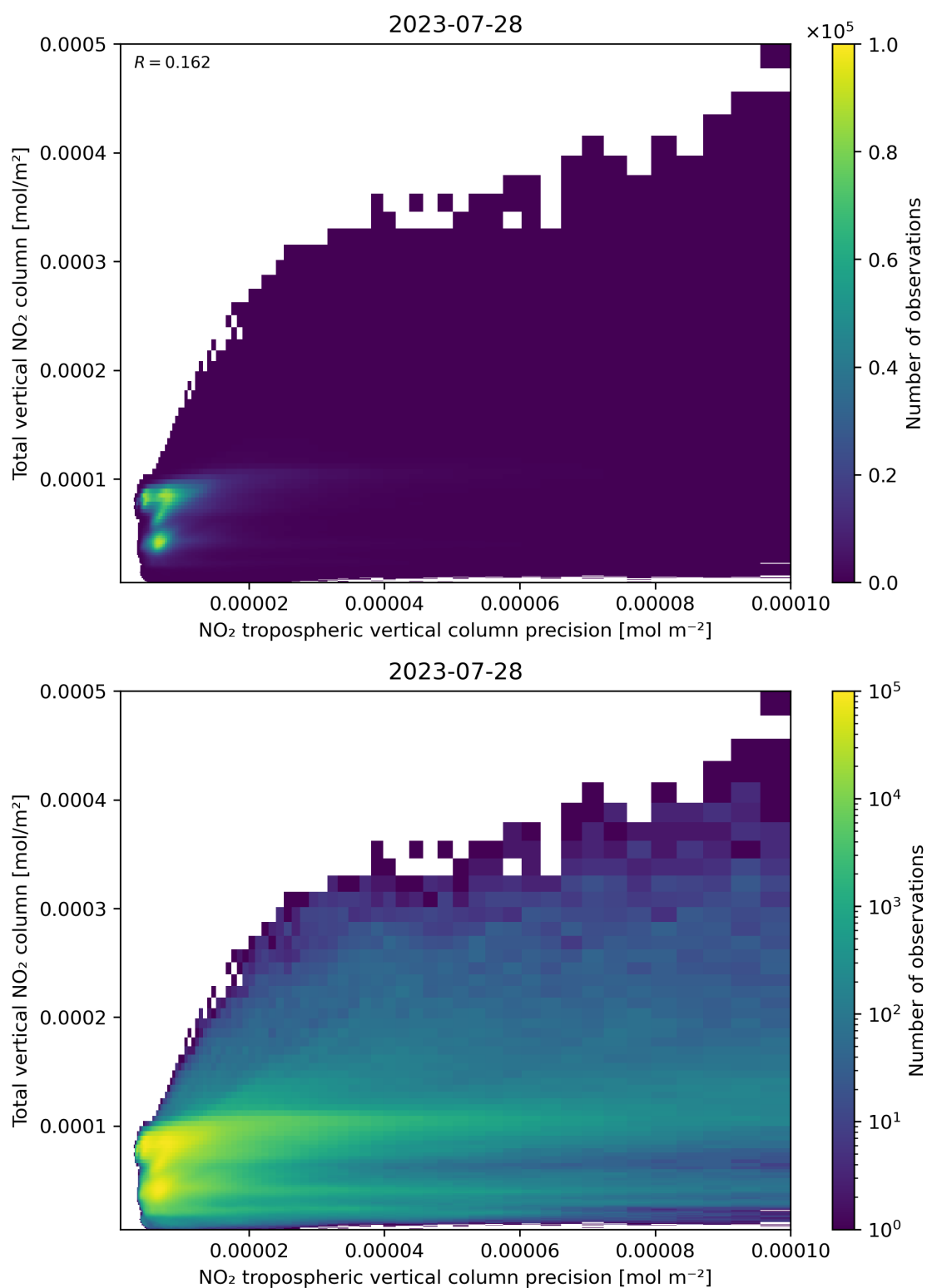
Figure 138: Scatter density plot of “NO 2 tropospheric vertical column precision” against “Total vertical NO 2 column” for 2023-07-27 to 2023-07-29.
