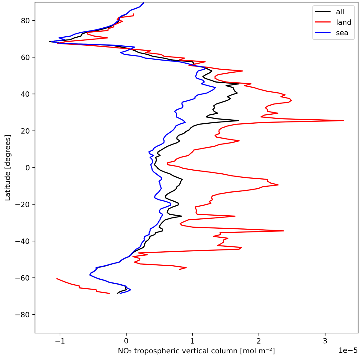
Figure 12: Zonal average of “NO 2 tropospheric vertical column” for 2023-07-27 to 2023-07-29.
