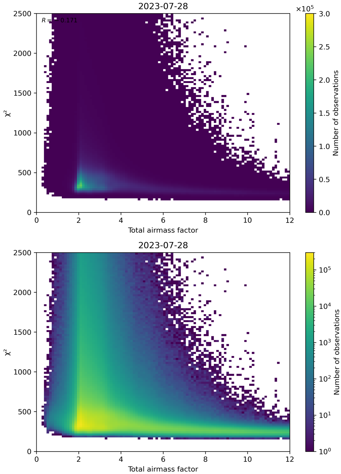
Figure 63: Scatter density plot of “Total airmass factor” against “ \chi^2 ” for 2023-07-27 to 2023-07-29.
