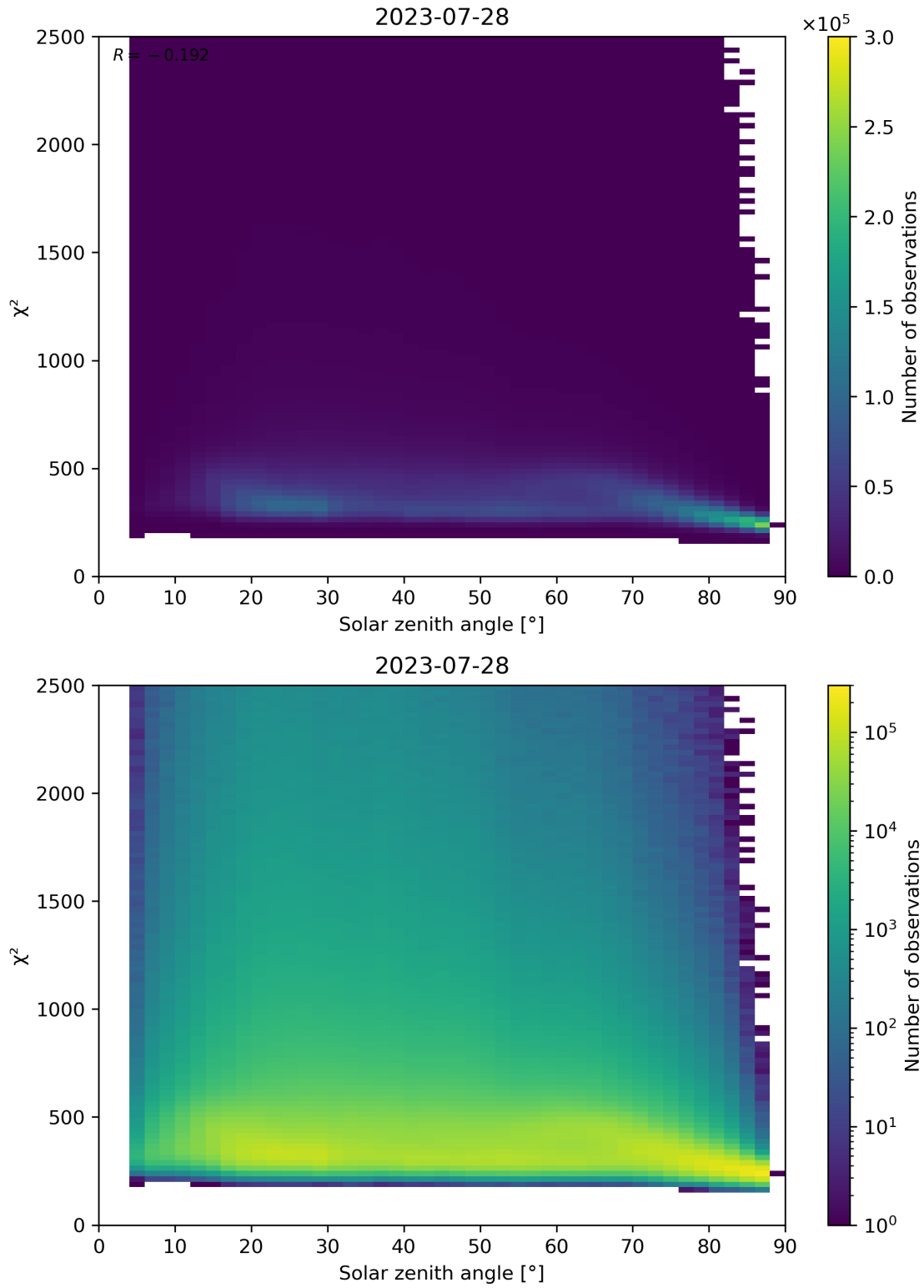
Figure 148: Scatter density plot of “Solar zenith angle” against “ \chi^2 ” for 2023-07-27 to 2023-07-29.
