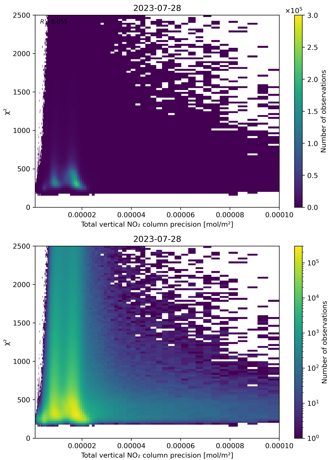
Figure 116: Scatter density plot of “Total vertical NO 2 column precision” against “ \chi^2 ” for 2023-07-27 to 2023-07-29.
