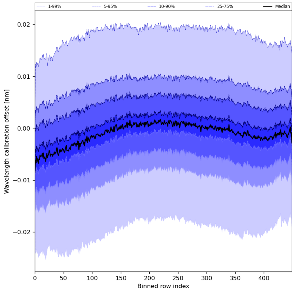
Figure 52: Along track statistics of “Wavelength calibration offset” for 2023-07-27 to 2023-07-29
