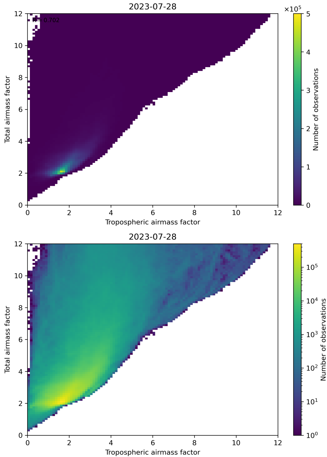
Figure 72: Scatter density plot of “Tropospheric airmass factor” against “Total airmass factor” for 2023-07-27 to 2023-07-29.
