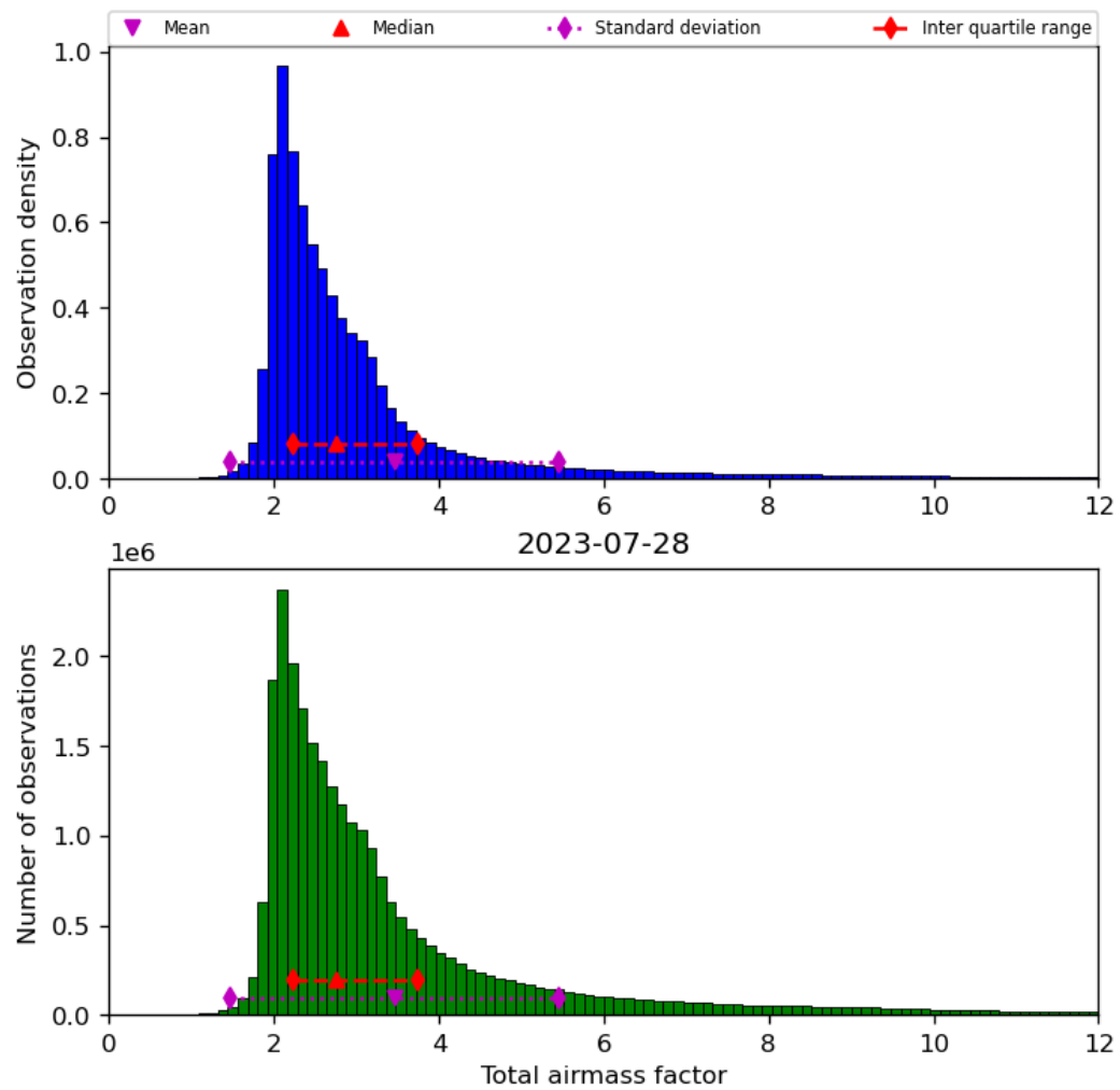
Figure 32: Histogram of “Total airmass factor” for 2023-07-27 to 2023-07-29
