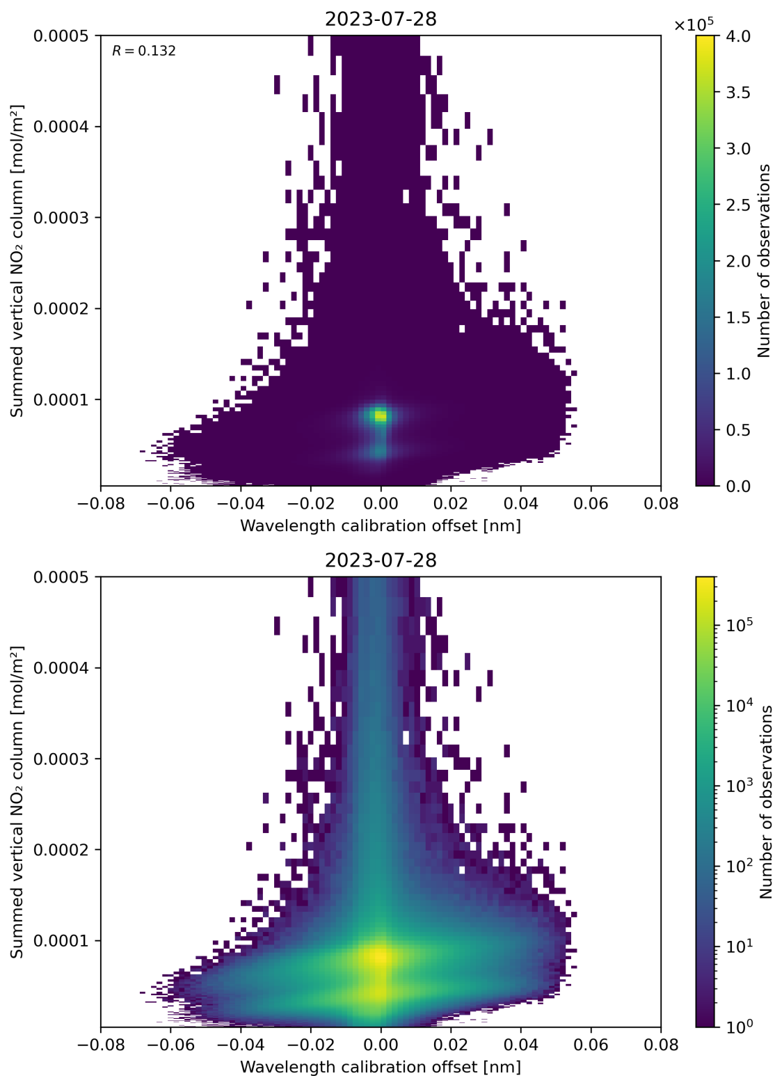
Figure 177: Scatter density plot of “Wavelength calibration offset” against “Summed vertical NO 2 column” for 2023-07-27 to 2023-07-29.
