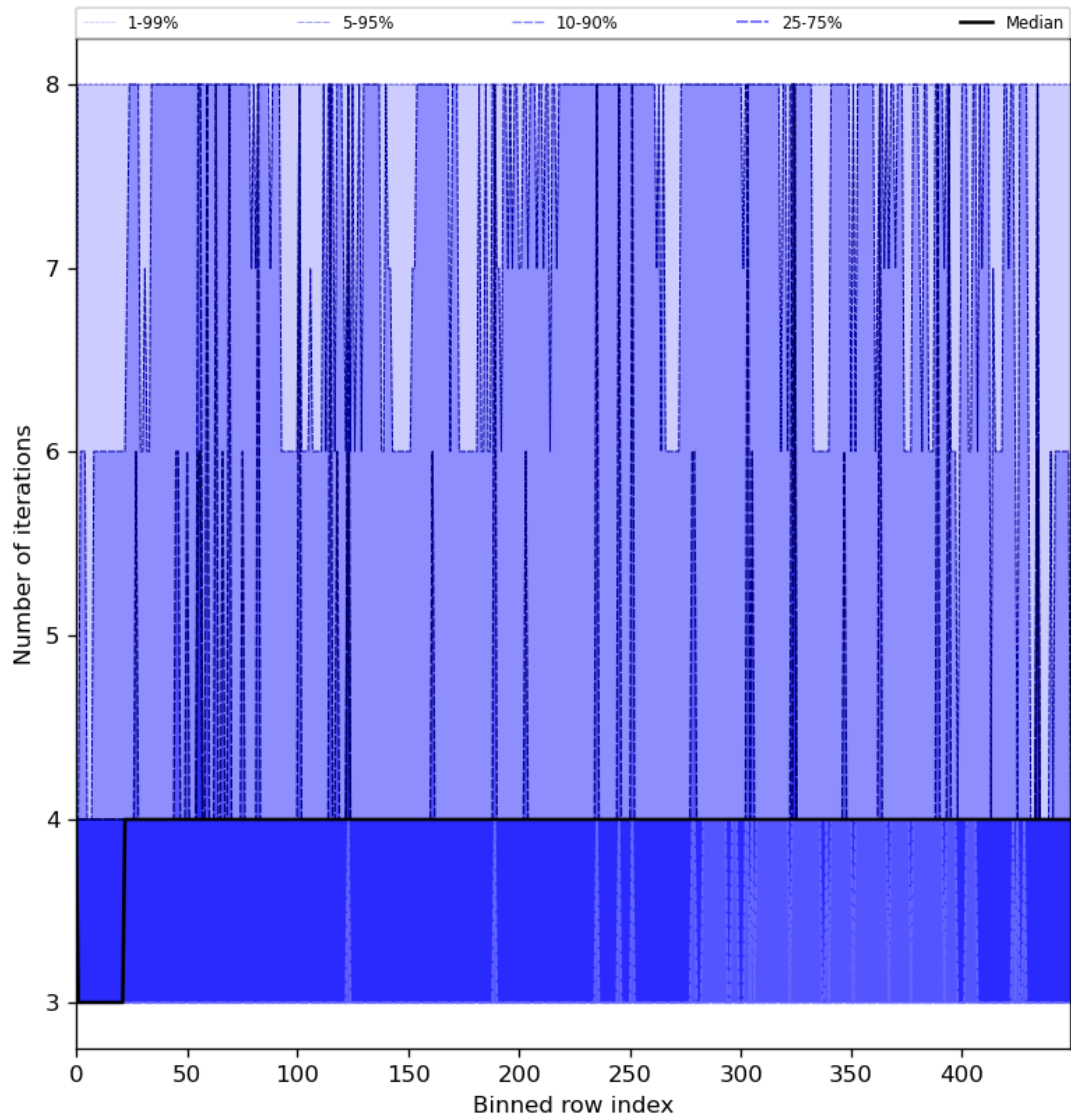
Figure 51: Along track statistics of “Number of iterations” for 2023-07-27 to 2023-07-29
