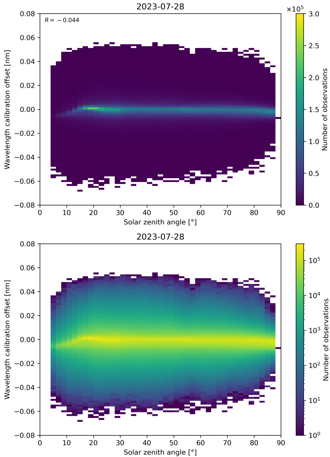
Figure 158: Scatter density plot of “Solar zenith angle” against “Wavelength calibration offset” for 2023-07-27 to 2023-07-29.
