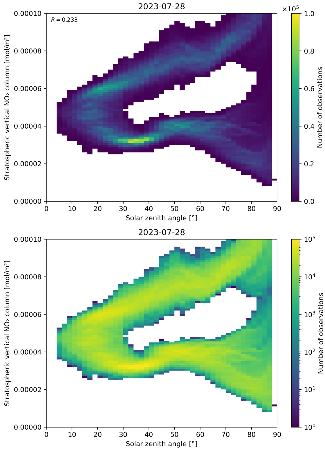
Figure 150: Scatter density plot of “Solar zenith angle” against “Stratospheric vertical NO 2 column” for 2023-07-27 to 2023-07-29.
