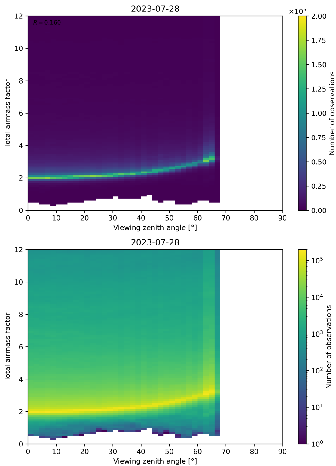
Figure 160: Scatter density plot of “Viewing zenith angle” against “Total airmass factor” for 2023-07-27 to 2023-07-29.
