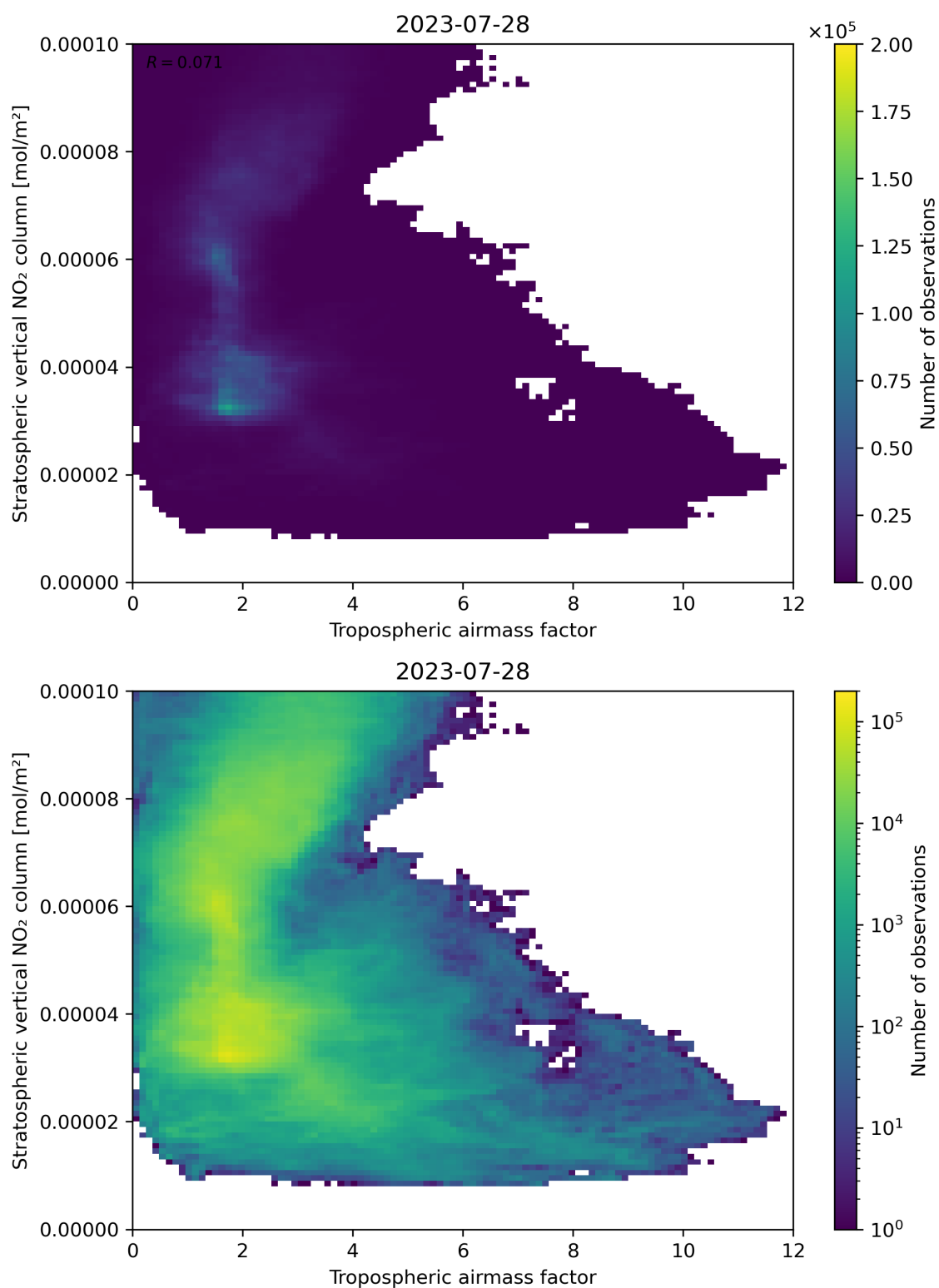
Figure 74: Scatter density plot of “Tropospheric airmass factor” against “Stratospheric vertical NO 2 column” for 2023-07-27 to 2023-07-29.
