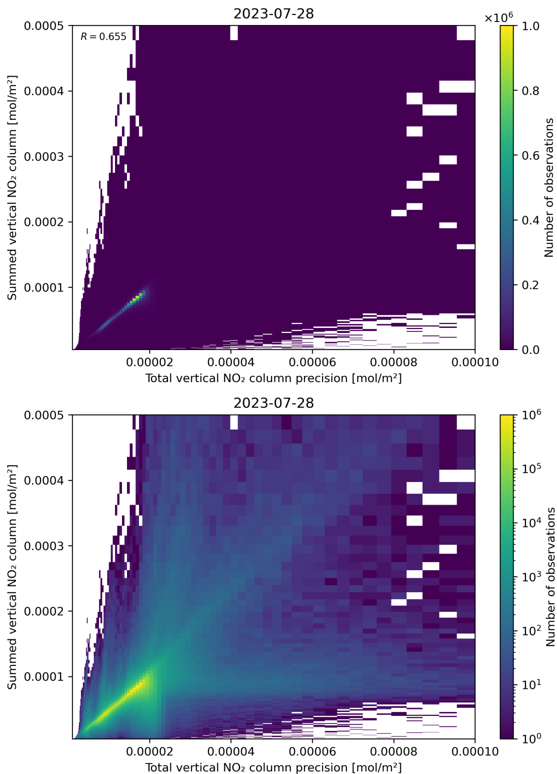
Figure 117: Scatter density plot of “Total vertical NO 2 column precision” against “Summed vertical NO 2 column” for 2023-07-27 to 2023-07-29.
