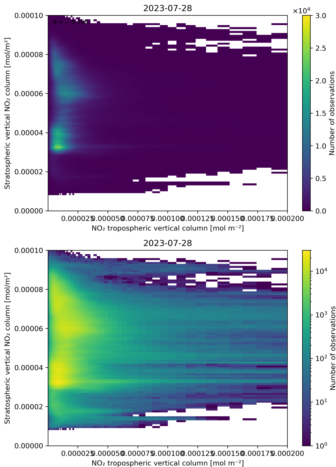
Figure 125: Scatter density plot of “NO 2 tropospheric vertical column” against “Stratospheric vertical NO 2 column” for 2023-07-27 to 2023-07-29.
