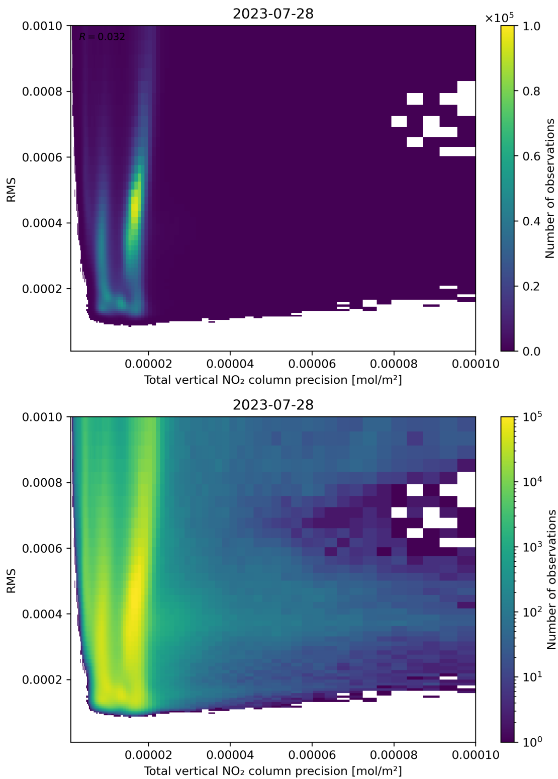
Figure 119: Scatter density plot of “Total vertical NO 2 column precision” against “RMS” for 2023-07-27 to 2023-07-29.
