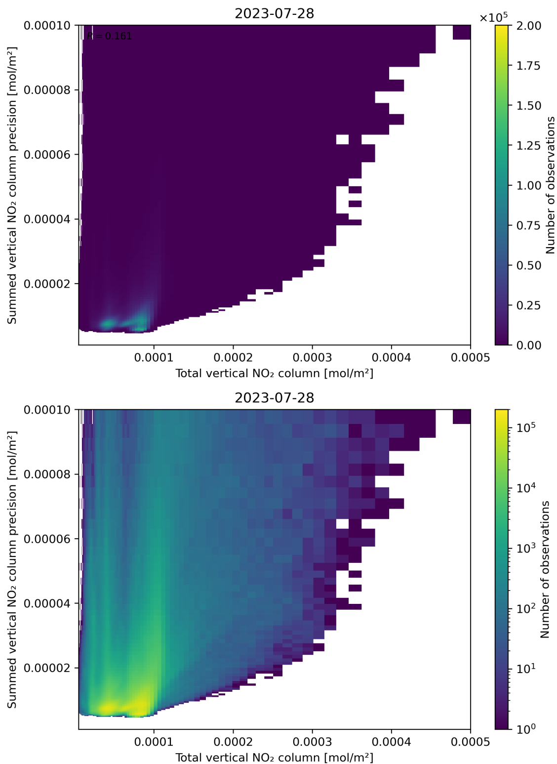
Figure 113: Scatter density plot of “Total vertical NO 2 column” against “Summed vertical NO 2 column precision” for 2023-07-27 to 2023-07-29.
