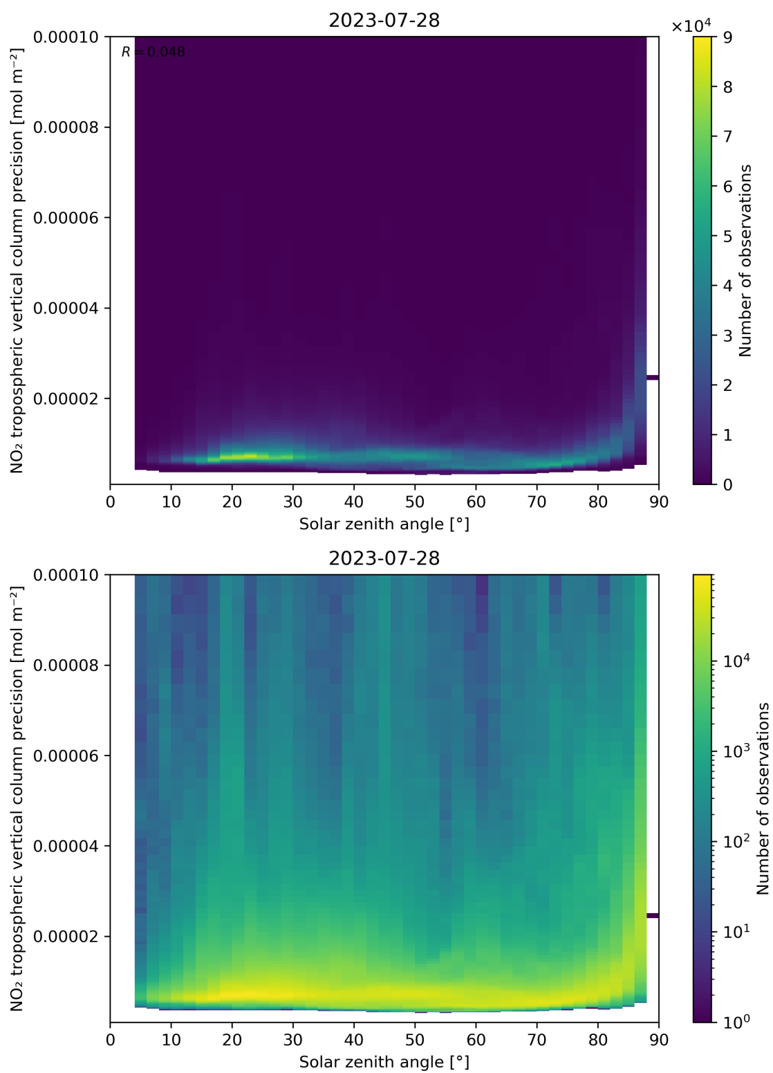
Figure 156: Scatter density plot of “Solar zenith angle” against “NO 2 tropospheric vertical column precision” for 2023-07-27 to 2023-07-29.
