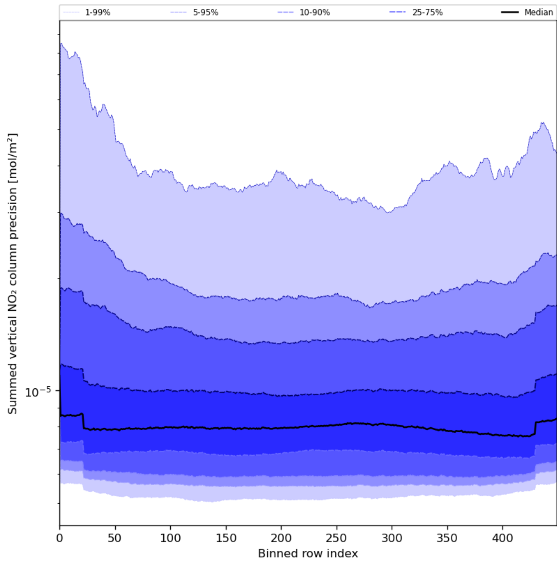
Figure 58: Along track statistics of “Summed vertical NO 2 column precision” for 2023-07-27 to 2023-07-29
