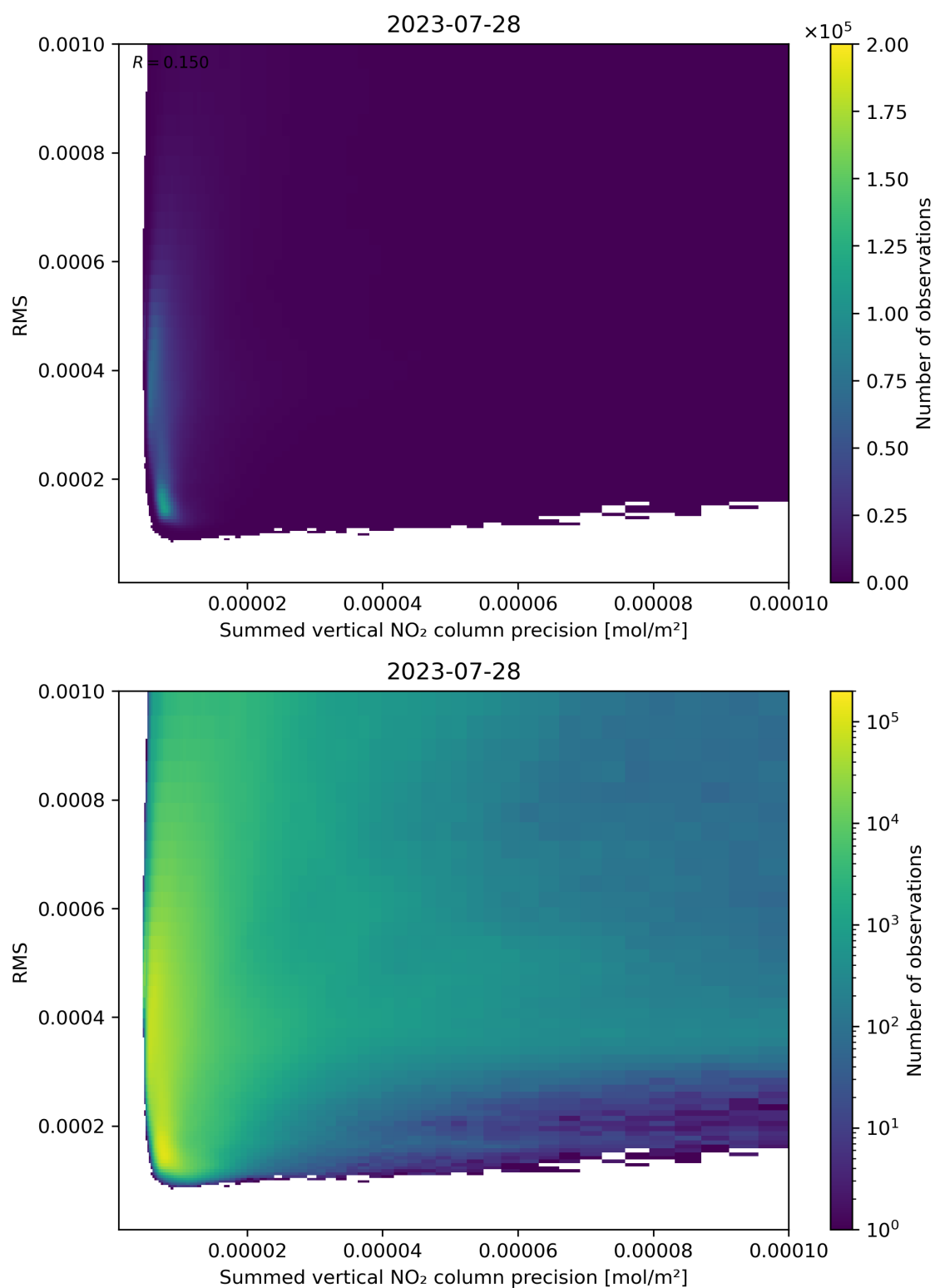
Figure 108: Scatter density plot of “Summed vertical NO 2 column precision” against “RMS” for 2023-07-27 to 2023-07-29.
