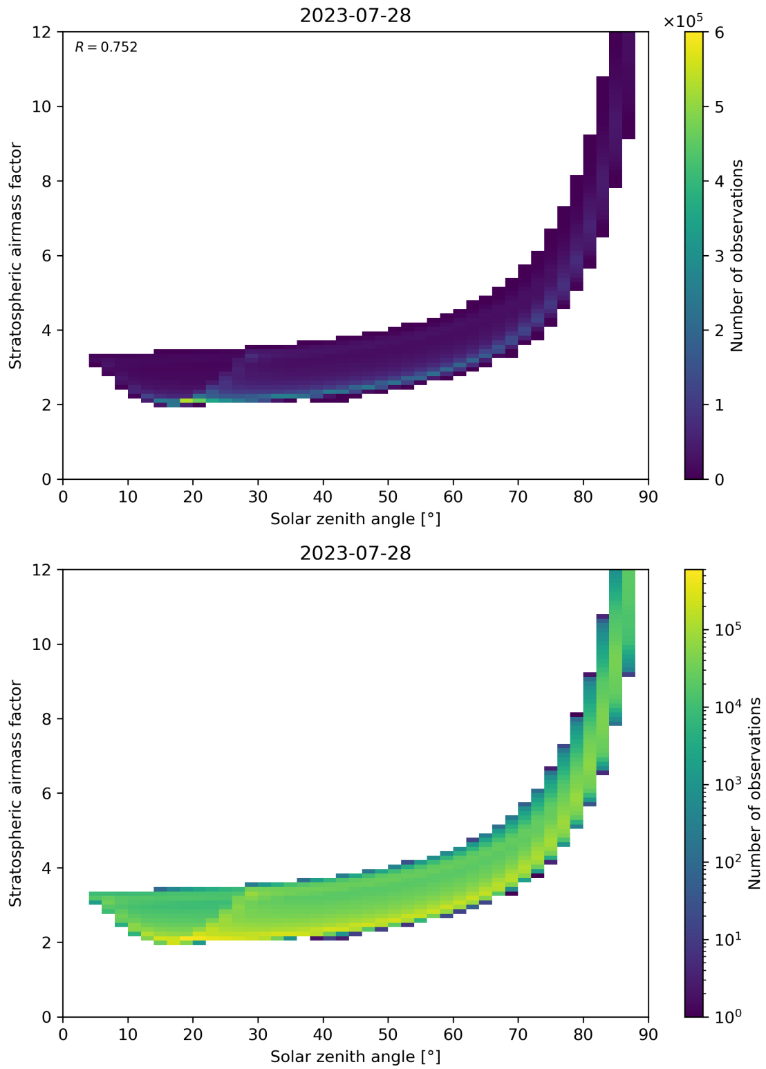
Figure 145: Scatter density plot of “Solar zenith angle” against “Stratospheric airmass factor” for 2023-07-27 to 2023-07-29.
