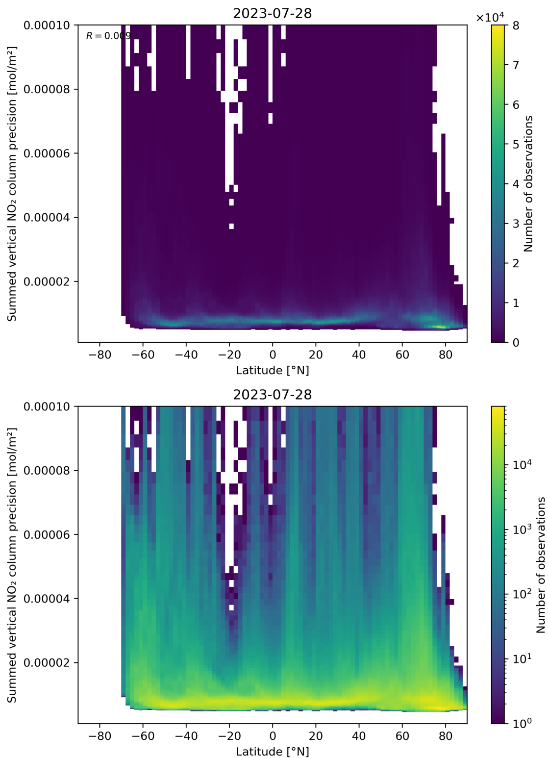
Figure 89: Scatter density plot of “Latitude” against “Summed vertical NO 2 column precision” for 2023-07-27 to 2023-07-29.
