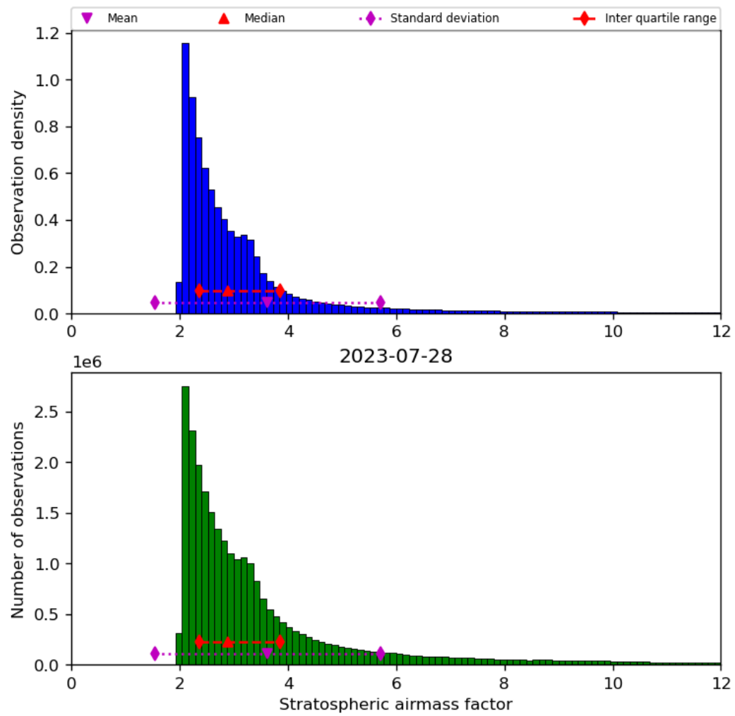
Figure 44: Histogram of “Stratospheric airmass factor” for 2023-07-27 to 2023-07-29
