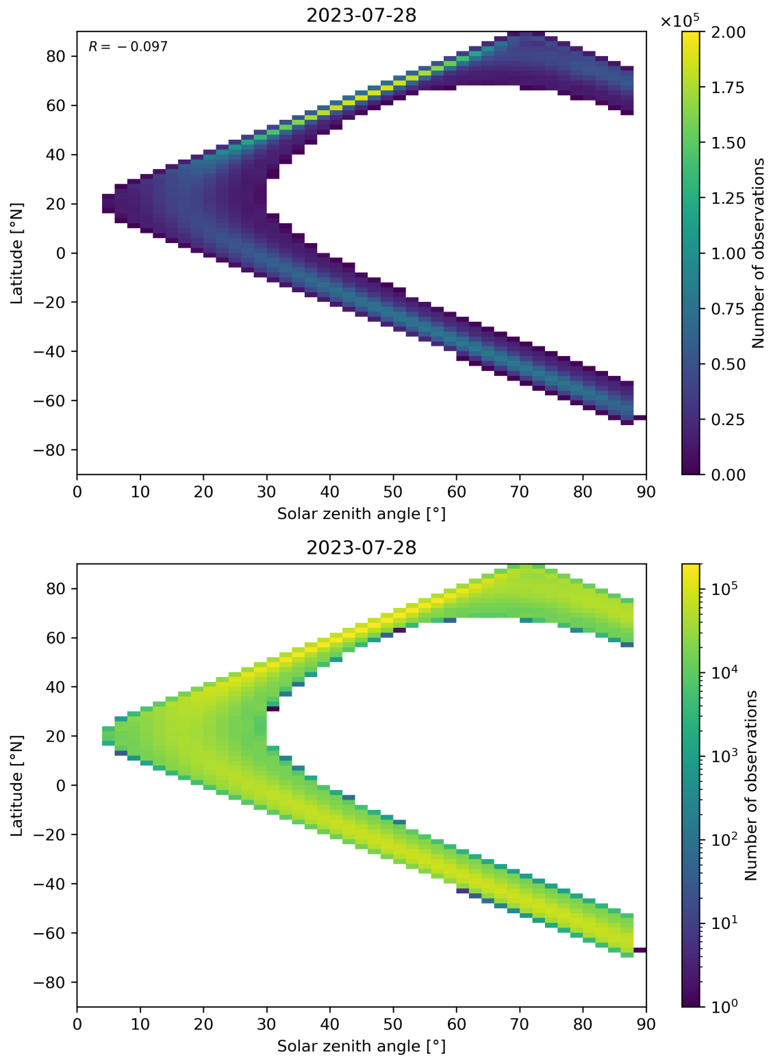
Figure 149: Scatter density plot of “Solar zenith angle” against “Latitude” for 2023-07-27 to 2023-07-29.
