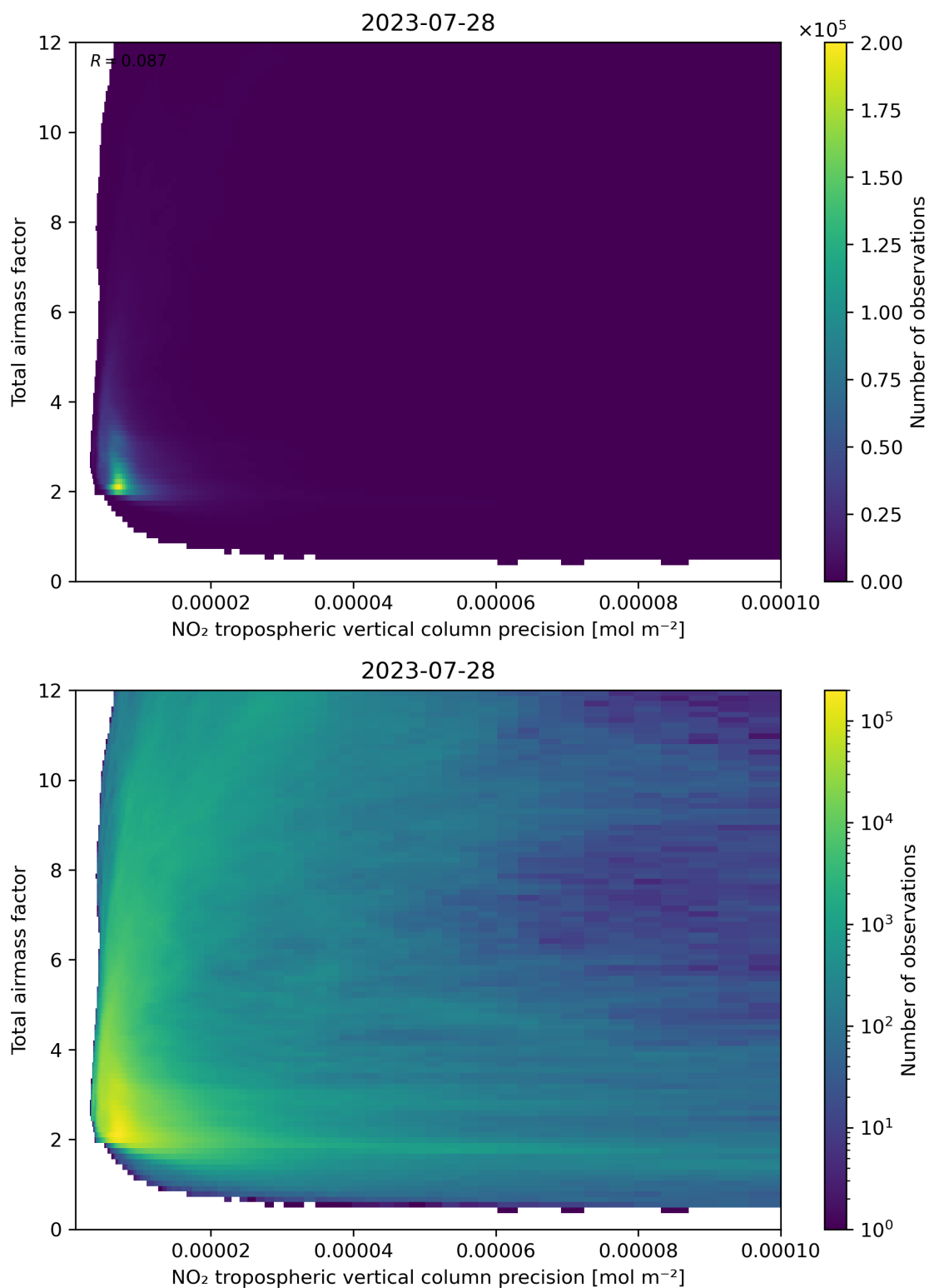
Figure 132: Scatter density plot of “NO 2 tropospheric vertical column precision” against “Total air mass factor” for 2023-07-27 to 2023-07-29.
