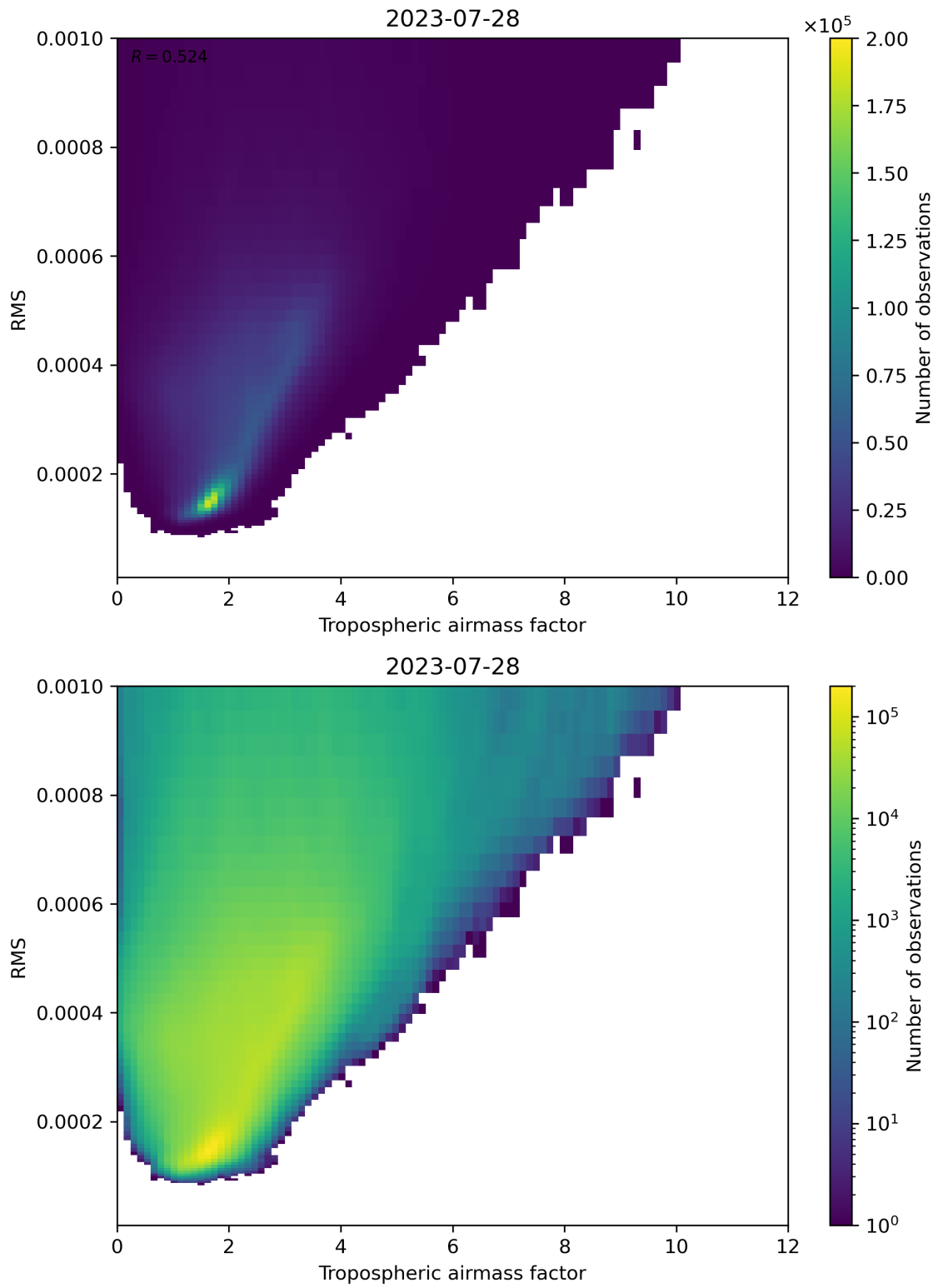
Figure 79: Scatter density plot of “Tropospheric airmass factor” against “RMS” for 2023-07-27 to 2023-07-29.
