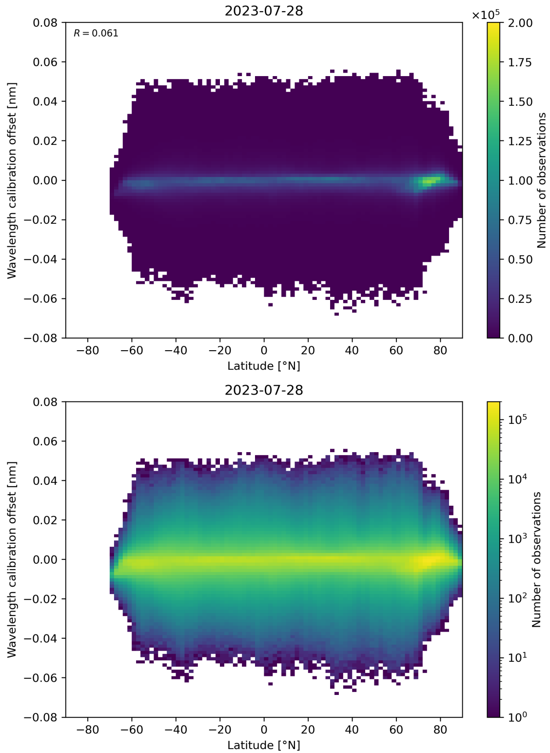
Figure 95: Scatter density plot of “Latitude” against “Wavelength calibration offset” for 2023-07-27 to 2023-07-29.
