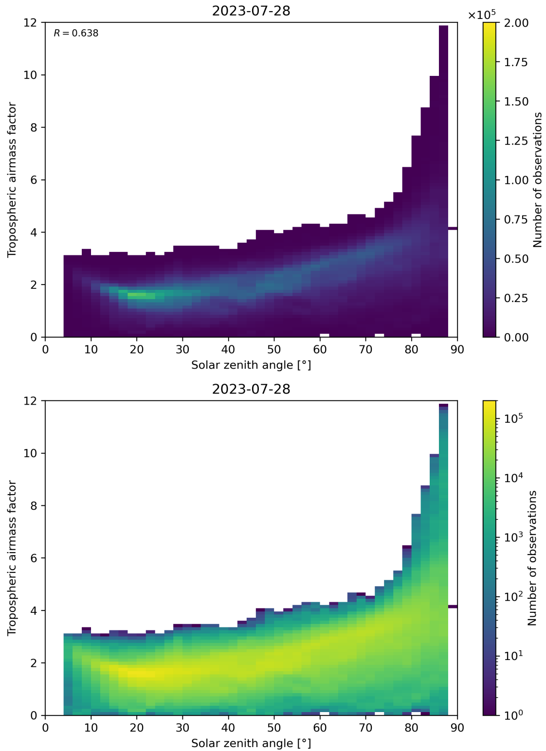
Figure 147: Scatter density plot of “Solar zenith angle” against “Tropospheric airmass factor” for 2023-07-27 to 2023-07-29.
