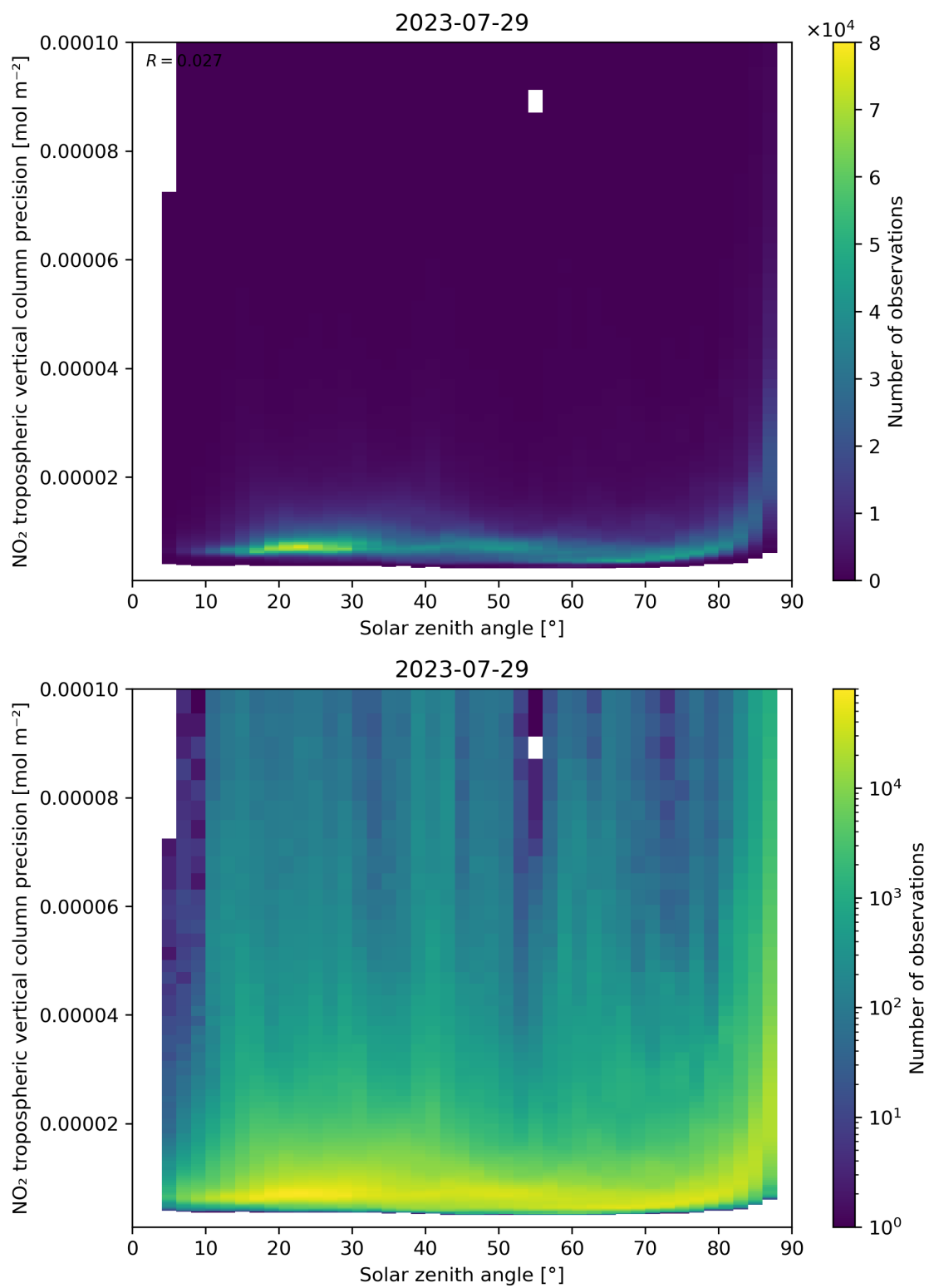
Figure 156: Scatter density plot of “Solar zenith angle” against “NO 2 tropospheric vertical column precision” for 2023-07-29 to 2023-07-30.
