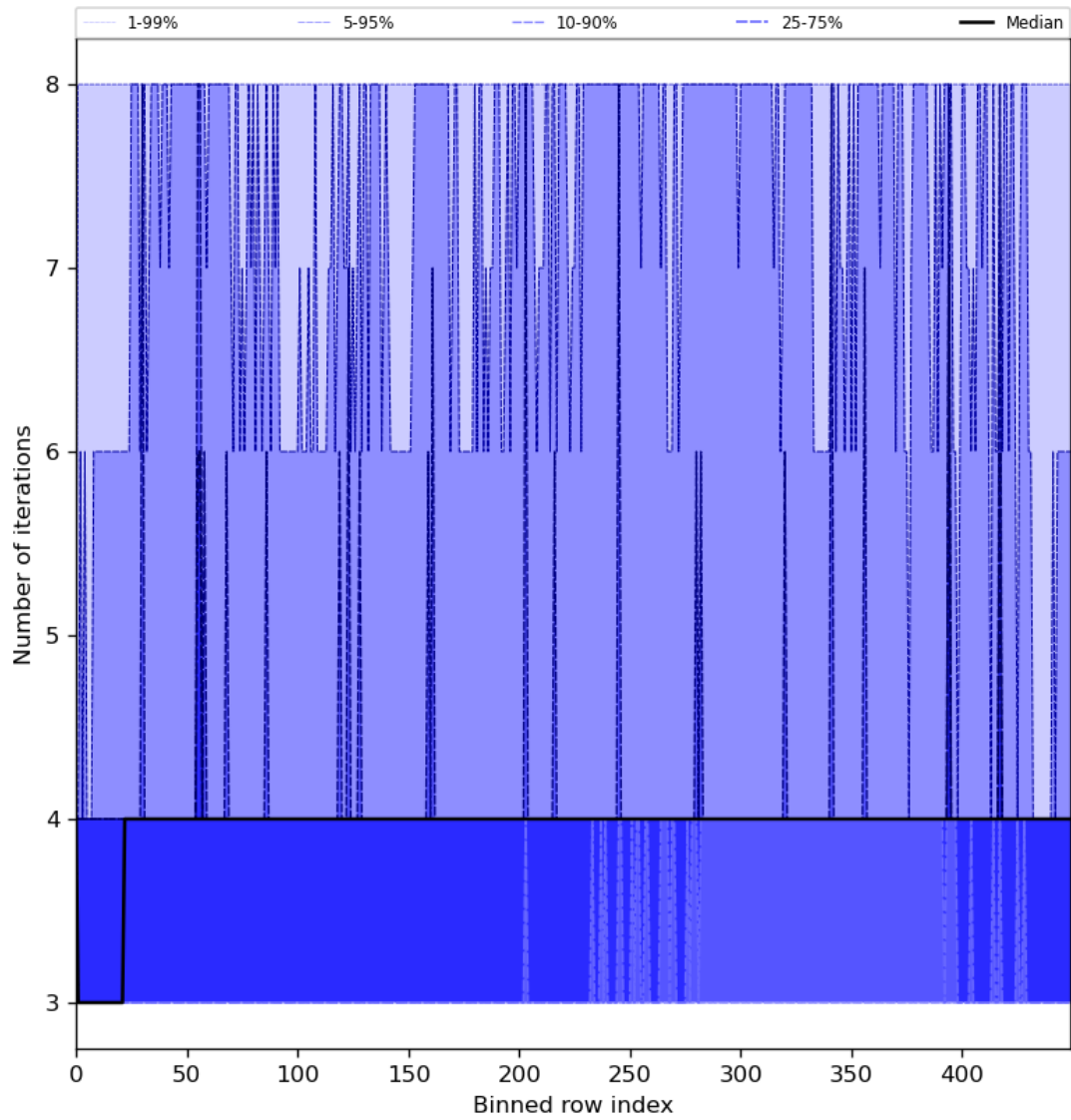
Figure 51: Along track statistics of “Number of iterations” for 2023-07-29 to 2023-07-30
