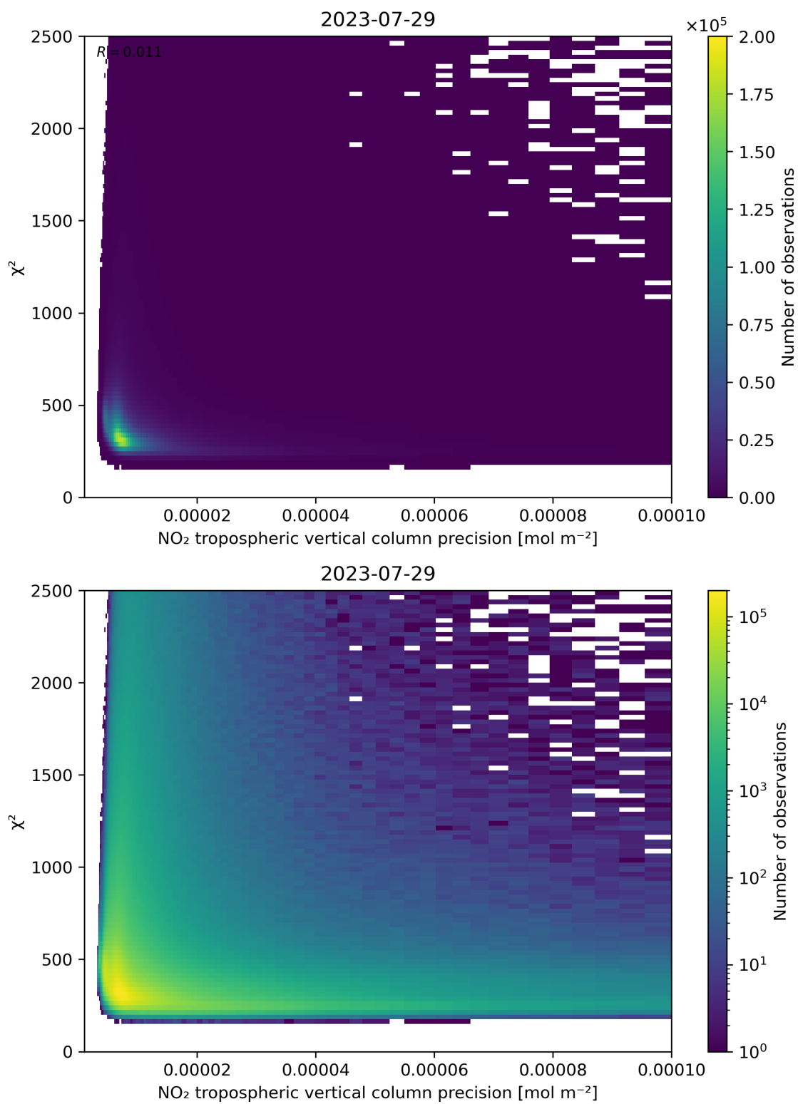
Figure 134: Scatter density plot of “NO 2 tropospheric vertical column precision” against “ \chi^2 ” for 2023-07-29 to 2023-07-30.
