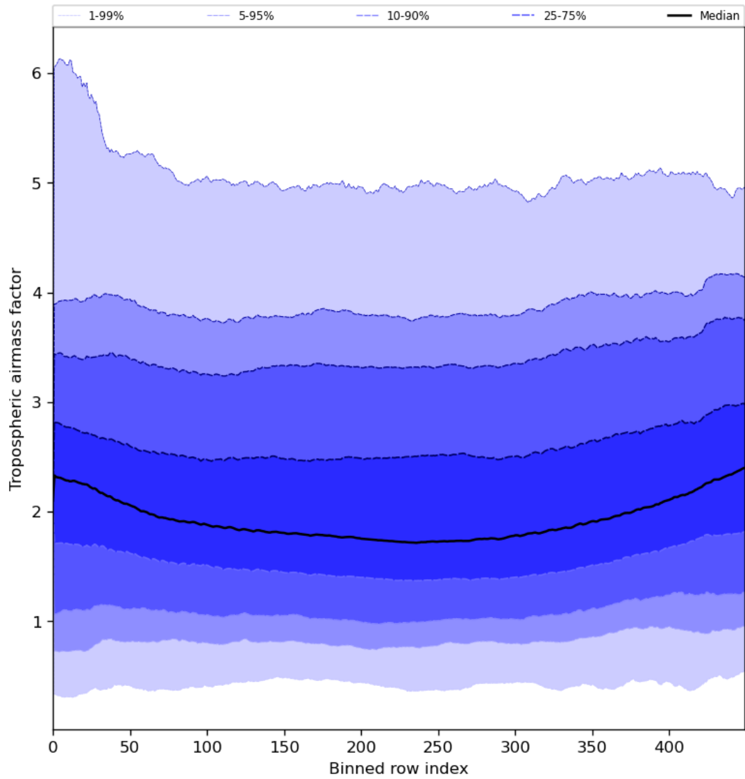
Figure 48: Along track statistics of “Tropospheric airmass factor” for 2023-07-29 to 2023-07-30
