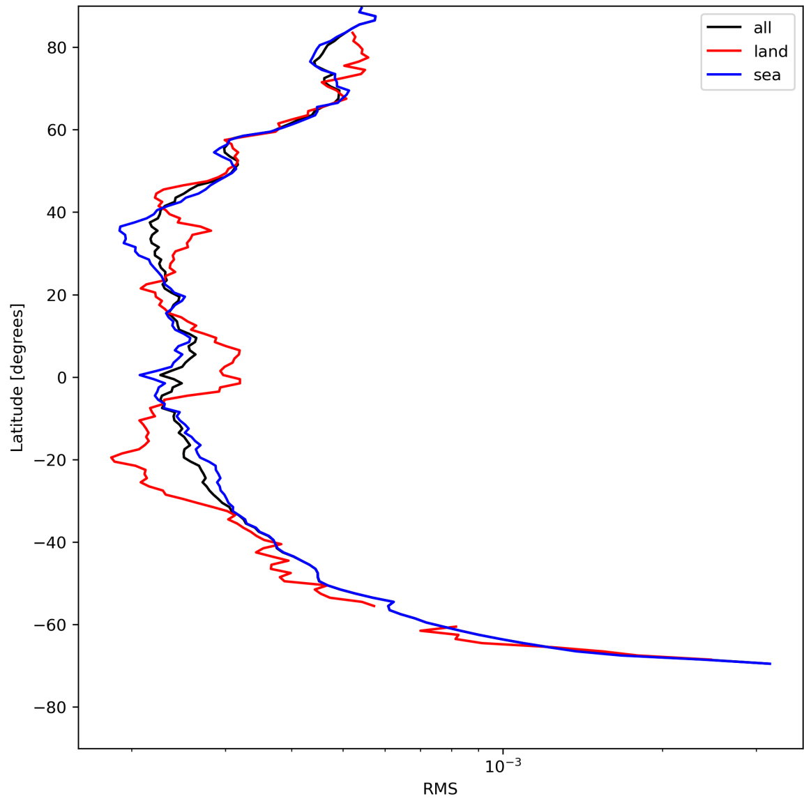
Figure 26: Zonal average of “RMS” for 2023-07-29 to 2023-07-30.
