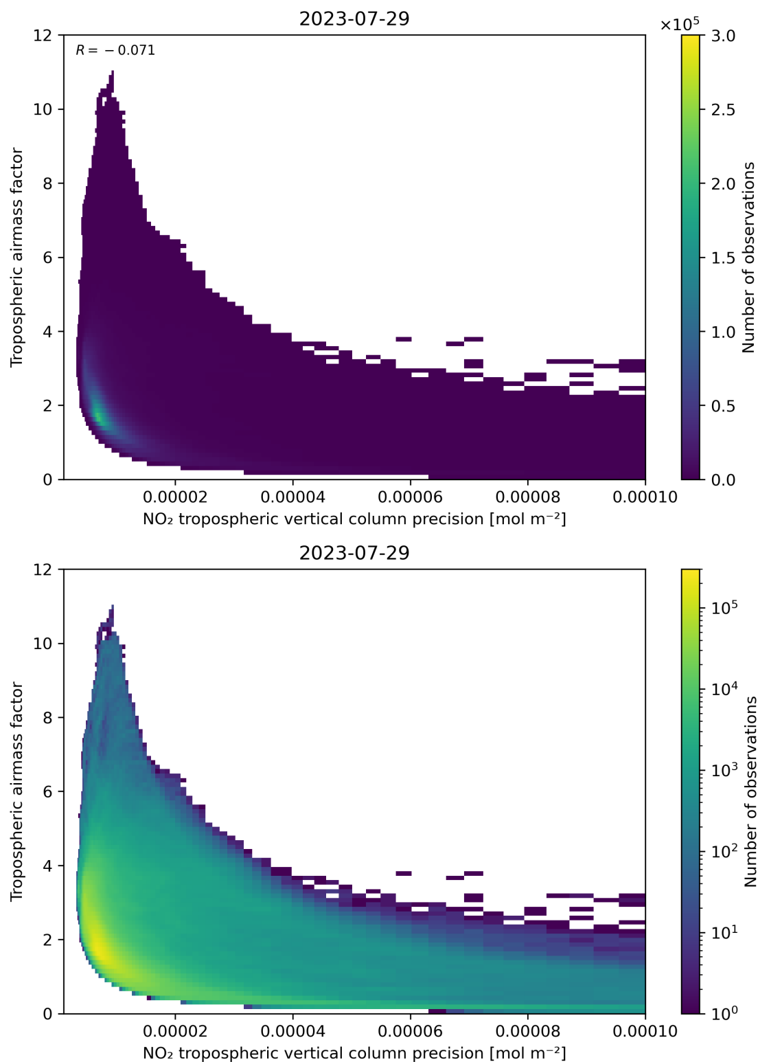
Figure 133: Scatter density plot of “NO 2 tropospheric vertical column precision” against “Tropospheric airmass factor” for 2023-07-29 to 2023-07-30.
