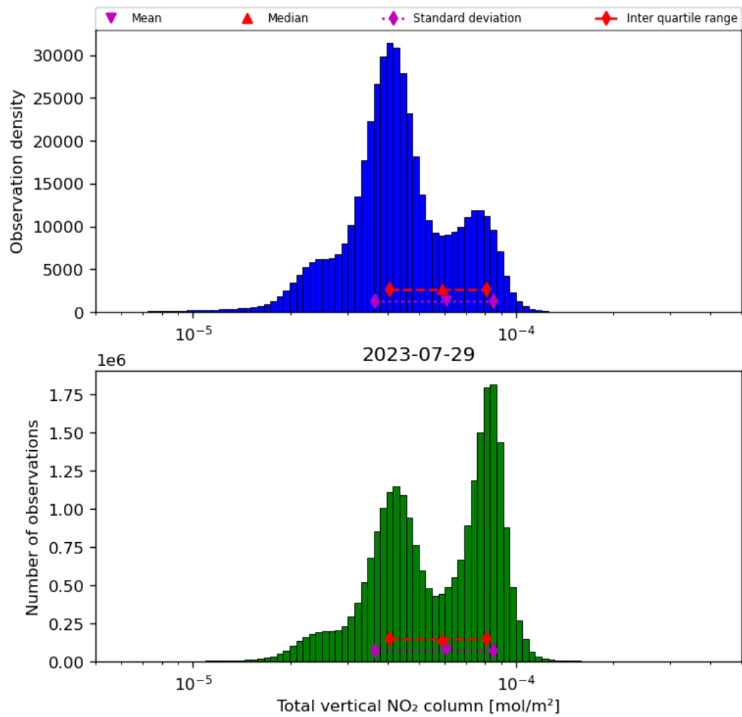
Figure 38: Histogram of “Total vertical NO 2 column” for 2023-07-29 to 2023-07-30
