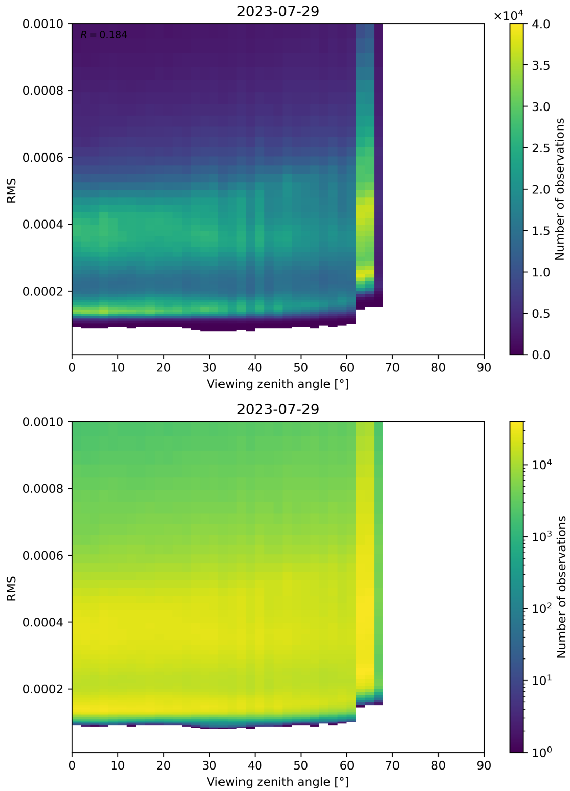
Figure 171: Scatter density plot of “Viewing zenith angle” against “RMS” for 2023-07-29 to 2023-07-30.
