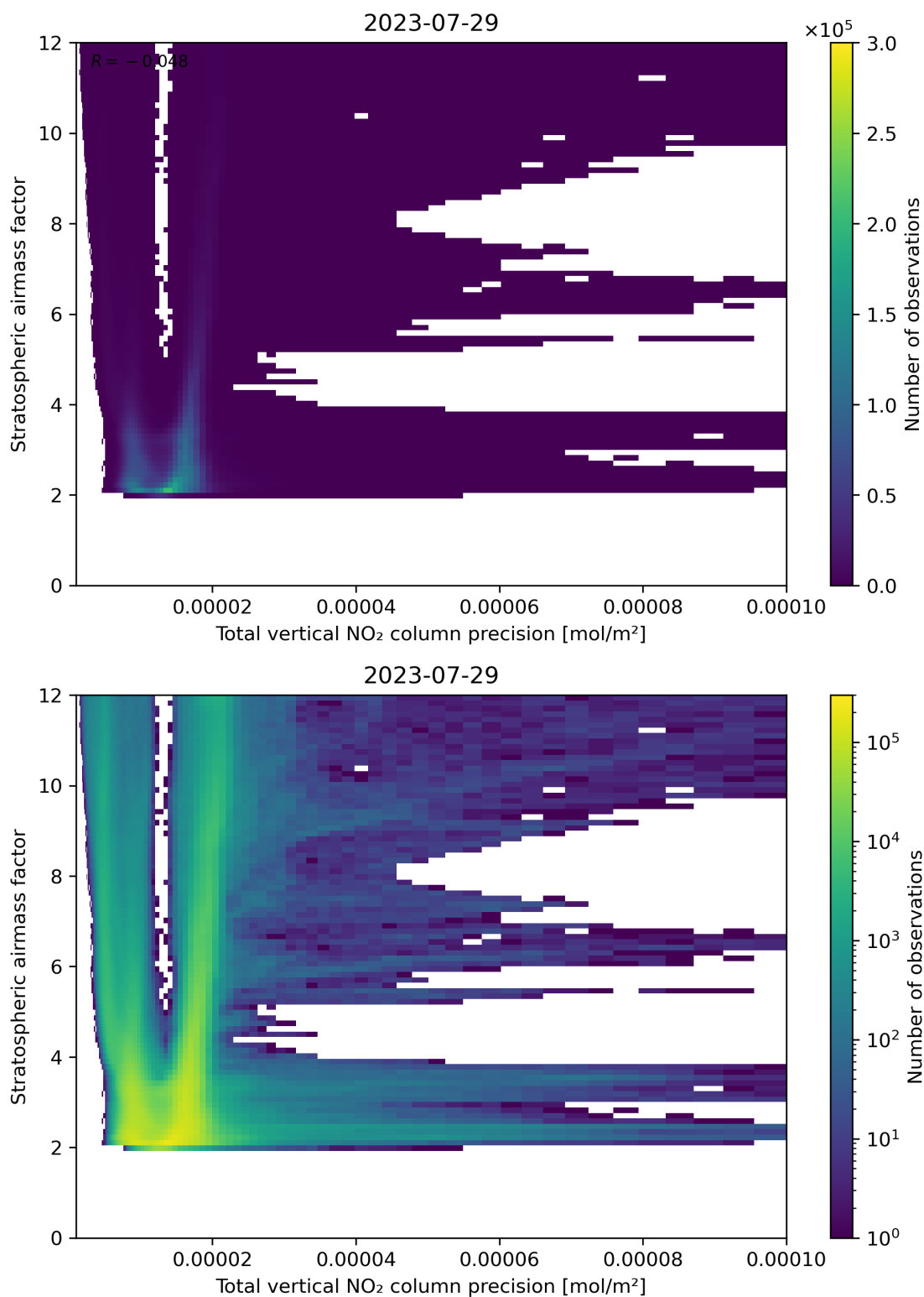
Figure 115: Scatter density plot of “Total vertical NO 2 column precision” against “Stratospheric air mass factor” for 2023-07-29 to 2023-07-30.
