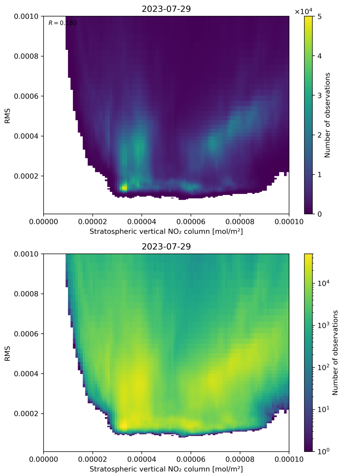
Figure 102: Scatter density plot of “Stratospheric vertical NO 2 column” against “RMS” for 2023-07-29 to 2023-07-30.
