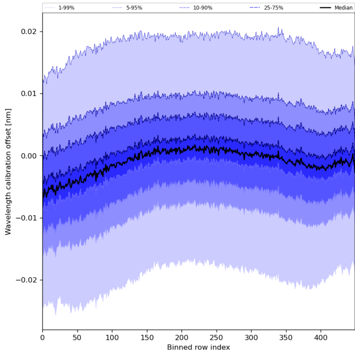
Figure 52: Along track statistics of “Wavelength calibration offset” for 2023-07-29 to 2023-07-30
