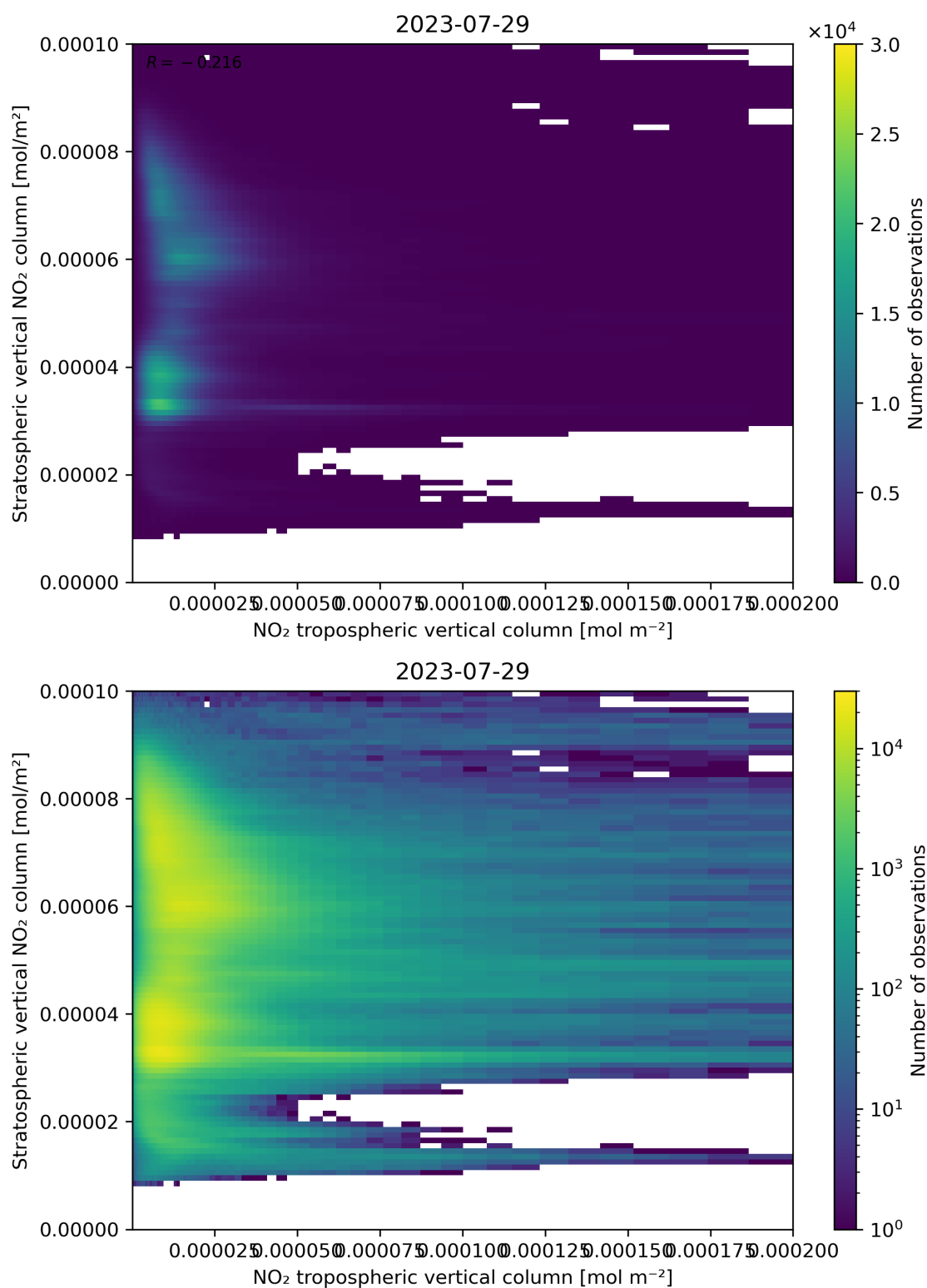
Figure 125: Scatter density plot of “NO 2 tropospheric vertical column” against “Stratospheric vertical NO 2 column” for 2023-07-29 to 2023-07-30.
