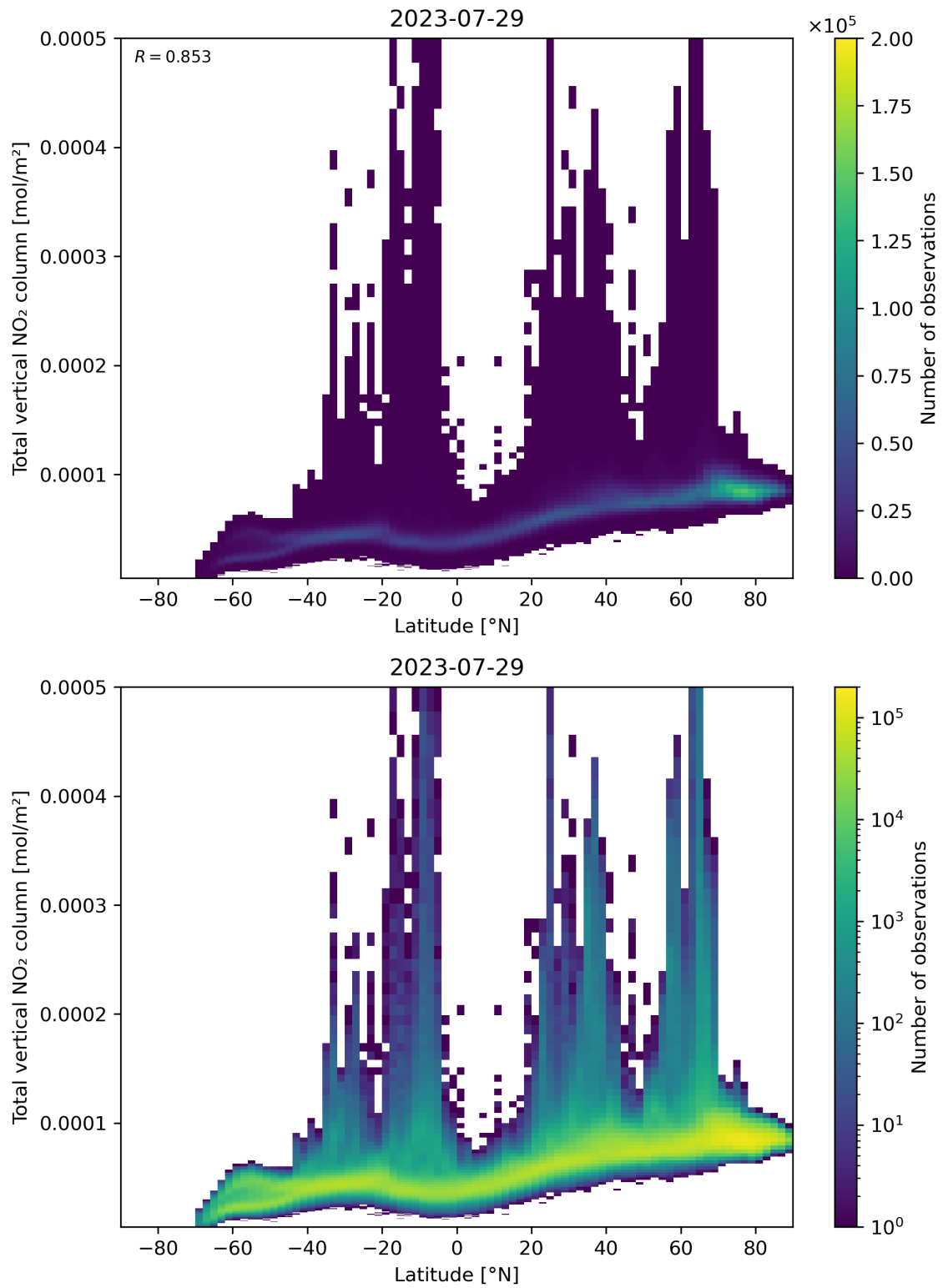
Figure 90: Scatter density plot of “Latitude” against “Total vertical NO 2 column” for 2023-07-29 to 2023-07-30.
