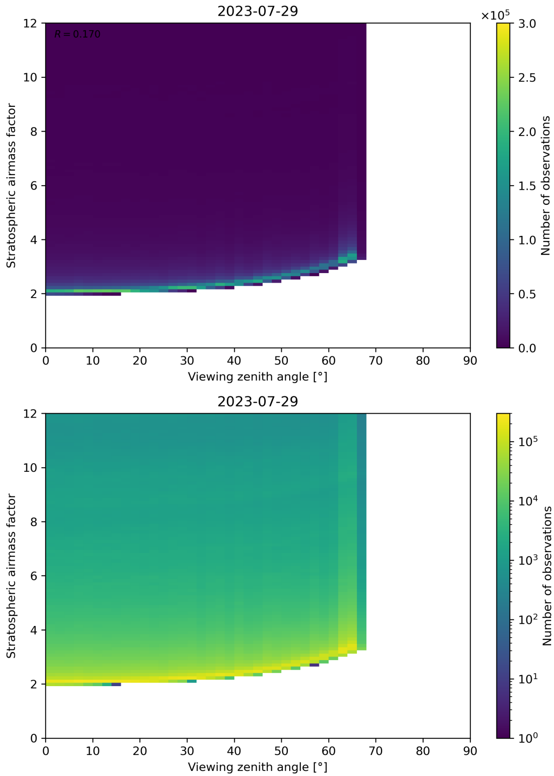
Figure 159: Scatter density plot of “Viewing zenith angle” against “Stratospheric airmass factor” for 2023-07-29 to 2023-07-30.
