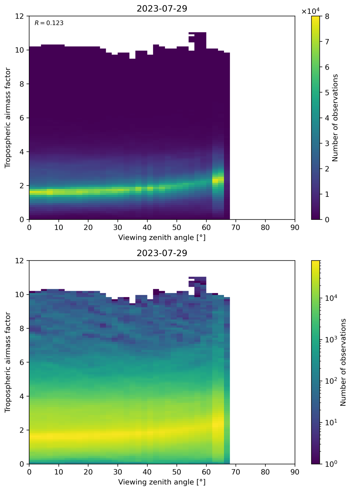
Figure 161: Scatter density plot of “Viewing zenith angle” against “Tropospheric airmass factor” for 2023-07-29 to 2023-07-30.
