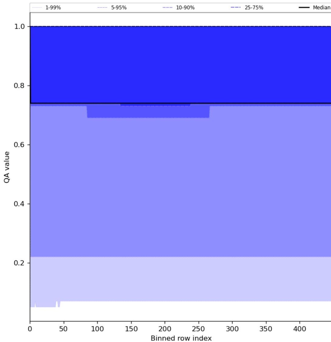
Figure 45: Along track statistics of “QA value” for 2023-07-29 to 2023-07-30
