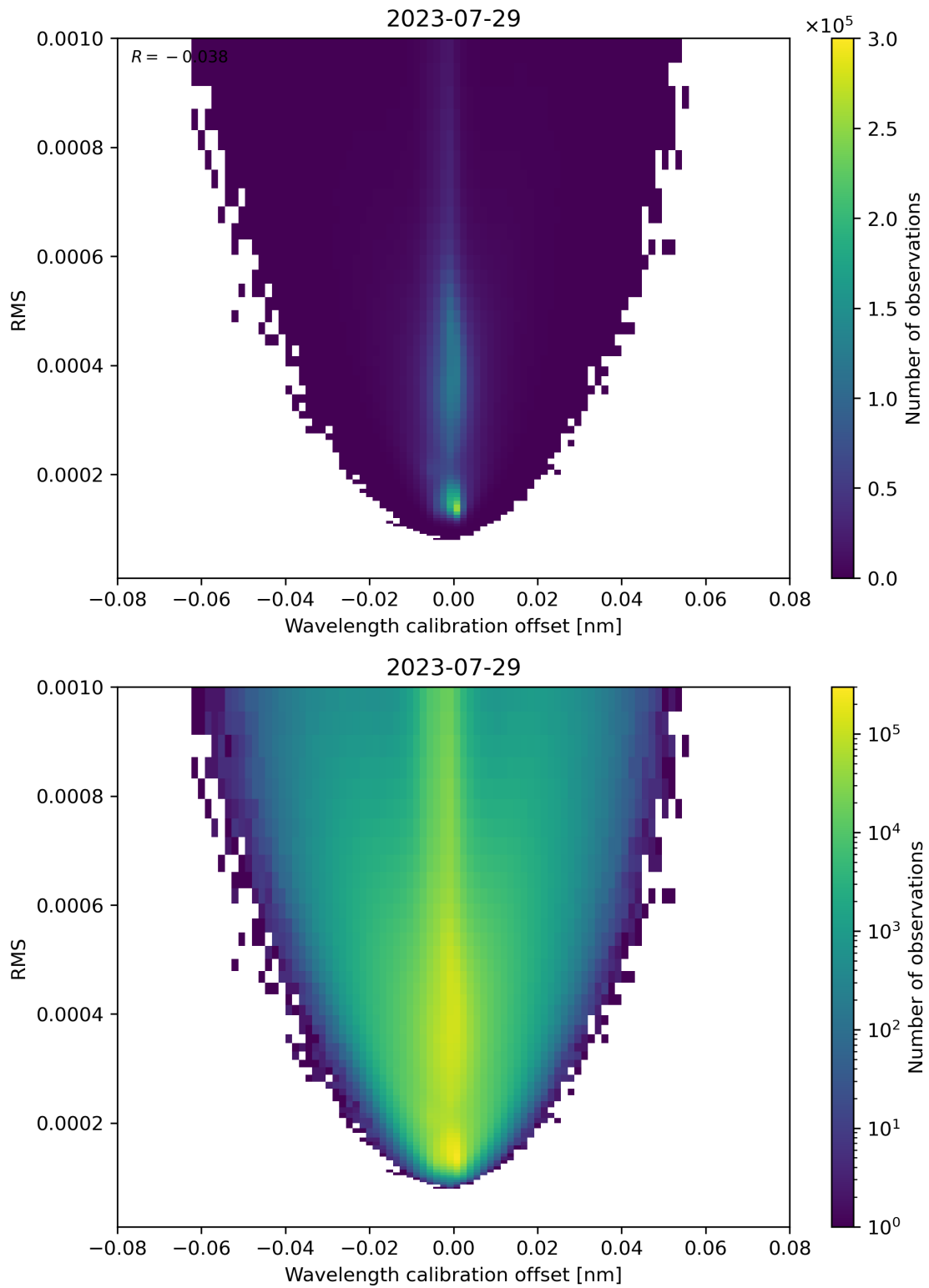
Figure 181: Scatter density plot of “Wavelength calibration offset” against “RMS” for 2023-07-29 to 2023-07-30.
