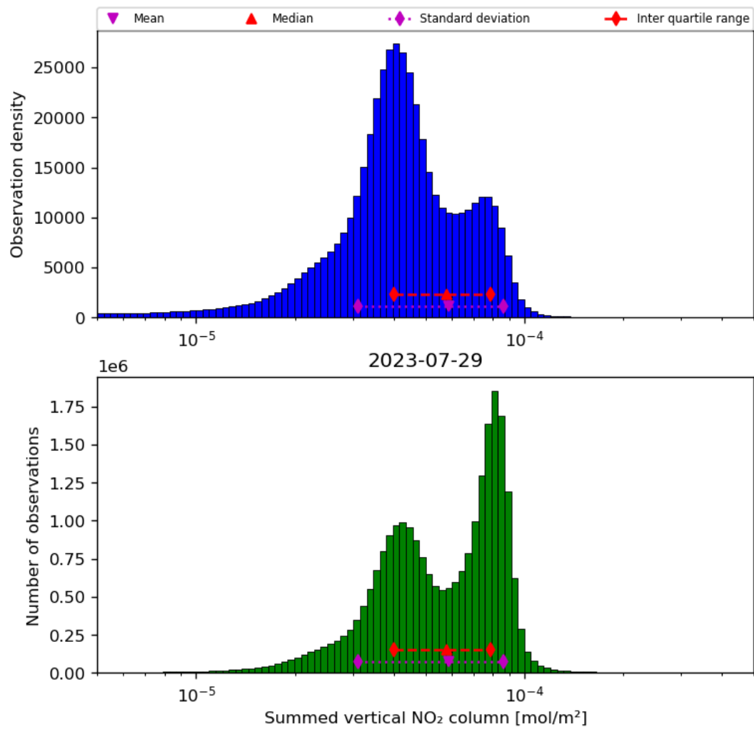
Figure 40: Histogram of “Summed vertical NO 2 column” for 2023-07-29 to 2023-07-30
