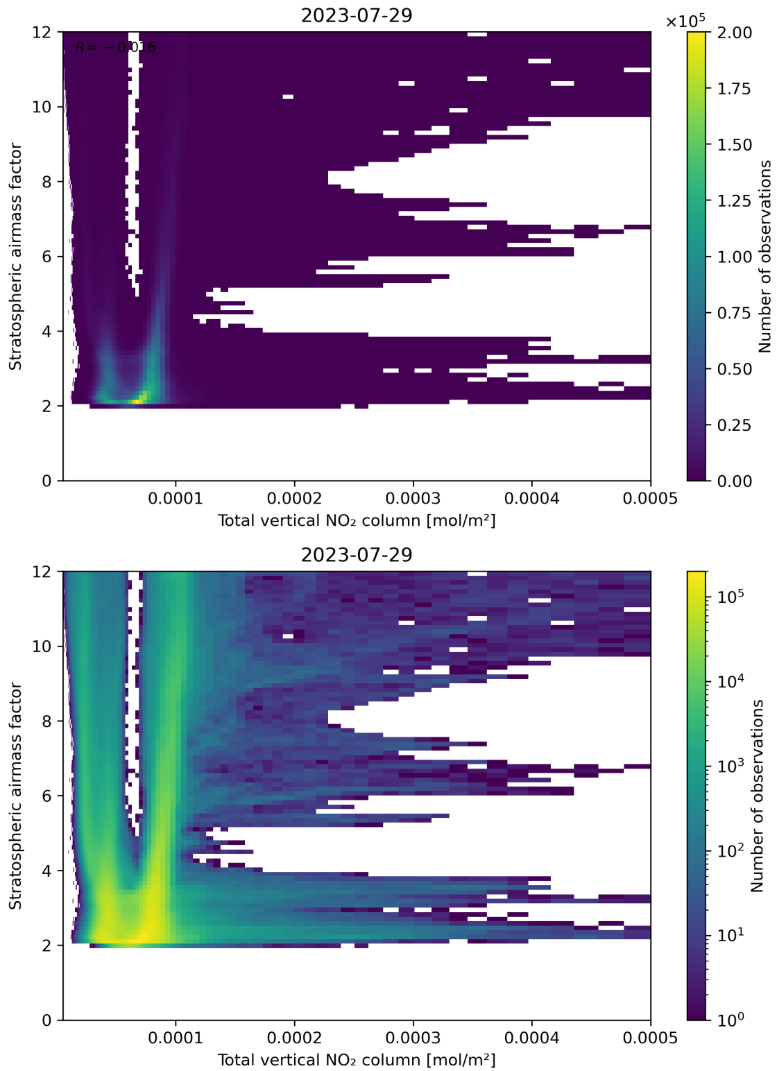
Figure 110: Scatter density plot of “Total vertical NO 2 column” against “Stratospheric airmass factor” for 2023-07-29 to 2023-07-30.
