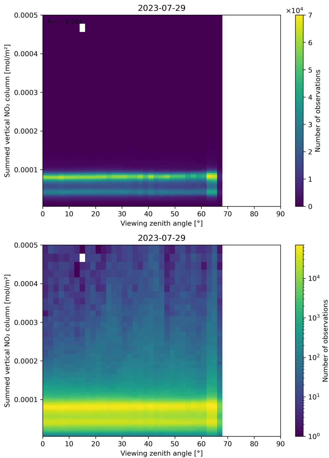
Figure 165: Scatter density plot of “Viewing zenith angle” against “Summed vertical NO 2 column” for 2023-07-29 to 2023-07-30.
