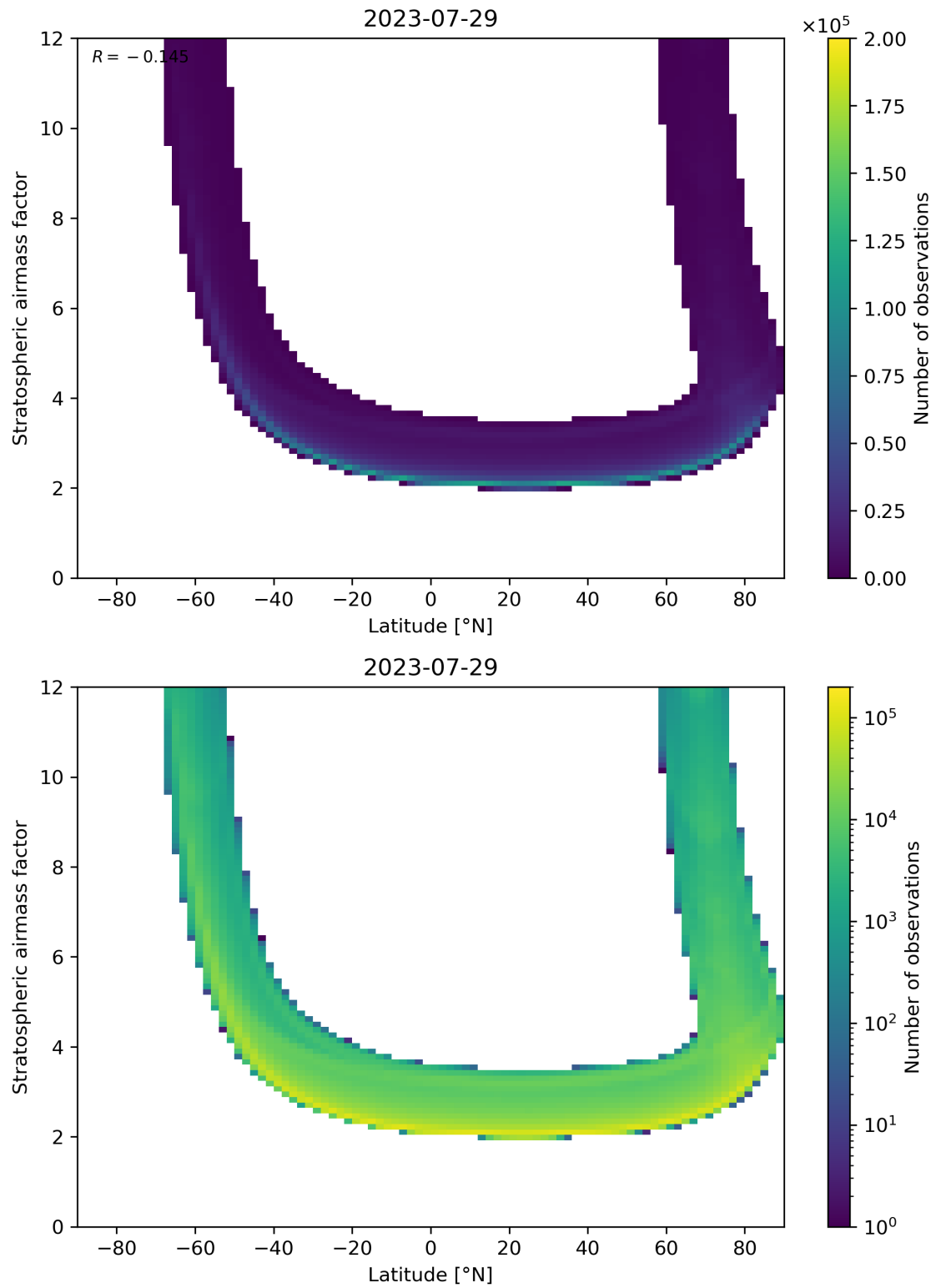
Figure 83: Scatter density plot of “Latitude” against “Stratospheric air mass factor” for 2023-07-29 to 2023-07-30.
