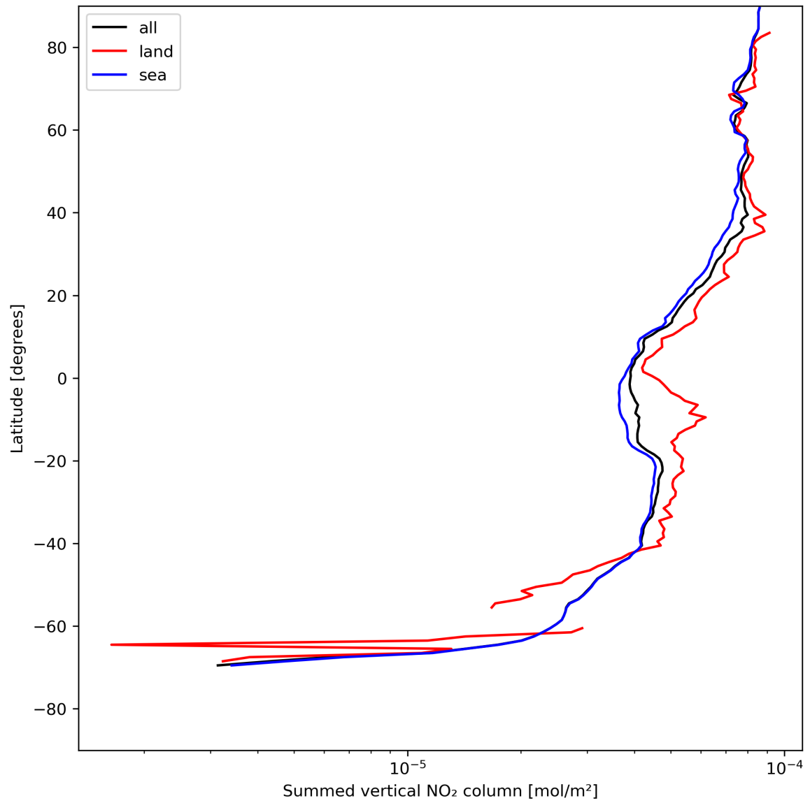
Figure 23: Zonal average of “Summed vertical NO 2 column” for 2023-07-29 to 2023-07-30.
