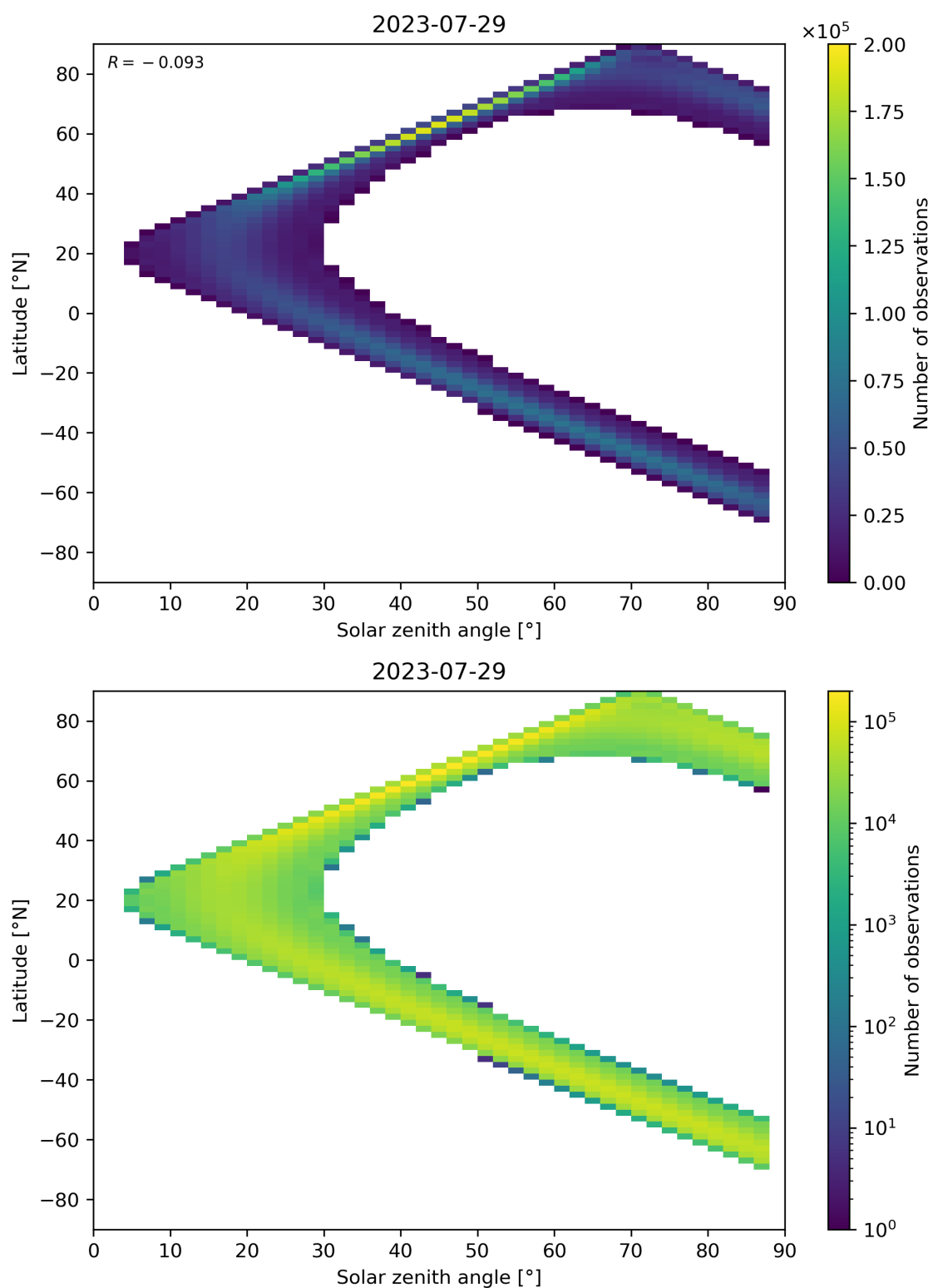
Figure 149: Scatter density plot of “Solar zenith angle” against “Latitude” for 2023-07-29 to 2023-07-30.
