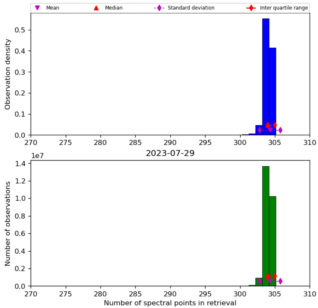
Figure 33: Histogram of “Number of spectral points in retrieval” for 2023-07-29 to 2023-07-30
