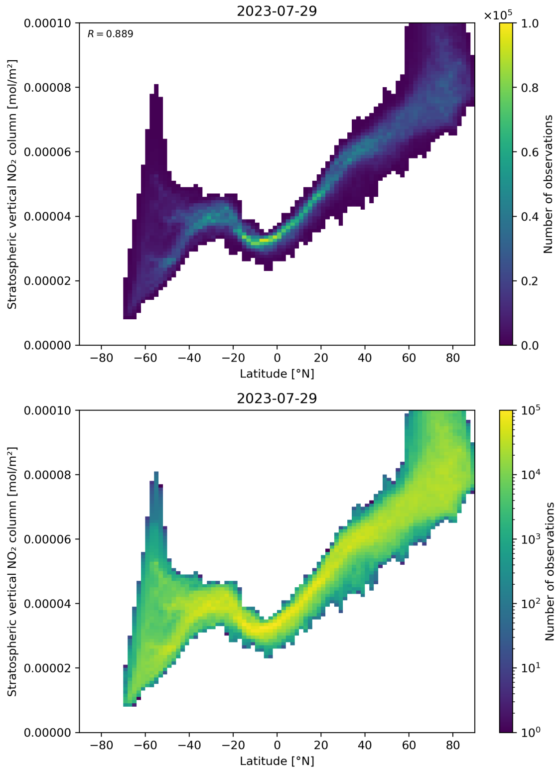
Figure 87: Scatter density plot of “Latitude” against “Stratospheric vertical \text{NO}_2 column” for 2023-07-29 to 2023-07-30.
