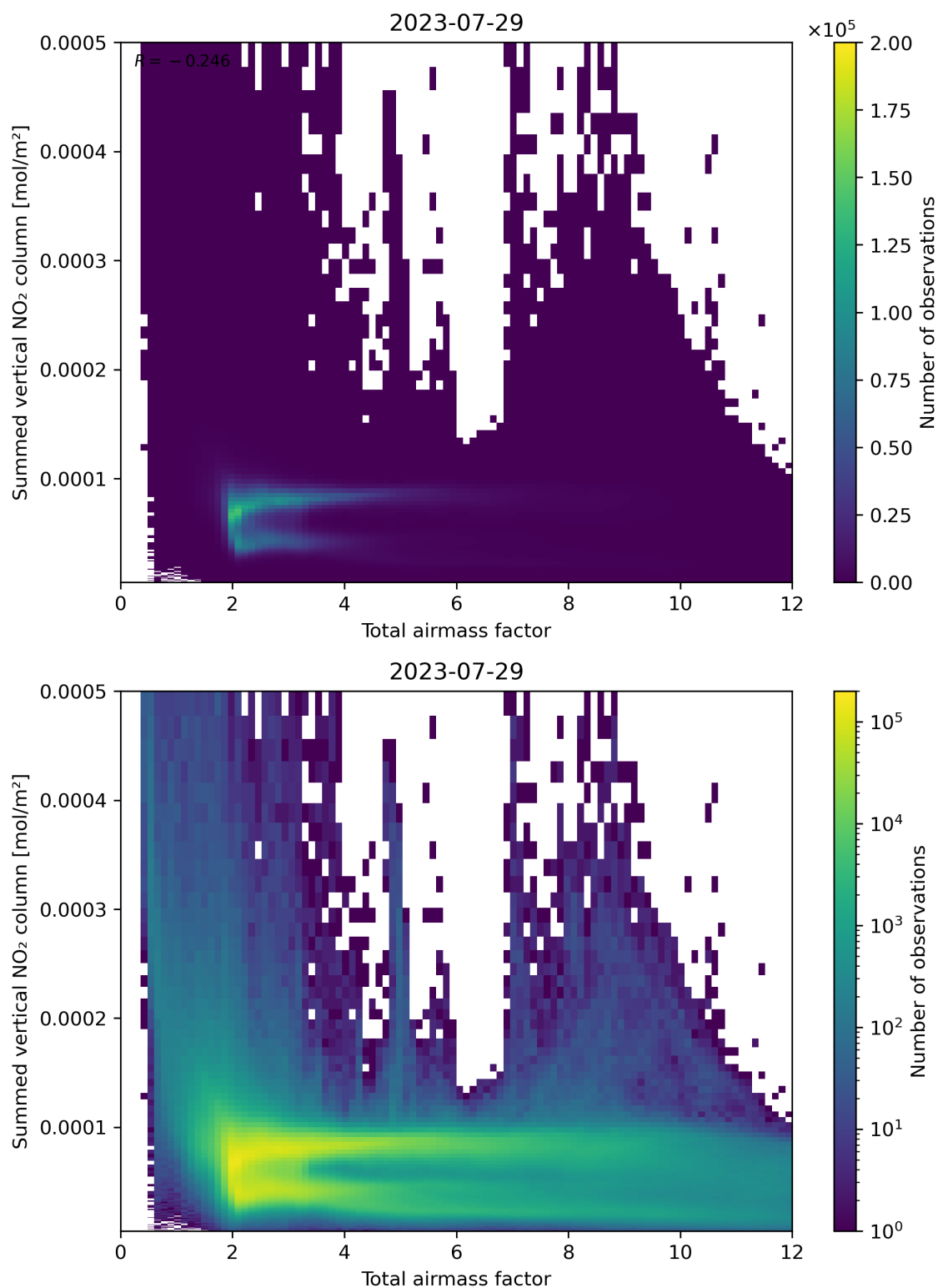
Figure 65: Scatter density plot of “Total airmass factor” against “Summed vertical NO 2 column” for 2023-07-29 to 2023-07-30.
