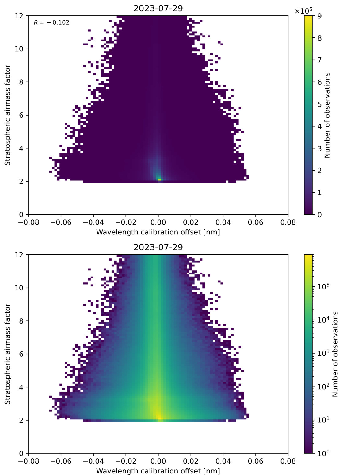
Figure 174: Scatter density plot of “Wavelength calibration offset” against “Stratospheric air mass factor” for 2023-07-29 to 2023-07-30.
