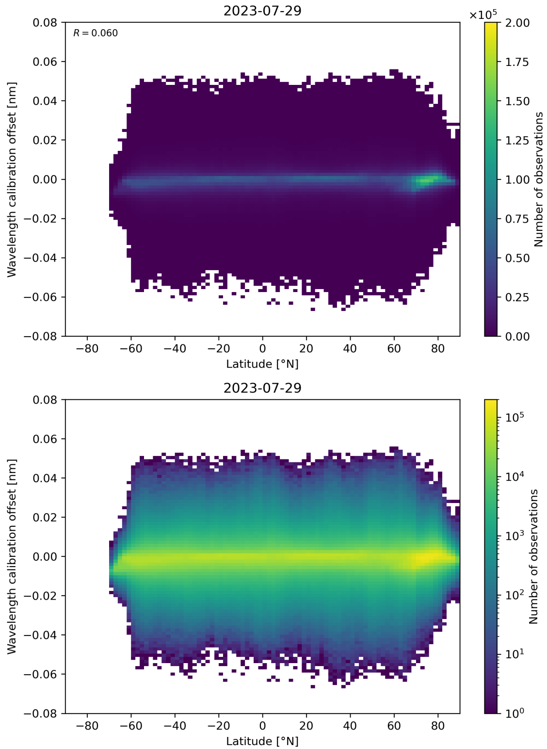
Figure 95: Scatter density plot of “Latitude” against “Wavelength calibration offset” for 2023-07-29 to 2023-07-30.
