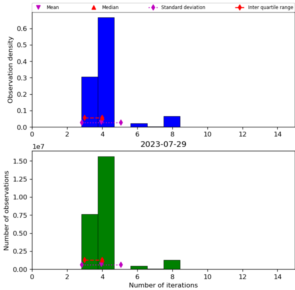
Figure 34: Histogram of “Number of iterations” for 2023-07-29 to 2023-07-30
