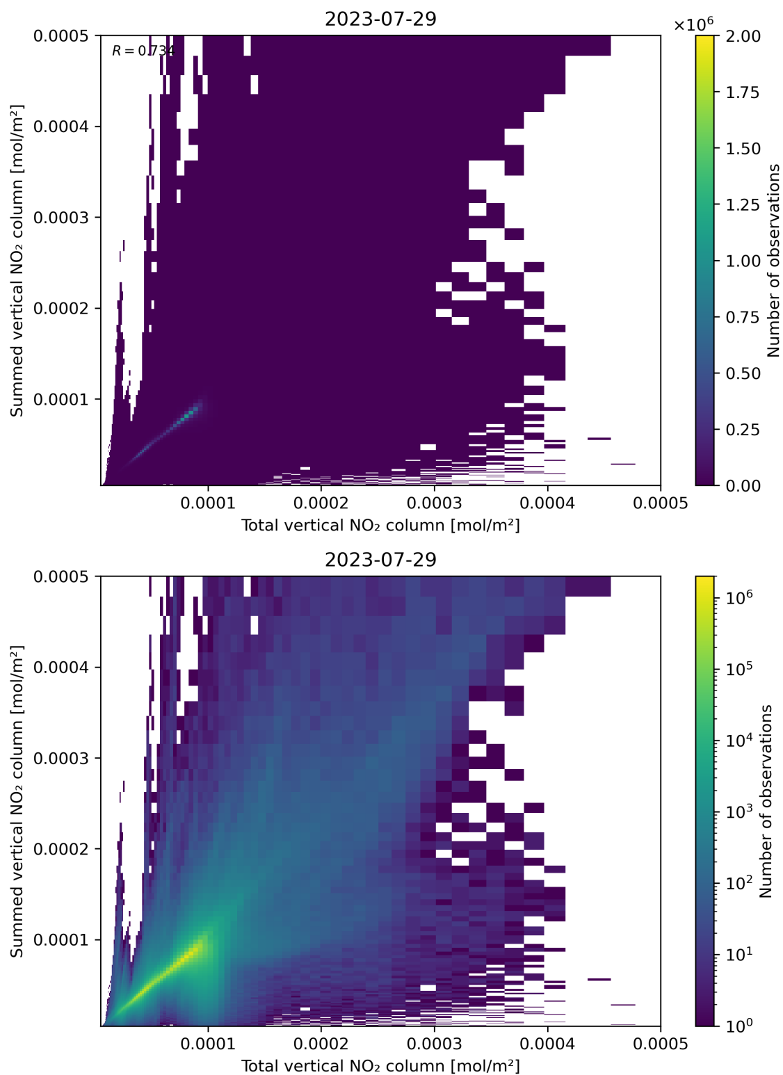
Figure 112: Scatter density plot of “Total vertical NO 2 column” against “Summed vertical NO 2 column” for 2023-07-29 to 2023-07-30.
