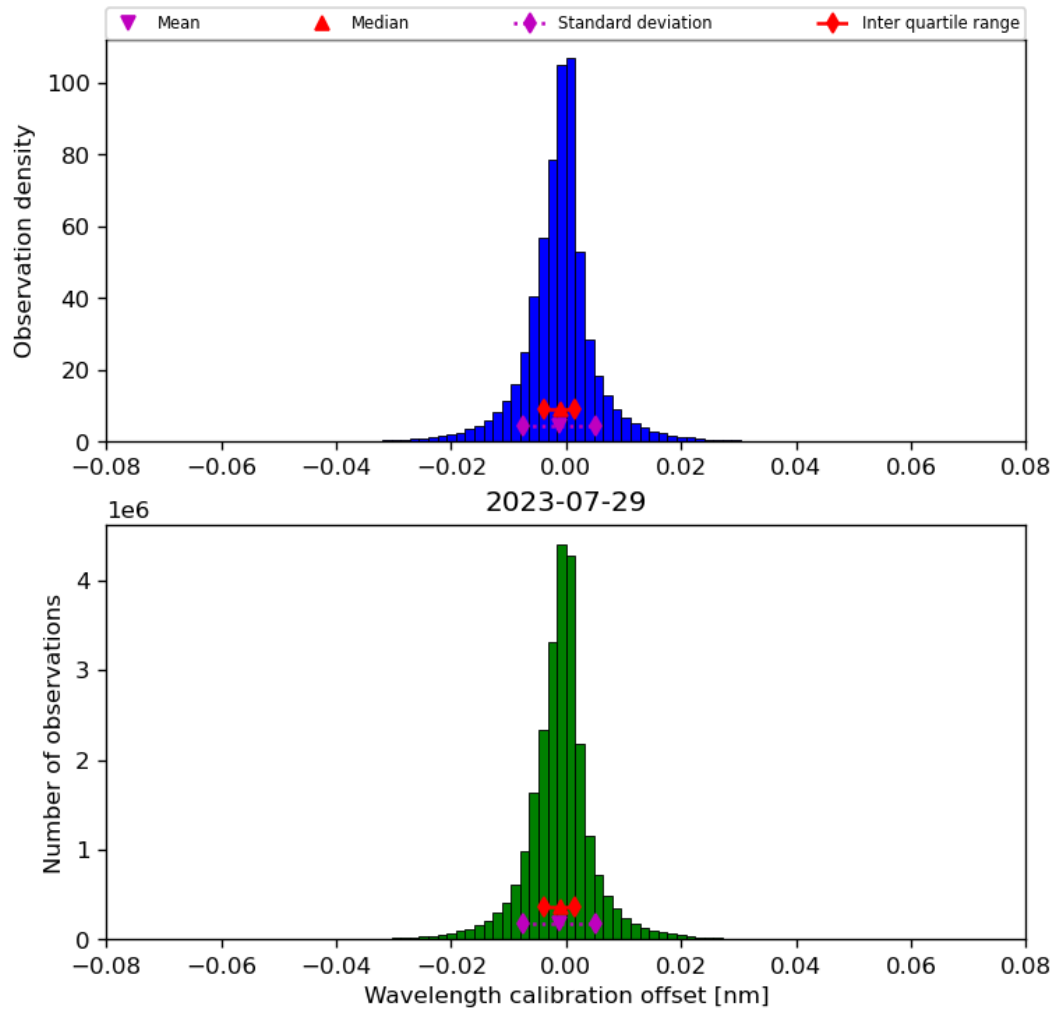
Figure 35: Histogram of “Wavelength calibration offset” for 2023-07-29 to 2023-07-30
