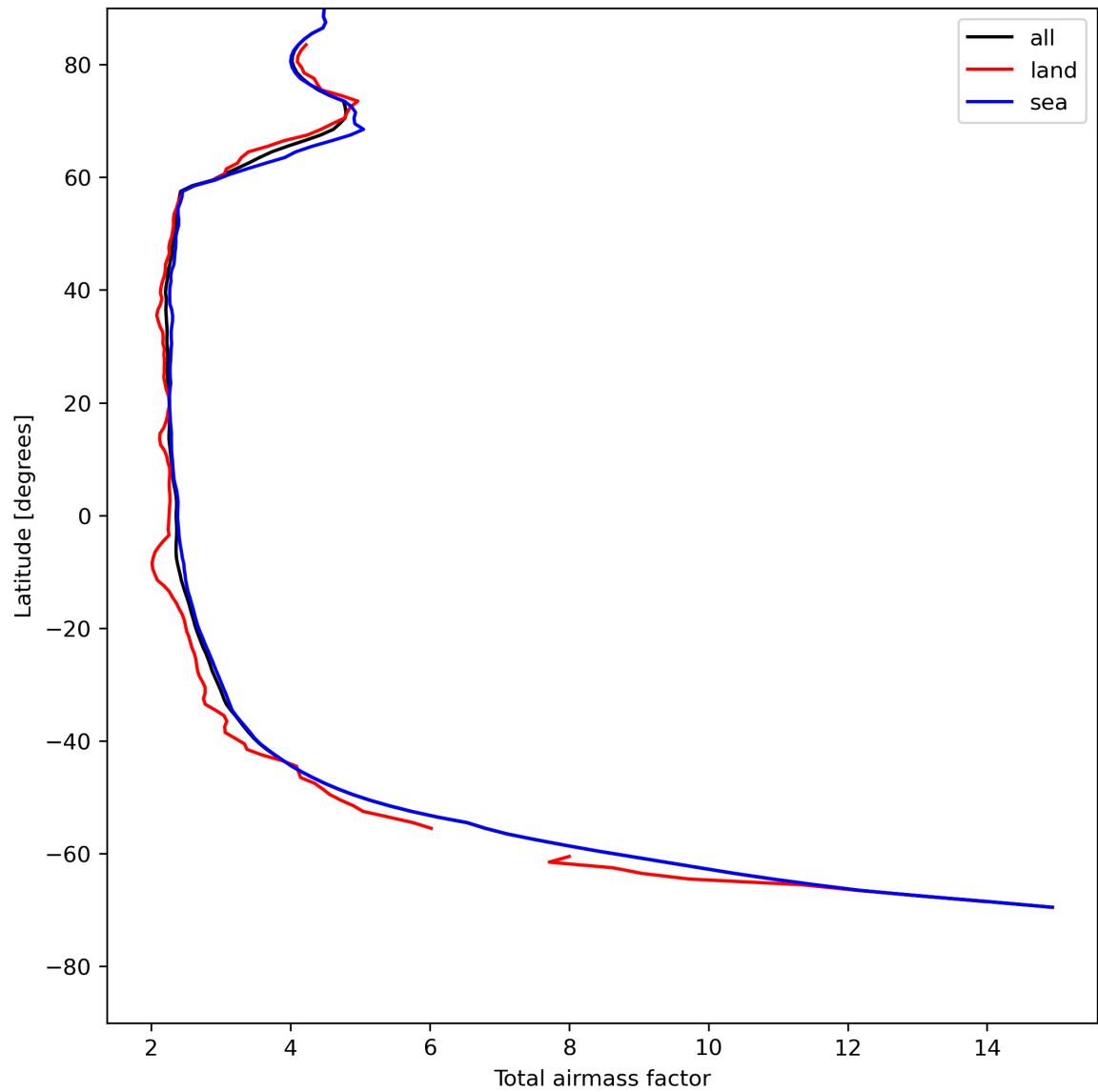
Figure 15: Zonal average of “Total airmass factor” for 2023-07-29 to 2023-07-30.
