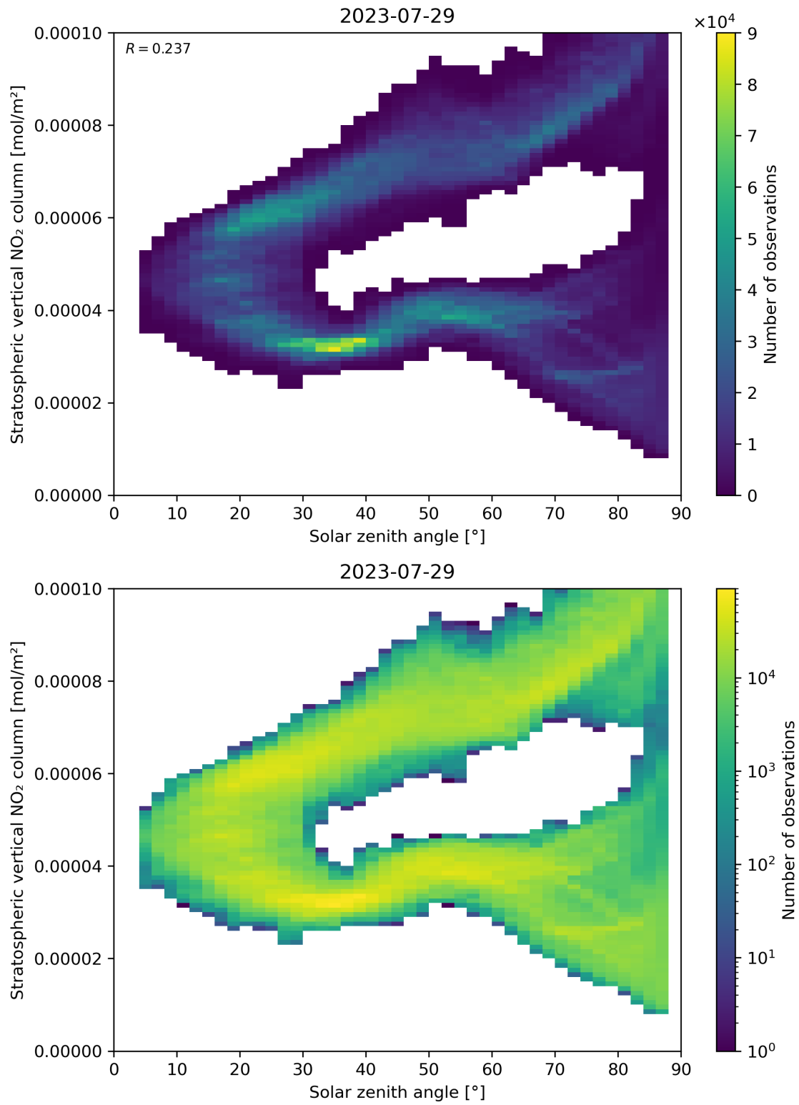
Figure 150: Scatter density plot of “Solar zenith angle” against “Stratospheric vertical NO 2 column” for 2023-07-29 to 2023-07-30.
