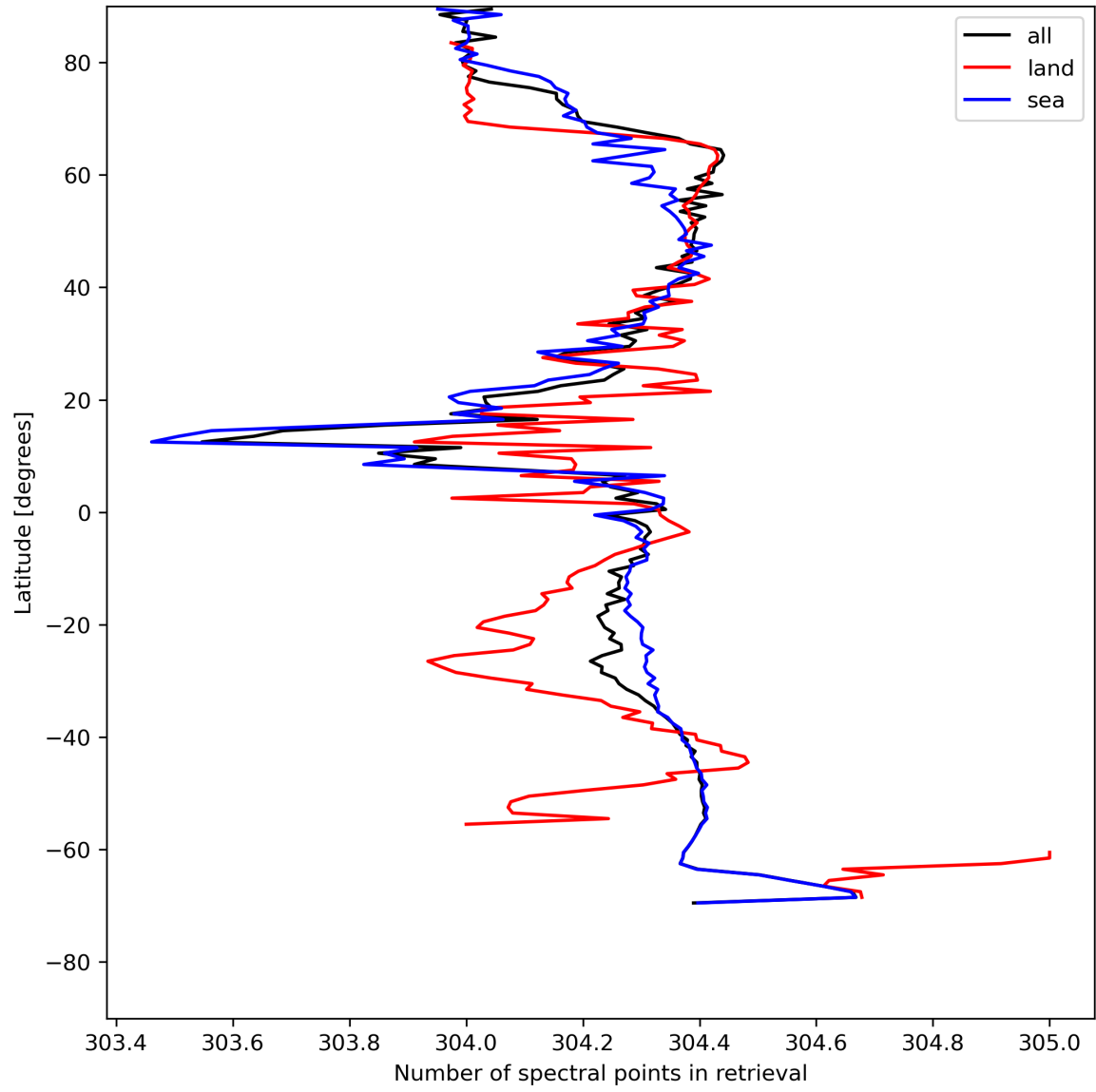
Figure 16: Zonal average of “Number of spectral points in retrieval” for 2023-07-29 to 2023-07-30.
