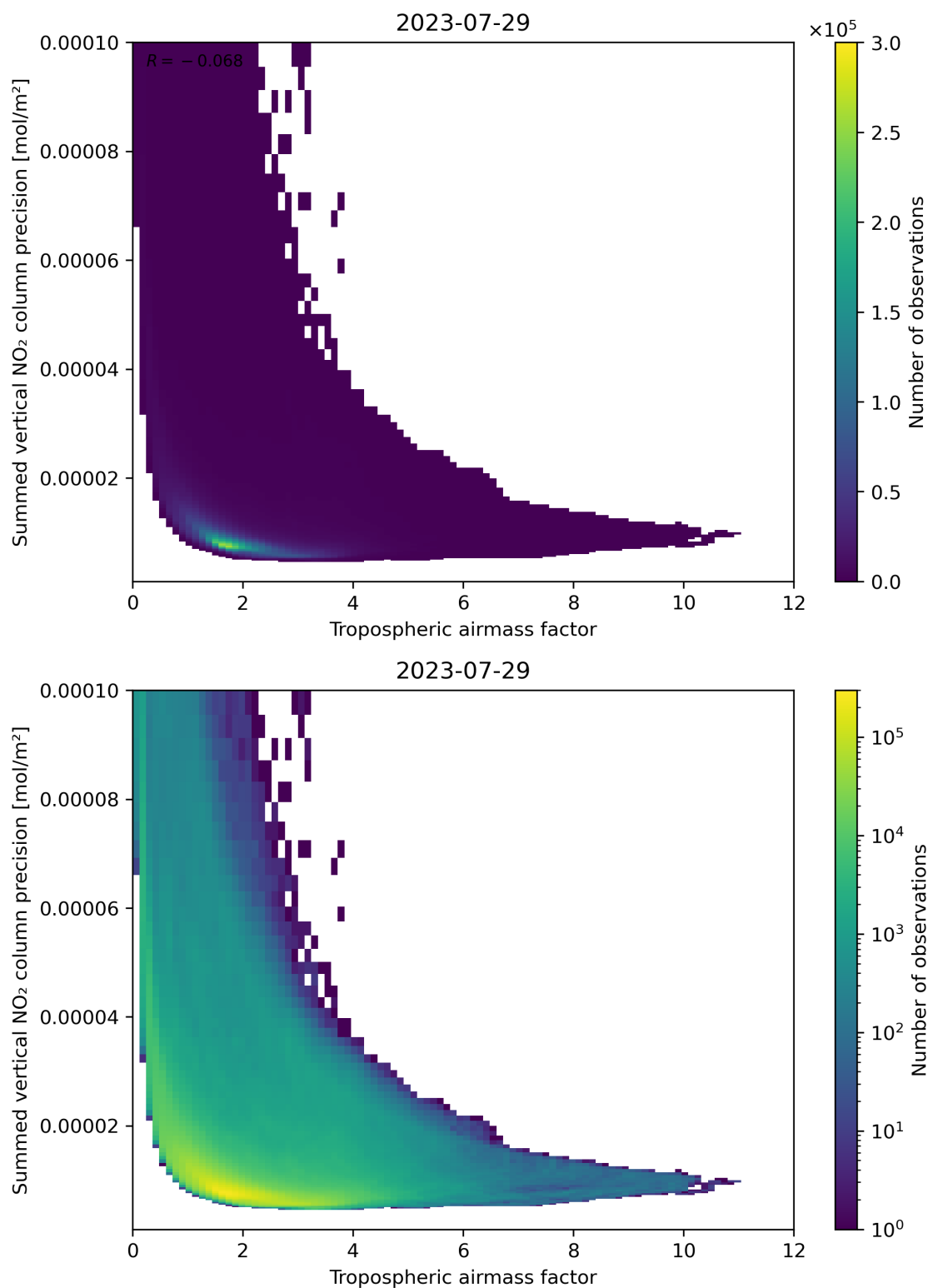
Figure 76: Scatter density plot of “Tropospheric air mass factor” against “Summed vertical NO 2 column precision” for 2023-07-29 to 2023-07-30.
