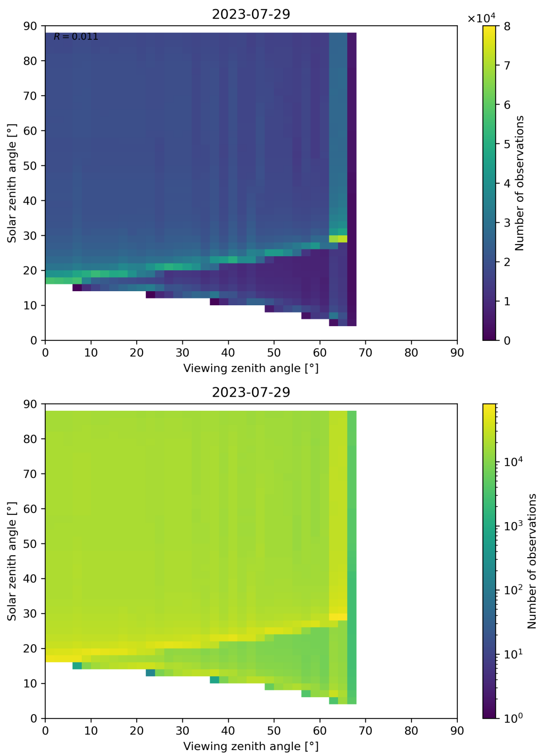
Figure 172: Scatter density plot of “Viewing zenith angle” against “Solar zenith angle” for 2023-07-29 to 2023-07-30.
