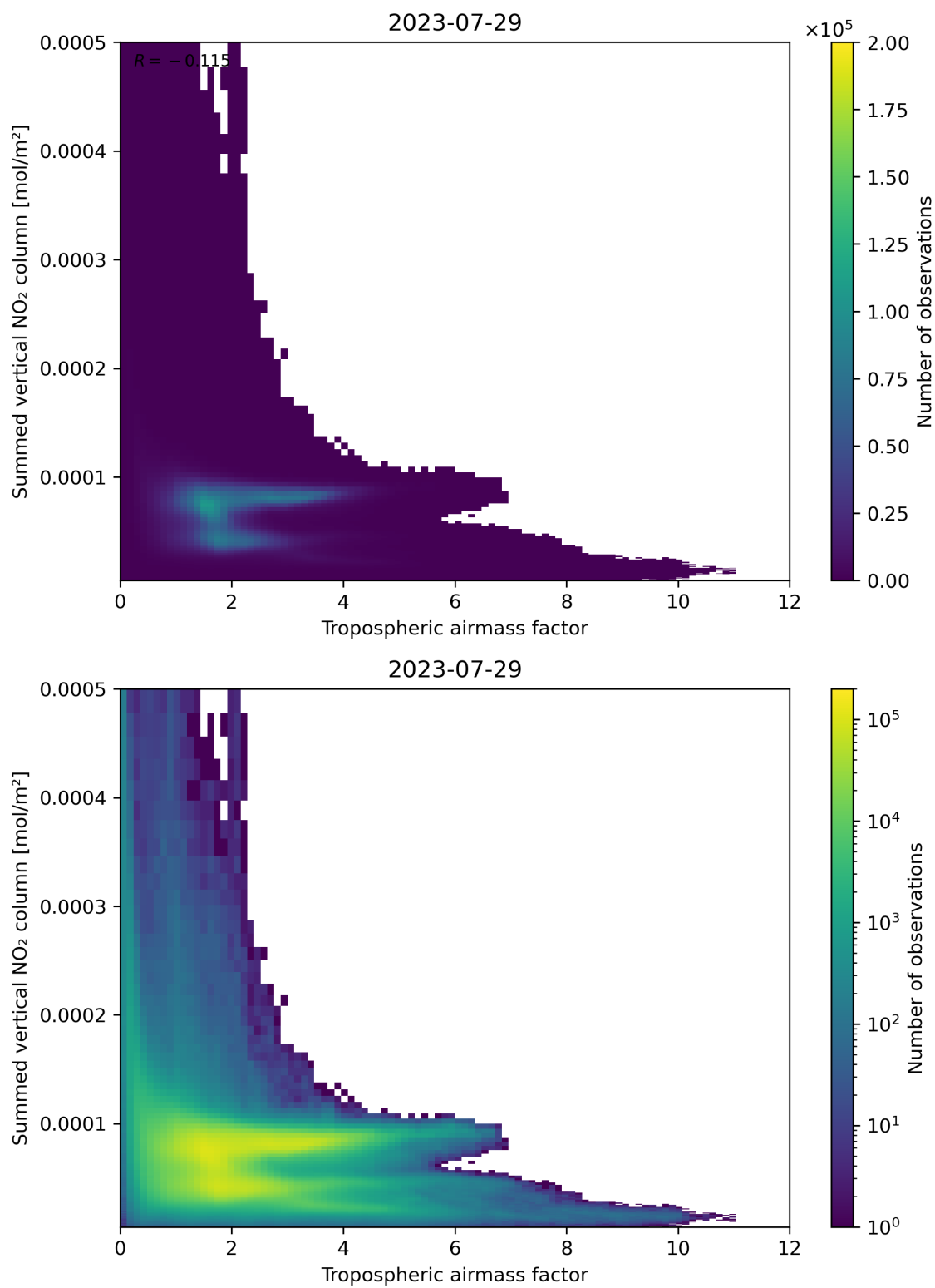
Figure 75: Scatter density plot of “Tropospheric airmass factor” against “Summed vertical NO 2 column” for 2023-07-29 to 2023-07-30.
