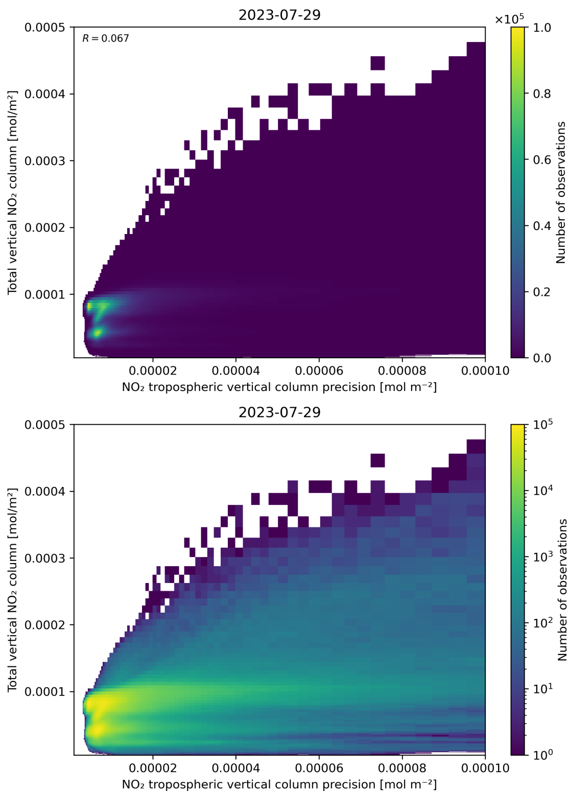
Figure 138: Scatter density plot of “NO 2 tropospheric vertical column precision” against “Total vertical NO 2 column” for 2023-07-29 to 2023-07-30.
