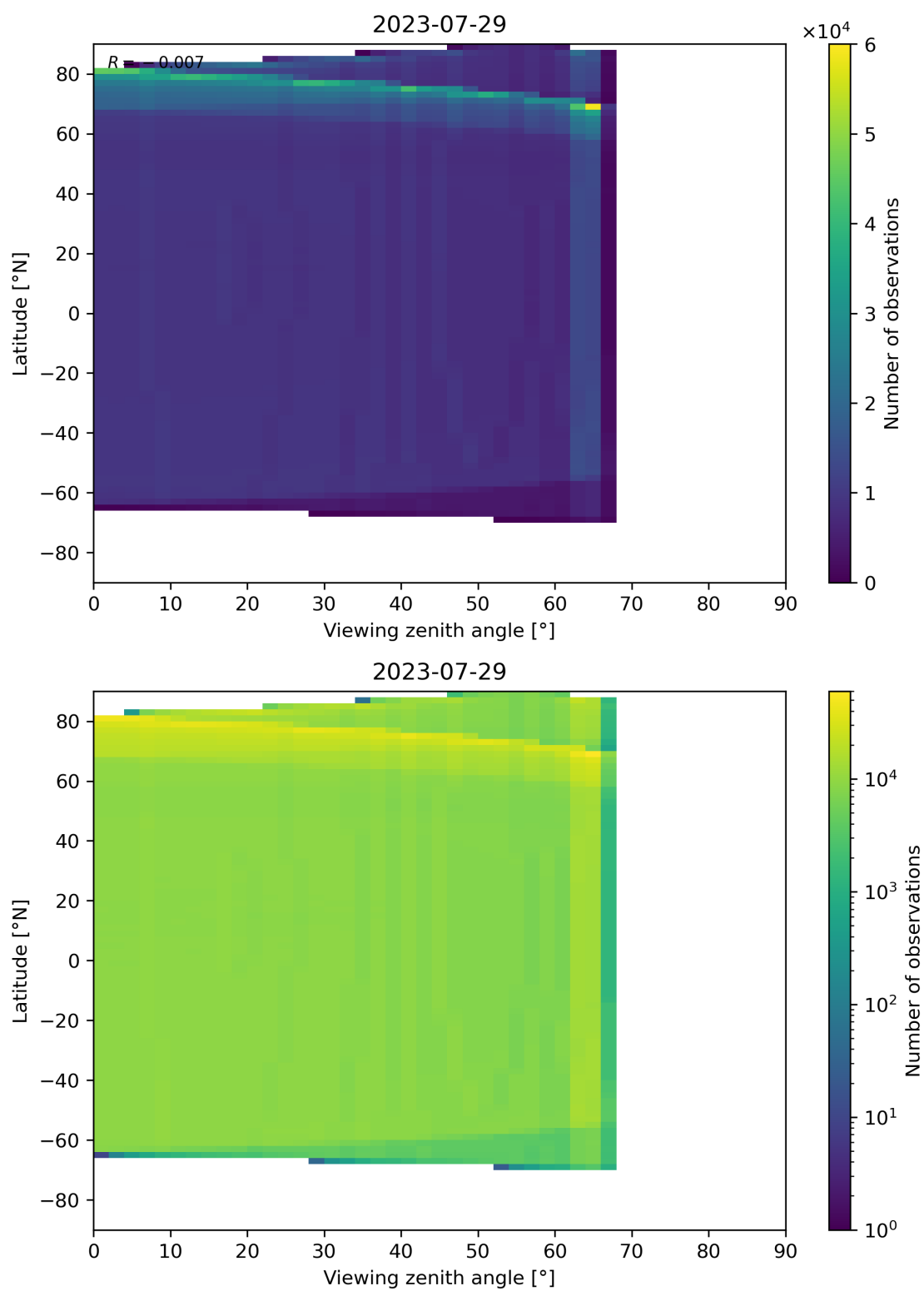
Figure 163: Scatter density plot of “Viewing zenith angle” against “Latitude” for 2023-07-29 to 2023-07-30.
