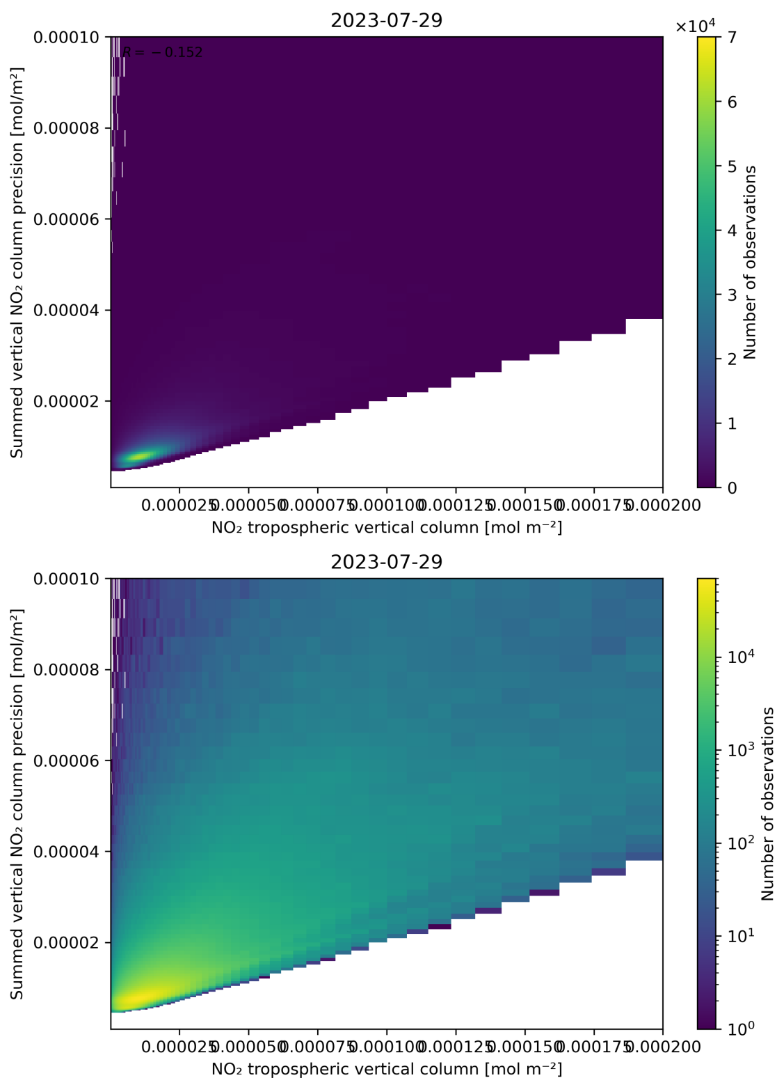
Figure 127: Scatter density plot of “NO 2 tropospheric vertical column” against “Summed vertical NO 2 column precision” for 2023-07-29 to 2023-07-30.
