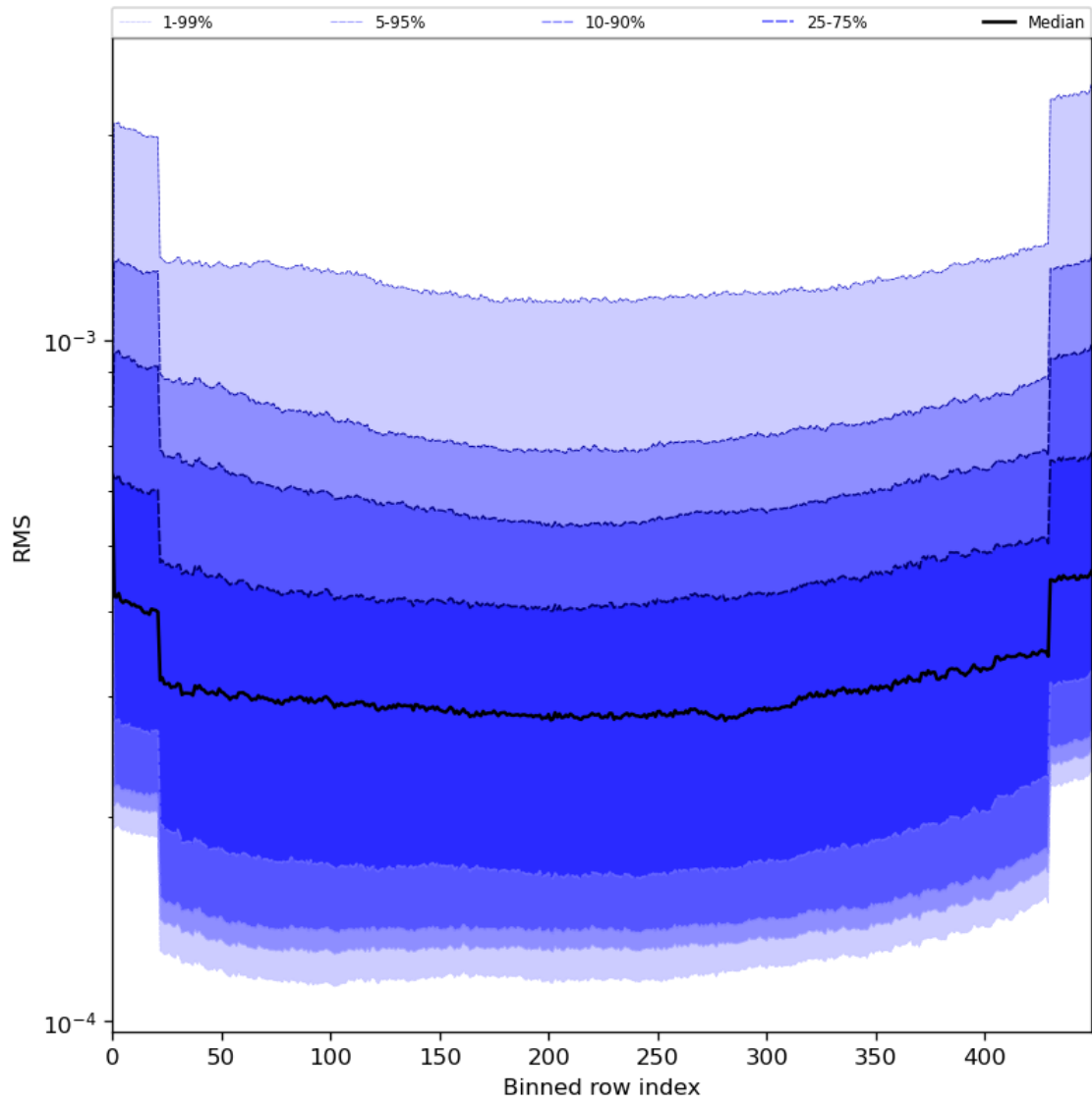
Figure 60: Along track statistics of “RMS” for 2023-07-29 to 2023-07-30
