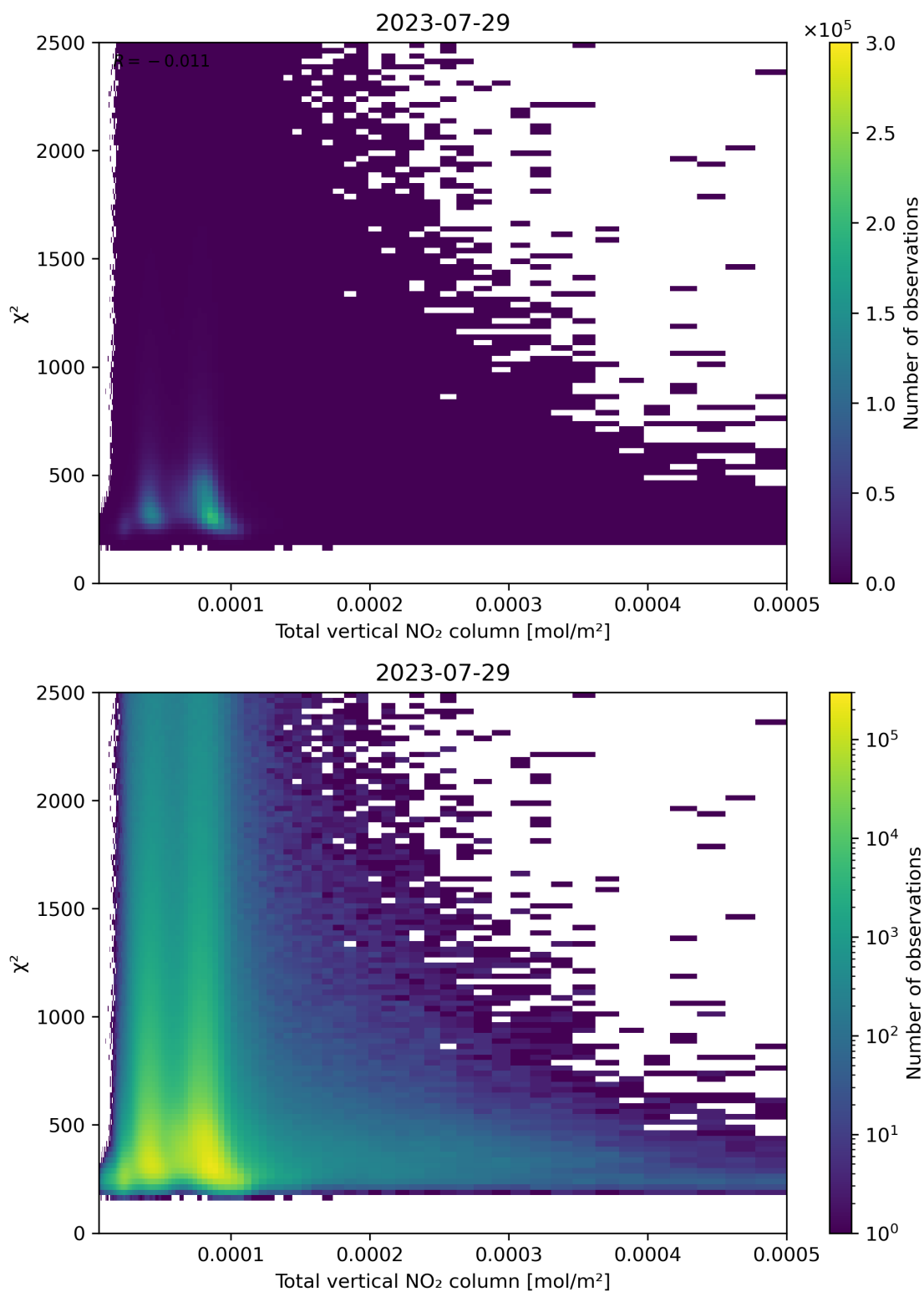
Figure 111: Scatter density plot of “Total vertical NO 2 column” against “ \chi^2 ” for 2023-07-29 to 2023-07-30.
