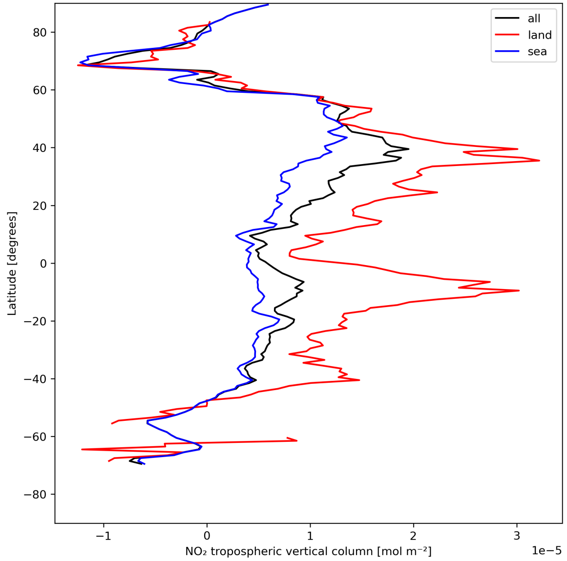
Figure 12: Zonal average of “NO 2 tropospheric vertical column” for 2023-07-29 to 2023-07-30.
