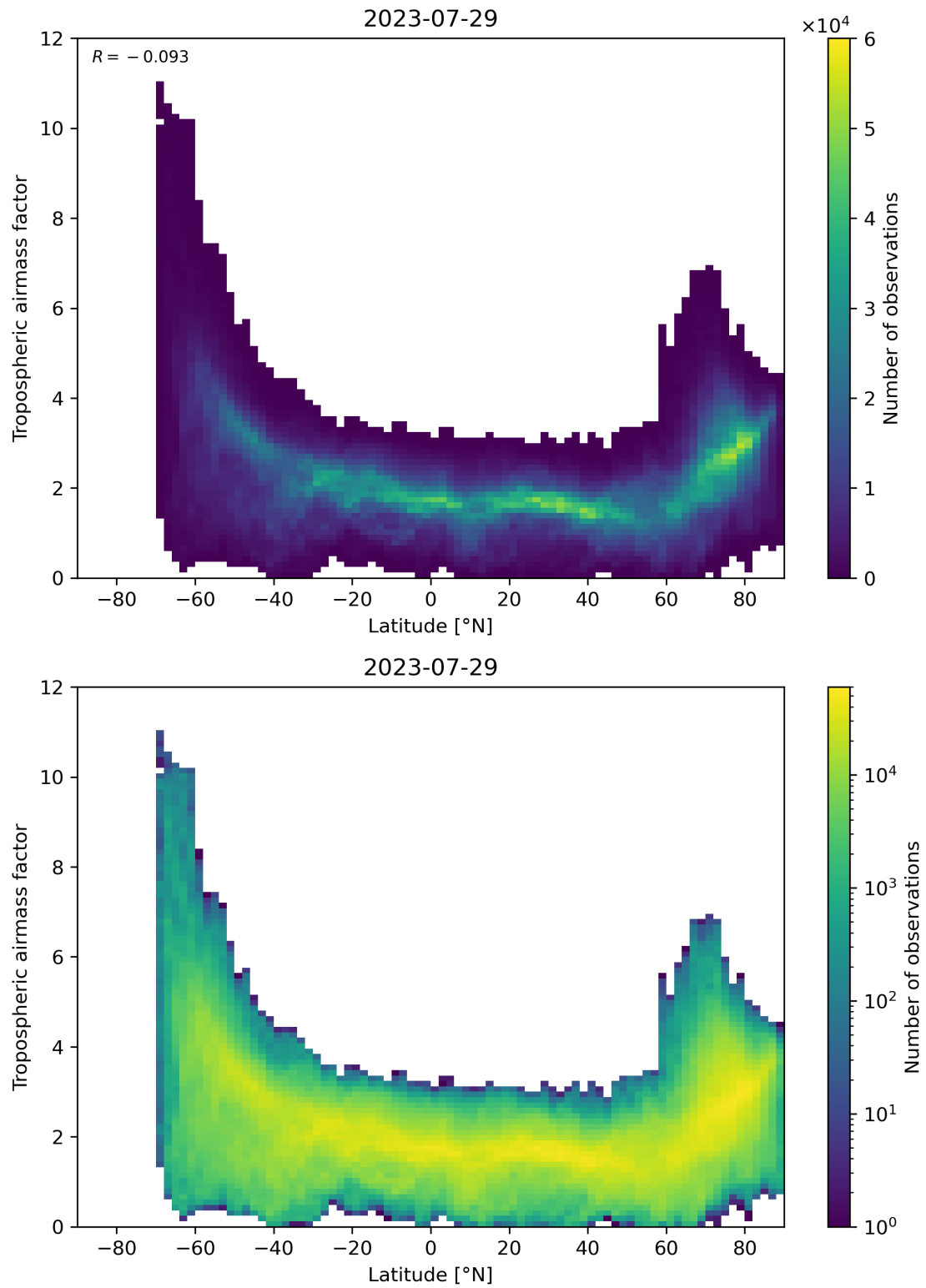
Figure 85: Scatter density plot of “Latitude” against “Tropospheric air mass factor” for 2023-07-29 to 2023-07-30.
