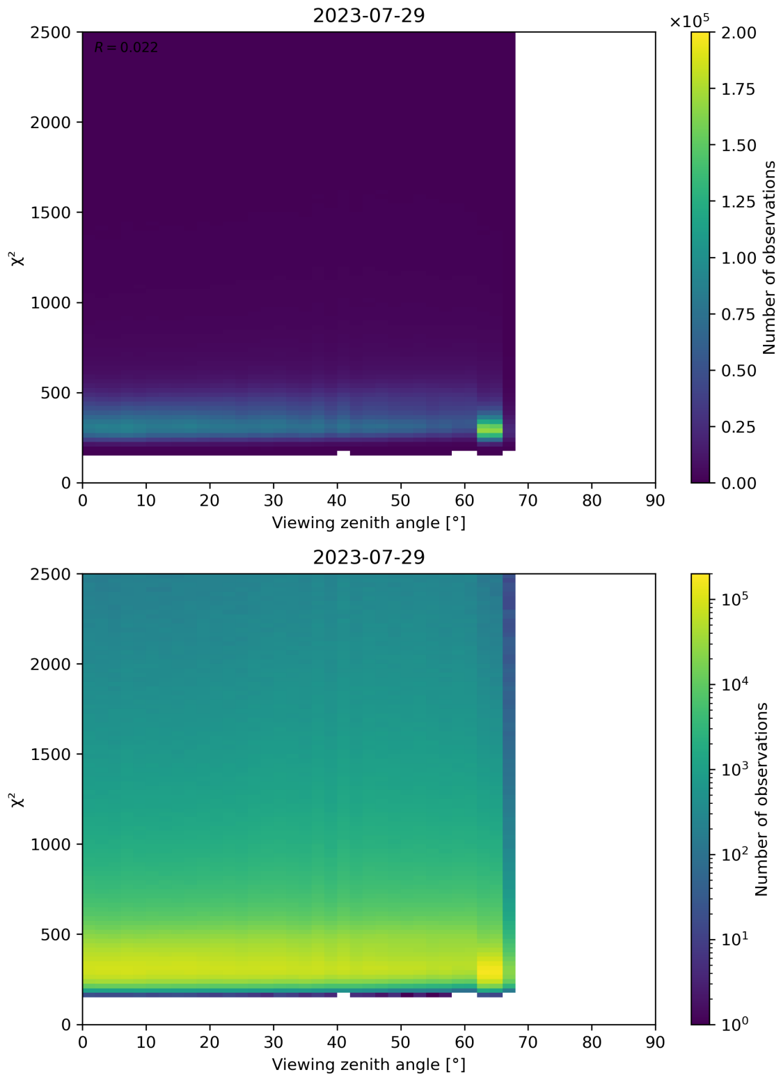
Figure 162: Scatter density plot of “Viewing zenith angle” against “ \chi^2 ” for 2023-07-29 to 2023-07-30.
