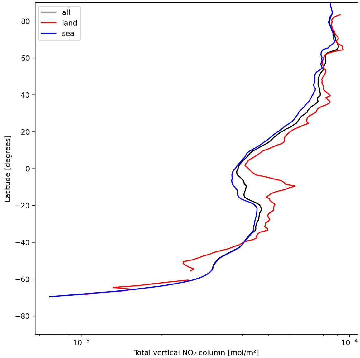
Figure 21: Zonal average of “Total vertical NO 2 column” for 2023-07-29 to 2023-07-30.
