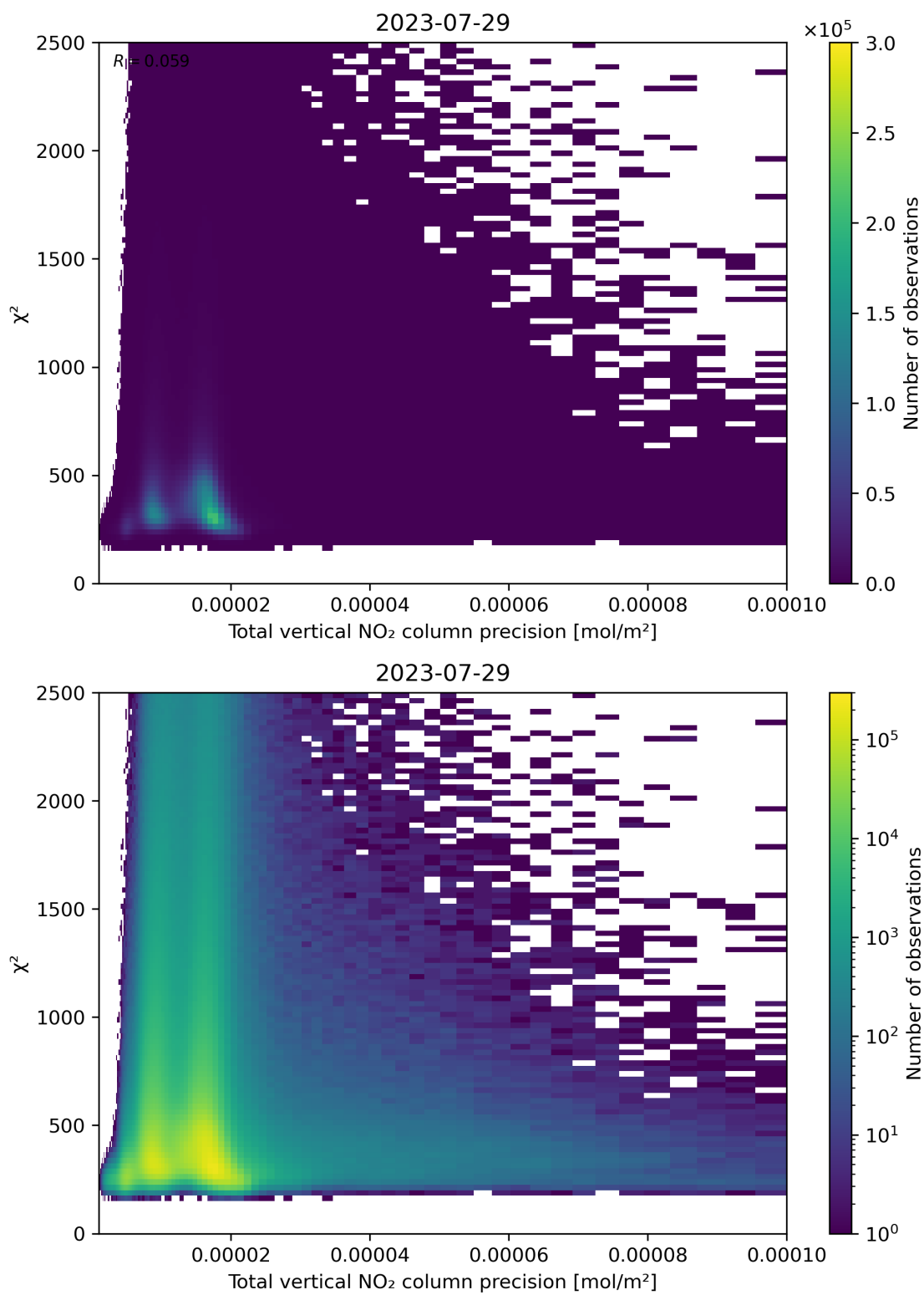
Figure 116: Scatter density plot of “Total vertical NO 2 column precision” against “ \chi^2 ” for 2023-07-29 to 2023-07-30.
