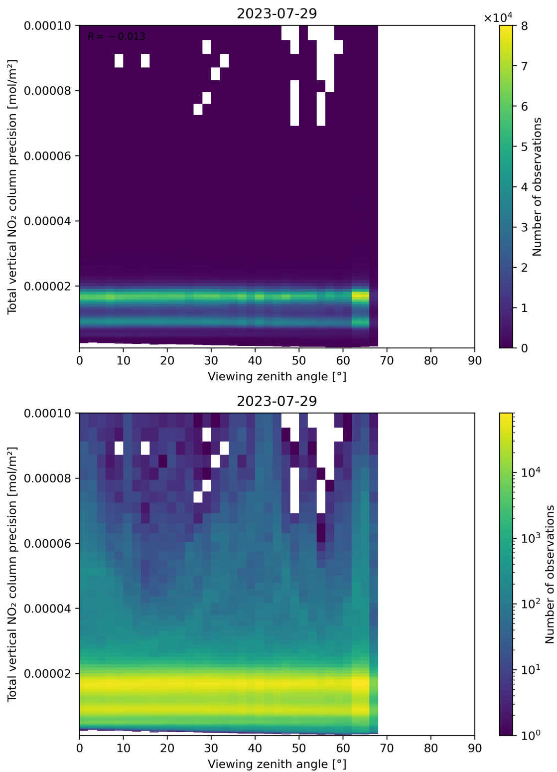
Figure 168: Scatter density plot of “Viewing zenith angle” against “Total vertical NO 2 column precision” for 2023-07-29 to 2023-07-30.
