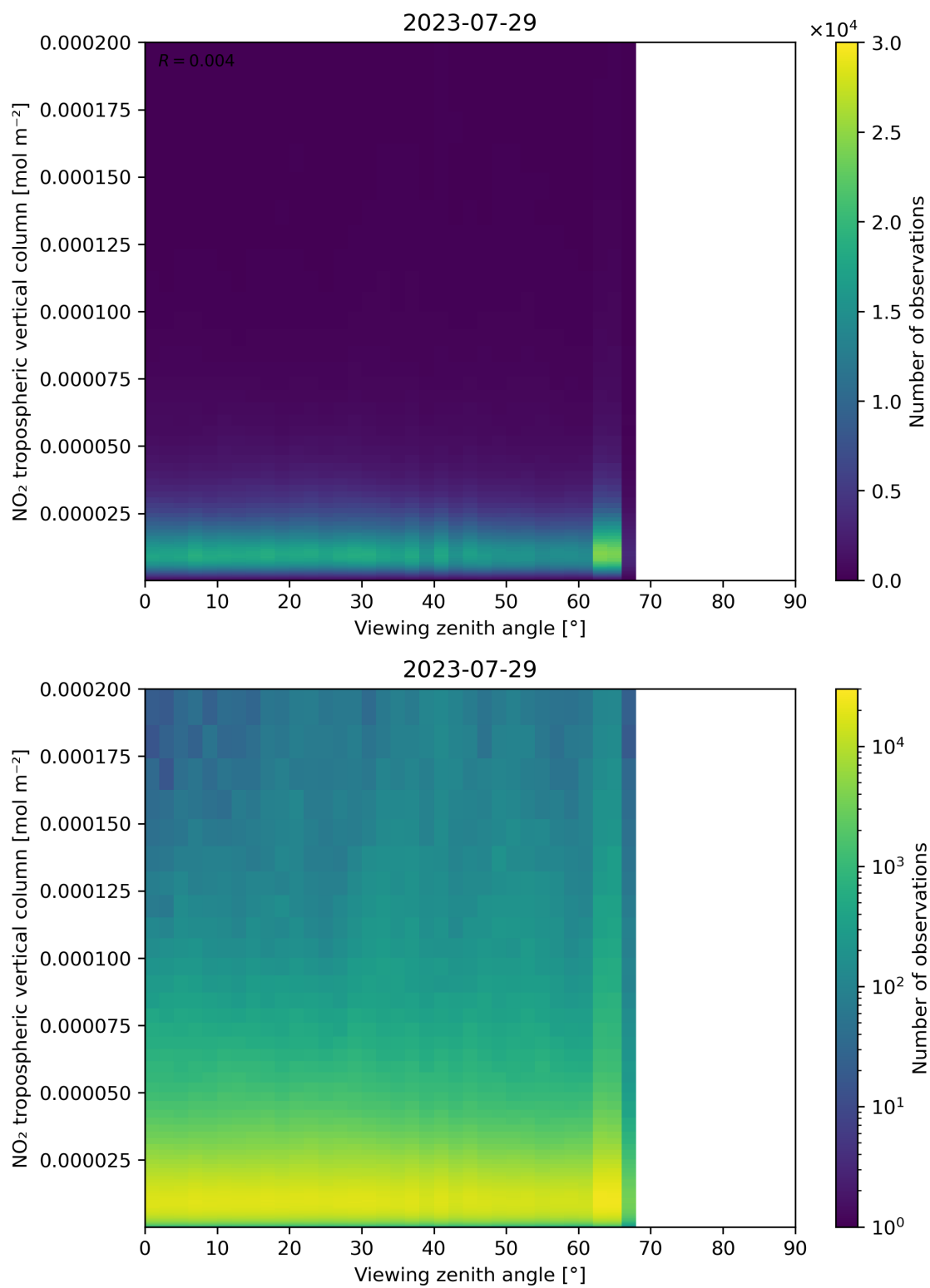
Figure 169: Scatter density plot of “Viewing zenith angle” against “NO 2 tropospheric vertical column” for 2023-07-29 to 2023-07-30.
