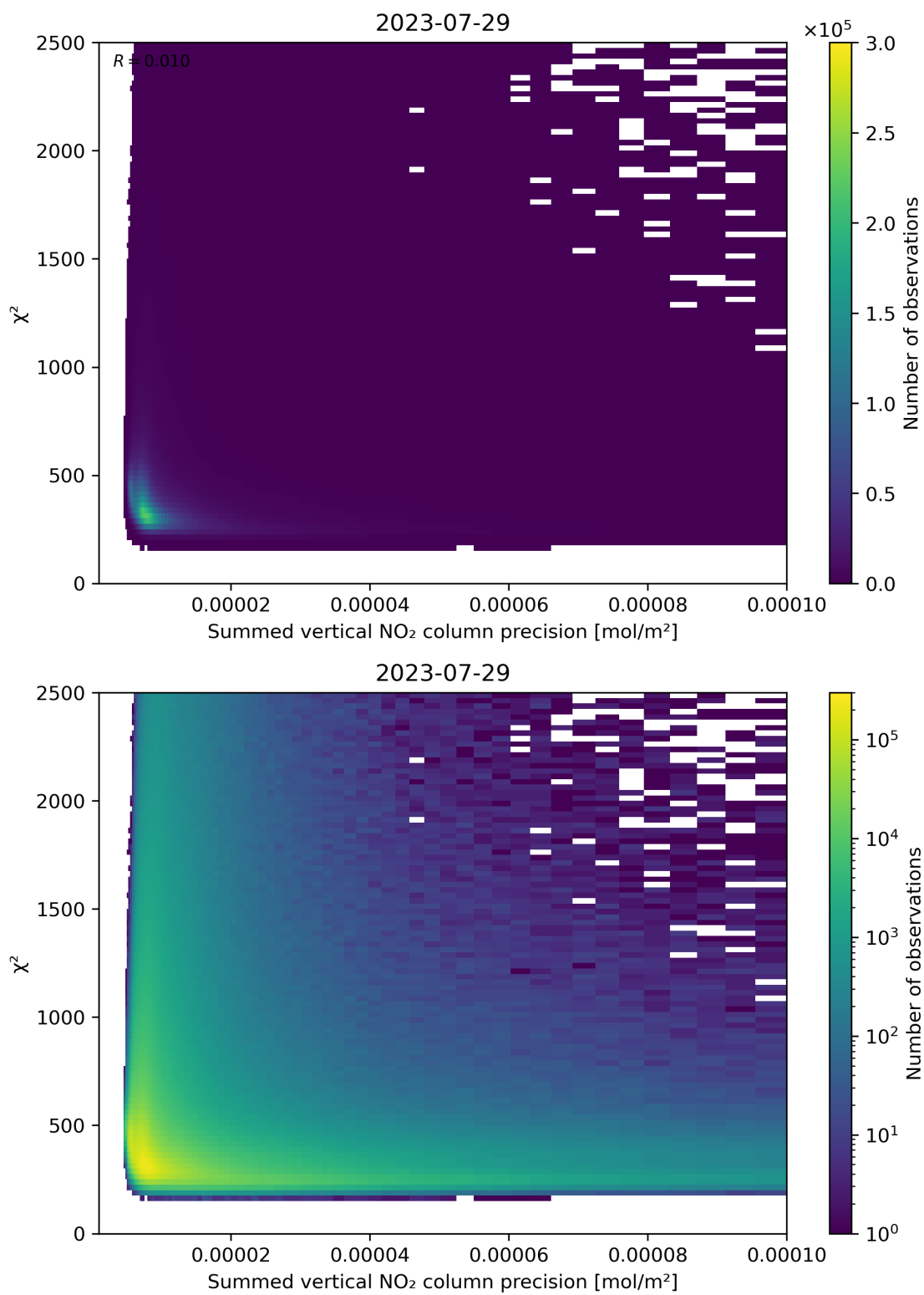
Figure 107: Scatter density plot of “Summed vertical NO 2 column precision” against “ \chi^2 ” for 2023-07-29 to 2023-07-30.
