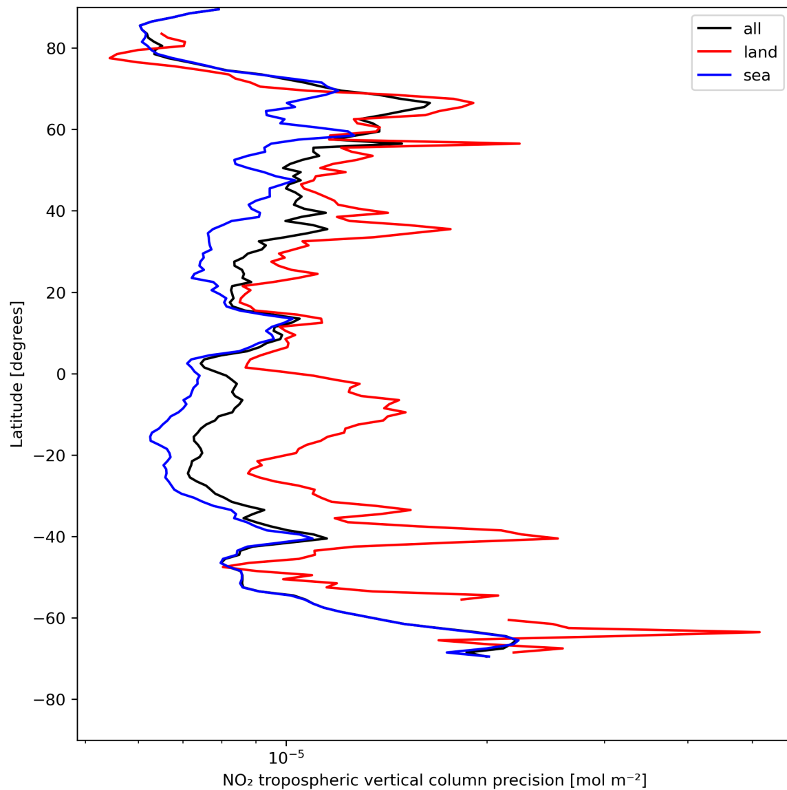
Figure 13: Zonal average of “NO 2 tropospheric vertical column precision” for 2023-07-29 to 2023-07-30.
