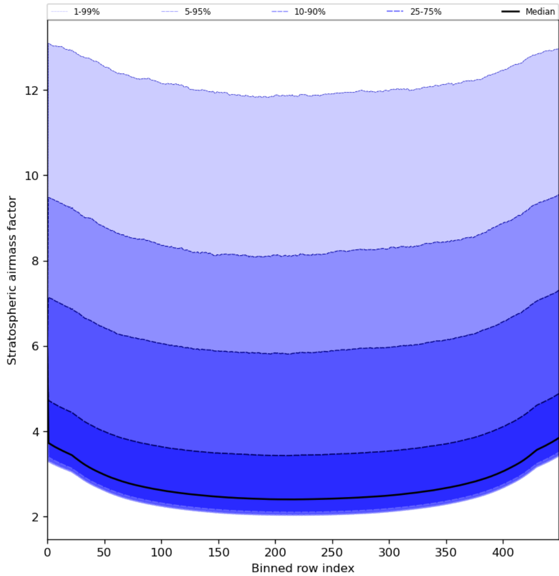
Figure 61: Along track statistics of “Stratospheric air mass factor” for 2023-07-29 to 2023-07-30
