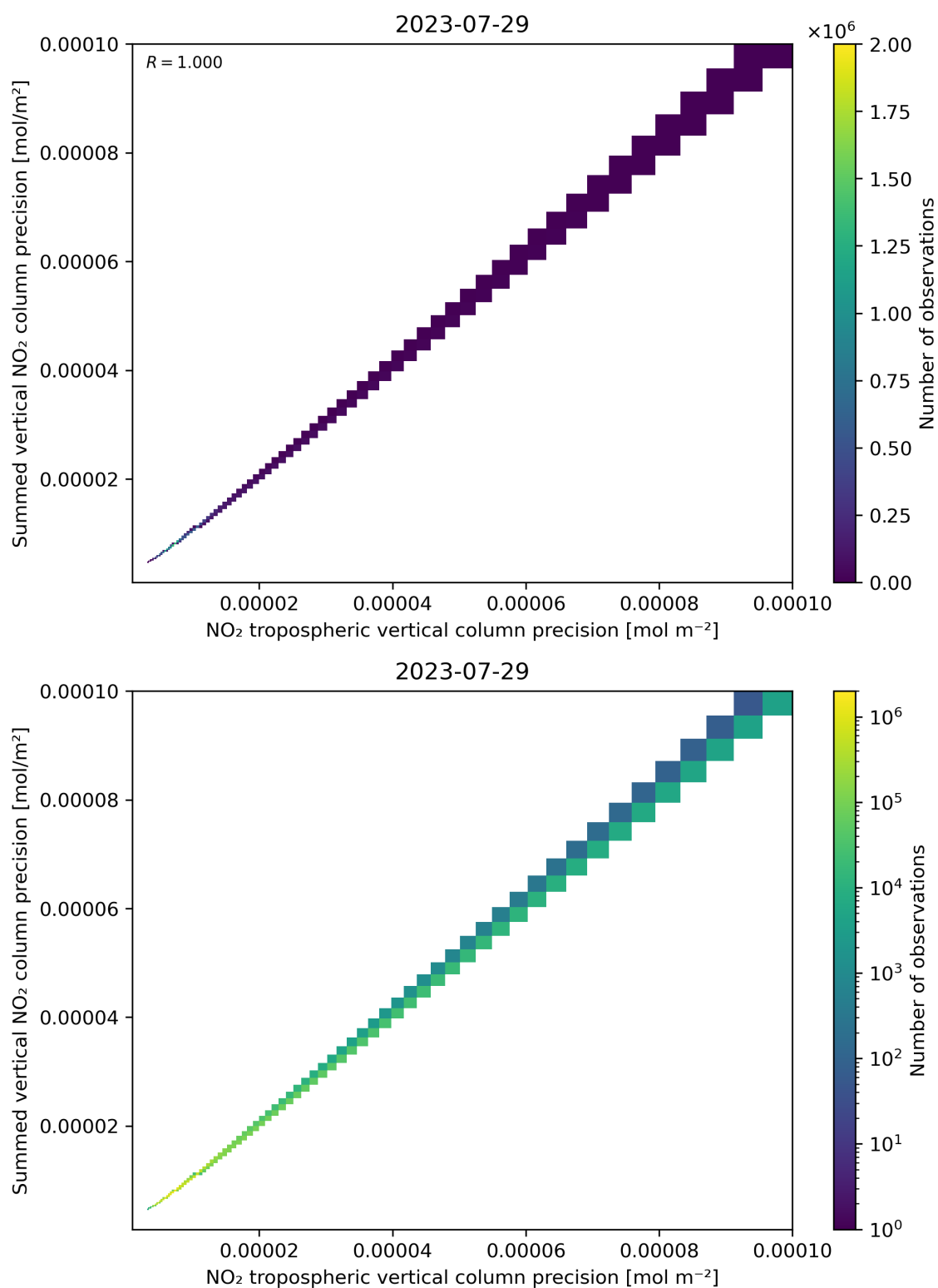
Figure 137: Scatter density plot of “NO 2 tropospheric vertical column precision” against “Summed vertical NO 2 column precision” for 2023-07-29 to 2023-07-30.
