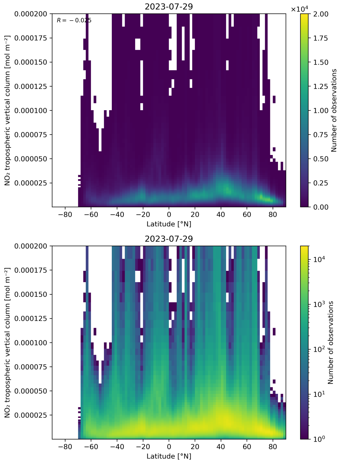
Figure 92: Scatter density plot of “Latitude” against “NO 2 tropospheric vertical column” for 2023-07-29 to 2023-07-30.
