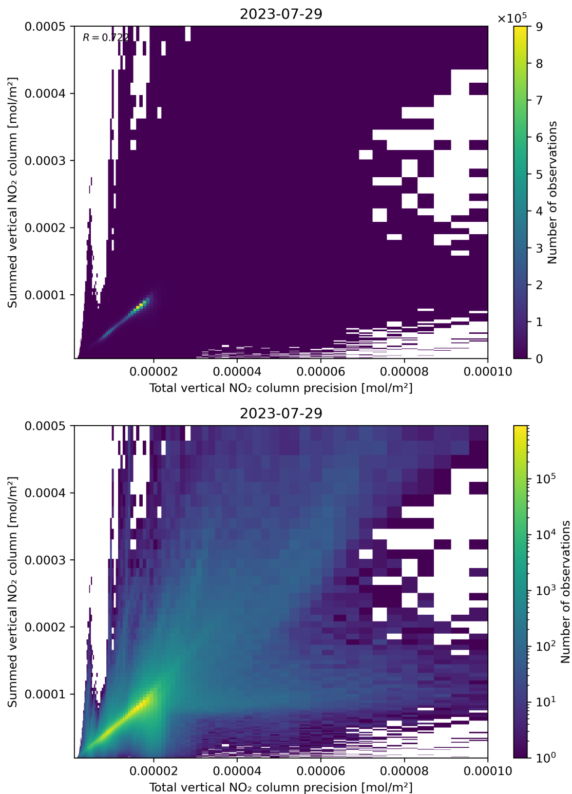
Figure 117: Scatter density plot of “Total vertical NO 2 column precision” against “Summed vertical NO 2 column” for 2023-07-29 to 2023-07-30.
