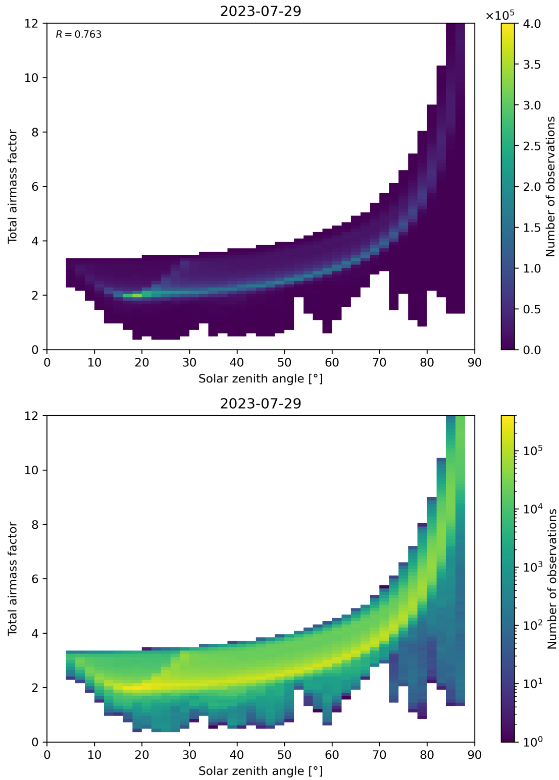
Figure 146: Scatter density plot of “Solar zenith angle” against “Total air mass factor” for 2023-07-29 to 2023-07-30.
