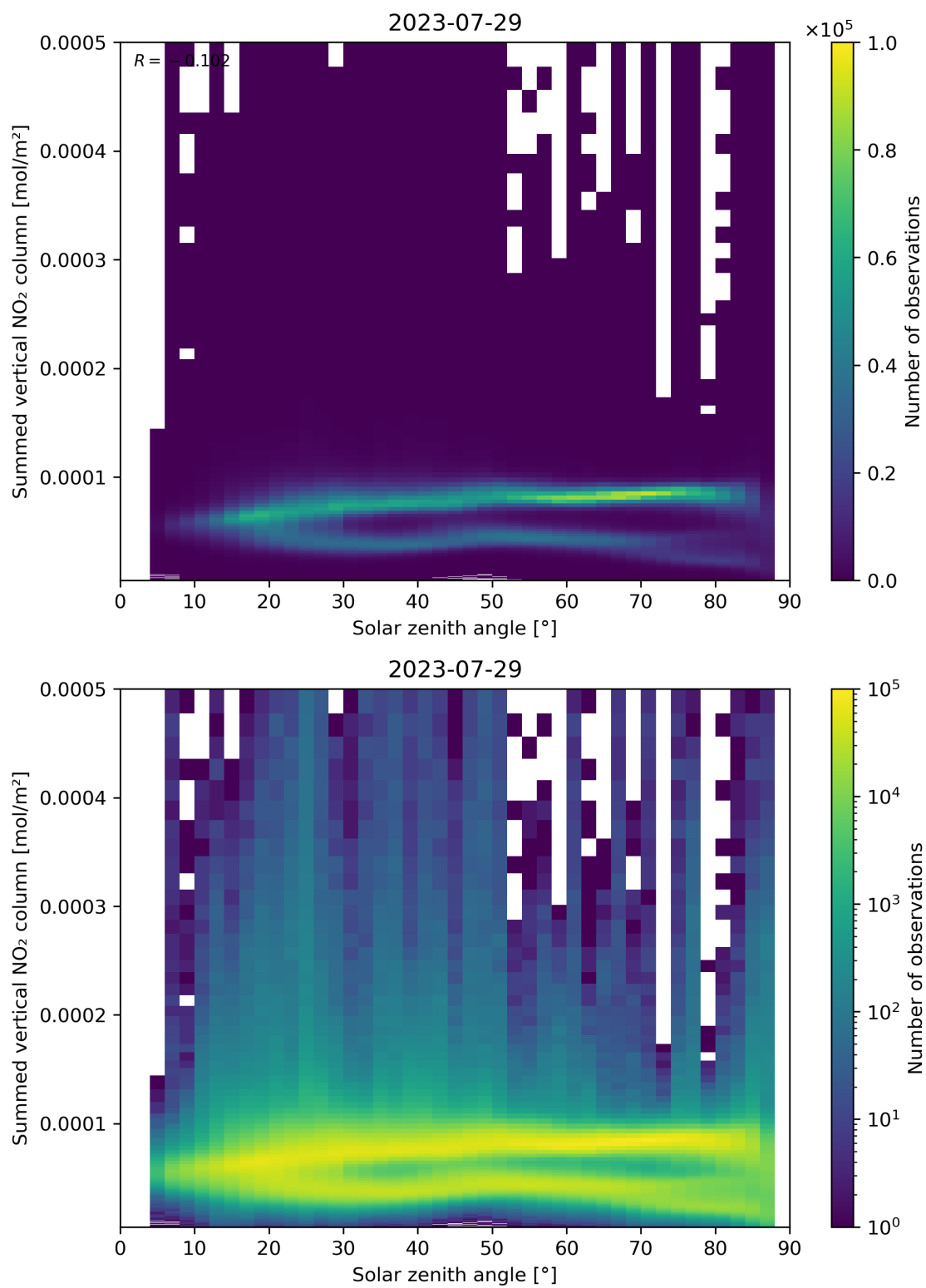
Figure 151: Scatter density plot of “Solar zenith angle” against “Summed vertical NO 2 column” for 2023-07-29 to 2023-07-30.
