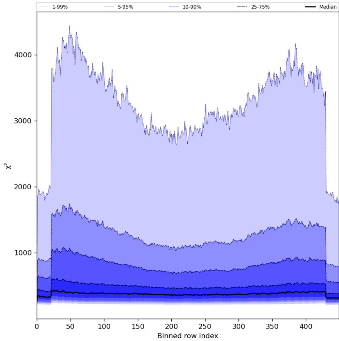
Figure 59: Along track statistics of “ \chi^2 ” for 2023-07-29 to 2023-07-30
