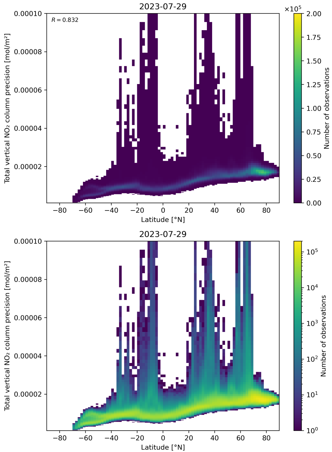
Figure 91: Scatter density plot of “Latitude” against “Total vertical NO 2 column precision” for 2023-07-29 to 2023-07-30.
