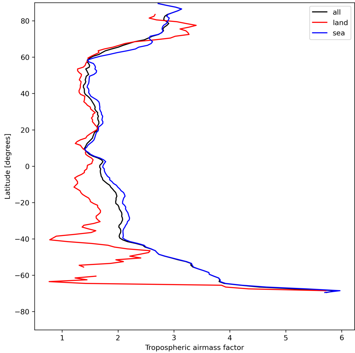
Figure 14: Zonal average of “Tropospheric airmass factor” for 2023-07-29 to 2023-07-30.
