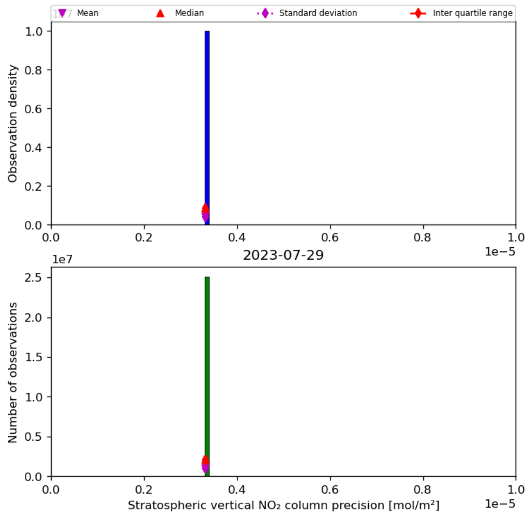
Figure 37: Histogram of “Stratospheric vertical NO 2 column precision” for 2023-07-29 to 2023-07-30
