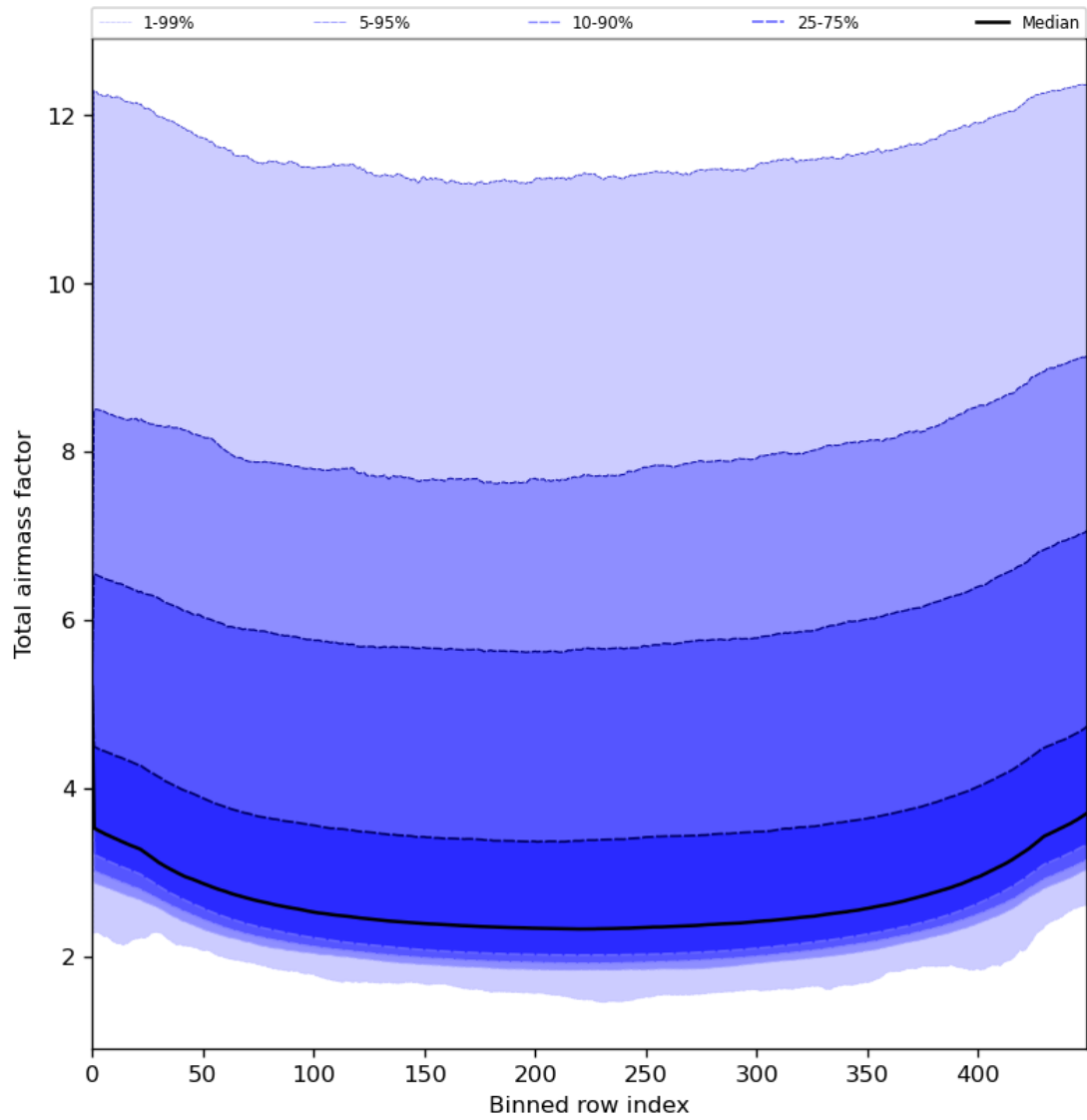
Figure 49: Along track statistics of “Total airmass factor” for 2023-07-29 to 2023-07-30
