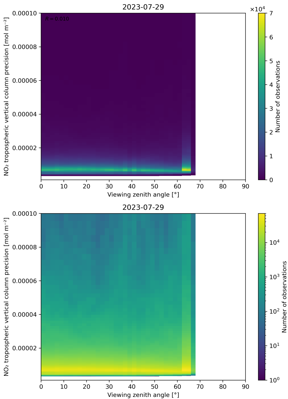
Figure 170: Scatter density plot of “Viewing zenith angle” against “NO 2 tropospheric vertical column precision” for 2023-07-29 to 2023-07-30.
