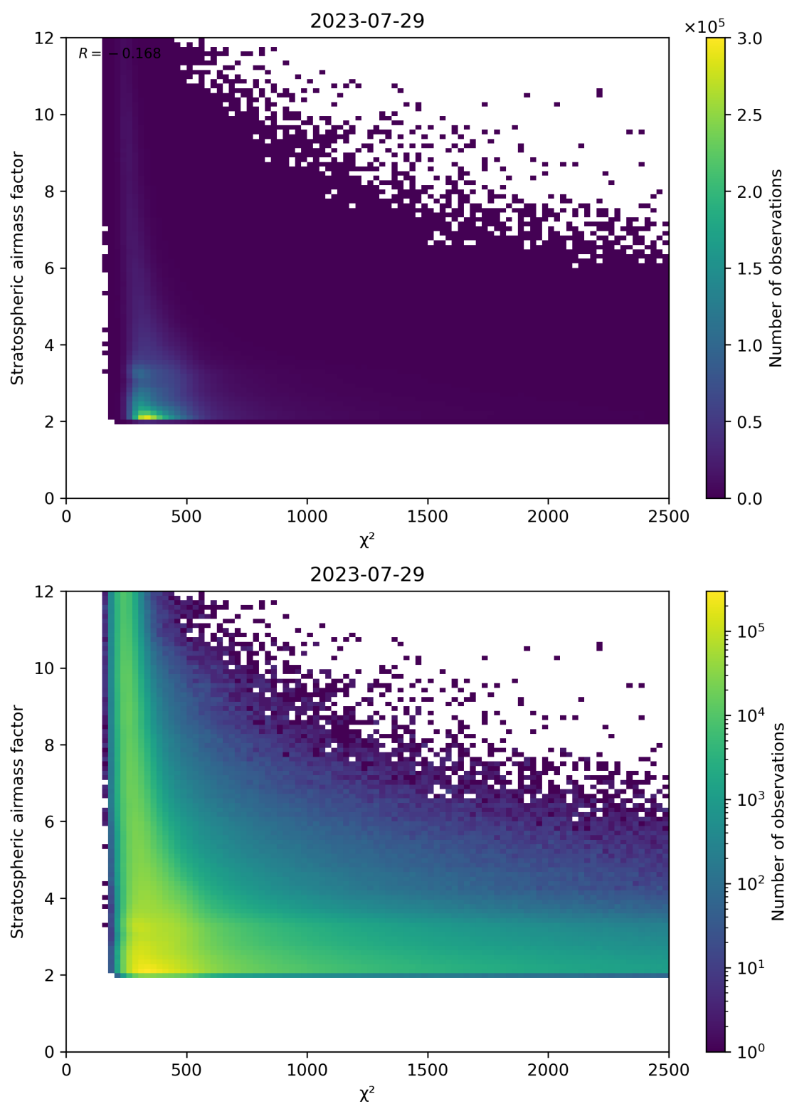
Figure 81: Scatter density plot of “ \chi^2 ” against “Stratospheric airmass factor” for 2023-07-29 to 2023-07-30.
