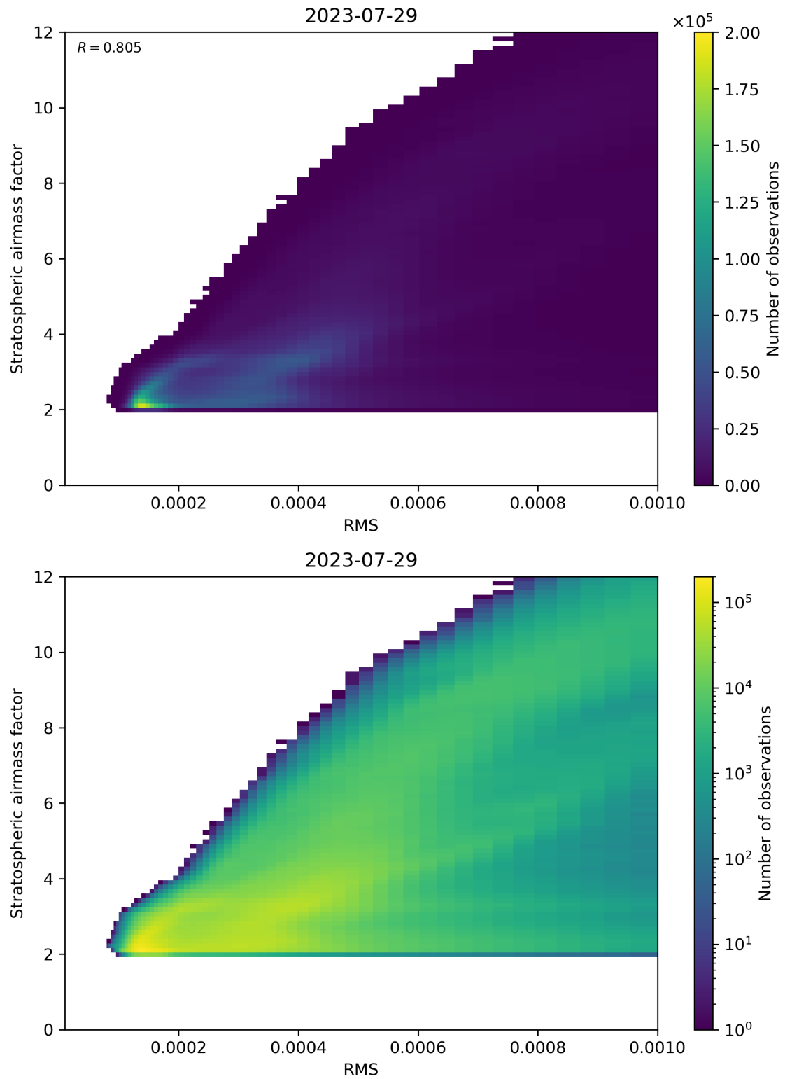
Figure 144: Scatter density plot of “RMS” against “Stratospheric airmass factor” for 2023-07-29 to 2023-07-30.
