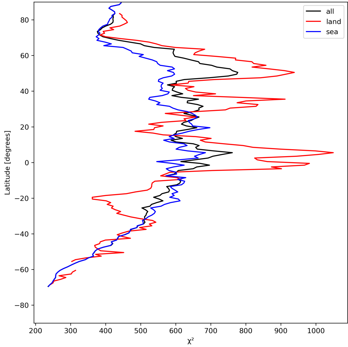
Figure 25: Zonal average of “ \chi^2 ” for 2023-07-29 to 2023-07-30.
