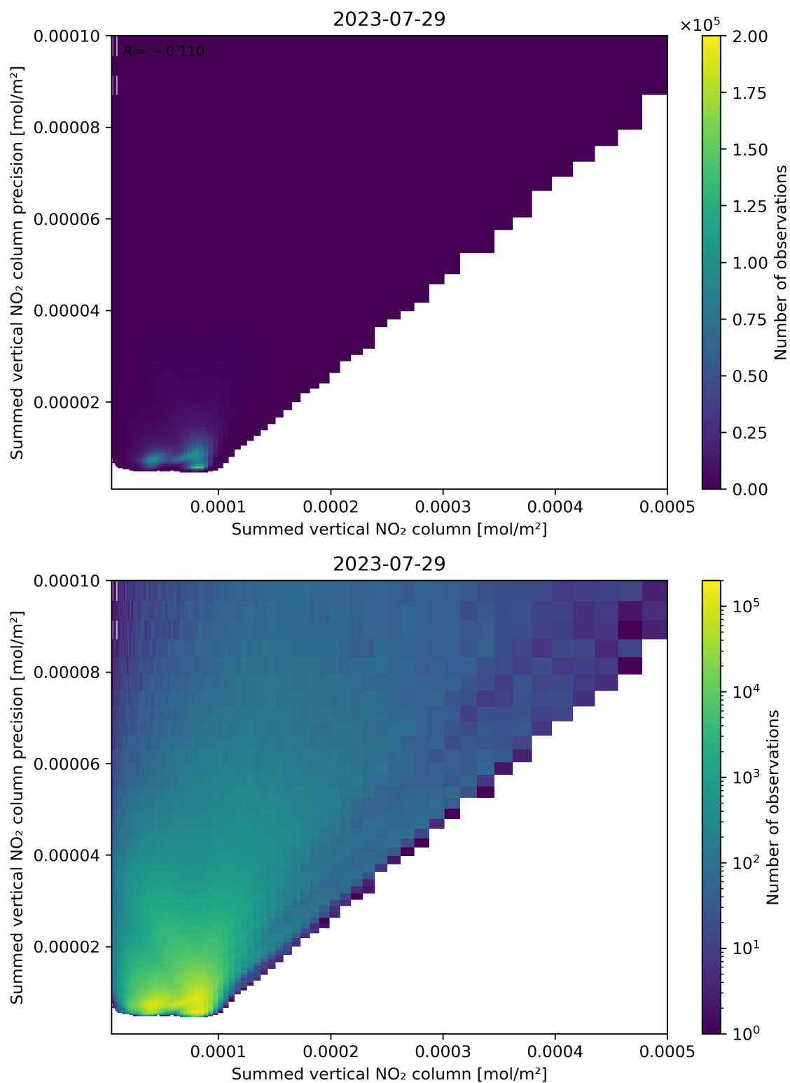
Figure 105: Scatter density plot of “Summed vertical NO 2 column” against “Summed vertical NO 2 column precision” for 2023-07-29 to 2023-07-30.
