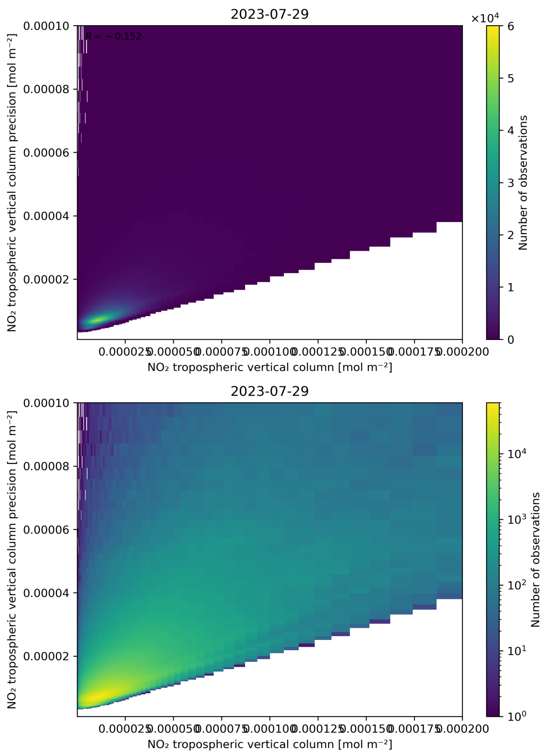
Figure 130: Scatter density plot of “NO 2 tropospheric vertical column” against “NO 2 tropospheric vertical column precision” for 2023-07-29 to 2023-07-30.
