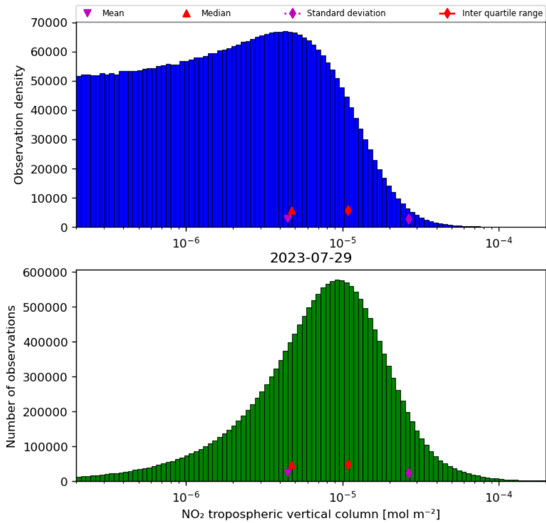
Figure 29: Histogram of “NO 2 tropospheric vertical column” for 2023-07-29 to 2023-07-30
