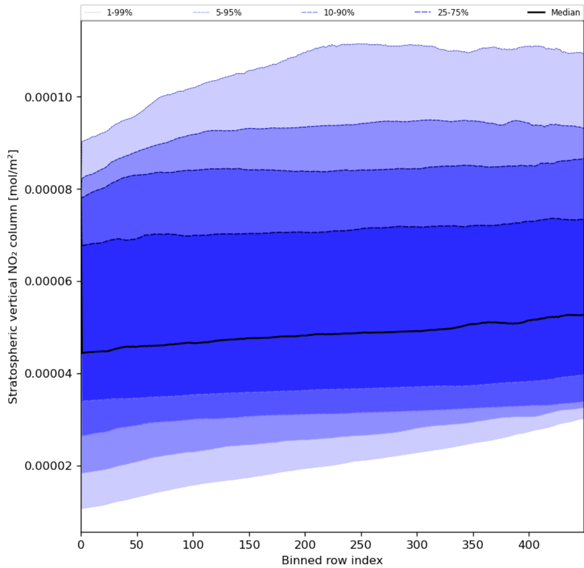
Figure 53: Along track statistics of “Stratospheric vertical NO 2 column” for 2023-07-29 to 2023-07-30
