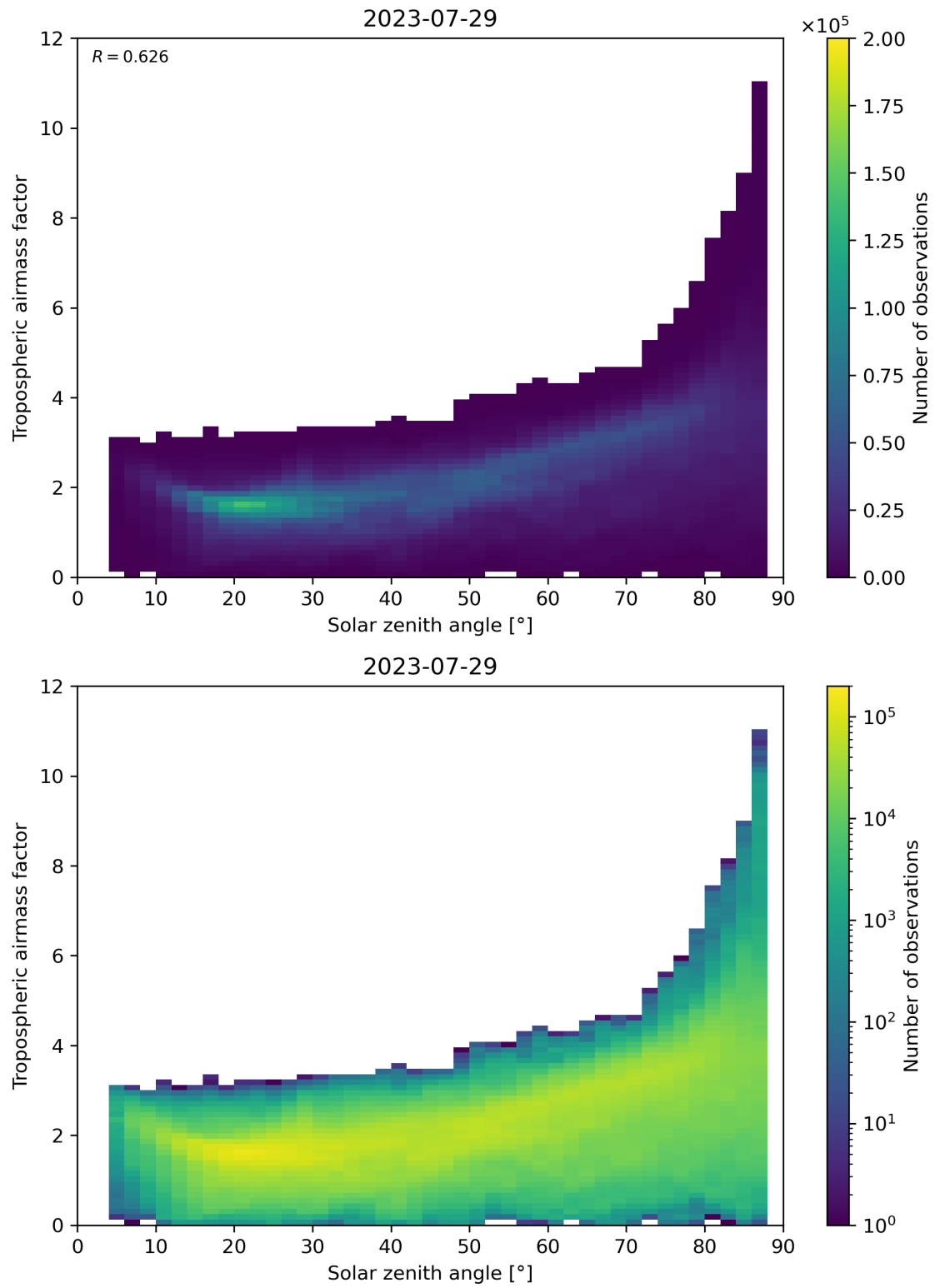
Figure 147: Scatter density plot of “Solar zenith angle” against “Tropospheric airmass factor” for 2023-07-29 to 2023-07-30.
