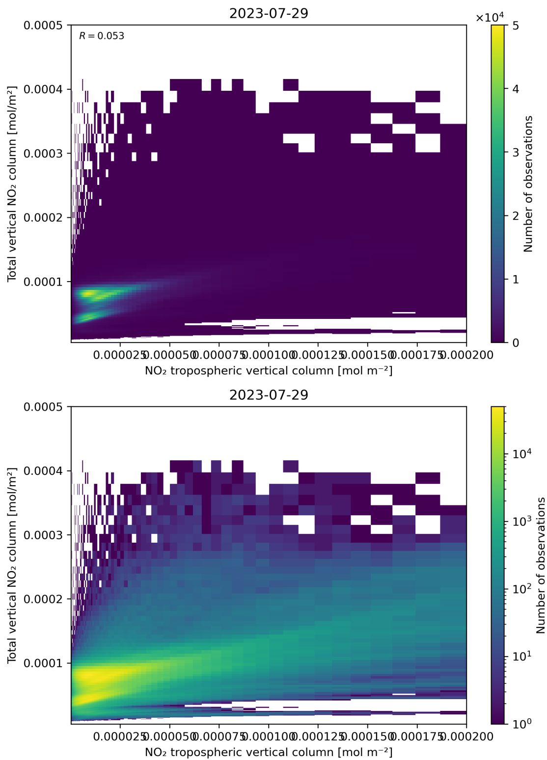
Figure 128: Scatter density plot of “NO 2 tropospheric vertical column” against “Total vertical NO 2 column” for 2023-07-29 to 2023-07-30.
