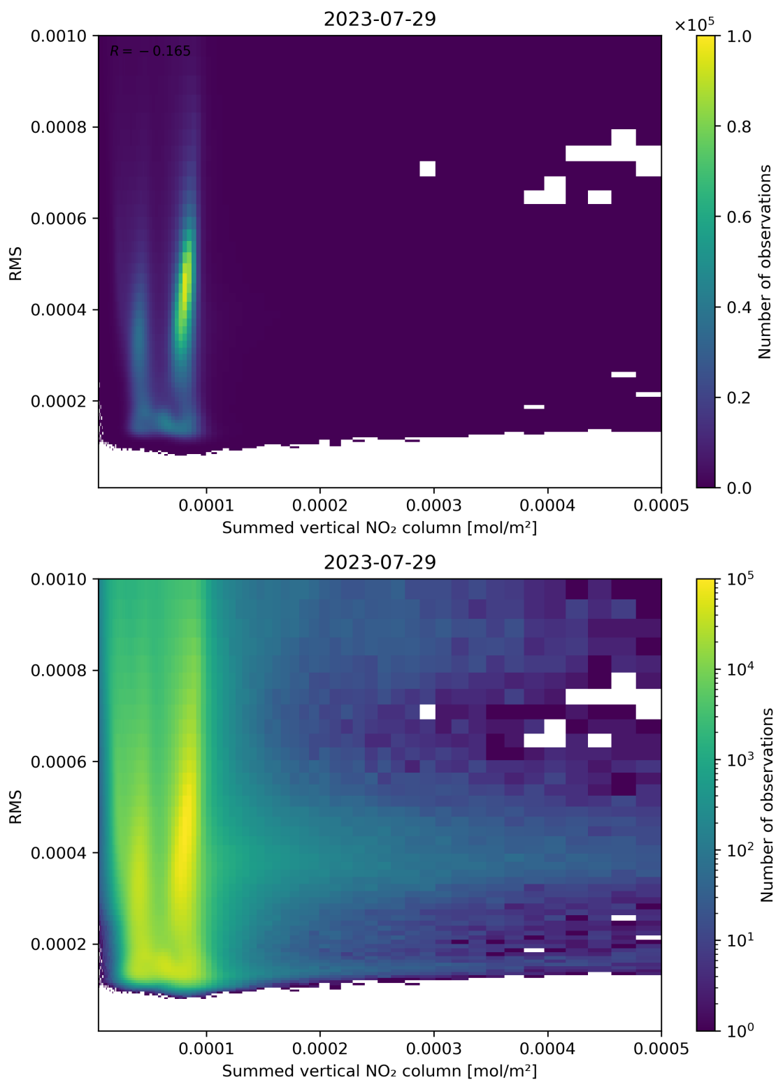
Figure 109: Scatter density plot of “Summed vertical NO 2 column” against “RMS” for 2023-07-29 to 2023-07-30.
