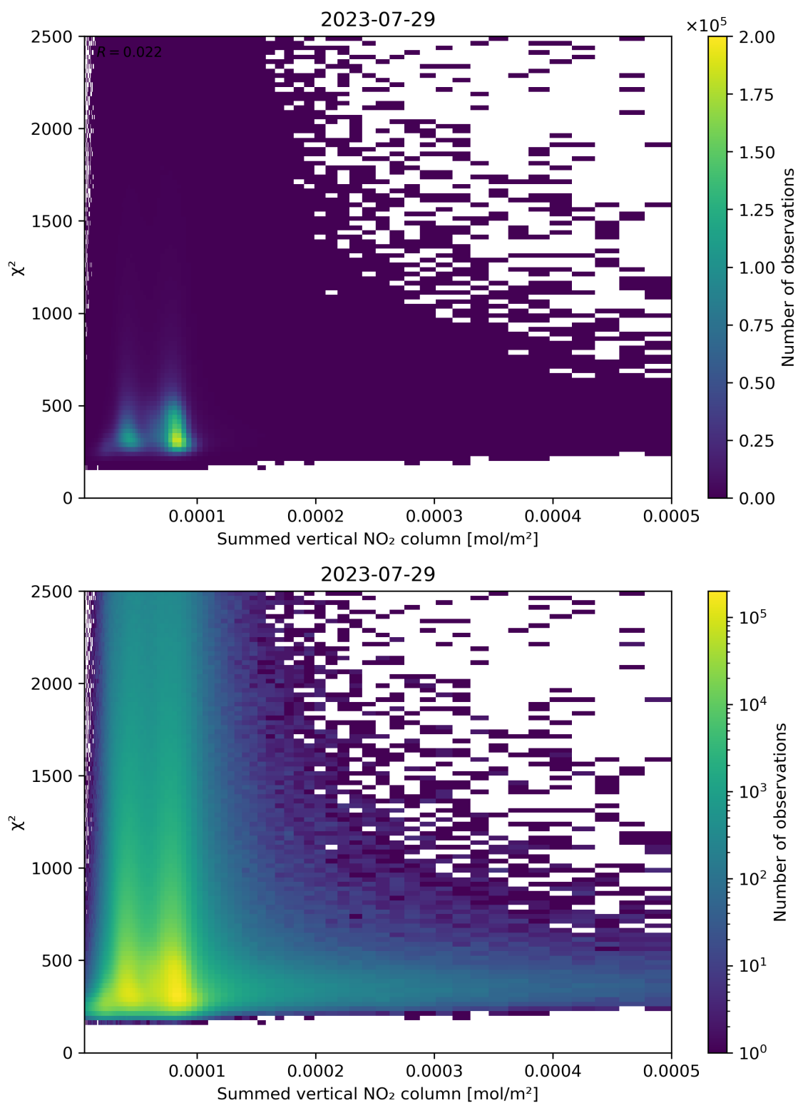
Figure 104: Scatter density plot of “Summed vertical NO 2 column” against “ \chi^2 ” for 2023-07-29 to 2023-07-30.
