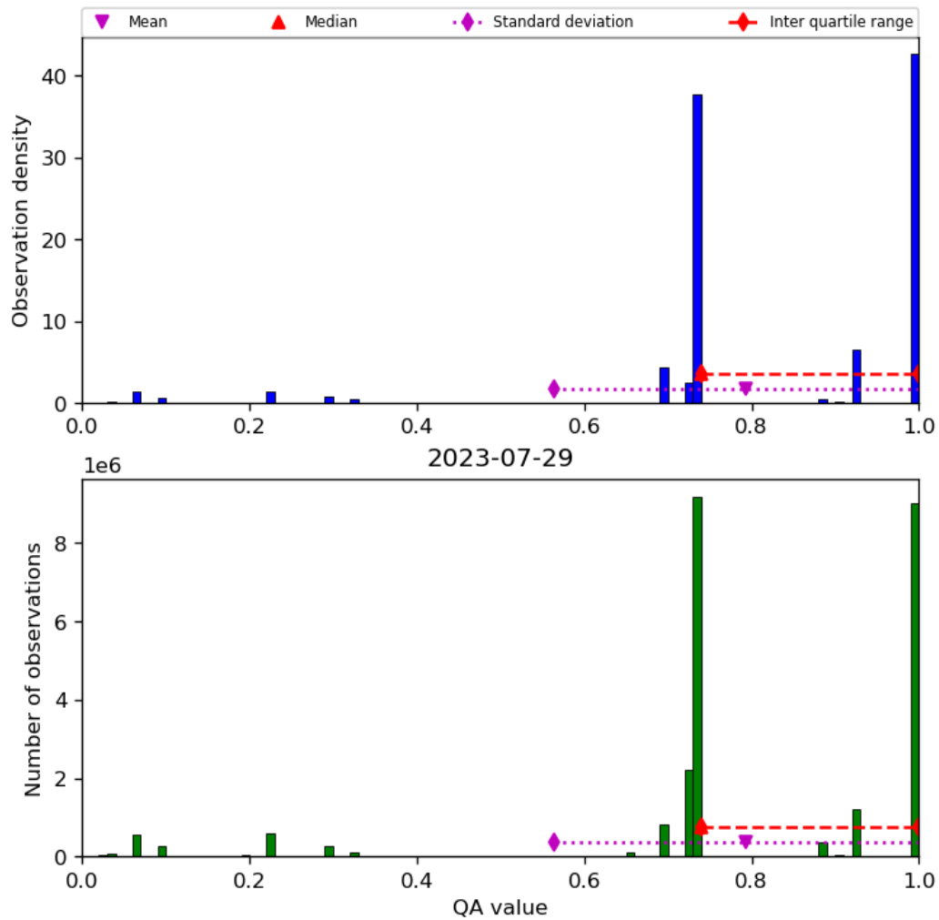
Figure 28: Histogram of “QA value” for 2023-07-29 to 2023-07-30
