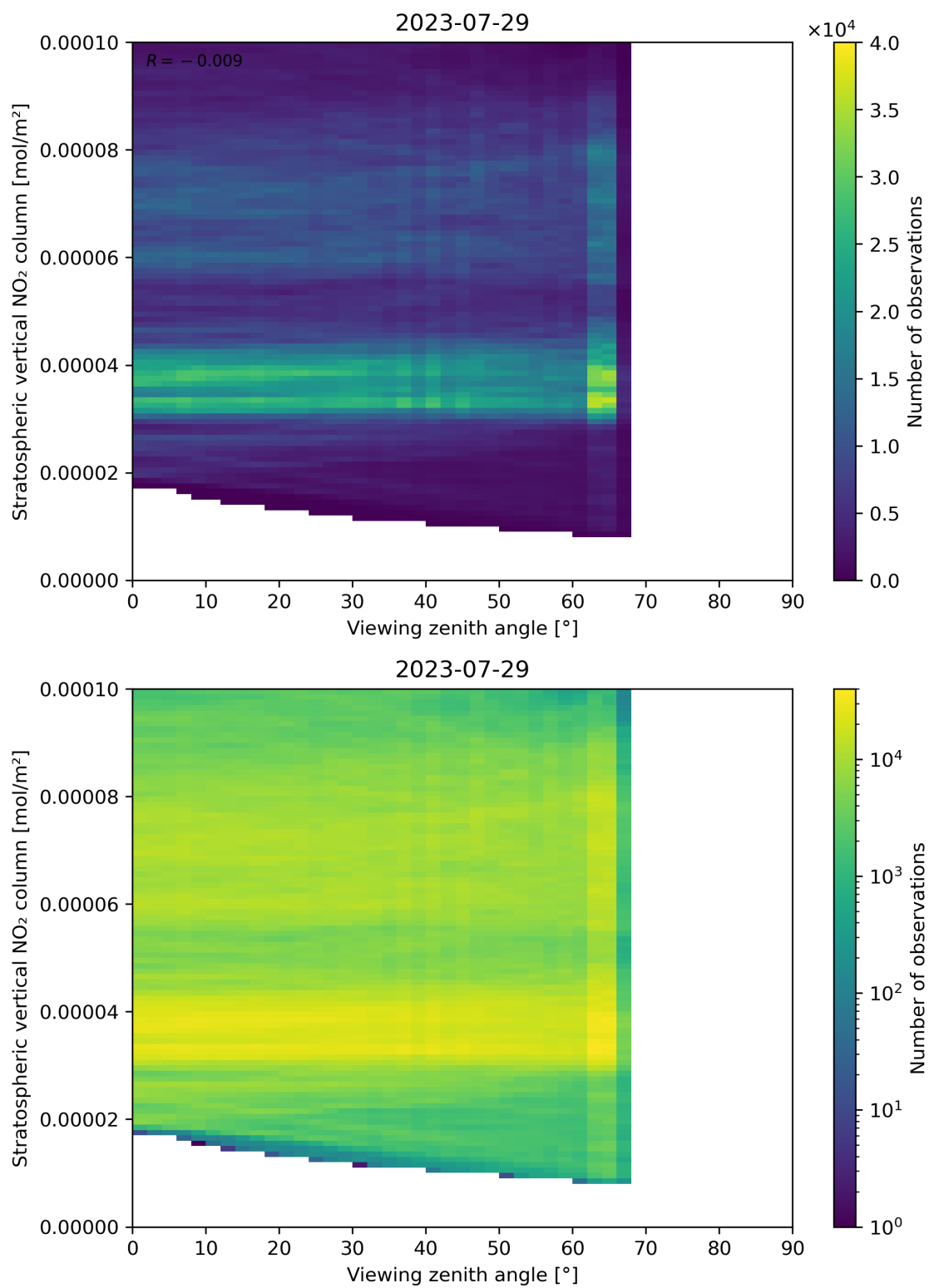
Figure 164: Scatter density plot of “Viewing zenith angle” against “Stratospheric vertical NO 2 column” for 2023-07-29 to 2023-07-30.
