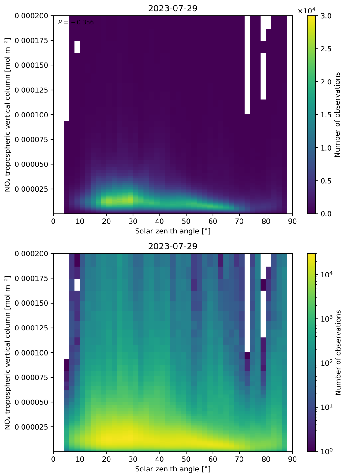
Figure 155: Scatter density plot of “Solar zenith angle” against “NO 2 tropospheric vertical column” for 2023-07-29 to 2023-07-30.
