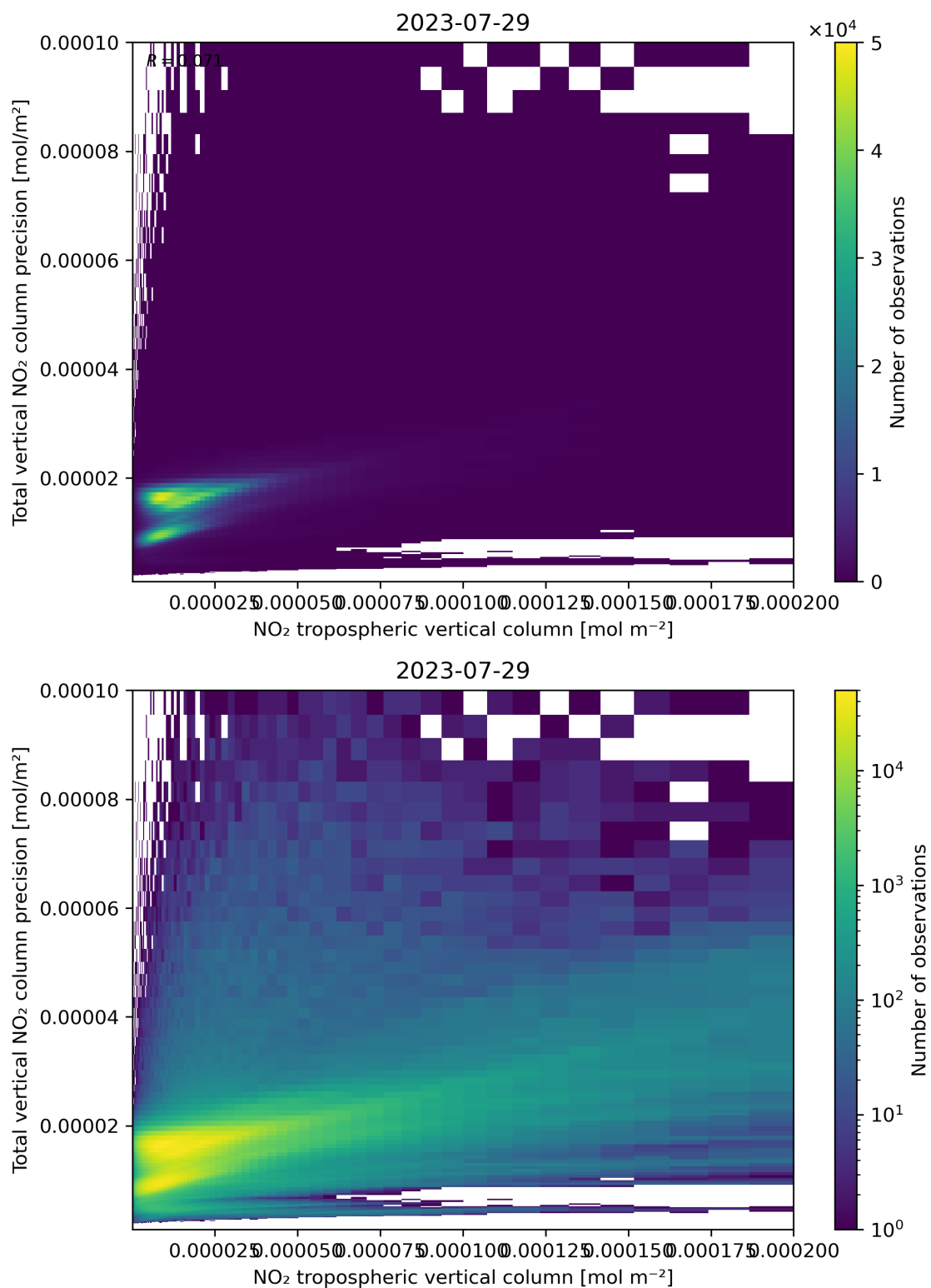
Figure 129: Scatter density plot of “NO 2 tropospheric vertical column” against “Total vertical NO 2 column precision” for 2023-07-29 to 2023-07-30.
