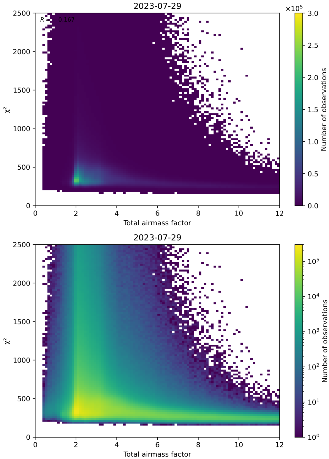
Figure 63: Scatter density plot of “Total airmass factor” against “ \chi^2 ” for 2023-07-29 to 2023-07-30.
