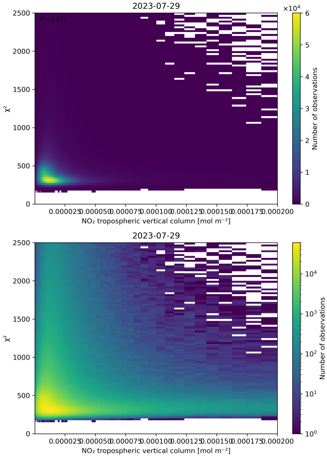
Figure 124: Scatter density plot of “NO 2 tropospheric vertical column” against “ \chi^2 ” for 2023-07-29 to 2023-07-30.
