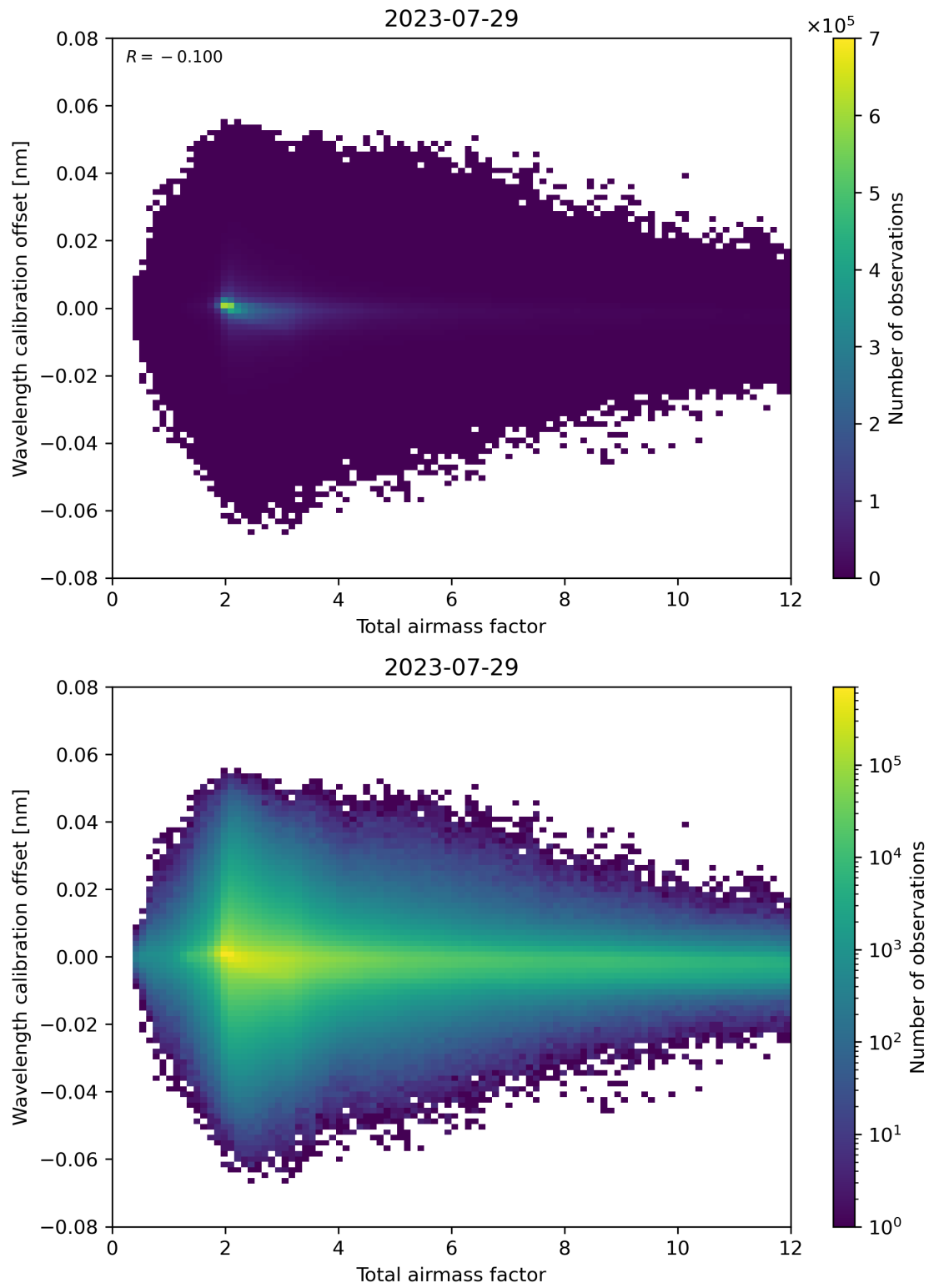
Figure 70: Scatter density plot of “Total airmass factor” against “Wavelength calibration offset” for 2023-07-29 to 2023-07-30.
