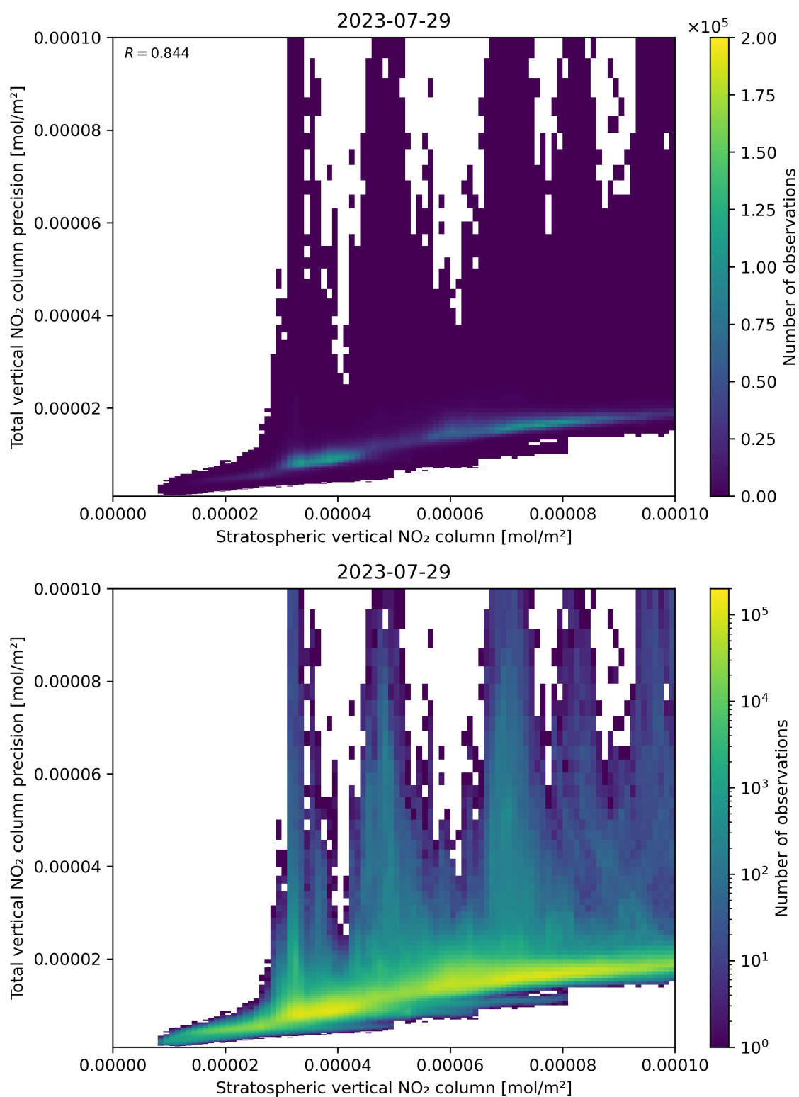
Figure 101: Scatter density plot of “Stratospheric vertical NO 2 column” against “Total vertical NO 2 column precision” for 2023-07-29 to 2023-07-30.
