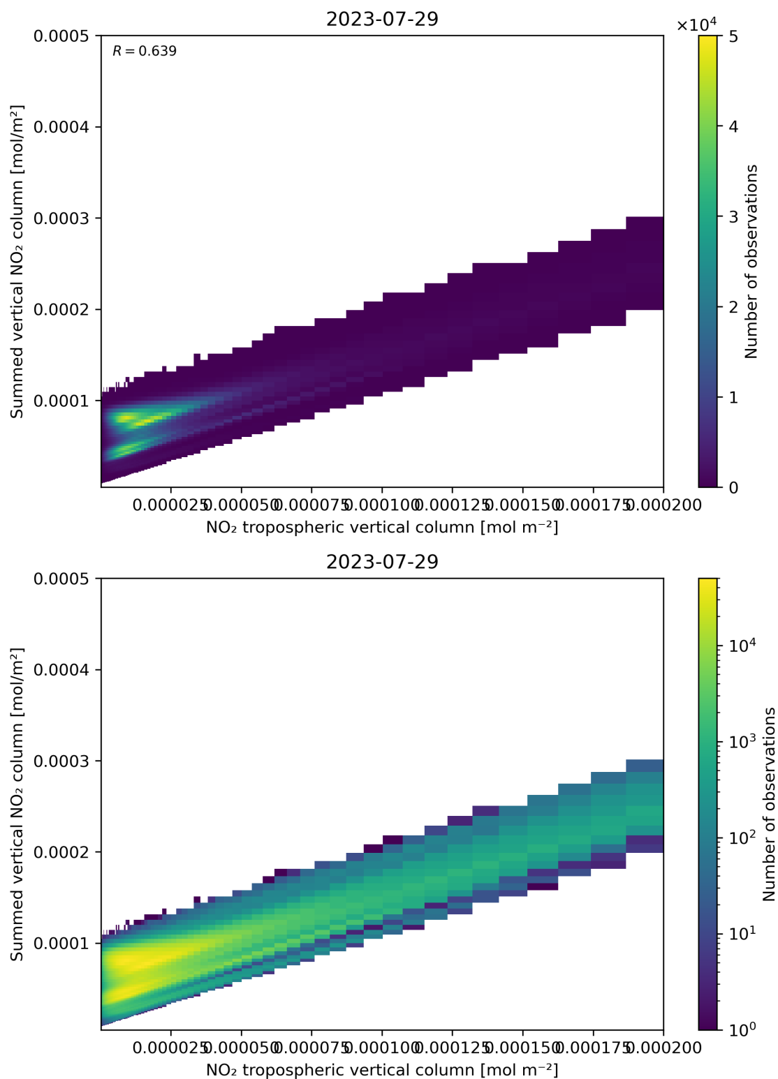
Figure 126: Scatter density plot of “NO 2 tropospheric vertical column” against “Summed vertical NO 2 column” for 2023-07-29 to 2023-07-30.
