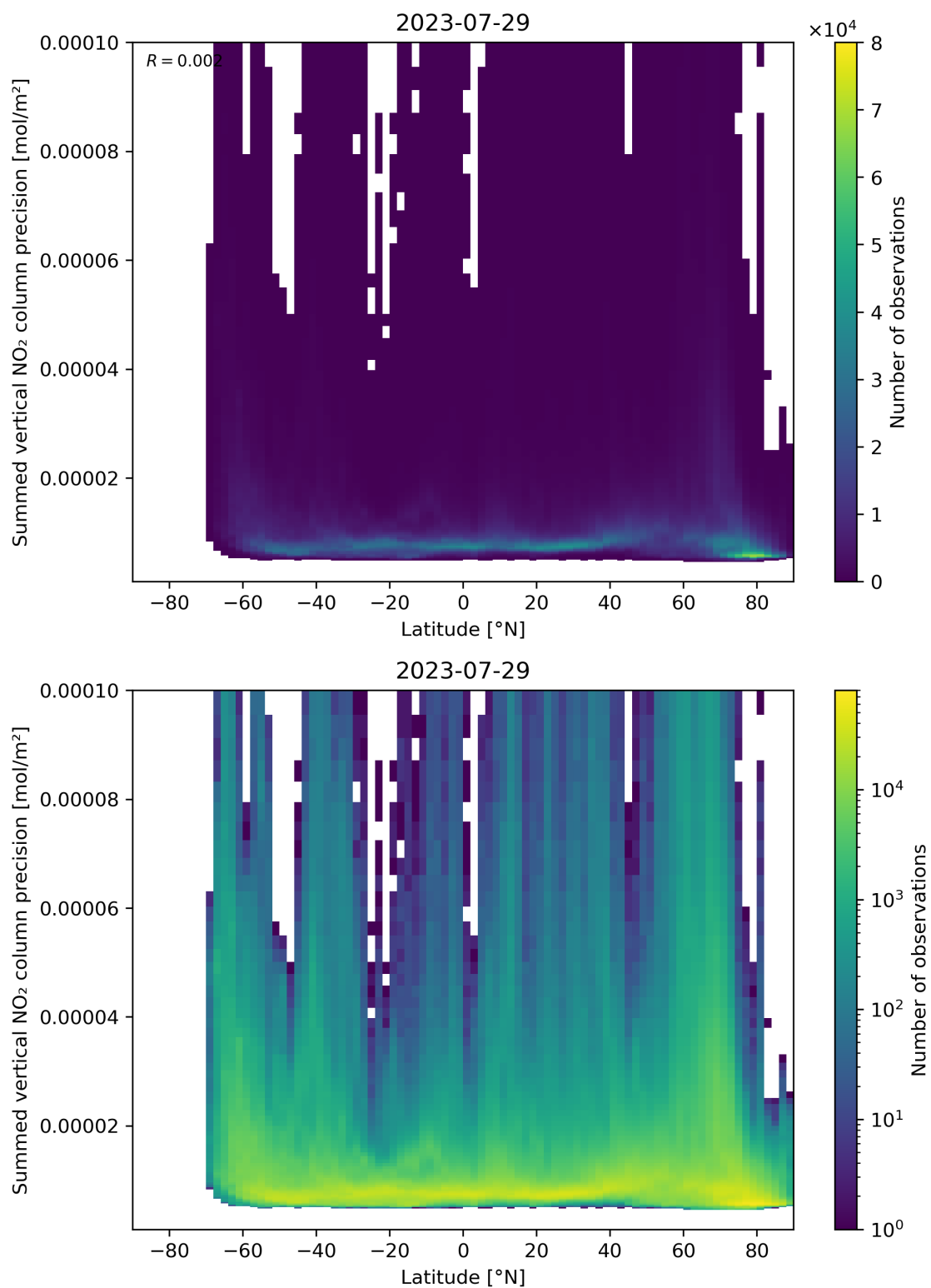
Figure 89: Scatter density plot of “Latitude” against “Summed vertical NO 2 column precision” for 2023-07-29 to 2023-07-30.
