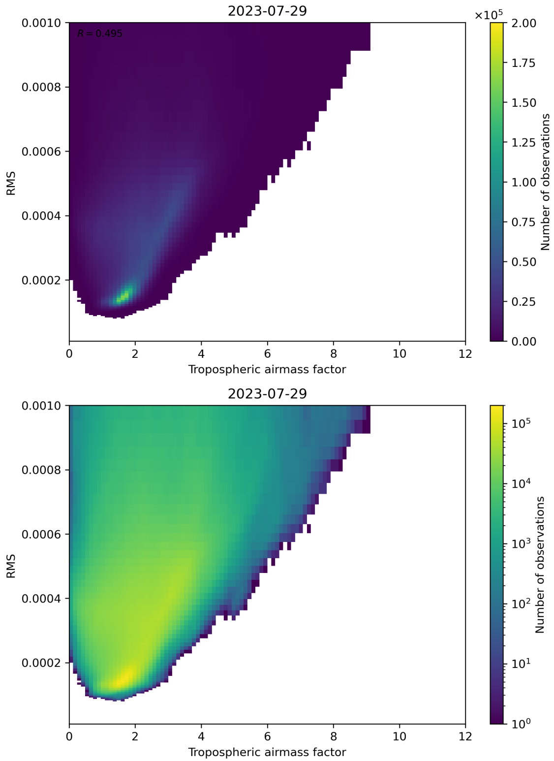
Figure 79: Scatter density plot of “Tropospheric airmass factor” against “RMS” for 2023-07-29 to 2023-07-30.
