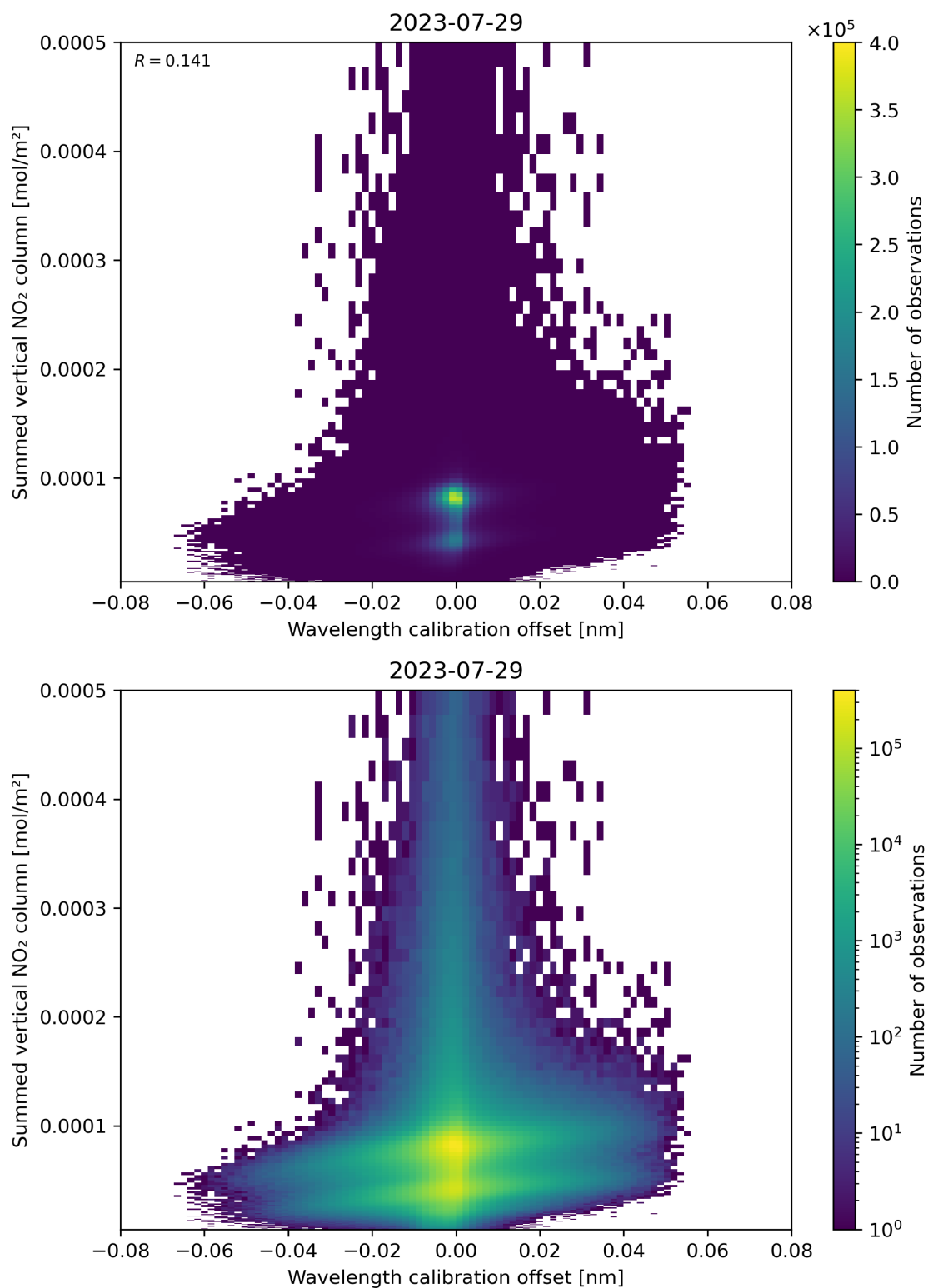
Figure 177: Scatter density plot of “Wavelength calibration offset” against “Summed vertical NO 2 column” for 2023-07-29 to 2023-07-30.
