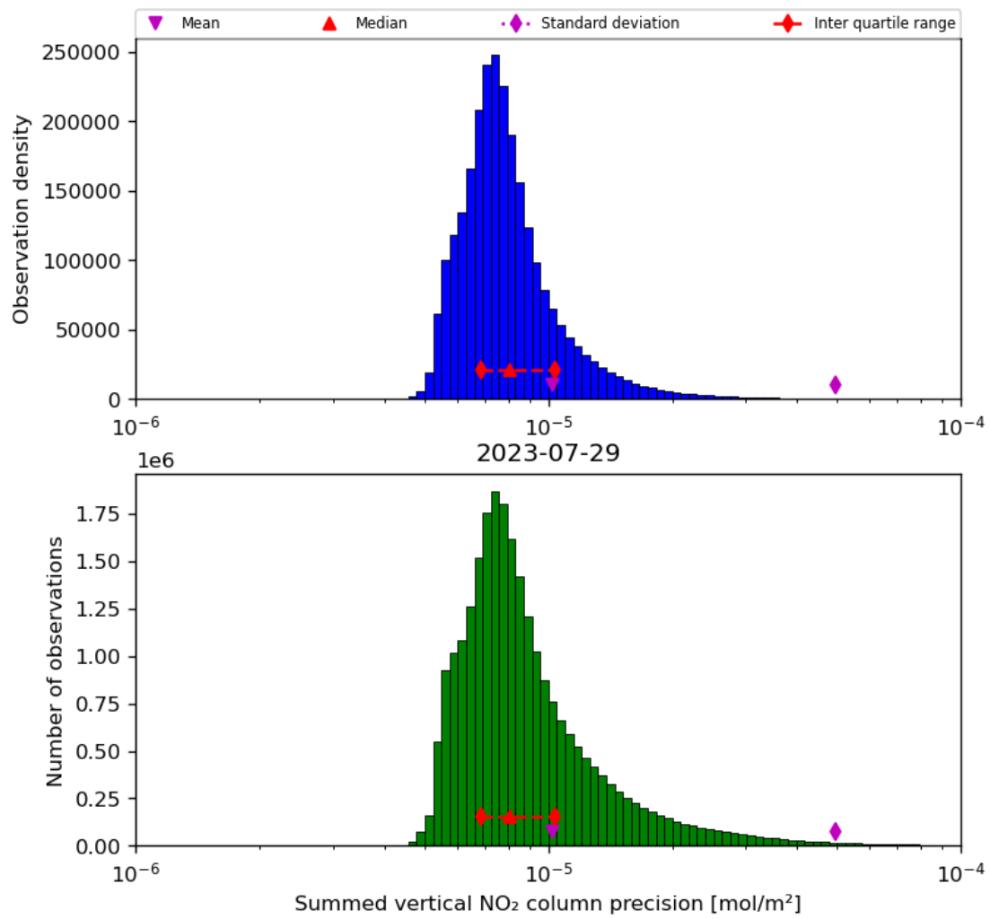
Figure 41: Histogram of "Summed vertical NO 2 column precision" for 2023-07-29 to 2023-07-30
