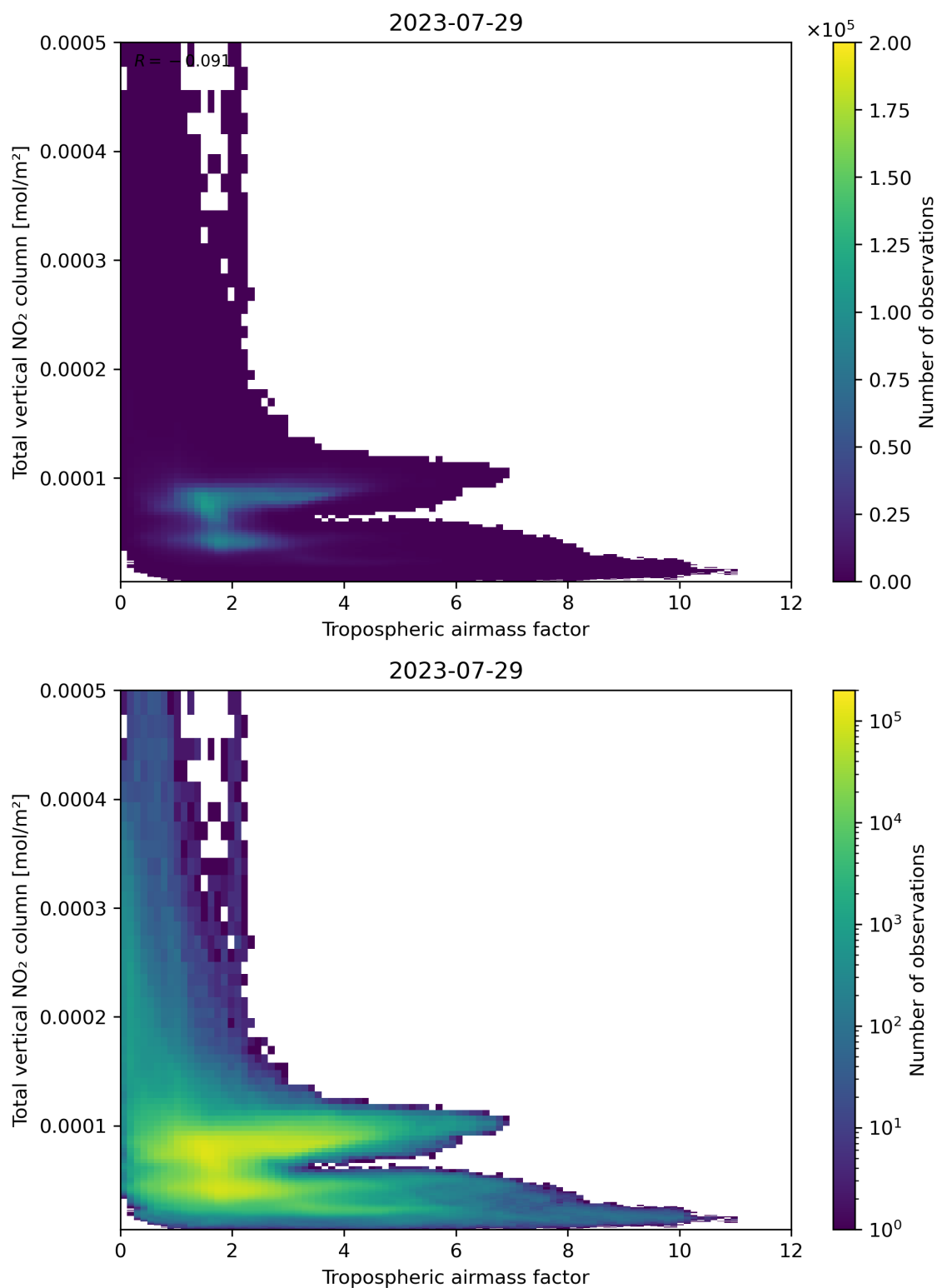
Figure 77: Scatter density plot of “Tropospheric airmass factor” against “Total vertical NO 2 column” for 2023-07-29 to 2023-07-30.
