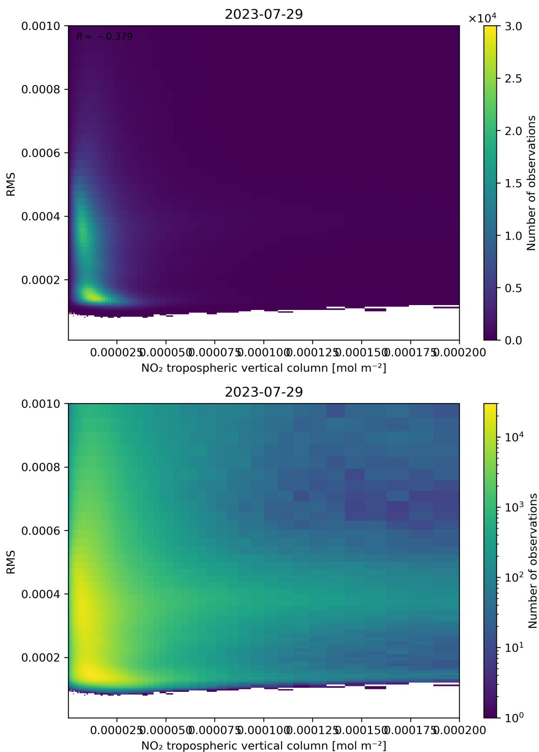
Figure 142: Scatter density plot of “NO 2 tropospheric vertical column” against “RMS” for 2023-07-29 to 2023-07-30.
