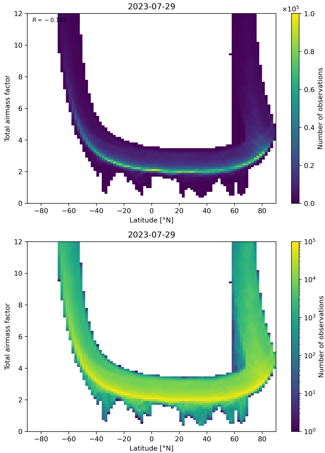
Figure 84: Scatter density plot of “Latitude” against “Total airmass factor” for 2023-07-29 to 2023-07-30.
