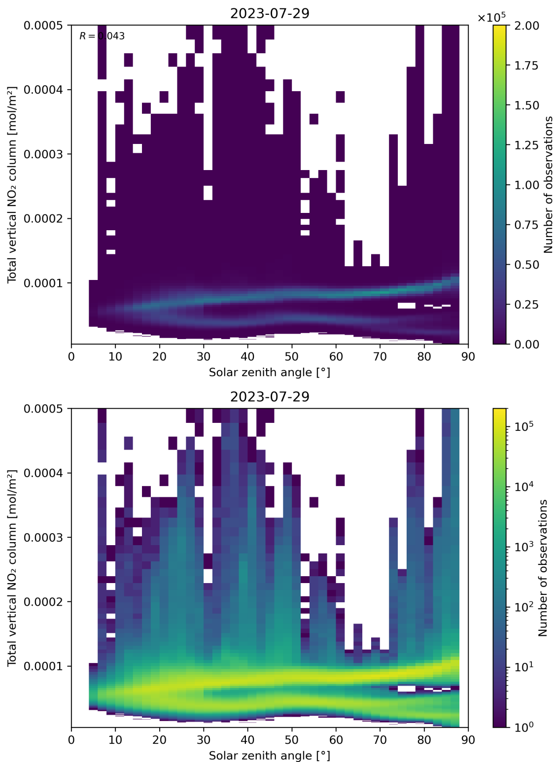
Figure 153: Scatter density plot of “Solar zenith angle” against “Total vertical NO 2 column” for 2023-07-29 to 2023-07-30.
