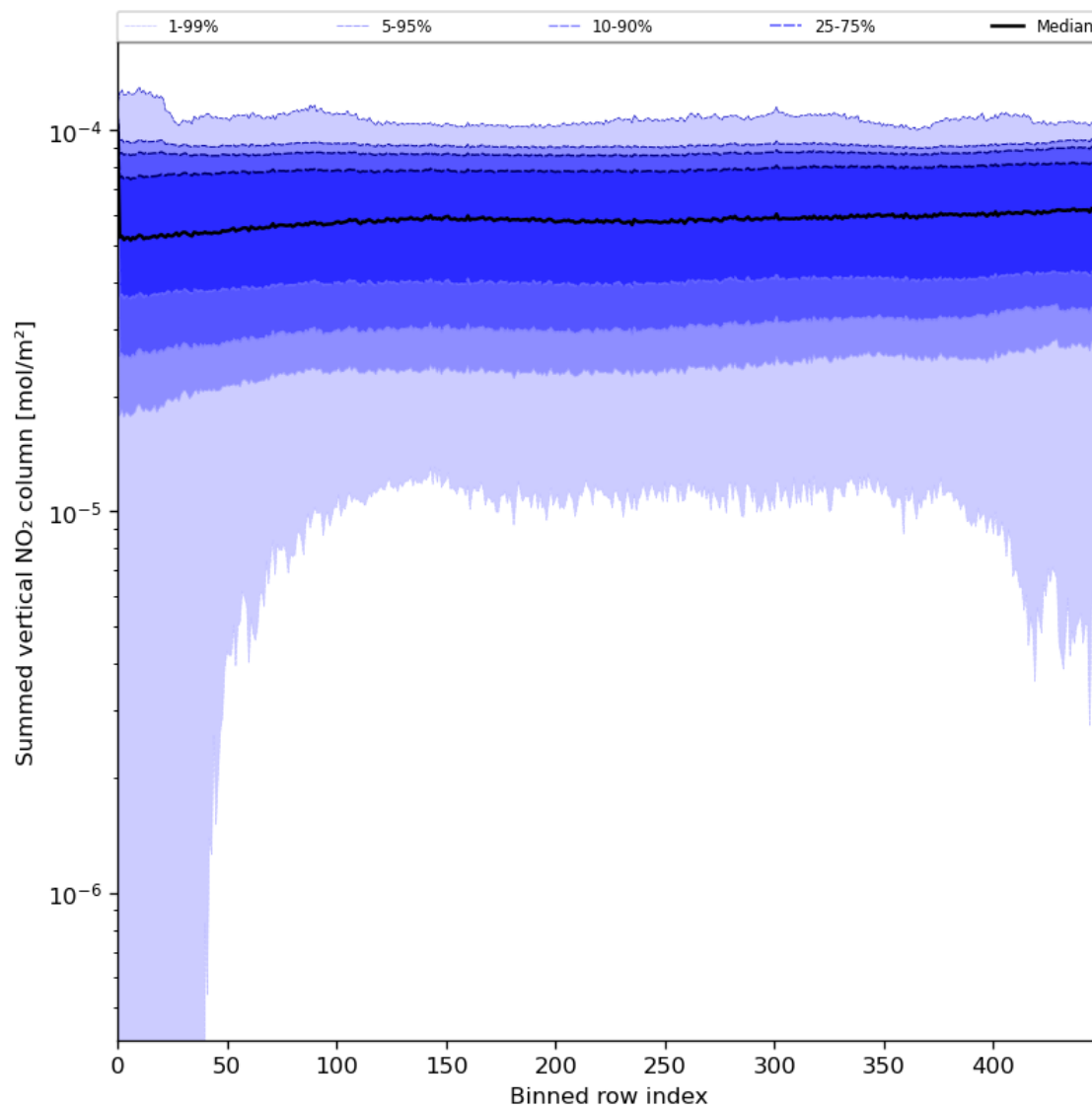
Figure 57: Along track statistics of “Summed vertical NO 2 column” for 2023-07-29 to 2023-07-30
