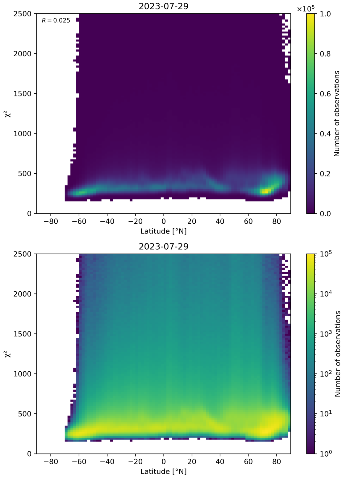
Figure 86: Scatter density plot of “Latitude” against “ \chi^2 ” for 2023-07-29 to 2023-07-30.
