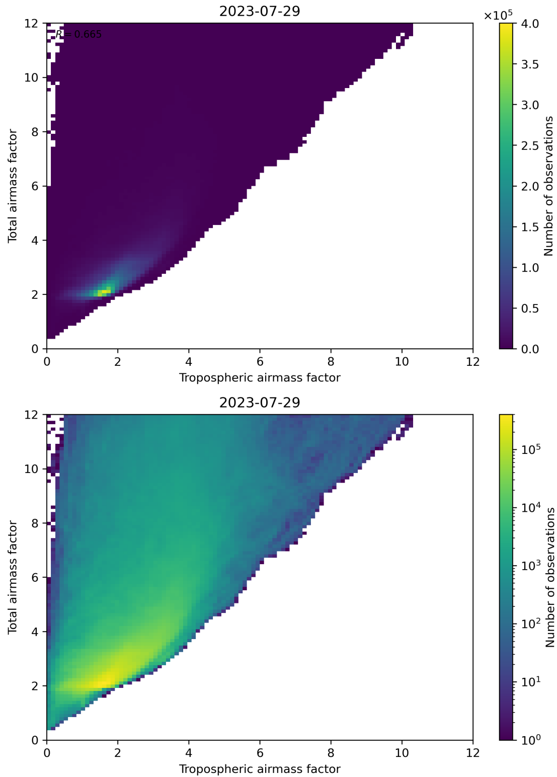
Figure 72: Scatter density plot of “Tropospheric airmass factor” against “Total airmass factor” for 2023-07-29 to 2023-07-30.
