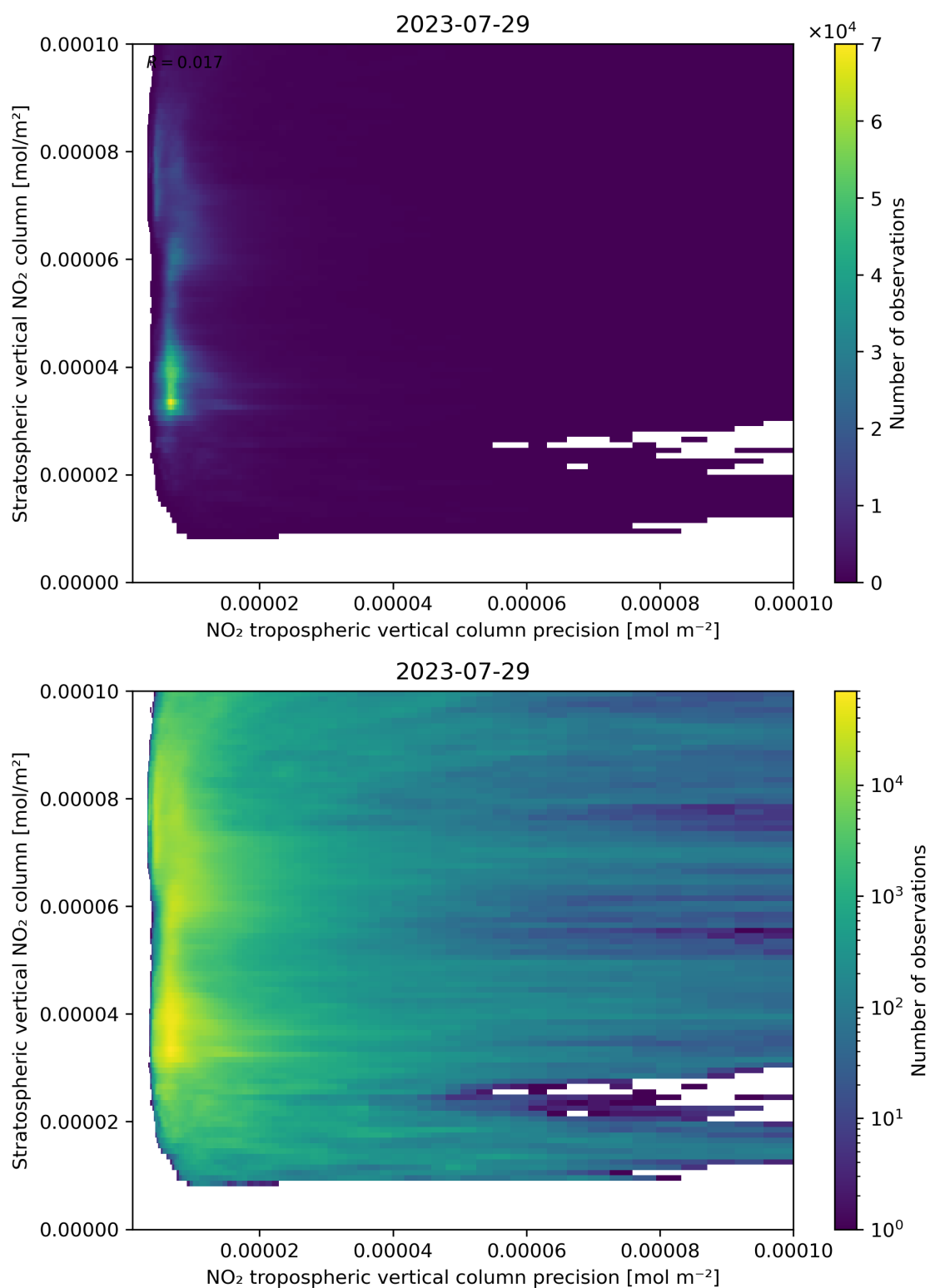
Figure 135: Scatter density plot of “NO 2 tropospheric vertical column precision” against “Stratospheric vertical NO 2 column” for 2023-07-29 to 2023-07-30.
