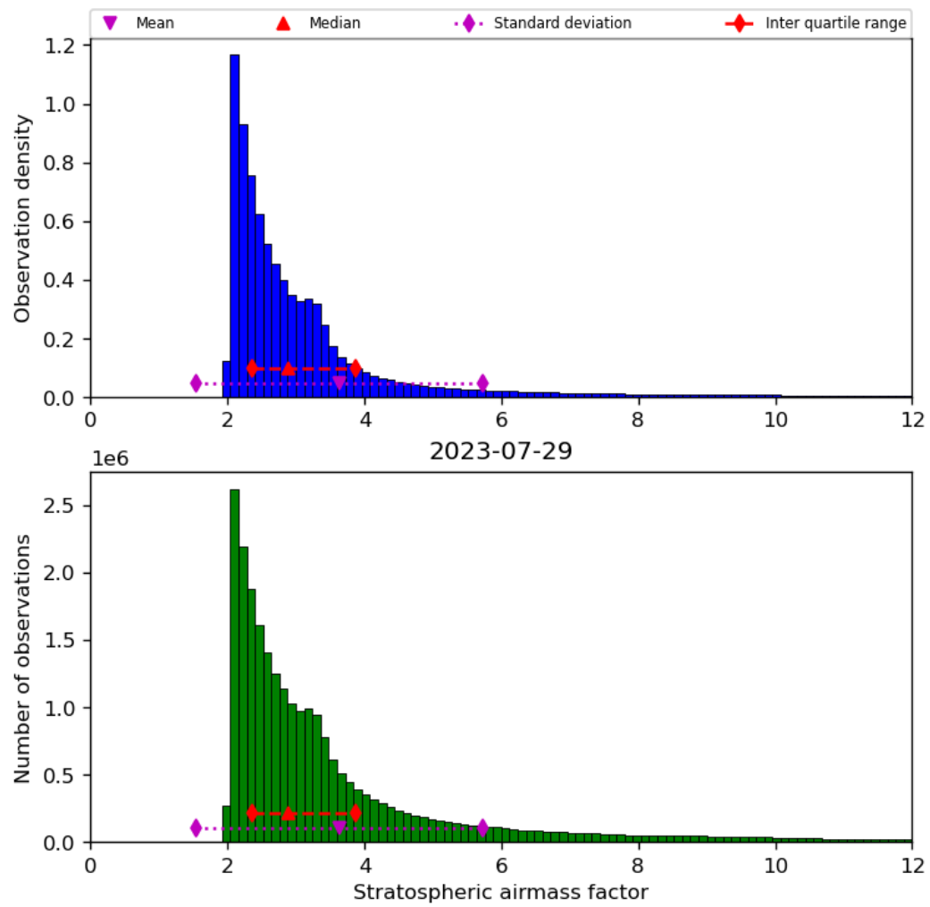
Figure 44: Histogram of “Stratospheric airmass factor” for 2023-07-29 to 2023-07-30
