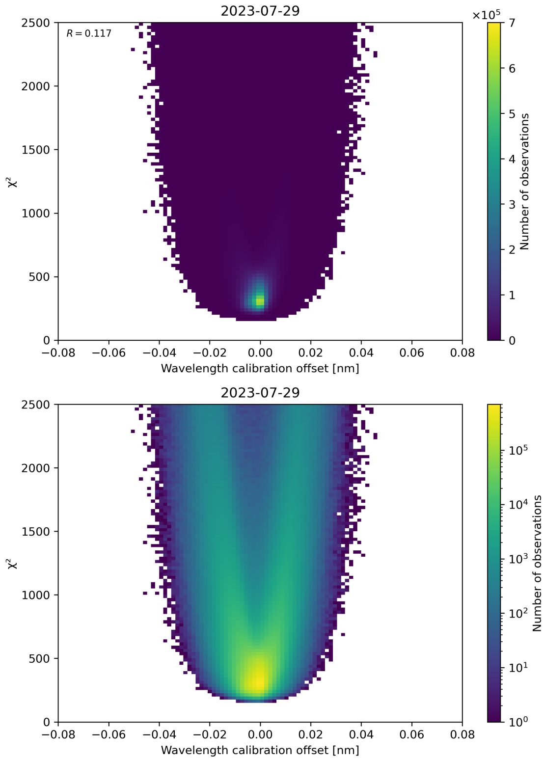
Figure 175: Scatter density plot of “Wavelength calibration offset” against “ \chi^2 ” for 2023-07-29 to 2023-07-30.
