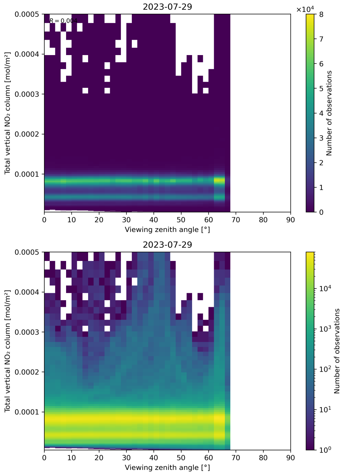
Figure 167: Scatter density plot of “Viewing zenith angle” against “Total vertical NO 2 column” for 2023-07-29 to 2023-07-30.
