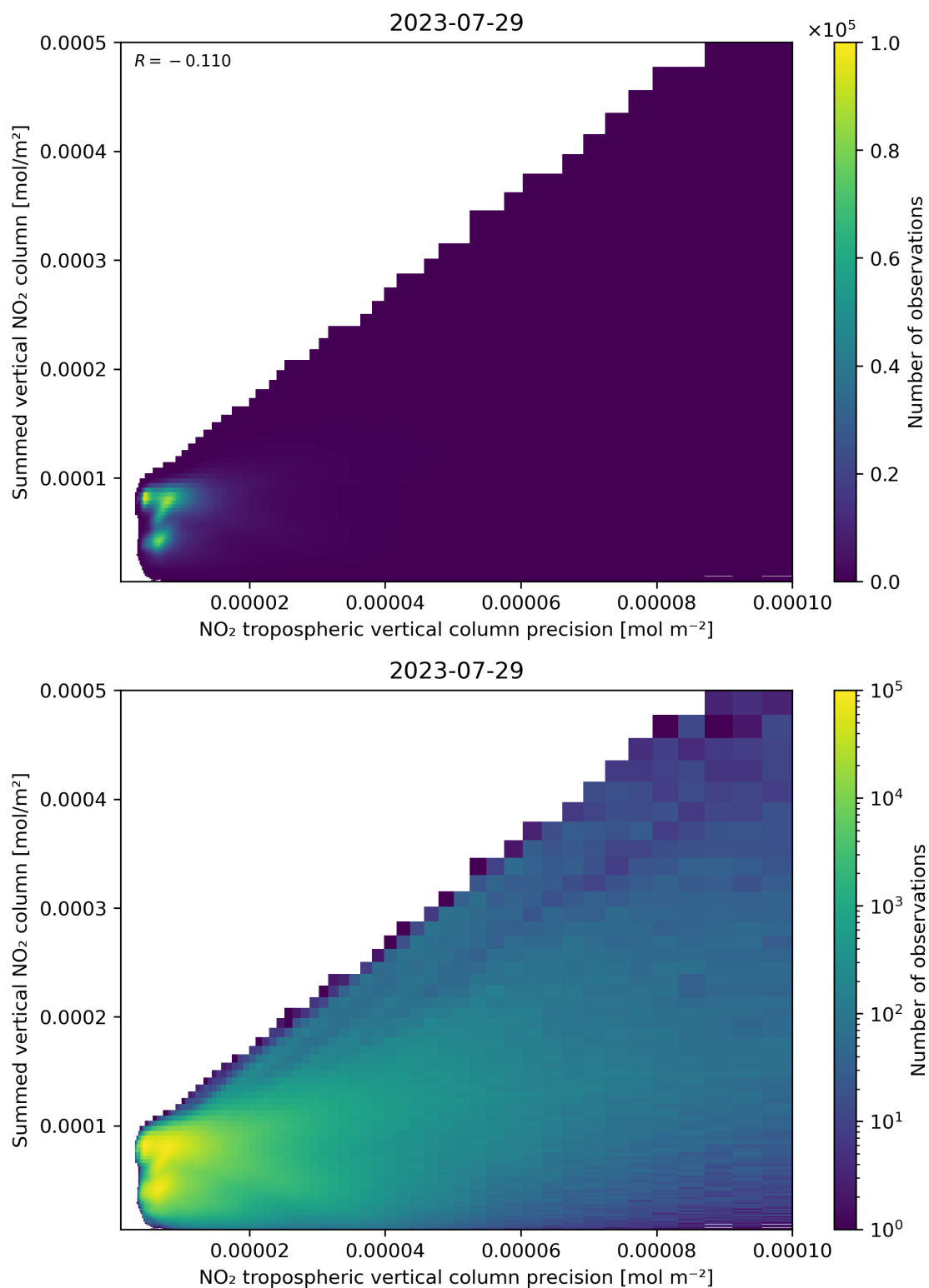
Figure 136: Scatter density plot of “NO 2 tropospheric vertical column precision” against “Summed vertical NO 2 column” for 2023-07-29 to 2023-07-30.
