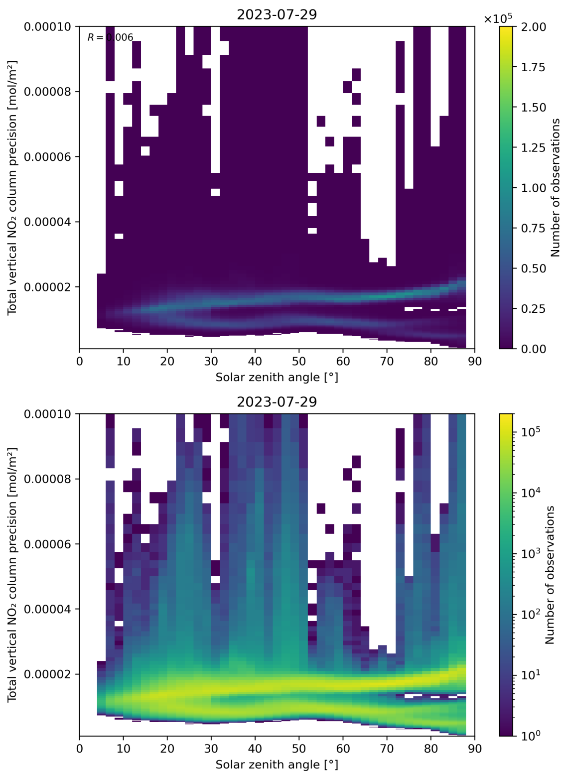
Figure 154: Scatter density plot of “Solar zenith angle” against “Total vertical NO 2 column precision” for 2023-07-29 to 2023-07-30.
