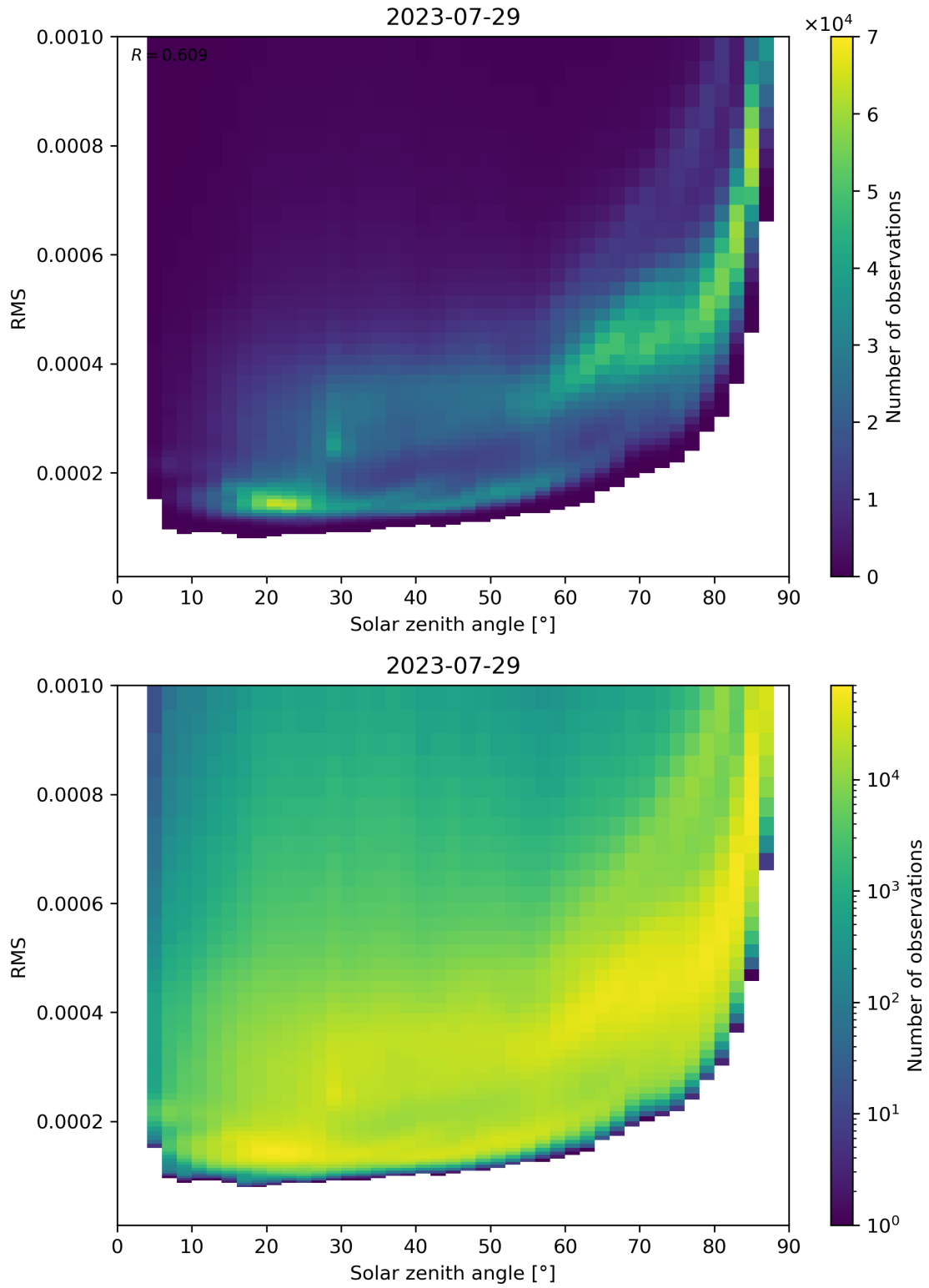
Figure 157: Scatter density plot of “Solar zenith angle” against “RMS” for 2023-07-29 to 2023-07-30.
