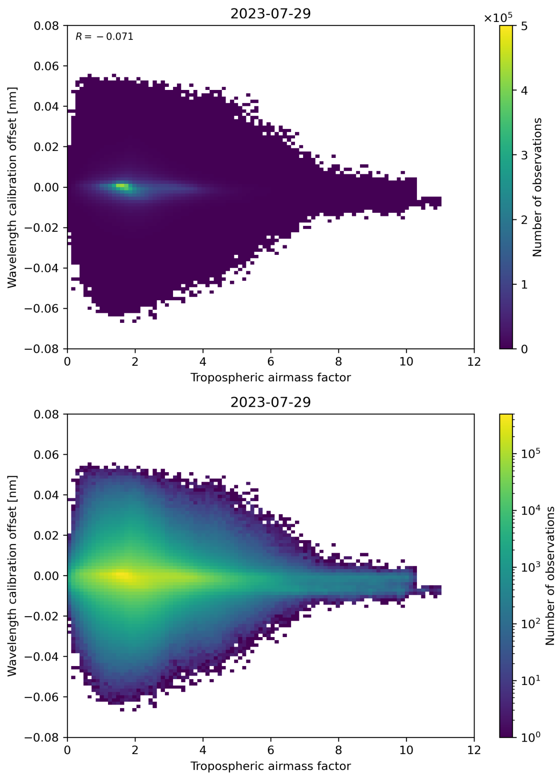
Figure 80: Scatter density plot of “Tropospheric air mass factor” against “Wavelength calibration offset” for 2023-07-29 to 2023-07-30.
