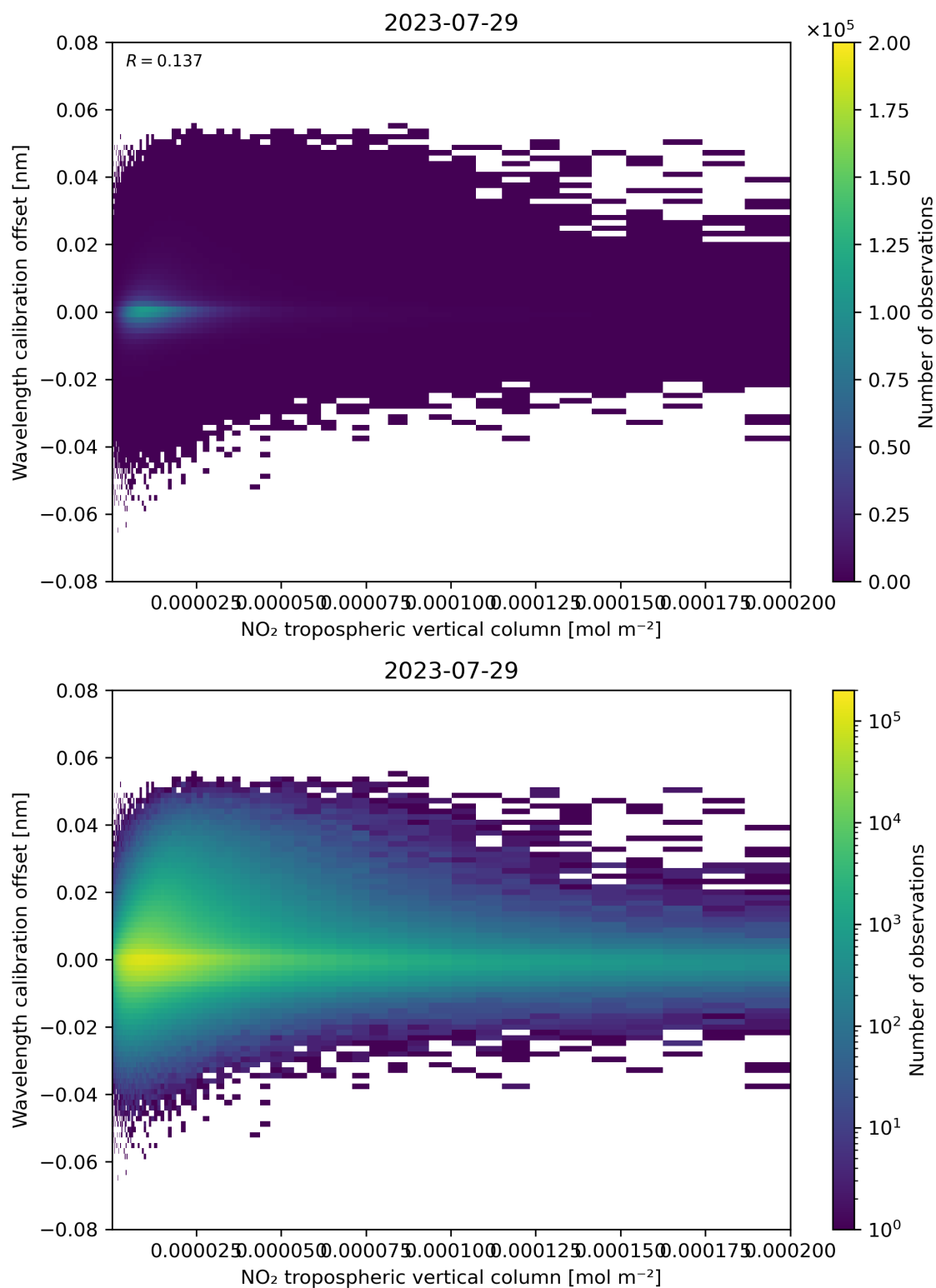
Figure 143: Scatter density plot of “NO 2 tropospheric vertical column” against “Wavelength calibration offset” for 2023-07-29 to 2023-07-30.
