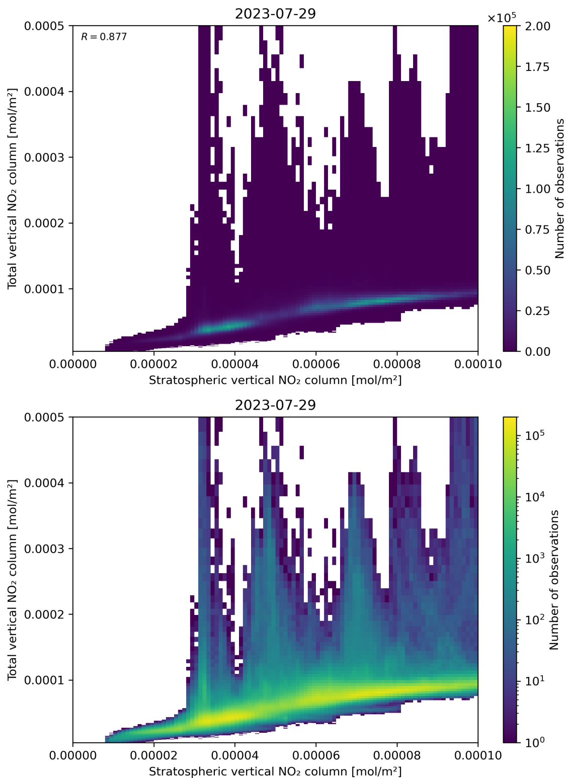
Figure 100: Scatter density plot of “Stratospheric vertical NO 2 column” against “Total vertical NO 2 column” for 2023-07-29 to 2023-07-30.
