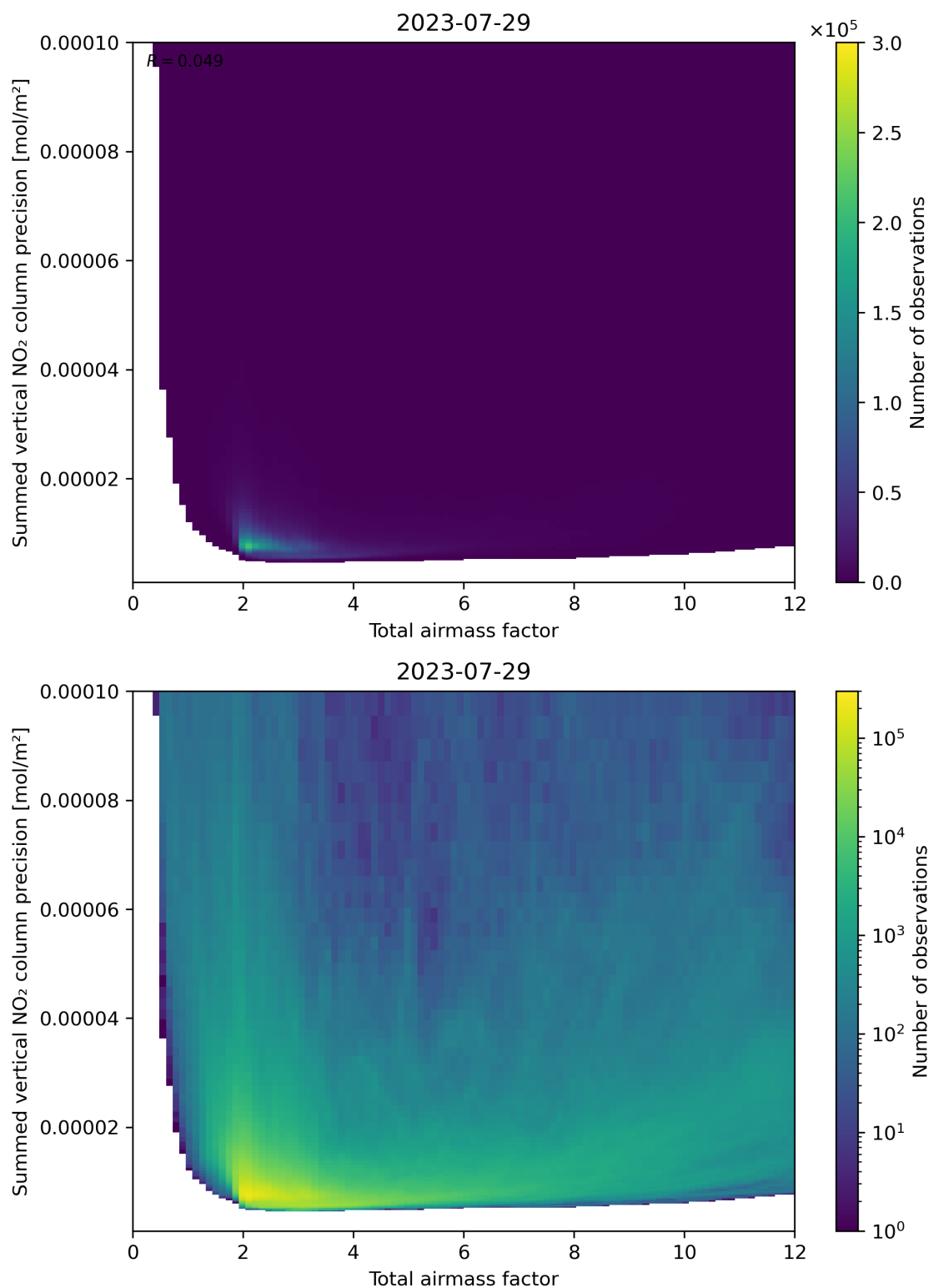
Figure 66: Scatter density plot of “Total airmass factor” against “Summed vertical NO 2 column precision” for 2023-07-29 to 2023-07-30.
