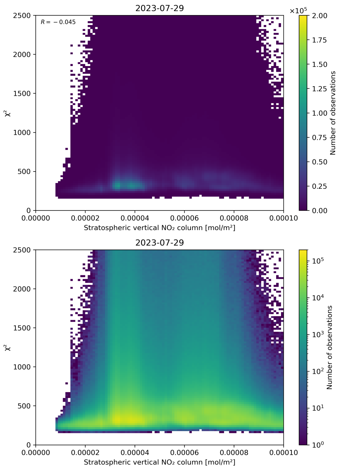
Figure 97: Scatter density plot of “Stratospheric vertical NO 2 column” against “ \chi^2 ” for 2023-07-29 to 2023-07-30.
