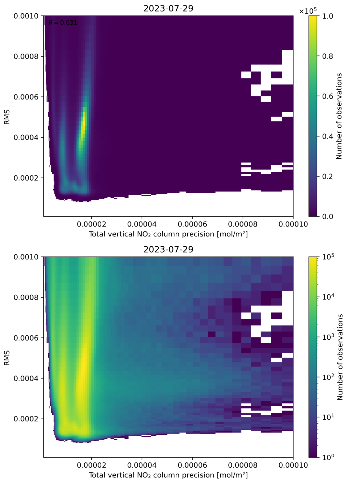
Figure 119: Scatter density plot of “Total vertical NO 2 column precision” against “RMS” for 2023-07-29 to 2023-07-30.
