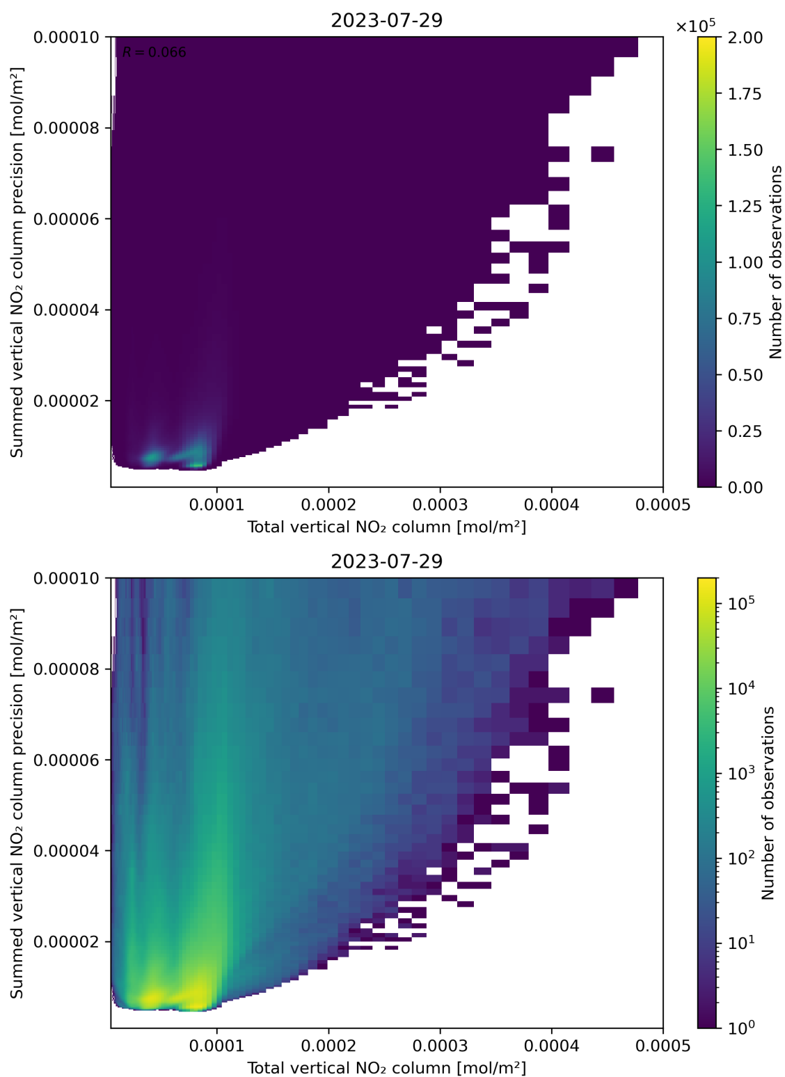
Figure 113: Scatter density plot of “Total vertical NO 2 column” against “Summed vertical NO 2 column precision” for 2023-07-29 to 2023-07-30.
