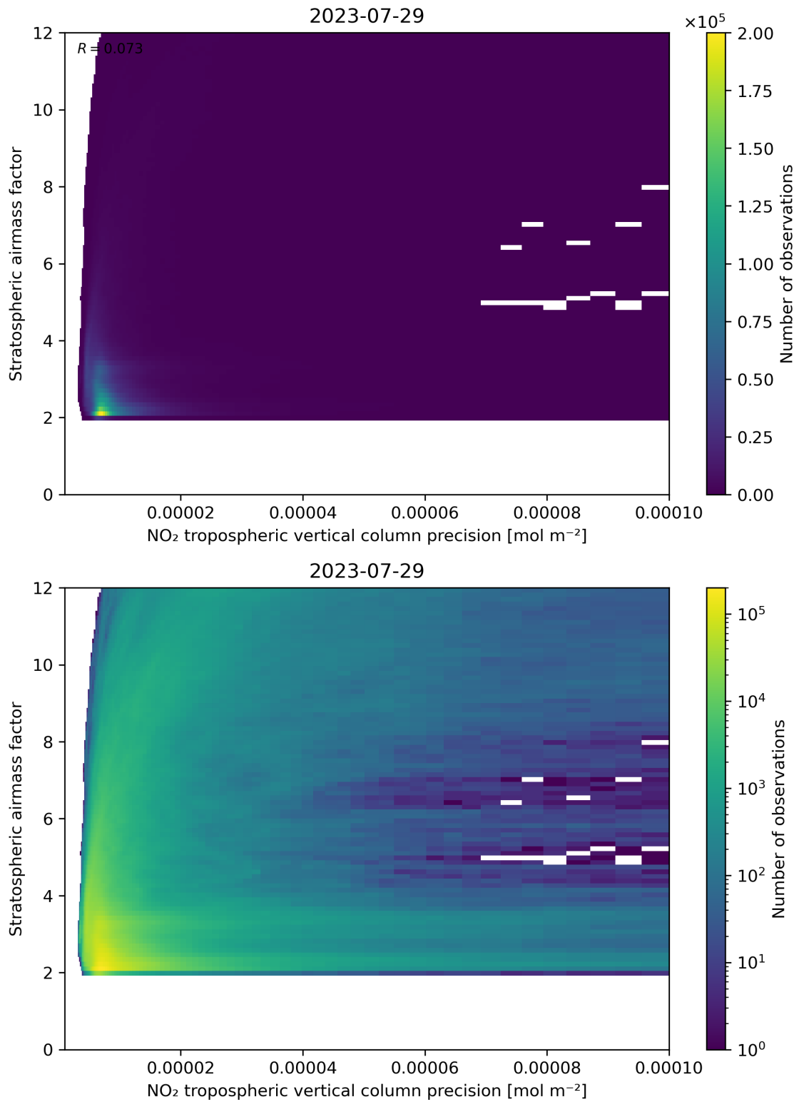
Figure 131: Scatter density plot of “NO 2 tropospheric vertical column precision” against “Stratospheric airmass factor” for 2023-07-29 to 2023-07-30.
