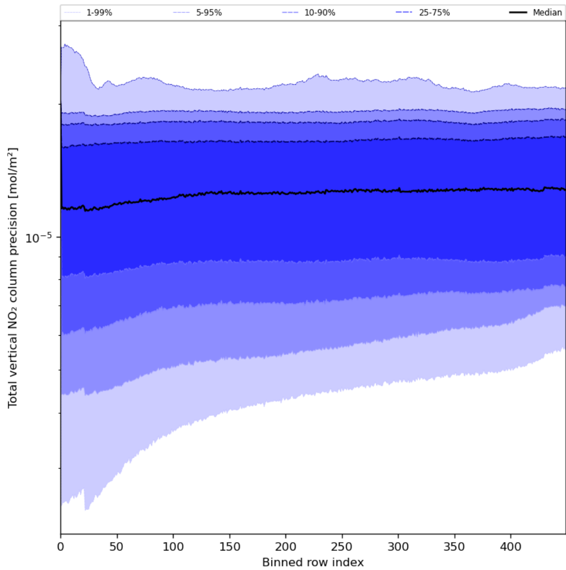
Figure 56: Along track statistics of “Total vertical NO 2 column precision” for 2023-07-29 to 2023-07-30
