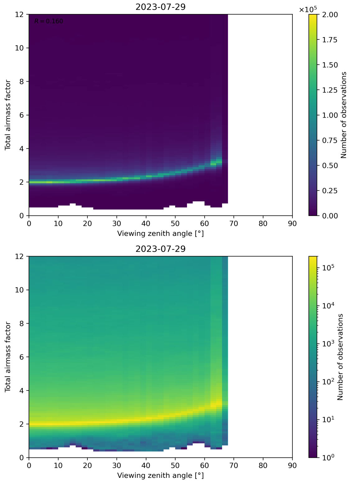
Figure 160: Scatter density plot of “Viewing zenith angle” against “Total airmass factor” for 2023-07-29 to 2023-07-30.
