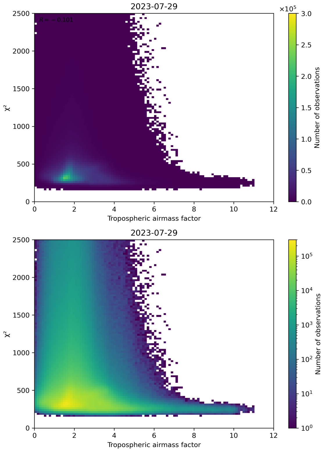
Figure 73: Scatter density plot of “Tropospheric airmass factor” against “ \chi^2 ” for 2023-07-29 to 2023-07-30.
