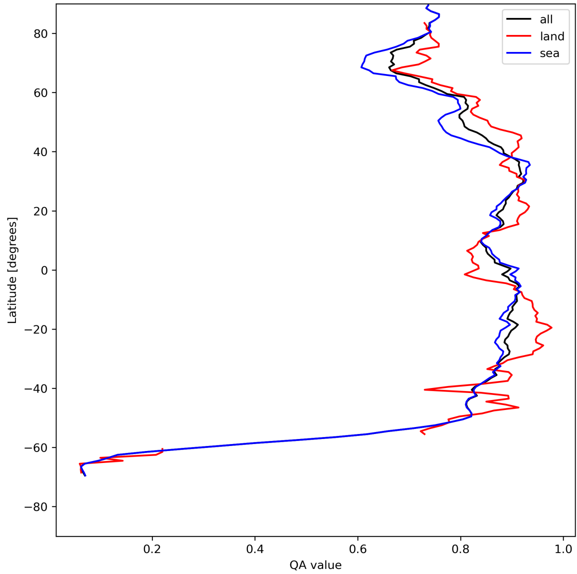
Figure 11: Zonal average of “QA value” for 2023-07-29 to 2023-07-30.
