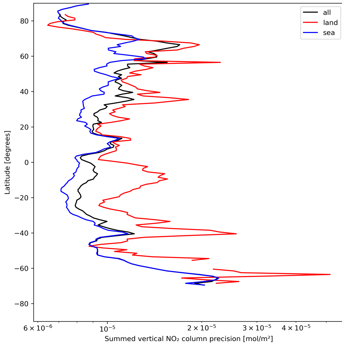
Figure 24: Zonal average of “Summed vertical NO 2 column precision” for 2023-07-29 to 2023-07-30.
