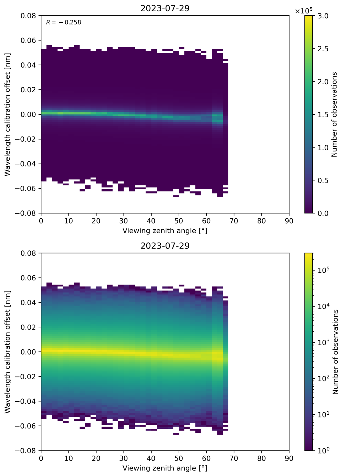
Figure 173: Scatter density plot of “Viewing zenith angle” against “Wavelength calibration offset” for 2023-07-29 to 2023-07-30.
