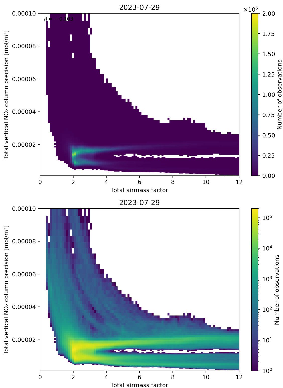
Figure 68: Scatter density plot of “Total airmass factor” against “Total vertical NO 2 column precision” for 2023-07-29 to 2023-07-30.
