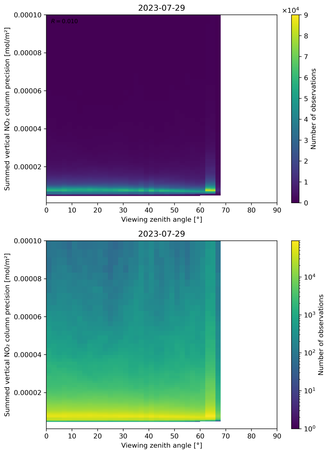
Figure 166: Scatter density plot of “Viewing zenith angle” against “Summed vertical NO 2 column precision” for 2023-07-29 to 2023-07-30.
