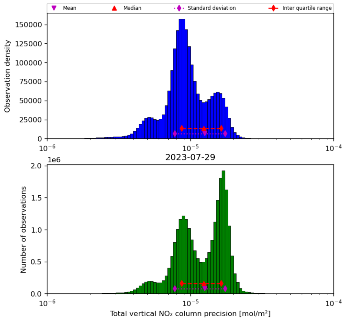
Figure 39: Histogram of "Total vertical NO 2 column precision" for 2023-07-29 to 2023-07-30
