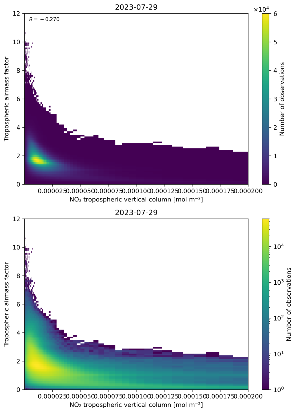
Figure 123: Scatter density plot of “NO 2 tropospheric vertical column” against “Tropospheric airmass factor” for 2023-07-29 to 2023-07-30.
