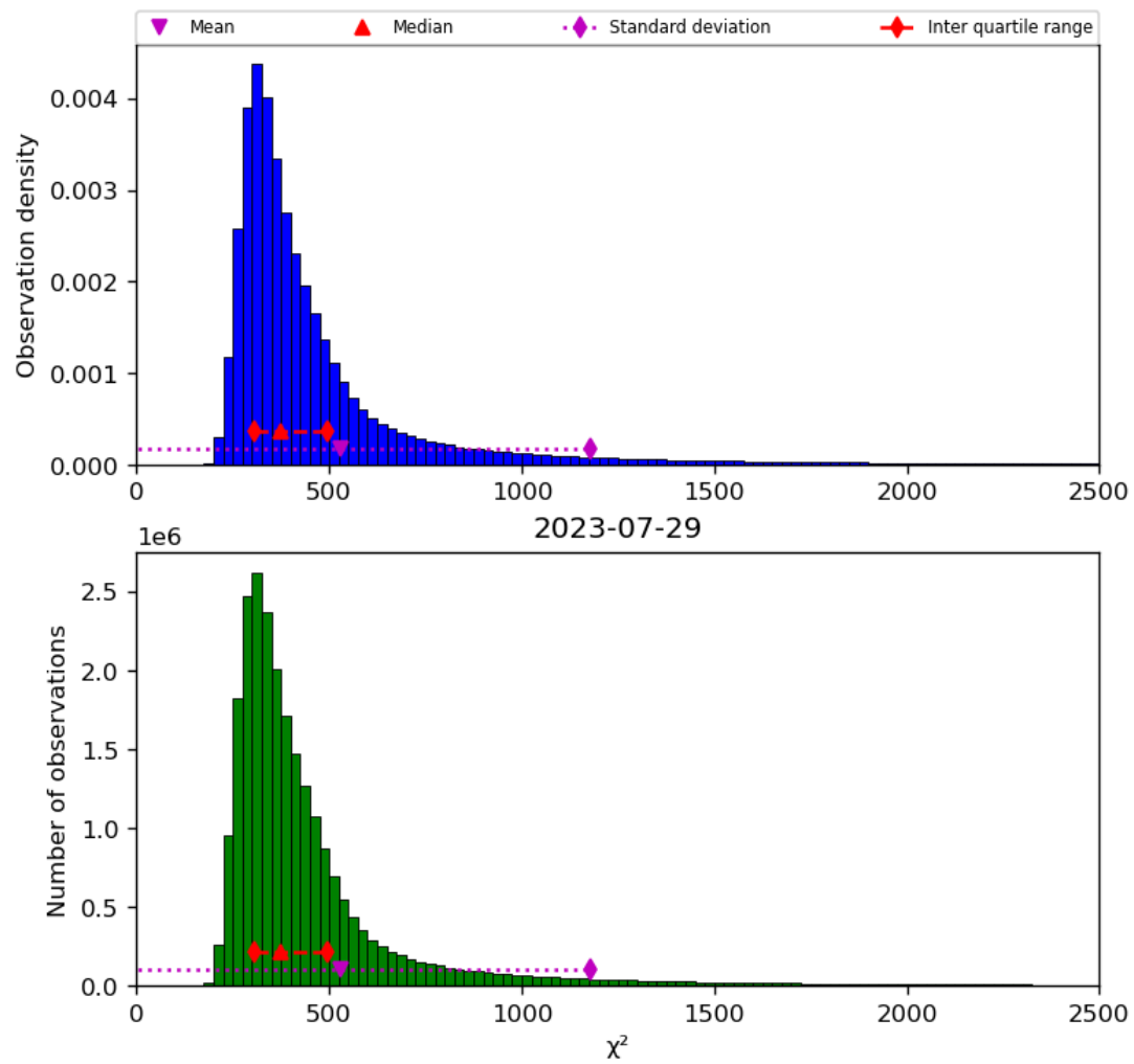
Figure 42: Histogram of “ \chi^2 ” for 2023-07-29 to 2023-07-30
