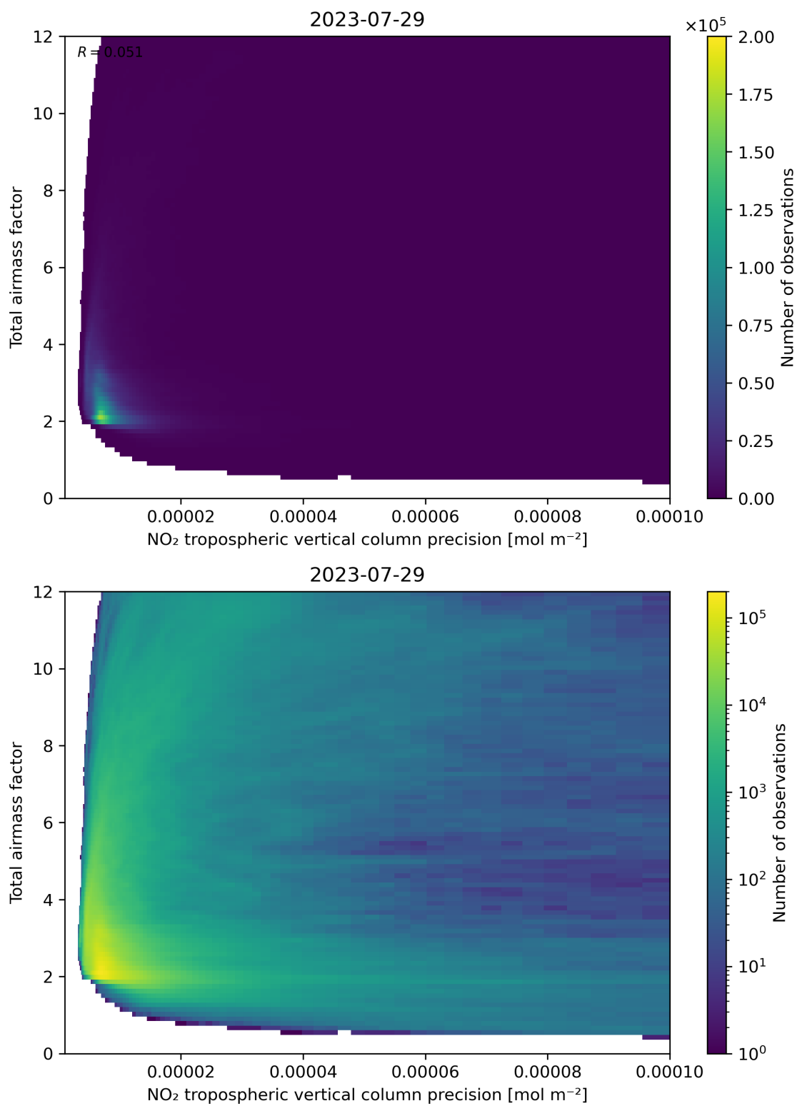
Figure 132: Scatter density plot of “NO 2 tropospheric vertical column precision” against “Total air mass factor” for 2023-07-29 to 2023-07-30.
