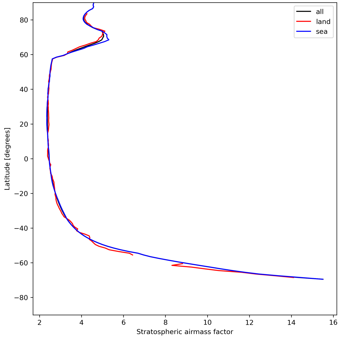
Figure 27: Zonal average of “Stratospheric airmass factor” for 2023-07-29 to 2023-07-30.
