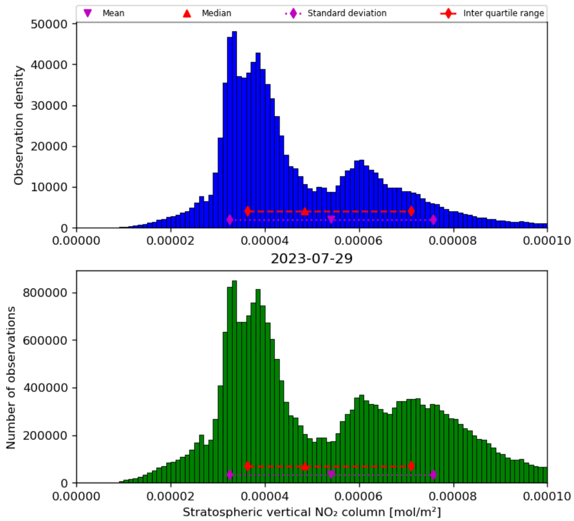
Figure 36: Histogram of “Stratospheric vertical NO 2 column” for 2023-07-29 to 2023-07-30
