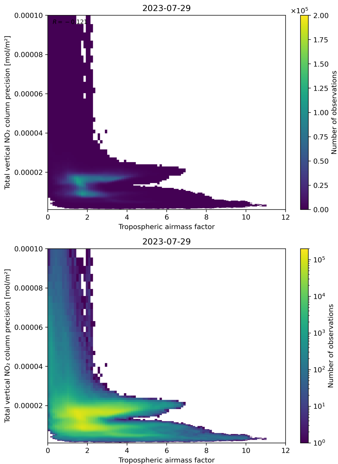
Figure 78: Scatter density plot of “Tropospheric airmass factor” against “Total vertical NO 2 column precision” for 2023-07-29 to 2023-07-30.
