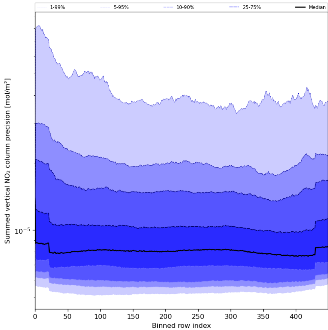
Figure 58: Along track statistics of “Summed vertical NO 2 column precision” for 2023-07-29 to 2023-07-30
