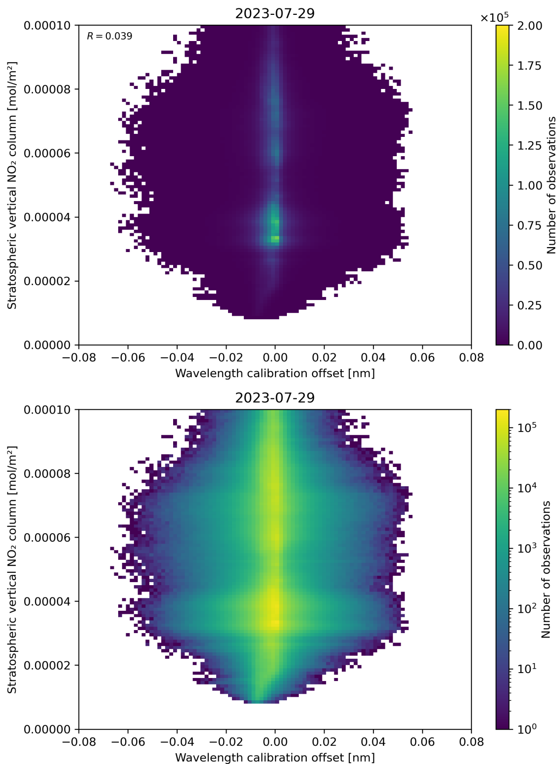
Figure 176: Scatter density plot of “Wavelength calibration offset” against “Stratospheric vertical NO 2 column” for 2023-07-29 to 2023-07-30.
