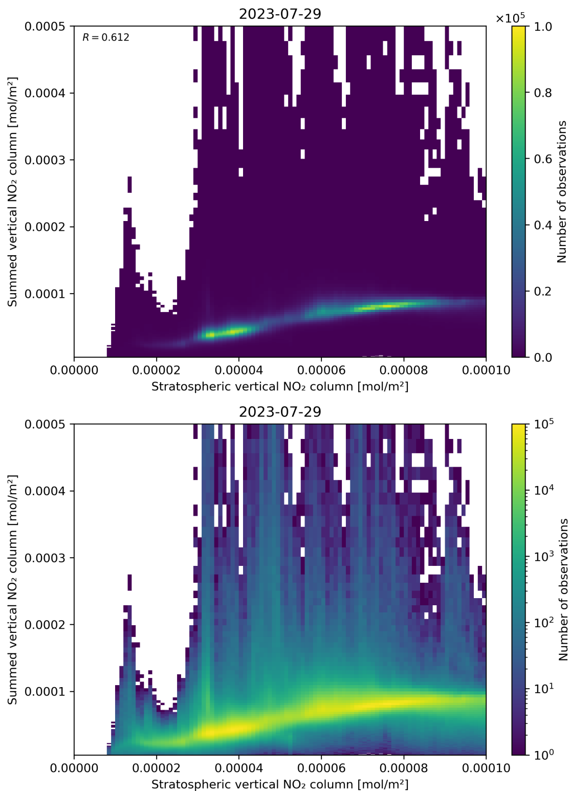
Figure 98: Scatter density plot of “Stratospheric vertical NO 2 column” against “Summed vertical NO 2 column” for 2023-07-29 to 2023-07-30.
