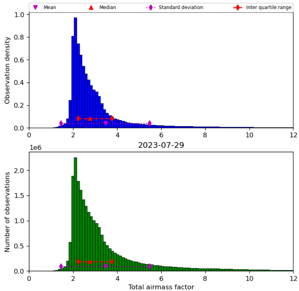
Figure 32: Histogram of “Total airmass factor” for 2023-07-29 to 2023-07-30
