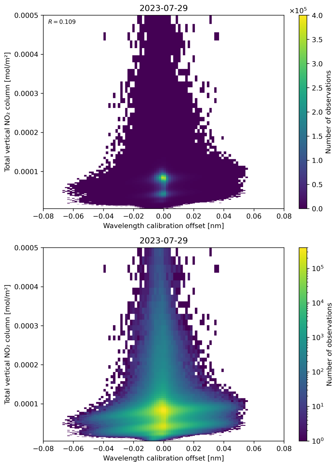
Figure 179: Scatter density plot of “Wavelength calibration offset” against “Total vertical NO 2 column” for 2023-07-29 to 2023-07-30.
