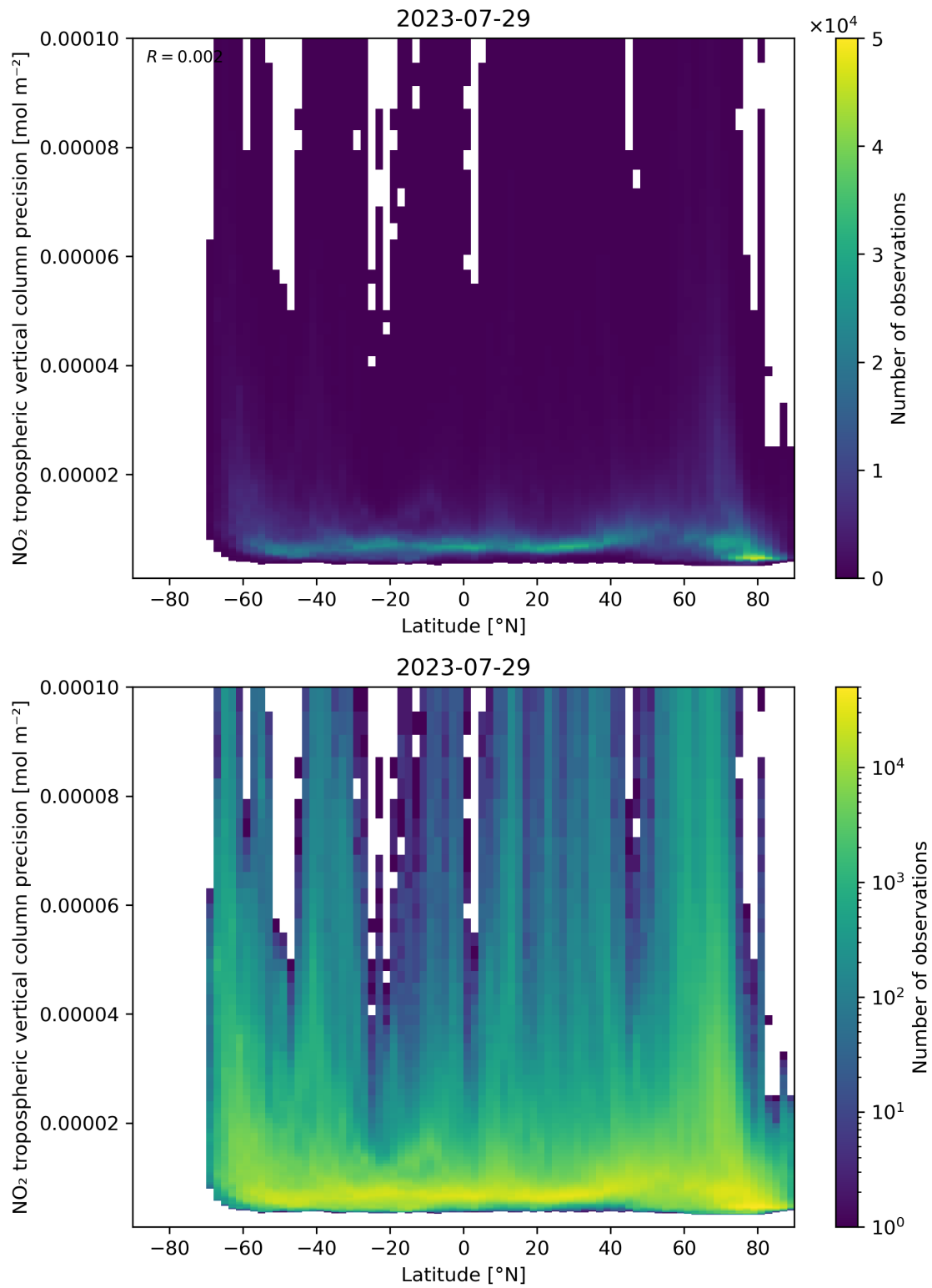
Figure 93: Scatter density plot of “Latitude” against “NO 2 tropospheric vertical column precision” for 2023-07-29 to 2023-07-30.
