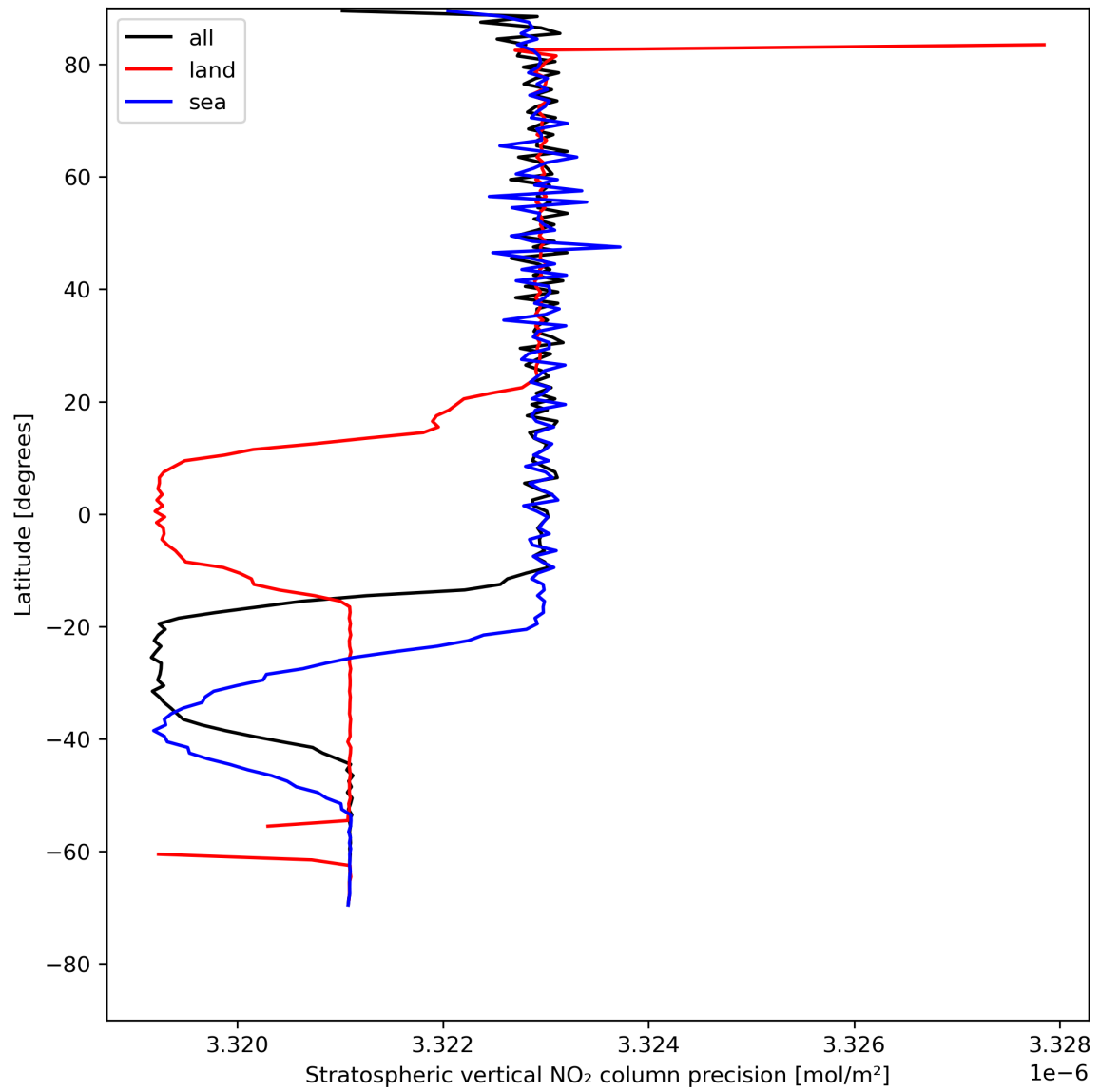
Figure 20: Zonal average of “Stratospheric vertical NO 2 column precision” for 2023-07-29 to 2023-07-30.
