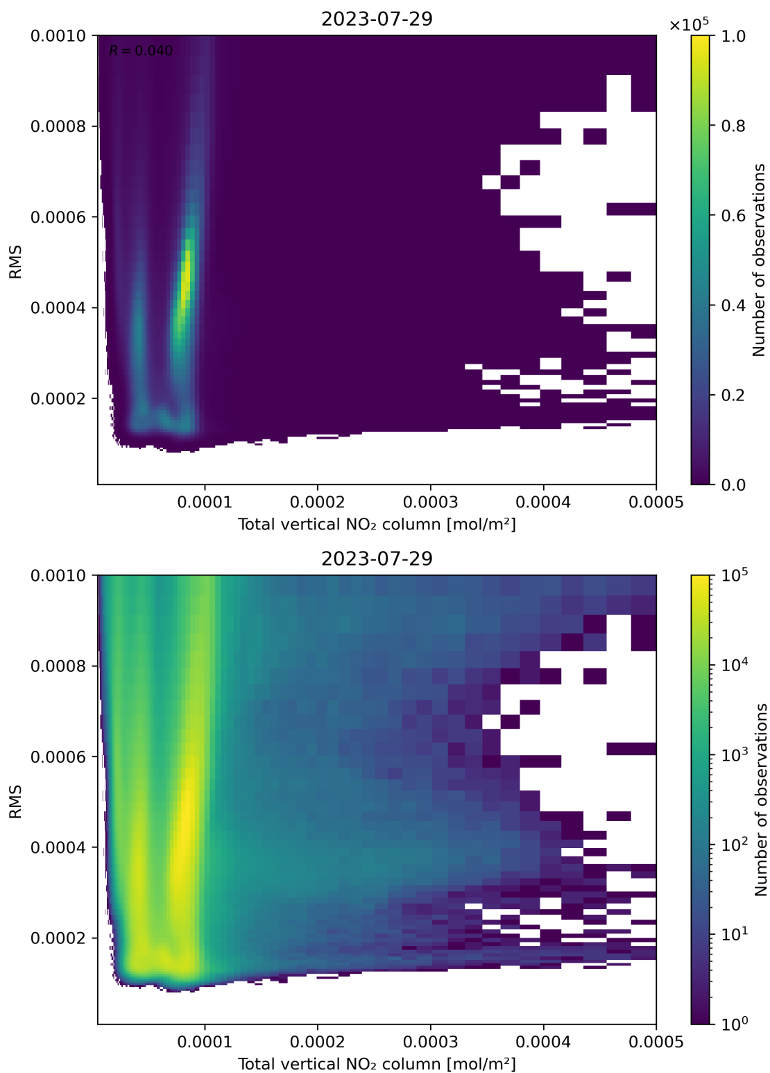
Figure 120: Scatter density plot of “Total vertical NO 2 column” against “RMS” for 2023-07-29 to 2023-07-30.
