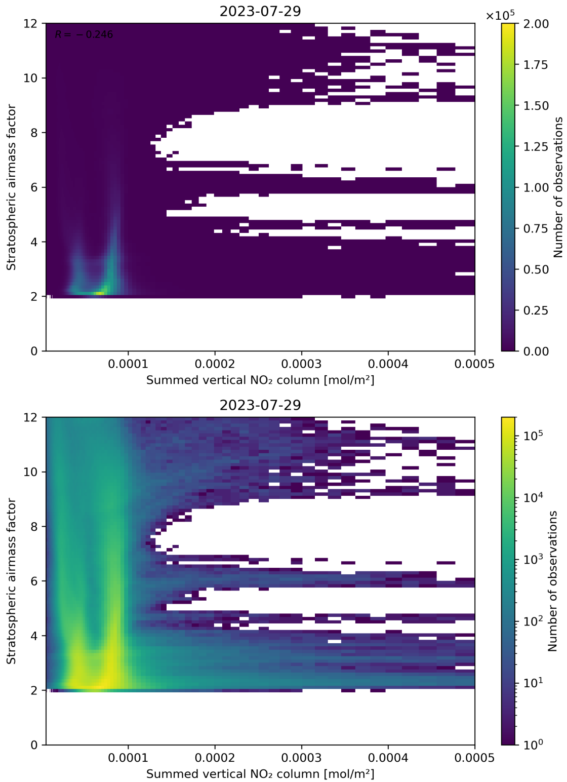
Figure 103: Scatter density plot of “Summed vertical NO 2 column” against “Stratospheric air mass factor” for 2023-07-29 to 2023-07-30.
