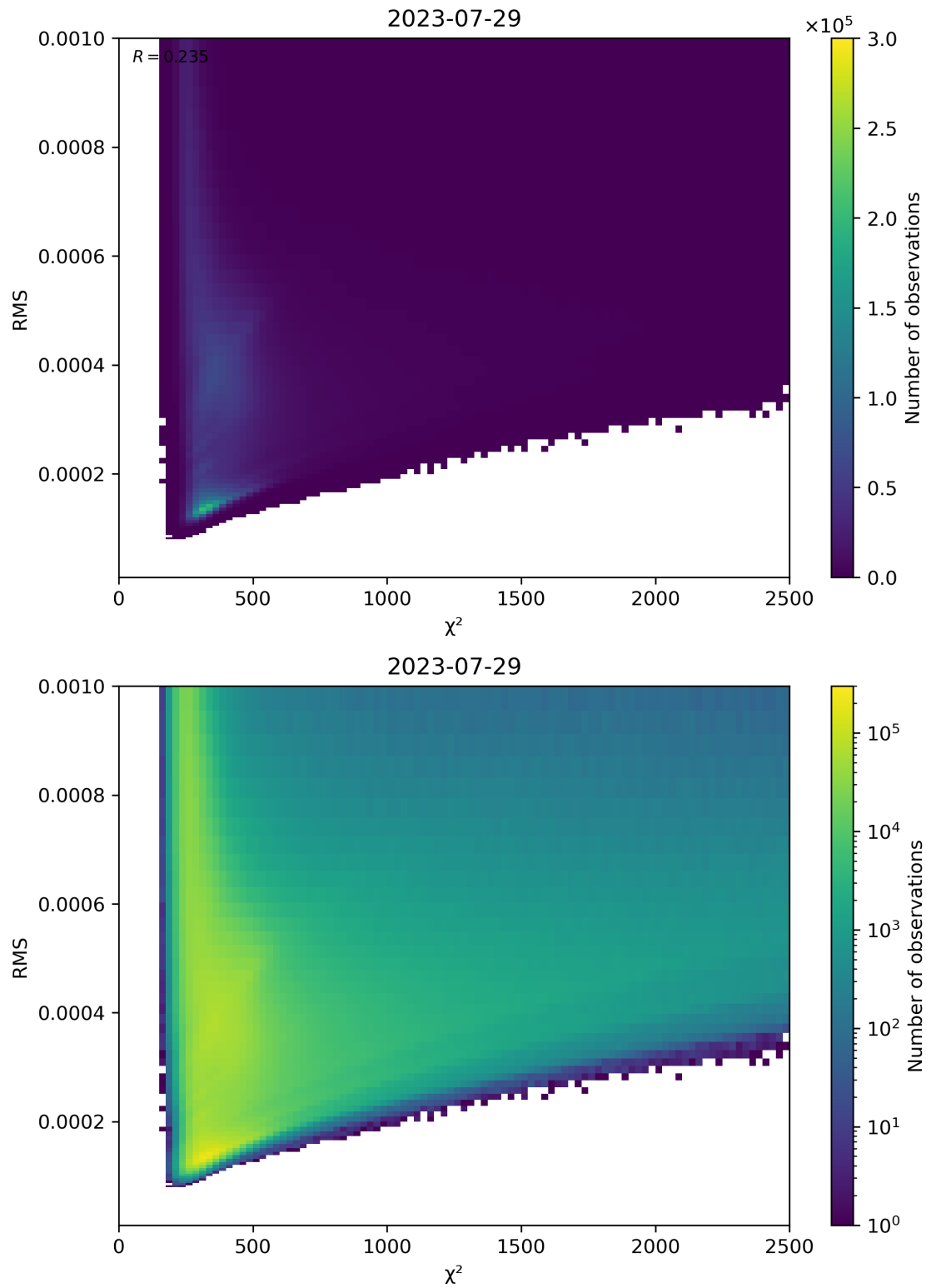
Figure 82: Scatter density plot of “ \chi^2 ” against “RMS” for 2023-07-29 to 2023-07-30.
