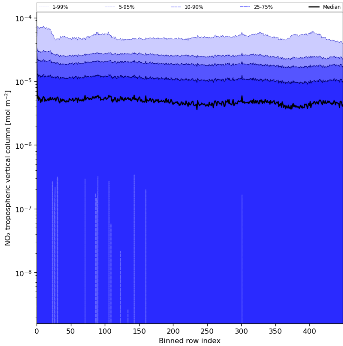
Figure 46: Along track statistics of “NO 2 tropospheric vertical column” for 2023-07-29 to 2023-07-30
