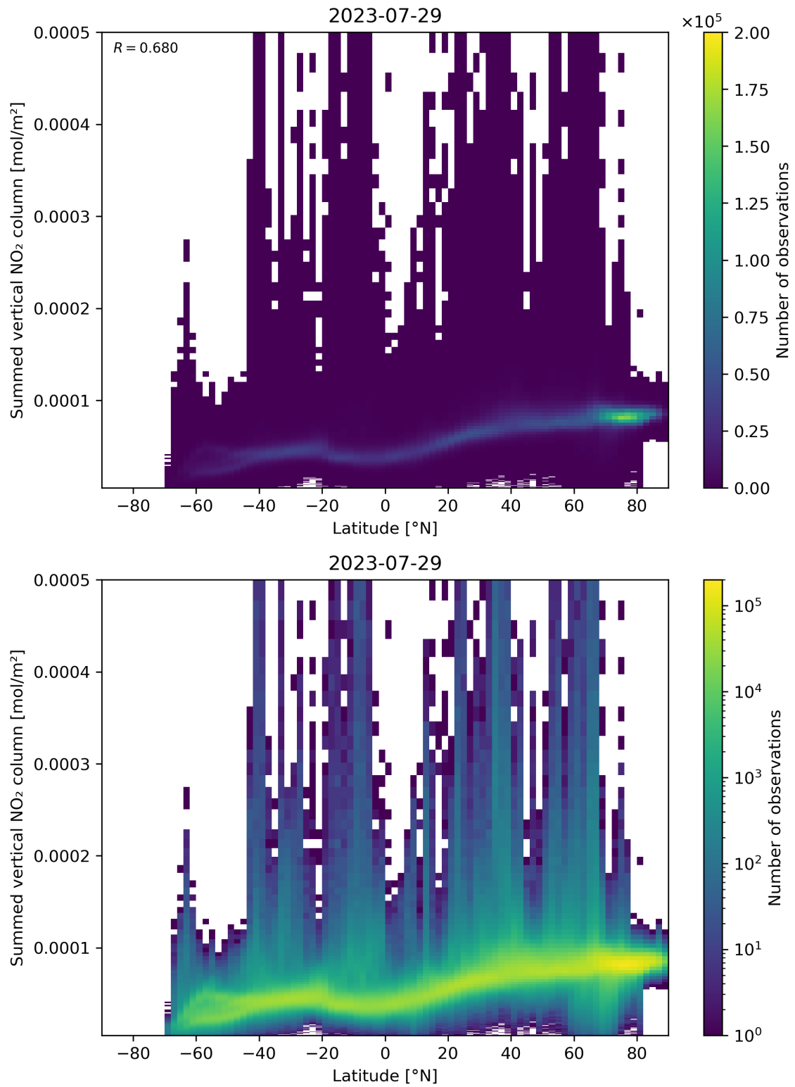
Figure 88: Scatter density plot of “Latitude” against “Summed vertical NO 2 column” for 2023-07-29 to 2023-07-30.
