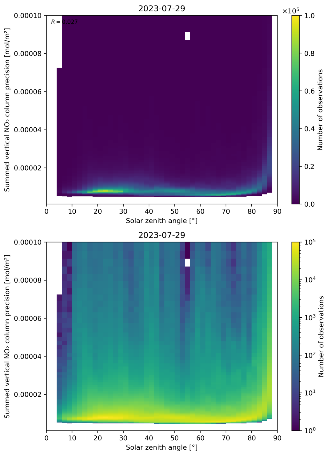
Figure 152: Scatter density plot of “Solar zenith angle” against “Summed vertical NO 2 column precision” for 2023-07-29 to 2023-07-30.
