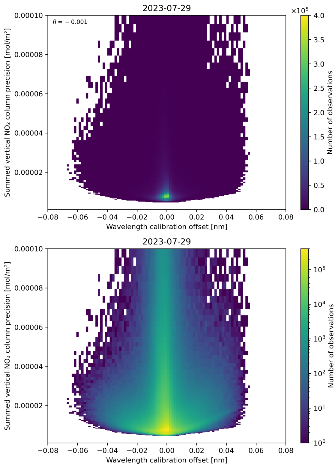
Figure 178: Scatter density plot of “Wavelength calibration offset” against “Summed vertical NO 2 column precision” for 2023-07-29 to 2023-07-30.
