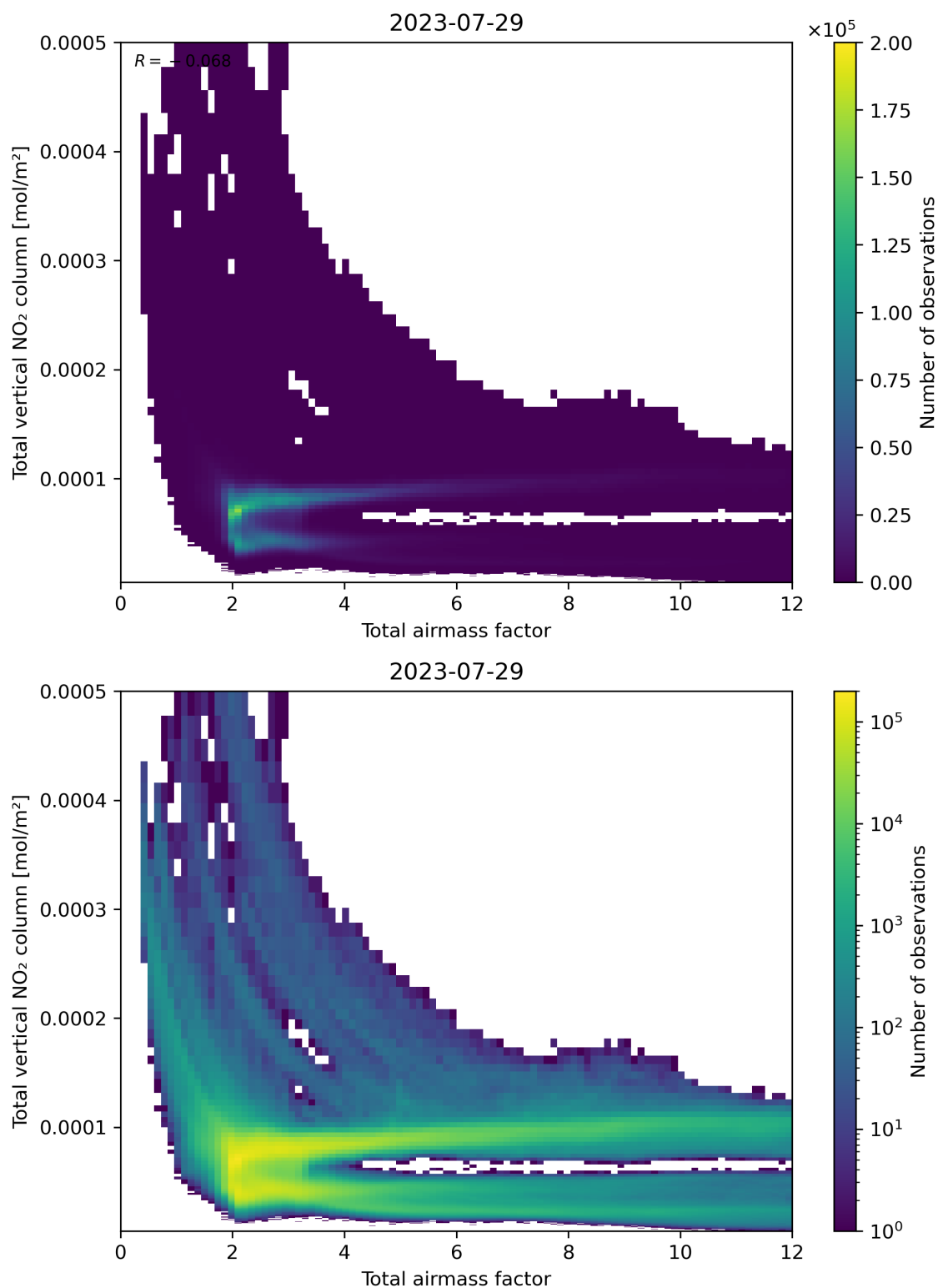
Figure 67: Scatter density plot of “Total airmass factor” against “Total vertical NO 2 column” for 2023-07-29 to 2023-07-30.
