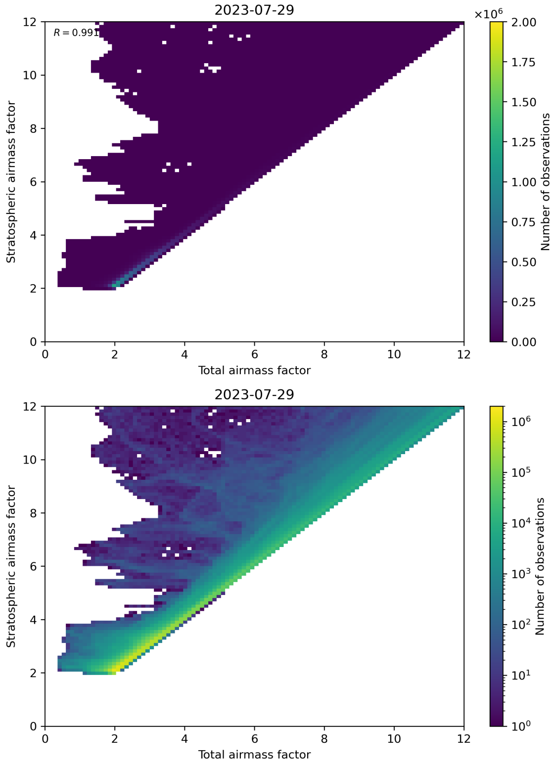
Figure 62: Scatter density plot of “Total air mass factor” against “Stratospheric air mass factor” for 2023-07-29 to 2023-07-30.
