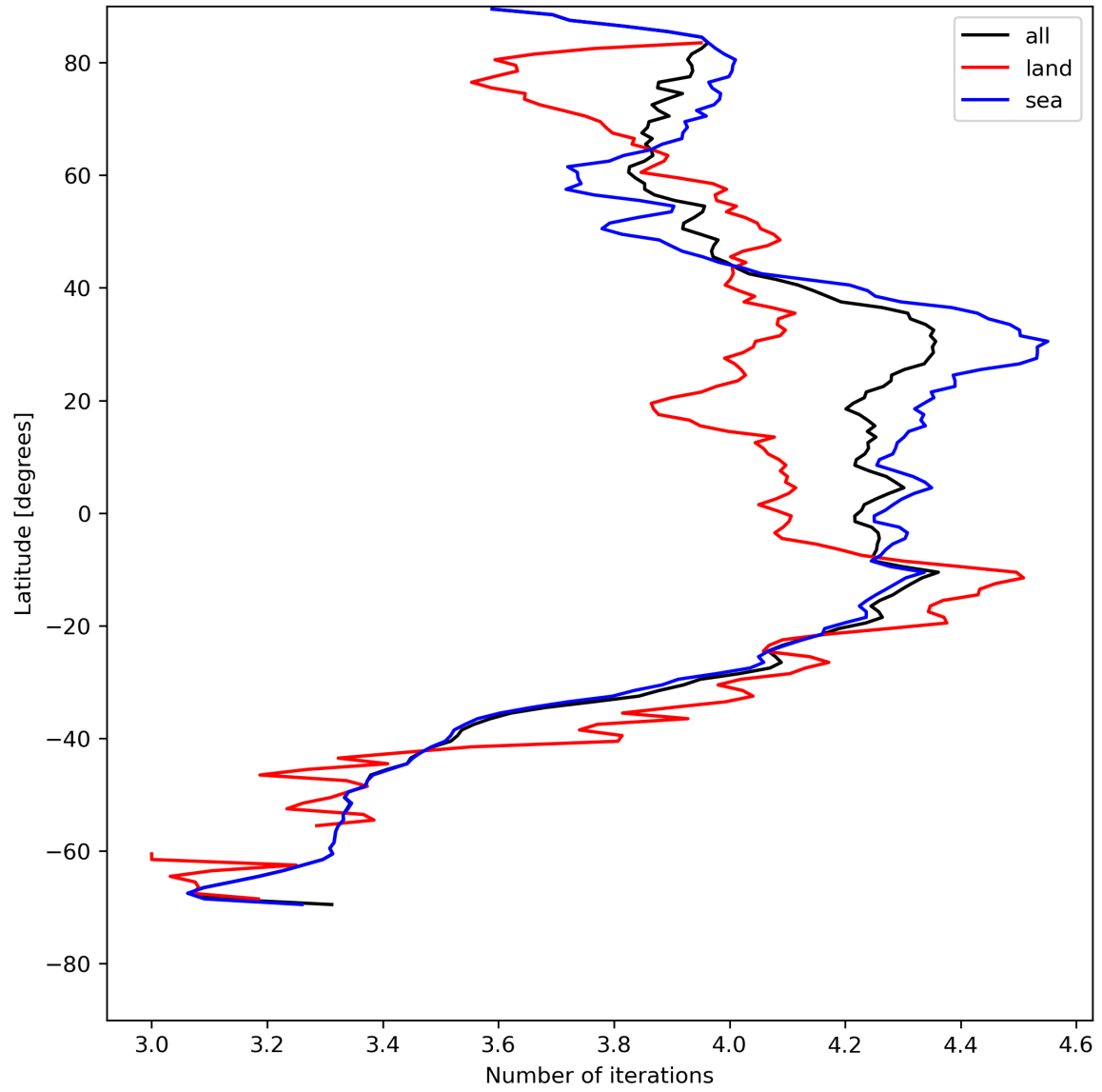
Figure 17: Zonal average of “Number of iterations” for 2023-07-29 to 2023-07-30.
