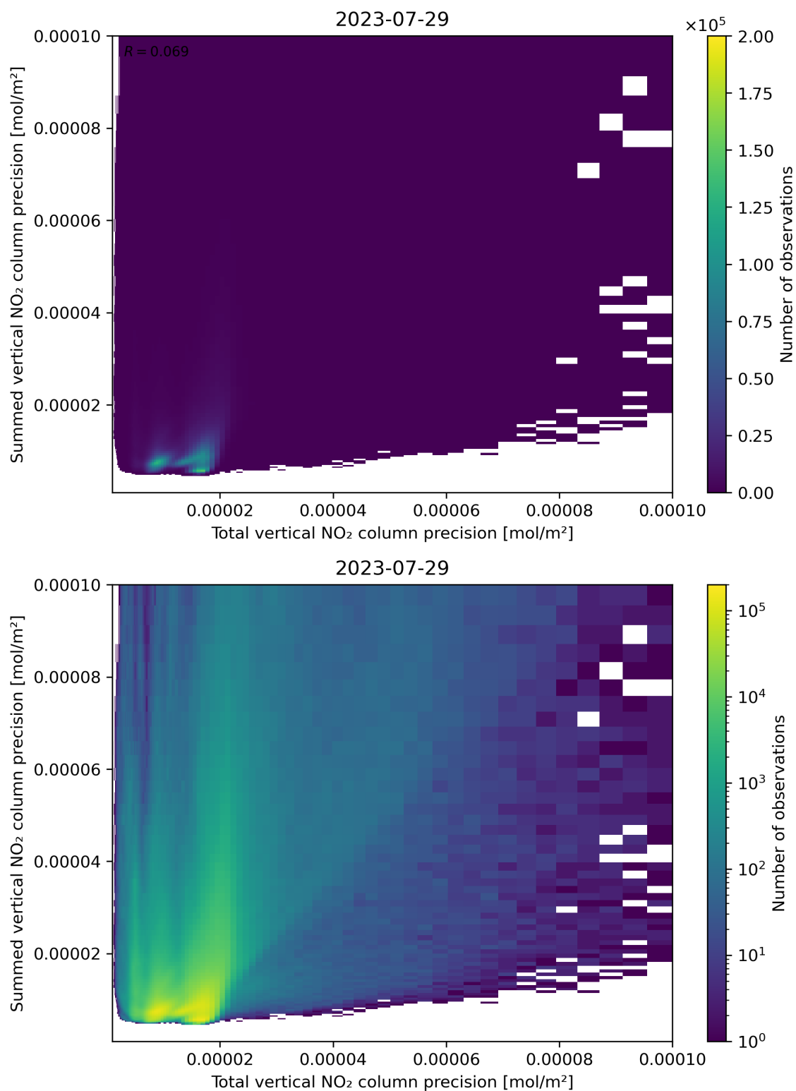
Figure 118: Scatter density plot of “Total vertical NO 2 column precision” against “Summed vertical NO 2 column precision” for 2023-07-29 to 2023-07-30.
