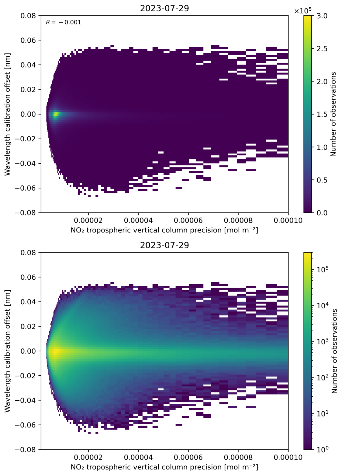
Figure 141: Scatter density plot of “NO 2 tropospheric vertical column precision” against “Wavelength calibration offset” for 2023-07-29 to 2023-07-30.
