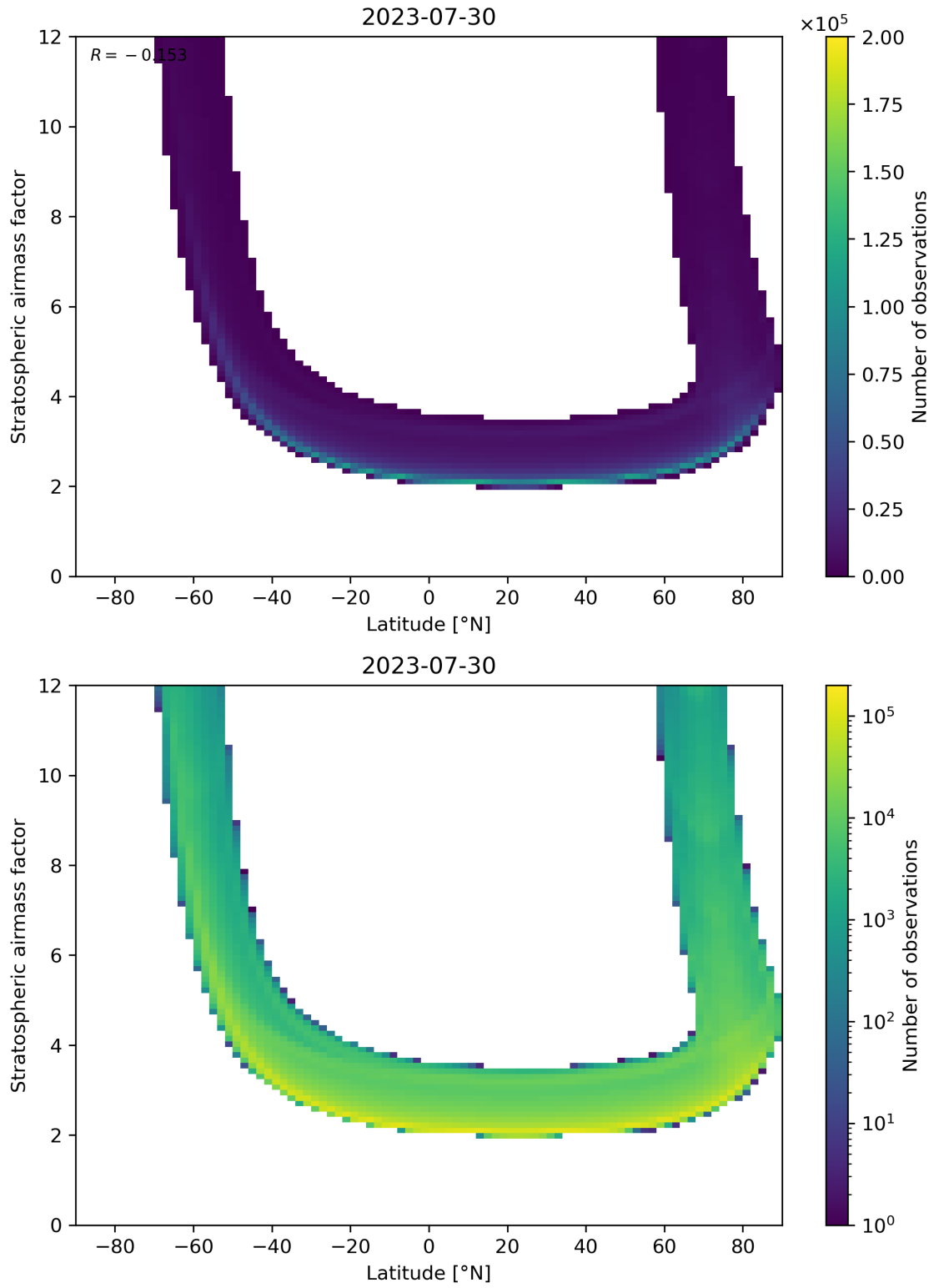
Figure 83: Scatter density plot of “Latitude” against “Stratospheric air mass factor” for 2023-07-29 to 2023-07-31.
