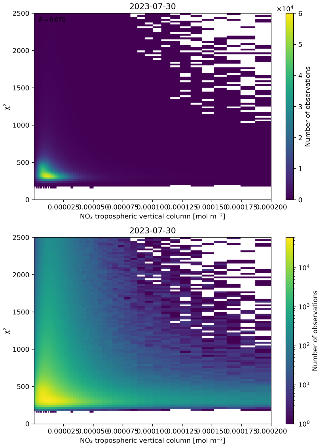
Figure 124: Scatter density plot of “NO 2 tropospheric vertical column” against “ \chi^2 ” for 2023-07-29 to 2023-07-31.
