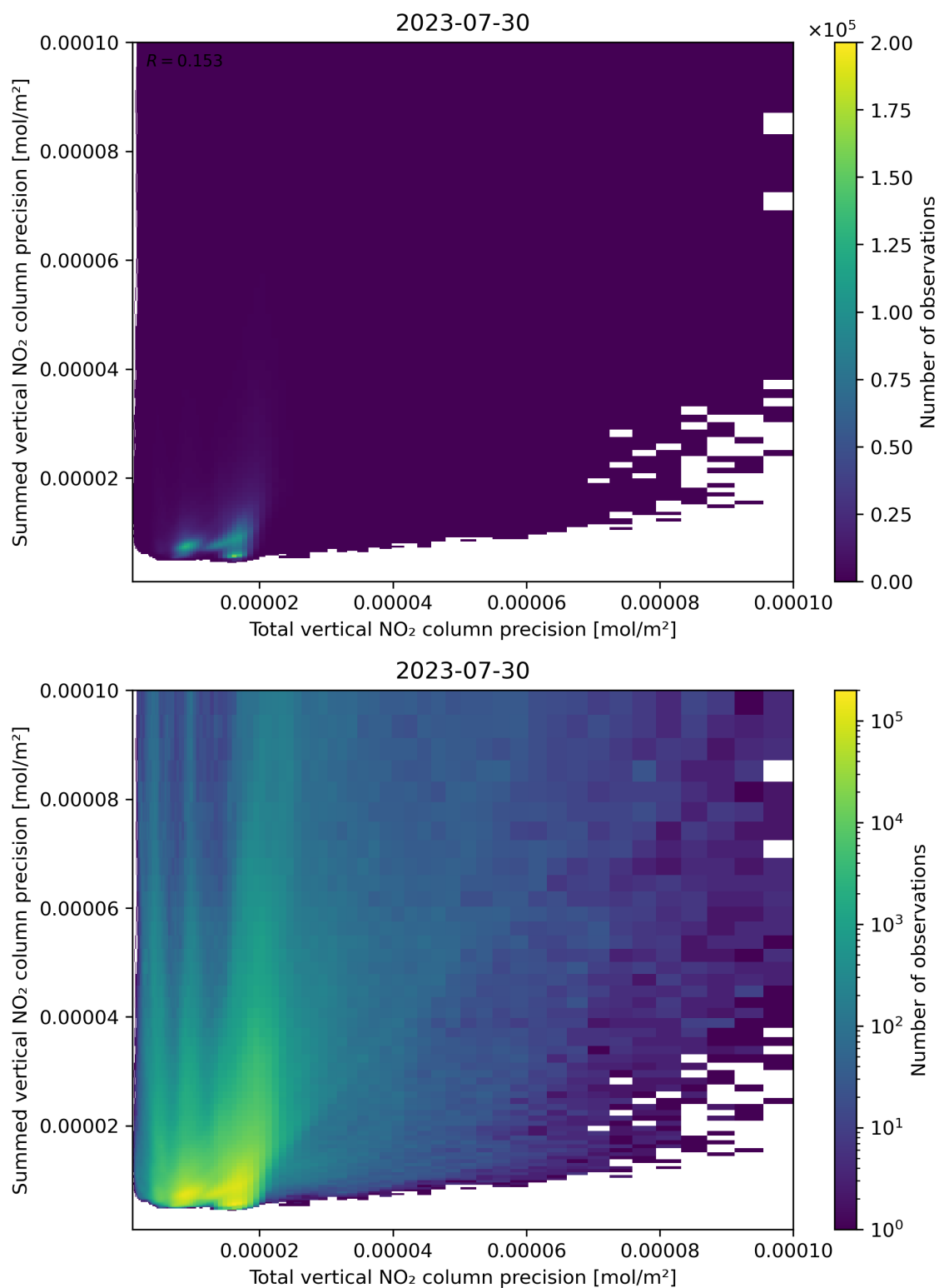
Figure 118: Scatter density plot of “Total vertical NO 2 column precision” against “Summed vertical NO 2 column precision” for 2023-07-29 to 2023-07-31.
