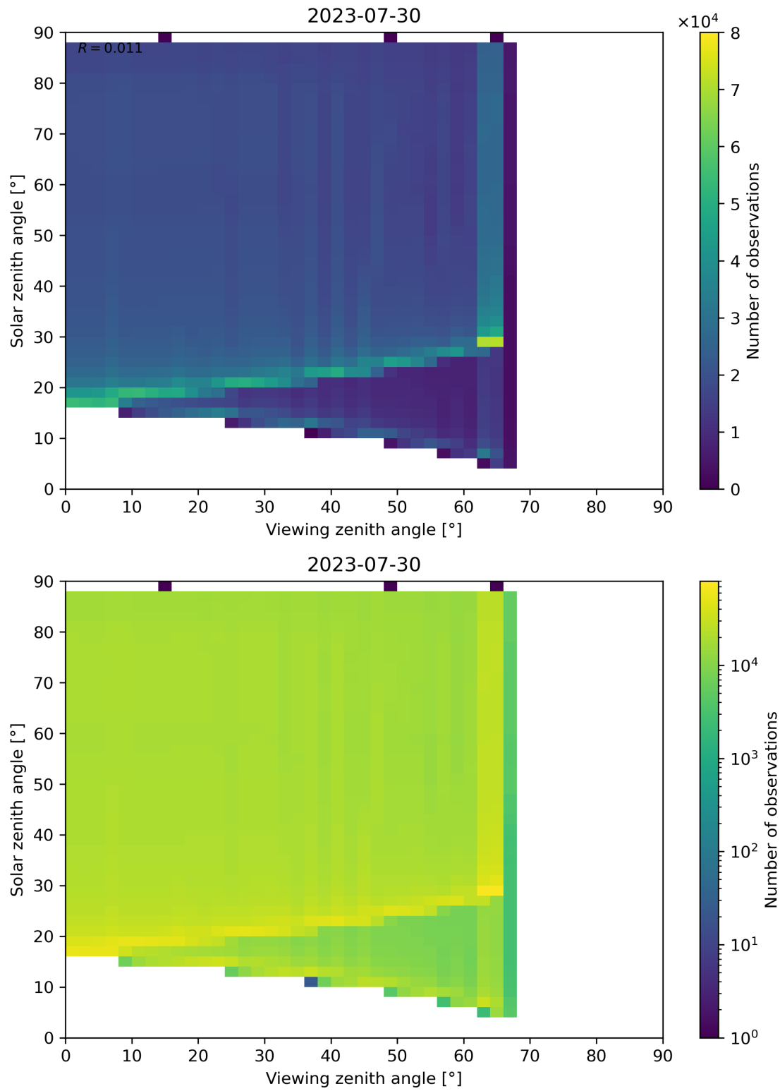
Figure 172: Scatter density plot of “Viewing zenith angle” against “Solar zenith angle” for 2023-07-29 to 2023-07-31.
