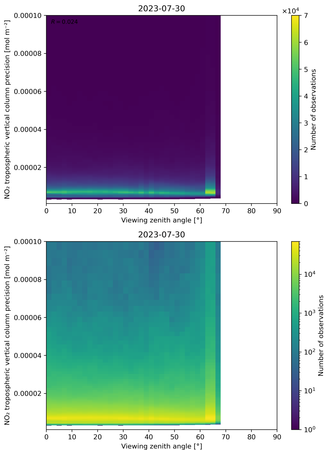
Figure 170: Scatter density plot of “Viewing zenith angle” against “NO 2 tropospheric vertical column precision” for 2023-07-29 to 2023-07-31.
