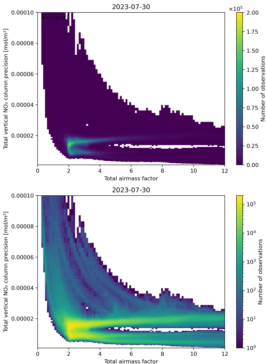
Figure 68: Scatter density plot of “Total airmass factor” against “Total vertical NO 2 column precision” for 2023-07-29 to 2023-07-31.
