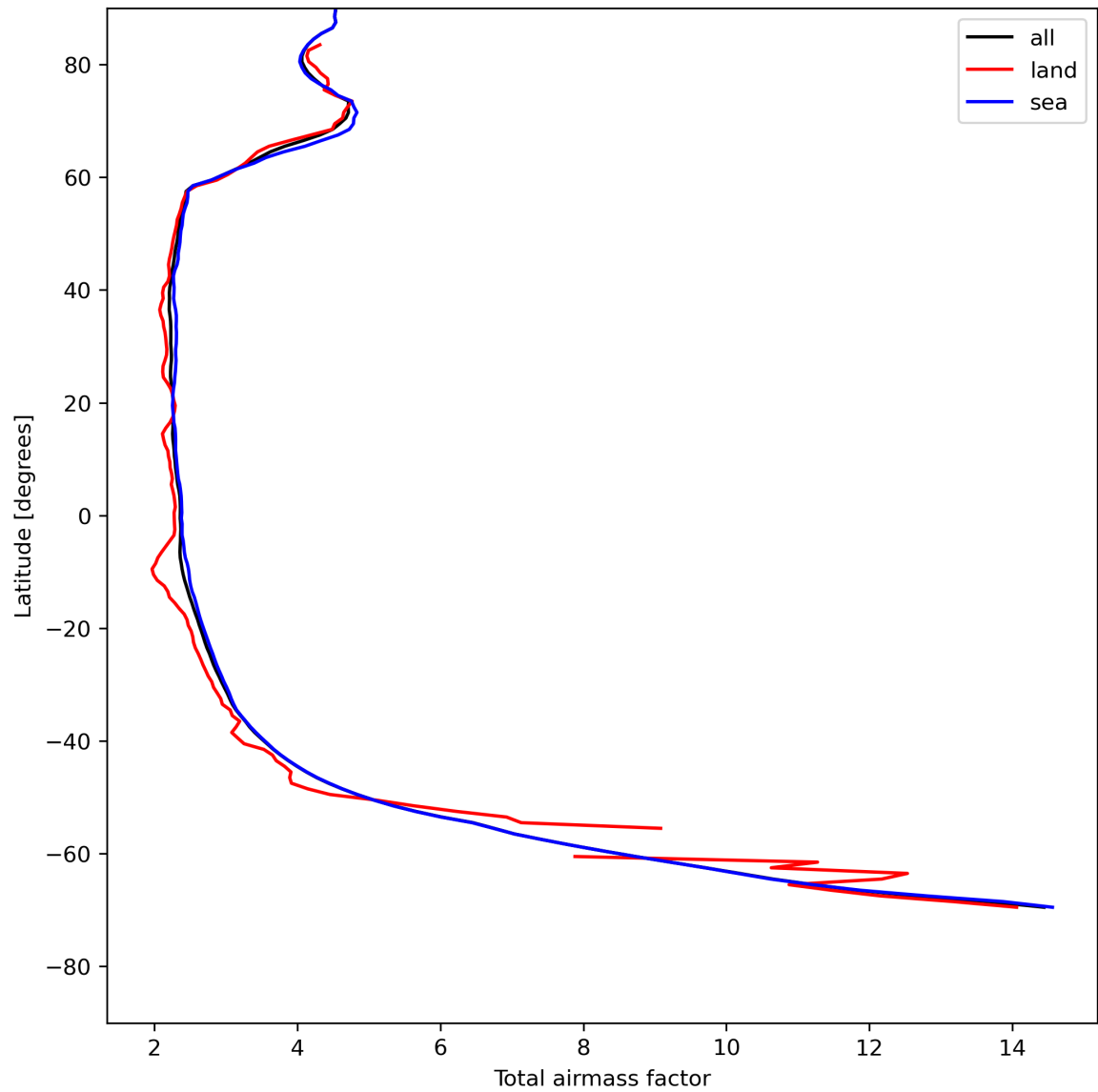
Figure 15: Zonal average of “Total airmass factor” for 2023-07-29 to 2023-07-31.
