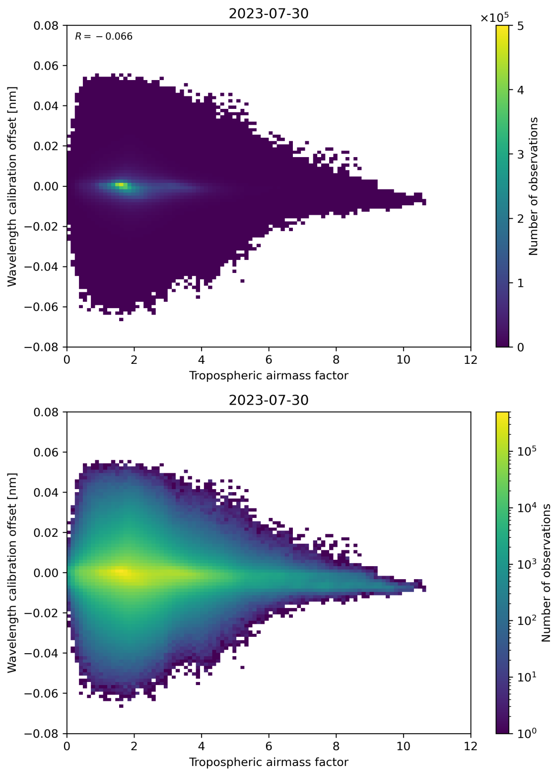
Figure 80: Scatter density plot of “Tropospheric airmass factor” against “Wavelength calibration offset” for 2023-07-29 to 2023-07-31.
