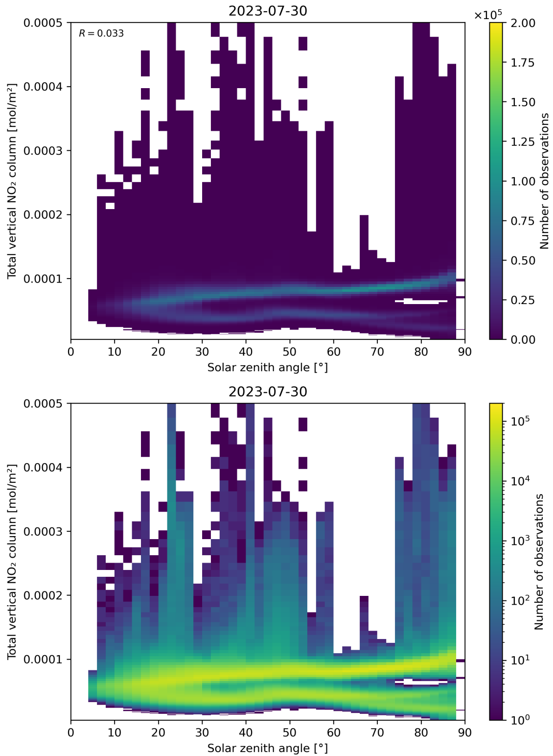
Figure 153: Scatter density plot of “Solar zenith angle” against “Total vertical \text{NO}_2 column” for 2023-07-29 to 2023-07-31.
