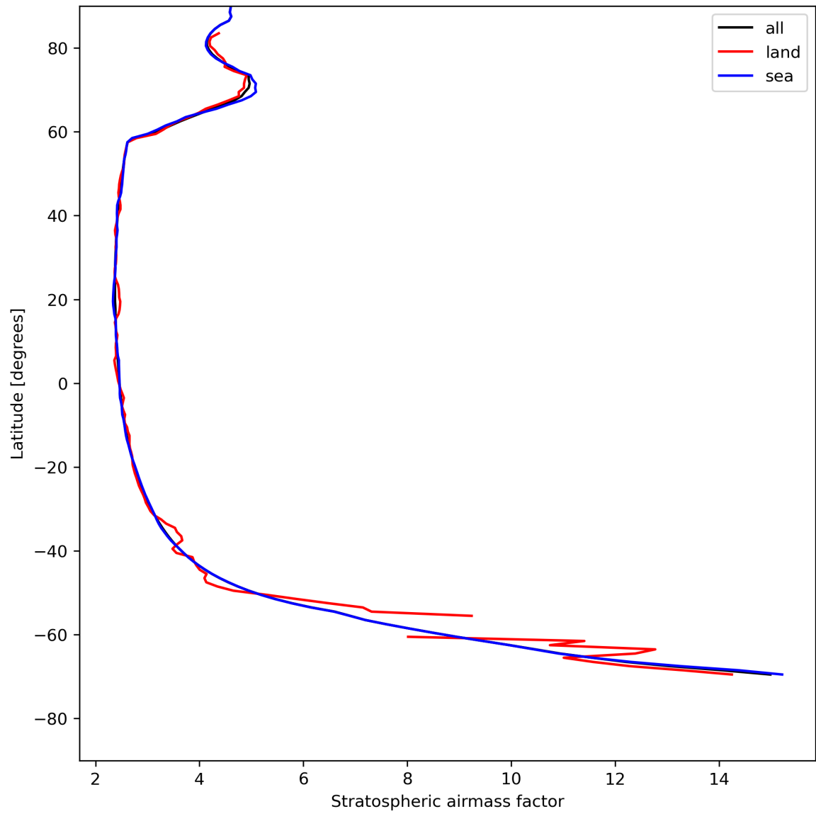
Figure 27: Zonal average of “Stratospheric air mass factor” for 2023-07-29 to 2023-07-31.
