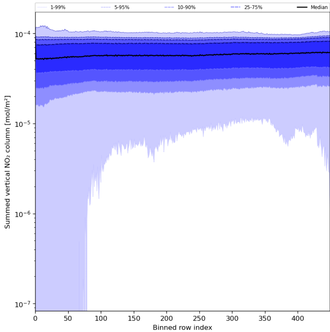
Figure 57: Along track statistics of “Summed vertical NO 2 column” for 2023-07-29 to 2023-07-31
