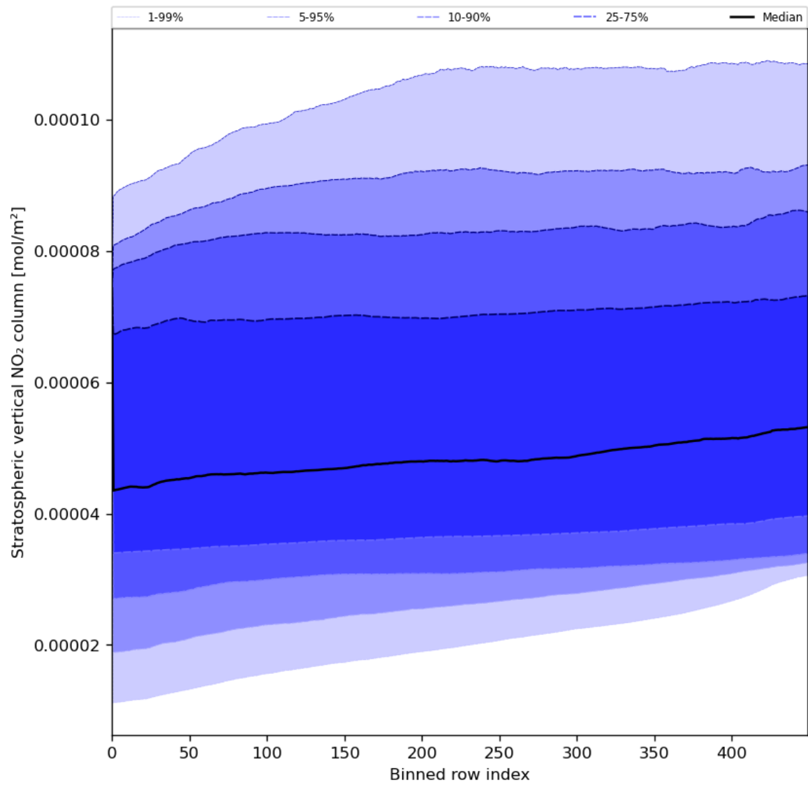
Figure 53: Along track statistics of “Stratospheric vertical NO 2 column” for 2023-07-29 to 2023-07-31
