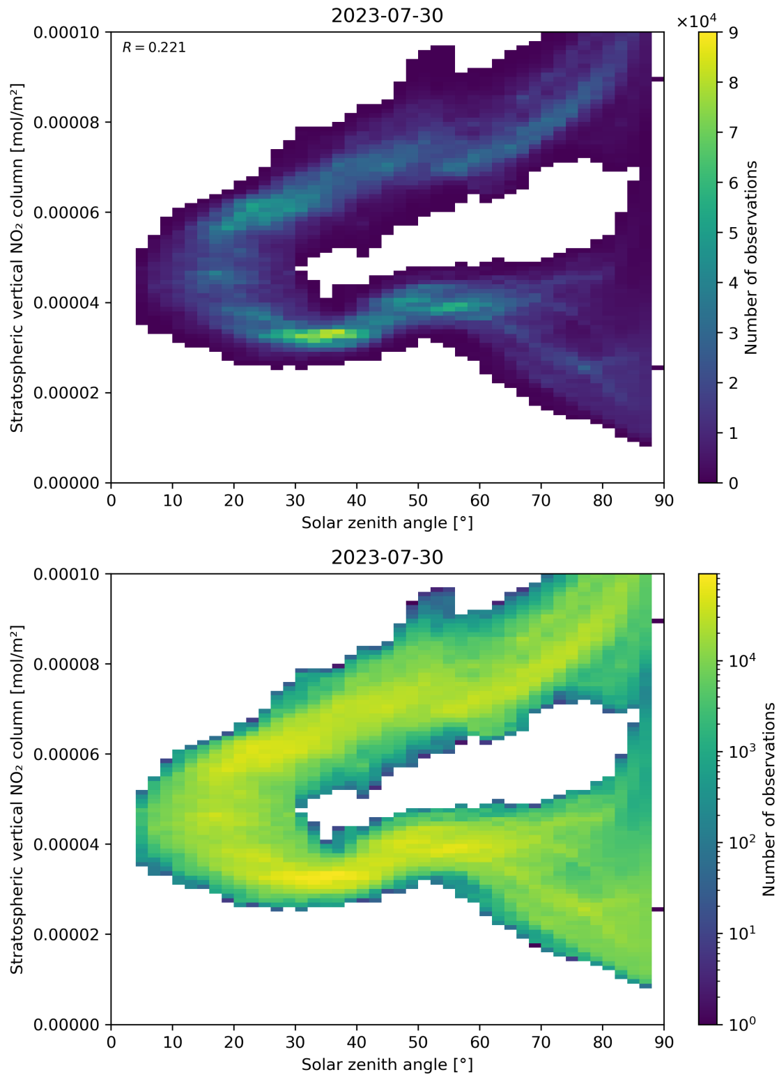
Figure 150: Scatter density plot of “Solar zenith angle” against “Stratospheric vertical NO 2 column” for 2023-07-29 to 2023-07-31.
