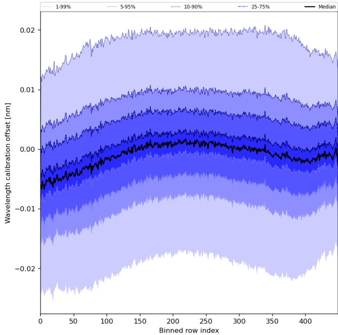
Figure 52: Along track statistics of “Wavelength calibration offset” for 2023-07-29 to 2023-07-31
