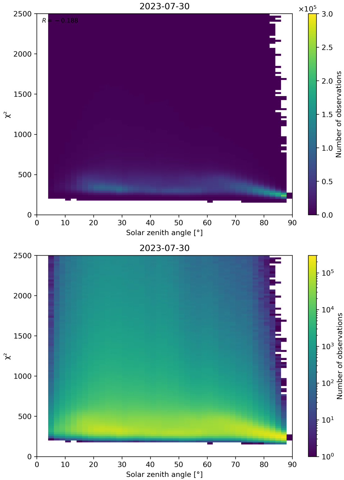
Figure 148: Scatter density plot of “Solar zenith angle” against “ \chi^2 ” for 2023-07-29 to 2023-07-31.
