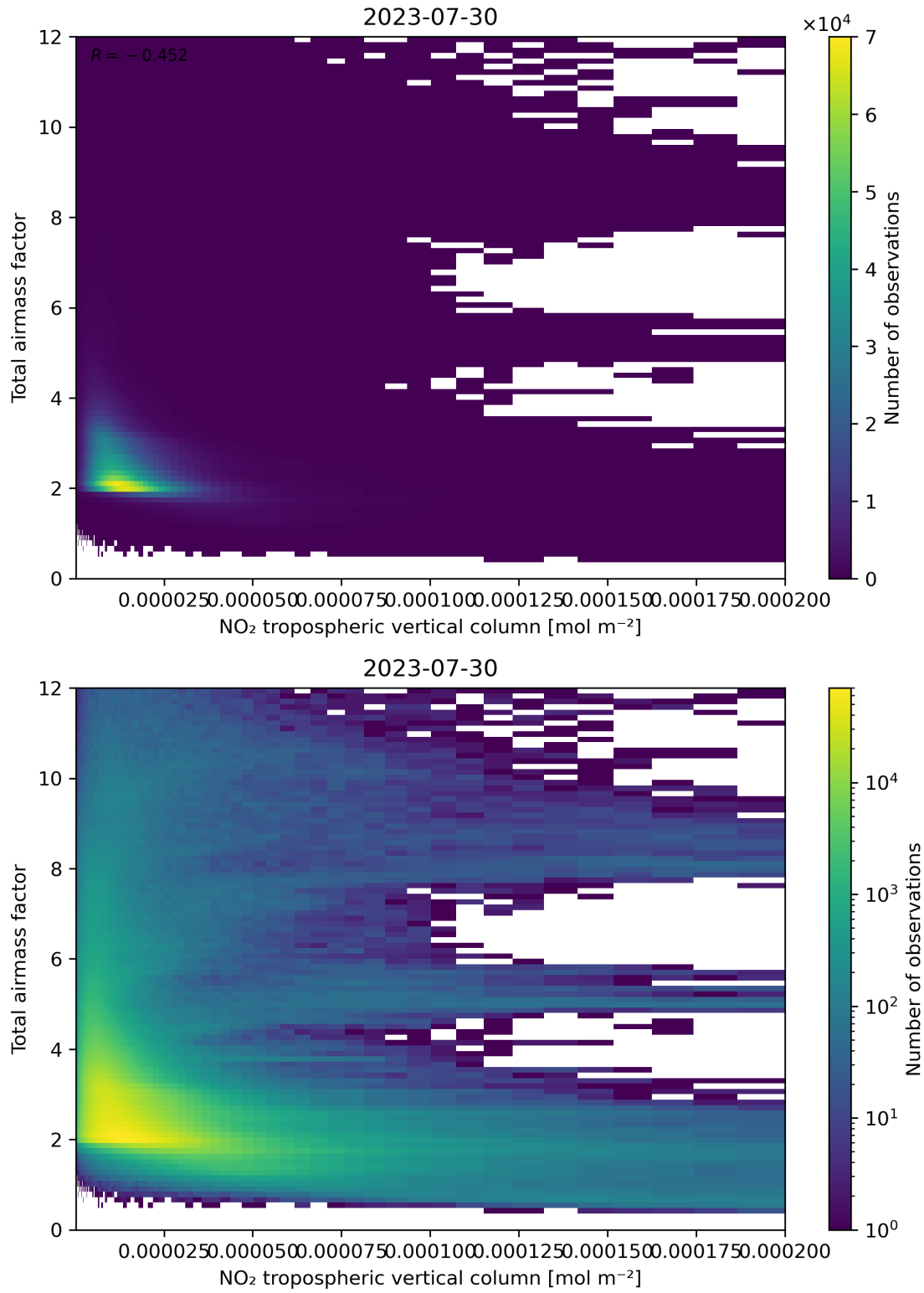
Figure 122: Scatter density plot of “NO 2 tropospheric vertical column” against “Total air mass factor” for 2023-07-29 to 2023-07-31.
