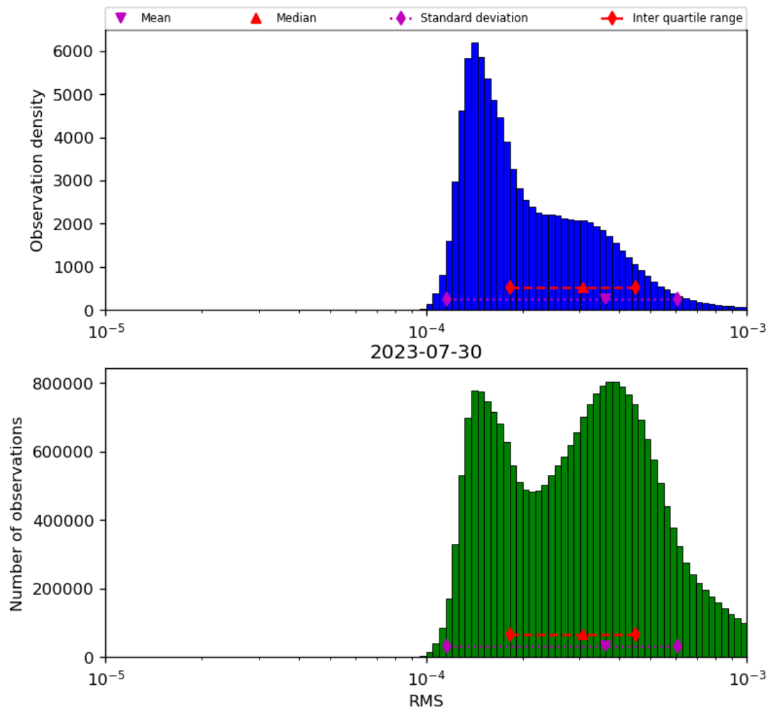
Figure 43: Histogram of “RMS” for 2023-07-29 to 2023-07-31
