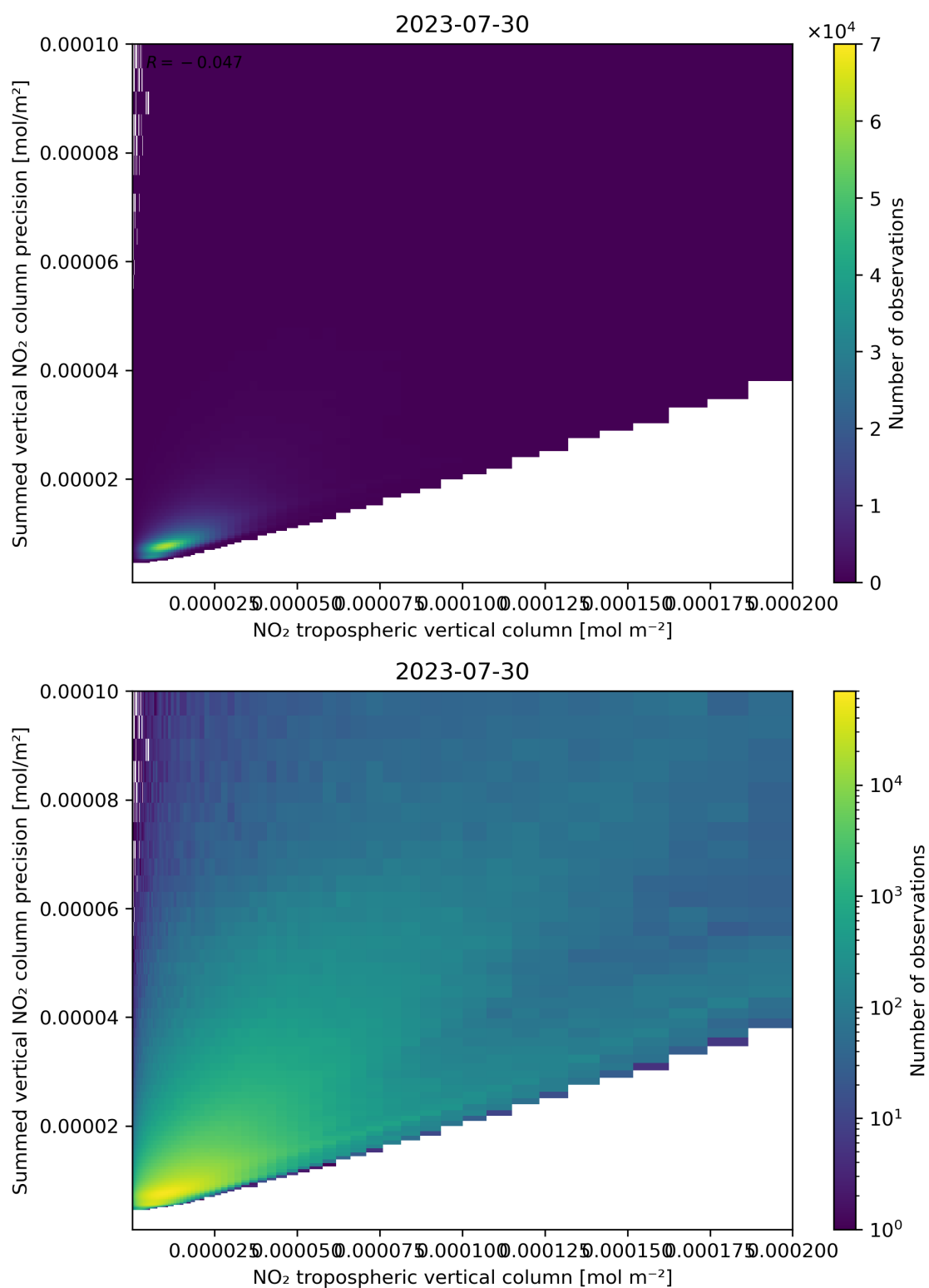
Figure 127: Scatter density plot of “NO 2 tropospheric vertical column” against “Summed vertical NO 2 column precision” for 2023-07-29 to 2023-07-31.
