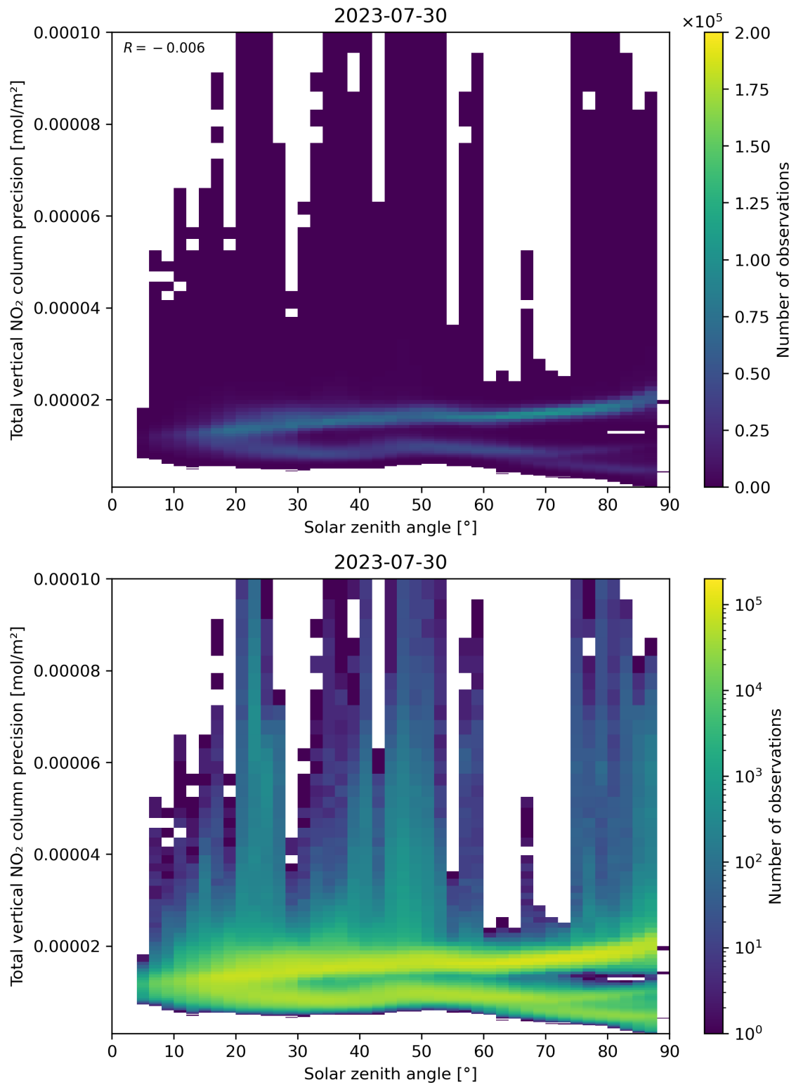
Figure 154: Scatter density plot of “Solar zenith angle” against “Total vertical NO 2 column precision” for 2023-07-29 to 2023-07-31.
