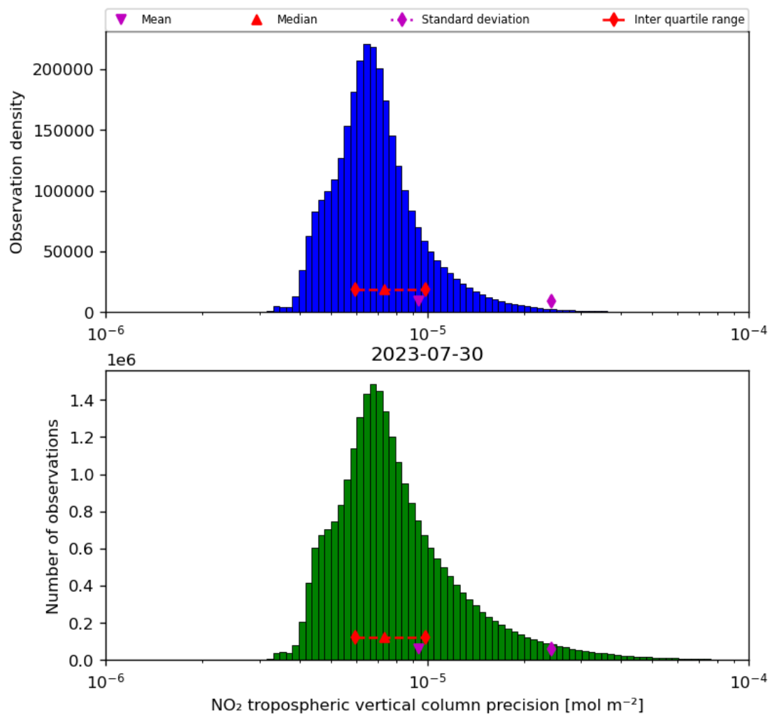
Figure 30: Histogram of “NO 2 tropospheric vertical column precision” for 2023-07-29 to 2023-07-31
