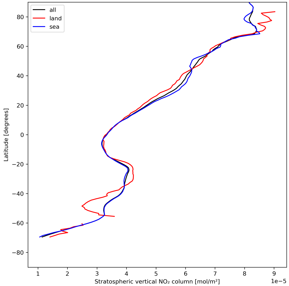
Figure 19: Zonal average of “Stratospheric vertical NO 2 column” for 2023-07-29 to 2023-07-31.
