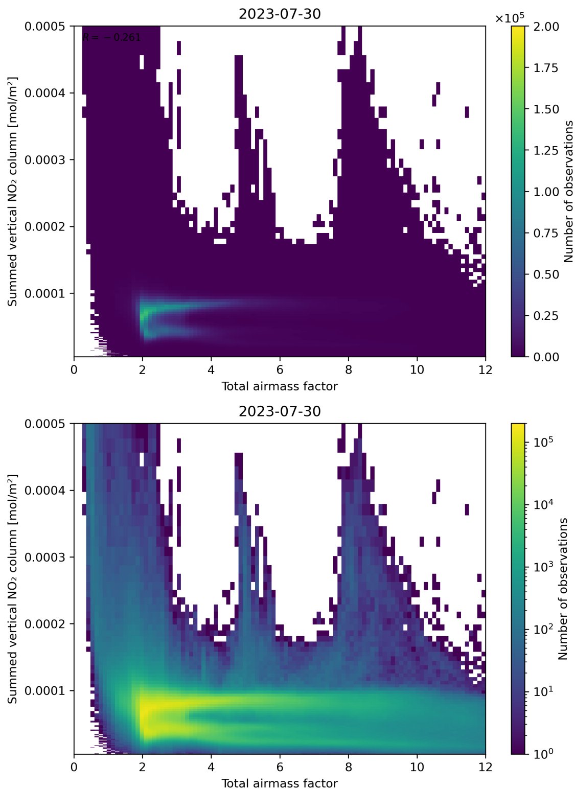
Figure 65: Scatter density plot of “Total airmass factor” against “Summed vertical NO 2 column” for 2023-07-29 to 2023-07-31.
