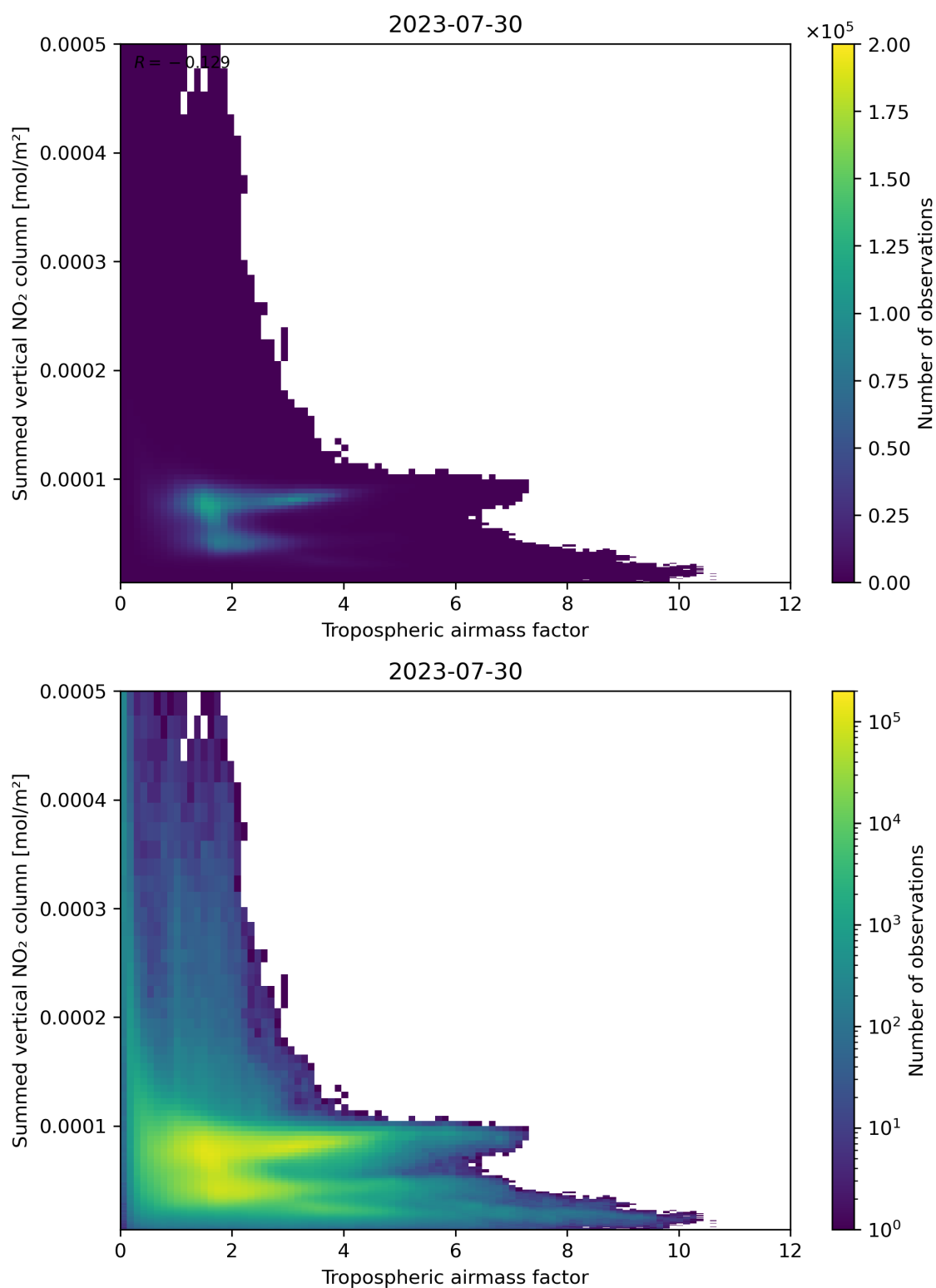
Figure 75: Scatter density plot of “Tropospheric airmass factor” against “Summed vertical NO 2 column” for 2023-07-29 to 2023-07-31.
