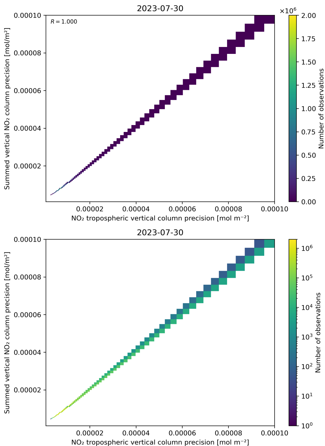
Figure 137: Scatter density plot of “NO 2 tropospheric vertical column precision” against “Summed vertical NO 2 column precision” for 2023-07-29 to 2023-07-31.
