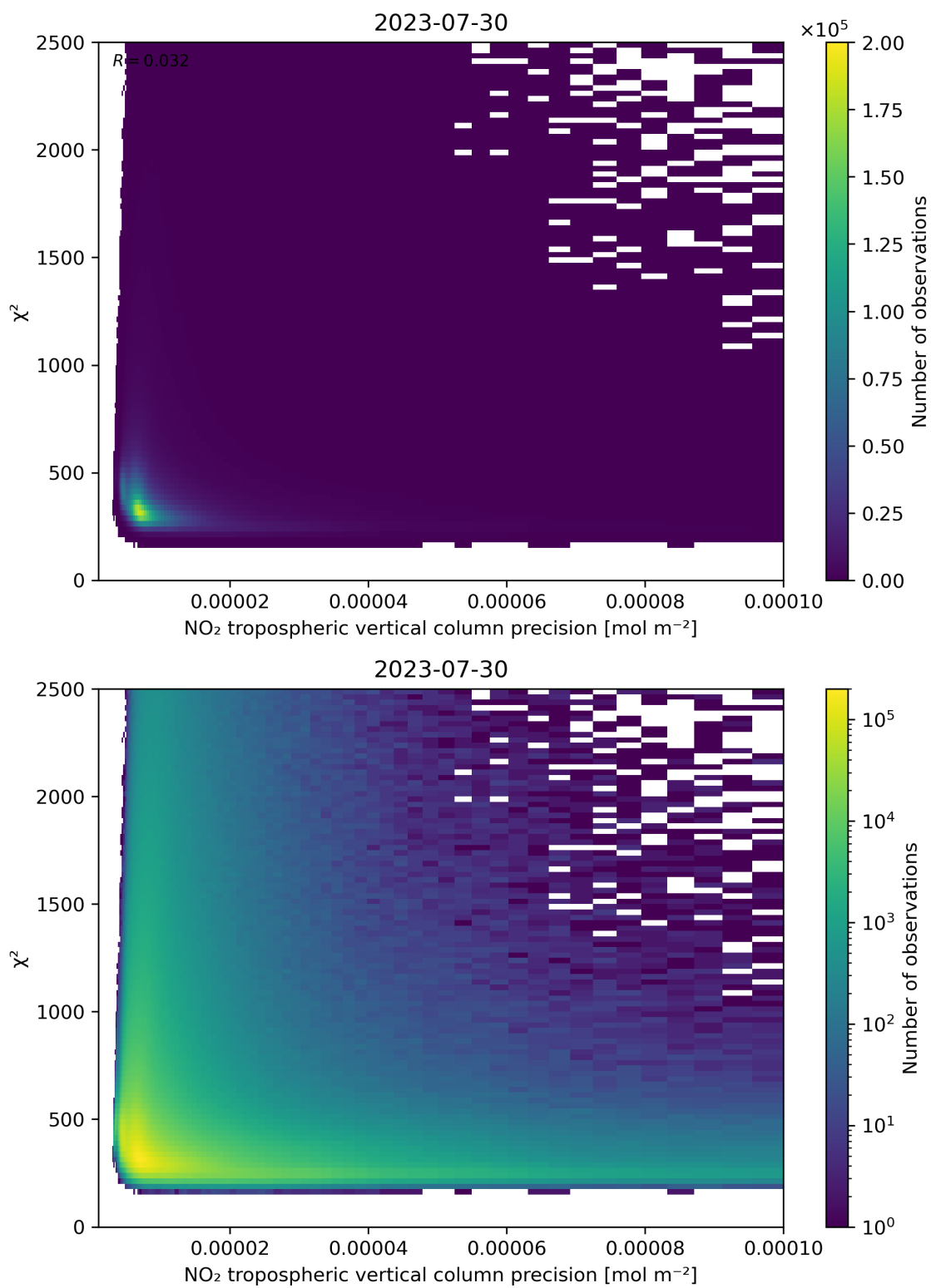
Figure 134: Scatter density plot of “NO 2 tropospheric vertical column precision” against “ \chi^2 ” for 2023-07-29 to 2023-07-31.
