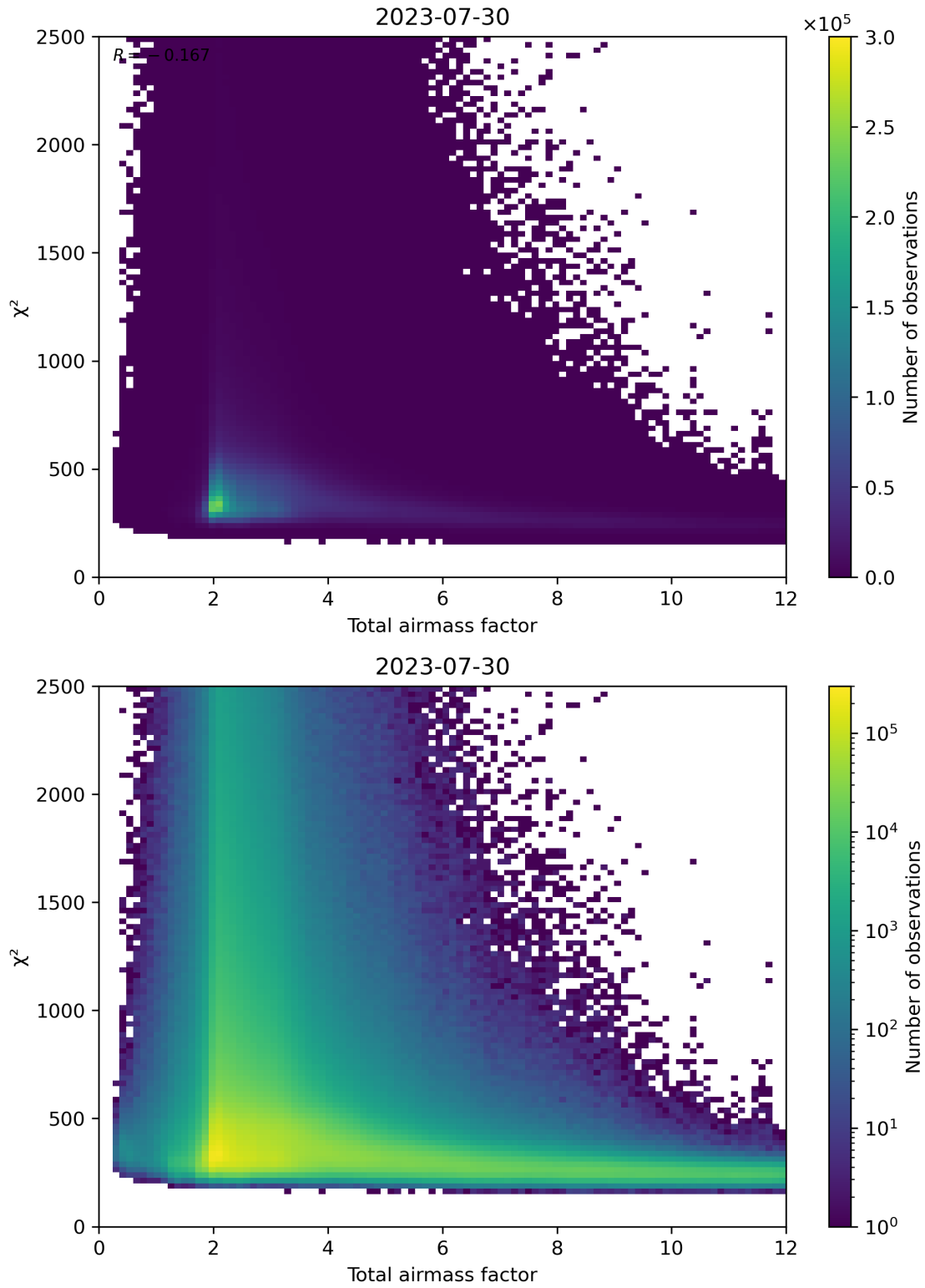
Figure 63: Scatter density plot of “Total airmass factor” against “ \chi^2 ” for 2023-07-29 to 2023-07-31.
