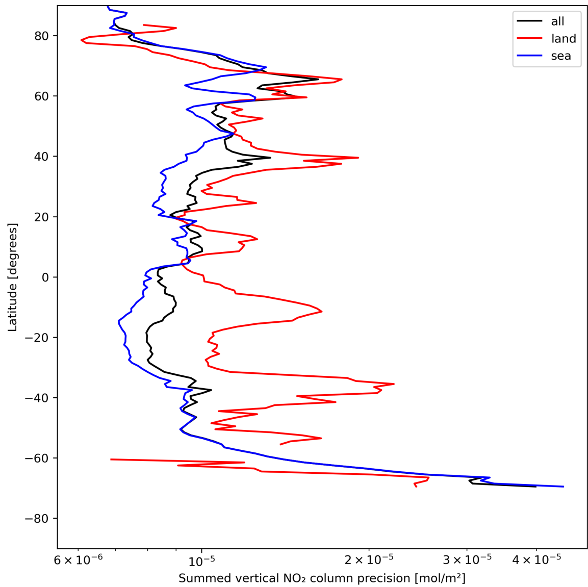
Figure 24: Zonal average of “Summed vertical NO 2 column precision” for 2023-07-29 to 2023-07-31.
