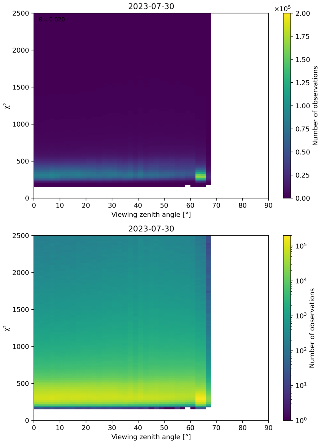
Figure 162: Scatter density plot of “Viewing zenith angle” against “ \chi^2 ” for 2023-07-29 to 2023-07-31.
