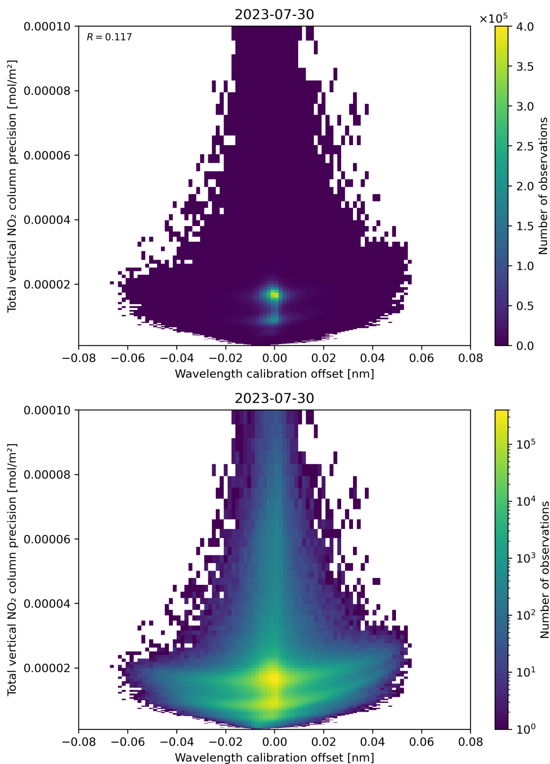
Figure 180: Scatter density plot of “Wavelength calibration offset” against “Total vertical NO 2 column precision” for 2023-07-29 to 2023-07-31.
