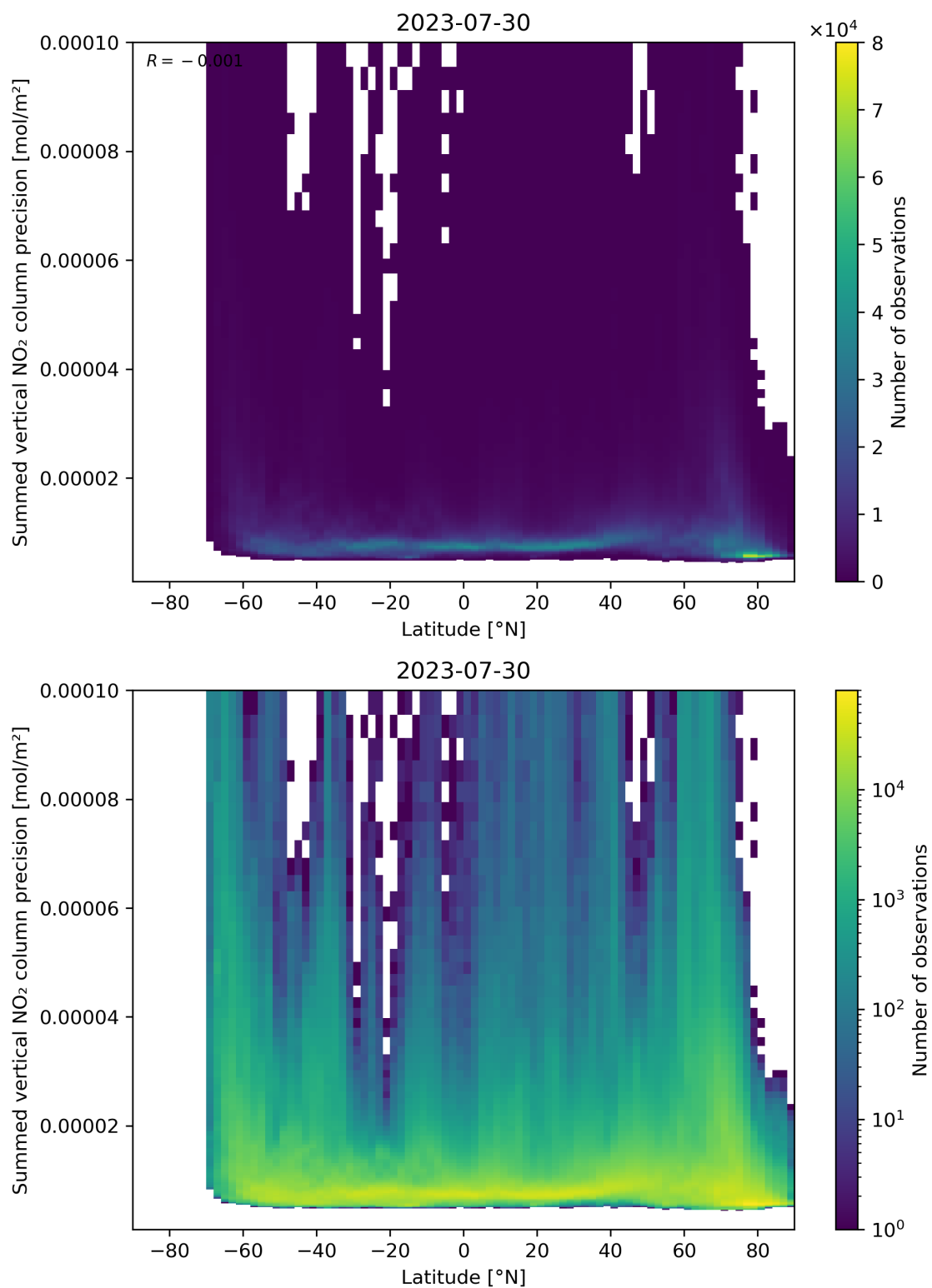
Figure 89: Scatter density plot of “Latitude” against “Summed vertical NO 2 column precision” for 2023-07-29 to 2023-07-31.
