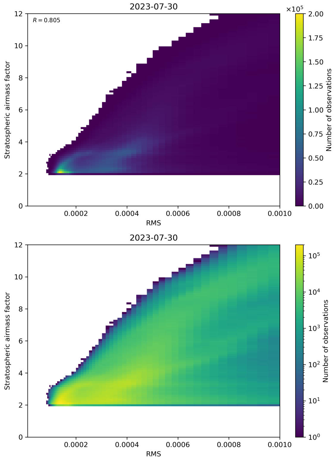
Figure 144: Scatter density plot of “RMS” against “Stratospheric airmass factor” for 2023-07-29 to 2023-07-31.
