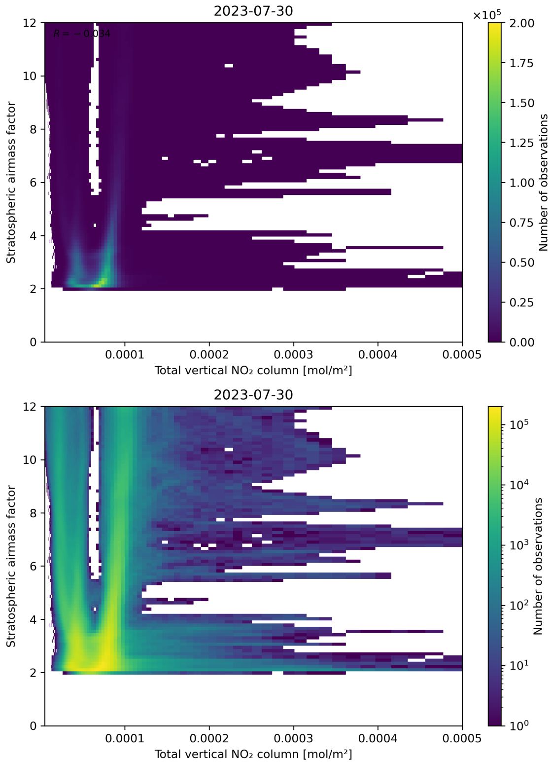
Figure 110: Scatter density plot of “Total vertical NO 2 column” against “Stratospheric airmass factor” for 2023-07-29 to 2023-07-31.
