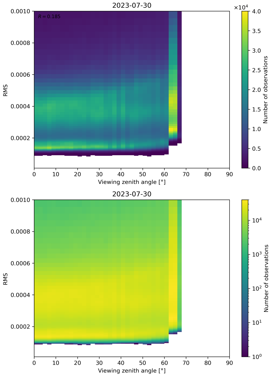
Figure 171: Scatter density plot of “Viewing zenith angle” against “RMS” for 2023-07-29 to 2023-07-31.
