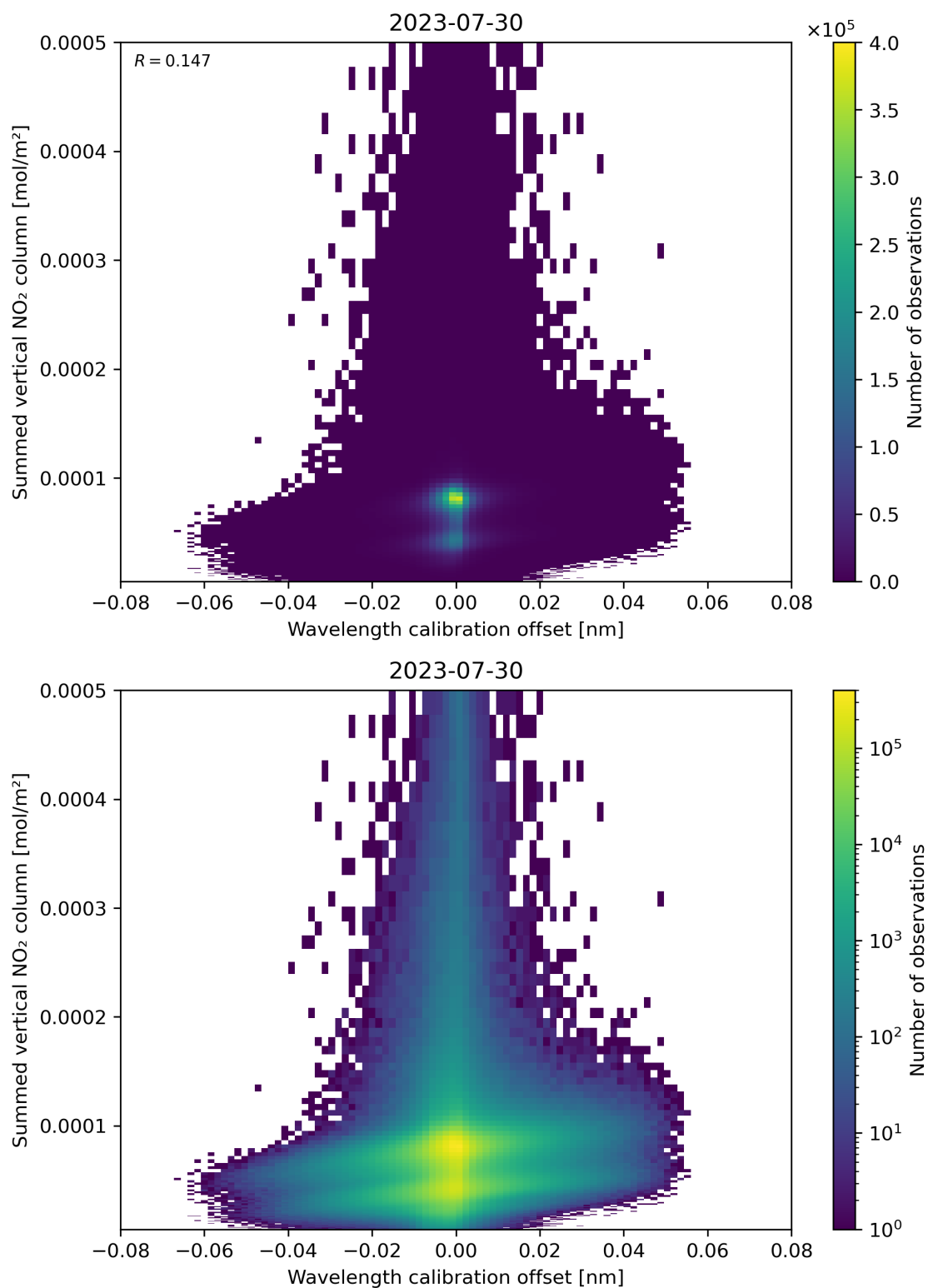
Figure 177: Scatter density plot of “Wavelength calibration offset” against “Summed vertical NO 2 column” for 2023-07-29 to 2023-07-31.
