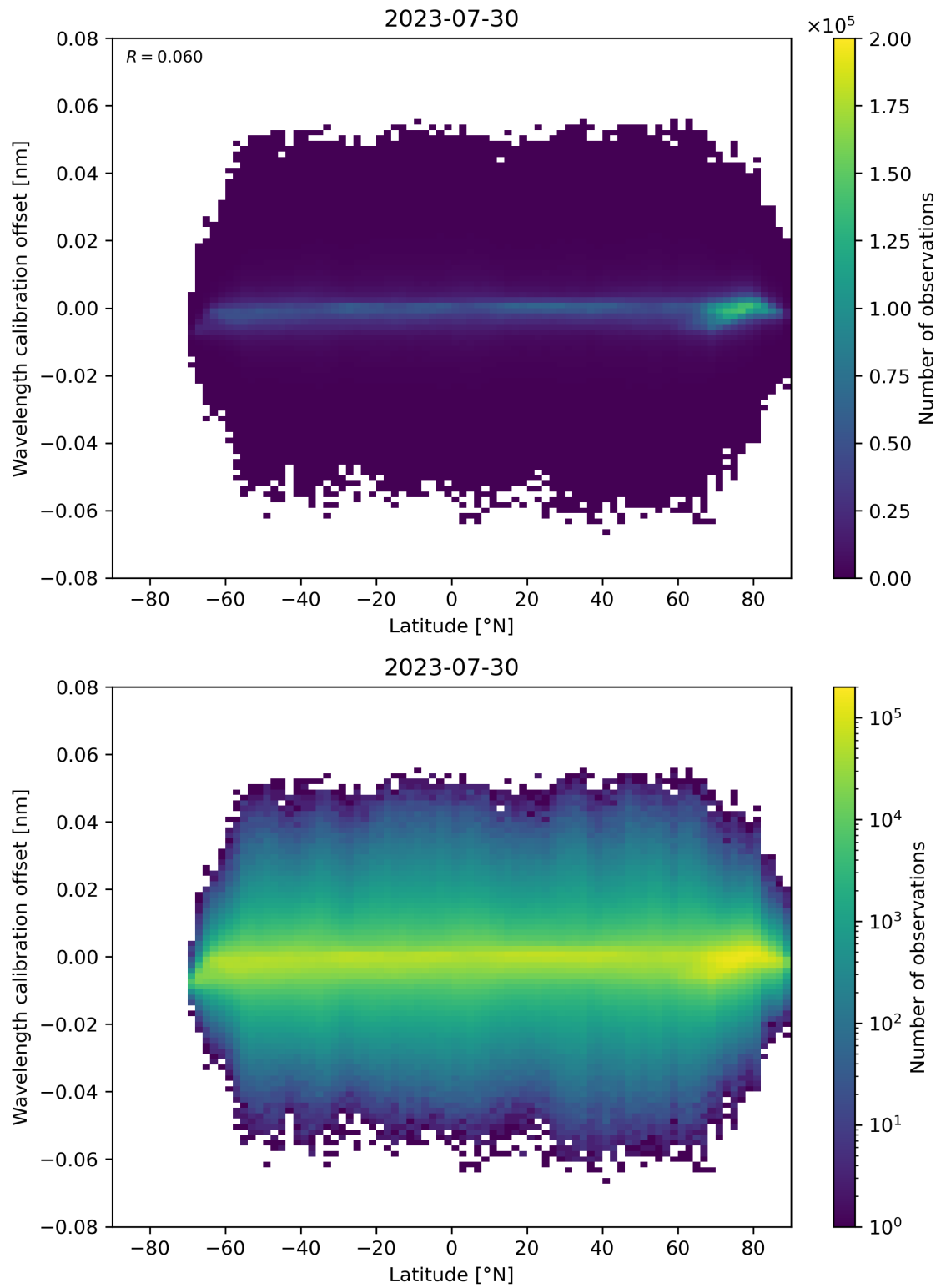
Figure 95: Scatter density plot of “Latitude” against “Wavelength calibration offset” for 2023-07-29 to 2023-07-31.
