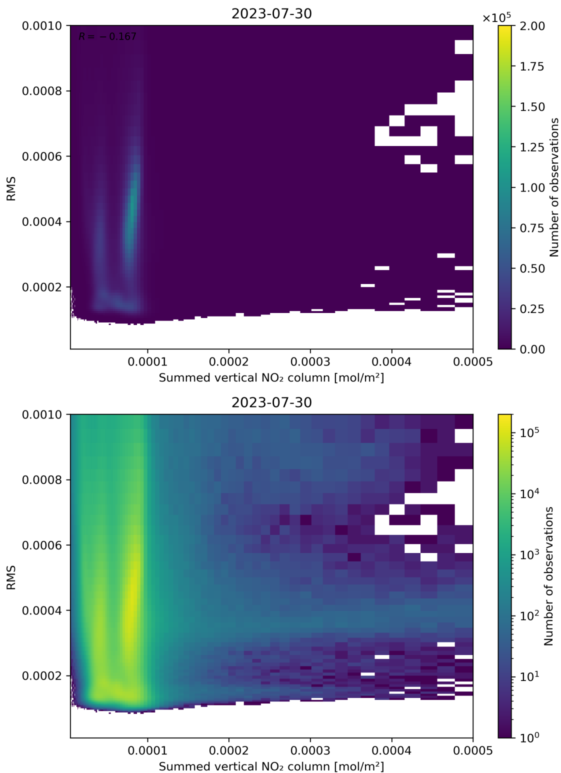
Figure 109: Scatter density plot of “Summed vertical NO 2 column” against “RMS” for 2023-07-29 to 2023-07-31.
