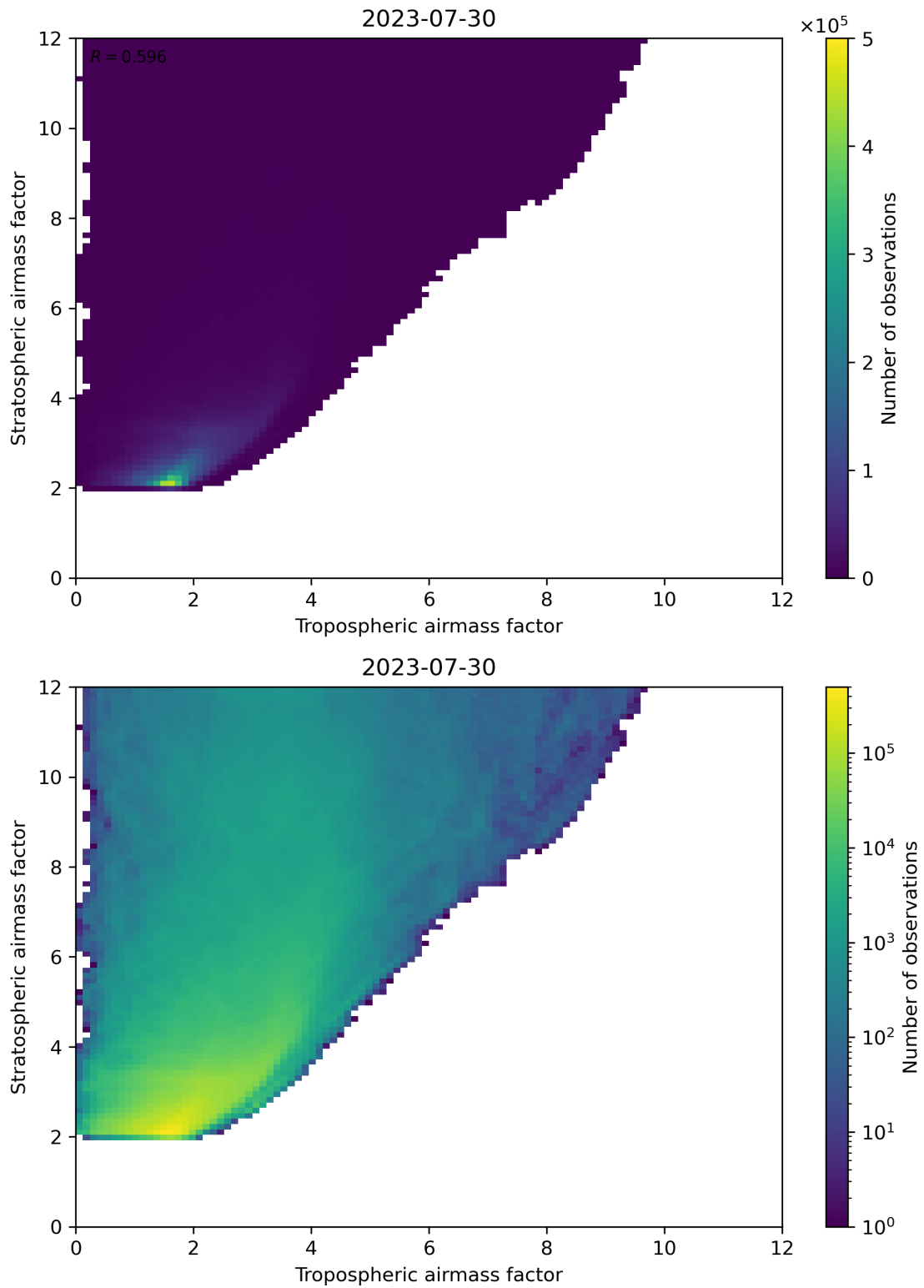
Figure 71: Scatter density plot of “Tropospheric airmass factor” against “Stratospheric airmass factor” for 2023-07-29 to 2023-07-31.
