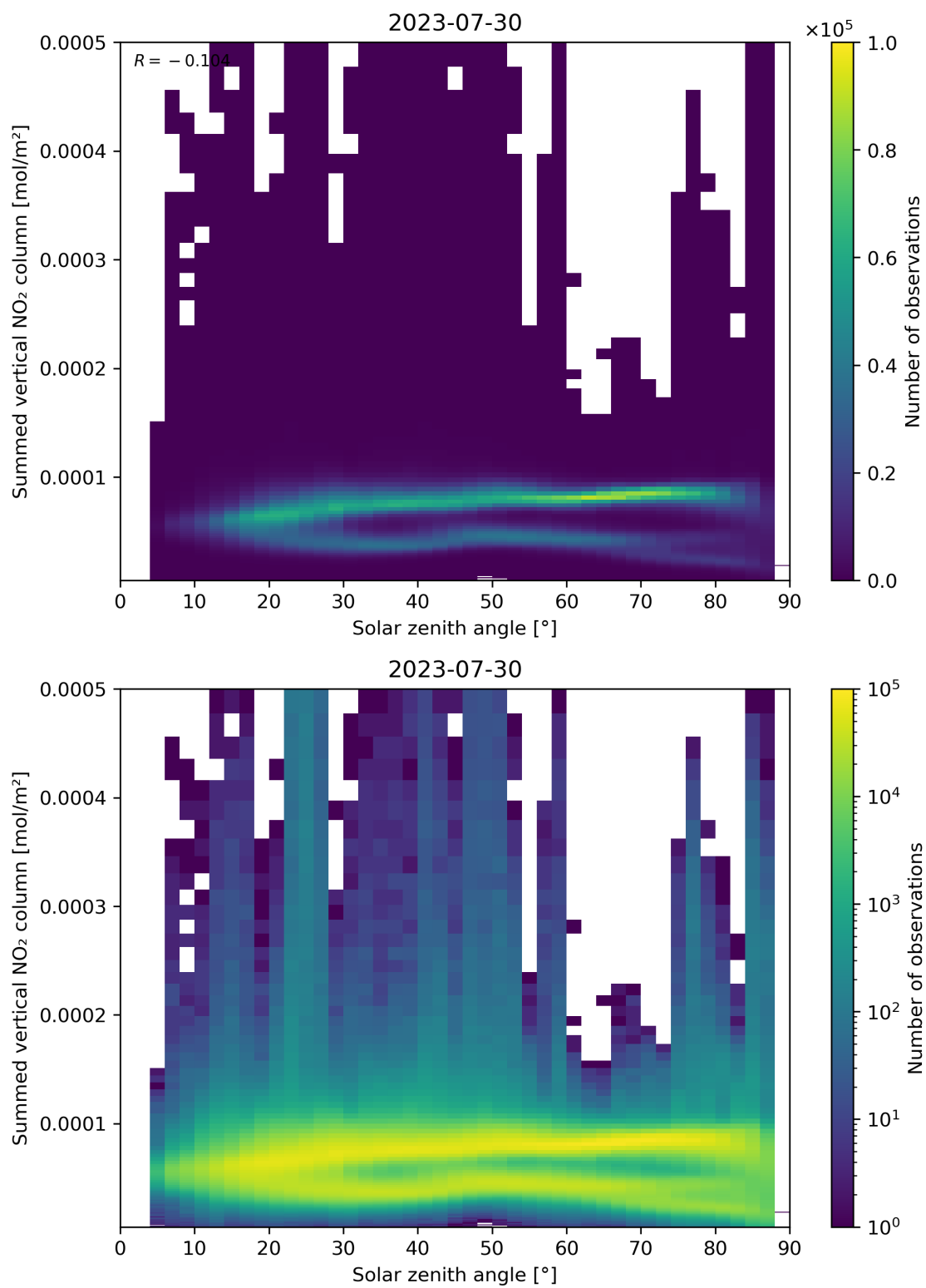
Figure 151: Scatter density plot of “Solar zenith angle” against “Summed vertical NO 2 column” for 2023-07-29 to 2023-07-31.
