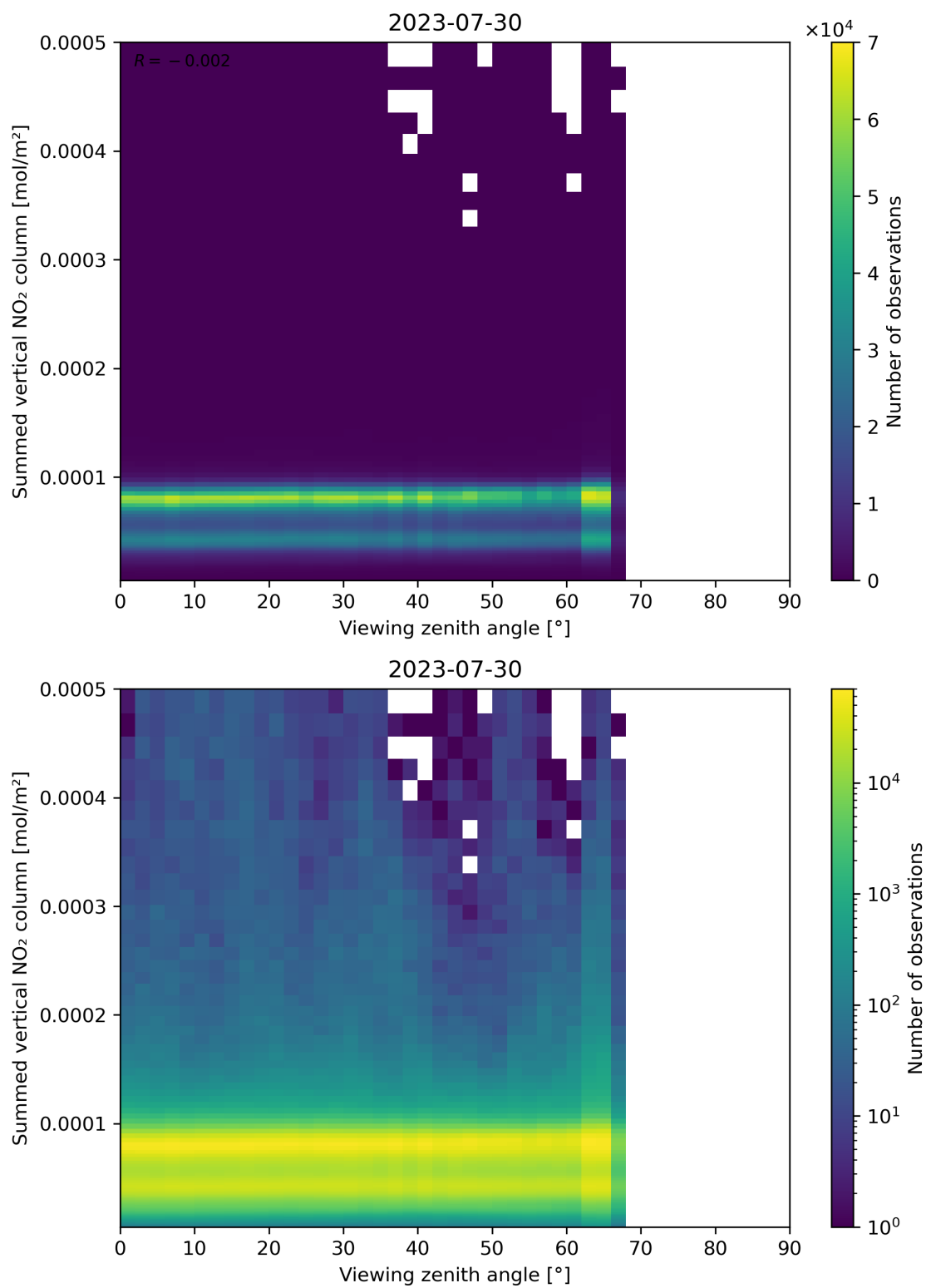
Figure 165: Scatter density plot of “Viewing zenith angle” against “Summed vertical NO 2 column” for 2023-07-29 to 2023-07-31.
