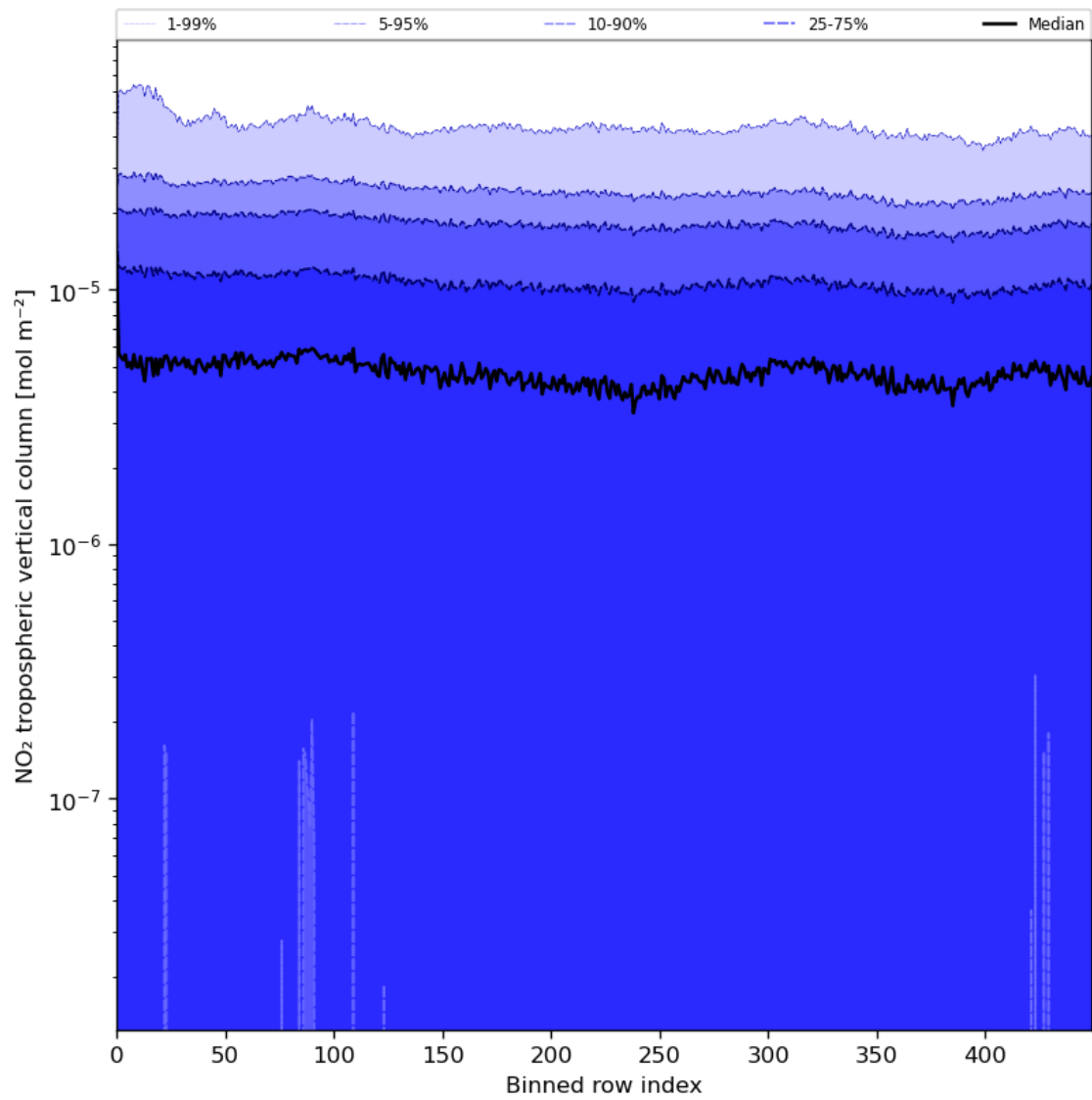
Figure 46: Along track statistics of “NO 2 tropospheric vertical column” for 2023-07-29 to 2023-07-31
