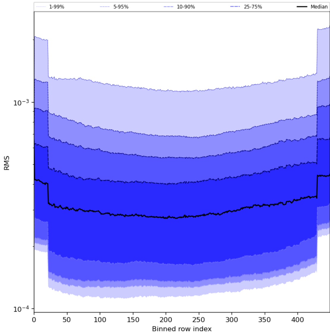
Figure 60: Along track statistics of “RMS” for 2023-07-29 to 2023-07-31
