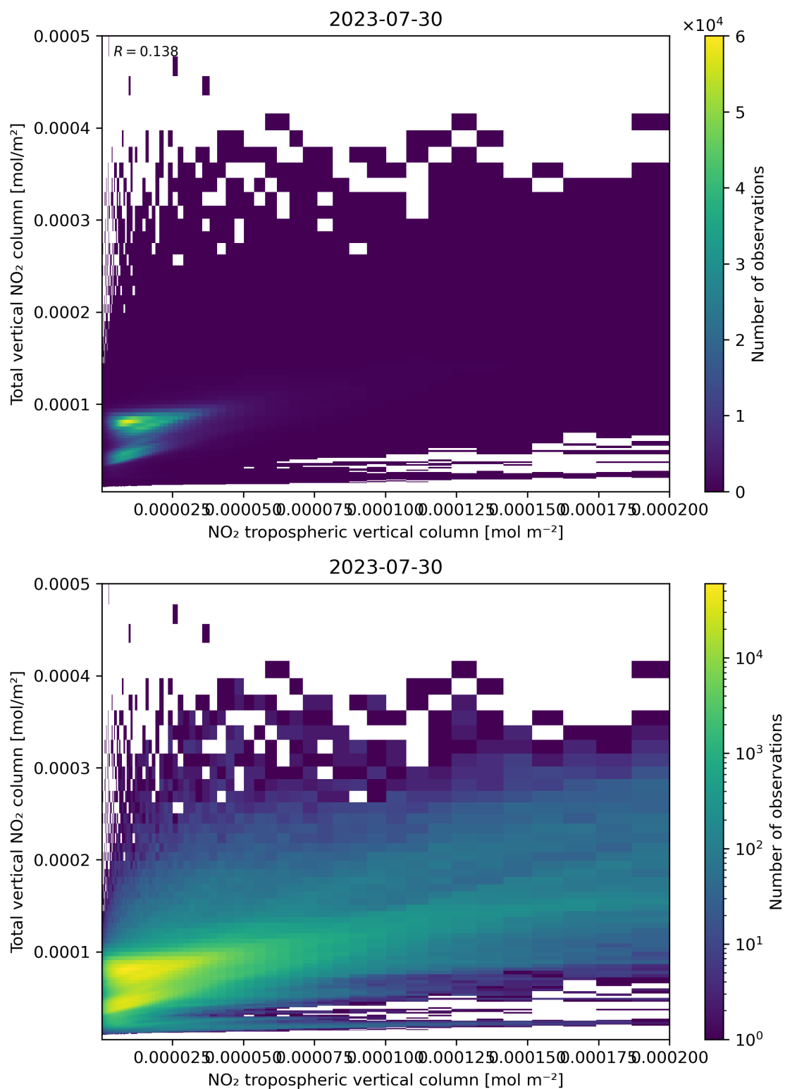
Figure 128: Scatter density plot of “NO 2 tropospheric vertical column” against “Total vertical NO 2 column” for 2023-07-29 to 2023-07-31.
