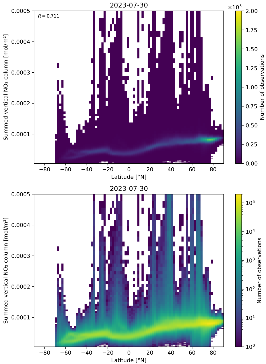
Figure 88: Scatter density plot of “Latitude” against “Summed vertical NO 2 column” for 2023-07-29 to 2023-07-31.
