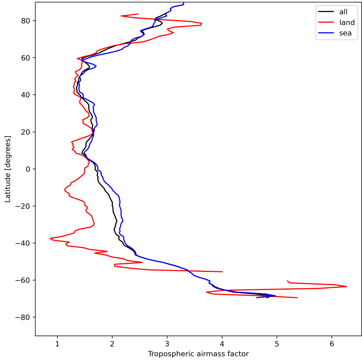
Figure 14: Zonal average of “Tropospheric airmass factor” for 2023-07-29 to 2023-07-31.
