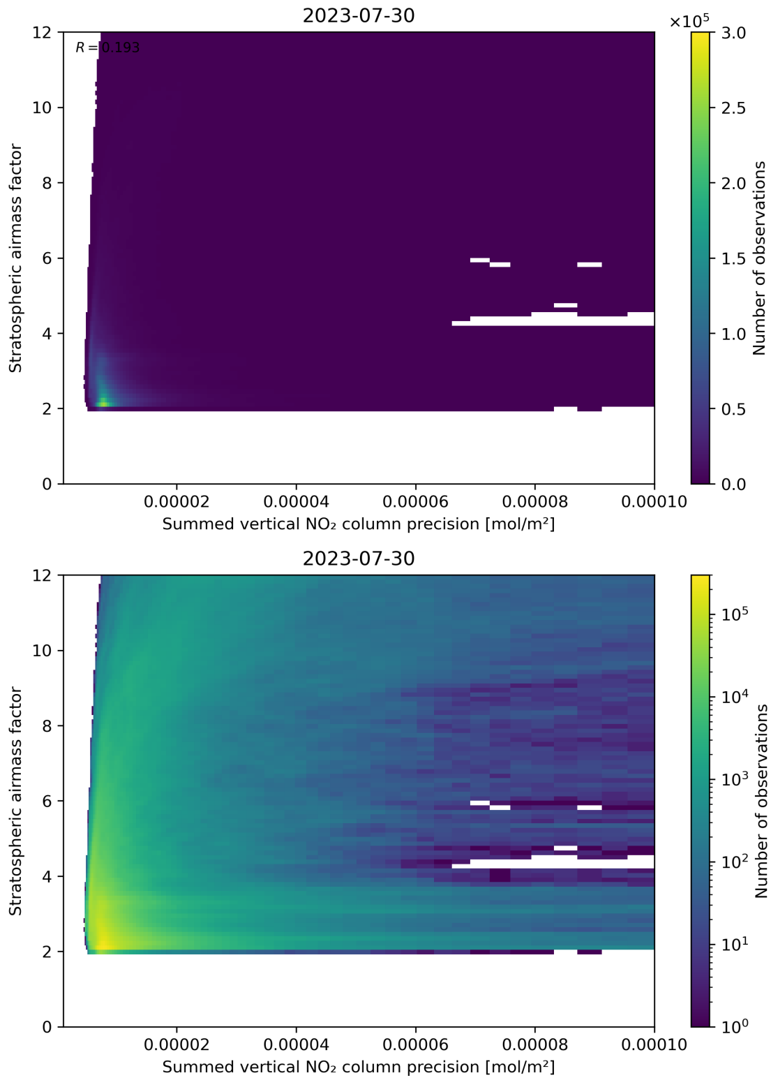
Figure 106: Scatter density plot of “Summed vertical NO 2 column precision” against “Stratospheric airmass factor” for 2023-07-29 to 2023-07-31.
