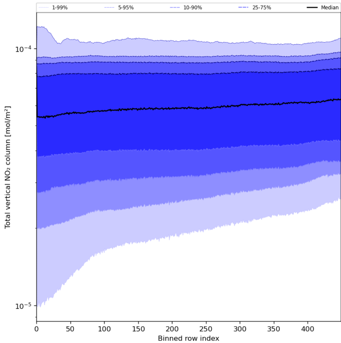
Figure 55: Along track statistics of “Total vertical NO 2 column” for 2023-07-29 to 2023-07-31
