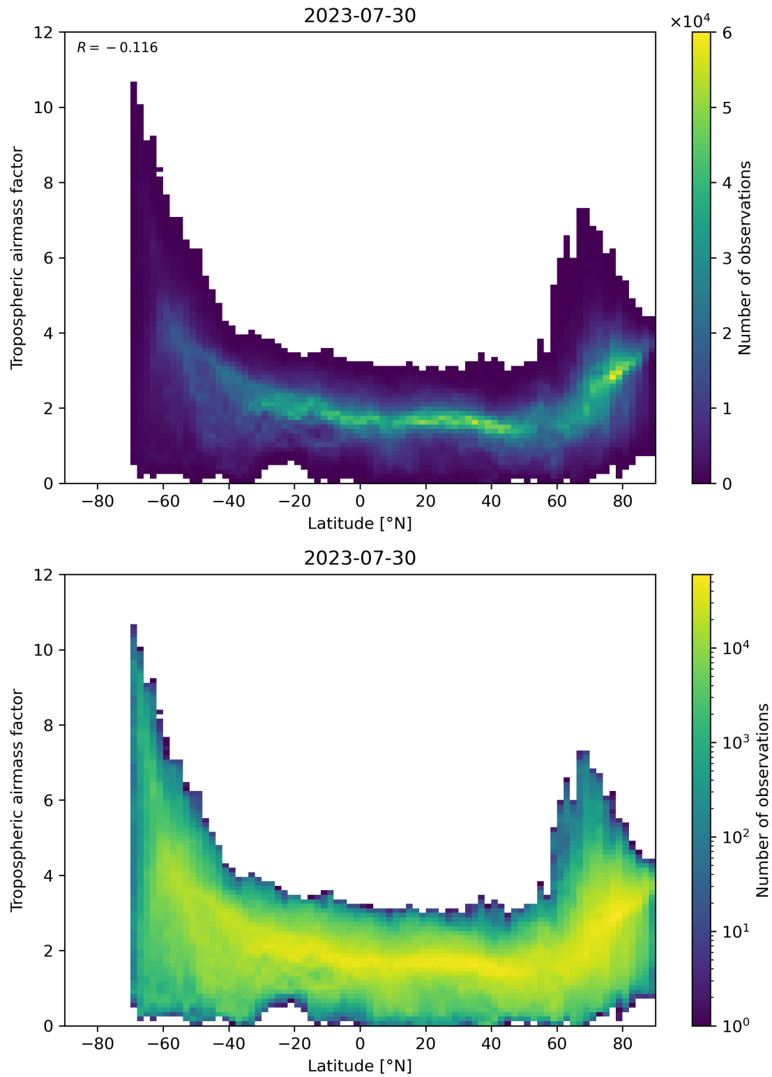
Figure 85: Scatter density plot of “Latitude” against “Tropospheric airmass factor” for 2023-07-29 to 2023-07-31.
