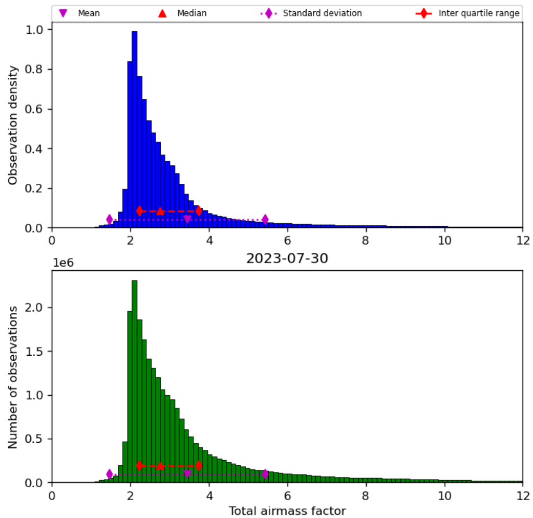
Figure 32: Histogram of “Total airmass factor” for 2023-07-29 to 2023-07-31
