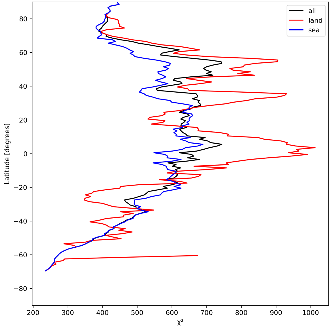
Figure 25: Zonal average of “ \chi^2 ” for 2023-07-29 to 2023-07-31.
