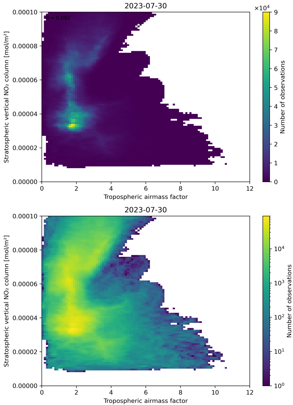
Figure 74: Scatter density plot of “Tropospheric air mass factor” against “Stratospheric vertical NO 2 column” for 2023-07-29 to 2023-07-31.
