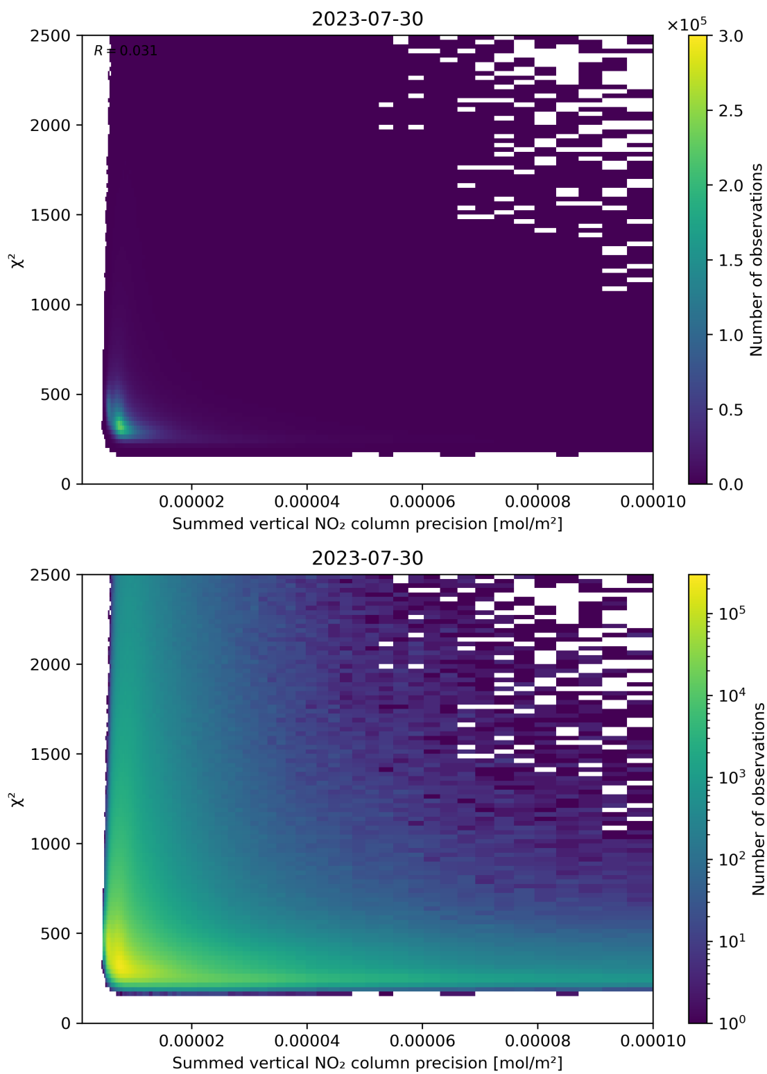
Figure 107: Scatter density plot of “Summed vertical NO 2 column precision” against “ \chi^2 ” for 2023-07-29 to 2023-07-31.
