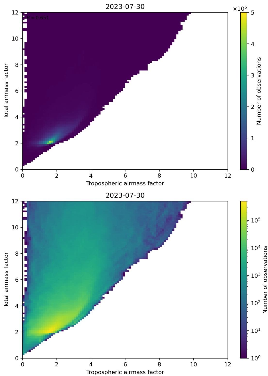
Figure 72: Scatter density plot of “Tropospheric airmass factor” against “Total airmass factor” for 2023-07-29 to 2023-07-31.
