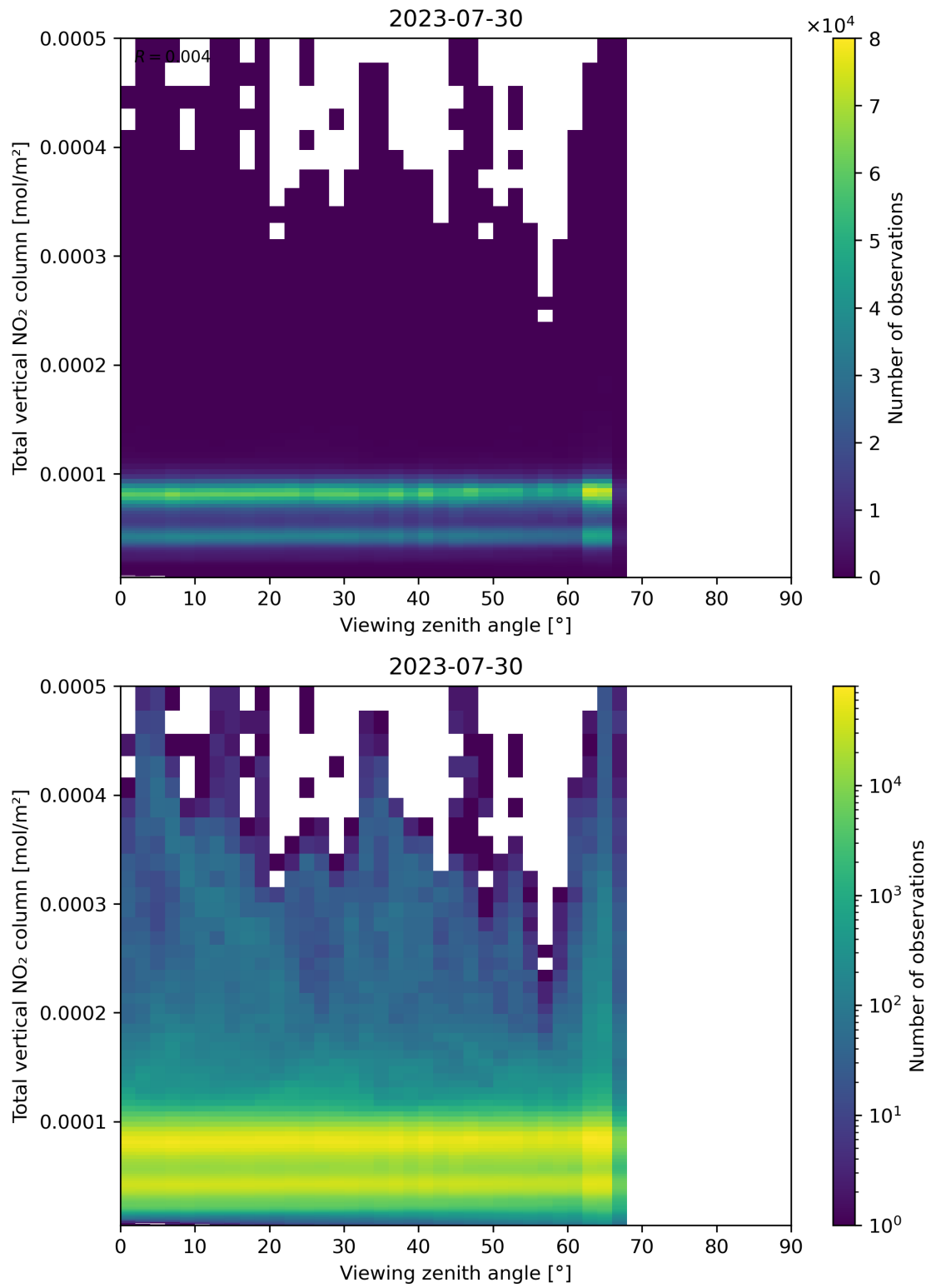
Figure 167: Scatter density plot of “Viewing zenith angle” against “Total vertical NO 2 column” for 2023-07-29 to 2023-07-31.
