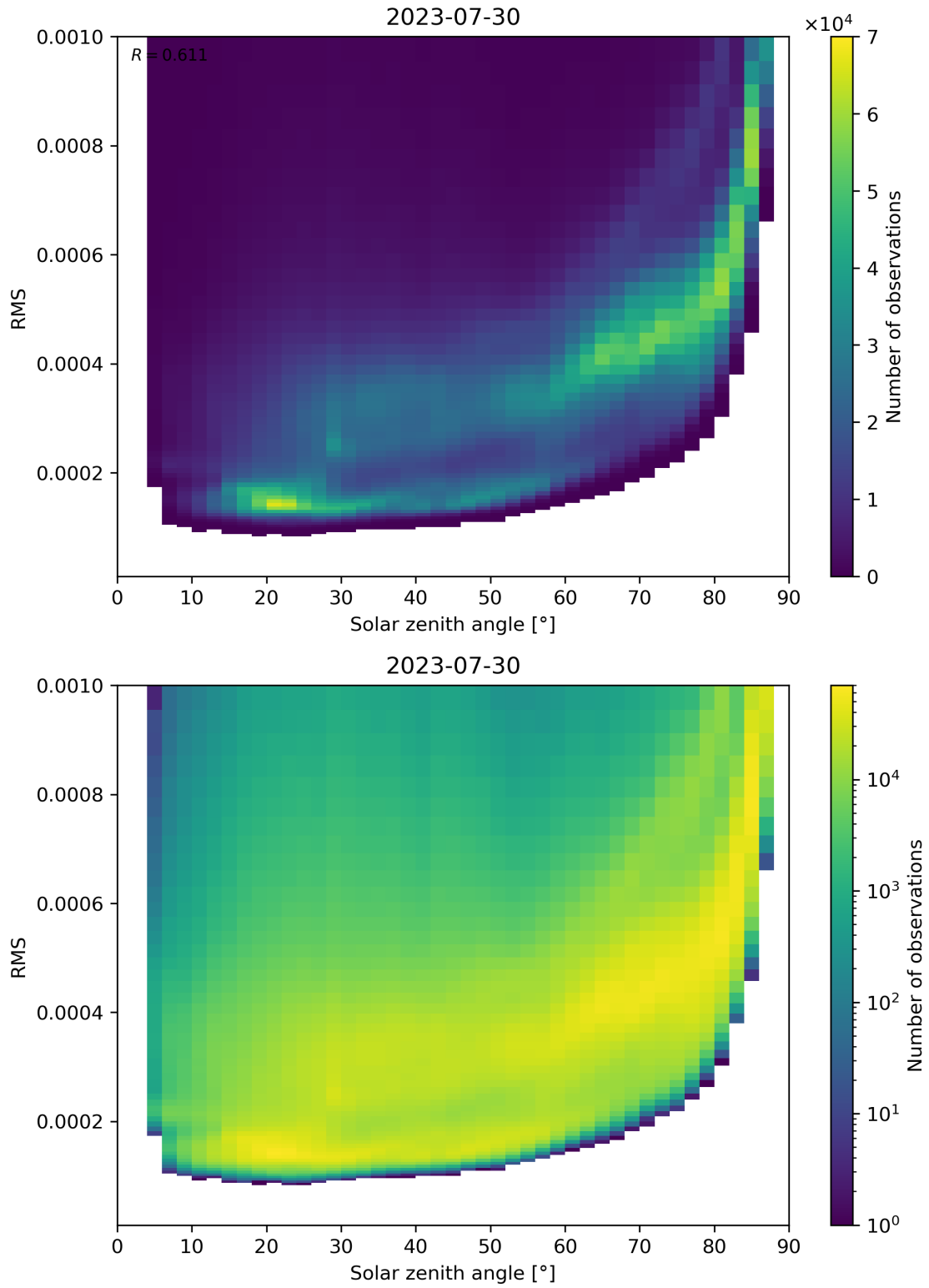
Figure 157: Scatter density plot of “Solar zenith angle” against “RMS” for 2023-07-29 to 2023-07-31.
