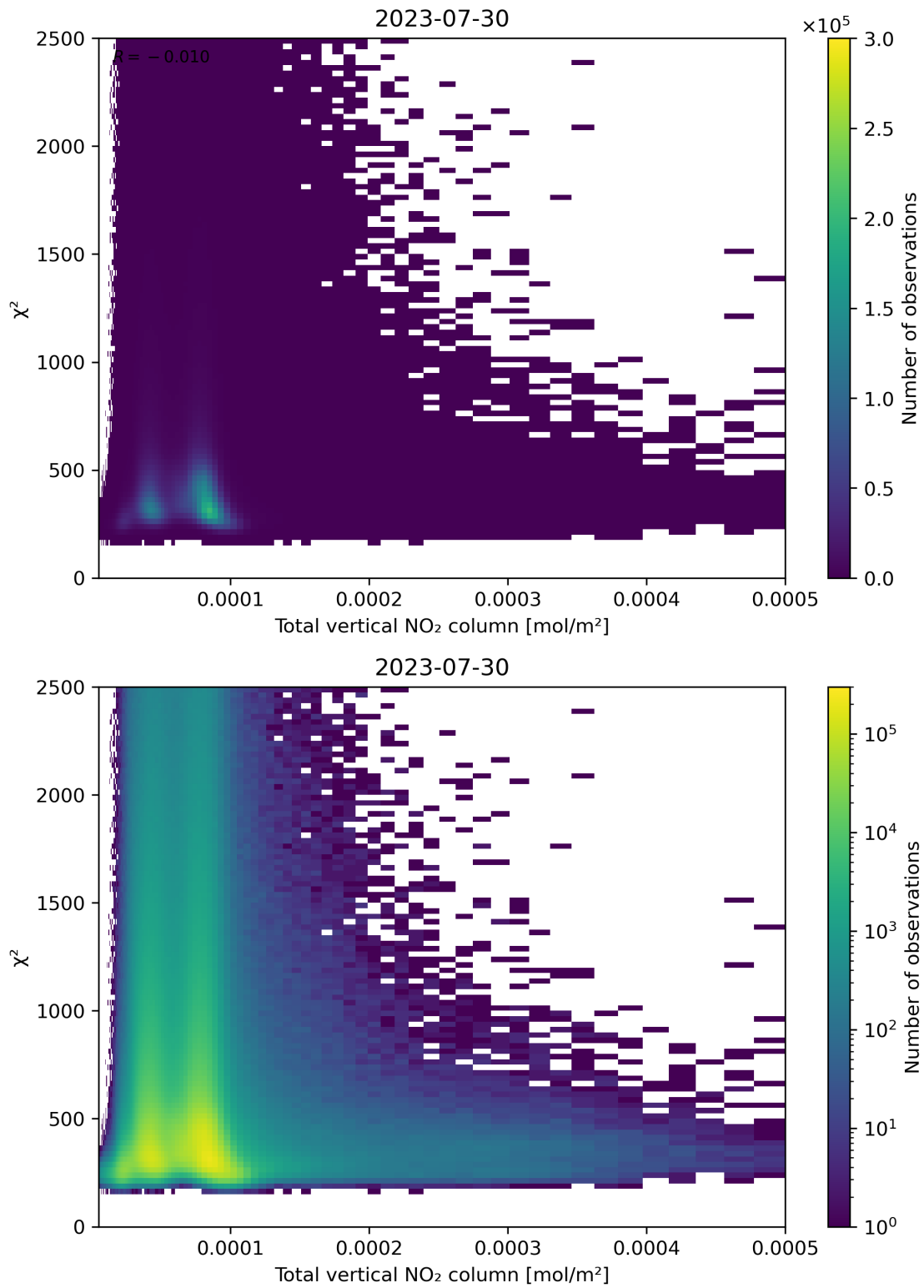
Figure 111: Scatter density plot of “Total vertical NO 2 column” against “ \chi^2 ” for 2023-07-29 to 2023-07-31.
