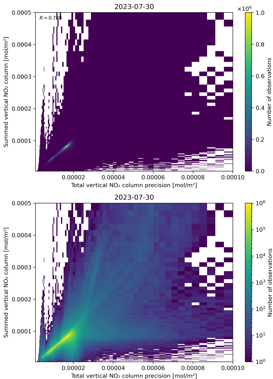
Figure 117: Scatter density plot of “Total vertical NO 2 column precision” against “Summed vertical NO 2 column” for 2023-07-29 to 2023-07-31.
