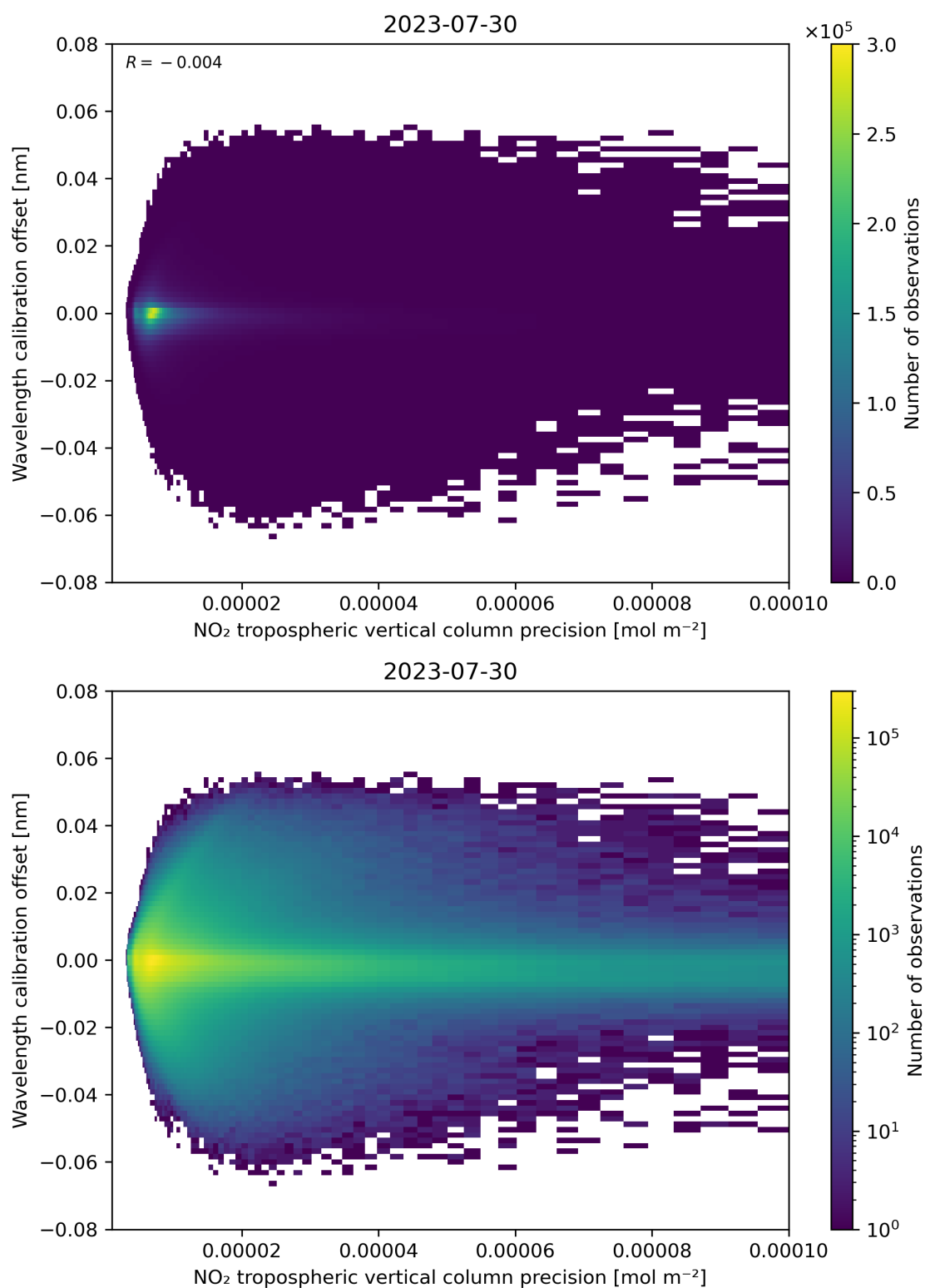
Figure 141: Scatter density plot of “NO 2 tropospheric vertical column precision” against “Wavelength calibration offset” for 2023-07-29 to 2023-07-31.
