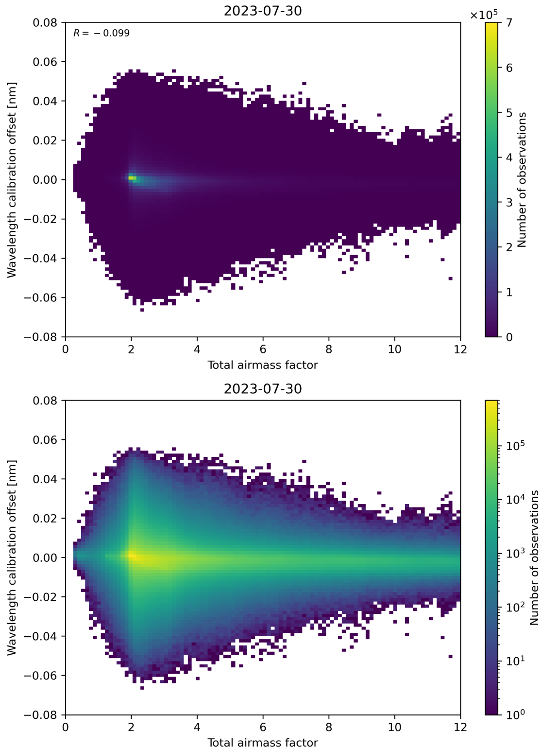
Figure 70: Scatter density plot of “Total airmass factor” against “Wavelength calibration offset” for 2023-07-29 to 2023-07-31.
