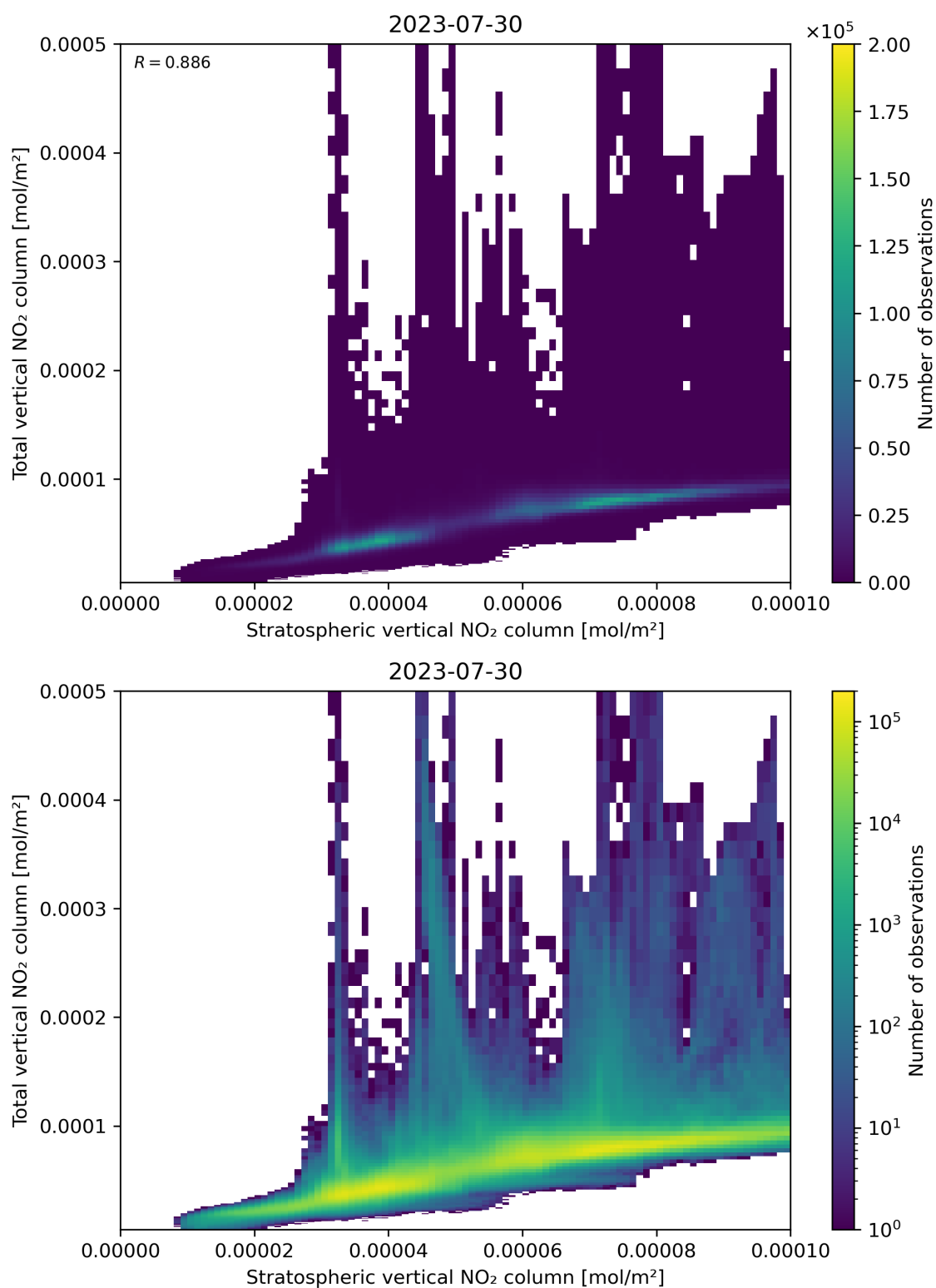
Figure 100: Scatter density plot of “Stratospheric vertical NO 2 column” against “Total vertical NO 2 column” for 2023-07-29 to 2023-07-31.
