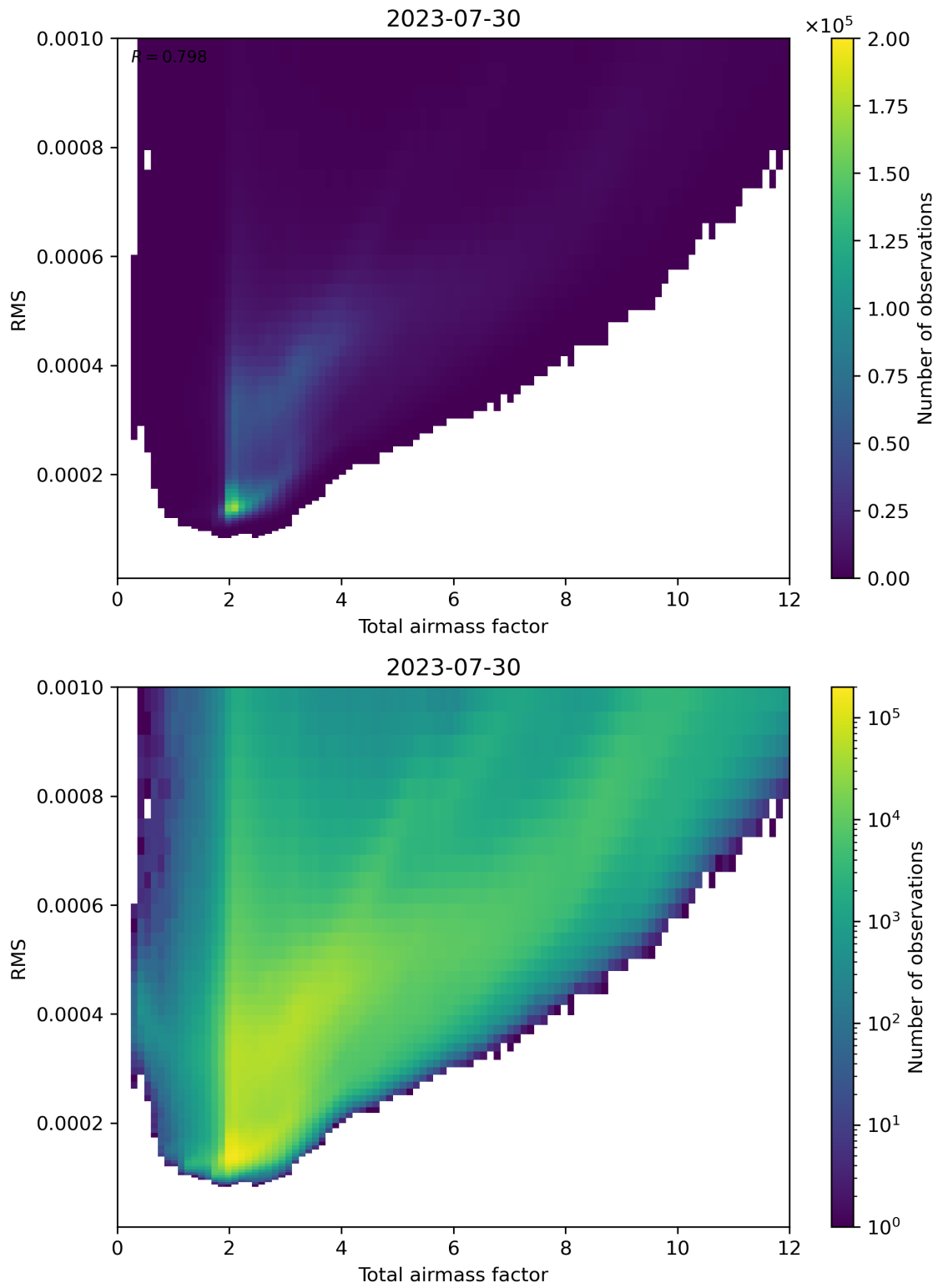
Figure 69: Scatter density plot of “Total airmass factor” against “RMS” for 2023-07-29 to 2023-07-31.
