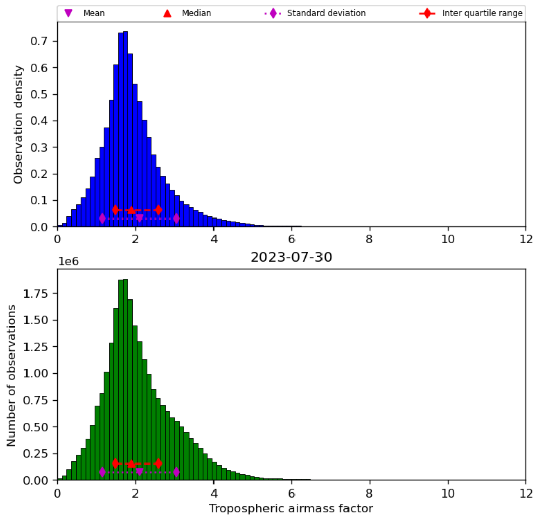
Figure 31: Histogram of “Tropospheric airmass factor” for 2023-07-29 to 2023-07-31
