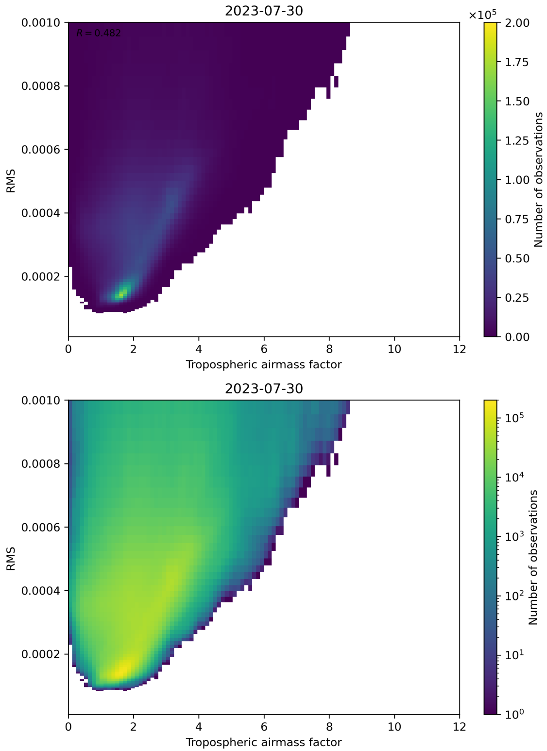
Figure 79: Scatter density plot of “Tropospheric airmass factor” against “RMS” for 2023-07-29 to 2023-07-31.
