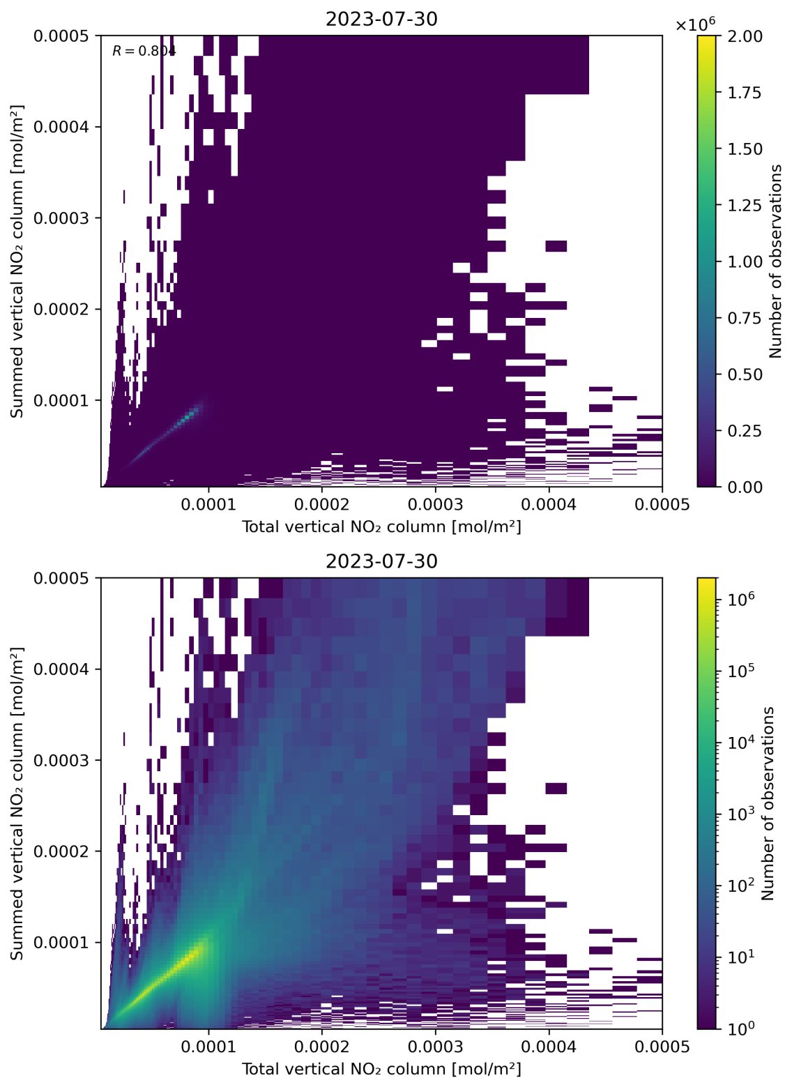
Figure 112: Scatter density plot of “Total vertical NO 2 column” against “Summed vertical NO 2 column” for 2023-07-29 to 2023-07-31.
