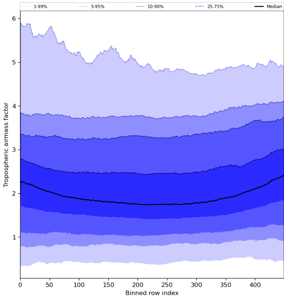
Figure 48: Along track statistics of “Tropospheric airmass factor” for 2023-07-29 to 2023-07-31
