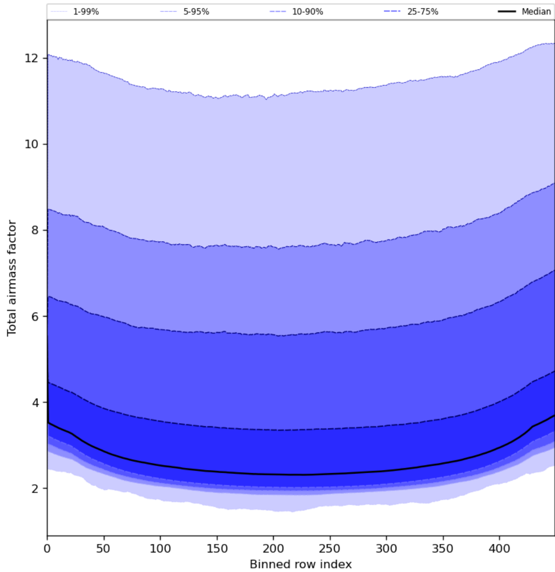
Figure 49: Along track statistics of “Total airmass factor” for 2023-07-29 to 2023-07-31
