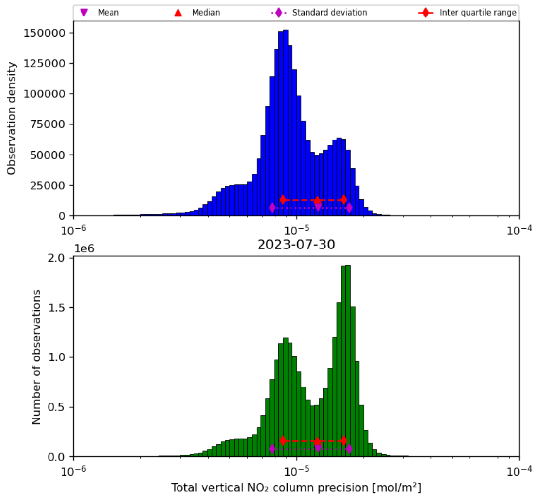
Figure 39: Histogram of “Total vertical NO 2 column precision” for 2023-07-29 to 2023-07-31
