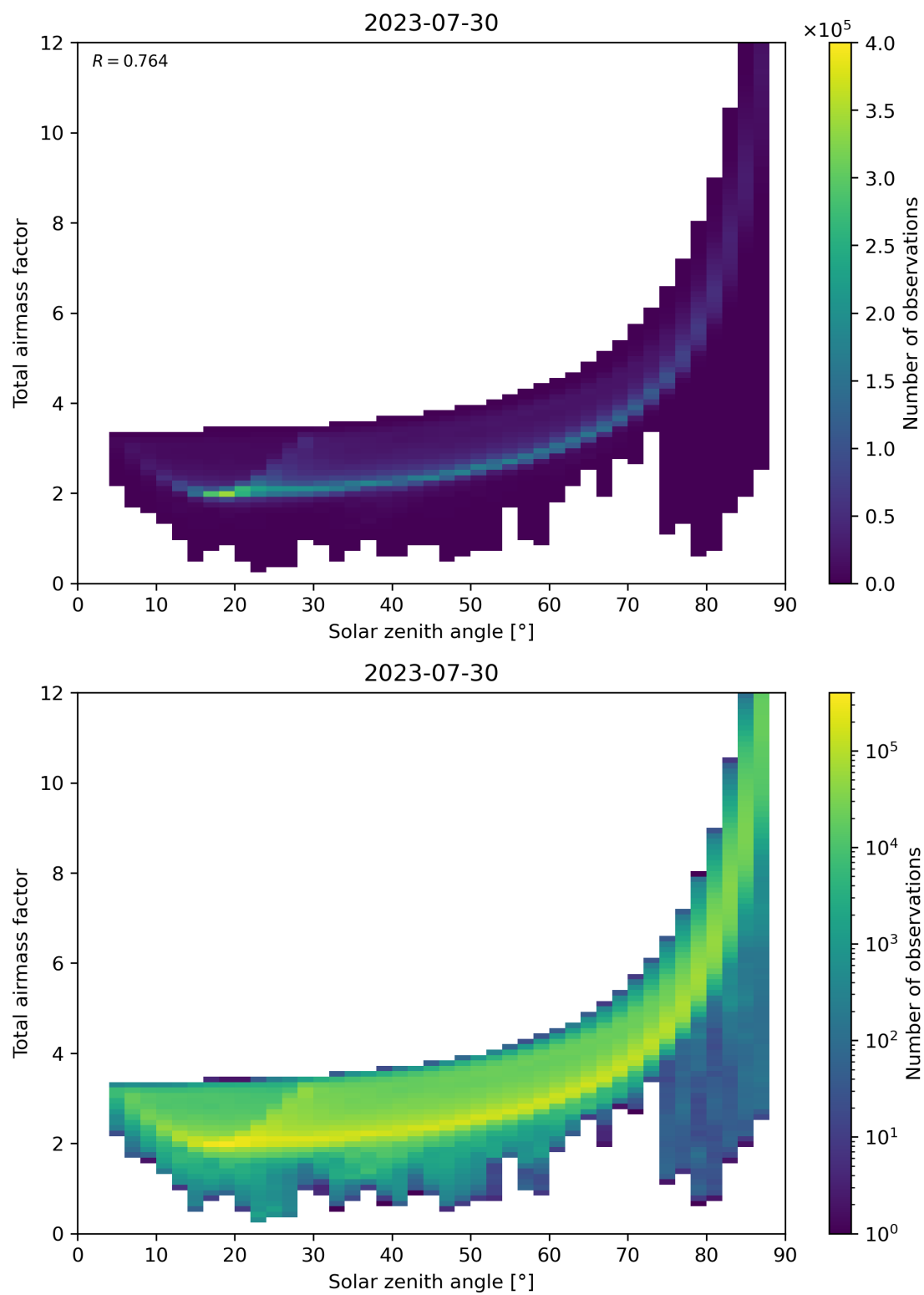
Figure 146: Scatter density plot of “Solar zenith angle” against “Total air mass factor” for 2023-07-29 to 2023-07-31.
