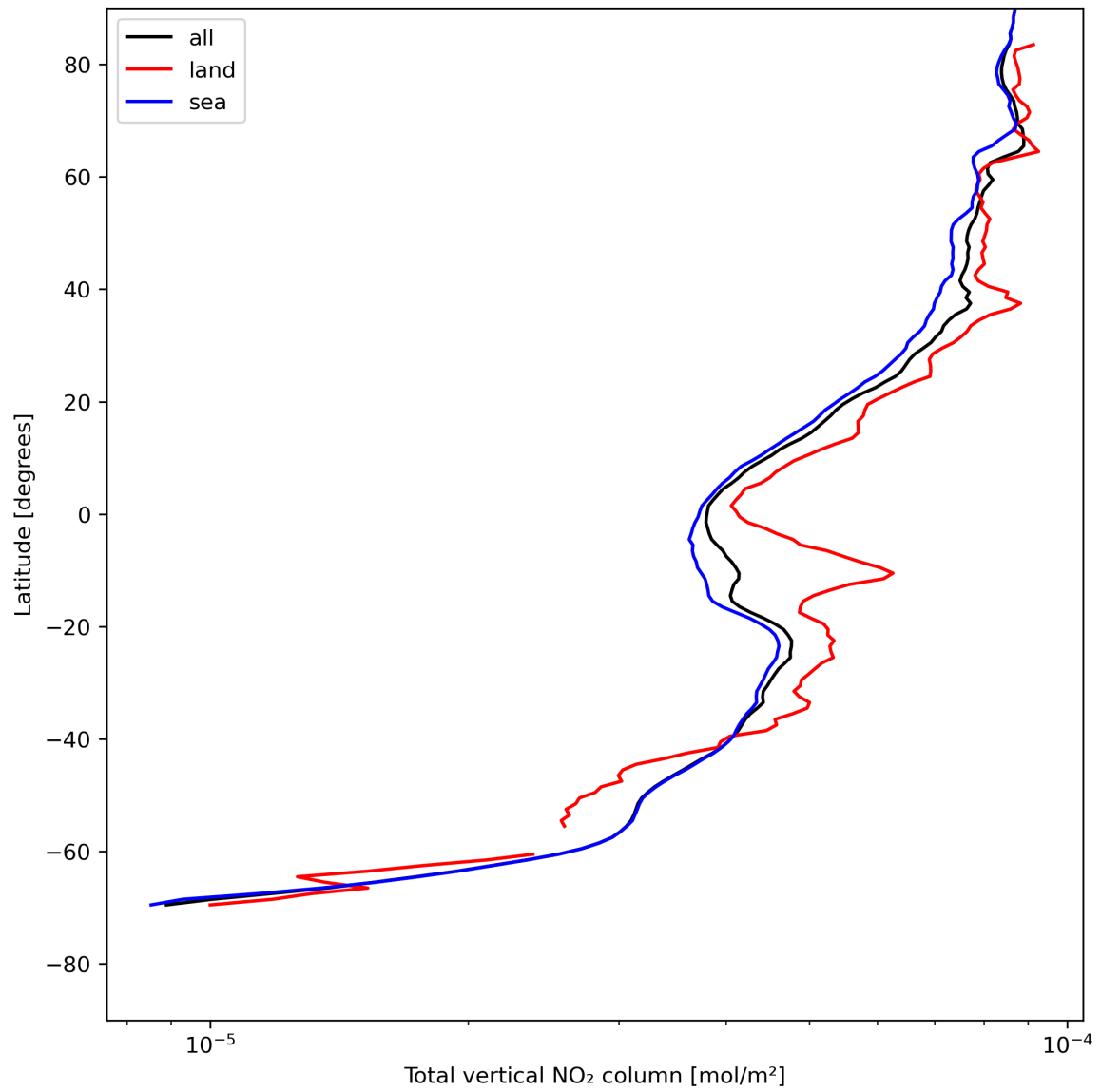
Figure 21: Zonal average of “Total vertical NO 2 column” for 2023-07-29 to 2023-07-31.
