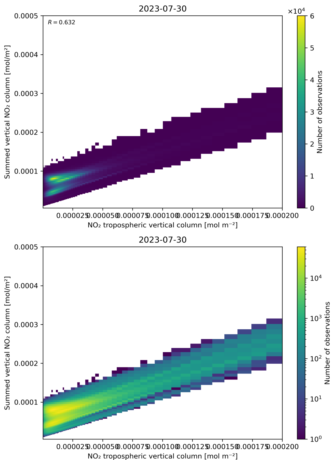
Figure 126: Scatter density plot of “NO 2 tropospheric vertical column” against “Summed vertical NO 2 column” for 2023-07-29 to 2023-07-31.
