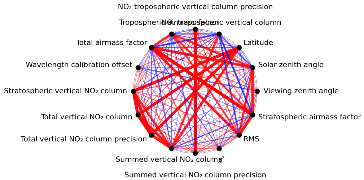
Figure 1: Map of correlation graph for 2023-07-29 to 2023-07-31.
