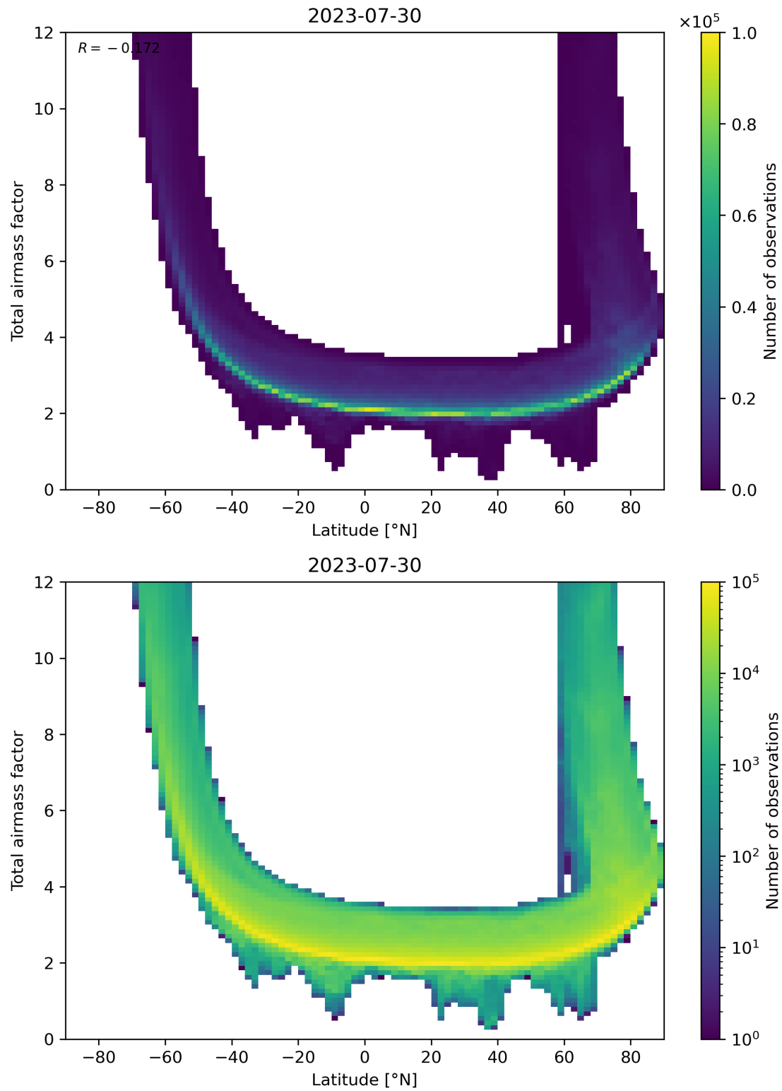
Figure 84: Scatter density plot of “Latitude” against “Total airmass factor” for 2023-07-29 to 2023-07-31.
