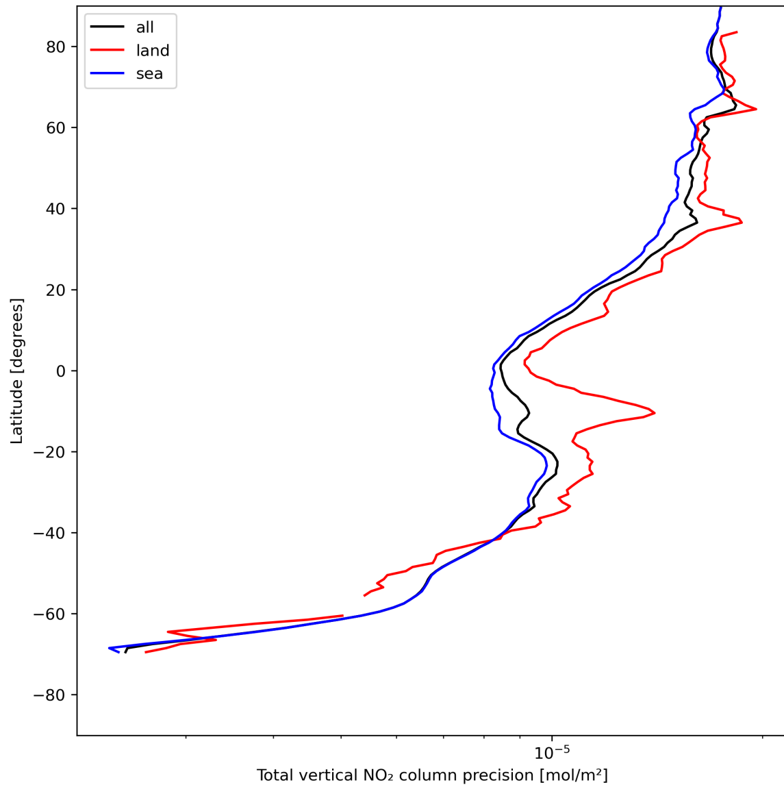
Figure 22: Zonal average of “Total vertical NO 2 column precision” for 2023-07-29 to 2023-07-31.
