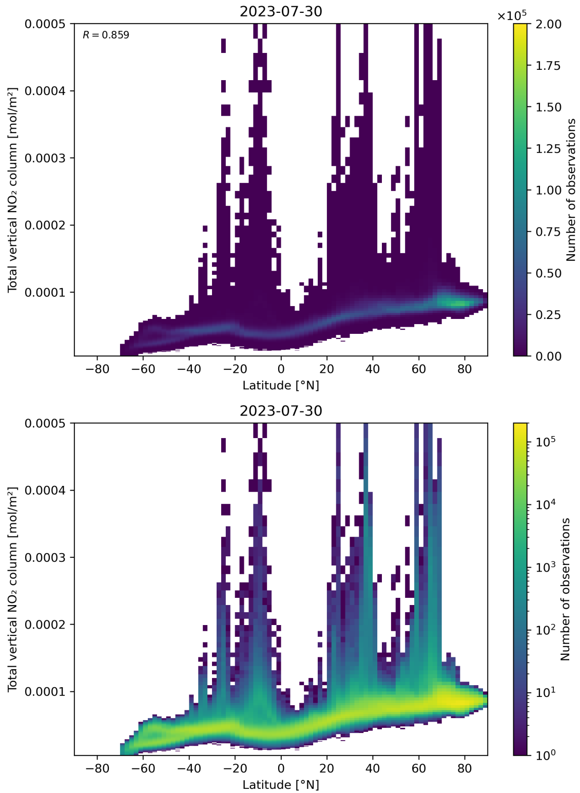
Figure 90: Scatter density plot of “Latitude” against “Total vertical NO 2 column” for 2023-07-29 to 2023-07-31.
