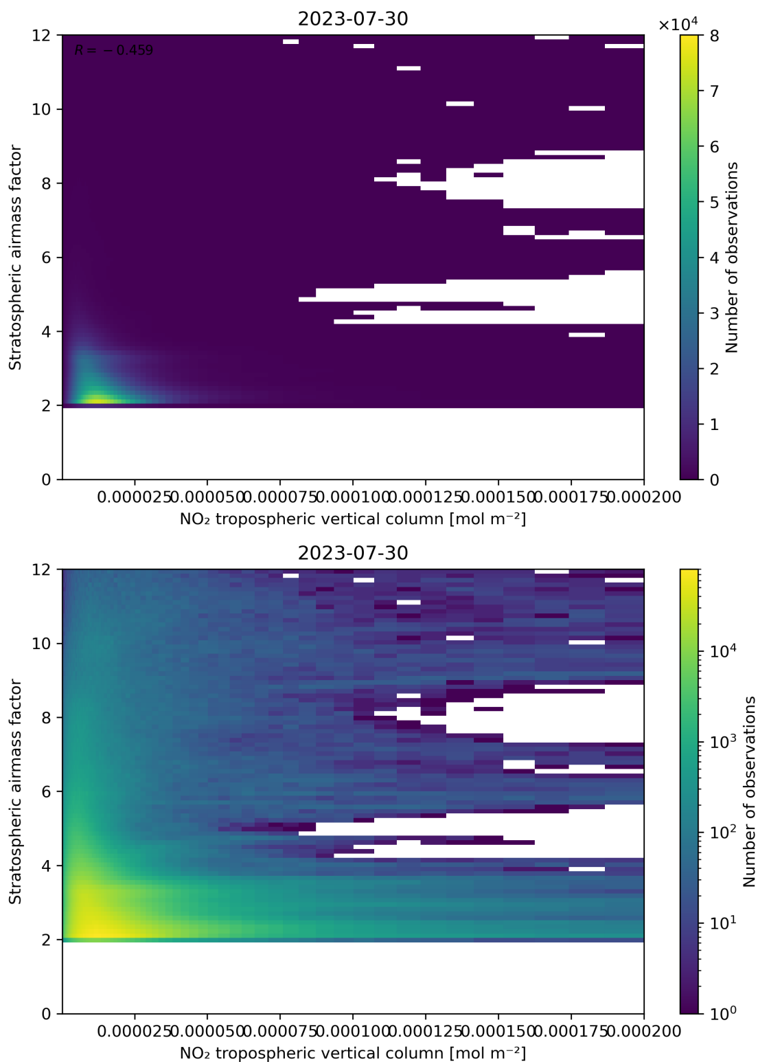
Figure 121: Scatter density plot of “NO 2 tropospheric vertical column” against “Stratospheric air mass factor” for 2023-07-29 to 2023-07-31.
