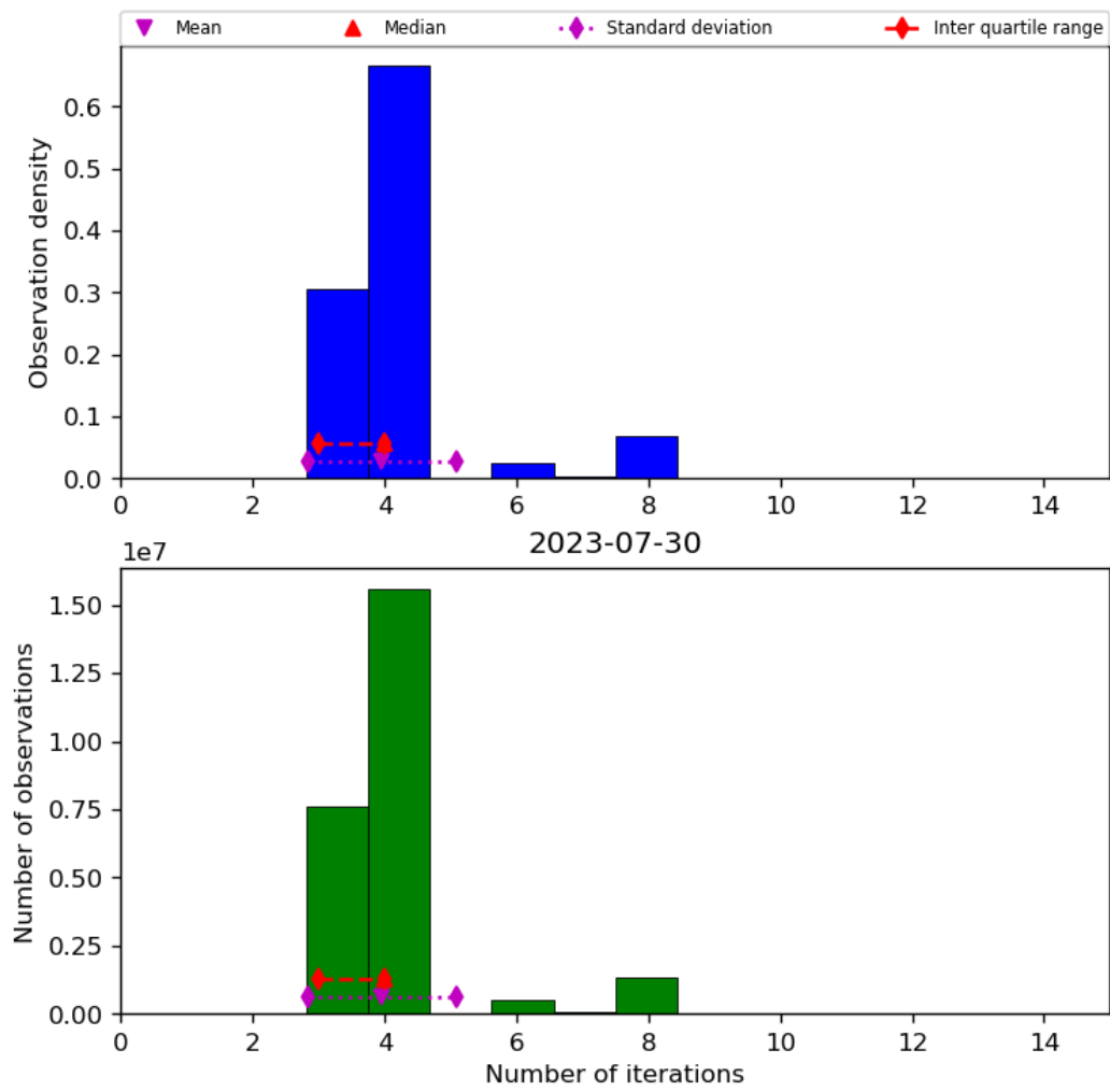
Figure 34: Histogram of “Number of iterations” for 2023-07-29 to 2023-07-31
