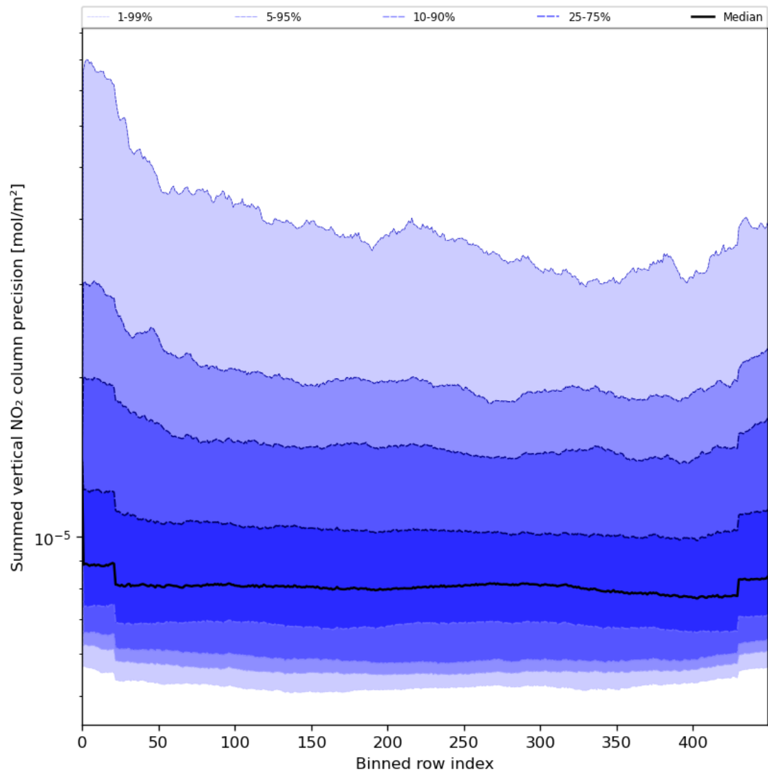
Figure 58: Along track statistics of “Summed vertical NO 2 column precision” for 2023-07-29 to 2023-07-31
