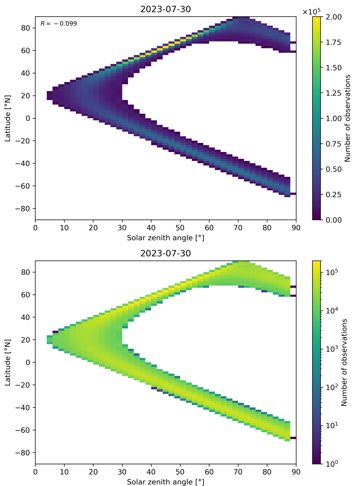
Figure 149: Scatter density plot of “Solar zenith angle” against “Latitude” for 2023-07-29 to 2023-07-31.
