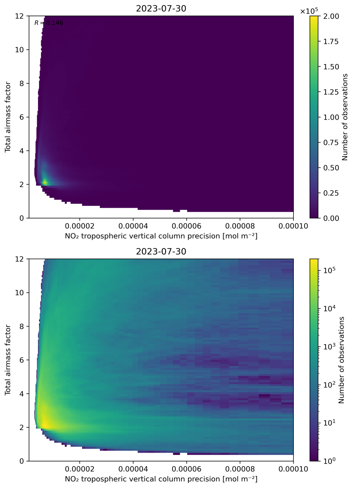
Figure 132: Scatter density plot of “NO 2 tropospheric vertical column precision” against “Total air mass factor” for 2023-07-29 to 2023-07-31.
