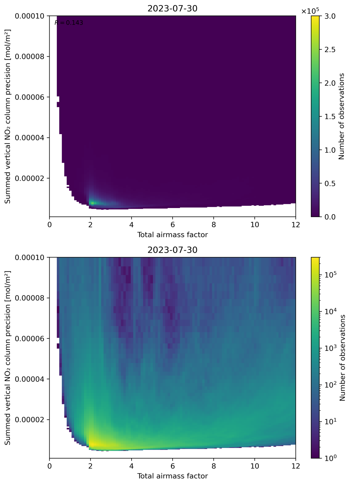
Figure 66: Scatter density plot of “Total airmass factor” against “Summed vertical NO 2 column precision” for 2023-07-29 to 2023-07-31.
