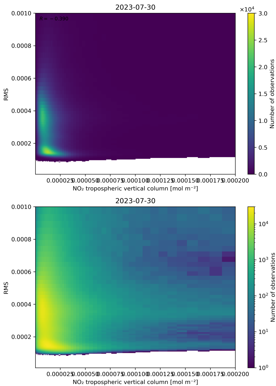
Figure 142: Scatter density plot of “NO 2 tropospheric vertical column” against “RMS” for 2023-07-29 to 2023-07-31.
