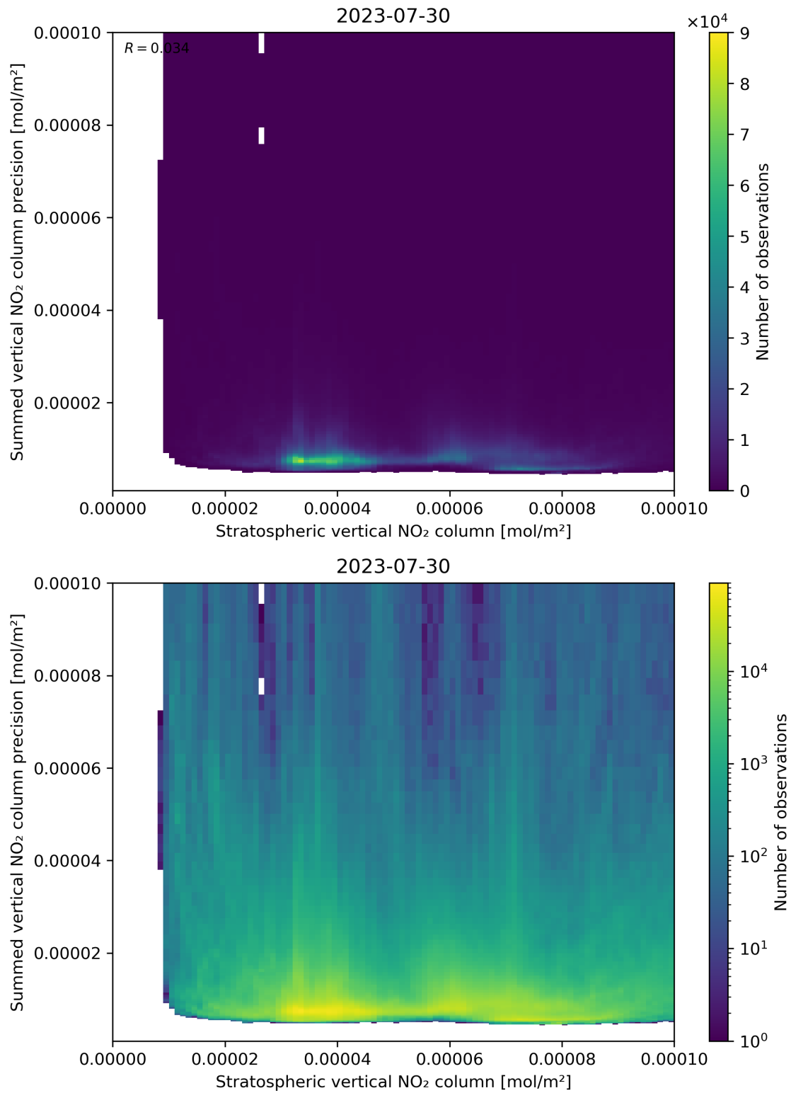
Figure 99: Scatter density plot of “Stratospheric vertical NO 2 column” against “Summed vertical NO 2 column precision” for 2023-07-29 to 2023-07-31.
