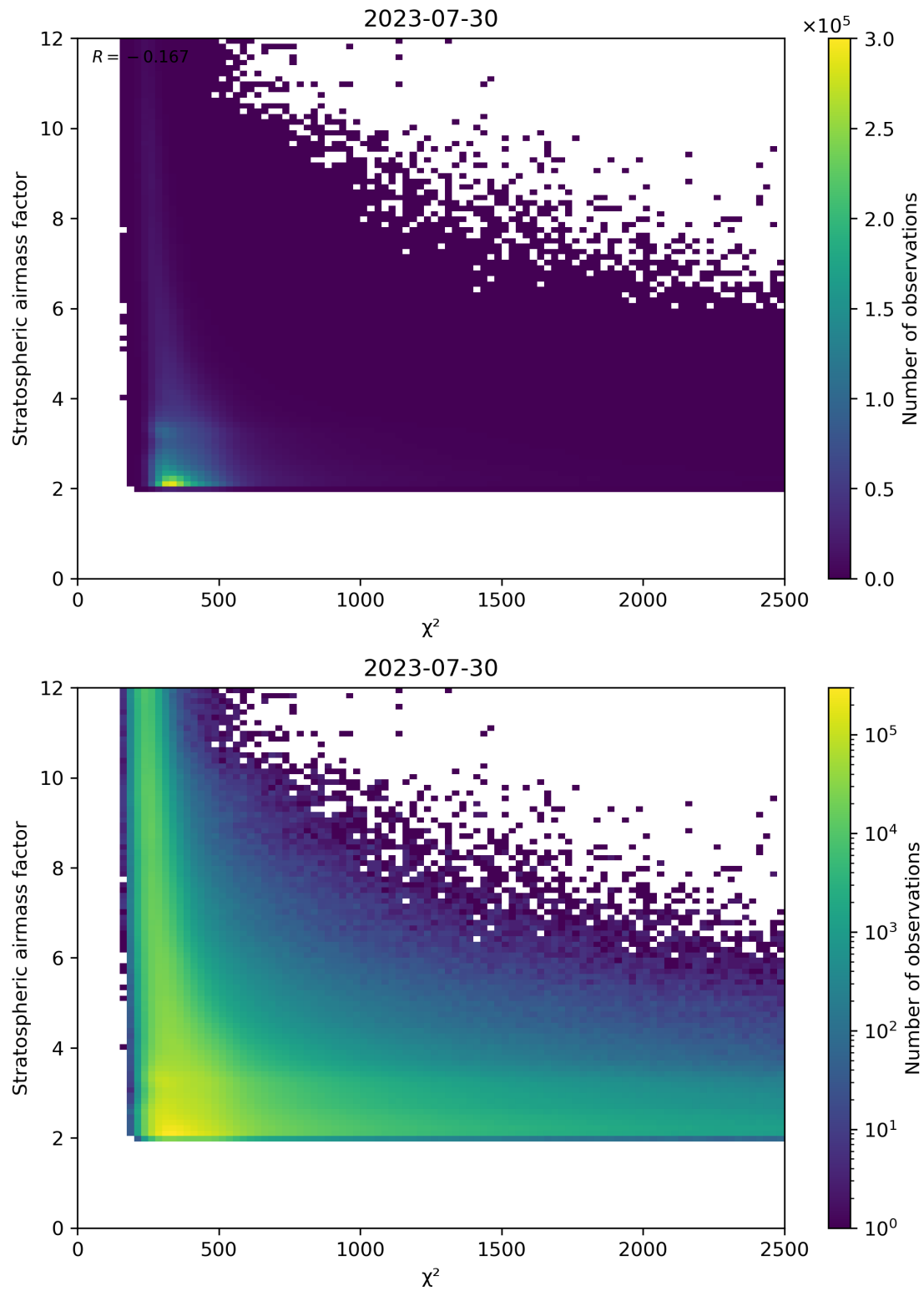
Figure 81: Scatter density plot of “ \chi^2 ” against “Stratospheric airmass factor” for 2023-07-29 to 2023-07-31.
