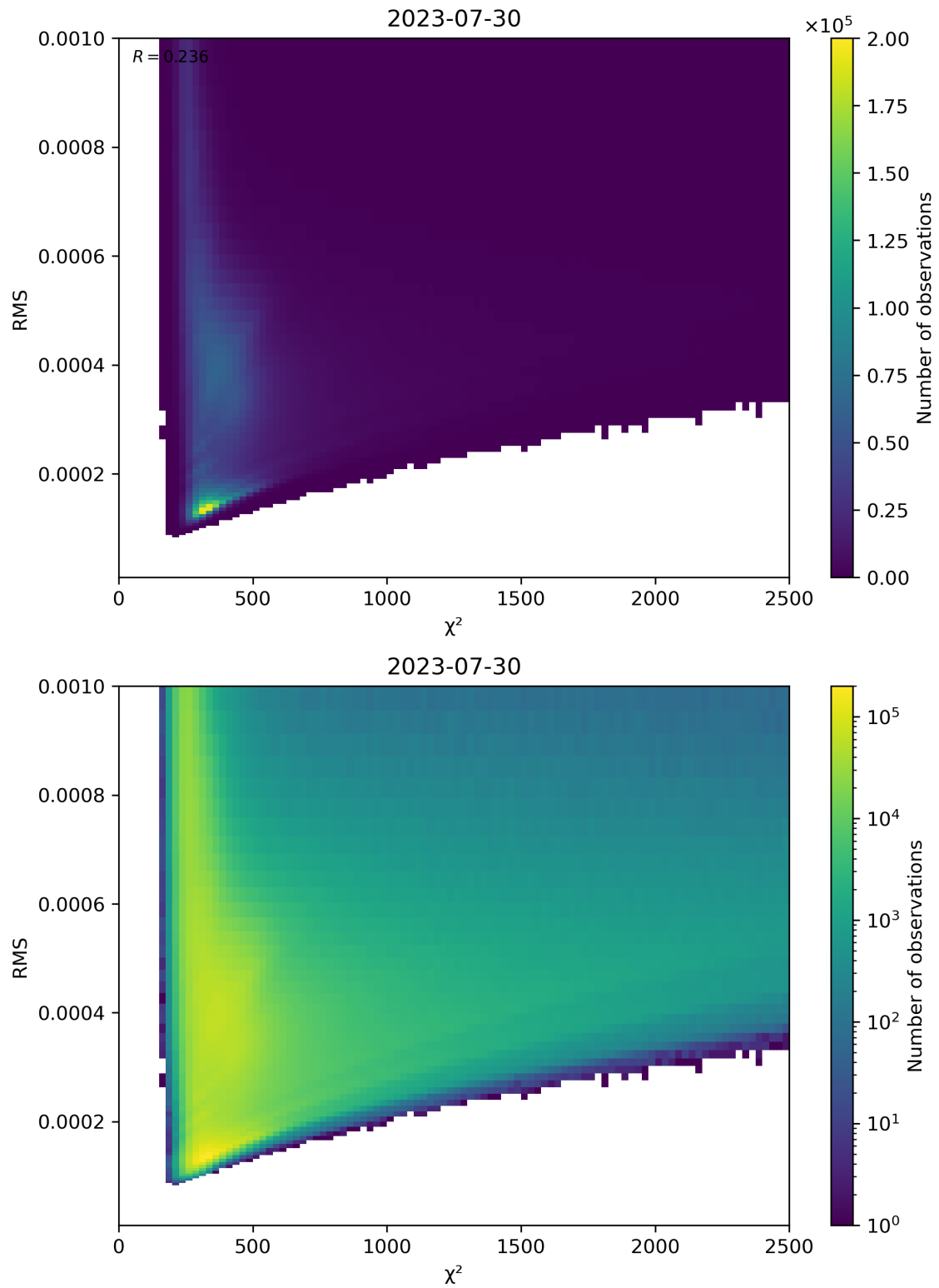
Figure 82: Scatter density plot of “ \chi^2 ” against “RMS” for 2023-07-29 to 2023-07-31.
