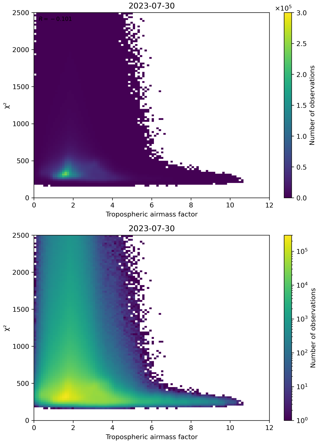
Figure 73: Scatter density plot of “Tropospheric airmass factor” against “ \chi^2 ” for 2023-07-29 to 2023-07-31.
