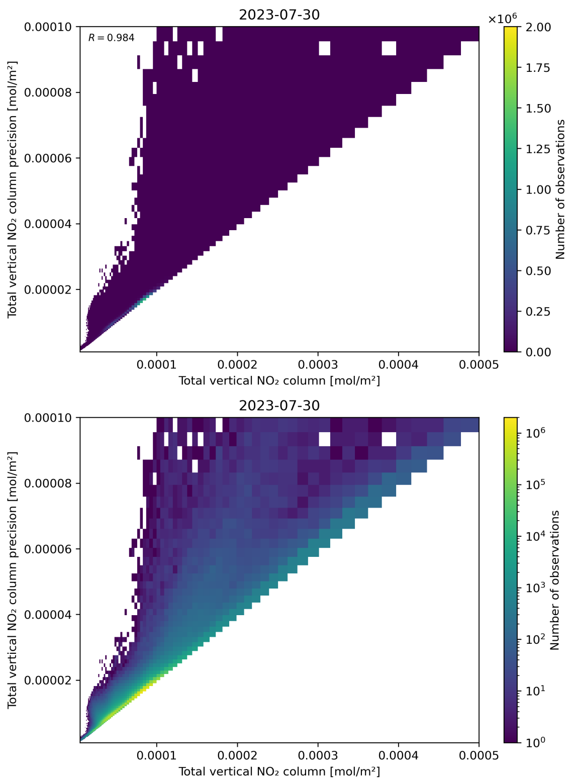
Figure 114: Scatter density plot of “Total vertical NO 2 column” against “Total vertical NO 2 column precision” for 2023-07-29 to 2023-07-31.
