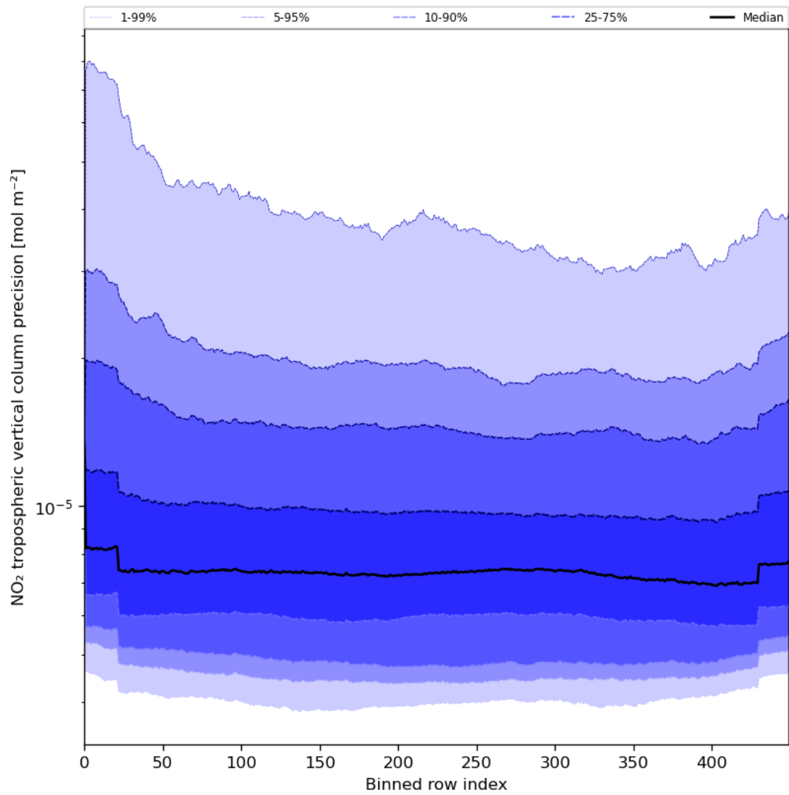
Figure 47: Along track statistics of “NO 2 tropospheric vertical column precision” for 2023-07-29 to 2023-07-31
