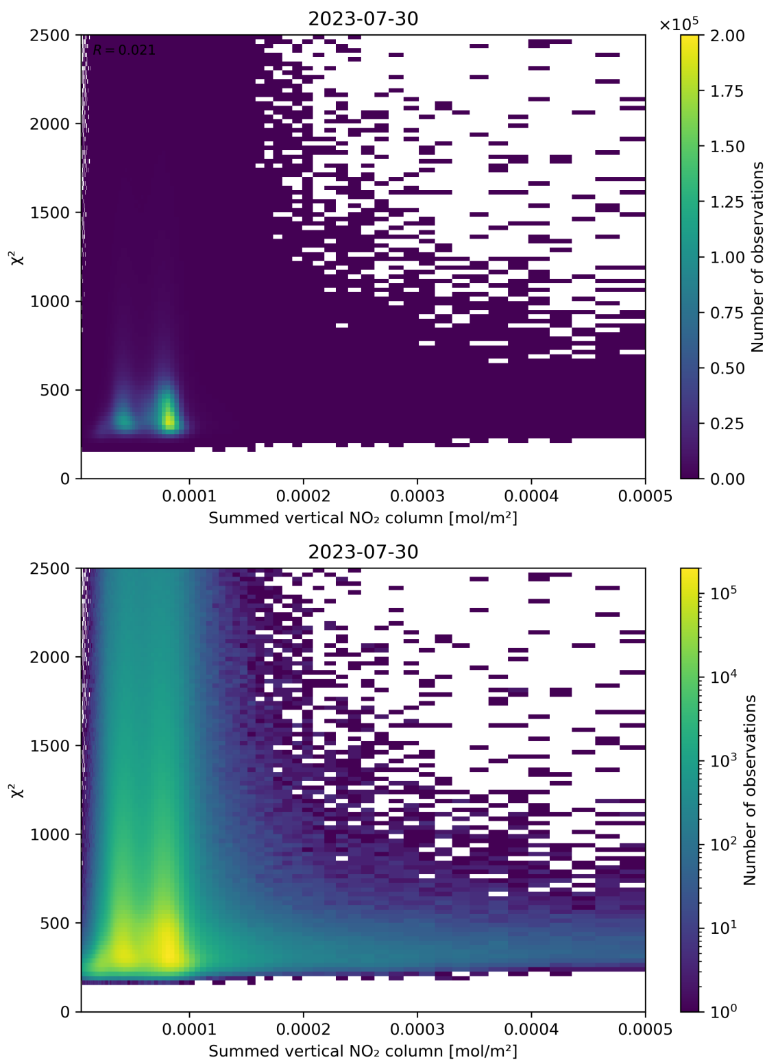
Figure 104: Scatter density plot of “Summed vertical NO 2 column” against “ \chi^2 ” for 2023-07-29 to 2023-07-31.
