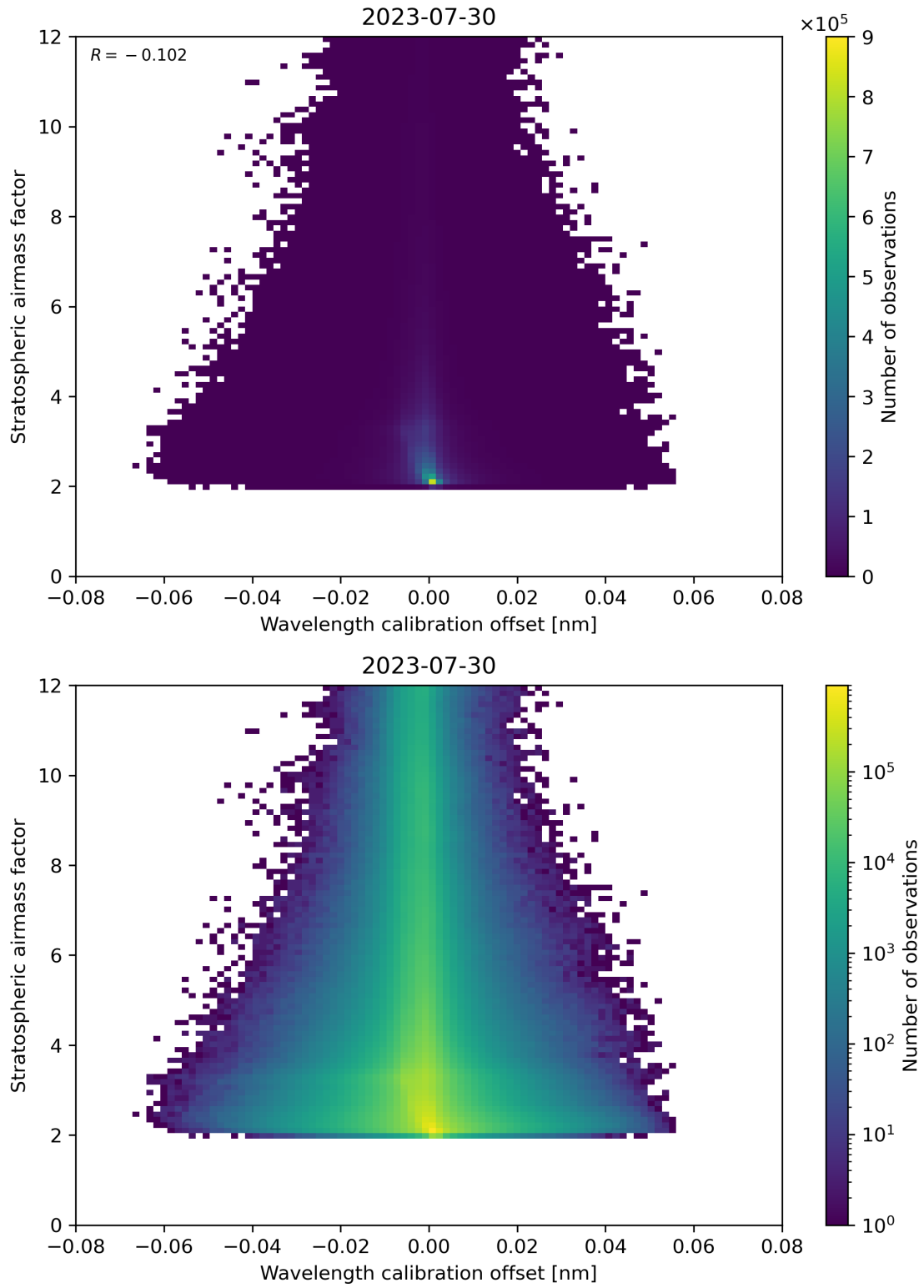
Figure 174: Scatter density plot of “Wavelength calibration offset” against “Stratospheric airmass factor” for 2023-07-29 to 2023-07-31.
