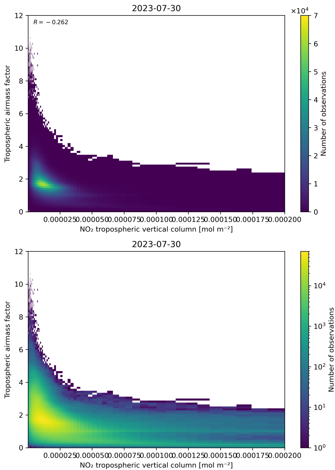
Figure 123: Scatter density plot of “NO 2 tropospheric vertical column” against “Tropospheric air mass factor” for 2023-07-29 to 2023-07-31.
