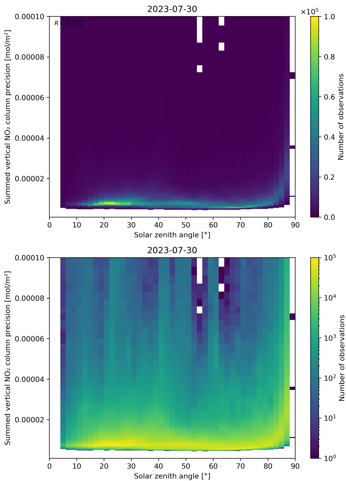
Figure 152: Scatter density plot of “Solar zenith angle” against “Summed vertical NO 2 column precision” for 2023-07-29 to 2023-07-31.
