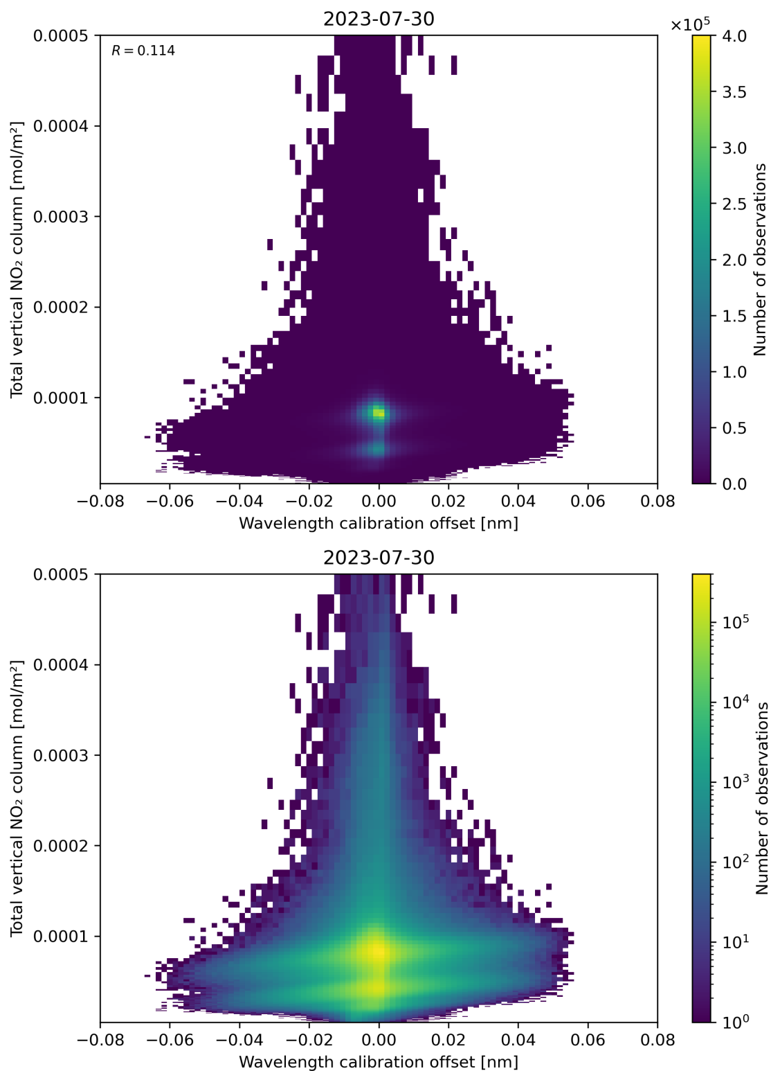
Figure 179: Scatter density plot of “Wavelength calibration offset” against “Total vertical NO 2 column” for 2023-07-29 to 2023-07-31.
