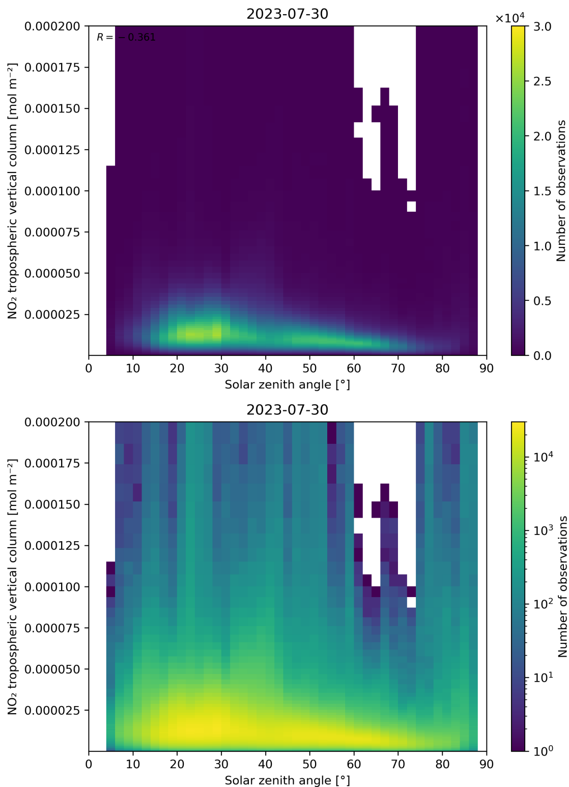
Figure 155: Scatter density plot of “Solar zenith angle” against “NO 2 tropospheric vertical column” for 2023-07-29 to 2023-07-31.
