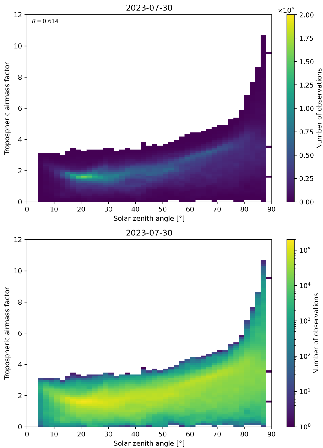
Figure 147: Scatter density plot of “Solar zenith angle” against “Tropospheric airmass factor” for 2023-07-29 to 2023-07-31.
