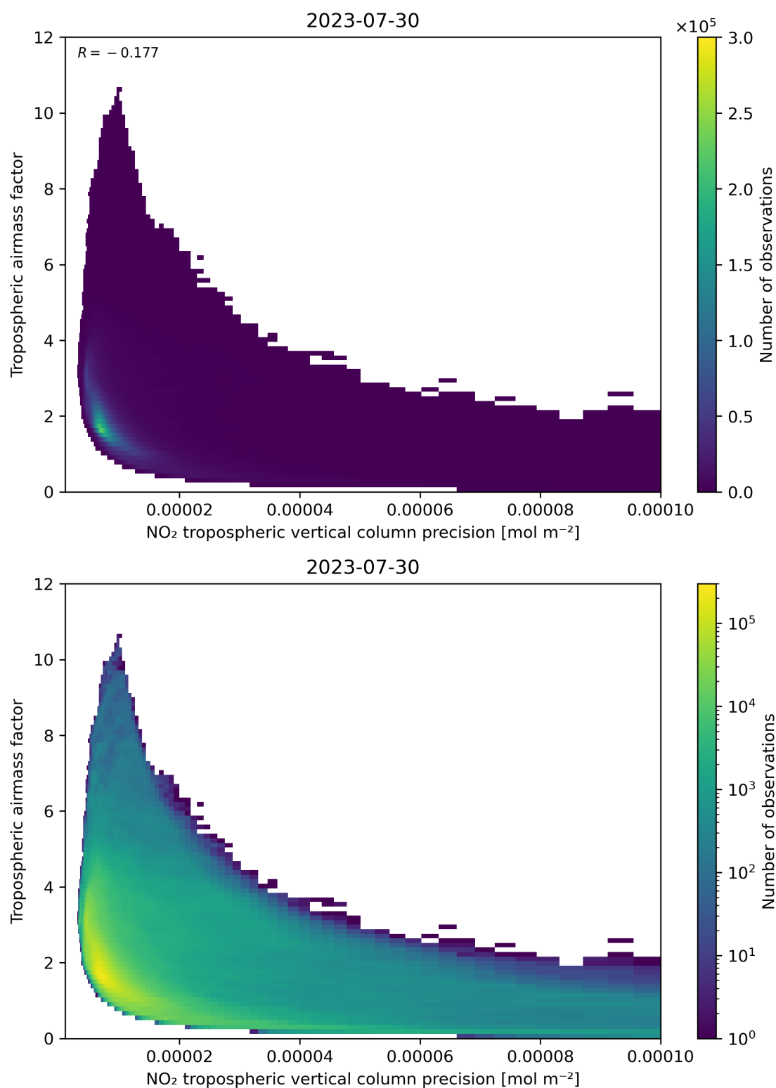
Figure 133: Scatter density plot of “NO 2 tropospheric vertical column precision” against “Tropospheric airmass factor” for 2023-07-29 to 2023-07-31.
