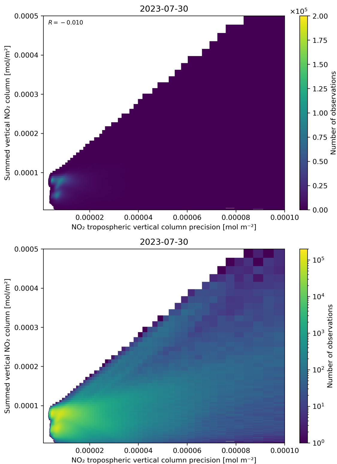
Figure 136: Scatter density plot of “NO 2 tropospheric vertical column precision” against “Summed vertical NO 2 column” for 2023-07-29 to 2023-07-31.
