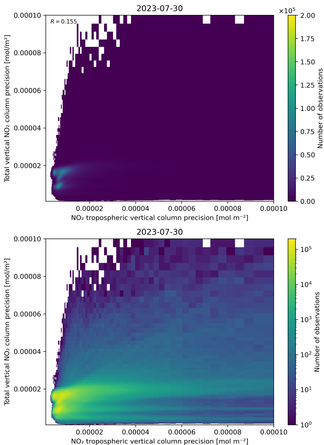
Figure 139: Scatter density plot of “NO 2 tropospheric vertical column precision” against “Total vertical NO 2 column precision” for 2023-07-29 to 2023-07-31.
