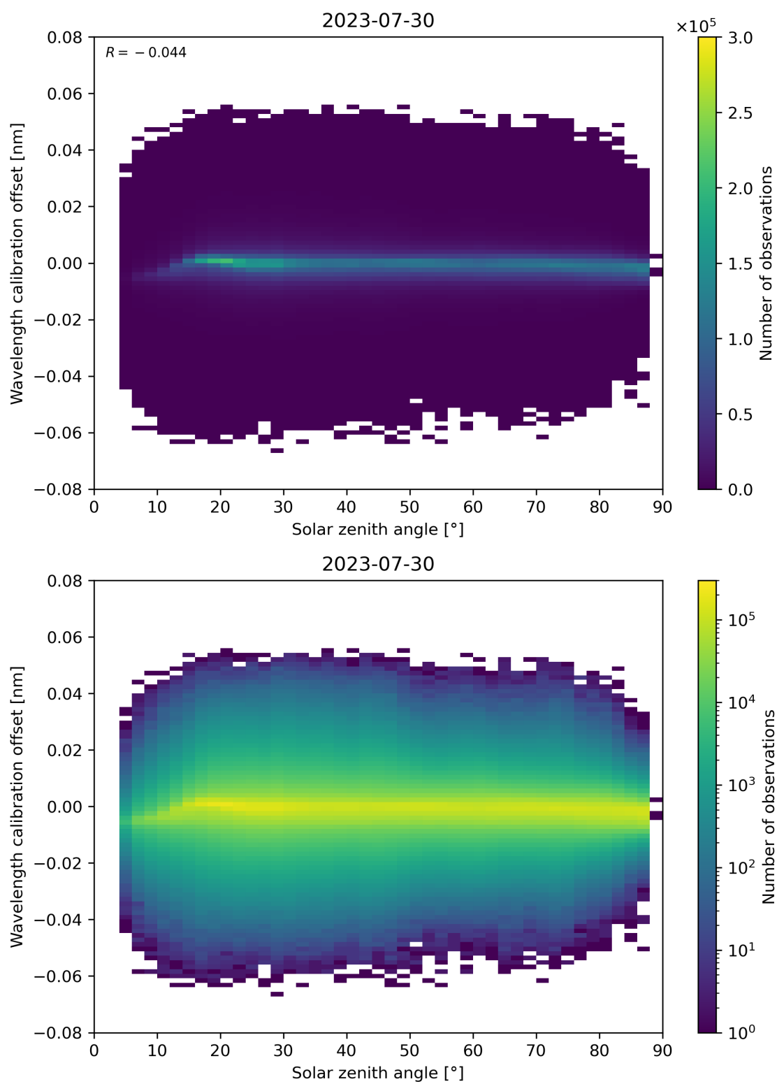
Figure 158: Scatter density plot of “Solar zenith angle” against “Wavelength calibration offset” for 2023-07-29 to 2023-07-31.
