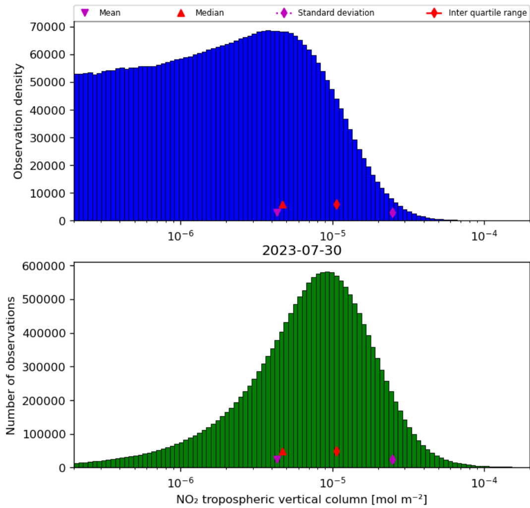
Figure 29: Histogram of “NO 2 tropospheric vertical column” for 2023-07-29 to 2023-07-31
