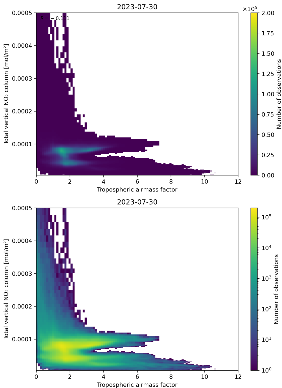
Figure 77: Scatter density plot of “Tropospheric airmass factor” against “Total vertical NO 2 column” for 2023-07-29 to 2023-07-31.
