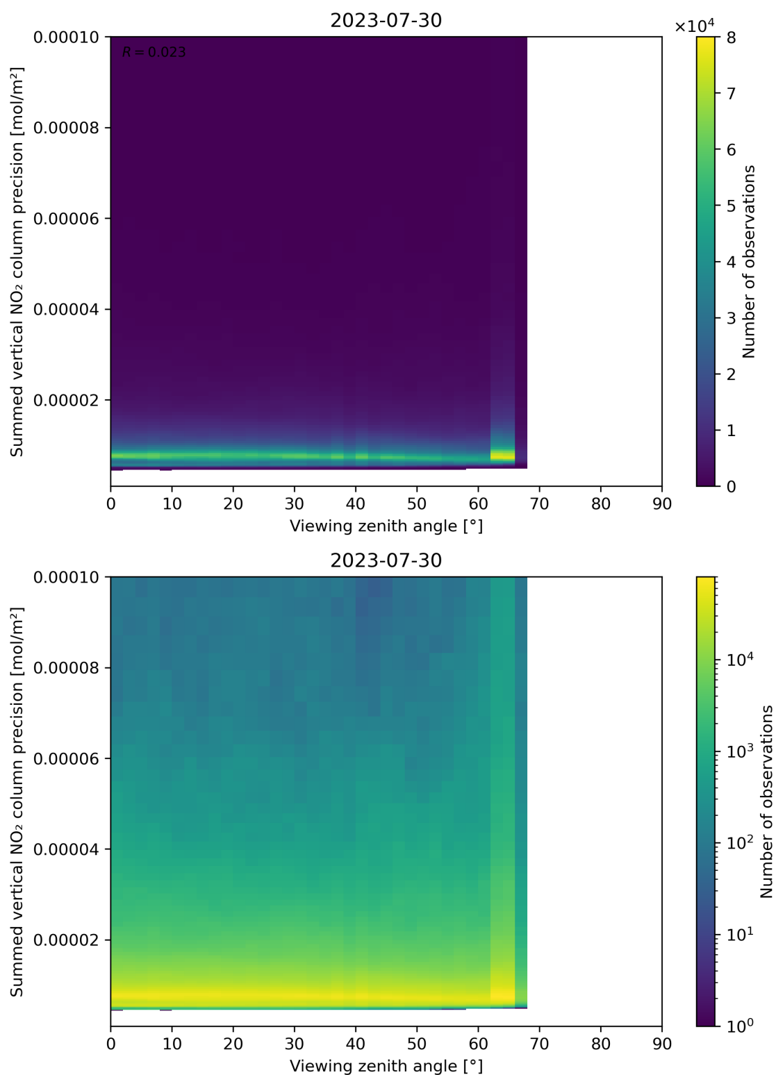
Figure 166: Scatter density plot of “Viewing zenith angle” against “Summed vertical NO 2 column precision” for 2023-07-29 to 2023-07-31.
