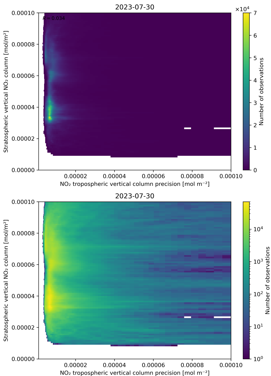
Figure 135: Scatter density plot of “NO 2 tropospheric vertical column precision” against “Stratospheric vertical NO 2 column” for 2023-07-29 to 2023-07-31.
