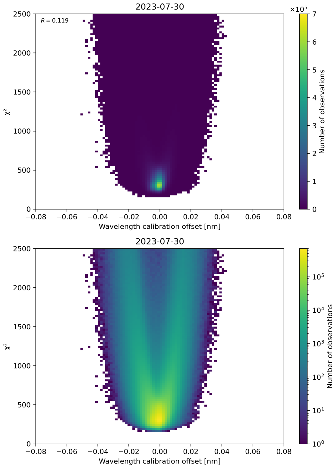
Figure 175: Scatter density plot of “Wavelength calibration offset” against “ \chi^2 ” for 2023-07-29 to 2023-07-31.
