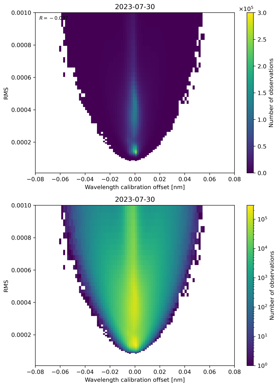
Figure 181: Scatter density plot of “Wavelength calibration offset” against “RMS” for 2023-07-29 to 2023-07-31.
