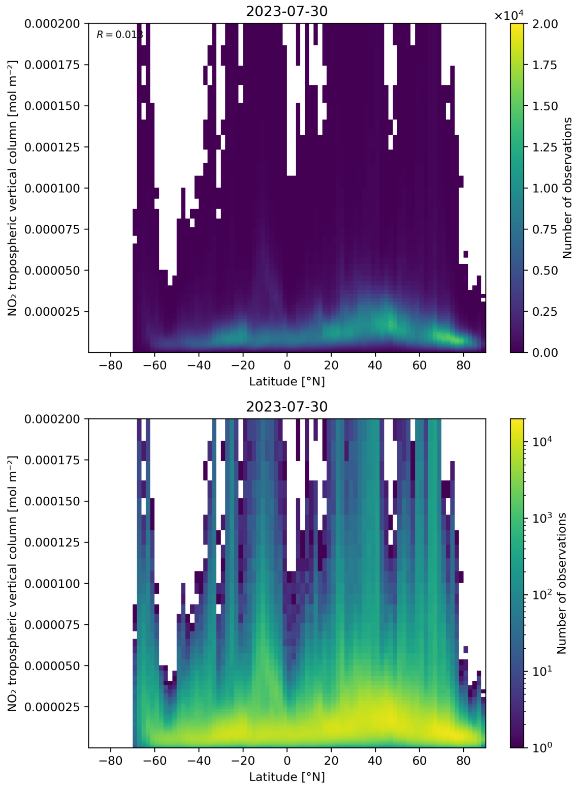
Figure 92: Scatter density plot of “Latitude” against “NO 2 tropospheric vertical column” for 2023-07-29 to 2023-07-31.
