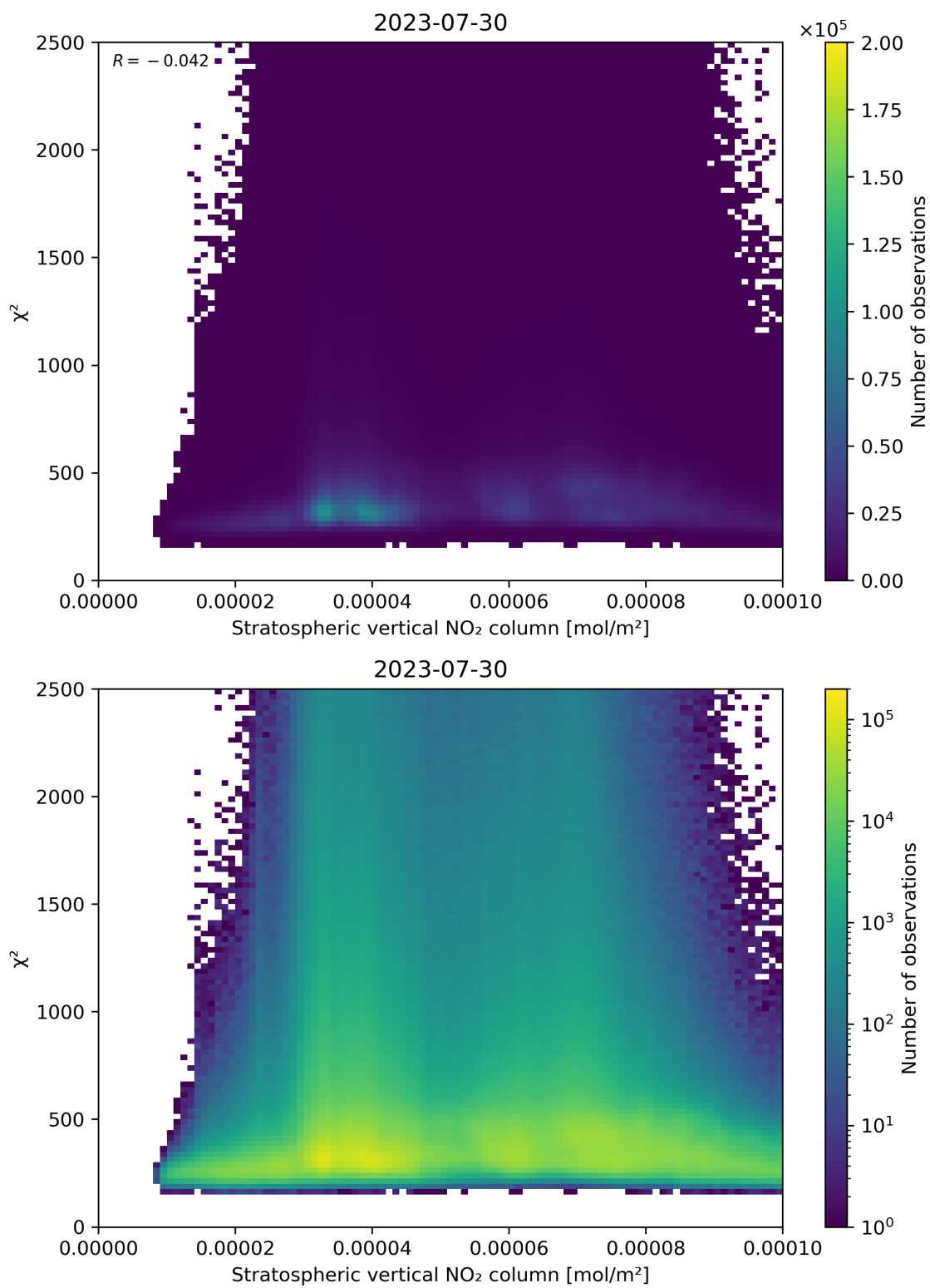
Figure 97: Scatter density plot of “Stratospheric vertical NO 2 column” against “ \chi^2 ” for 2023-07-29 to 2023-07-31.
