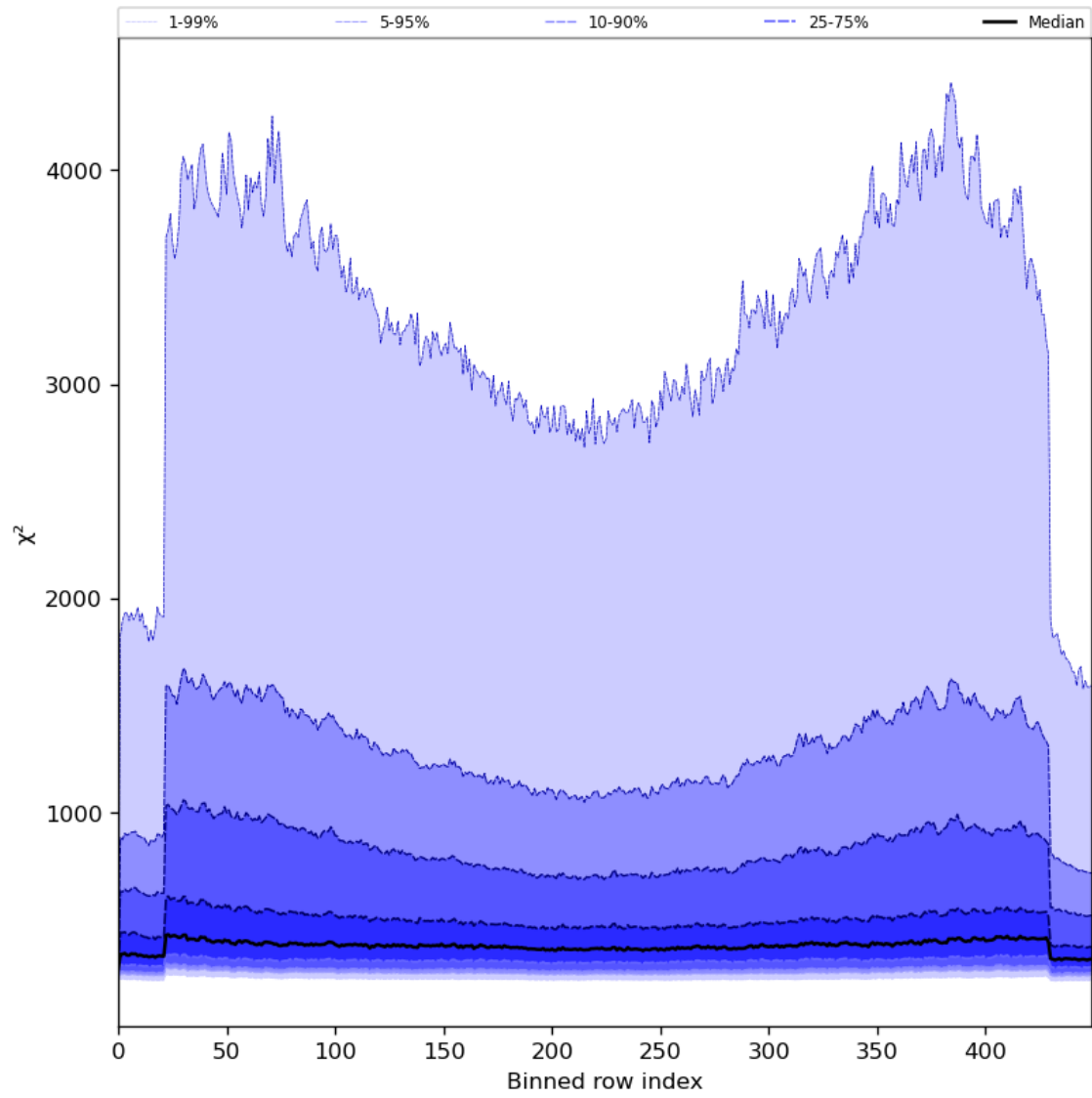
Figure 59: Along track statistics of “ \chi^2 ” for 2023-07-29 to 2023-07-31
