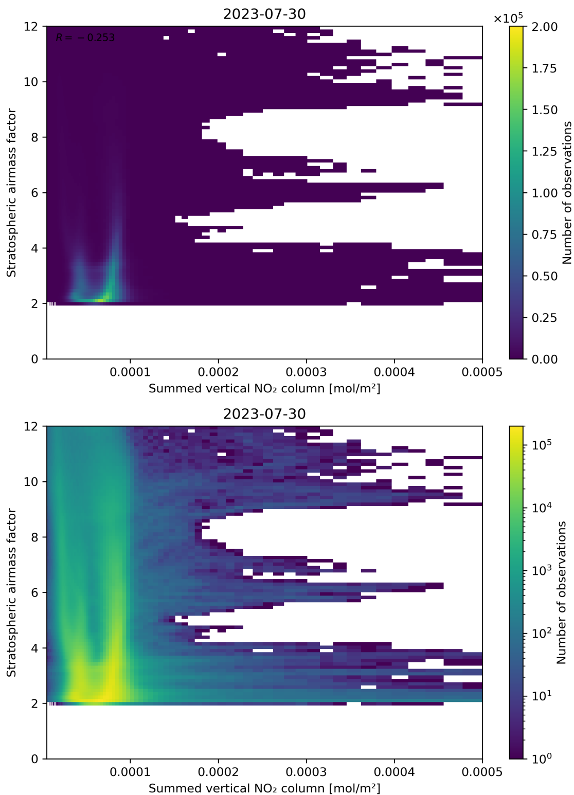
Figure 103: Scatter density plot of “Summed vertical NO 2 column” against “Stratospheric air mass factor” for 2023-07-29 to 2023-07-31.
