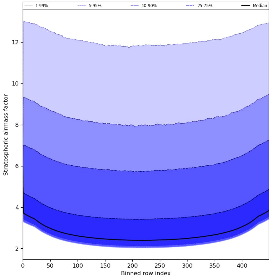
Figure 61: Along track statistics of “Stratospheric air mass factor” for 2023-07-29 to 2023-07-31
