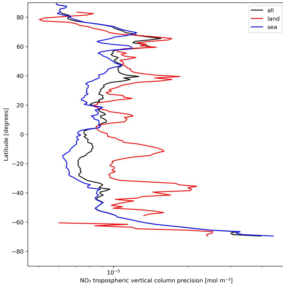
Figure 13: Zonal average of “NO 2 tropospheric vertical column precision” for 2023-07-29 to 2023-07-31.
