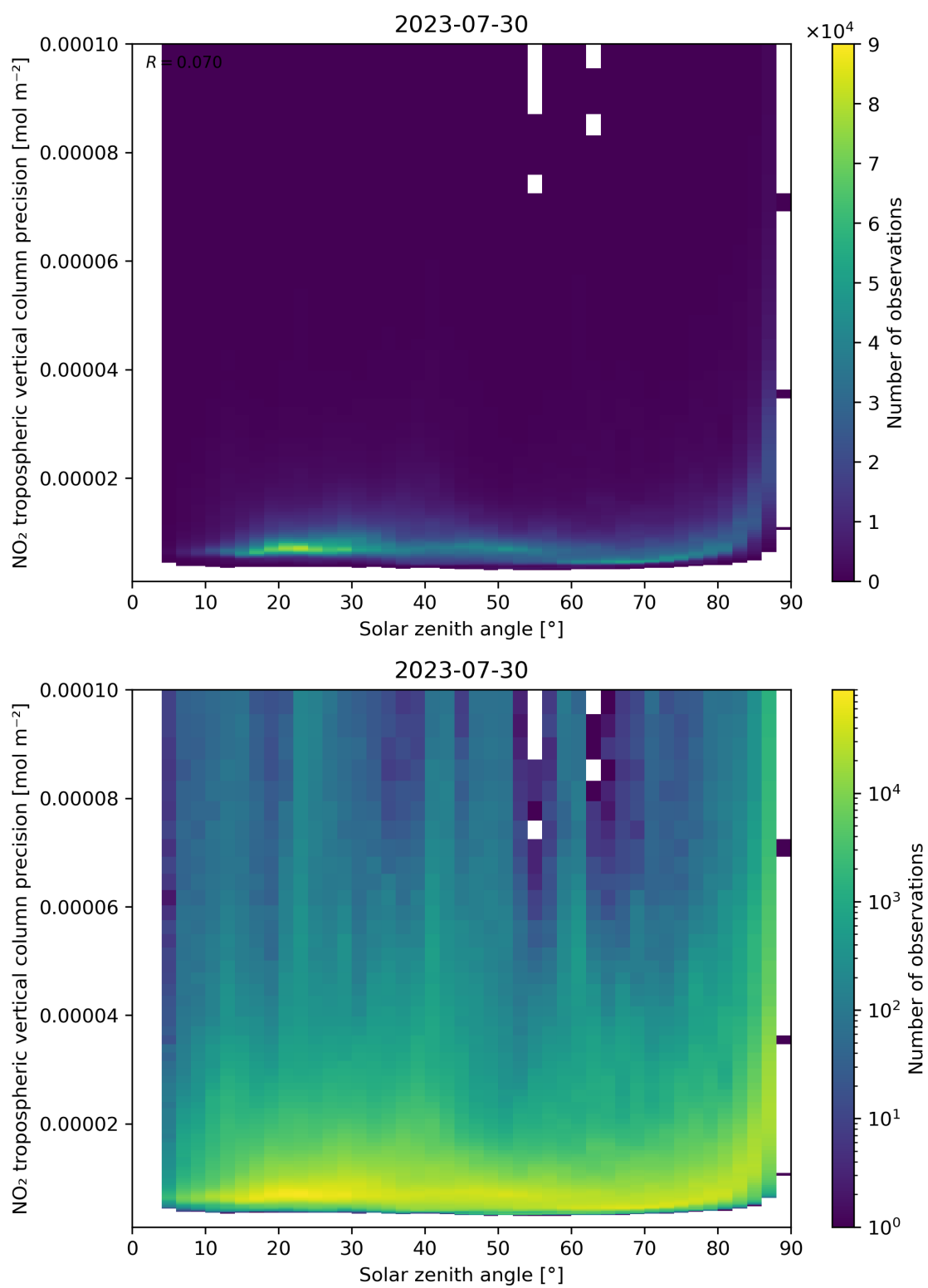
Figure 156: Scatter density plot of “Solar zenith angle” against “NO 2 tropospheric vertical column precision” for 2023-07-29 to 2023-07-31.
