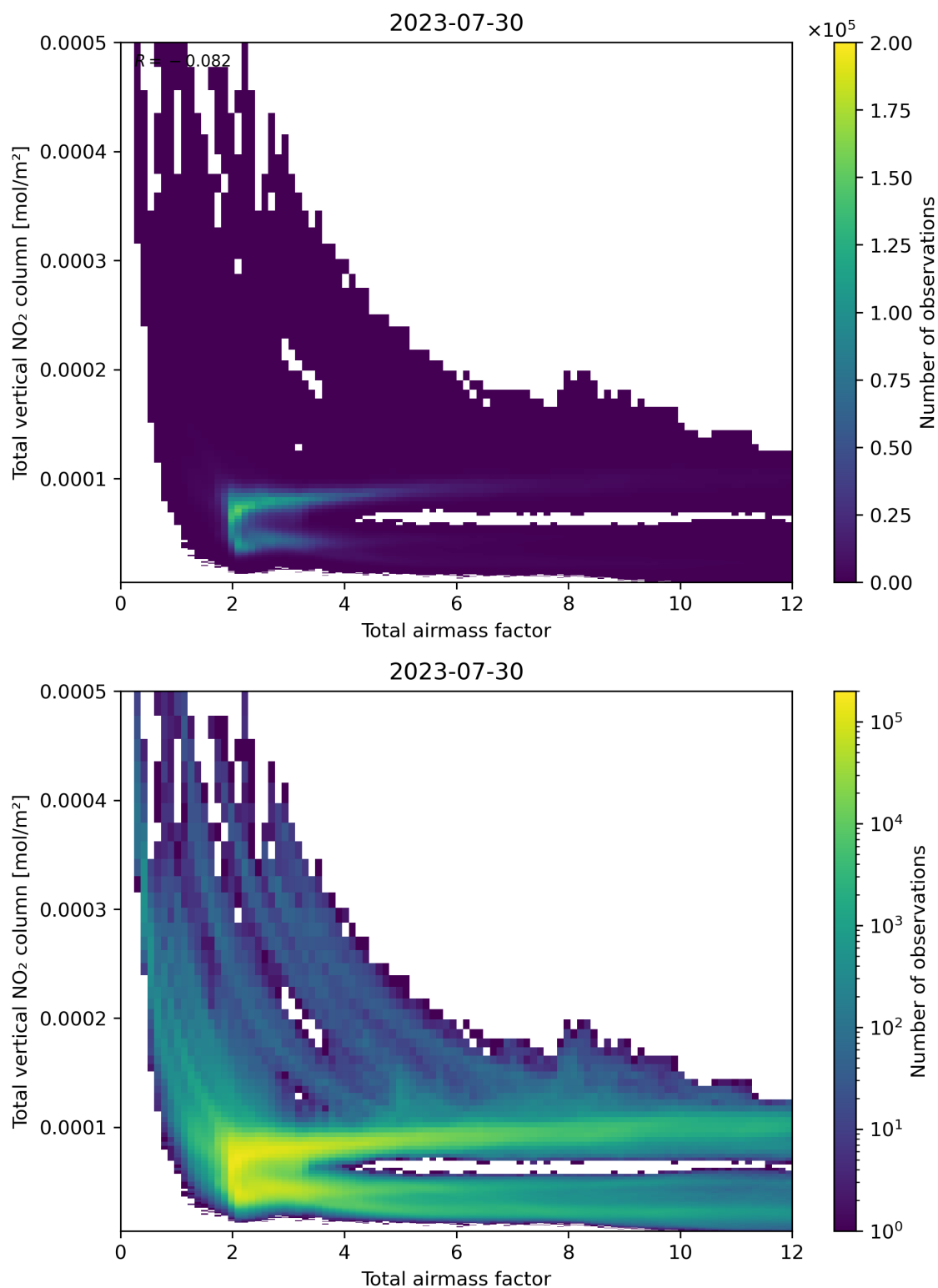
Figure 67: Scatter density plot of “Total airmass factor” against “Total vertical NO 2 column” for 2023-07-29 to 2023-07-31.
