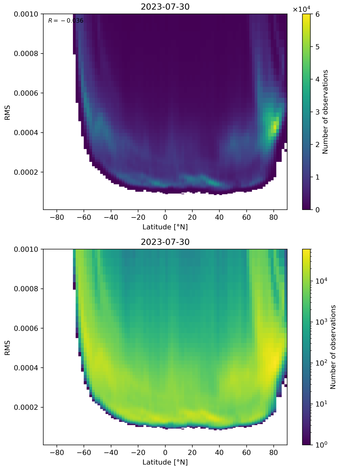
Figure 94: Scatter density plot of “Latitude” against “RMS” for 2023-07-29 to 2023-07-31.
