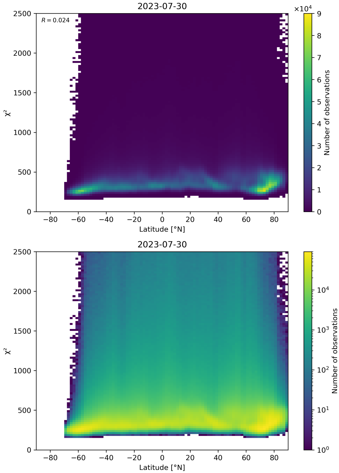
Figure 86: Scatter density plot of “Latitude” against “ \chi^2 ” for 2023-07-29 to 2023-07-31.
