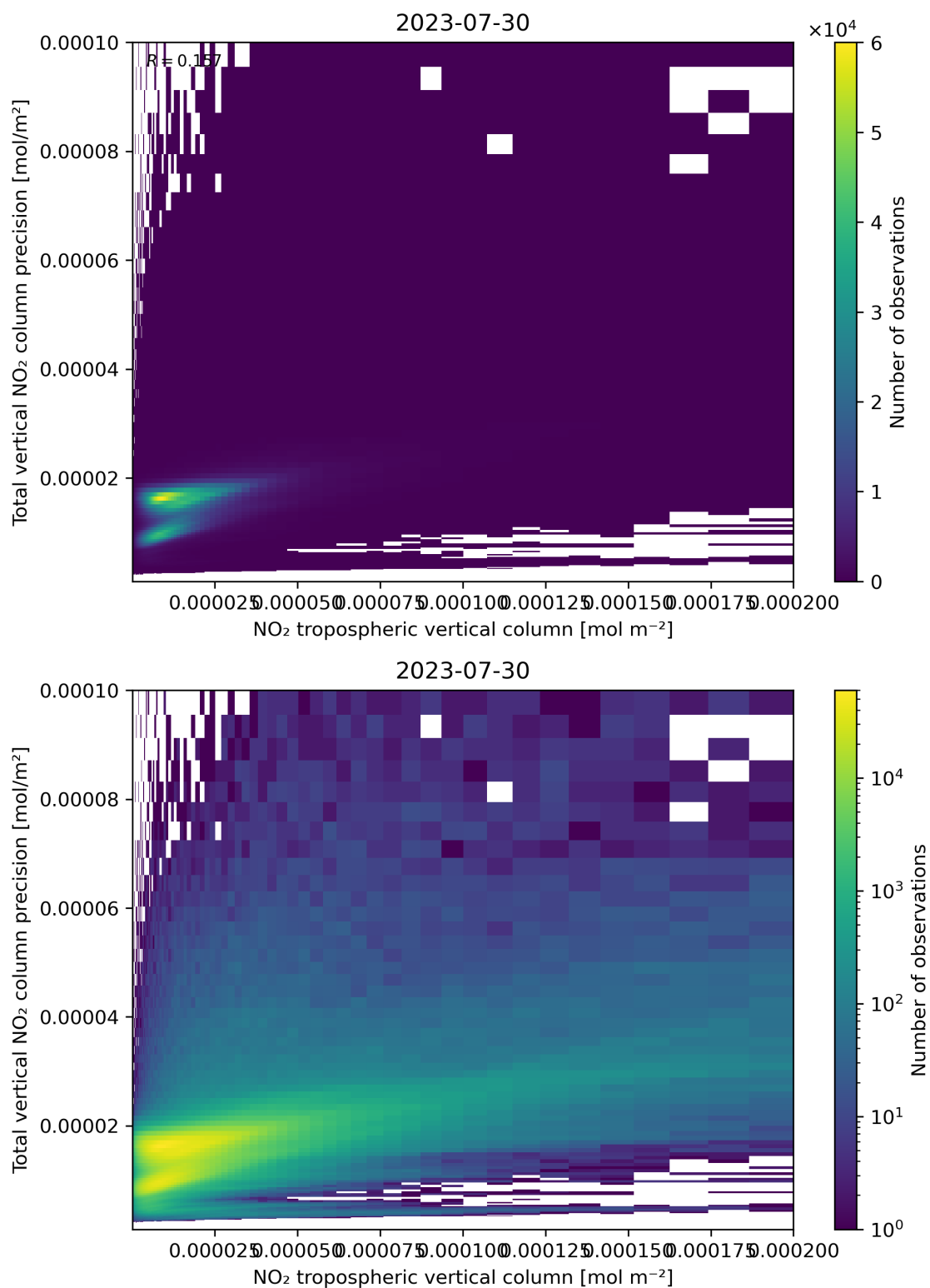
Figure 129: Scatter density plot of “NO 2 tropospheric vertical column” against “Total vertical NO 2 column precision” for 2023-07-29 to 2023-07-31.
