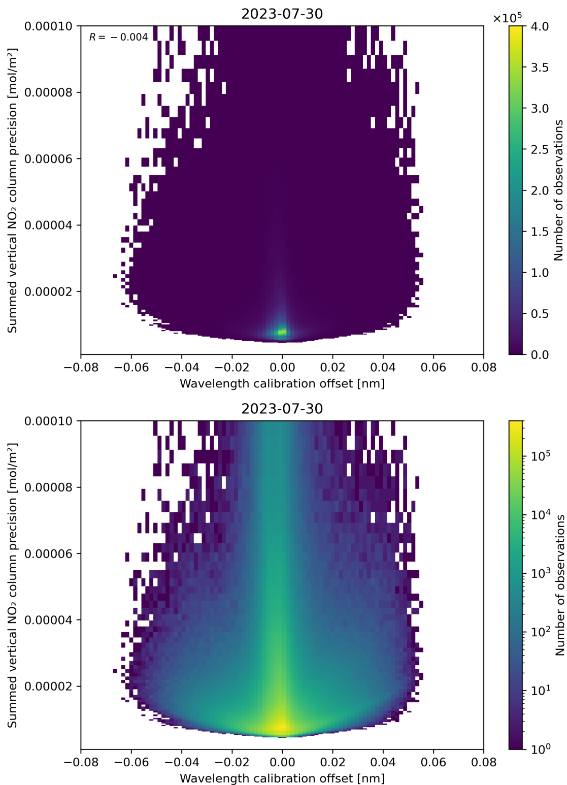
Figure 178: Scatter density plot of “Wavelength calibration offset” against “Summed vertical NO 2 column precision” for 2023-07-29 to 2023-07-31.
