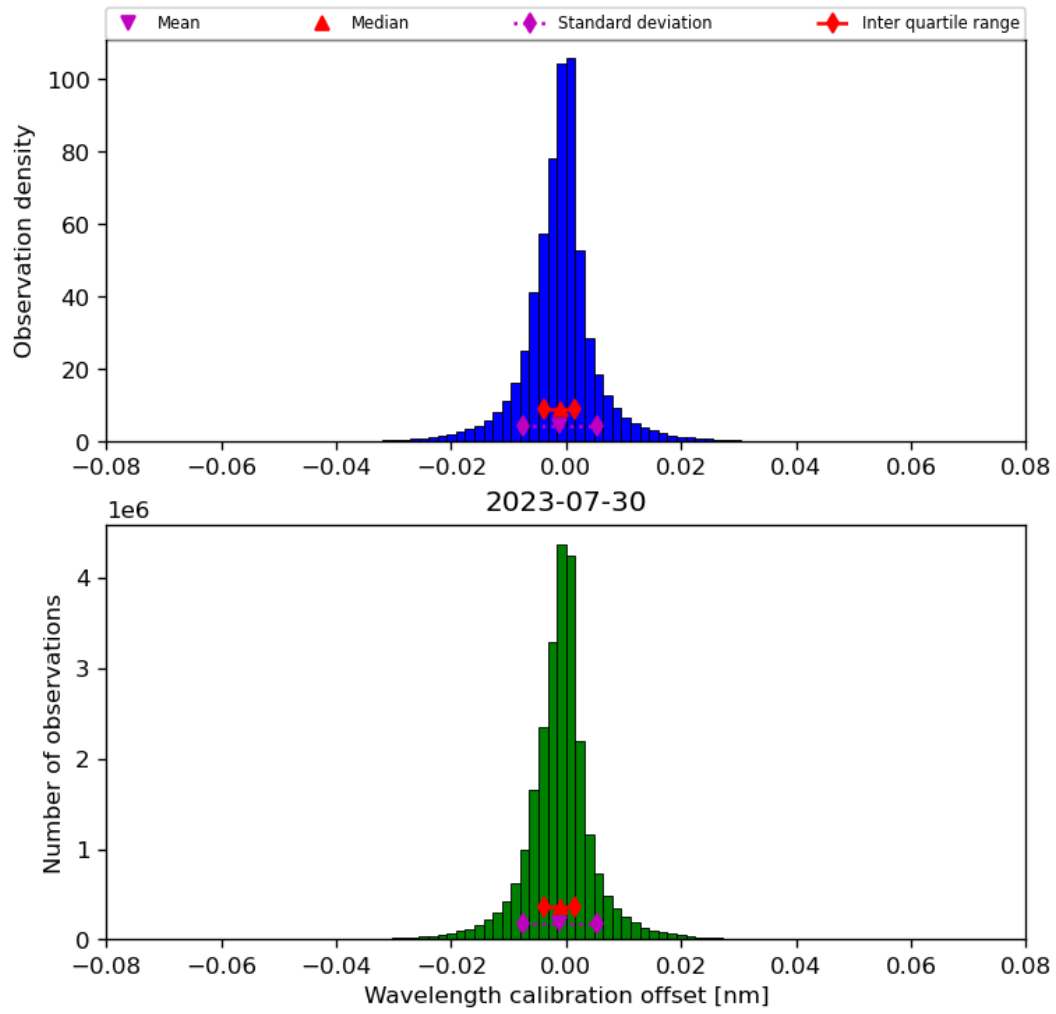
Figure 35: Histogram of “Wavelength calibration offset” for 2023-07-29 to 2023-07-31
