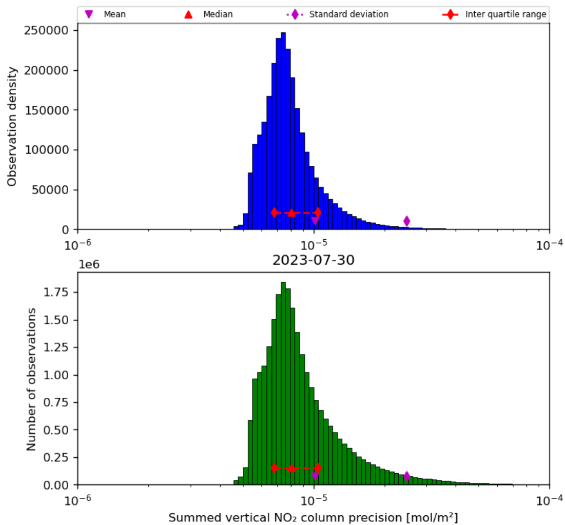
Figure 41: Histogram of “Summed vertical NO 2 column precision” for 2023-07-29 to 2023-07-31
