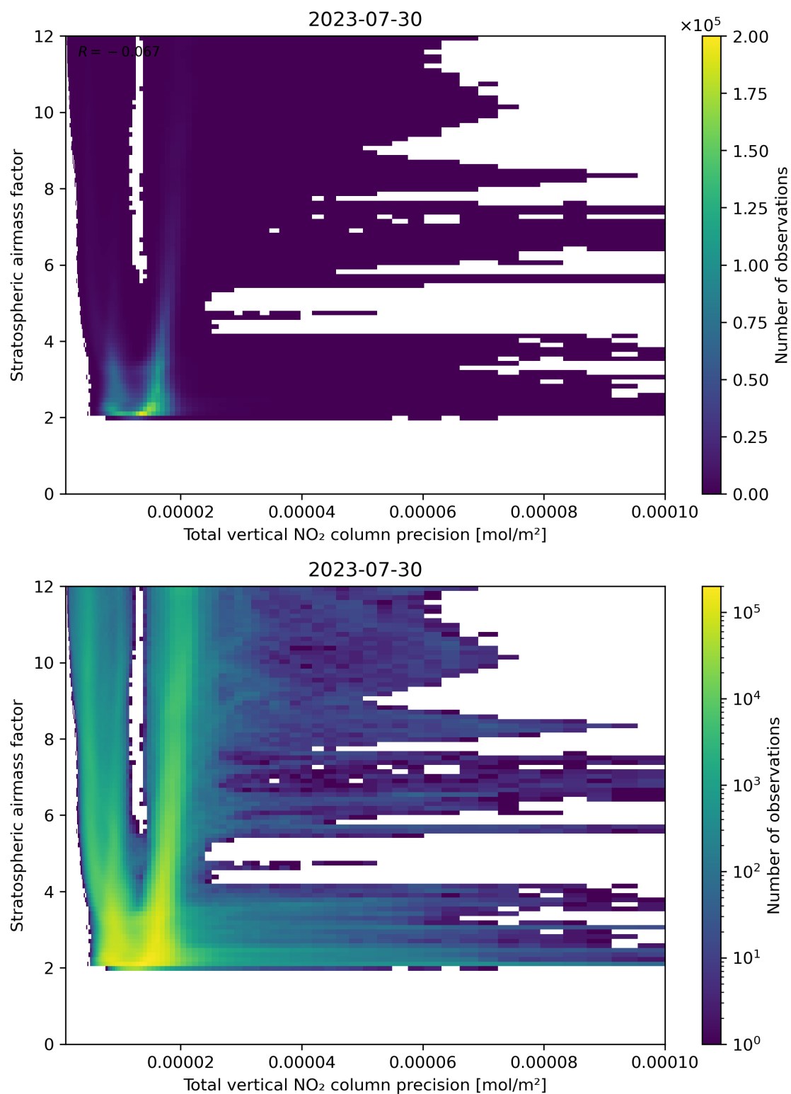
Figure 115: Scatter density plot of “Total vertical NO 2 column precision” against “Stratospheric air mass factor” for 2023-07-29 to 2023-07-31.
