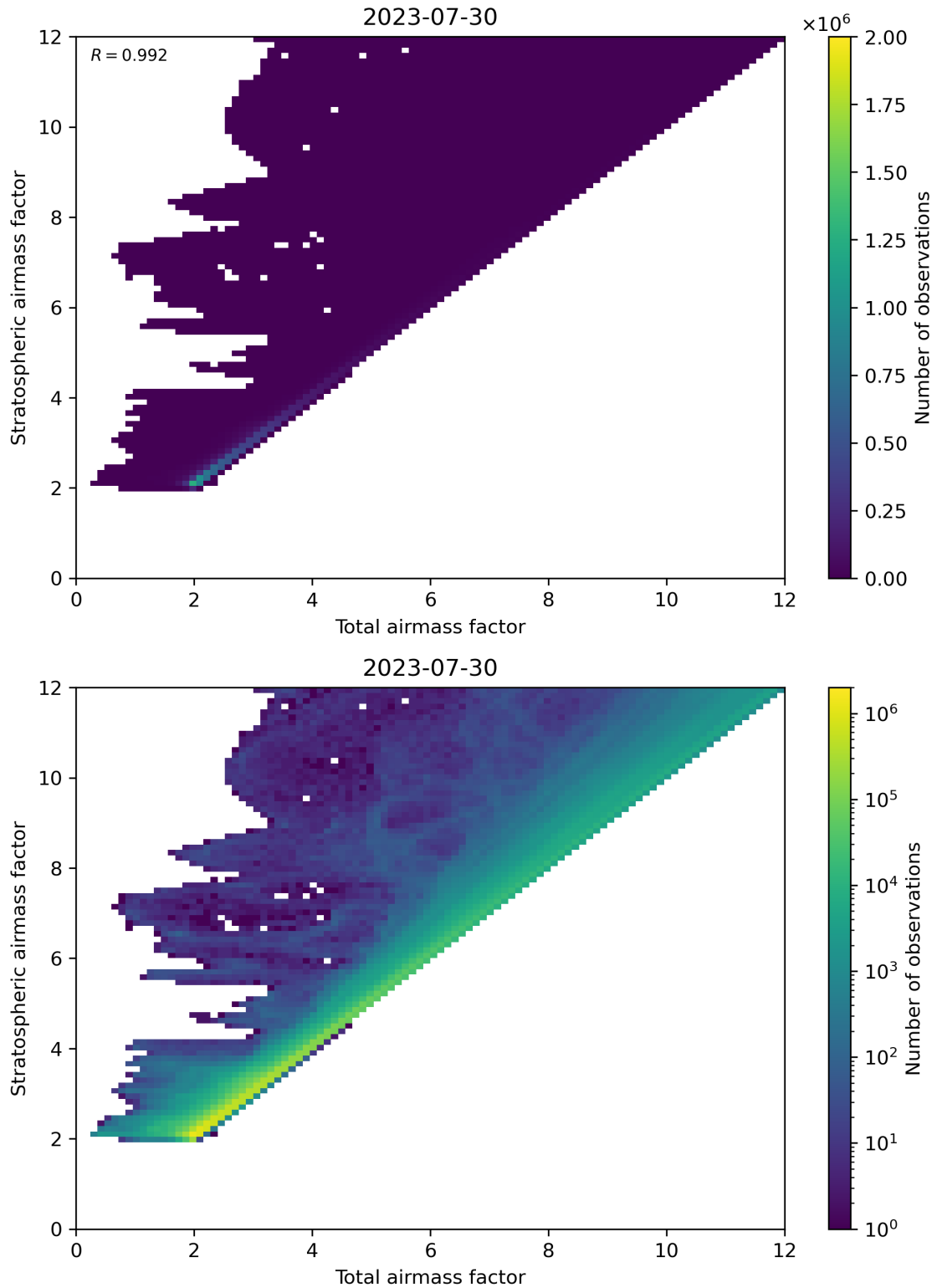
Figure 62: Scatter density plot of “Total airmass factor” against “Stratospheric airmass factor” for 2023-07-29 to 2023-07-31.
