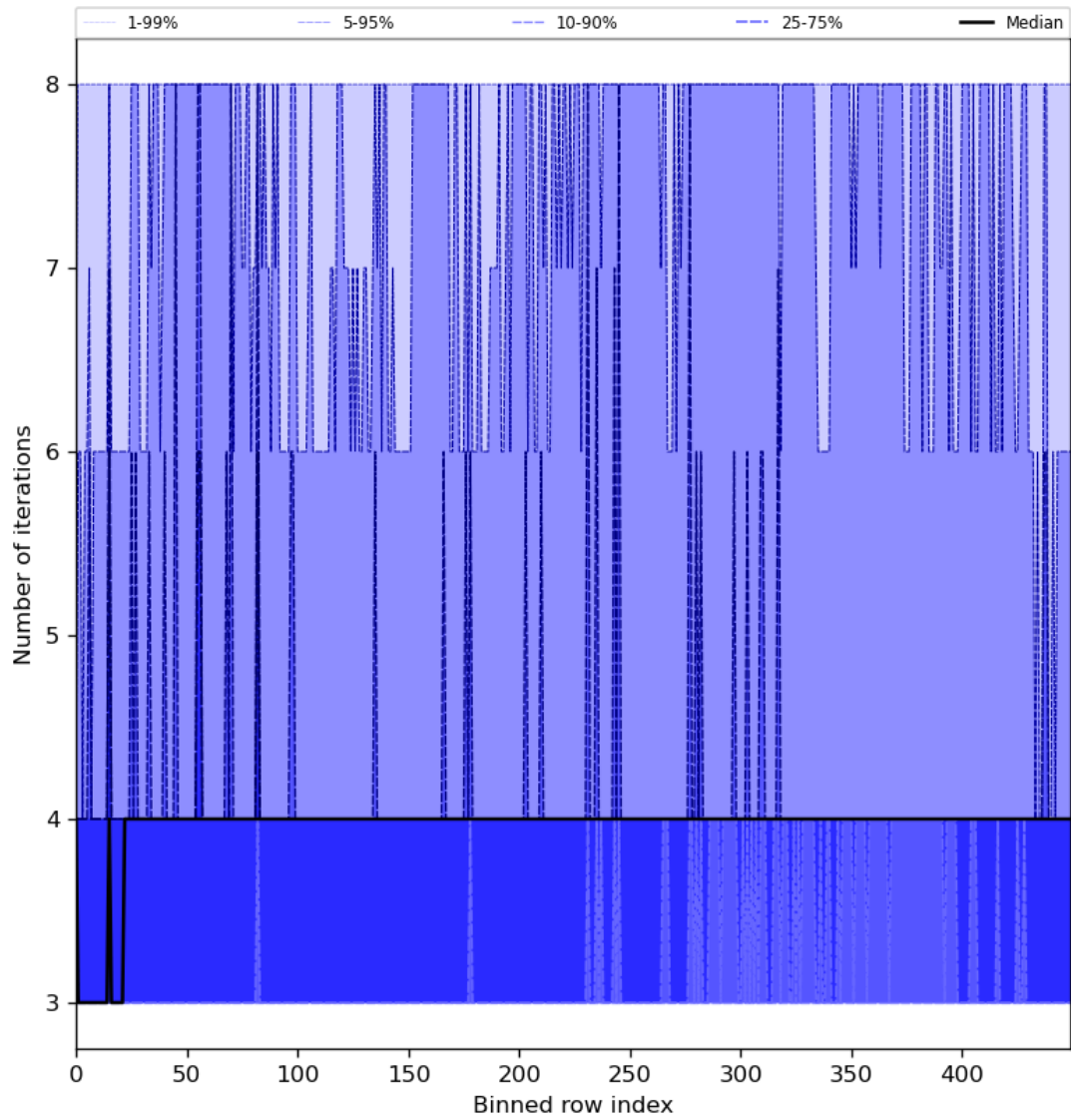
Figure 51: Along track statistics of “Number of iterations” for 2023-07-29 to 2023-07-31
