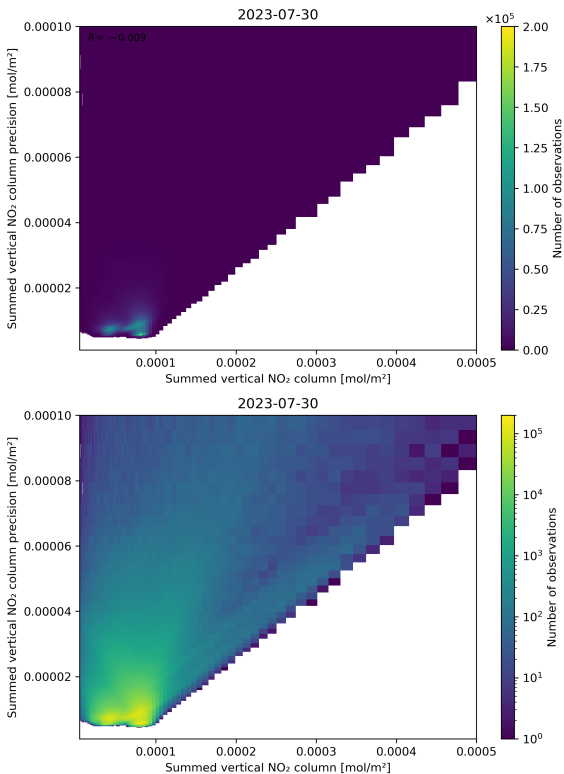
Figure 105: Scatter density plot of “Summed vertical NO 2 column” against “Summed vertical NO 2 column precision” for 2023-07-29 to 2023-07-31.
