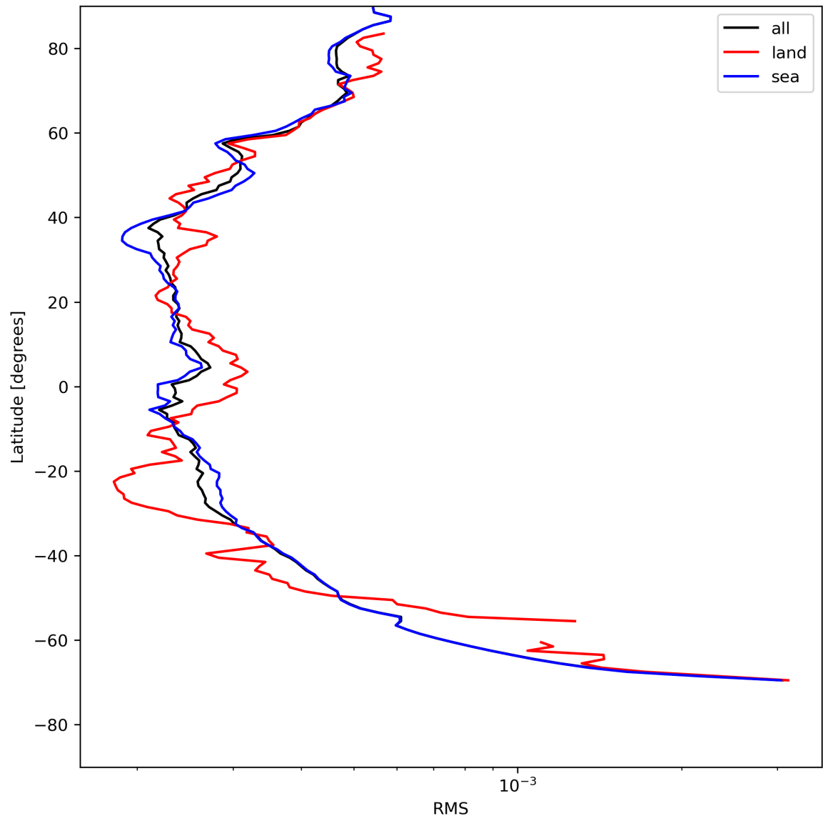
Figure 26: Zonal average of “RMS” for 2023-07-29 to 2023-07-31.
