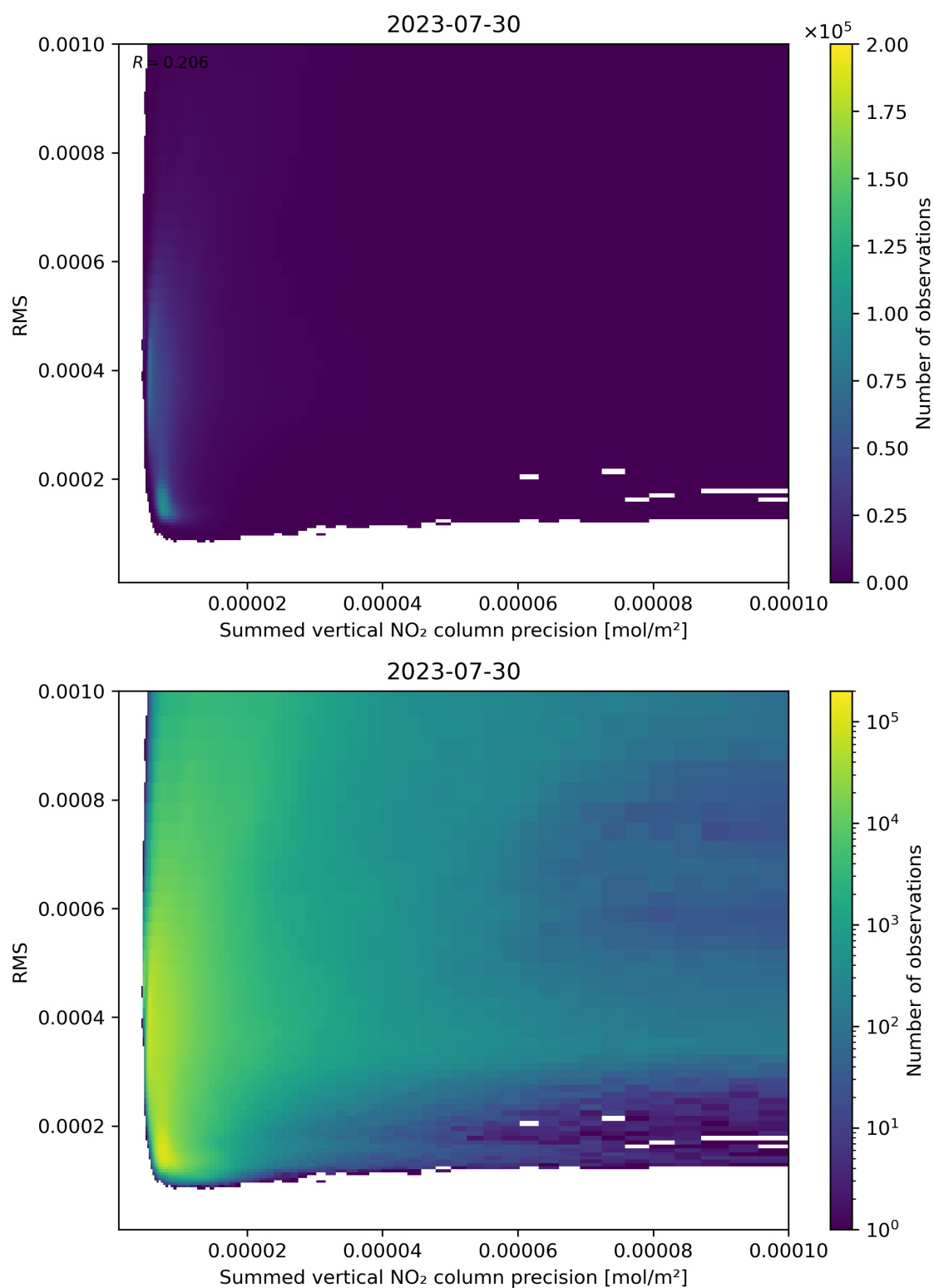
Figure 108: Scatter density plot of “Summed vertical NO 2 column precision” against “RMS” for 2023-07-29 to 2023-07-31.
