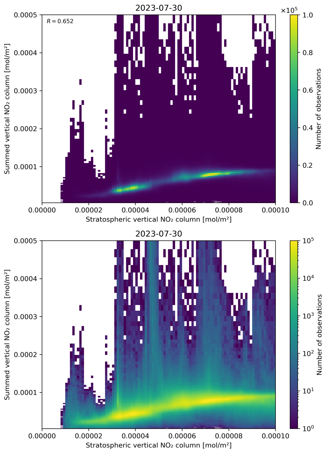
Figure 98: Scatter density plot of “Stratospheric vertical NO 2 column” against “Summed vertical NO 2 column” for 2023-07-29 to 2023-07-31.
