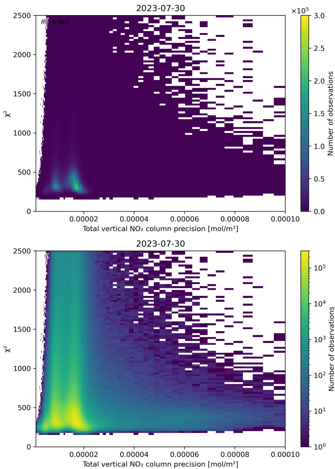
Figure 116: Scatter density plot of “Total vertical NO 2 column precision” against “ \chi^2 ” for 2023-07-29 to 2023-07-31.
