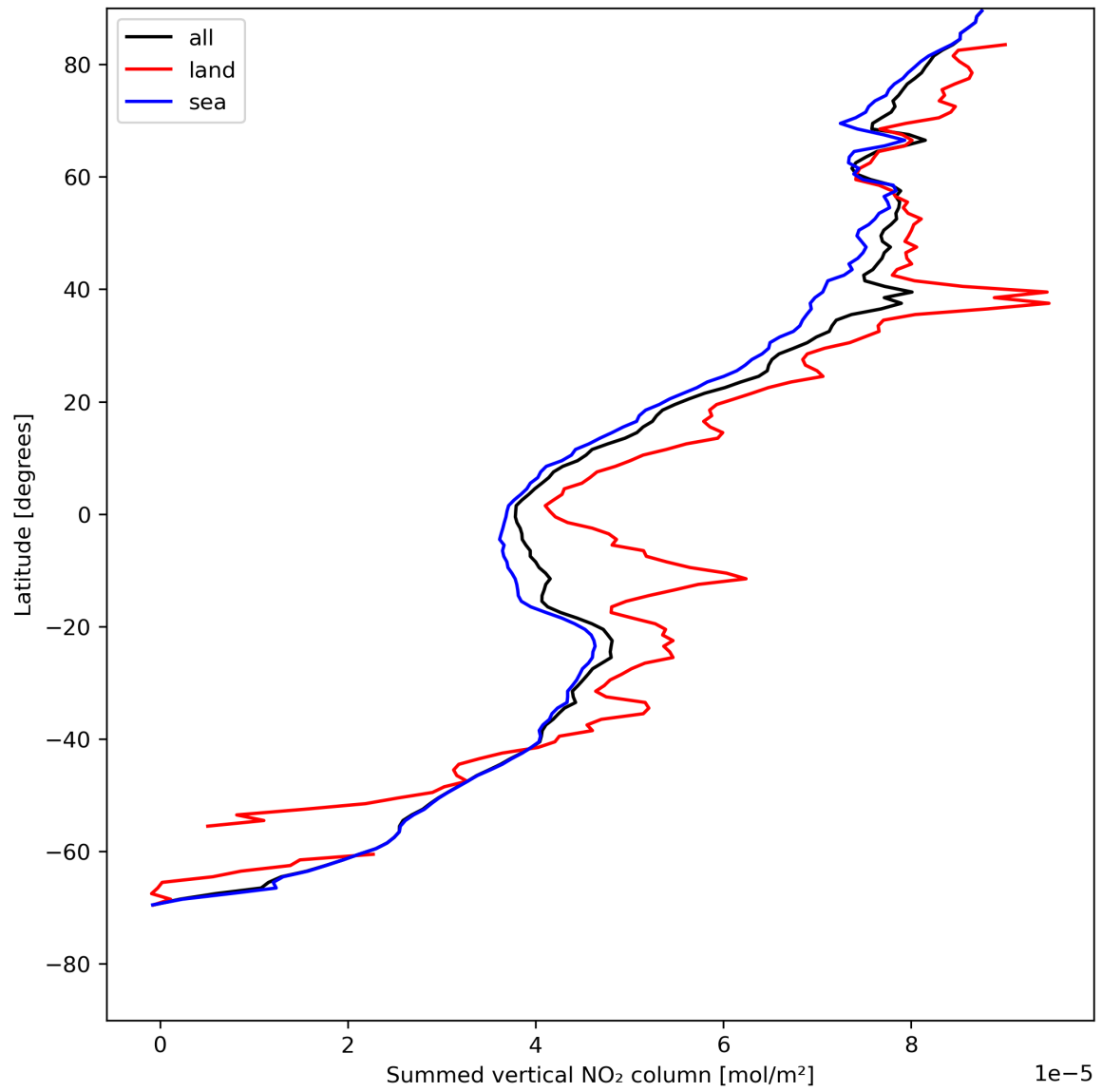
Figure 23: Zonal average of “Summed vertical NO 2 column” for 2023-07-29 to 2023-07-31.
