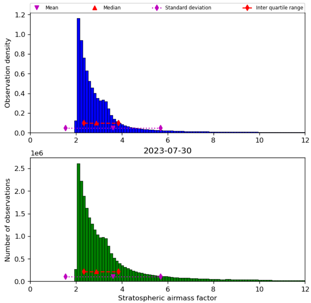
Figure 44: Histogram of “Stratospheric airmass factor” for 2023-07-29 to 2023-07-31
