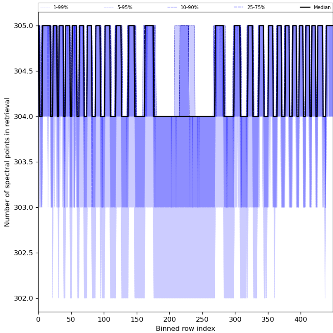
Figure 50: Along track statistics of “Number of spectral points in retrieval” for 2023-07-29 to 2023-07-31
