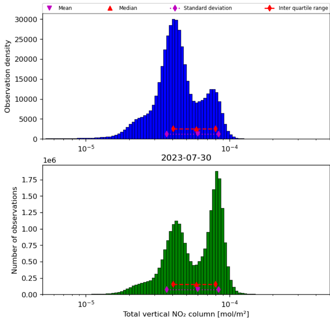
Figure 38: Histogram of “Total vertical NO 2 column” for 2023-07-29 to 2023-07-31
