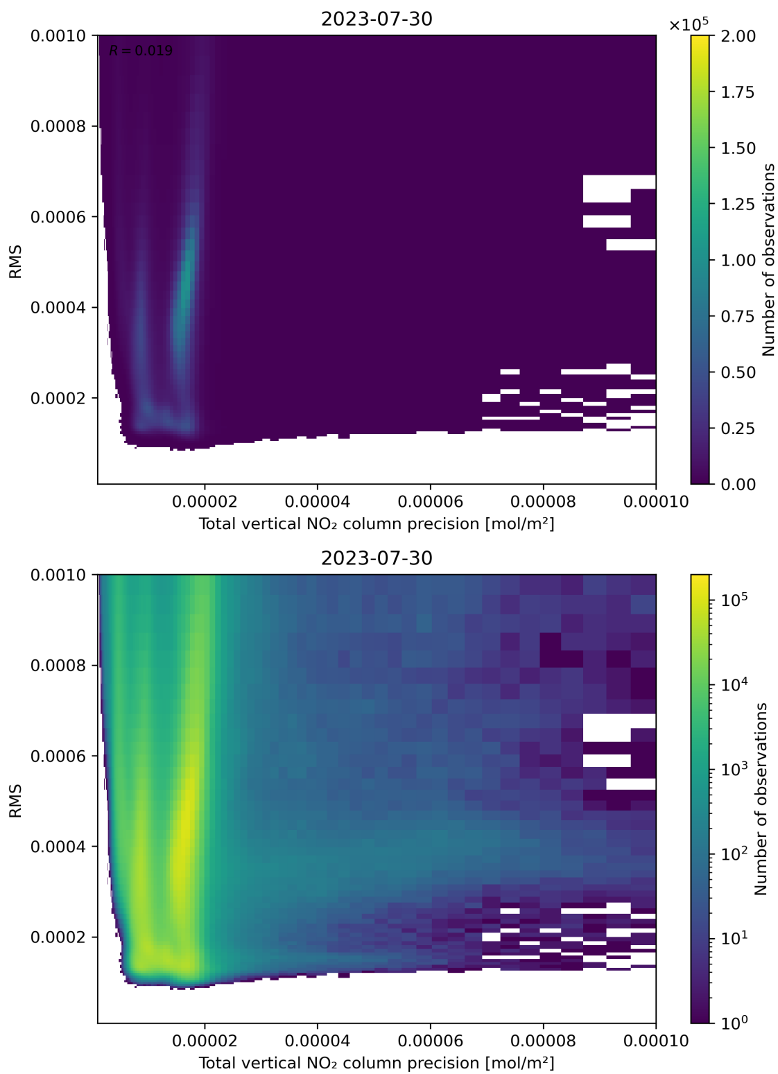
Figure 119: Scatter density plot of “Total vertical NO 2 column precision” against “RMS” for 2023-07-29 to 2023-07-31.
