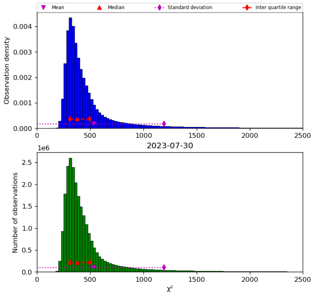
Figure 42: Histogram of " \chi^2 " for 2023-07-29 to 2023-07-31
