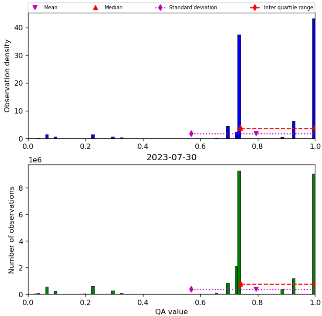
Figure 28: Histogram of “QA value” for 2023-07-29 to 2023-07-31
