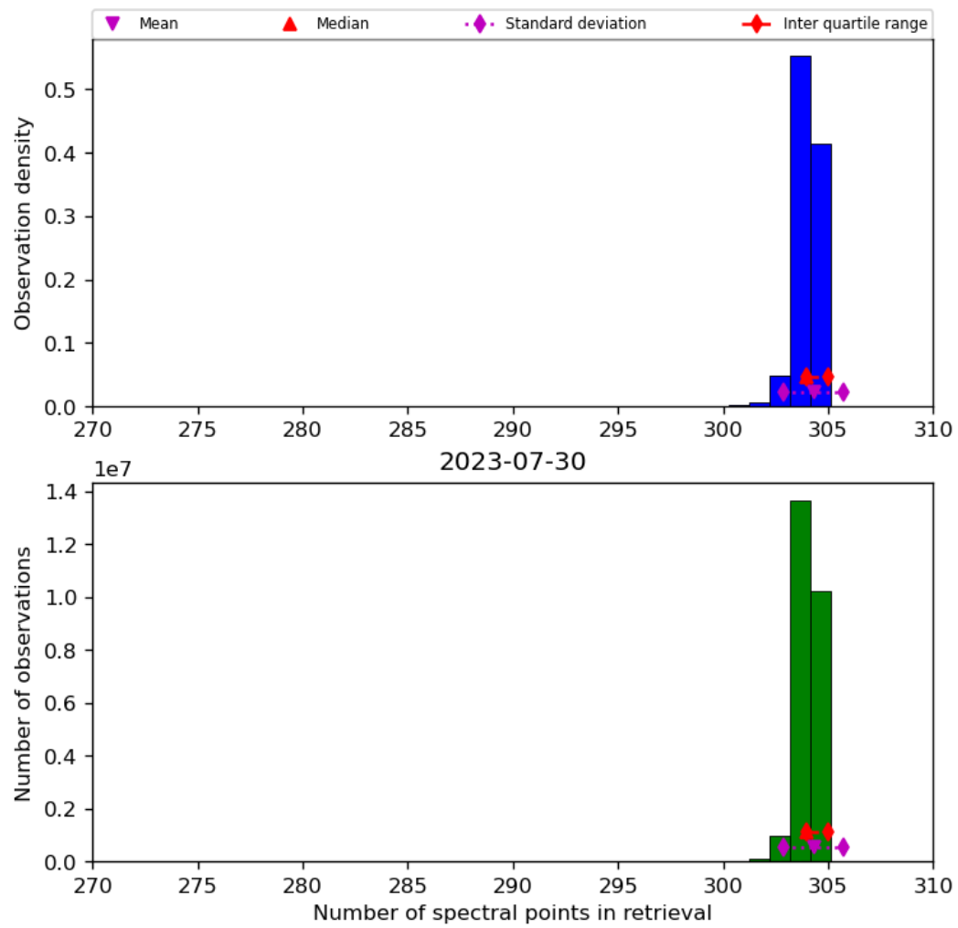
Figure 33: Histogram of “Number of spectral points in retrieval” for 2023-07-29 to 2023-07-31
