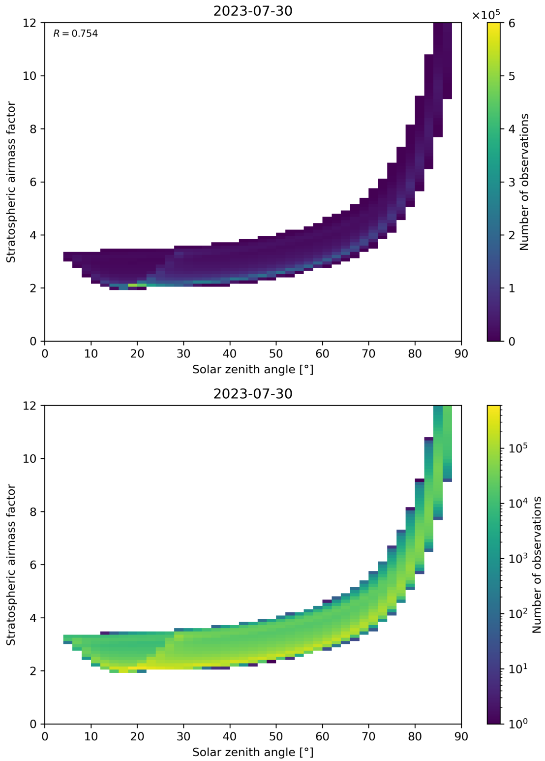
Figure 145: Scatter density plot of “Solar zenith angle” against “Stratospheric airmass factor” for 2023-07-29 to 2023-07-31.
