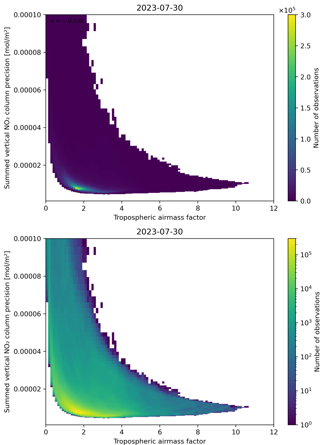
Figure 76: Scatter density plot of “Tropospheric air mass factor” against “Summed vertical NO 2 column precision” for 2023-07-29 to 2023-07-31.
