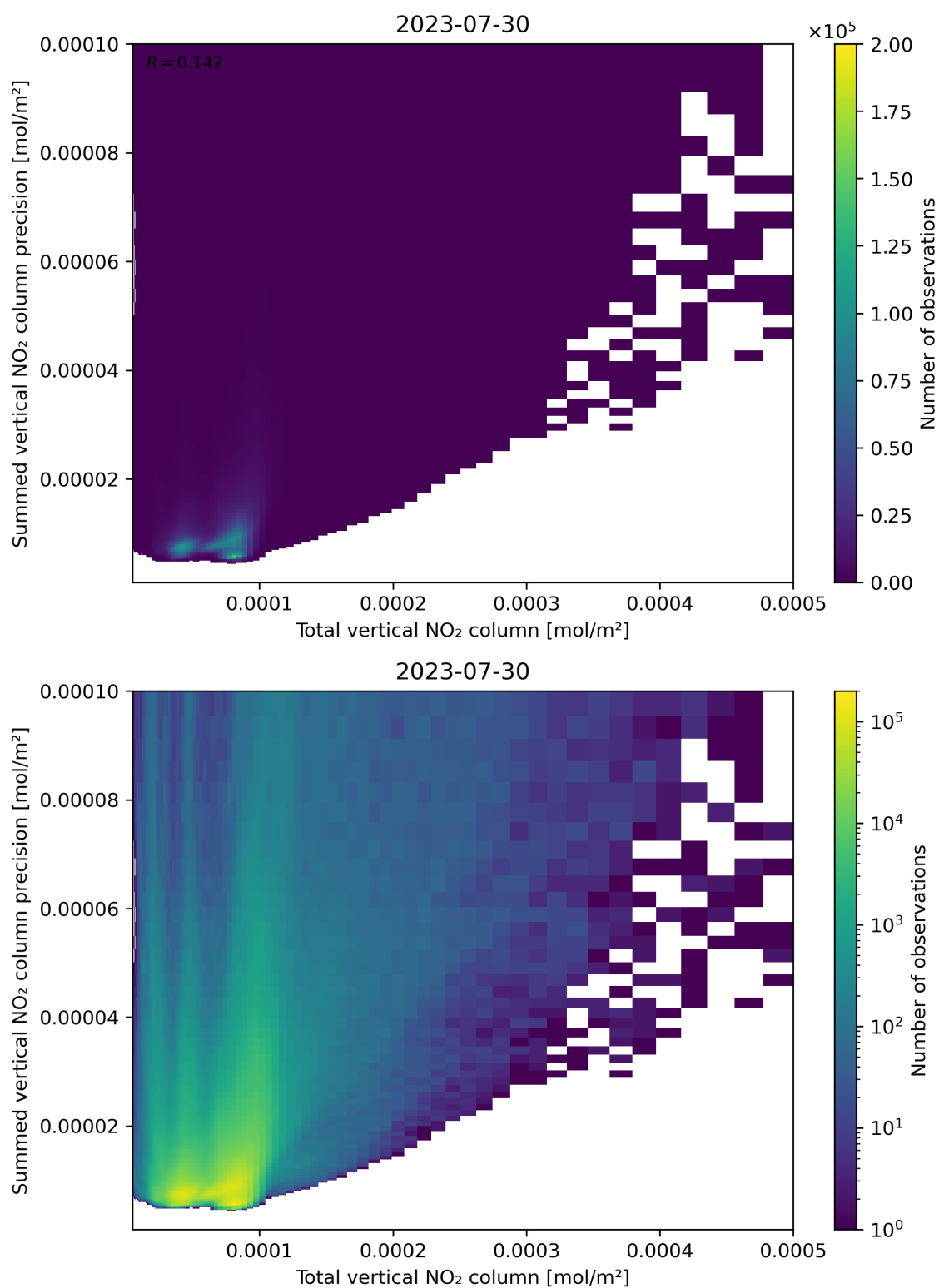
Figure 113: Scatter density plot of “Total vertical NO 2 column” against “Summed vertical NO 2 column precision” for 2023-07-29 to 2023-07-31.
