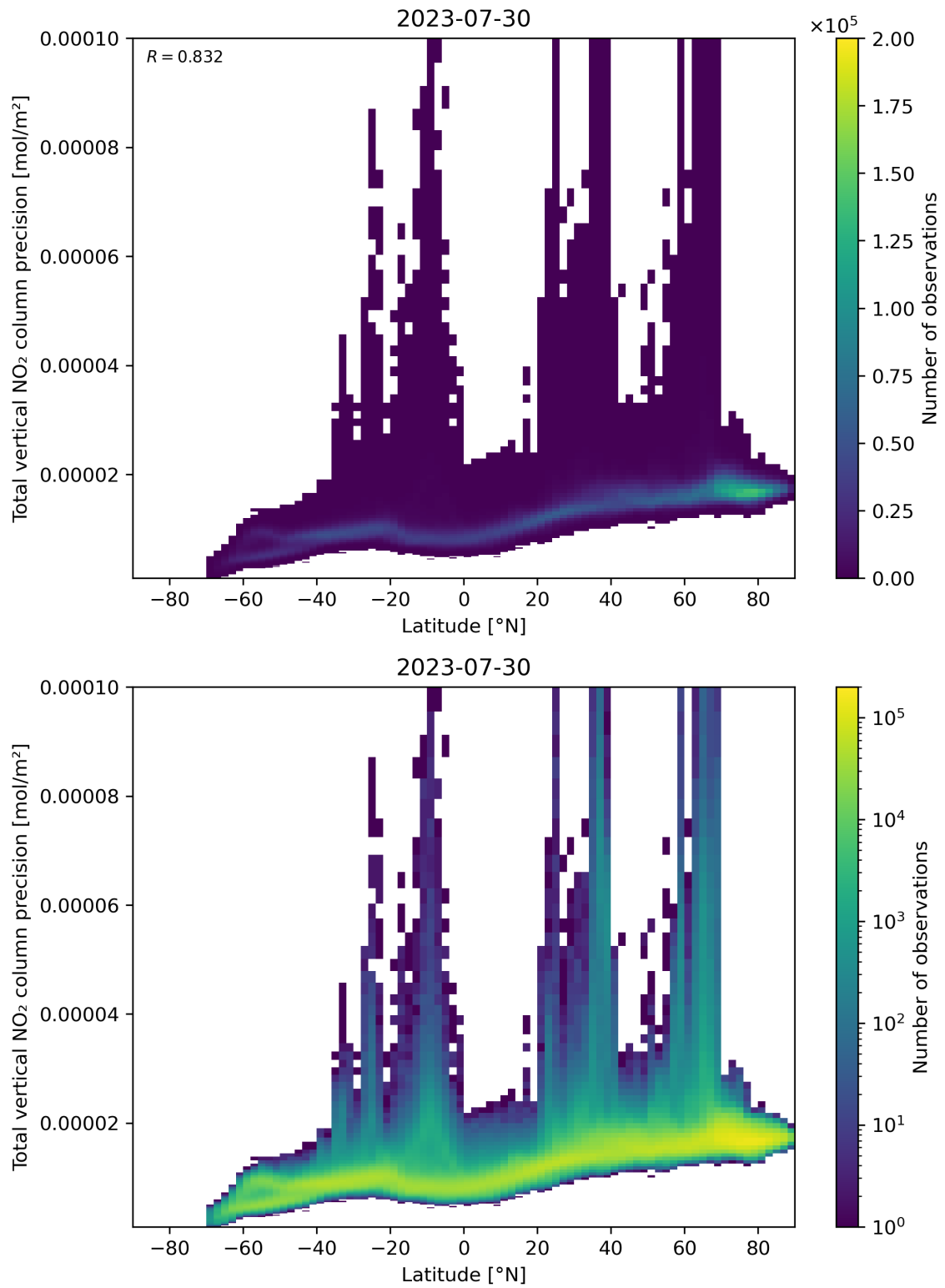
Figure 91: Scatter density plot of “Latitude” against “Total vertical NO 2 column precision” for 2023-07-29 to 2023-07-31.
