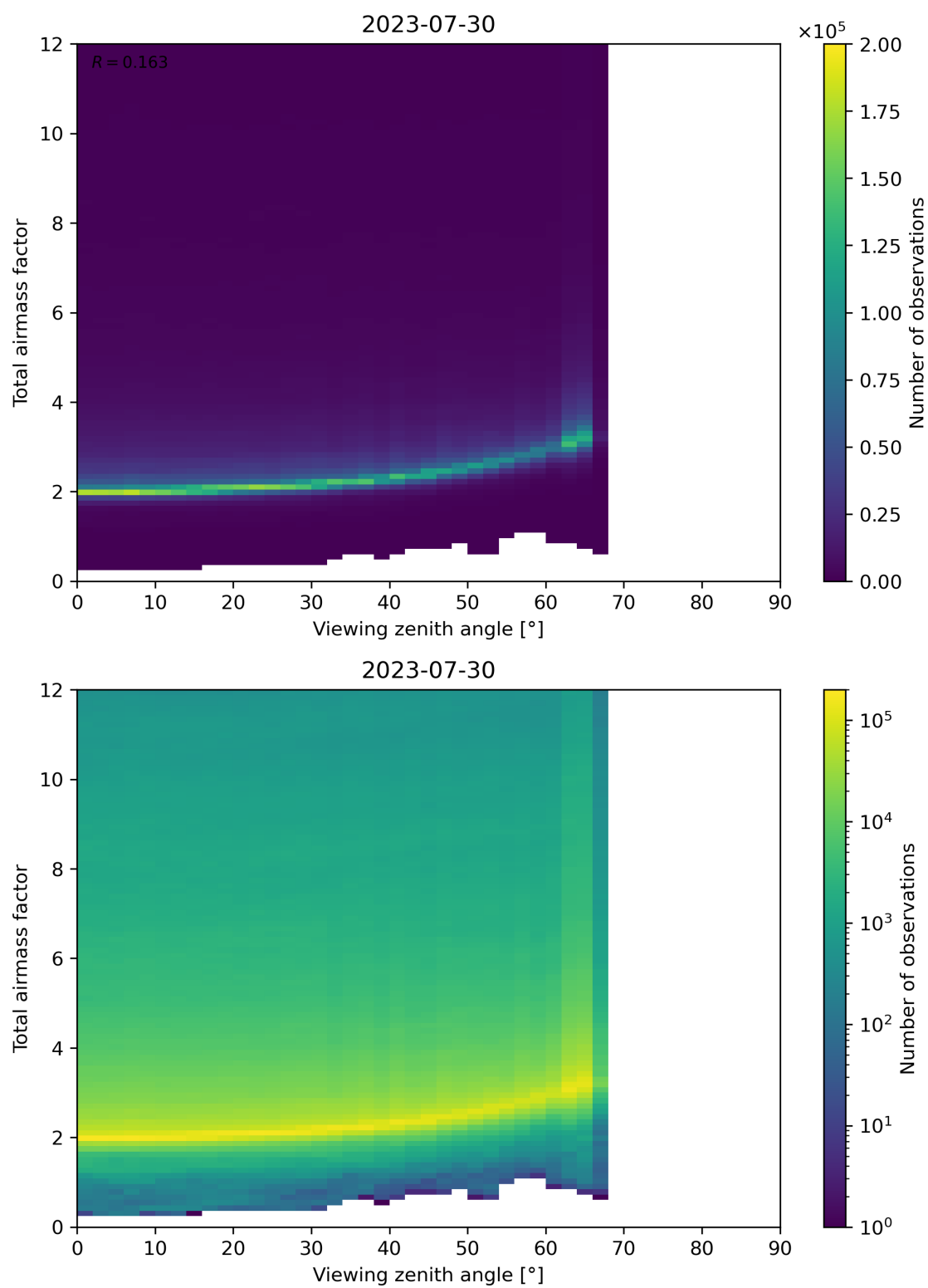
Figure 160: Scatter density plot of “Viewing zenith angle” against “Total airmass factor” for 2023-07-29 to 2023-07-31.
