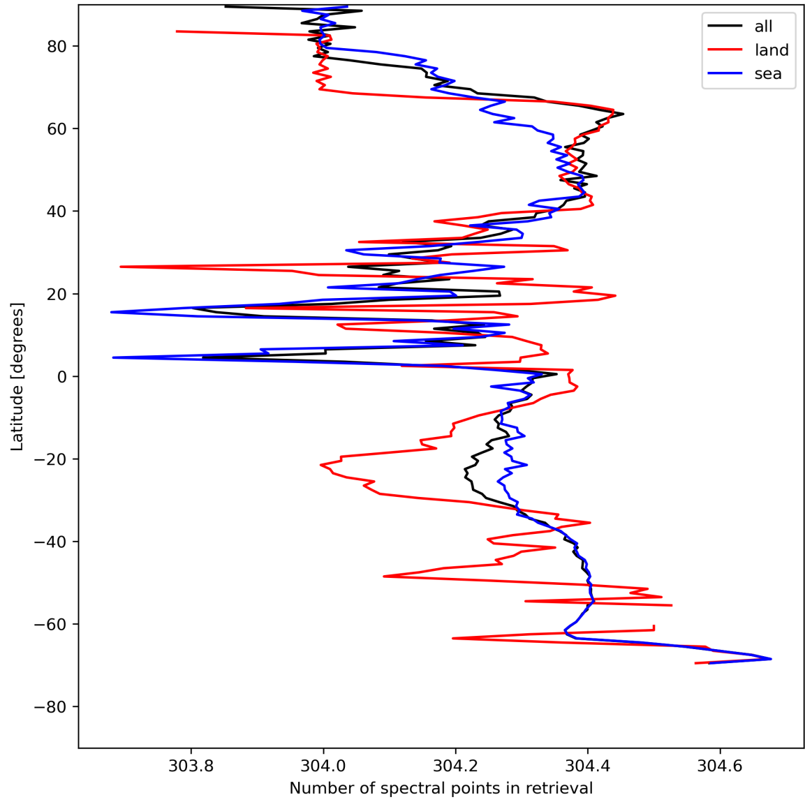
Figure 16: Zonal average of “Number of spectral points in retrieval” for 2023-07-29 to 2023-07-31.
