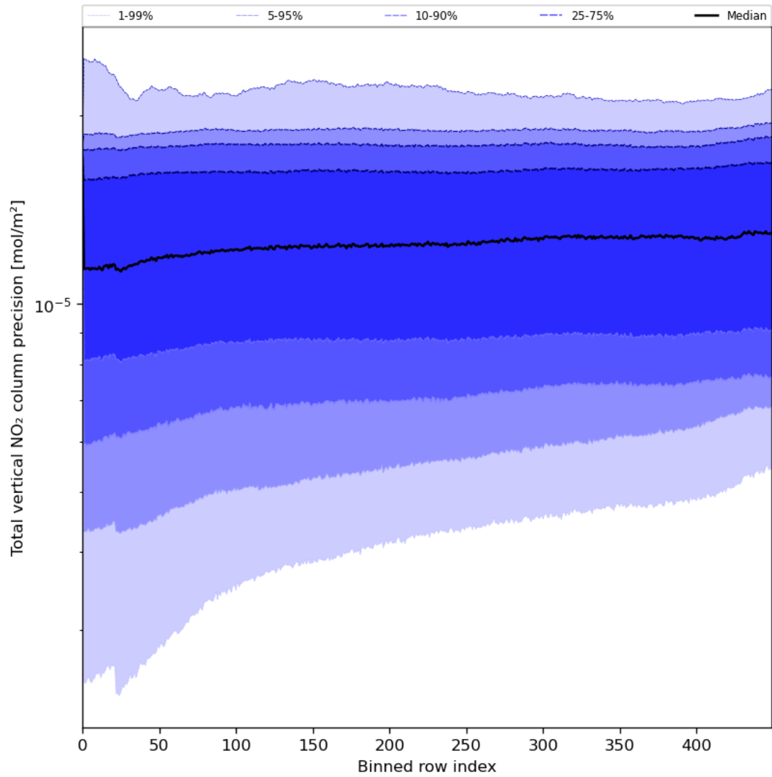
Figure 56: Along track statistics of “Total vertical NO 2 column precision” for 2023-07-29 to 2023-07-31
