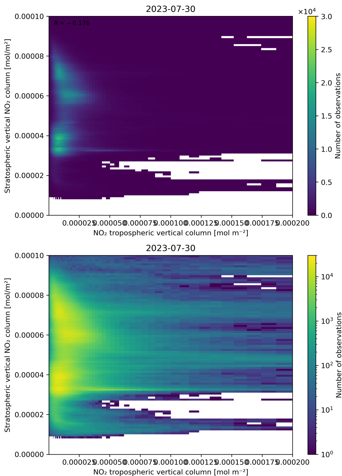
Figure 125: Scatter density plot of “NO 2 tropospheric vertical column” against “Stratospheric vertical NO 2 column” for 2023-07-29 to 2023-07-31.
