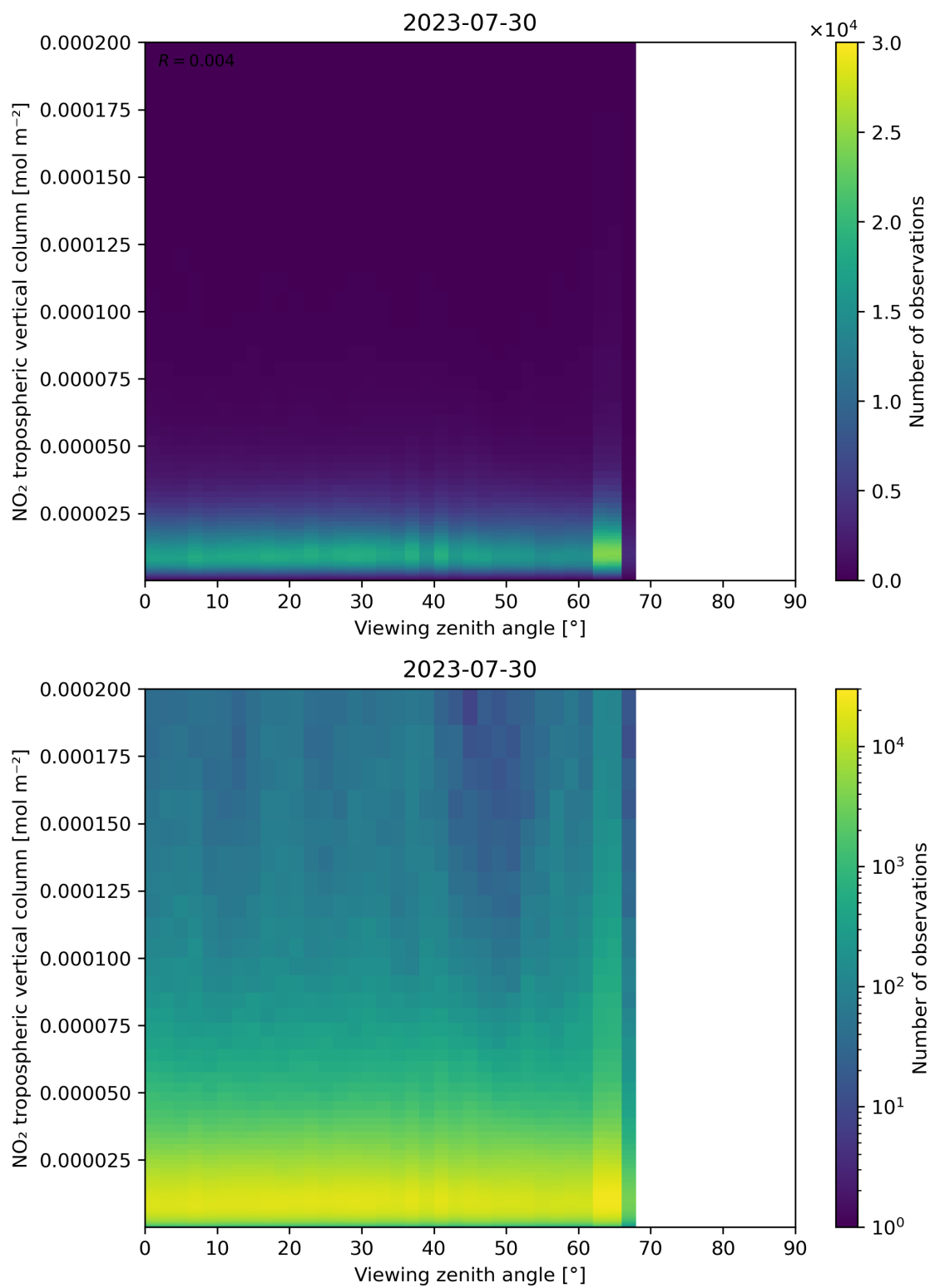
Figure 169: Scatter density plot of “Viewing zenith angle” against “NO 2 tropospheric vertical column” for 2023-07-29 to 2023-07-31.
