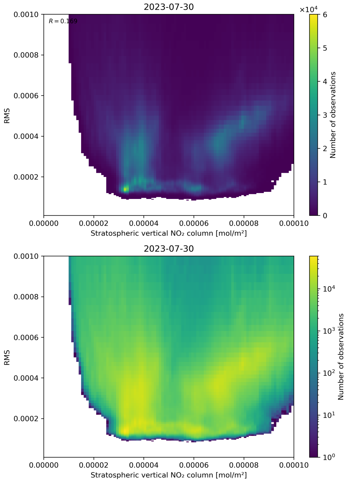
Figure 102: Scatter density plot of “Stratospheric vertical NO 2 column” against “RMS” for 2023-07-29 to 2023-07-31.
