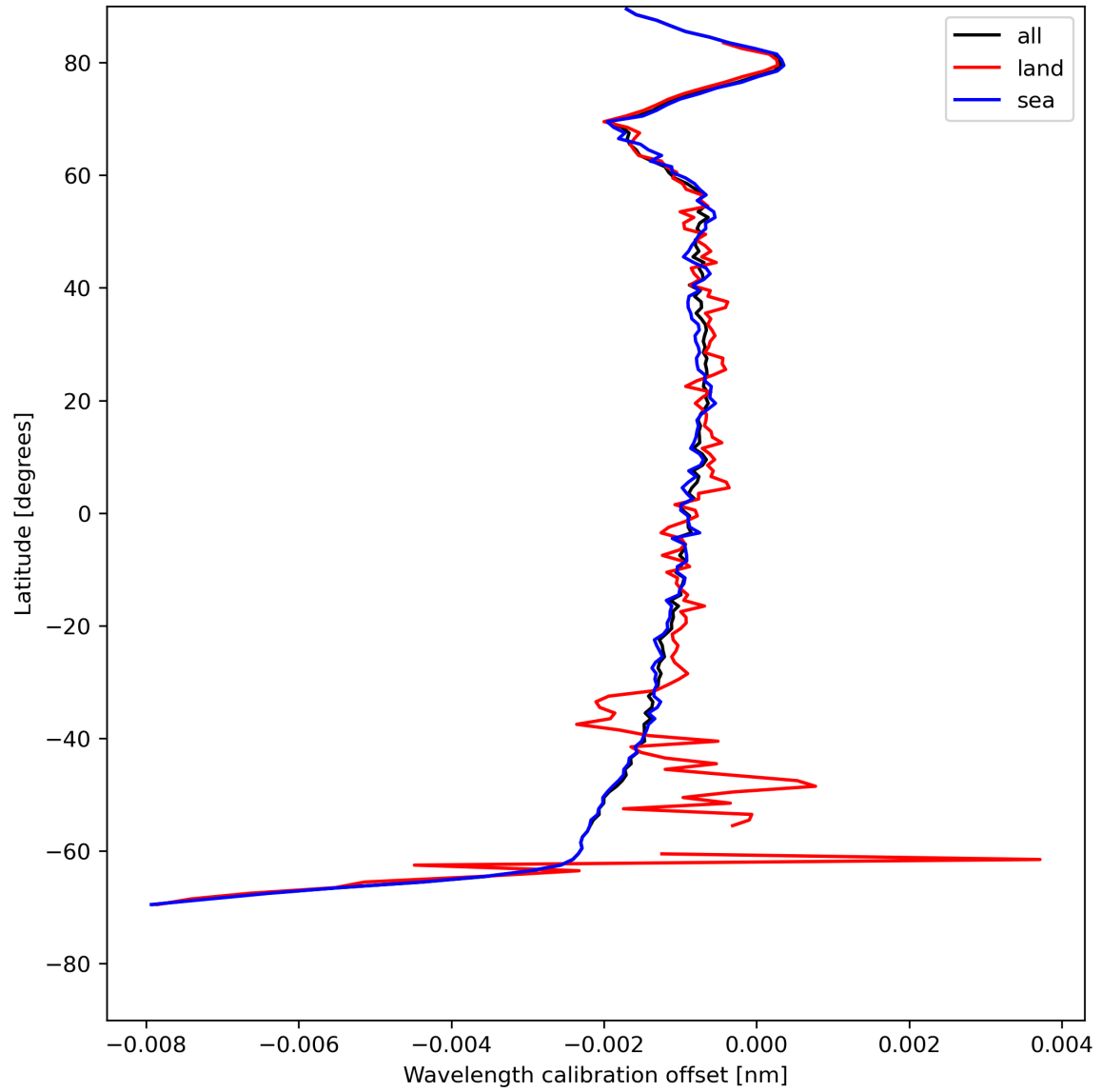
Figure 18: Zonal average of “Wavelength calibration offset” for 2023-07-29 to 2023-07-31.
