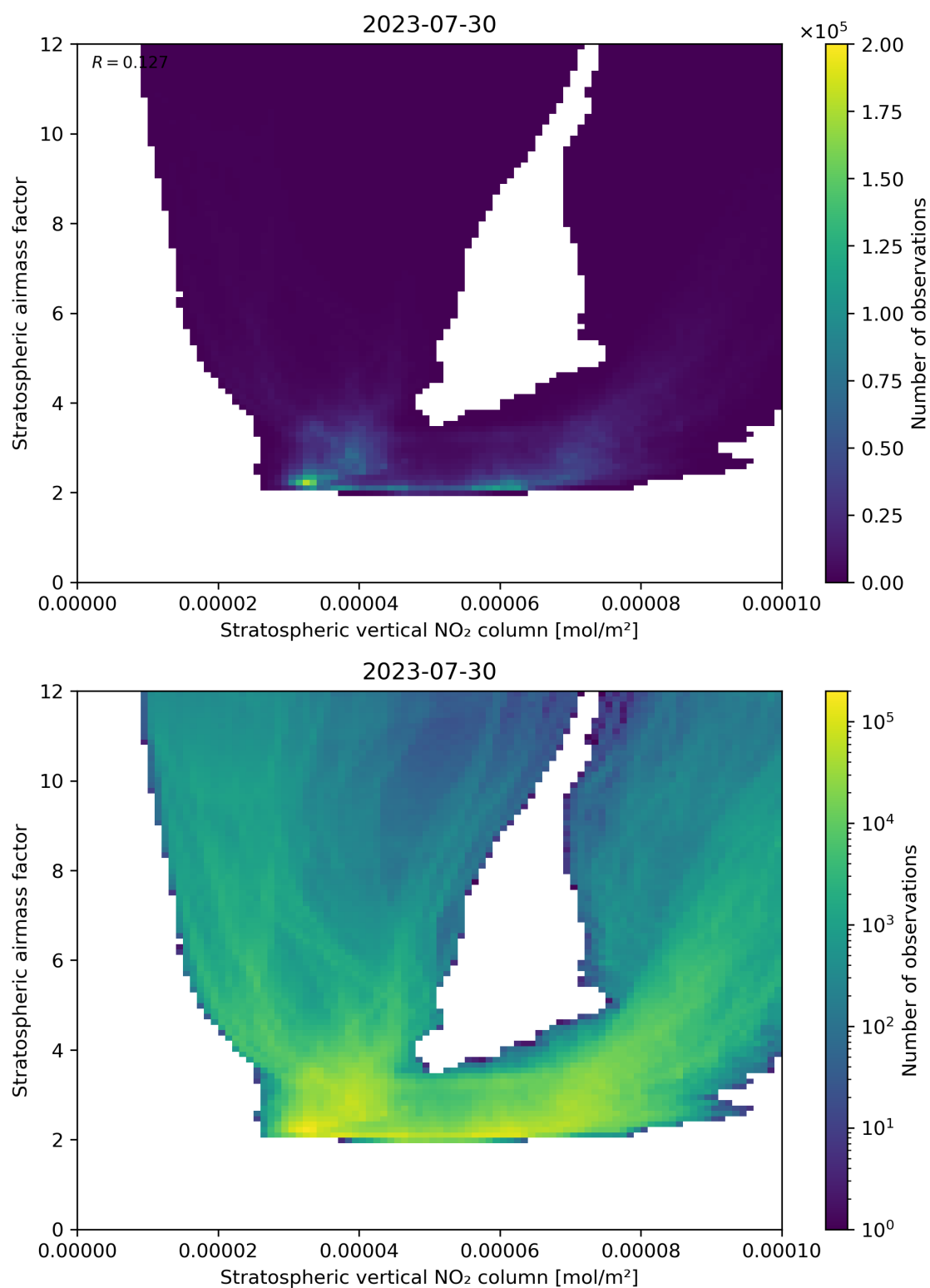
Figure 96: Scatter density plot of “Stratospheric vertical NO 2 column” against “Stratospheric airmass factor” for 2023-07-29 to 2023-07-31.
