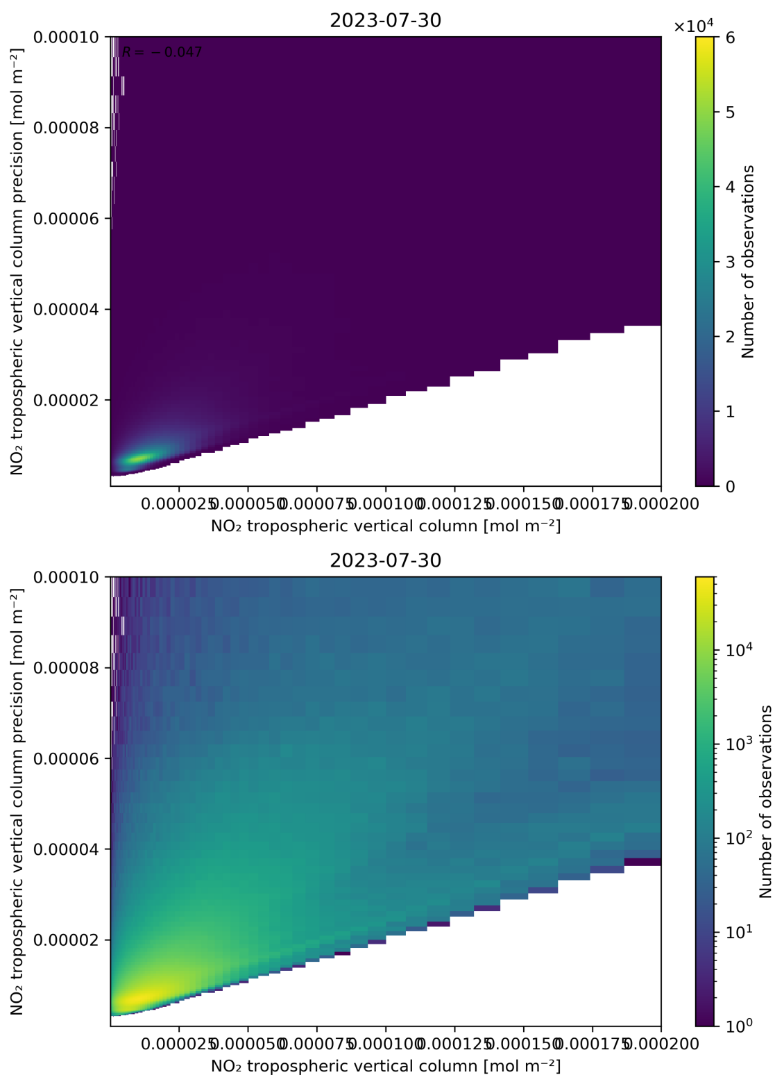
Figure 130: Scatter density plot of “NO 2 tropospheric vertical column” against “NO 2 tropospheric vertical column precision” for 2023-07-29 to 2023-07-31.
