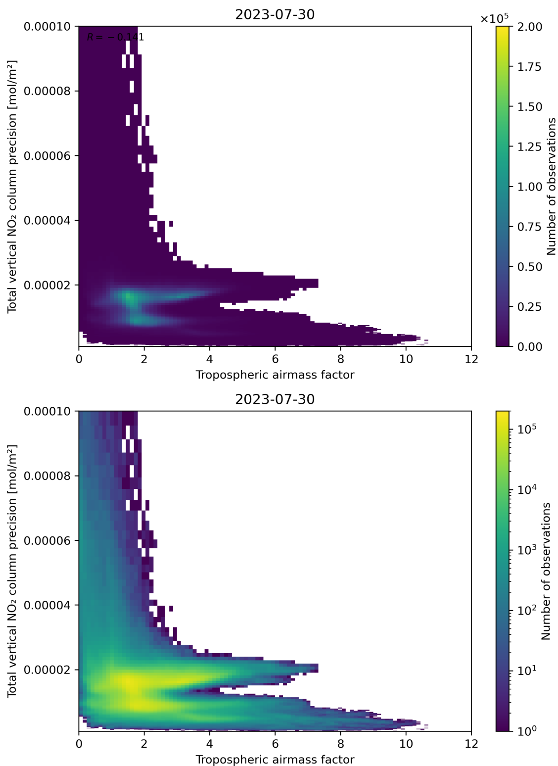
Figure 78: Scatter density plot of “Tropospheric air mass factor” against “Total vertical NO 2 column precision” for 2023-07-29 to 2023-07-31.
