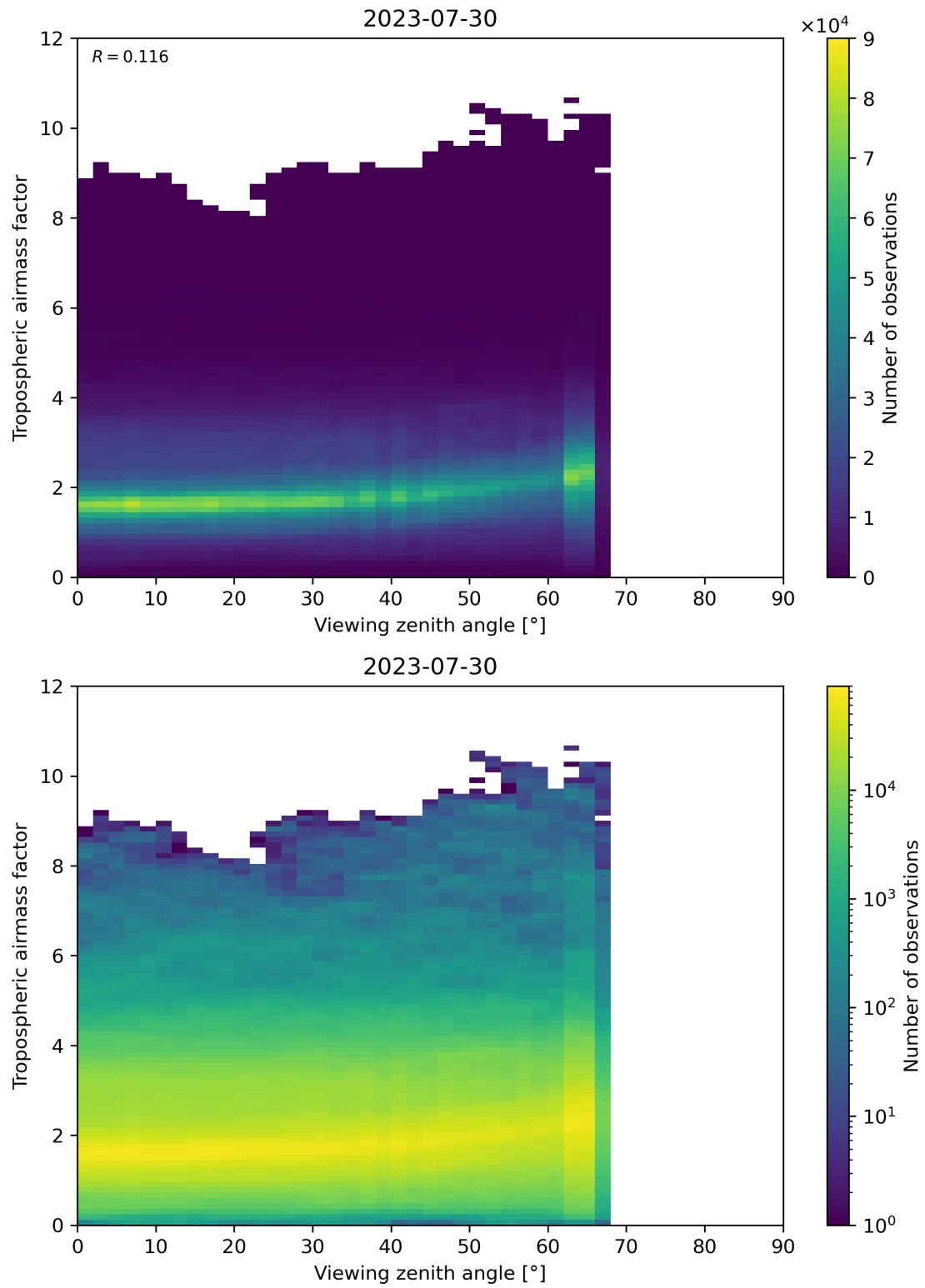
Figure 161: Scatter density plot of “Viewing zenith angle” against “Tropospheric airmass factor” for 2023-07-29 to 2023-07-31.
