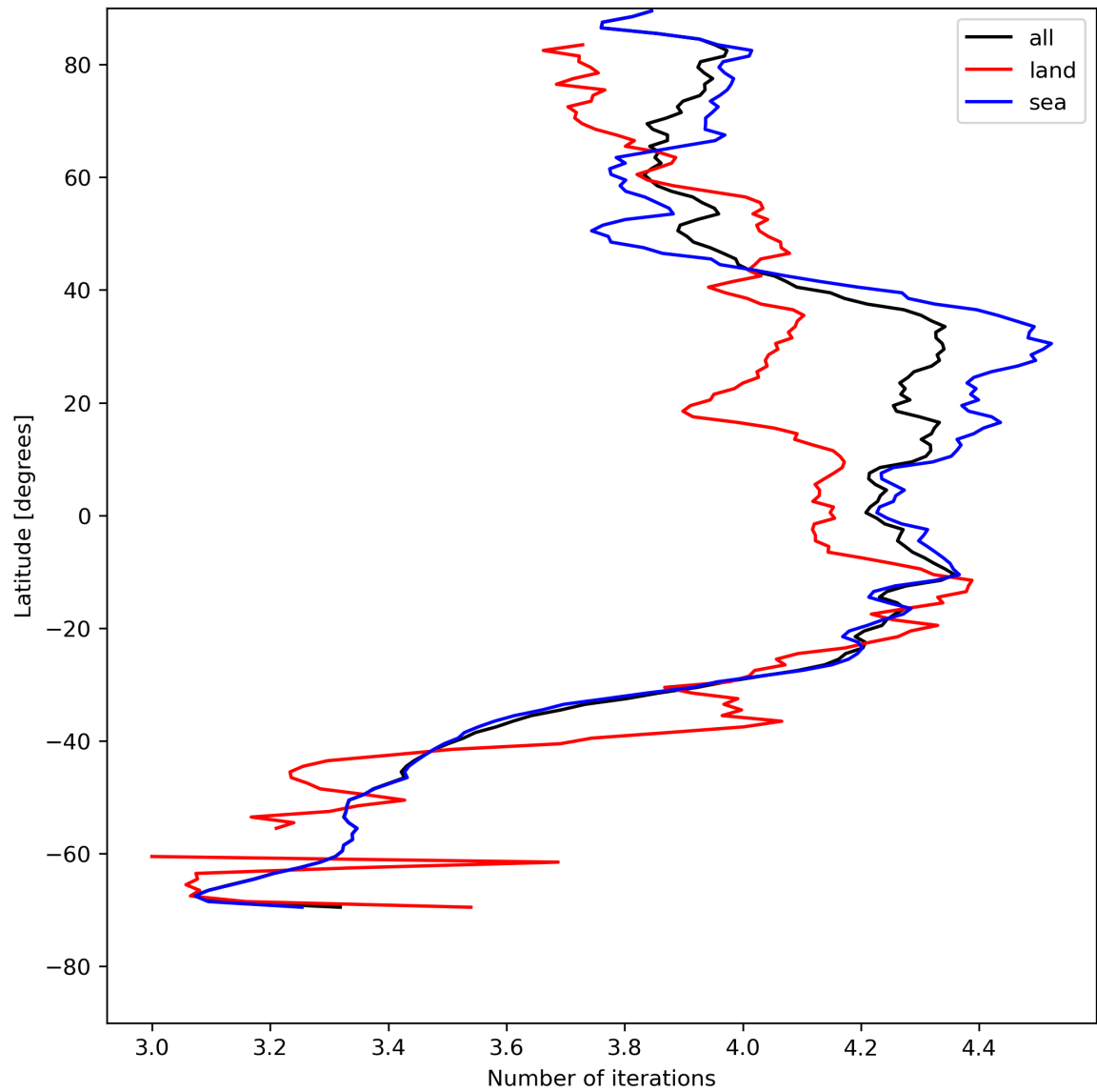
Figure 17: Zonal average of “Number of iterations” for 2023-07-29 to 2023-07-31.
