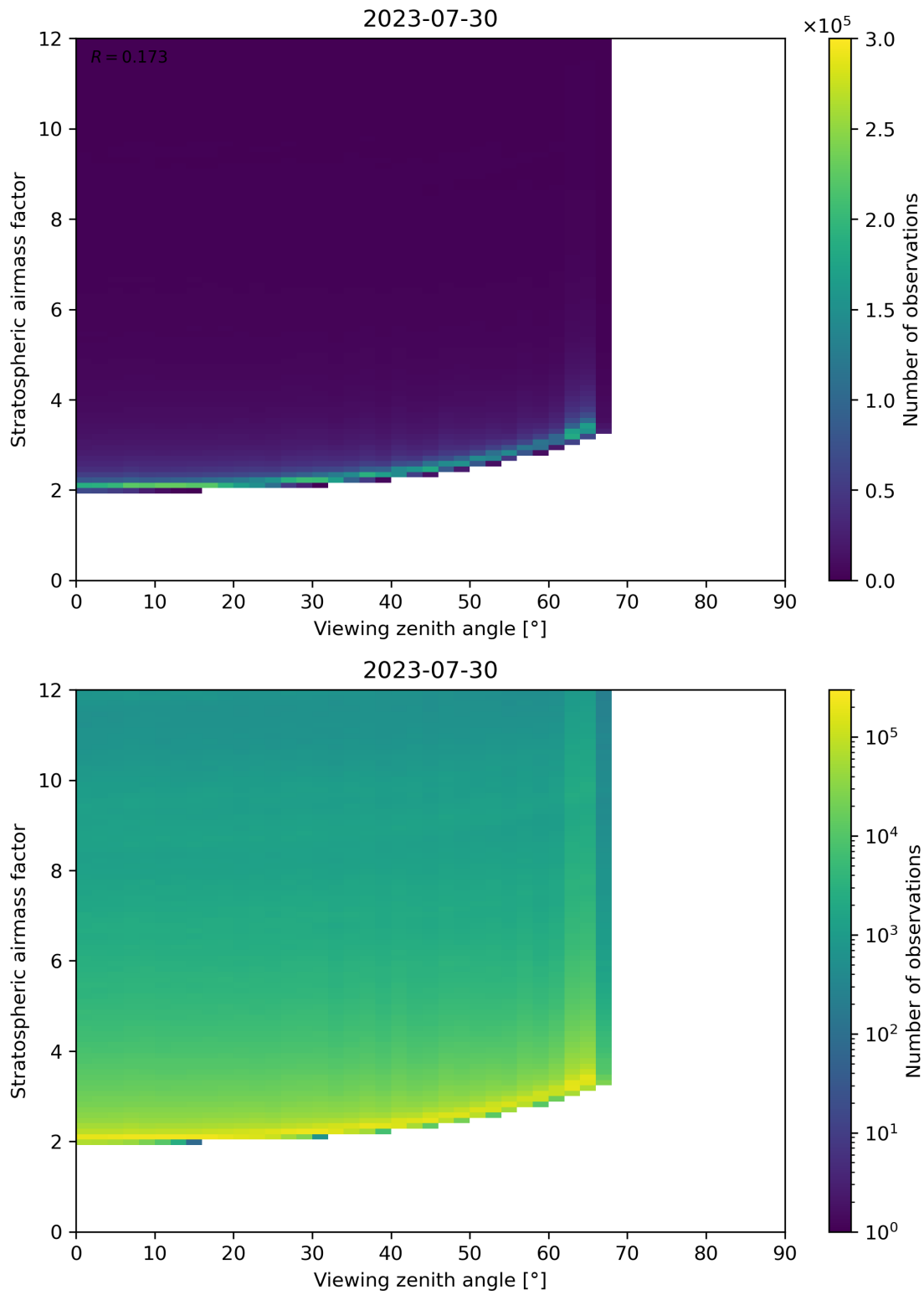
Figure 159: Scatter density plot of “Viewing zenith angle” against “Stratospheric airmass factor” for 2023-07-29 to 2023-07-31.
