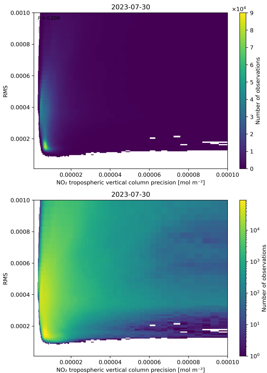
Figure 140: Scatter density plot of “NO 2 tropospheric vertical column precision” against “RMS” for 2023-07-29 to 2023-07-31.
