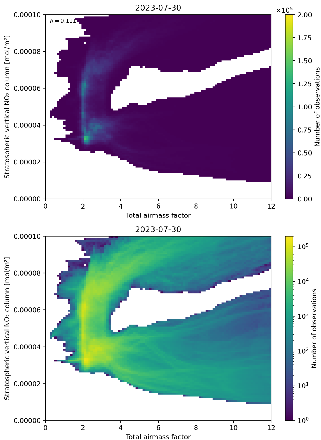
Figure 64: Scatter density plot of “Total airmass factor” against “Stratospheric vertical NO 2 column” for 2023-07-29 to 2023-07-31.
