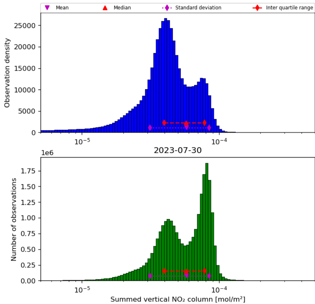
Figure 40: Histogram of “Summed vertical NO 2 column” for 2023-07-29 to 2023-07-31
