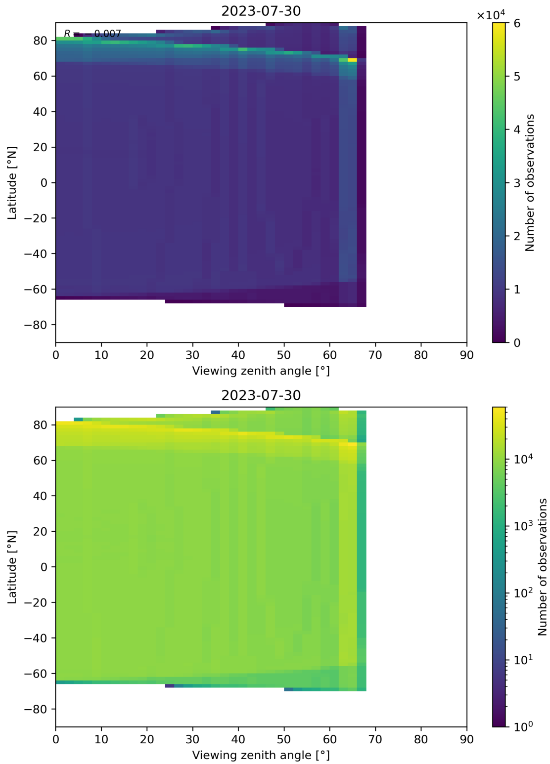
Figure 163: Scatter density plot of “Viewing zenith angle” against “Latitude” for 2023-07-29 to 2023-07-31.
