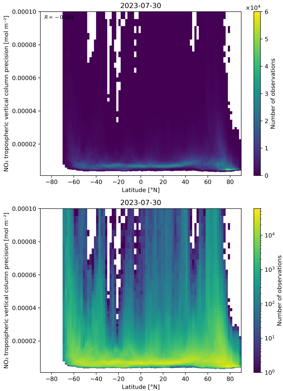
Figure 93: Scatter density plot of “Latitude” against “NO 2 tropospheric vertical column precision” for 2023-07-29 to 2023-07-31.
