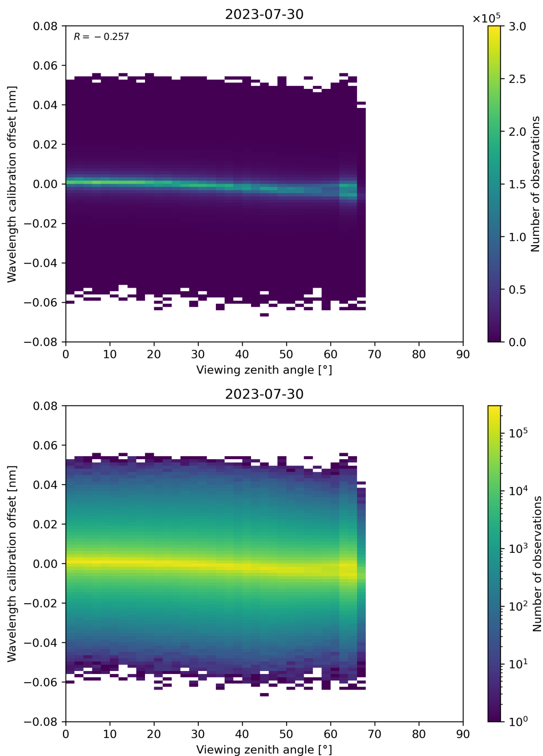
Figure 173: Scatter density plot of “Viewing zenith angle” against “Wavelength calibration offset” for 2023-07-29 to 2023-07-31.
