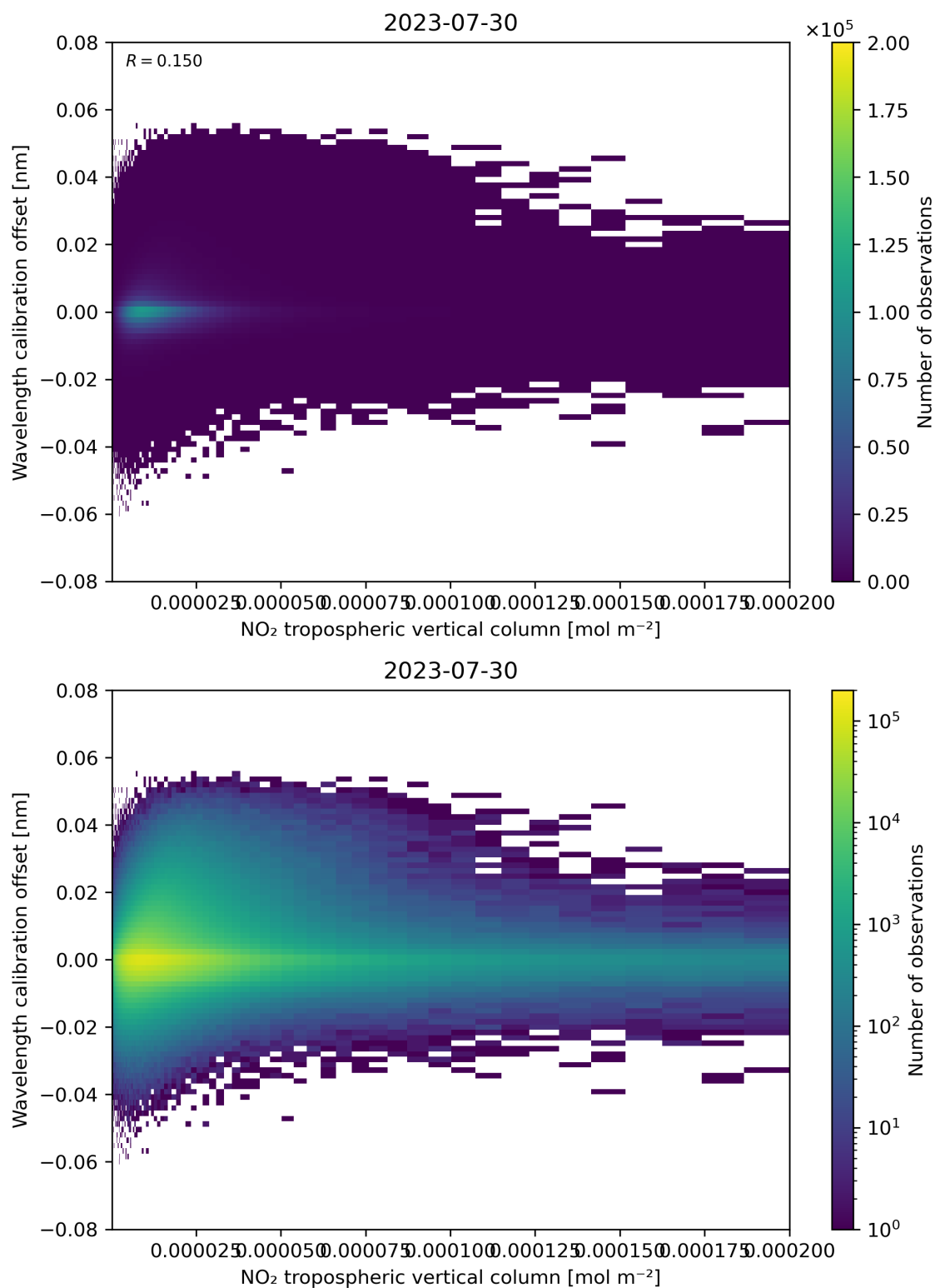
Figure 143: Scatter density plot of “NO 2 tropospheric vertical column” against “Wavelength calibration offset” for 2023-07-29 to 2023-07-31.
