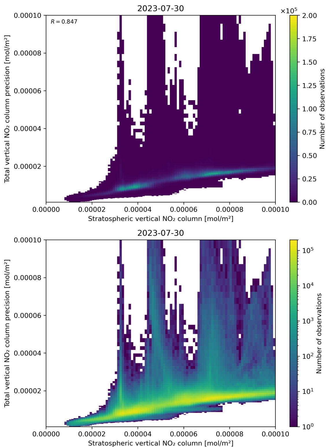
Figure 101: Scatter density plot of “Stratospheric vertical NO 2 column” against “Total vertical NO 2 column precision” for 2023-07-29 to 2023-07-31.
