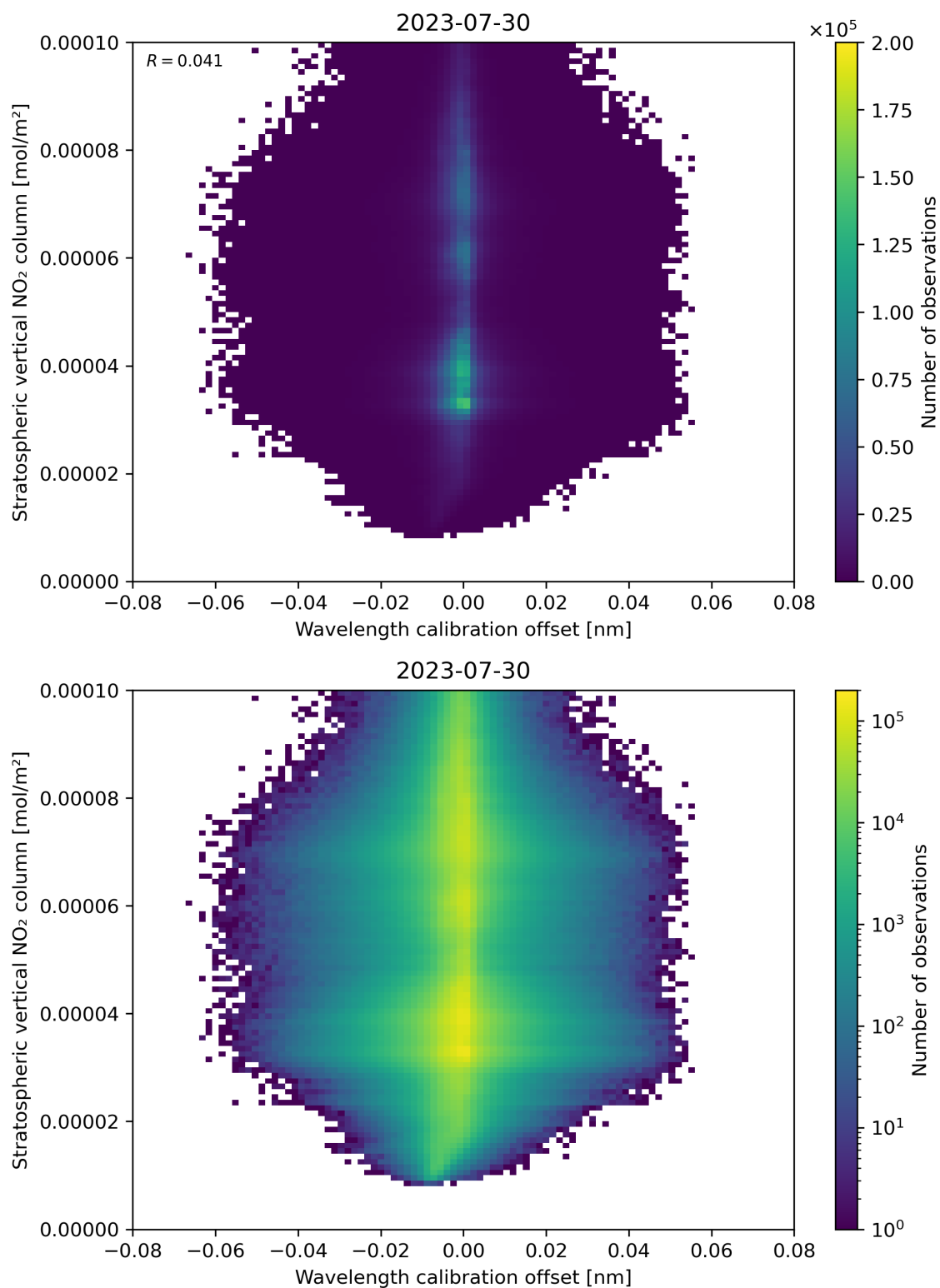
Figure 176: Scatter density plot of “Wavelength calibration offset” against “Stratospheric vertical NO 2 column” for 2023-07-29 to 2023-07-31.
