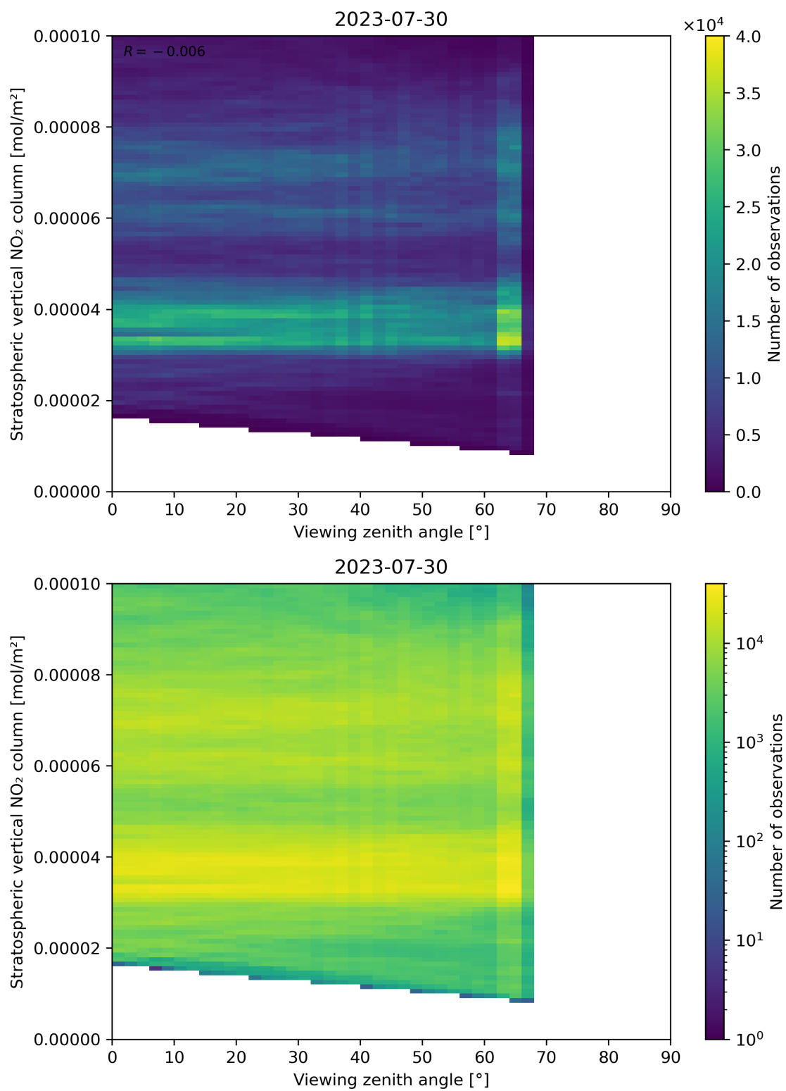
Figure 164: Scatter density plot of “Viewing zenith angle” against “Stratospheric vertical NO 2 column” for 2023-07-29 to 2023-07-31.
