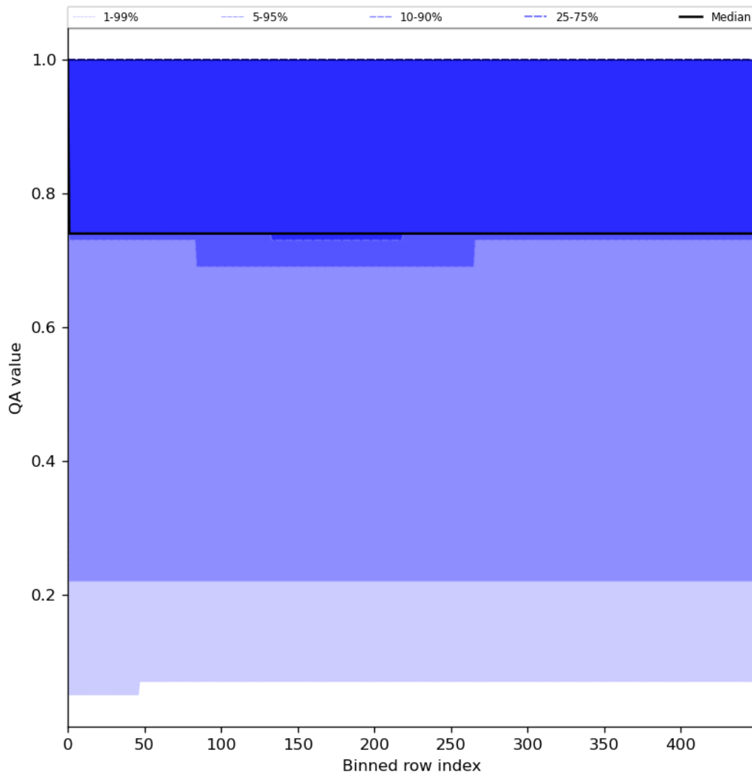
Figure 45: Along track statistics of “QA value” for 2023-07-29 to 2023-07-31
