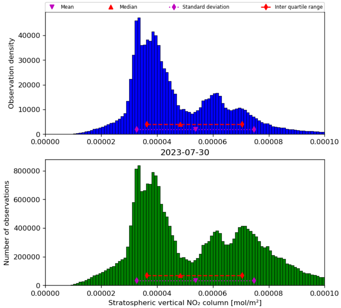
Figure 36: Histogram of “Stratospheric vertical NO 2 column” for 2023-07-29 to 2023-07-31
