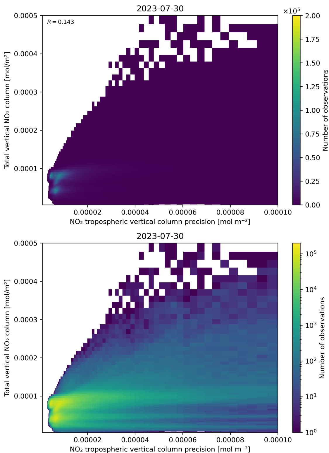
Figure 138: Scatter density plot of “NO 2 tropospheric vertical column precision” against “Total vertical NO 2 column” for 2023-07-29 to 2023-07-31.
