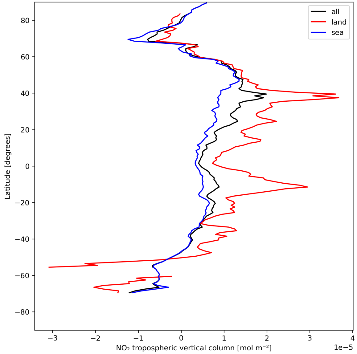
Figure 12: Zonal average of “NO 2 tropospheric vertical column” for 2023-07-29 to 2023-07-31.
