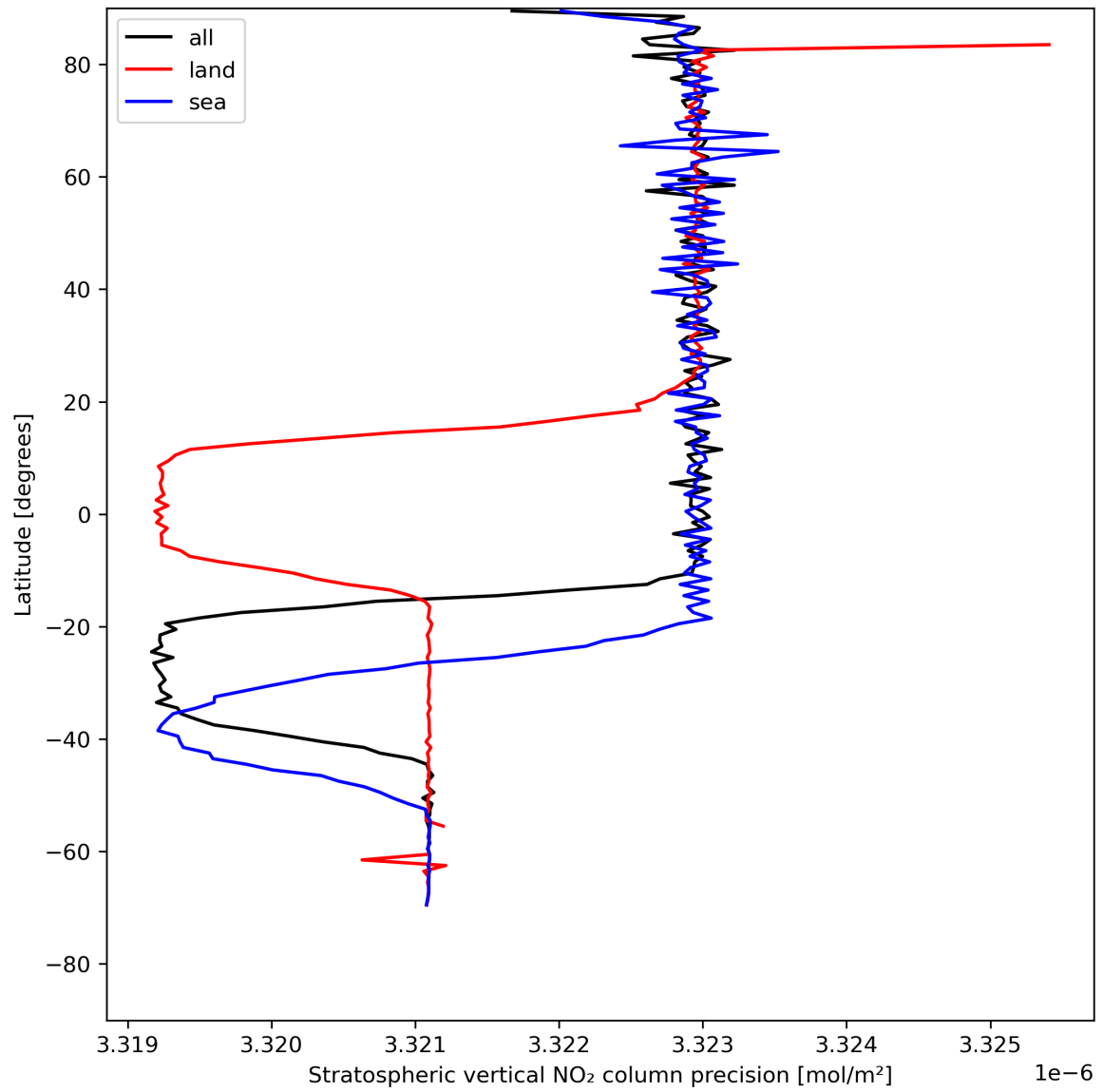
Figure 20: Zonal average of “Stratospheric vertical NO 2 column precision” for 2023-07-29 to 2023-07-31.
