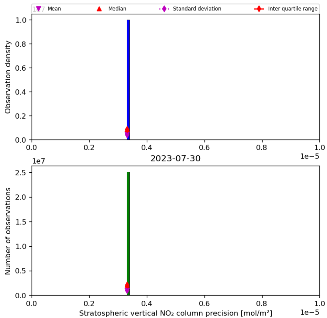
Figure 37: Histogram of “Stratospheric vertical NO 2 column precision” for 2023-07-29 to 2023-07-31
