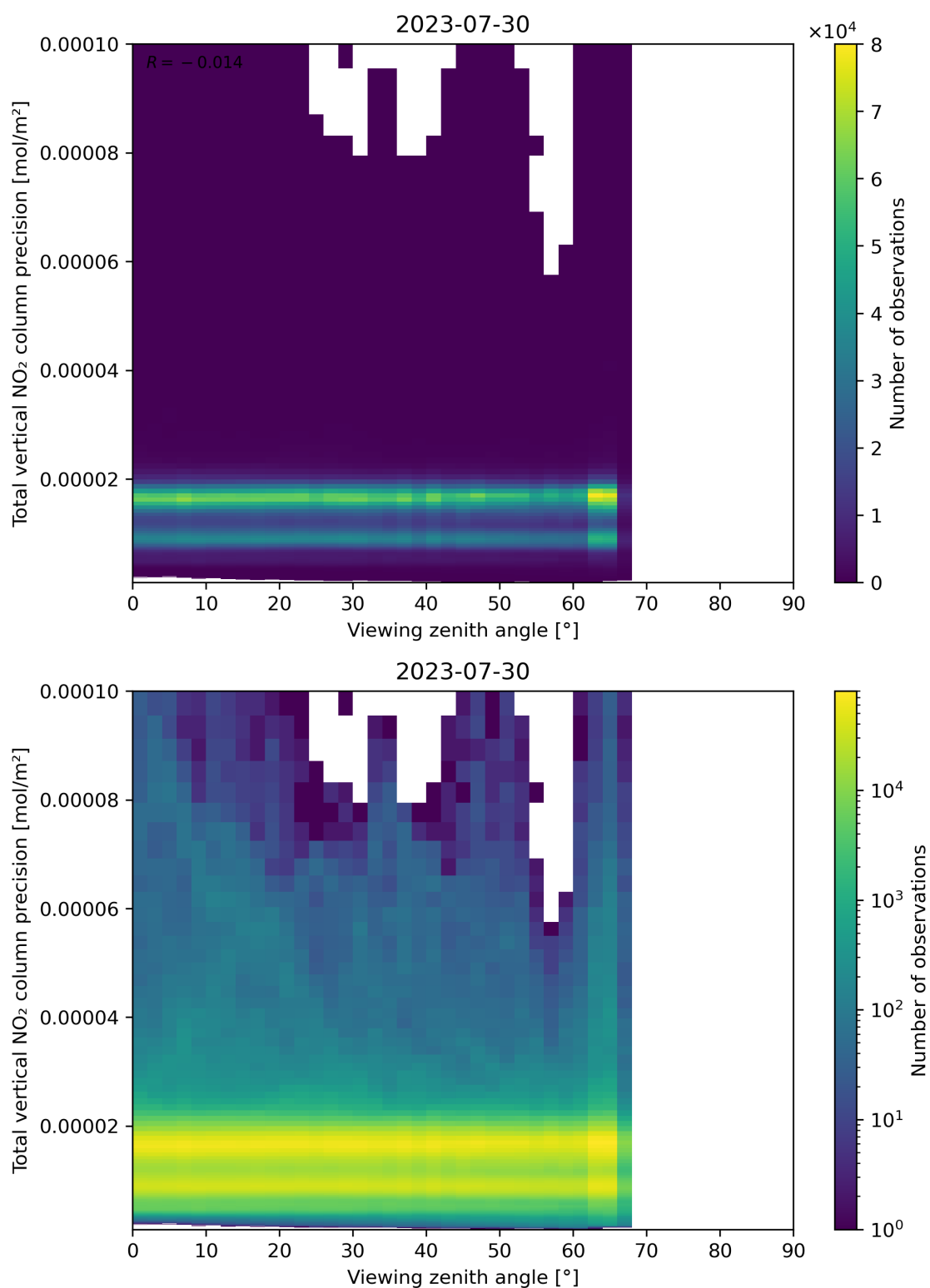
Figure 168: Scatter density plot of “Viewing zenith angle” against “Total vertical NO 2 column precision” for 2023-07-29 to 2023-07-31.
