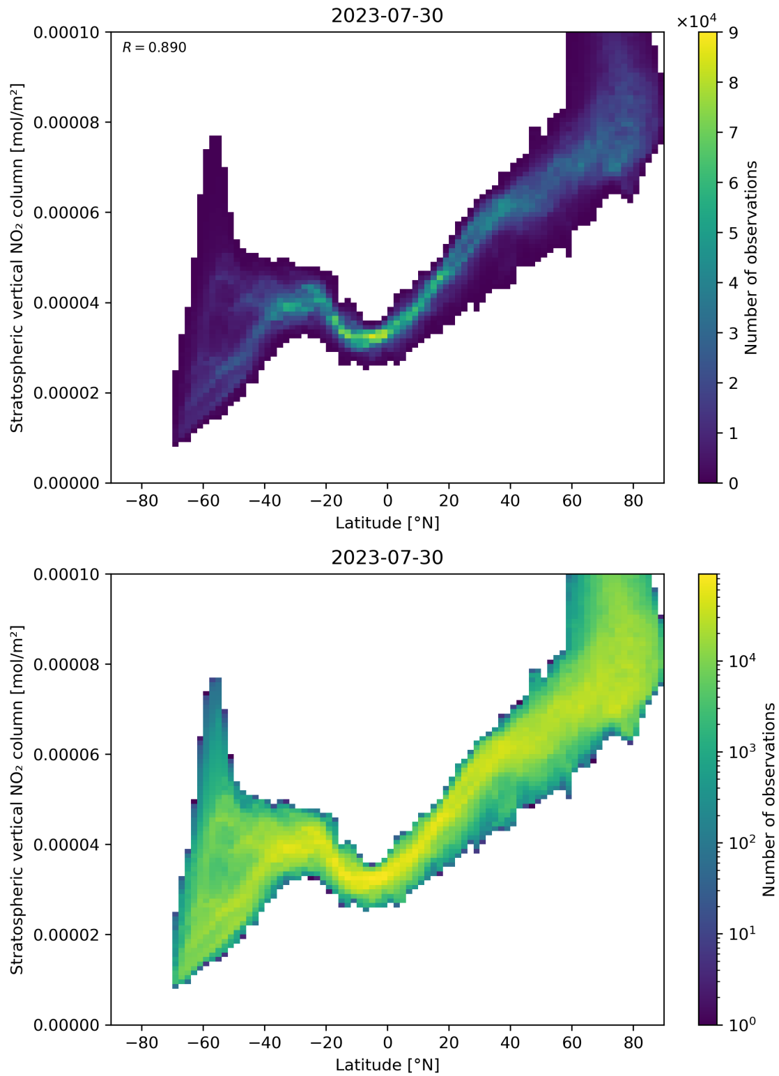
Figure 87: Scatter density plot of “Latitude” against “Stratospheric vertical NO 2 column” for 2023-07-29 to 2023-07-31.
