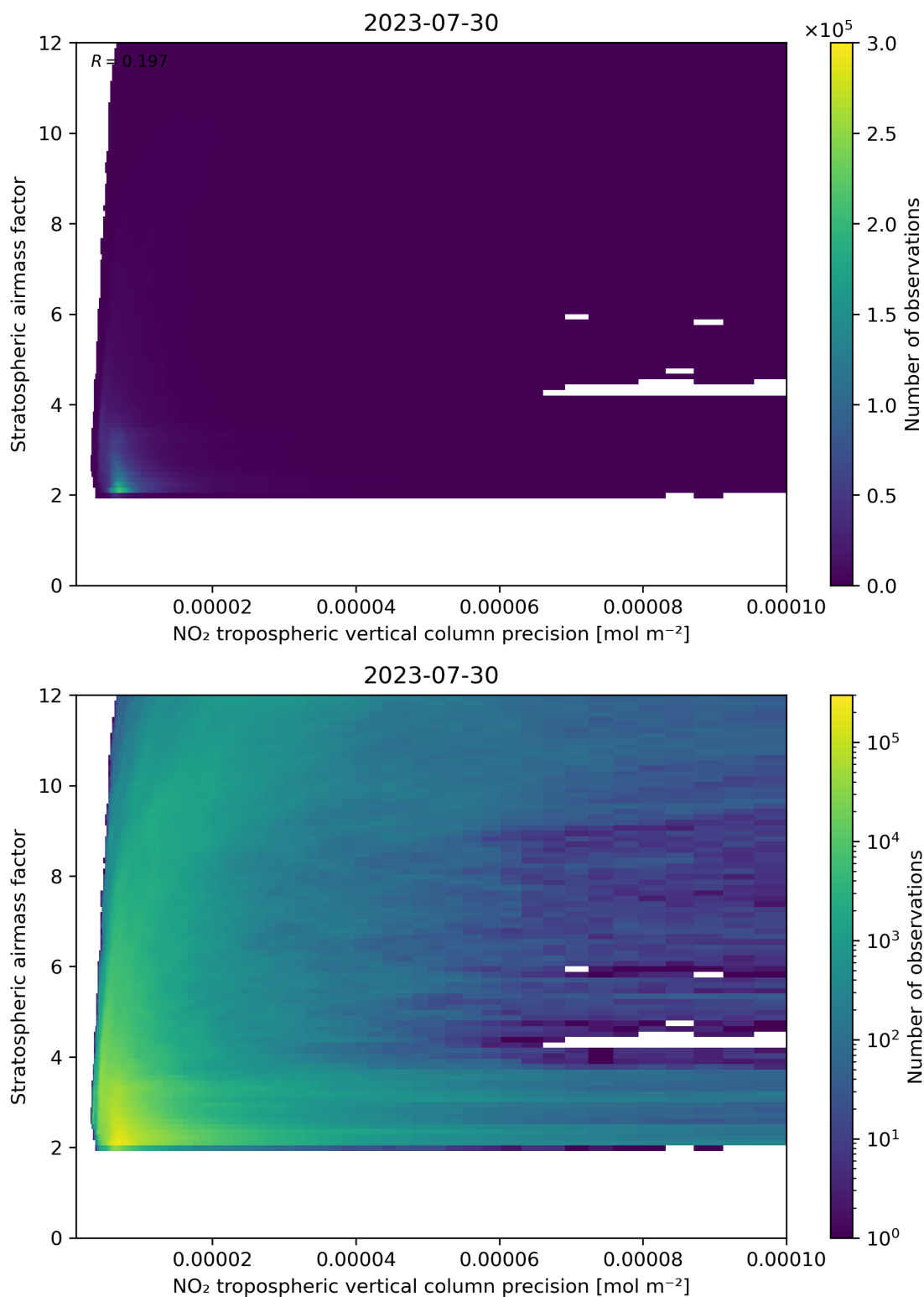
Figure 131: Scatter density plot of “NO 2 tropospheric vertical column precision” against “Stratospheric airmass factor” for 2023-07-29 to 2023-07-31.
