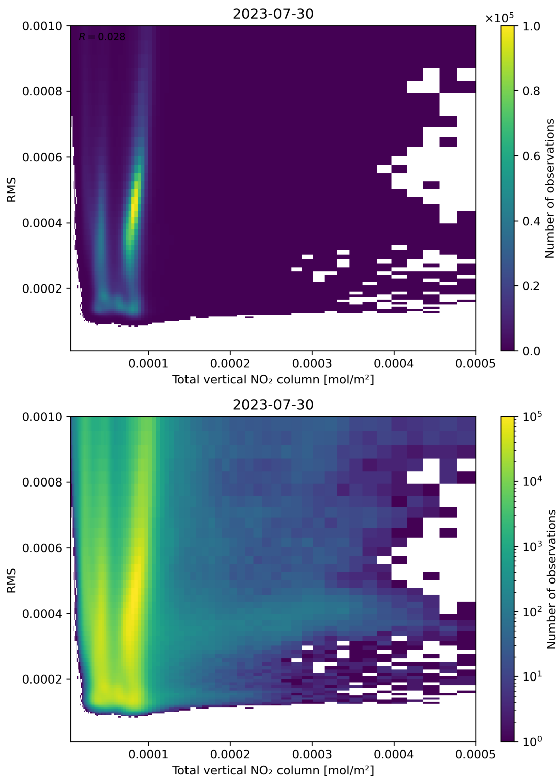
Figure 120: Scatter density plot of “Total vertical NO 2 column” against “RMS” for 2023-07-29 to 2023-07-31.
