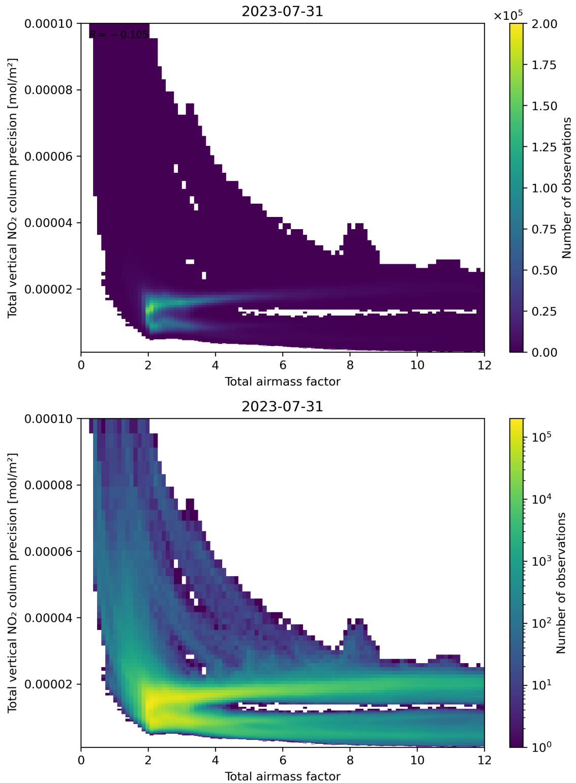
Figure 68: Scatter density plot of “Total airmass factor” against “Total vertical NO 2 column precision” for 2023-07-30 to 2023-08-01.
