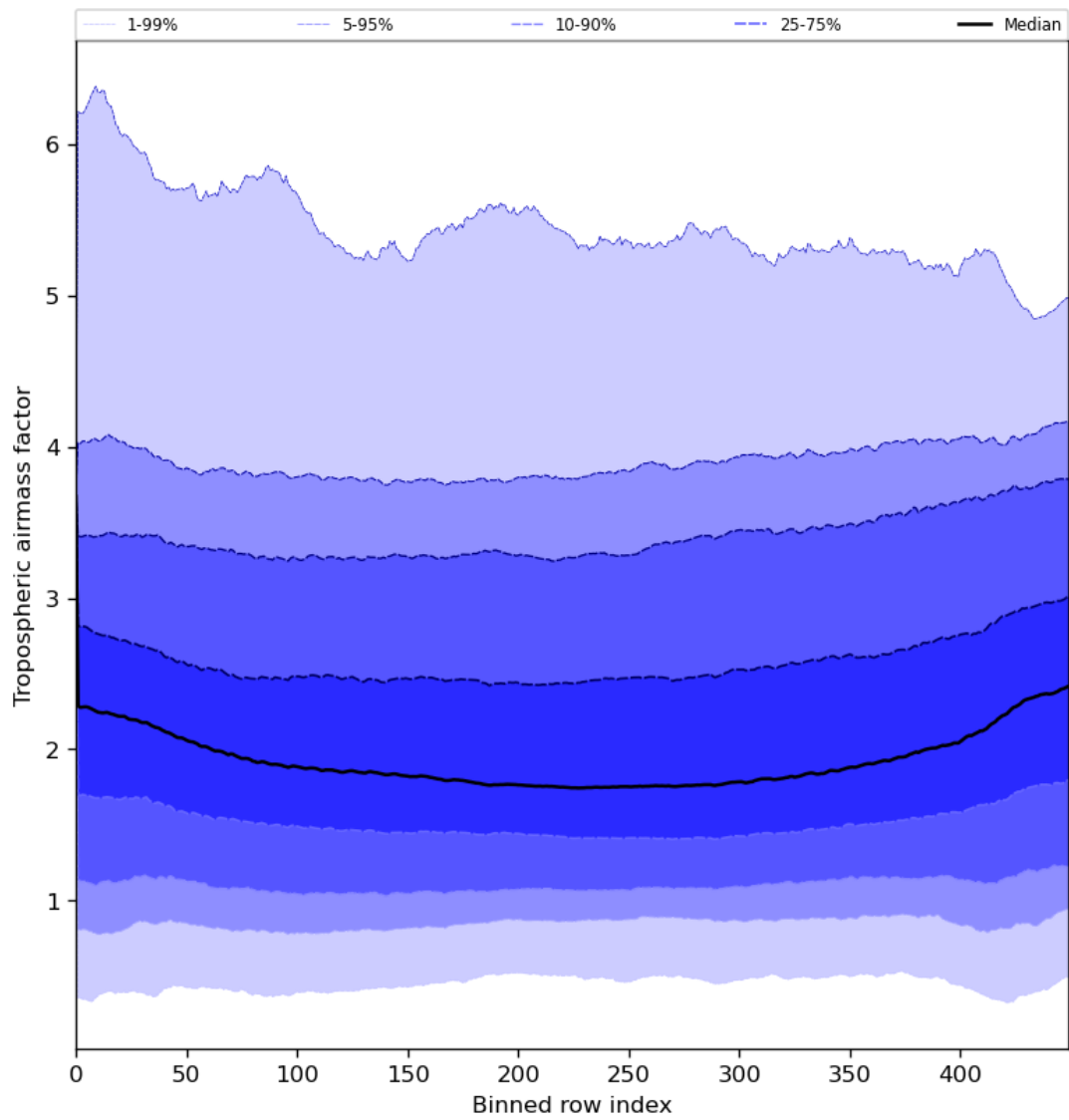
Figure 48: Along track statistics of “Tropospheric airmass factor” for 2023-07-30 to 2023-08-01
