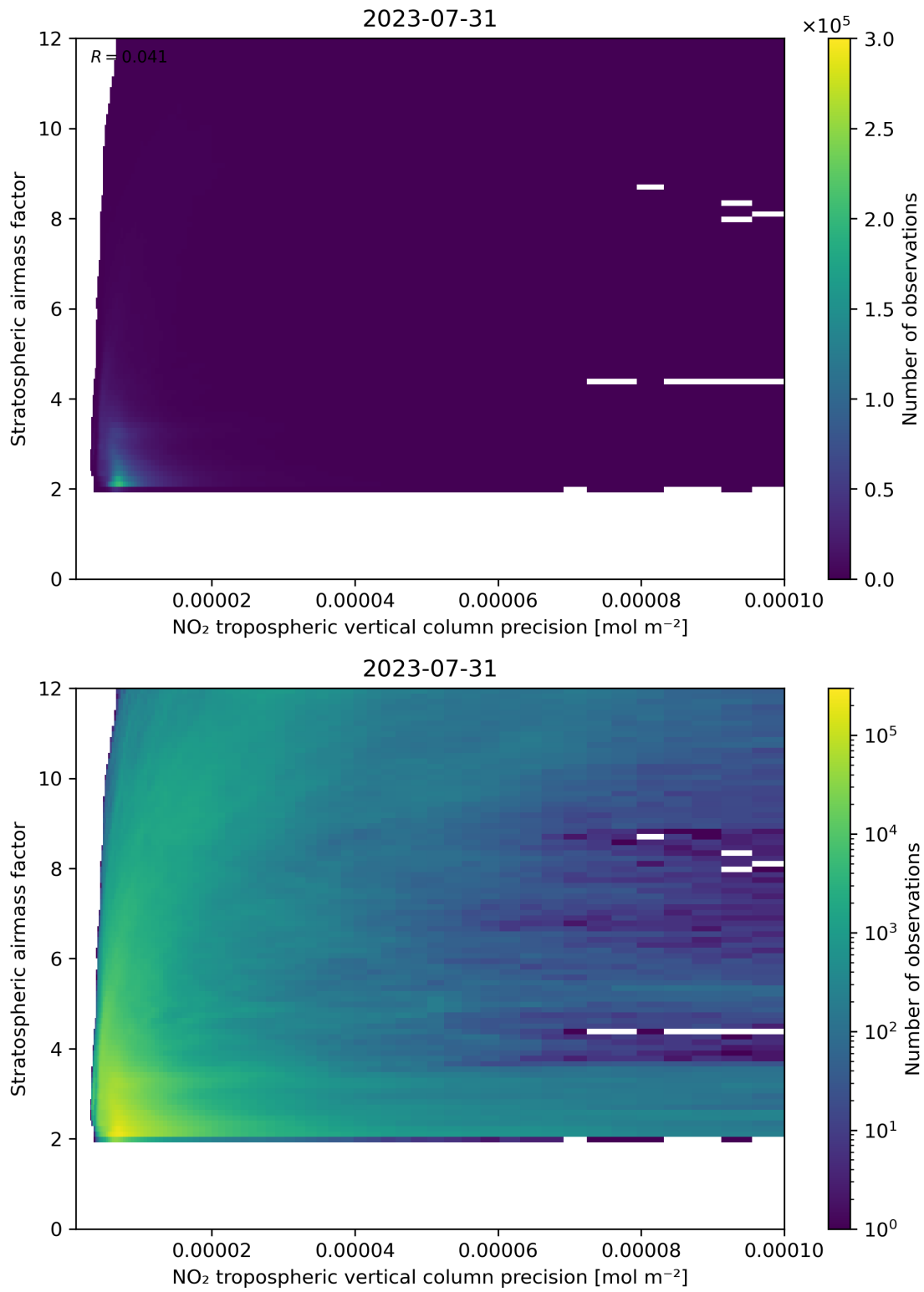
Figure 131: Scatter density plot of “NO 2 tropospheric vertical column precision” against “Stratospheric airmass factor” for 2023-07-30 to 2023-08-01.
