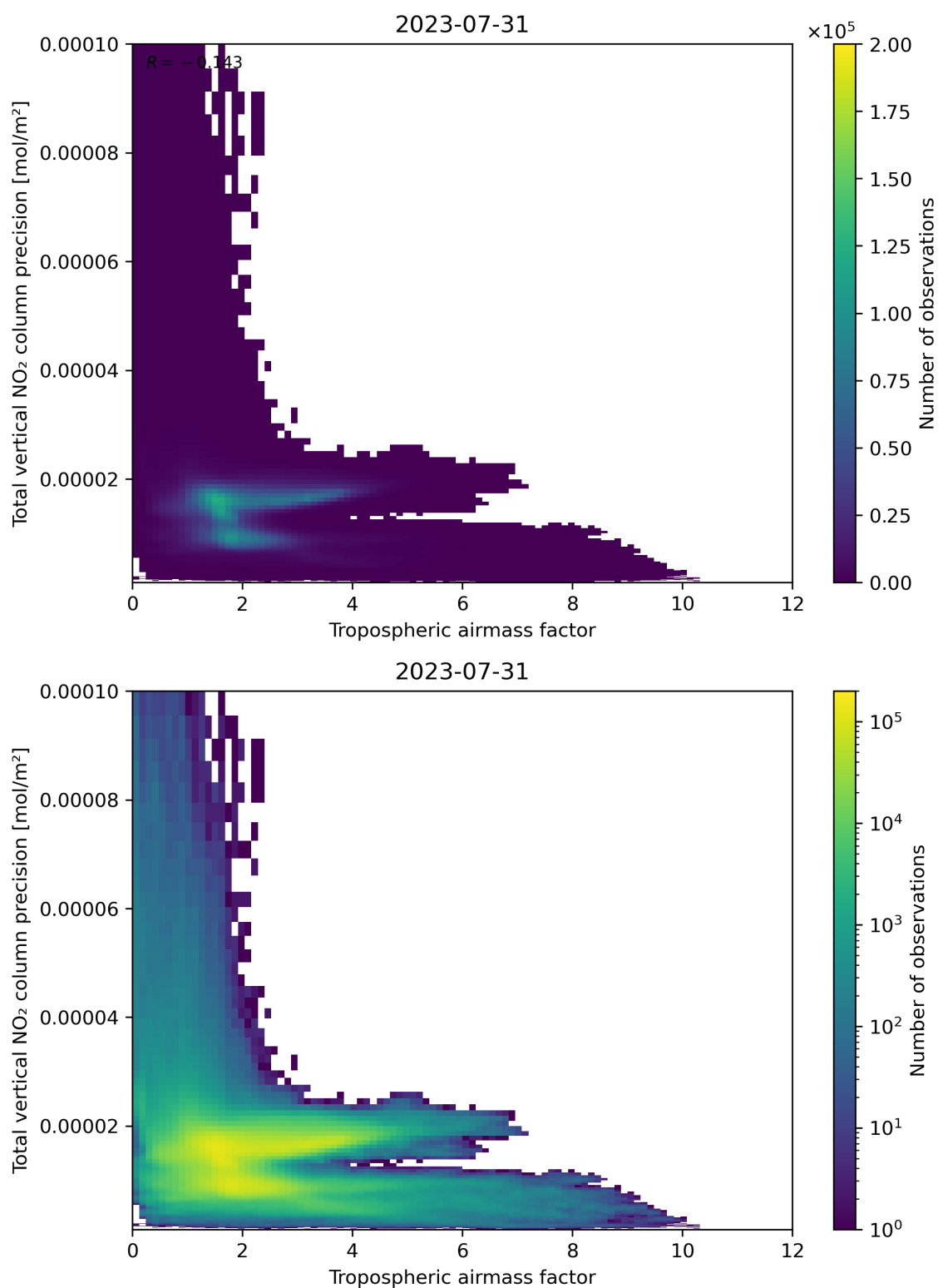
Figure 78: Scatter density plot of “Tropospheric air mass factor” against “Total vertical NO 2 column precision” for 2023-07-30 to 2023-08-01.
