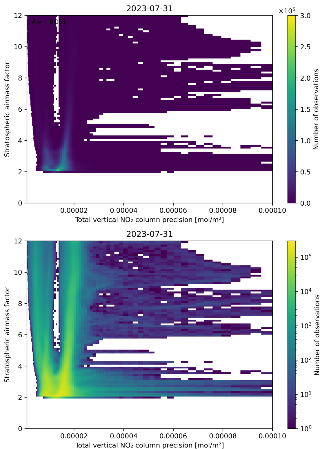
Figure 115: Scatter density plot of “Total vertical NO 2 column precision” against “Stratospheric air mass factor” for 2023-07-30 to 2023-08-01.
