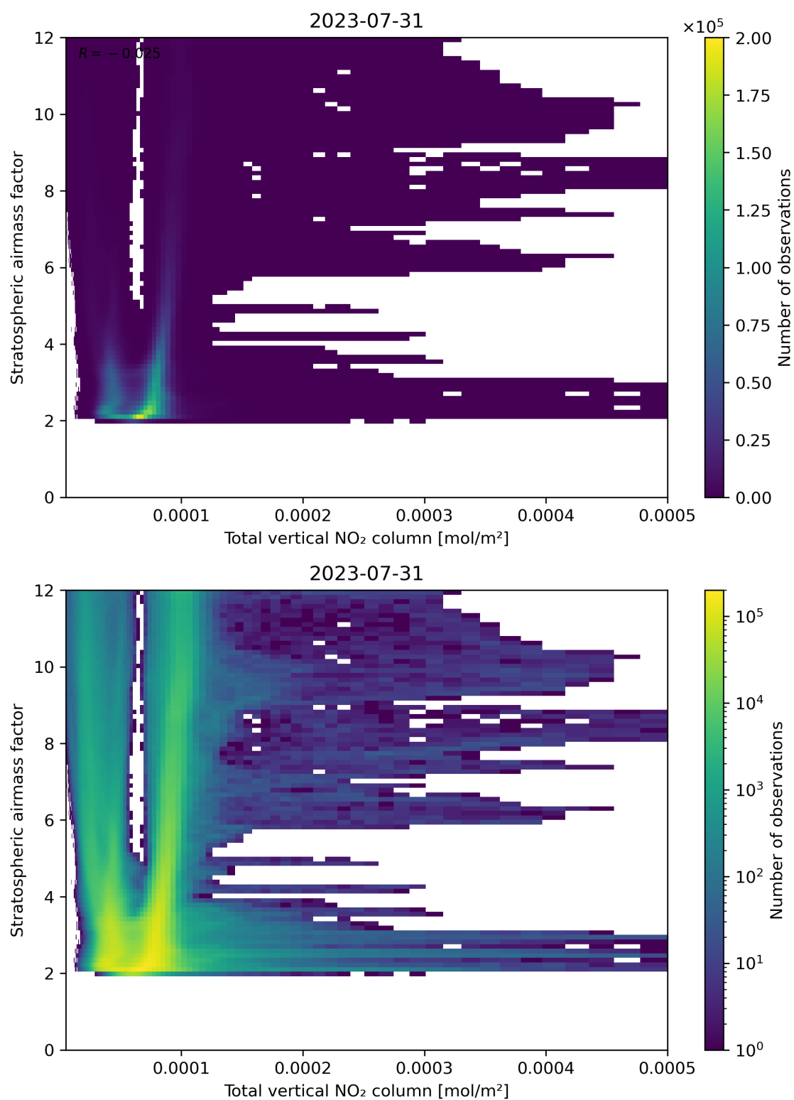
Figure 110: Scatter density plot of “Total vertical NO 2 column” against “Stratospheric airmass factor” for 2023-07-30 to 2023-08-01.
