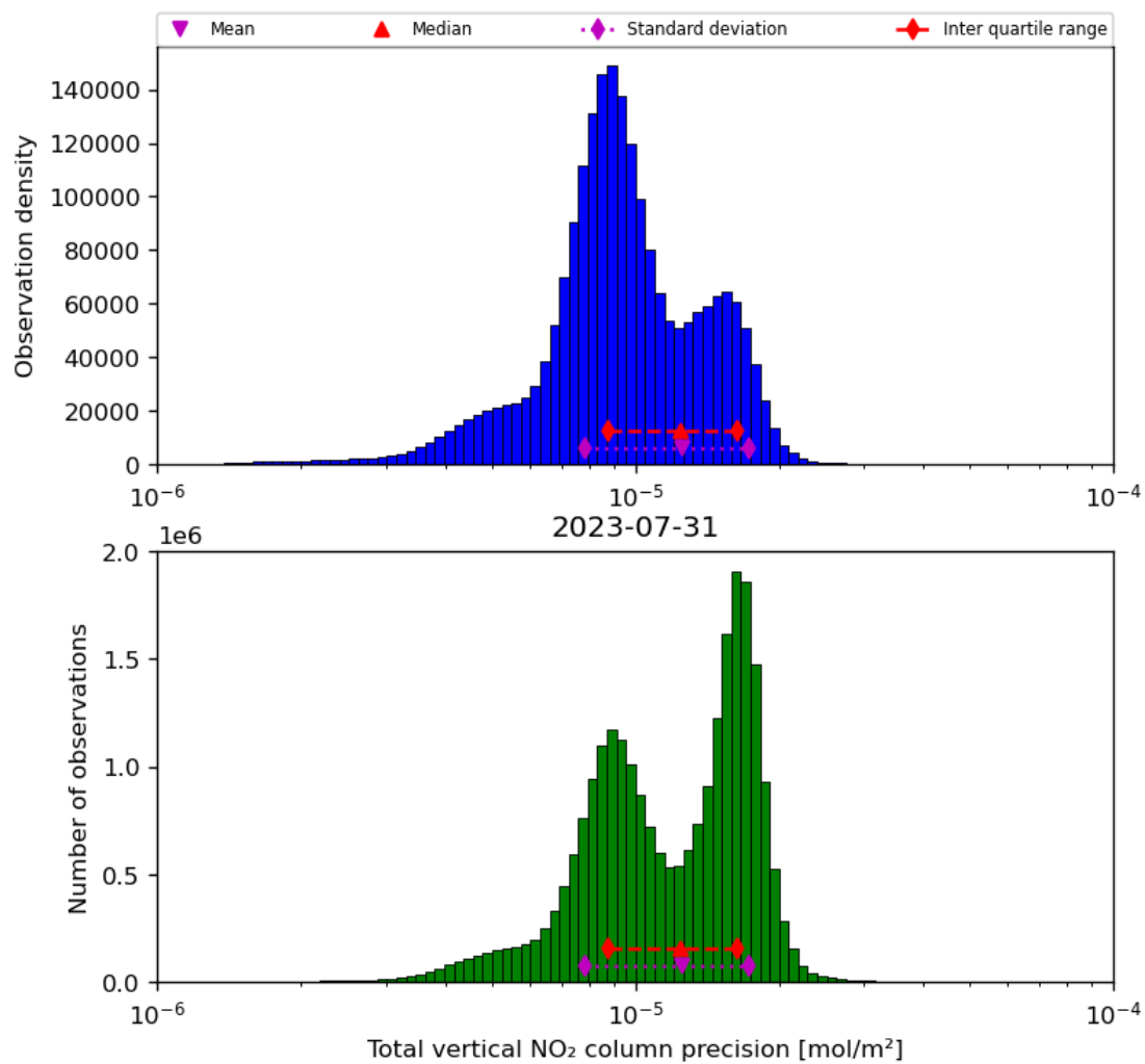
Figure 39: Histogram of "Total vertical NO 2 column precision" for 2023-07-30 to 2023-08-01
