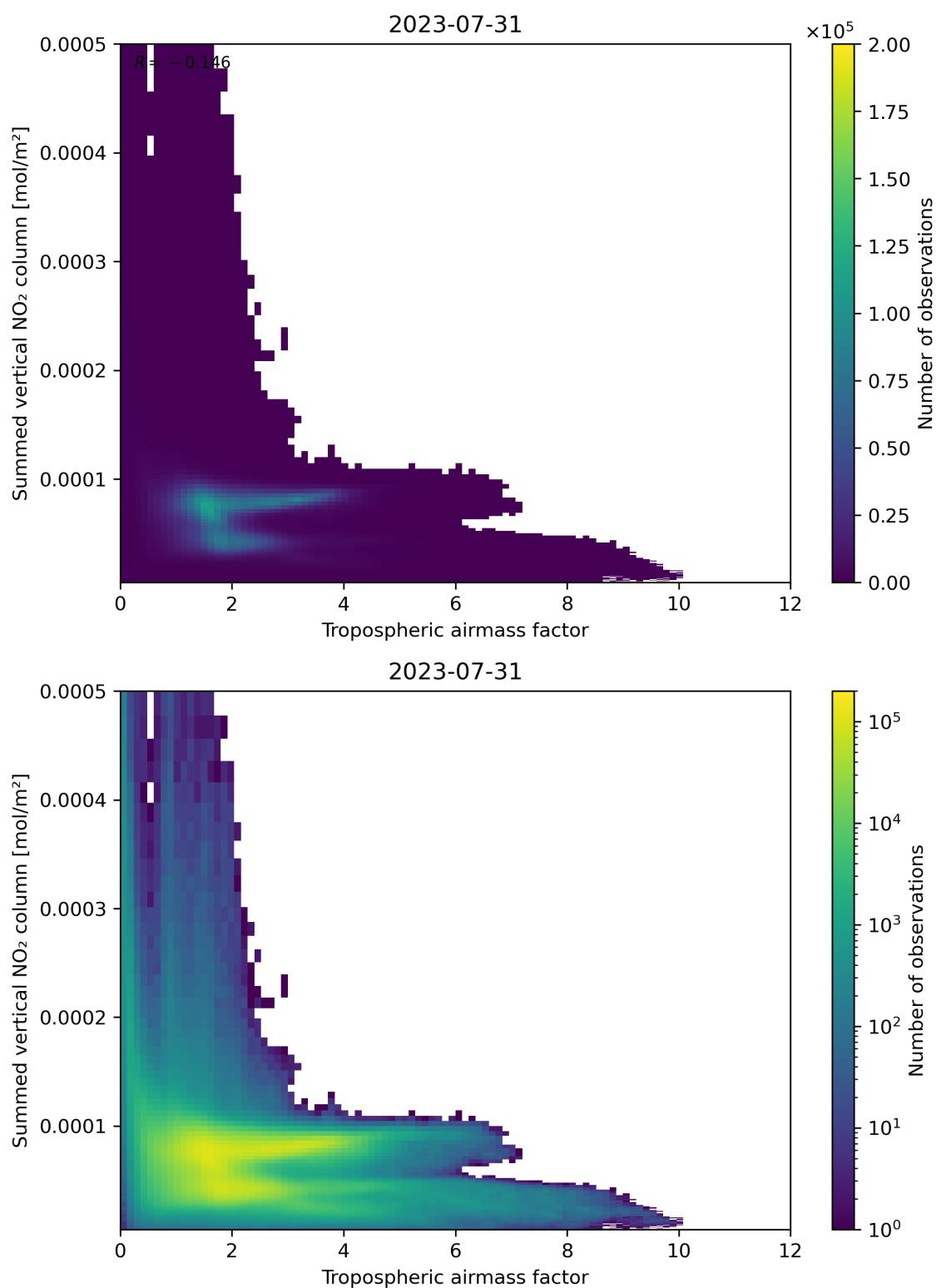
Figure 75: Scatter density plot of “Tropospheric airmass factor” against “Summed vertical NO 2 column” for 2023-07-30 to 2023-08-01.
