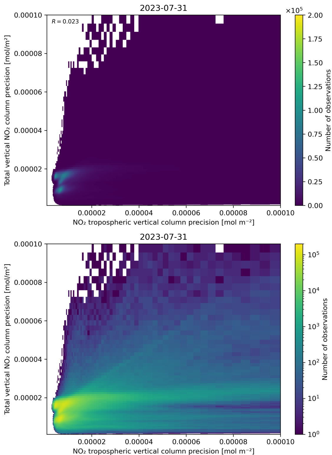
Figure 139: Scatter density plot of “NO 2 tropospheric vertical column precision” against “Total vertical NO 2 column precision” for 2023-07-30 to 2023-08-01.
