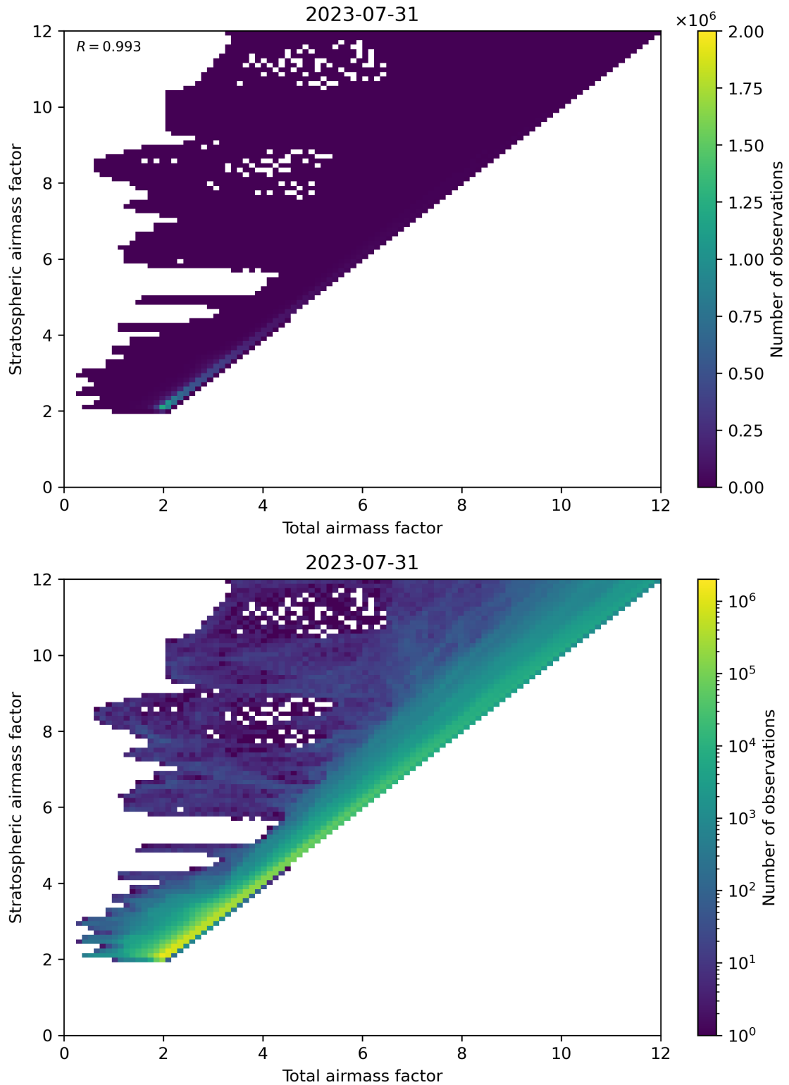
Figure 62: Scatter density plot of “Total airmass factor” against “Stratospheric airmass factor” for 2023-07-30 to 2023-08-01.
