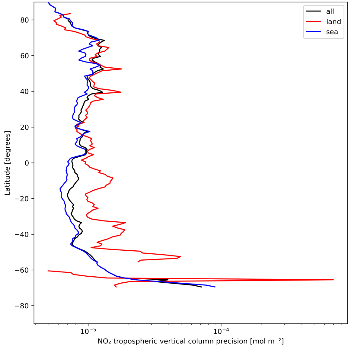
Figure 13: Zonal average of “NO 2 tropospheric vertical column precision” for 2023-07-30 to 2023-08-01.
