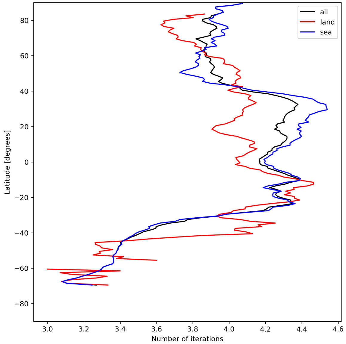
Figure 17: Zonal average of “Number of iterations” for 2023-07-30 to 2023-08-01.
