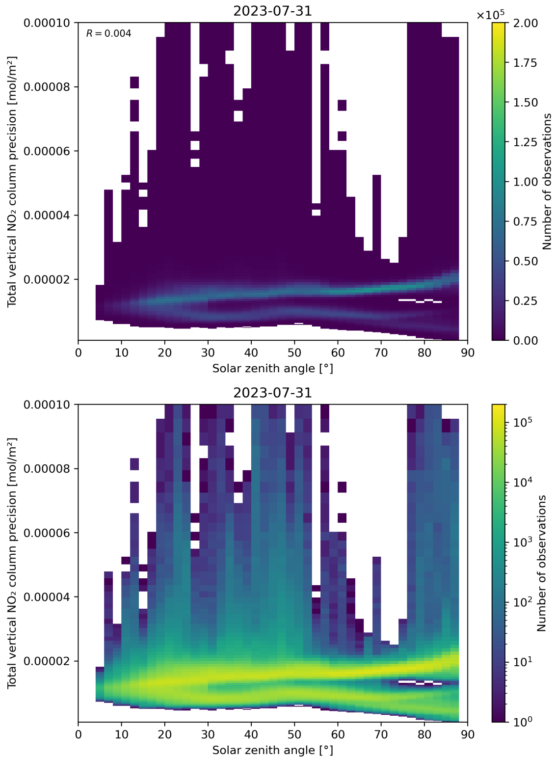
Figure 154: Scatter density plot of “Solar zenith angle” against “Total vertical NO 2 column precision” for 2023-07-30 to 2023-08-01.
