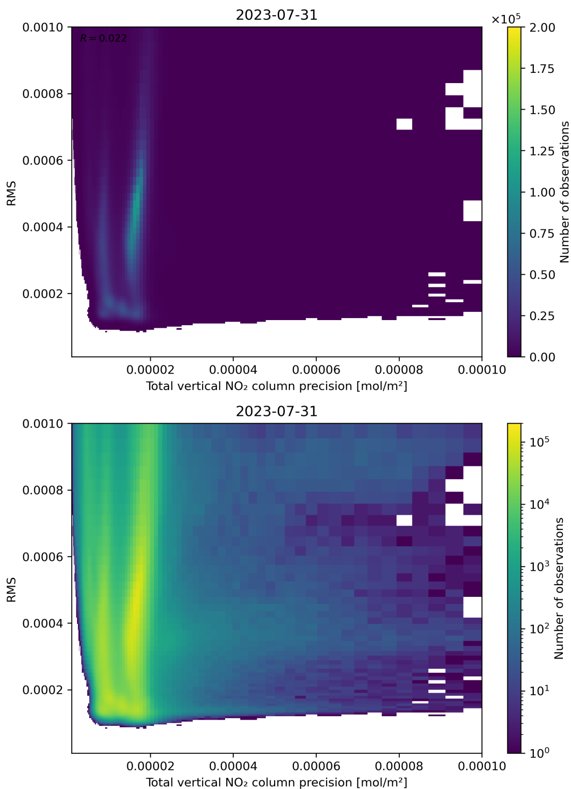
Figure 119: Scatter density plot of “Total vertical NO 2 column precision” against “RMS” for 2023-07-30 to 2023-08-01.
