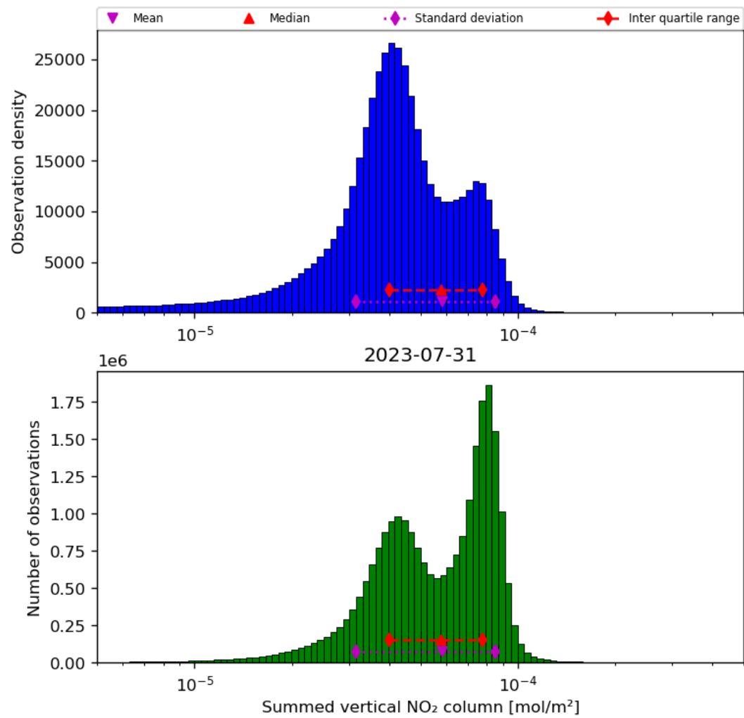
Figure 40: Histogram of “Summed vertical NO 2 column” for 2023-07-30 to 2023-08-01
