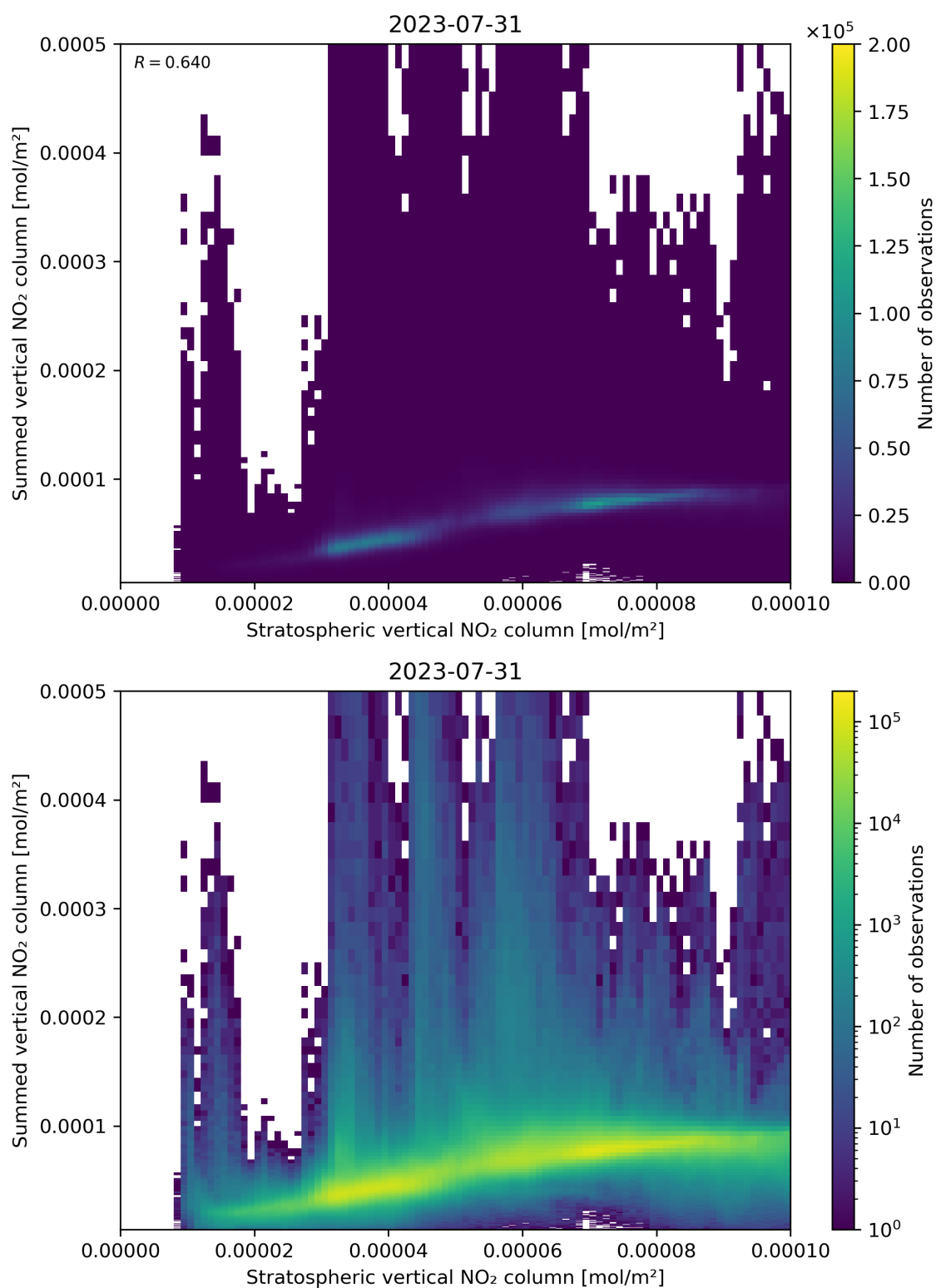
Figure 98: Scatter density plot of “Stratospheric vertical NO 2 column” against “Summed vertical NO 2 column” for 2023-07-30 to 2023-08-01.
