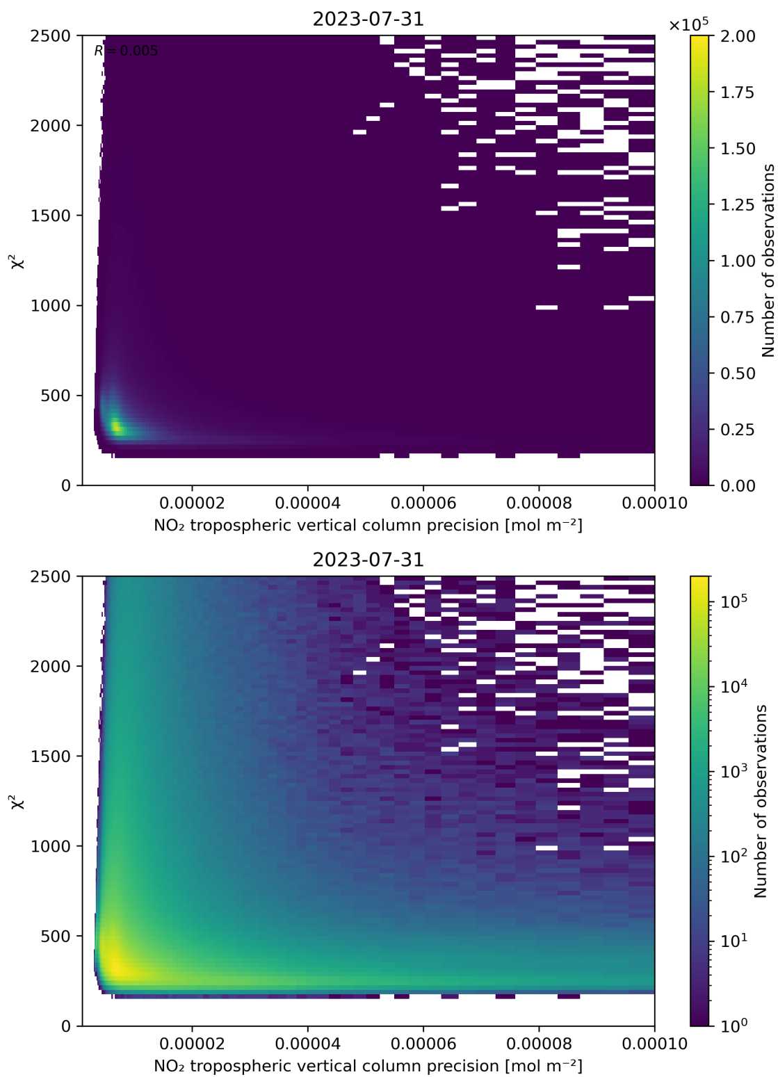
Figure 134: Scatter density plot of “NO 2 tropospheric vertical column precision” against “ \chi^2 ” for 2023-07-30 to 2023-08-01.
