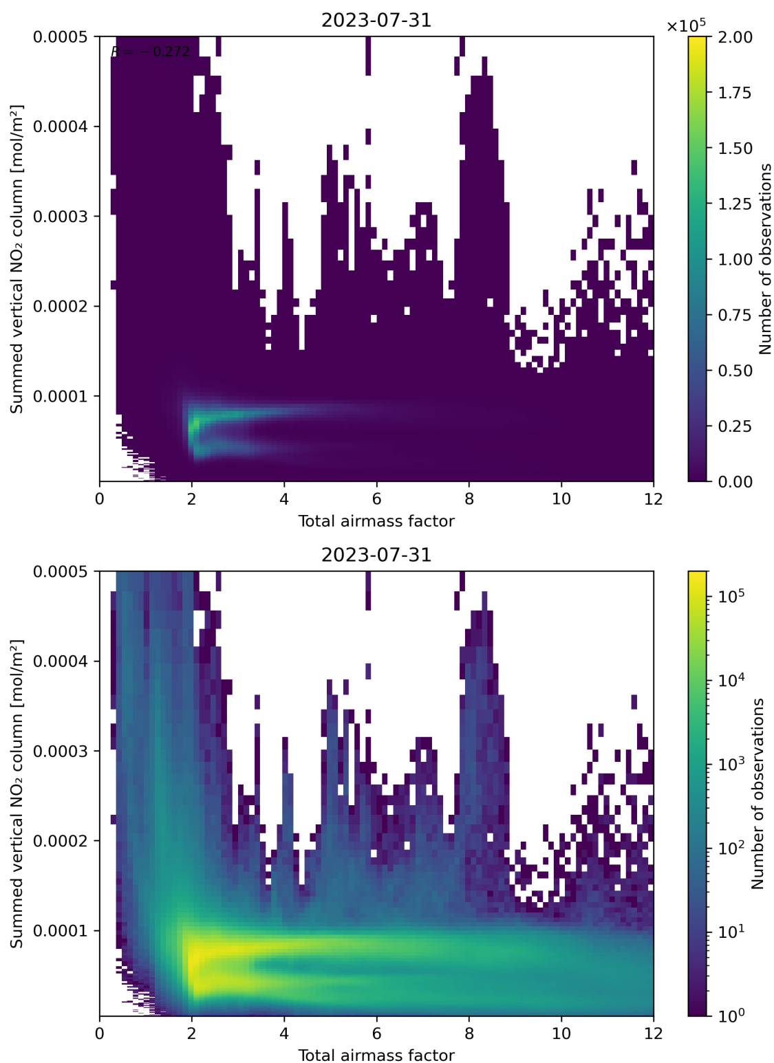
Figure 65: Scatter density plot of “Total airmass factor” against “Summed vertical NO 2 column” for 2023-07-30 to 2023-08-01.
