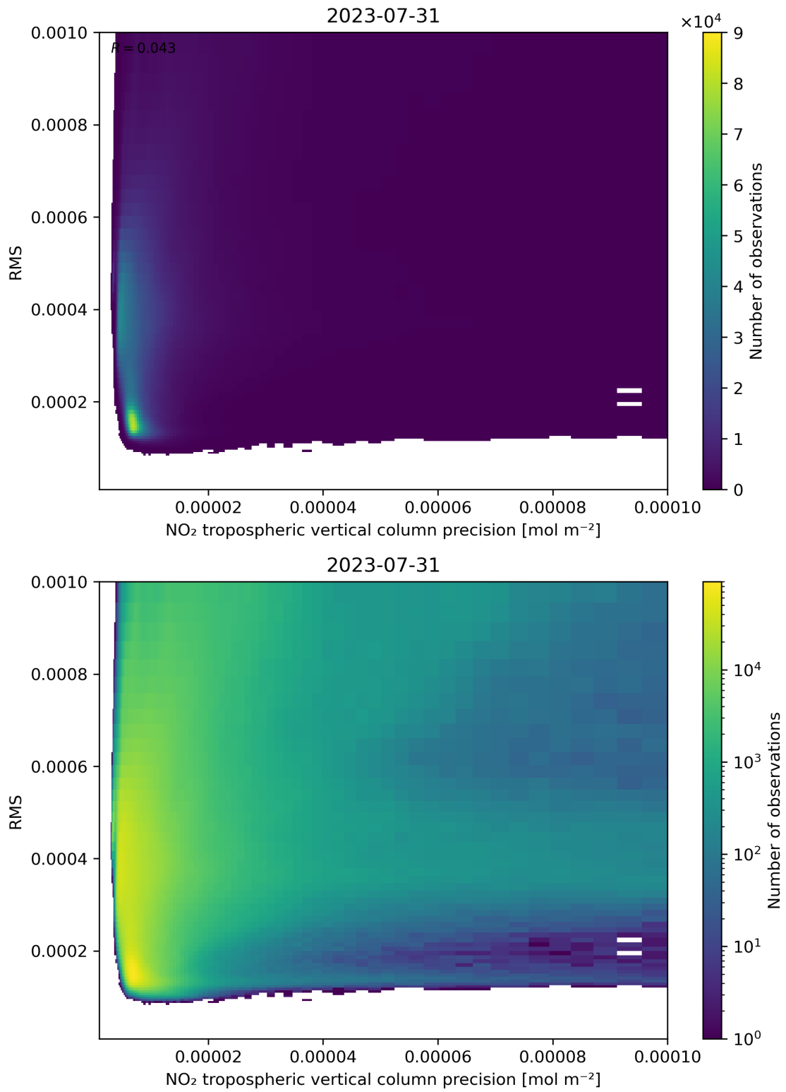
Figure 140: Scatter density plot of “NO 2 tropospheric vertical column precision” against “RMS” for 2023-07-30 to 2023-08-01.
