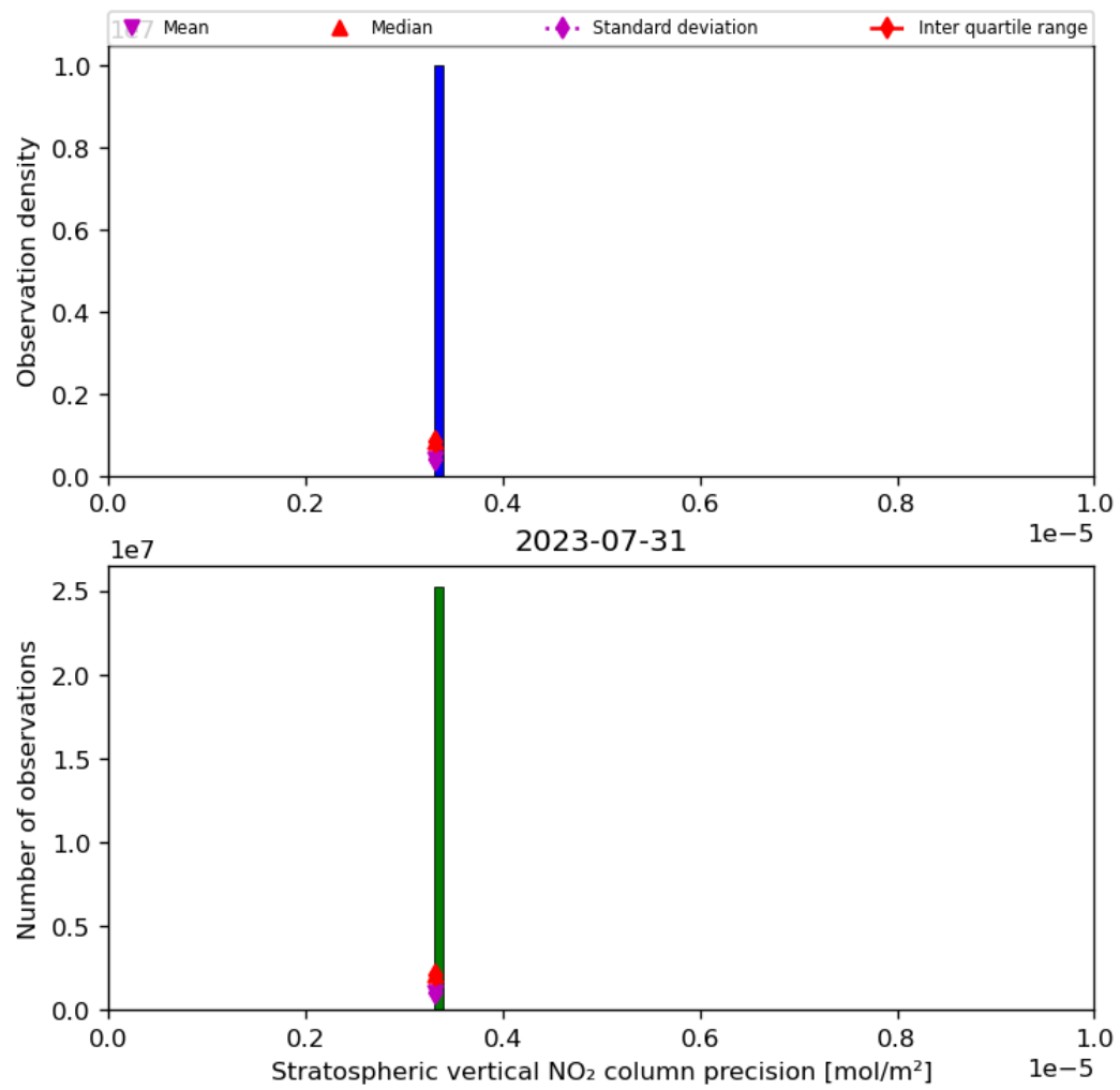
Figure 37: Histogram of “Stratospheric vertical NO 2 column precision” for 2023-07-30 to 2023-08-01
