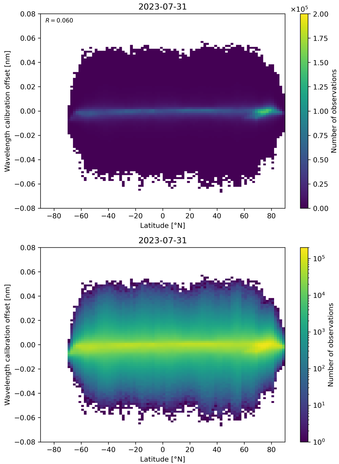
Figure 95: Scatter density plot of “Latitude” against “Wavelength calibration offset” for 2023-07-30 to 2023-08-01.
