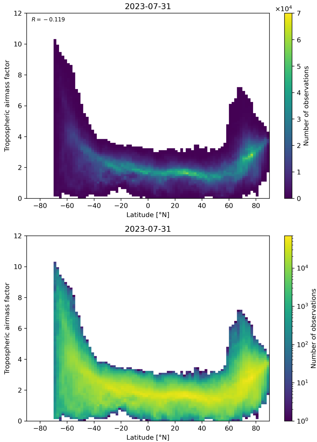
Figure 85: Scatter density plot of “Latitude” against “Tropospheric airmass factor” for 2023-07-30 to 2023-08-01.
