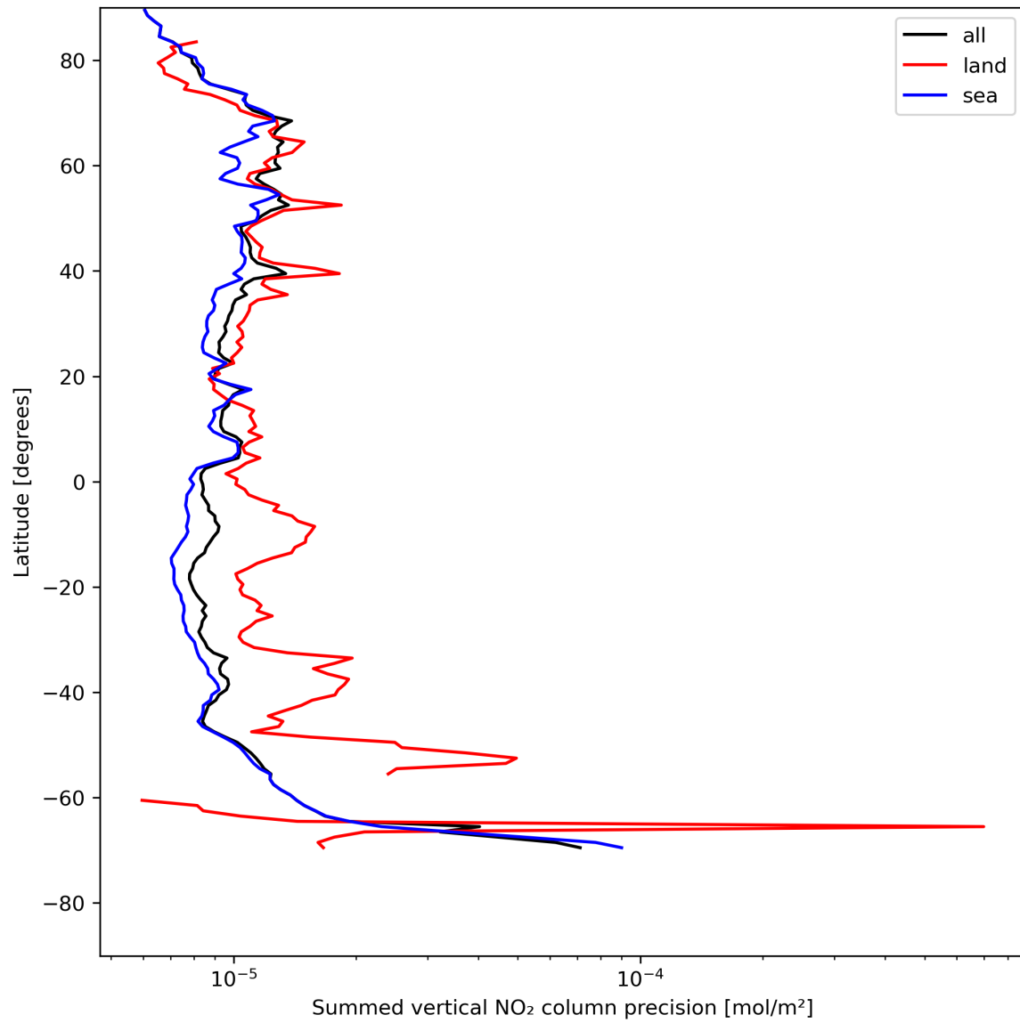
Figure 24: Zonal average of “Summed vertical NO 2 column precision” for 2023-07-30 to 2023-08-01.
