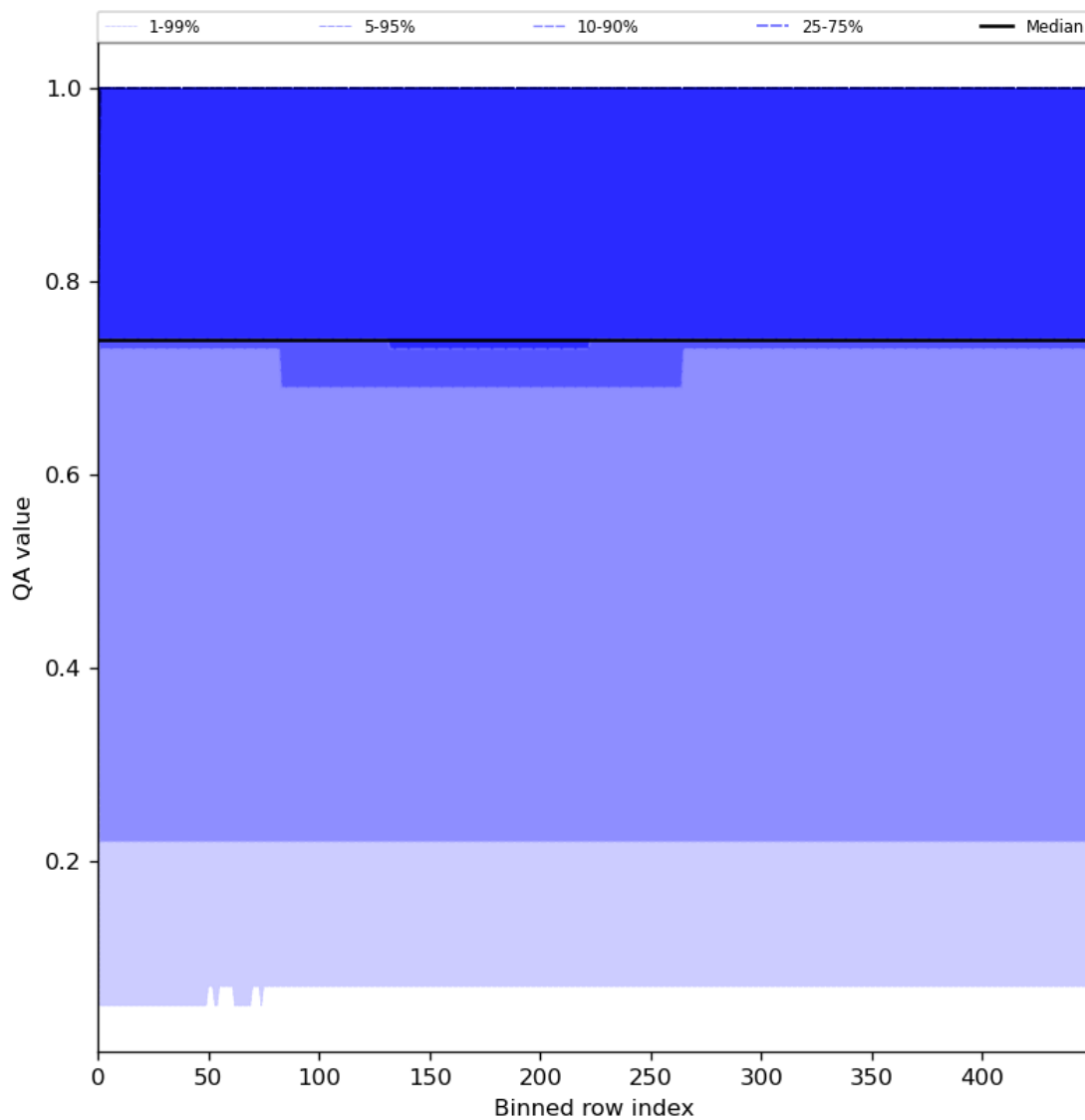
Figure 45: Along track statistics of “QA value” for 2023-07-30 to 2023-08-01
