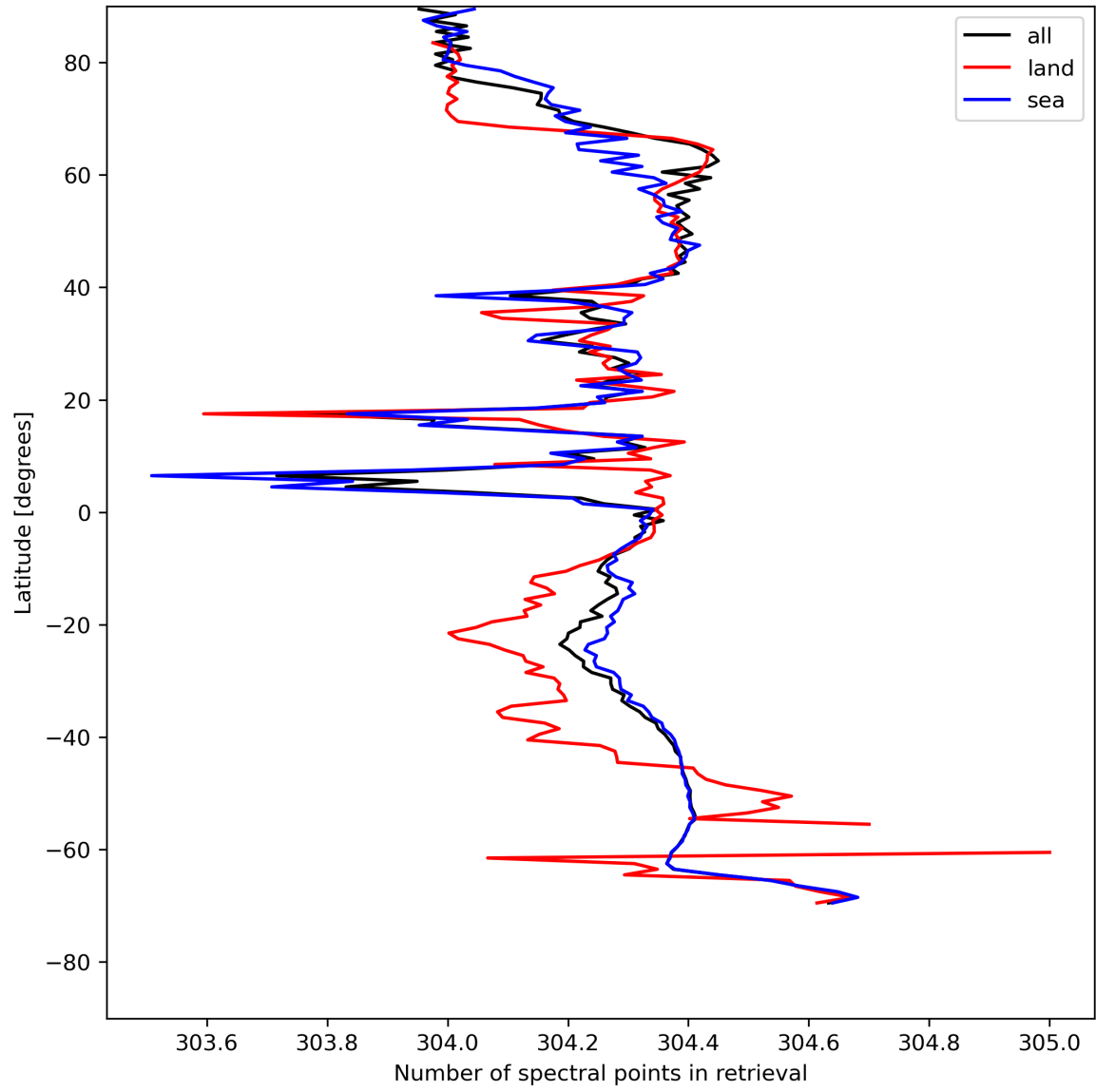
Figure 16: Zonal average of “Number of spectral points in retrieval” for 2023-07-30 to 2023-08-01.
