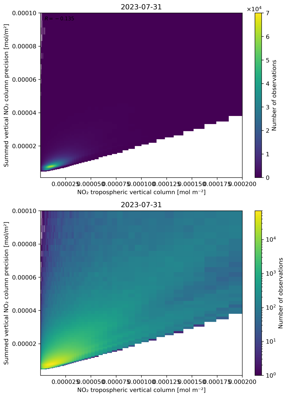
Figure 127: Scatter density plot of “NO 2 tropospheric vertical column” against “Summed vertical NO 2 column precision” for 2023-07-30 to 2023-08-01.
