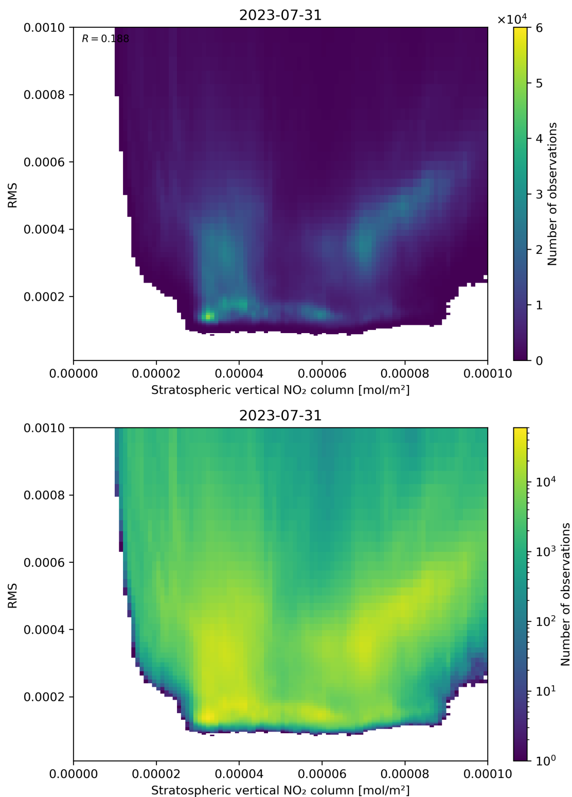
Figure 102: Scatter density plot of “Stratospheric vertical NO 2 column” against “RMS” for 2023-07-30 to 2023-08-01.
