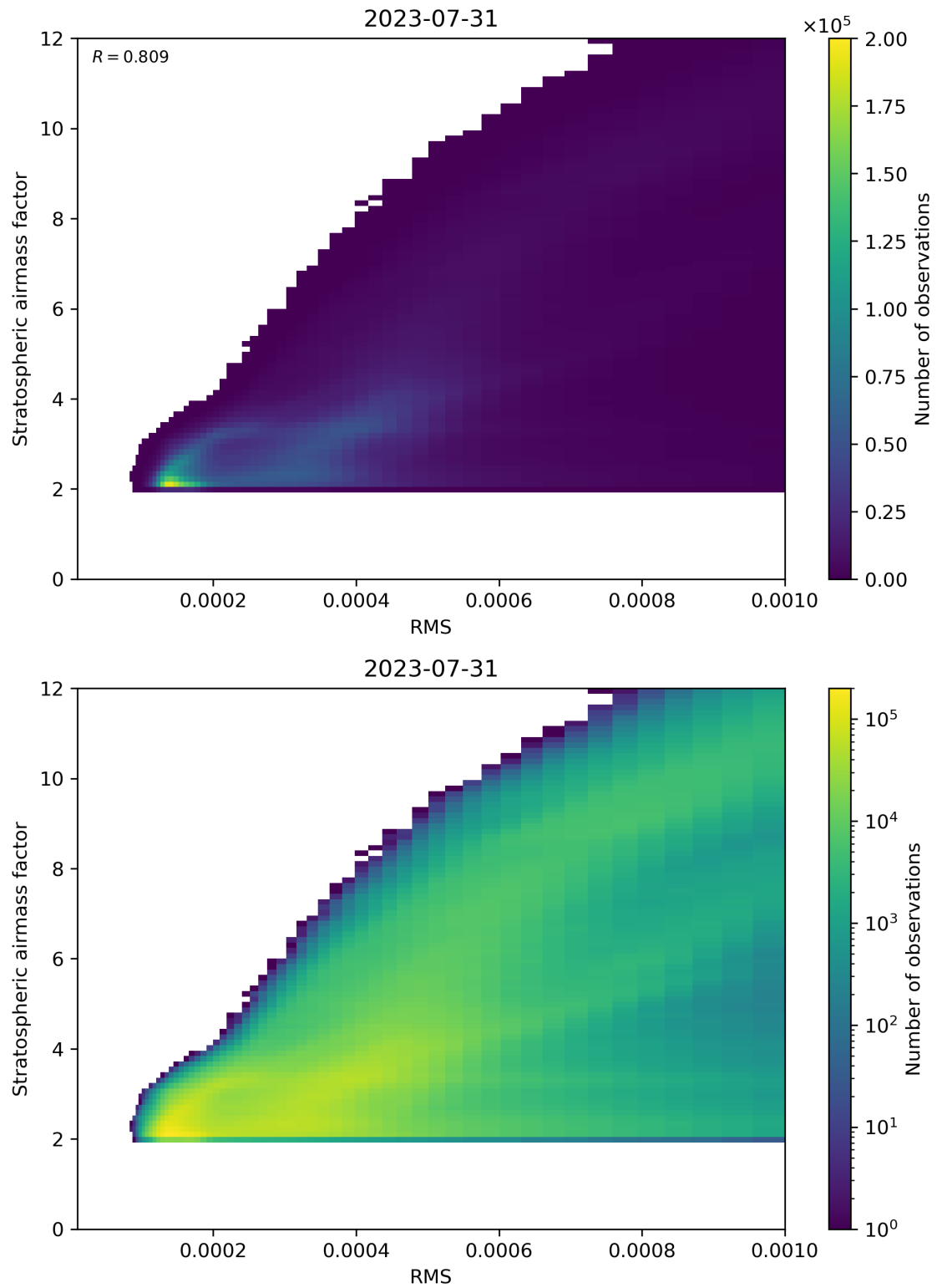
Figure 144: Scatter density plot of “RMS” against “Stratospheric airmass factor” for 2023-07-30 to 2023-08-01.
