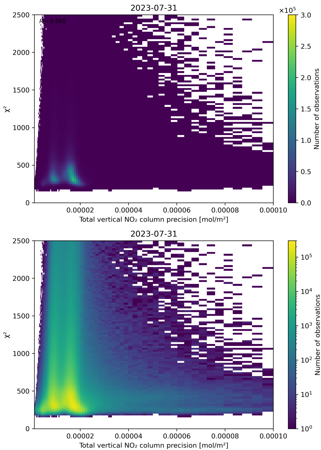
Figure 116: Scatter density plot of “Total vertical NO 2 column precision” against “ \chi^2 ” for 2023-07-30 to 2023-08-01.
