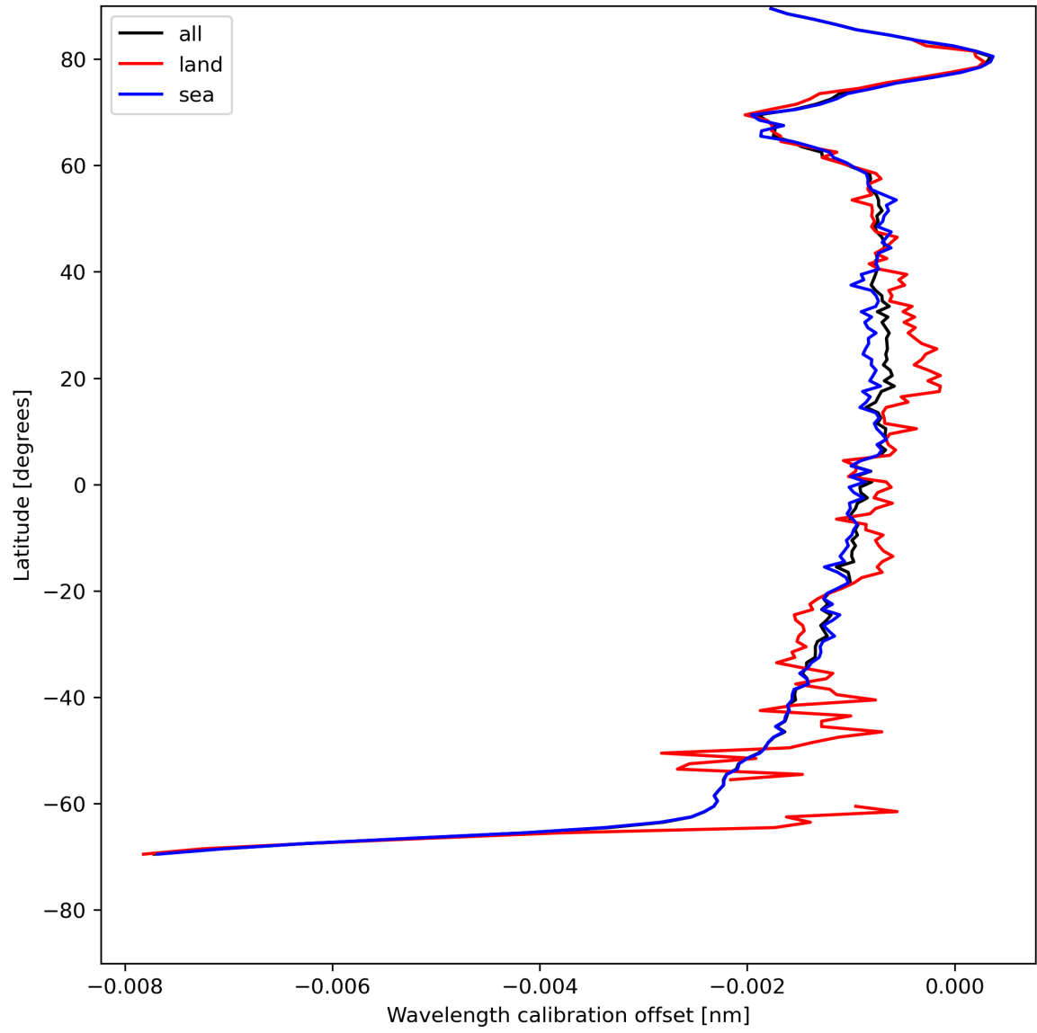
Figure 18: Zonal average of “Wavelength calibration offset” for 2023-07-30 to 2023-08-01.
