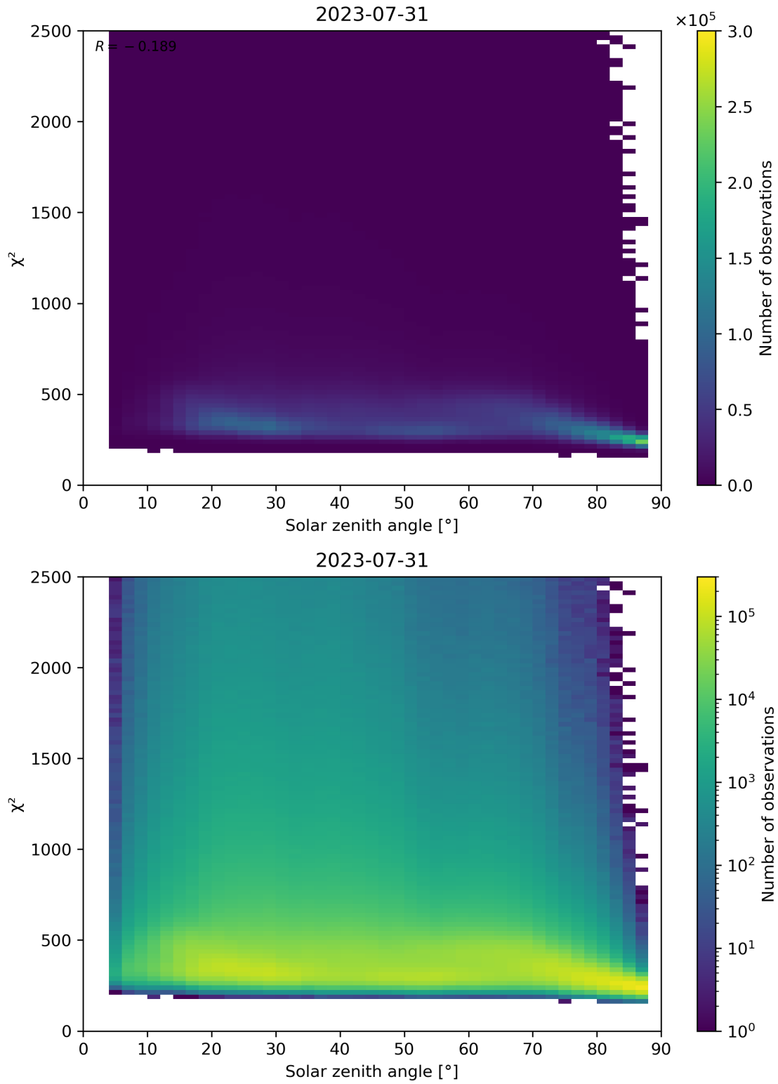
Figure 148: Scatter density plot of “Solar zenith angle” against “ \chi^2 ” for 2023-07-30 to 2023-08-01.
