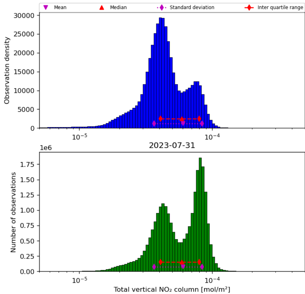
Figure 38: Histogram of “Total vertical NO 2 column” for 2023-07-30 to 2023-08-01
