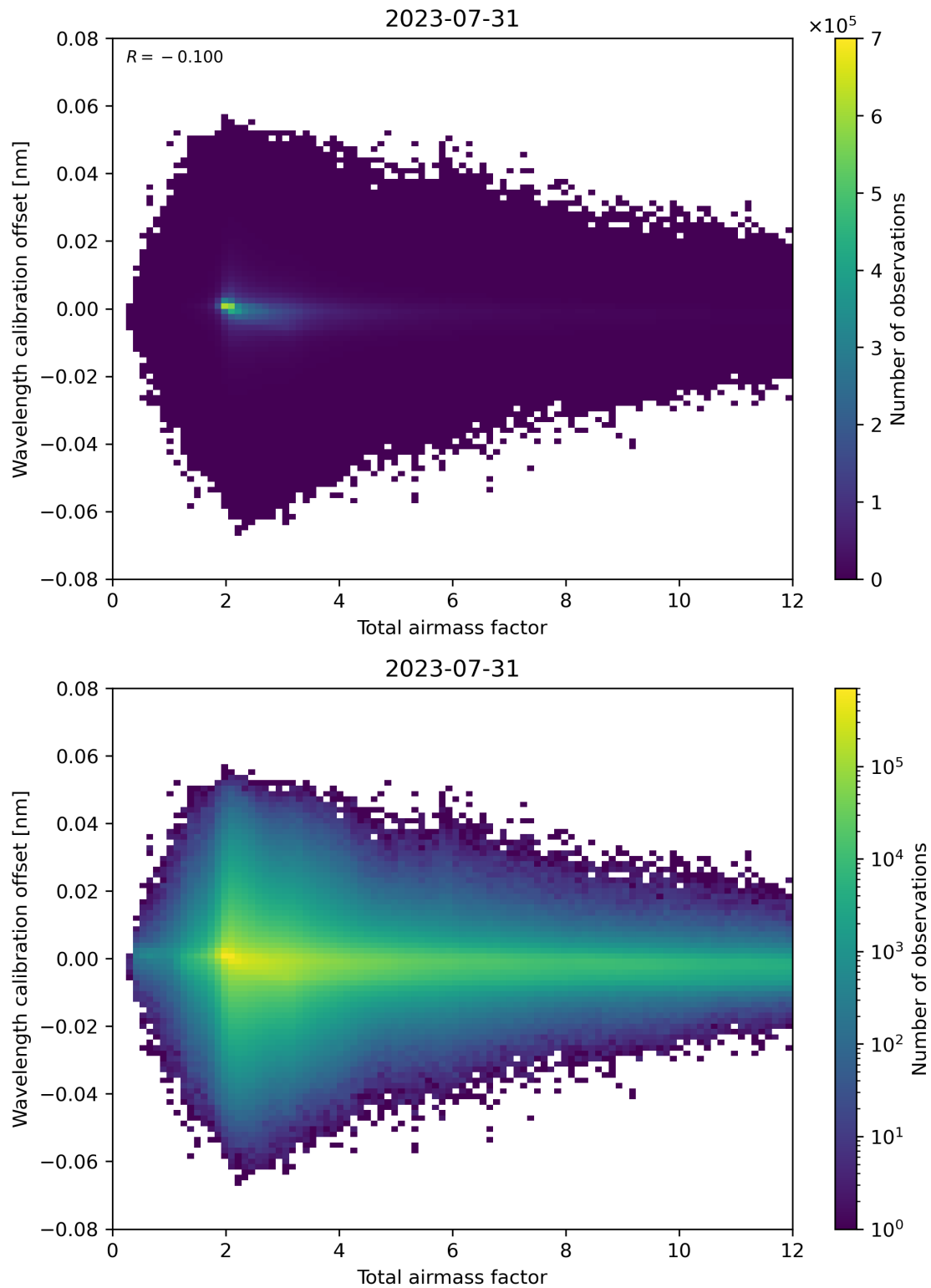
Figure 70: Scatter density plot of “Total airmass factor” against “Wavelength calibration offset” for 2023-07-30 to 2023-08-01.
