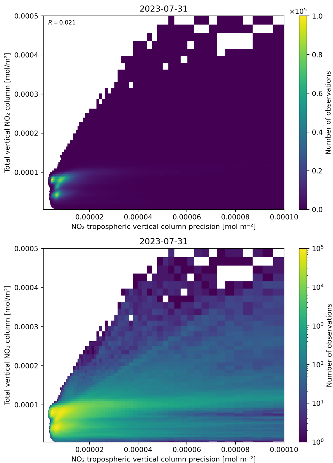
Figure 138: Scatter density plot of “NO 2 tropospheric vertical column precision” against “Total vertical NO 2 column” for 2023-07-30 to 2023-08-01.
