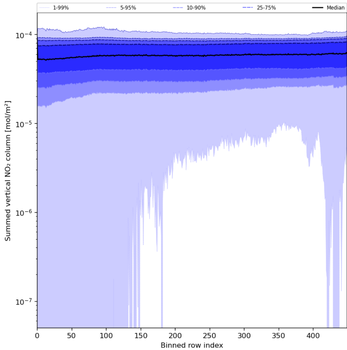
Figure 57: Along track statistics of “Summed vertical NO 2 column” for 2023-07-30 to 2023-08-01
