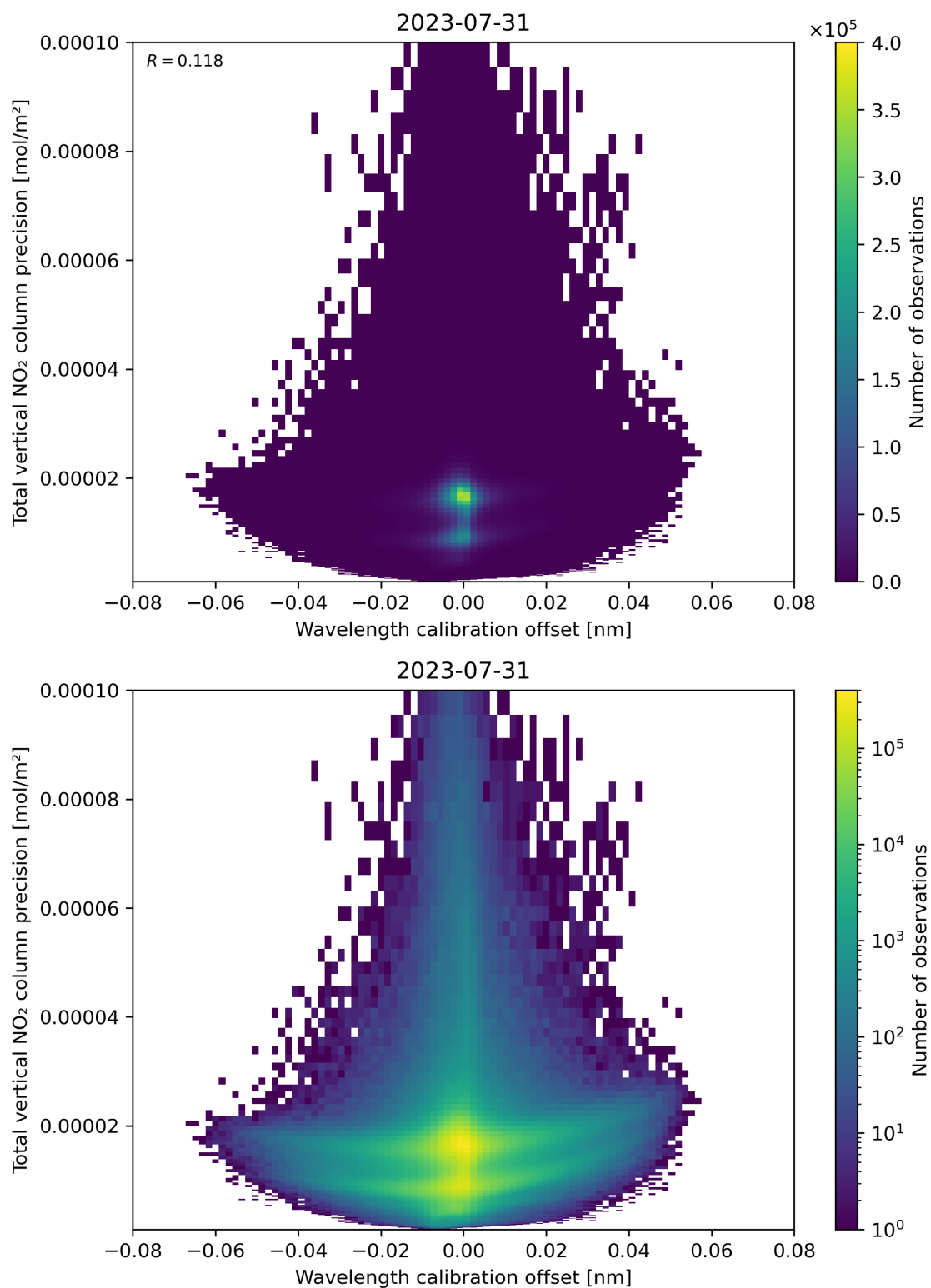
Figure 180: Scatter density plot of “Wavelength calibration offset” against “Total vertical NO 2 column precision” for 2023-07-30 to 2023-08-01.
