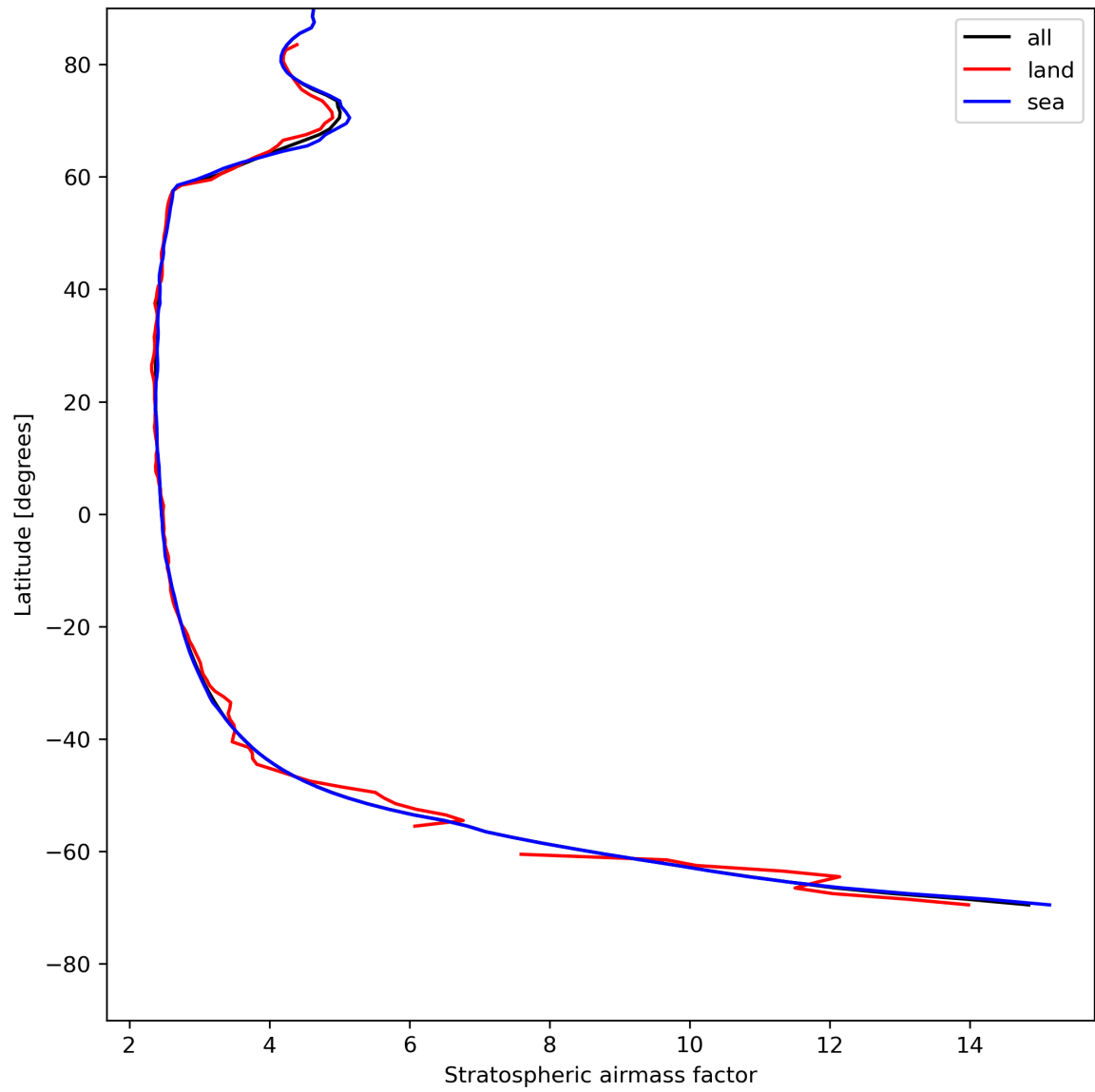
Figure 27: Zonal average of “Stratospheric air mass factor” for 2023-07-30 to 2023-08-01.
