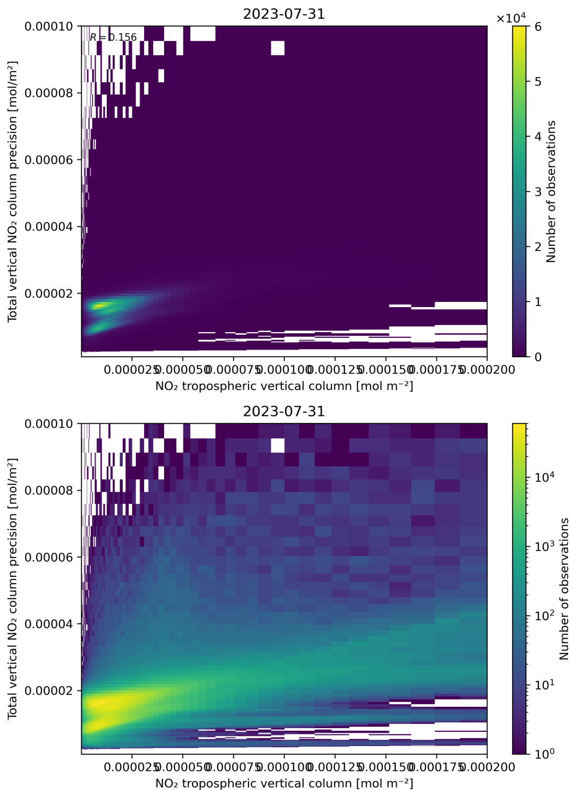
Figure 129: Scatter density plot of “NO 2 tropospheric vertical column” against “Total vertical NO 2 column precision” for 2023-07-30 to 2023-08-01.
