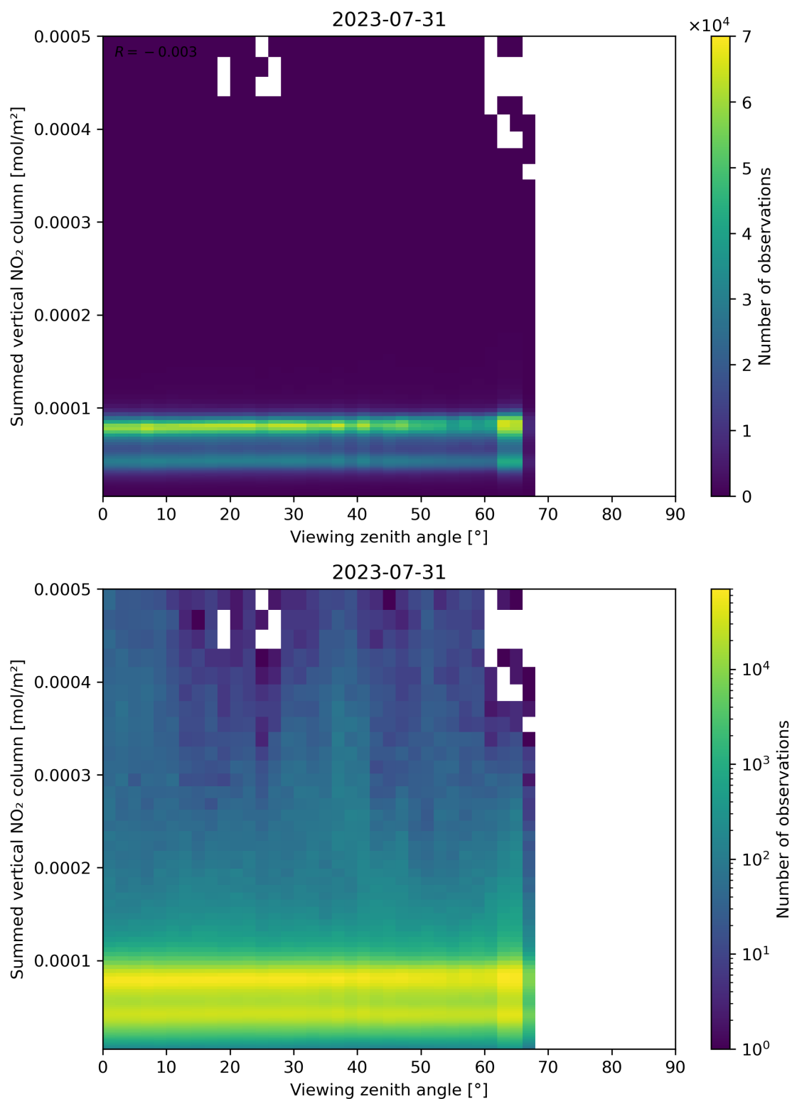
Figure 165: Scatter density plot of “Viewing zenith angle” against “Summed vertical NO 2 column” for 2023-07-30 to 2023-08-01.
