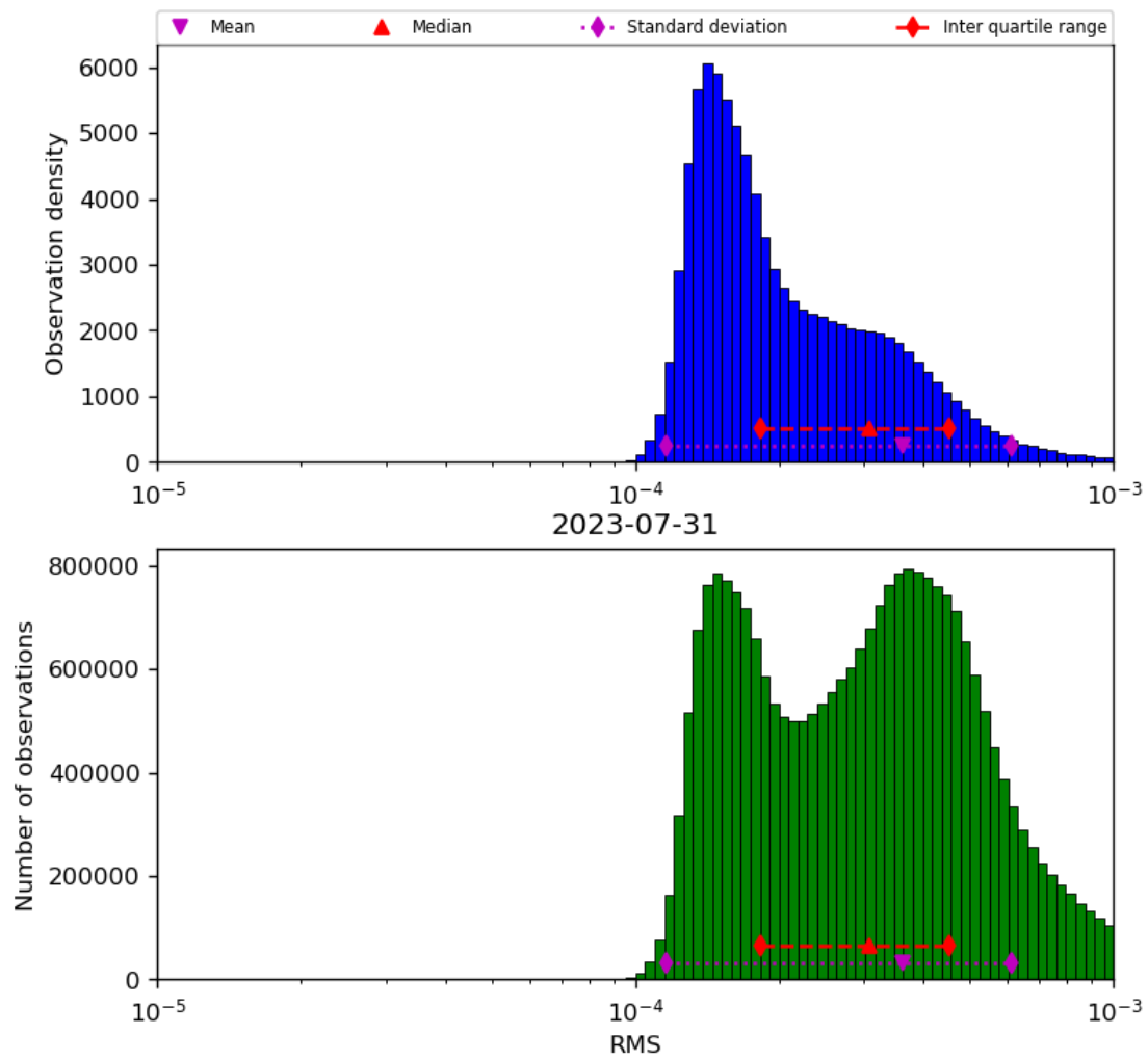
Figure 43: Histogram of “RMS” for 2023-07-30 to 2023-08-01
