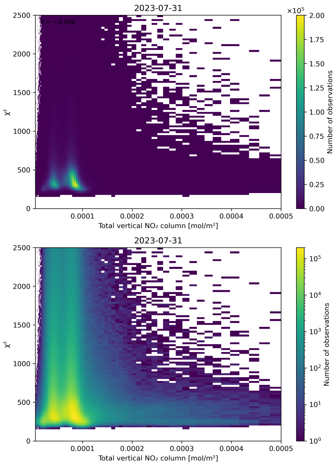
Figure 111: Scatter density plot of “Total vertical NO 2 column” against “ \chi^2 ” for 2023-07-30 to 2023-08-01.
