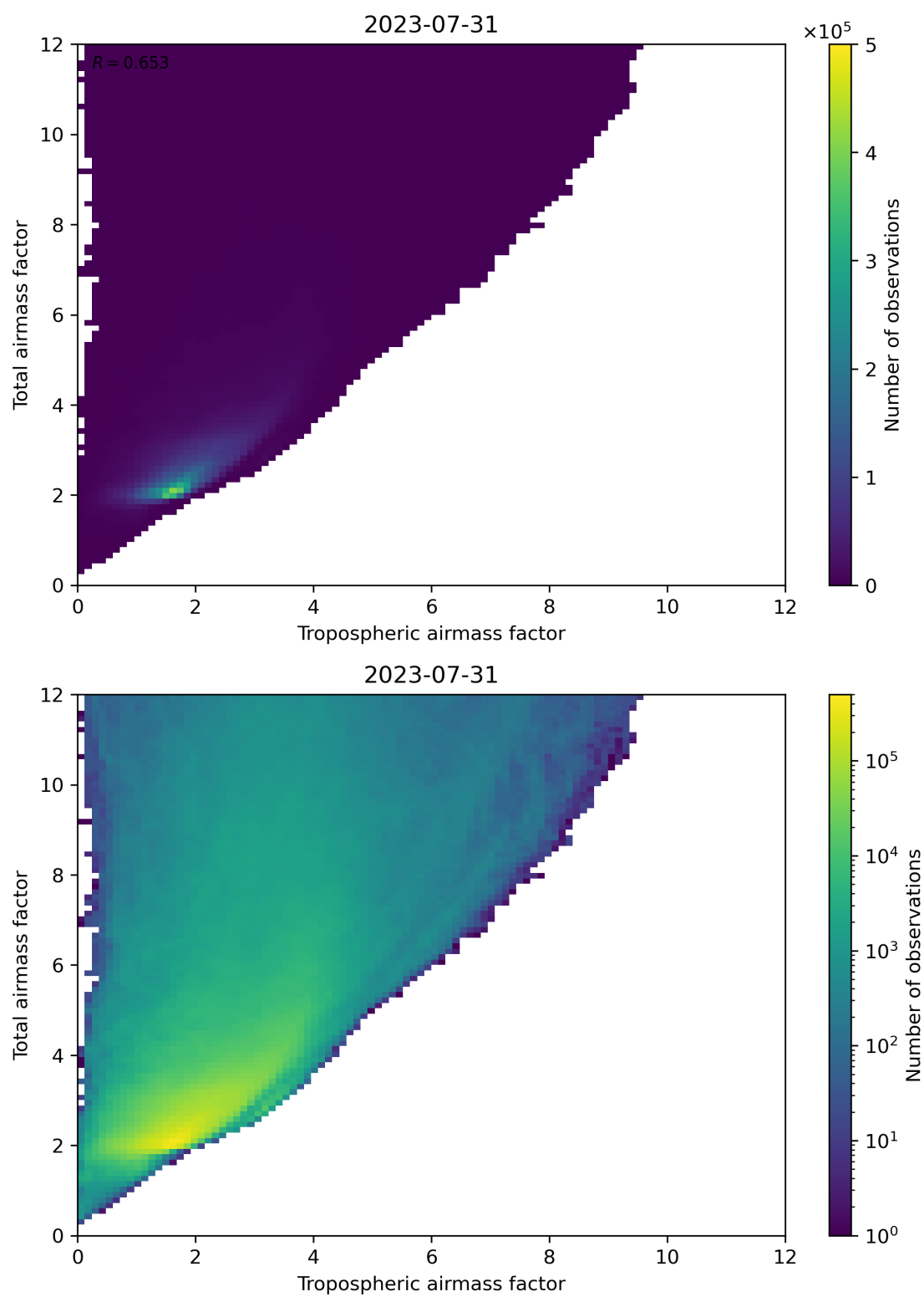
Figure 72: Scatter density plot of “Tropospheric airmass factor” against “Total airmass factor” for 2023-07-30 to 2023-08-01.
