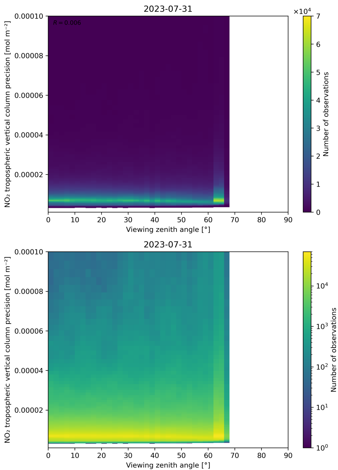
Figure 170: Scatter density plot of “Viewing zenith angle” against “NO 2 tropospheric vertical column precision” for 2023-07-30 to 2023-08-01.
