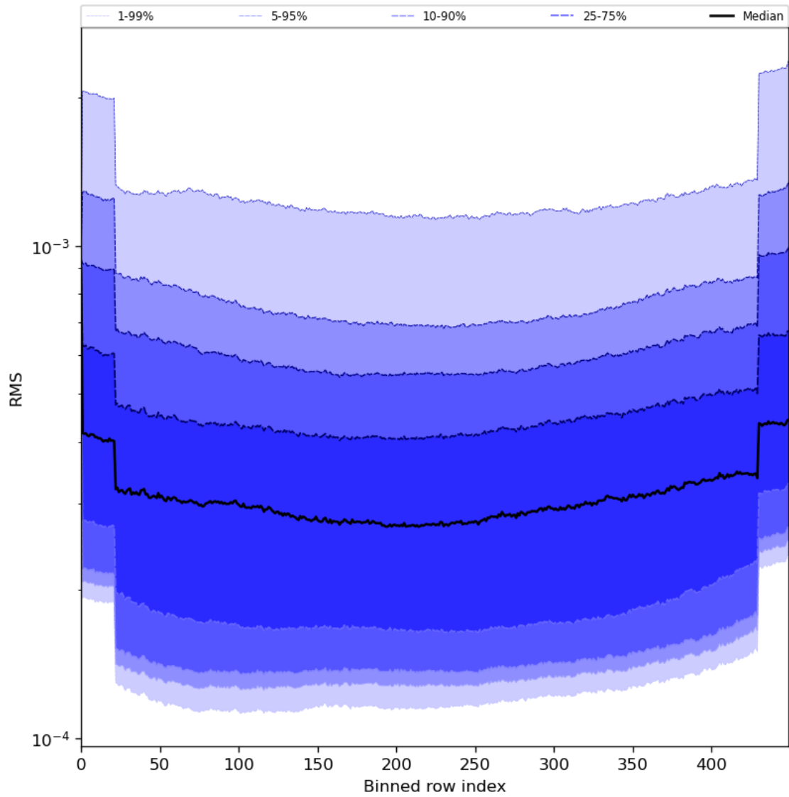
Figure 60: Along track statistics of “RMS” for 2023-07-30 to 2023-08-01
