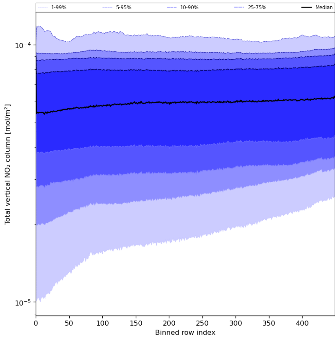
Figure 55: Along track statistics of “Total vertical NO 2 column” for 2023-07-30 to 2023-08-01
