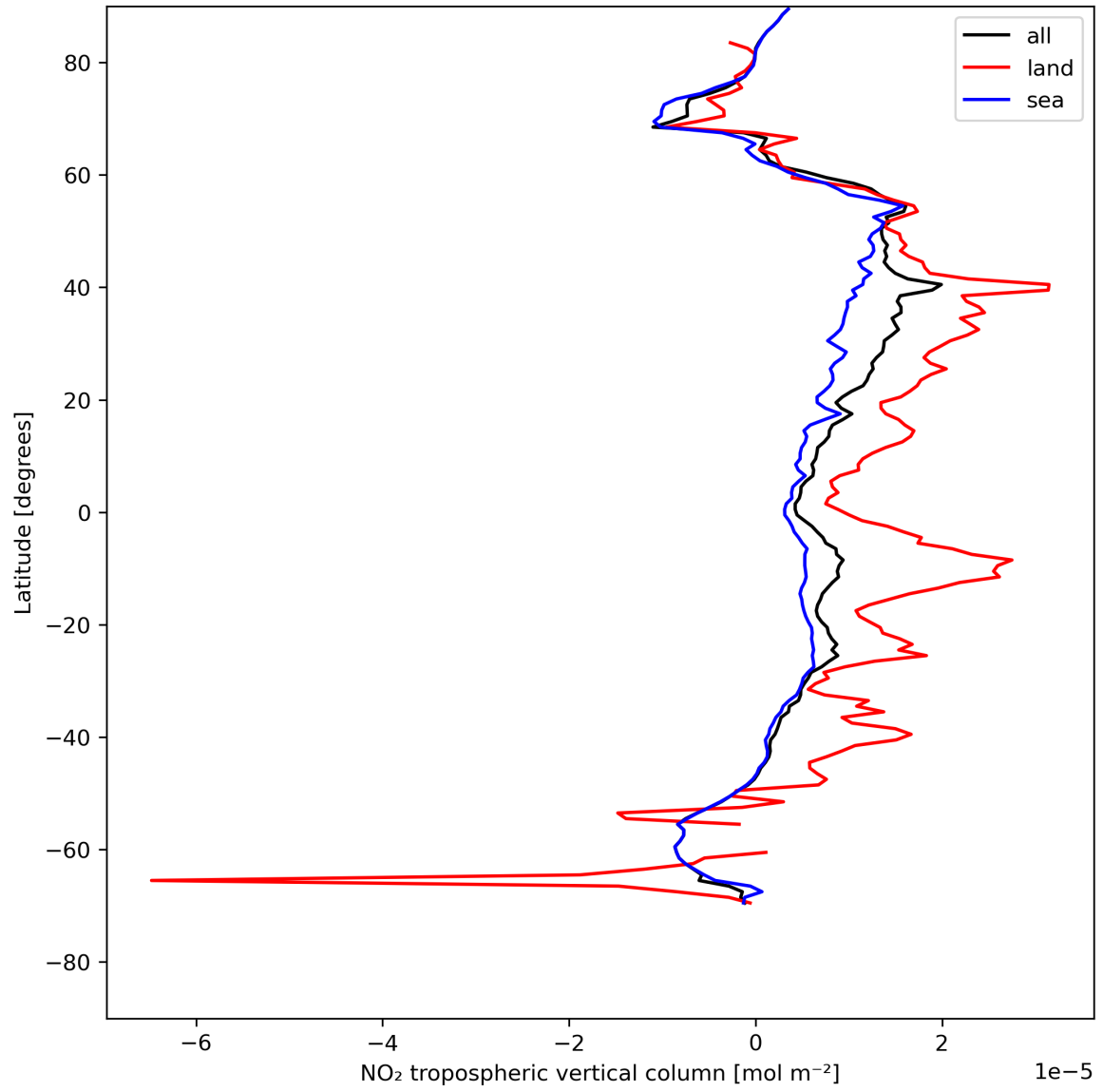
Figure 12: Zonal average of “NO 2 tropospheric vertical column” for 2023-07-30 to 2023-08-01.
