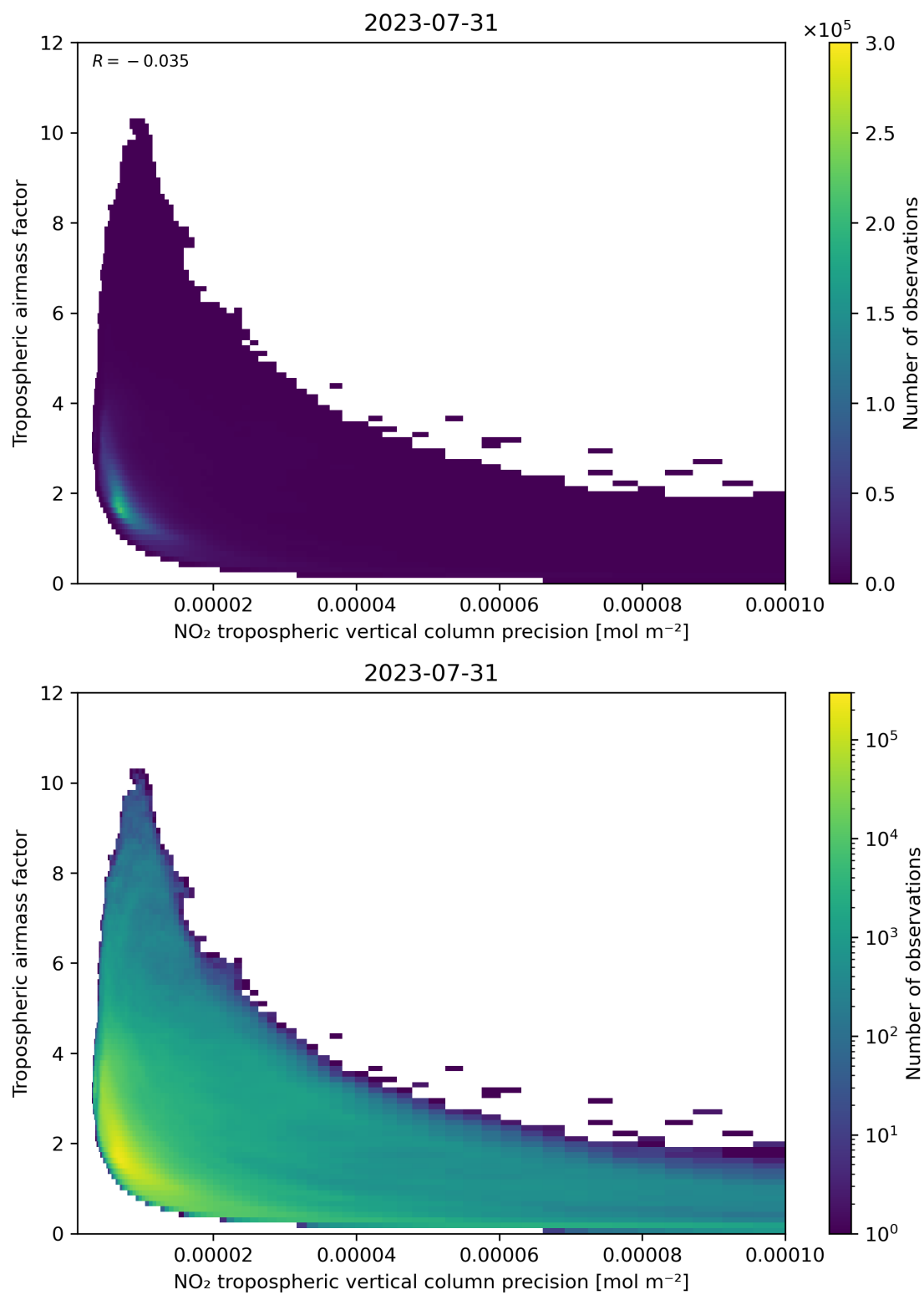
Figure 133: Scatter density plot of “NO 2 tropospheric vertical column precision” against “Tropospheric airmass factor” for 2023-07-30 to 2023-08-01.
