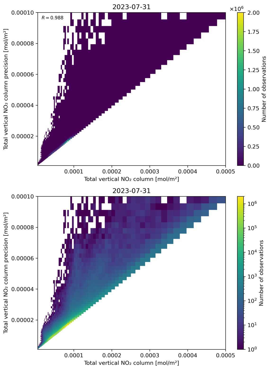
Figure 114: Scatter density plot of “Total vertical NO 2 column” against “Total vertical NO 2 column precision” for 2023-07-30 to 2023-08-01.
