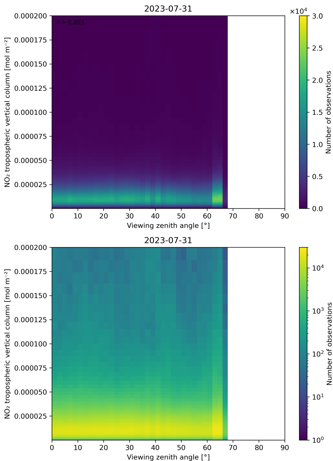
Figure 169: Scatter density plot of “Viewing zenith angle” against “NO 2 tropospheric vertical column” for 2023-07-30 to 2023-08-01.
