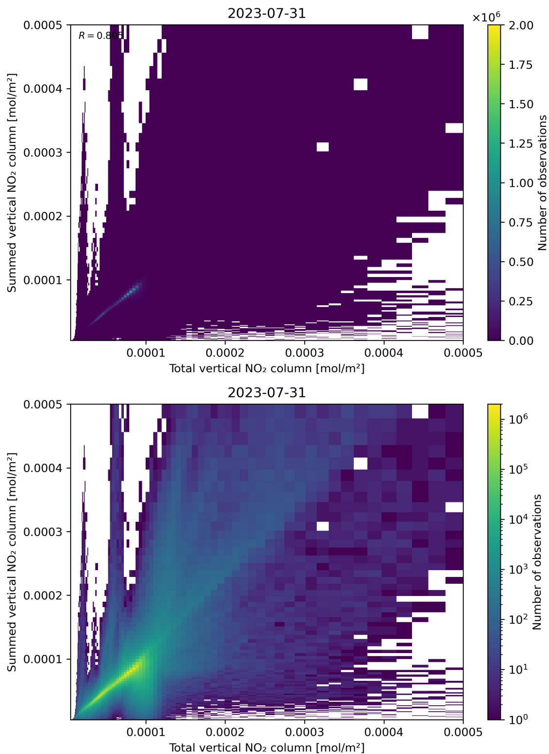
Figure 112: Scatter density plot of “Total vertical NO 2 column” against “Summed vertical NO 2 column” for 2023-07-30 to 2023-08-01.
