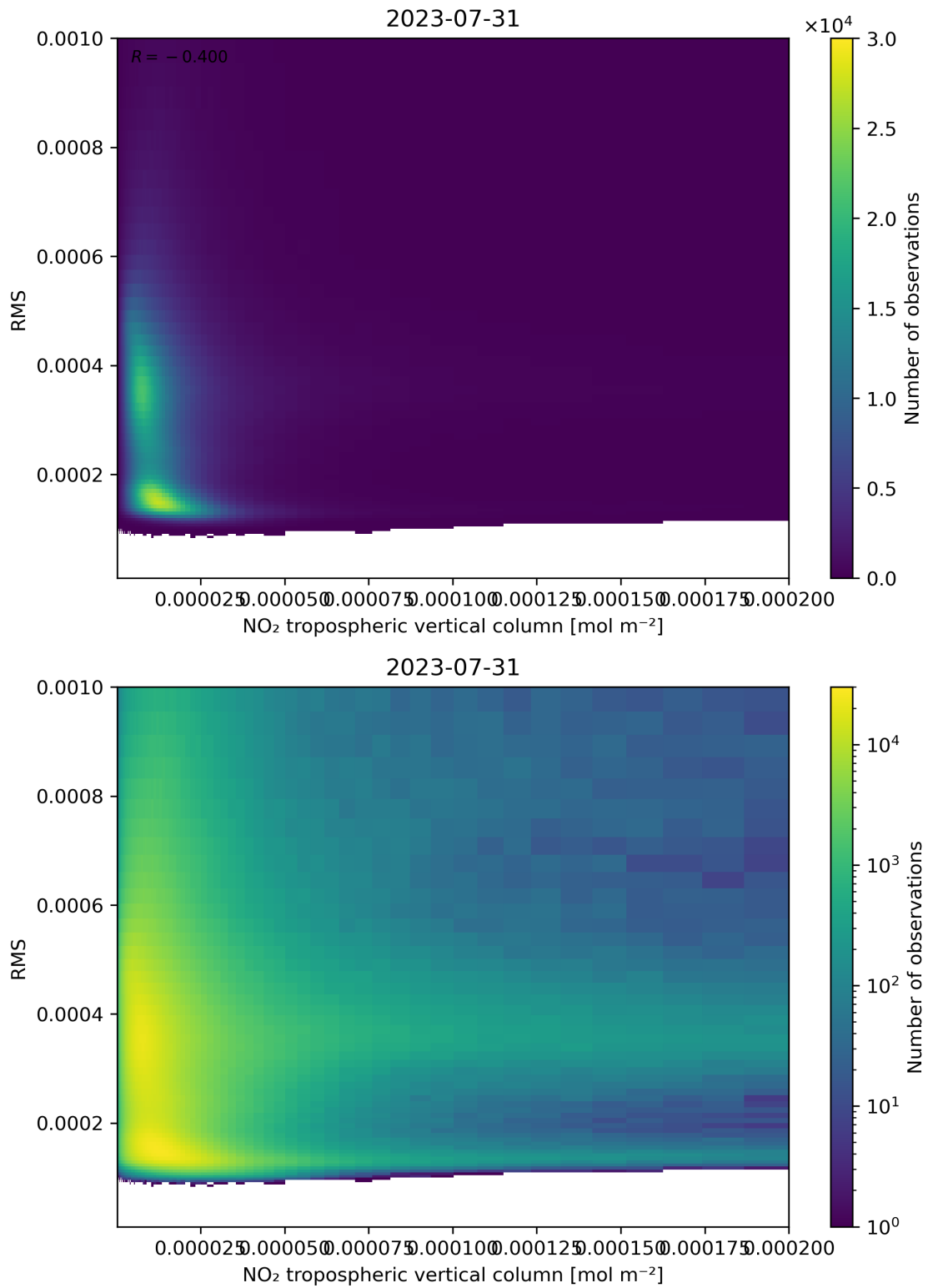
Figure 142: Scatter density plot of “NO 2 tropospheric vertical column” against “RMS” for 2023-07-30 to 2023-08-01.
