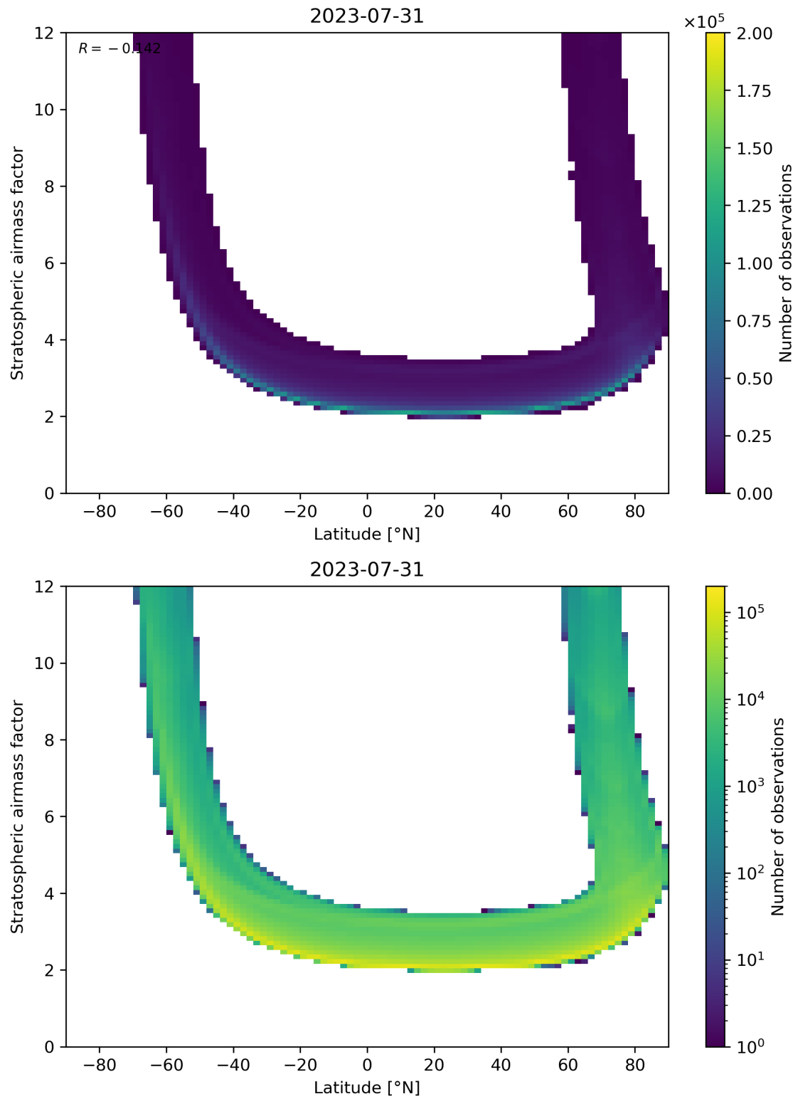
Figure 83: Scatter density plot of “Latitude” against “Stratospheric air mass factor” for 2023-07-30 to 2023-08-01.
