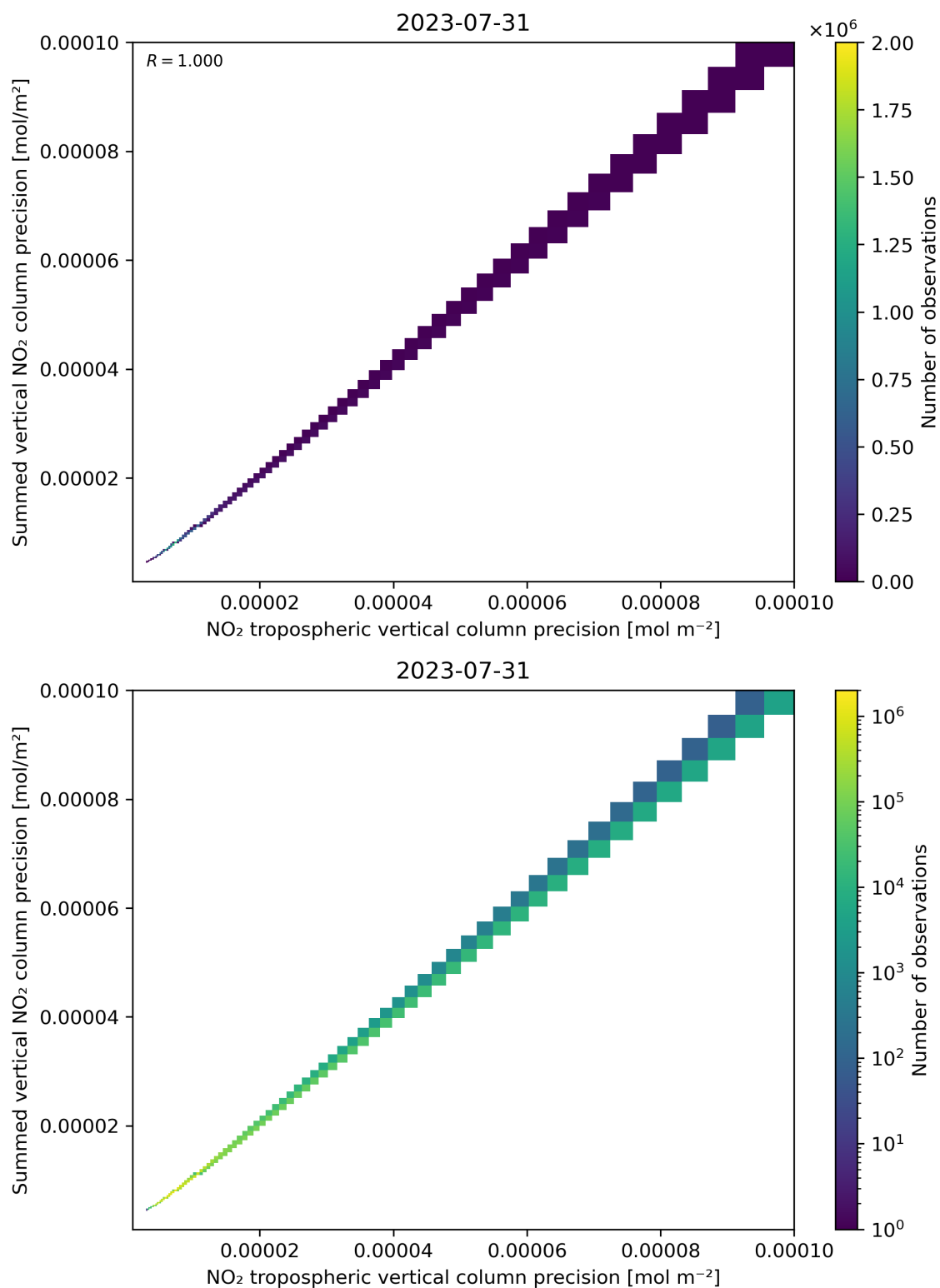
Figure 137: Scatter density plot of “NO 2 tropospheric vertical column precision” against “Summed vertical NO 2 column precision” for 2023-07-30 to 2023-08-01.
