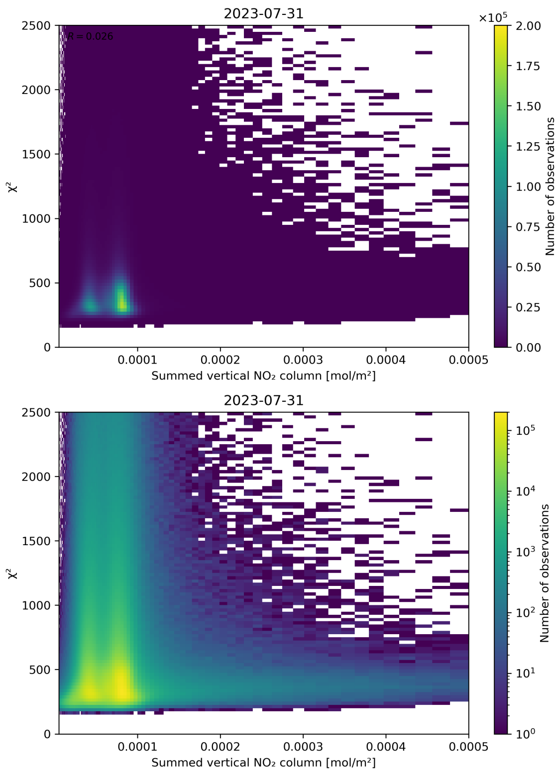
Figure 104: Scatter density plot of “Summed vertical NO 2 column” against “ \chi^2 ” for 2023-07-30 to 2023-08-01.
