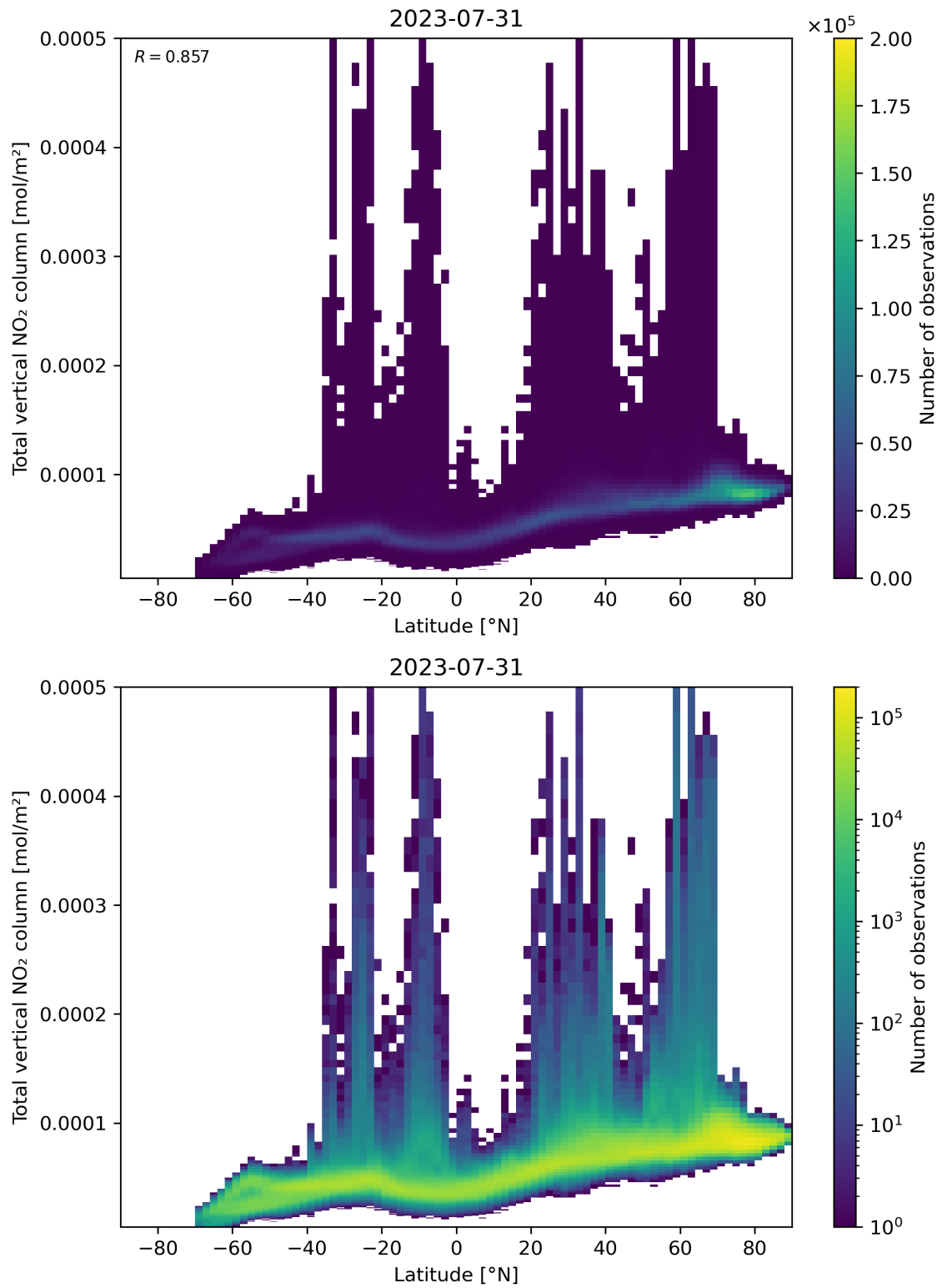
Figure 90: Scatter density plot of “Latitude” against “Total vertical NO 2 column” for 2023-07-30 to 2023-08-01.
