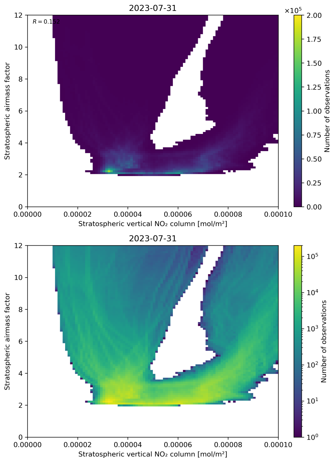
Figure 96: Scatter density plot of “Stratospheric vertical NO 2 column” against “Stratospheric airmass factor” for 2023-07-30 to 2023-08-01.
