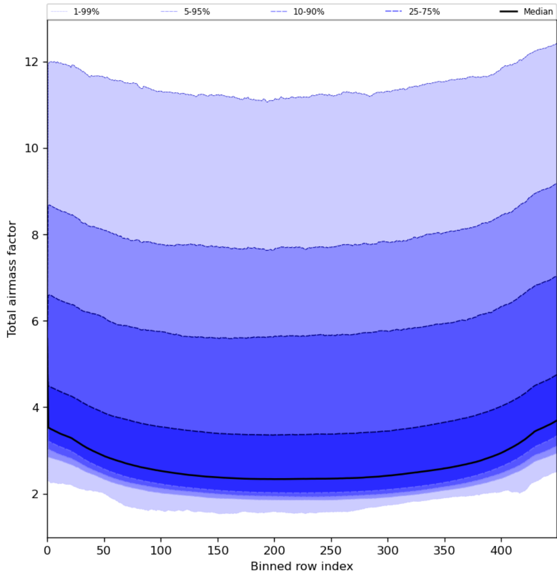
Figure 49: Along track statistics of “Total airmass factor” for 2023-07-30 to 2023-08-01
