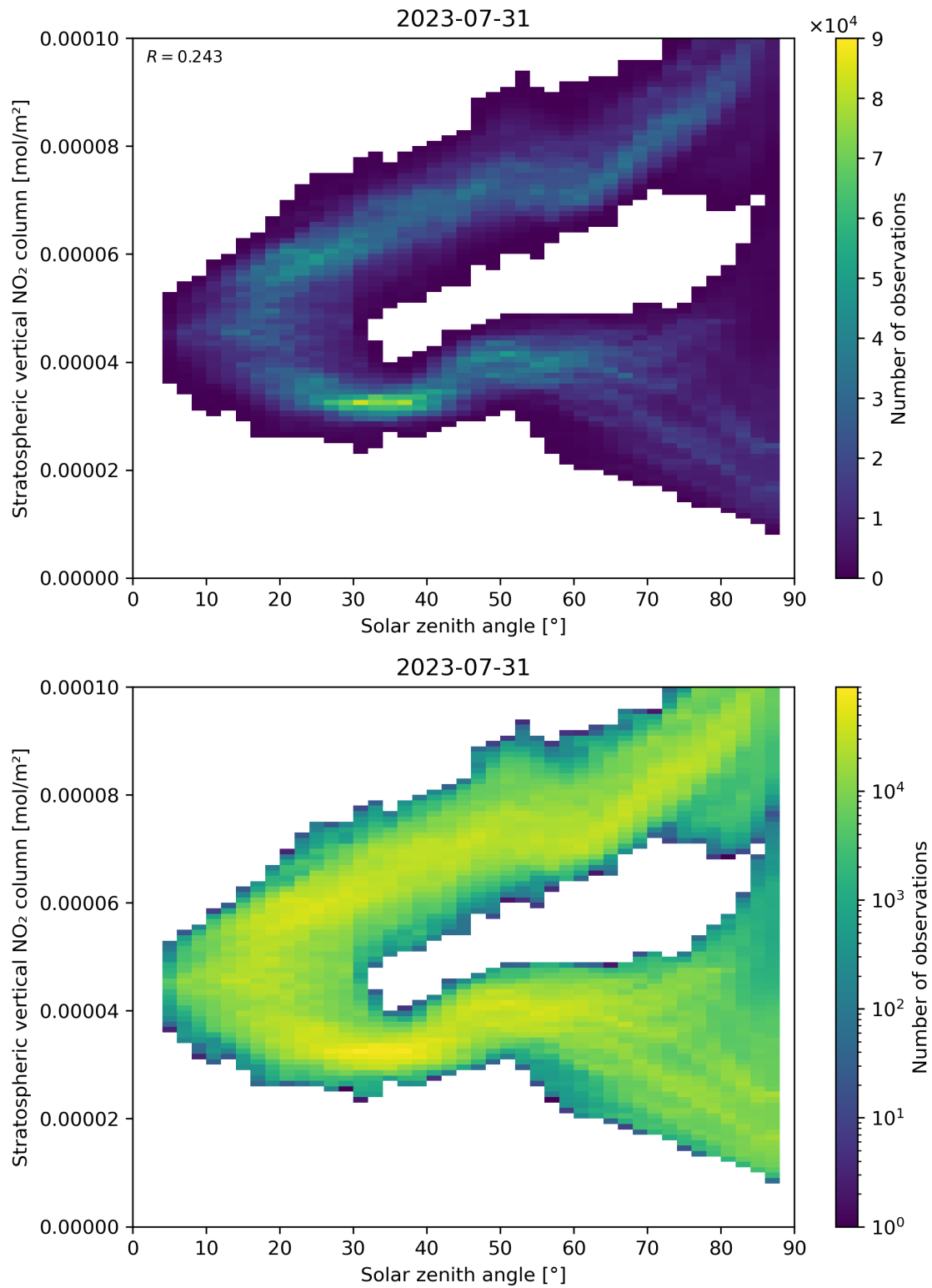
Figure 150: Scatter density plot of “Solar zenith angle” against “Stratospheric vertical NO 2 column” for 2023-07-30 to 2023-08-01.
