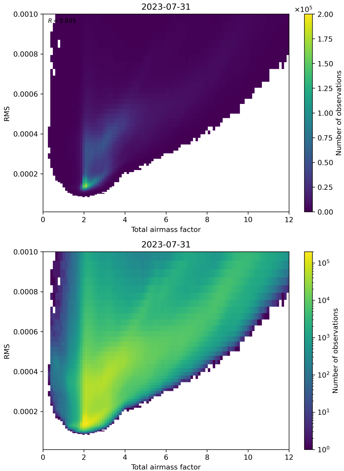
Figure 69: Scatter density plot of “Total airmass factor” against “RMS” for 2023-07-30 to 2023-08-01.
