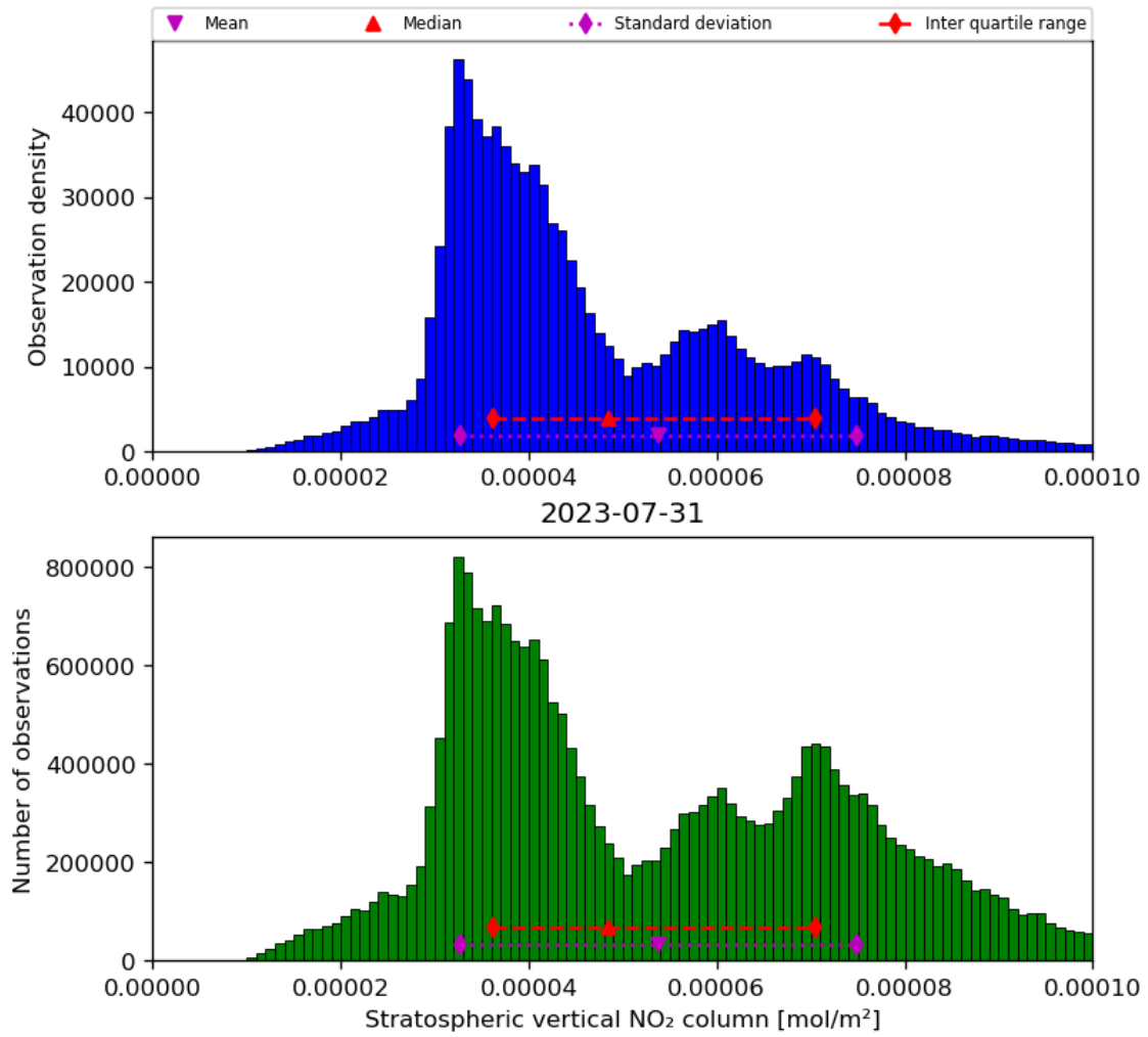
Figure 36: Histogram of “Stratospheric vertical NO 2 column” for 2023-07-30 to 2023-08-01
