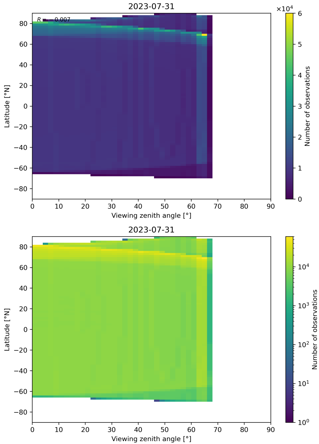
Figure 163: Scatter density plot of “Viewing zenith angle” against “Latitude” for 2023-07-30 to 2023-08-01.
