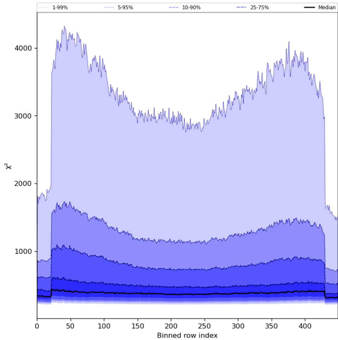
Figure 59: Along track statistics of “ \chi^2 ” for 2023-07-30 to 2023-08-01
