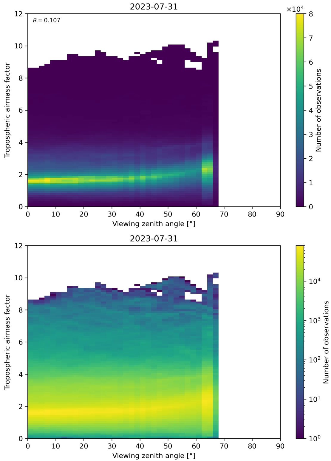
Figure 161: Scatter density plot of “Viewing zenith angle” against “Tropospheric airmass factor” for 2023-07-30 to 2023-08-01.
