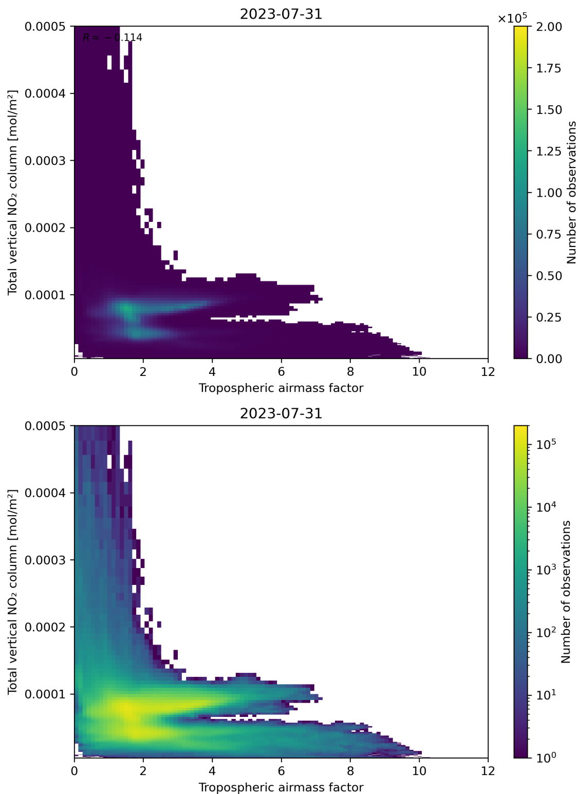
Figure 77: Scatter density plot of “Tropospheric airmass factor” against “Total vertical NO 2 column” for 2023-07-30 to 2023-08-01.
