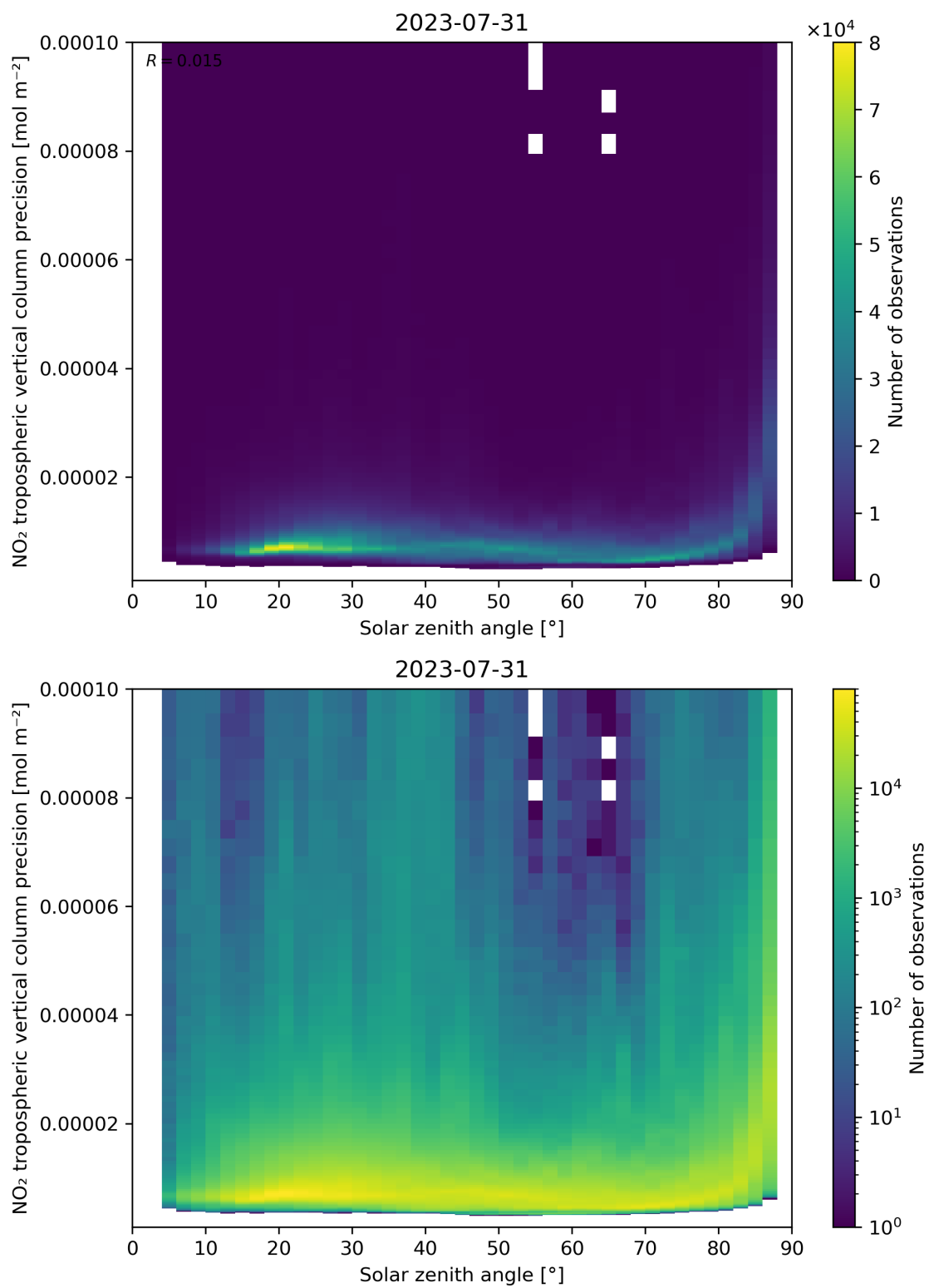
Figure 156: Scatter density plot of “Solar zenith angle” against “NO 2 tropospheric vertical column precision” for 2023-07-30 to 2023-08-01.
