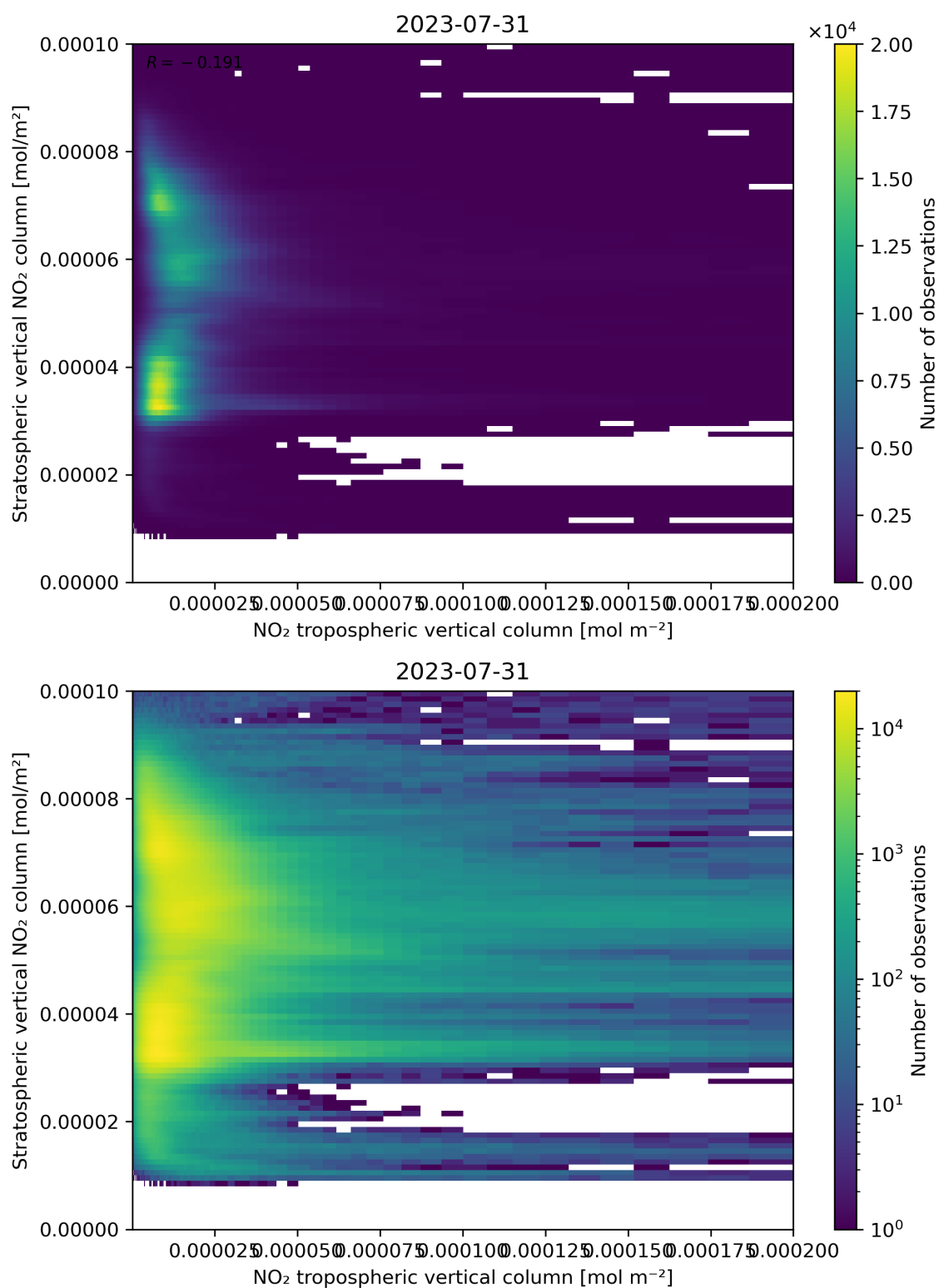
Figure 125: Scatter density plot of “NO 2 tropospheric vertical column” against “Stratospheric vertical NO 2 column” for 2023-07-30 to 2023-08-01.
