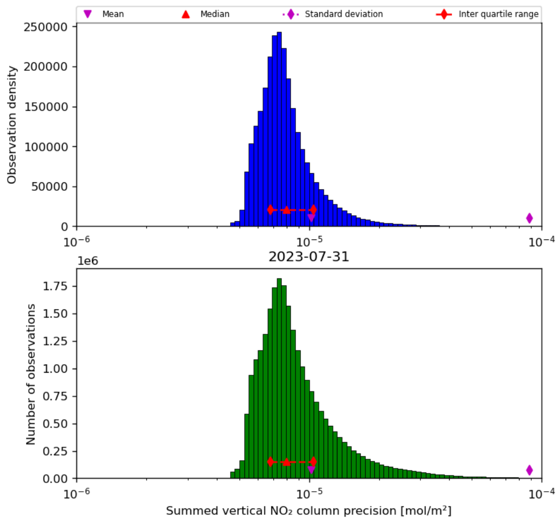
Figure 41: Histogram of "Summed vertical NO 2 column precision" for 2023-07-30 to 2023-08-01
