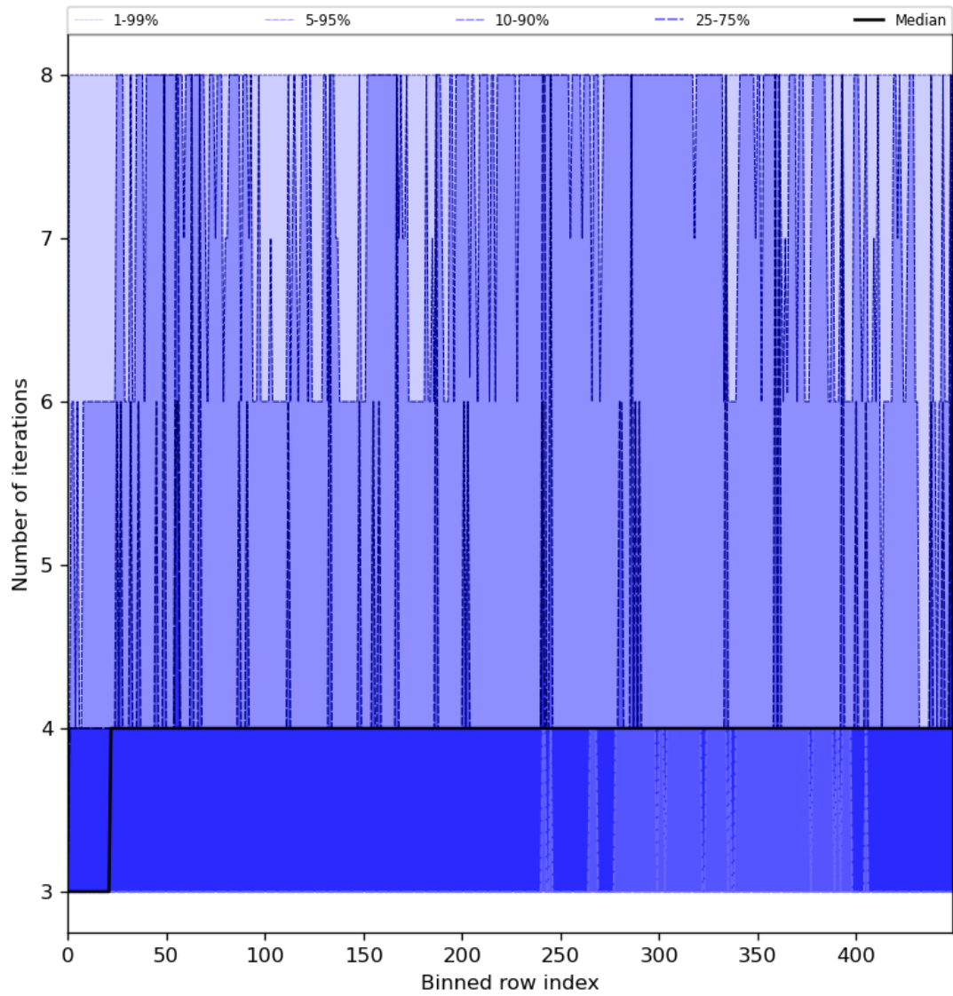
Figure 51: Along track statistics of “Number of iterations” for 2023-07-30 to 2023-08-01
