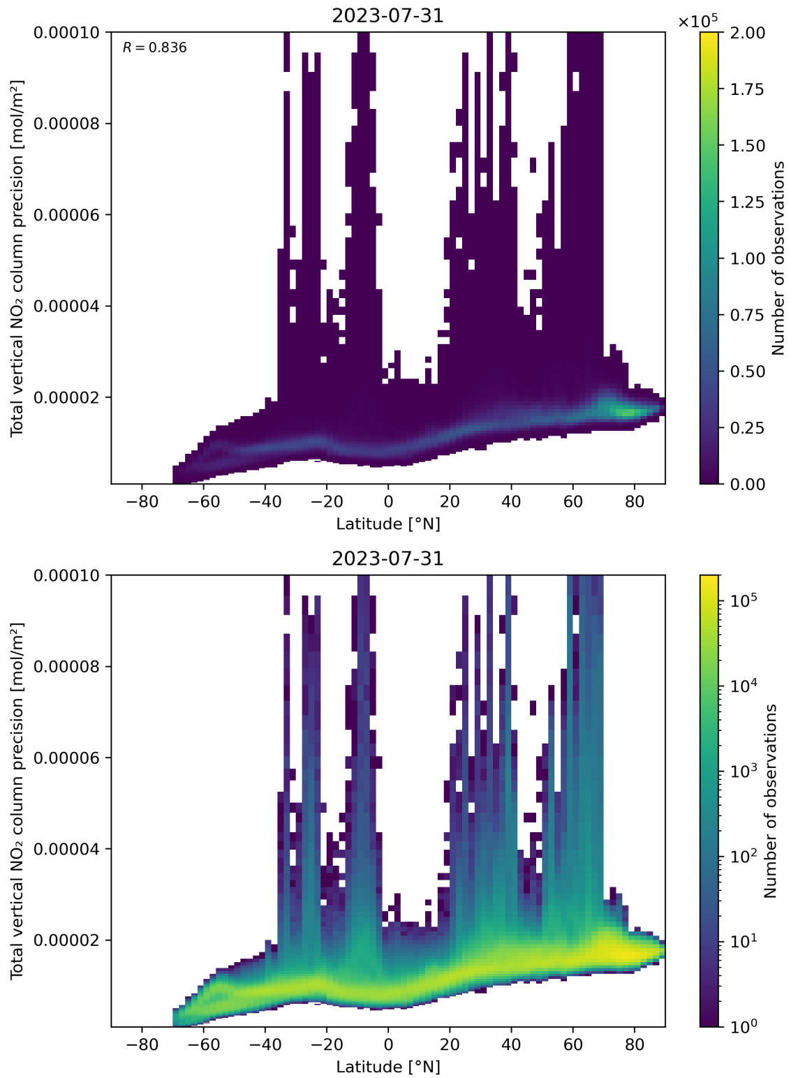
Figure 91: Scatter density plot of “Latitude” against “Total vertical NO 2 column precision” for 2023-07-30 to 2023-08-01.
