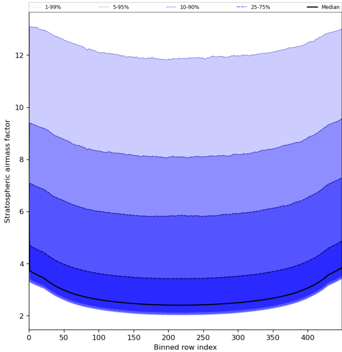
Figure 61: Along track statistics of “Stratospheric airmass factor” for 2023-07-30 to 2023-08-01
