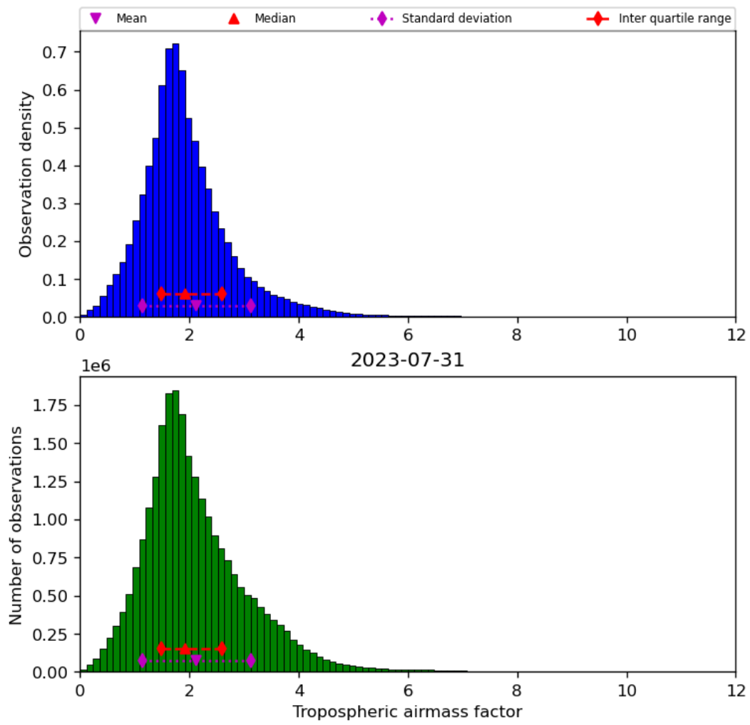
Figure 31: Histogram of “Tropospheric airmass factor” for 2023-07-30 to 2023-08-01
