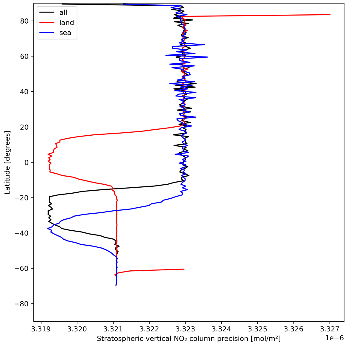
Figure 20: Zonal average of “Stratospheric vertical NO 2 column precision” for 2023-07-30 to 2023-08-01.
