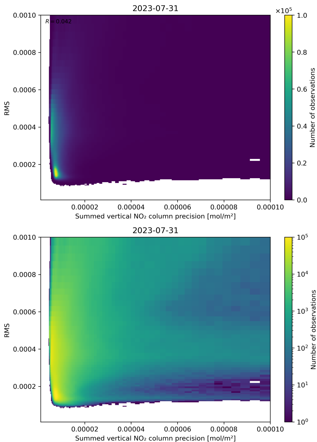
Figure 108: Scatter density plot of “Summed vertical NO 2 column precision” against “RMS” for 2023-07-30 to 2023-08-01.
