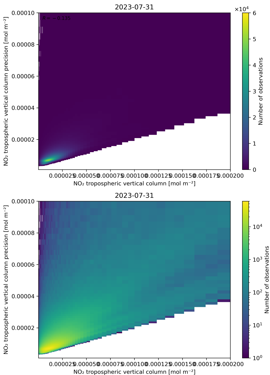
Figure 130: Scatter density plot of “NO 2 tropospheric vertical column” against “NO 2 tropospheric vertical column precision” for 2023-07-30 to 2023-08-01.
