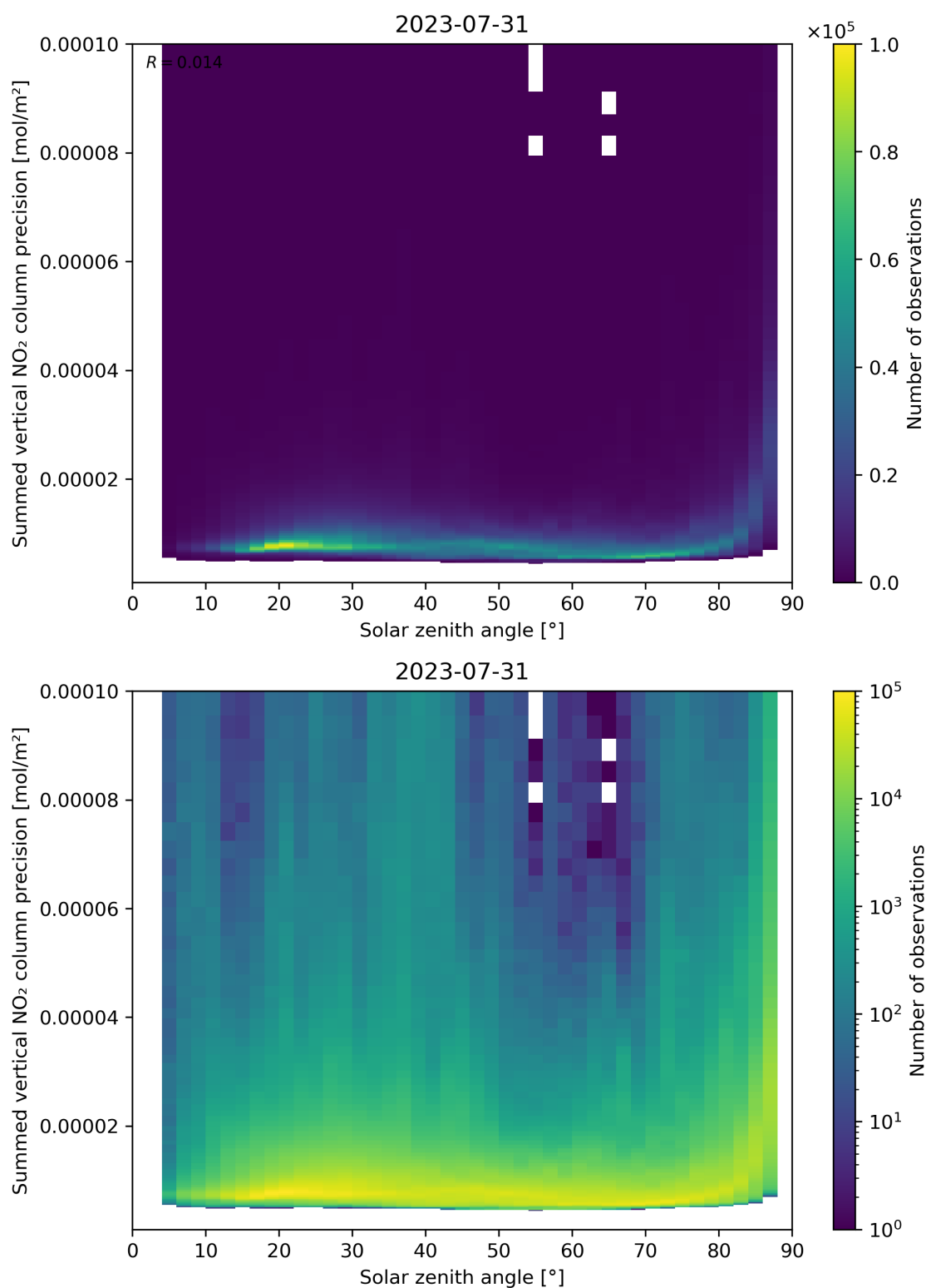
Figure 152: Scatter density plot of “Solar zenith angle” against “Summed vertical NO 2 column precision” for 2023-07-30 to 2023-08-01.
