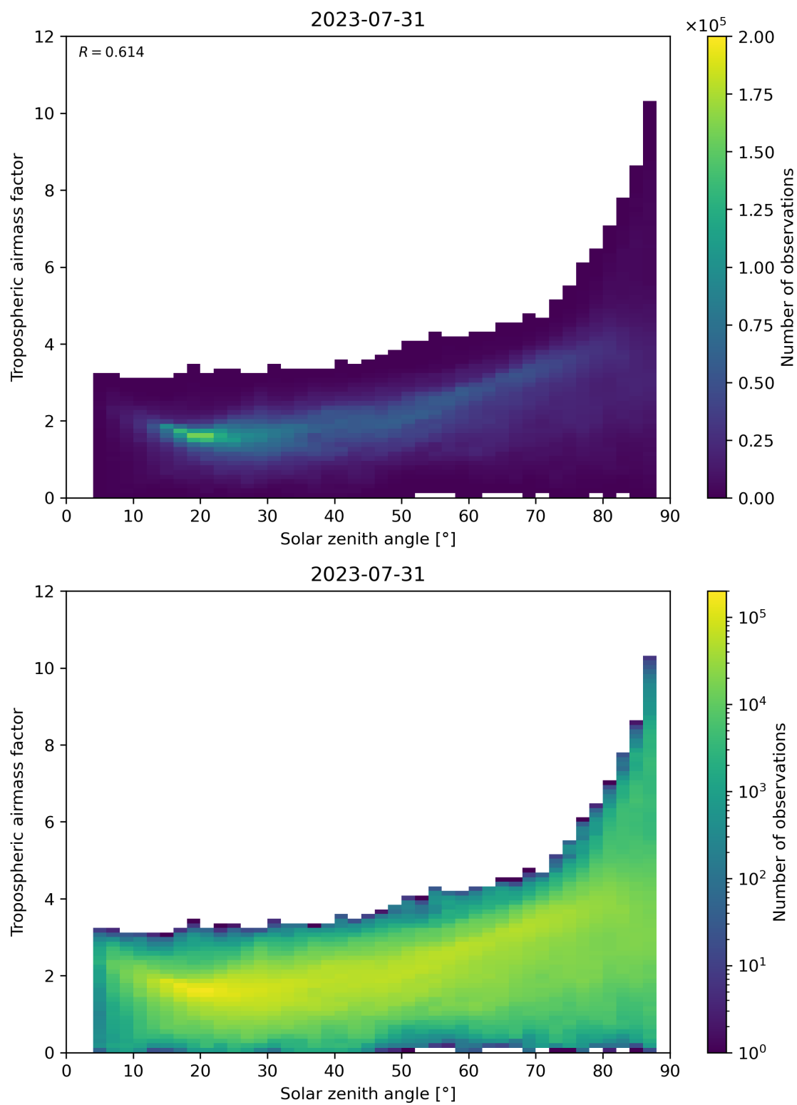
Figure 147: Scatter density plot of “Solar zenith angle” against “Tropospheric airmass factor” for 2023-07-30 to 2023-08-01.
