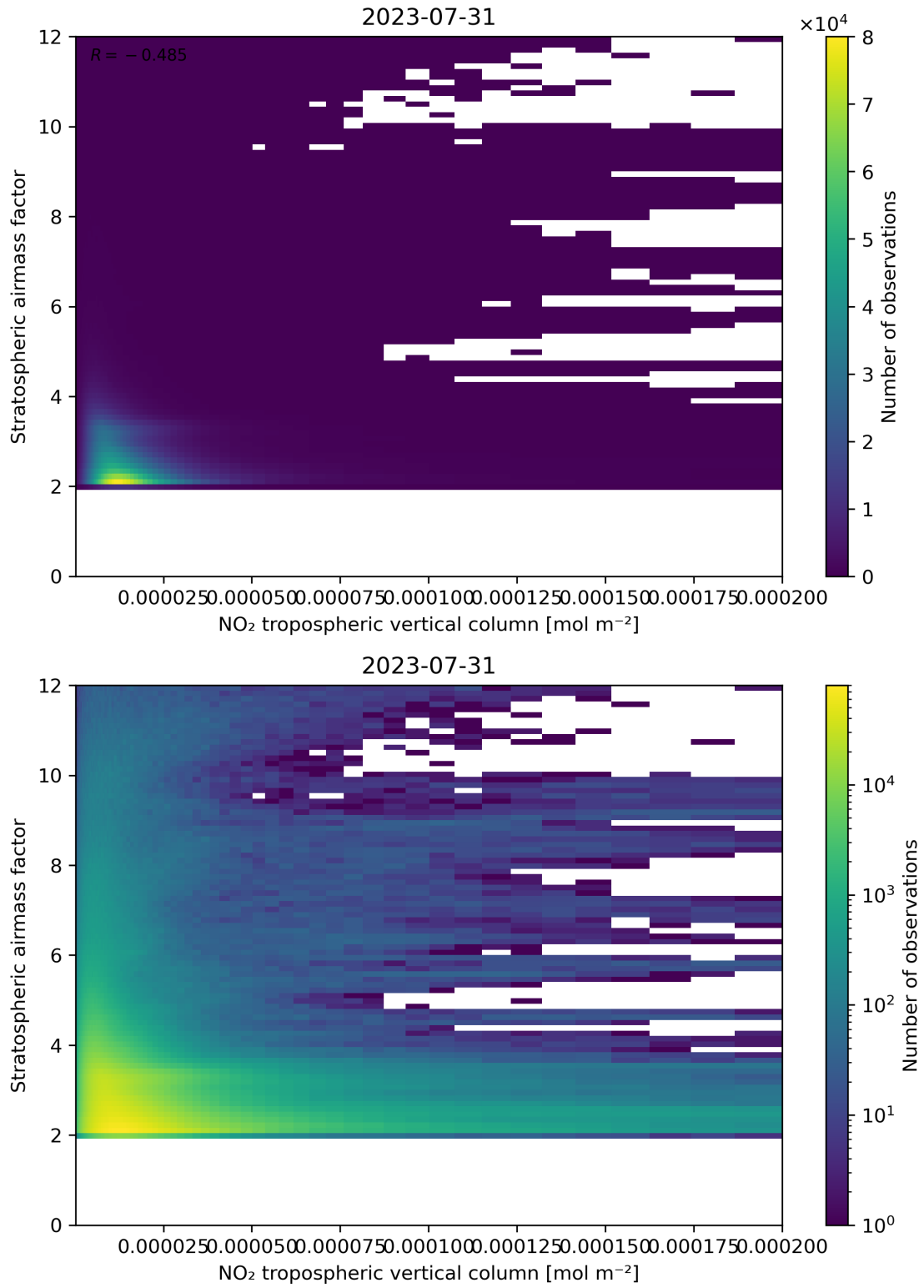
Figure 121: Scatter density plot of “NO 2 tropospheric vertical column” against “Stratospheric air mass factor” for 2023-07-30 to 2023-08-01.
