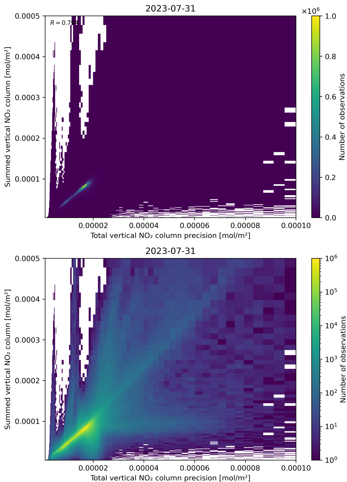
Figure 117: Scatter density plot of “Total vertical NO 2 column precision” against “Summed vertical NO 2 column” for 2023-07-30 to 2023-08-01.
