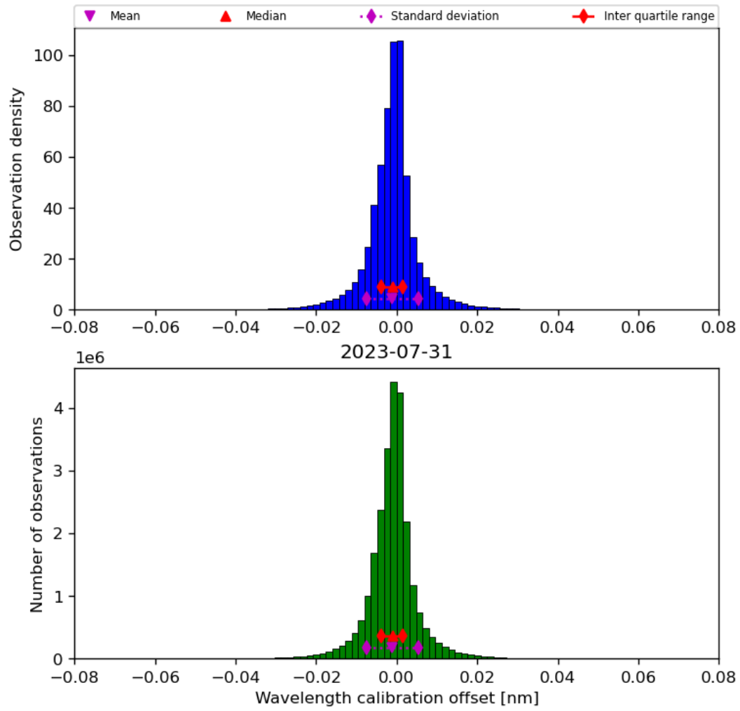
Figure 35: Histogram of “Wavelength calibration offset” for 2023-07-30 to 2023-08-01
