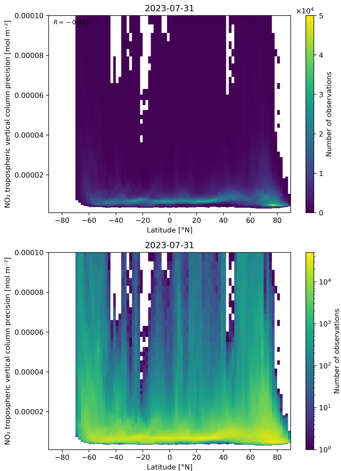
Figure 93: Scatter density plot of “Latitude” against “NO 2 tropospheric vertical column precision” for 2023-07-30 to 2023-08-01.
