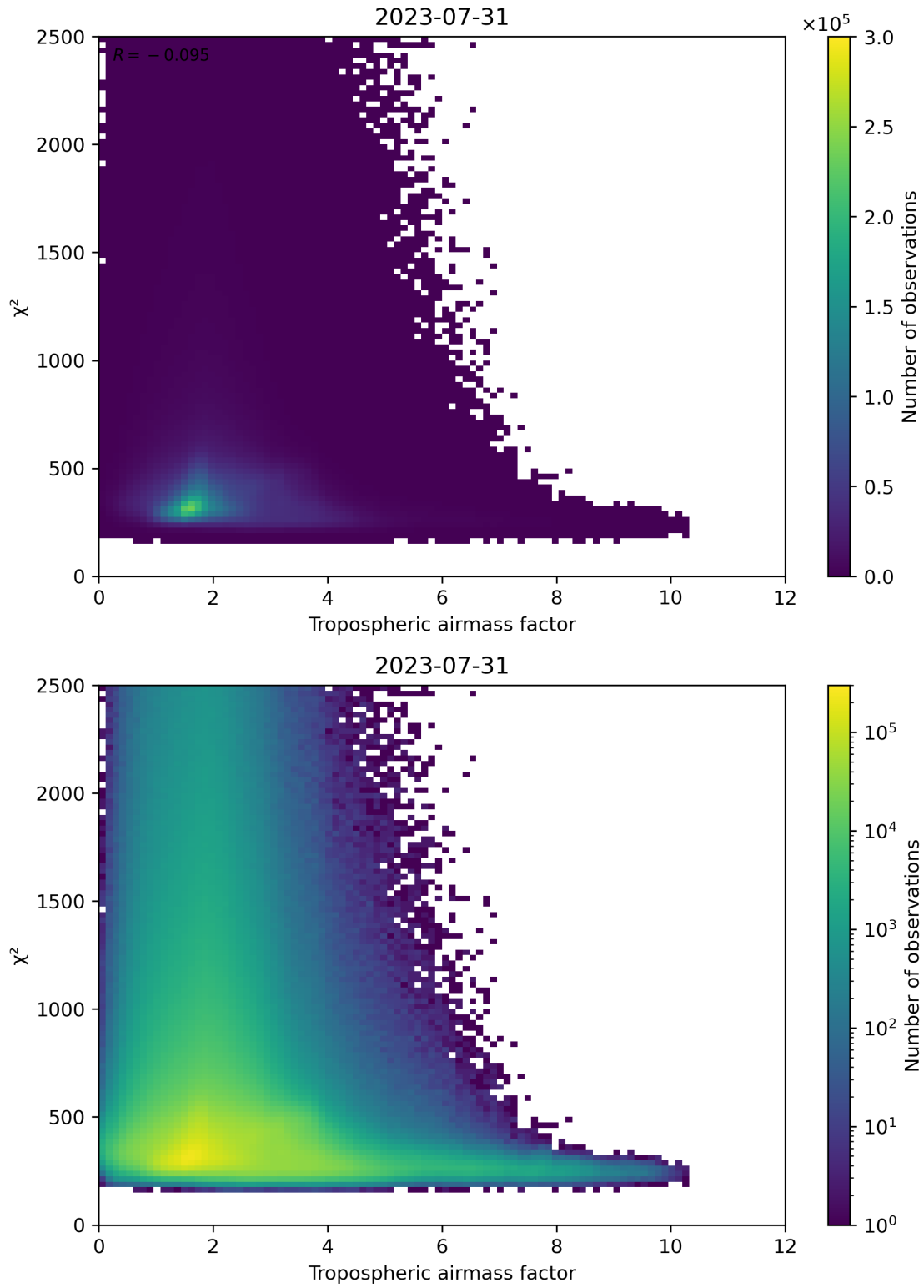
Figure 73: Scatter density plot of “Tropospheric airmass factor” against “ \chi^2 ” for 2023-07-30 to 2023-08-01.
