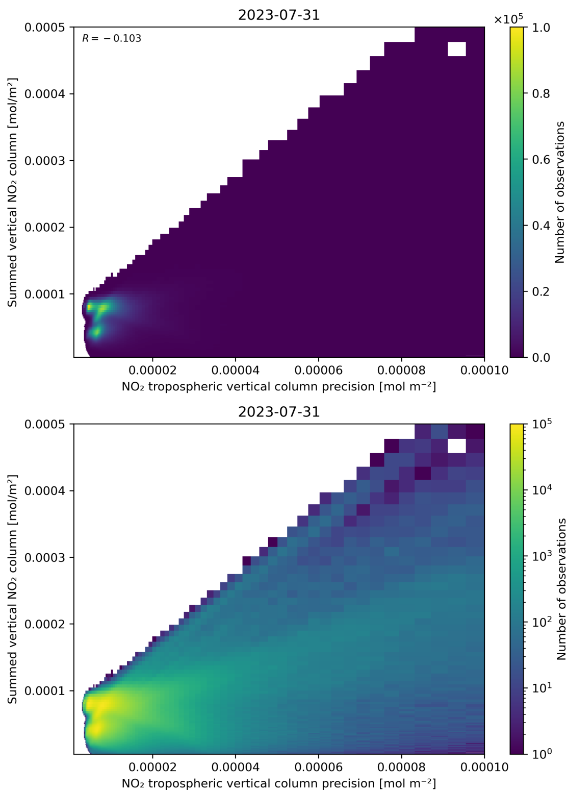
Figure 136: Scatter density plot of “NO 2 tropospheric vertical column precision” against “Summed vertical NO 2 column” for 2023-07-30 to 2023-08-01.
