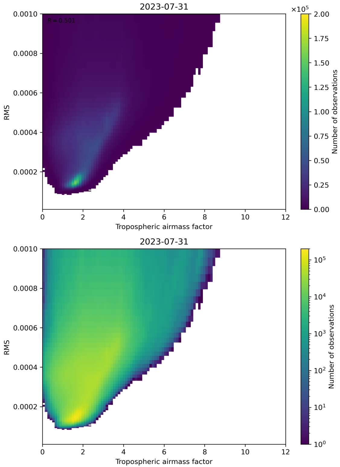
Figure 79: Scatter density plot of “Tropospheric airmass factor” against “RMS” for 2023-07-30 to 2023-08-01.
