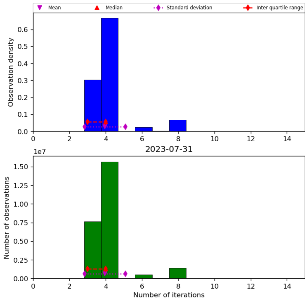
Figure 34: Histogram of “Number of iterations” for 2023-07-30 to 2023-08-01
