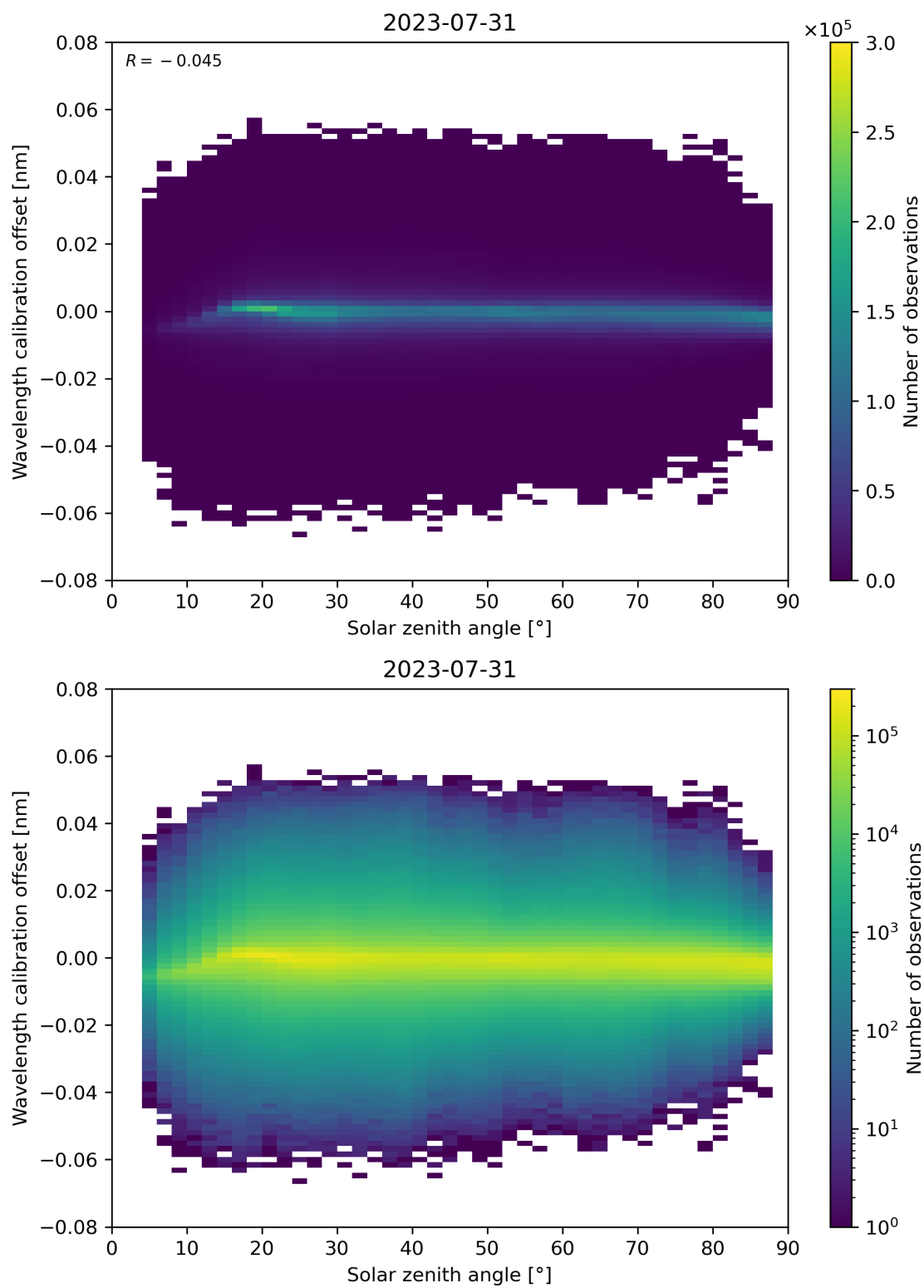
Figure 158: Scatter density plot of “Solar zenith angle” against “Wavelength calibration offset” for 2023-07-30 to 2023-08-01.
