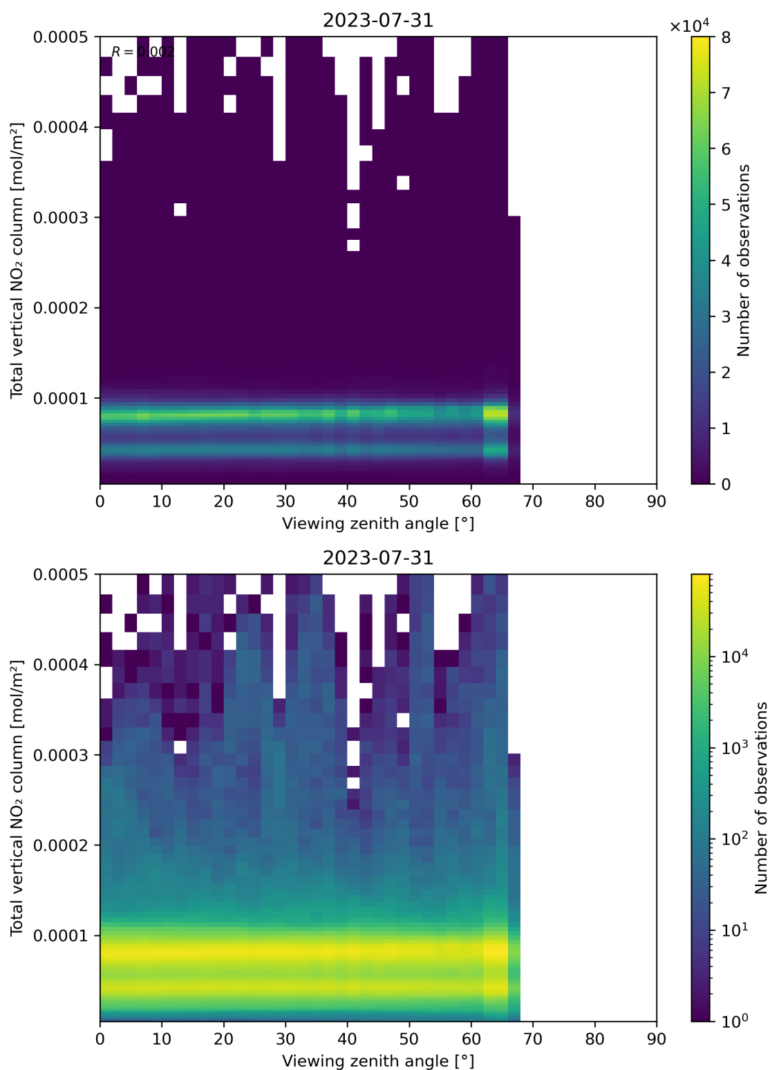
Figure 167: Scatter density plot of “Viewing zenith angle” against “Total vertical NO 2 column” for 2023-07-30 to 2023-08-01.
