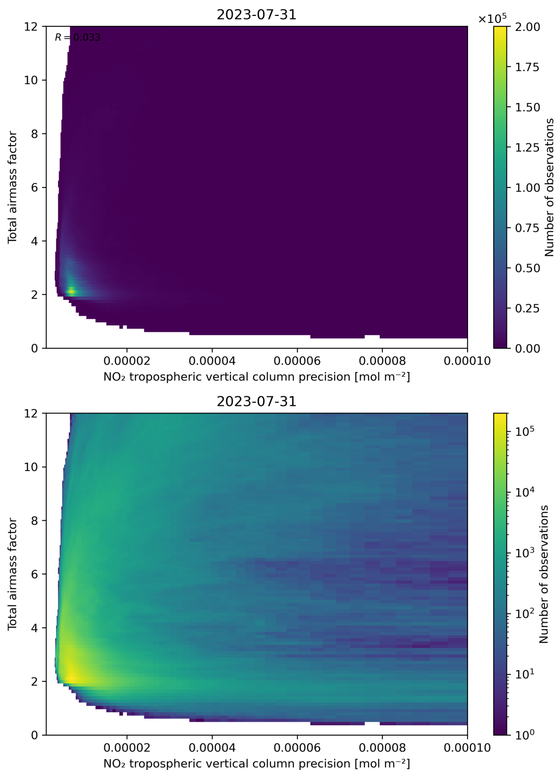
Figure 132: Scatter density plot of “NO 2 tropospheric vertical column precision” against “Total air mass factor” for 2023-07-30 to 2023-08-01.
