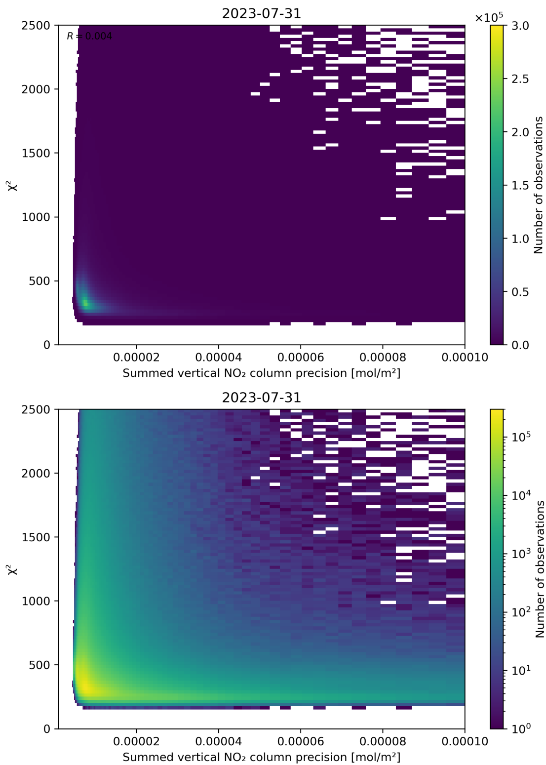
Figure 107: Scatter density plot of “Summed vertical NO 2 column precision” against “ \chi^2 ” for 2023-07-30 to 2023-08-01.
