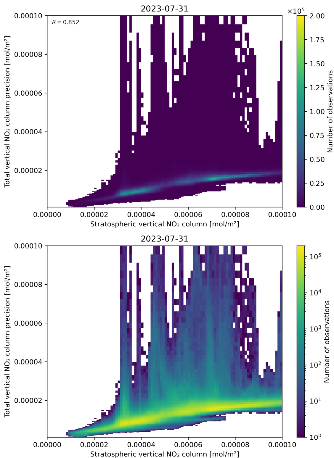
Figure 101: Scatter density plot of “Stratospheric vertical NO 2 column” against “Total vertical NO 2 column precision” for 2023-07-30 to 2023-08-01.
