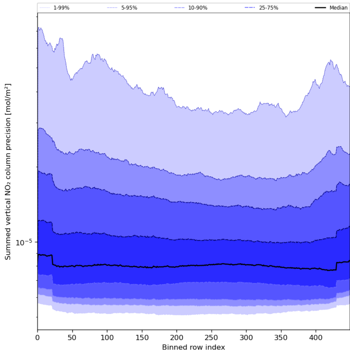
Figure 58: Along track statistics of “Summed vertical NO 2 column precision” for 2023-07-30 to 2023-08-01
