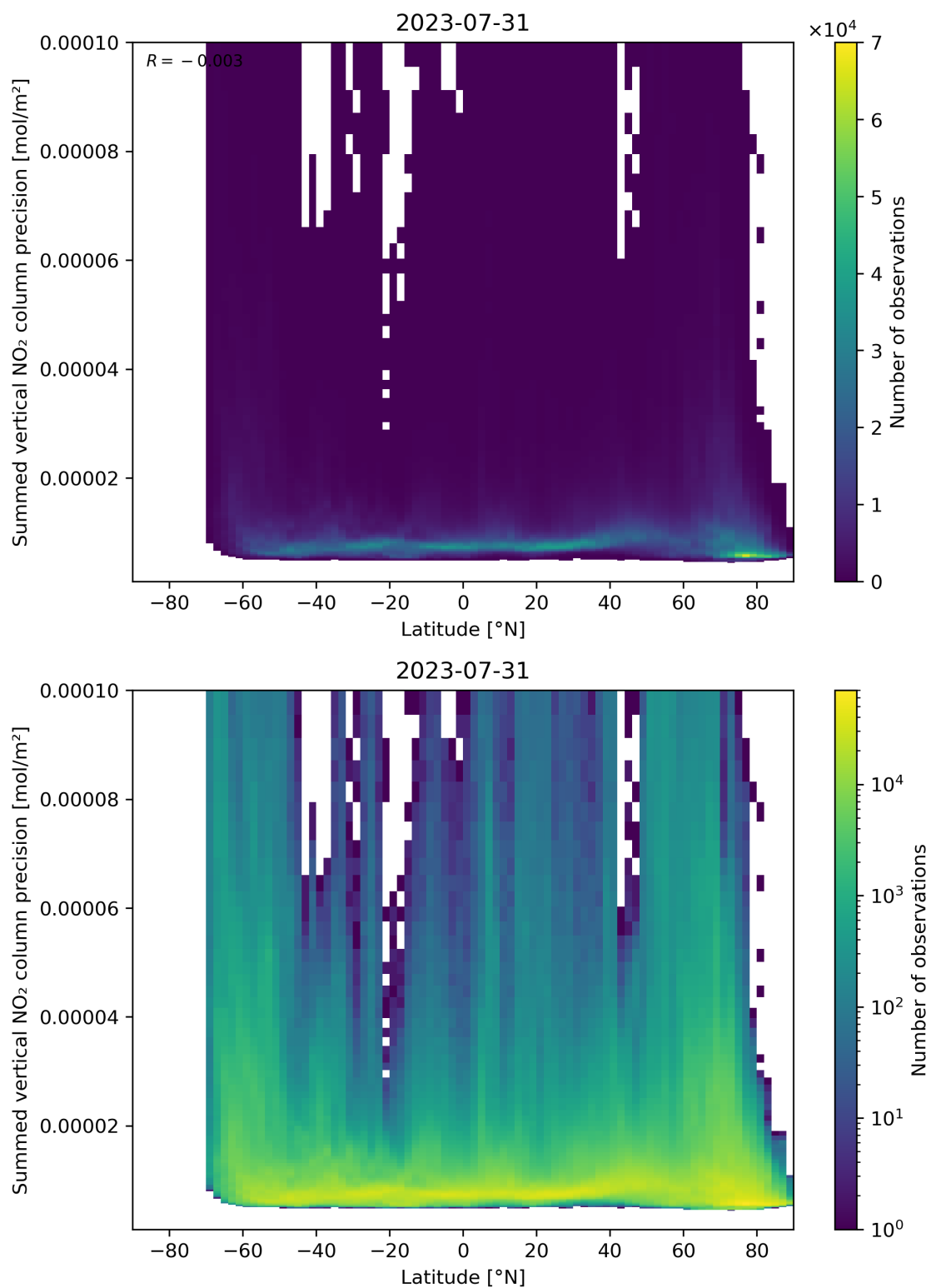
Figure 89: Scatter density plot of “Latitude” against “Summed vertical NO 2 column precision” for 2023-07-30 to 2023-08-01.
