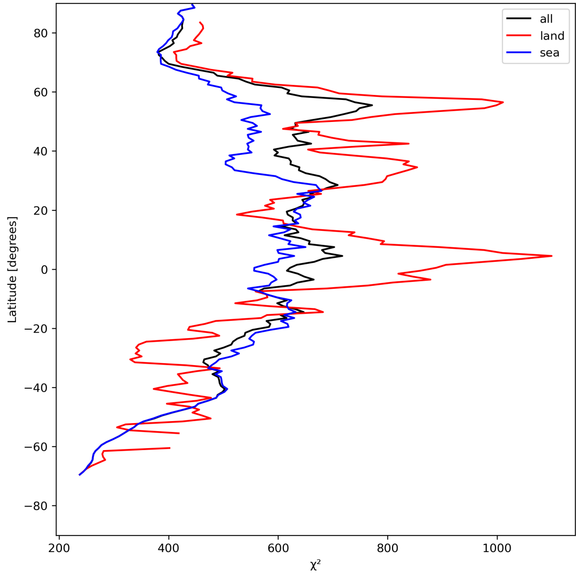
Figure 25: Zonal average of “ \chi^2 ” for 2023-07-30 to 2023-08-01.
