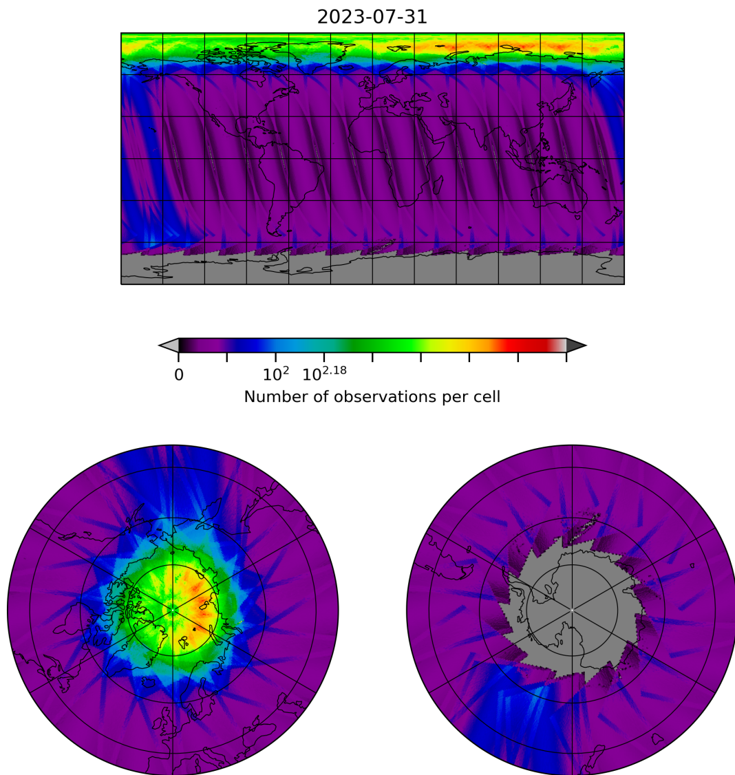
Figure 10: Map of the number of observations for 2023-07-30 to 2023-08-01
