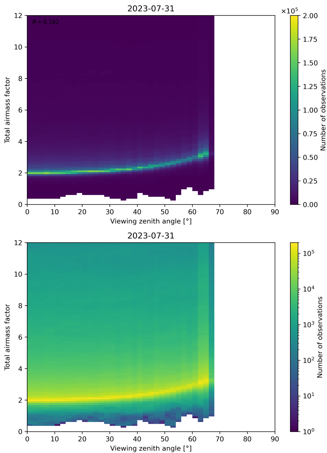
Figure 160: Scatter density plot of “Viewing zenith angle” against “Total airmass factor” for 2023-07-30 to 2023-08-01.
