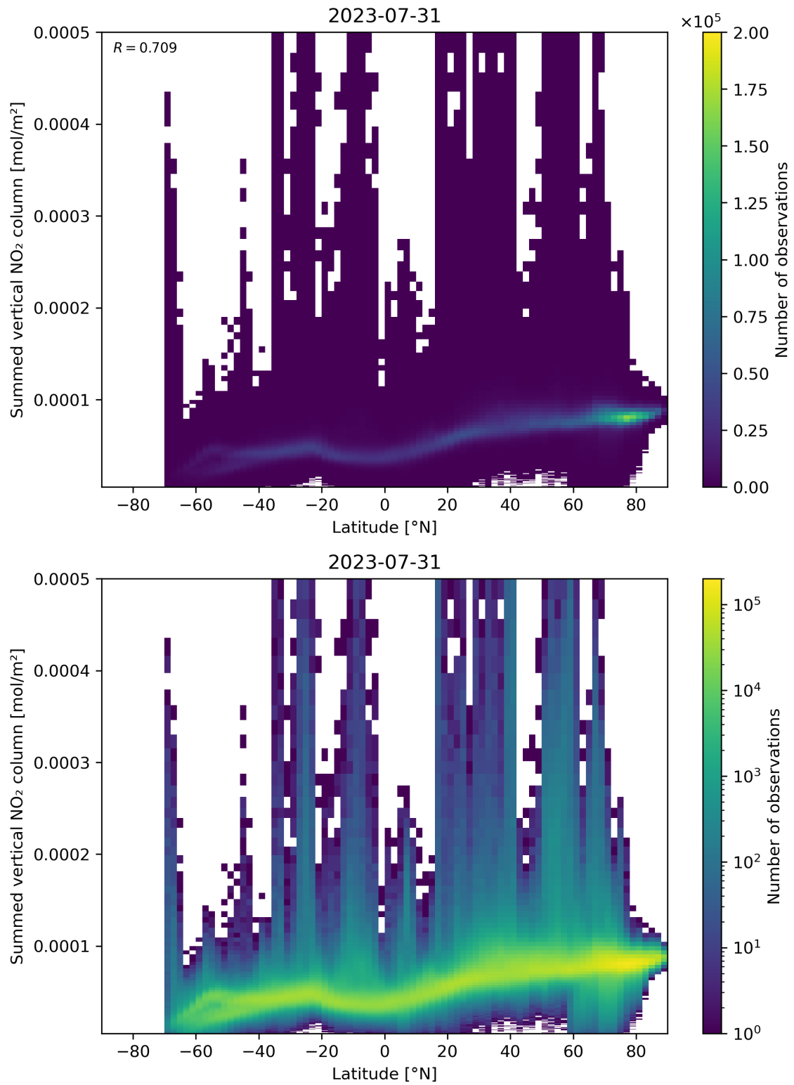
Figure 88: Scatter density plot of “Latitude” against “Summed vertical NO 2 column” for 2023-07-30 to 2023-08-01.
