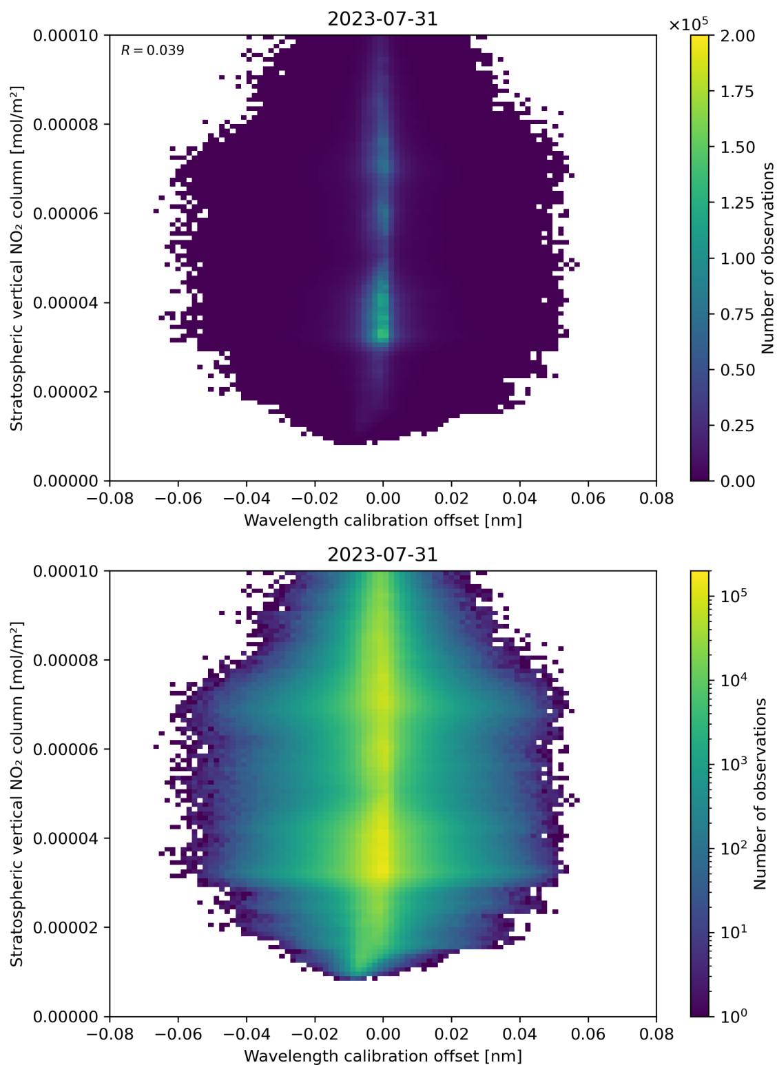
Figure 176: Scatter density plot of “Wavelength calibration offset” against “Stratospheric vertical NO 2 column” for 2023-07-30 to 2023-08-01.
