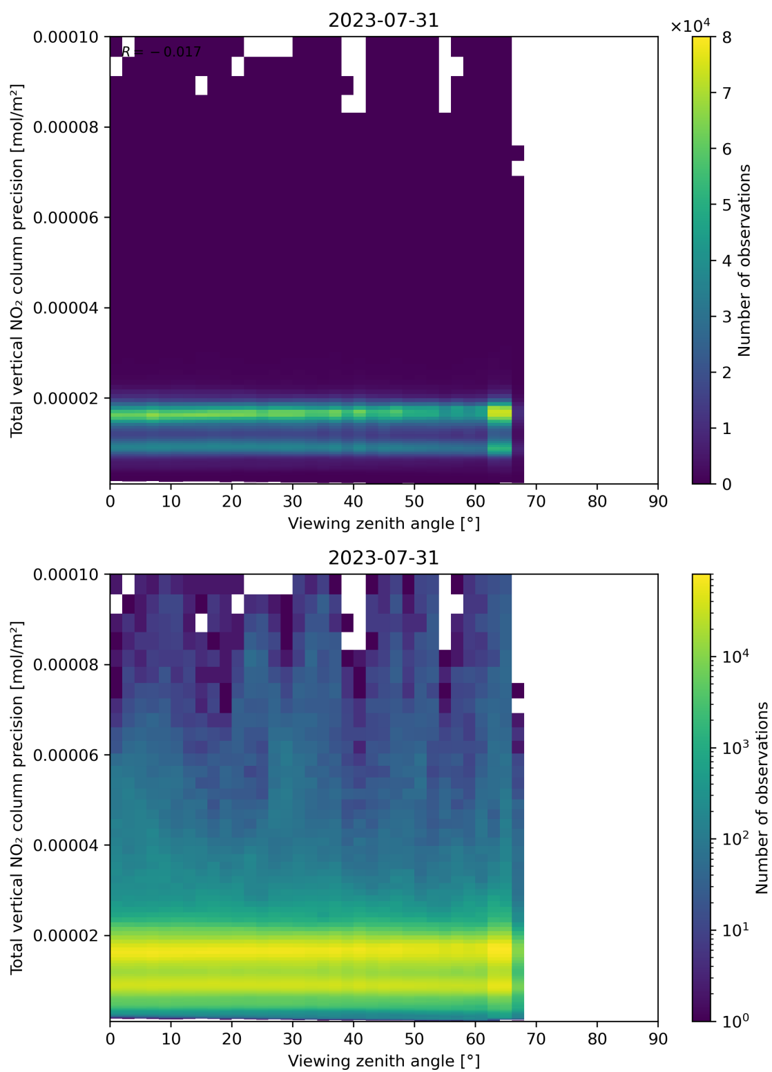
Figure 168: Scatter density plot of “Viewing zenith angle” against “Total vertical NO 2 column precision” for 2023-07-30 to 2023-08-01.
