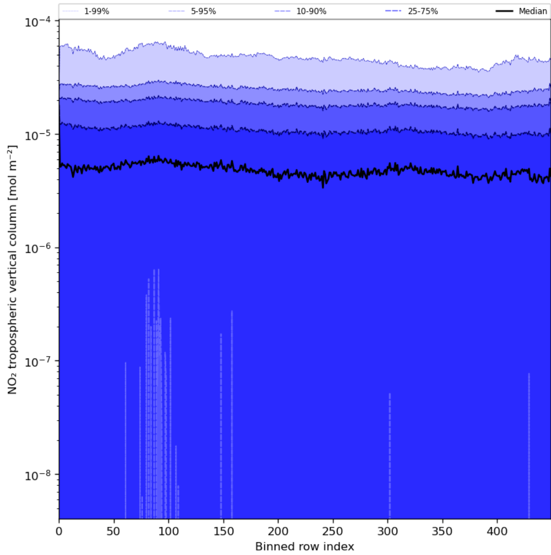
Figure 46: Along track statistics of “NO 2 tropospheric vertical column” for 2023-07-30 to 2023-08-01
