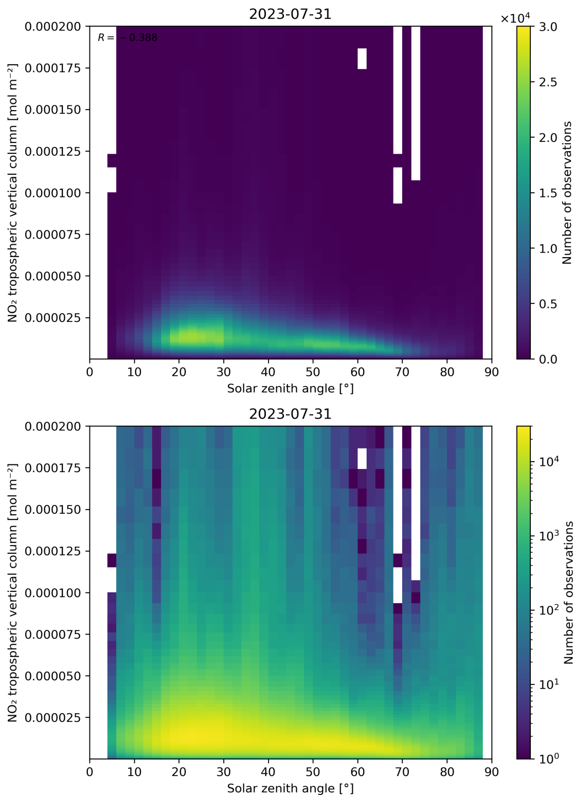
Figure 155: Scatter density plot of “Solar zenith angle” against “NO 2 tropospheric vertical column” for 2023-07-30 to 2023-08-01.
