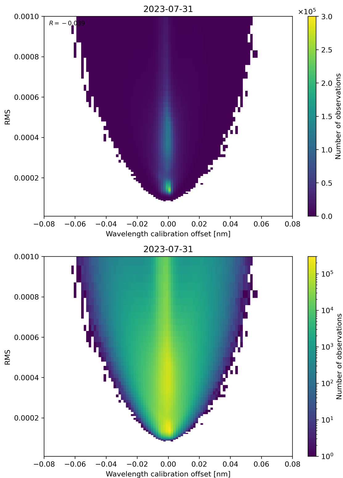
Figure 181: Scatter density plot of “Wavelength calibration offset” against “RMS” for 2023-07-30 to 2023-08-01.
