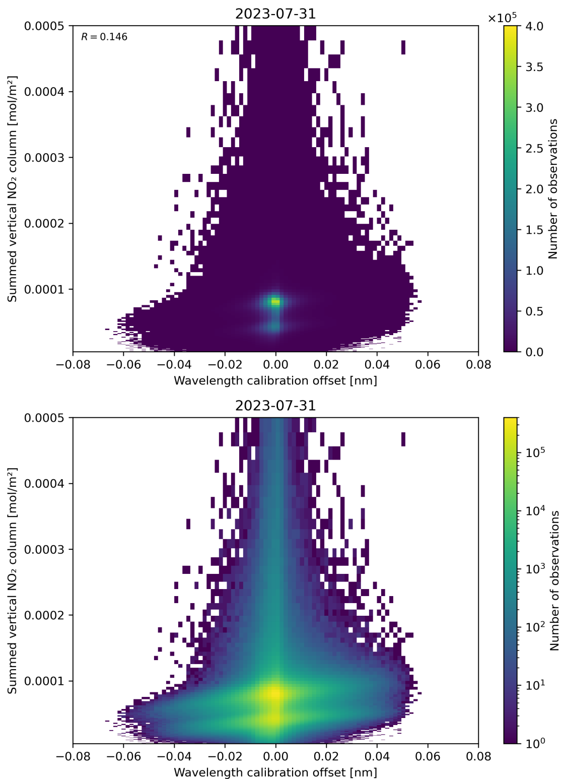
Figure 177: Scatter density plot of “Wavelength calibration offset” against “Summed vertical NO 2 column” for 2023-07-30 to 2023-08-01.
