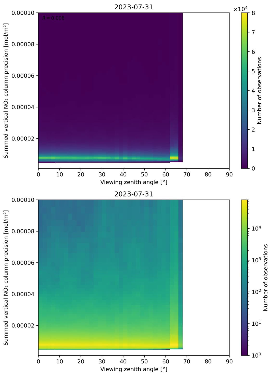
Figure 166: Scatter density plot of “Viewing zenith angle” against “Summed vertical NO 2 column precision” for 2023-07-30 to 2023-08-01.
