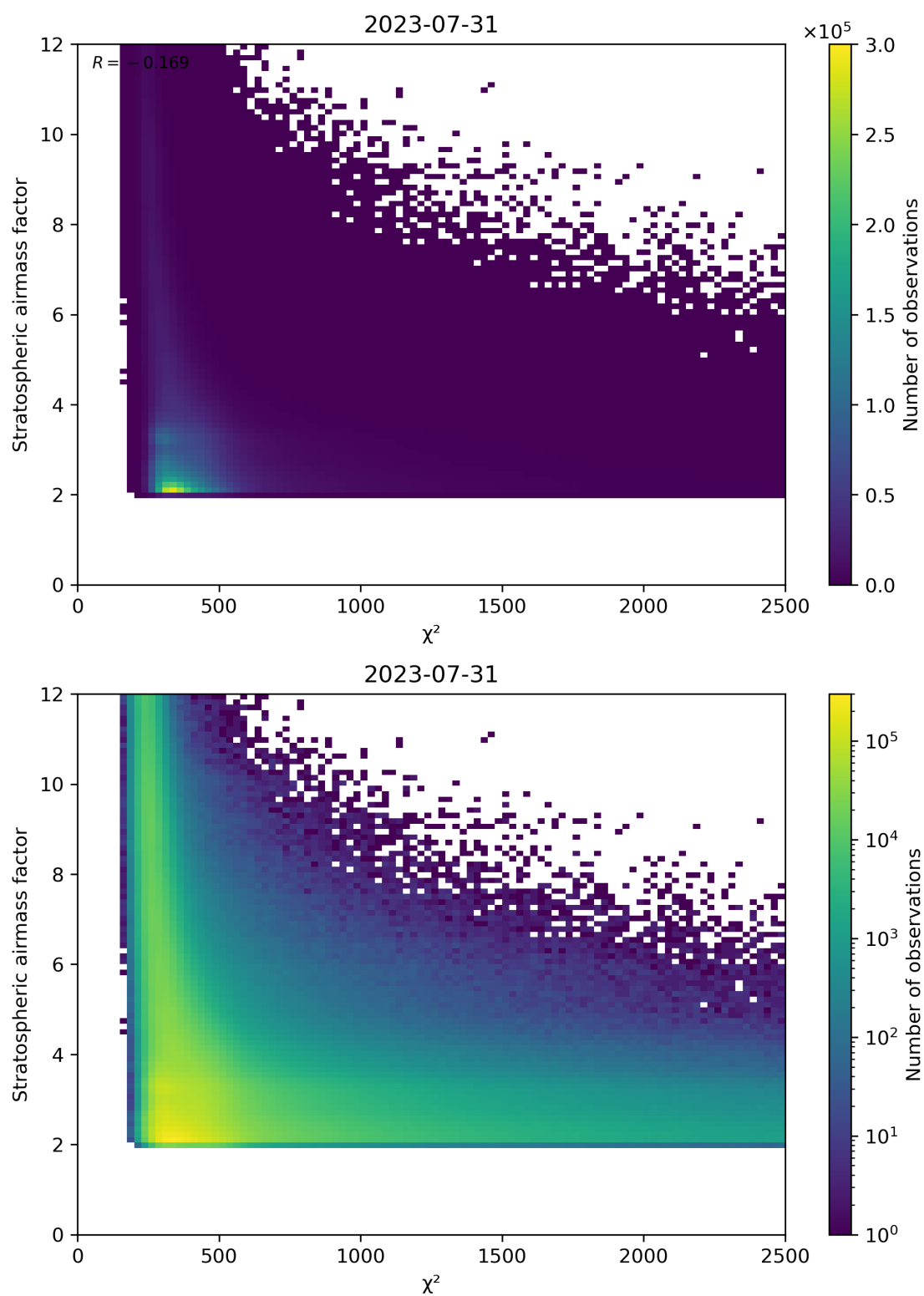
Figure 81: Scatter density plot of “ \chi^2 ” against “Stratospheric airmass factor” for 2023-07-30 to 2023-08-01.
