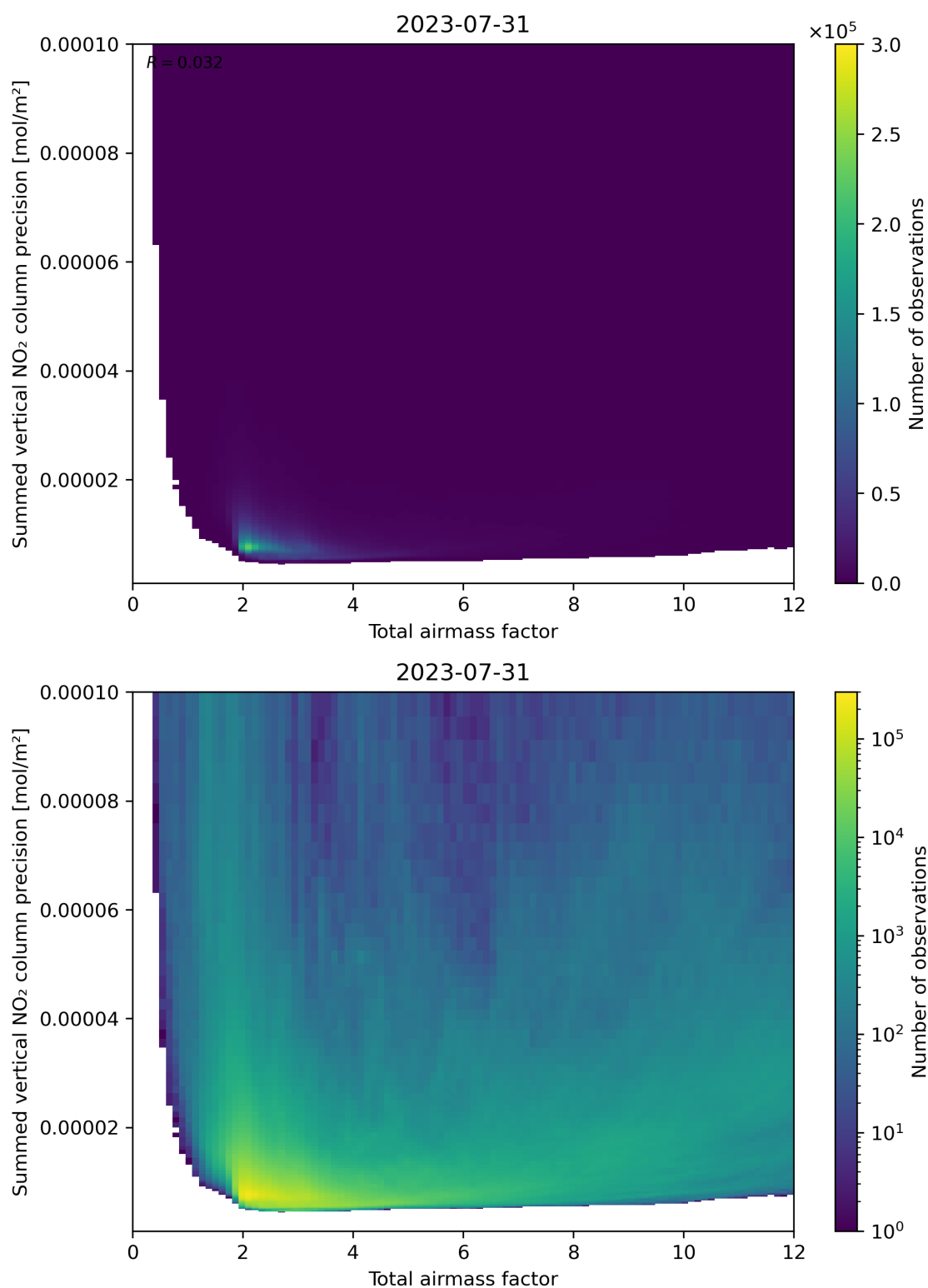
Figure 66: Scatter density plot of “Total airmass factor” against “Summed vertical NO 2 column precision” for 2023-07-30 to 2023-08-01.
