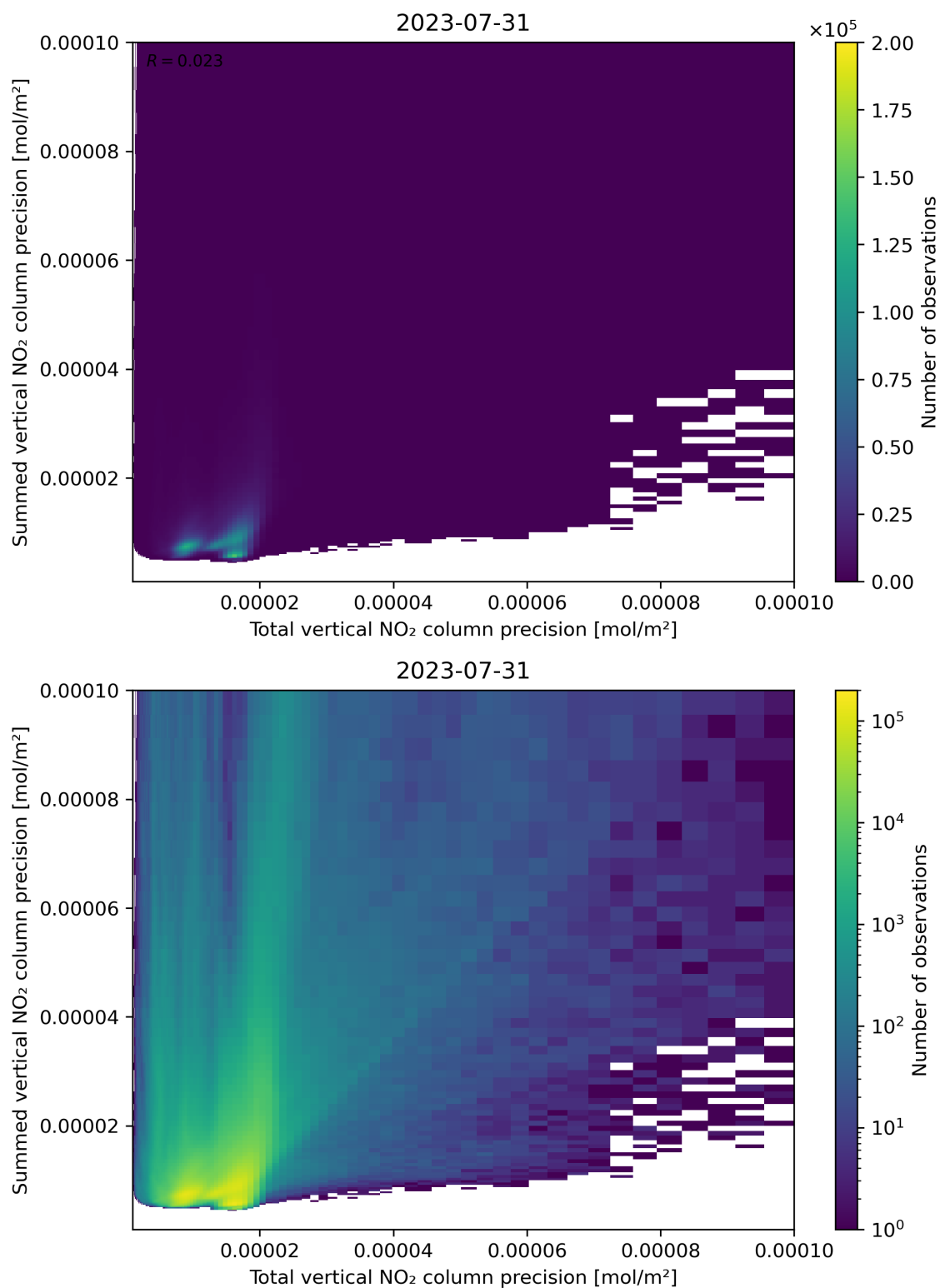
Figure 118: Scatter density plot of “Total vertical NO 2 column precision” against “Summed vertical NO 2 column precision” for 2023-07-30 to 2023-08-01.
