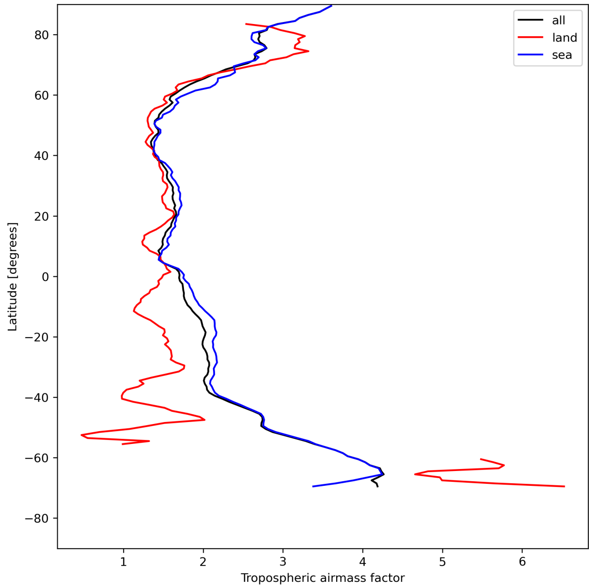
Figure 14: Zonal average of “Tropospheric airmass factor” for 2023-07-30 to 2023-08-01.
