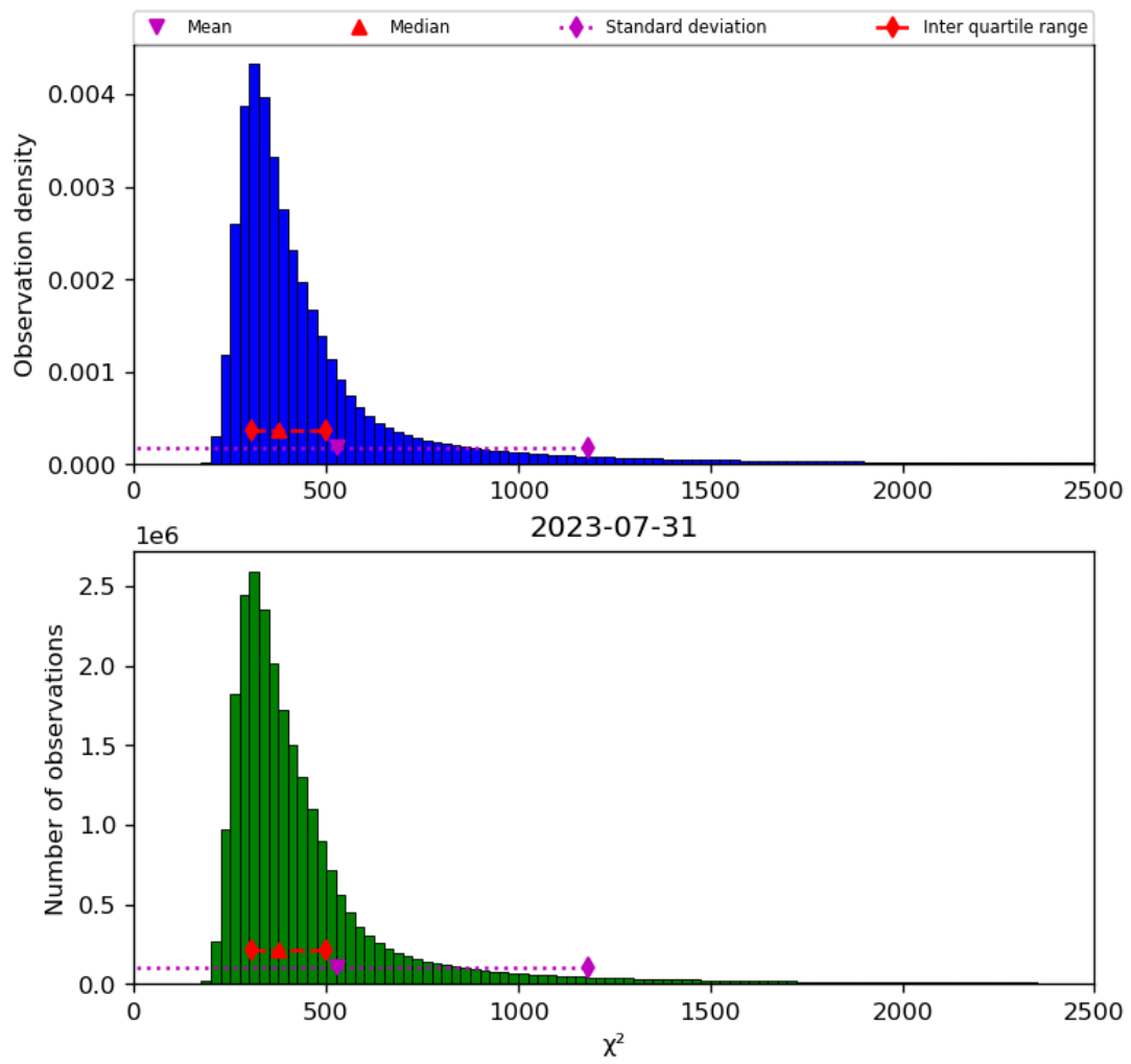
Figure 42: Histogram of " \chi^2 " for 2023-07-30 to 2023-08-01
