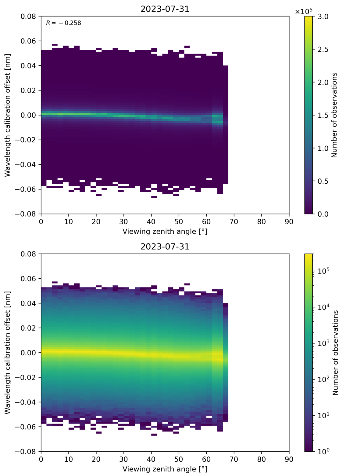
Figure 173: Scatter density plot of “Viewing zenith angle” against “Wavelength calibration offset” for 2023-07-30 to 2023-08-01.
