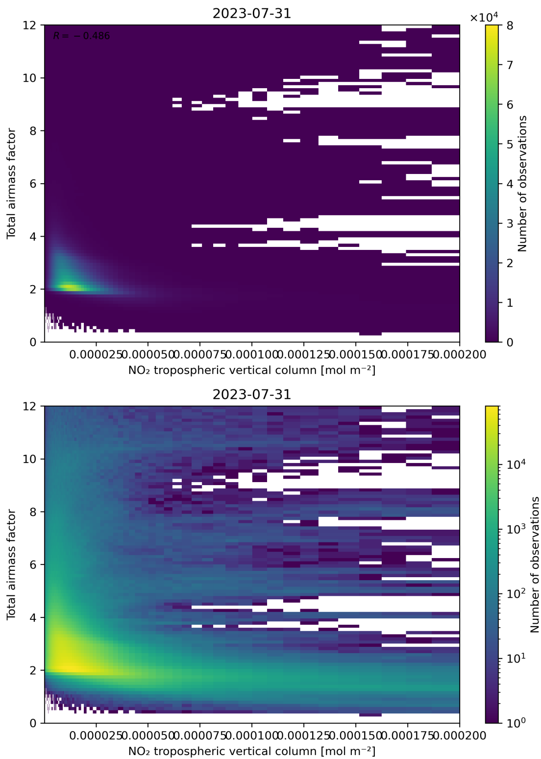
Figure 122: Scatter density plot of “NO 2 tropospheric vertical column” against “Total air mass factor” for 2023-07-30 to 2023-08-01.
