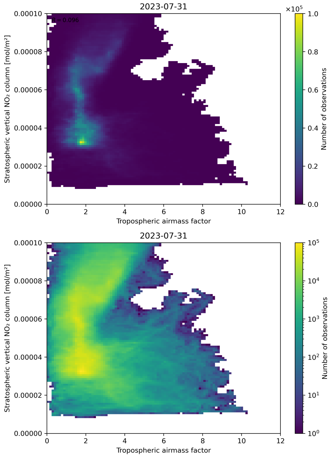
Figure 74: Scatter density plot of “Tropospheric air mass factor” against “Stratospheric vertical NO 2 column” for 2023-07-30 to 2023-08-01.
