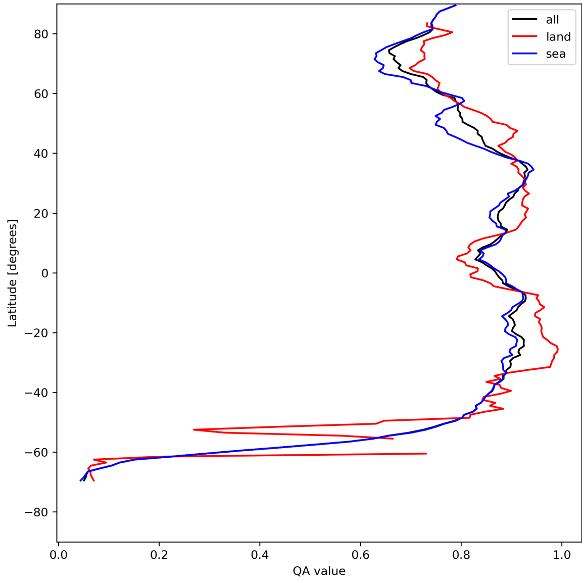
Figure 11: Zonal average of “QA value” for 2023-07-30 to 2023-08-01.
