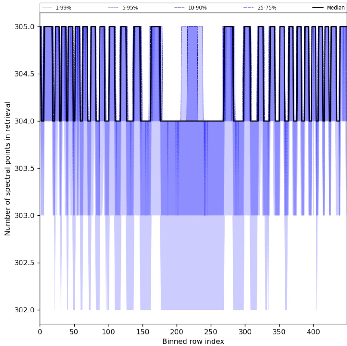
Figure 50: Along track statistics of “Number of spectral points in retrieval” for 2023-07-30 to 2023-08-01
