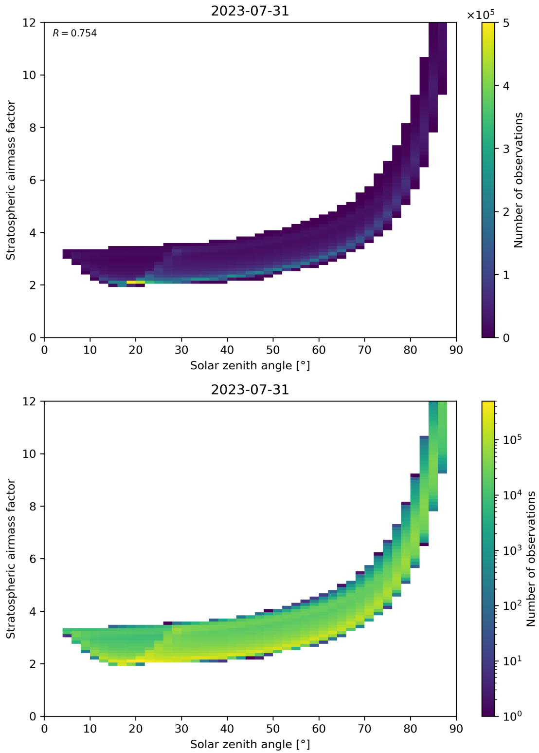
Figure 145: Scatter density plot of “Solar zenith angle” against “Stratospheric airmass factor” for 2023-07-30 to 2023-08-01.
