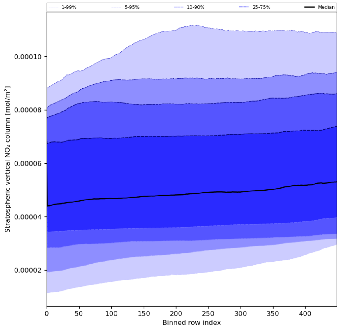
Figure 53: Along track statistics of “Stratospheric vertical NO 2 column” for 2023-07-30 to 2023-08-01
