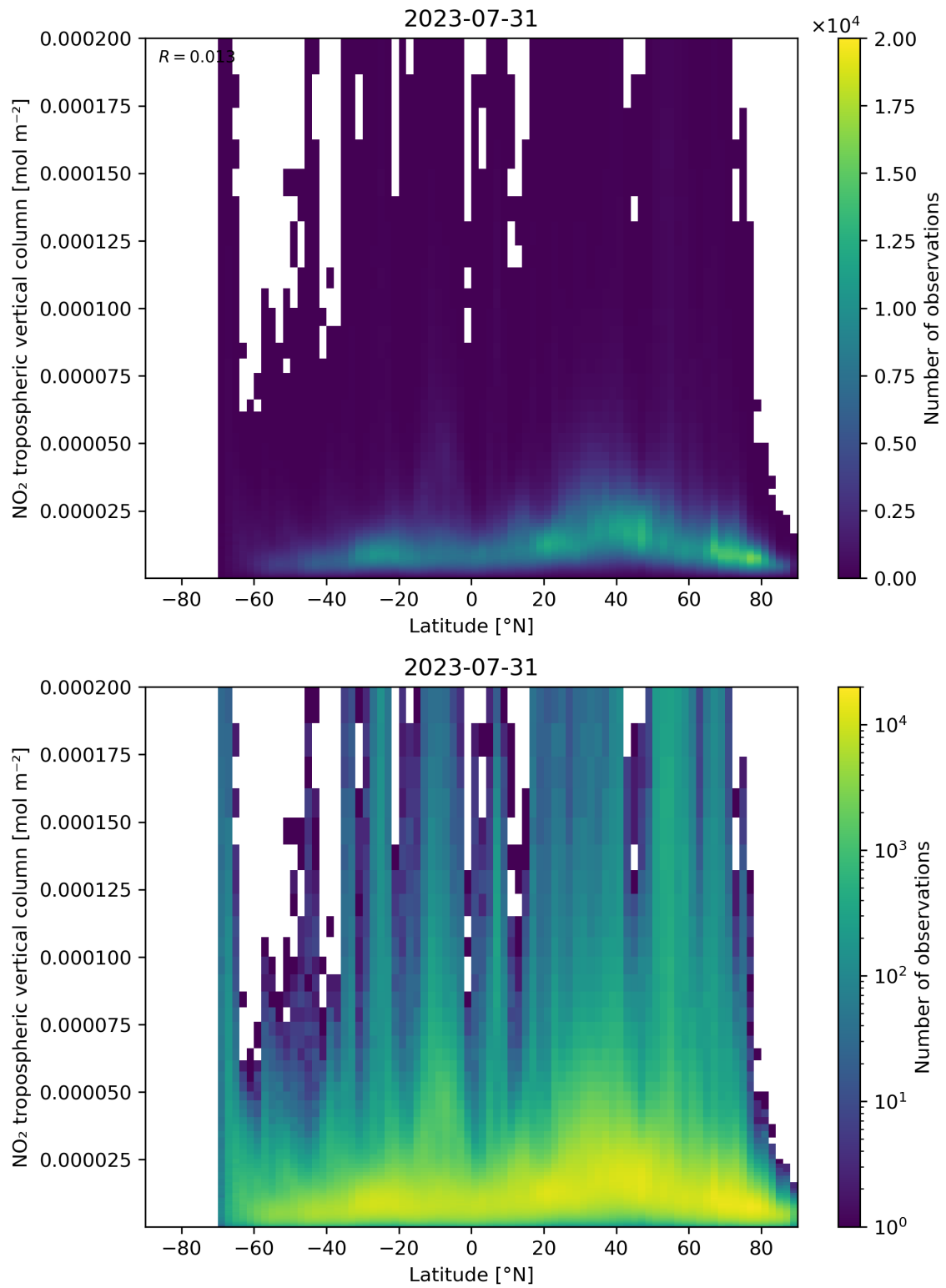
Figure 92: Scatter density plot of “Latitude” against “NO 2 tropospheric vertical column” for 2023-07-30 to 2023-08-01.
