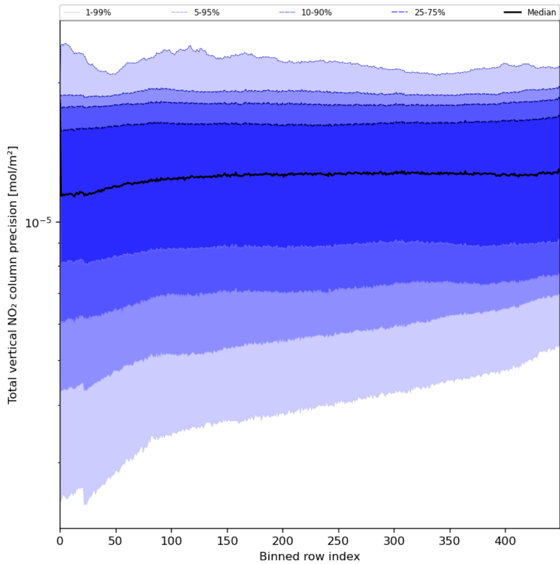
Figure 56: Along track statistics of “Total vertical NO 2 column precision” for 2023-07-30 to 2023-08-01
