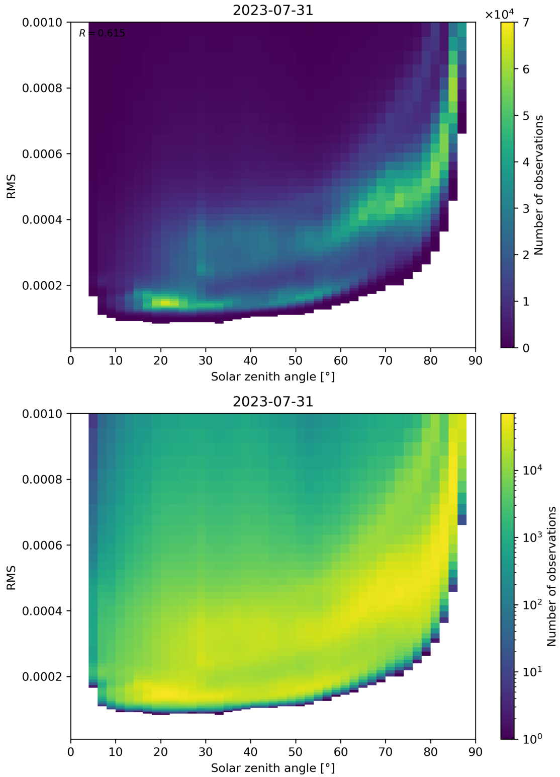
Figure 157: Scatter density plot of “Solar zenith angle” against “RMS” for 2023-07-30 to 2023-08-01.
