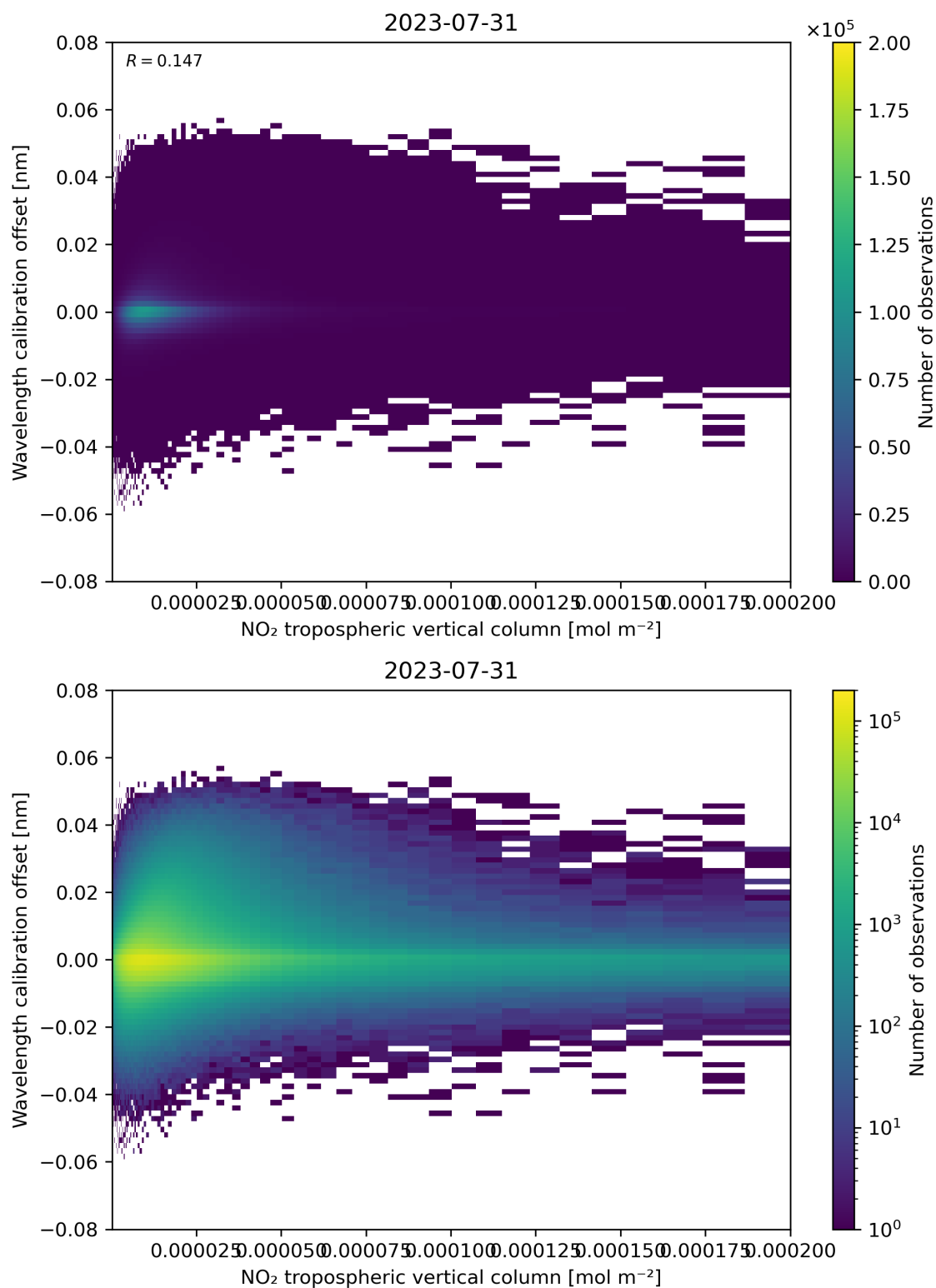
Figure 143: Scatter density plot of “NO 2 tropospheric vertical column” against “Wavelength calibration offset” for 2023-07-30 to 2023-08-01.
