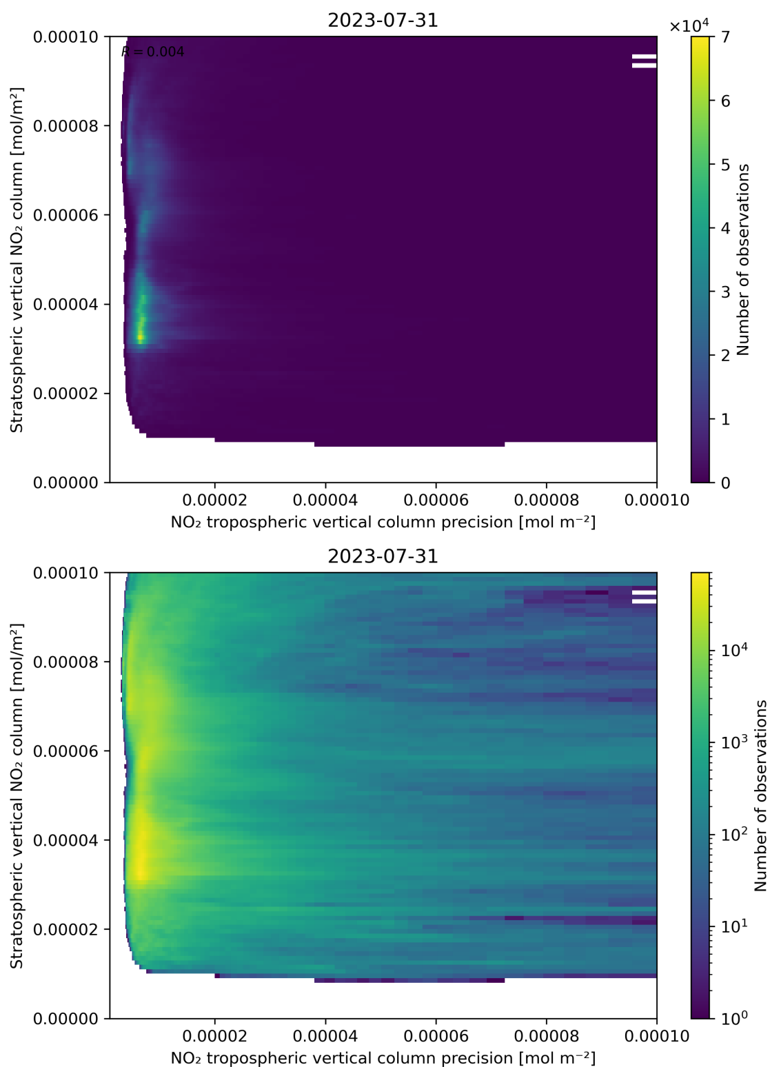
Figure 135: Scatter density plot of “NO 2 tropospheric vertical column precision” against “Stratospheric vertical NO 2 column” for 2023-07-30 to 2023-08-01.
