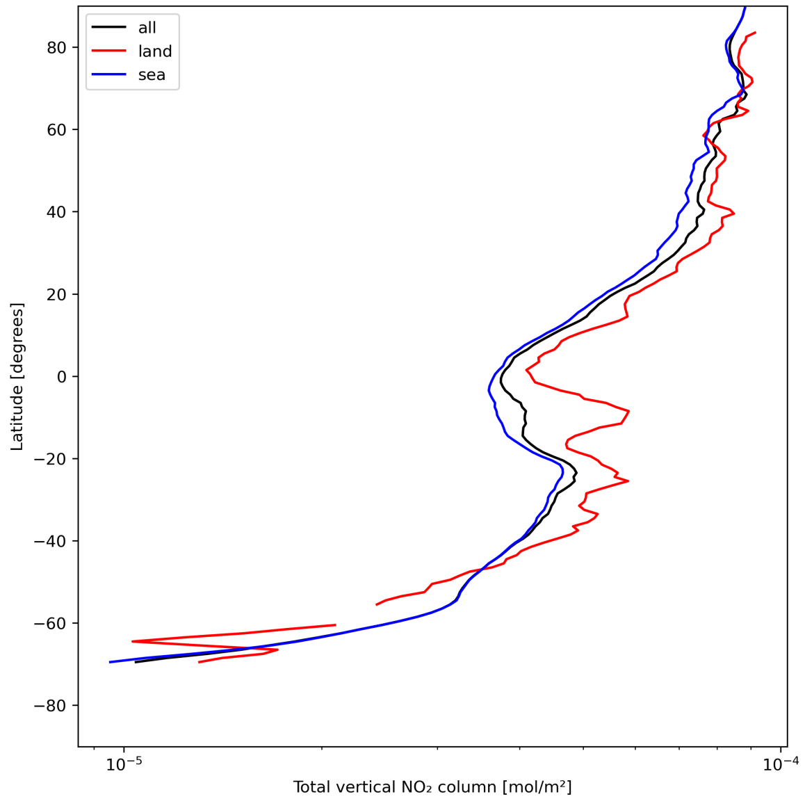
Figure 21: Zonal average of “Total vertical NO 2 column” for 2023-07-30 to 2023-08-01.
