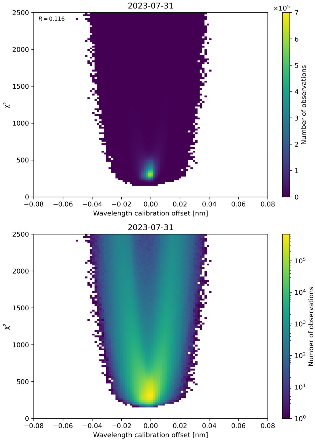
Figure 175: Scatter density plot of “Wavelength calibration offset” against “ \chi^2 ” for 2023-07-30 to 2023-08-01.
