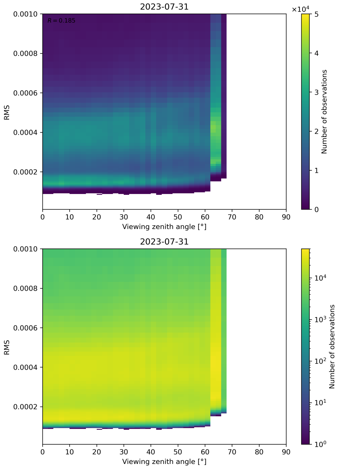
Figure 171: Scatter density plot of “Viewing zenith angle” against “RMS” for 2023-07-30 to 2023-08-01.
