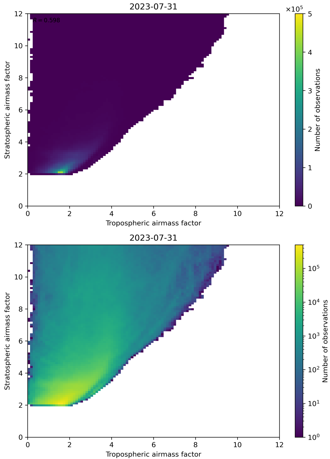
Figure 71: Scatter density plot of “Tropospheric airmass factor” against “Stratospheric airmass factor” for 2023-07-30 to 2023-08-01.
