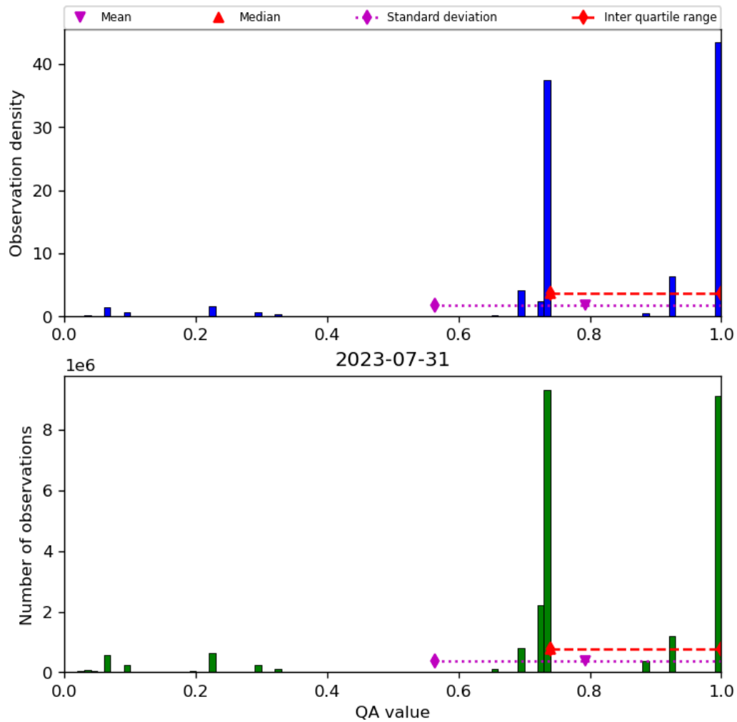
Figure 28: Histogram of “QA value” for 2023-07-30 to 2023-08-01
