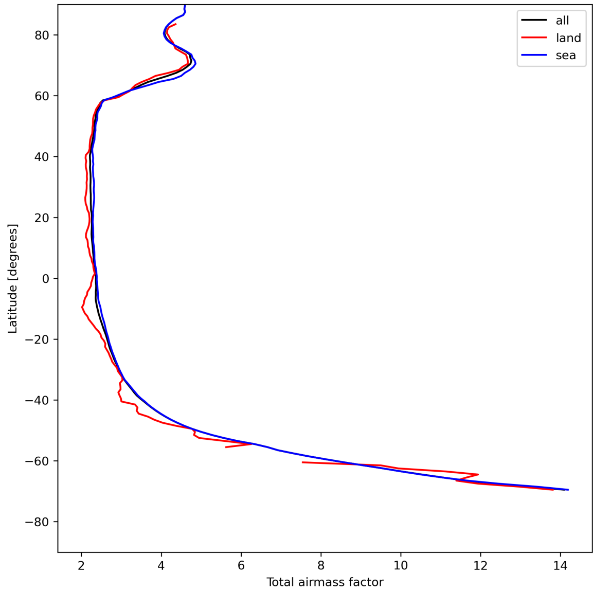
Figure 15: Zonal average of “Total airmass factor” for 2023-07-30 to 2023-08-01.
