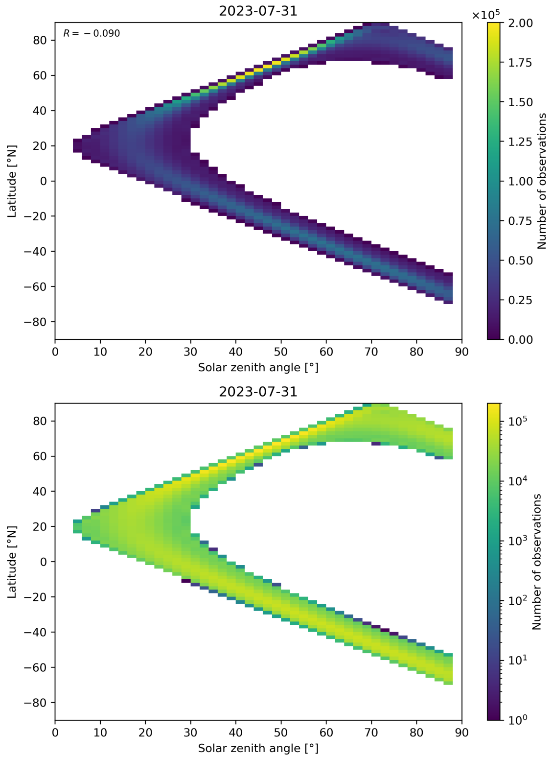
Figure 149: Scatter density plot of “Solar zenith angle” against “Latitude” for 2023-07-30 to 2023-08-01.
