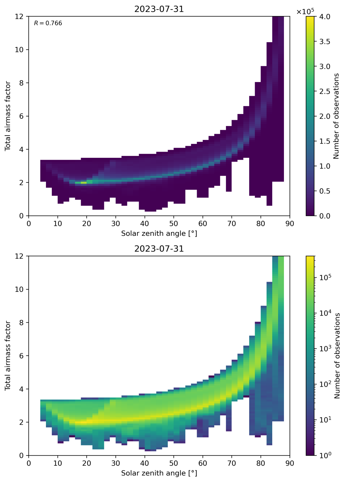
Figure 146: Scatter density plot of “Solar zenith angle” against “Total air mass factor” for 2023-07-30 to 2023-08-01.
