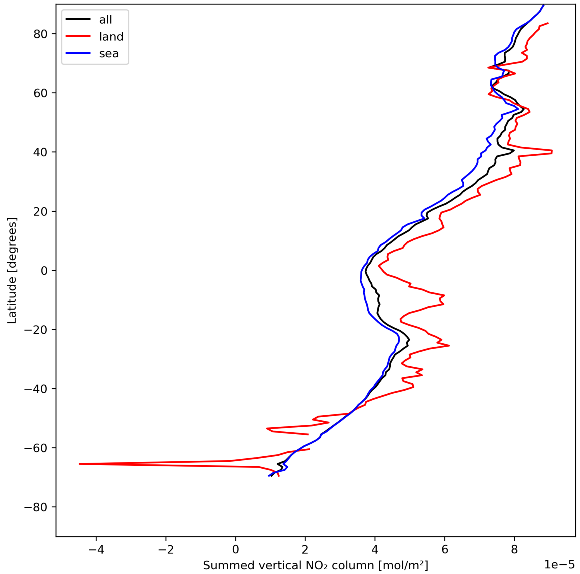
Figure 23: Zonal average of “Summed vertical NO 2 column” for 2023-07-30 to 2023-08-01.
