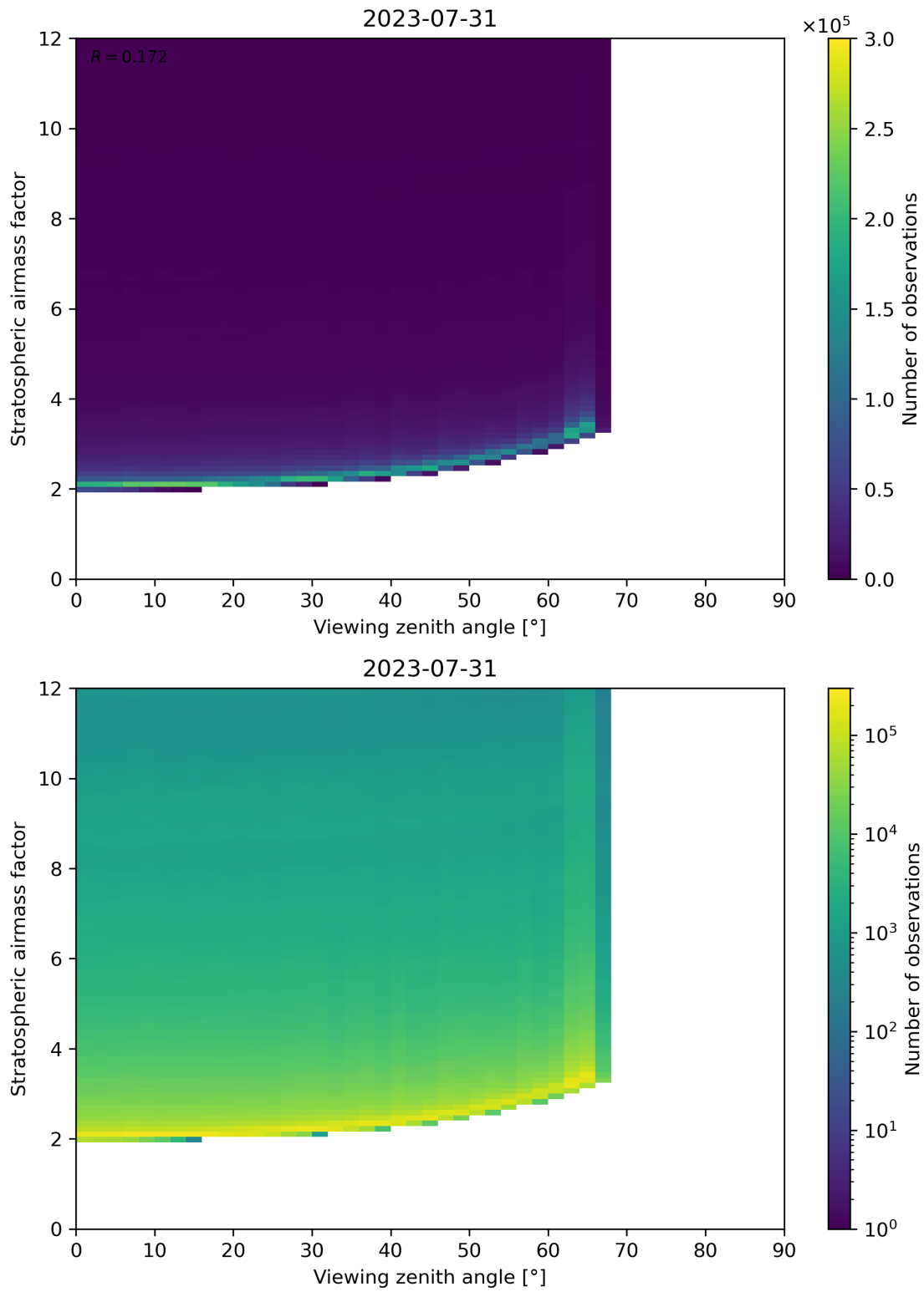
Figure 159: Scatter density plot of “Viewing zenith angle” against “Stratospheric airmass factor” for 2023-07-30 to 2023-08-01.
