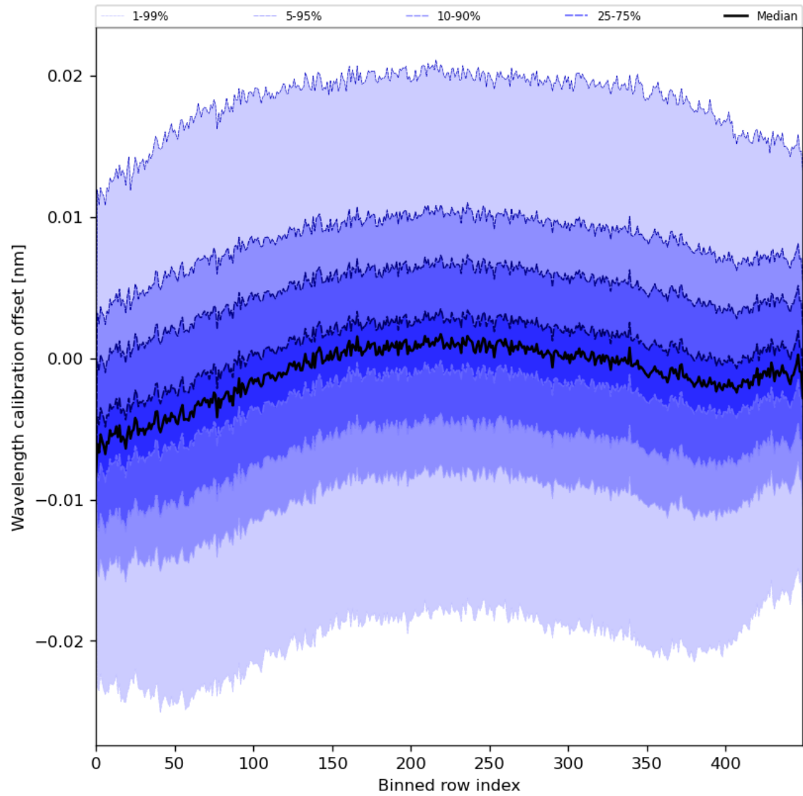
Figure 52: Along track statistics of “Wavelength calibration offset” for 2023-07-30 to 2023-08-01
