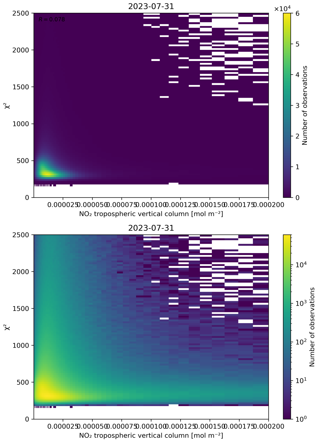
Figure 124: Scatter density plot of “NO 2 tropospheric vertical column” against “ \chi^2 ” for 2023-07-30 to 2023-08-01.
