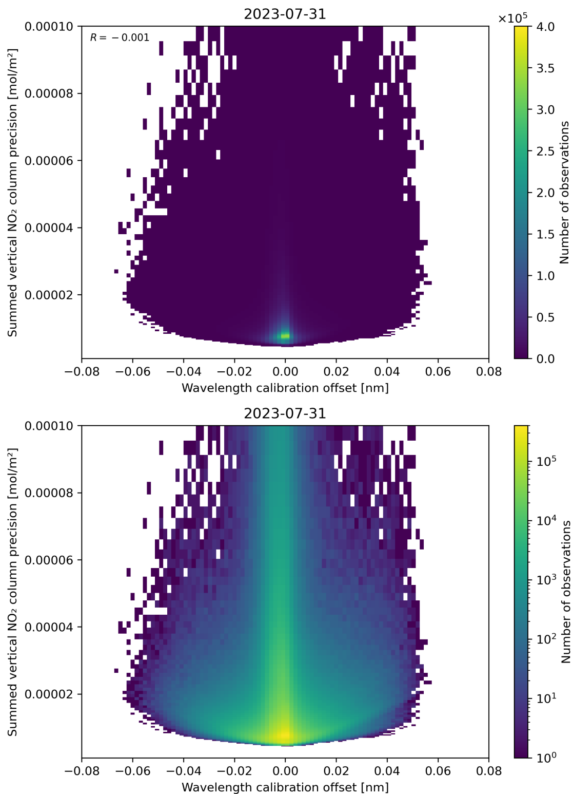
Figure 178: Scatter density plot of “Wavelength calibration offset” against “Summed vertical NO 2 column precision” for 2023-07-30 to 2023-08-01.
