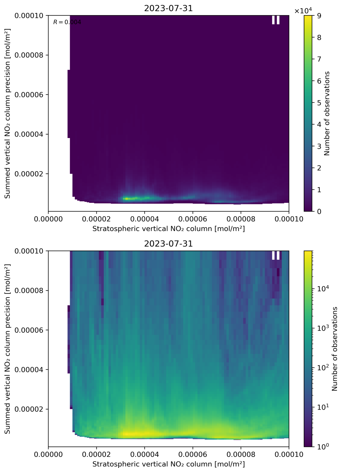
Figure 99: Scatter density plot of “Stratospheric vertical NO 2 column” against “Summed vertical NO 2 column precision” for 2023-07-30 to 2023-08-01.
