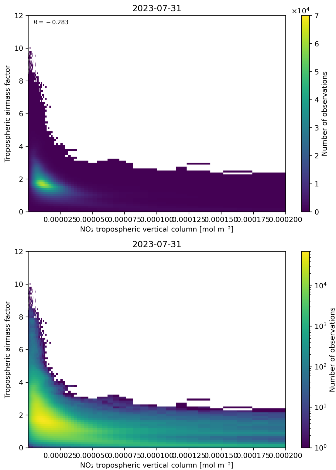
Figure 123: Scatter density plot of “NO 2 tropospheric vertical column” against “Tropospheric air mass factor” for 2023-07-30 to 2023-08-01.
