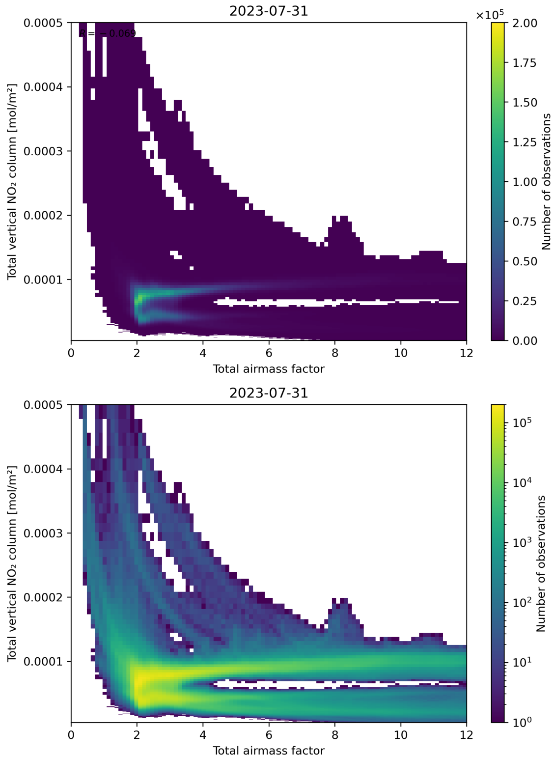
Figure 67: Scatter density plot of “Total airmass factor” against “Total vertical NO 2 column” for 2023-07-30 to 2023-08-01.
