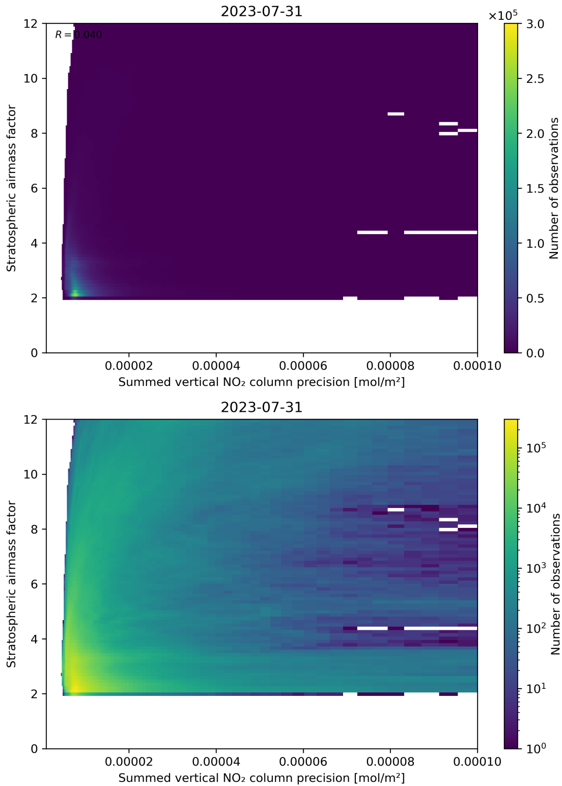
Figure 106: Scatter density plot of “Summed vertical NO 2 column precision” against “Stratospheric airmass factor” for 2023-07-30 to 2023-08-01.
