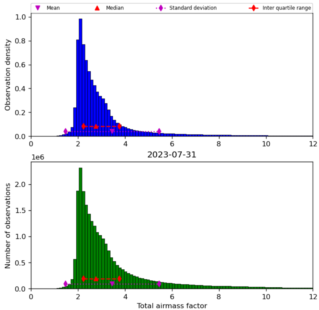
Figure 32: Histogram of “Total airmass factor” for 2023-07-30 to 2023-08-01
