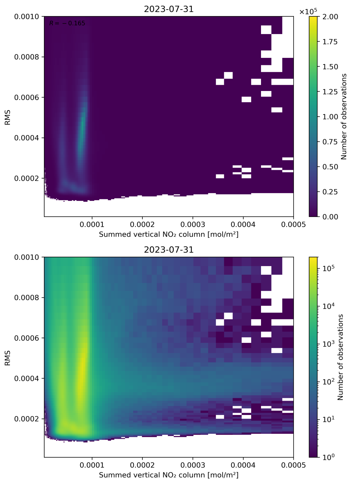
Figure 109: Scatter density plot of “Summed vertical NO 2 column” against “RMS” for 2023-07-30 to 2023-08-01.
