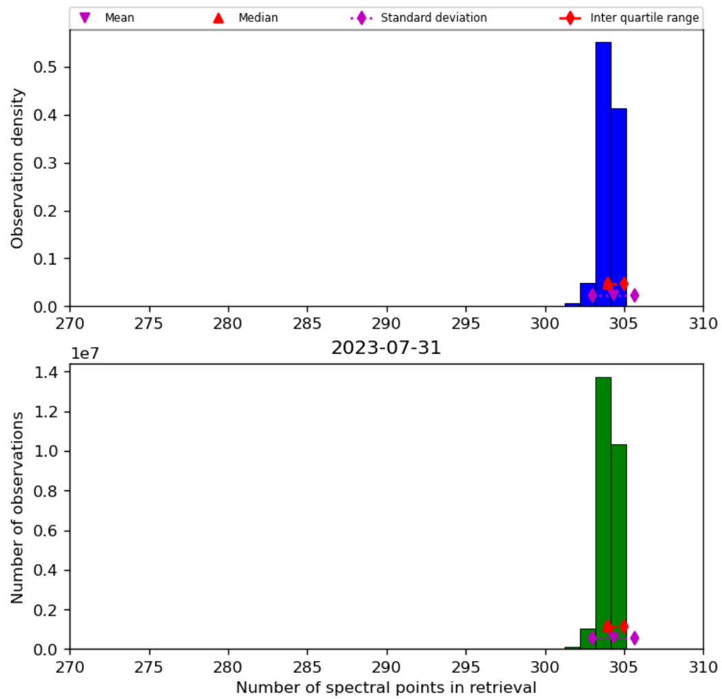
Figure 33: Histogram of “Number of spectral points in retrieval” for 2023-07-30 to 2023-08-01
