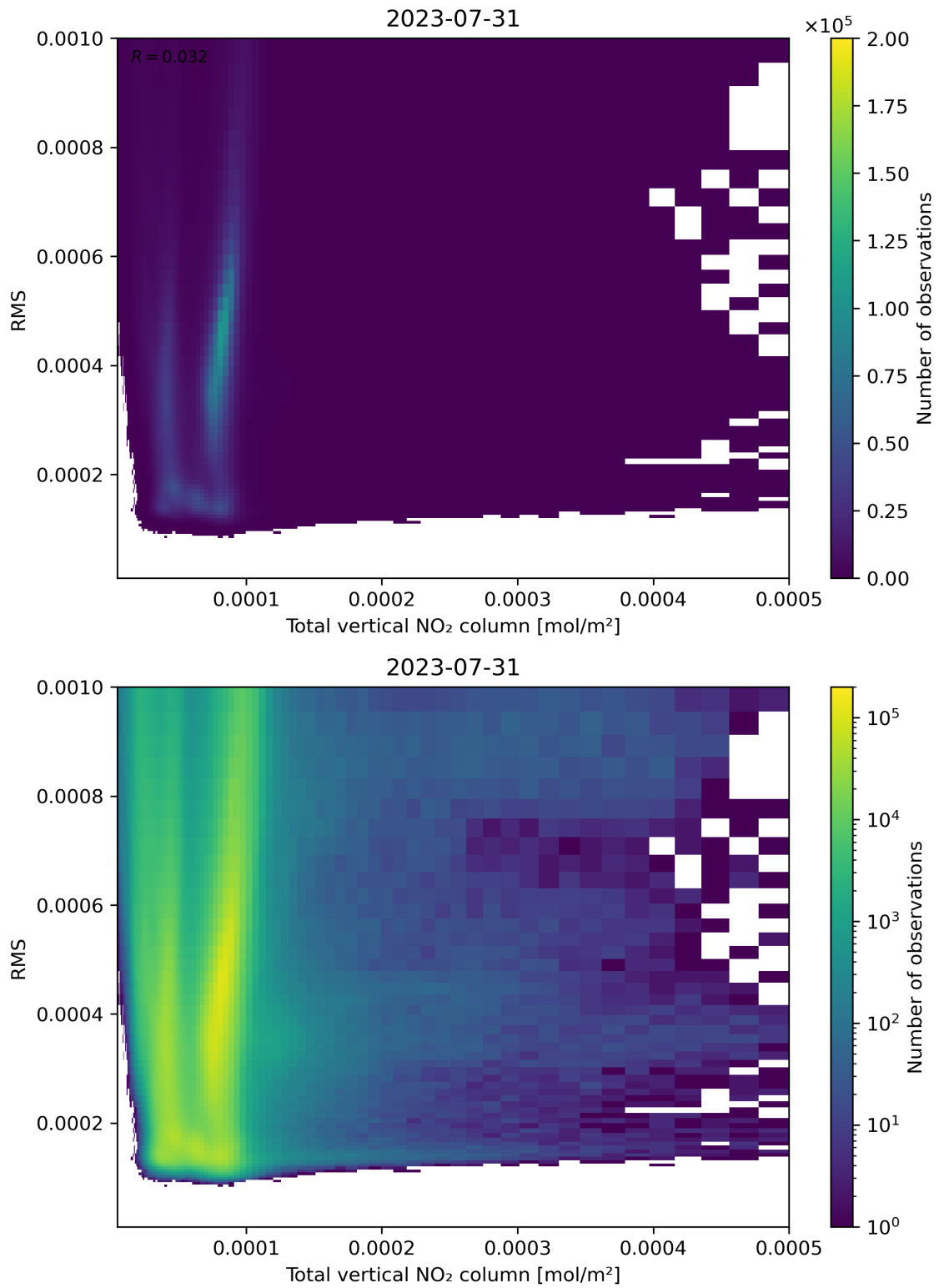
Figure 120: Scatter density plot of “Total vertical NO 2 column” against “RMS” for 2023-07-30 to 2023-08-01.
