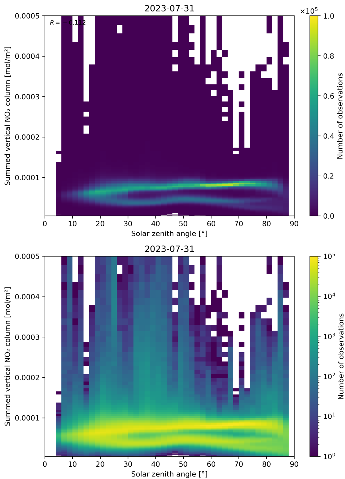
Figure 151: Scatter density plot of “Solar zenith angle” against “Summed vertical NO 2 column” for 2023-07-30 to 2023-08-01.
