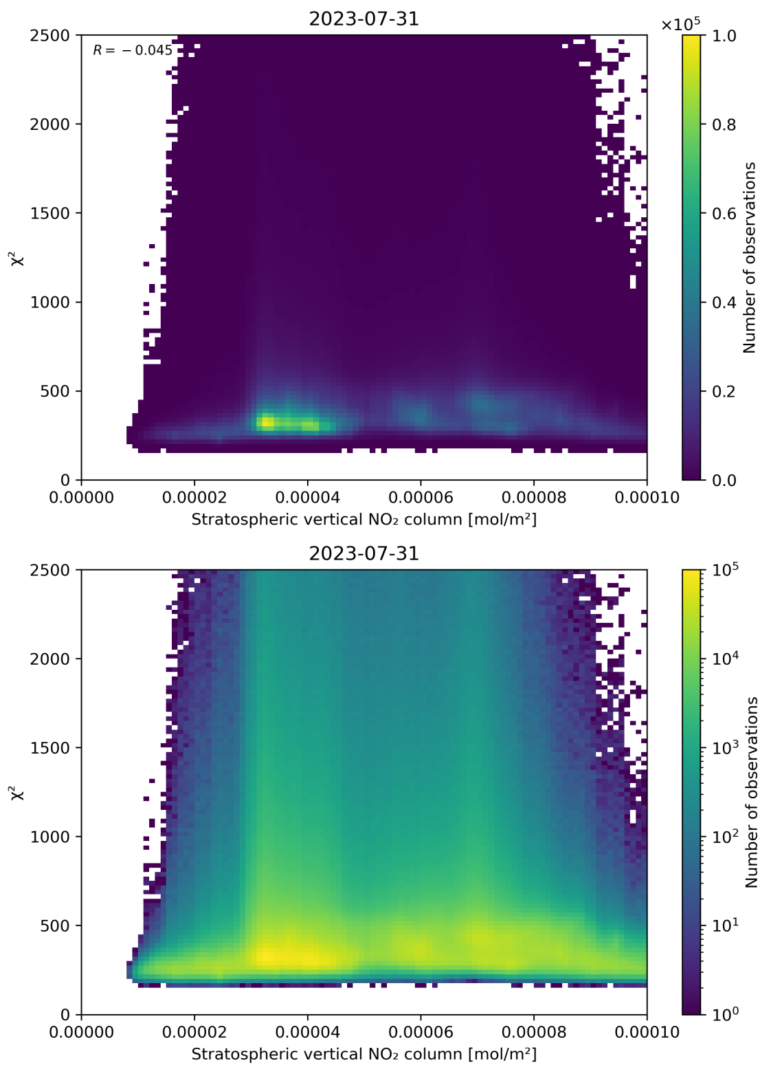
Figure 97: Scatter density plot of “Stratospheric vertical NO 2 column” against “ \chi^2 ” for 2023-07-30 to 2023-08-01.
