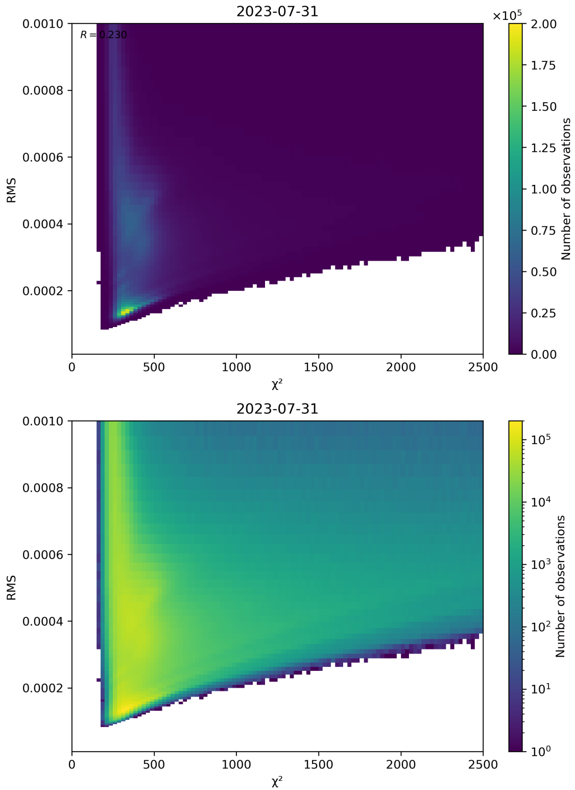
Figure 82: Scatter density plot of “ \chi^2 ” against “RMS” for 2023-07-30 to 2023-08-01.
