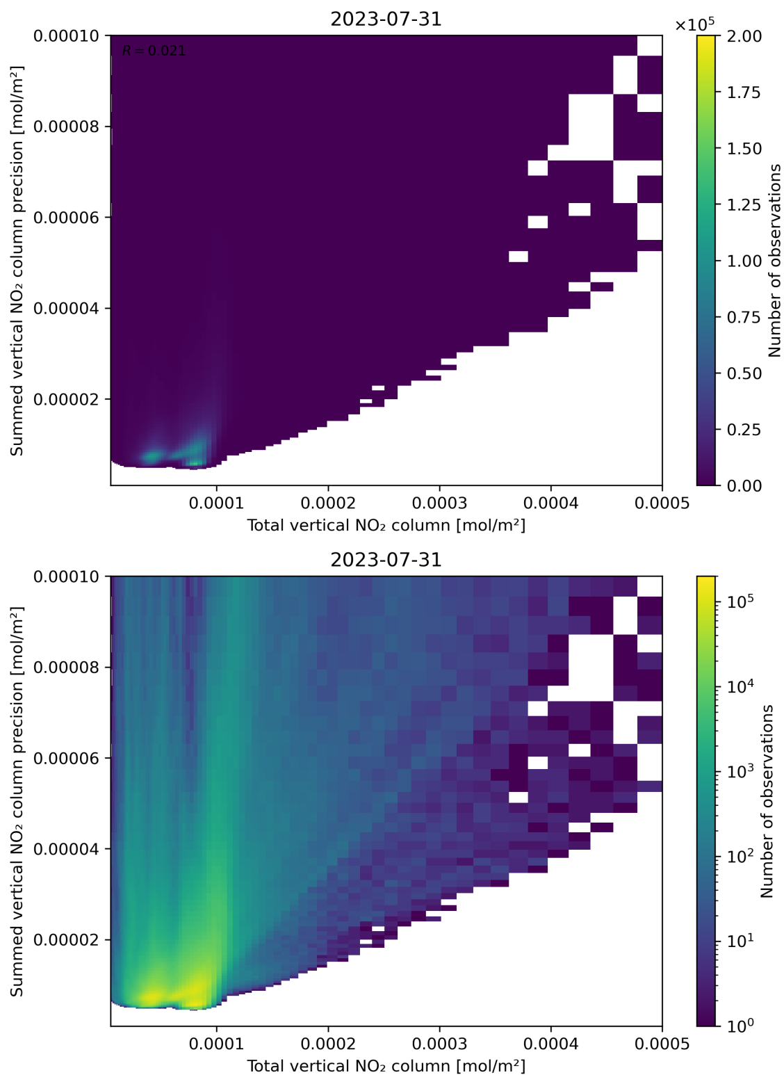
Figure 113: Scatter density plot of “Total vertical NO 2 column” against “Summed vertical NO 2 column precision” for 2023-07-30 to 2023-08-01.
