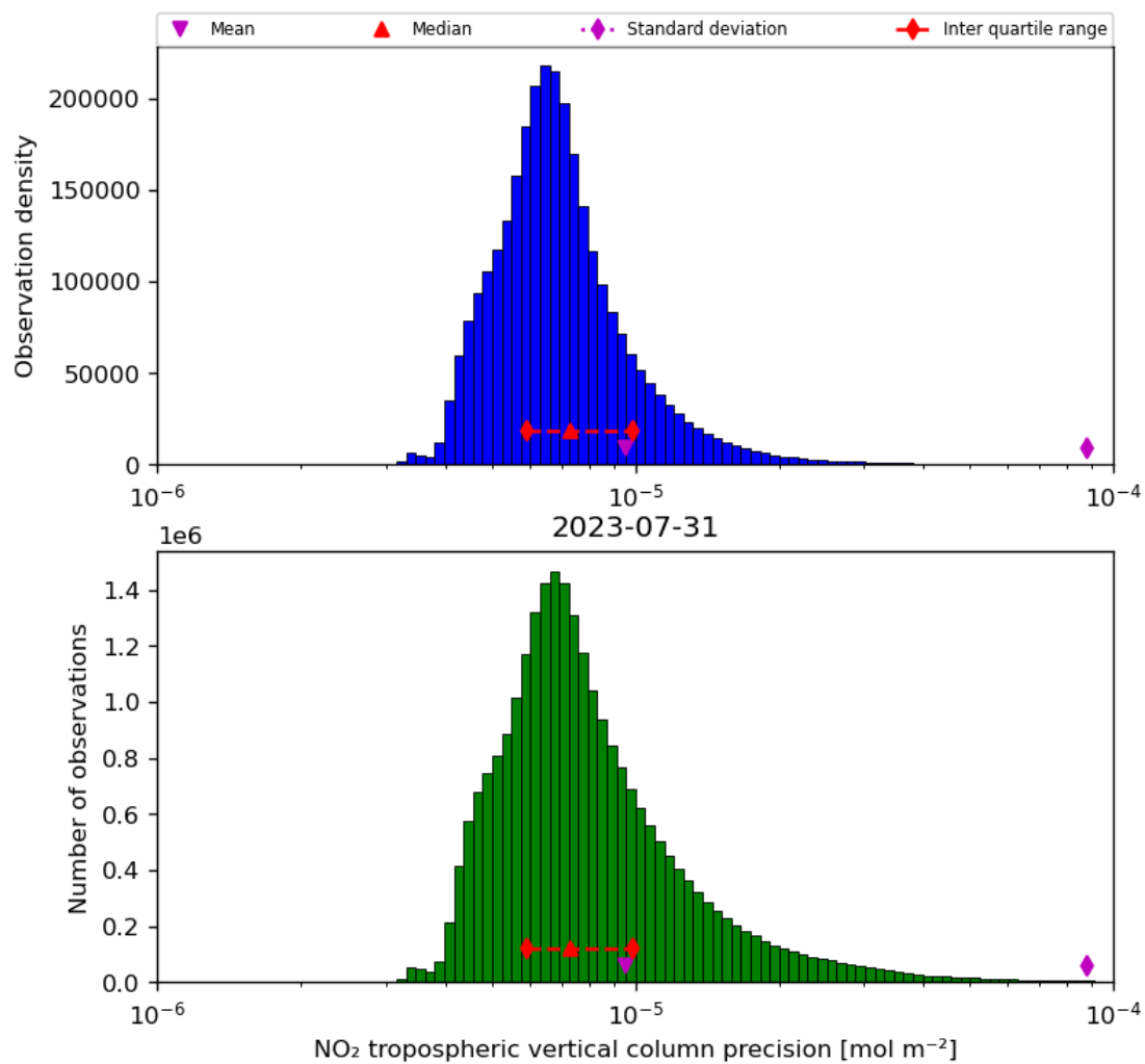
Figure 30: Histogram of “NO 2 tropospheric vertical column precision” for 2023-07-30 to 2023-08-01
