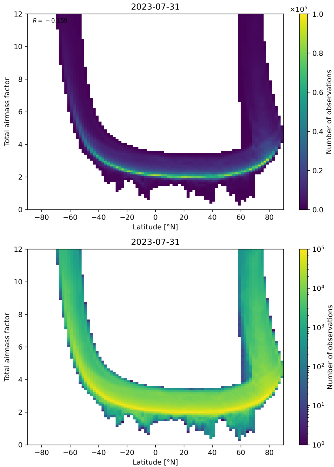
Figure 84: Scatter density plot of “Latitude” against “Total airmass factor” for 2023-07-30 to 2023-08-01.
