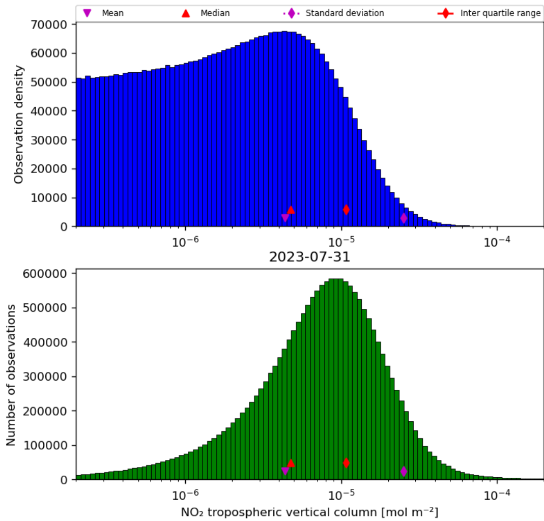
Figure 29: Histogram of “NO 2 tropospheric vertical column” for 2023-07-30 to 2023-08-01
