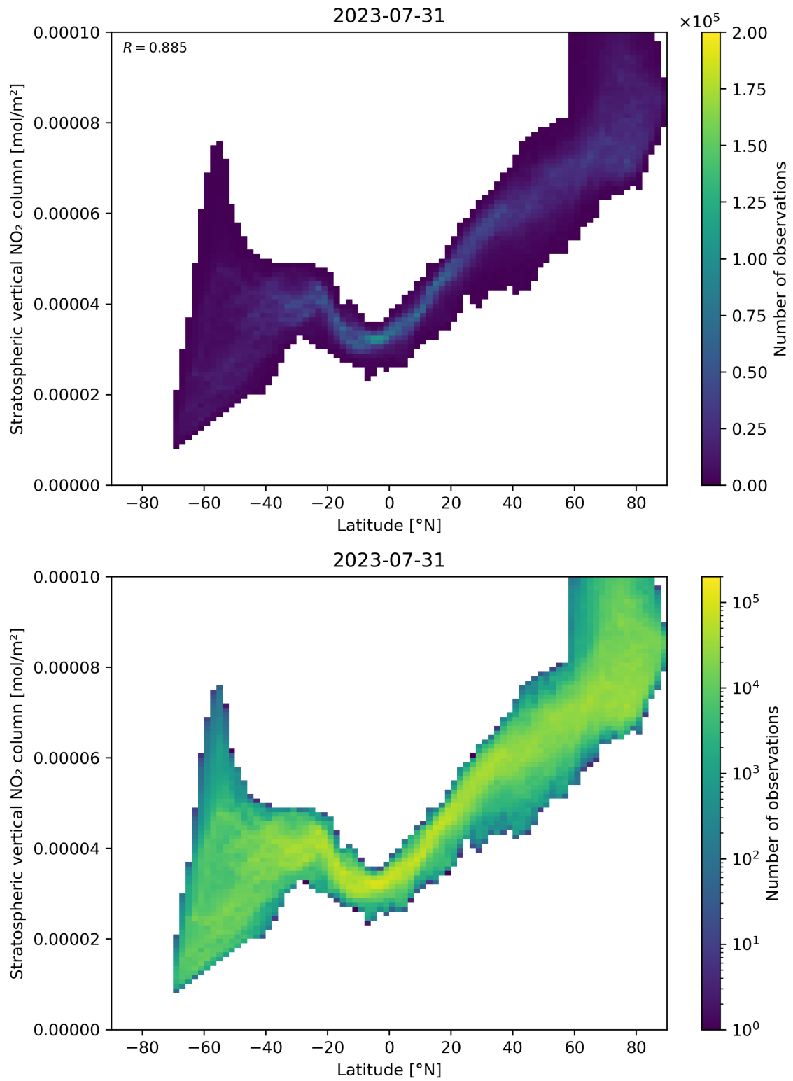
Figure 87: Scatter density plot of “Latitude” against “Stratospheric vertical NO 2 column” for 2023-07-30 to 2023-08-01.
