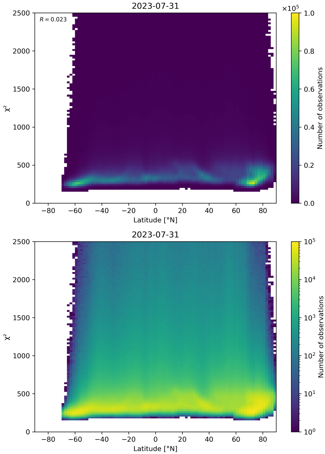
Figure 86: Scatter density plot of “Latitude” against “ \chi^2 ” for 2023-07-30 to 2023-08-01.
