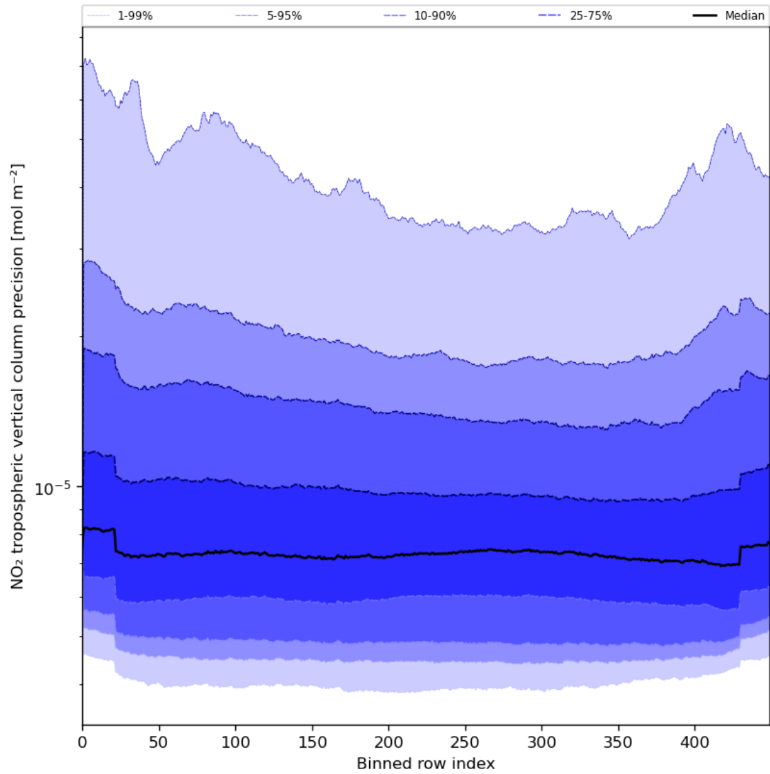
Figure 47: Along track statistics of “NO 2 tropospheric vertical column precision” for 2023-07-30 to 2023-08-01
