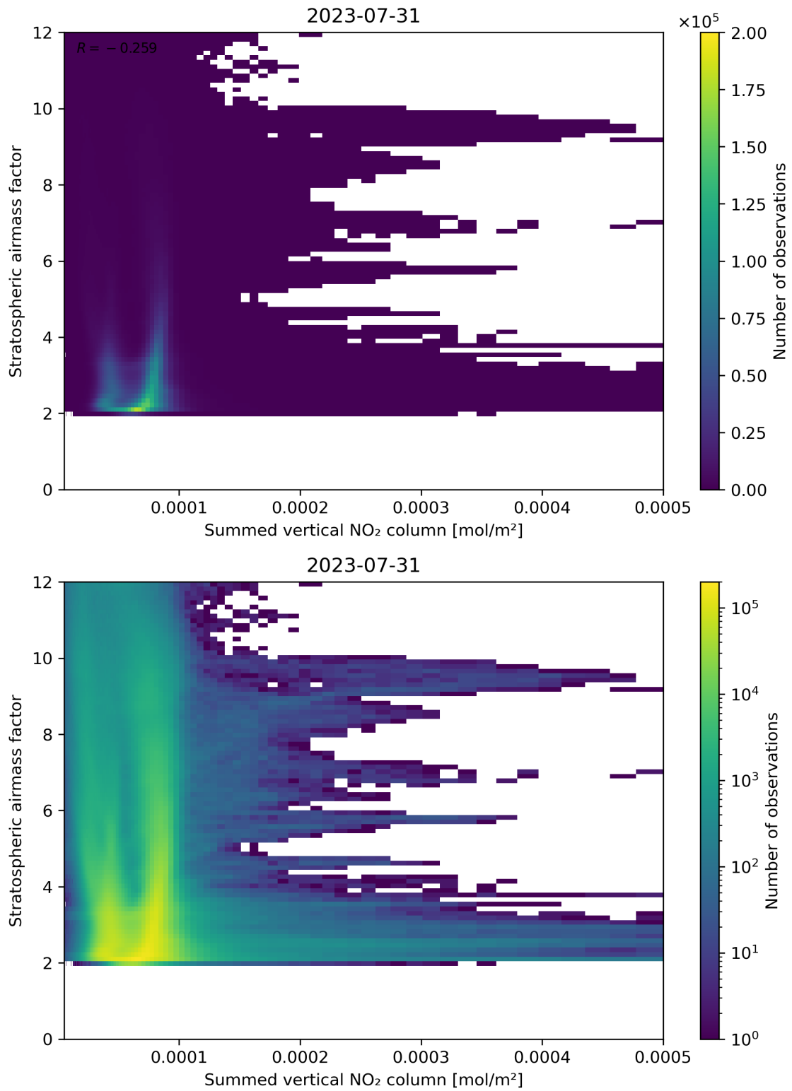
Figure 103: Scatter density plot of “Summed vertical NO 2 column” against “Stratospheric air mass factor” for 2023-07-30 to 2023-08-01.
