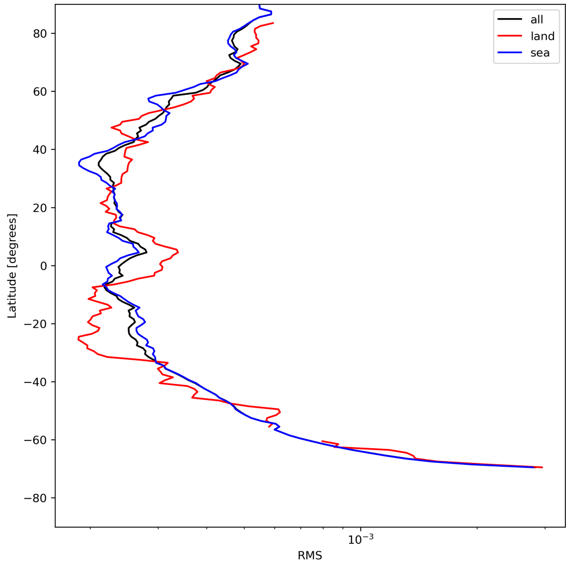
Figure 26: Zonal average of “RMS” for 2023-07-30 to 2023-08-01.
