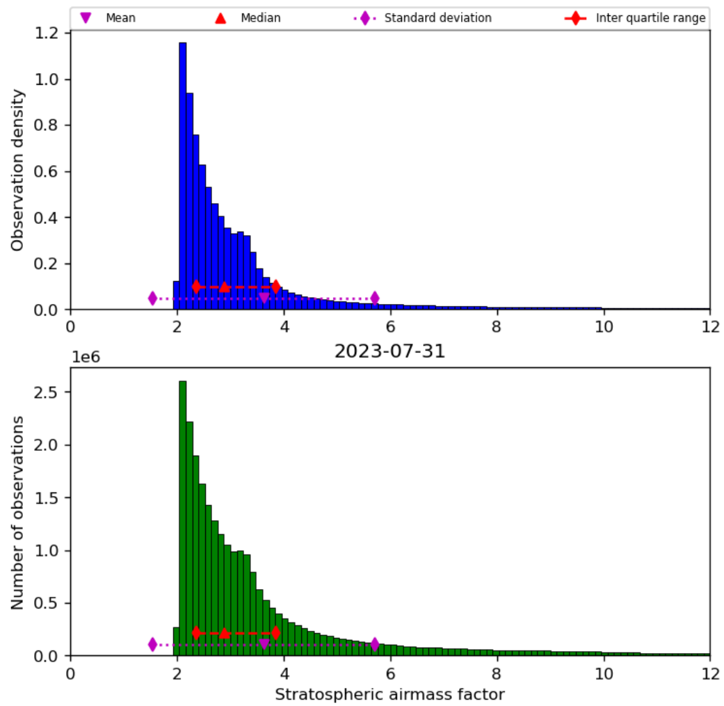
Figure 44: Histogram of “Stratospheric airmass factor” for 2023-07-30 to 2023-08-01
