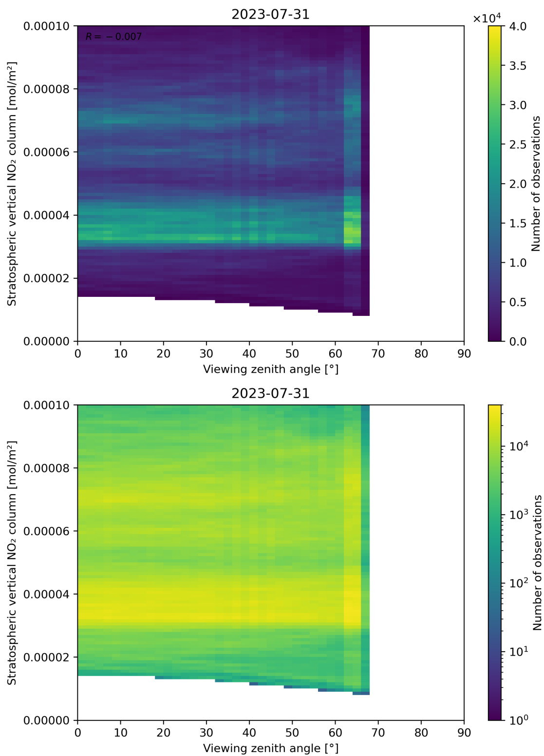
Figure 164: Scatter density plot of “Viewing zenith angle” against “Stratospheric vertical NO 2 column” for 2023-07-30 to 2023-08-01.
