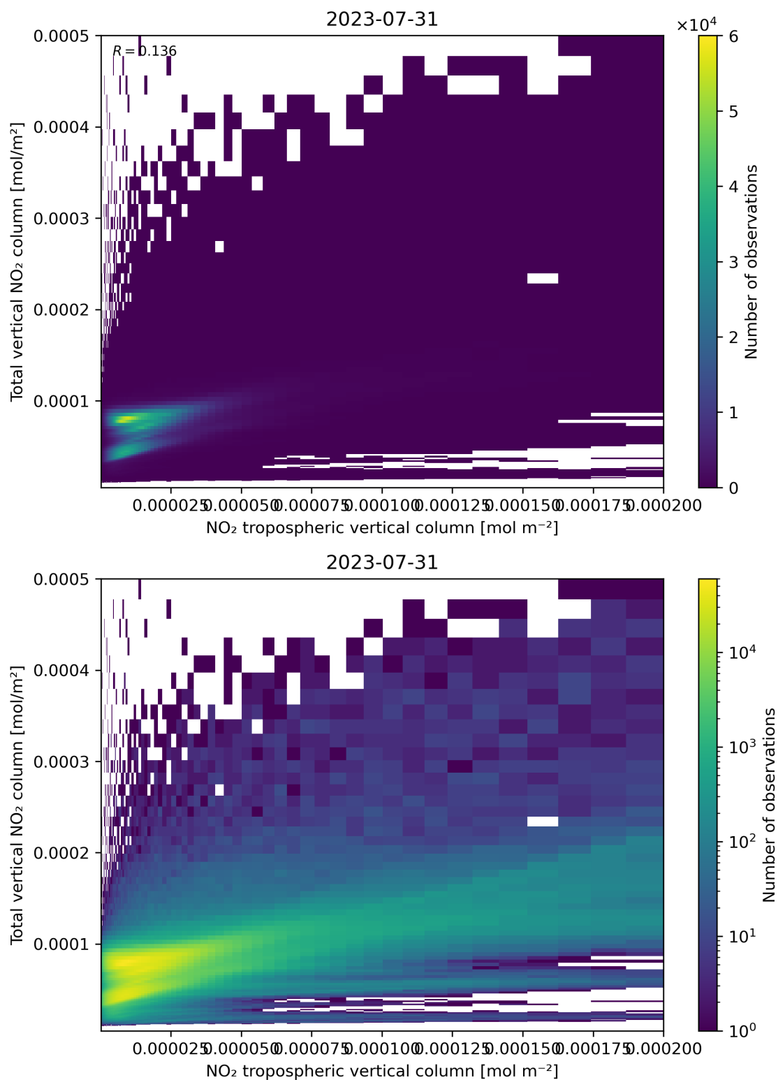
Figure 128: Scatter density plot of “NO 2 tropospheric vertical column” against “Total vertical NO 2 column” for 2023-07-30 to 2023-08-01.
