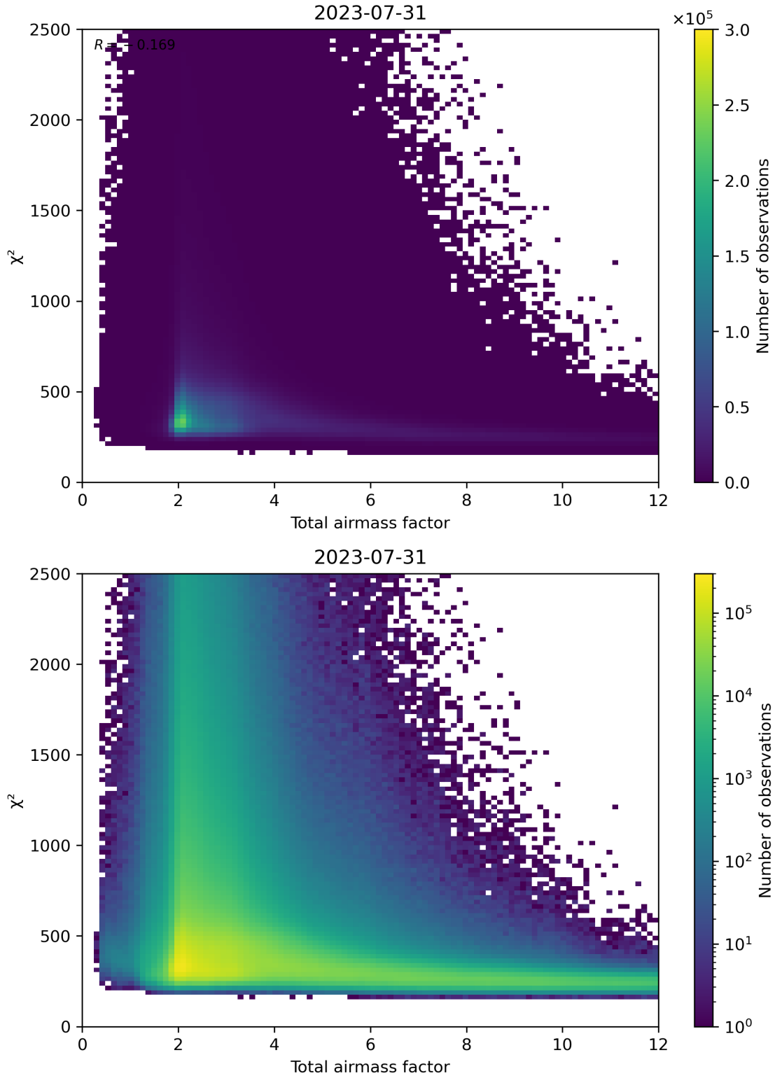
Figure 63: Scatter density plot of “Total airmass factor” against “ \chi^2 ” for 2023-07-30 to 2023-08-01.
