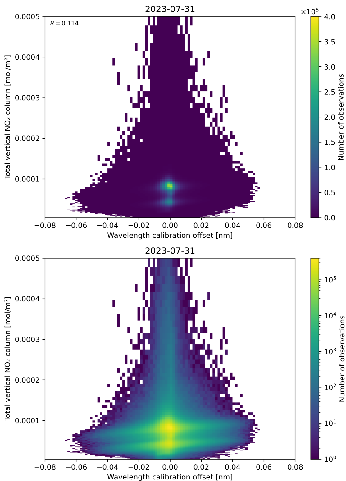
Figure 179: Scatter density plot of “Wavelength calibration offset” against “Total vertical NO 2 column” for 2023-07-30 to 2023-08-01.
