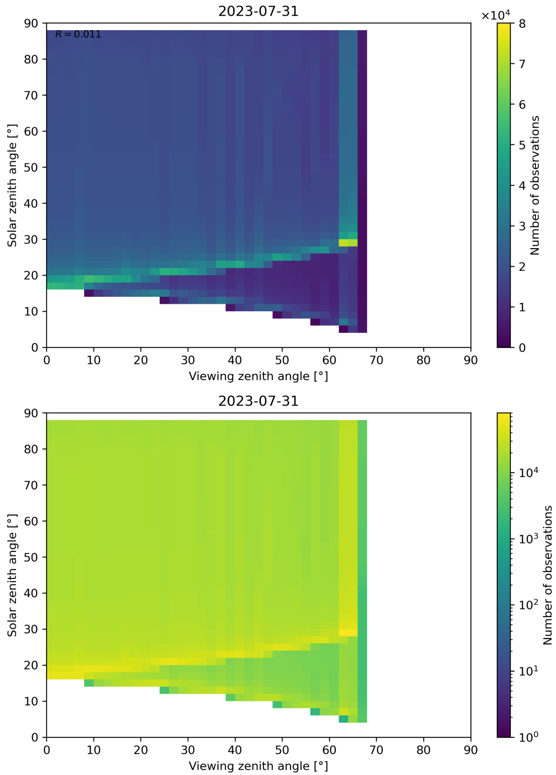
Figure 172: Scatter density plot of “Viewing zenith angle” against “Solar zenith angle” for 2023-07-30 to 2023-08-01.
