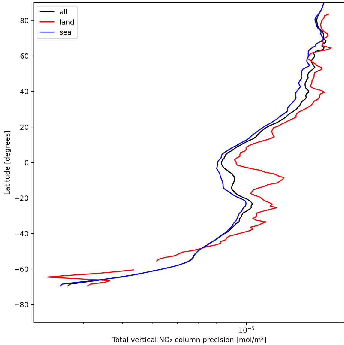
Figure 22: Zonal average of “Total vertical NO 2 column precision” for 2023-07-30 to 2023-08-01.
