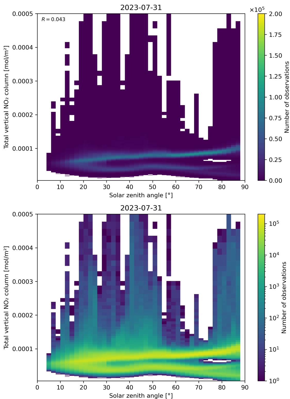
Figure 153: Scatter density plot of “Solar zenith angle” against “Total vertical NO 2 column” for 2023-07-30 to 2023-08-01.
