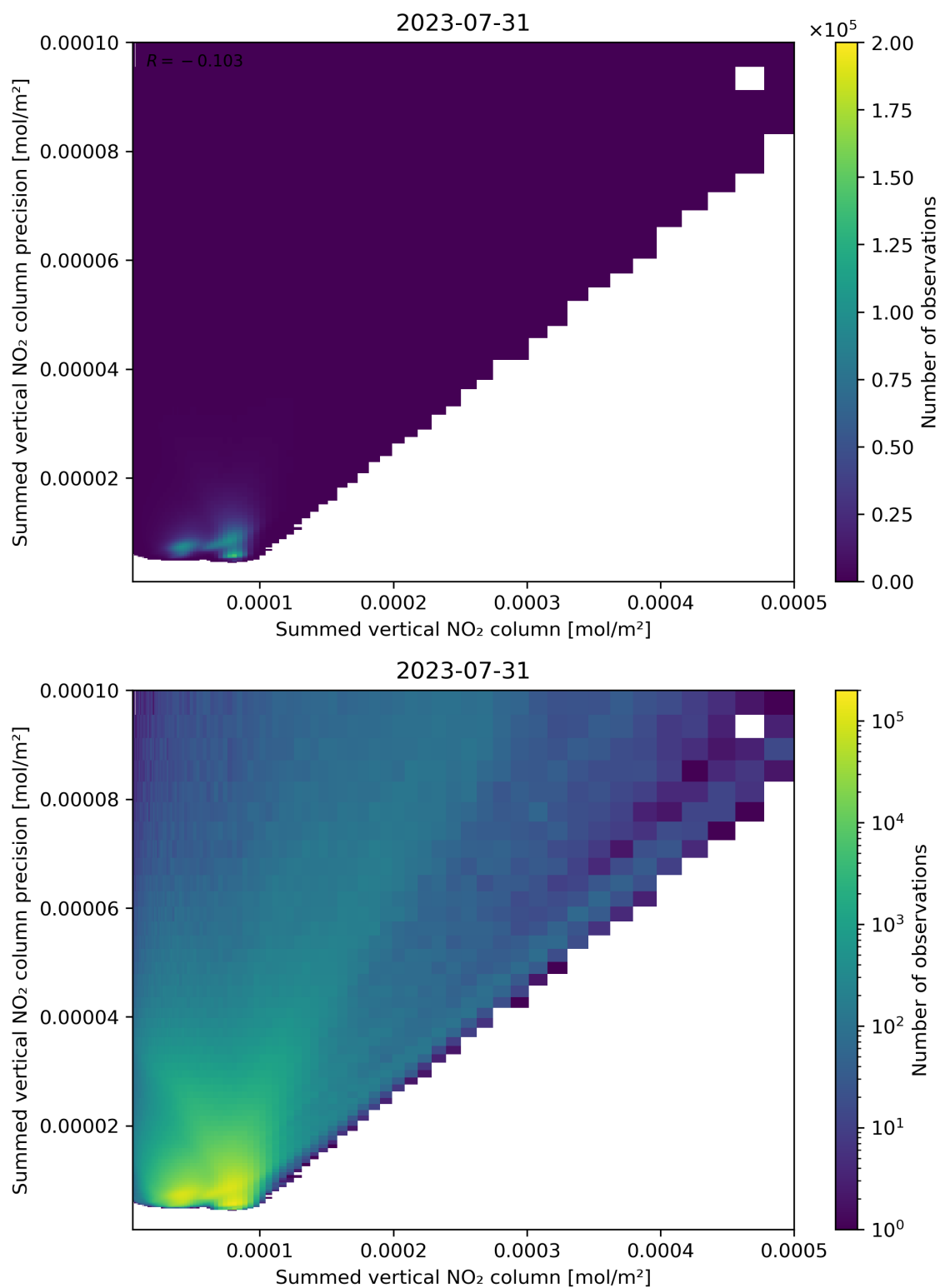
Figure 105: Scatter density plot of “Summed vertical NO 2 column” against “Summed vertical NO 2 column precision” for 2023-07-30 to 2023-08-01.
