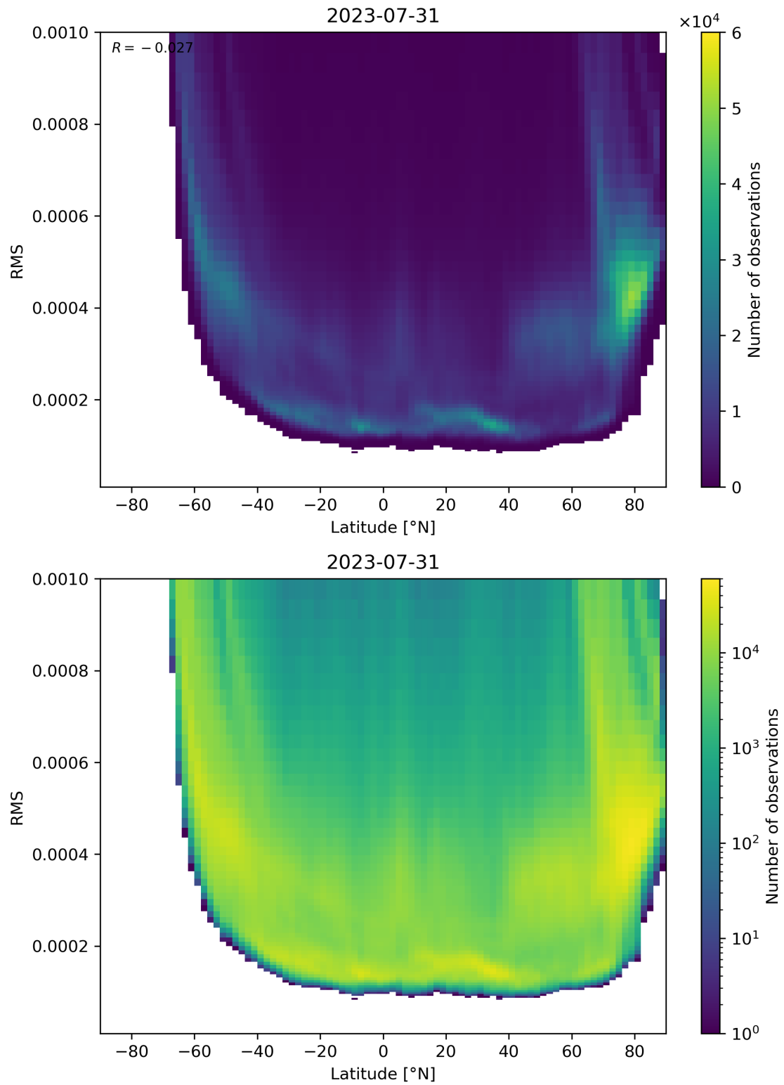
Figure 94: Scatter density plot of “Latitude” against “RMS” for 2023-07-30 to 2023-08-01.
