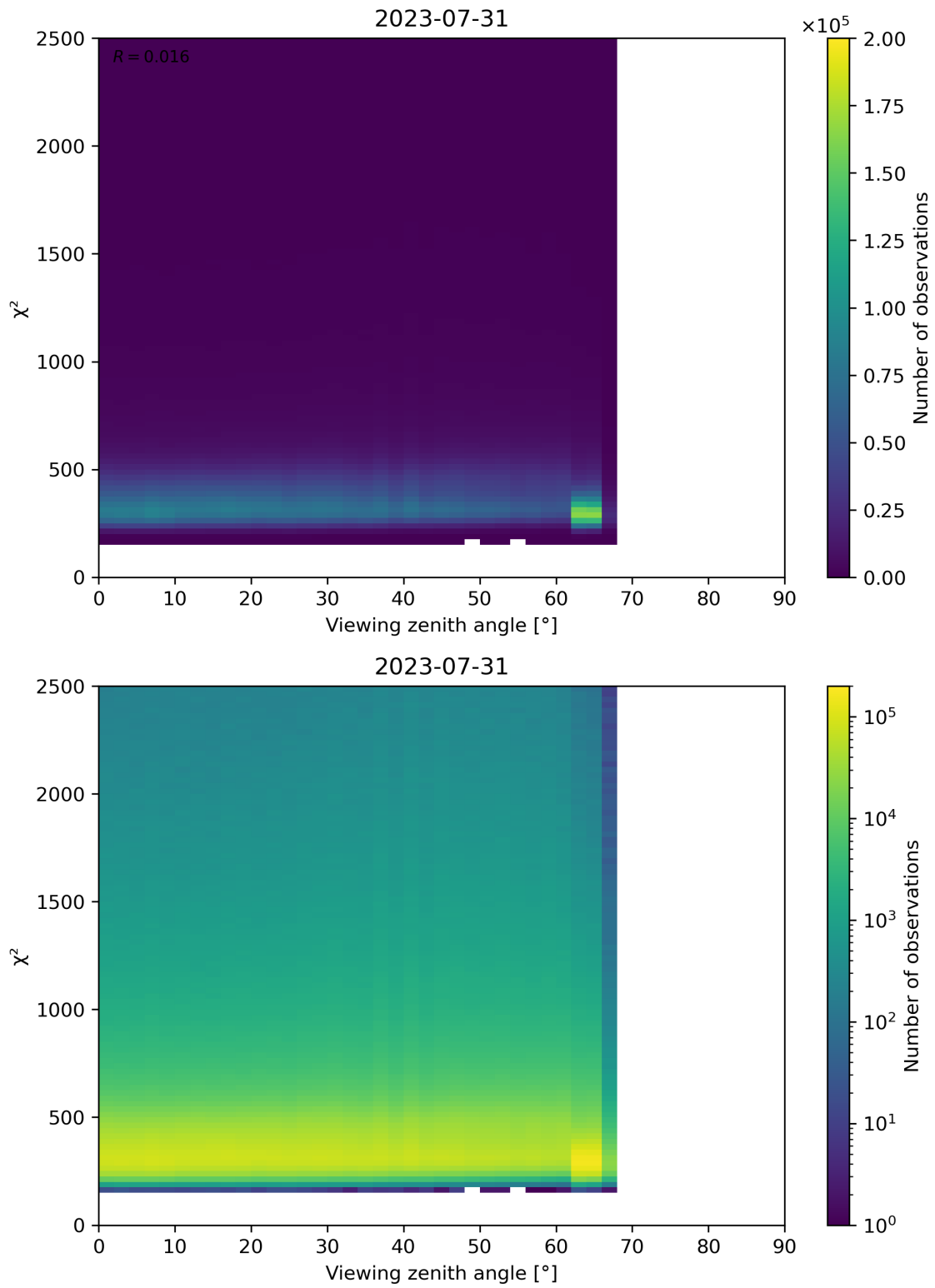
Figure 162: Scatter density plot of “Viewing zenith angle” against “ \chi^2 ” for 2023-07-30 to 2023-08-01.
