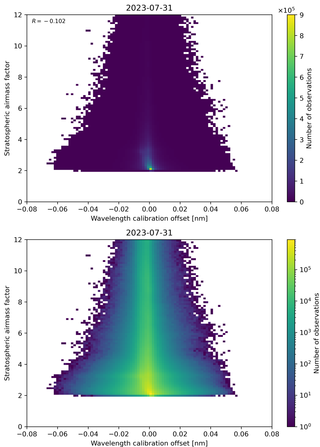
Figure 174: Scatter density plot of “Wavelength calibration offset” against “Stratospheric air mass factor” for 2023-07-30 to 2023-08-01.
