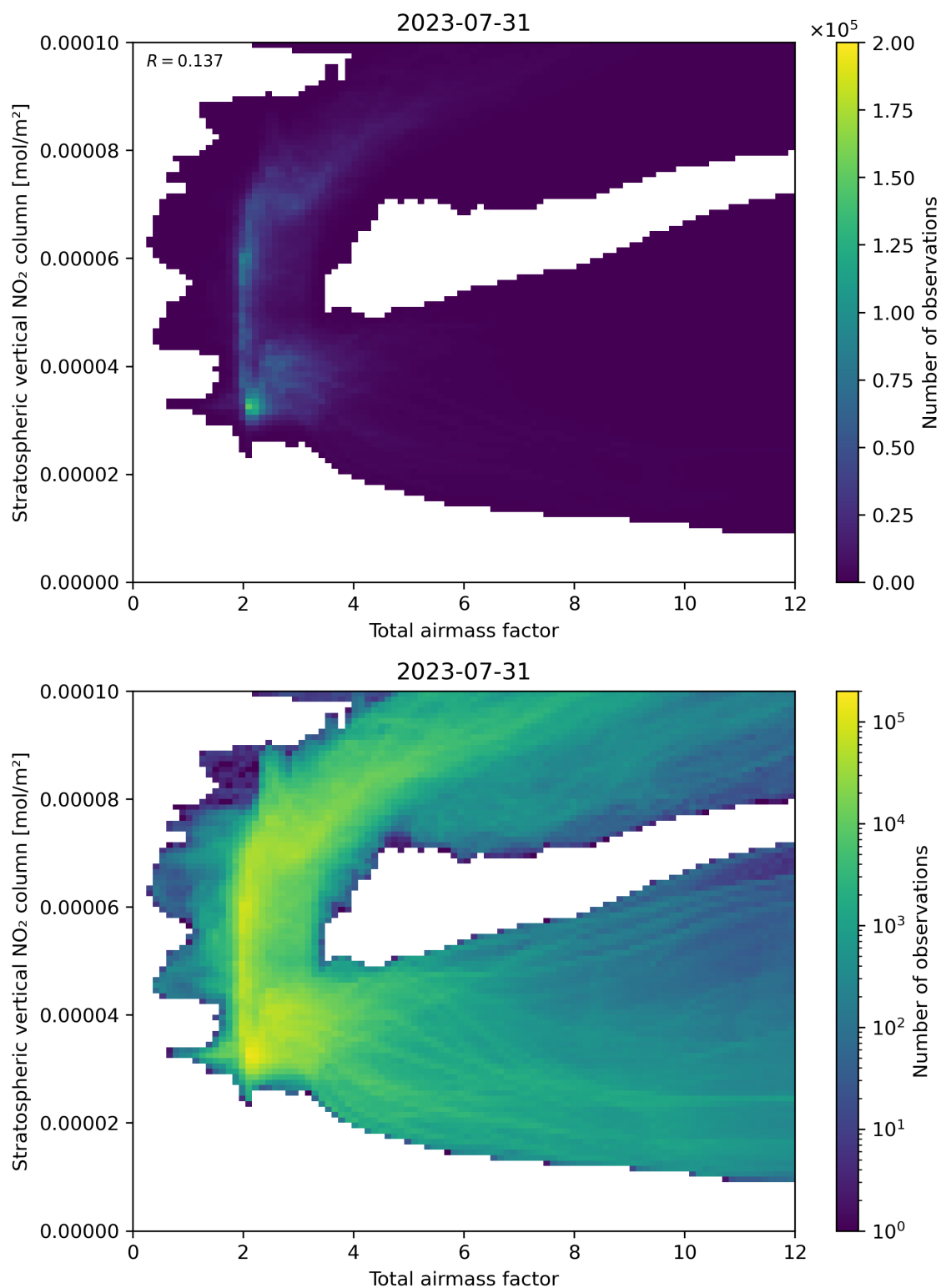
Figure 64: Scatter density plot of “Total airmass factor” against “Stratospheric vertical NO 2 column” for 2023-07-30 to 2023-08-01.
