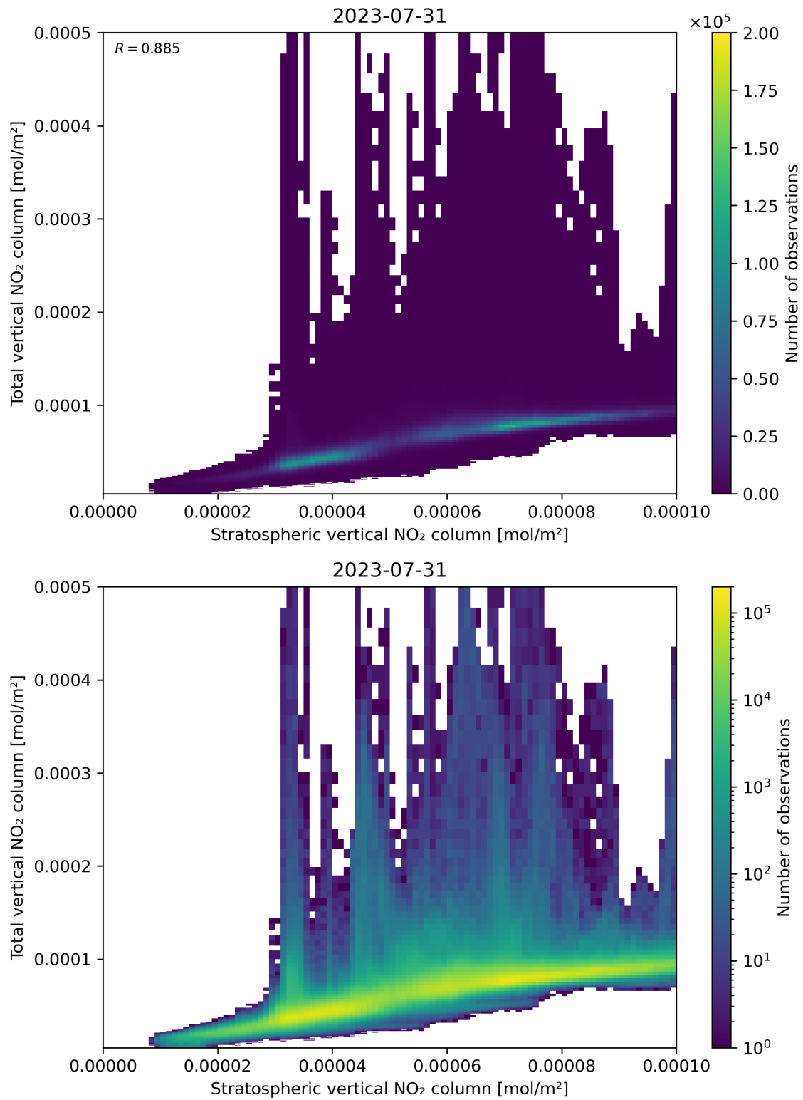
Figure 100: Scatter density plot of “Stratospheric vertical NO 2 column” against “Total vertical NO 2 column” for 2023-07-30 to 2023-08-01.
