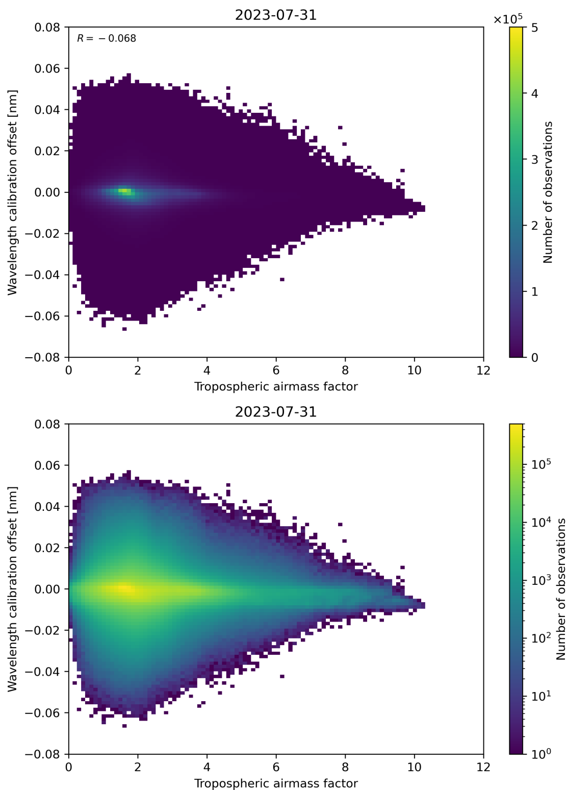
Figure 80: Scatter density plot of “Tropospheric airmass factor” against “Wavelength calibration offset” for 2023-07-30 to 2023-08-01.
