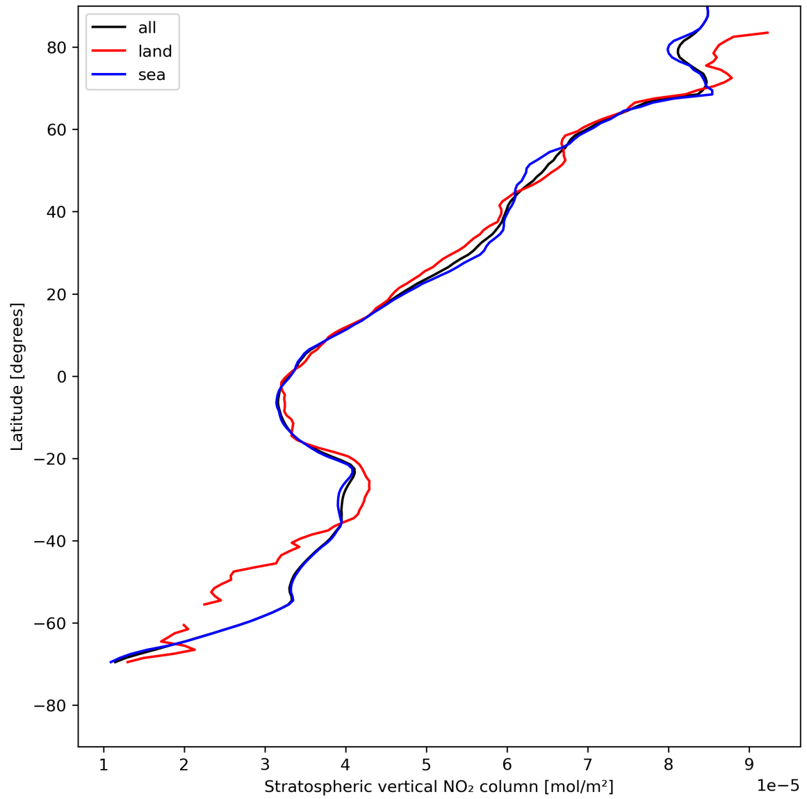
Figure 19: Zonal average of “Stratospheric vertical NO 2 column” for 2023-07-30 to 2023-08-01.
