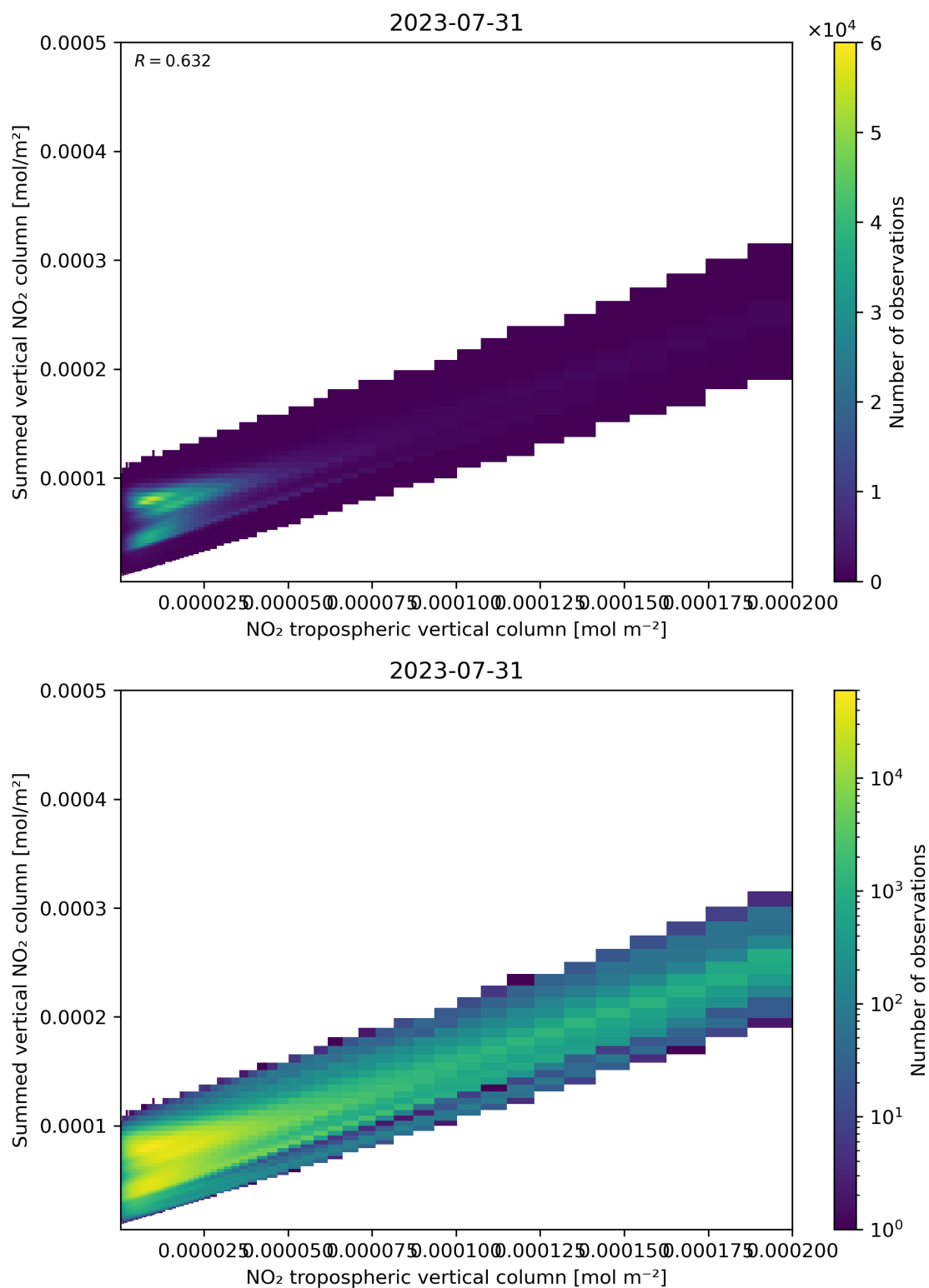
Figure 126: Scatter density plot of “NO 2 tropospheric vertical column” against “Summed vertical NO 2 column” for 2023-07-30 to 2023-08-01.
