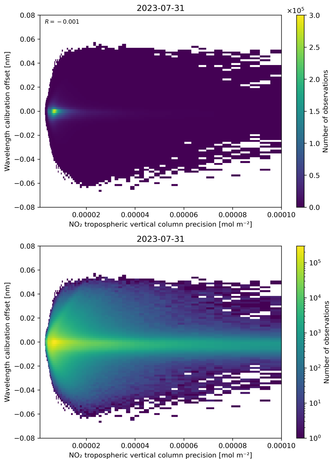
Figure 141: Scatter density plot of “NO 2 tropospheric vertical column precision” against “Wavelength calibration offset” for 2023-07-30 to 2023-08-01.
