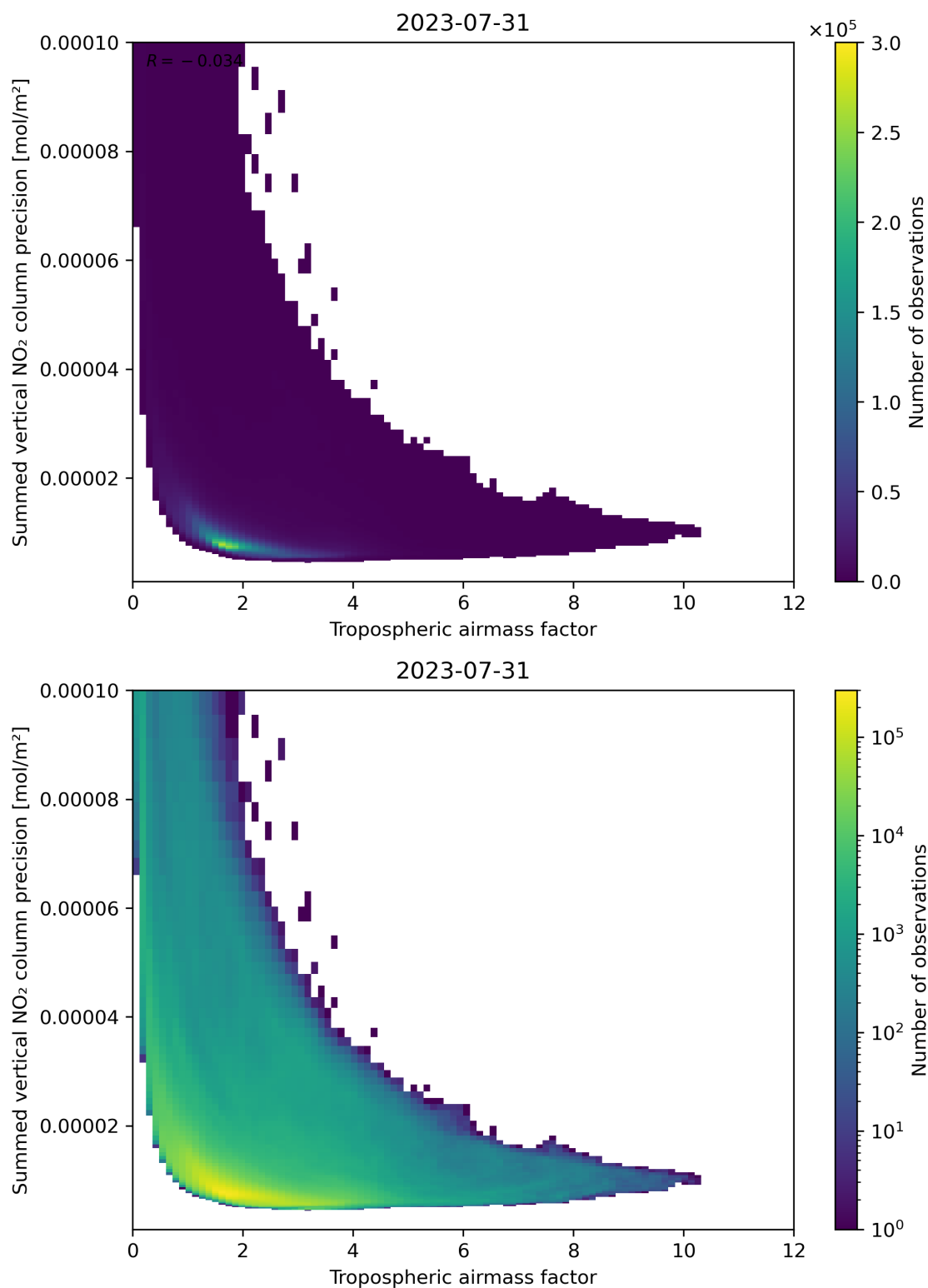
Figure 76: Scatter density plot of “Tropospheric air mass factor” against “Summed vertical NO 2 column precision” for 2023-07-30 to 2023-08-01.
