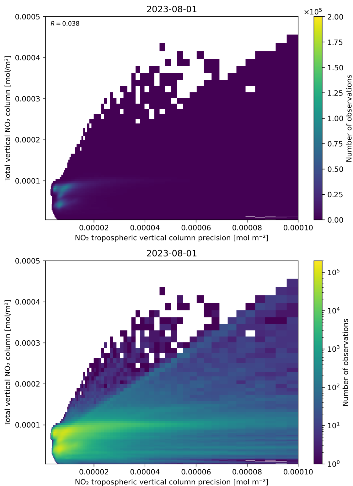
Figure 138: Scatter density plot of “NO 2 tropospheric vertical column precision” against “Total vertical NO 2 column” for 2023-07-31 to 2023-08-02.
