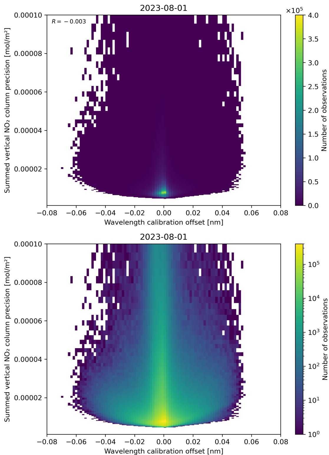
Figure 178: Scatter density plot of “Wavelength calibration offset” against “Summed vertical NO 2 column precision” for 2023-07-31 to 2023-08-02.
