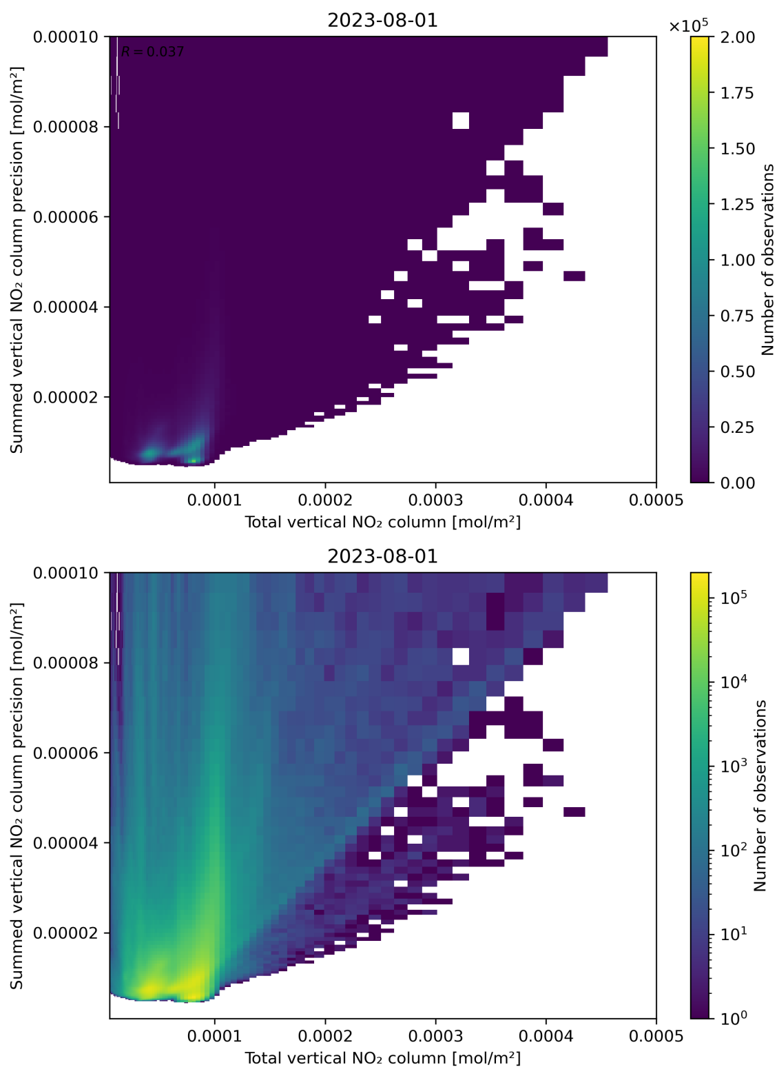
Figure 113: Scatter density plot of “Total vertical NO 2 column” against “Summed vertical NO 2 column precision” for 2023-07-31 to 2023-08-02.
