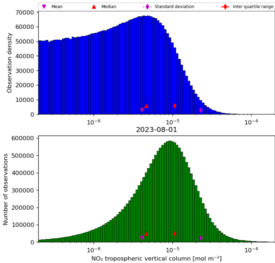
Figure 29: Histogram of “NO 2 tropospheric vertical column” for 2023-07-31 to 2023-08-02
