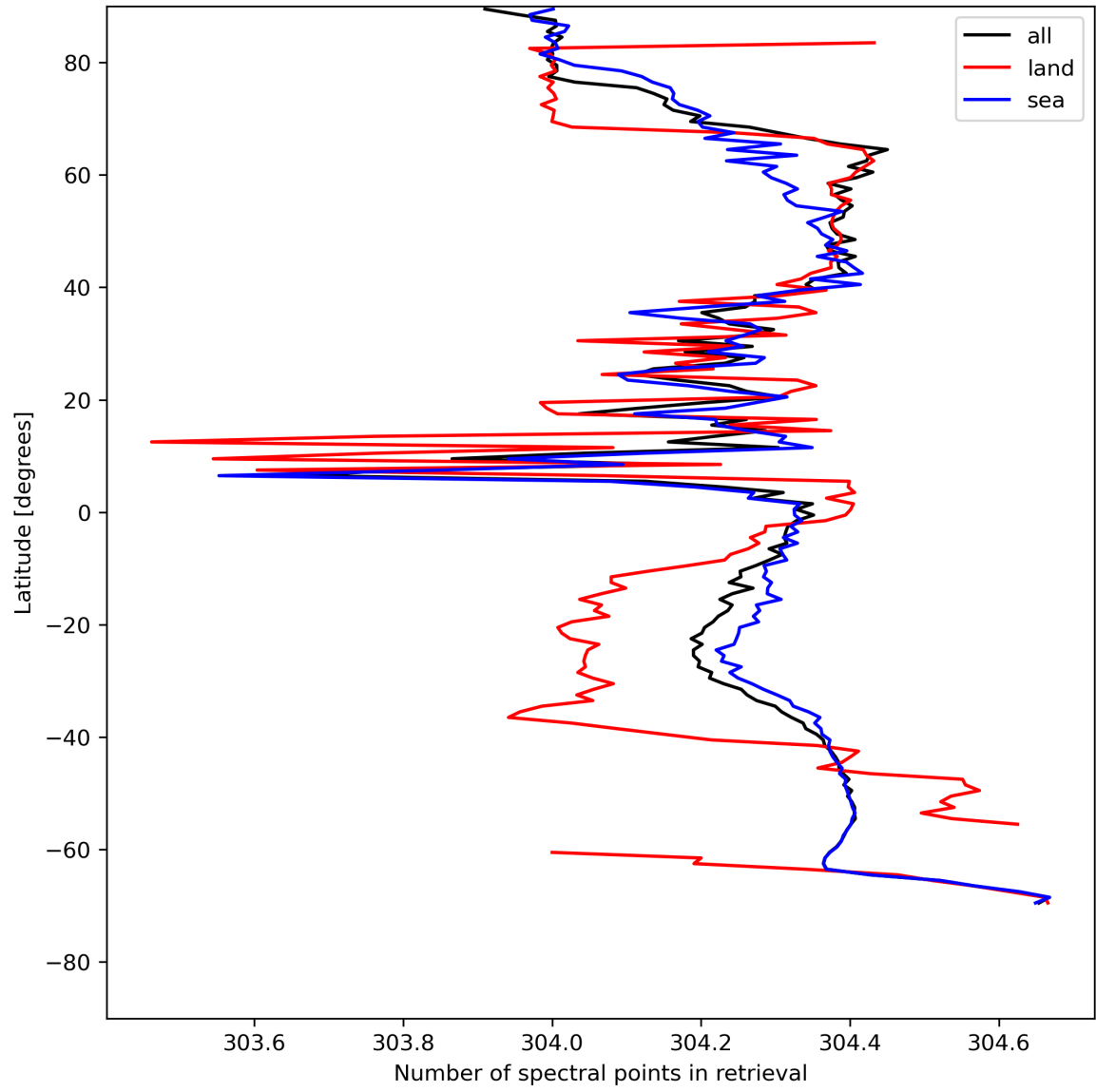
Figure 16: Zonal average of “Number of spectral points in retrieval” for 2023-07-31 to 2023-08-02.
