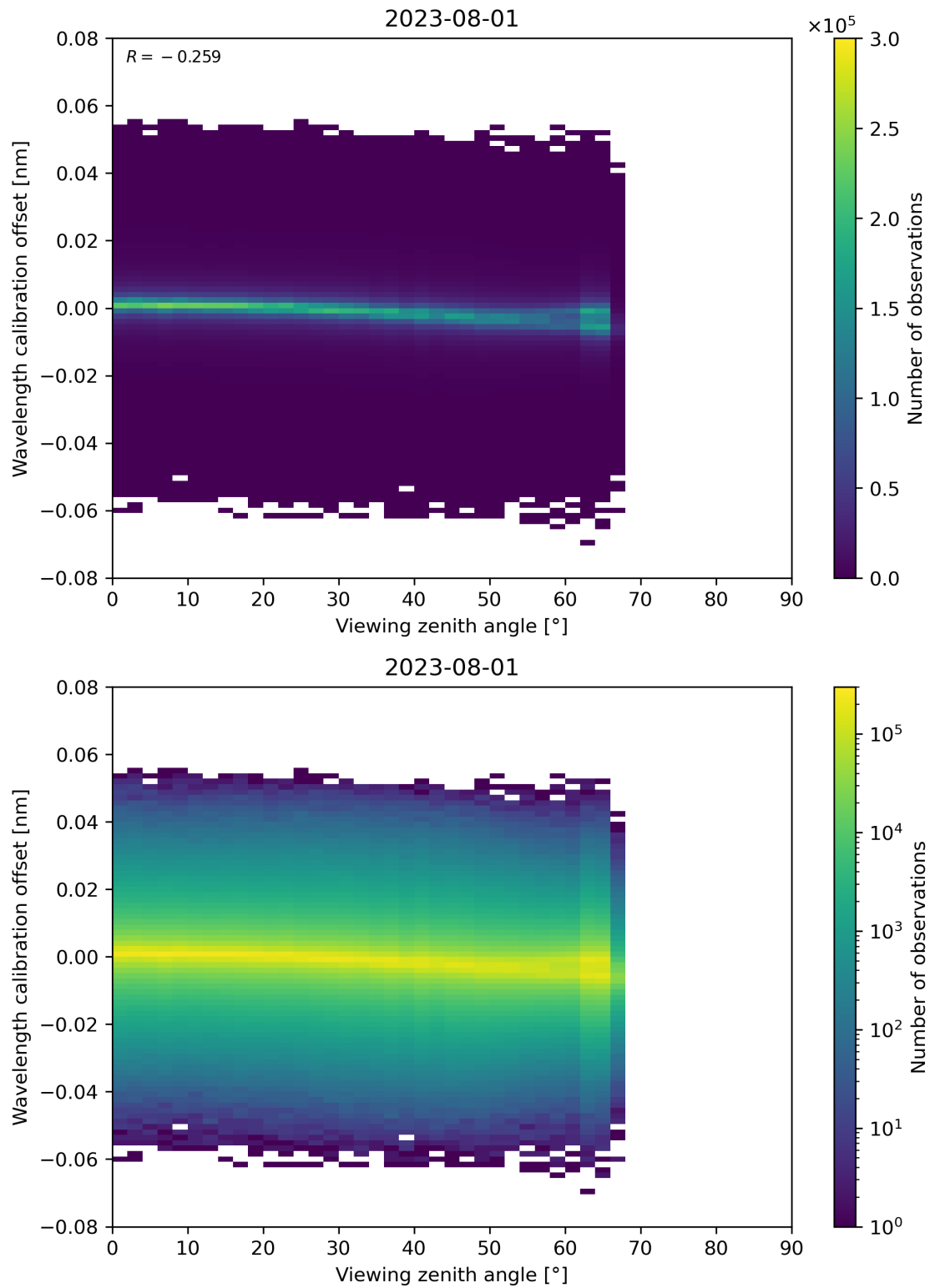
Figure 173: Scatter density plot of “Viewing zenith angle” against “Wavelength calibration offset” for 2023-07-31 to 2023-08-02.
