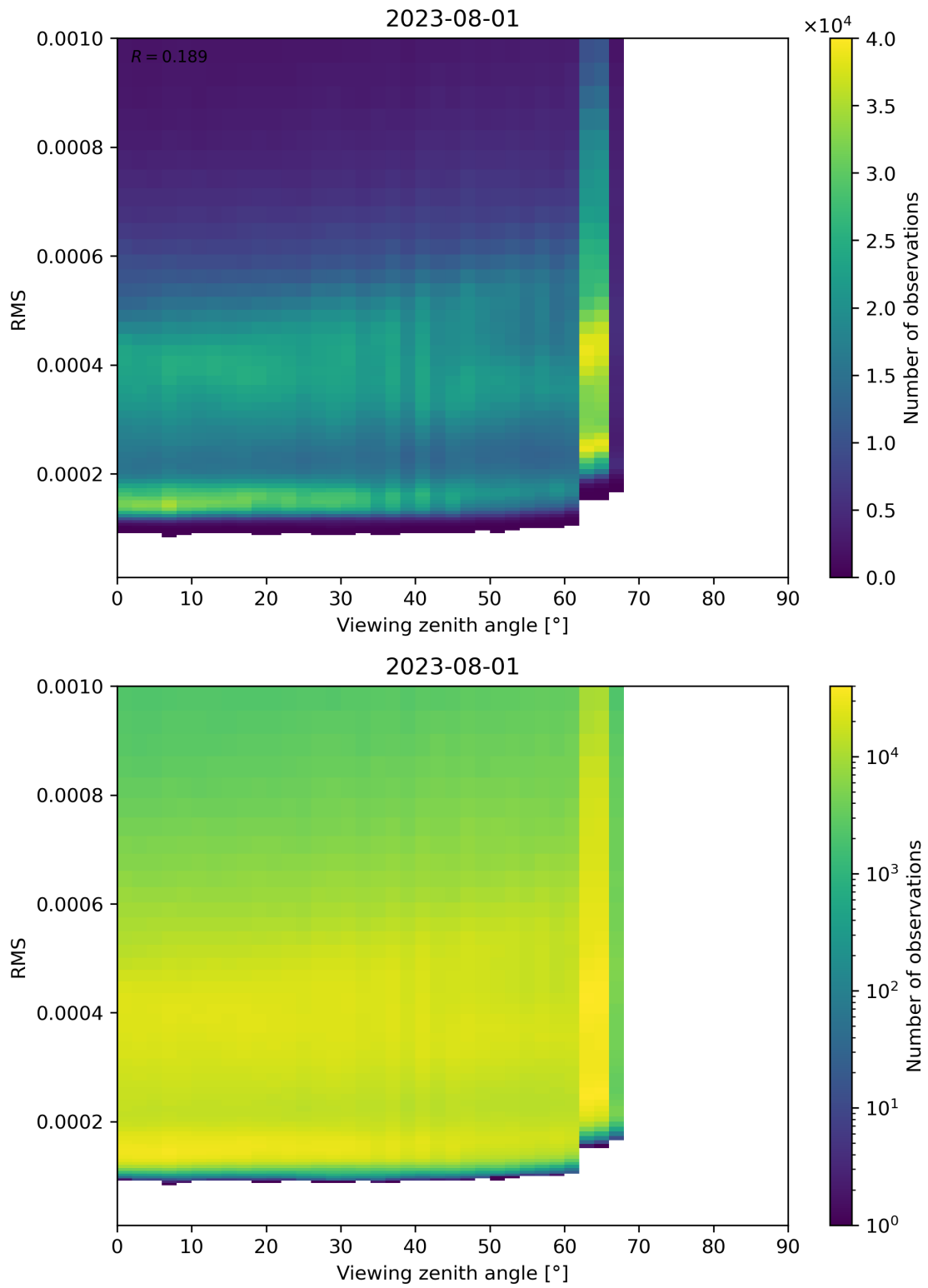
Figure 171: Scatter density plot of “Viewing zenith angle” against “RMS” for 2023-07-31 to 2023-08-02.
