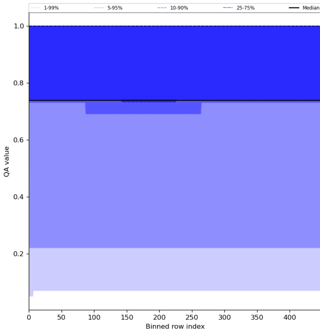
Figure 45: Along track statistics of “QA value” for 2023-07-31 to 2023-08-02
