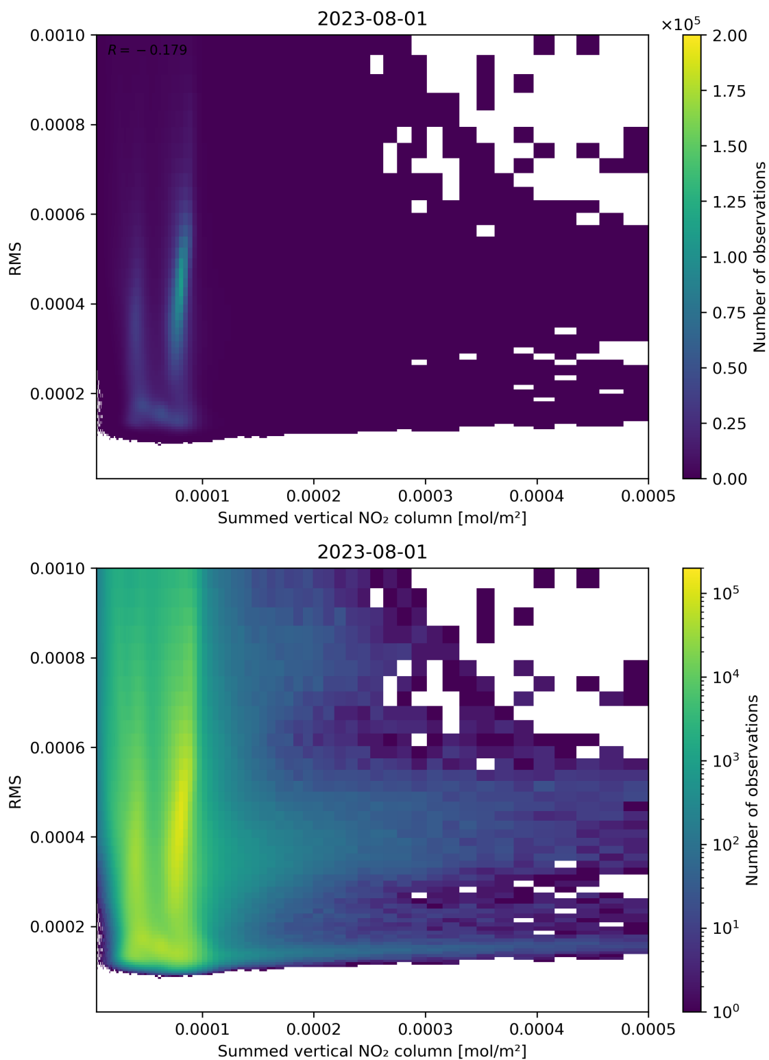
Figure 109: Scatter density plot of “Summed vertical NO 2 column” against “RMS” for 2023-07-31 to 2023-08-02.
