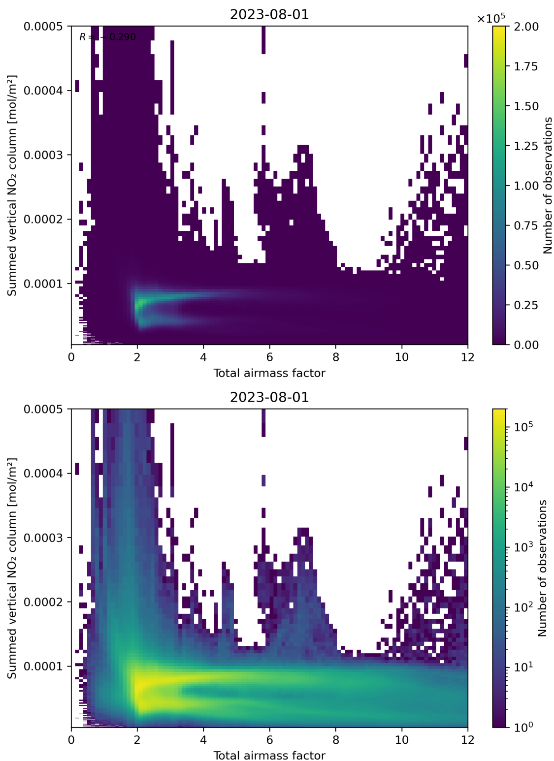
Figure 65: Scatter density plot of “Total airmass factor” against “Summed vertical NO 2 column” for 2023-07-31 to 2023-08-02.
