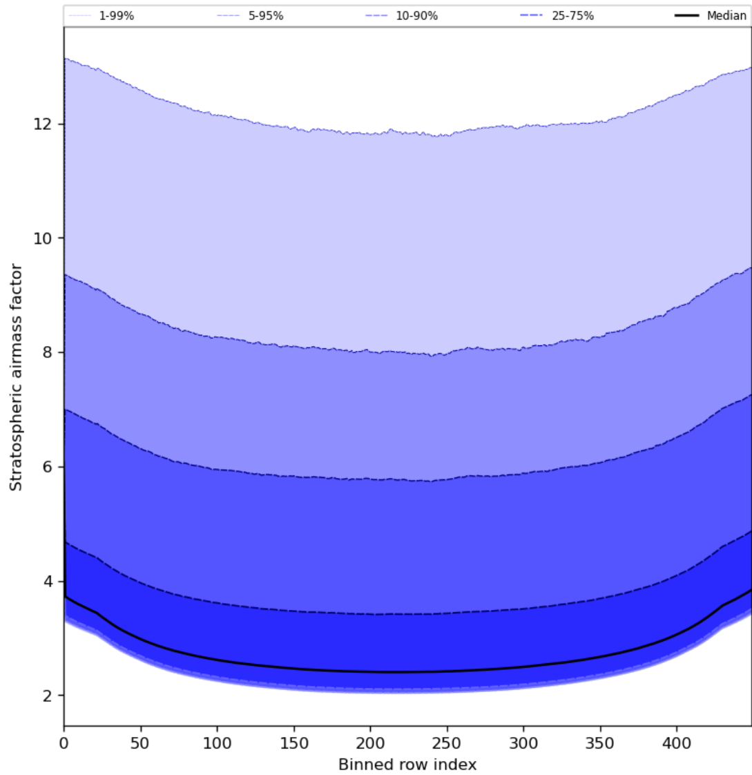
Figure 61: Along track statistics of “Stratospheric airmass factor” for 2023-07-31 to 2023-08-02
