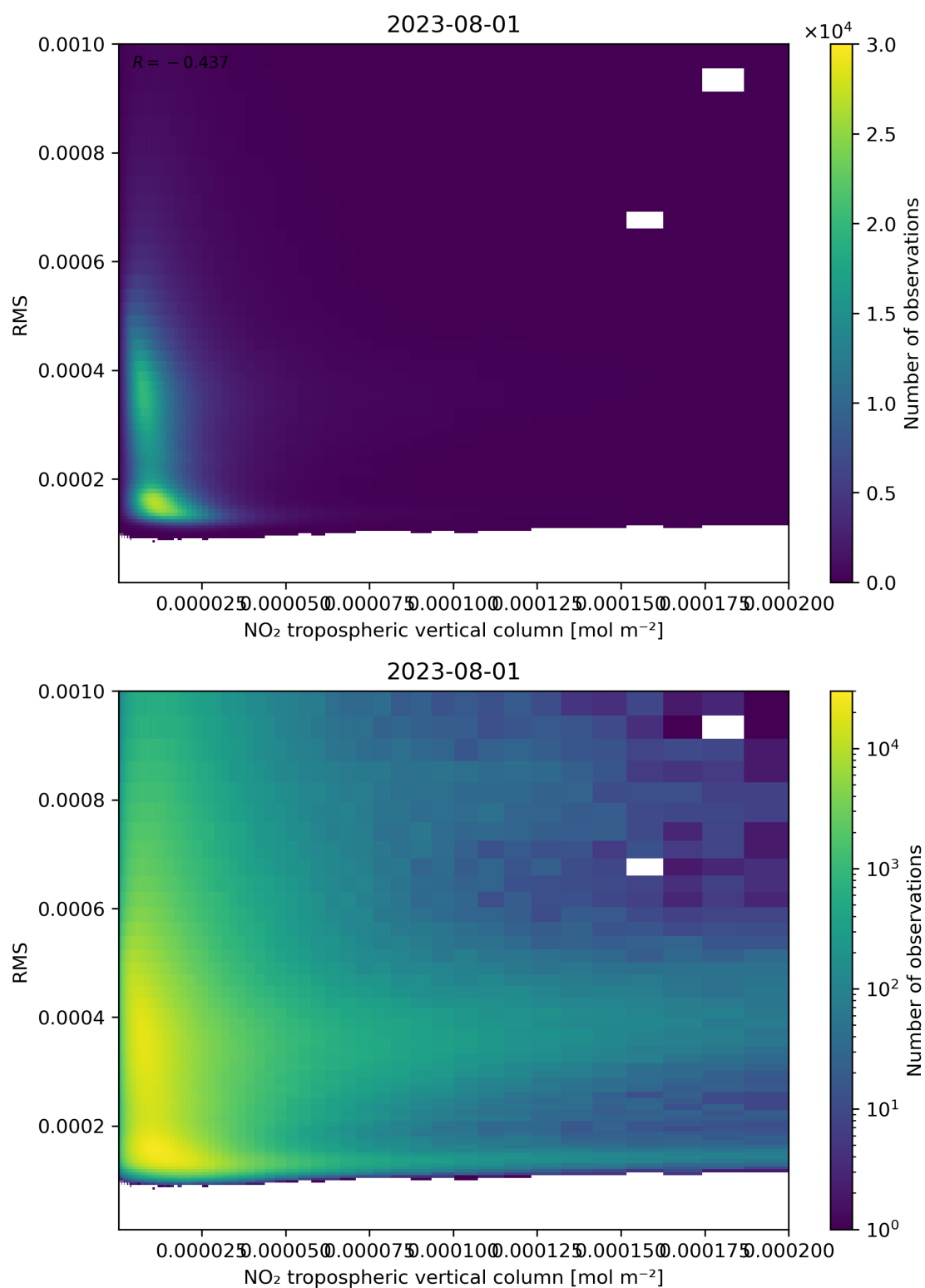
Figure 142: Scatter density plot of “NO 2 tropospheric vertical column” against “RMS” for 2023-07-31 to 2023-08-02.
