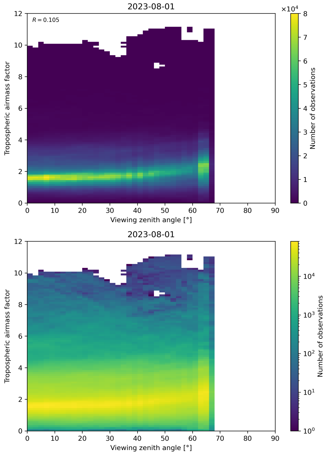
Figure 161: Scatter density plot of “Viewing zenith angle” against “Tropospheric airmass factor” for 2023-07-31 to 2023-08-02.
