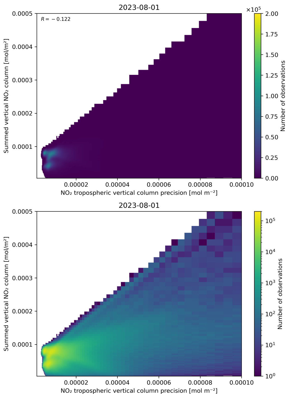
Figure 136: Scatter density plot of “NO 2 tropospheric vertical column precision” against “Summed vertical NO 2 column” for 2023-07-31 to 2023-08-02.
