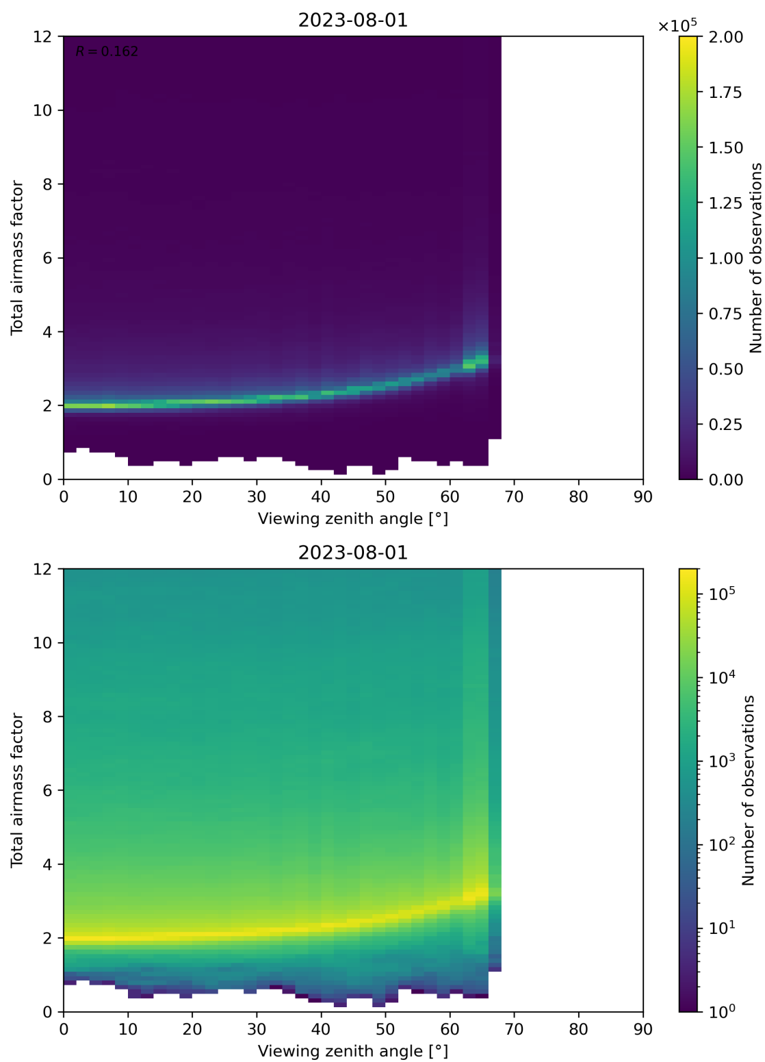
Figure 160: Scatter density plot of “Viewing zenith angle” against “Total airmass factor” for 2023-07-31 to 2023-08-02.
