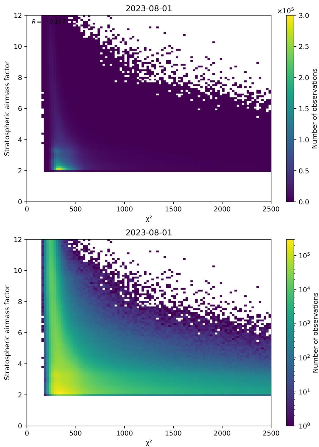
Figure 81: Scatter density plot of “ \chi^2 ” against “Stratospheric airmass factor” for 2023-07-31 to 2023-08-02.
