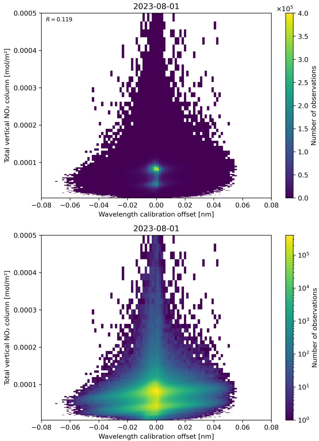
Figure 179: Scatter density plot of “Wavelength calibration offset” against “Total vertical NO 2 column” for 2023-07-31 to 2023-08-02.
