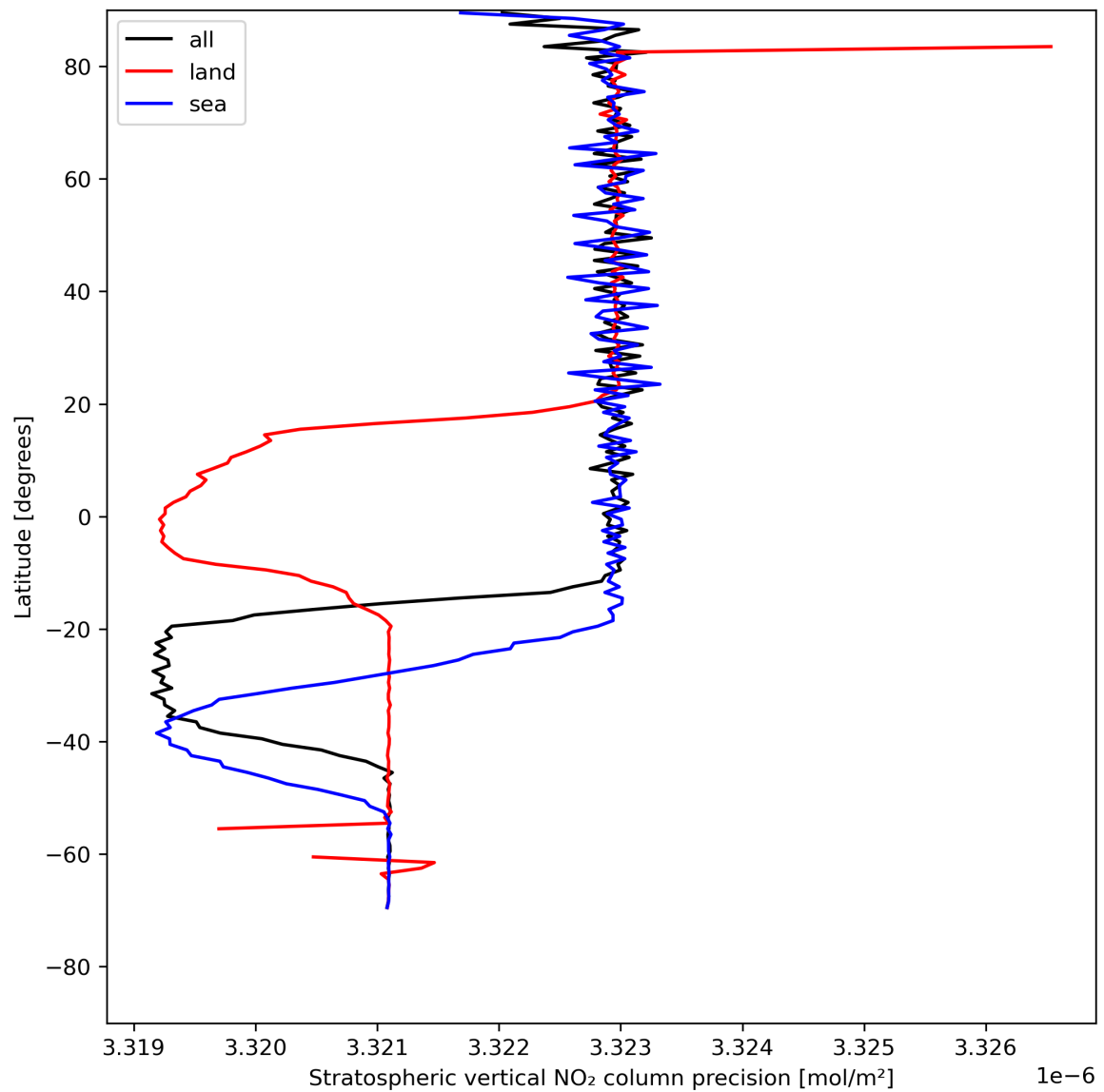
Figure 20: Zonal average of “Stratospheric vertical NO 2 column precision” for 2023-07-31 to 2023-08-02.
