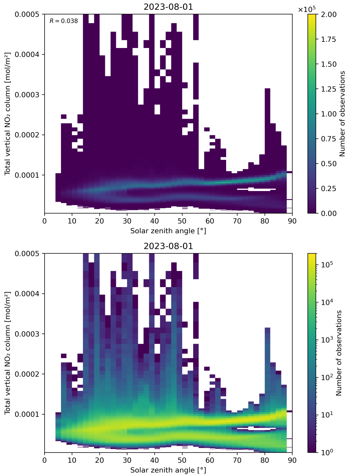
Figure 153: Scatter density plot of “Solar zenith angle” against “Total vertical \text{NO}_2 column” for 2023-07-31 to 2023-08-02.
