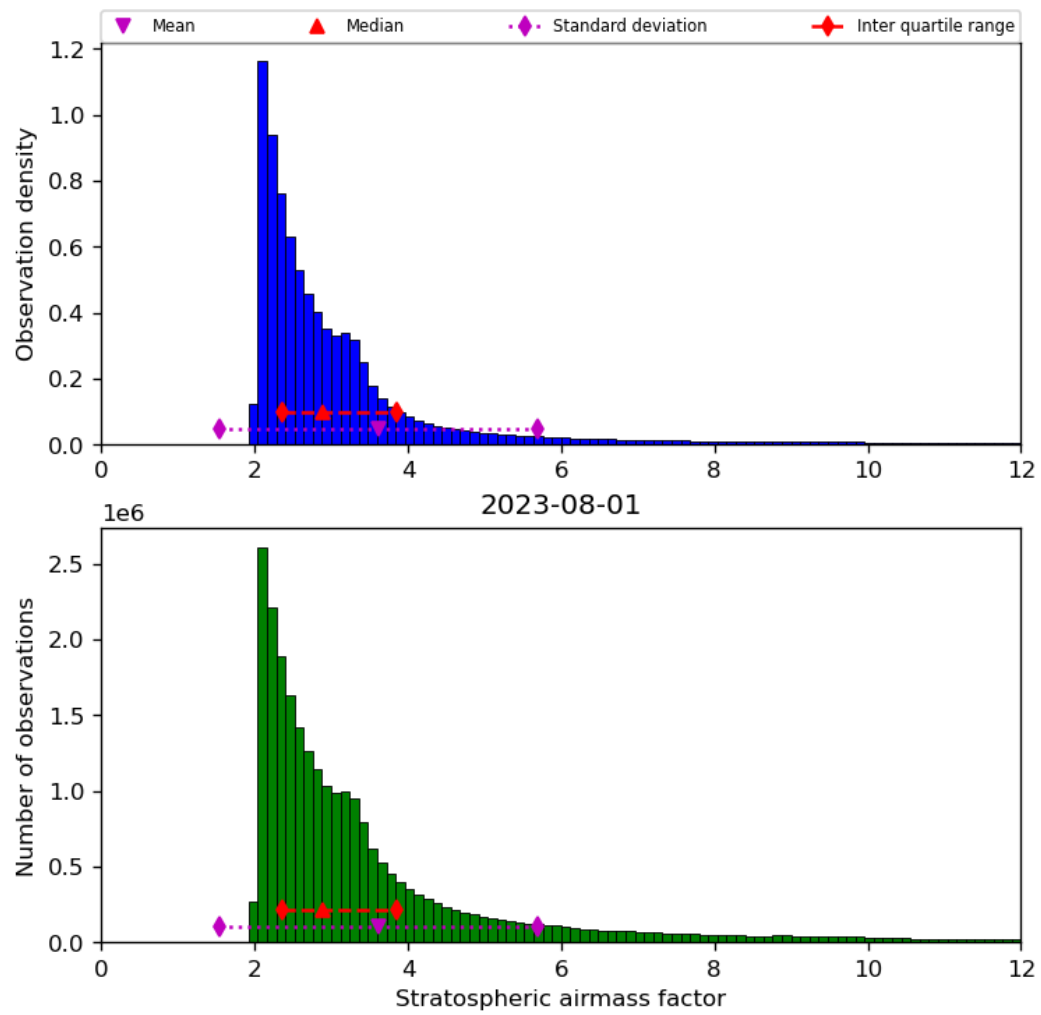
Figure 44: Histogram of “Stratospheric airmass factor” for 2023-07-31 to 2023-08-02
