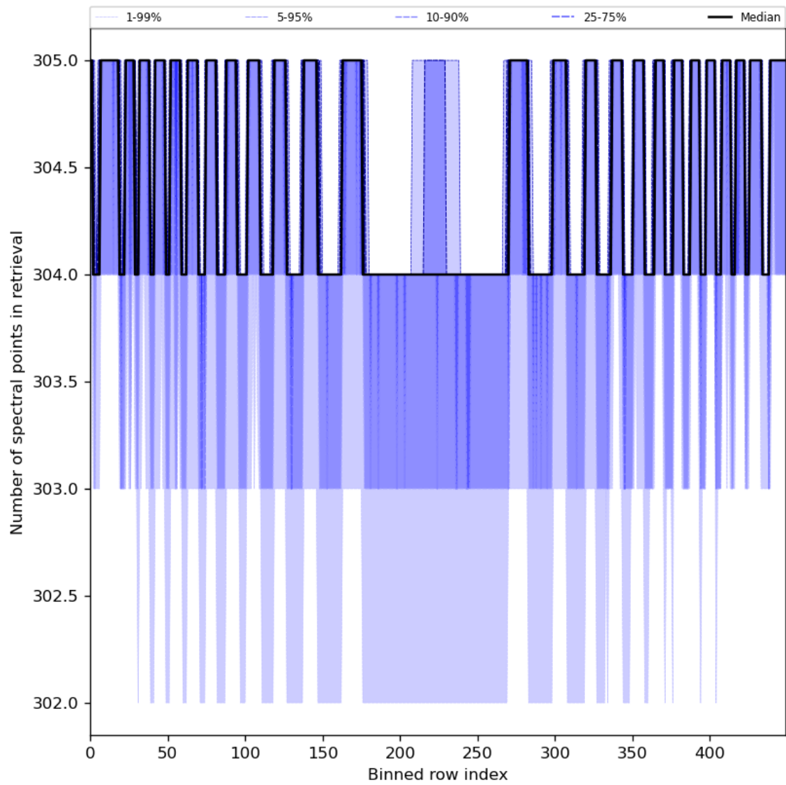
Figure 50: Along track statistics of “Number of spectral points in retrieval” for 2023-07-31 to 2023-08-02
