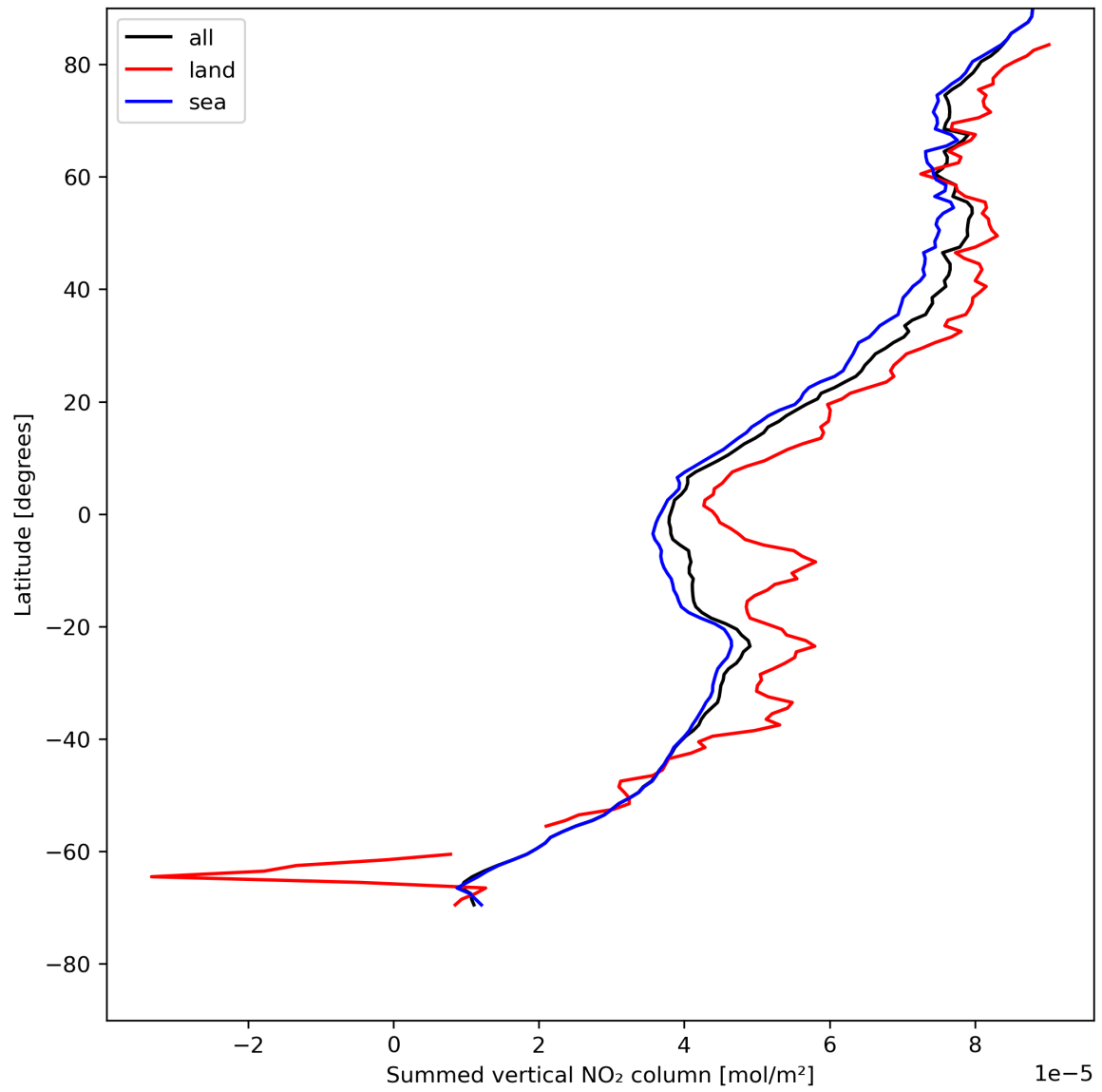
Figure 23: Zonal average of “Summed vertical NO 2 column” for 2023-07-31 to 2023-08-02.
