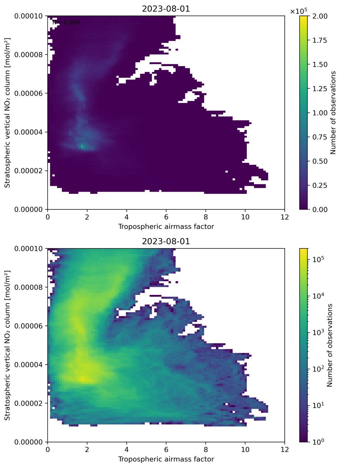
Figure 74: Scatter density plot of “Tropospheric air mass factor” against “Stratospheric vertical NO 2 column” for 2023-07-31 to 2023-08-02.
