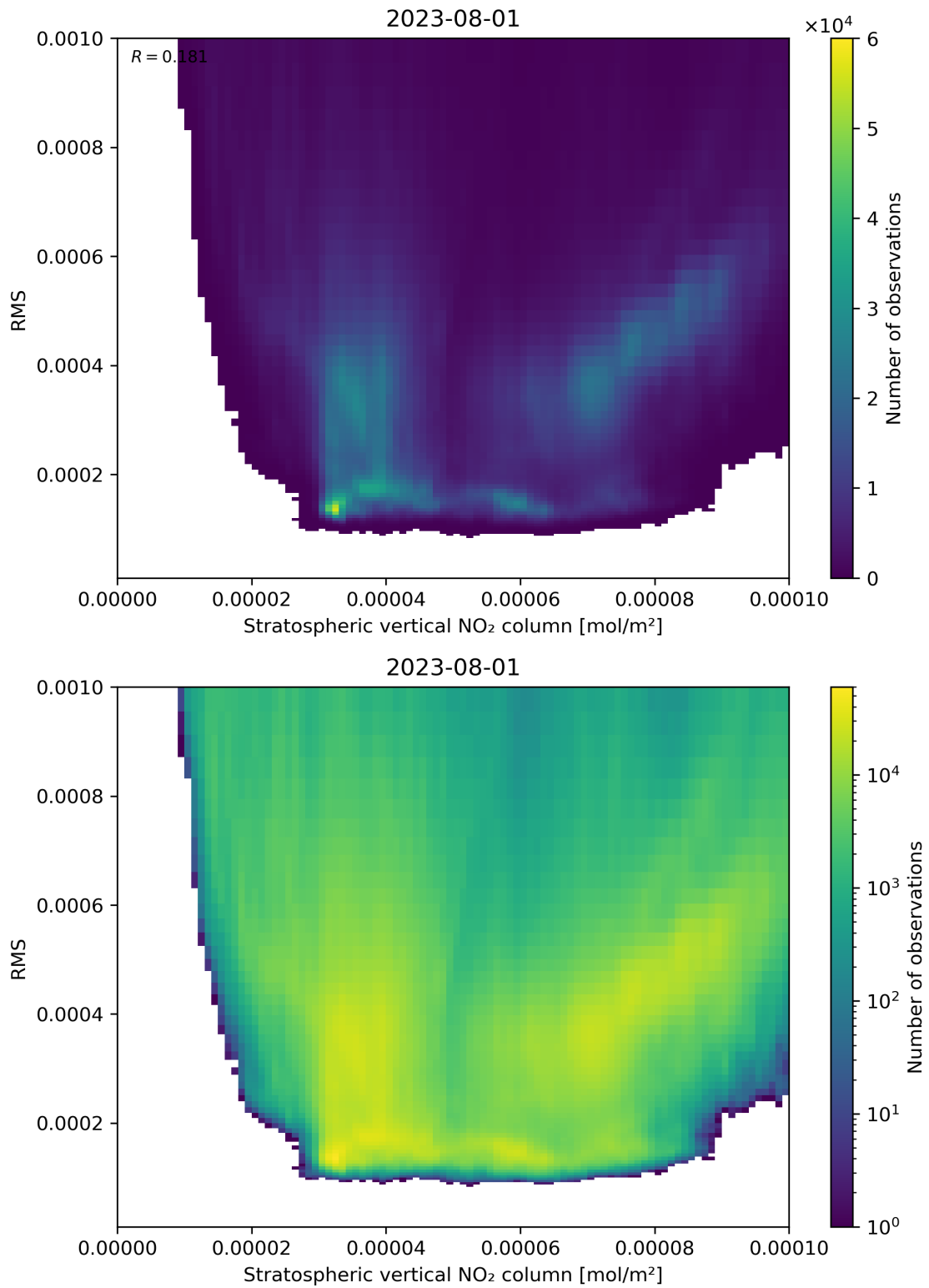
Figure 102: Scatter density plot of “Stratospheric vertical NO 2 column” against “RMS” for 2023-07-31 to 2023-08-02.
