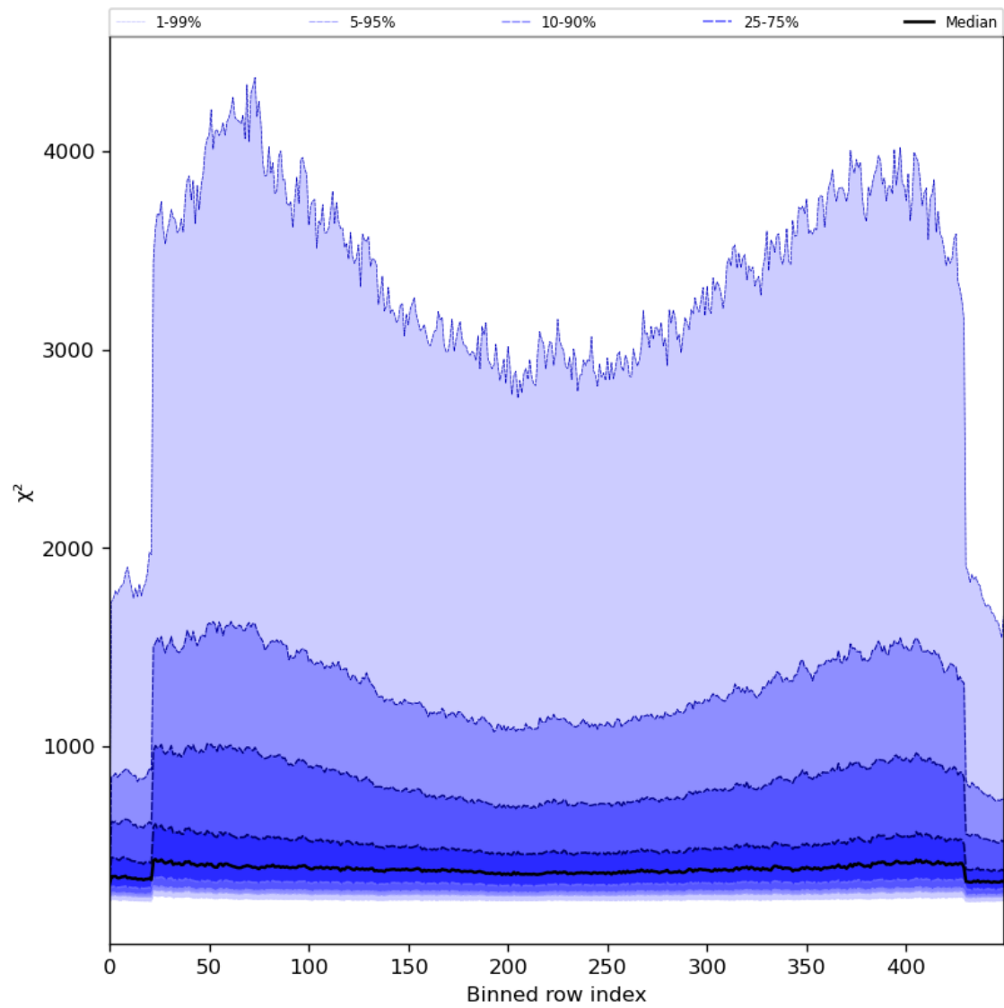
Figure 59: Along track statistics of “ \chi^2 ” for 2023-07-31 to 2023-08-02
