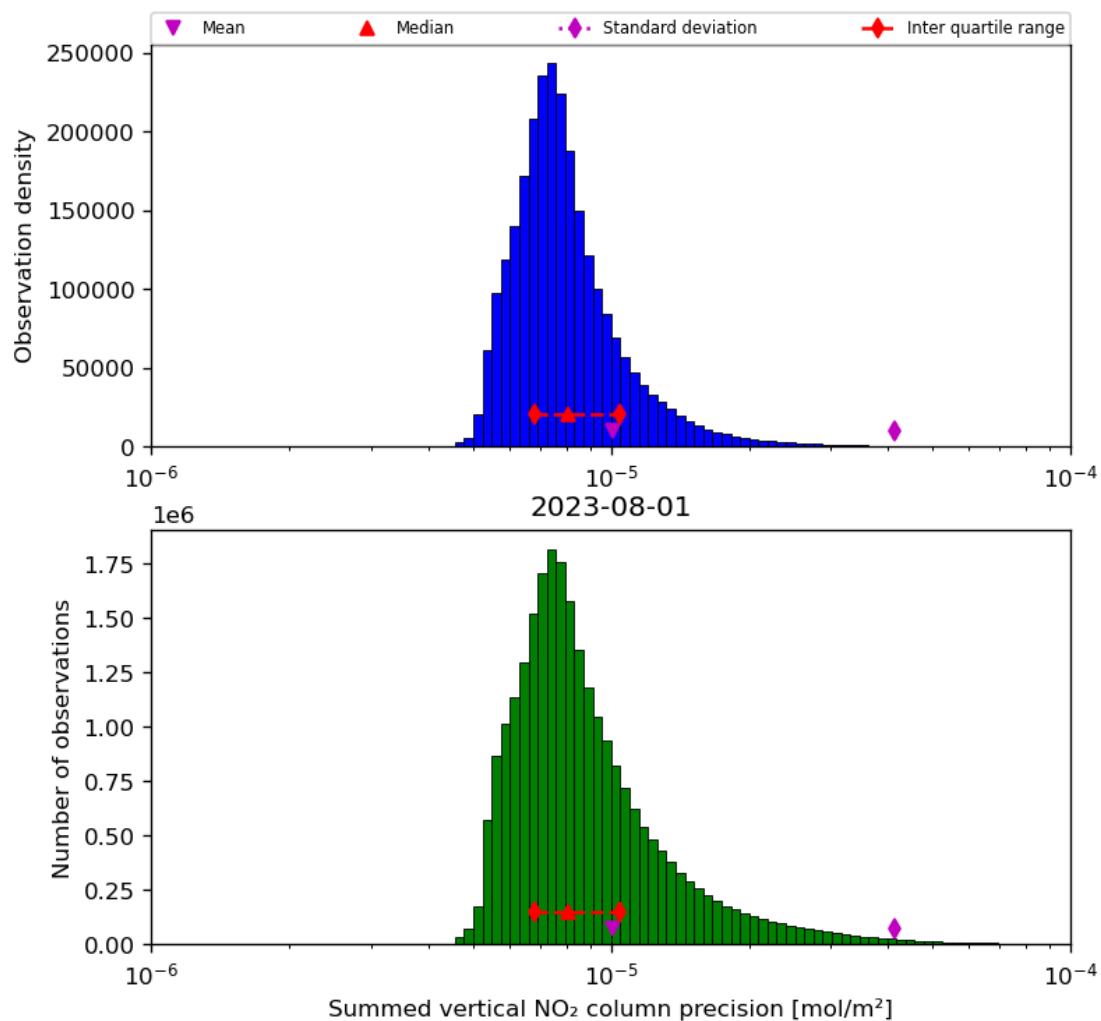
Figure 41: Histogram of "Summed vertical NO 2 column precision" for 2023-07-31 to 2023-08-02
