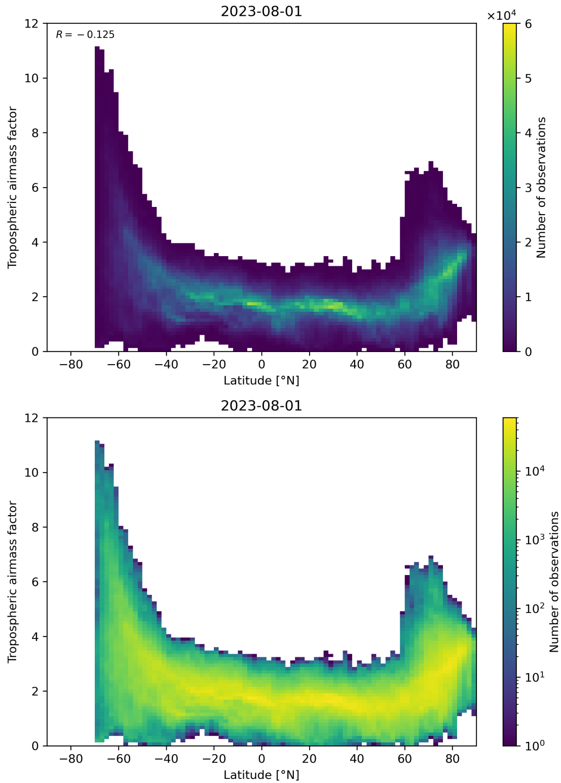
Figure 85: Scatter density plot of “Latitude” against “Tropospheric airmass factor” for 2023-07-31 to 2023-08-02.
