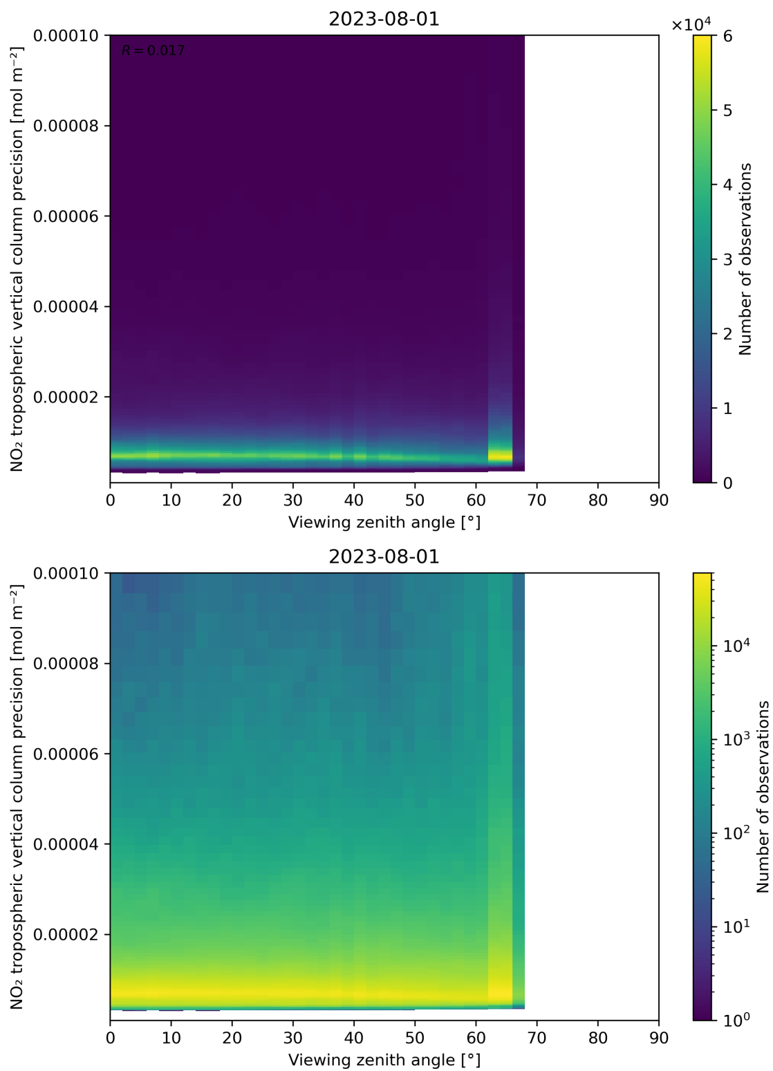
Figure 170: Scatter density plot of “Viewing zenith angle” against “NO 2 tropospheric vertical column precision” for 2023-07-31 to 2023-08-02.
