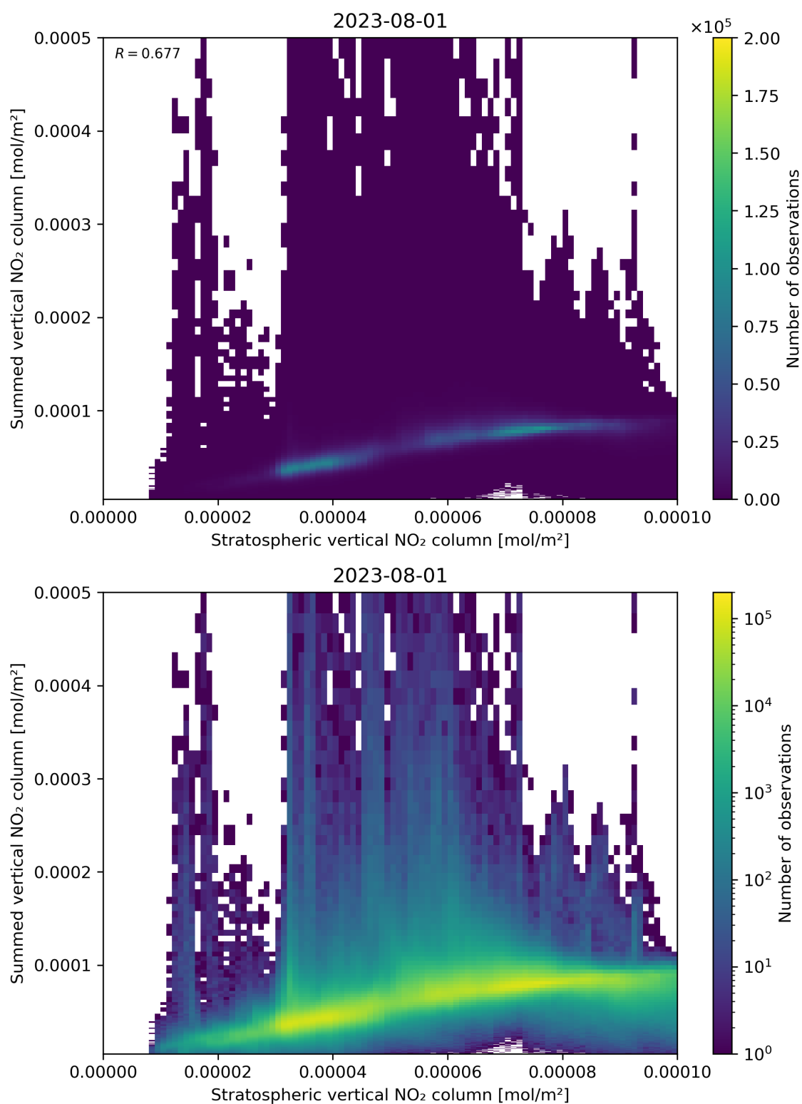
Figure 98: Scatter density plot of “Stratospheric vertical NO 2 column” against “Summed vertical NO 2 column” for 2023-07-31 to 2023-08-02.
