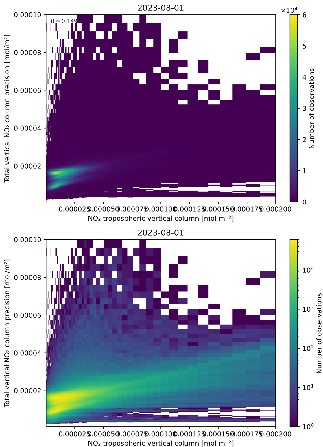
Figure 129: Scatter density plot of “NO 2 tropospheric vertical column” against “Total vertical NO 2 column precision” for 2023-07-31 to 2023-08-02.
