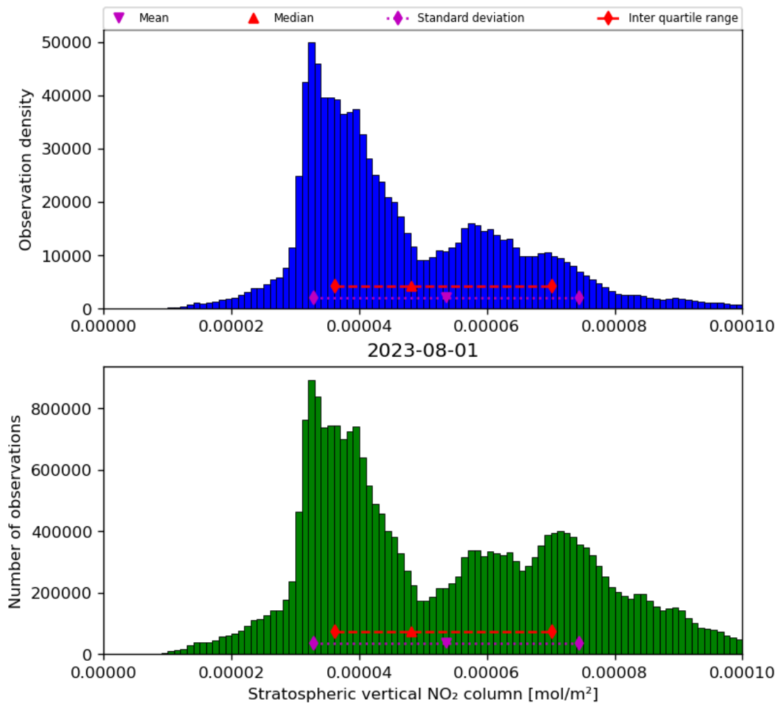
Figure 36: Histogram of “Stratospheric vertical NO 2 column” for 2023-07-31 to 2023-08-02
