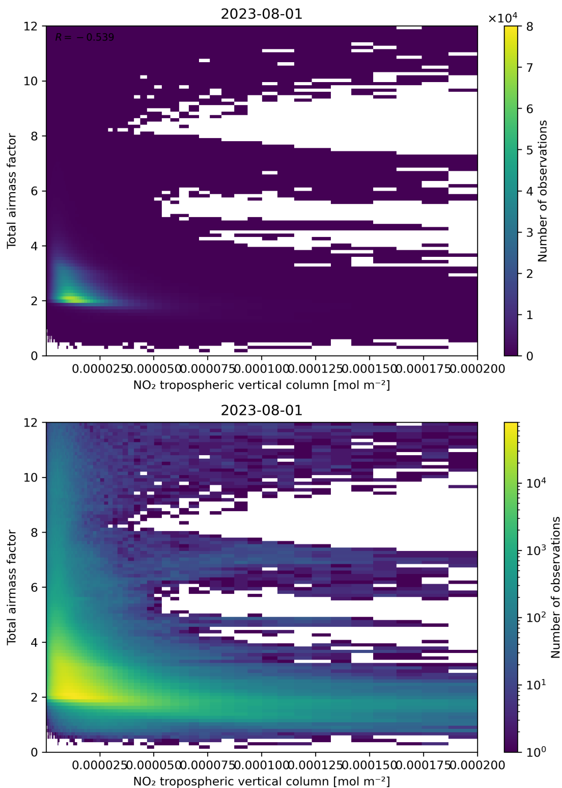
Figure 122: Scatter density plot of “NO 2 tropospheric vertical column” against “Total air mass factor” for 2023-07-31 to 2023-08-02.
