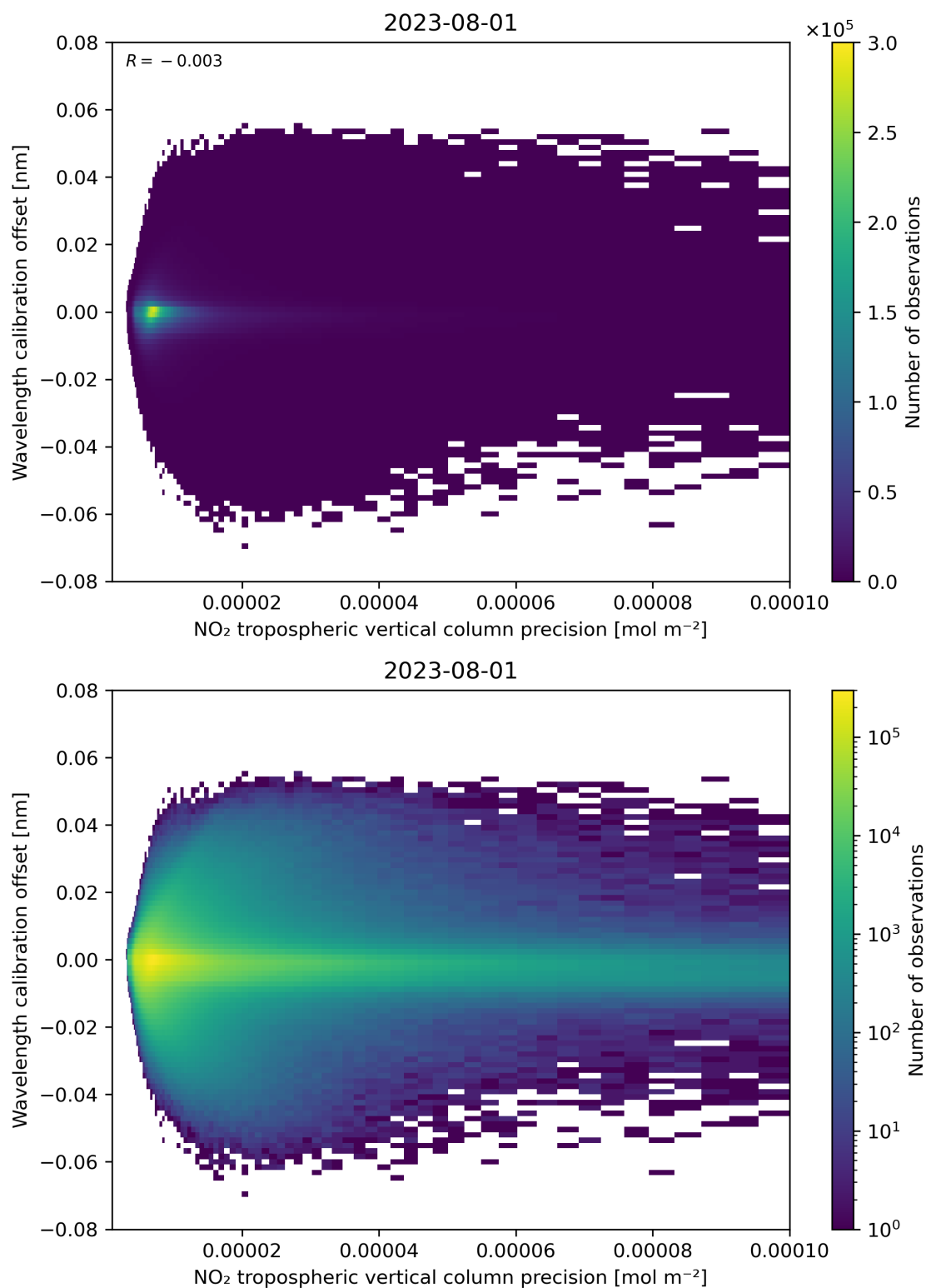
Figure 141: Scatter density plot of “NO 2 tropospheric vertical column precision” against “Wavelength calibration offset” for 2023-07-31 to 2023-08-02.
