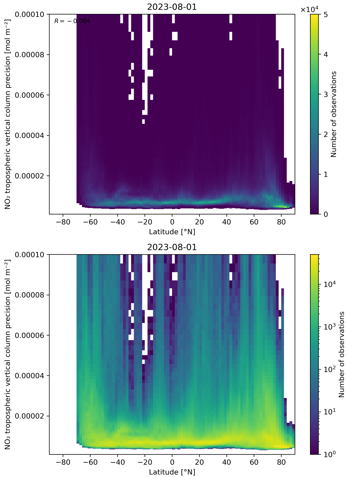
Figure 93: Scatter density plot of “Latitude” against “NO 2 tropospheric vertical column precision” for 2023-07-31 to 2023-08-02.
