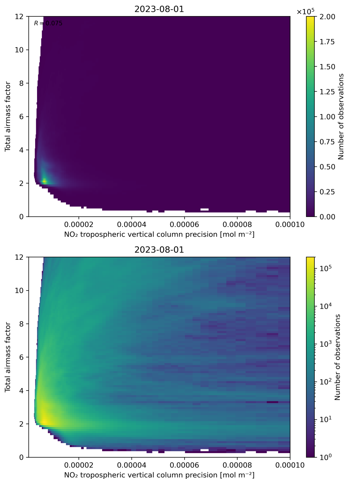
Figure 132: Scatter density plot of “NO 2 tropospheric vertical column precision” against “Total air mass factor” for 2023-07-31 to 2023-08-02.
