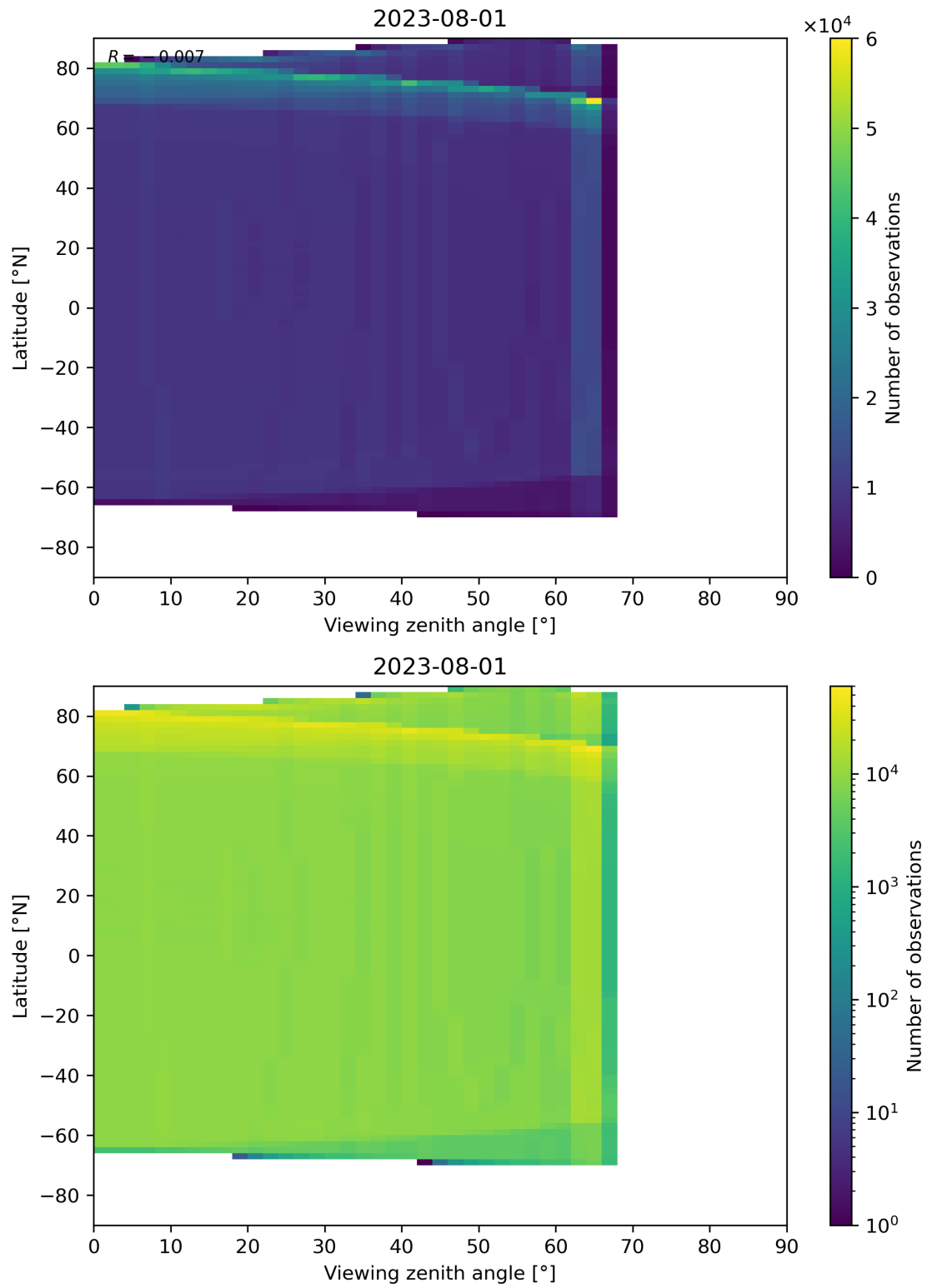
Figure 163: Scatter density plot of “Viewing zenith angle” against “Latitude” for 2023-07-31 to 2023-08-02.
