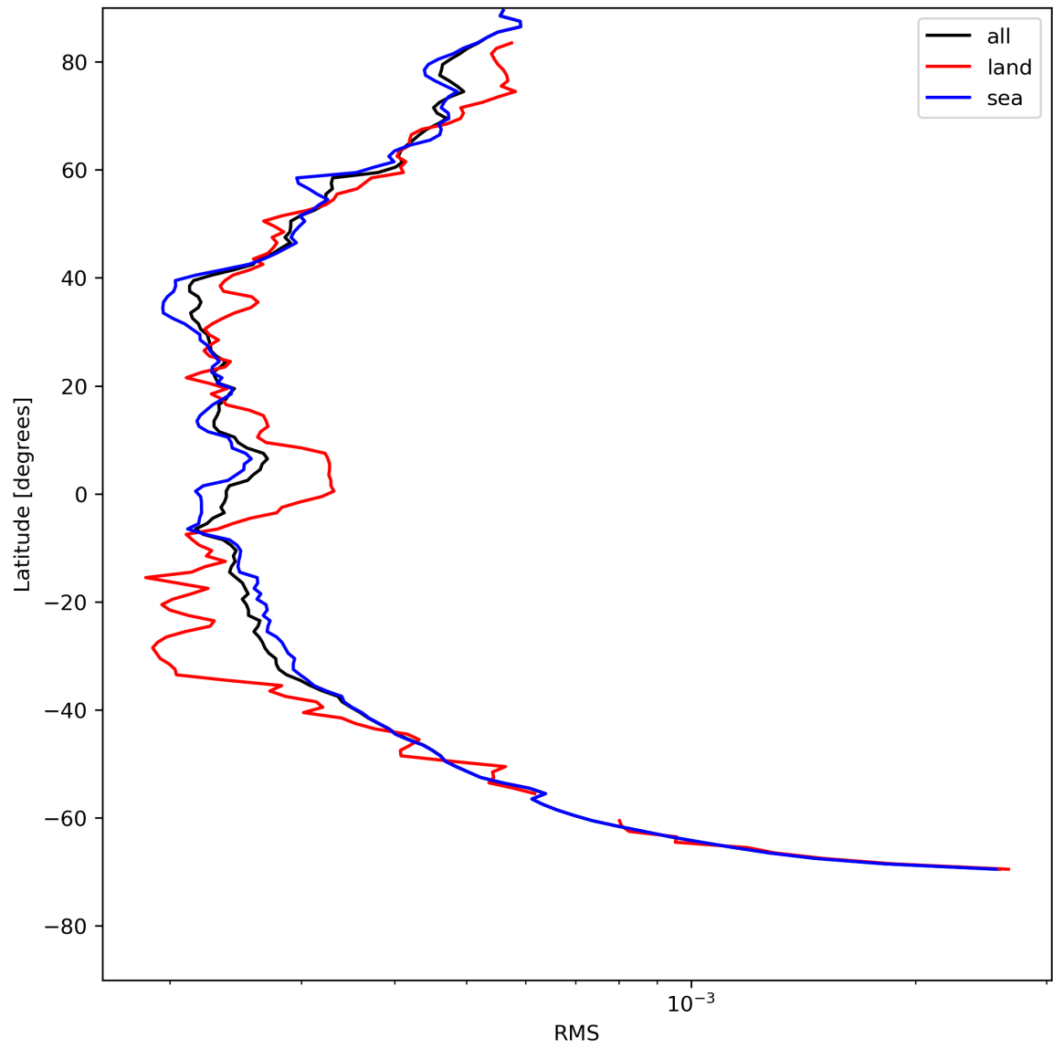
Figure 26: Zonal average of “RMS” for 2023-07-31 to 2023-08-02.
