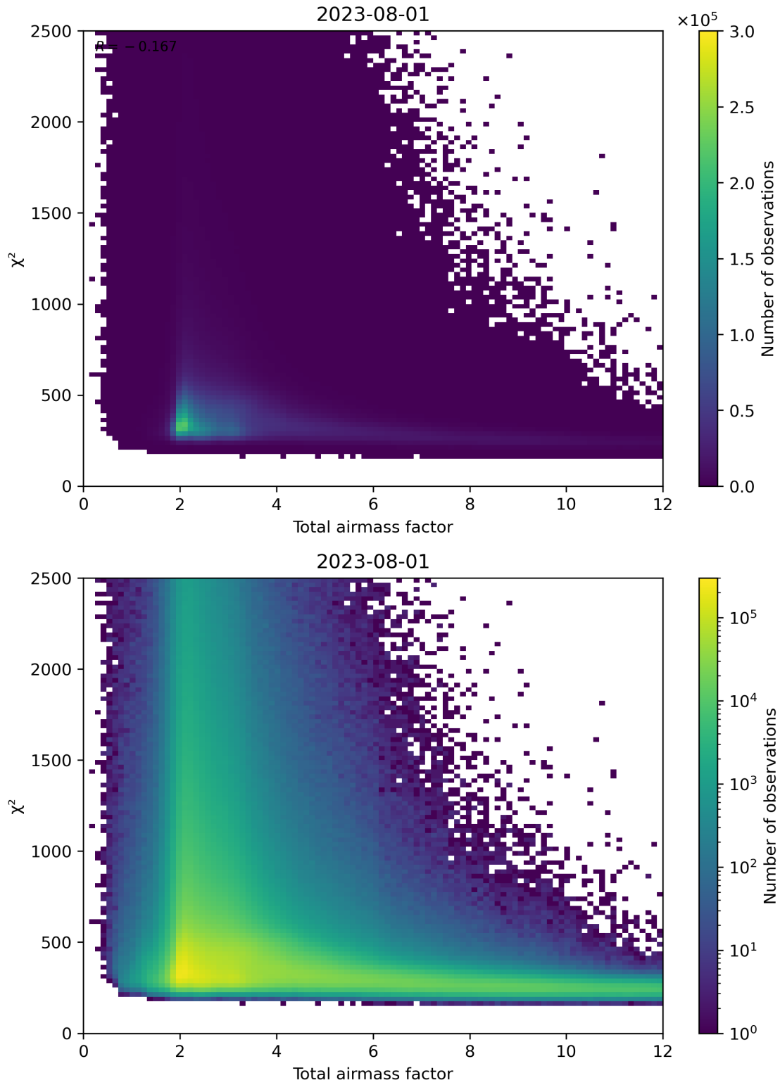
Figure 63: Scatter density plot of “Total airmass factor” against “ \chi^2 ” for 2023-07-31 to 2023-08-02.
