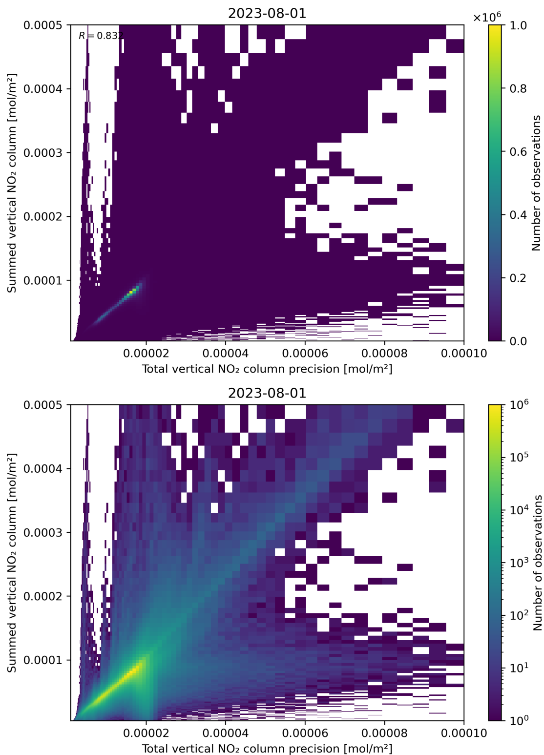
Figure 117: Scatter density plot of “Total vertical NO 2 column precision” against “Summed vertical NO 2 column” for 2023-07-31 to 2023-08-02.
