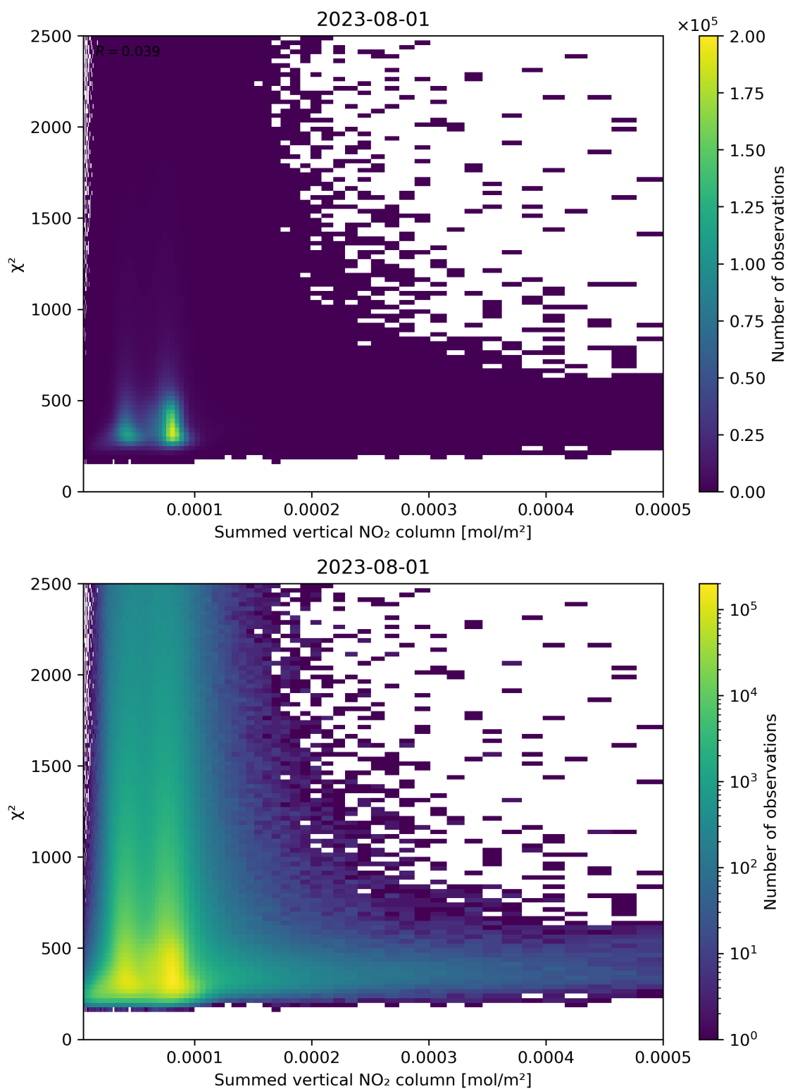
Figure 104: Scatter density plot of “Summed vertical NO 2 column” against “ \chi^2 ” for 2023-07-31 to 2023-08-02.
