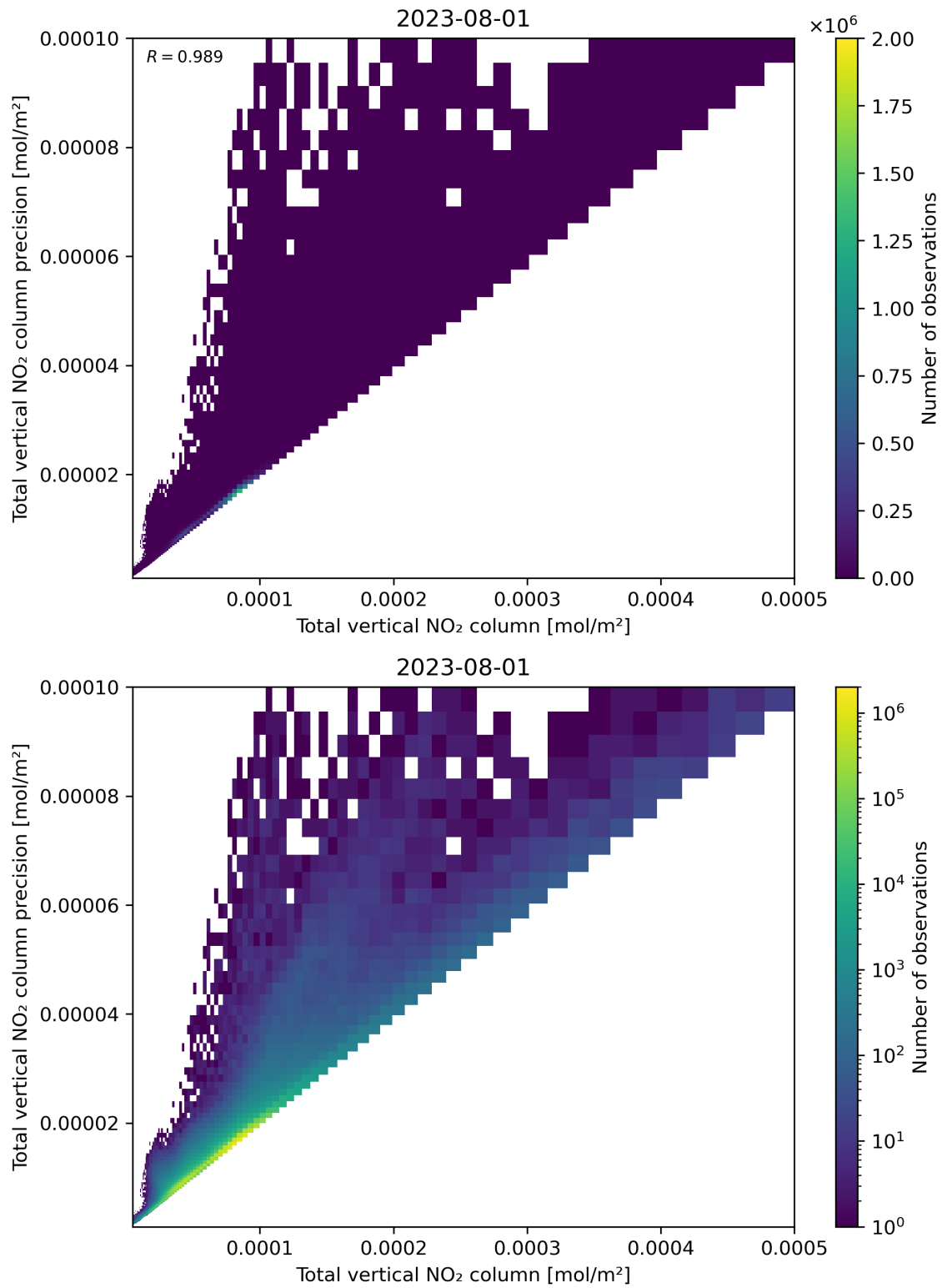
Figure 114: Scatter density plot of “Total vertical NO 2 column” against “Total vertical NO 2 column precision” for 2023-07-31 to 2023-08-02.
