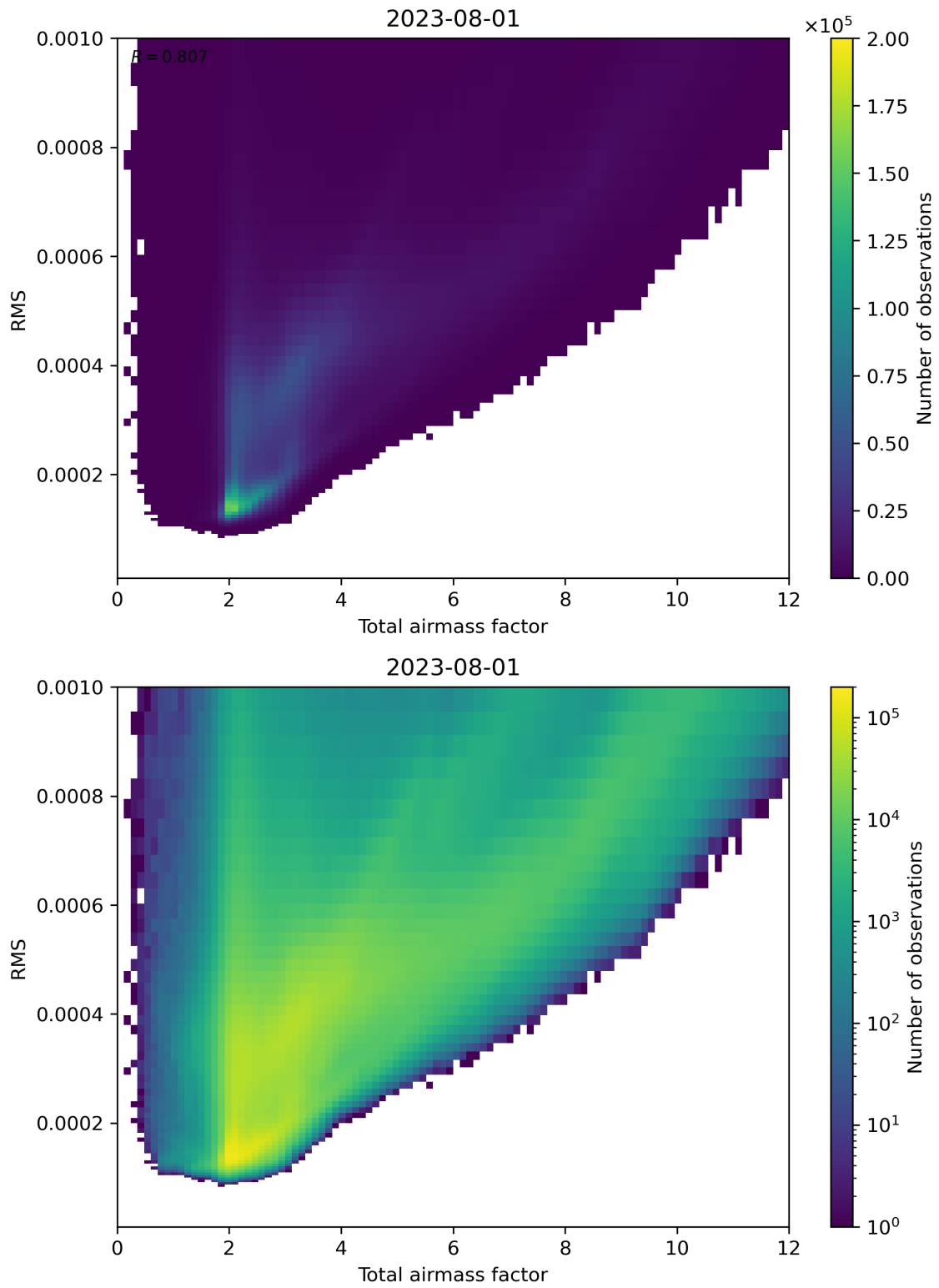
Figure 69: Scatter density plot of “Total airmass factor” against “RMS” for 2023-07-31 to 2023-08-02.
