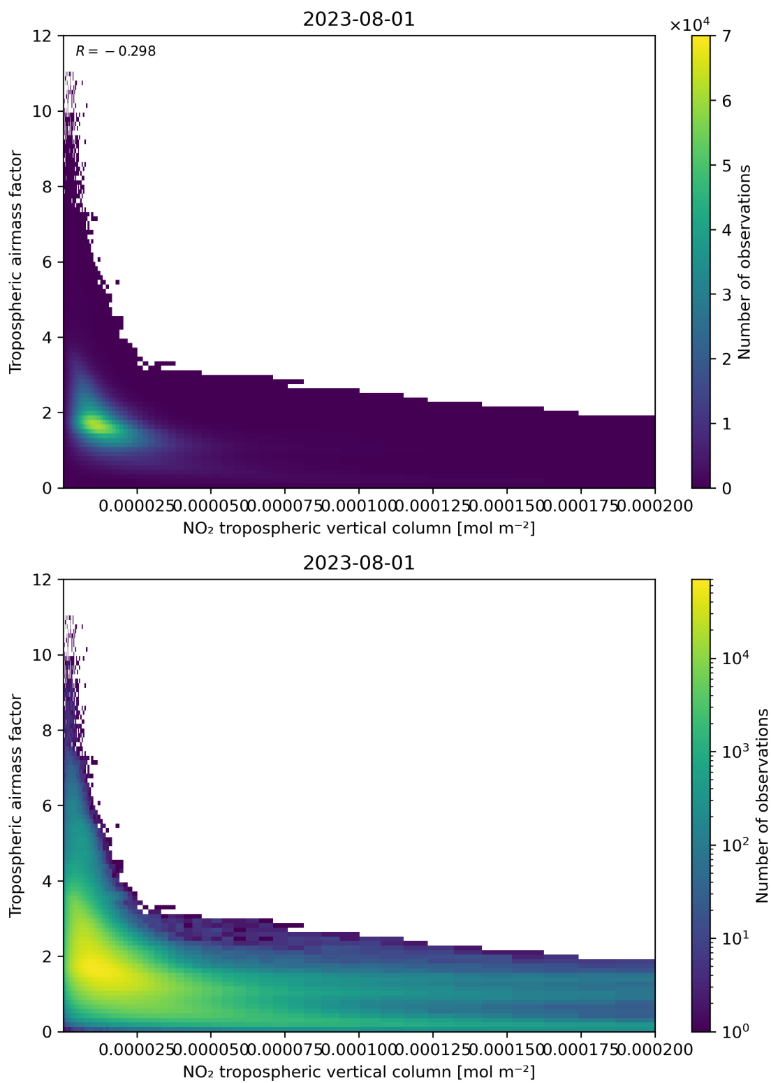
Figure 123: Scatter density plot of “NO 2 tropospheric vertical column” against “Tropospheric air mass factor” for 2023-07-31 to 2023-08-02.
