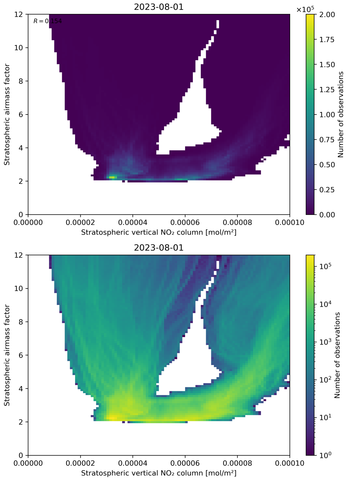
Figure 96: Scatter density plot of “Stratospheric vertical NO 2 column” against “Stratospheric airmass factor” for 2023-07-31 to 2023-08-02.
