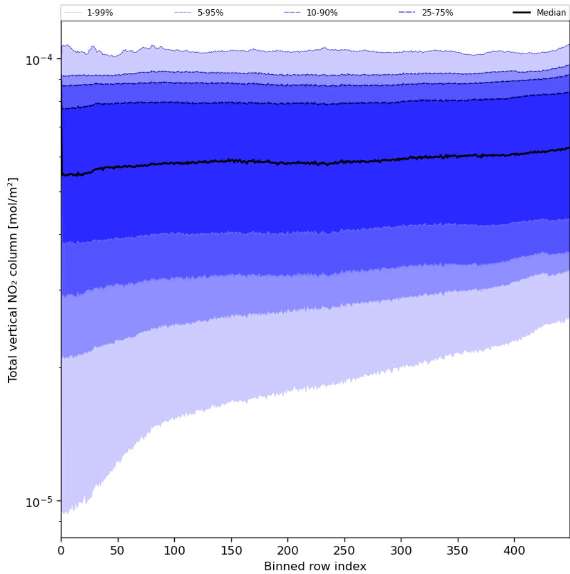
Figure 55: Along track statistics of “Total vertical NO 2 column” for 2023-07-31 to 2023-08-02
