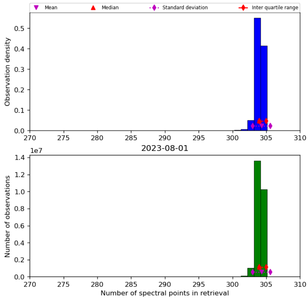
Figure 33: Histogram of “Number of spectral points in retrieval” for 2023-07-31 to 2023-08-02
