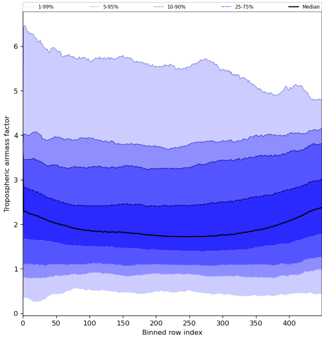
Figure 48: Along track statistics of “Tropospheric air mass factor” for 2023-07-31 to 2023-08-02
