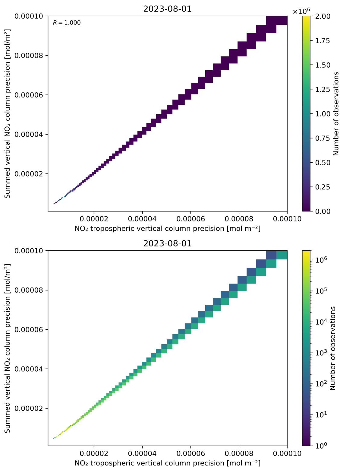
Figure 137: Scatter density plot of “NO 2 tropospheric vertical column precision” against “Summed vertical NO 2 column precision” for 2023-07-31 to 2023-08-02.
