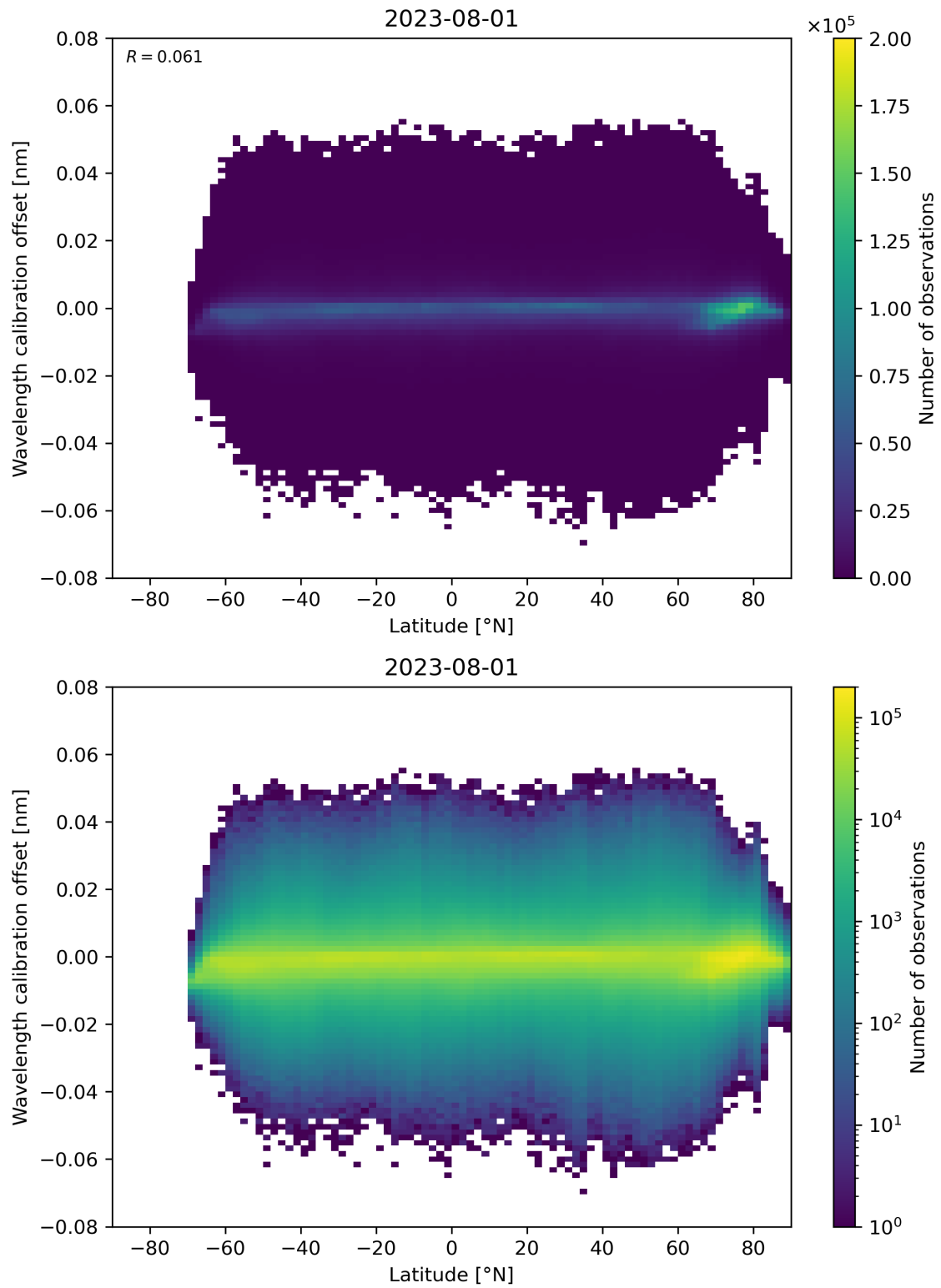
Figure 95: Scatter density plot of “Latitude” against “Wavelength calibration offset” for 2023-07-31 to 2023-08-02.
