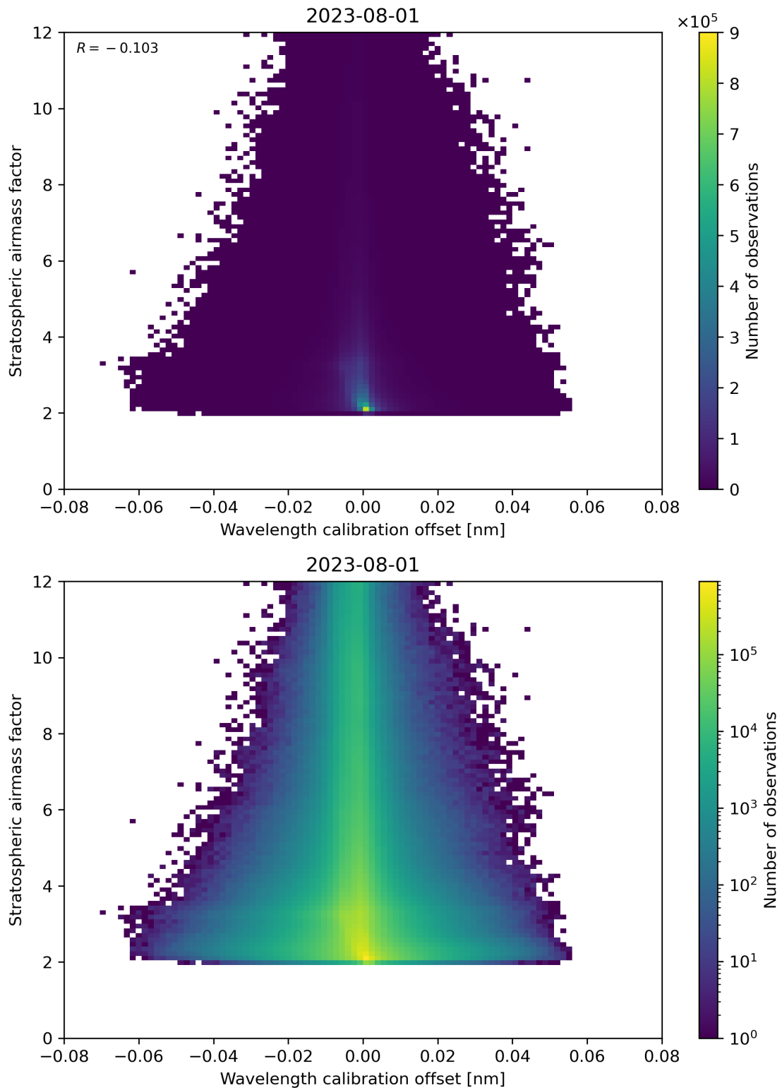
Figure 174: Scatter density plot of “Wavelength calibration offset” against “Stratospheric airmass factor” for 2023-07-31 to 2023-08-02.
