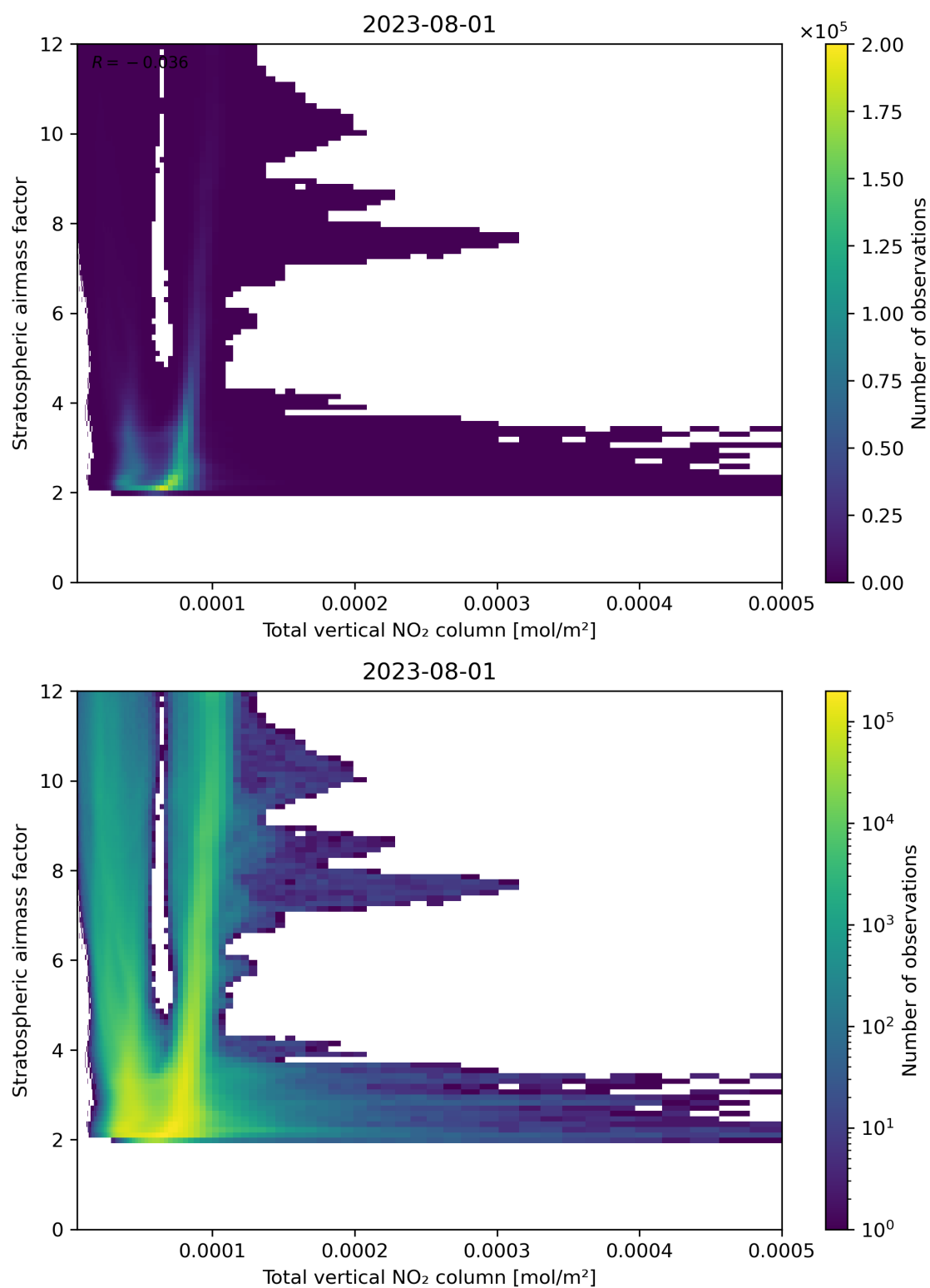
Figure 110: Scatter density plot of “Total vertical NO 2 column” against “Stratospheric airmass factor” for 2023-07-31 to 2023-08-02.
