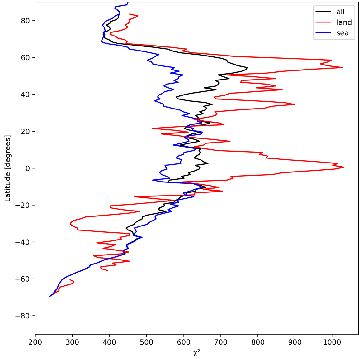
Figure 25: Zonal average of " \chi^2 " for 2023-07-31 to 2023-08-02.
