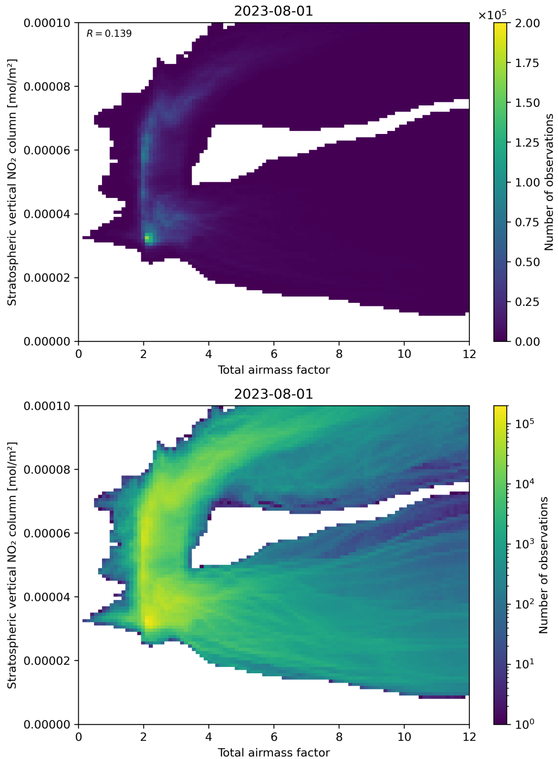
Figure 64: Scatter density plot of “Total airmass factor” against “Stratospheric vertical NO 2 column” for 2023-07-31 to 2023-08-02.
