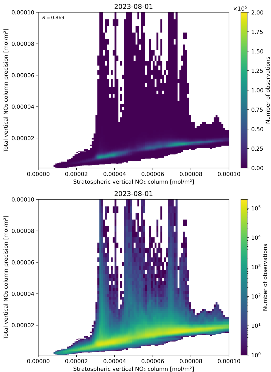
Figure 101: Scatter density plot of “Stratospheric vertical NO 2 column” against “Total vertical NO 2 column precision” for 2023-07-31 to 2023-08-02.
