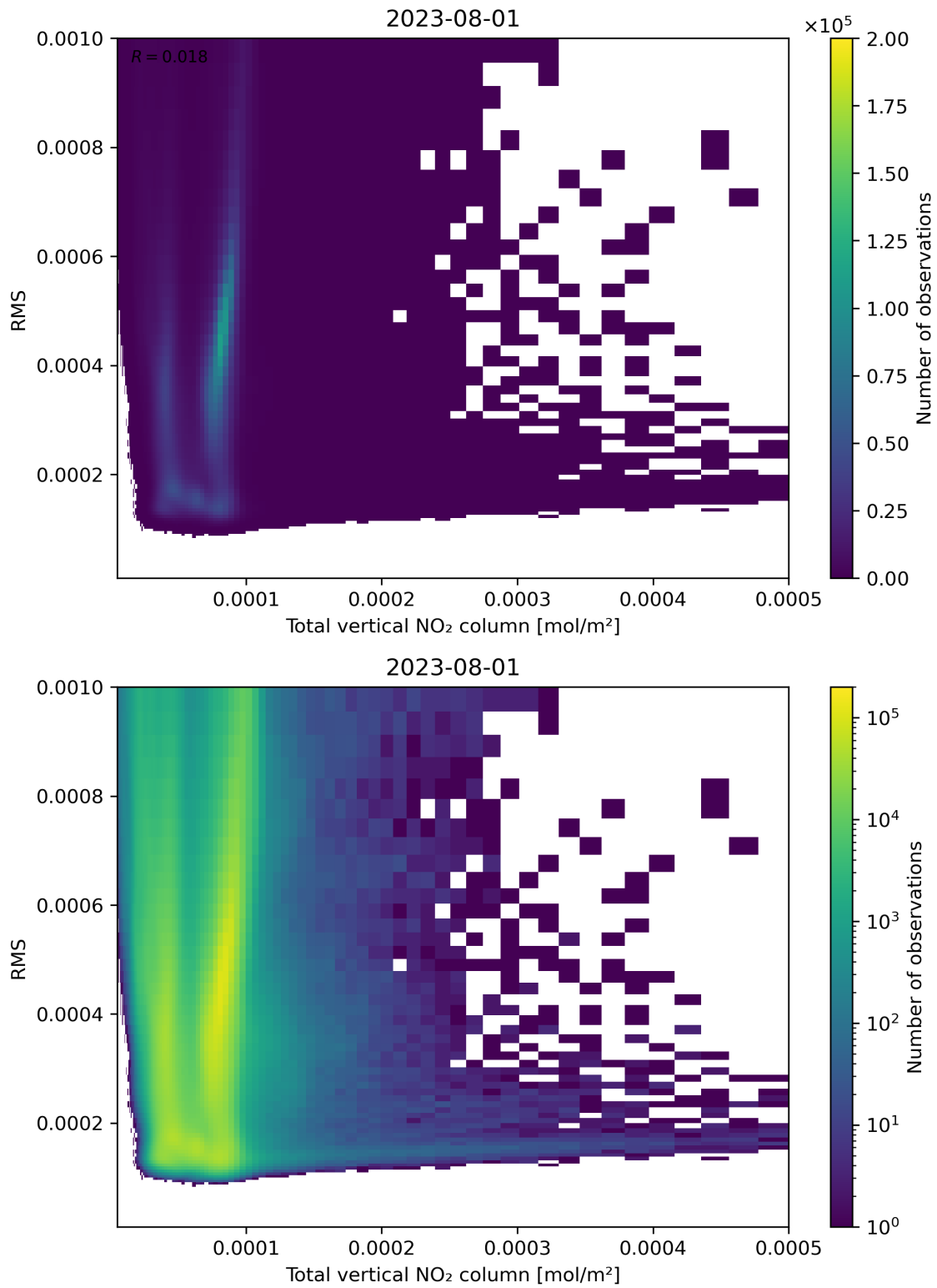
Figure 120: Scatter density plot of “Total vertical NO 2 column” against “RMS” for 2023-07-31 to 2023-08-02.
