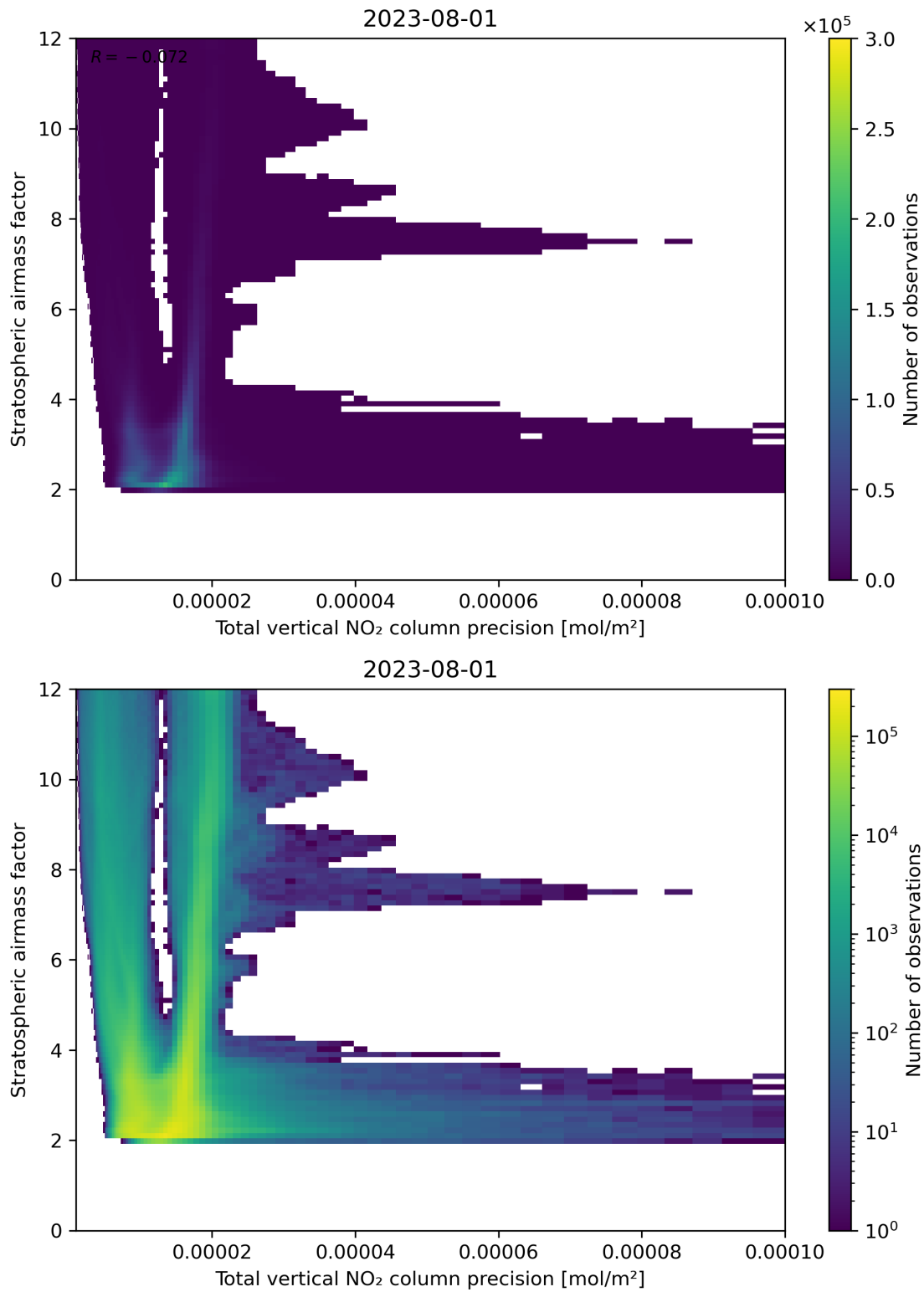
Figure 115: Scatter density plot of “Total vertical NO 2 column precision” against “Stratospheric air mass factor” for 2023-07-31 to 2023-08-02.
