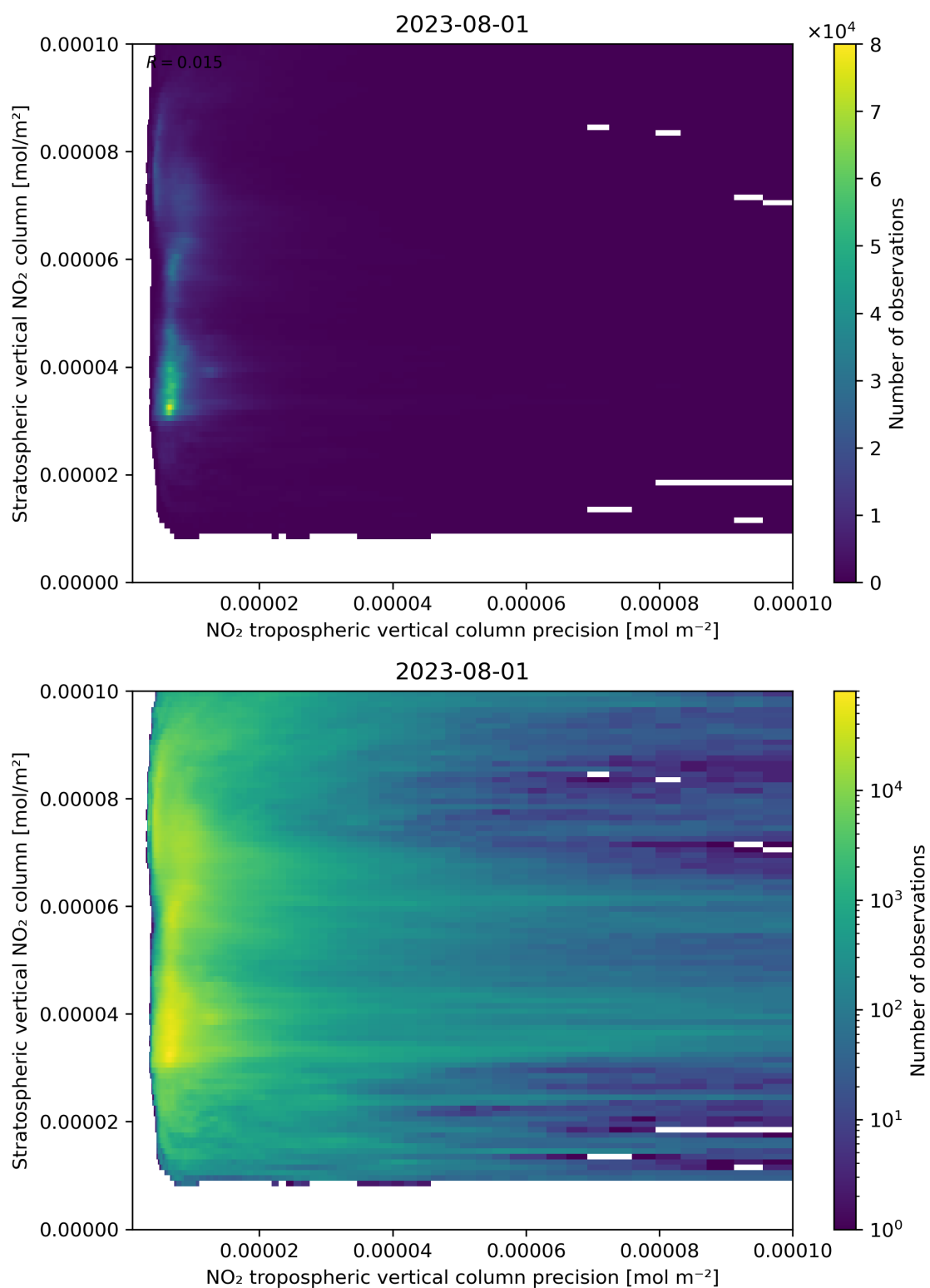
Figure 135: Scatter density plot of “NO 2 tropospheric vertical column precision” against “Stratospheric vertical NO 2 column” for 2023-07-31 to 2023-08-02.
