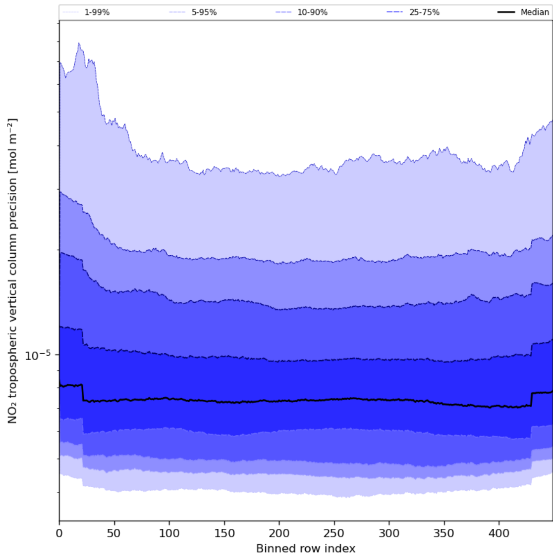
Figure 47: Along track statistics of “NO 2 tropospheric vertical column precision” for 2023-07-31 to 2023-08-02
