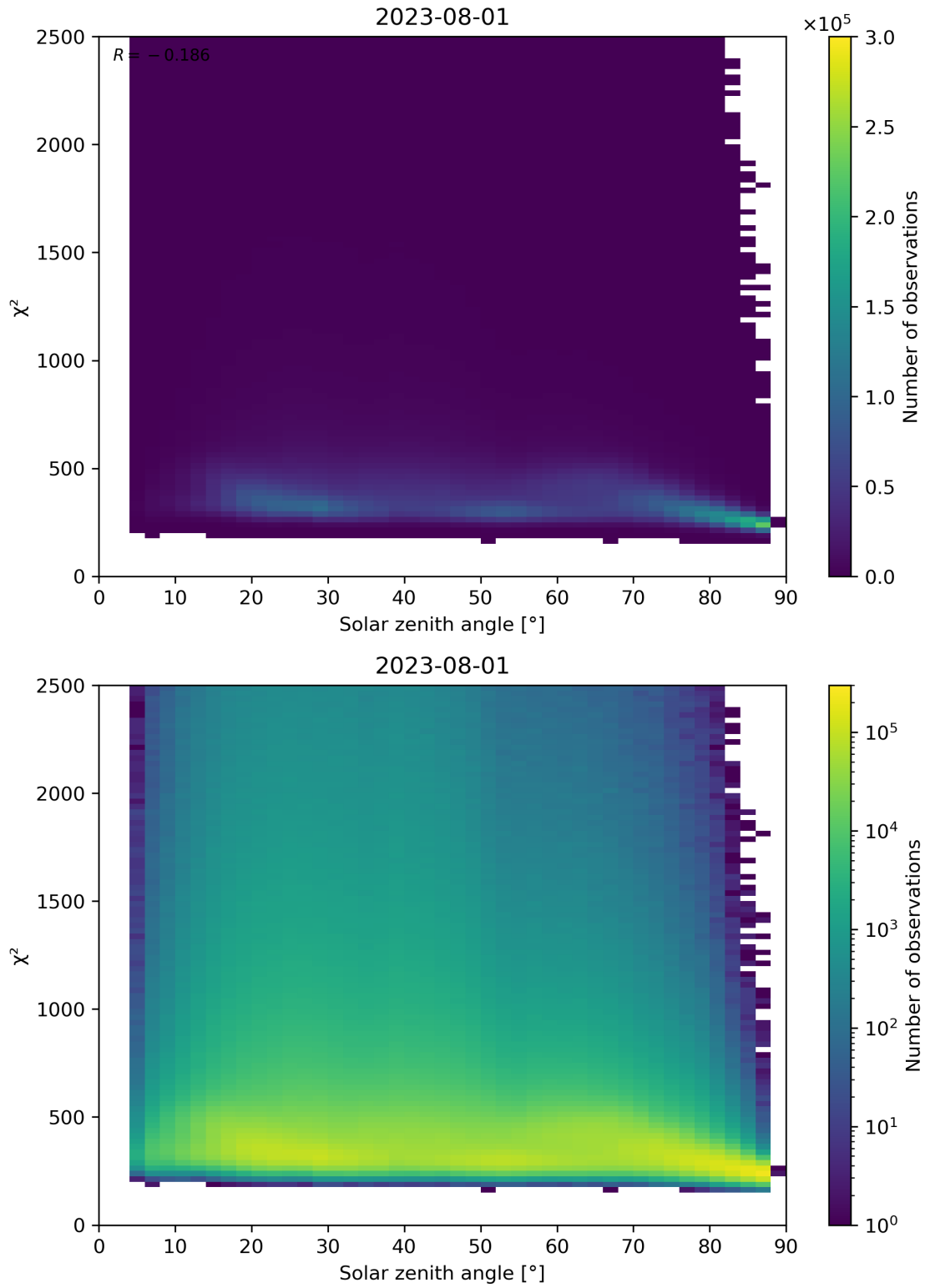
Figure 148: Scatter density plot of “Solar zenith angle” against “ \chi^2 ” for 2023-07-31 to 2023-08-02.
