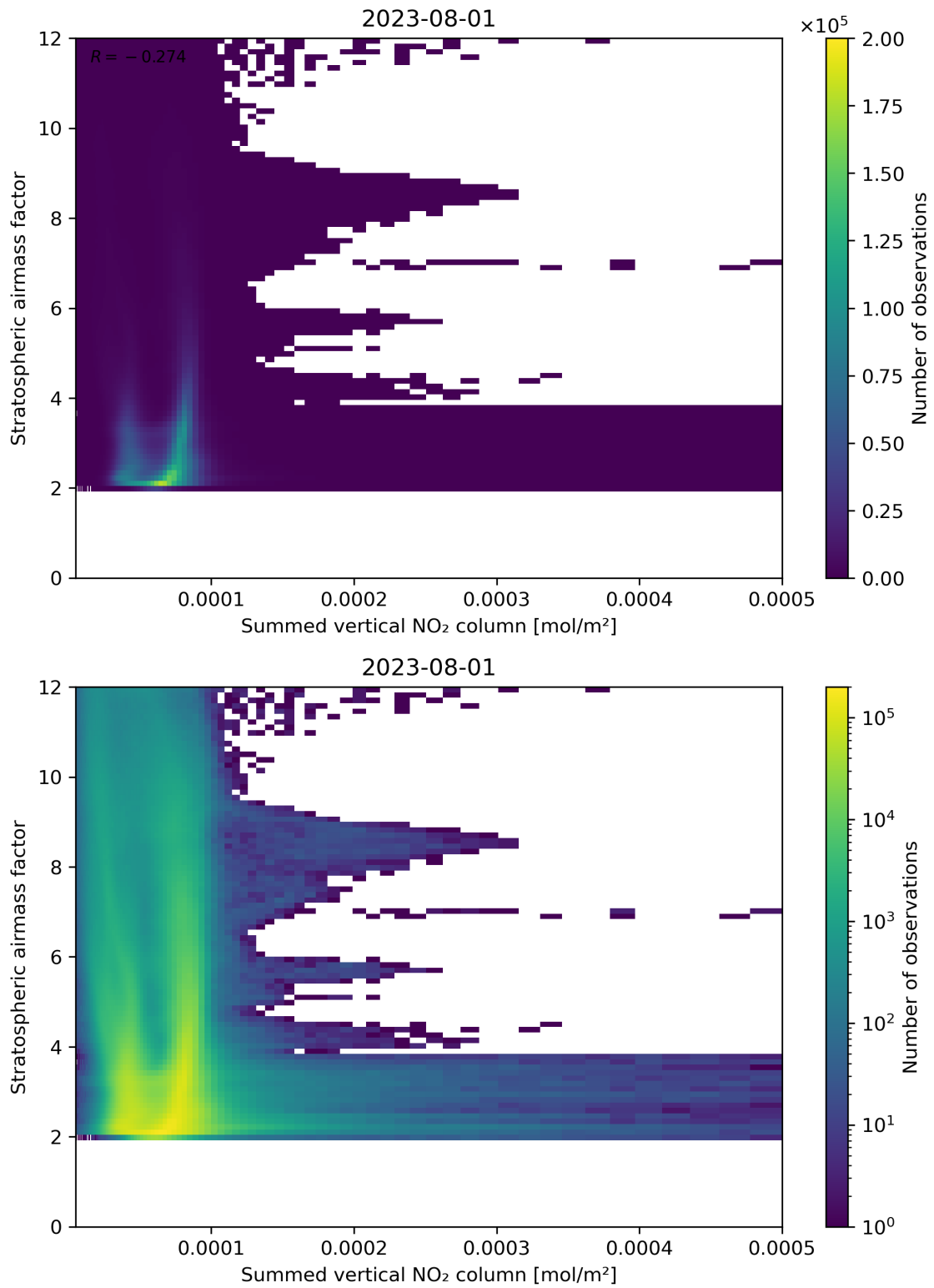
Figure 103: Scatter density plot of “Summed vertical NO 2 column” against “Stratospheric air mass factor” for 2023-07-31 to 2023-08-02.
