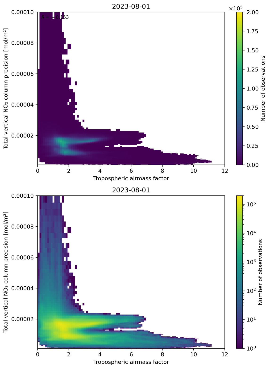
Figure 78: Scatter density plot of “Tropospheric air mass factor” against “Total vertical NO 2 column precision” for 2023-07-31 to 2023-08-02.
