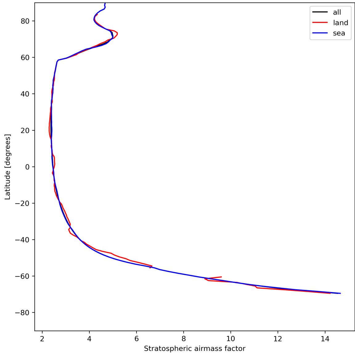
Figure 27: Zonal average of “Stratospheric air mass factor” for 2023-07-31 to 2023-08-02.
