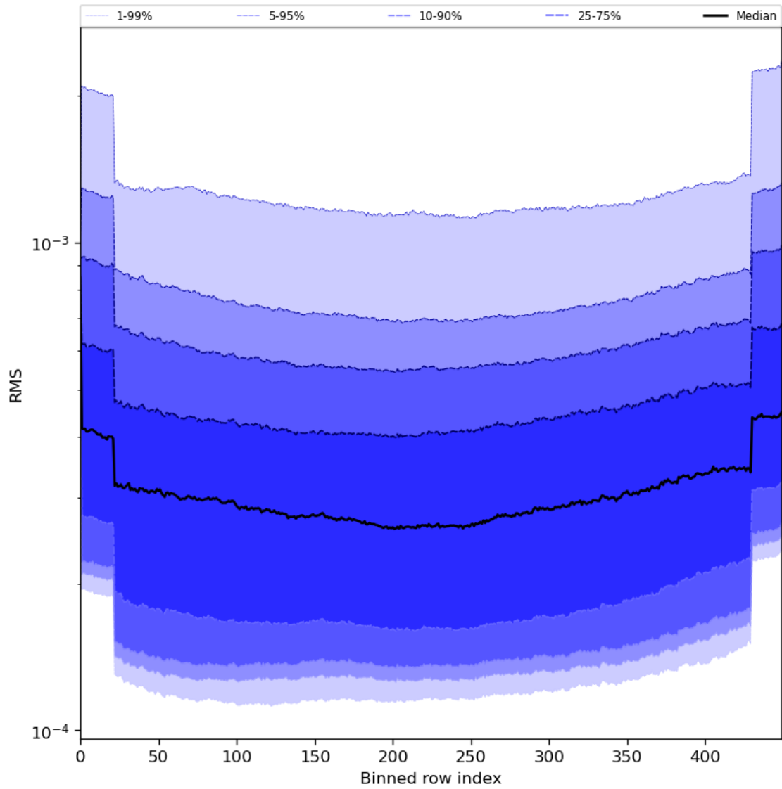
Figure 60: Along track statistics of “RMS” for 2023-07-31 to 2023-08-02
