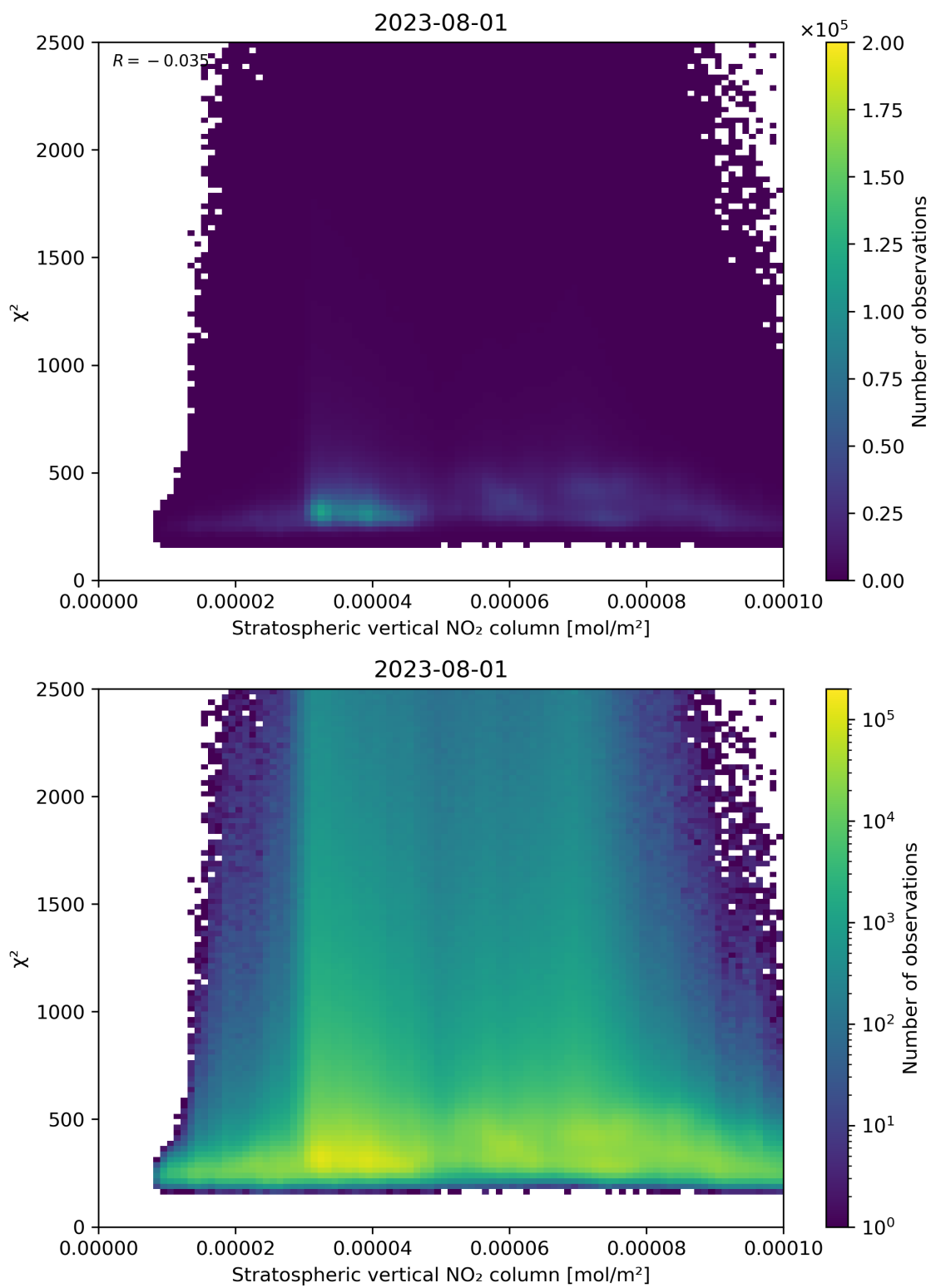
Figure 97: Scatter density plot of “Stratospheric vertical NO 2 column” against “ \chi^2 ” for 2023-07-31 to 2023-08-02.
