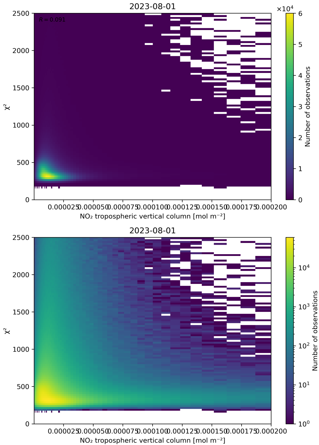
Figure 124: Scatter density plot of “NO 2 tropospheric vertical column” against “ \chi^2 ” for 2023-07-31 to 2023-08-02.
