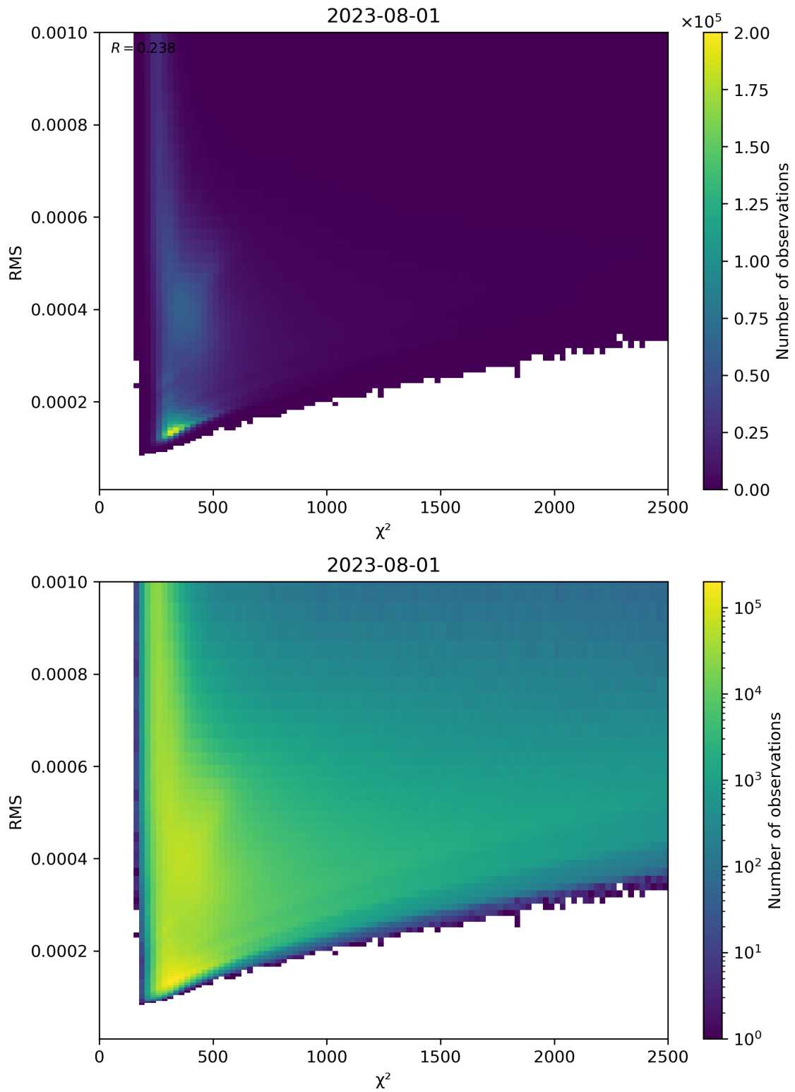
Figure 82: Scatter density plot of “ \chi^2 ” against “RMS” for 2023-07-31 to 2023-08-02.
