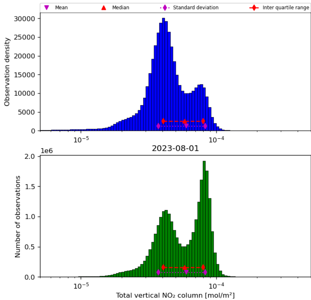
Figure 38: Histogram of “Total vertical NO 2 column” for 2023-07-31 to 2023-08-02
