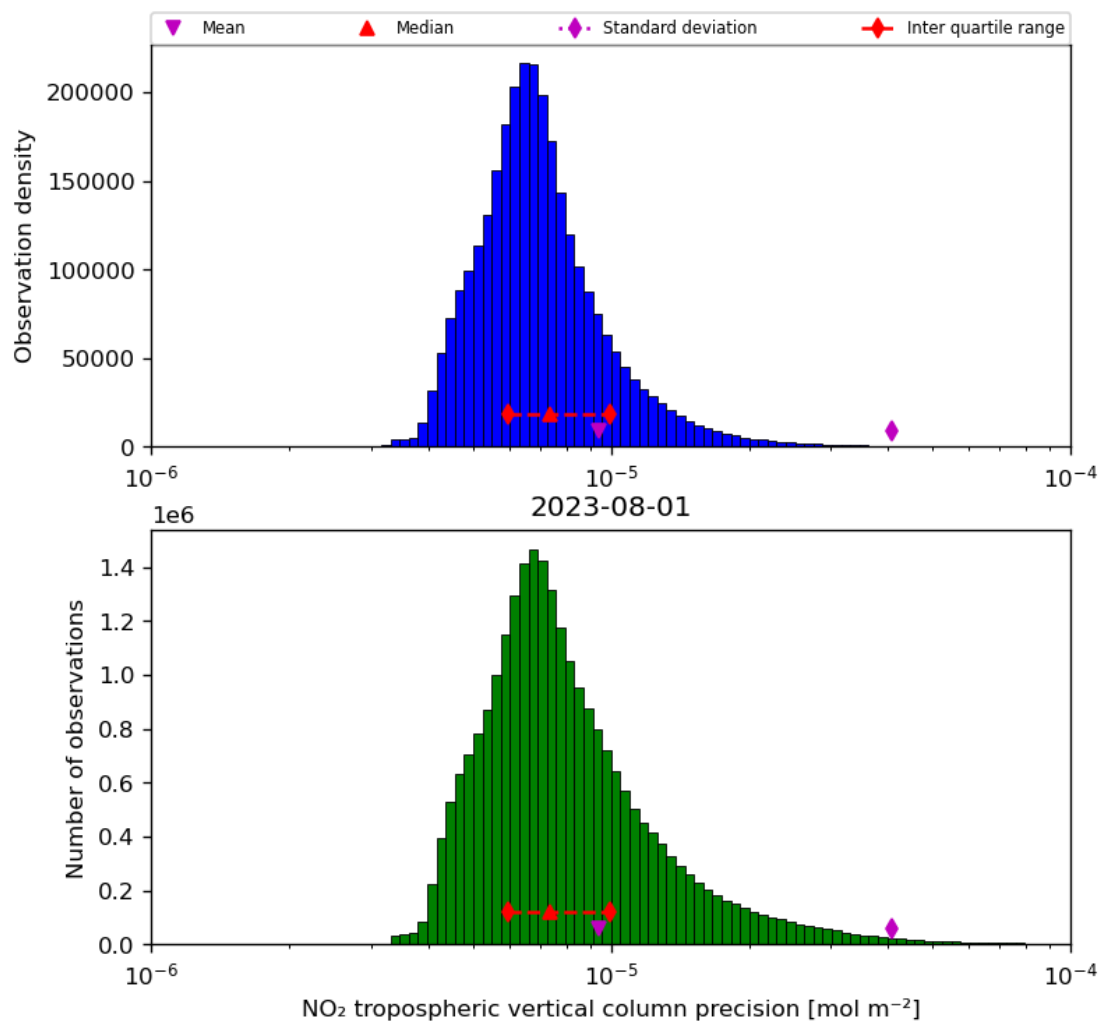
Figure 30: Histogram of “NO 2 tropospheric vertical column precision” for 2023-07-31 to 2023-08-02
