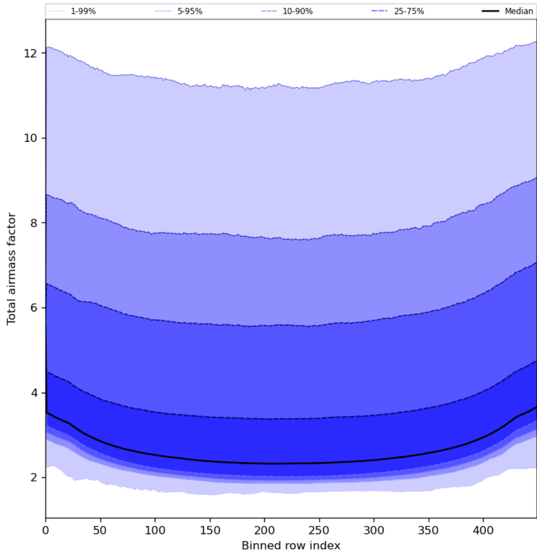
Figure 49: Along track statistics of “Total airmass factor” for 2023-07-31 to 2023-08-02
