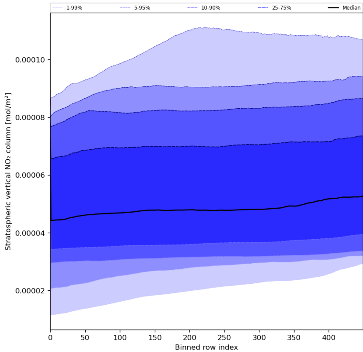
Figure 53: Along track statistics of “Stratospheric vertical NO 2 column” for 2023-07-31 to 2023-08-02
