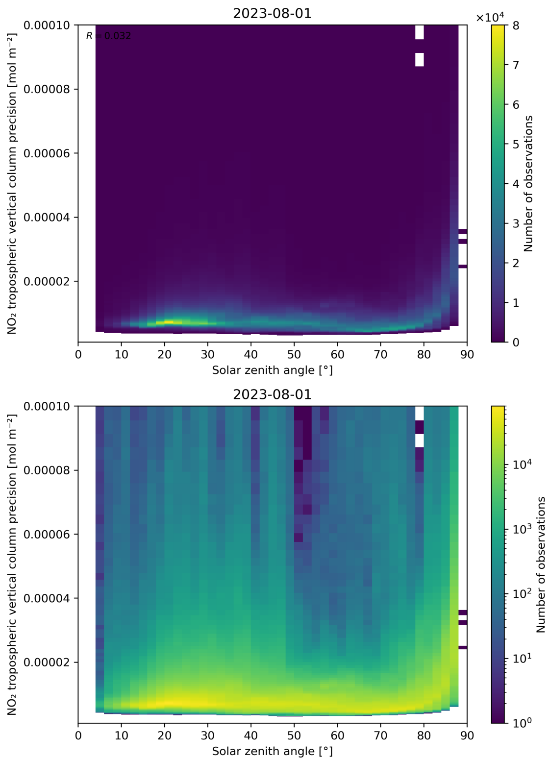
Figure 156: Scatter density plot of “Solar zenith angle” against “NO 2 tropospheric vertical column precision” for 2023-07-31 to 2023-08-02.
