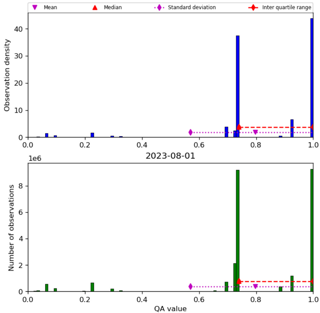
Figure 28: Histogram of “QA value” for 2023-07-31 to 2023-08-02
