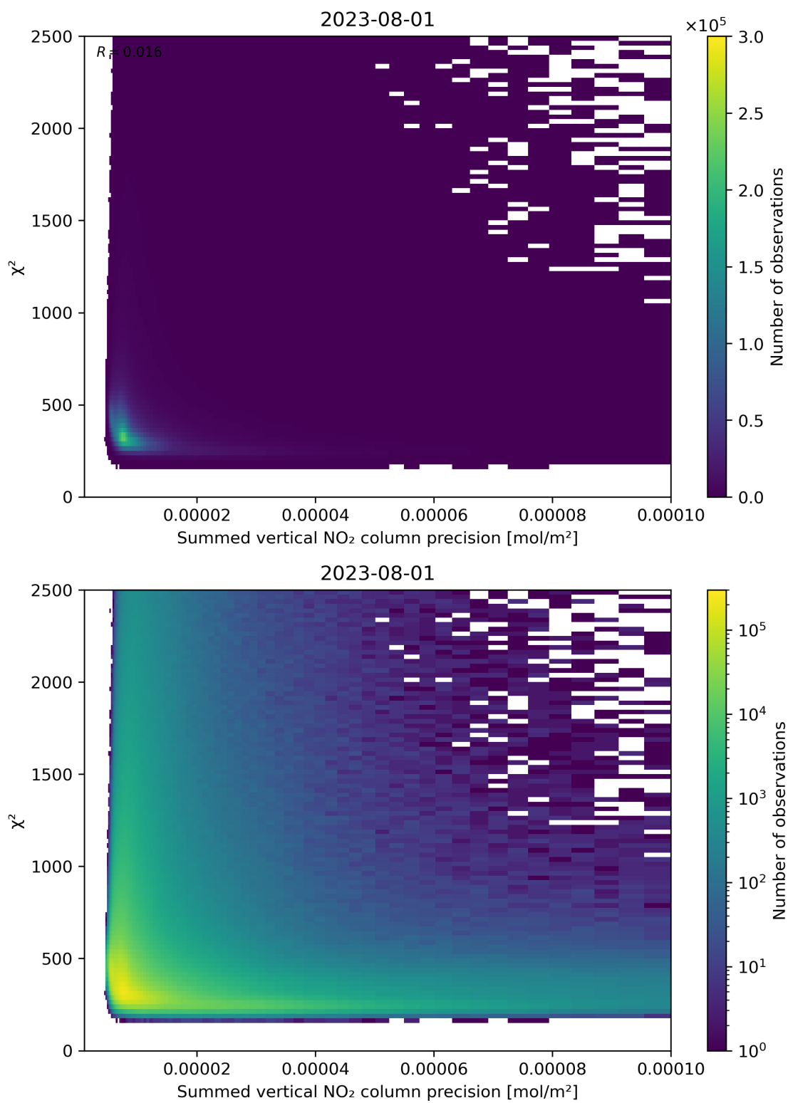
Figure 107: Scatter density plot of “Summed vertical NO 2 column precision” against “ \chi^2 ” for 2023-07-31 to 2023-08-02.
