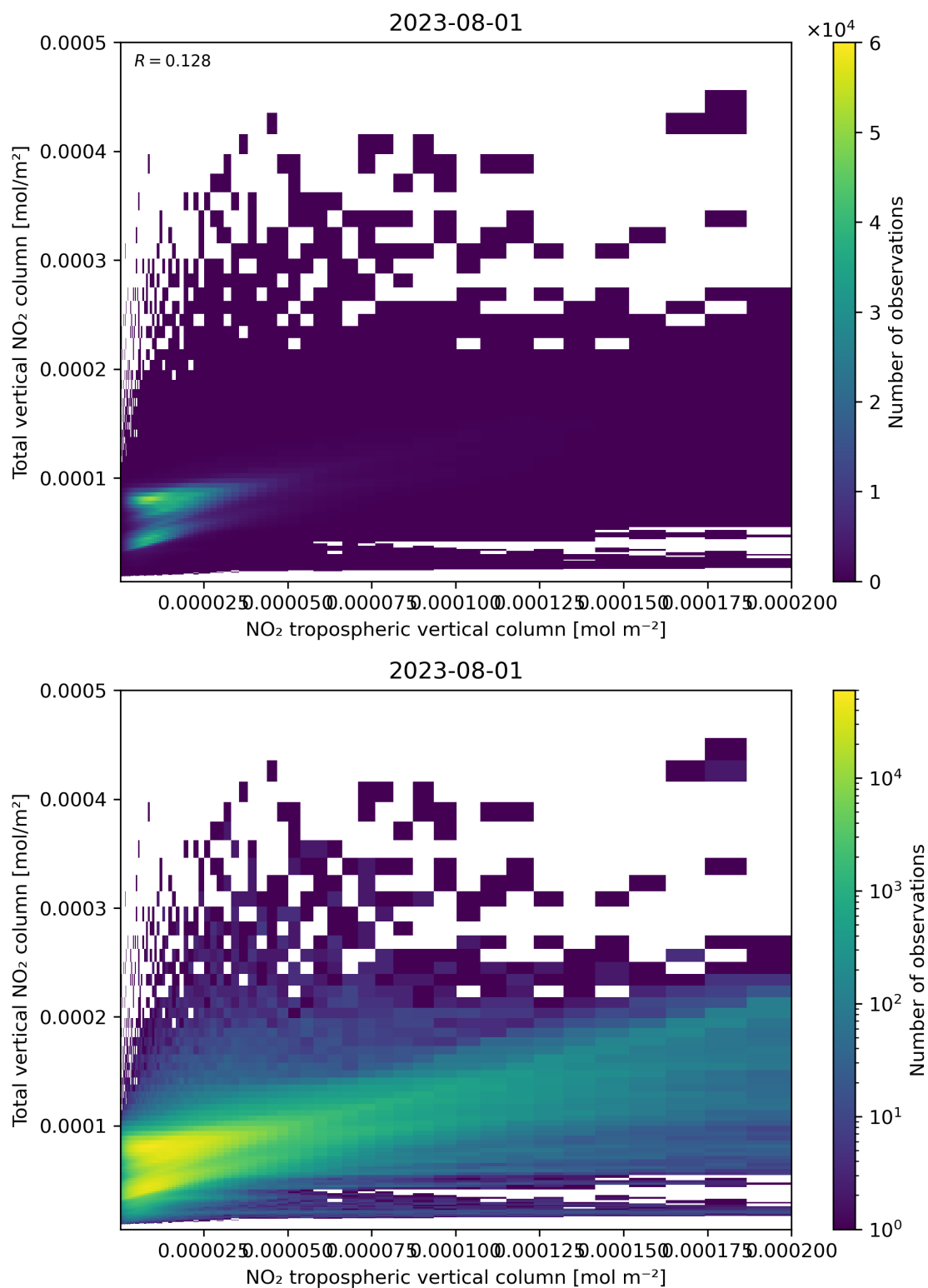
Figure 128: Scatter density plot of “NO 2 tropospheric vertical column” against “Total vertical NO 2 column” for 2023-07-31 to 2023-08-02.
