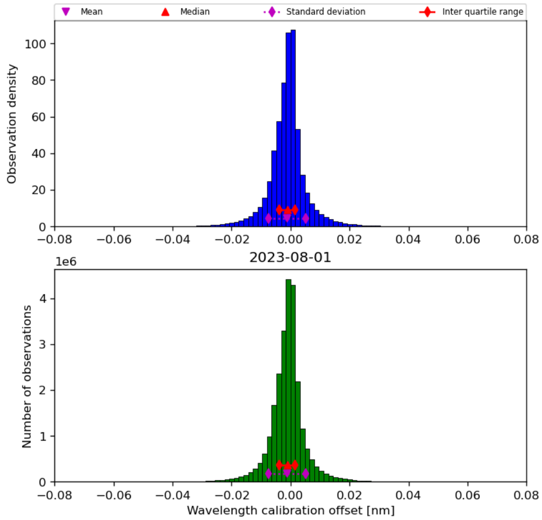
Figure 35: Histogram of “Wavelength calibration offset” for 2023-07-31 to 2023-08-02
