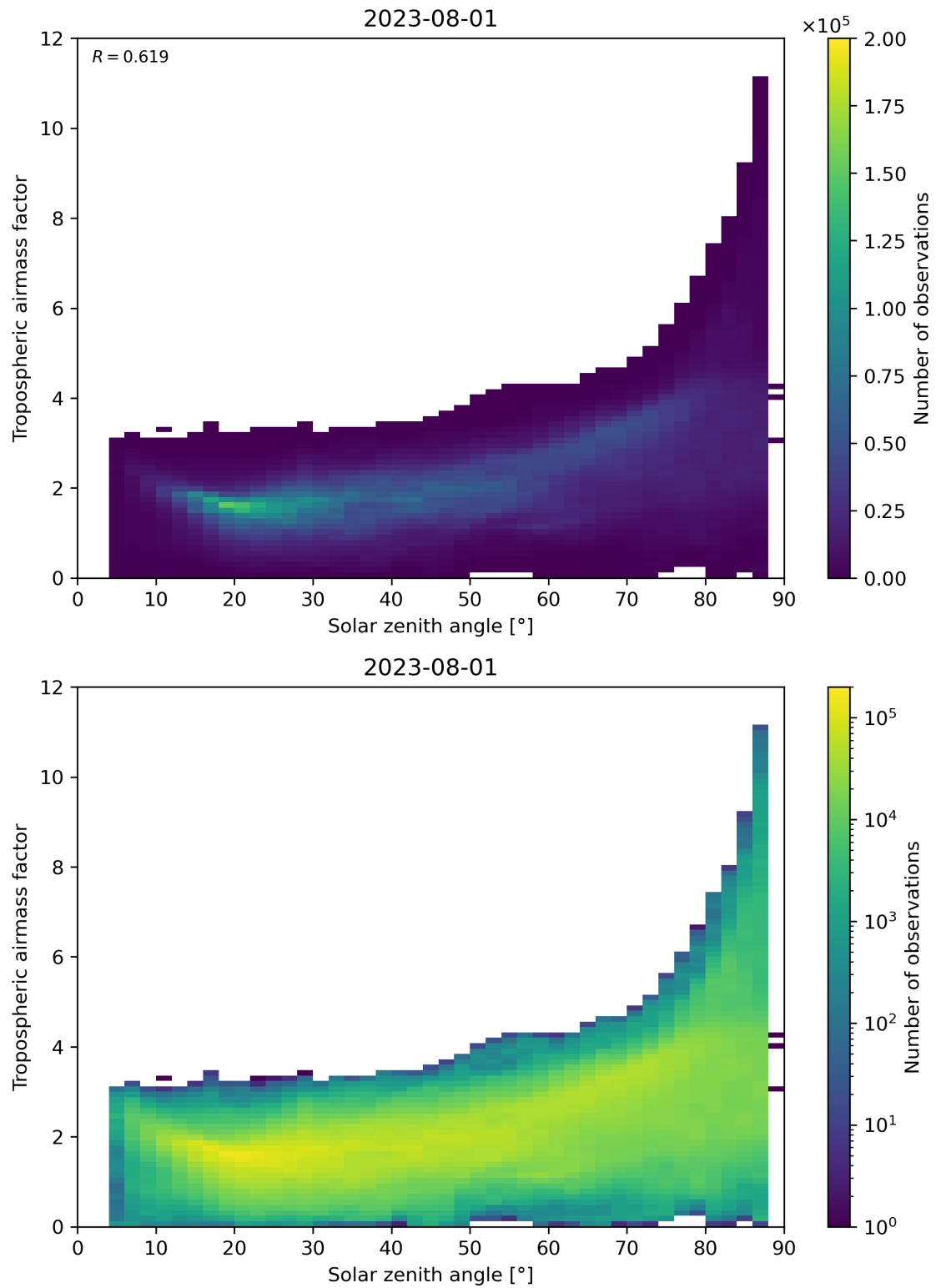
Figure 147: Scatter density plot of “Solar zenith angle” against “Tropospheric airmass factor” for 2023-07-31 to 2023-08-02.
