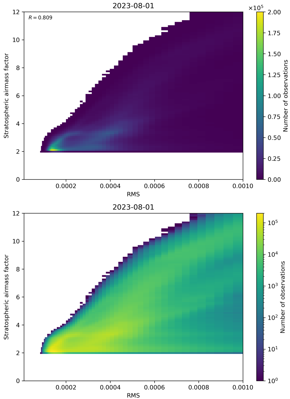
Figure 144: Scatter density plot of “RMS” against “Stratospheric airmass factor” for 2023-07-31 to 2023-08-02.
