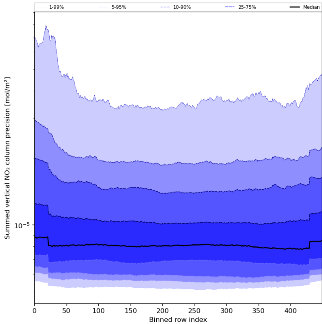
Figure 58: Along track statistics of “Summed vertical NO 2 column precision” for 2023-07-31 to 2023-08-02
