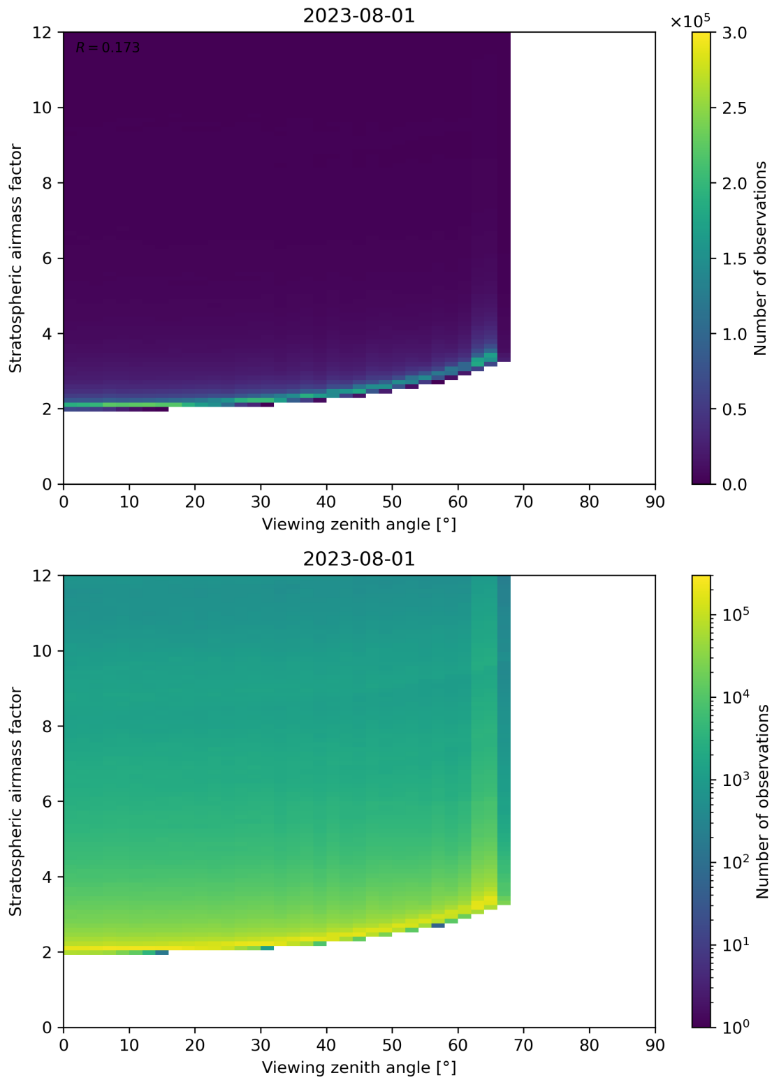
Figure 159: Scatter density plot of “Viewing zenith angle” against “Stratospheric airmass factor” for 2023-07-31 to 2023-08-02.
