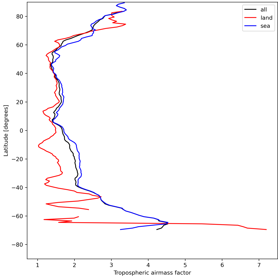
Figure 14: Zonal average of “Tropospheric air mass factor” for 2023-07-31 to 2023-08-02.
