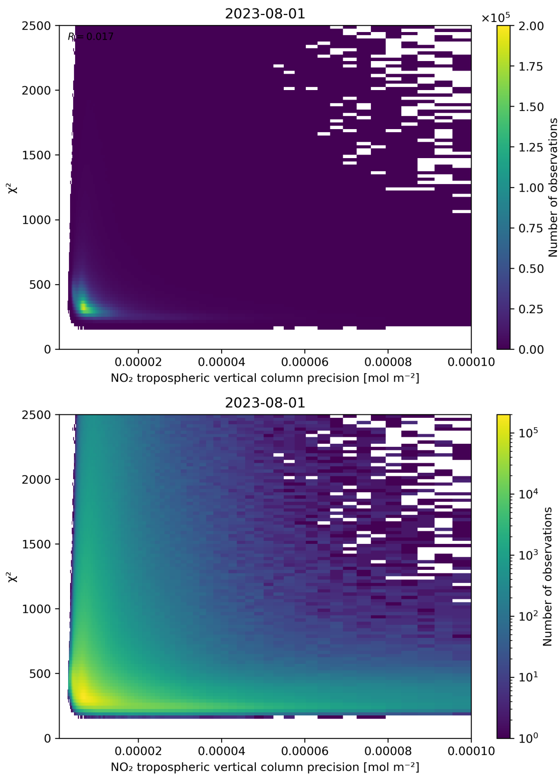
Figure 134: Scatter density plot of “NO 2 tropospheric vertical column precision” against “ \chi^2 ” for 2023-07-31 to 2023-08-02.
