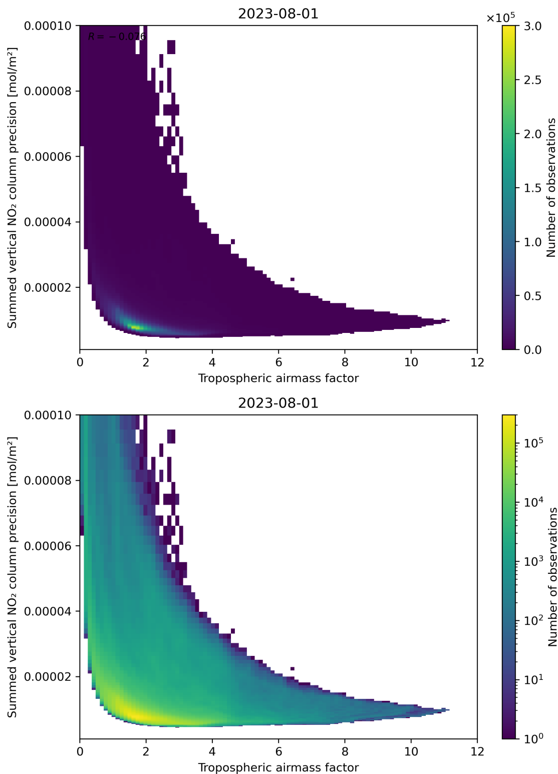
Figure 76: Scatter density plot of “Tropospheric air mass factor” against “Summed vertical NO 2 column precision” for 2023-07-31 to 2023-08-02.
