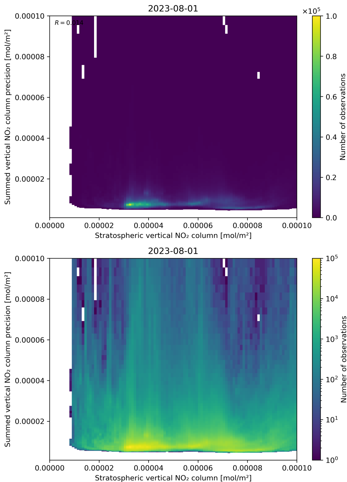
Figure 99: Scatter density plot of “Stratospheric vertical NO 2 column” against “Summed vertical NO 2 column precision” for 2023-07-31 to 2023-08-02.
