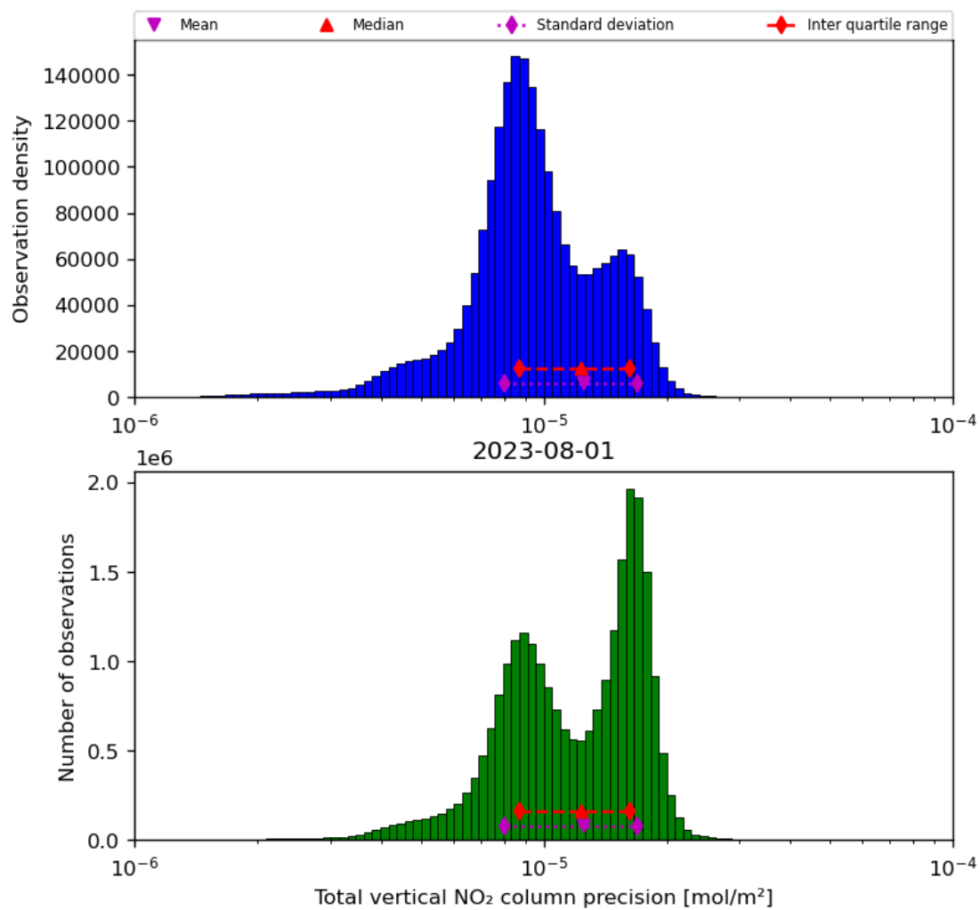
Figure 39: Histogram of “Total vertical NO 2 column precision” for 2023-07-31 to 2023-08-02
