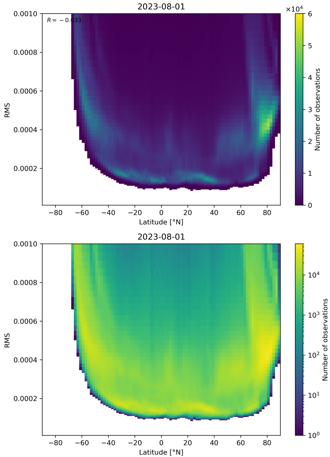
Figure 94: Scatter density plot of “Latitude” against “RMS” for 2023-07-31 to 2023-08-02.
