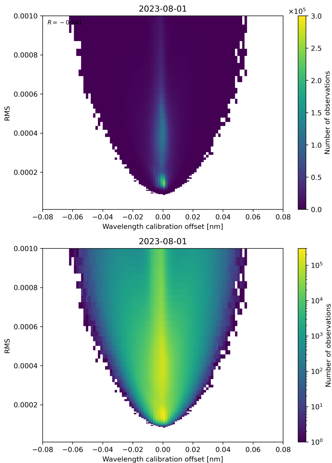
Figure 181: Scatter density plot of “Wavelength calibration offset” against “RMS” for 2023-07-31 to 2023-08-02.
