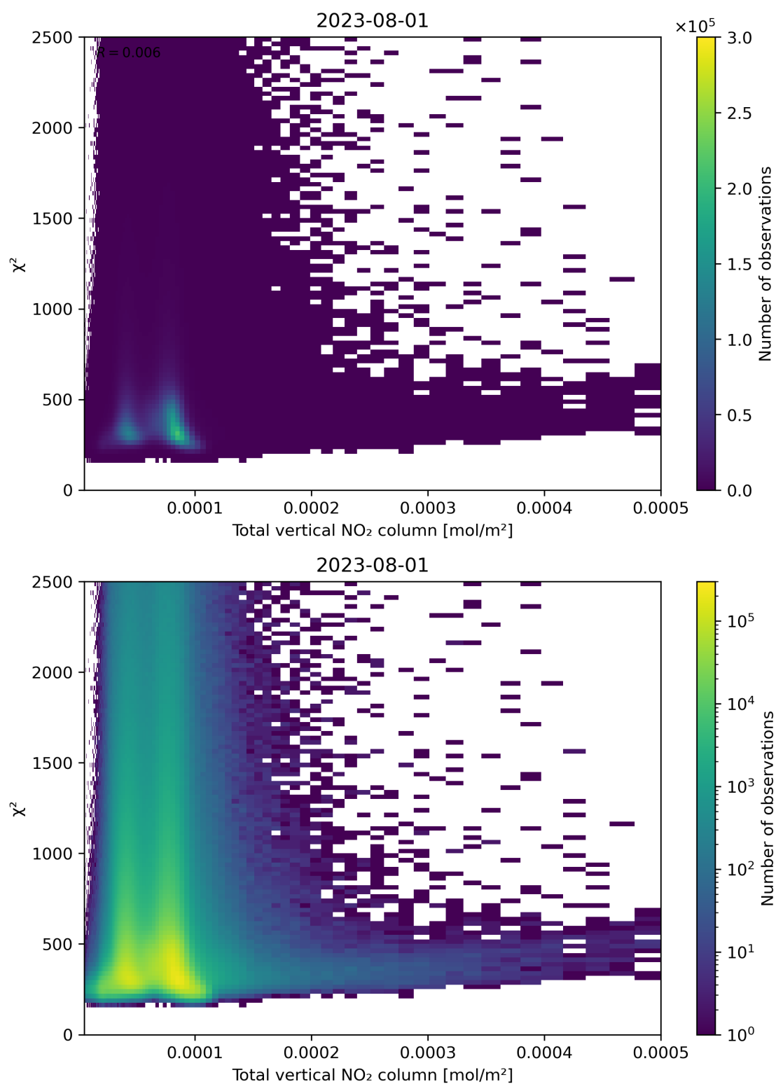
Figure 111: Scatter density plot of “Total vertical NO 2 column” against “ \chi^2 ” for 2023-07-31 to 2023-08-02.
