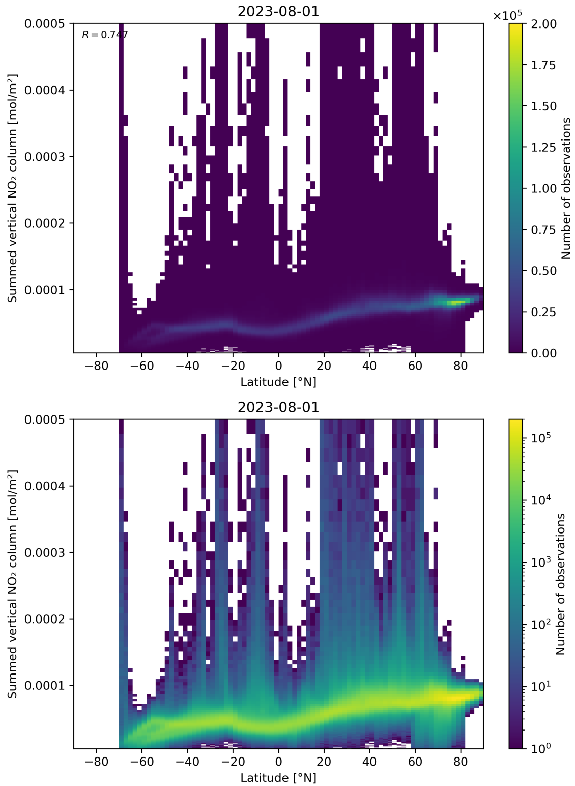
Figure 88: Scatter density plot of “Latitude” against “Summed vertical NO 2 column” for 2023-07-31 to 2023-08-02.
