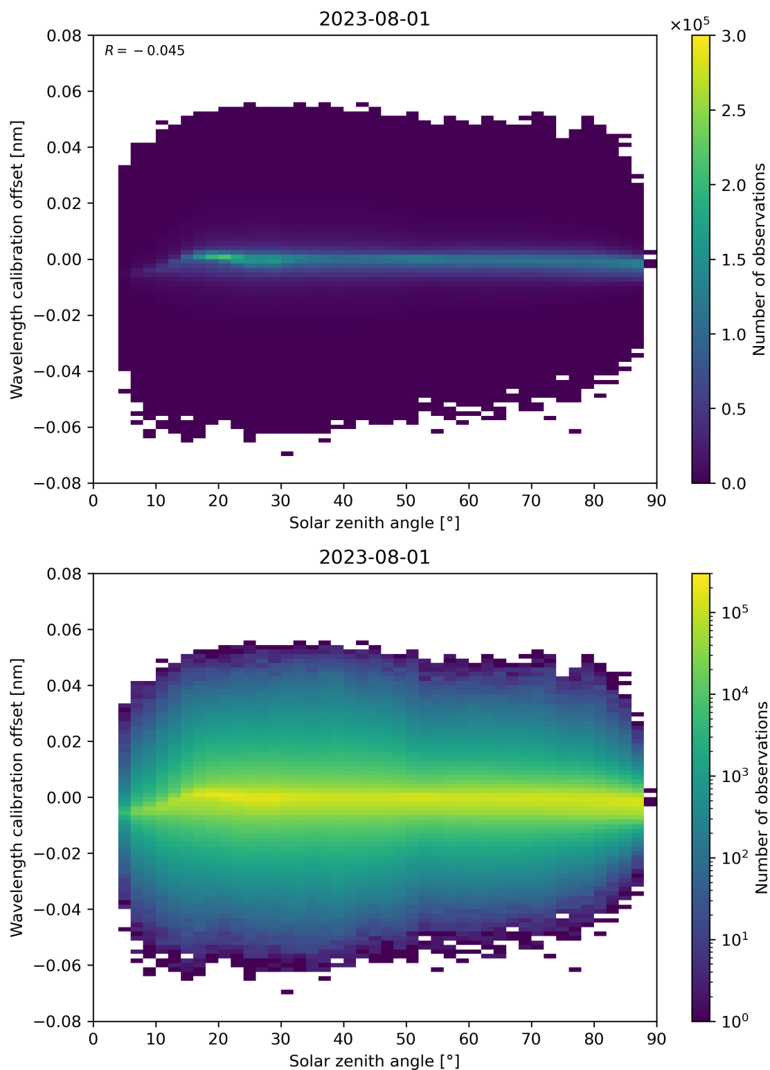
Figure 158: Scatter density plot of “Solar zenith angle” against “Wavelength calibration offset” for 2023-07-31 to 2023-08-02.
