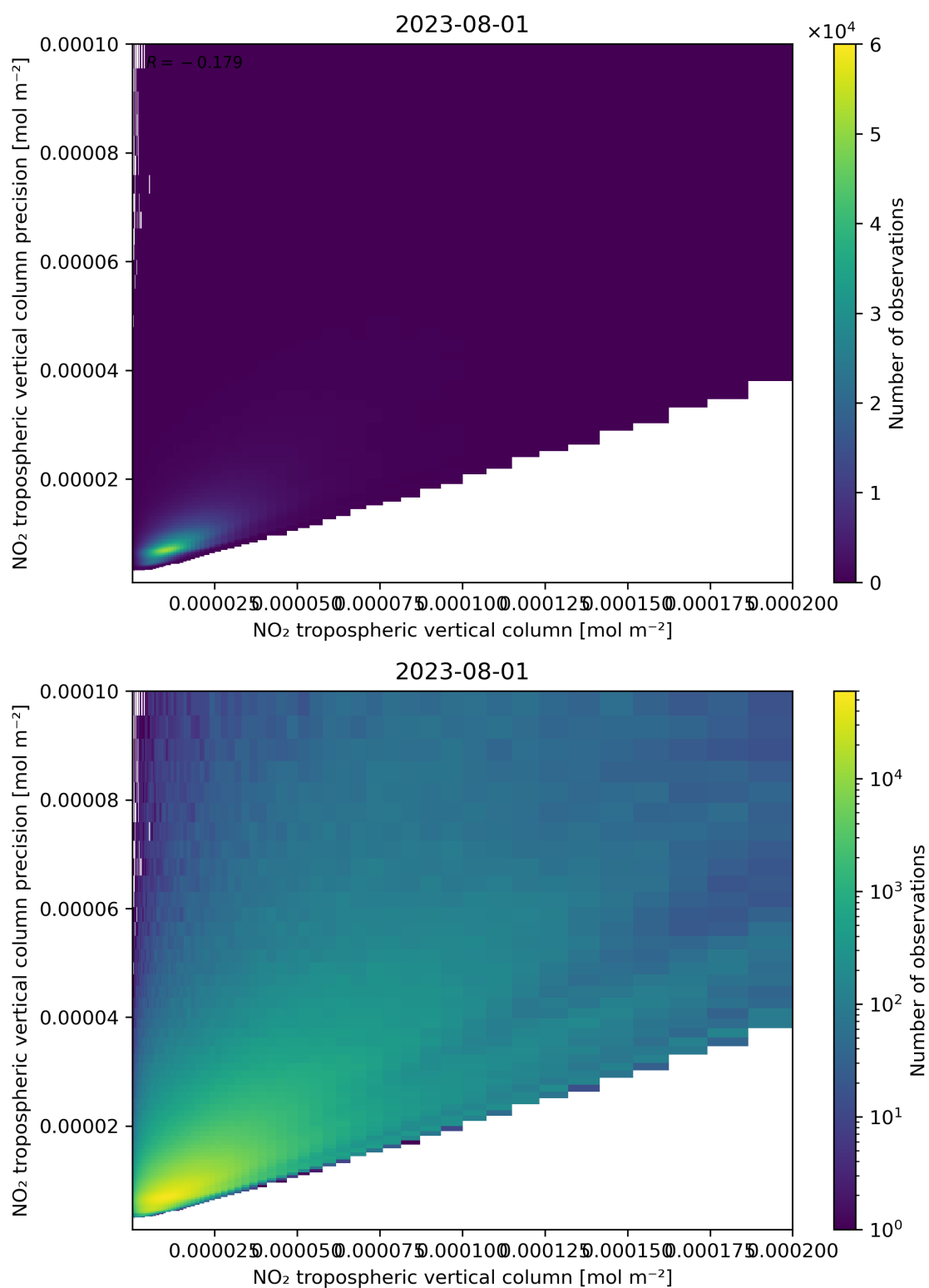
Figure 130: Scatter density plot of “NO 2 tropospheric vertical column” against “NO 2 tropospheric vertical column precision” for 2023-07-31 to 2023-08-02.
