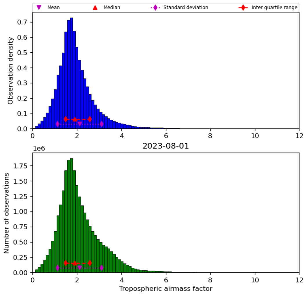
Figure 31: Histogram of “Tropospheric airmass factor” for 2023-07-31 to 2023-08-02
