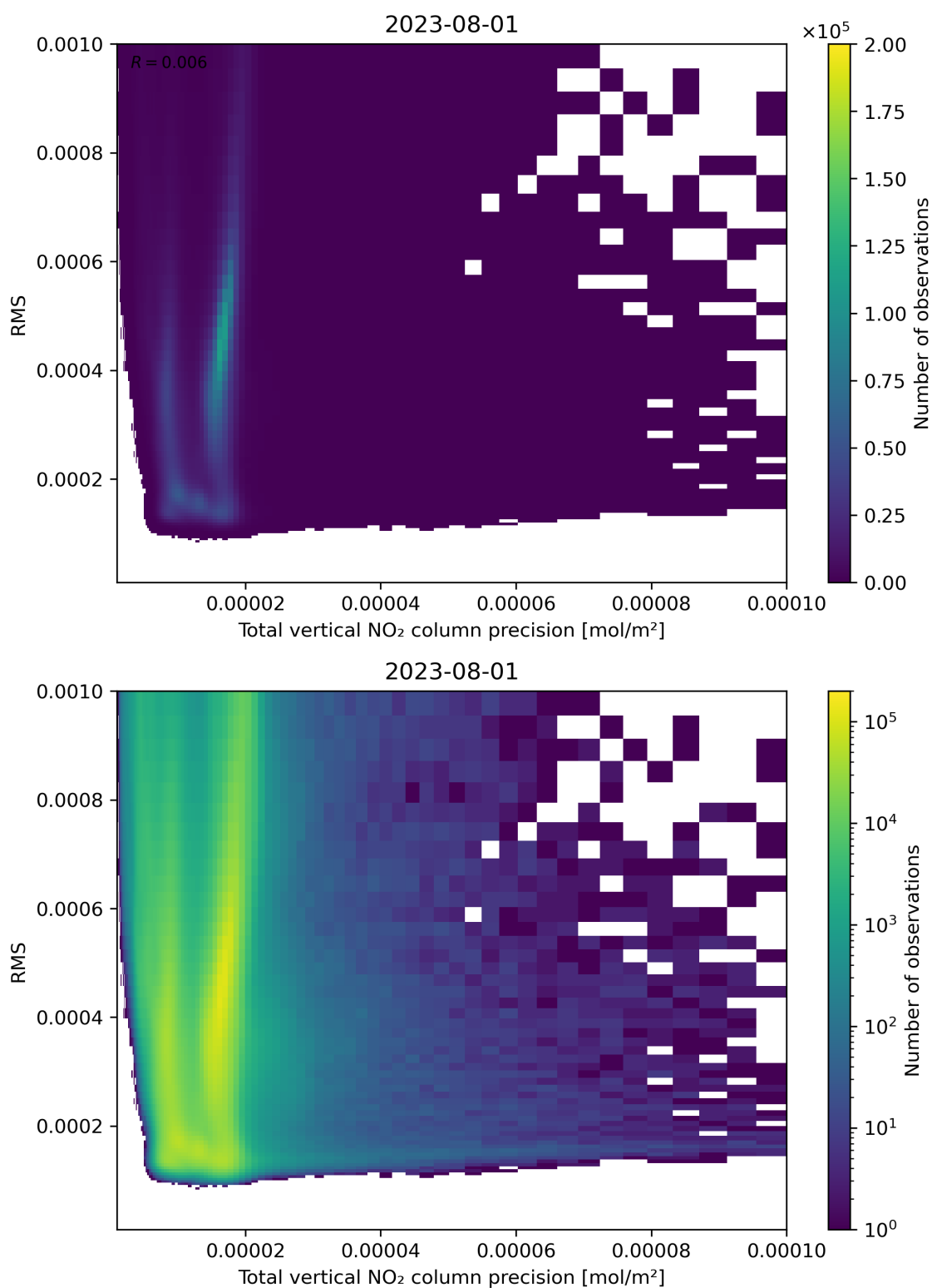
Figure 119: Scatter density plot of “Total vertical NO 2 column precision” against “RMS” for 2023-07-31 to 2023-08-02.
