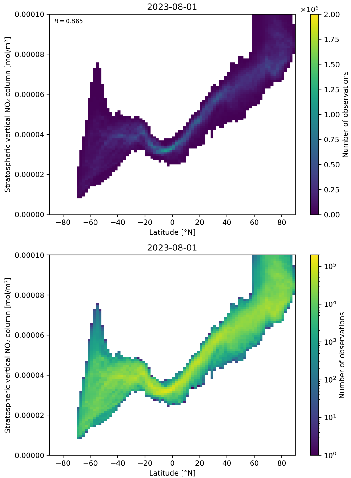
Figure 87: Scatter density plot of “Latitude” against “Stratospheric vertical NO 2 column” for 2023-07-31 to 2023-08-02.
