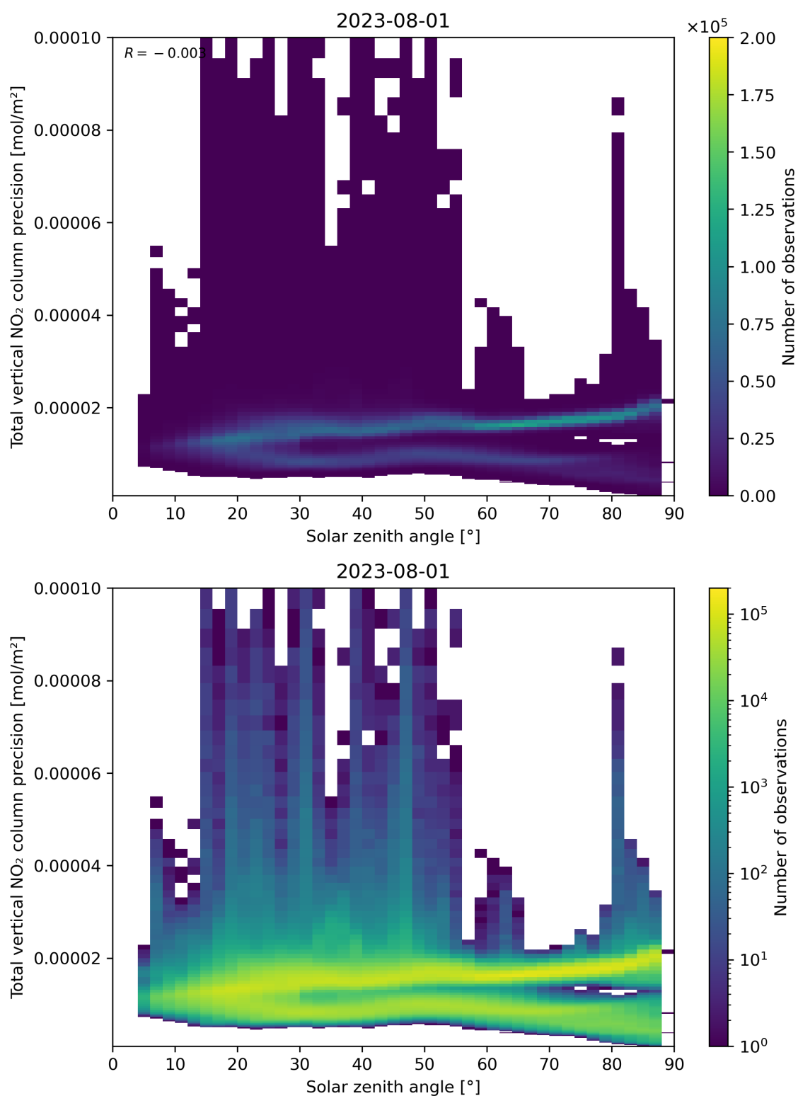
Figure 154: Scatter density plot of “Solar zenith angle” against “Total vertical NO 2 column precision” for 2023-07-31 to 2023-08-02.
