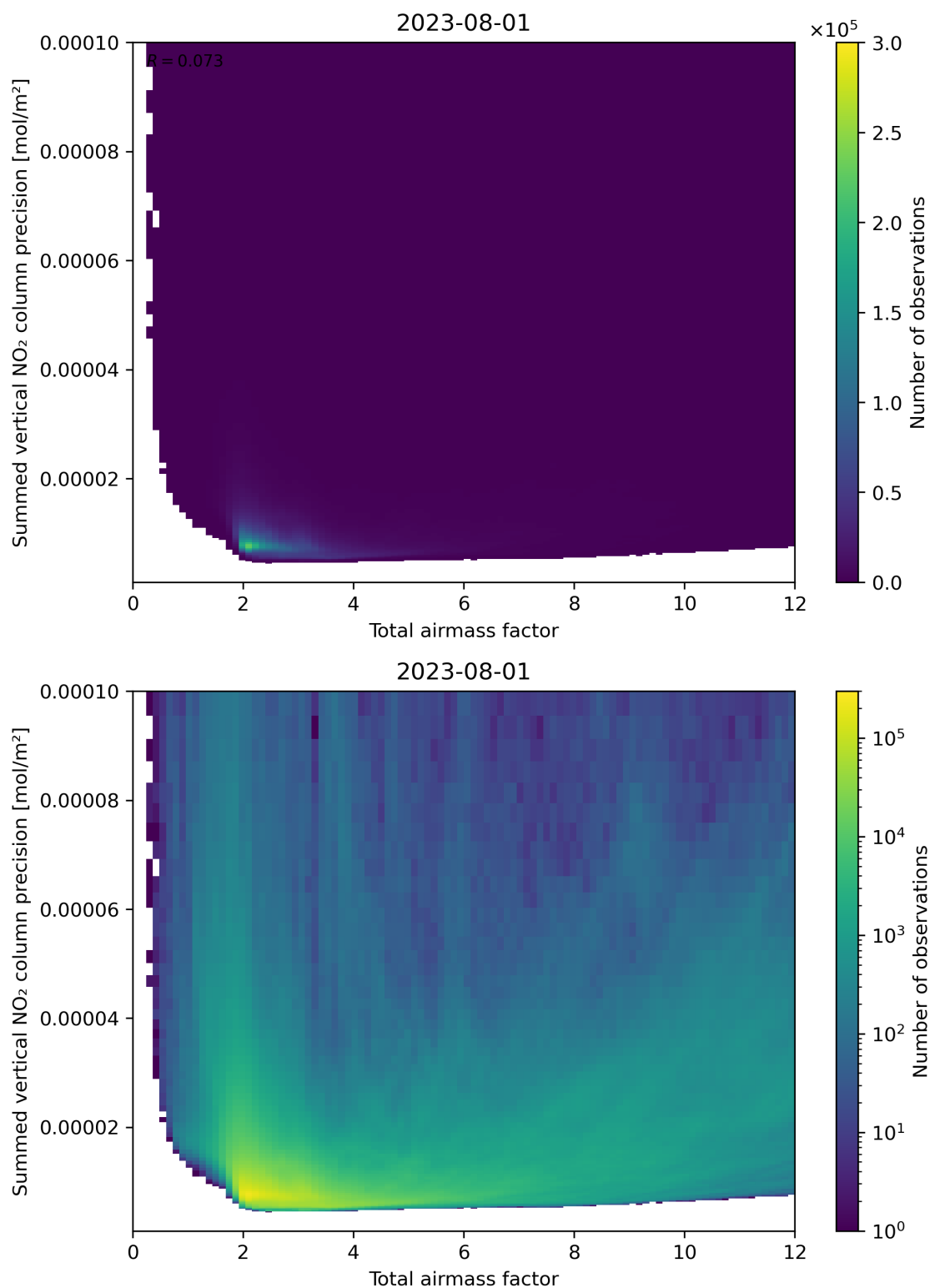
Figure 66: Scatter density plot of “Total airmass factor” against “Summed vertical NO 2 column precision” for 2023-07-31 to 2023-08-02.
