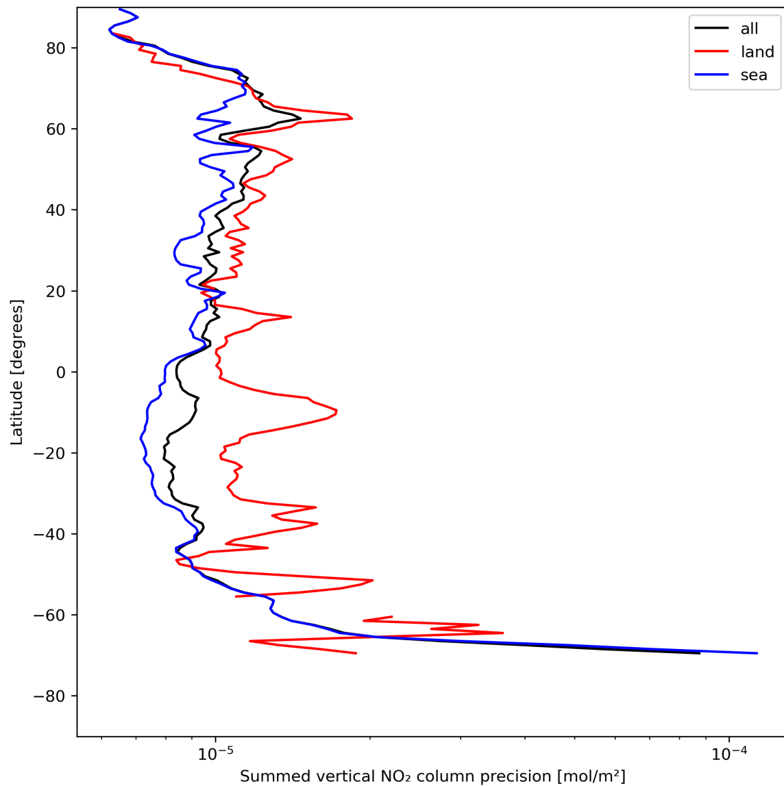
Figure 24: Zonal average of “Summed vertical NO 2 column precision” for 2023-07-31 to 2023-08-02.
