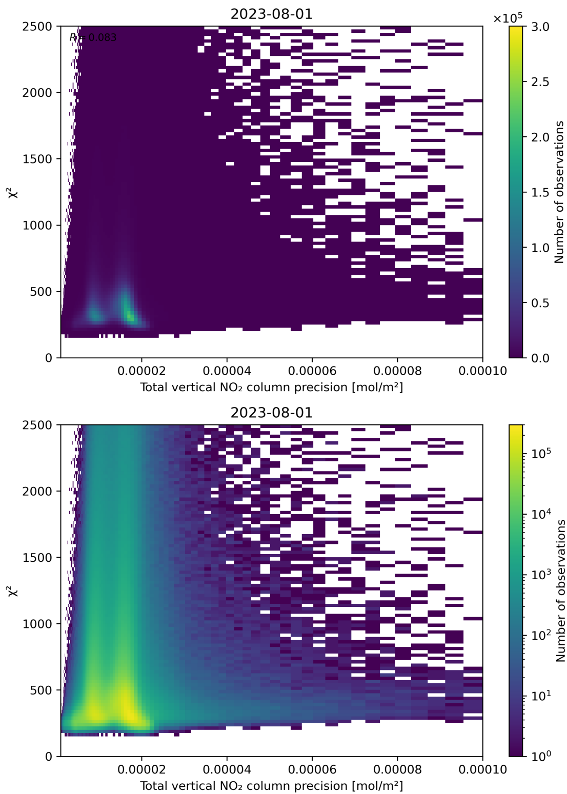
Figure 116: Scatter density plot of “Total vertical NO 2 column precision” against “ \chi^2 ” for 2023-07-31 to 2023-08-02.
