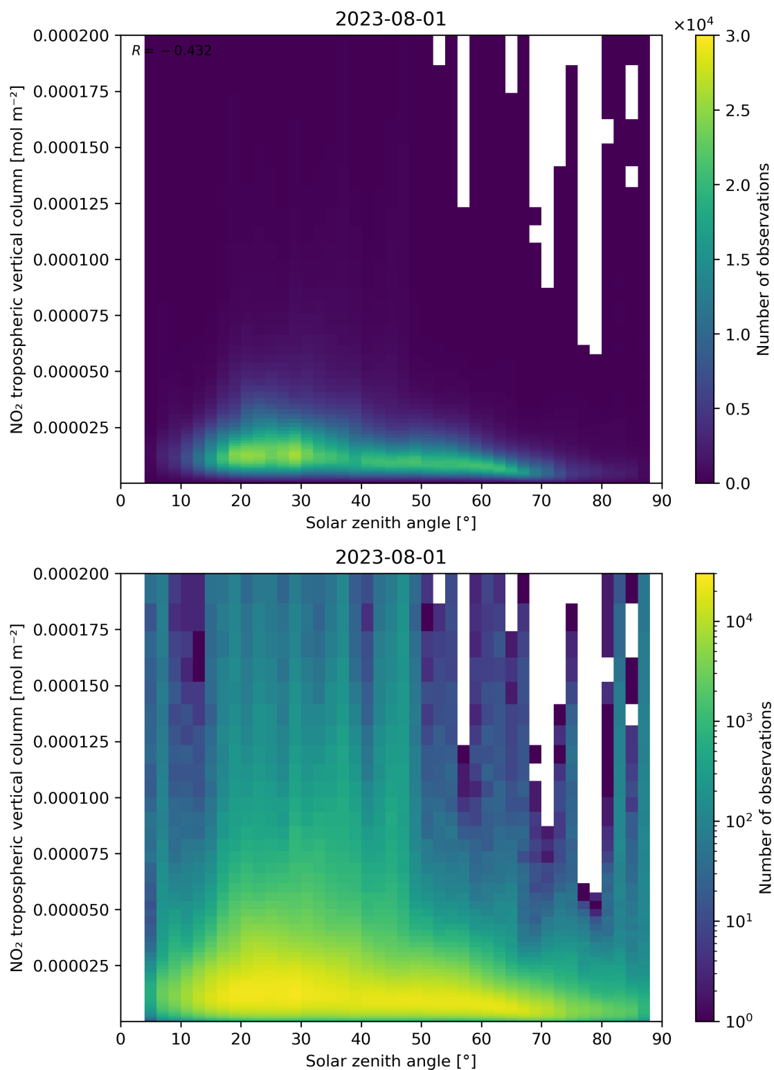
Figure 155: Scatter density plot of “Solar zenith angle” against “NO 2 tropospheric vertical column” for 2023-07-31 to 2023-08-02.
