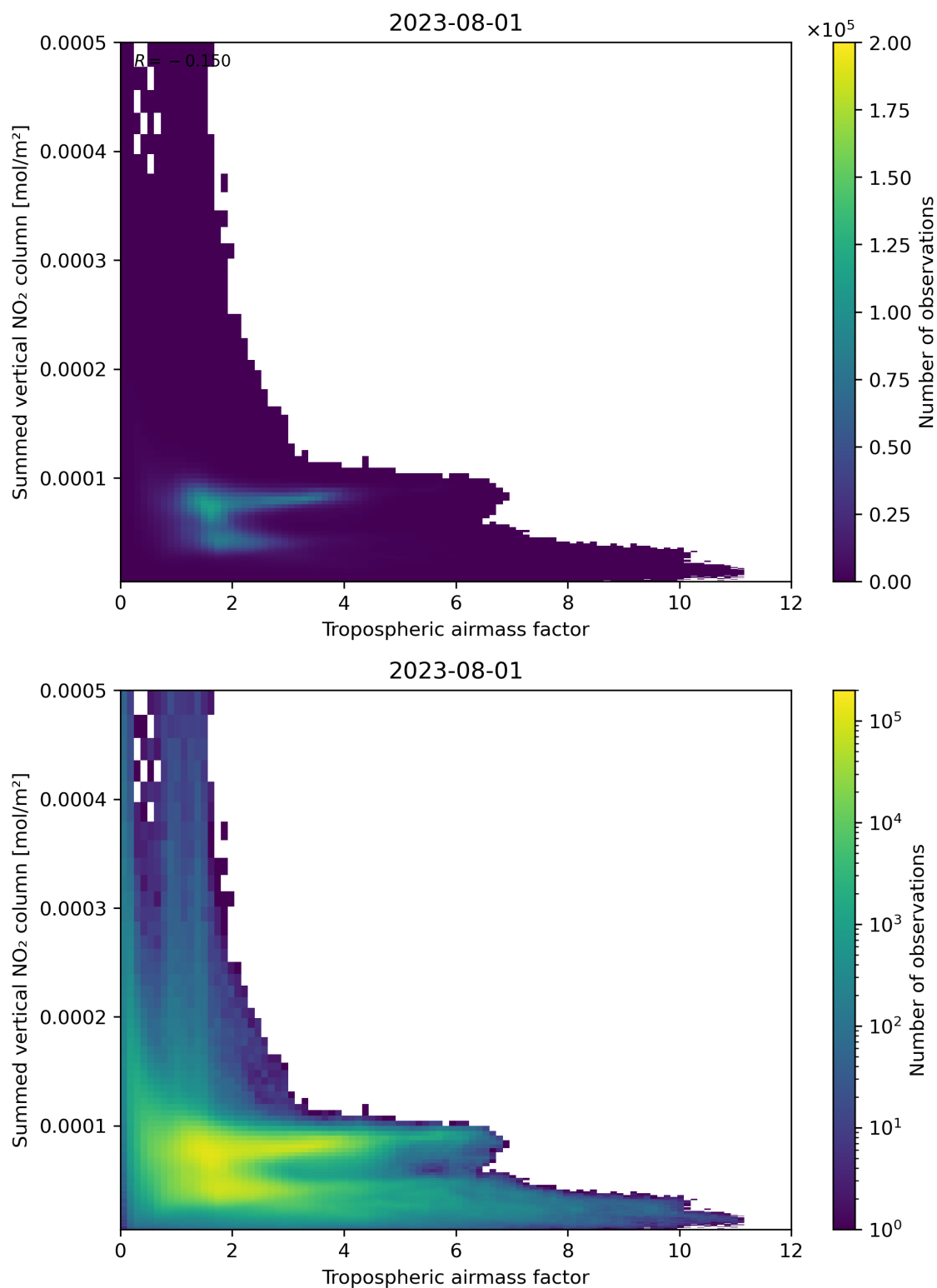
Figure 75: Scatter density plot of “Tropospheric airmass factor” against “Summed vertical NO 2 column” for 2023-07-31 to 2023-08-02.
