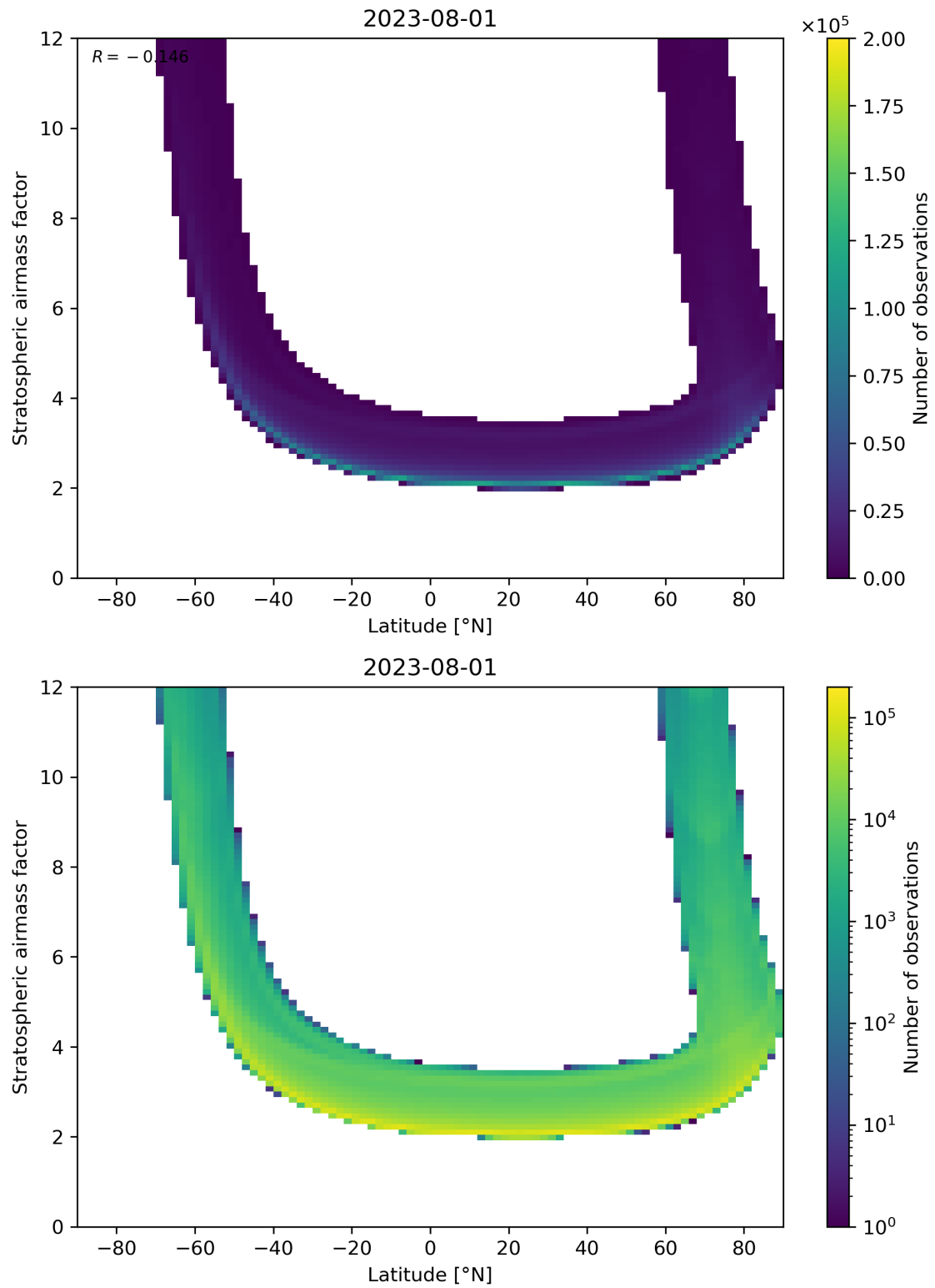
Figure 83: Scatter density plot of “Latitude” against “Stratospheric air mass factor” for 2023-07-31 to 2023-08-02.
