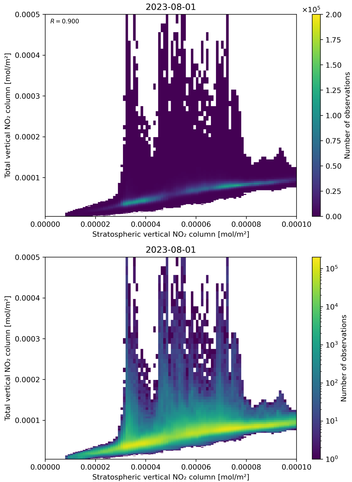
Figure 100: Scatter density plot of “Stratospheric vertical NO 2 column” against “Total vertical NO 2 column” for 2023-07-31 to 2023-08-02.
