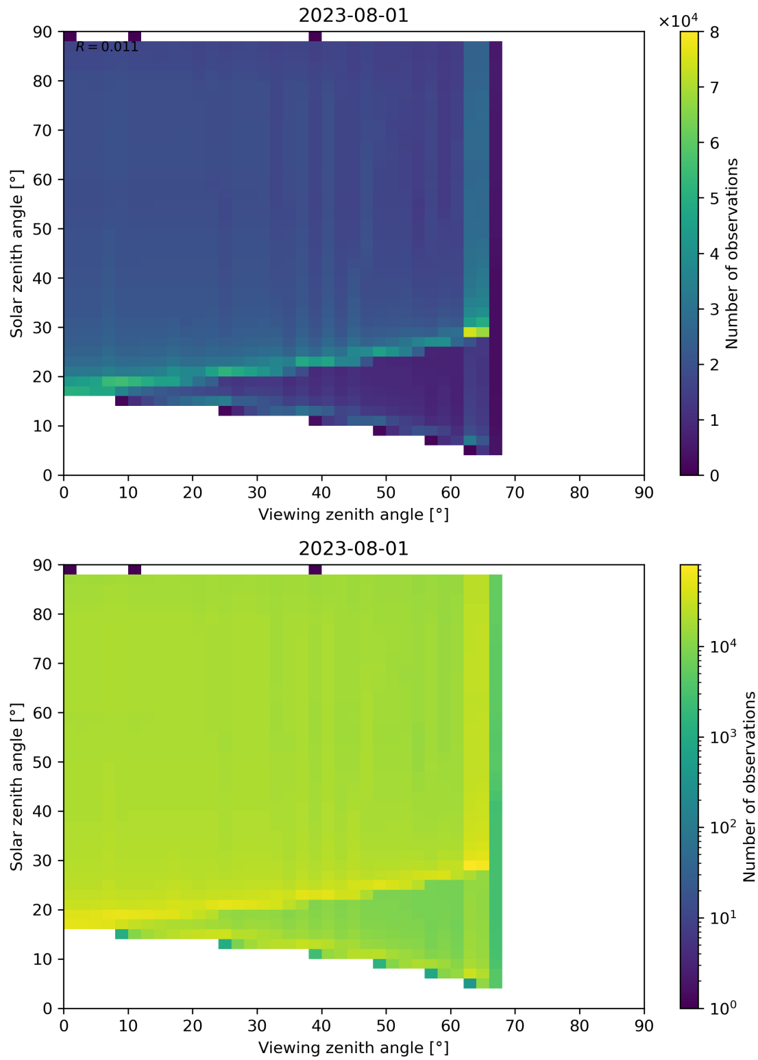
Figure 172: Scatter density plot of “Viewing zenith angle” against “Solar zenith angle” for 2023-07-31 to 2023-08-02.
