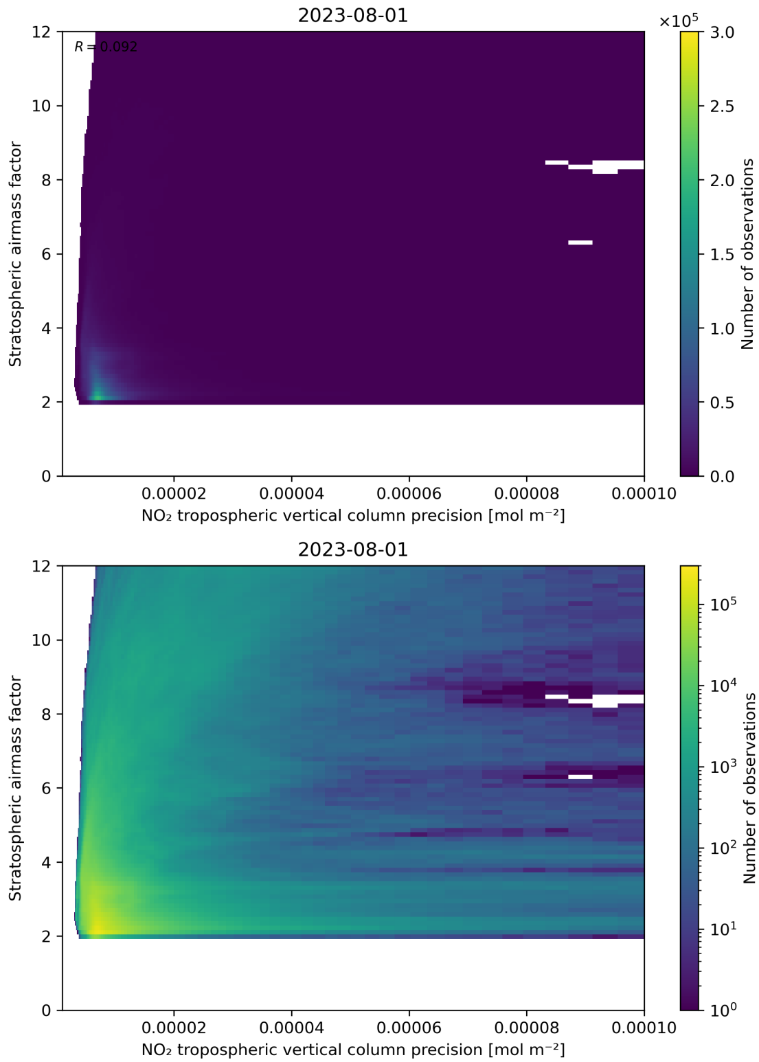
Figure 131: Scatter density plot of “NO 2 tropospheric vertical column precision” against “Stratospheric airmass factor” for 2023-07-31 to 2023-08-02.
