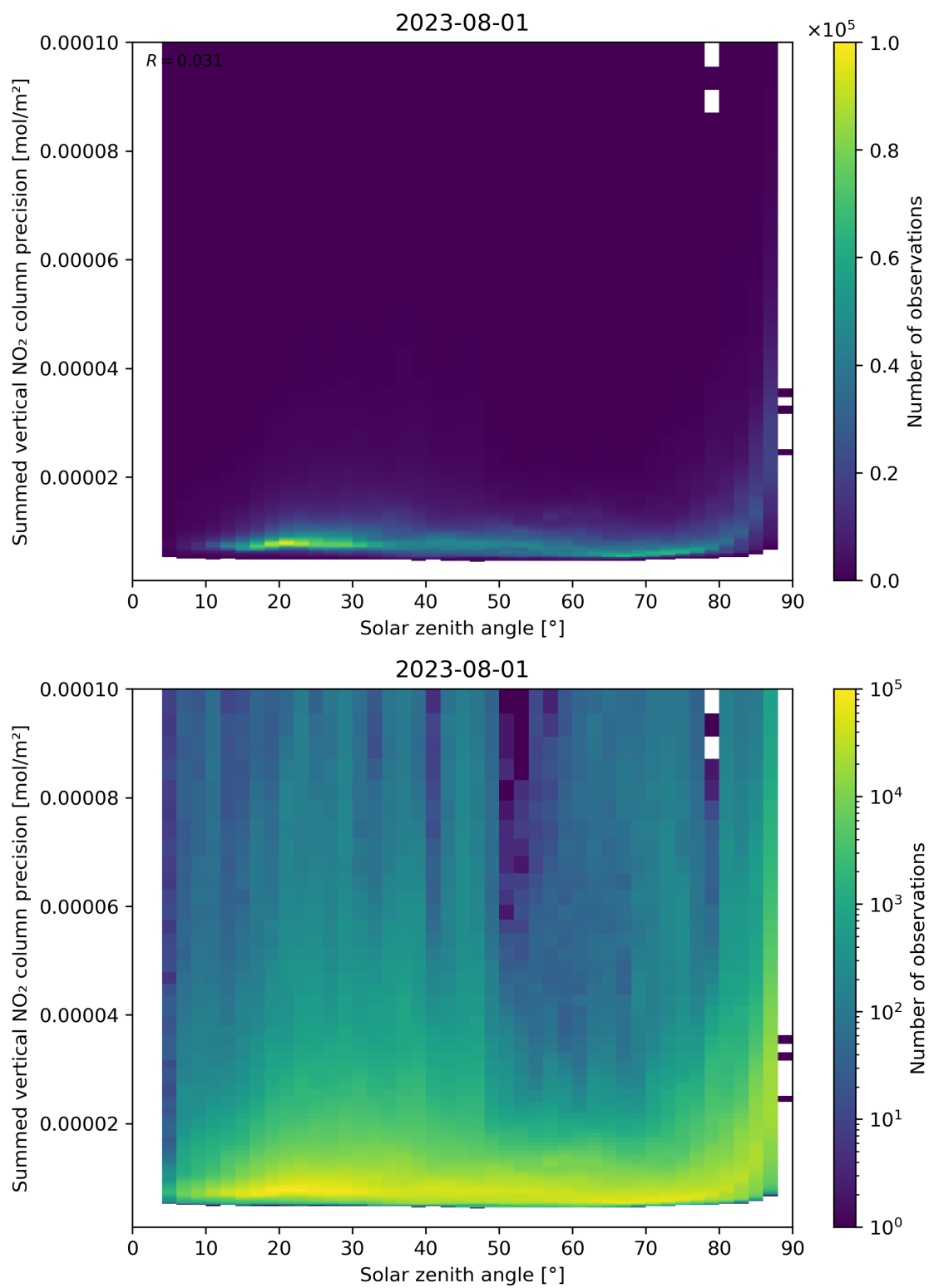
Figure 152: Scatter density plot of “Solar zenith angle” against “Summed vertical NO 2 column precision” for 2023-07-31 to 2023-08-02.
