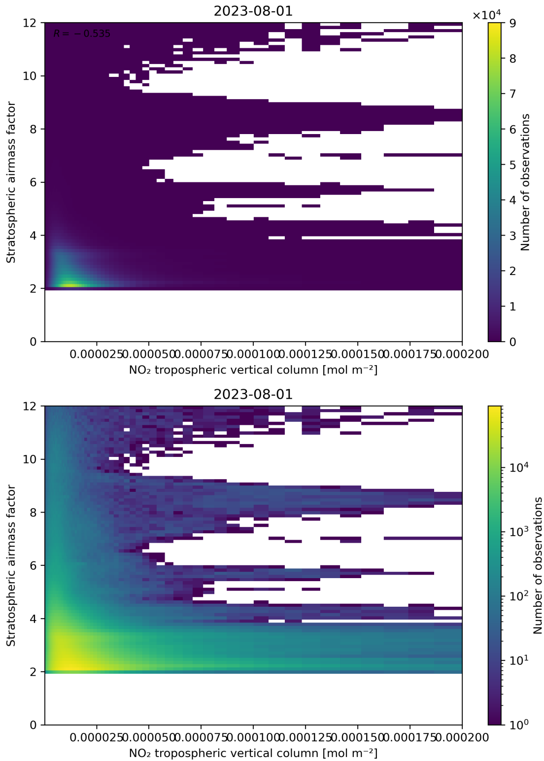
Figure 121: Scatter density plot of “NO 2 tropospheric vertical column” against “Stratospheric air mass factor” for 2023-07-31 to 2023-08-02.
