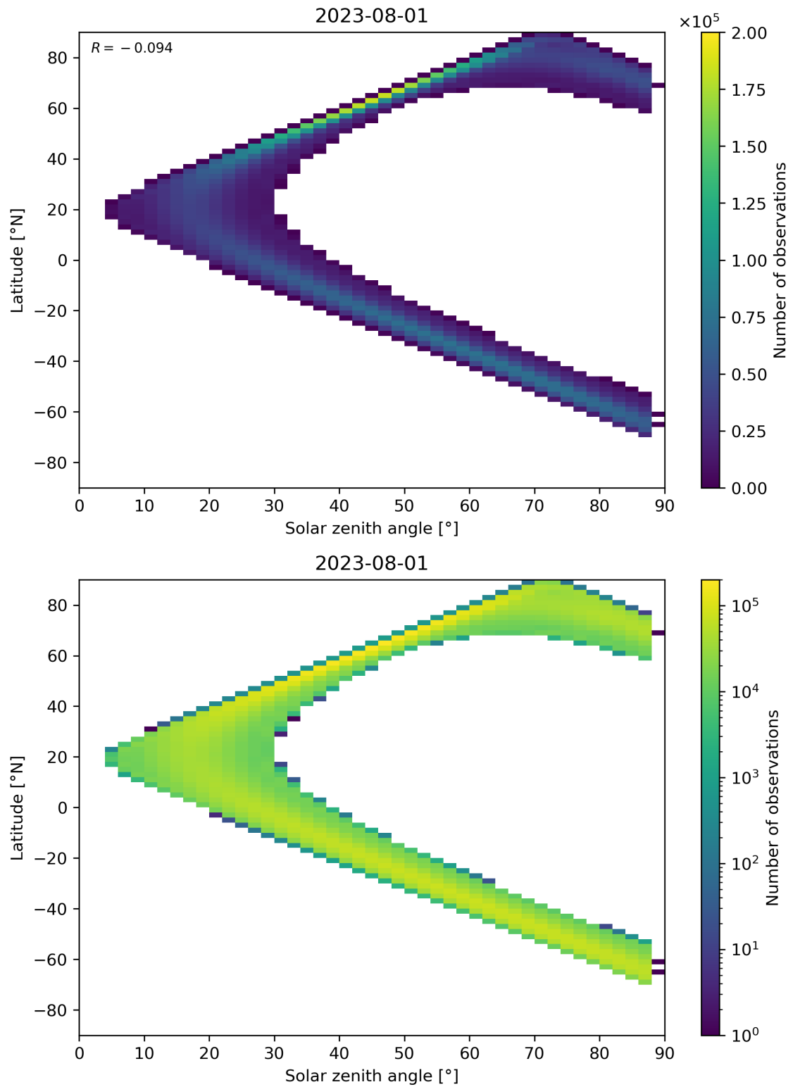
Figure 149: Scatter density plot of “Solar zenith angle” against “Latitude” for 2023-07-31 to 2023-08-02.
