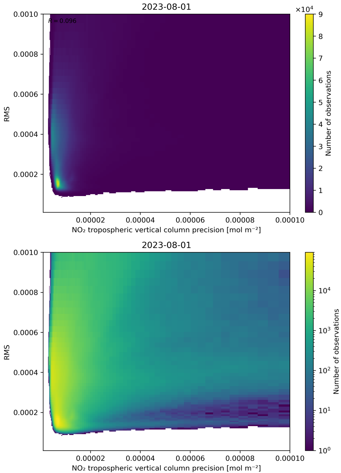
Figure 140: Scatter density plot of “NO 2 tropospheric vertical column precision” against “RMS” for 2023-07-31 to 2023-08-02.
