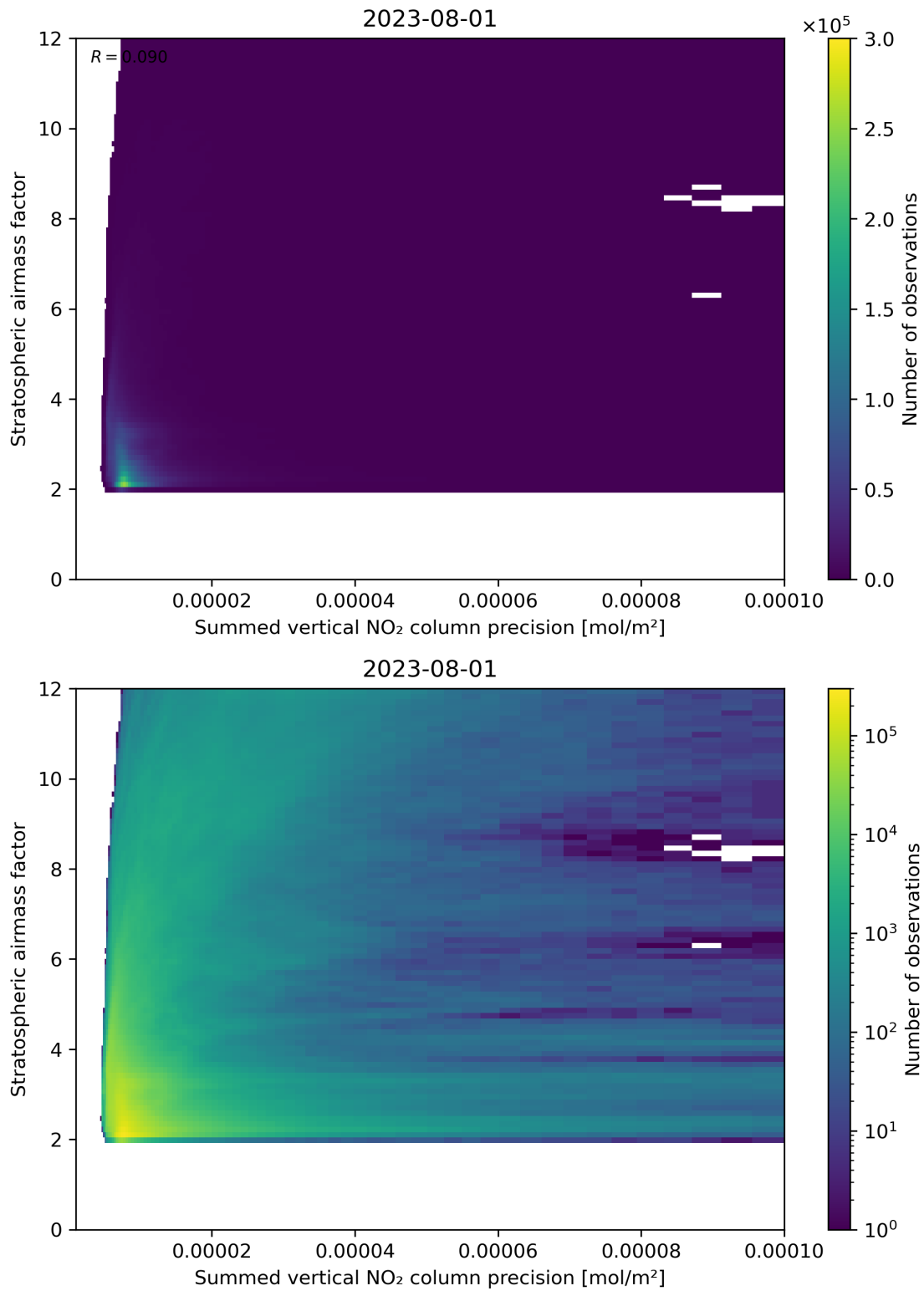
Figure 106: Scatter density plot of “Summed vertical NO 2 column precision” against “Stratospheric airmass factor” for 2023-07-31 to 2023-08-02.
