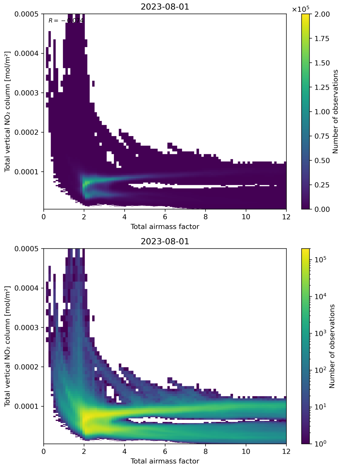
Figure 67: Scatter density plot of “Total airmass factor” against “Total vertical NO 2 column” for 2023-07-31 to 2023-08-02.
