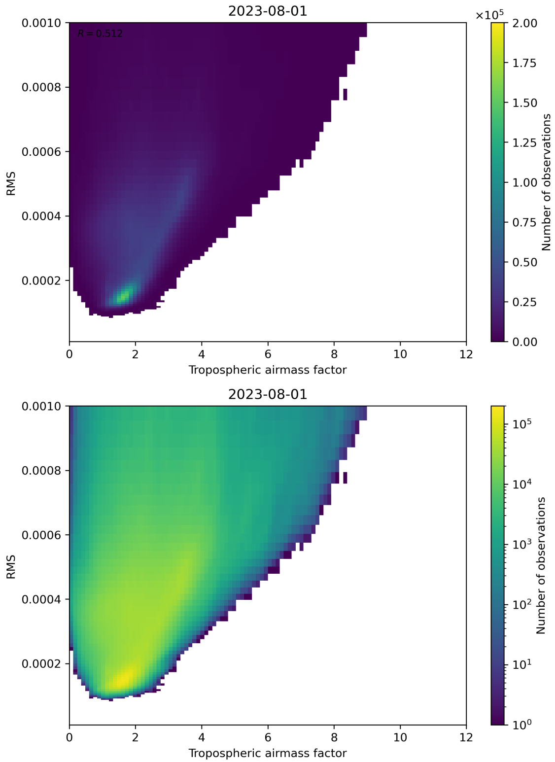
Figure 79: Scatter density plot of “Tropospheric airmass factor” against “RMS” for 2023-07-31 to 2023-08-02.
