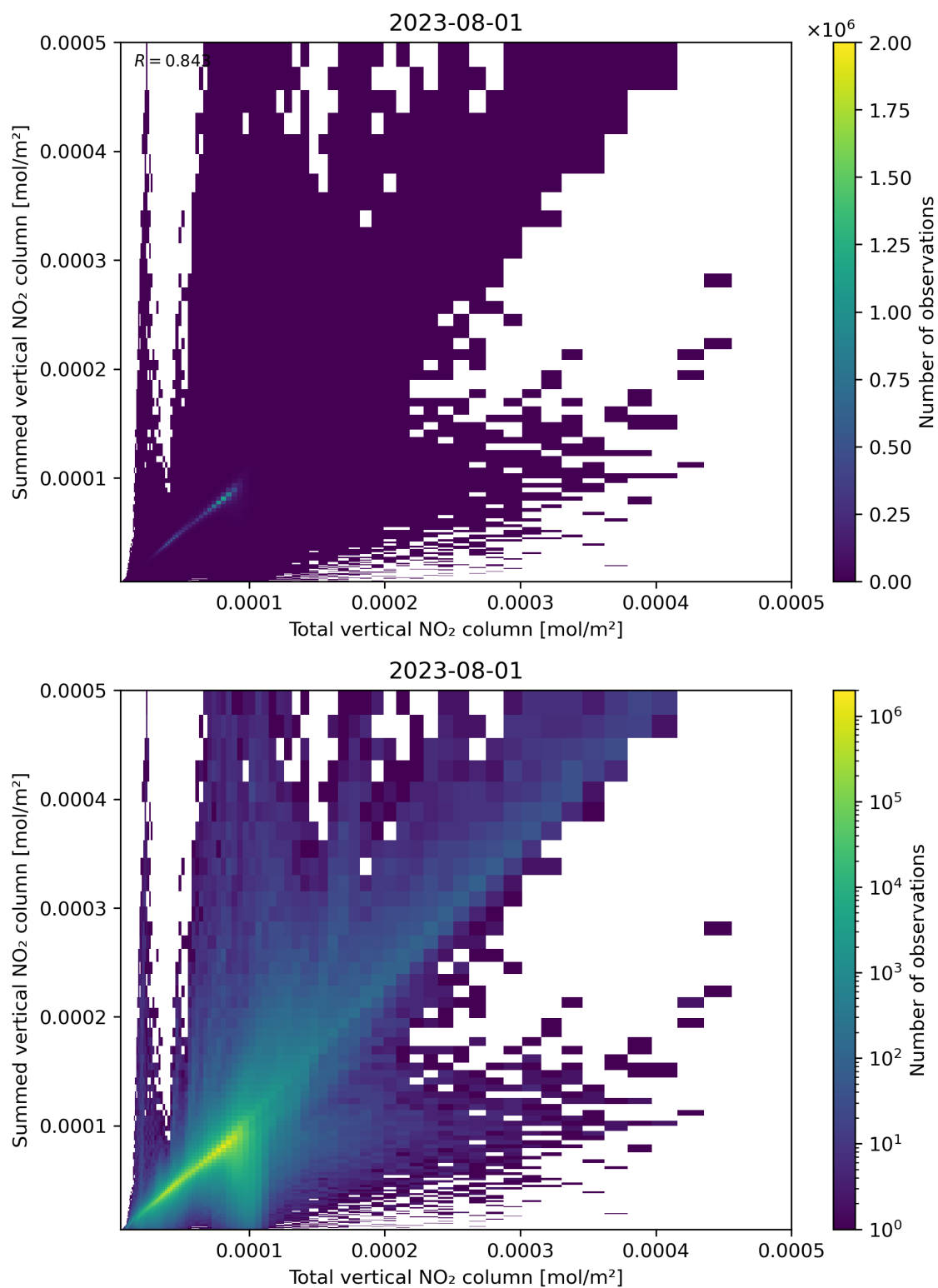
Figure 112: Scatter density plot of “Total vertical NO 2 column” against “Summed vertical NO 2 column” for 2023-07-31 to 2023-08-02.
