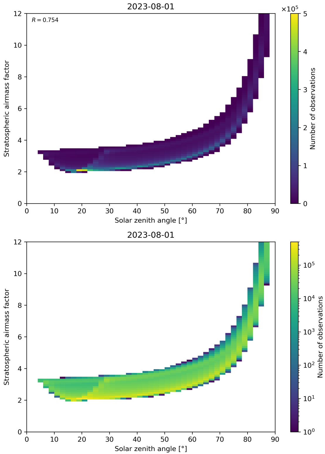
Figure 145: Scatter density plot of “Solar zenith angle” against “Stratospheric airmass factor” for 2023-07-31 to 2023-08-02.
