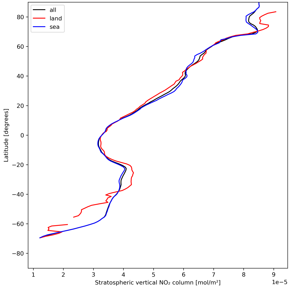
Figure 19: Zonal average of “Stratospheric vertical NO 2 column” for 2023-07-31 to 2023-08-02.
