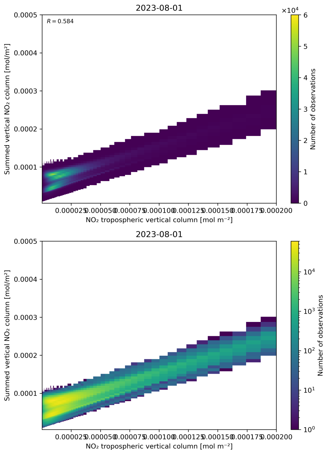
Figure 126: Scatter density plot of “NO 2 tropospheric vertical column” against “Summed vertical NO 2 column” for 2023-07-31 to 2023-08-02.
