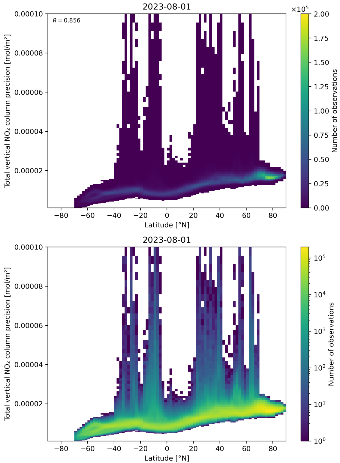
Figure 91: Scatter density plot of “Latitude” against “Total vertical NO 2 column precision” for 2023-07-31 to 2023-08-02.
