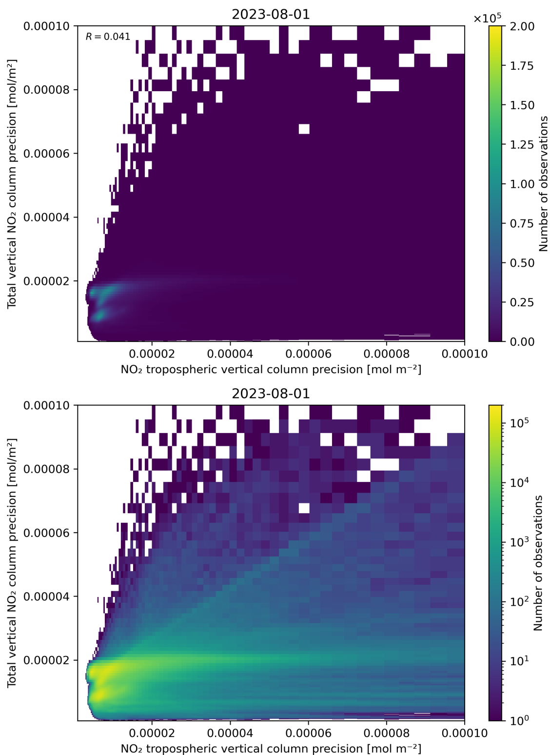
Figure 139: Scatter density plot of “NO 2 tropospheric vertical column precision” against “Total vertical NO 2 column precision” for 2023-07-31 to 2023-08-02.
