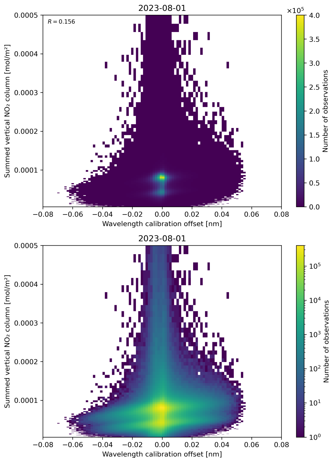
Figure 177: Scatter density plot of “Wavelength calibration offset” against “Summed vertical NO 2 column” for 2023-07-31 to 2023-08-02.
