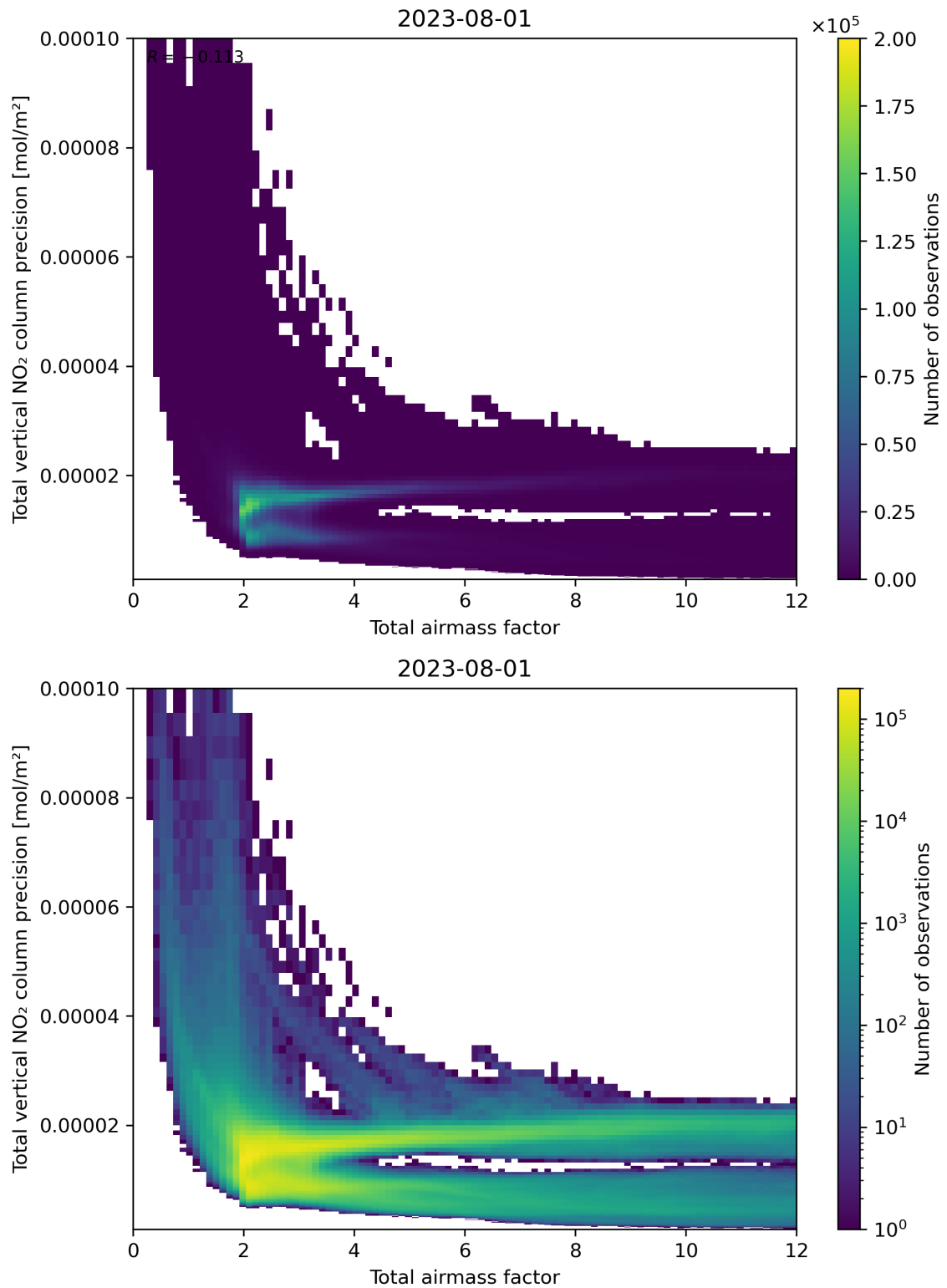
Figure 68: Scatter density plot of “Total airmass factor” against “Total vertical NO 2 column precision” for 2023-07-31 to 2023-08-02.
