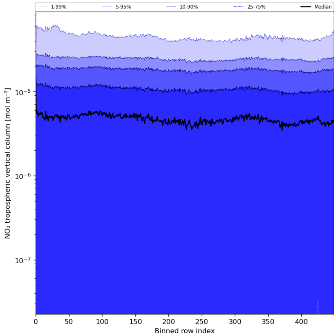
Figure 46: Along track statistics of “NO 2 tropospheric vertical column” for 2023-07-31 to 2023-08-02
