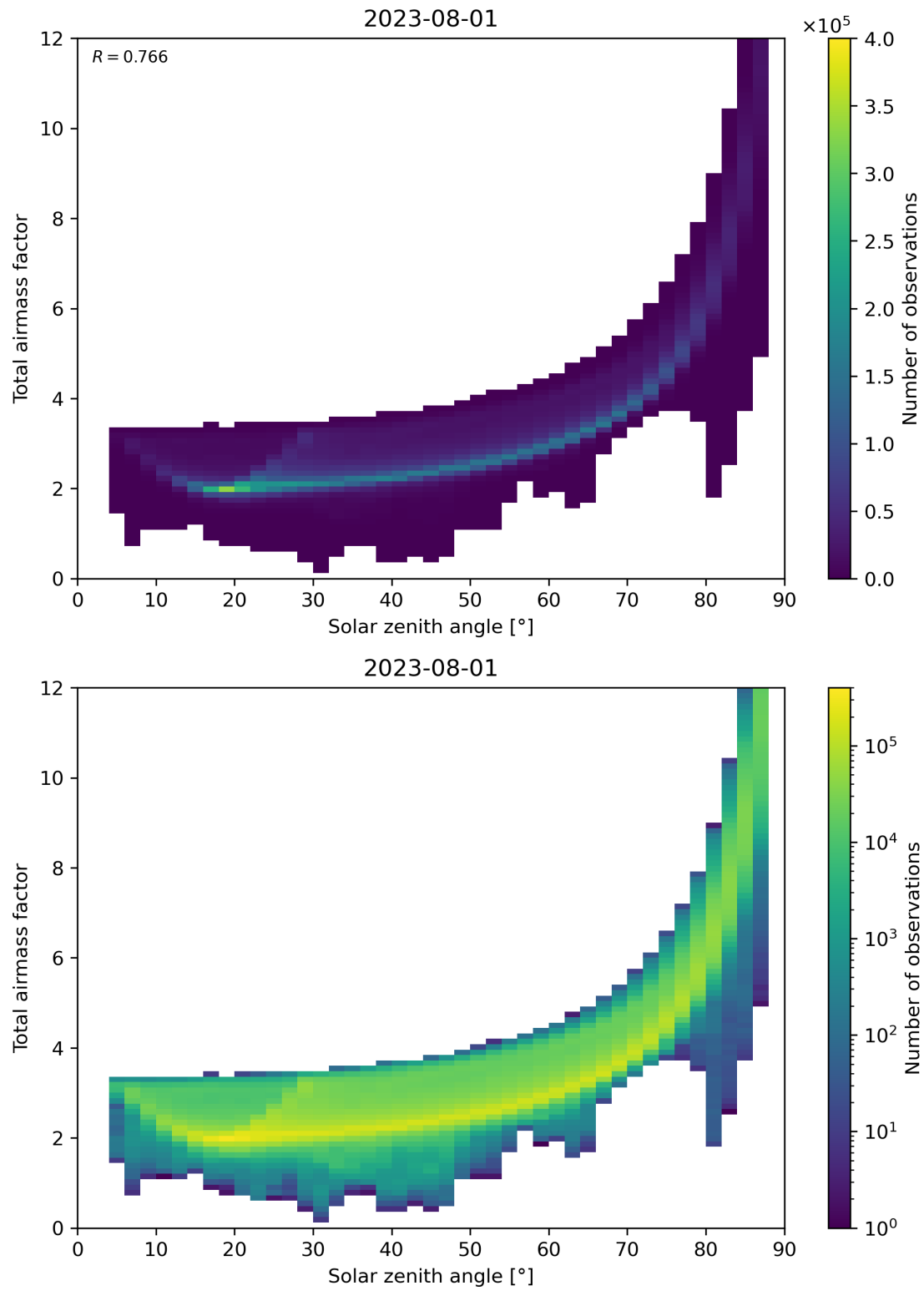
Figure 146: Scatter density plot of “Solar zenith angle” against “Total air mass factor” for 2023-07-31 to 2023-08-02.
