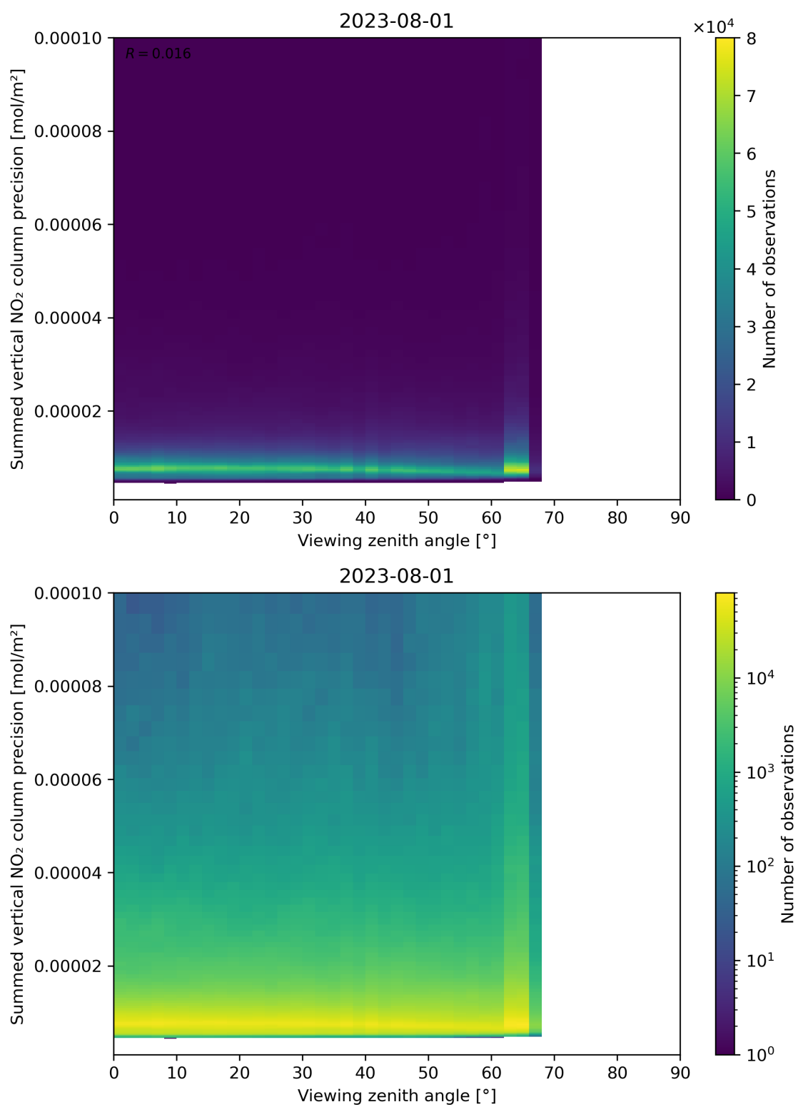
Figure 166: Scatter density plot of “Viewing zenith angle” against “Summed vertical NO 2 column precision” for 2023-07-31 to 2023-08-02.
