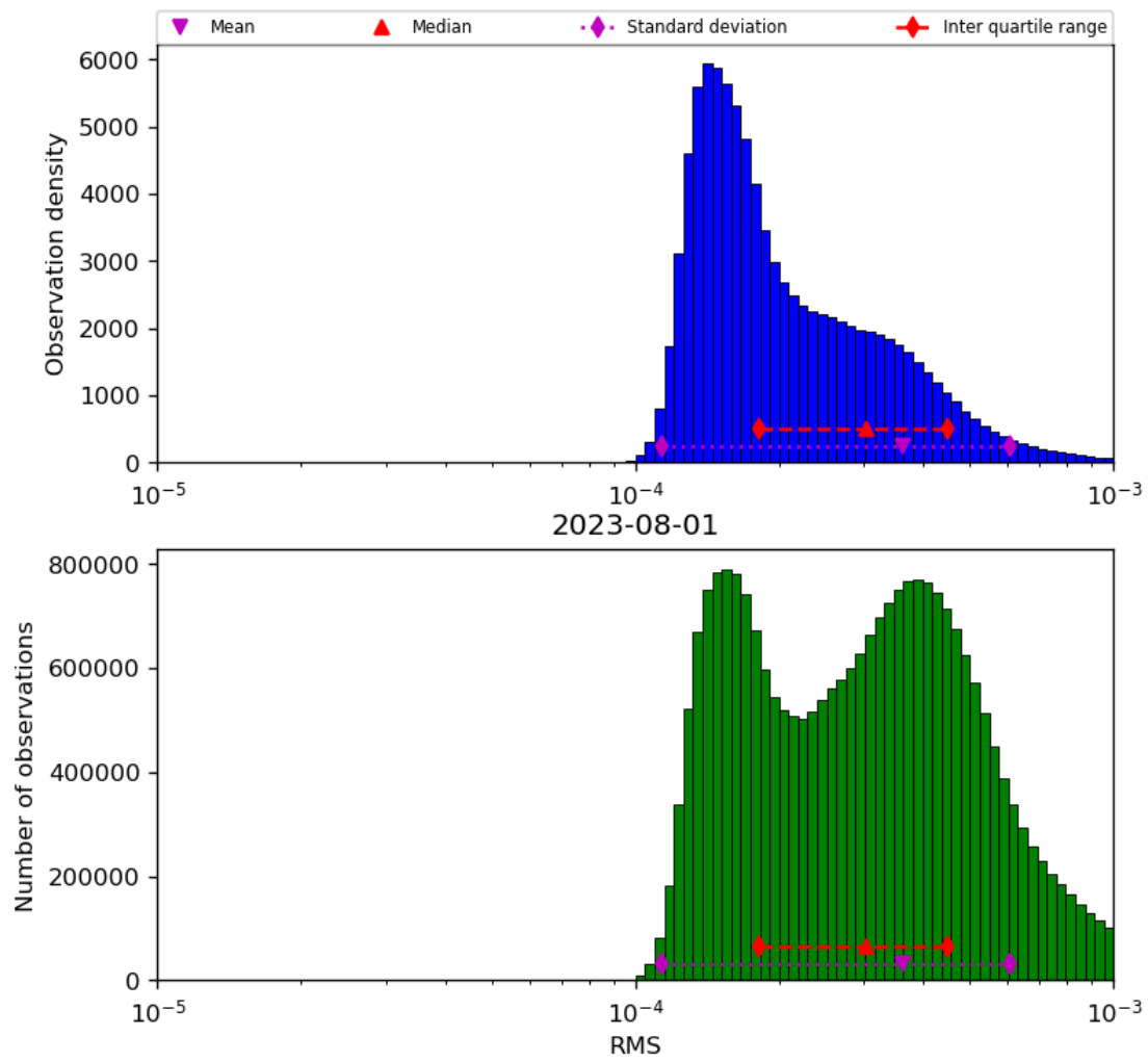
Figure 43: Histogram of “RMS” for 2023-07-31 to 2023-08-02
