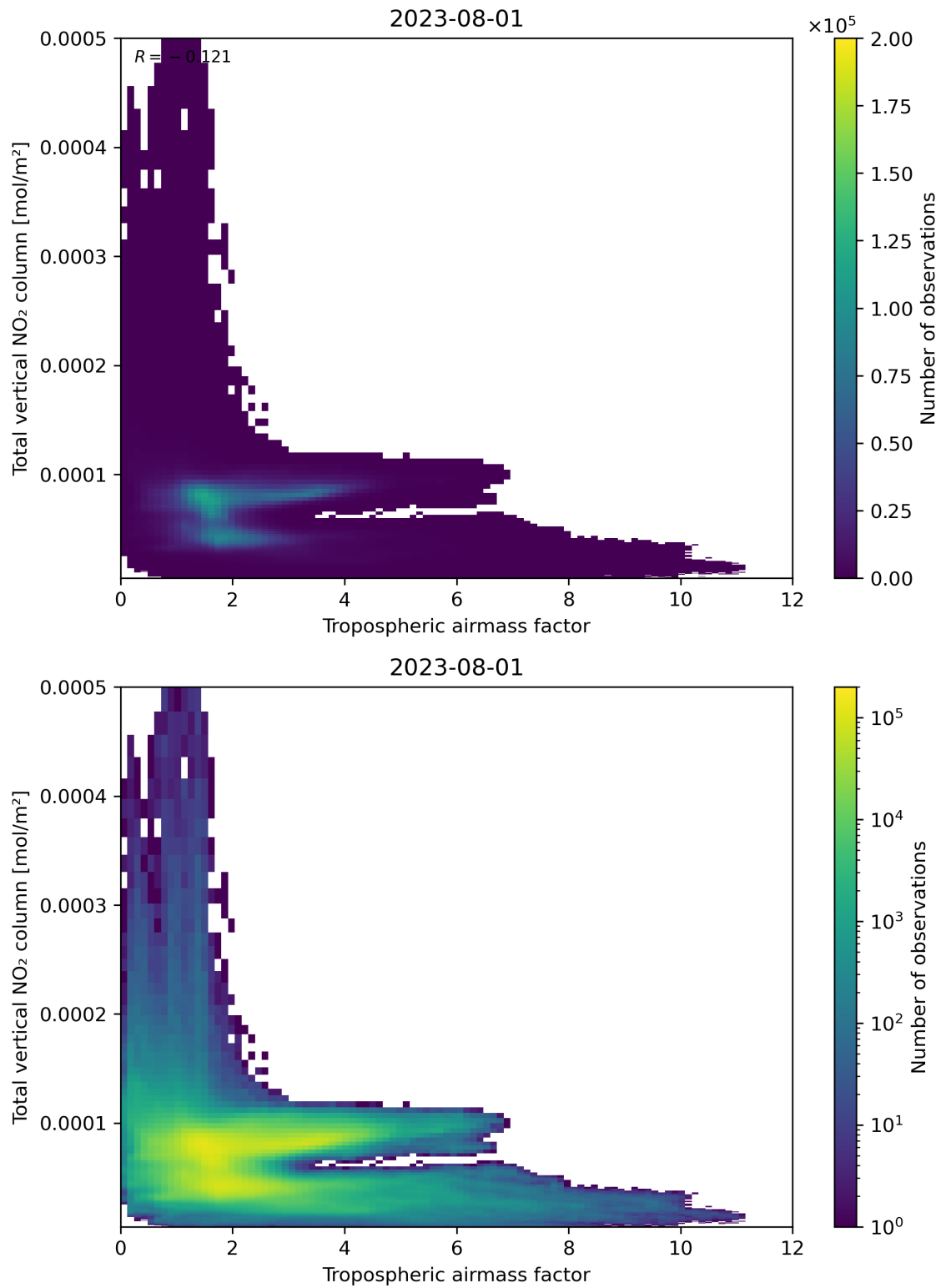
Figure 77: Scatter density plot of “Tropospheric airmass factor” against “Total vertical NO 2 column” for 2023-07-31 to 2023-08-02.
