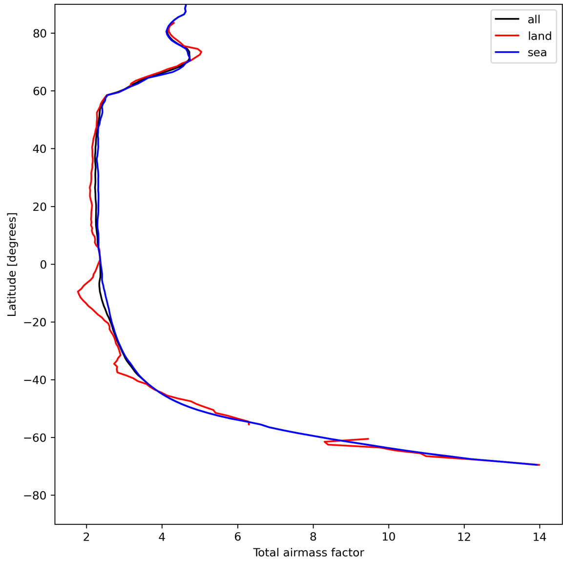
Figure 15: Zonal average of “Total airmass factor” for 2023-07-31 to 2023-08-02.
