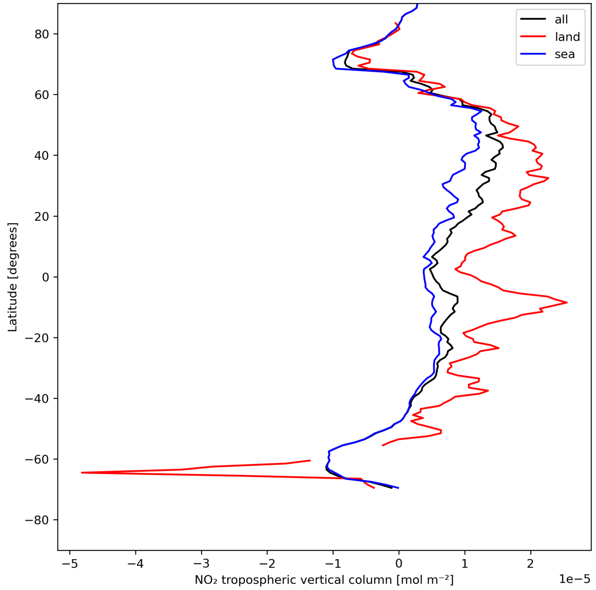
Figure 12: Zonal average of “NO 2 tropospheric vertical column” for 2023-07-31 to 2023-08-02.
