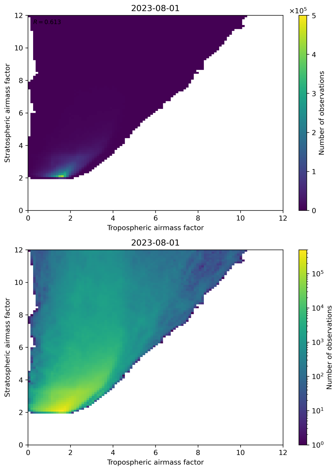
Figure 71: Scatter density plot of “Tropospheric airmass factor” against “Stratospheric airmass factor” for 2023-07-31 to 2023-08-02.
