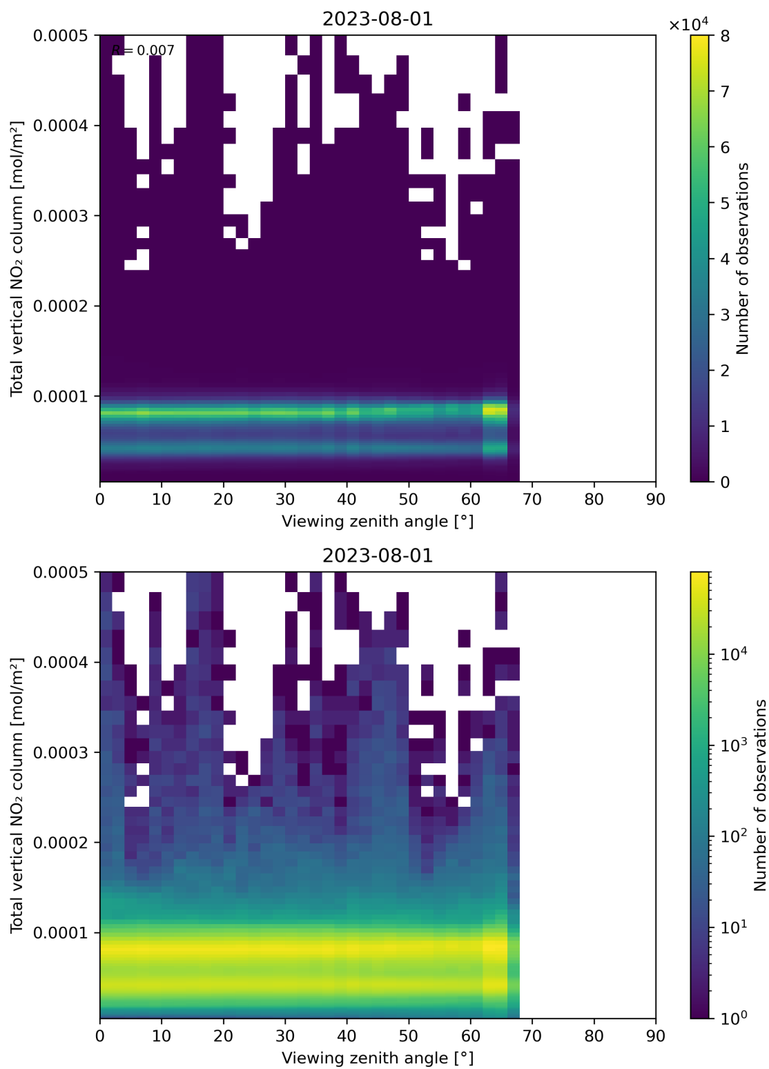
Figure 167: Scatter density plot of “Viewing zenith angle” against “Total vertical NO 2 column” for 2023-07-31 to 2023-08-02.
