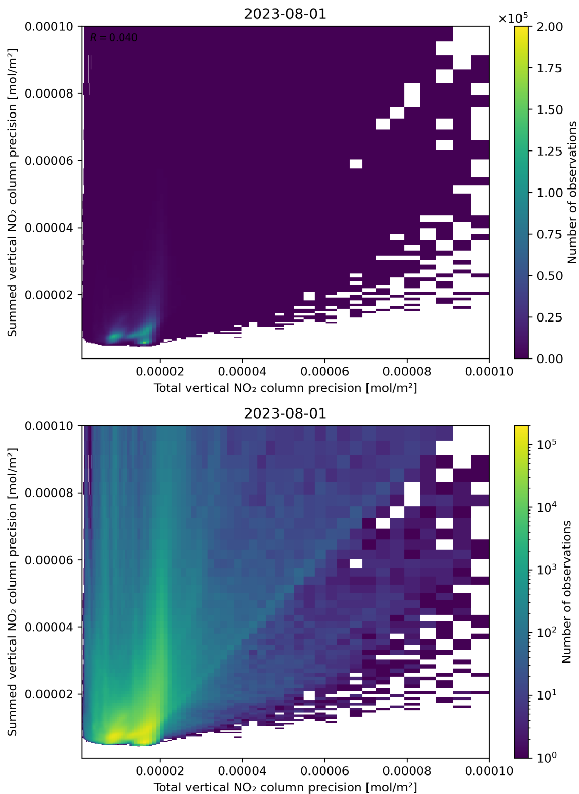
Figure 118: Scatter density plot of “Total vertical NO 2 column precision” against “Summed vertical NO 2 column precision” for 2023-07-31 to 2023-08-02.
