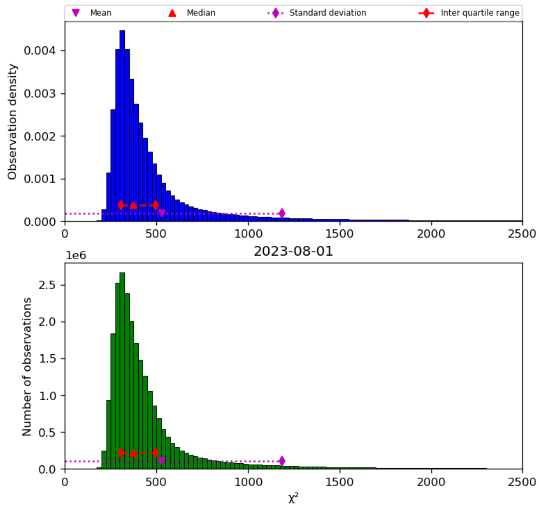
Figure 42: Histogram of “ \chi^2 ” for 2023-07-31 to 2023-08-02
