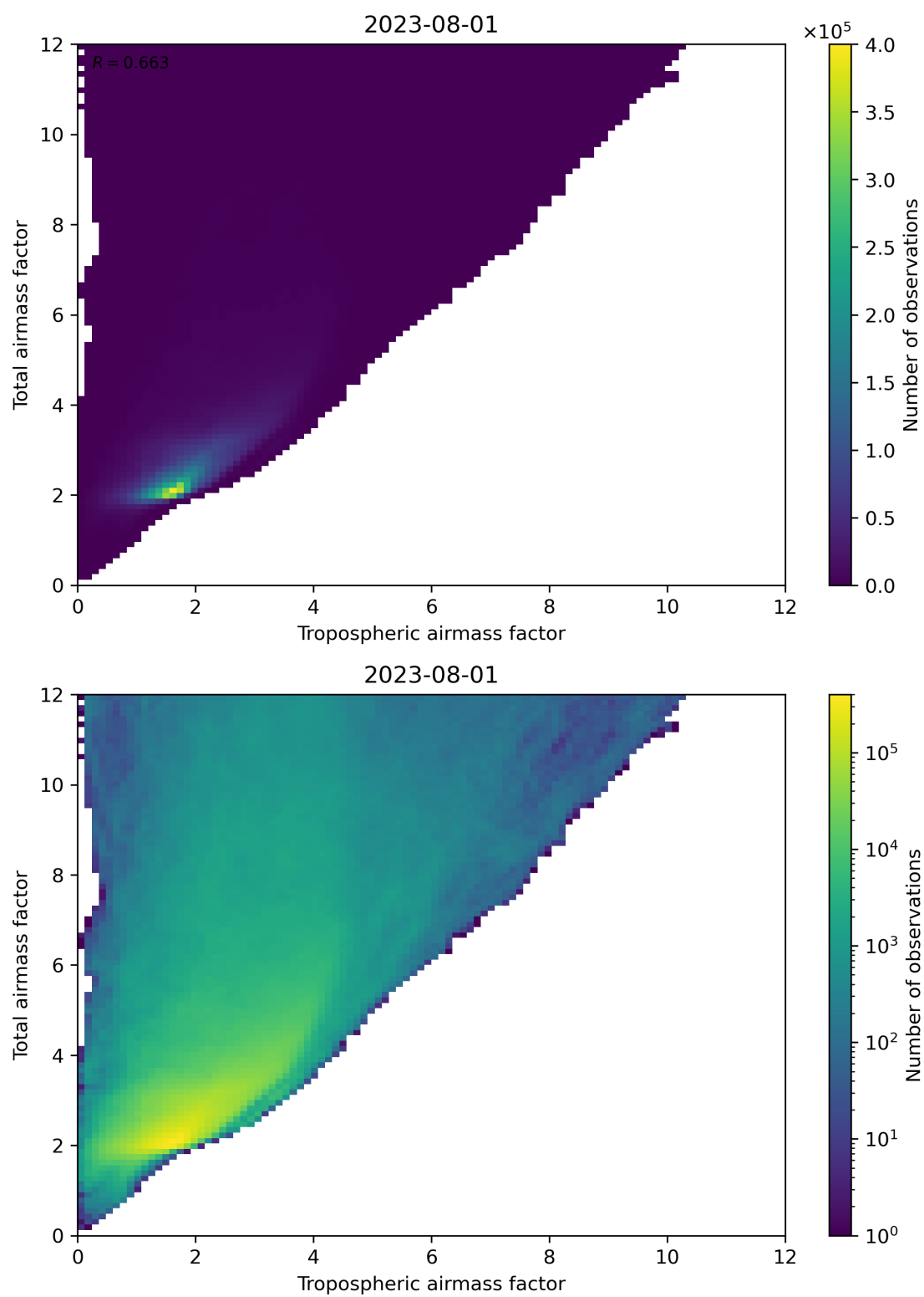
Figure 72: Scatter density plot of “Tropospheric airmass factor” against “Total airmass factor” for 2023-07-31 to 2023-08-02.
