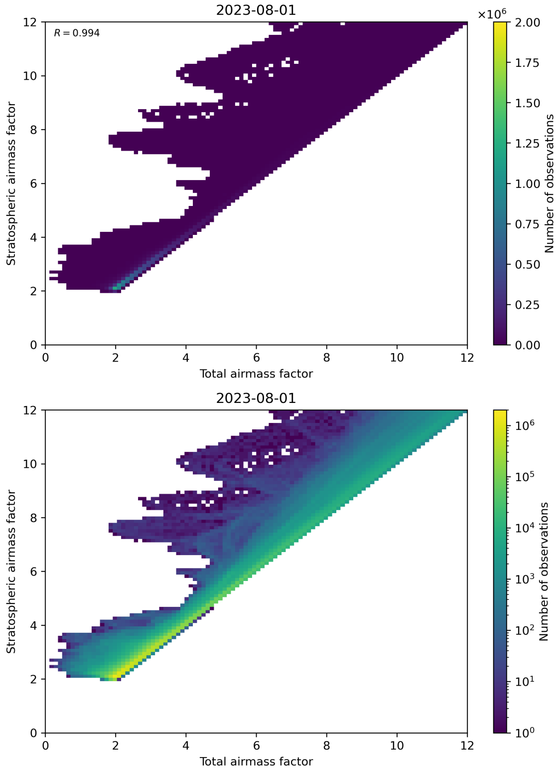
Figure 62: Scatter density plot of “Total airmass factor” against “Stratospheric airmass factor” for 2023-07-31 to 2023-08-02.
