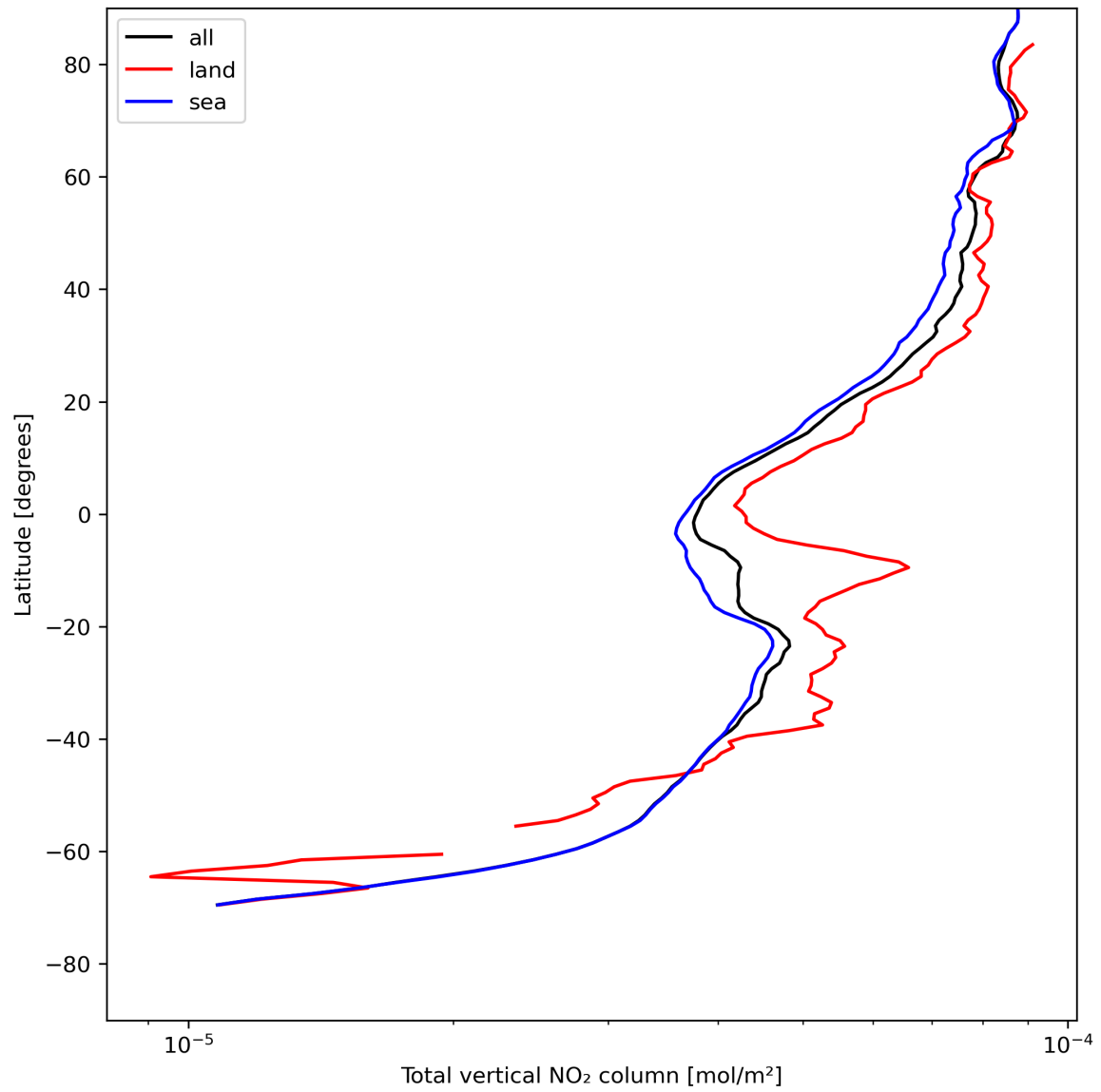
Figure 21: Zonal average of “Total vertical NO 2 column” for 2023-07-31 to 2023-08-02.
