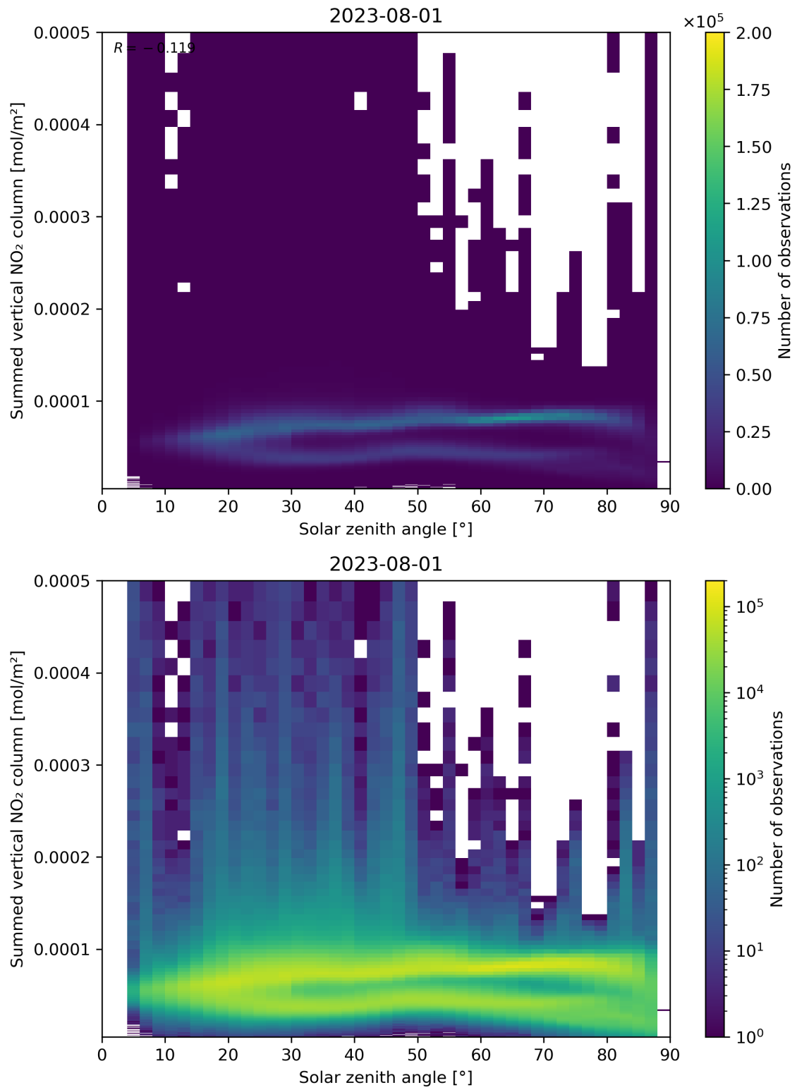
Figure 151: Scatter density plot of “Solar zenith angle” against “Summed vertical NO 2 column” for 2023-07-31 to 2023-08-02.
