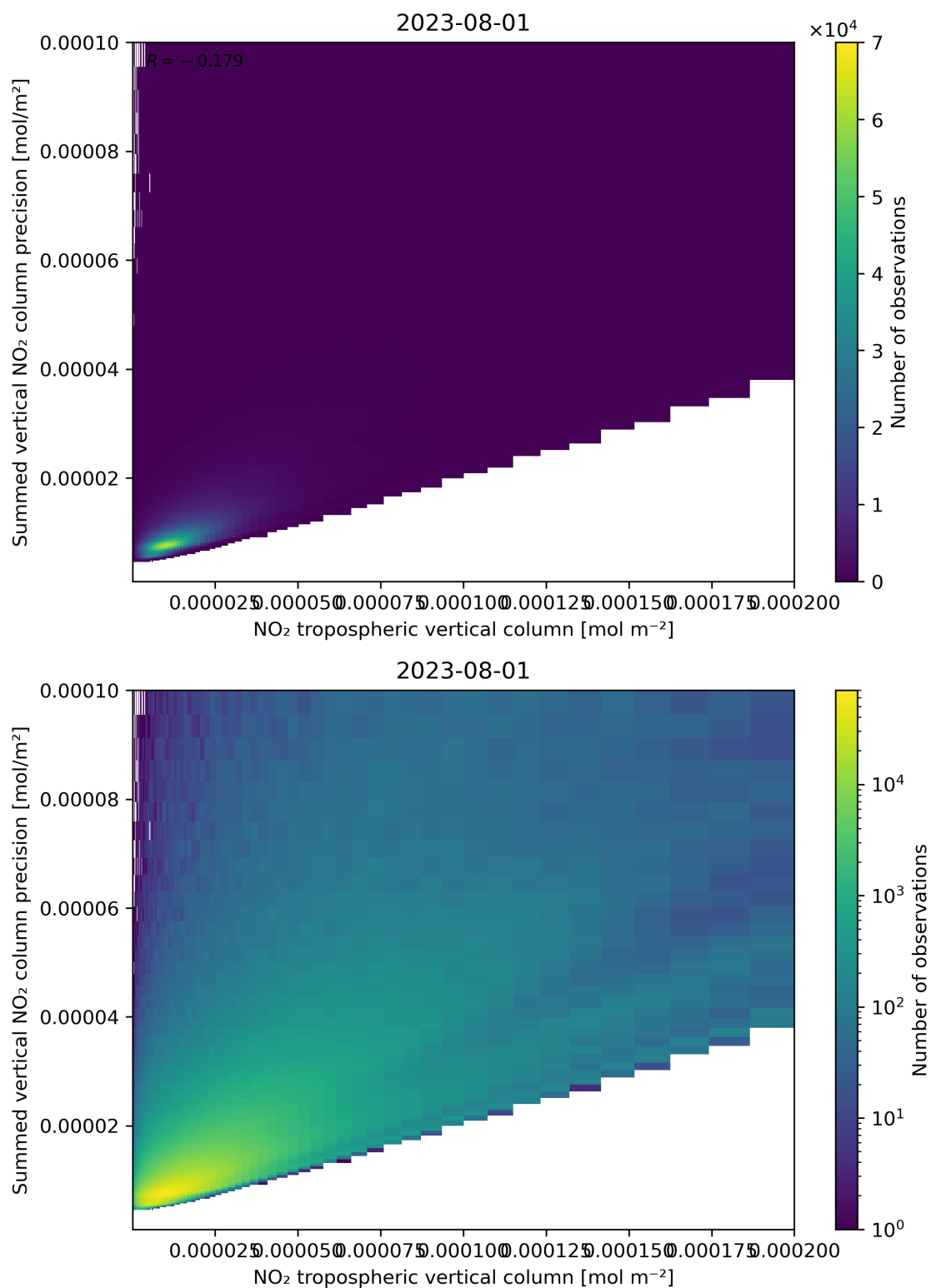
Figure 127: Scatter density plot of “NO 2 tropospheric vertical column” against “Summed vertical NO 2 column precision” for 2023-07-31 to 2023-08-02.
