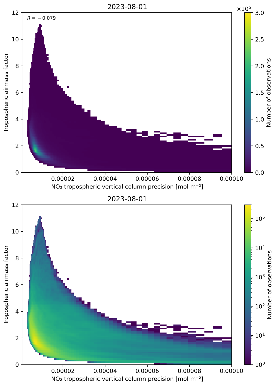
Figure 133: Scatter density plot of “NO 2 tropospheric vertical column precision” against “Tropospheric airmass factor” for 2023-07-31 to 2023-08-02.
