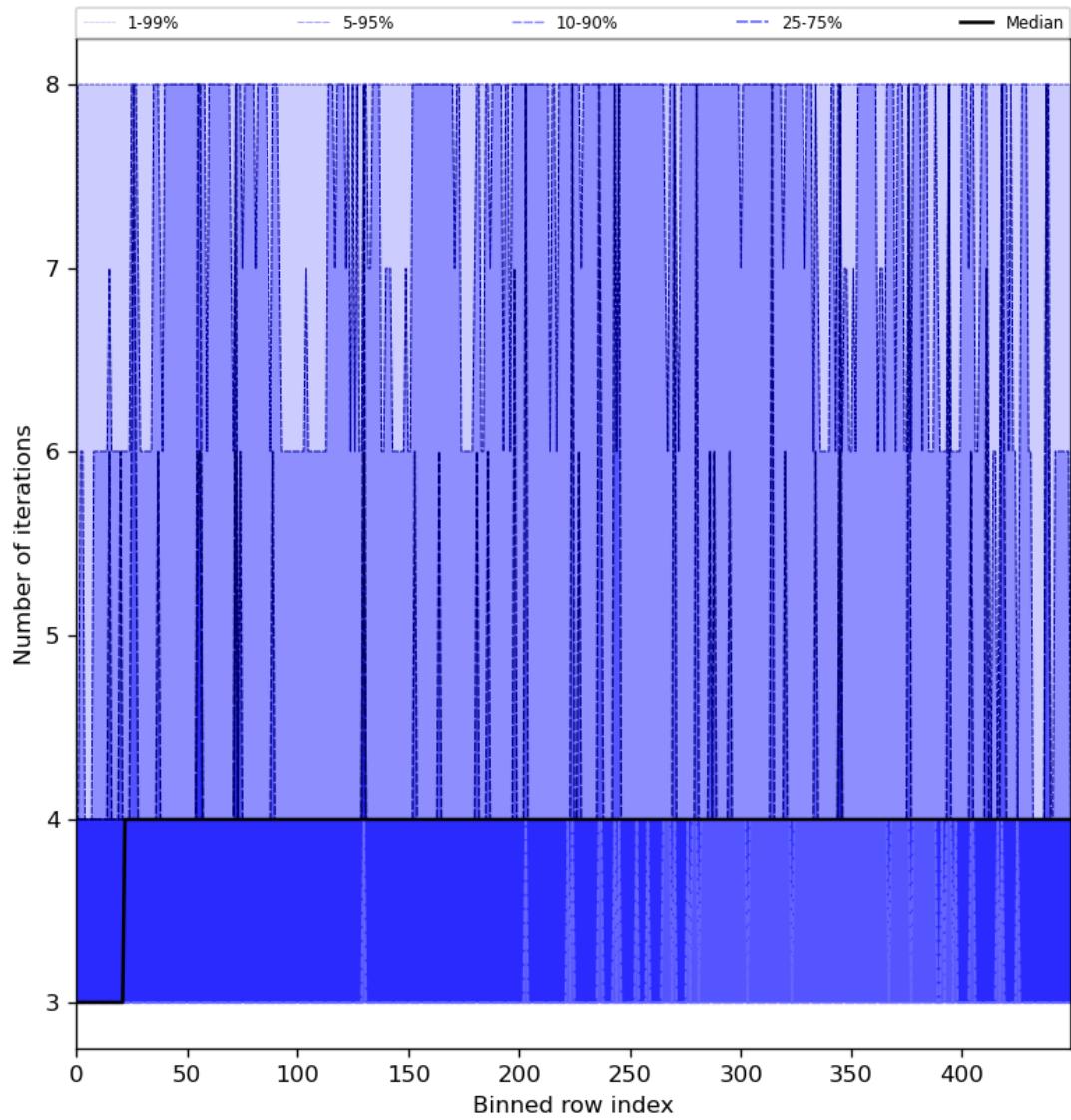
Figure 51: Along track statistics of “Number of iterations” for 2023-07-31 to 2023-08-02
