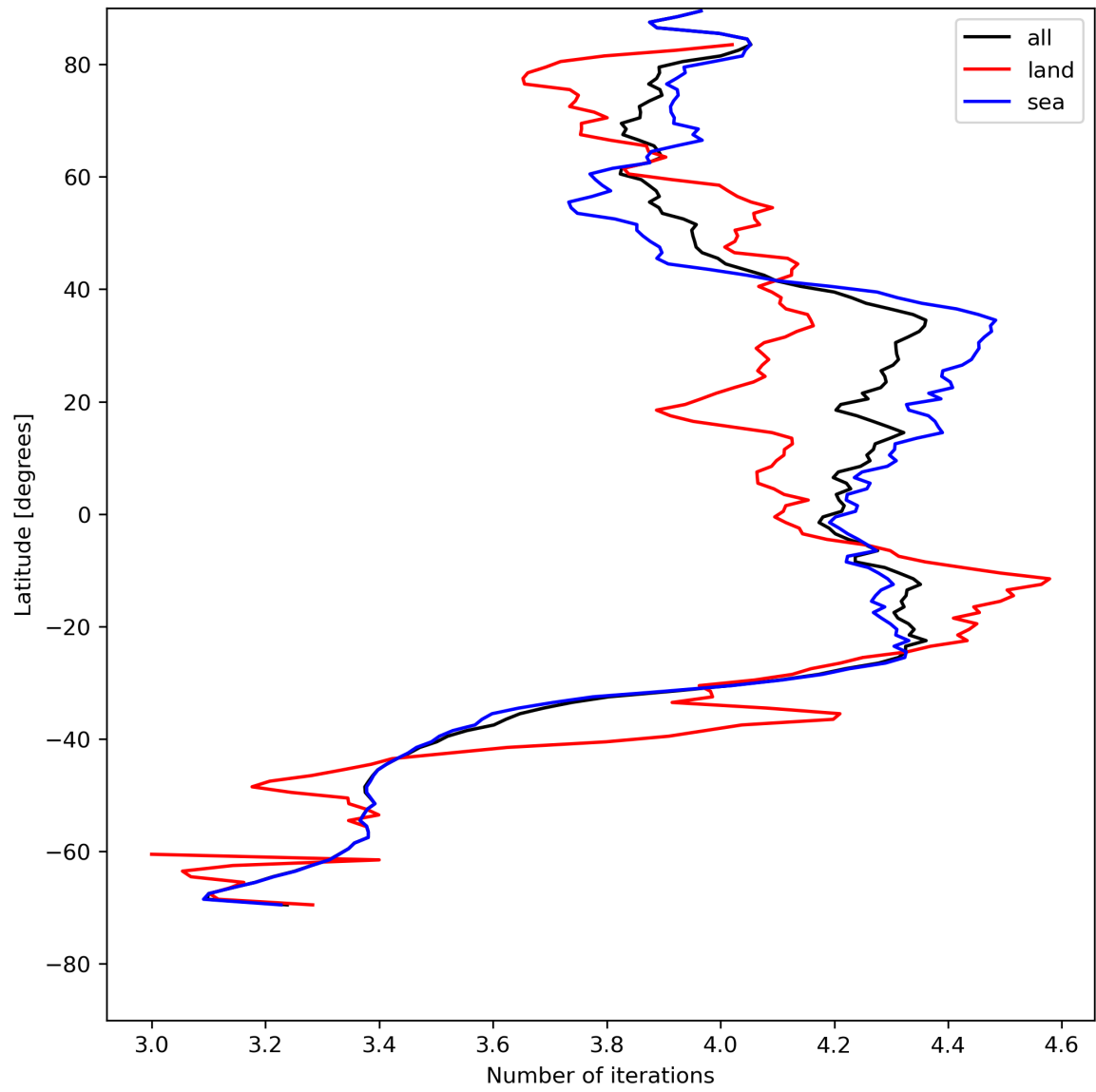
Figure 17: Zonal average of “Number of iterations” for 2023-07-31 to 2023-08-02.
