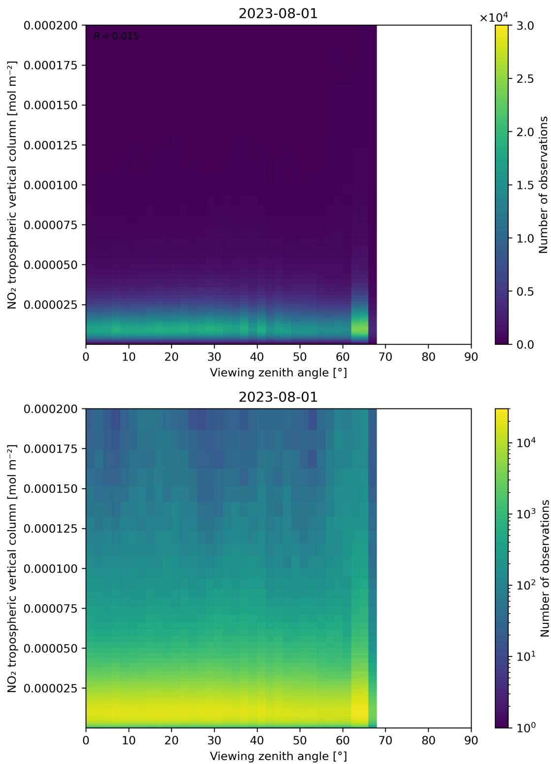
Figure 169: Scatter density plot of “Viewing zenith angle” against “NO 2 tropospheric vertical column” for 2023-07-31 to 2023-08-02.
