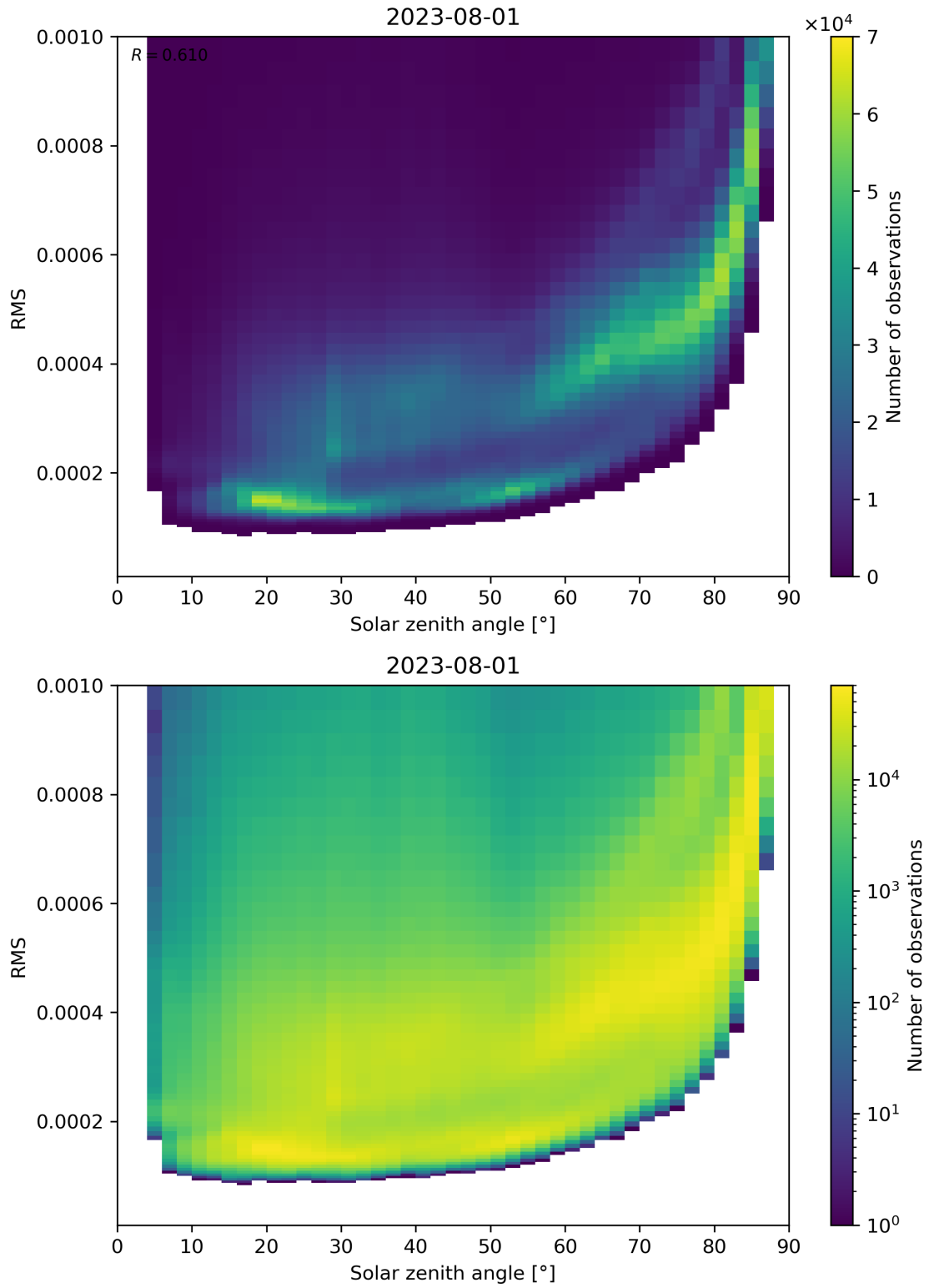
Figure 157: Scatter density plot of “Solar zenith angle” against “RMS” for 2023-07-31 to 2023-08-02.
