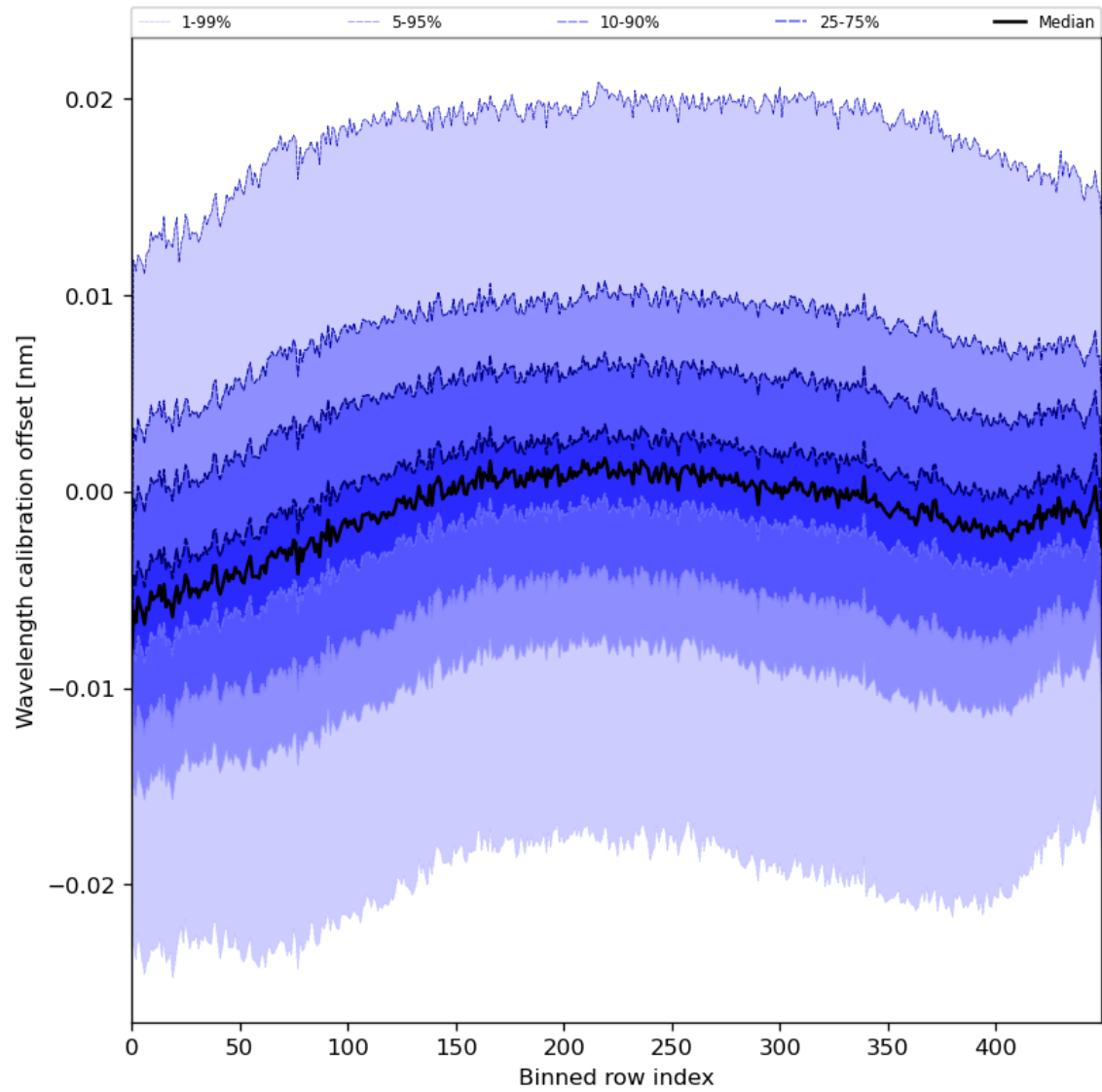
Figure 52: Along track statistics of “Wavelength calibration offset” for 2023-07-31 to 2023-08-02
