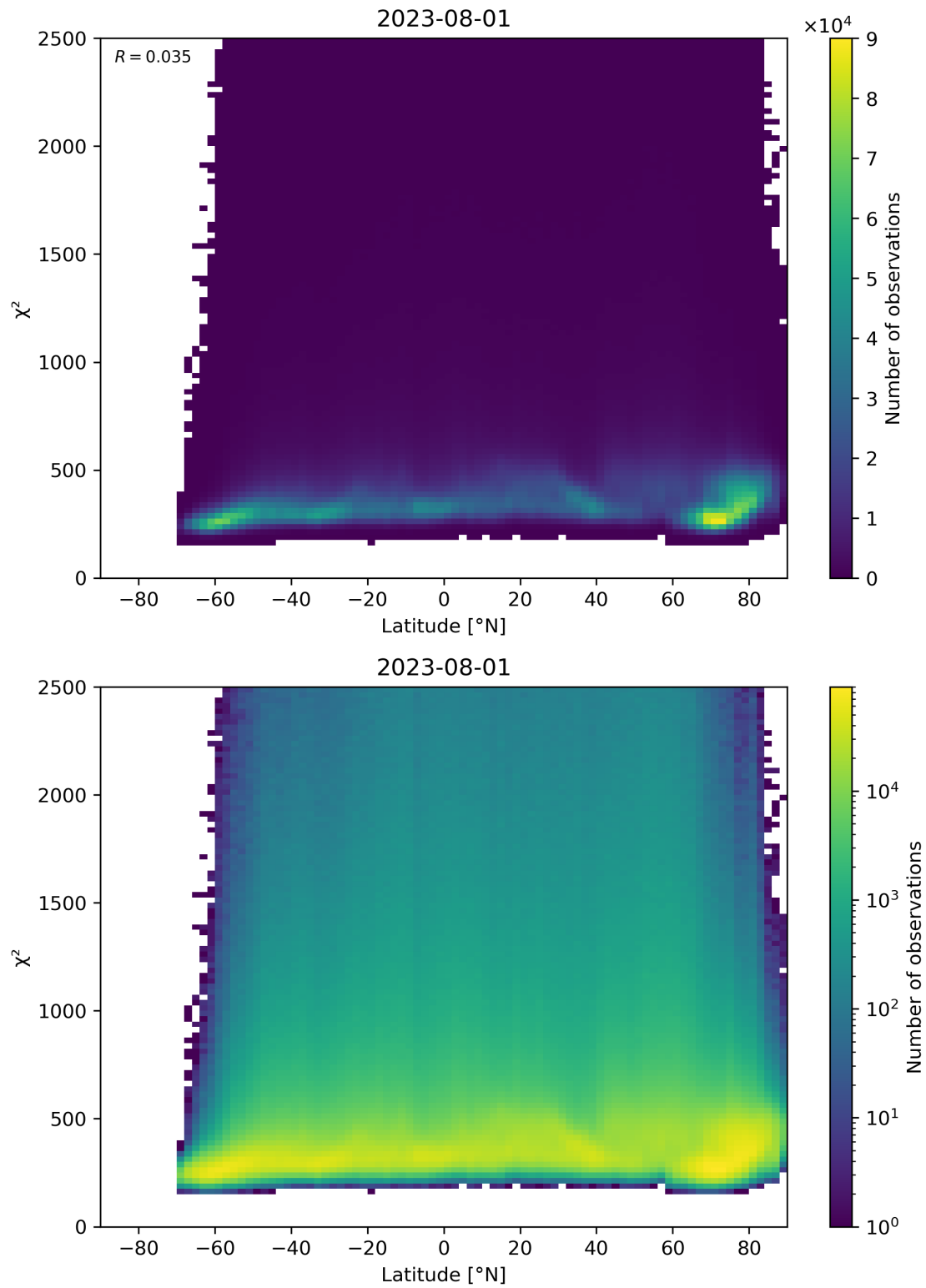
Figure 86: Scatter density plot of “Latitude” against “ \chi^2 ” for 2023-07-31 to 2023-08-02.
