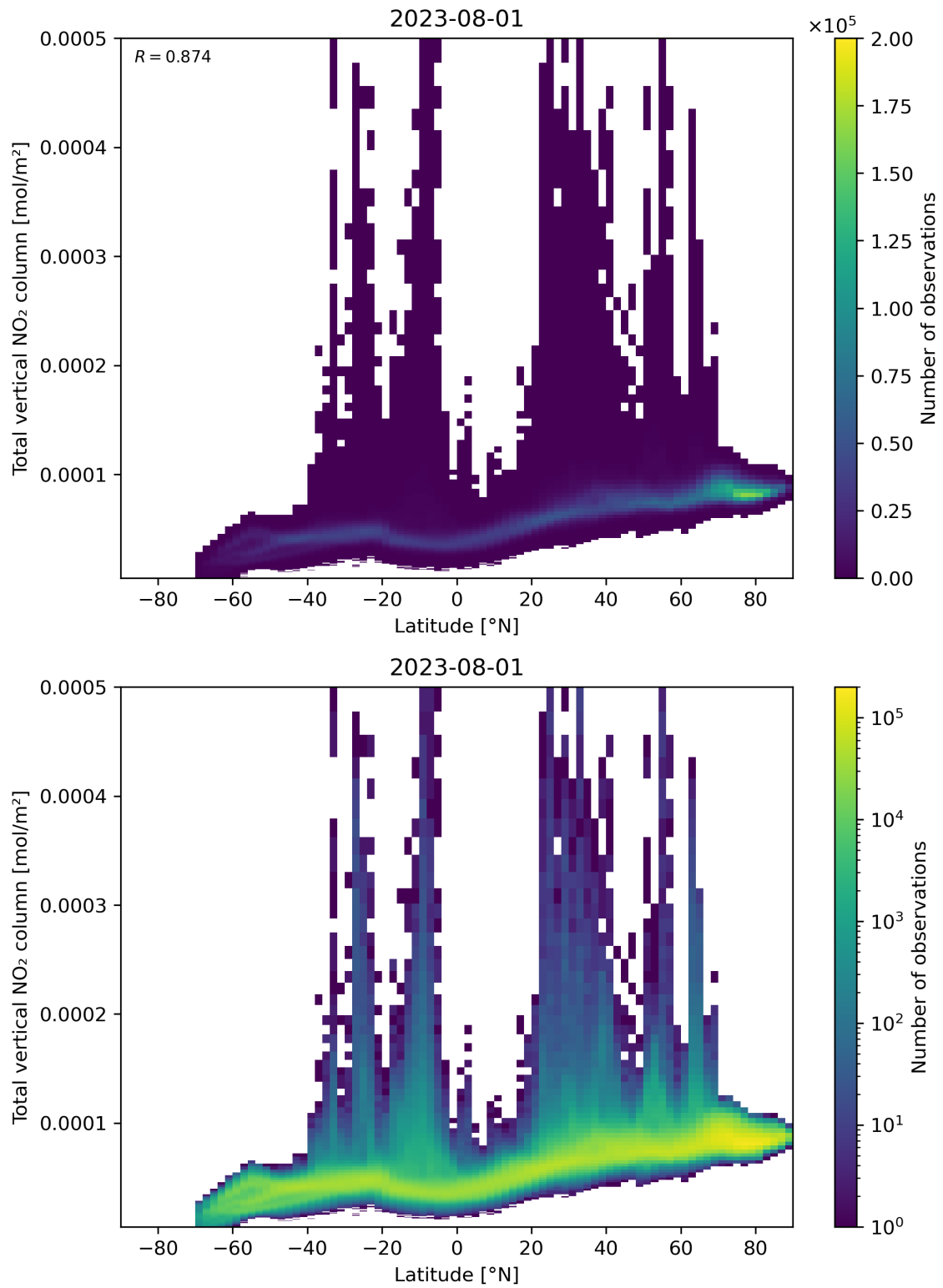
Figure 90: Scatter density plot of “Latitude” against “Total vertical NO 2 column” for 2023-07-31 to 2023-08-02.
