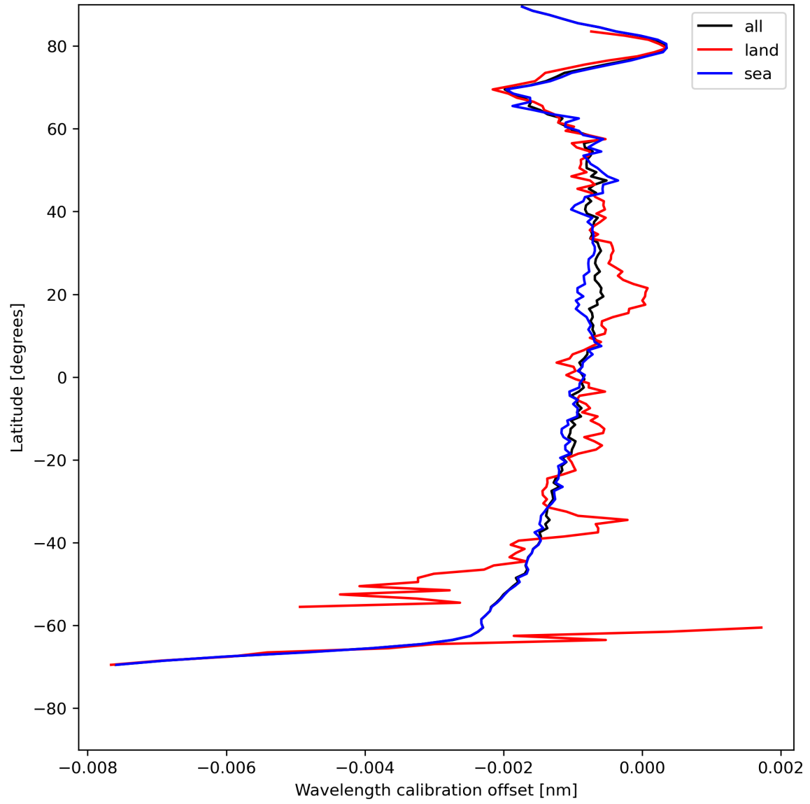
Figure 18: Zonal average of “Wavelength calibration offset” for 2023-07-31 to 2023-08-02.
