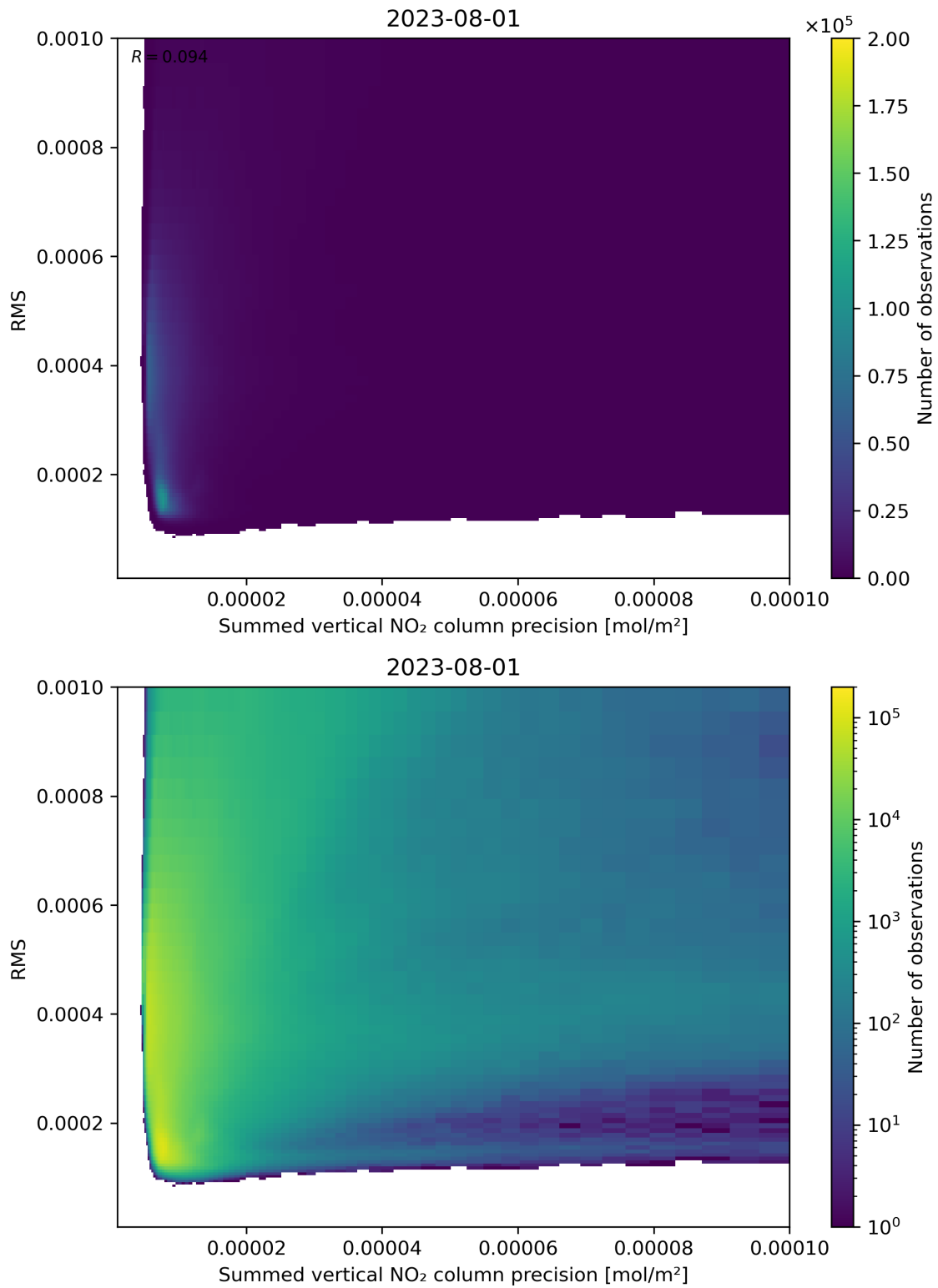
Figure 108: Scatter density plot of “Summed vertical NO 2 column precision” against “RMS” for 2023-07-31 to 2023-08-02.
