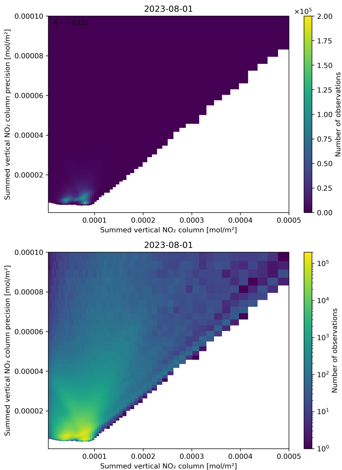
Figure 105: Scatter density plot of “Summed vertical NO 2 column” against “Summed vertical NO 2 column precision” for 2023-07-31 to 2023-08-02.
