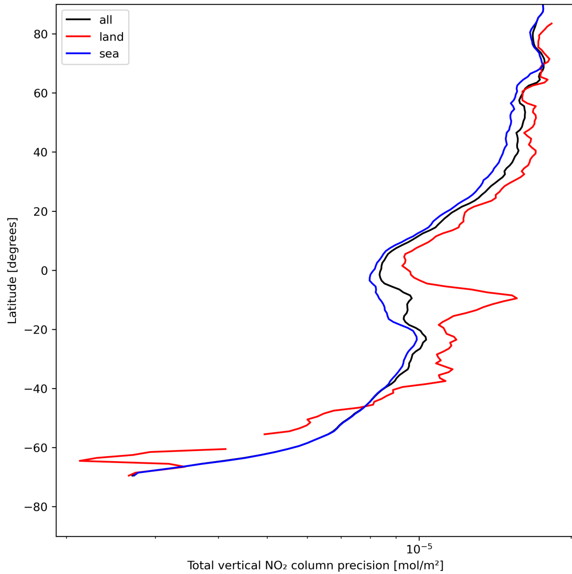
Figure 22: Zonal average of “Total vertical NO 2 column precision” for 2023-07-31 to 2023-08-02.
