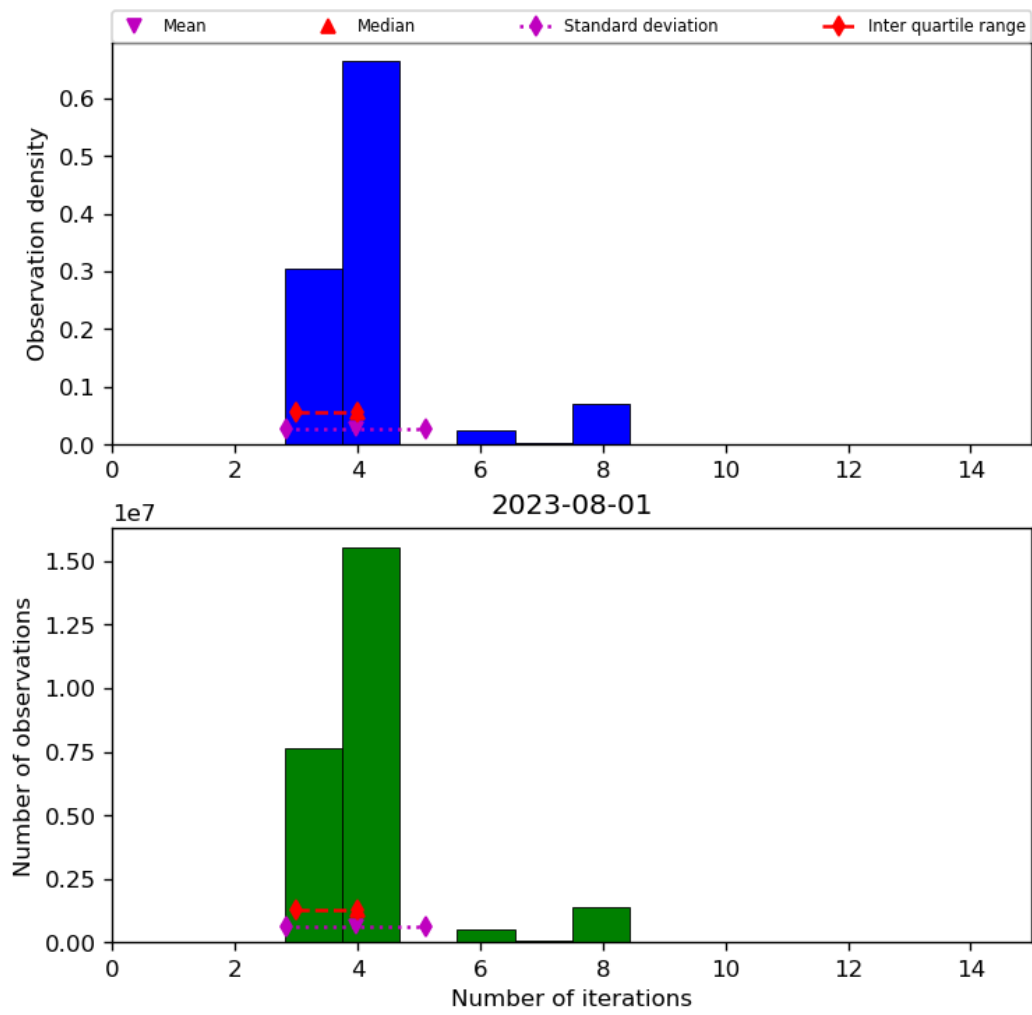
Figure 34: Histogram of "Number of iterations" for 2023-07-31 to 2023-08-02
