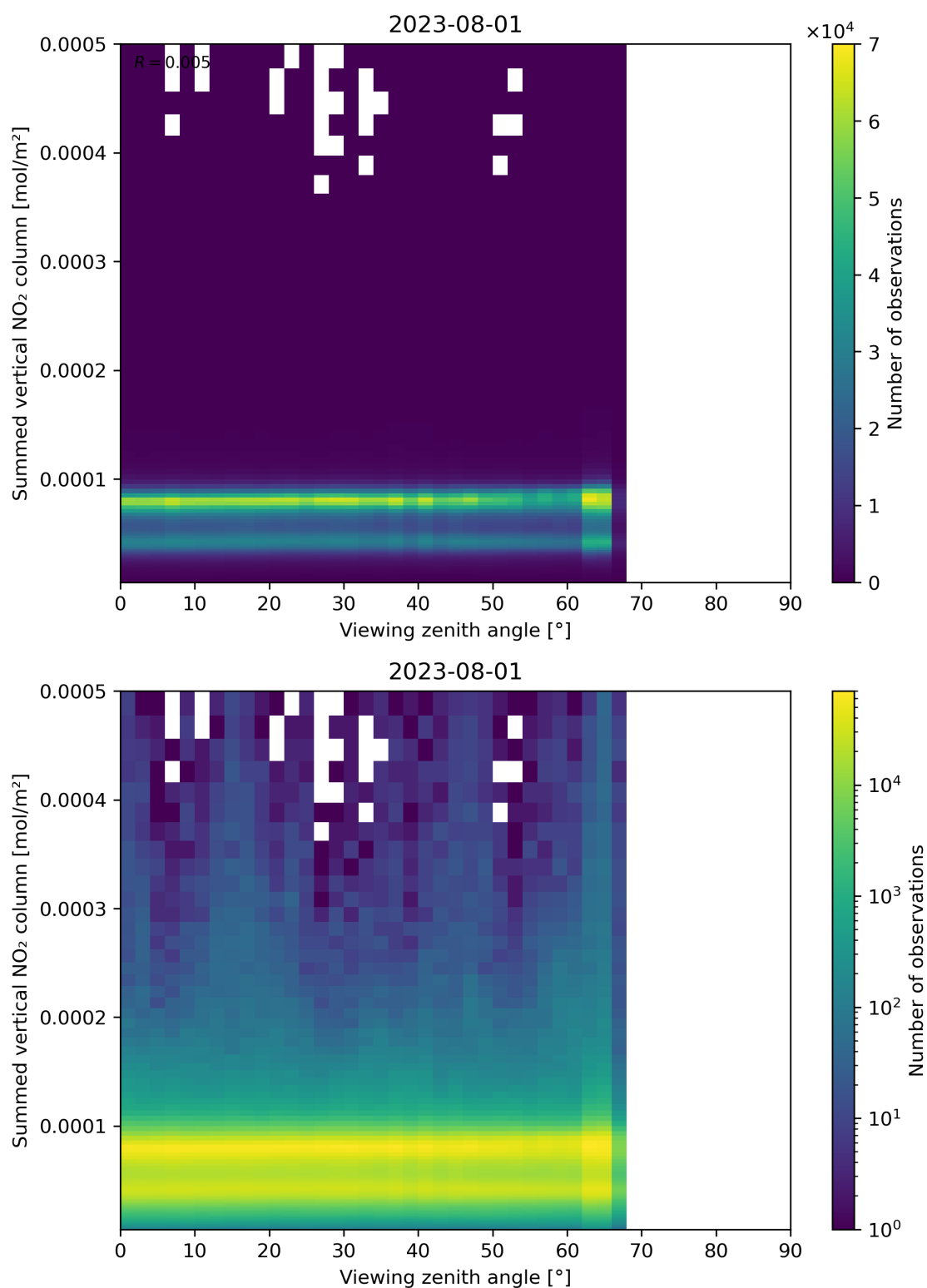
Figure 165: Scatter density plot of “Viewing zenith angle” against “Summed vertical NO 2 column” for 2023-07-31 to 2023-08-02.
