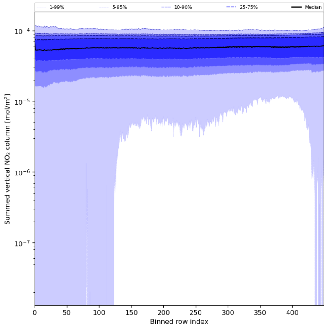
Figure 57: Along track statistics of “Summed vertical NO 2 column” for 2023-07-31 to 2023-08-02
