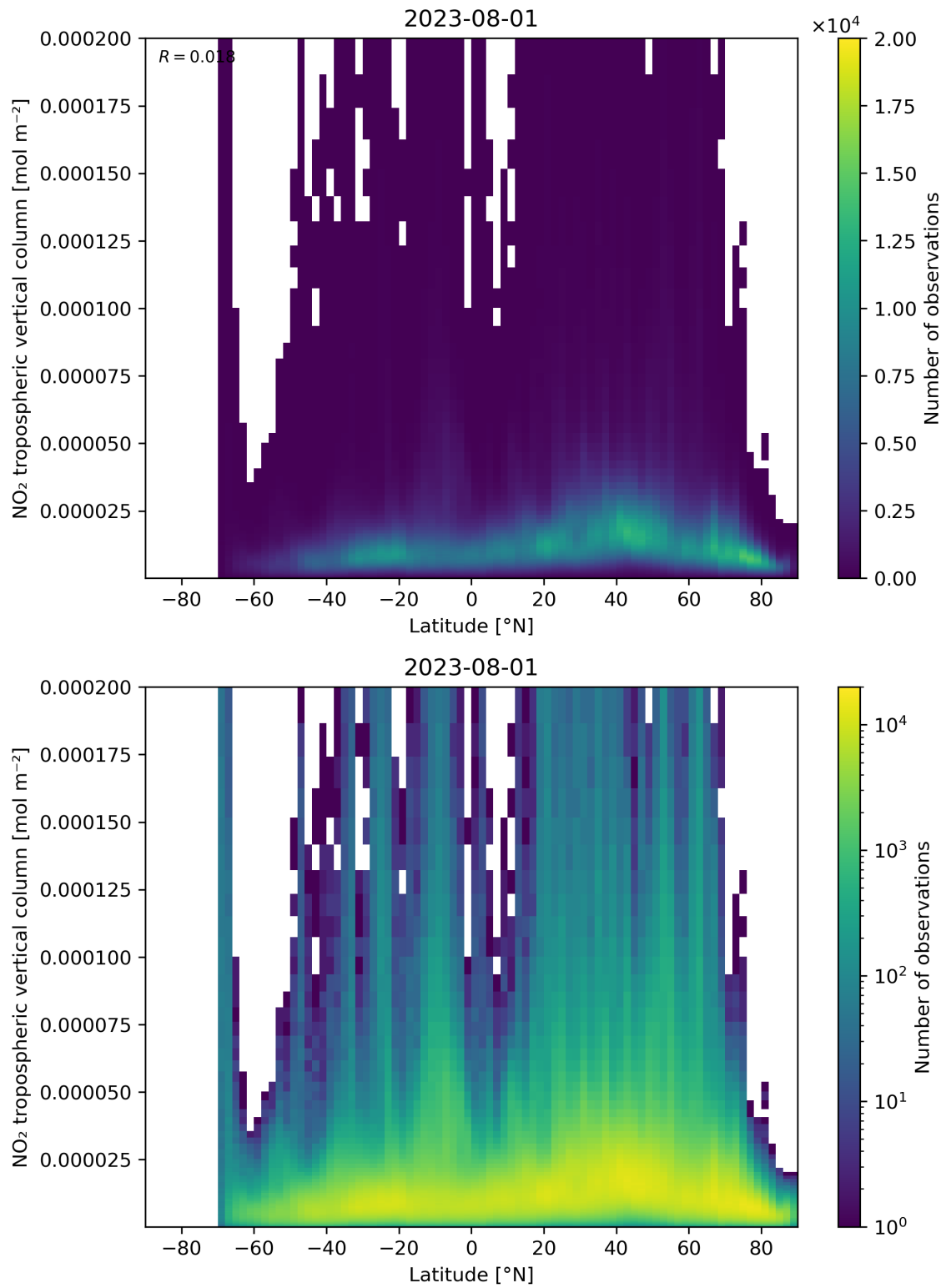
Figure 92: Scatter density plot of “Latitude” against “NO 2 tropospheric vertical column” for 2023-07-31 to 2023-08-02.
