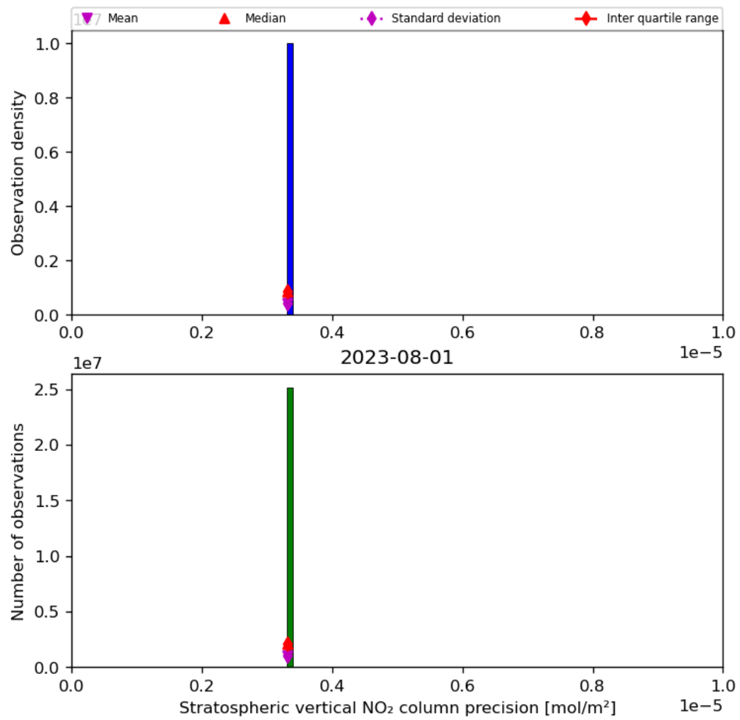
Figure 37: Histogram of “Stratospheric vertical NO 2 column precision” for 2023-07-31 to 2023-08-02
