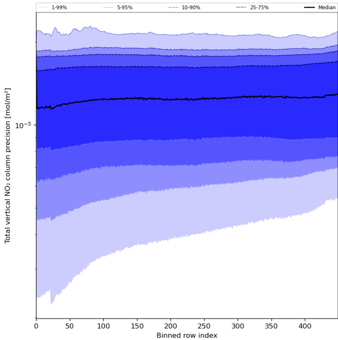
Figure 56: Along track statistics of “Total vertical NO 2 column precision” for 2023-07-31 to 2023-08-02
