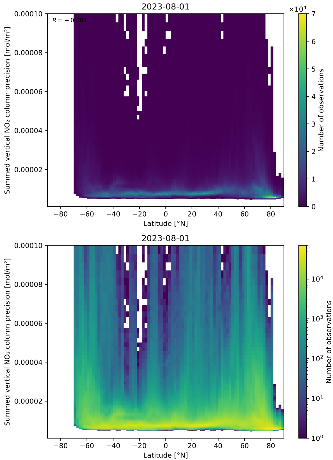
Figure 89: Scatter density plot of “Latitude” against “Summed vertical NO 2 column precision” for 2023-07-31 to 2023-08-02.
