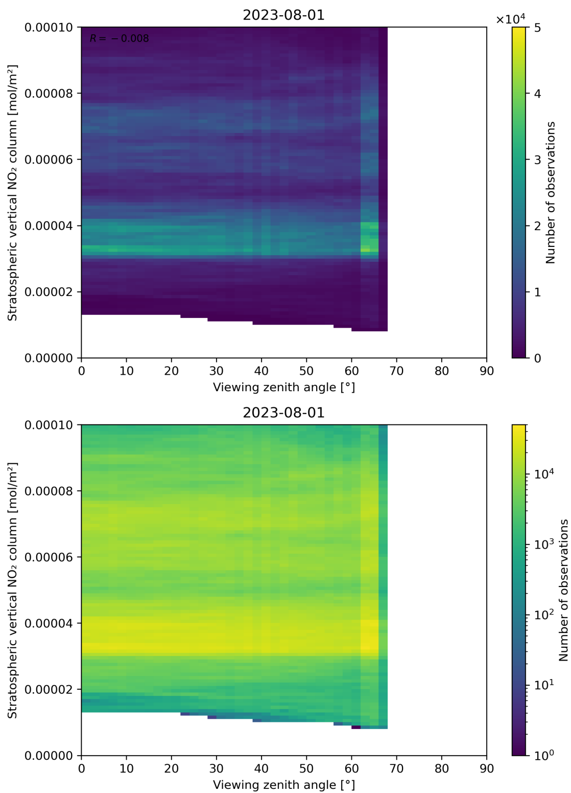
Figure 164: Scatter density plot of “Viewing zenith angle” against “Stratospheric vertical NO 2 column” for 2023-07-31 to 2023-08-02.
