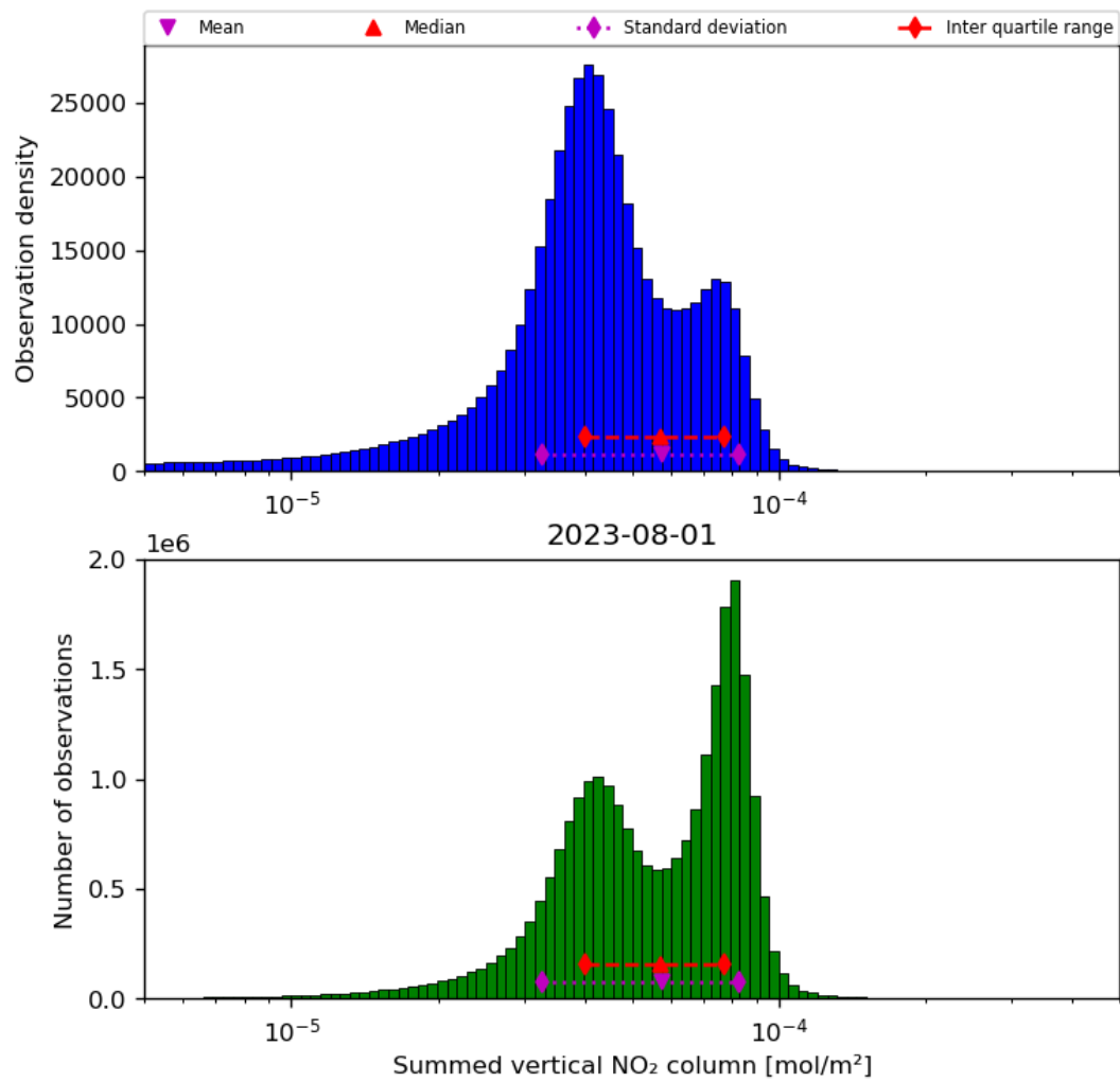
Figure 40: Histogram of “Summed vertical NO 2 column” for 2023-07-31 to 2023-08-02
