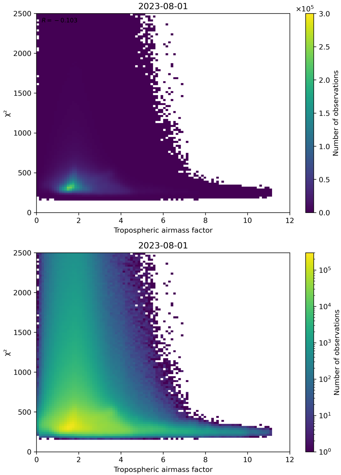
Figure 73: Scatter density plot of “Tropospheric airmass factor” against “ \chi^2 ” for 2023-07-31 to 2023-08-02.
