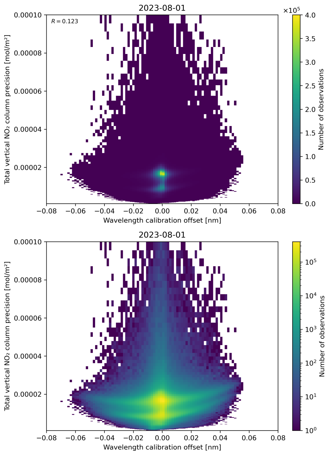
Figure 180: Scatter density plot of “Wavelength calibration offset” against “Total vertical NO 2 column precision” for 2023-07-31 to 2023-08-02.
