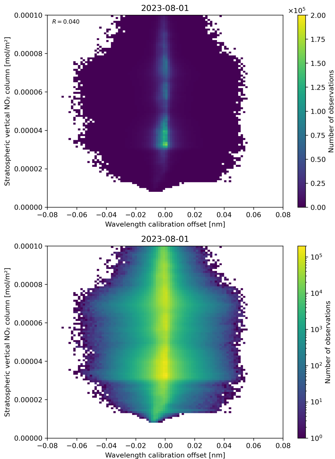
Figure 176: Scatter density plot of “Wavelength calibration offset” against “Stratospheric vertical NO 2 column” for 2023-07-31 to 2023-08-02.
