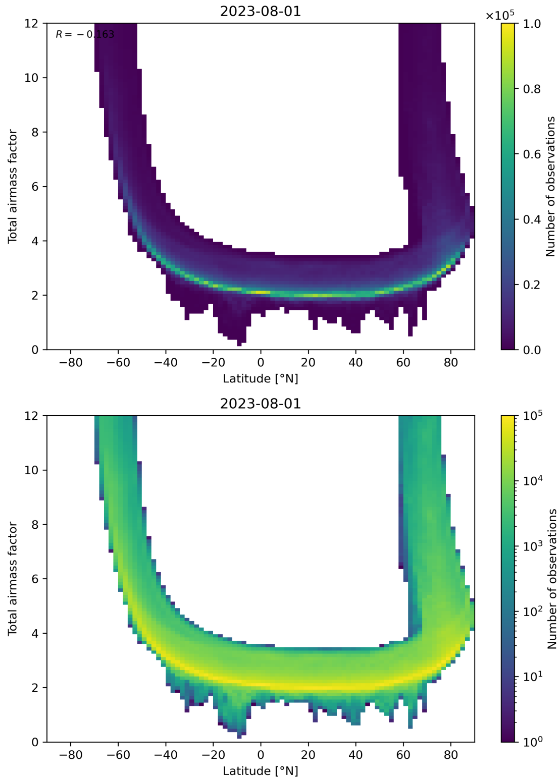
Figure 84: Scatter density plot of “Latitude” against “Total airmass factor” for 2023-07-31 to 2023-08-02.
