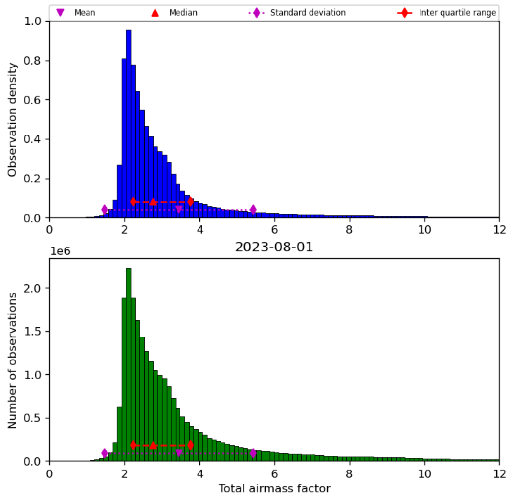
Figure 32: Histogram of “Total airmass factor” for 2023-07-31 to 2023-08-02
