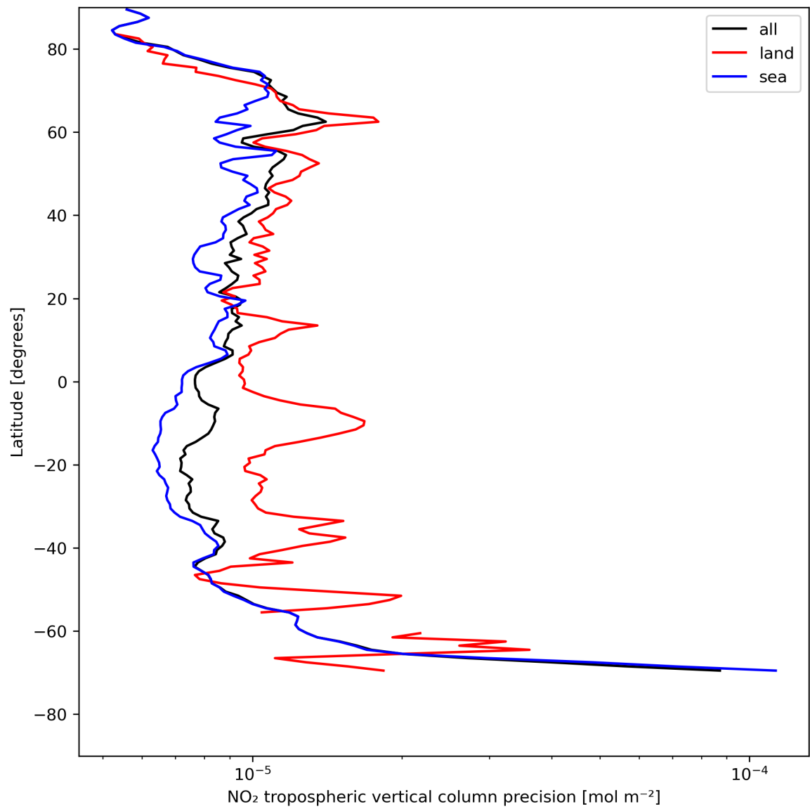
Figure 13: Zonal average of “NO 2 tropospheric vertical column precision” for 2023-07-31 to 2023-08-02.
