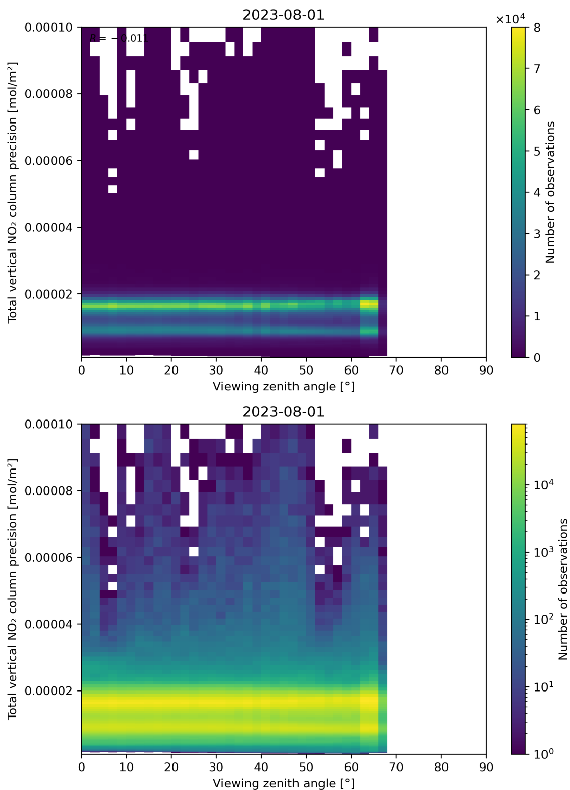
Figure 168: Scatter density plot of “Viewing zenith angle” against “Total vertical NO 2 column precision” for 2023-07-31 to 2023-08-02.
