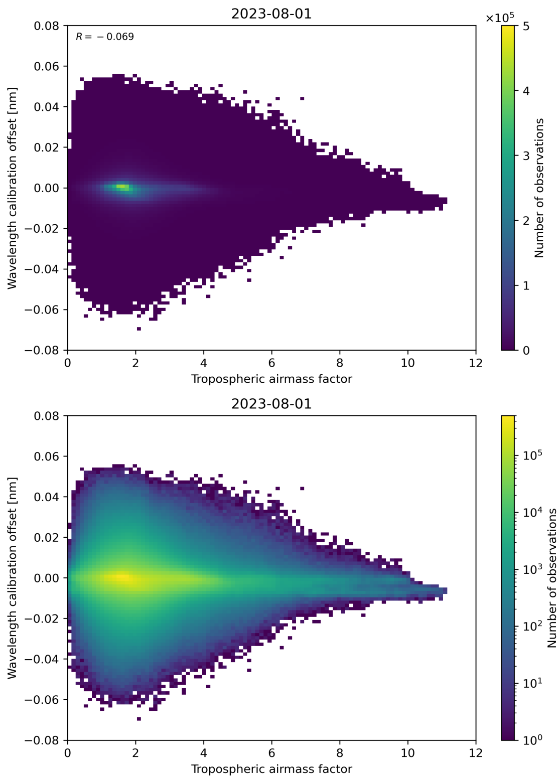
Figure 80: Scatter density plot of “Tropospheric air mass factor” against “Wavelength calibration offset” for 2023-07-31 to 2023-08-02.
