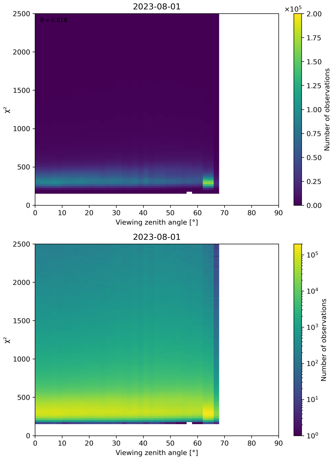
Figure 162: Scatter density plot of “Viewing zenith angle” against “ \chi^2 ” for 2023-07-31 to 2023-08-02.
