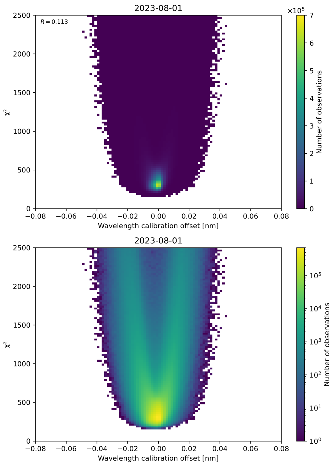
Figure 175: Scatter density plot of “Wavelength calibration offset” against “ \chi^2 ” for 2023-07-31 to 2023-08-02.
