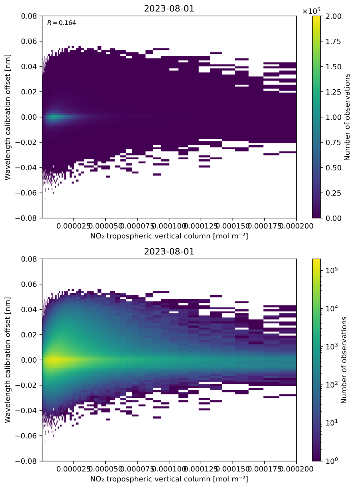
Figure 143: Scatter density plot of “NO 2 tropospheric vertical column” against “Wavelength calibration offset” for 2023-07-31 to 2023-08-02.
