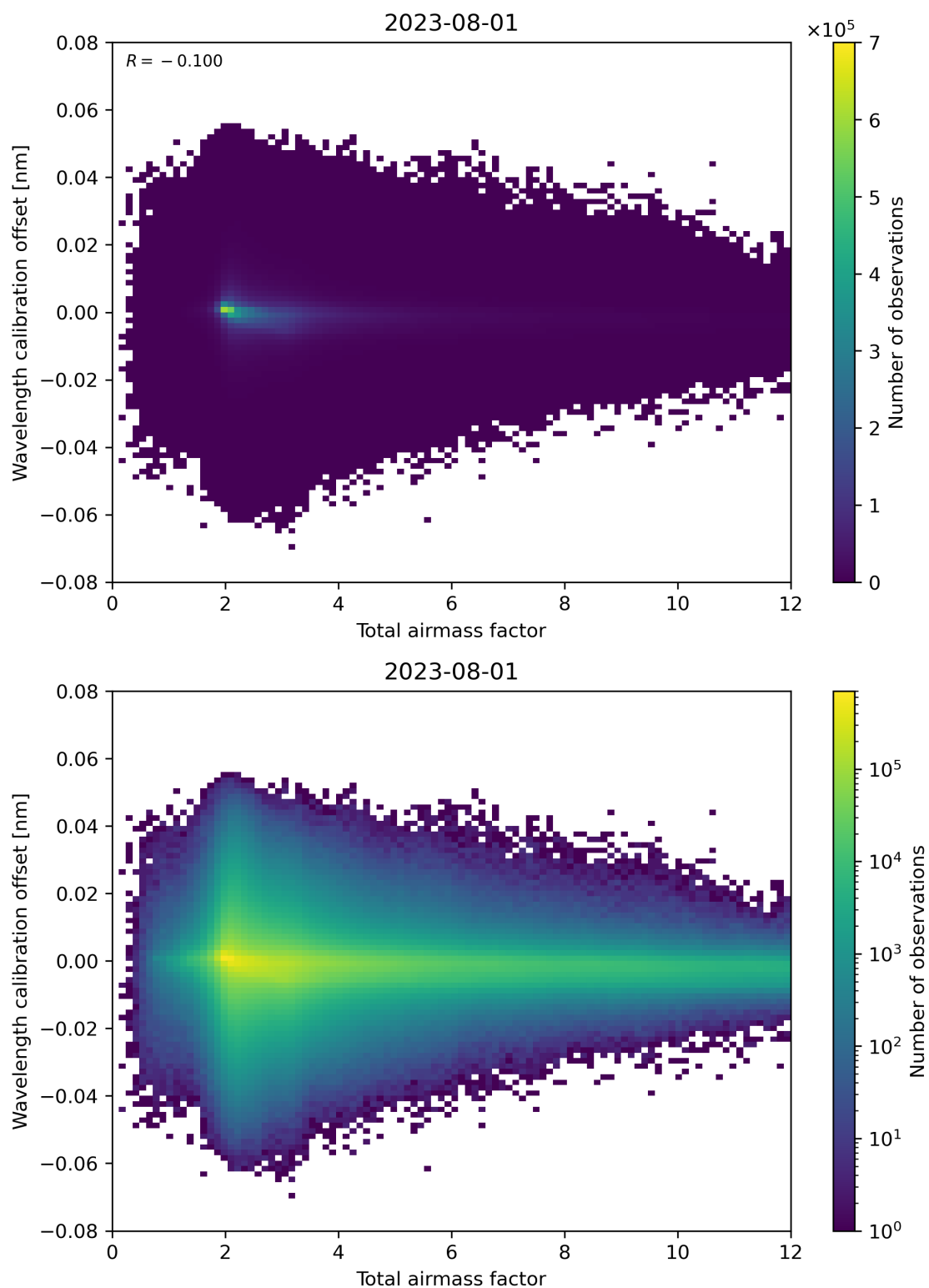
Figure 70: Scatter density plot of “Total airmass factor” against “Wavelength calibration offset” for 2023-07-31 to 2023-08-02.
