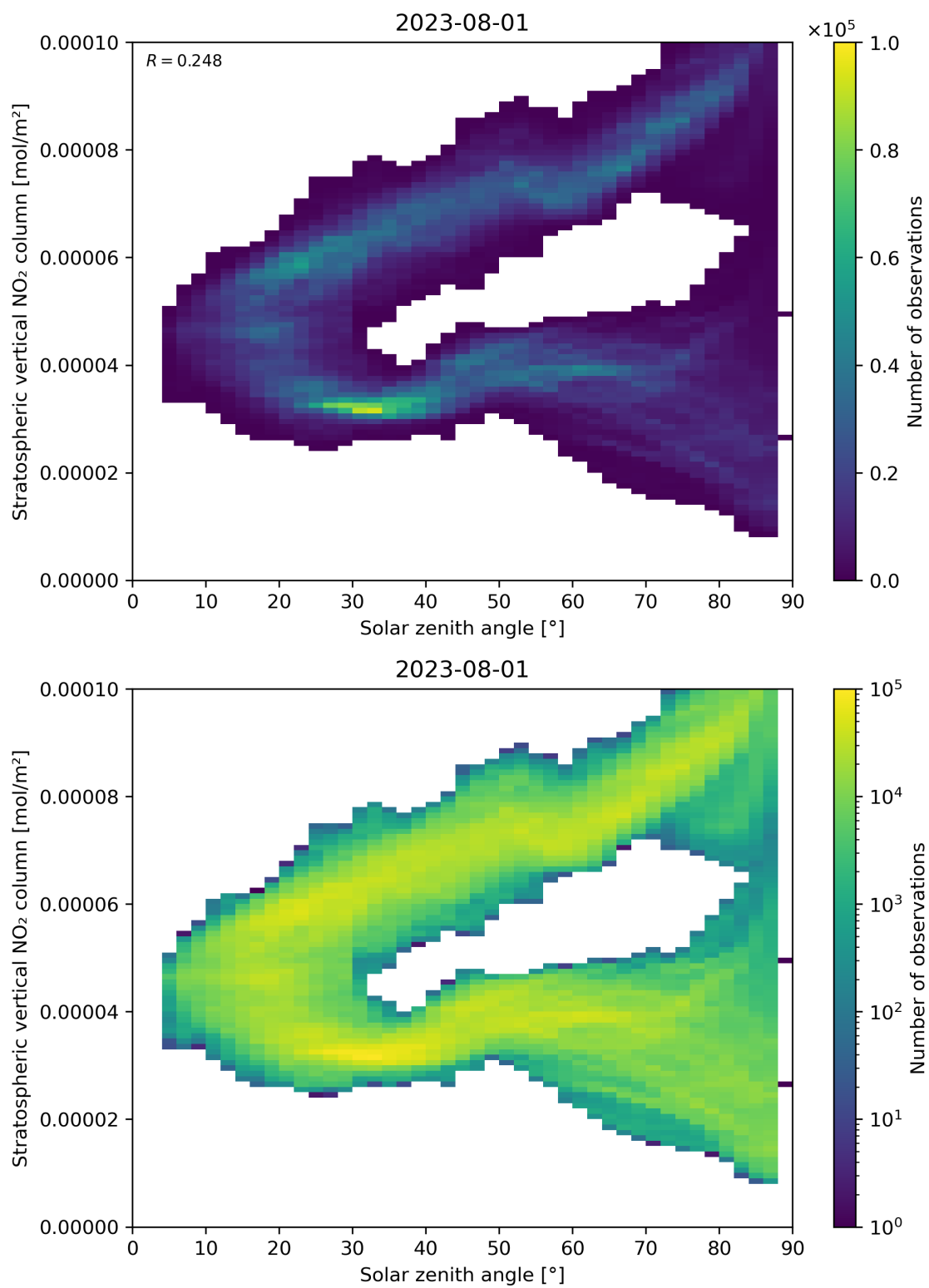
Figure 150: Scatter density plot of “Solar zenith angle” against “Stratospheric vertical NO 2 column” for 2023-07-31 to 2023-08-02.
