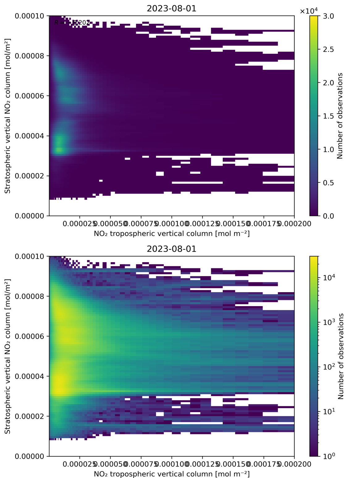
Figure 125: Scatter density plot of “NO 2 tropospheric vertical column” against “Stratospheric vertical NO 2 column” for 2023-07-31 to 2023-08-02.
