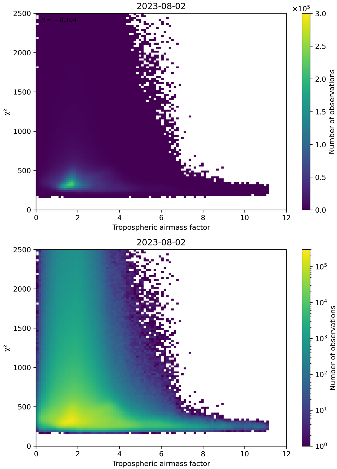
Figure 73: Scatter density plot of “Tropospheric airmass factor” against “ \chi^2 ” for 2023-08-01 to 2023-08-03.
