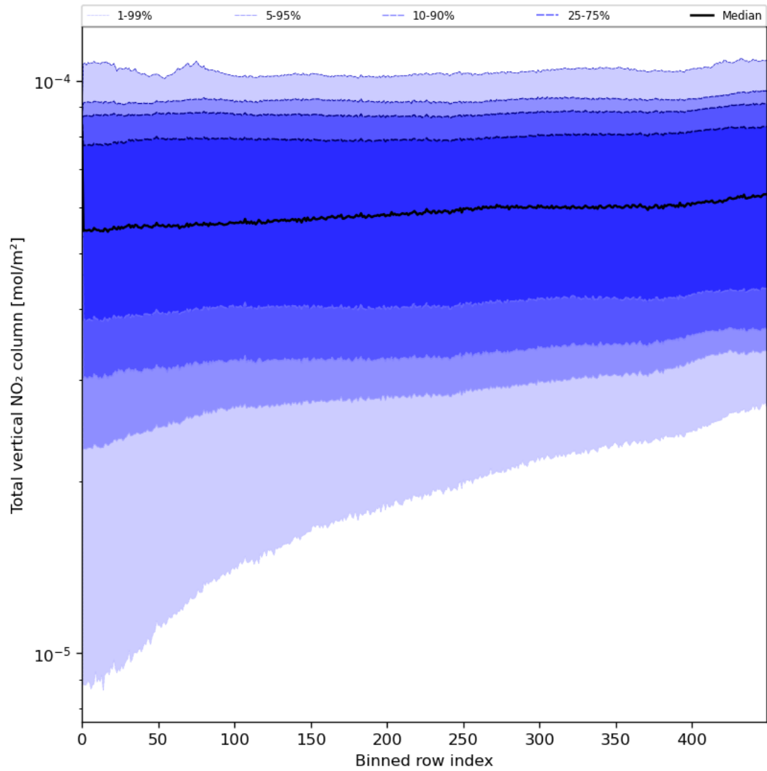
Figure 55: Along track statistics of “Total vertical NO 2 column” for 2023-08-01 to 2023-08-03
