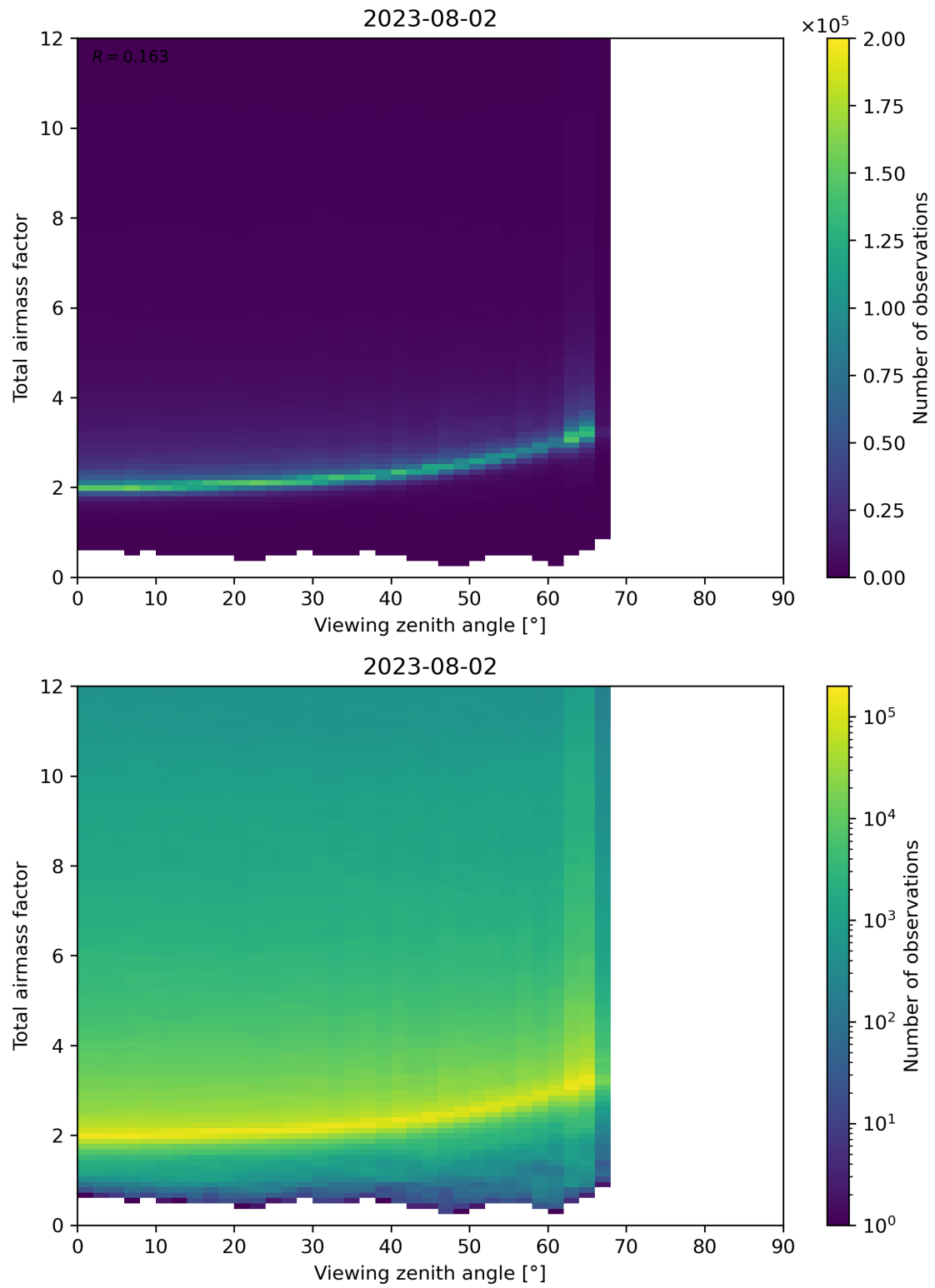
Figure 160: Scatter density plot of “Viewing zenith angle” against “Total airmass factor” for 2023-08-01 to 2023-08-03.
