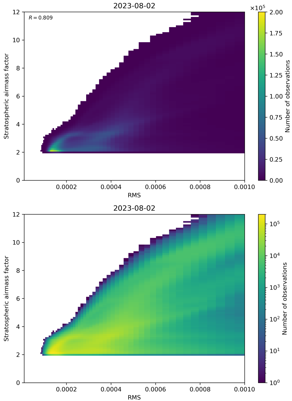
Figure 144: Scatter density plot of “RMS” against “Stratospheric airmass factor” for 2023-08-01 to 2023-08-03.
