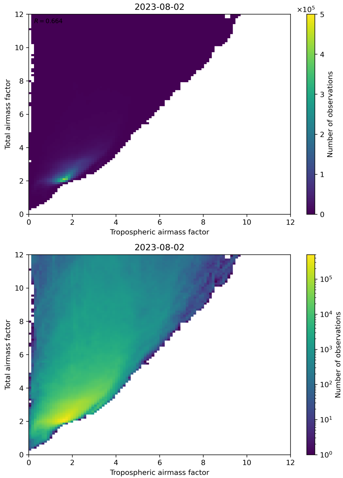
Figure 72: Scatter density plot of “Tropospheric airmass factor” against “Total airmass factor” for 2023-08-01 to 2023-08-03.
