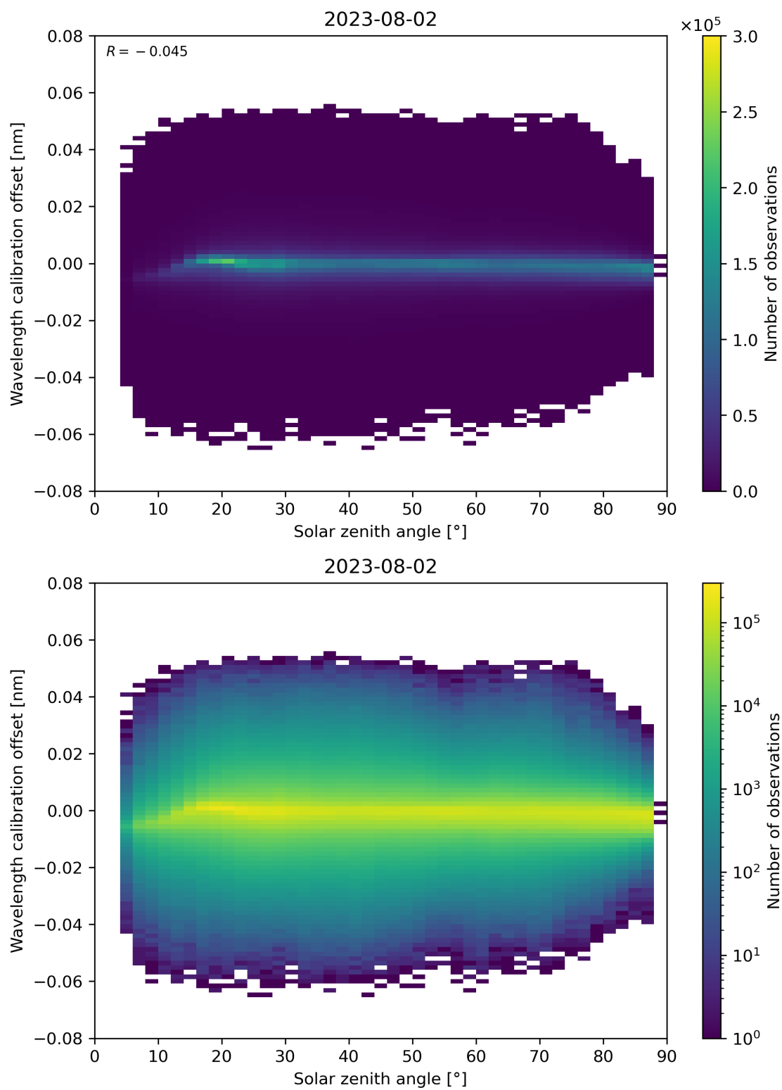
Figure 158: Scatter density plot of “Solar zenith angle” against “Wavelength calibration offset” for 2023-08-01 to 2023-08-03.
