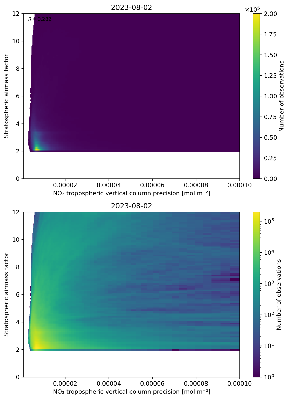
Figure 131: Scatter density plot of “NO 2 tropospheric vertical column precision” against “Stratospheric airmass factor” for 2023-08-01 to 2023-08-03.
