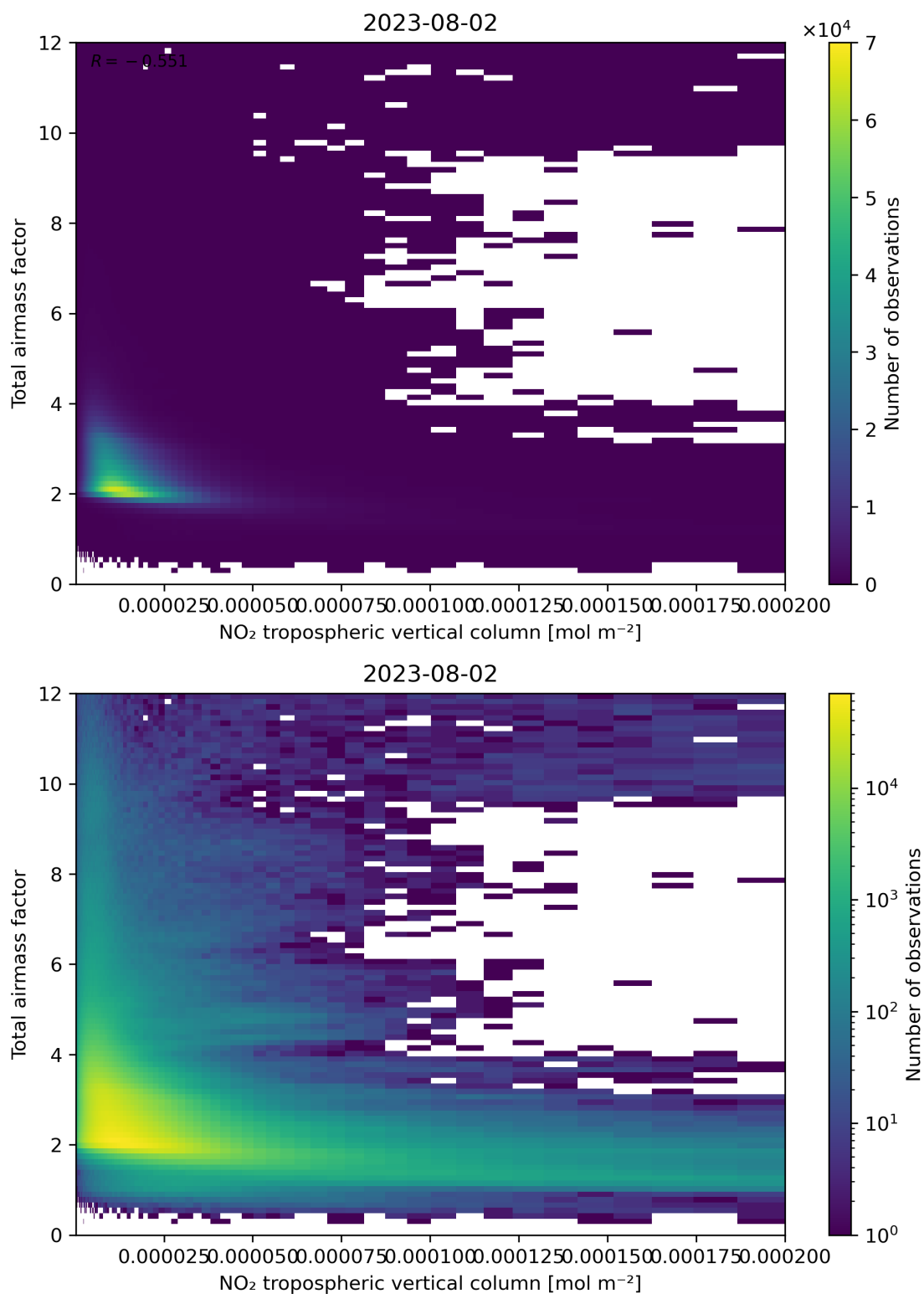
Figure 122: Scatter density plot of “NO 2 tropospheric vertical column” against “Total air mass factor” for 2023-08-01 to 2023-08-03.
