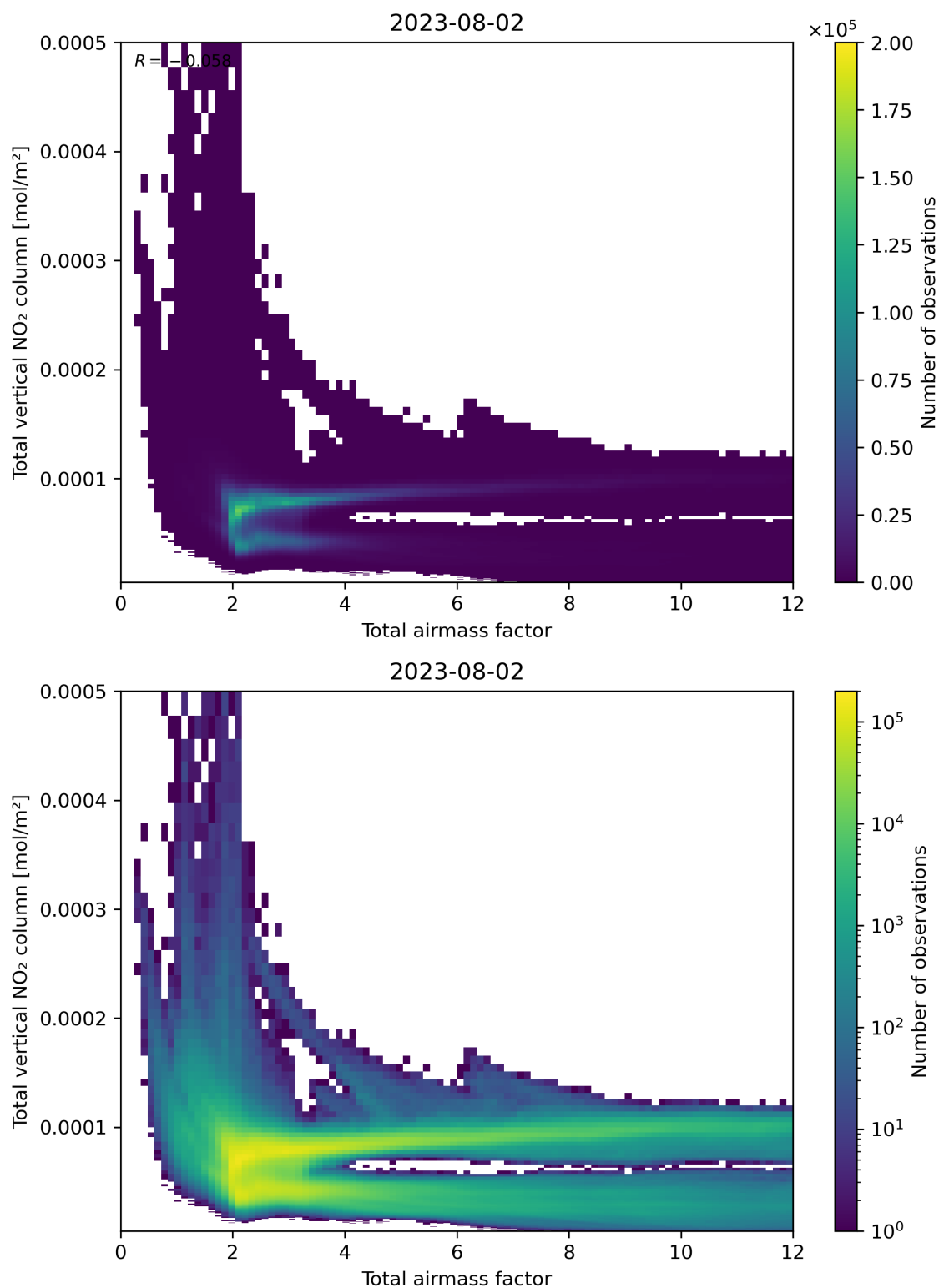
Figure 67: Scatter density plot of “Total airmass factor” against “Total vertical NO 2 column” for 2023-08-01 to 2023-08-03.
