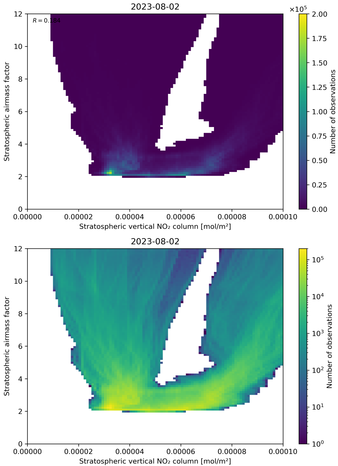
Figure 96: Scatter density plot of “Stratospheric vertical NO 2 column” against “Stratospheric airmass factor” for 2023-08-01 to 2023-08-03.
