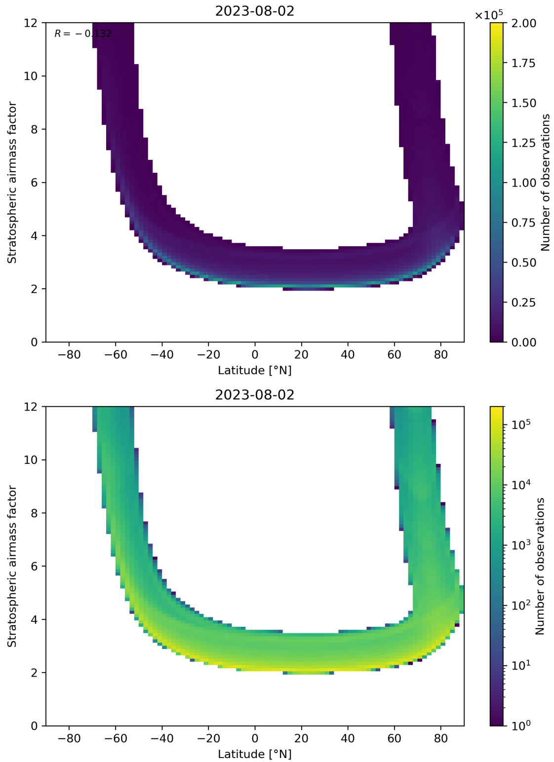
Figure 83: Scatter density plot of “Latitude” against “Stratospheric air mass factor” for 2023-08-01 to 2023-08-03.
