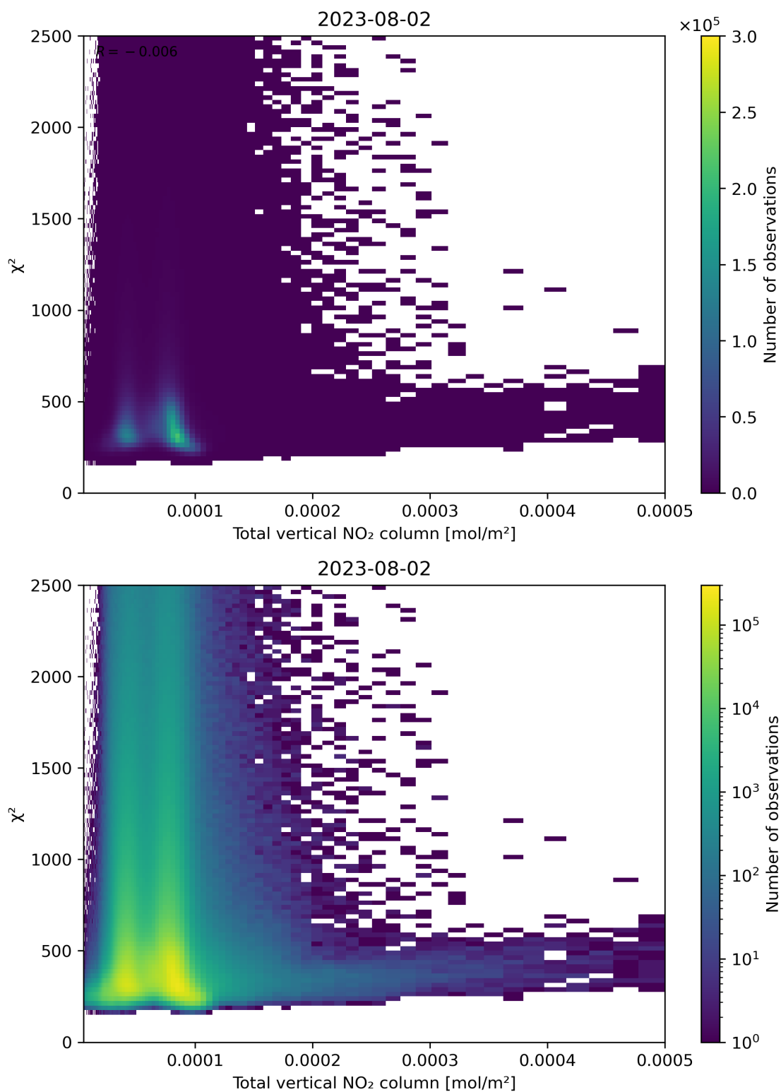
Figure 111: Scatter density plot of “Total vertical NO 2 column” against “ \chi^2 ” for 2023-08-01 to 2023-08-03.
