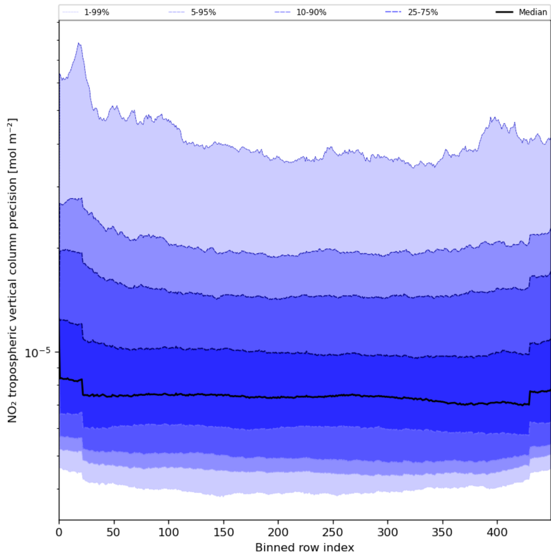
Figure 47: Along track statistics of “NO 2 tropospheric vertical column precision” for 2023-08-01 to 2023-08-03
