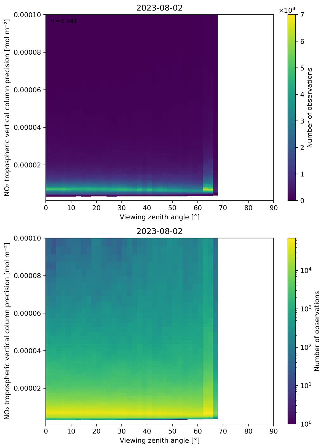
Figure 170: Scatter density plot of “Viewing zenith angle” against “NO 2 tropospheric vertical column precision” for 2023-08-01 to 2023-08-03.
