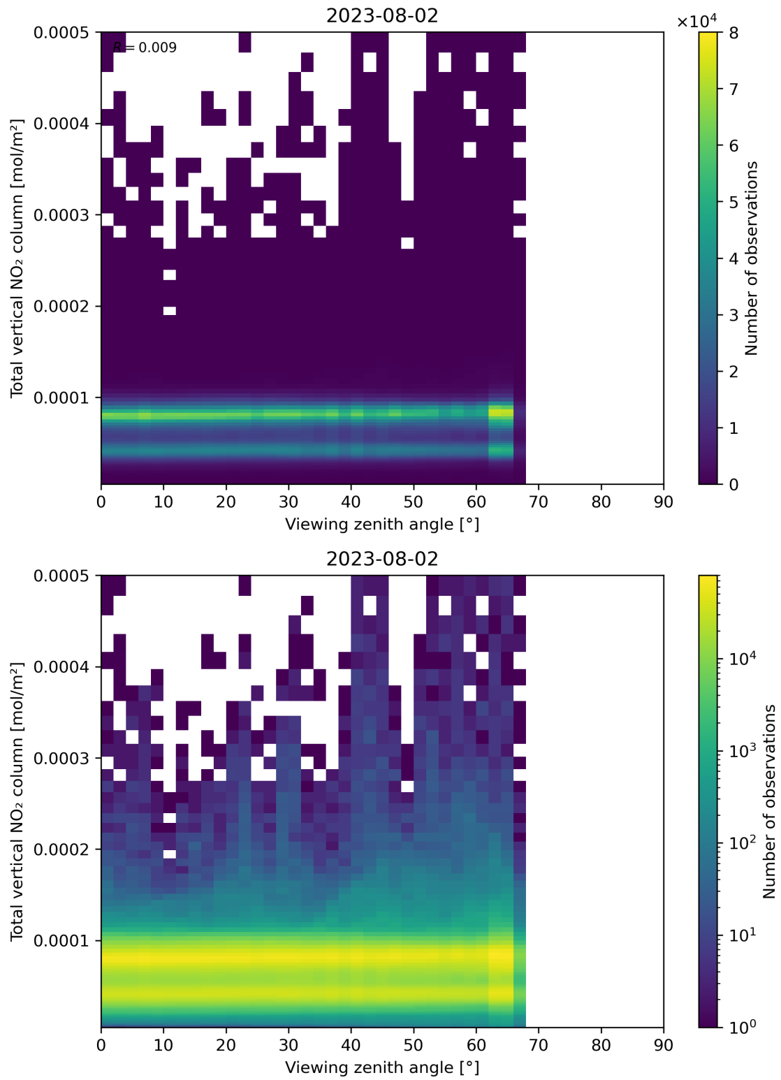
Figure 167: Scatter density plot of “Viewing zenith angle” against “Total vertical NO 2 column” for 2023-08-01 to 2023-08-03.
