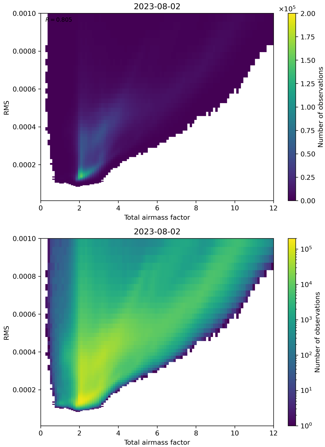
Figure 69: Scatter density plot of “Total airmass factor” against “RMS” for 2023-08-01 to 2023-08-03.
