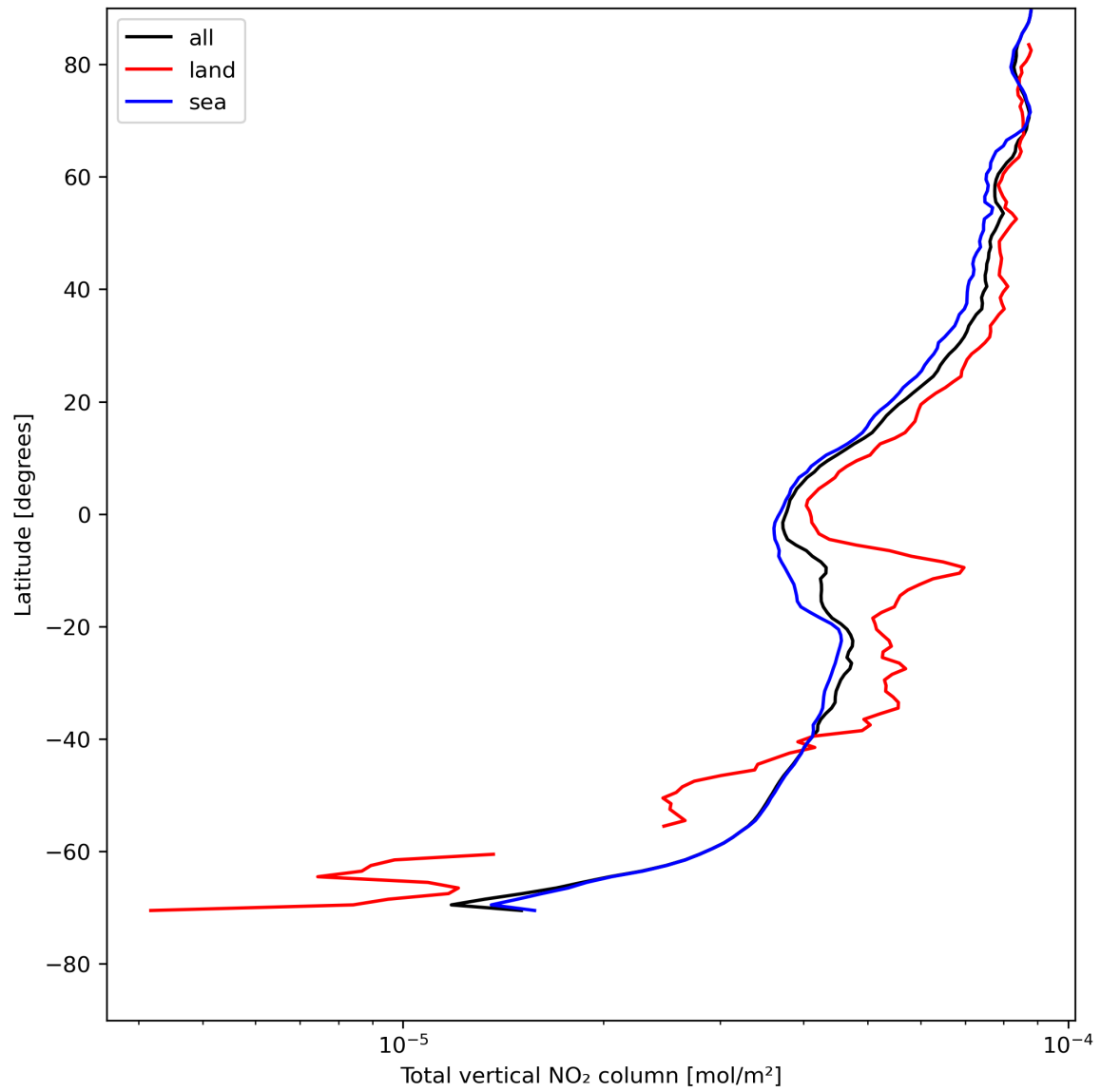
Figure 21: Zonal average of “Total vertical NO 2 column” for 2023-08-01 to 2023-08-03.
