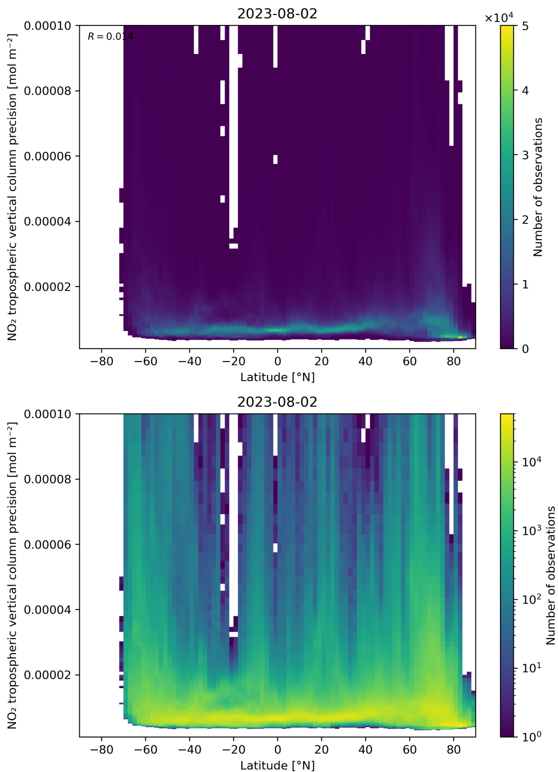
Figure 93: Scatter density plot of “Latitude” against “NO 2 tropospheric vertical column precision” for 2023-08-01 to 2023-08-03.
