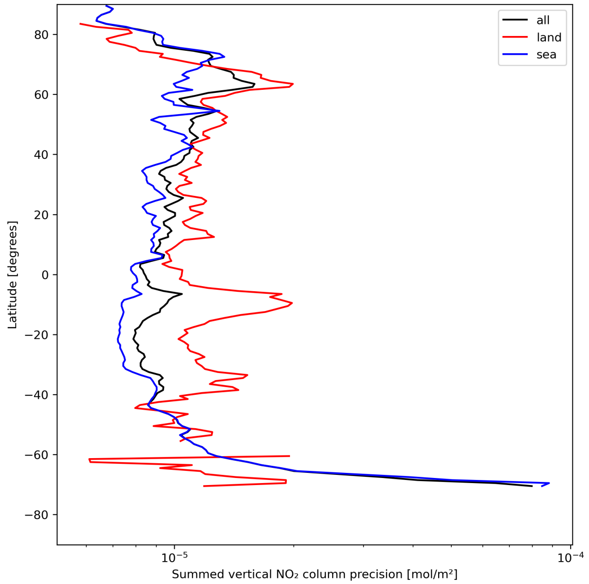
Figure 24: Zonal average of “Summed vertical NO 2 column precision” for 2023-08-01 to 2023-08-03.
