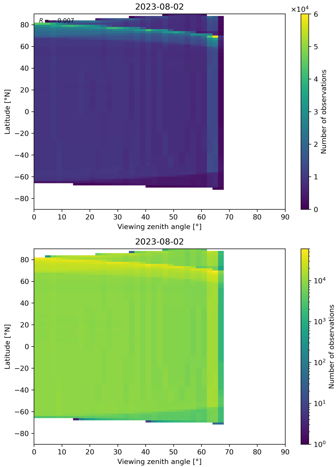
Figure 163: Scatter density plot of “Viewing zenith angle” against “Latitude” for 2023-08-01 to 2023-08-03.
