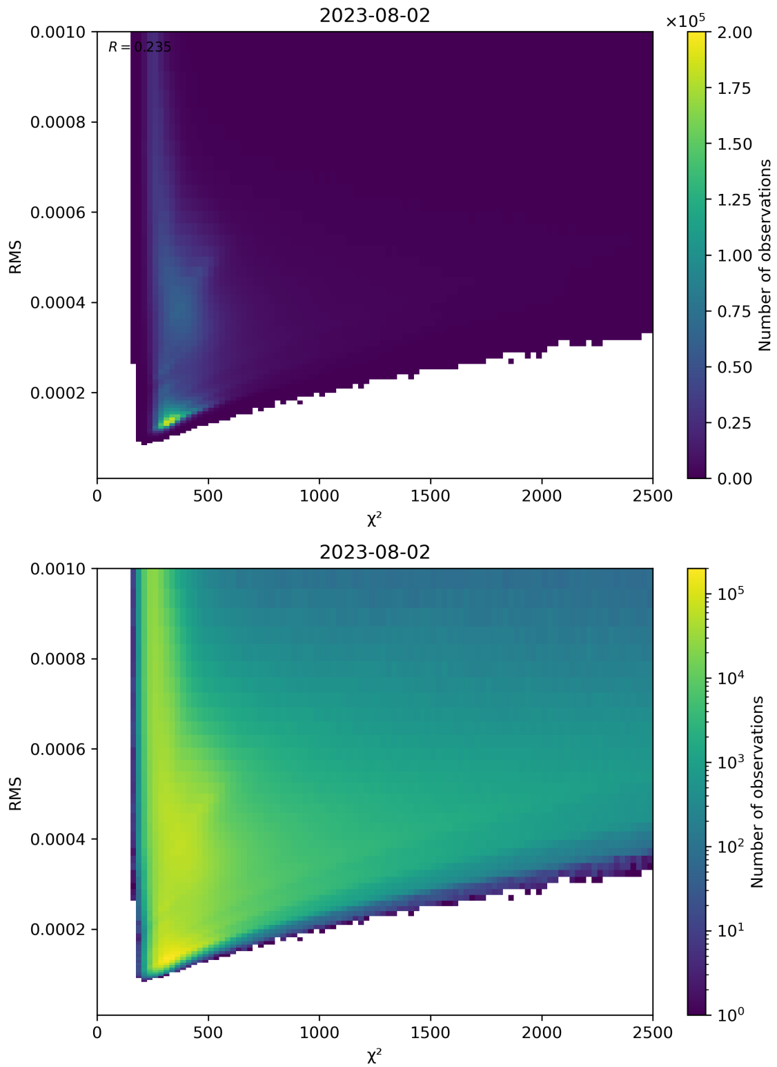
Figure 82: Scatter density plot of “ \chi^2 ” against “RMS” for 2023-08-01 to 2023-08-03.
