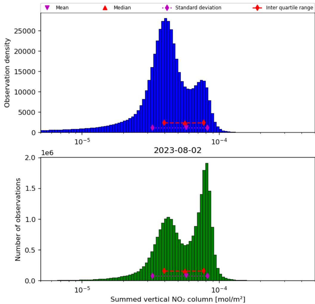
Figure 40: Histogram of “Summed vertical NO 2 column” for 2023-08-01 to 2023-08-03
