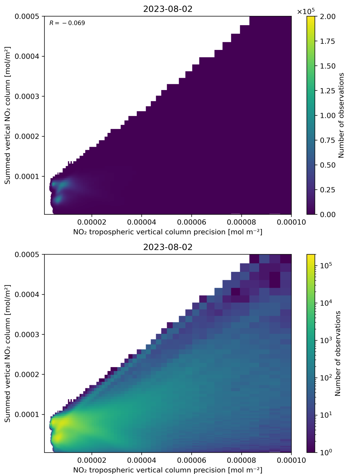
Figure 136: Scatter density plot of “NO 2 tropospheric vertical column precision” against “Summed vertical NO 2 column” for 2023-08-01 to 2023-08-03.
