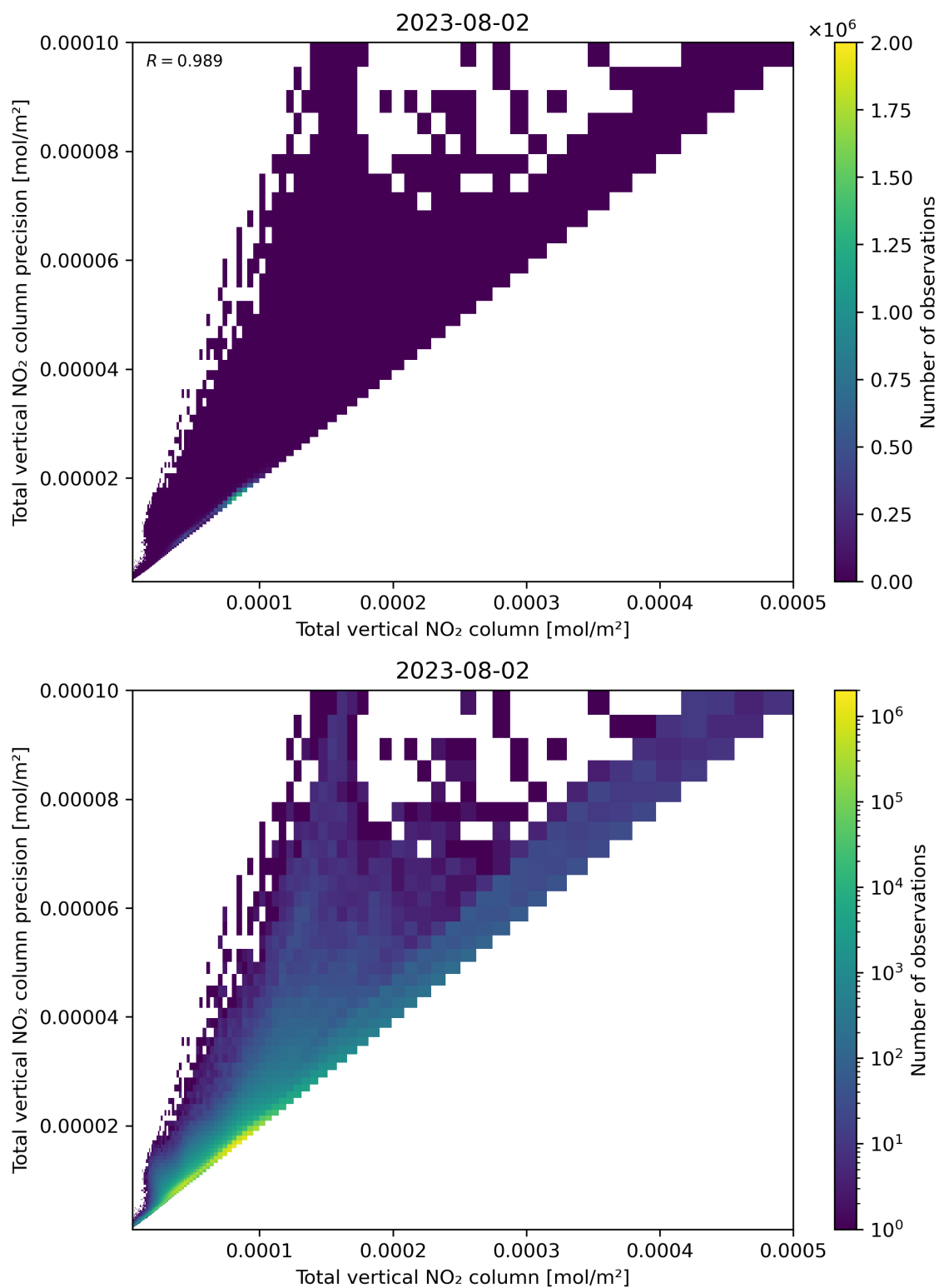
Figure 114: Scatter density plot of “Total vertical NO 2 column” against “Total vertical NO 2 column precision” for 2023-08-01 to 2023-08-03.
