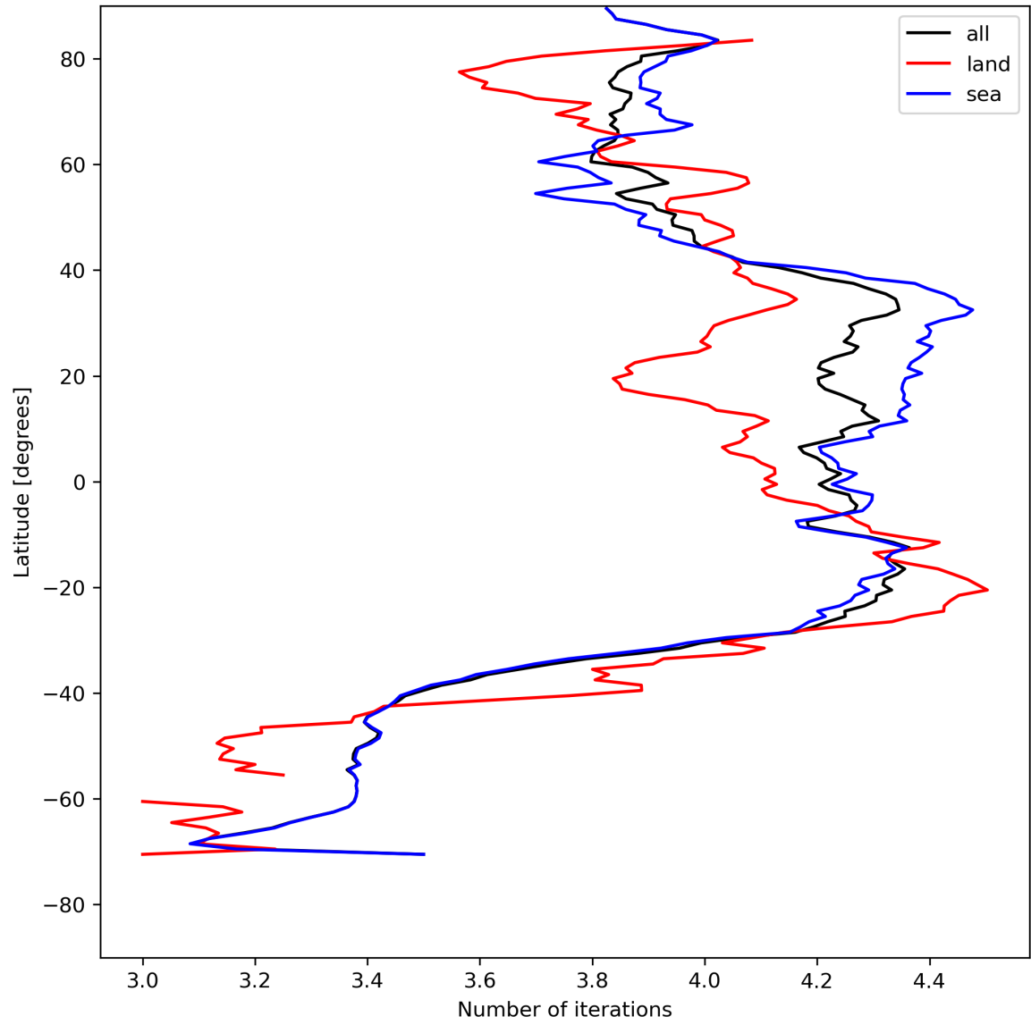
Figure 17: Zonal average of “Number of iterations” for 2023-08-01 to 2023-08-03.
