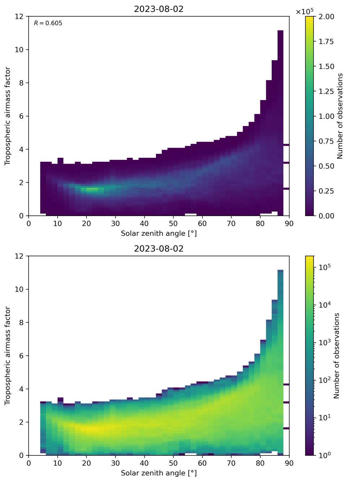
Figure 147: Scatter density plot of “Solar zenith angle” against “Tropospheric airmass factor” for 2023-08-01 to 2023-08-03.
