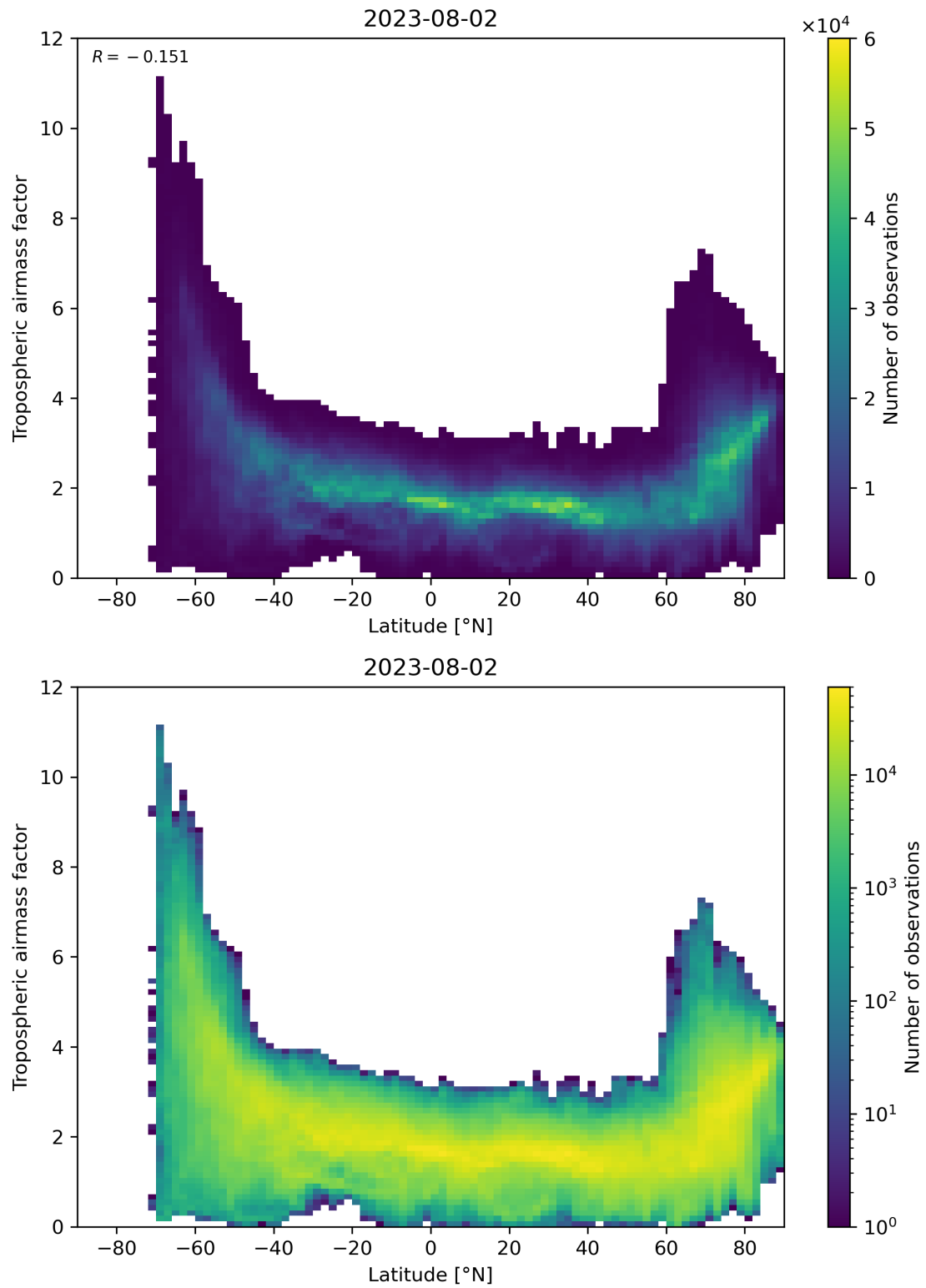
Figure 85: Scatter density plot of “Latitude” against “Tropospheric airmass factor” for 2023-08-01 to 2023-08-03.
