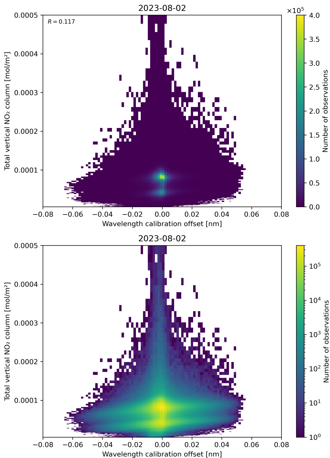
Figure 179: Scatter density plot of “Wavelength calibration offset” against “Total vertical NO 2 column” for 2023-08-01 to 2023-08-03.
