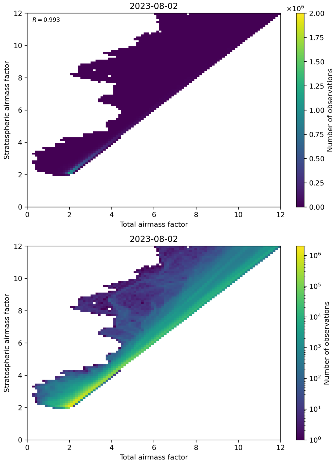
Figure 62: Scatter density plot of “Total airmass factor” against “Stratospheric airmass factor” for 2023-08-01 to 2023-08-03.
