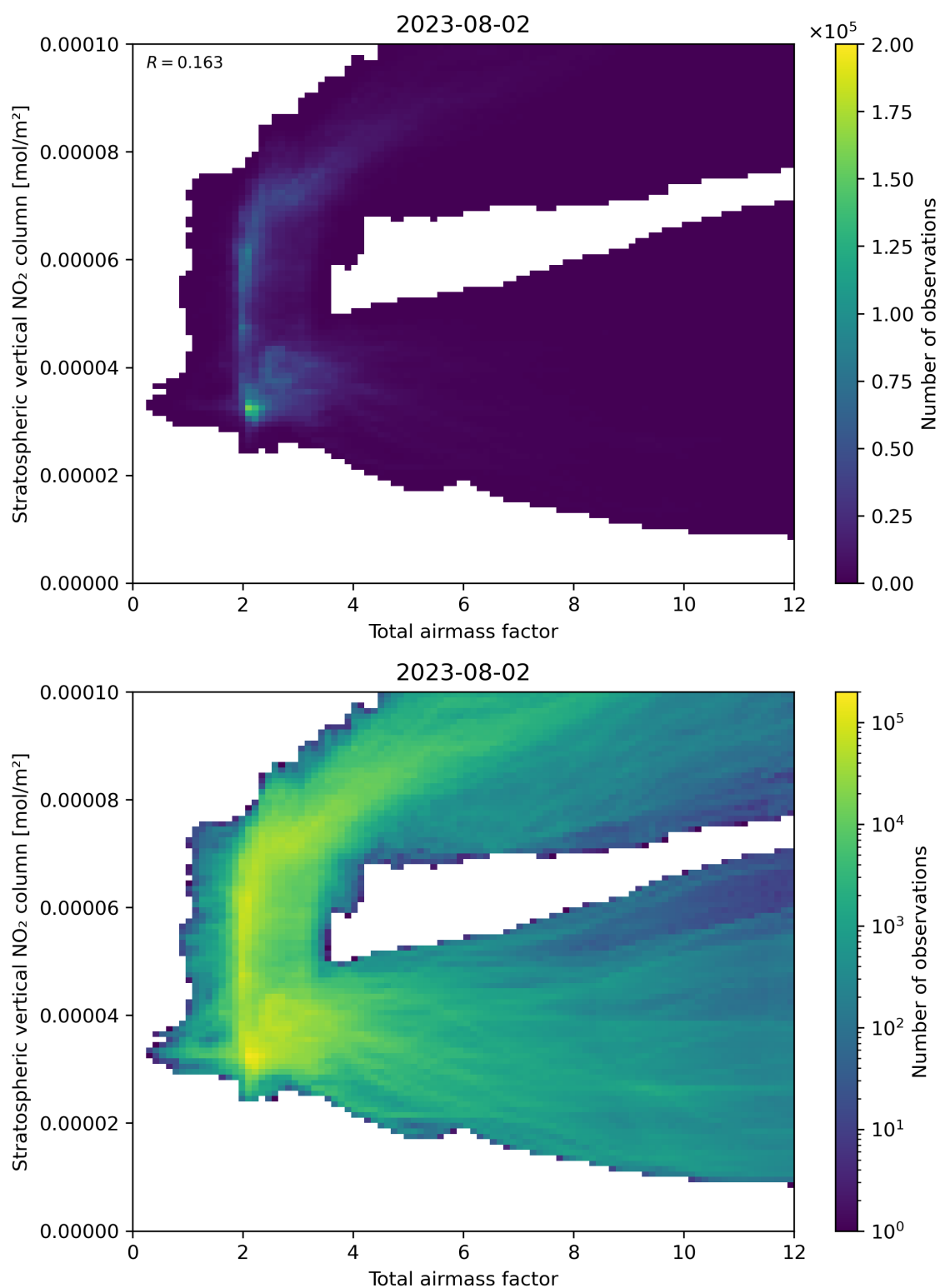
Figure 64: Scatter density plot of “Total airmass factor” against “Stratospheric vertical NO 2 column” for 2023-08-01 to 2023-08-03.
