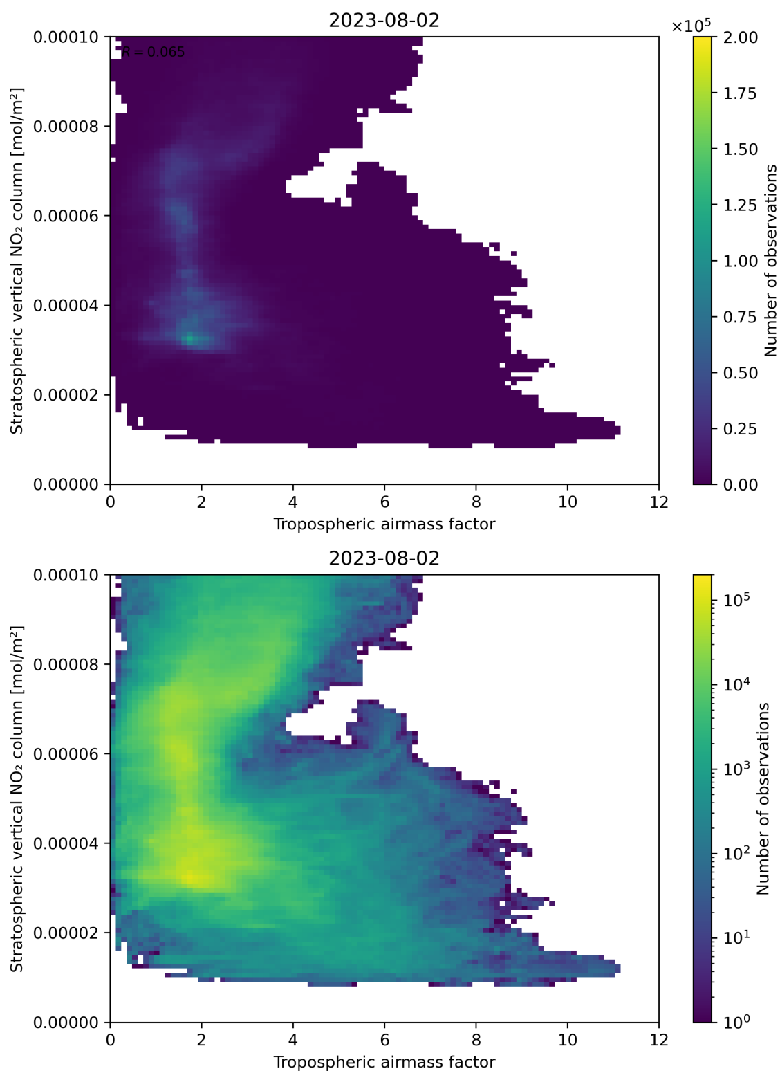
Figure 74: Scatter density plot of “Tropospheric air mass factor” against “Stratospheric vertical NO 2 column” for 2023-08-01 to 2023-08-03.
