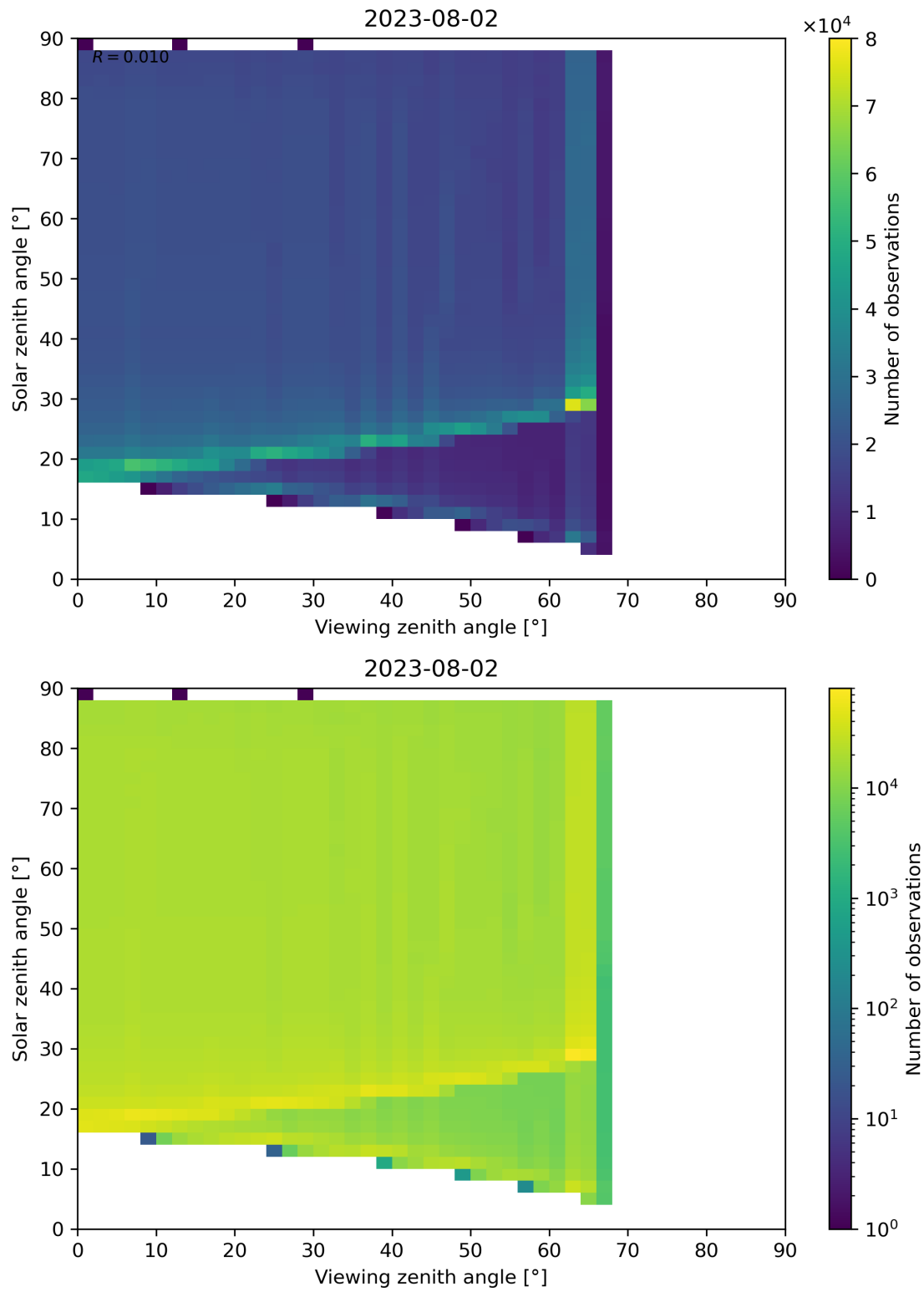
Figure 172: Scatter density plot of “Viewing zenith angle” against “Solar zenith angle” for 2023-08-01 to 2023-08-03.
