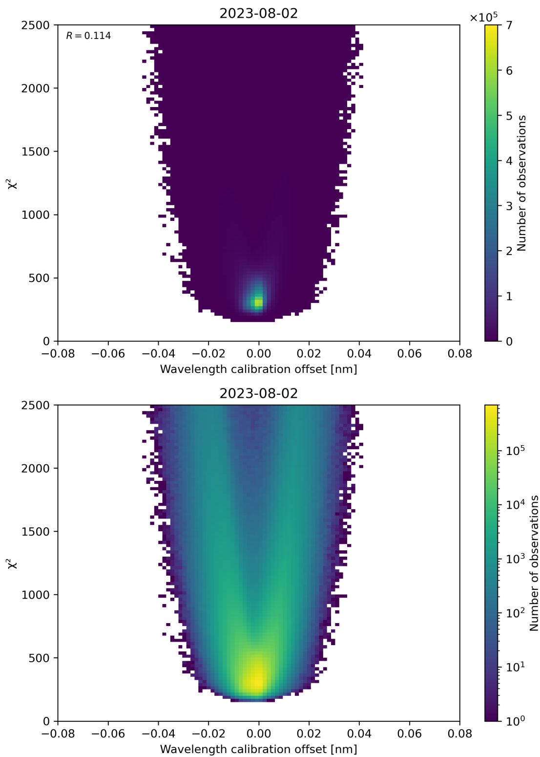
Figure 175: Scatter density plot of “Wavelength calibration offset” against “ \chi^2 ” for 2023-08-01 to 2023-08-03.
