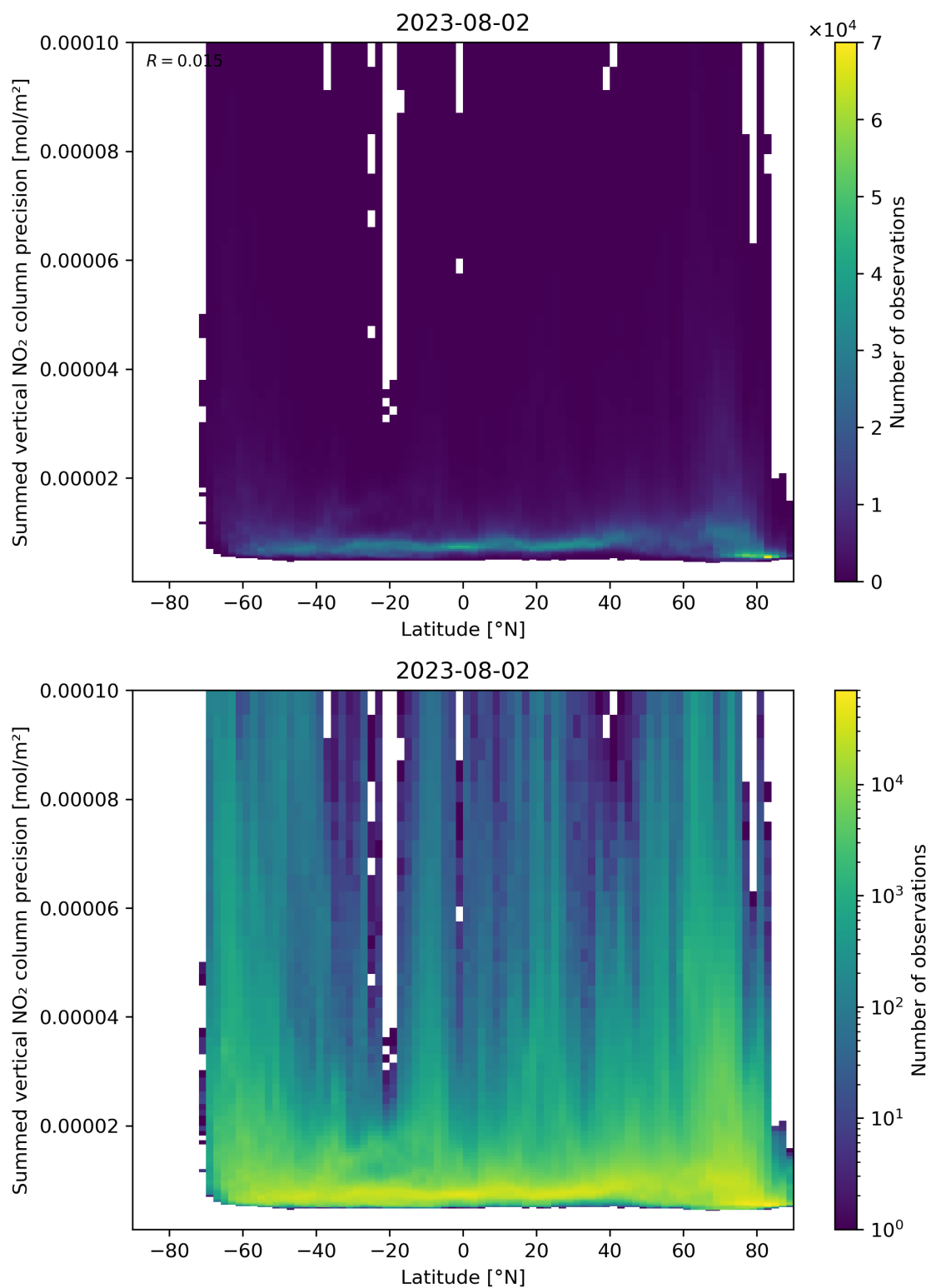
Figure 89: Scatter density plot of “Latitude” against “Summed vertical NO 2 column precision” for 2023-08-01 to 2023-08-03.
