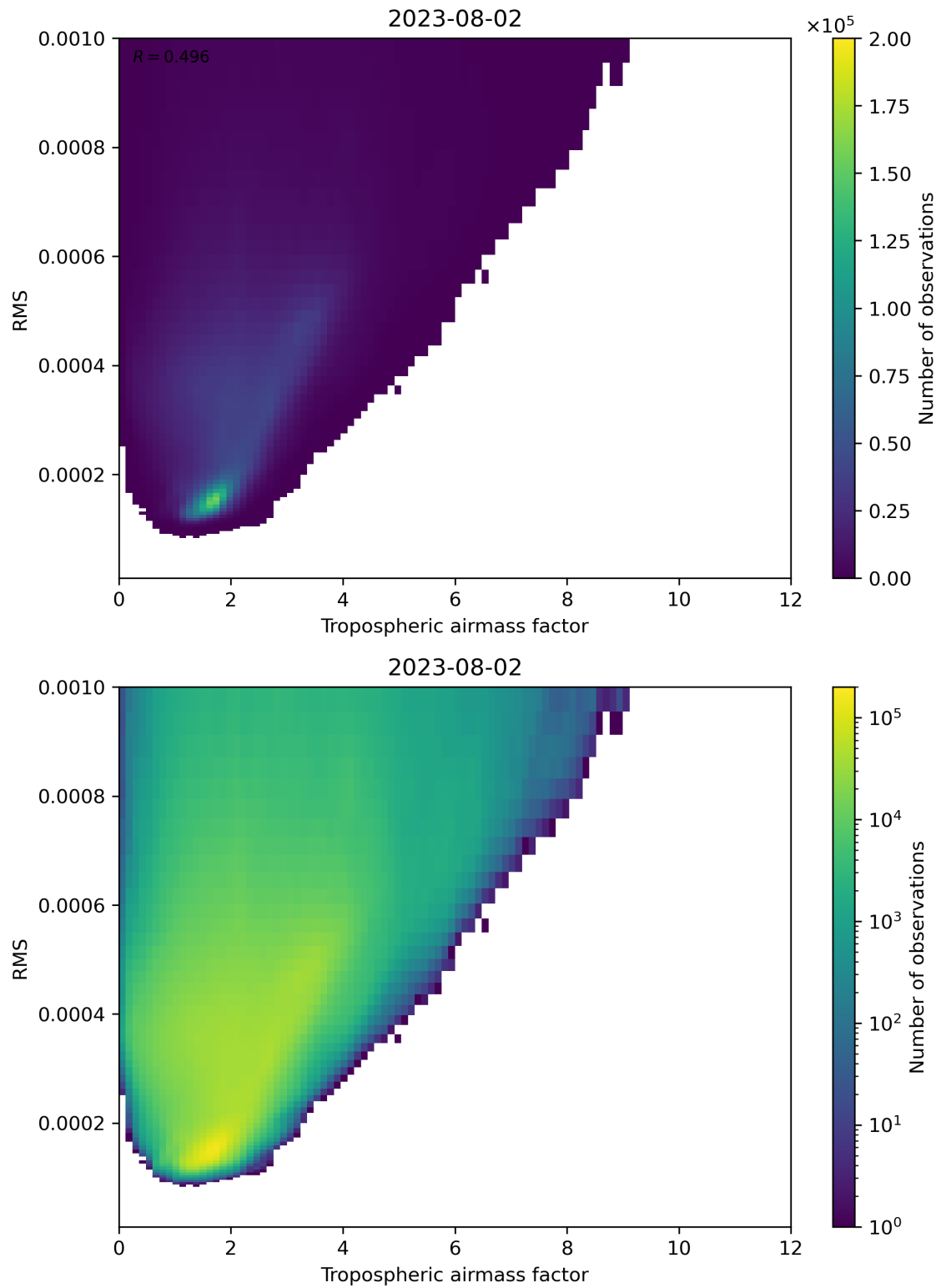
Figure 79: Scatter density plot of “Tropospheric airmass factor” against “RMS” for 2023-08-01 to 2023-08-03.
