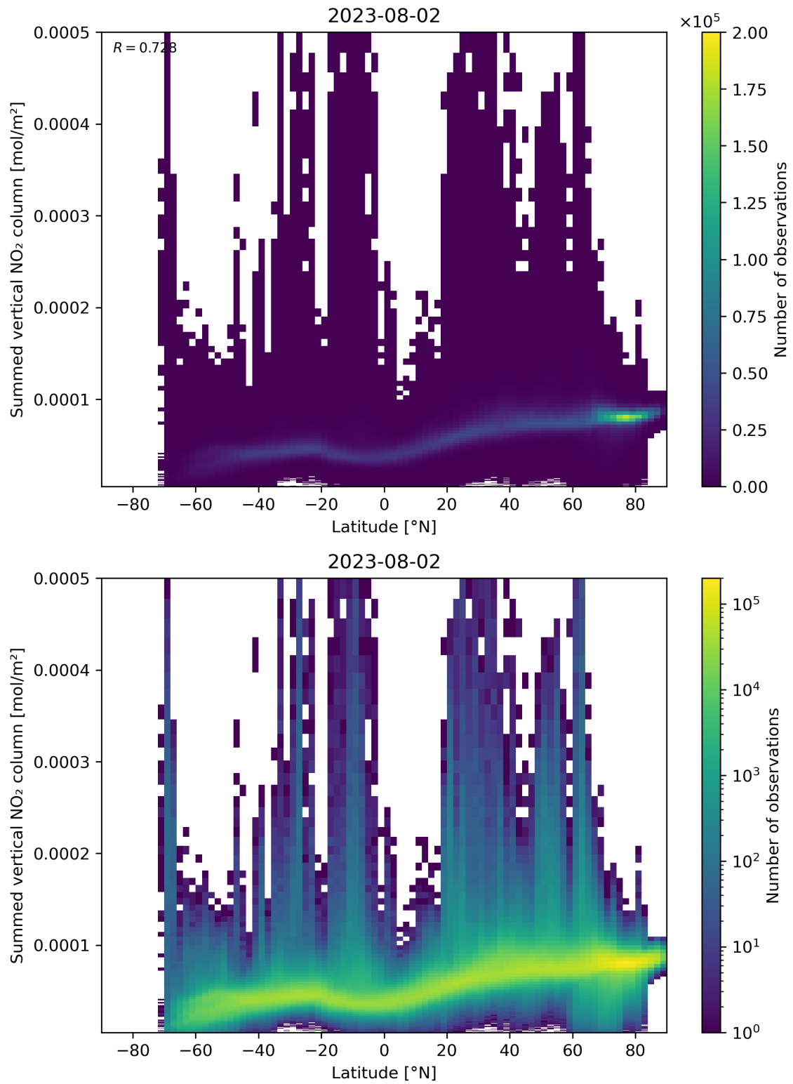
Figure 88: Scatter density plot of “Latitude” against “Summed vertical NO 2 column” for 2023-08-01 to 2023-08-03.
