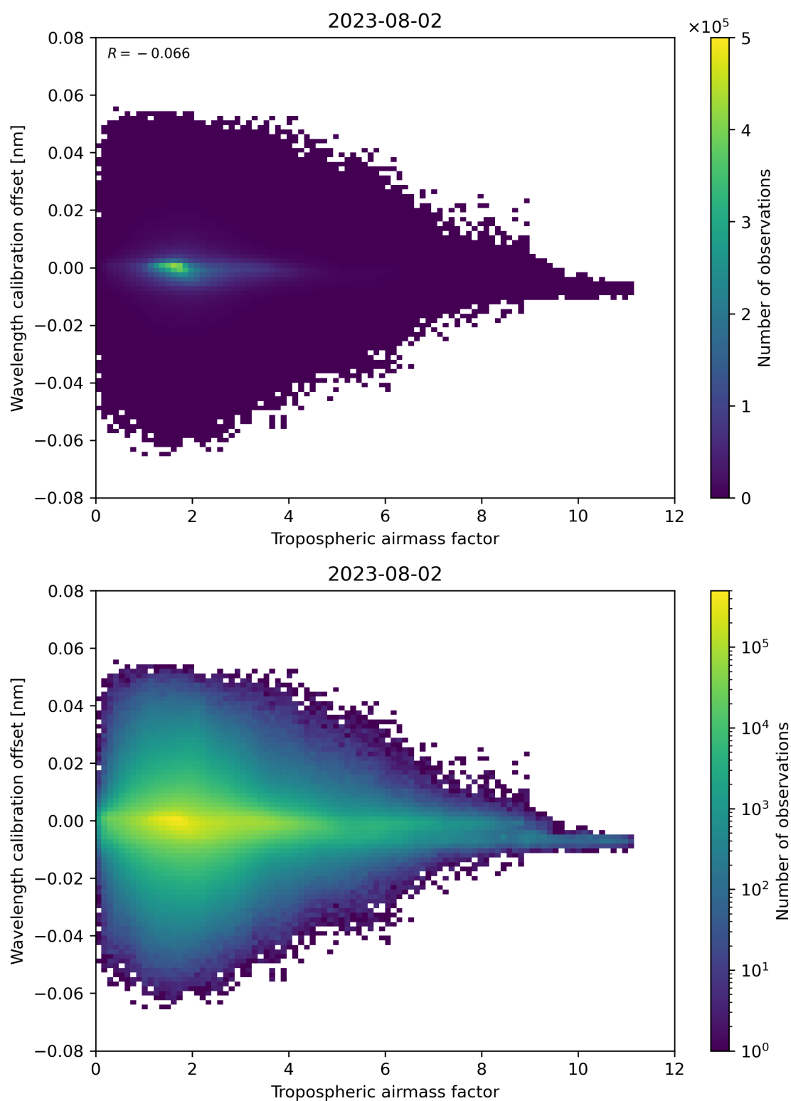
Figure 80: Scatter density plot of “Tropospheric airmass factor” against “Wavelength calibration offset” for 2023-08-01 to 2023-08-03.
