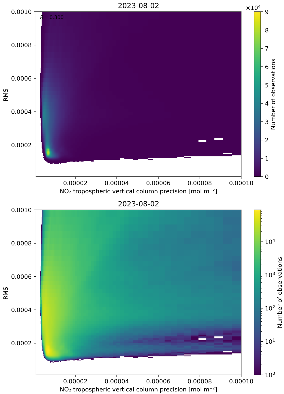
Figure 140: Scatter density plot of “NO 2 tropospheric vertical column precision” against “RMS” for 2023-08-01 to 2023-08-03.
