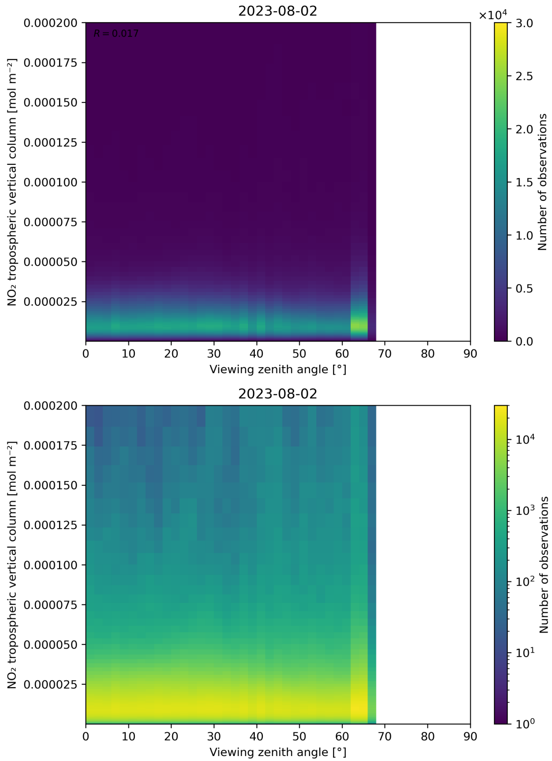
Figure 169: Scatter density plot of “Viewing zenith angle” against “NO 2 tropospheric vertical column” for 2023-08-01 to 2023-08-03.
