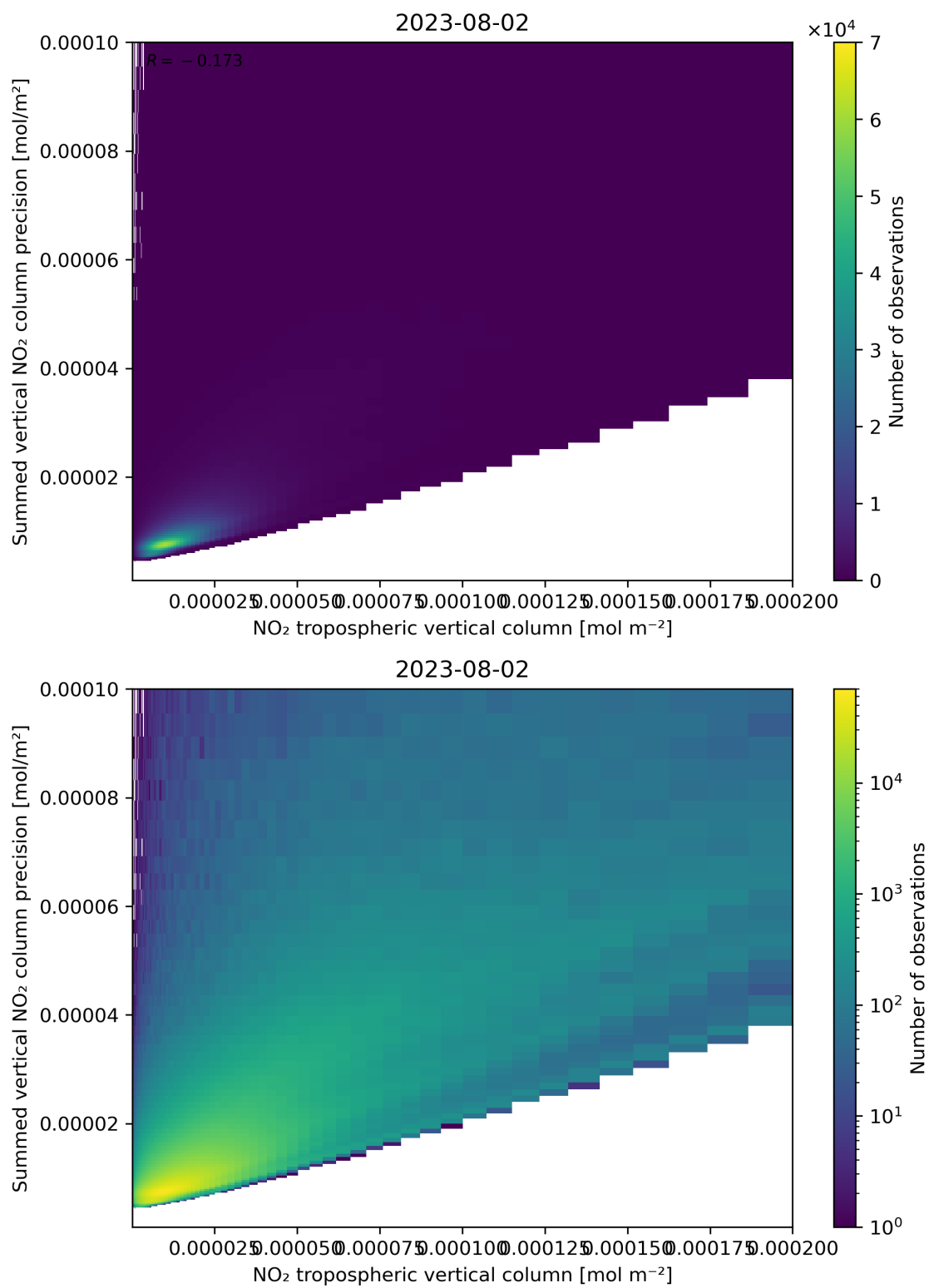
Figure 127: Scatter density plot of “NO 2 tropospheric vertical column” against “Summed vertical NO 2 column precision” for 2023-08-01 to 2023-08-03.
