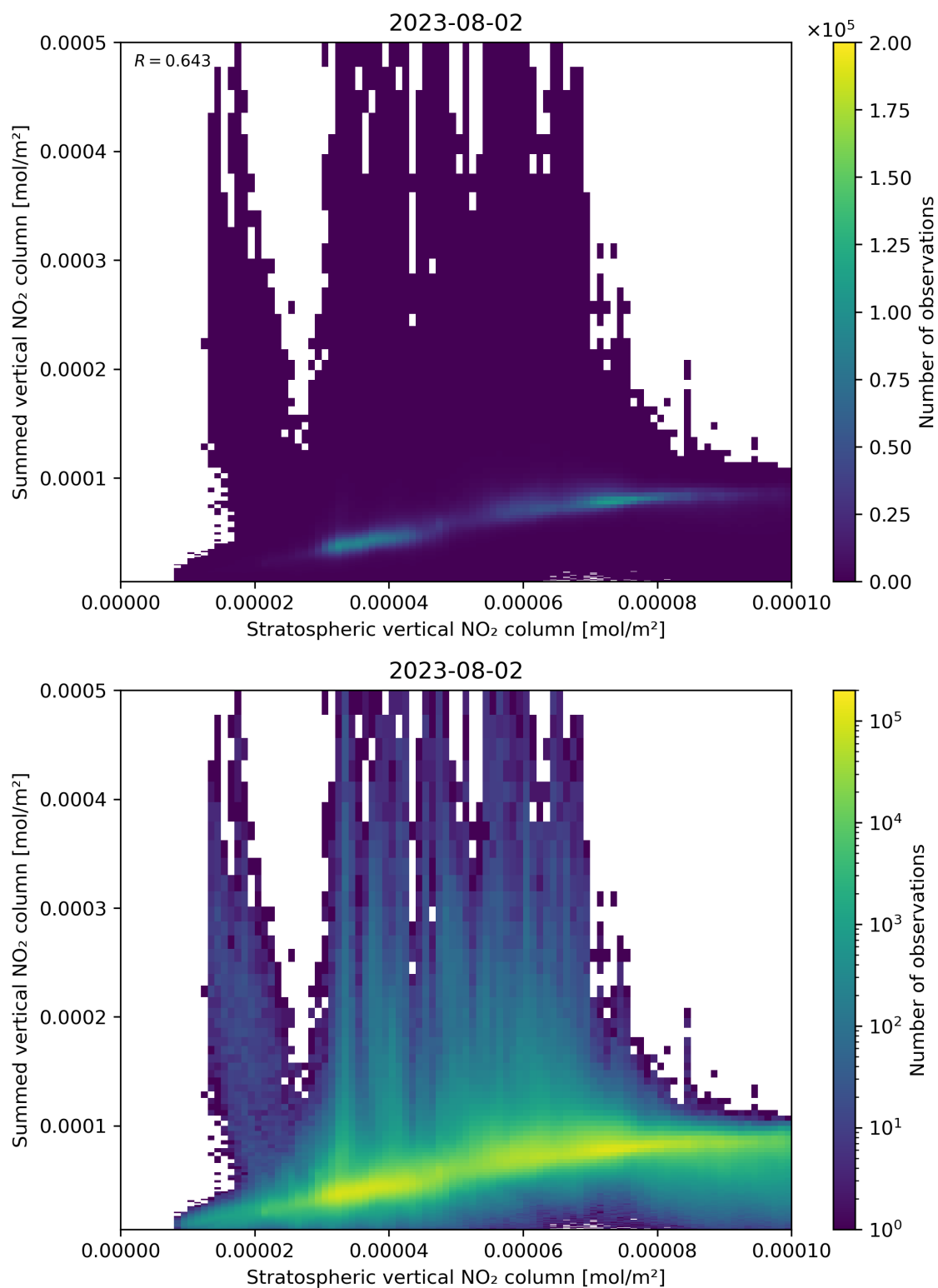
Figure 98: Scatter density plot of “Stratospheric vertical NO 2 column” against “Summed vertical NO 2 column” for 2023-08-01 to 2023-08-03.
