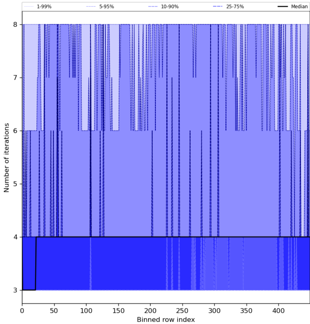
Figure 51: Along track statistics of “Number of iterations” for 2023-08-01 to 2023-08-03
