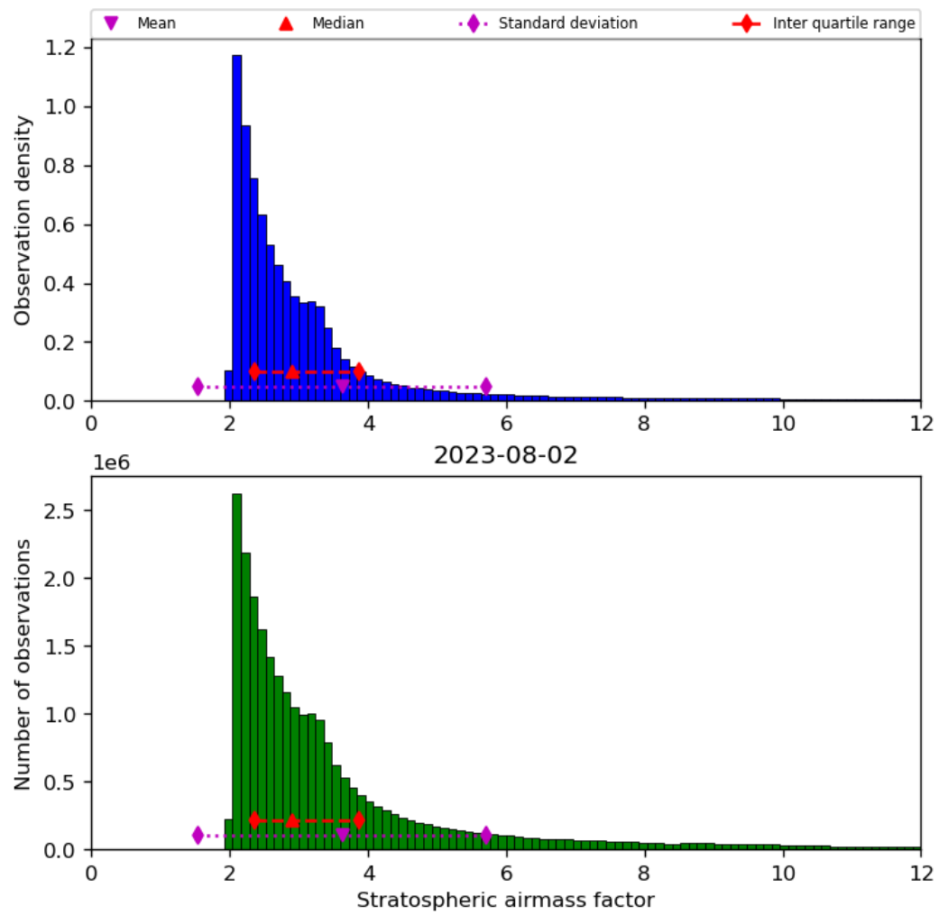
Figure 44: Histogram of “Stratospheric airmass factor” for 2023-08-01 to 2023-08-03
