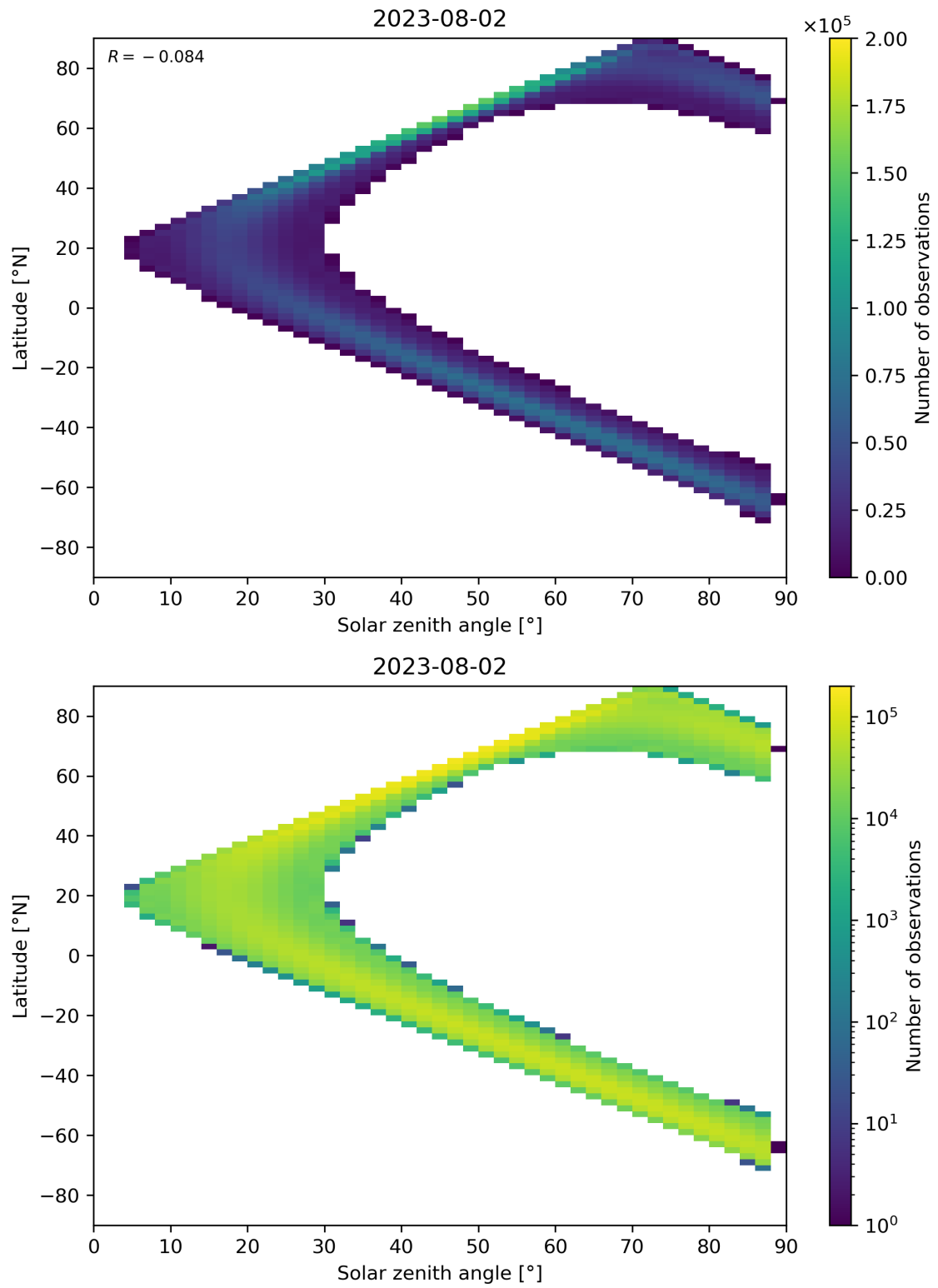
Figure 149: Scatter density plot of “Solar zenith angle” against “Latitude” for 2023-08-01 to 2023-08-03.
