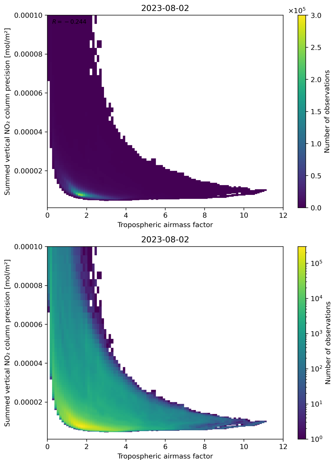
Figure 76: Scatter density plot of “Tropospheric air mass factor” against “Summed vertical NO 2 column precision” for 2023-08-01 to 2023-08-03.
