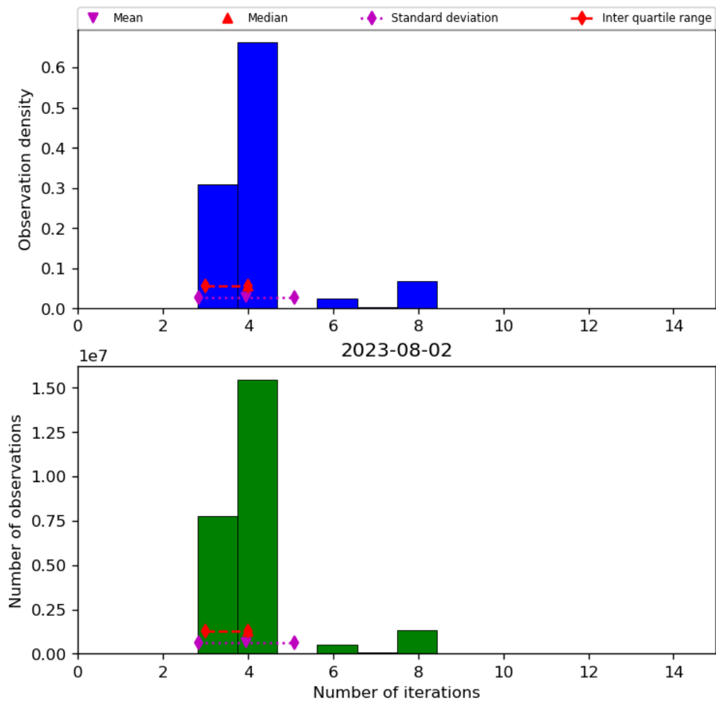
Figure 34: Histogram of “Number of iterations” for 2023-08-01 to 2023-08-03
