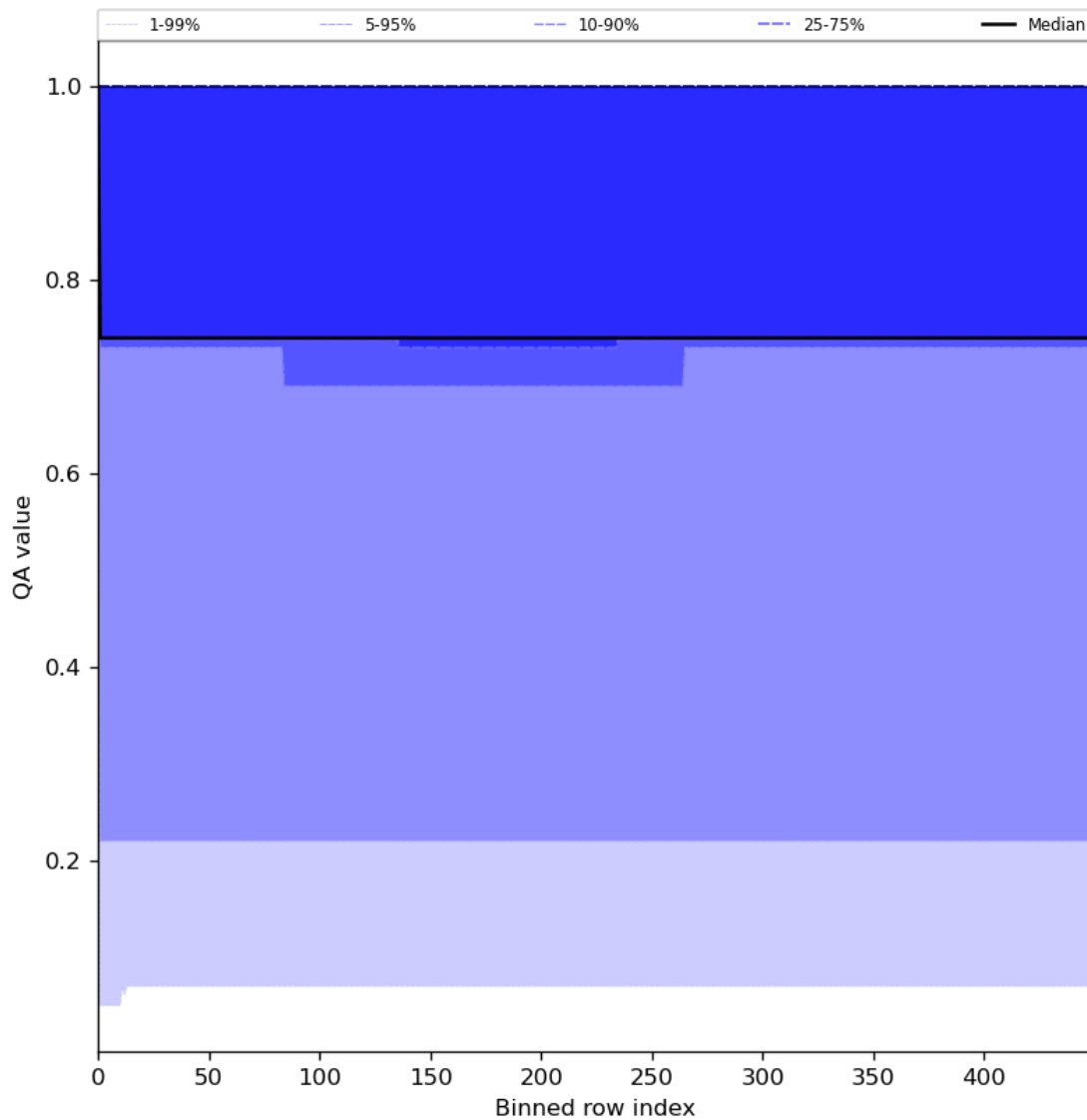
Figure 45: Along track statistics of “QA value” for 2023-08-01 to 2023-08-03
