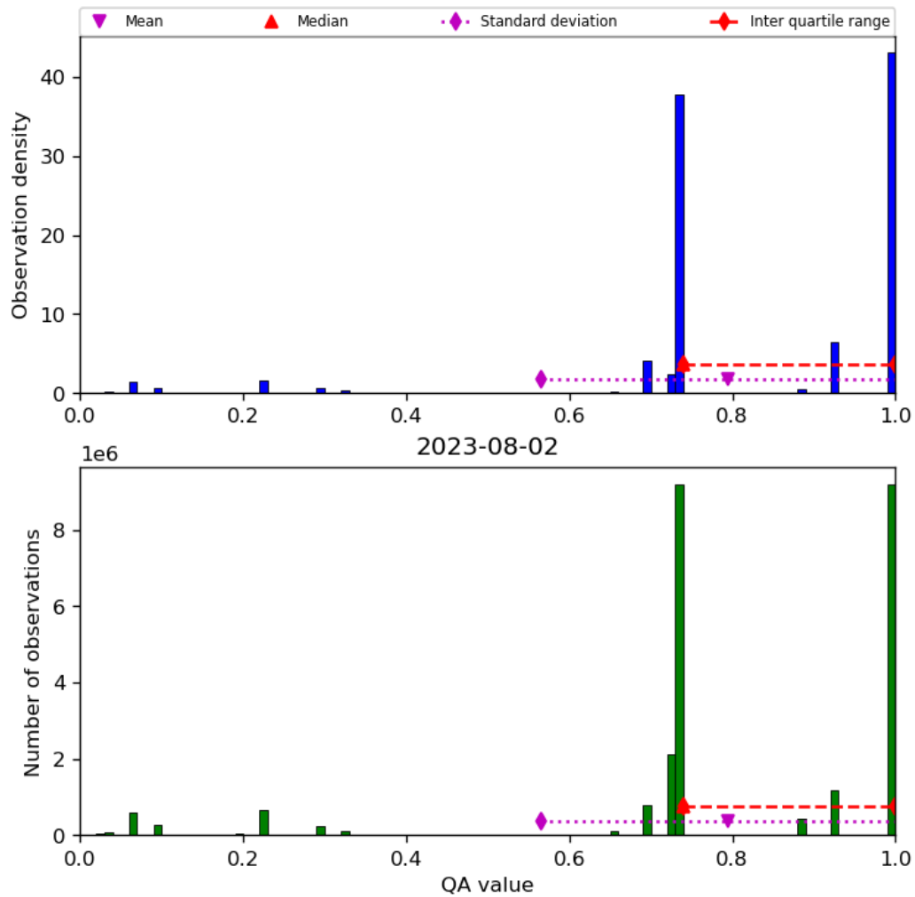
Figure 28: Histogram of “QA value” for 2023-08-01 to 2023-08-03
