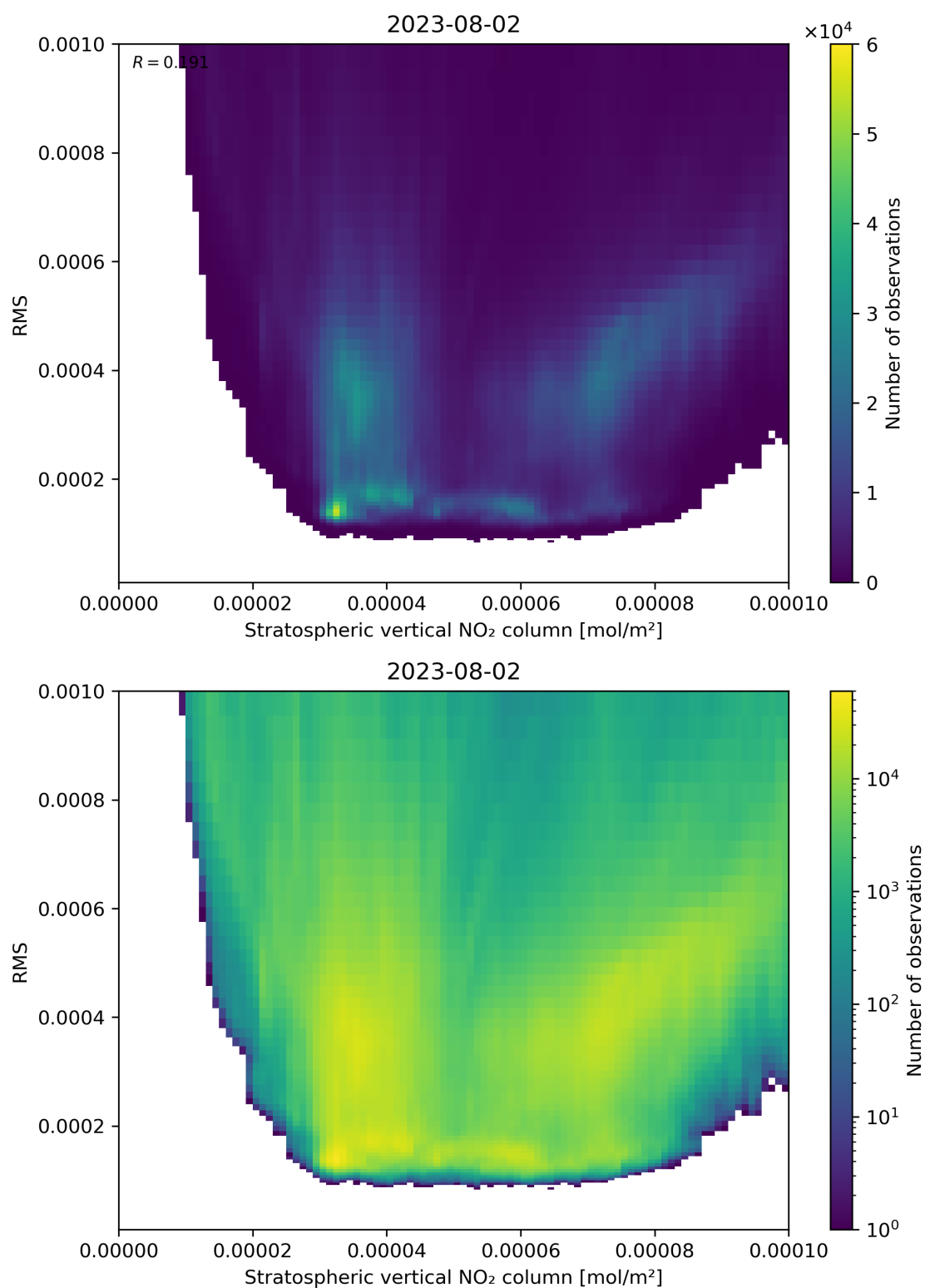
Figure 102: Scatter density plot of “Stratospheric vertical NO 2 column” against “RMS” for 2023-08-01 to 2023-08-03.
