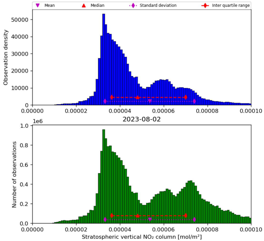
Figure 36: Histogram of “Stratospheric vertical NO 2 column” for 2023-08-01 to 2023-08-03
