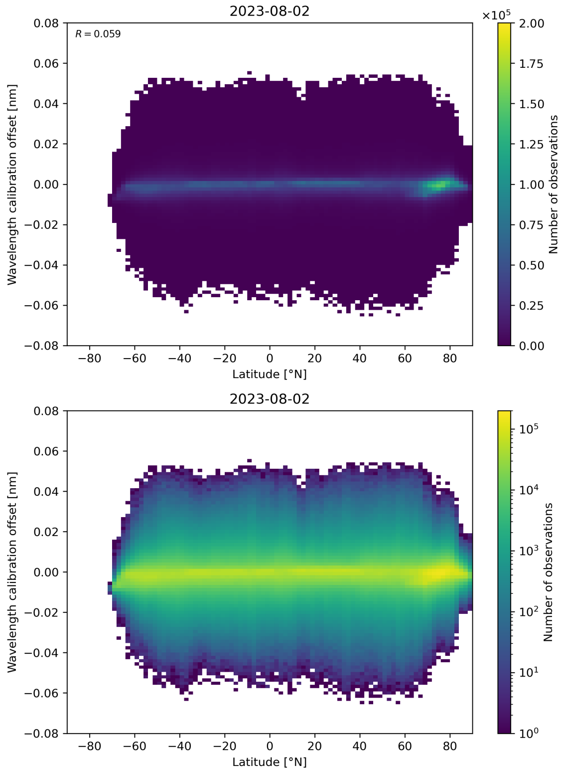
Figure 95: Scatter density plot of “Latitude” against “Wavelength calibration offset” for 2023-08-01 to 2023-08-03.
