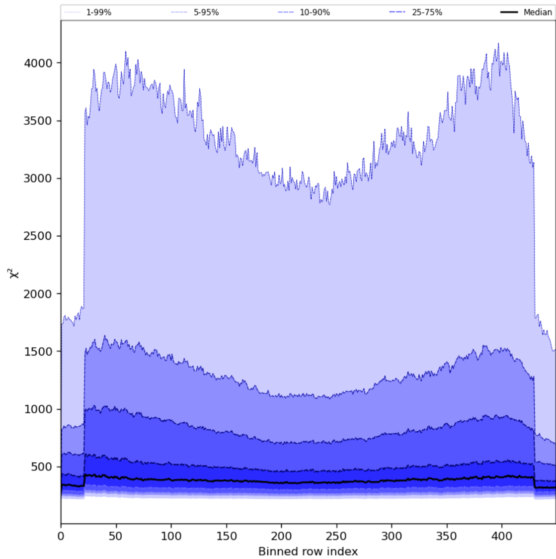
Figure 59: Along track statistics of " \chi^2 " for 2023-08-01 to 2023-08-03
