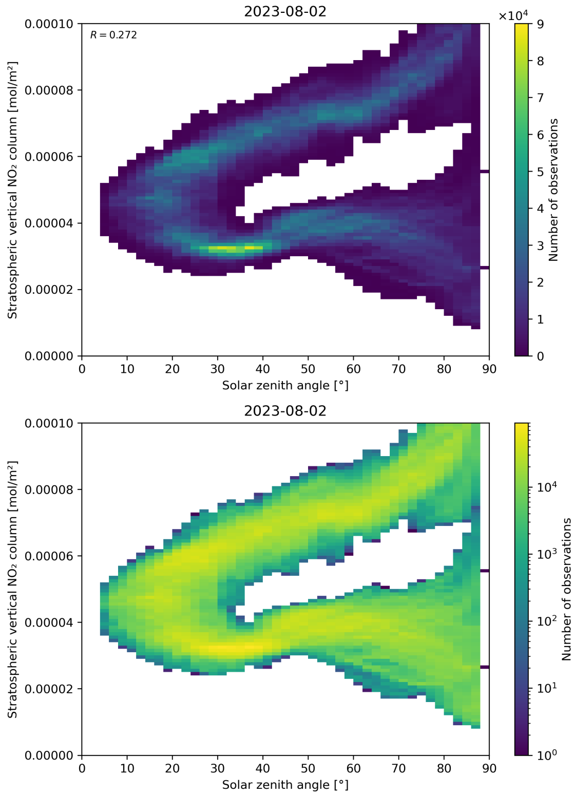
Figure 150: Scatter density plot of “Solar zenith angle” against “Stratospheric vertical NO 2 column” for 2023-08-01 to 2023-08-03.
