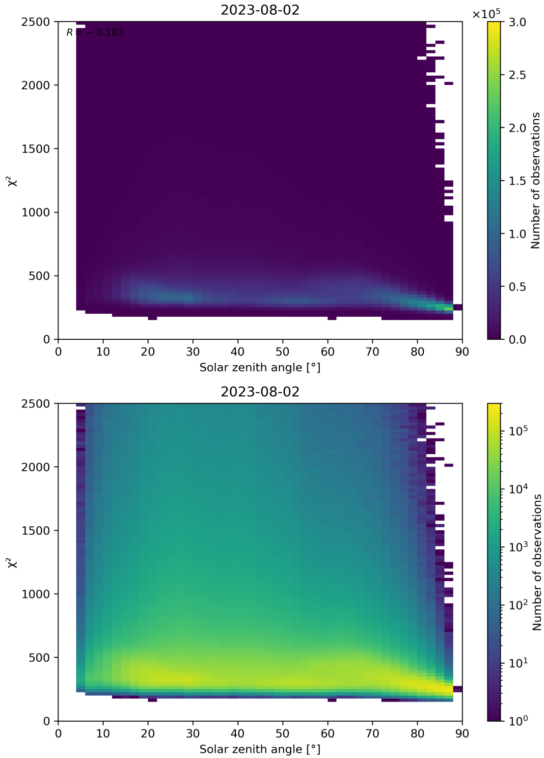
Figure 148: Scatter density plot of “Solar zenith angle” against “ \chi^2 ” for 2023-08-01 to 2023-08-03.
