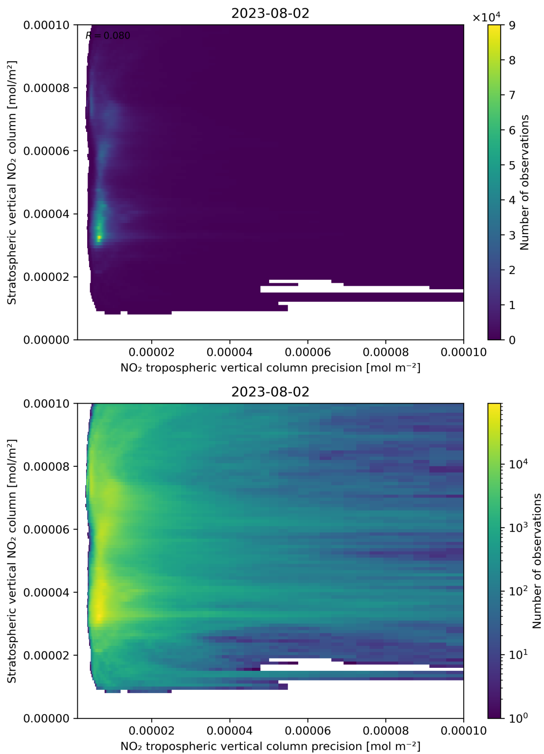
Figure 135: Scatter density plot of “NO 2 tropospheric vertical column precision” against “Stratospheric vertical NO 2 column” for 2023-08-01 to 2023-08-03.
