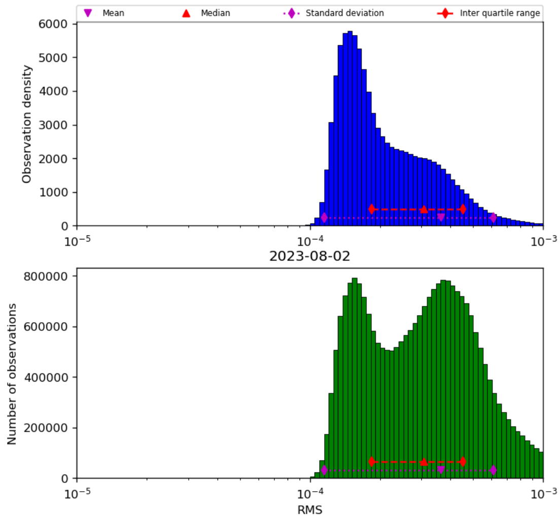
Figure 43: Histogram of “RMS” for 2023-08-01 to 2023-08-03
