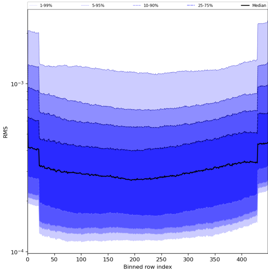
Figure 60: Along track statistics of “RMS” for 2023-08-01 to 2023-08-03
