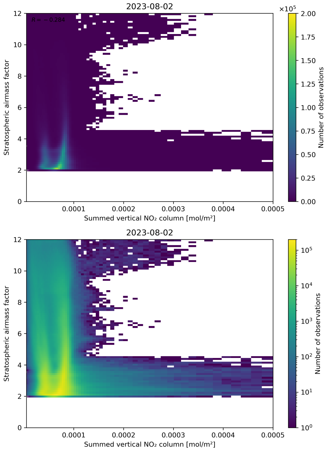
Figure 103: Scatter density plot of “Summed vertical NO 2 column” against “Stratospheric air mass factor” for 2023-08-01 to 2023-08-03.
