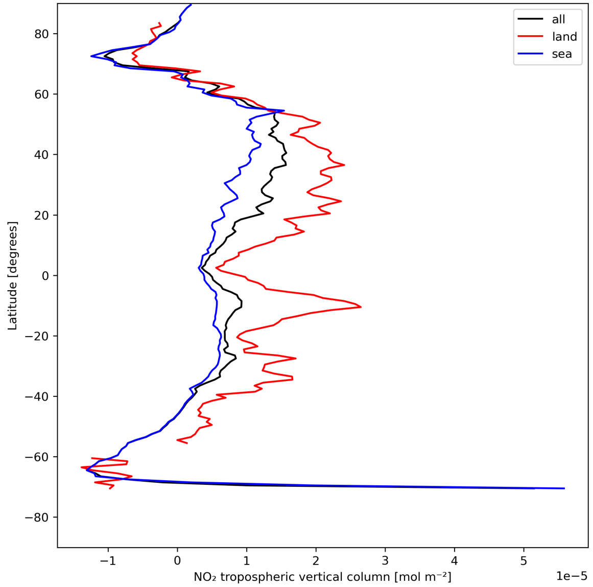
Figure 12: Zonal average of “NO 2 tropospheric vertical column” for 2023-08-01 to 2023-08-03.
