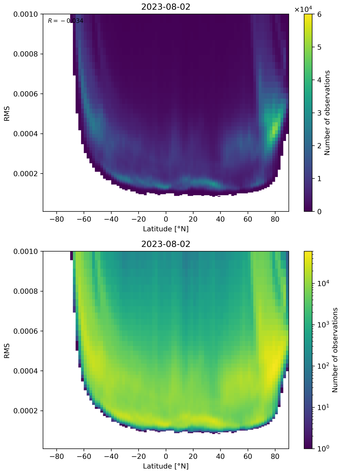
Figure 94: Scatter density plot of “Latitude” against “RMS” for 2023-08-01 to 2023-08-03.
