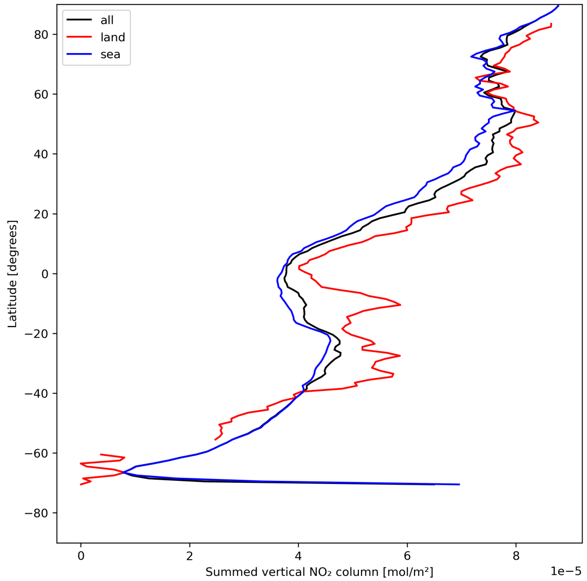
Figure 23: Zonal average of “Summed vertical NO 2 column” for 2023-08-01 to 2023-08-03.
