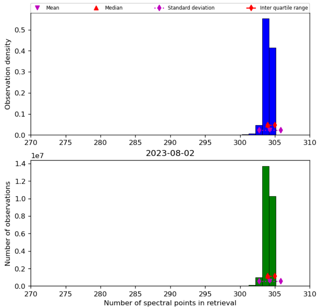
Figure 33: Histogram of “Number of spectral points in retrieval” for 2023-08-01 to 2023-08-03
