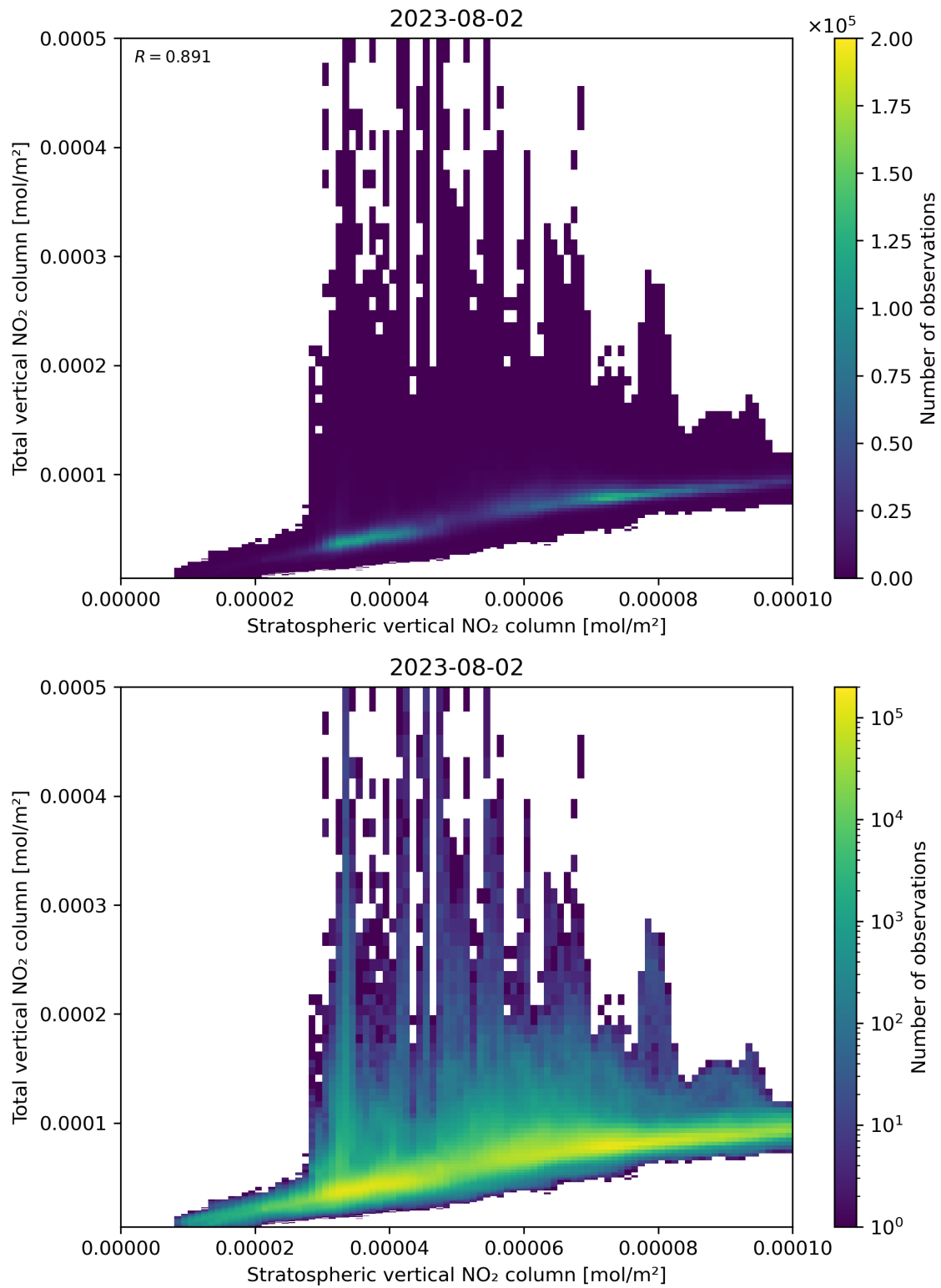
Figure 100: Scatter density plot of “Stratospheric vertical NO 2 column” against “Total vertical NO 2 column” for 2023-08-01 to 2023-08-03.
