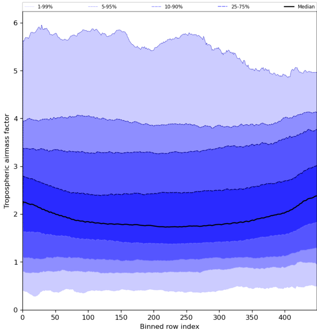
Figure 48: Along track statistics of “Tropospheric airmass factor” for 2023-08-01 to 2023-08-03
