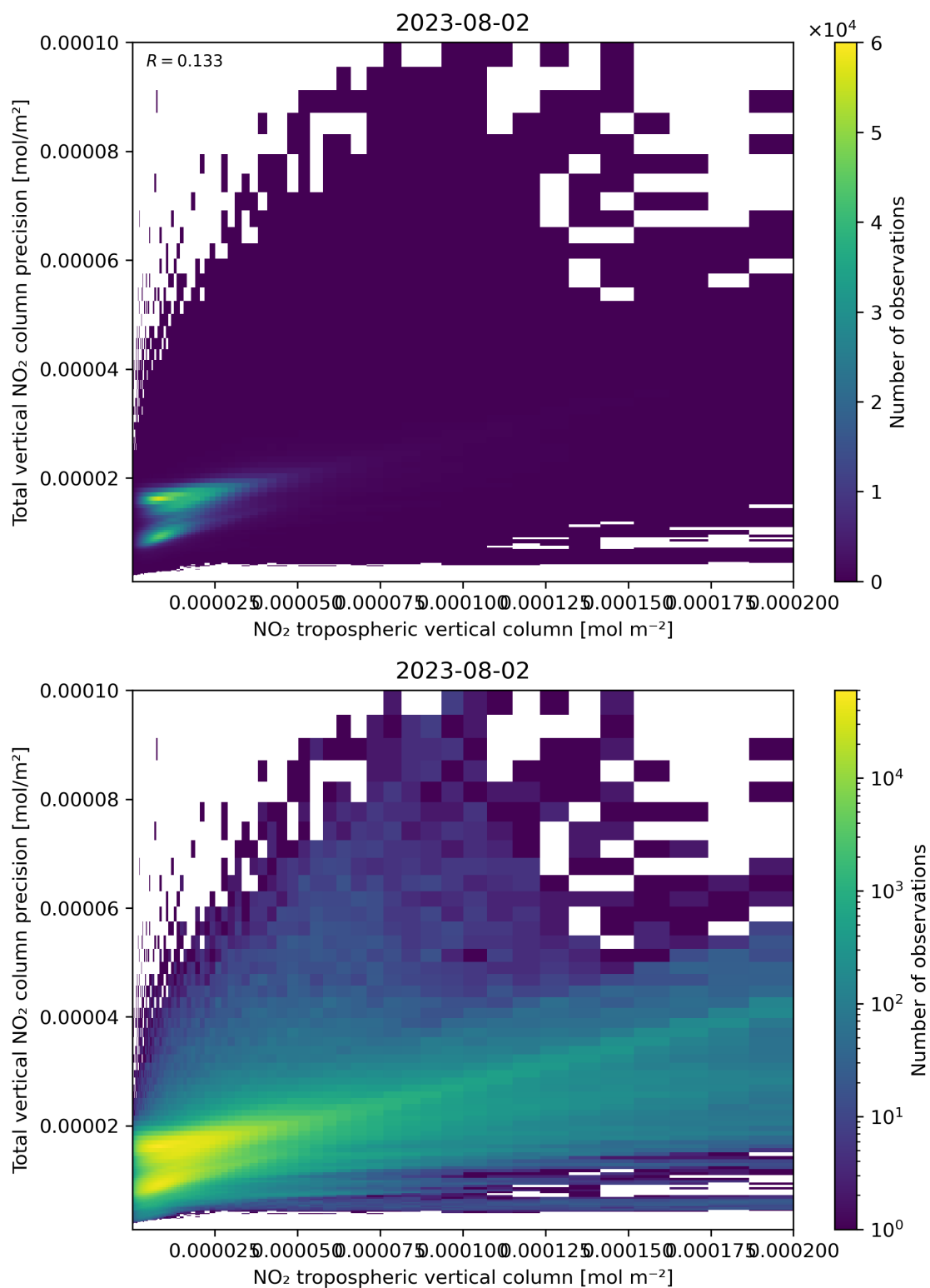
Figure 129: Scatter density plot of “NO 2 tropospheric vertical column” against “Total vertical NO 2 column precision” for 2023-08-01 to 2023-08-03.
