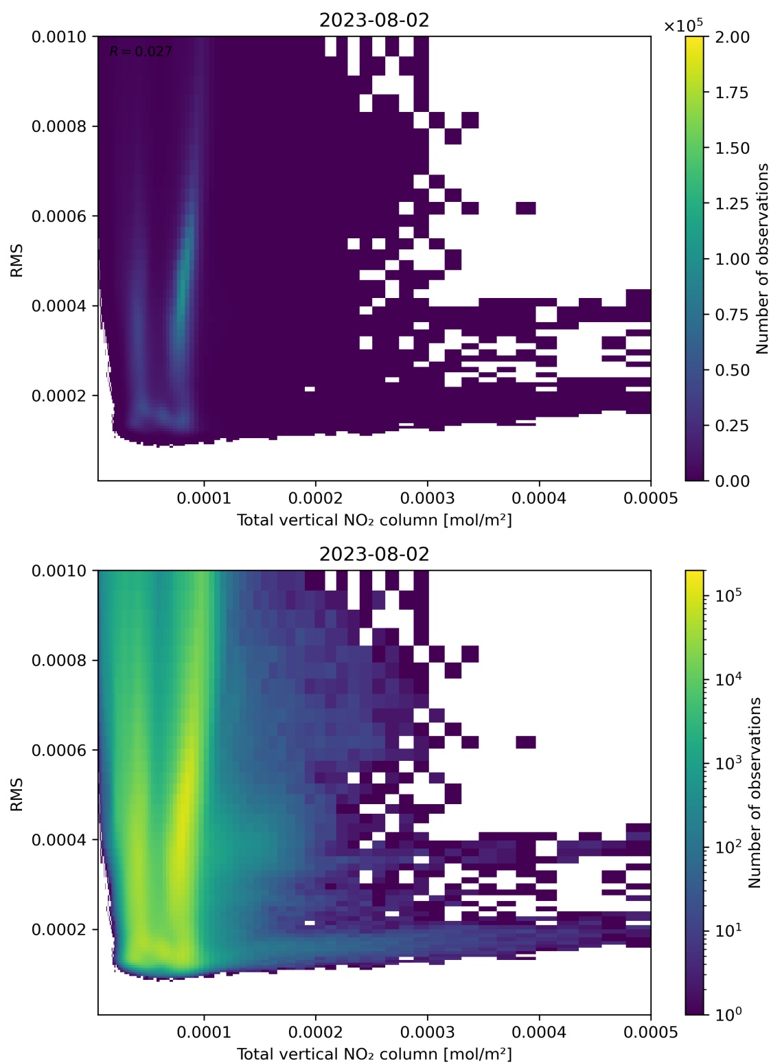
Figure 120: Scatter density plot of “Total vertical NO 2 column” against “RMS” for 2023-08-01 to 2023-08-03.
