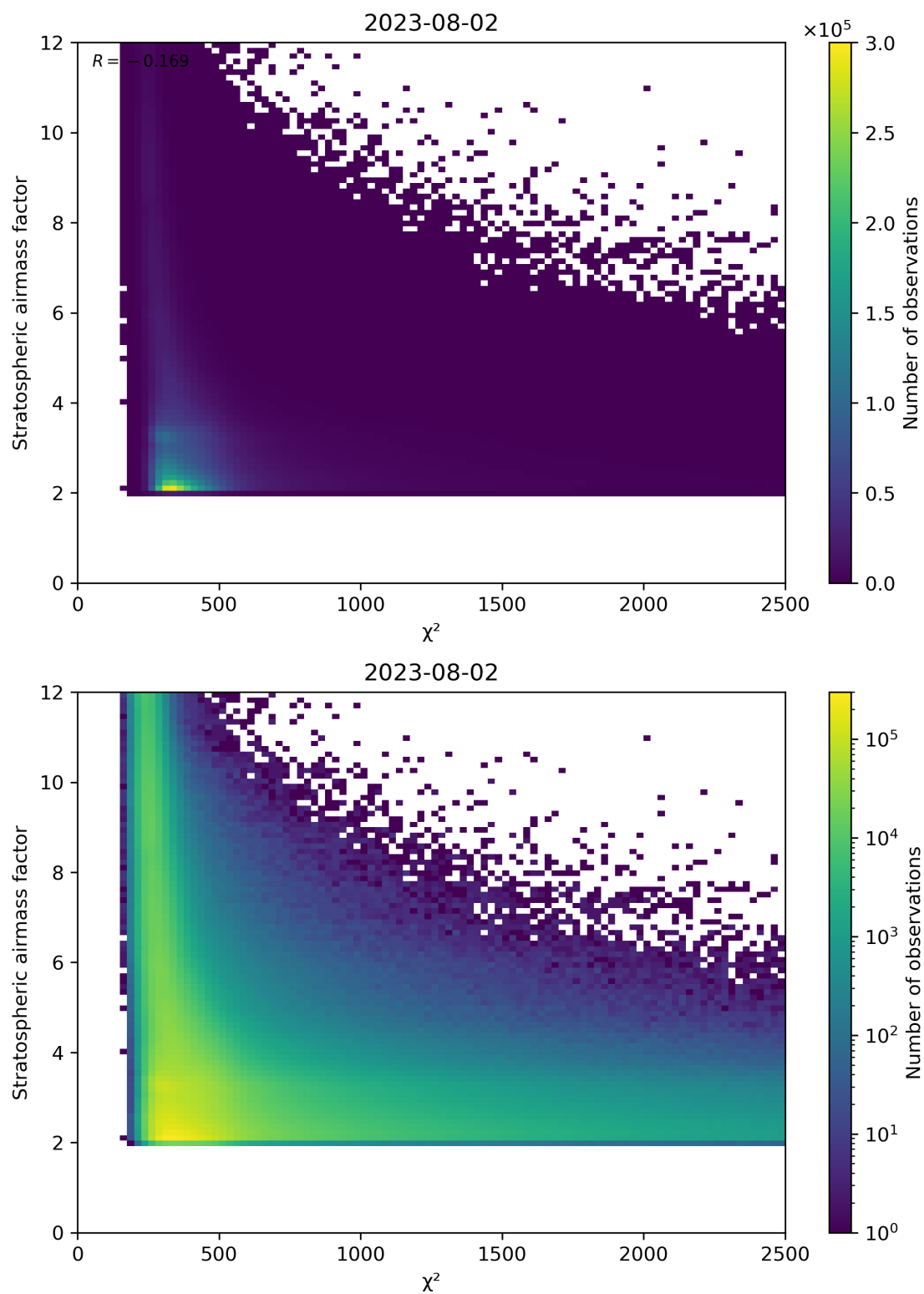
Figure 81: Scatter density plot of “ \chi^2 ” against “Stratospheric airmass factor” for 2023-08-01 to 2023-08-03.
