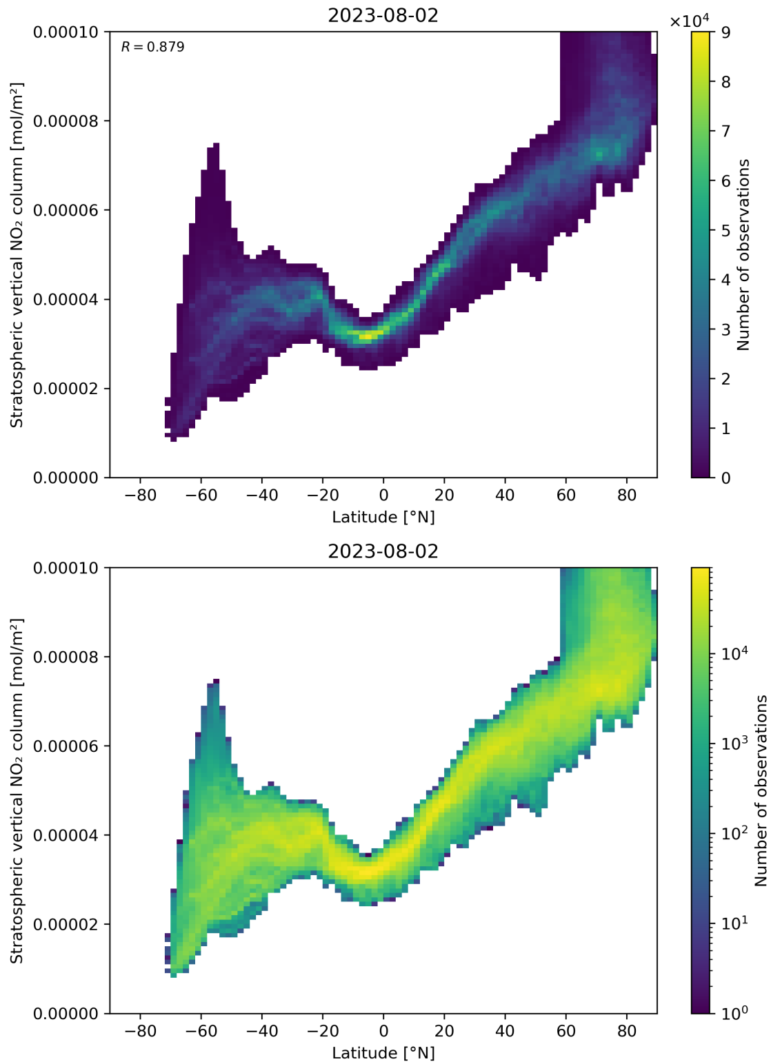
Figure 87: Scatter density plot of “Latitude” against “Stratospheric vertical NO 2 column” for 2023-08-01 to 2023-08-03.
