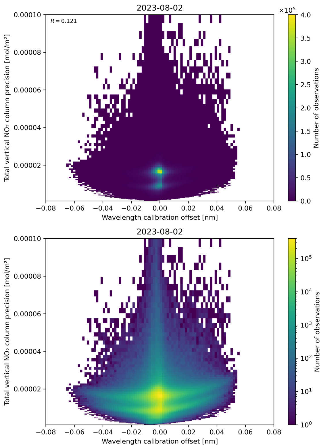
Figure 180: Scatter density plot of “Wavelength calibration offset” against “Total vertical NO 2 column precision” for 2023-08-01 to 2023-08-03.
