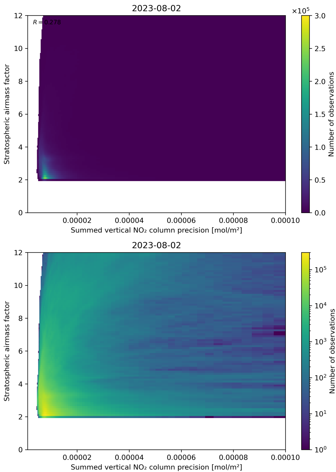
Figure 106: Scatter density plot of “Summed vertical NO 2 column precision” against “Stratospheric airmass factor” for 2023-08-01 to 2023-08-03.
