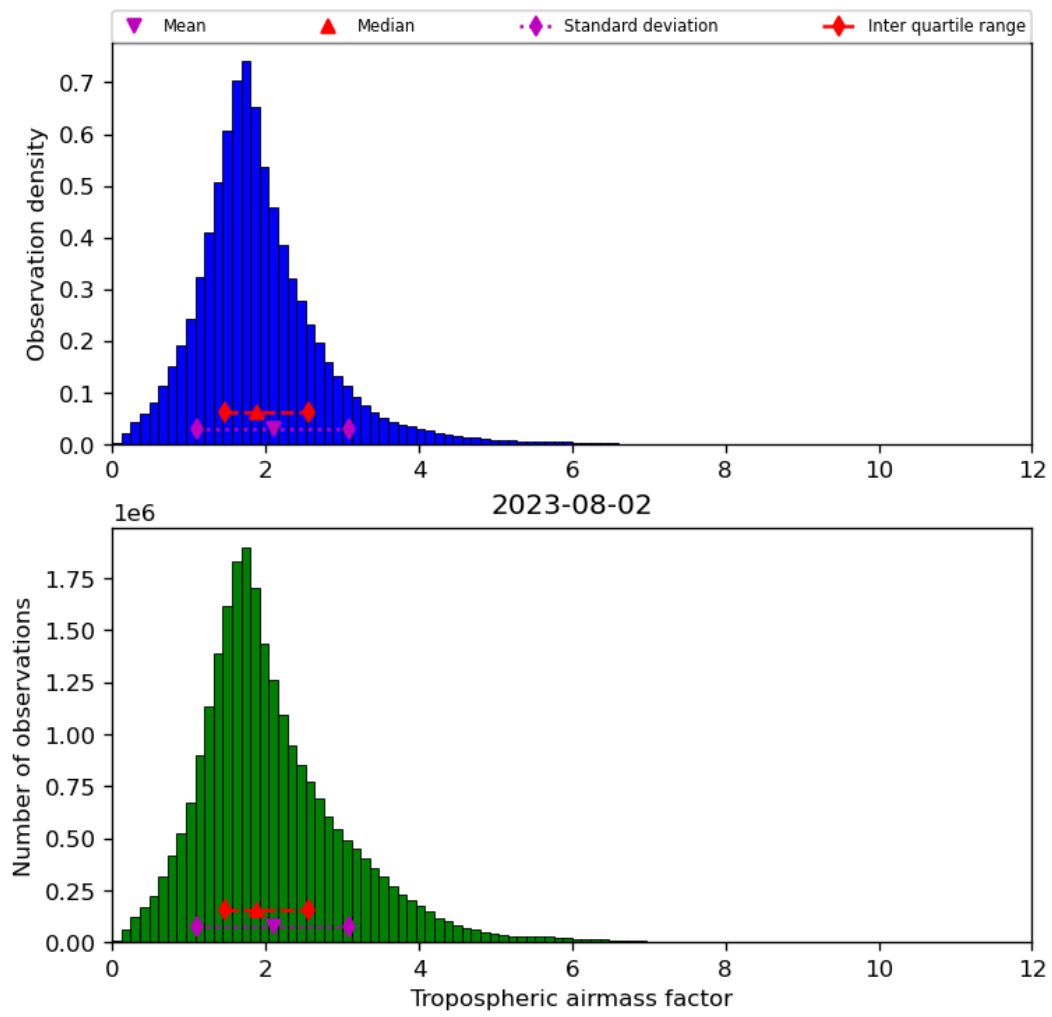
Figure 31: Histogram of “Tropospheric airmass factor” for 2023-08-01 to 2023-08-03
