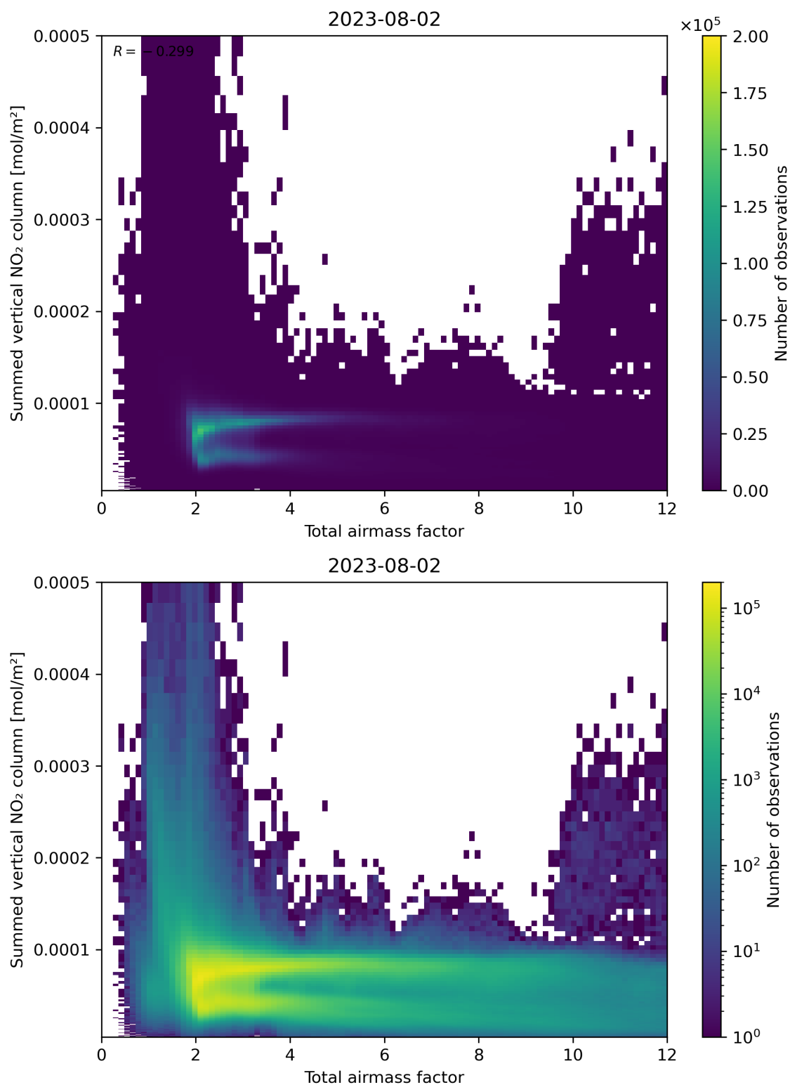
Figure 65: Scatter density plot of “Total airmass factor” against “Summed vertical NO 2 column” for 2023-08-01 to 2023-08-03.
