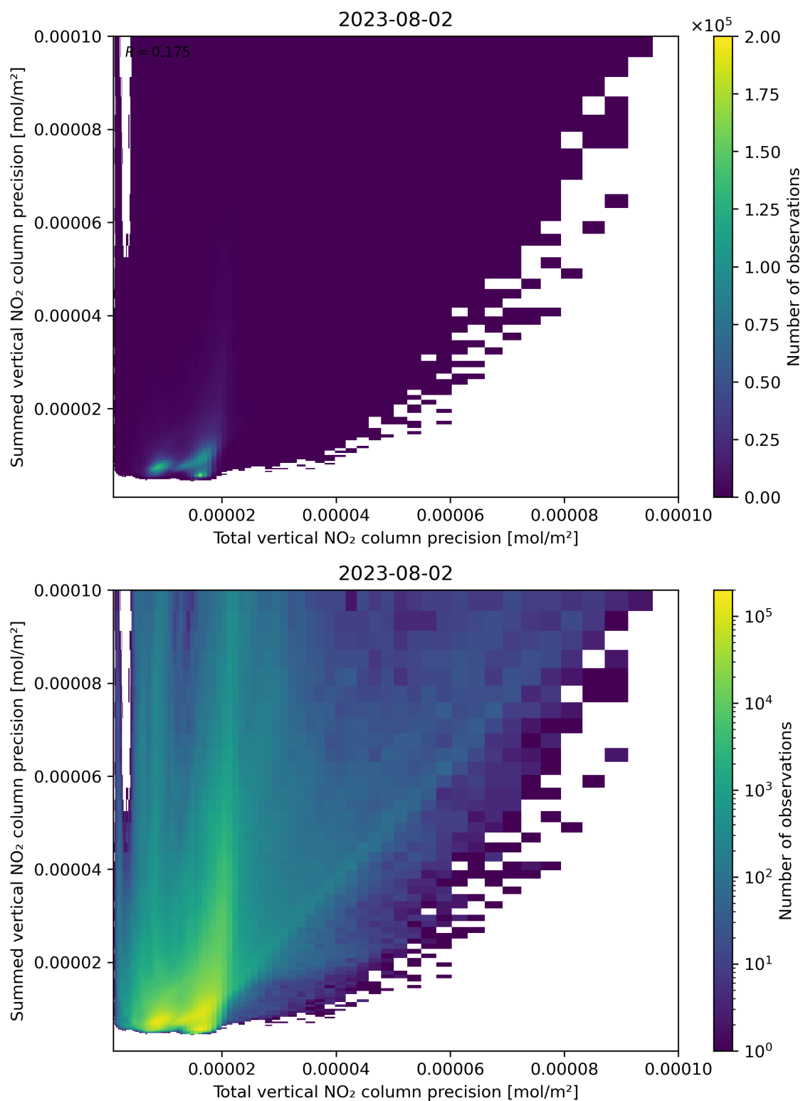
Figure 118: Scatter density plot of “Total vertical NO 2 column precision” against “Summed vertical NO 2 column precision” for 2023-08-01 to 2023-08-03.
