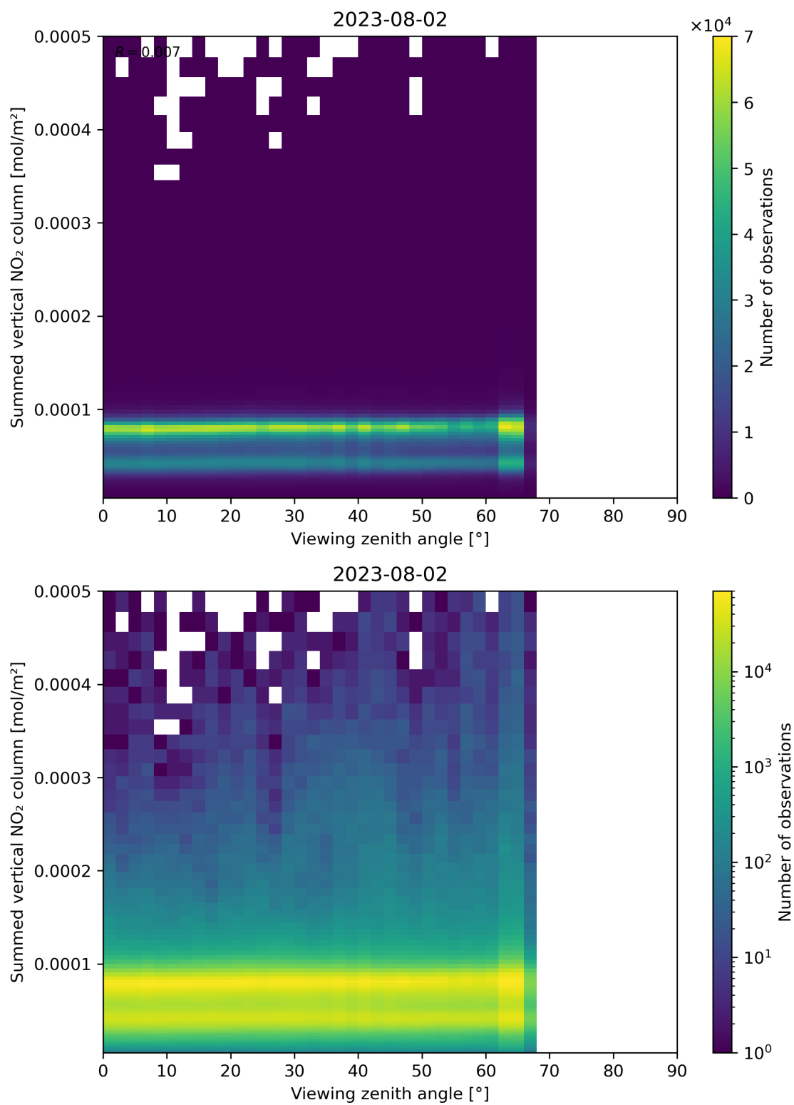
Figure 165: Scatter density plot of “Viewing zenith angle” against “Summed vertical NO 2 column” for 2023-08-01 to 2023-08-03.
