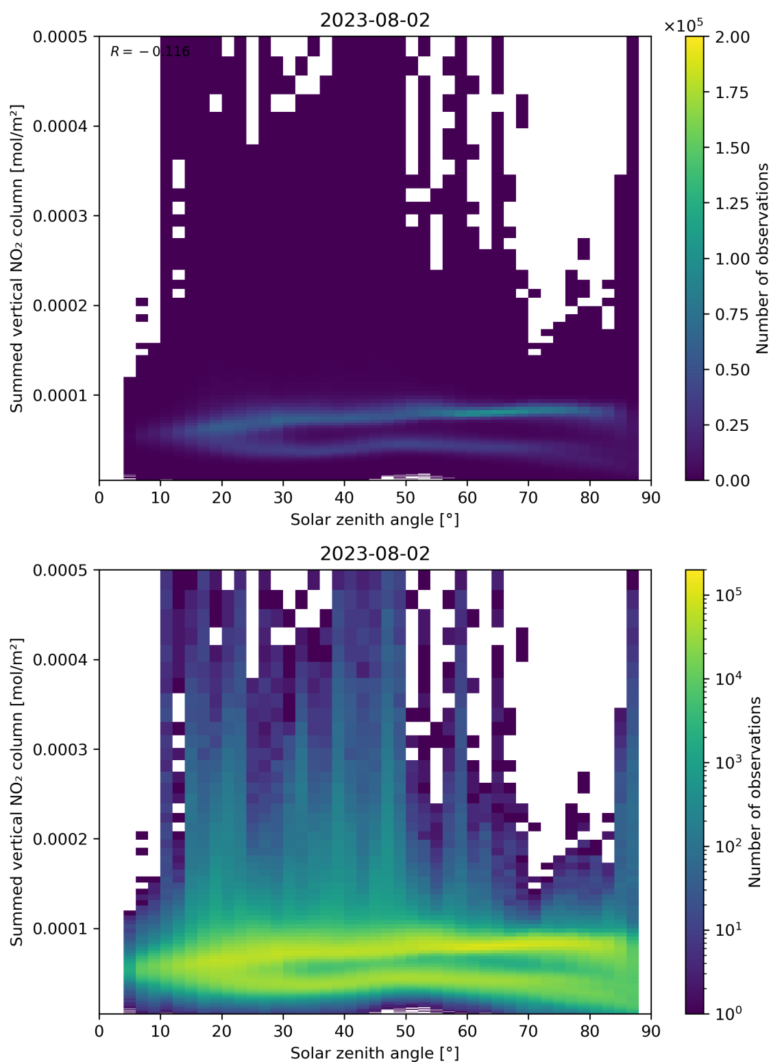
Figure 151: Scatter density plot of “Solar zenith angle” against “Summed vertical NO 2 column” for 2023-08-01 to 2023-08-03.
