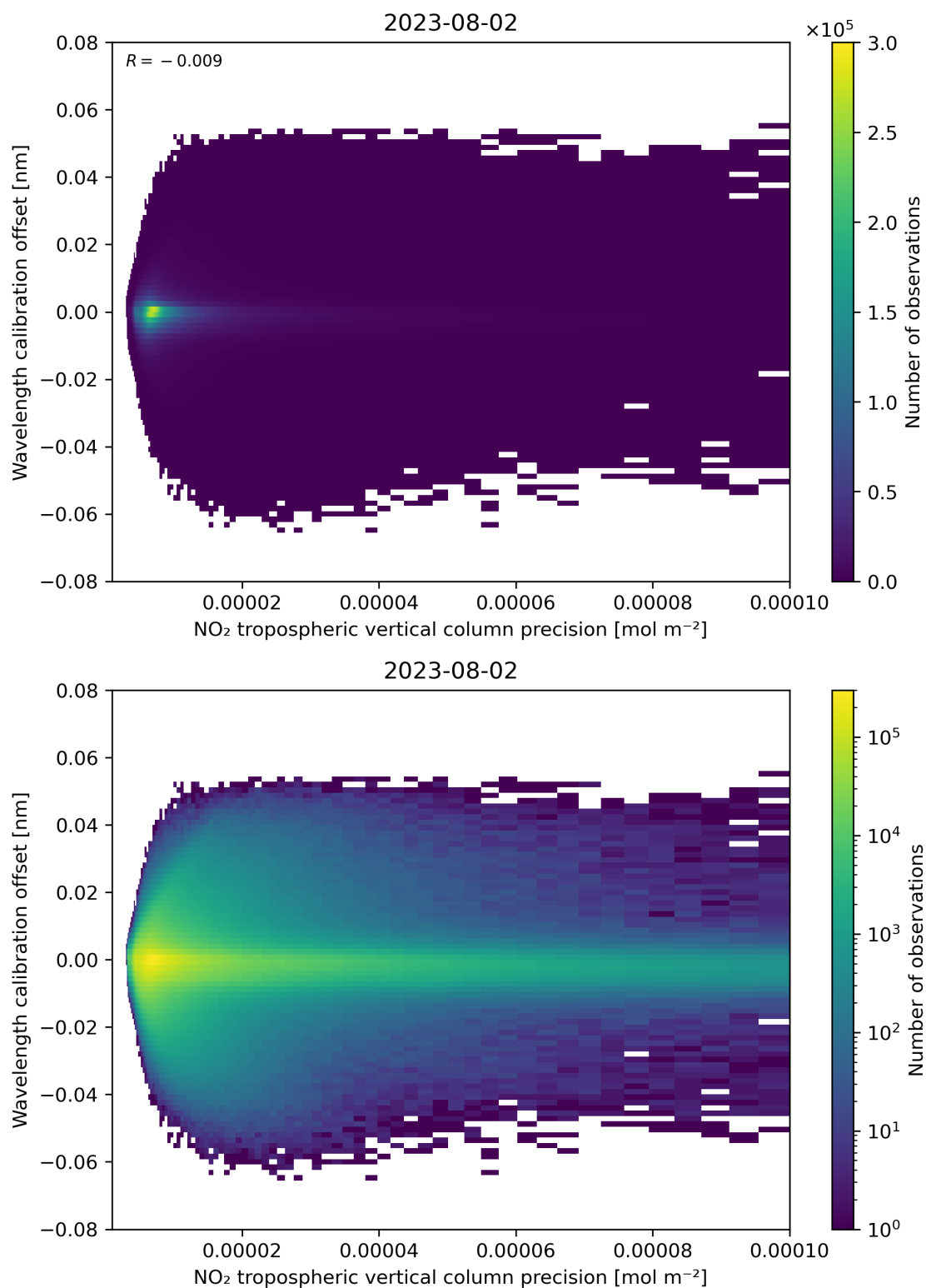
Figure 141: Scatter density plot of “NO 2 tropospheric vertical column precision” against “Wavelength calibration offset” for 2023-08-01 to 2023-08-03.
