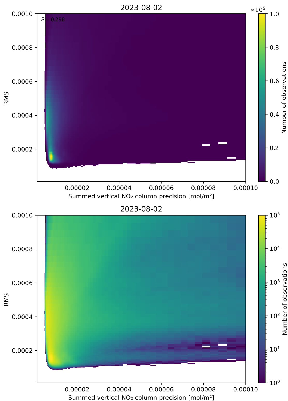
Figure 108: Scatter density plot of “Summed vertical NO 2 column precision” against “RMS” for 2023-08-01 to 2023-08-03.
