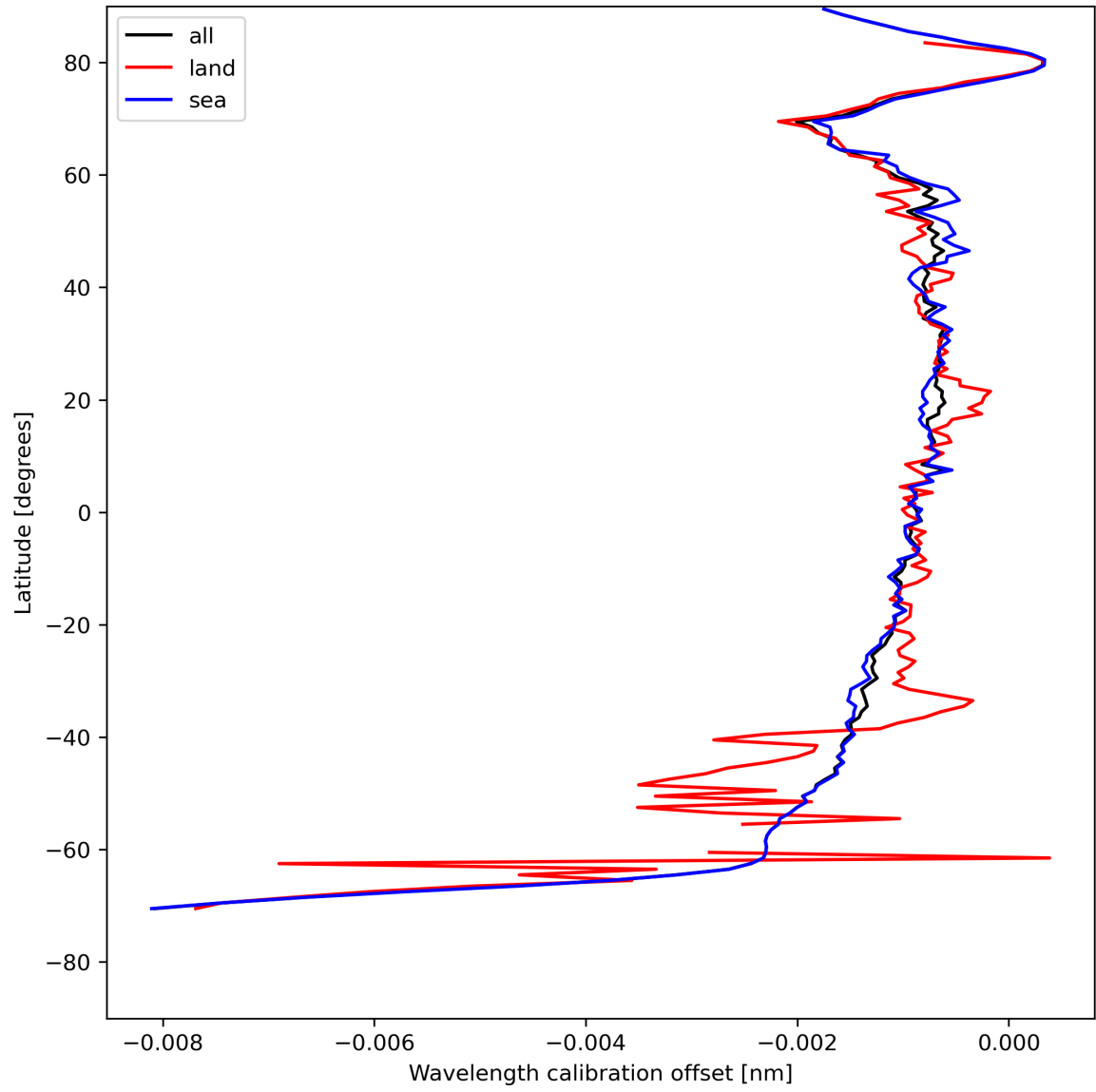
Figure 18: Zonal average of “Wavelength calibration offset” for 2023-08-01 to 2023-08-03.
