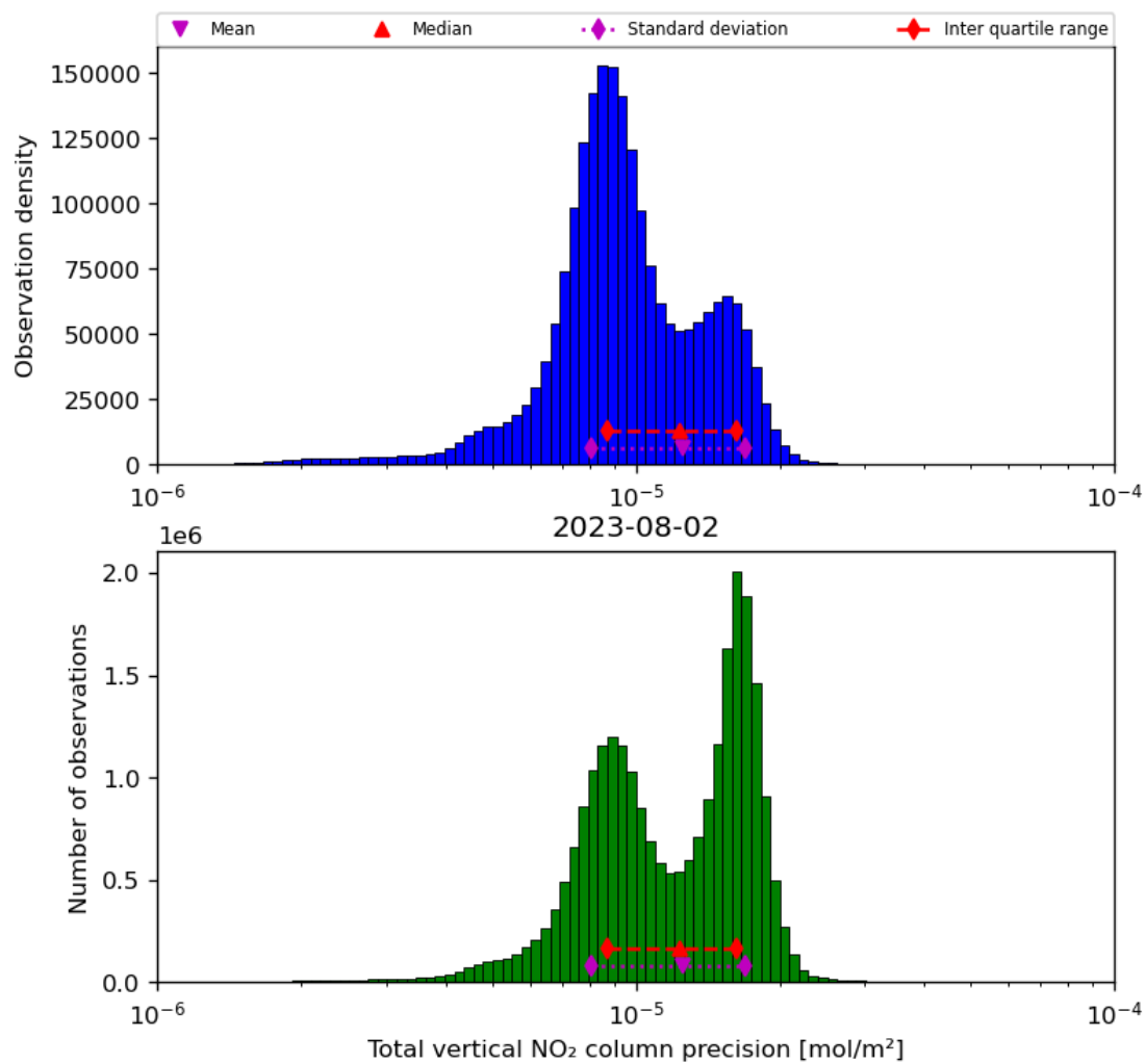
Figure 39: Histogram of “Total vertical NO 2 column precision” for 2023-08-01 to 2023-08-03
