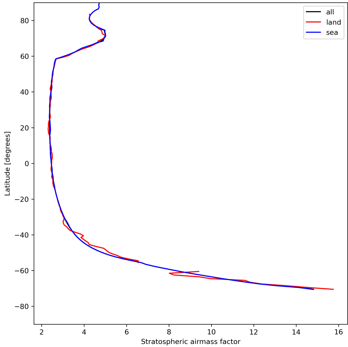
Figure 27: Zonal average of “Stratospheric airmass factor” for 2023-08-01 to 2023-08-03.
