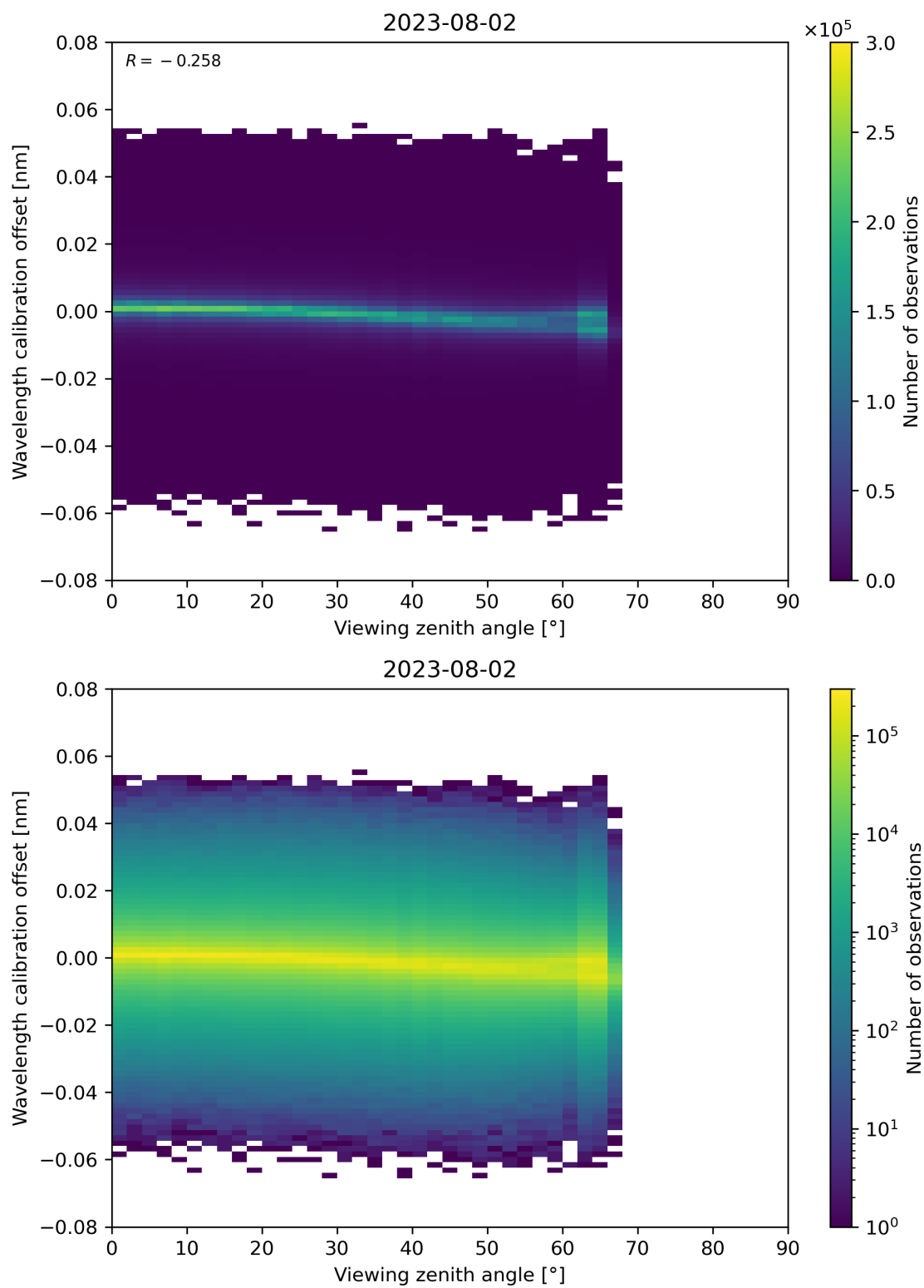
Figure 173: Scatter density plot of “Viewing zenith angle” against “Wavelength calibration offset” for 2023-08-01 to 2023-08-03.
