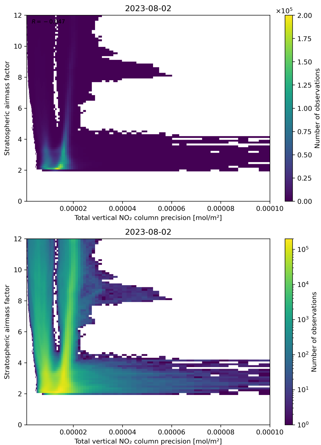
Figure 115: Scatter density plot of “Total vertical NO 2 column precision” against “Stratospheric air mass factor” for 2023-08-01 to 2023-08-03.
