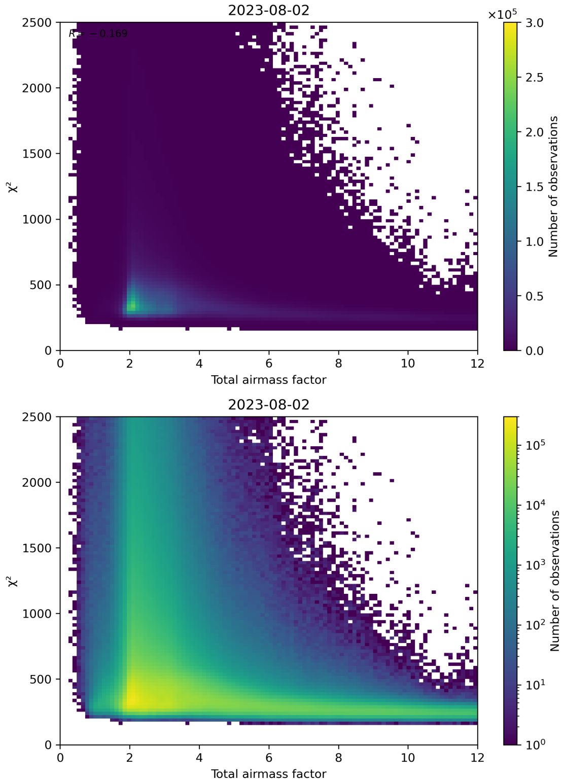
Figure 63: Scatter density plot of “Total airmass factor” against “ \chi^2 ” for 2023-08-01 to 2023-08-03.
