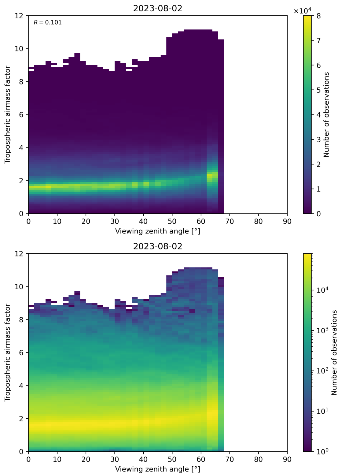
Figure 161: Scatter density plot of “Viewing zenith angle” against “Tropospheric airmass factor” for 2023-08-01 to 2023-08-03.
