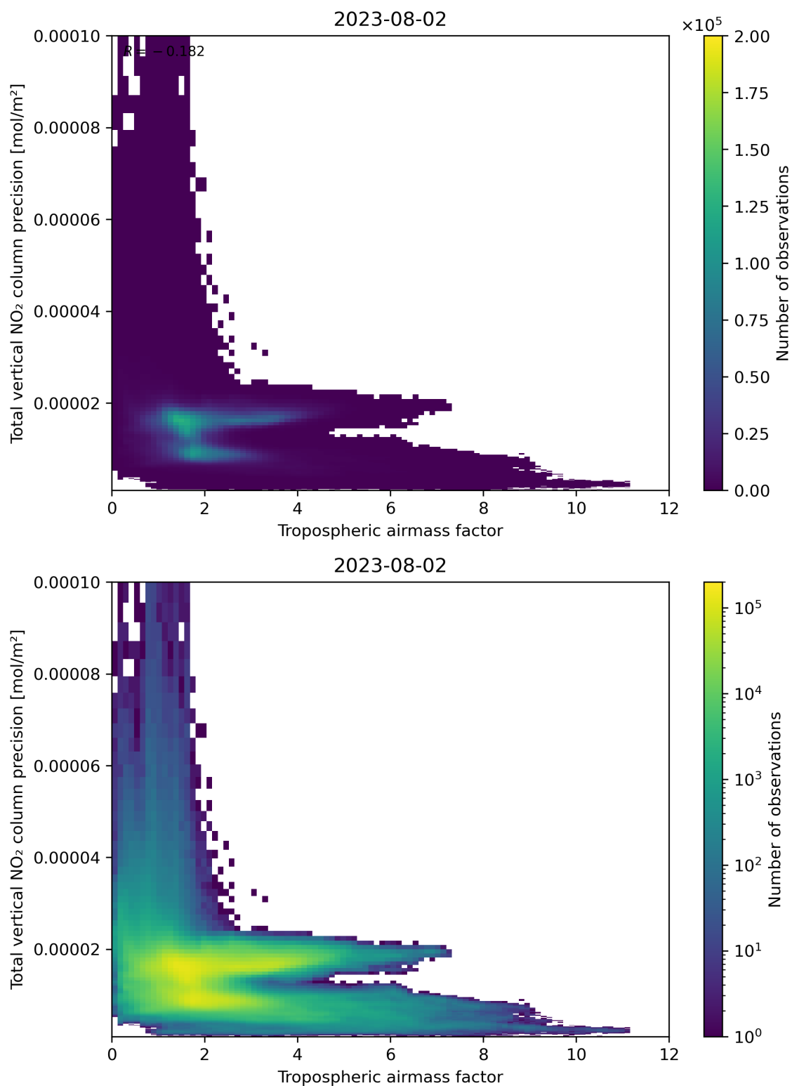
Figure 78: Scatter density plot of “Tropospheric air mass factor” against “Total vertical NO 2 column precision” for 2023-08-01 to 2023-08-03.
