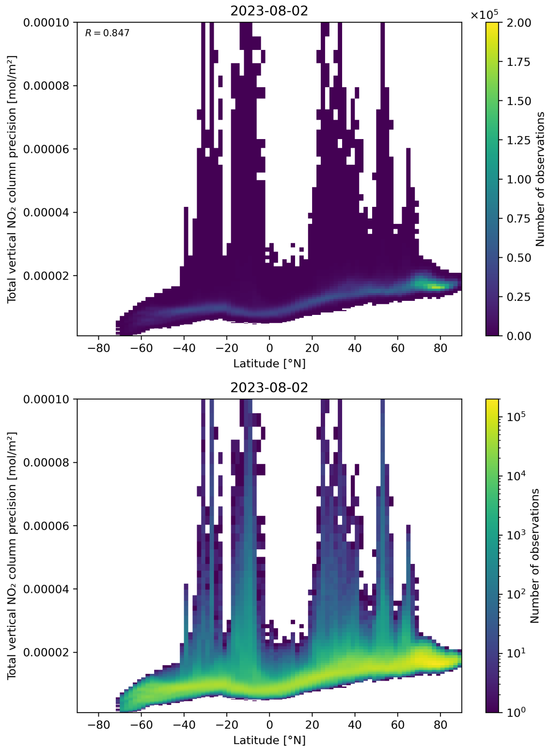
Figure 91: Scatter density plot of “Latitude” against “Total vertical NO 2 column precision” for 2023-08-01 to 2023-08-03.
