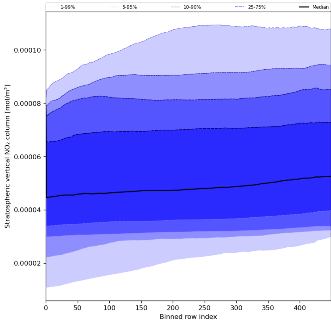
Figure 53: Along track statistics of “Stratospheric vertical NO 2 column” for 2023-08-01 to 2023-08-03
