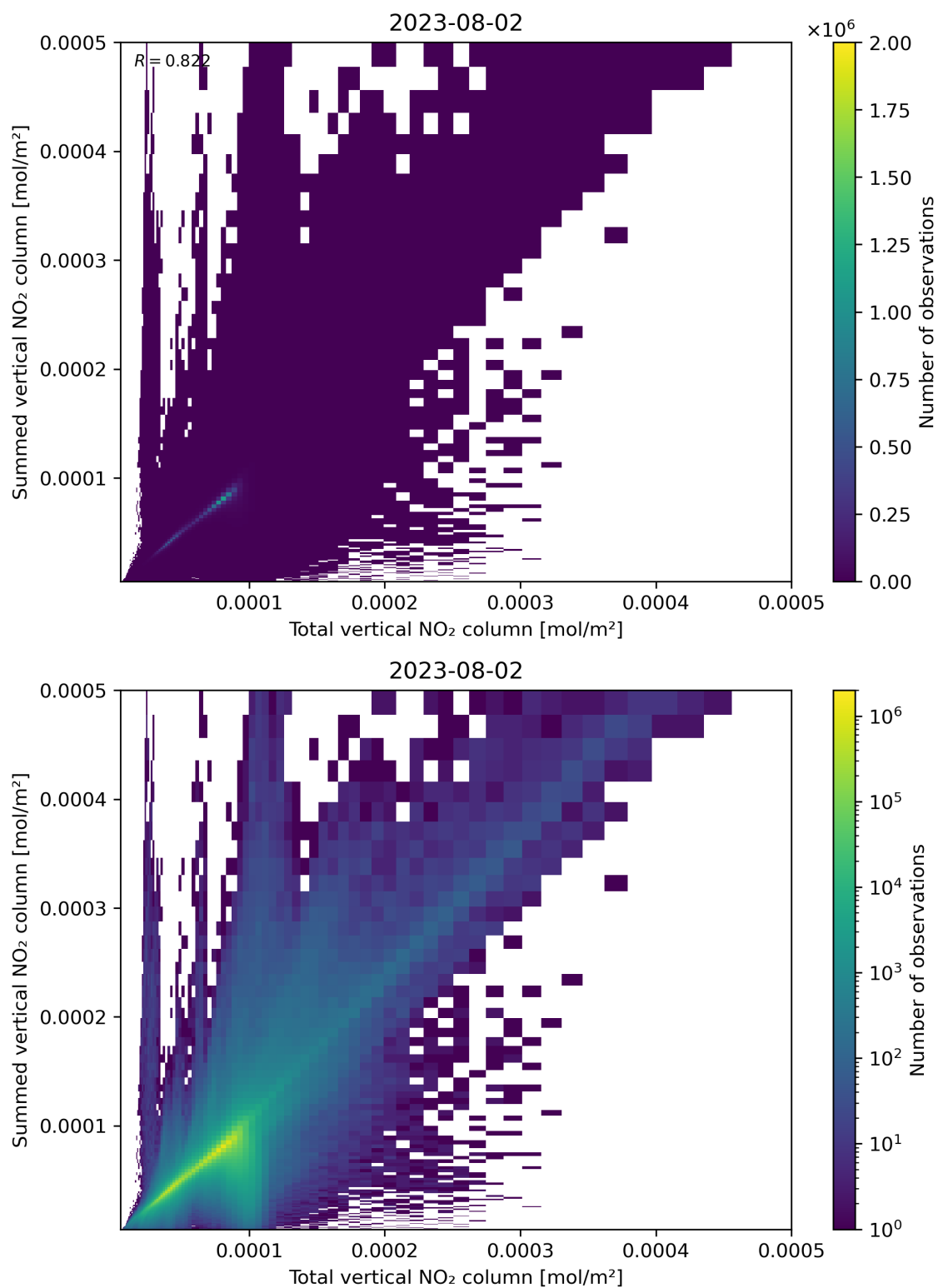
Figure 112: Scatter density plot of “Total vertical NO 2 column” against “Summed vertical NO 2 column” for 2023-08-01 to 2023-08-03.
