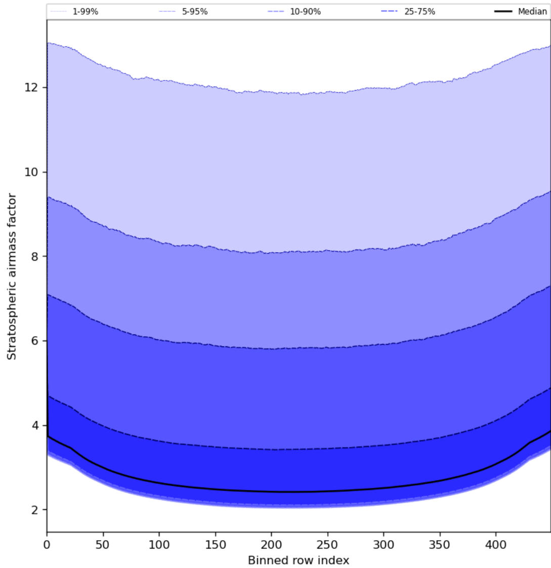
Figure 61: Along track statistics of “Stratospheric airmass factor” for 2023-08-01 to 2023-08-03
