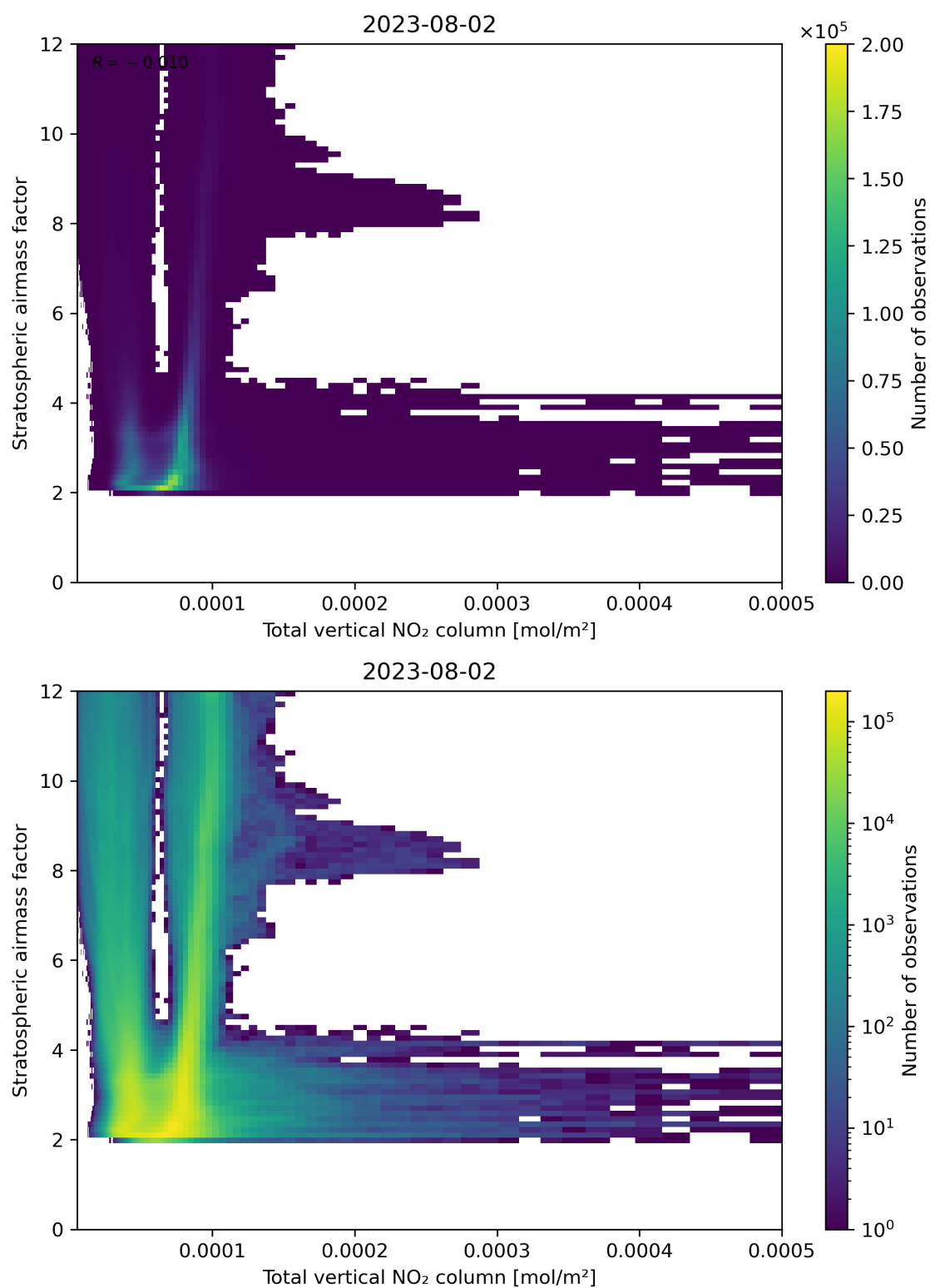
Figure 110: Scatter density plot of “Total vertical NO 2 column” against “Stratospheric airmass factor” for 2023-08-01 to 2023-08-03.
