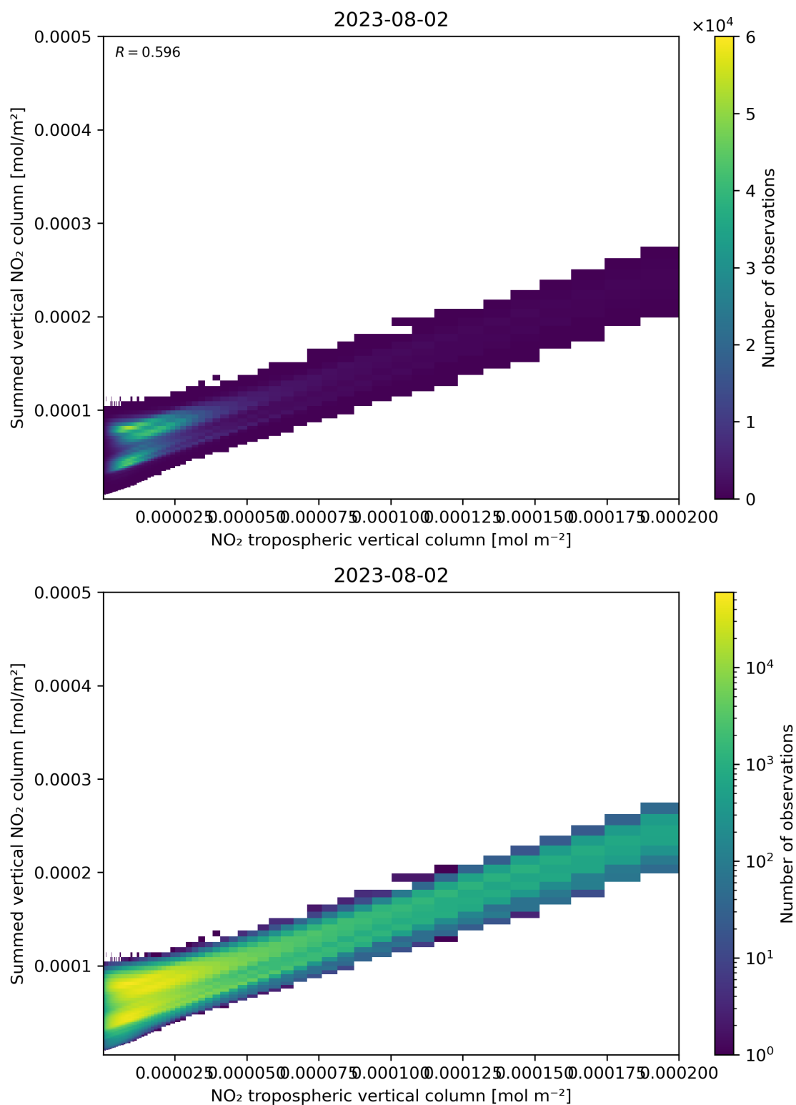
Figure 126: Scatter density plot of “NO 2 tropospheric vertical column” against “Summed vertical NO 2 column” for 2023-08-01 to 2023-08-03.
