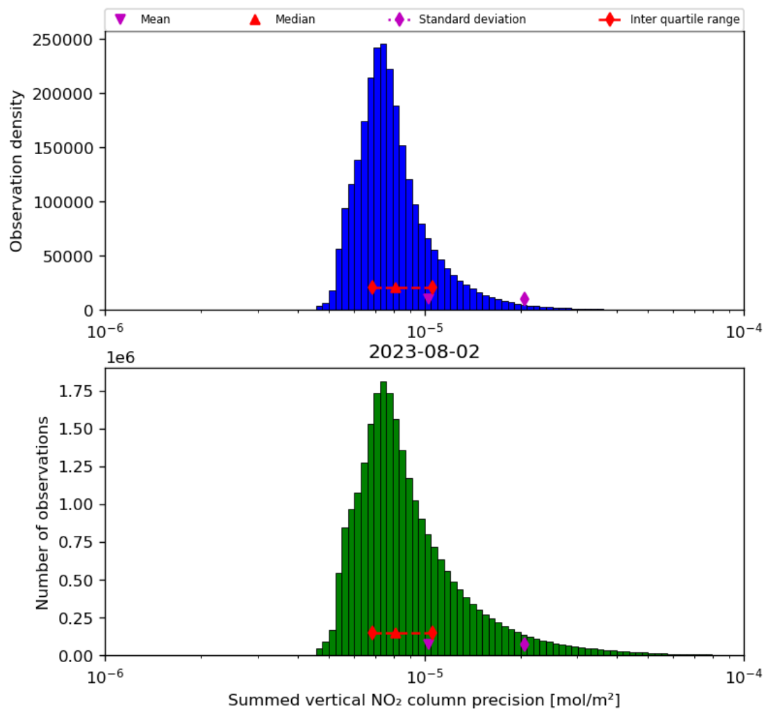
Figure 41: Histogram of "Summed vertical NO 2 column precision" for 2023-08-01 to 2023-08-03
