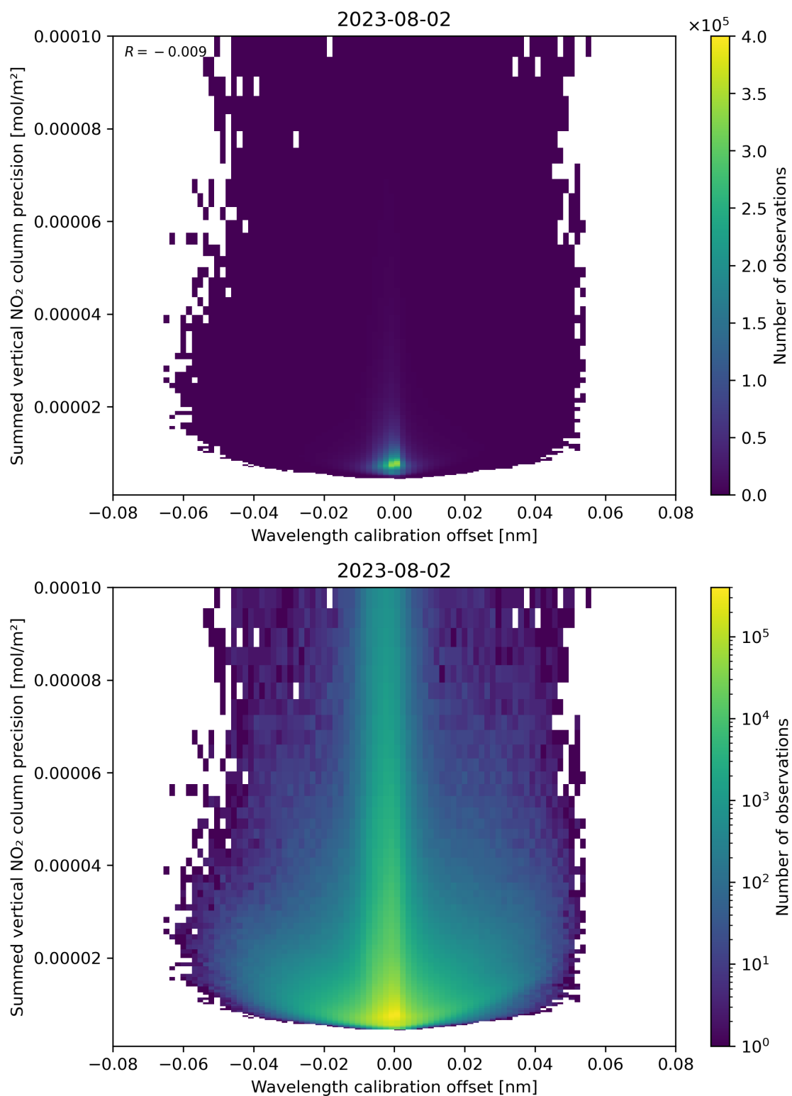
Figure 178: Scatter density plot of “Wavelength calibration offset” against “Summed vertical NO 2 column precision” for 2023-08-01 to 2023-08-03.
