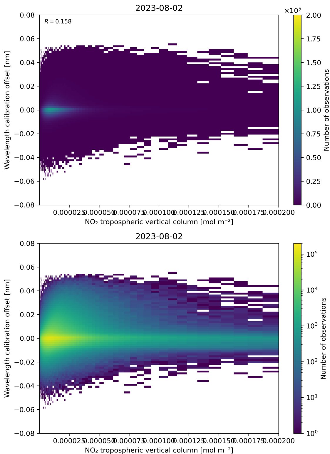
Figure 143: Scatter density plot of “NO 2 tropospheric vertical column” against “Wavelength calibration offset” for 2023-08-01 to 2023-08-03.
