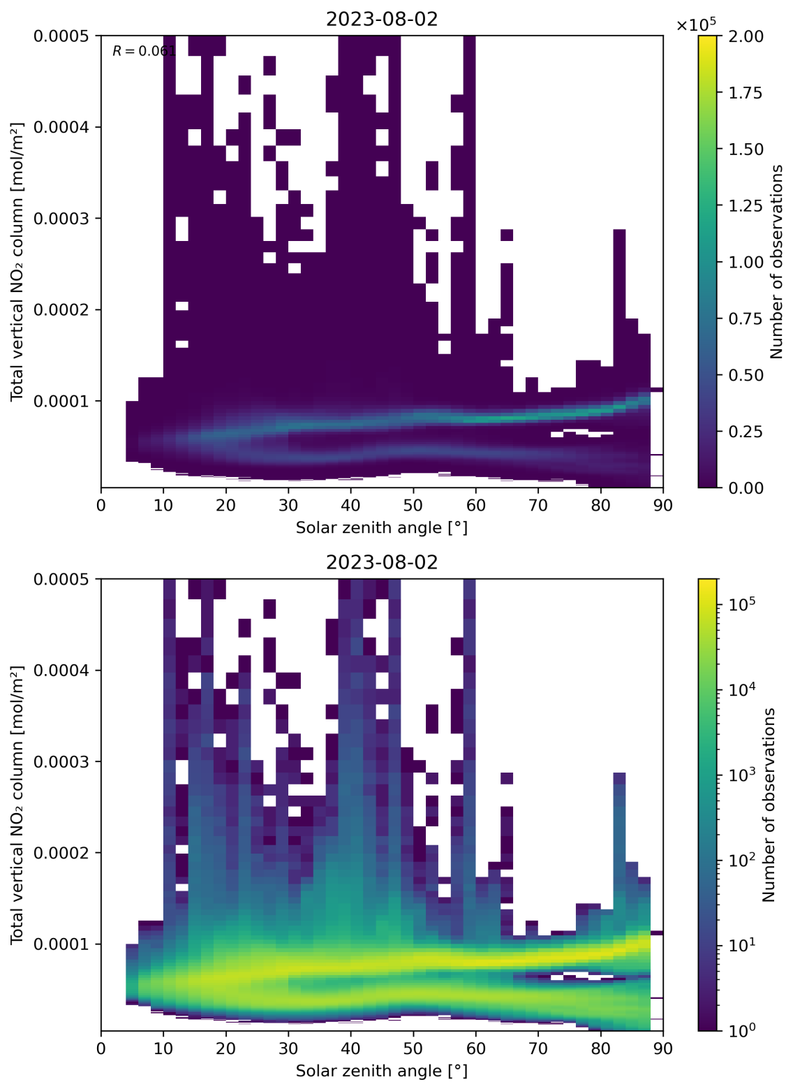
Figure 153: Scatter density plot of “Solar zenith angle” against “Total vertical NO 2 column” for 2023-08-01 to 2023-08-03.
