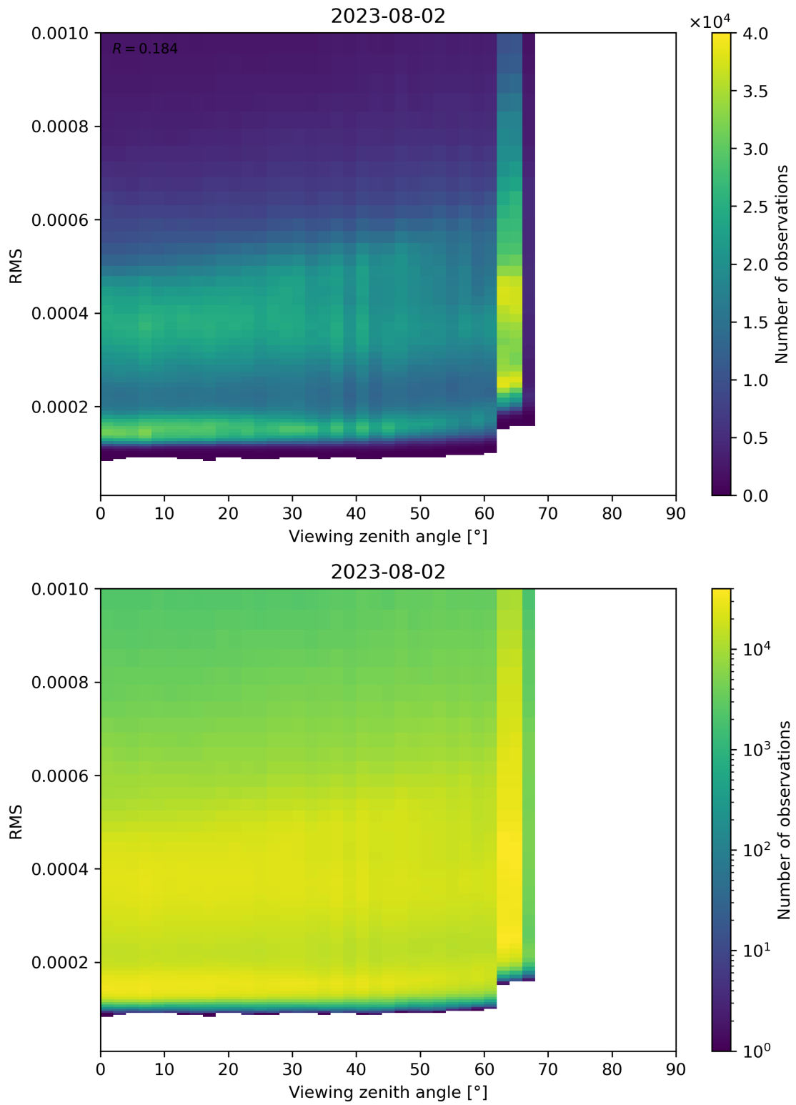
Figure 171: Scatter density plot of “Viewing zenith angle” against “RMS” for 2023-08-01 to 2023-08-03.
