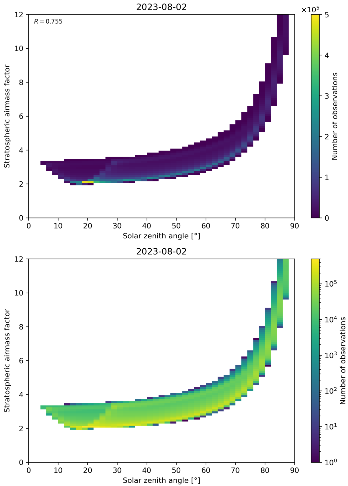
Figure 145: Scatter density plot of “Solar zenith angle” against “Stratospheric airmass factor” for 2023-08-01 to 2023-08-03.
