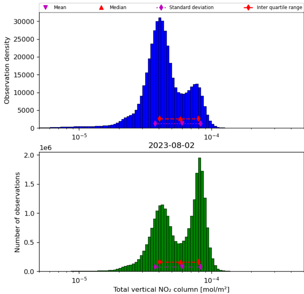
Figure 38: Histogram of “Total vertical NO 2 column” for 2023-08-01 to 2023-08-03
