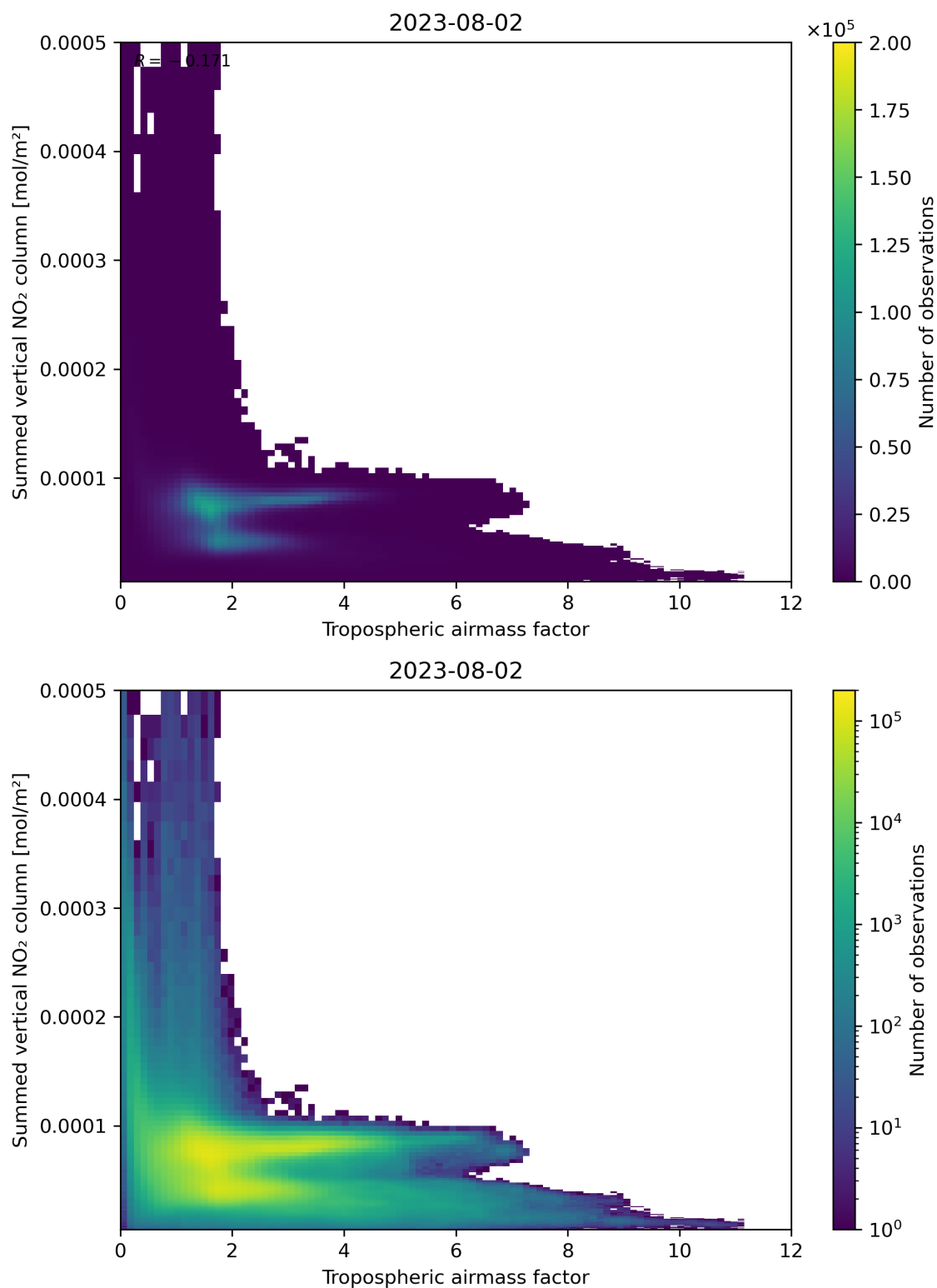
Figure 75: Scatter density plot of “Tropospheric airmass factor” against “Summed vertical NO 2 column” for 2023-08-01 to 2023-08-03.
