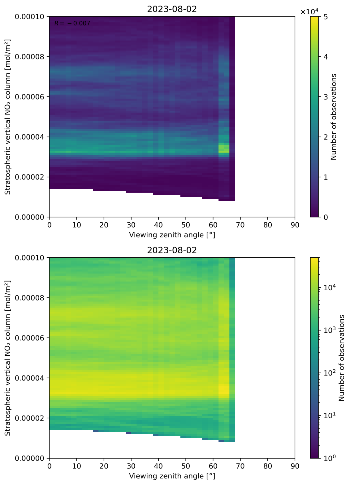
Figure 164: Scatter density plot of “Viewing zenith angle” against “Stratospheric vertical NO 2 column” for 2023-08-01 to 2023-08-03.
