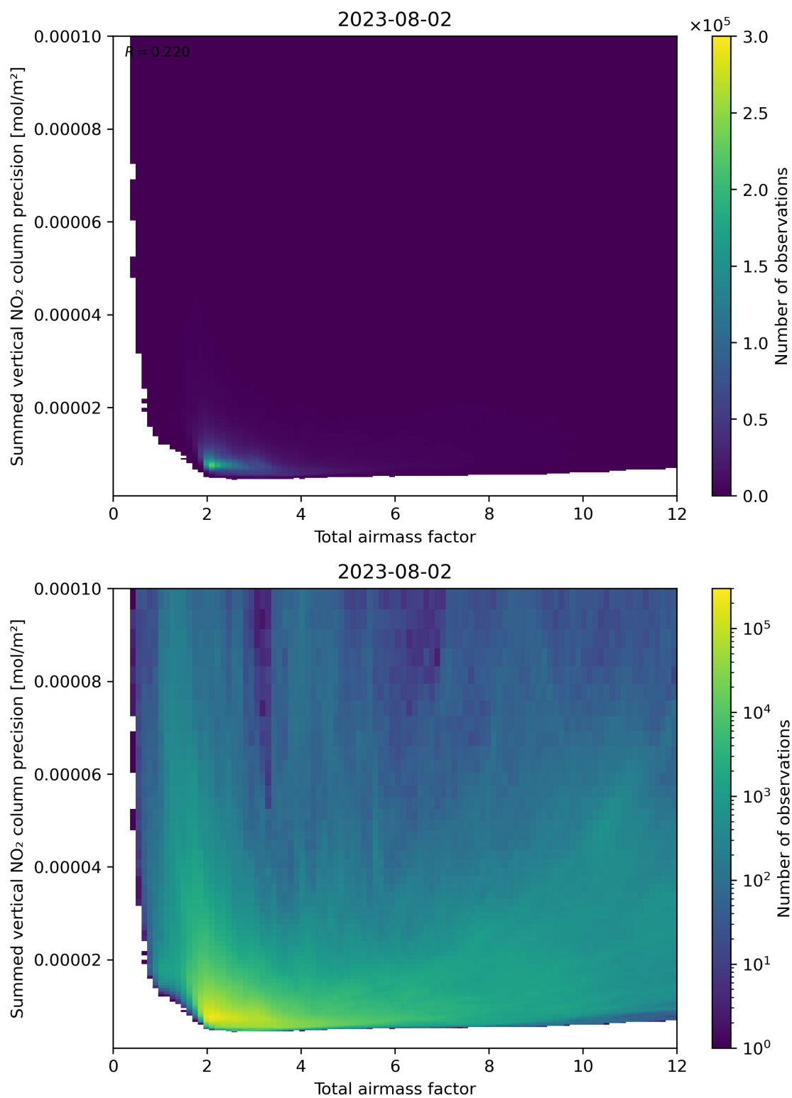
Figure 66: Scatter density plot of “Total airmass factor” against “Summed vertical NO 2 column precision” for 2023-08-01 to 2023-08-03.
