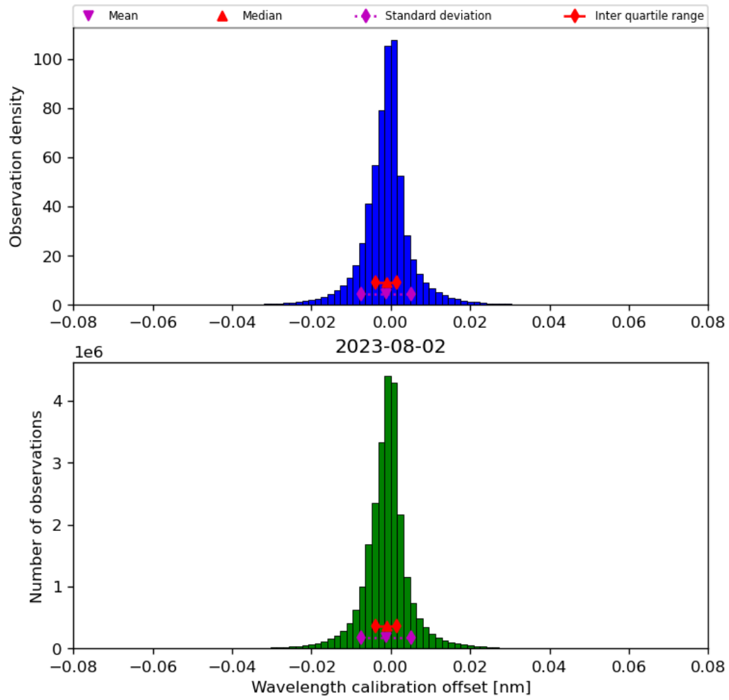
Figure 35: Histogram of “Wavelength calibration offset” for 2023-08-01 to 2023-08-03
