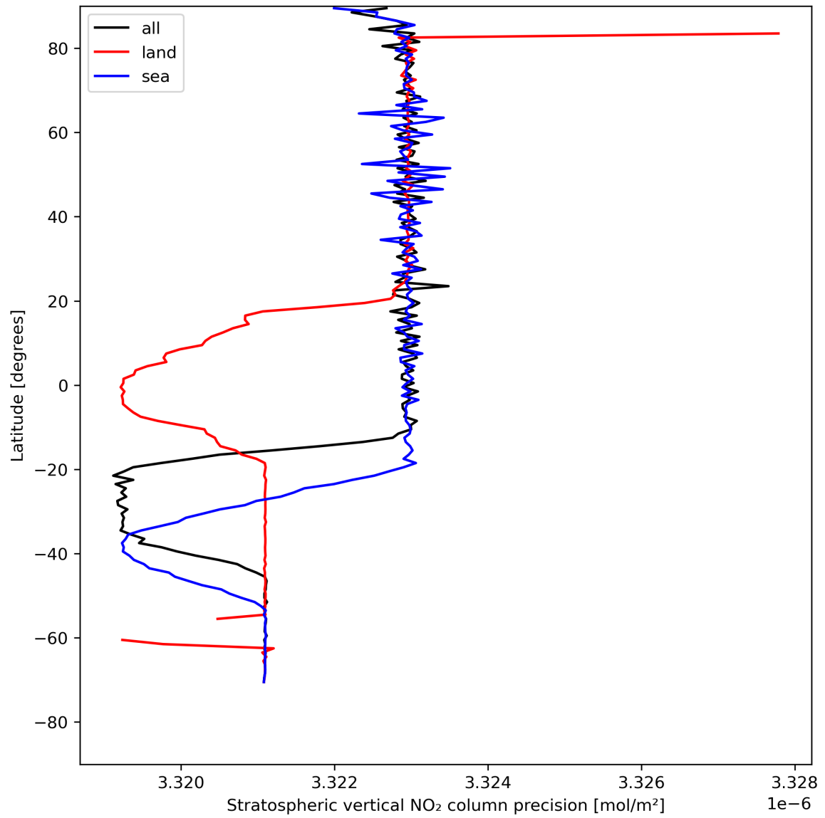
Figure 20: Zonal average of “Stratospheric vertical NO 2 column precision” for 2023-08-01 to 2023-08-03.
