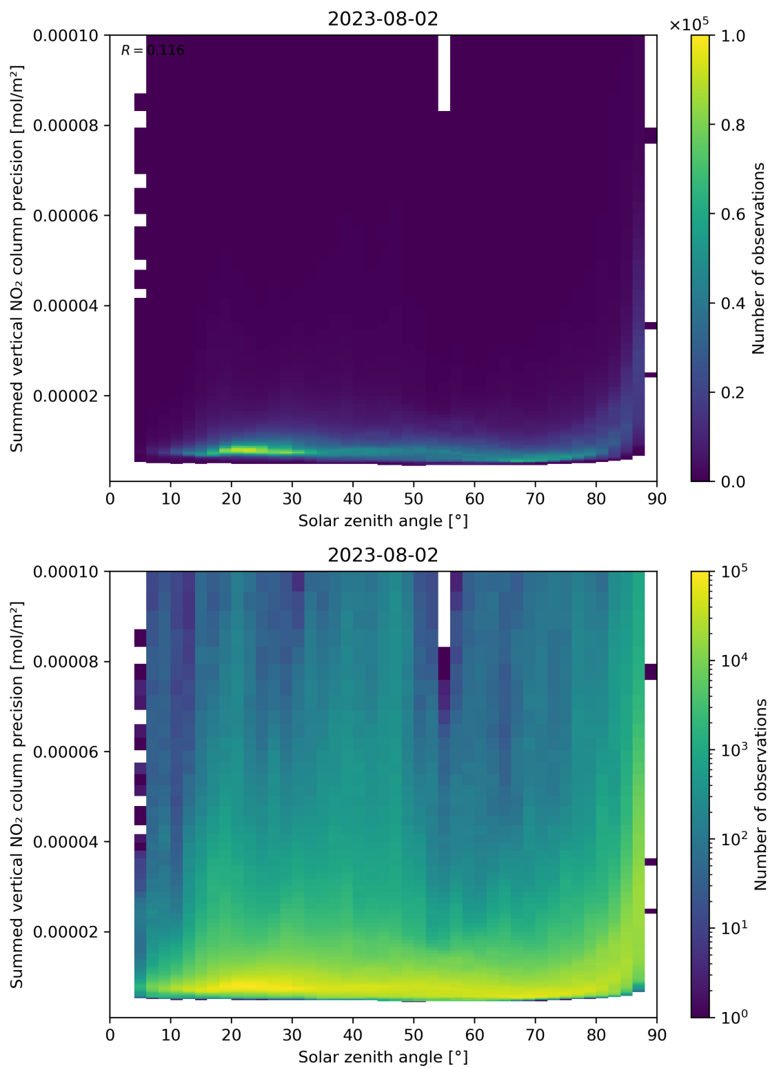
Figure 152: Scatter density plot of “Solar zenith angle” against “Summed vertical NO 2 column precision” for 2023-08-01 to 2023-08-03.
