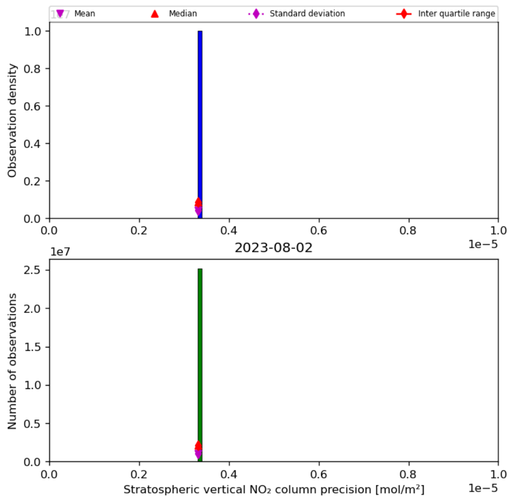
Figure 37: Histogram of “Stratospheric vertical NO 2 column precision” for 2023-08-01 to 2023-08-03
