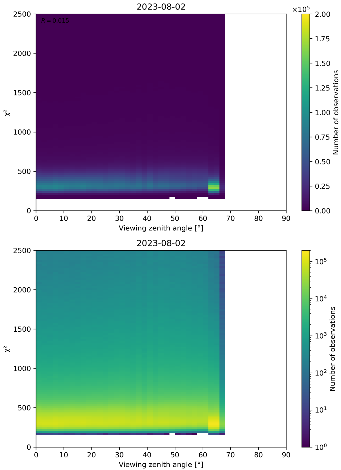
Figure 162: Scatter density plot of “Viewing zenith angle” against “ \chi^2 ” for 2023-08-01 to 2023-08-03.
