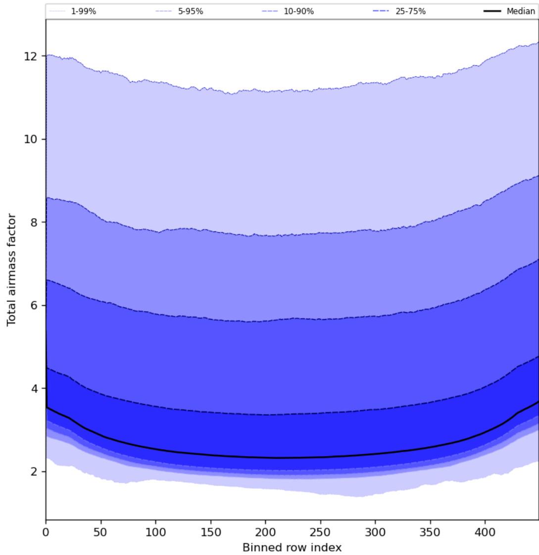
Figure 49: Along track statistics of “Total airmass factor” for 2023-08-01 to 2023-08-03
