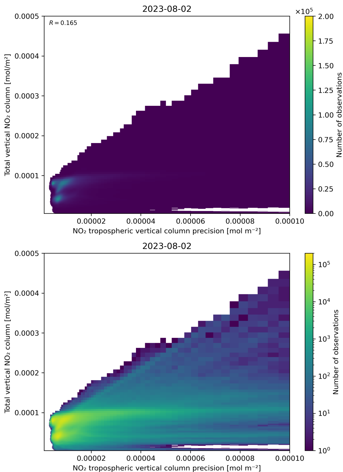
Figure 138: Scatter density plot of “NO 2 tropospheric vertical column precision” against “Total vertical NO 2 column” for 2023-08-01 to 2023-08-03.
