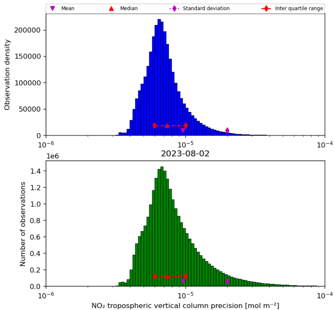
Figure 30: Histogram of “NO 2 tropospheric vertical column precision” for 2023-08-01 to 2023-08-03
