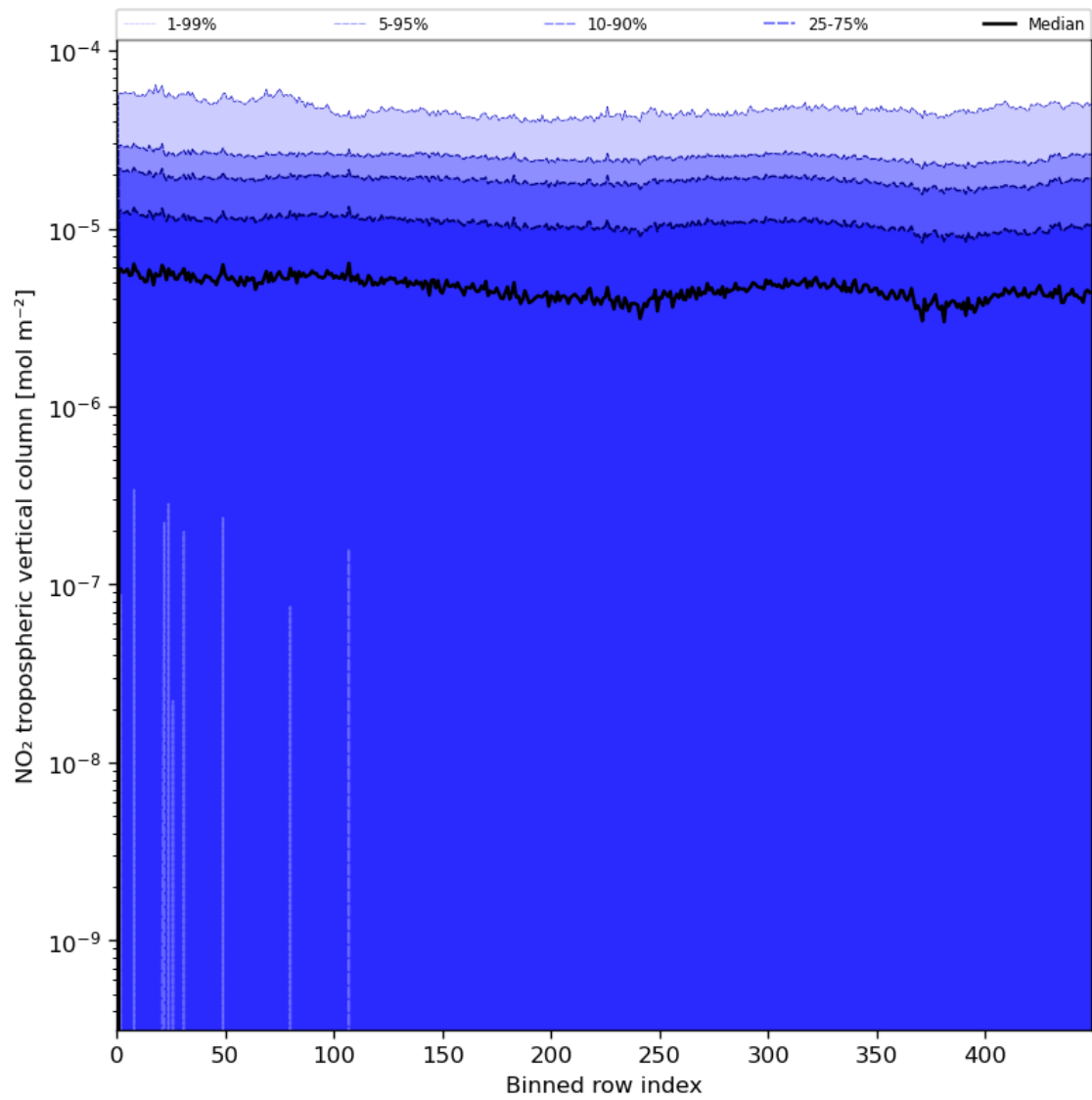
Figure 46: Along track statistics of “NO 2 tropospheric vertical column” for 2023-08-01 to 2023-08-03
