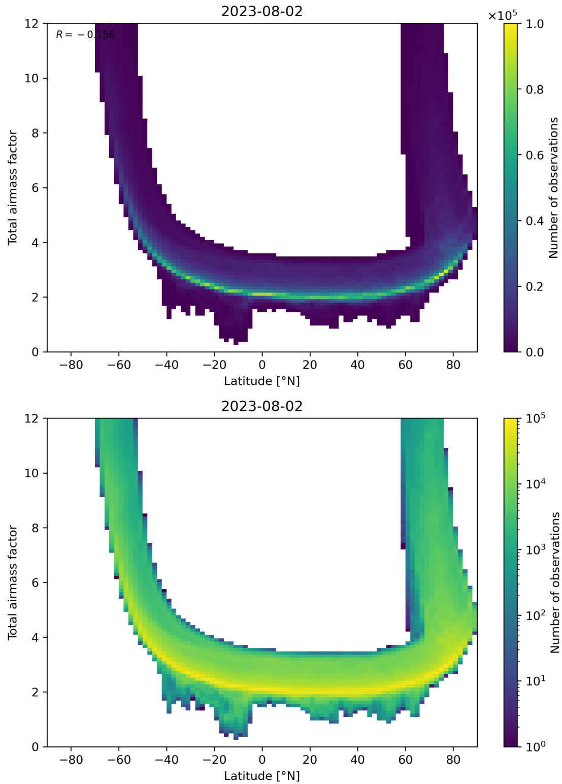
Figure 84: Scatter density plot of “Latitude” against “Total airmass factor” for 2023-08-01 to 2023-08-03.
