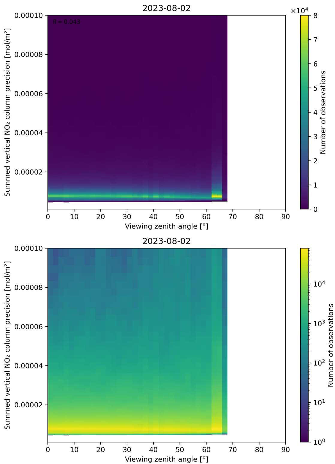
Figure 166: Scatter density plot of “Viewing zenith angle” against “Summed vertical NO 2 column precision” for 2023-08-01 to 2023-08-03.
