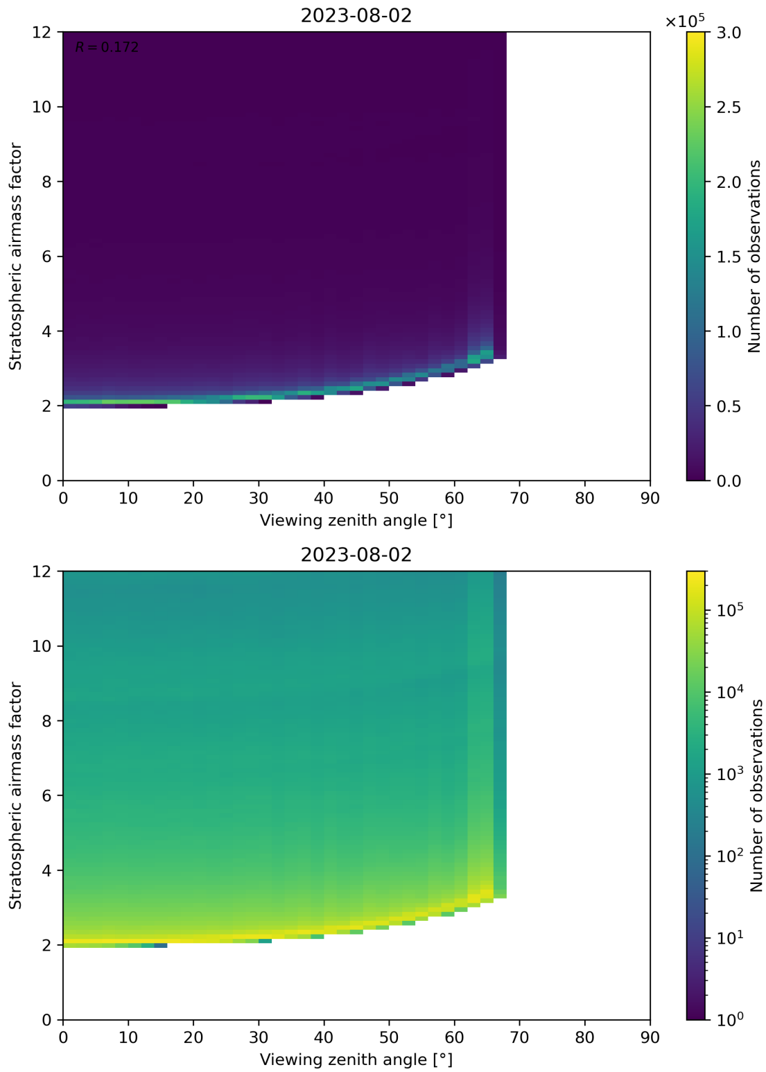
Figure 159: Scatter density plot of “Viewing zenith angle” against “Stratospheric airmass factor” for 2023-08-01 to 2023-08-03.
