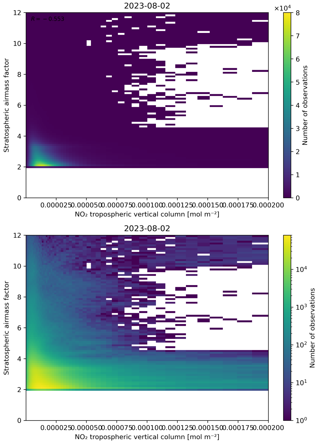
Figure 121: Scatter density plot of “NO 2 tropospheric vertical column” against “Stratospheric air mass factor” for 2023-08-01 to 2023-08-03.
