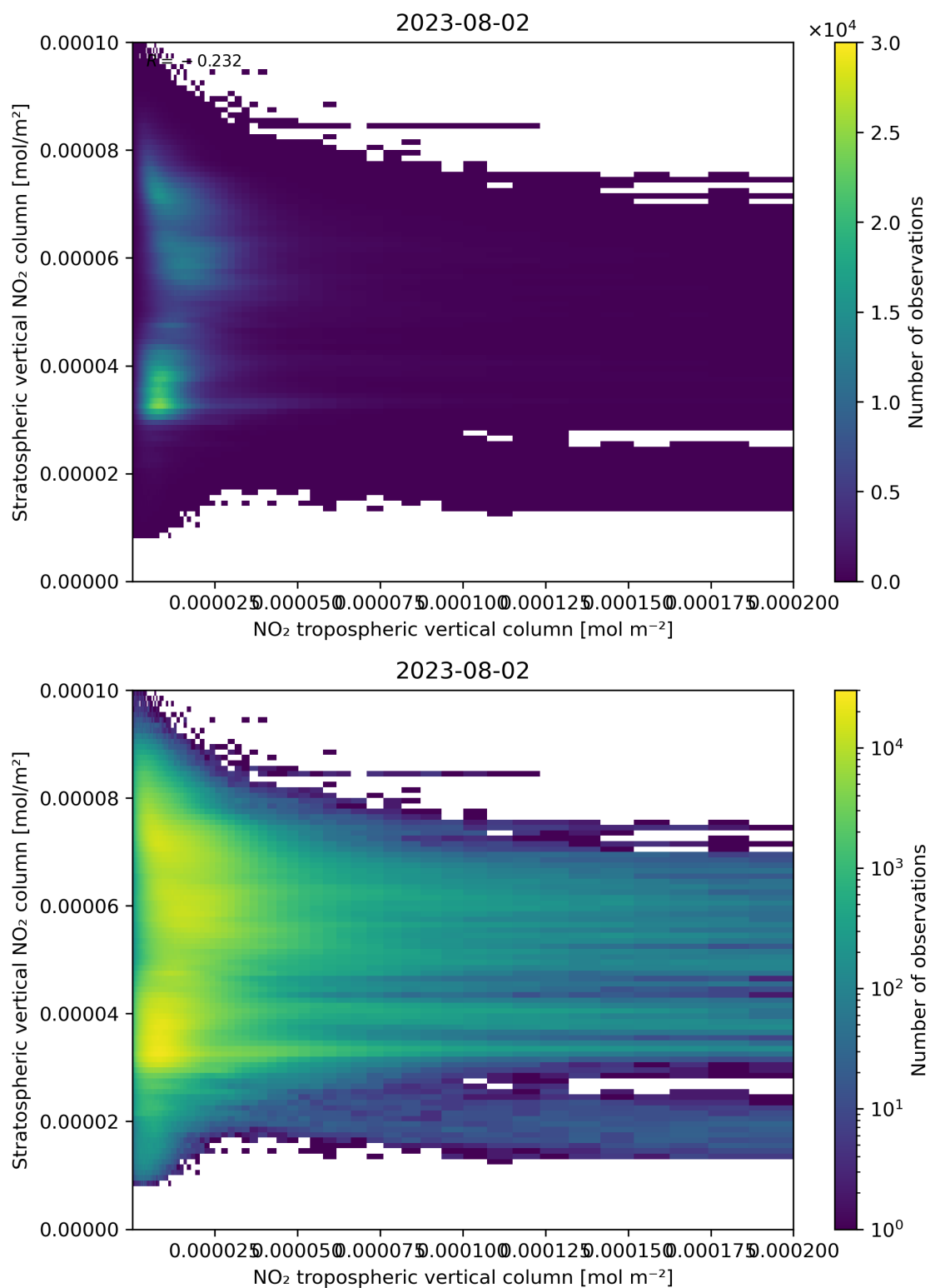
Figure 125: Scatter density plot of “NO 2 tropospheric vertical column” against “Stratospheric vertical NO 2 column” for 2023-08-01 to 2023-08-03.
