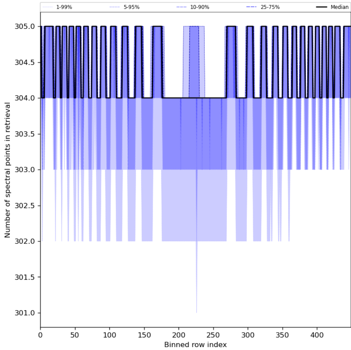
Figure 50: Along track statistics of “Number of spectral points in retrieval” for 2023-08-01 to 2023-08-03
