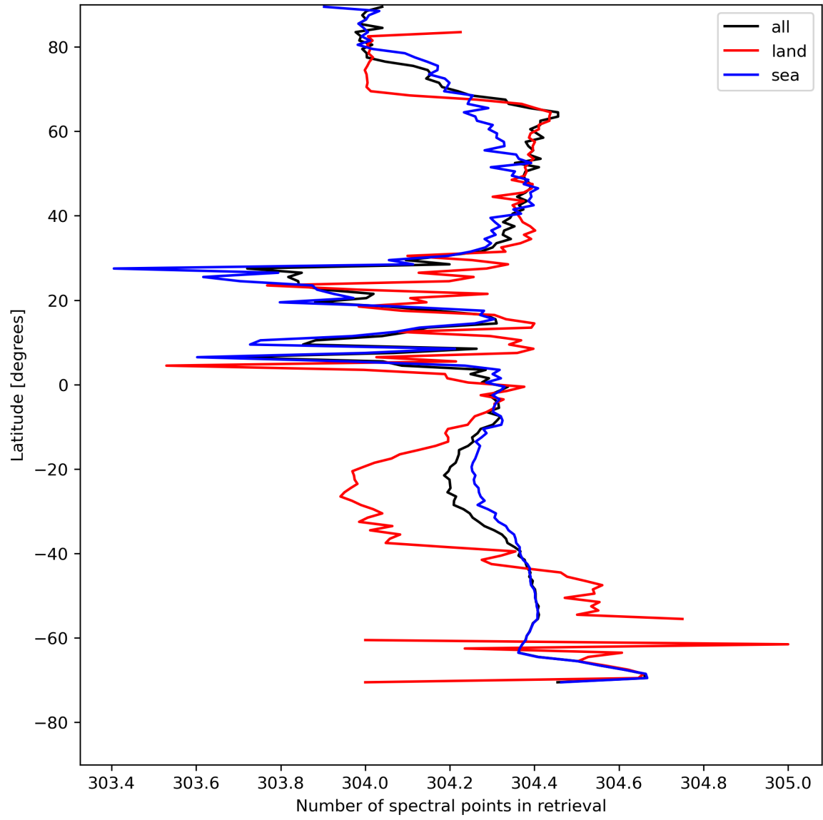
Figure 16: Zonal average of “Number of spectral points in retrieval” for 2023-08-01 to 2023-08-03.
