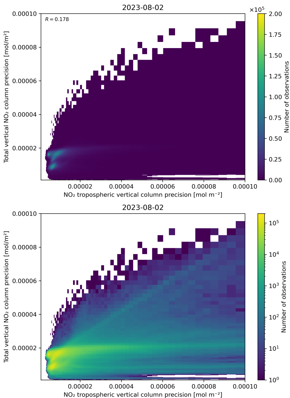
Figure 139: Scatter density plot of “NO 2 tropospheric vertical column precision” against “Total vertical NO 2 column precision” for 2023-08-01 to 2023-08-03.
