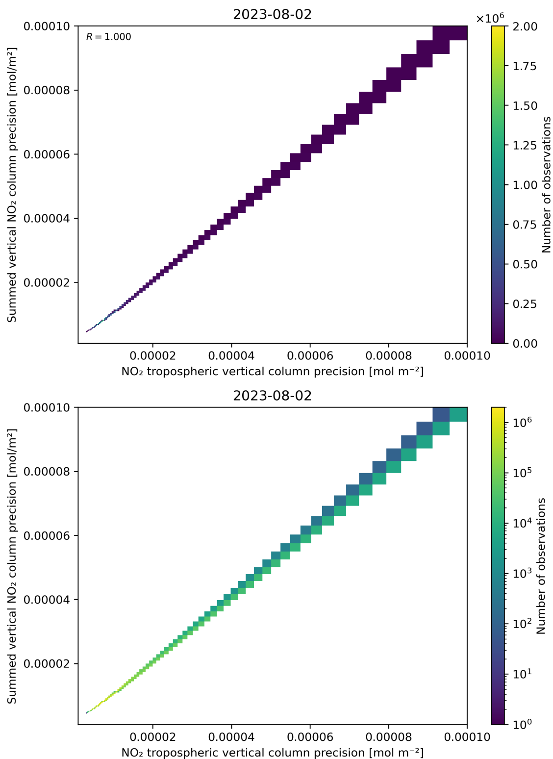
Figure 137: Scatter density plot of “NO 2 tropospheric vertical column precision” against “Summed vertical NO 2 column precision” for 2023-08-01 to 2023-08-03.
