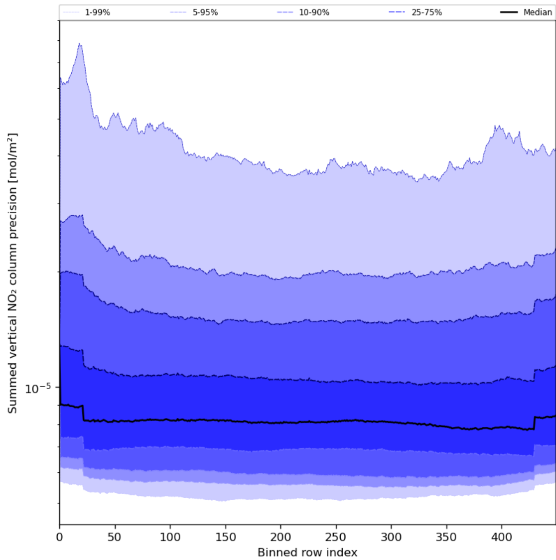
Figure 58: Along track statistics of “Summed vertical NO 2 column precision” for 2023-08-01 to 2023-08-03
