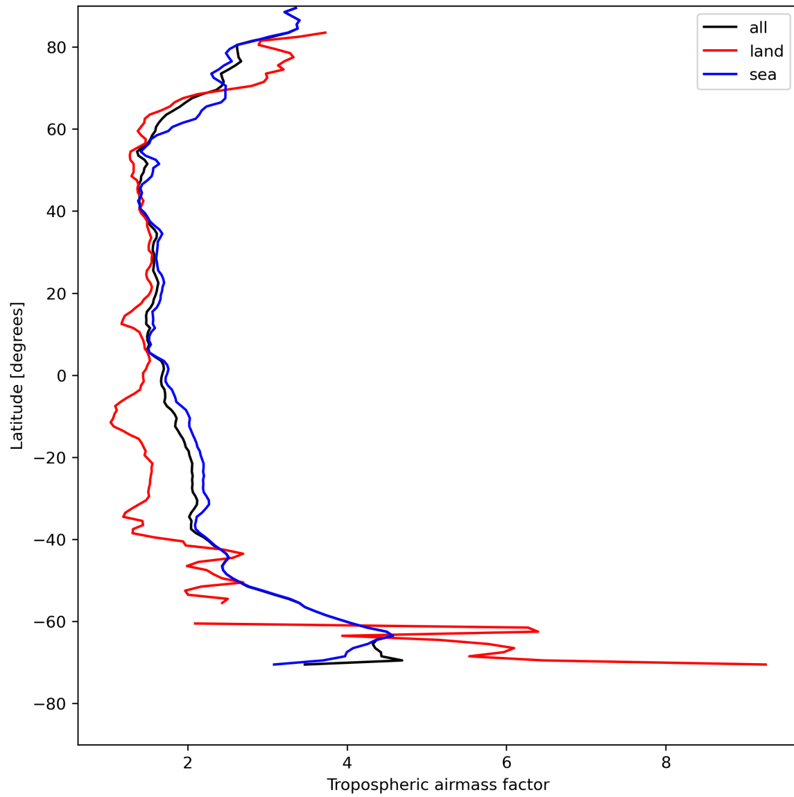
Figure 14: Zonal average of “Tropospheric airmass factor” for 2023-08-01 to 2023-08-03.
