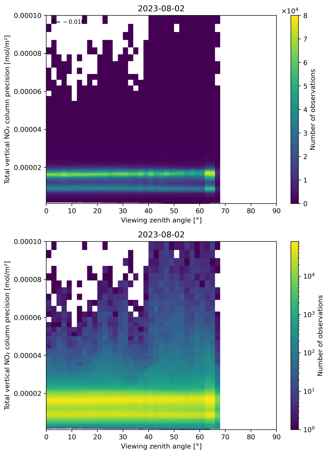
Figure 168: Scatter density plot of “Viewing zenith angle” against “Total vertical NO 2 column precision” for 2023-08-01 to 2023-08-03.
