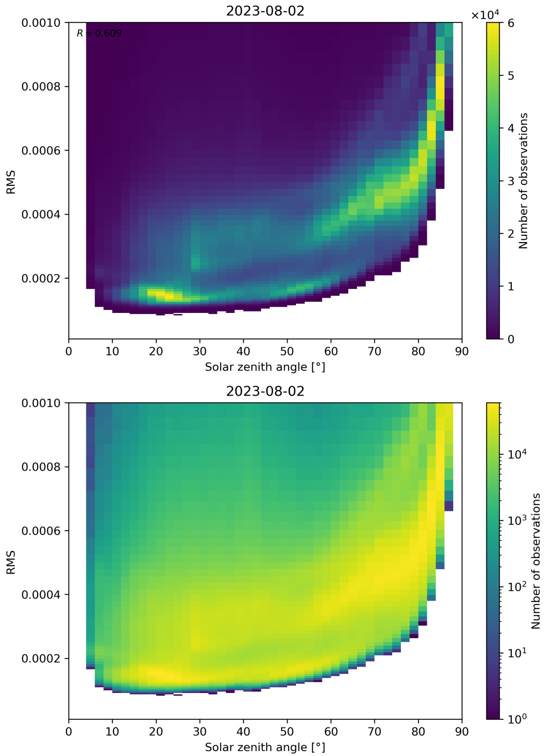
Figure 157: Scatter density plot of “Solar zenith angle” against “RMS” for 2023-08-01 to 2023-08-03.
