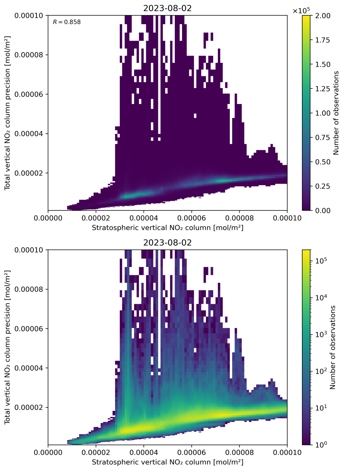
Figure 101: Scatter density plot of “Stratospheric vertical NO 2 column” against “Total vertical NO 2 column precision” for 2023-08-01 to 2023-08-03.
