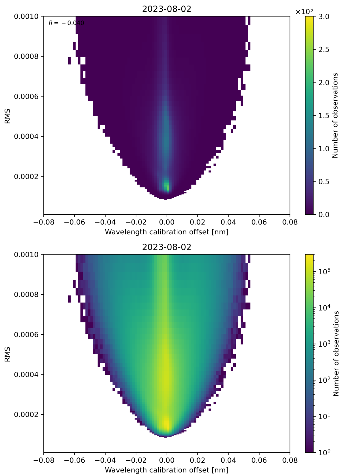
Figure 181: Scatter density plot of “Wavelength calibration offset” against “RMS” for 2023-08-01 to 2023-08-03.
