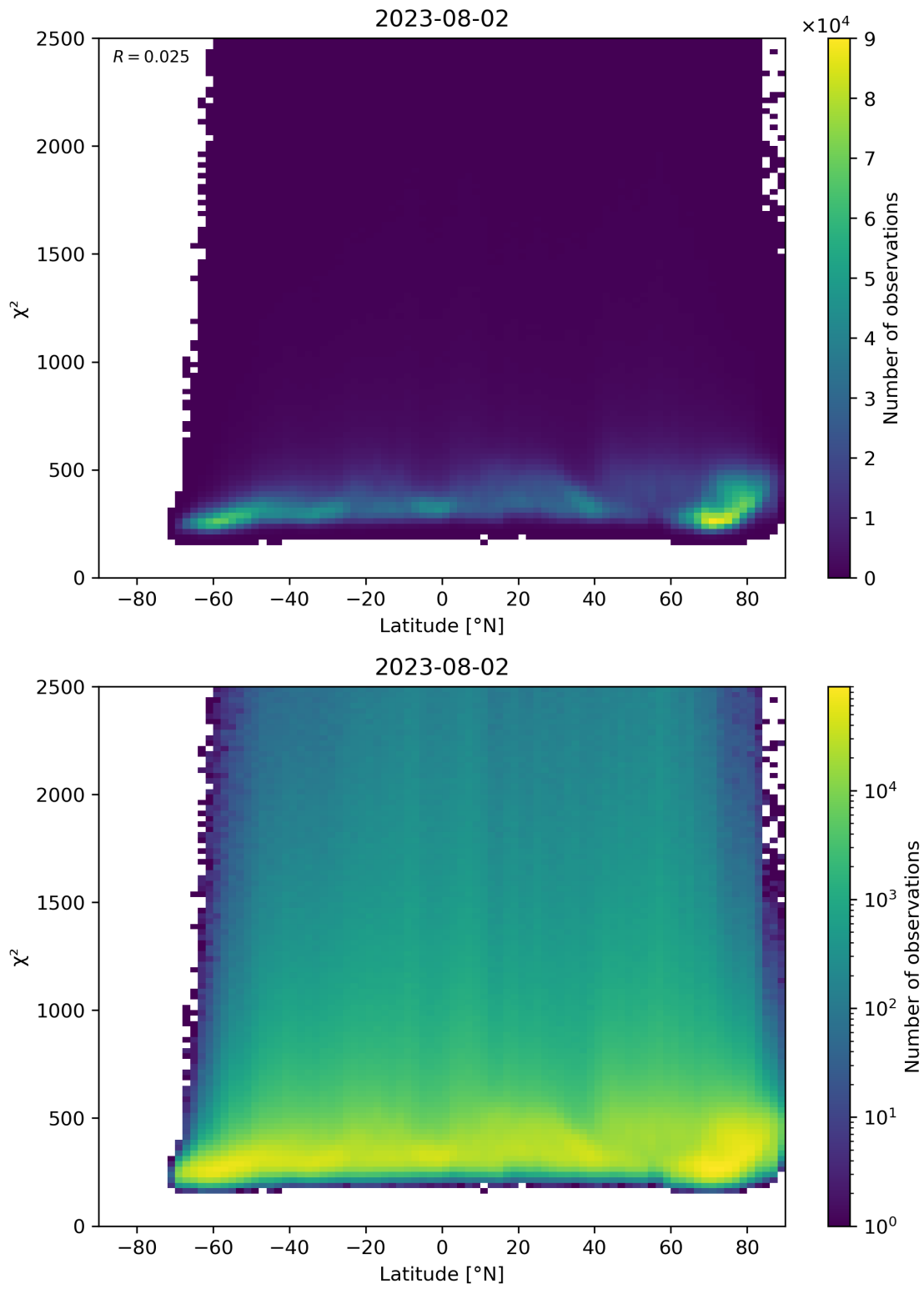
Figure 86: Scatter density plot of “Latitude” against “ \chi^2 ” for 2023-08-01 to 2023-08-03.
