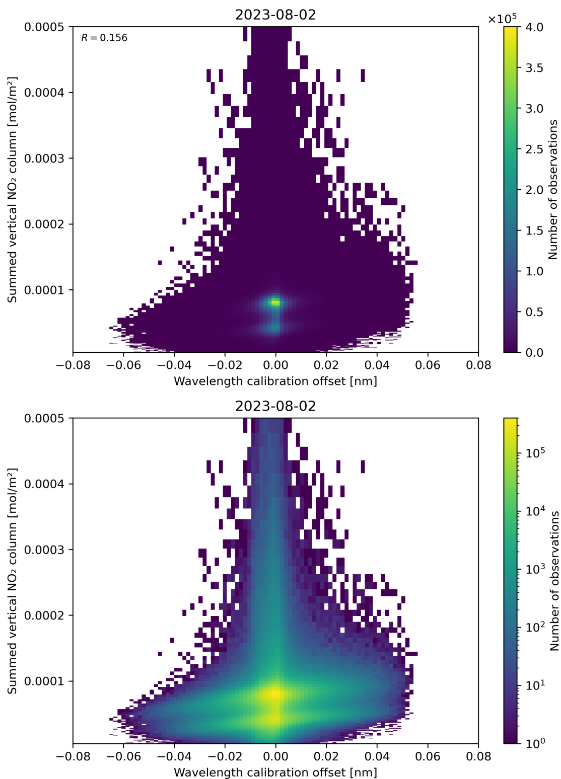
Figure 177: Scatter density plot of “Wavelength calibration offset” against “Summed vertical NO 2 column” for 2023-08-01 to 2023-08-03.
