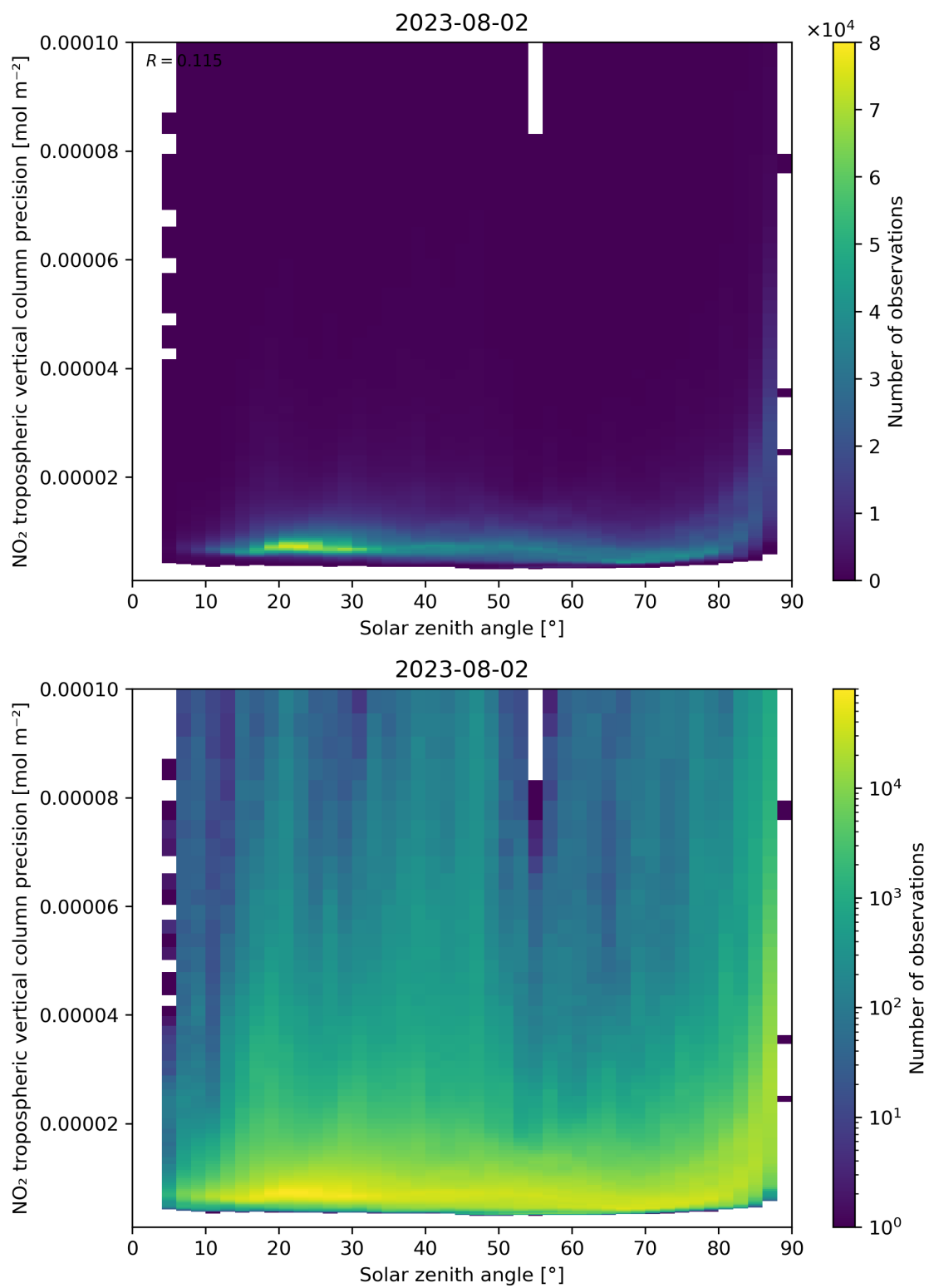
Figure 156: Scatter density plot of “Solar zenith angle” against “NO 2 tropospheric vertical column precision” for 2023-08-01 to 2023-08-03.
