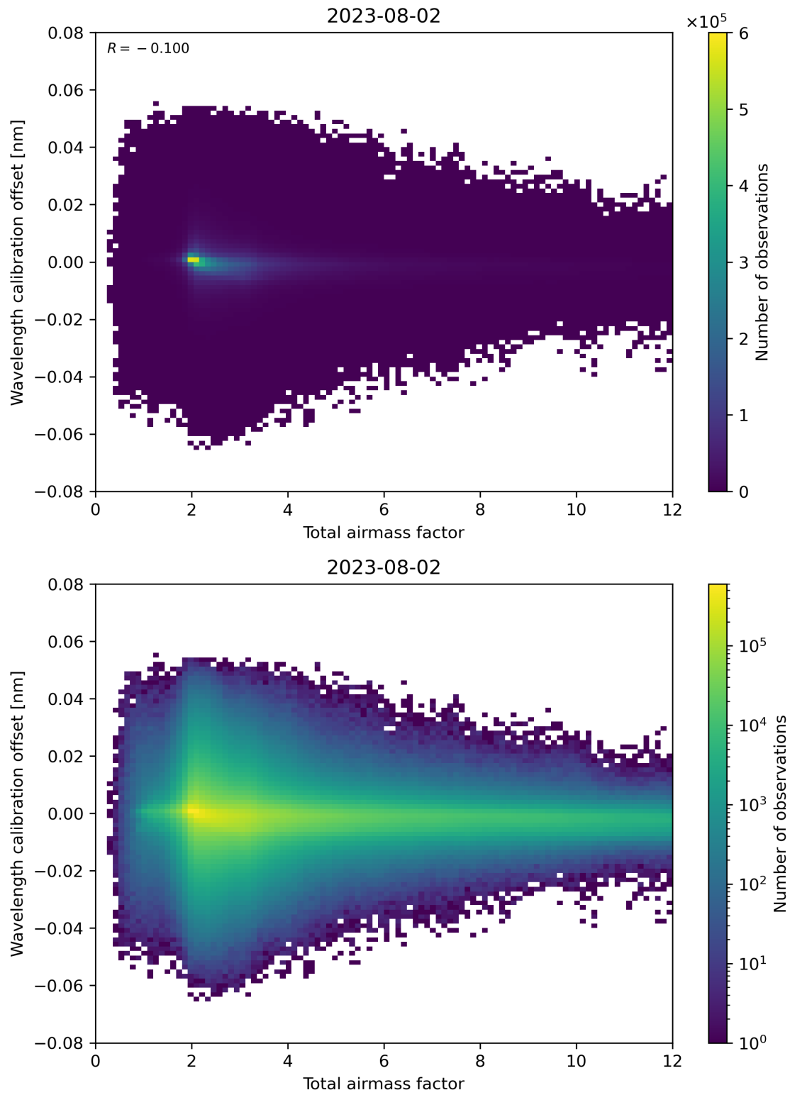
Figure 70: Scatter density plot of “Total airmass factor” against “Wavelength calibration offset” for 2023-08-01 to 2023-08-03.
