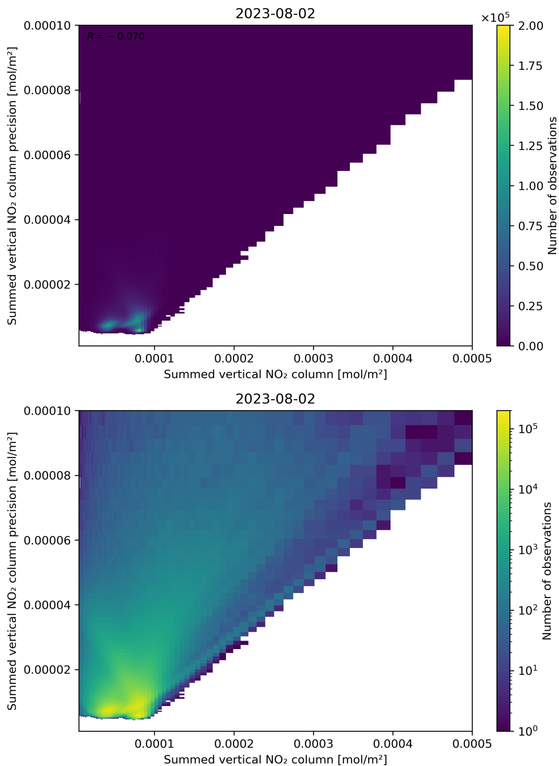
Figure 105: Scatter density plot of “Summed vertical NO 2 column” against “Summed vertical NO 2 column precision” for 2023-08-01 to 2023-08-03.
