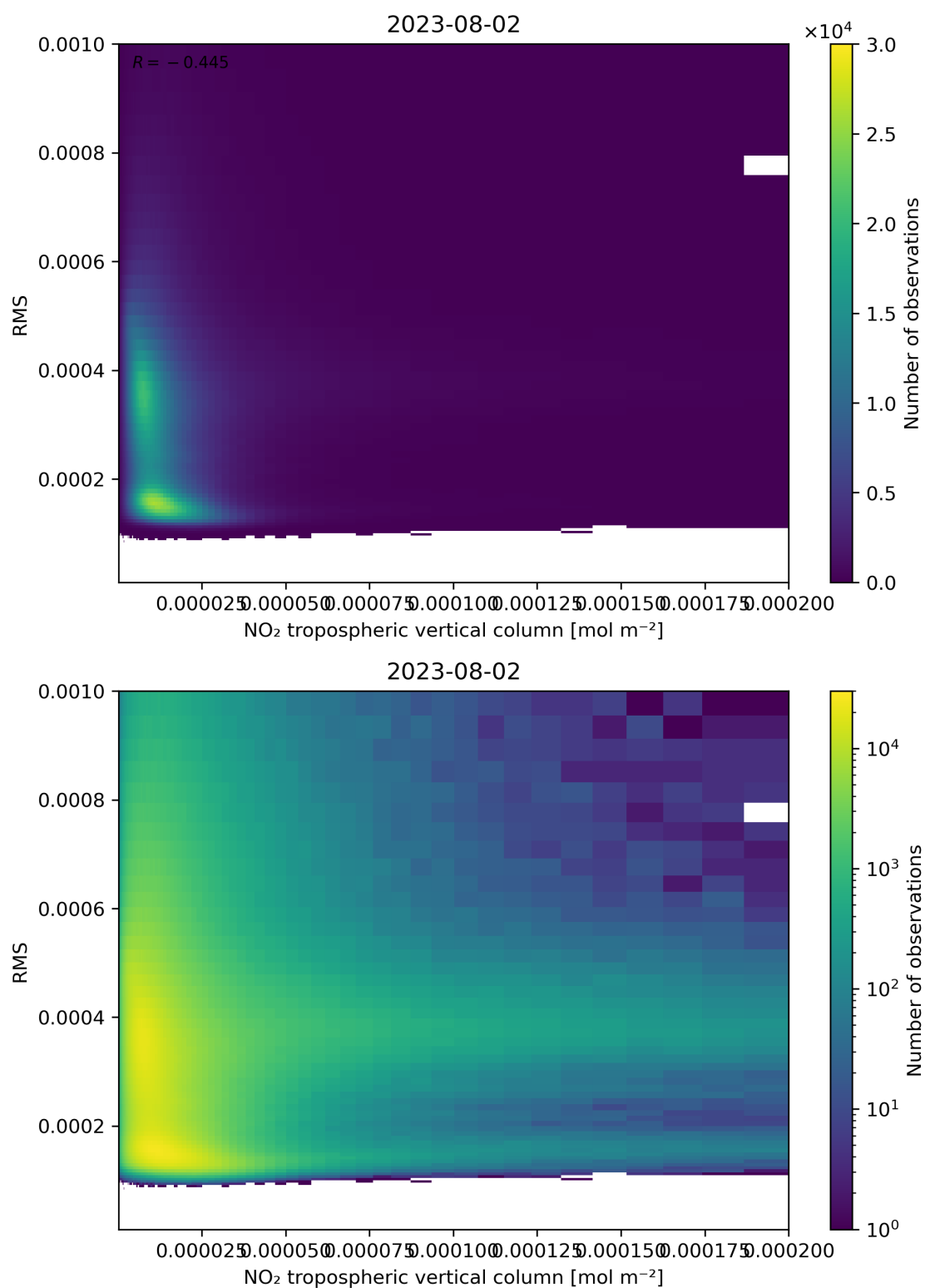
Figure 142: Scatter density plot of “NO 2 tropospheric vertical column” against “RMS” for 2023-08-01 to 2023-08-03.
