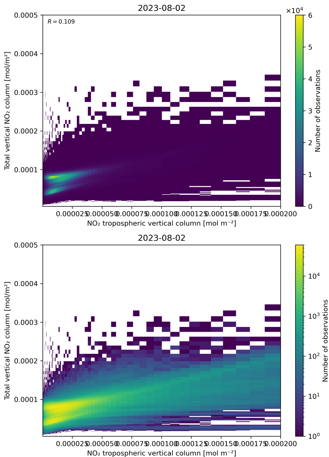
Figure 128: Scatter density plot of “NO 2 tropospheric vertical column” against “Total vertical NO 2 column” for 2023-08-01 to 2023-08-03.
