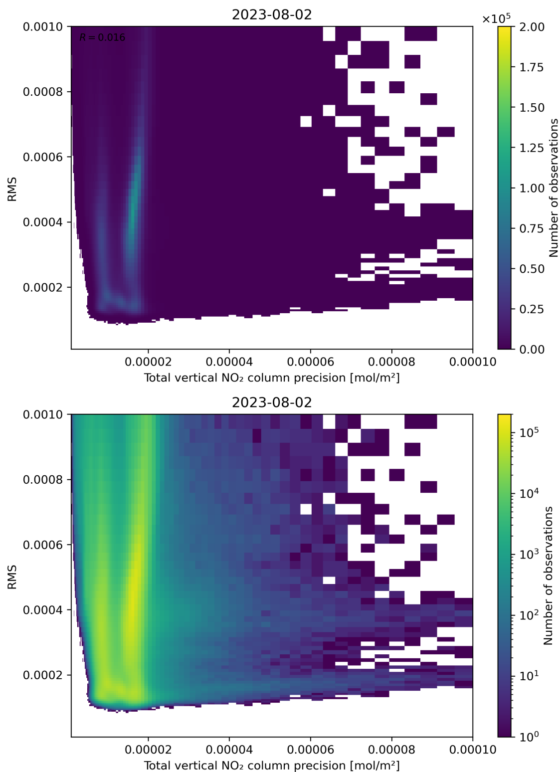
Figure 119: Scatter density plot of “Total vertical NO 2 column precision” against “RMS” for 2023-08-01 to 2023-08-03.
