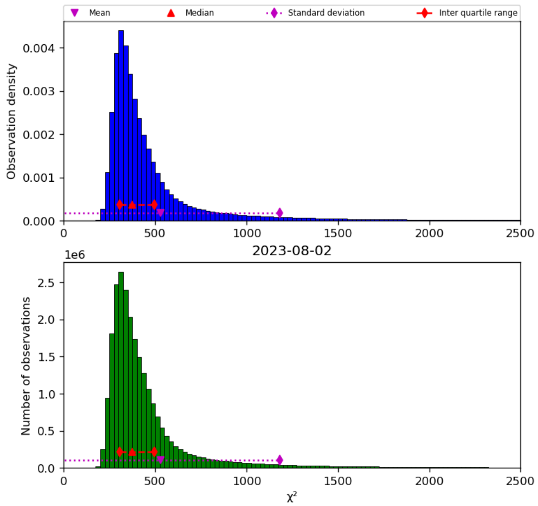
Figure 42: Histogram of “ \chi^2 ” for 2023-08-01 to 2023-08-03
