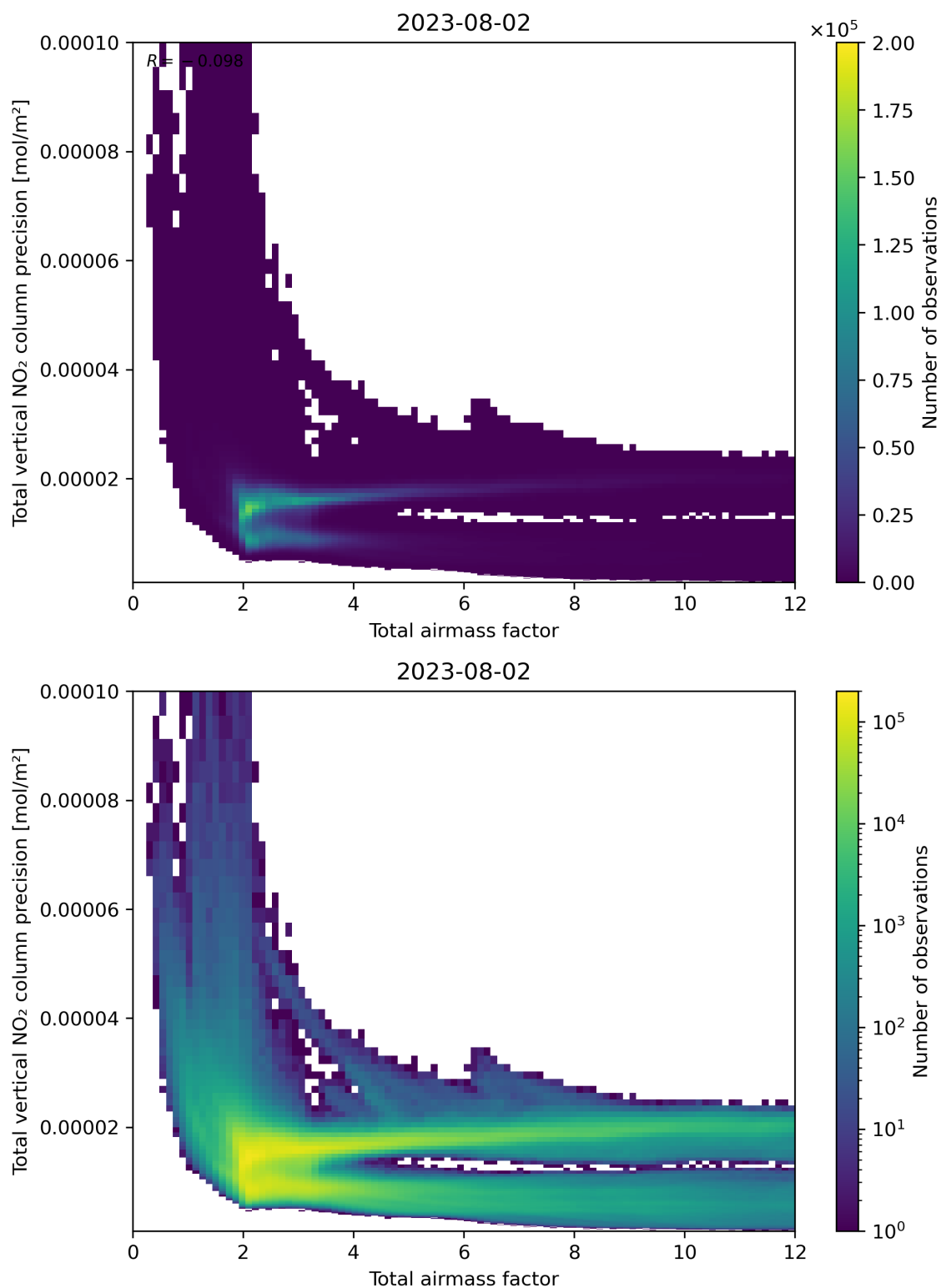
Figure 68: Scatter density plot of “Total airmass factor” against “Total vertical NO 2 column precision” for 2023-08-01 to 2023-08-03.
