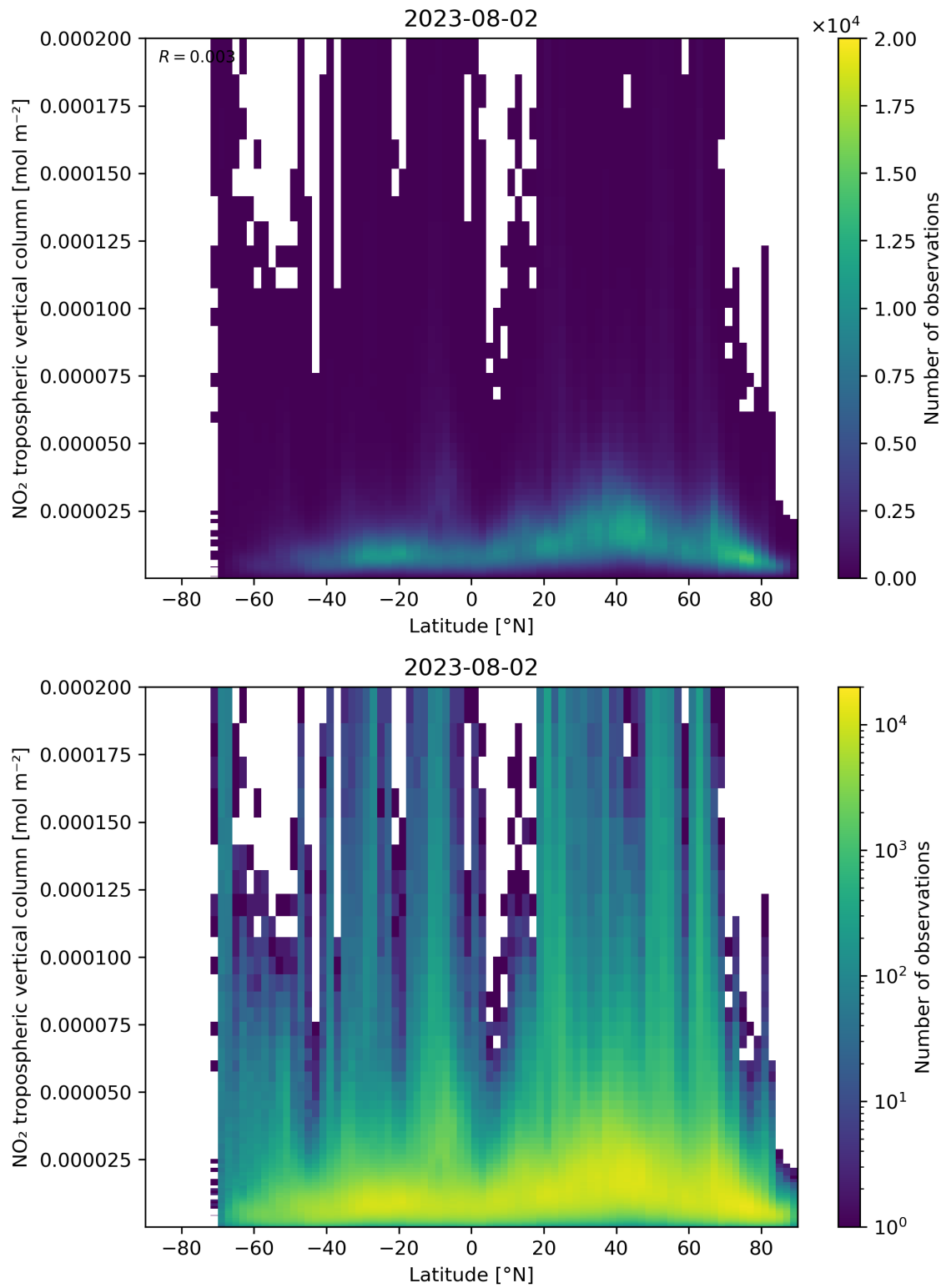
Figure 92: Scatter density plot of “Latitude” against “NO 2 tropospheric vertical column” for 2023-08-01 to 2023-08-03.
