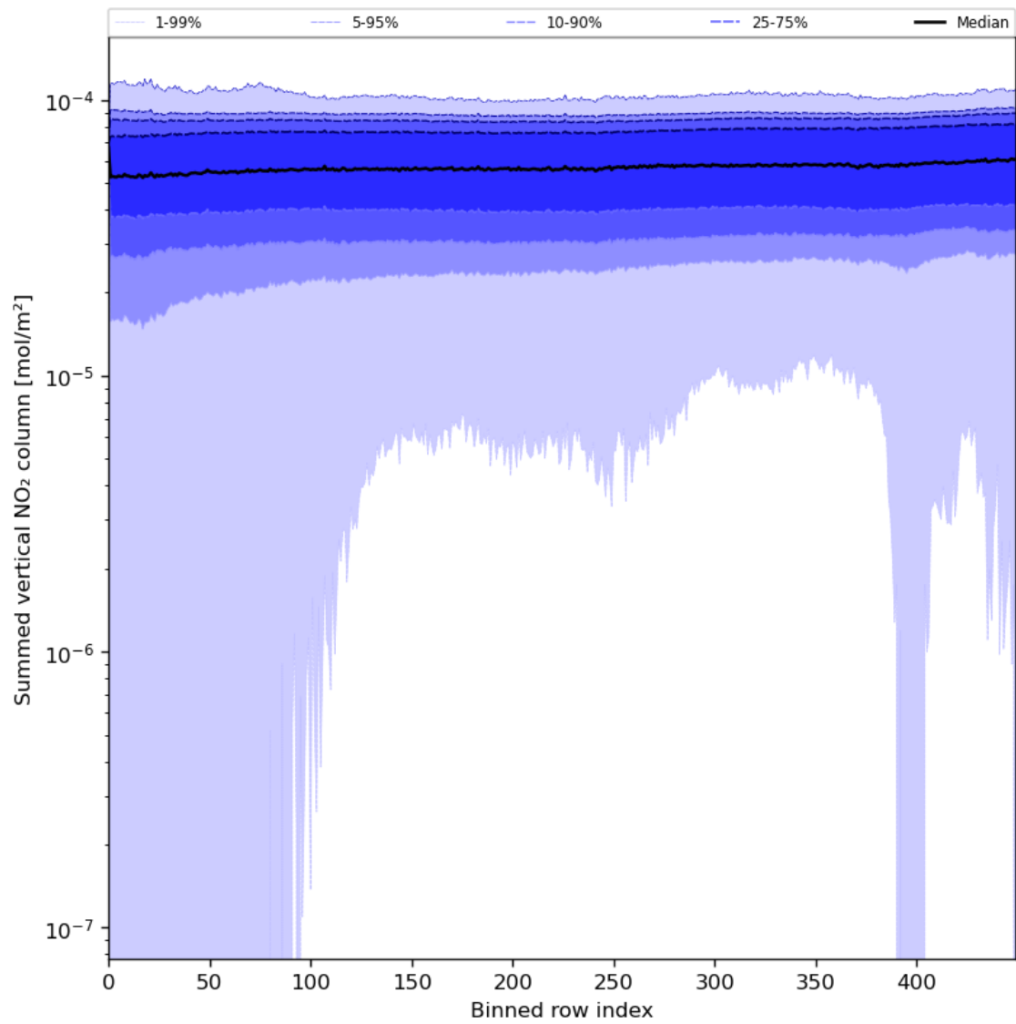
Figure 57: Along track statistics of “Summed vertical NO 2 column” for 2023-08-01 to 2023-08-03
