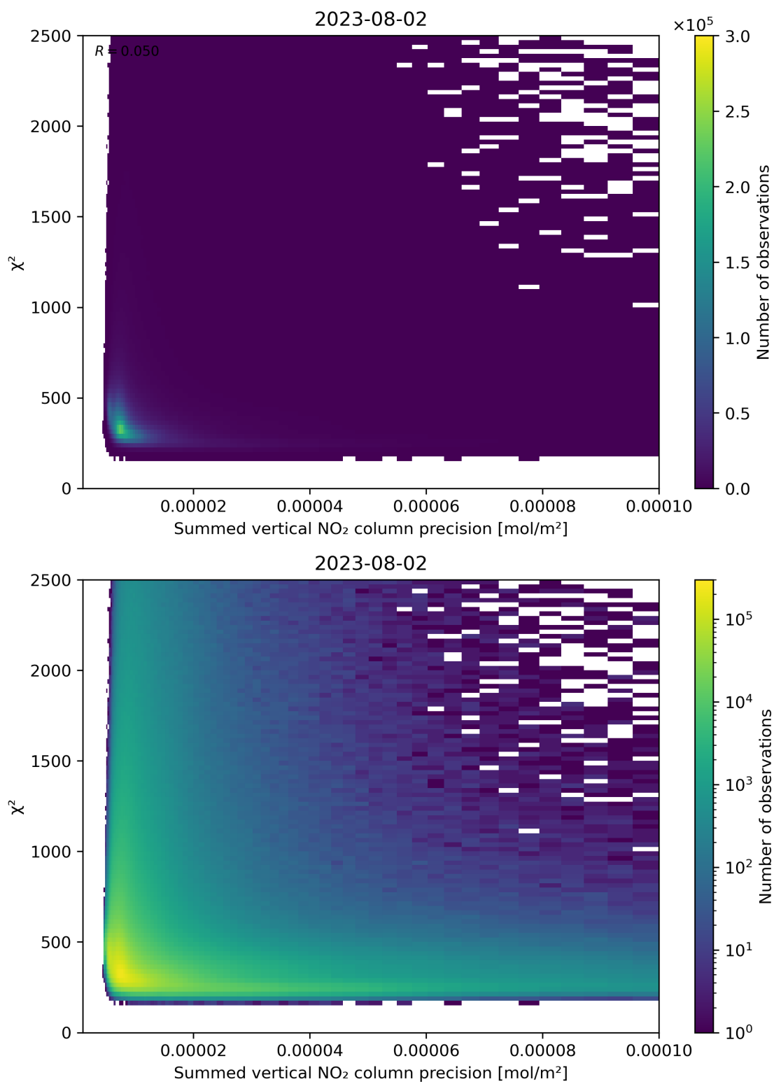
Figure 107: Scatter density plot of “Summed vertical NO 2 column precision” against “ \chi^2 ” for 2023-08-01 to 2023-08-03.
