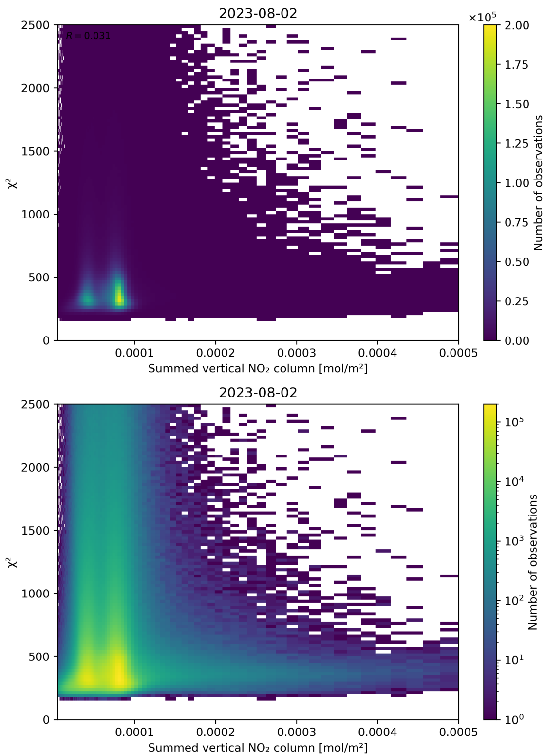
Figure 104: Scatter density plot of “Summed vertical NO 2 column” against “ \chi^2 ” for 2023-08-01 to 2023-08-03.
