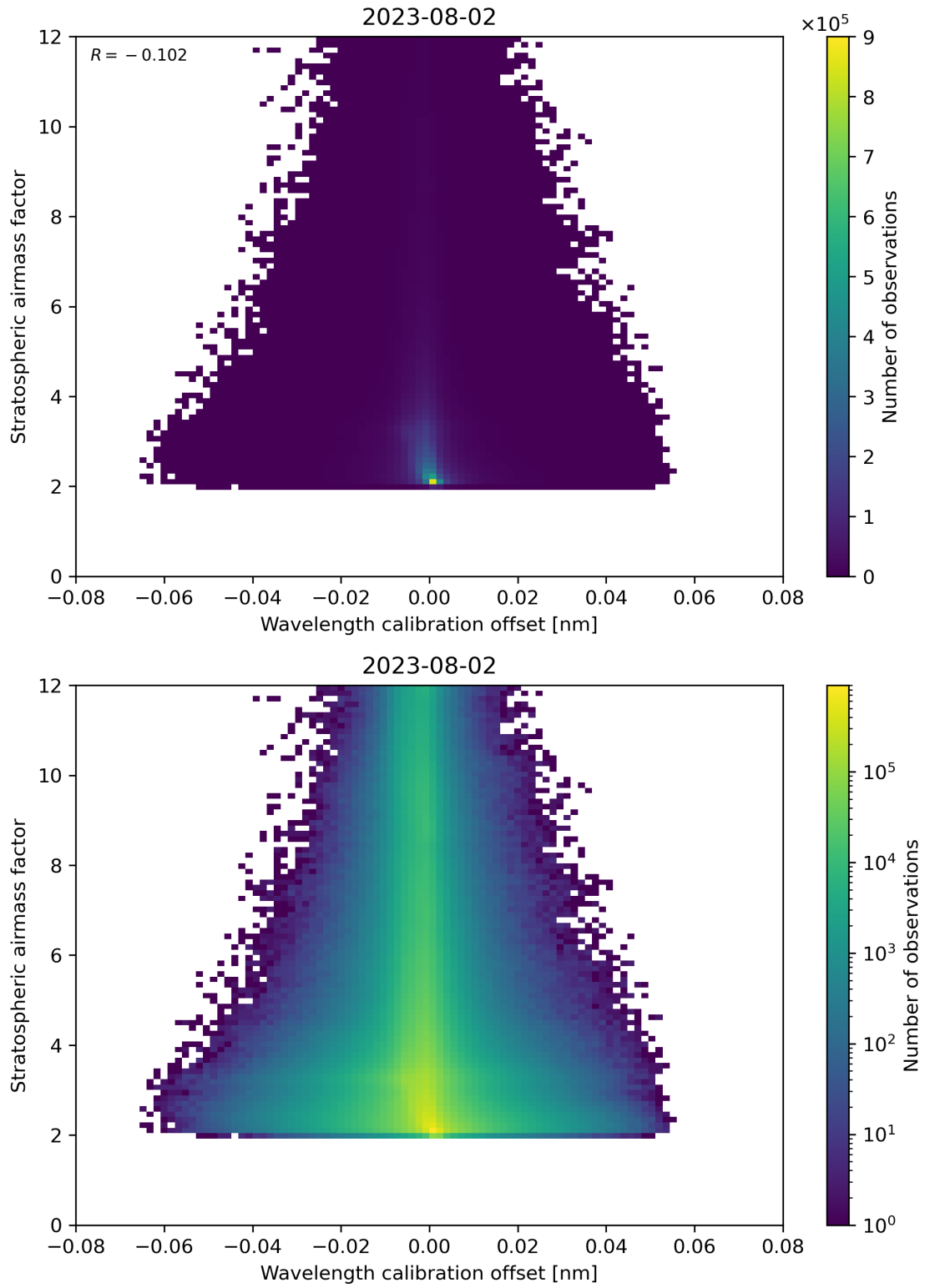
Figure 174: Scatter density plot of “Wavelength calibration offset” against “Stratospheric airmass factor” for 2023-08-01 to 2023-08-03.
