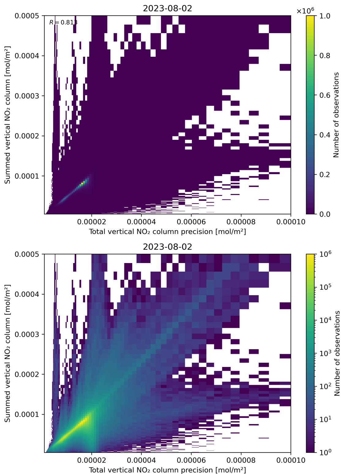
Figure 117: Scatter density plot of “Total vertical NO 2 column precision” against “Summed vertical NO 2 column” for 2023-08-01 to 2023-08-03.
