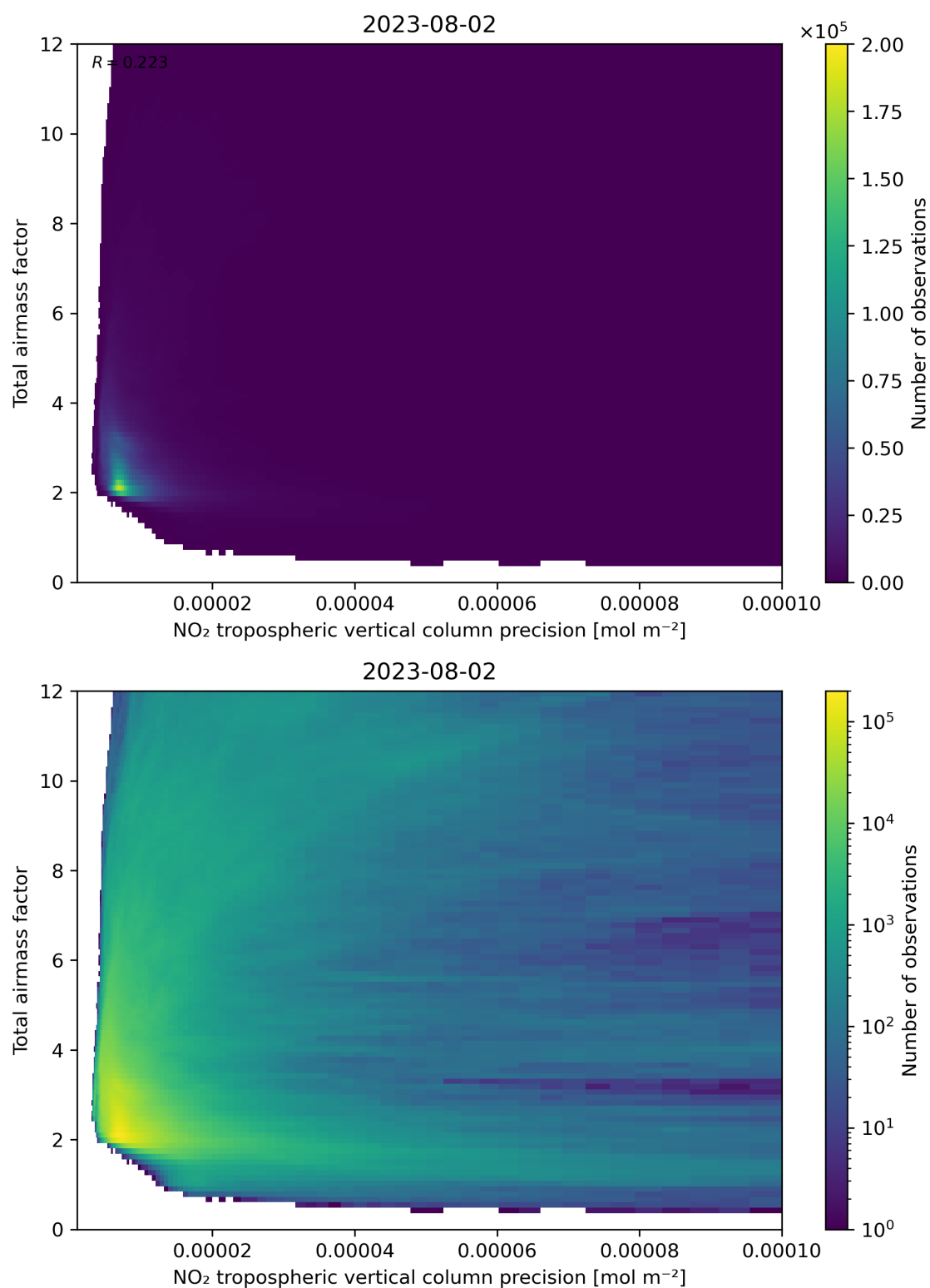
Figure 132: Scatter density plot of “NO 2 tropospheric vertical column precision” against “Total air mass factor” for 2023-08-01 to 2023-08-03.
