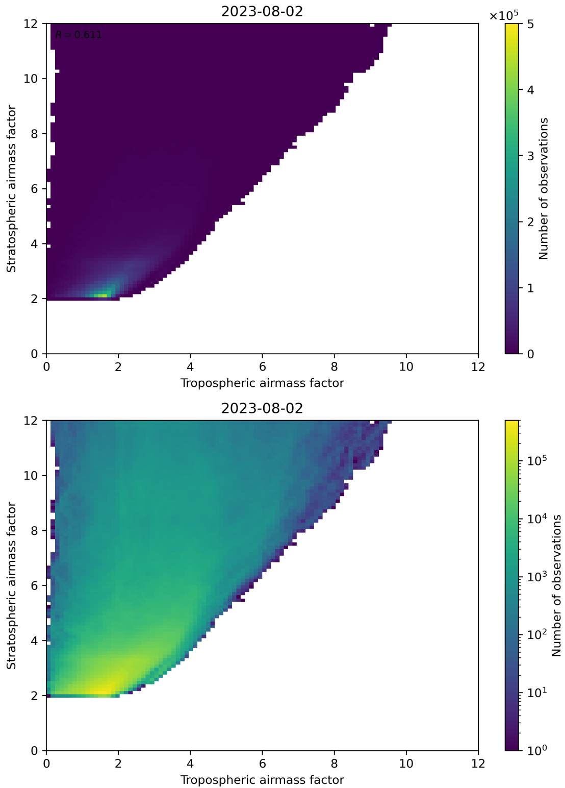
Figure 71: Scatter density plot of “Tropospheric airmass factor” against “Stratospheric airmass factor” for 2023-08-01 to 2023-08-03.
