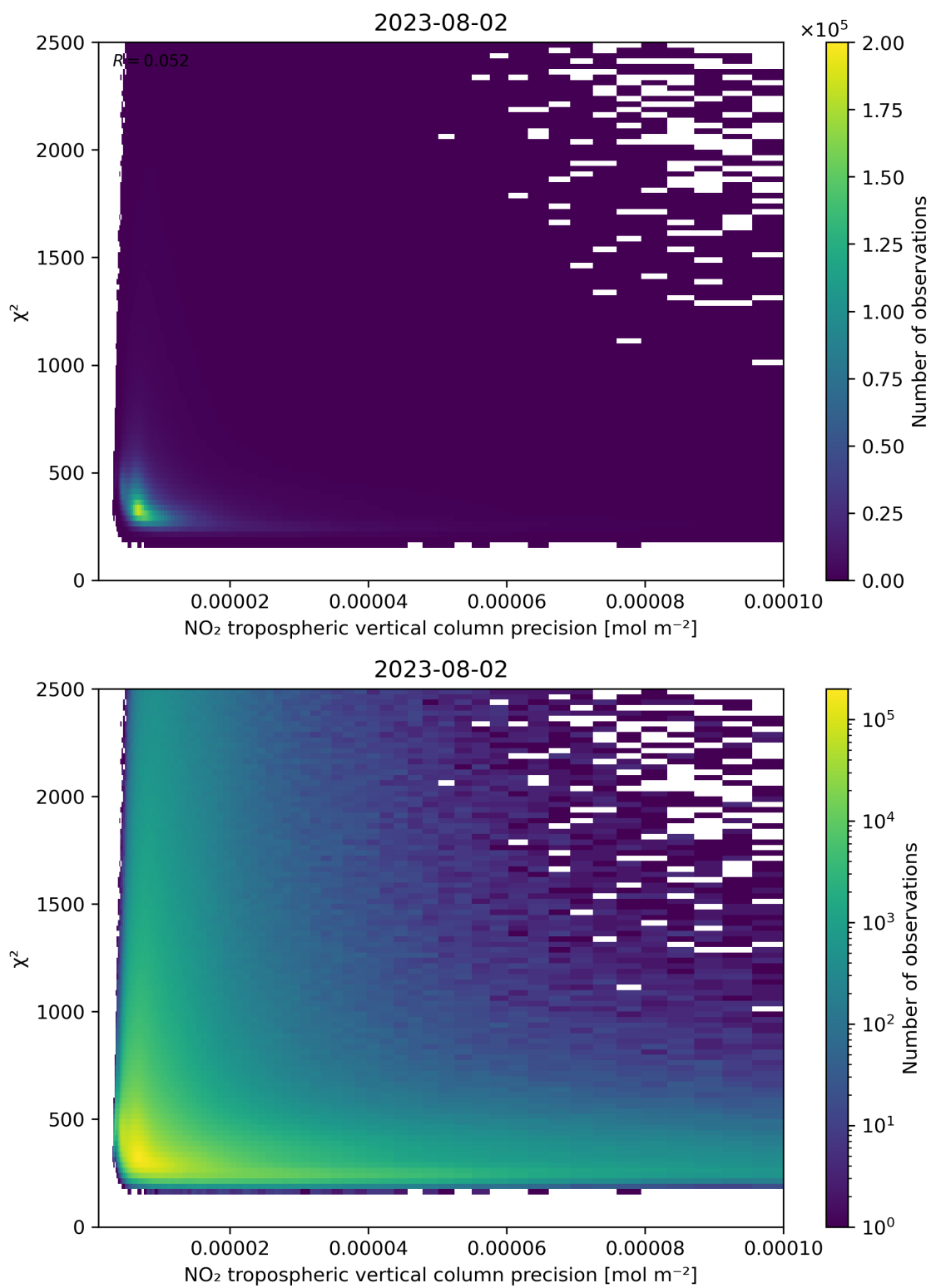
Figure 134: Scatter density plot of “NO 2 tropospheric vertical column precision” against “ \chi^2 ” for 2023-08-01 to 2023-08-03.
