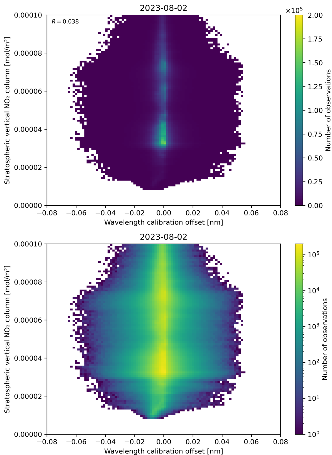
Figure 176: Scatter density plot of “Wavelength calibration offset” against “Stratospheric vertical NO 2 column” for 2023-08-01 to 2023-08-03.
