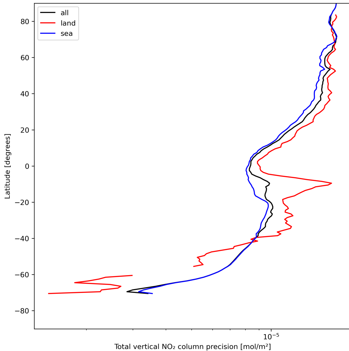
Figure 22: Zonal average of “Total vertical NO 2 column precision” for 2023-08-01 to 2023-08-03.
