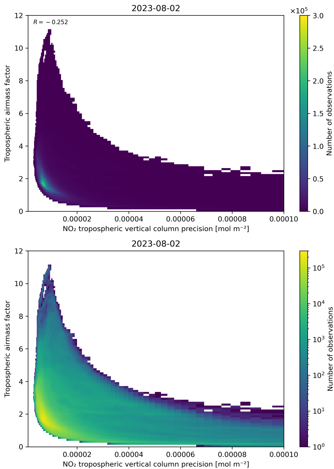
Figure 133: Scatter density plot of “NO 2 tropospheric vertical column precision” against “Tropospheric airmass factor” for 2023-08-01 to 2023-08-03.
