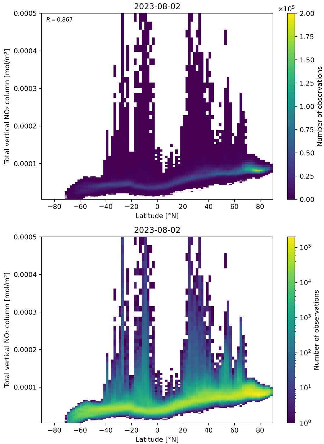
Figure 90: Scatter density plot of “Latitude” against “Total vertical NO 2 column” for 2023-08-01 to 2023-08-03.
