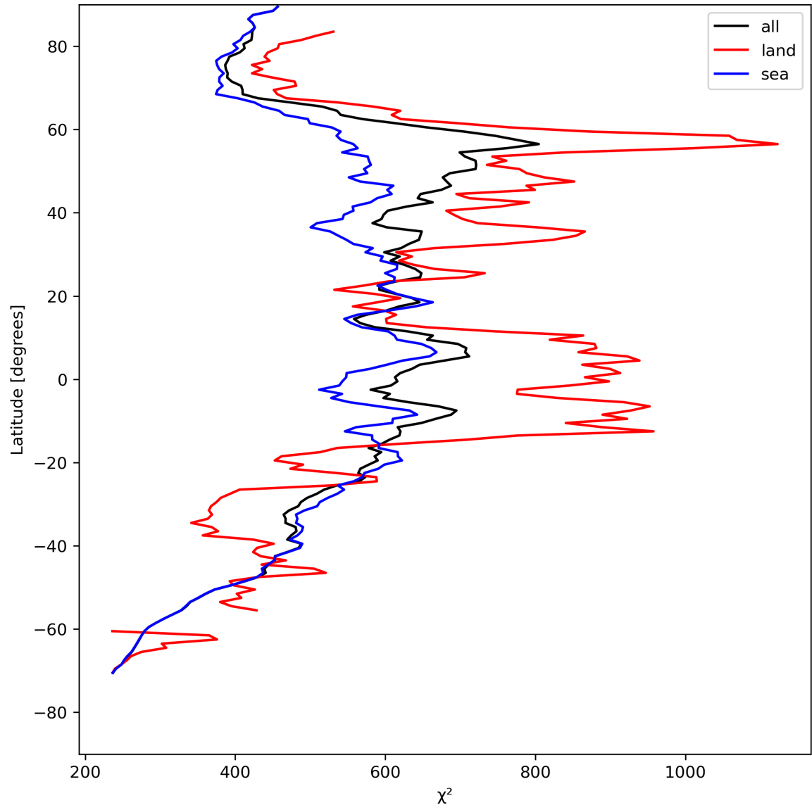
Figure 25: Zonal average of “ \chi^2 ” for 2023-08-01 to 2023-08-03.
