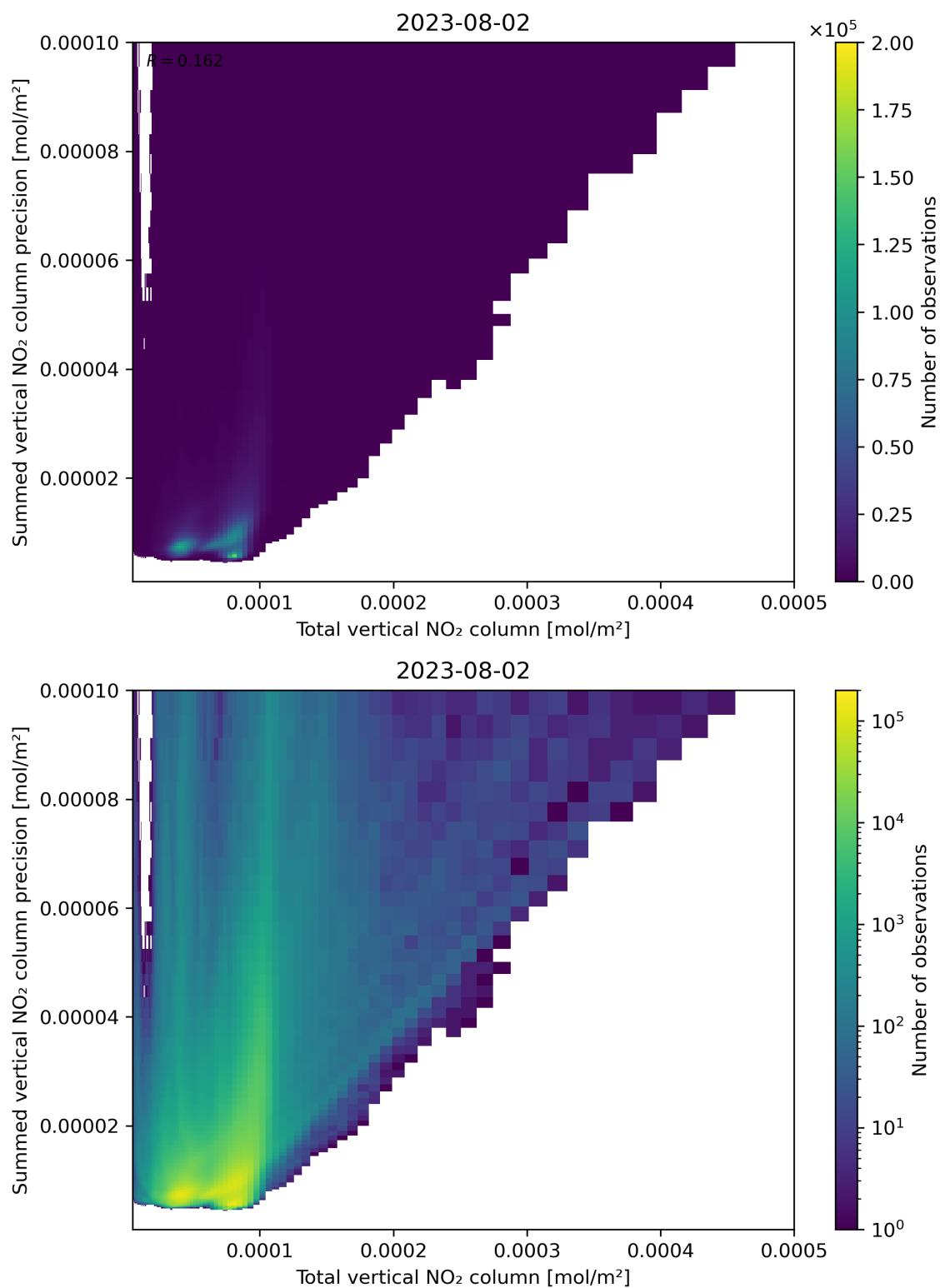
Figure 113: Scatter density plot of “Total vertical NO 2 column” against “Summed vertical NO 2 column precision” for 2023-08-01 to 2023-08-03.
