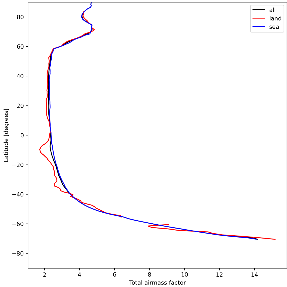
Figure 15: Zonal average of “Total airmass factor” for 2023-08-01 to 2023-08-03.
