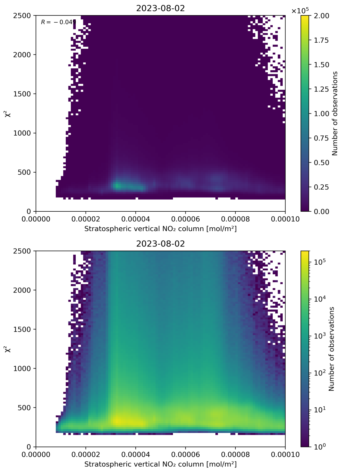
Figure 97: Scatter density plot of “Stratospheric vertical NO 2 column” against “ \chi^2 ” for 2023-08-01 to 2023-08-03.
