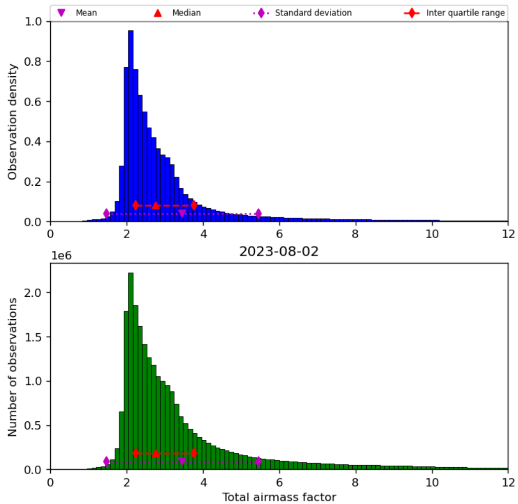
Figure 32: Histogram of “Total airmass factor” for 2023-08-01 to 2023-08-03
