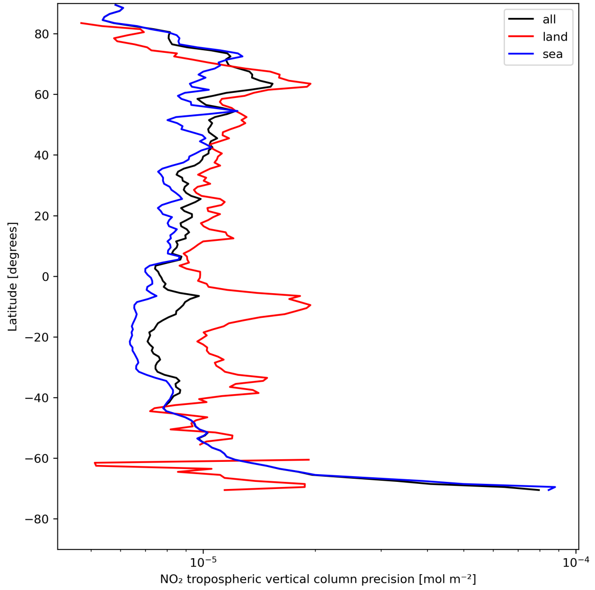
Figure 13: Zonal average of “NO 2 tropospheric vertical column precision” for 2023-08-01 to 2023-08-03.
