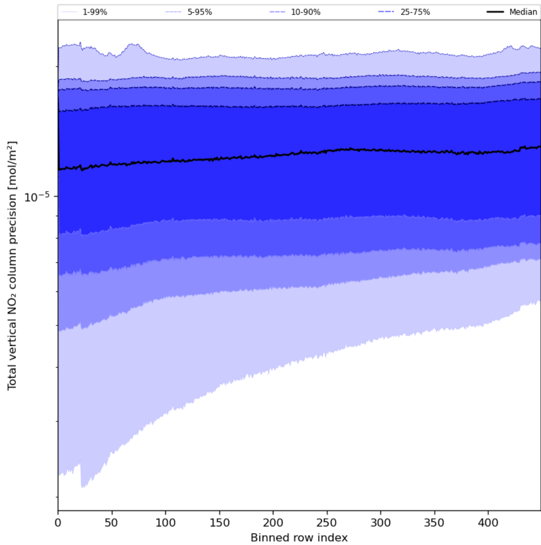
Figure 56: Along track statistics of “Total vertical NO 2 column precision” for 2023-08-01 to 2023-08-03
