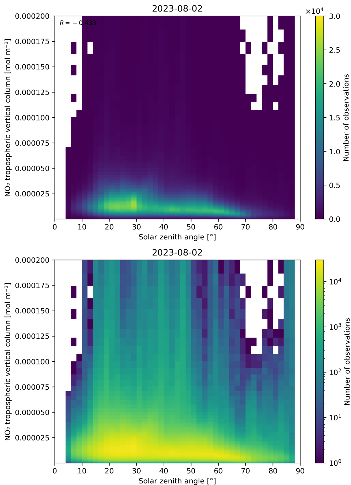
Figure 155: Scatter density plot of “Solar zenith angle” against “NO 2 tropospheric vertical column” for 2023-08-01 to 2023-08-03.
