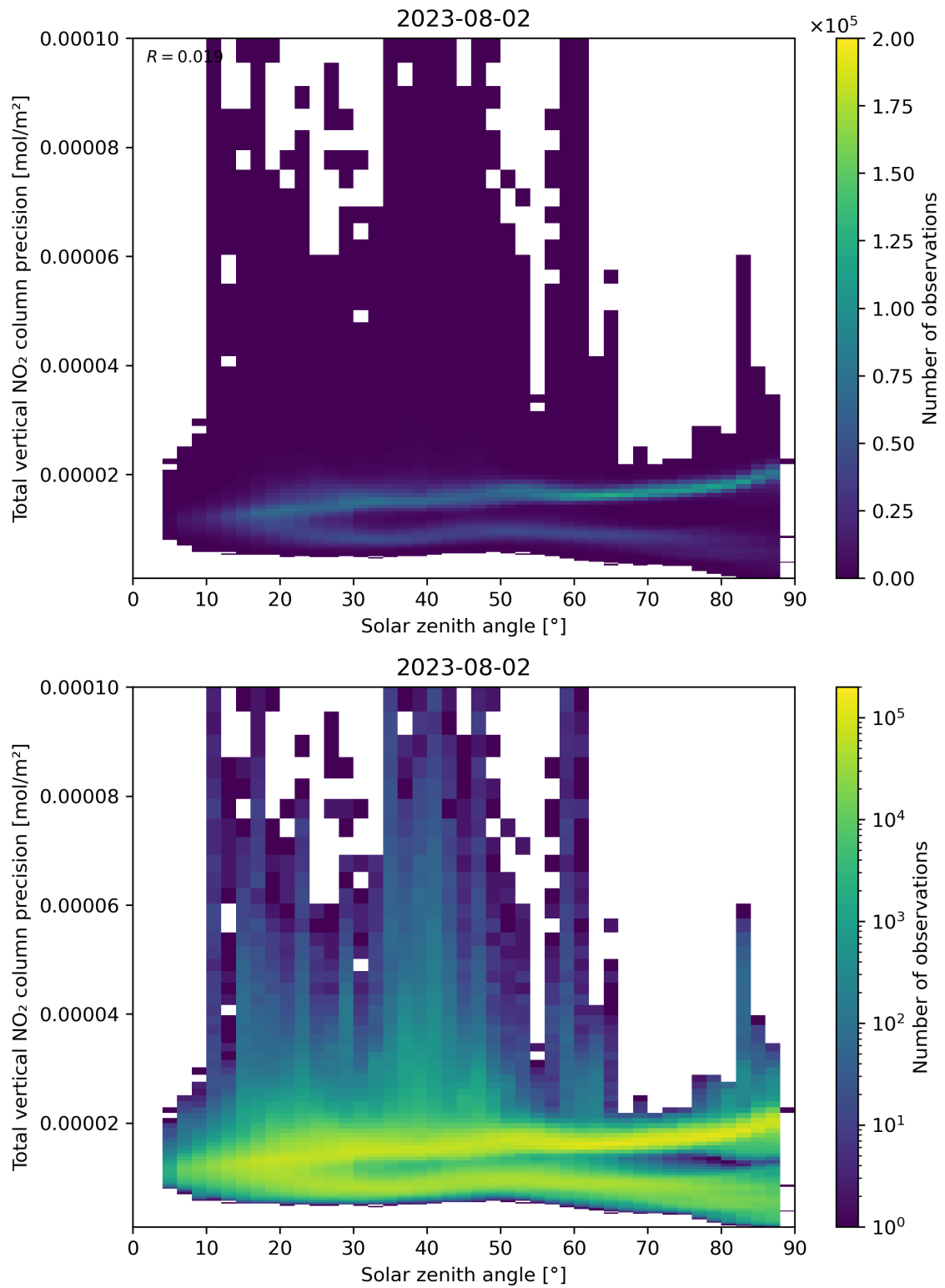
Figure 154: Scatter density plot of “Solar zenith angle” against “Total vertical NO 2 column precision” for 2023-08-01 to 2023-08-03.
