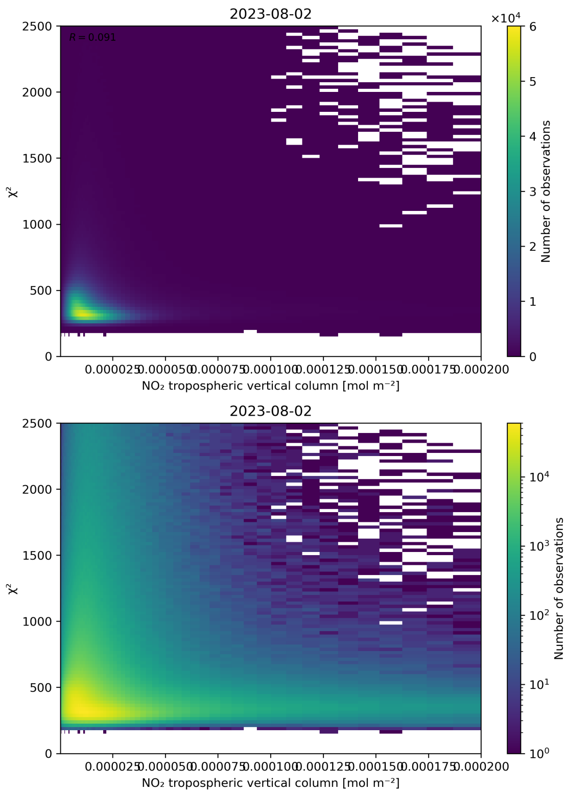
Figure 124: Scatter density plot of “NO 2 tropospheric vertical column” against “ \chi^2 ” for 2023-08-01 to 2023-08-03.
