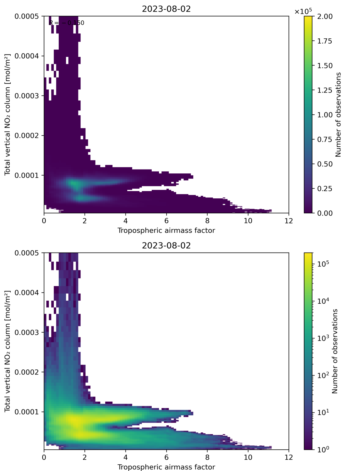
Figure 77: Scatter density plot of “Tropospheric airmass factor” against “Total vertical NO 2 column” for 2023-08-01 to 2023-08-03.
