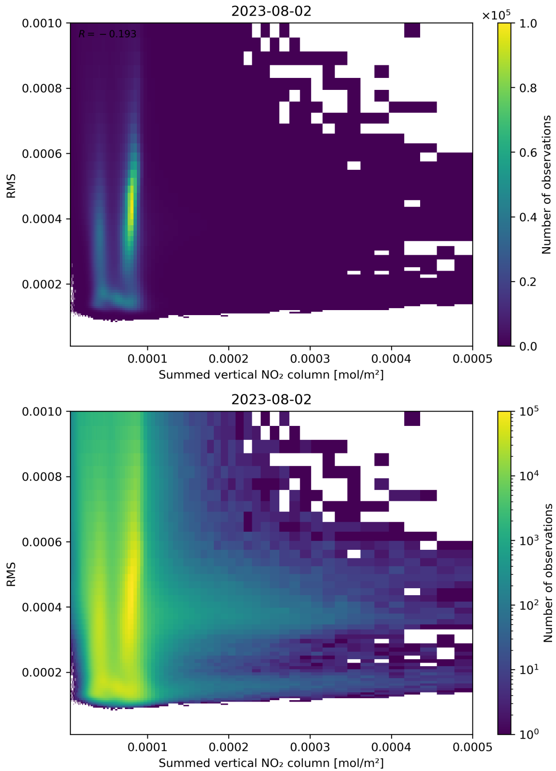
Figure 109: Scatter density plot of “Summed vertical NO 2 column” against “RMS” for 2023-08-01 to 2023-08-03.
