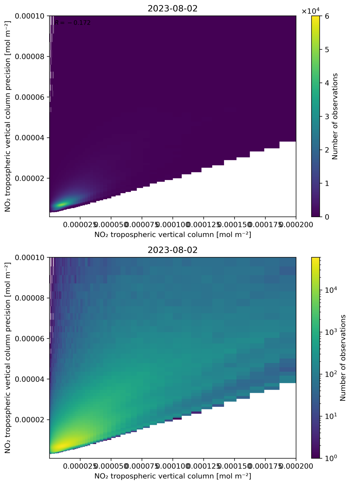
Figure 130: Scatter density plot of “NO 2 tropospheric vertical column” against “NO 2 tropospheric vertical column precision” for 2023-08-01 to 2023-08-03.
