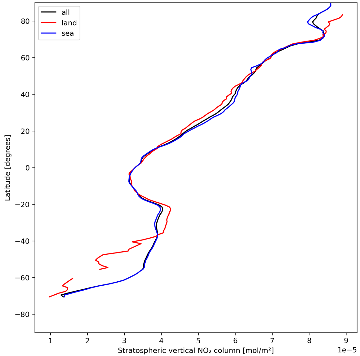
Figure 19: Zonal average of “Stratospheric vertical NO 2 column” for 2023-08-01 to 2023-08-03.
