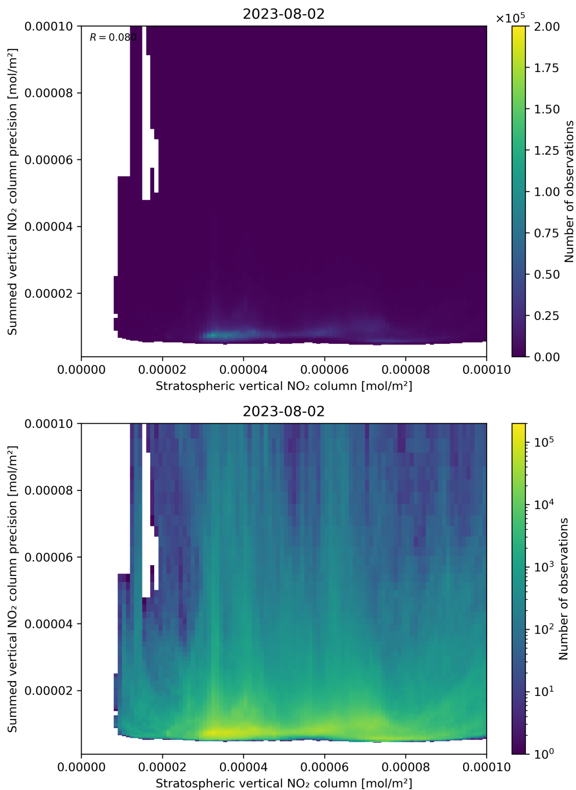
Figure 99: Scatter density plot of “Stratospheric vertical NO 2 column” against “Summed vertical NO 2 column precision” for 2023-08-01 to 2023-08-03.
