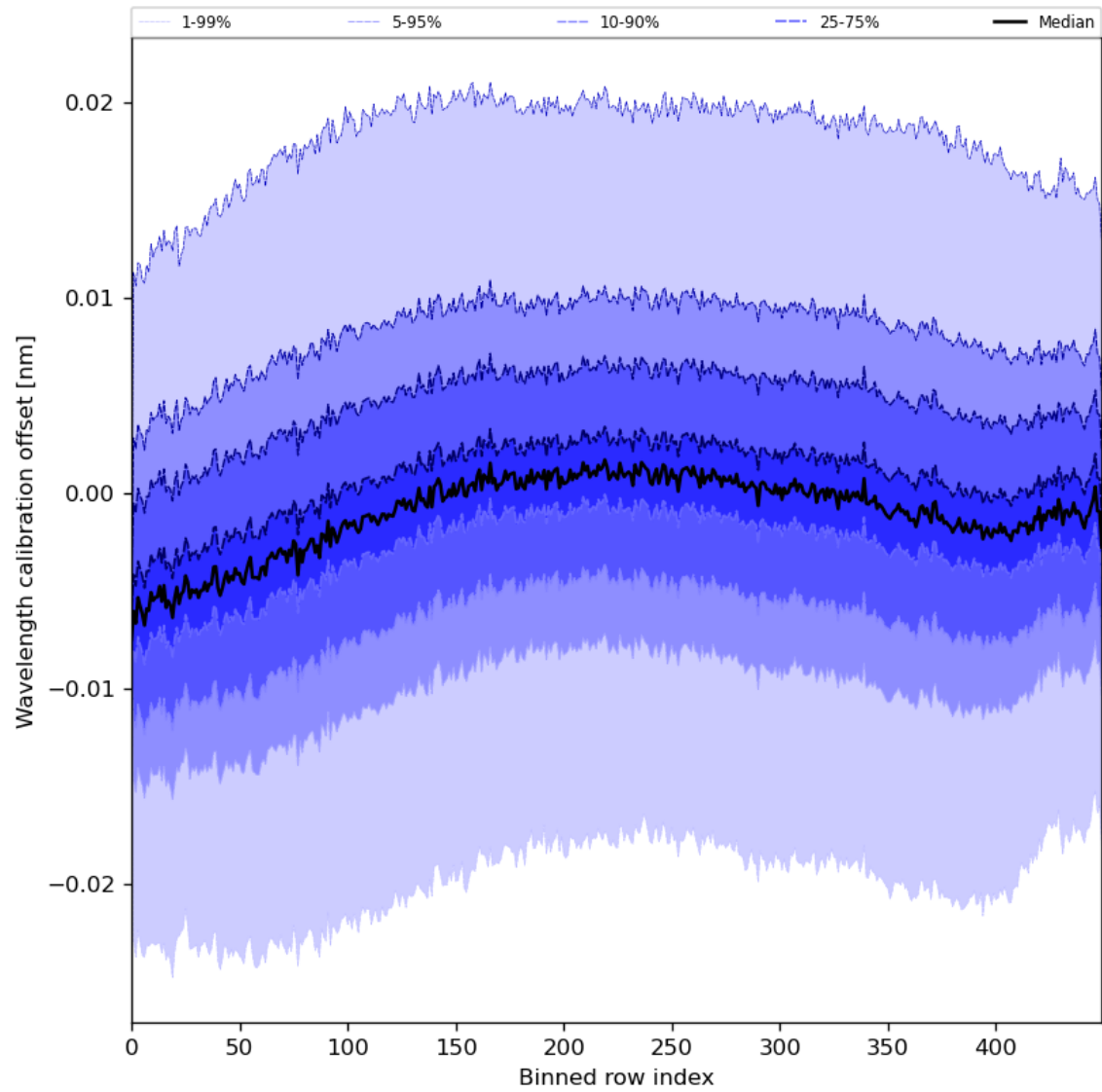
Figure 52: Along track statistics of “Wavelength calibration offset” for 2023-08-01 to 2023-08-03
