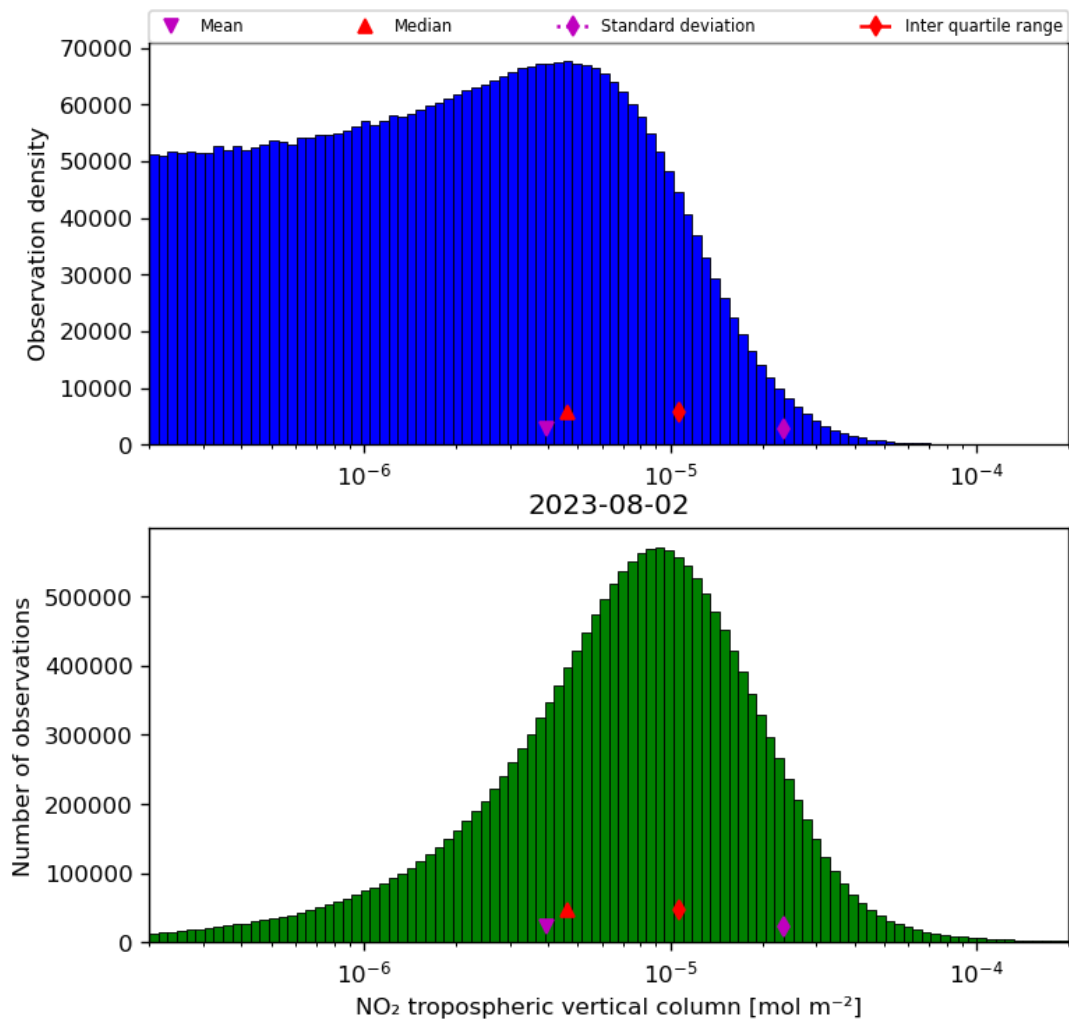
Figure 29: Histogram of “NO 2 tropospheric vertical column” for 2023-08-01 to 2023-08-03
