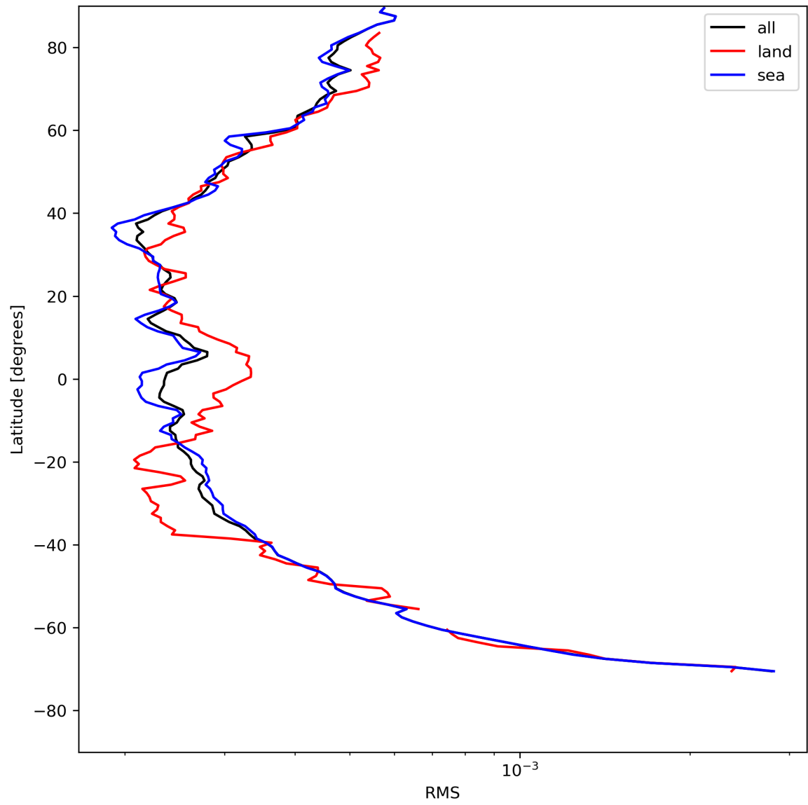
Figure 26: Zonal average of “RMS” for 2023-08-01 to 2023-08-03.
