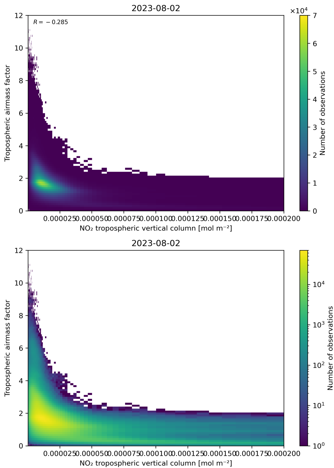
Figure 123: Scatter density plot of “NO 2 tropospheric vertical column” against “Tropospheric air mass factor” for 2023-08-01 to 2023-08-03.
