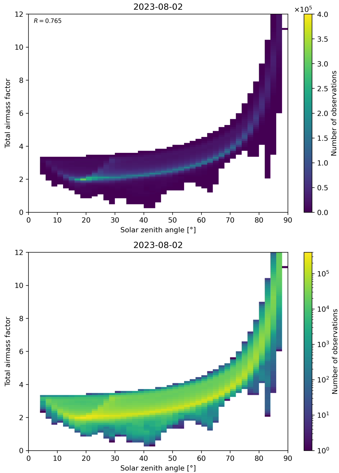
Figure 146: Scatter density plot of “Solar zenith angle” against “Total air mass factor” for 2023-08-01 to 2023-08-03.
