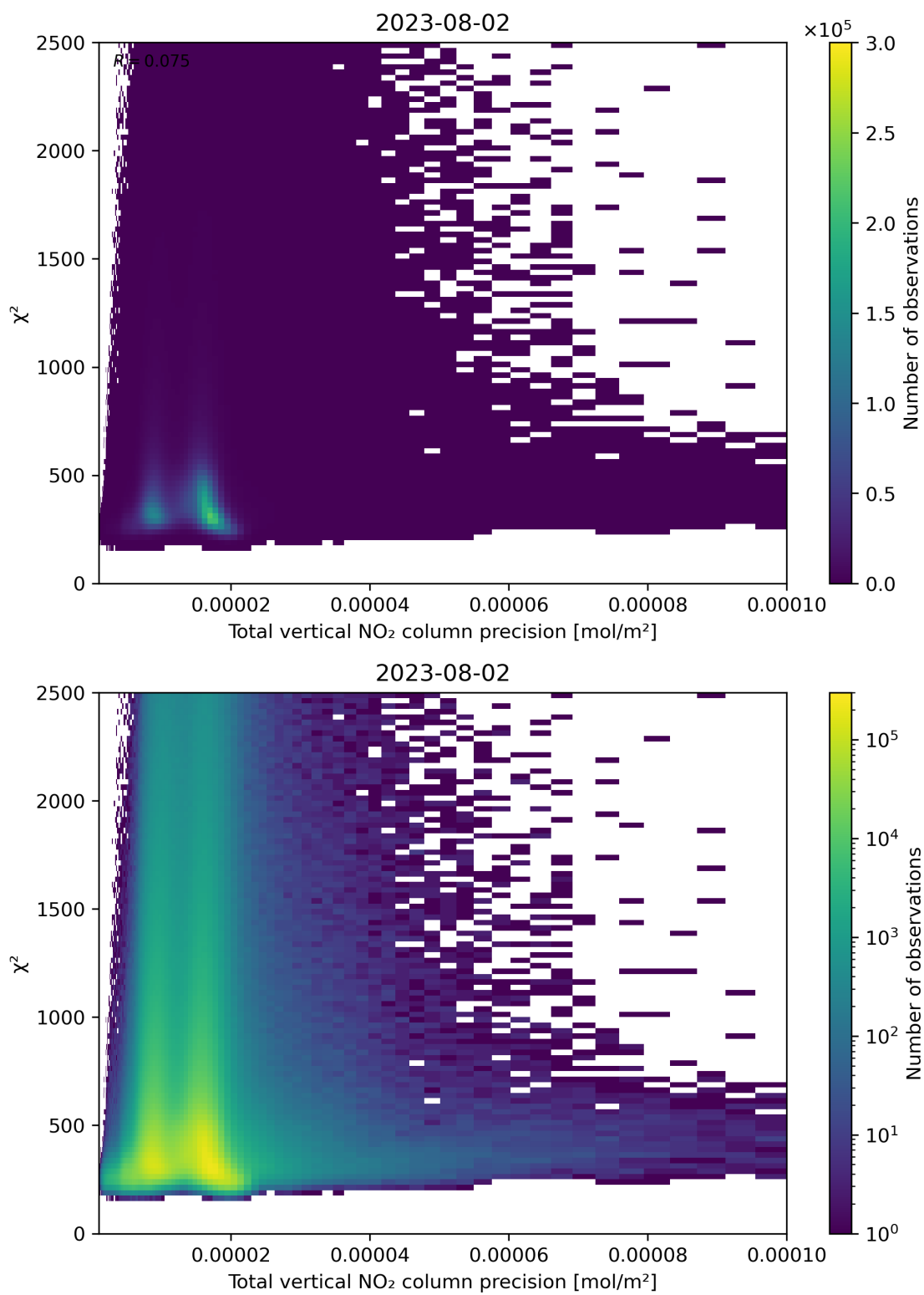
Figure 116: Scatter density plot of “Total vertical NO 2 column precision” against “ \chi^2 ” for 2023-08-01 to 2023-08-03.
