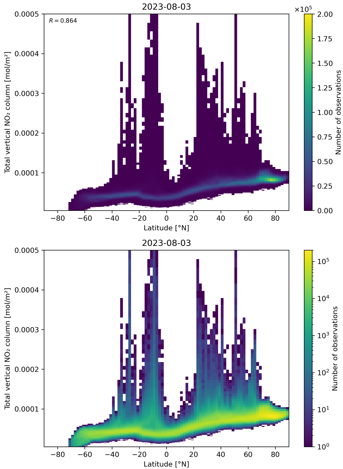
Figure 90: Scatter density plot of “Latitude” against “Total vertical NO 2 column” for 2023-08-02 to 2023-08-04.
