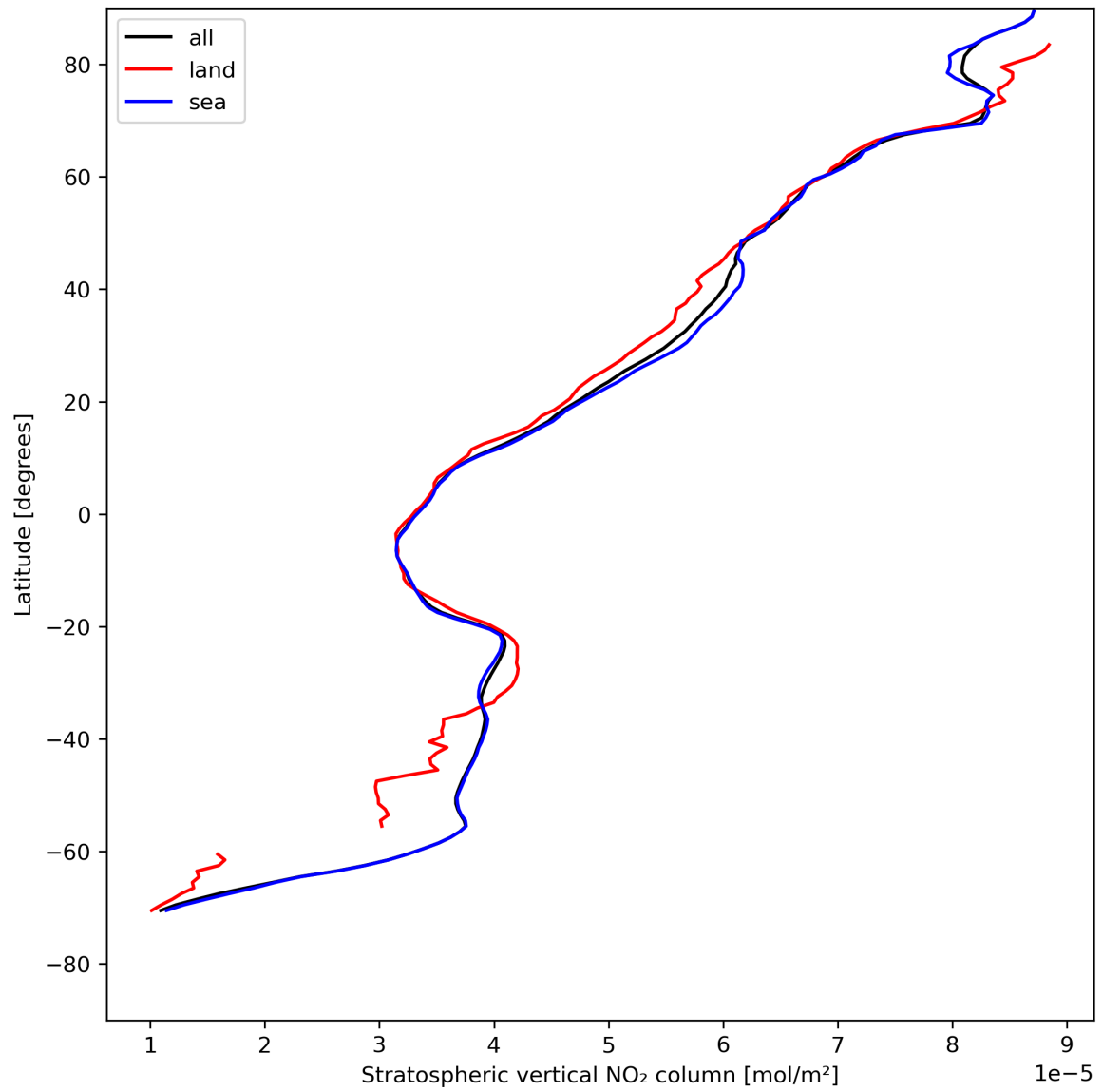
Figure 19: Zonal average of “Stratospheric vertical NO 2 column” for 2023-08-02 to 2023-08-04.
