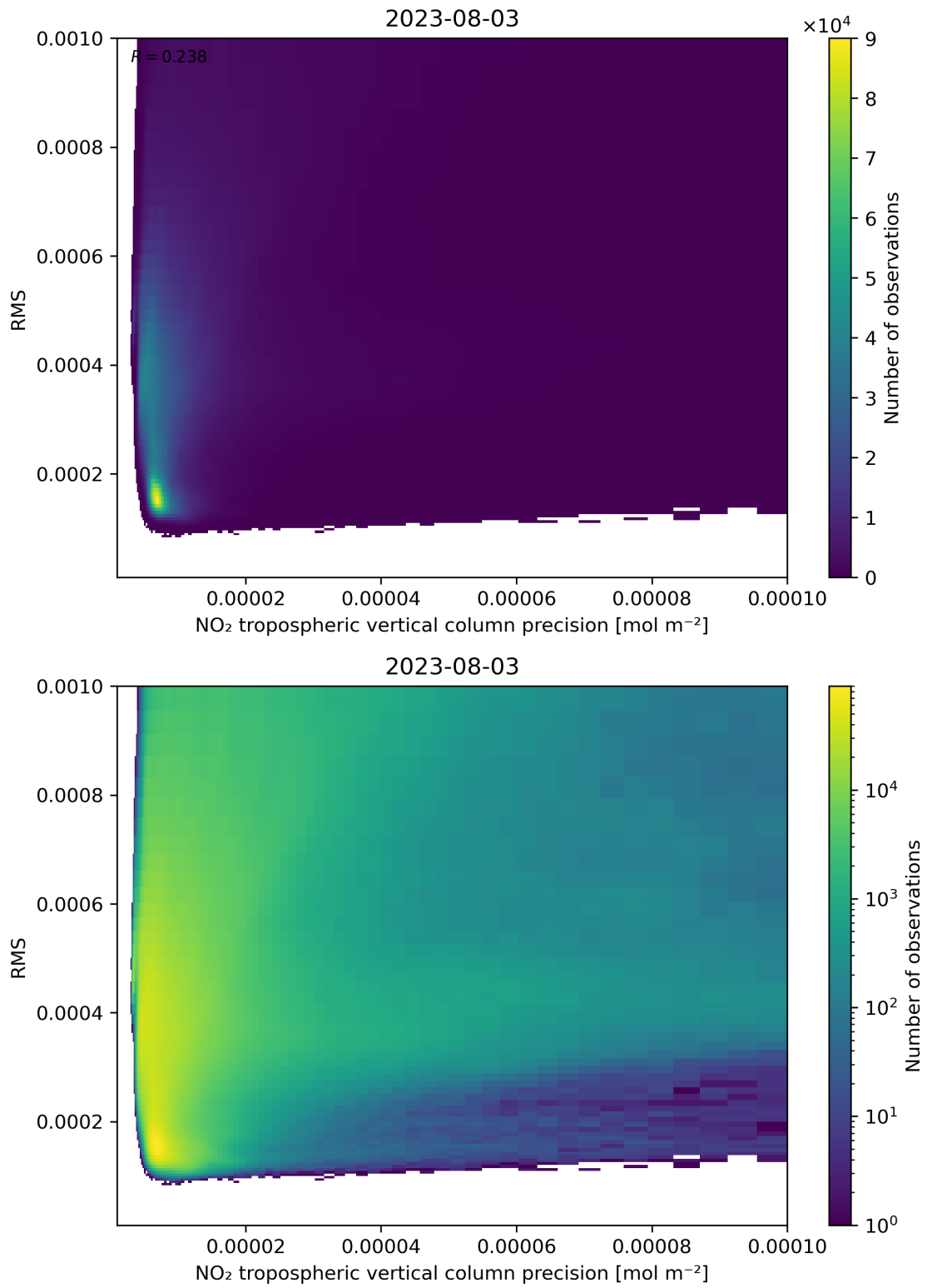
Figure 140: Scatter density plot of “NO 2 tropospheric vertical column precision” against “RMS” for 2023-08-02 to 2023-08-04.
