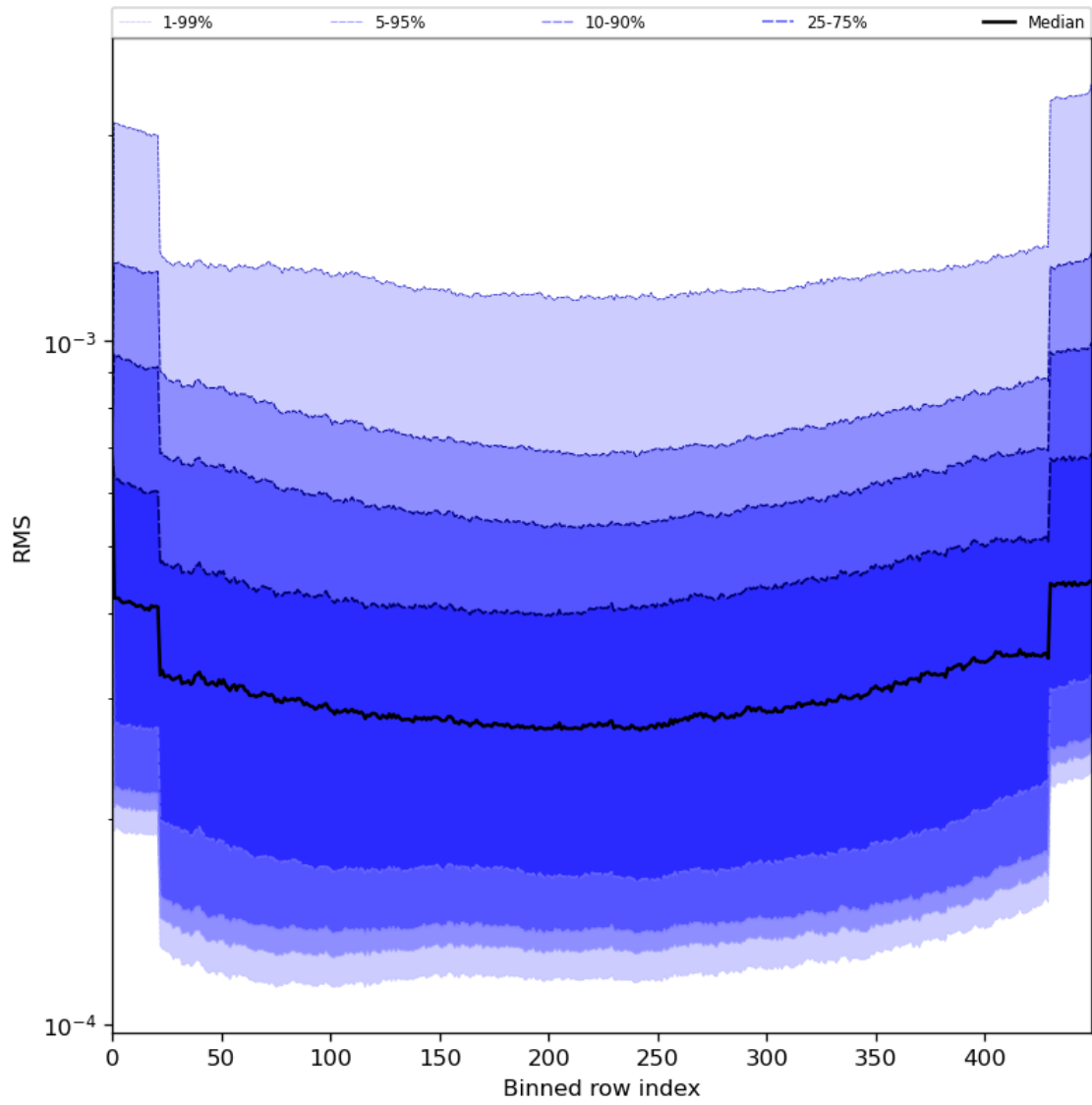
Figure 60: Along track statistics of “RMS” for 2023-08-02 to 2023-08-04
