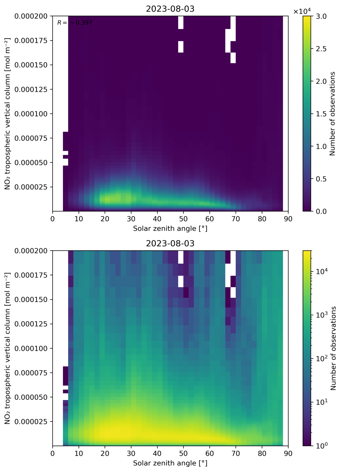
Figure 155: Scatter density plot of “Solar zenith angle” against “NO 2 tropospheric vertical column” for 2023-08-02 to 2023-08-04.
