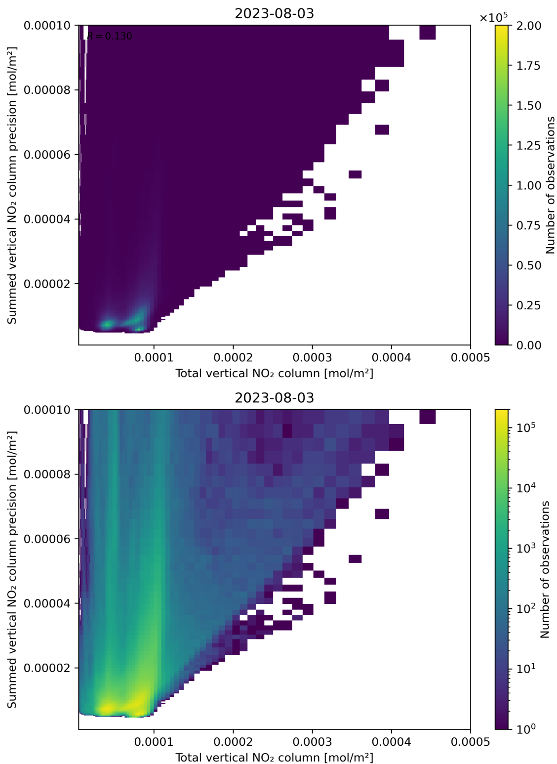
Figure 113: Scatter density plot of “Total vertical NO 2 column” against “Summed vertical NO 2 column precision” for 2023-08-02 to 2023-08-04.
