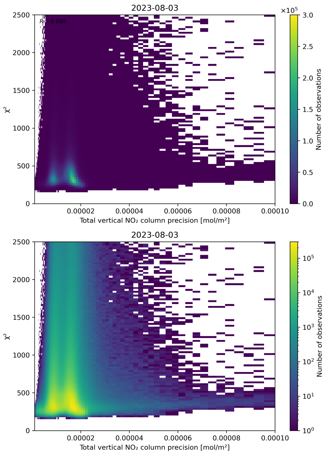
Figure 116: Scatter density plot of “Total vertical NO 2 column precision” against “ \chi^2 ” for 2023-08-02 to 2023-08-04.
