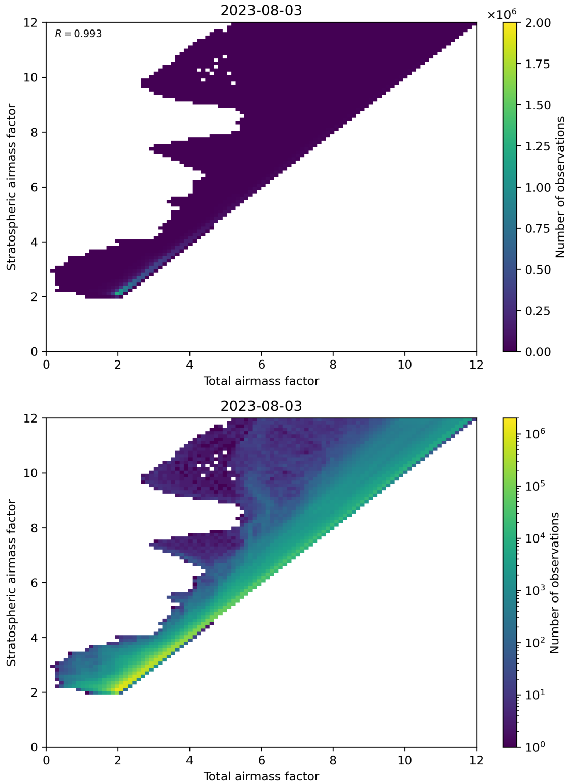
Figure 62: Scatter density plot of “Total airmass factor” against “Stratospheric airmass factor” for 2023-08-02 to 2023-08-04.
