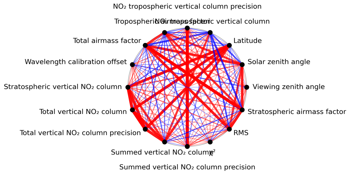
Figure 1: Map of correlation graph for 2023-08-02 to 2023-08-04.
