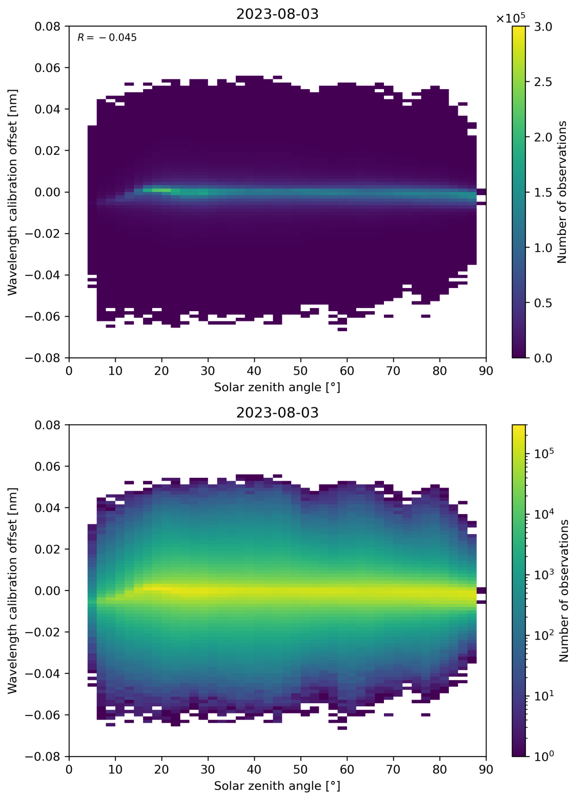
Figure 158: Scatter density plot of “Solar zenith angle” against “Wavelength calibration offset” for 2023-08-02 to 2023-08-04.
