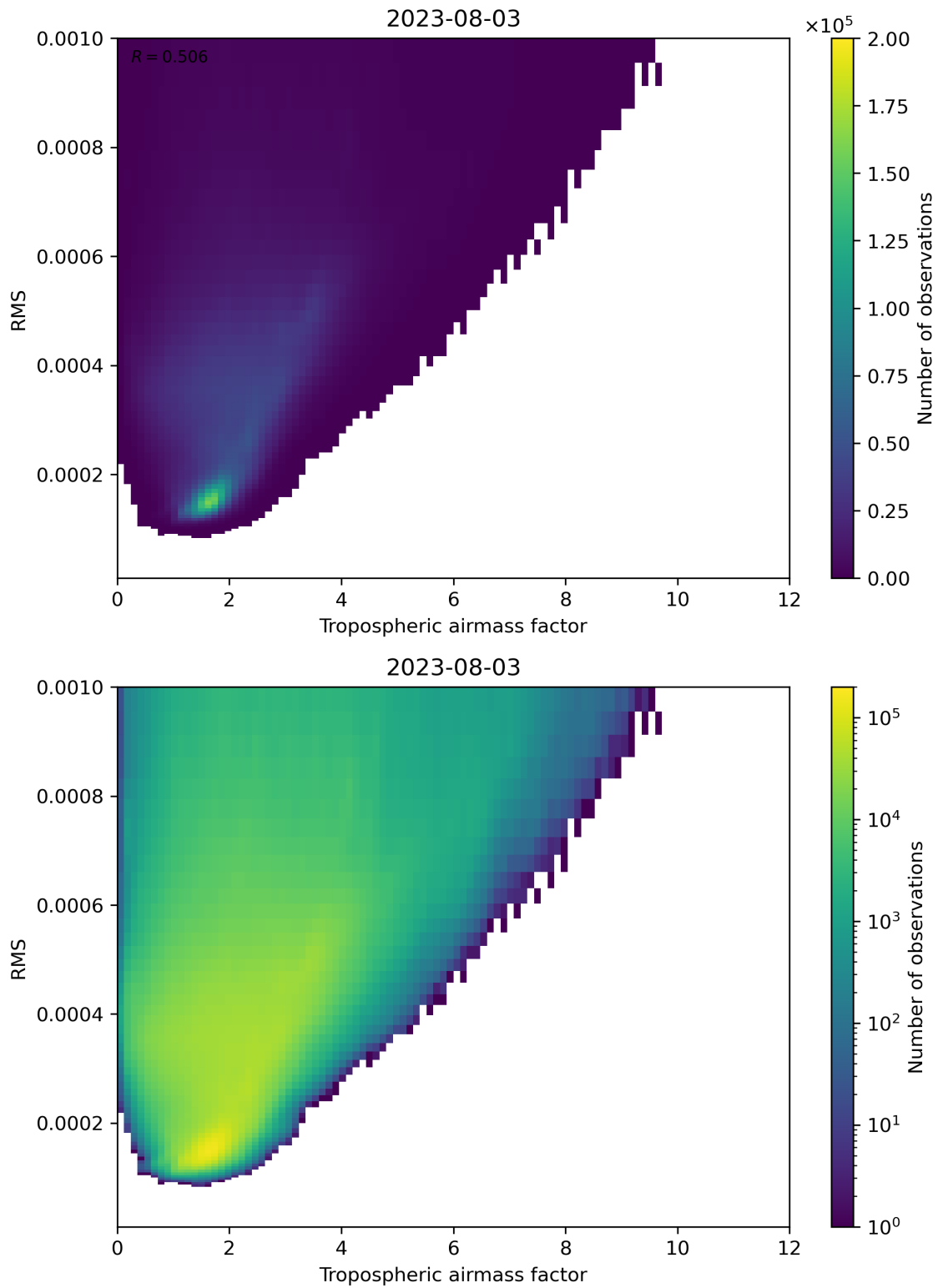
Figure 79: Scatter density plot of “Tropospheric airmass factor” against “RMS” for 2023-08-02 to 2023-08-04.
