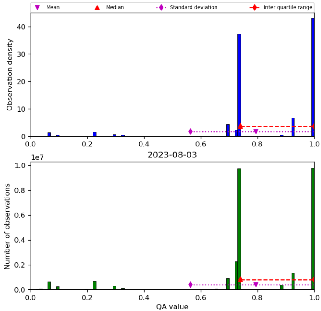
Figure 28: Histogram of “QA value” for 2023-08-02 to 2023-08-04
