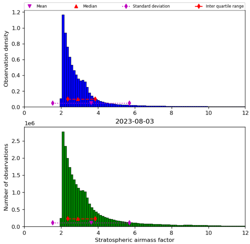
Figure 44: Histogram of “Stratospheric airmass factor” for 2023-08-02 to 2023-08-04
