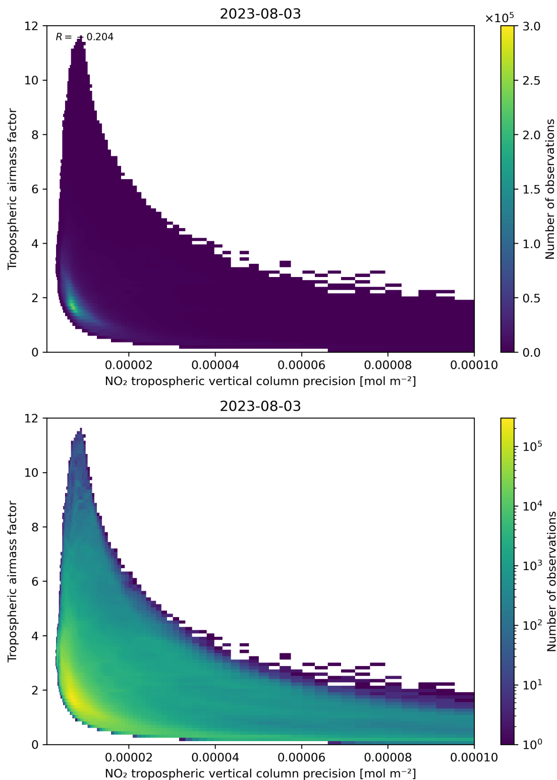
Figure 133: Scatter density plot of “NO 2 tropospheric vertical column precision” against “Tropospheric air mass factor” for 2023-08-02 to 2023-08-04.
