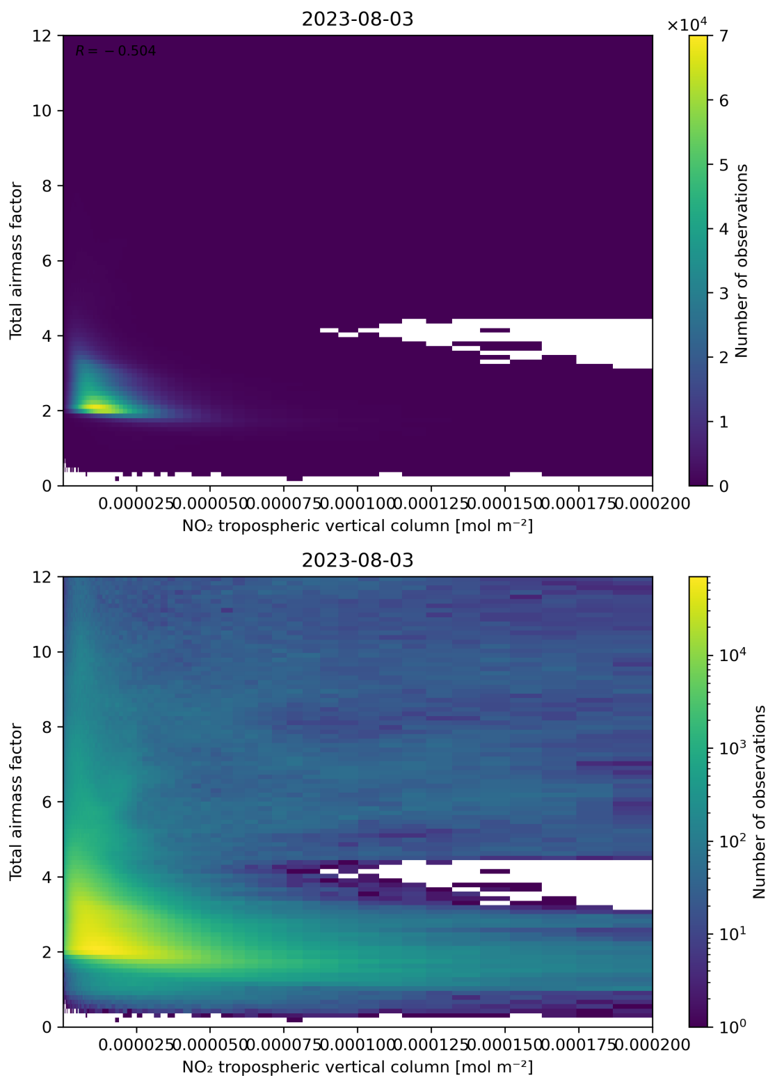
Figure 122: Scatter density plot of “NO 2 tropospheric vertical column” against “Total air mass factor” for 2023-08-02 to 2023-08-04.
