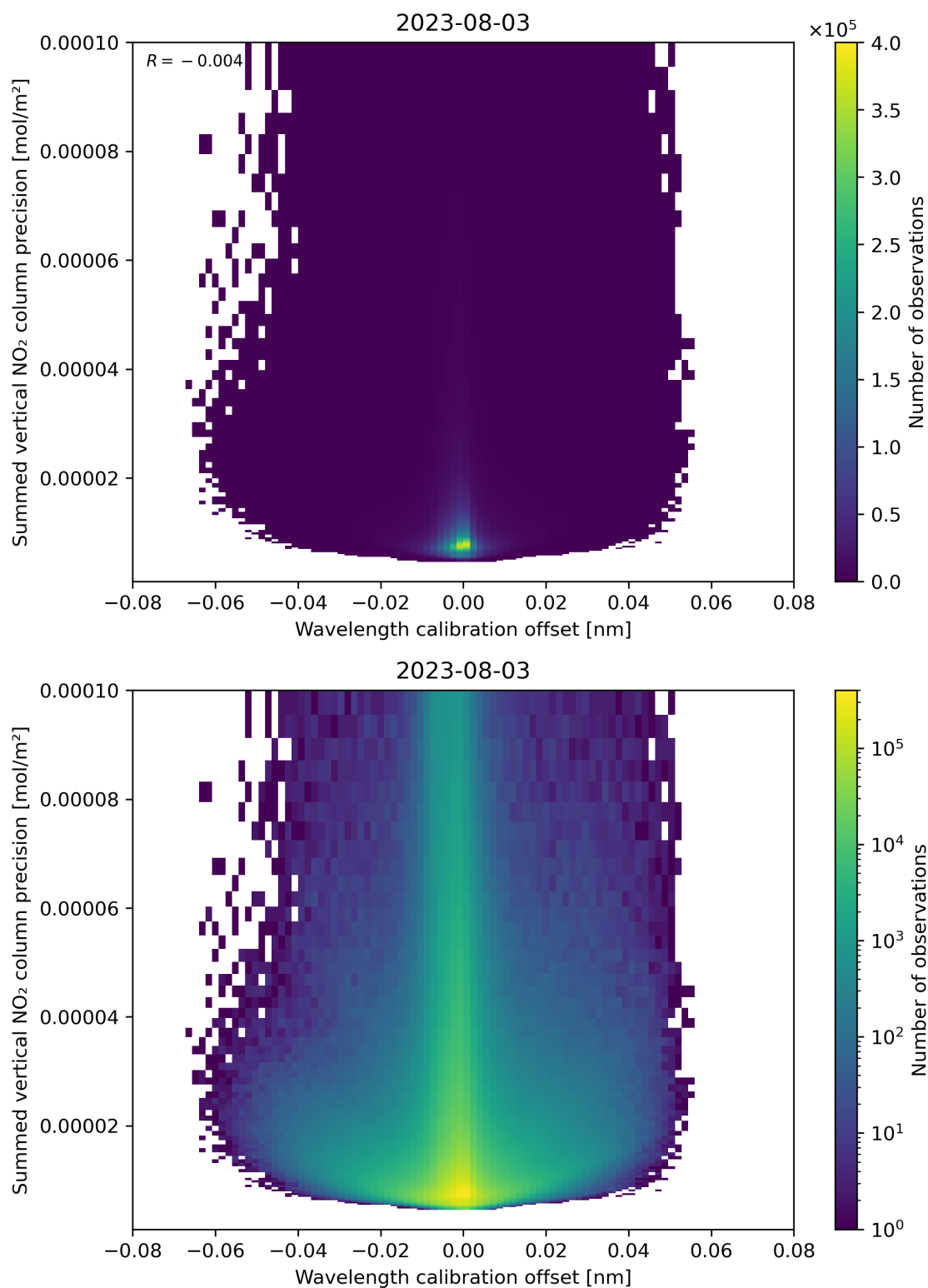
Figure 178: Scatter density plot of “Wavelength calibration offset” against “Summed vertical NO 2 column precision” for 2023-08-02 to 2023-08-04.
