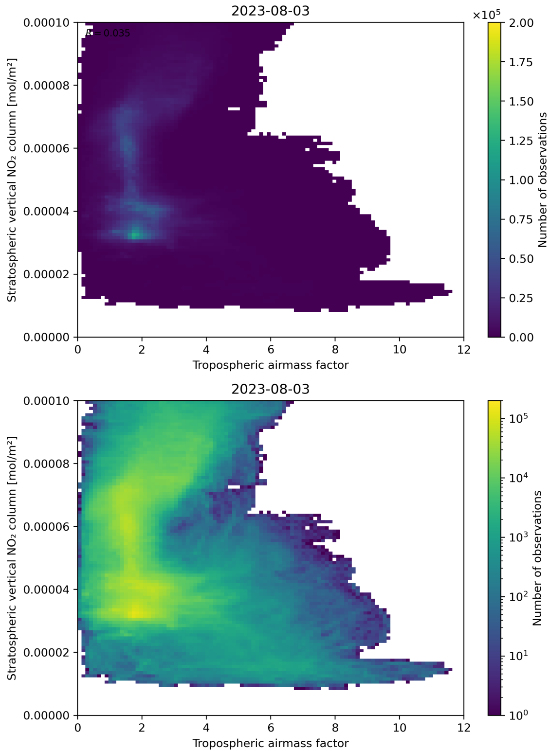
Figure 74: Scatter density plot of “Tropospheric air mass factor” against “Stratospheric vertical NO 2 column” for 2023-08-02 to 2023-08-04.
