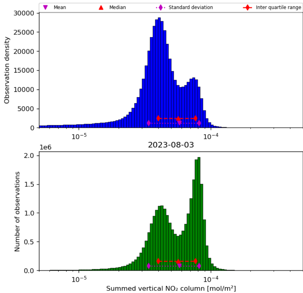
Figure 40: Histogram of “Summed vertical NO 2 column” for 2023-08-02 to 2023-08-04
