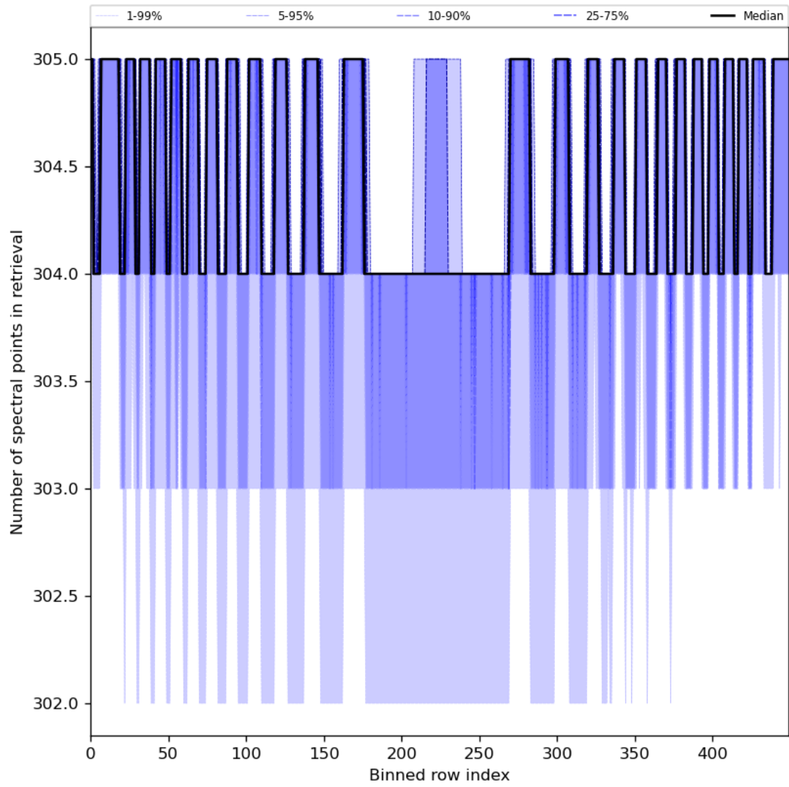
Figure 50: Along track statistics of “Number of spectral points in retrieval” for 2023-08-02 to 2023-08-04
