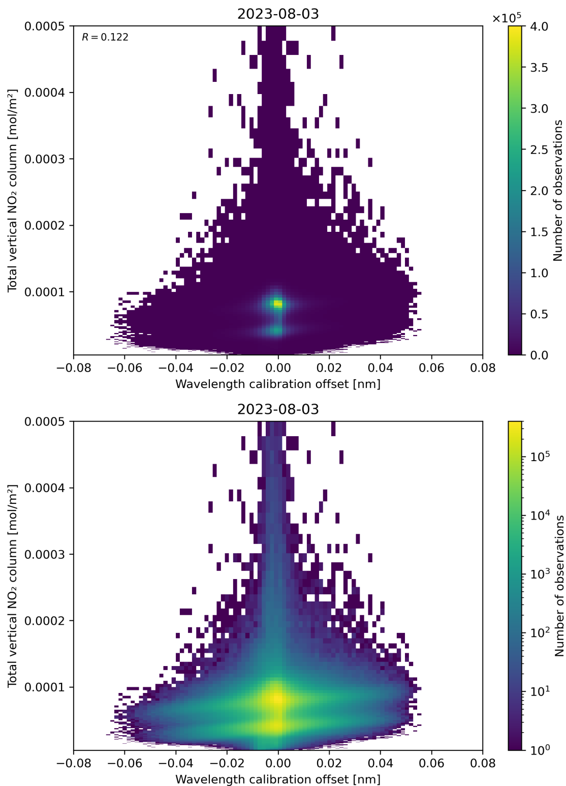
Figure 179: Scatter density plot of “Wavelength calibration offset” against “Total vertical NO 2 column” for 2023-08-02 to 2023-08-04.
