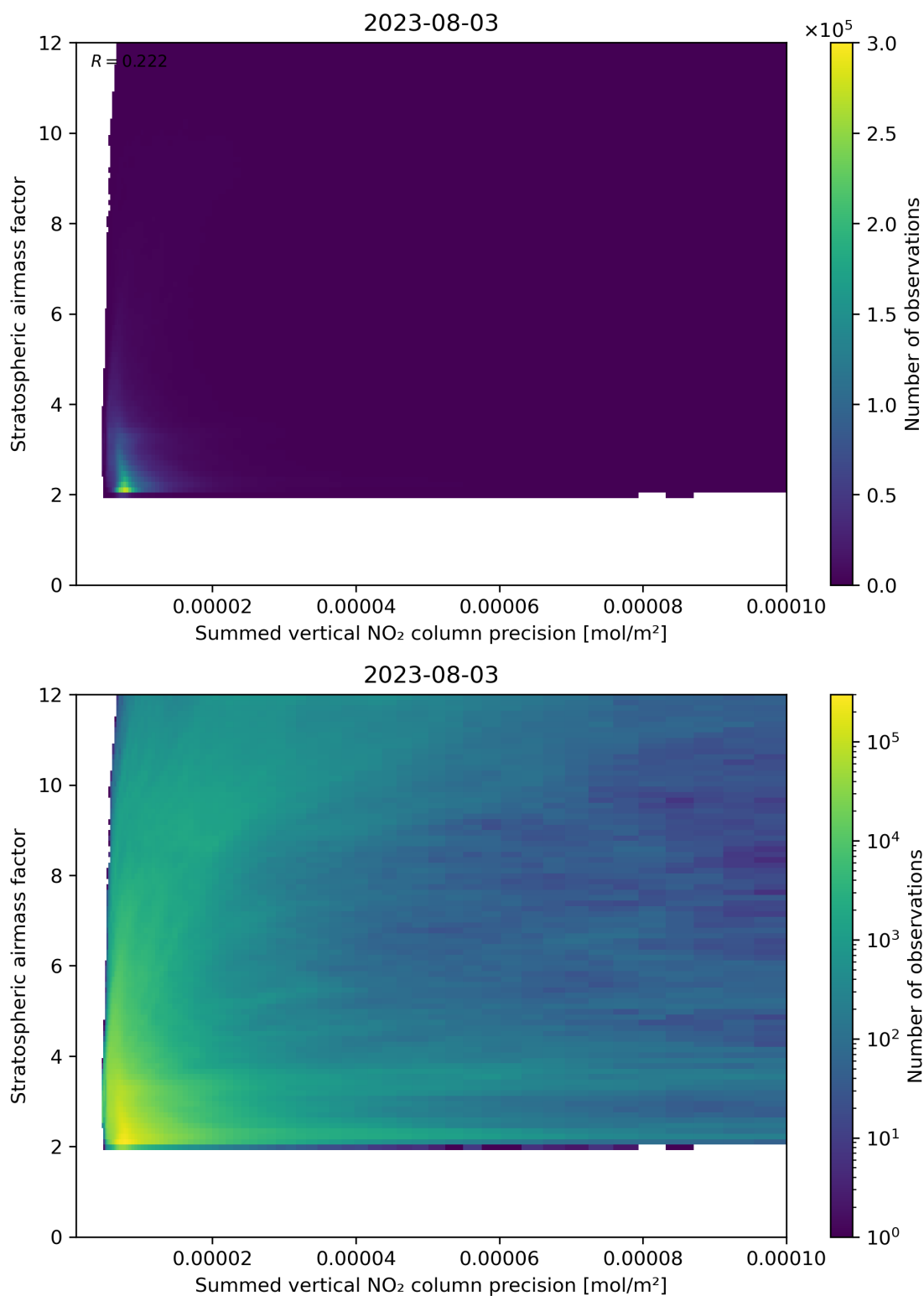
Figure 106: Scatter density plot of “Summed vertical NO 2 column precision” against “Stratospheric airmass factor” for 2023-08-02 to 2023-08-04.
