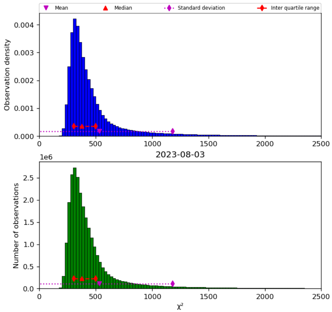
Figure 42: Histogram of “ \chi^2 ” for 2023-08-02 to 2023-08-04
