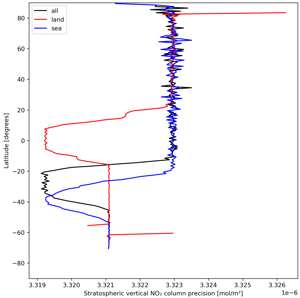
Figure 20: Zonal average of “Stratospheric vertical NO 2 column precision” for 2023-08-02 to 2023-08-04.
