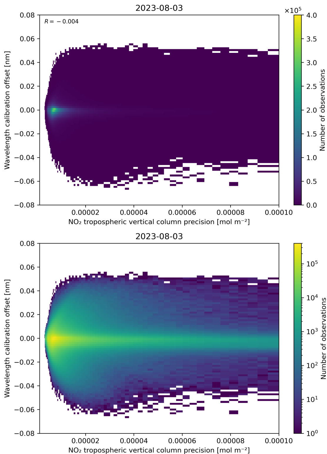
Figure 141: Scatter density plot of “NO 2 tropospheric vertical column precision” against “Wavelength calibration offset” for 2023-08-02 to 2023-08-04.
