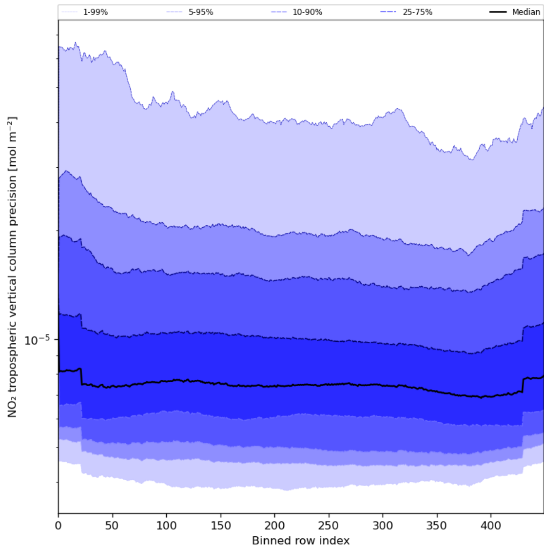
Figure 47: Along track statistics of “NO 2 tropospheric vertical column precision” for 2023-08-02 to 2023-08-04
