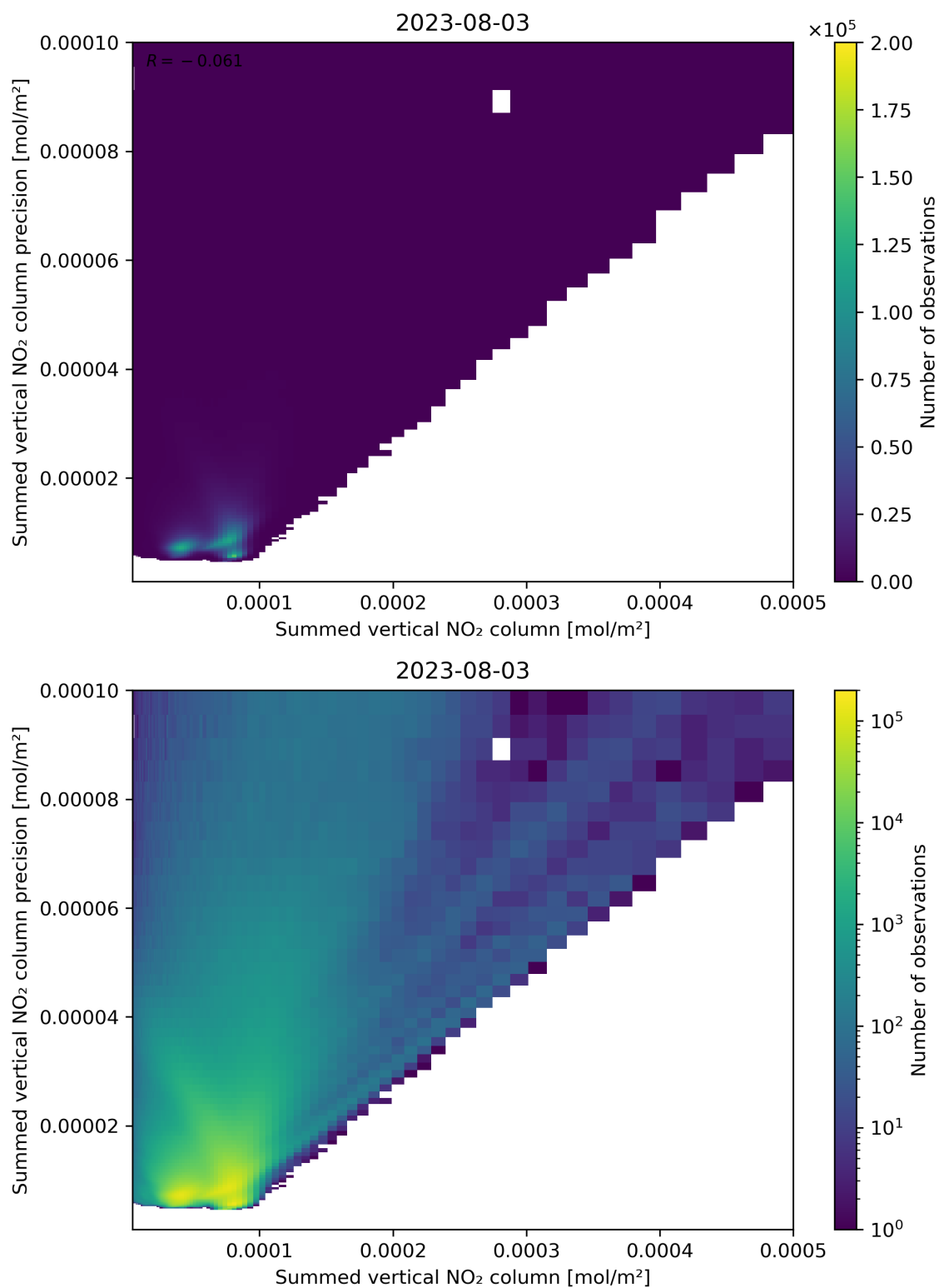
Figure 105: Scatter density plot of “Summed vertical NO 2 column” against “Summed vertical NO 2 column precision” for 2023-08-02 to 2023-08-04.
