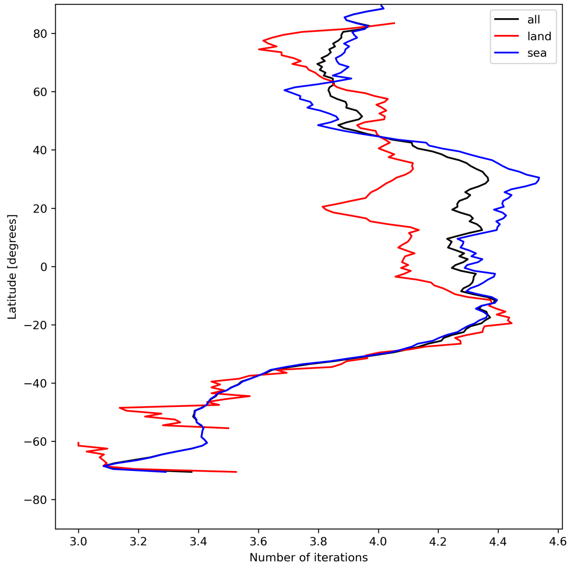
Figure 17: Zonal average of “Number of iterations” for 2023-08-02 to 2023-08-04.
