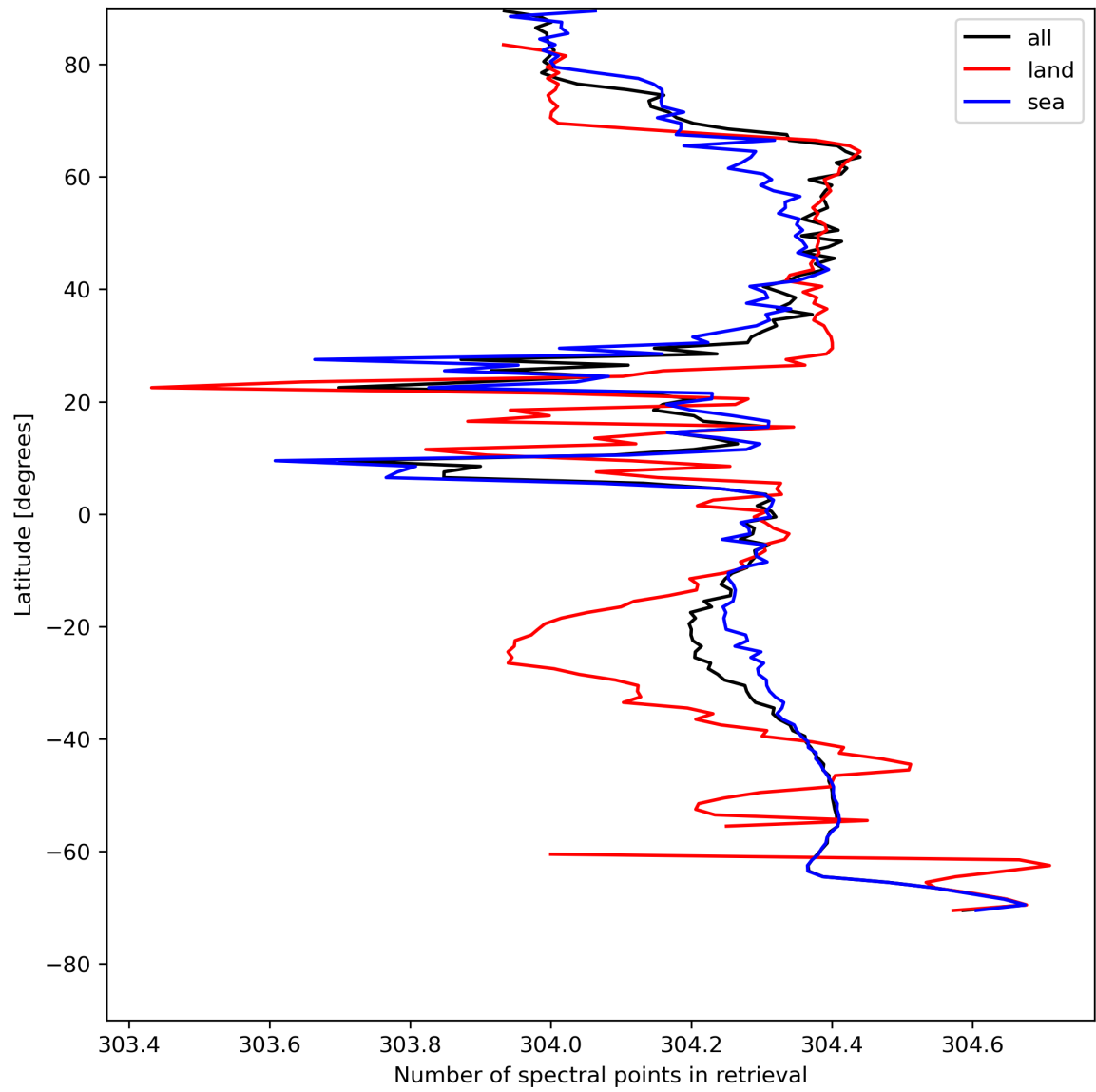
Figure 16: Zonal average of “Number of spectral points in retrieval” for 2023-08-02 to 2023-08-04.
