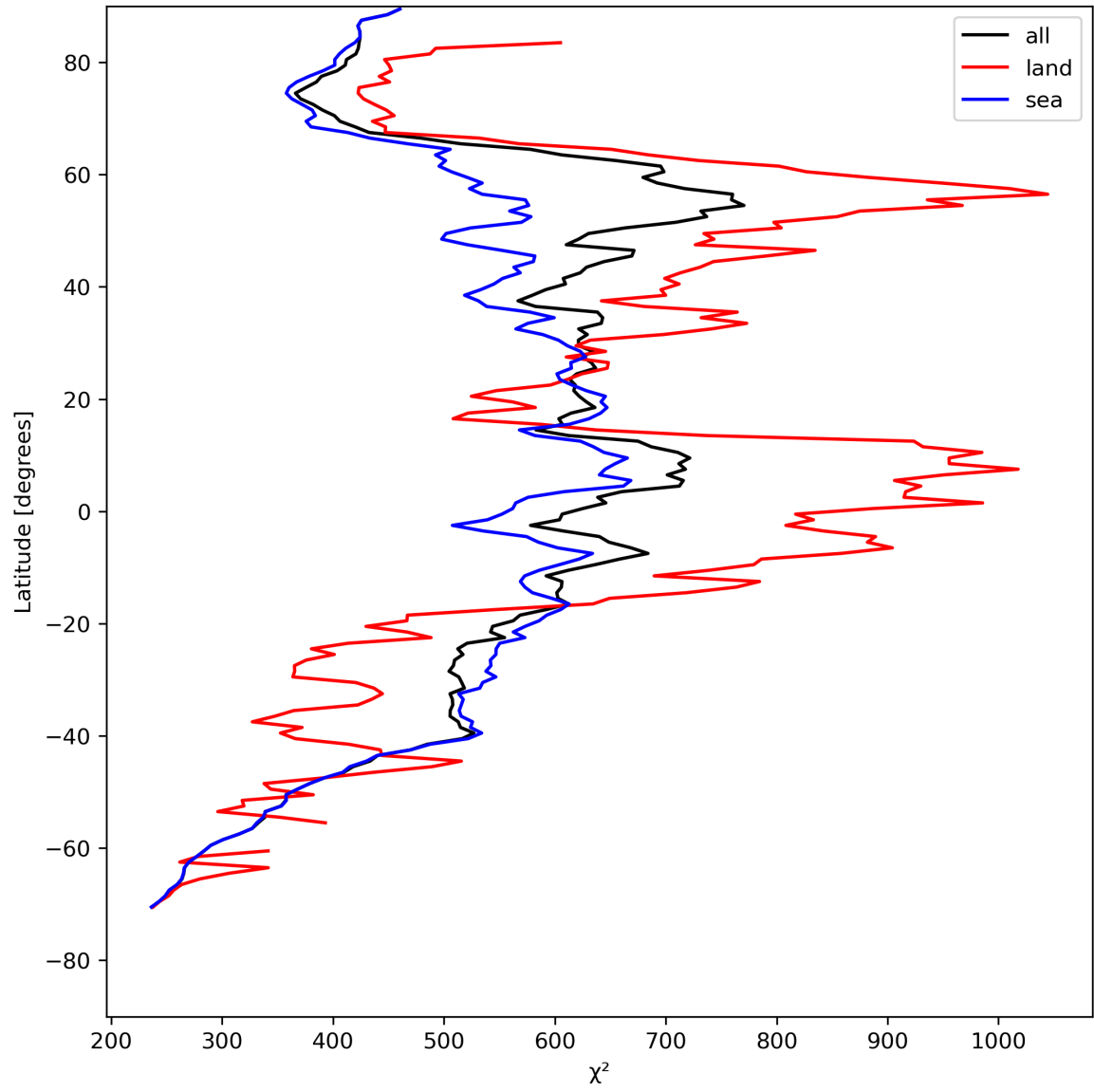
Figure 25: Zonal average of “ \chi^2 ” for 2023-08-02 to 2023-08-04.
