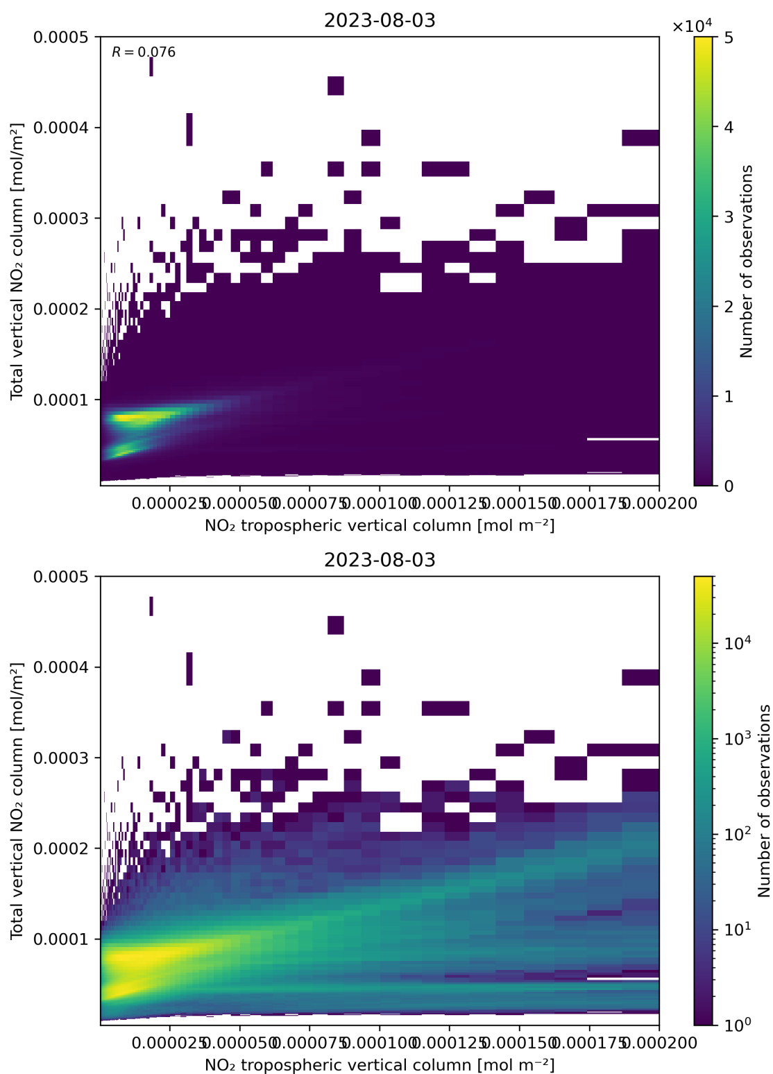
Figure 128: Scatter density plot of “NO 2 tropospheric vertical column” against “Total vertical NO 2 column” for 2023-08-02 to 2023-08-04.
