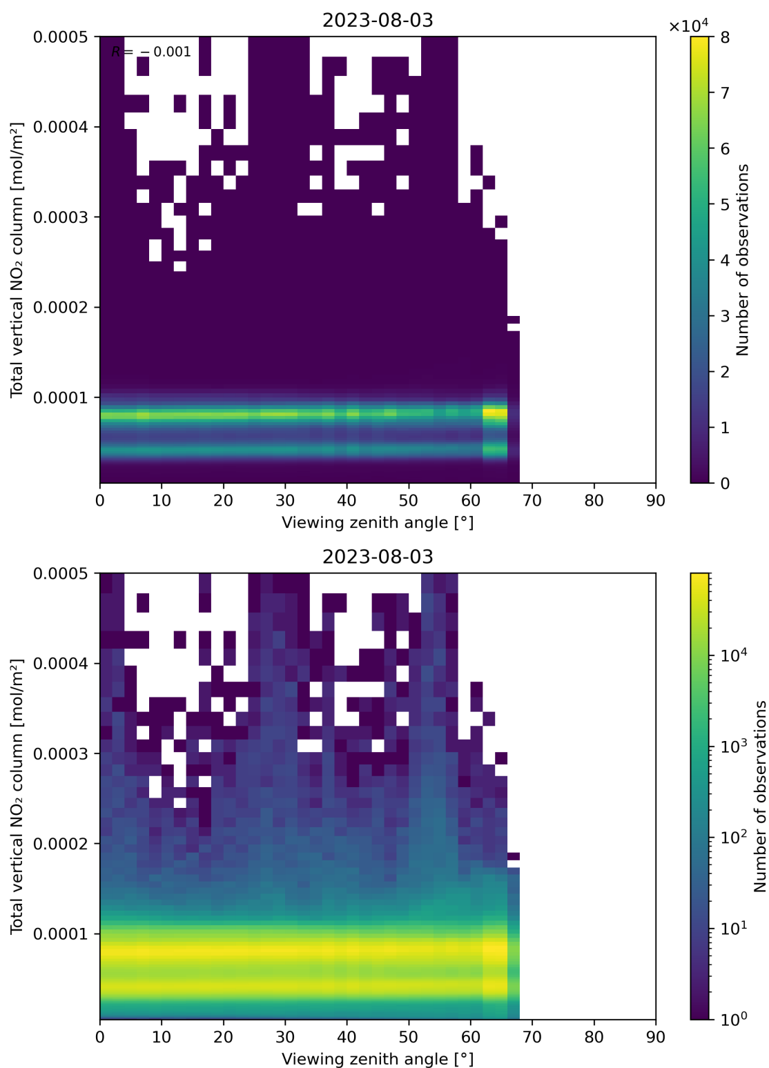
Figure 167: Scatter density plot of “Viewing zenith angle” against “Total vertical NO 2 column” for 2023-08-02 to 2023-08-04.
