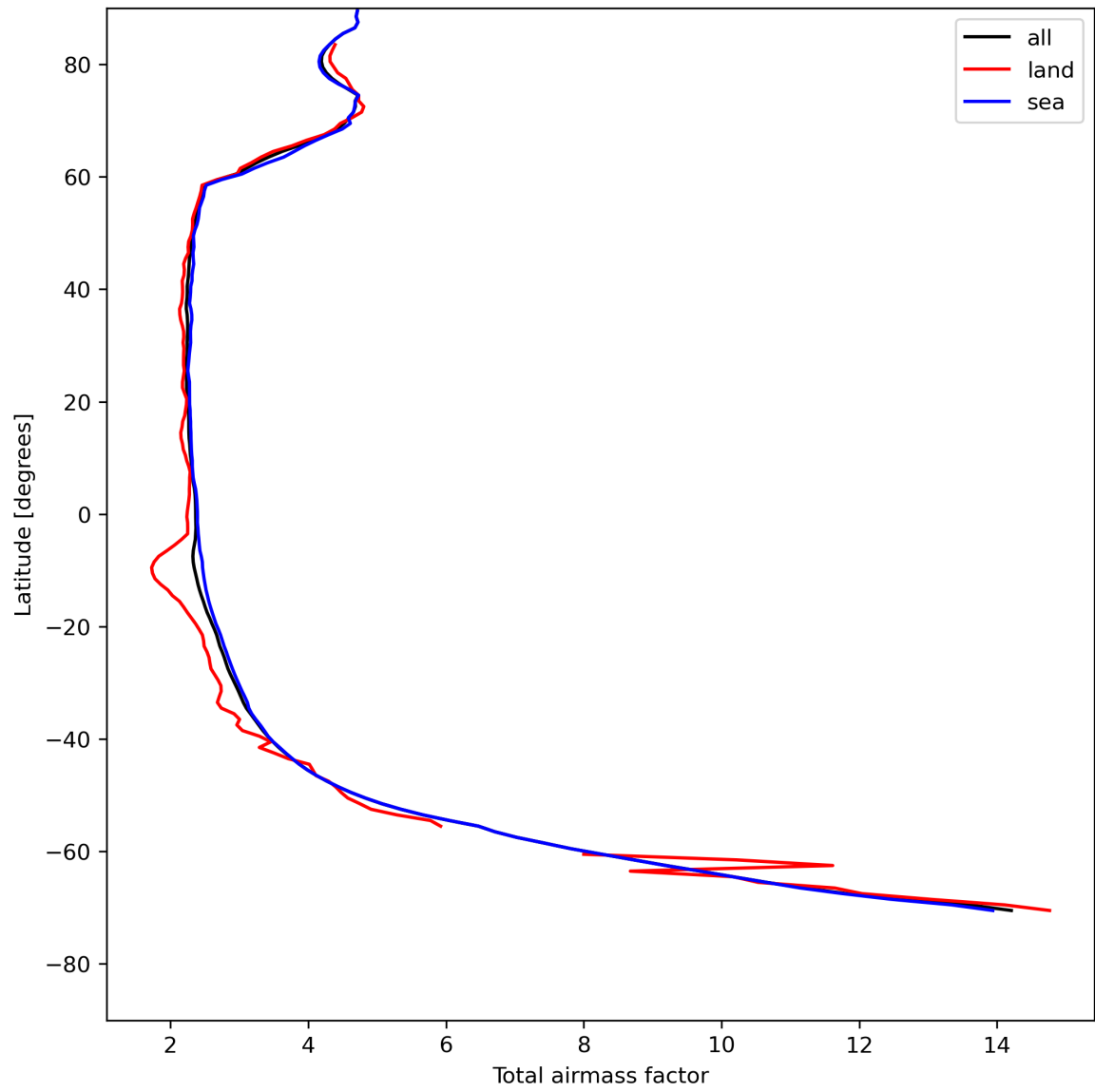
Figure 15: Zonal average of “Total airmass factor” for 2023-08-02 to 2023-08-04.
