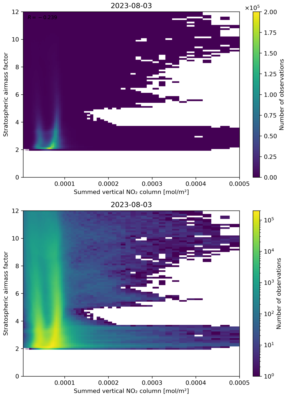
Figure 103: Scatter density plot of “Summed vertical NO 2 column” against “Stratospheric air mass factor” for 2023-08-02 to 2023-08-04.
