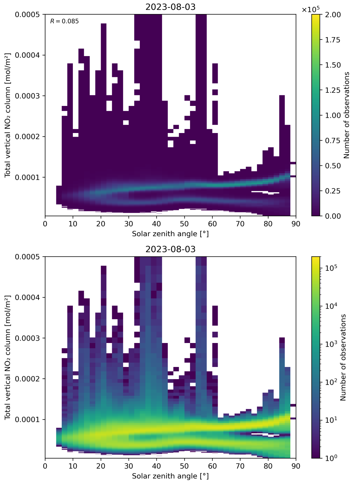
Figure 153: Scatter density plot of “Solar zenith angle” against “Total vertical NO 2 column” for 2023-08-02 to 2023-08-04.
