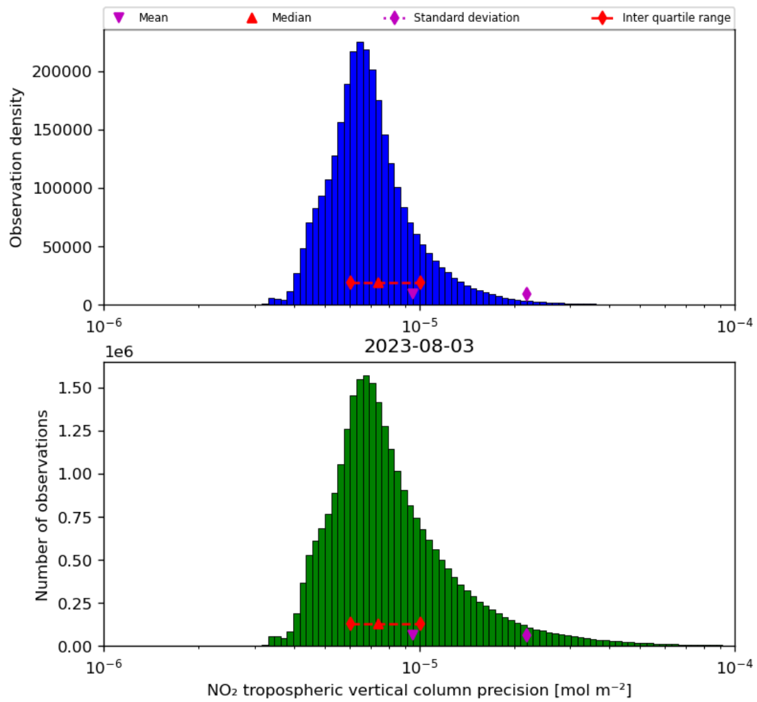
Figure 30: Histogram of “NO 2 tropospheric vertical column precision” for 2023-08-02 to 2023-08-04
