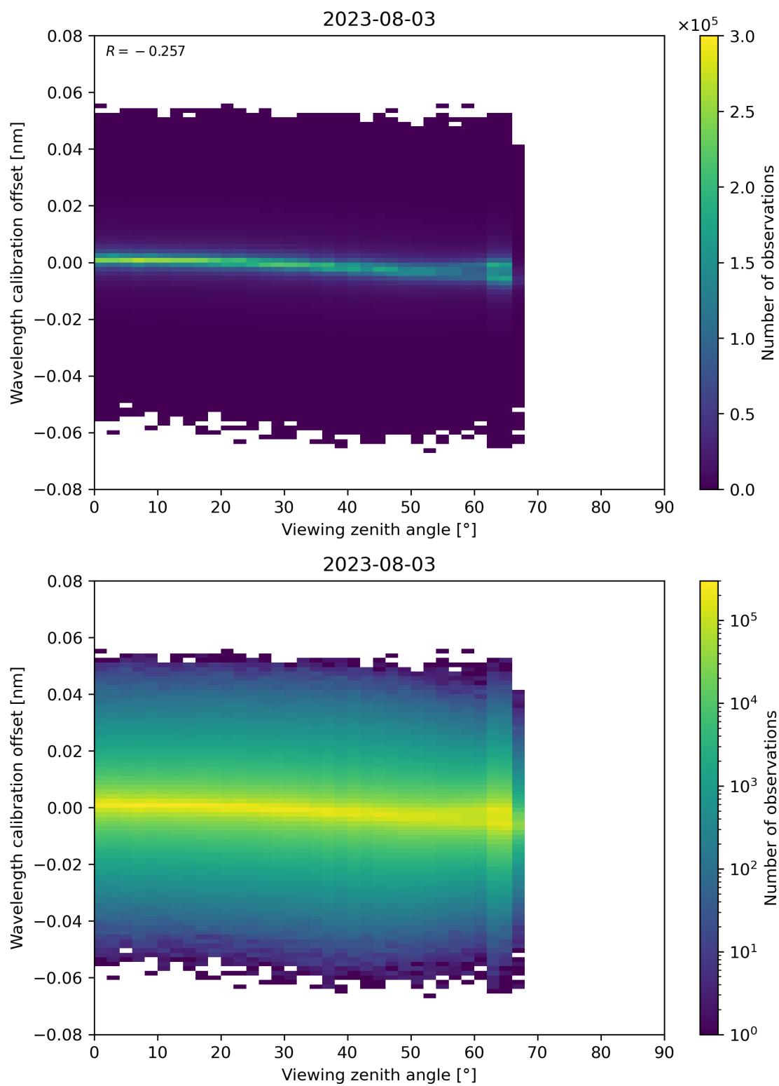
Figure 173: Scatter density plot of “Viewing zenith angle” against “Wavelength calibration offset” for 2023-08-02 to 2023-08-04.
