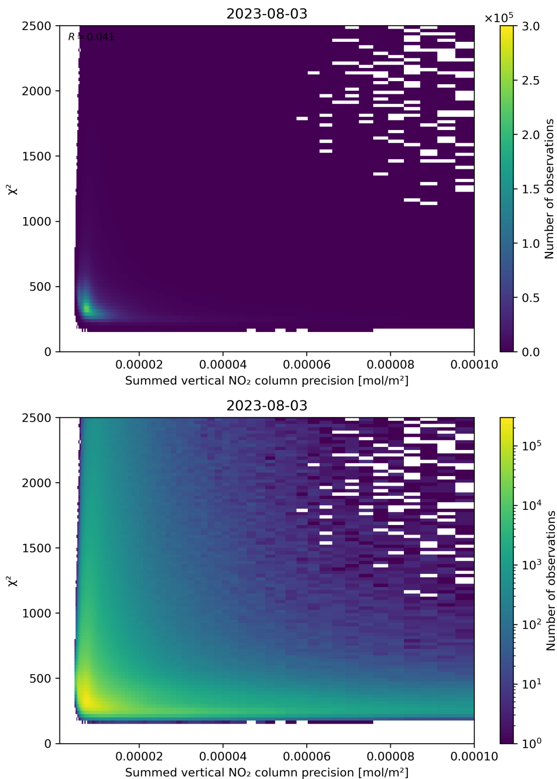
Figure 107: Scatter density plot of “Summed vertical NO 2 column precision” against “ \chi^2 ” for 2023-08-02 to 2023-08-04.
