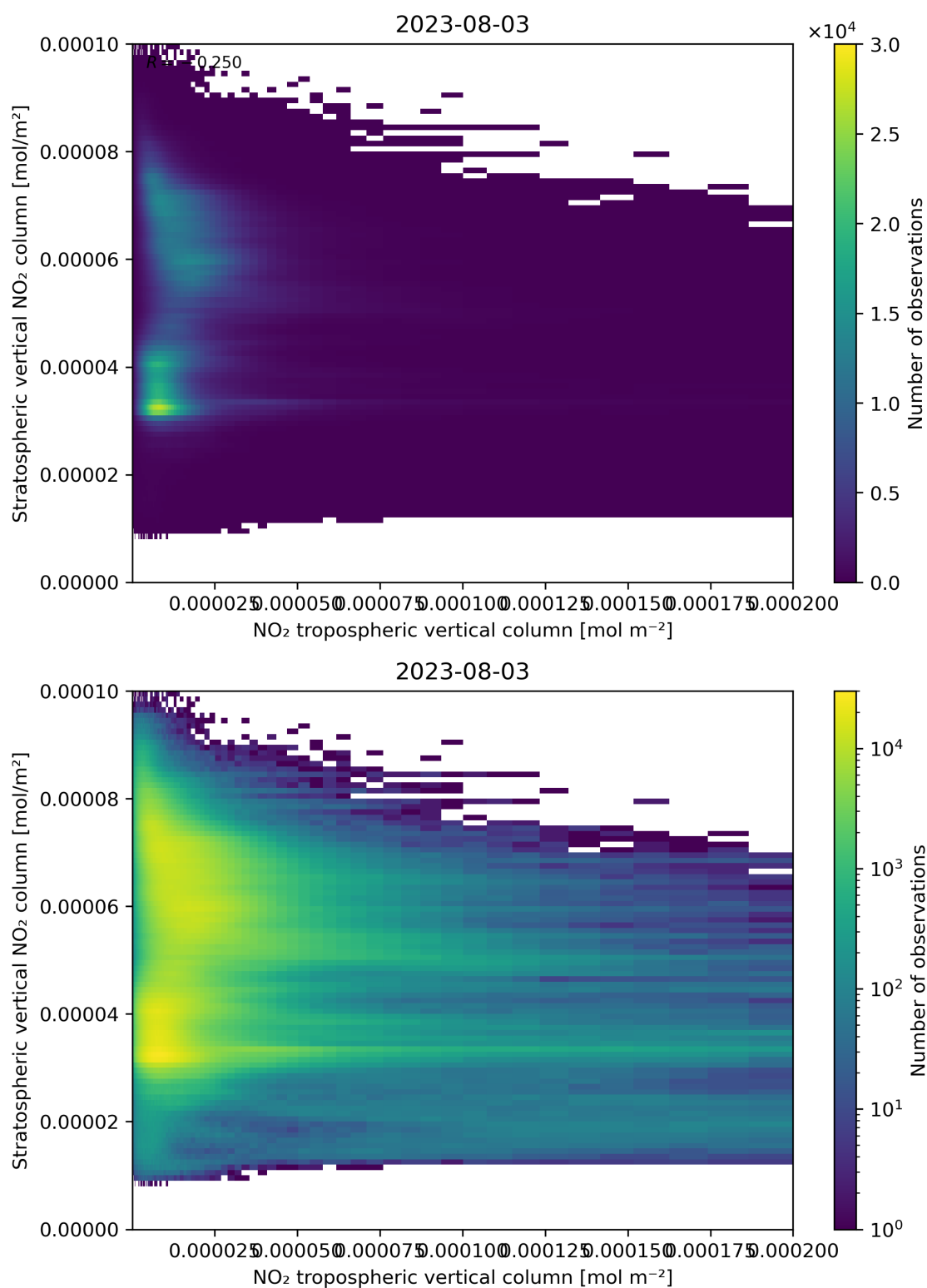
Figure 125: Scatter density plot of “NO 2 tropospheric vertical column” against “Stratospheric vertical NO 2 column” for 2023-08-02 to 2023-08-04.
