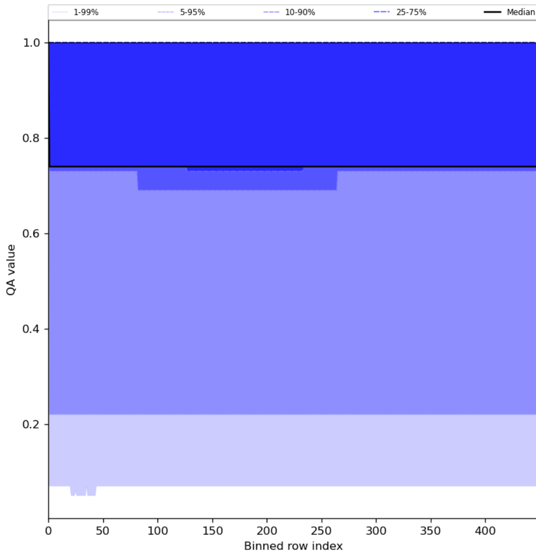
Figure 45: Along track statistics of “QA value” for 2023-08-02 to 2023-08-04
