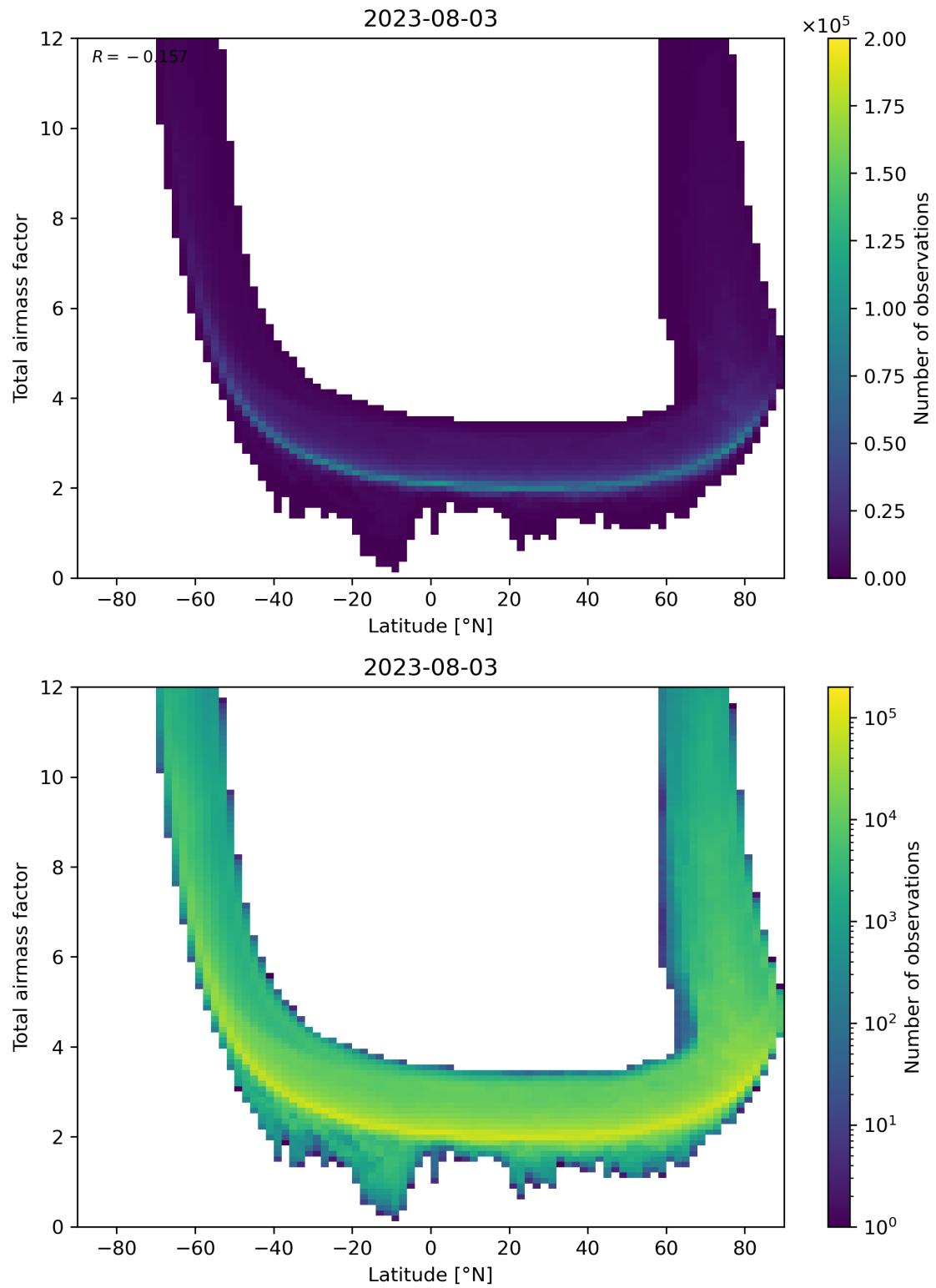
Figure 84: Scatter density plot of “Latitude” against “Total airmass factor” for 2023-08-02 to 2023-08-04.
