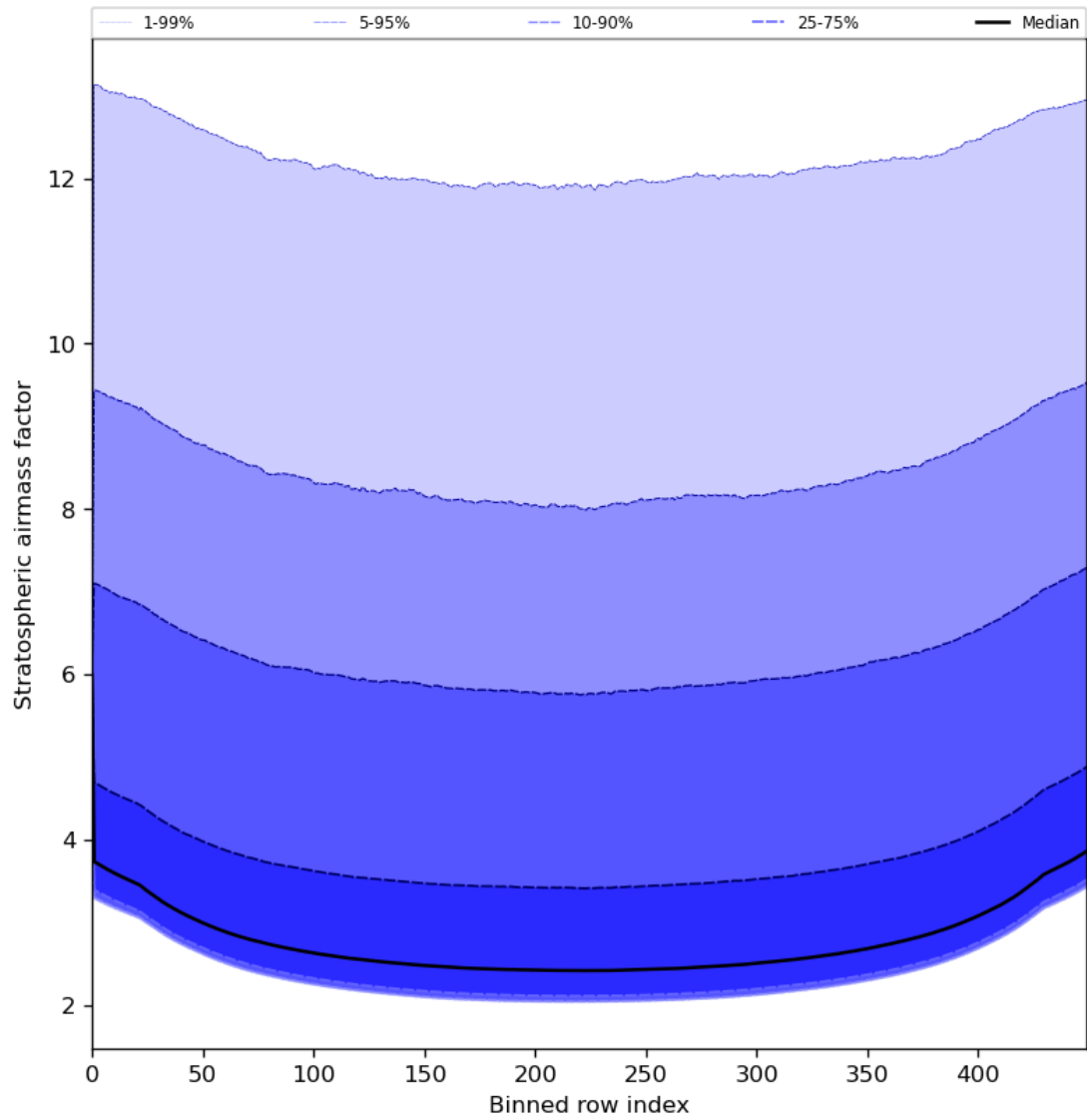
Figure 61: Along track statistics of “Stratospheric airmass factor” for 2023-08-02 to 2023-08-04
