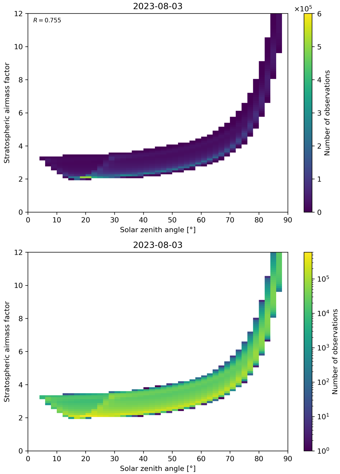
Figure 145: Scatter density plot of “Solar zenith angle” against “Stratospheric airmass factor” for 2023-08-02 to 2023-08-04.
