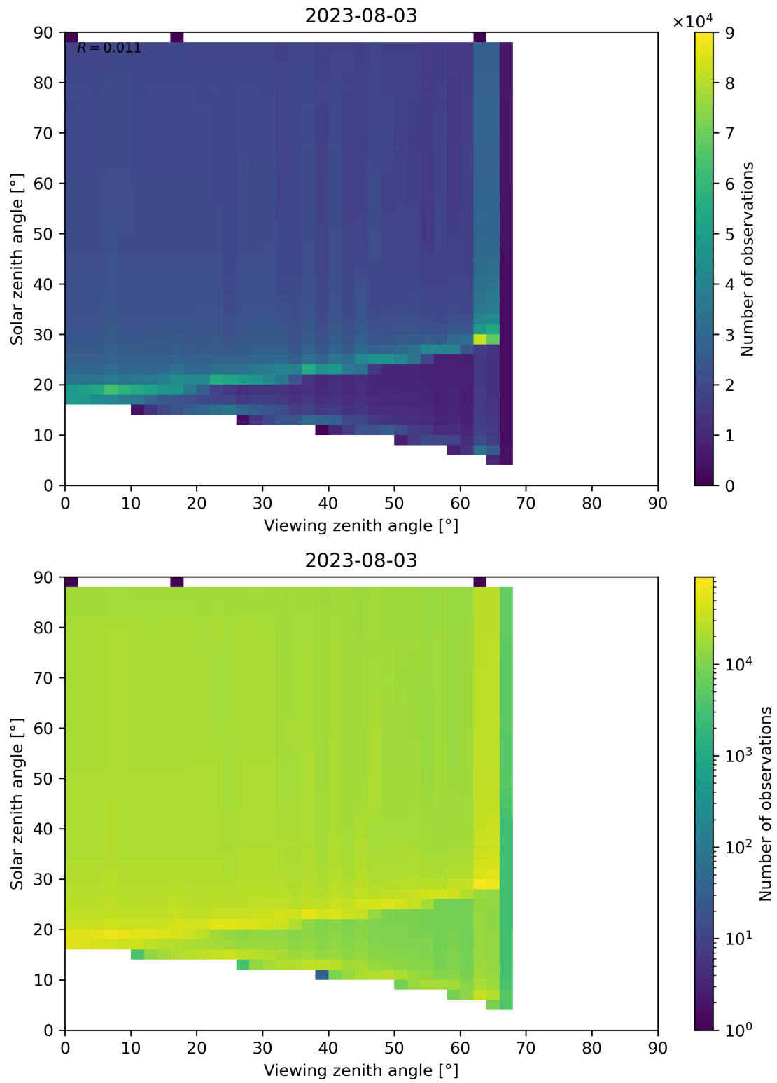
Figure 172: Scatter density plot of “Viewing zenith angle” against “Solar zenith angle” for 2023-08-02 to 2023-08-04.
