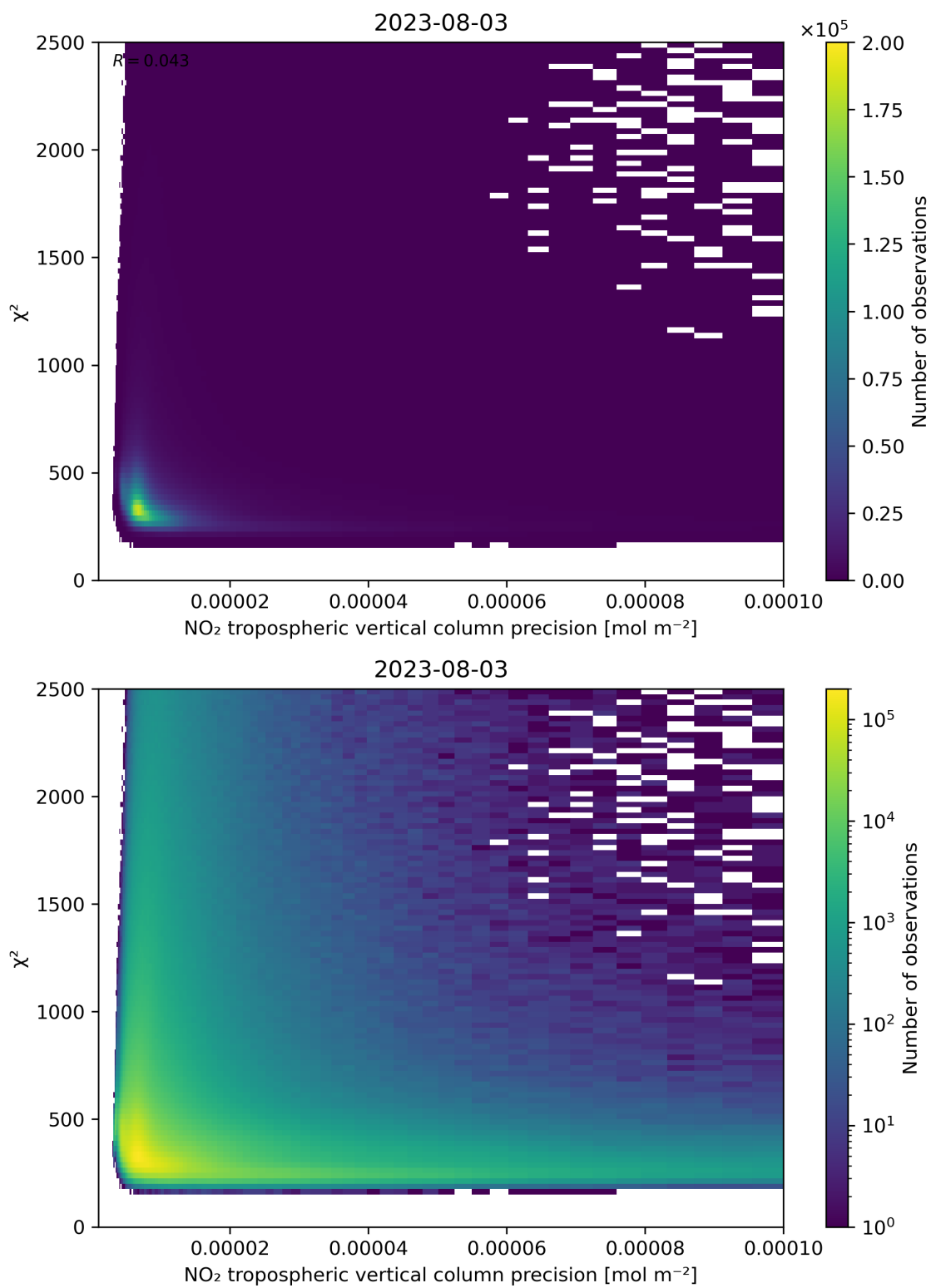
Figure 134: Scatter density plot of “NO 2 tropospheric vertical column precision” against “ \chi^2 ” for 2023-08-02 to 2023-08-04.
