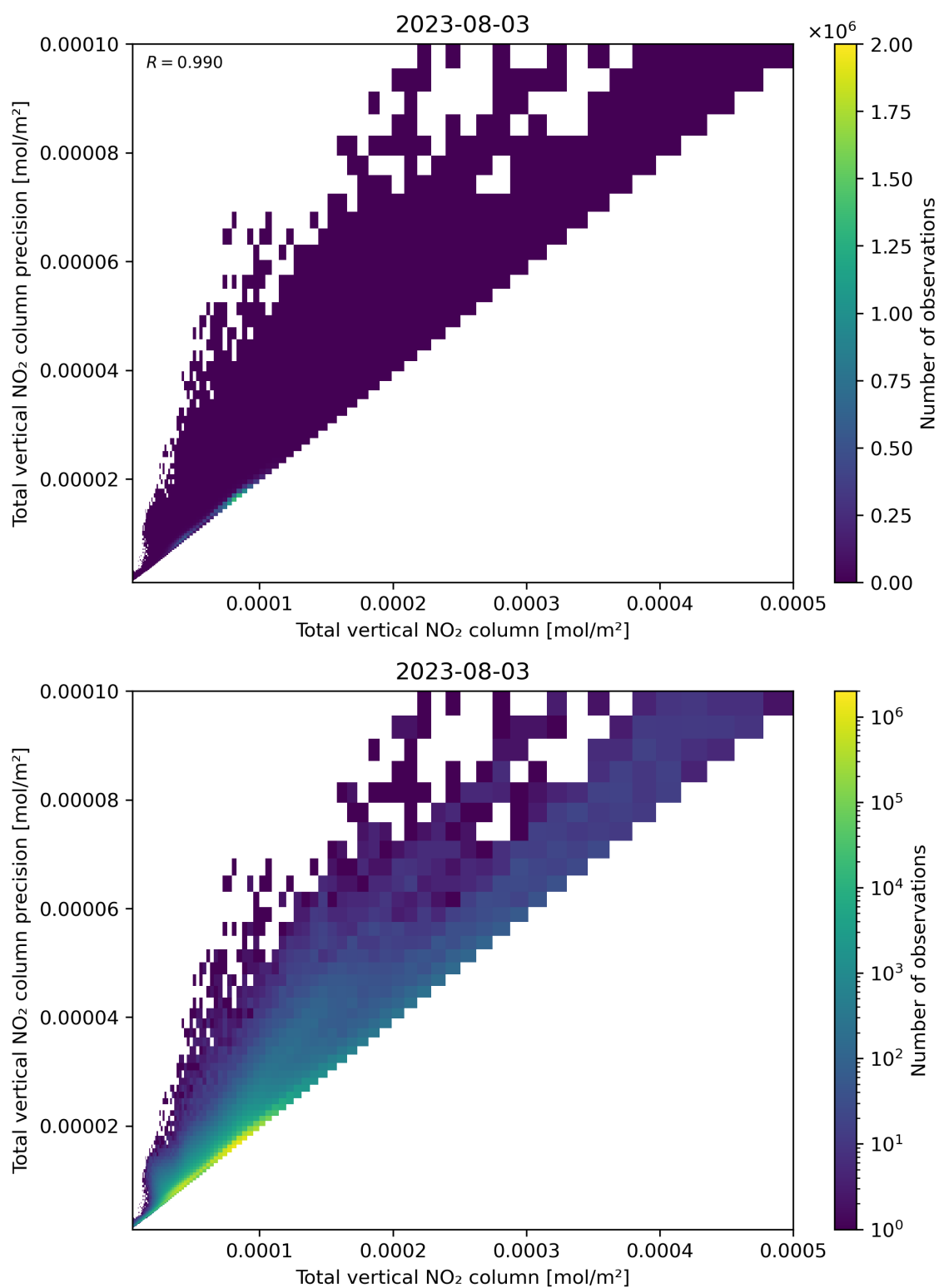
Figure 114: Scatter density plot of “Total vertical NO 2 column” against “Total vertical NO 2 column precision” for 2023-08-02 to 2023-08-04.
