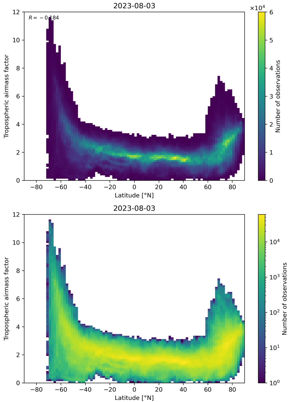
Figure 85: Scatter density plot of “Latitude” against “Tropospheric airmass factor” for 2023-08-02 to 2023-08-04.
