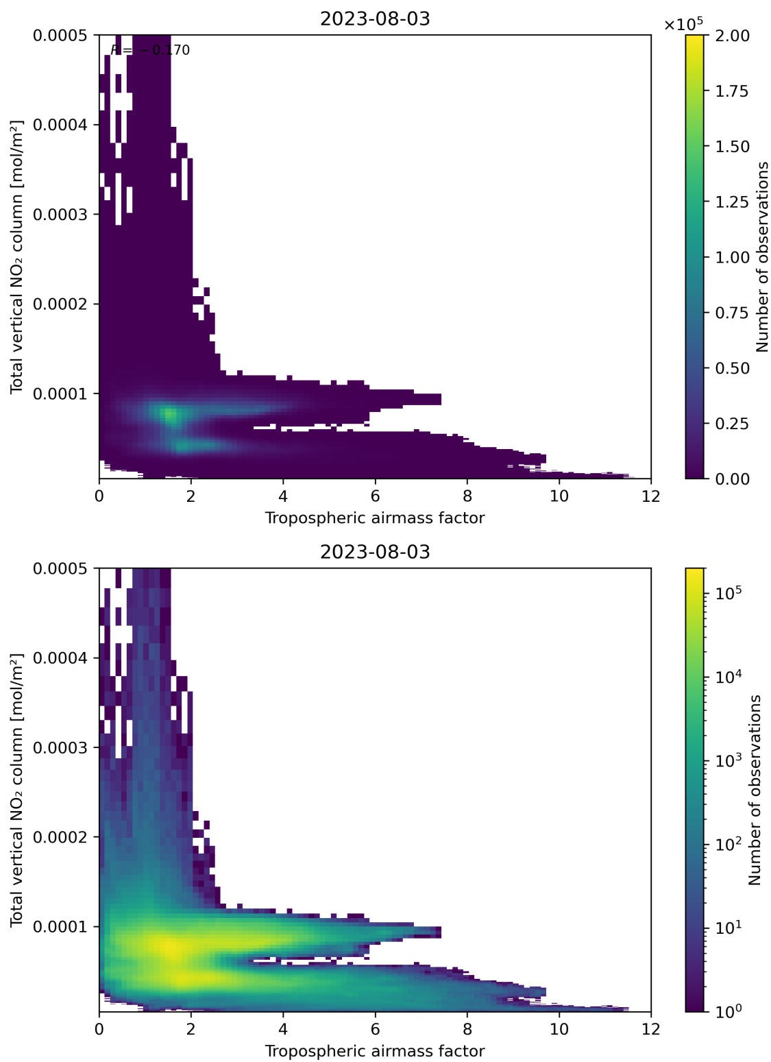
Figure 77: Scatter density plot of “Tropospheric airmass factor” against “Total vertical NO 2 column” for 2023-08-02 to 2023-08-04.
