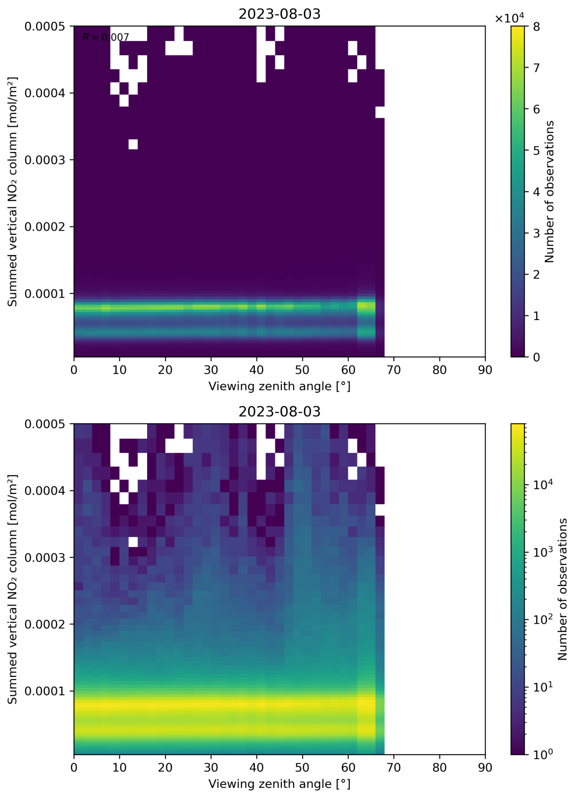
Figure 165: Scatter density plot of “Viewing zenith angle” against “Summed vertical NO 2 column” for 2023-08-02 to 2023-08-04.
