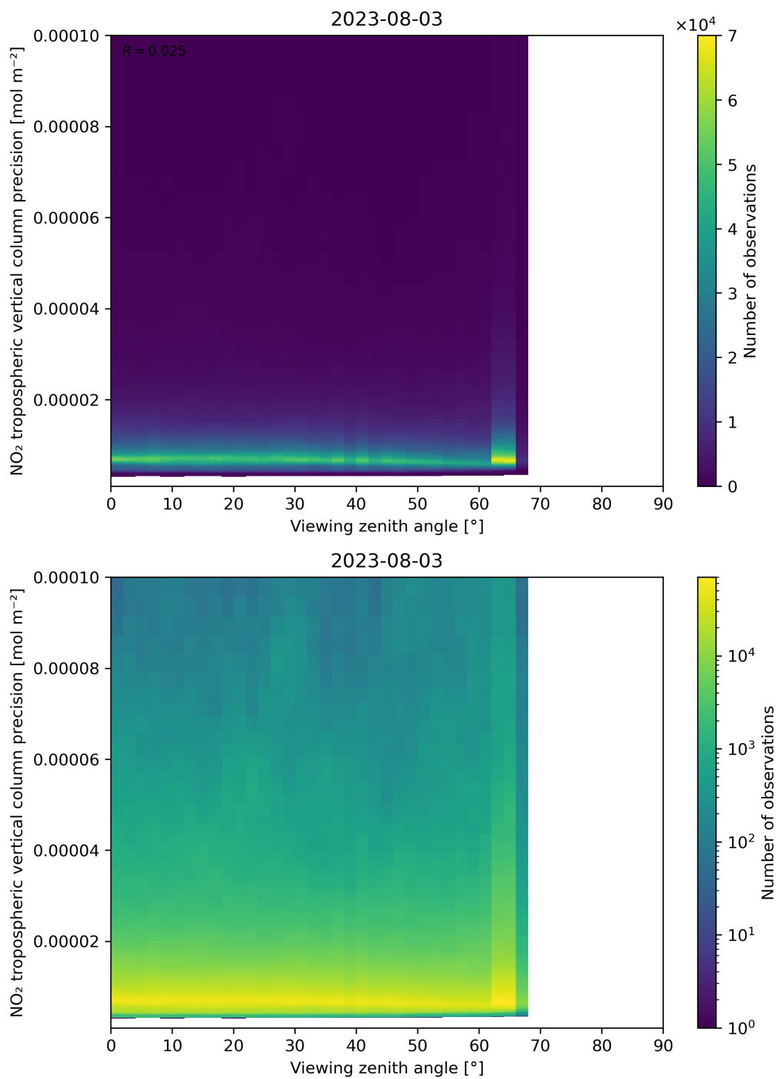
Figure 170: Scatter density plot of “Viewing zenith angle” against “NO 2 tropospheric vertical column precision” for 2023-08-02 to 2023-08-04.
