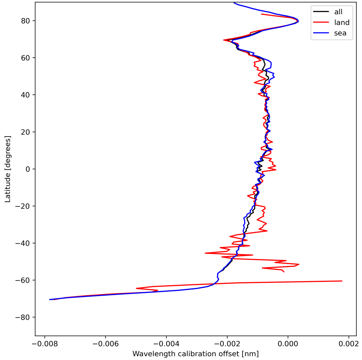
Figure 18: Zonal average of “Wavelength calibration offset” for 2023-08-02 to 2023-08-04.
