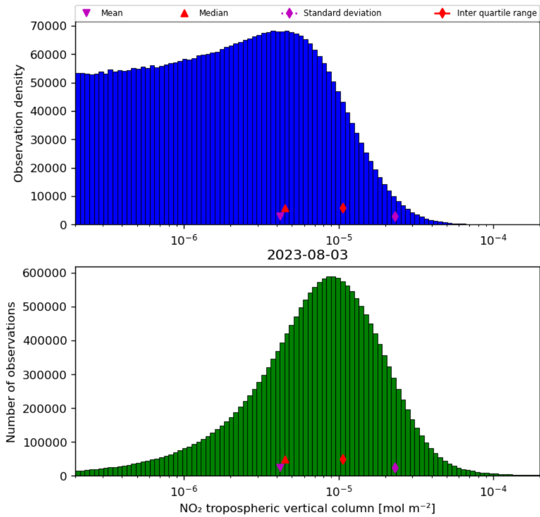
Figure 29: Histogram of “NO 2 tropospheric vertical column” for 2023-08-02 to 2023-08-04
