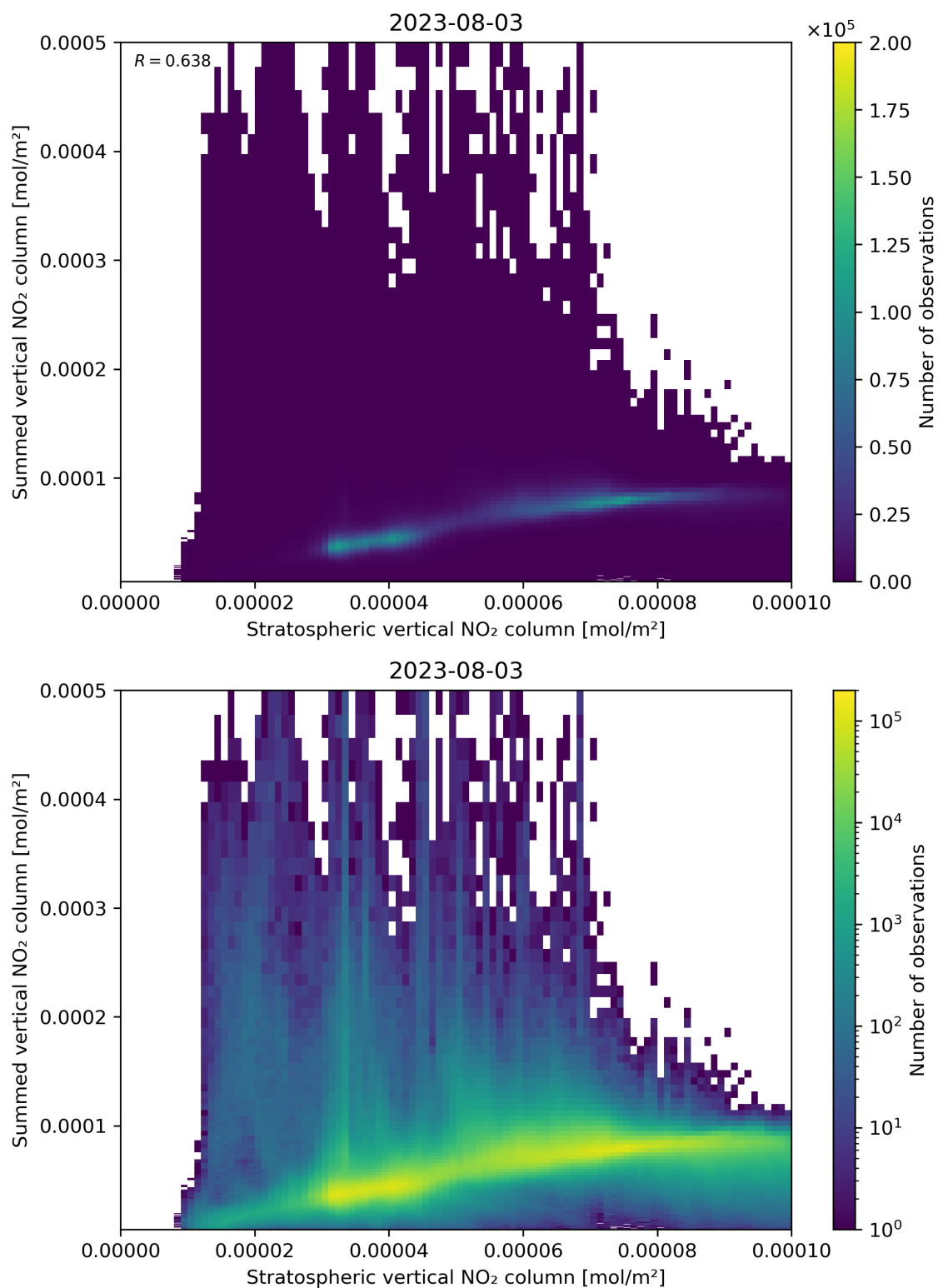
Figure 98: Scatter density plot of “Stratospheric vertical NO 2 column” against “Summed vertical NO 2 column” for 2023-08-02 to 2023-08-04.
