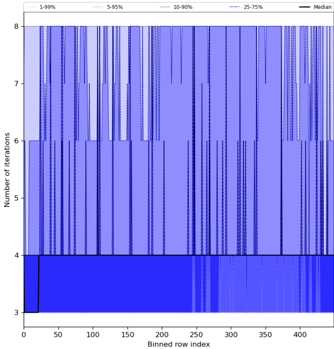
Figure 51: Along track statistics of “Number of iterations” for 2023-08-02 to 2023-08-04
