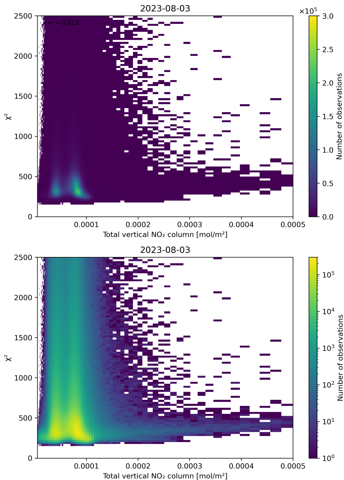
Figure 111: Scatter density plot of “Total vertical NO 2 column” against “ \chi^2 ” for 2023-08-02 to 2023-08-04.
