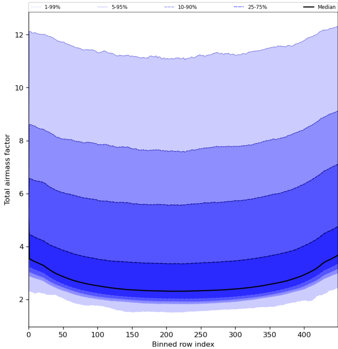
Figure 49: Along track statistics of “Total airmass factor” for 2023-08-02 to 2023-08-04
