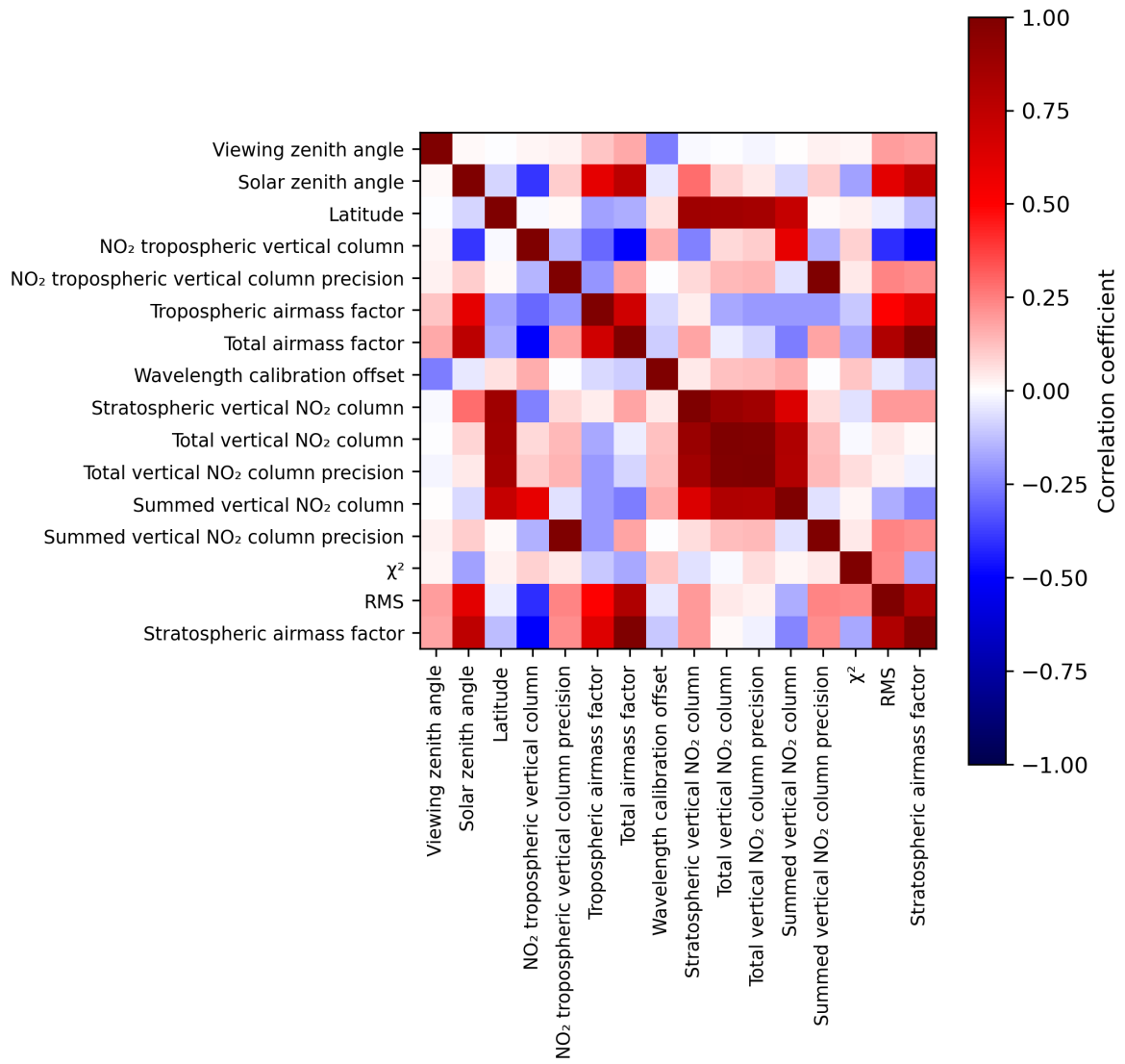
Figure 2: Map of correlation matrix for 2023-08-02 to 2023-08-04.
