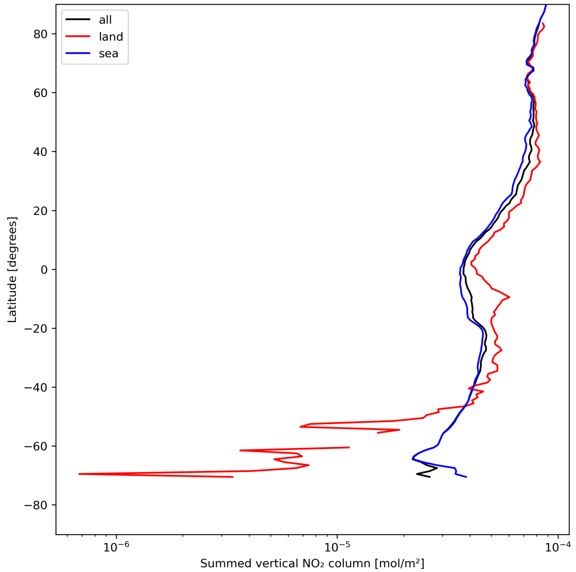
Figure 23: Zonal average of “Summed vertical NO 2 column” for 2023-08-02 to 2023-08-04.
