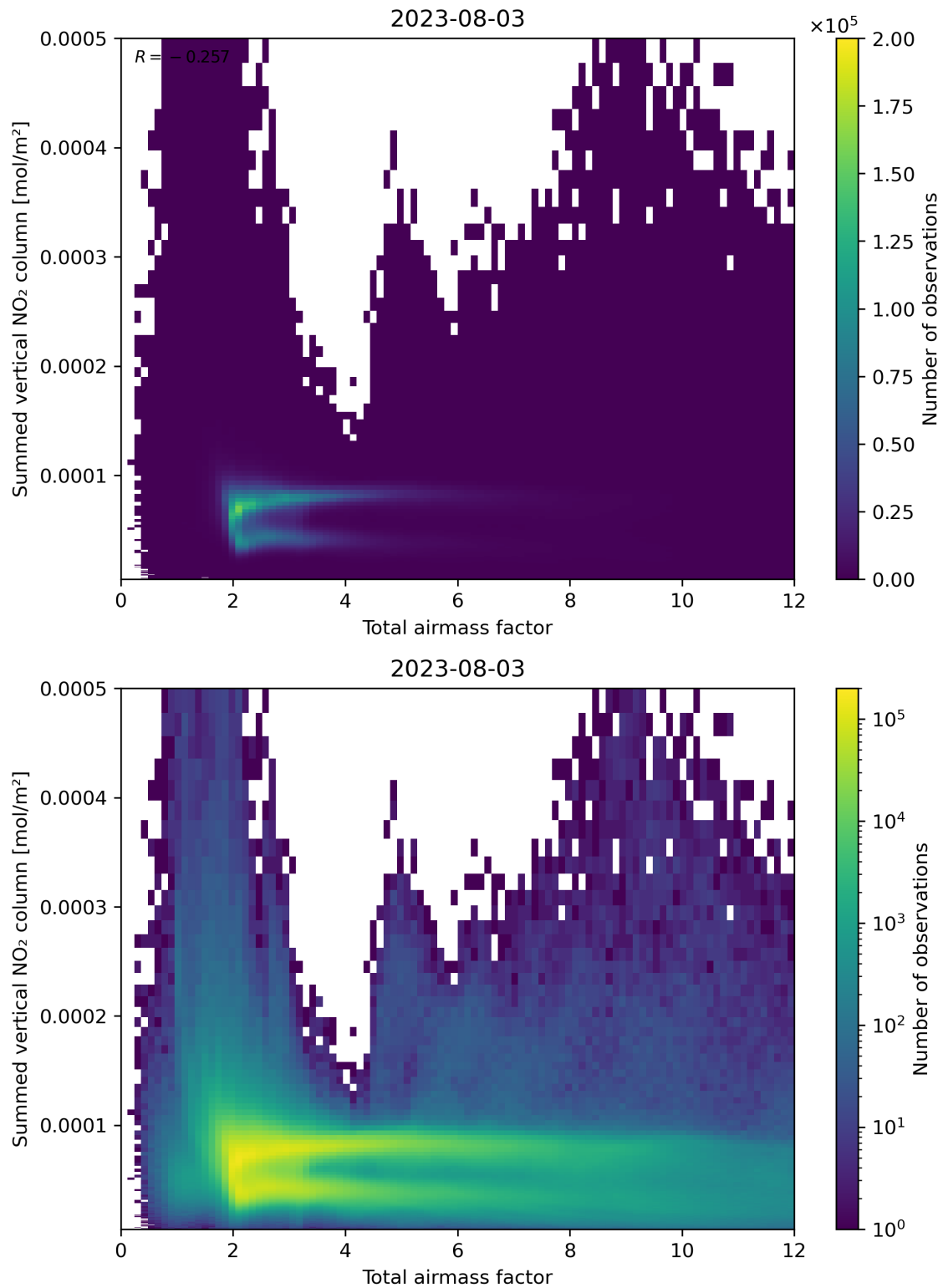
Figure 65: Scatter density plot of “Total airmass factor” against “Summed vertical NO 2 column” for 2023-08-02 to 2023-08-04.
