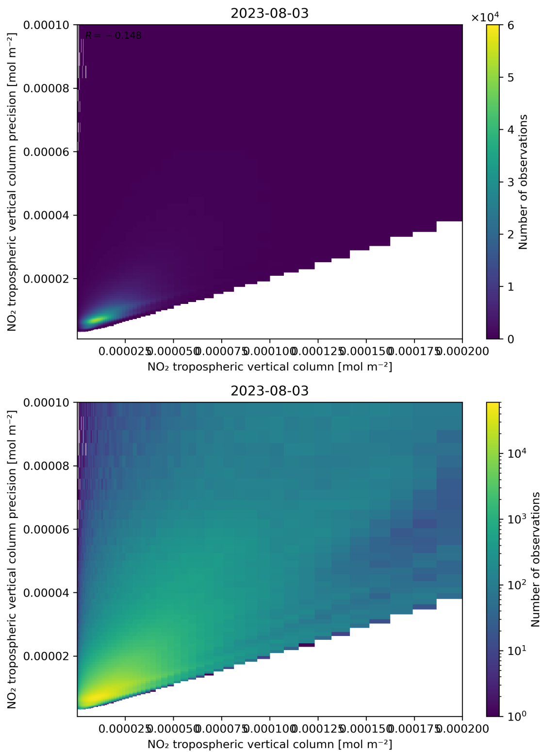
Figure 130: Scatter density plot of “NO 2 tropospheric vertical column” against “NO 2 tropospheric vertical column precision” for 2023-08-02 to 2023-08-04.
