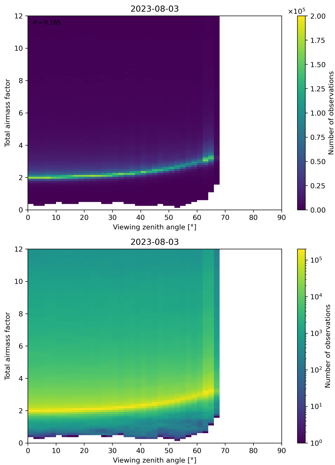
Figure 160: Scatter density plot of “Viewing zenith angle” against “Total airmass factor” for 2023-08-02 to 2023-08-04.
