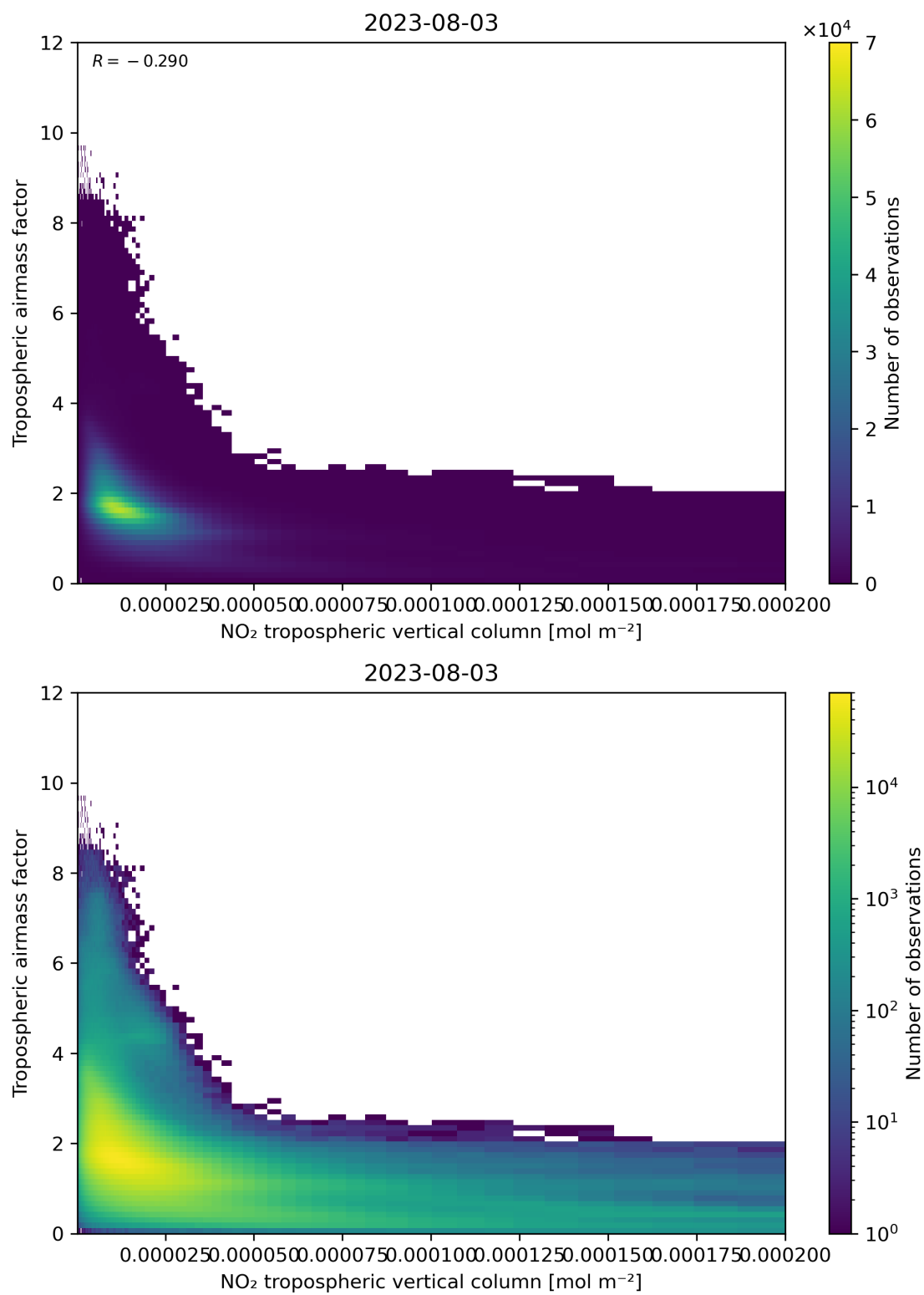
Figure 123: Scatter density plot of “NO 2 tropospheric vertical column” against “Tropospheric air mass factor” for 2023-08-02 to 2023-08-04.
