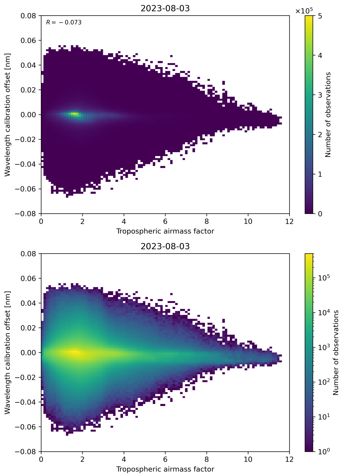
Figure 80: Scatter density plot of “Tropospheric airmass factor” against “Wavelength calibration offset” for 2023-08-02 to 2023-08-04.
