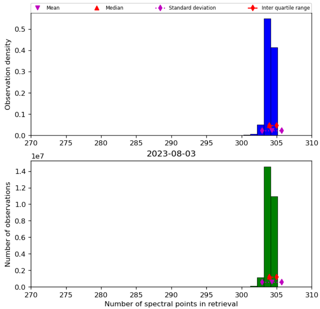
Figure 33: Histogram of “Number of spectral points in retrieval” for 2023-08-02 to 2023-08-04
