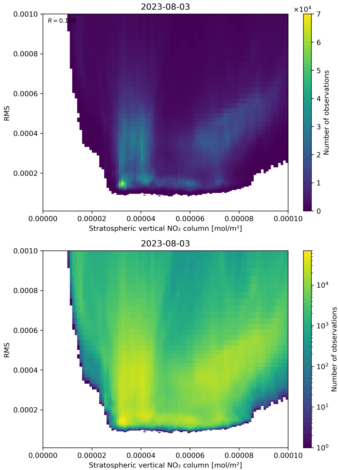
Figure 102: Scatter density plot of “Stratospheric vertical NO 2 column” against “RMS” for 2023-08-02 to 2023-08-04.
