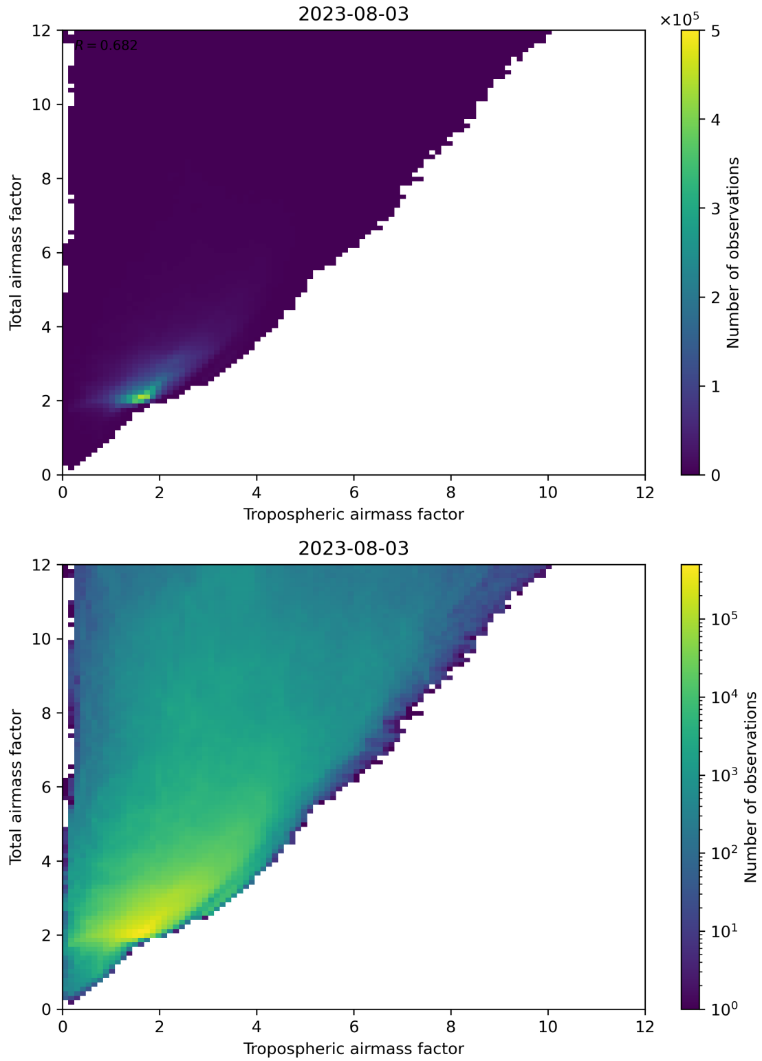
Figure 72: Scatter density plot of “Tropospheric airmass factor” against “Total airmass factor” for 2023-08-02 to 2023-08-04.
