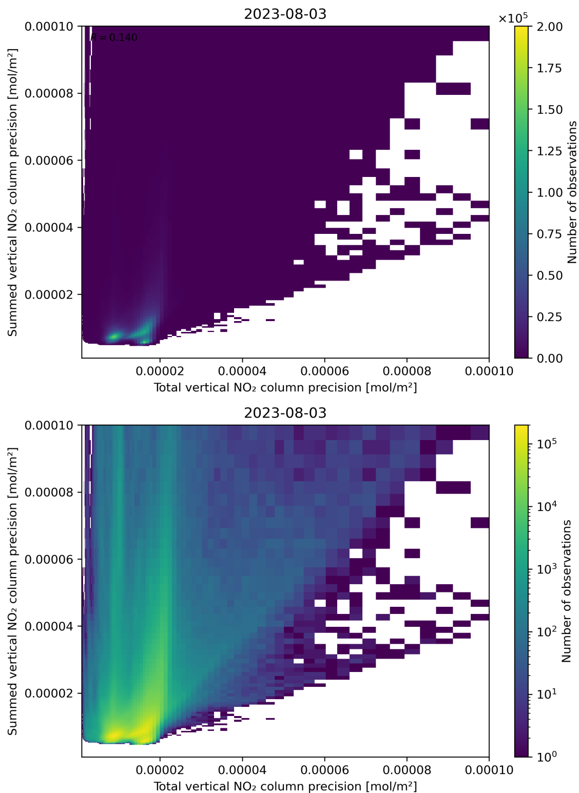
Figure 118: Scatter density plot of “Total vertical NO 2 column precision” against “Summed vertical NO 2 column precision” for 2023-08-02 to 2023-08-04.
