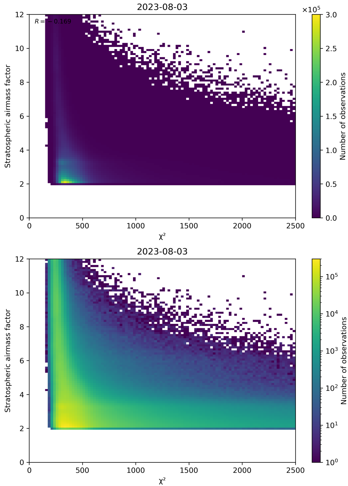
Figure 81: Scatter density plot of “ \chi^2 ” against “Stratospheric airmass factor” for 2023-08-02 to 2023-08-04.
