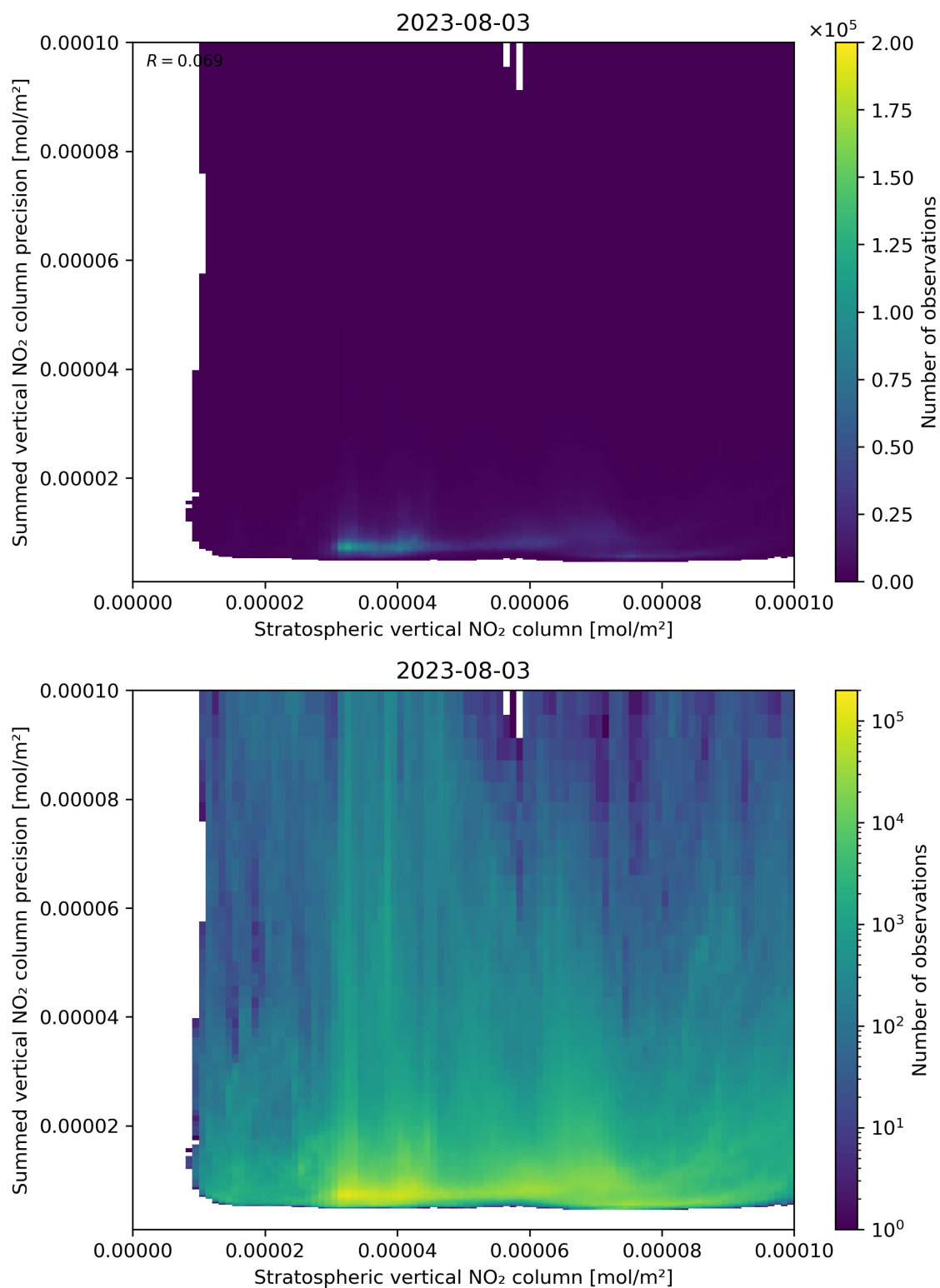
Figure 99: Scatter density plot of “Stratospheric vertical NO 2 column” against “Summed vertical NO 2 column precision” for 2023-08-02 to 2023-08-04.
