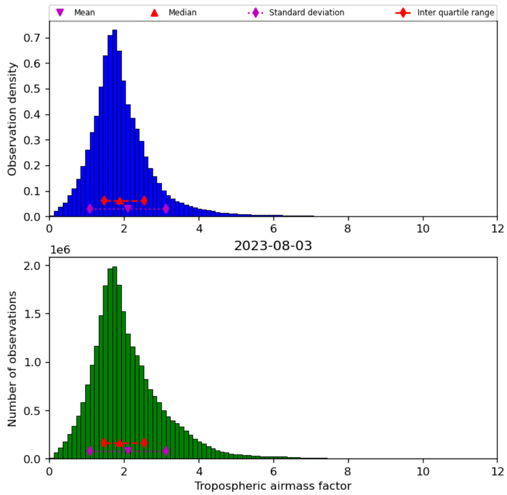
Figure 31: Histogram of “Tropospheric airmass factor” for 2023-08-02 to 2023-08-04
