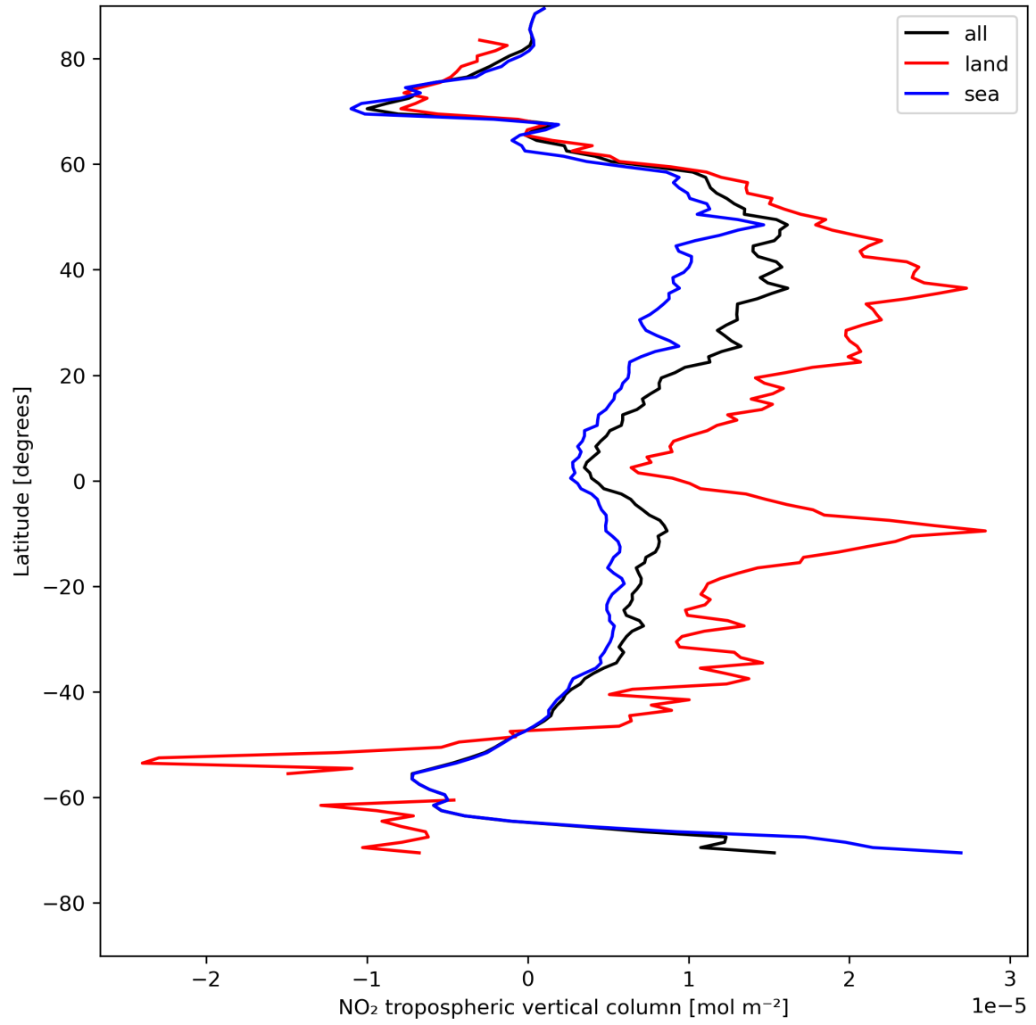
Figure 12: Zonal average of “NO 2 tropospheric vertical column” for 2023-08-02 to 2023-08-04.
