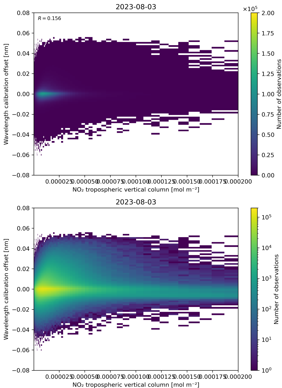
Figure 143: Scatter density plot of “NO 2 tropospheric vertical column” against “Wavelength calibration offset” for 2023-08-02 to 2023-08-04.
