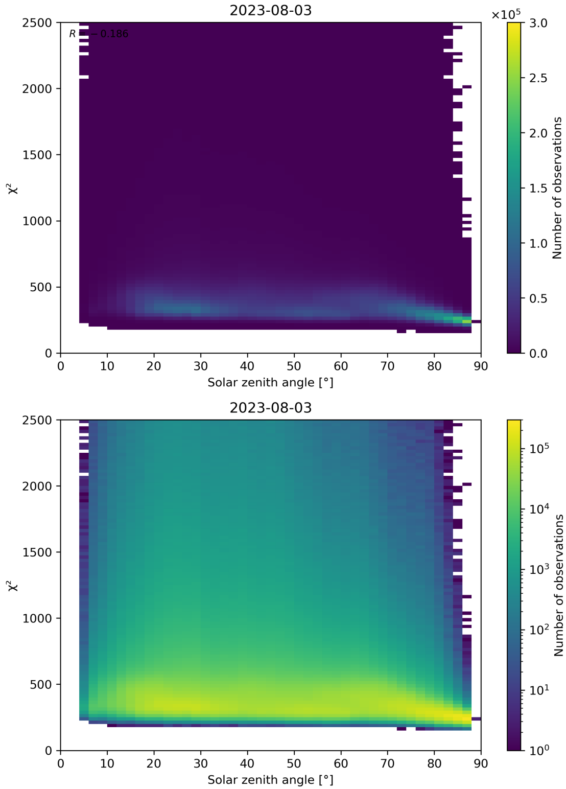
Figure 148: Scatter density plot of “Solar zenith angle” against “ \chi^2 ” for 2023-08-02 to 2023-08-04.
