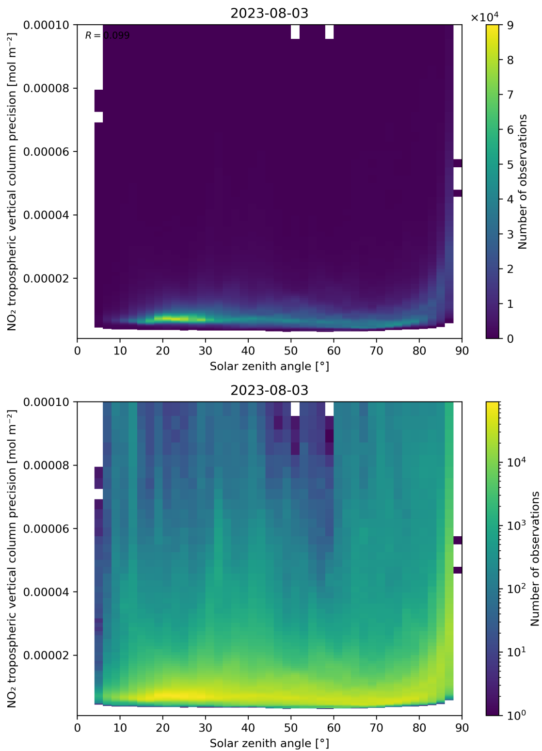
Figure 156: Scatter density plot of “Solar zenith angle” against “NO 2 tropospheric vertical column precision” for 2023-08-02 to 2023-08-04.
