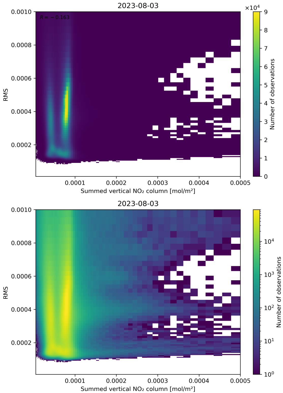
Figure 109: Scatter density plot of “Summed vertical NO 2 column” against “RMS” for 2023-08-02 to 2023-08-04.
