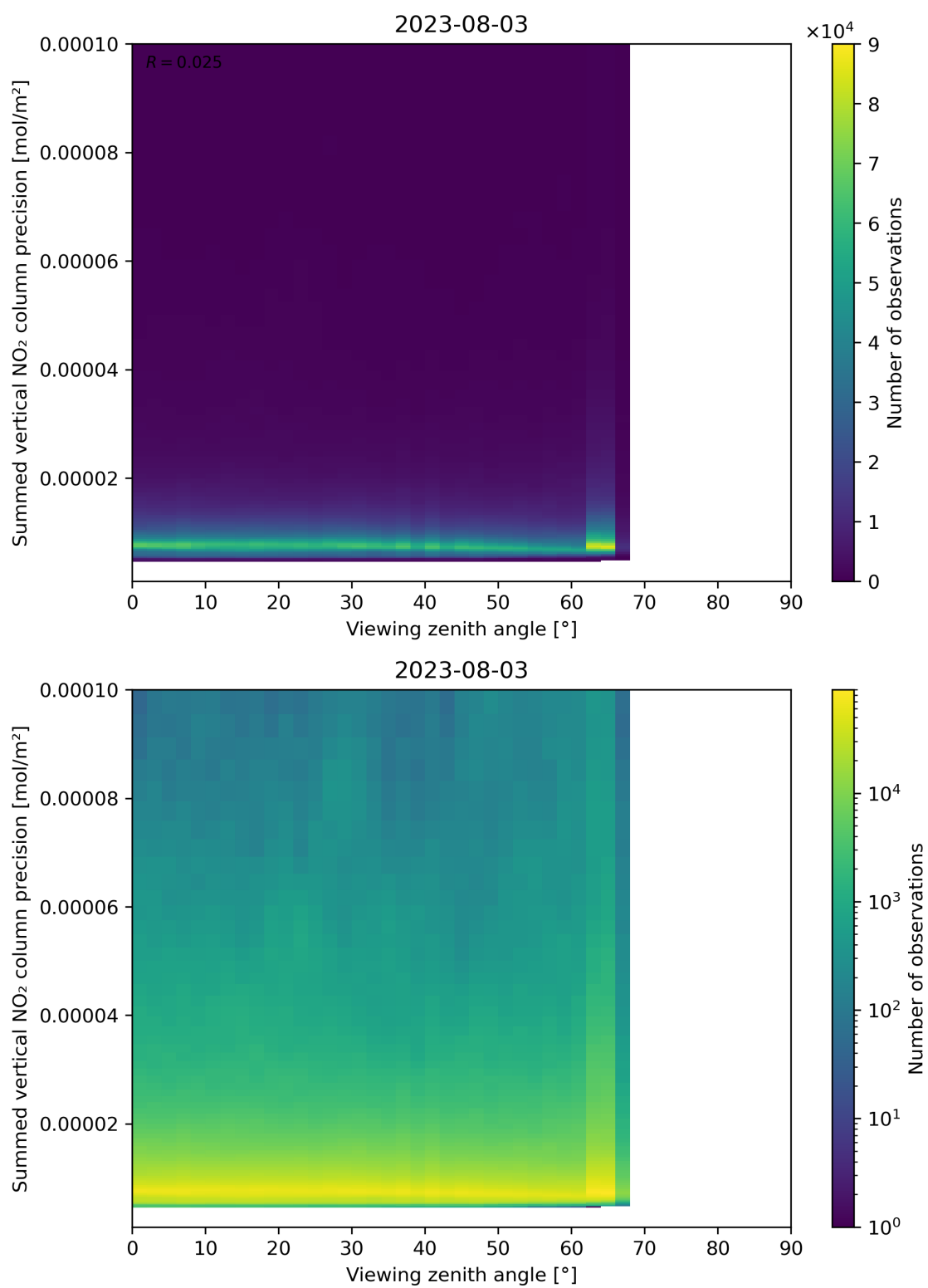
Figure 166: Scatter density plot of “Viewing zenith angle” against “Summed vertical NO 2 column precision” for 2023-08-02 to 2023-08-04.
