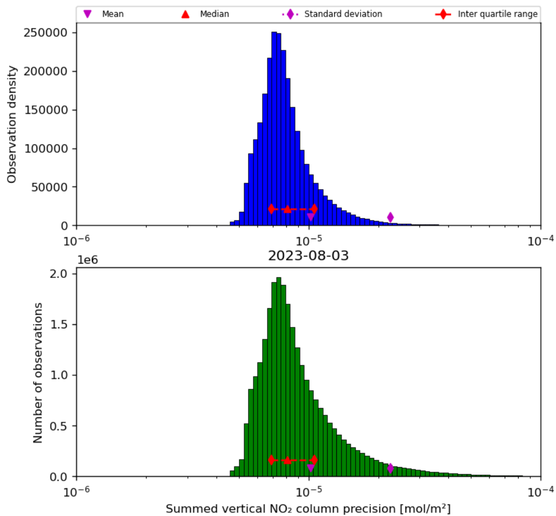
Figure 41: Histogram of “Summed vertical NO 2 column precision” for 2023-08-02 to 2023-08-04
