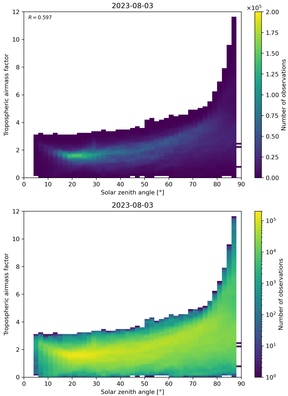
Figure 147: Scatter density plot of “Solar zenith angle” against “Tropospheric airmass factor” for 2023-08-02 to 2023-08-04.
