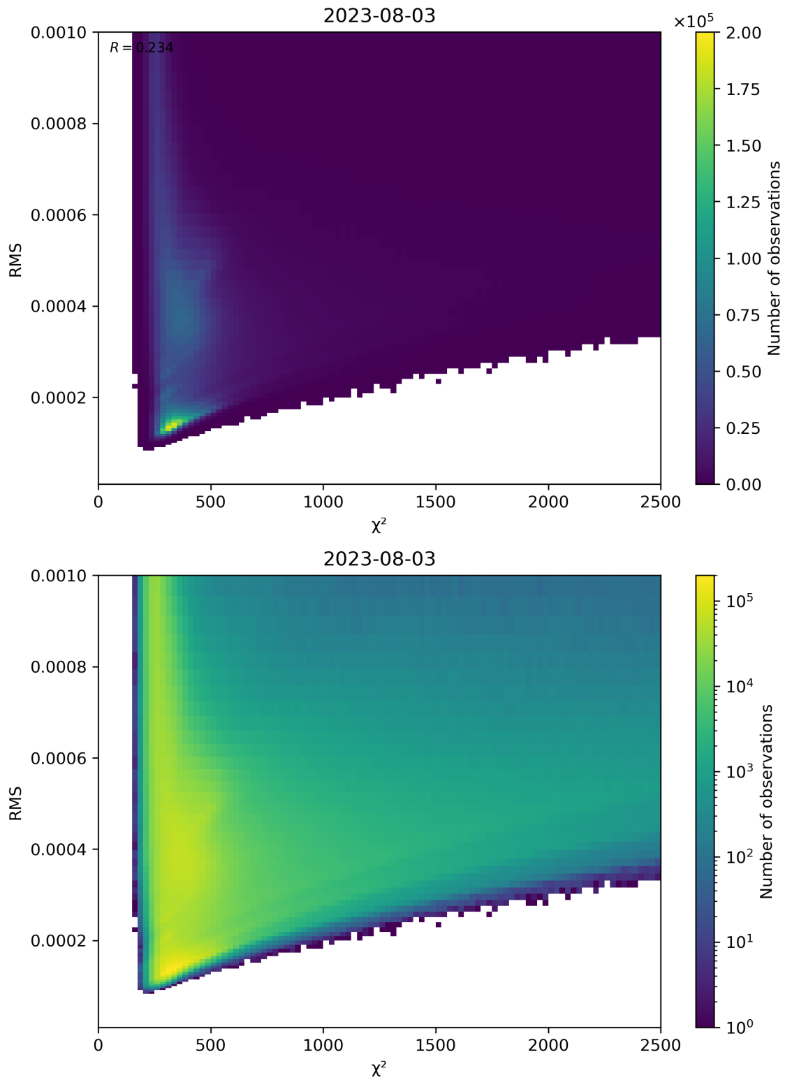
Figure 82: Scatter density plot of “ \chi^2 ” against “RMS” for 2023-08-02 to 2023-08-04.
