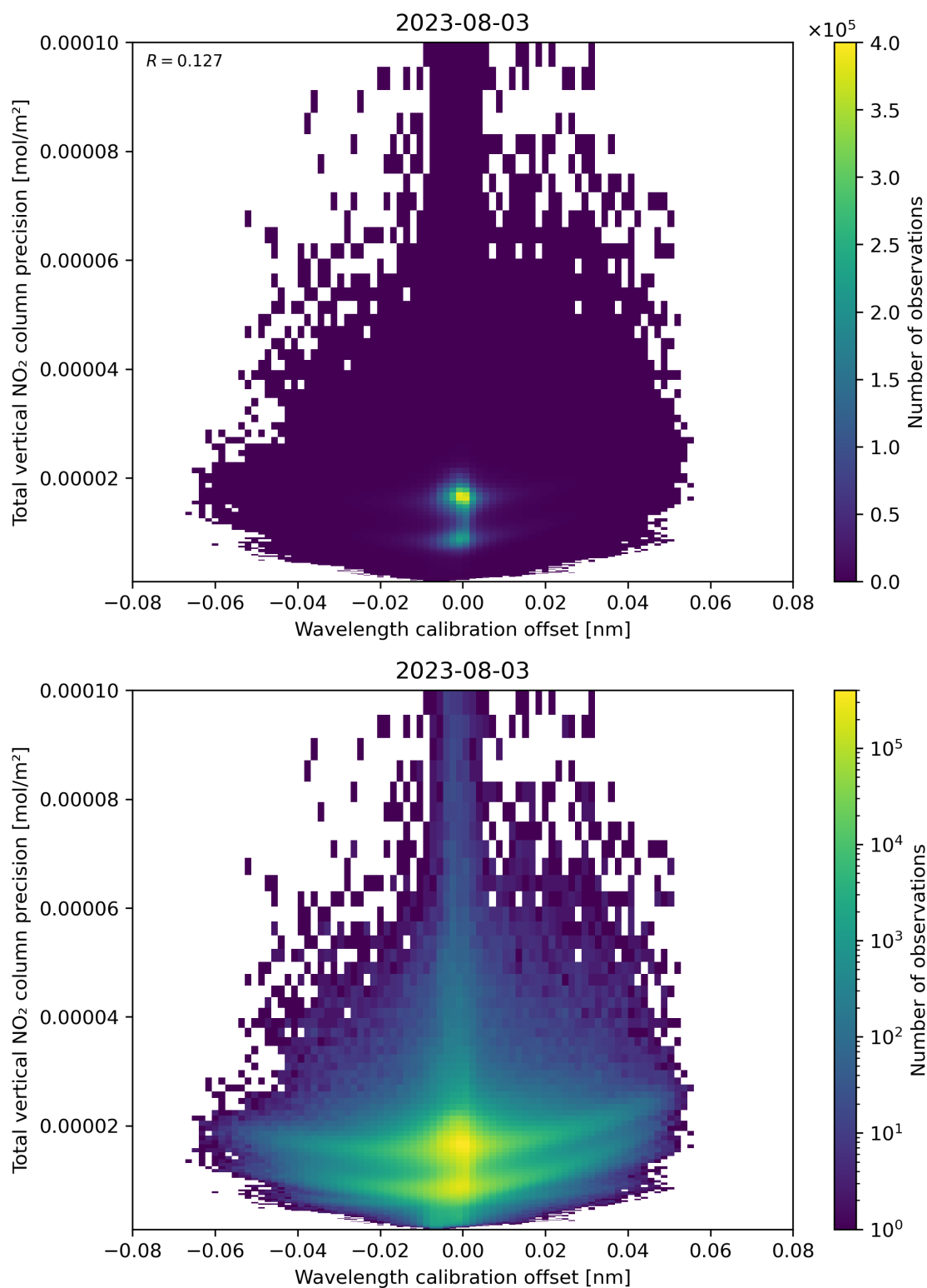
Figure 180: Scatter density plot of “Wavelength calibration offset” against “Total vertical NO 2 column precision” for 2023-08-02 to 2023-08-04.
