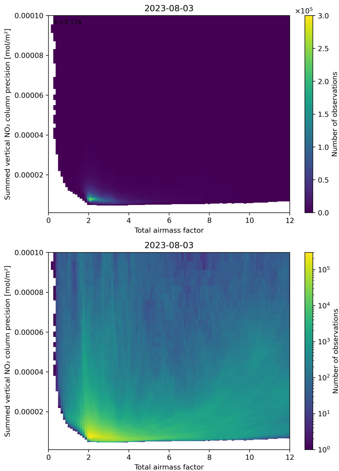
Figure 66: Scatter density plot of “Total airmass factor” against “Summed vertical NO 2 column precision” for 2023-08-02 to 2023-08-04.
