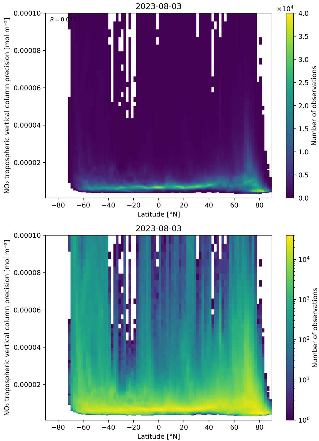
Figure 93: Scatter density plot of “Latitude” against “NO 2 tropospheric vertical column precision” for 2023-08-02 to 2023-08-04.
