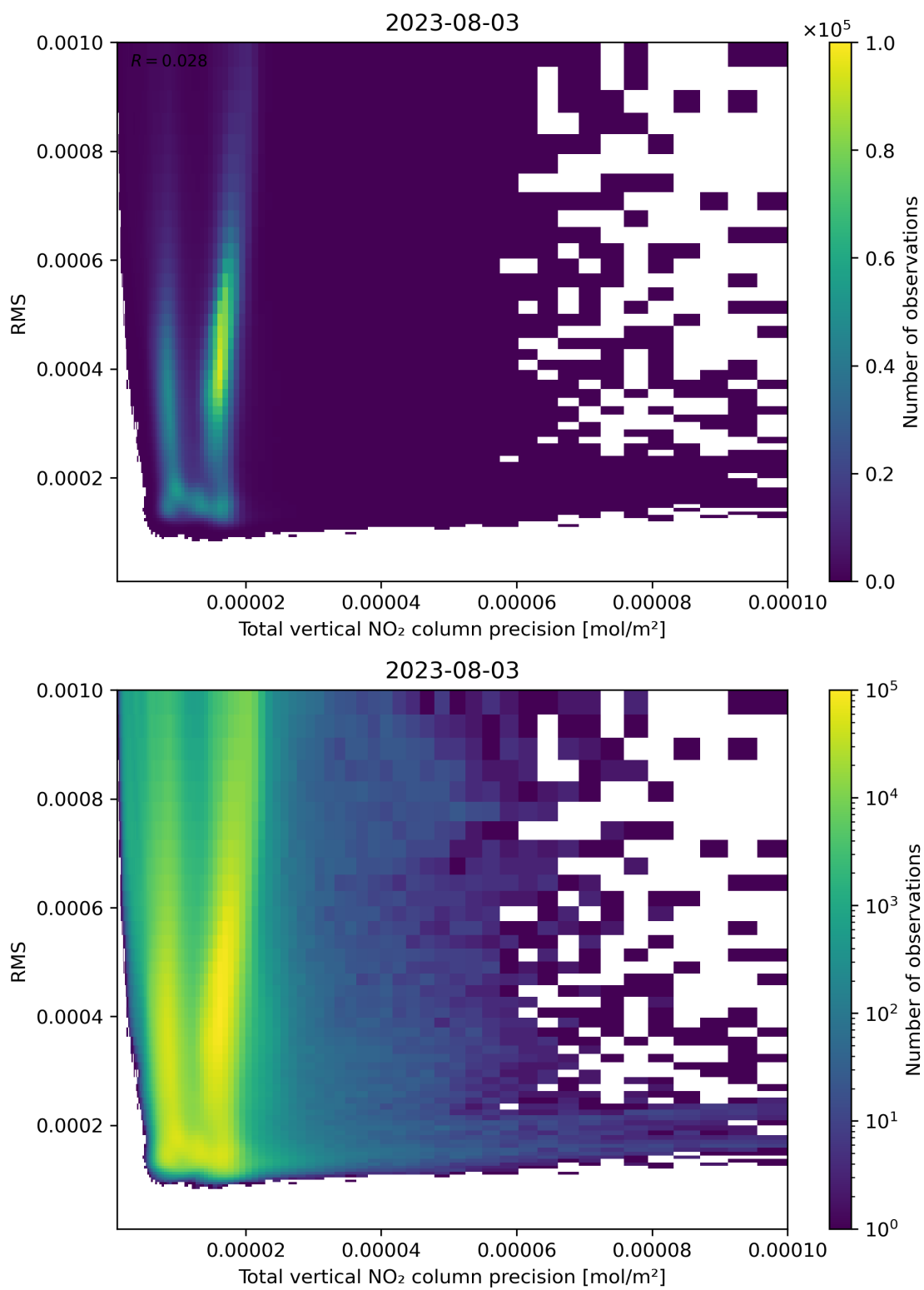
Figure 119: Scatter density plot of “Total vertical NO 2 column precision” against “RMS” for 2023-08-02 to 2023-08-04.
