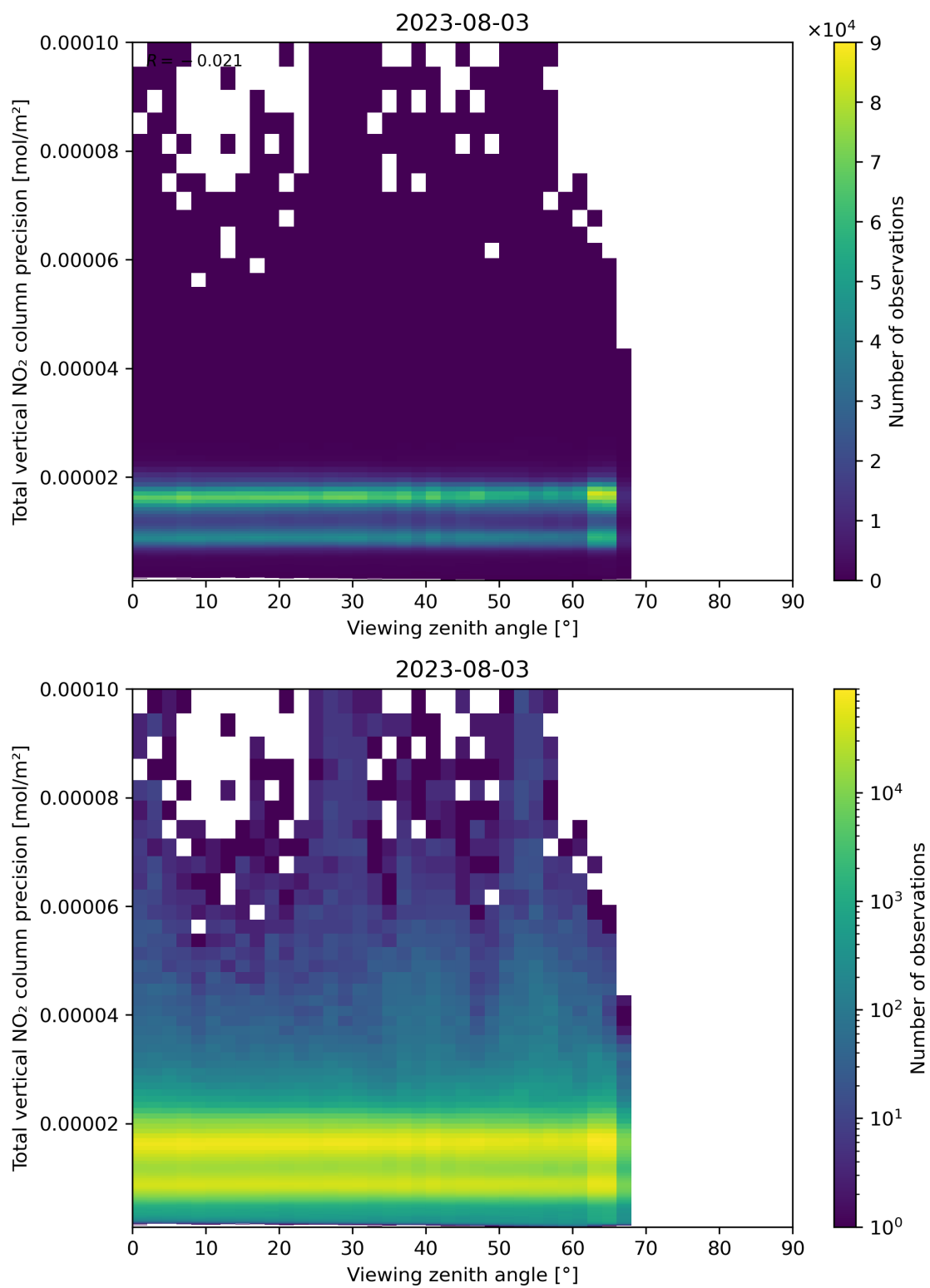
Figure 168: Scatter density plot of “Viewing zenith angle” against “Total vertical NO 2 column precision” for 2023-08-02 to 2023-08-04.
