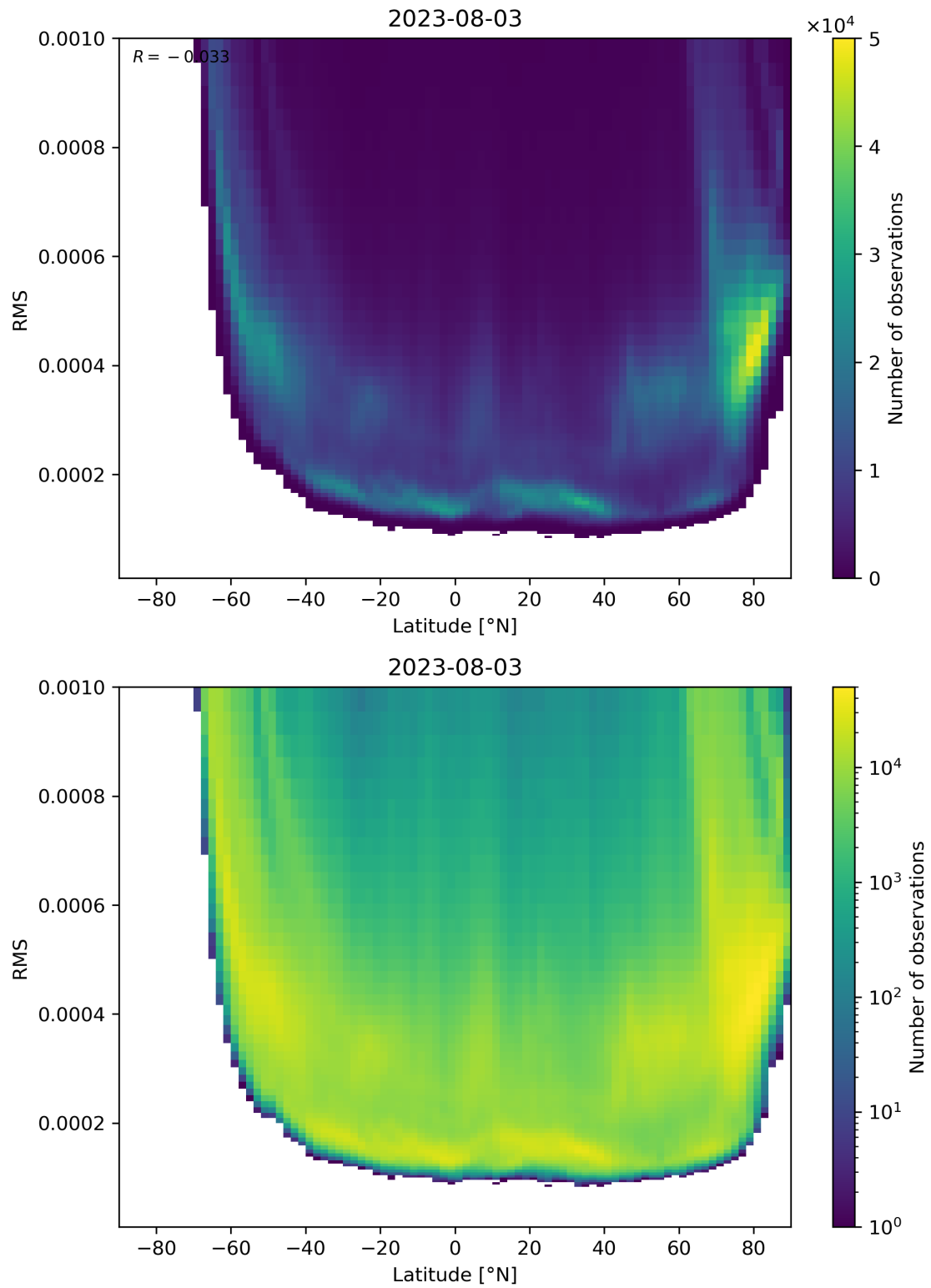
Figure 94: Scatter density plot of “Latitude” against “RMS” for 2023-08-02 to 2023-08-04.
