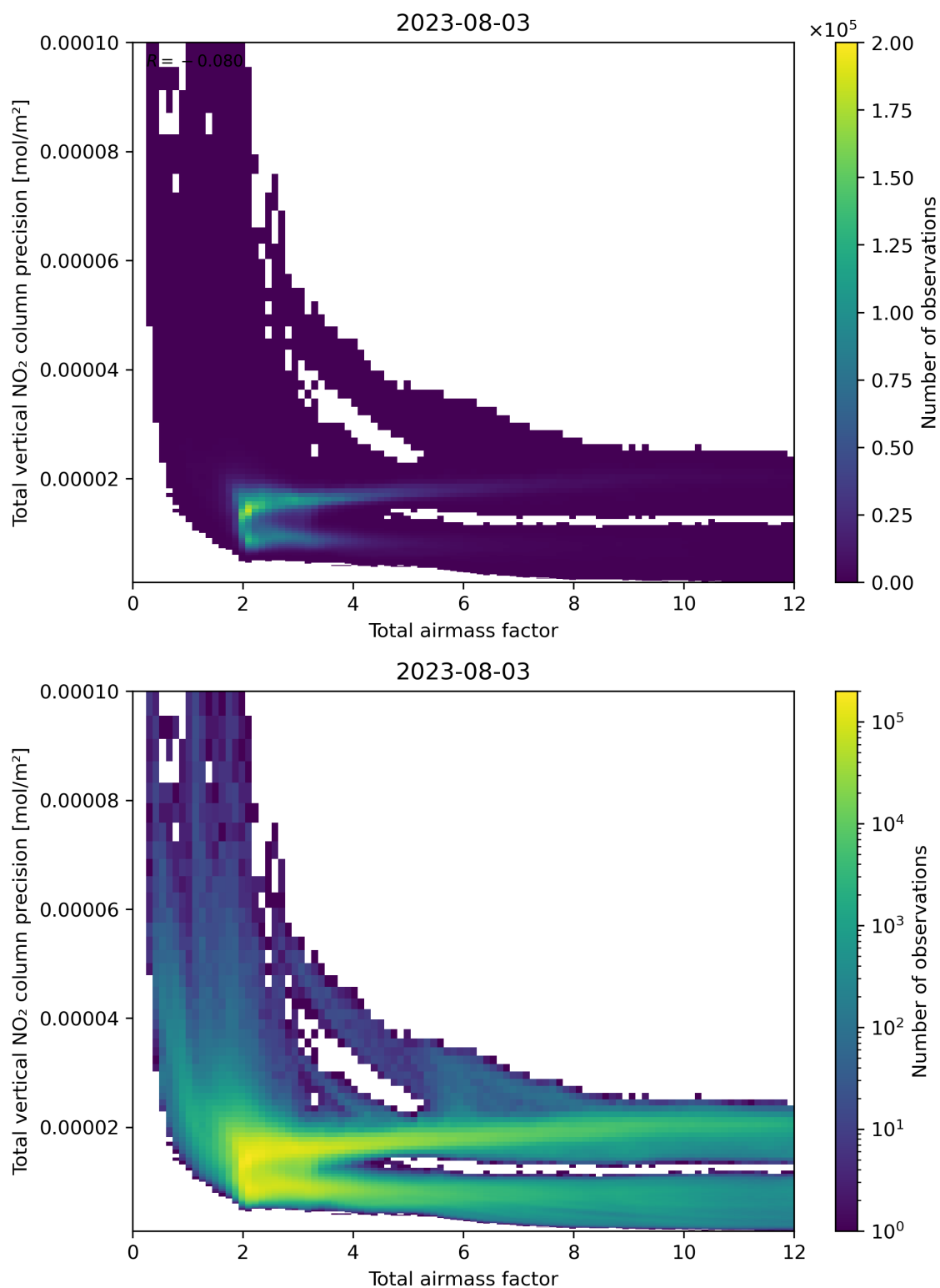
Figure 68: Scatter density plot of “Total airmass factor” against “Total vertical NO 2 column precision” for 2023-08-02 to 2023-08-04.
