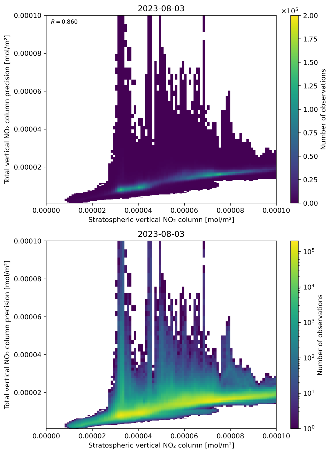
Figure 101: Scatter density plot of “Stratospheric vertical NO 2 column” against “Total vertical NO 2 column precision” for 2023-08-02 to 2023-08-04.
