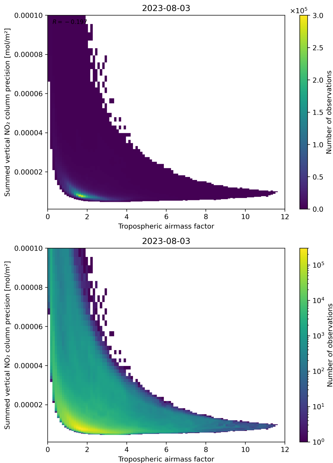
Figure 76: Scatter density plot of “Tropospheric air mass factor” against “Summed vertical NO 2 column precision” for 2023-08-02 to 2023-08-04.
