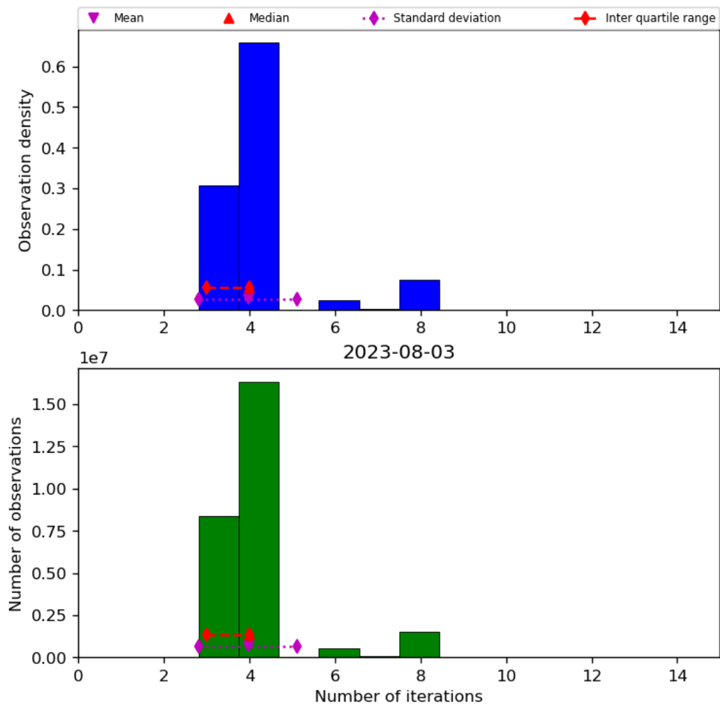
Figure 34: Histogram of “Number of iterations” for 2023-08-02 to 2023-08-04
