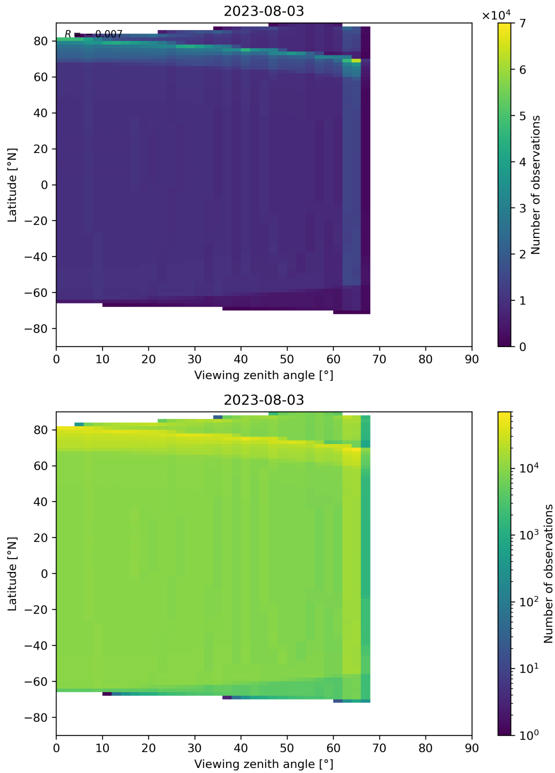
Figure 163: Scatter density plot of “Viewing zenith angle” against “Latitude” for 2023-08-02 to 2023-08-04.
