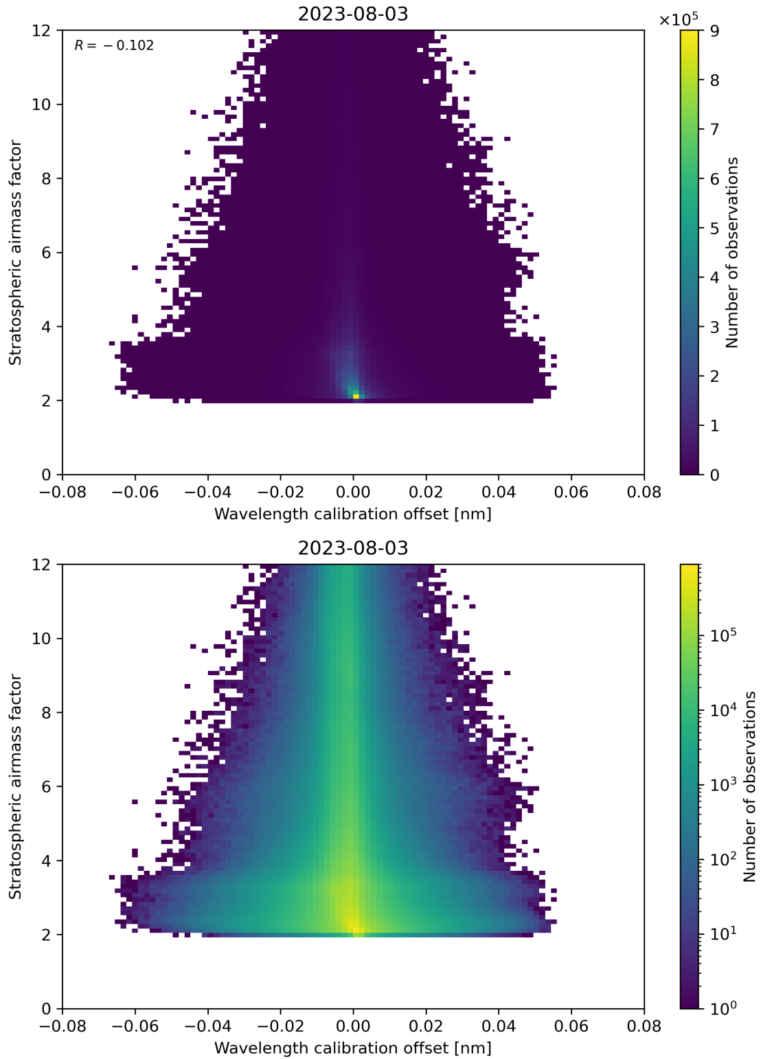
Figure 174: Scatter density plot of “Wavelength calibration offset” against “Stratospheric airmass factor” for 2023-08-02 to 2023-08-04.
