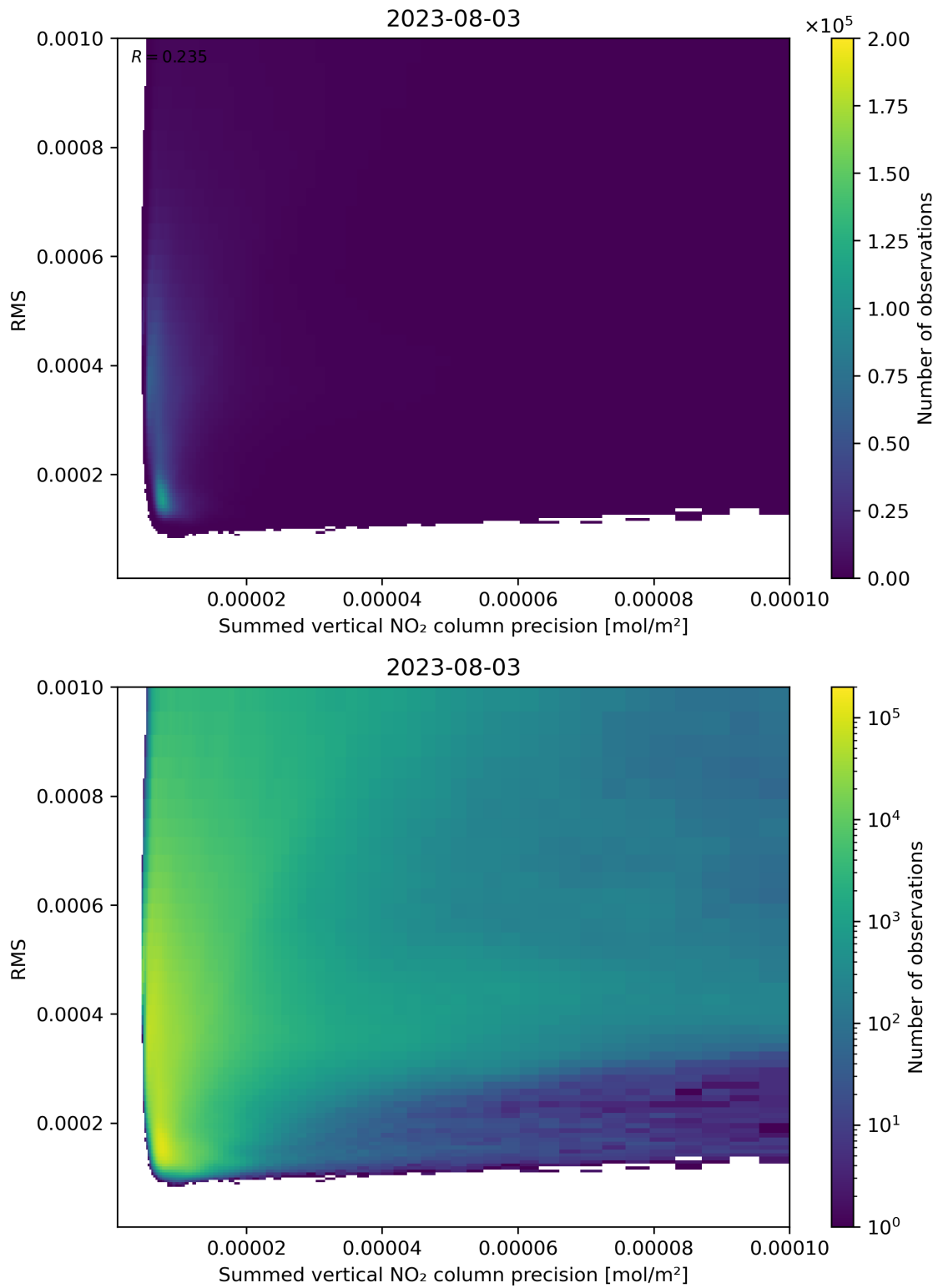
Figure 108: Scatter density plot of “Summed vertical NO 2 column precision” against “RMS” for 2023-08-02 to 2023-08-04.
