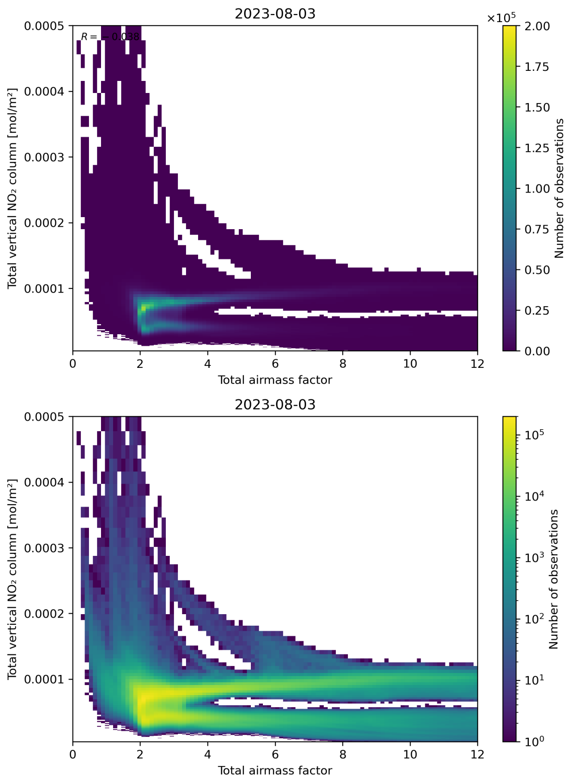
Figure 67: Scatter density plot of “Total airmass factor” against “Total vertical NO 2 column” for 2023-08-02 to 2023-08-04.
