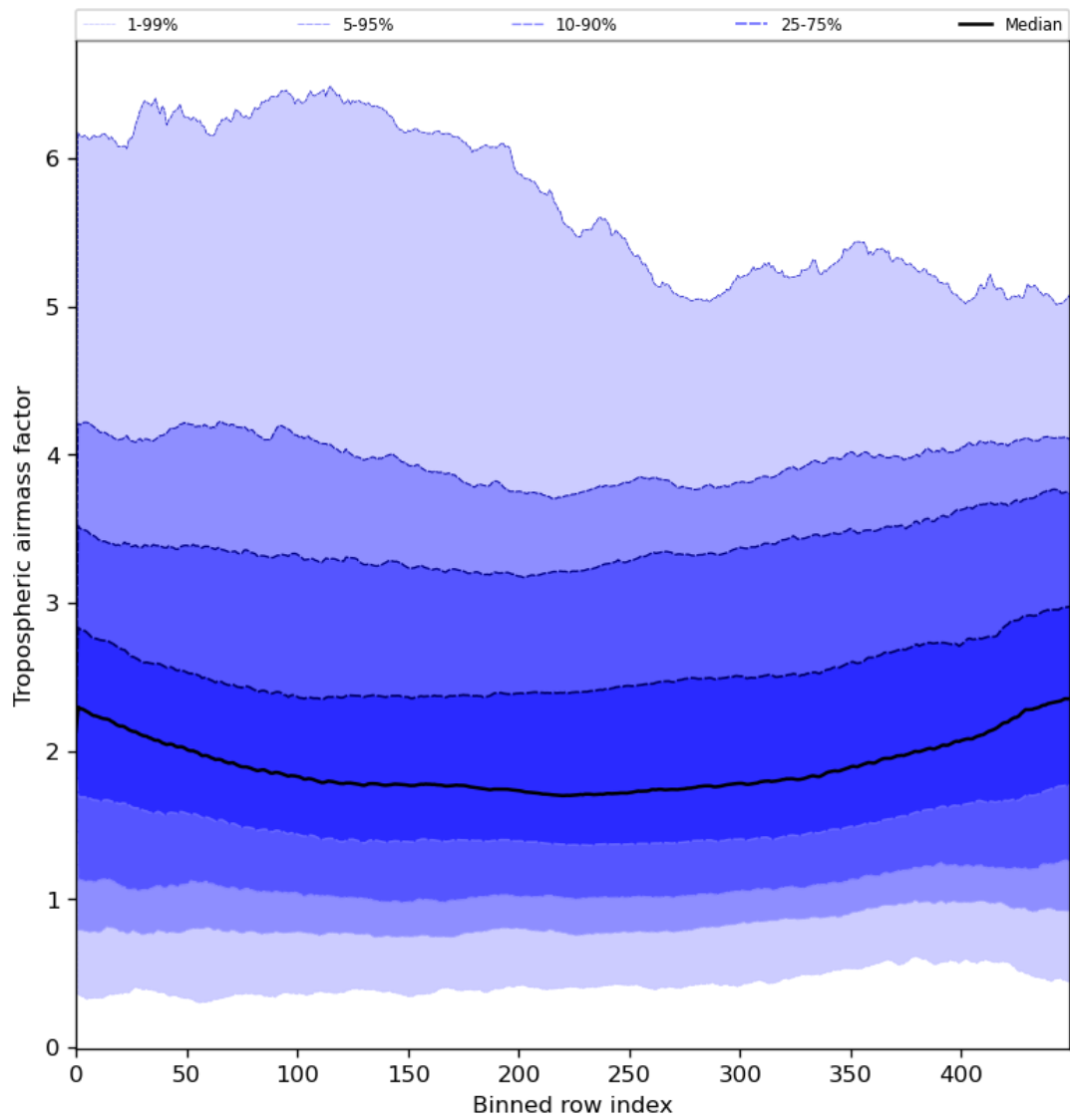
Figure 48: Along track statistics of “Tropospheric air mass factor” for 2023-08-02 to 2023-08-04
