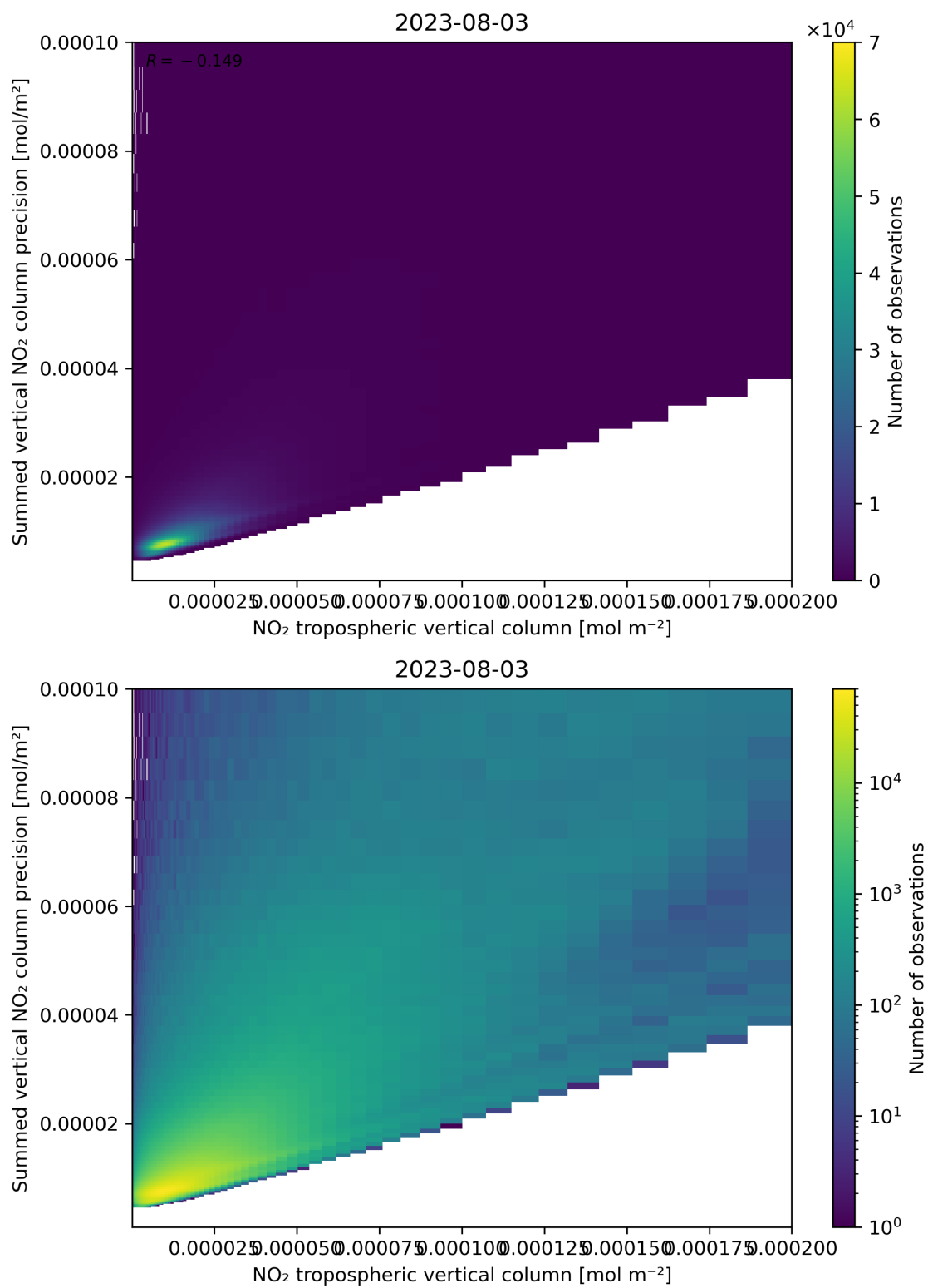
Figure 127: Scatter density plot of “NO 2 tropospheric vertical column” against “Summed vertical NO 2 column precision” for 2023-08-02 to 2023-08-04.
