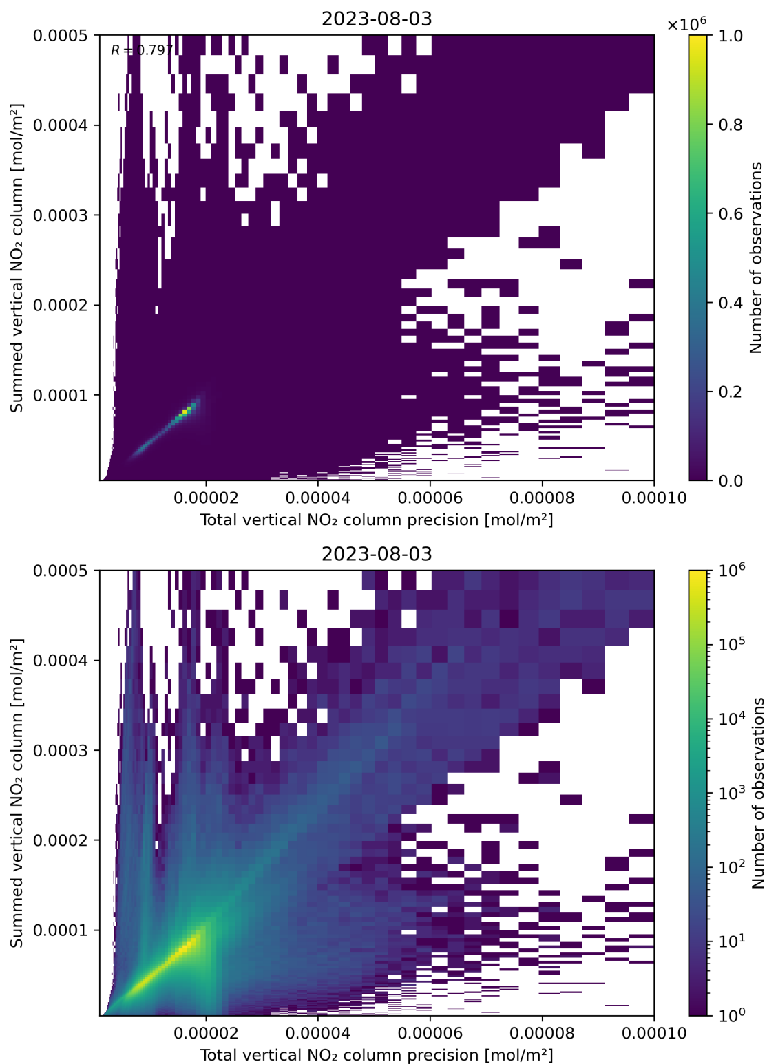
Figure 117: Scatter density plot of “Total vertical NO 2 column precision” against “Summed vertical NO 2 column” for 2023-08-02 to 2023-08-04.
