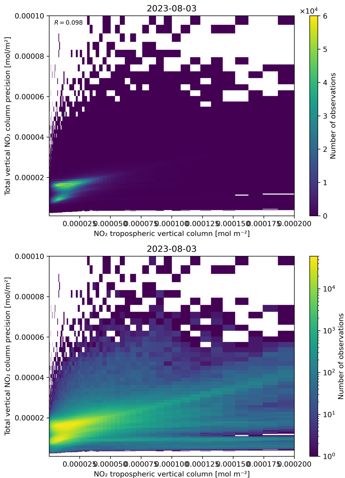
Figure 129: Scatter density plot of “NO 2 tropospheric vertical column” against “Total vertical NO 2 column precision” for 2023-08-02 to 2023-08-04.
