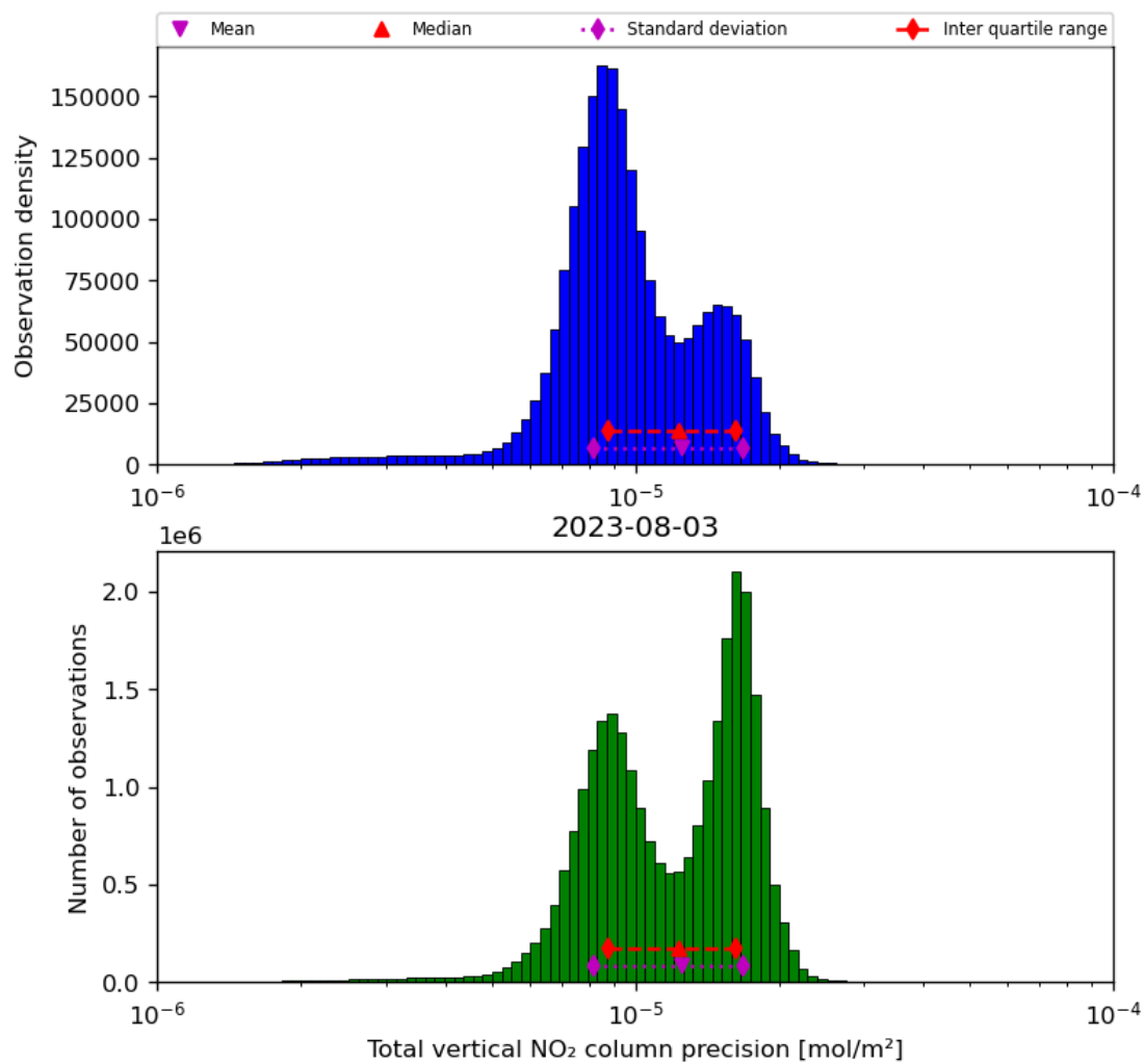
Figure 39: Histogram of “Total vertical NO 2 column precision” for 2023-08-02 to 2023-08-04
