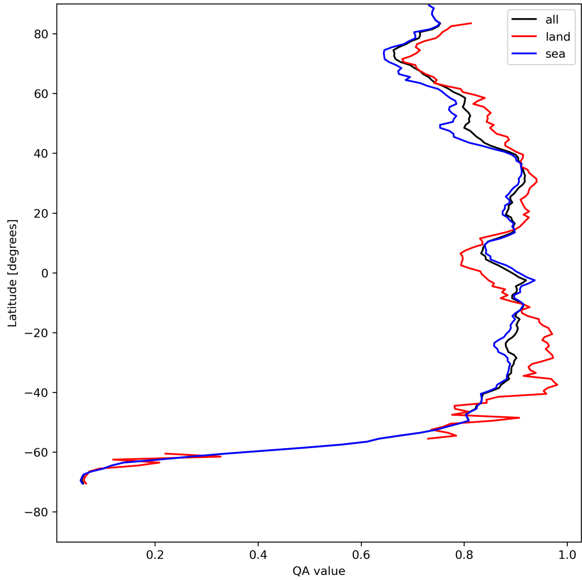
Figure 11: Zonal average of “QA value” for 2023-08-02 to 2023-08-04.
