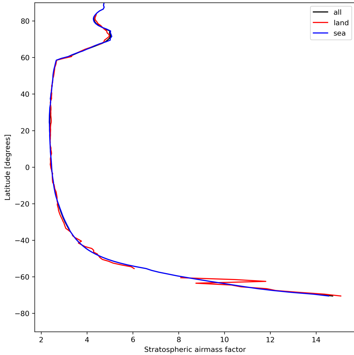
Figure 27: Zonal average of “Stratospheric airmass factor” for 2023-08-02 to 2023-08-04.
