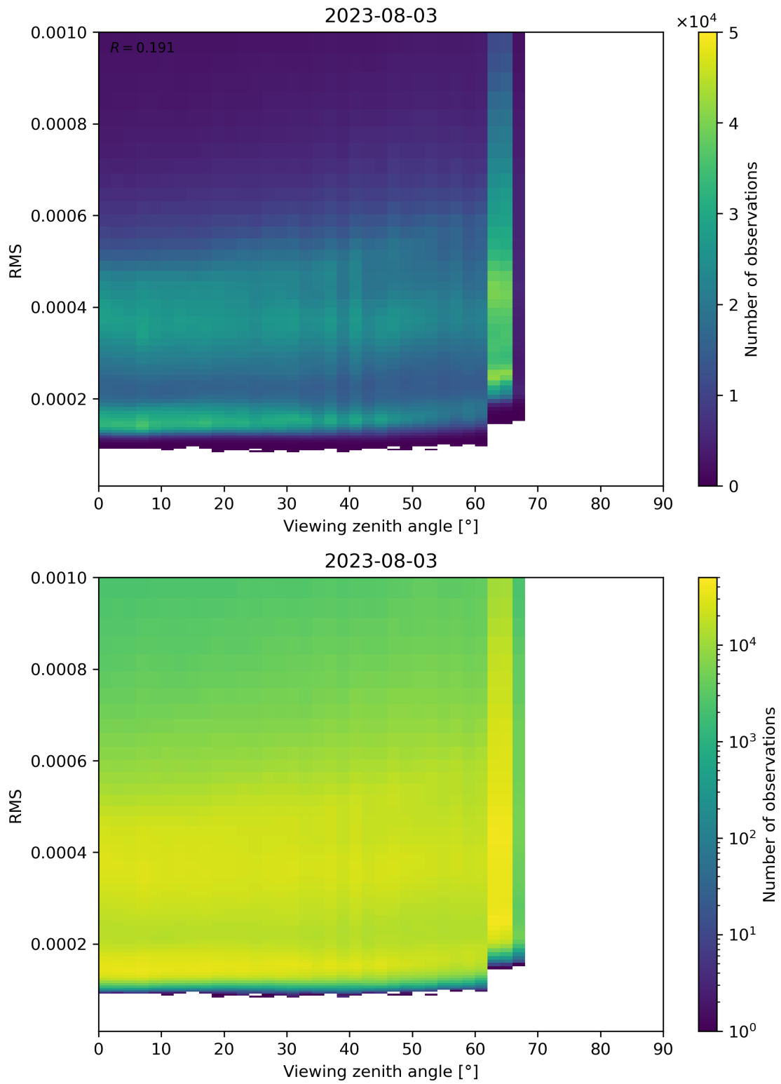
Figure 171: Scatter density plot of “Viewing zenith angle” against “RMS” for 2023-08-02 to 2023-08-04.
