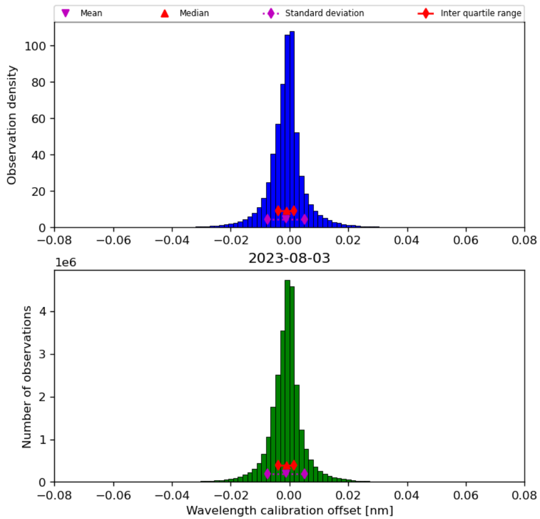
Figure 35: Histogram of “Wavelength calibration offset” for 2023-08-02 to 2023-08-04
