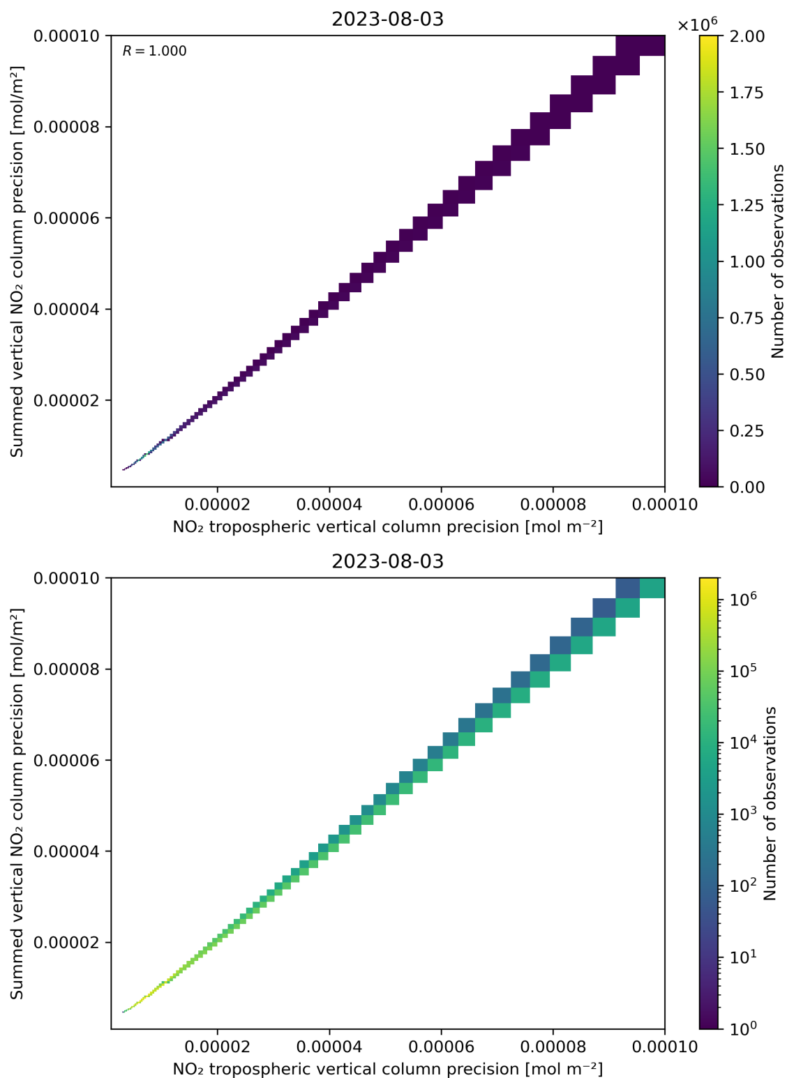
Figure 137: Scatter density plot of “NO 2 tropospheric vertical column precision” against “Summed vertical NO 2 column precision” for 2023-08-02 to 2023-08-04.
