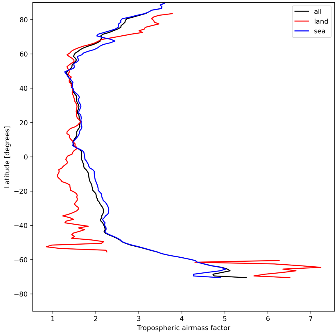
Figure 14: Zonal average of “Tropospheric airmass factor” for 2023-08-02 to 2023-08-04.
