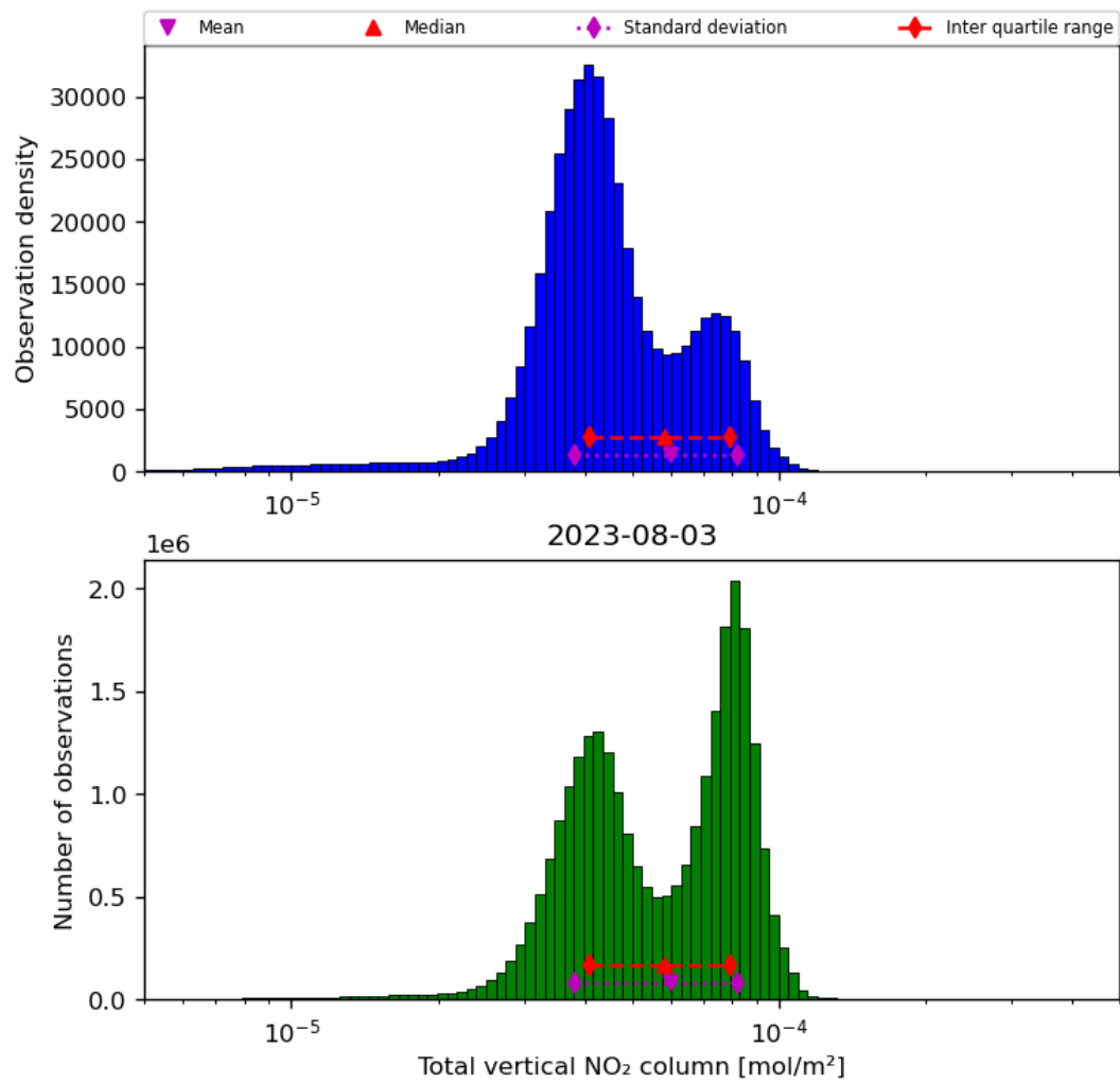
Figure 38: Histogram of “Total vertical NO 2 column” for 2023-08-02 to 2023-08-04
