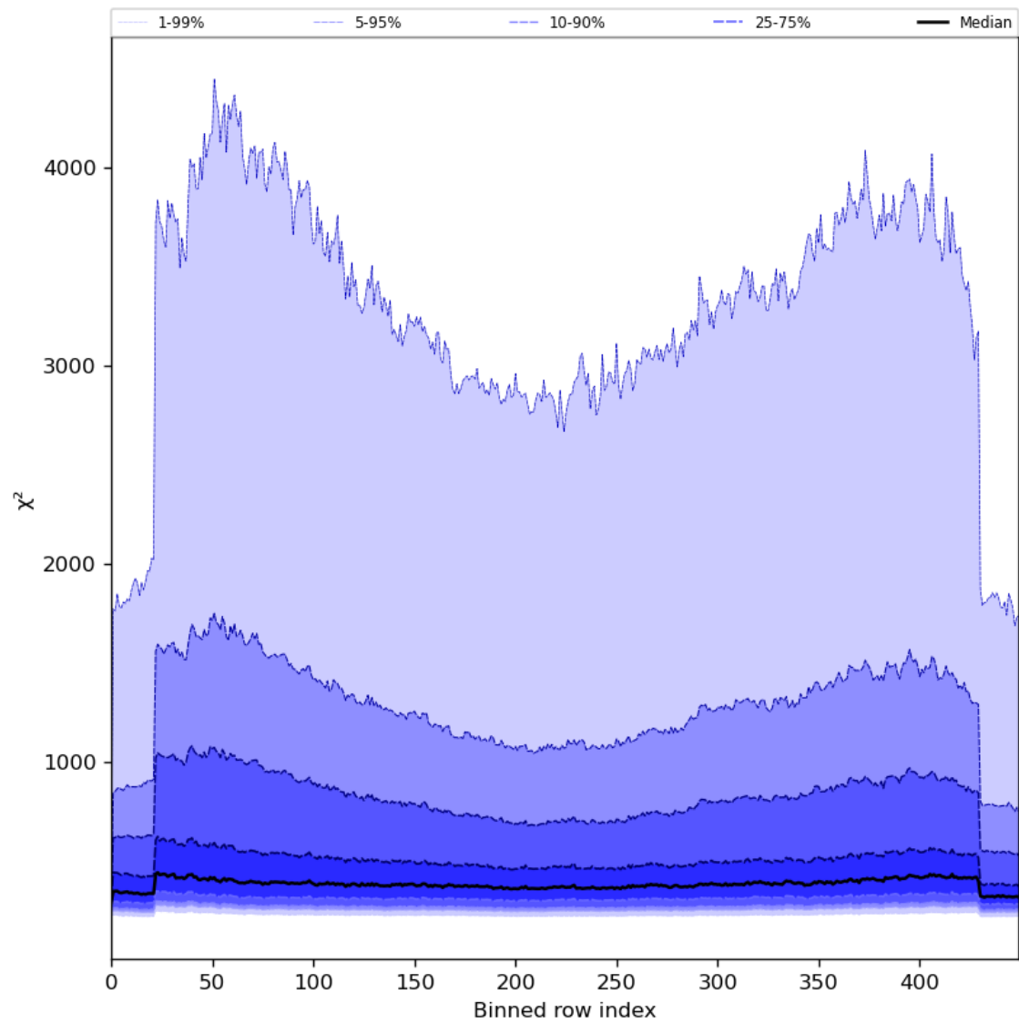
Figure 59: Along track statistics of “ \chi^2 ” for 2023-08-02 to 2023-08-04
