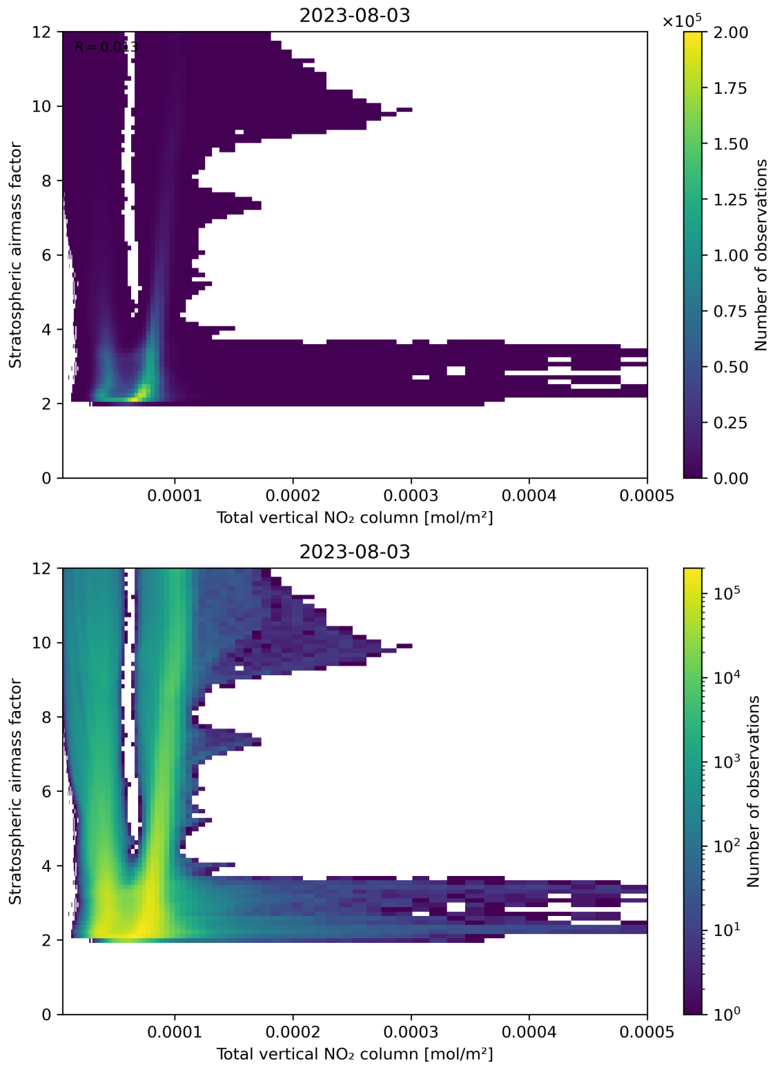
Figure 110: Scatter density plot of “Total vertical NO 2 column” against “Stratospheric airmass factor” for 2023-08-02 to 2023-08-04.
