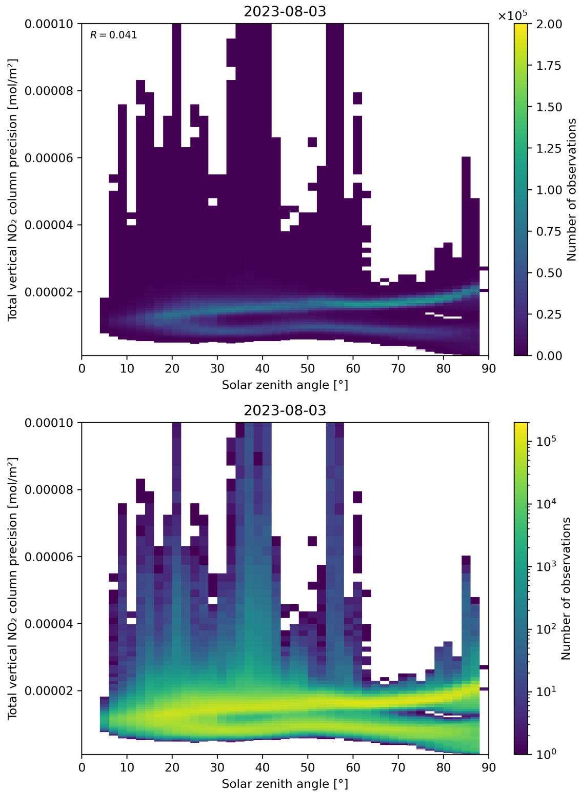
Figure 154: Scatter density plot of “Solar zenith angle” against “Total vertical NO 2 column precision” for 2023-08-02 to 2023-08-04.
