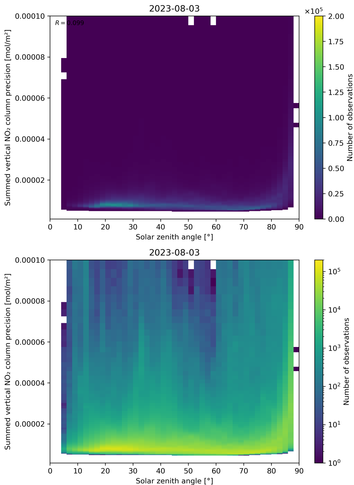
Figure 152: Scatter density plot of “Solar zenith angle” against “Summed vertical NO 2 column precision” for 2023-08-02 to 2023-08-04.
