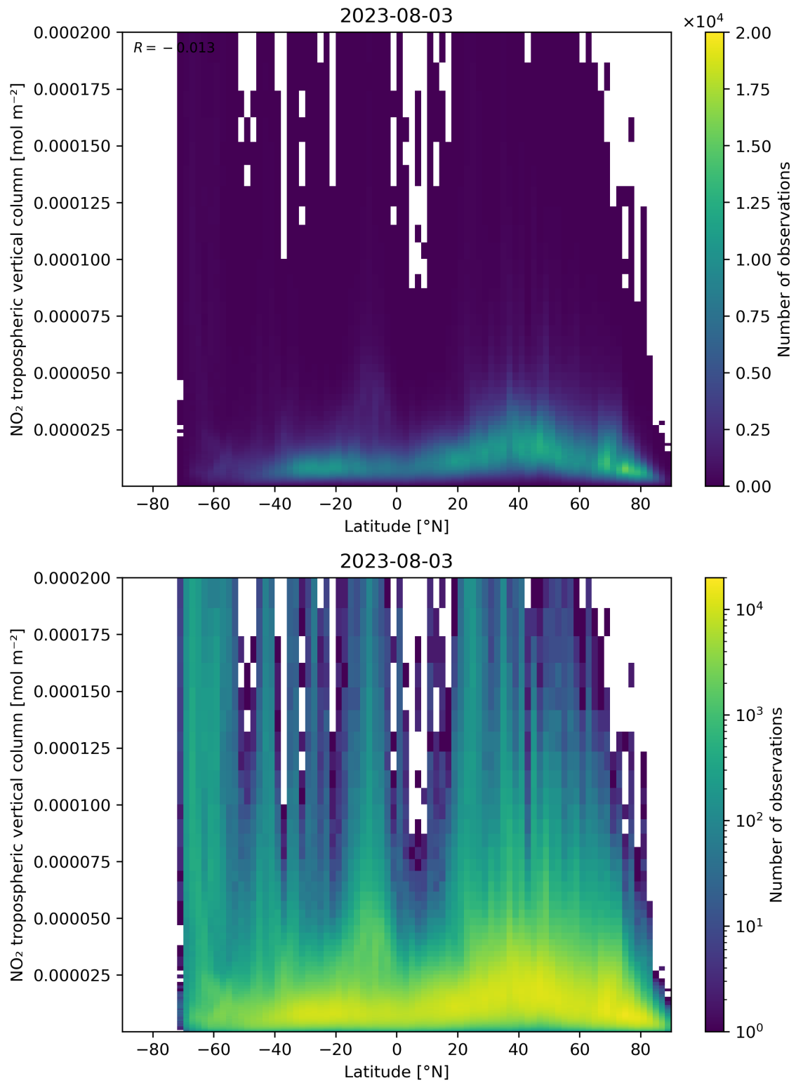
Figure 92: Scatter density plot of “Latitude” against “NO 2 tropospheric vertical column” for 2023-08-02 to 2023-08-04.
