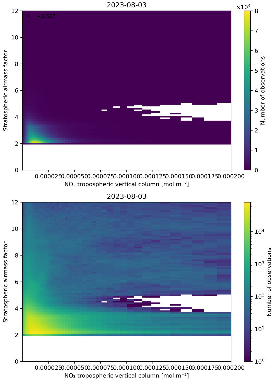
Figure 121: Scatter density plot of “NO 2 tropospheric vertical column” against “Stratospheric air mass factor” for 2023-08-02 to 2023-08-04.
