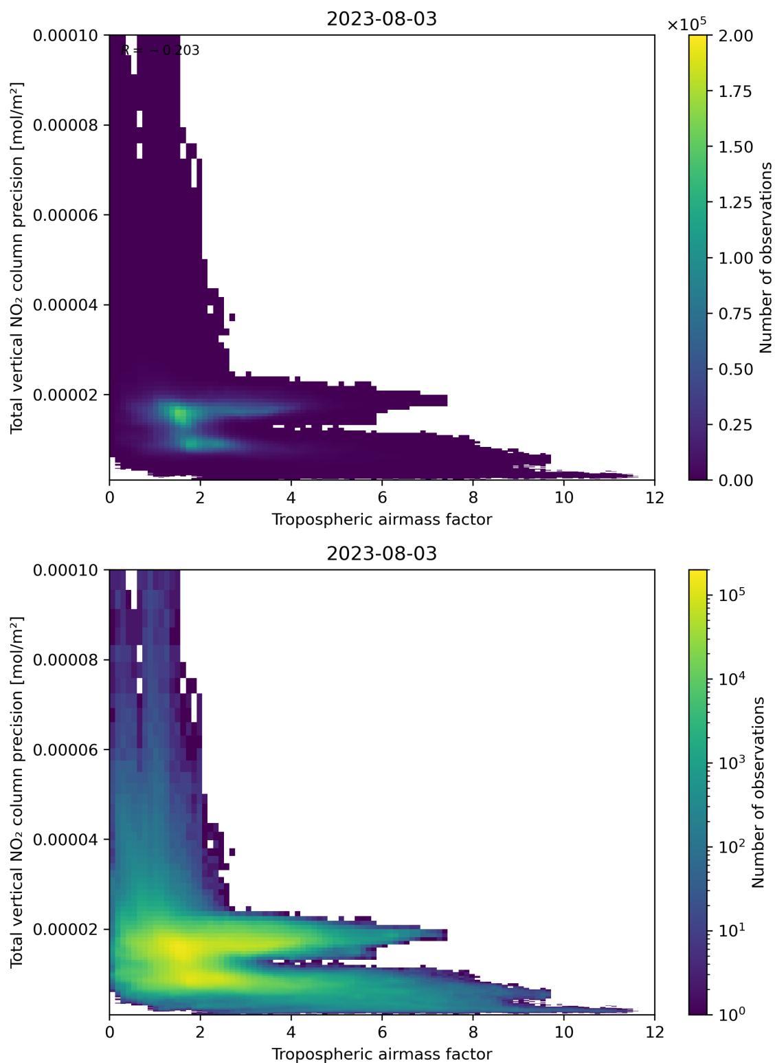
Figure 78: Scatter density plot of “Tropospheric air mass factor” against “Total vertical NO 2 column precision” for 2023-08-02 to 2023-08-04.
