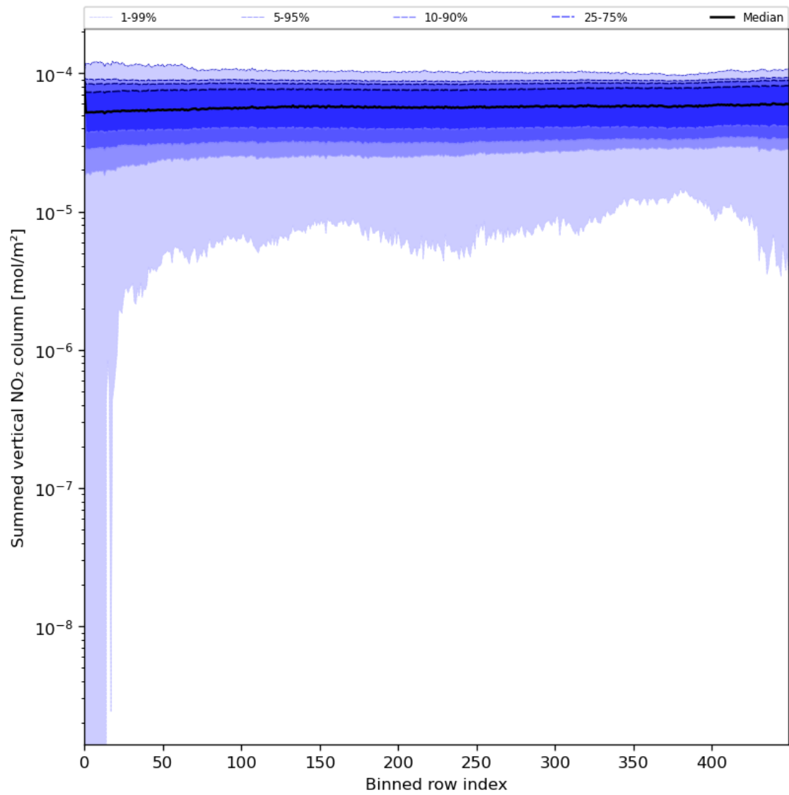
Figure 57: Along track statistics of “Summed vertical NO 2 column” for 2023-08-02 to 2023-08-04
