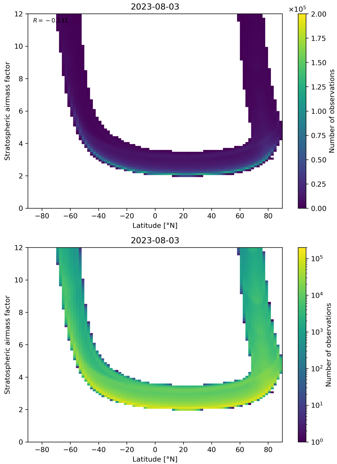
Figure 83: Scatter density plot of “Latitude” against “Stratospheric air mass factor” for 2023-08-02 to 2023-08-04.
