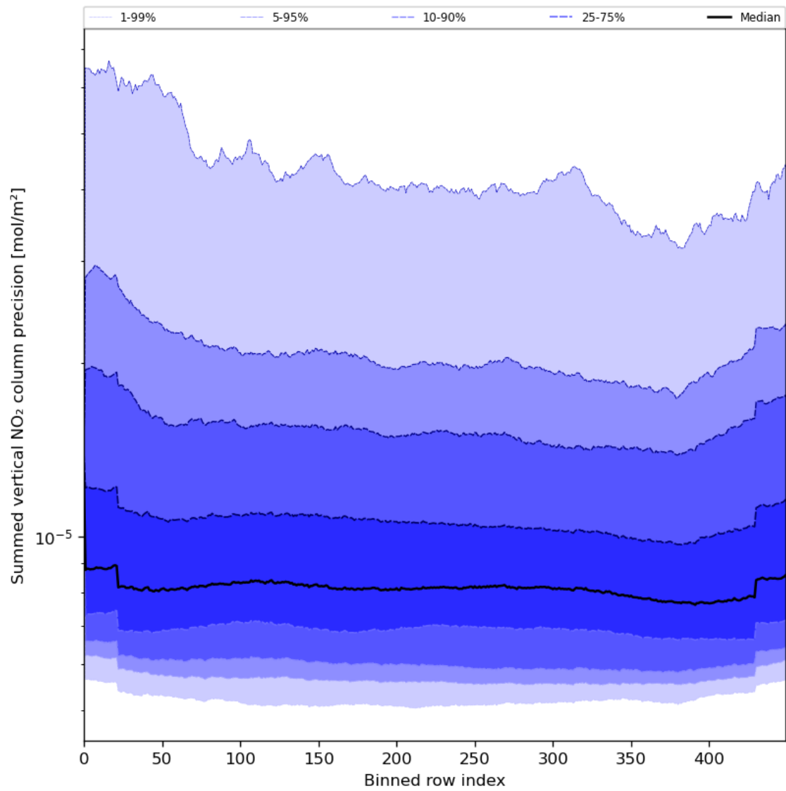
Figure 58: Along track statistics of “Summed vertical NO 2 column precision” for 2023-08-02 to 2023-08-04
