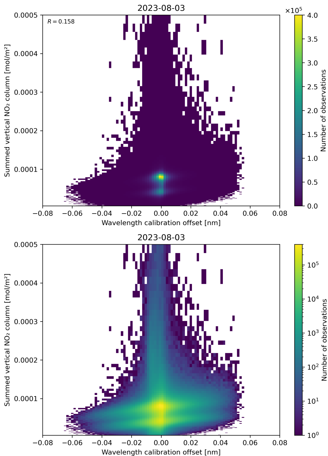
Figure 177: Scatter density plot of “Wavelength calibration offset” against “Summed vertical NO 2 column” for 2023-08-02 to 2023-08-04.
