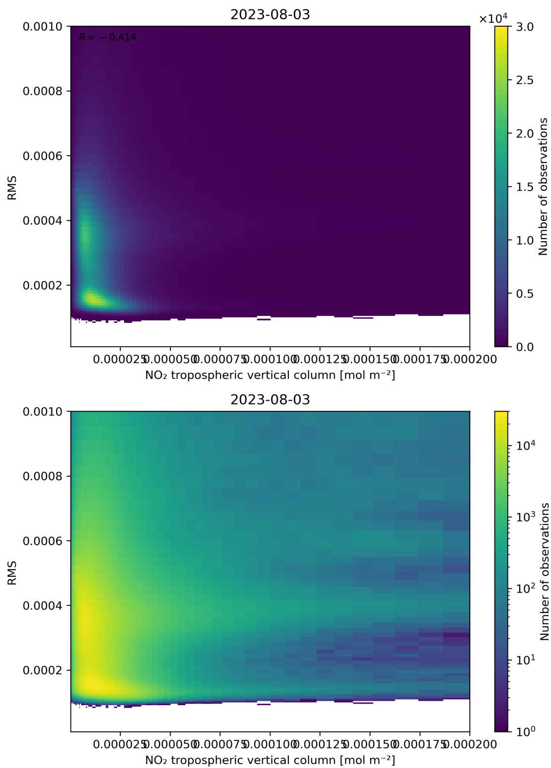
Figure 142: Scatter density plot of “NO 2 tropospheric vertical column” against “RMS” for 2023-08-02 to 2023-08-04.
