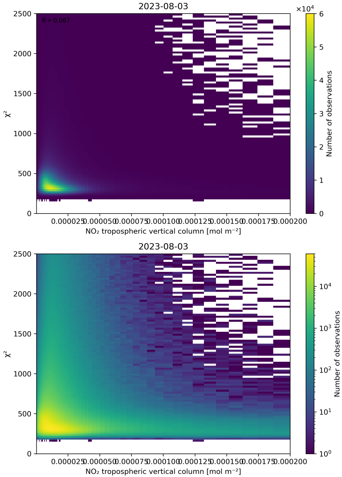
Figure 124: Scatter density plot of “NO 2 tropospheric vertical column” against “ \chi^2 ” for 2023-08-02 to 2023-08-04.
