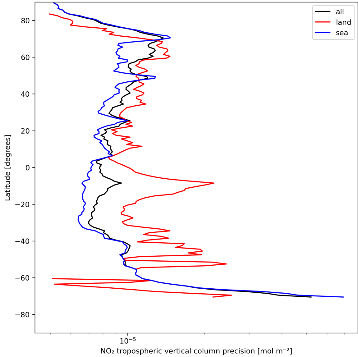
Figure 13: Zonal average of "NO 2 tropospheric vertical column precision" for 2023-08-02 to 2023-08-04.
