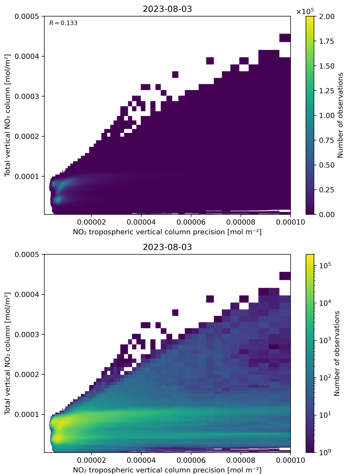
Figure 138: Scatter density plot of “NO 2 tropospheric vertical column precision” against “Total vertical NO 2 column” for 2023-08-02 to 2023-08-04.
