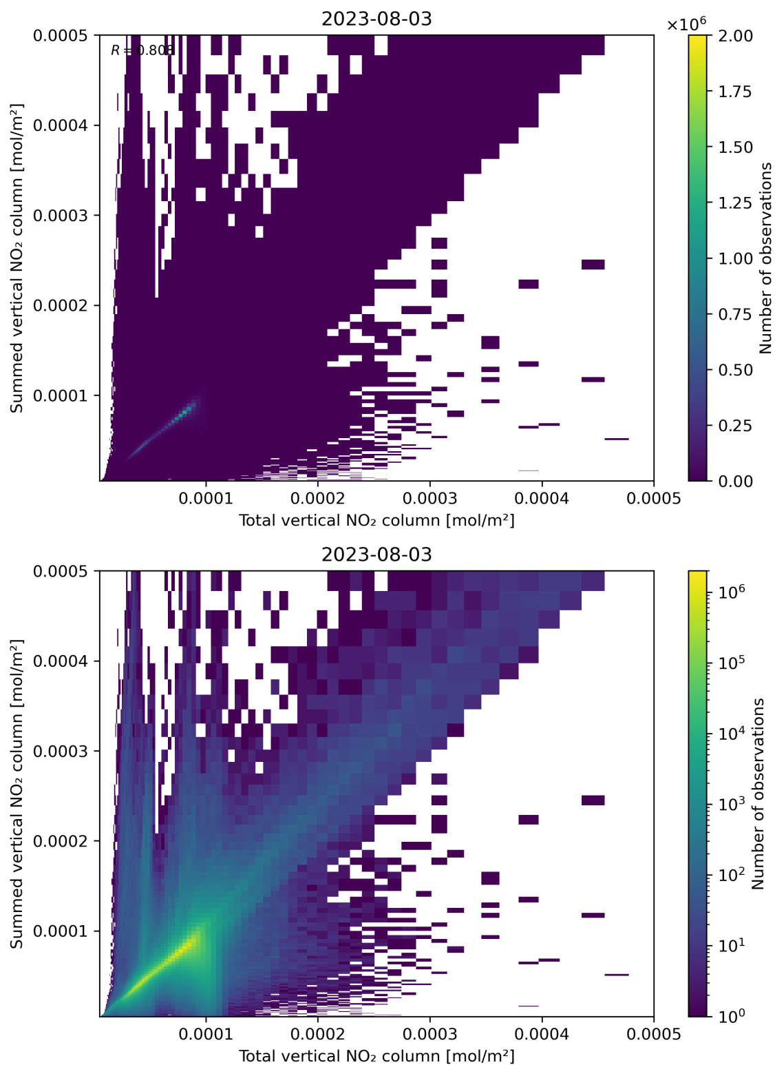
Figure 112: Scatter density plot of “Total vertical NO 2 column” against “Summed vertical NO 2 column” for 2023-08-02 to 2023-08-04.
