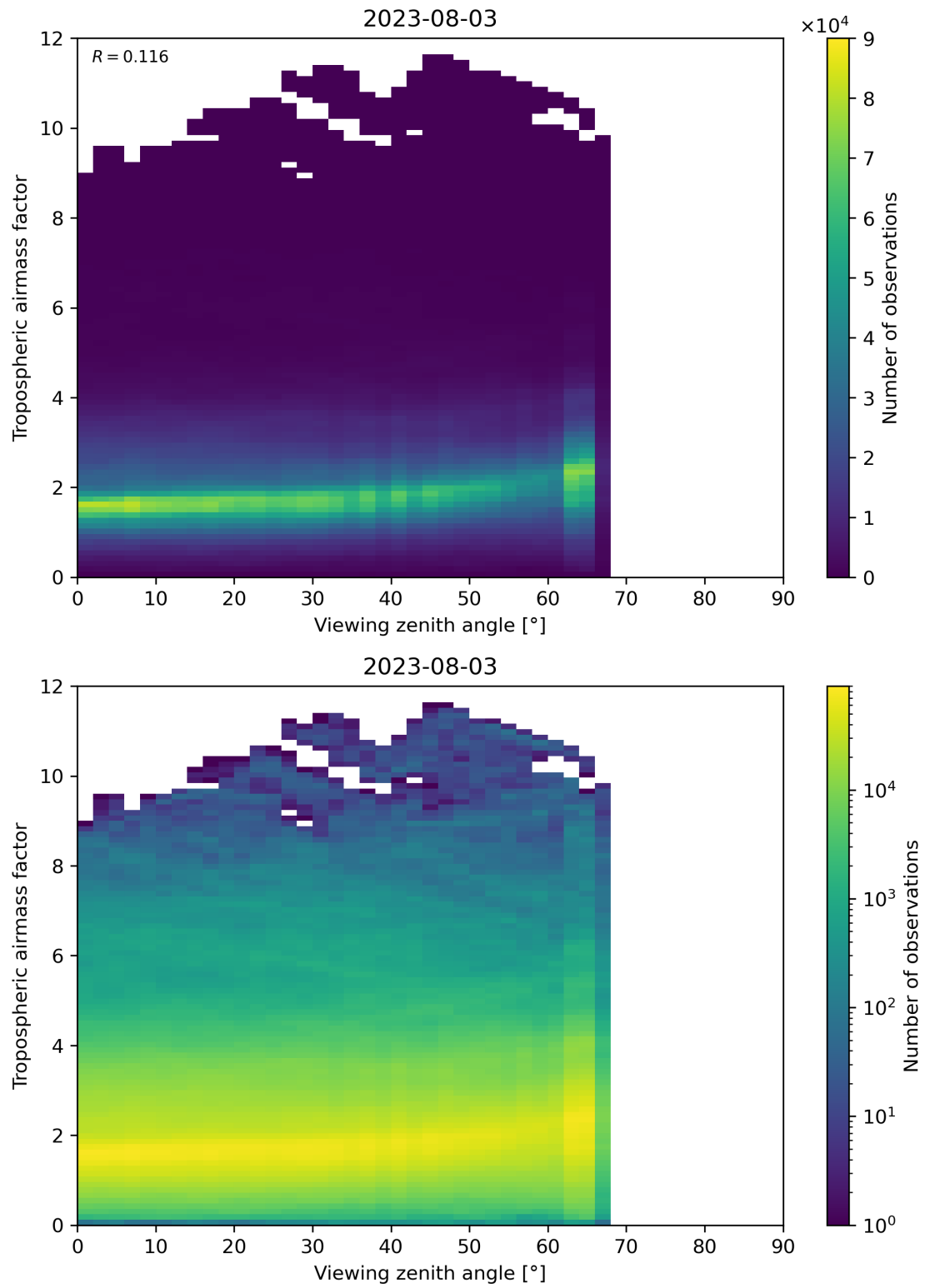
Figure 161: Scatter density plot of “Viewing zenith angle” against “Tropospheric airmass factor” for 2023-08-02 to 2023-08-04.
