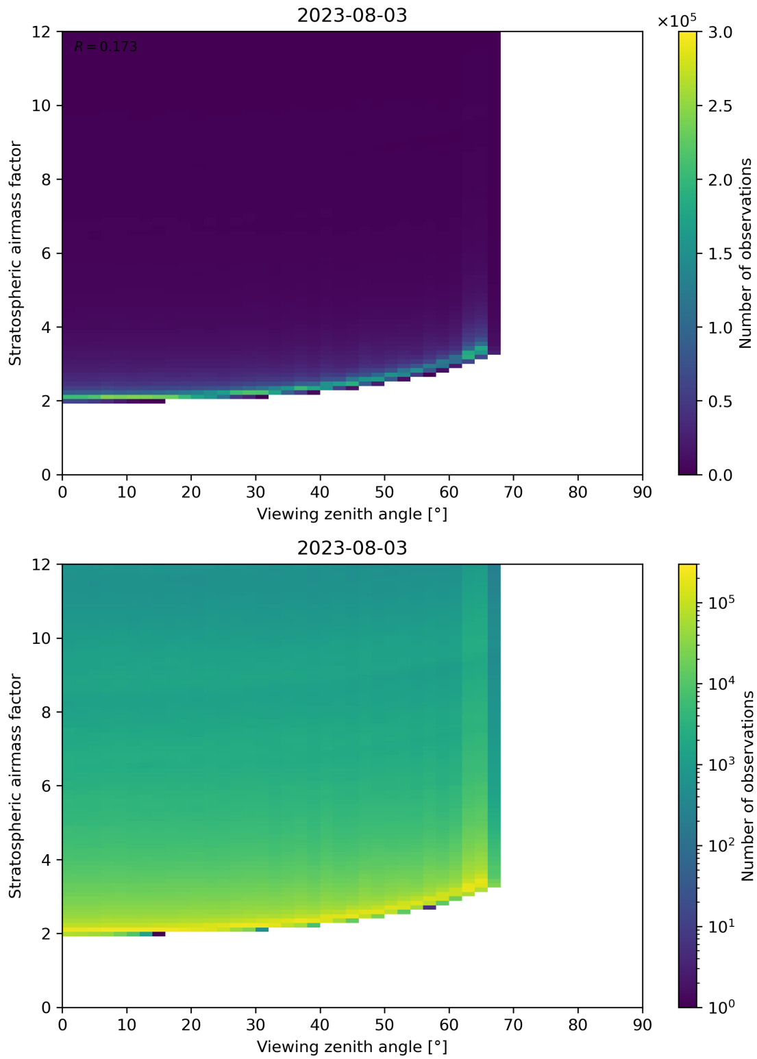
Figure 159: Scatter density plot of “Viewing zenith angle” against “Stratospheric airmass factor” for 2023-08-02 to 2023-08-04.
