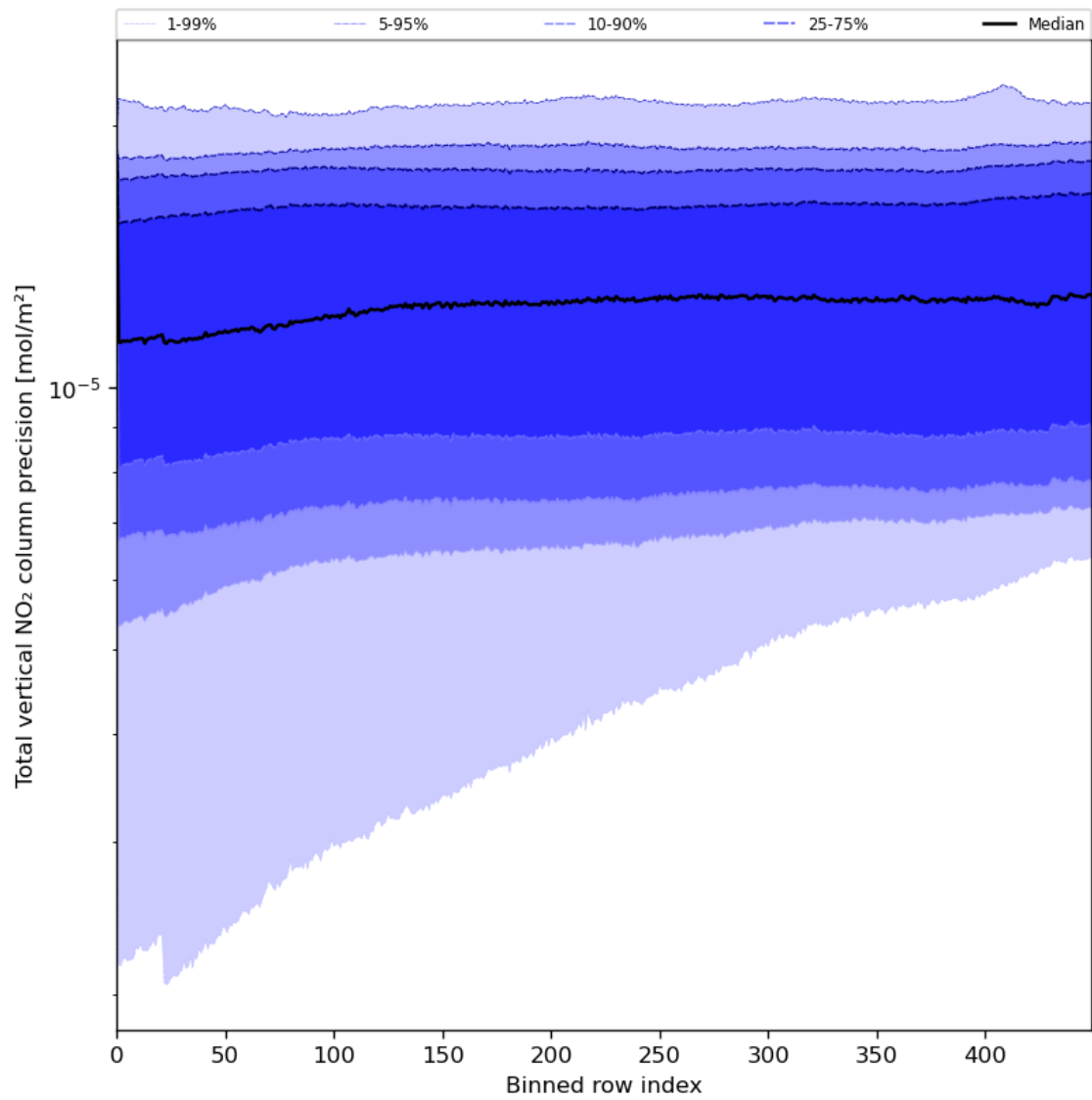
Figure 56: Along track statistics of “Total vertical NO 2 column precision” for 2023-08-02 to 2023-08-04
