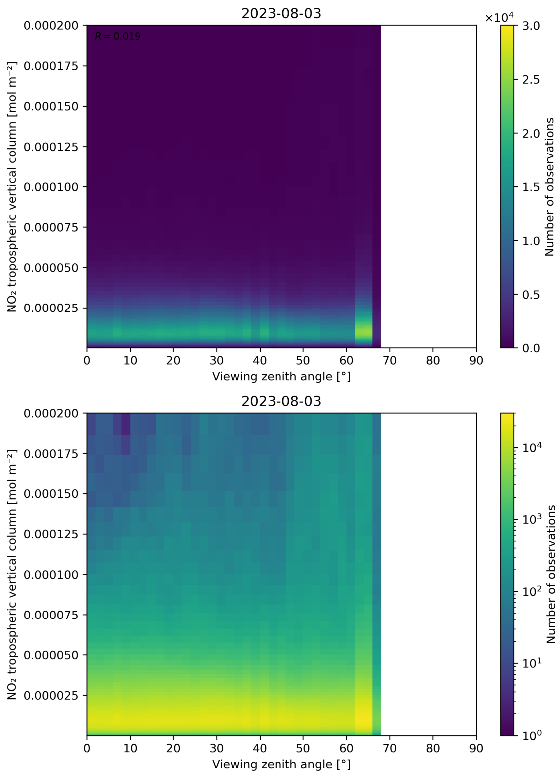
Figure 169: Scatter density plot of “Viewing zenith angle” against “NO 2 tropospheric vertical column” for 2023-08-02 to 2023-08-04.
