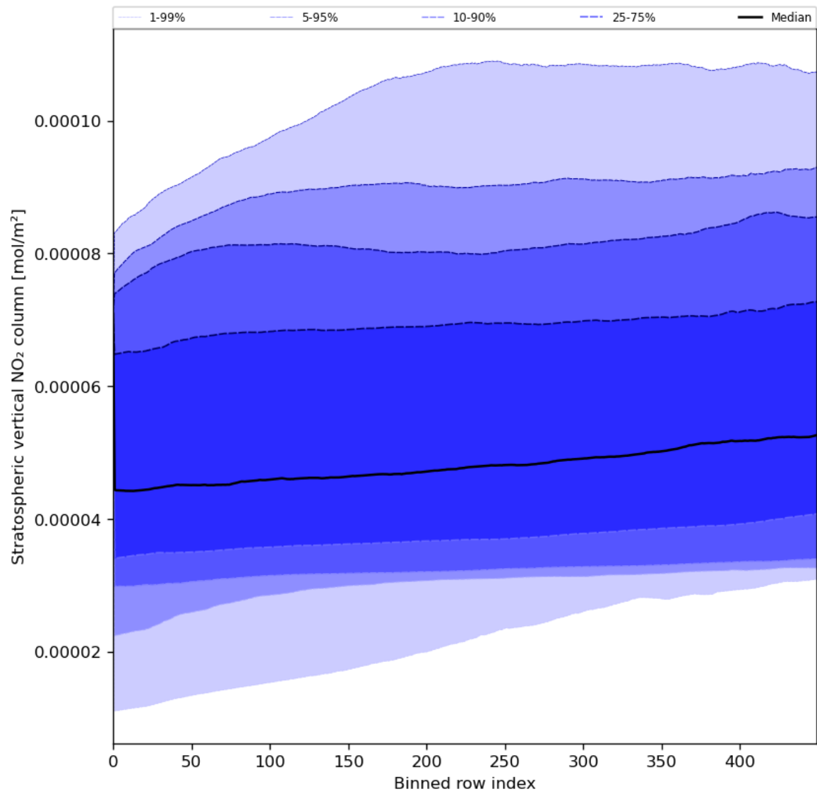
Figure 53: Along track statistics of “Stratospheric vertical NO 2 column” for 2023-08-02 to 2023-08-04
