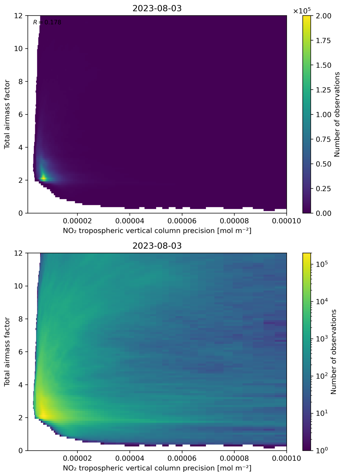
Figure 132: Scatter density plot of “NO 2 tropospheric vertical column precision” against “Total air mass factor” for 2023-08-02 to 2023-08-04.
