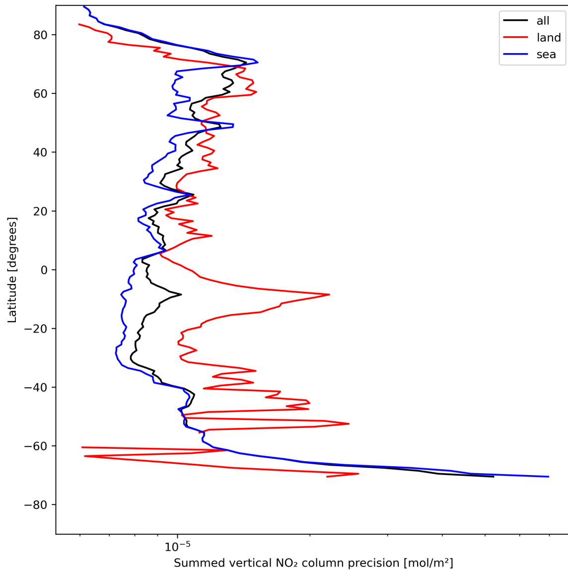
Figure 24: Zonal average of “Summed vertical NO 2 column precision” for 2023-08-02 to 2023-08-04.
