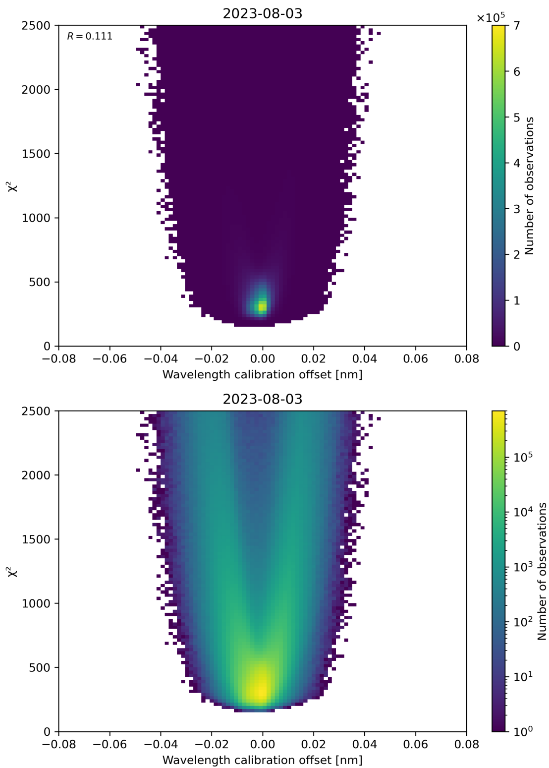
Figure 175: Scatter density plot of “Wavelength calibration offset” against “ \chi^2 ” for 2023-08-02 to 2023-08-04.
