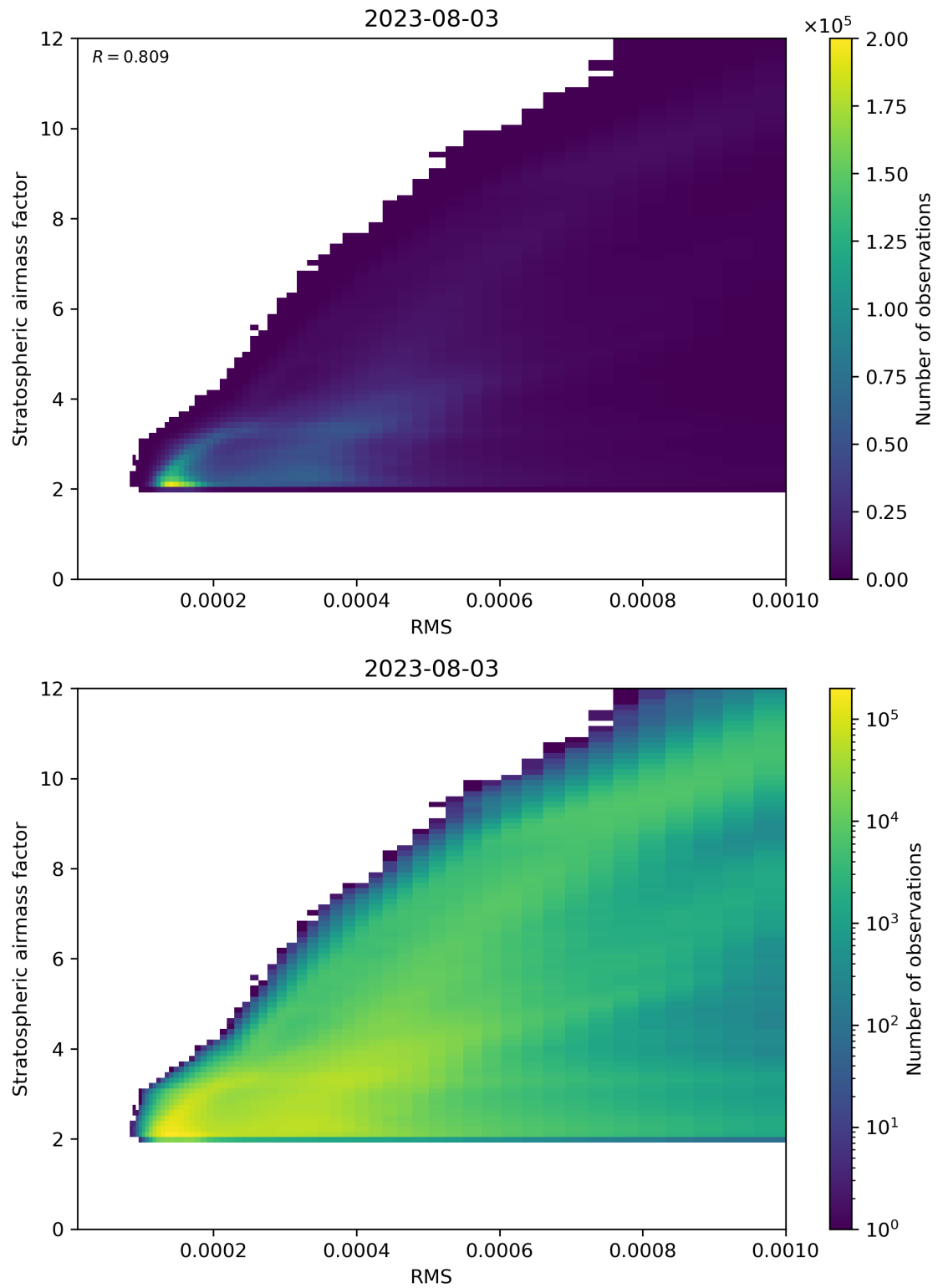
Figure 144: Scatter density plot of “RMS” against “Stratospheric airmass factor” for 2023-08-02 to 2023-08-04.
