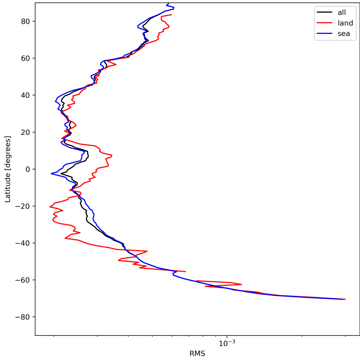
Figure 26: Zonal average of “RMS” for 2023-08-02 to 2023-08-04.
