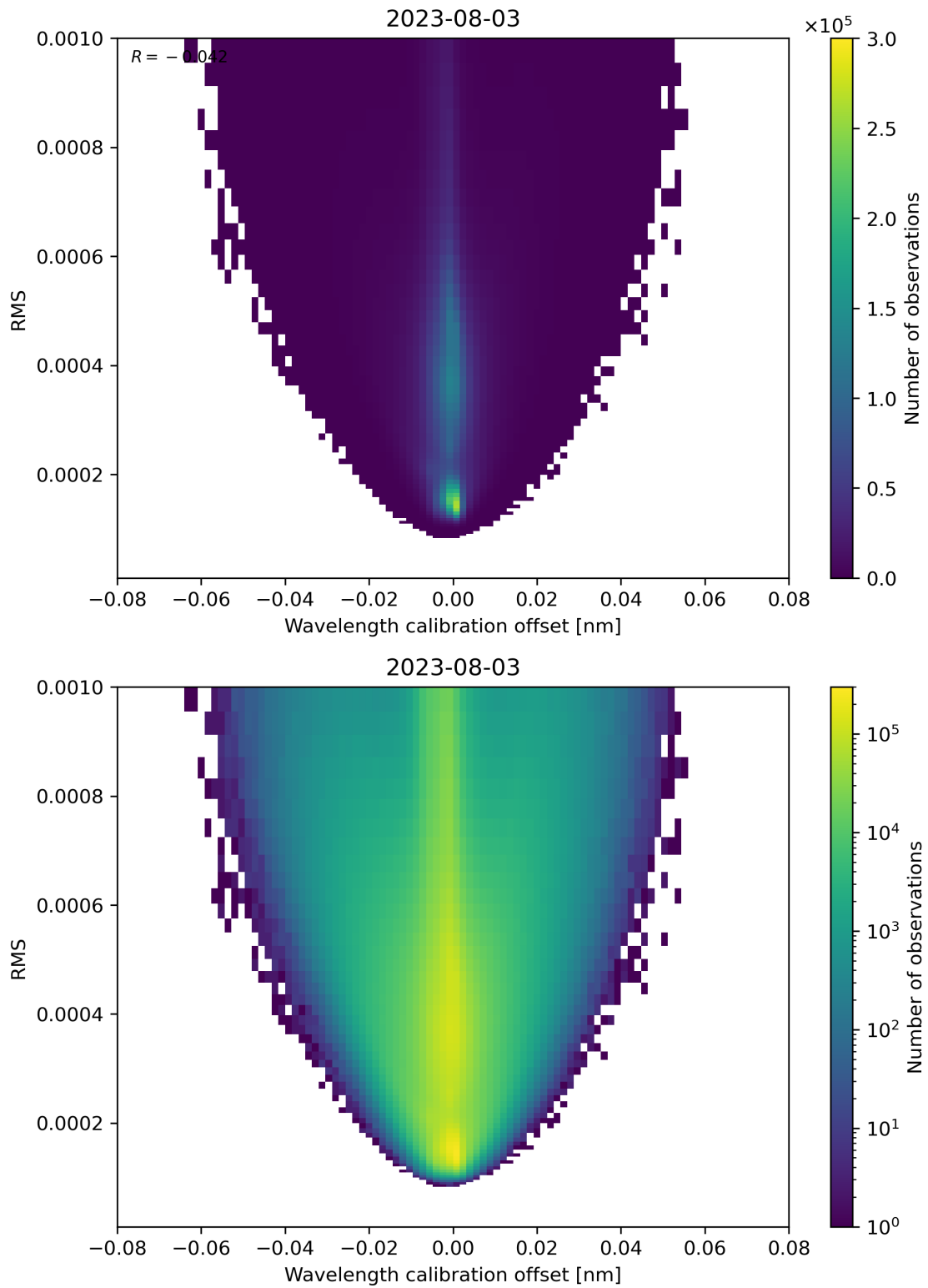
Figure 181: Scatter density plot of “Wavelength calibration offset” against “RMS” for 2023-08-02 to 2023-08-04.
