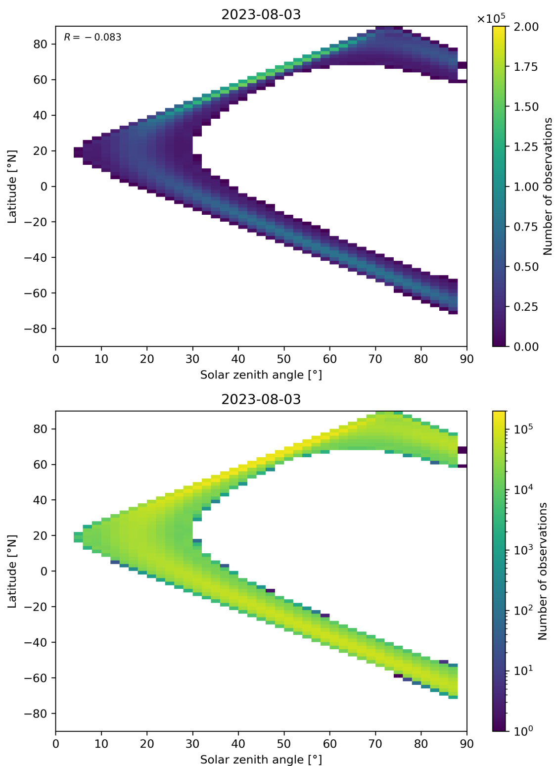
Figure 149: Scatter density plot of “Solar zenith angle” against “Latitude” for 2023-08-02 to 2023-08-04.
