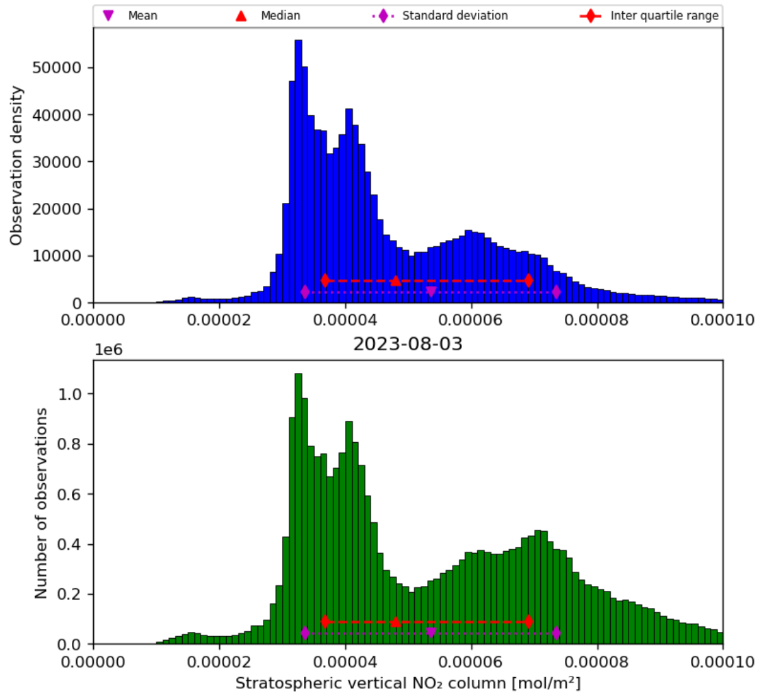
Figure 36: Histogram of “Stratospheric vertical NO 2 column” for 2023-08-02 to 2023-08-04
