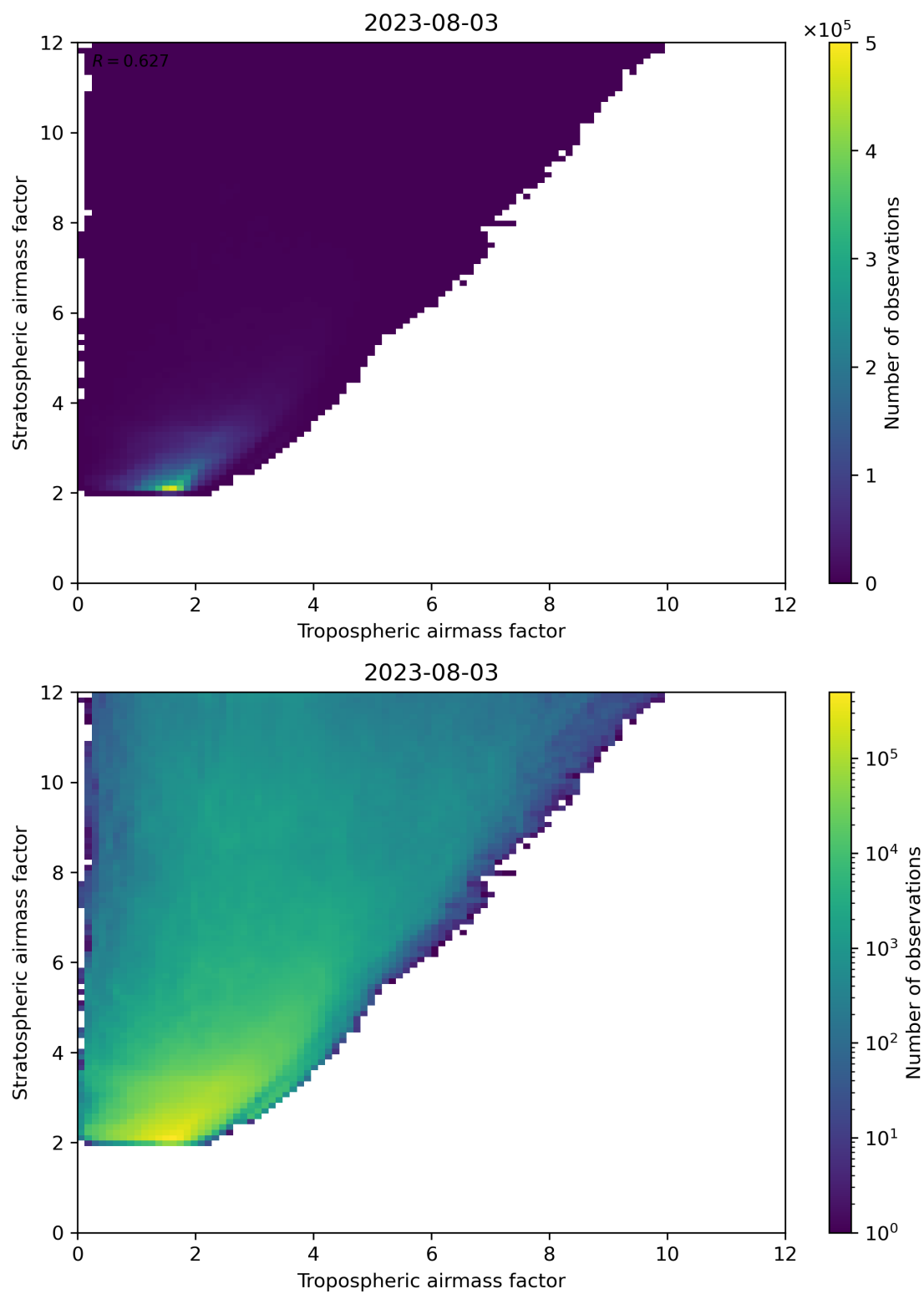
Figure 71: Scatter density plot of “Tropospheric airmass factor” against “Stratospheric airmass factor” for 2023-08-02 to 2023-08-04.
