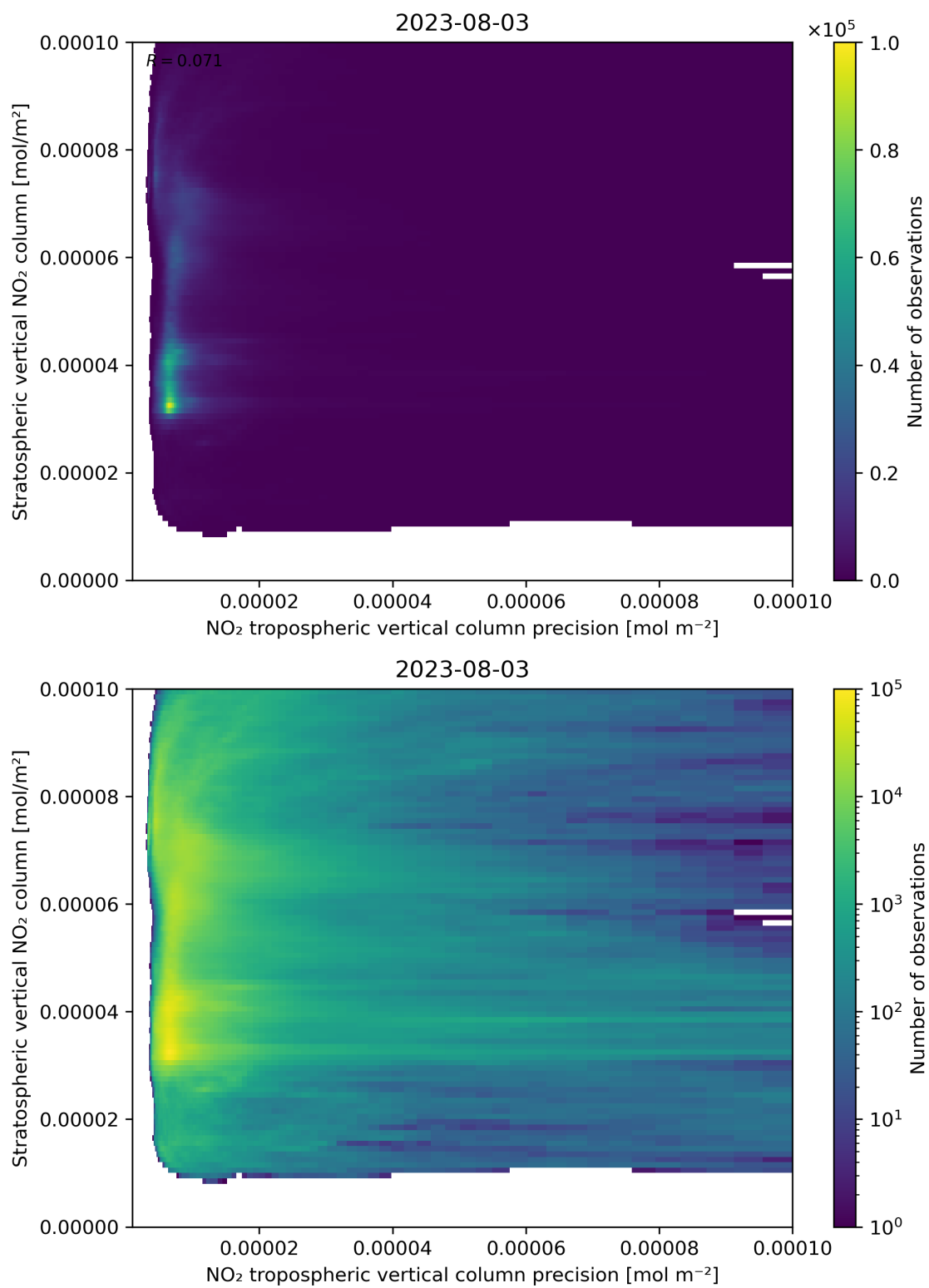
Figure 135: Scatter density plot of “NO 2 tropospheric vertical column precision” against “Stratospheric vertical NO 2 column” for 2023-08-02 to 2023-08-04.
