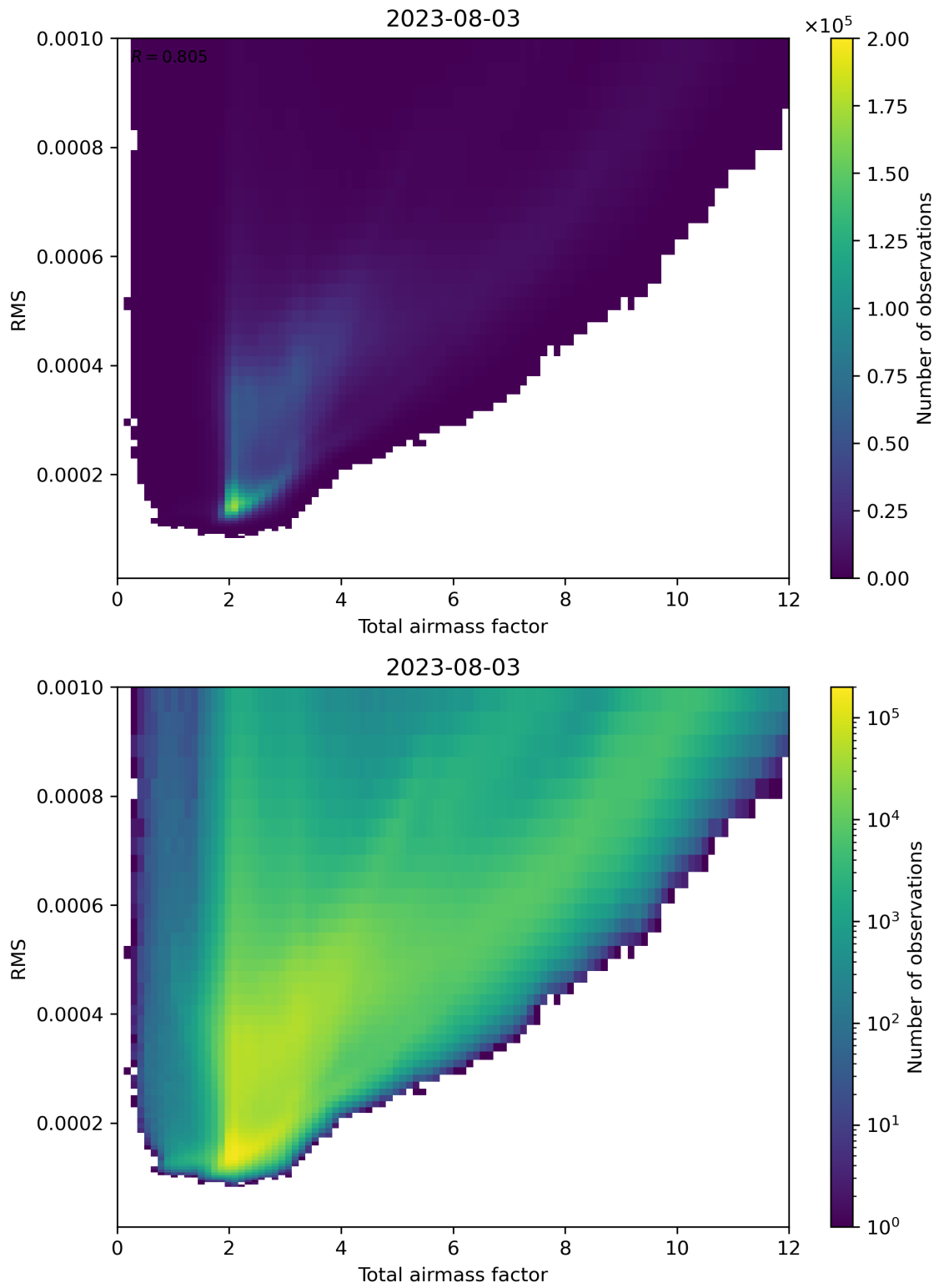
Figure 69: Scatter density plot of “Total airmass factor” against “RMS” for 2023-08-02 to 2023-08-04.
