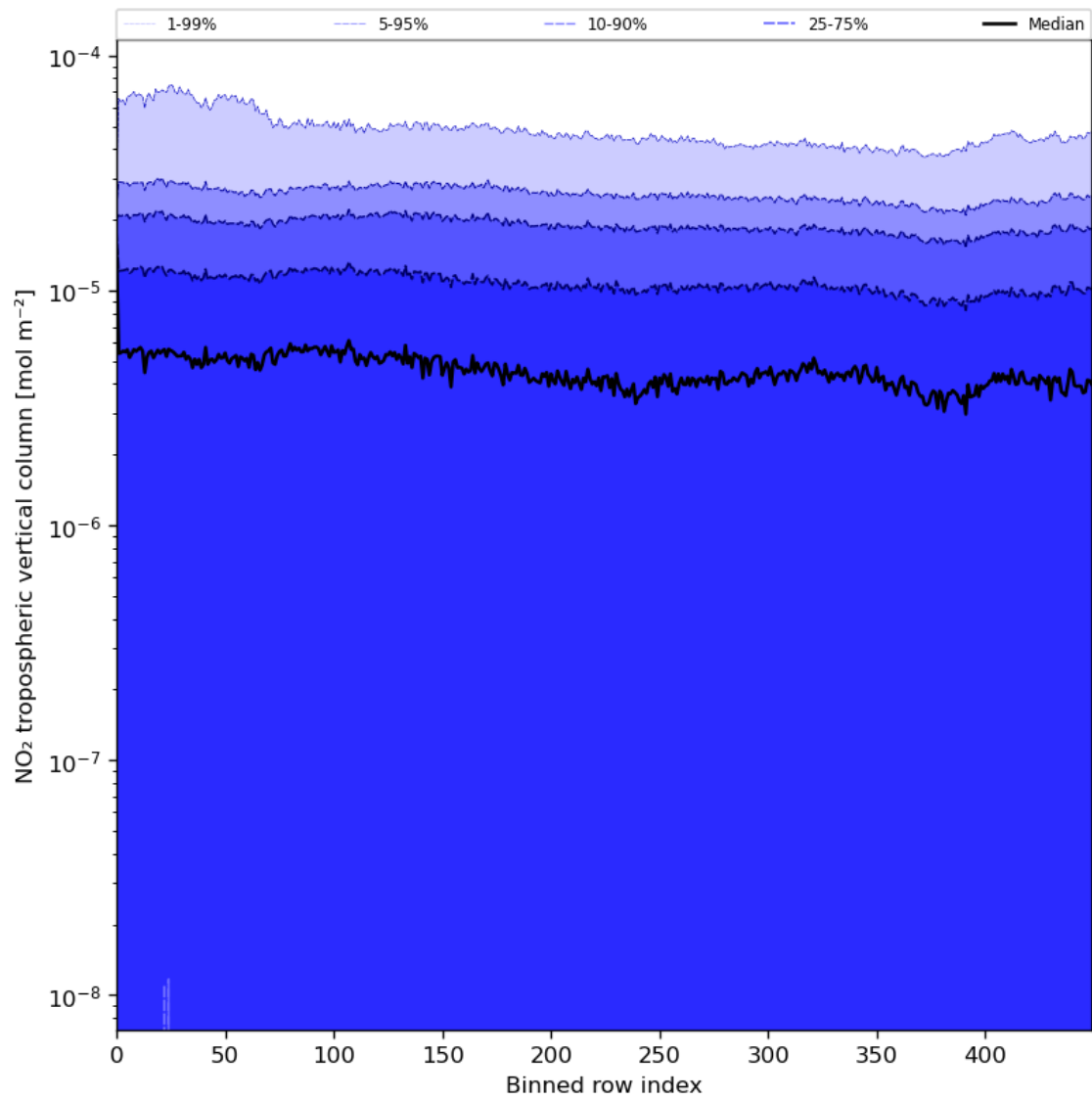
Figure 46: Along track statistics of "NO 2 tropospheric vertical column" for 2023-08-02 to 2023-08-04
