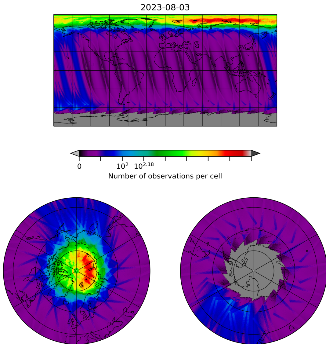
Figure 10: Map of the number of observations for 2023-08-02 to 2023-08-04
