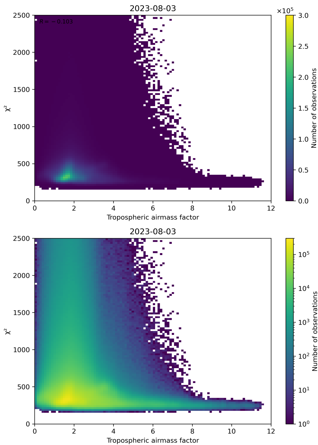
Figure 73: Scatter density plot of “Tropospheric airmass factor” against “ \chi^2 ” for 2023-08-02 to 2023-08-04.
