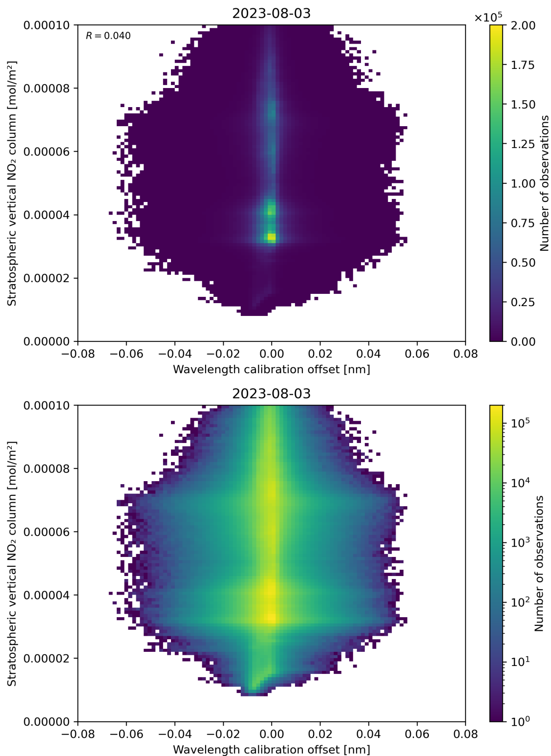
Figure 176: Scatter density plot of “Wavelength calibration offset” against “Stratospheric vertical NO 2 column” for 2023-08-02 to 2023-08-04.
