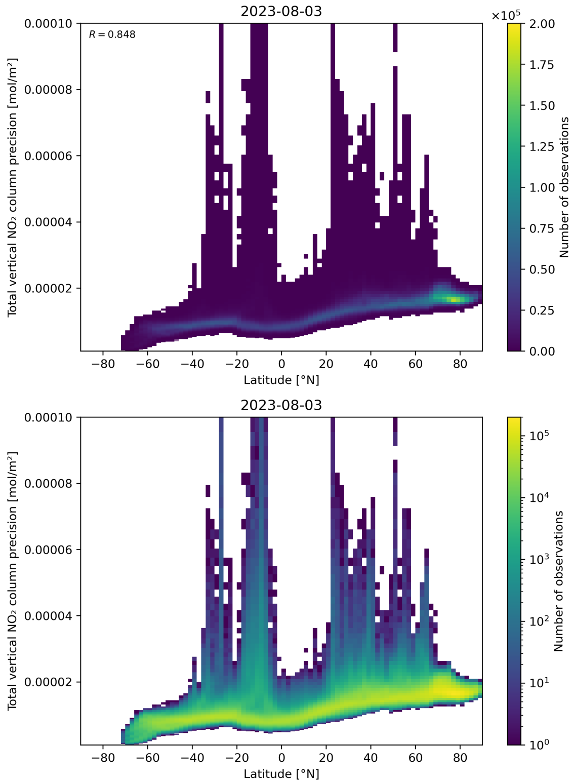
Figure 91: Scatter density plot of “Latitude” against “Total vertical NO 2 column precision” for 2023-08-02 to 2023-08-04.
