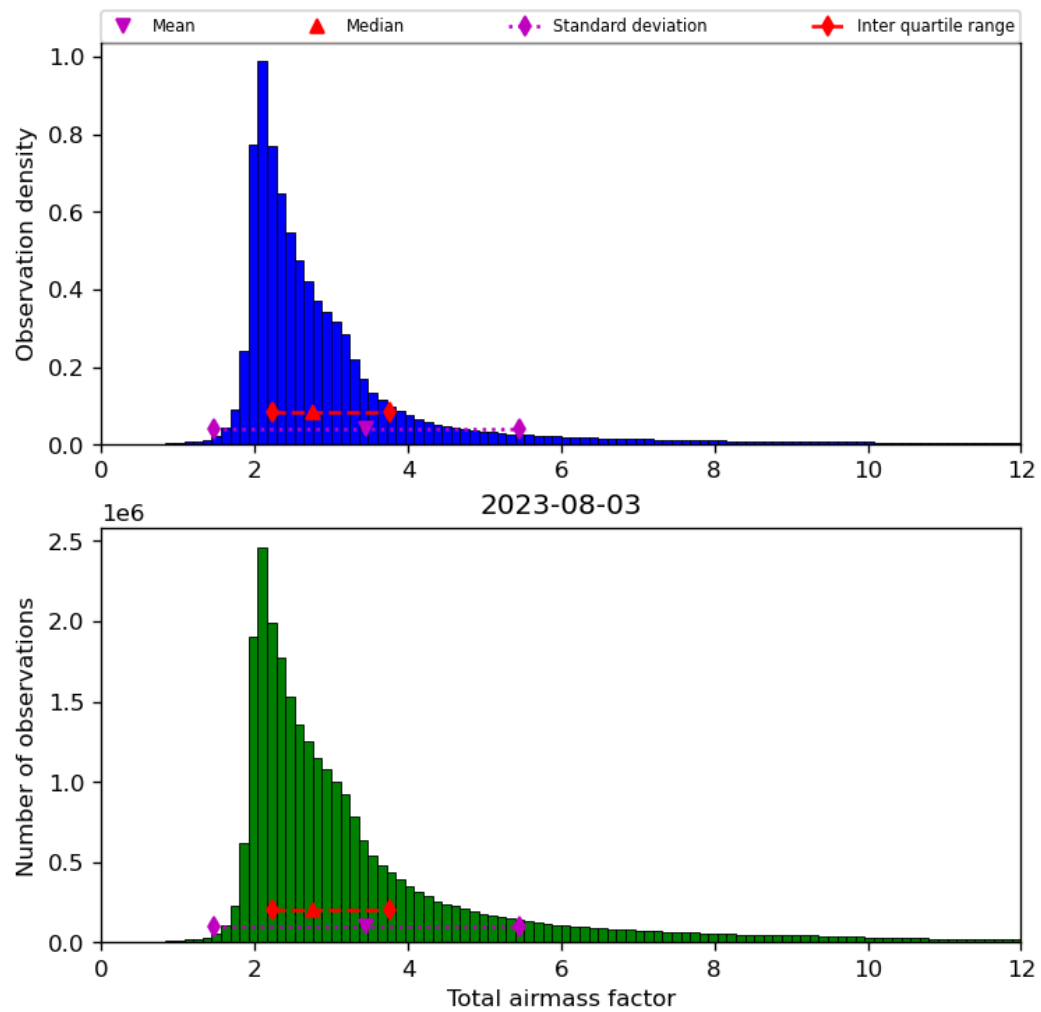
Figure 32: Histogram of “Total airmass factor” for 2023-08-02 to 2023-08-04
