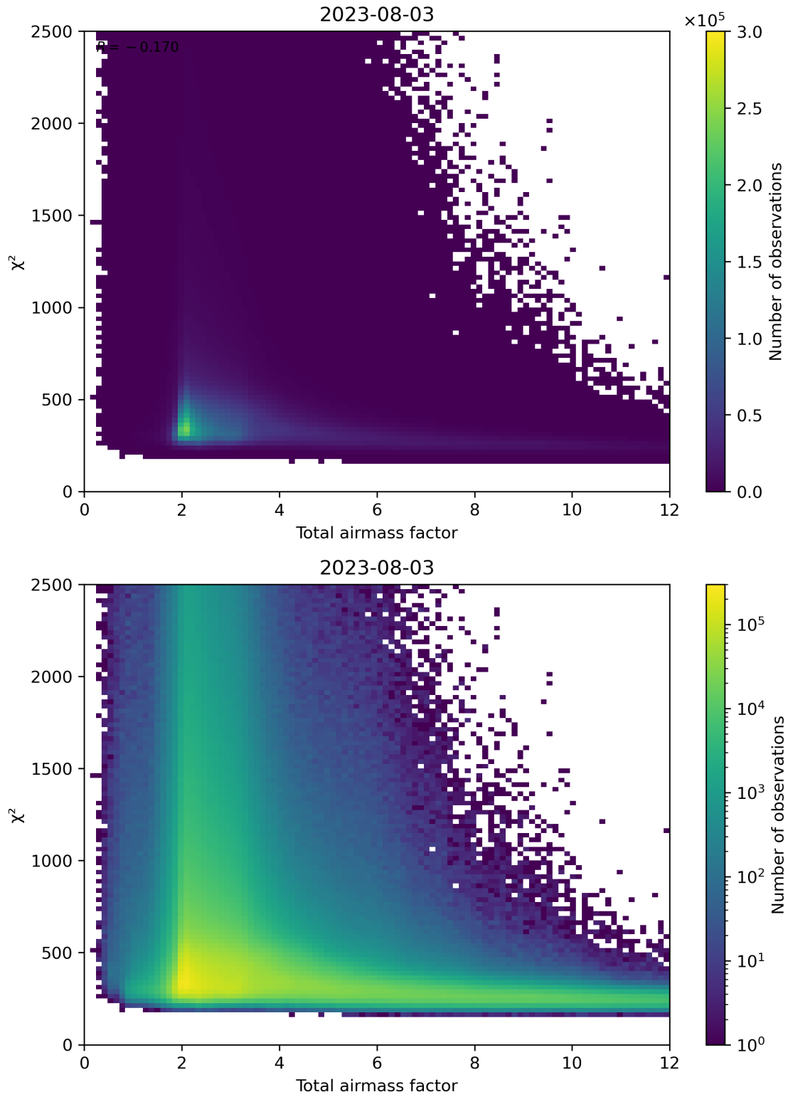
Figure 63: Scatter density plot of “Total airmass factor” against “ \chi^2 ” for 2023-08-02 to 2023-08-04.
