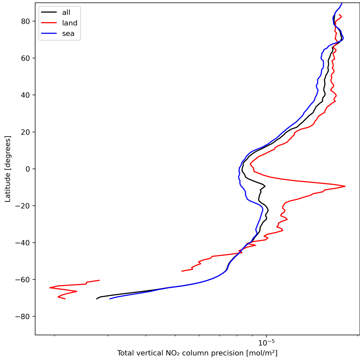
Figure 22: Zonal average of “Total vertical NO 2 column precision” for 2023-08-02 to 2023-08-04.
