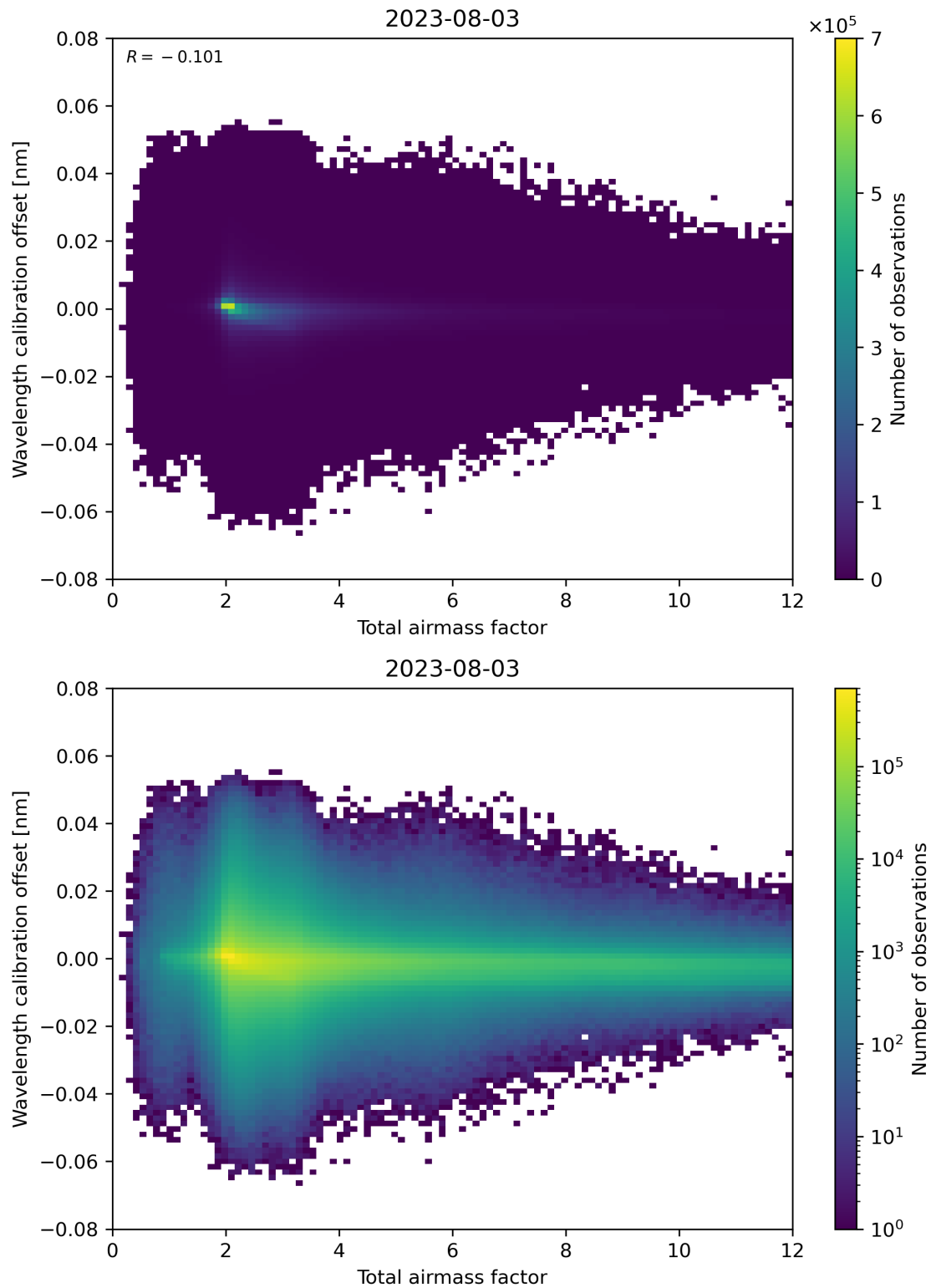
Figure 70: Scatter density plot of “Total airmass factor” against “Wavelength calibration offset” for 2023-08-02 to 2023-08-04.
