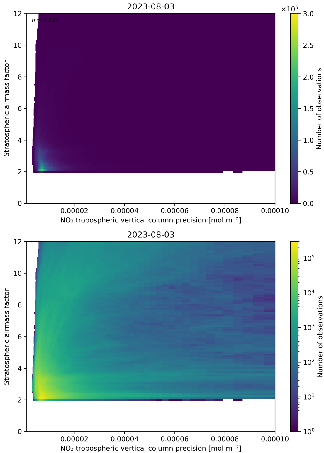
Figure 131: Scatter density plot of “NO 2 tropospheric vertical column precision” against “Stratospheric airmass factor” for 2023-08-02 to 2023-08-04.
