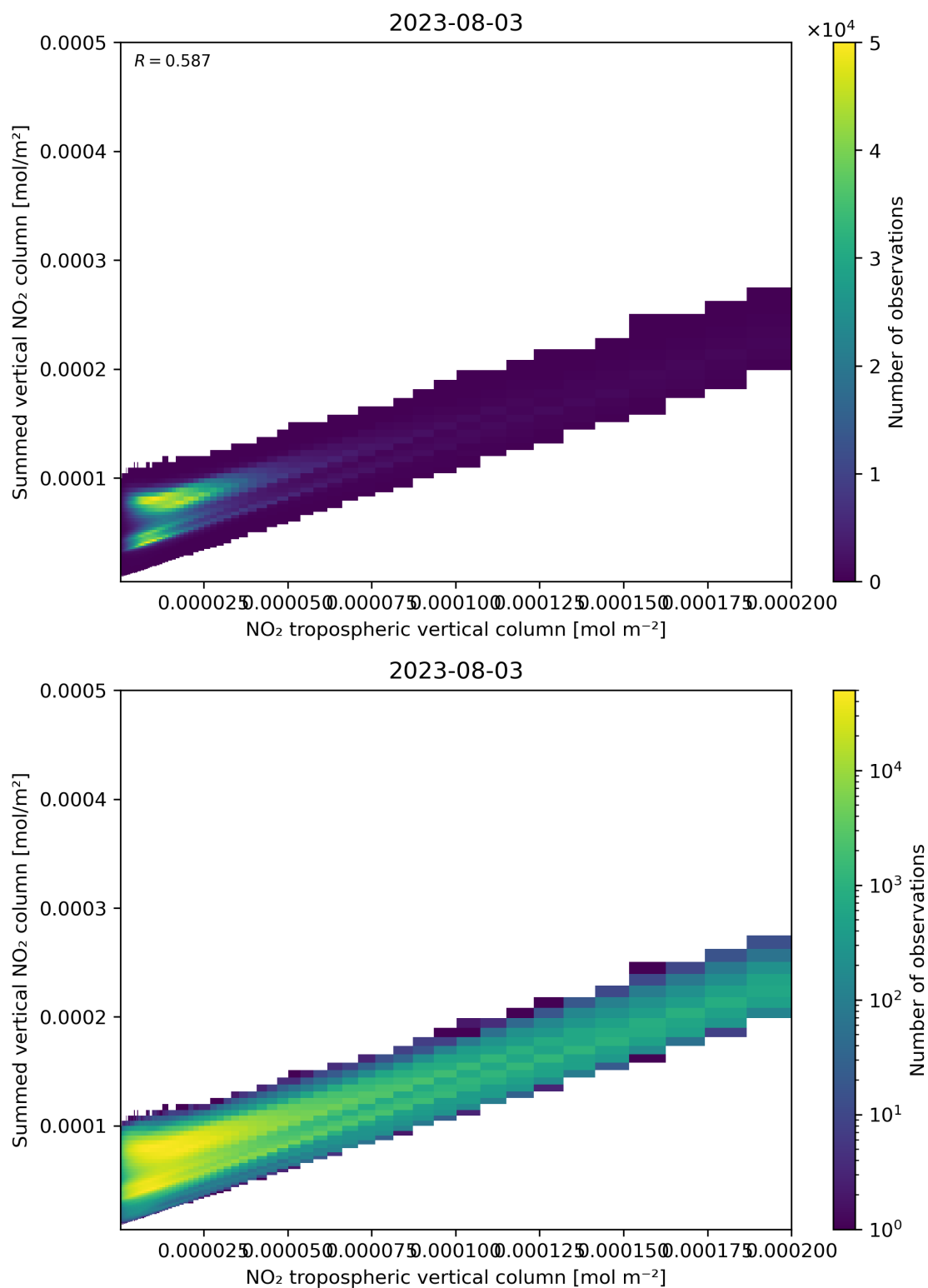
Figure 126: Scatter density plot of “NO 2 tropospheric vertical column” against “Summed vertical NO 2 column” for 2023-08-02 to 2023-08-04.
