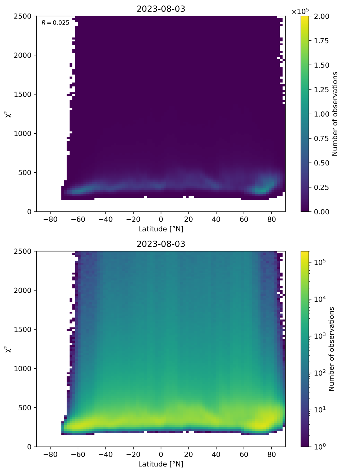
Figure 86: Scatter density plot of “Latitude” against “ \chi^2 ” for 2023-08-02 to 2023-08-04.
