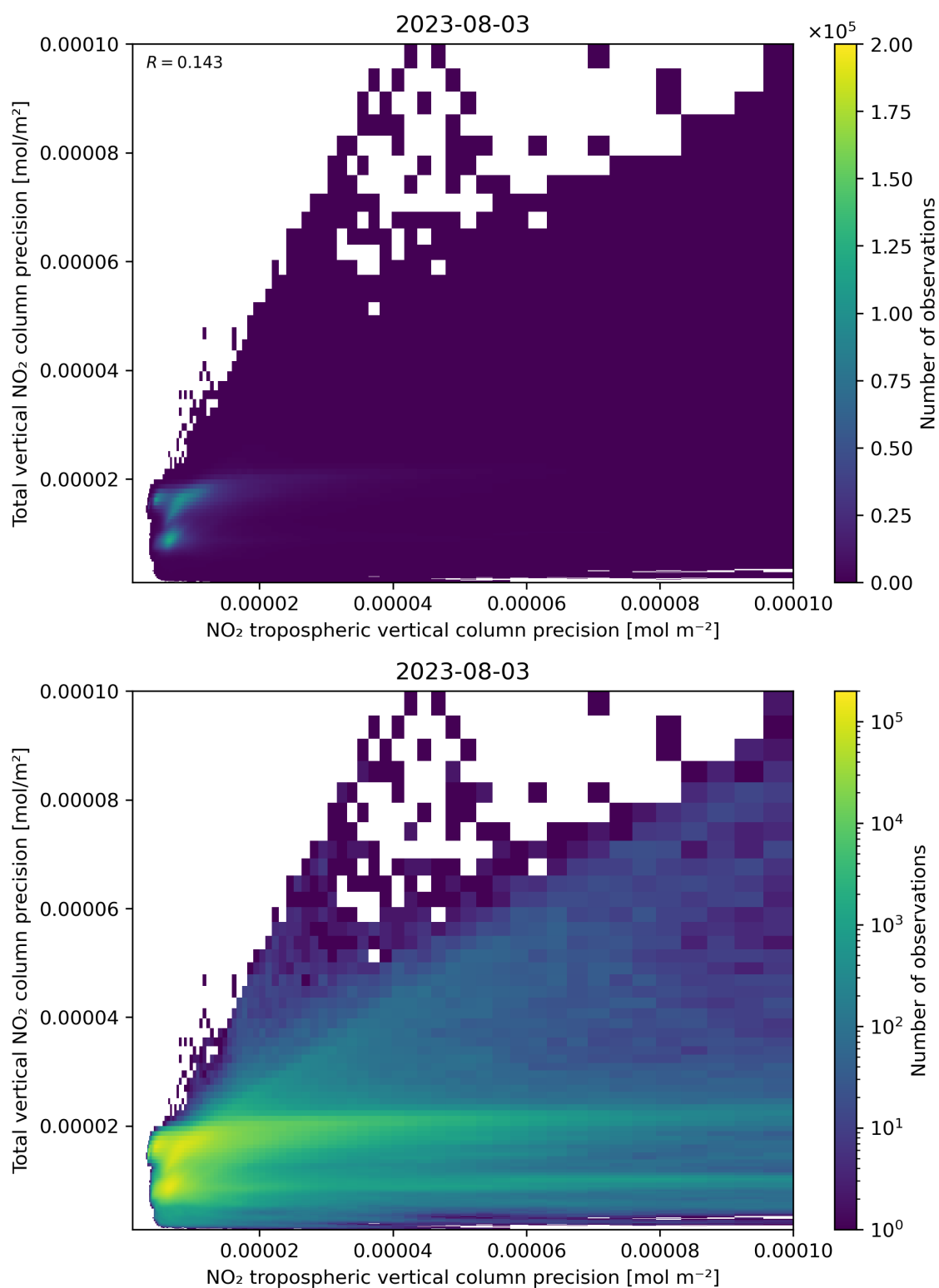
Figure 139: Scatter density plot of “NO 2 tropospheric vertical column precision” against “Total vertical NO 2 column precision” for 2023-08-02 to 2023-08-04.
