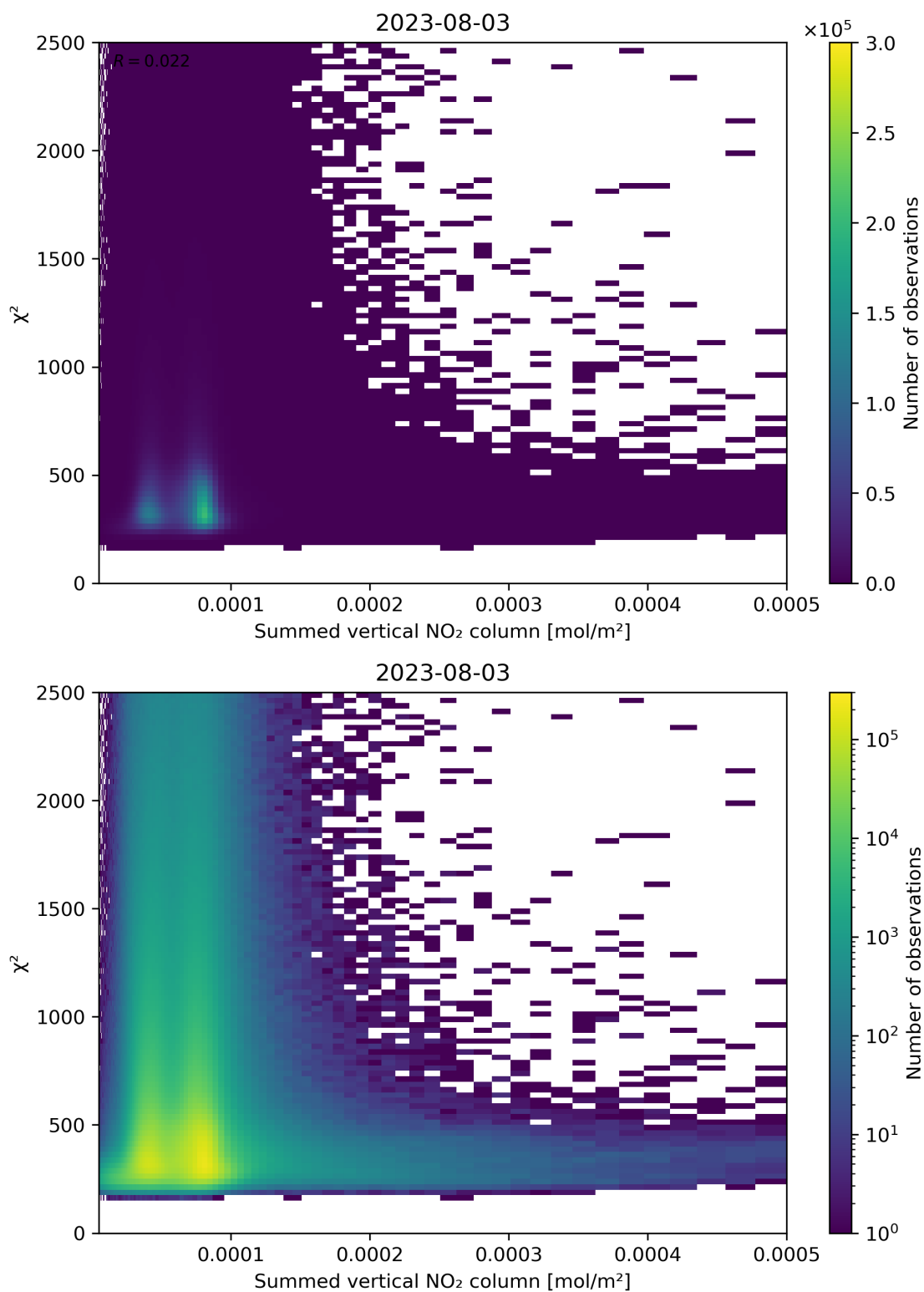
Figure 104: Scatter density plot of “Summed vertical NO 2 column” against “ \chi^2 ” for 2023-08-02 to 2023-08-04.
