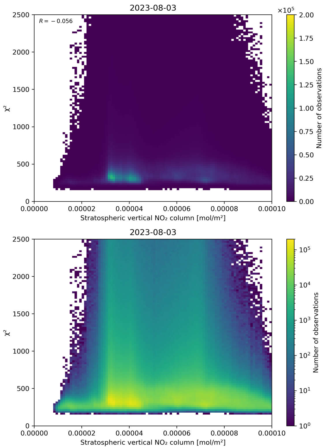
Figure 97: Scatter density plot of “Stratospheric vertical NO 2 column” against “ \chi^2 ” for 2023-08-02 to 2023-08-04.
