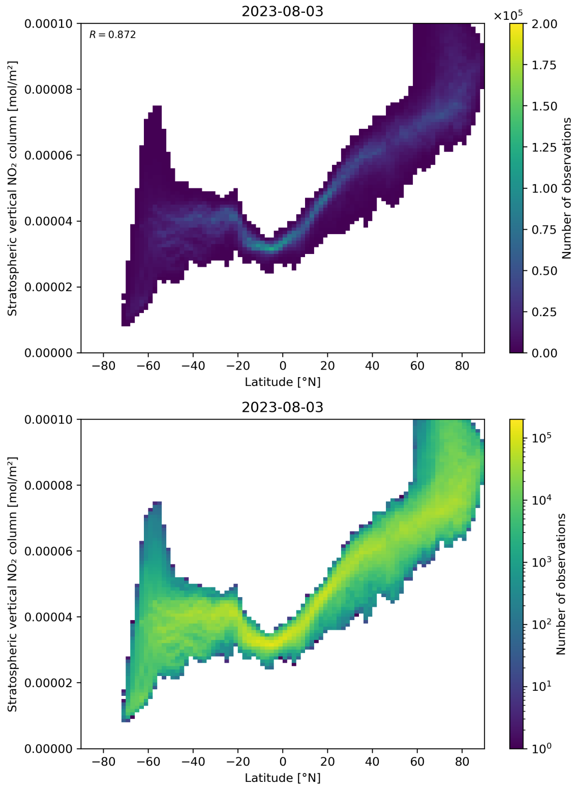
Figure 87: Scatter density plot of “Latitude” against “Stratospheric vertical NO 2 column” for 2023-08-02 to 2023-08-04.
