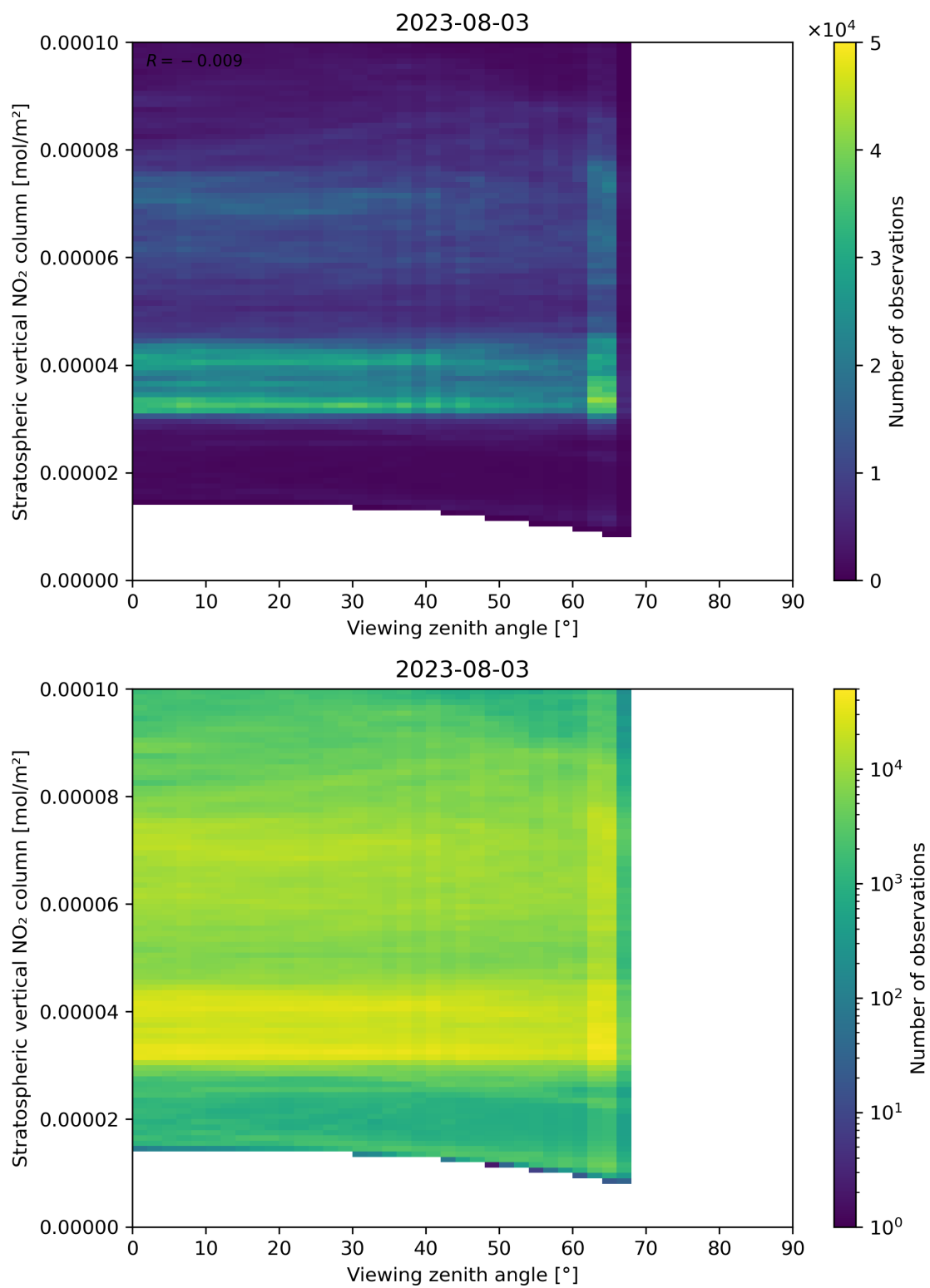
Figure 164: Scatter density plot of “Viewing zenith angle” against “Stratospheric vertical NO 2 column” for 2023-08-02 to 2023-08-04.
