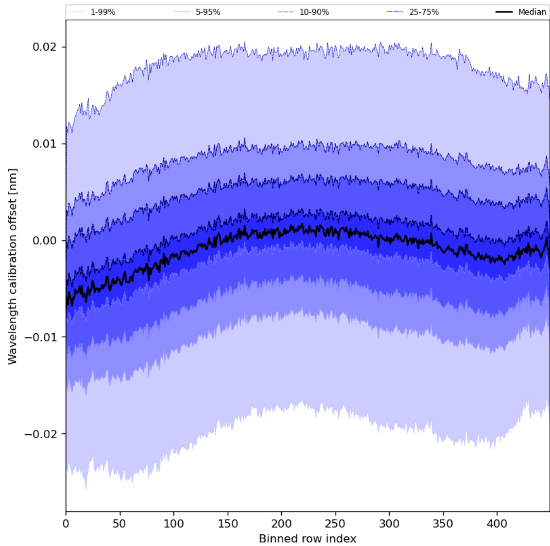
Figure 52: Along track statistics of “Wavelength calibration offset” for 2023-08-02 to 2023-08-04
