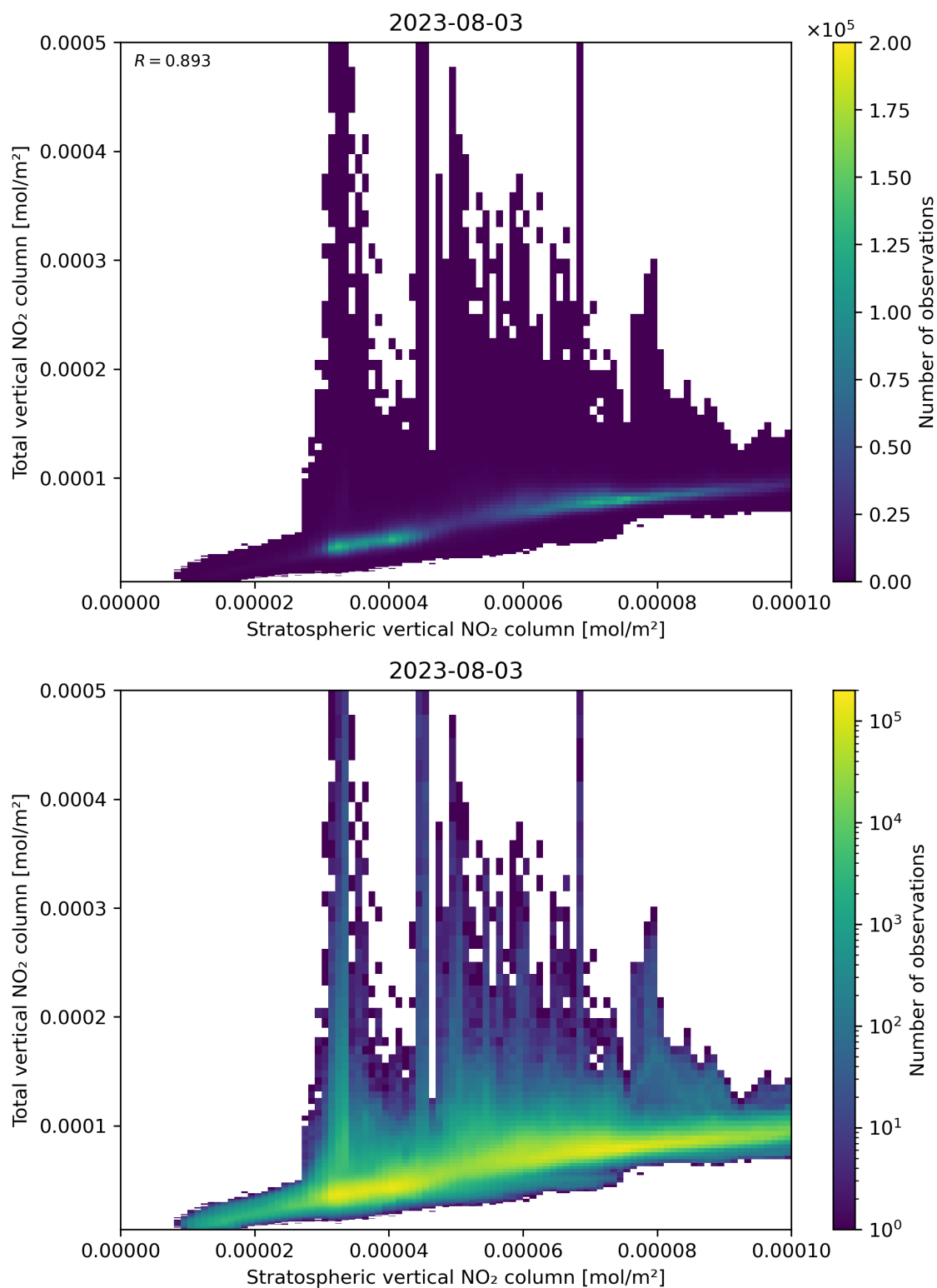
Figure 100: Scatter density plot of “Stratospheric vertical NO 2 column” against “Total vertical NO 2 column” for 2023-08-02 to 2023-08-04.
