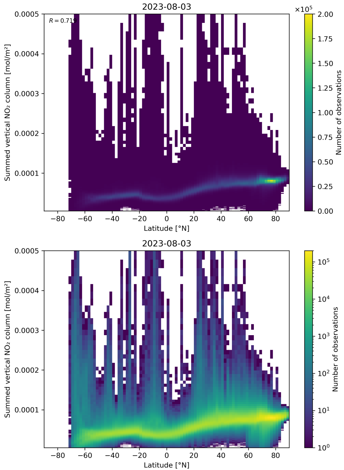
Figure 88: Scatter density plot of “Latitude” against “Summed vertical NO 2 column” for 2023-08-02 to 2023-08-04.
