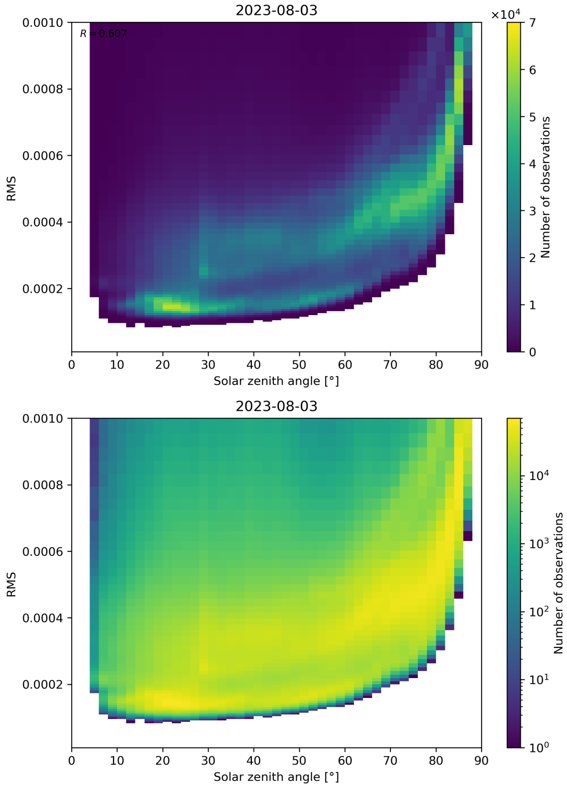
Figure 157: Scatter density plot of “Solar zenith angle” against “RMS” for 2023-08-02 to 2023-08-04.
