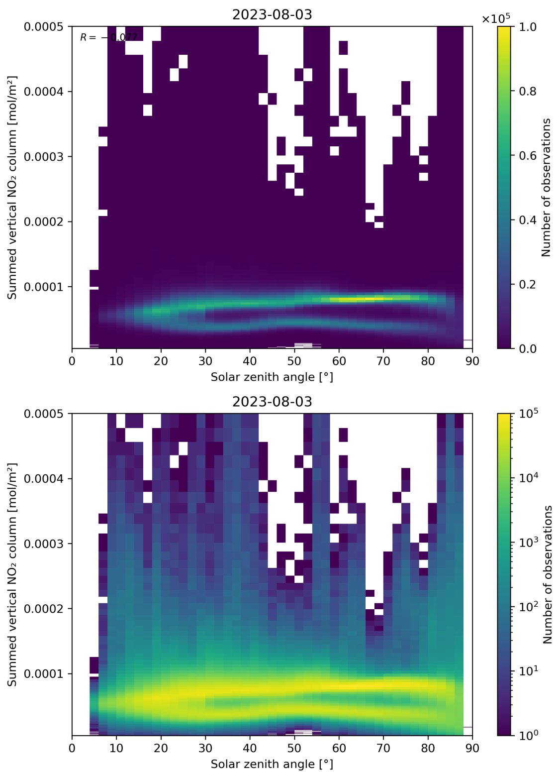
Figure 151: Scatter density plot of “Solar zenith angle” against “Summed vertical NO 2 column” for 2023-08-02 to 2023-08-04.
