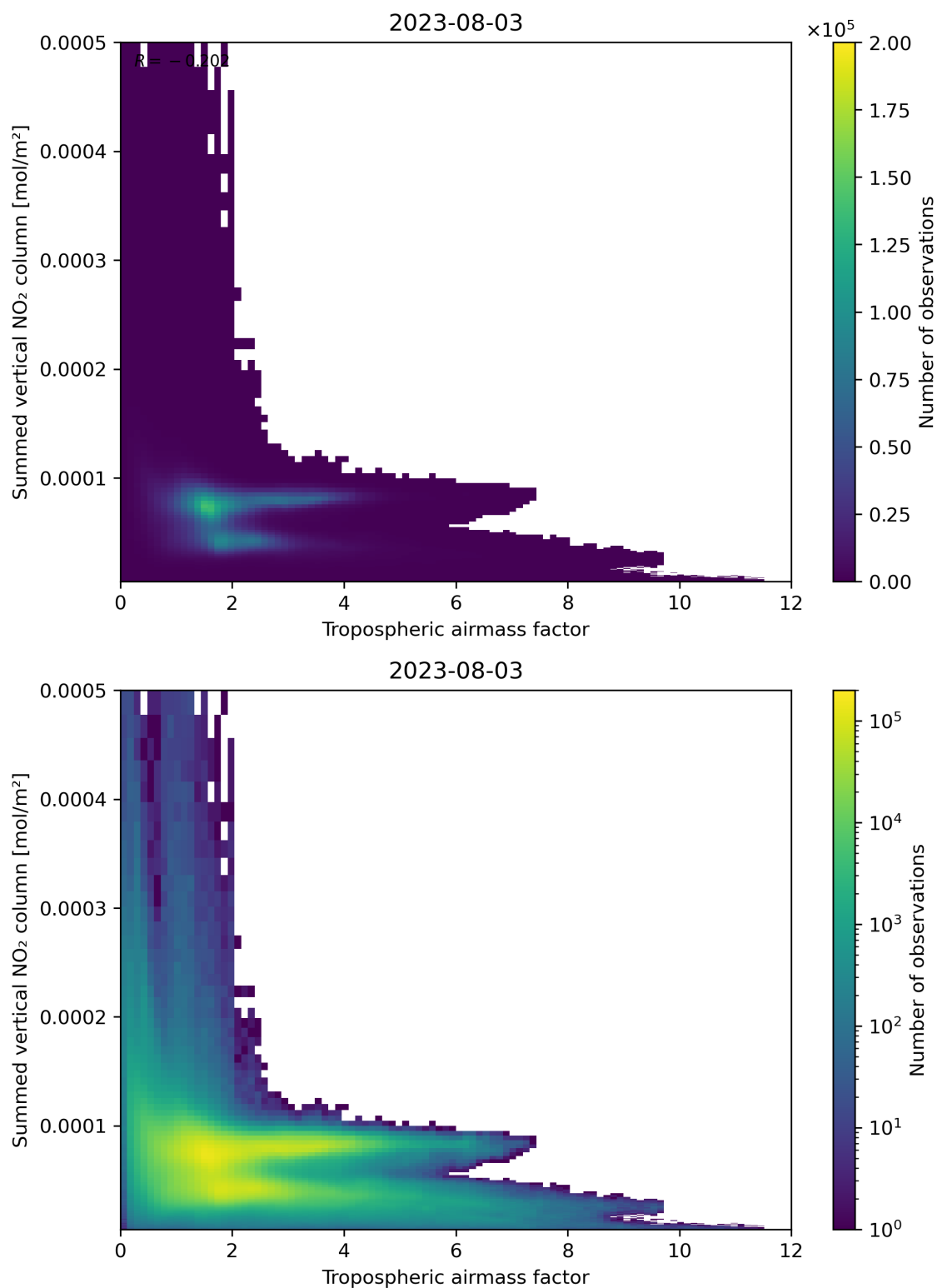
Figure 75: Scatter density plot of “Tropospheric airmass factor” against “Summed vertical NO 2 column” for 2023-08-02 to 2023-08-04.
