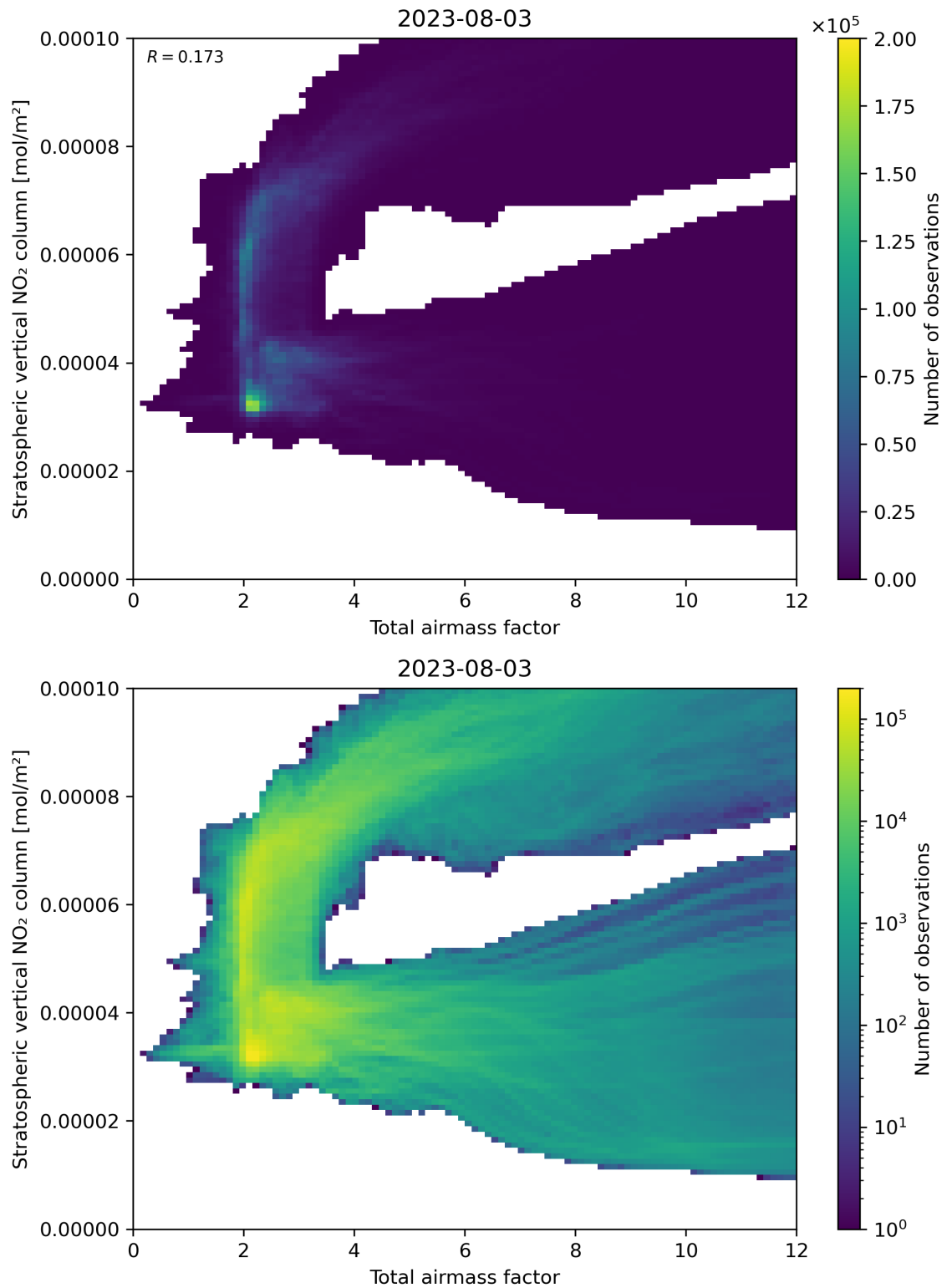
Figure 64: Scatter density plot of “Total airmass factor” against “Stratospheric vertical \text{NO}_2 column” for 2023-08-02 to 2023-08-04.
