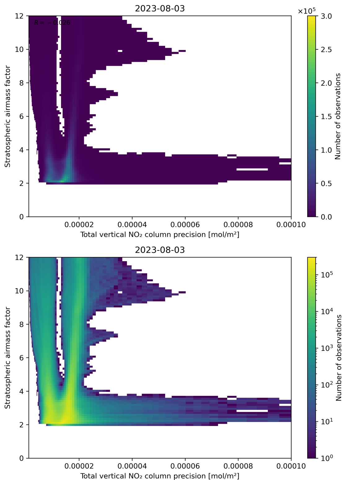
Figure 115: Scatter density plot of “Total vertical NO 2 column precision” against “Stratospheric air mass factor” for 2023-08-02 to 2023-08-04.
