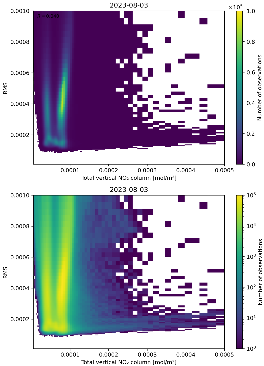
Figure 120: Scatter density plot of “Total vertical NO 2 column” against “RMS” for 2023-08-02 to 2023-08-04.
