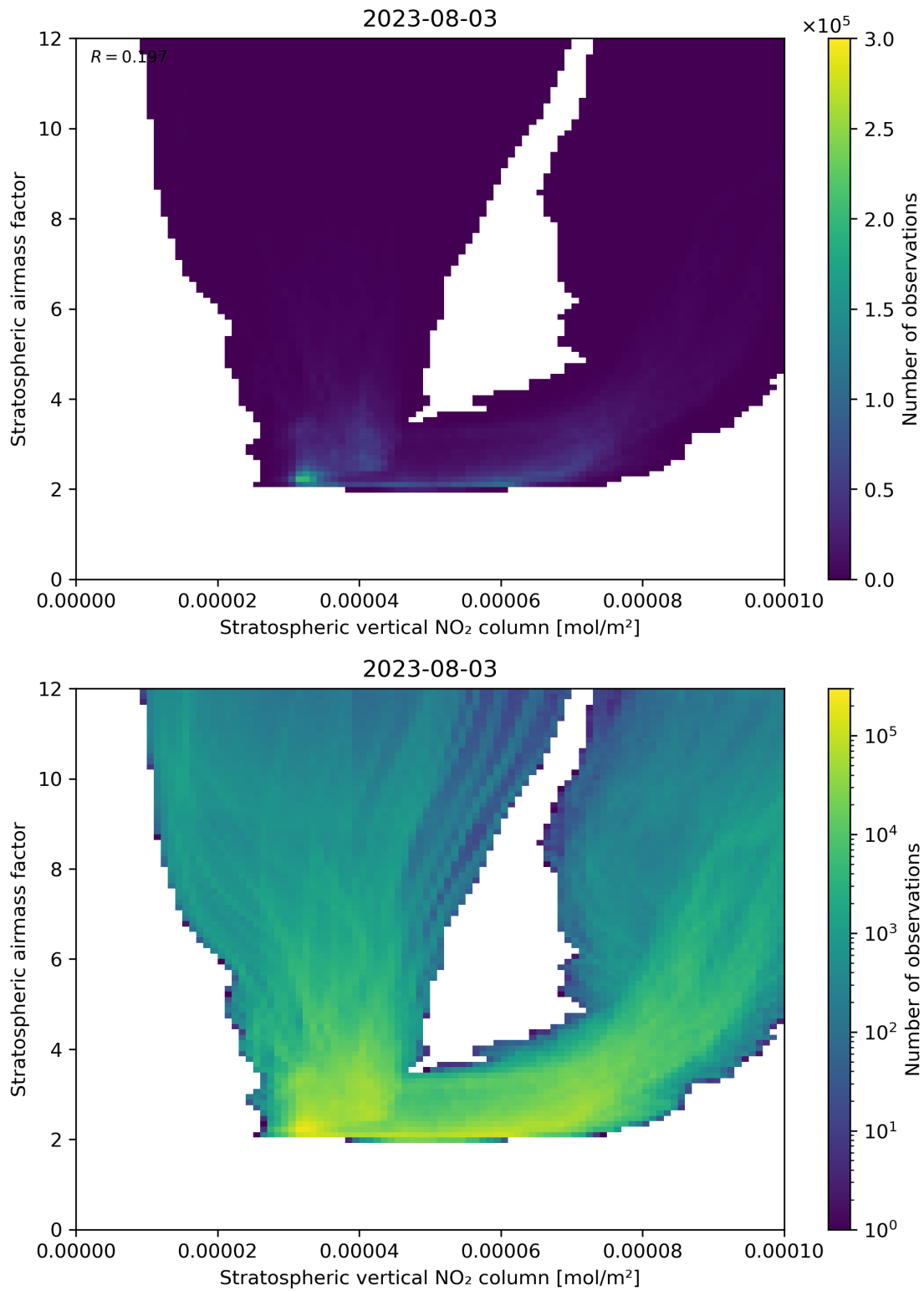
Figure 96: Scatter density plot of “Stratospheric vertical NO 2 column” against “Stratospheric airmass factor” for 2023-08-02 to 2023-08-04.
