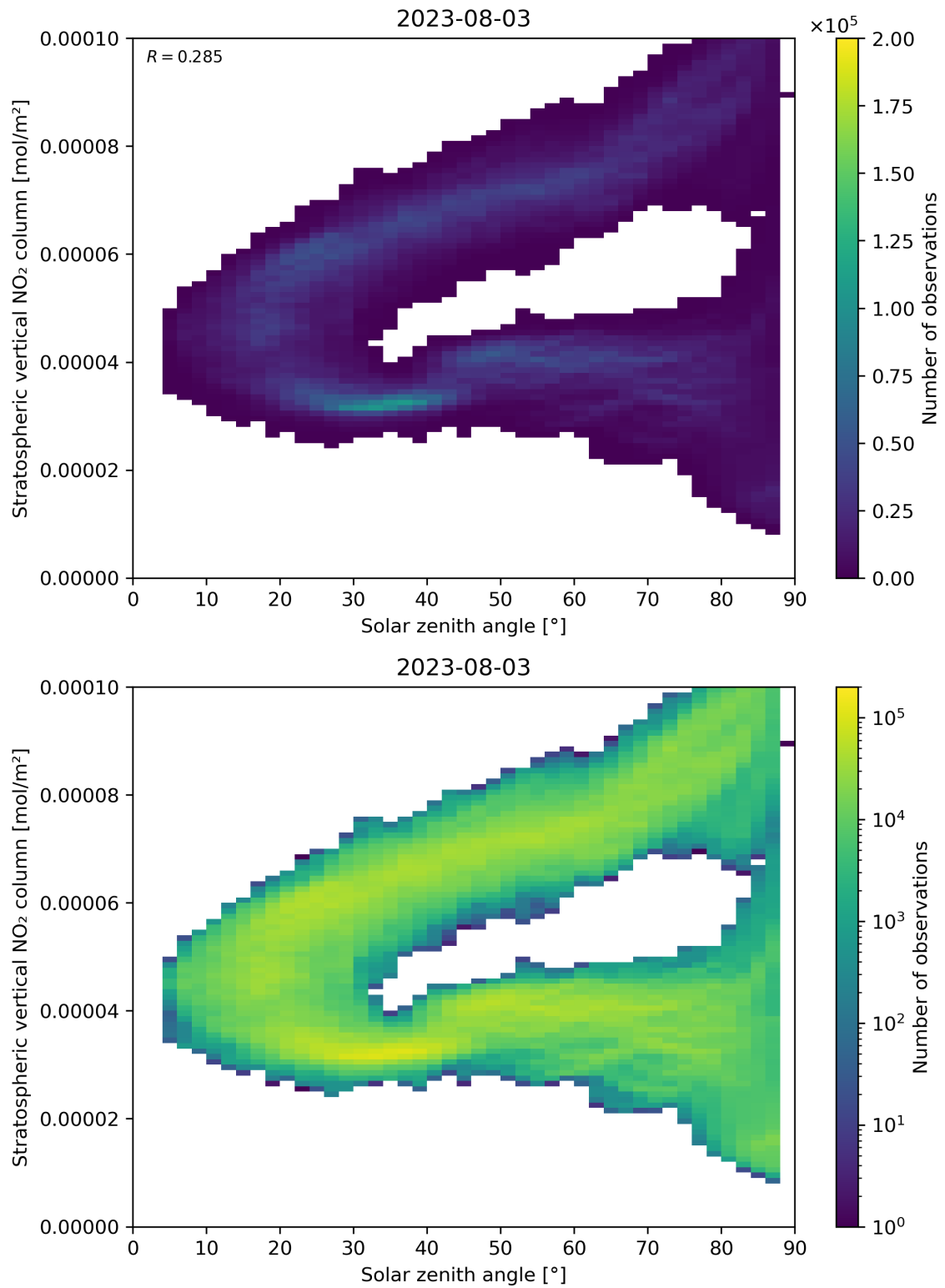
Figure 150: Scatter density plot of “Solar zenith angle” against “Stratospheric vertical NO 2 column” for 2023-08-02 to 2023-08-04.
