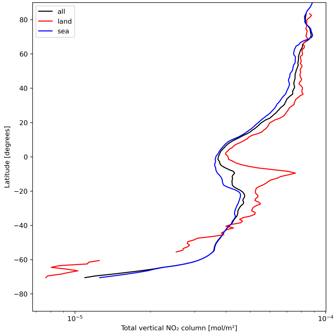
Figure 21: Zonal average of “Total vertical NO 2 column” for 2023-08-02 to 2023-08-04.
