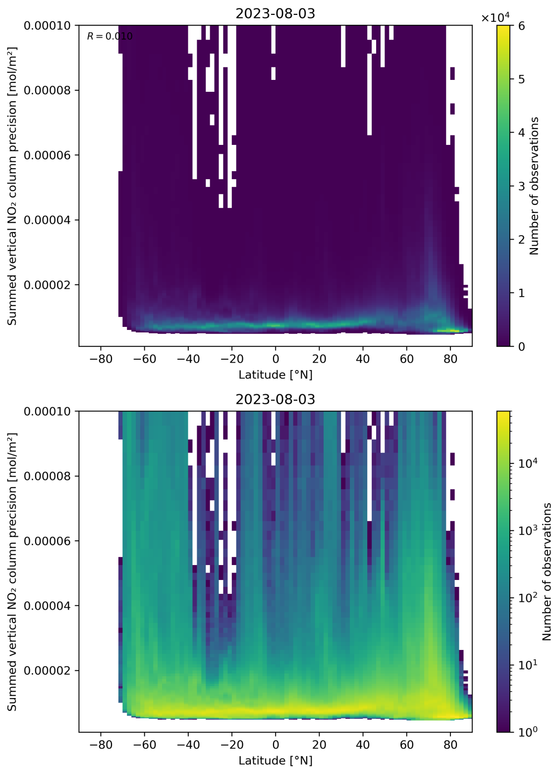
Figure 89: Scatter density plot of “Latitude” against “Summed vertical NO 2 column precision” for 2023-08-02 to 2023-08-04.
