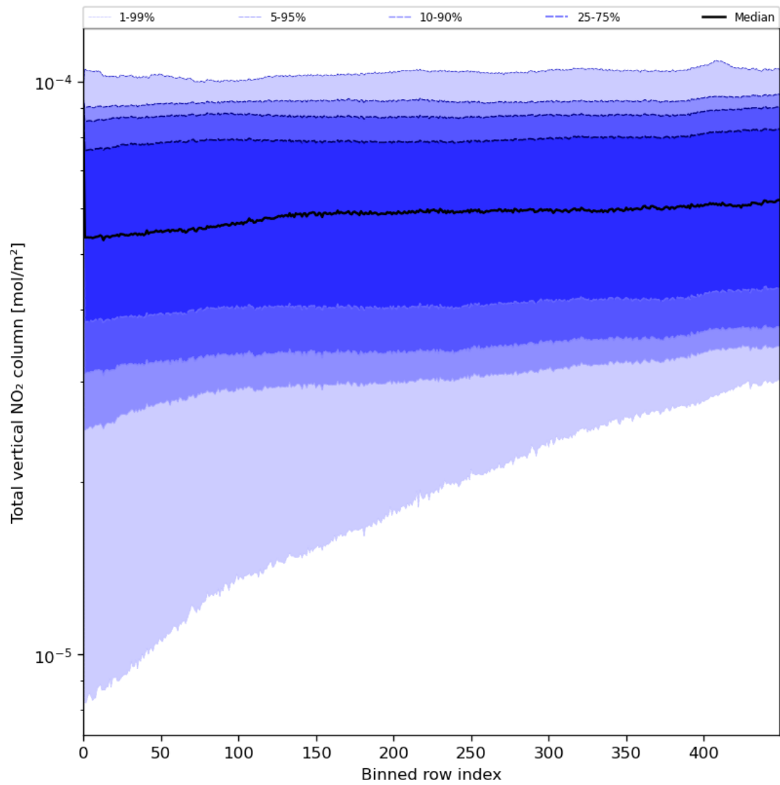
Figure 55: Along track statistics of “Total vertical NO 2 column” for 2023-08-02 to 2023-08-04
