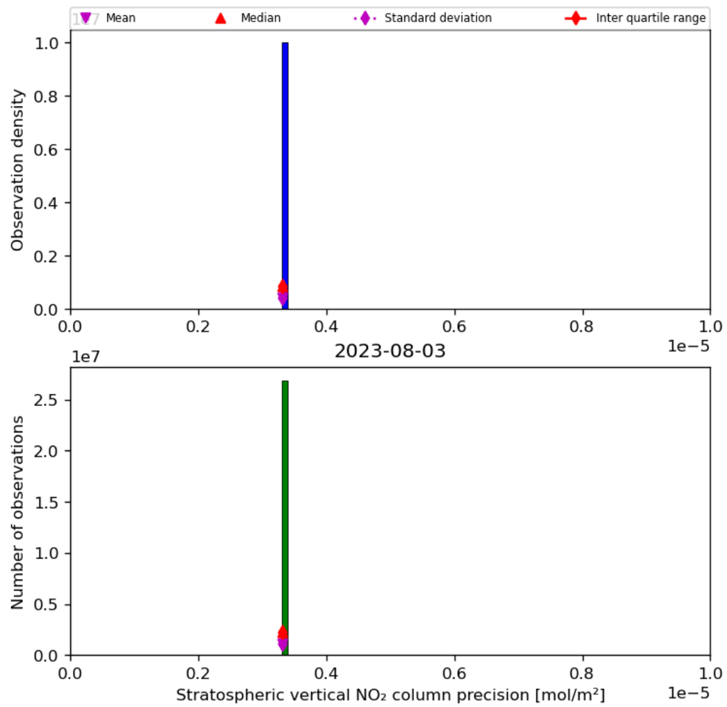
Figure 37: Histogram of “Stratospheric vertical NO 2 column precision” for 2023-08-02 to 2023-08-04
