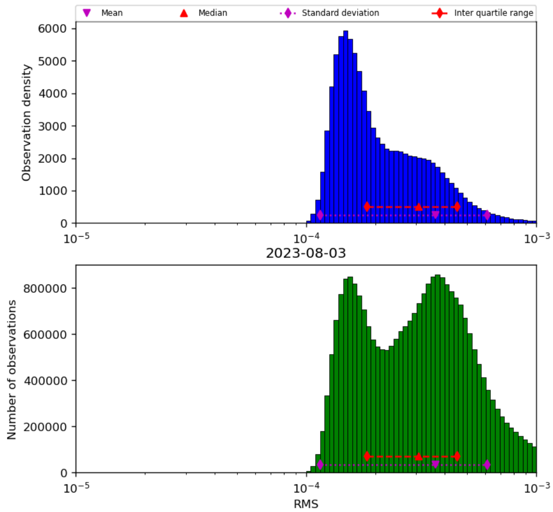
Figure 43: Histogram of “RMS” for 2023-08-02 to 2023-08-04
