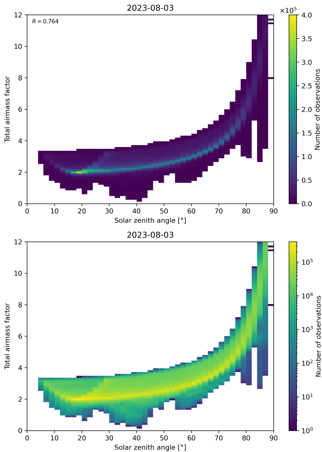
Figure 146: Scatter density plot of “Solar zenith angle” against “Total air mass factor” for 2023-08-02 to 2023-08-04.
