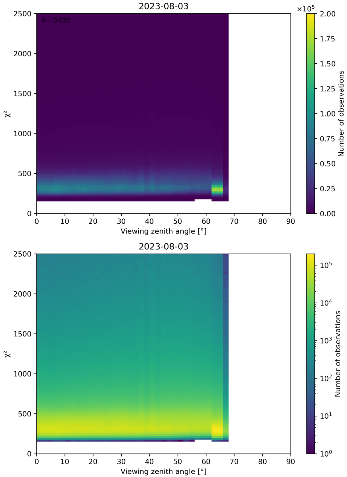
Figure 162: Scatter density plot of “Viewing zenith angle” against “ \chi^2 ” for 2023-08-02 to 2023-08-04.
