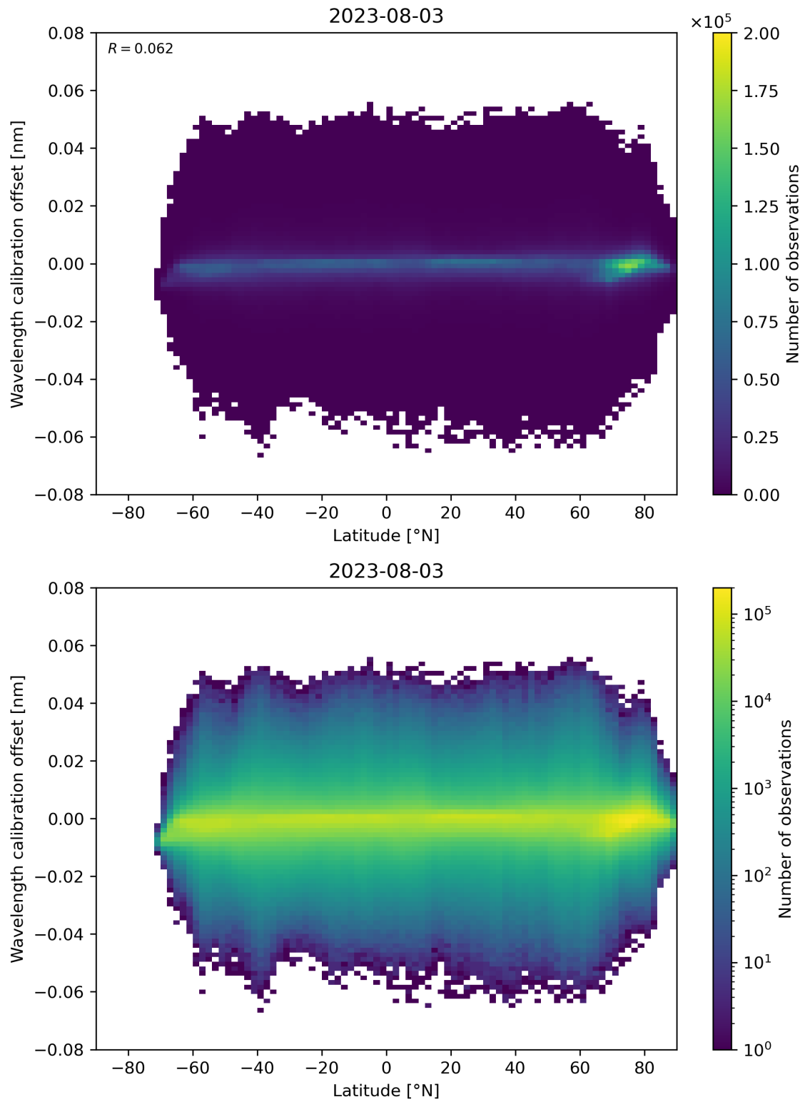
Figure 95: Scatter density plot of “Latitude” against “Wavelength calibration offset” for 2023-08-02 to 2023-08-04.
