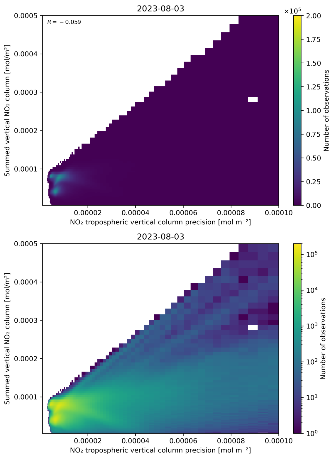
Figure 136: Scatter density plot of “NO 2 tropospheric vertical column precision” against “Summed vertical NO 2 column” for 2023-08-02 to 2023-08-04.
