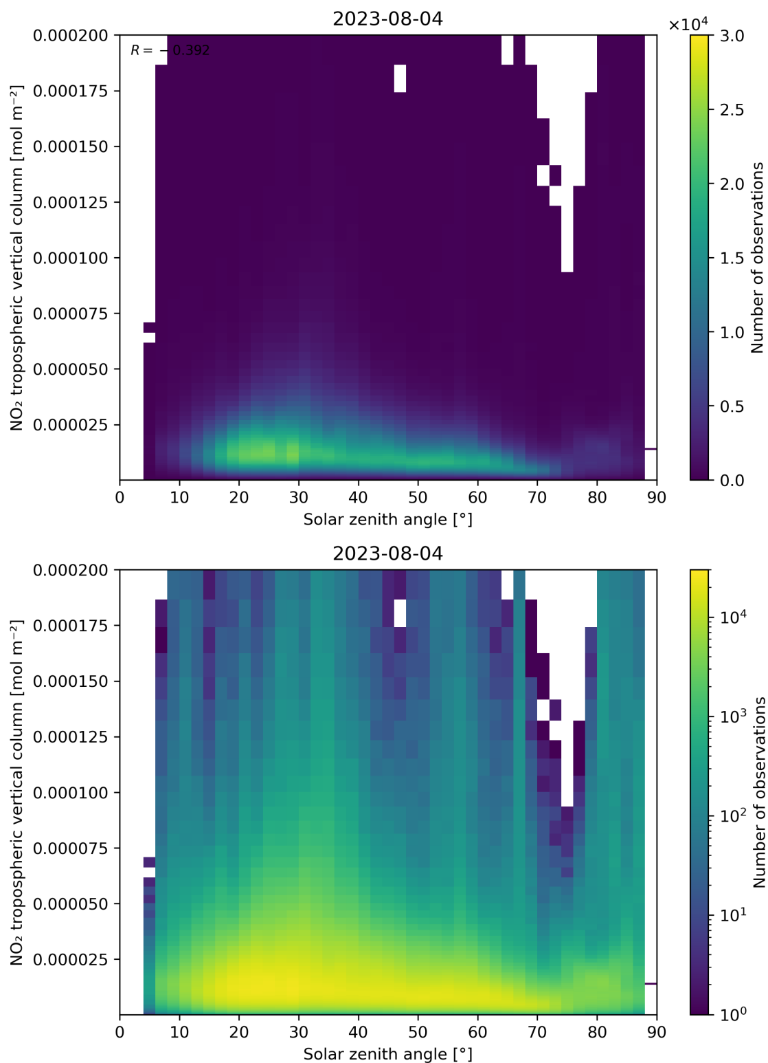
Figure 155: Scatter density plot of “Solar zenith angle” against “NO 2 tropospheric vertical column” for 2023-08-04 to 2023-08-05.
