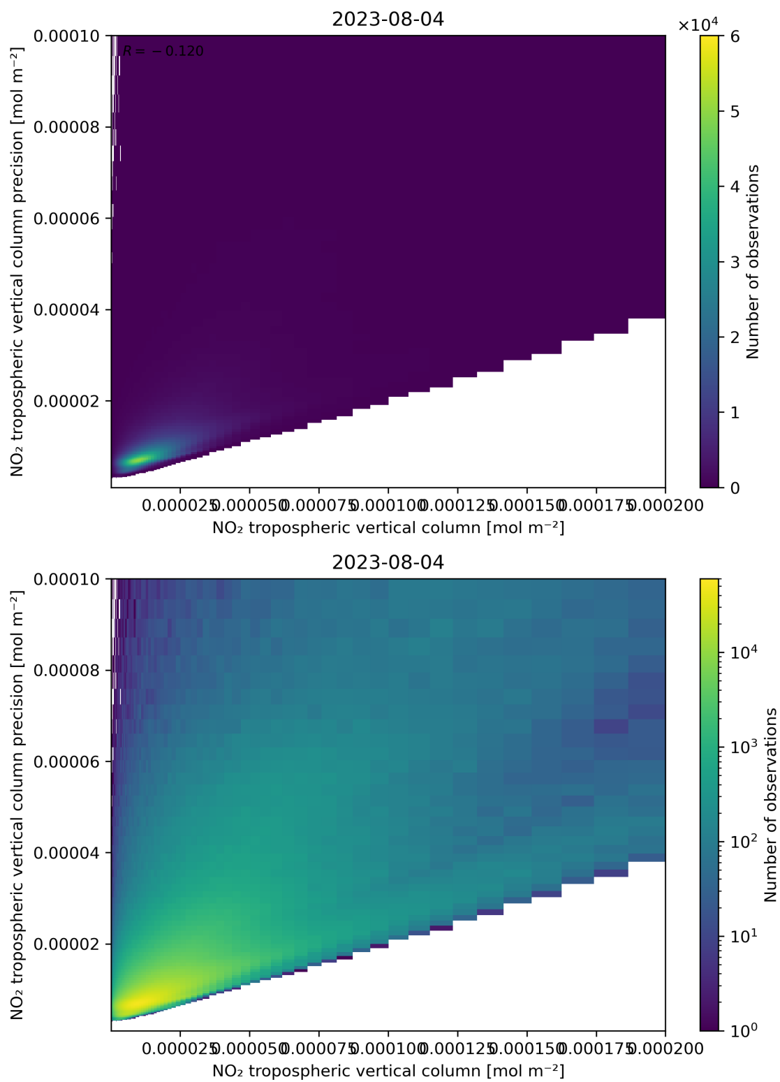
Figure 130: Scatter density plot of “NO 2 tropospheric vertical column” against “NO 2 tropospheric vertical column precision” for 2023-08-04 to 2023-08-05.
