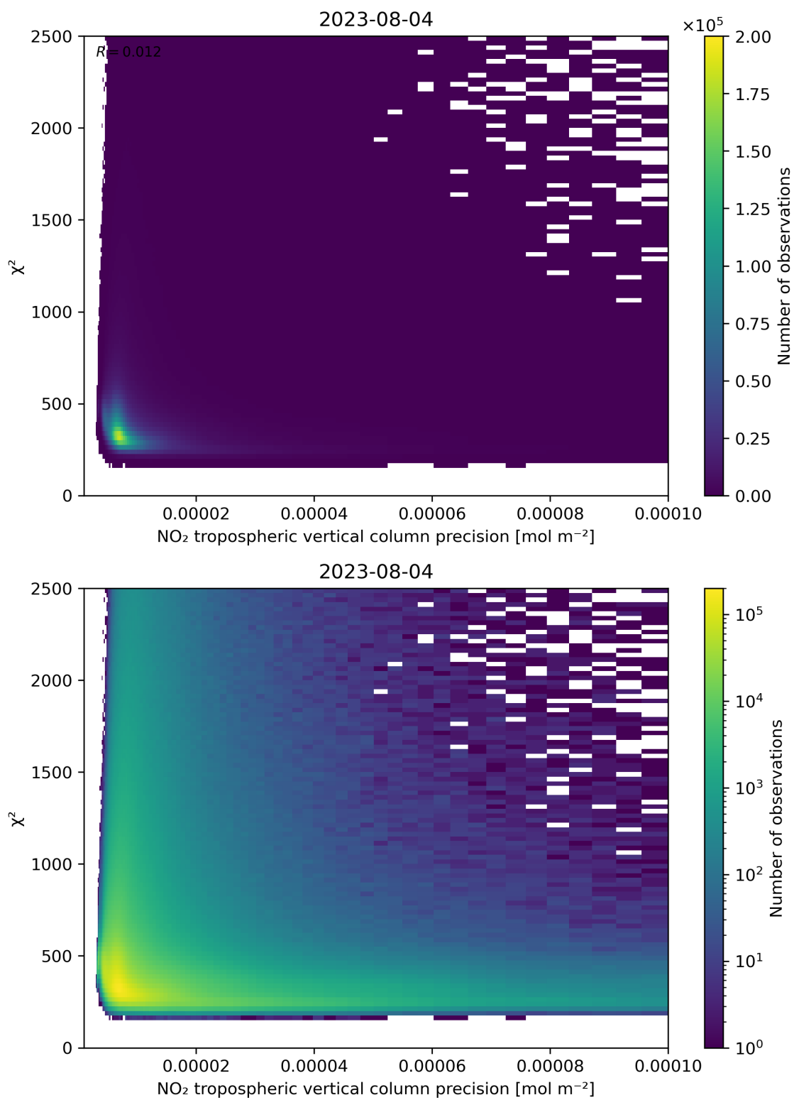
Figure 134: Scatter density plot of “NO 2 tropospheric vertical column precision” against “ \chi^2 ” for 2023-08-04 to 2023-08-05.
