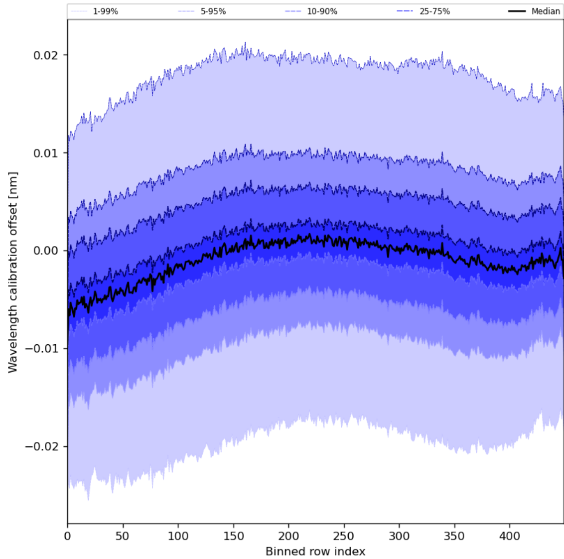
Figure 52: Along track statistics of “Wavelength calibration offset” for 2023-08-04 to 2023-08-05
