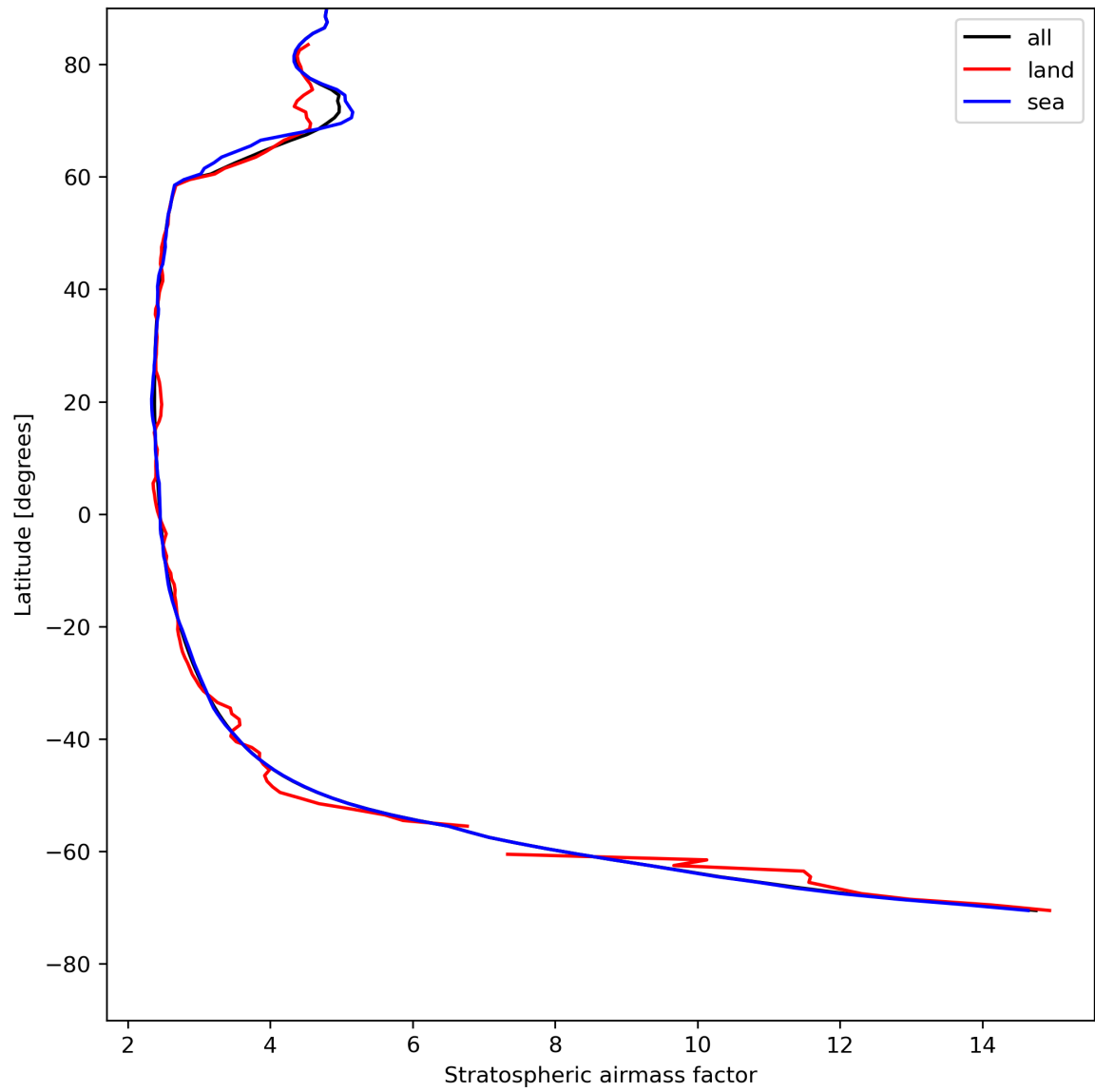
Figure 27: Zonal average of “Stratospheric air mass factor” for 2023-08-04 to 2023-08-05.
