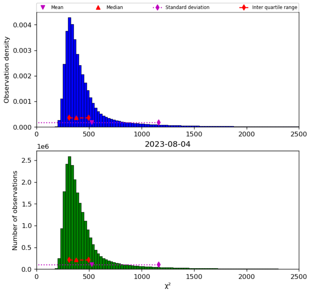
Figure 42: Histogram of “ \chi^2 ” for 2023-08-04 to 2023-08-05
