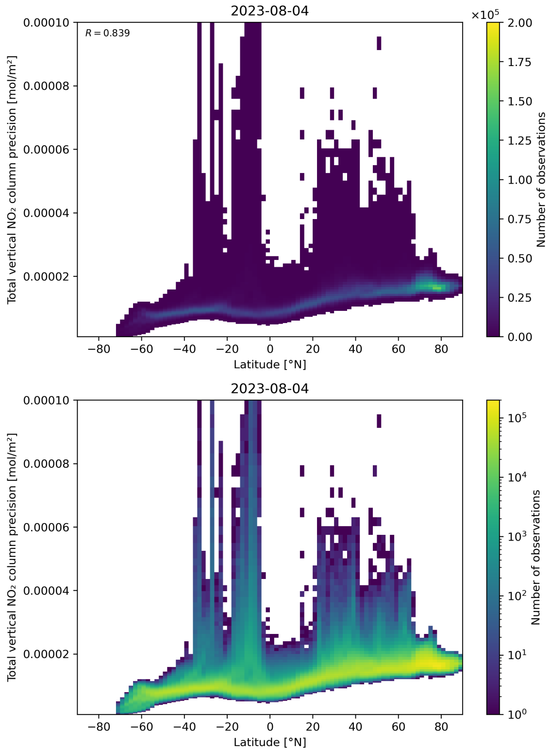
Figure 91: Scatter density plot of “Latitude” against “Total vertical NO 2 column precision” for 2023-08-04 to 2023-08-05.
