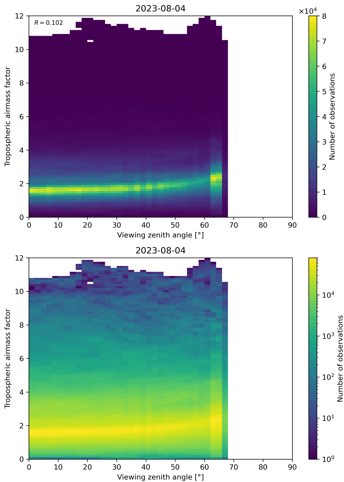
Figure 161: Scatter density plot of “Viewing zenith angle” against “Tropospheric airmass factor” for 2023-08-04 to 2023-08-05.
