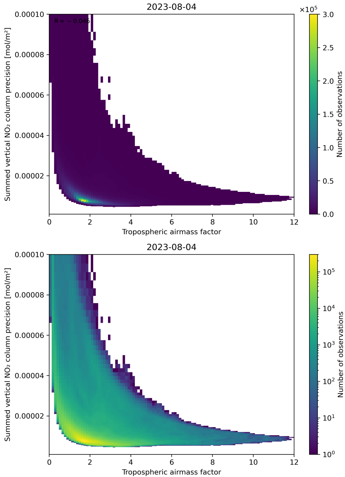
Figure 76: Scatter density plot of “Tropospheric air mass factor” against “Summed vertical NO 2 column precision” for 2023-08-04 to 2023-08-05.
