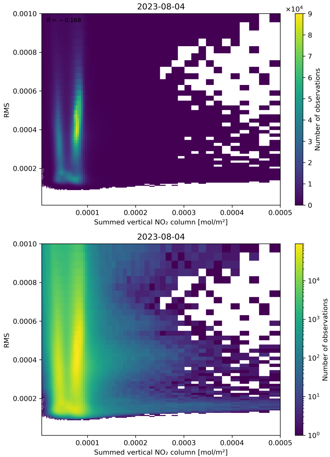
Figure 109: Scatter density plot of “Summed vertical NO 2 column” against “RMS” for 2023-08-04 to 2023-08-05.
