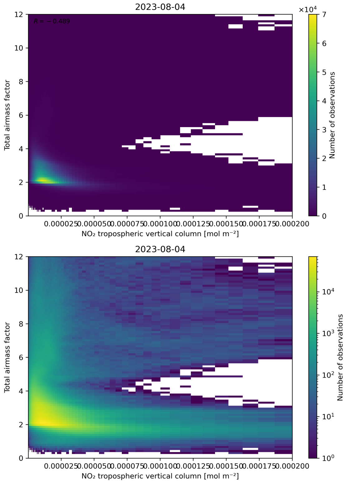
Figure 122: Scatter density plot of “NO 2 tropospheric vertical column” against “Total air mass factor” for 2023-08-04 to 2023-08-05.
