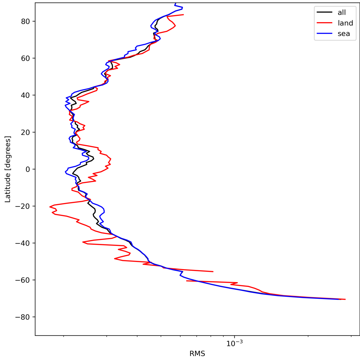
Figure 26: Zonal average of “RMS” for 2023-08-04 to 2023-08-05.
