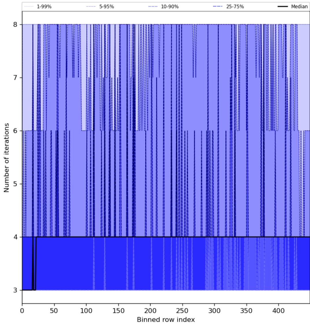
Figure 51: Along track statistics of “Number of iterations” for 2023-08-04 to 2023-08-05
