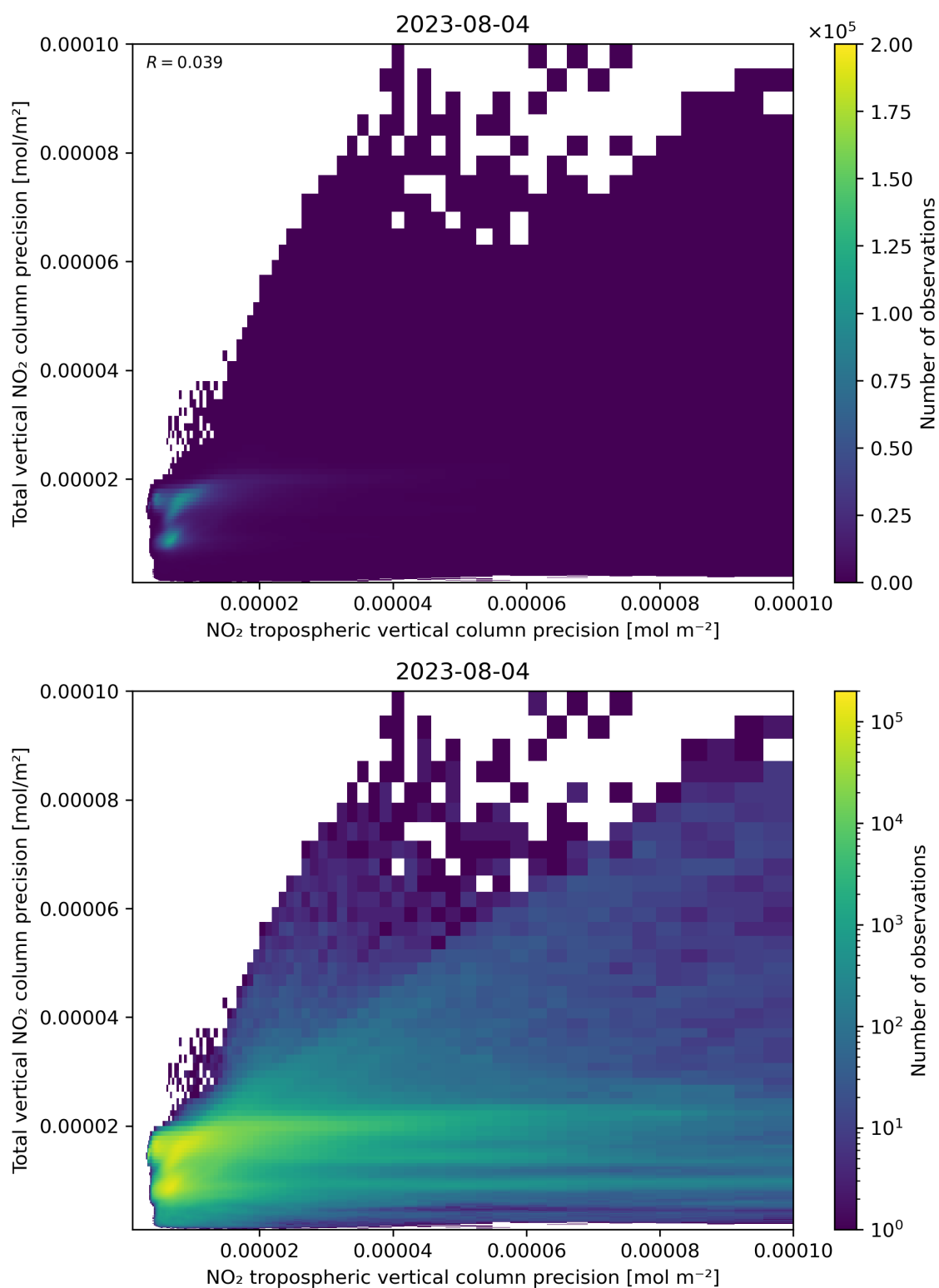
Figure 139: Scatter density plot of “NO 2 tropospheric vertical column precision” against “Total vertical NO 2 column precision” for 2023-08-04 to 2023-08-05.
