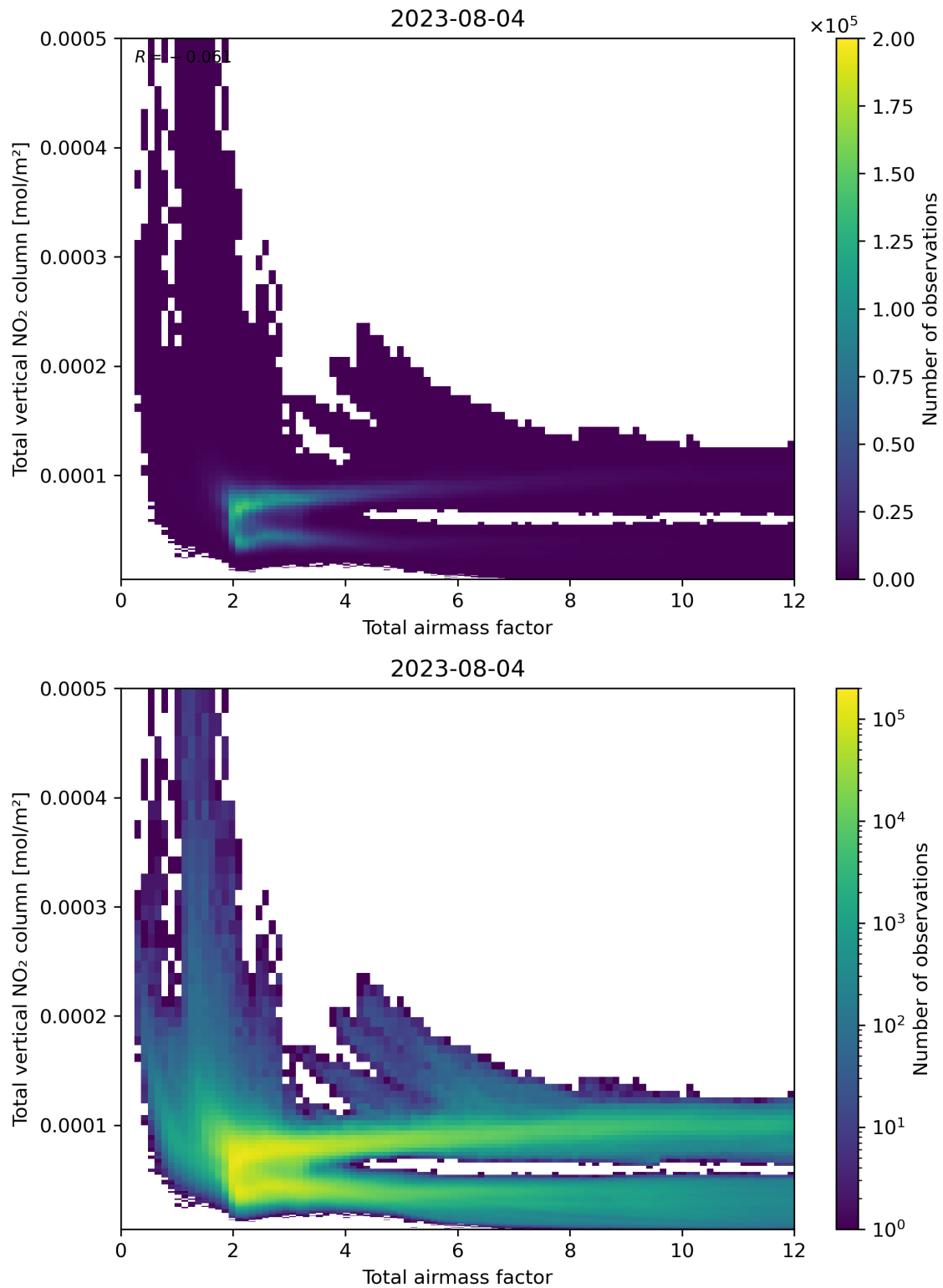
Figure 67: Scatter density plot of “Total airmass factor” against “Total vertical NO 2 column” for 2023-08-04 to 2023-08-05.
