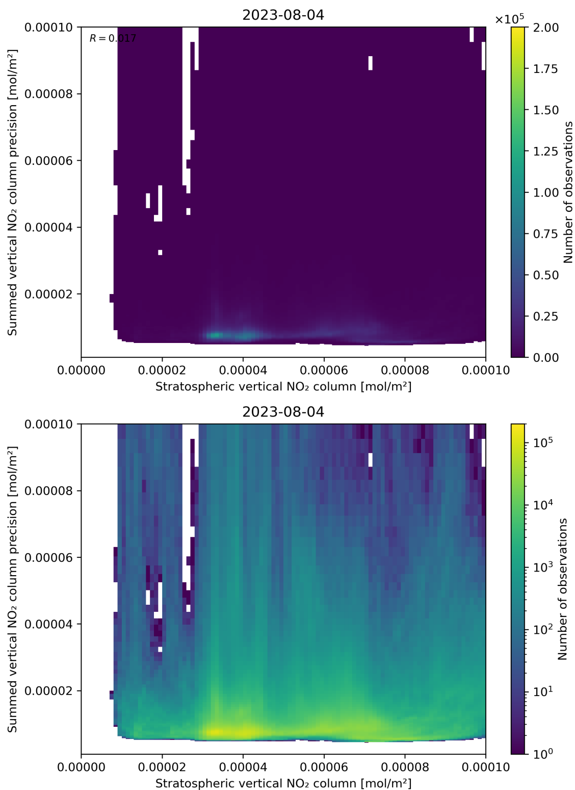
Figure 99: Scatter density plot of “Stratospheric vertical NO 2 column” against “Summed vertical NO 2 column precision” for 2023-08-04 to 2023-08-05.
