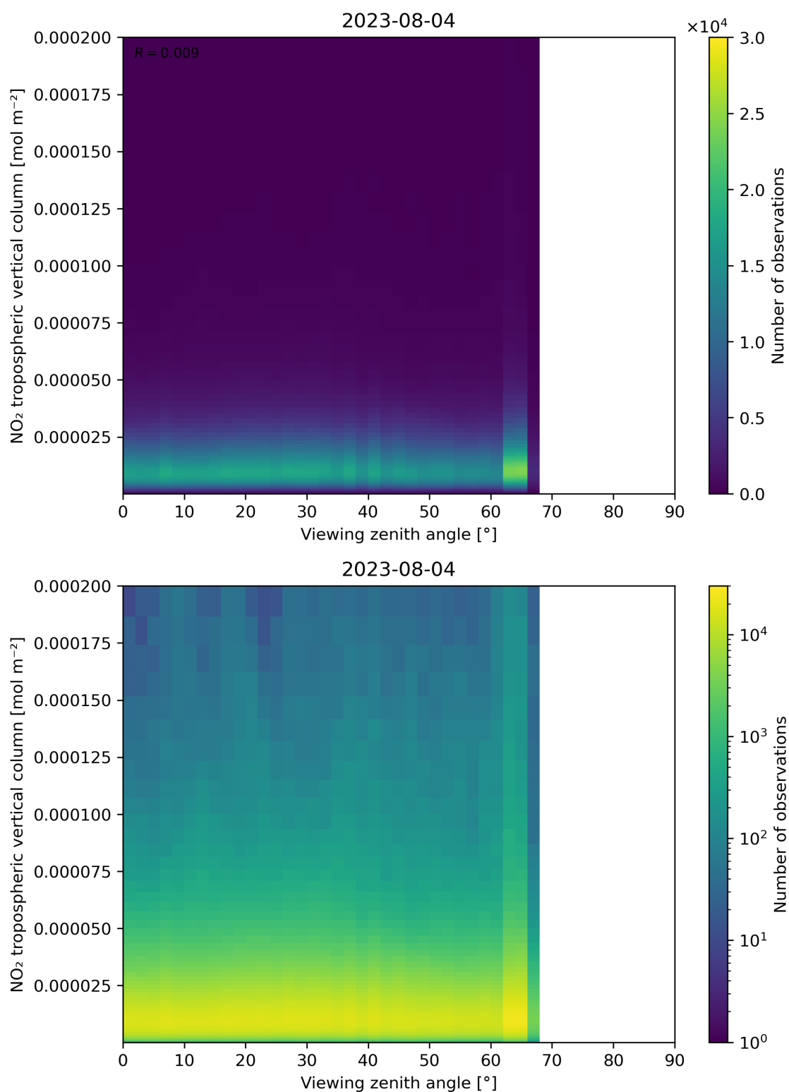
Figure 169: Scatter density plot of “Viewing zenith angle” against “NO 2 tropospheric vertical column” for 2023-08-04 to 2023-08-05.
