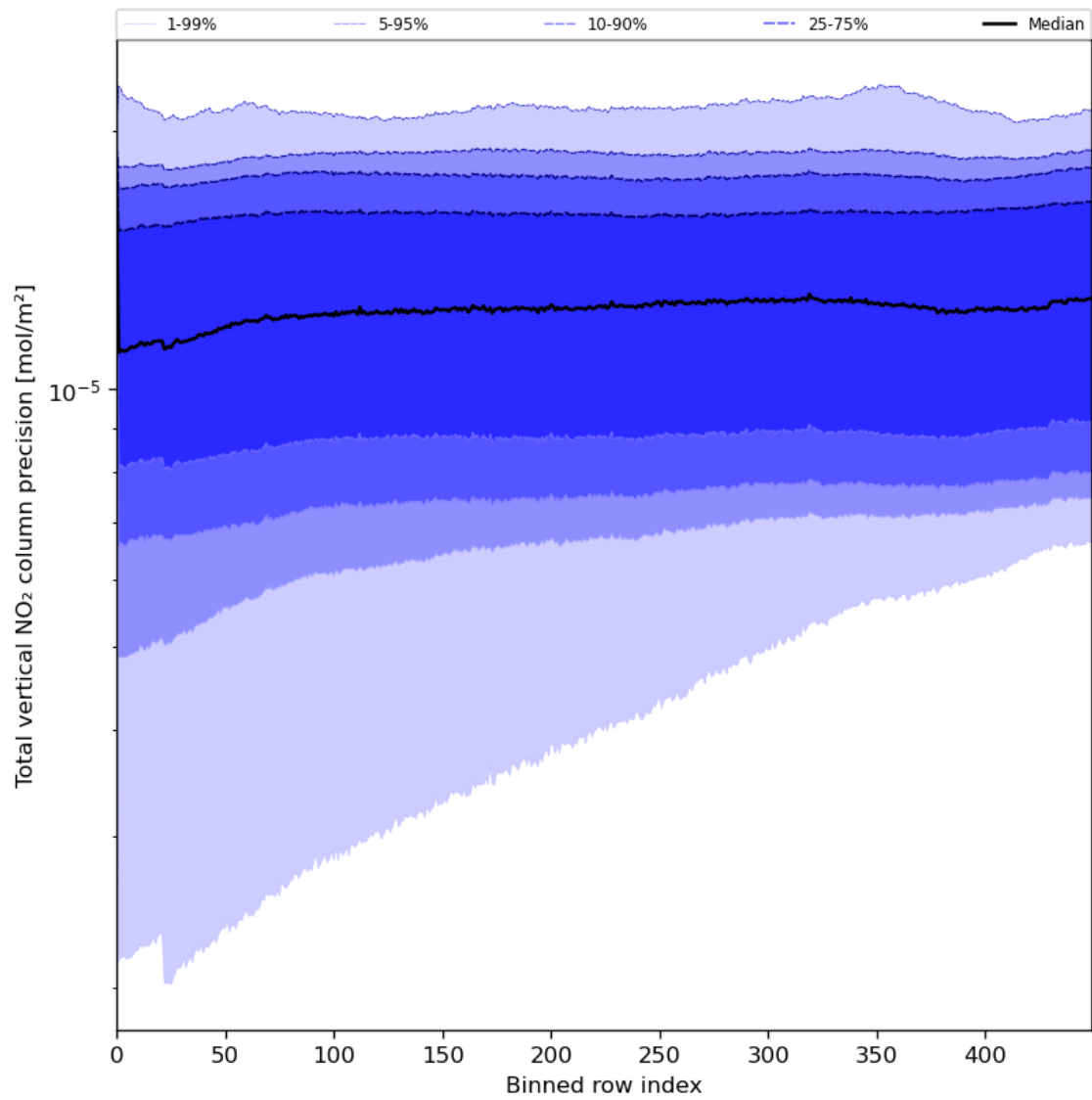
Figure 56: Along track statistics of “Total vertical NO 2 column precision” for 2023-08-04 to 2023-08-05
