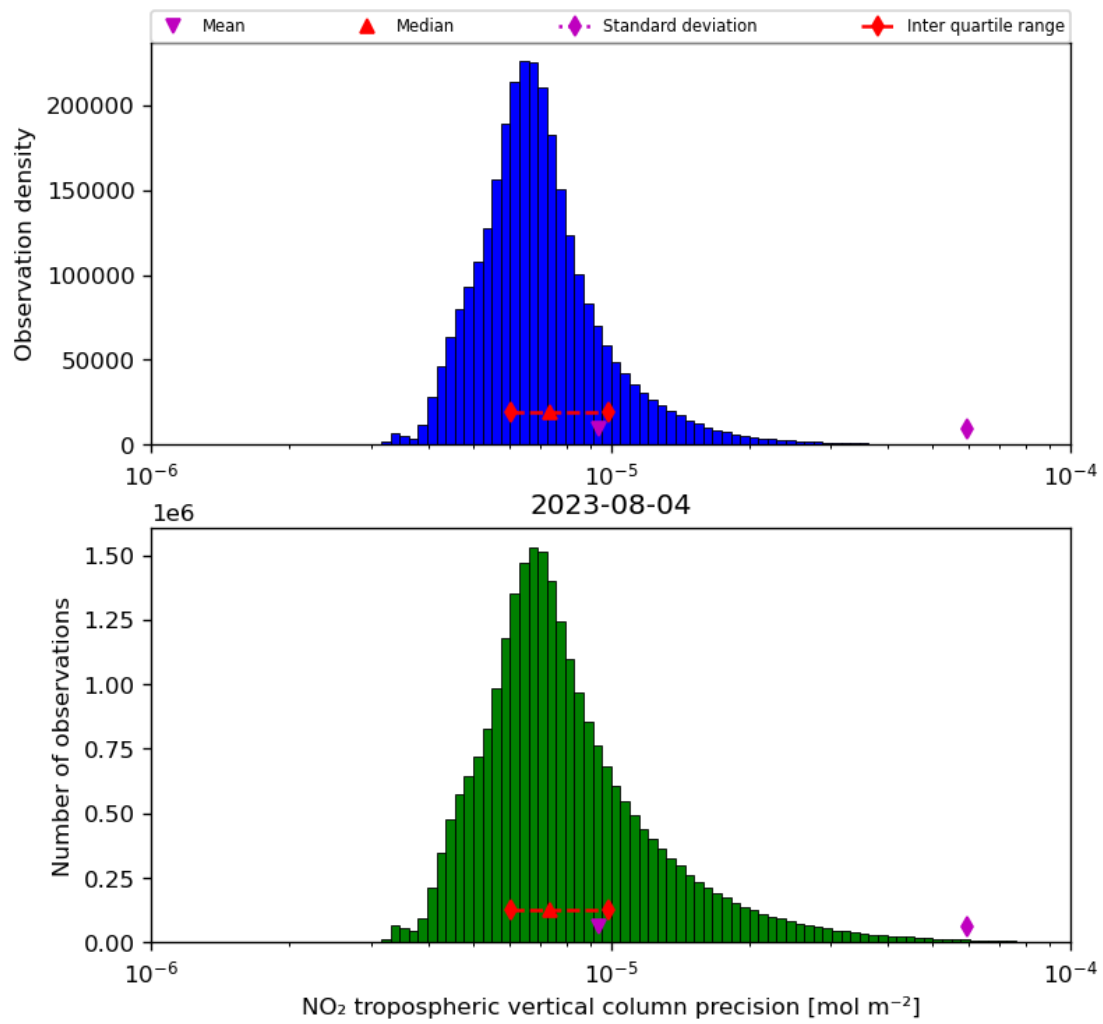
Figure 30: Histogram of “NO 2 tropospheric vertical column precision” for 2023-08-04 to 2023-08-05
