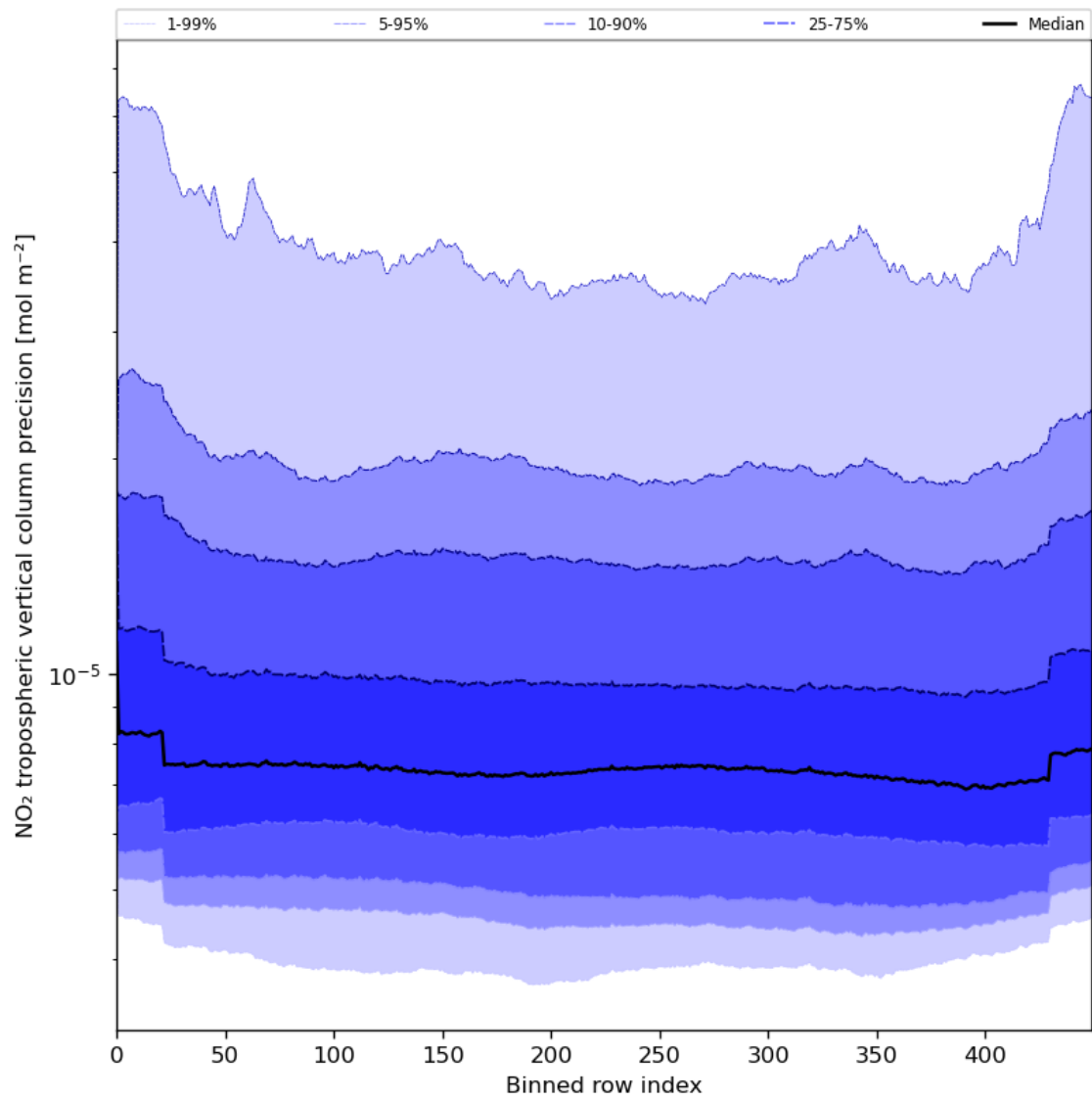
Figure 47: Along track statistics of “NO 2 tropospheric vertical column precision” for 2023-08-04 to 2023-08-05
