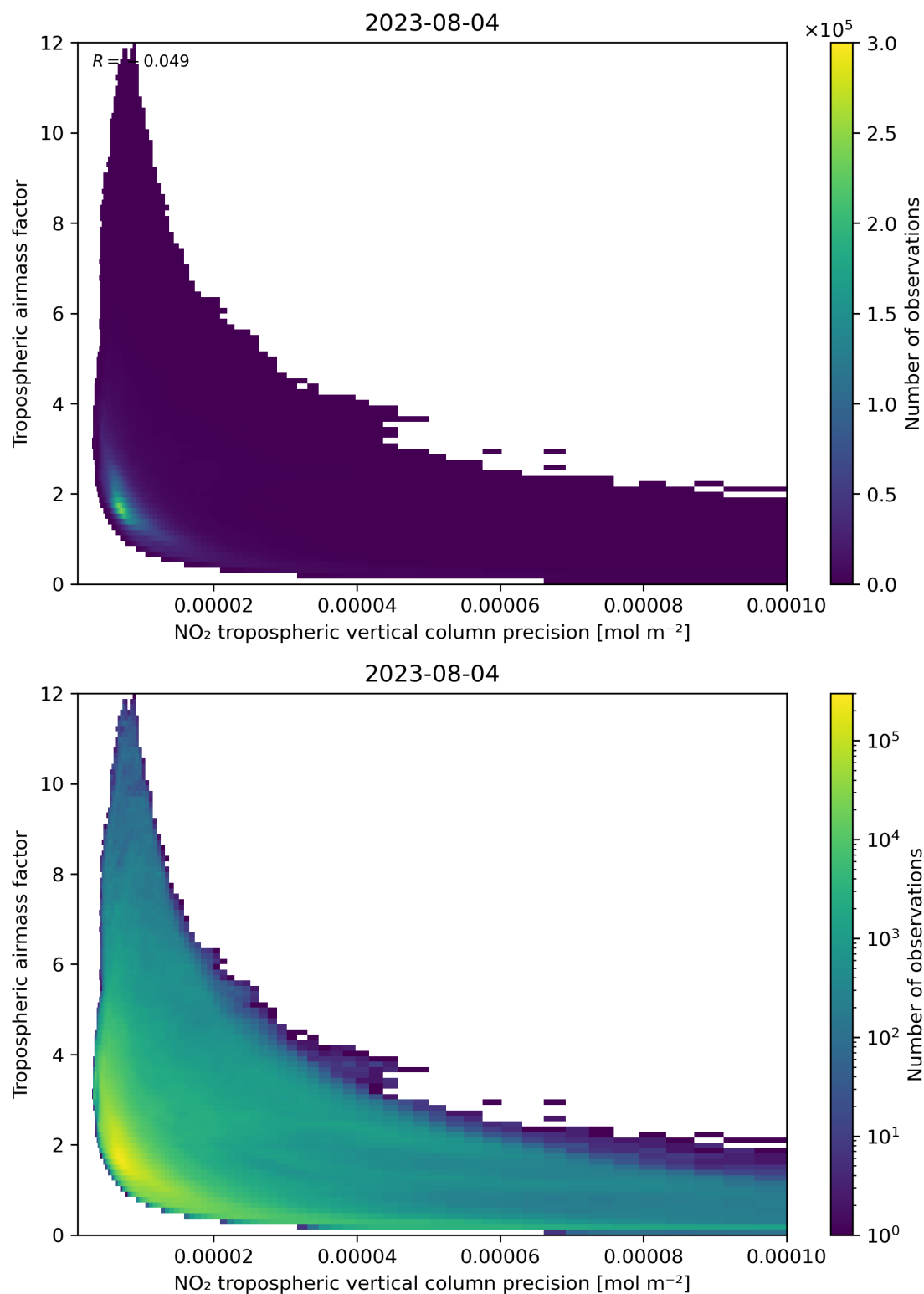
Figure 133: Scatter density plot of “NO 2 tropospheric vertical column precision” against “Tropospheric airmass factor” for 2023-08-04 to 2023-08-05.
