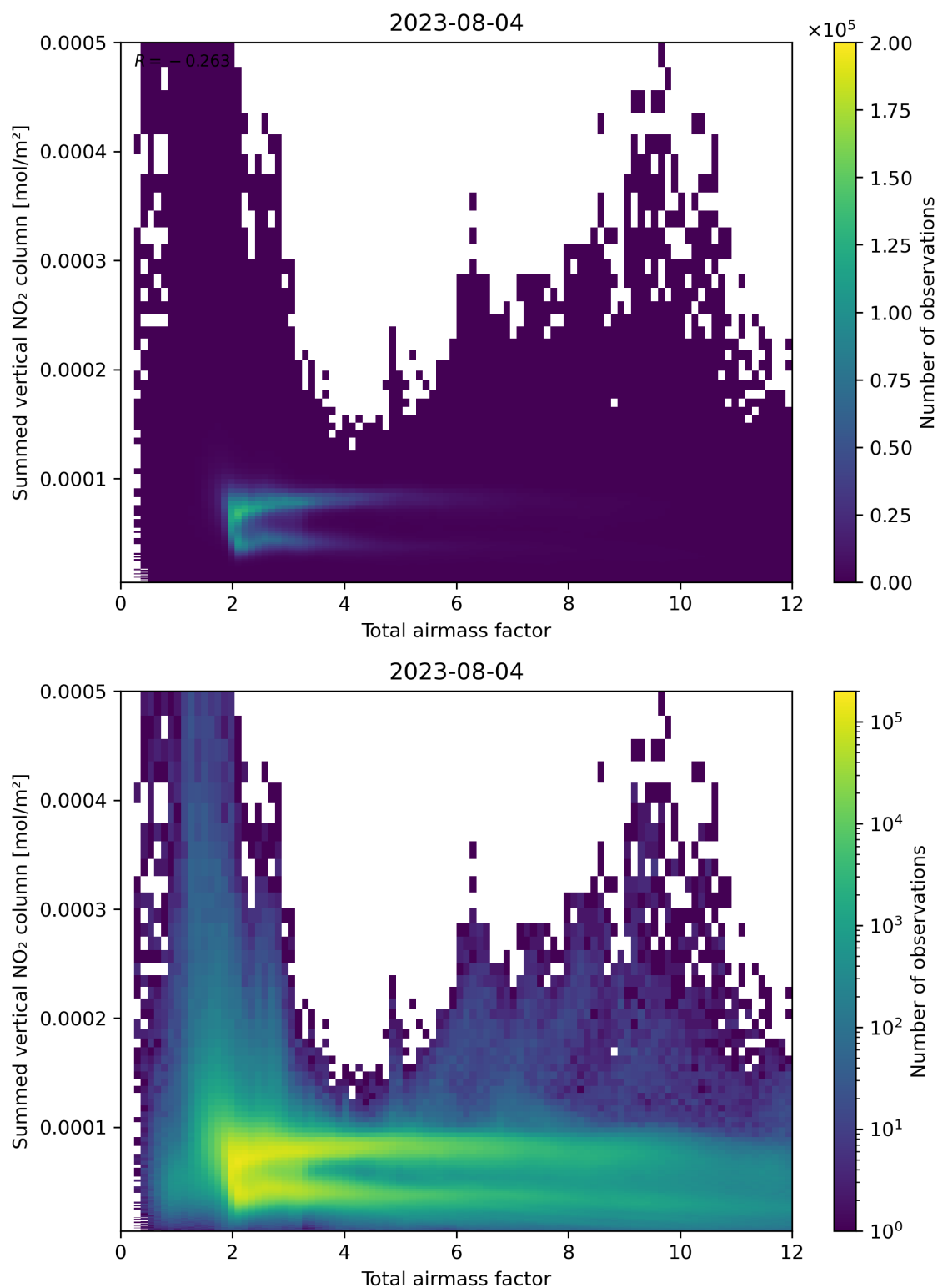
Figure 65: Scatter density plot of “Total airmass factor” against “Summed vertical NO 2 column” for 2023-08-04 to 2023-08-05.
