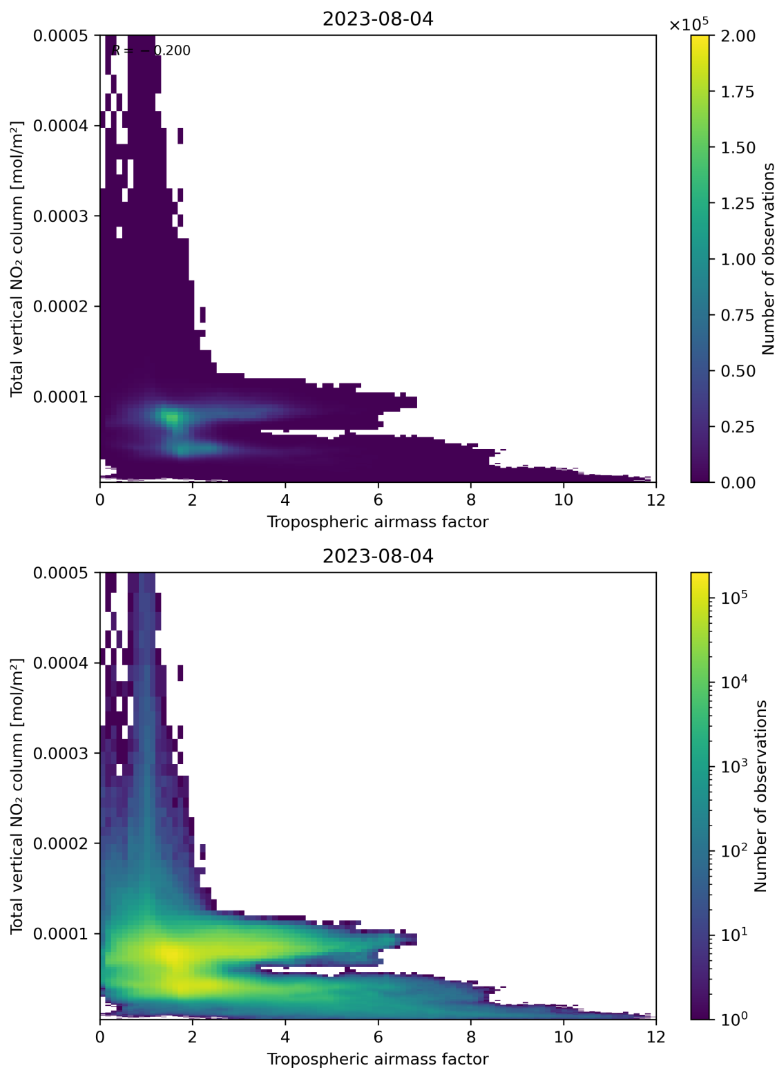
Figure 77: Scatter density plot of “Tropospheric airmass factor” against “Total vertical NO 2 column” for 2023-08-04 to 2023-08-05.
