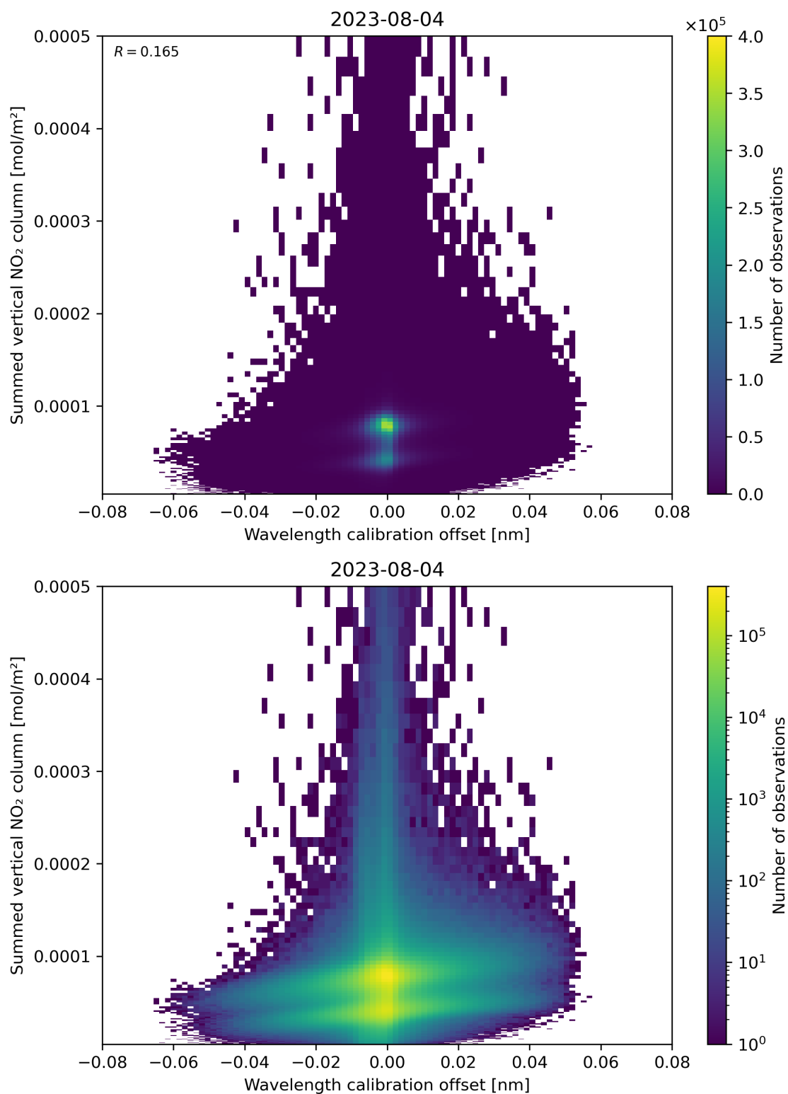
Figure 177: Scatter density plot of “Wavelength calibration offset” against “Summed vertical NO 2 column” for 2023-08-04 to 2023-08-05.
