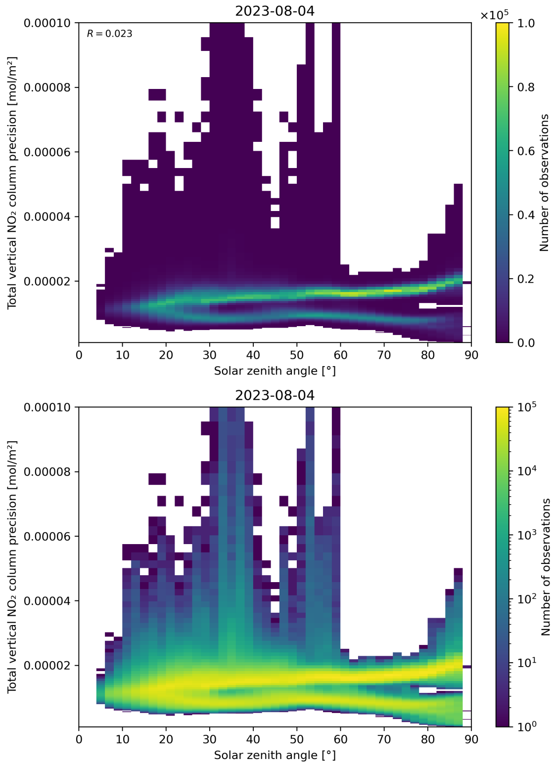
Figure 154: Scatter density plot of “Solar zenith angle” against “Total vertical NO 2 column precision” for 2023-08-04 to 2023-08-05.
