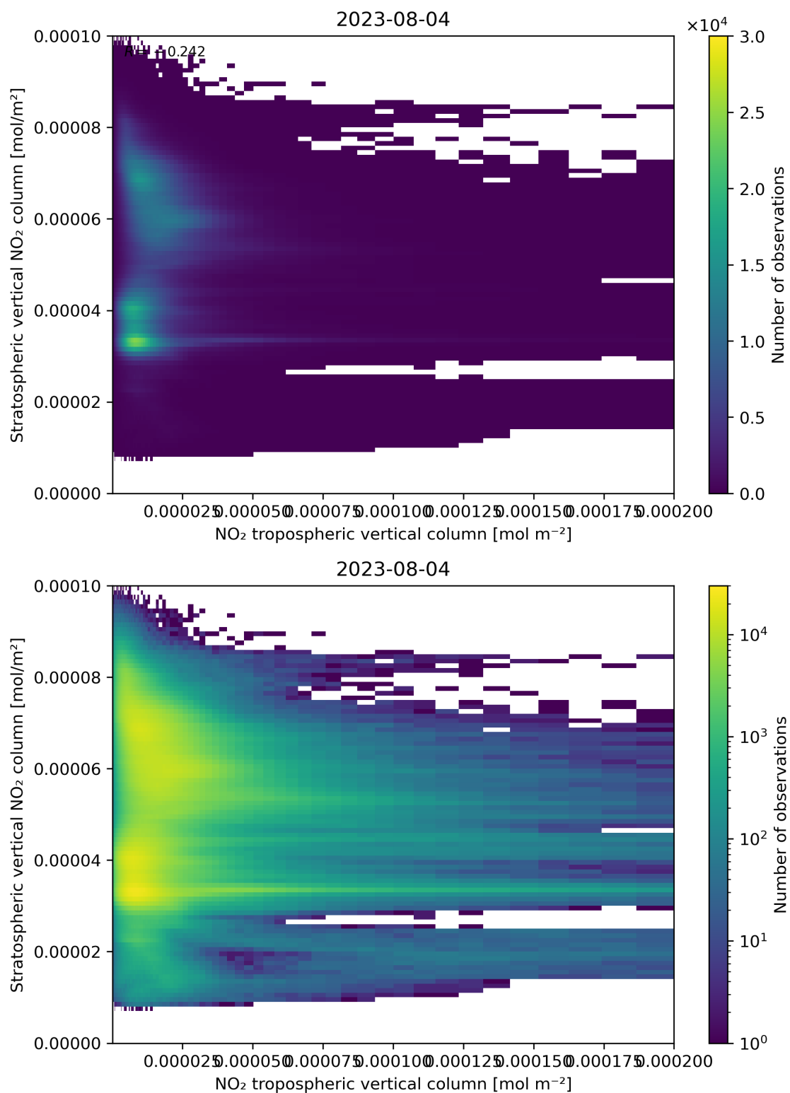
Figure 125: Scatter density plot of “NO 2 tropospheric vertical column” against “Stratospheric vertical NO 2 column” for 2023-08-04 to 2023-08-05.
