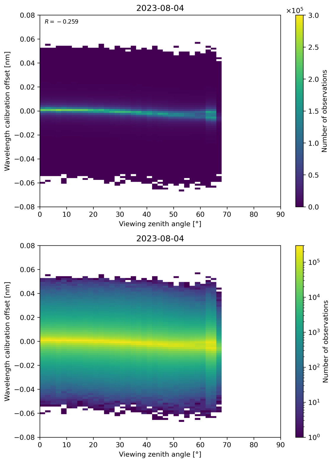
Figure 173: Scatter density plot of “Viewing zenith angle” against “Wavelength calibration offset” for 2023-08-04 to 2023-08-05.
