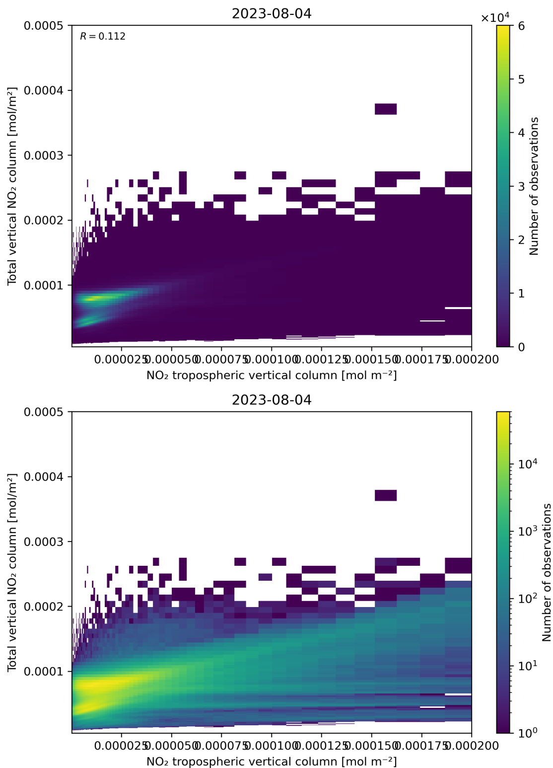
Figure 128: Scatter density plot of “NO 2 tropospheric vertical column” against “Total vertical NO 2 column” for 2023-08-04 to 2023-08-05.
