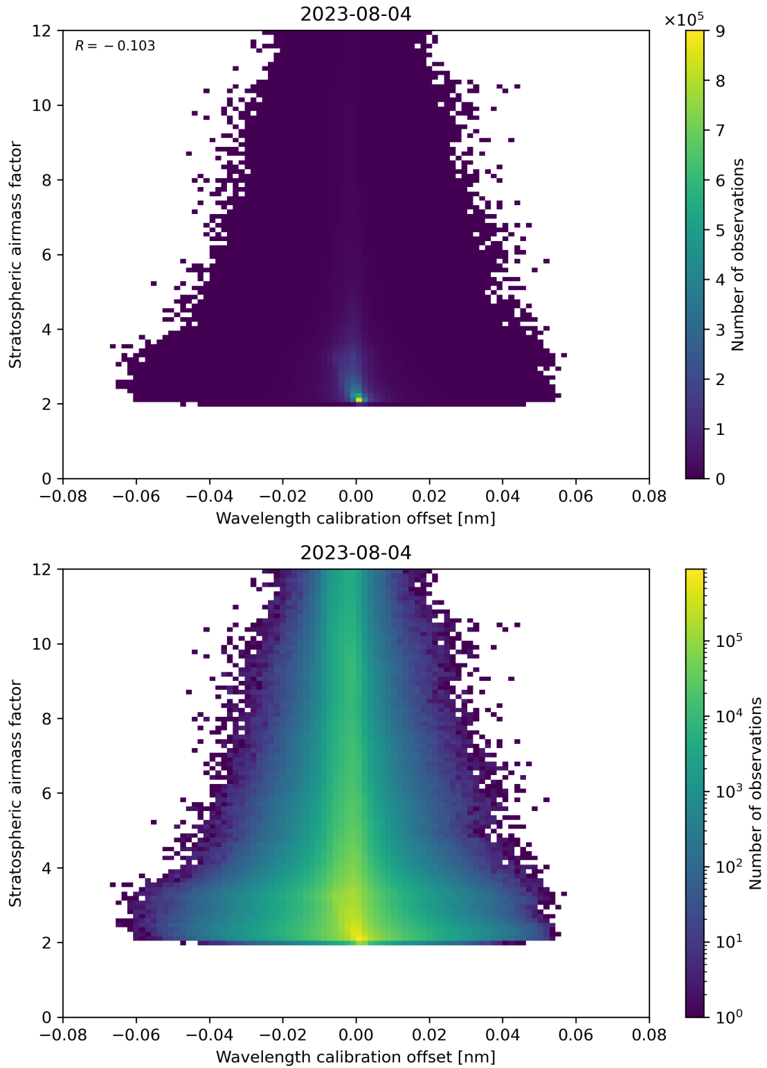
Figure 174: Scatter density plot of “Wavelength calibration offset” against “Stratospheric air mass factor” for 2023-08-04 to 2023-08-05.
