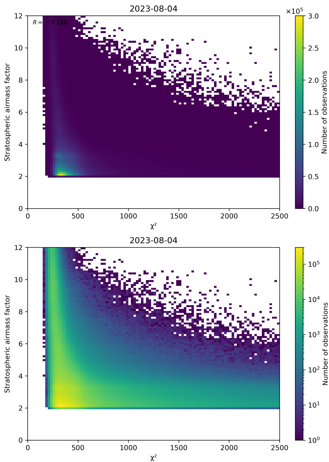
Figure 81: Scatter density plot of “ \chi^2 ” against “Stratospheric airmass factor” for 2023-08-04 to 2023-08-05.
