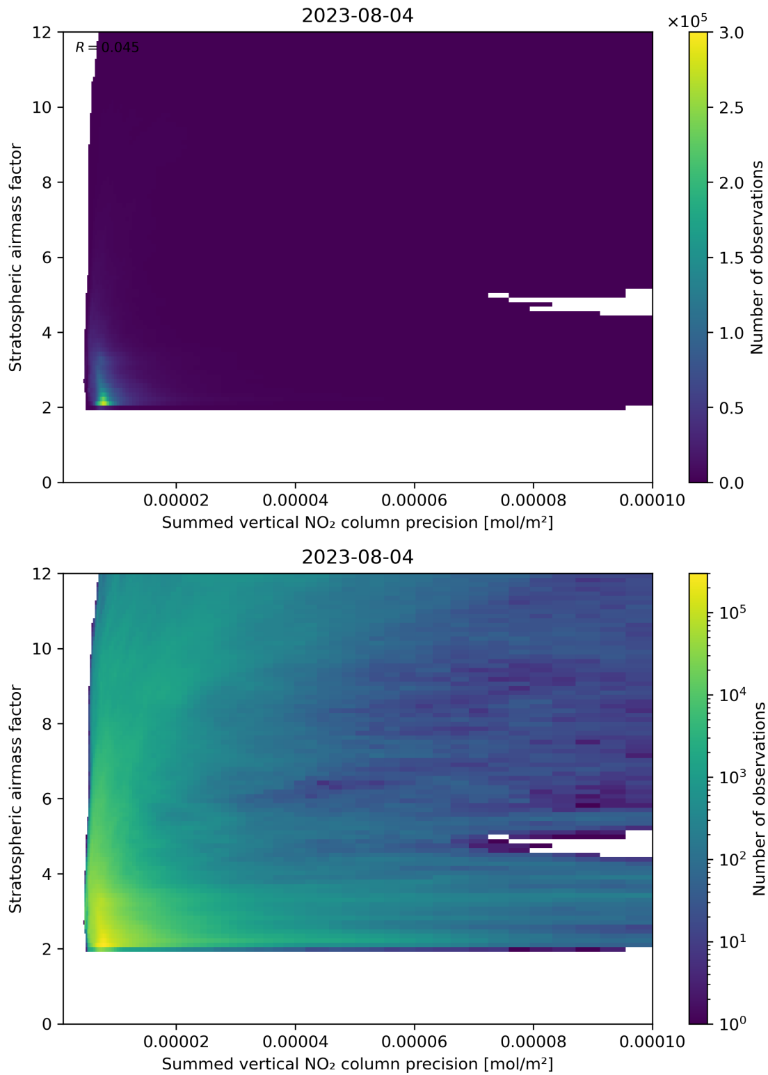
Figure 106: Scatter density plot of “Summed vertical NO 2 column precision” against “Stratospheric airmass factor” for 2023-08-04 to 2023-08-05.
