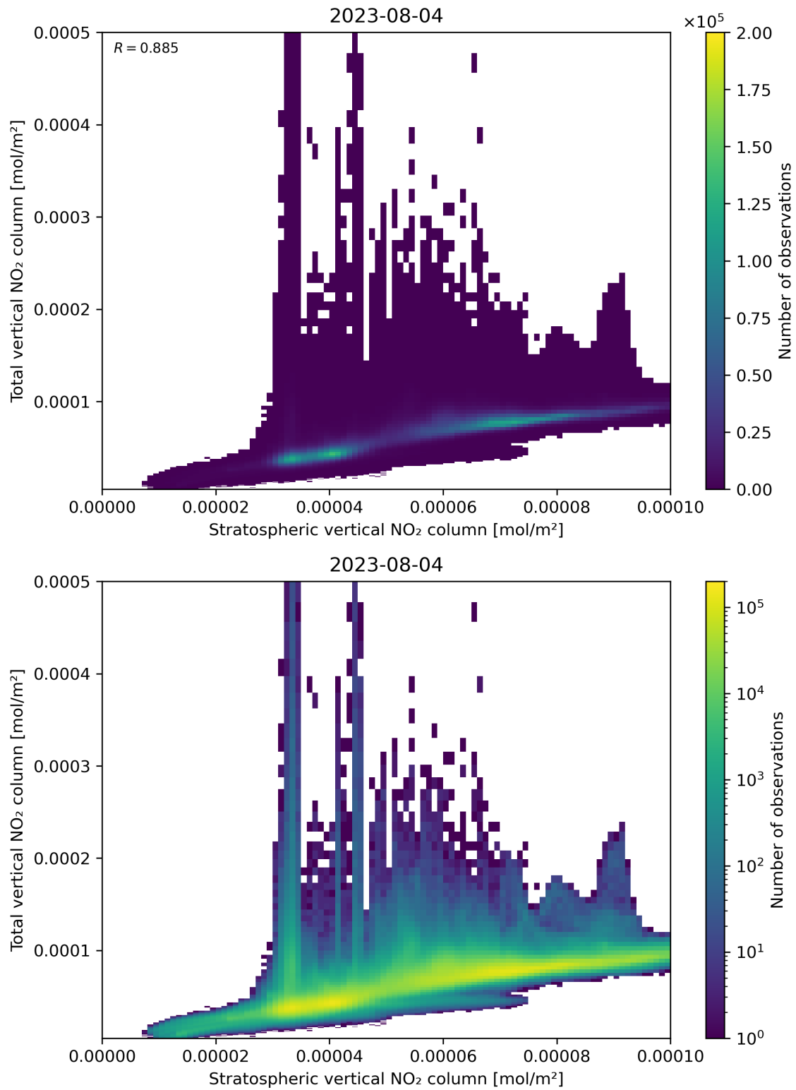
Figure 100: Scatter density plot of “Stratospheric vertical NO 2 column” against “Total vertical NO 2 column” for 2023-08-04 to 2023-08-05.
