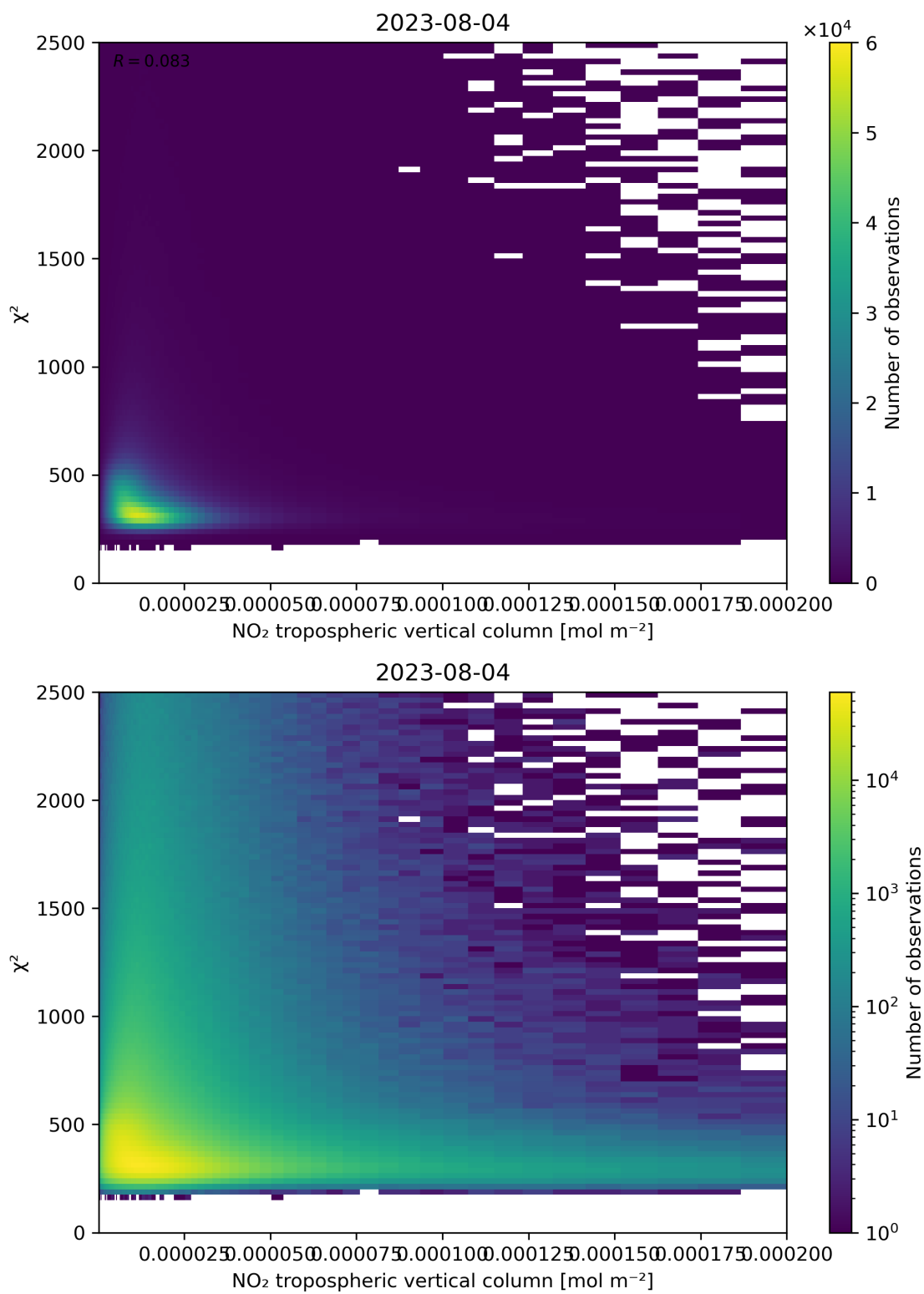
Figure 124: Scatter density plot of “NO 2 tropospheric vertical column” against “ \chi^2 ” for 2023-08-04 to 2023-08-05.
