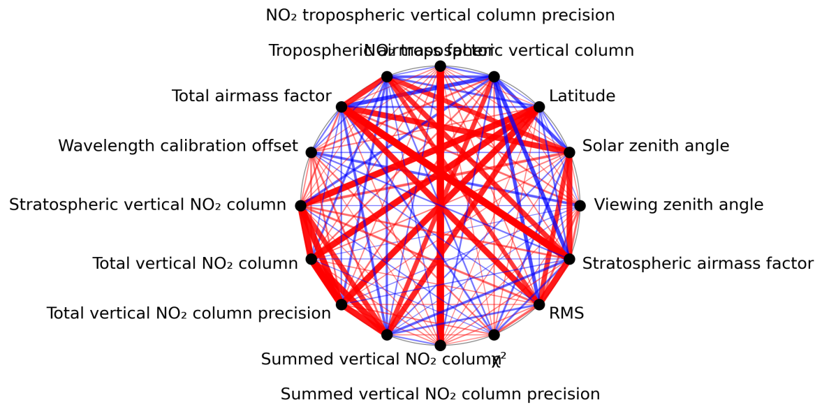
Figure 1: Map of correlation graph for 2023-08-04 to 2023-08-05.
