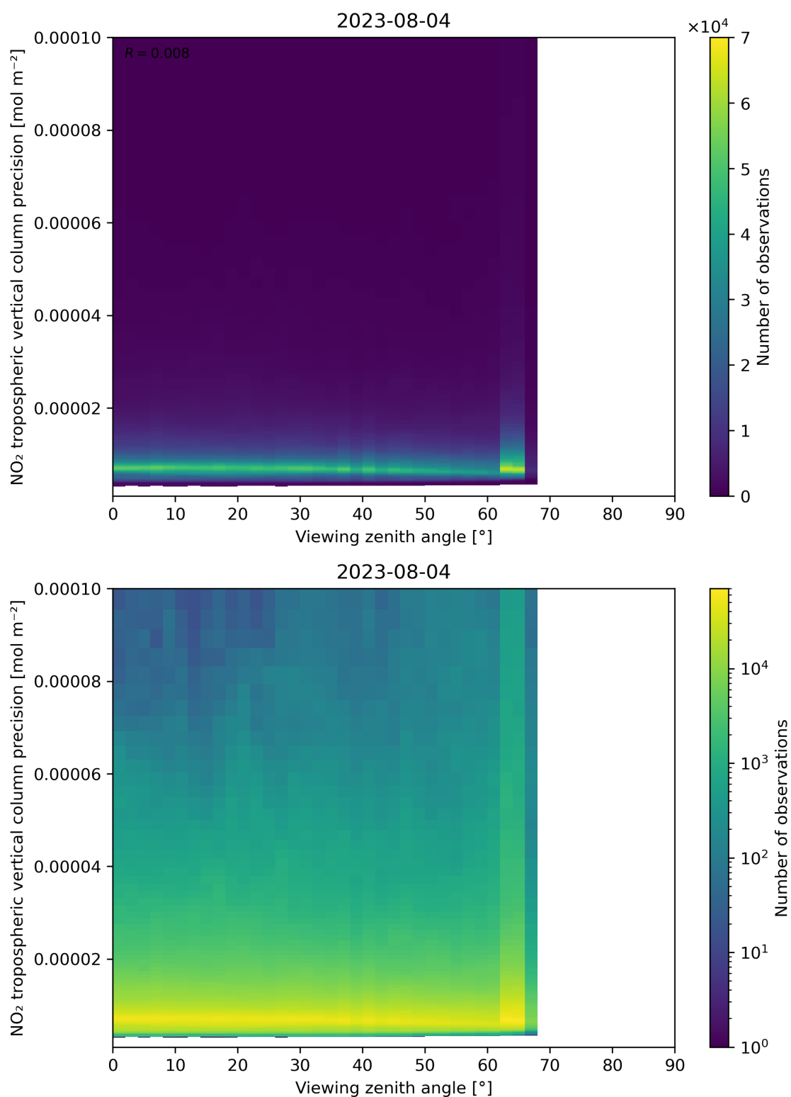
Figure 170: Scatter density plot of “Viewing zenith angle” against “NO 2 tropospheric vertical column precision” for 2023-08-04 to 2023-08-05.
