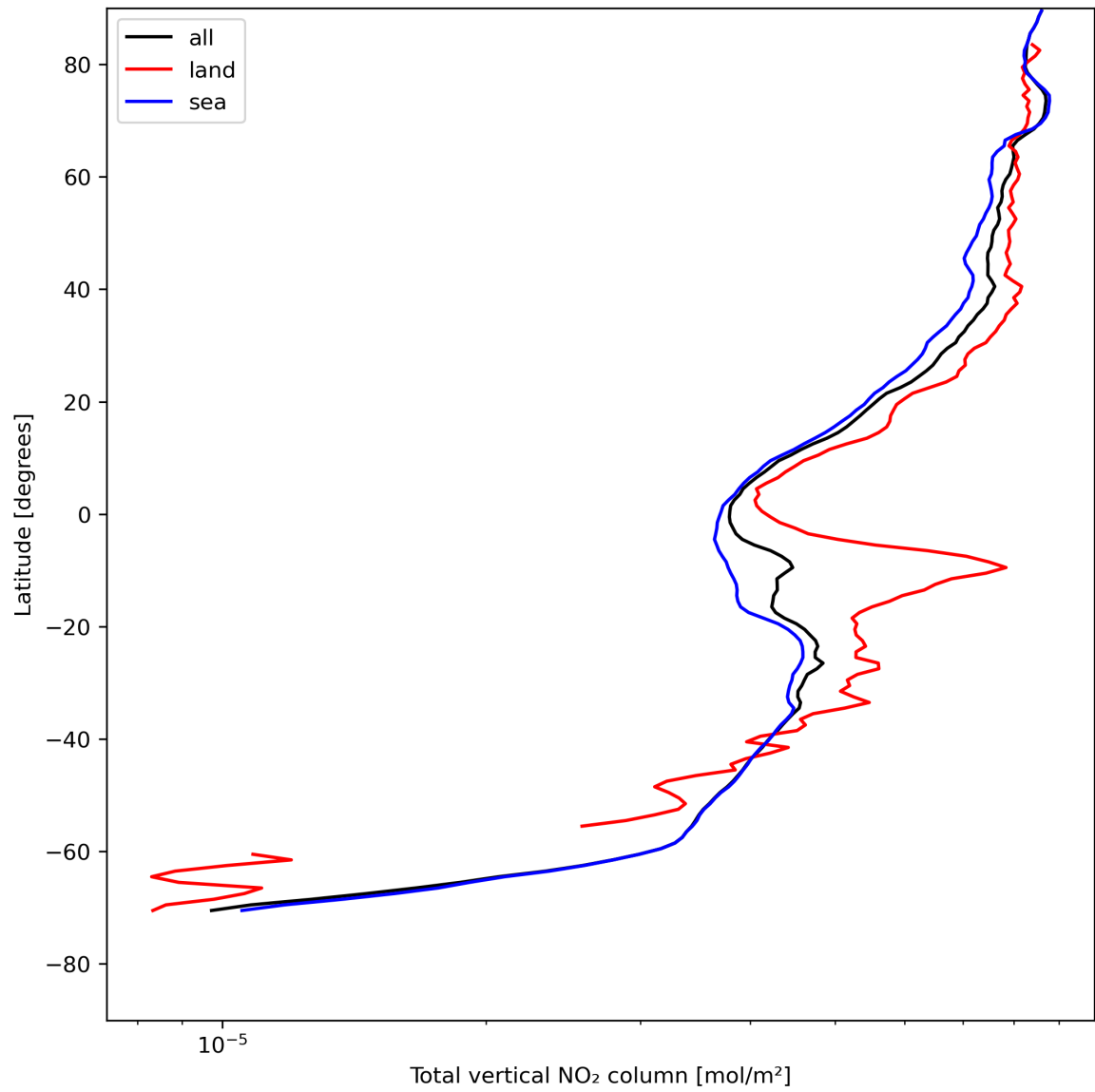
Figure 21: Zonal average of “Total vertical NO 2 column” for 2023-08-04 to 2023-08-05.
