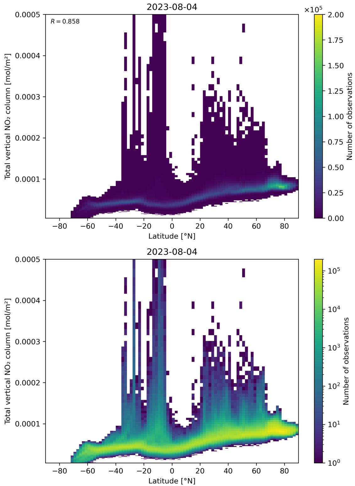
Figure 90: Scatter density plot of “Latitude” against “Total vertical NO 2 column” for 2023-08-04 to 2023-08-05.
