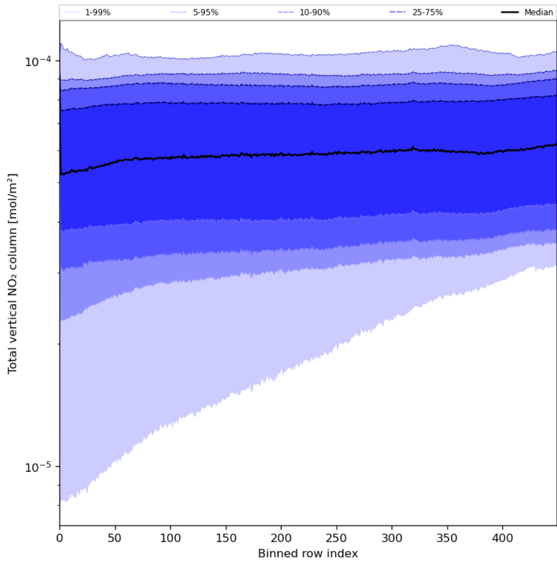
Figure 55: Along track statistics of “Total vertical NO 2 column” for 2023-08-04 to 2023-08-05
