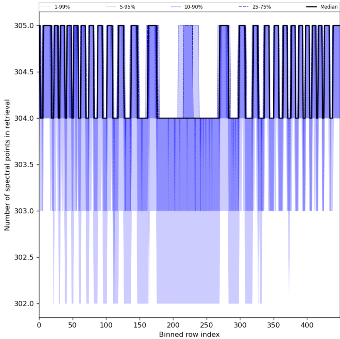
Figure 50: Along track statistics of “Number of spectral points in retrieval” for 2023-08-04 to 2023-08-05
