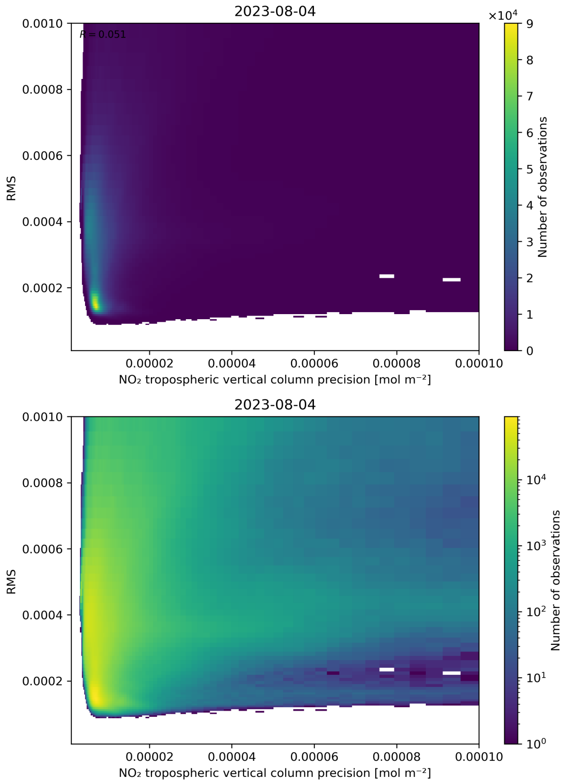
Figure 140: Scatter density plot of “NO 2 tropospheric vertical column precision” against “RMS” for 2023-08-04 to 2023-08-05.
