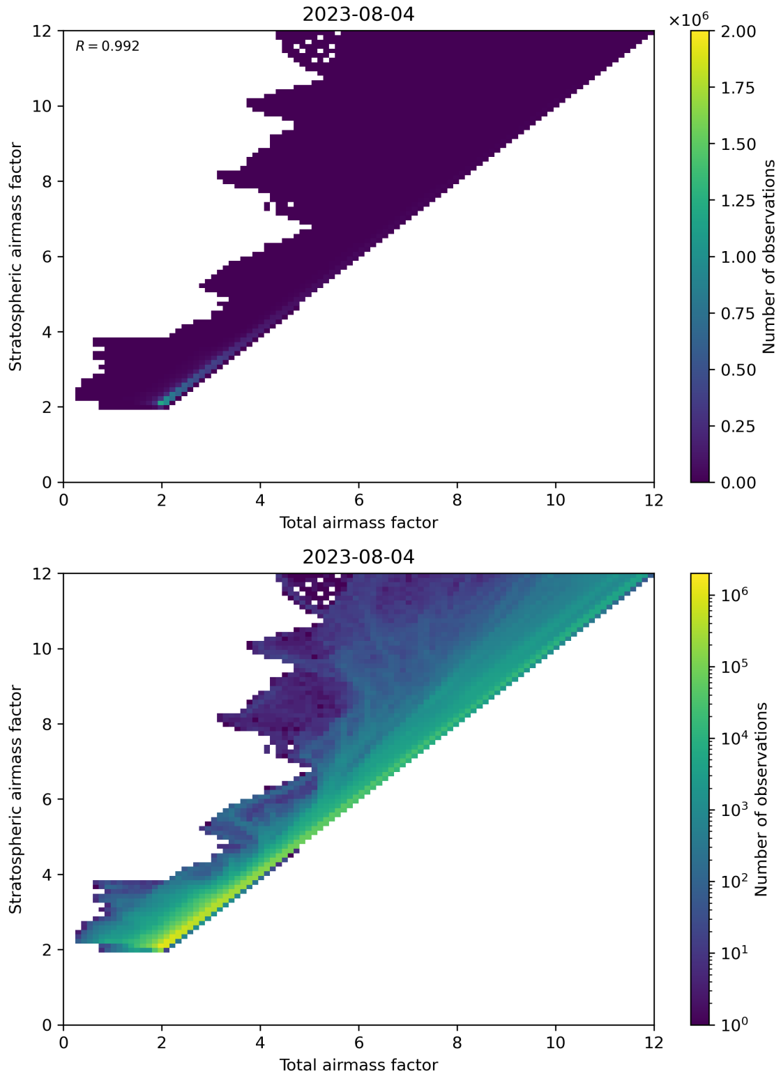
Figure 62: Scatter density plot of “Total airmass factor” against “Stratospheric airmass factor” for 2023-08-04 to 2023-08-05.
