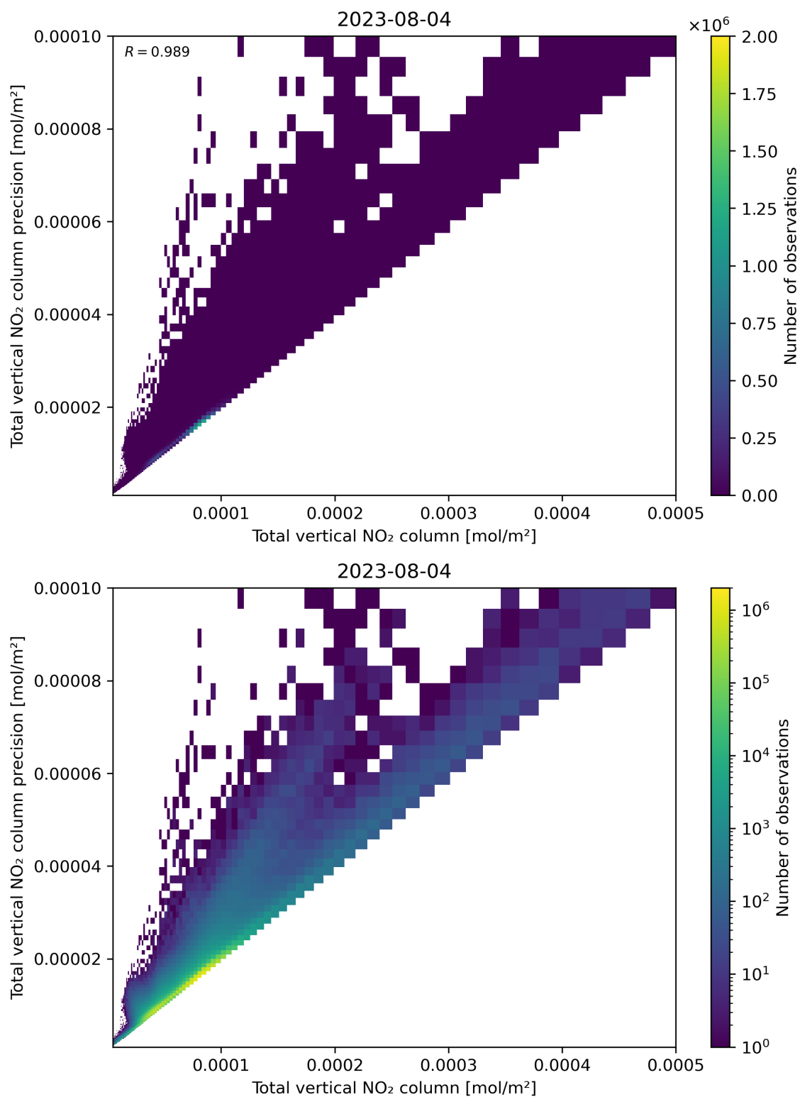
Figure 114: Scatter density plot of “Total vertical NO 2 column” against “Total vertical NO 2 column precision” for 2023-08-04 to 2023-08-05.
