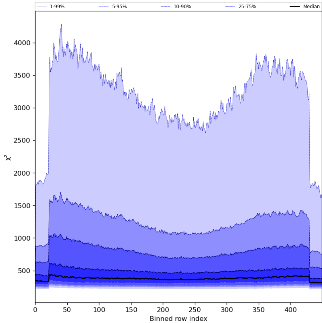
Figure 59: Along track statistics of “ \chi^2 ” for 2023-08-04 to 2023-08-05
