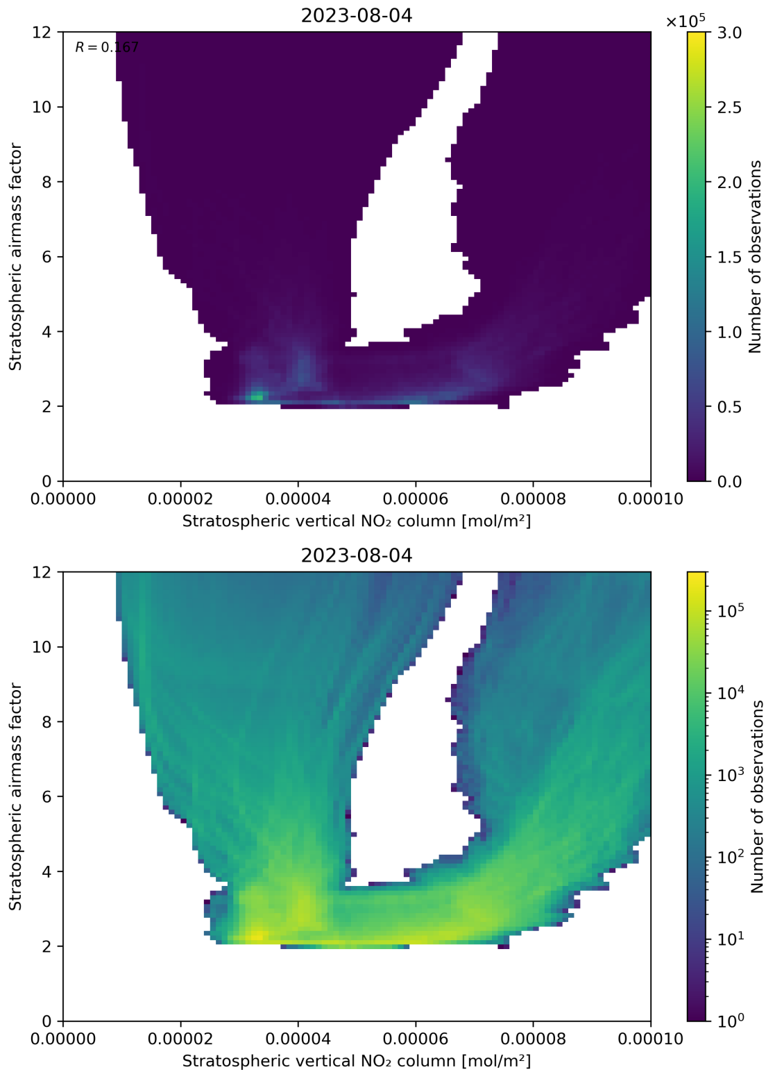
Figure 96: Scatter density plot of “Stratospheric vertical NO 2 column” against “Stratospheric airmass factor” for 2023-08-04 to 2023-08-05.
