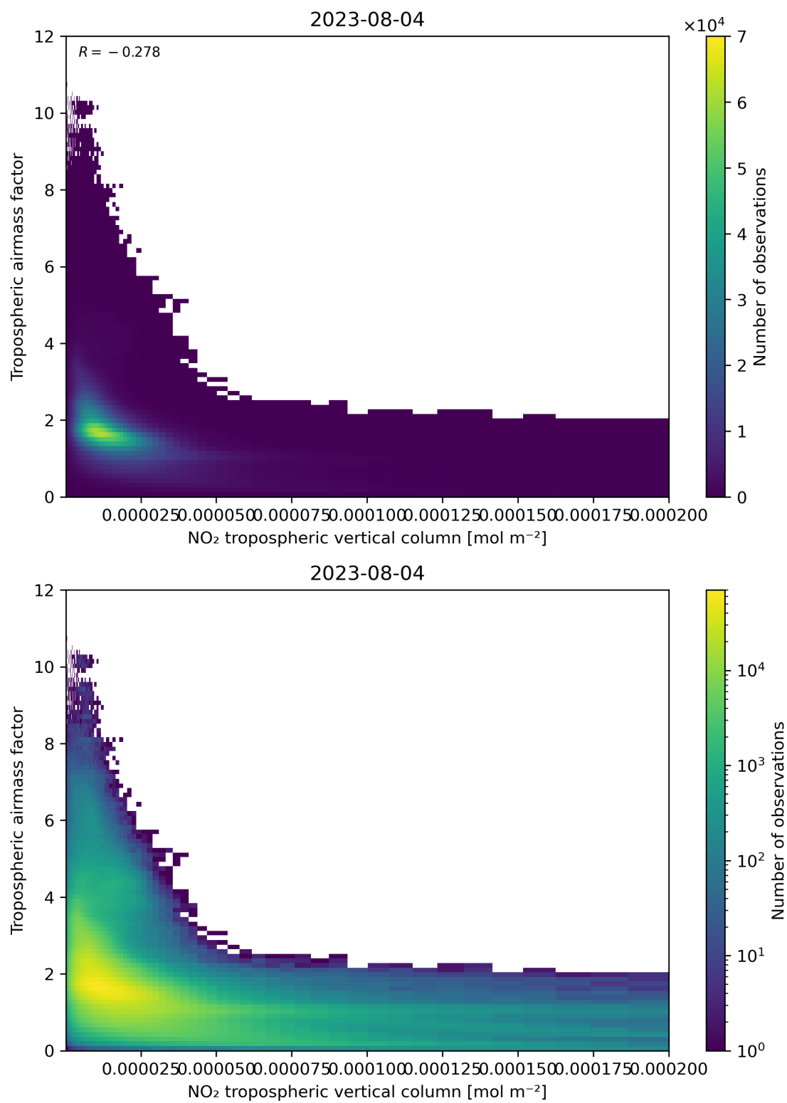
Figure 123: Scatter density plot of “NO 2 tropospheric vertical column” against “Tropospheric airmass factor” for 2023-08-04 to 2023-08-05.
