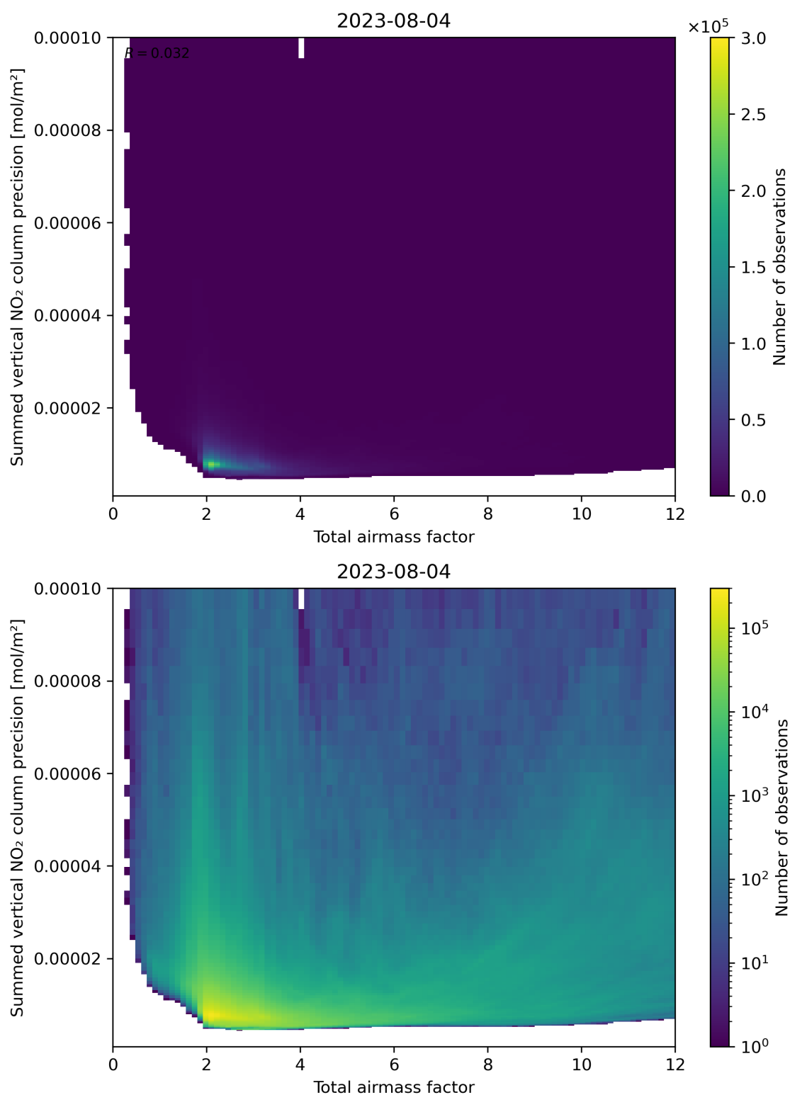
Figure 66: Scatter density plot of “Total airmass factor” against “Summed vertical NO 2 column precision” for 2023-08-04 to 2023-08-05.
