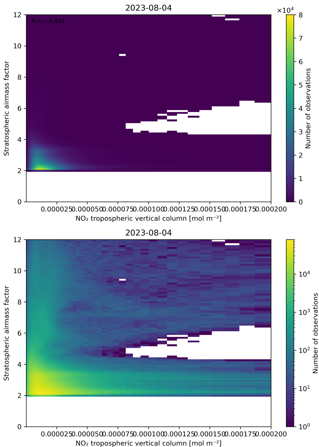
Figure 121: Scatter density plot of “NO 2 tropospheric vertical column” against “Stratospheric air mass factor” for 2023-08-04 to 2023-08-05.
