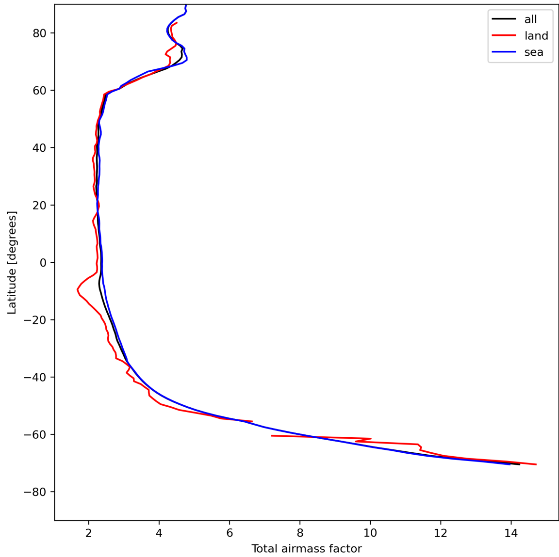
Figure 15: Zonal average of “Total airmass factor” for 2023-08-04 to 2023-08-05.
