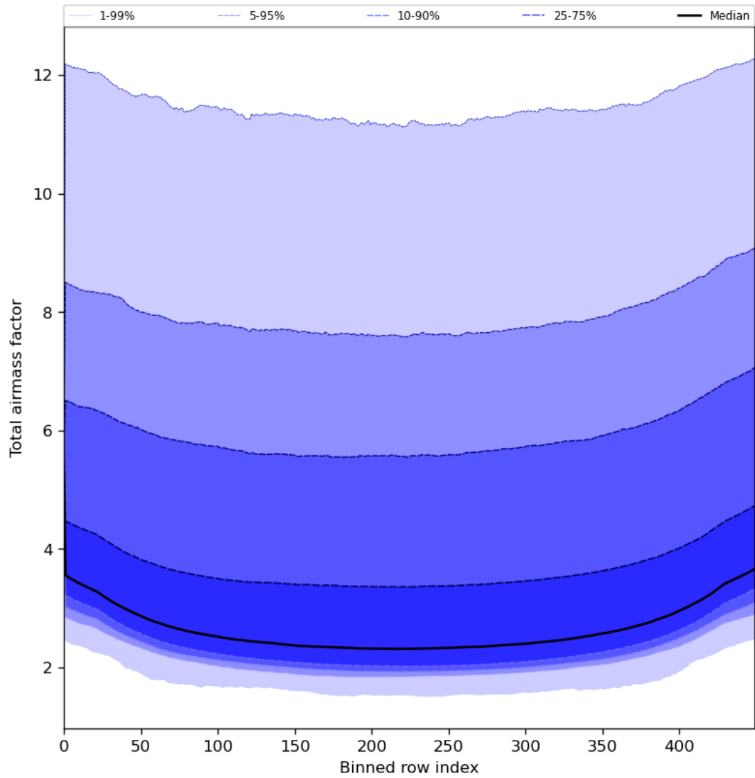
Figure 49: Along track statistics of “Total airmass factor” for 2023-08-04 to 2023-08-05
