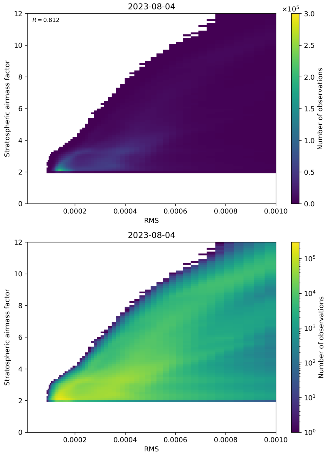
Figure 144: Scatter density plot of “RMS” against “Stratospheric airmass factor” for 2023-08-04 to 2023-08-05.
