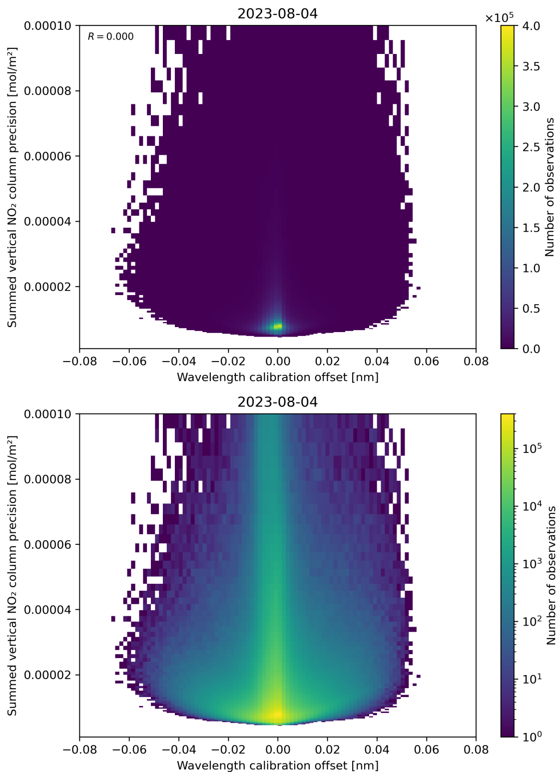
Figure 178: Scatter density plot of “Wavelength calibration offset” against “Summed vertical NO 2 column precision” for 2023-08-04 to 2023-08-05.
