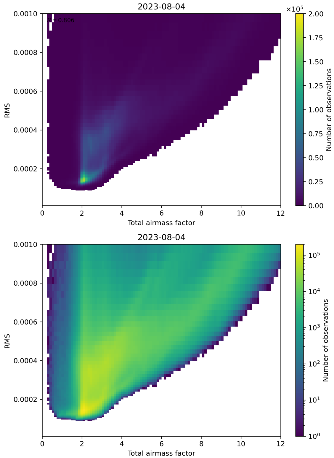
Figure 69: Scatter density plot of “Total airmass factor” against “RMS” for 2023-08-04 to 2023-08-05.
