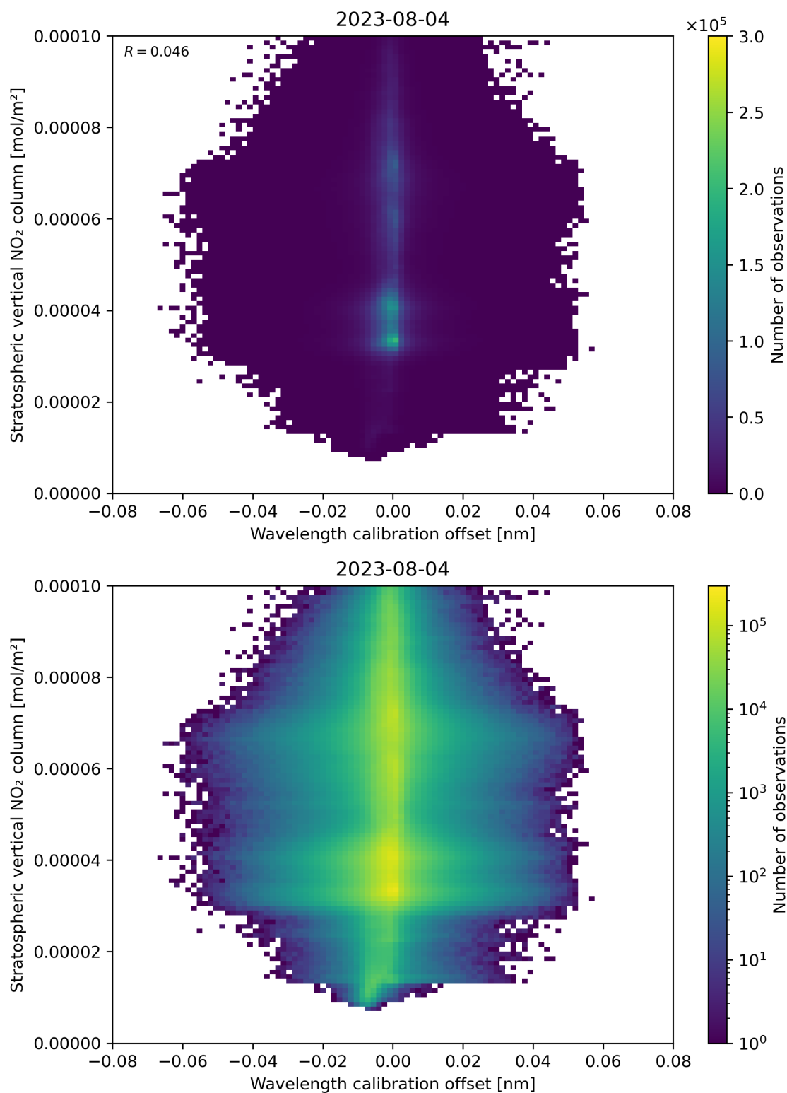
Figure 176: Scatter density plot of “Wavelength calibration offset” against “Stratospheric vertical NO 2 column” for 2023-08-04 to 2023-08-05.
