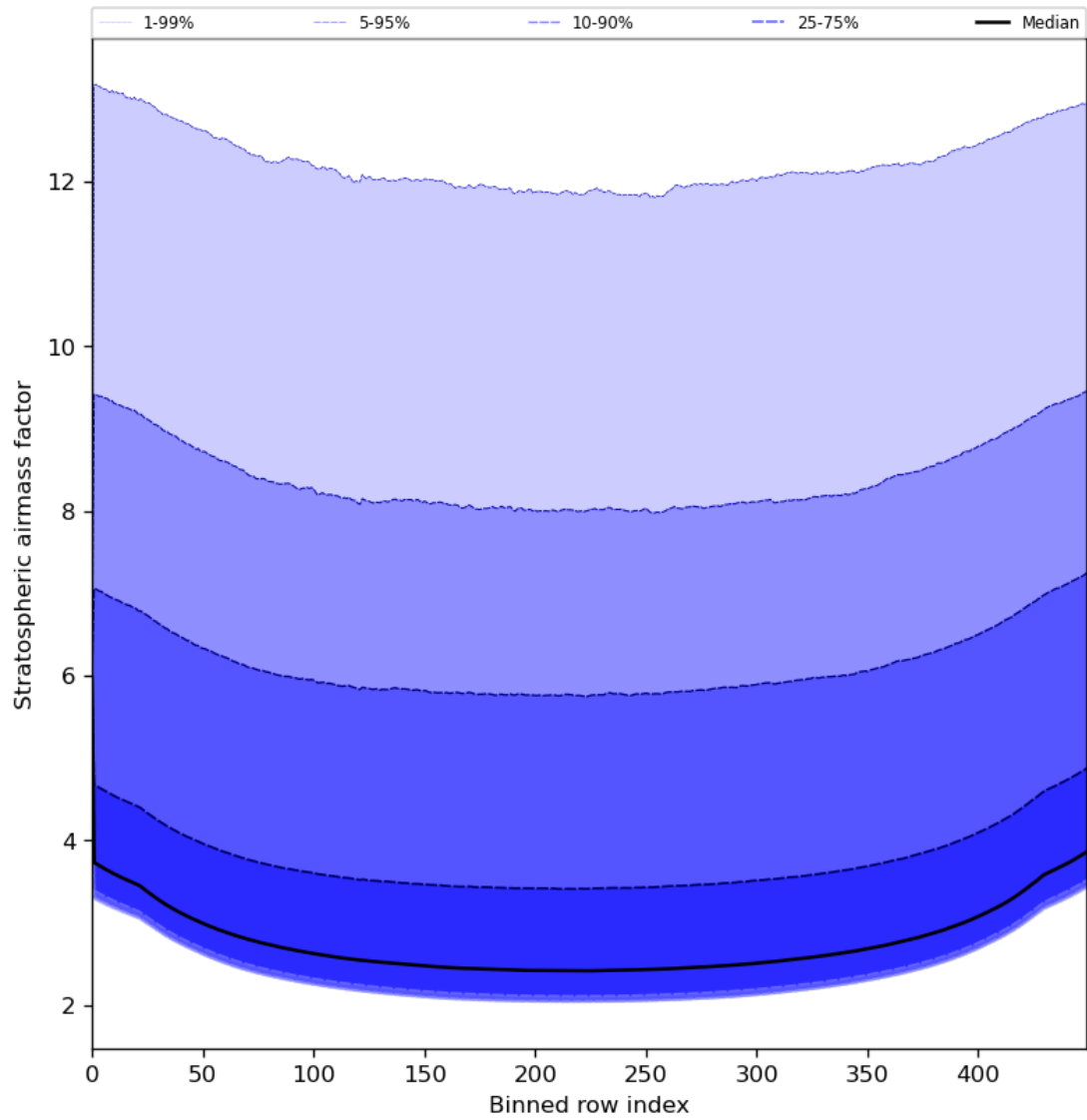
Figure 61: Along track statistics of “Stratospheric airmass factor” for 2023-08-04 to 2023-08-05
