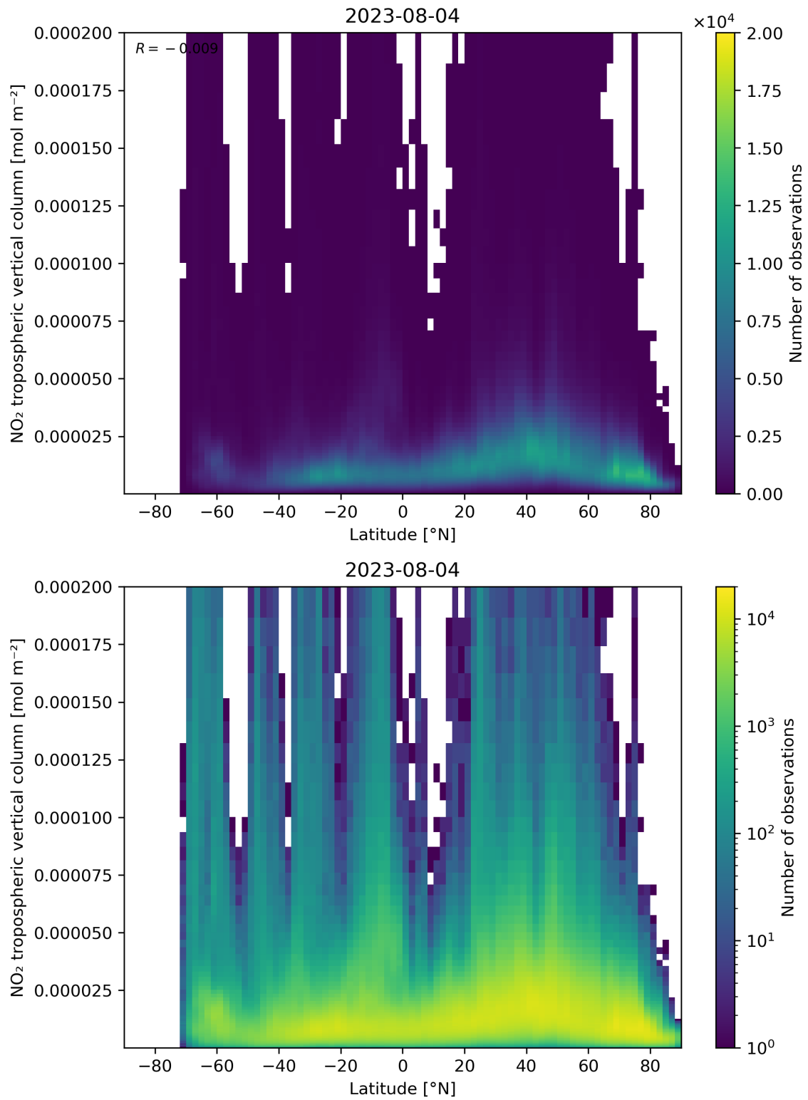
Figure 92: Scatter density plot of “Latitude” against “NO 2 tropospheric vertical column” for 2023-08-04 to 2023-08-05.
