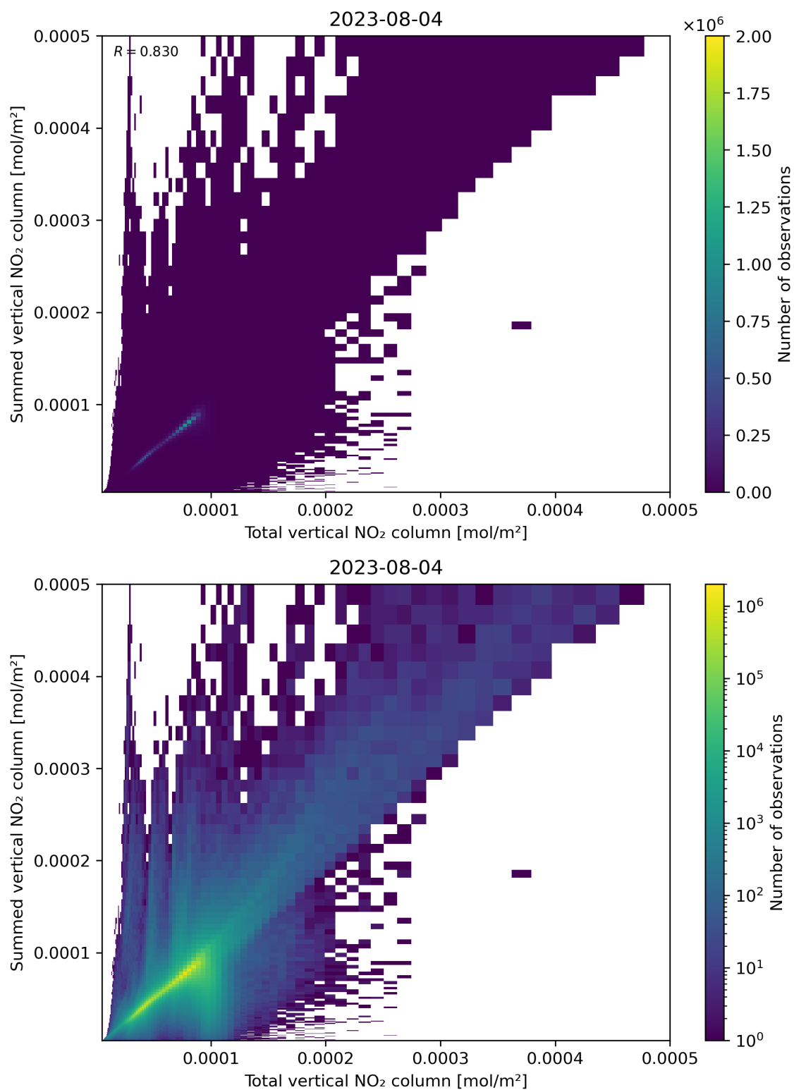
Figure 112: Scatter density plot of “Total vertical NO 2 column” against “Summed vertical NO 2 column” for 2023-08-04 to 2023-08-05.
