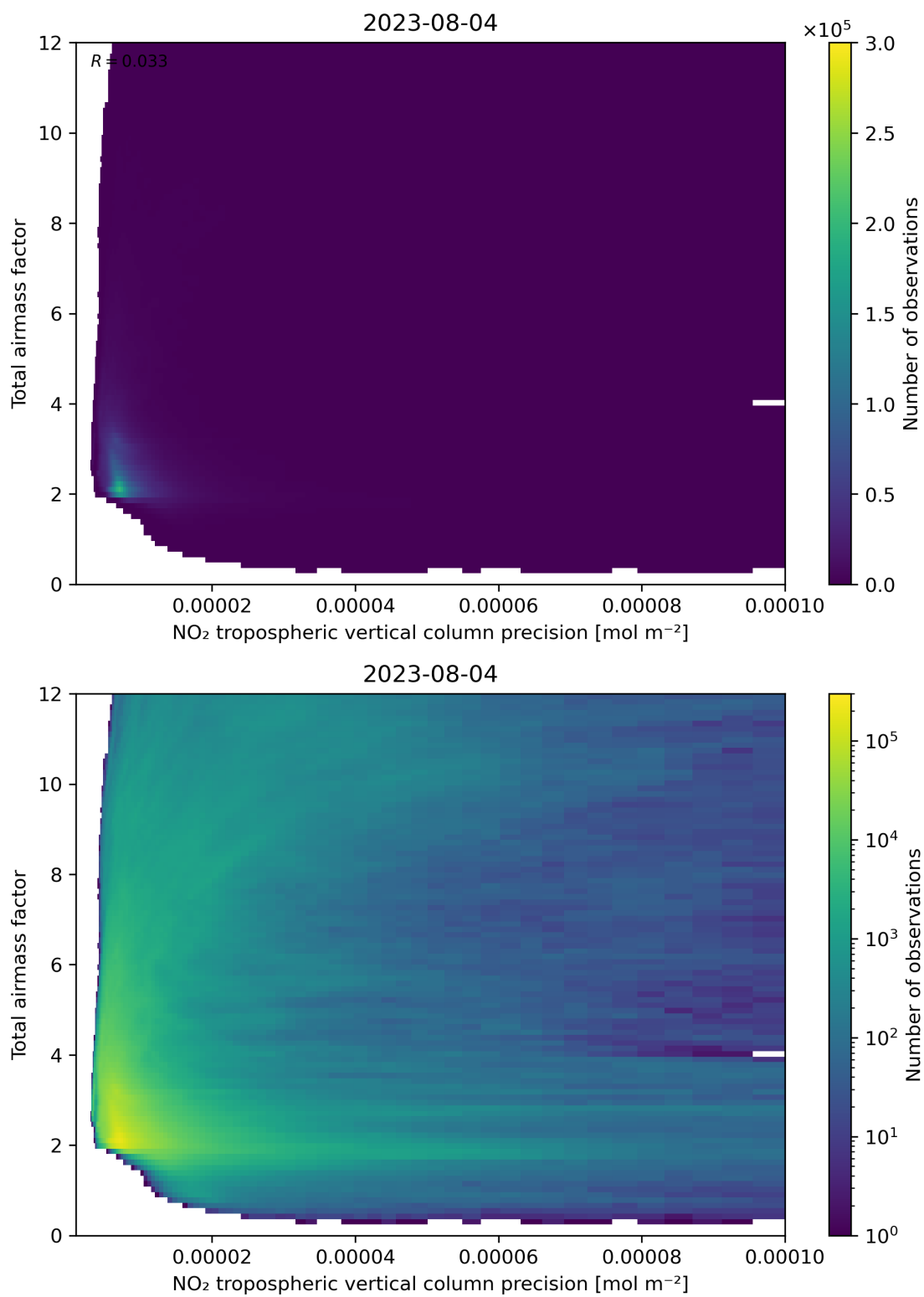
Figure 132: Scatter density plot of “NO 2 tropospheric vertical column precision” against “Total air mass factor” for 2023-08-04 to 2023-08-05.
