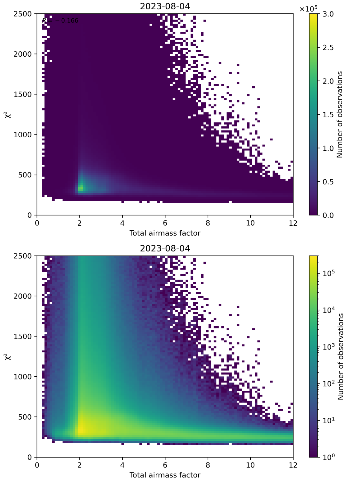
Figure 63: Scatter density plot of “Total airmass factor” against “ \chi^2 ” for 2023-08-04 to 2023-08-05.
