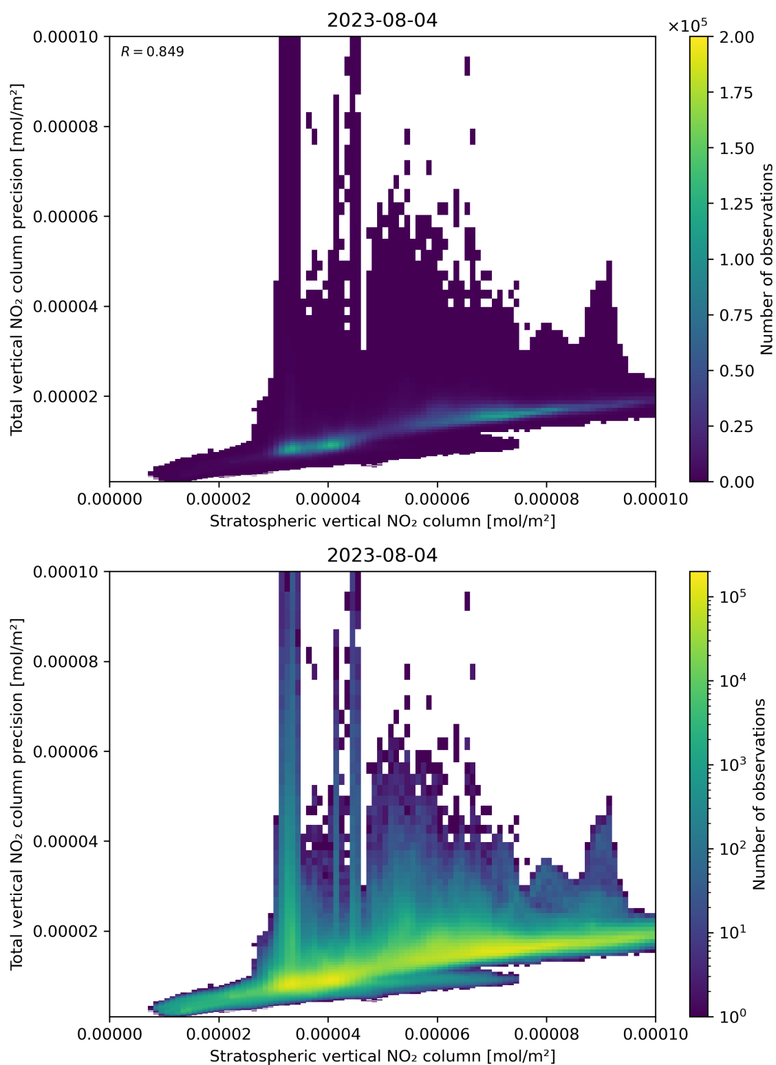
Figure 101: Scatter density plot of “Stratospheric vertical NO 2 column” against “Total vertical NO 2 column precision” for 2023-08-04 to 2023-08-05.
