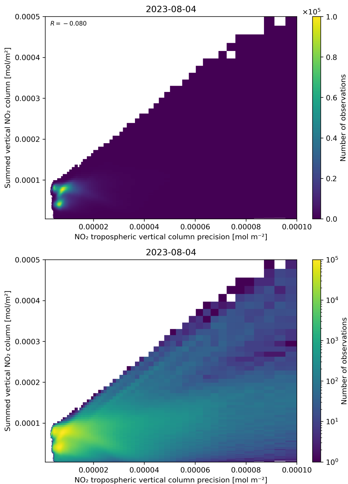
Figure 136: Scatter density plot of “NO 2 tropospheric vertical column precision” against “Summed vertical NO 2 column” for 2023-08-04 to 2023-08-05.
