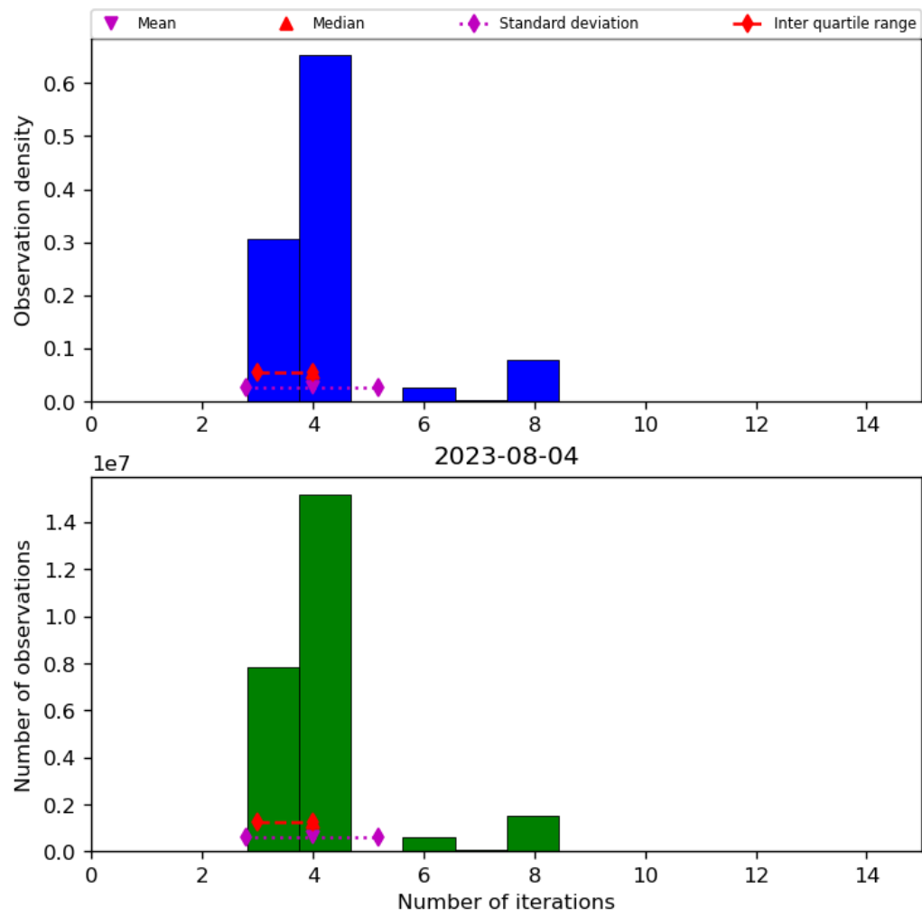
Figure 34: Histogram of “Number of iterations” for 2023-08-04 to 2023-08-05
