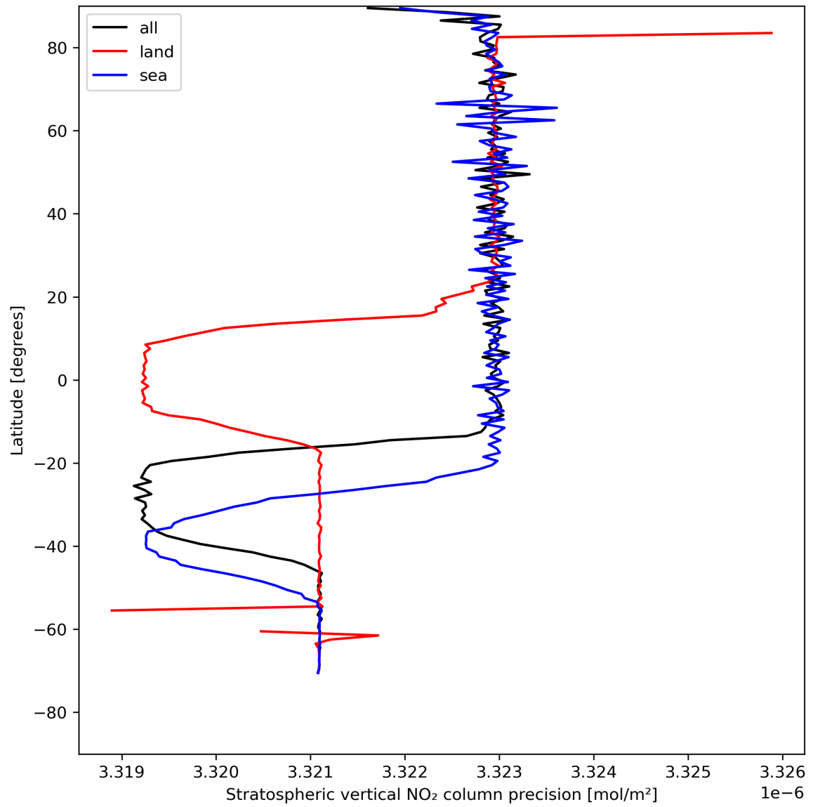
Figure 20: Zonal average of “Stratospheric vertical NO 2 column precision” for 2023-08-04 to 2023-08-05.
