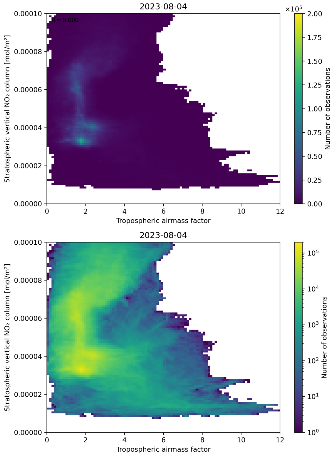
Figure 74: Scatter density plot of “Tropospheric air mass factor” against “Stratospheric vertical NO 2 column” for 2023-08-04 to 2023-08-05.
