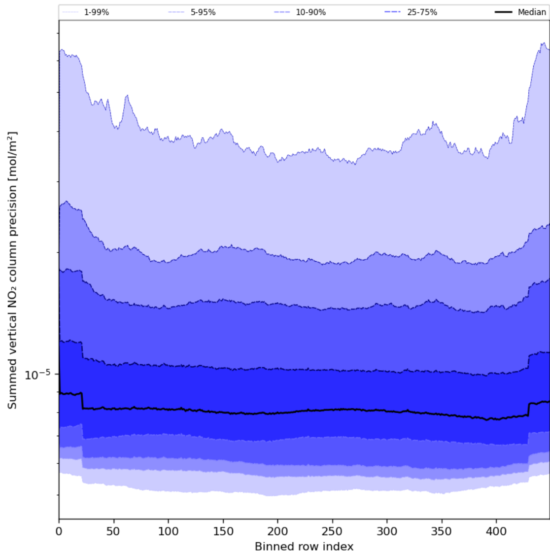
Figure 58: Along track statistics of “Summed vertical NO 2 column precision” for 2023-08-04 to 2023-08-05
