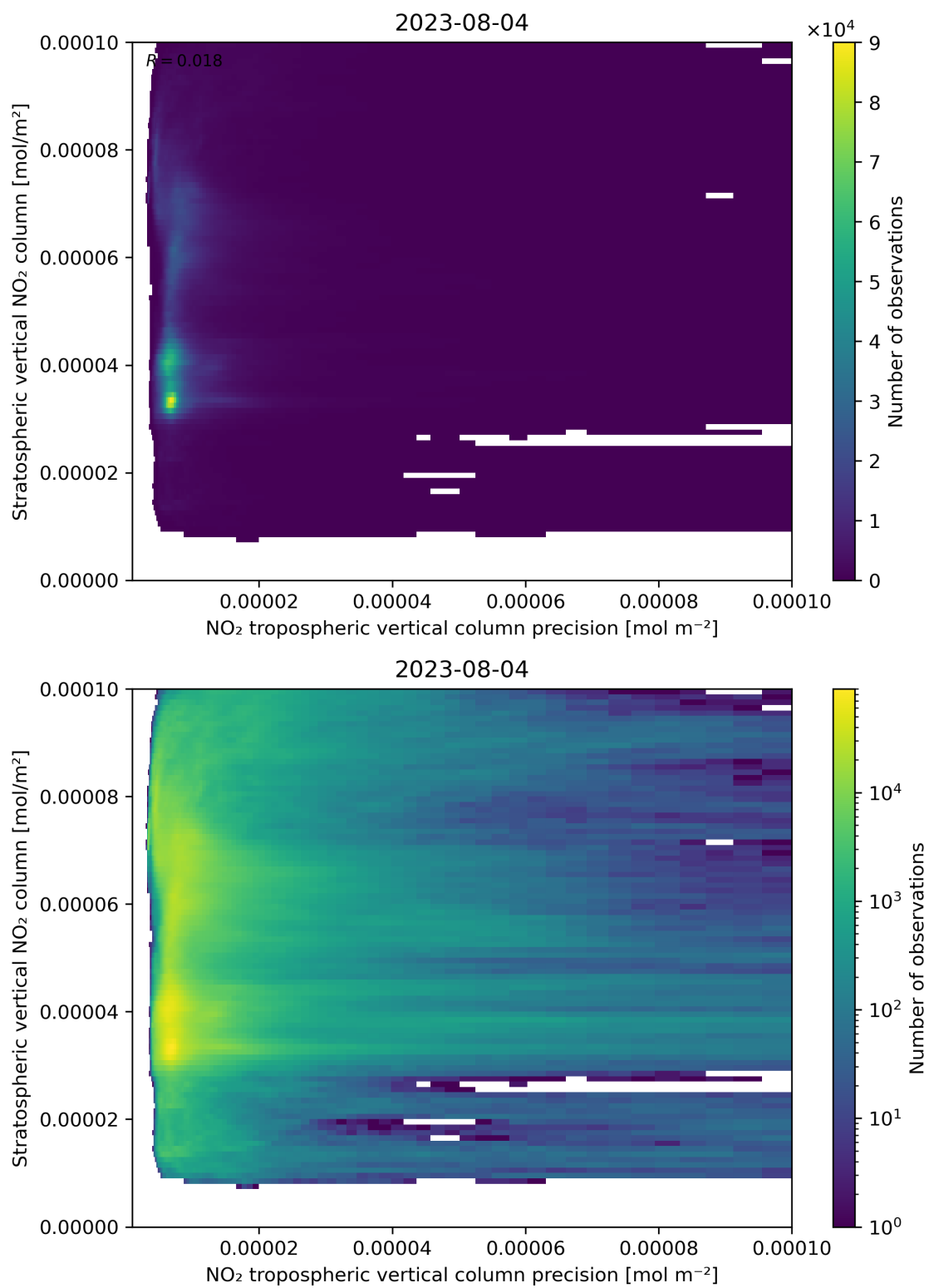
Figure 135: Scatter density plot of “NO 2 tropospheric vertical column precision” against “Stratospheric vertical NO 2 column” for 2023-08-04 to 2023-08-05.
