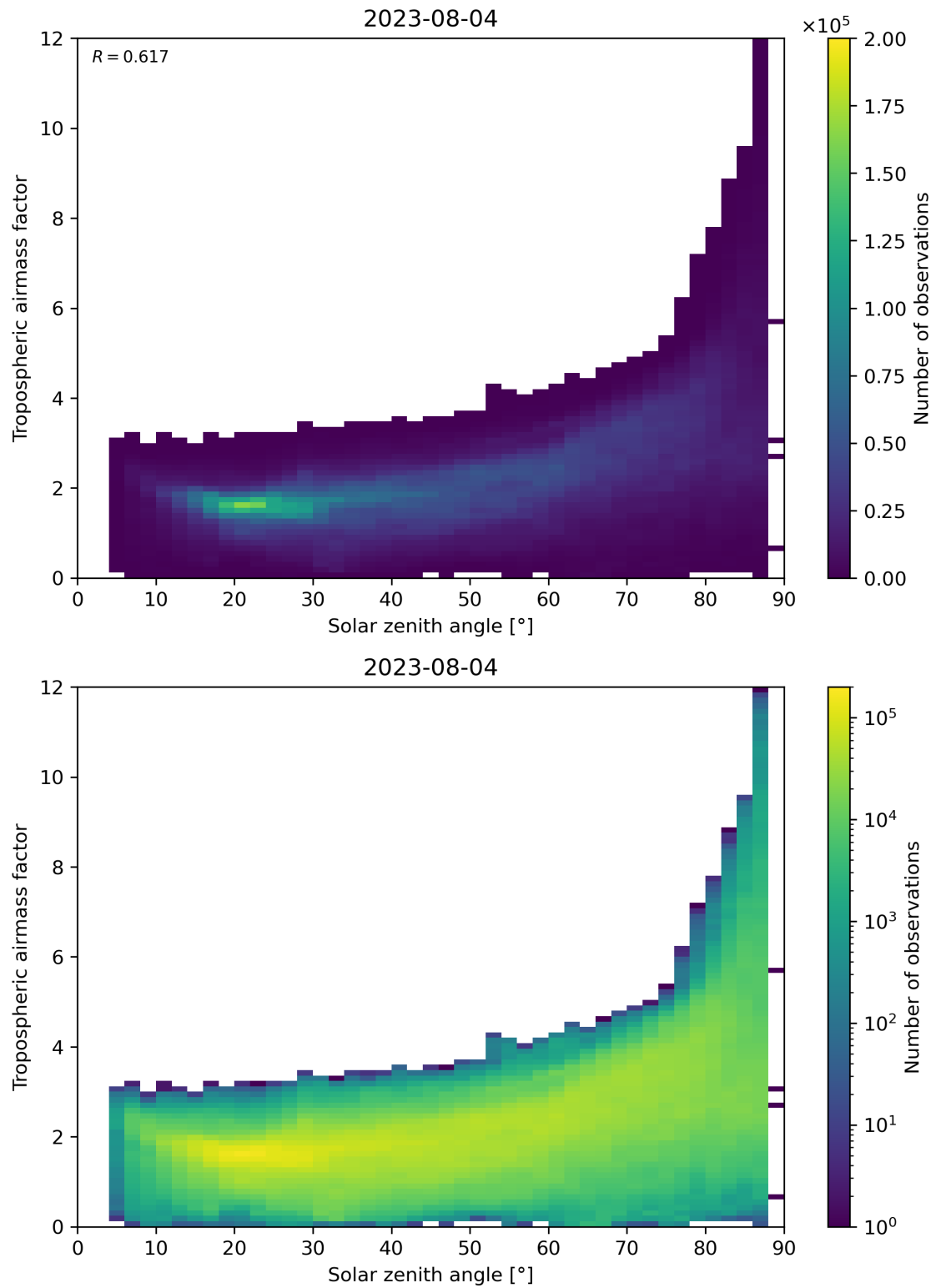
Figure 147: Scatter density plot of “Solar zenith angle” against “Tropospheric airmass factor” for 2023-08-04 to 2023-08-05.
