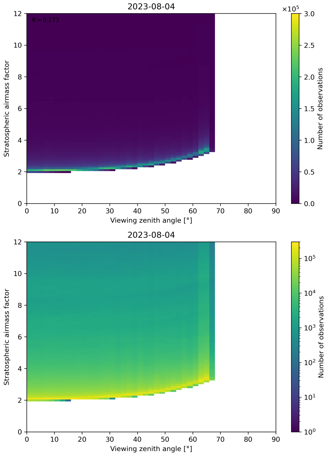
Figure 159: Scatter density plot of “Viewing zenith angle” against “Stratospheric airmass factor” for 2023-08-04 to 2023-08-05.
