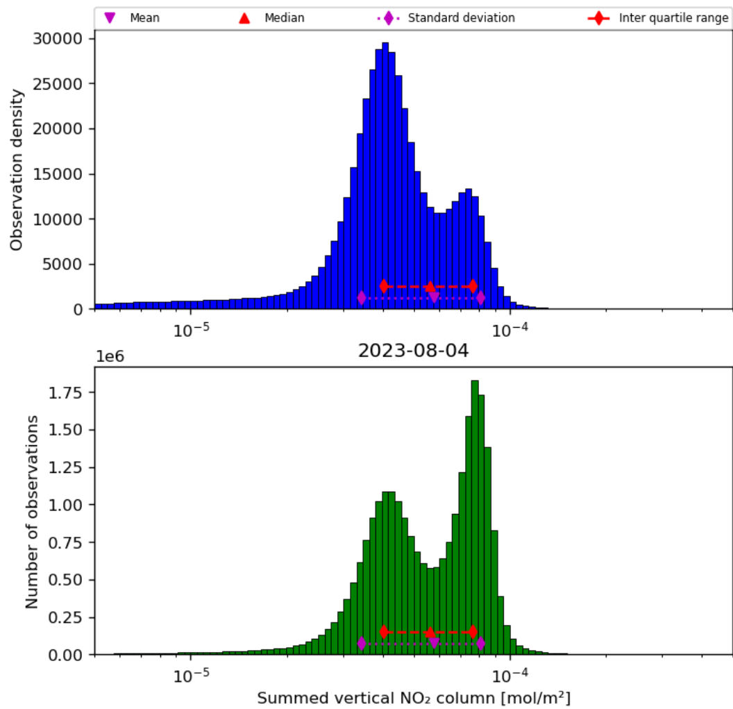
Figure 40: Histogram of "Summed vertical NO 2 column" for 2023-08-04 to 2023-08-05
