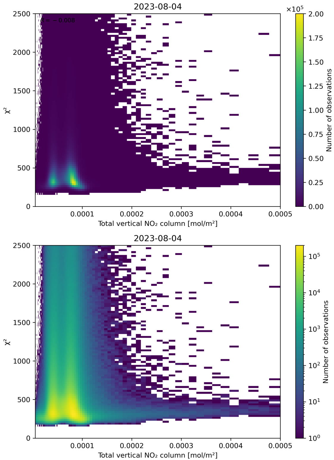
Figure 111: Scatter density plot of “Total vertical NO 2 column” against “ \chi^2 ” for 2023-08-04 to 2023-08-05.
