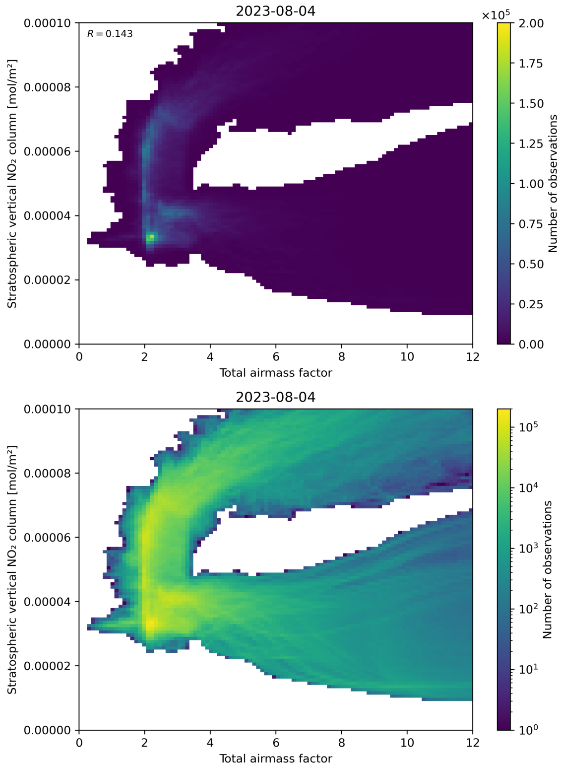
Figure 64: Scatter density plot of “Total airmass factor” against “Stratospheric vertical \text{NO}_2 column” for 2023-08-04 to 2023-08-05.
