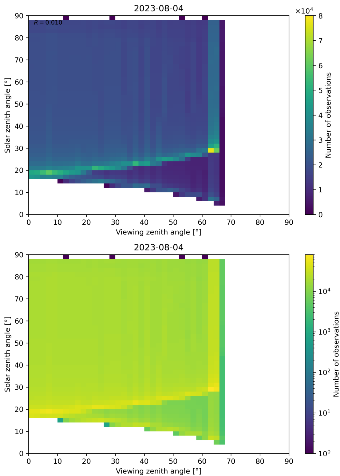
Figure 172: Scatter density plot of “Viewing zenith angle” against “Solar zenith angle” for 2023-08-04 to 2023-08-05.
