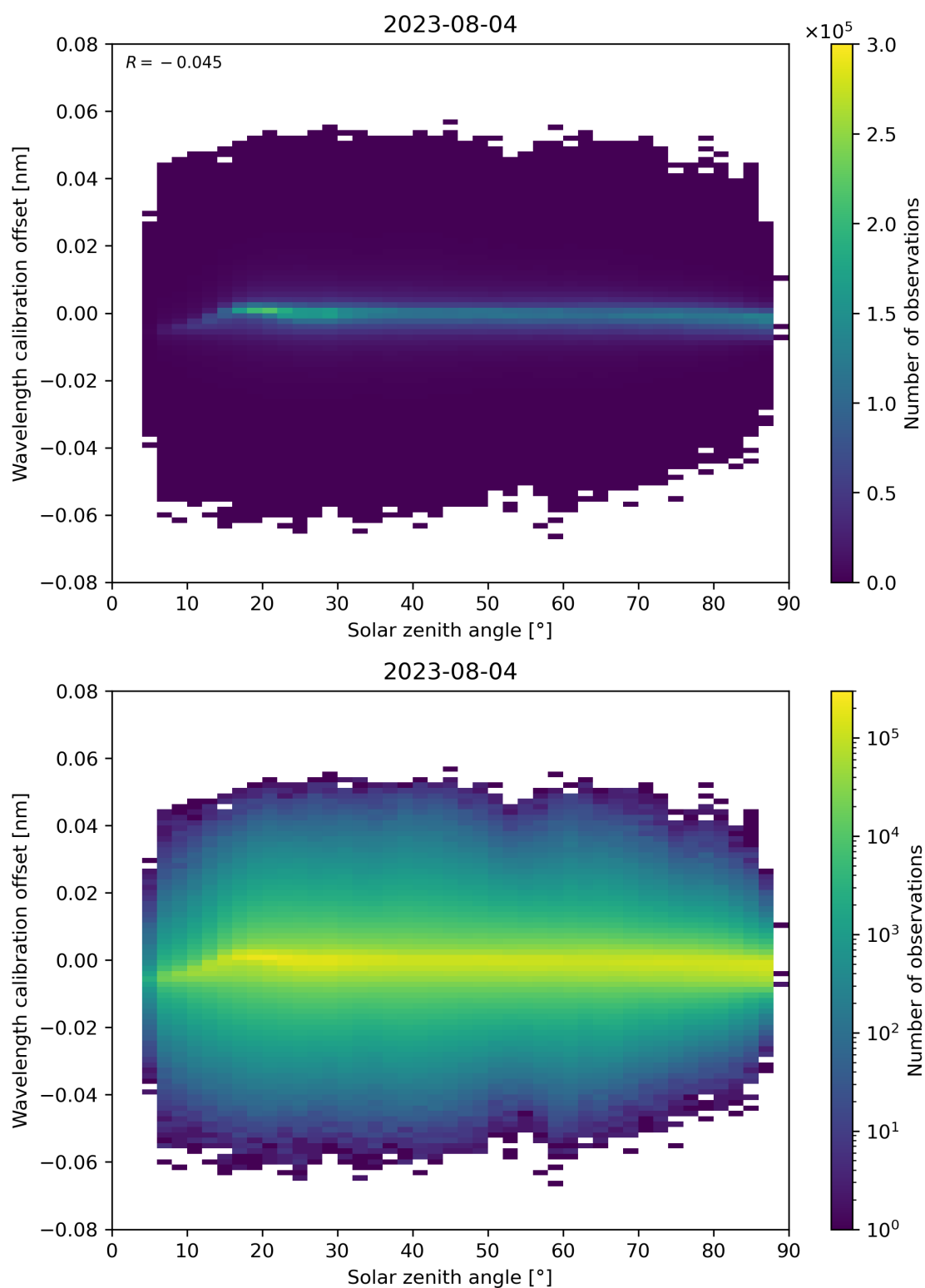
Figure 158: Scatter density plot of “Solar zenith angle” against “Wavelength calibration offset” for 2023-08-04 to 2023-08-05.
