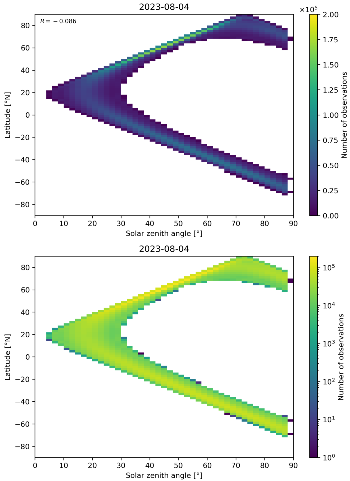
Figure 149: Scatter density plot of “Solar zenith angle” against “Latitude” for 2023-08-04 to 2023-08-05.
