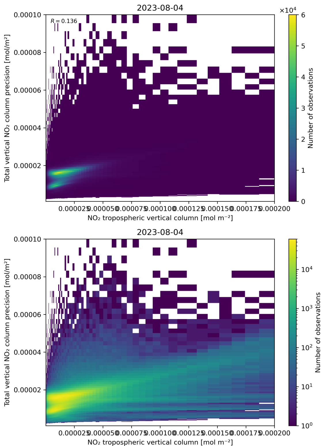
Figure 129: Scatter density plot of “NO 2 tropospheric vertical column” against “Total vertical NO 2 column precision” for 2023-08-04 to 2023-08-05.
