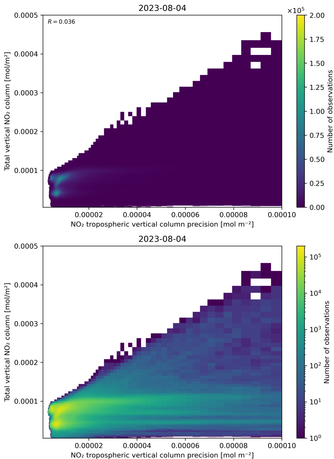
Figure 138: Scatter density plot of “NO 2 tropospheric vertical column precision” against “Total vertical NO 2 column” for 2023-08-04 to 2023-08-05.
