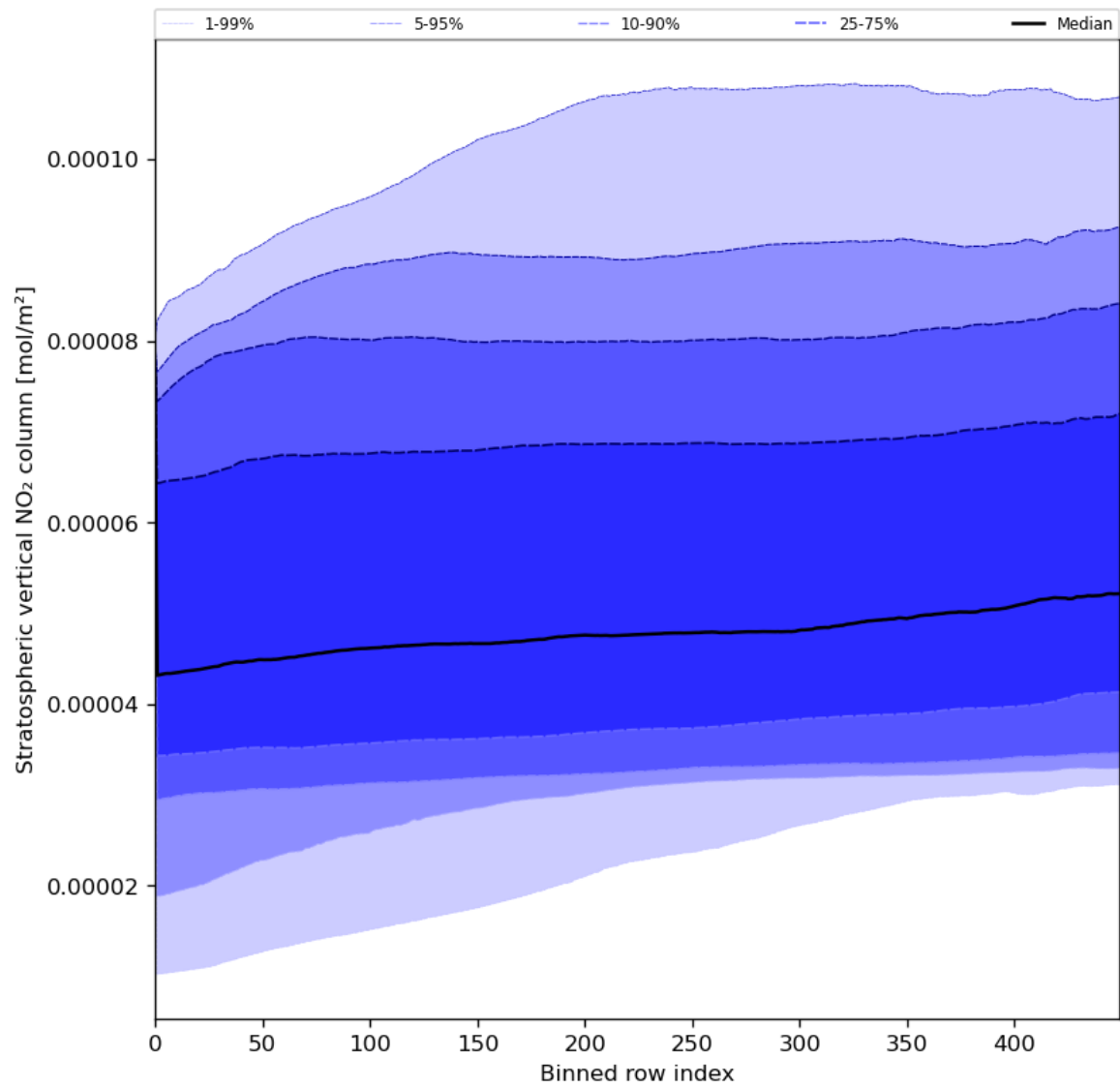
Figure 53: Along track statistics of “Stratospheric vertical NO 2 column” for 2023-08-04 to 2023-08-05
