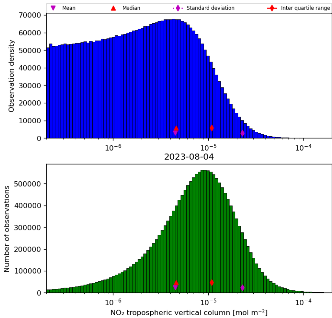
Figure 29: Histogram of “NO 2 tropospheric vertical column” for 2023-08-04 to 2023-08-05
