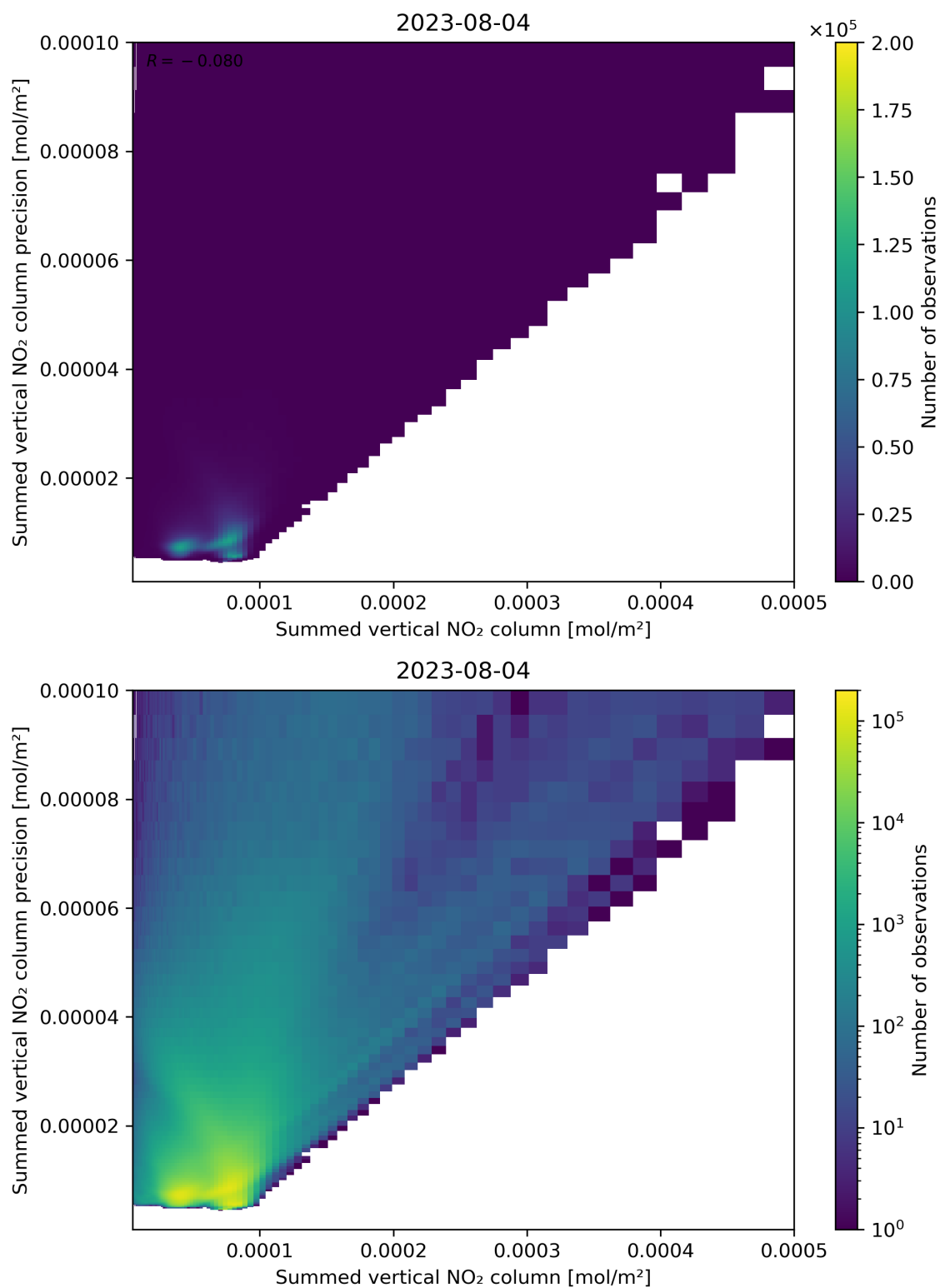
Figure 105: Scatter density plot of “Summed vertical NO 2 column” against “Summed vertical NO 2 column precision” for 2023-08-04 to 2023-08-05.
