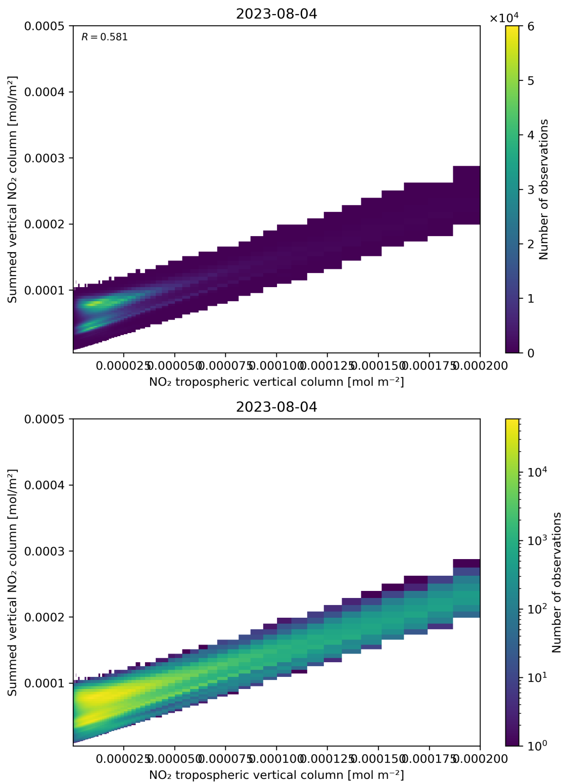
Figure 126: Scatter density plot of “NO 2 tropospheric vertical column” against “Summed vertical NO 2 column” for 2023-08-04 to 2023-08-05.
