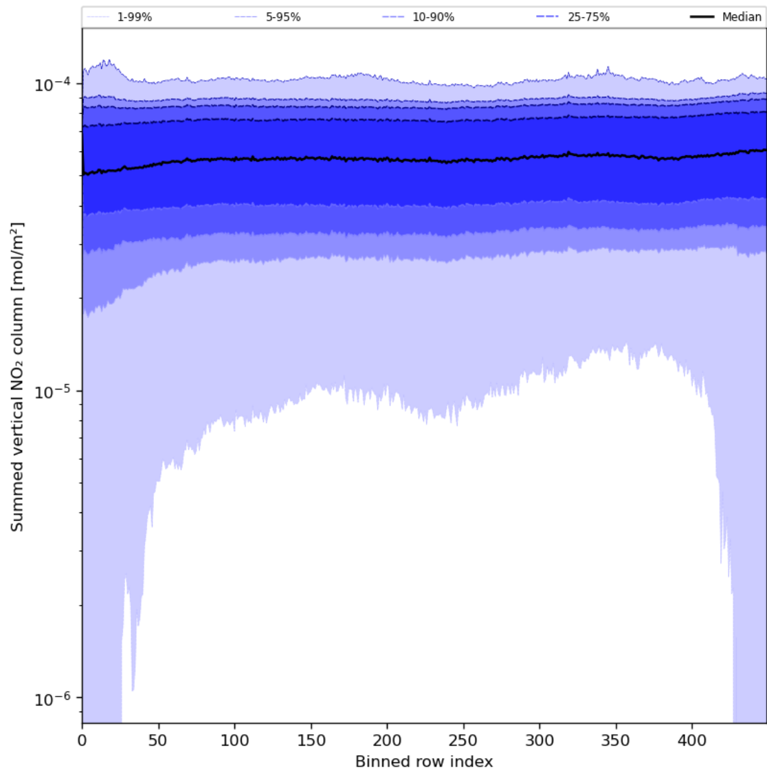
Figure 57: Along track statistics of “Summed vertical NO 2 column” for 2023-08-04 to 2023-08-05
