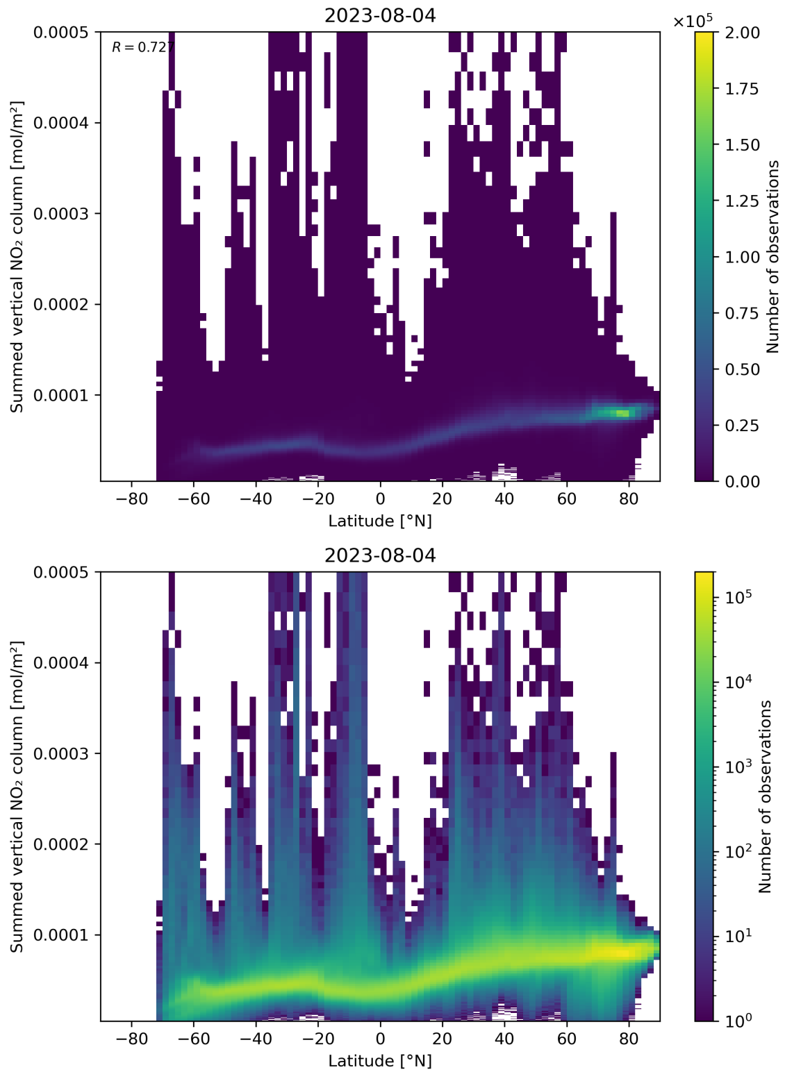
Figure 88: Scatter density plot of “Latitude” against “Summed vertical NO 2 column” for 2023-08-04 to 2023-08-05.
