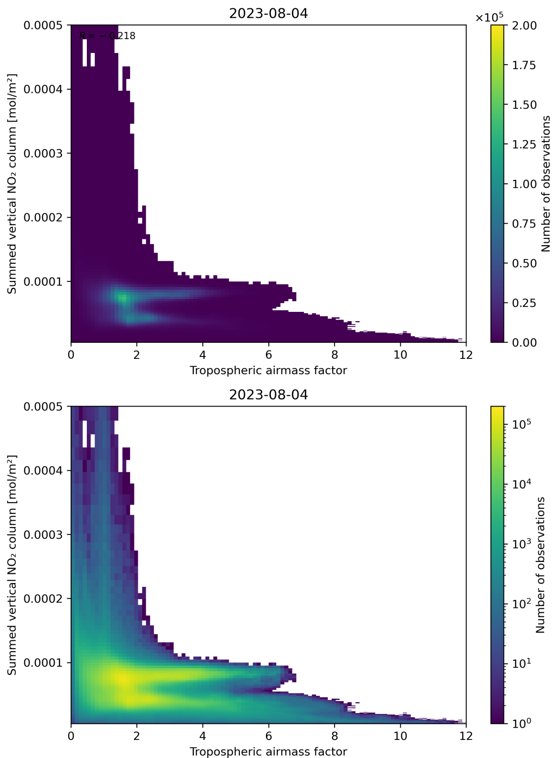
Figure 75: Scatter density plot of “Tropospheric air mass factor” against “Summed vertical NO 2 column” for 2023-08-04 to 2023-08-05.
