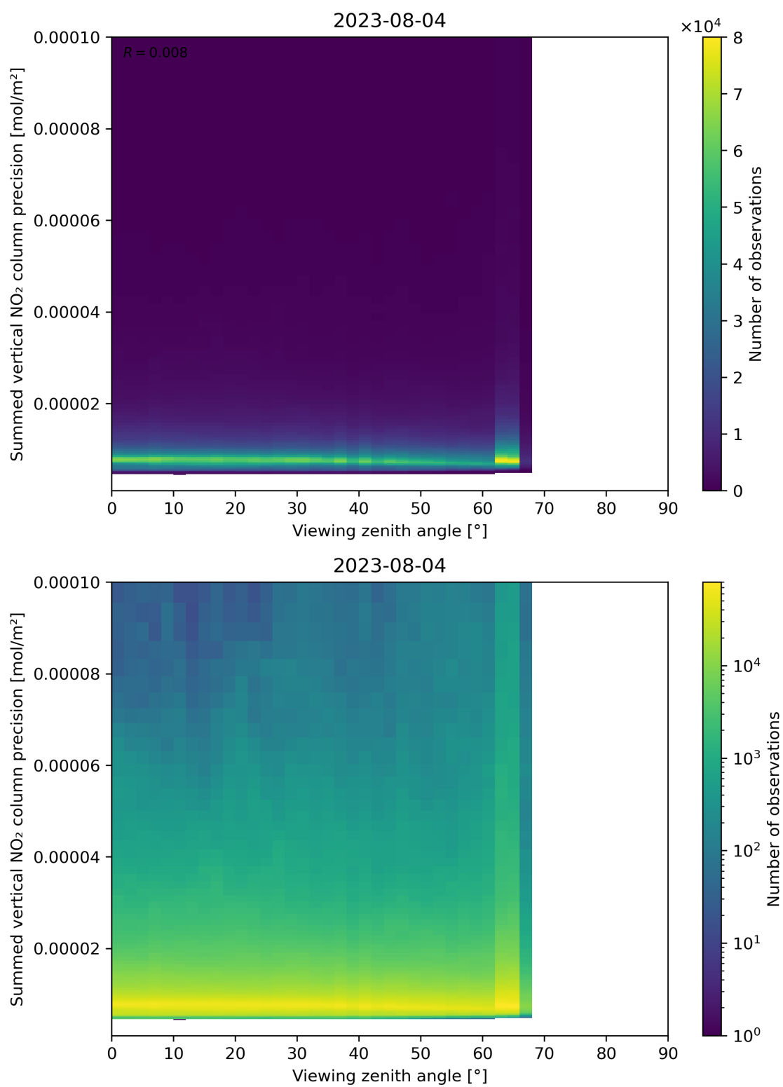
Figure 166: Scatter density plot of “Viewing zenith angle” against “Summed vertical NO 2 column precision” for 2023-08-04 to 2023-08-05.
