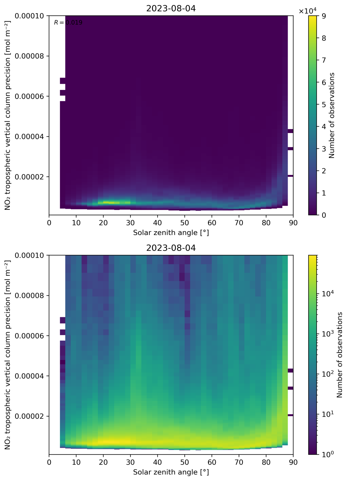
Figure 156: Scatter density plot of “Solar zenith angle” against “NO 2 tropospheric vertical column precision” for 2023-08-04 to 2023-08-05.
