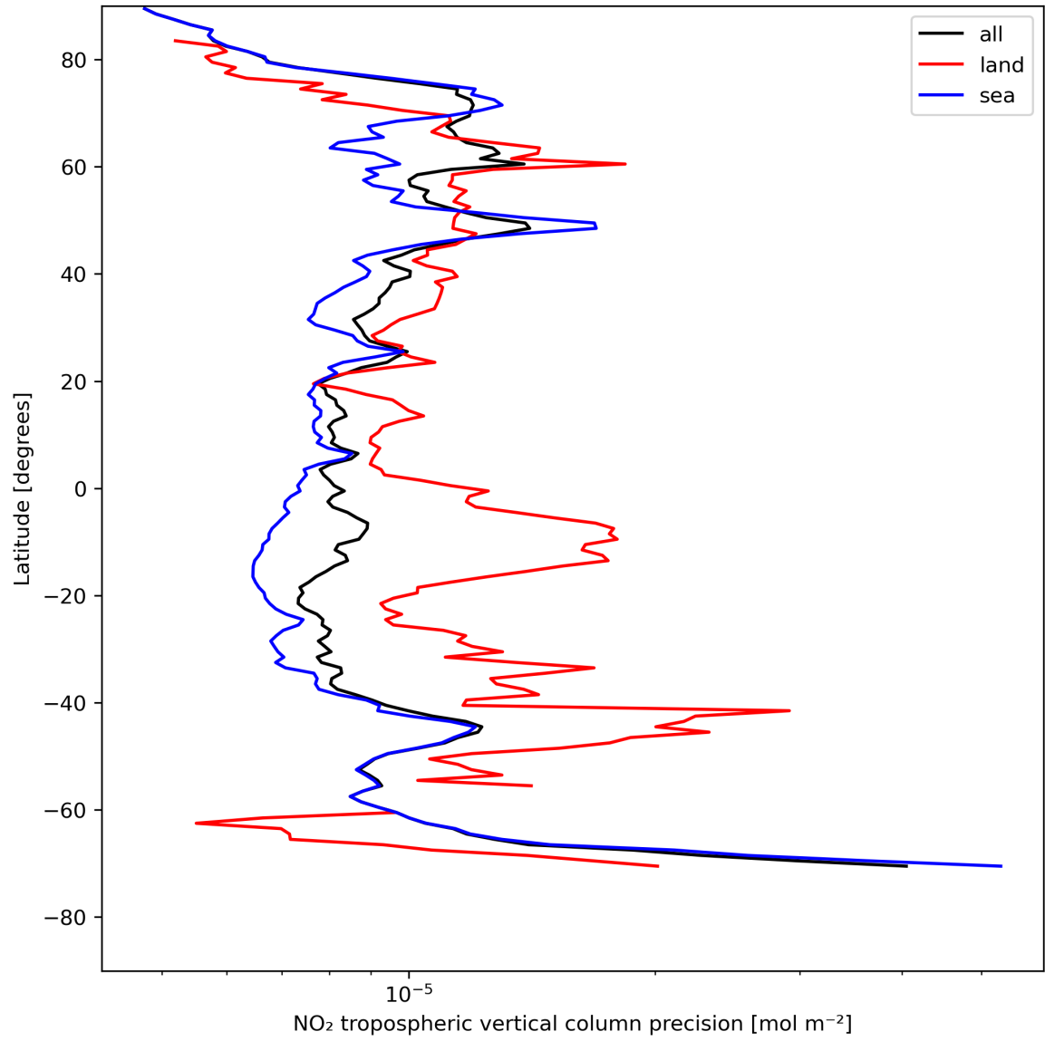
Figure 13: Zonal average of “NO 2 tropospheric vertical column precision” for 2023-08-04 to 2023-08-05.
