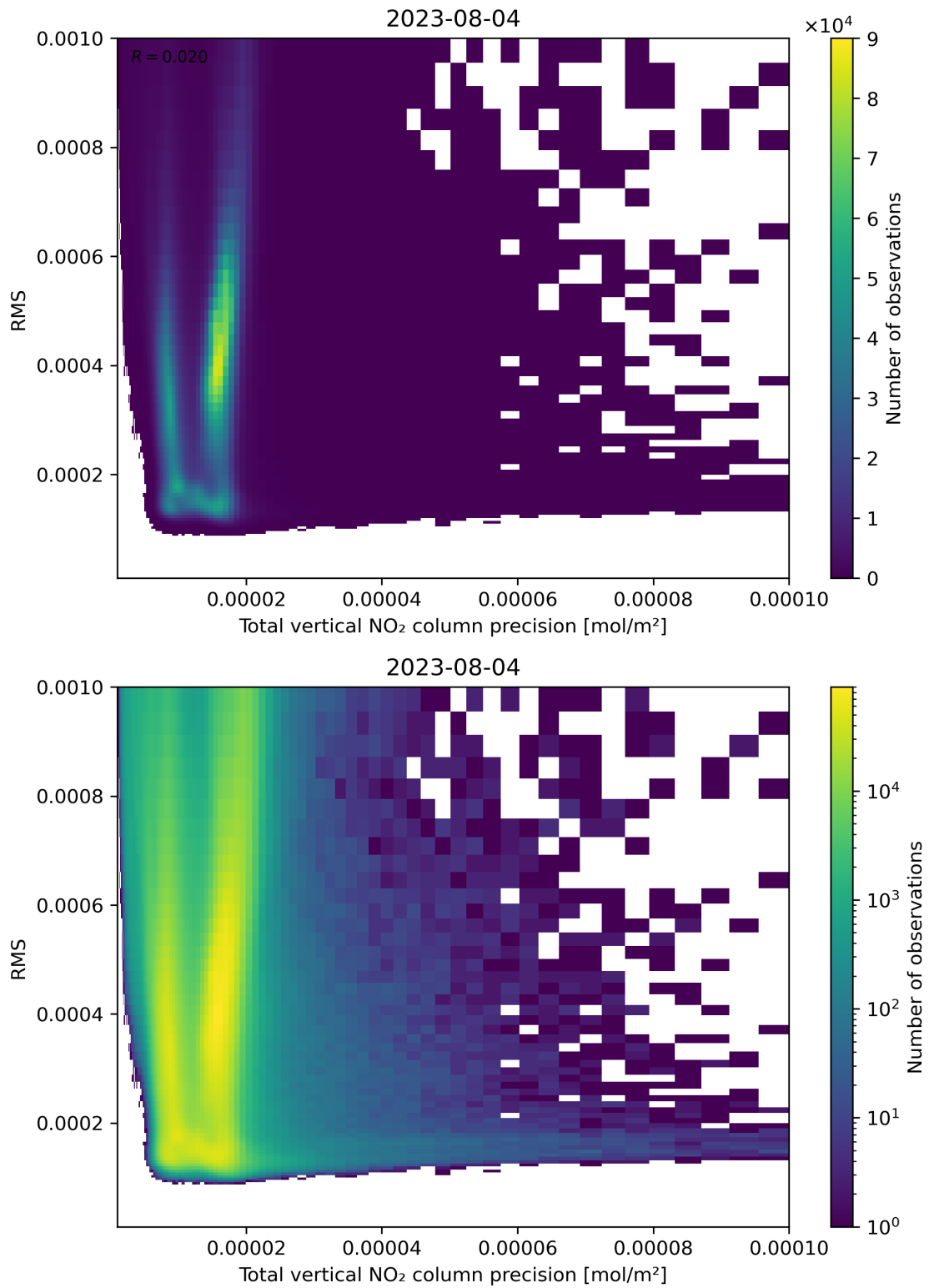
Figure 119: Scatter density plot of “Total vertical NO 2 column precision” against “RMS” for 2023-08-04 to 2023-08-05.
