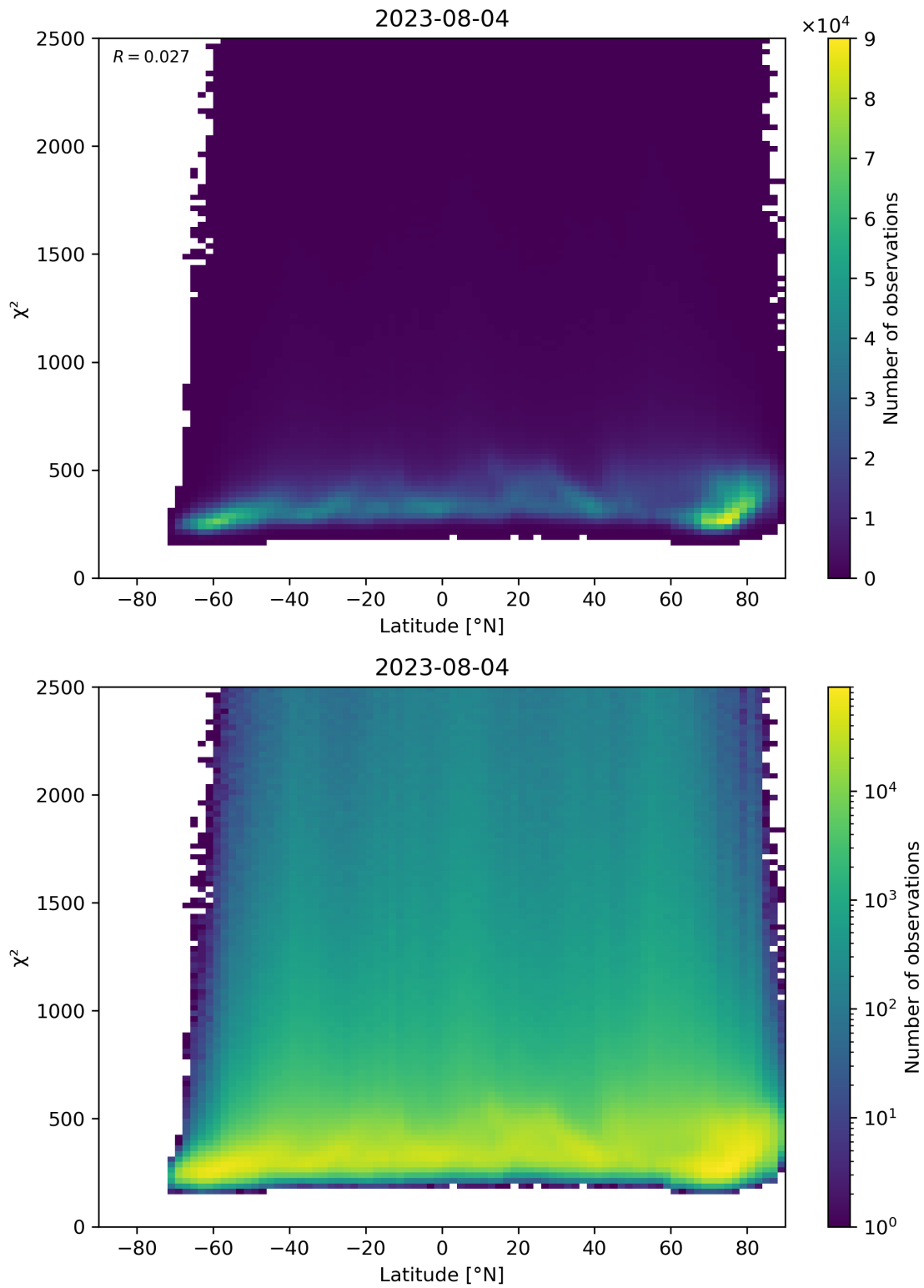
Figure 86: Scatter density plot of “Latitude” against “ \chi^2 ” for 2023-08-04 to 2023-08-05.
