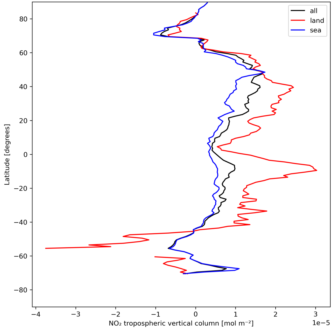
Figure 12: Zonal average of “NO 2 tropospheric vertical column” for 2023-08-04 to 2023-08-05.
