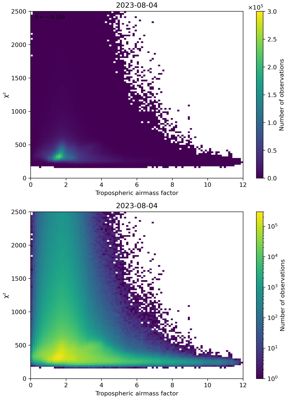
Figure 73: Scatter density plot of “Tropospheric airmass factor” against “ \chi^2 ” for 2023-08-04 to 2023-08-05.
