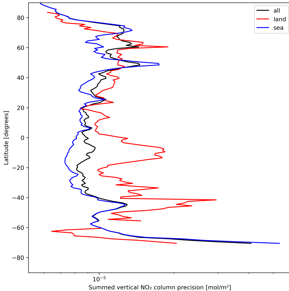
Figure 24: Zonal average of “Summed vertical NO 2 column precision” for 2023-08-04 to 2023-08-05.
