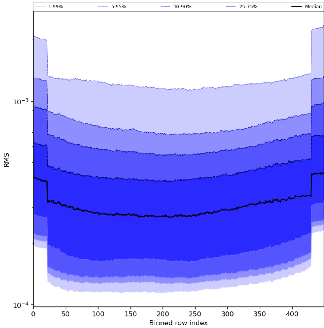
Figure 60: Along track statistics of “RMS” for 2023-08-04 to 2023-08-05
