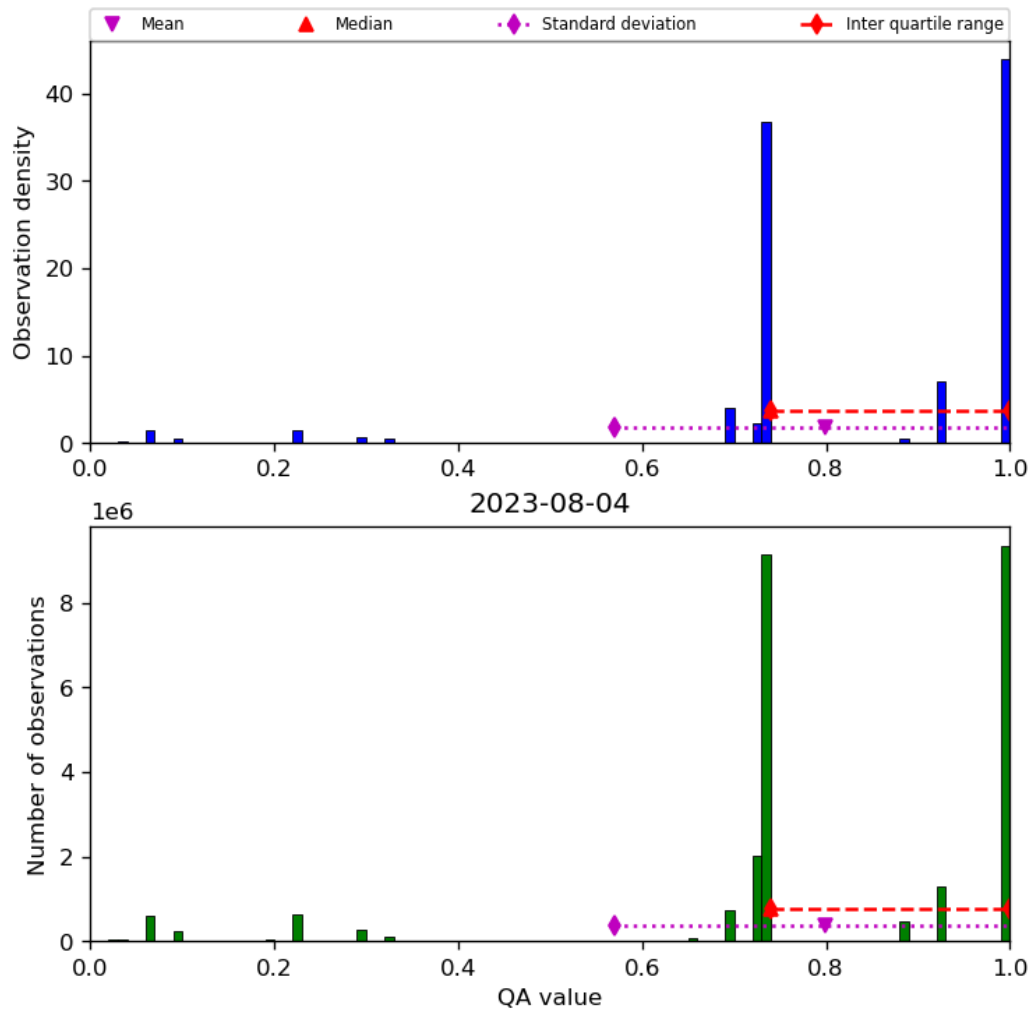
Figure 28: Histogram of “QA value” for 2023-08-04 to 2023-08-05
