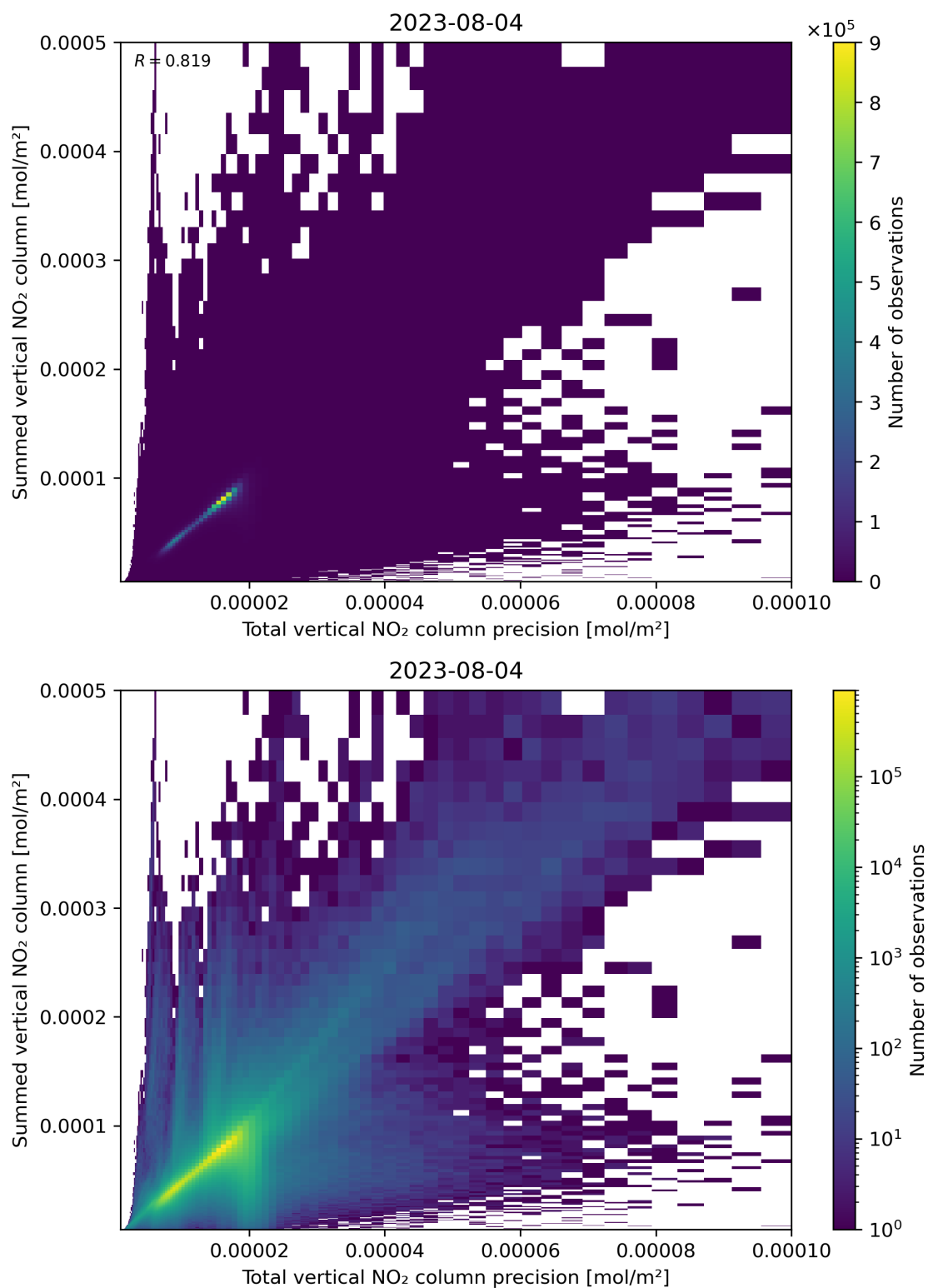
Figure 117: Scatter density plot of “Total vertical NO 2 column precision” against “Summed vertical NO 2 column” for 2023-08-04 to 2023-08-05.
