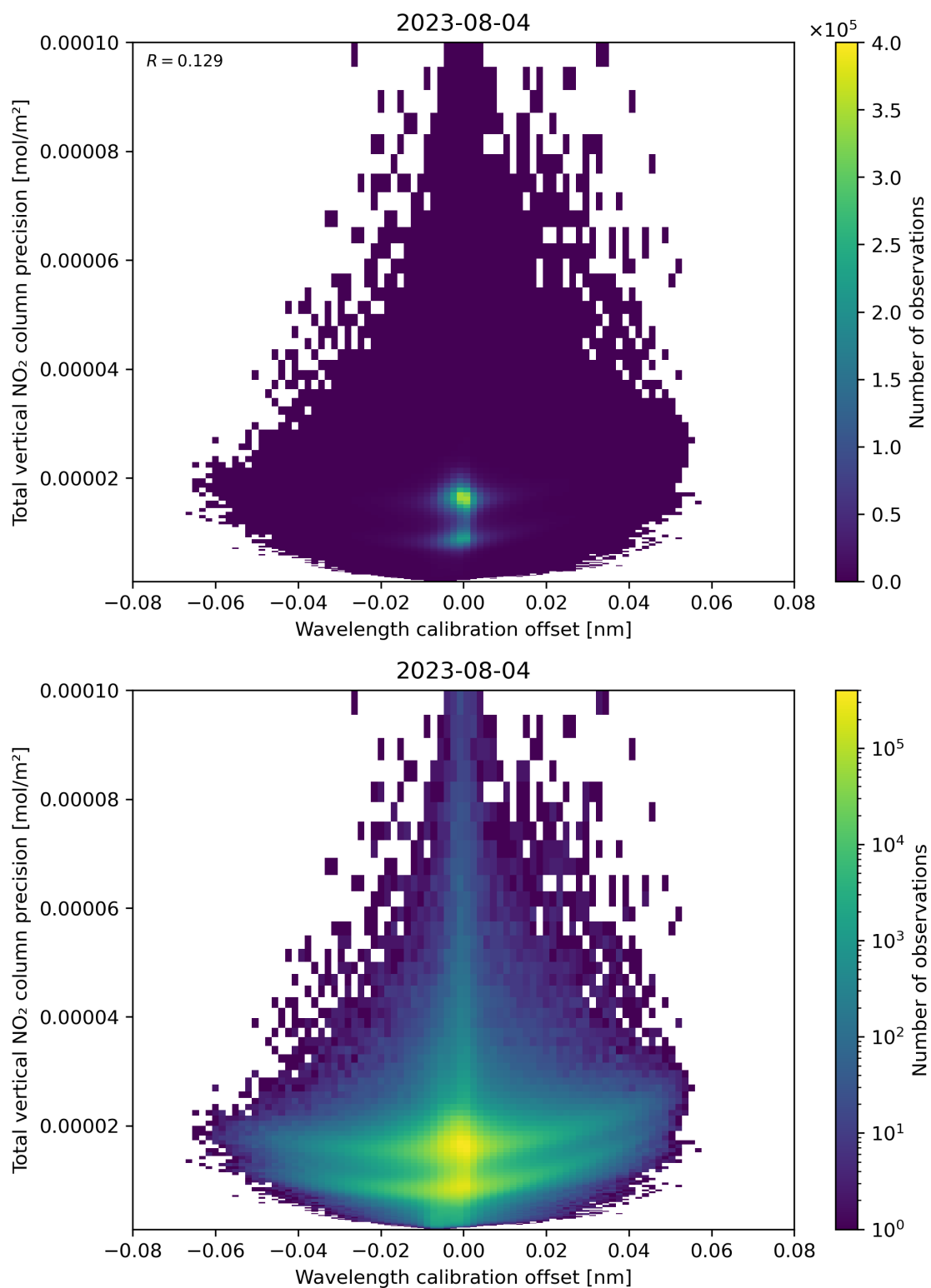
Figure 180: Scatter density plot of “Wavelength calibration offset” against “Total vertical NO 2 column precision” for 2023-08-04 to 2023-08-05.
