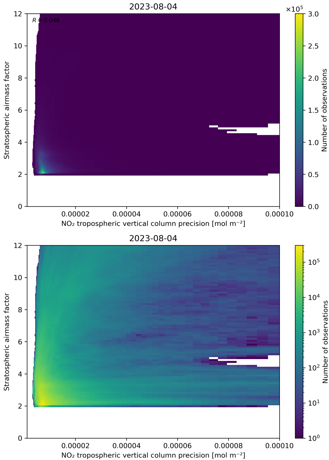
Figure 131: Scatter density plot of “NO 2 tropospheric vertical column precision” against “Stratospheric airmass factor” for 2023-08-04 to 2023-08-05.
