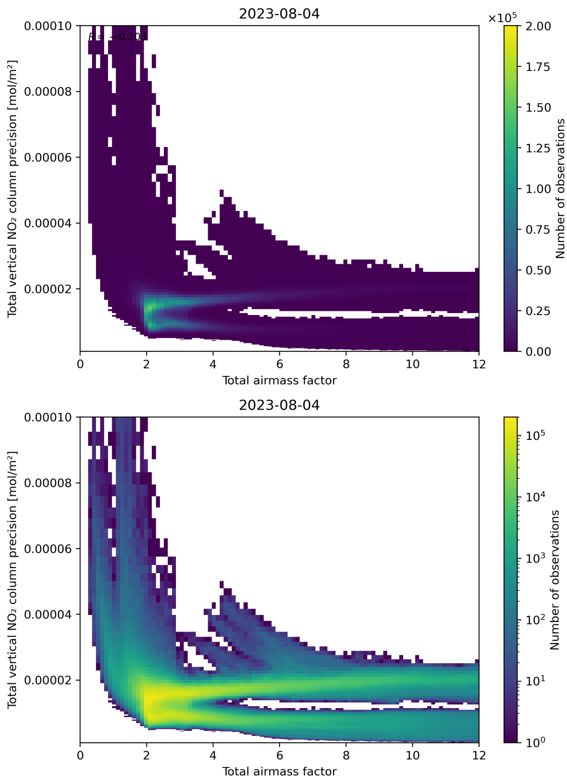
Figure 68: Scatter density plot of “Total airmass factor” against “Total vertical NO 2 column precision” for 2023-08-04 to 2023-08-05.
