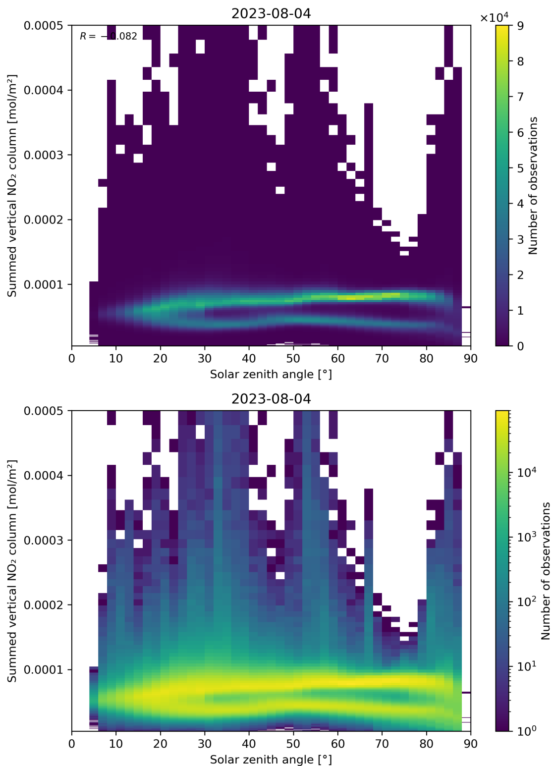
Figure 151: Scatter density plot of “Solar zenith angle” against “Summed vertical NO 2 column” for 2023-08-04 to 2023-08-05.
