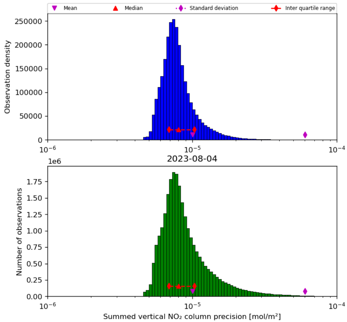
Figure 41: Histogram of “Summed vertical NO 2 column precision” for 2023-08-04 to 2023-08-05
