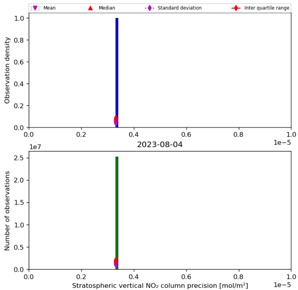
Figure 37: Histogram of “Stratospheric vertical NO 2 column precision” for 2023-08-04 to 2023-08-05
