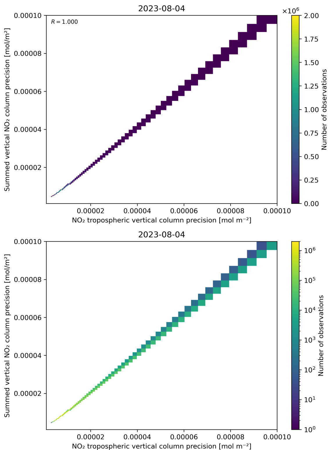
Figure 137: Scatter density plot of “NO 2 tropospheric vertical column precision” against “Summed vertical NO 2 column precision” for 2023-08-04 to 2023-08-05.
