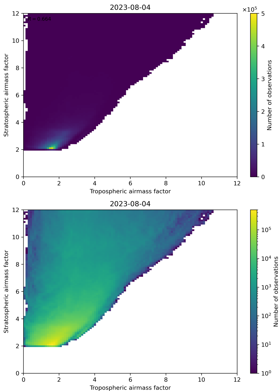
Figure 71: Scatter density plot of “Tropospheric airmass factor” against “Stratospheric airmass factor” for 2023-08-04 to 2023-08-05.
