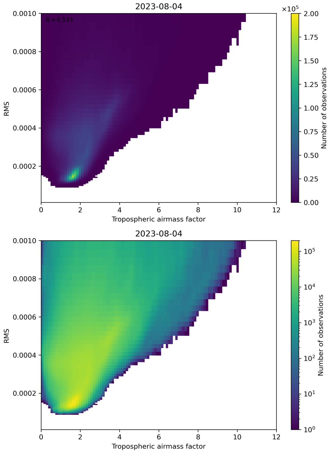
Figure 79: Scatter density plot of “Tropospheric airmass factor” against “RMS” for 2023-08-04 to 2023-08-05.
