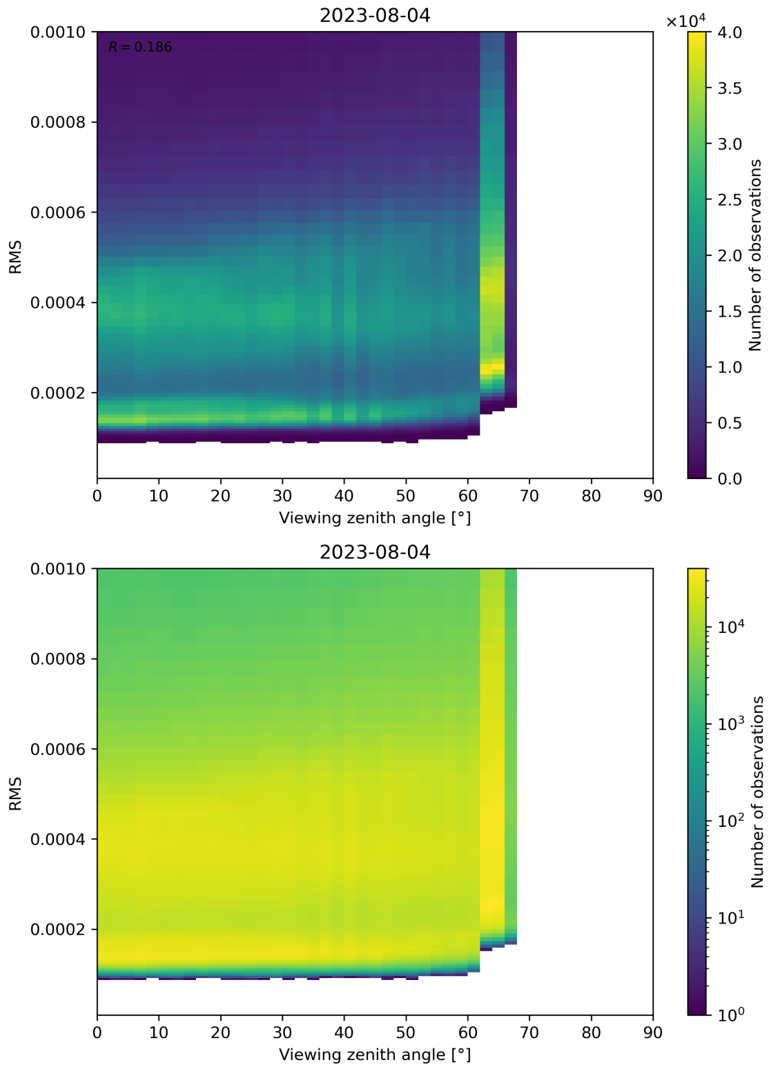
Figure 171: Scatter density plot of “Viewing zenith angle” against “RMS” for 2023-08-04 to 2023-08-05.
