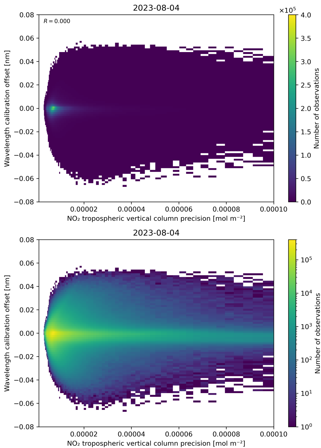
Figure 141: Scatter density plot of “NO 2 tropospheric vertical column precision” against “Wavelength calibration offset” for 2023-08-04 to 2023-08-05.
