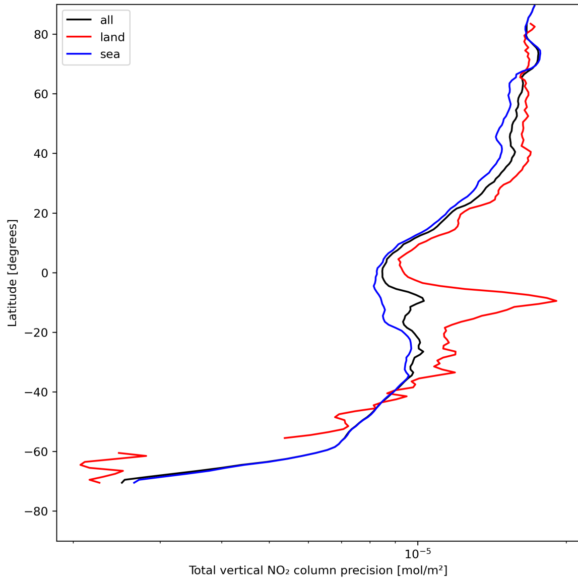
Figure 22: Zonal average of “Total vertical NO 2 column precision” for 2023-08-04 to 2023-08-05.
