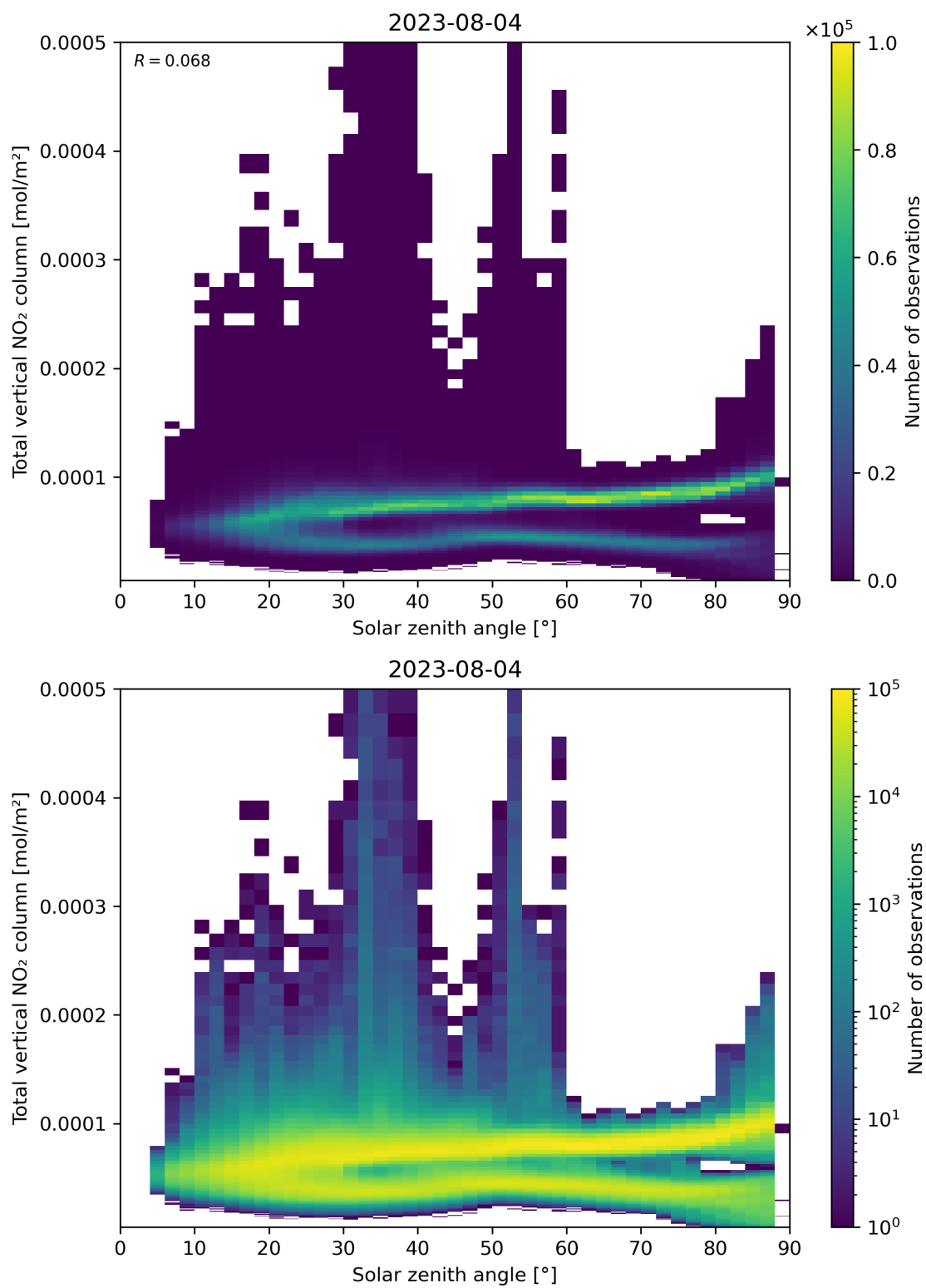
Figure 153: Scatter density plot of “Solar zenith angle” against “Total vertical NO 2 column” for 2023-08-04 to 2023-08-05.
