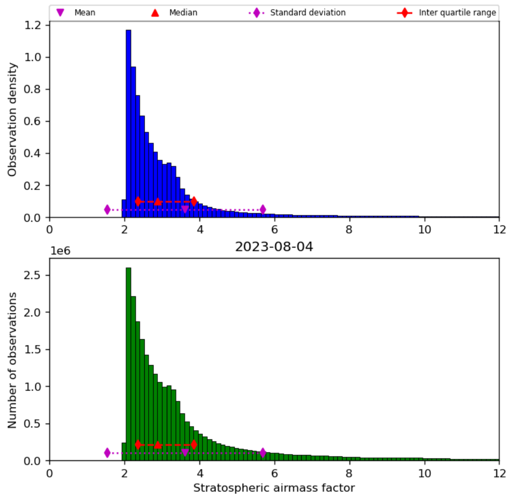
Figure 44: Histogram of “Stratospheric airmass factor” for 2023-08-04 to 2023-08-05
