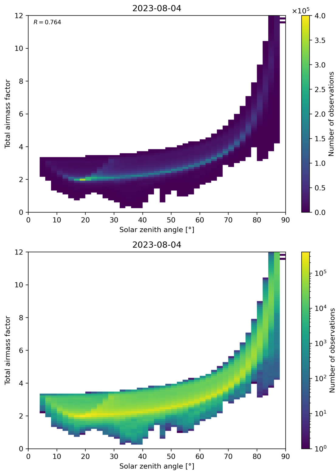
Figure 146: Scatter density plot of “Solar zenith angle” against “Total air mass factor” for 2023-08-04 to 2023-08-05.
