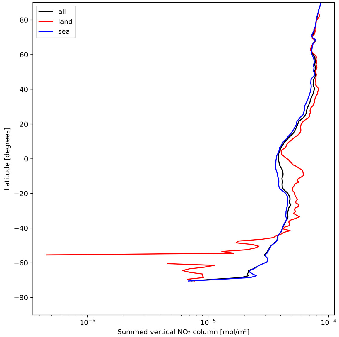
Figure 23: Zonal average of “Summed vertical NO 2 column” for 2023-08-04 to 2023-08-05.
