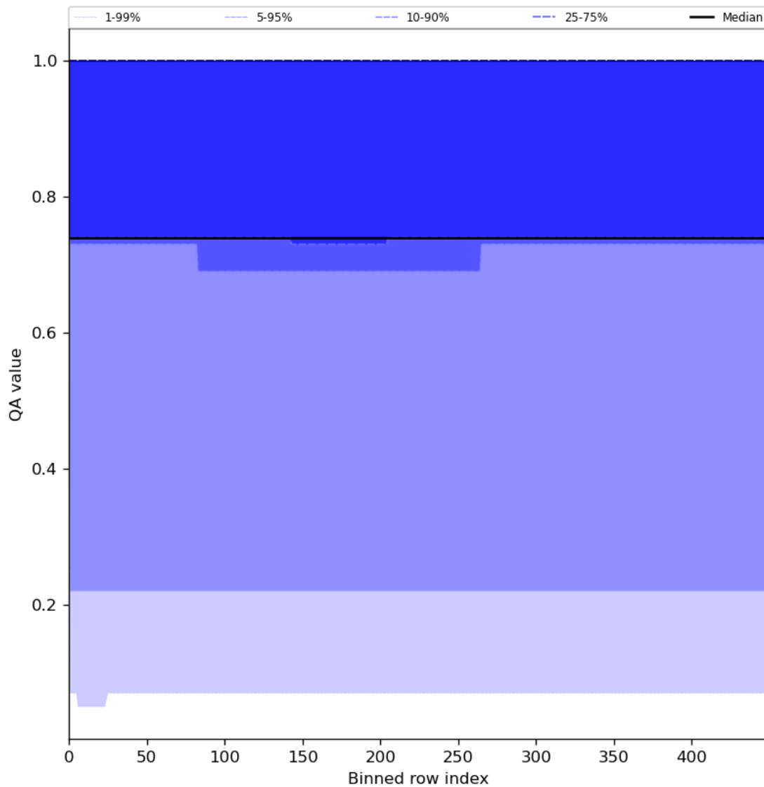
Figure 45: Along track statistics of “QA value” for 2023-08-04 to 2023-08-05
