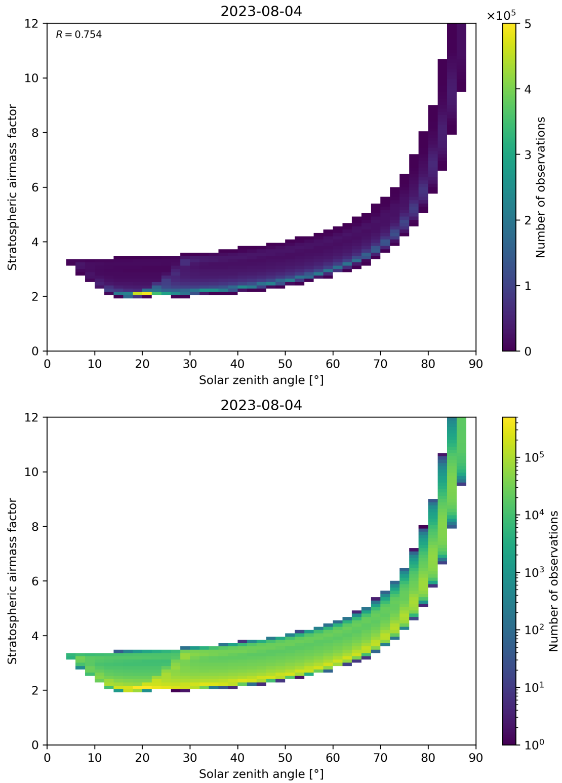
Figure 145: Scatter density plot of “Solar zenith angle” against “Stratospheric airmass factor” for 2023-08-04 to 2023-08-05.
