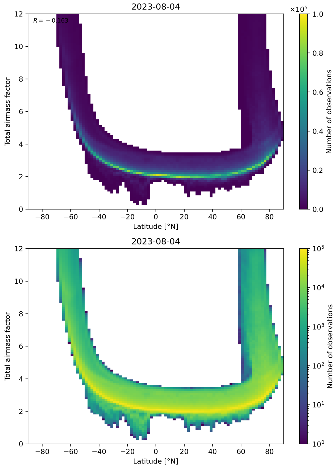
Figure 84: Scatter density plot of “Latitude” against “Total airmass factor” for 2023-08-04 to 2023-08-05.
