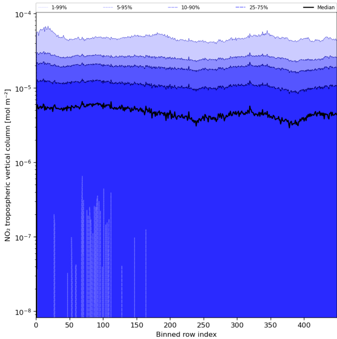
Figure 46: Along track statistics of “NO 2 tropospheric vertical column” for 2023-08-04 to 2023-08-05
