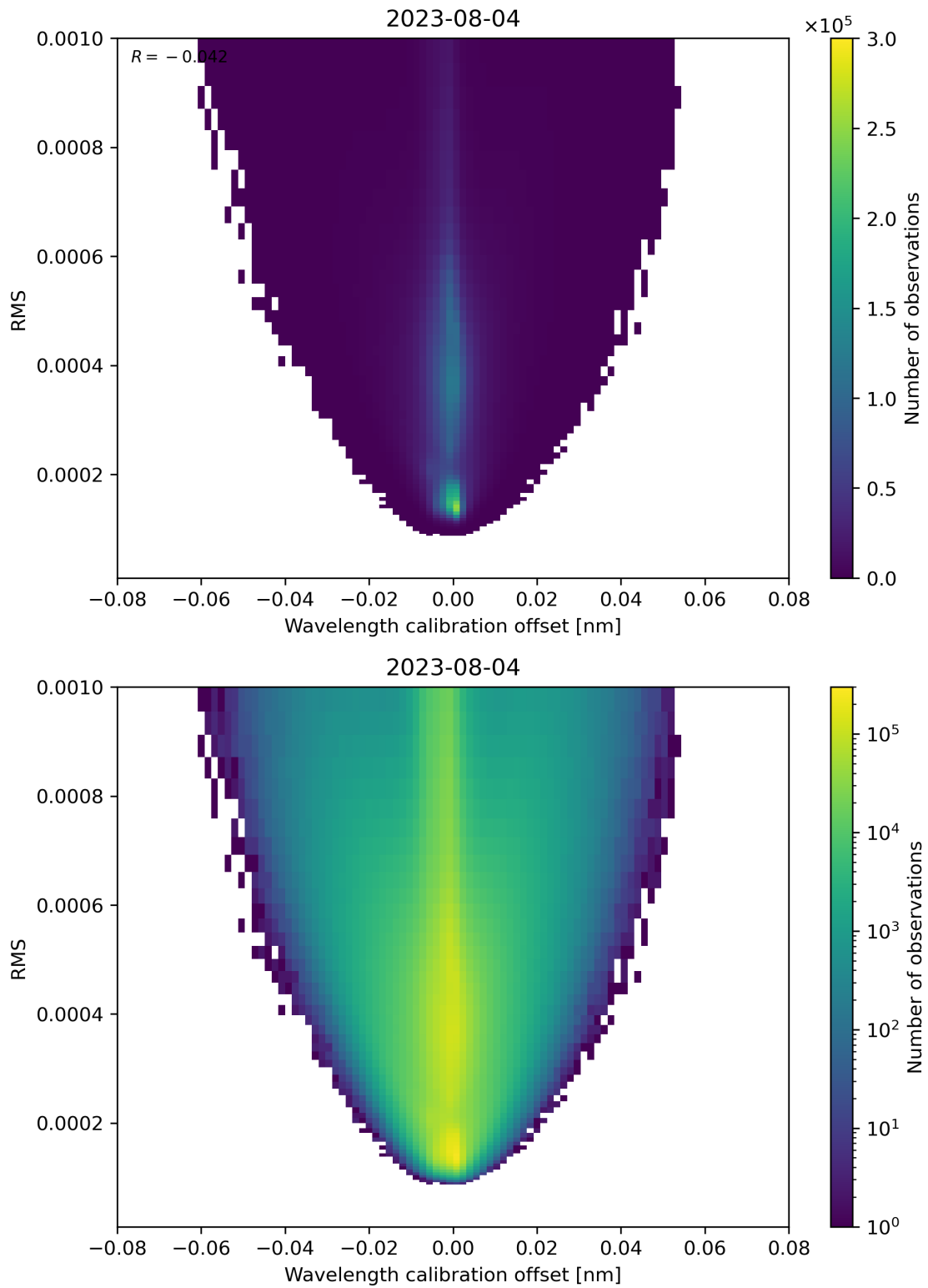
Figure 181: Scatter density plot of “Wavelength calibration offset” against “RMS” for 2023-08-04 to 2023-08-05.
