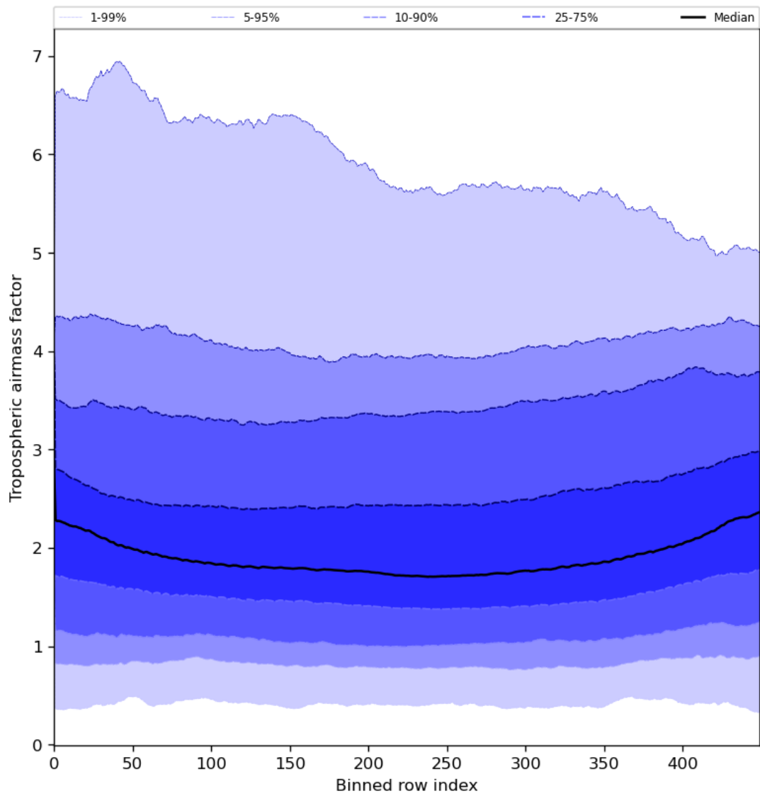
Figure 48: Along track statistics of “Tropospheric airmass factor” for 2023-08-04 to 2023-08-05
