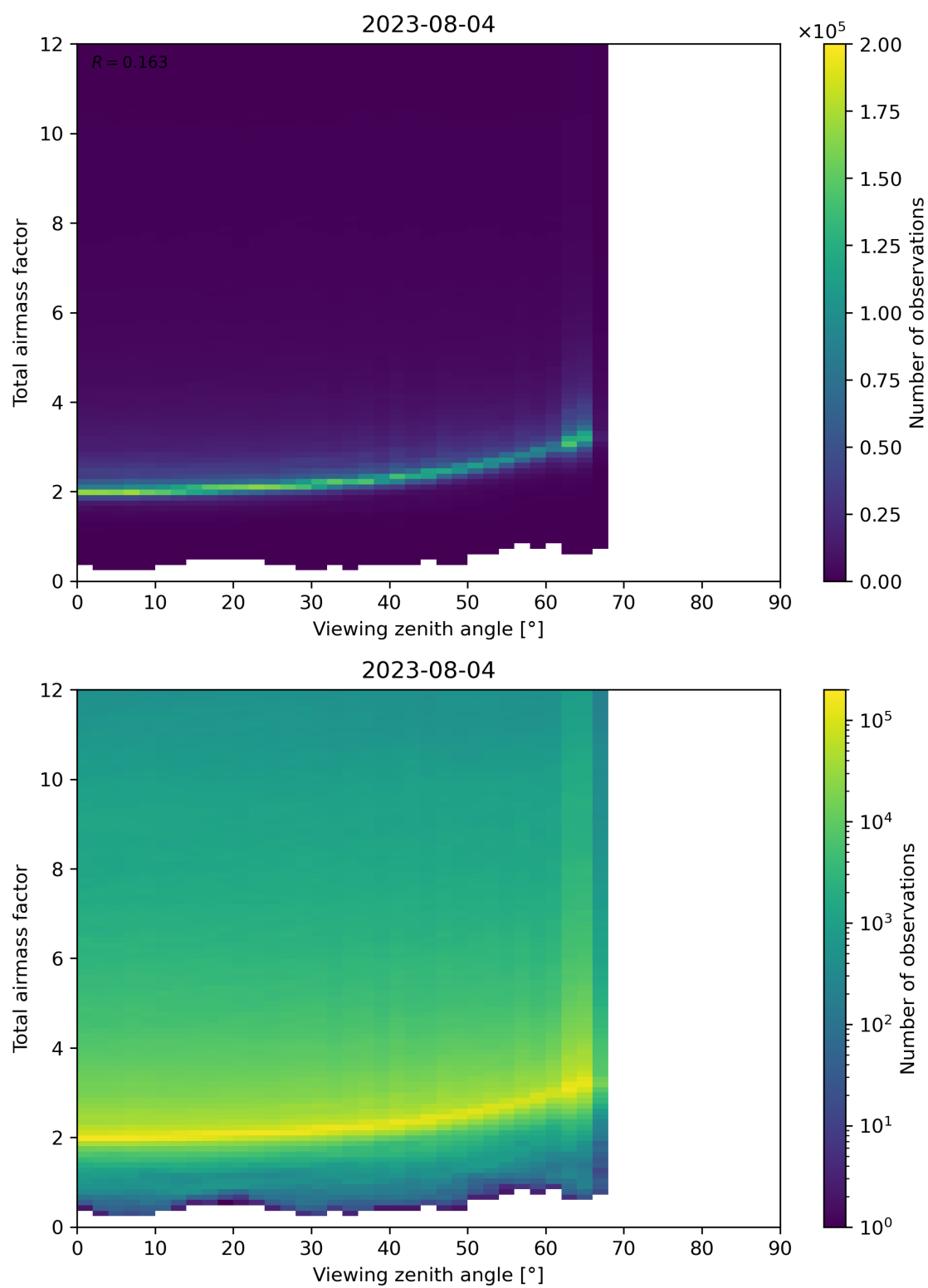
Figure 160: Scatter density plot of “Viewing zenith angle” against “Total airmass factor” for 2023-08-04 to 2023-08-05.
