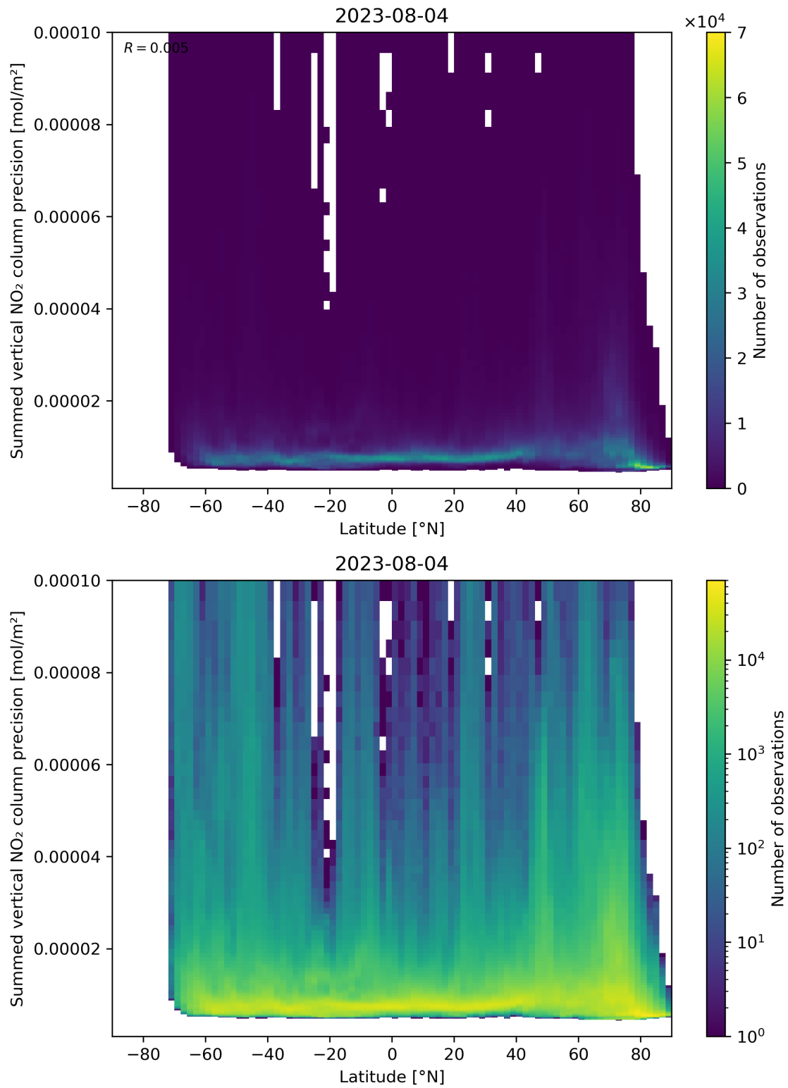
Figure 89: Scatter density plot of “Latitude” against “Summed vertical NO 2 column precision” for 2023-08-04 to 2023-08-05.
