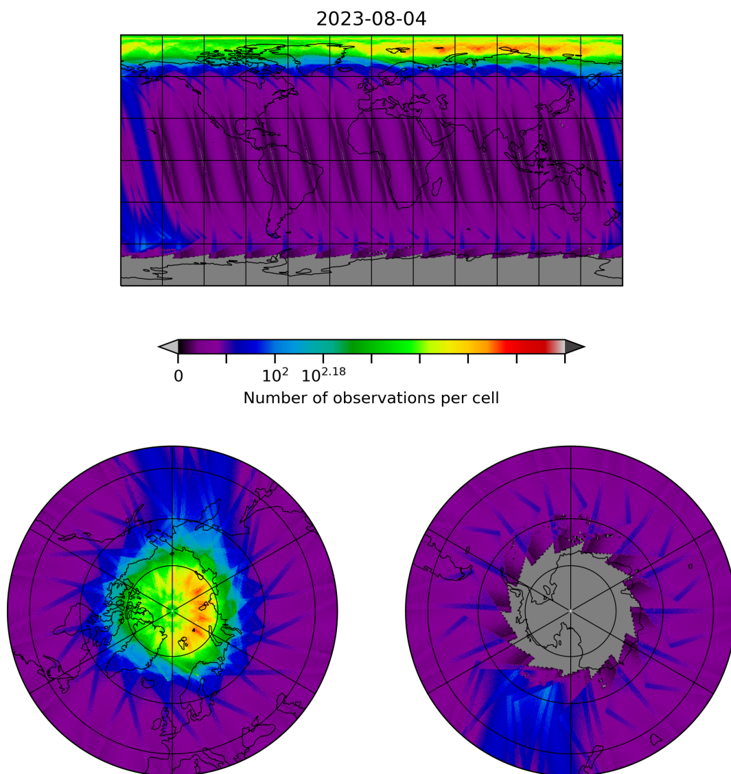
Figure 10: Map of the number of observations for 2023-08-04 to 2023-08-05
