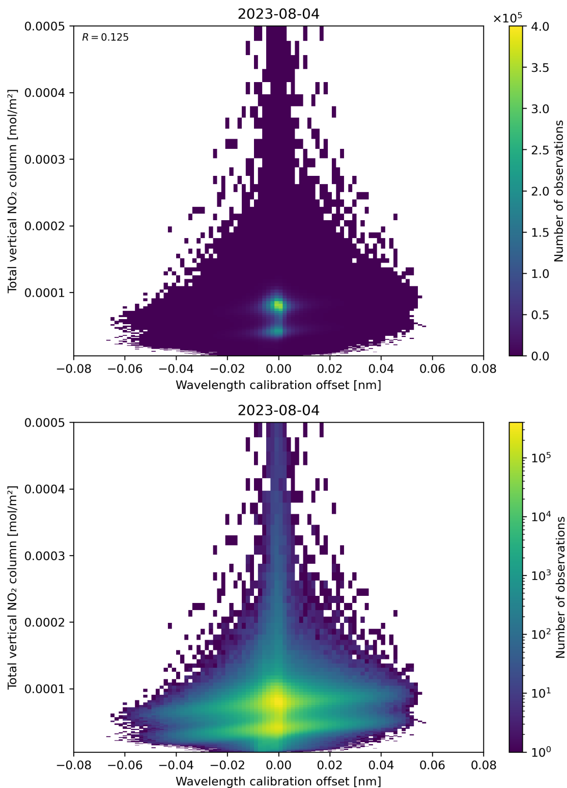
Figure 179: Scatter density plot of “Wavelength calibration offset” against “Total vertical NO 2 column” for 2023-08-04 to 2023-08-05.
