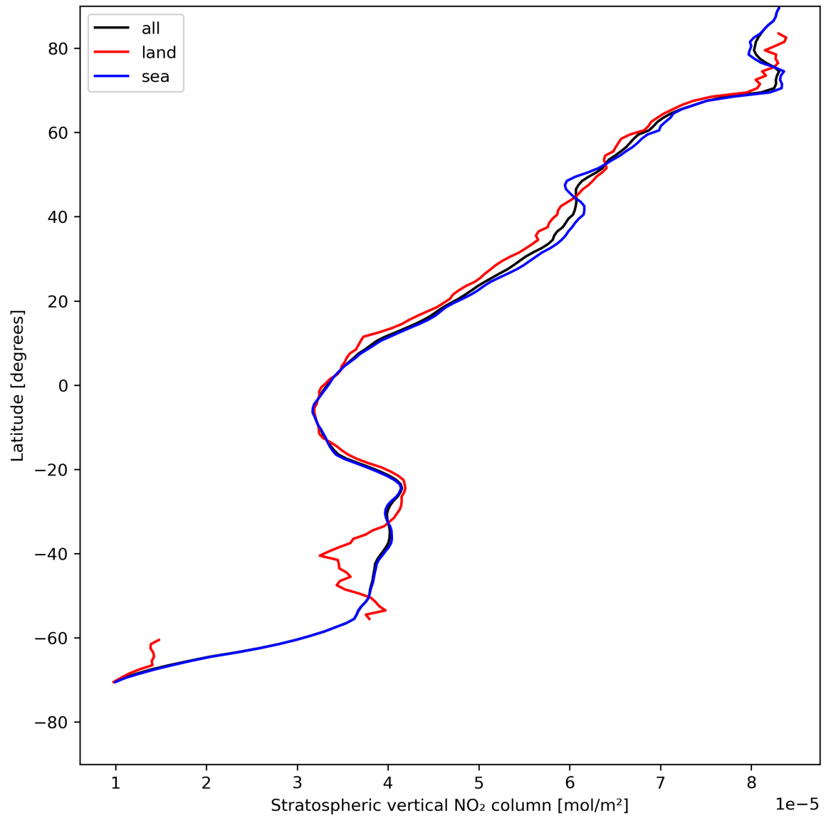
Figure 19: Zonal average of “Stratospheric vertical NO 2 column” for 2023-08-04 to 2023-08-05.
