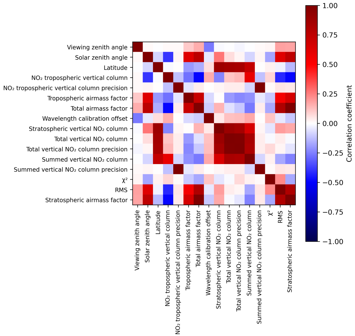
Figure 2: Map of correlation matrix for 2023-08-04 to 2023-08-05.
