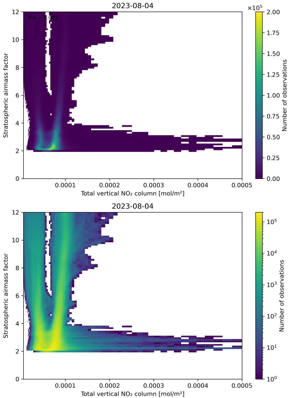
Figure 110: Scatter density plot of “Total vertical NO 2 column” against “Stratospheric airmass factor” for 2023-08-04 to 2023-08-05.
