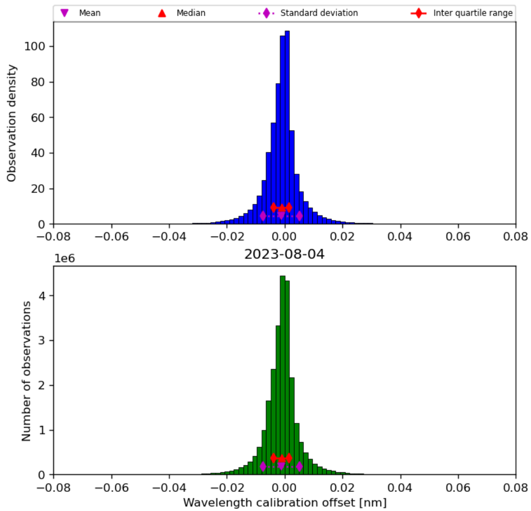
Figure 35: Histogram of “Wavelength calibration offset” for 2023-08-04 to 2023-08-05
