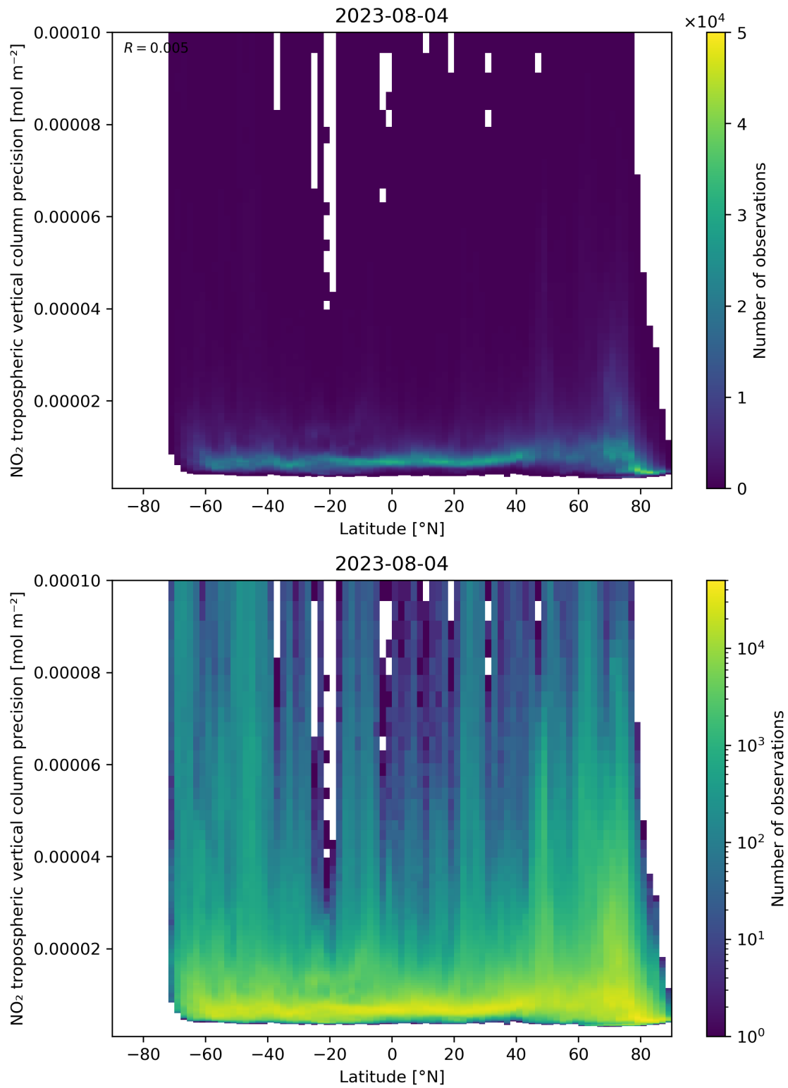
Figure 93: Scatter density plot of “Latitude” against “NO 2 tropospheric vertical column precision” for 2023-08-04 to 2023-08-05.
