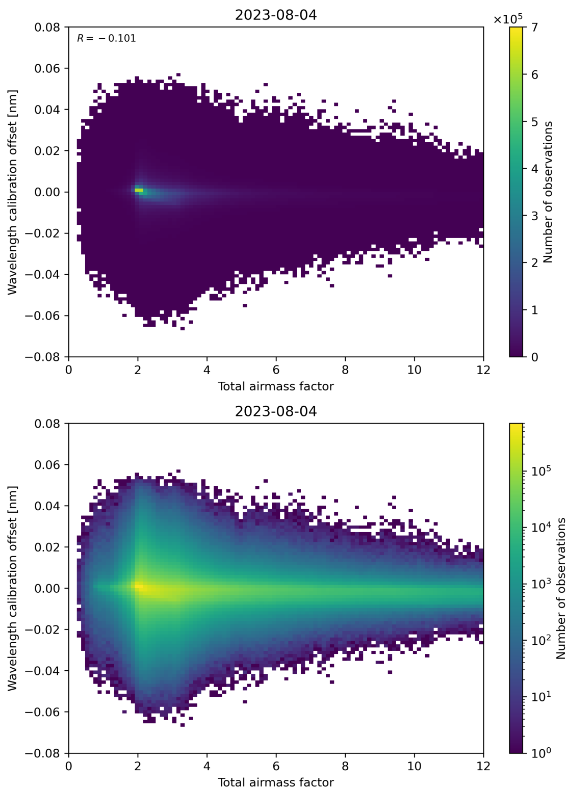
Figure 70: Scatter density plot of “Total airmass factor” against “Wavelength calibration offset” for 2023-08-04 to 2023-08-05.
