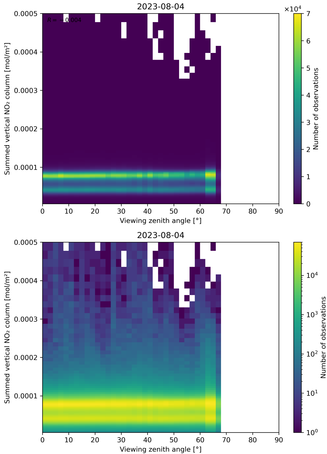
Figure 165: Scatter density plot of “Viewing zenith angle” against “Summed vertical NO 2 column” for 2023-08-04 to 2023-08-05.
