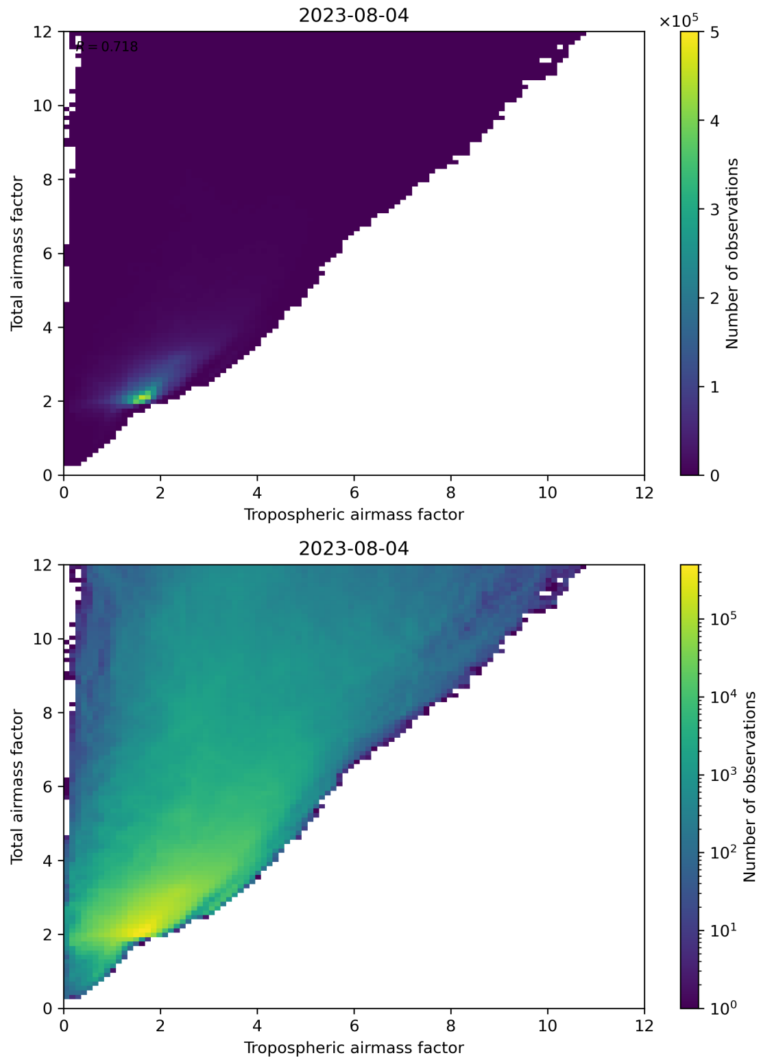
Figure 72: Scatter density plot of “Tropospheric airmass factor” against “Total airmass factor” for 2023-08-04 to 2023-08-05.
