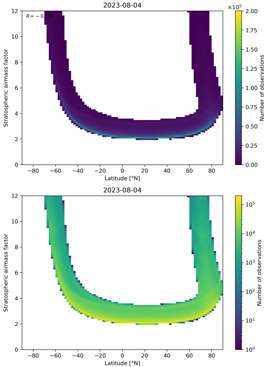
Figure 83: Scatter density plot of “Latitude” against “Stratospheric air mass factor” for 2023-08-04 to 2023-08-05.
