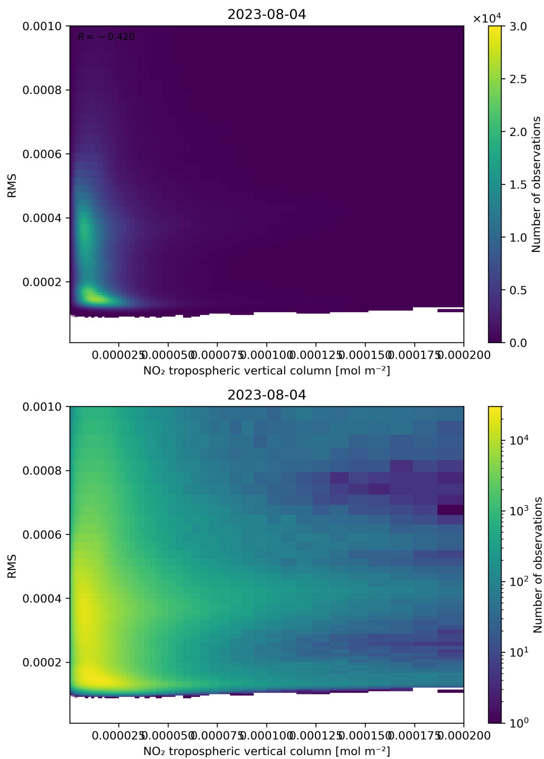
Figure 142: Scatter density plot of “NO 2 tropospheric vertical column” against “RMS” for 2023-08-04 to 2023-08-05.
