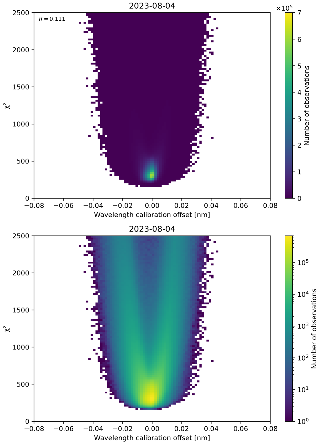
Figure 175: Scatter density plot of “Wavelength calibration offset” against “ \chi^2 ” for 2023-08-04 to 2023-08-05.
