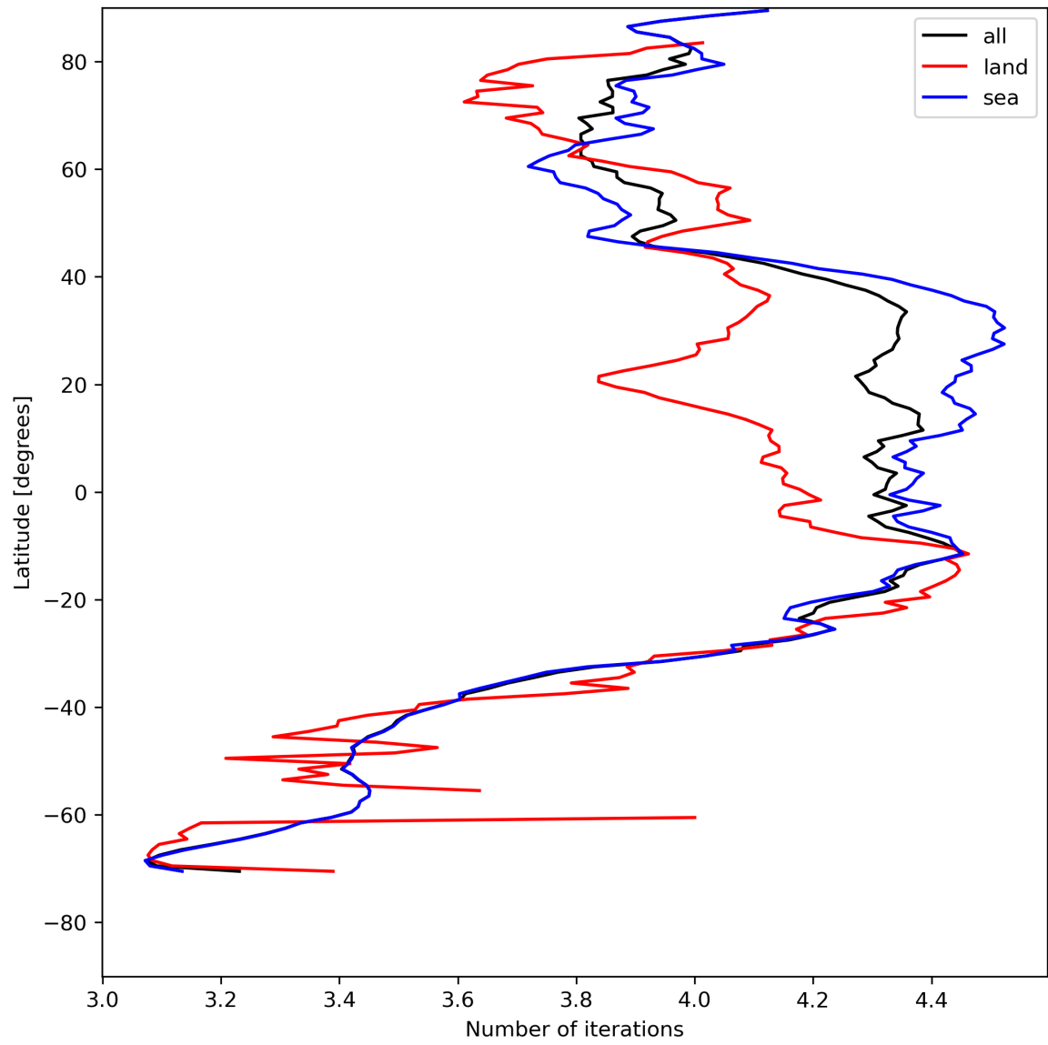
Figure 17: Zonal average of “Number of iterations” for 2023-08-04 to 2023-08-05.
