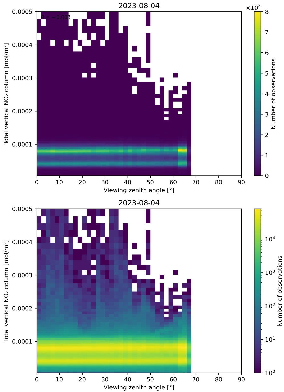
Figure 167: Scatter density plot of “Viewing zenith angle” against “Total vertical NO 2 column” for 2023-08-04 to 2023-08-05.
