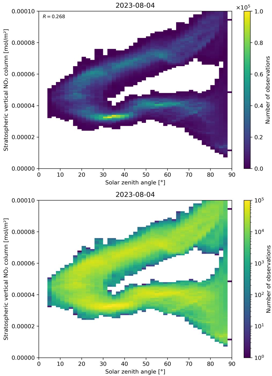
Figure 150: Scatter density plot of “Solar zenith angle” against “Stratospheric vertical NO 2 column” for 2023-08-04 to 2023-08-05.
