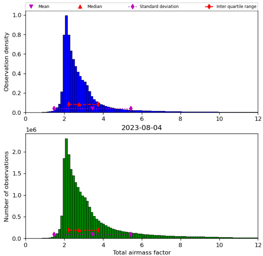
Figure 32: Histogram of “Total airmass factor” for 2023-08-04 to 2023-08-05
