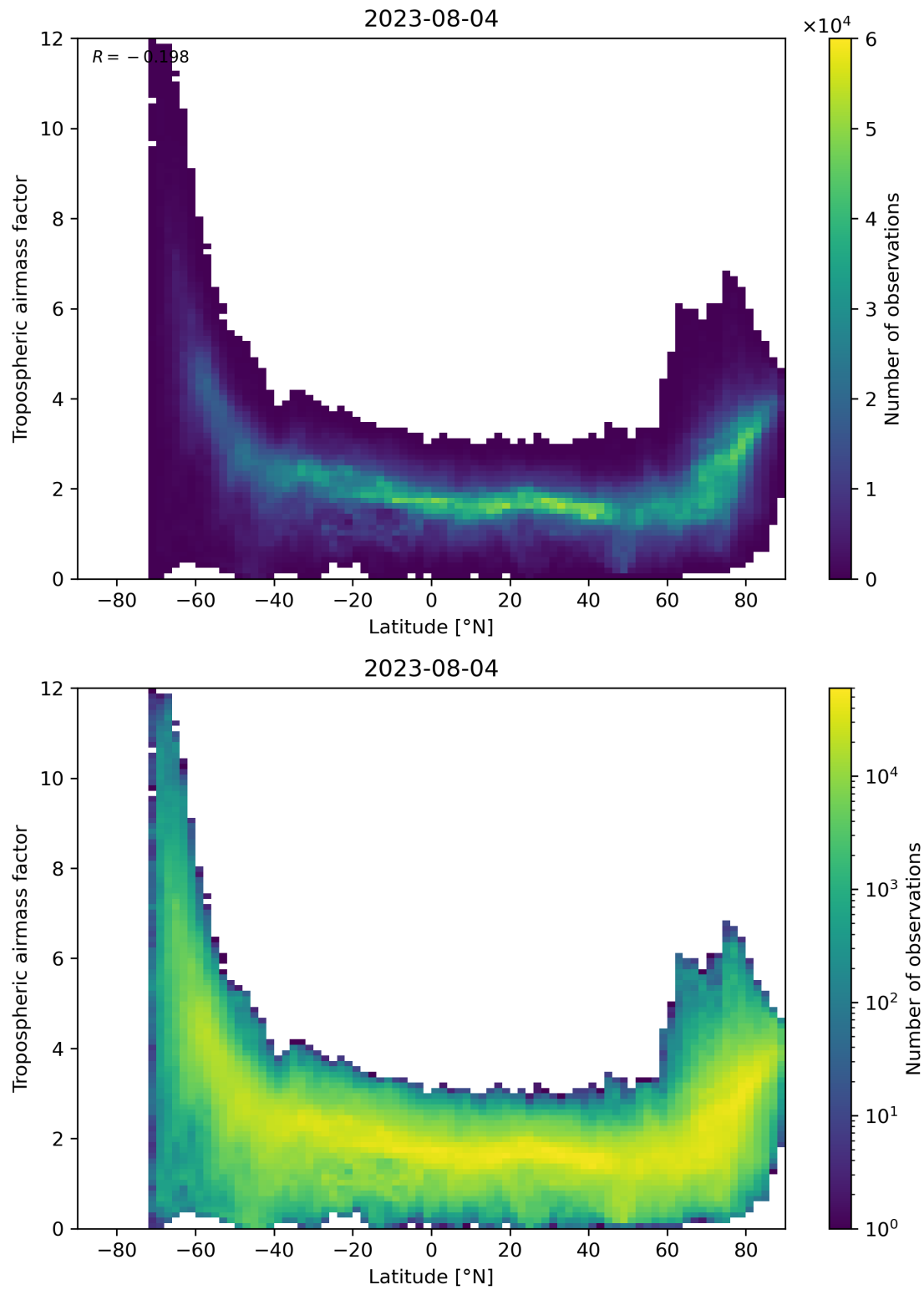
Figure 85: Scatter density plot of “Latitude” against “Tropospheric airmass factor” for 2023-08-04 to 2023-08-05.
