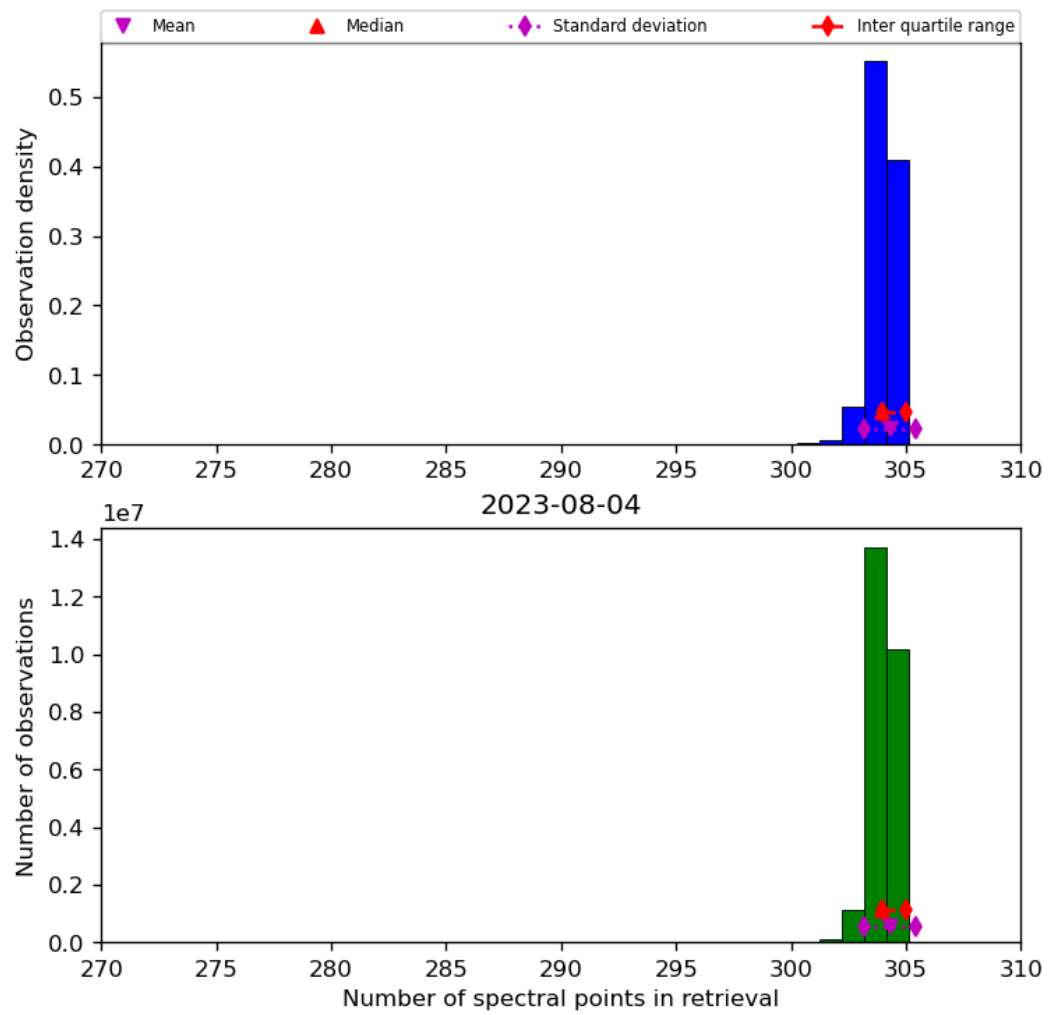
Figure 33: Histogram of “Number of spectral points in retrieval” for 2023-08-04 to 2023-08-05
