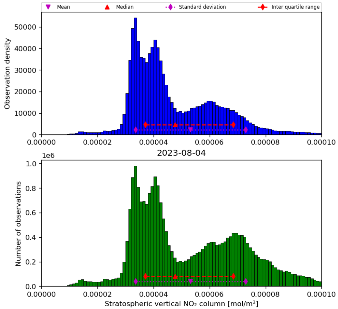
Figure 36: Histogram of “Stratospheric vertical NO 2 column” for 2023-08-04 to 2023-08-05
