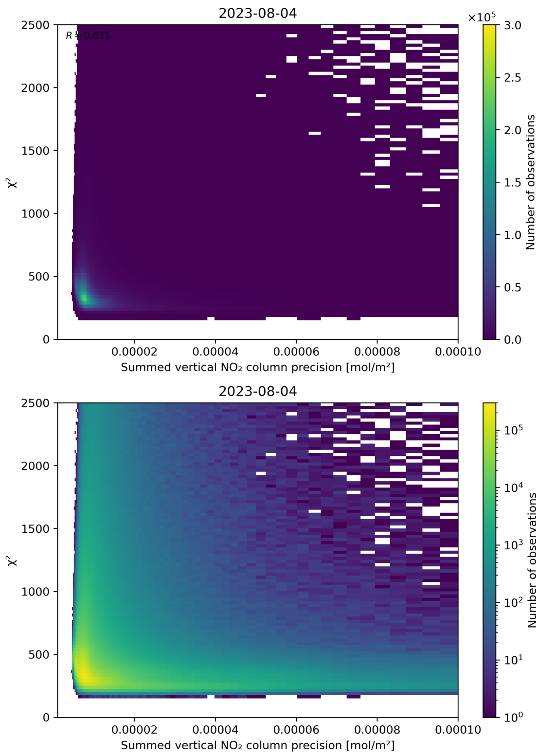
Figure 107: Scatter density plot of “Summed vertical NO 2 column precision” against “ \chi^2 ” for 2023-08-04 to 2023-08-05.
