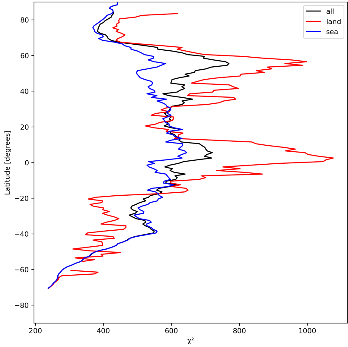
Figure 25: Zonal average of “ \chi^2 ” for 2023-08-04 to 2023-08-05.
