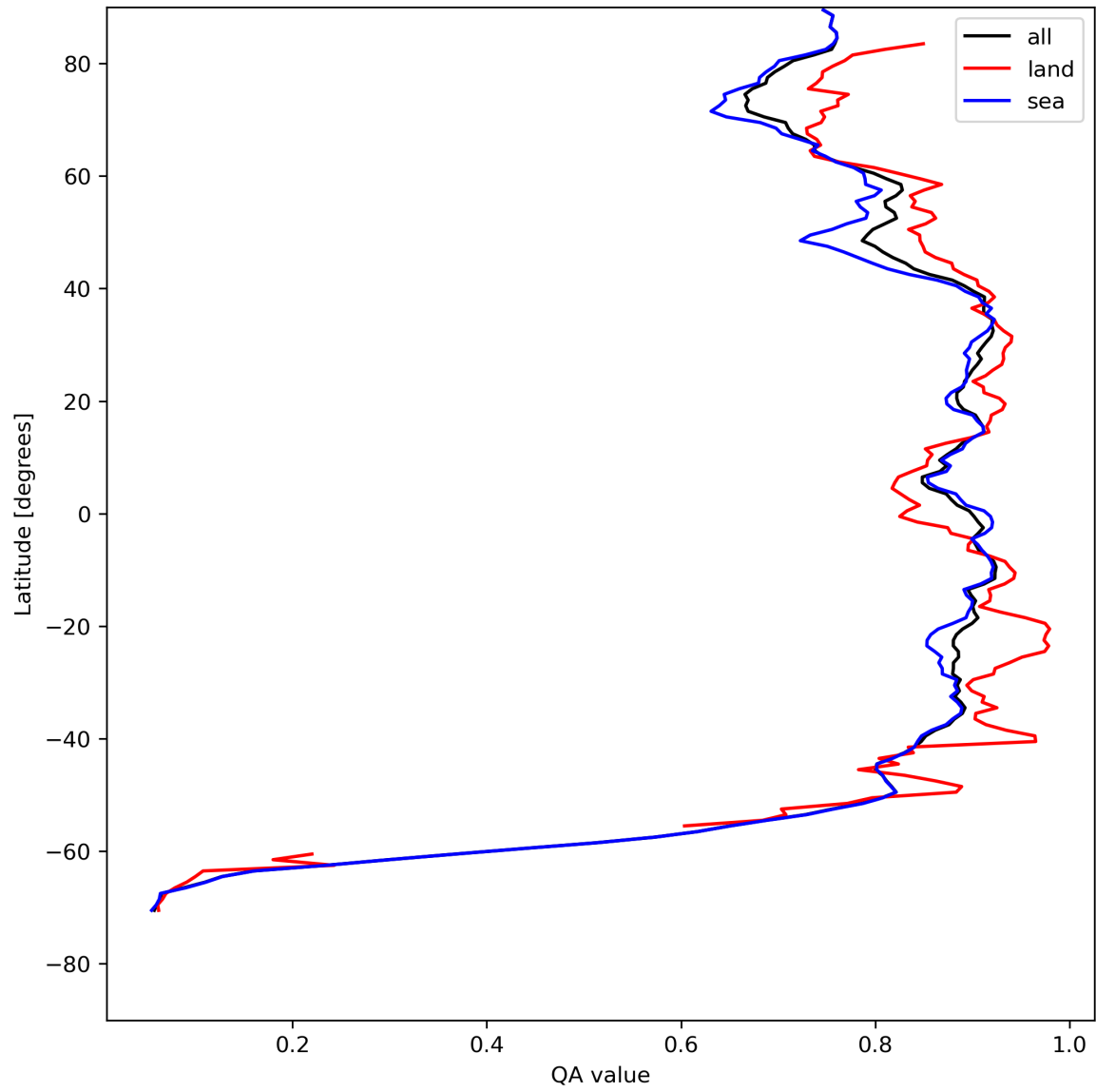
Figure 11: Zonal average of “QA value” for 2023-08-04 to 2023-08-05.
