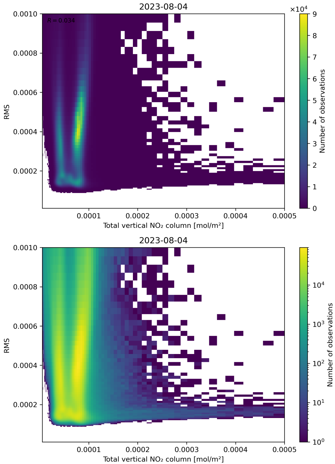
Figure 120: Scatter density plot of “Total vertical NO 2 column” against “RMS” for 2023-08-04 to 2023-08-05.
