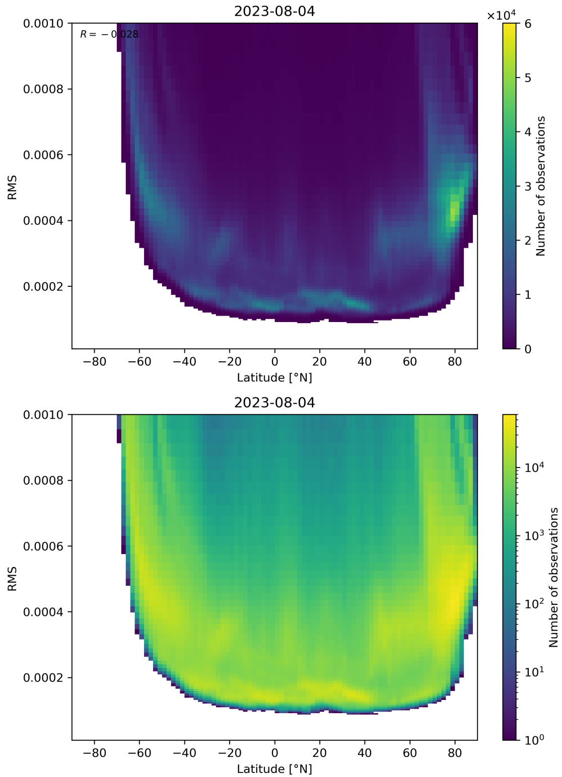
Figure 94: Scatter density plot of “Latitude” against “RMS” for 2023-08-04 to 2023-08-05.
