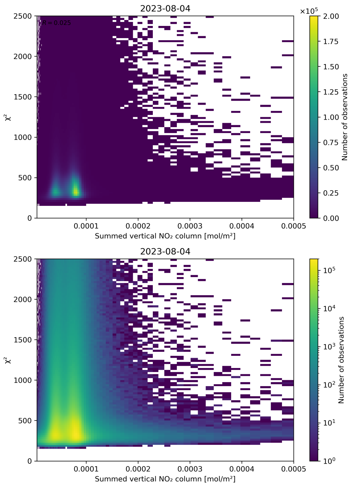
Figure 104: Scatter density plot of “Summed vertical NO 2 column” against “ \chi^2 ” for 2023-08-04 to 2023-08-05.
