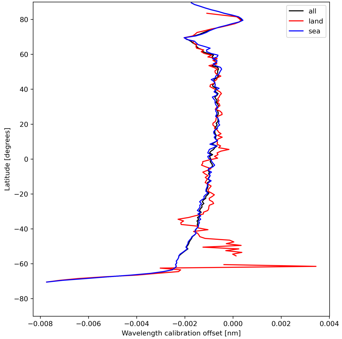
Figure 18: Zonal average of “Wavelength calibration offset” for 2023-08-04 to 2023-08-05.
