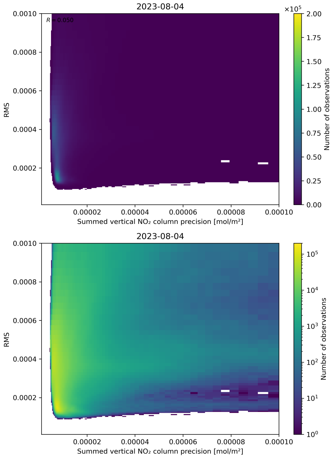
Figure 108: Scatter density plot of “Summed vertical NO 2 column precision” against “RMS” for 2023-08-04 to 2023-08-05.
