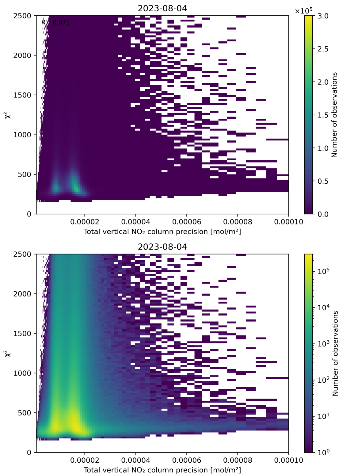
Figure 116: Scatter density plot of “Total vertical NO 2 column precision” against “ \chi^2 ” for 2023-08-04 to 2023-08-05.
