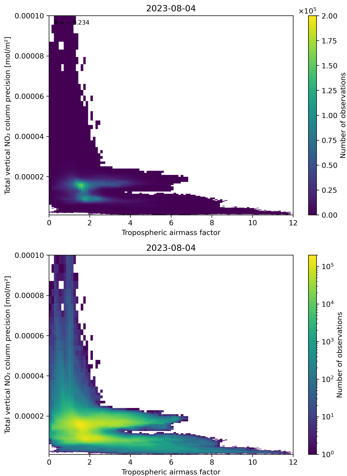
Figure 78: Scatter density plot of “Tropospheric air mass factor” against “Total vertical NO 2 column precision” for 2023-08-04 to 2023-08-05.
