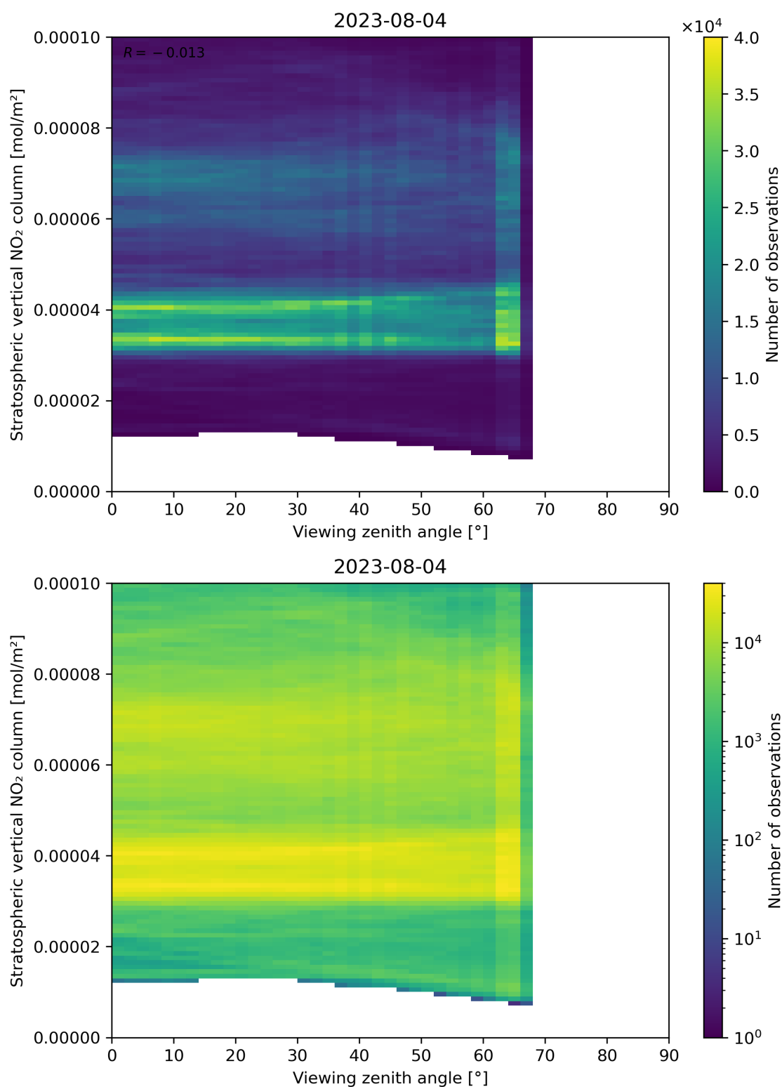
Figure 164: Scatter density plot of “Viewing zenith angle” against “Stratospheric vertical NO 2 column” for 2023-08-04 to 2023-08-05.
