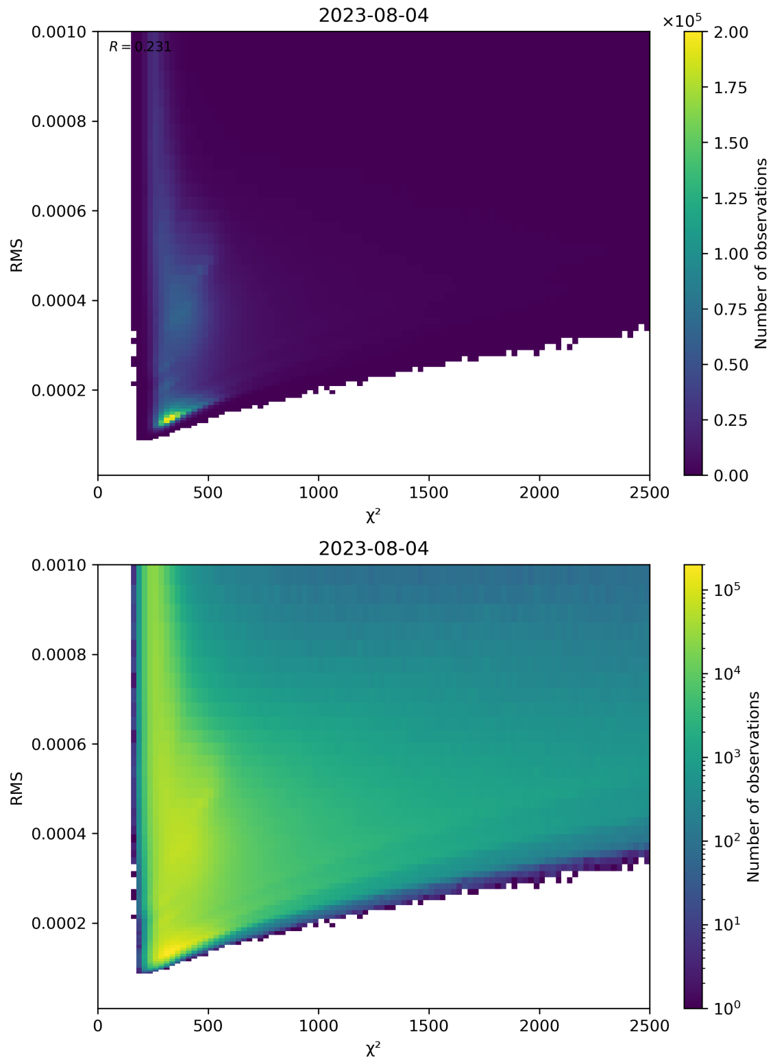
Figure 82: Scatter density plot of “ \chi^2 ” against “RMS” for 2023-08-04 to 2023-08-05.
