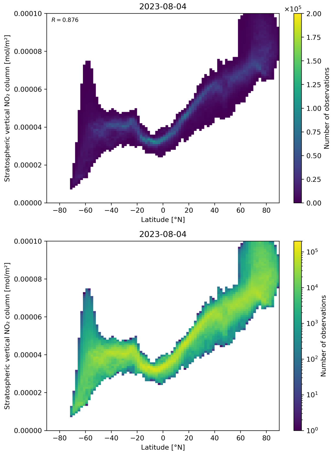
Figure 87: Scatter density plot of “Latitude” against “Stratospheric vertical NO 2 column” for 2023-08-04 to 2023-08-05.
