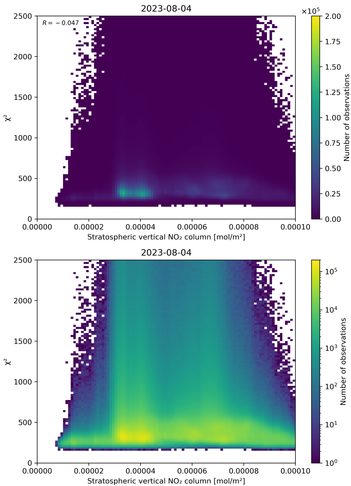
Figure 97: Scatter density plot of “Stratospheric vertical NO 2 column” against “ \chi^2 ” for 2023-08-04 to 2023-08-05.
