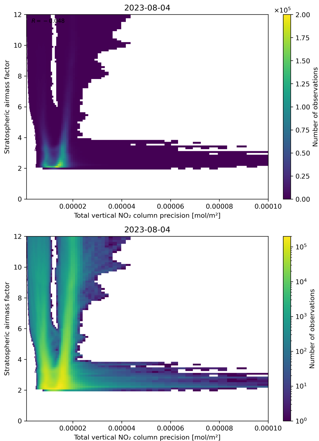
Figure 115: Scatter density plot of “Total vertical NO 2 column precision” against “Stratospheric air mass factor” for 2023-08-04 to 2023-08-05.
