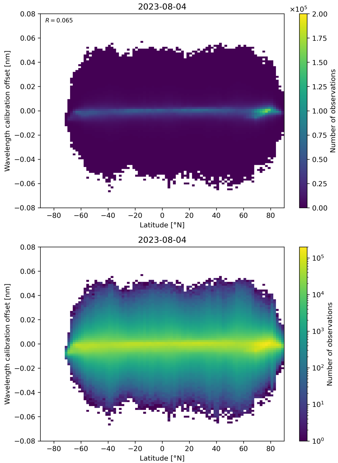
Figure 95: Scatter density plot of “Latitude” against “Wavelength calibration offset” for 2023-08-04 to 2023-08-05.
