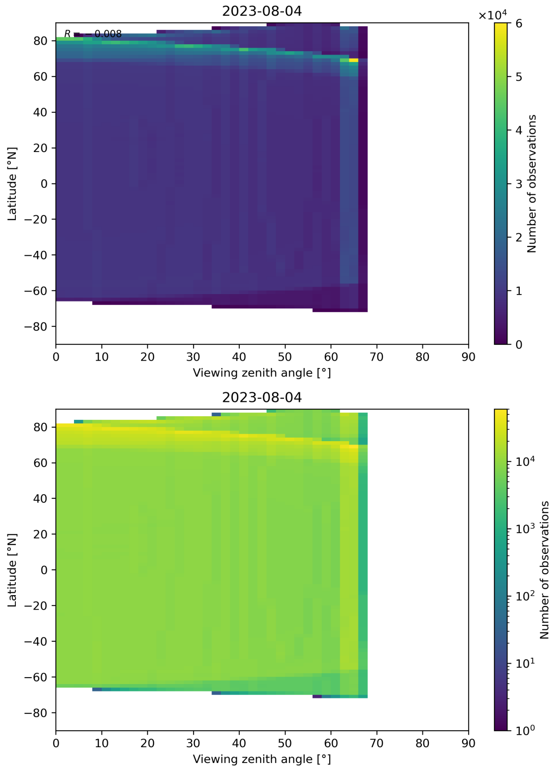
Figure 163: Scatter density plot of “Viewing zenith angle” against “Latitude” for 2023-08-04 to 2023-08-05.
