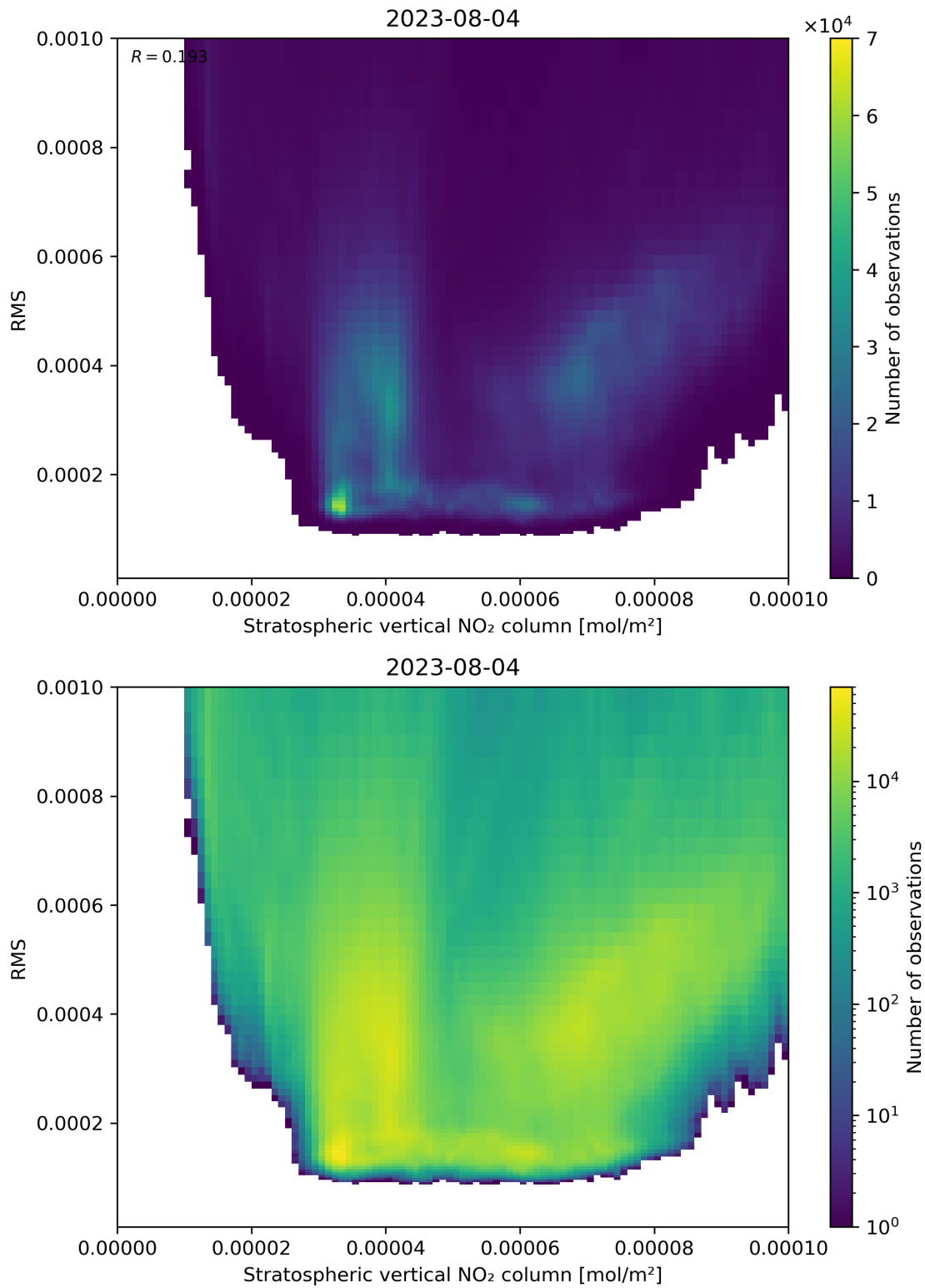
Figure 102: Scatter density plot of “Stratospheric vertical NO 2 column” against “RMS” for 2023-08-04 to 2023-08-05.
