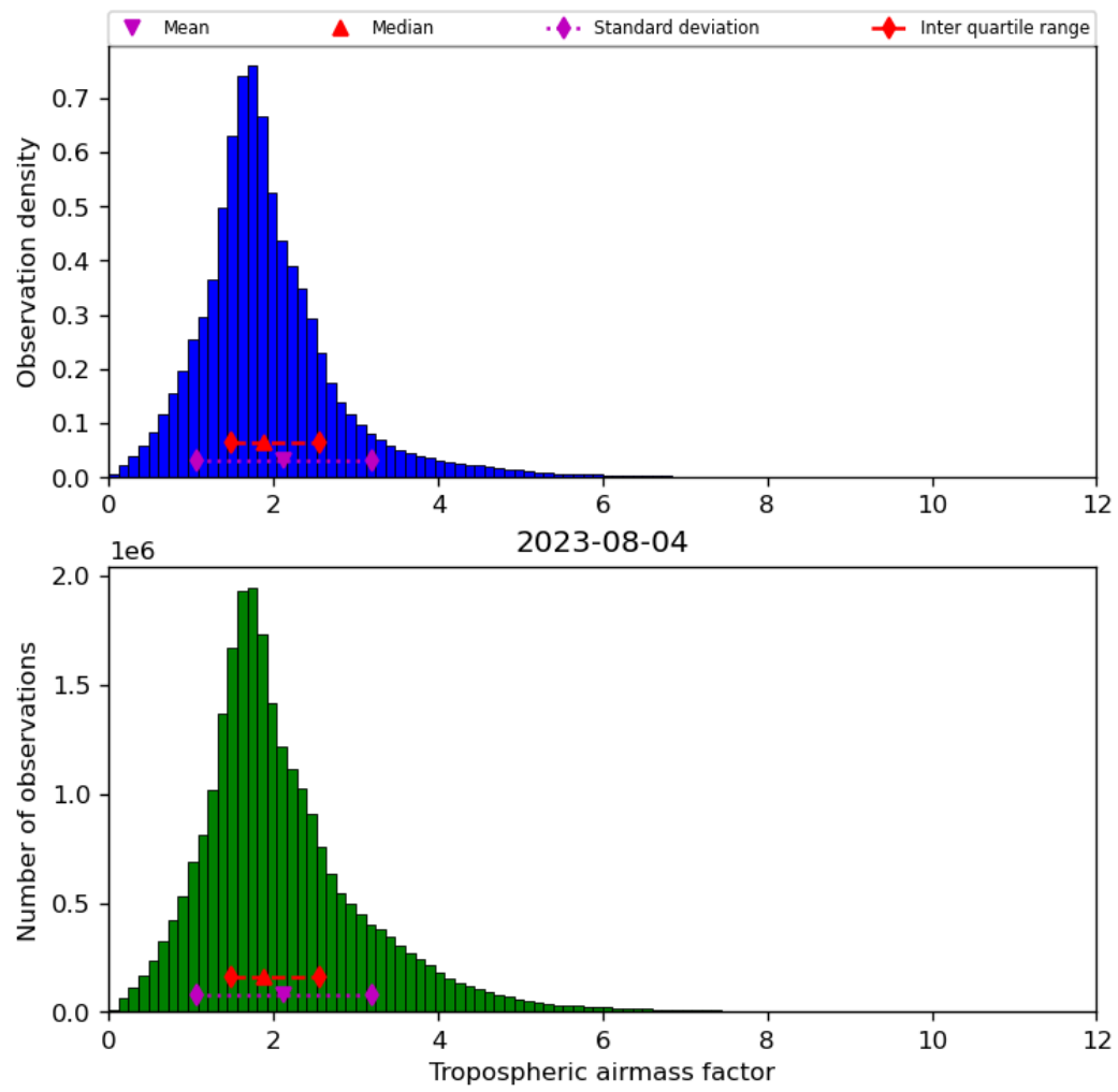
Figure 31: Histogram of “Tropospheric airmass factor” for 2023-08-04 to 2023-08-05
