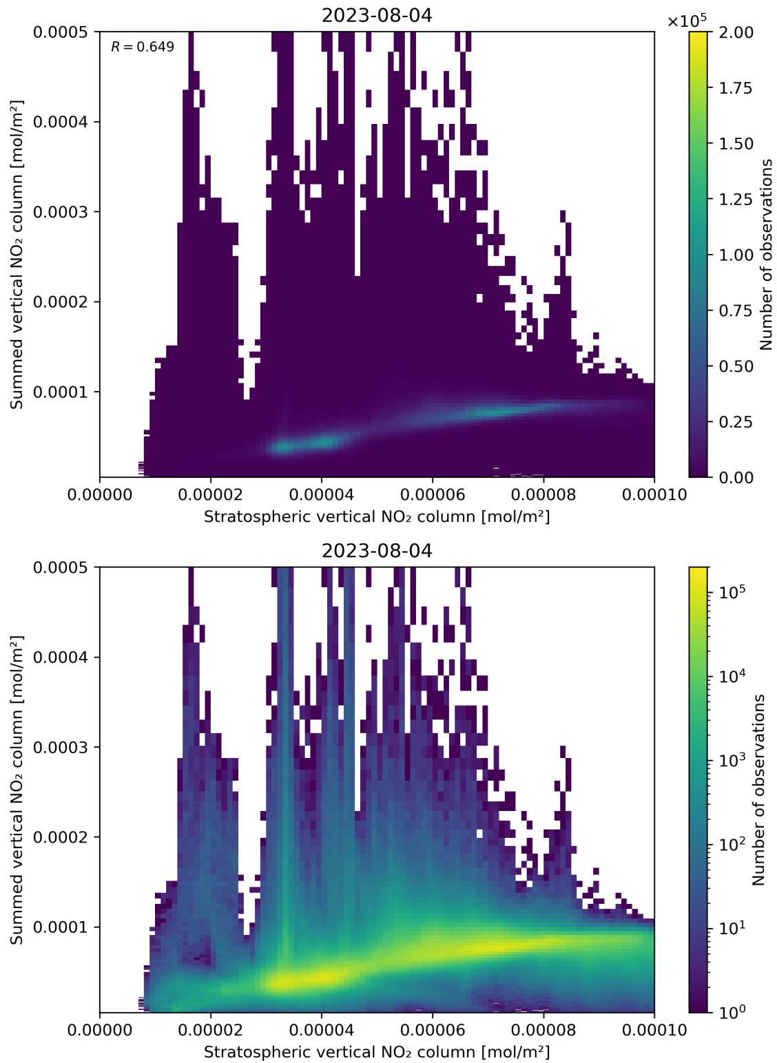
Figure 98: Scatter density plot of “Stratospheric vertical NO 2 column” against “Summed vertical NO 2 column” for 2023-08-04 to 2023-08-05.
