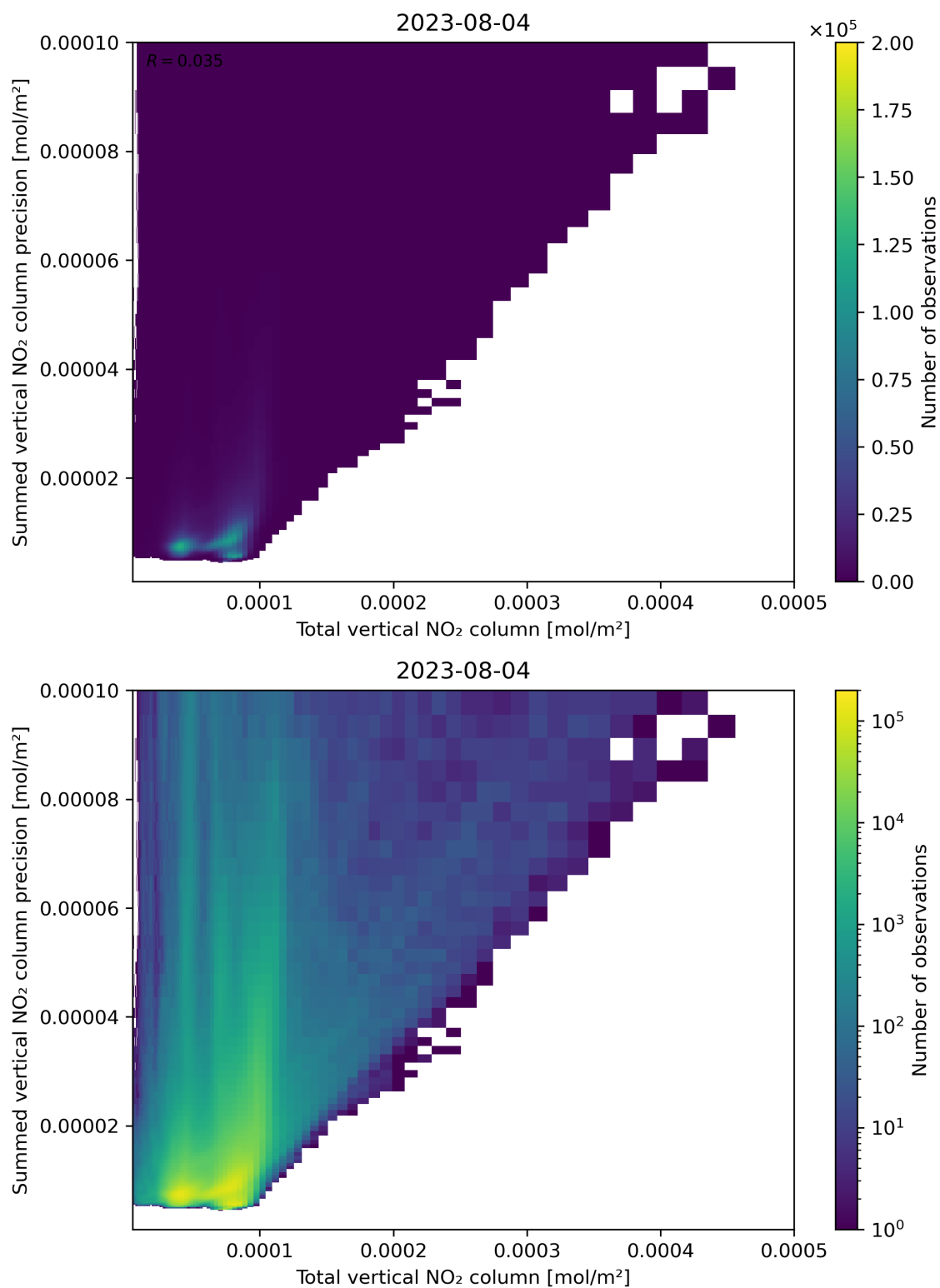
Figure 113: Scatter density plot of “Total vertical NO 2 column” against “Summed vertical NO 2 column precision” for 2023-08-04 to 2023-08-05.
