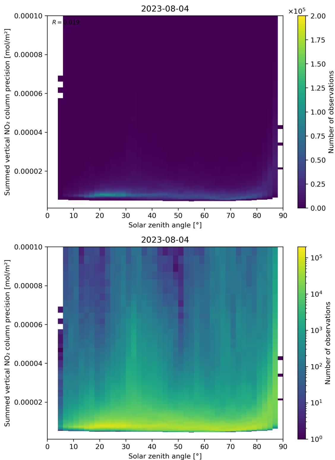
Figure 152: Scatter density plot of “Solar zenith angle” against “Summed vertical NO 2 column precision” for 2023-08-04 to 2023-08-05.
