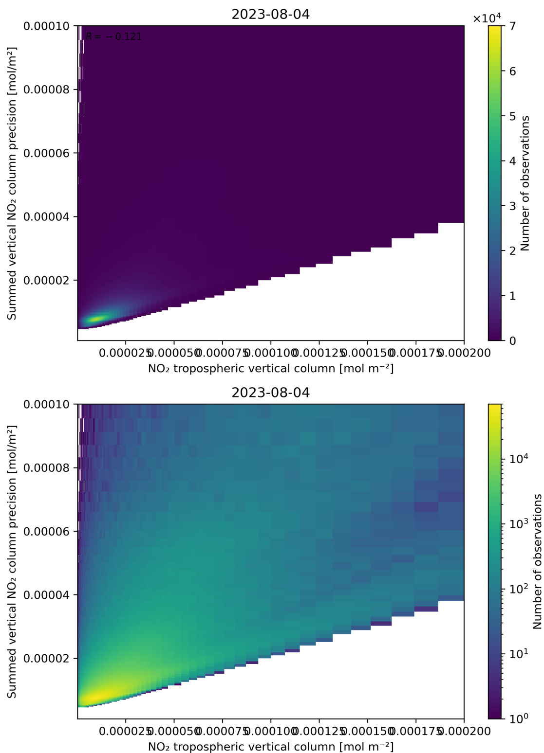
Figure 127: Scatter density plot of “NO 2 tropospheric vertical column” against “Summed vertical NO 2 column precision” for 2023-08-04 to 2023-08-05.
