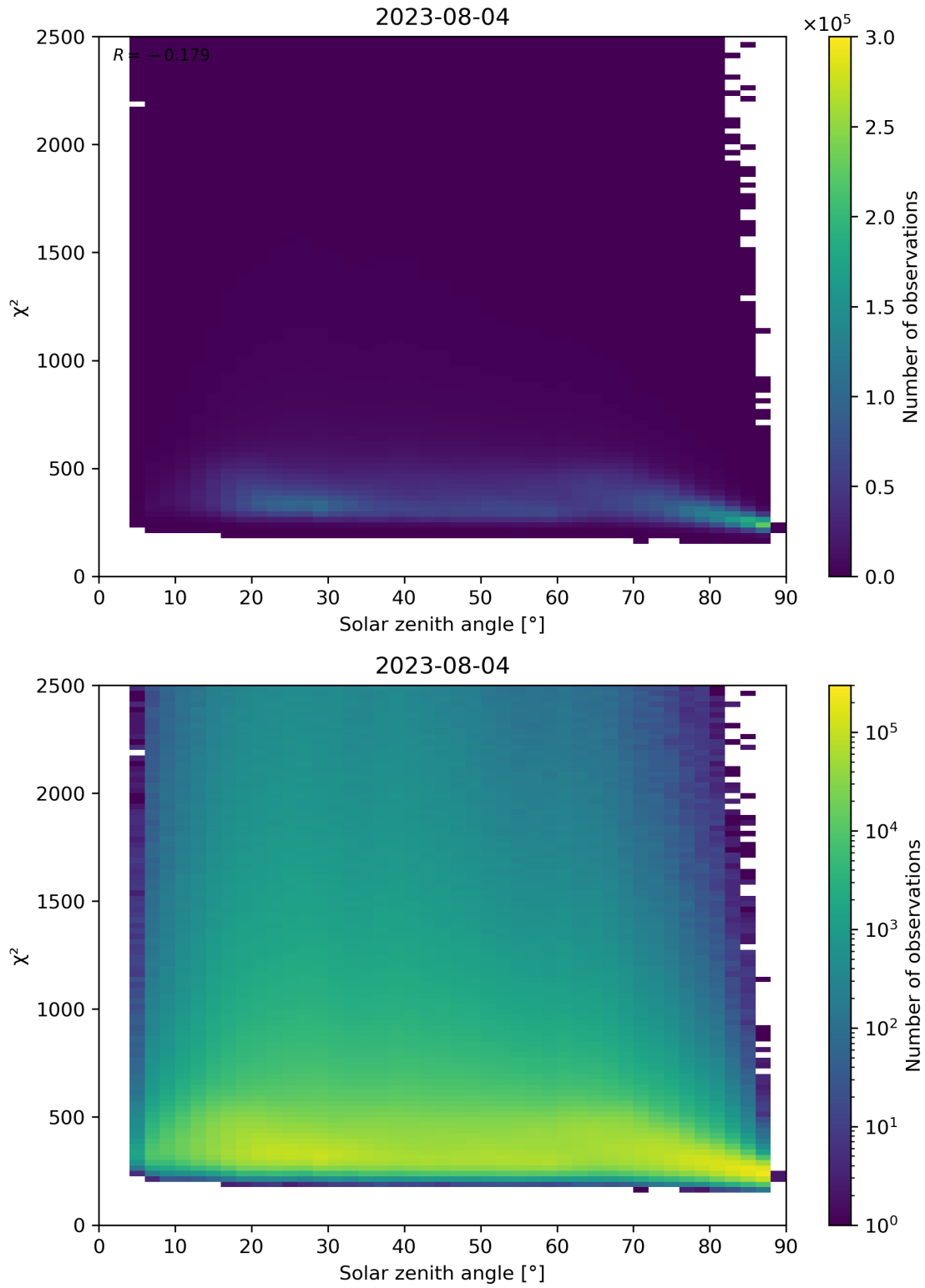
Figure 148: Scatter density plot of “Solar zenith angle” against “ \chi^2 ” for 2023-08-04 to 2023-08-05.
