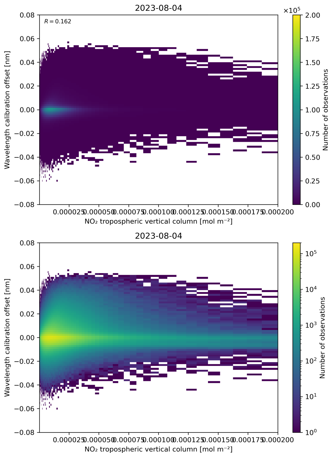
Figure 143: Scatter density plot of “NO 2 tropospheric vertical column” against “Wavelength calibration offset” for 2023-08-04 to 2023-08-05.
