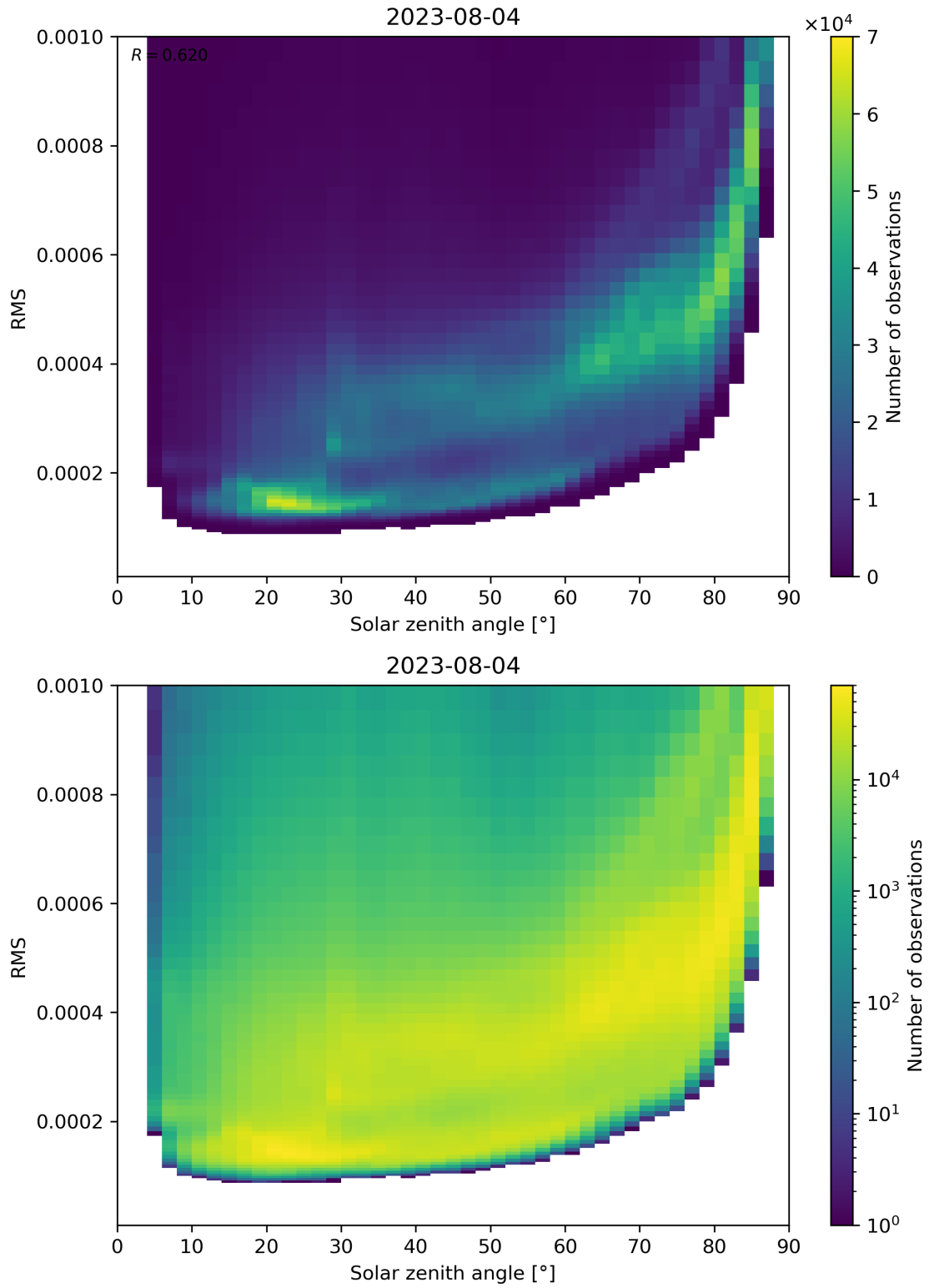
Figure 157: Scatter density plot of “Solar zenith angle” against “RMS” for 2023-08-04 to 2023-08-05.
