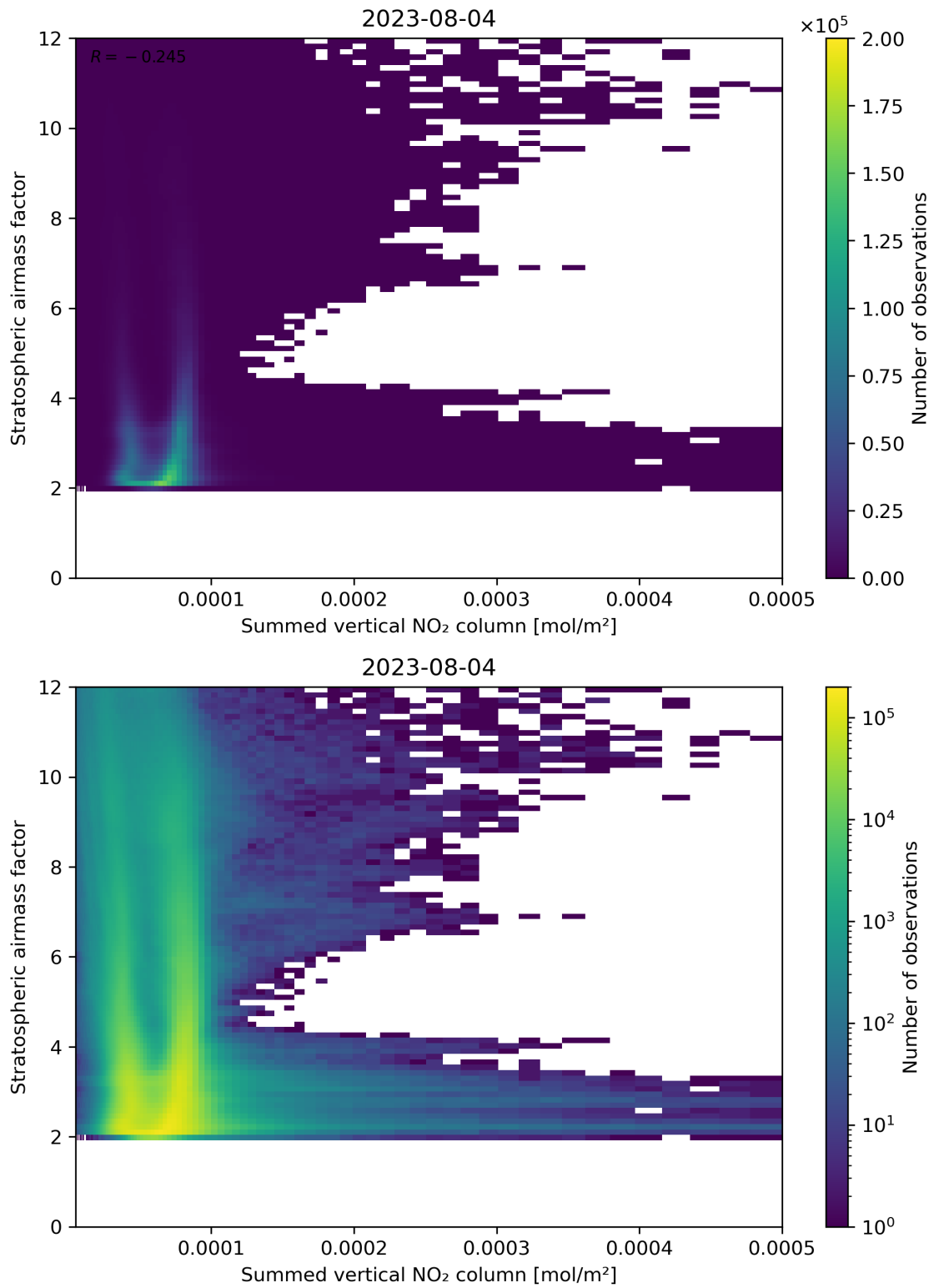
Figure 103: Scatter density plot of “Summed vertical NO 2 column” against “Stratospheric air mass factor” for 2023-08-04 to 2023-08-05.
