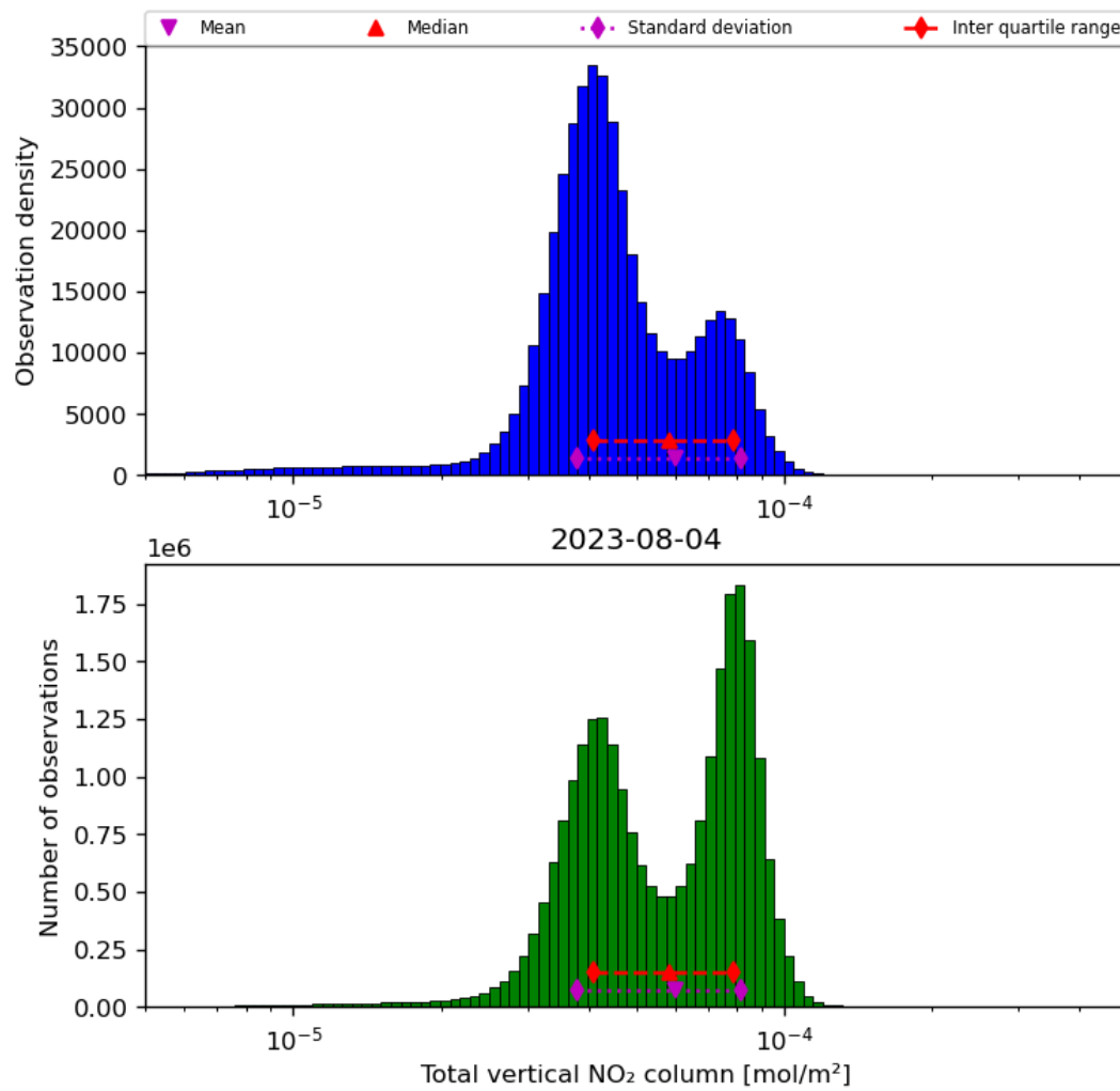
Figure 38: Histogram of “Total vertical NO 2 column” for 2023-08-04 to 2023-08-05
