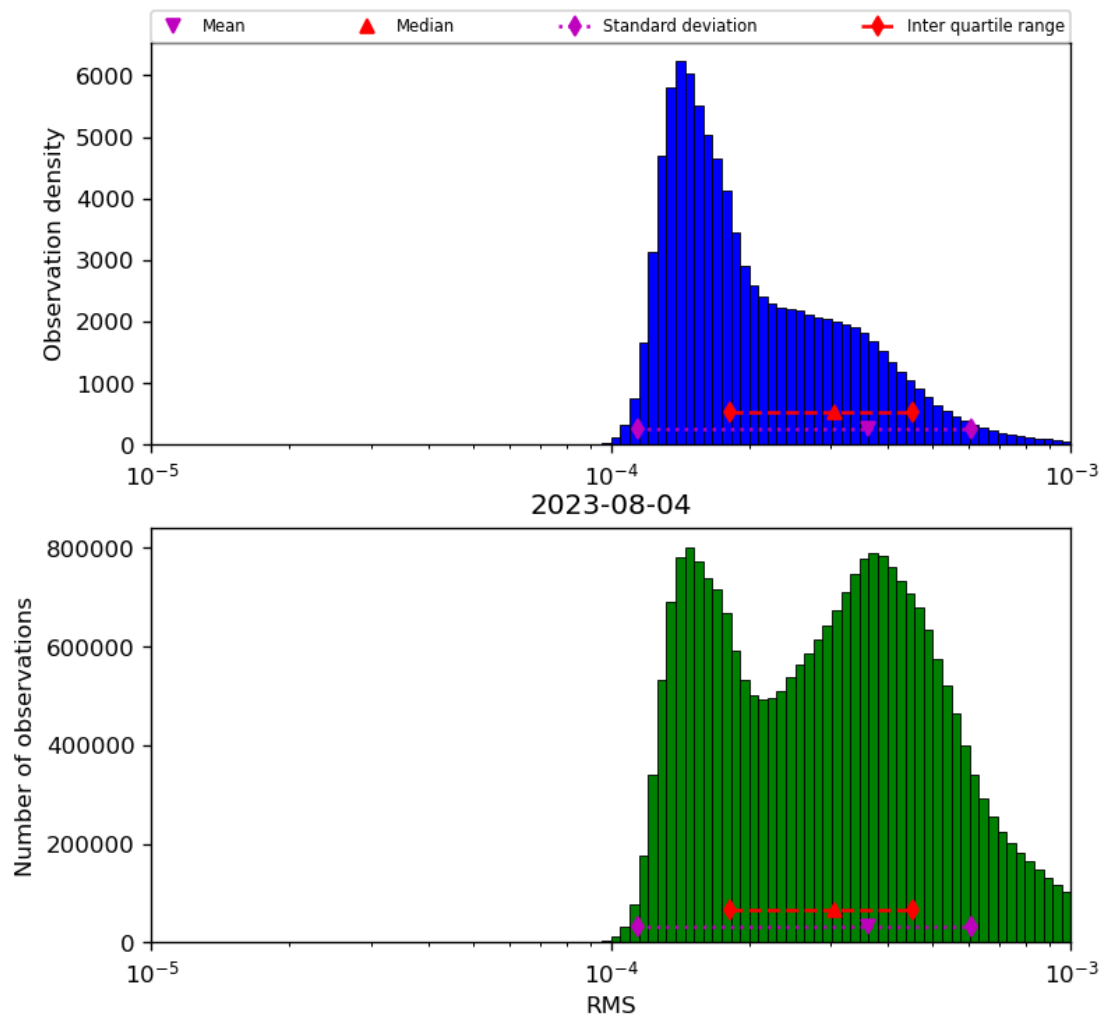
Figure 43: Histogram of “RMS” for 2023-08-04 to 2023-08-05
