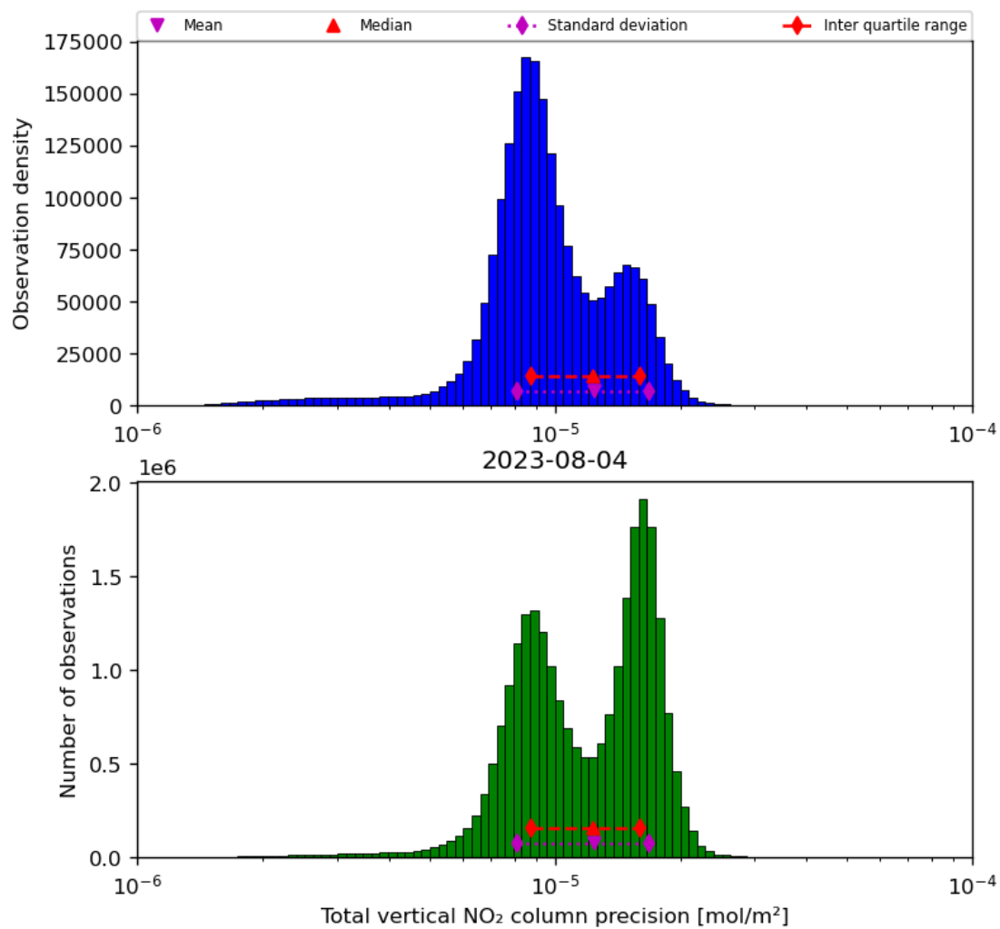
Figure 39: Histogram of “Total vertical NO 2 column precision” for 2023-08-04 to 2023-08-05
