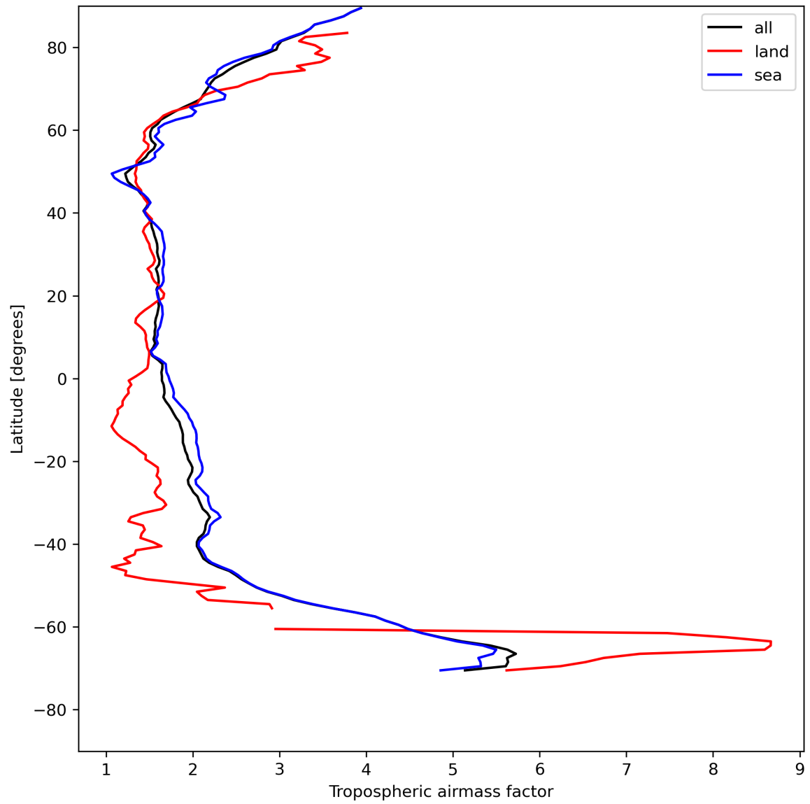
Figure 14: Zonal average of “Tropospheric air mass factor” for 2023-08-04 to 2023-08-05.
