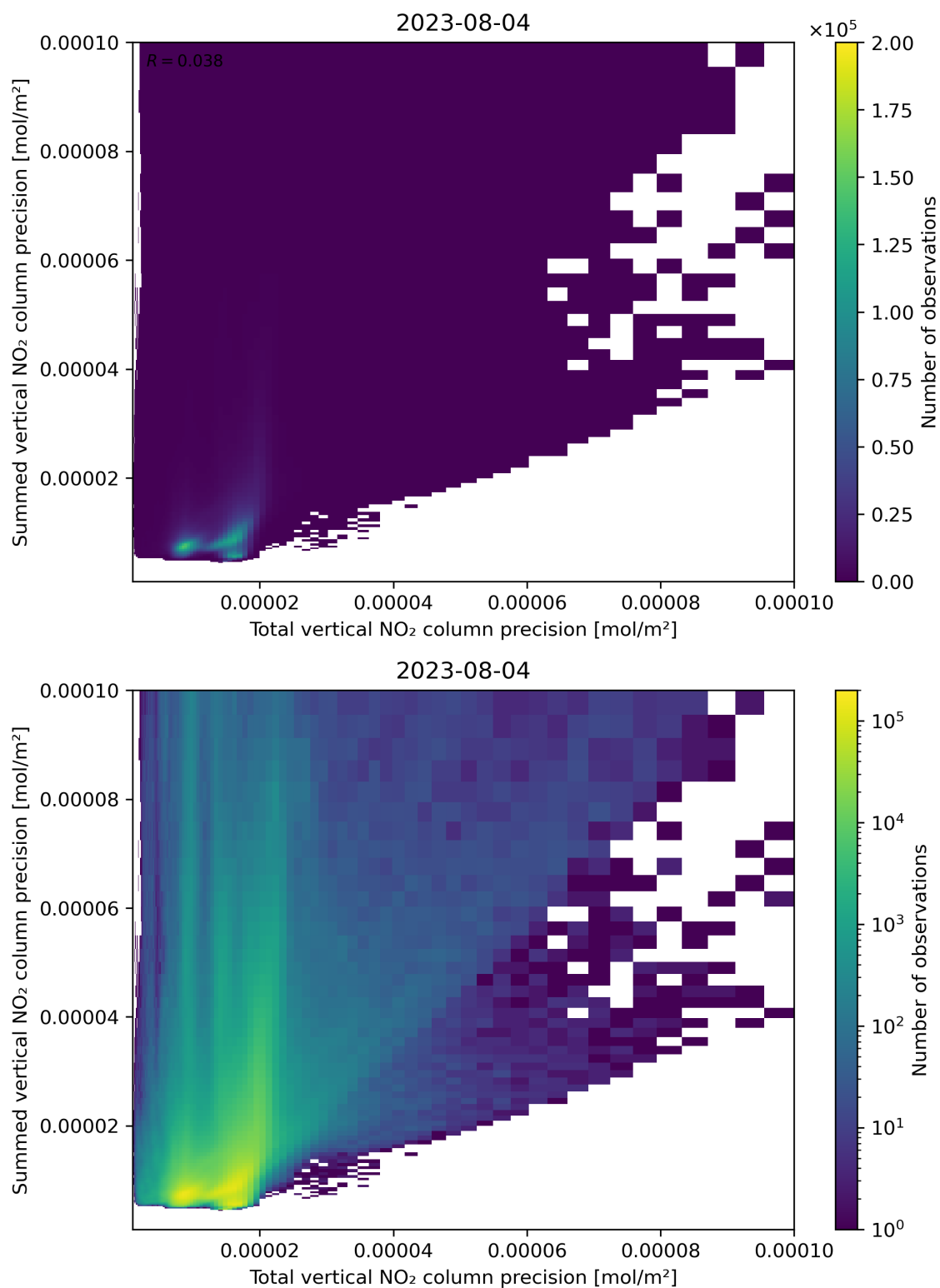
Figure 118: Scatter density plot of “Total vertical NO 2 column precision” against “Summed vertical NO 2 column precision” for 2023-08-04 to 2023-08-05.
