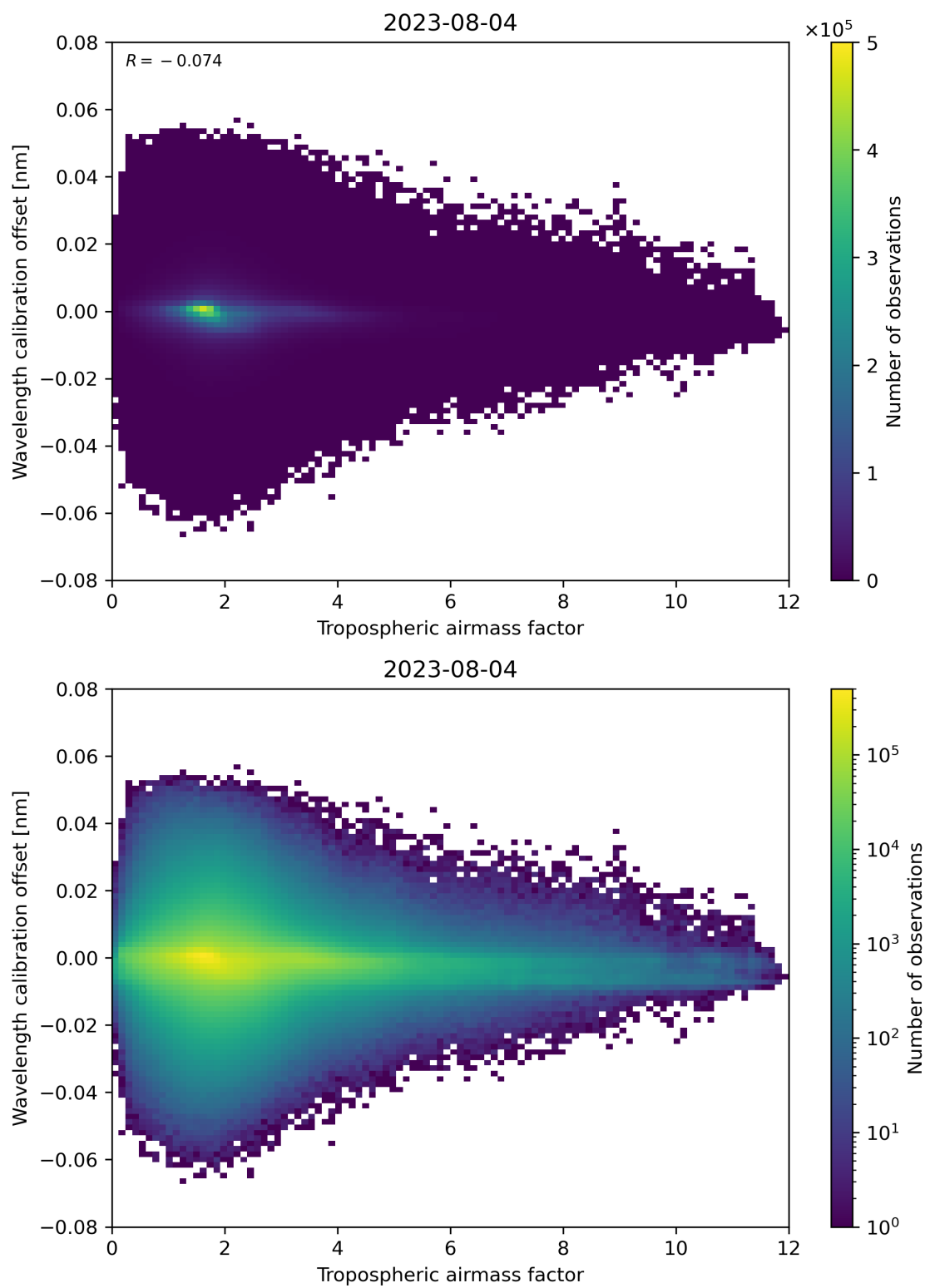
Figure 80: Scatter density plot of “Tropospheric airmass factor” against “Wavelength calibration offset” for 2023-08-04 to 2023-08-05.
