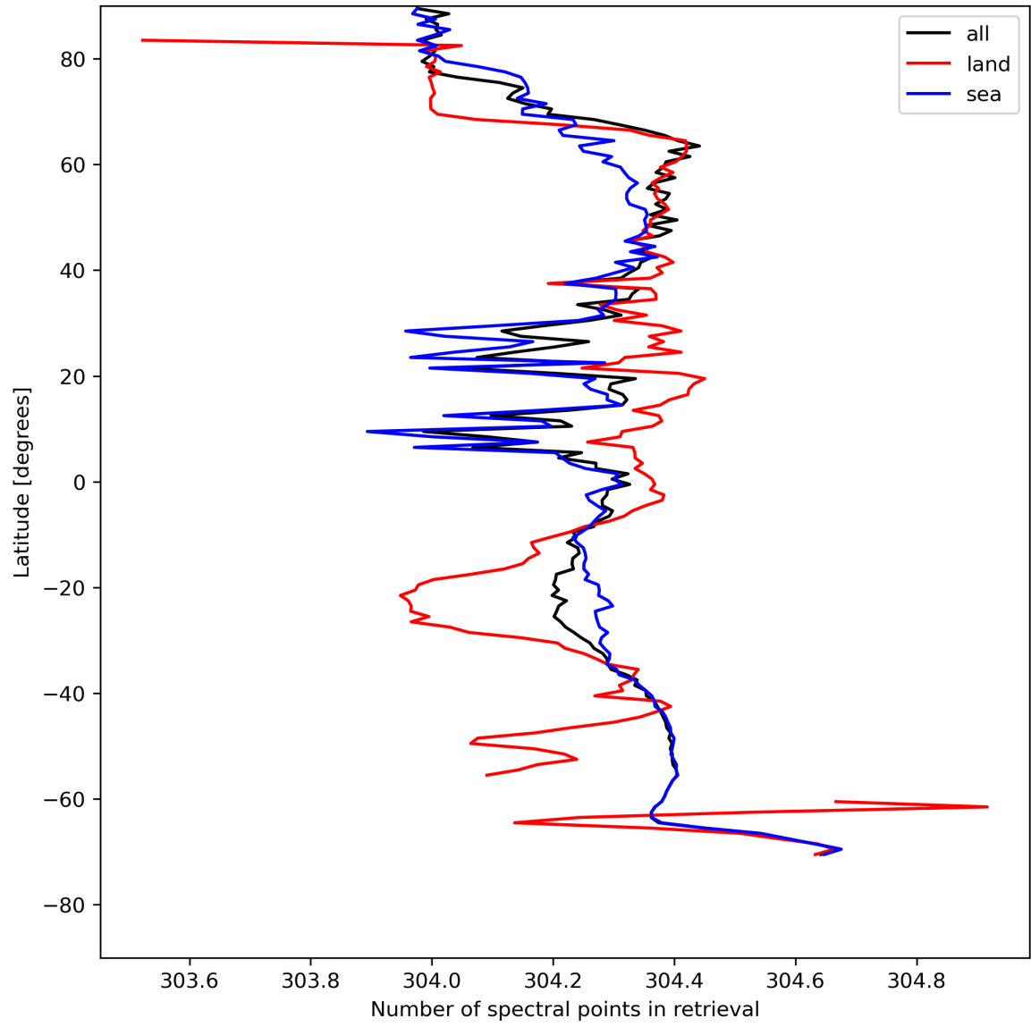
Figure 16: Zonal average of “Number of spectral points in retrieval” for 2023-08-04 to 2023-08-05.
