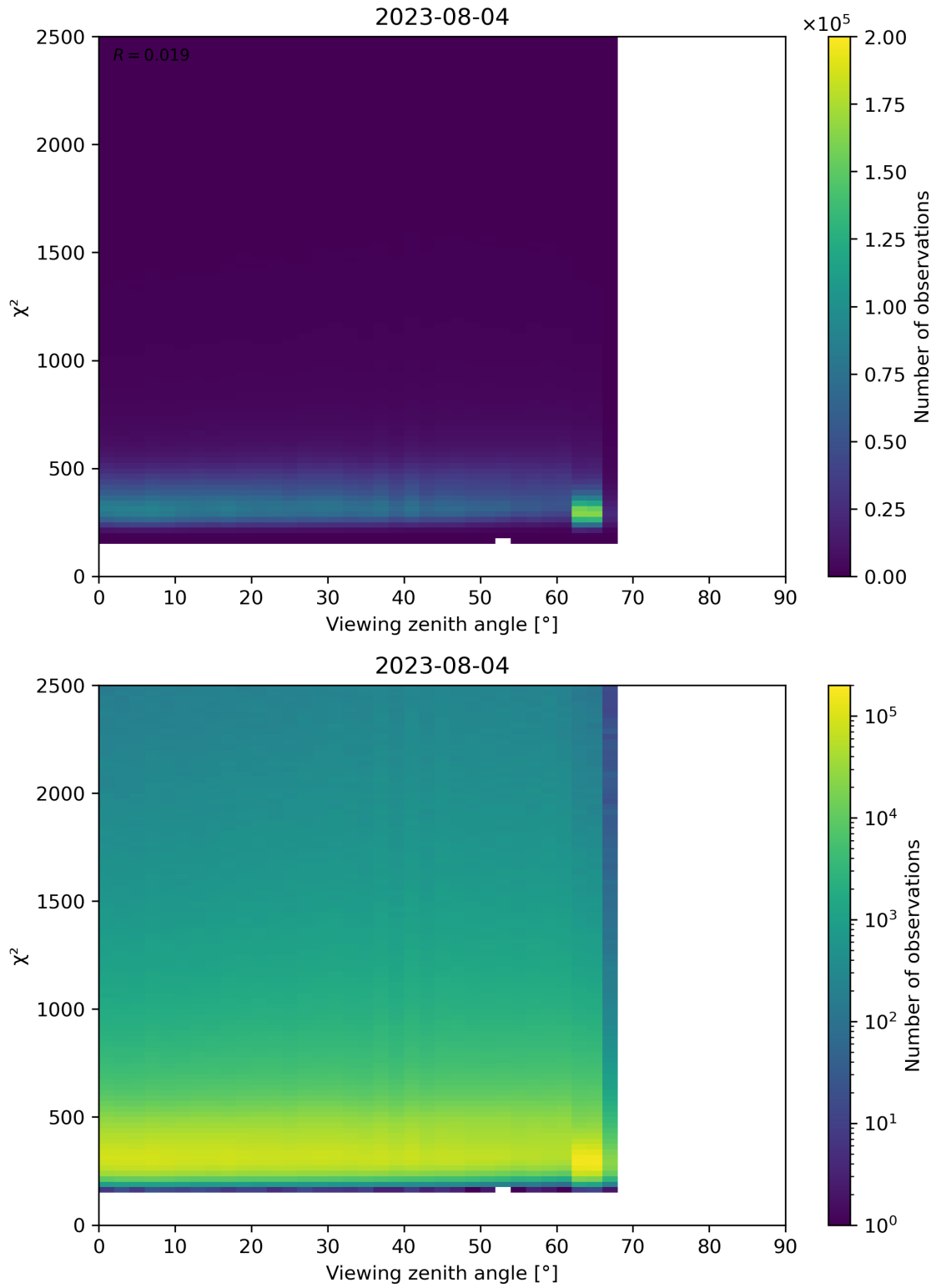
Figure 162: Scatter density plot of “Viewing zenith angle” against “ \chi^2 ” for 2023-08-04 to 2023-08-05.
