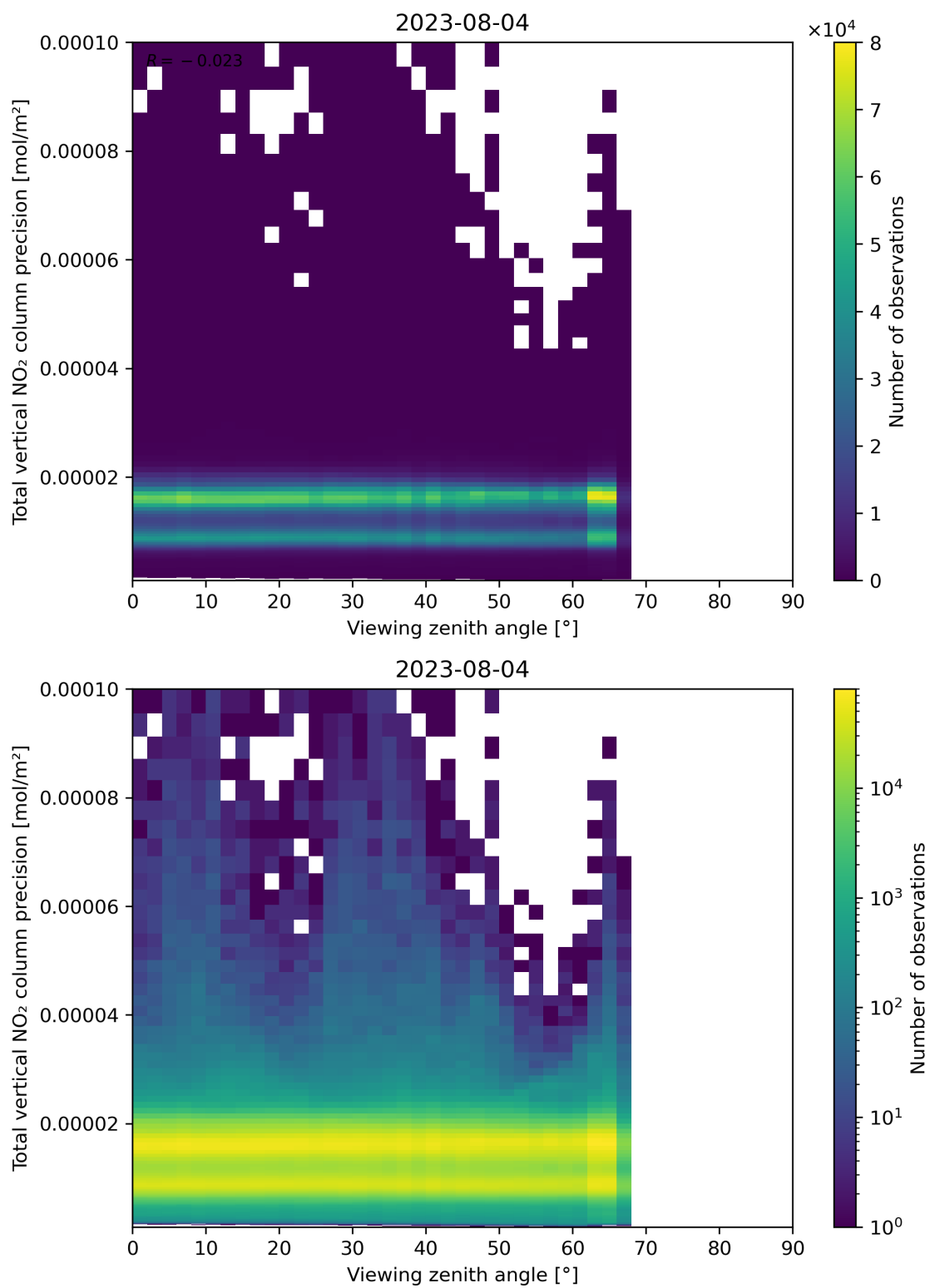
Figure 168: Scatter density plot of “Viewing zenith angle” against “Total vertical NO 2 column precision” for 2023-08-04 to 2023-08-05.
