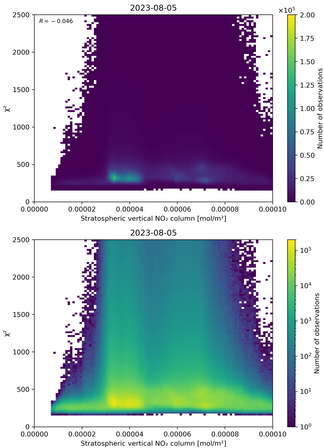
Figure 97: Scatter density plot of “Stratospheric vertical NO 2 column” against “ \chi^2 ” for 2023-08-04 to 2023-08-06.
