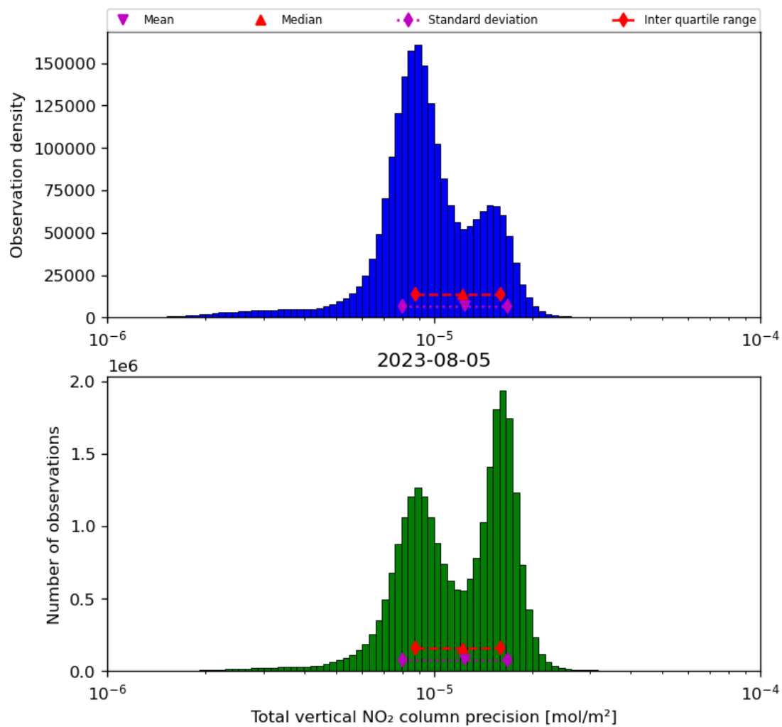
Figure 39: Histogram of "Total vertical NO 2 column precision" for 2023-08-04 to 2023-08-06
