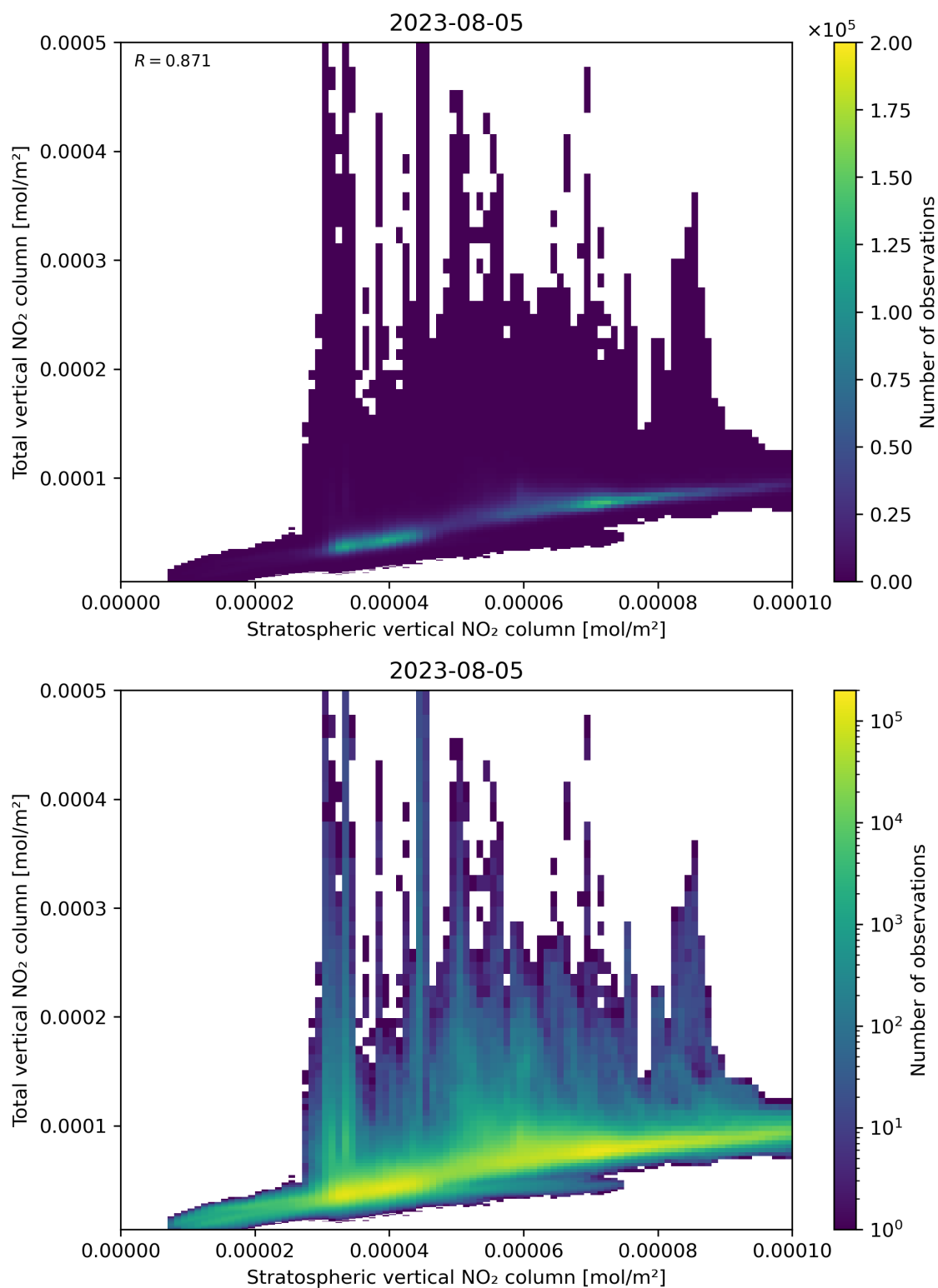
Figure 100: Scatter density plot of “Stratospheric vertical NO 2 column” against “Total vertical NO 2 column” for 2023-08-04 to 2023-08-06.
