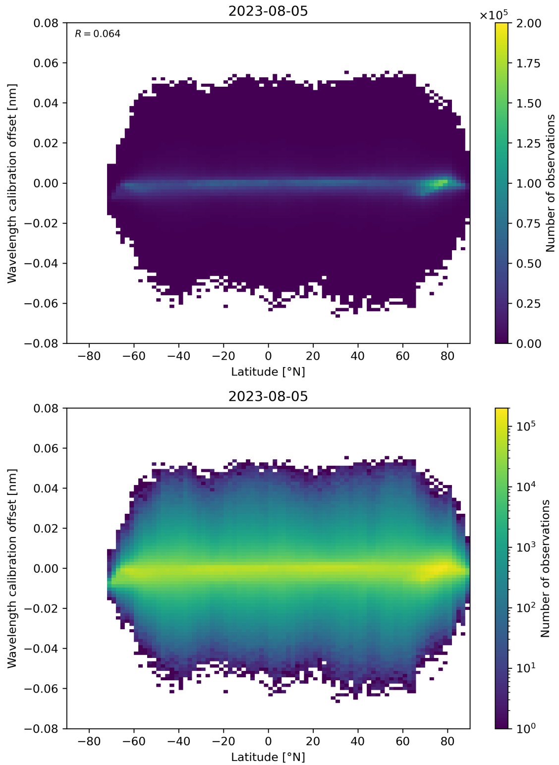
Figure 95: Scatter density plot of “Latitude” against “Wavelength calibration offset” for 2023-08-04 to 2023-08-06.
