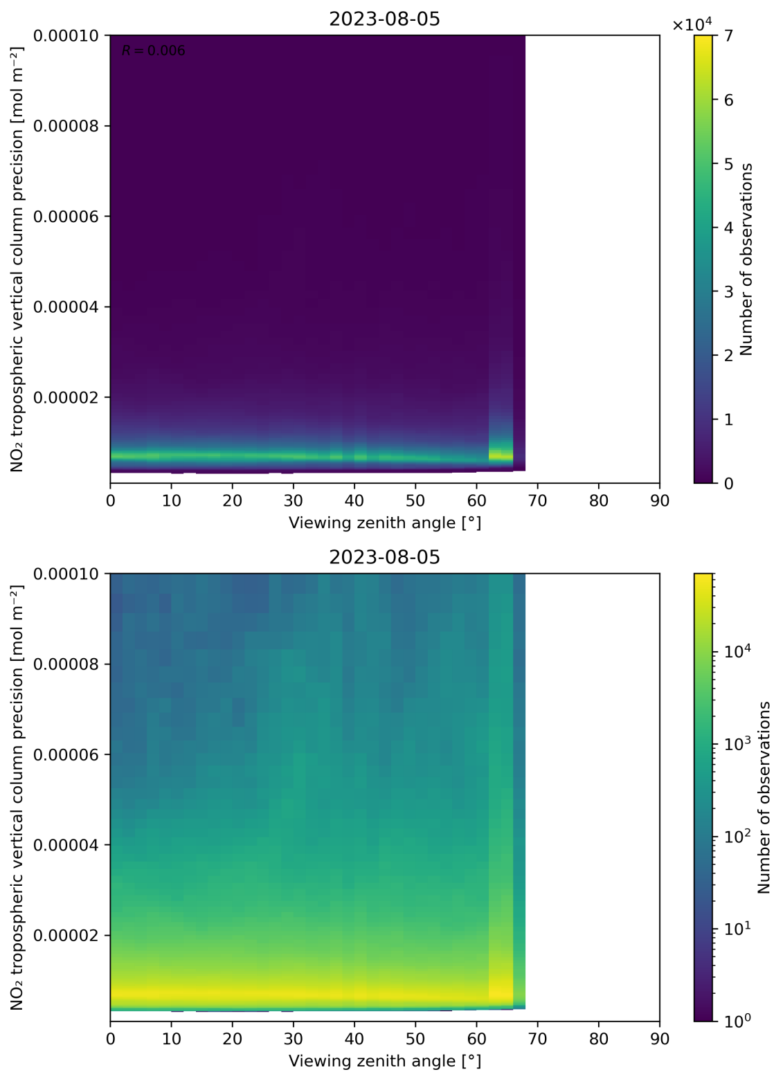
Figure 170: Scatter density plot of “Viewing zenith angle” against “NO 2 tropospheric vertical column precision” for 2023-08-04 to 2023-08-06.
