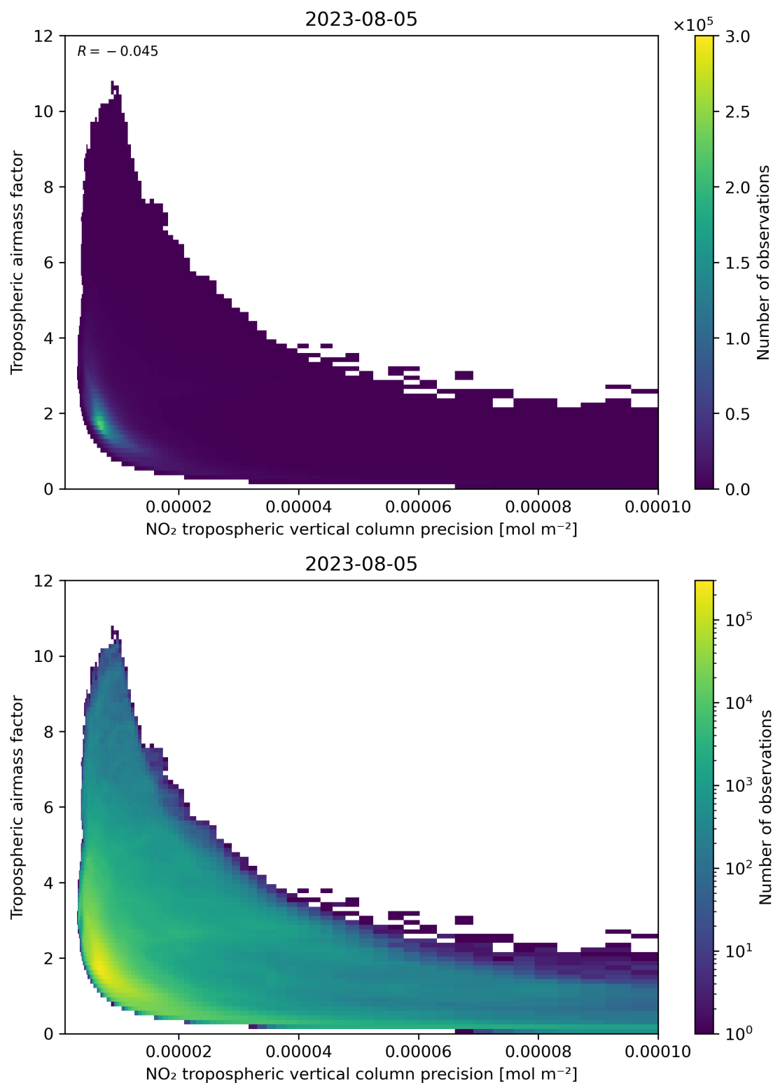
Figure 133: Scatter density plot of “NO 2 tropospheric vertical column precision” against “Tropospheric airmass factor” for 2023-08-04 to 2023-08-06.
