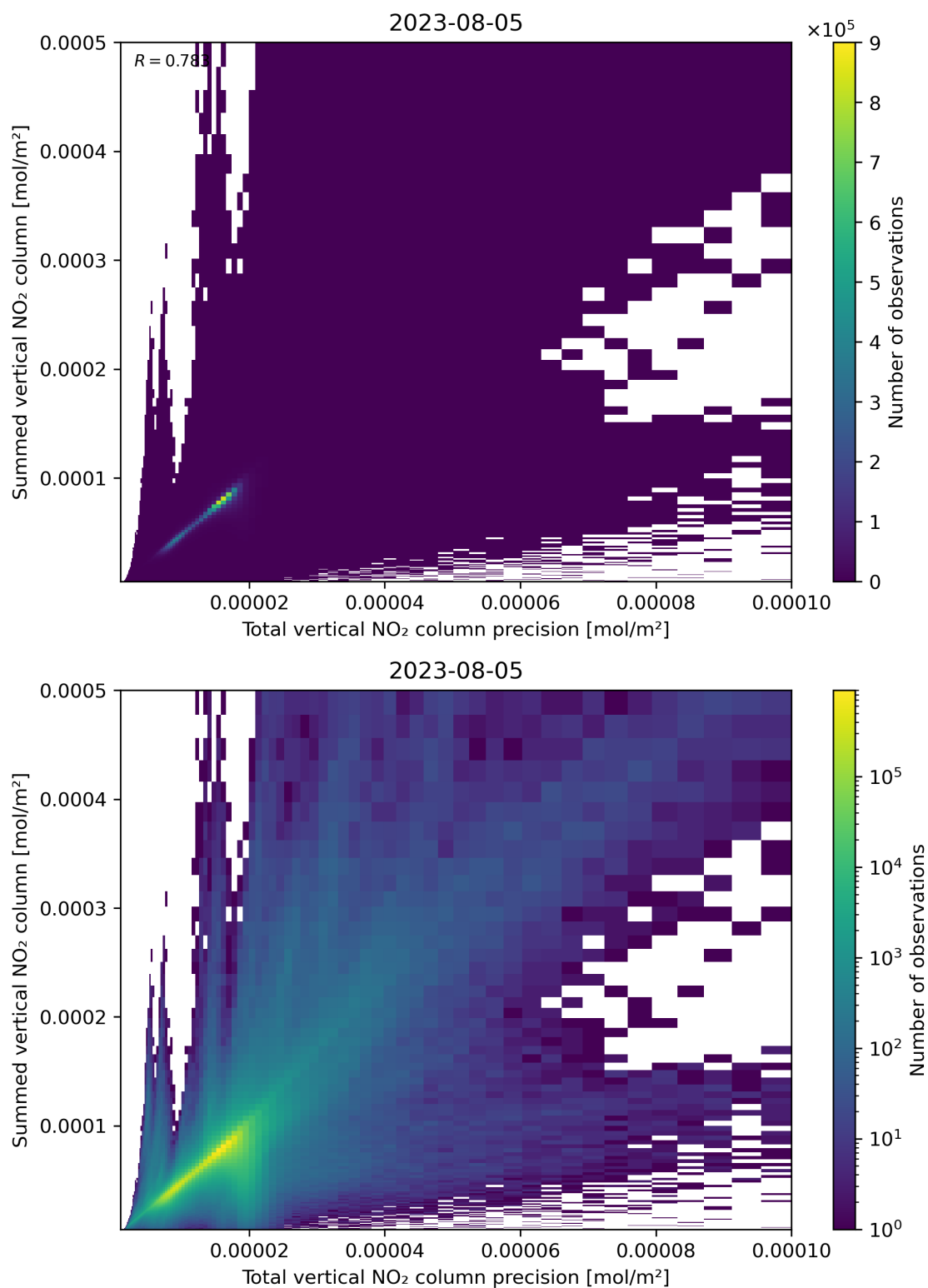
Figure 117: Scatter density plot of “Total vertical NO 2 column precision” against “Summed vertical NO 2 column” for 2023-08-04 to 2023-08-06.
