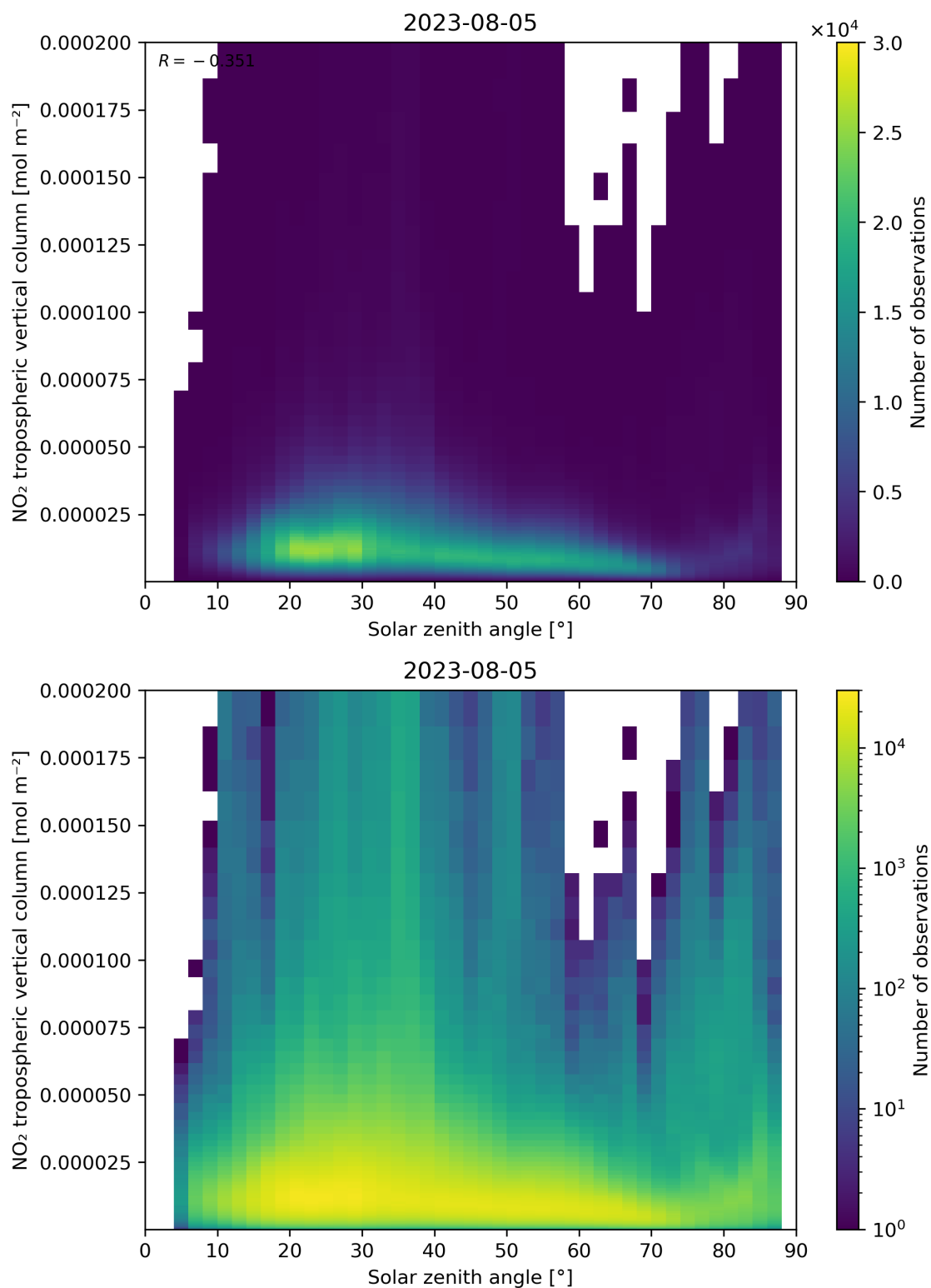
Figure 155: Scatter density plot of “Solar zenith angle” against “NO 2 tropospheric vertical column” for 2023-08-04 to 2023-08-06.
