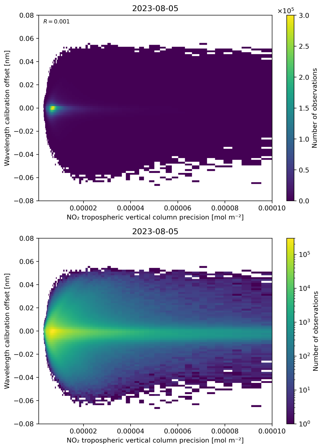
Figure 141: Scatter density plot of “NO 2 tropospheric vertical column precision” against “Wavelength calibration offset” for 2023-08-04 to 2023-08-06.
