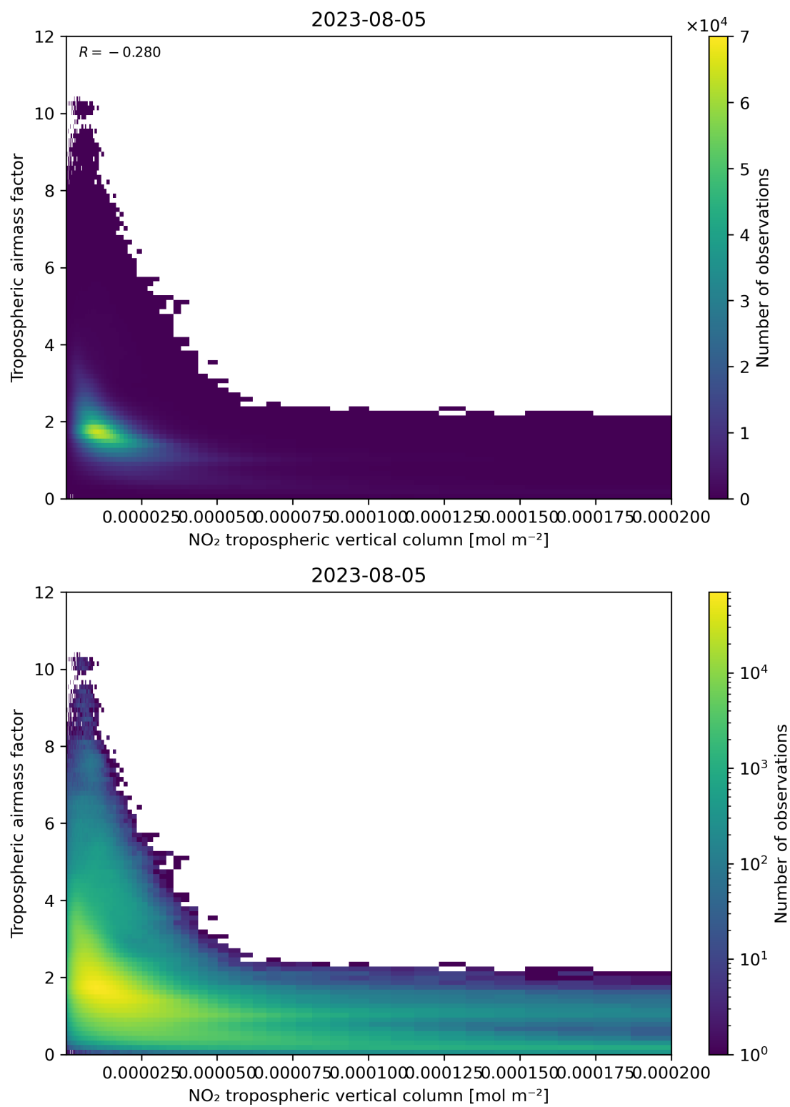
Figure 123: Scatter density plot of “NO 2 tropospheric vertical column” against “Tropospheric air mass factor” for 2023-08-04 to 2023-08-06.
