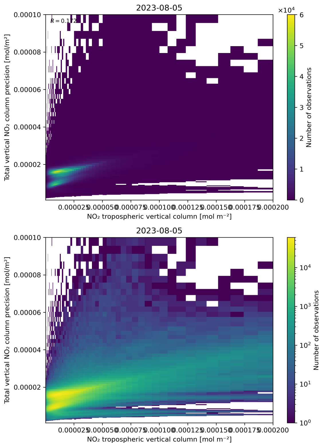
Figure 129: Scatter density plot of “NO 2 tropospheric vertical column” against “Total vertical NO 2 column precision” for 2023-08-04 to 2023-08-06.
