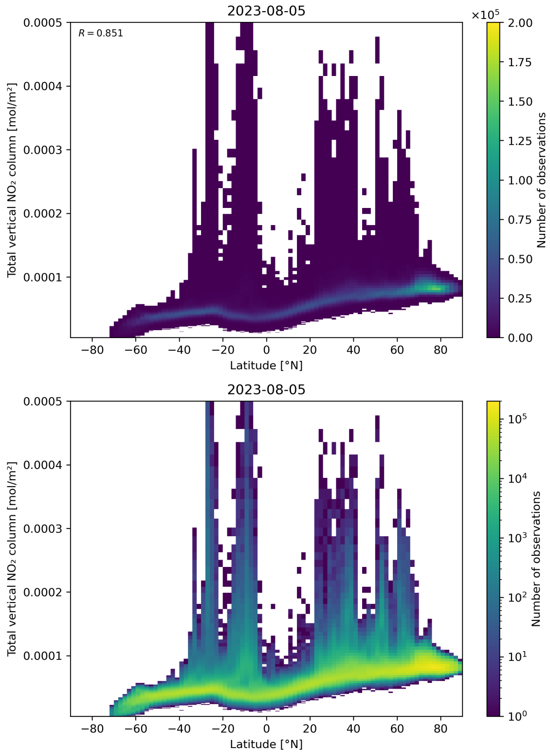
Figure 90: Scatter density plot of “Latitude” against “Total vertical NO 2 column” for 2023-08-04 to 2023-08-06.
