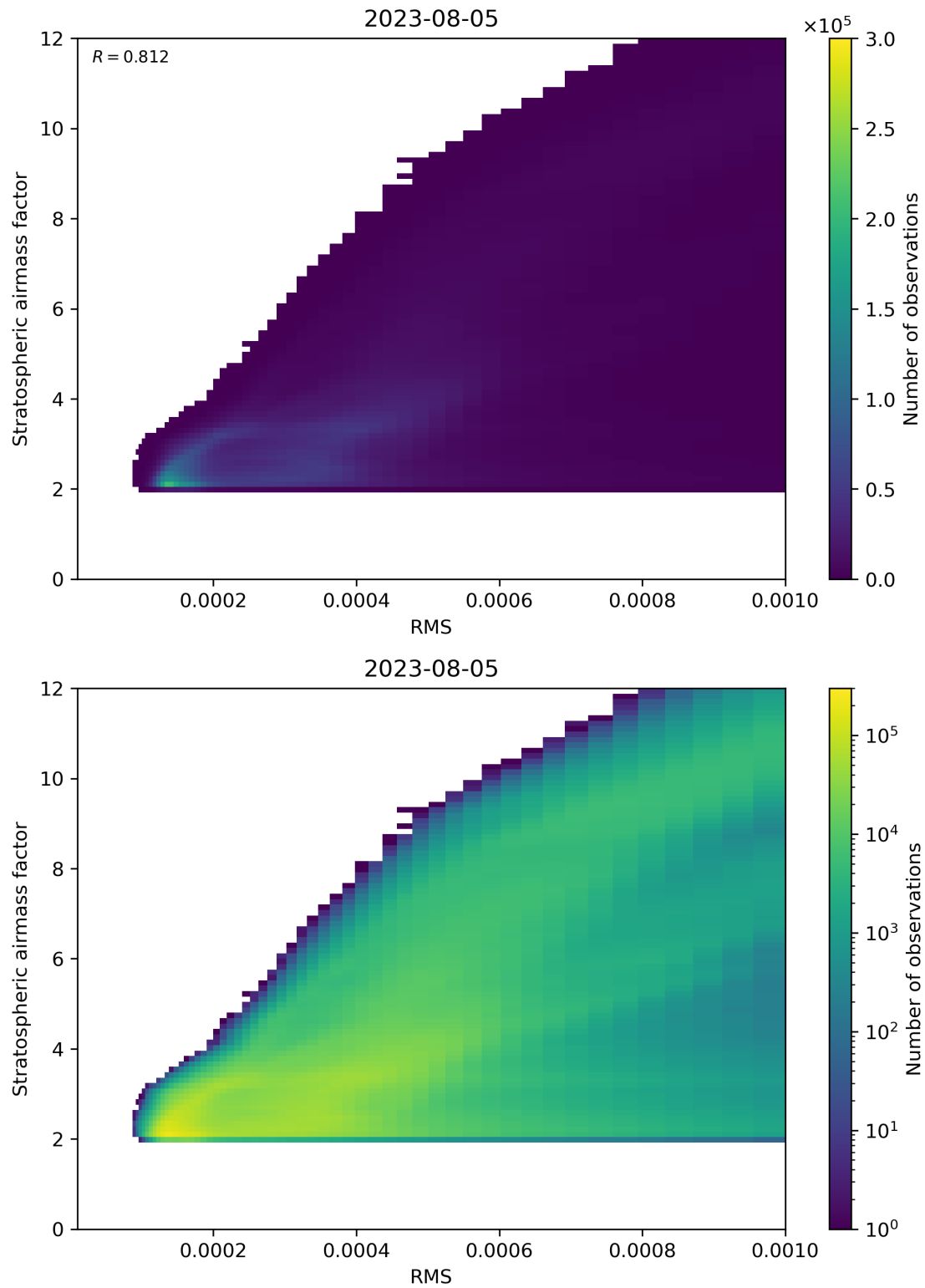
Figure 144: Scatter density plot of “RMS” against “Stratospheric airmass factor” for 2023-08-04 to 2023-08-06.
