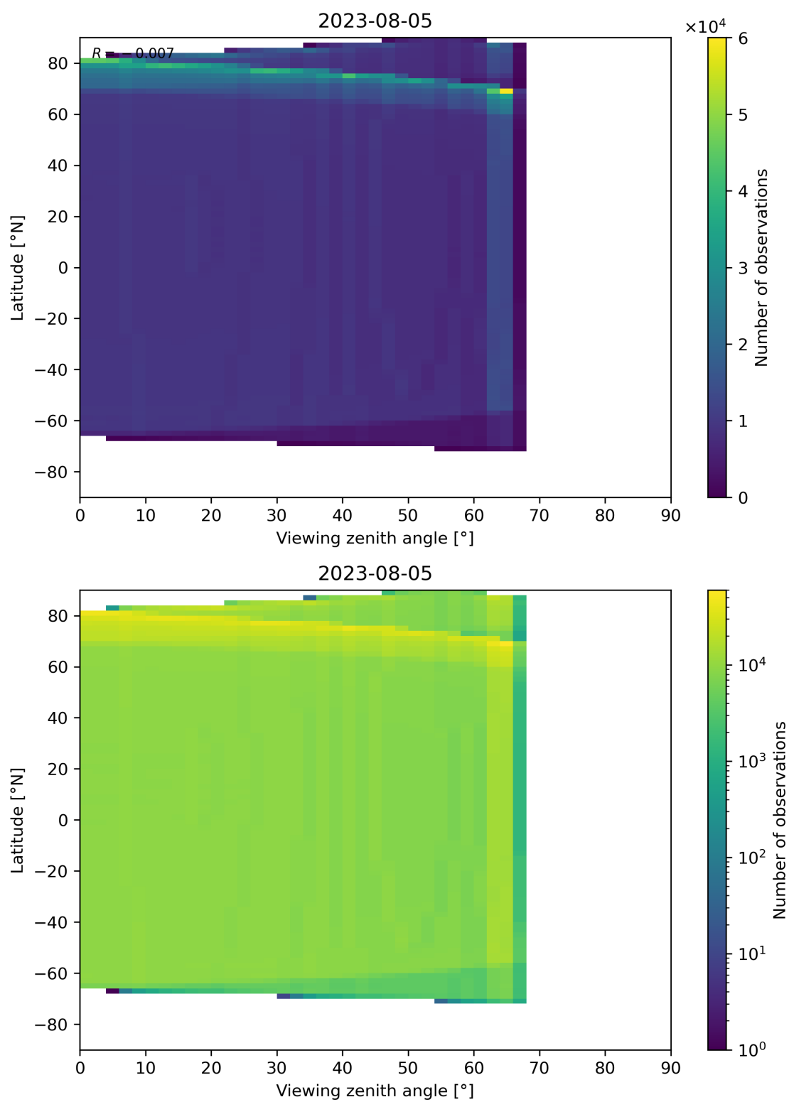
Figure 163: Scatter density plot of “Viewing zenith angle” against “Latitude” for 2023-08-04 to 2023-08-06.
