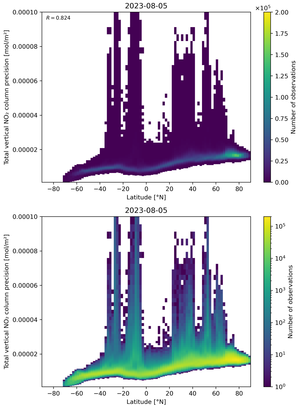
Figure 91: Scatter density plot of “Latitude” against “Total vertical NO 2 column precision” for 2023-08-04 to 2023-08-06.
