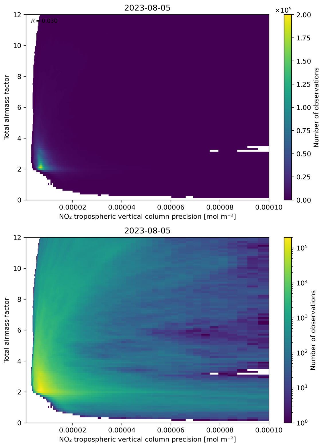
Figure 132: Scatter density plot of “NO 2 tropospheric vertical column precision” against “Total air mass factor” for 2023-08-04 to 2023-08-06.
