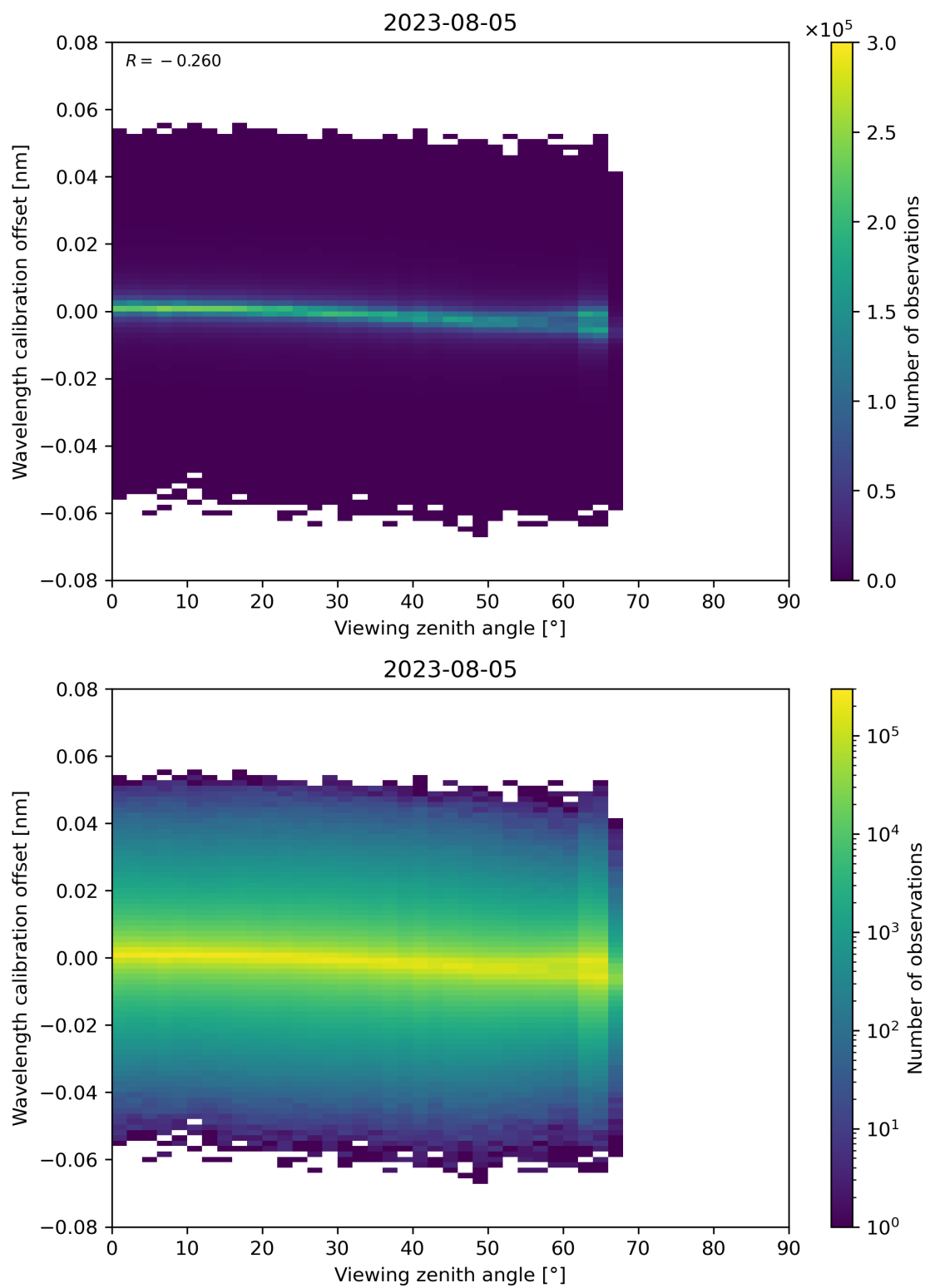
Figure 173: Scatter density plot of “Viewing zenith angle” against “Wavelength calibration offset” for 2023-08-04 to 2023-08-06.
