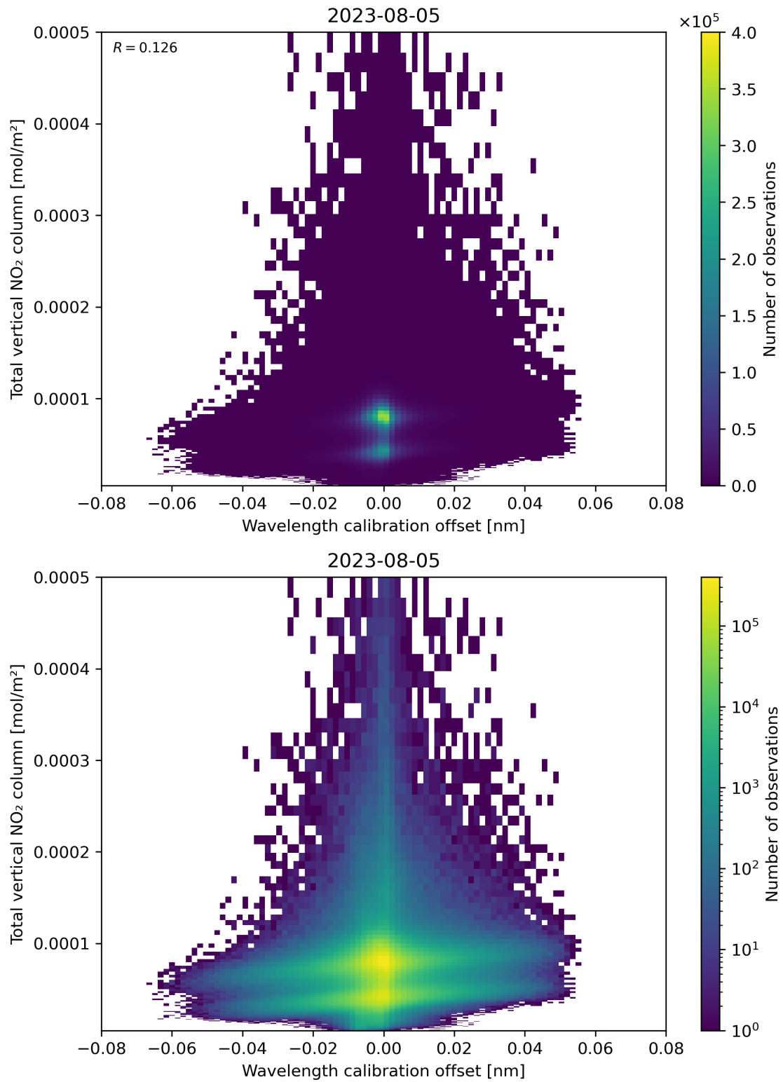
Figure 179: Scatter density plot of “Wavelength calibration offset” against “Total vertical NO 2 column” for 2023-08-04 to 2023-08-06.
