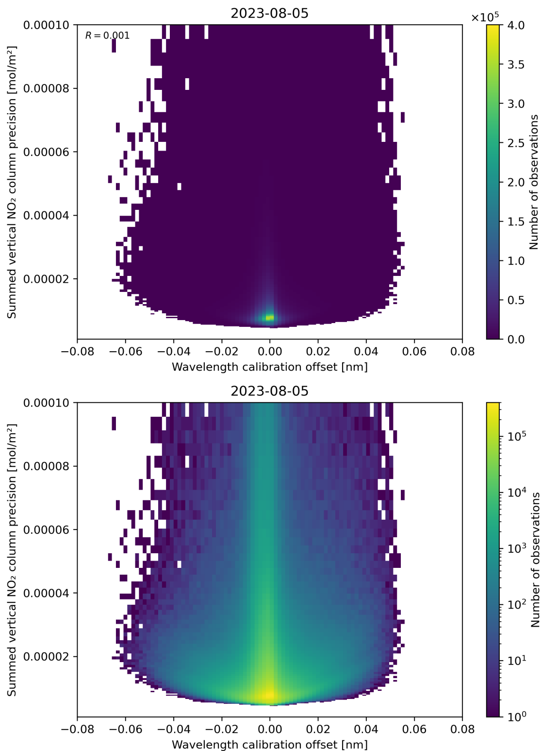
Figure 178: Scatter density plot of “Wavelength calibration offset” against “Summed vertical NO 2 column precision” for 2023-08-04 to 2023-08-06.
