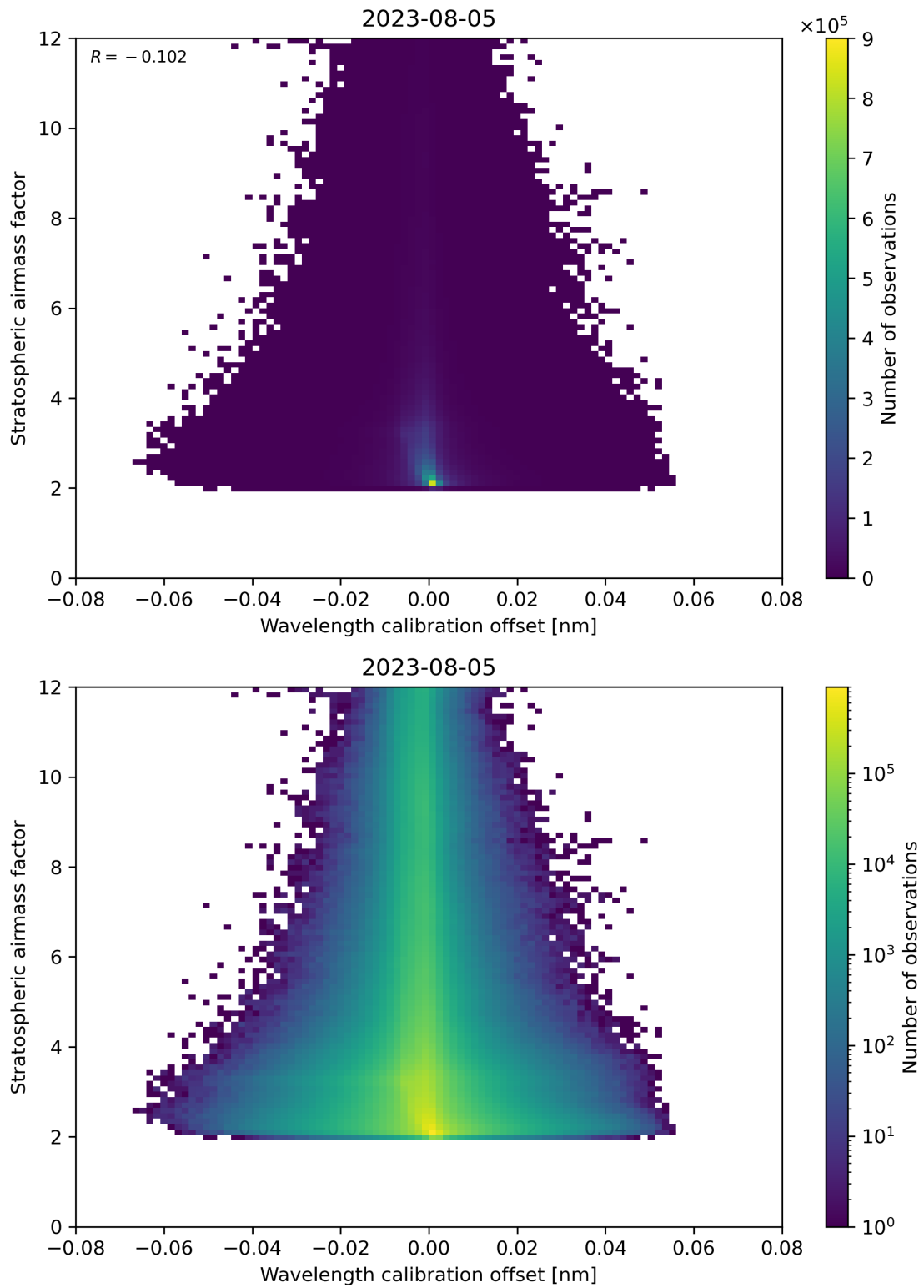
Figure 174: Scatter density plot of “Wavelength calibration offset” against “Stratospheric airmass factor” for 2023-08-04 to 2023-08-06.
