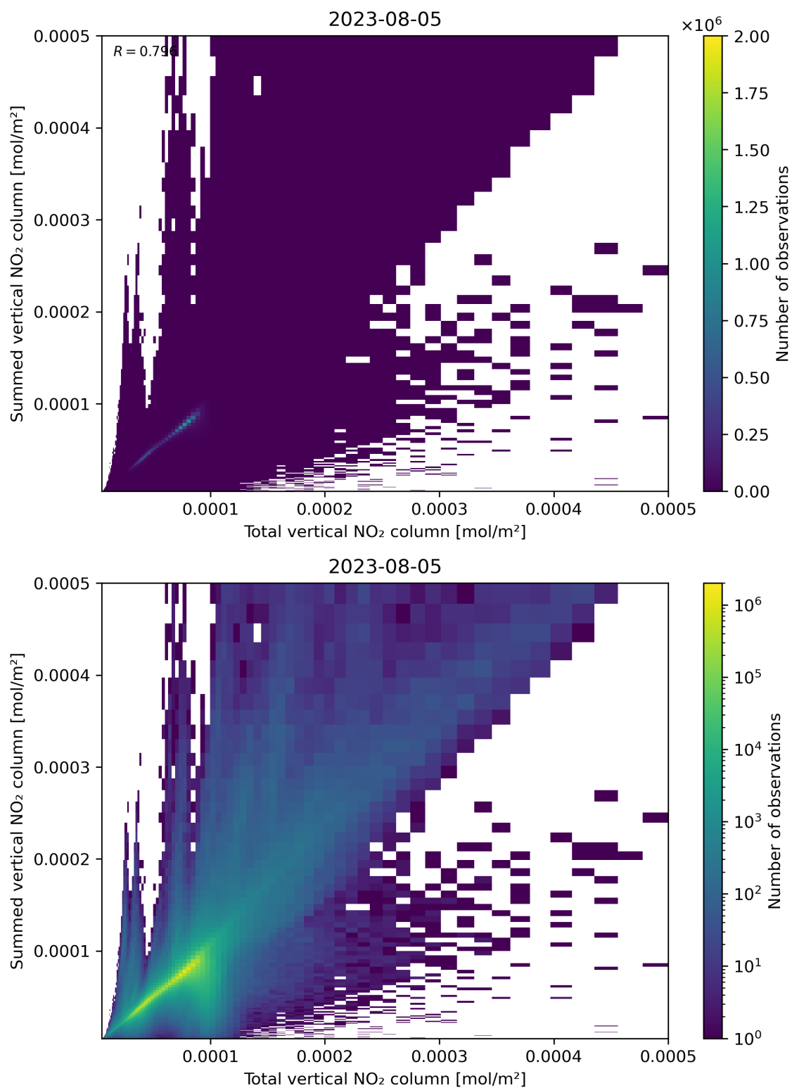
Figure 112: Scatter density plot of “Total vertical NO 2 column” against “Summed vertical NO 2 column” for 2023-08-04 to 2023-08-06.
