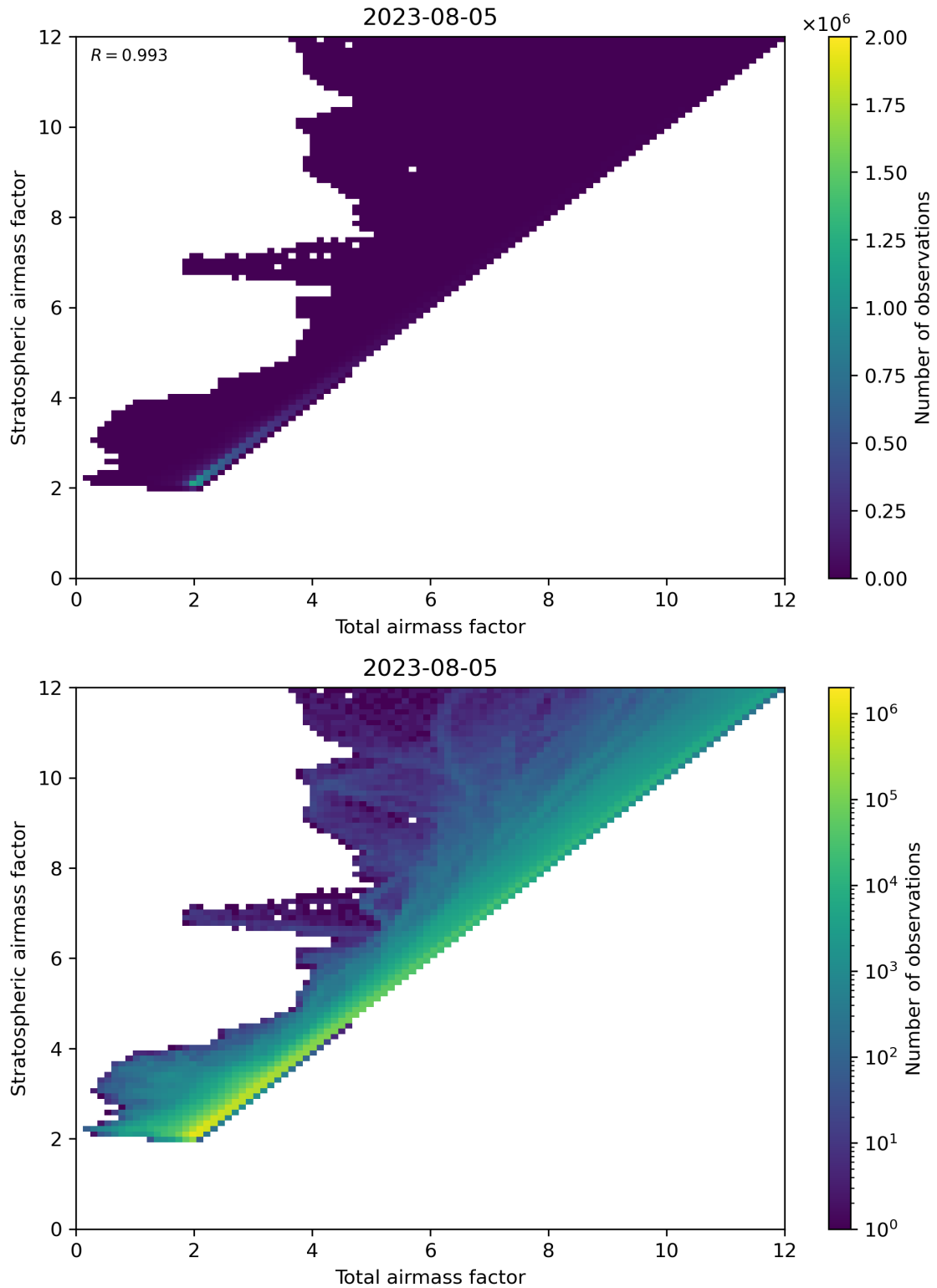
Figure 62: Scatter density plot of “Total airmass factor” against “Stratospheric airmass factor” for 2023-08-04 to 2023-08-06.
