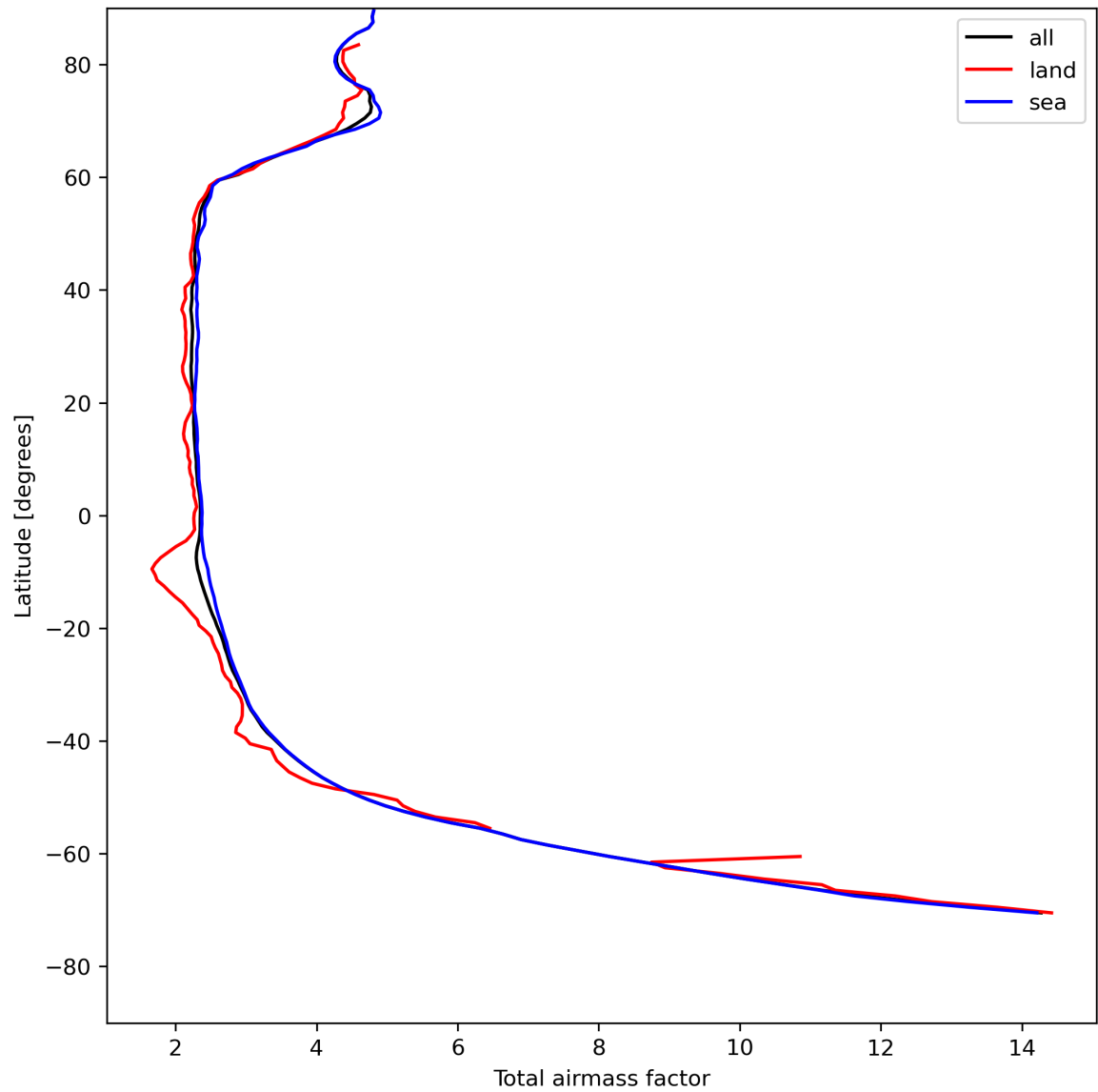
Figure 15: Zonal average of “Total airmass factor” for 2023-08-04 to 2023-08-06.
