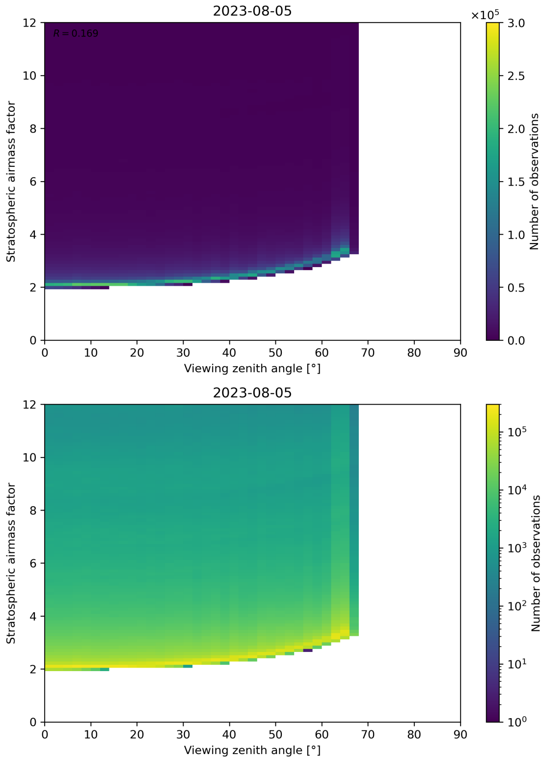
Figure 159: Scatter density plot of “Viewing zenith angle” against “Stratospheric airmass factor” for 2023-08-04 to 2023-08-06.
