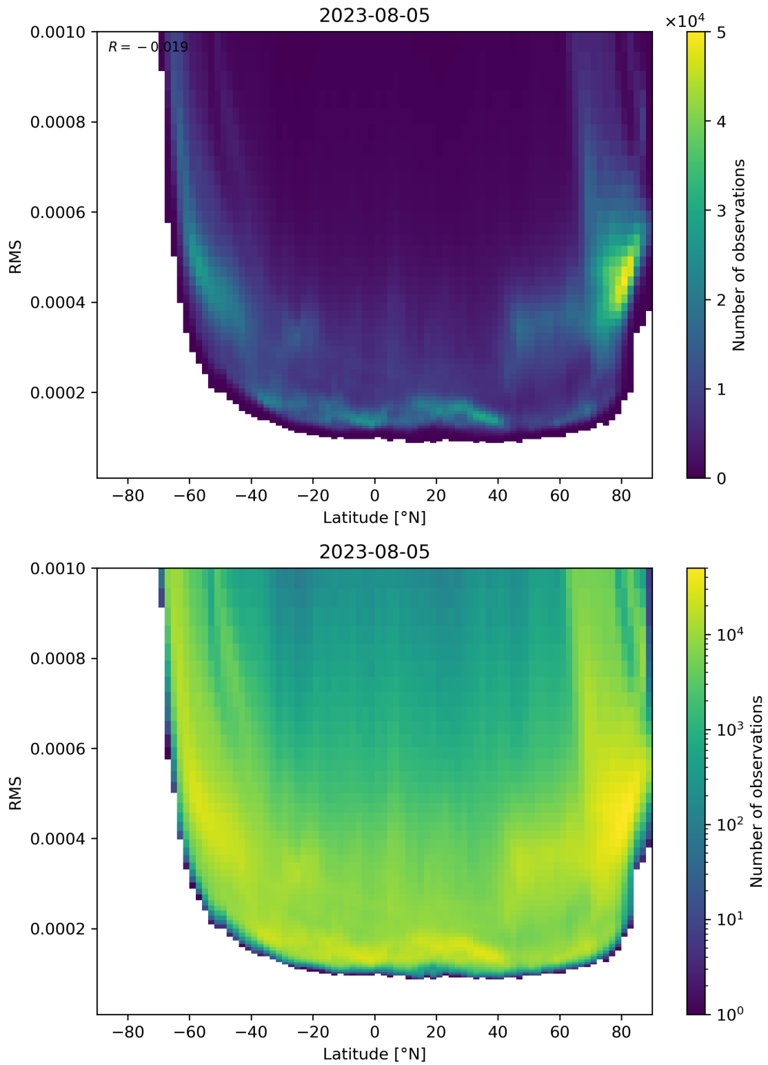
Figure 94: Scatter density plot of “Latitude” against “RMS” for 2023-08-04 to 2023-08-06.
