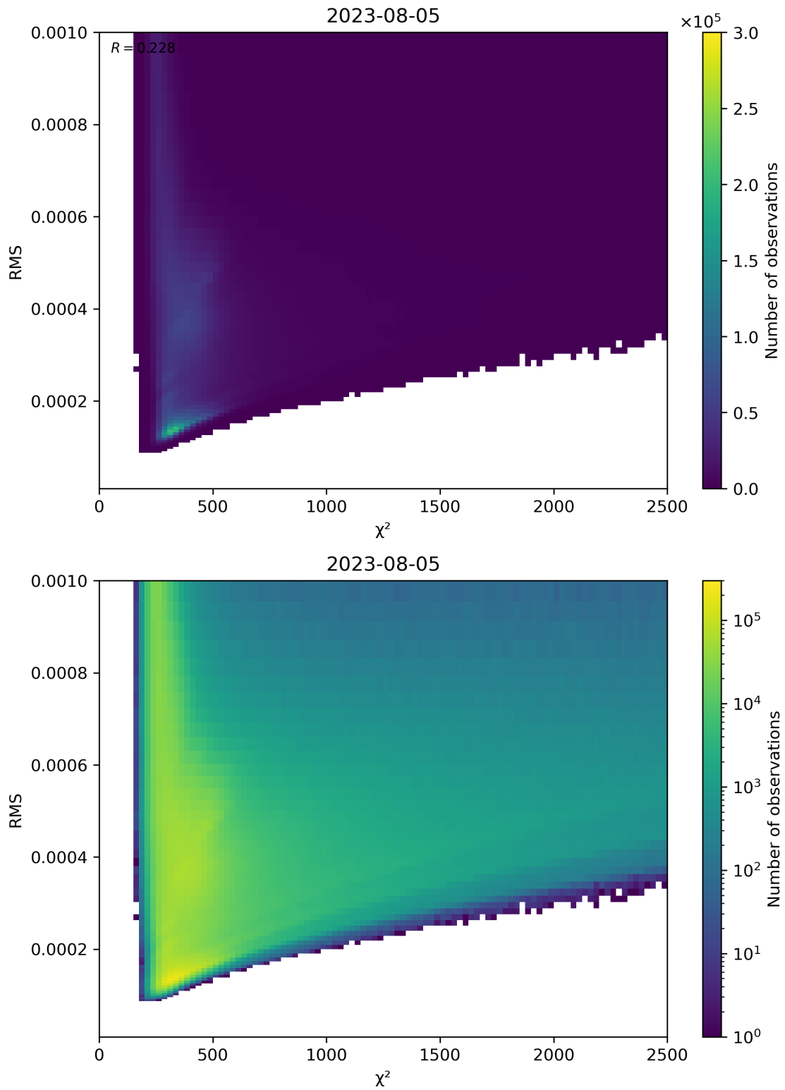
Figure 82: Scatter density plot of “ \chi^2 ” against “RMS” for 2023-08-04 to 2023-08-06.
