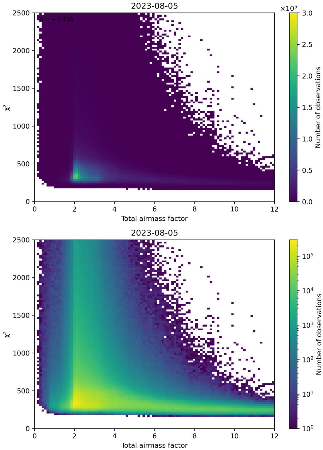
Figure 63: Scatter density plot of “Total airmass factor” against “ \chi^2 ” for 2023-08-04 to 2023-08-06.
