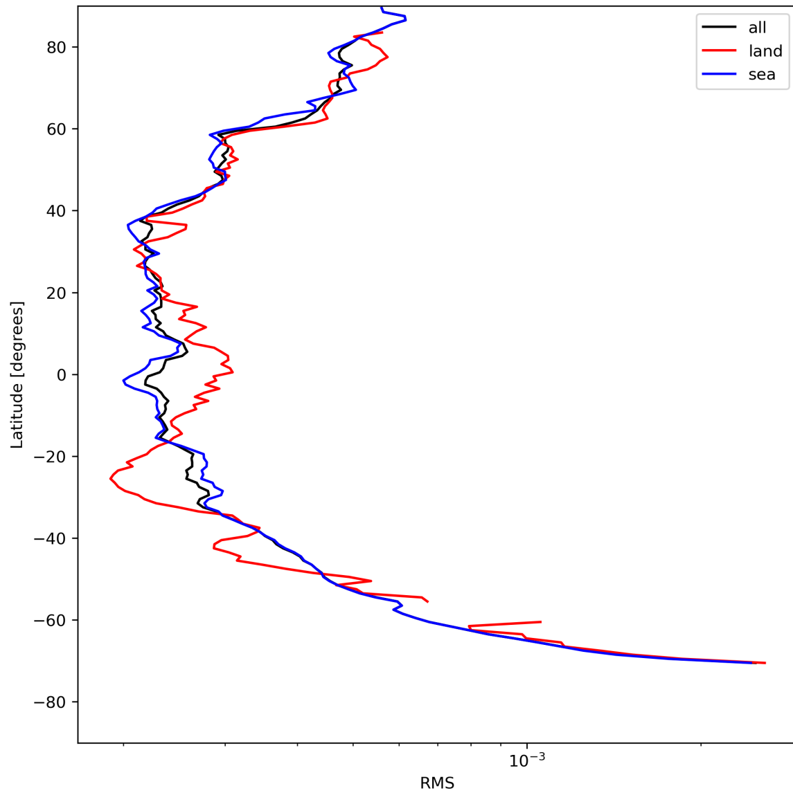
Figure 26: Zonal average of “RMS” for 2023-08-04 to 2023-08-06.
