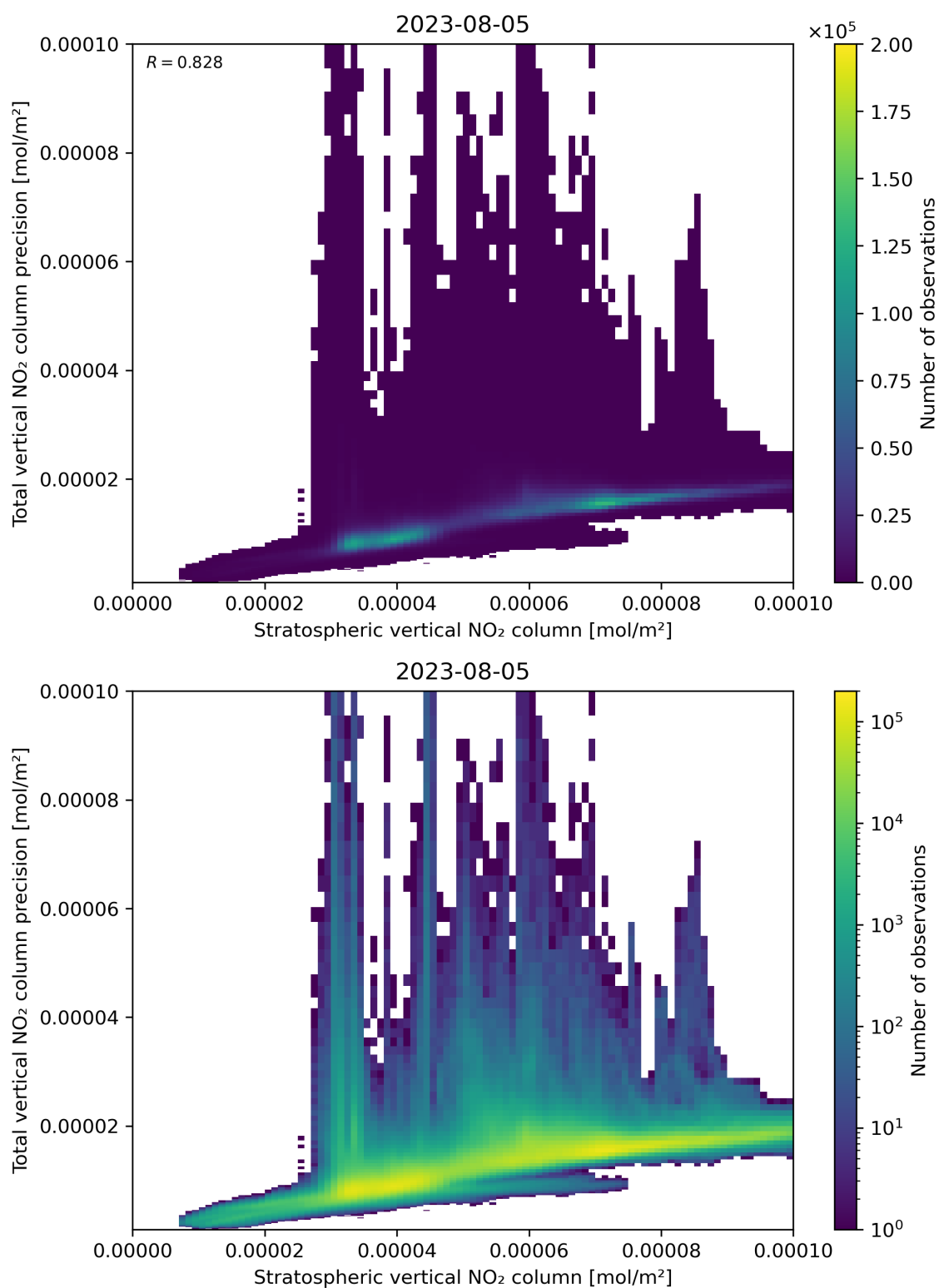
Figure 101: Scatter density plot of “Stratospheric vertical NO 2 column” against “Total vertical NO 2 column precision” for 2023-08-04 to 2023-08-06.
