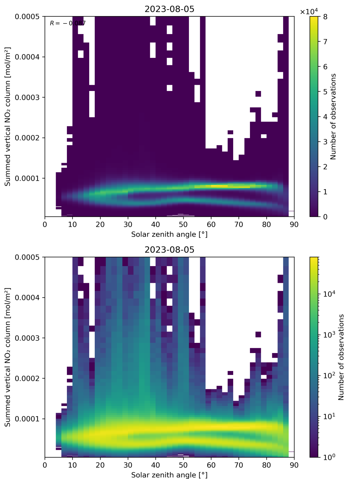
Figure 151: Scatter density plot of “Solar zenith angle” against “Summed vertical NO 2 column” for 2023-08-04 to 2023-08-06.
