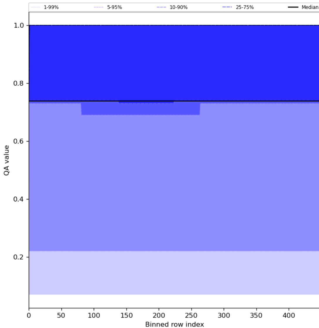
Figure 45: Along track statistics of “QA value” for 2023-08-04 to 2023-08-06
