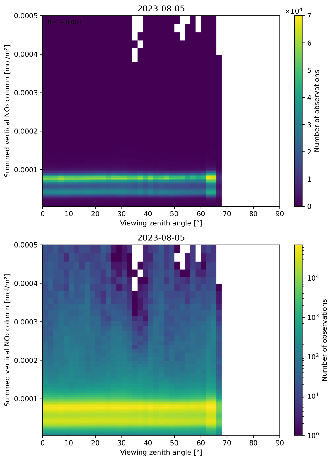
Figure 165: Scatter density plot of “Viewing zenith angle” against “Summed vertical NO 2 column” for 2023-08-04 to 2023-08-06.
