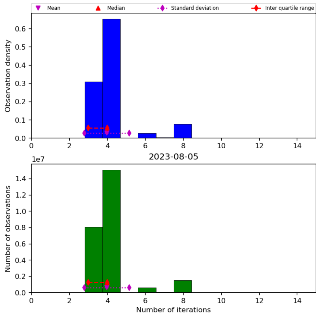
Figure 34: Histogram of “Number of iterations” for 2023-08-04 to 2023-08-06
