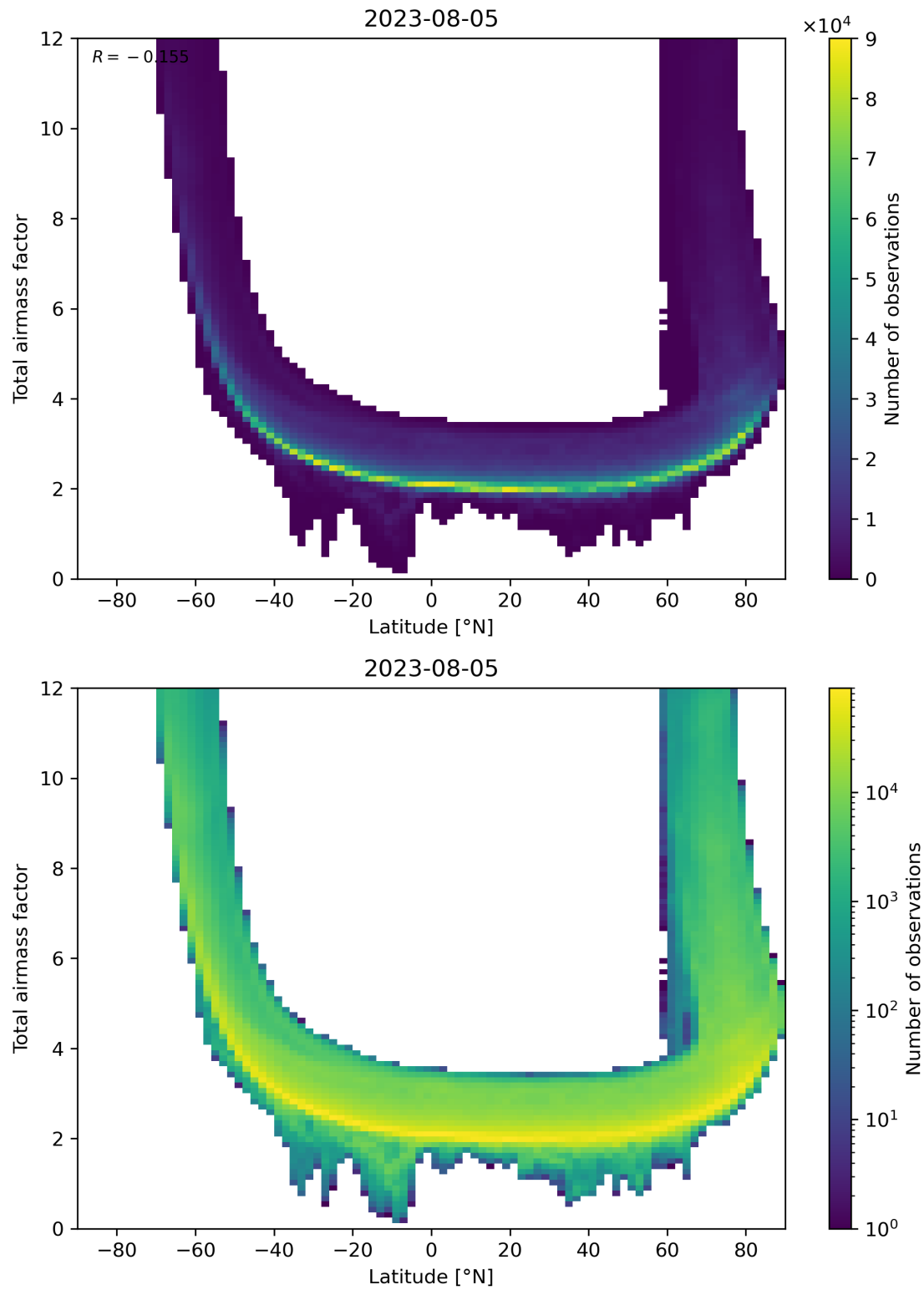
Figure 84: Scatter density plot of “Latitude” against “Total air mass factor” for 2023-08-04 to 2023-08-06.
