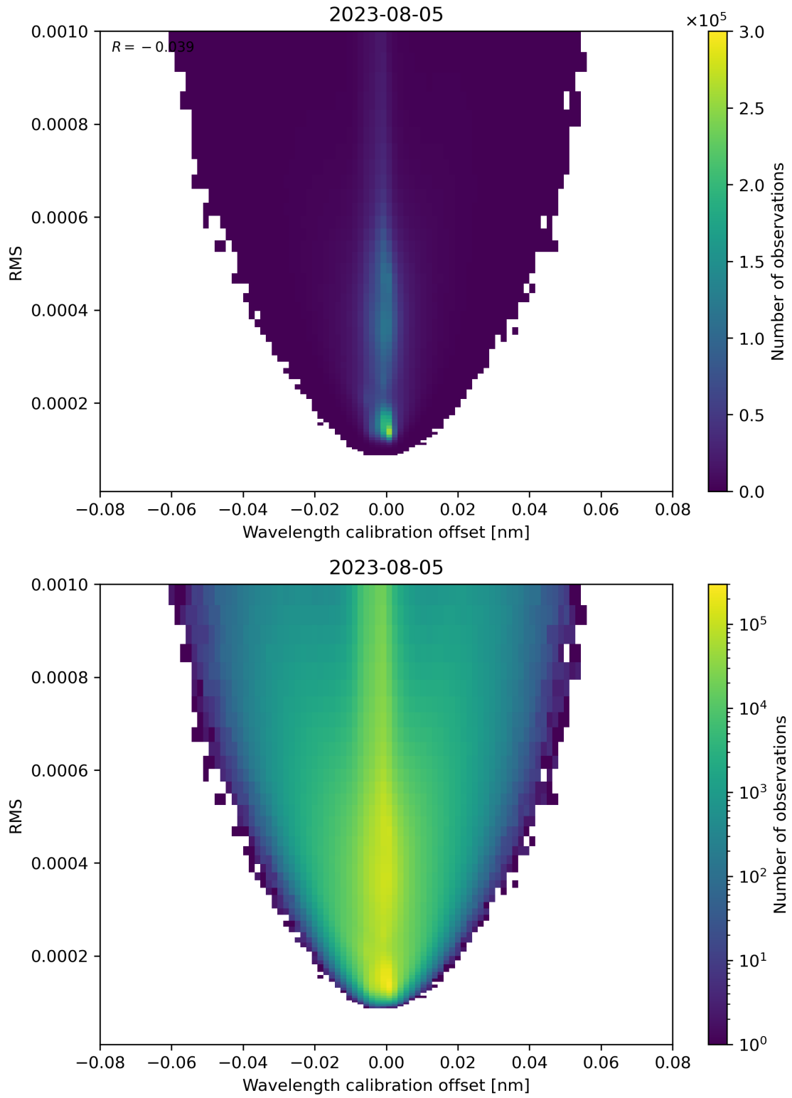
Figure 181: Scatter density plot of “Wavelength calibration offset” against “RMS” for 2023-08-04 to 2023-08-06.
