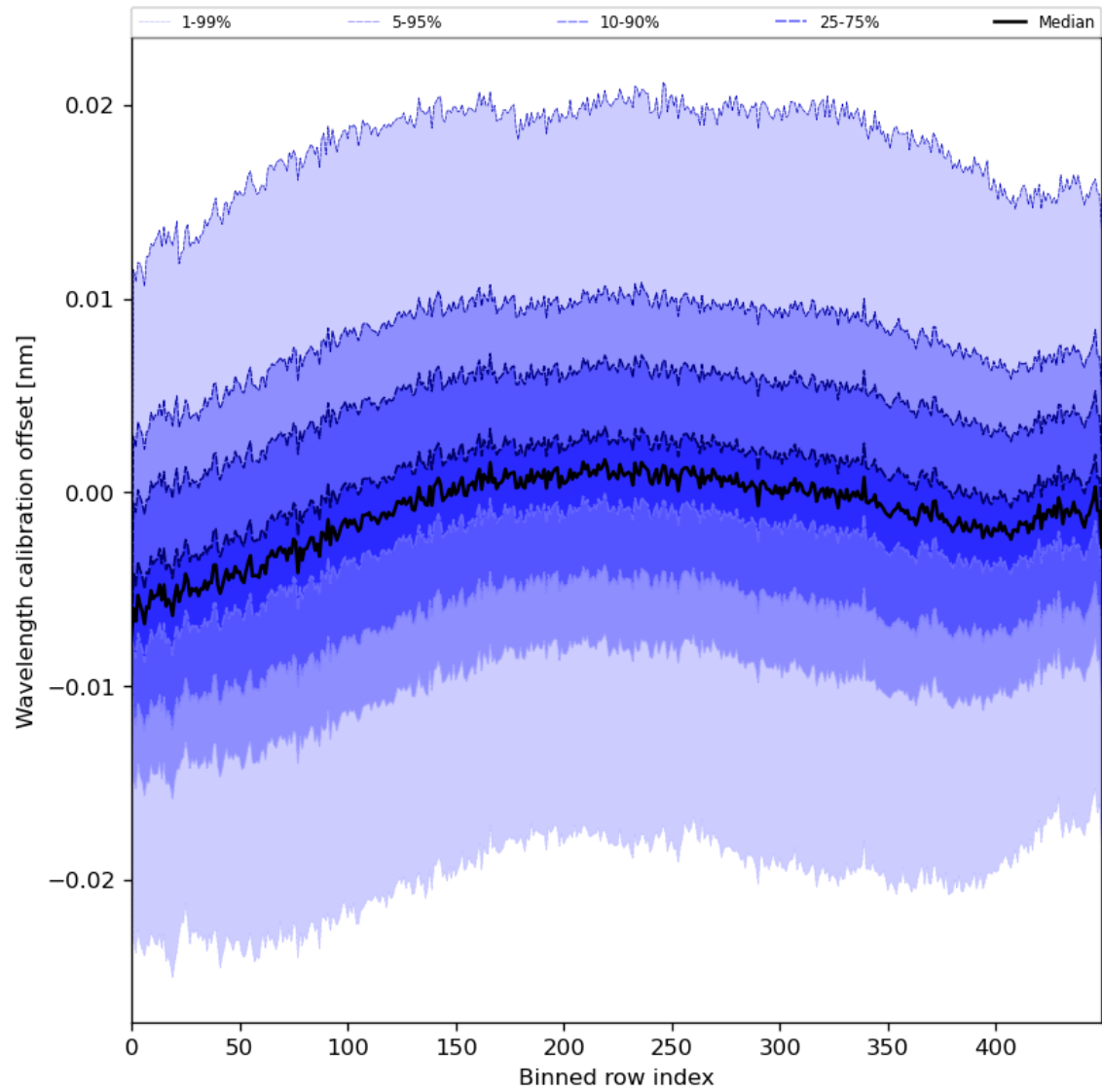
Figure 52: Along track statistics of “Wavelength calibration offset” for 2023-08-04 to 2023-08-06
