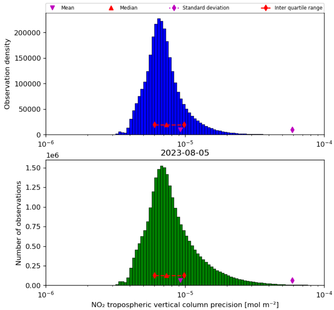
Figure 30: Histogram of “NO 2 tropospheric vertical column precision” for 2023-08-04 to 2023-08-06
