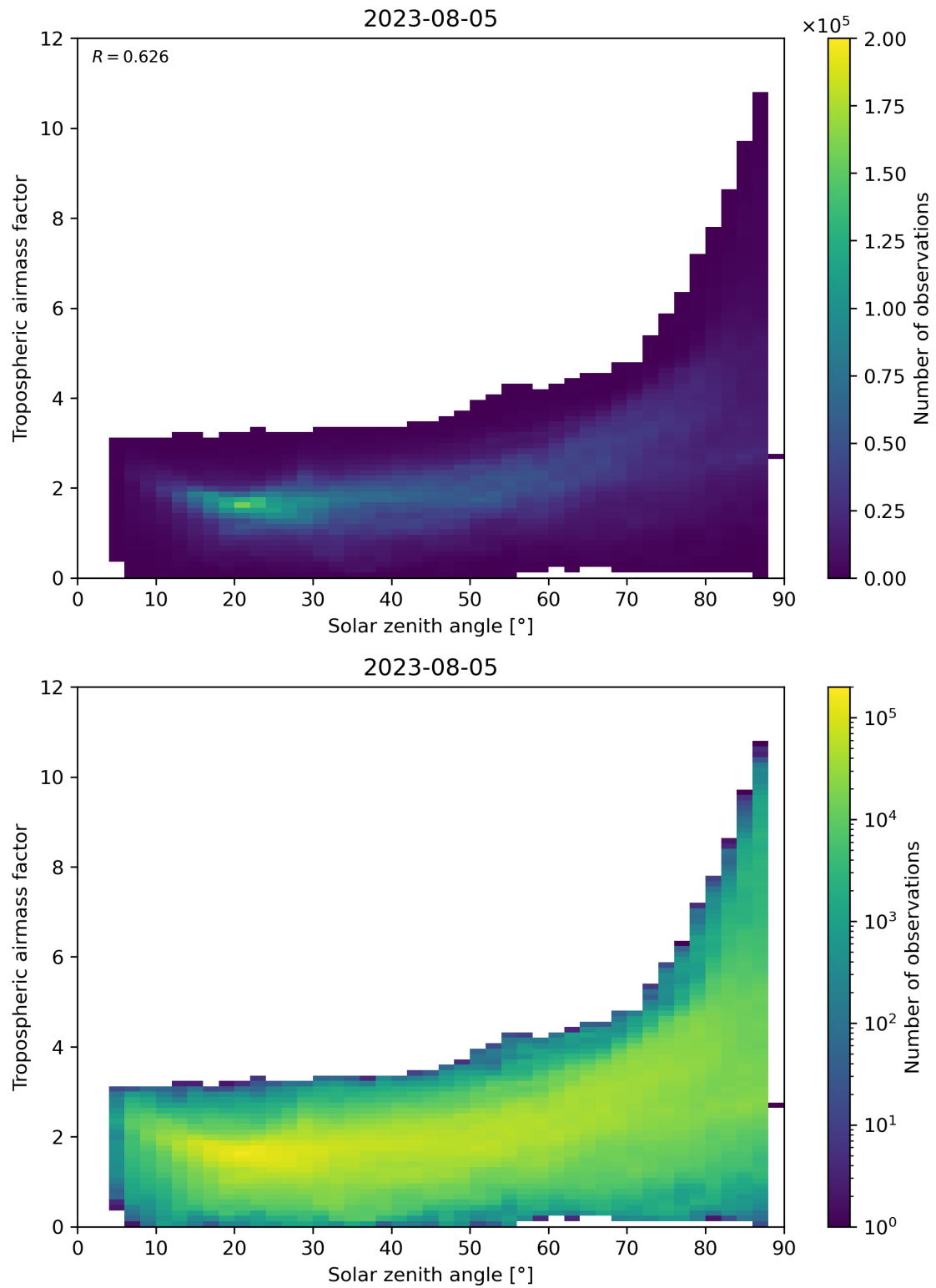
Figure 147: Scatter density plot of “Solar zenith angle” against “Tropospheric airmass factor” for 2023-08-04 to 2023-08-06.
