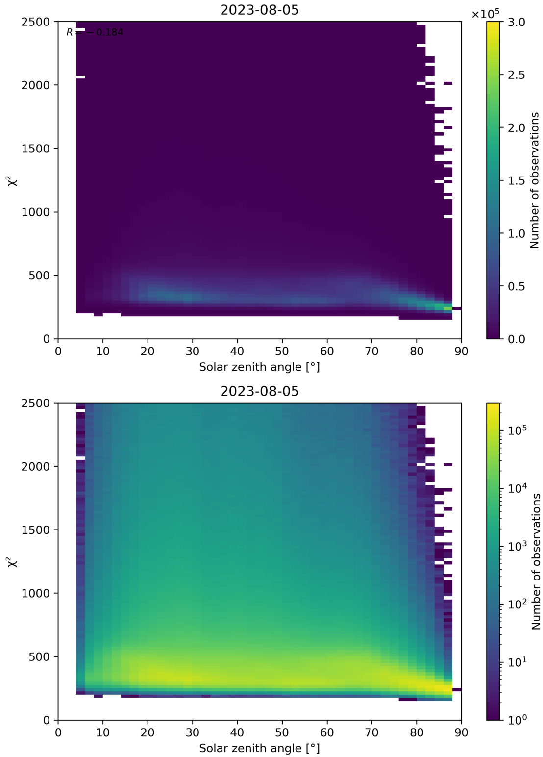
Figure 148: Scatter density plot of “Solar zenith angle” against “ \chi^2 ” for 2023-08-04 to 2023-08-06.
