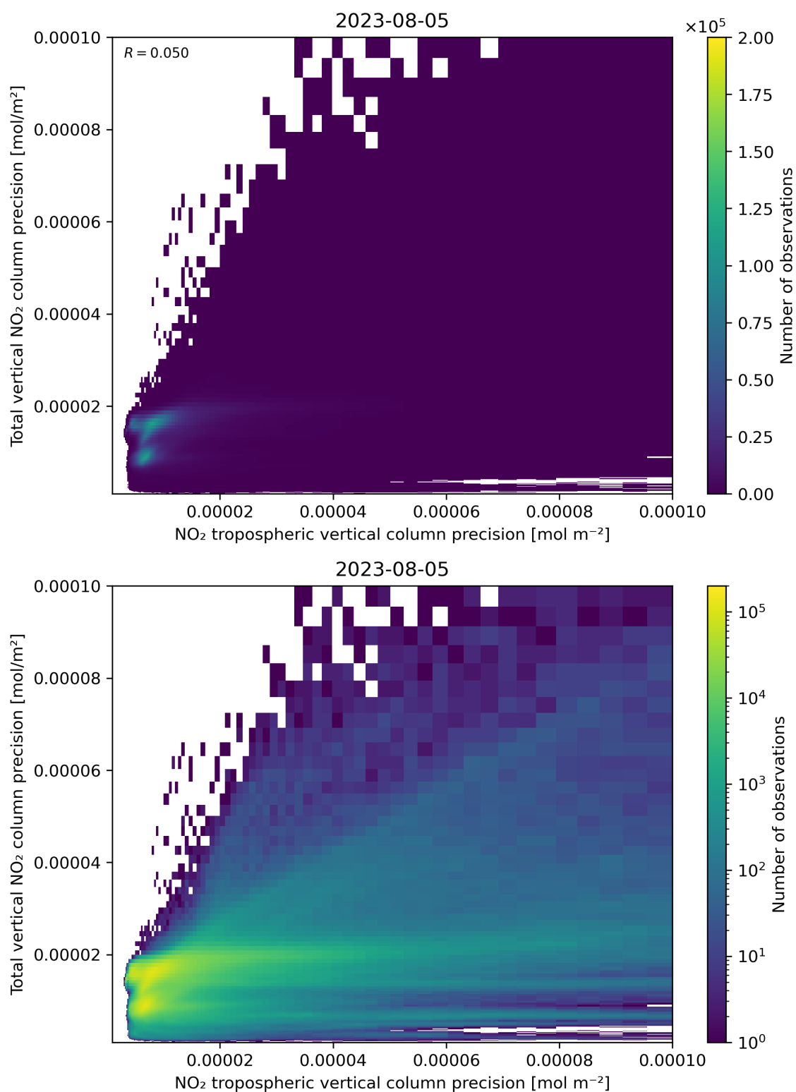
Figure 139: Scatter density plot of “NO 2 tropospheric vertical column precision” against “Total vertical NO 2 column precision” for 2023-08-04 to 2023-08-06.
