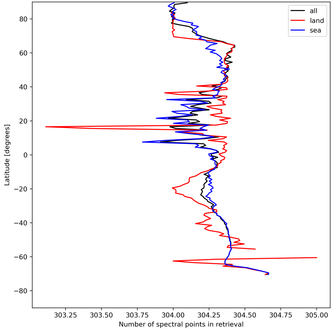
Figure 16: Zonal average of “Number of spectral points in retrieval” for 2023-08-04 to 2023-08-06.
