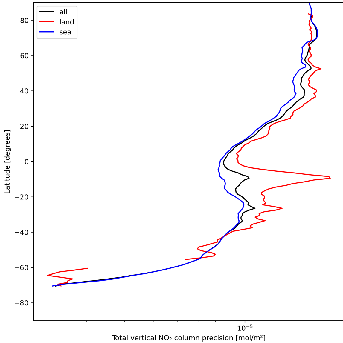
Figure 22: Zonal average of “Total vertical NO 2 column precision” for 2023-08-04 to 2023-08-06.
