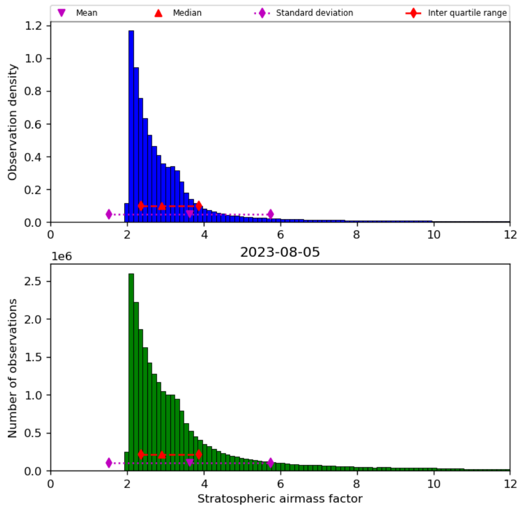
Figure 44: Histogram of “Stratospheric airmass factor” for 2023-08-04 to 2023-08-06
