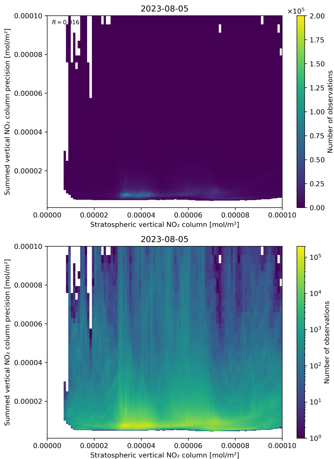
Figure 99: Scatter density plot of “Stratospheric vertical NO 2 column” against “Summed vertical NO 2 column precision” for 2023-08-04 to 2023-08-06.
