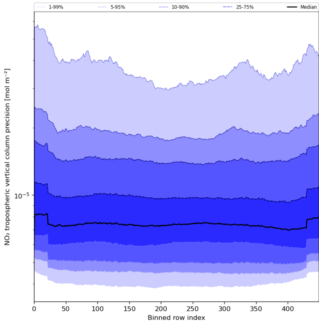
Figure 47: Along track statistics of “NO 2 tropospheric vertical column precision” for 2023-08-04 to 2023-08-06
