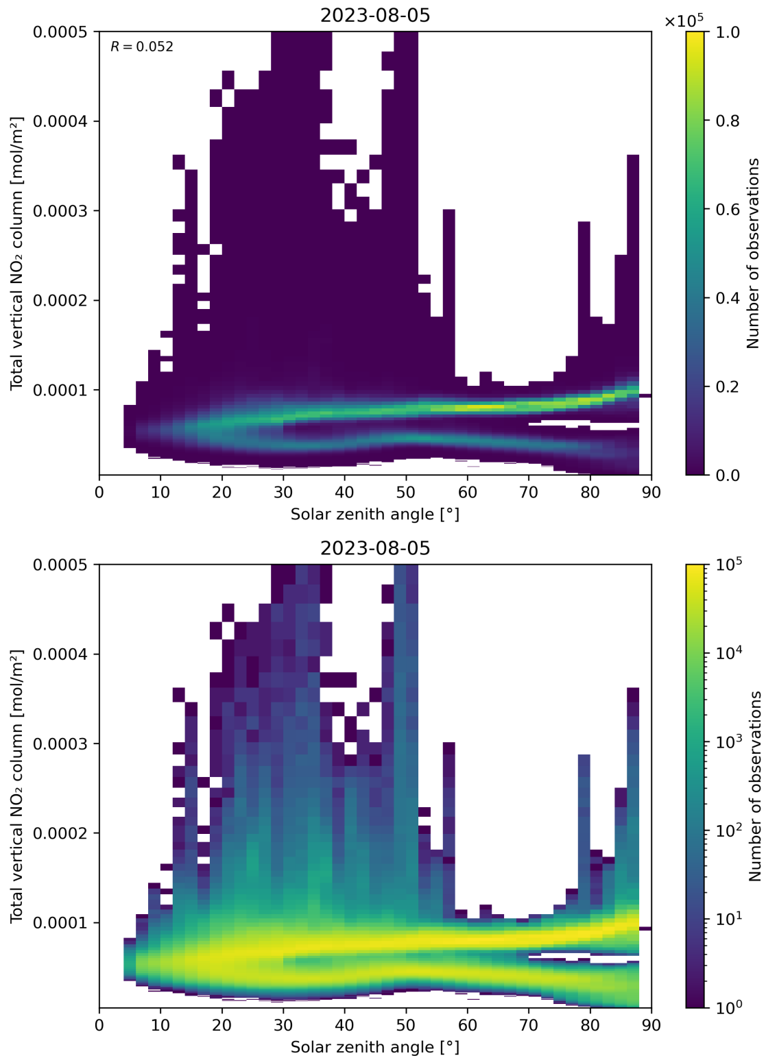
Figure 153: Scatter density plot of “Solar zenith angle” against “Total vertical NO 2 column” for 2023-08-04 to 2023-08-06.
