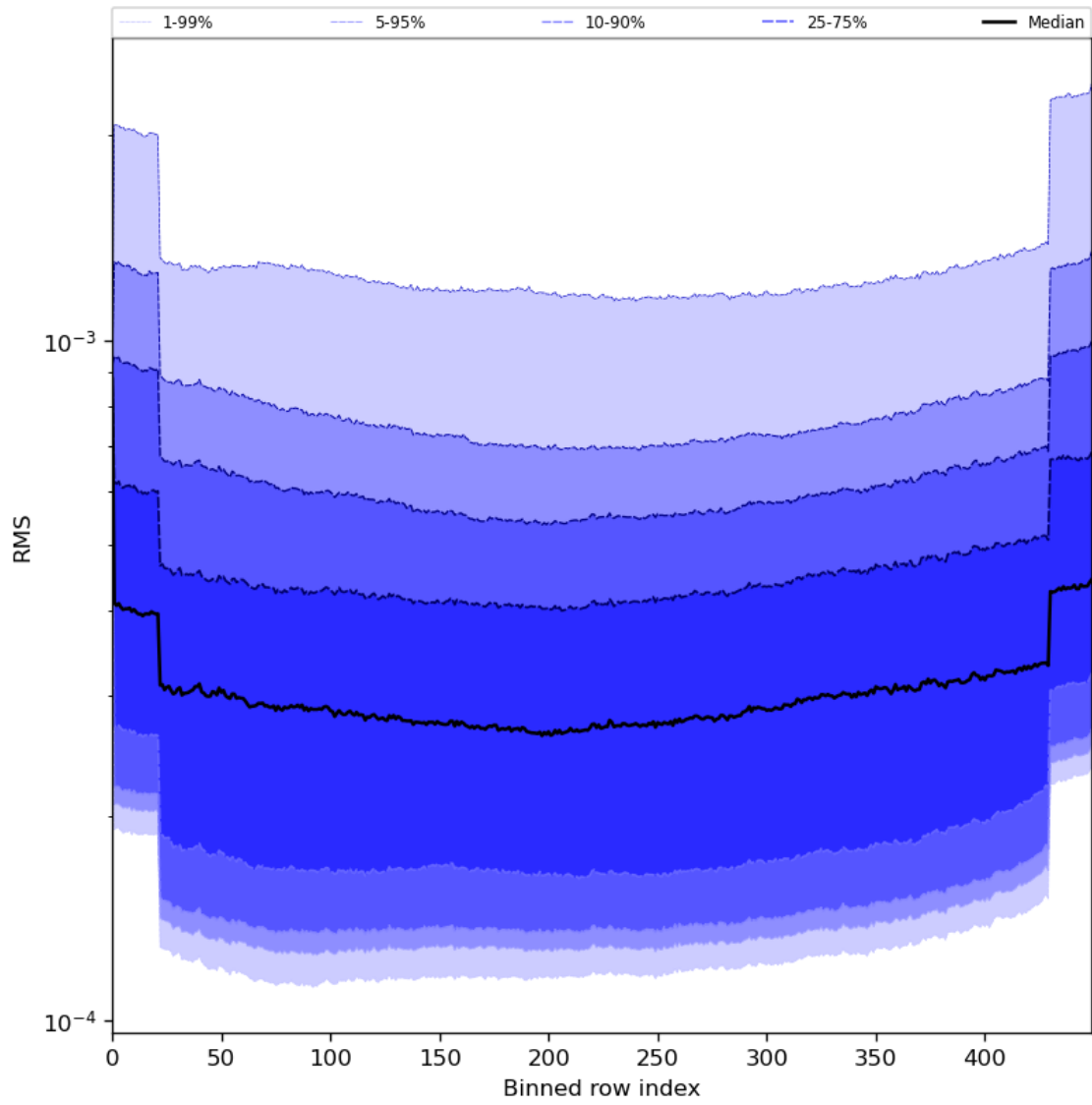
Figure 60: Along track statistics of “RMS” for 2023-08-04 to 2023-08-06
