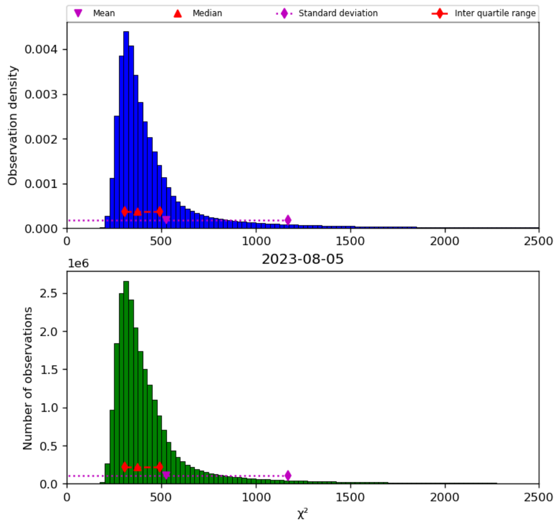
Figure 42: Histogram of “ \chi^2 ” for 2023-08-04 to 2023-08-06
