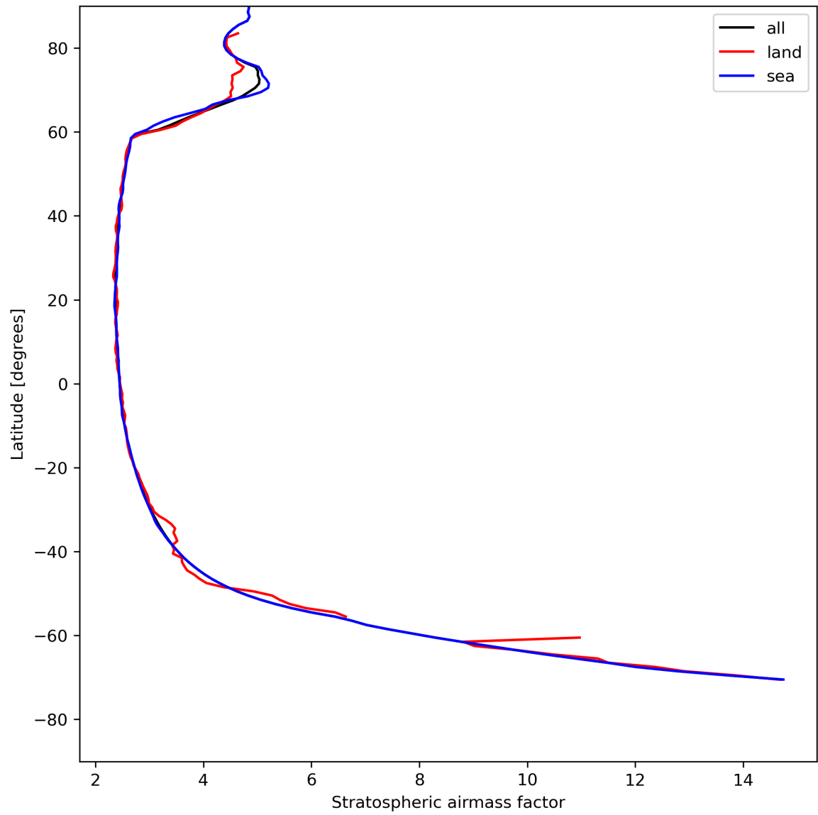
Figure 27: Zonal average of “Stratospheric air mass factor” for 2023-08-04 to 2023-08-06.
