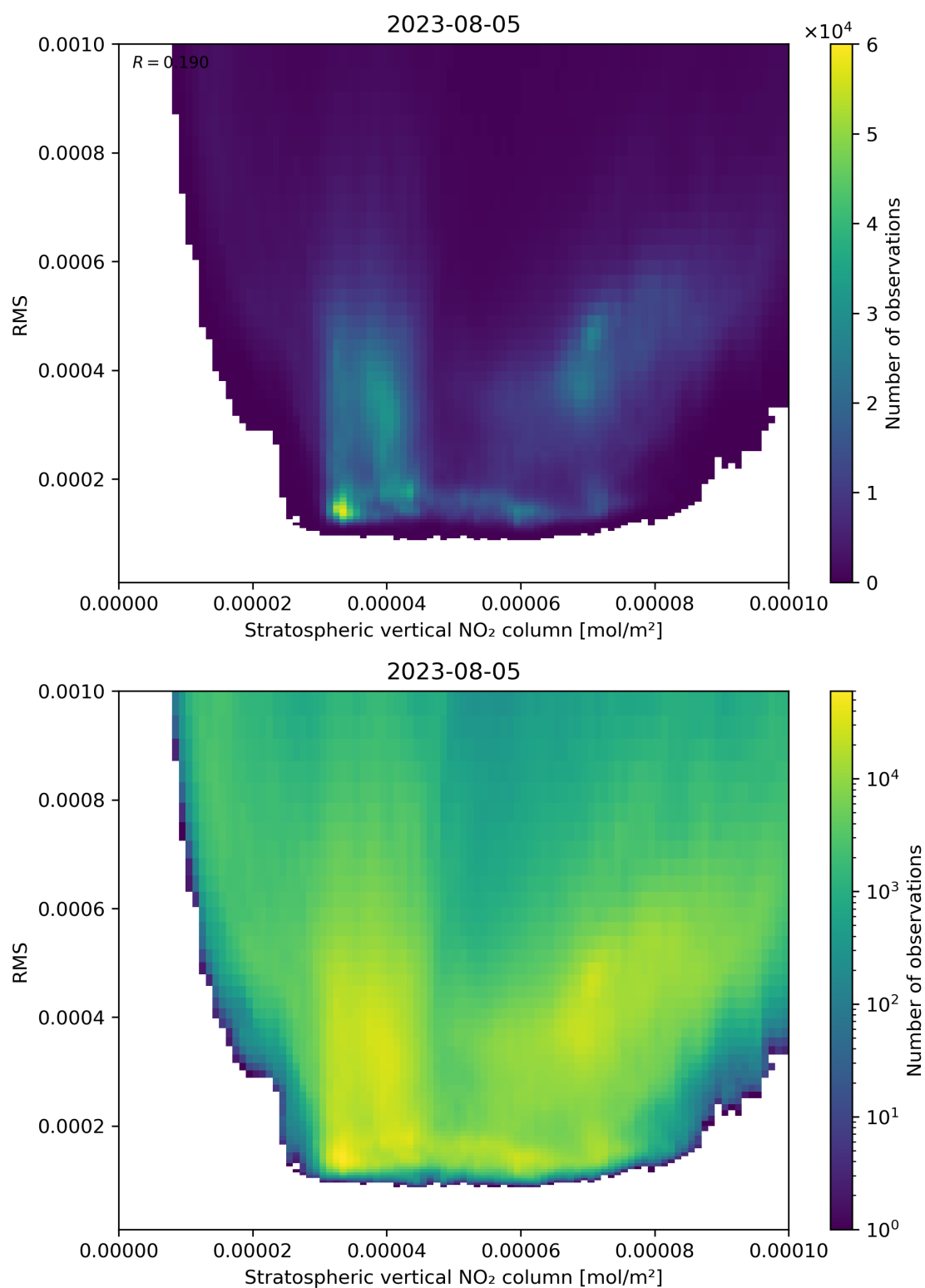
Figure 102: Scatter density plot of “Stratospheric vertical NO 2 column” against “RMS” for 2023-08-04 to 2023-08-06.
