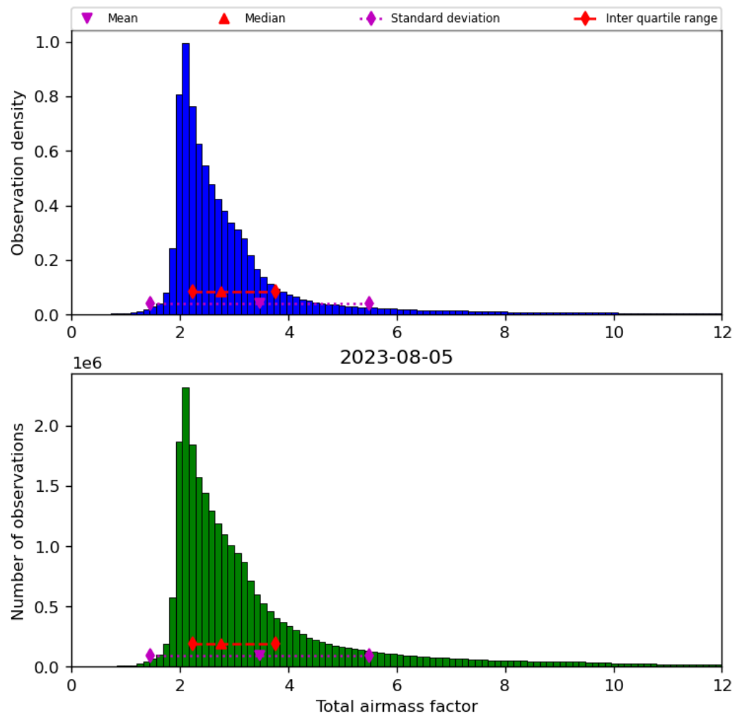
Figure 32: Histogram of “Total airmass factor” for 2023-08-04 to 2023-08-06
