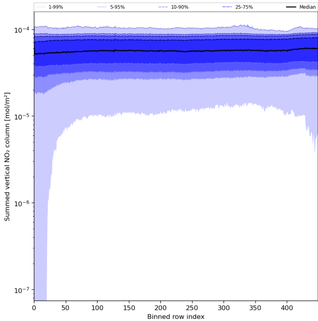
Figure 57: Along track statistics of “Summed vertical NO 2 column” for 2023-08-04 to 2023-08-06
