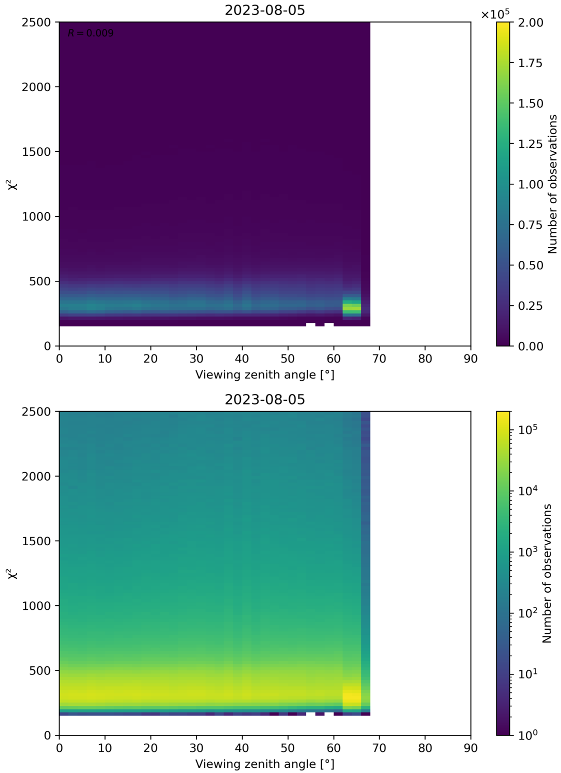
Figure 162: Scatter density plot of “Viewing zenith angle” against “ \chi^2 ” for 2023-08-04 to 2023-08-06.
