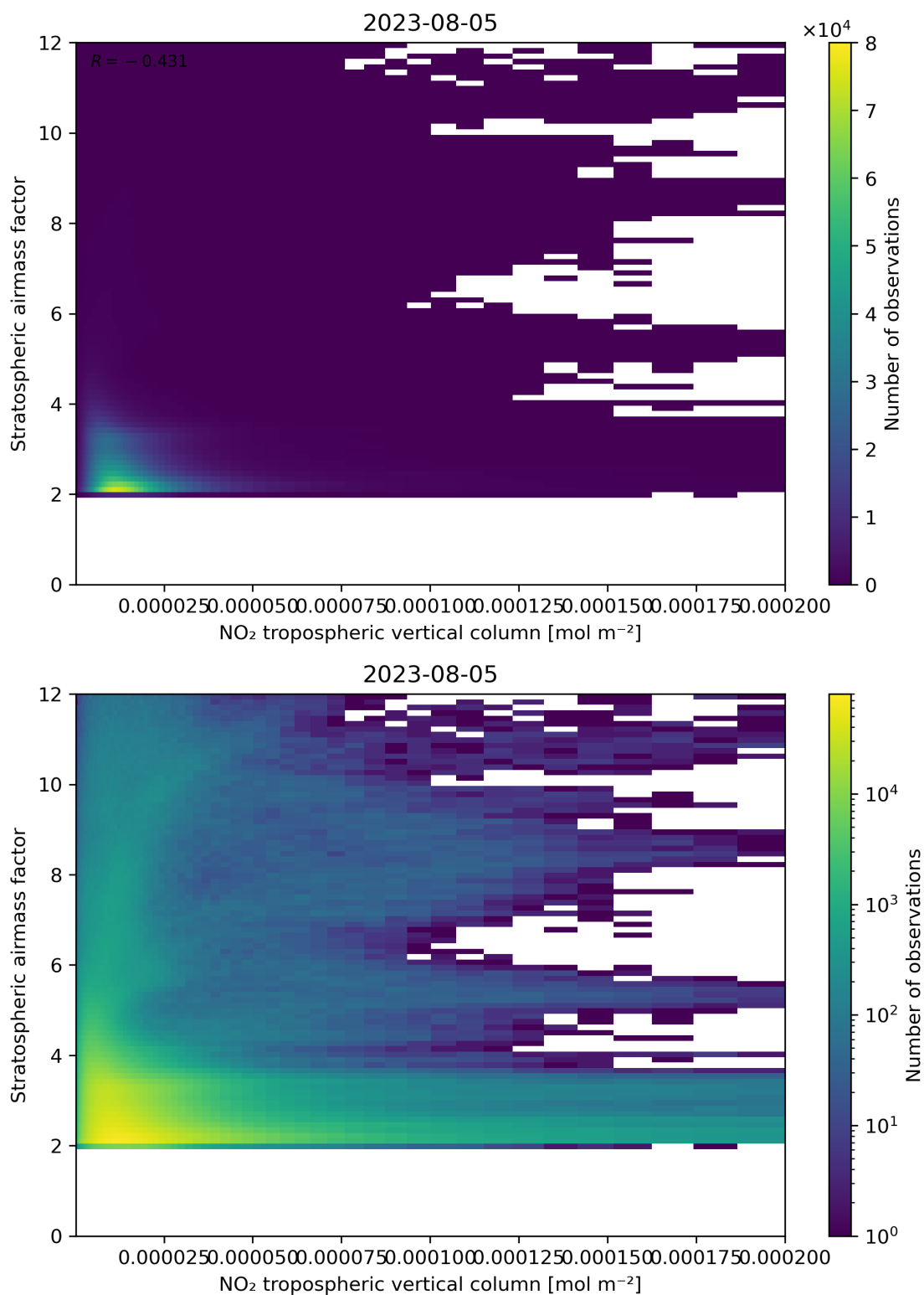
Figure 121: Scatter density plot of “NO 2 tropospheric vertical column” against “Stratospheric air mass factor” for 2023-08-04 to 2023-08-06.
