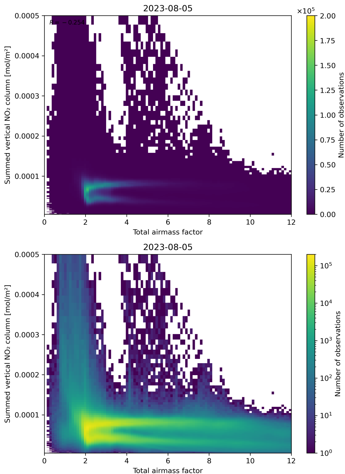
Figure 65: Scatter density plot of “Total airmass factor” against “Summed vertical NO 2 column” for 2023-08-04 to 2023-08-06.
