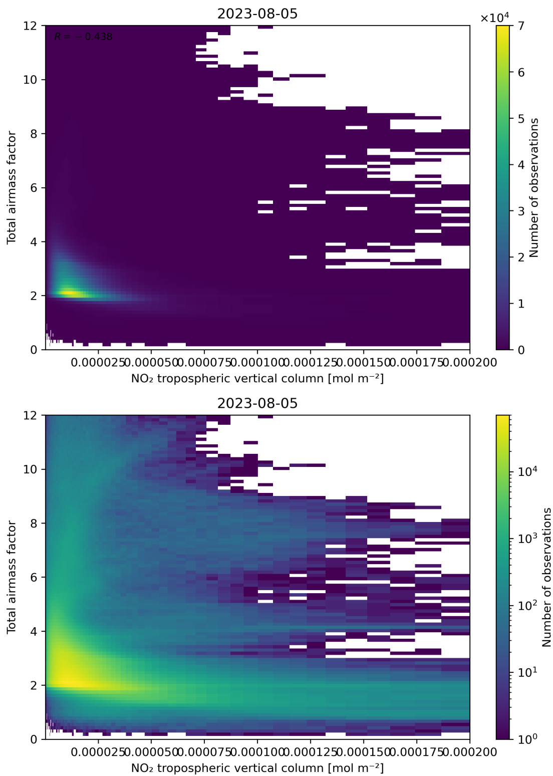
Figure 122: Scatter density plot of “NO 2 tropospheric vertical column” against “Total air mass factor” for 2023-08-04 to 2023-08-06.
