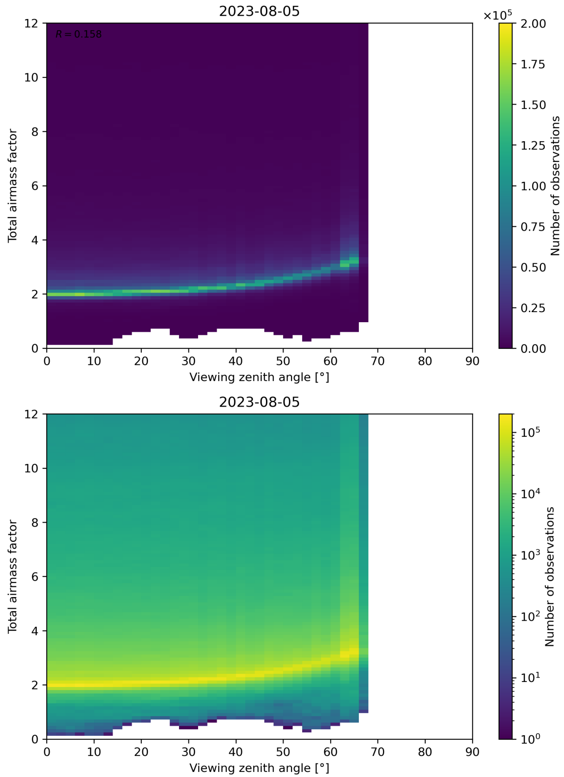
Figure 160: Scatter density plot of “Viewing zenith angle” against “Total airmass factor” for 2023-08-04 to 2023-08-06.
