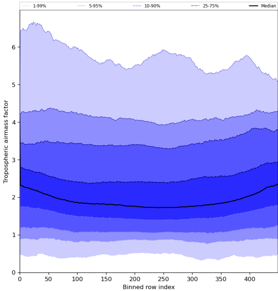
Figure 48: Along track statistics of “Tropospheric airmass factor” for 2023-08-04 to 2023-08-06
