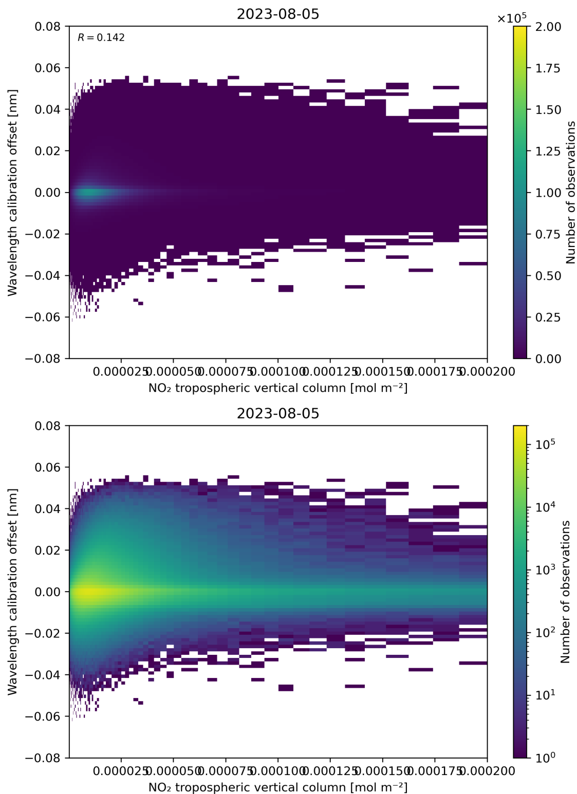
Figure 143: Scatter density plot of “NO 2 tropospheric vertical column” against “Wavelength calibration offset” for 2023-08-04 to 2023-08-06.
