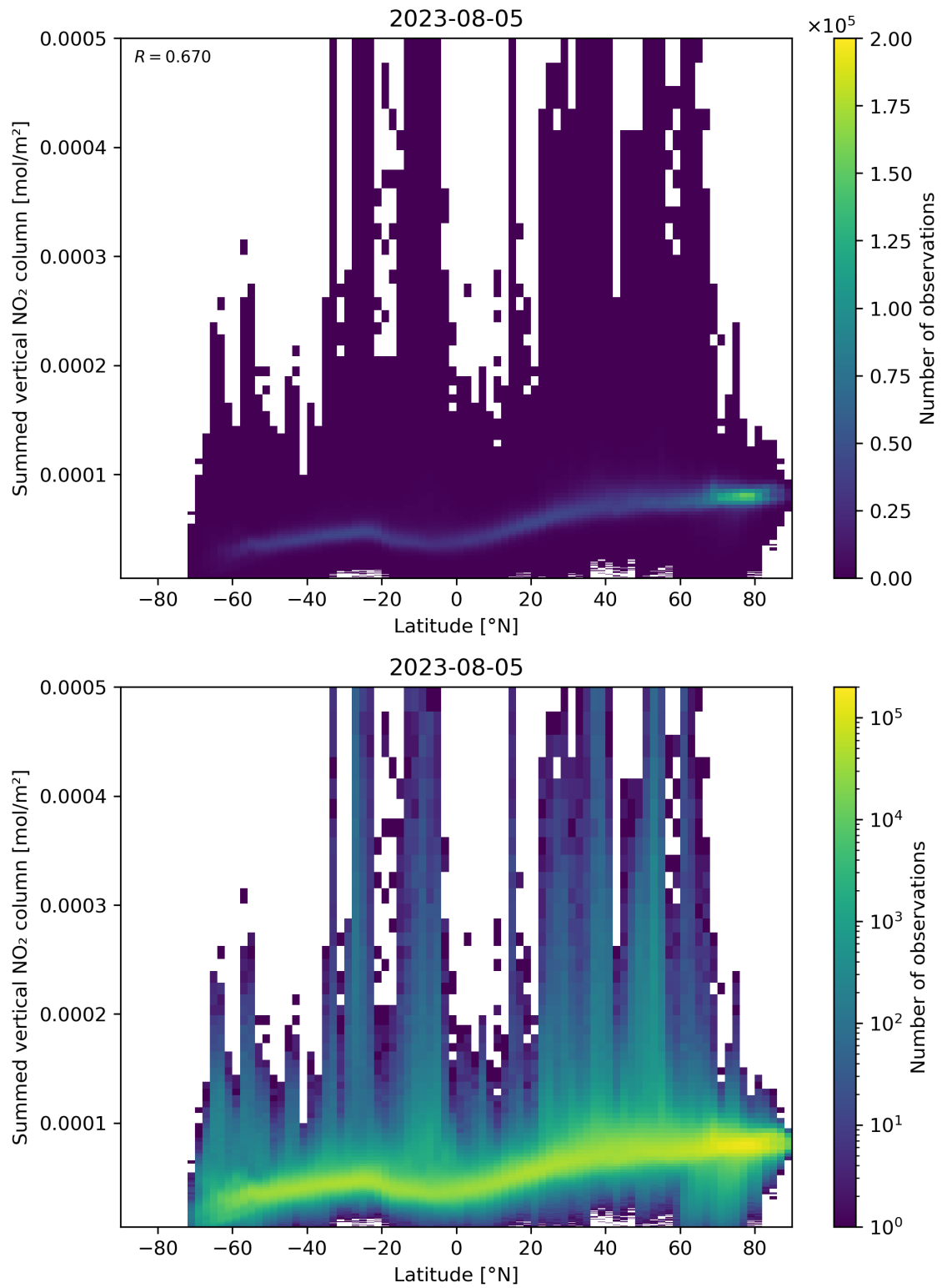
Figure 88: Scatter density plot of “Latitude” against “Summed vertical NO 2 column” for 2023-08-04 to 2023-08-06.
