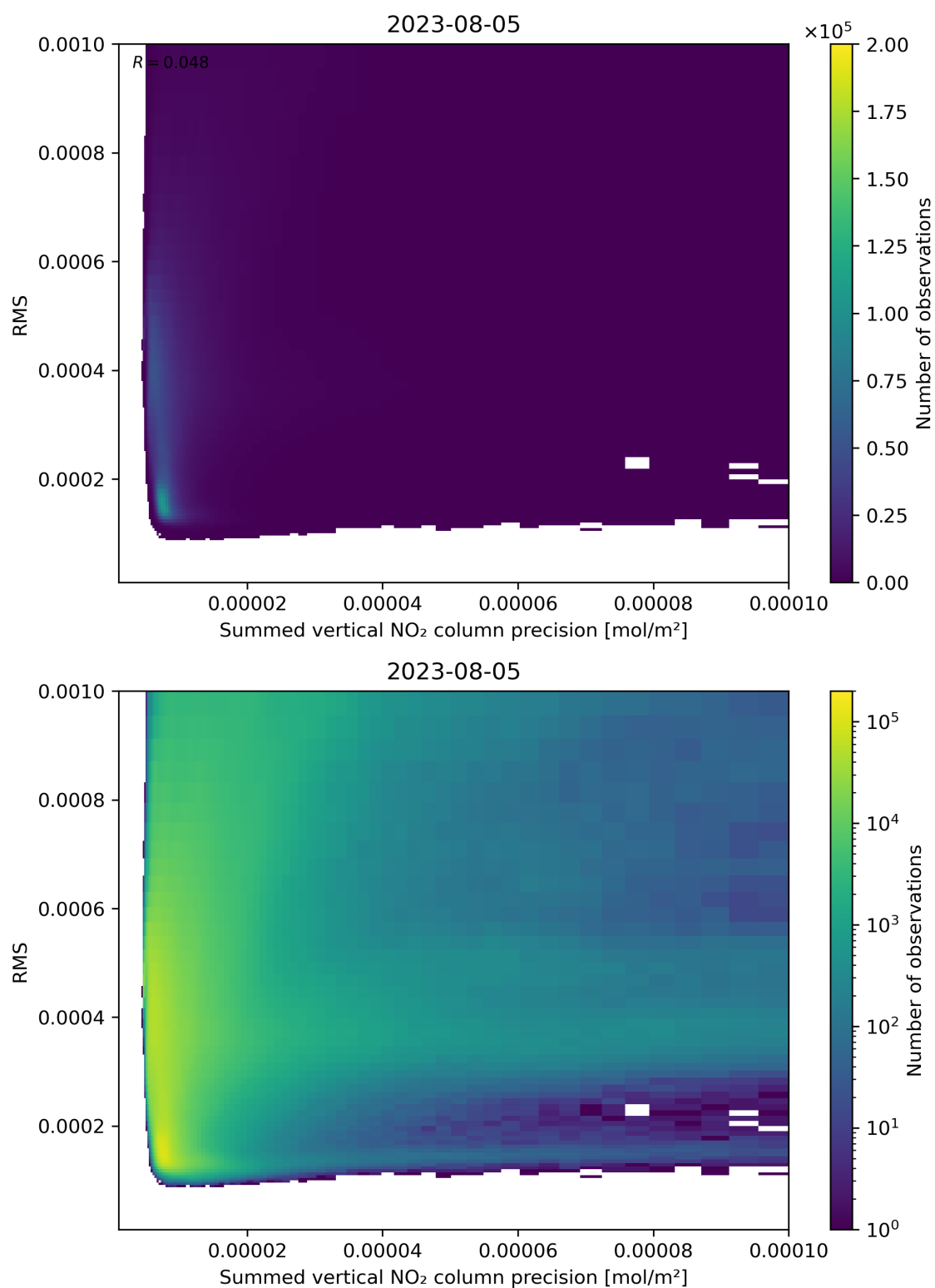
Figure 108: Scatter density plot of “Summed vertical NO 2 column precision” against “RMS” for 2023-08-04 to 2023-08-06.
