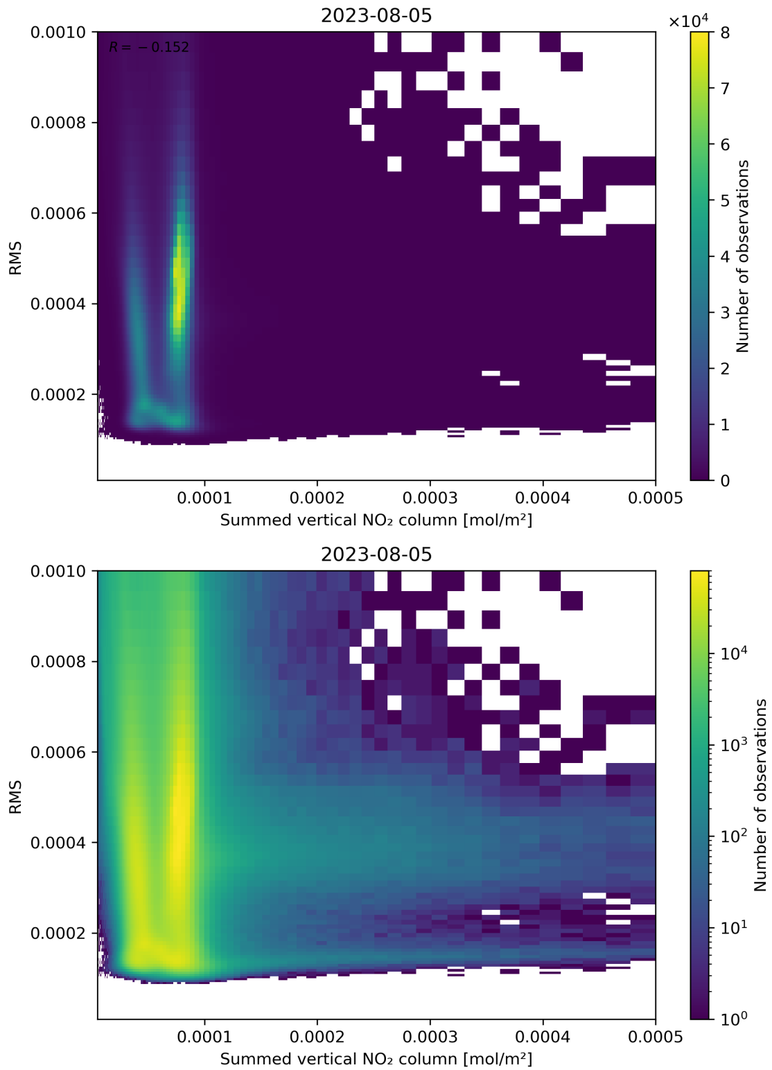
Figure 109: Scatter density plot of “Summed vertical NO 2 column” against “RMS” for 2023-08-04 to 2023-08-06.
