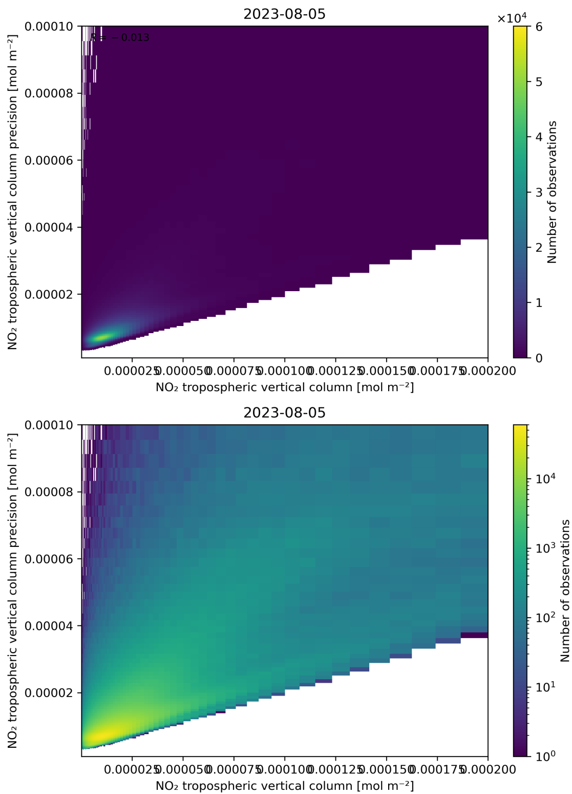
Figure 130: Scatter density plot of “NO 2 tropospheric vertical column” against “NO 2 tropospheric vertical column precision” for 2023-08-04 to 2023-08-06.
