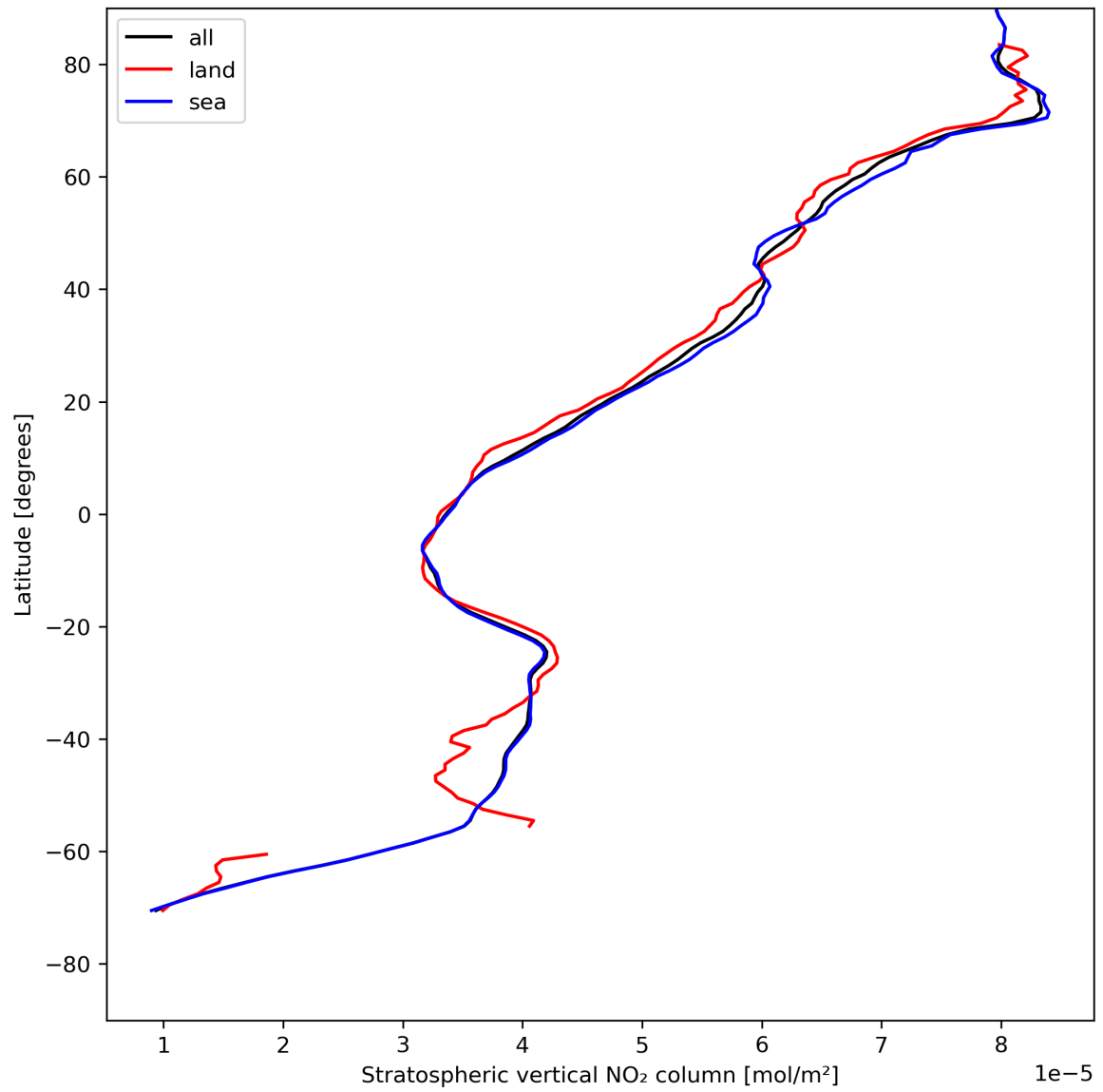
Figure 19: Zonal average of “Stratospheric vertical NO 2 column” for 2023-08-04 to 2023-08-06.
