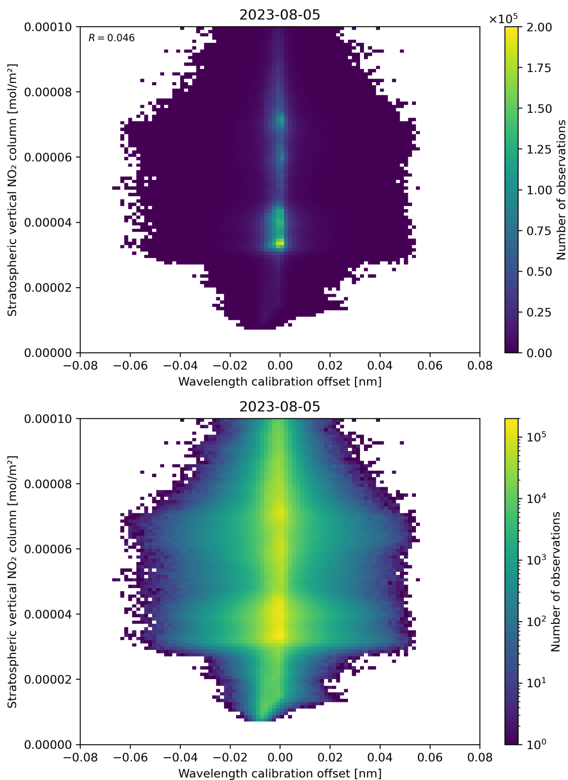
Figure 176: Scatter density plot of “Wavelength calibration offset” against “Stratospheric vertical NO 2 column” for 2023-08-04 to 2023-08-06.
