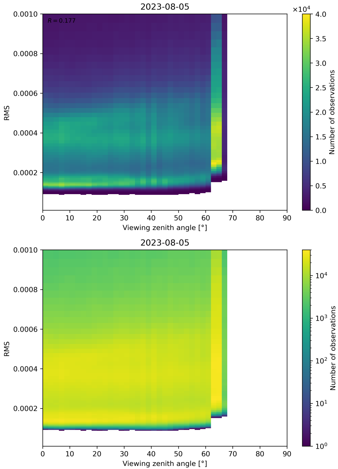
Figure 171: Scatter density plot of “Viewing zenith angle” against “RMS” for 2023-08-04 to 2023-08-06.
