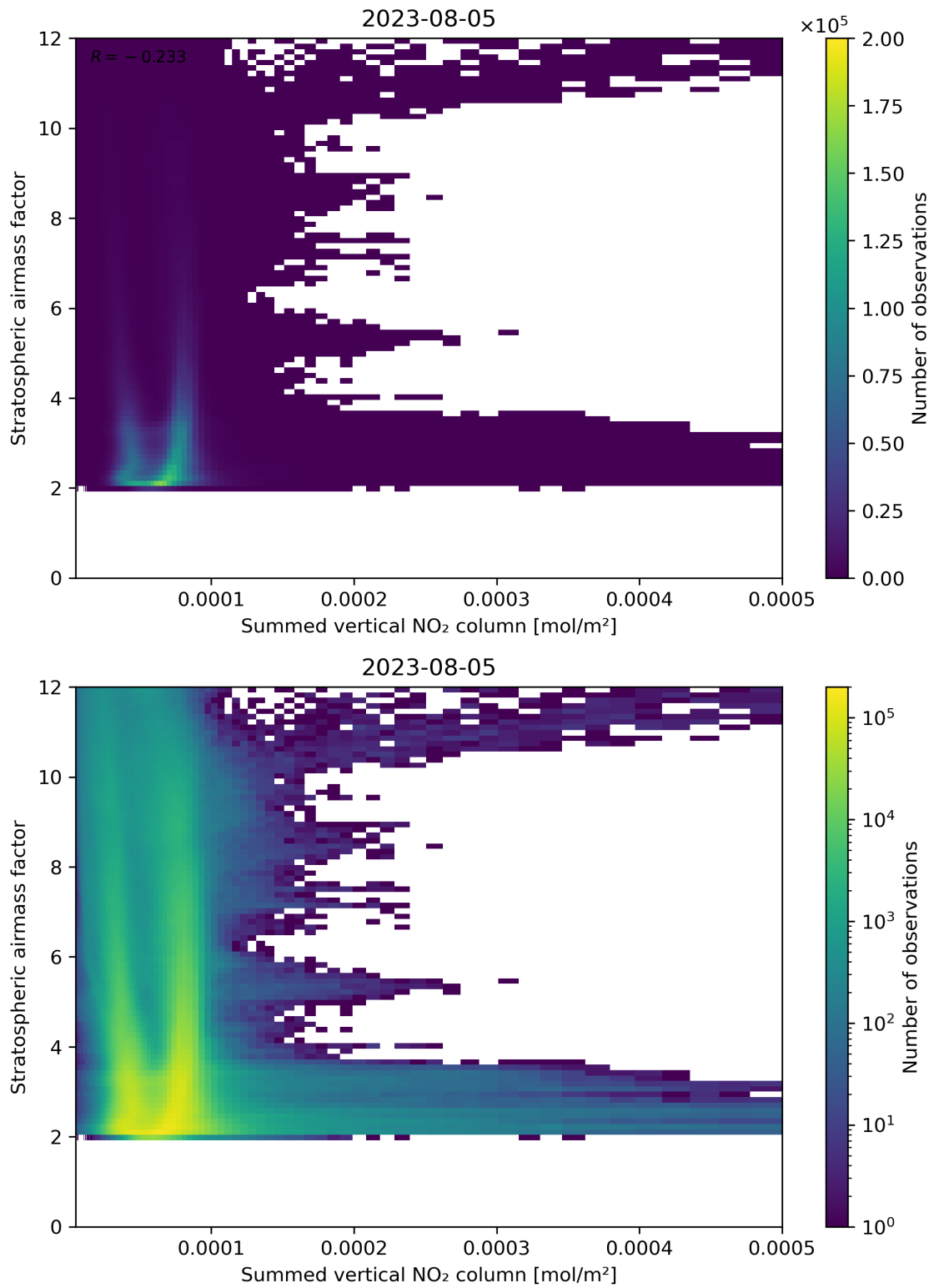
Figure 103: Scatter density plot of “Summed vertical NO 2 column” against “Stratospheric air mass factor” for 2023-08-04 to 2023-08-06.
