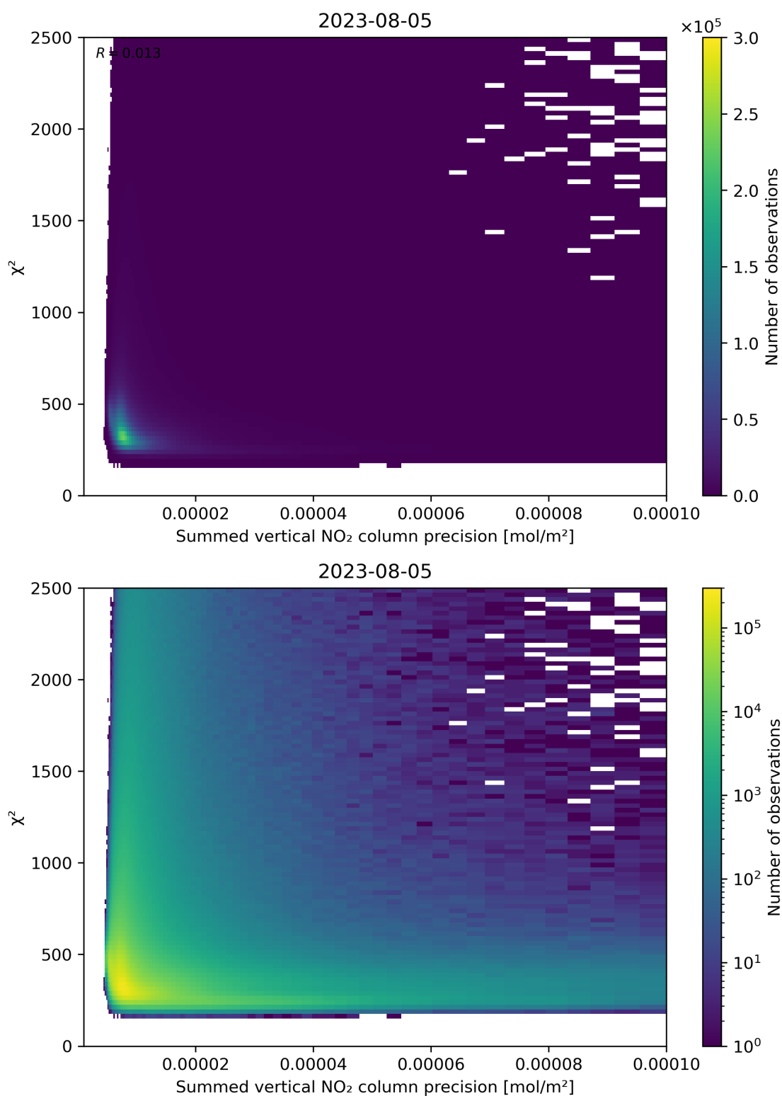
Figure 107: Scatter density plot of “Summed vertical NO 2 column precision” against “ \chi^2 ” for 2023-08-04 to 2023-08-06.
