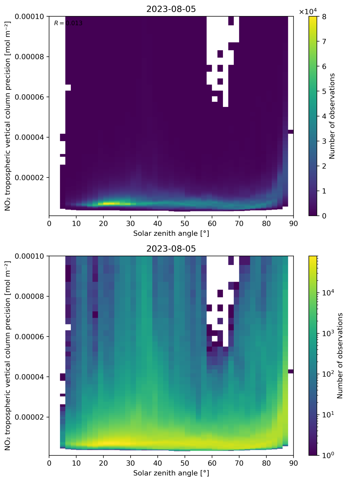
Figure 156: Scatter density plot of “Solar zenith angle” against “NO 2 tropospheric vertical column precision” for 2023-08-04 to 2023-08-06.
