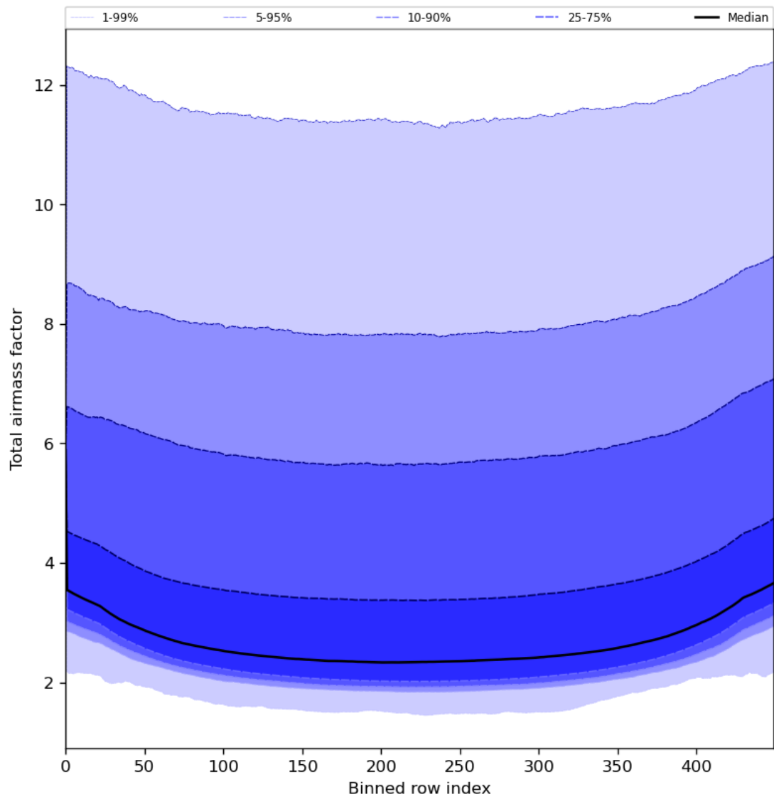
Figure 49: Along track statistics of “Total airmass factor” for 2023-08-04 to 2023-08-06
