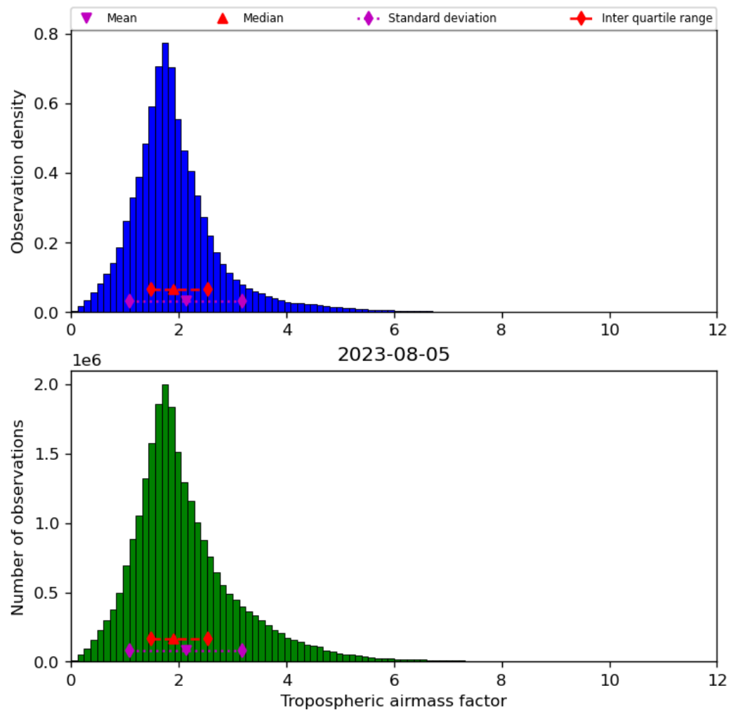
Figure 31: Histogram of “Tropospheric airmass factor” for 2023-08-04 to 2023-08-06
