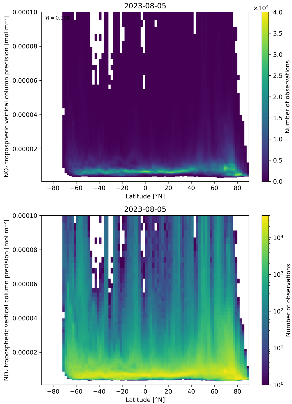
Figure 93: Scatter density plot of “Latitude” against “NO 2 tropospheric vertical column precision” for 2023-08-04 to 2023-08-06.
