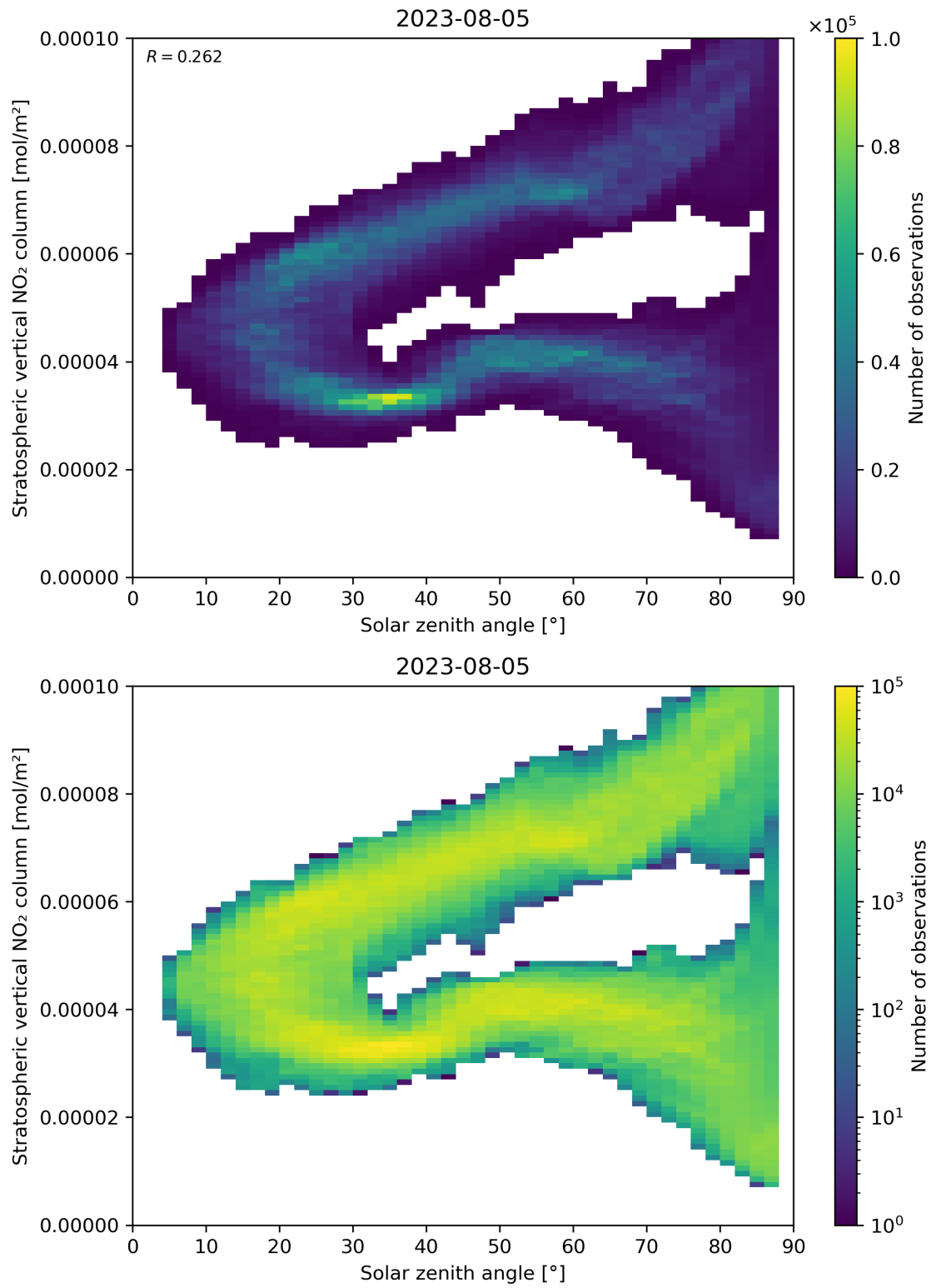
Figure 150: Scatter density plot of “Solar zenith angle” against “Stratospheric vertical NO 2 column” for 2023-08-04 to 2023-08-06.
