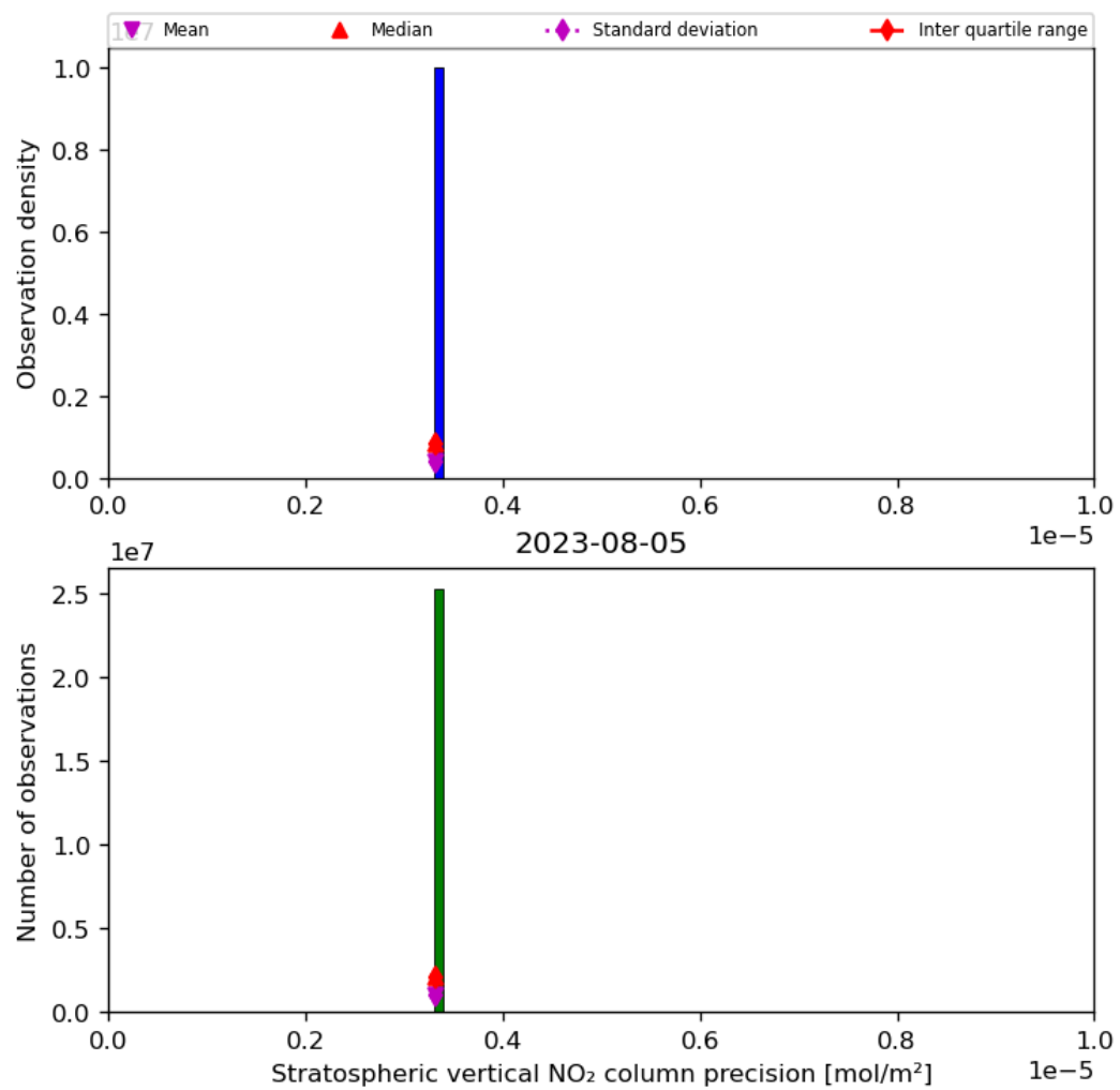
Figure 37: Histogram of “Stratospheric vertical NO 2 column precision” for 2023-08-04 to 2023-08-06
