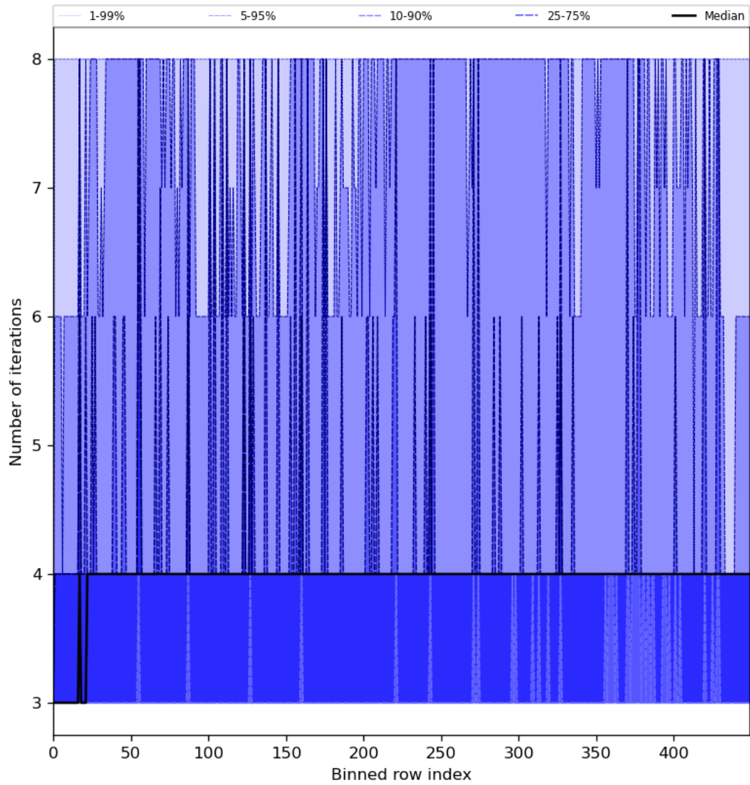
Figure 51: Along track statistics of “Number of iterations” for 2023-08-04 to 2023-08-06
