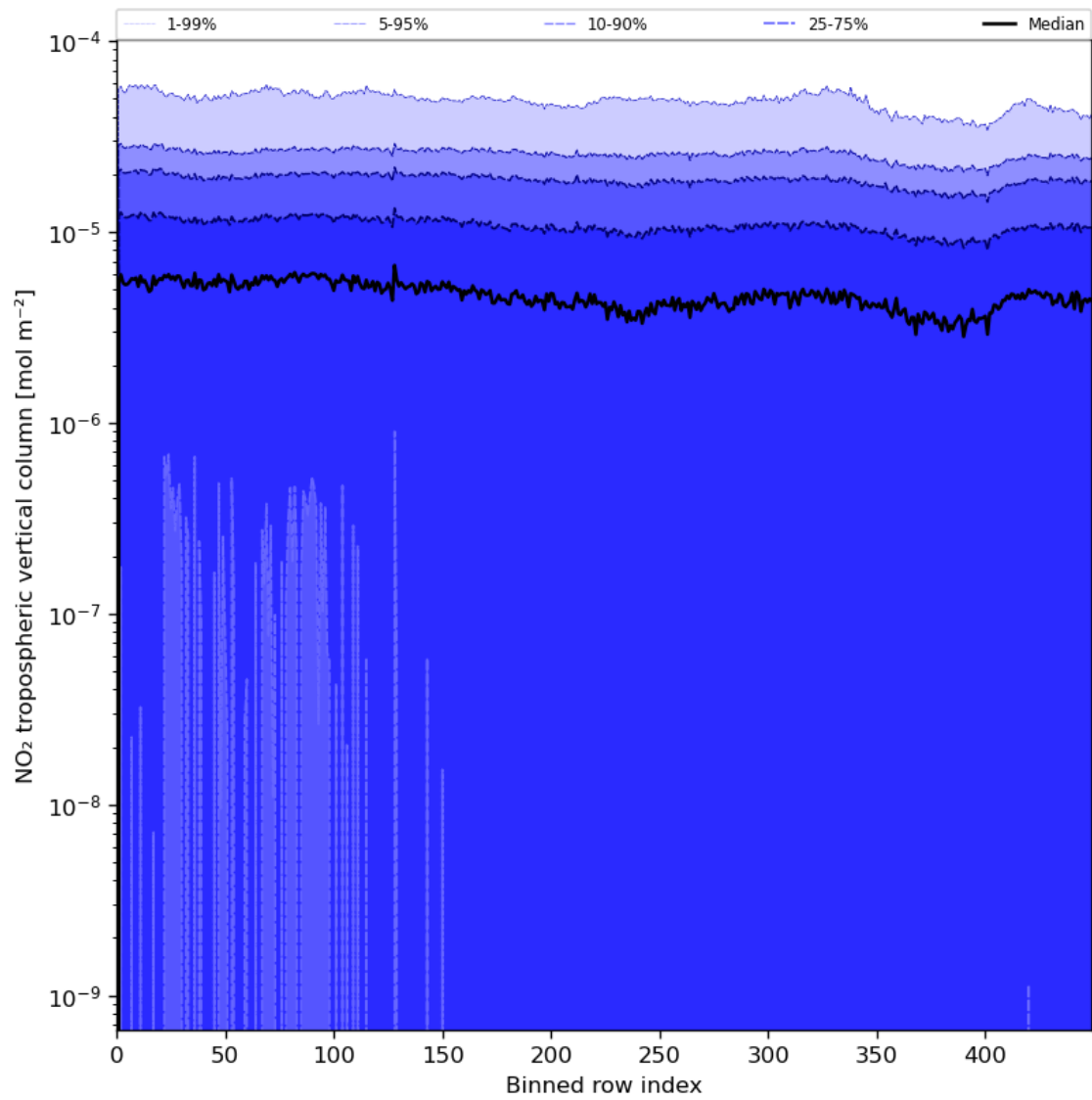
Figure 46: Along track statistics of “ \text{NO}_2 tropospheric vertical column” for 2023-08-04 to 2023-08-06
