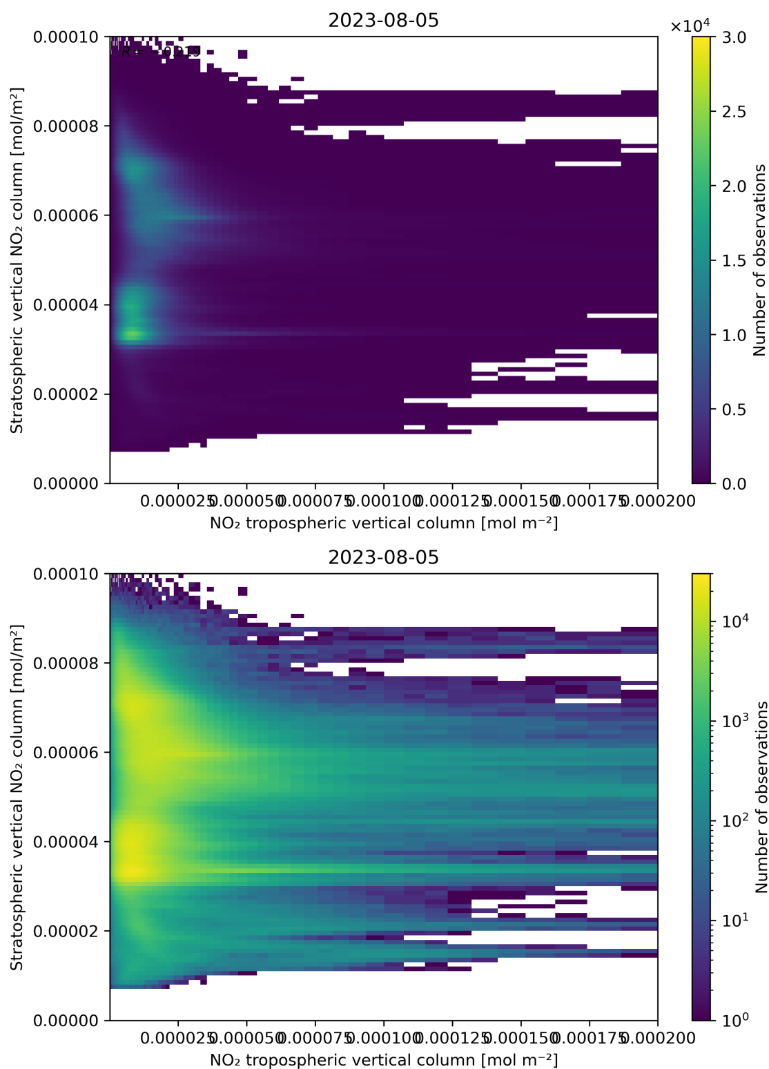
Figure 125: Scatter density plot of “NO 2 tropospheric vertical column” against “Stratospheric vertical NO 2 column” for 2023-08-04 to 2023-08-06.
