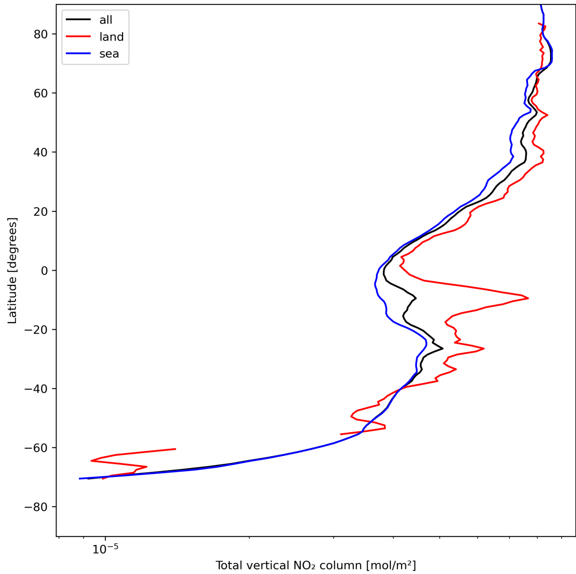
Figure 21: Zonal average of “Total vertical NO 2 column” for 2023-08-04 to 2023-08-06.
