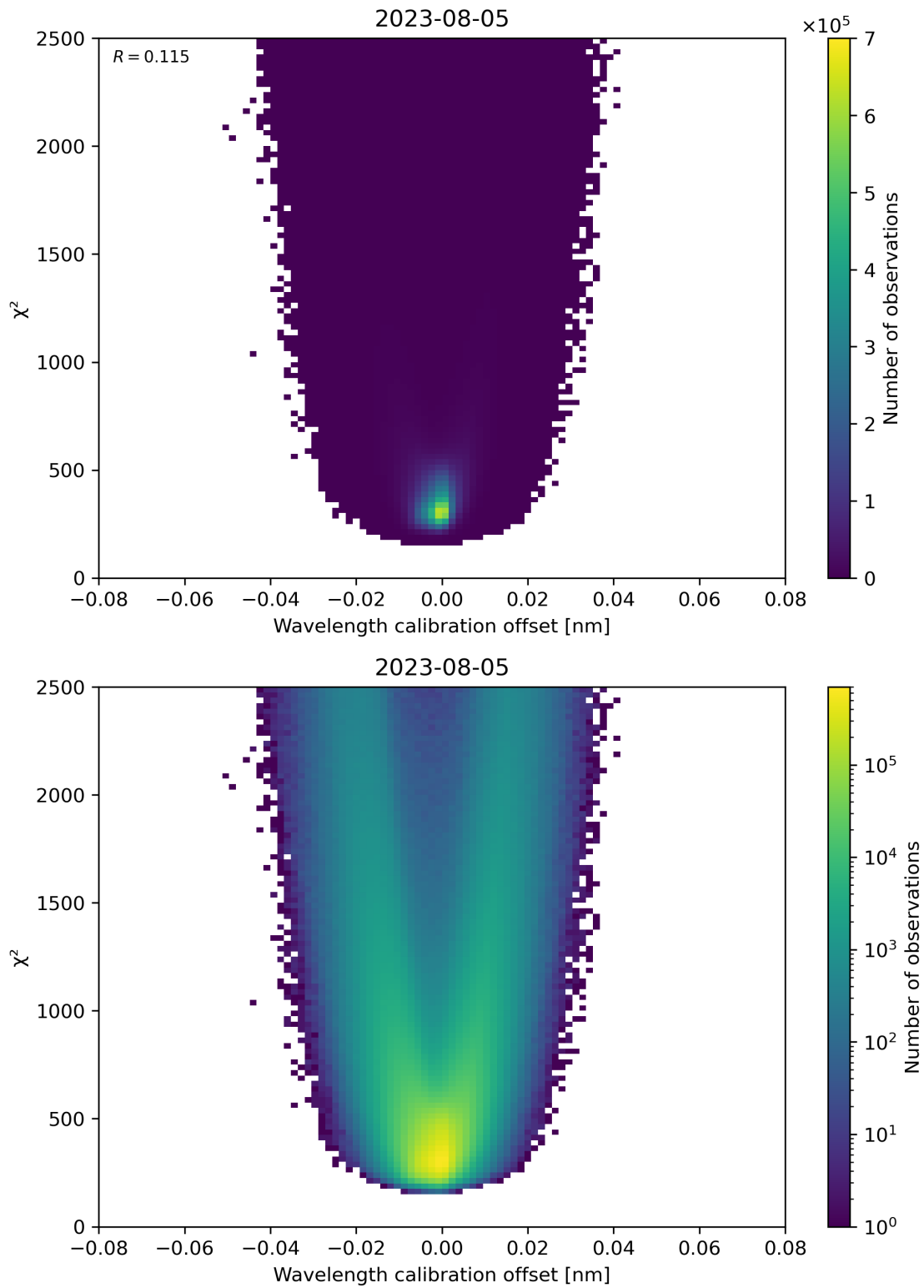
Figure 175: Scatter density plot of “Wavelength calibration offset” against “ \chi^2 ” for 2023-08-04 to 2023-08-06.
