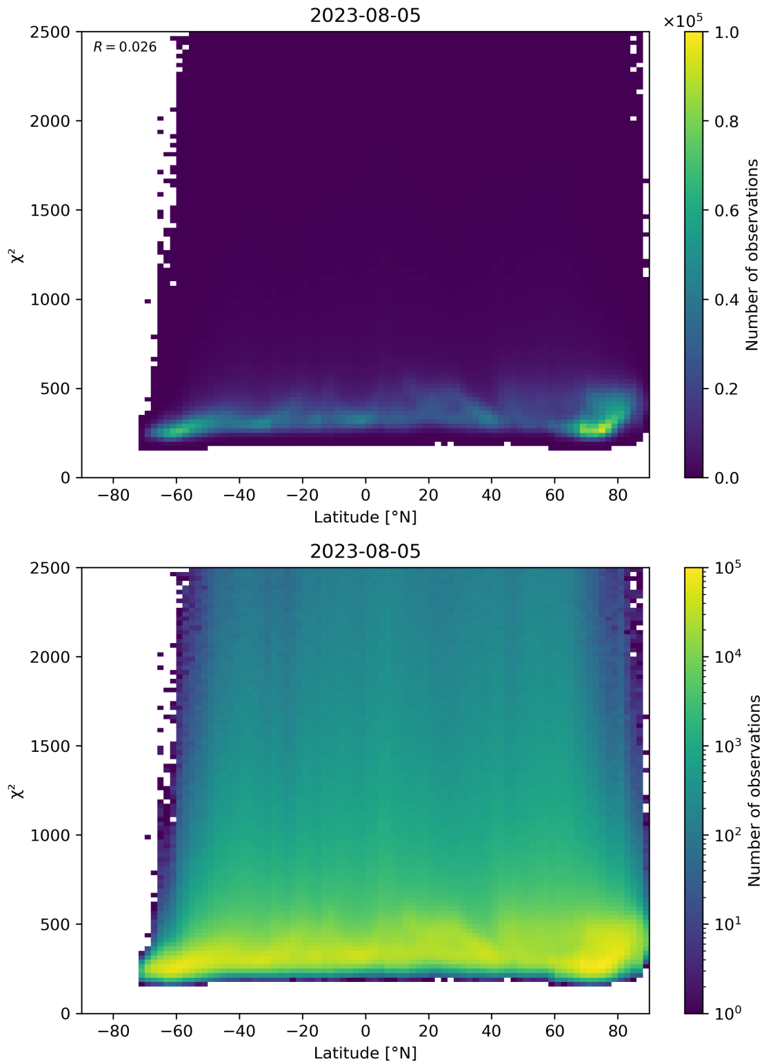
Figure 86: Scatter density plot of “Latitude” against “ \chi^2 ” for 2023-08-04 to 2023-08-06.
