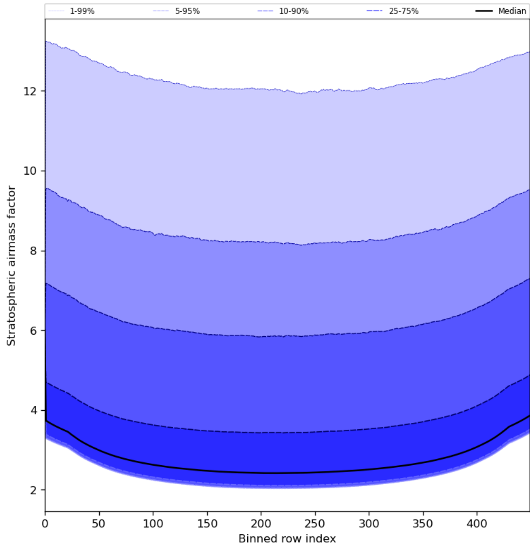
Figure 61: Along track statistics of “Stratospheric airmass factor” for 2023-08-04 to 2023-08-06
