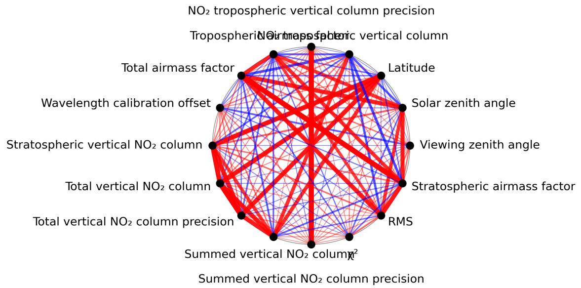
Figure 1: Map of correlation graph for 2023-08-04 to 2023-08-06.
