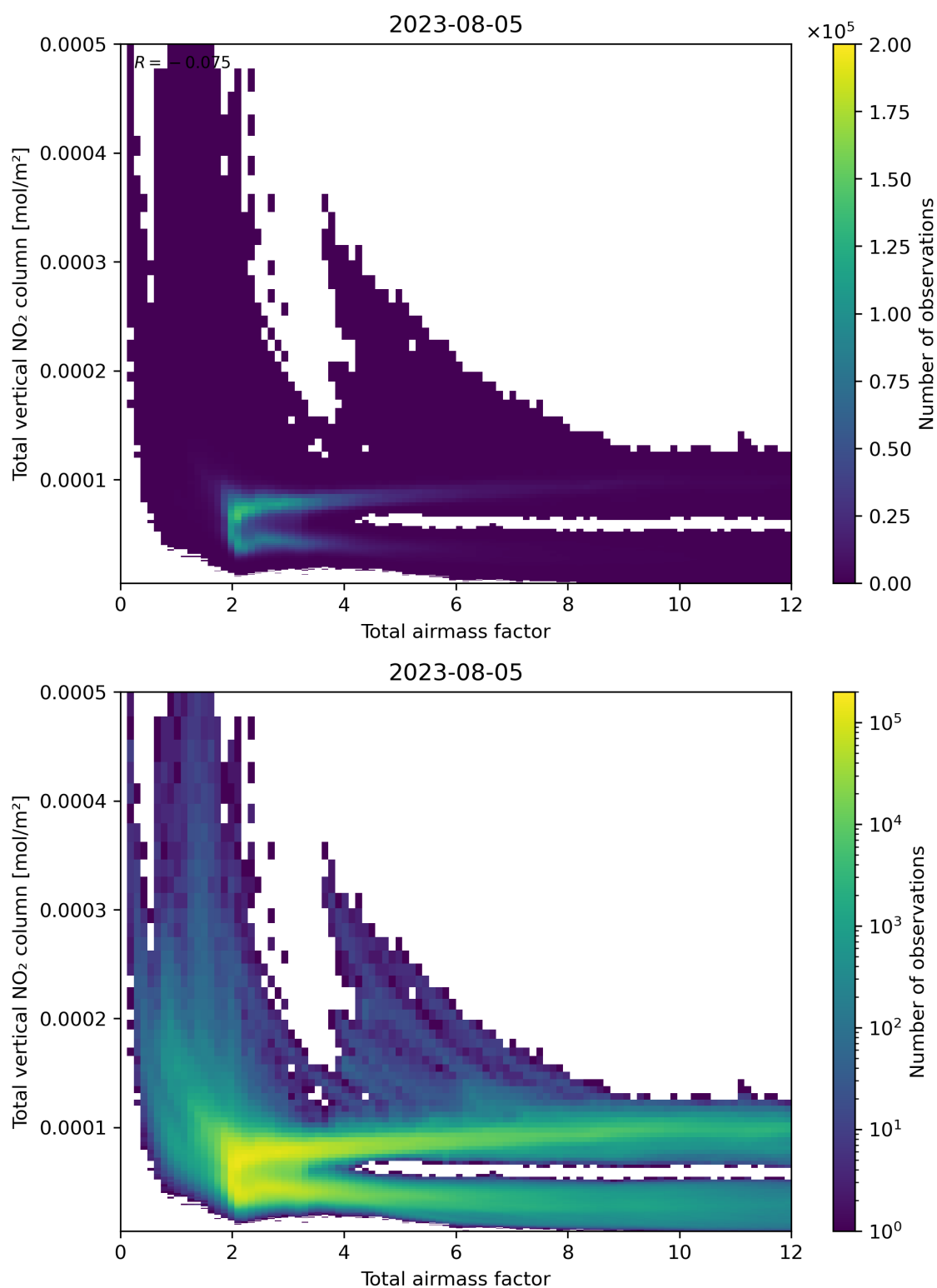
Figure 67: Scatter density plot of “Total airmass factor” against “Total vertical NO 2 column” for 2023-08-04 to 2023-08-06.
