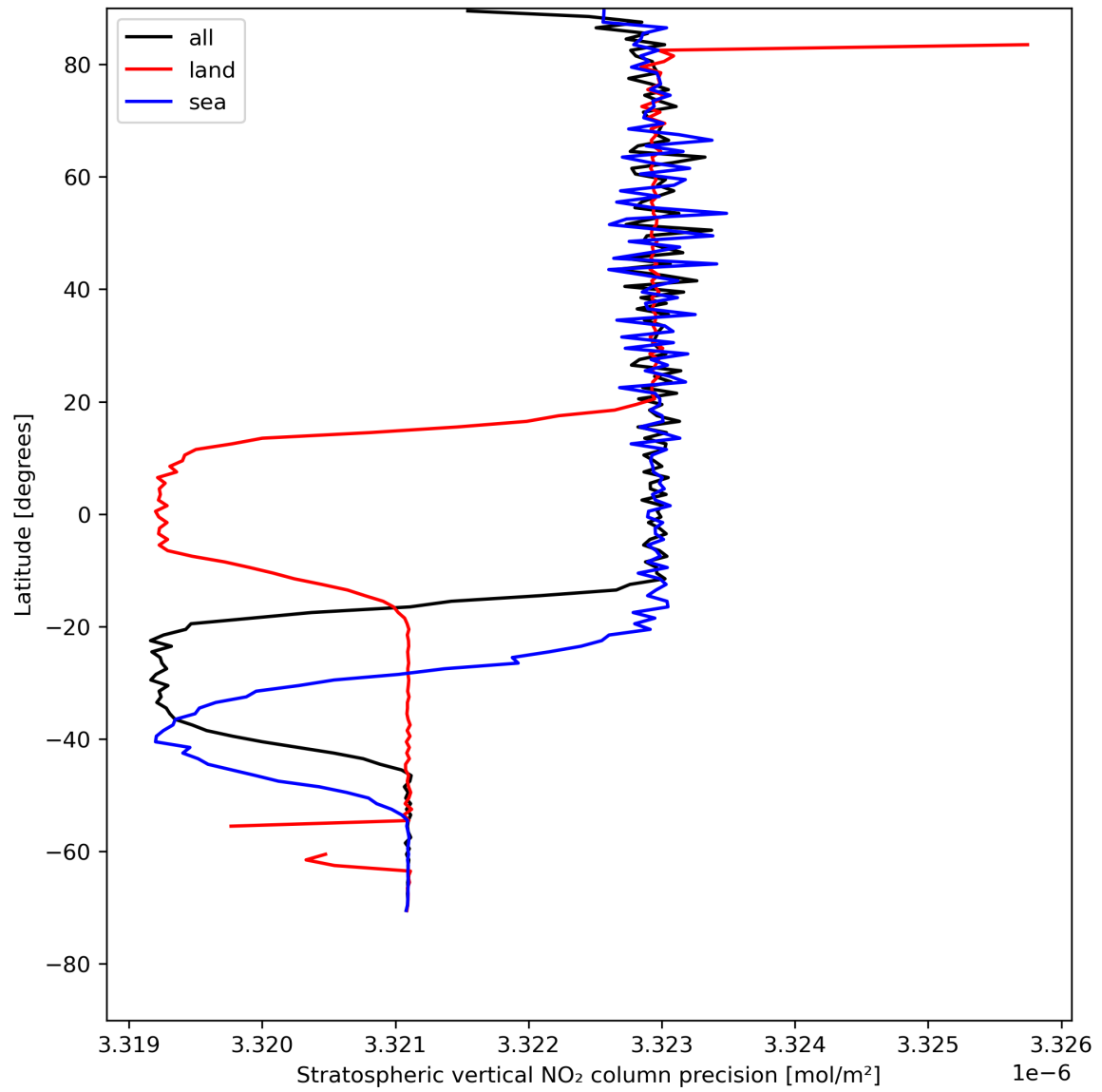
Figure 20: Zonal average of “Stratospheric vertical NO 2 column precision” for 2023-08-04 to 2023-08-06.
