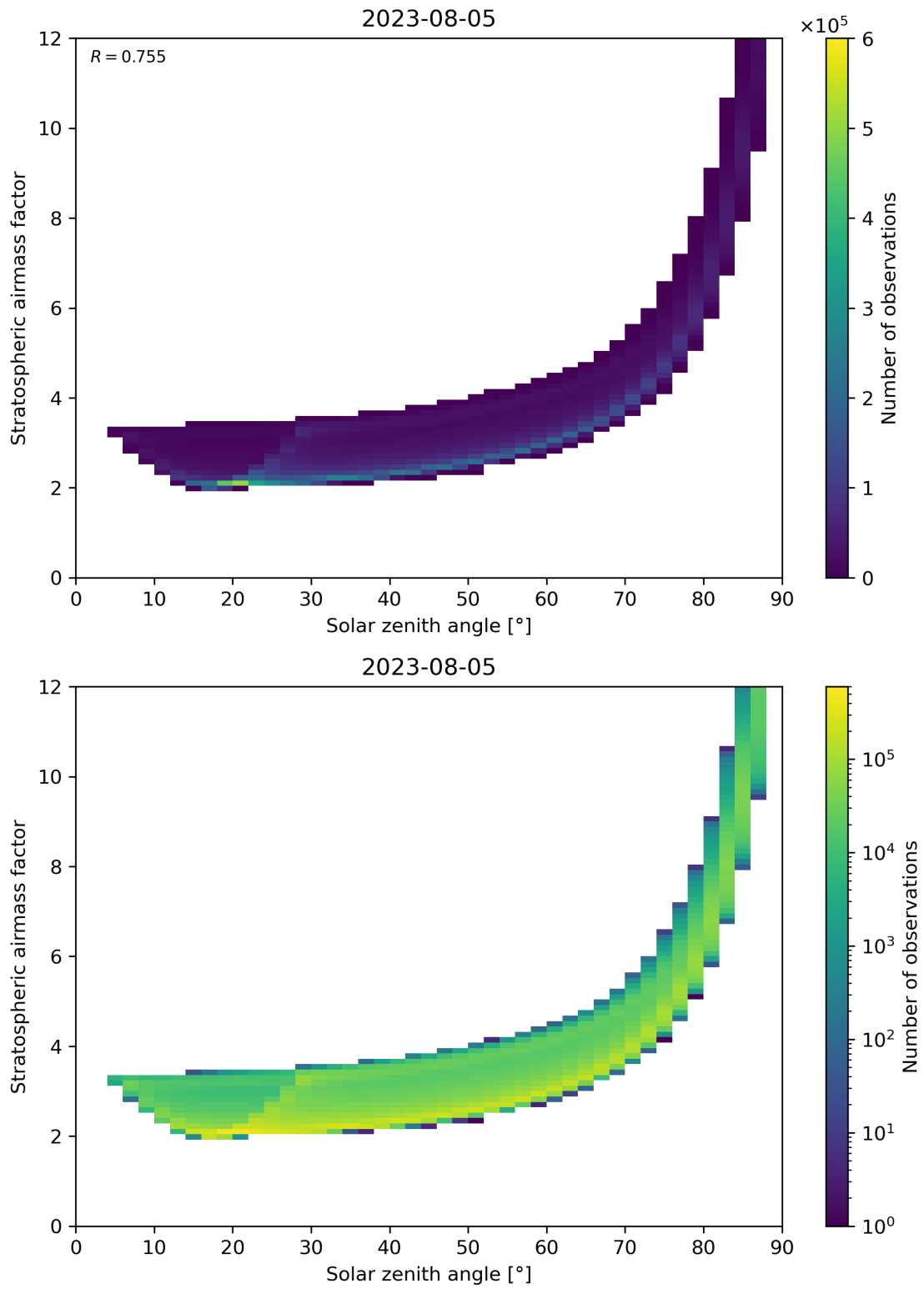
Figure 145: Scatter density plot of “Solar zenith angle” against “Stratospheric airmass factor” for 2023-08-04 to 2023-08-06.
