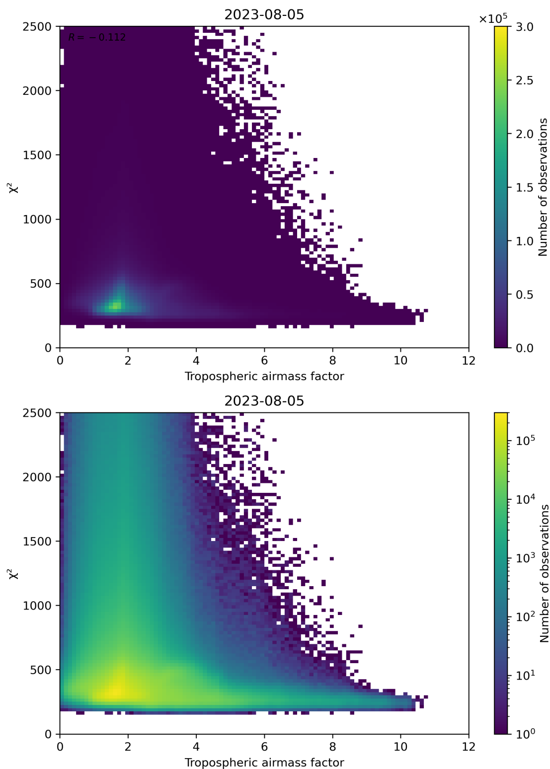
Figure 73: Scatter density plot of “Tropospheric airmass factor” against “ \chi^2 ” for 2023-08-04 to 2023-08-06.
