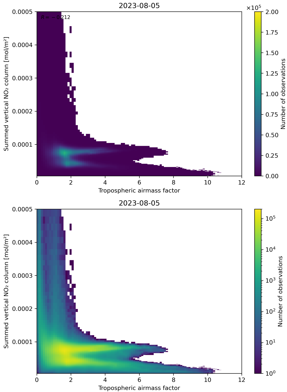
Figure 75: Scatter density plot of “Tropospheric airmass factor” against “Summed vertical NO 2 column” for 2023-08-04 to 2023-08-06.
