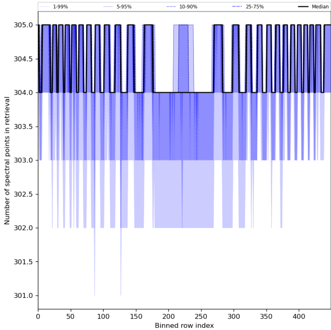
Figure 50: Along track statistics of “Number of spectral points in retrieval” for 2023-08-04 to 2023-08-06
