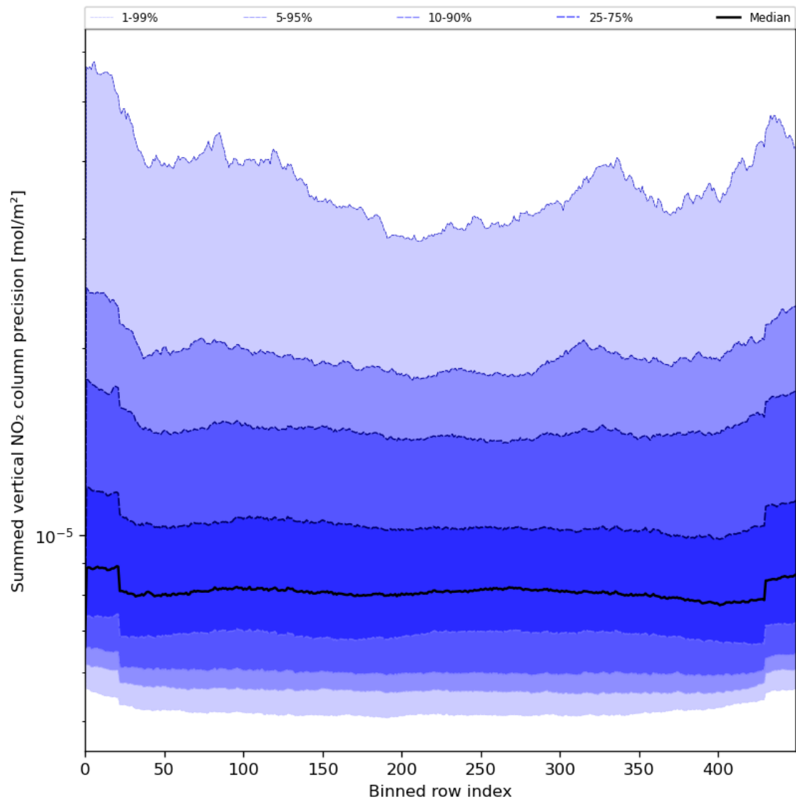
Figure 58: Along track statistics of “Summed vertical NO 2 column precision” for 2023-08-04 to 2023-08-06
