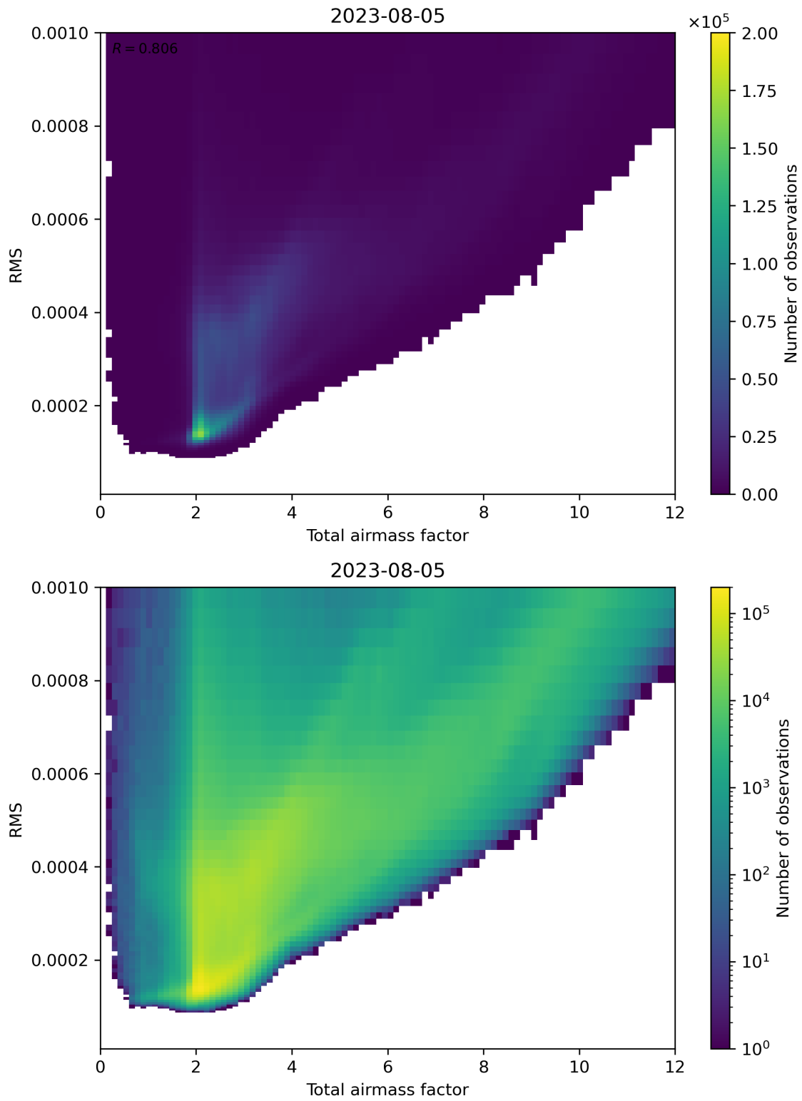
Figure 69: Scatter density plot of “Total airmass factor” against “RMS” for 2023-08-04 to 2023-08-06.
