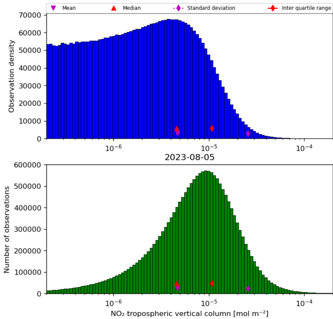
Figure 29: Histogram of “NO 2 tropospheric vertical column” for 2023-08-04 to 2023-08-06
