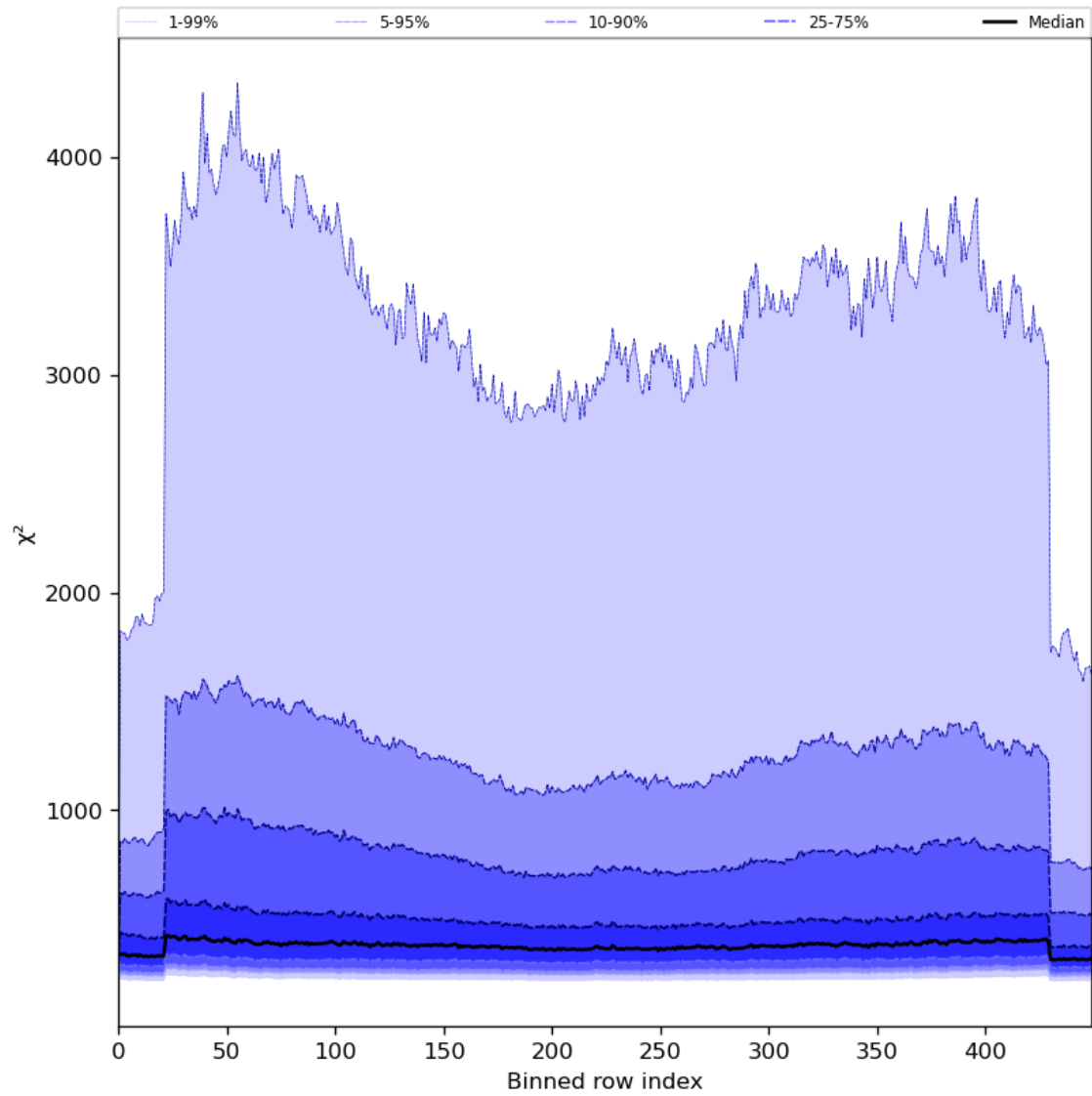
Figure 59: Along track statistics of “ \chi^2 ” for 2023-08-04 to 2023-08-06
