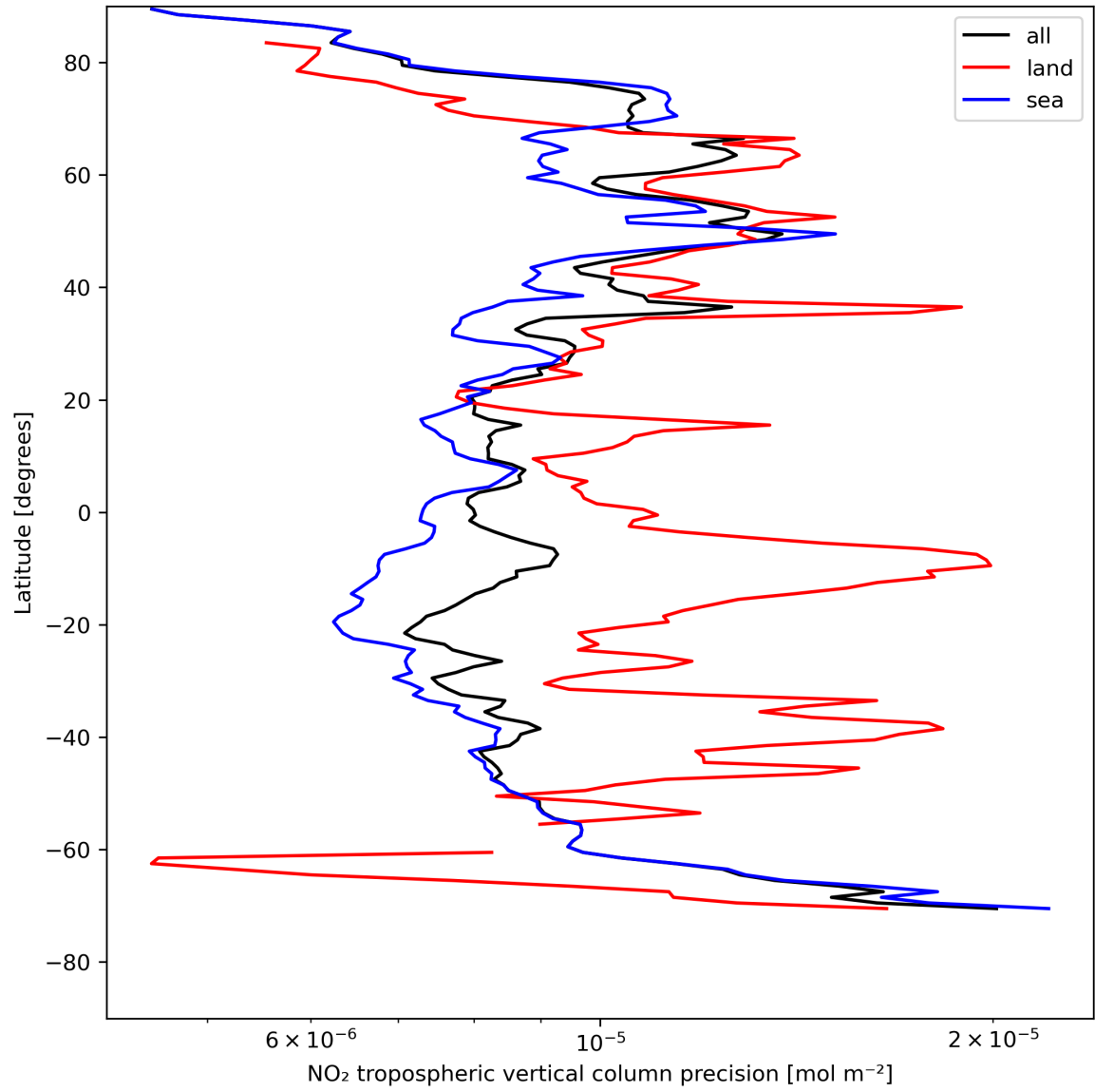
Figure 13: Zonal average of “NO 2 tropospheric vertical column precision” for 2023-08-04 to 2023-08-06.
