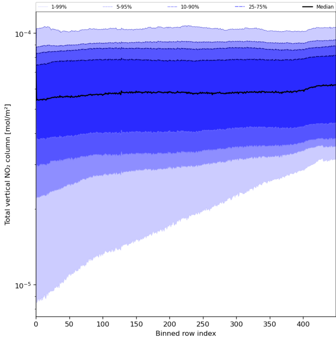
Figure 55: Along track statistics of “Total vertical NO 2 column” for 2023-08-04 to 2023-08-06
