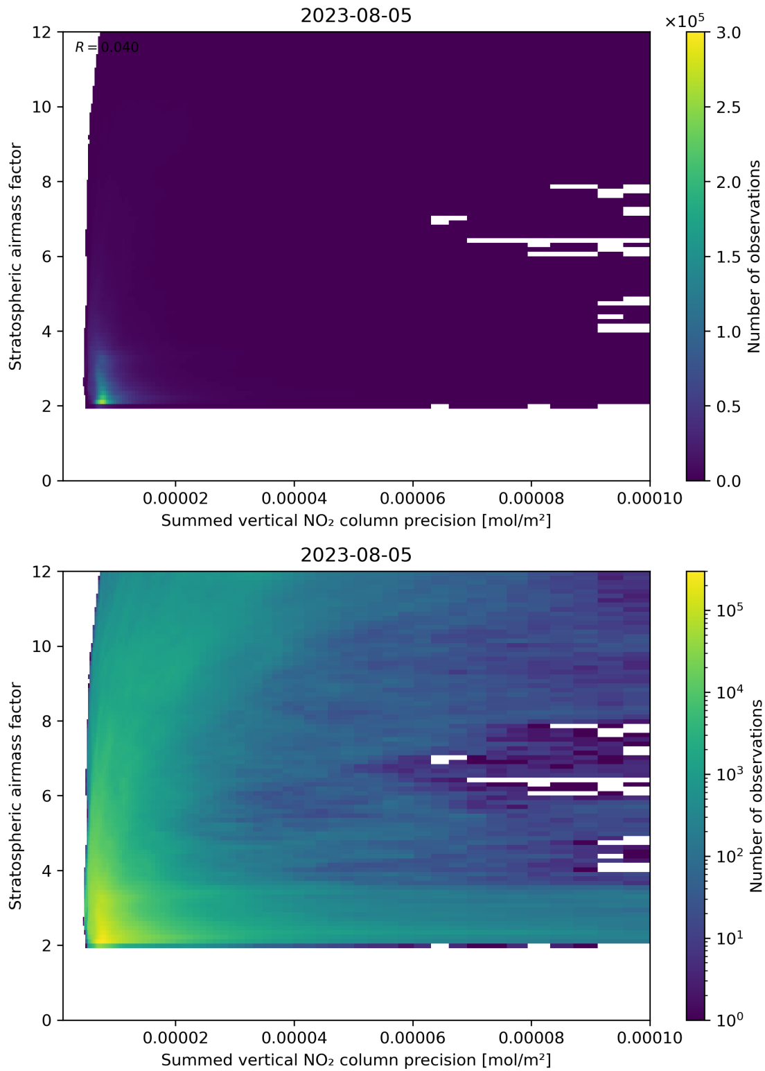
Figure 106: Scatter density plot of “Summed vertical NO 2 column precision” against “Stratospheric airmass factor” for 2023-08-04 to 2023-08-06.
