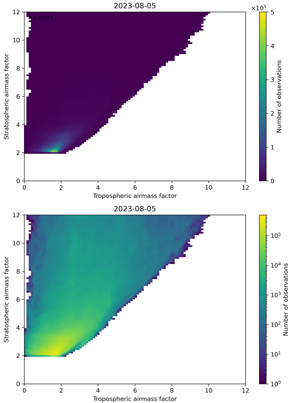
Figure 71: Scatter density plot of “Tropospheric airmass factor” against “Stratospheric airmass factor” for 2023-08-04 to 2023-08-06.
