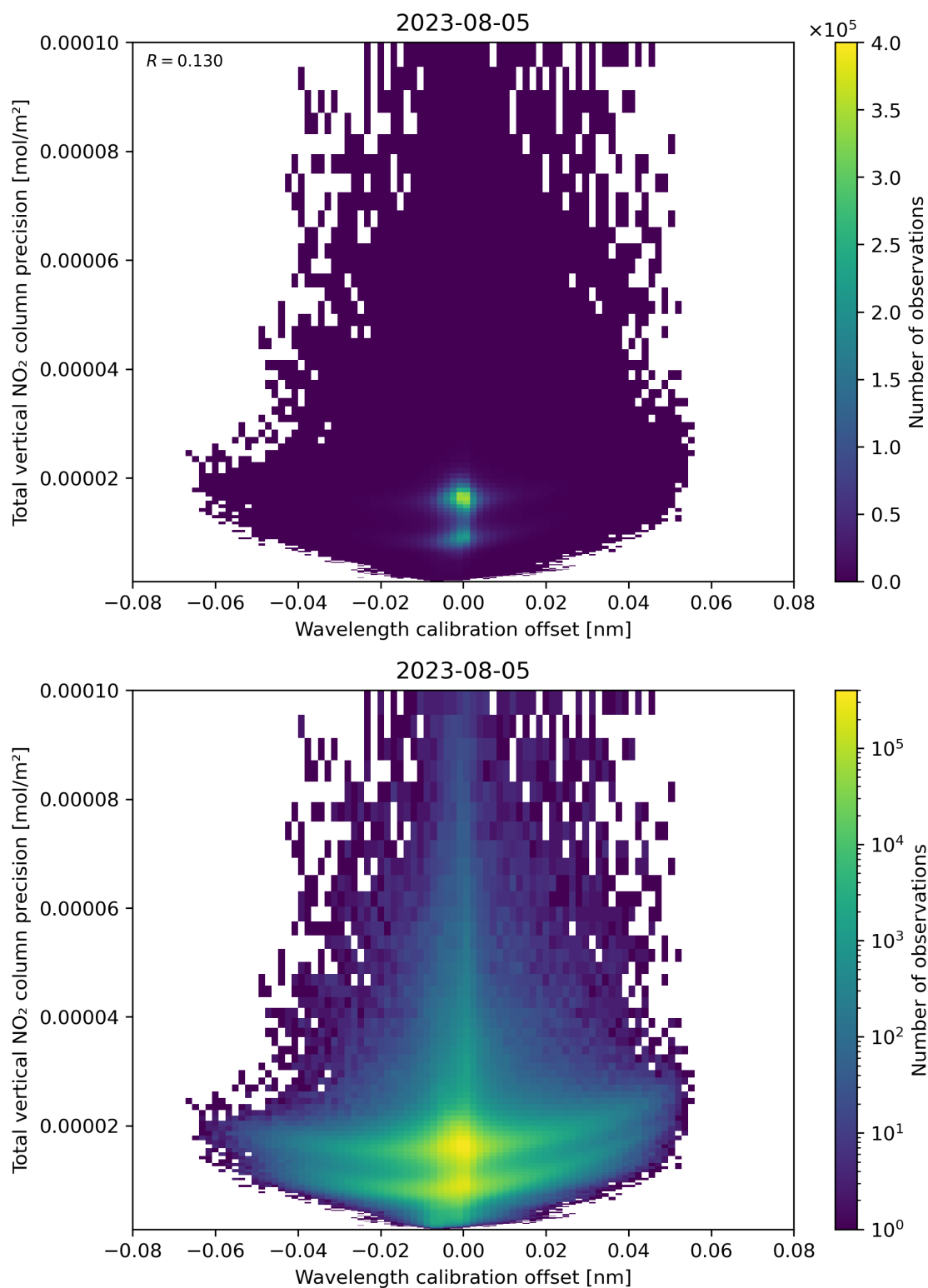
Figure 180: Scatter density plot of “Wavelength calibration offset” against “Total vertical NO 2 column precision” for 2023-08-04 to 2023-08-06.
