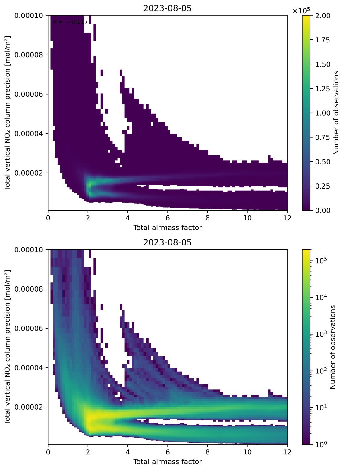
Figure 68: Scatter density plot of “Total airmass factor” against “Total vertical NO 2 column precision” for 2023-08-04 to 2023-08-06.
