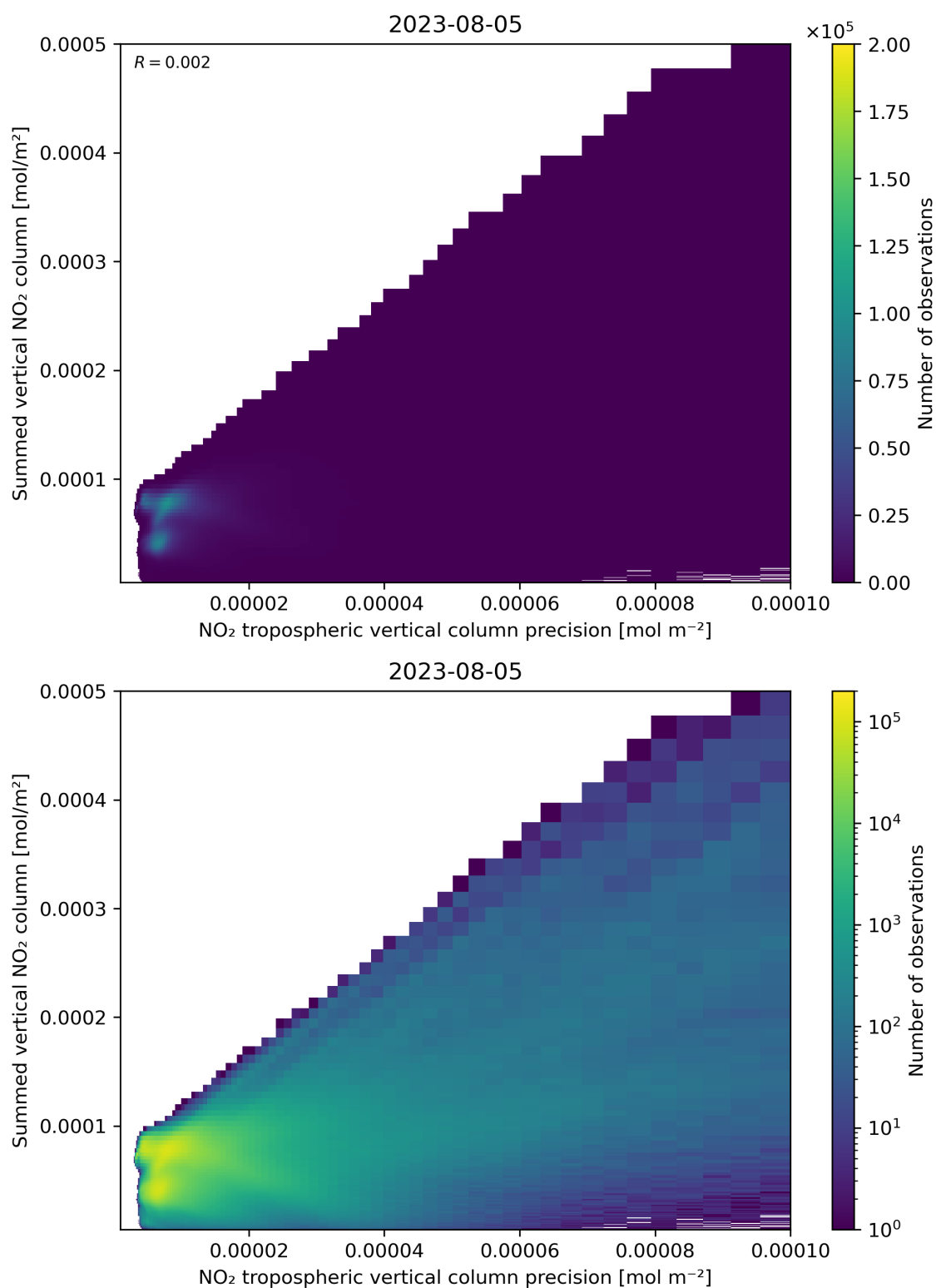
Figure 136: Scatter density plot of “NO 2 tropospheric vertical column precision” against “Summed vertical NO 2 column” for 2023-08-04 to 2023-08-06.
