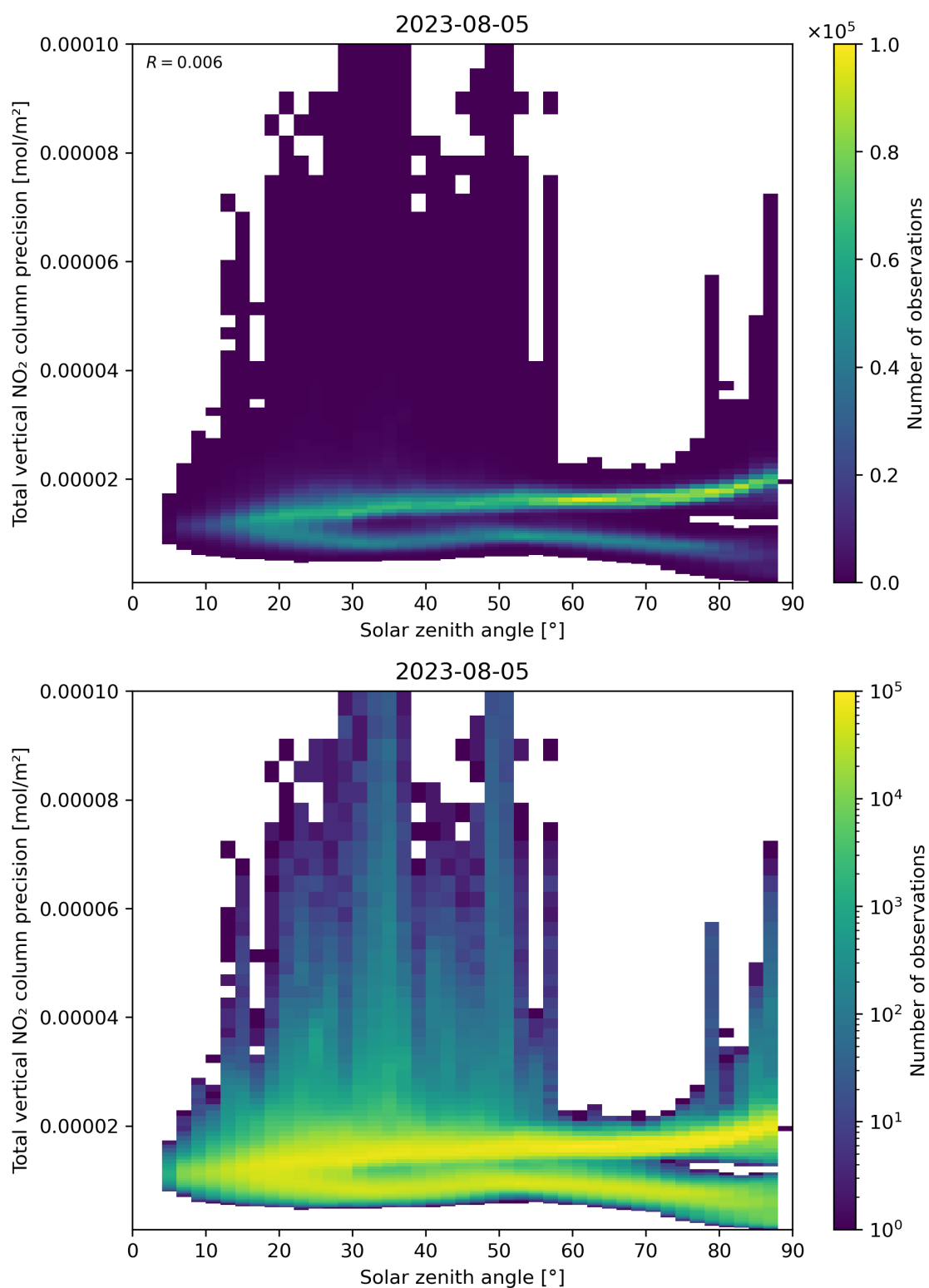
Figure 154: Scatter density plot of “Solar zenith angle” against “Total vertical NO 2 column precision” for 2023-08-04 to 2023-08-06.
