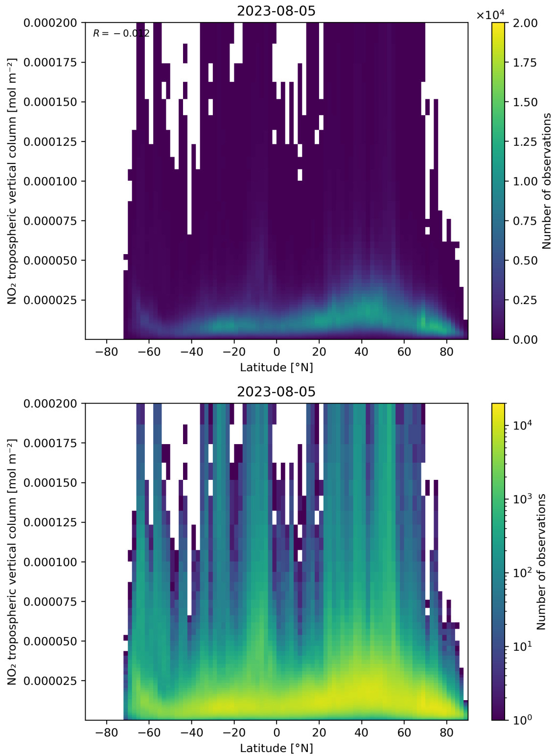
Figure 92: Scatter density plot of “Latitude” against “NO 2 tropospheric vertical column” for 2023-08-04 to 2023-08-06.
