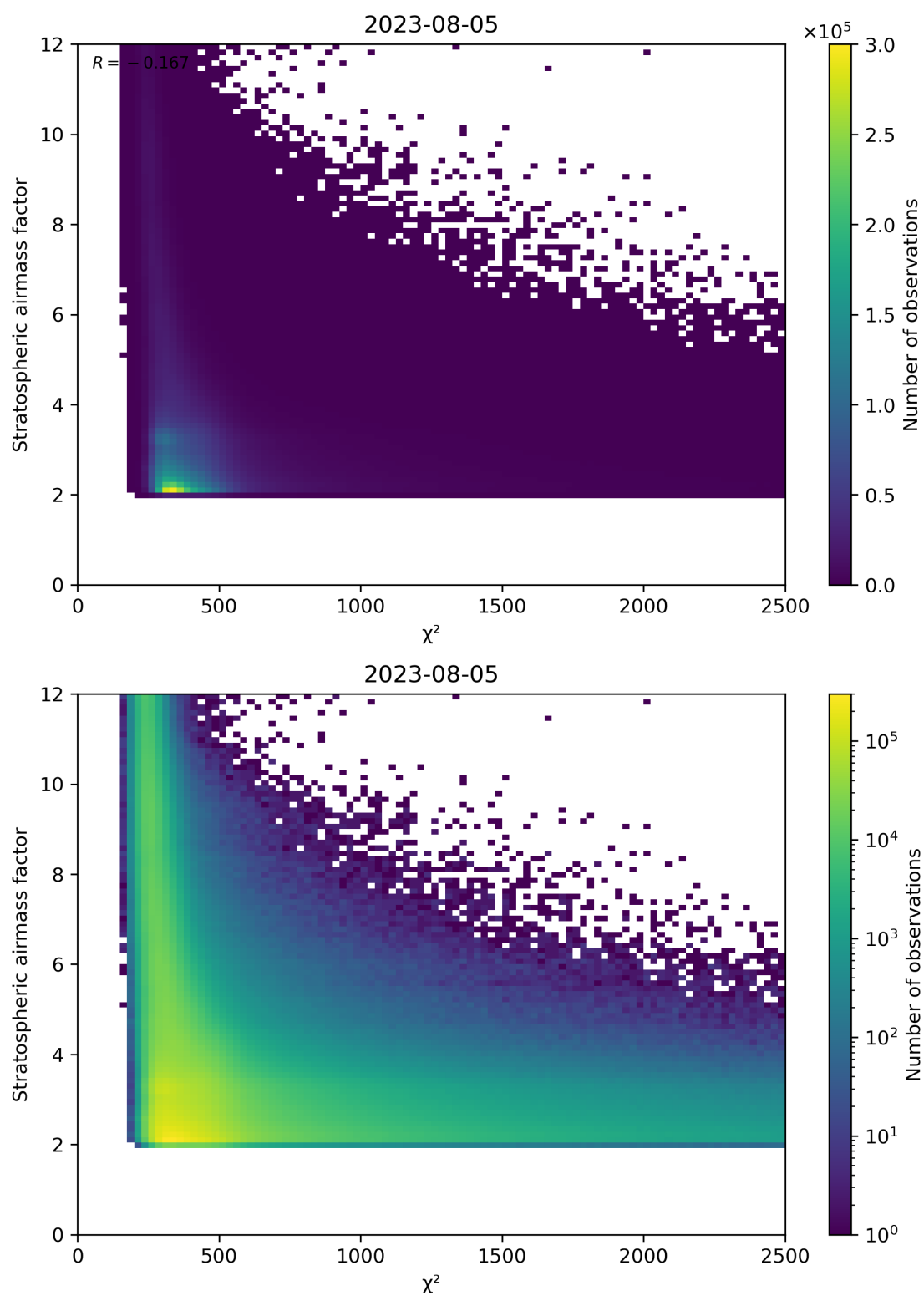
Figure 81: Scatter density plot of “ \chi^2 ” against “Stratospheric airmass factor” for 2023-08-04 to 2023-08-06.
