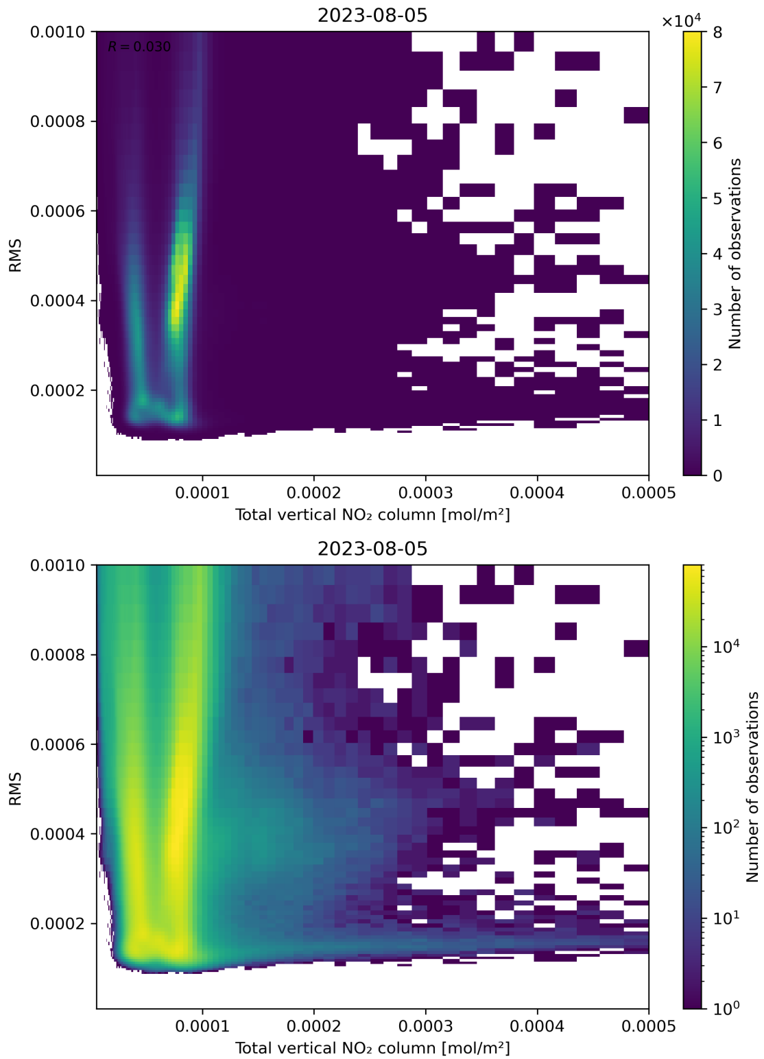
Figure 120: Scatter density plot of “Total vertical NO 2 column” against “RMS” for 2023-08-04 to 2023-08-06.
