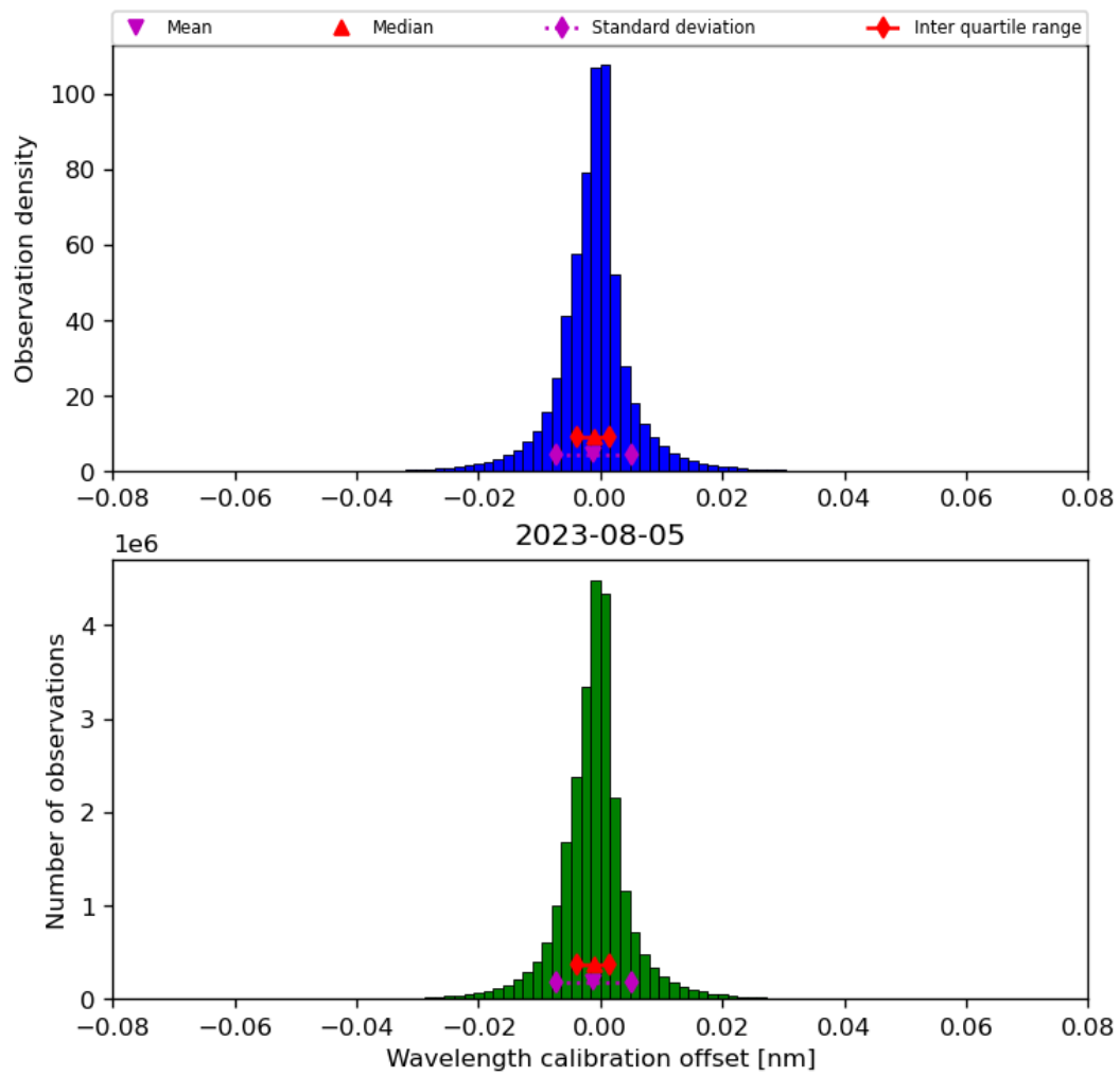
Figure 35: Histogram of “Wavelength calibration offset” for 2023-08-04 to 2023-08-06
