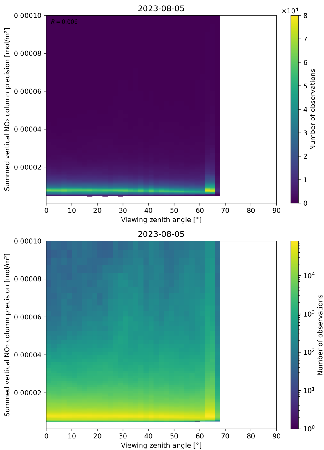
Figure 166: Scatter density plot of “Viewing zenith angle” against “Summed vertical NO 2 column precision” for 2023-08-04 to 2023-08-06.
