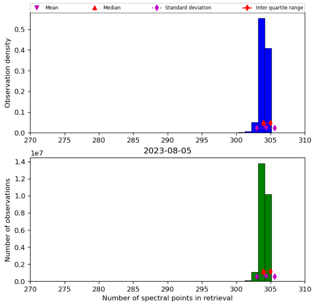
Figure 33: Histogram of “Number of spectral points in retrieval” for 2023-08-04 to 2023-08-06
