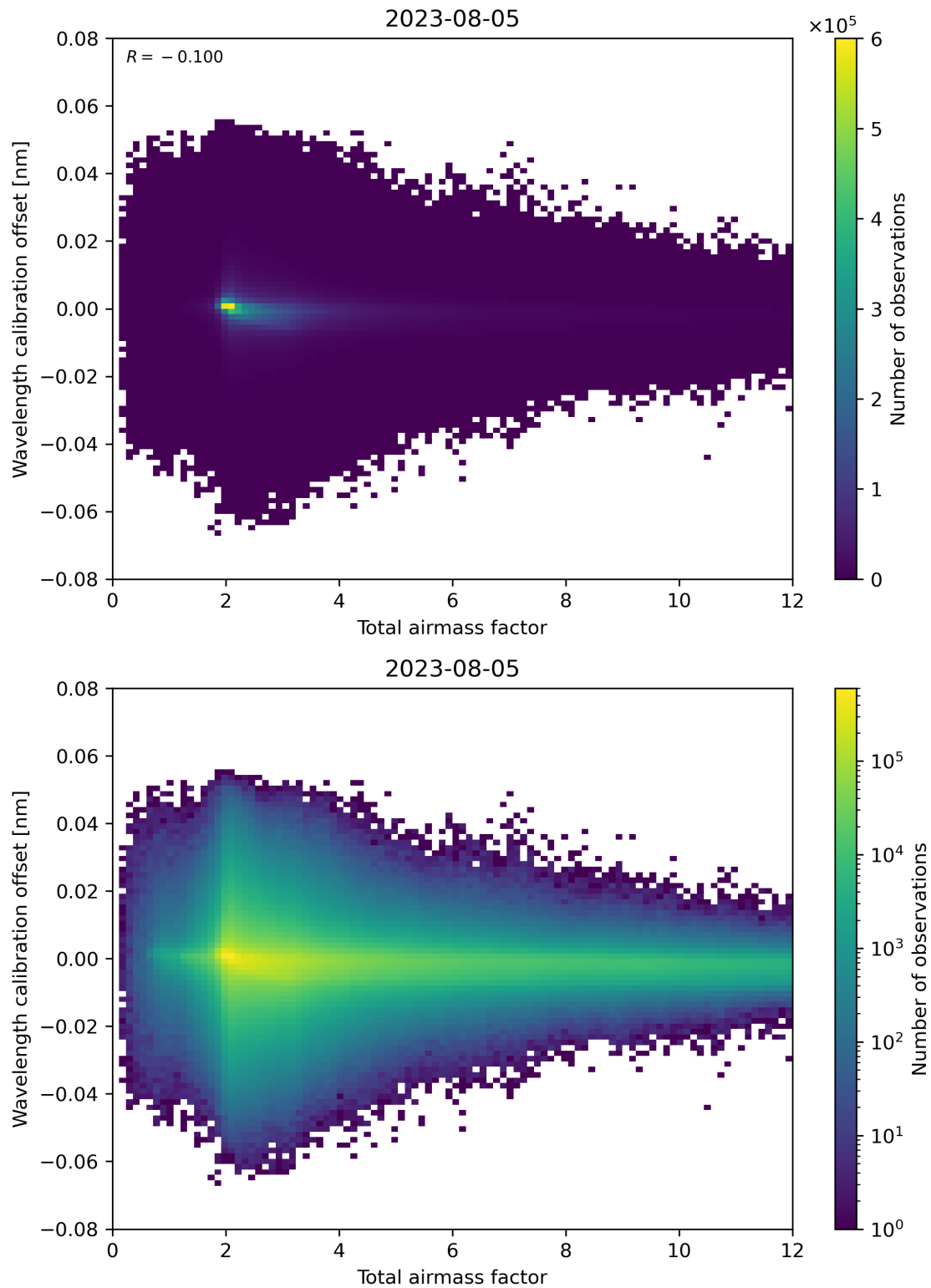
Figure 70: Scatter density plot of “Total airmass factor” against “Wavelength calibration offset” for 2023-08-04 to 2023-08-06.
