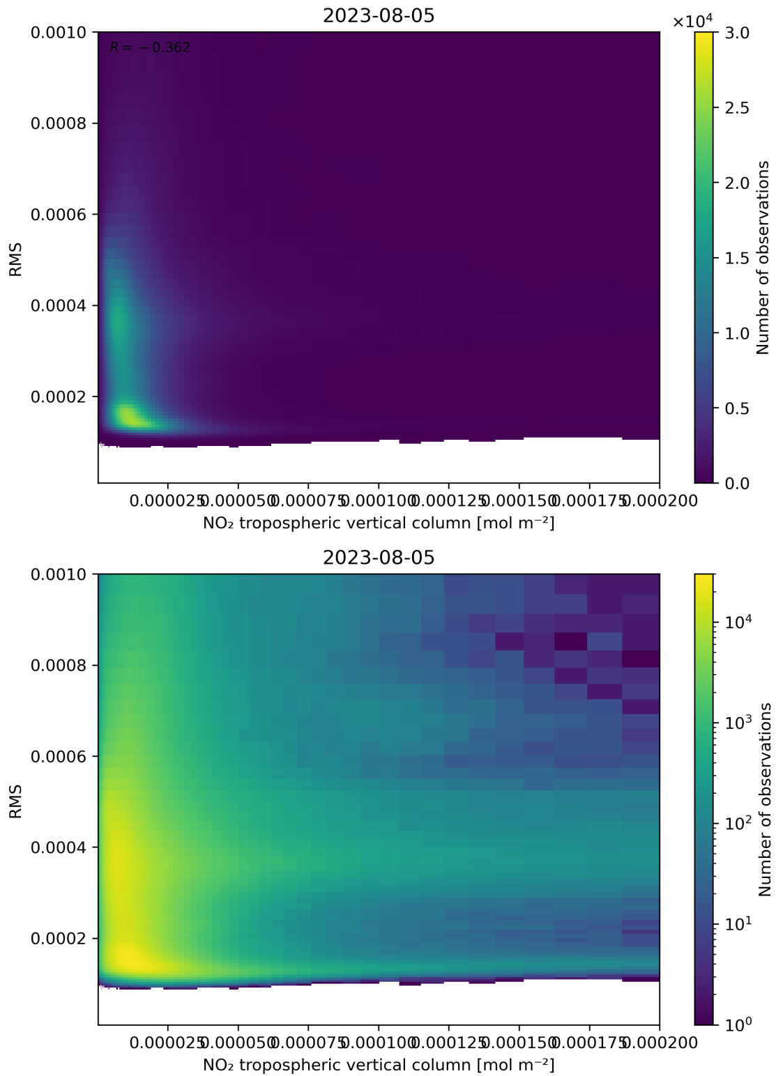
Figure 142: Scatter density plot of “NO 2 tropospheric vertical column” against “RMS” for 2023-08-04 to 2023-08-06.
