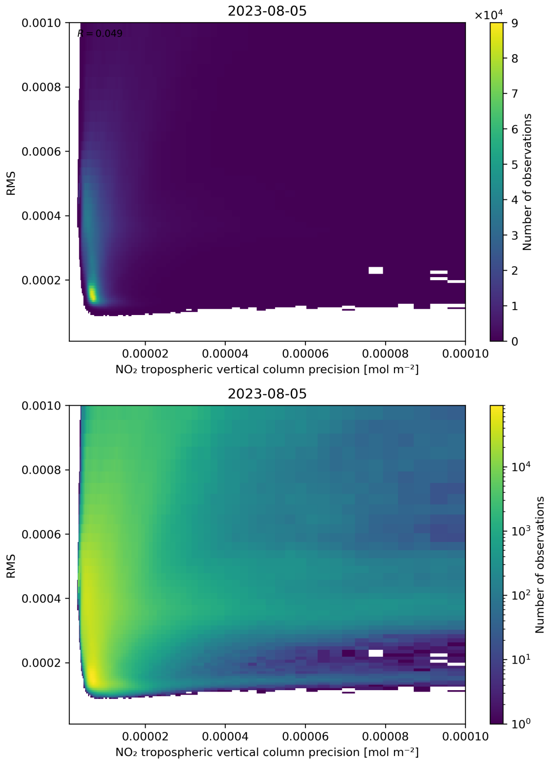
Figure 140: Scatter density plot of “NO 2 tropospheric vertical column precision” against “RMS” for 2023-08-04 to 2023-08-06.
