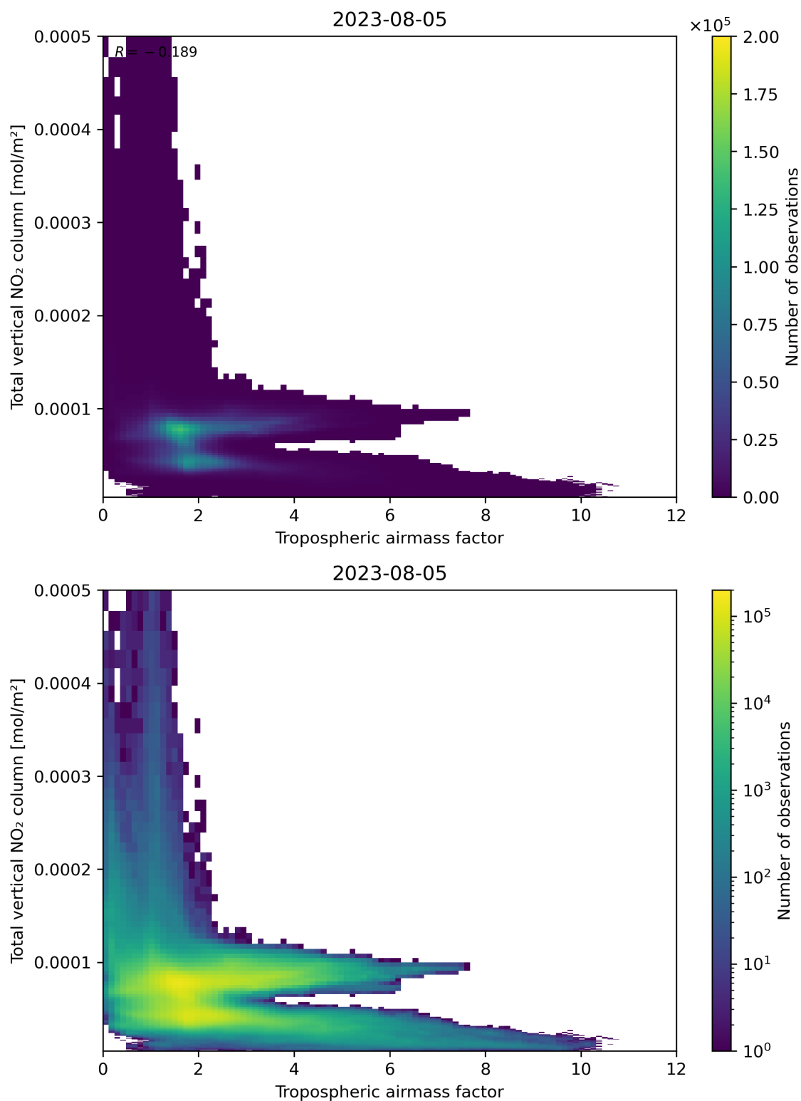
Figure 77: Scatter density plot of “Tropospheric airmass factor” against “Total vertical NO 2 column” for 2023-08-04 to 2023-08-06.
