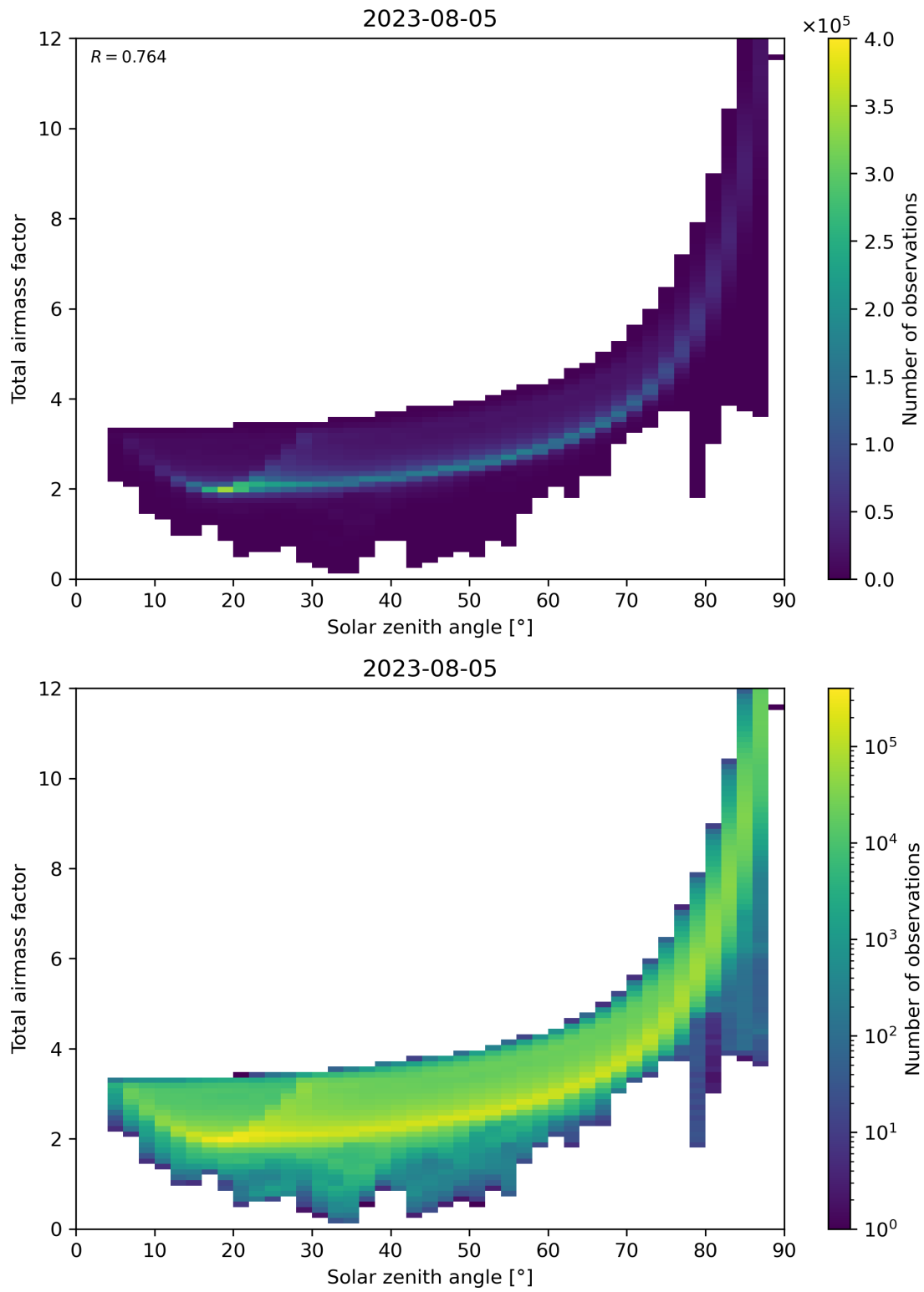
Figure 146: Scatter density plot of “Solar zenith angle” against “Total air mass factor” for 2023-08-04 to 2023-08-06.
