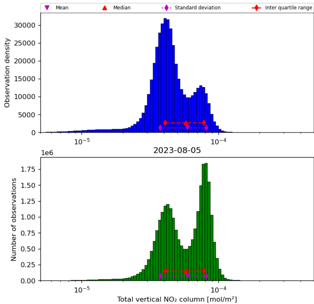
Figure 38: Histogram of “Total vertical NO 2 column” for 2023-08-04 to 2023-08-06
