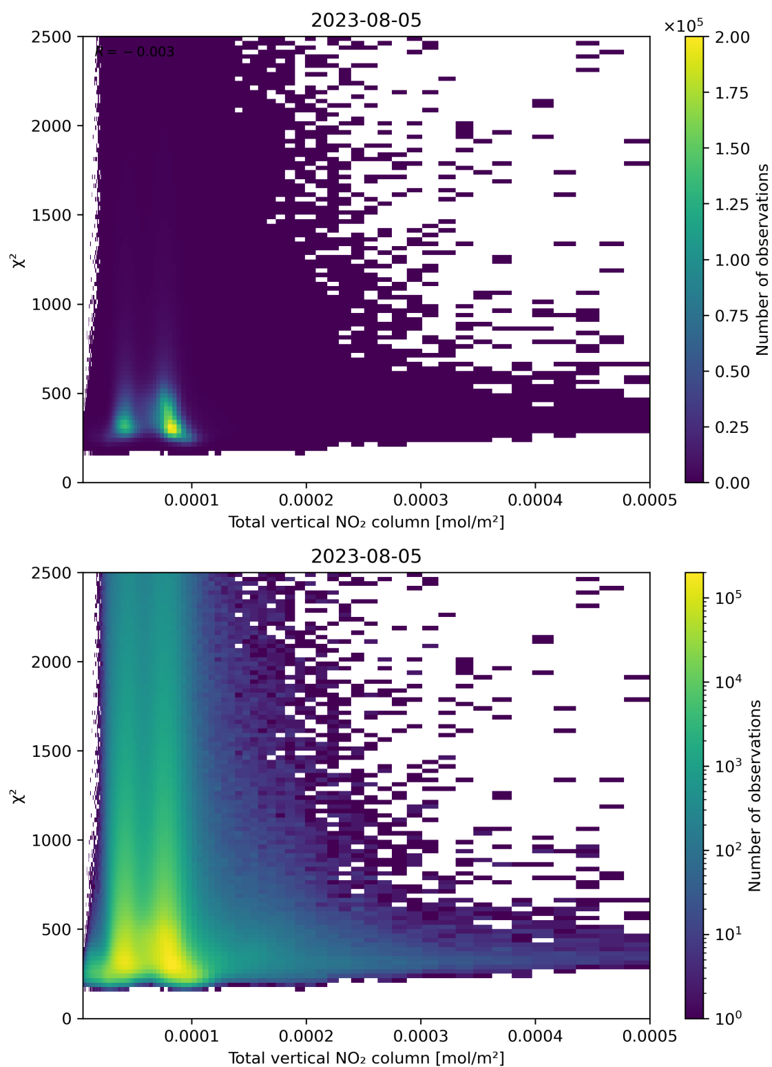
Figure 111: Scatter density plot of “Total vertical NO 2 column” against “ \chi^2 ” for 2023-08-04 to 2023-08-06.
