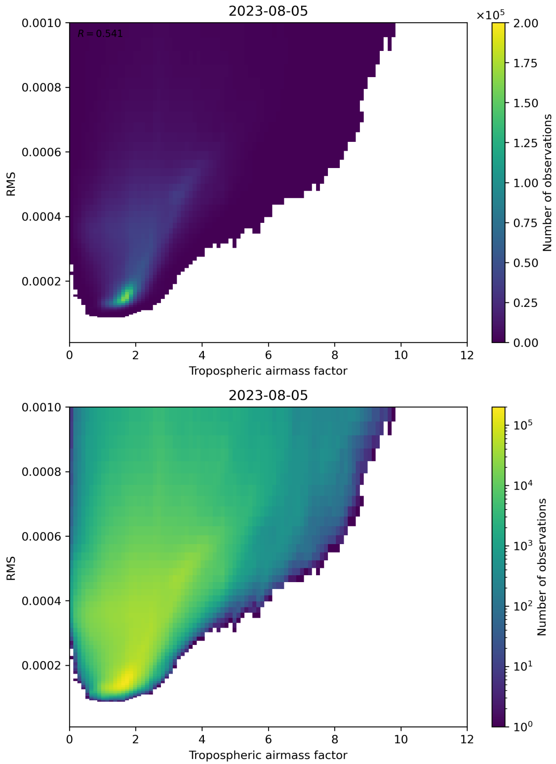
Figure 79: Scatter density plot of “Tropospheric airmass factor” against “RMS” for 2023-08-04 to 2023-08-06.
