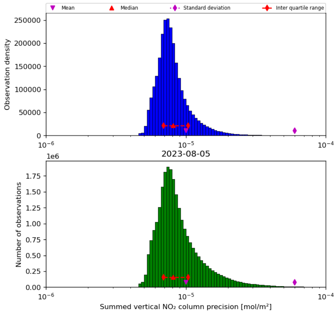
Figure 41: Histogram of “Summed vertical NO 2 column precision” for 2023-08-04 to 2023-08-06
