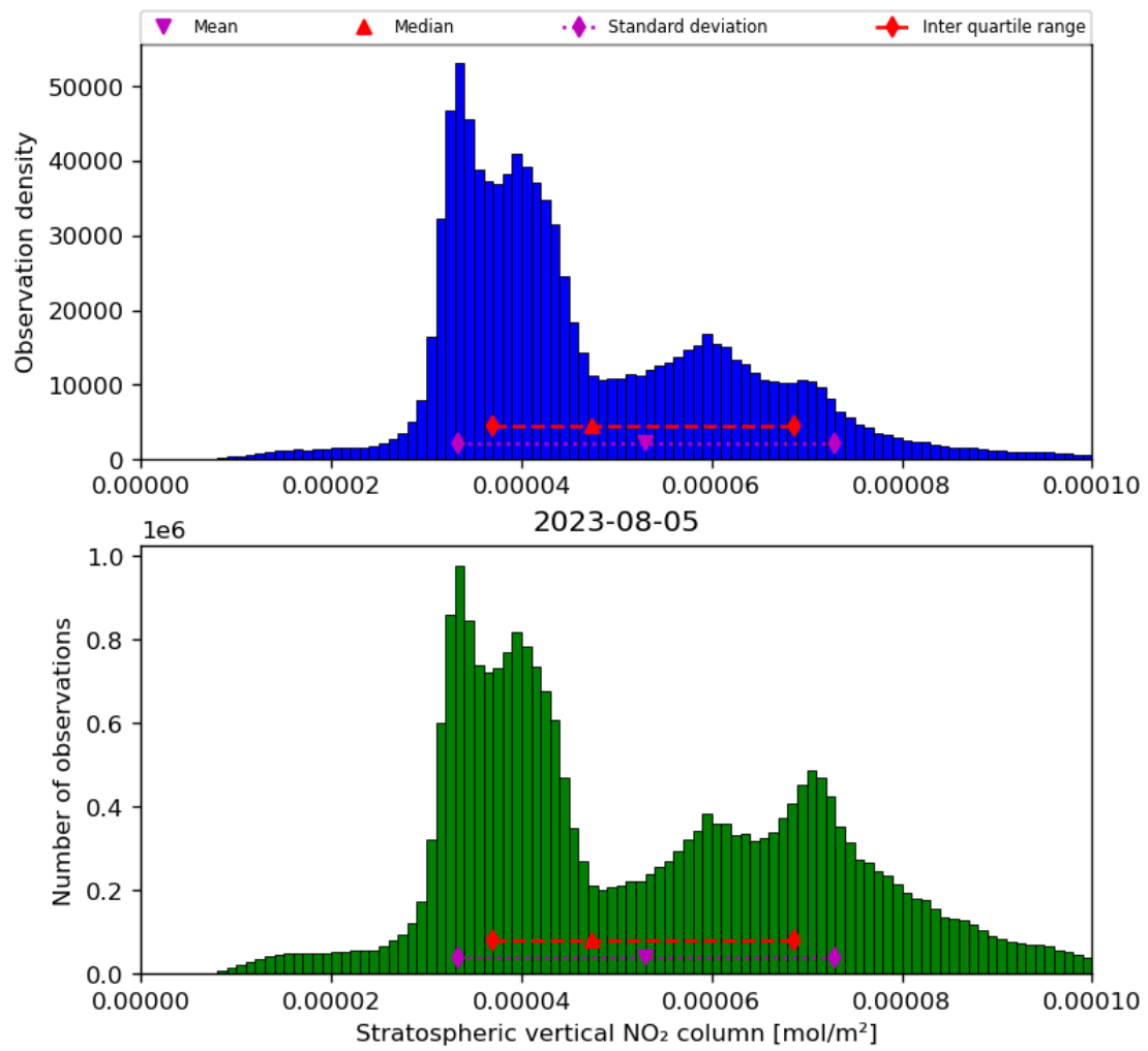
Figure 36: Histogram of “Stratospheric vertical NO 2 column” for 2023-08-04 to 2023-08-06
