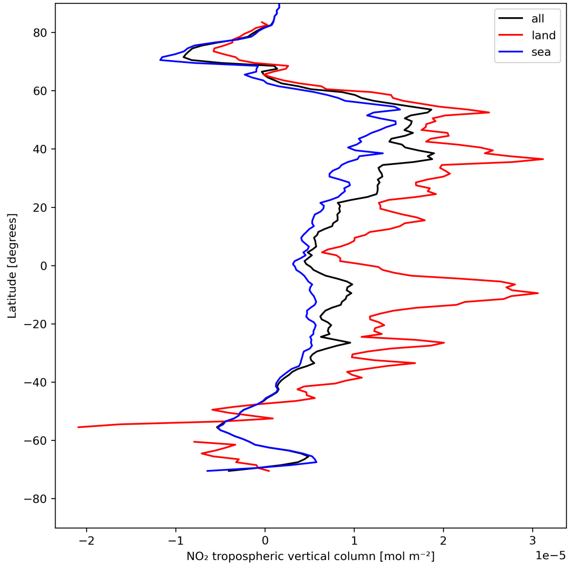
Figure 12: Zonal average of “NO 2 tropospheric vertical column” for 2023-08-04 to 2023-08-06.
