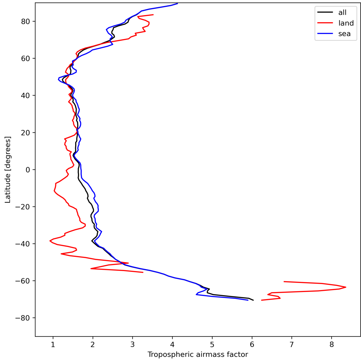
Figure 14: Zonal average of “Tropospheric airmass factor” for 2023-08-04 to 2023-08-06.
