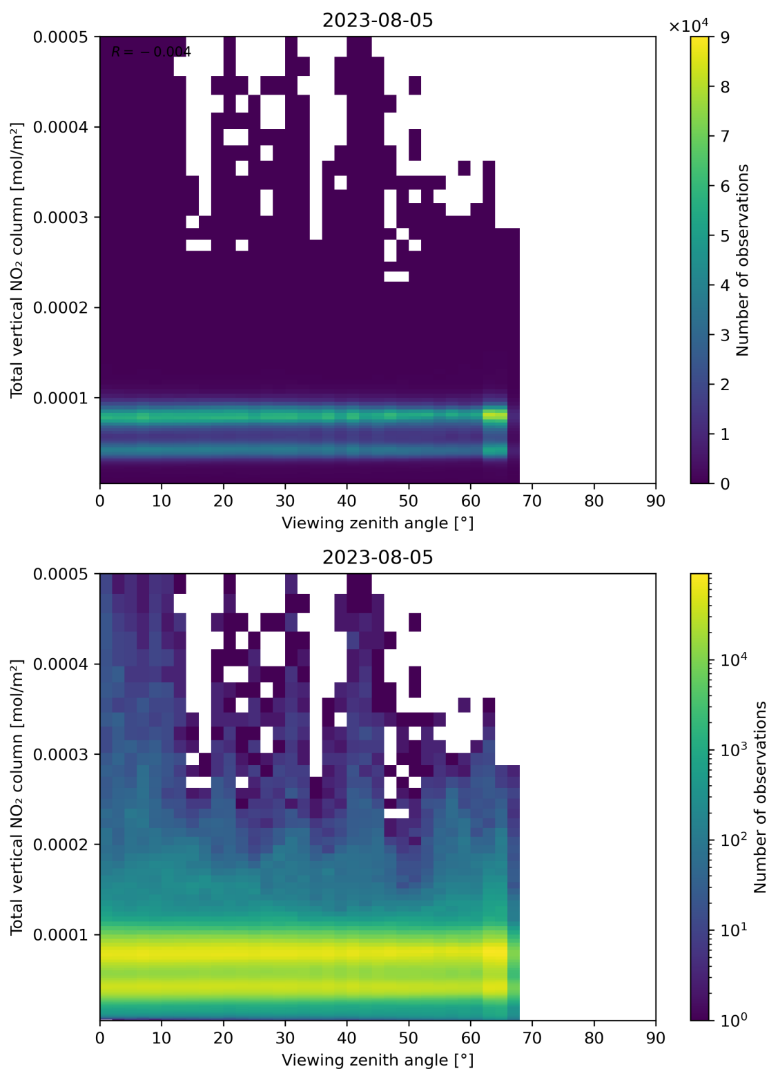
Figure 167: Scatter density plot of “Viewing zenith angle” against “Total vertical NO 2 column” for 2023-08-04 to 2023-08-06.
