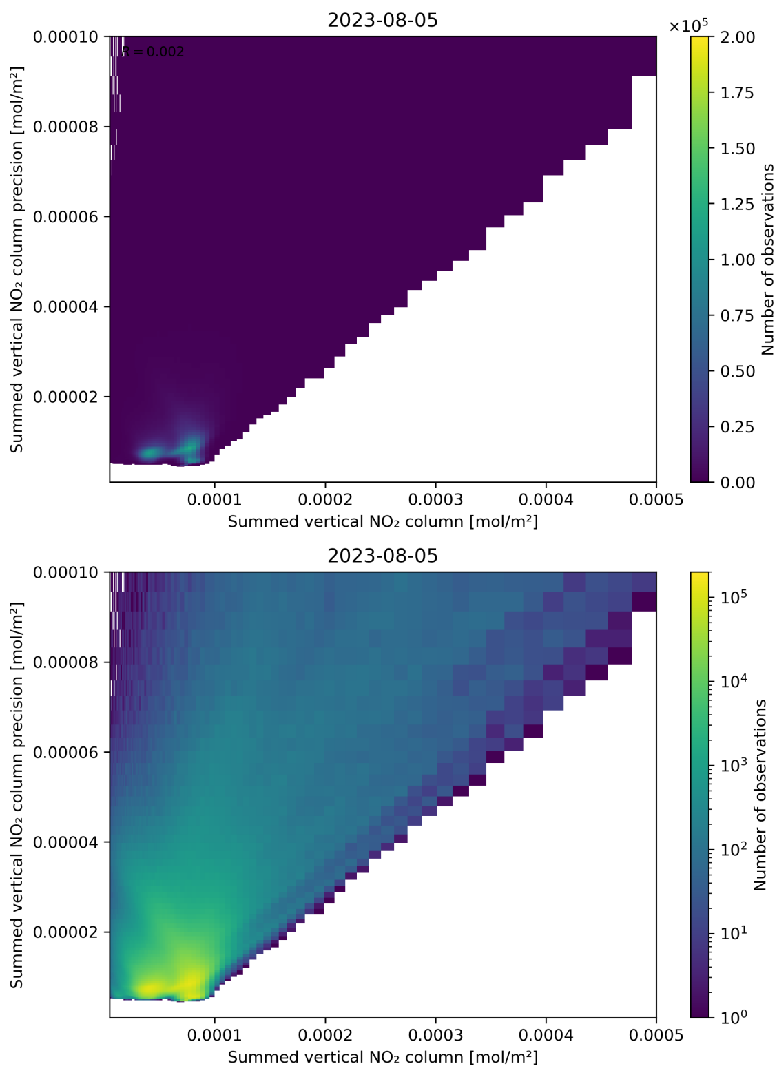
Figure 105: Scatter density plot of “Summed vertical NO 2 column” against “Summed vertical NO 2 column precision” for 2023-08-04 to 2023-08-06.
