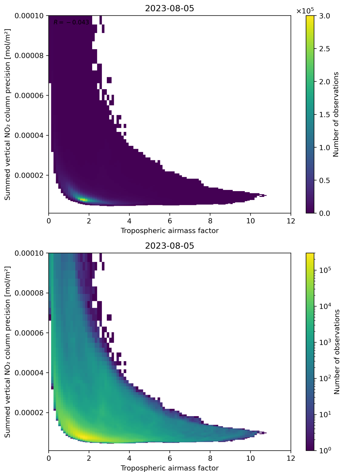
Figure 76: Scatter density plot of “Tropospheric air mass factor” against “Summed vertical NO 2 column precision” for 2023-08-04 to 2023-08-06.
