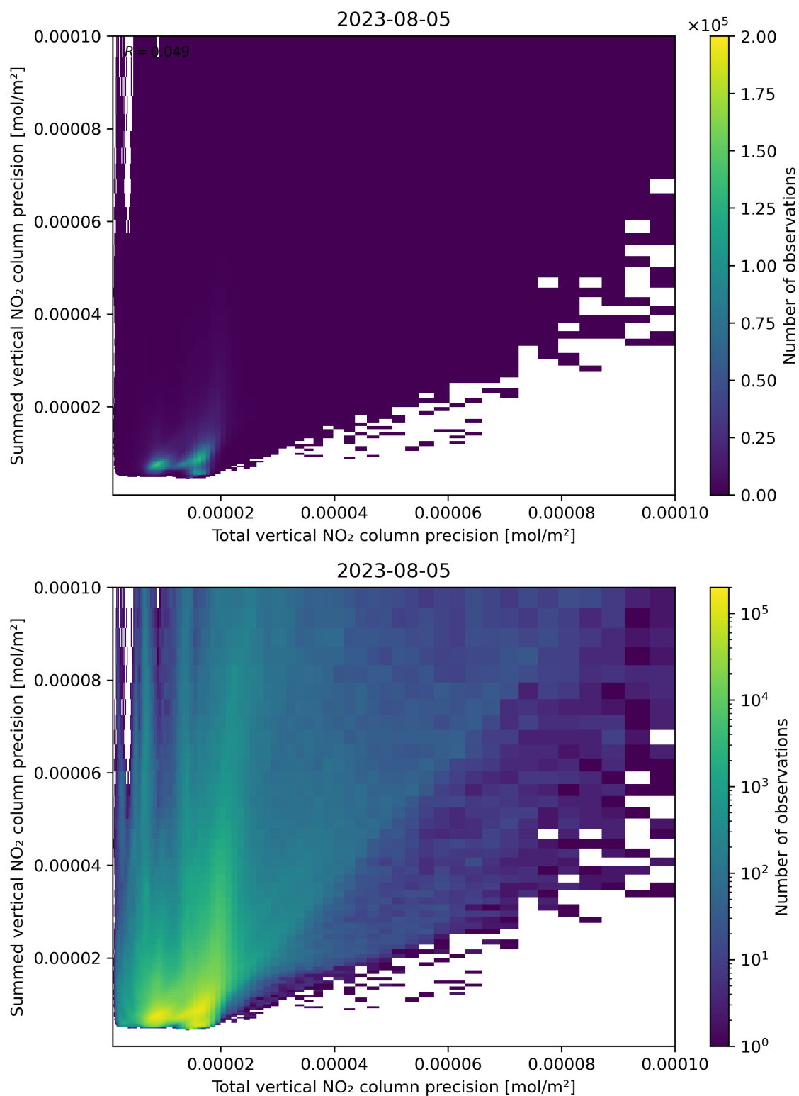
Figure 118: Scatter density plot of “Total vertical NO 2 column precision” against “Summed vertical NO 2 column precision” for 2023-08-04 to 2023-08-06.
