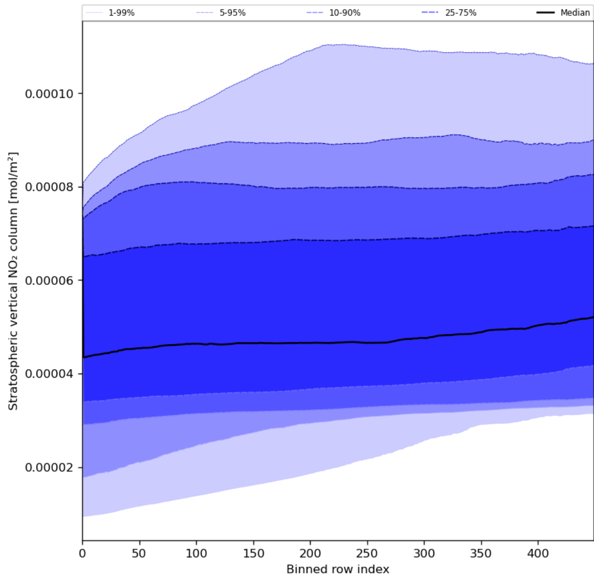
Figure 53: Along track statistics of “Stratospheric vertical NO 2 column” for 2023-08-04 to 2023-08-06
