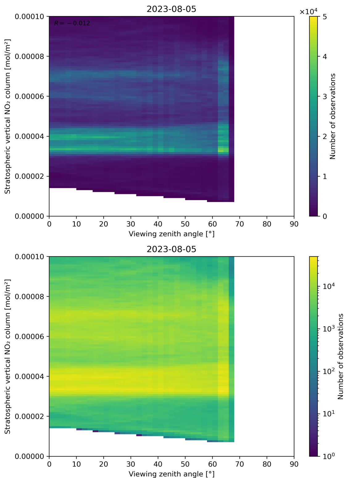
Figure 164: Scatter density plot of “Viewing zenith angle” against “Stratospheric vertical NO 2 column” for 2023-08-04 to 2023-08-06.
