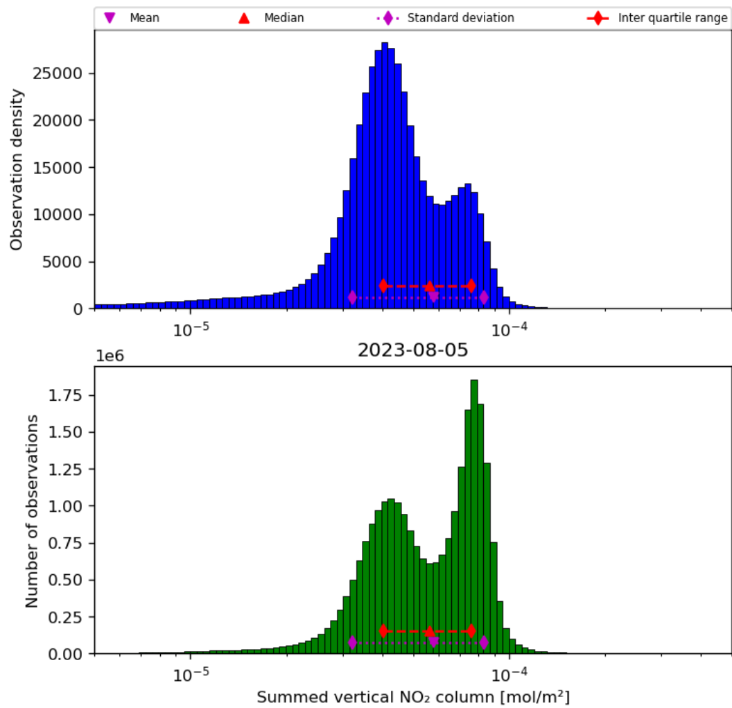
Figure 40: Histogram of “Summed vertical NO 2 column” for 2023-08-04 to 2023-08-06
