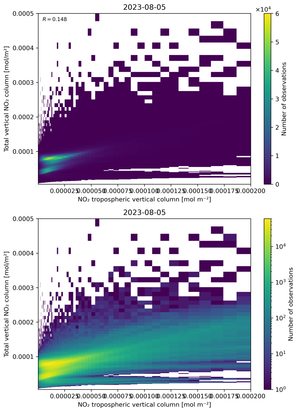
Figure 128: Scatter density plot of “NO 2 tropospheric vertical column” against “Total vertical NO 2 column” for 2023-08-04 to 2023-08-06.
