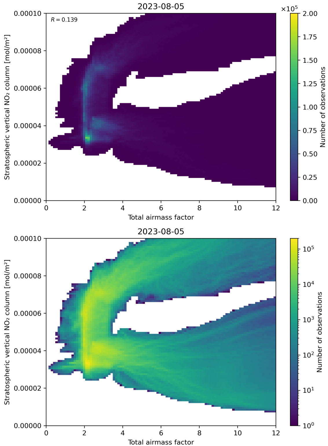
Figure 64: Scatter density plot of “Total airmass factor” against “Stratospheric vertical NO 2 column” for 2023-08-04 to 2023-08-06.
