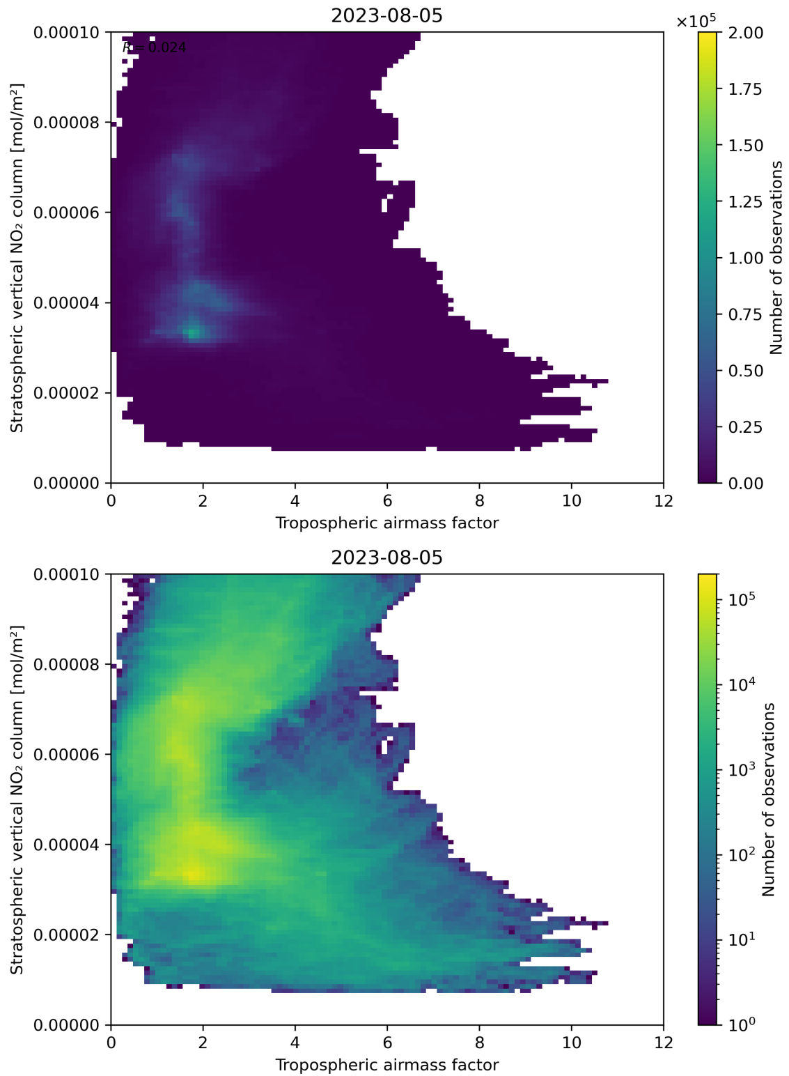
Figure 74: Scatter density plot of “Tropospheric airmass factor” against “Stratospheric vertical NO 2 column” for 2023-08-04 to 2023-08-06.
