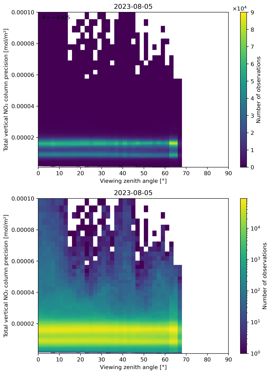
Figure 168: Scatter density plot of “Viewing zenith angle” against “Total vertical NO 2 column precision” for 2023-08-04 to 2023-08-06.
