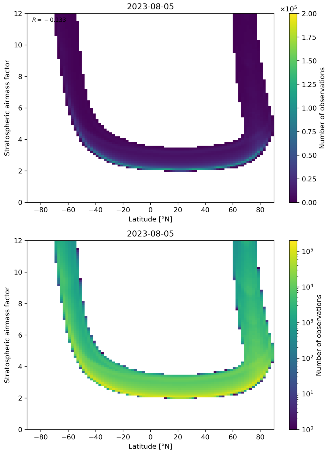
Figure 83: Scatter density plot of “Latitude” against “Stratospheric air mass factor” for 2023-08-04 to 2023-08-06.
