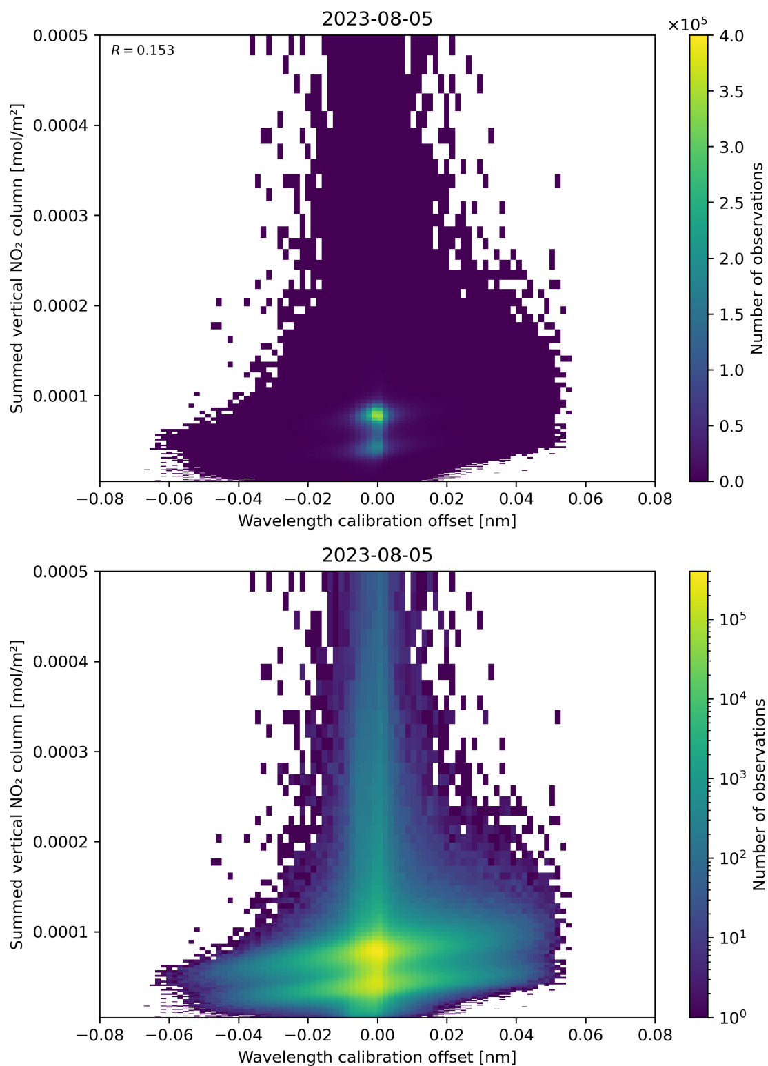
Figure 177: Scatter density plot of “Wavelength calibration offset” against “Summed vertical NO 2 column” for 2023-08-04 to 2023-08-06.
