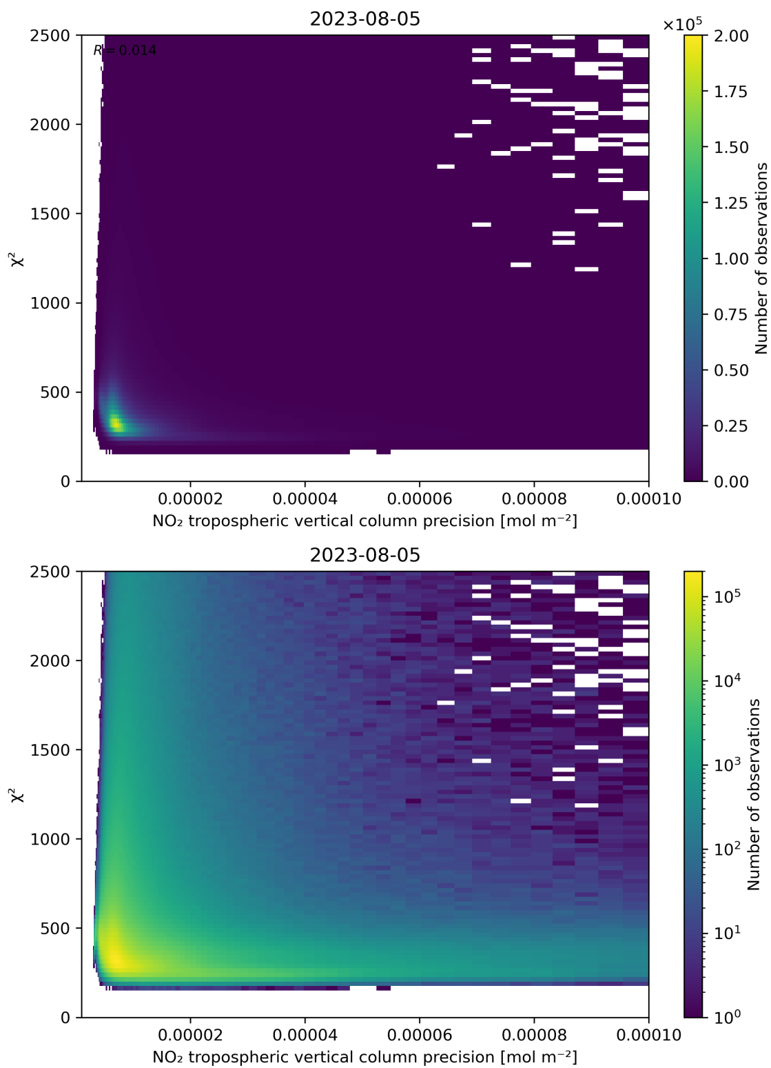
Figure 134: Scatter density plot of “NO 2 tropospheric vertical column precision” against “ \chi^2 ” for 2023-08-04 to 2023-08-06.
