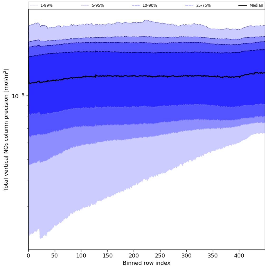
Figure 56: Along track statistics of “Total vertical NO 2 column precision” for 2023-08-04 to 2023-08-06
