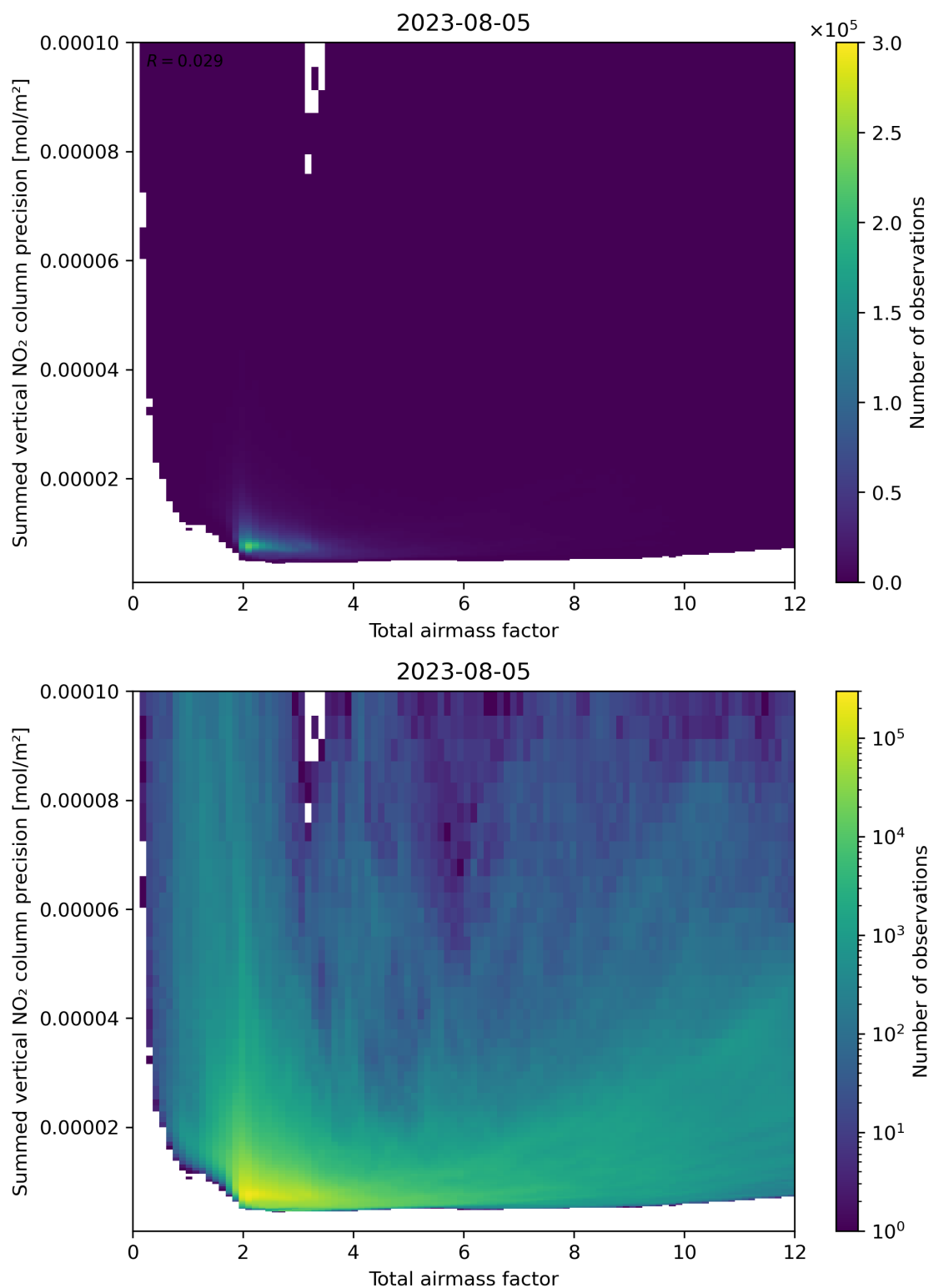
Figure 66: Scatter density plot of “Total airmass factor” against “Summed vertical NO 2 column precision” for 2023-08-04 to 2023-08-06.
