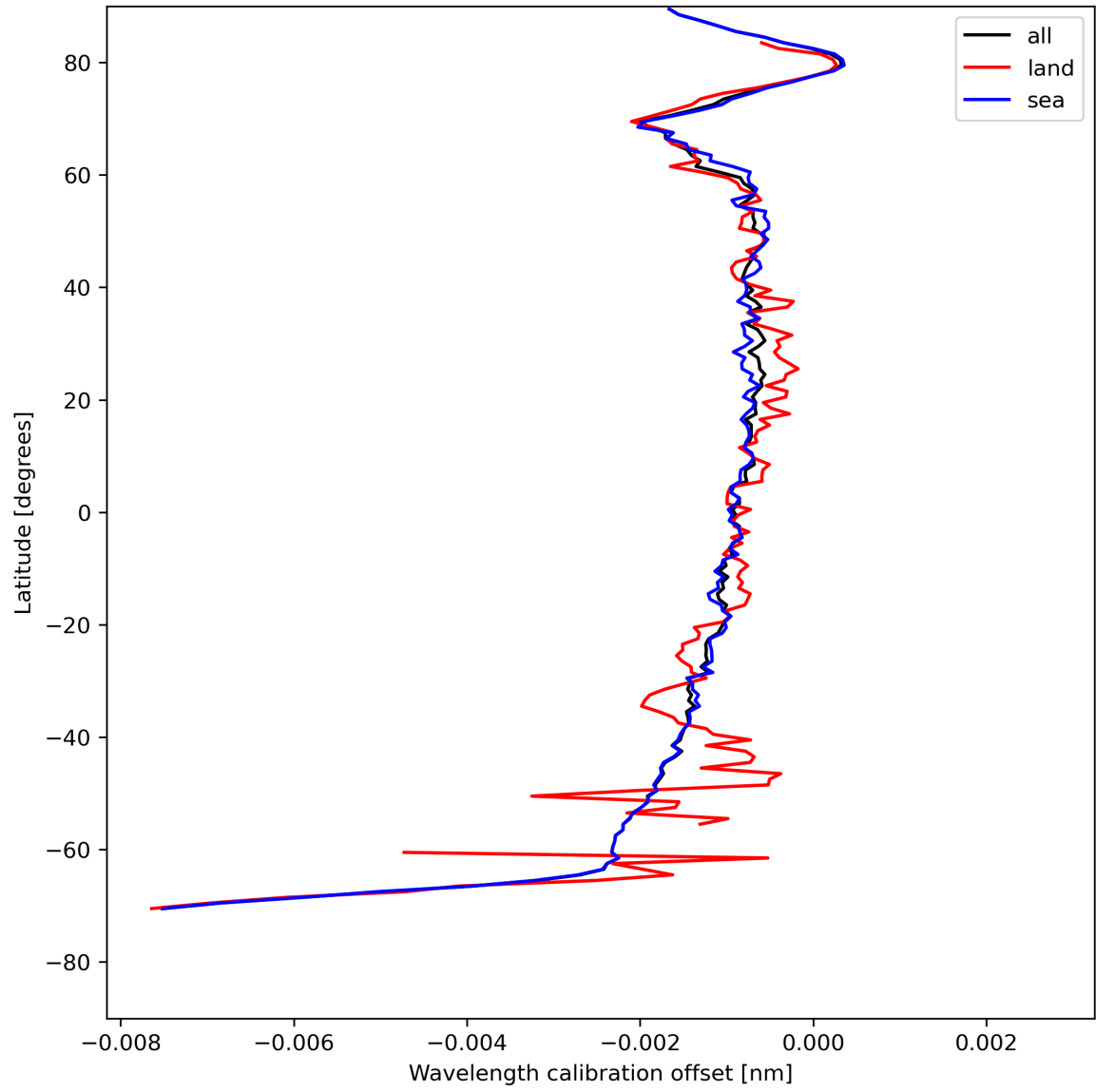
Figure 18: Zonal average of “Wavelength calibration offset” for 2023-08-04 to 2023-08-06.
