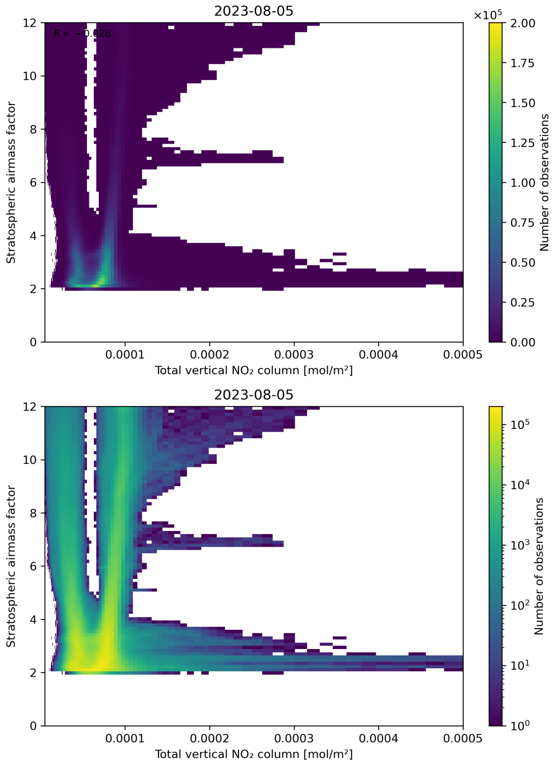
Figure 110: Scatter density plot of “Total vertical NO 2 column” against “Stratospheric air mass factor” for 2023-08-04 to 2023-08-06.
