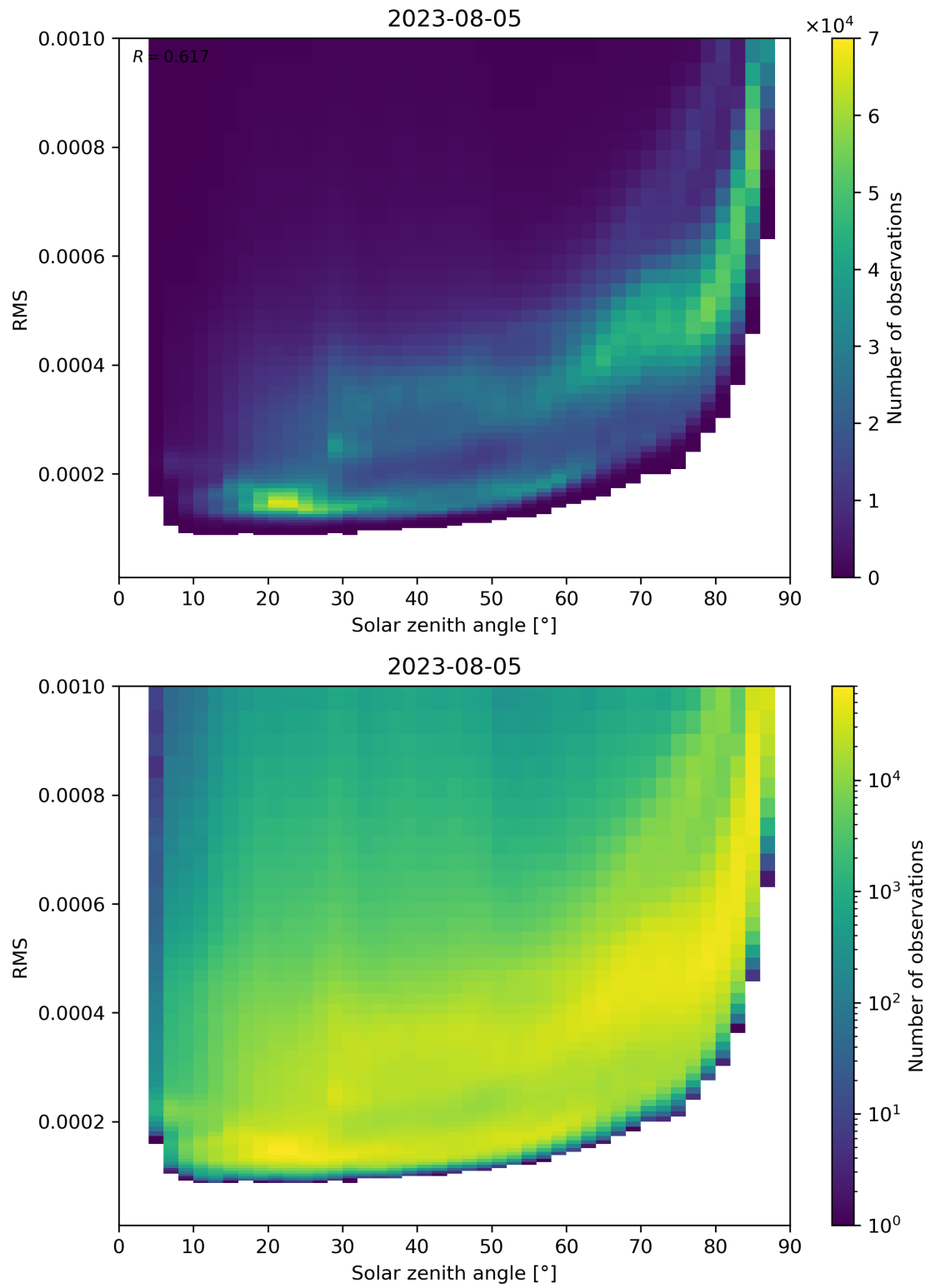
Figure 157: Scatter density plot of “Solar zenith angle” against “RMS” for 2023-08-04 to 2023-08-06.
