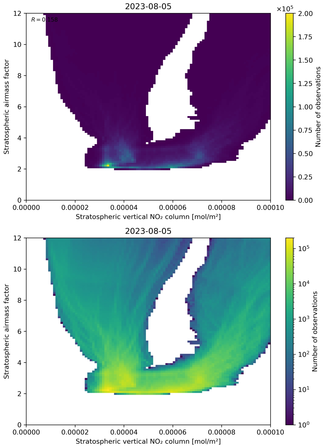
Figure 96: Scatter density plot of “Stratospheric vertical NO 2 column” against “Stratospheric airmass factor” for 2023-08-04 to 2023-08-06.
