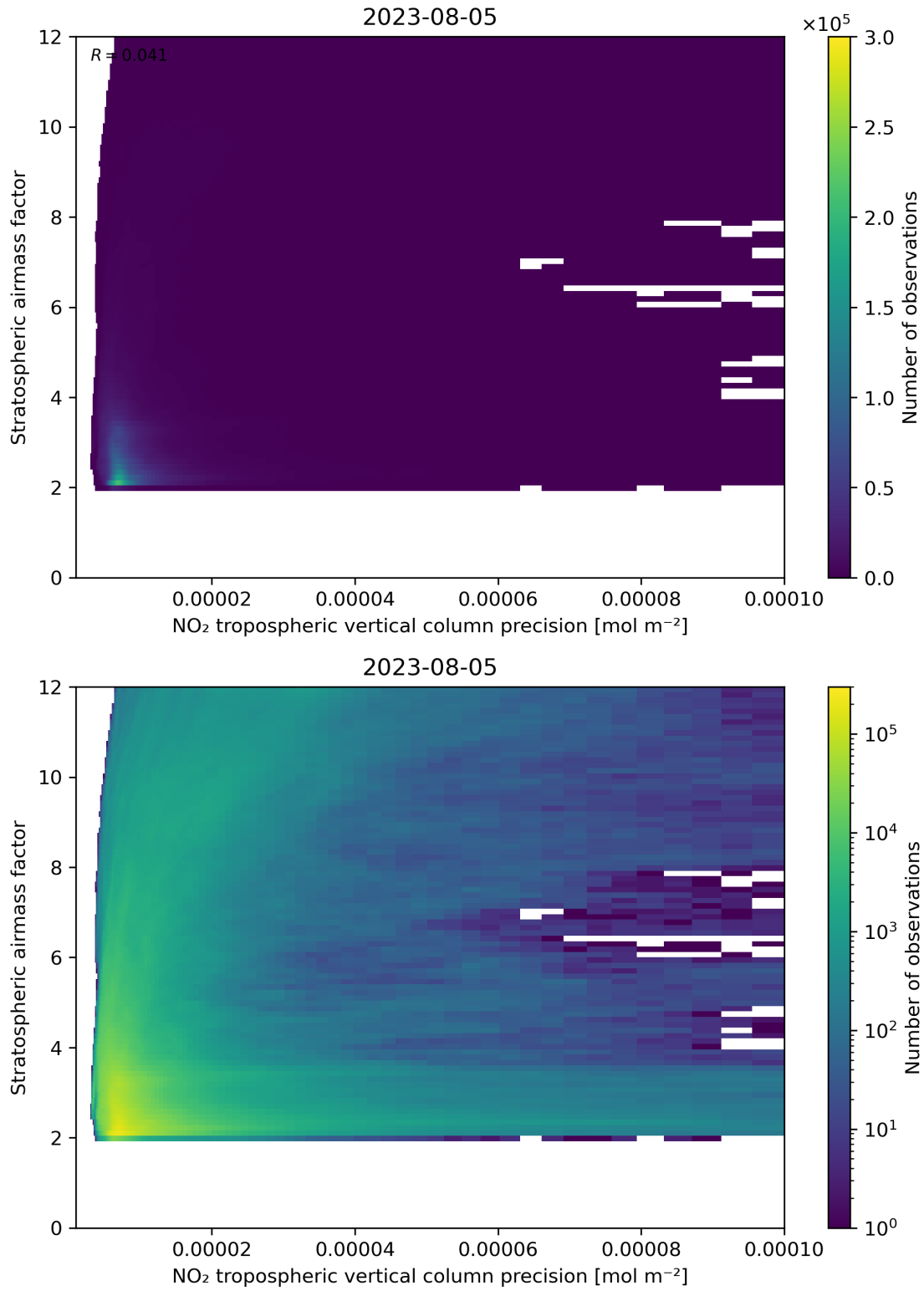
Figure 131: Scatter density plot of “NO 2 tropospheric vertical column precision” against “Stratospheric airmass factor” for 2023-08-04 to 2023-08-06.
