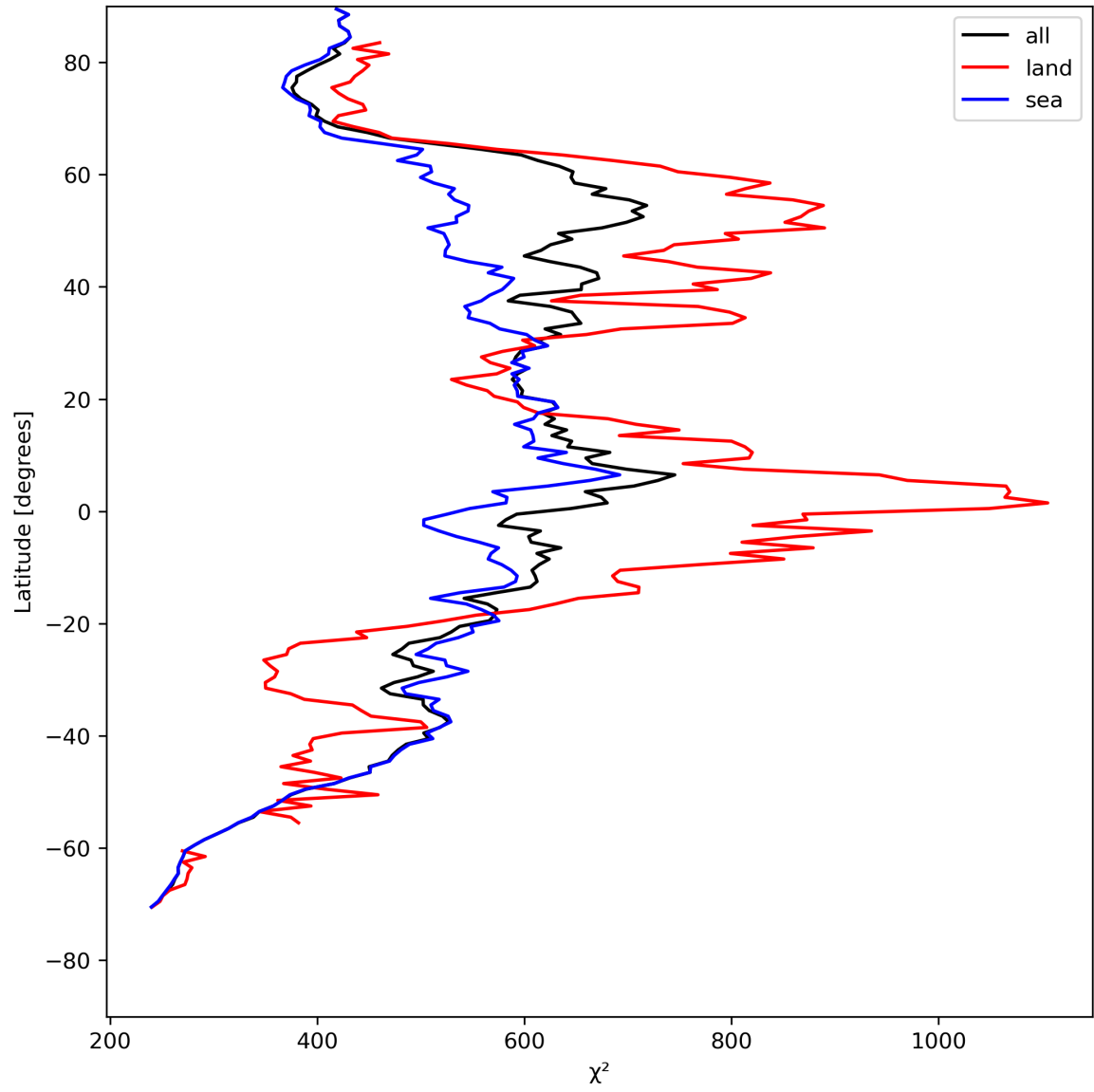
Figure 25: Zonal average of “ \chi^2 ” for 2023-08-04 to 2023-08-06.
