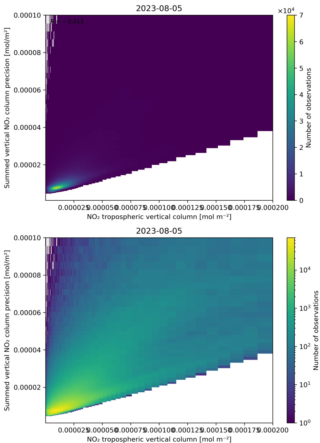
Figure 127: Scatter density plot of “NO 2 tropospheric vertical column” against “Summed vertical NO 2 column precision” for 2023-08-04 to 2023-08-06.
