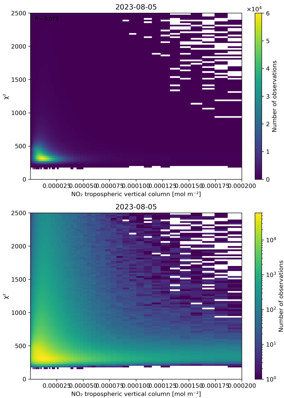
Figure 124: Scatter density plot of “NO 2 tropospheric vertical column” against “ \chi^2 ” for 2023-08-04 to 2023-08-06.
