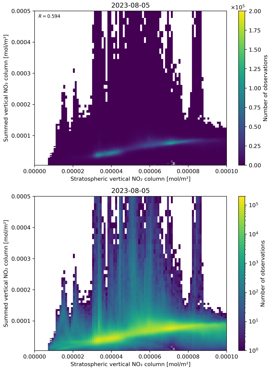
Figure 98: Scatter density plot of “Stratospheric vertical NO 2 column” against “Summed vertical NO 2 column” for 2023-08-04 to 2023-08-06.
