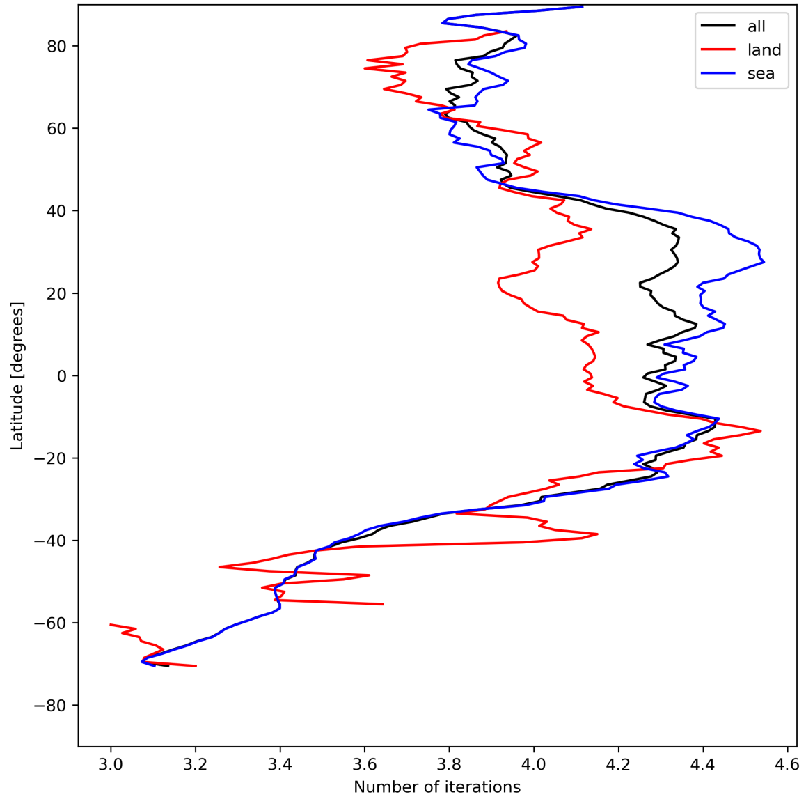
Figure 17: Zonal average of “Number of iterations” for 2023-08-04 to 2023-08-06.
