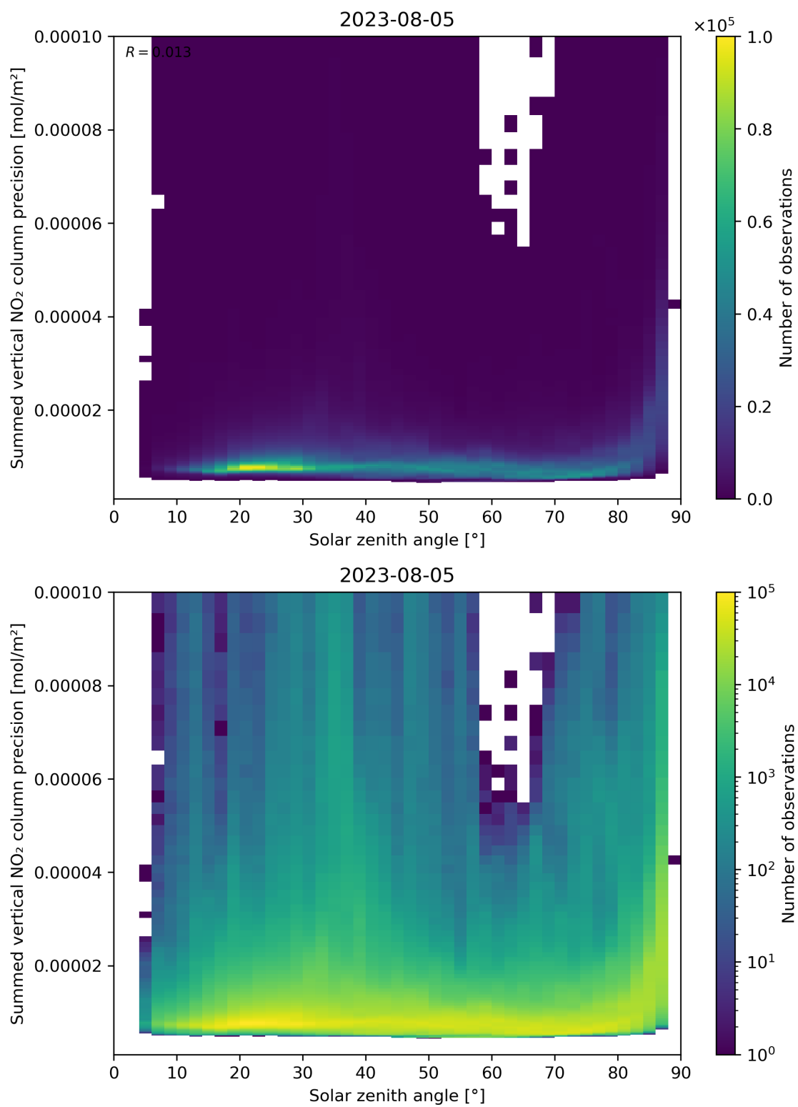
Figure 152: Scatter density plot of “Solar zenith angle” against “Summed vertical NO 2 column precision” for 2023-08-04 to 2023-08-06.
