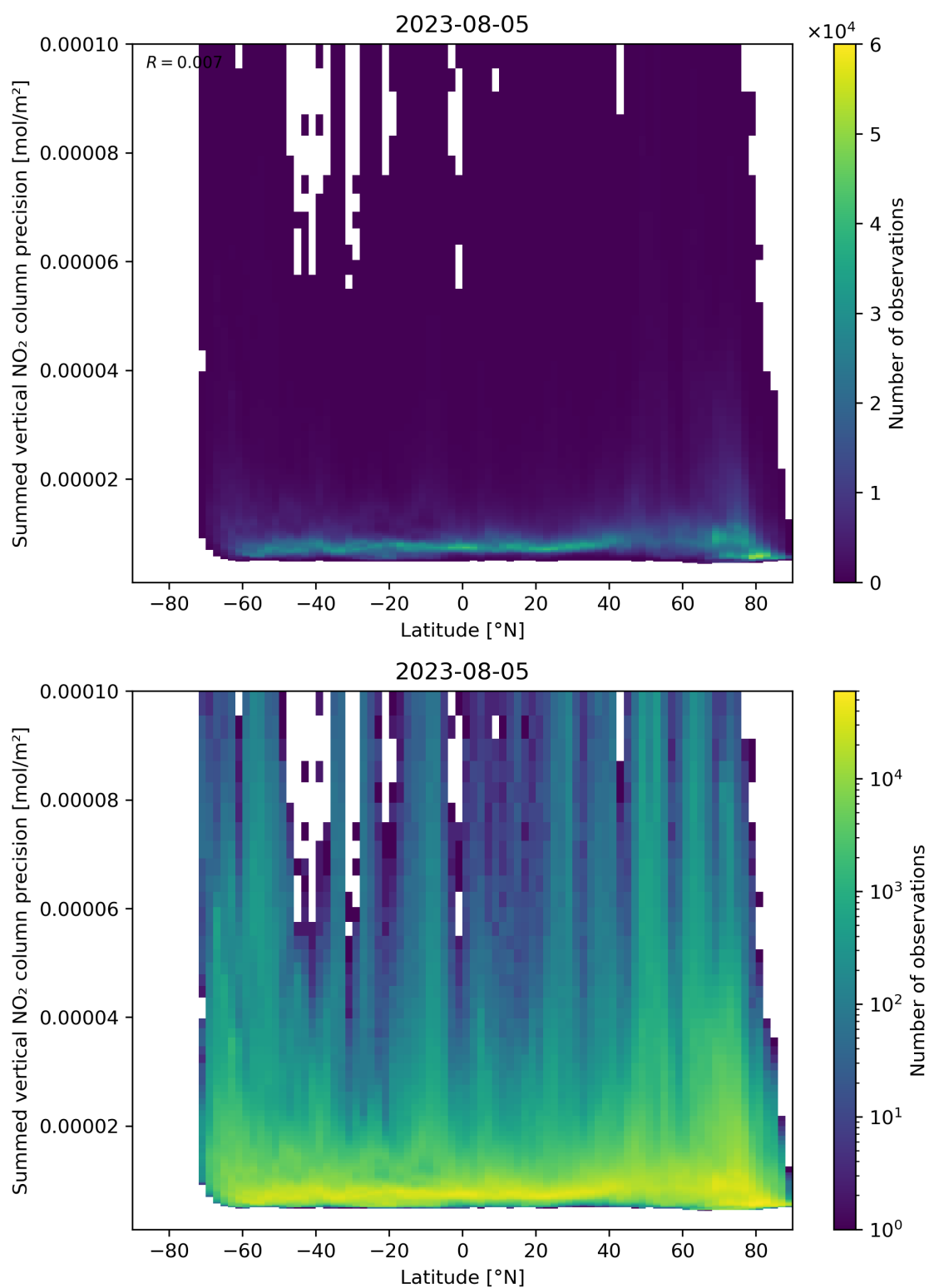
Figure 89: Scatter density plot of “Latitude” against “Summed vertical NO 2 column precision” for 2023-08-04 to 2023-08-06.
