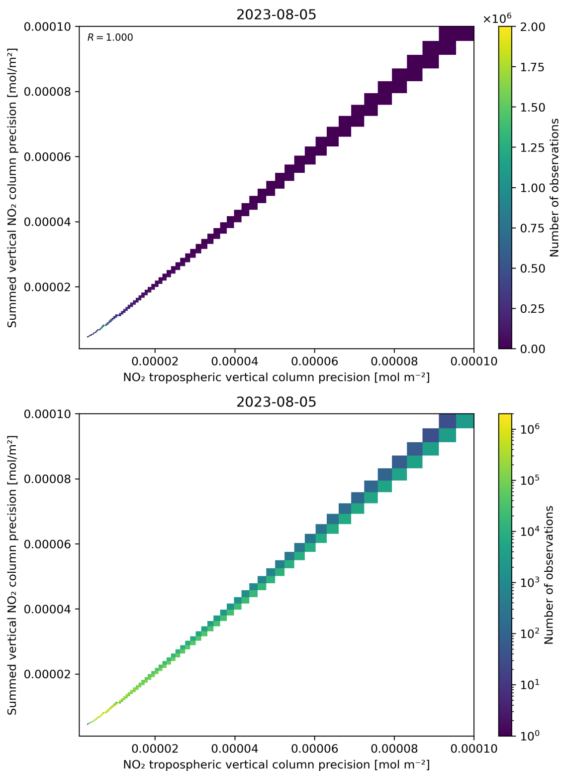
Figure 137: Scatter density plot of “NO 2 tropospheric vertical column precision” against “Summed vertical NO 2 column precision” for 2023-08-04 to 2023-08-06.
