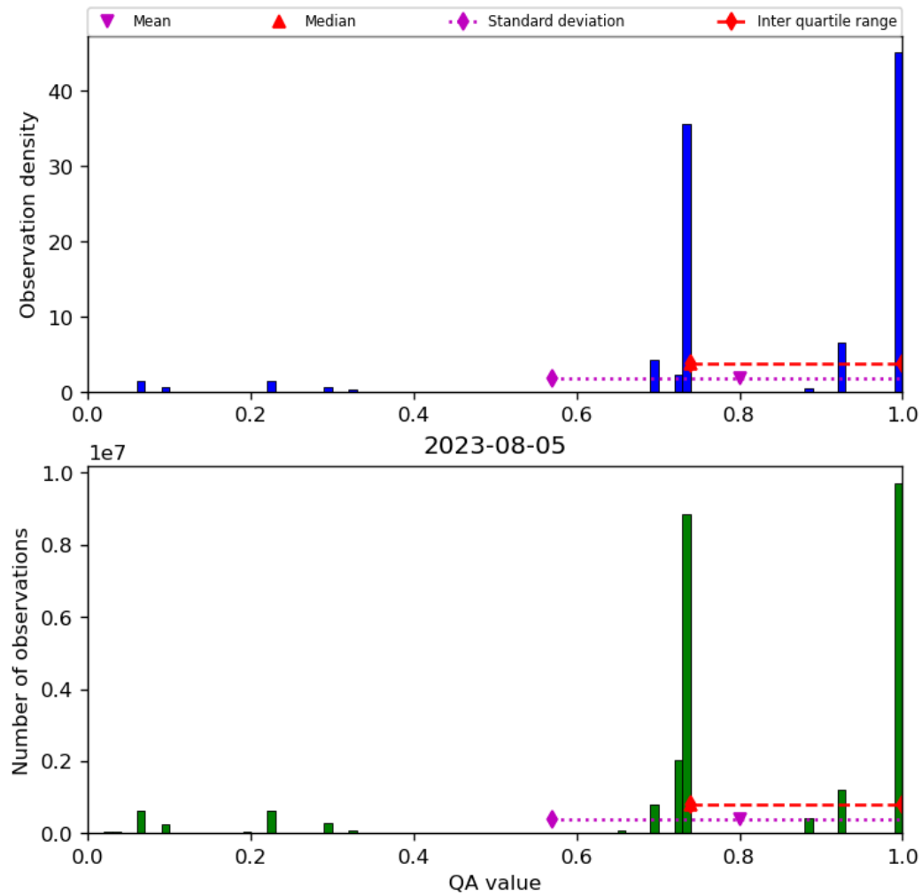
Figure 28: Histogram of “QA value” for 2023-08-04 to 2023-08-06
