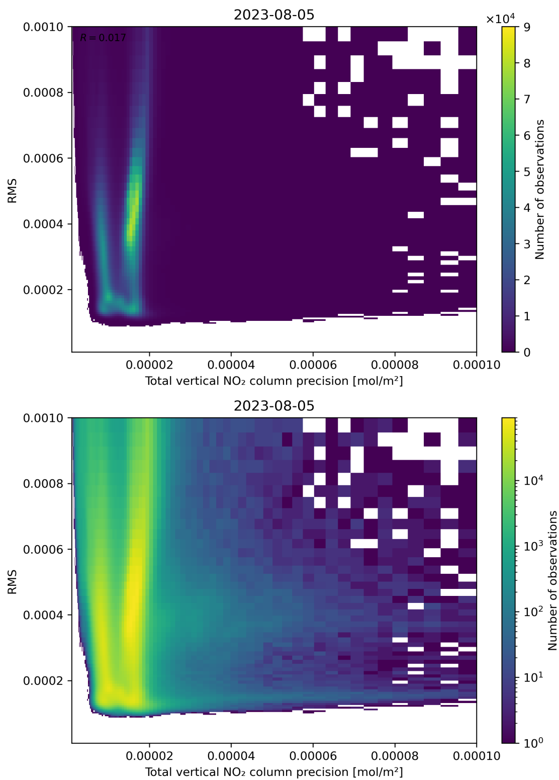
Figure 119: Scatter density plot of “Total vertical NO 2 column precision” against “RMS” for 2023-08-04 to 2023-08-06.
