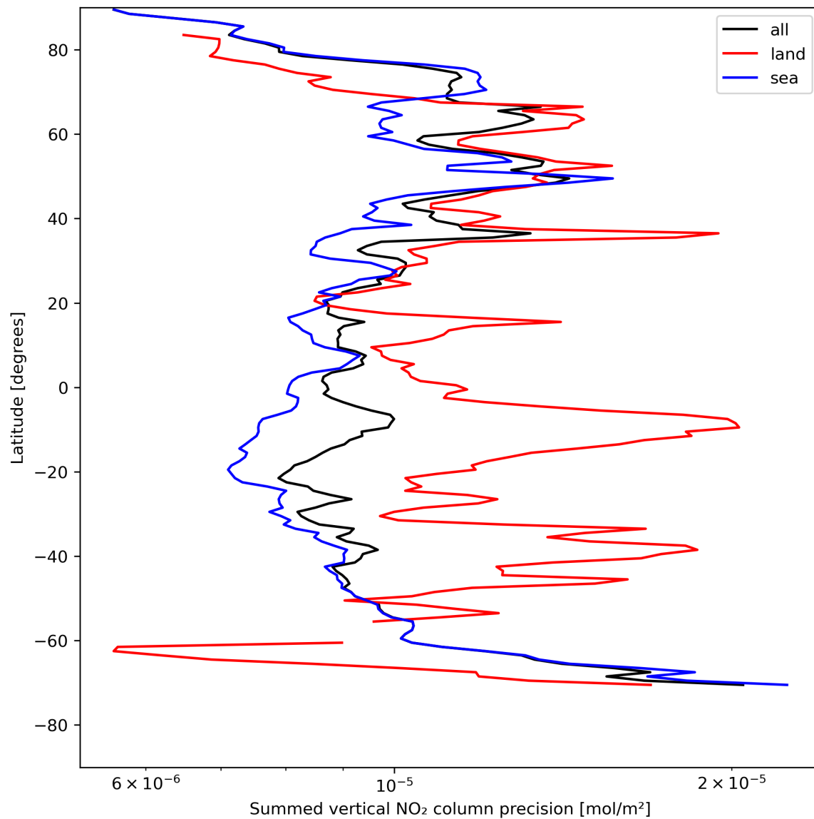
Figure 24: Zonal average of “Summed vertical NO 2 column precision” for 2023-08-04 to 2023-08-06.
