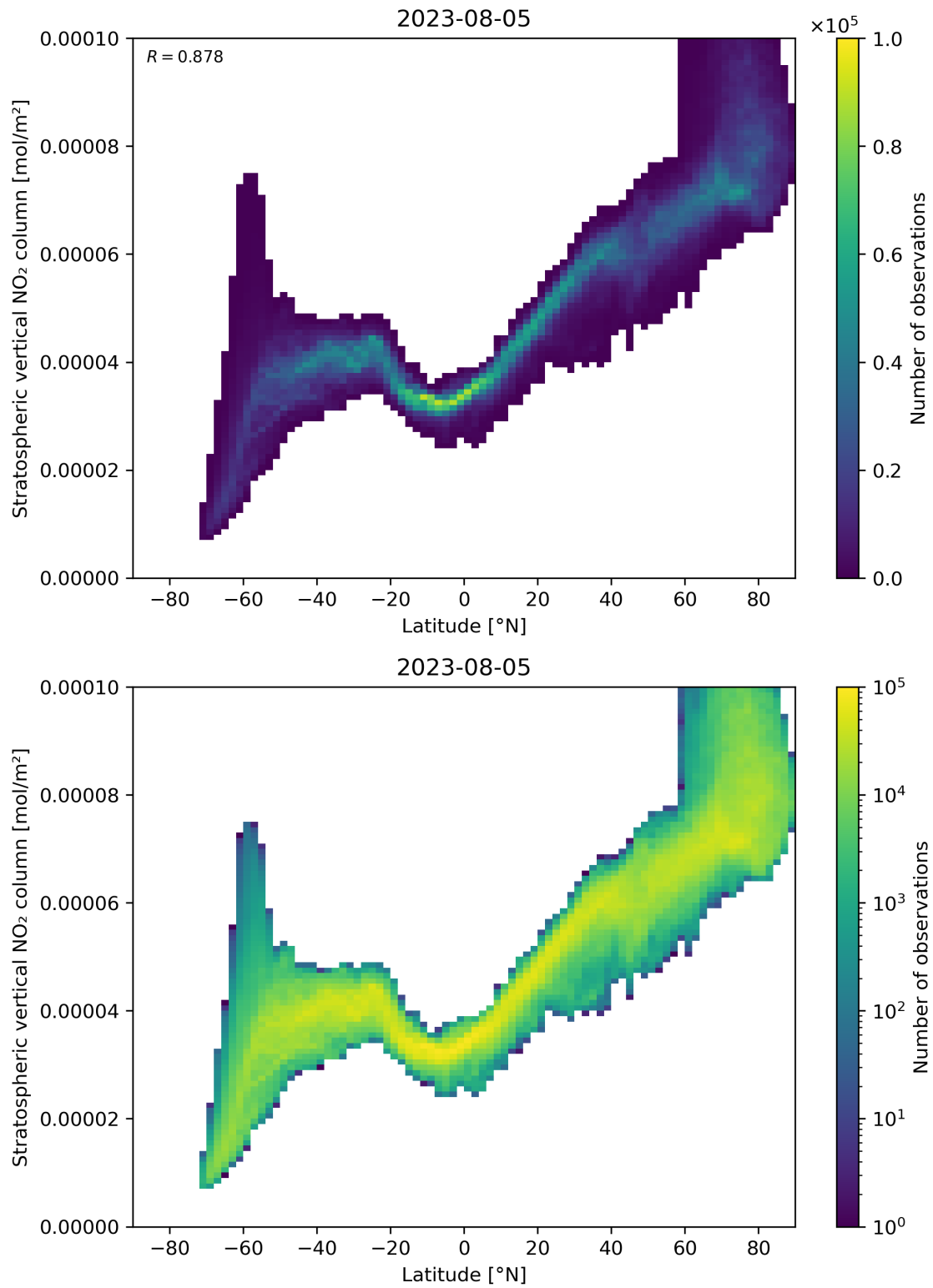
Figure 87: Scatter density plot of “Latitude” against “Stratospheric vertical NO 2 column” for 2023-08-04 to 2023-08-06.
