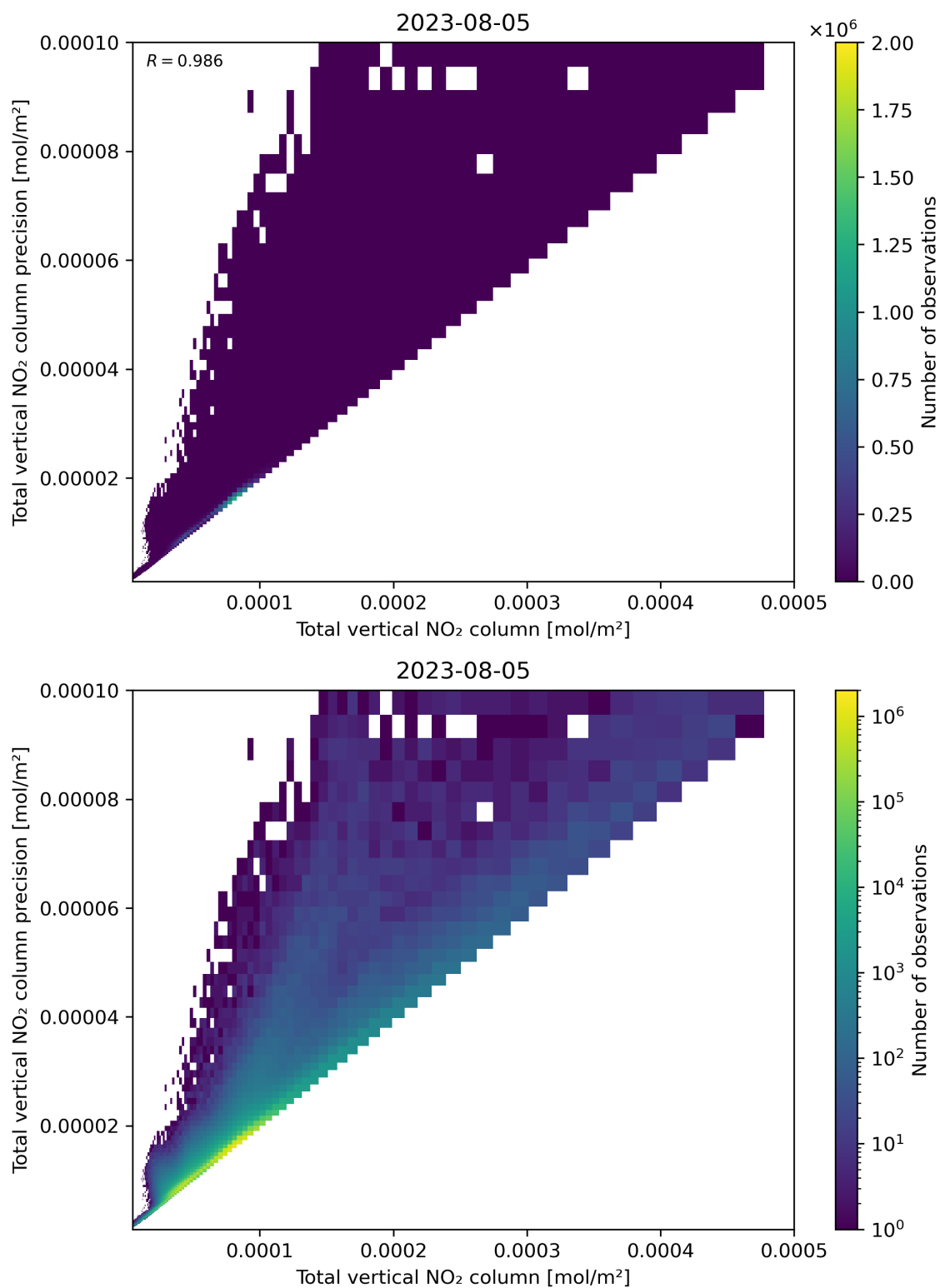
Figure 114: Scatter density plot of “Total vertical NO 2 column” against “Total vertical NO 2 column precision” for 2023-08-04 to 2023-08-06.
