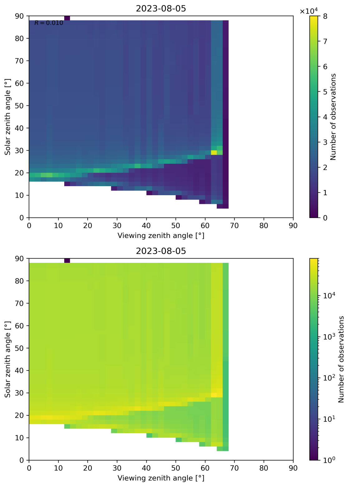
Figure 172: Scatter density plot of “Viewing zenith angle” against “Solar zenith angle” for 2023-08-04 to 2023-08-06.
