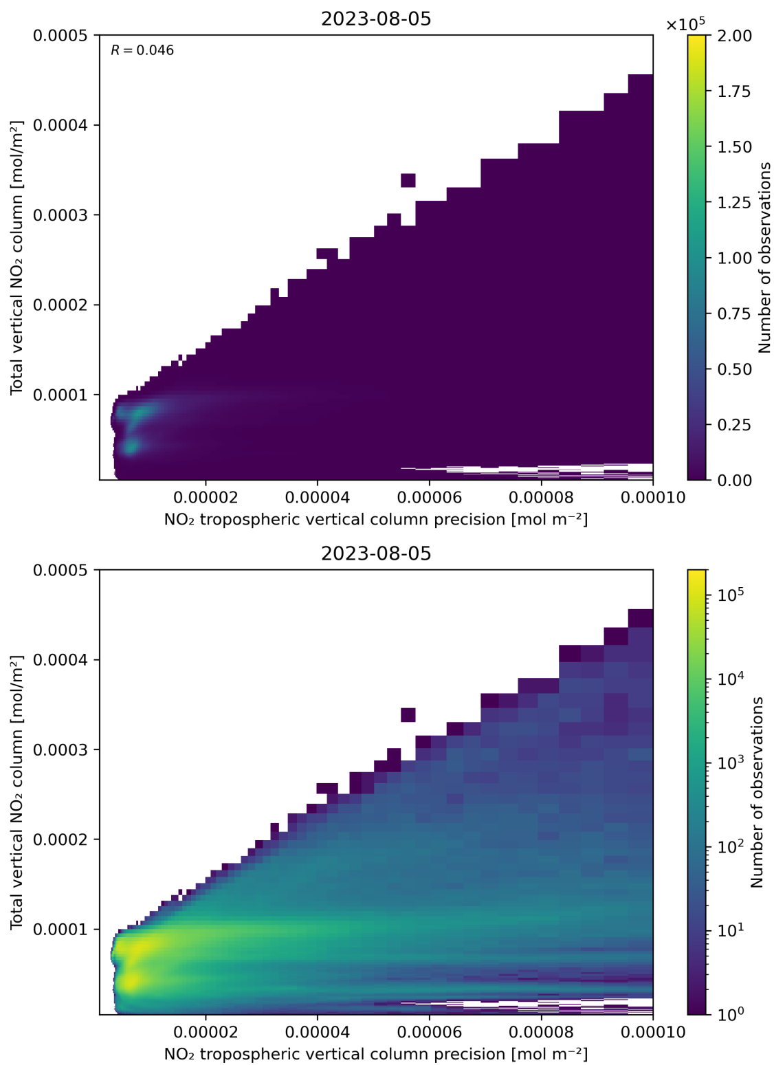
Figure 138: Scatter density plot of “NO 2 tropospheric vertical column precision” against “Total vertical NO 2 column” for 2023-08-04 to 2023-08-06.
