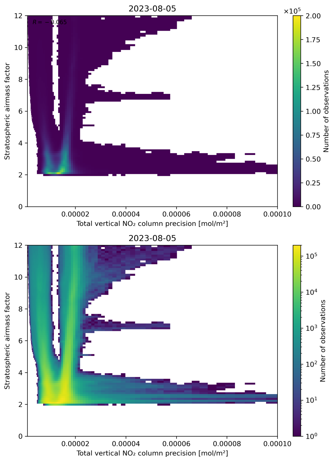
Figure 115: Scatter density plot of “Total vertical NO 2 column precision” against “Stratospheric air mass factor” for 2023-08-04 to 2023-08-06.
