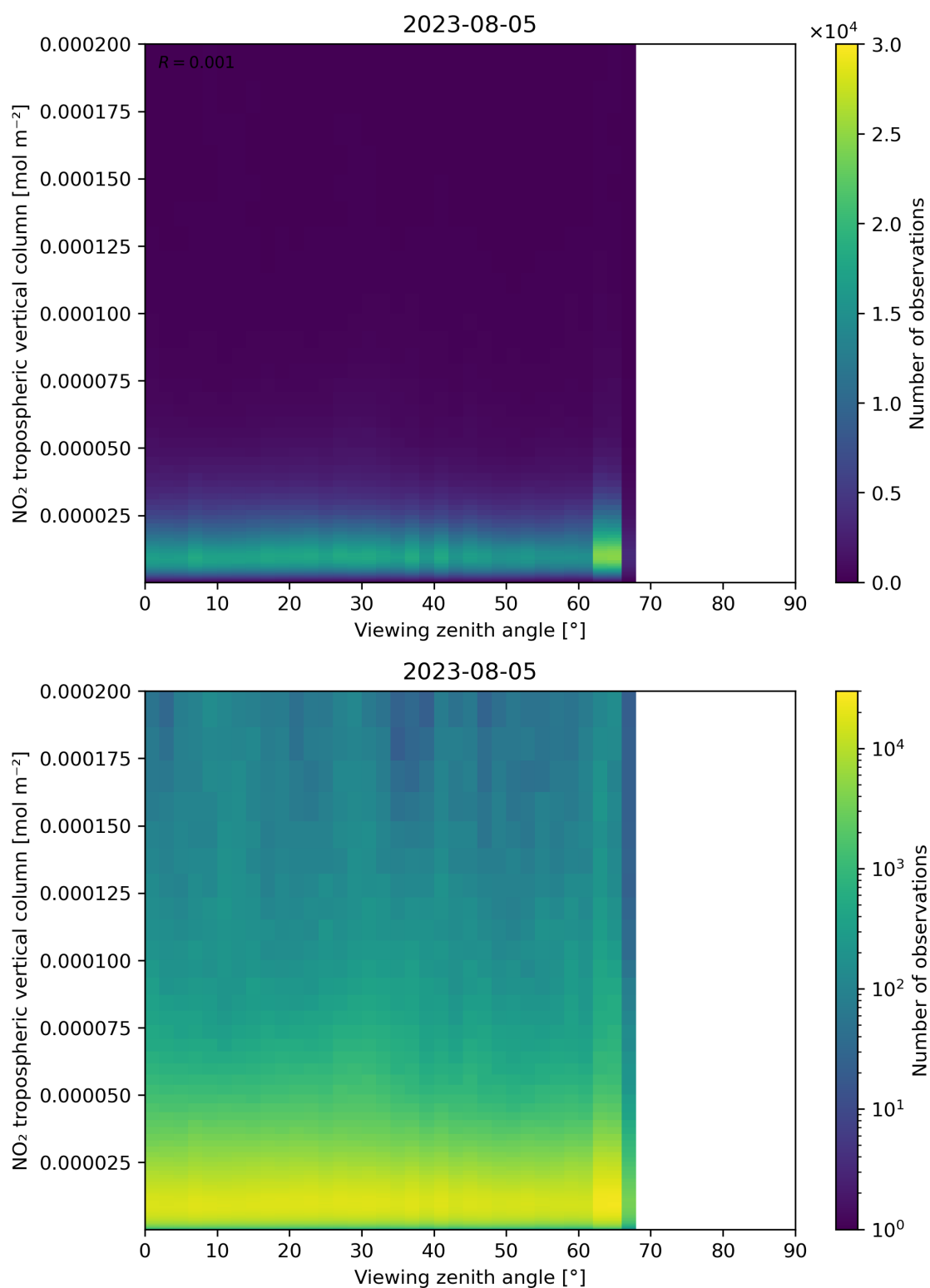
Figure 169: Scatter density plot of “Viewing zenith angle” against “NO 2 tropospheric vertical column” for 2023-08-04 to 2023-08-06.
