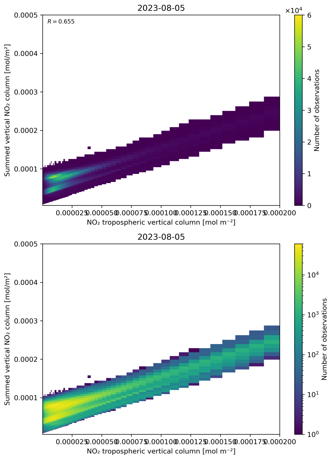
Figure 126: Scatter density plot of “NO 2 tropospheric vertical column” against “Summed vertical NO 2 column” for 2023-08-04 to 2023-08-06.
