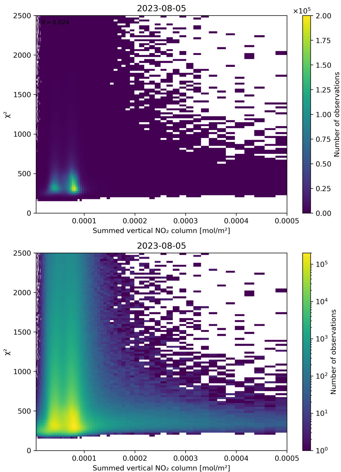
Figure 104: Scatter density plot of “Summed vertical NO 2 column” against “ \chi^2 ” for 2023-08-04 to 2023-08-06.
