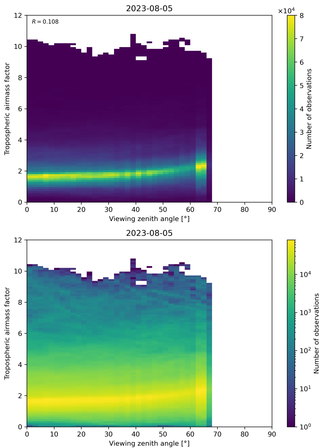
Figure 161: Scatter density plot of “Viewing zenith angle” against “Tropospheric airmass factor” for 2023-08-04 to 2023-08-06.
