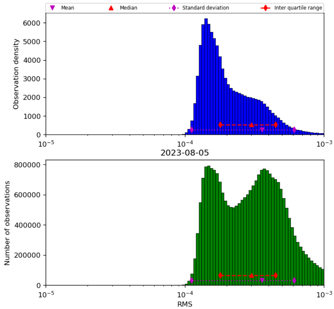
Figure 43: Histogram of “RMS” for 2023-08-04 to 2023-08-06
