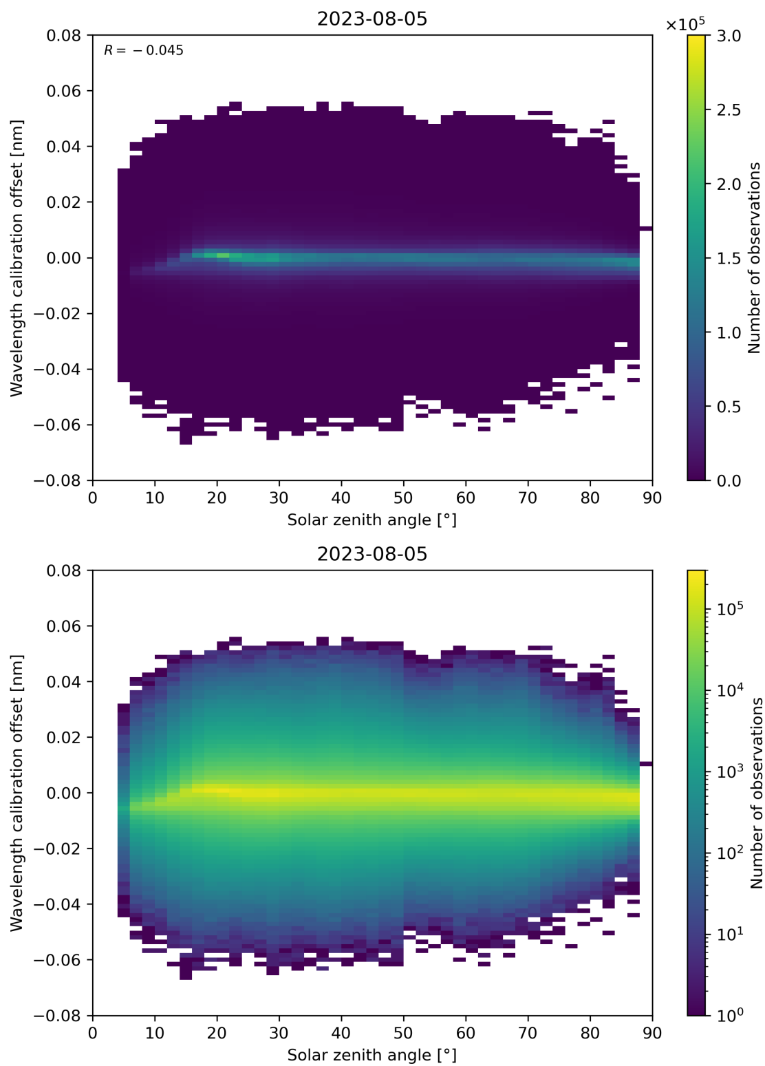
Figure 158: Scatter density plot of “Solar zenith angle” against “Wavelength calibration offset” for 2023-08-04 to 2023-08-06.
