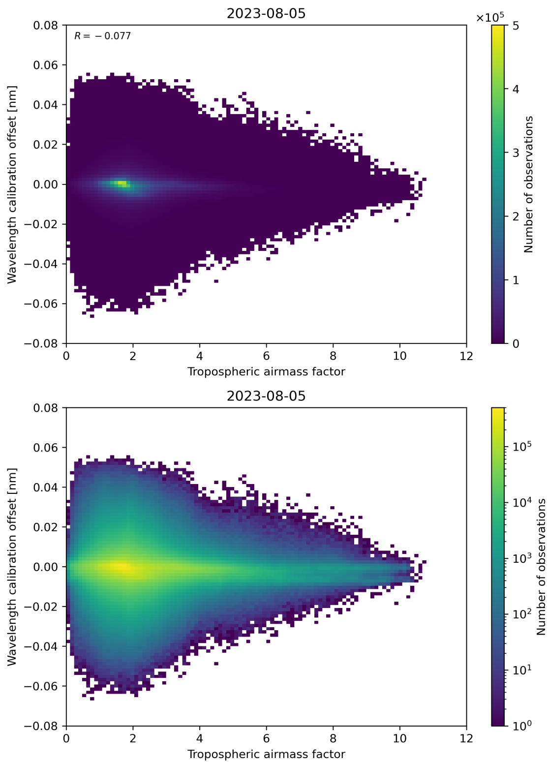
Figure 80: Scatter density plot of “Tropospheric air mass factor” against “Wavelength calibration offset” for 2023-08-04 to 2023-08-06.
