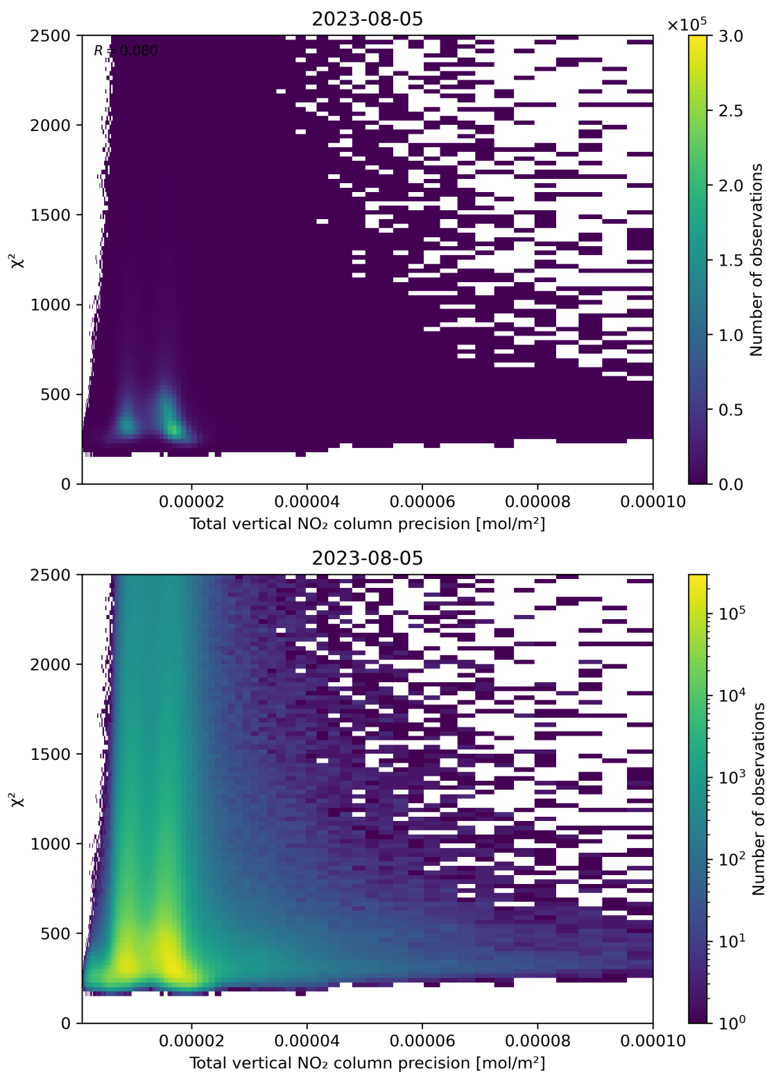
Figure 116: Scatter density plot of “Total vertical NO 2 column precision” against “ \chi^2 ” for 2023-08-04 to 2023-08-06.
