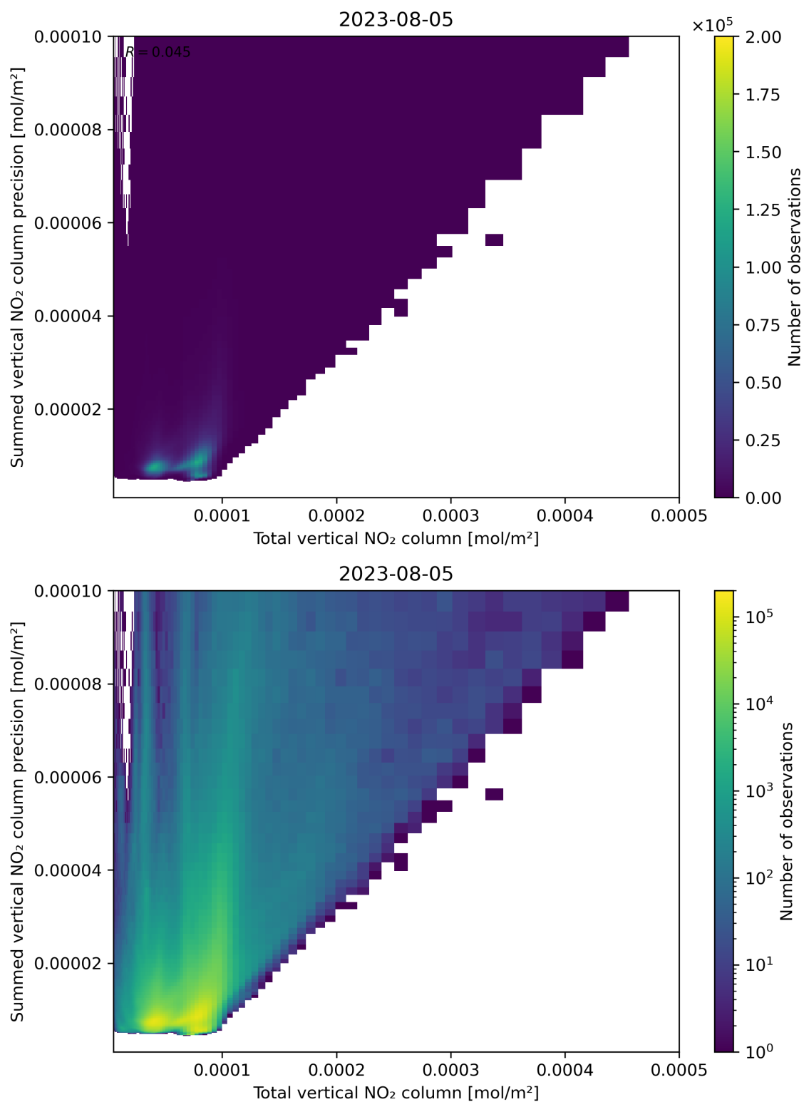
Figure 113: Scatter density plot of “Total vertical NO 2 column” against “Summed vertical NO 2 column precision” for 2023-08-04 to 2023-08-06.
