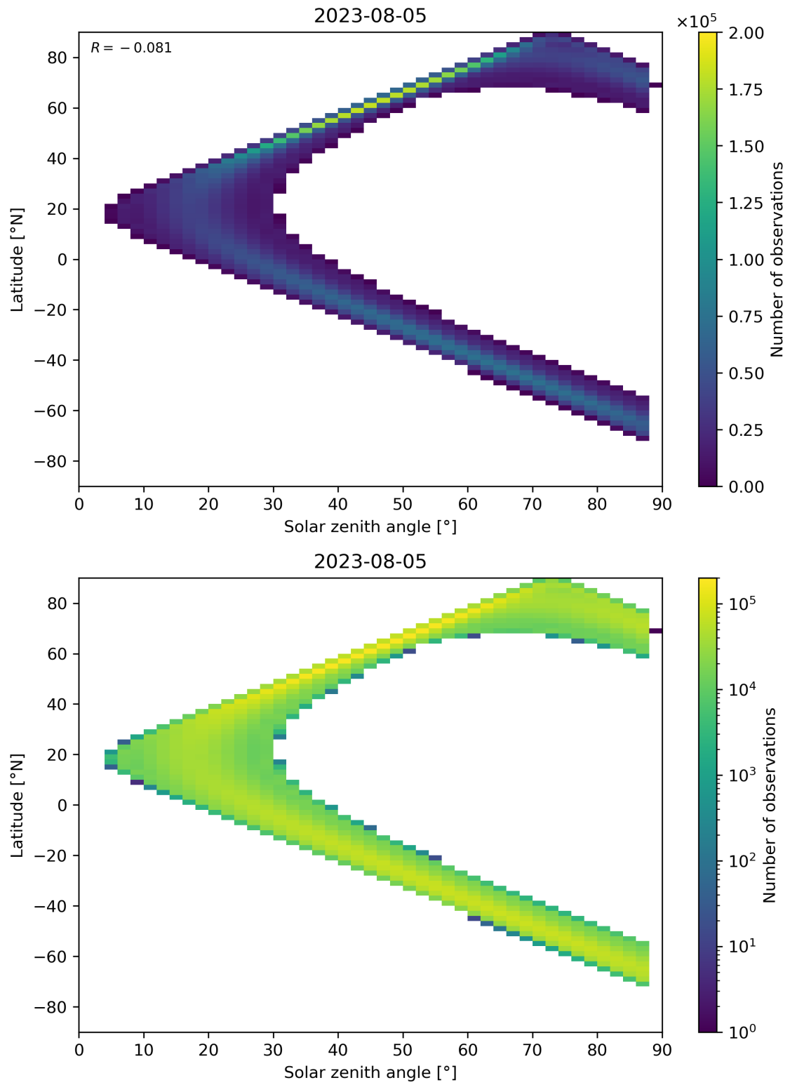
Figure 149: Scatter density plot of “Solar zenith angle” against “Latitude” for 2023-08-04 to 2023-08-06.
