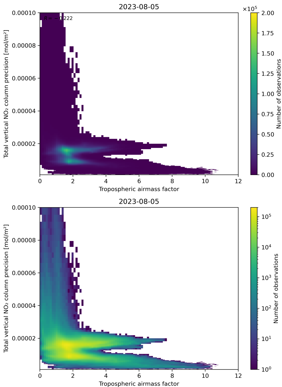
Figure 78: Scatter density plot of “Tropospheric air mass factor” against “Total vertical NO 2 column precision” for 2023-08-04 to 2023-08-06.
