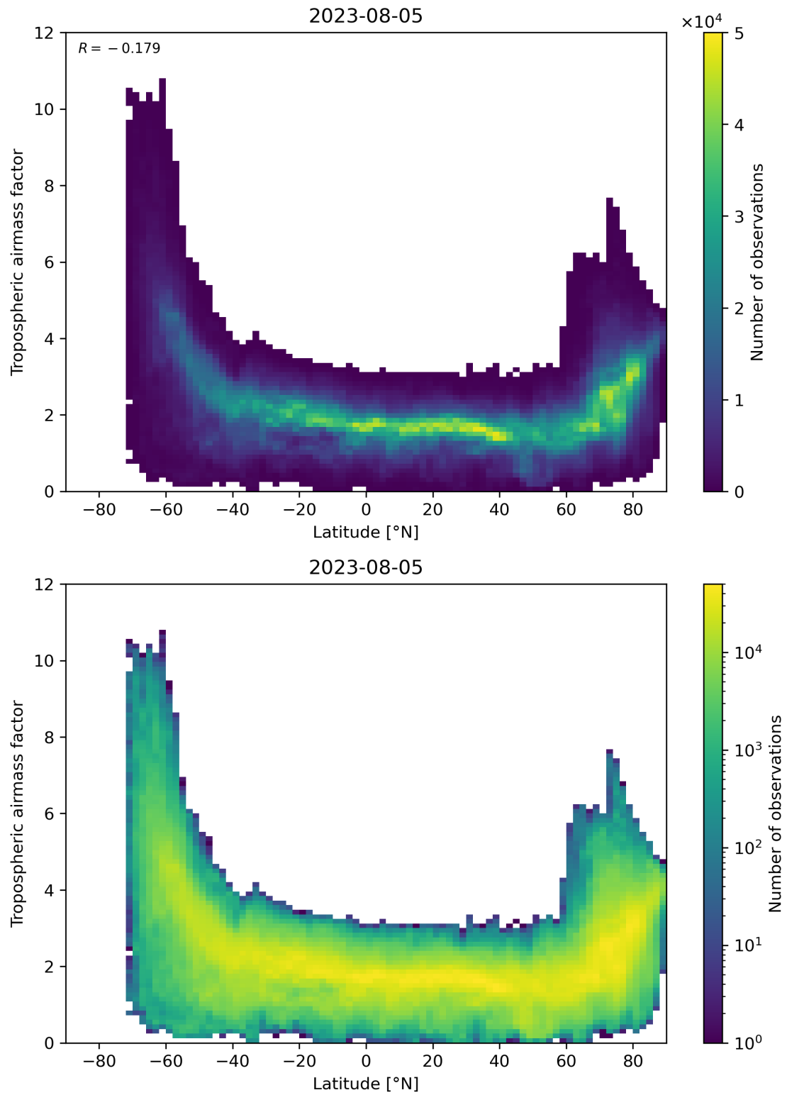
Figure 85: Scatter density plot of “Latitude” against “Tropospheric airmass factor” for 2023-08-04 to 2023-08-06.
