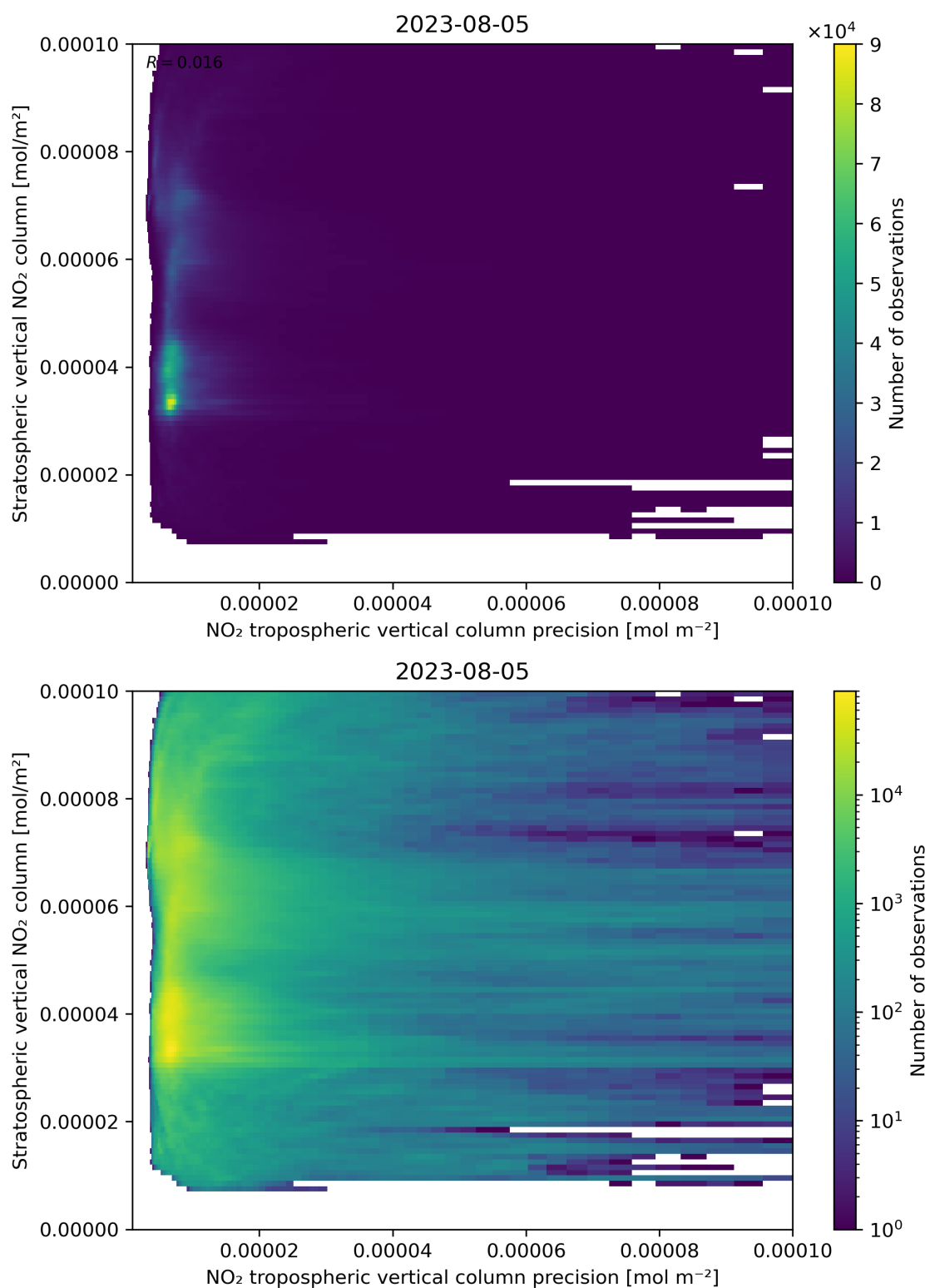
Figure 135: Scatter density plot of “NO 2 tropospheric vertical column precision” against “Stratospheric vertical NO 2 column” for 2023-08-04 to 2023-08-06.
