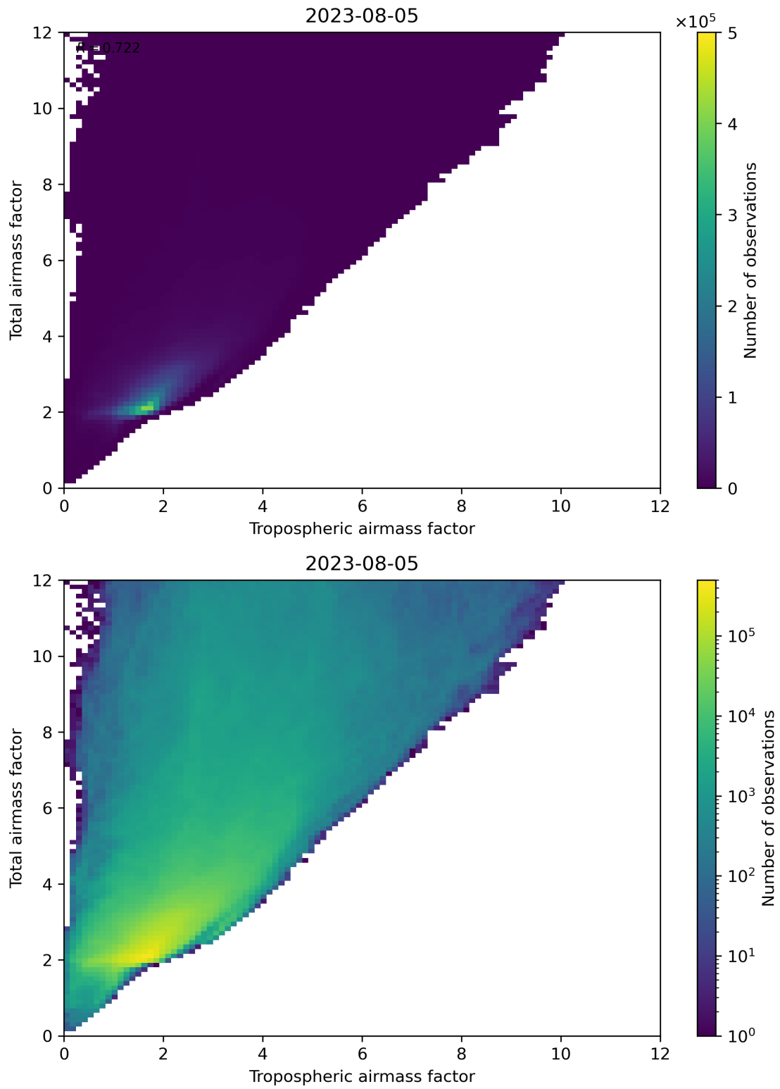
Figure 72: Scatter density plot of “Tropospheric airmass factor” against “Total airmass factor” for 2023-08-04 to 2023-08-06.
