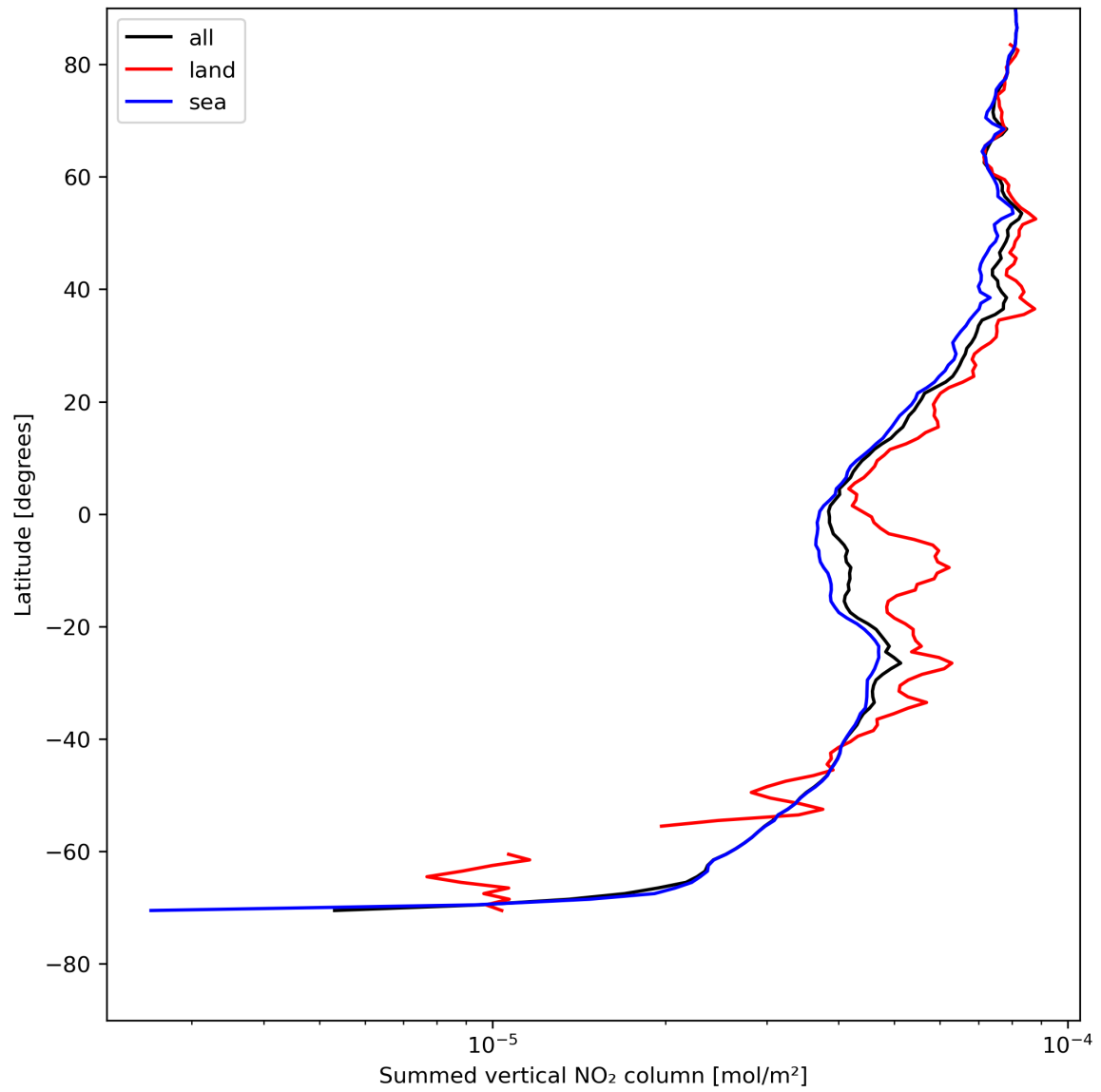
Figure 23: Zonal average of “Summed vertical NO 2 column” for 2023-08-04 to 2023-08-06.
