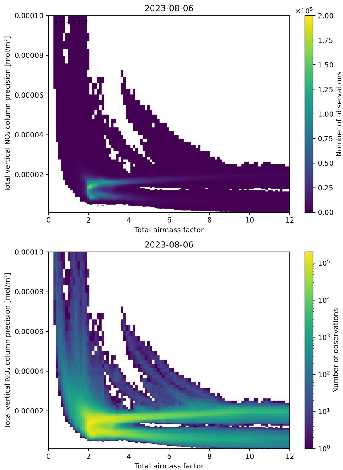
Figure 68: Scatter density plot of “Total airmass factor” against “Total vertical NO 2 column precision” for 2023-08-05 to 2023-08-07.
