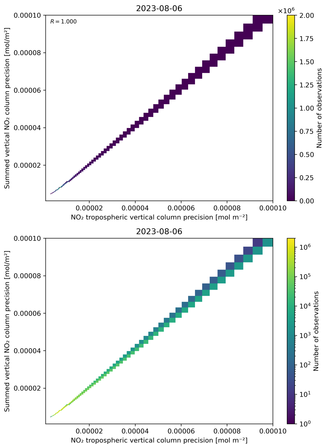
Figure 137: Scatter density plot of “NO 2 tropospheric vertical column precision” against “Summed vertical NO 2 column precision” for 2023-08-05 to 2023-08-07.
