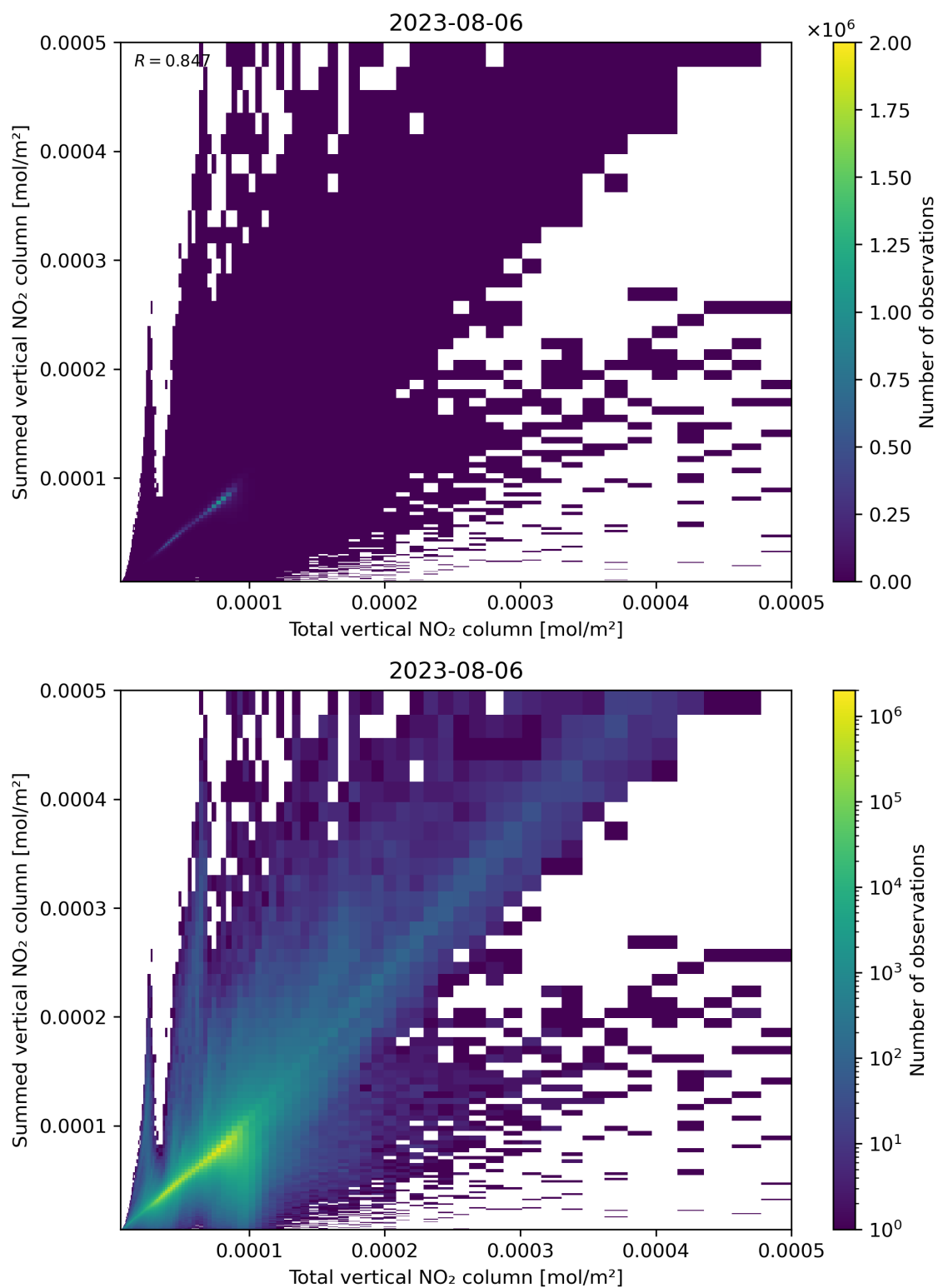
Figure 112: Scatter density plot of “Total vertical NO 2 column” against “Summed vertical NO 2 column” for 2023-08-05 to 2023-08-07.
