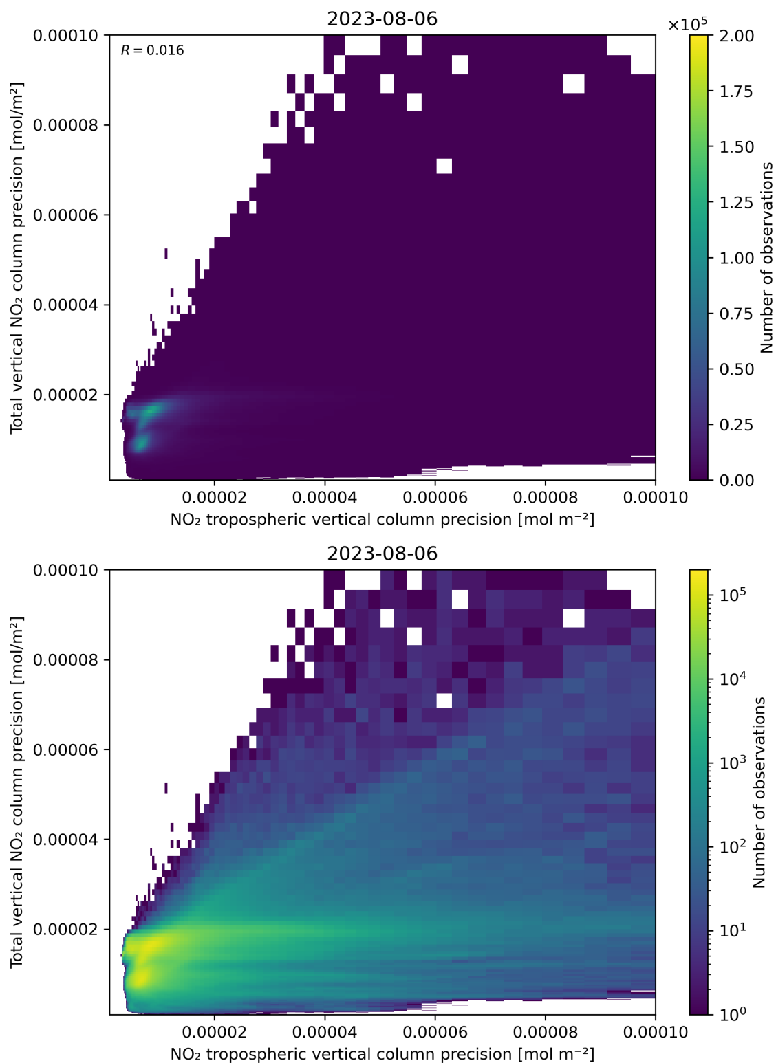
Figure 139: Scatter density plot of “NO 2 tropospheric vertical column precision” against “Total vertical NO 2 column precision” for 2023-08-05 to 2023-08-07.
