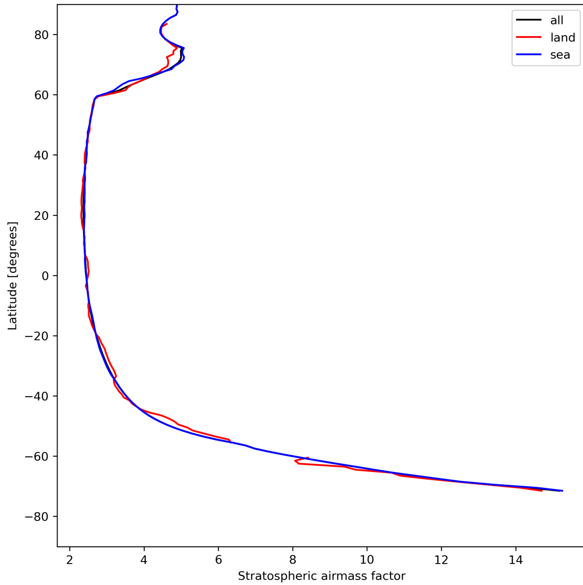
Figure 27: Zonal average of “Stratospheric airmass factor” for 2023-08-05 to 2023-08-07.
