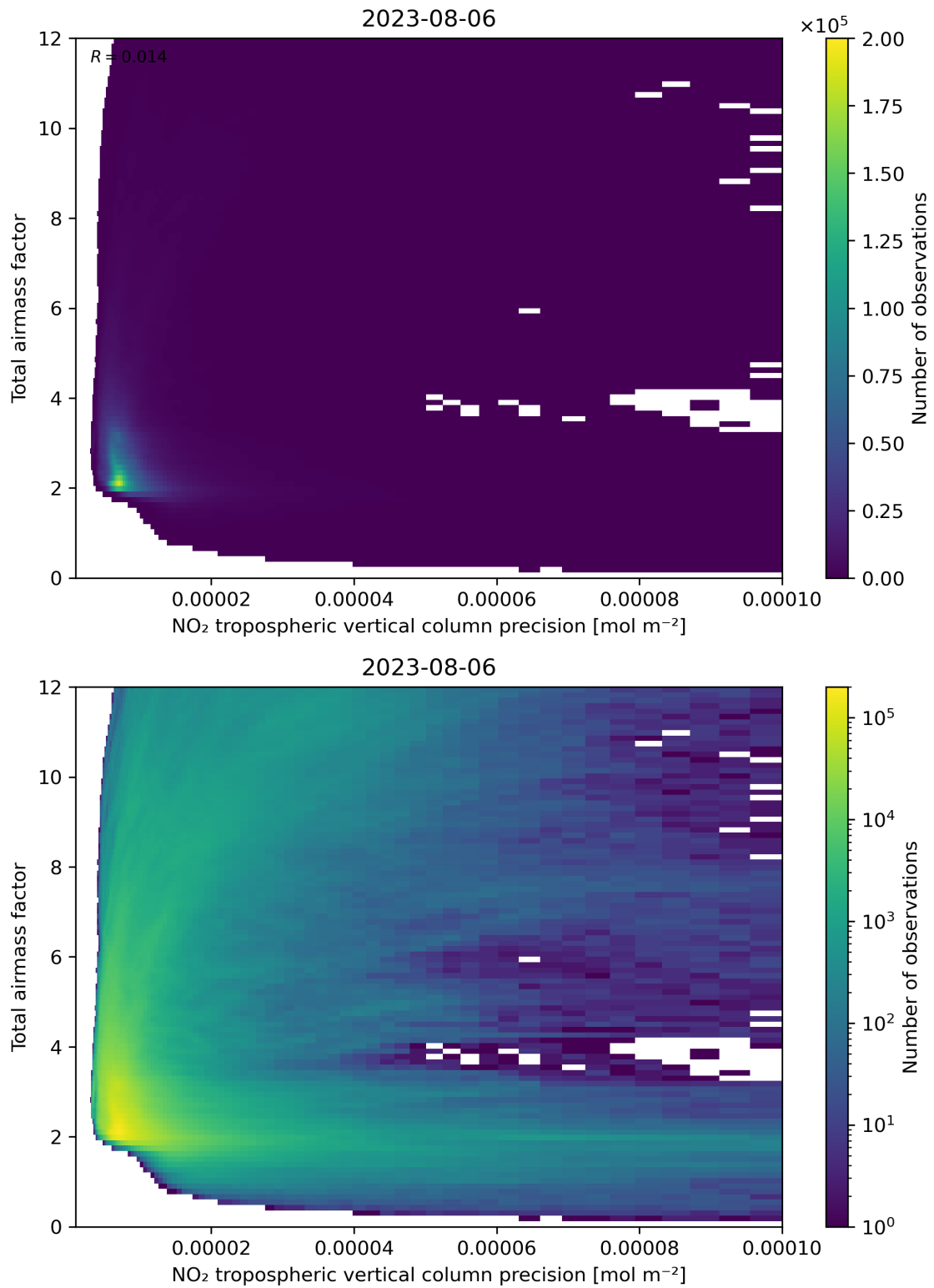
Figure 132: Scatter density plot of “NO 2 tropospheric vertical column precision” against “Total air mass factor” for 2023-08-05 to 2023-08-07.
