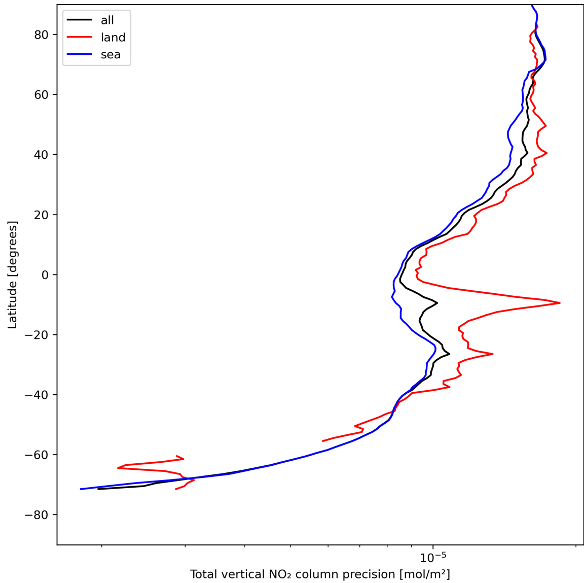
Figure 22: Zonal average of “Total vertical NO 2 column precision” for 2023-08-05 to 2023-08-07.
