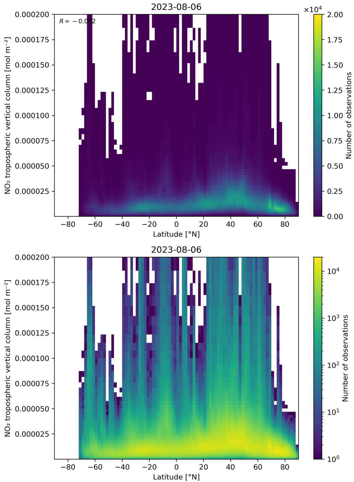
Figure 92: Scatter density plot of “Latitude” against “NO 2 tropospheric vertical column” for 2023-08-05 to 2023-08-07.
