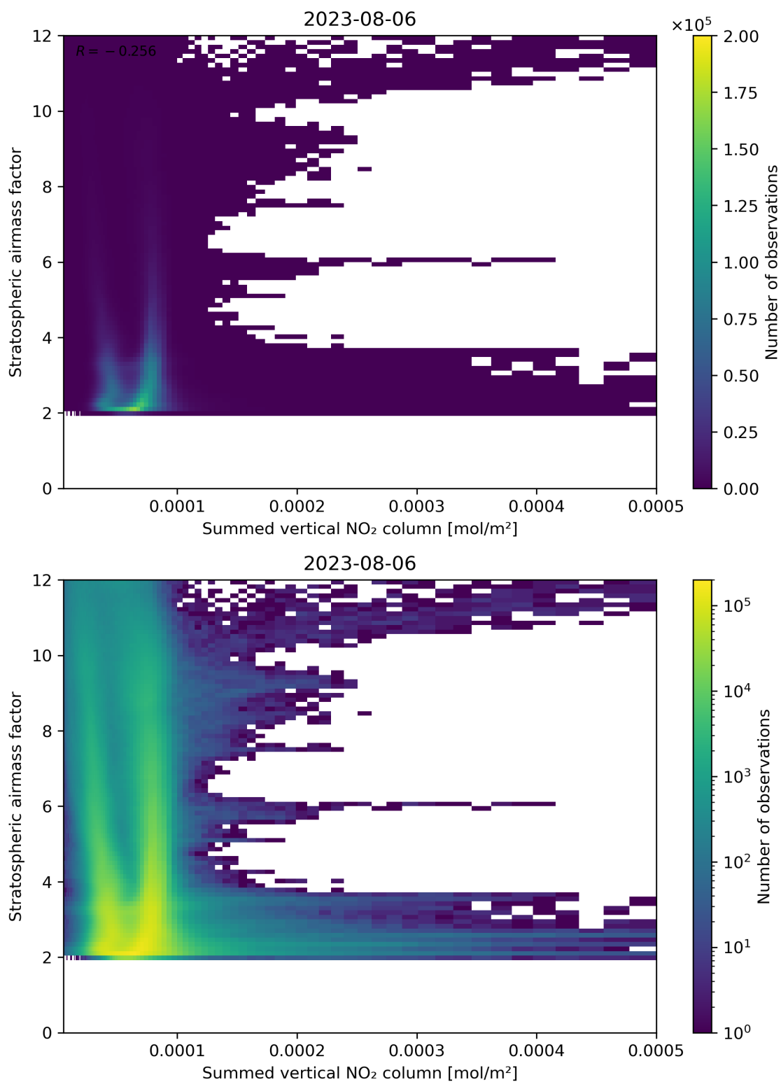
Figure 103: Scatter density plot of “Summed vertical NO 2 column” against “Stratospheric airmass factor” for 2023-08-05 to 2023-08-07.
