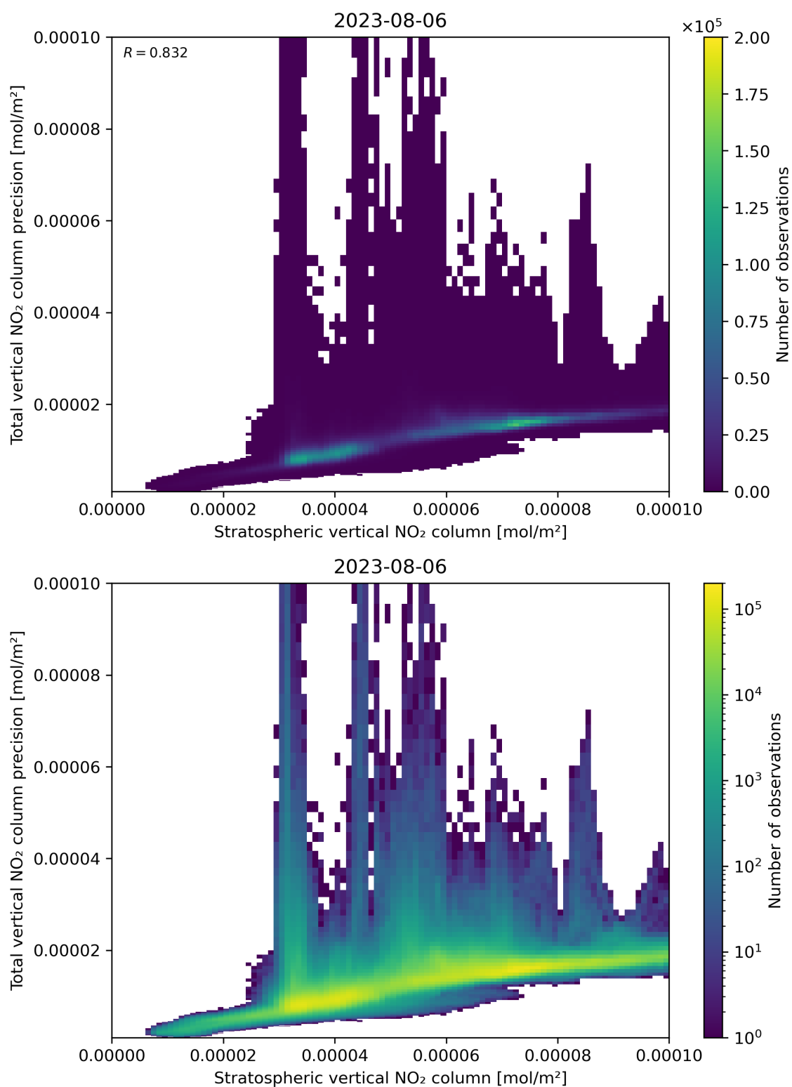
Figure 101: Scatter density plot of “Stratospheric vertical NO 2 column” against “Total vertical NO 2 column precision” for 2023-08-05 to 2023-08-07.
