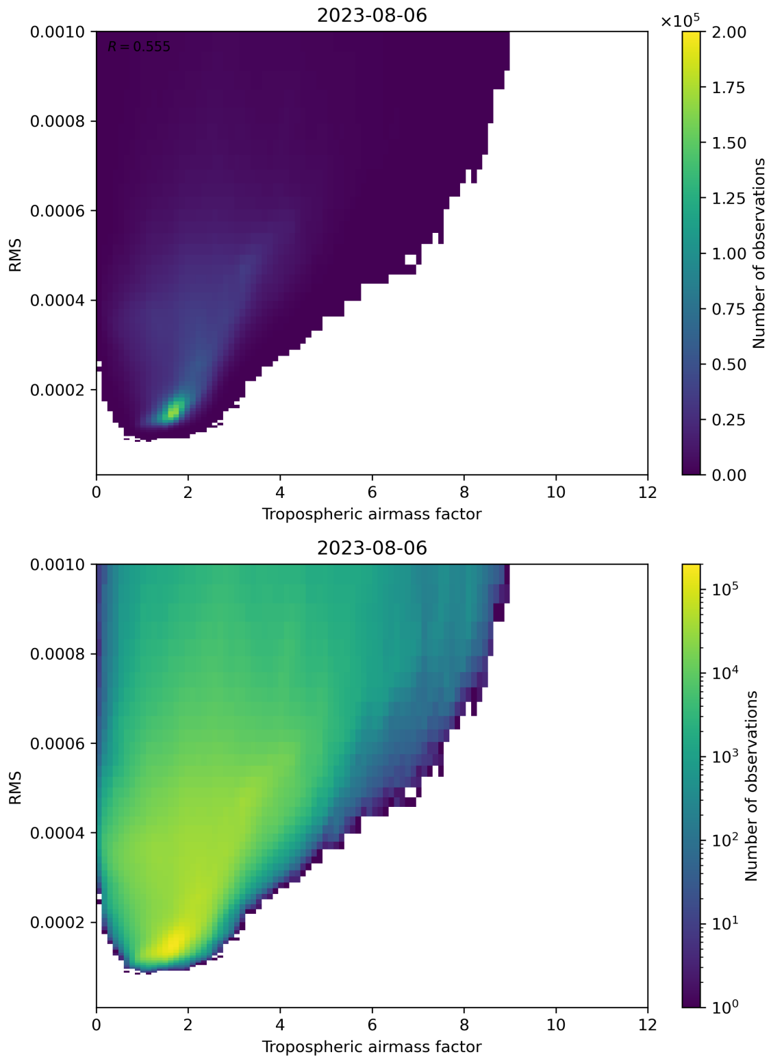
Figure 79: Scatter density plot of “Tropospheric airmass factor” against “RMS” for 2023-08-05 to 2023-08-07.
