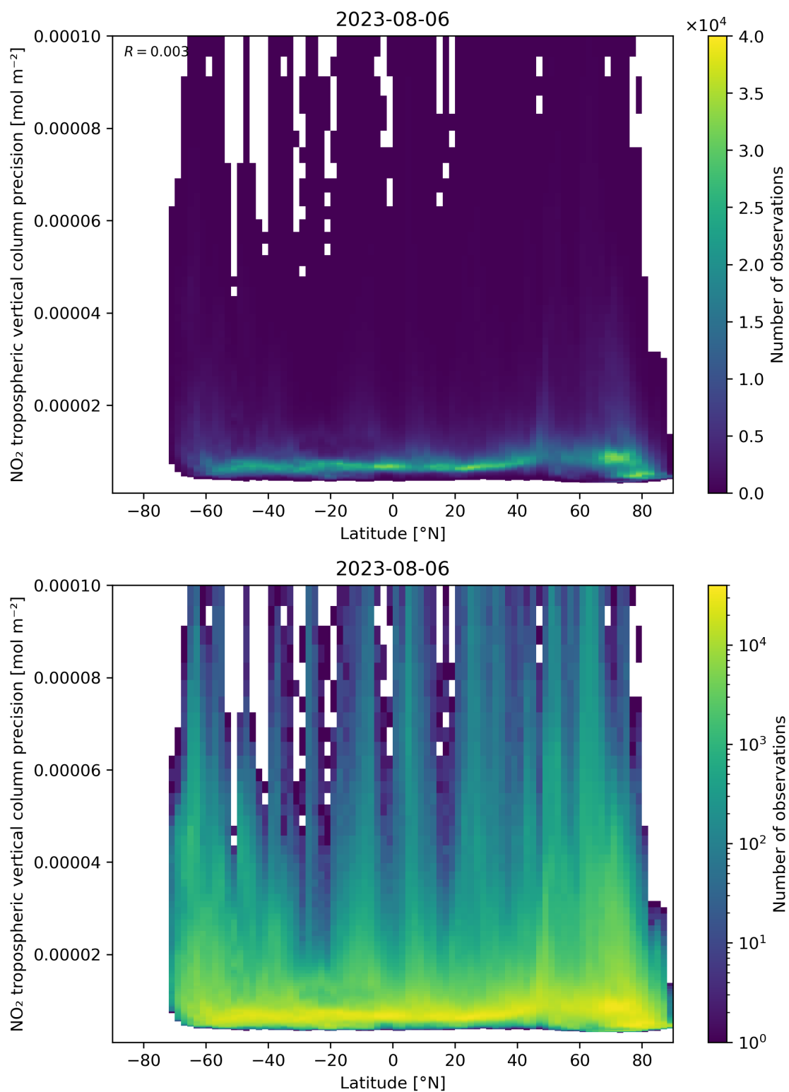
Figure 93: Scatter density plot of “Latitude” against “NO 2 tropospheric vertical column precision” for 2023-08-05 to 2023-08-07.
