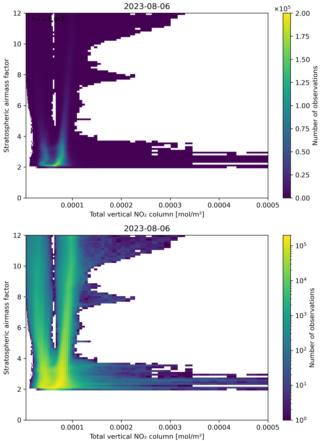
Figure 110: Scatter density plot of “Total vertical NO 2 column” against “Stratospheric airmass factor” for 2023-08-05 to 2023-08-07.
