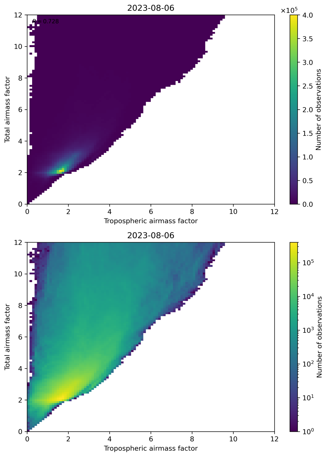
Figure 72: Scatter density plot of “Tropospheric airmass factor” against “Total airmass factor” for 2023-08-05 to 2023-08-07.
