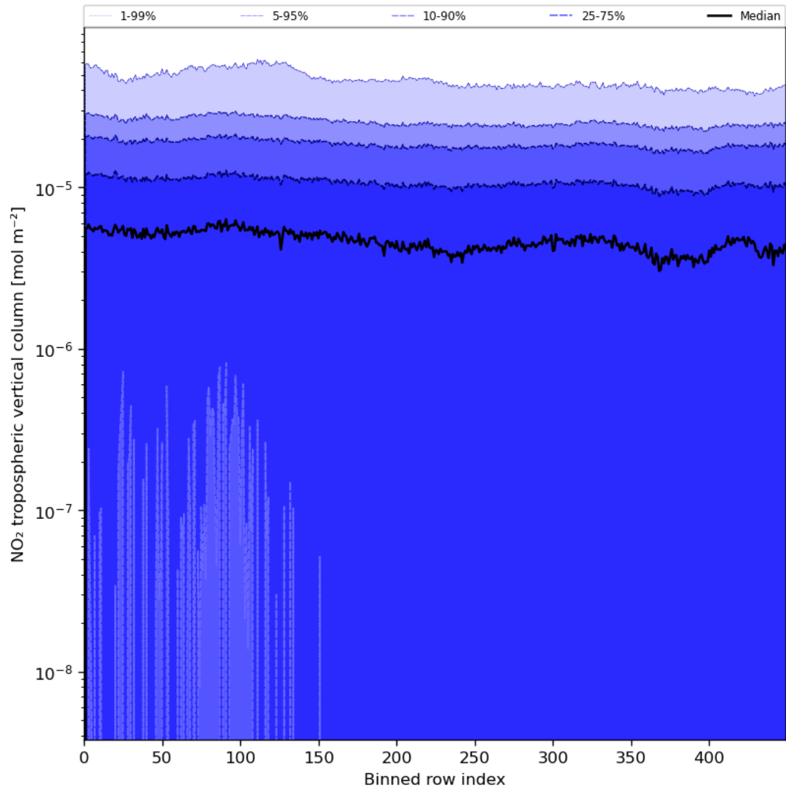
Figure 46: Along track statistics of “NO 2 tropospheric vertical column” for 2023-08-05 to 2023-08-07
