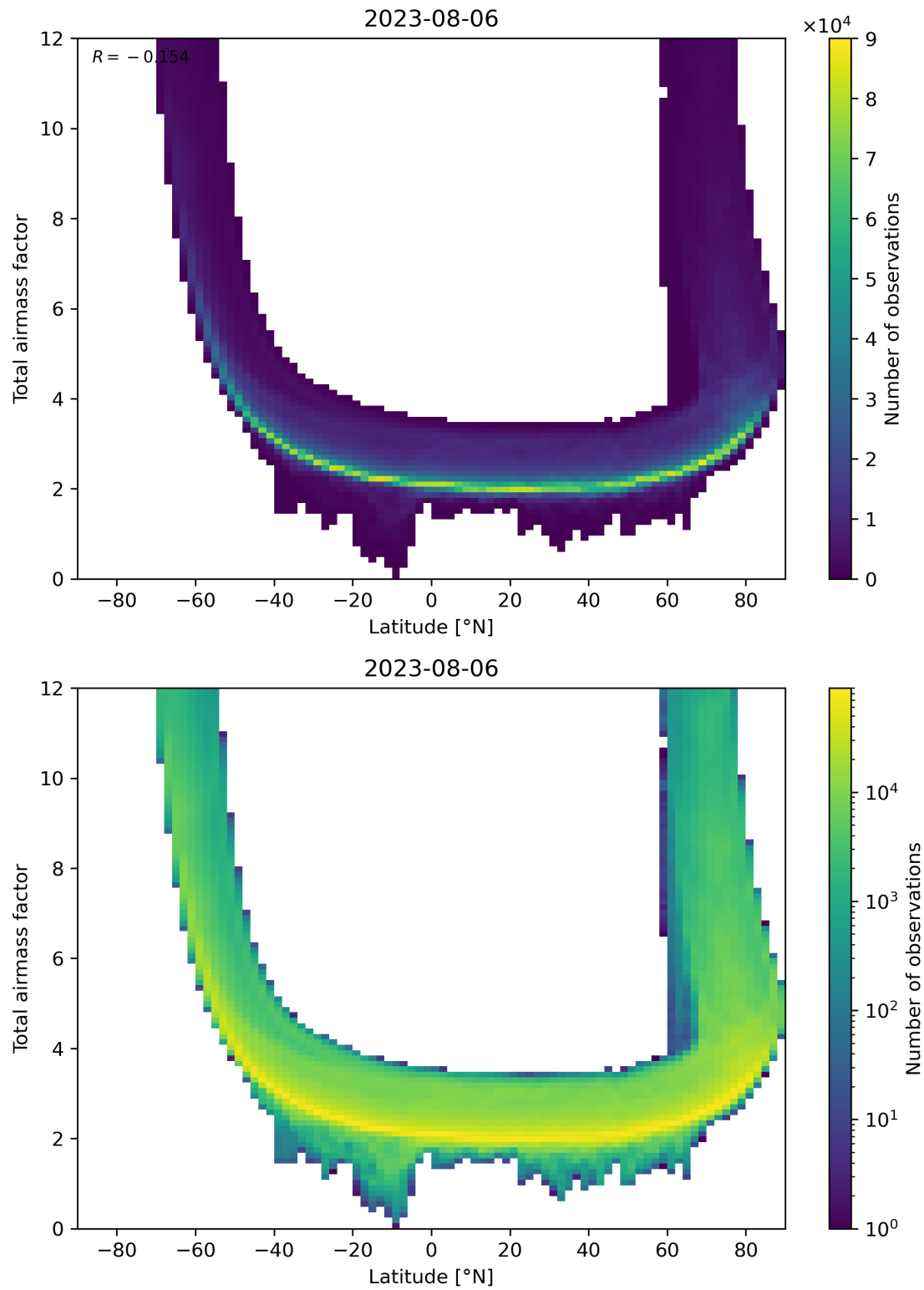
Figure 84: Scatter density plot of “Latitude” against “Total airmass factor” for 2023-08-05 to 2023-08-07.
