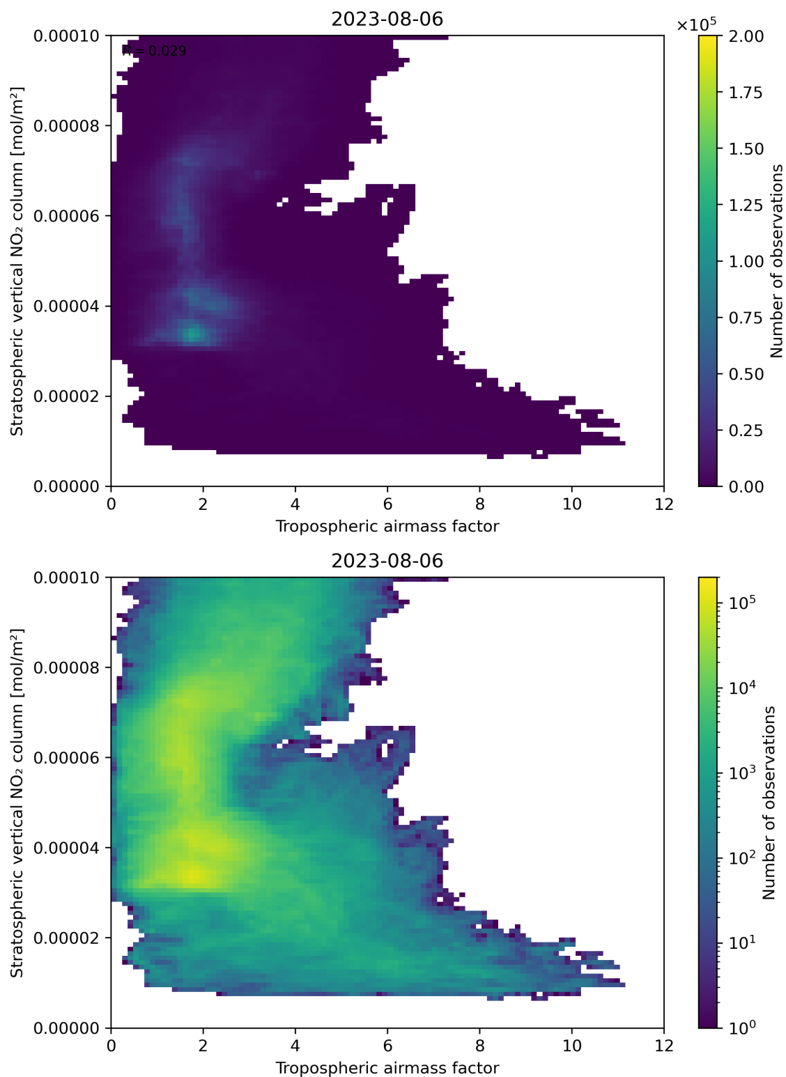
Figure 74: Scatter density plot of “Tropospheric air mass factor” against “Stratospheric vertical NO 2 column” for 2023-08-05 to 2023-08-07.
