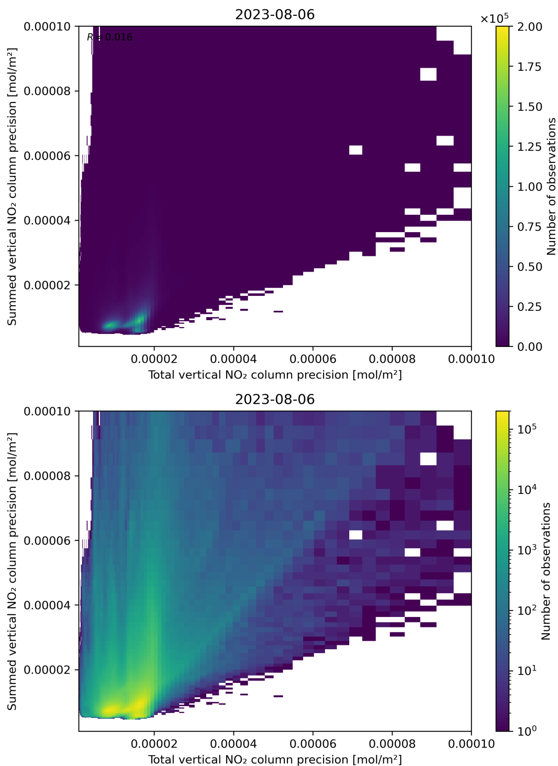
Figure 118: Scatter density plot of “Total vertical NO 2 column precision” against “Summed vertical NO 2 column precision” for 2023-08-05 to 2023-08-07.
