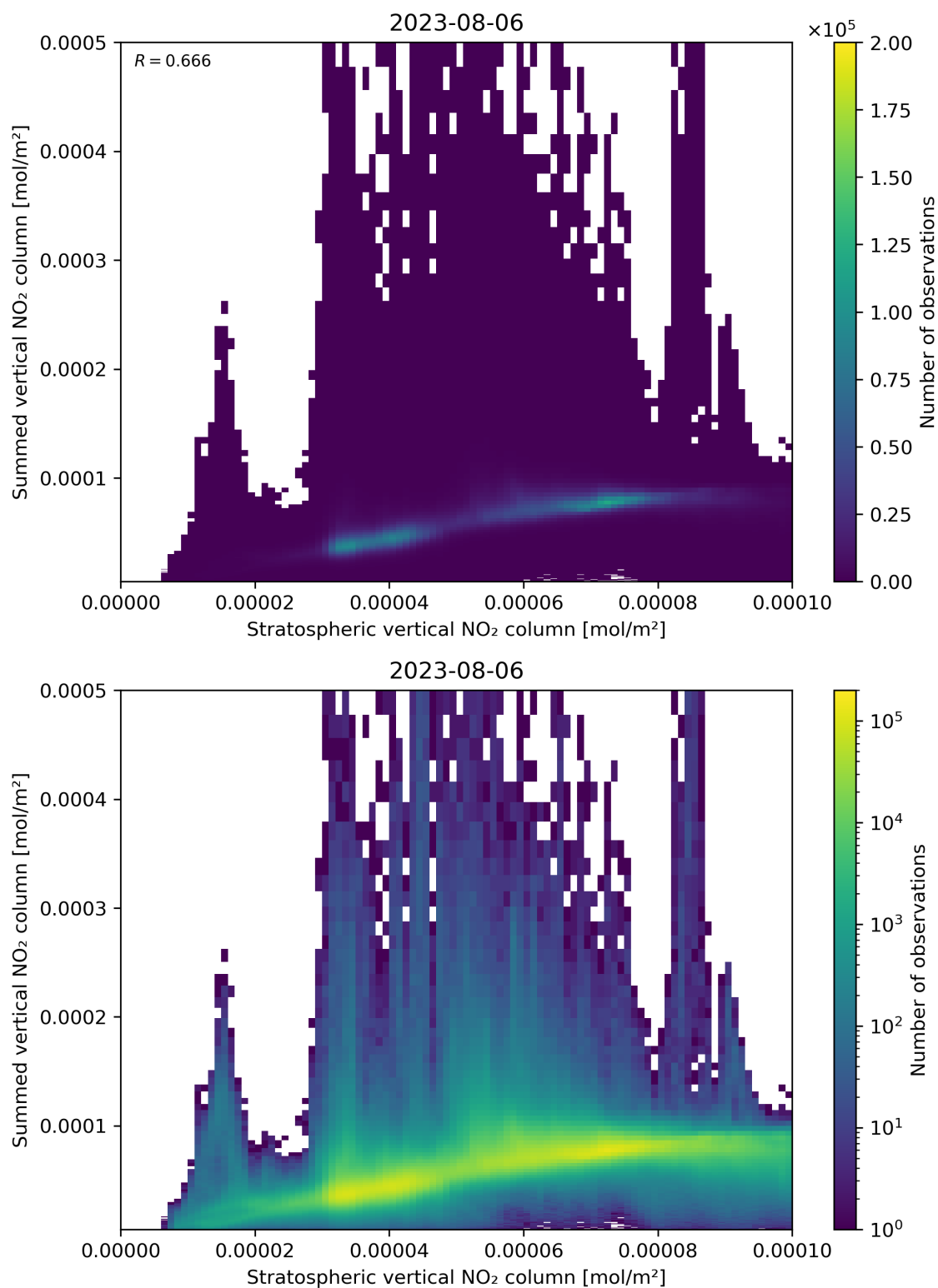
Figure 98: Scatter density plot of “Stratospheric vertical NO 2 column” against “Summed vertical NO 2 column” for 2023-08-05 to 2023-08-07.
