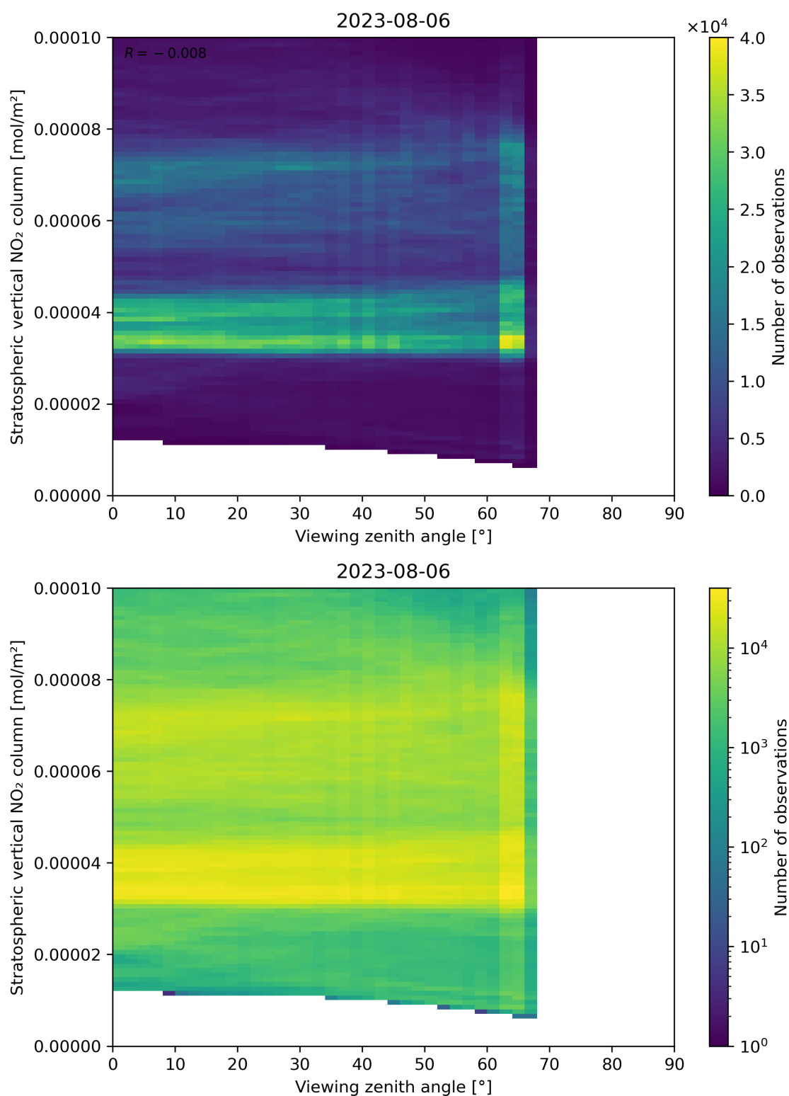
Figure 164: Scatter density plot of “Viewing zenith angle” against “Stratospheric vertical NO 2 column” for 2023-08-05 to 2023-08-07.
