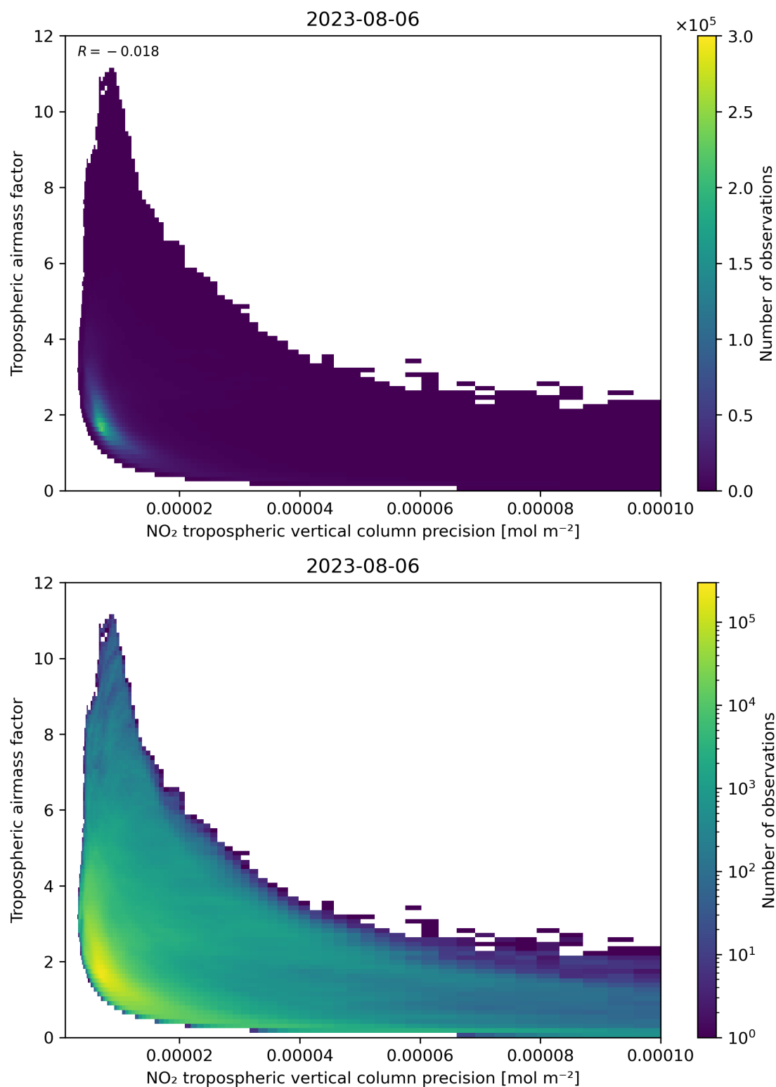
Figure 133: Scatter density plot of “NO 2 tropospheric vertical column precision” against “Tropospheric airmass factor” for 2023-08-05 to 2023-08-07.
