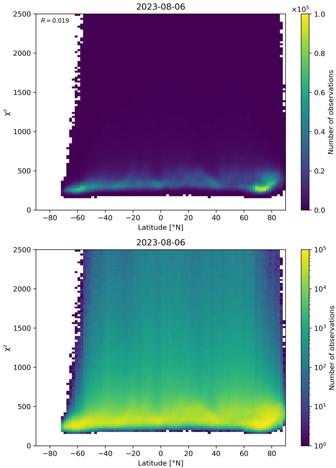
Figure 86: Scatter density plot of “Latitude” against “ \chi^2 ” for 2023-08-05 to 2023-08-07.
