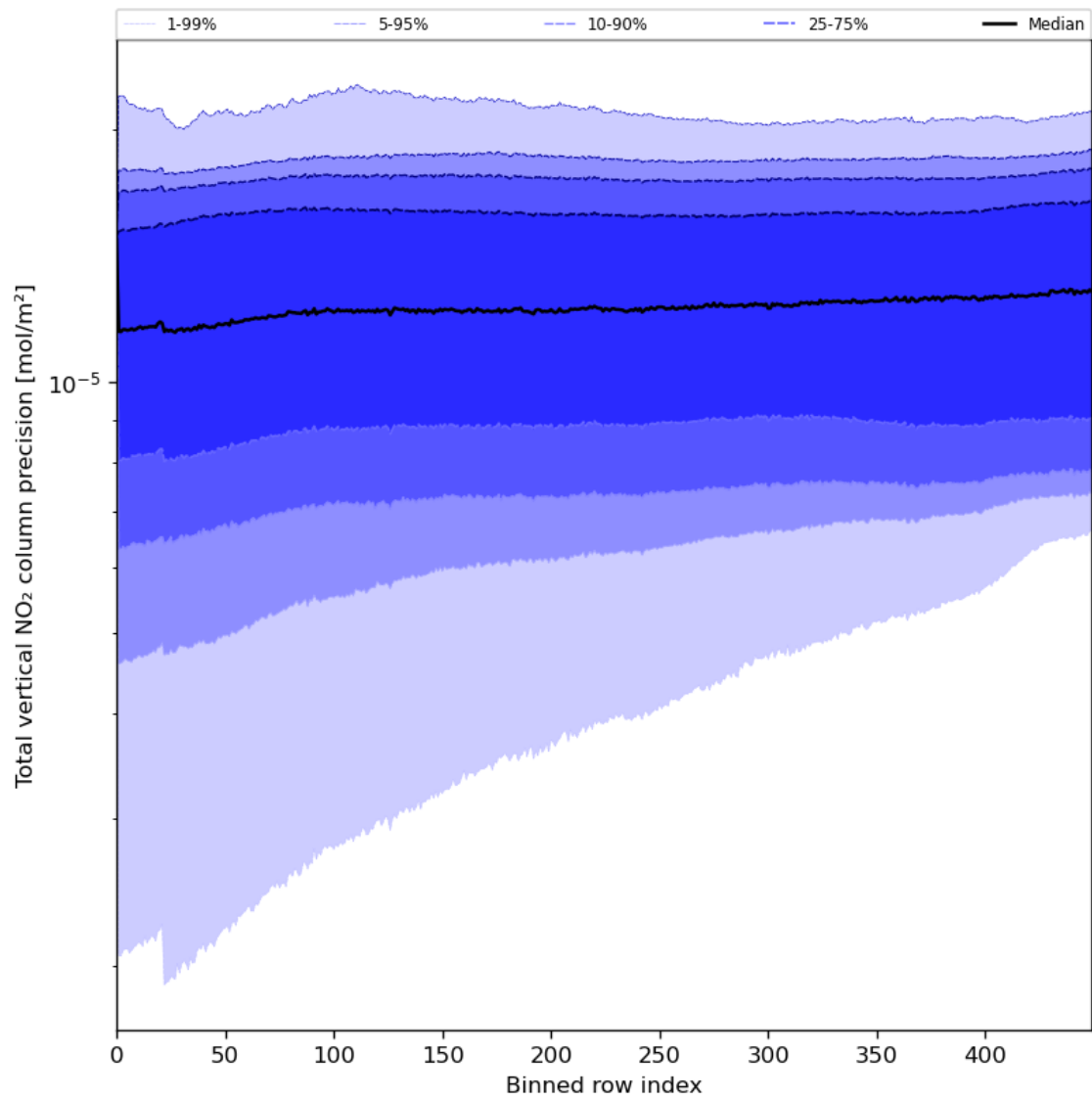
Figure 56: Along track statistics of “Total vertical NO 2 column precision” for 2023-08-05 to 2023-08-07
