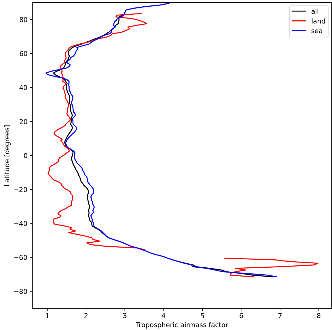
Figure 14: Zonal average of “Tropospheric airmass factor” for 2023-08-05 to 2023-08-07.
