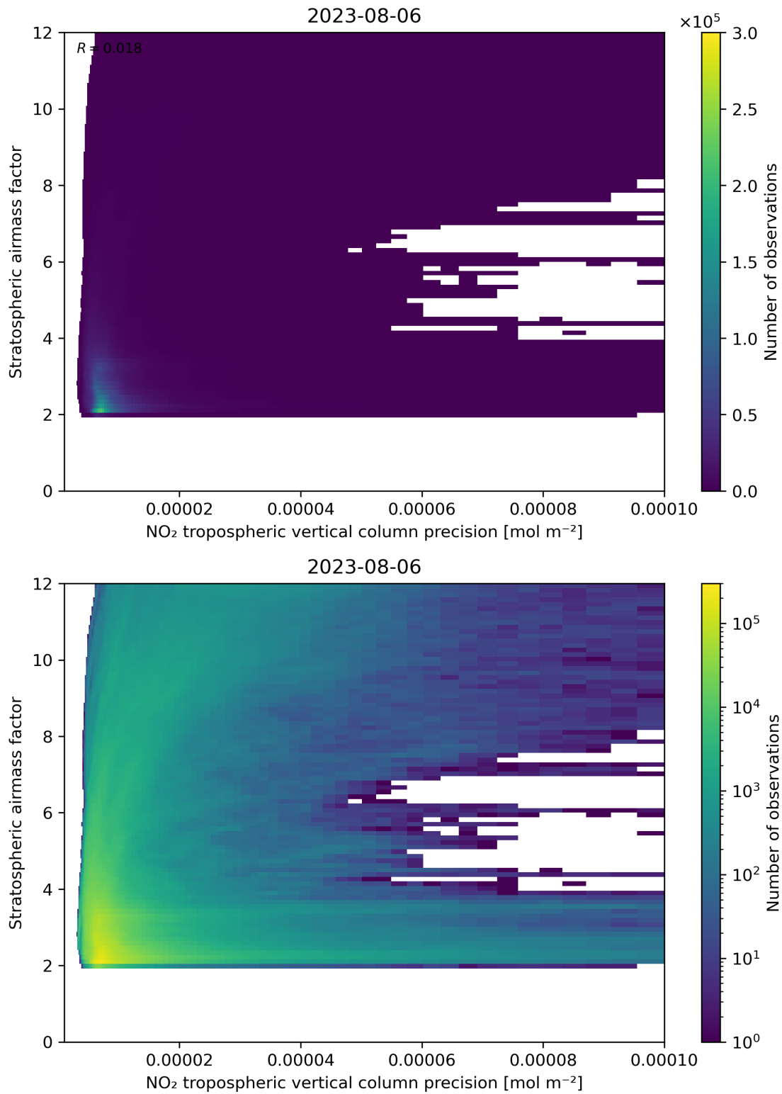
Figure 131: Scatter density plot of “NO 2 tropospheric vertical column precision” against “Stratospheric airmass factor” for 2023-08-05 to 2023-08-07.
