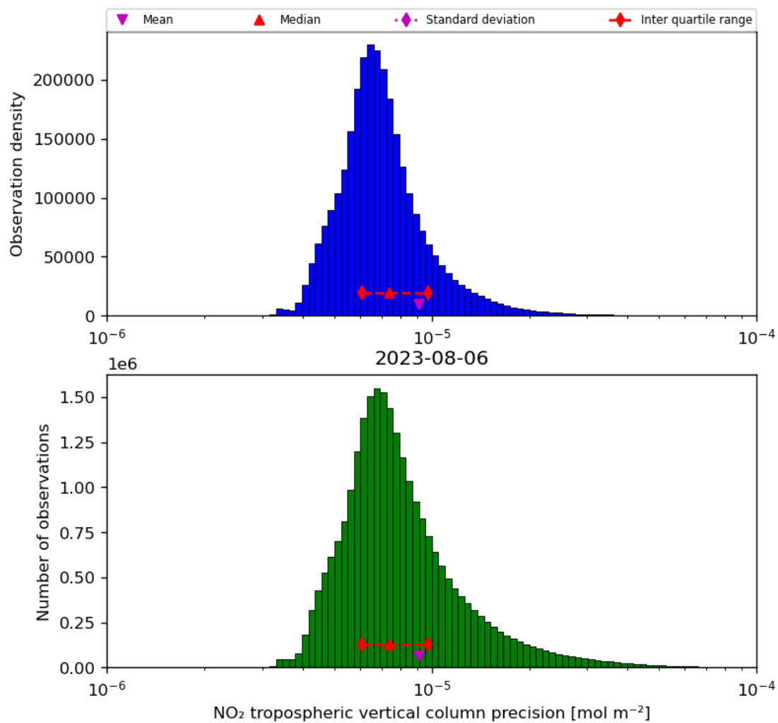
Figure 30: Histogram of “NO 2 tropospheric vertical column precision” for 2023-08-05 to 2023-08-07
