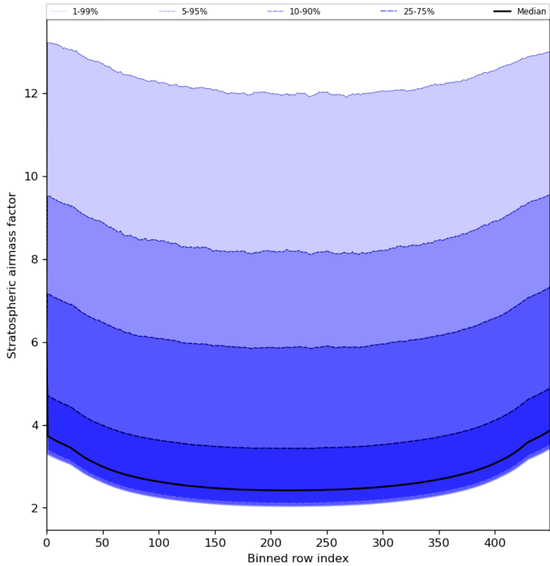
Figure 61: Along track statistics of “Stratospheric air mass factor” for 2023-08-05 to 2023-08-07
