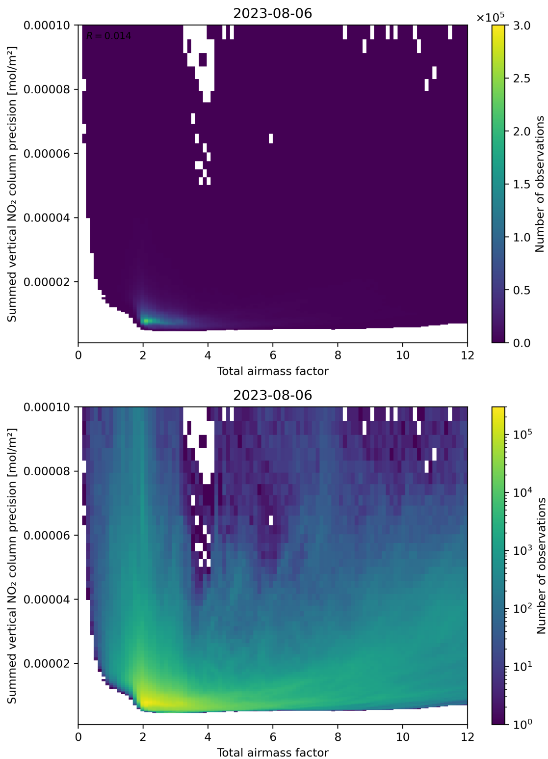
Figure 66: Scatter density plot of “Total airmass factor” against “Summed vertical NO 2 column precision” for 2023-08-05 to 2023-08-07.
