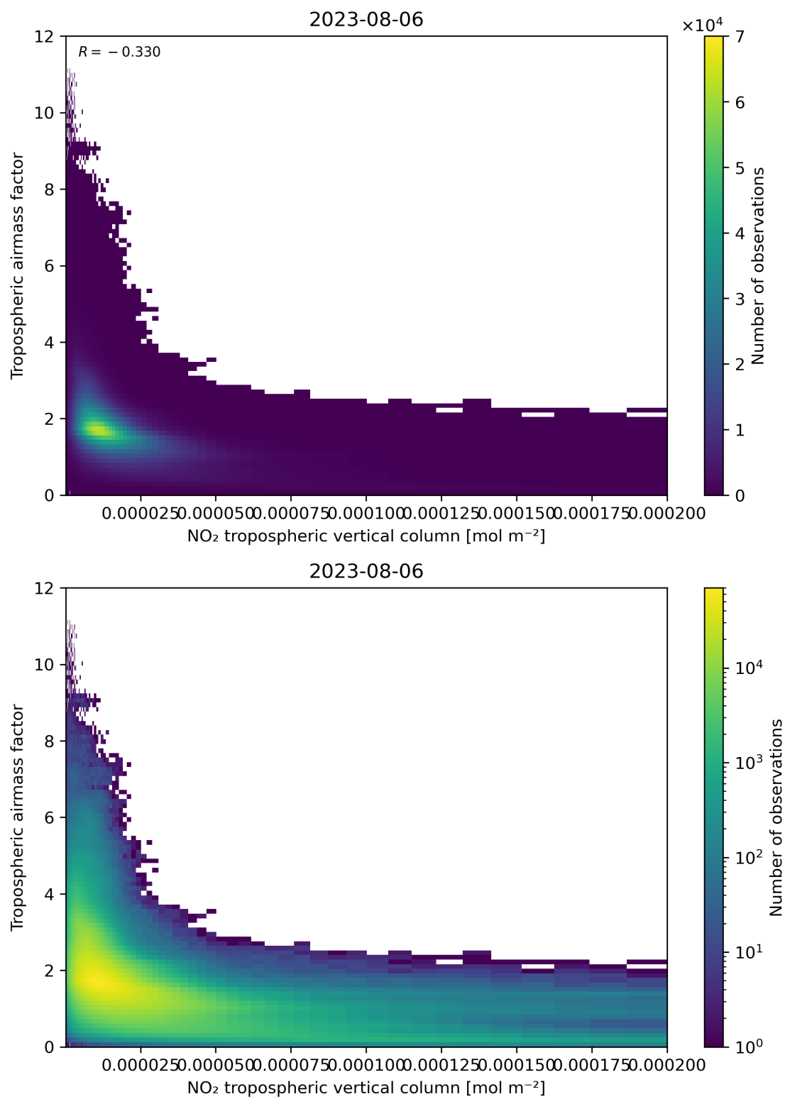
Figure 123: Scatter density plot of “NO 2 tropospheric vertical column” against “Tropospheric air mass factor” for 2023-08-05 to 2023-08-07.
