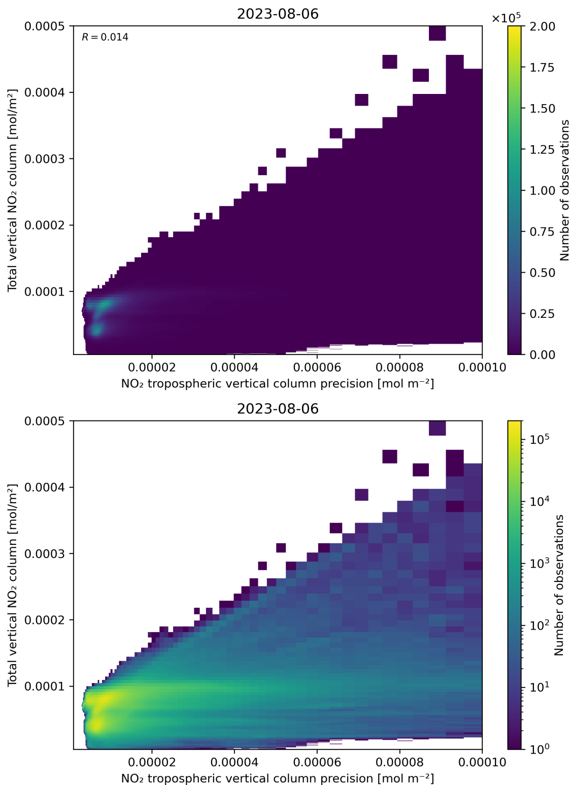
Figure 138: Scatter density plot of “NO 2 tropospheric vertical column precision” against “Total vertical NO 2 column” for 2023-08-05 to 2023-08-07.
