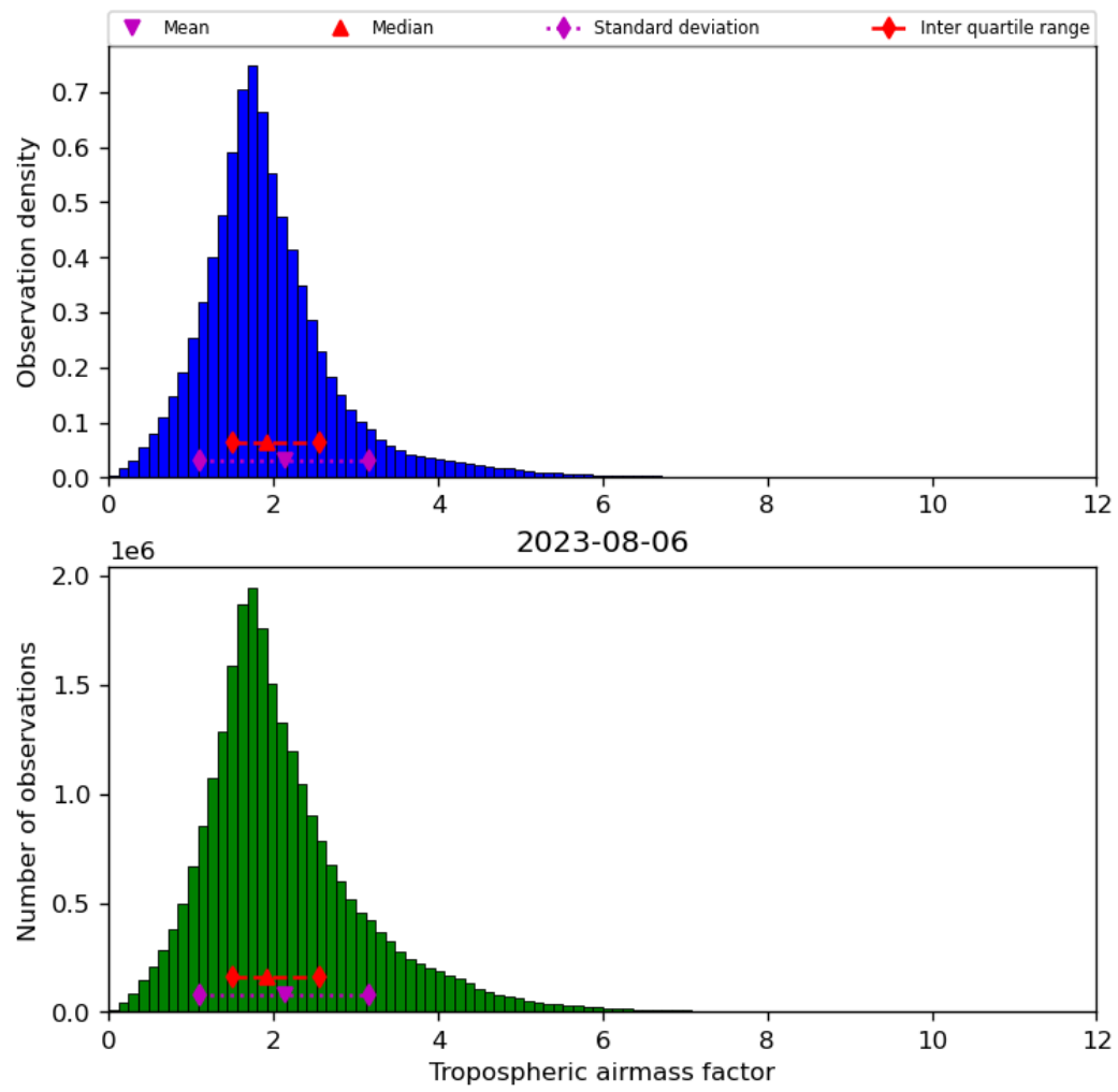
Figure 31: Histogram of “Tropospheric airmass factor” for 2023-08-05 to 2023-08-07
