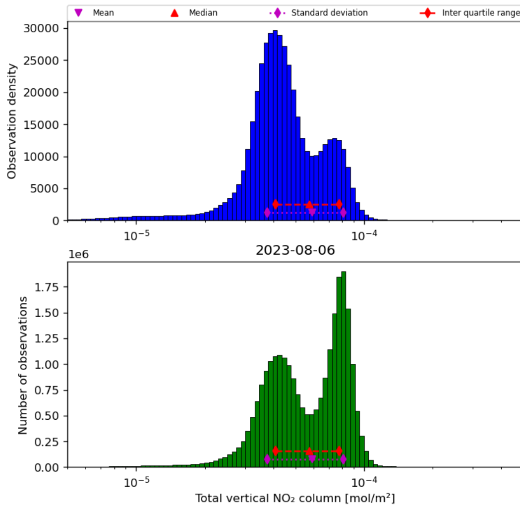
Figure 38: Histogram of “Total vertical NO 2 column” for 2023-08-05 to 2023-08-07
