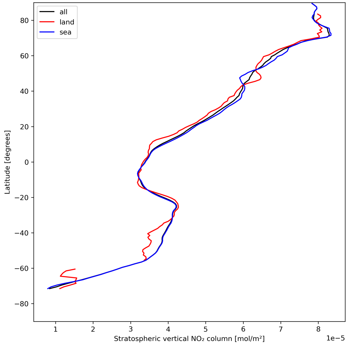
Figure 19: Zonal average of “Stratospheric vertical NO 2 column” for 2023-08-05 to 2023-08-07.
