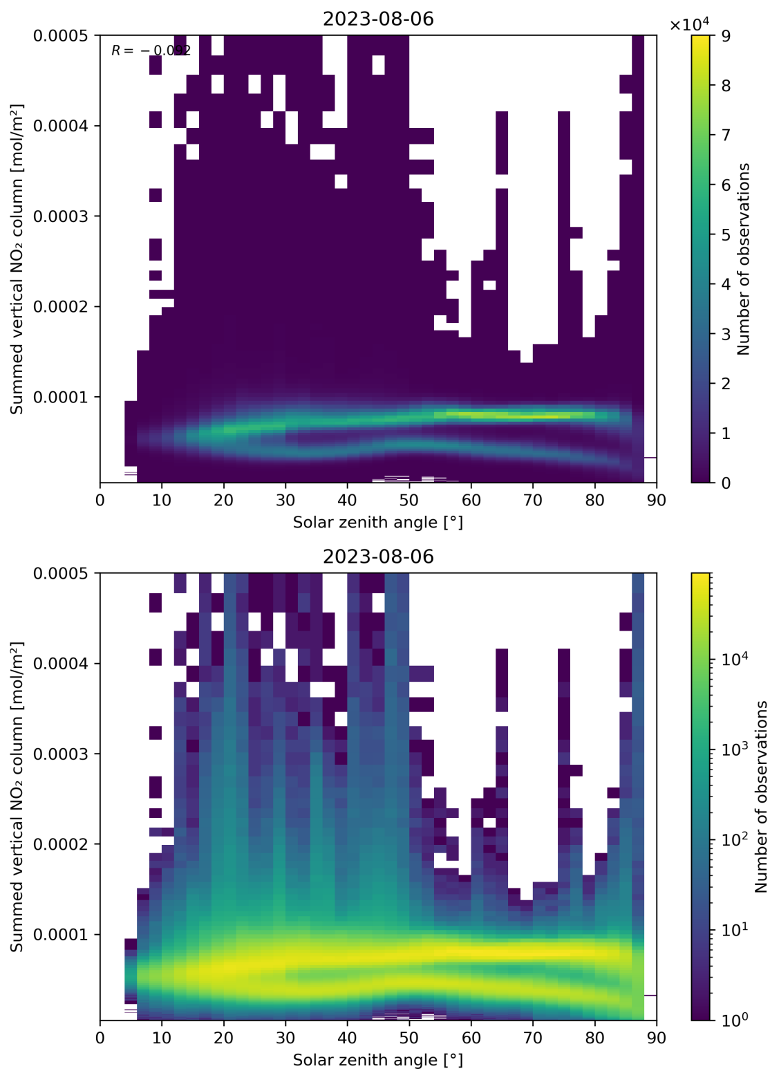
Figure 151: Scatter density plot of “Solar zenith angle” against “Summed vertical NO 2 column” for 2023-08-05 to 2023-08-07.
