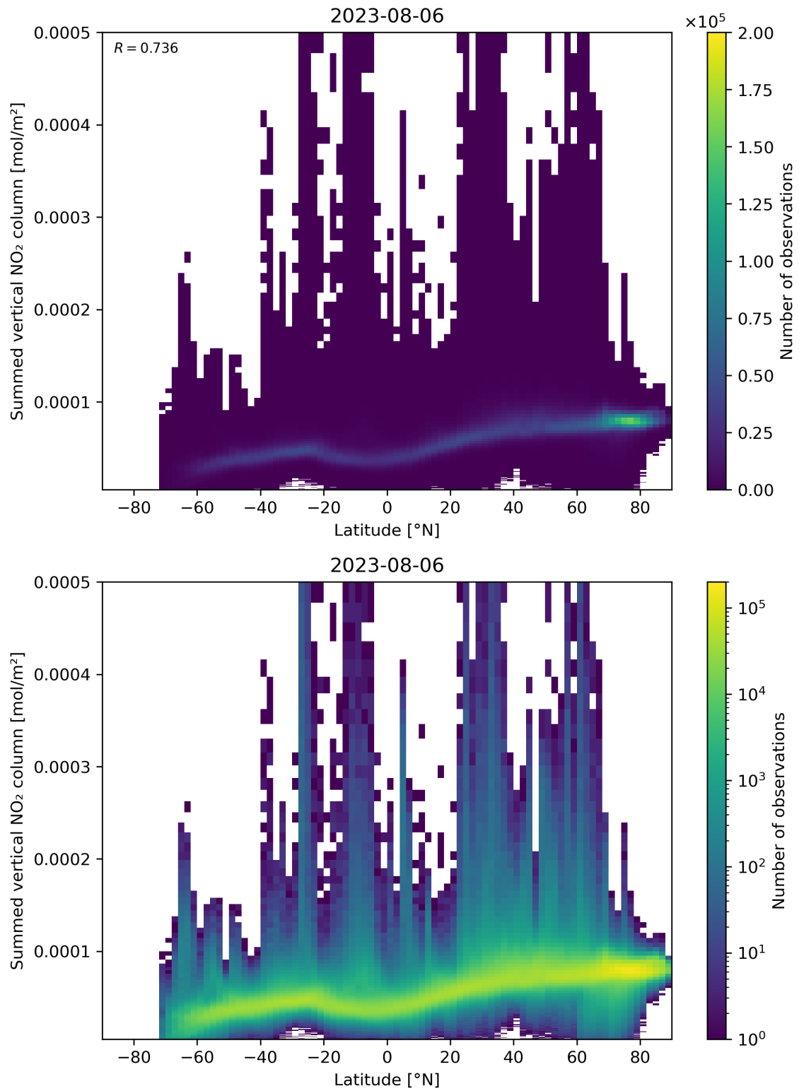
Figure 88: Scatter density plot of “Latitude” against “Summed vertical NO 2 column” for 2023-08-05 to 2023-08-07.
