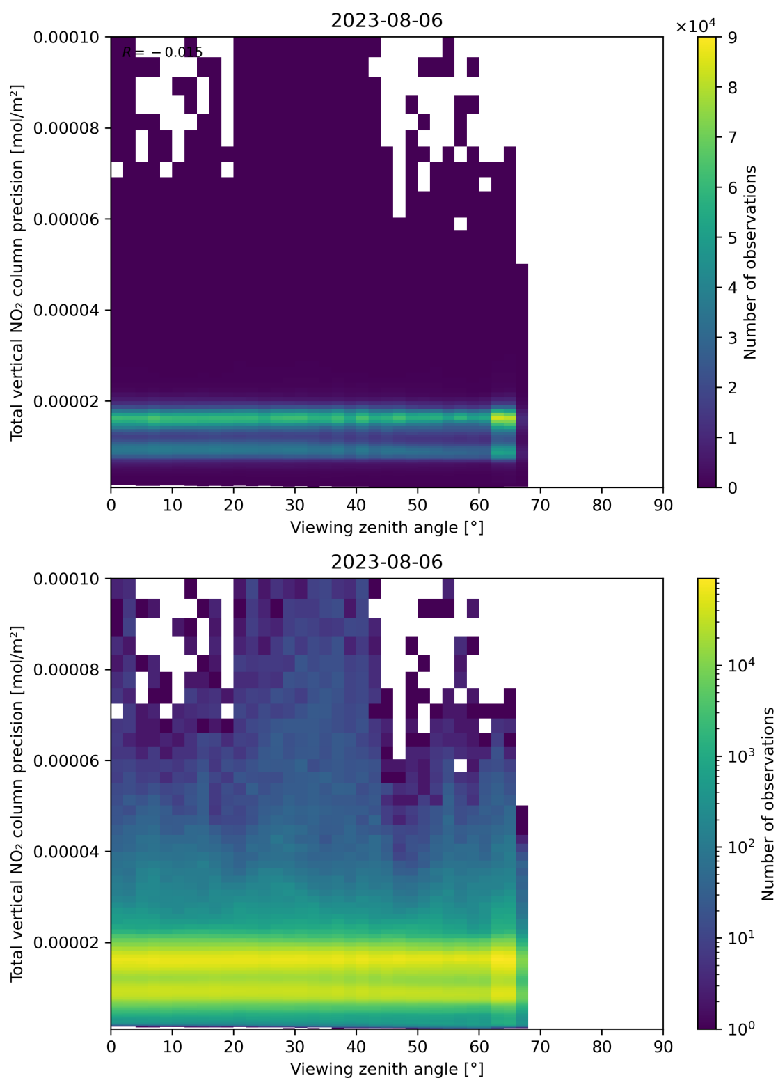
Figure 168: Scatter density plot of “Viewing zenith angle” against “Total vertical NO 2 column precision” for 2023-08-05 to 2023-08-07.
