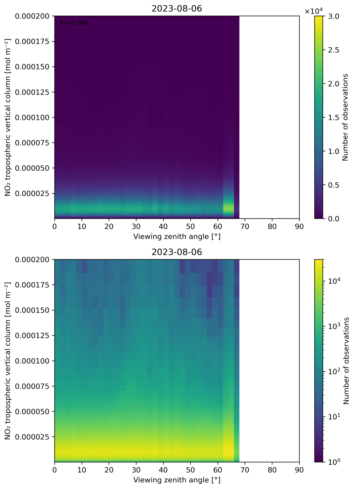
Figure 169: Scatter density plot of “Viewing zenith angle” against “NO 2 tropospheric vertical column” for 2023-08-05 to 2023-08-07.
