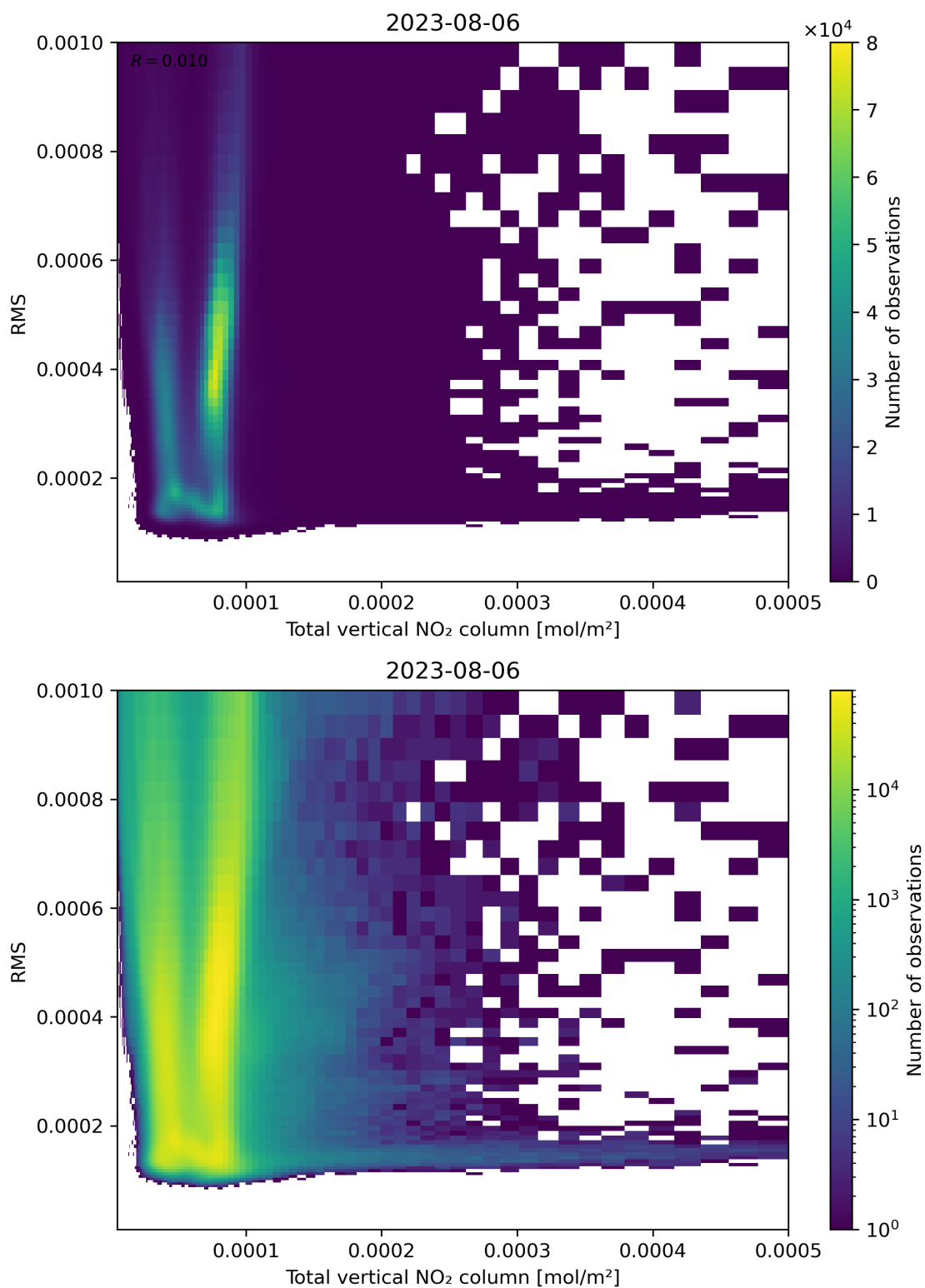
Figure 120: Scatter density plot of “Total vertical NO 2 column” against “RMS” for 2023-08-05 to 2023-08-07.
