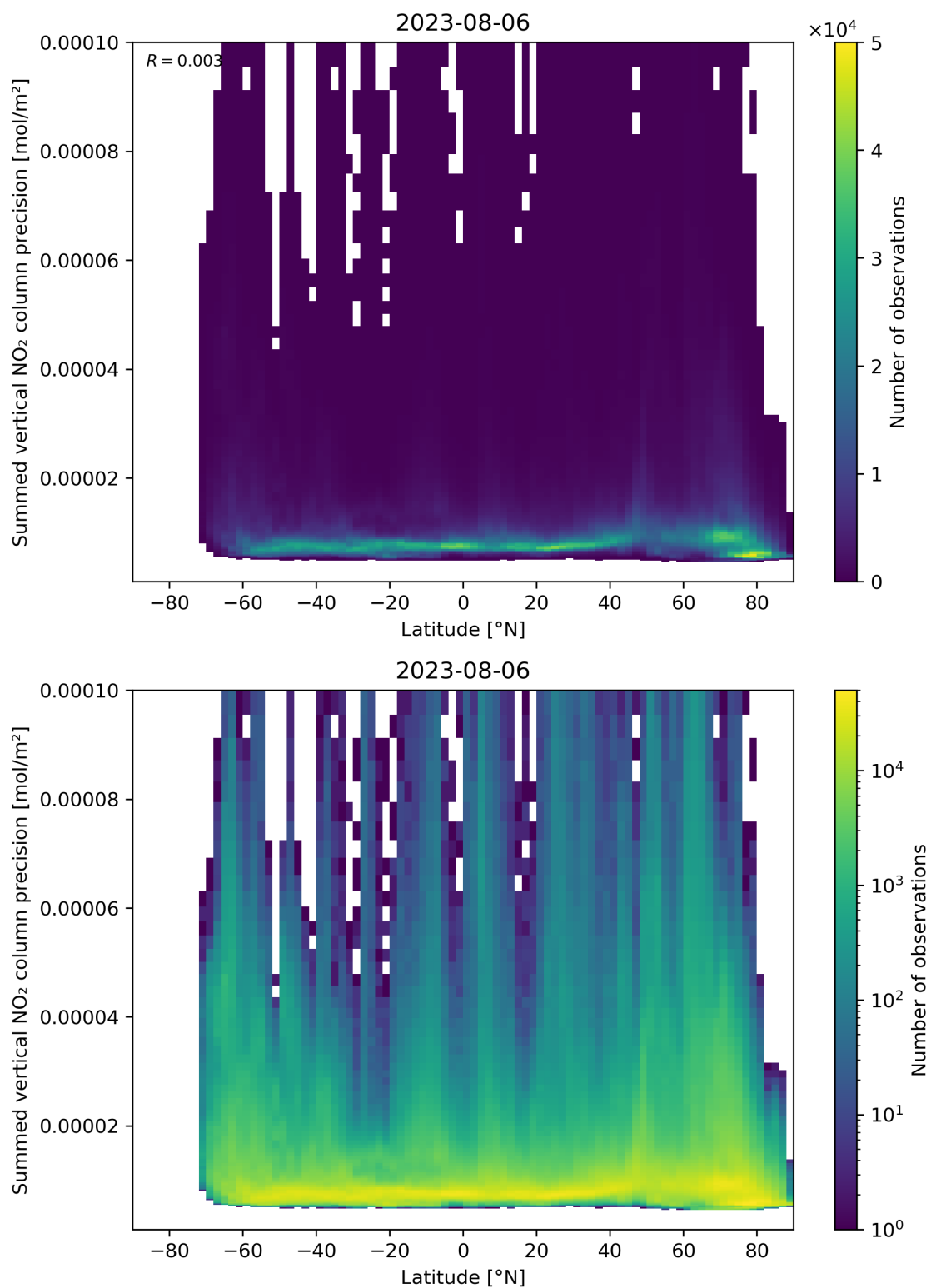
Figure 89: Scatter density plot of “Latitude” against “Summed vertical NO 2 column precision” for 2023-08-05 to 2023-08-07.
