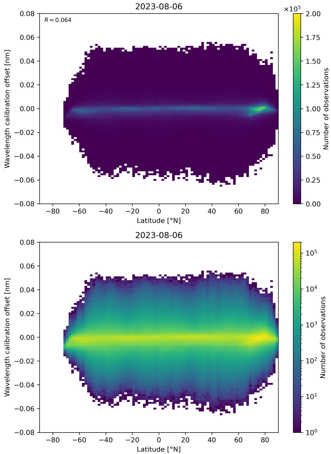
Figure 95: Scatter density plot of “Latitude” against “Wavelength calibration offset” for 2023-08-05 to 2023-08-07.
