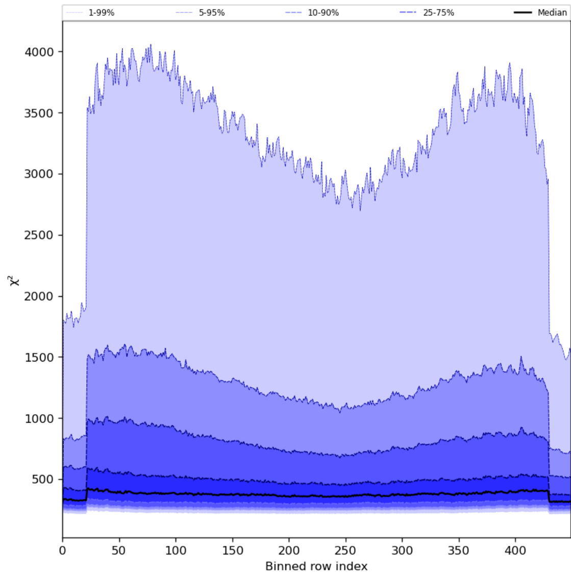
Figure 59: Along track statistics of “ \chi^2 ” for 2023-08-05 to 2023-08-07
