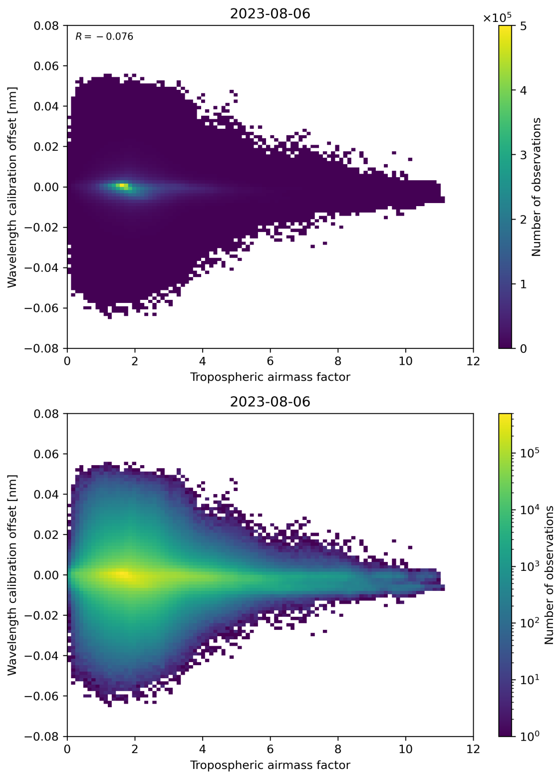
Figure 80: Scatter density plot of “Tropospheric airmass factor” against “Wavelength calibration offset” for 2023-08-05 to 2023-08-07.
