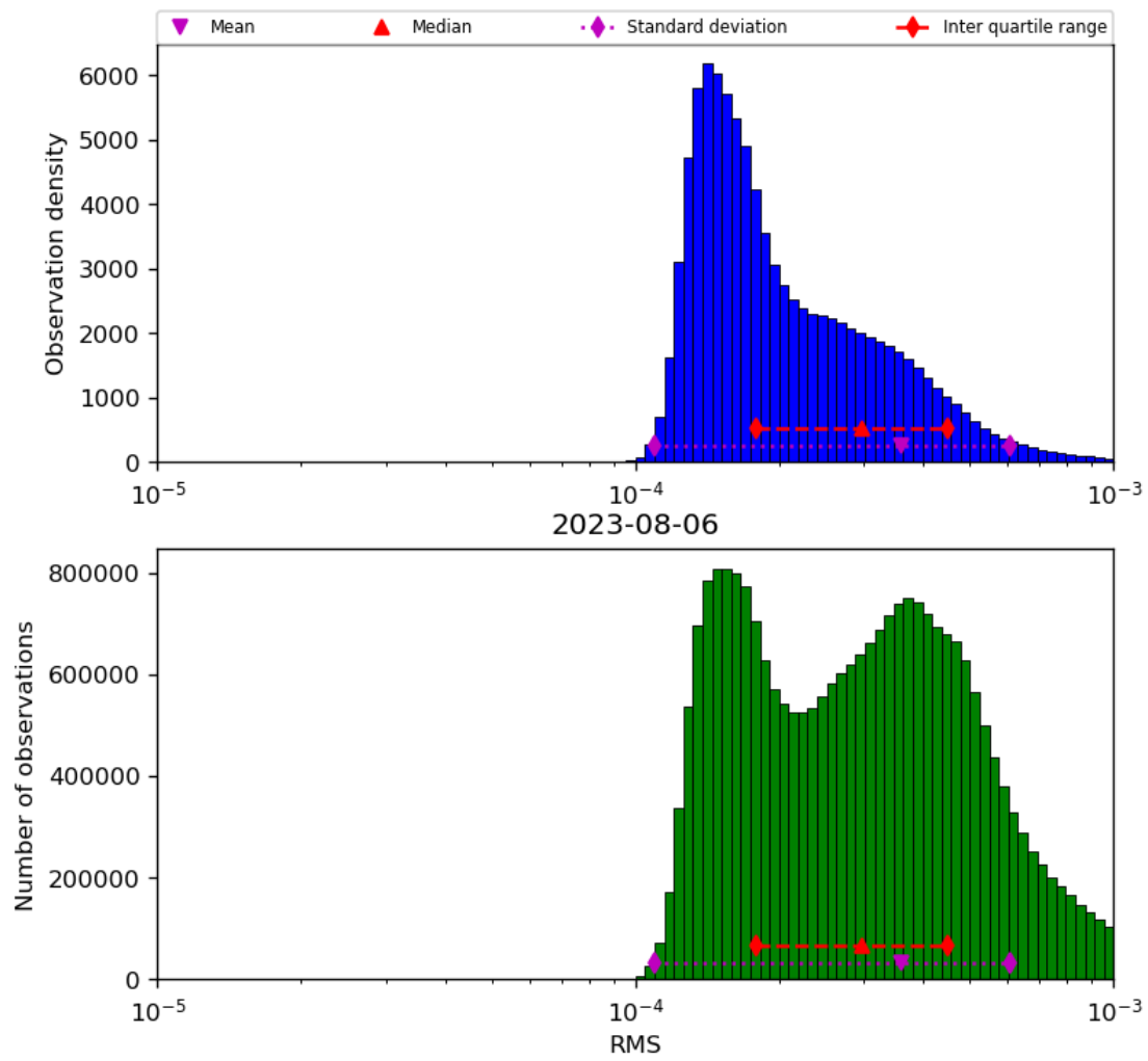
Figure 43: Histogram of “RMS” for 2023-08-05 to 2023-08-07
