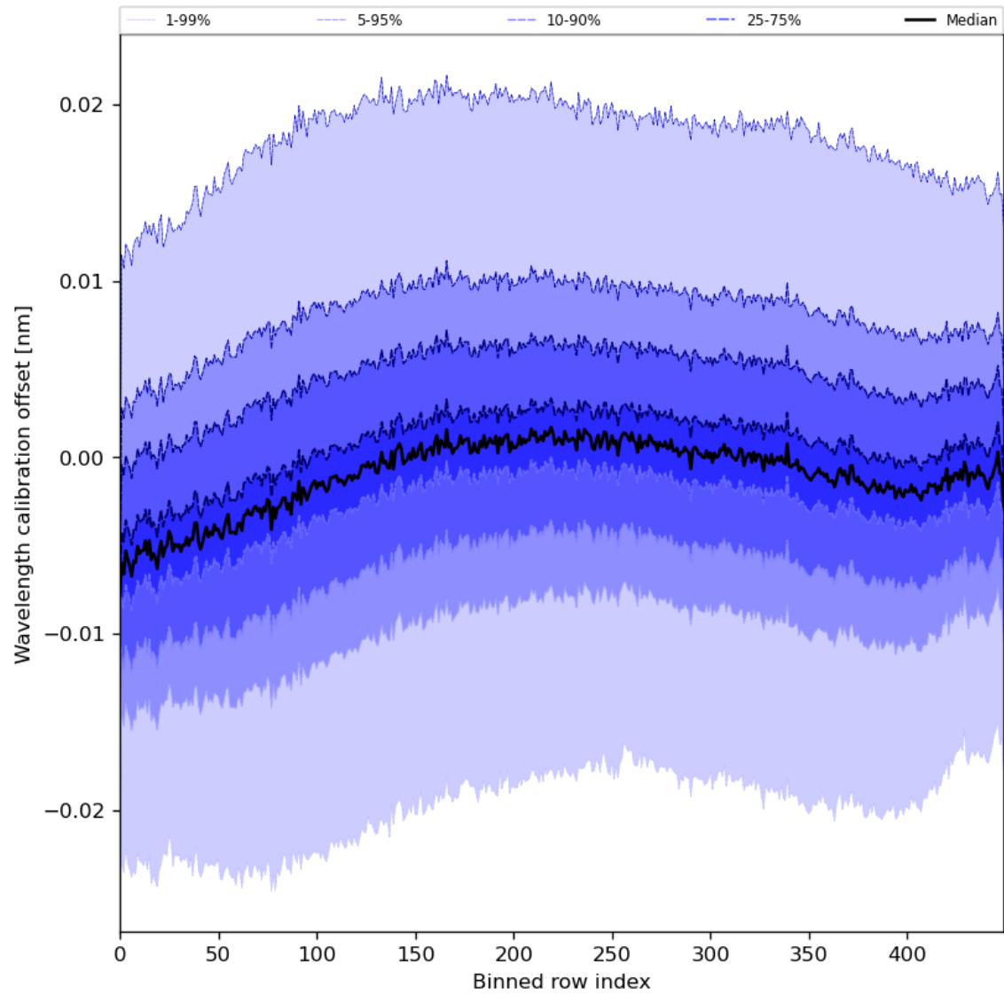
Figure 52: Along track statistics of “Wavelength calibration offset” for 2023-08-05 to 2023-08-07
