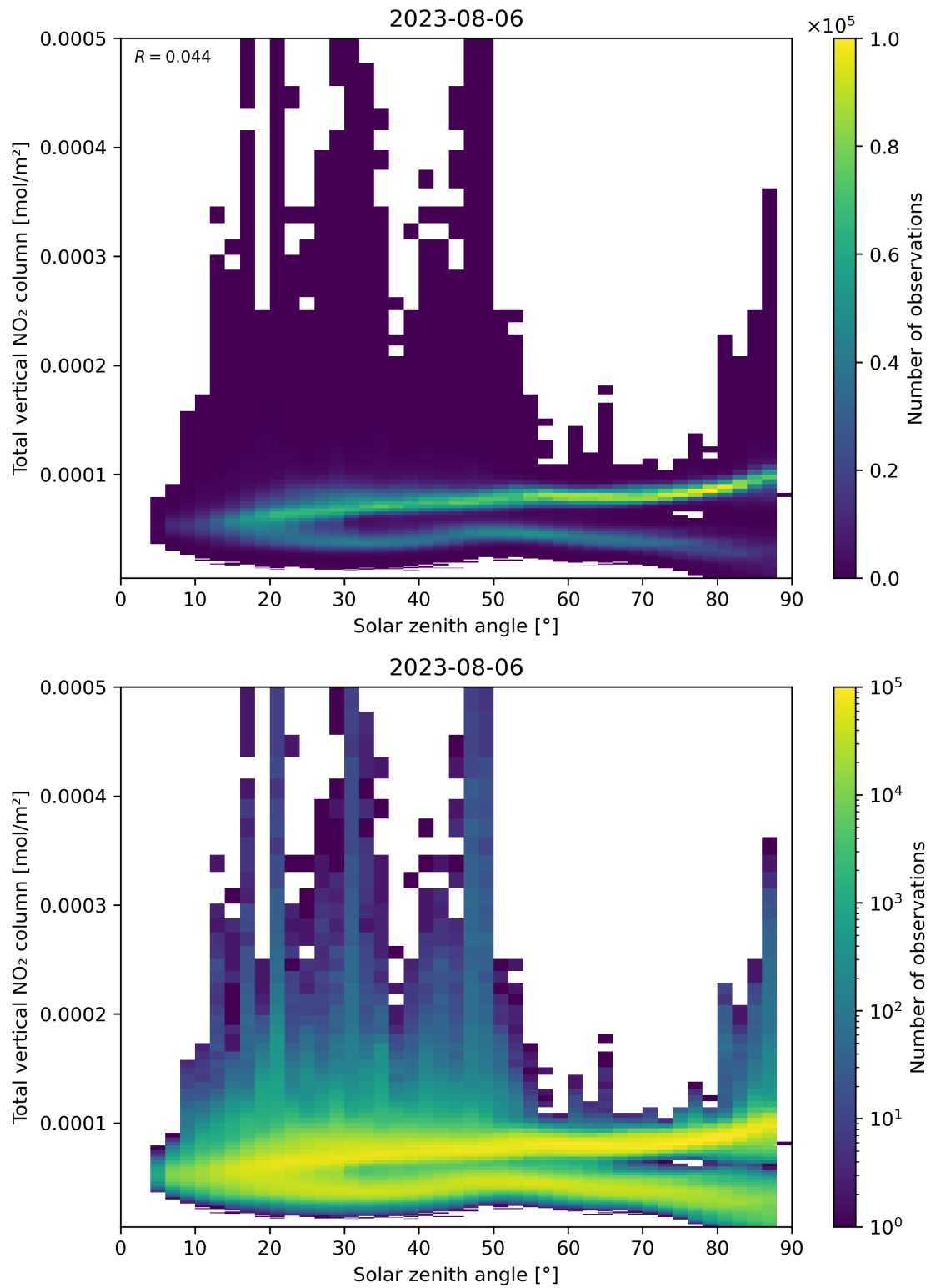
Figure 153: Scatter density plot of “Solar zenith angle” against “Total vertical NO 2 column” for 2023-08-05 to 2023-08-07.
