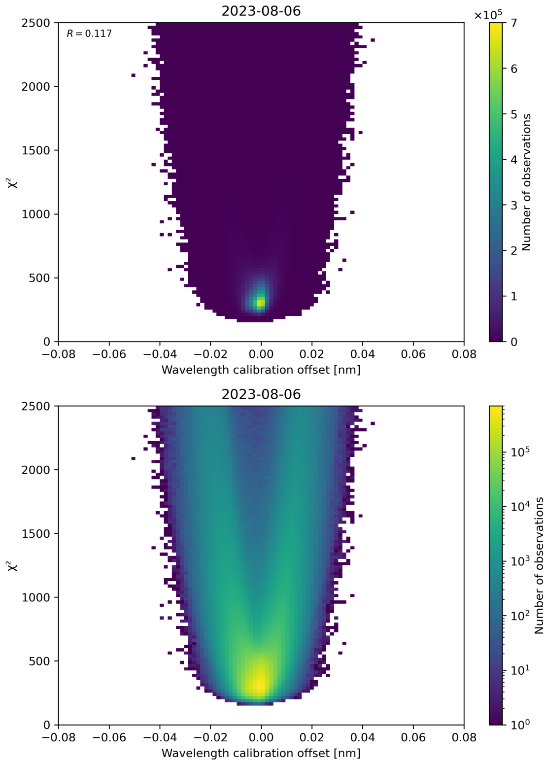
Figure 175: Scatter density plot of “Wavelength calibration offset” against “ \chi^2 ” for 2023-08-05 to 2023-08-07.
