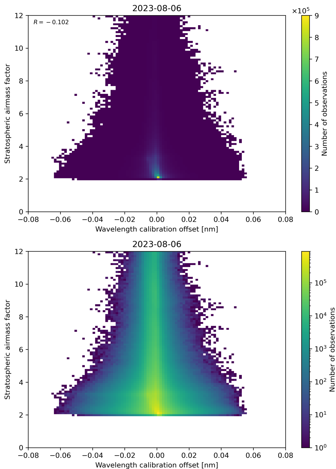
Figure 174: Scatter density plot of “Wavelength calibration offset” against “Stratospheric airmass factor” for 2023-08-05 to 2023-08-07.
