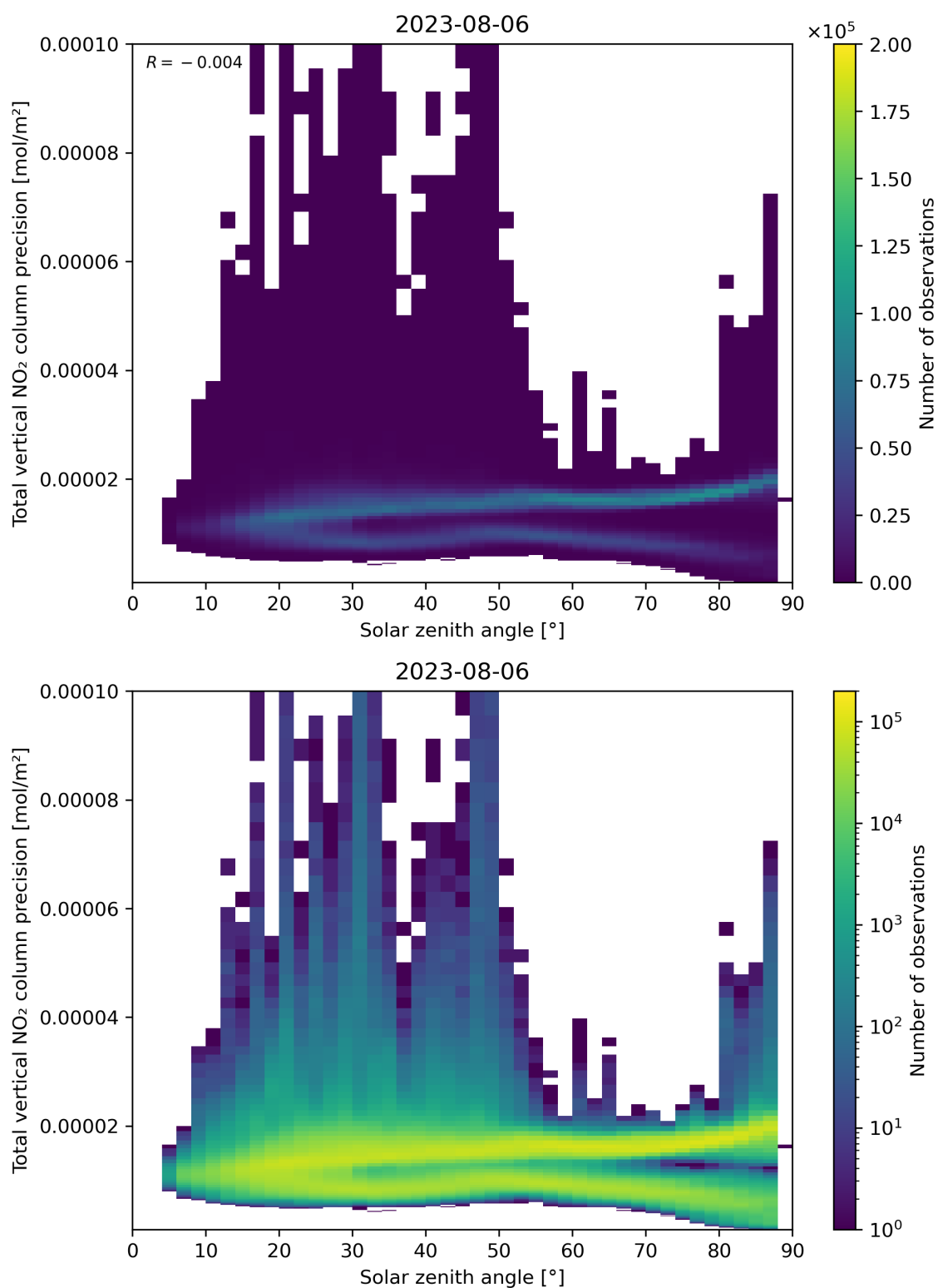
Figure 154: Scatter density plot of “Solar zenith angle” against “Total vertical NO 2 column precision” for 2023-08-05 to 2023-08-07.
