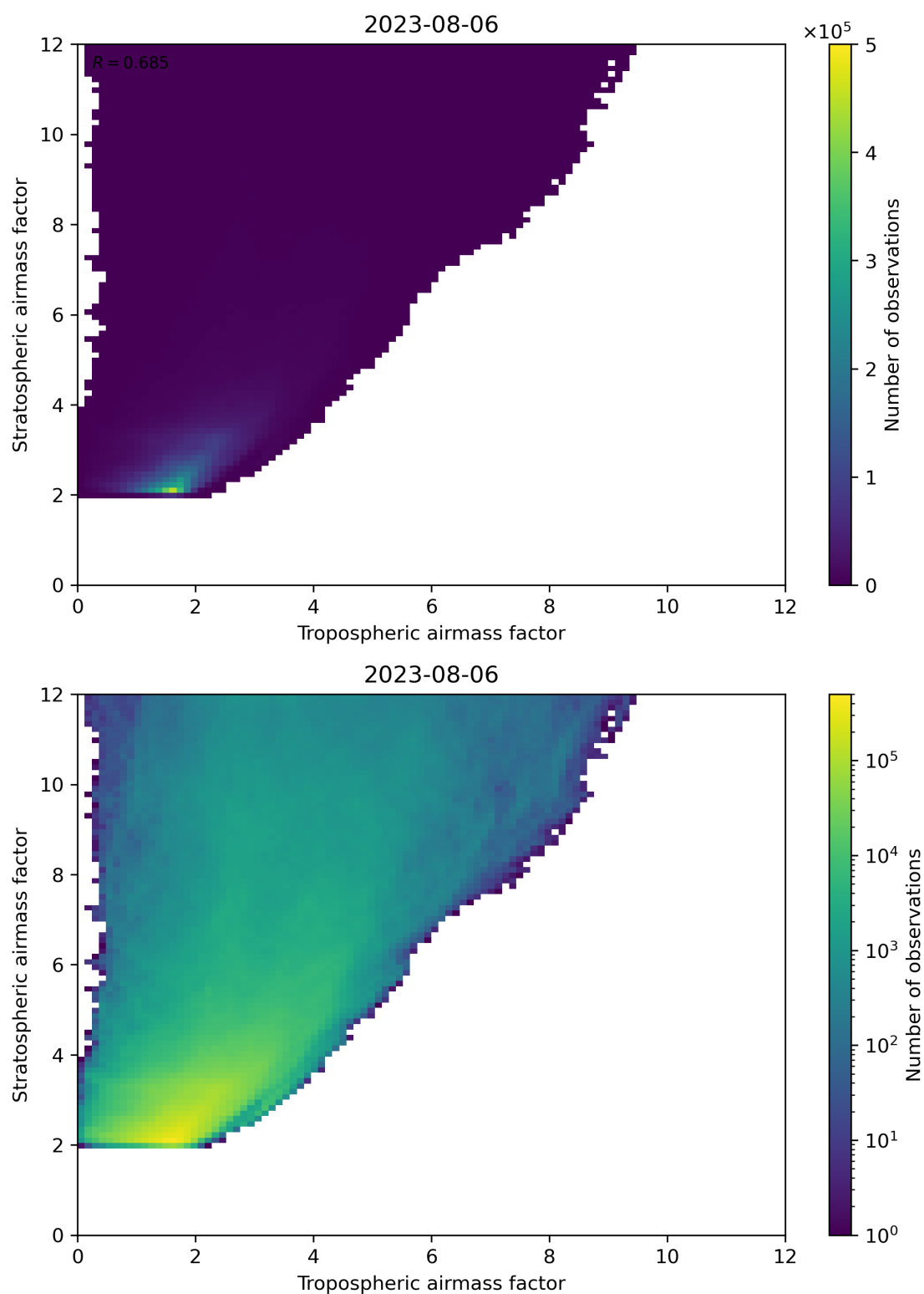
Figure 71: Scatter density plot of “Tropospheric airmass factor” against “Stratospheric airmass factor” for 2023-08-05 to 2023-08-07.
