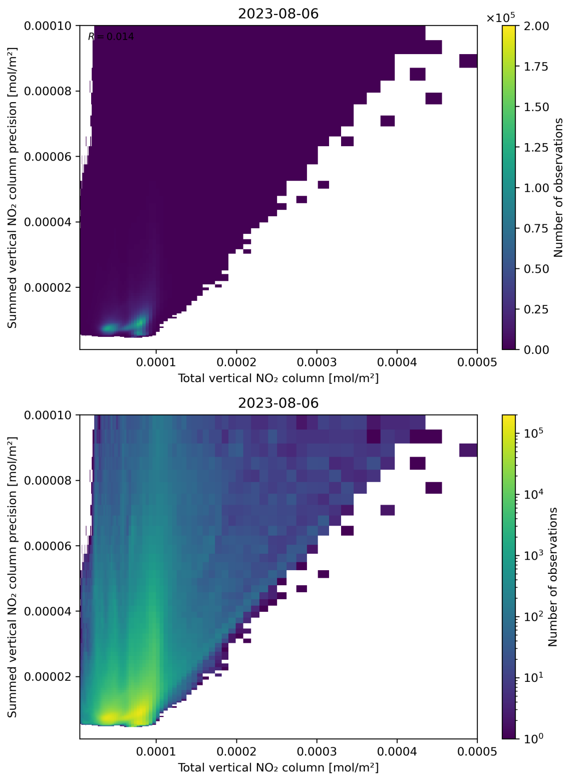
Figure 113: Scatter density plot of “Total vertical NO 2 column” against “Summed vertical NO 2 column precision” for 2023-08-05 to 2023-08-07.
