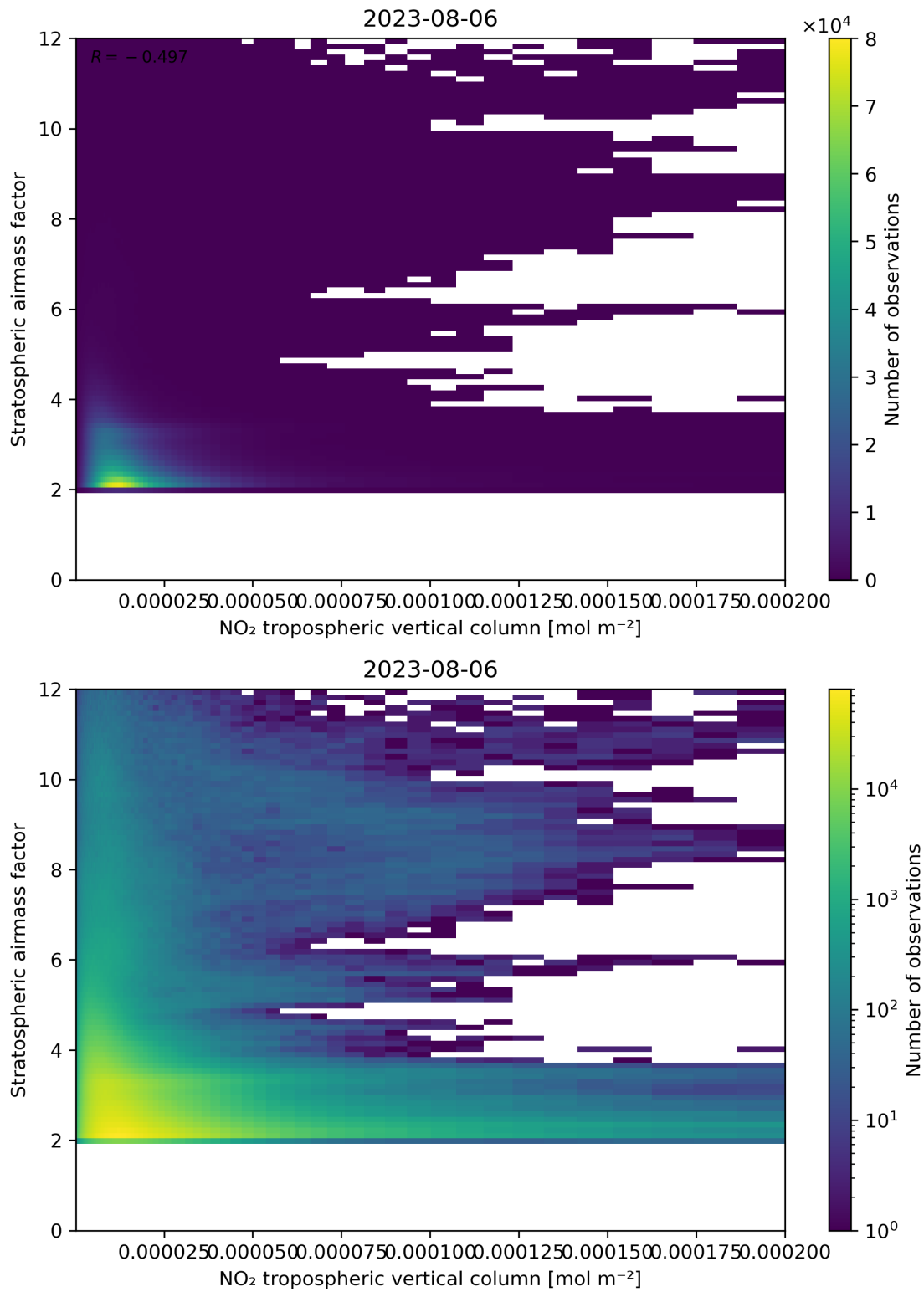
Figure 121: Scatter density plot of “NO 2 tropospheric vertical column” against “Stratospheric air mass factor” for 2023-08-05 to 2023-08-07.
