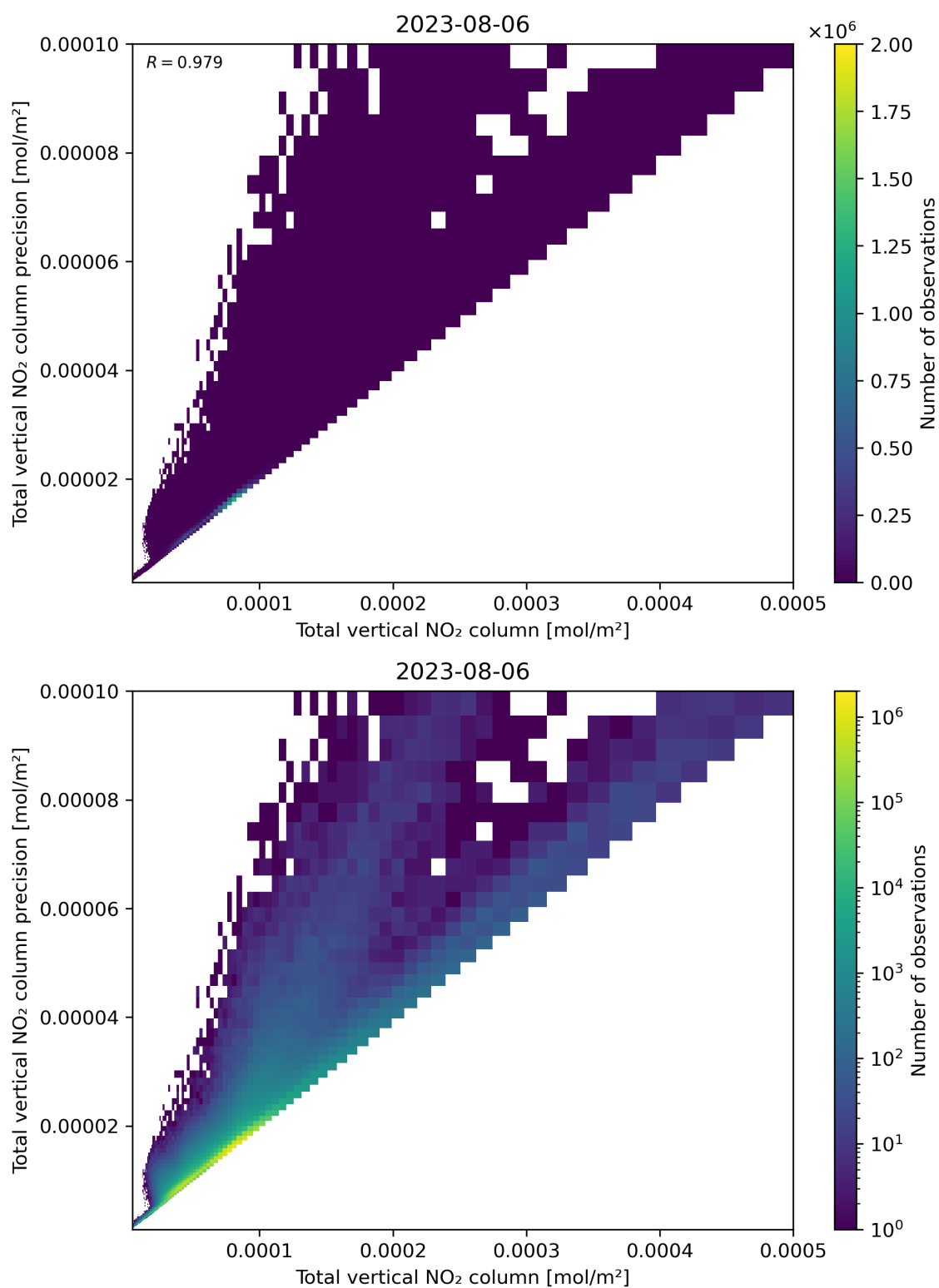
Figure 114: Scatter density plot of “Total vertical NO 2 column” against “Total vertical NO 2 column precision” for 2023-08-05 to 2023-08-07.
