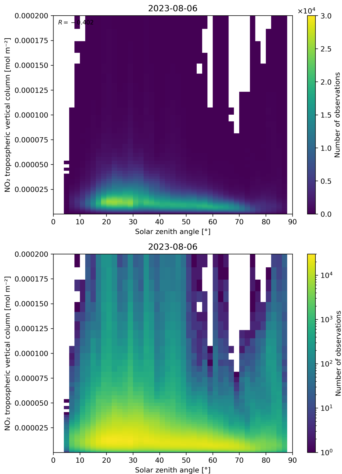
Figure 155: Scatter density plot of “Solar zenith angle” against “NO 2 tropospheric vertical column” for 2023-08-05 to 2023-08-07.
