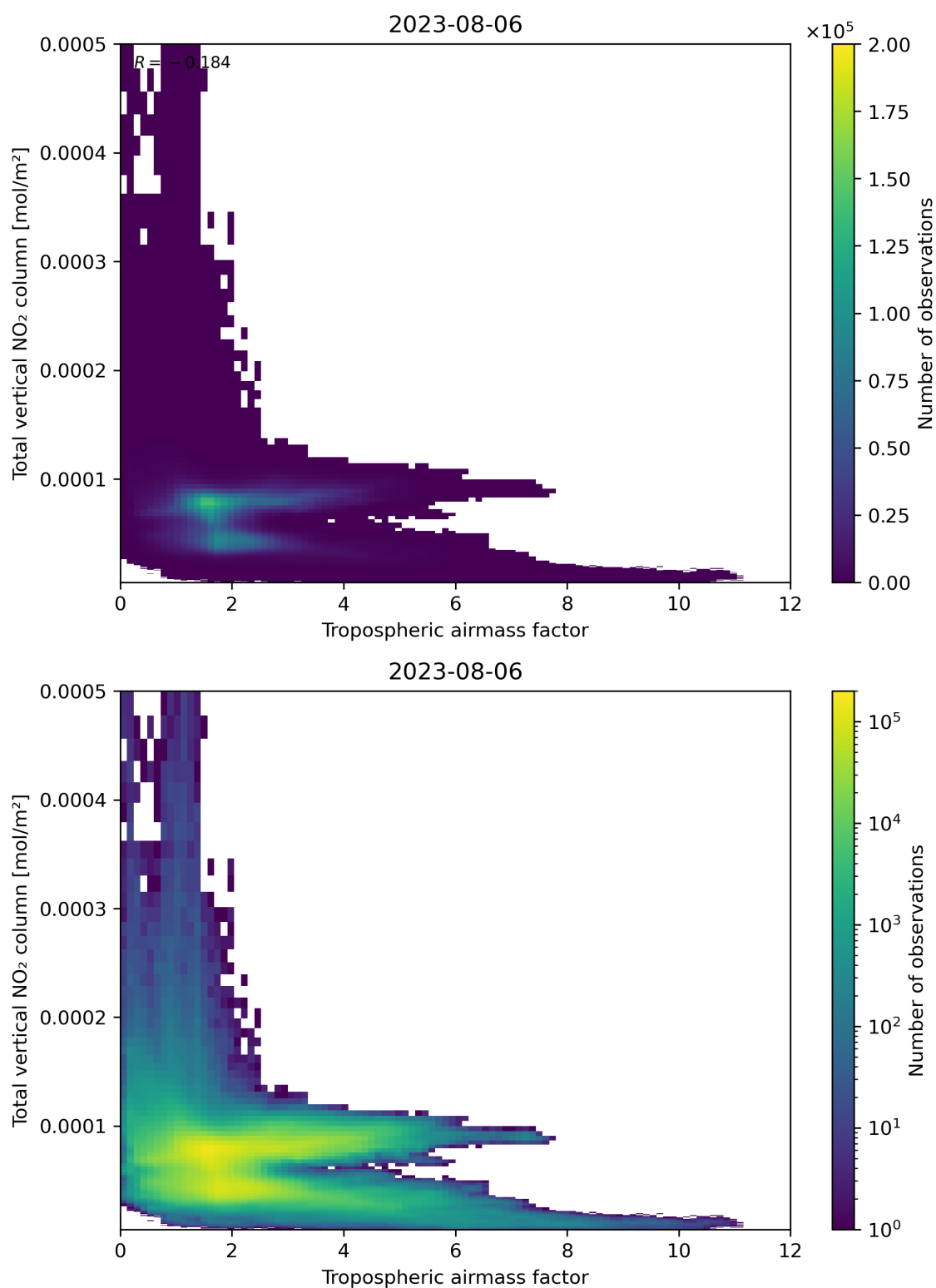
Figure 77: Scatter density plot of “Tropospheric airmass factor” against “Total vertical NO 2 column” for 2023-08-05 to 2023-08-07.
