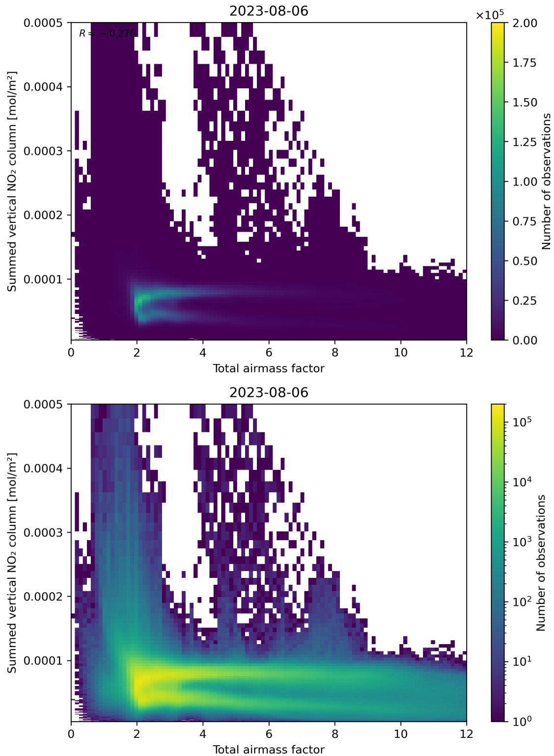
Figure 65: Scatter density plot of “Total airmass factor” against “Summed vertical NO 2 column” for 2023-08-05 to 2023-08-07.
