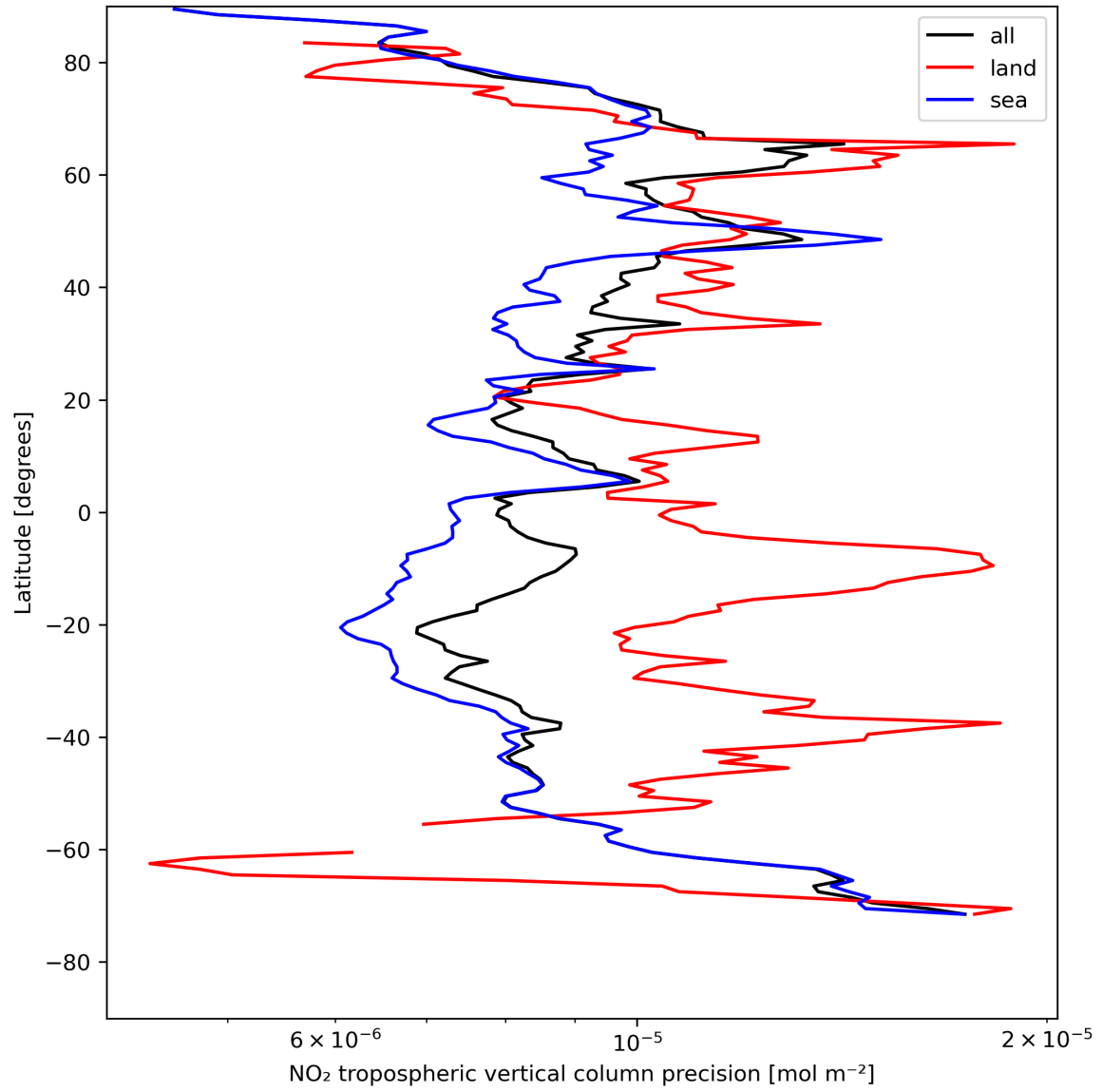
Figure 13: Zonal average of “NO 2 tropospheric vertical column precision” for 2023-08-05 to 2023-08-07.
