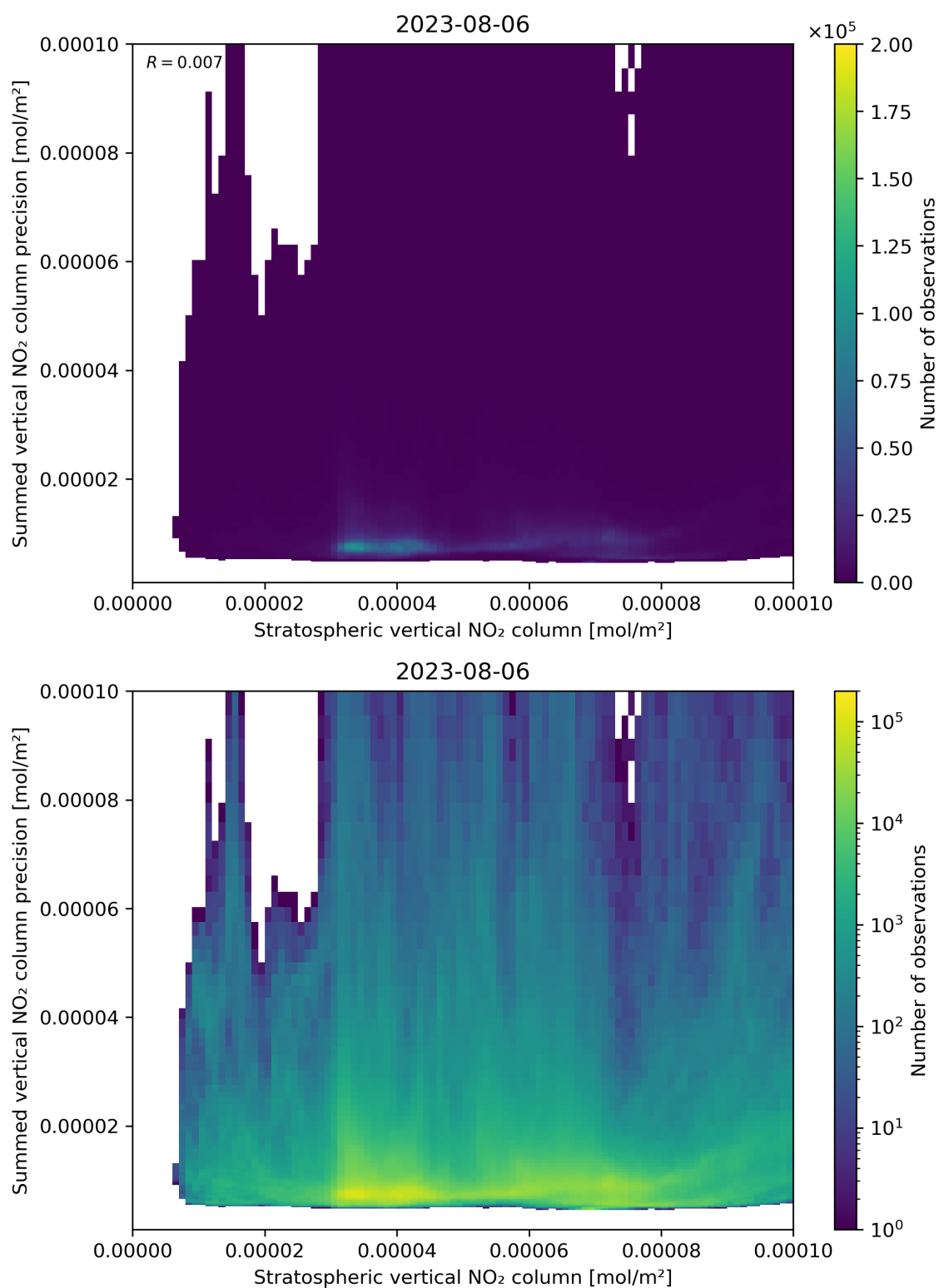
Figure 99: Scatter density plot of “Stratospheric vertical NO 2 column” against “Summed vertical NO 2 column precision” for 2023-08-05 to 2023-08-07.
