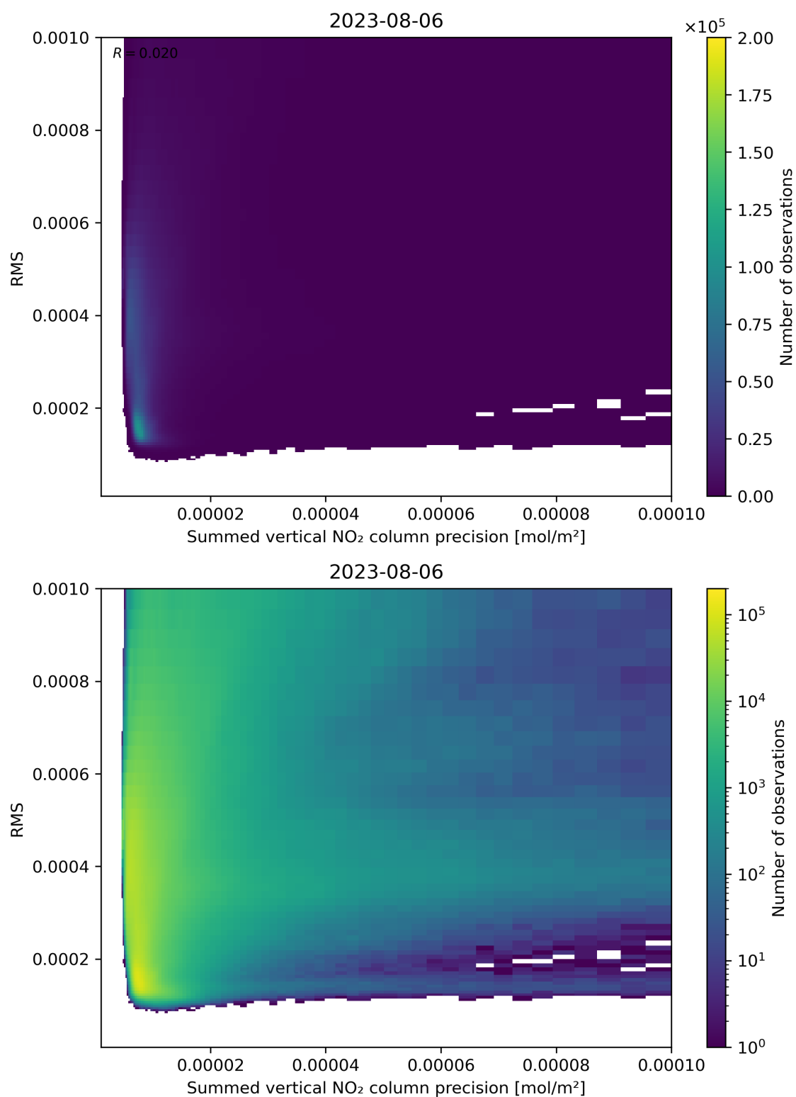
Figure 108: Scatter density plot of “Summed vertical NO 2 column precision” against “RMS” for 2023-08-05 to 2023-08-07.
