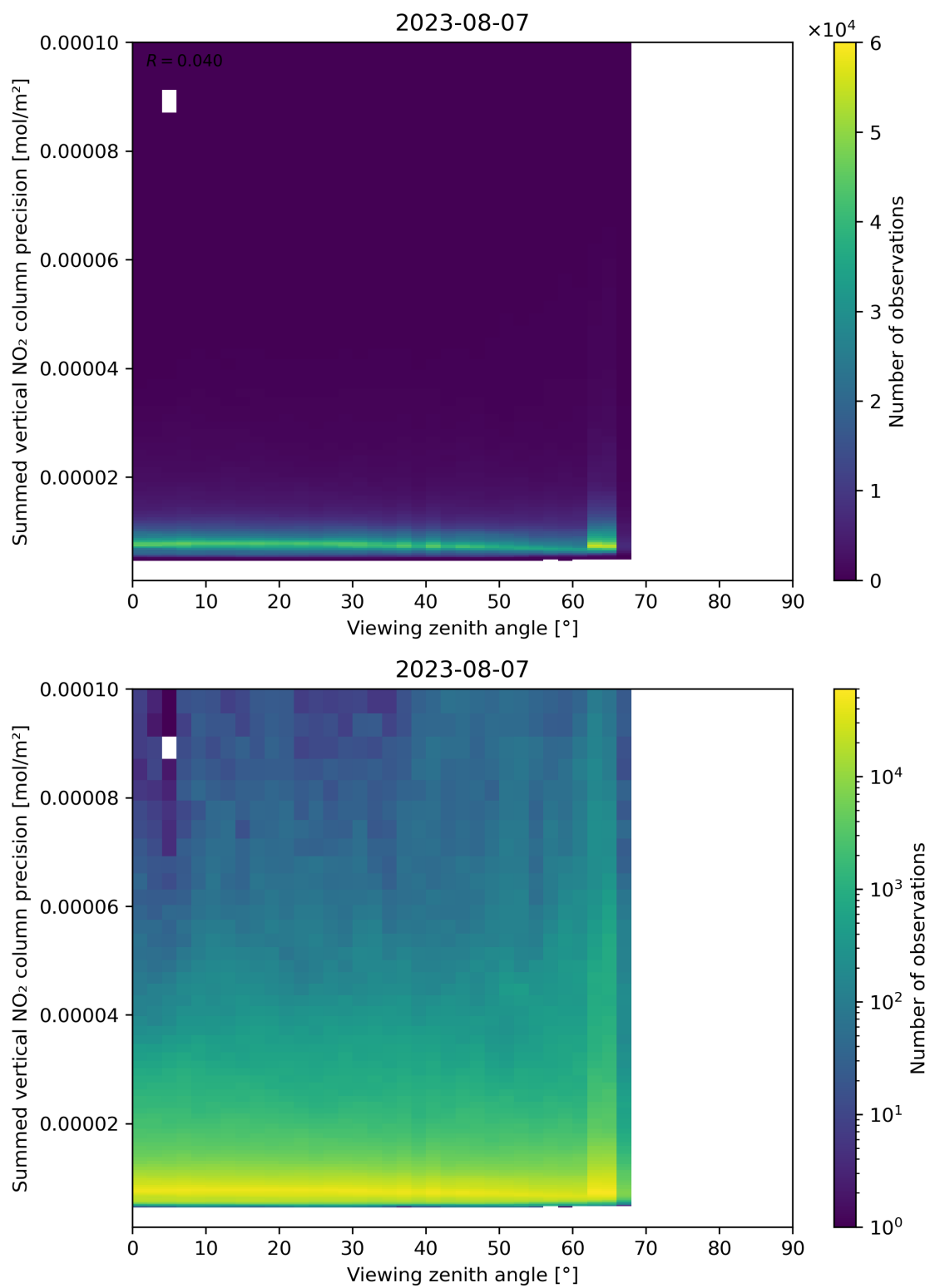
Figure 166: Scatter density plot of “Viewing zenith angle” against “Summed vertical NO 2 column precision” for 2023-08-06 to 2023-08-08.
