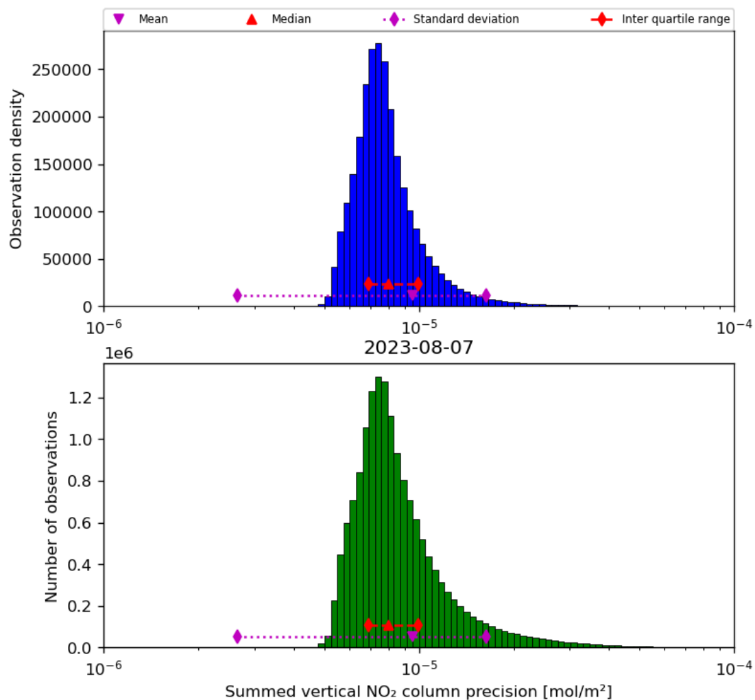
Figure 41: Histogram of "Summed vertical NO 2 column precision" for 2023-08-06 to 2023-08-08
