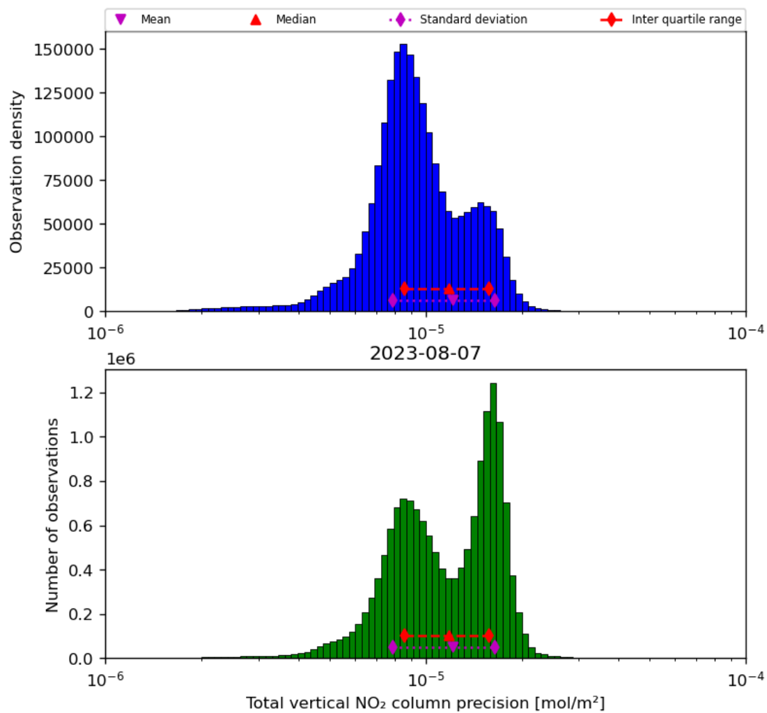
Figure 39: Histogram of “Total vertical NO 2 column precision” for 2023-08-06 to 2023-08-08
