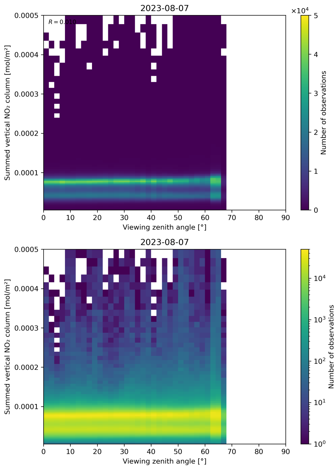
Figure 165: Scatter density plot of “Viewing zenith angle” against “Summed vertical NO 2 column” for 2023-08-06 to 2023-08-08.
