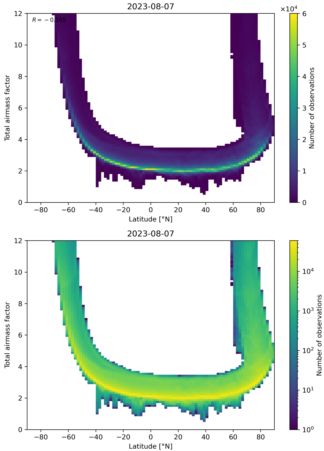
Figure 84: Scatter density plot of “Latitude” against “Total airmass factor” for 2023-08-06 to 2023-08-08.
