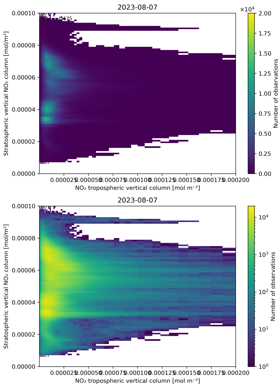
Figure 125: Scatter density plot of “NO 2 tropospheric vertical column” against “Stratospheric vertical NO 2 column” for 2023-08-06 to 2023-08-08.
