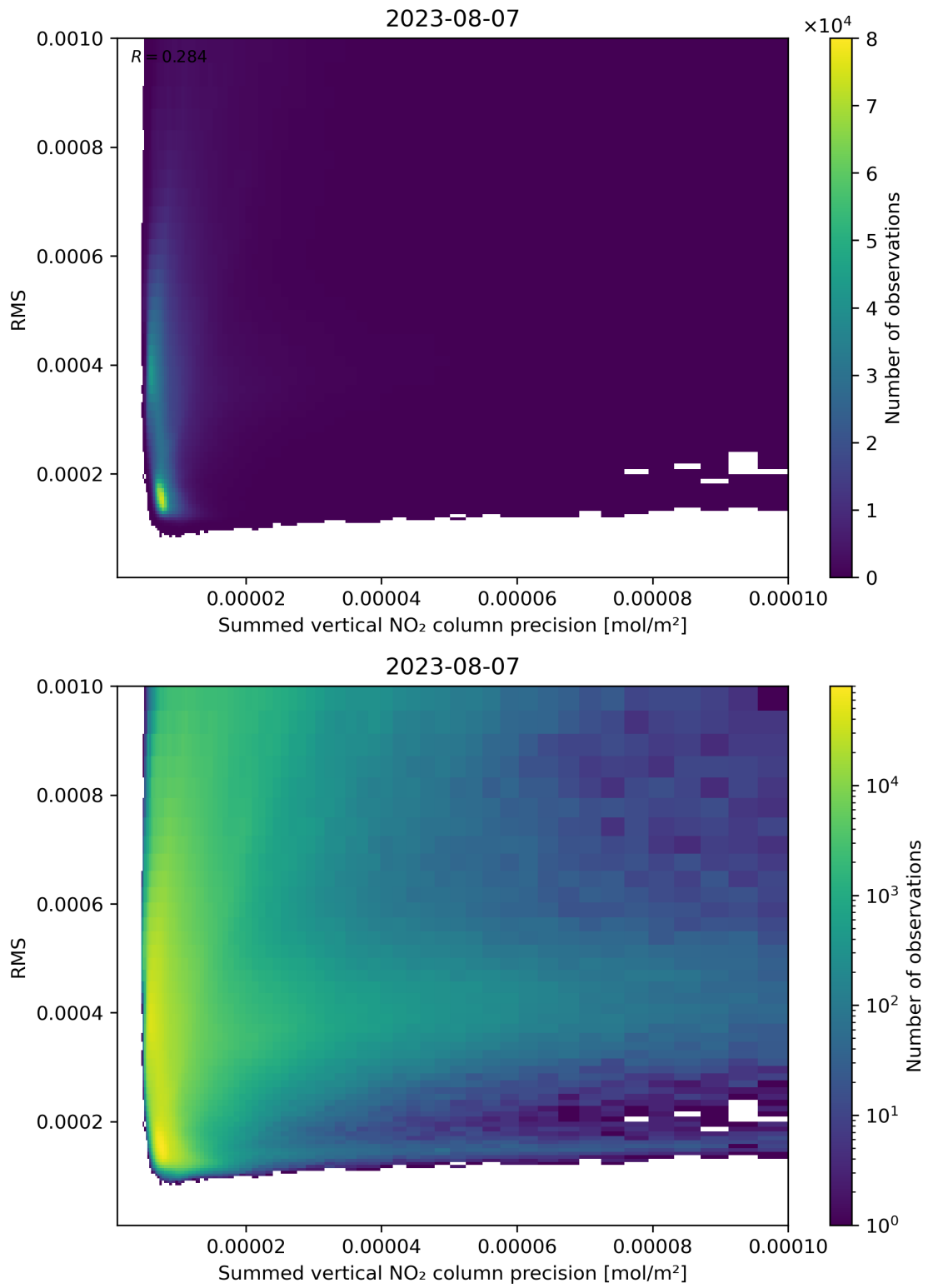
Figure 108: Scatter density plot of “Summed vertical NO 2 column precision” against “RMS” for 2023-08-06 to 2023-08-08.
