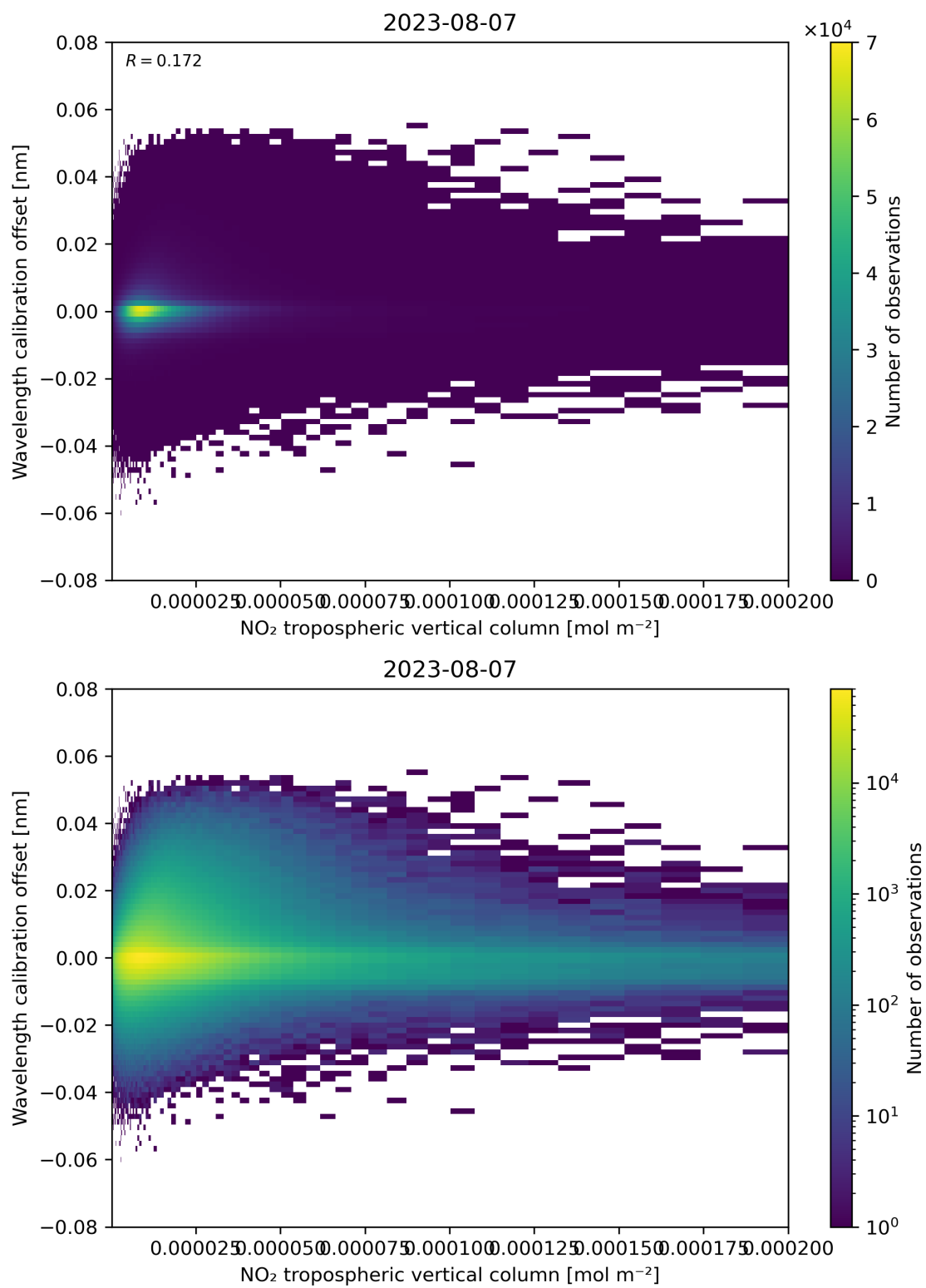
Figure 143: Scatter density plot of “NO 2 tropospheric vertical column” against “Wavelength calibration offset” for 2023-08-06 to 2023-08-08.
