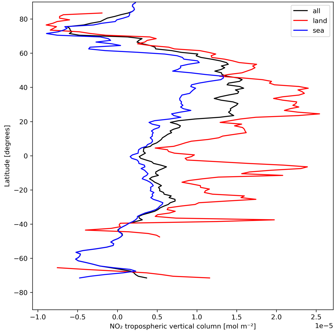
Figure 12: Zonal average of “NO 2 tropospheric vertical column” for 2023-08-06 to 2023-08-08.
