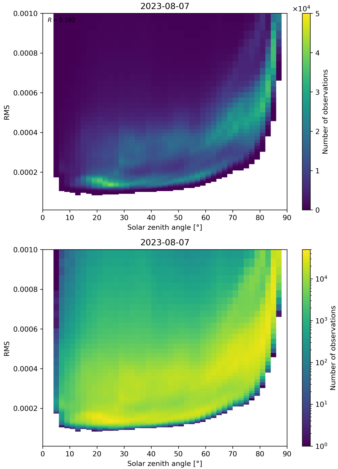
Figure 157: Scatter density plot of “Solar zenith angle” against “RMS” for 2023-08-06 to 2023-08-08.
