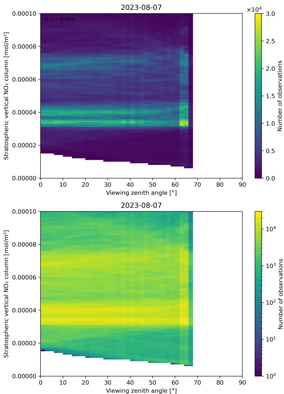
Figure 164: Scatter density plot of “Viewing zenith angle” against “Stratospheric vertical NO 2 column” for 2023-08-06 to 2023-08-08.
