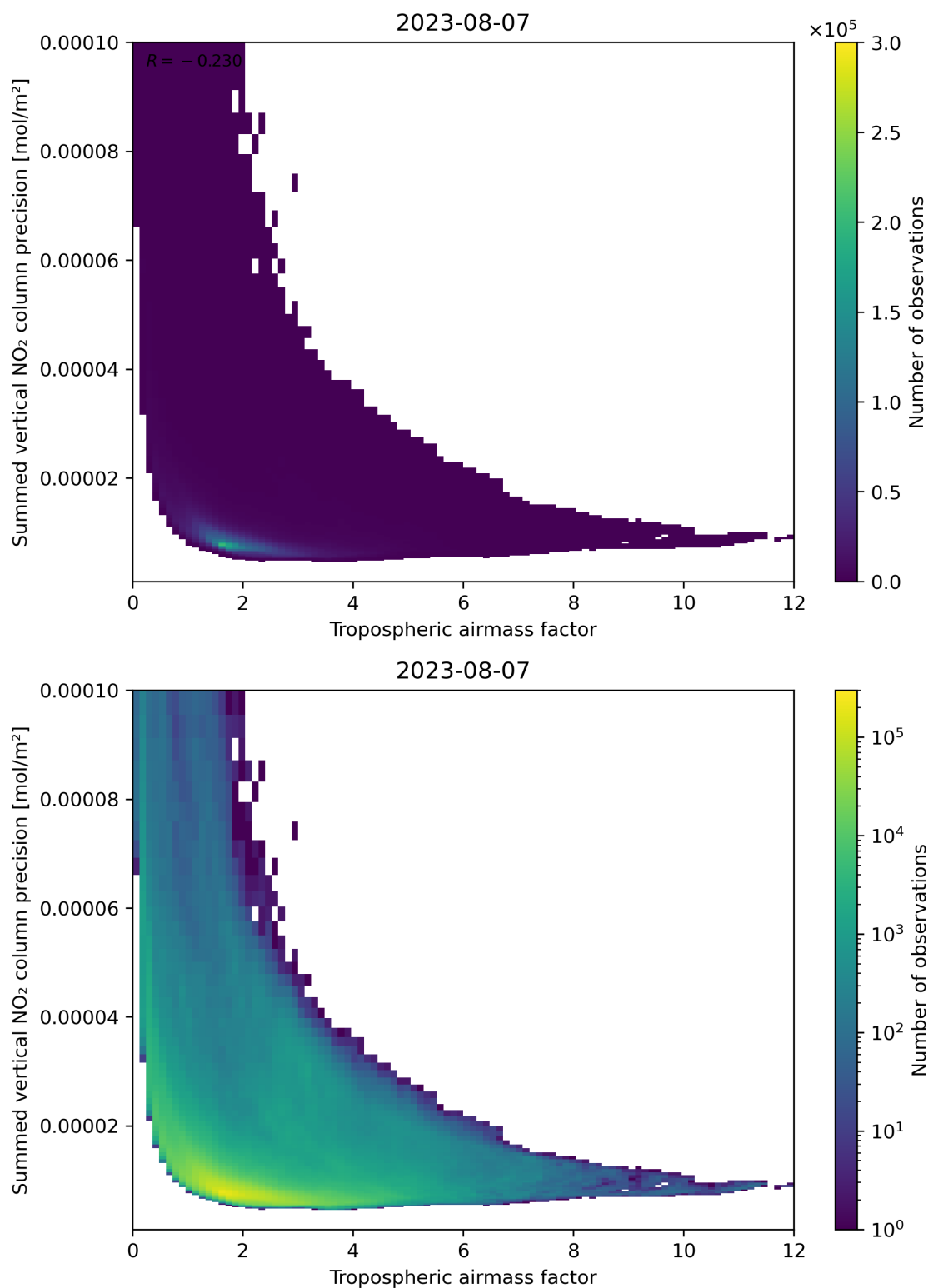
Figure 76: Scatter density plot of “Tropospheric air mass factor” against “Summed vertical NO 2 column precision” for 2023-08-06 to 2023-08-08.
