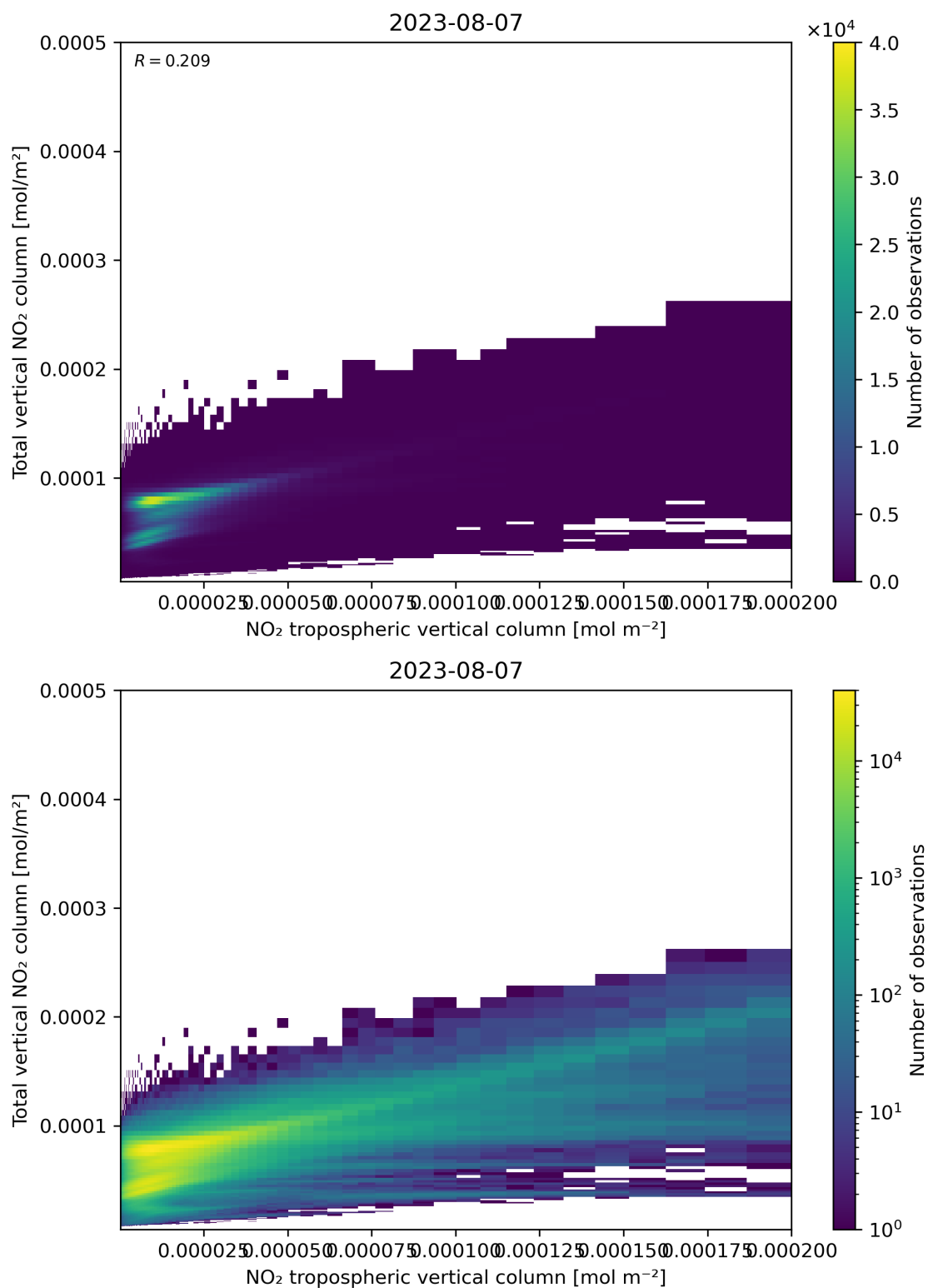
Figure 128: Scatter density plot of “NO 2 tropospheric vertical column” against “Total vertical NO 2 column” for 2023-08-06 to 2023-08-08.
