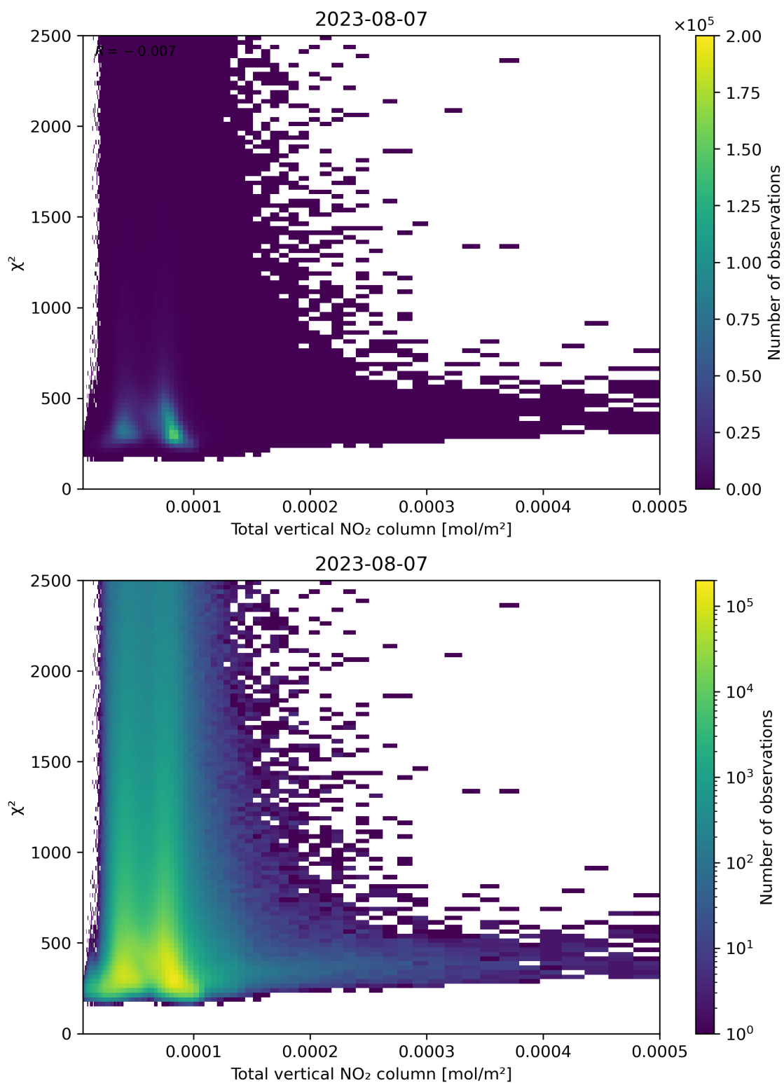
Figure 111: Scatter density plot of “Total vertical NO 2 column” against “ \chi^2 ” for 2023-08-06 to 2023-08-08.
