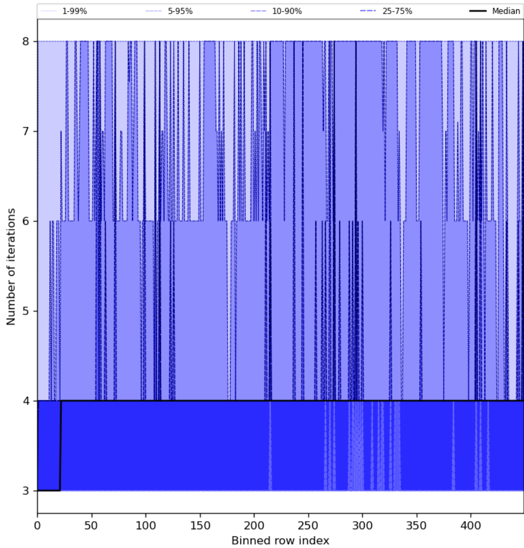
Figure 51: Along track statistics of “Number of iterations” for 2023-08-06 to 2023-08-08
