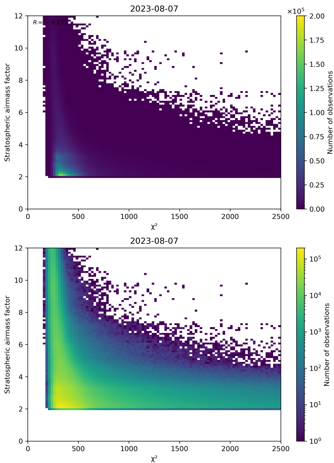
Figure 81: Scatter density plot of “ \chi^2 ” against “Stratospheric airmass factor” for 2023-08-06 to 2023-08-08.
