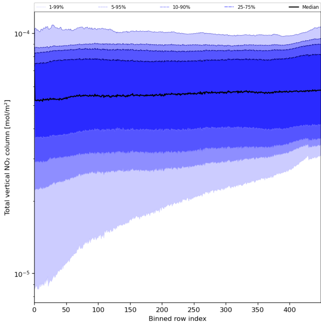
Figure 55: Along track statistics of “Total vertical NO 2 column” for 2023-08-06 to 2023-08-08
