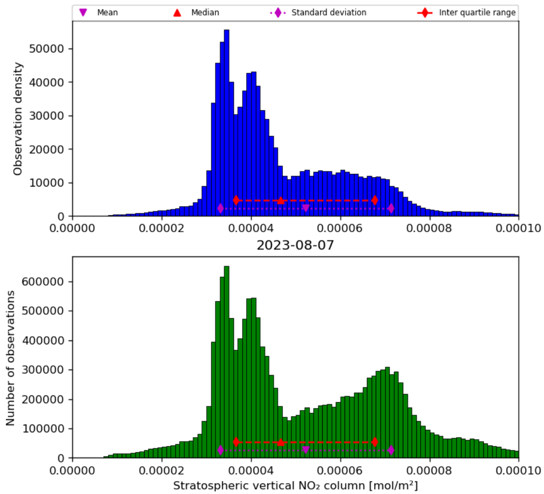
Figure 36: Histogram of “Stratospheric vertical NO 2 column” for 2023-08-06 to 2023-08-08
