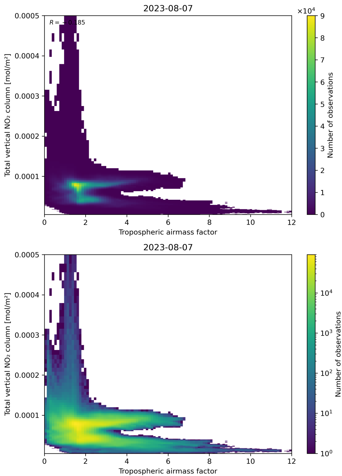
Figure 77: Scatter density plot of “Tropospheric airmass factor” against “Total vertical NO 2 column” for 2023-08-06 to 2023-08-08.
