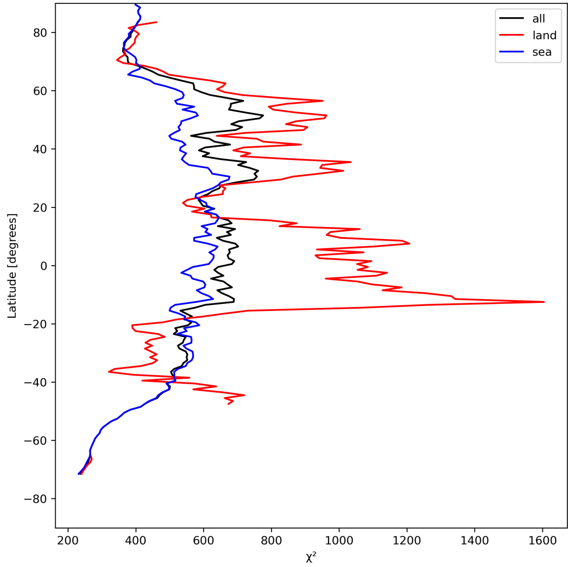
Figure 25: Zonal average of “ \chi^2 ” for 2023-08-06 to 2023-08-08.
