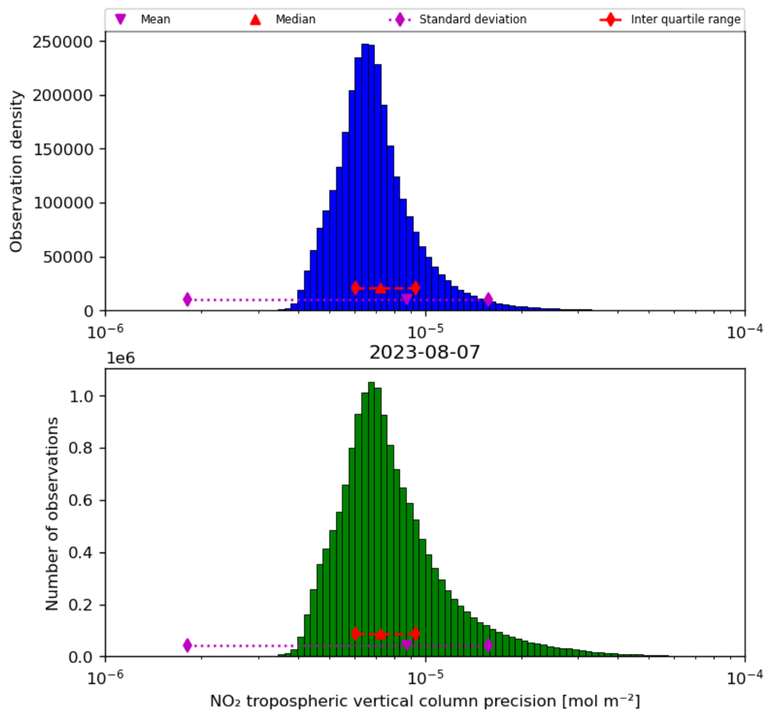
Figure 30: Histogram of “NO 2 tropospheric vertical column precision” for 2023-08-06 to 2023-08-08
