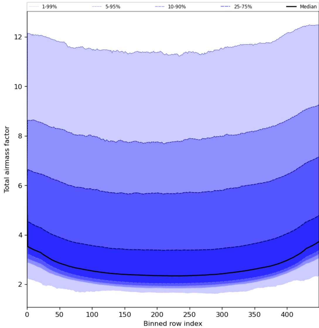
Figure 49: Along track statistics of “Total airmass factor” for 2023-08-06 to 2023-08-08
