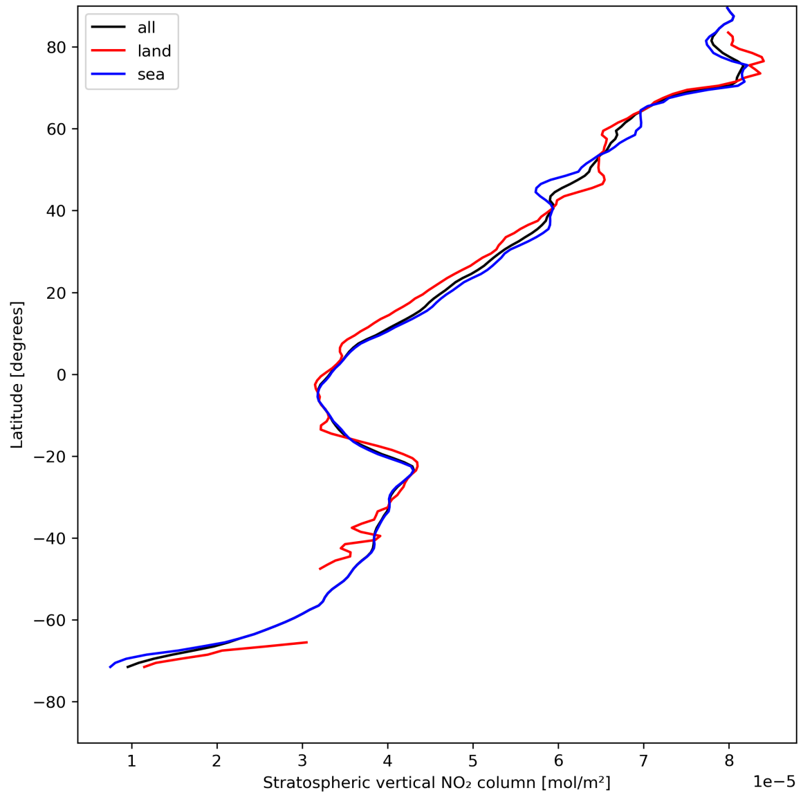
Figure 19: Zonal average of “Stratospheric vertical NO 2 column” for 2023-08-06 to 2023-08-08.
