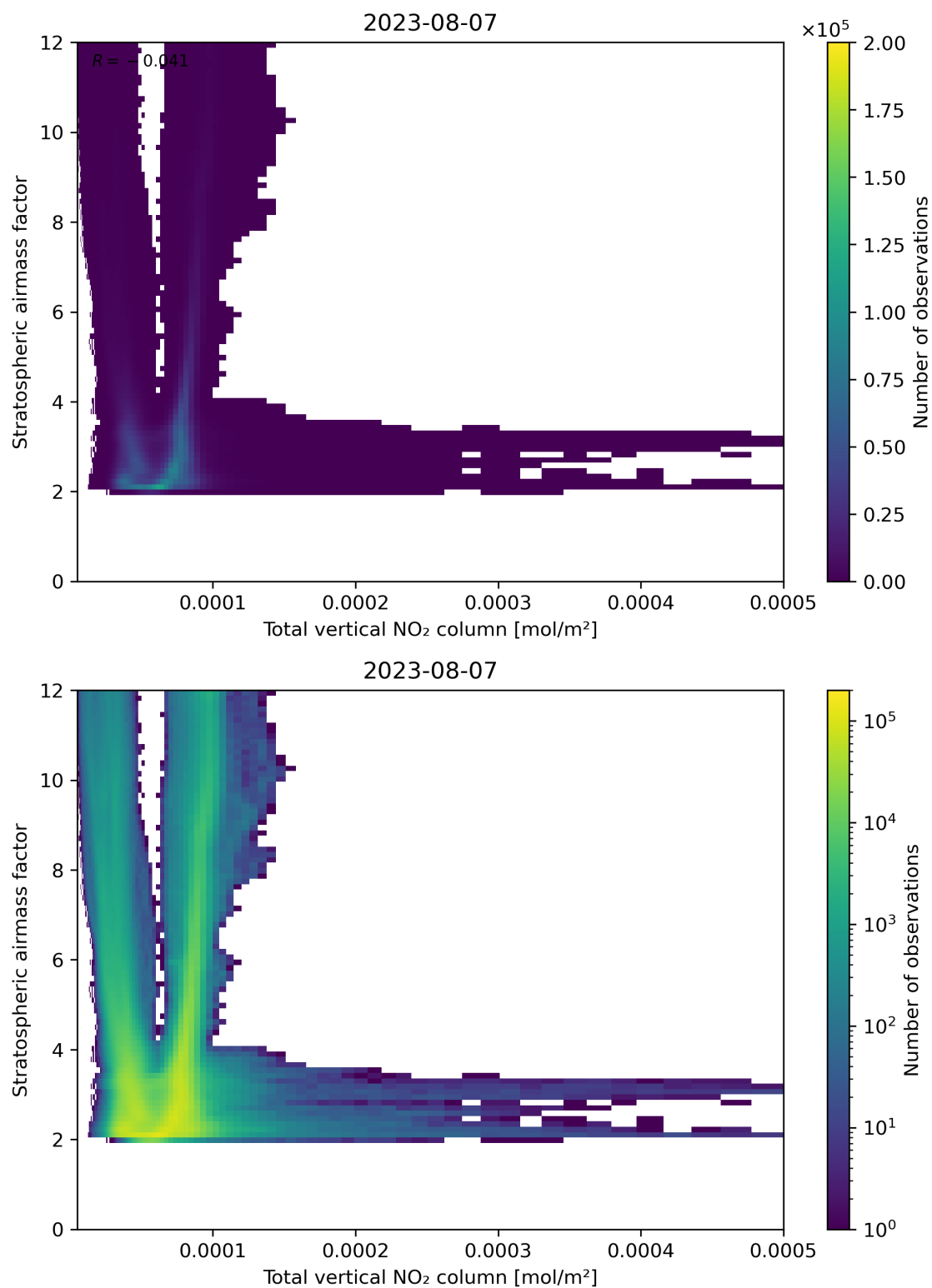
Figure 110: Scatter density plot of “Total vertical NO 2 column” against “Stratospheric airmass factor” for 2023-08-06 to 2023-08-08.
