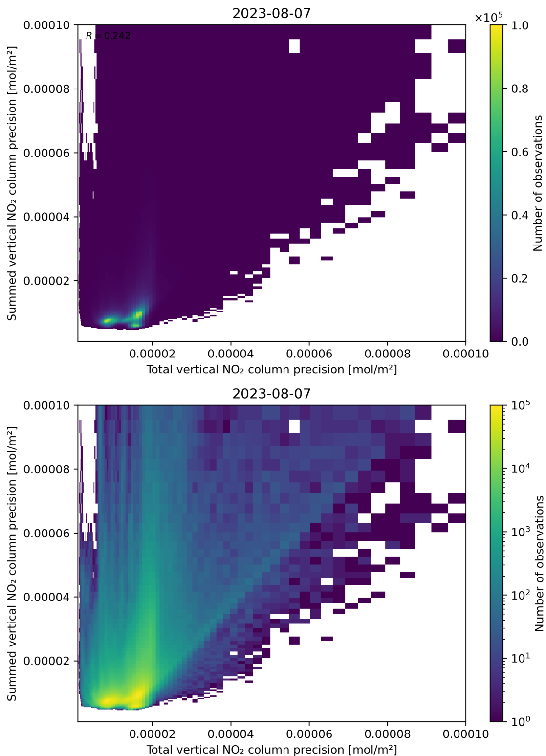
Figure 118: Scatter density plot of “Total vertical NO 2 column precision” against “Summed vertical NO 2 column precision” for 2023-08-06 to 2023-08-08.
