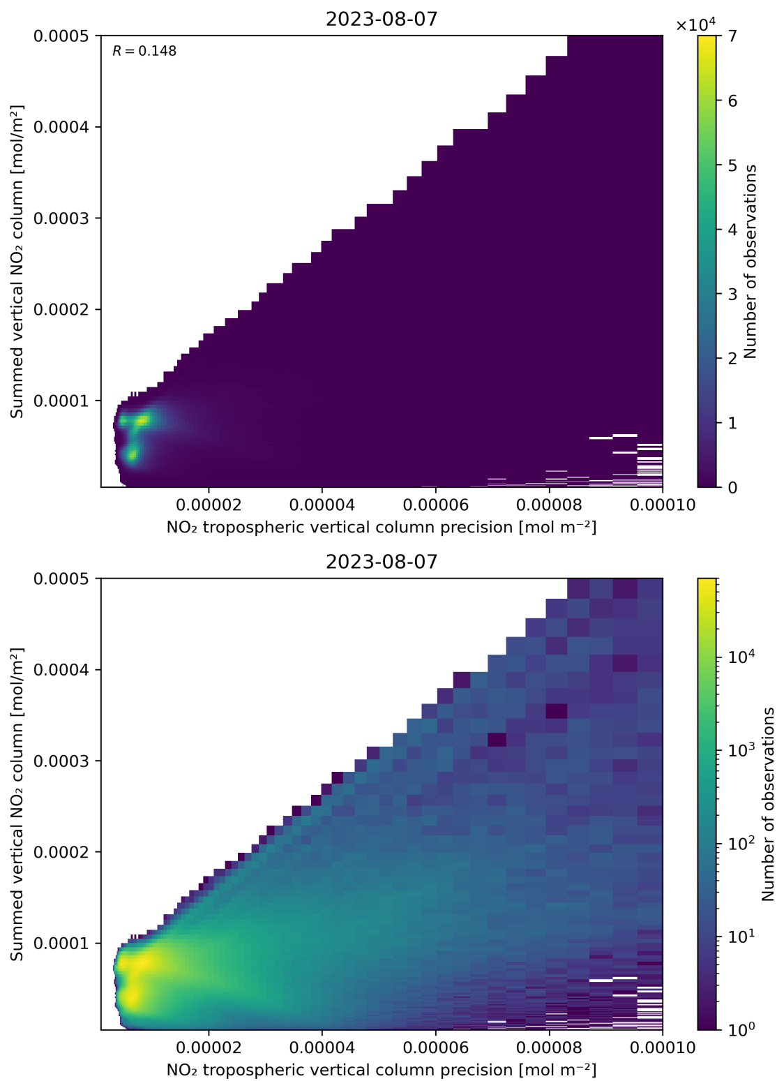
Figure 136: Scatter density plot of “NO 2 tropospheric vertical column precision” against “Summed vertical NO 2 column” for 2023-08-06 to 2023-08-08.
