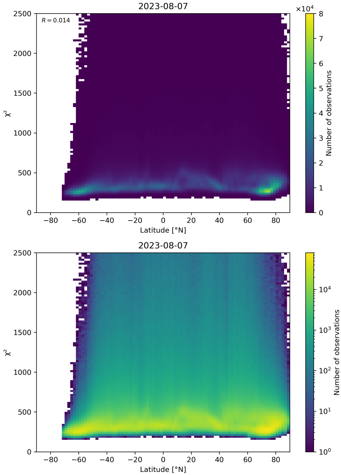
Figure 86: Scatter density plot of “Latitude” against “ \chi^2 ” for 2023-08-06 to 2023-08-08.
