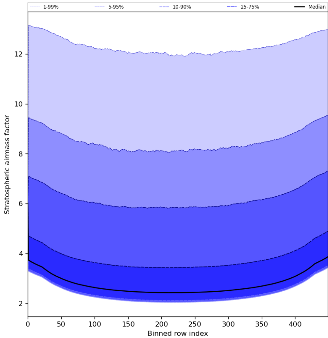
Figure 61: Along track statistics of “Stratospheric airmass factor” for 2023-08-06 to 2023-08-08
