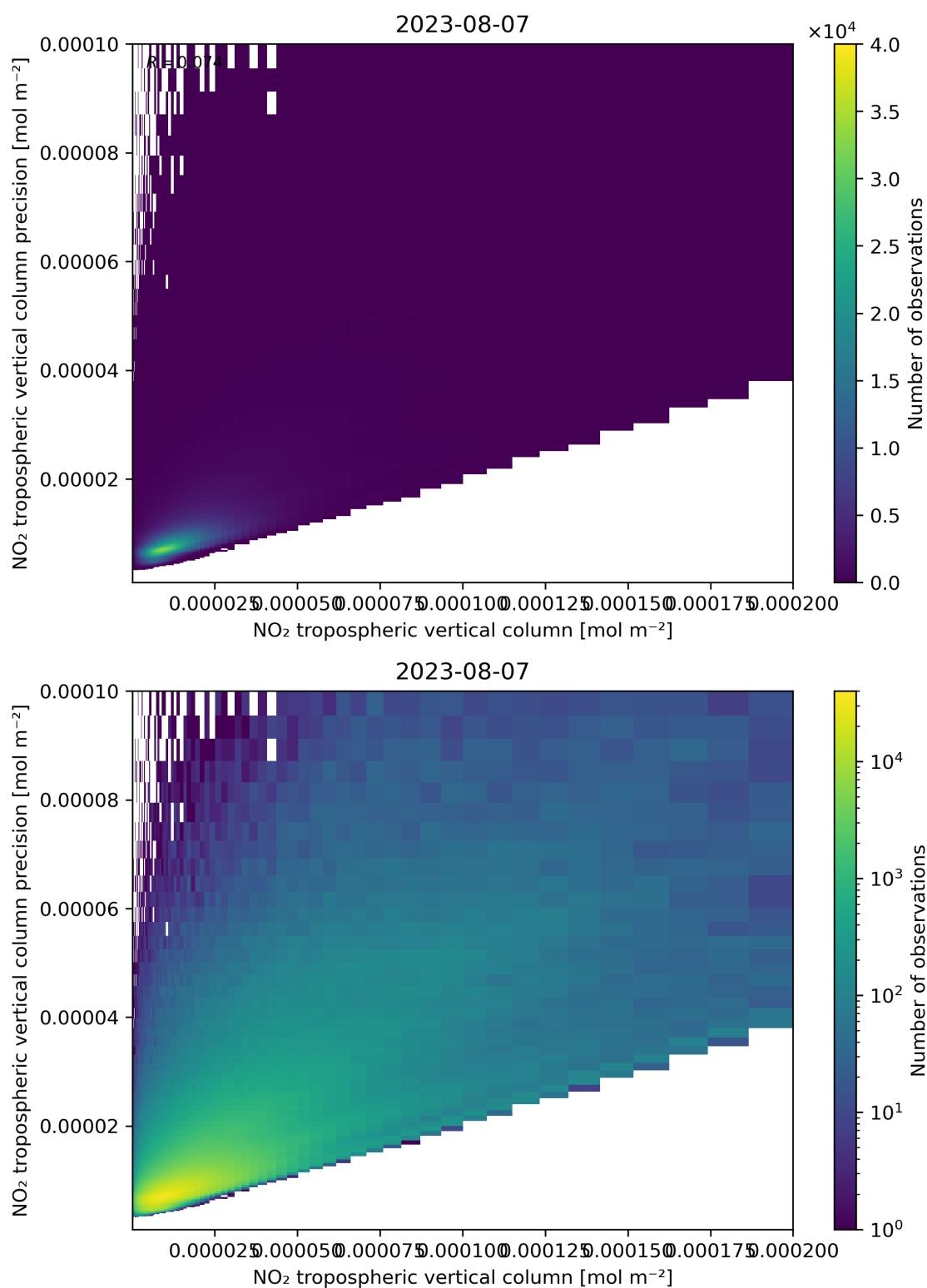
Figure 130: Scatter density plot of “NO 2 tropospheric vertical column” against “NO 2 tropospheric vertical column precision” for 2023-08-06 to 2023-08-08.
