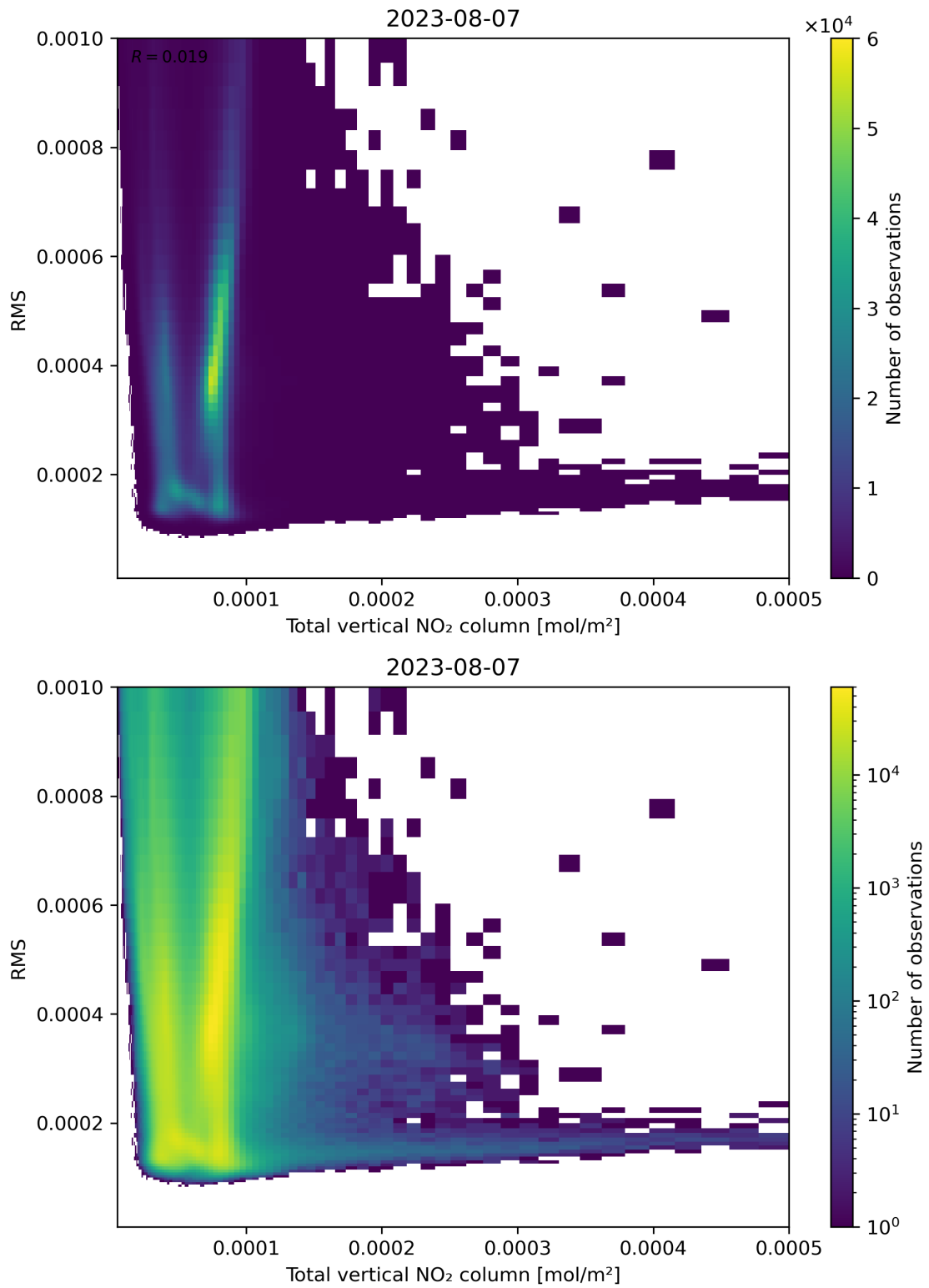
Figure 120: Scatter density plot of “Total vertical NO 2 column” against “RMS” for 2023-08-06 to 2023-08-08.
