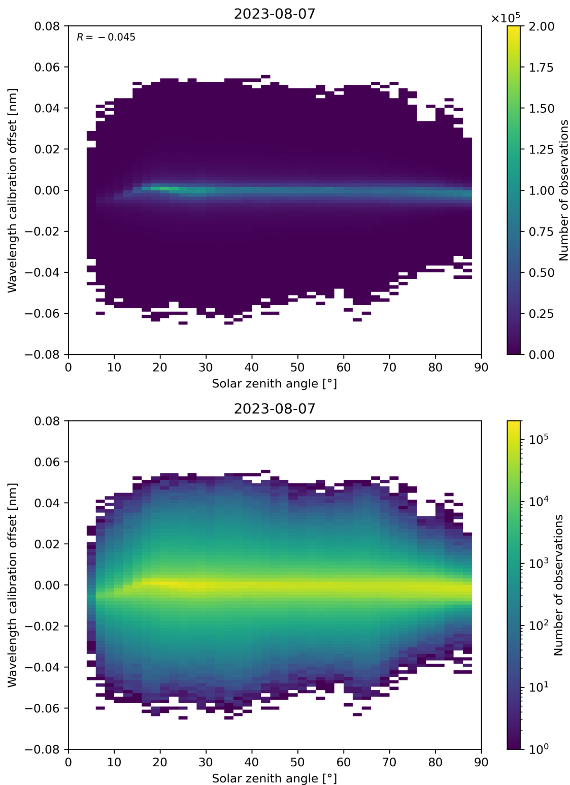
Figure 158: Scatter density plot of “Solar zenith angle” against “Wavelength calibration offset” for 2023-08-06 to 2023-08-08.
