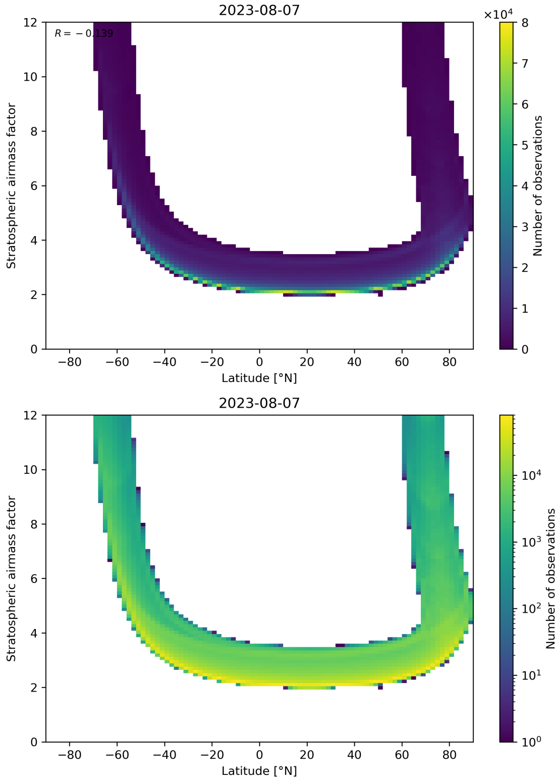
Figure 83: Scatter density plot of “Latitude” against “Stratospheric airmass factor” for 2023-08-06 to 2023-08-08.
