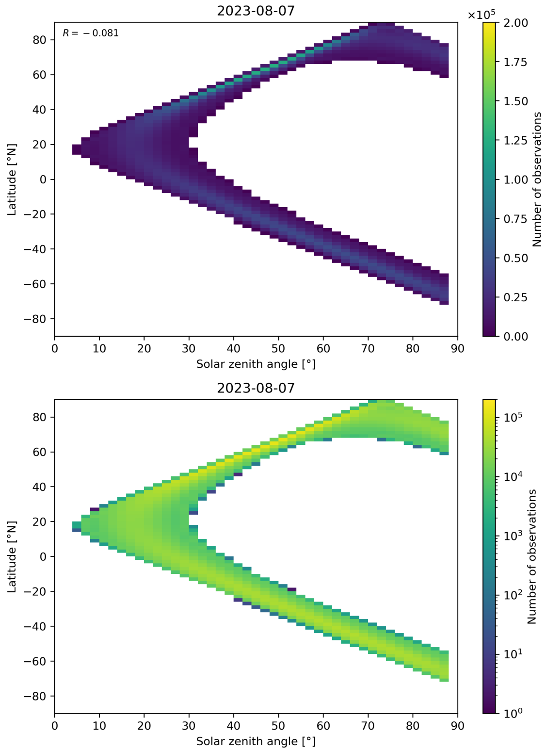
Figure 149: Scatter density plot of “Solar zenith angle” against “Latitude” for 2023-08-06 to 2023-08-08.
