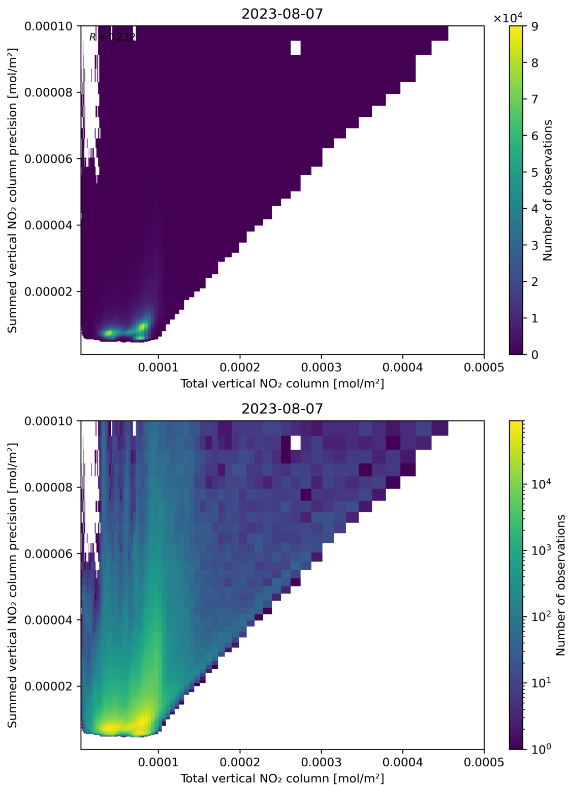
Figure 113: Scatter density plot of “Total vertical NO 2 column” against “Summed vertical NO 2 column precision” for 2023-08-06 to 2023-08-08.
