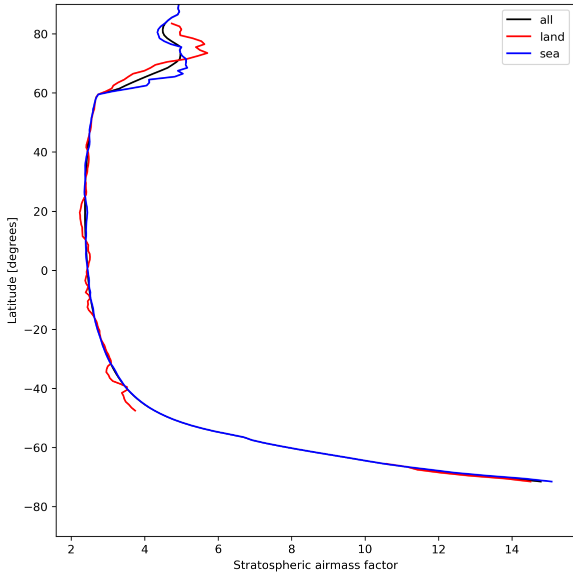
Figure 27: Zonal average of “Stratospheric air mass factor” for 2023-08-06 to 2023-08-08.
