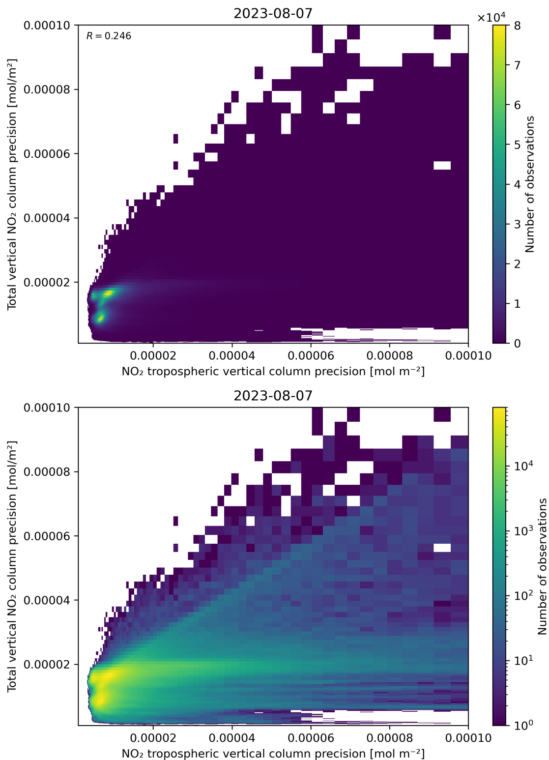
Figure 139: Scatter density plot of “NO 2 tropospheric vertical column precision” against “Total vertical NO 2 column precision” for 2023-08-06 to 2023-08-08.
