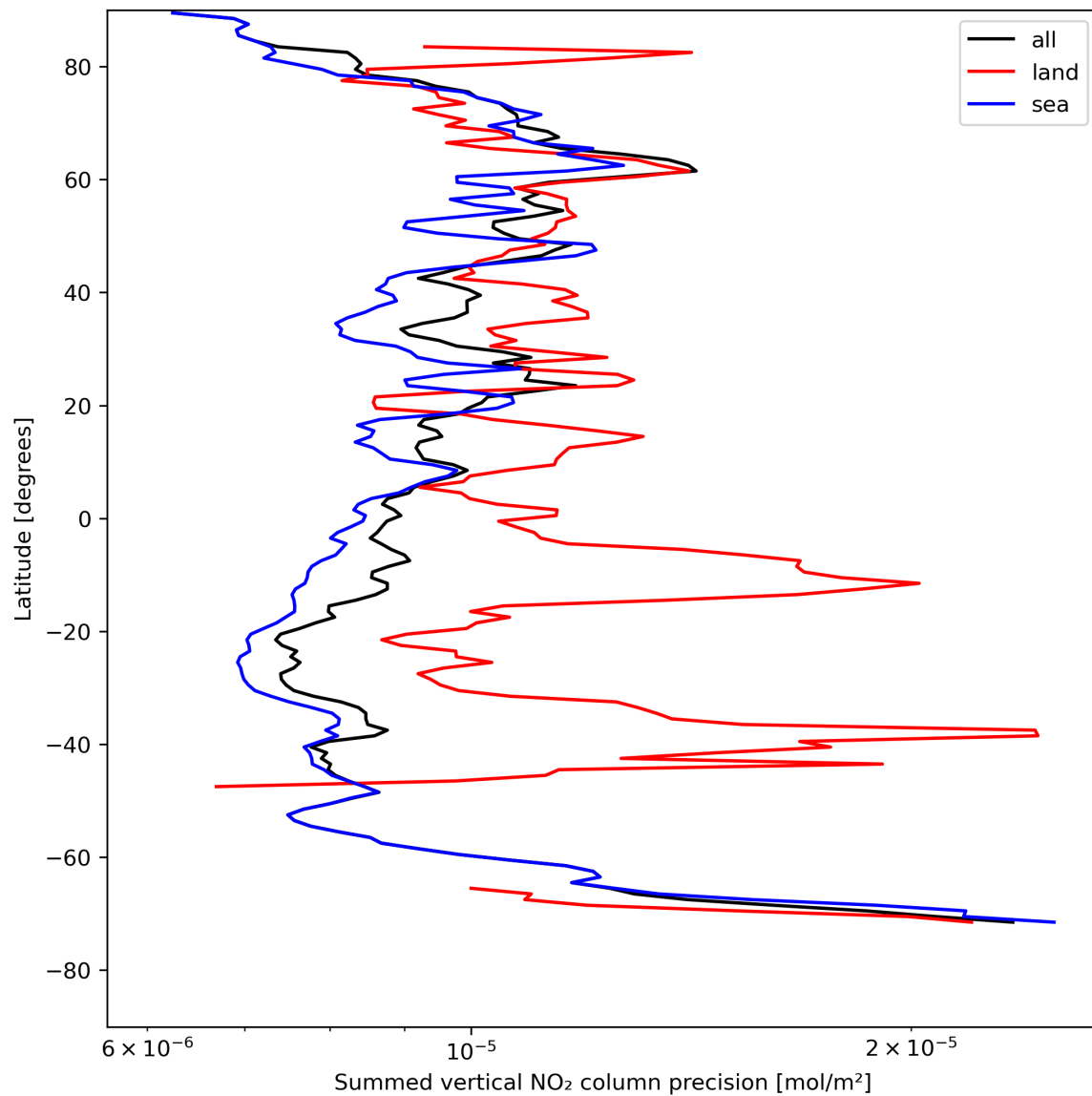
Figure 24: Zonal average of “Summed vertical NO 2 column precision” for 2023-08-06 to 2023-08-08.
