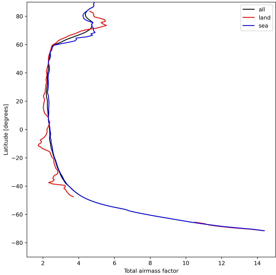
Figure 15: Zonal average of “Total airmass factor” for 2023-08-06 to 2023-08-08.
