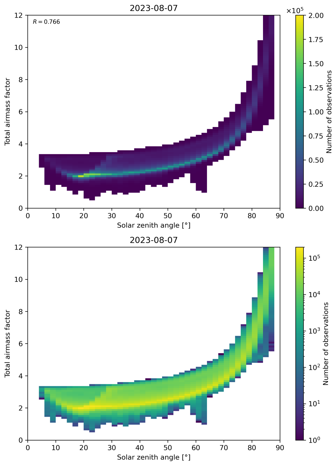
Figure 146: Scatter density plot of “Solar zenith angle” against “Total air mass factor” for 2023-08-06 to 2023-08-08.
