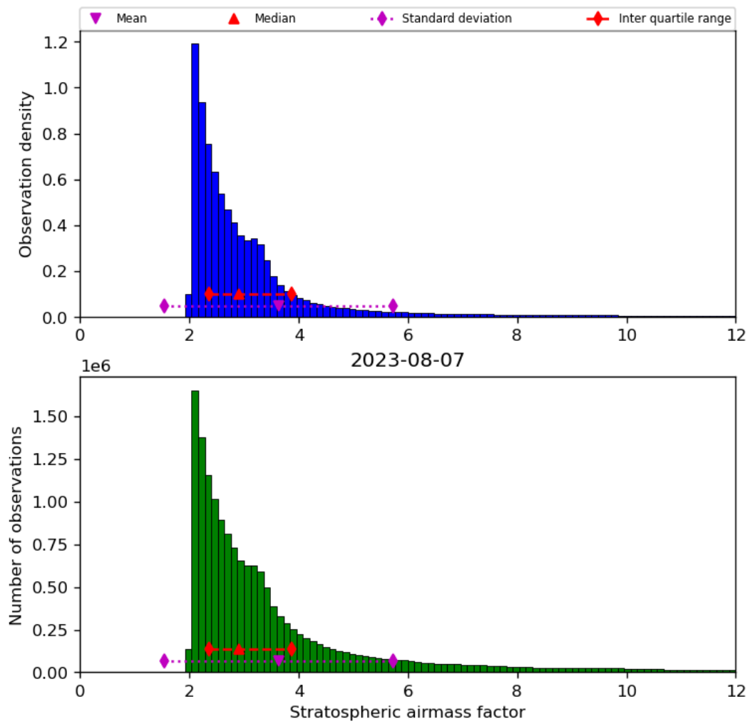
Figure 44: Histogram of “Stratospheric airmass factor” for 2023-08-06 to 2023-08-08
