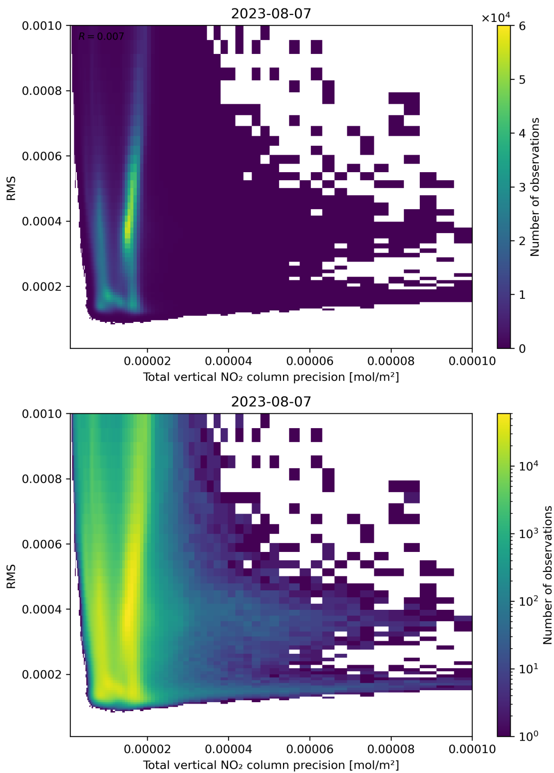
Figure 119: Scatter density plot of “Total vertical NO 2 column precision” against “RMS” for 2023-08-06 to 2023-08-08.
