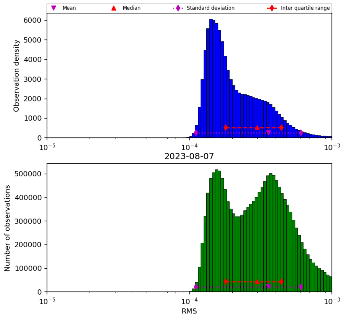
Figure 43: Histogram of “RMS” for 2023-08-06 to 2023-08-08
