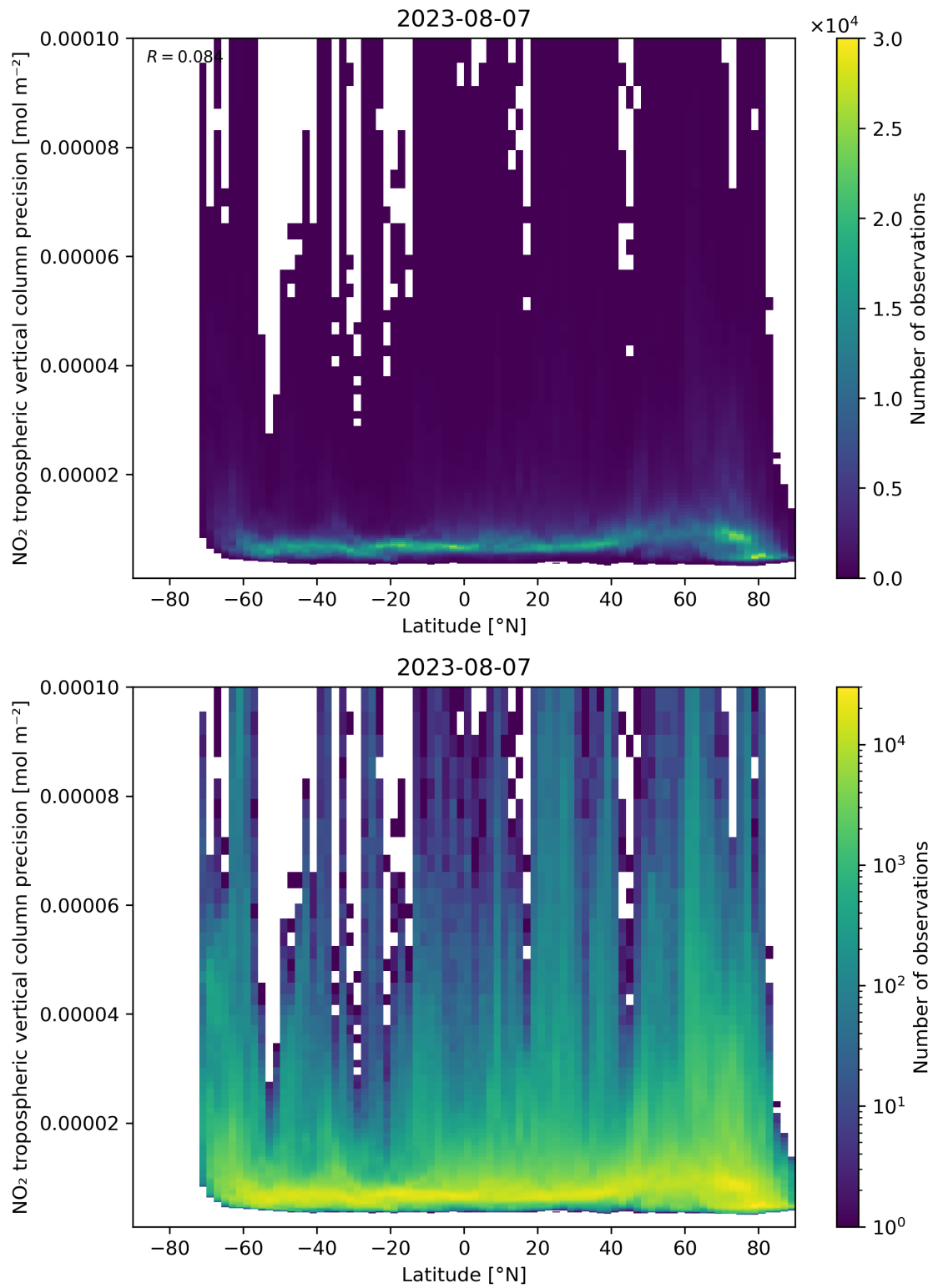
Figure 93: Scatter density plot of “Latitude” against “NO 2 tropospheric vertical column precision” for 2023-08-06 to 2023-08-08.
