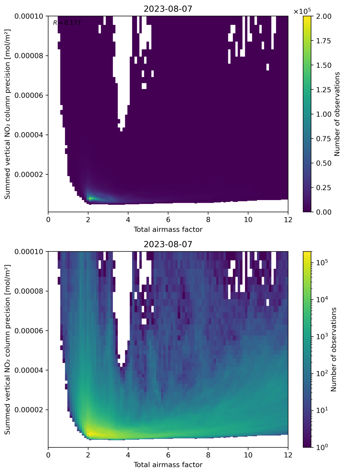
Figure 66: Scatter density plot of “Total airmass factor” against “Summed vertical NO 2 column precision” for 2023-08-06 to 2023-08-08.
