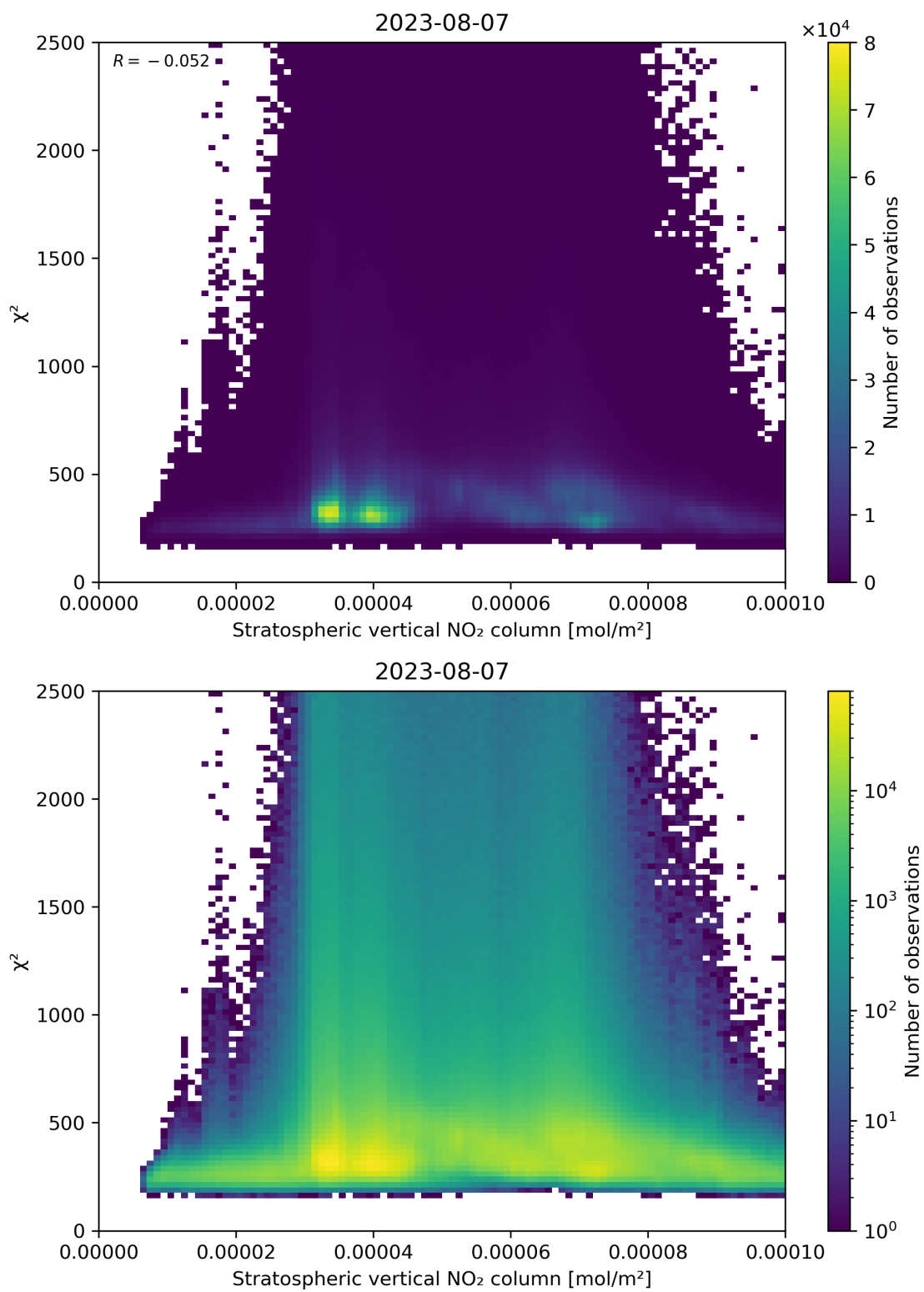
Figure 97: Scatter density plot of “Stratospheric vertical NO 2 column” against “ \chi^2 ” for 2023-08-06 to 2023-08-08.
