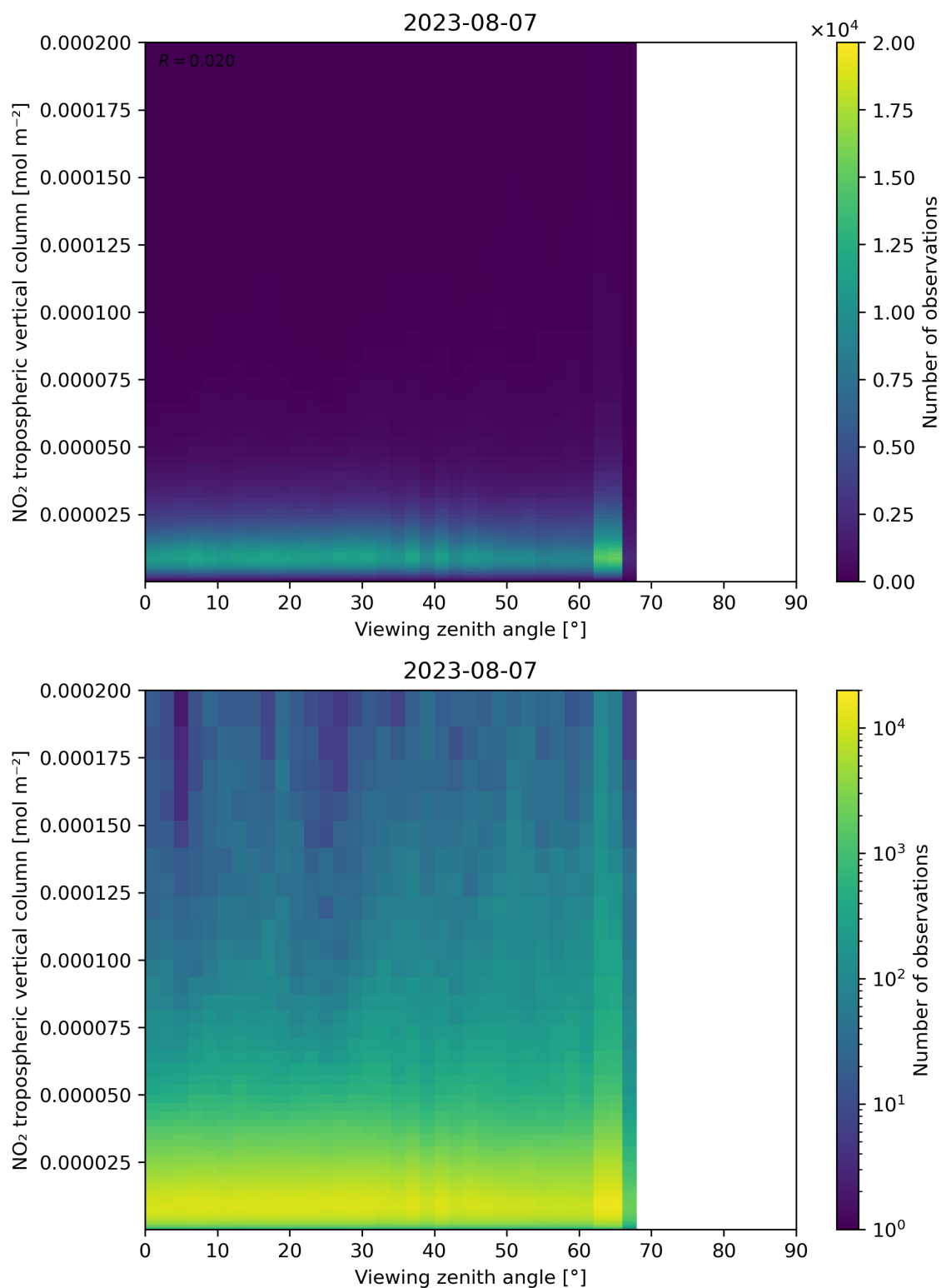
Figure 169: Scatter density plot of “Viewing zenith angle” against “NO 2 tropospheric vertical column” for 2023-08-06 to 2023-08-08.
