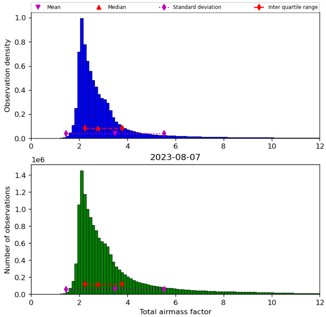
Figure 32: Histogram of “Total airmass factor” for 2023-08-06 to 2023-08-08
