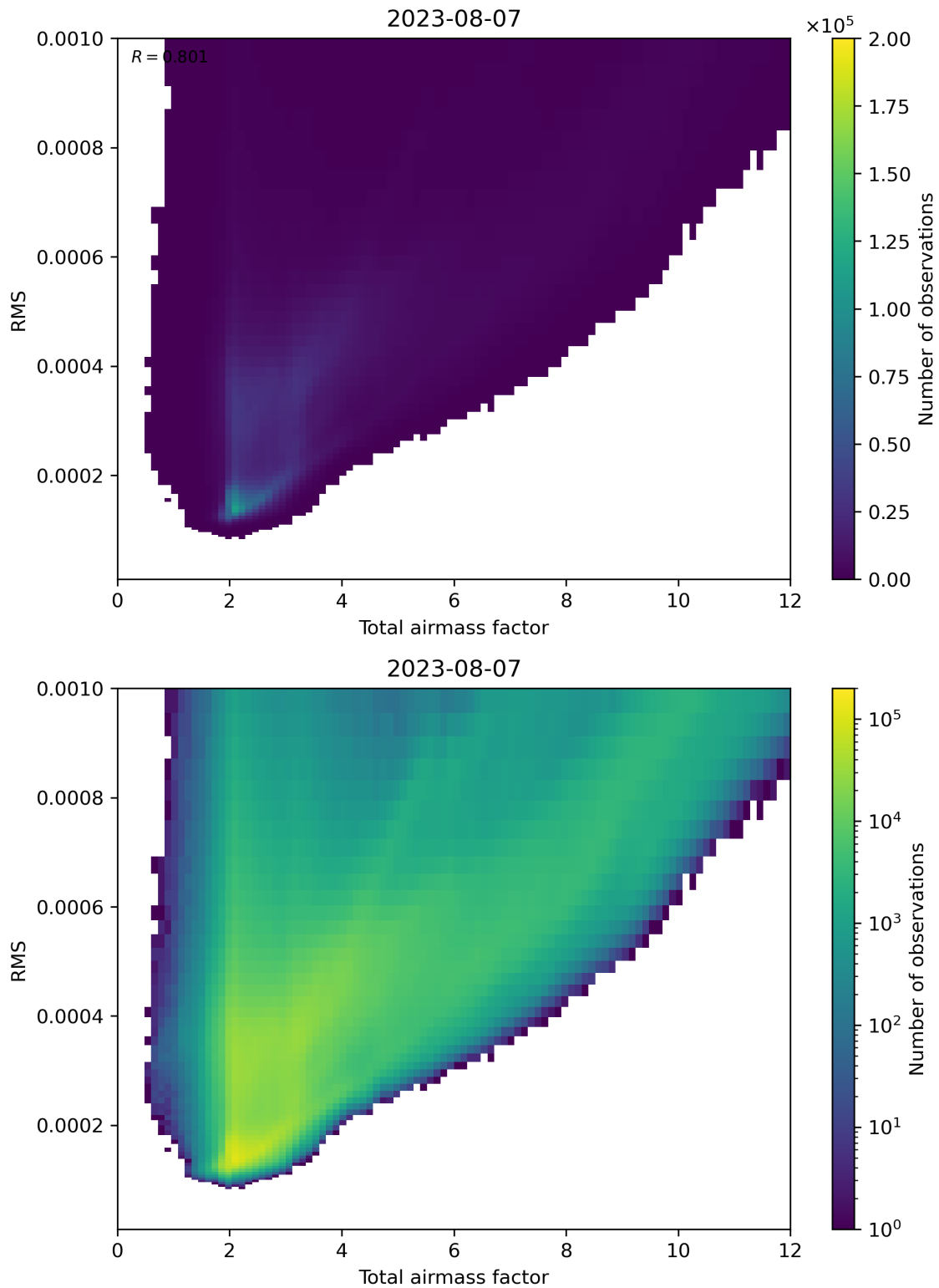
Figure 69: Scatter density plot of “Total airmass factor” against “RMS” for 2023-08-06 to 2023-08-08.
