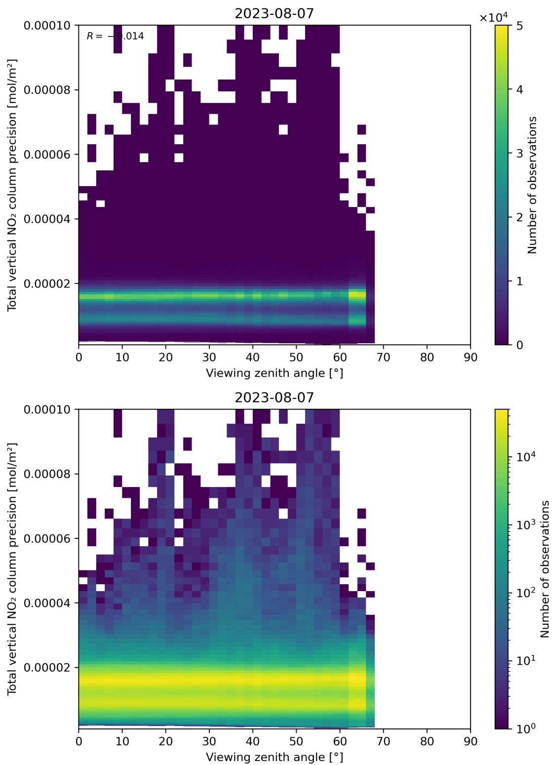
Figure 168: Scatter density plot of “Viewing zenith angle” against “Total vertical NO 2 column precision” for 2023-08-06 to 2023-08-08.
