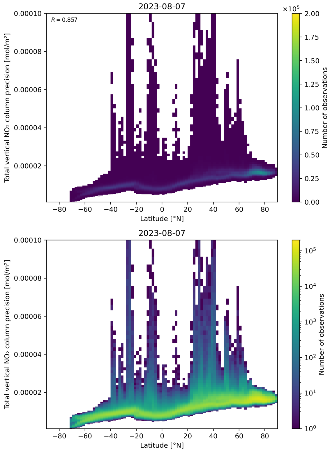
Figure 91: Scatter density plot of “Latitude” against “Total vertical NO 2 column precision” for 2023-08-06 to 2023-08-08.
