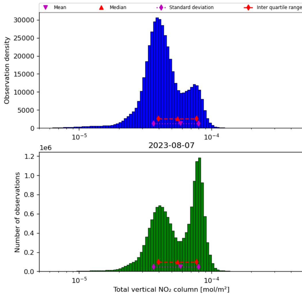
Figure 38: Histogram of “Total vertical NO 2 column” for 2023-08-06 to 2023-08-08
