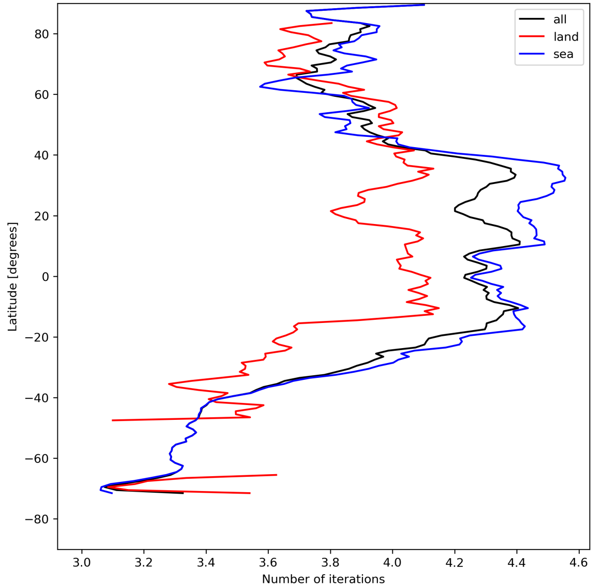
Figure 17: Zonal average of “Number of iterations” for 2023-08-06 to 2023-08-08.
