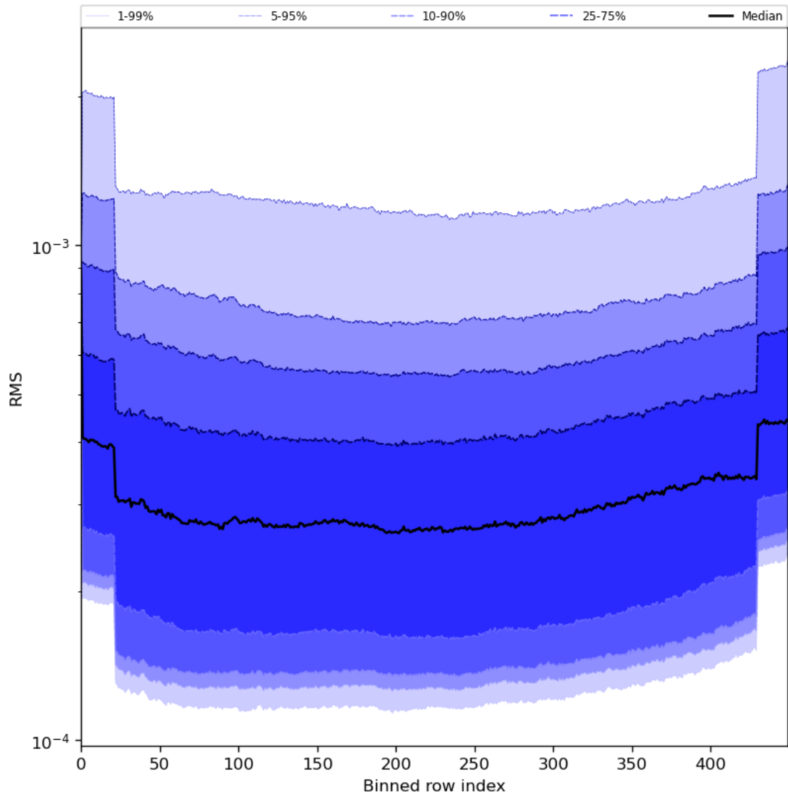
Figure 60: Along track statistics of “RMS” for 2023-08-06 to 2023-08-08
