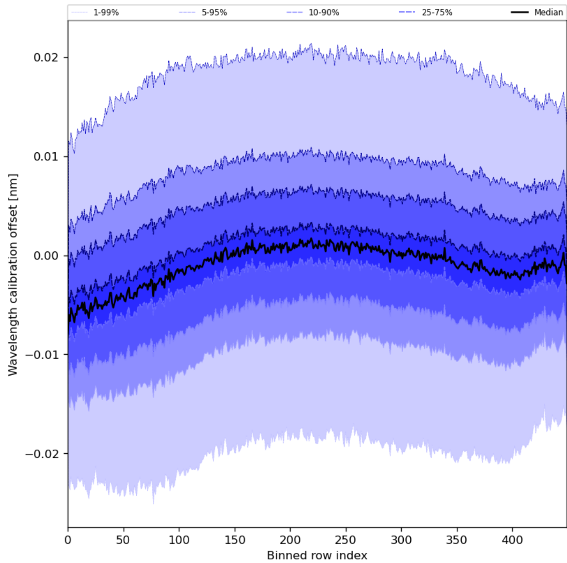
Figure 52: Along track statistics of “Wavelength calibration offset” for 2023-08-06 to 2023-08-08
