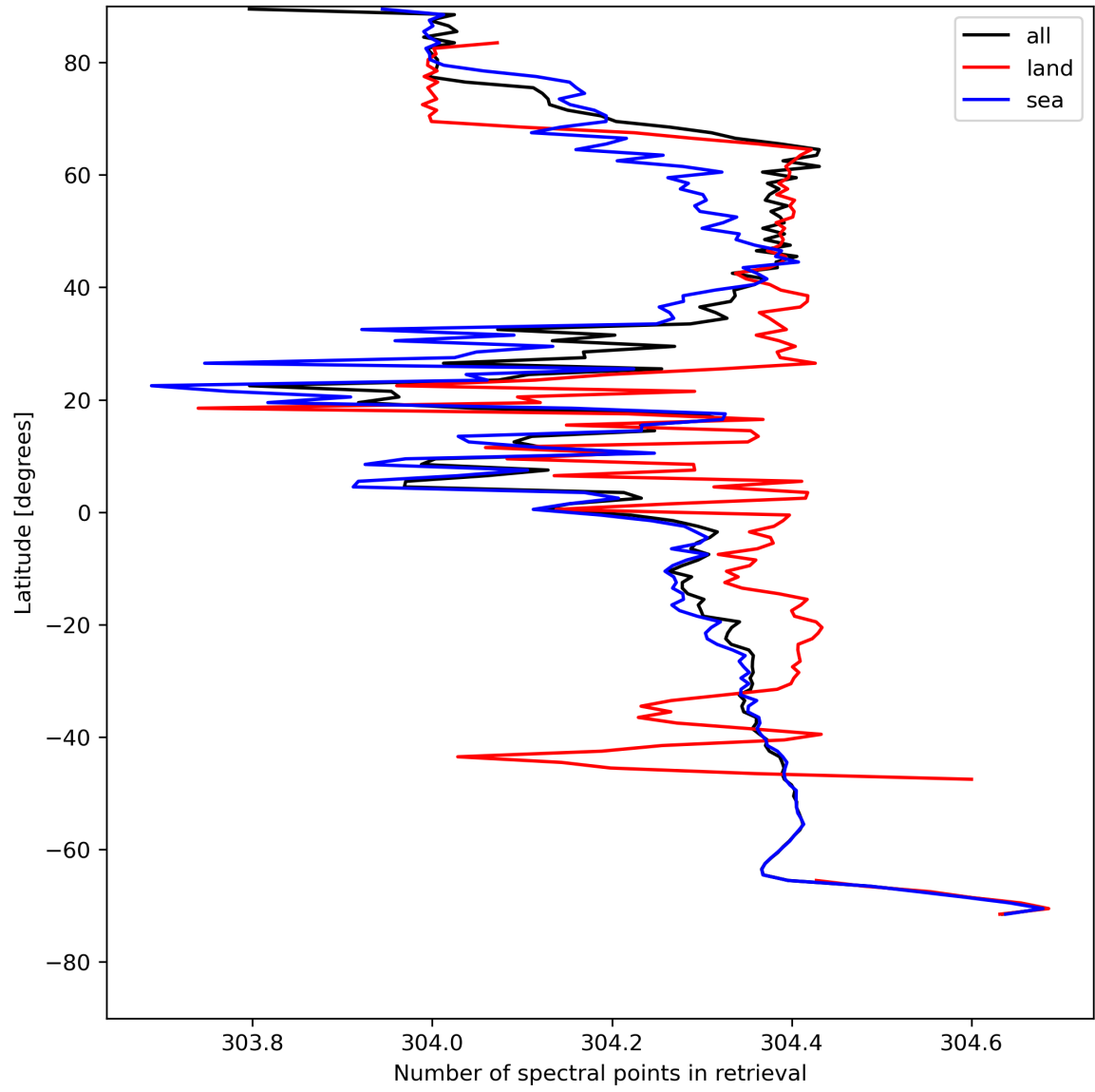
Figure 16: Zonal average of “Number of spectral points in retrieval” for 2023-08-06 to 2023-08-08.
