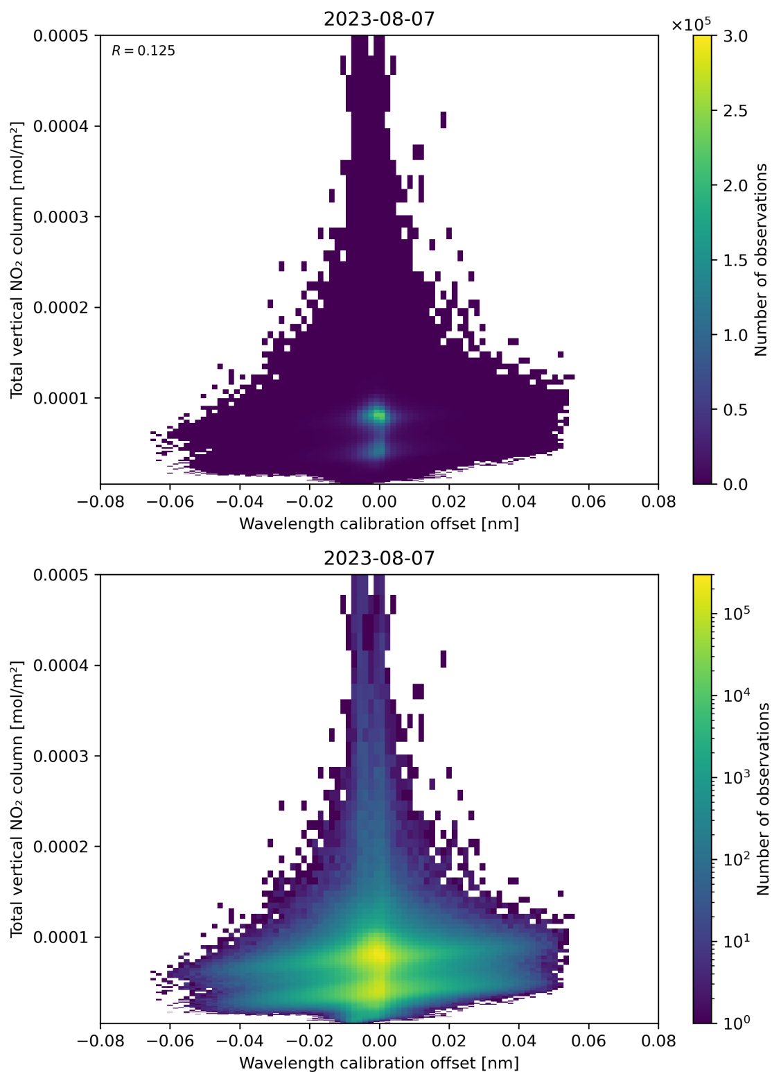
Figure 179: Scatter density plot of “Wavelength calibration offset” against “Total vertical NO 2 column” for 2023-08-06 to 2023-08-08.
