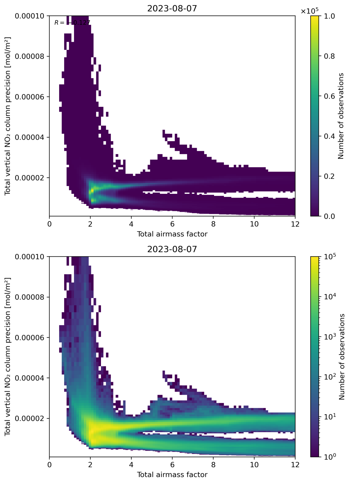
Figure 68: Scatter density plot of “Total airmass factor” against “Total vertical NO 2 column precision” for 2023-08-06 to 2023-08-08.
