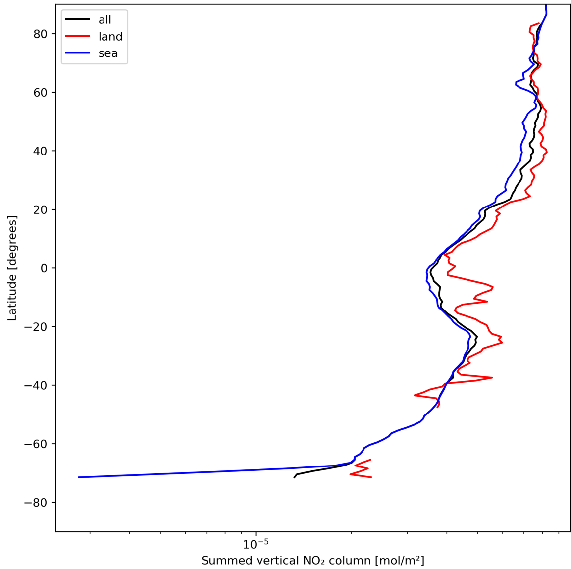
Figure 23: Zonal average of “Summed vertical NO 2 column” for 2023-08-06 to 2023-08-08.
