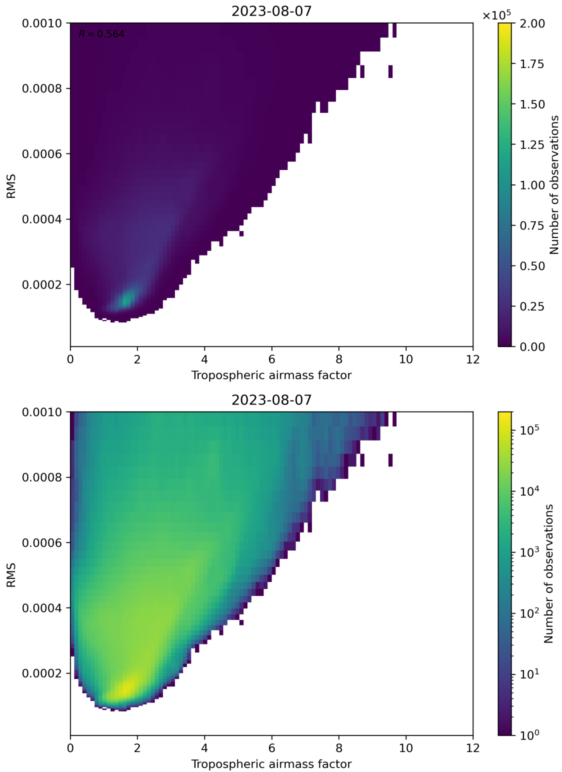
Figure 79: Scatter density plot of “Tropospheric airmass factor” against “RMS” for 2023-08-06 to 2023-08-08.
