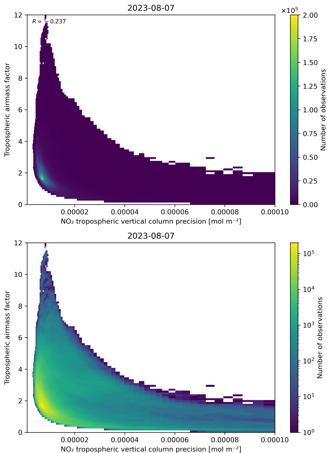
Figure 133: Scatter density plot of “NO 2 tropospheric vertical column precision” against “Tropospheric air mass factor” for 2023-08-06 to 2023-08-08.
