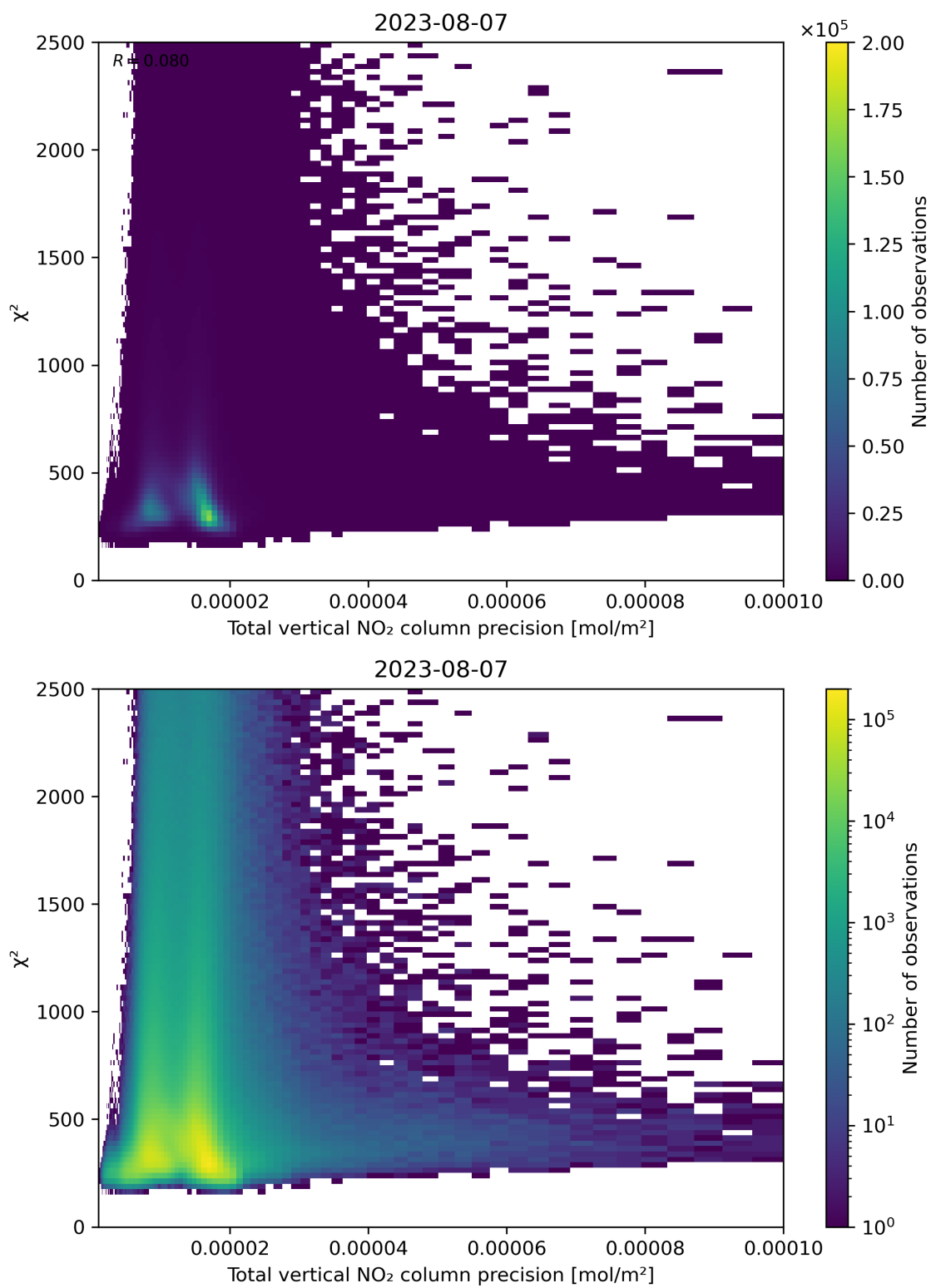
Figure 116: Scatter density plot of “Total vertical NO 2 column precision” against “ \chi^2 ” for 2023-08-06 to 2023-08-08.
