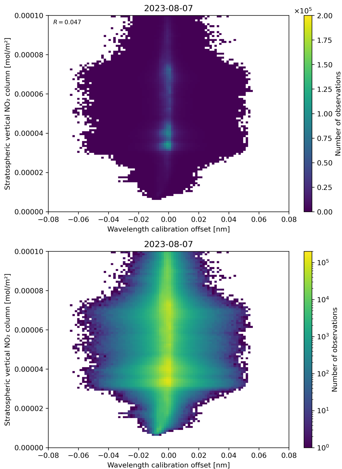
Figure 176: Scatter density plot of “Wavelength calibration offset” against “Stratospheric vertical NO 2 column” for 2023-08-06 to 2023-08-08.
