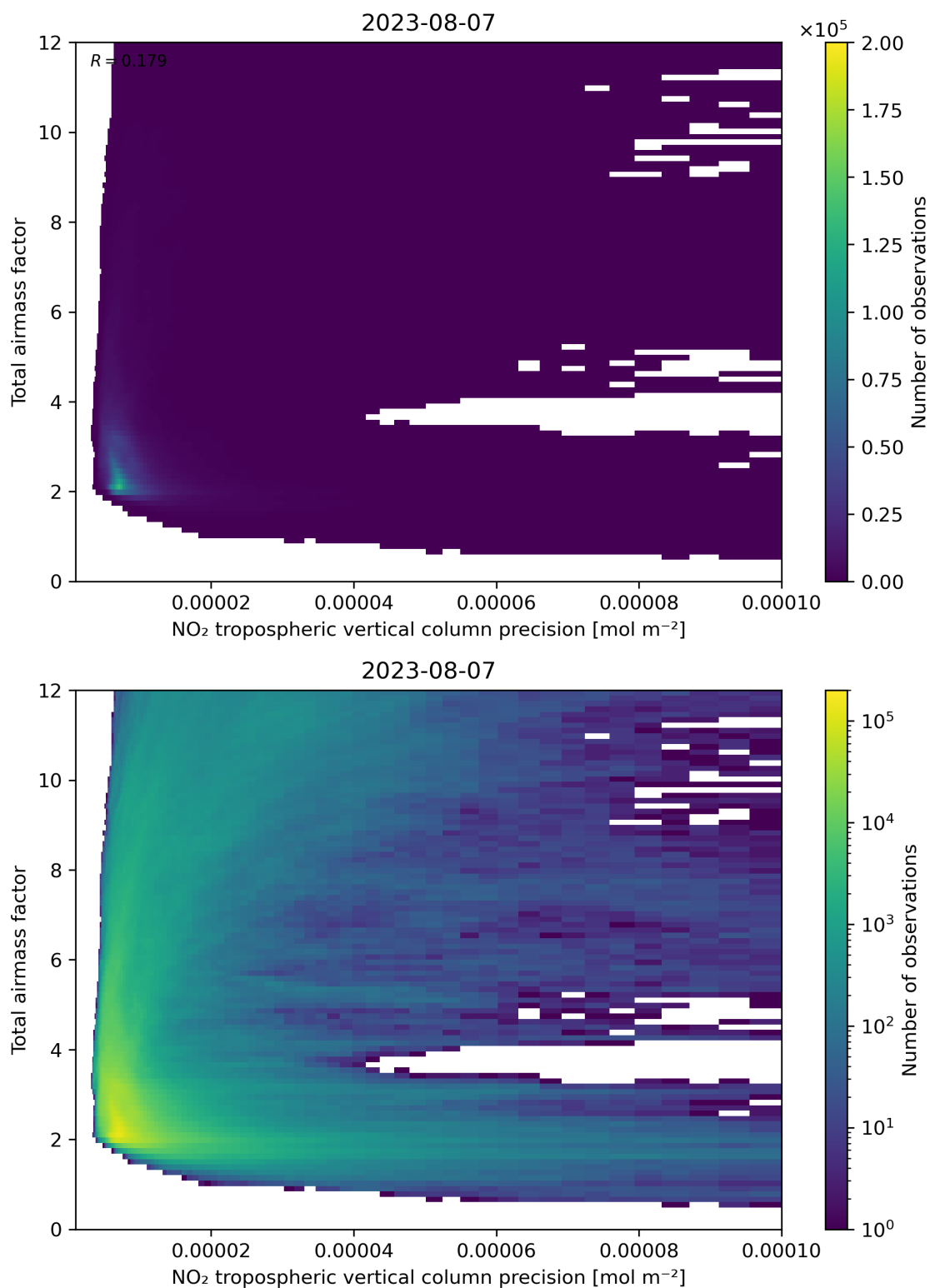
Figure 132: Scatter density plot of “NO 2 tropospheric vertical column precision” against “Total air mass factor” for 2023-08-06 to 2023-08-08.
