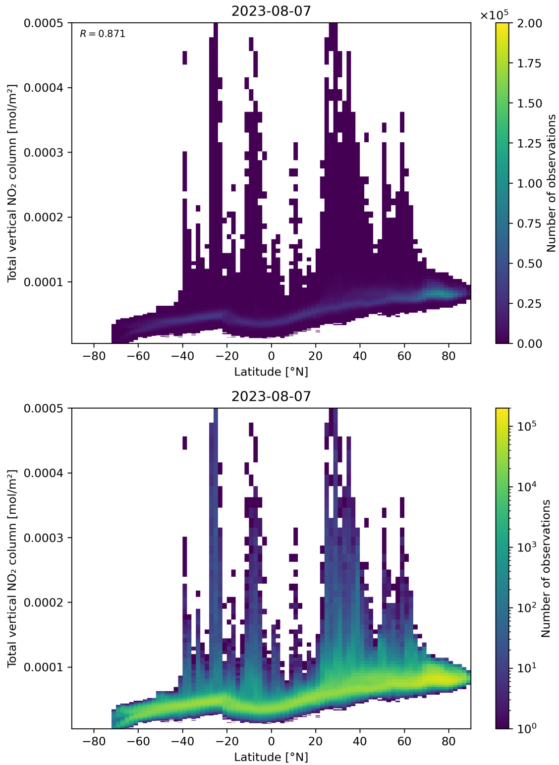
Figure 90: Scatter density plot of “Latitude” against “Total vertical NO 2 column” for 2023-08-06 to 2023-08-08.
