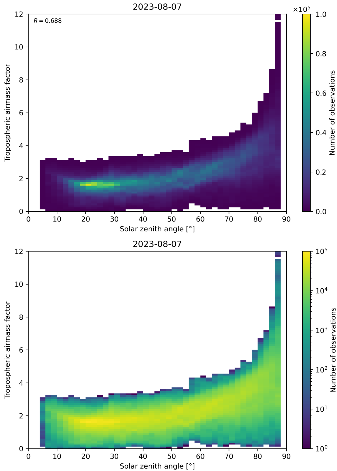
Figure 147: Scatter density plot of “Solar zenith angle” against “Tropospheric airmass factor” for 2023-08-06 to 2023-08-08.
