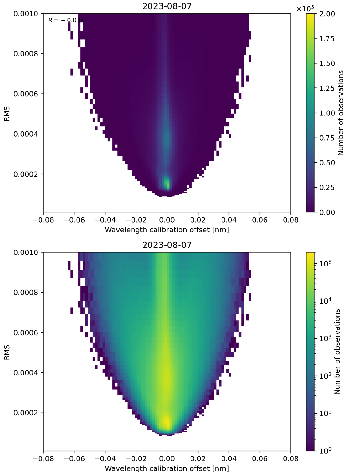
Figure 181: Scatter density plot of “Wavelength calibration offset” against “RMS” for 2023-08-06 to 2023-08-08.
