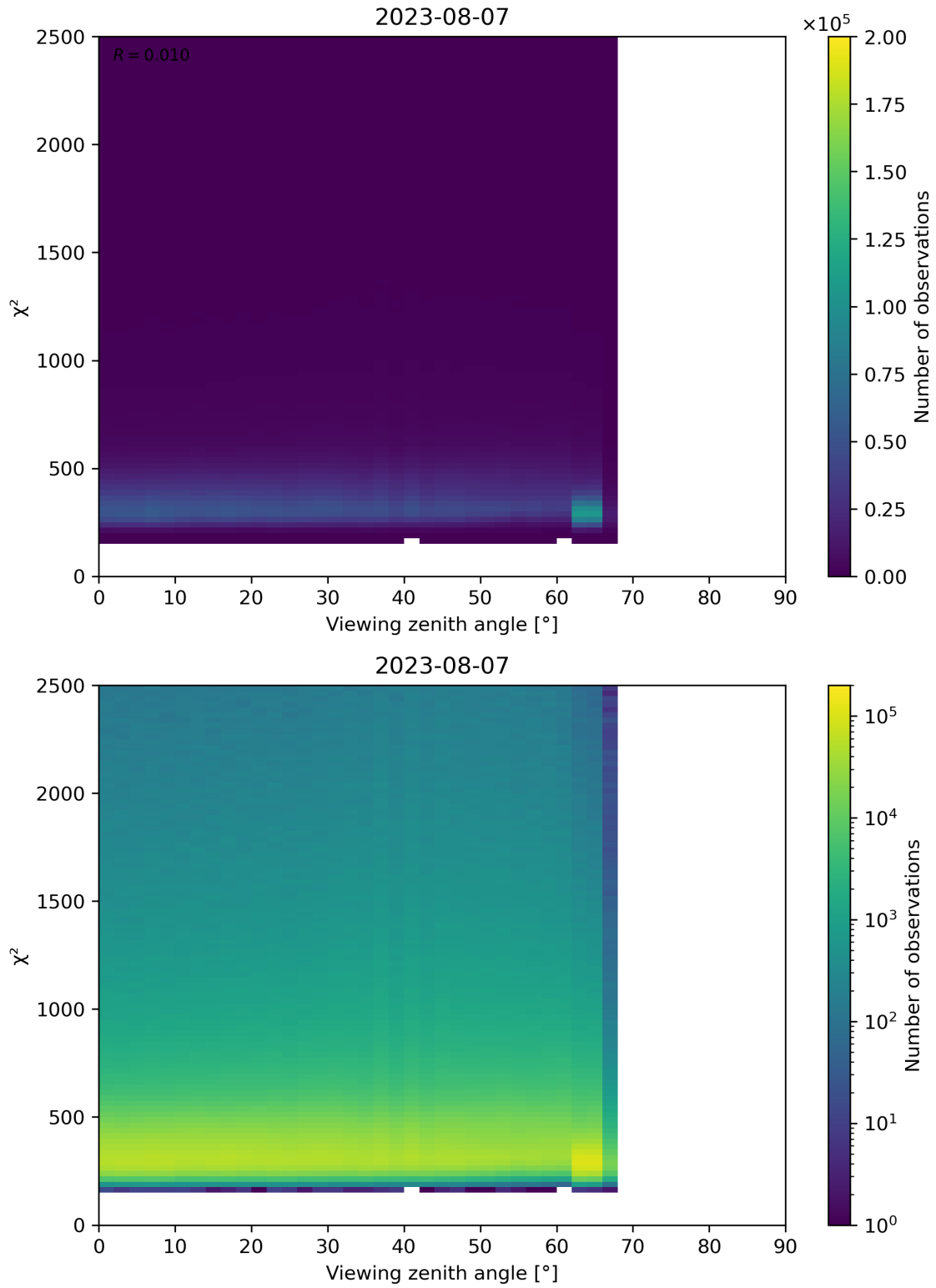
Figure 162: Scatter density plot of “Viewing zenith angle” against “ \chi^2 ” for 2023-08-06 to 2023-08-08.
