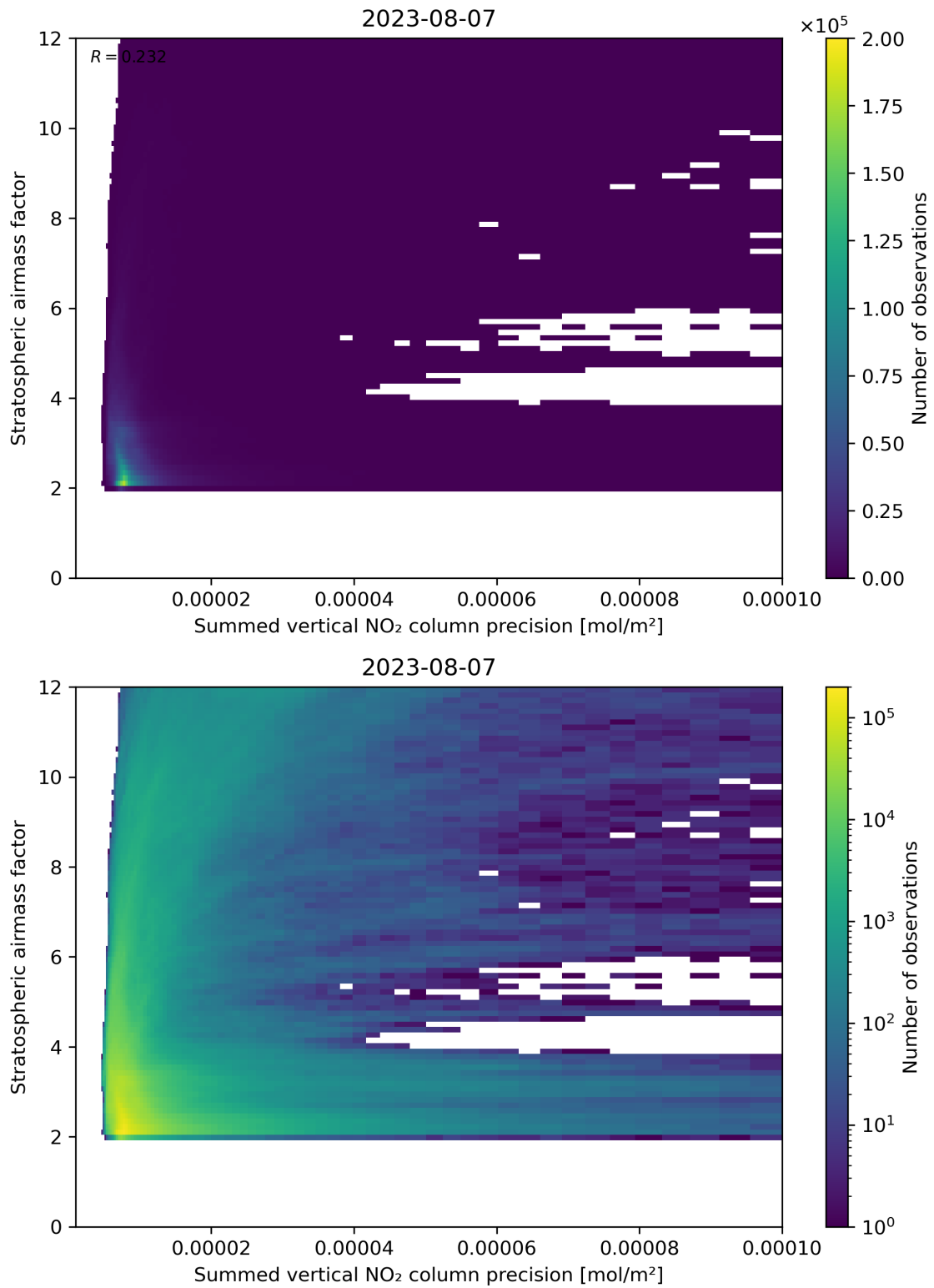
Figure 106: Scatter density plot of “Summed vertical NO 2 column precision” against “Stratospheric airmass factor” for 2023-08-06 to 2023-08-08.
