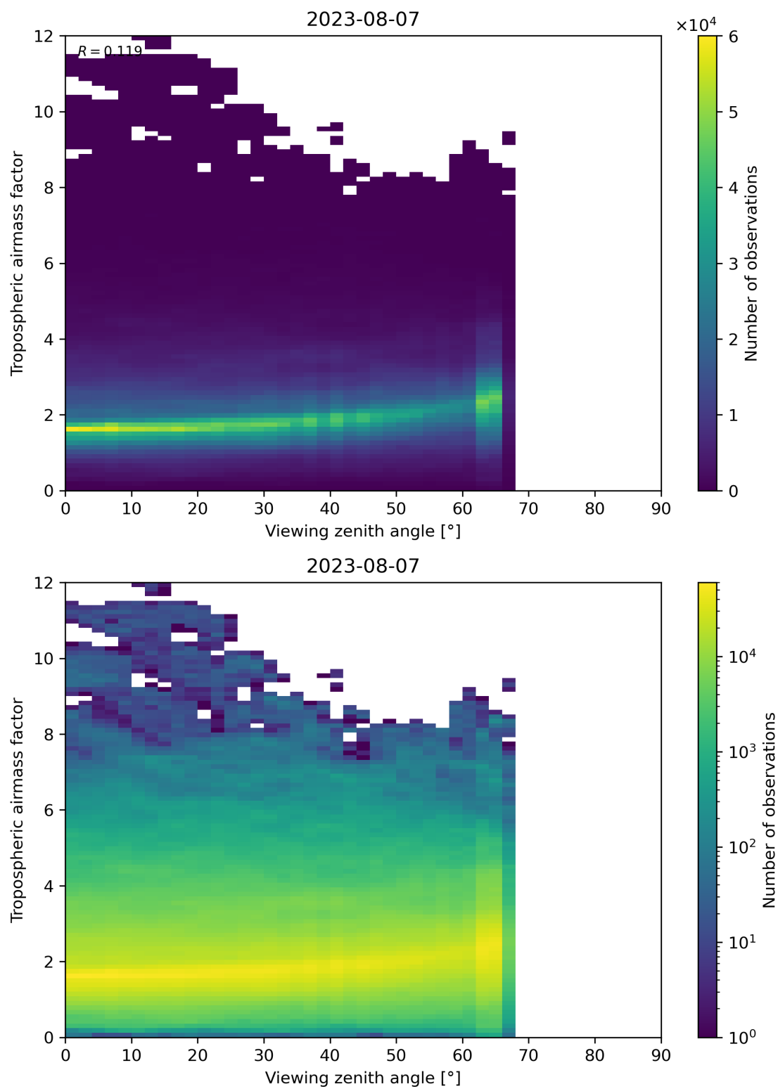
Figure 161: Scatter density plot of “Viewing zenith angle” against “Tropospheric airmass factor” for 2023-08-06 to 2023-08-08.
