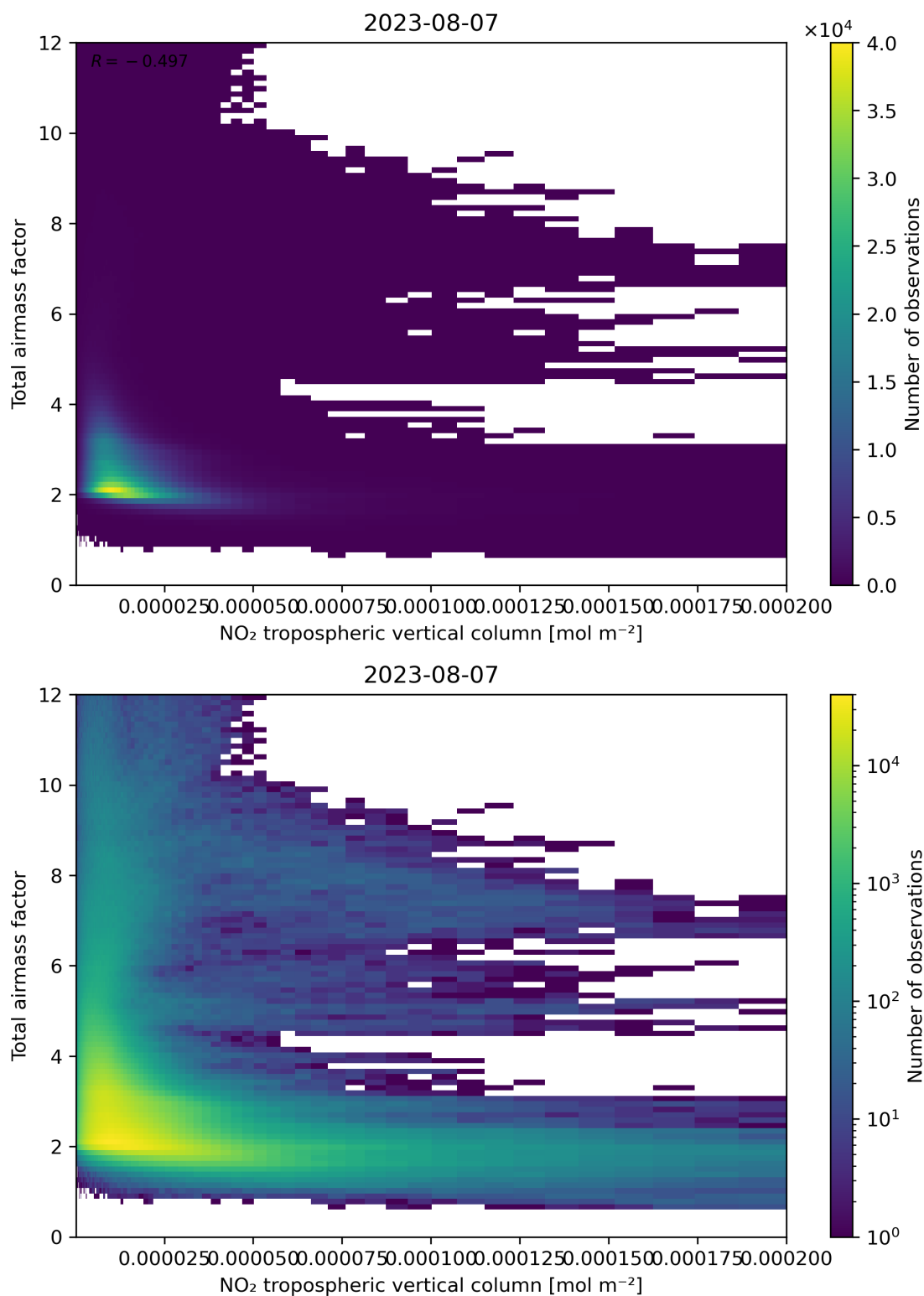
Figure 122: Scatter density plot of “NO 2 tropospheric vertical column” against “Total air mass factor” for 2023-08-06 to 2023-08-08.
