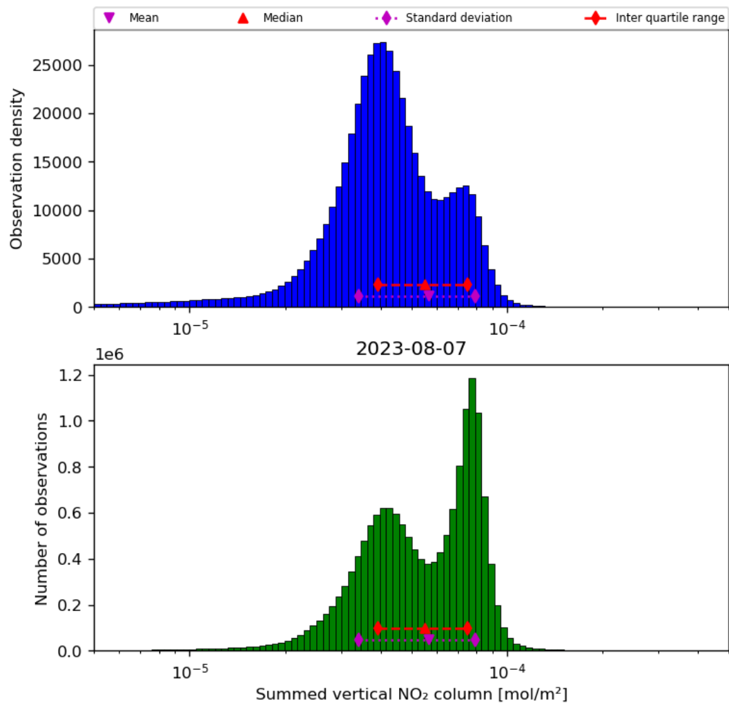
Figure 40: Histogram of “Summed vertical NO 2 column” for 2023-08-06 to 2023-08-08
