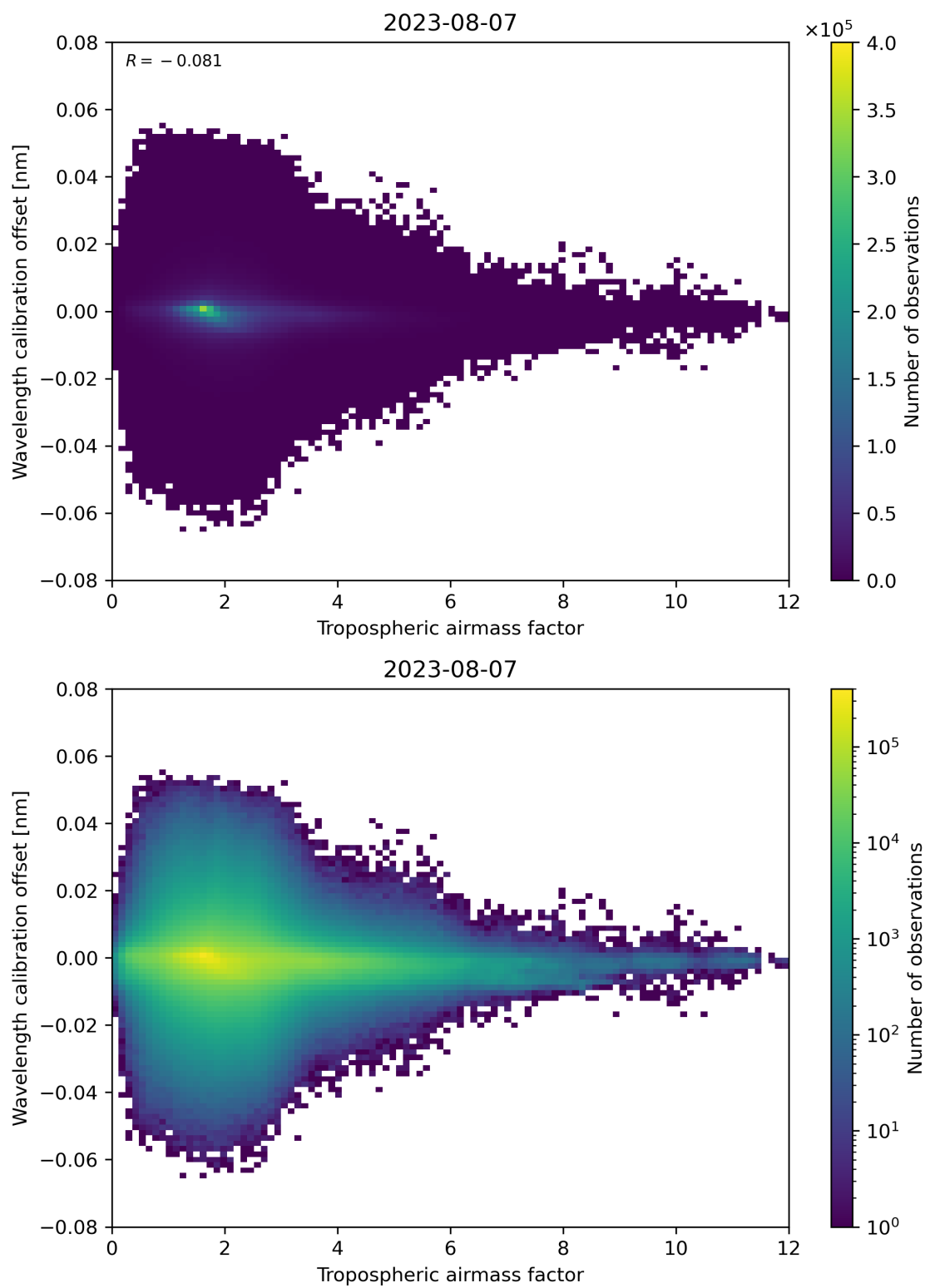
Figure 80: Scatter density plot of “Tropospheric airmass factor” against “Wavelength calibration offset” for 2023-08-06 to 2023-08-08.
