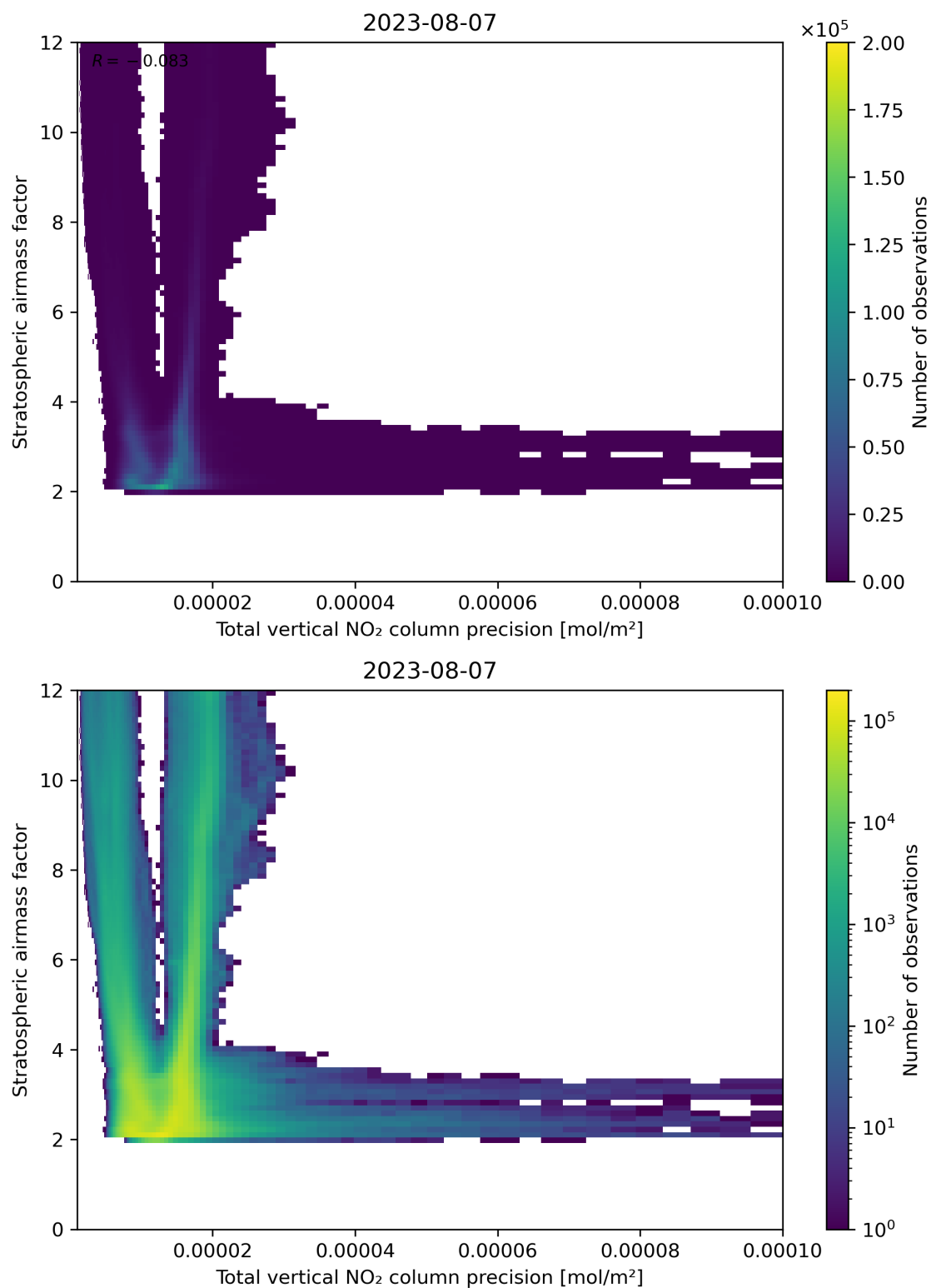
Figure 115: Scatter density plot of “Total vertical NO 2 column precision” against “Stratospheric air mass factor” for 2023-08-06 to 2023-08-08.
