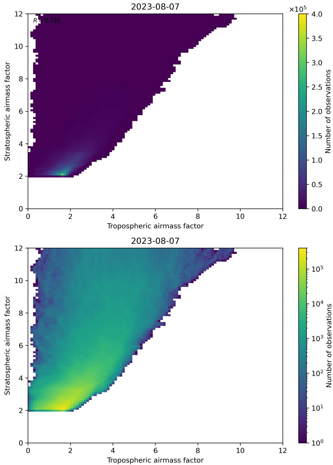
Figure 71: Scatter density plot of “Tropospheric airmass factor” against “Stratospheric airmass factor” for 2023-08-06 to 2023-08-08.
