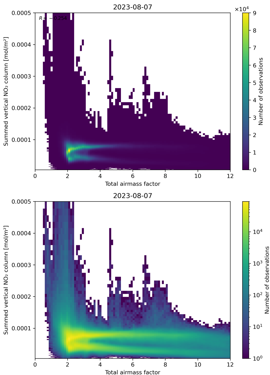
Figure 65: Scatter density plot of “Total airmass factor” against “Summed vertical NO 2 column” for 2023-08-06 to 2023-08-08.
