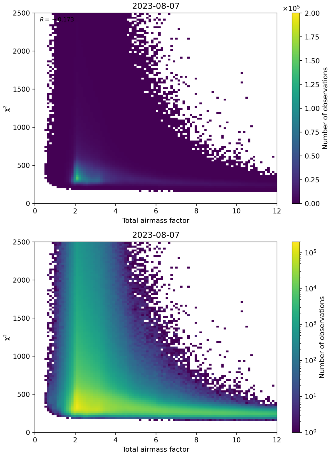
Figure 63: Scatter density plot of “Total airmass factor” against “ \chi^2 ” for 2023-08-06 to 2023-08-08.
