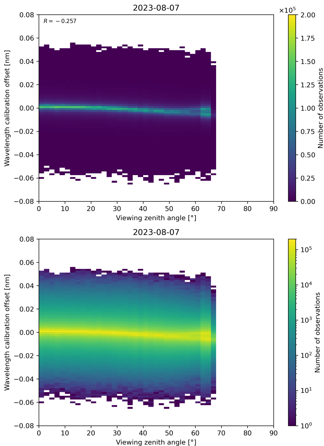
Figure 173: Scatter density plot of “Viewing zenith angle” against “Wavelength calibration offset” for 2023-08-06 to 2023-08-08.
