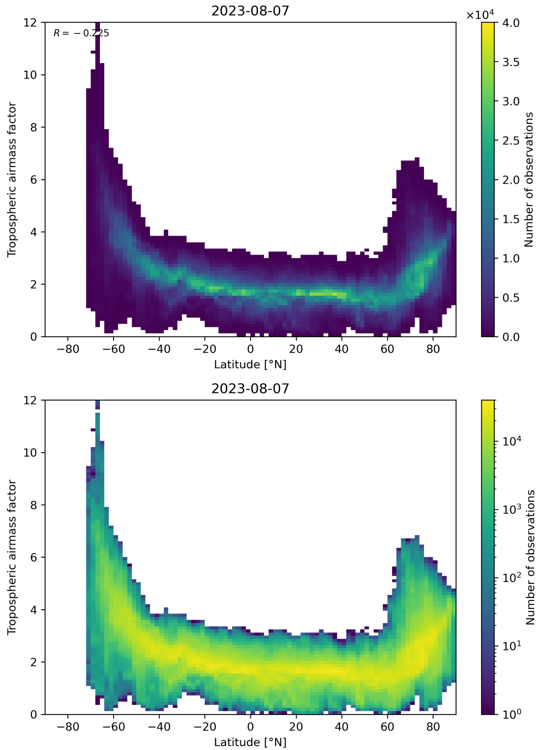
Figure 85: Scatter density plot of “Latitude” against “Tropospheric airmass factor” for 2023-08-06 to 2023-08-08.
