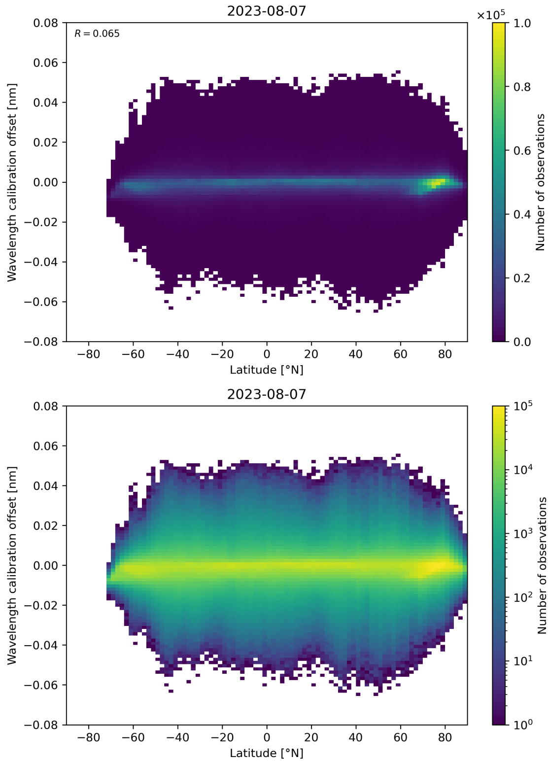
Figure 95: Scatter density plot of “Latitude” against “Wavelength calibration offset” for 2023-08-06 to 2023-08-08.
