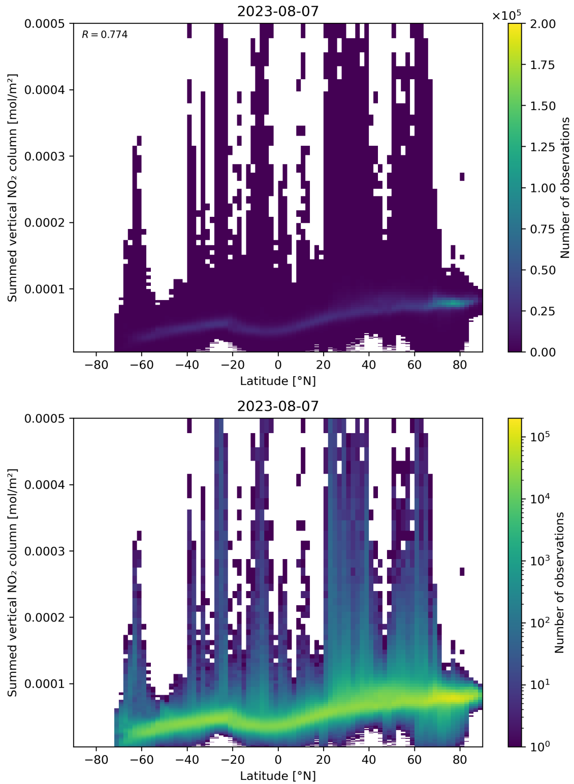
Figure 88: Scatter density plot of “Latitude” against “Summed vertical NO 2 column” for 2023-08-06 to 2023-08-08.
