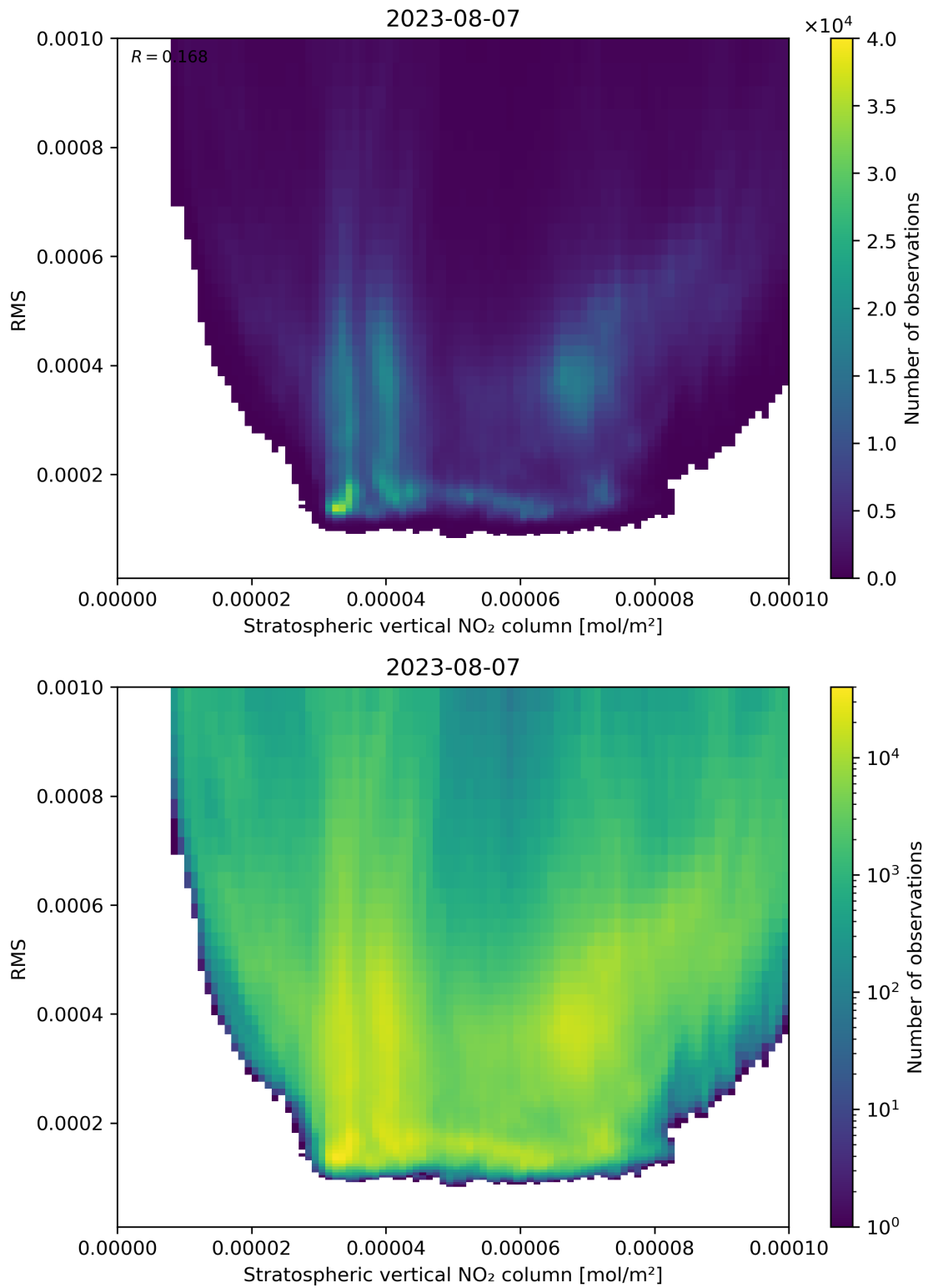
Figure 102: Scatter density plot of “Stratospheric vertical NO 2 column” against “RMS” for 2023-08-06 to 2023-08-08.
