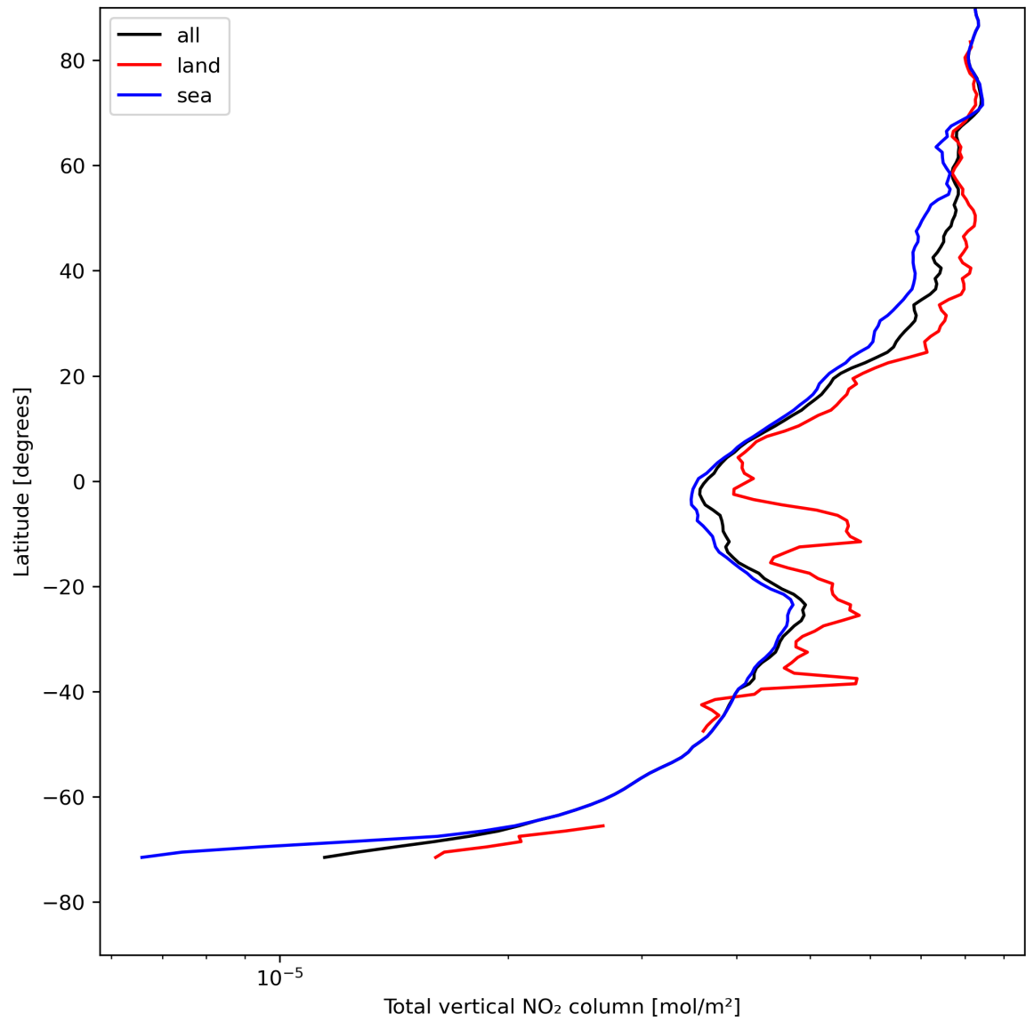
Figure 21: Zonal average of “Total vertical NO 2 column” for 2023-08-06 to 2023-08-08.
