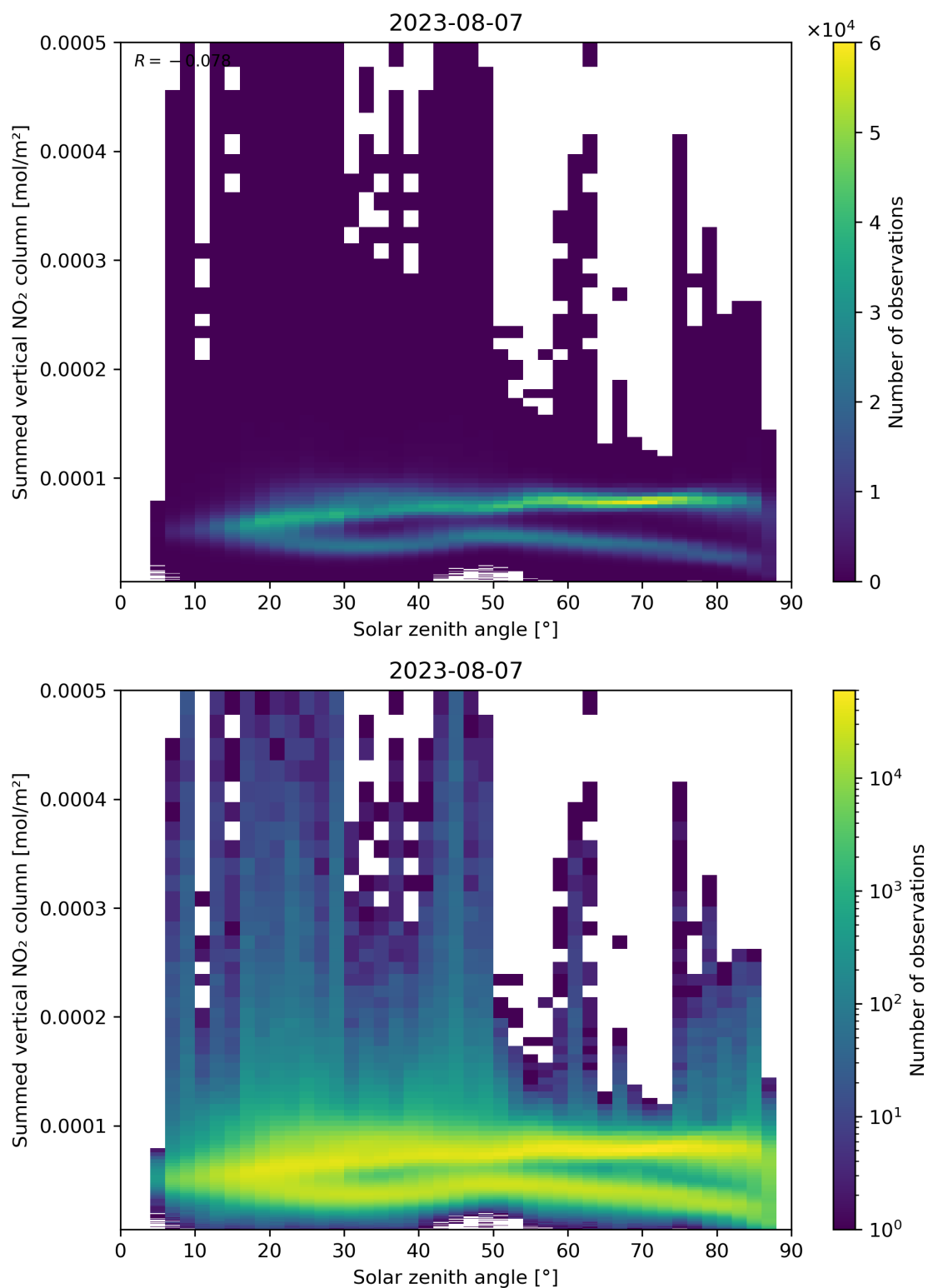
Figure 151: Scatter density plot of “Solar zenith angle” against “Summed vertical NO 2 column” for 2023-08-06 to 2023-08-08.
