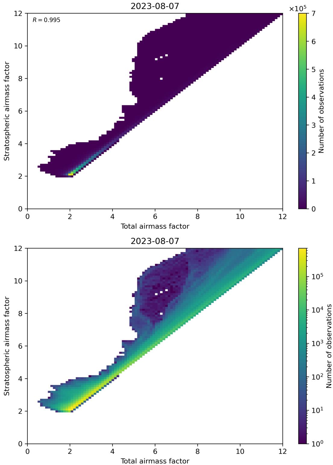
Figure 62: Scatter density plot of “Total airmass factor” against “Stratospheric airmass factor” for 2023-08-06 to 2023-08-08.
