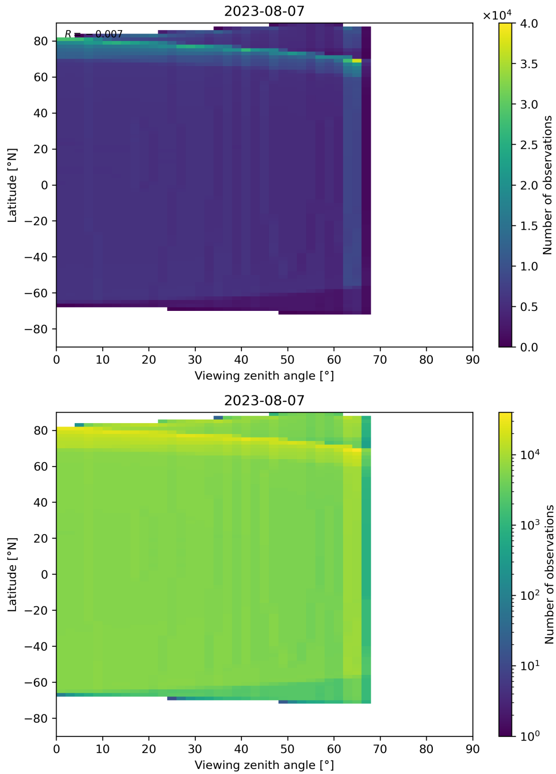
Figure 163: Scatter density plot of “Viewing zenith angle” against “Latitude” for 2023-08-06 to 2023-08-08.
