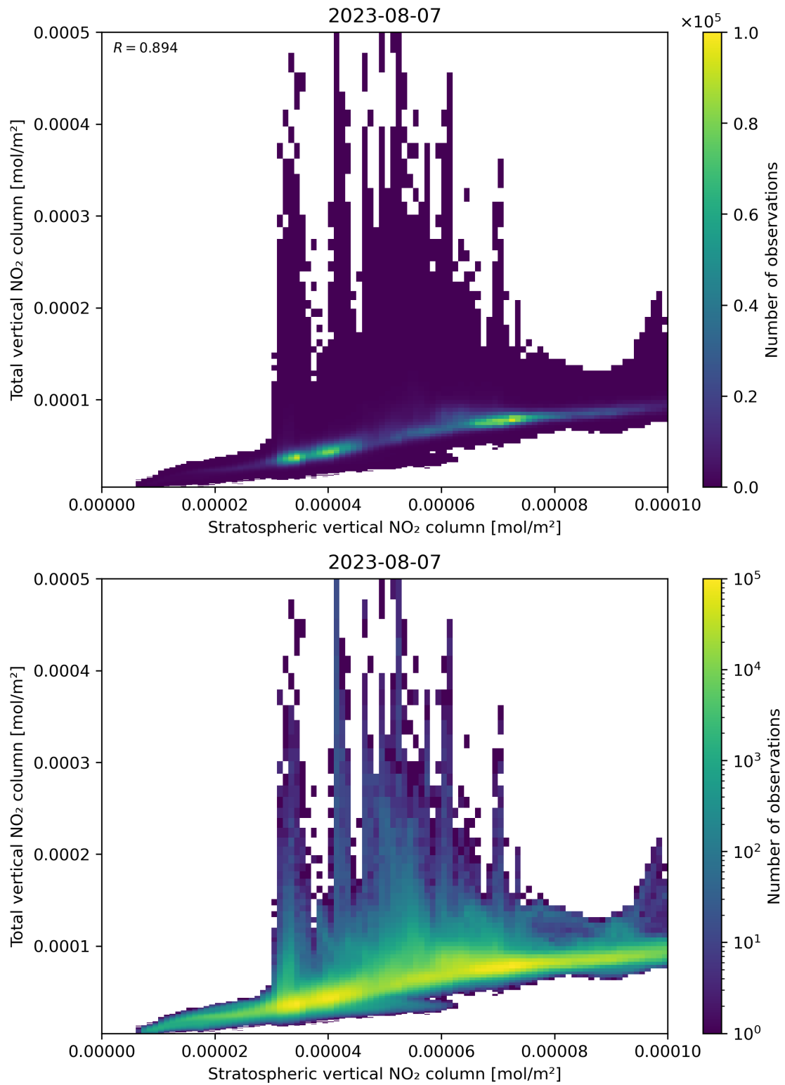
Figure 100: Scatter density plot of “Stratospheric vertical NO 2 column” against “Total vertical NO 2 column” for 2023-08-06 to 2023-08-08.
