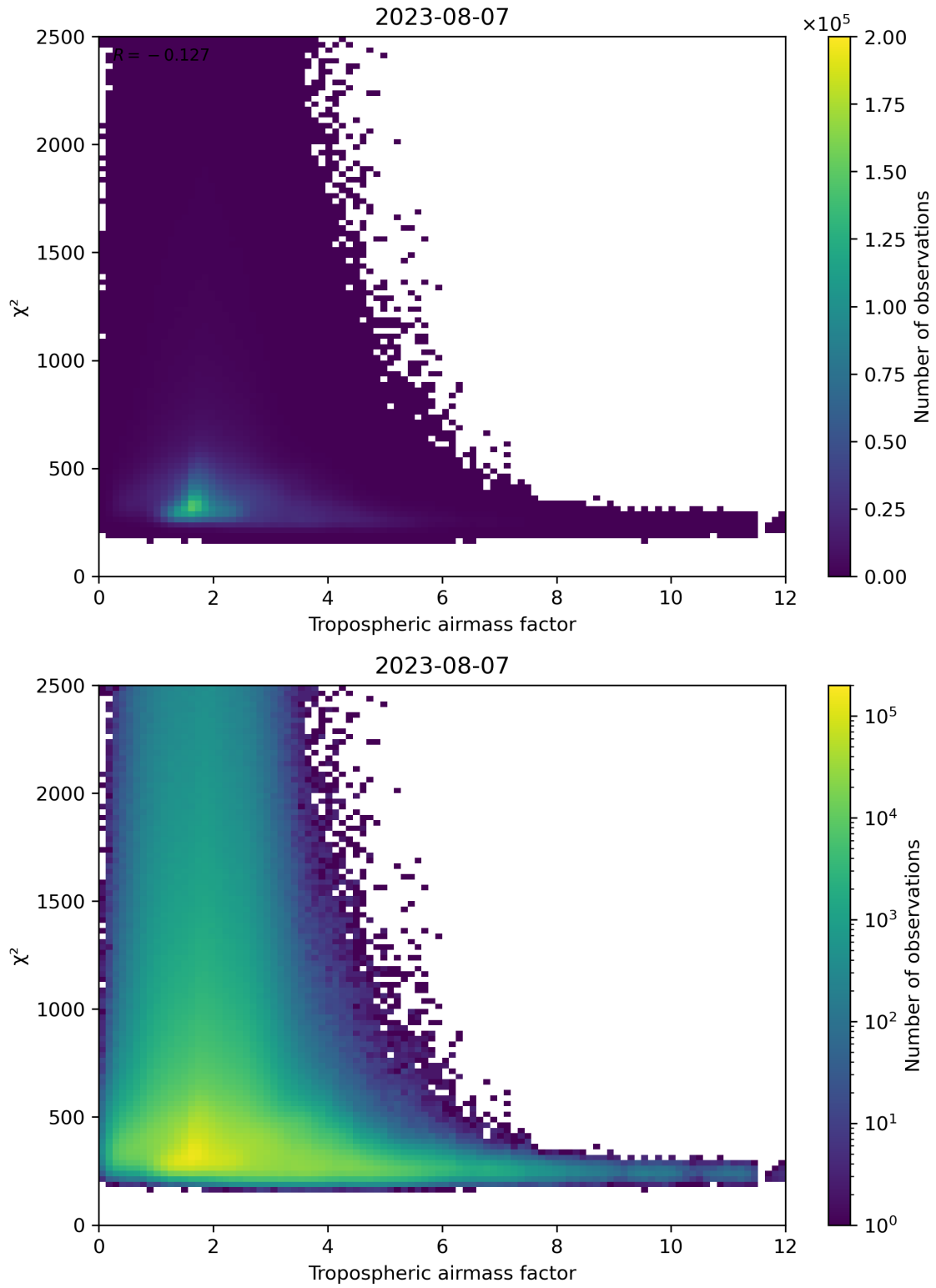
Figure 73: Scatter density plot of “Tropospheric airmass factor” against “ \chi^2 ” for 2023-08-06 to 2023-08-08.
