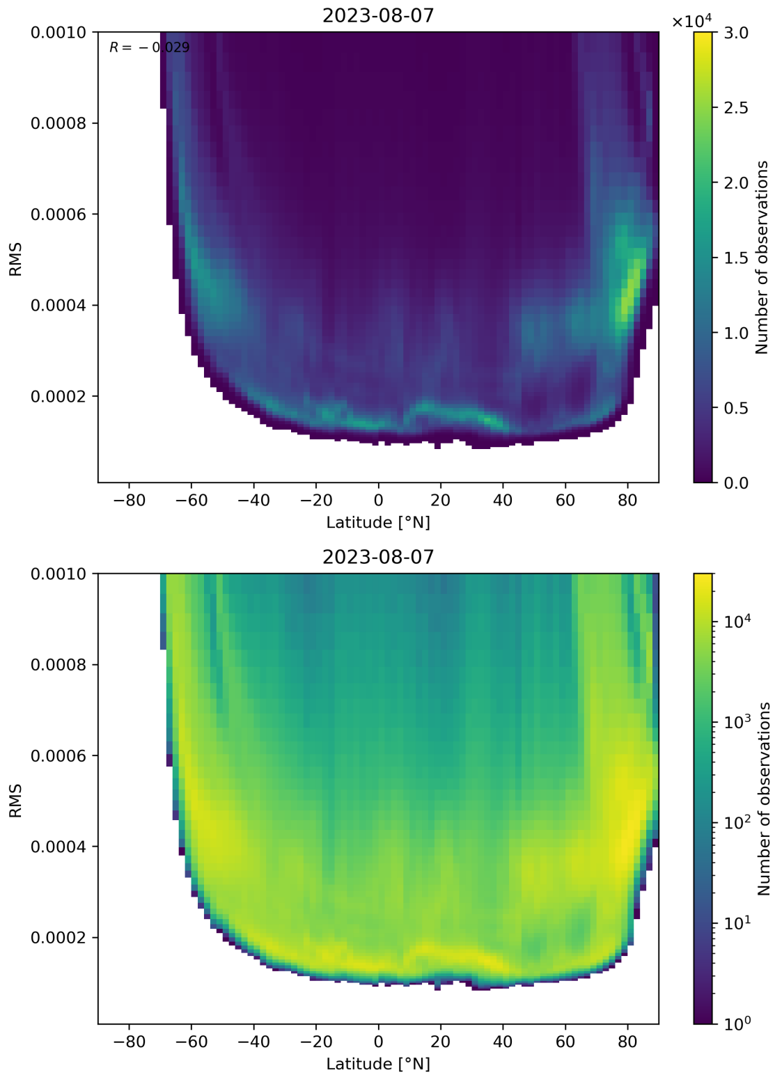
Figure 94: Scatter density plot of “Latitude” against “RMS” for 2023-08-06 to 2023-08-08.
