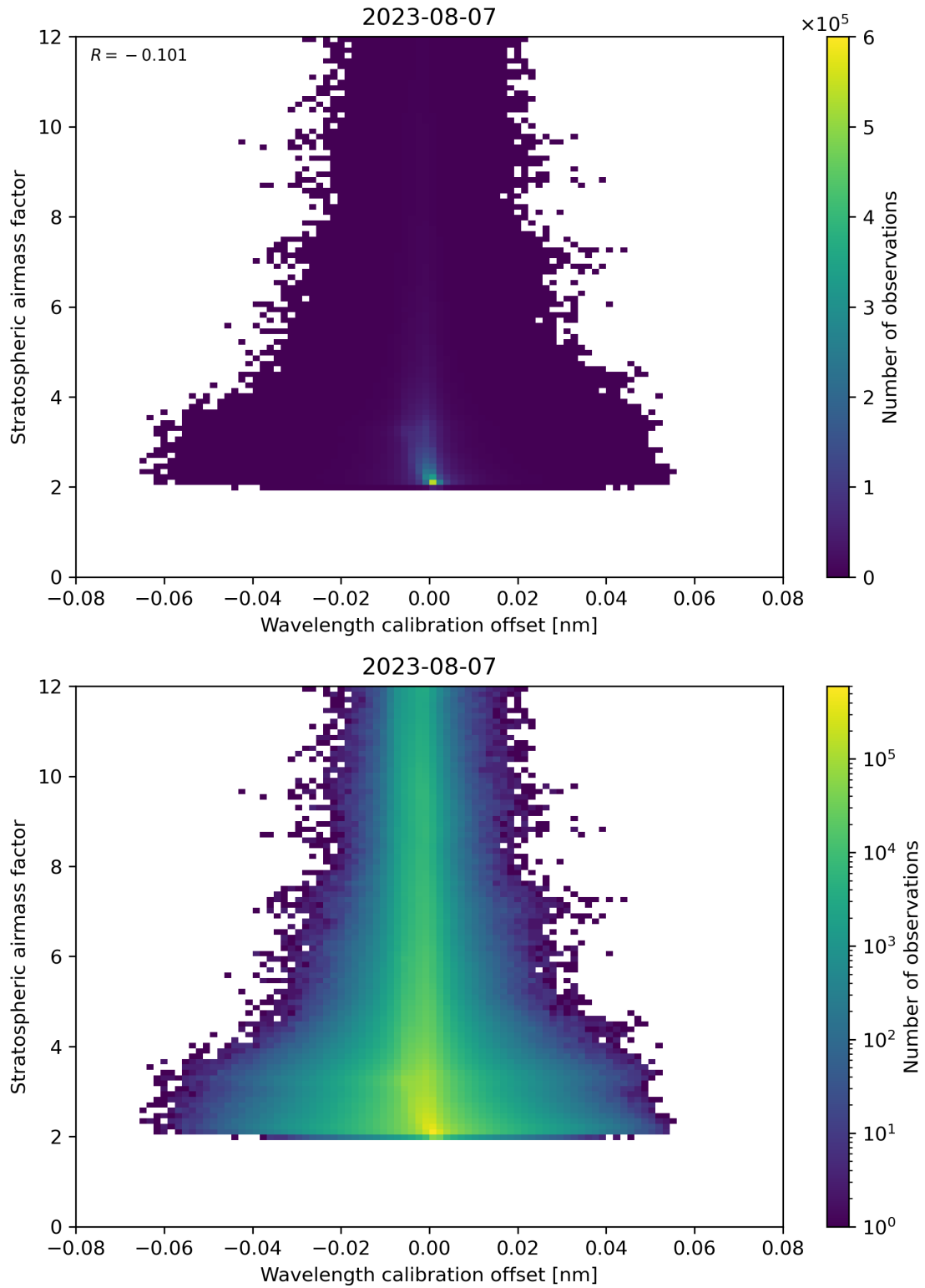
Figure 174: Scatter density plot of “Wavelength calibration offset” against “Stratospheric airmass factor” for 2023-08-06 to 2023-08-08.
