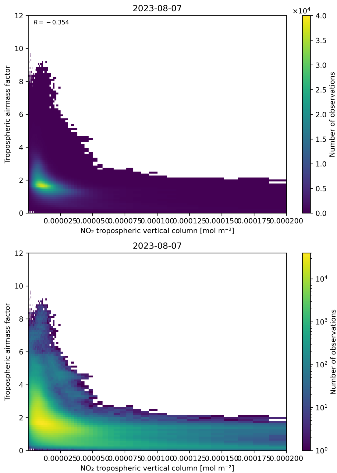
Figure 123: Scatter density plot of “NO 2 tropospheric vertical column” against “Tropospheric air mass factor” for 2023-08-06 to 2023-08-08.
