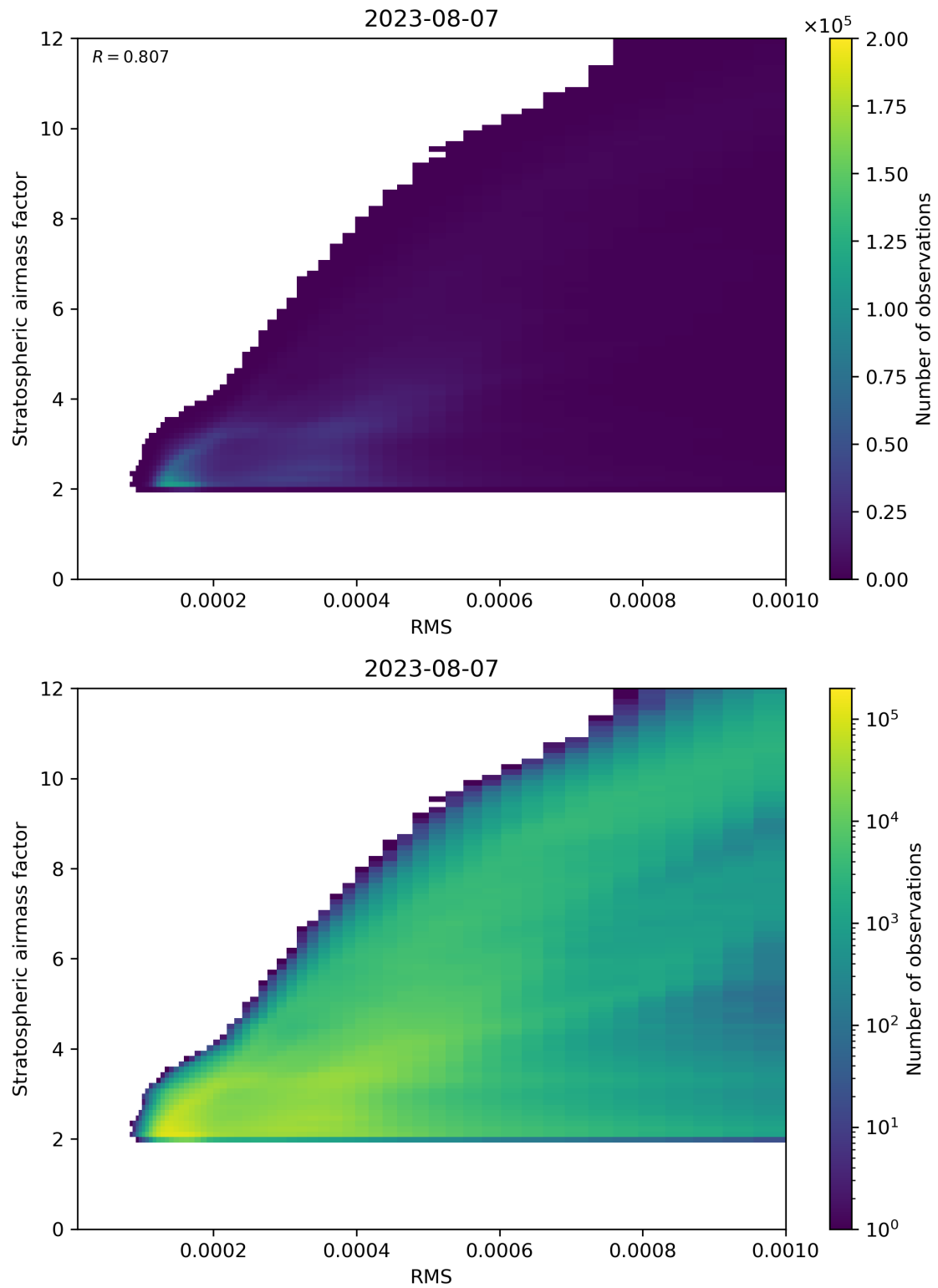
Figure 144: Scatter density plot of “RMS” against “Stratospheric airmass factor” for 2023-08-06 to 2023-08-08.
