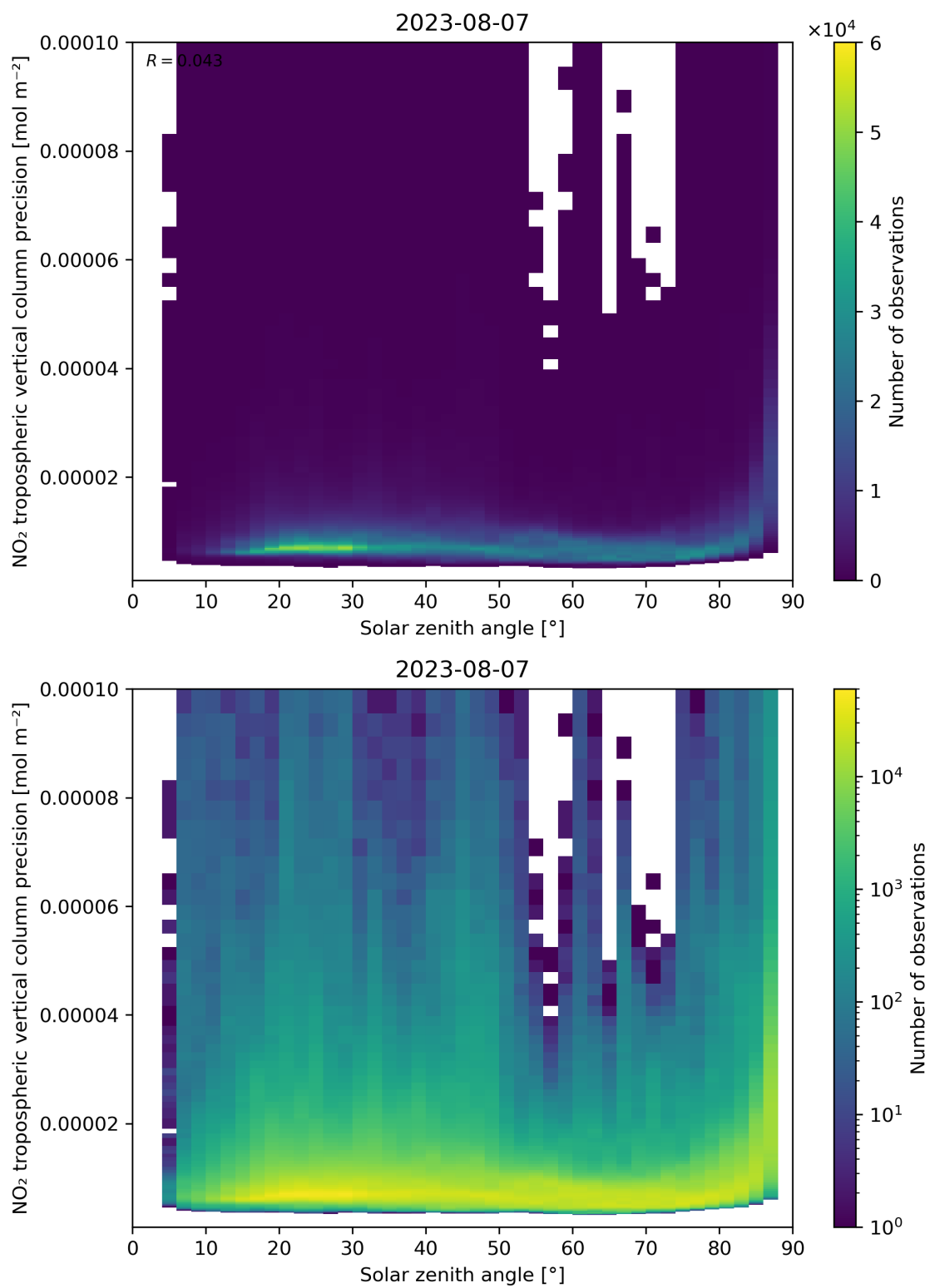
Figure 156: Scatter density plot of “Solar zenith angle” against “NO 2 tropospheric vertical column precision” for 2023-08-06 to 2023-08-08.
