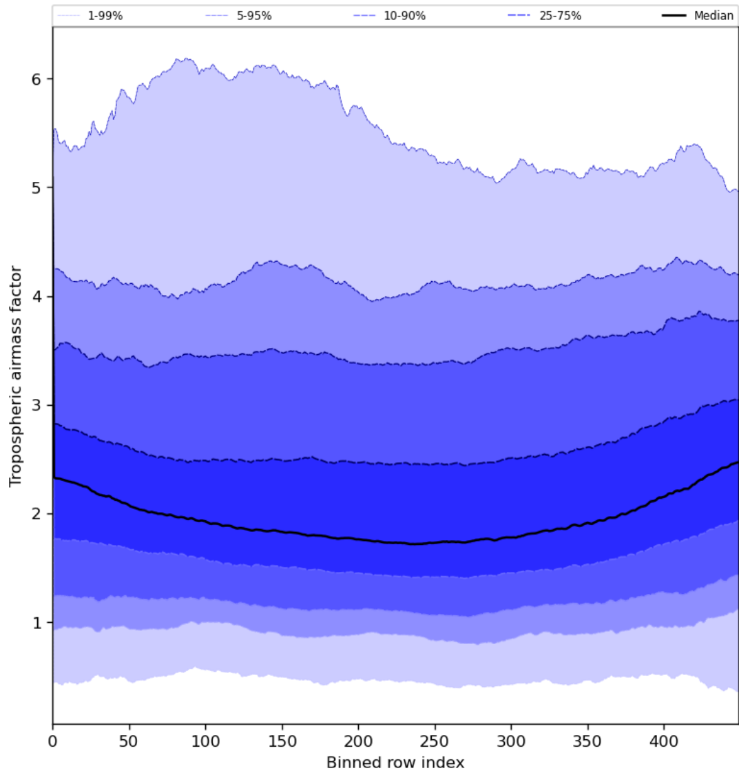
Figure 48: Along track statistics of “Tropospheric airmass factor” for 2023-08-06 to 2023-08-08
