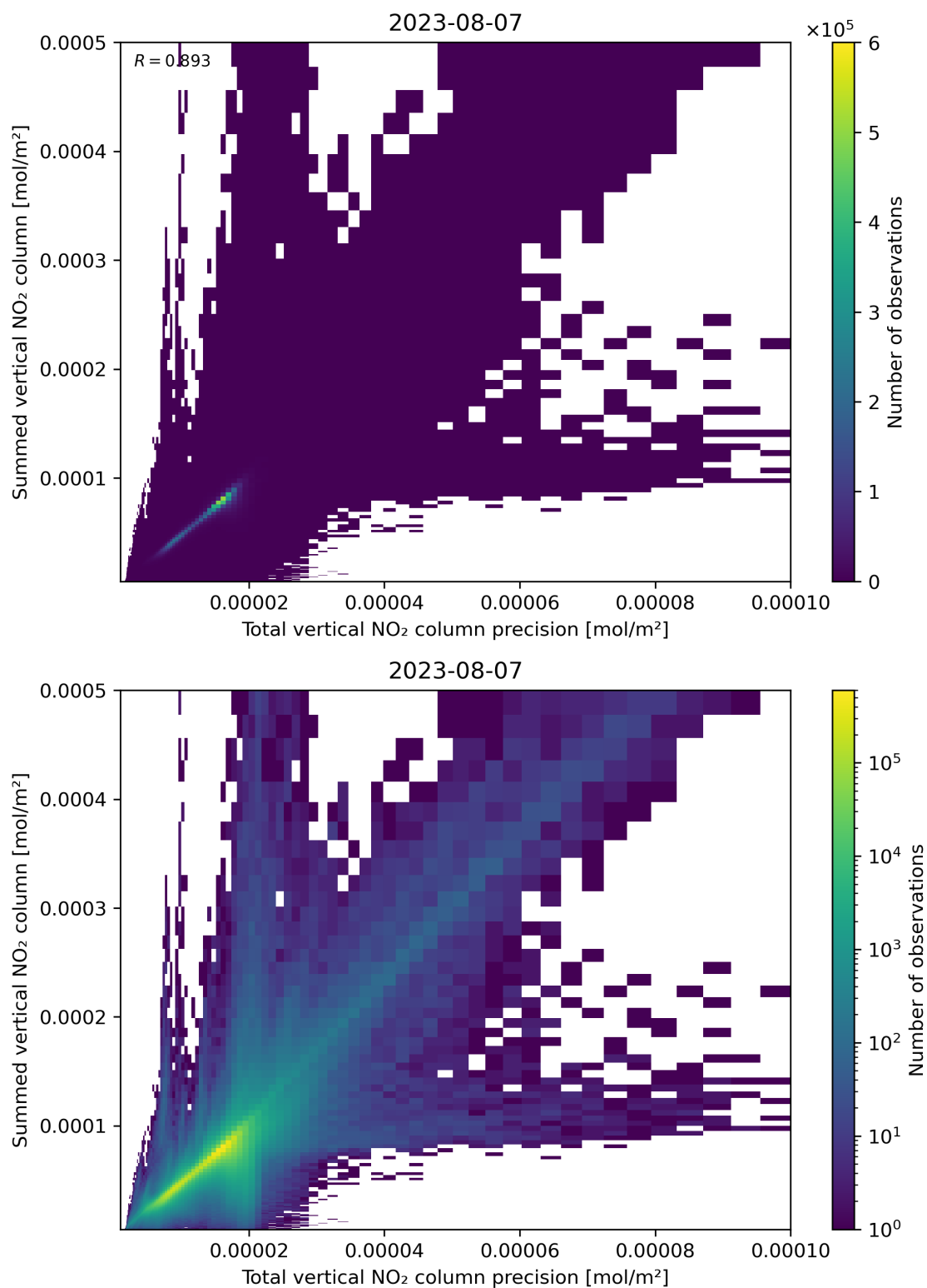
Figure 117: Scatter density plot of “Total vertical NO 2 column precision” against “Summed vertical NO 2 column” for 2023-08-06 to 2023-08-08.
