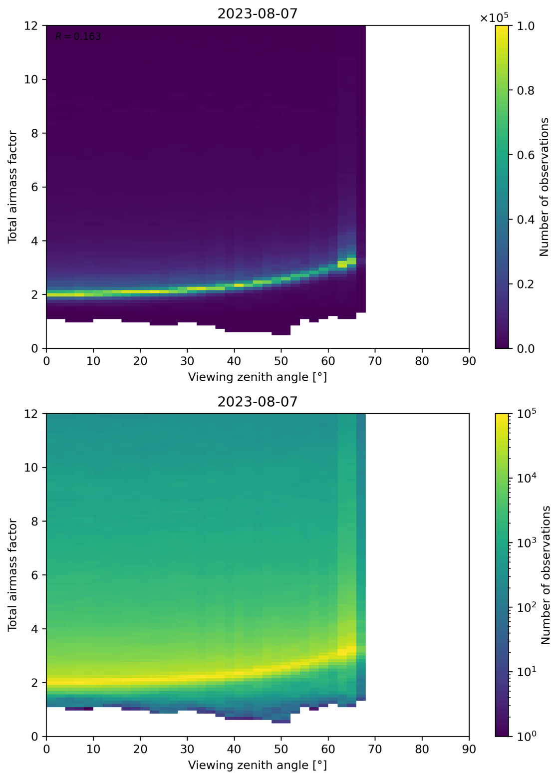
Figure 160: Scatter density plot of “Viewing zenith angle” against “Total airmass factor” for 2023-08-06 to 2023-08-08.
