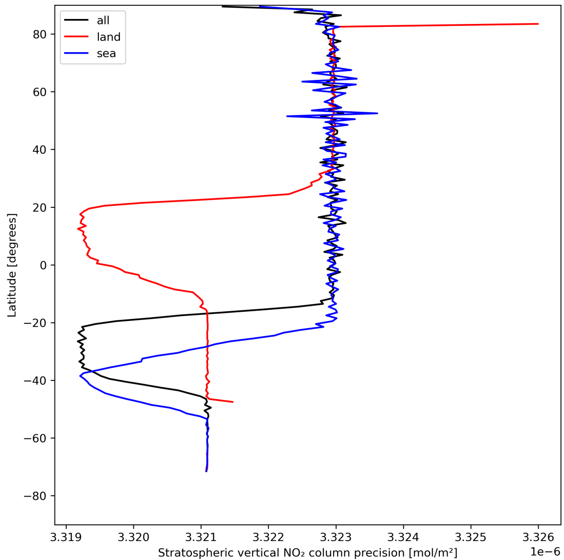
Figure 20: Zonal average of “Stratospheric vertical NO 2 column precision” for 2023-08-06 to 2023-08-08.
