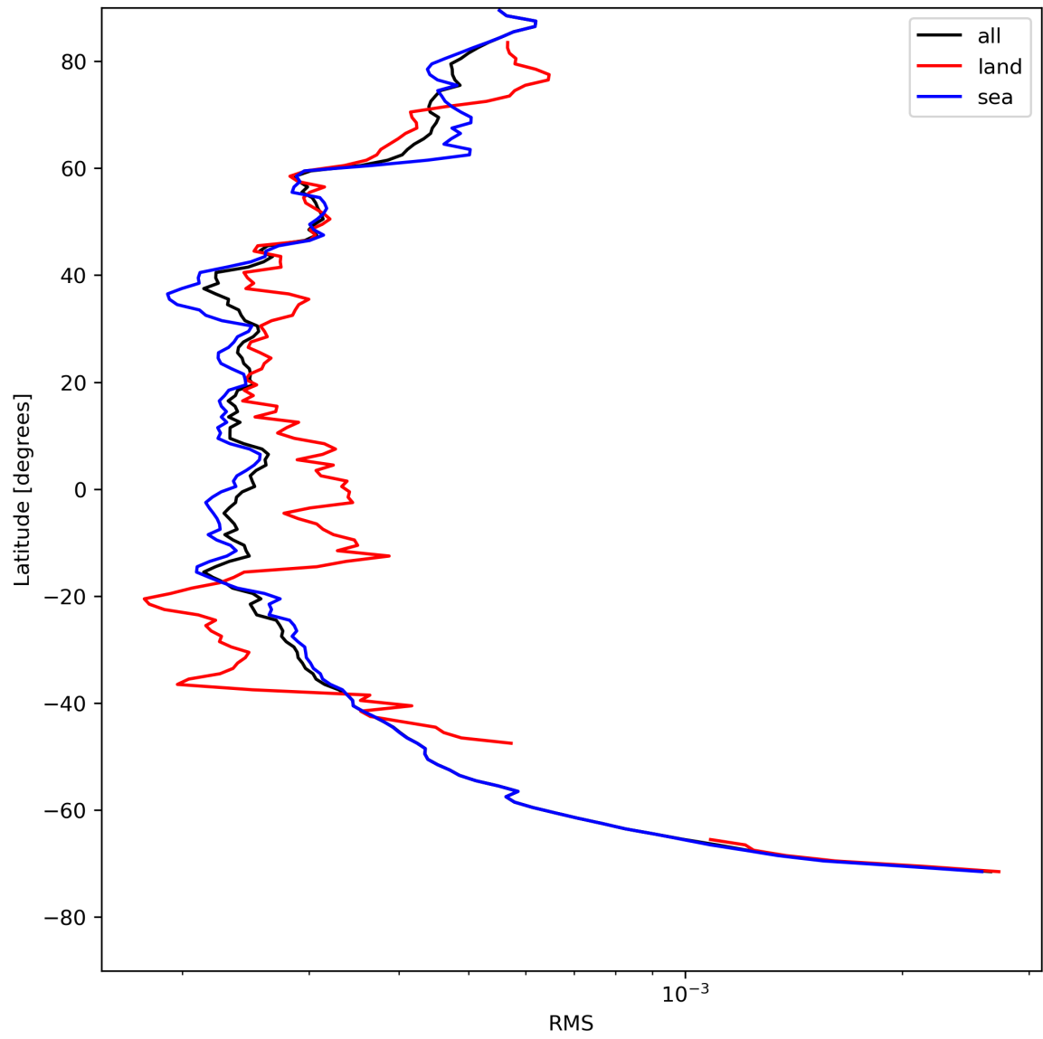
Figure 26: Zonal average of “RMS” for 2023-08-06 to 2023-08-08.
