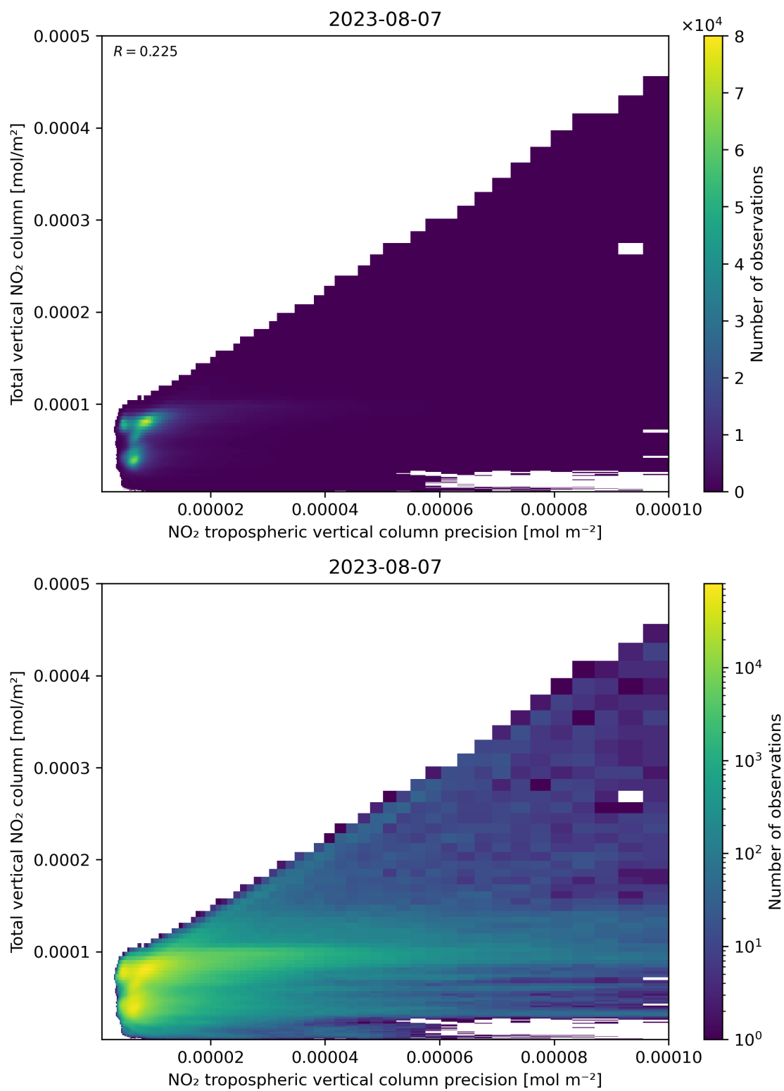
Figure 138: Scatter density plot of “NO 2 tropospheric vertical column precision” against “Total vertical NO 2 column” for 2023-08-06 to 2023-08-08.
