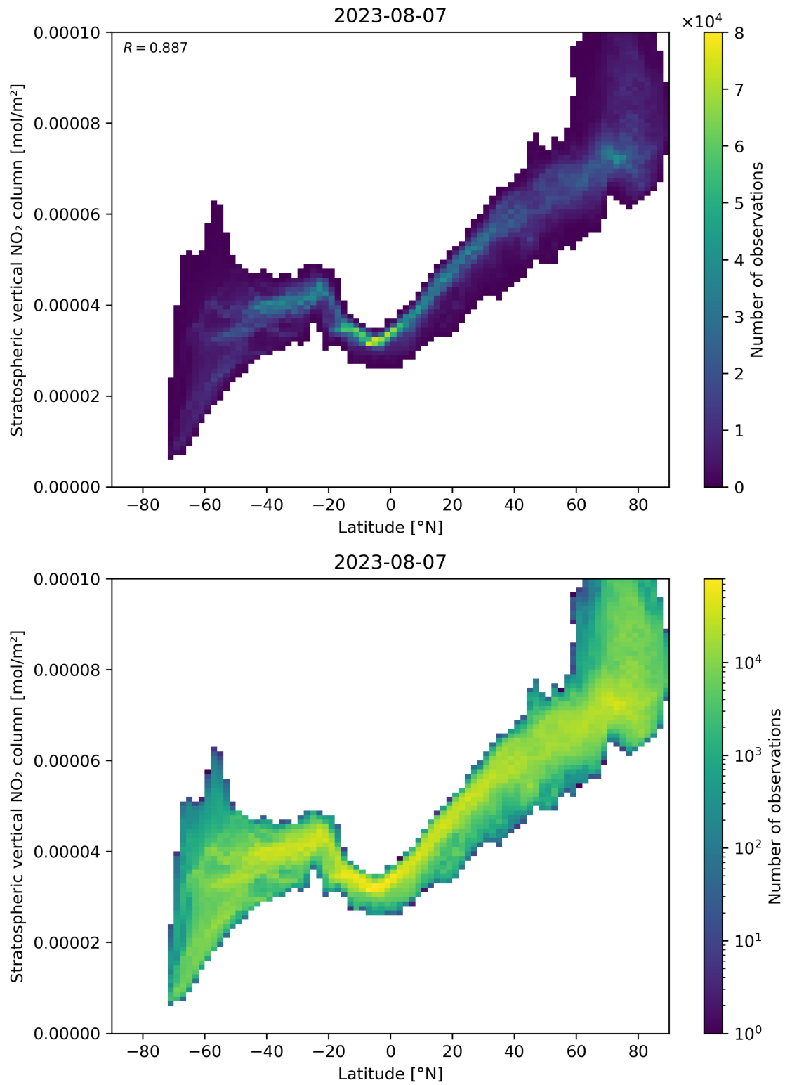
Figure 87: Scatter density plot of “Latitude” against “Stratospheric vertical NO 2 column” for 2023-08-06 to 2023-08-08.
