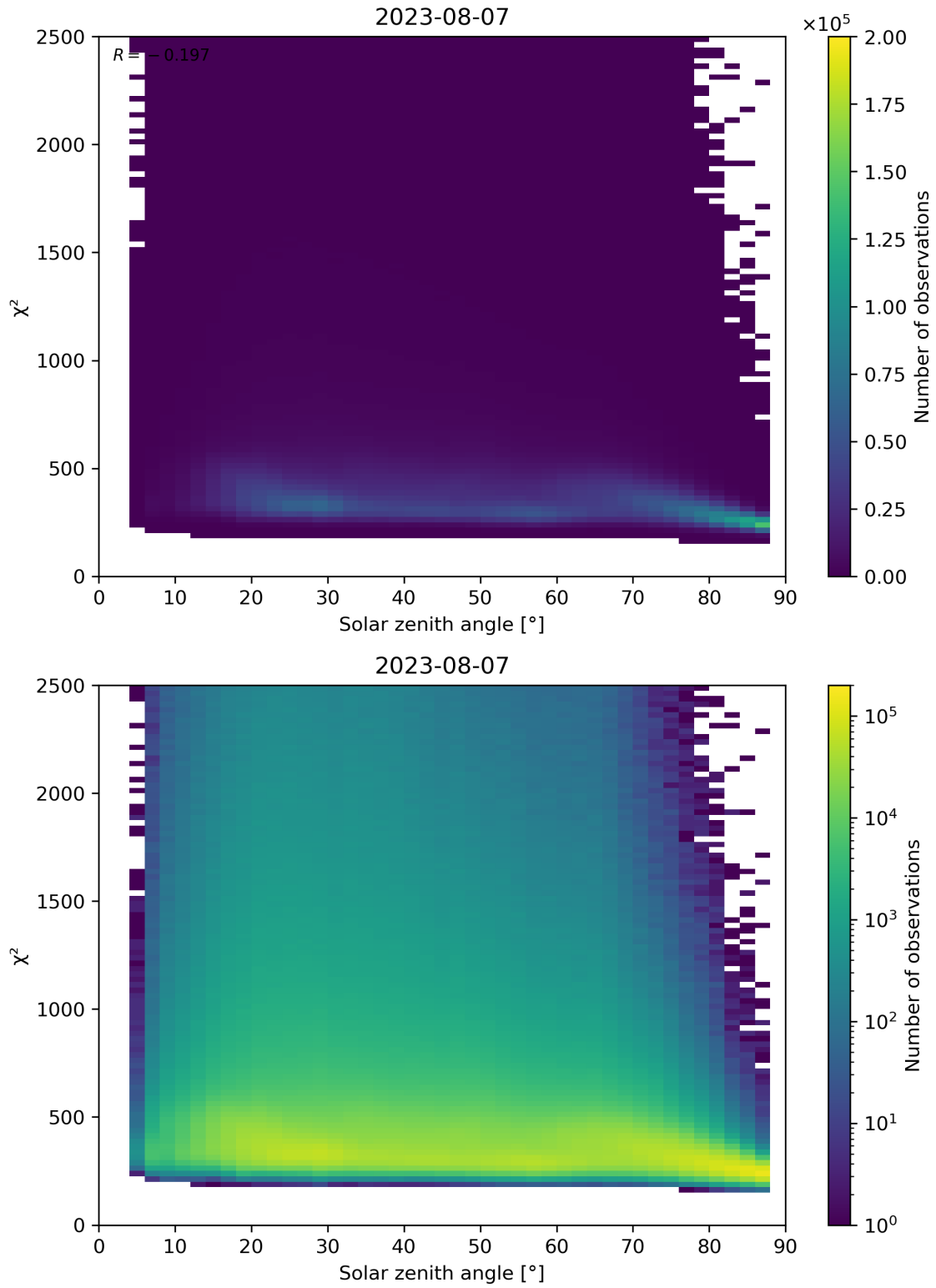
Figure 148: Scatter density plot of “Solar zenith angle” against “ \chi^2 ” for 2023-08-06 to 2023-08-08.
