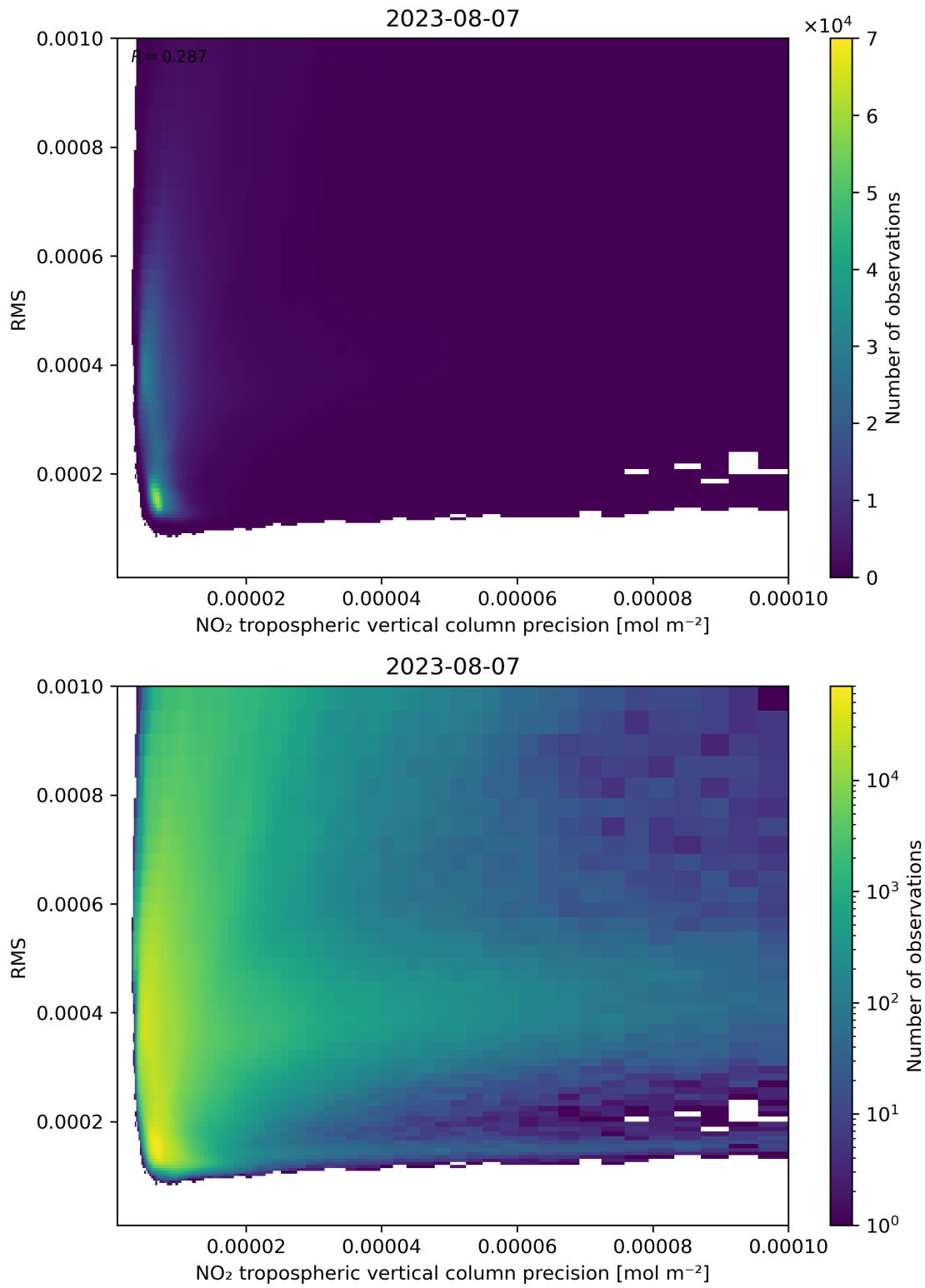
Figure 140: Scatter density plot of “NO 2 tropospheric vertical column precision” against “RMS” for 2023-08-06 to 2023-08-08.
