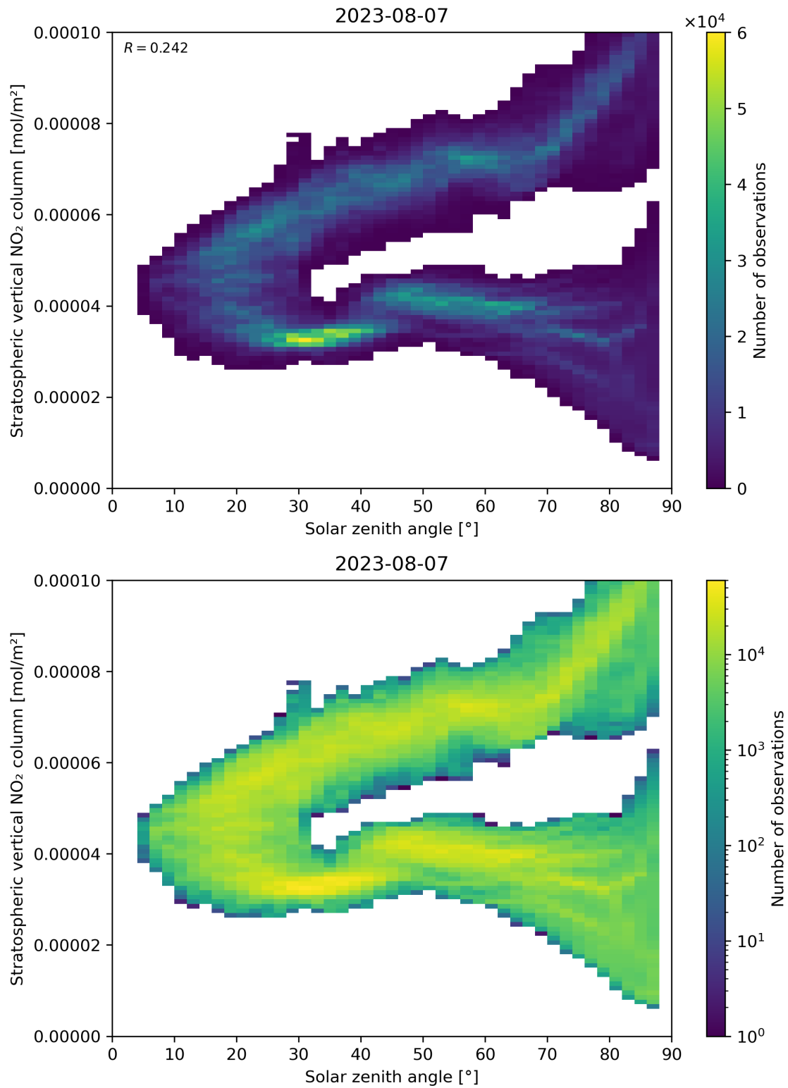
Figure 150: Scatter density plot of “Solar zenith angle” against “Stratospheric vertical NO 2 column” for 2023-08-06 to 2023-08-08.
