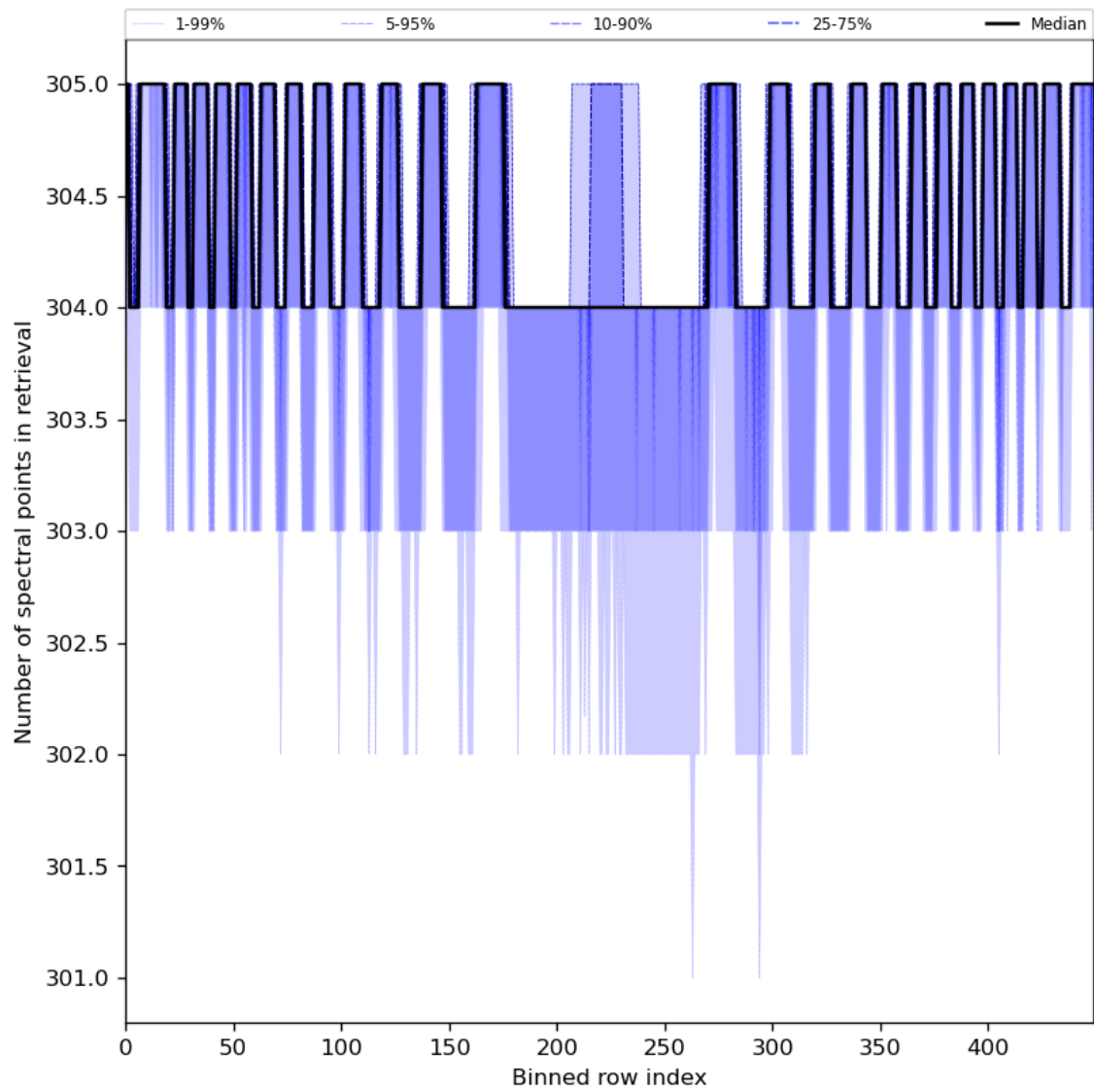
Figure 50: Along track statistics of “Number of spectral points in retrieval” for 2023-08-06 to 2023-08-08
