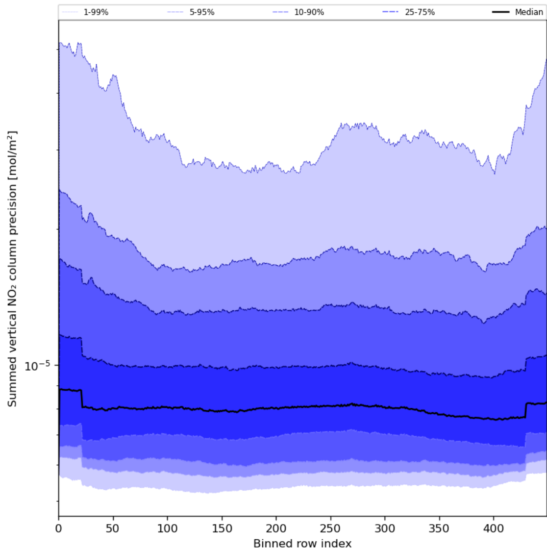
Figure 58: Along track statistics of “Summed vertical NO 2 column precision” for 2023-08-06 to 2023-08-08
