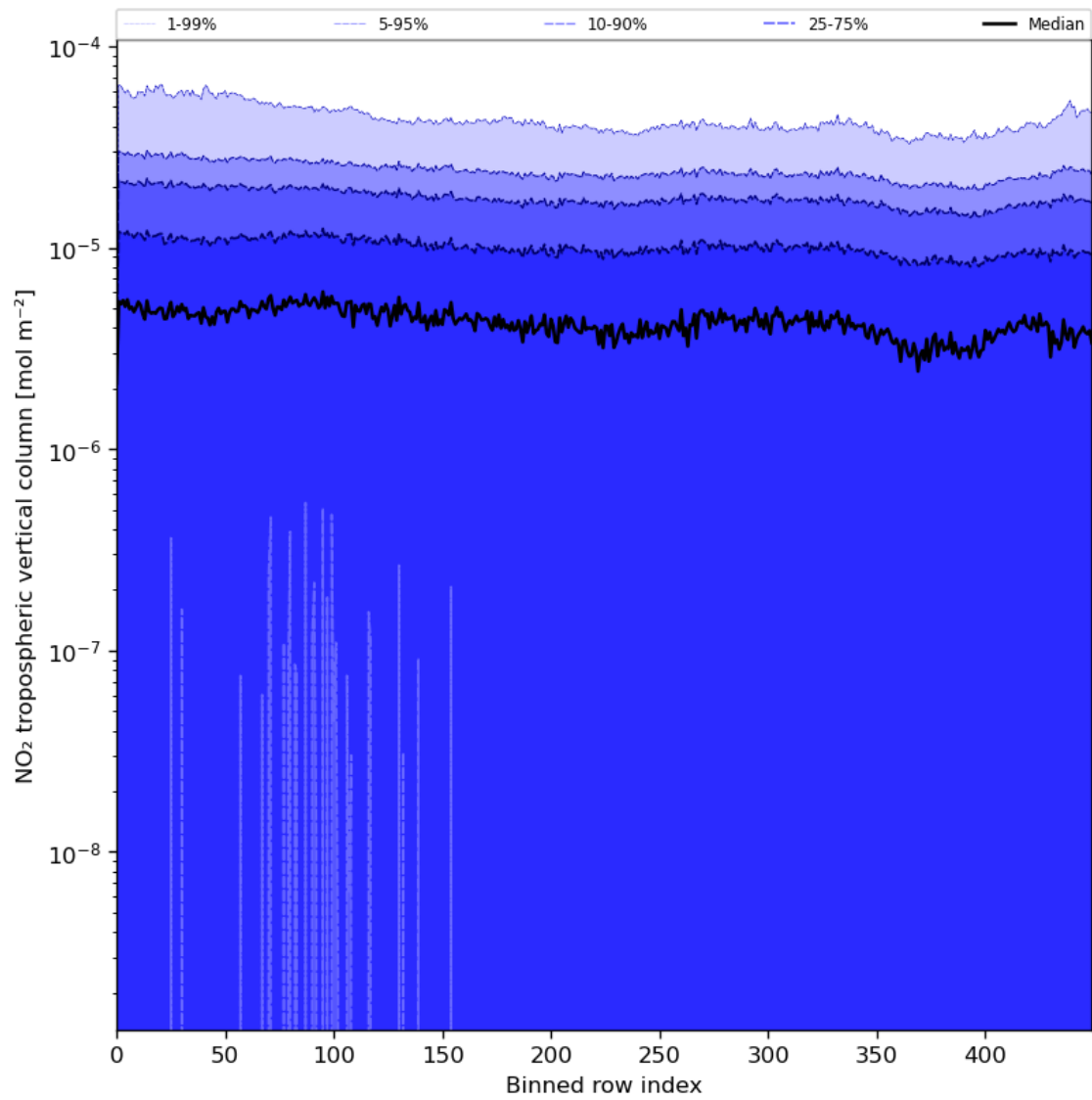
Figure 46: Along track statistics of “NO 2 tropospheric vertical column” for 2023-08-06 to 2023-08-08
