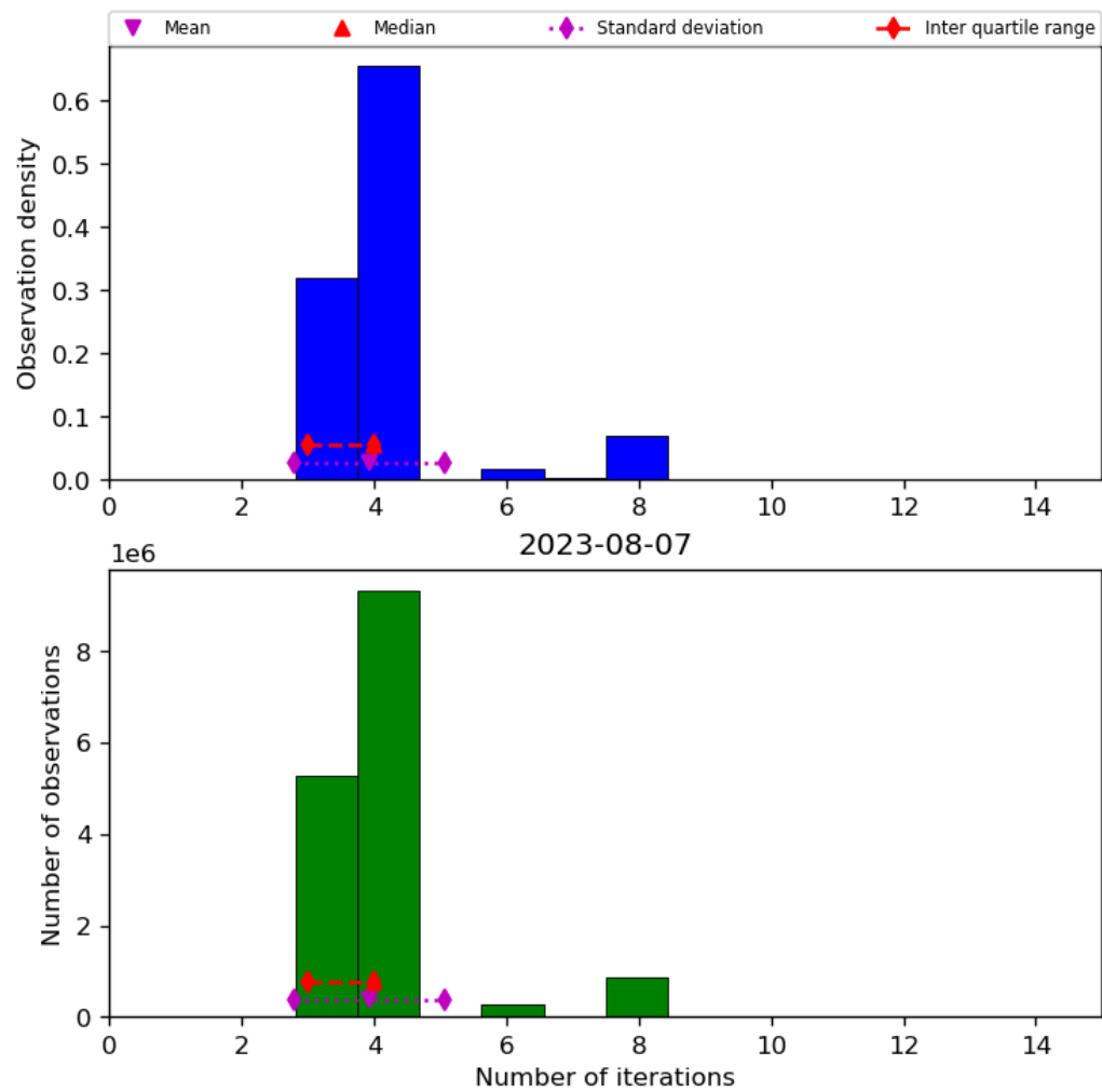
Figure 34: Histogram of “Number of iterations” for 2023-08-06 to 2023-08-08
