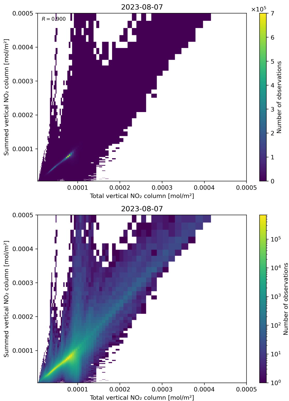
Figure 112: Scatter density plot of “Total vertical NO 2 column” against “Summed vertical NO 2 column” for 2023-08-06 to 2023-08-08.
