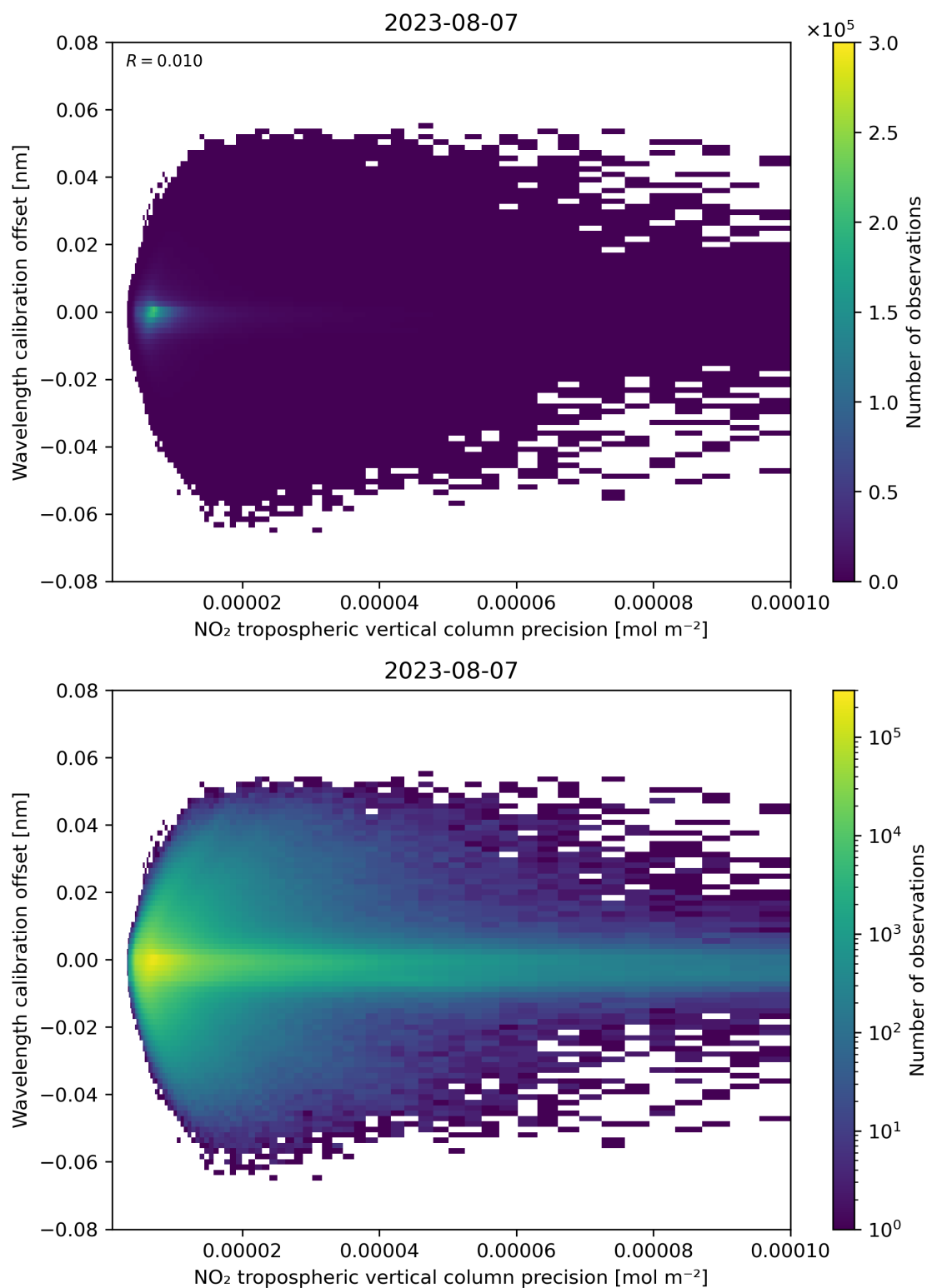
Figure 141: Scatter density plot of “NO 2 tropospheric vertical column precision” against “Wavelength calibration offset” for 2023-08-06 to 2023-08-08.
