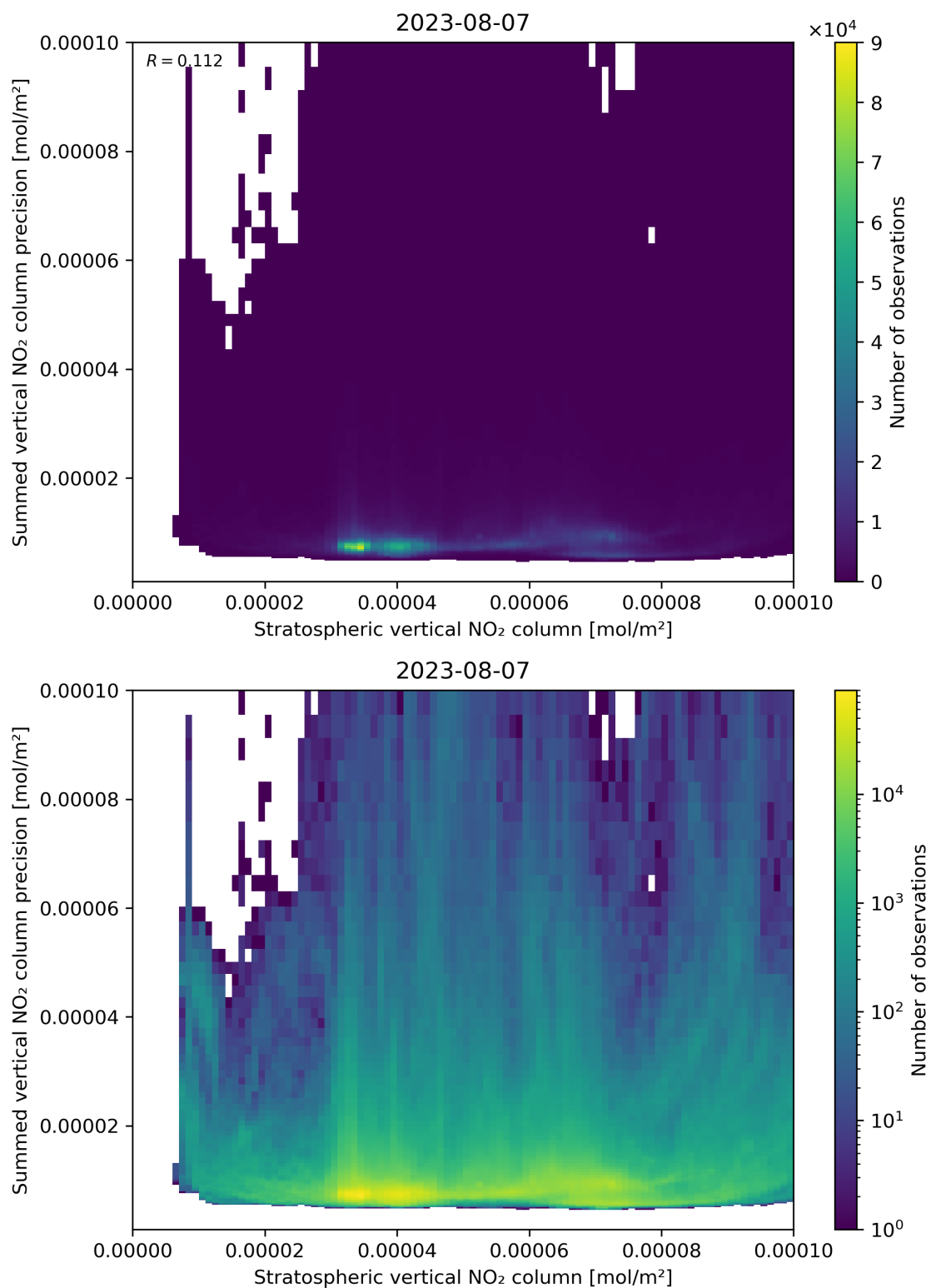
Figure 99: Scatter density plot of “Stratospheric vertical NO 2 column” against “Summed vertical NO 2 column precision” for 2023-08-06 to 2023-08-08.
