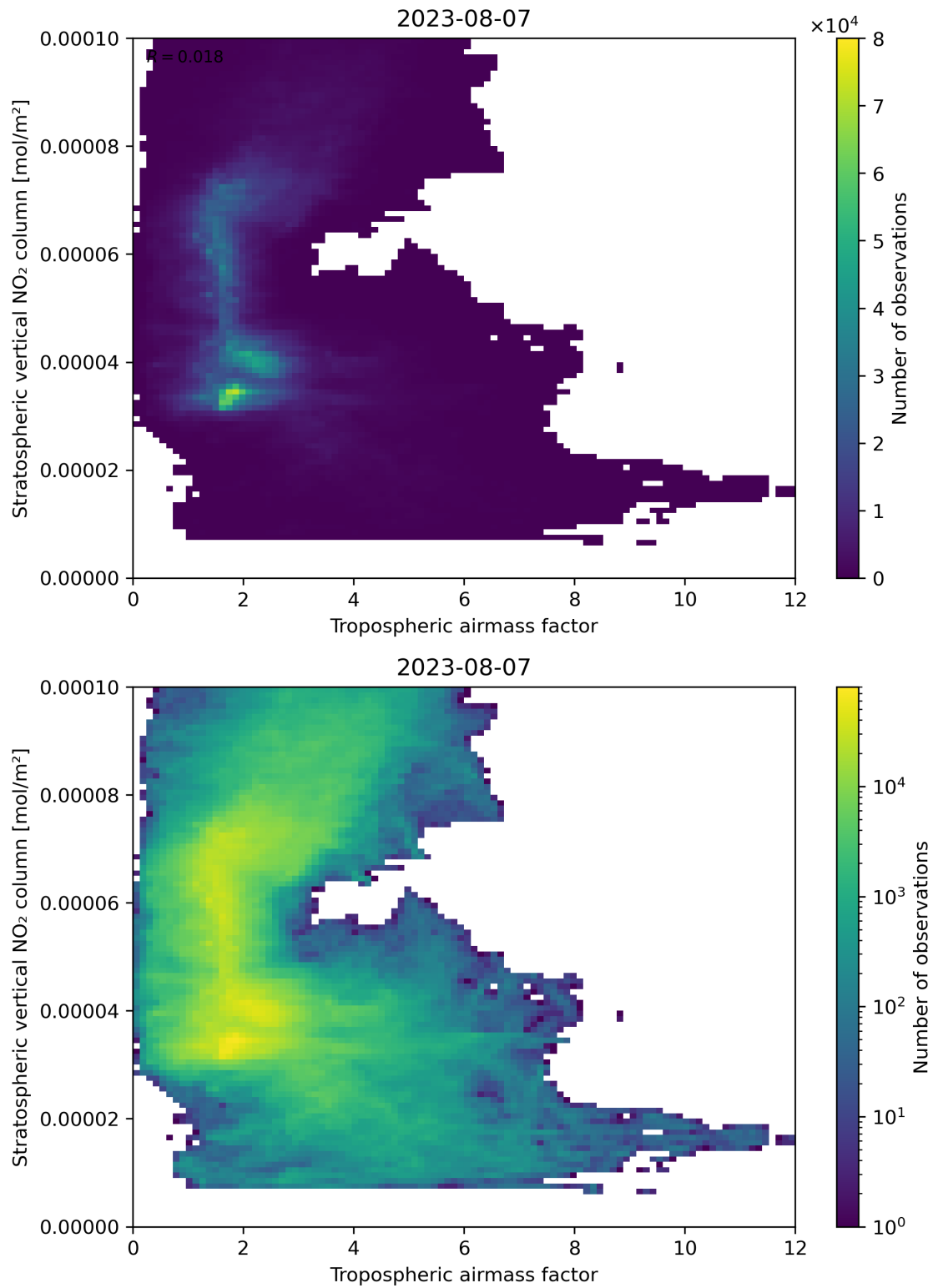
Figure 74: Scatter density plot of “Tropospheric air mass factor” against “Stratospheric vertical NO 2 column” for 2023-08-06 to 2023-08-08.
