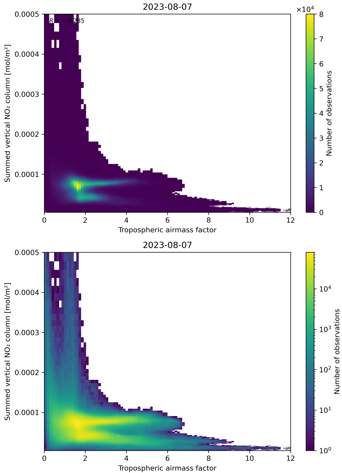
Figure 75: Scatter density plot of “Tropospheric air mass factor” against “Summed vertical NO 2 column” for 2023-08-06 to 2023-08-08.
