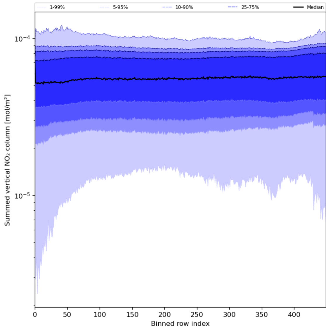
Figure 57: Along track statistics of “Summed vertical NO 2 column” for 2023-08-06 to 2023-08-08
