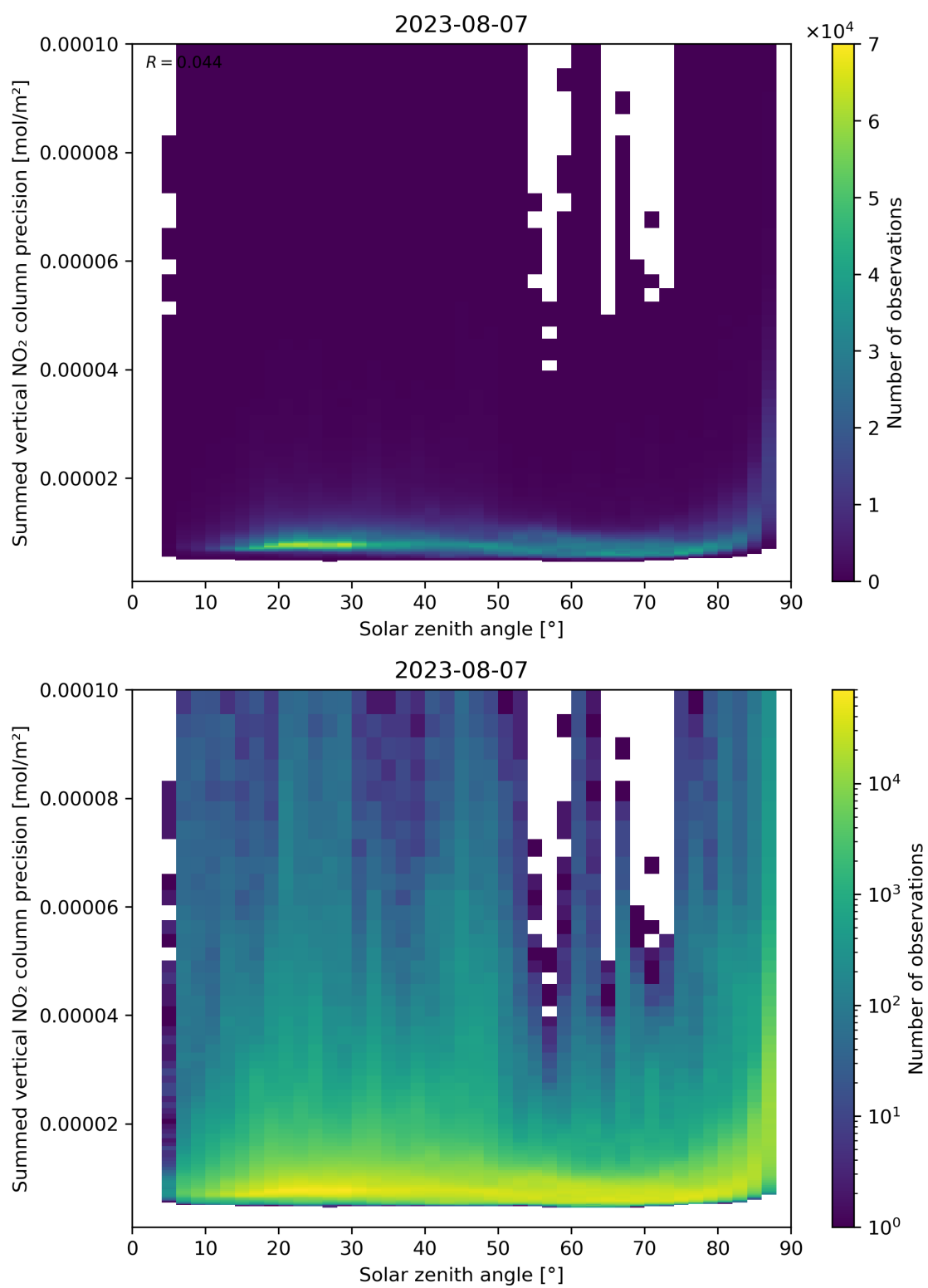
Figure 152: Scatter density plot of “Solar zenith angle” against “Summed vertical NO 2 column precision” for 2023-08-06 to 2023-08-08.
