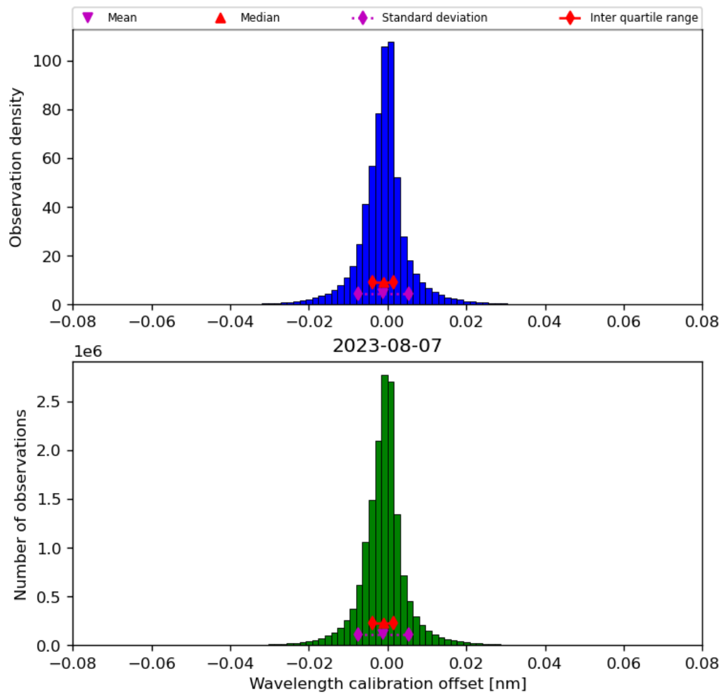
Figure 35: Histogram of “Wavelength calibration offset” for 2023-08-06 to 2023-08-08
