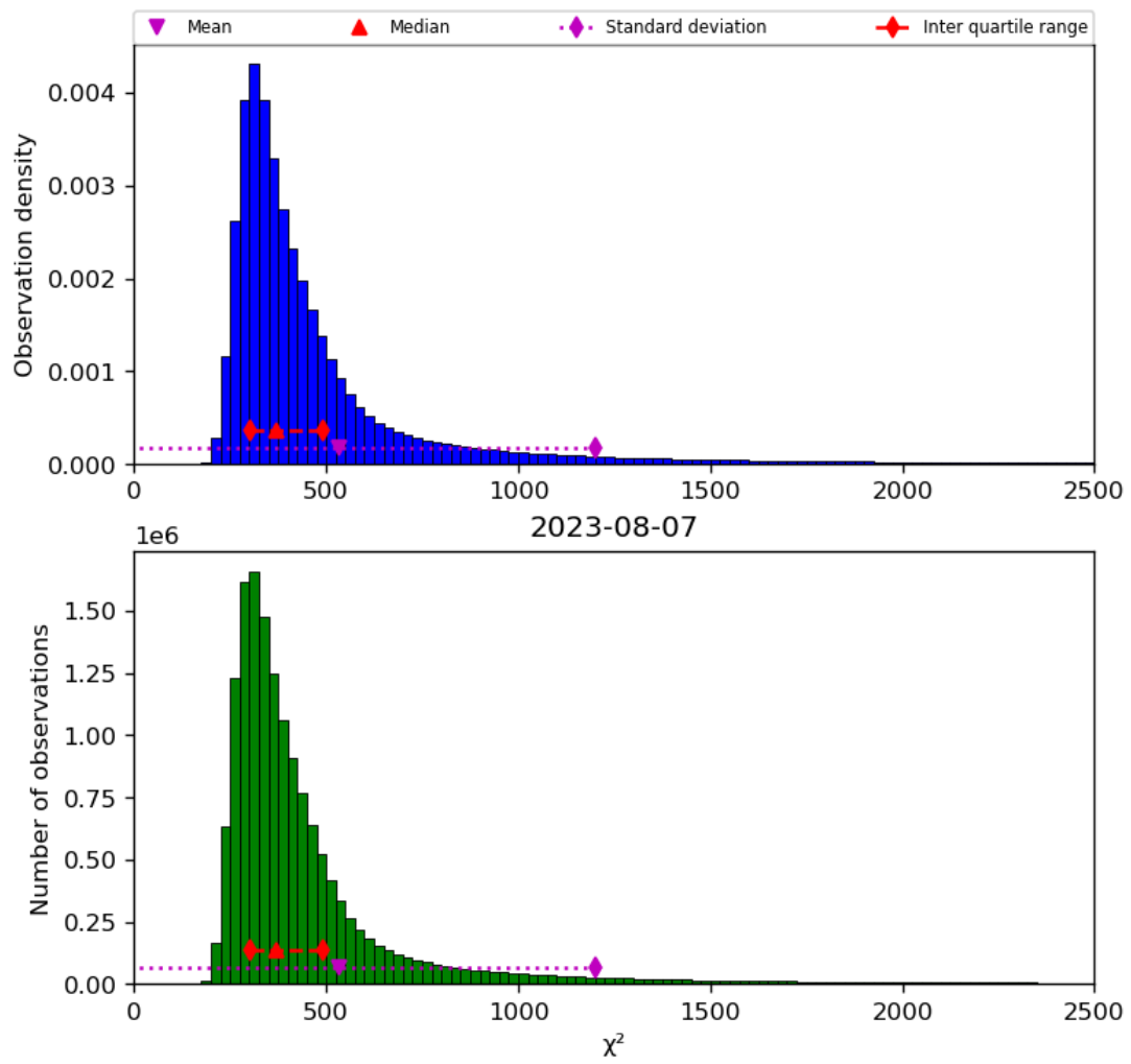
Figure 42: Histogram of “ \chi^2 ” for 2023-08-06 to 2023-08-08
