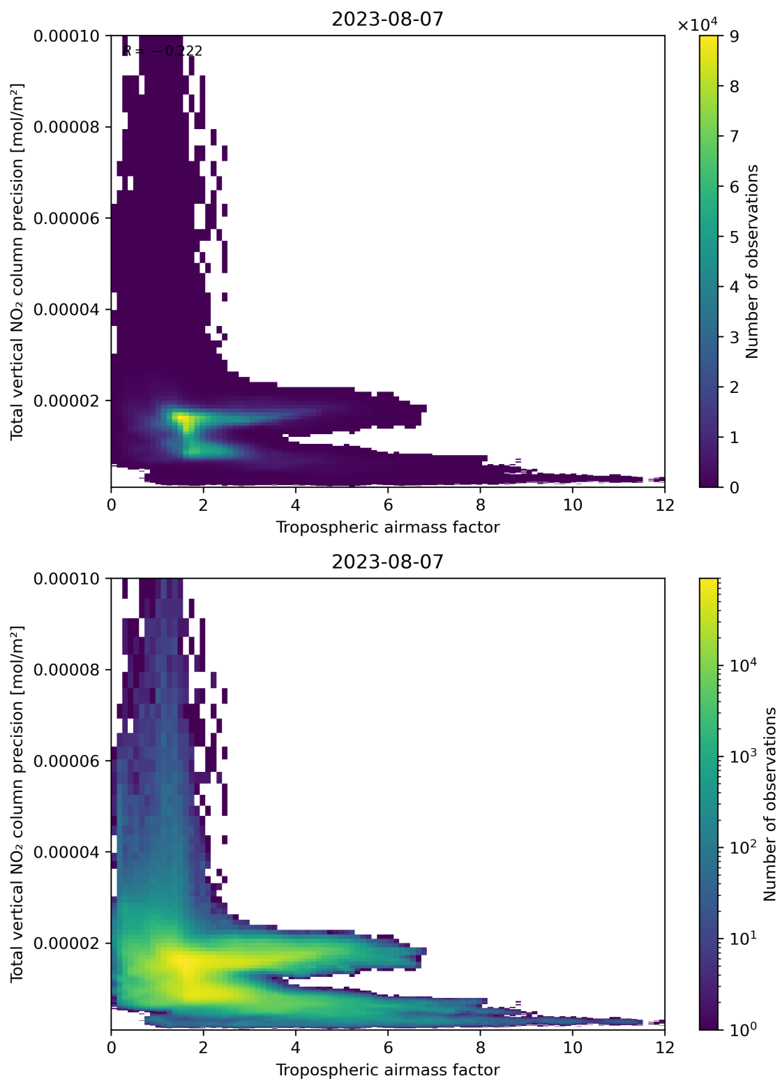
Figure 78: Scatter density plot of “Tropospheric air mass factor” against “Total vertical NO 2 column precision” for 2023-08-06 to 2023-08-08.
