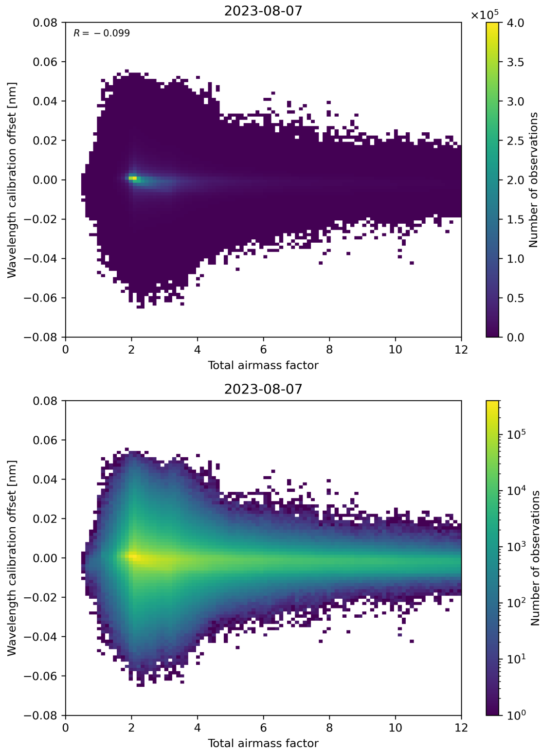
Figure 70: Scatter density plot of “Total airmass factor” against “Wavelength calibration offset” for 2023-08-06 to 2023-08-08.
