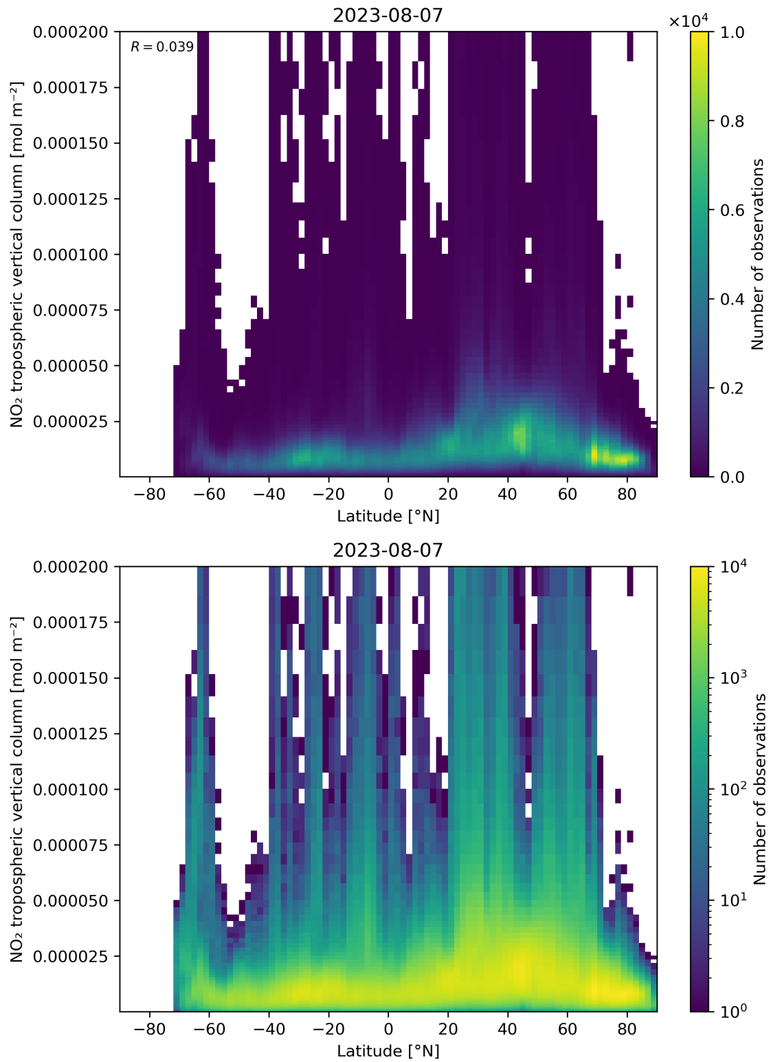
Figure 92: Scatter density plot of “Latitude” against “NO 2 tropospheric vertical column” for 2023-08-06 to 2023-08-08.
