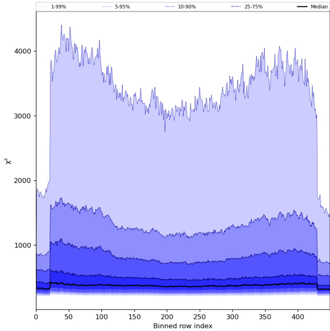
Figure 59: Along track statistics of “ \chi^2 ” for 2023-08-06 to 2023-08-08
