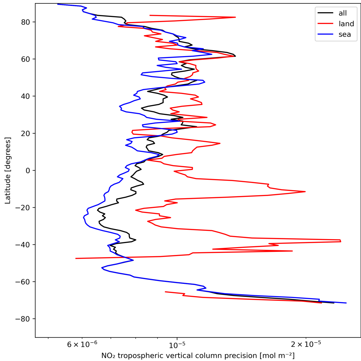
Figure 13: Zonal average of “NO 2 tropospheric vertical column precision” for 2023-08-06 to 2023-08-08.
