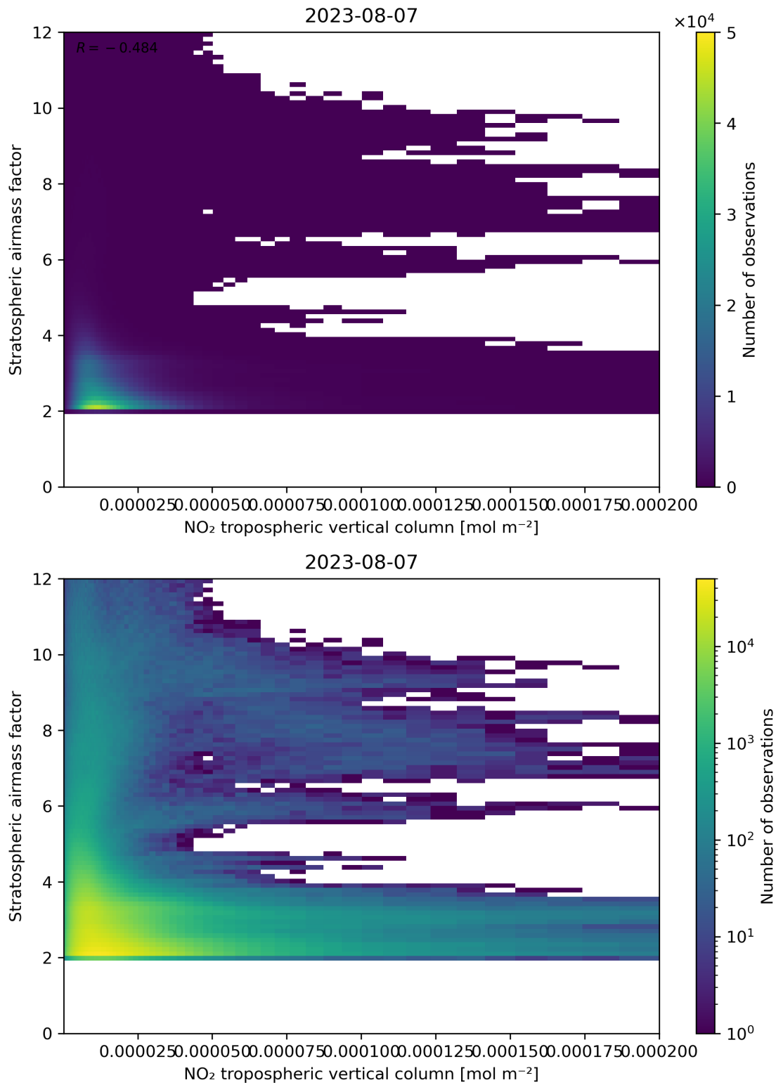
Figure 121: Scatter density plot of “NO 2 tropospheric vertical column” against “Stratospheric air mass factor” for 2023-08-06 to 2023-08-08.
