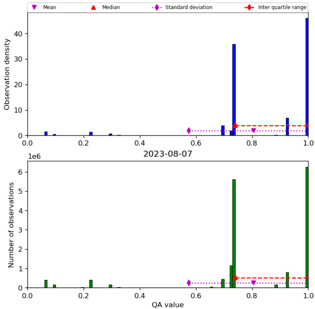
Figure 28: Histogram of “QA value” for 2023-08-06 to 2023-08-08
