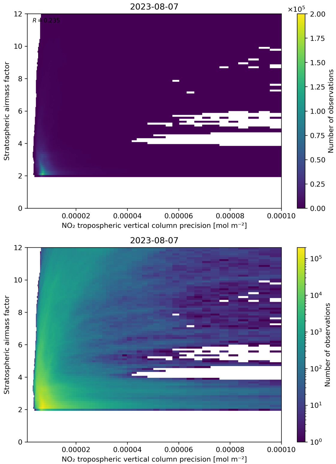
Figure 131: Scatter density plot of “NO 2 tropospheric vertical column precision” against “Stratospheric airmass factor” for 2023-08-06 to 2023-08-08.
