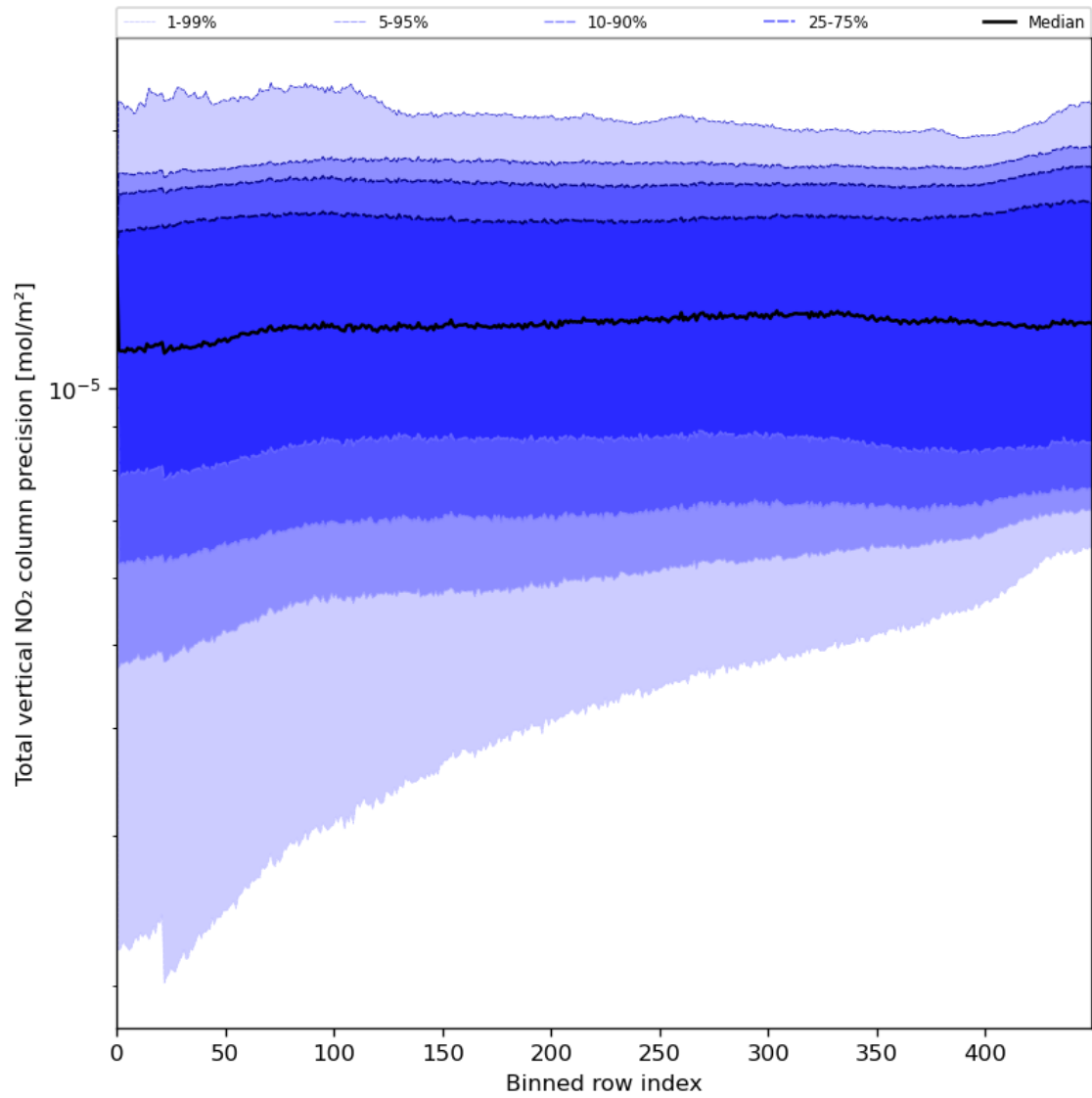
Figure 56: Along track statistics of “Total vertical NO 2 column precision” for 2023-08-06 to 2023-08-08
