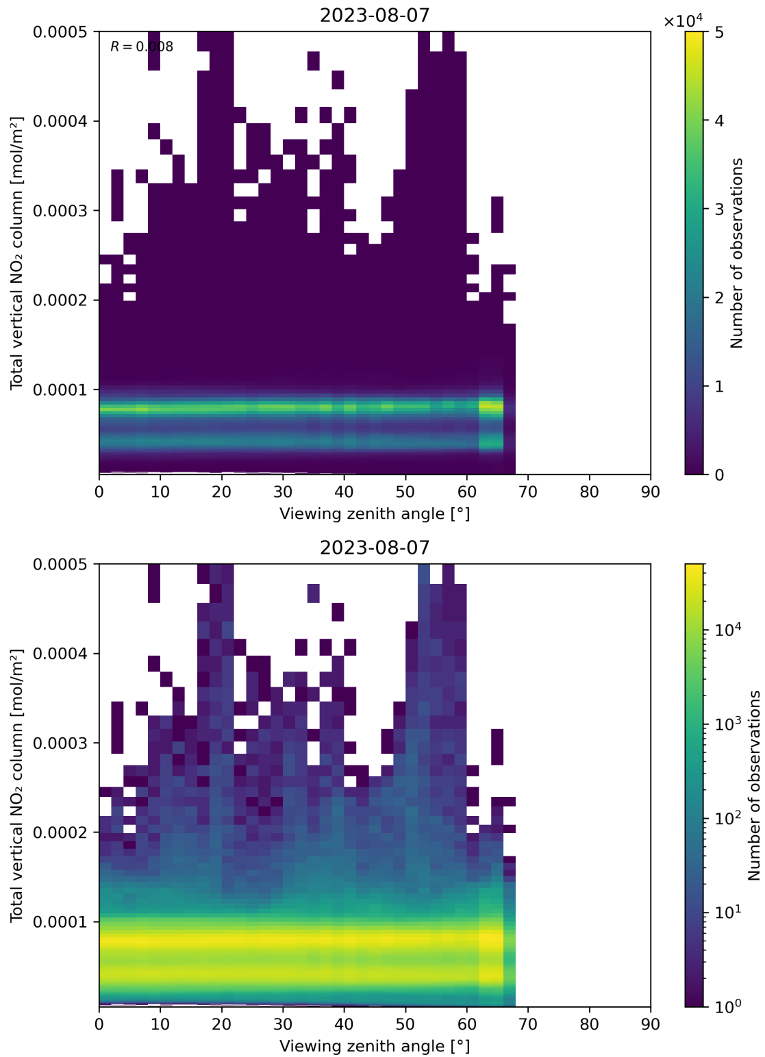
Figure 167: Scatter density plot of “Viewing zenith angle” against “Total vertical NO 2 column” for 2023-08-06 to 2023-08-08.
