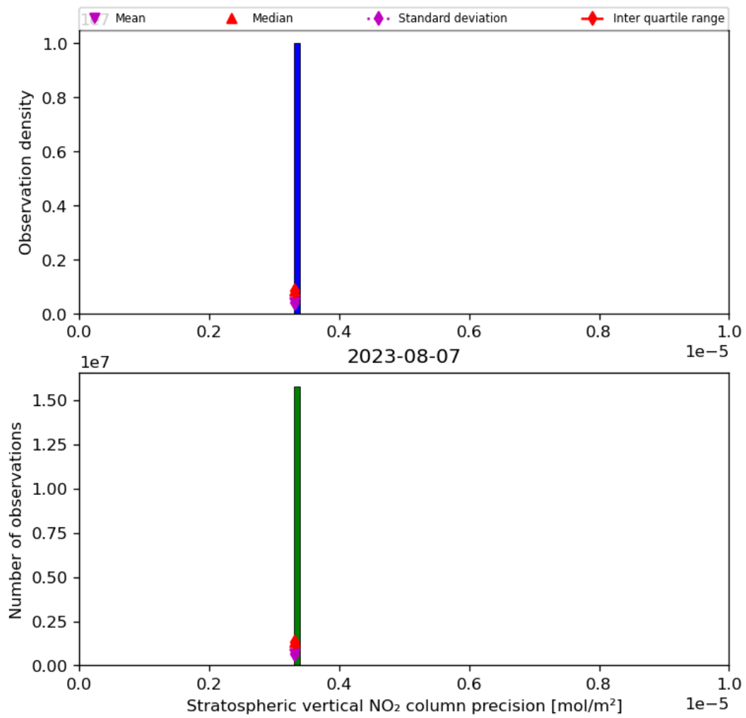
Figure 37: Histogram of “Stratospheric vertical NO 2 column precision” for 2023-08-06 to 2023-08-08
