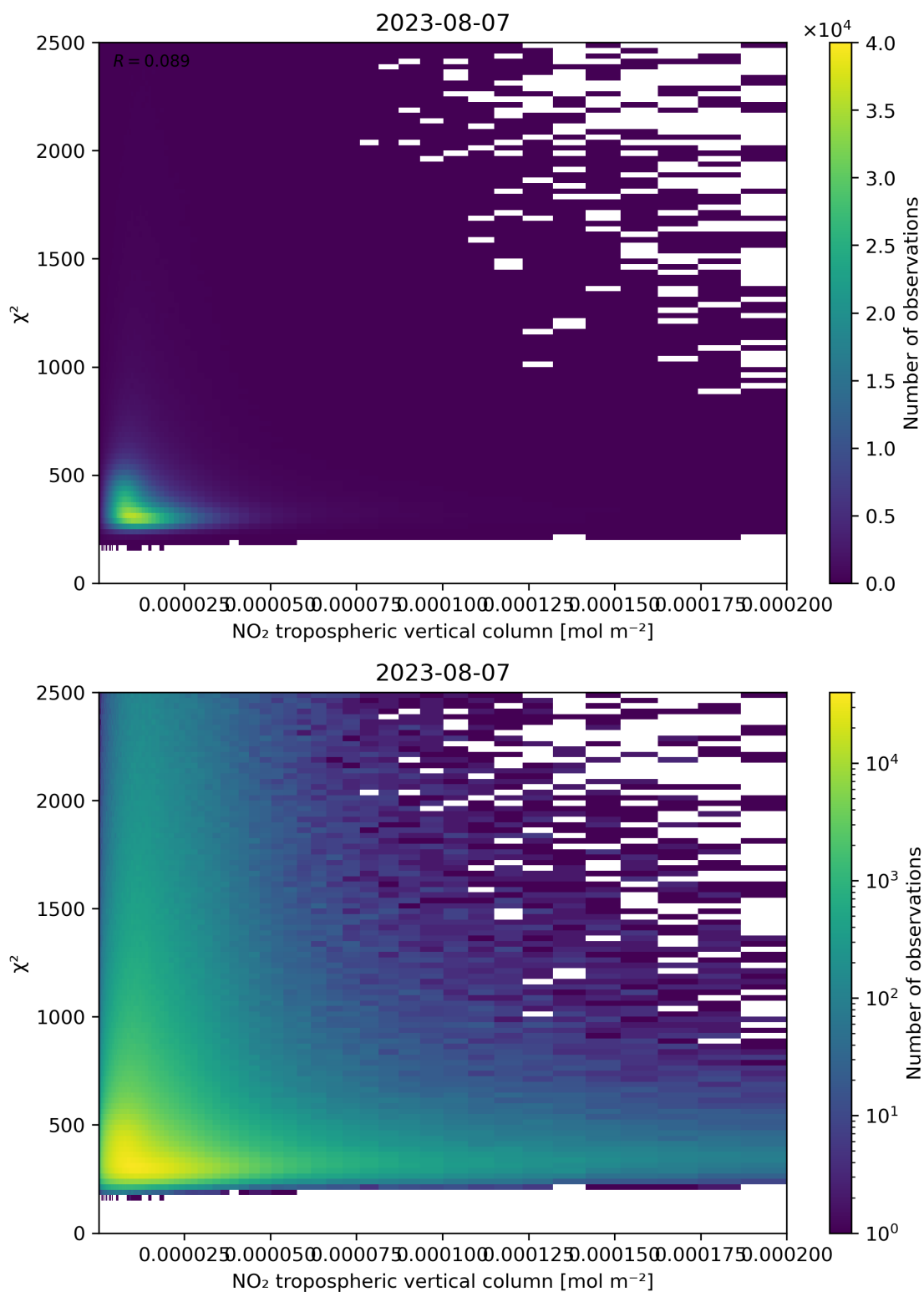
Figure 124: Scatter density plot of “NO 2 tropospheric vertical column” against “ \chi^2 ” for 2023-08-06 to 2023-08-08.
