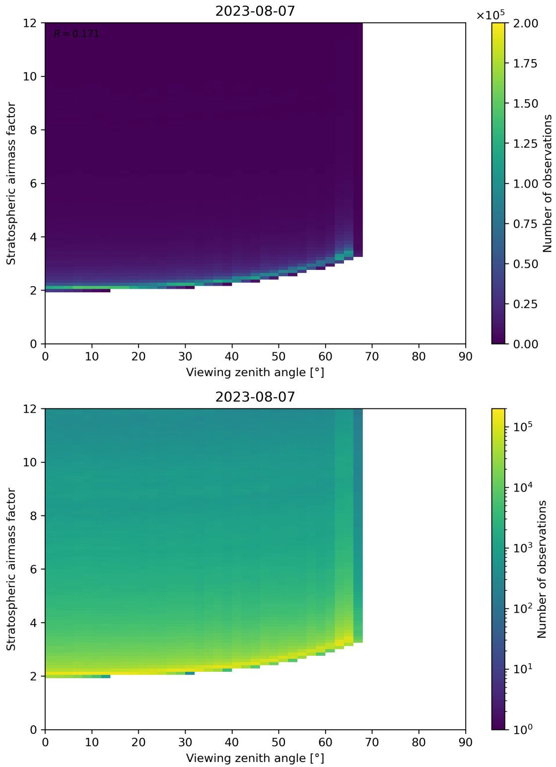
Figure 159: Scatter density plot of “Viewing zenith angle” against “Stratospheric airmass factor” for 2023-08-06 to 2023-08-08.
