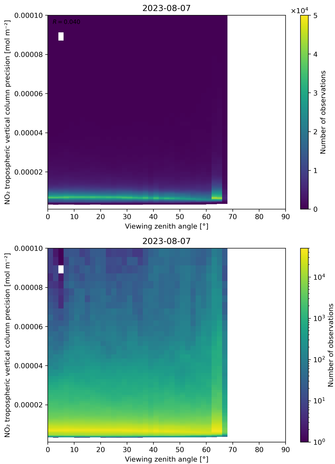
Figure 170: Scatter density plot of “Viewing zenith angle” against “NO 2 tropospheric vertical column precision” for 2023-08-06 to 2023-08-08.
