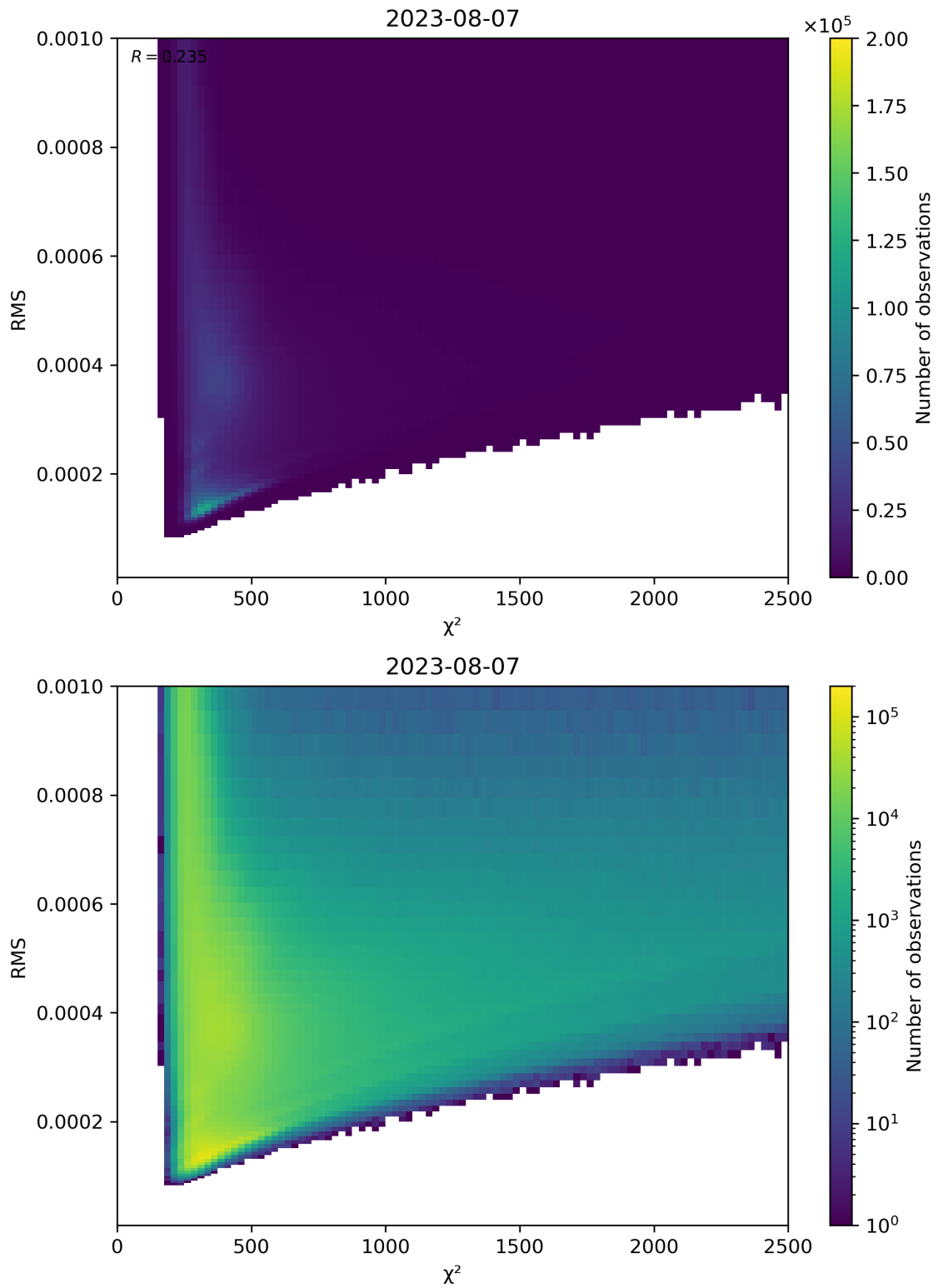
Figure 82: Scatter density plot of “ \chi^2 ” against “RMS” for 2023-08-06 to 2023-08-08.
