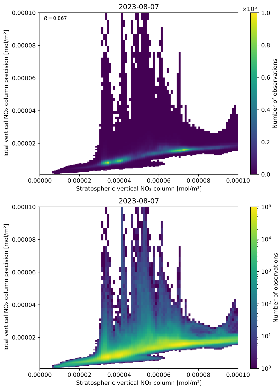
Figure 101: Scatter density plot of “Stratospheric vertical NO 2 column” against “Total vertical NO 2 column precision” for 2023-08-06 to 2023-08-08.
