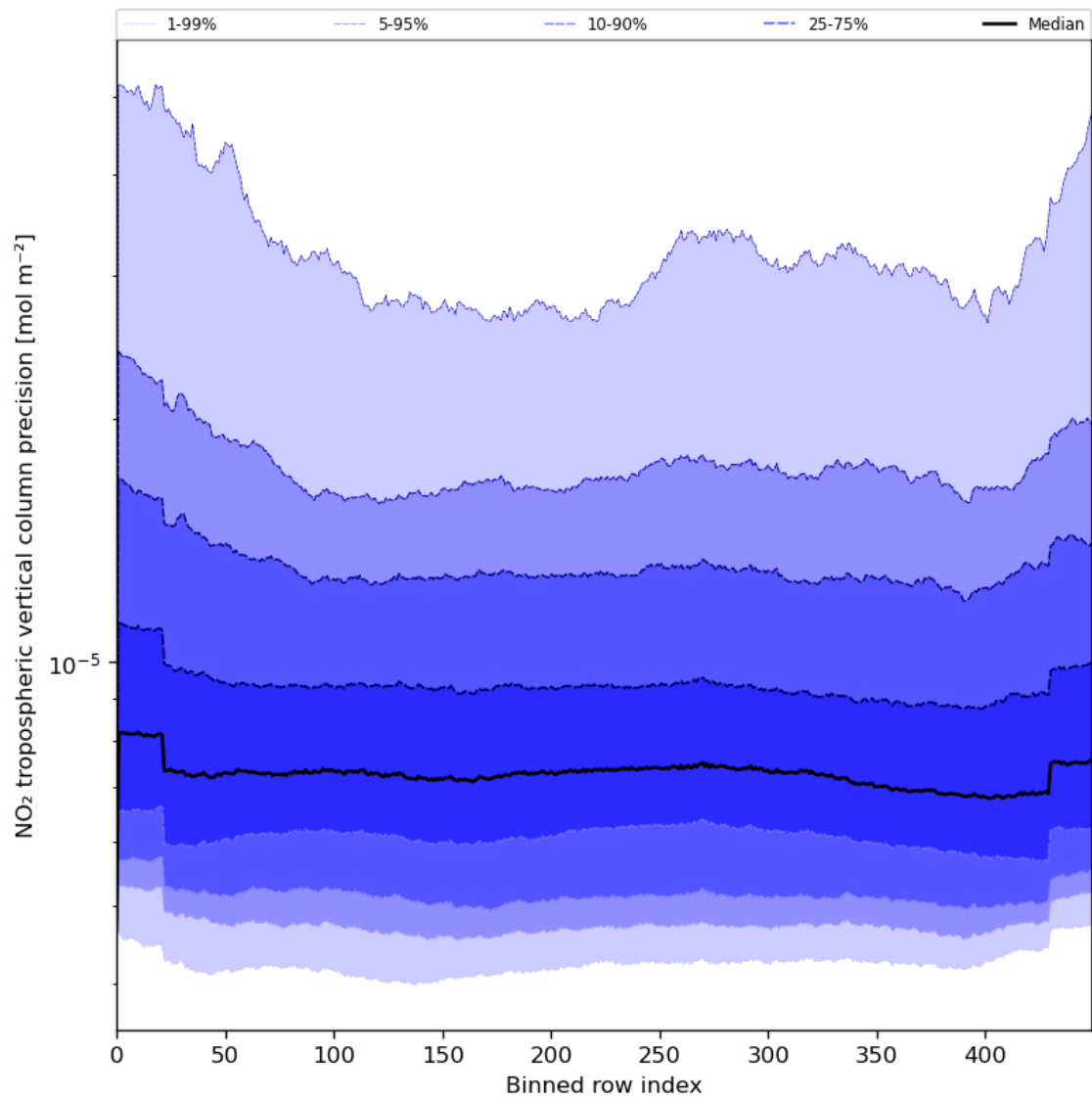
Figure 47: Along track statistics of “NO 2 tropospheric vertical column precision” for 2023-08-06 to 2023-08-08
