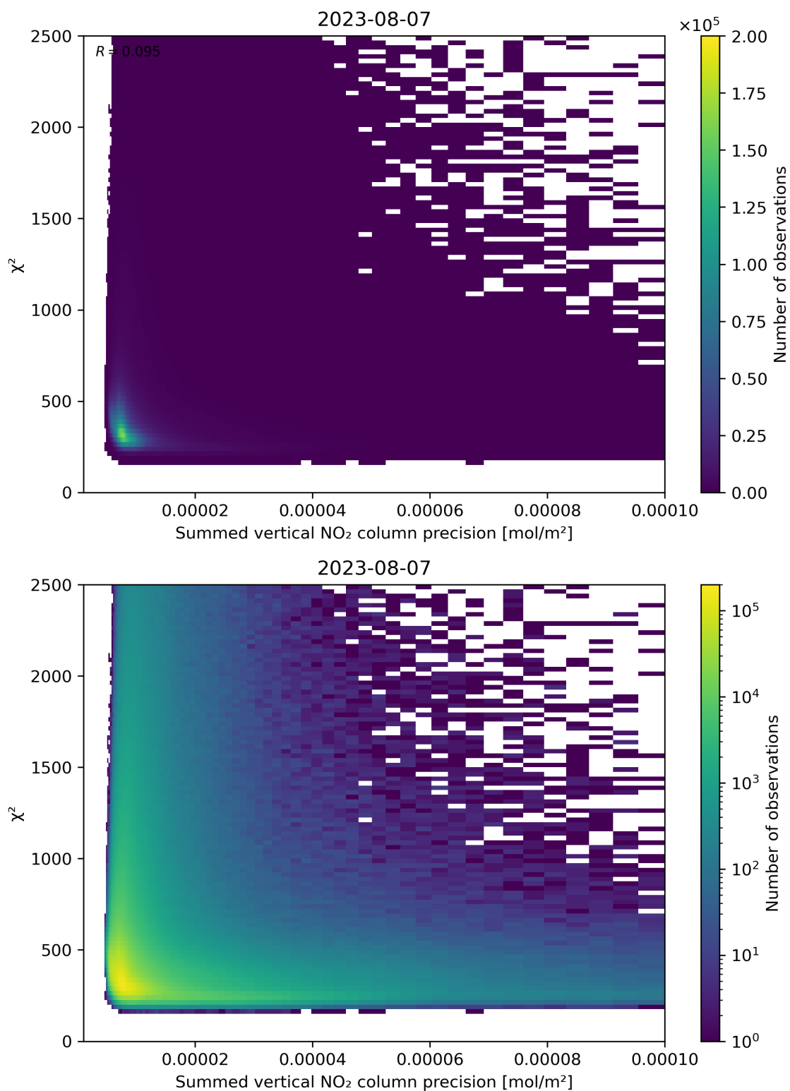
Figure 107: Scatter density plot of “Summed vertical NO 2 column precision” against “ \chi^2 ” for 2023-08-06 to 2023-08-08.
