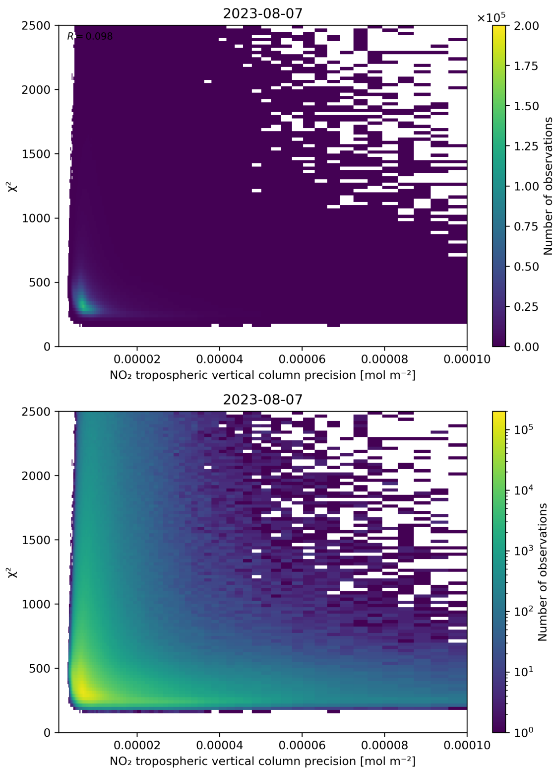
Figure 134: Scatter density plot of “NO 2 tropospheric vertical column precision” against “ \chi^2 ” for 2023-08-06 to 2023-08-08.
