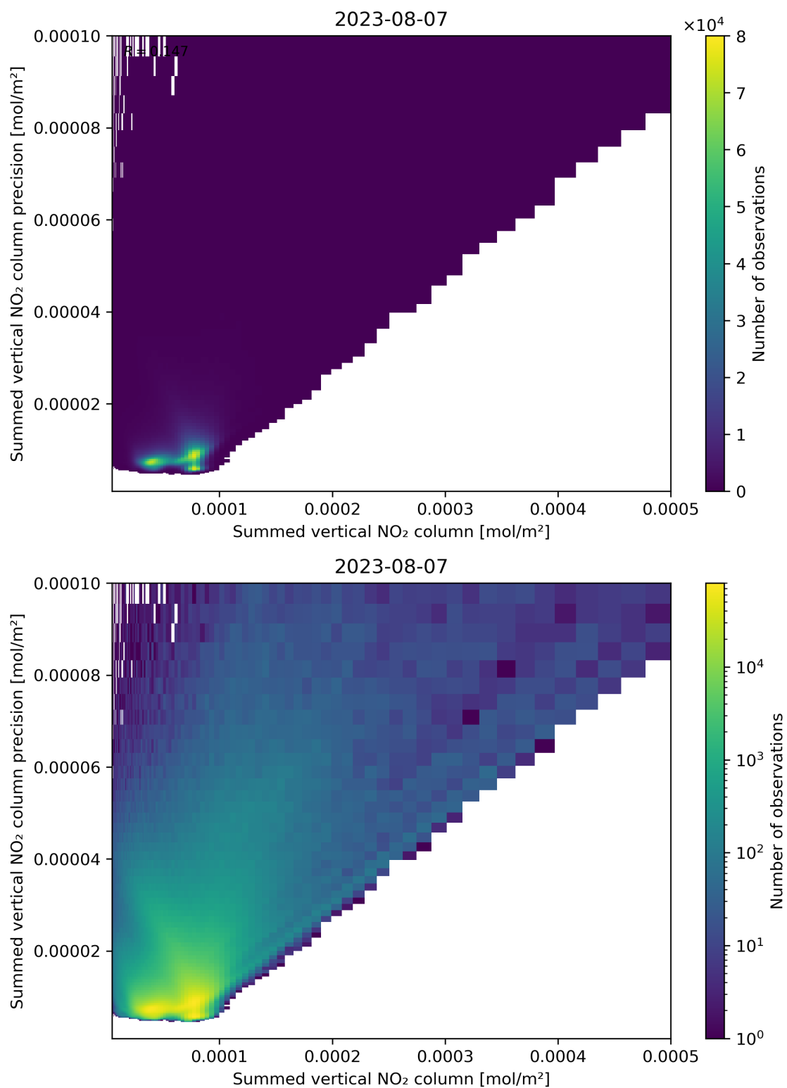
Figure 105: Scatter density plot of “Summed vertical NO 2 column” against “Summed vertical NO 2 column precision” for 2023-08-06 to 2023-08-08.
