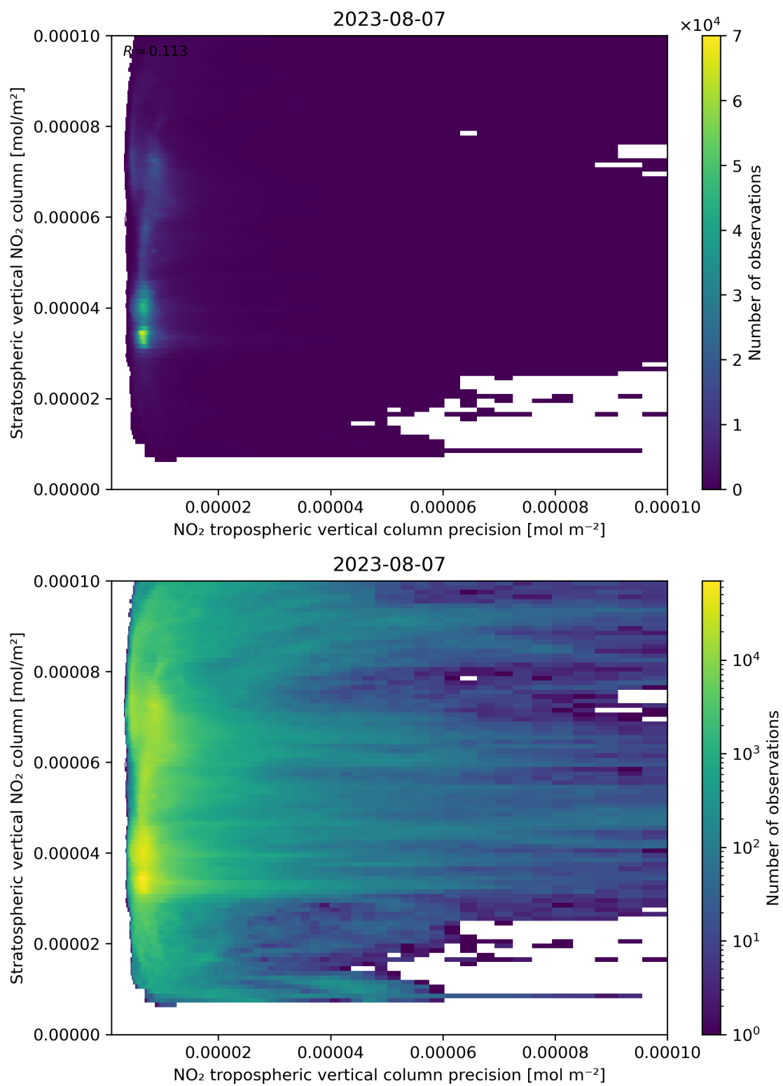
Figure 135: Scatter density plot of “NO 2 tropospheric vertical column precision” against “Stratospheric vertical NO 2 column” for 2023-08-06 to 2023-08-08.
