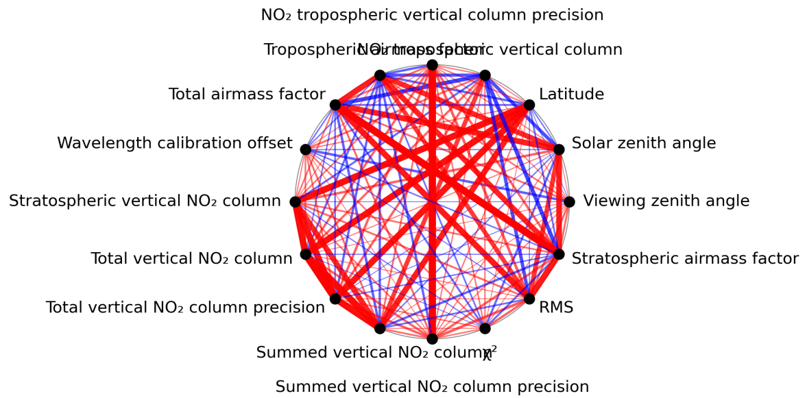
Figure 1: Map of correlation graph for 2023-08-06 to 2023-08-08.
