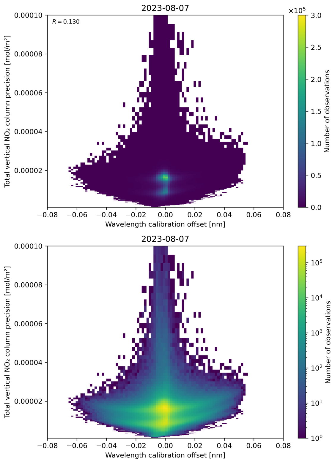
Figure 180: Scatter density plot of “Wavelength calibration offset” against “Total vertical NO 2 column precision” for 2023-08-06 to 2023-08-08.
