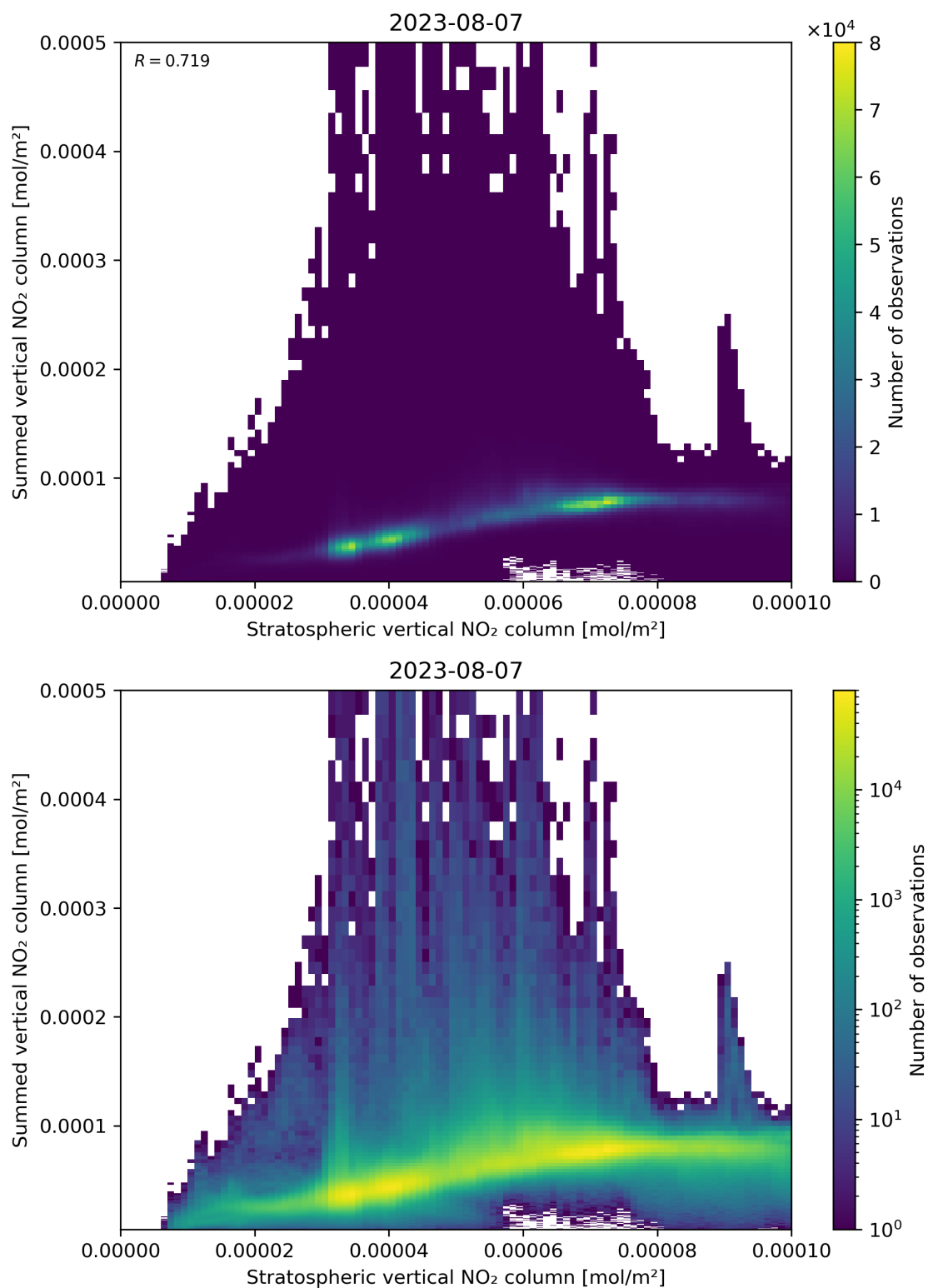
Figure 98: Scatter density plot of “Stratospheric vertical NO 2 column” against “Summed vertical NO 2 column” for 2023-08-06 to 2023-08-08.
