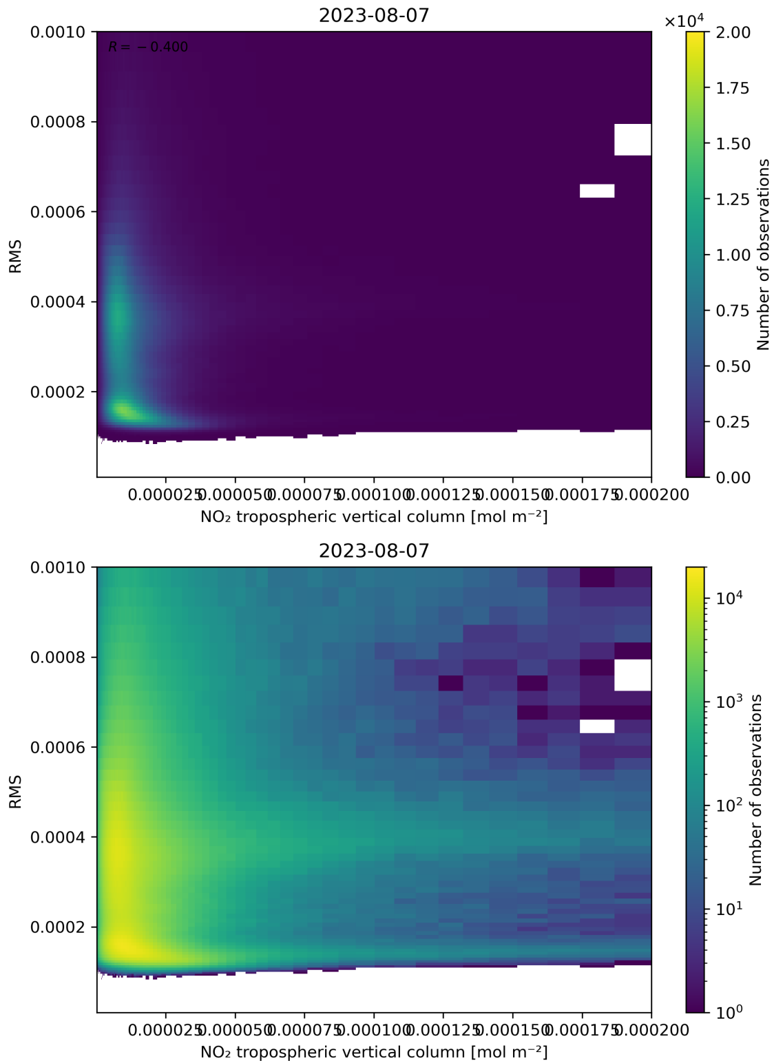
Figure 142: Scatter density plot of “NO 2 tropospheric vertical column” against “RMS” for 2023-08-06 to 2023-08-08.
