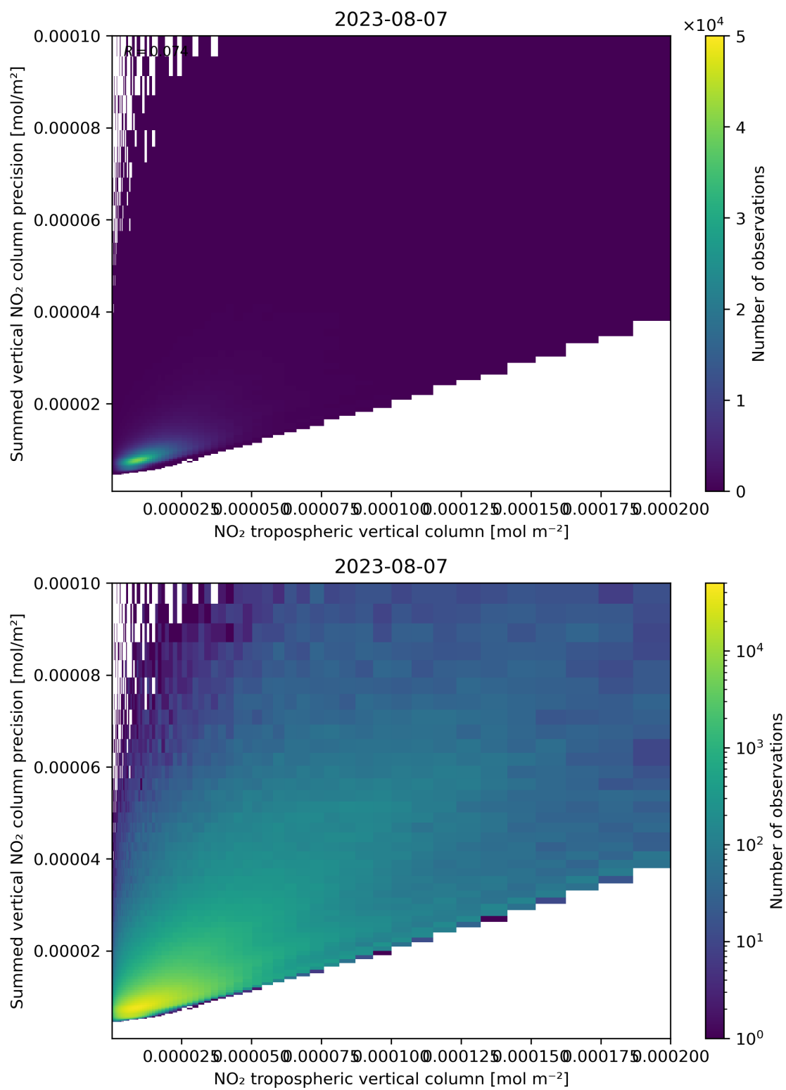
Figure 127: Scatter density plot of “NO 2 tropospheric vertical column” against “Summed vertical NO 2 column precision” for 2023-08-06 to 2023-08-08.
