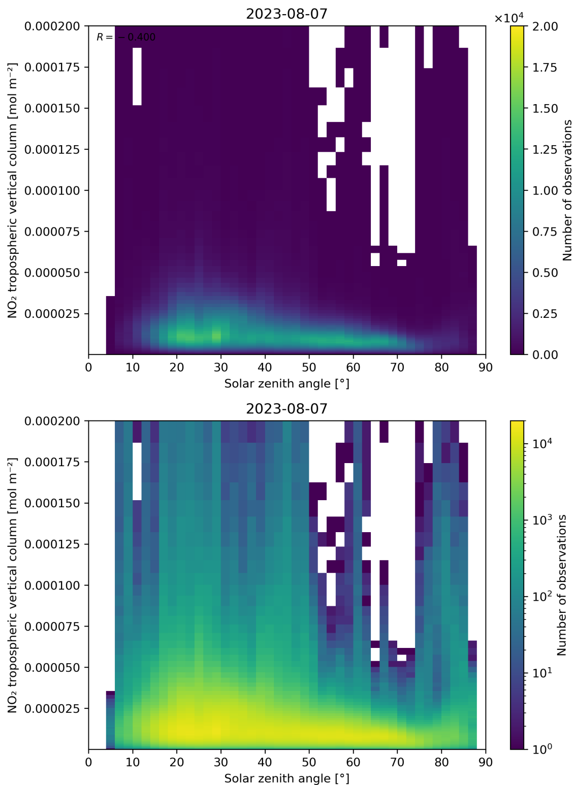
Figure 155: Scatter density plot of “Solar zenith angle” against “NO 2 tropospheric vertical column” for 2023-08-06 to 2023-08-08.
