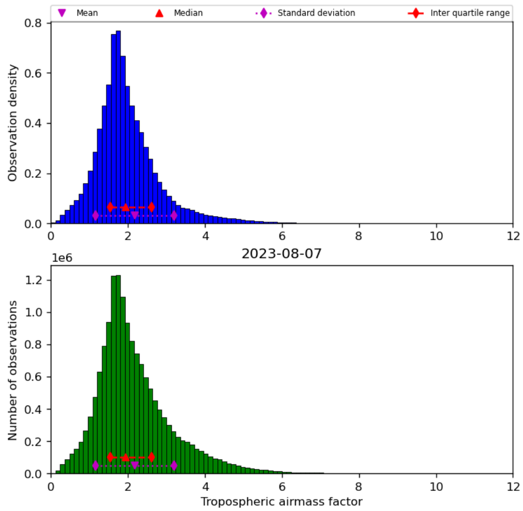
Figure 31: Histogram of “Tropospheric airmass factor” for 2023-08-06 to 2023-08-08
