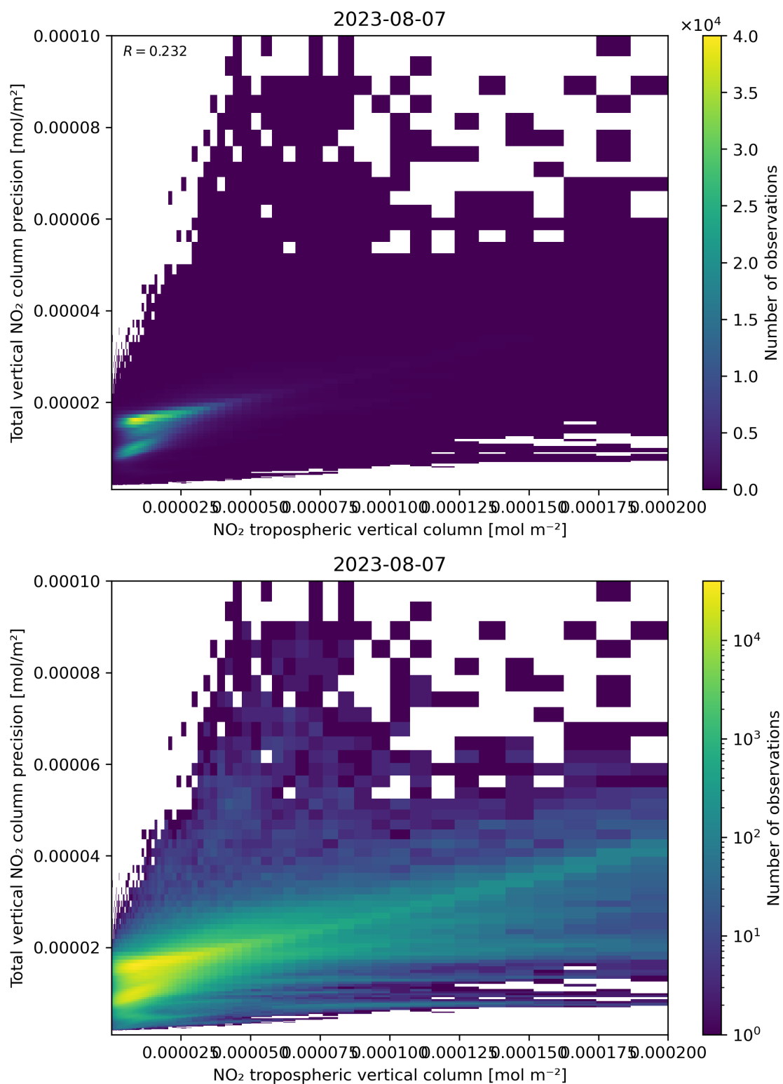
Figure 129: Scatter density plot of “NO 2 tropospheric vertical column” against “Total vertical NO 2 column precision” for 2023-08-06 to 2023-08-08.
