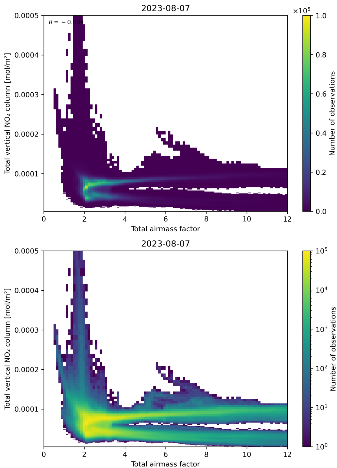
Figure 67: Scatter density plot of “Total airmass factor” against “Total vertical NO 2 column” for 2023-08-06 to 2023-08-08.
