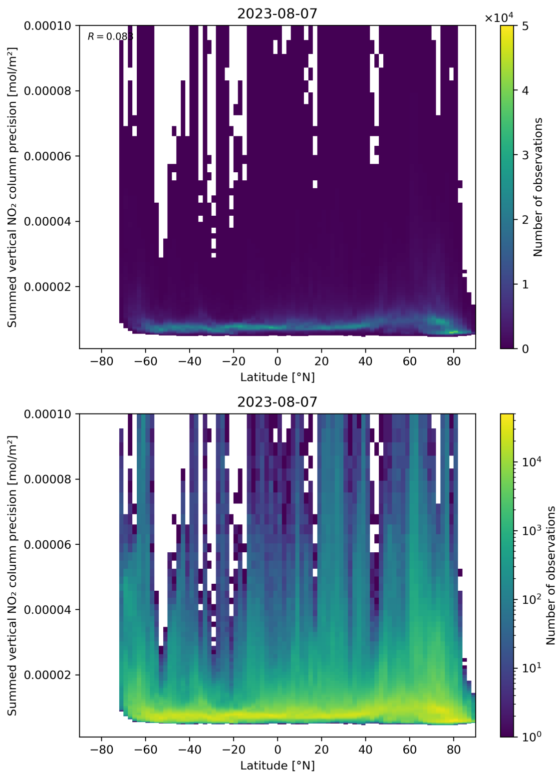
Figure 89: Scatter density plot of “Latitude” against “Summed vertical NO 2 column precision” for 2023-08-06 to 2023-08-08.
