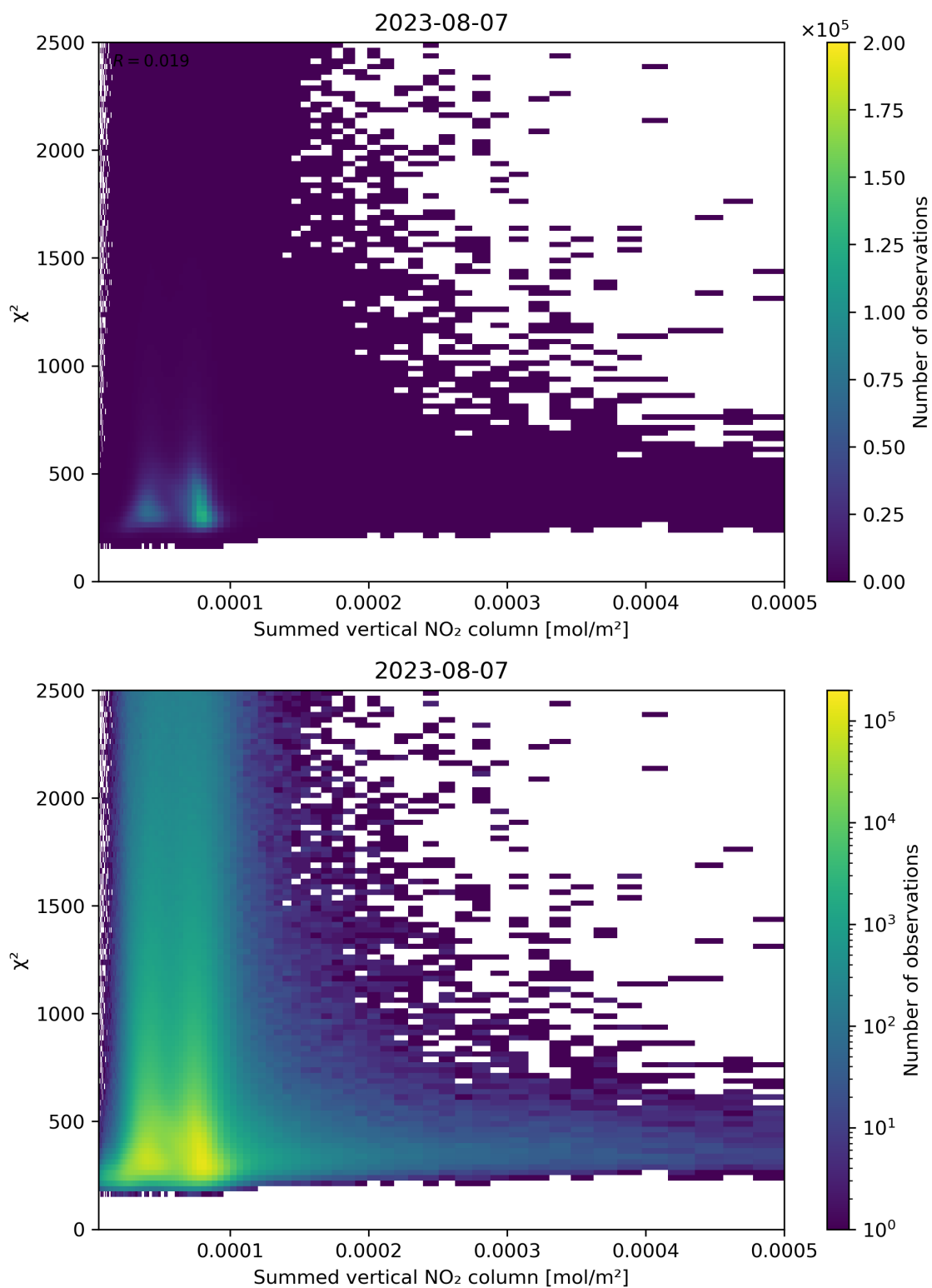
Figure 104: Scatter density plot of “Summed vertical NO 2 column” against “ \chi^2 ” for 2023-08-06 to 2023-08-08.
