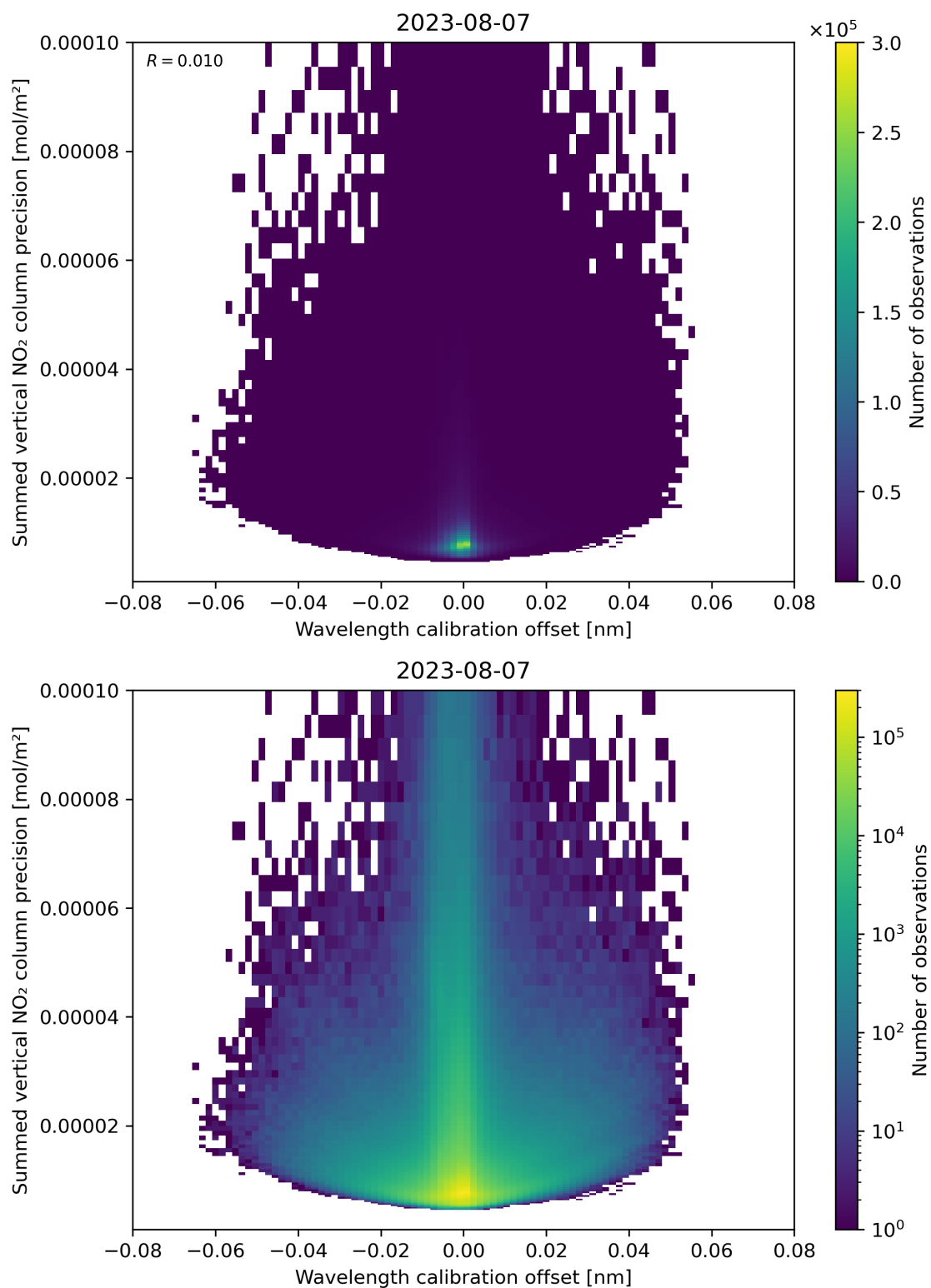
Figure 178: Scatter density plot of “Wavelength calibration offset” against “Summed vertical NO 2 column precision” for 2023-08-06 to 2023-08-08.
