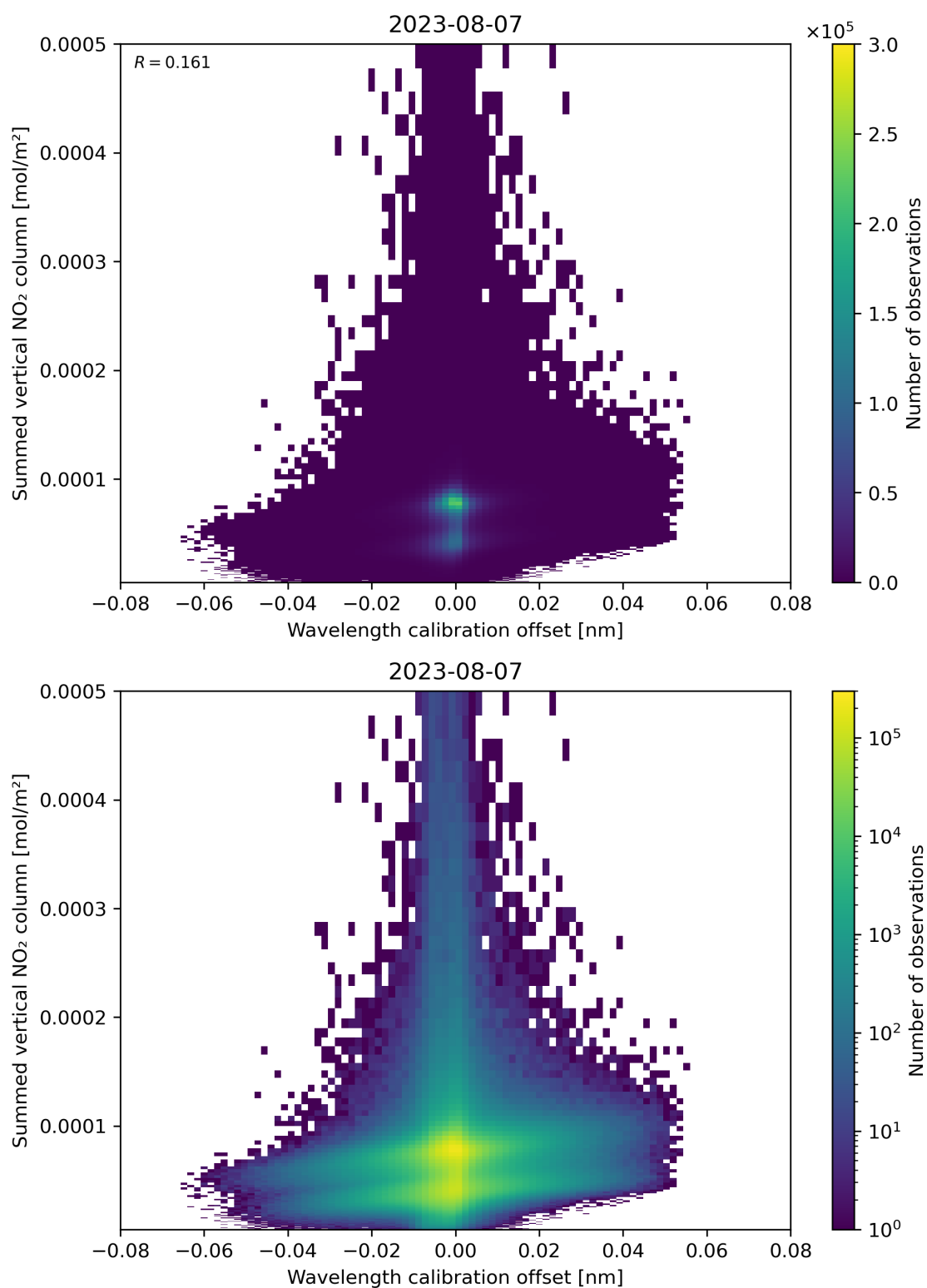
Figure 177: Scatter density plot of “Wavelength calibration offset” against “Summed vertical NO 2 column” for 2023-08-06 to 2023-08-08.
