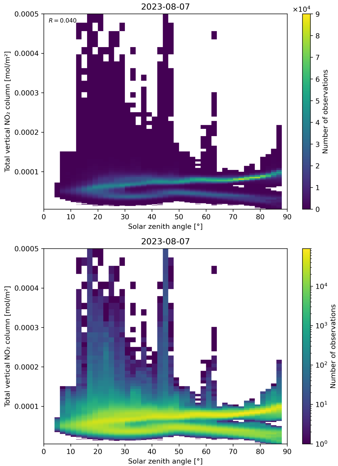
Figure 153: Scatter density plot of “Solar zenith angle” against “Total vertical NO 2 column” for 2023-08-06 to 2023-08-08.
