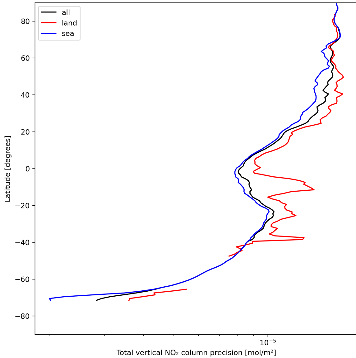
Figure 22: Zonal average of “Total vertical NO 2 column precision” for 2023-08-06 to 2023-08-08.
