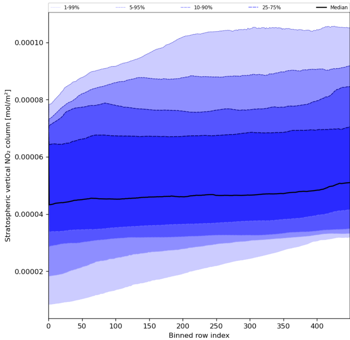
Figure 53: Along track statistics of “Stratospheric vertical NO 2 column” for 2023-08-06 to 2023-08-08
