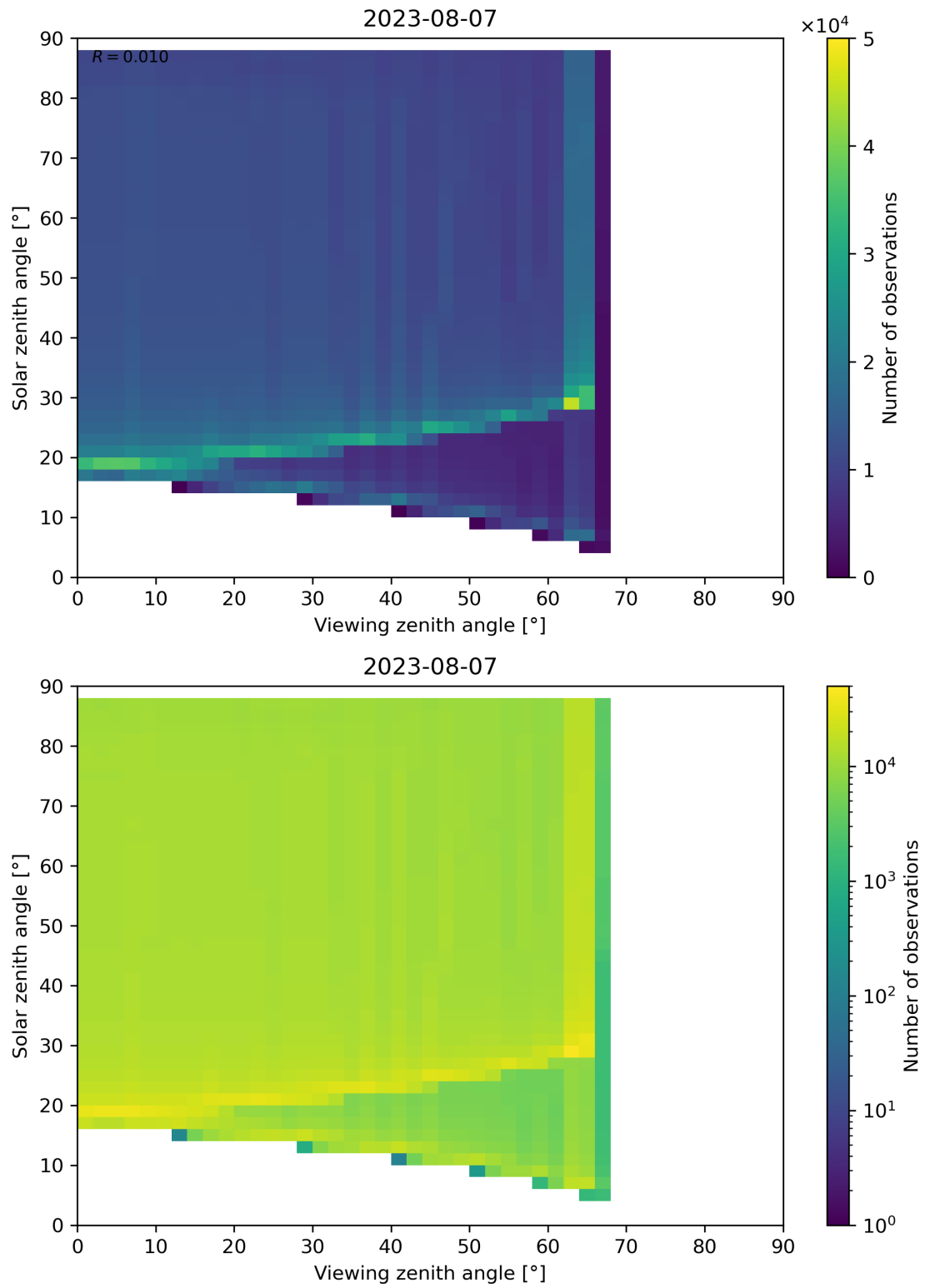
Figure 172: Scatter density plot of “Viewing zenith angle” against “Solar zenith angle” for 2023-08-06 to 2023-08-08.
