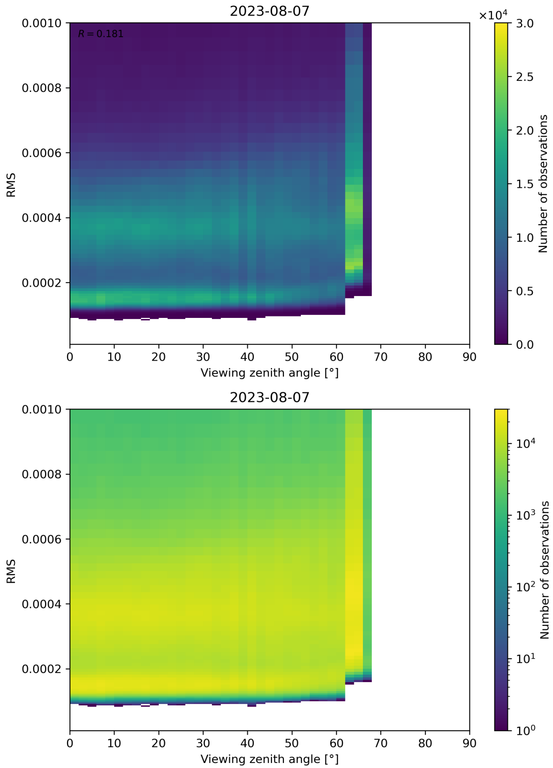
Figure 171: Scatter density plot of “Viewing zenith angle” against “RMS” for 2023-08-06 to 2023-08-08.
