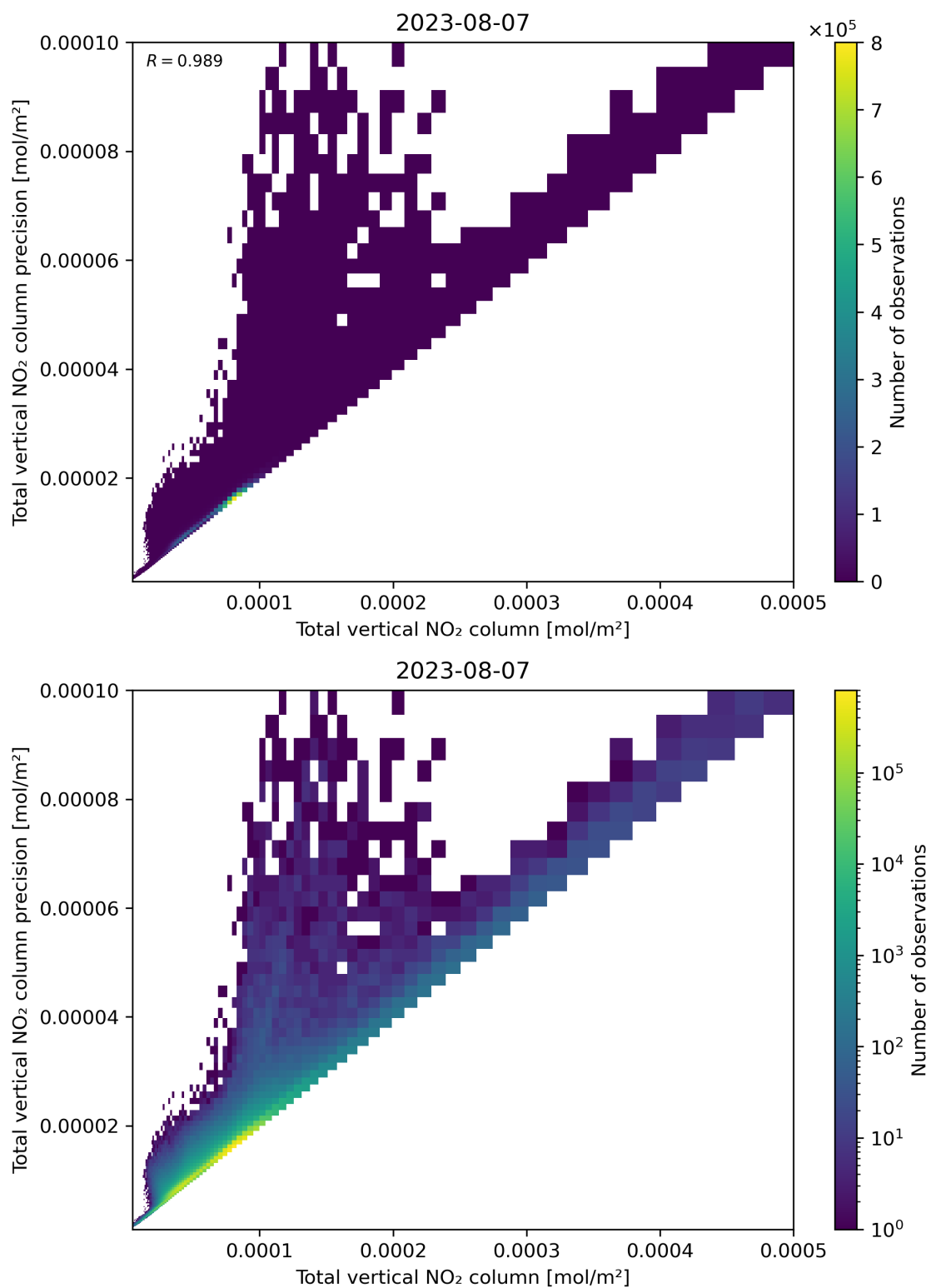
Figure 114: Scatter density plot of “Total vertical NO 2 column” against “Total vertical NO 2 column precision” for 2023-08-06 to 2023-08-08.
