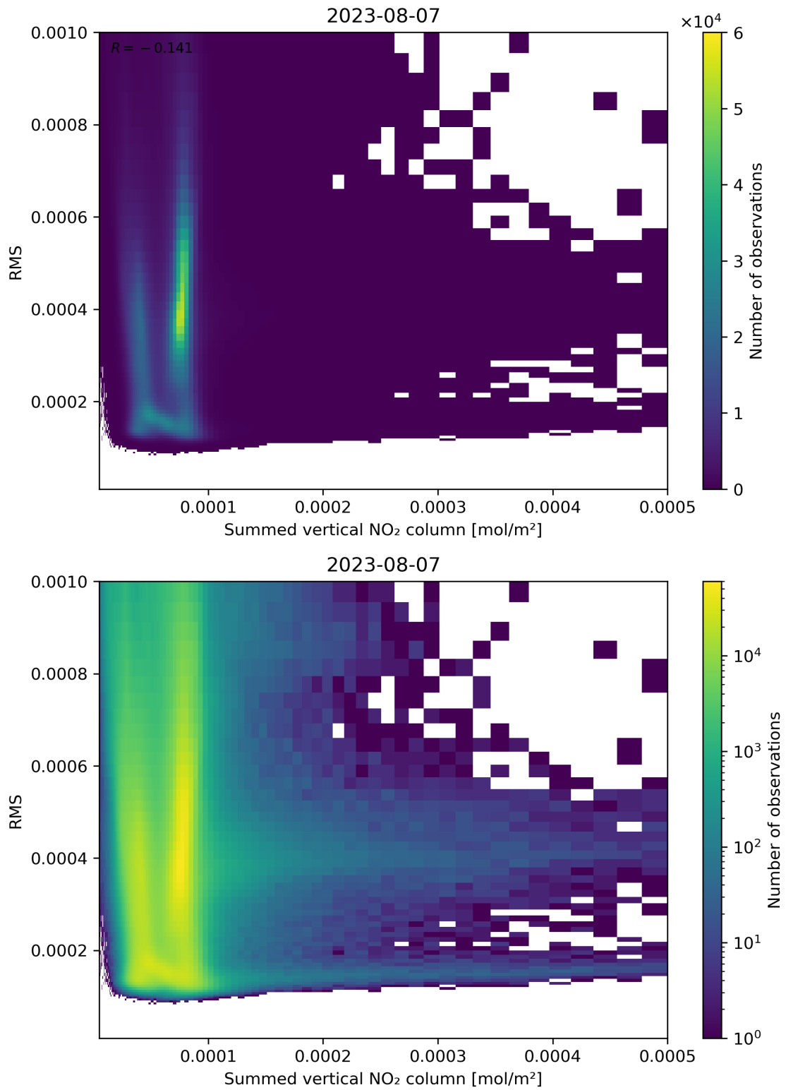
Figure 109: Scatter density plot of “Summed vertical NO 2 column” against “RMS” for 2023-08-06 to 2023-08-08.
