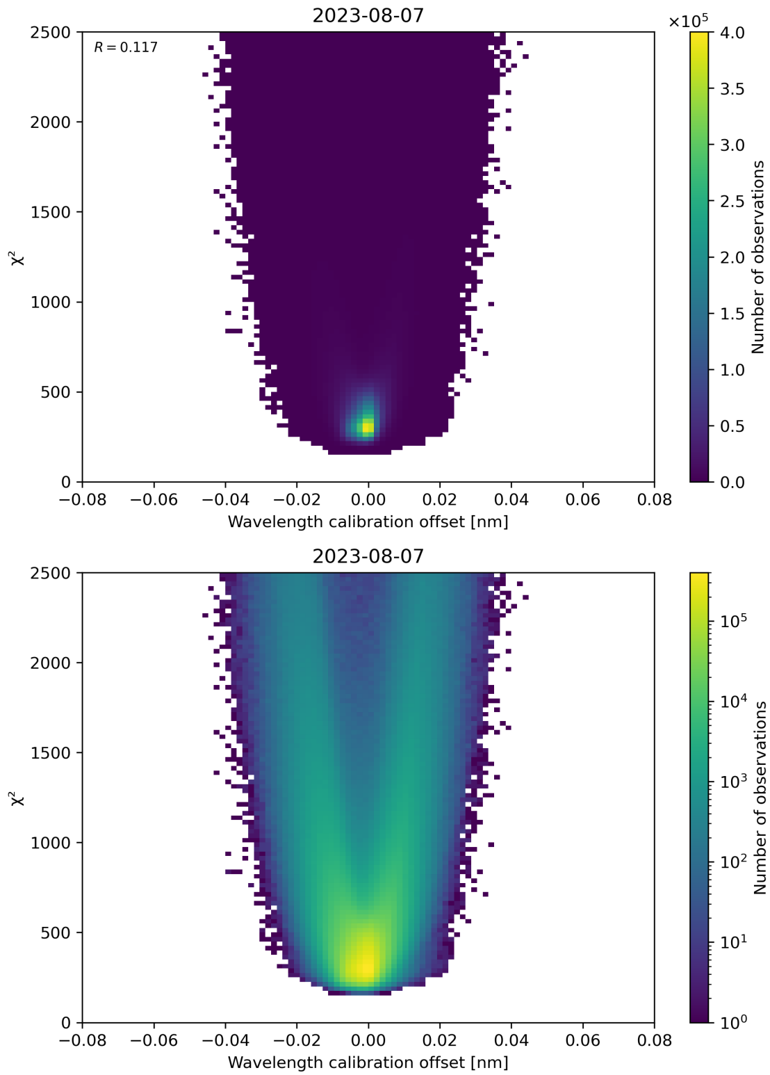
Figure 175: Scatter density plot of “Wavelength calibration offset” against “ \chi^2 ” for 2023-08-06 to 2023-08-08.
