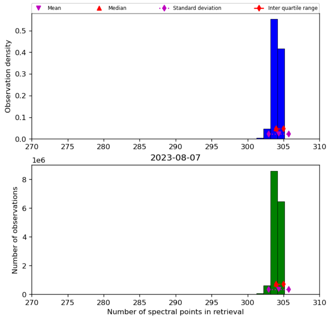
Figure 33: Histogram of “Number of spectral points in retrieval” for 2023-08-06 to 2023-08-08
