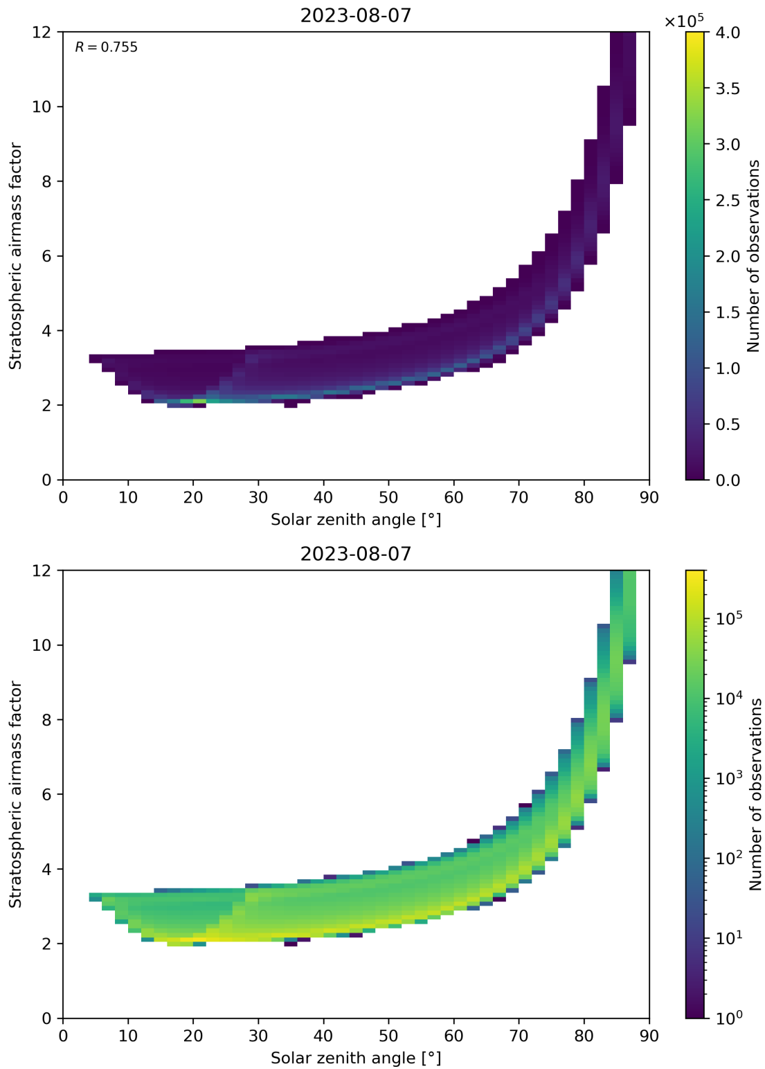
Figure 145: Scatter density plot of “Solar zenith angle” against “Stratospheric airmass factor” for 2023-08-06 to 2023-08-08.
