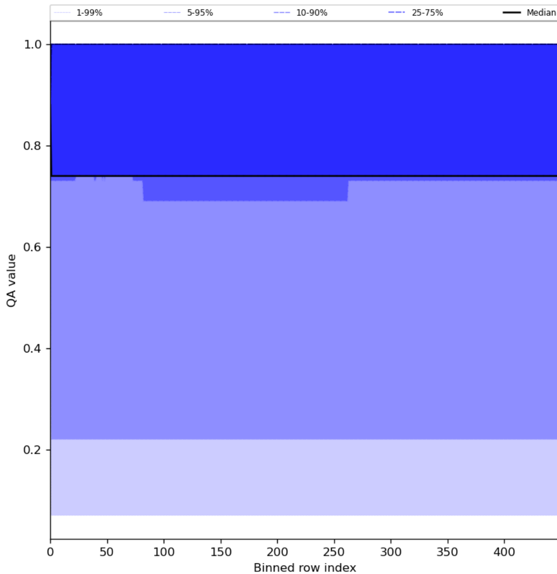
Figure 45: Along track statistics of “QA value” for 2023-08-06 to 2023-08-08
