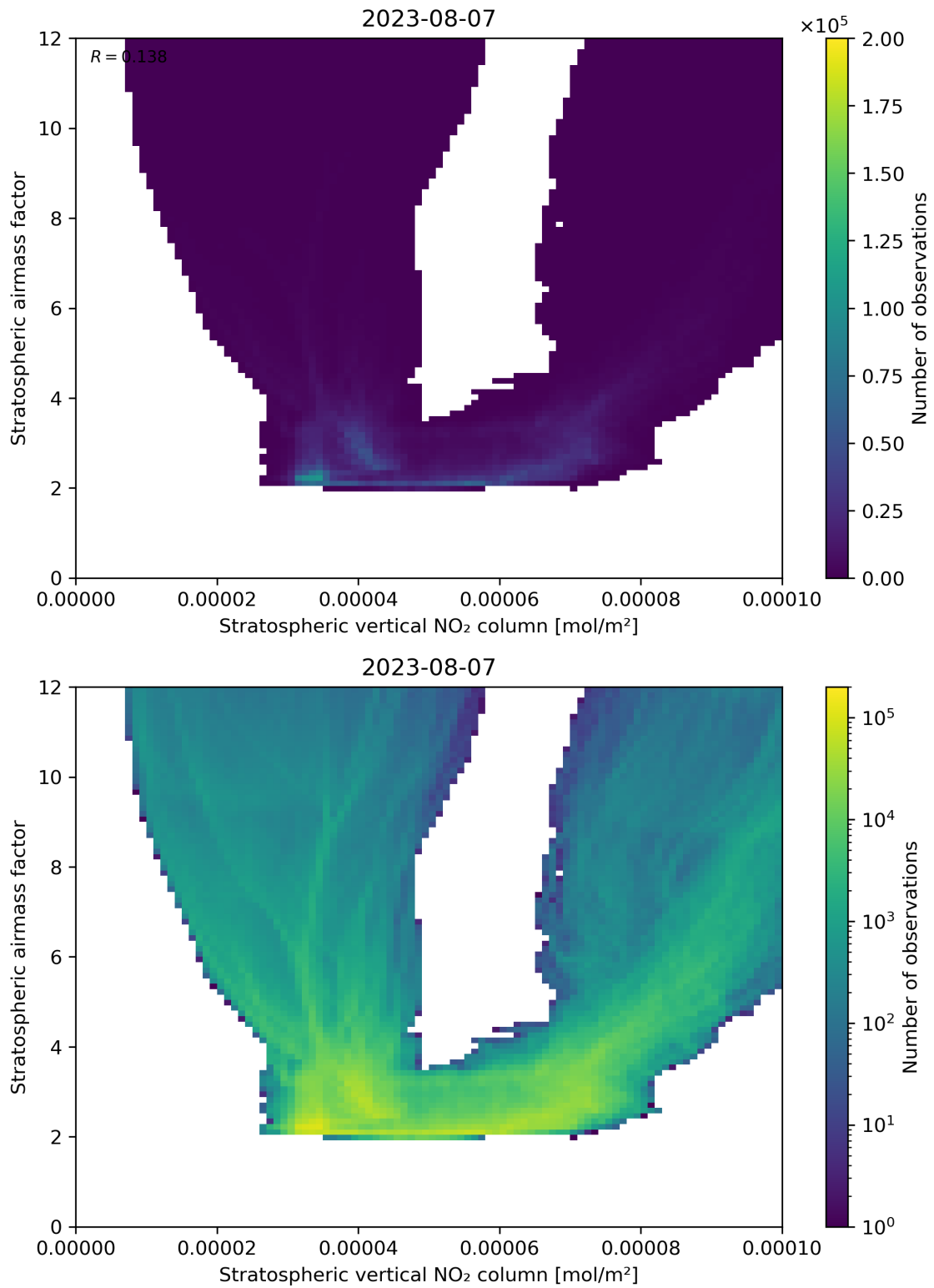
Figure 96: Scatter density plot of “Stratospheric vertical NO 2 column” against “Stratospheric airmass factor” for 2023-08-06 to 2023-08-08.
