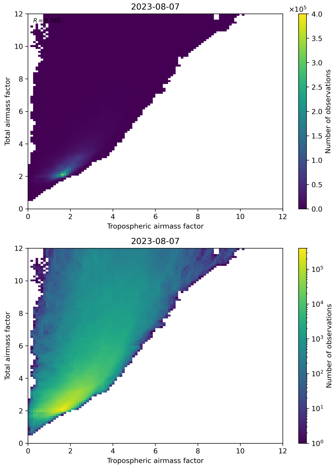
Figure 72: Scatter density plot of “Tropospheric airmass factor” against “Total airmass factor” for 2023-08-06 to 2023-08-08.
