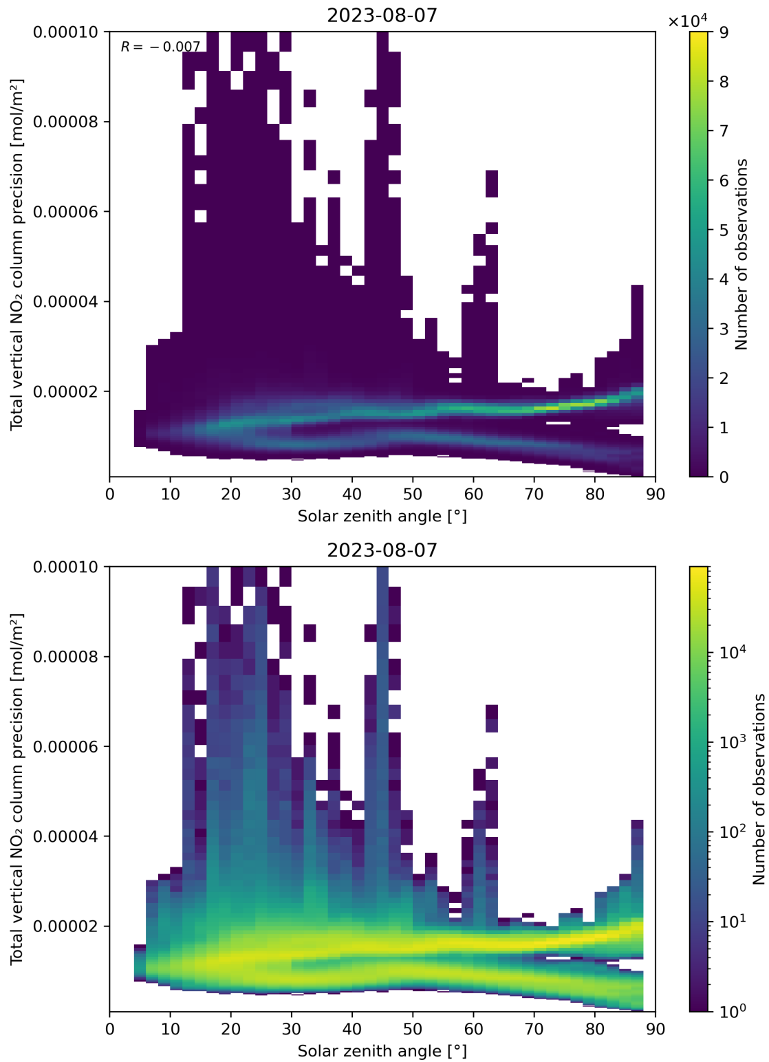
Figure 154: Scatter density plot of “Solar zenith angle” against “Total vertical NO 2 column precision” for 2023-08-06 to 2023-08-08.
