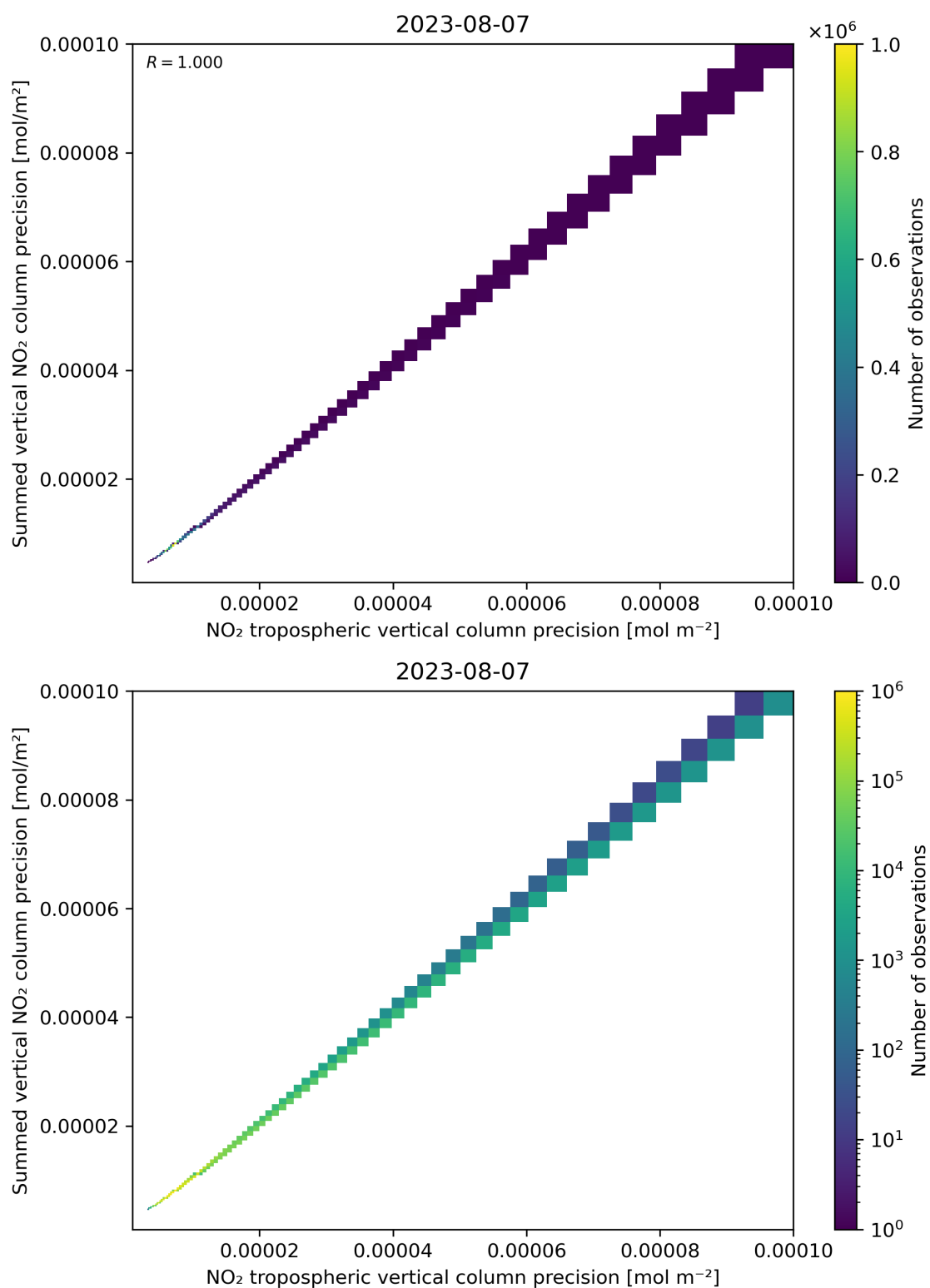
Figure 137: Scatter density plot of “NO 2 tropospheric vertical column precision” against “Summed vertical NO 2 column precision” for 2023-08-06 to 2023-08-08.
