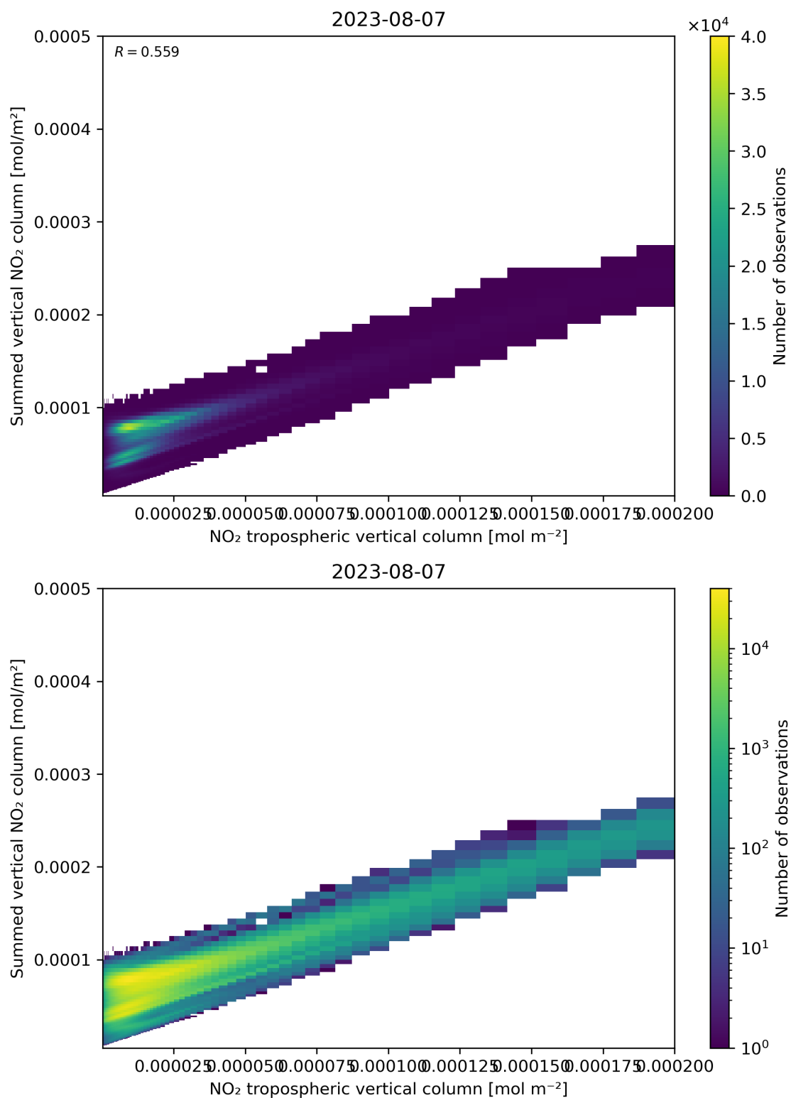
Figure 126: Scatter density plot of “NO 2 tropospheric vertical column” against “Summed vertical NO 2 column” for 2023-08-06 to 2023-08-08.
