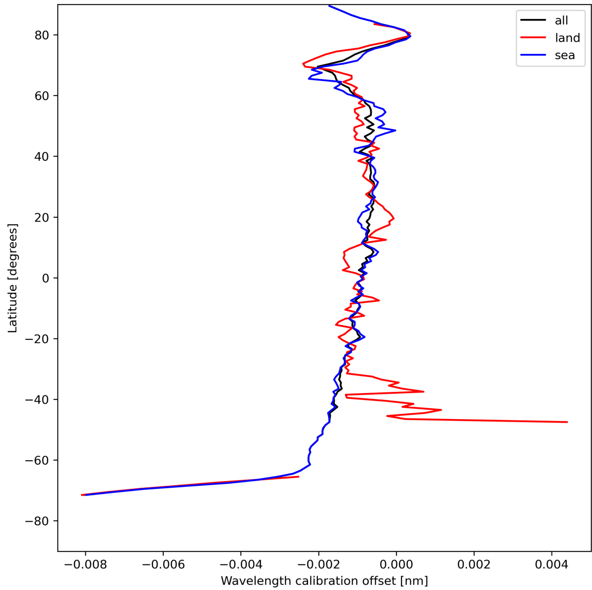
Figure 18: Zonal average of “Wavelength calibration offset” for 2023-08-06 to 2023-08-08.
