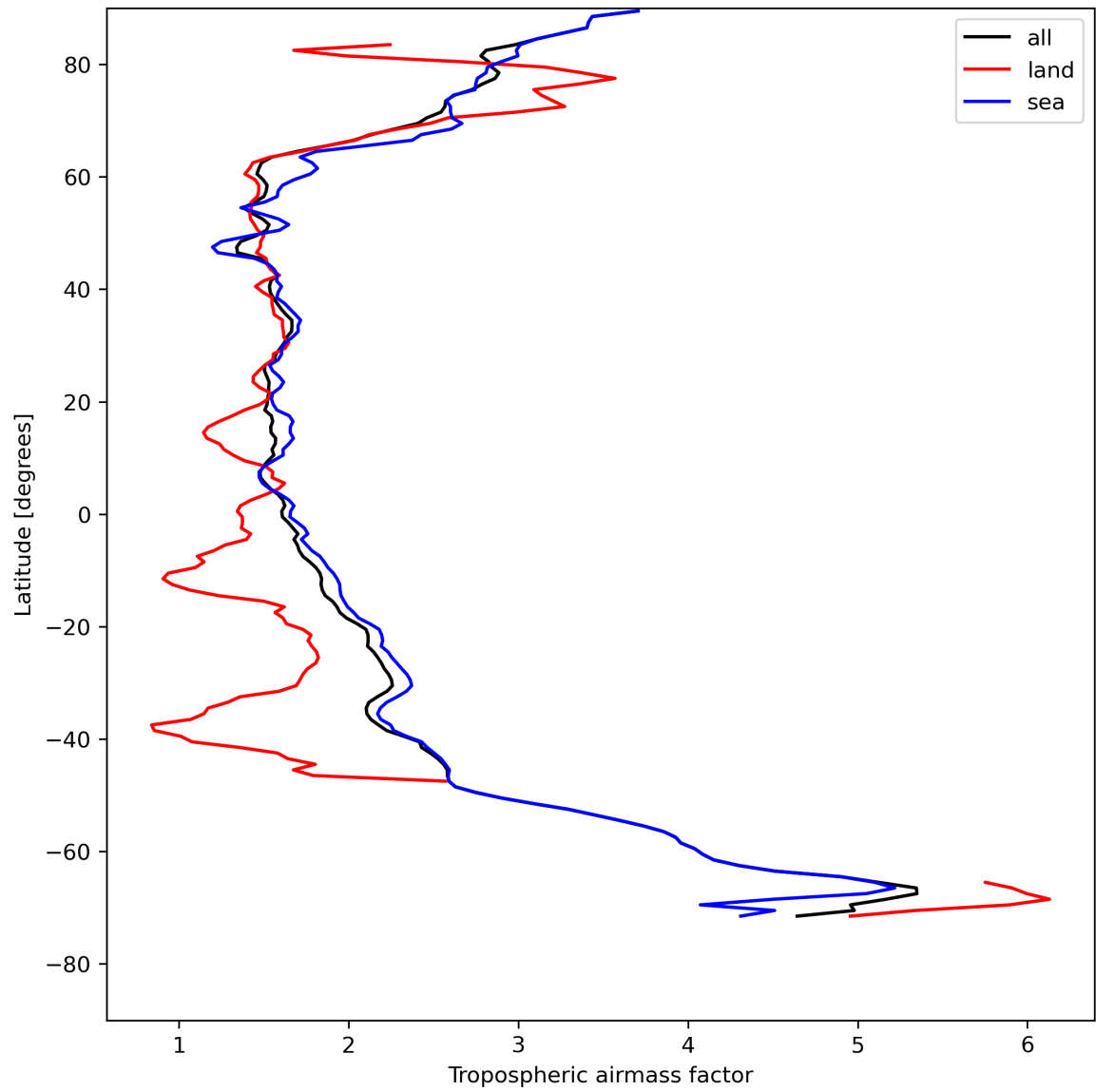
Figure 14: Zonal average of “Tropospheric airmass factor” for 2023-08-06 to 2023-08-08.
