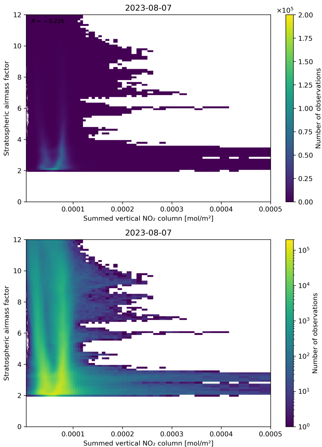
Figure 103: Scatter density plot of “Summed vertical NO 2 column” against “Stratospheric air mass factor” for 2023-08-06 to 2023-08-08.
