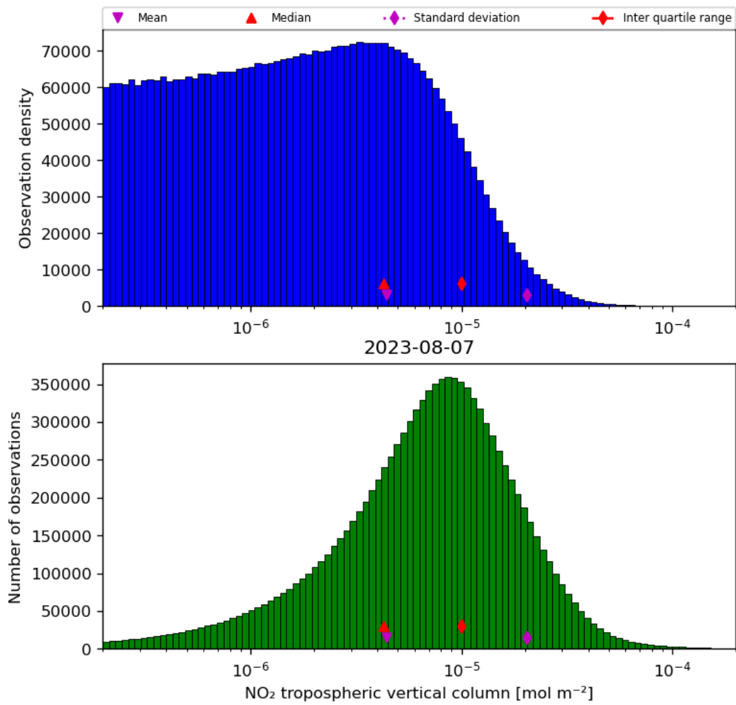
Figure 29: Histogram of “NO 2 tropospheric vertical column” for 2023-08-06 to 2023-08-08
