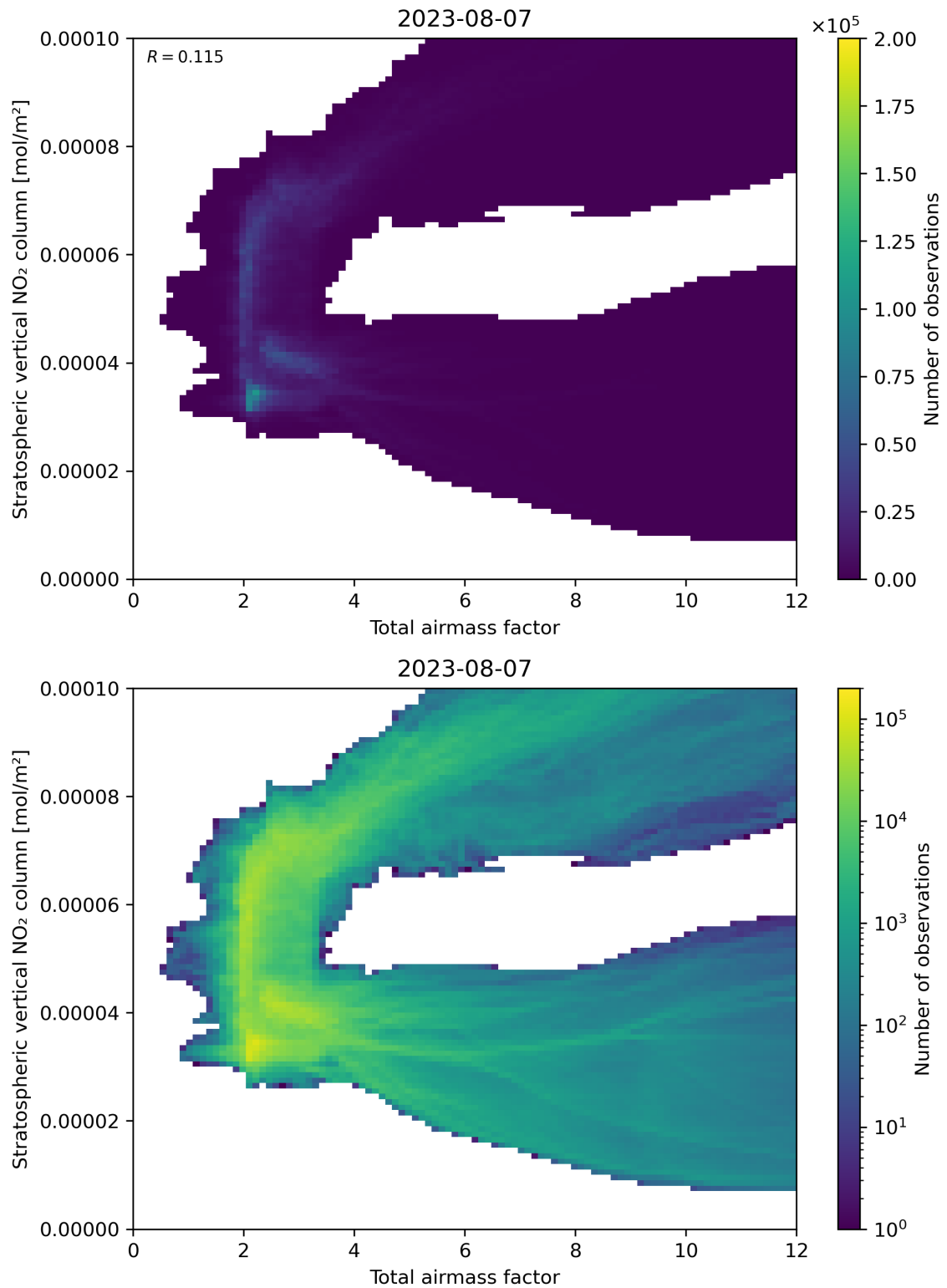
Figure 64: Scatter density plot of “Total airmass factor” against “Stratospheric vertical \text{NO}_2 column” for 2023-08-06 to 2023-08-08.
