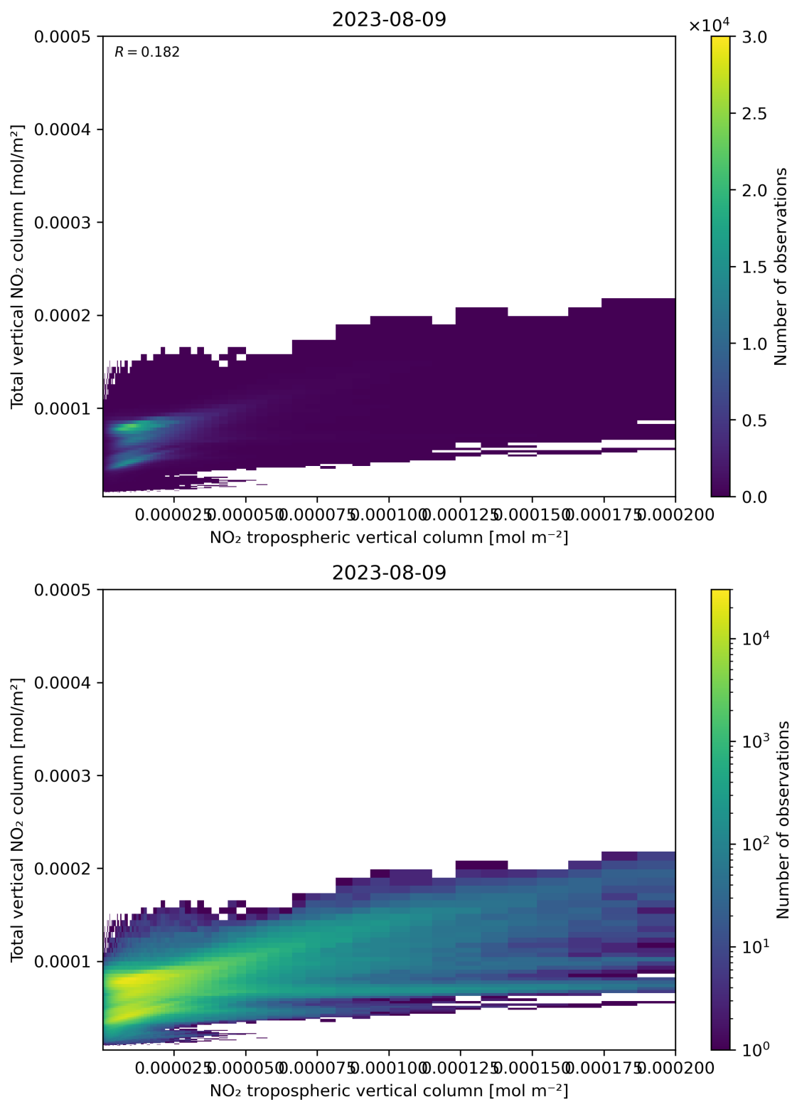
Figure 128: Scatter density plot of “NO 2 tropospheric vertical column” against “Total vertical NO 2 column” for 2023-08-09 to 2023-08-10.
