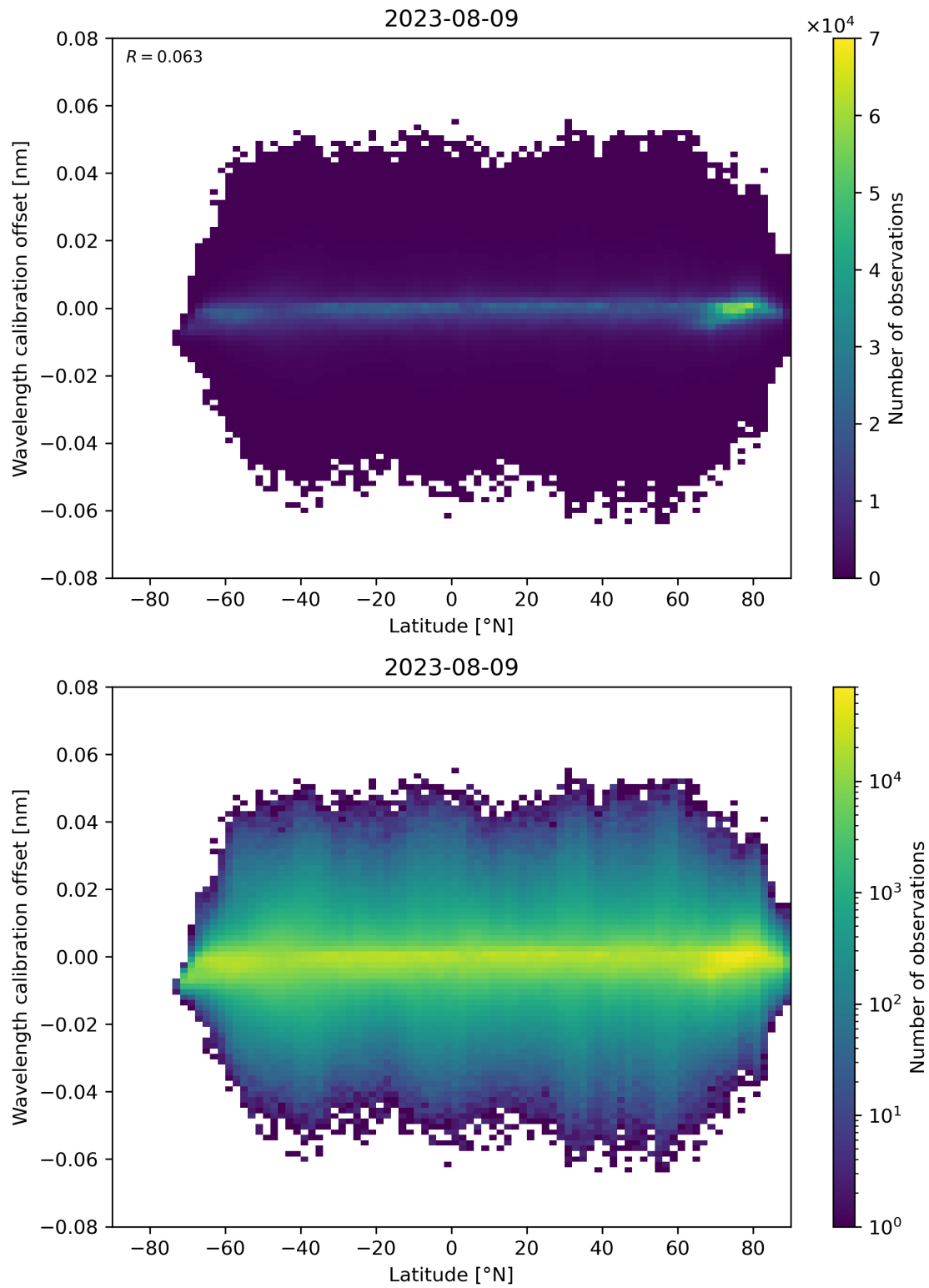
Figure 95: Scatter density plot of “Latitude” against “Wavelength calibration offset” for 2023-08-09 to 2023-08-10.
