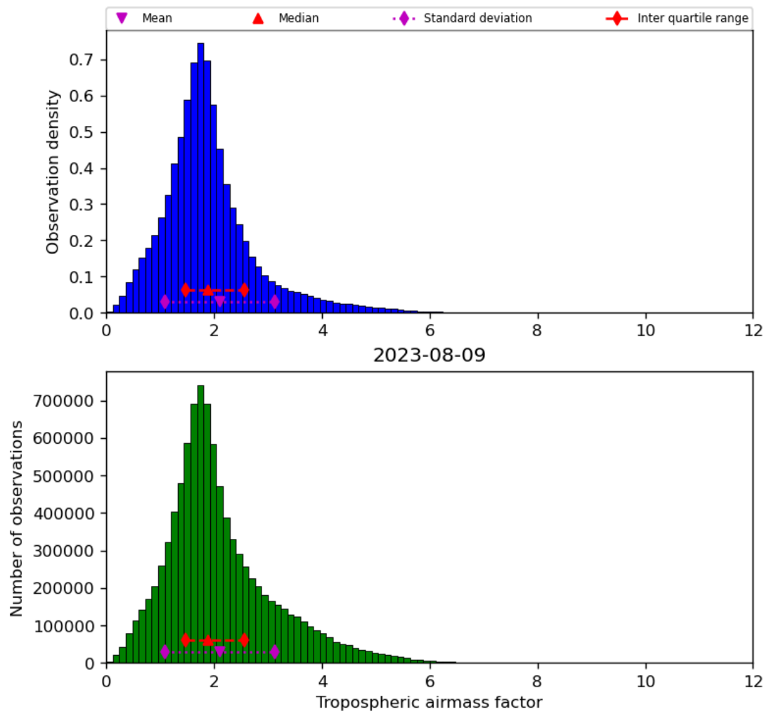
Figure 31: Histogram of “Tropospheric airmass factor” for 2023-08-09 to 2023-08-10
