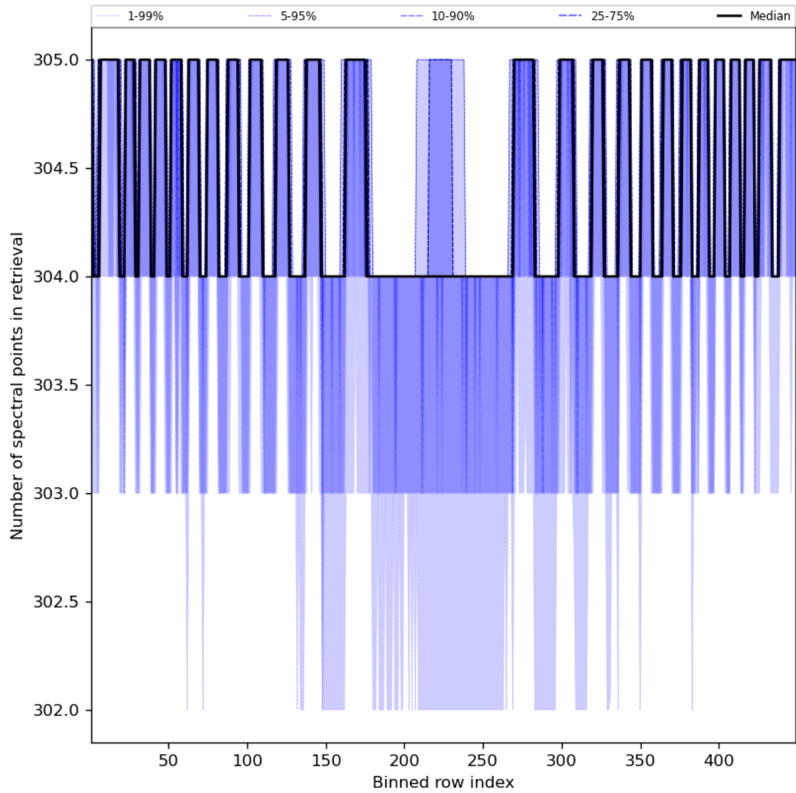
Figure 50: Along track statistics of “Number of spectral points in retrieval” for 2023-08-09 to 2023-08-10
