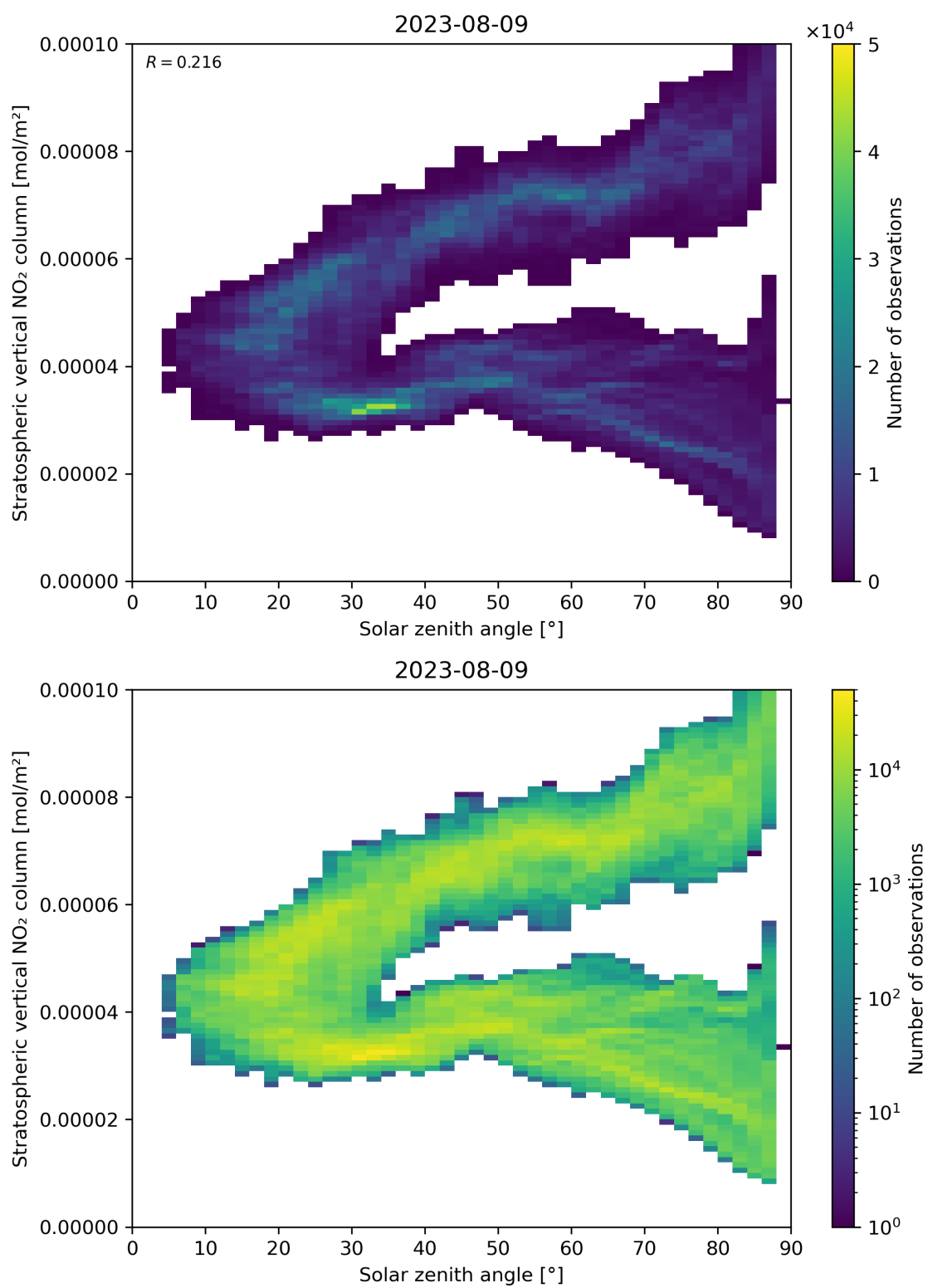
Figure 150: Scatter density plot of “Solar zenith angle” against “Stratospheric vertical NO 2 column” for 2023-08-09 to 2023-08-10.
