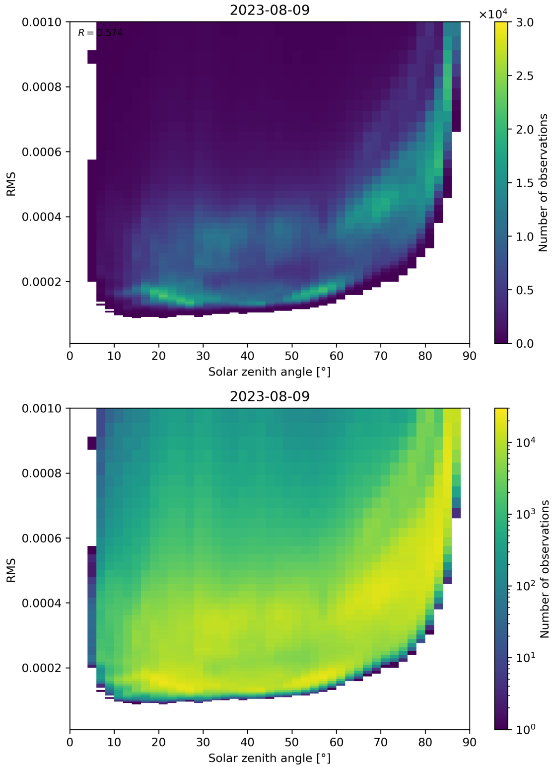
Figure 157: Scatter density plot of “Solar zenith angle” against “RMS” for 2023-08-09 to 2023-08-10.
