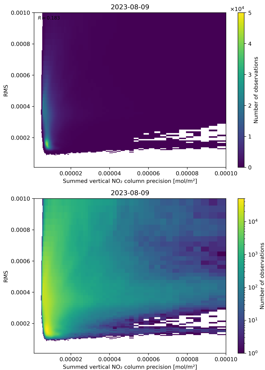
Figure 108: Scatter density plot of “Summed vertical NO 2 column precision” against “RMS” for 2023-08-09 to 2023-08-10.
