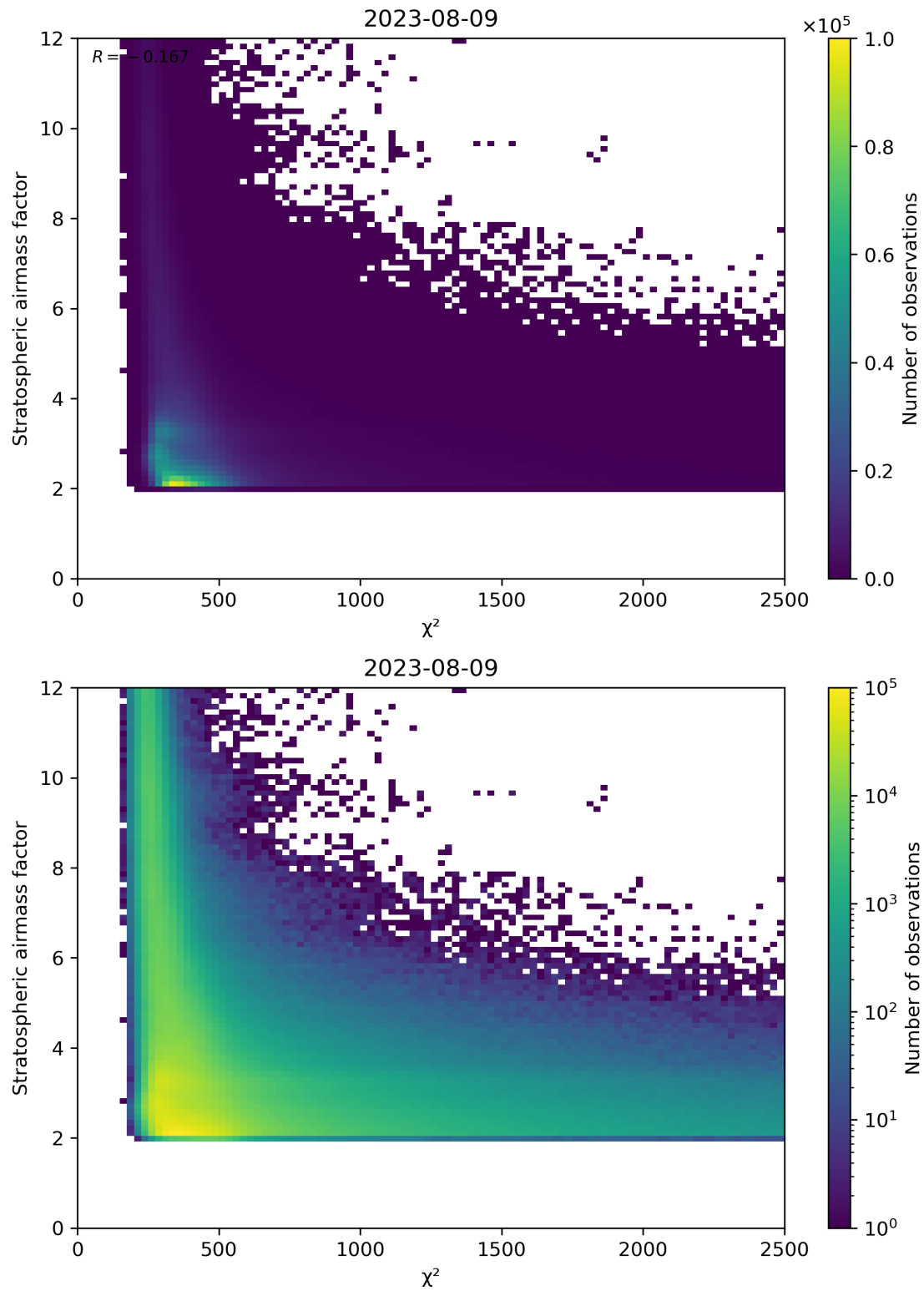
Figure 81: Scatter density plot of “ \chi^2 ” against “Stratospheric airmass factor” for 2023-08-09 to 2023-08-10.
