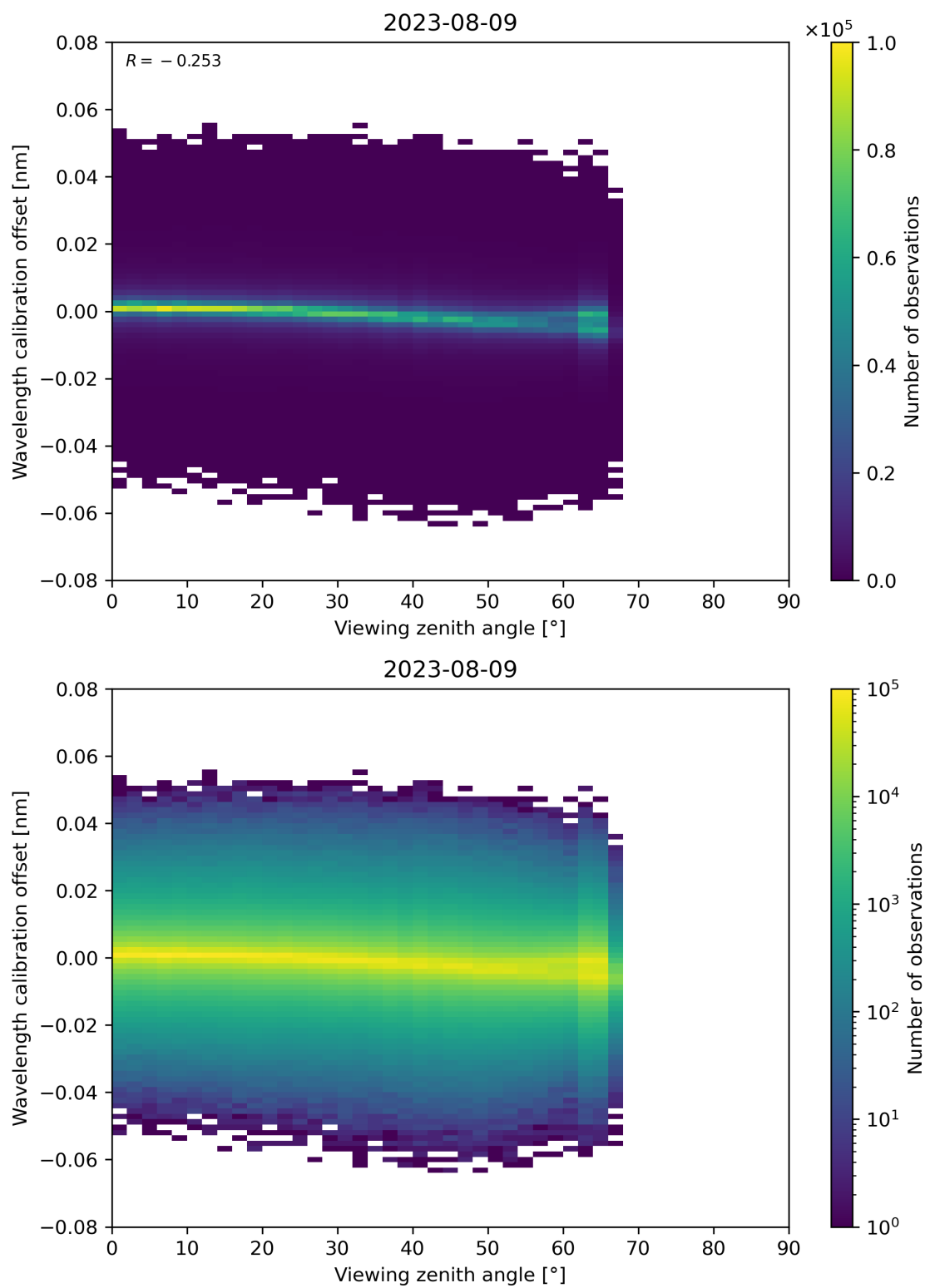
Figure 173: Scatter density plot of “Viewing zenith angle” against “Wavelength calibration offset” for 2023-08-09 to 2023-08-10.
