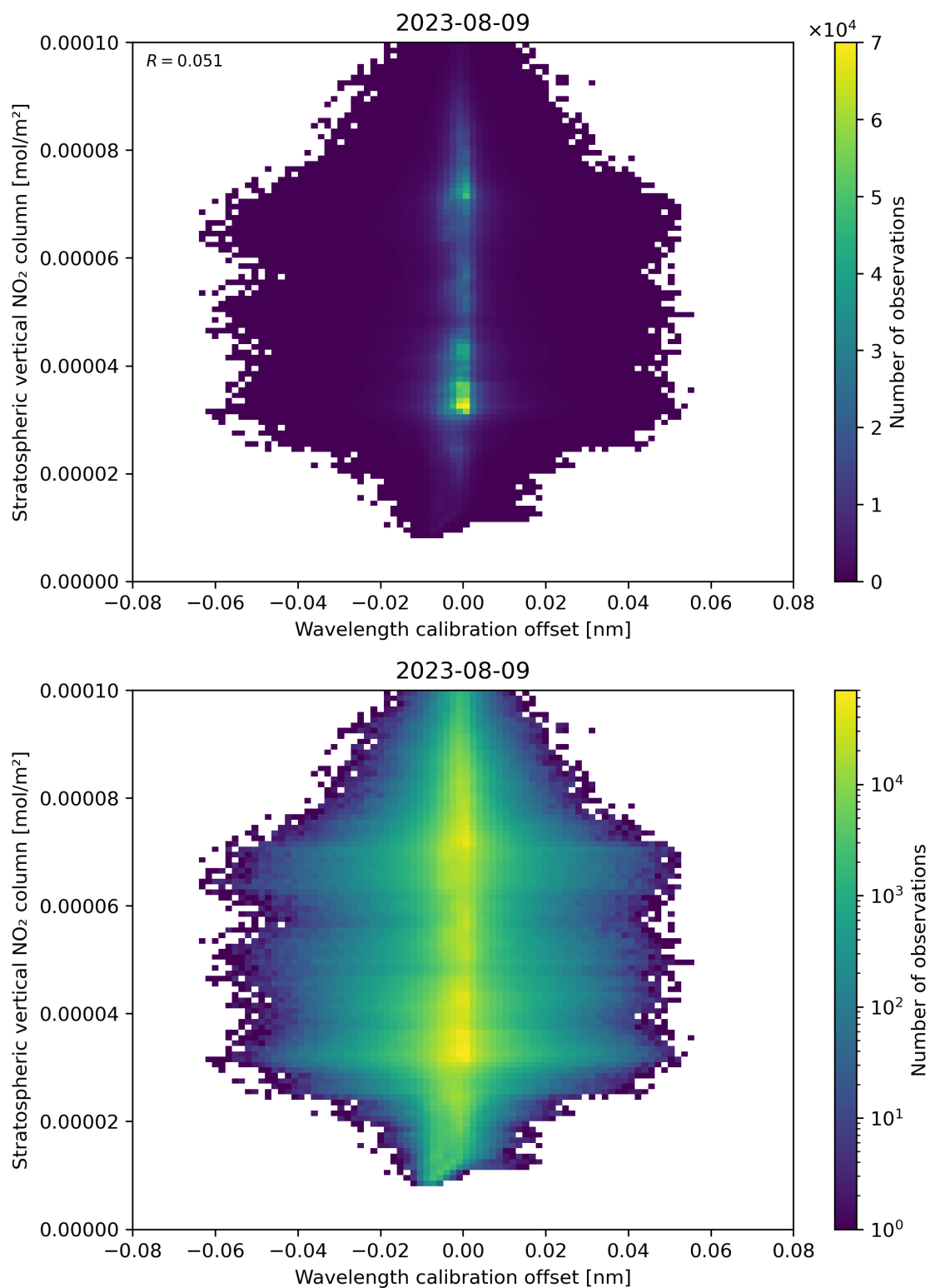
Figure 176: Scatter density plot of “Wavelength calibration offset” against “Stratospheric vertical NO 2 column” for 2023-08-09 to 2023-08-10.
