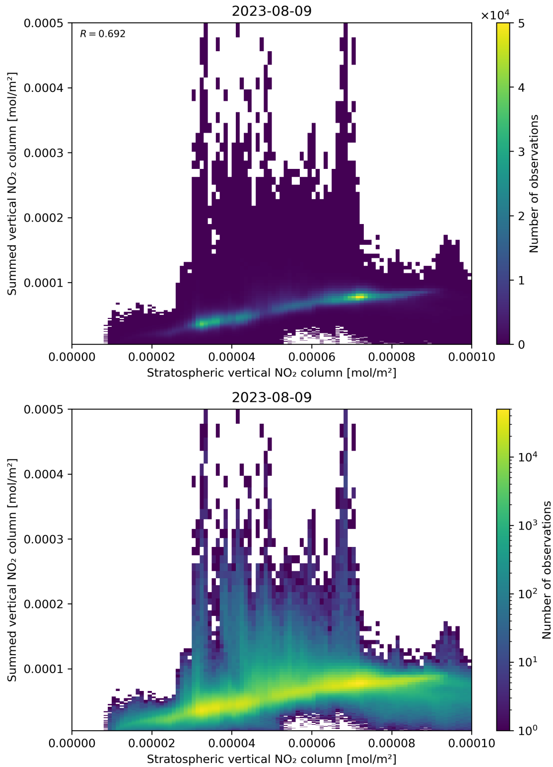
Figure 98: Scatter density plot of “Stratospheric vertical NO 2 column” against “Summed vertical NO 2 column” for 2023-08-09 to 2023-08-10.
