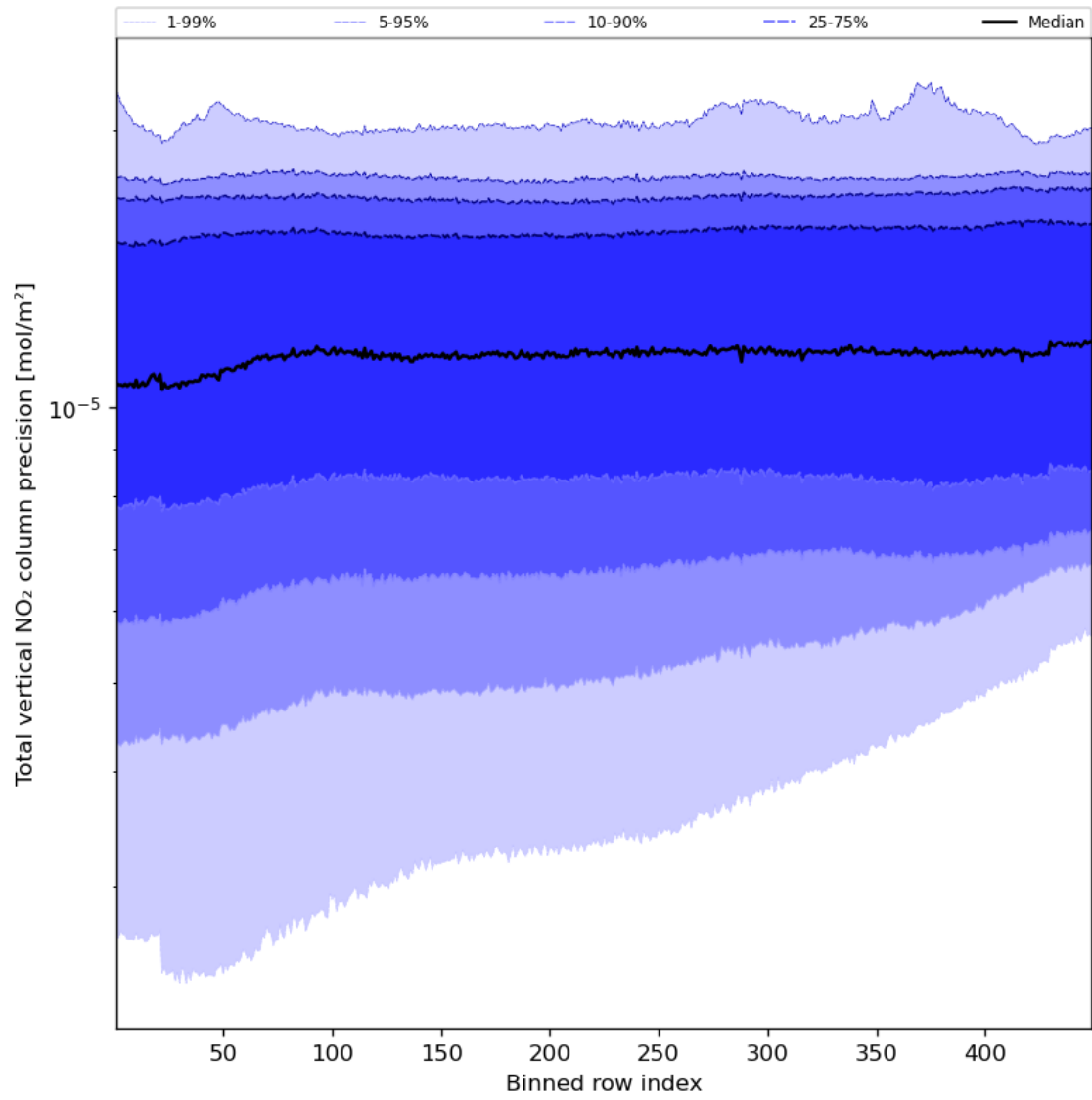
Figure 56: Along track statistics of “Total vertical NO 2 column precision” for 2023-08-09 to 2023-08-10
