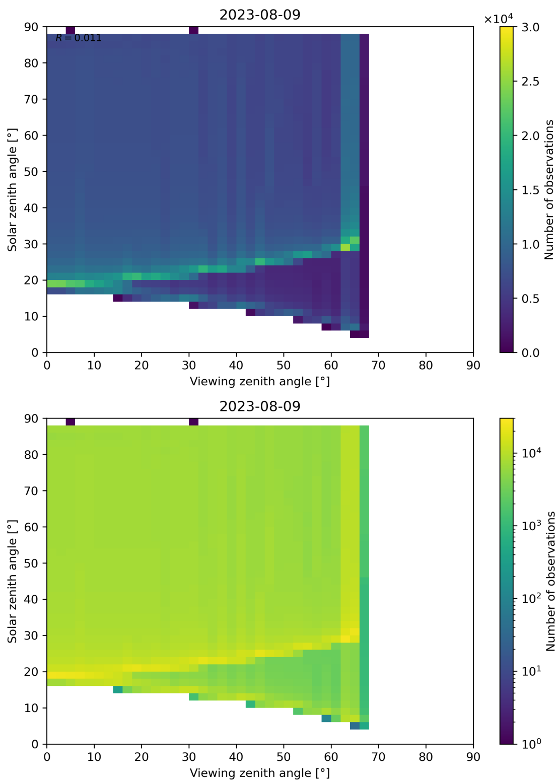
Figure 172: Scatter density plot of “Viewing zenith angle” against “Solar zenith angle” for 2023-08-09 to 2023-08-10.
