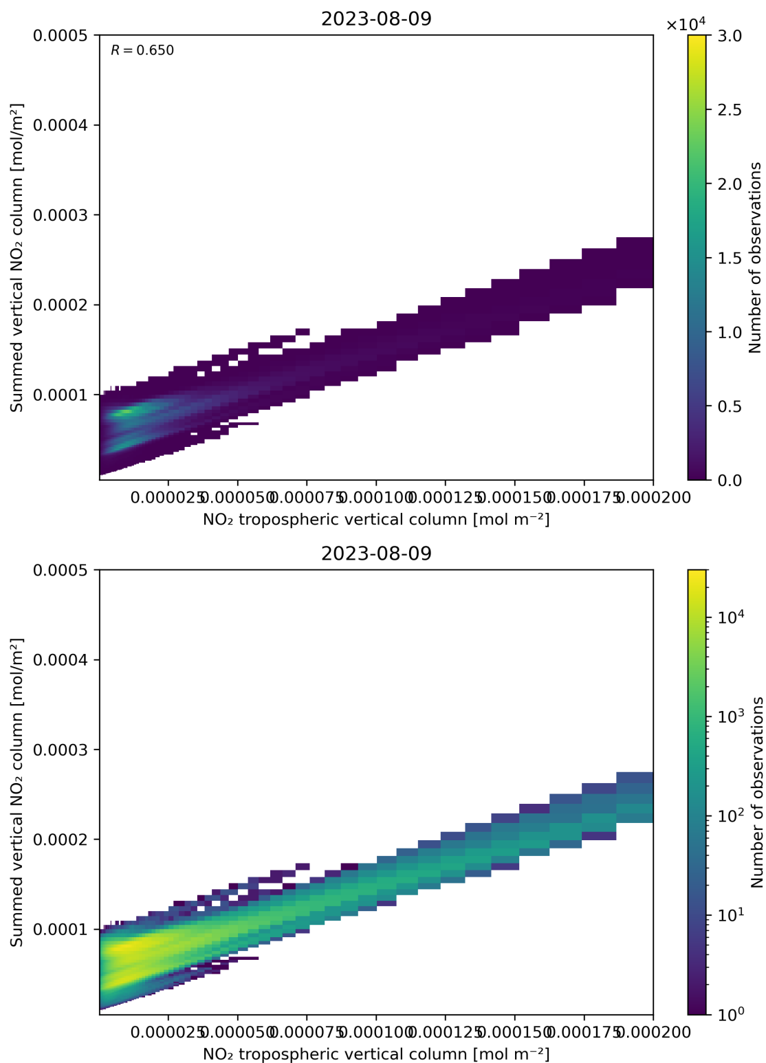
Figure 126: Scatter density plot of “NO 2 tropospheric vertical column” against “Summed vertical NO 2 column” for 2023-08-09 to 2023-08-10.
