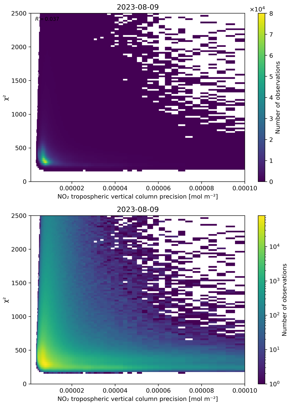
Figure 134: Scatter density plot of “NO 2 tropospheric vertical column precision” against “ \chi^2 ” for 2023-08-09 to 2023-08-10.
