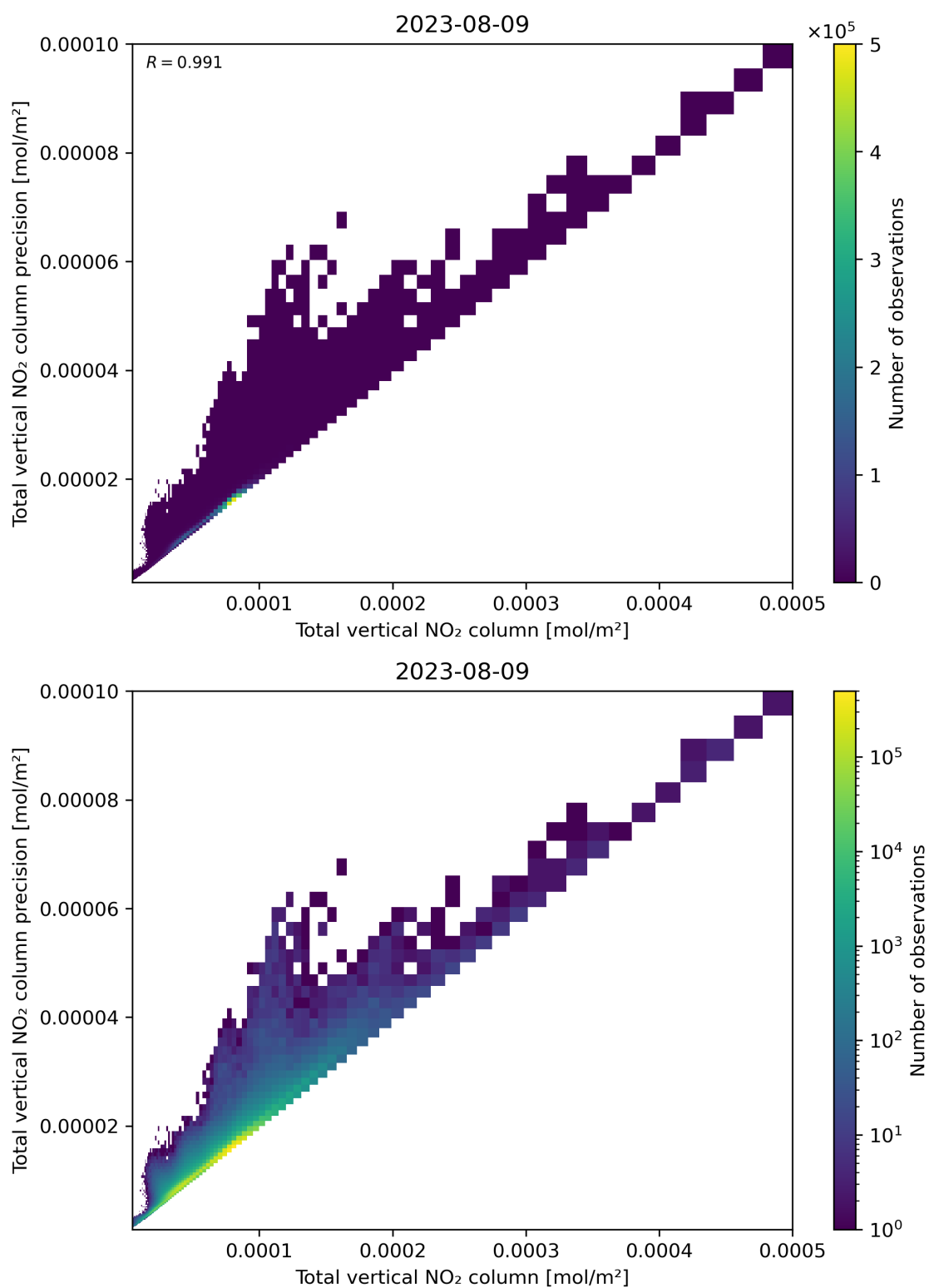
Figure 114: Scatter density plot of “Total vertical NO 2 column” against “Total vertical NO 2 column precision” for 2023-08-09 to 2023-08-10.
