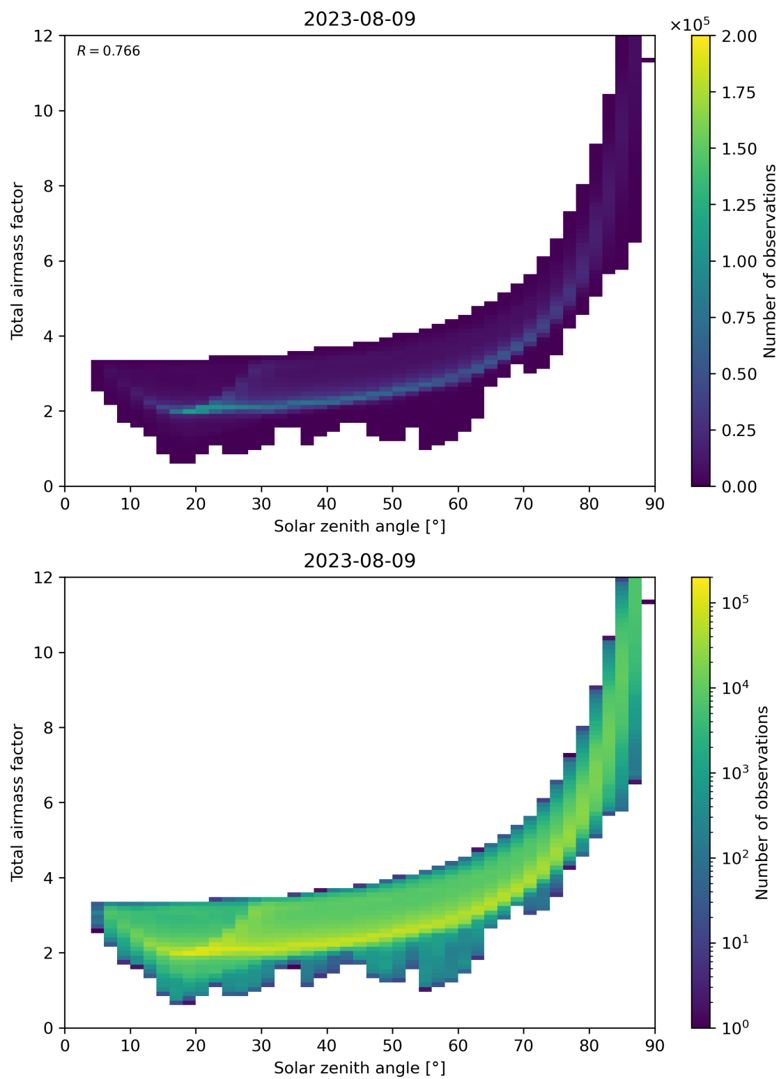
Figure 146: Scatter density plot of “Solar zenith angle” against “Total air mass factor” for 2023-08-09 to 2023-08-10.
