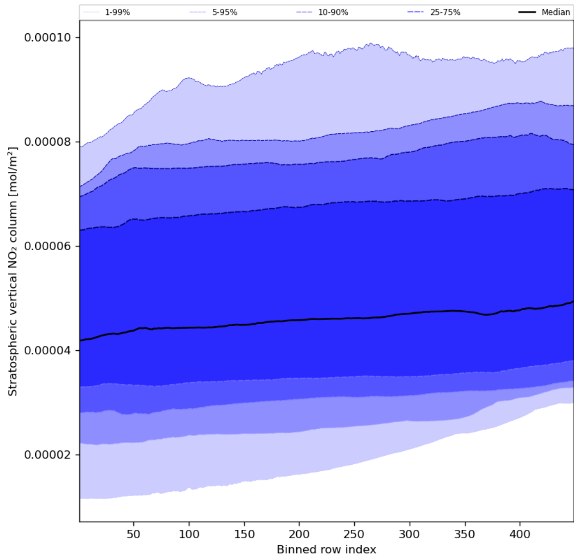
Figure 53: Along track statistics of “Stratospheric vertical NO 2 column” for 2023-08-09 to 2023-08-10
