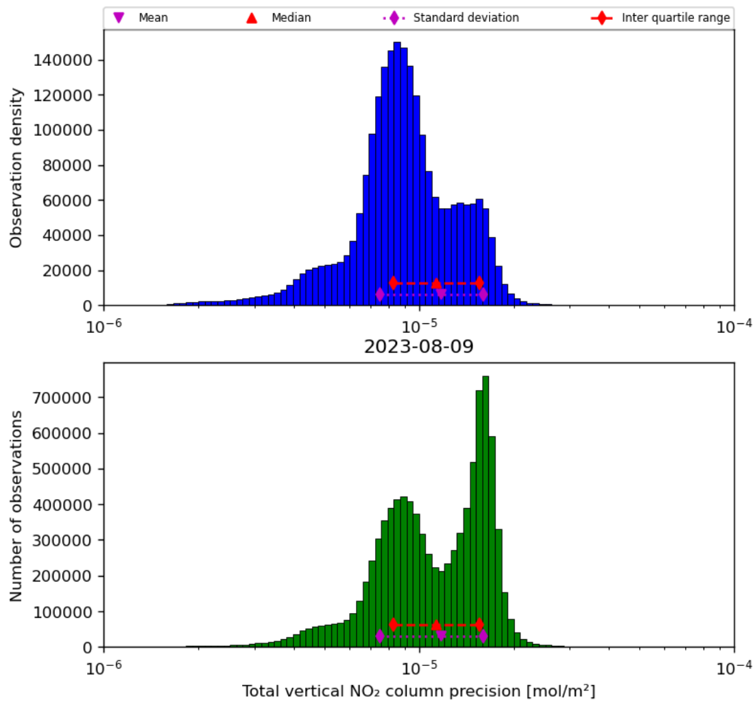
Figure 39: Histogram of “Total vertical NO 2 column precision” for 2023-08-09 to 2023-08-10
