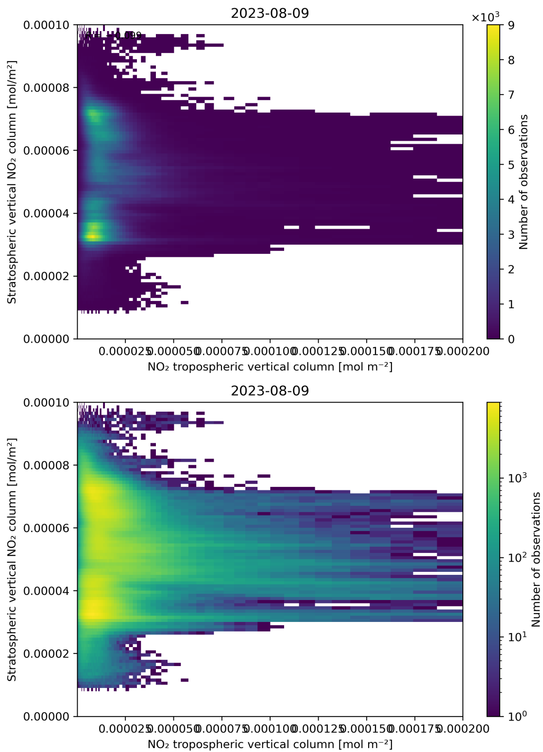
Figure 125: Scatter density plot of “NO 2 tropospheric vertical column” against “Stratospheric vertical NO 2 column” for 2023-08-09 to 2023-08-10.
