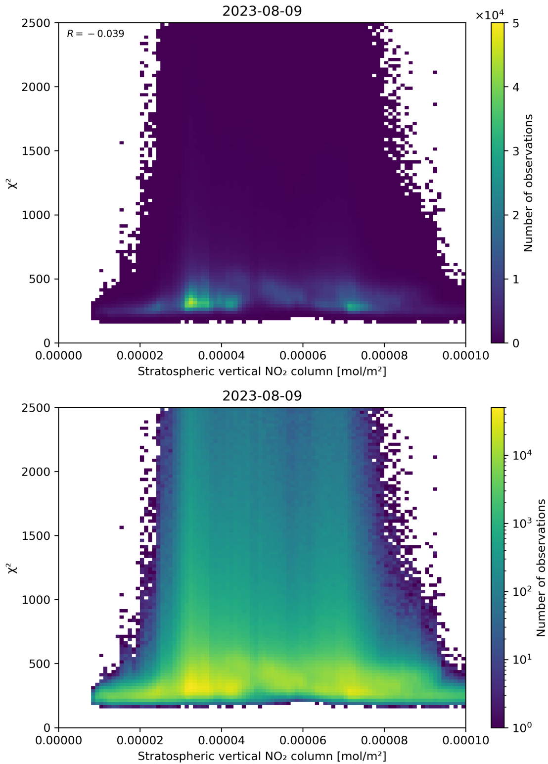
Figure 97: Scatter density plot of “Stratospheric vertical NO 2 column” against “ \chi^2 ” for 2023-08-09 to 2023-08-10.
