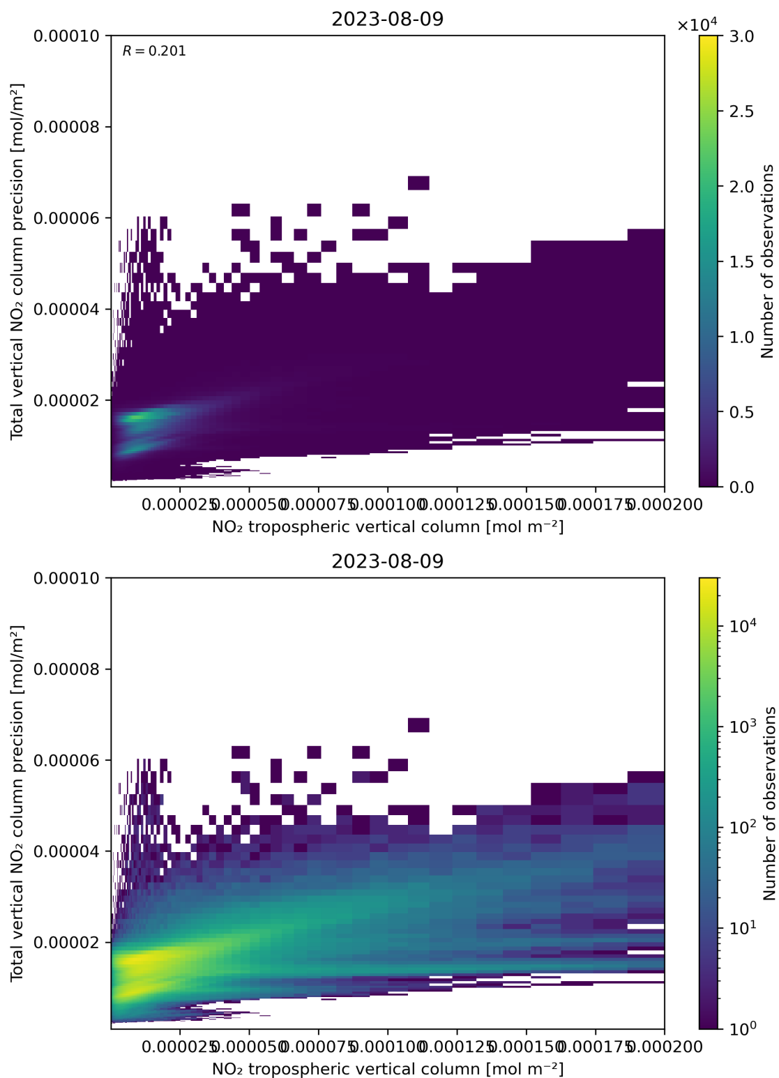
Figure 129: Scatter density plot of “NO 2 tropospheric vertical column” against “Total vertical NO 2 column precision” for 2023-08-09 to 2023-08-10.
