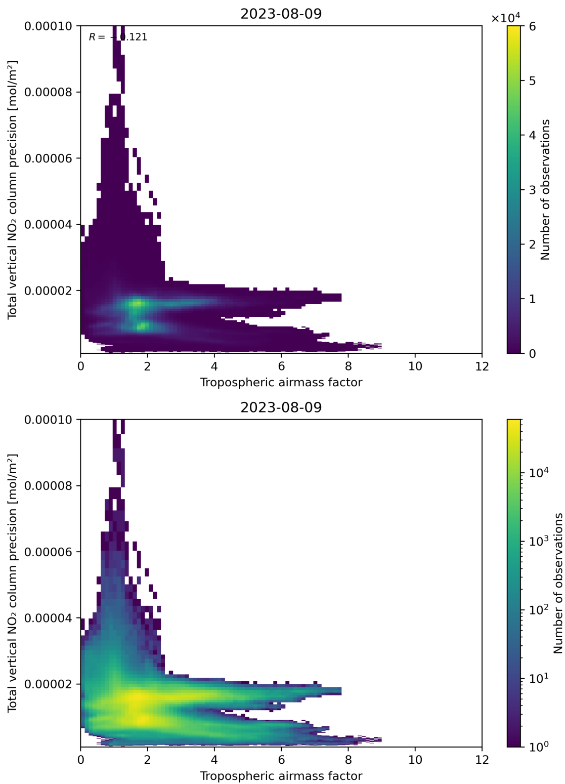
Figure 78: Scatter density plot of “Tropospheric air mass factor” against “Total vertical NO 2 column precision” for 2023-08-09 to 2023-08-10.
