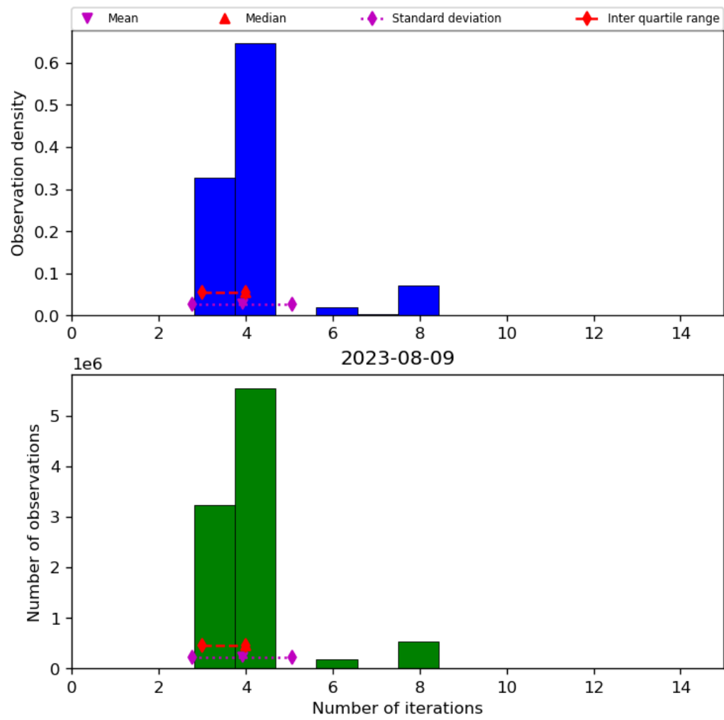
Figure 34: Histogram of “Number of iterations” for 2023-08-09 to 2023-08-10
