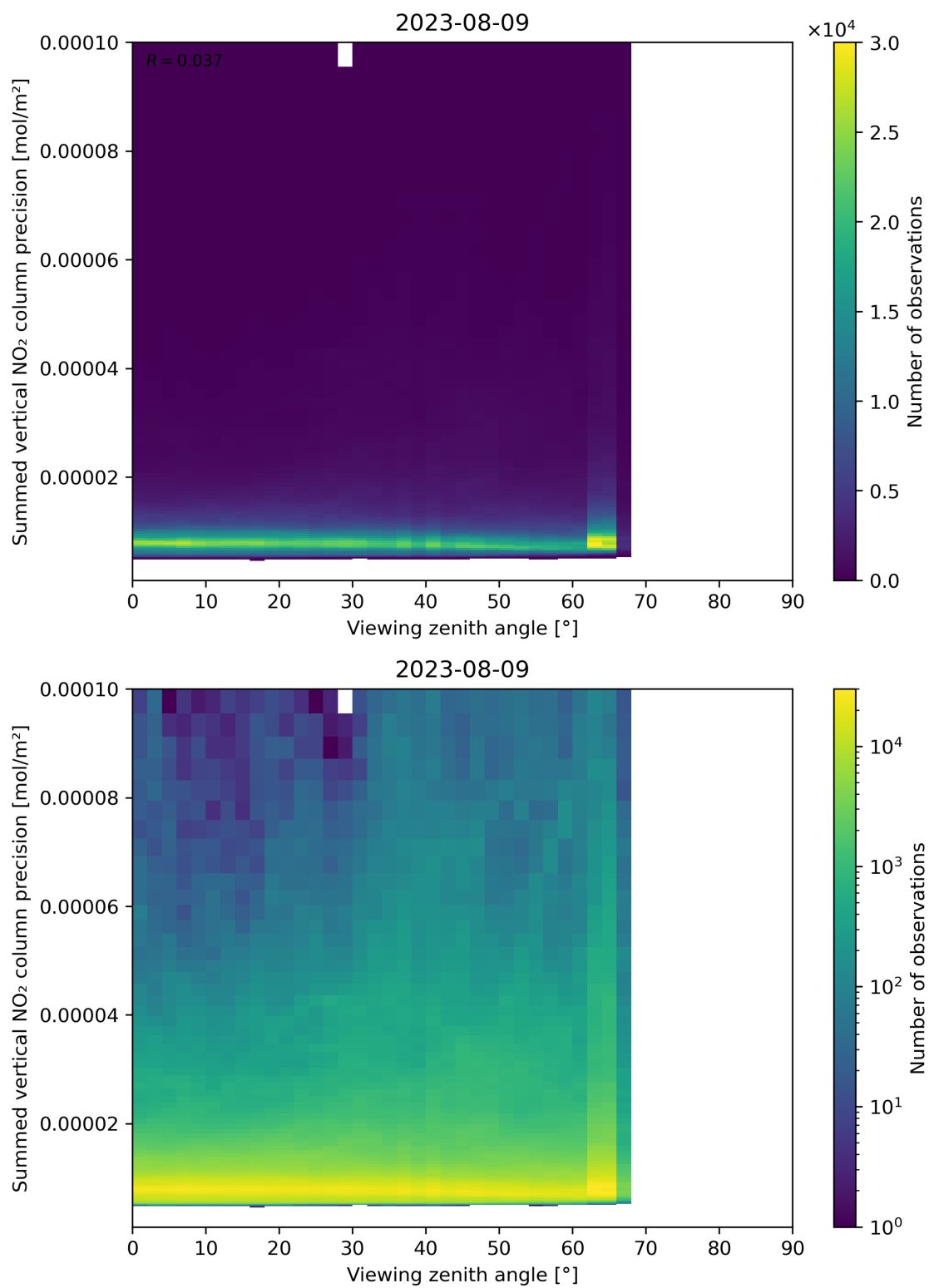
Figure 166: Scatter density plot of “Viewing zenith angle” against “Summed vertical NO 2 column precision” for 2023-08-09 to 2023-08-10.
