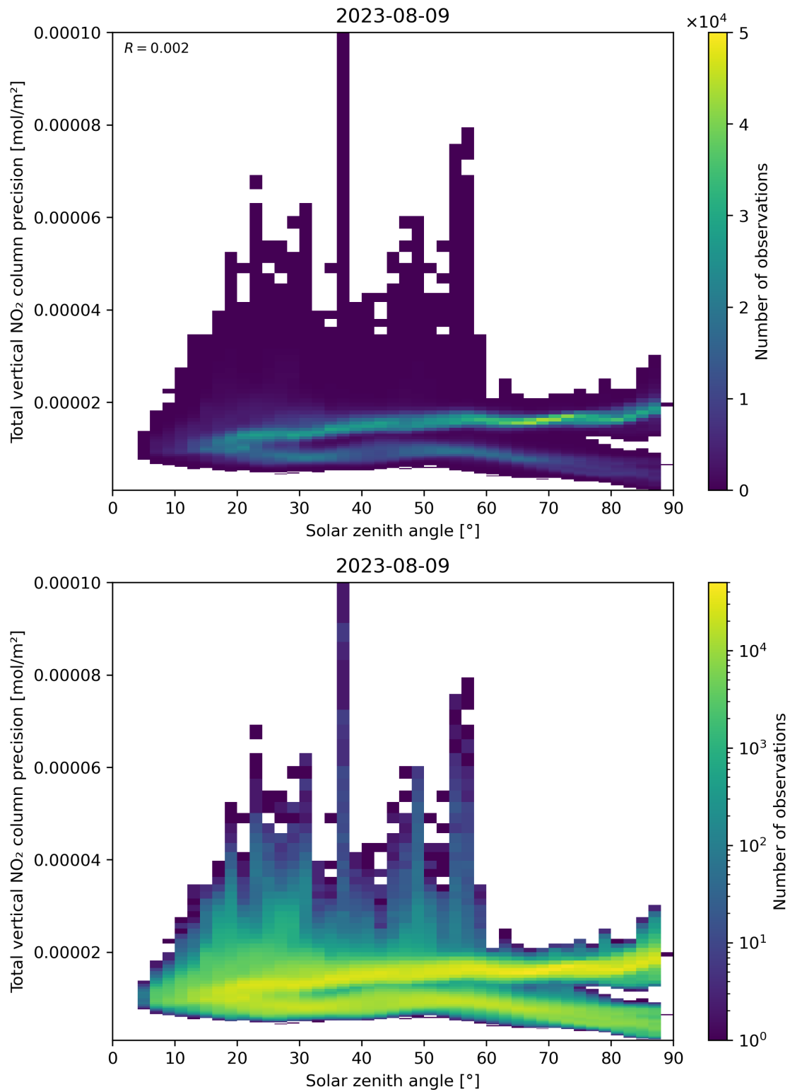
Figure 154: Scatter density plot of “Solar zenith angle” against “Total vertical NO 2 column precision” for 2023-08-09 to 2023-08-10.
