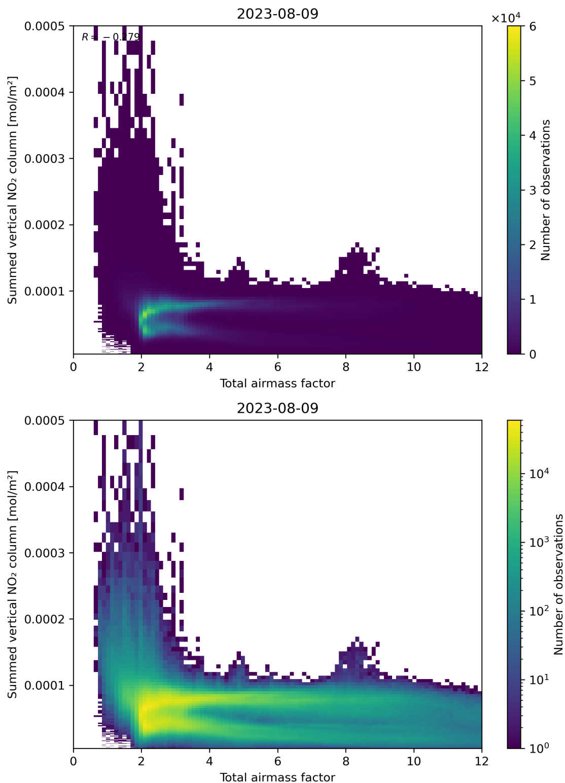
Figure 65: Scatter density plot of “Total airmass factor” against “Summed vertical NO 2 column” for 2023-08-09 to 2023-08-10.
