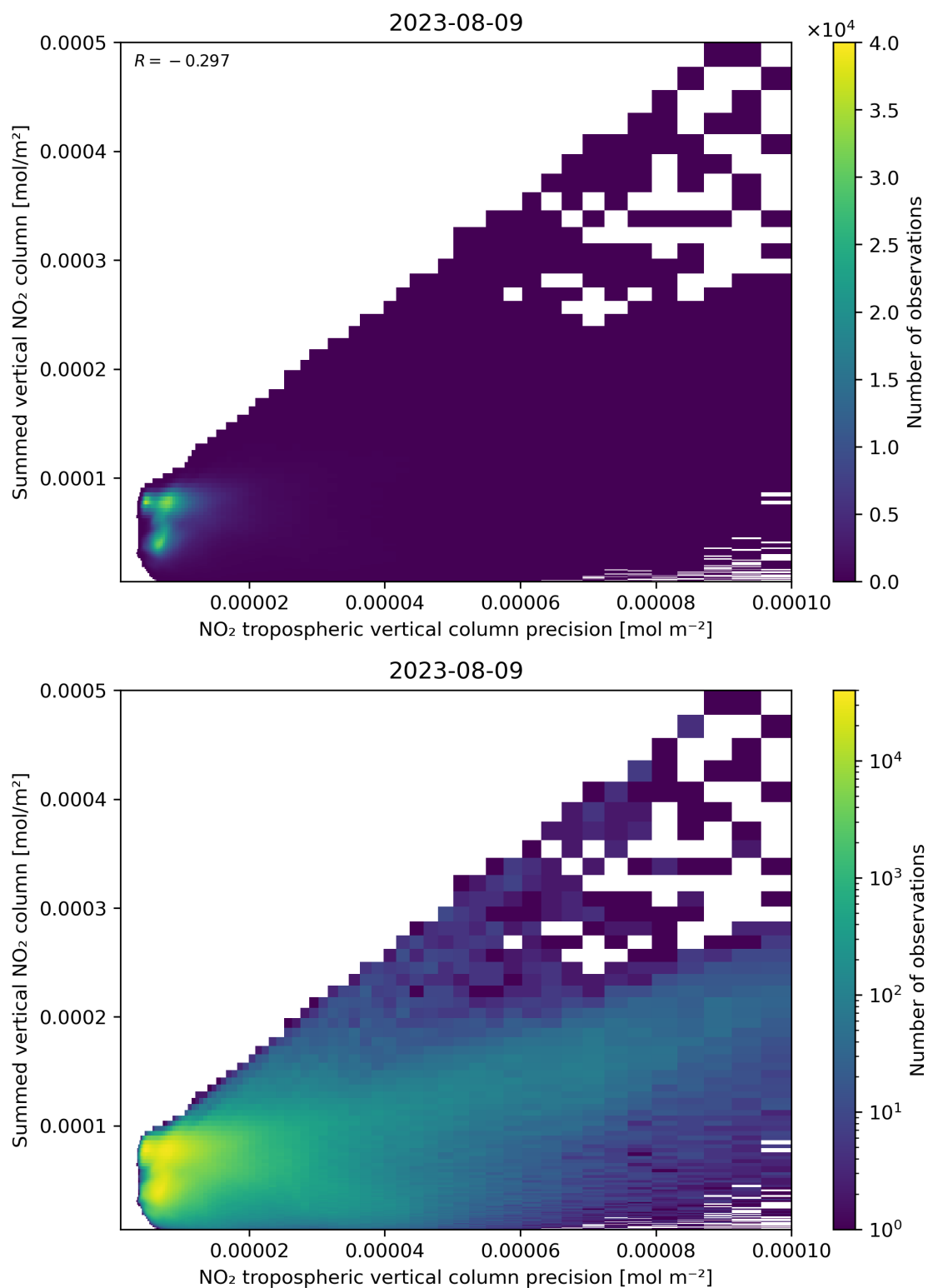
Figure 136: Scatter density plot of “NO 2 tropospheric vertical column precision” against “Summed vertical NO 2 column” for 2023-08-09 to 2023-08-10.
