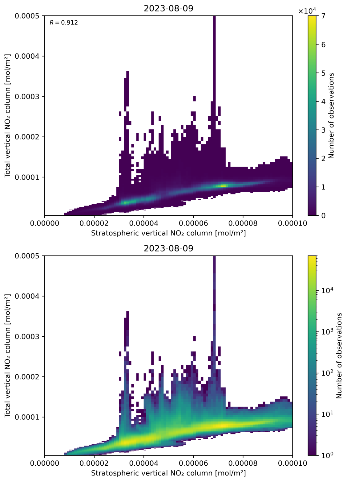
Figure 100: Scatter density plot of “Stratospheric vertical NO 2 column” against “Total vertical NO 2 column” for 2023-08-09 to 2023-08-10.
