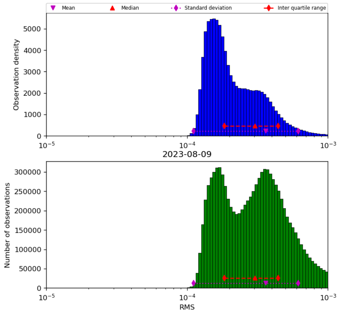
Figure 43: Histogram of “RMS” for 2023-08-09 to 2023-08-10
