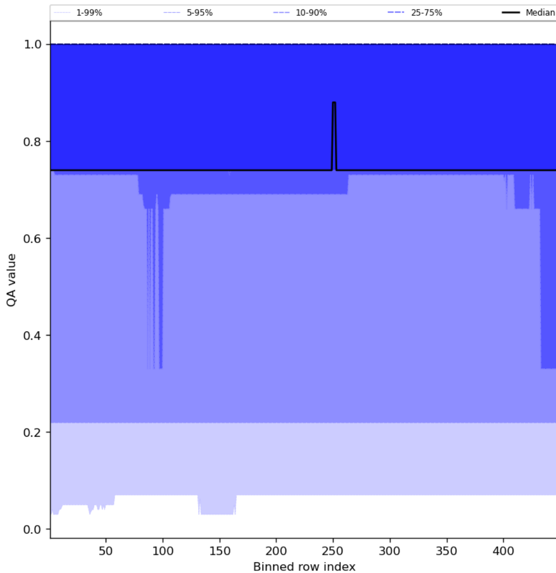
Figure 45: Along track statistics of “QA value” for 2023-08-09 to 2023-08-10
