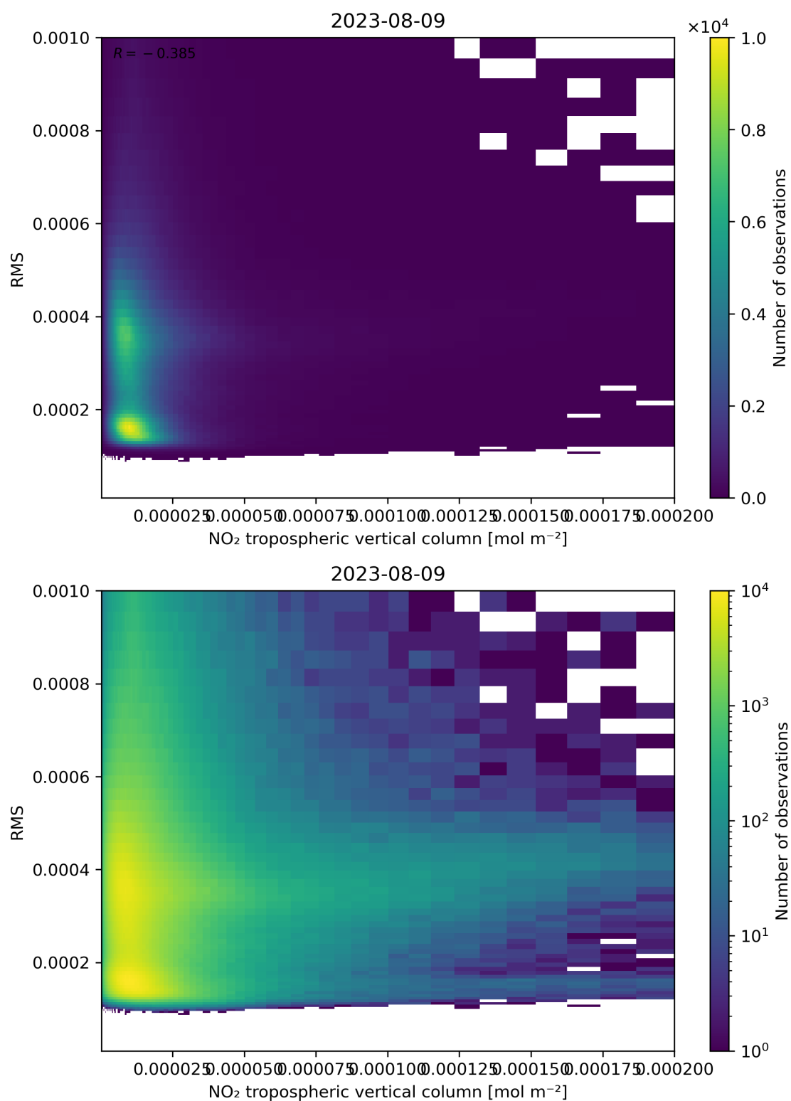
Figure 142: Scatter density plot of “NO 2 tropospheric vertical column” against “RMS” for 2023-08-09 to 2023-08-10.
