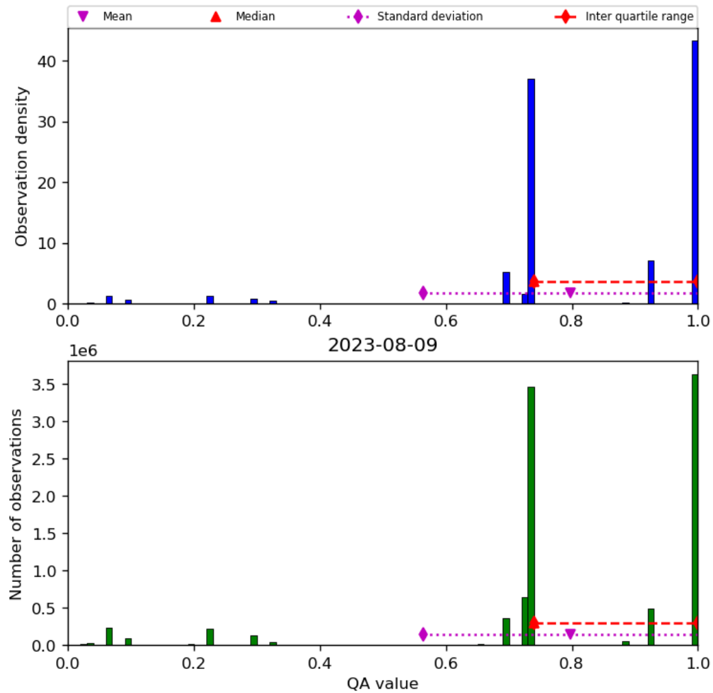
Figure 28: Histogram of “QA value” for 2023-08-09 to 2023-08-10
