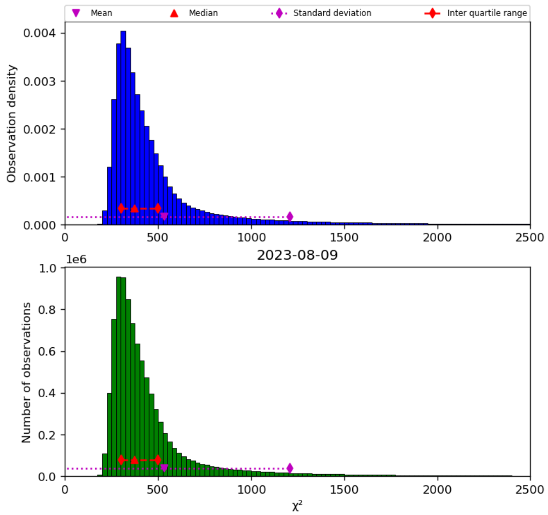
Figure 42: Histogram of “ \chi^2 ” for 2023-08-09 to 2023-08-10
