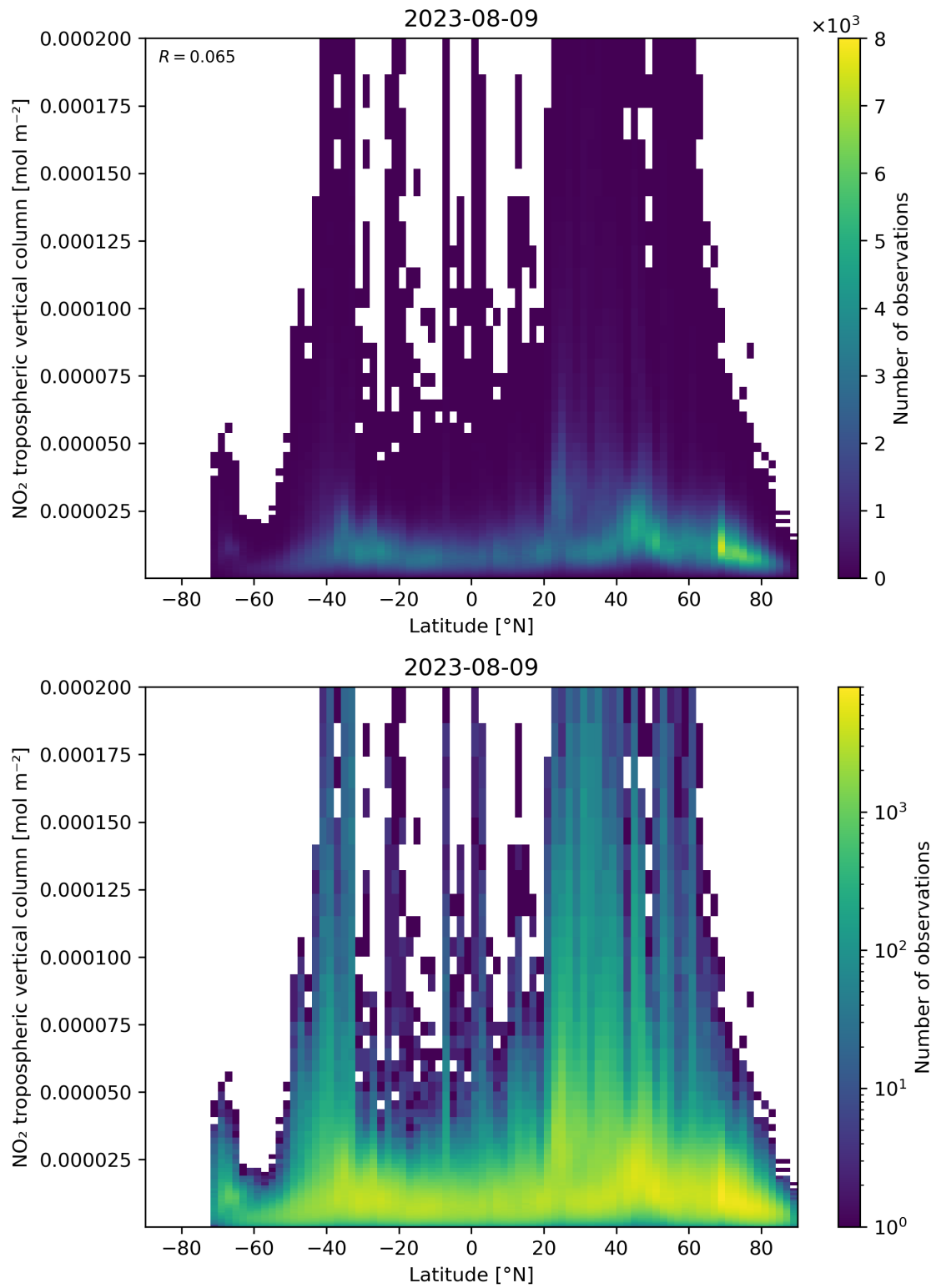
Figure 92: Scatter density plot of “Latitude” against “NO 2 tropospheric vertical column” for 2023-08-09 to 2023-08-10.
