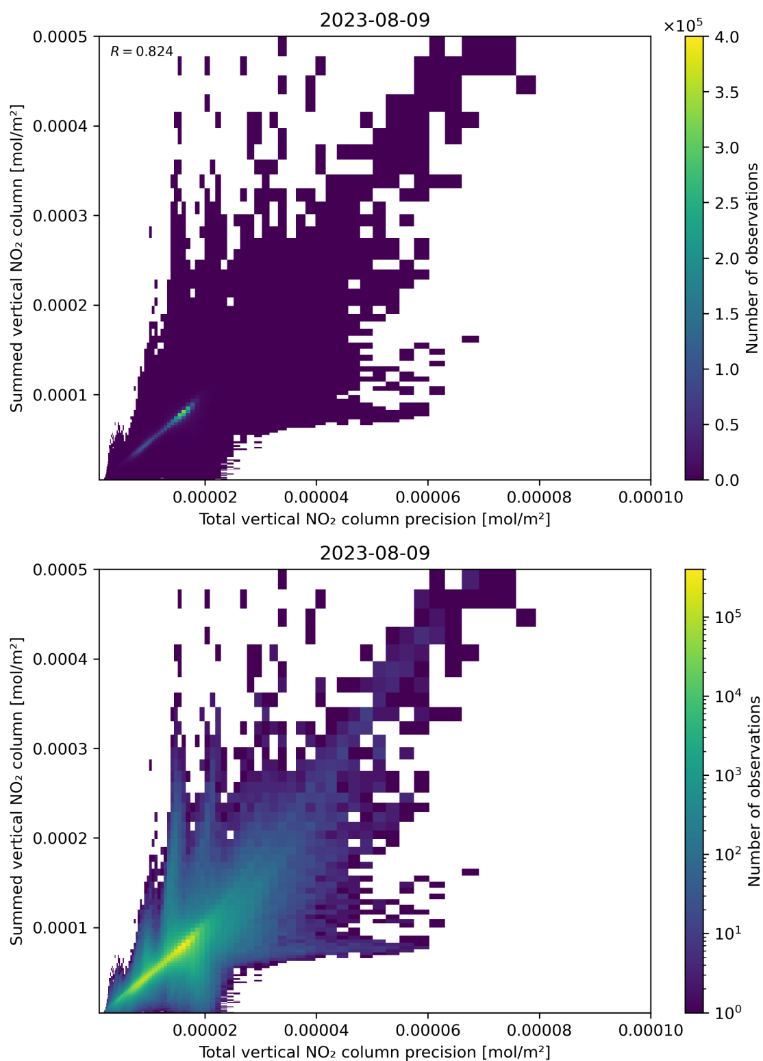
Figure 117: Scatter density plot of “Total vertical NO 2 column precision” against “Summed vertical NO 2 column” for 2023-08-09 to 2023-08-10.
