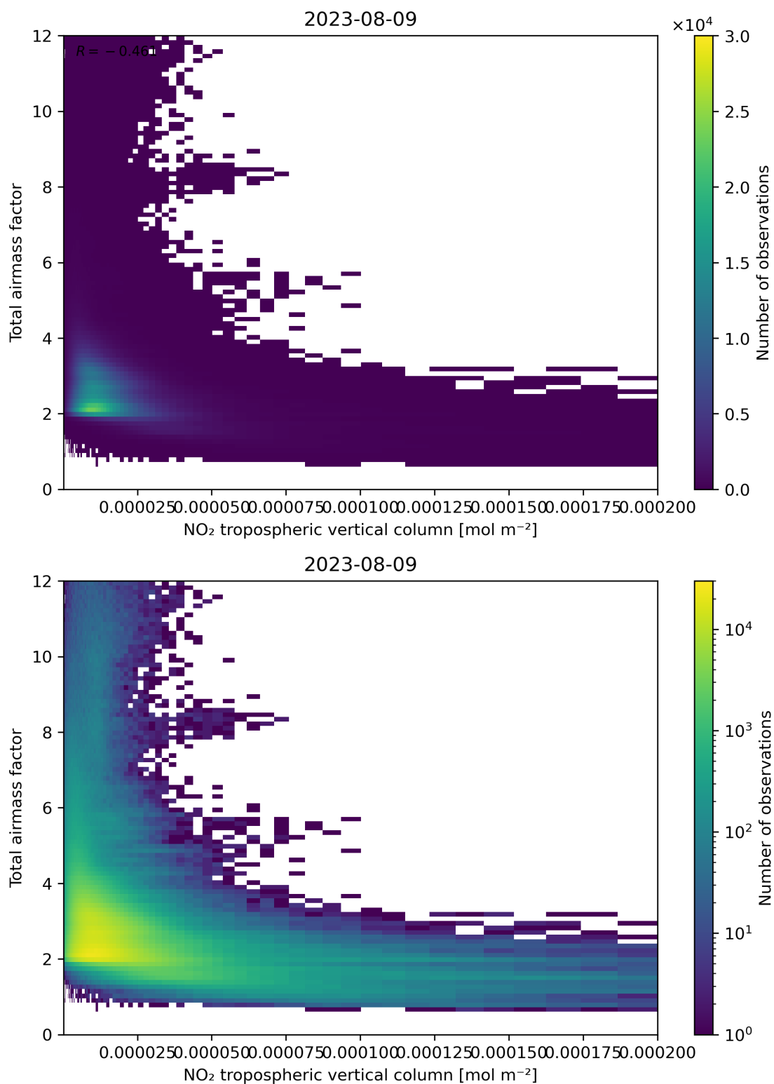
Figure 122: Scatter density plot of “NO 2 tropospheric vertical column” against “Total air mass factor” for 2023-08-09 to 2023-08-10.
