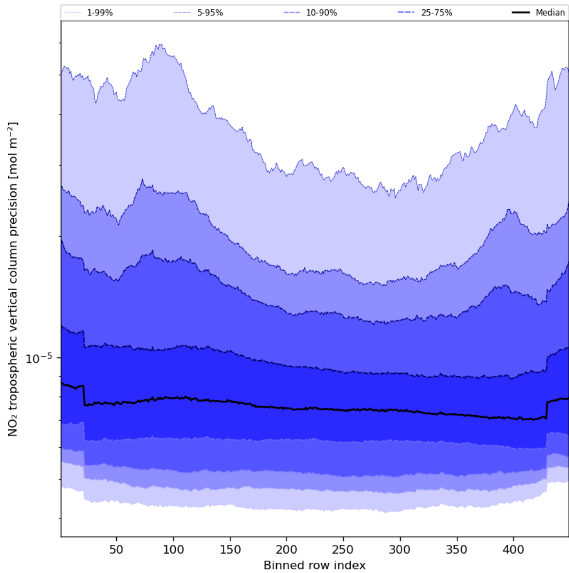
Figure 47: Along track statistics of “NO 2 tropospheric vertical column precision” for 2023-08-09 to 2023-08-10
