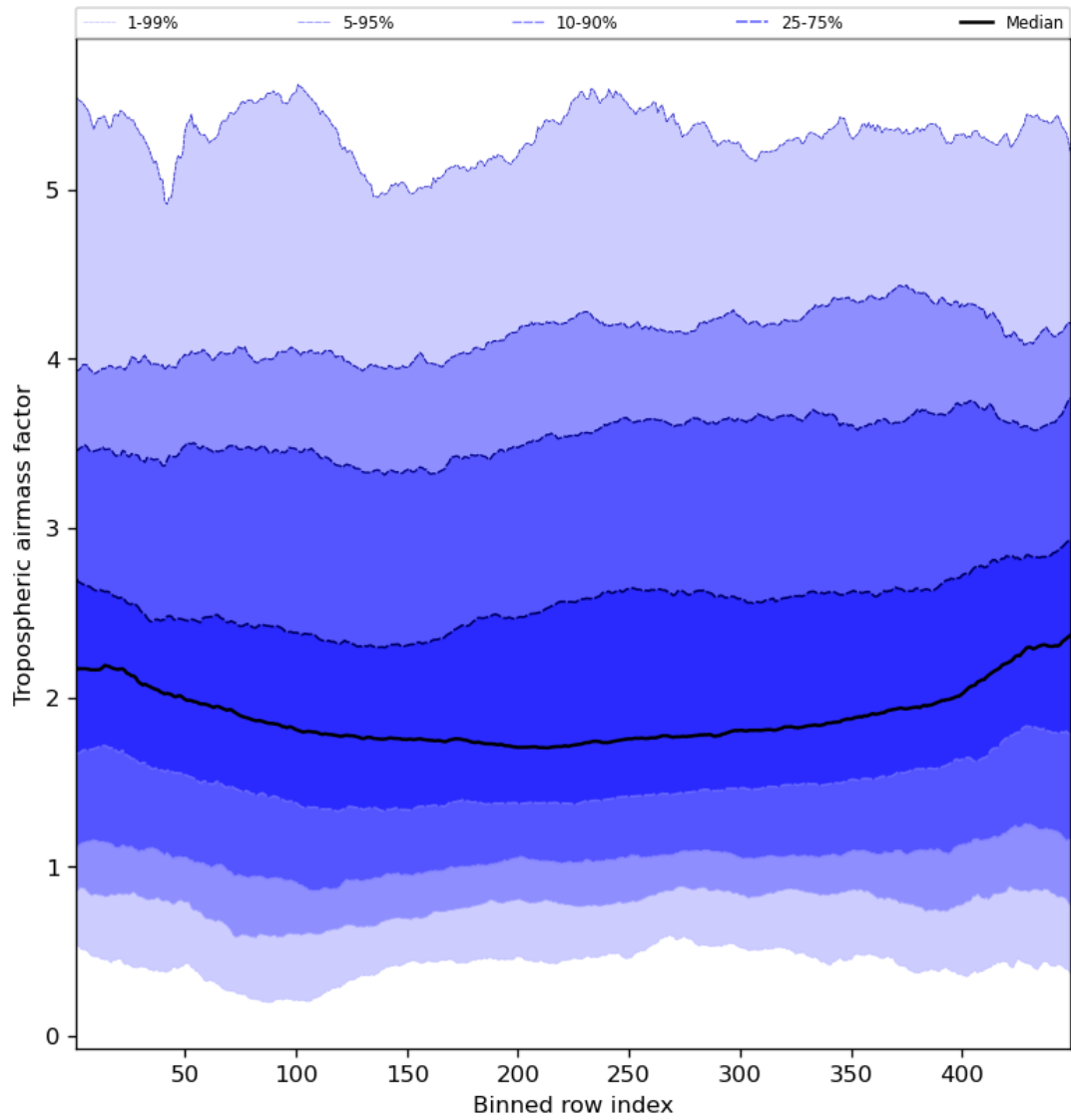
Figure 48: Along track statistics of “Tropospheric air mass factor” for 2023-08-09 to 2023-08-10
