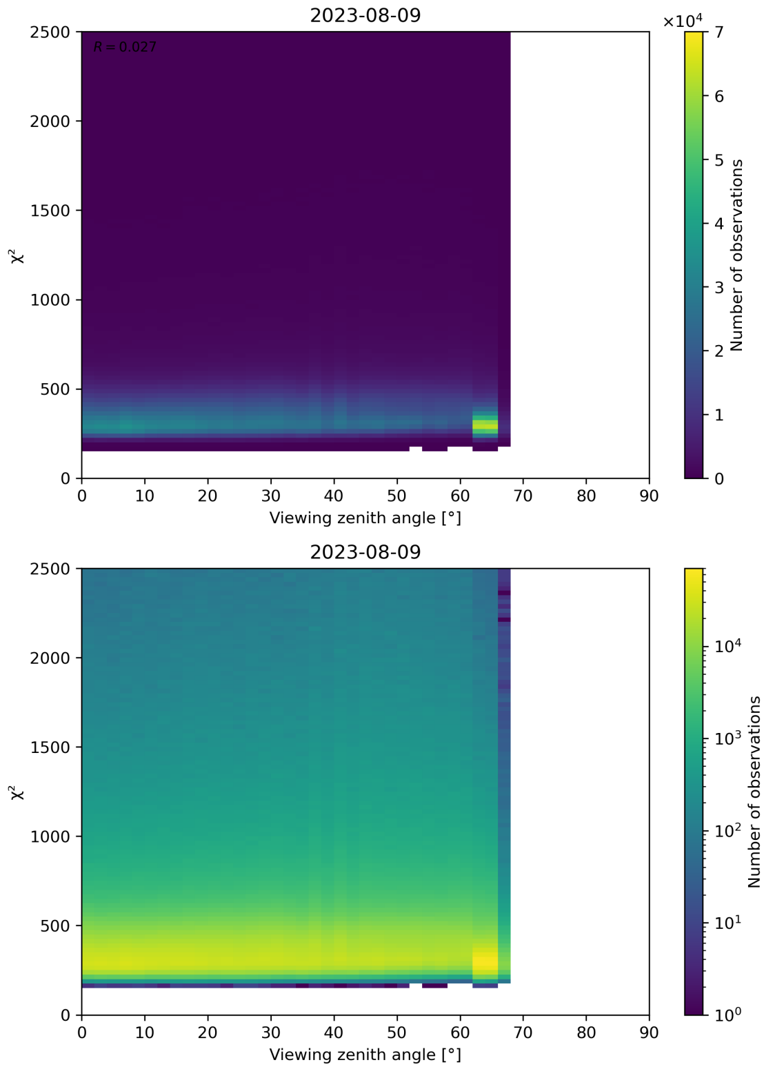
Figure 162: Scatter density plot of “Viewing zenith angle” against “ \chi^2 ” for 2023-08-09 to 2023-08-10.
