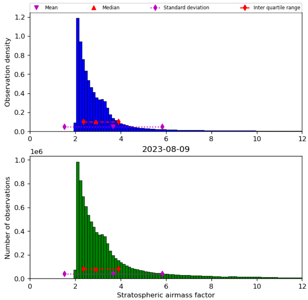
Figure 44: Histogram of “Stratospheric airmass factor” for 2023-08-09 to 2023-08-10
