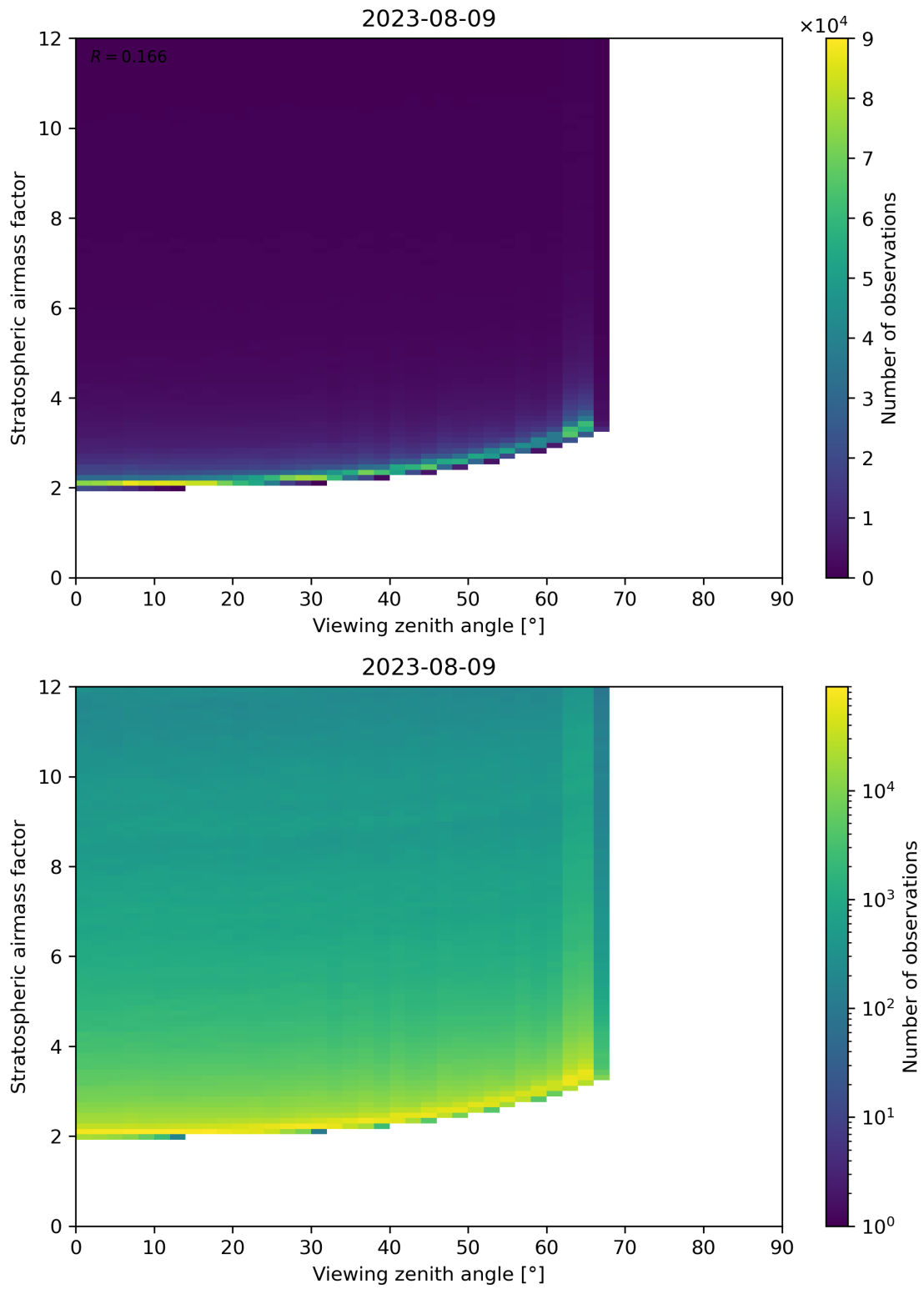
Figure 159: Scatter density plot of “Viewing zenith angle” against “Stratospheric airmass factor” for 2023-08-09 to 2023-08-10.
