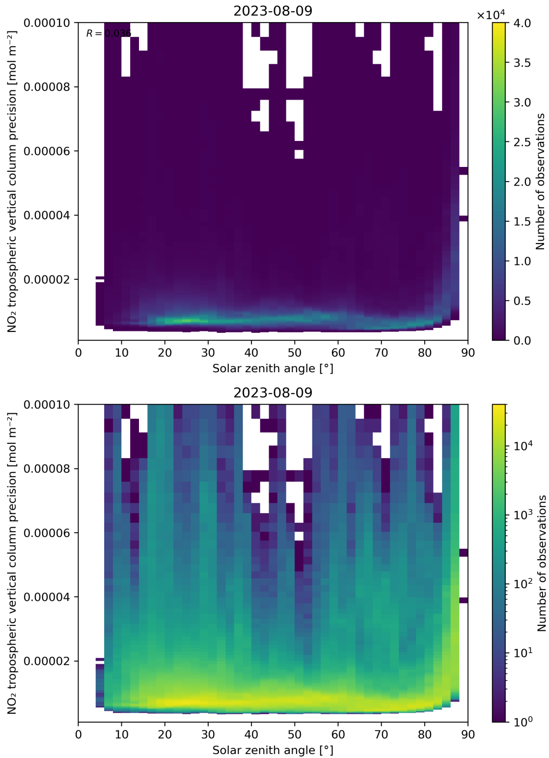
Figure 156: Scatter density plot of “Solar zenith angle” against “NO 2 tropospheric vertical column precision” for 2023-08-09 to 2023-08-10.
