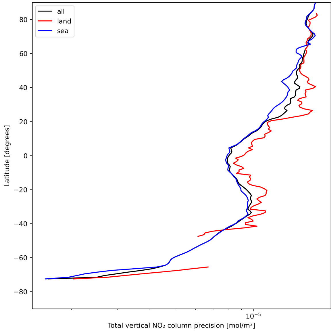
Figure 22: Zonal average of “Total vertical NO 2 column precision” for 2023-08-09 to 2023-08-10.
