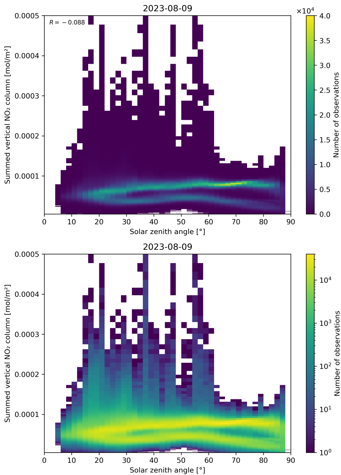
Figure 151: Scatter density plot of “Solar zenith angle” against “Summed vertical NO 2 column” for 2023-08-09 to 2023-08-10.
