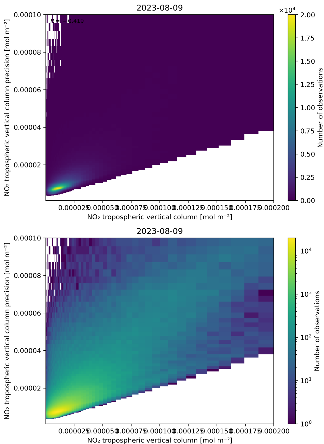
Figure 130: Scatter density plot of “NO 2 tropospheric vertical column” against “NO 2 tropospheric vertical column precision” for 2023-08-09 to 2023-08-10.
