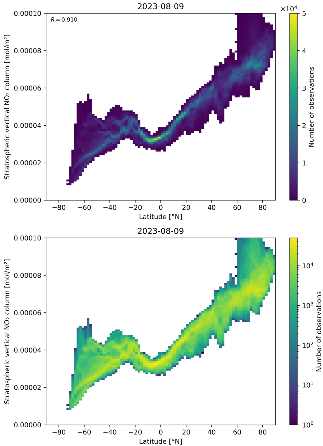
Figure 87: Scatter density plot of “Latitude” against “Stratospheric vertical \text{NO}_2 column” for 2023-08-09 to 2023-08-10.
