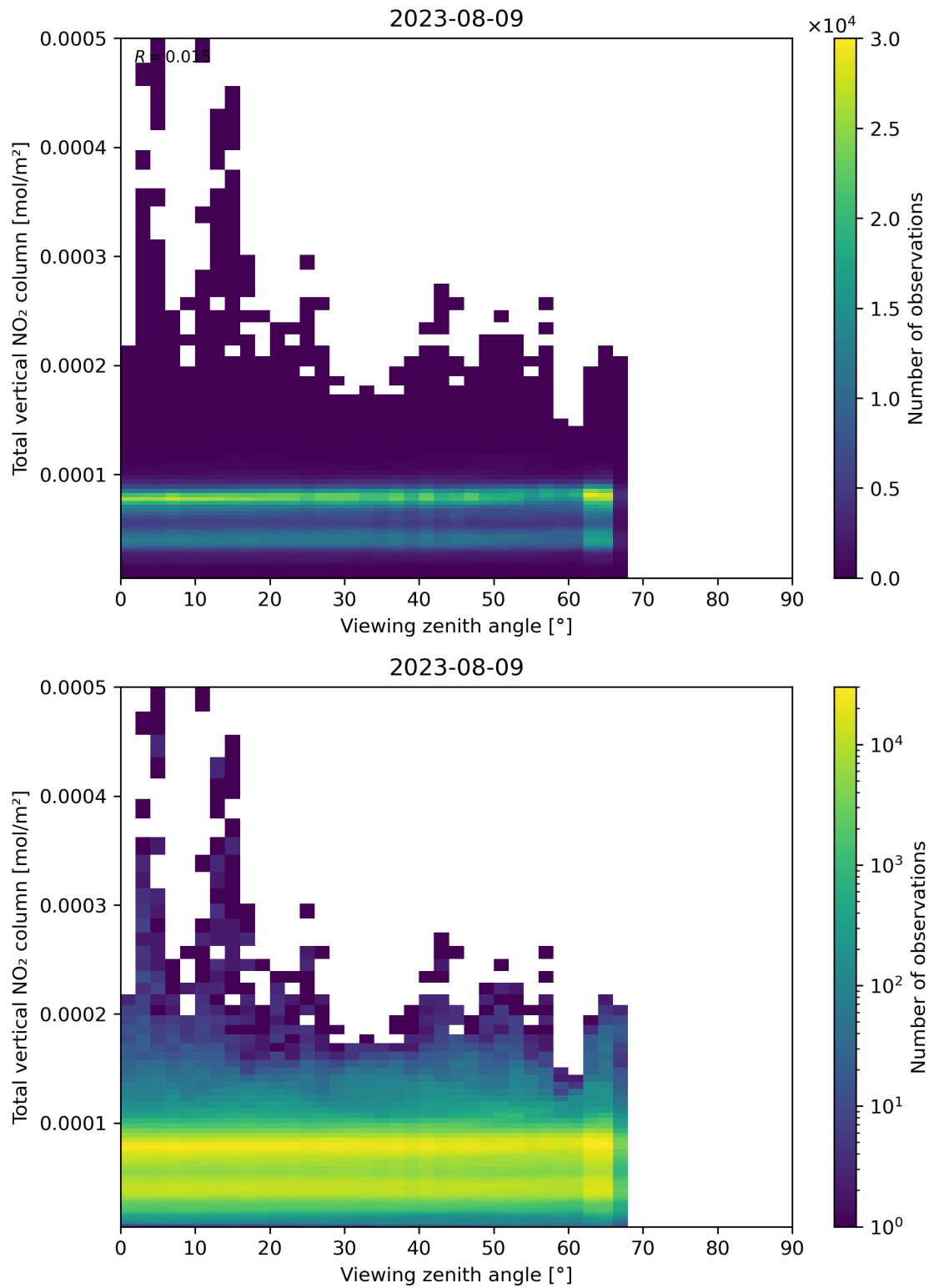
Figure 167: Scatter density plot of “Viewing zenith angle” against “Total vertical NO 2 column” for 2023-08-09 to 2023-08-10.
