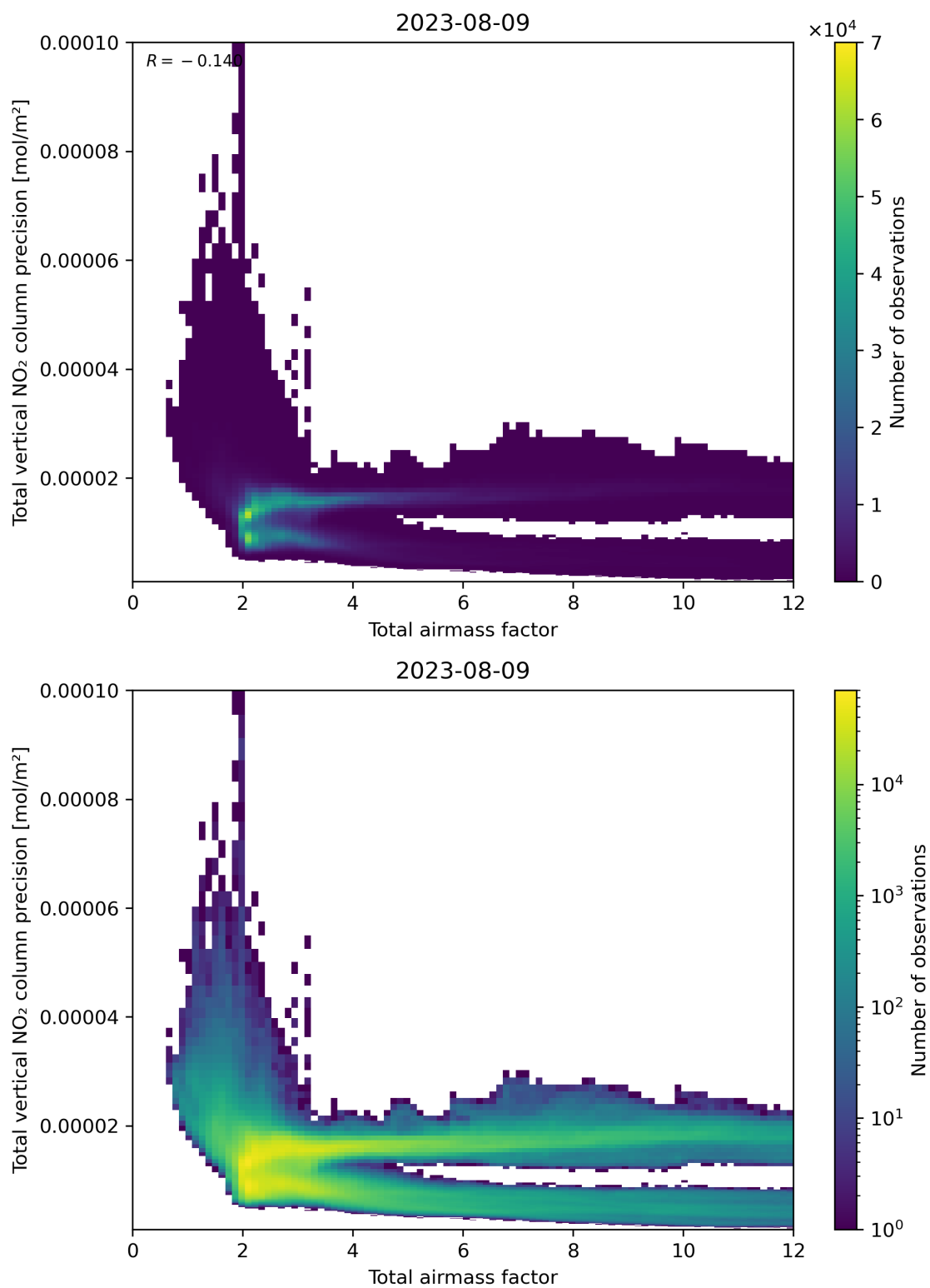
Figure 68: Scatter density plot of “Total airmass factor” against “Total vertical NO 2 column precision” for 2023-08-09 to 2023-08-10.
