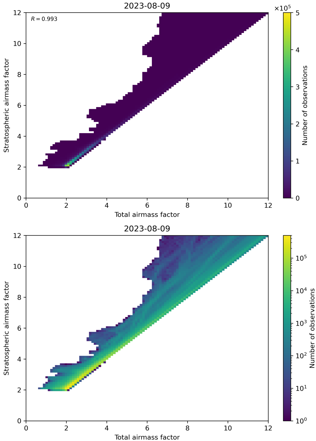
Figure 62: Scatter density plot of “Total airmass factor” against “Stratospheric airmass factor” for 2023-08-09 to 2023-08-10.
