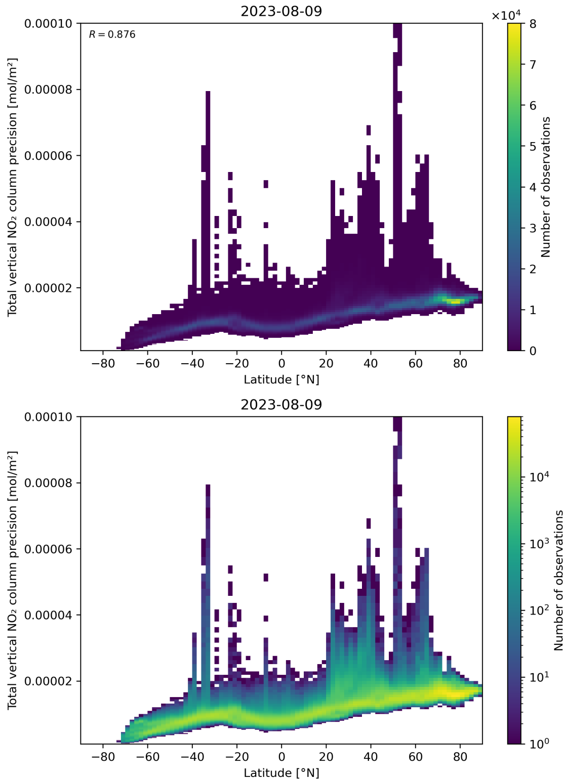
Figure 91: Scatter density plot of “Latitude” against “Total vertical NO 2 column precision” for 2023-08-09 to 2023-08-10.
