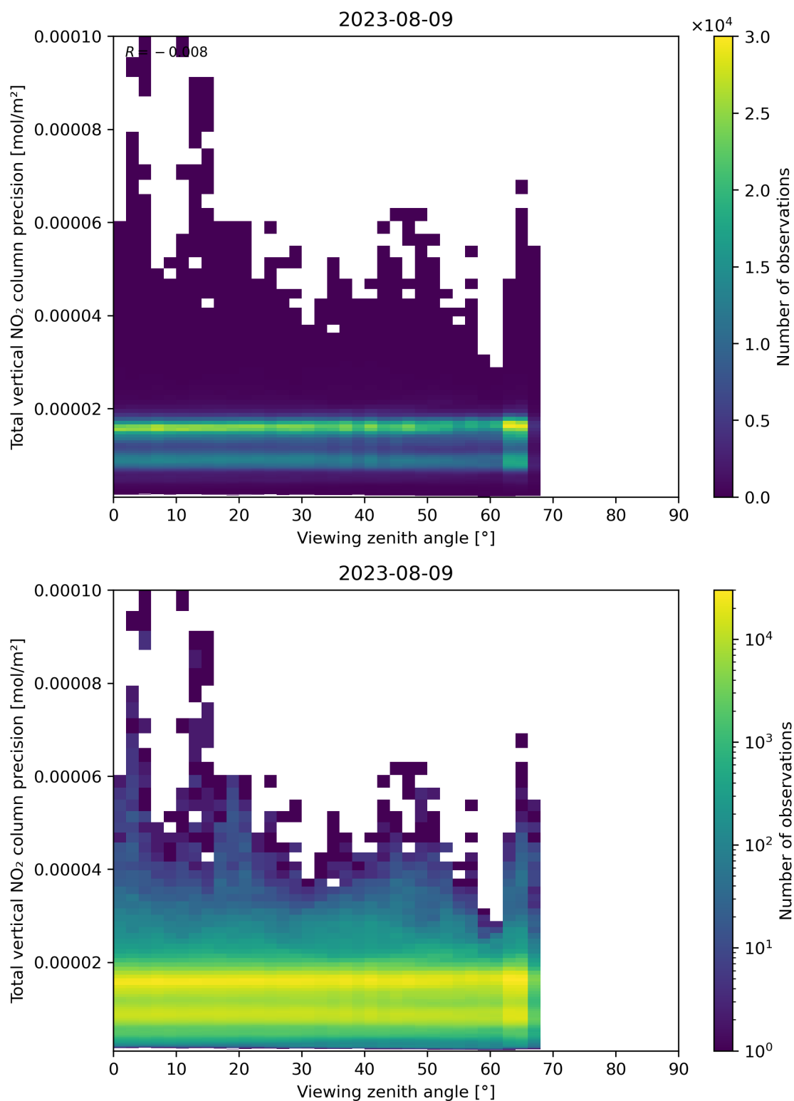
Figure 168: Scatter density plot of “Viewing zenith angle” against “Total vertical NO 2 column precision” for 2023-08-09 to 2023-08-10.
