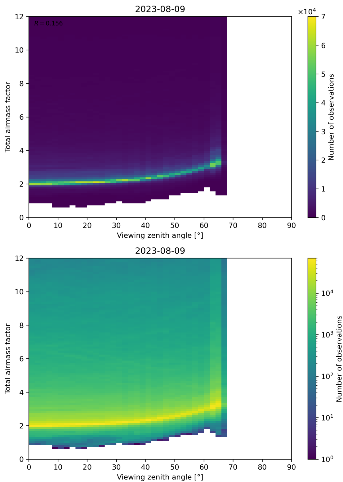
Figure 160: Scatter density plot of “Viewing zenith angle” against “Total airmass factor” for 2023-08-09 to 2023-08-10.
