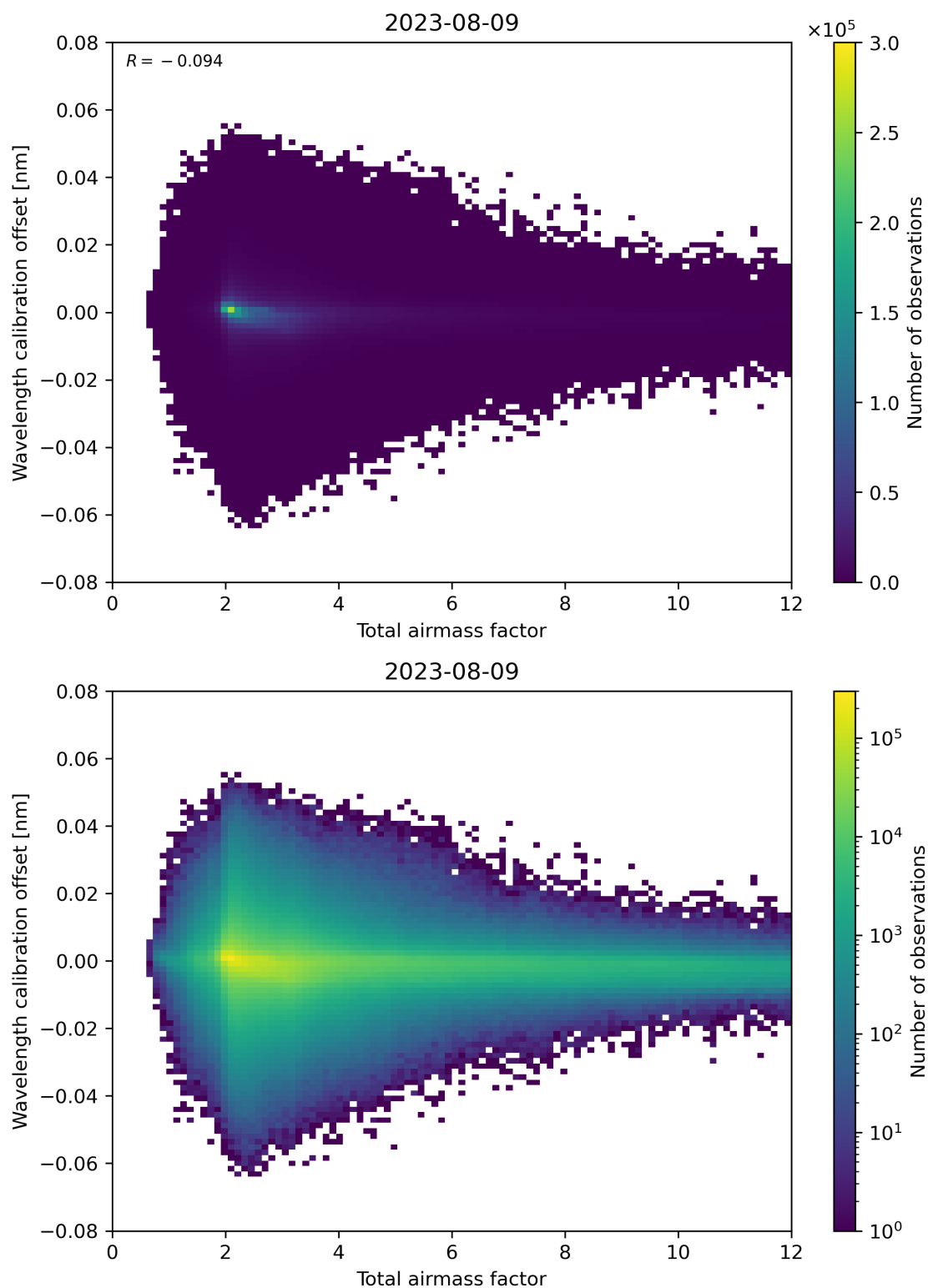
Figure 70: Scatter density plot of “Total airmass factor” against “Wavelength calibration offset” for 2023-08-09 to 2023-08-10.
