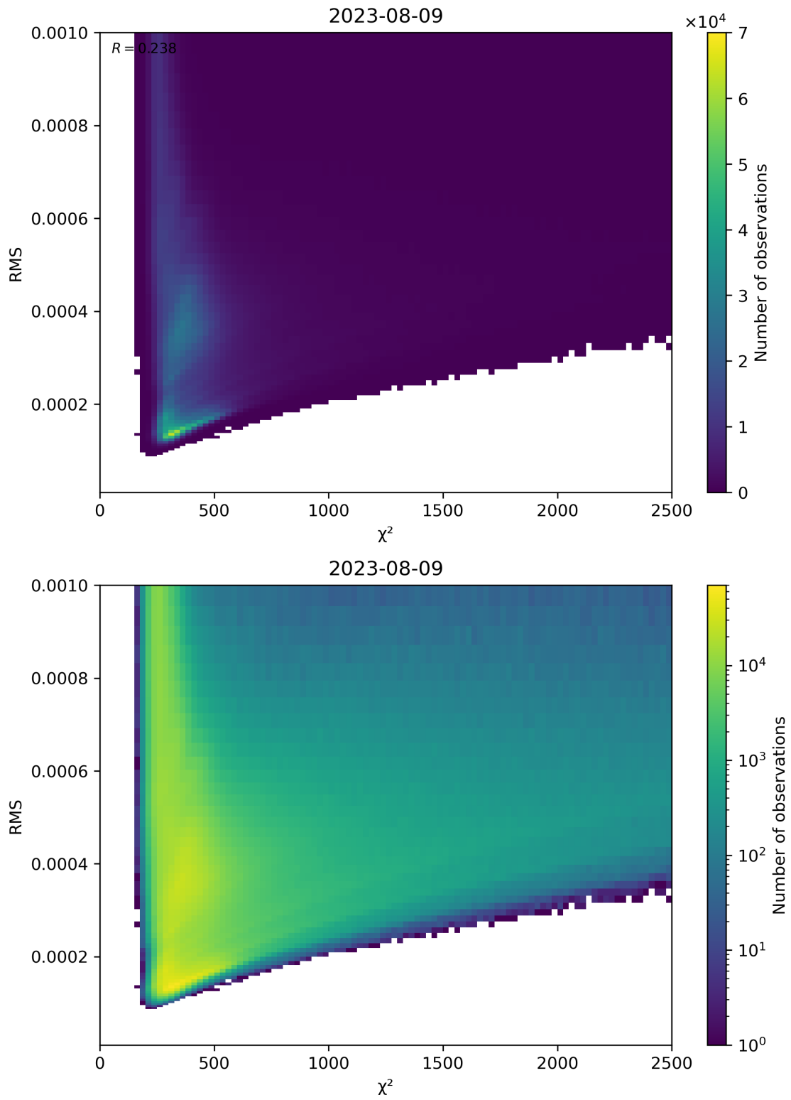
Figure 82: Scatter density plot of “ \chi^2 ” against “RMS” for 2023-08-09 to 2023-08-10.
