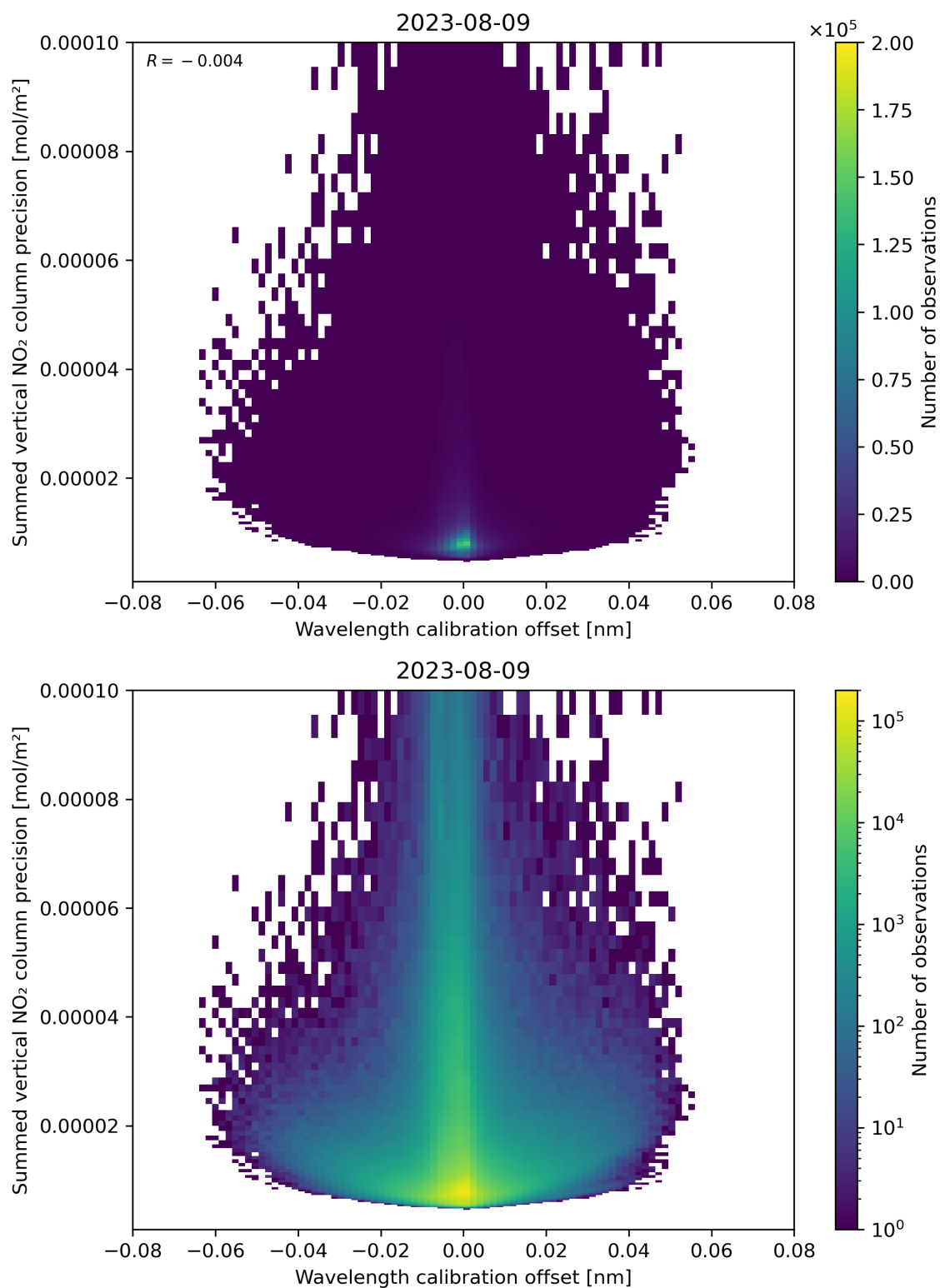
Figure 178: Scatter density plot of “Wavelength calibration offset” against “Summed vertical NO 2 column precision” for 2023-08-09 to 2023-08-10.
