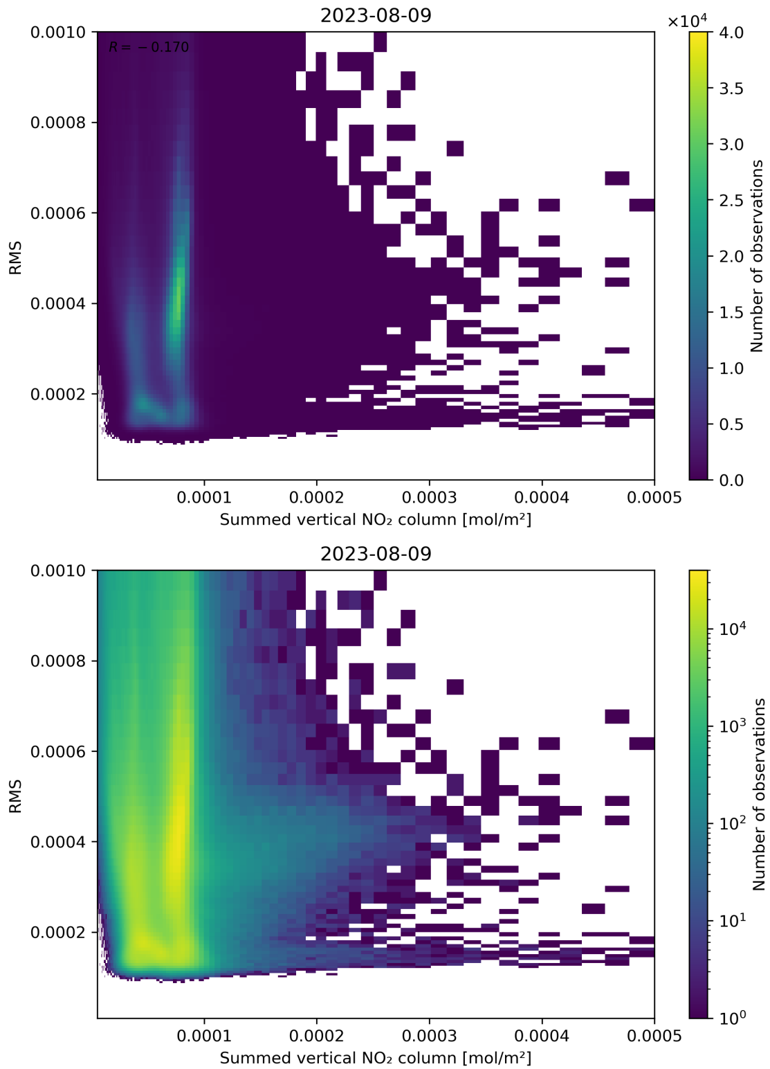
Figure 109: Scatter density plot of “Summed vertical NO 2 column” against “RMS” for 2023-08-09 to 2023-08-10.
