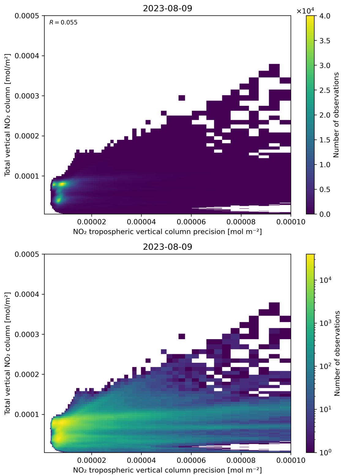
Figure 138: Scatter density plot of “NO 2 tropospheric vertical column precision” against “Total vertical NO 2 column” for 2023-08-09 to 2023-08-10.
