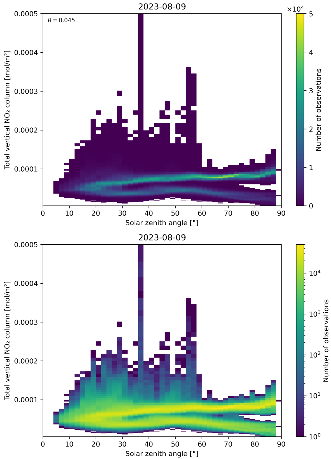
Figure 153: Scatter density plot of “Solar zenith angle” against “Total vertical NO 2 column” for 2023-08-09 to 2023-08-10.
