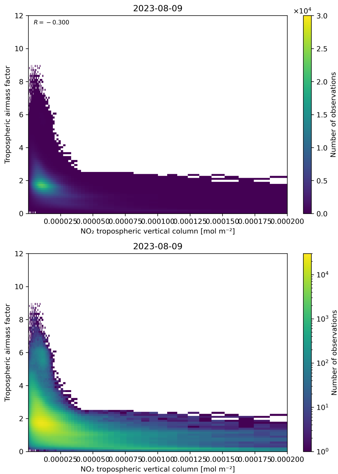
Figure 123: Scatter density plot of “NO 2 tropospheric vertical column” against “Tropospheric air mass factor” for 2023-08-09 to 2023-08-10.
