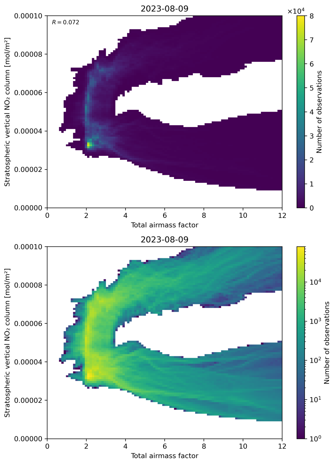
Figure 64: Scatter density plot of “Total airmass factor” against “Stratospheric vertical \text{NO}_2 column” for 2023-08-09 to 2023-08-10.
