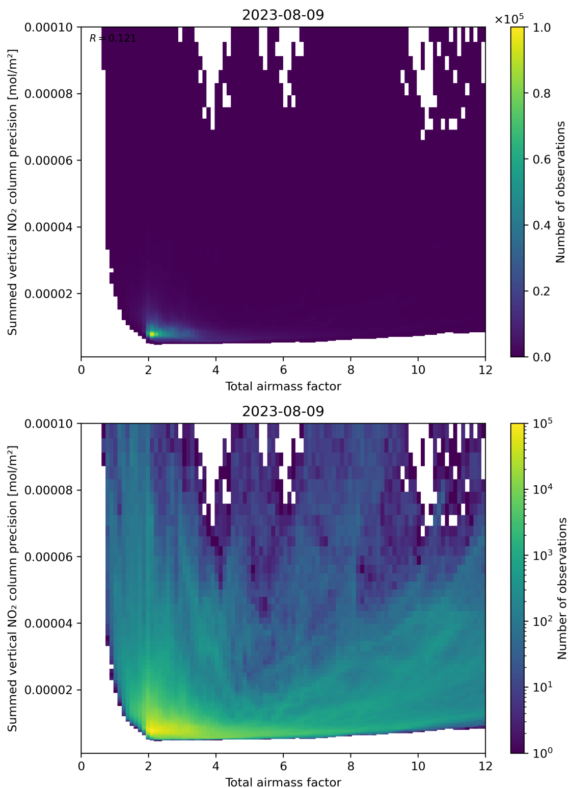
Figure 66: Scatter density plot of “Total airmass factor” against “Summed vertical NO 2 column precision” for 2023-08-09 to 2023-08-10.
