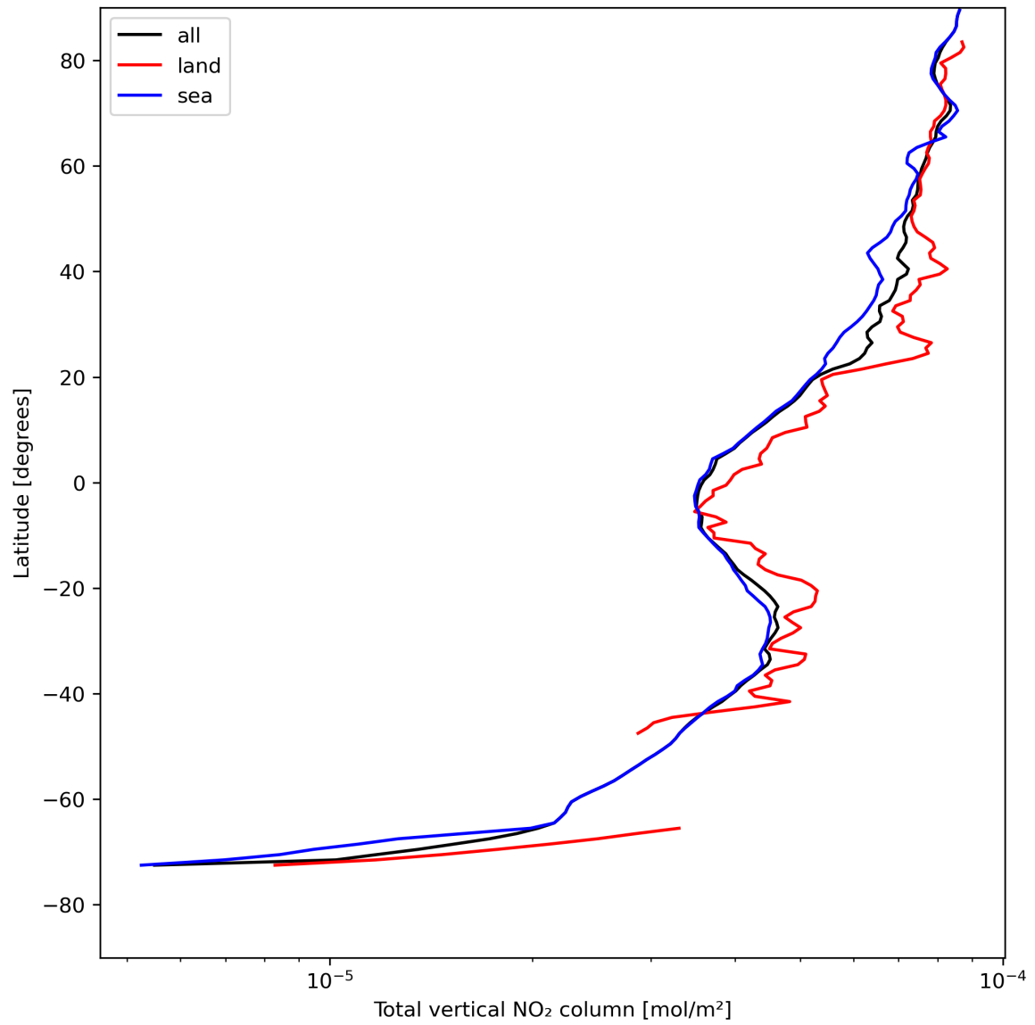
Figure 21: Zonal average of “Total vertical NO 2 column” for 2023-08-09 to 2023-08-10.
