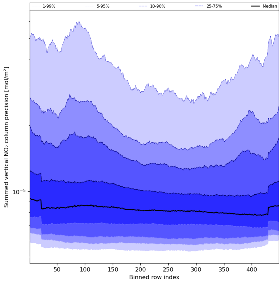
Figure 58: Along track statistics of “Summed vertical NO 2 column precision” for 2023-08-09 to 2023-08-10
