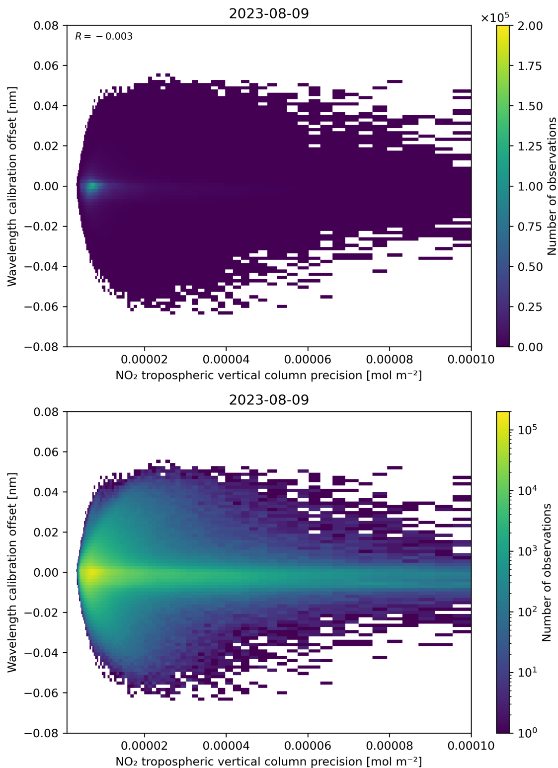
Figure 141: Scatter density plot of “NO 2 tropospheric vertical column precision” against “Wavelength calibration offset” for 2023-08-09 to 2023-08-10.
