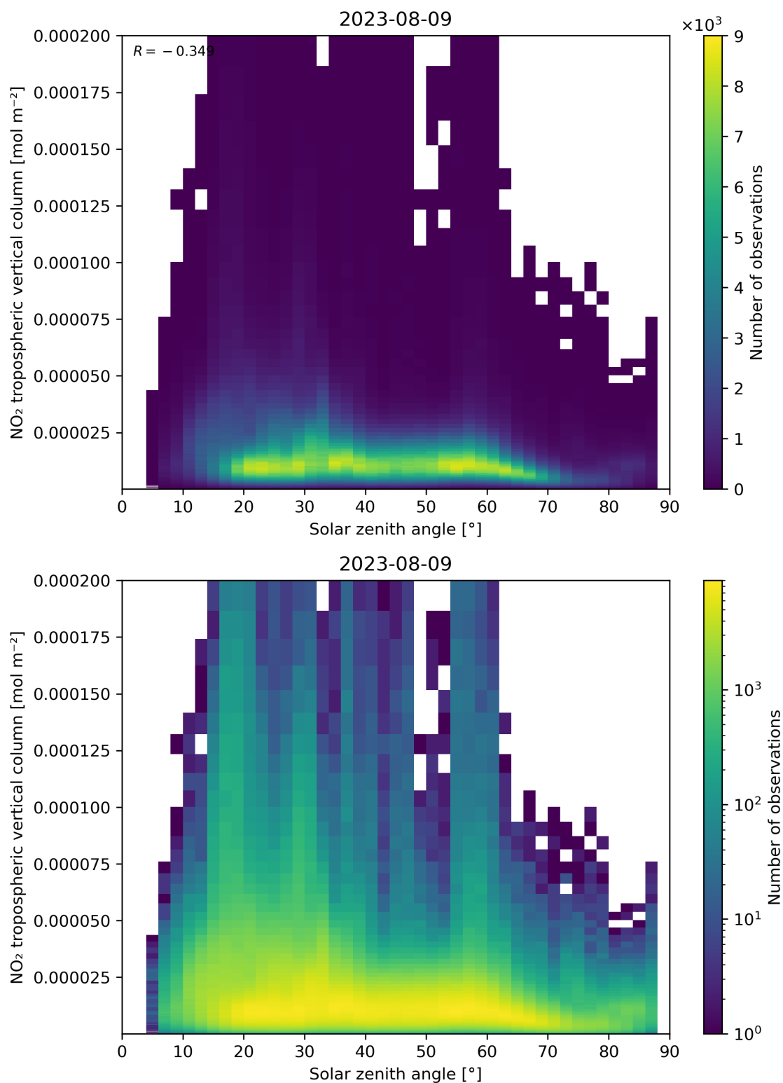
Figure 155: Scatter density plot of “Solar zenith angle” against “NO 2 tropospheric vertical column” for 2023-08-09 to 2023-08-10.
