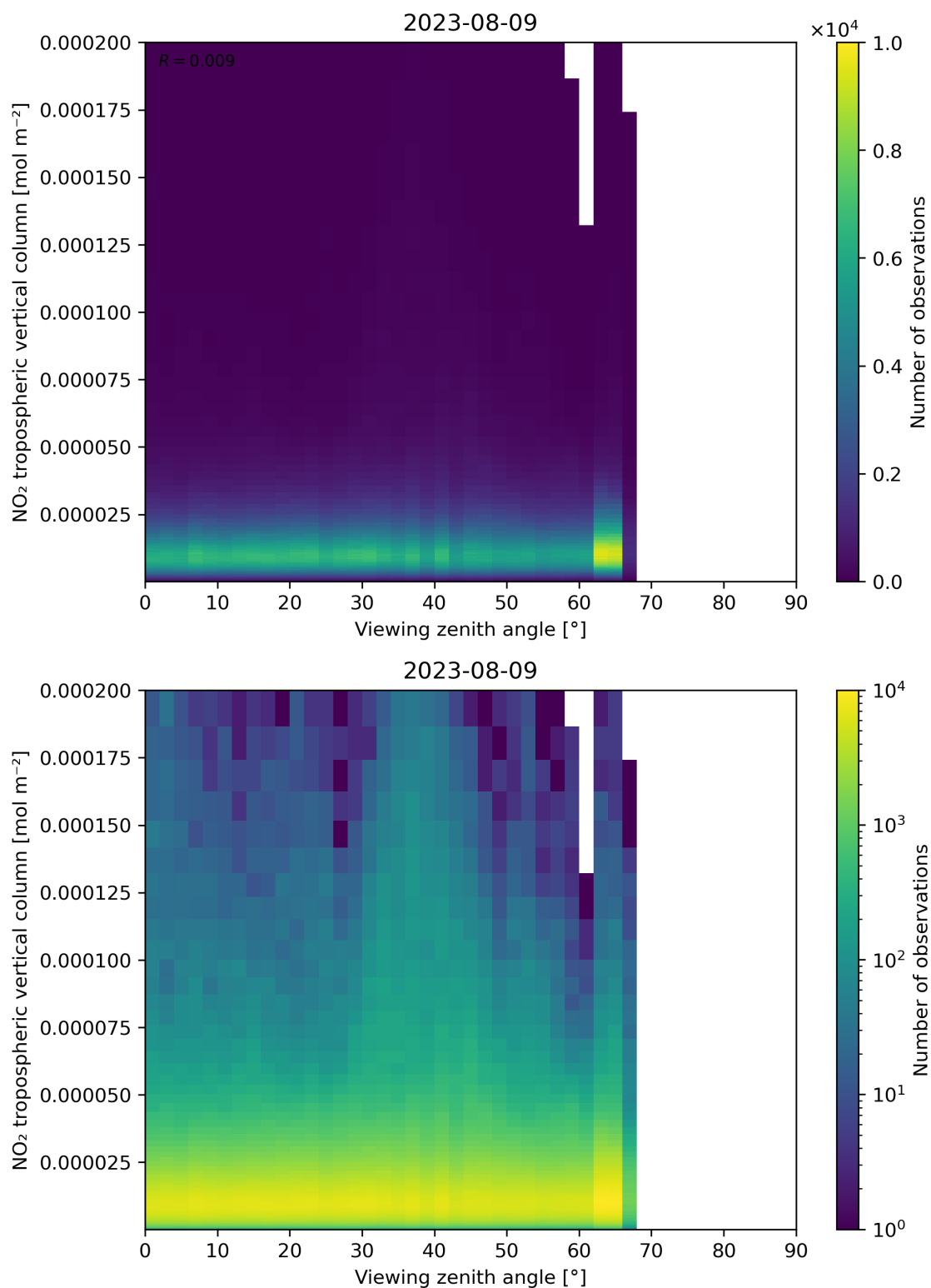
Figure 169: Scatter density plot of “Viewing zenith angle” against “NO 2 tropospheric vertical column” for 2023-08-09 to 2023-08-10.
