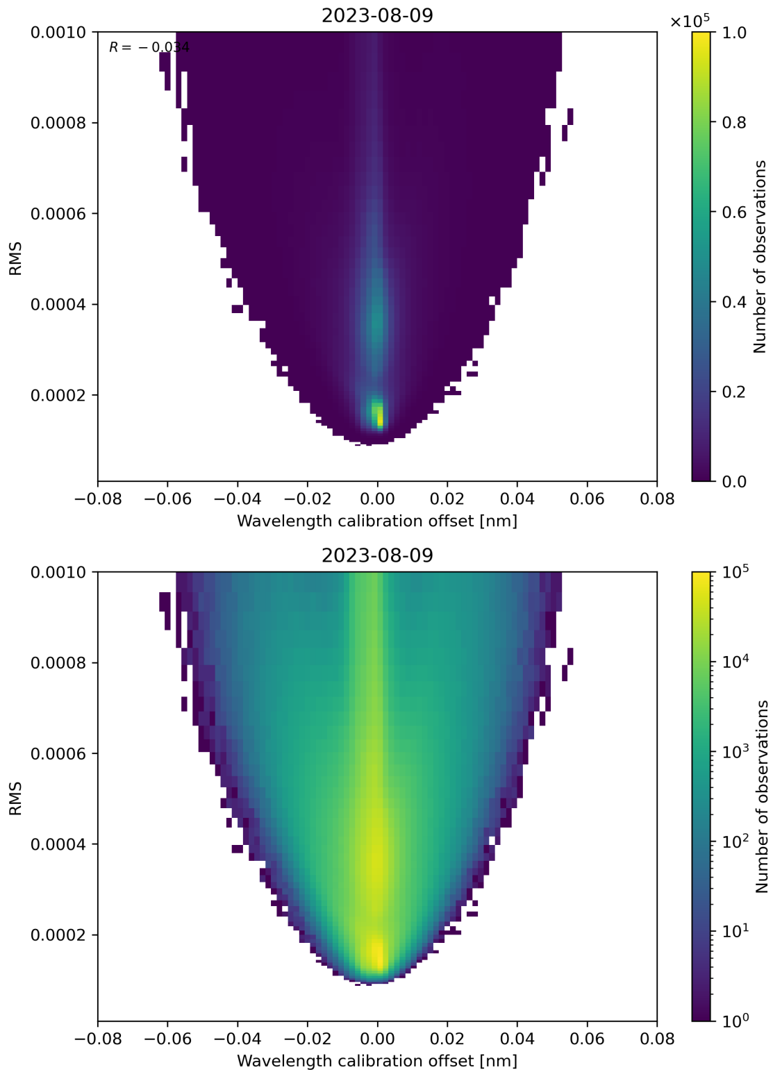
Figure 181: Scatter density plot of “Wavelength calibration offset” against “RMS” for 2023-08-09 to 2023-08-10.
