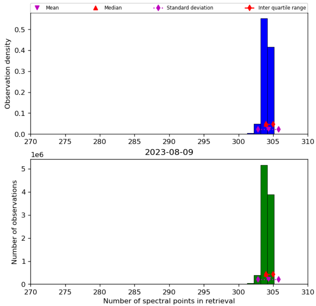
Figure 33: Histogram of “Number of spectral points in retrieval” for 2023-08-09 to 2023-08-10
