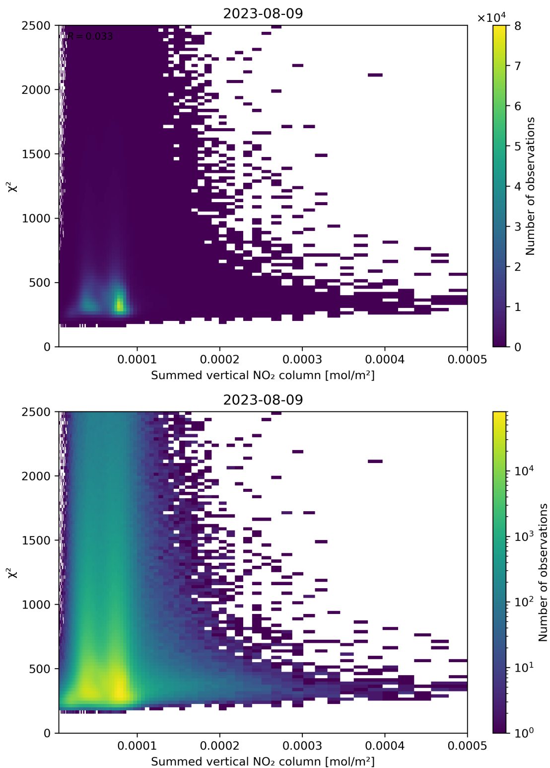
Figure 104: Scatter density plot of “Summed vertical NO 2 column” against “ \chi^2 ” for 2023-08-09 to 2023-08-10.
