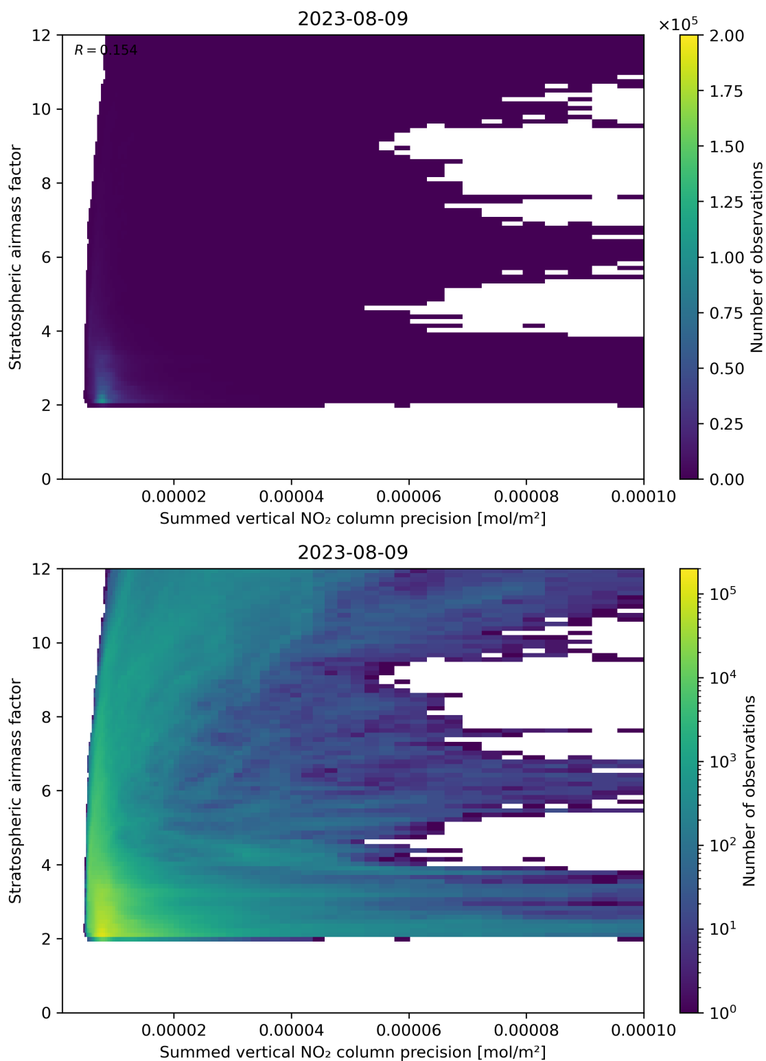
Figure 106: Scatter density plot of “Summed vertical NO 2 column precision” against “Stratospheric airmass factor” for 2023-08-09 to 2023-08-10.
