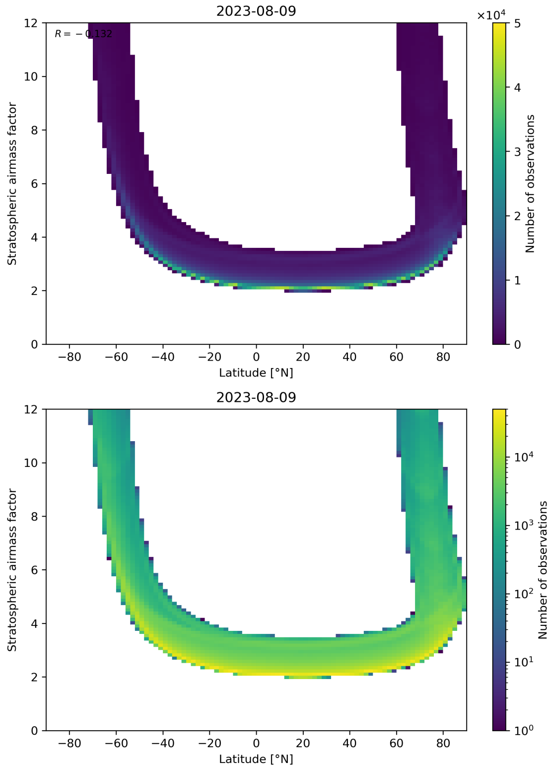
Figure 83: Scatter density plot of “Latitude” against “Stratospheric airmass factor” for 2023-08-09 to 2023-08-10.
