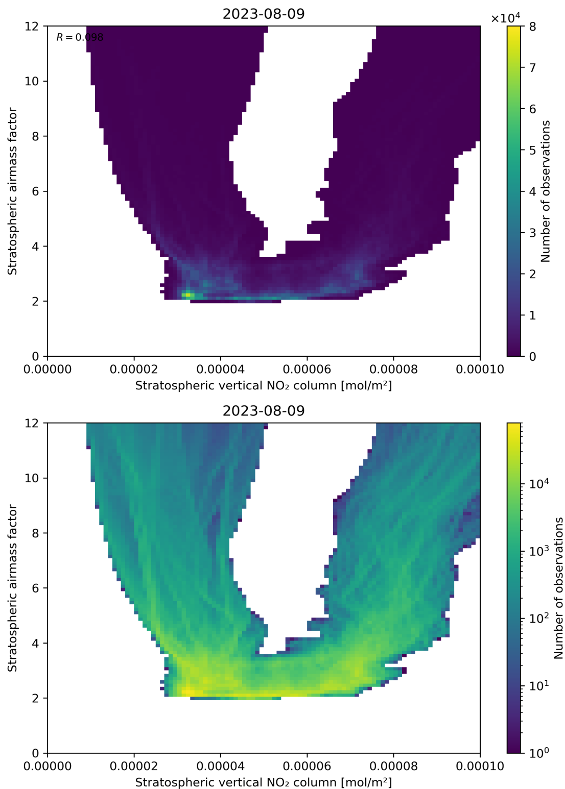
Figure 96: Scatter density plot of “Stratospheric vertical NO 2 column” against “Stratospheric airmass factor” for 2023-08-09 to 2023-08-10.
