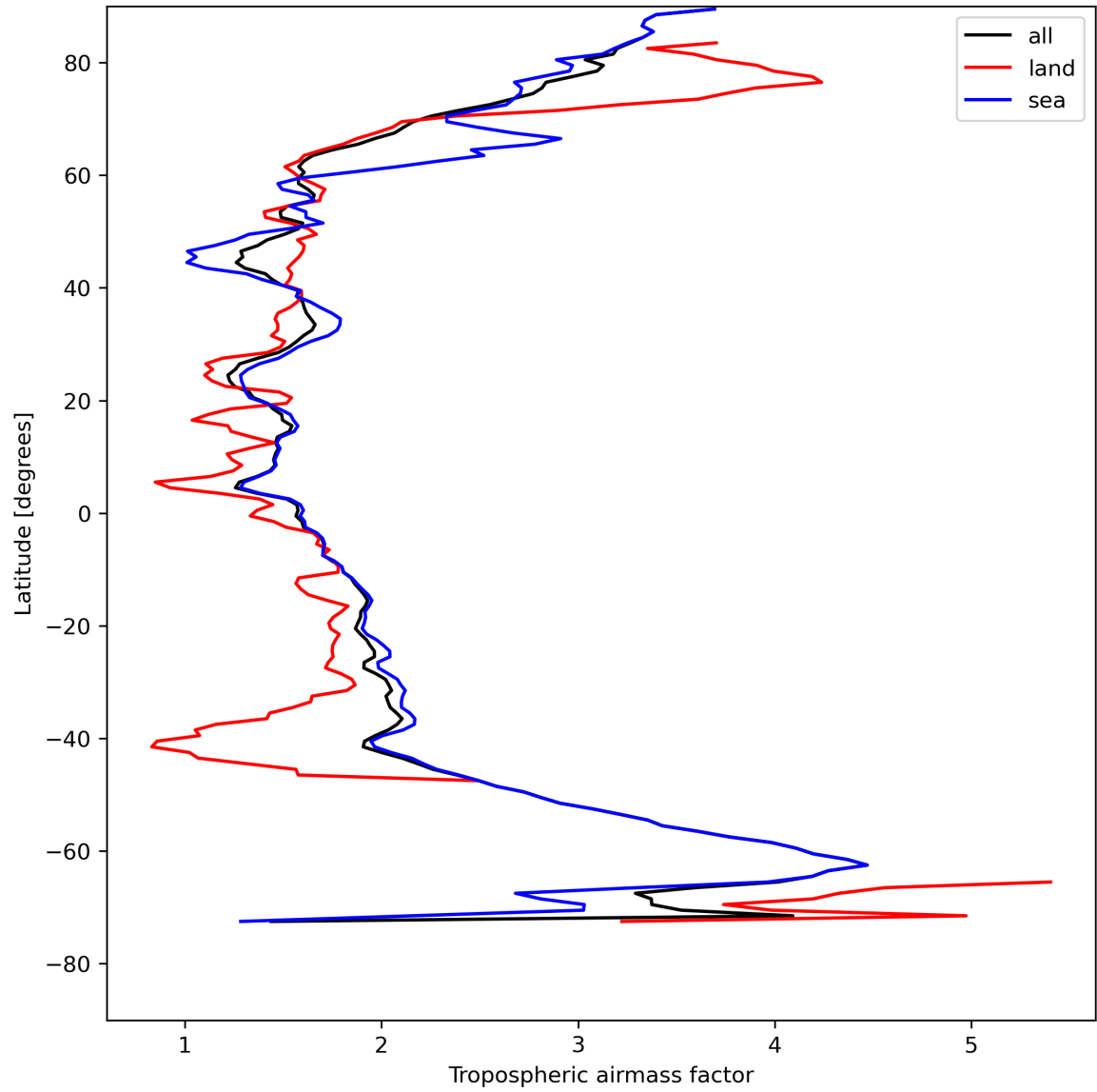
Figure 14: Zonal average of “Tropospheric airmass factor” for 2023-08-09 to 2023-08-10.
