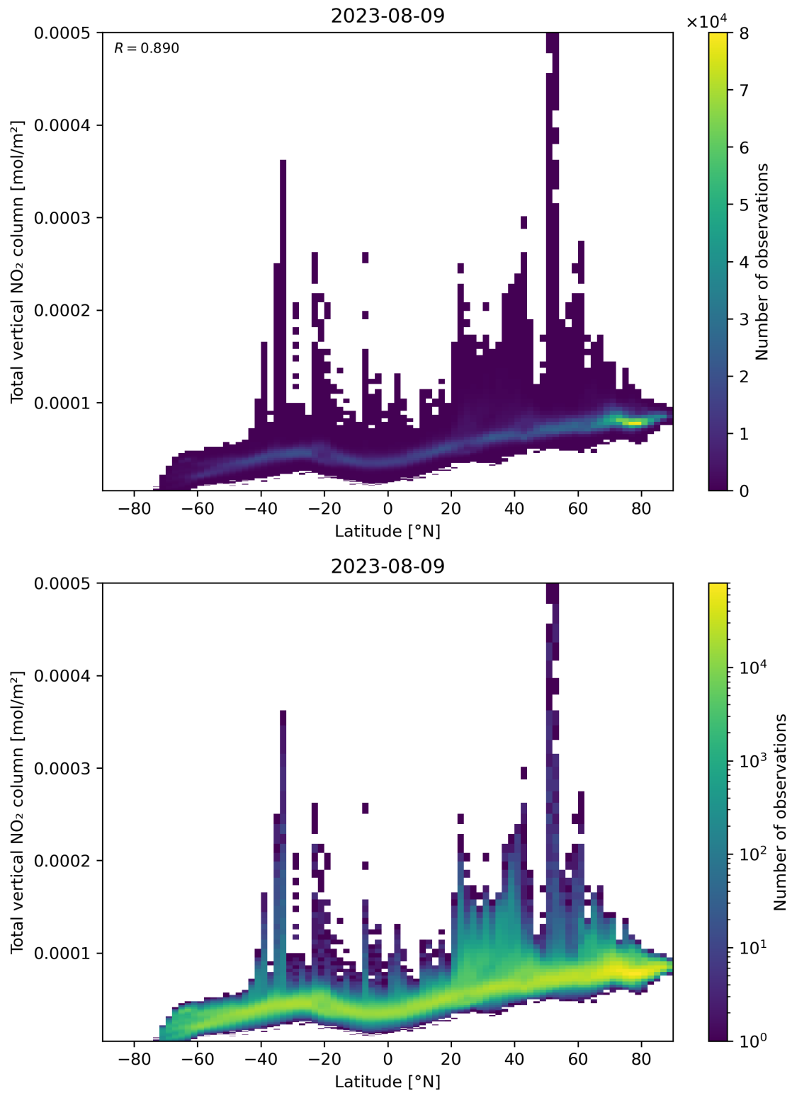
Figure 90: Scatter density plot of “Latitude” against “Total vertical NO 2 column” for 2023-08-09 to 2023-08-10.
