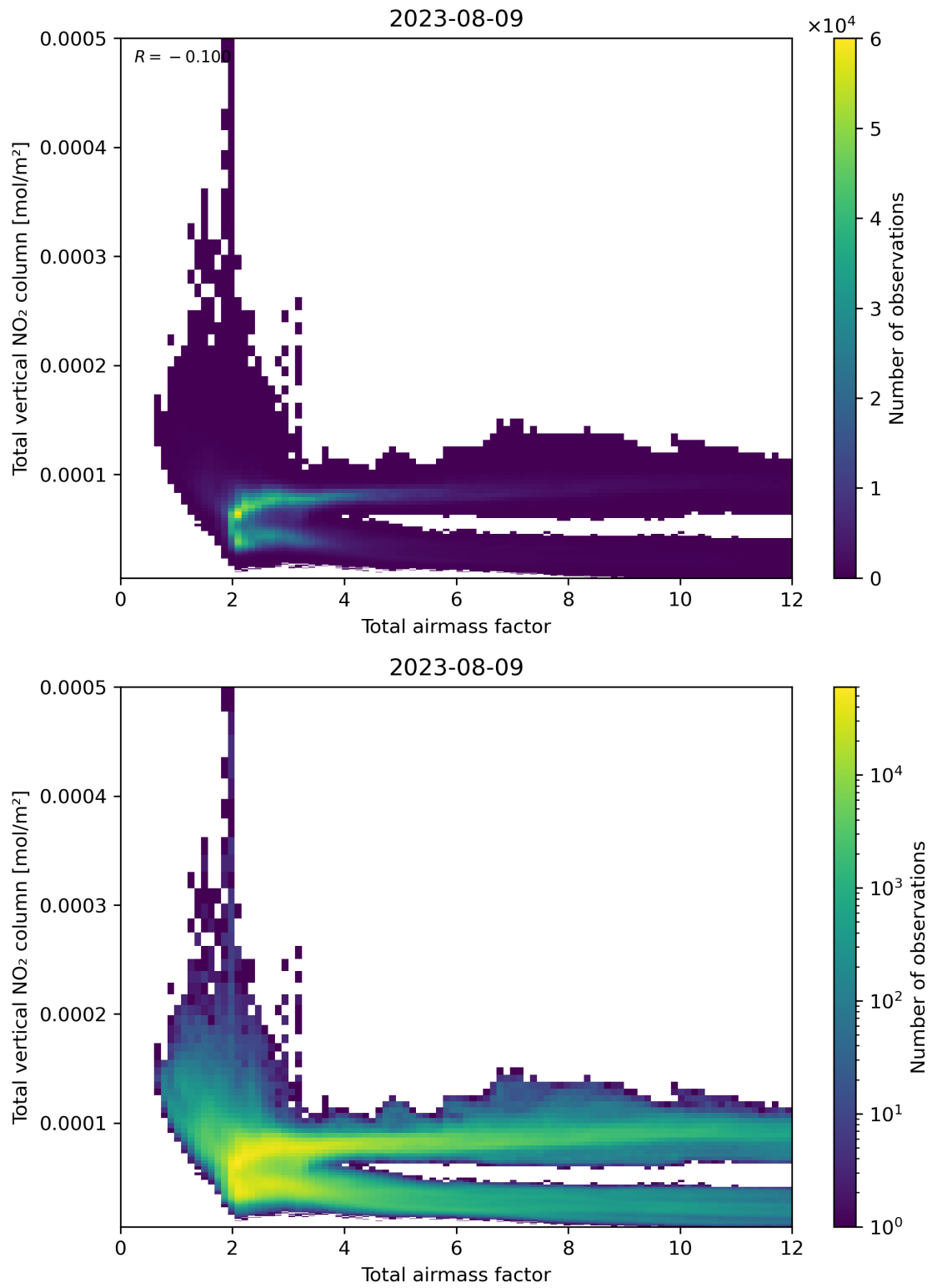
Figure 67: Scatter density plot of “Total airmass factor” against “Total vertical NO 2 column” for 2023-08-09 to 2023-08-10.
