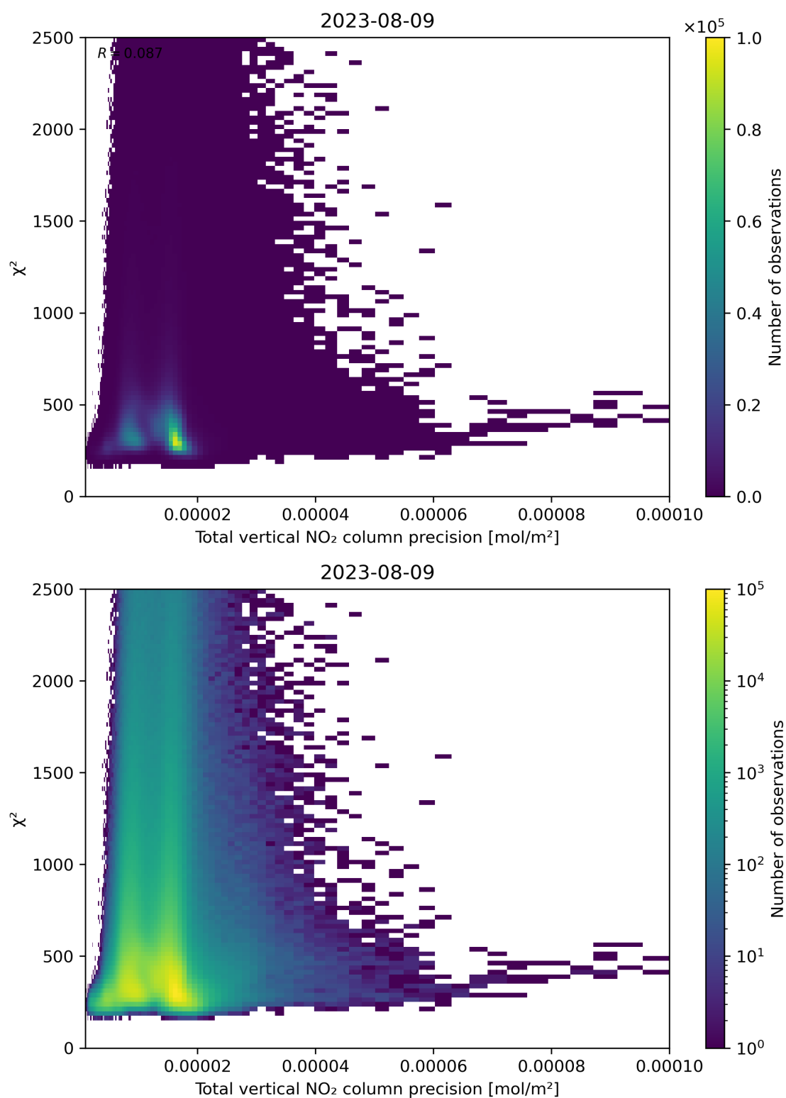
Figure 116: Scatter density plot of “Total vertical NO 2 column precision” against “ \chi^2 ” for 2023-08-09 to 2023-08-10.
