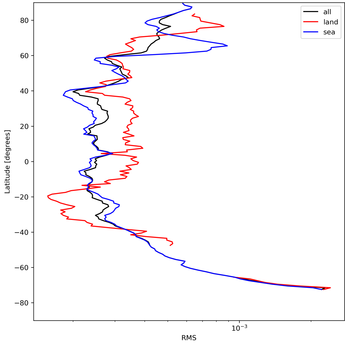
Figure 26: Zonal average of “RMS” for 2023-08-09 to 2023-08-10.
