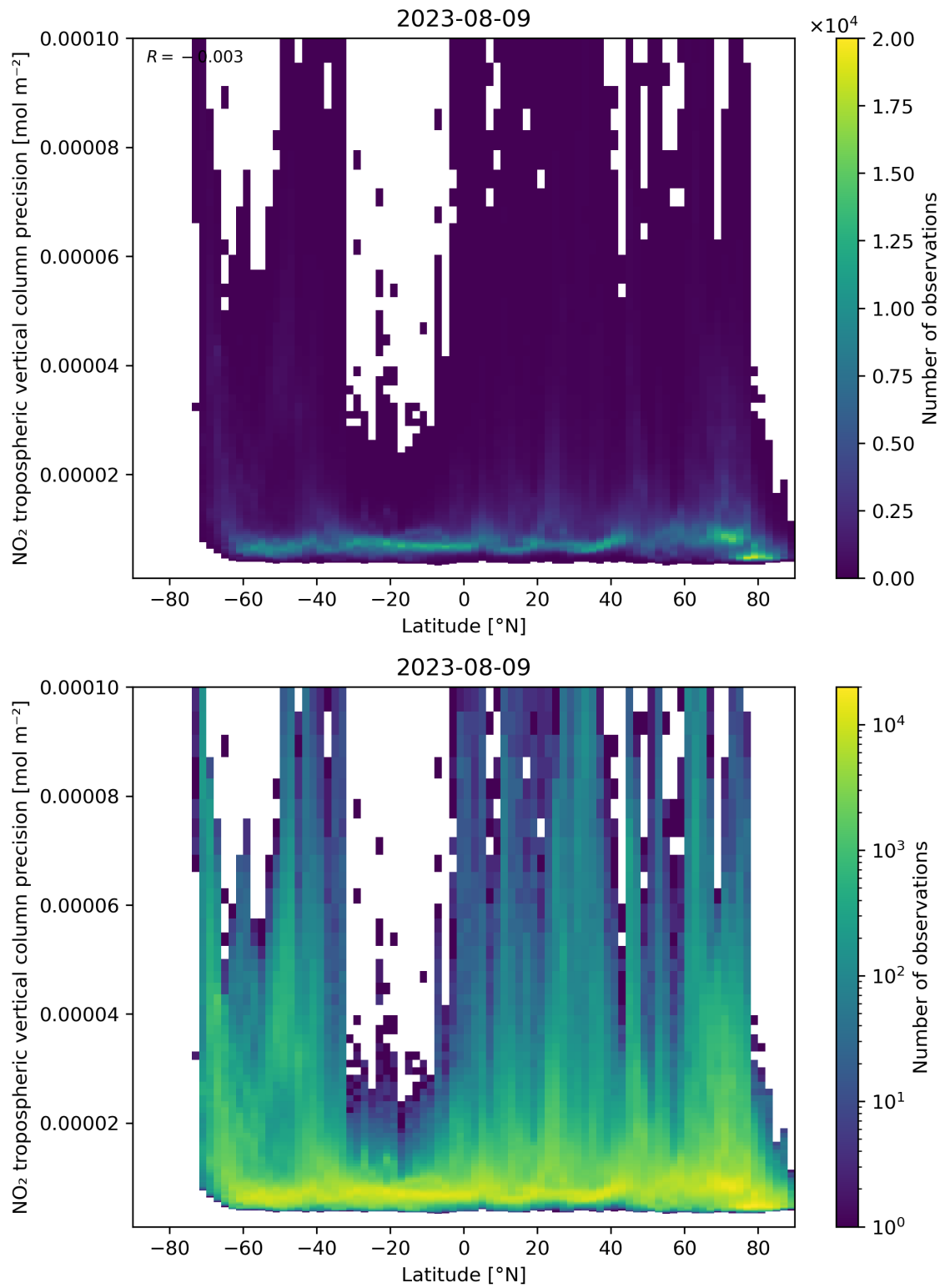
Figure 93: Scatter density plot of “Latitude” against “NO 2 tropospheric vertical column precision” for 2023-08-09 to 2023-08-10.
