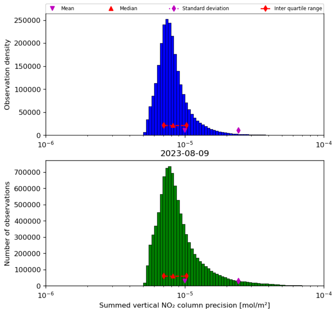
Figure 41: Histogram of “Summed vertical NO 2 column precision” for 2023-08-09 to 2023-08-10
