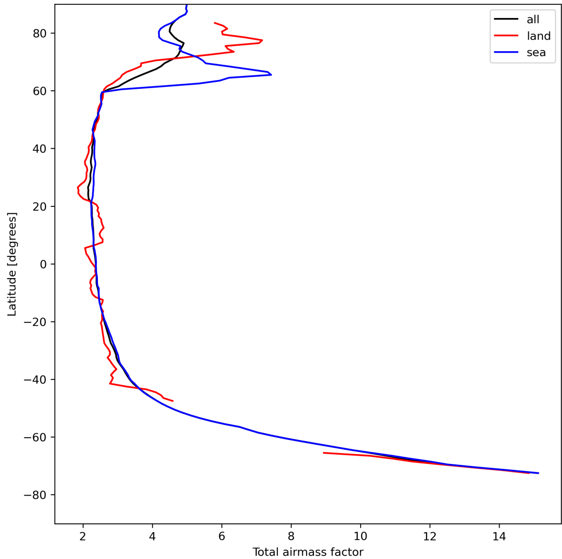
Figure 15: Zonal average of “Total airmass factor” for 2023-08-09 to 2023-08-10.
