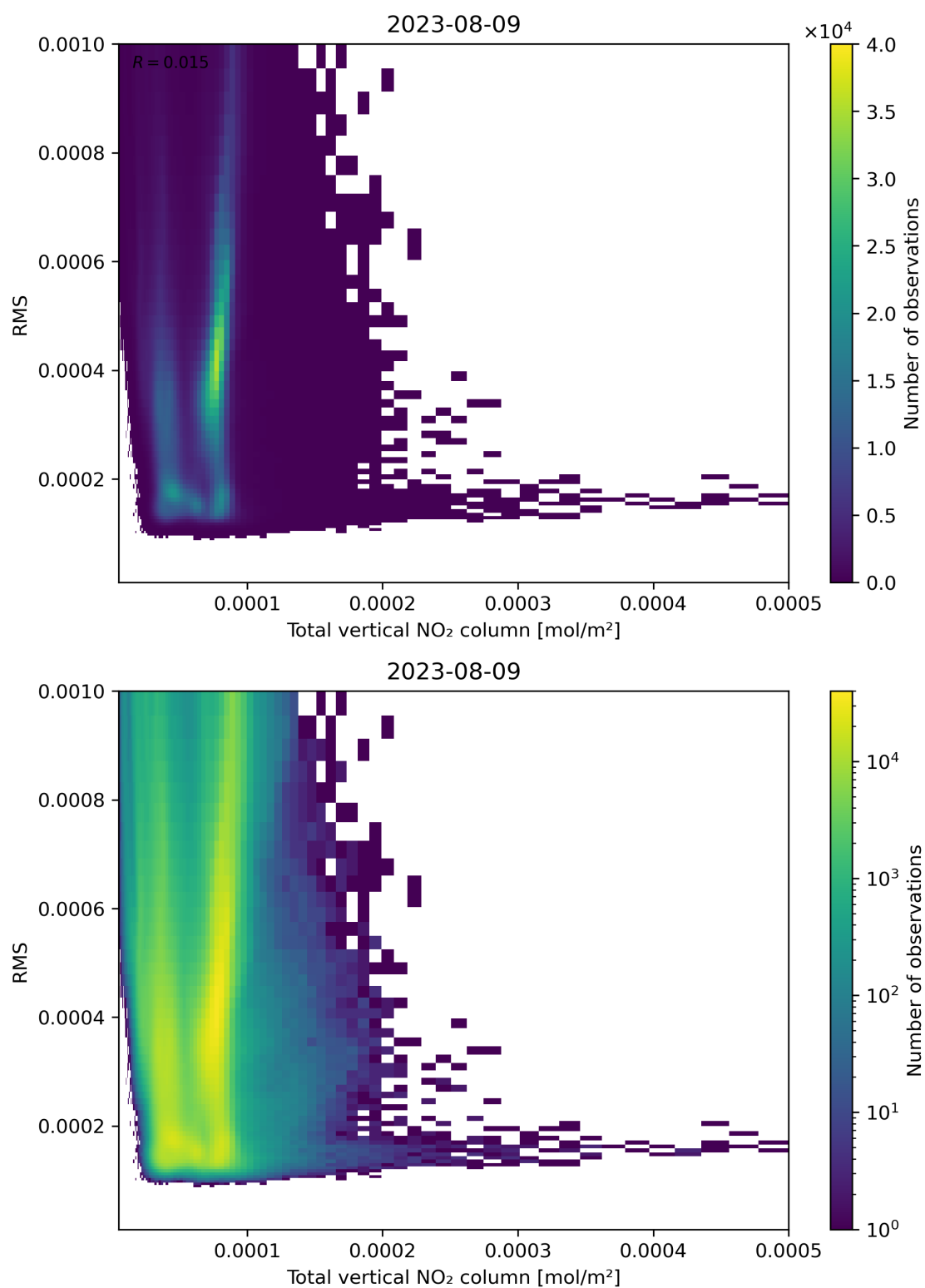
Figure 120: Scatter density plot of “Total vertical NO 2 column” against “RMS” for 2023-08-09 to 2023-08-10.
