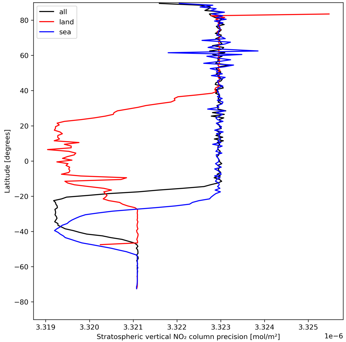
Figure 20: Zonal average of “Stratospheric vertical NO 2 column precision” for 2023-08-09 to 2023-08-10.
