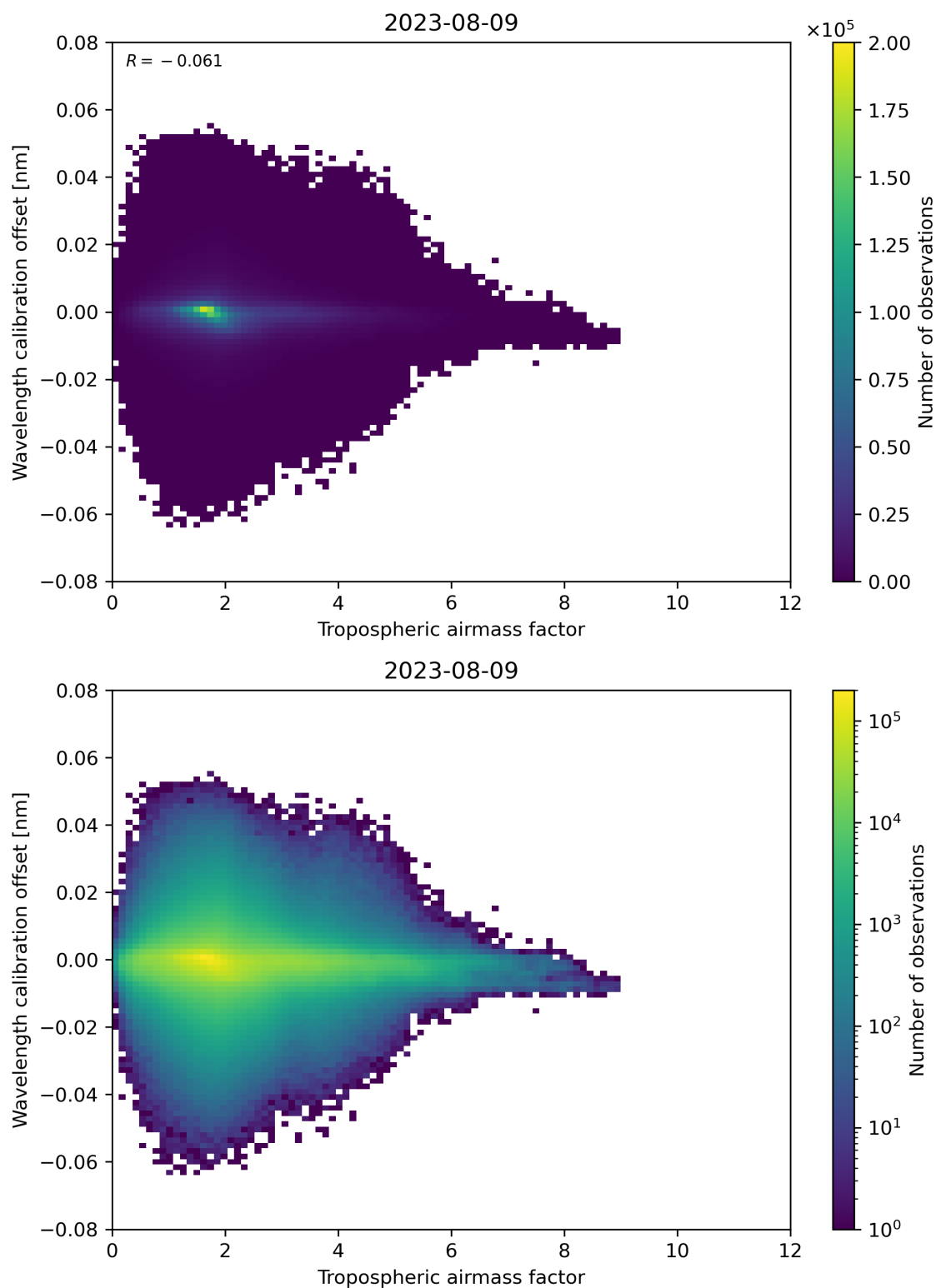
Figure 80: Scatter density plot of “Tropospheric airmass factor” against “Wavelength calibration offset” for 2023-08-09 to 2023-08-10.
