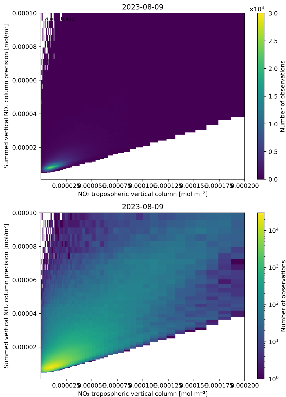
Figure 127: Scatter density plot of “NO 2 tropospheric vertical column” against “Summed vertical NO 2 column precision” for 2023-08-09 to 2023-08-10.
