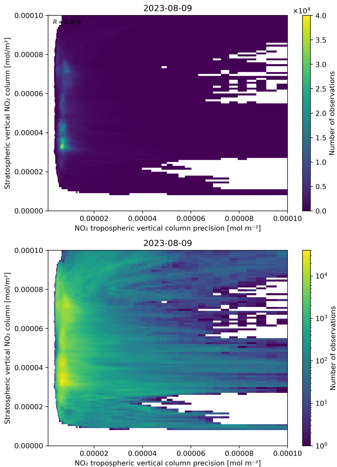
Figure 135: Scatter density plot of “NO 2 tropospheric vertical column precision” against “Stratospheric vertical NO 2 column” for 2023-08-09 to 2023-08-10.
