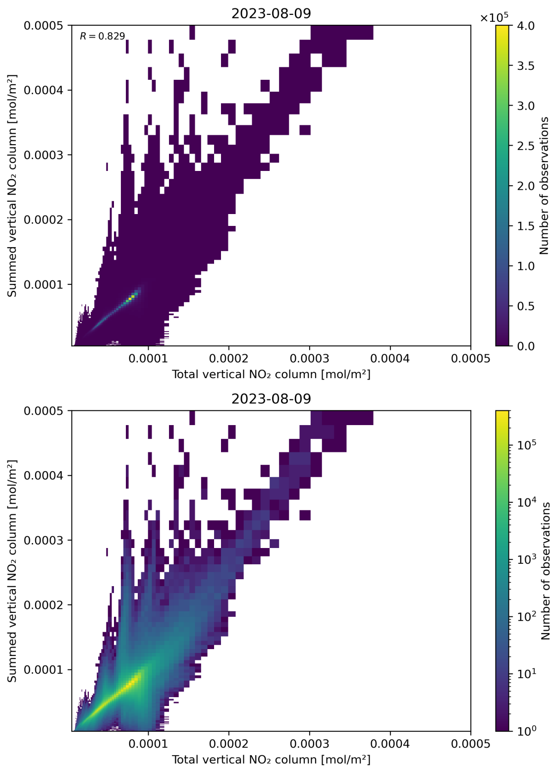
Figure 112: Scatter density plot of “Total vertical NO 2 column” against “Summed vertical NO 2 column” for 2023-08-09 to 2023-08-10.
