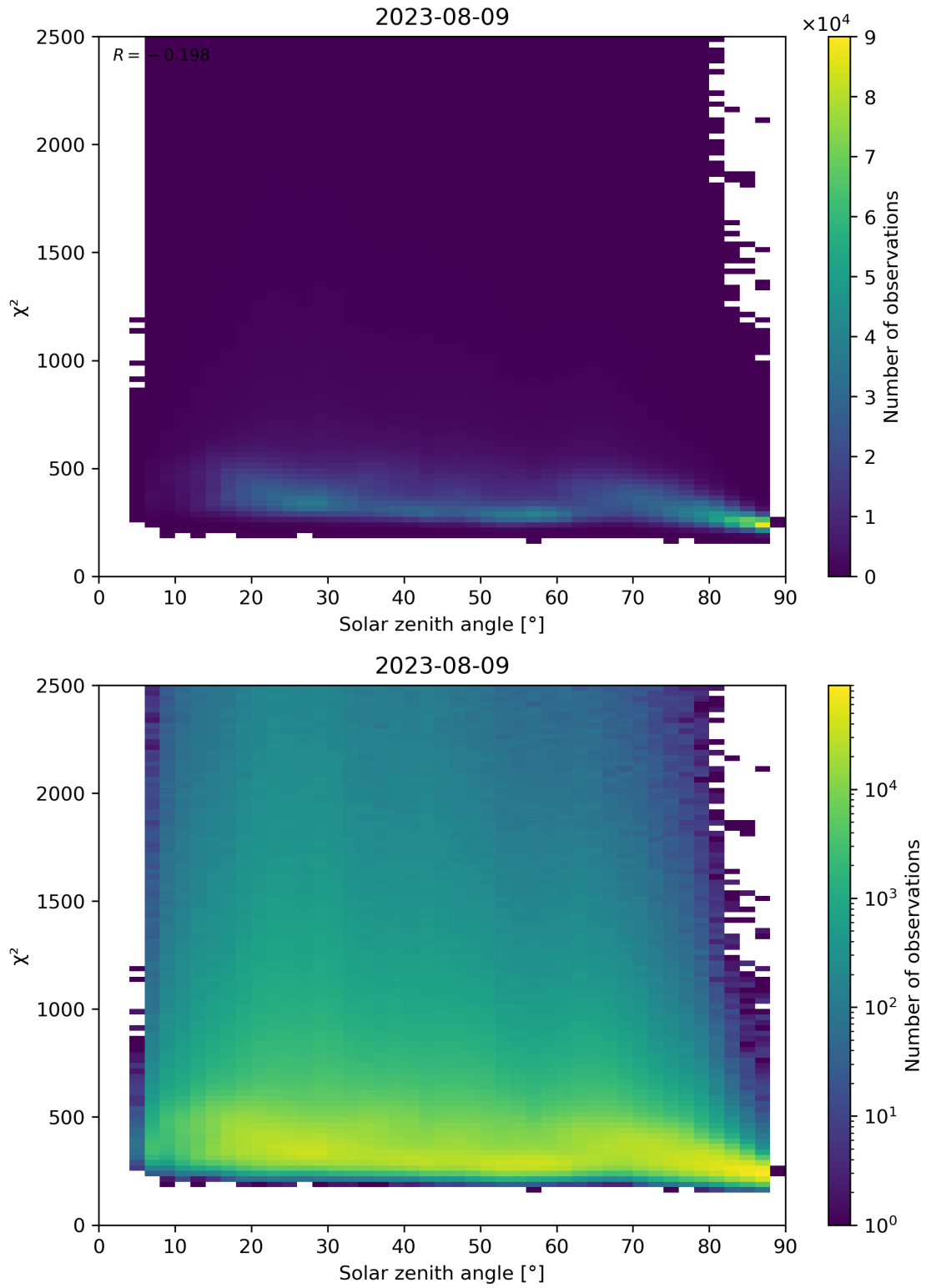
Figure 148: Scatter density plot of “Solar zenith angle” against “ \chi^2 ” for 2023-08-09 to 2023-08-10.
