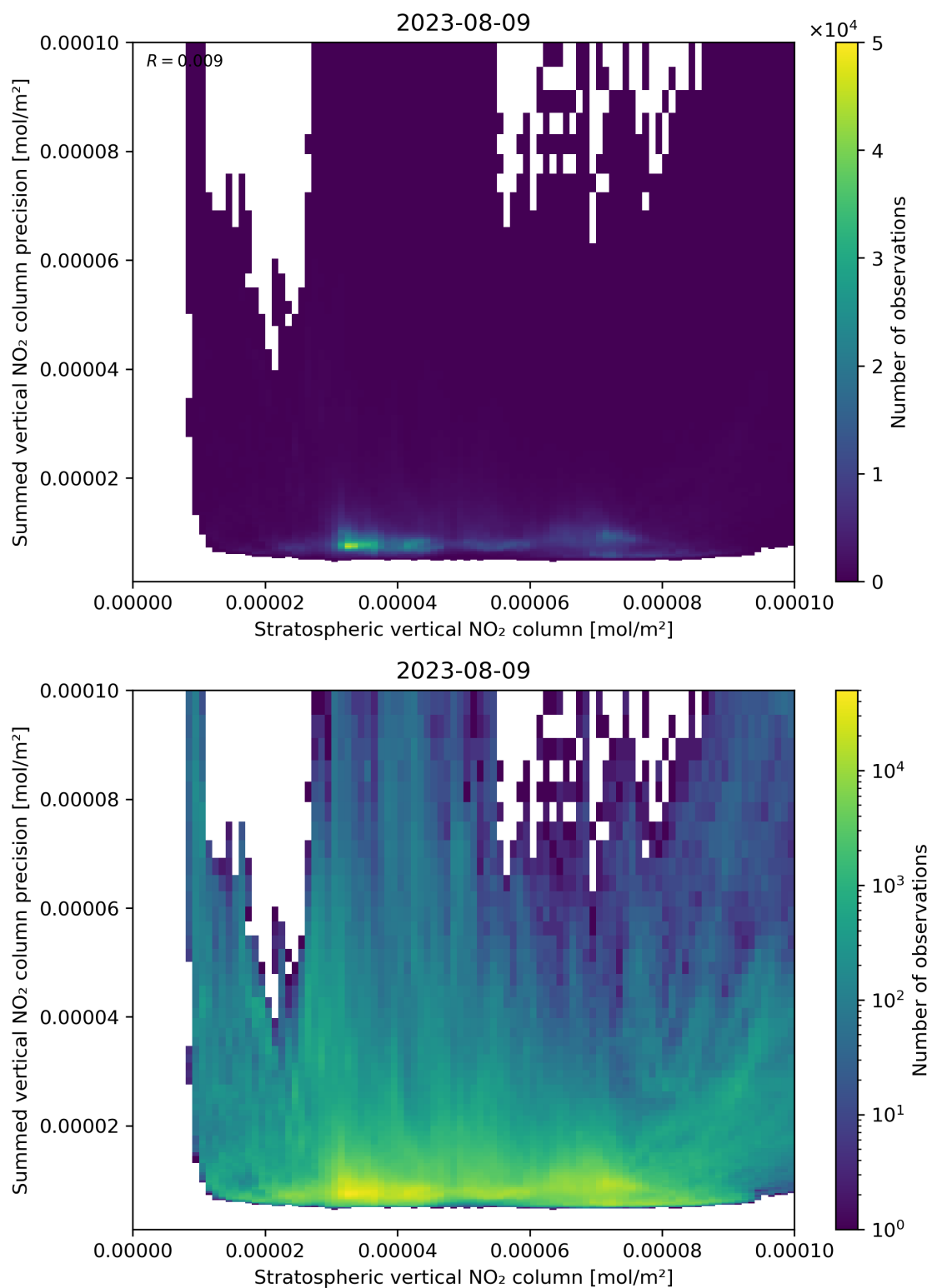
Figure 99: Scatter density plot of “Stratospheric vertical NO 2 column” against “Summed vertical NO 2 column precision” for 2023-08-09 to 2023-08-10.
