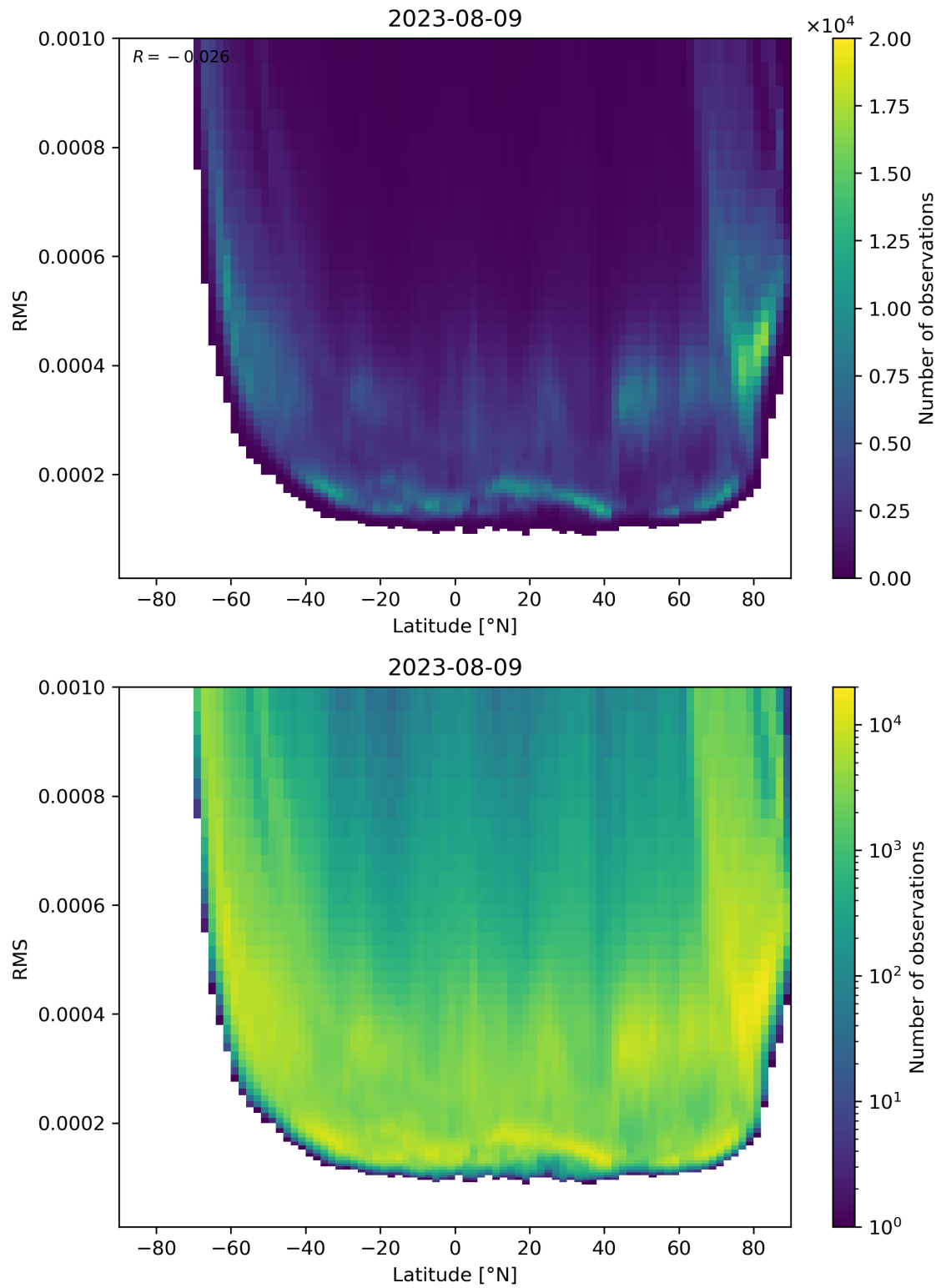
Figure 94: Scatter density plot of “Latitude” against “RMS” for 2023-08-09 to 2023-08-10.
