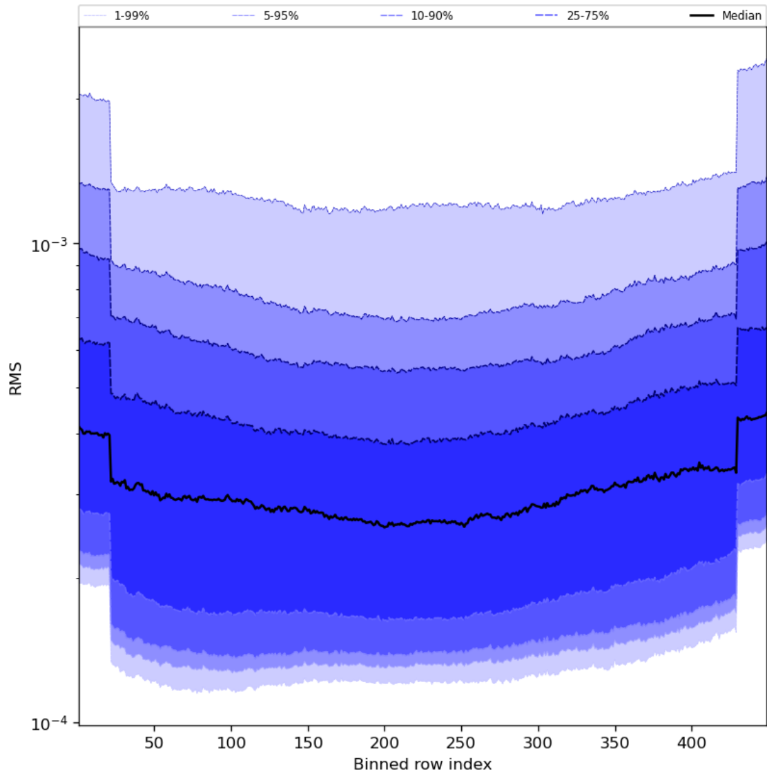
Figure 60: Along track statistics of “RMS” for 2023-08-09 to 2023-08-10
