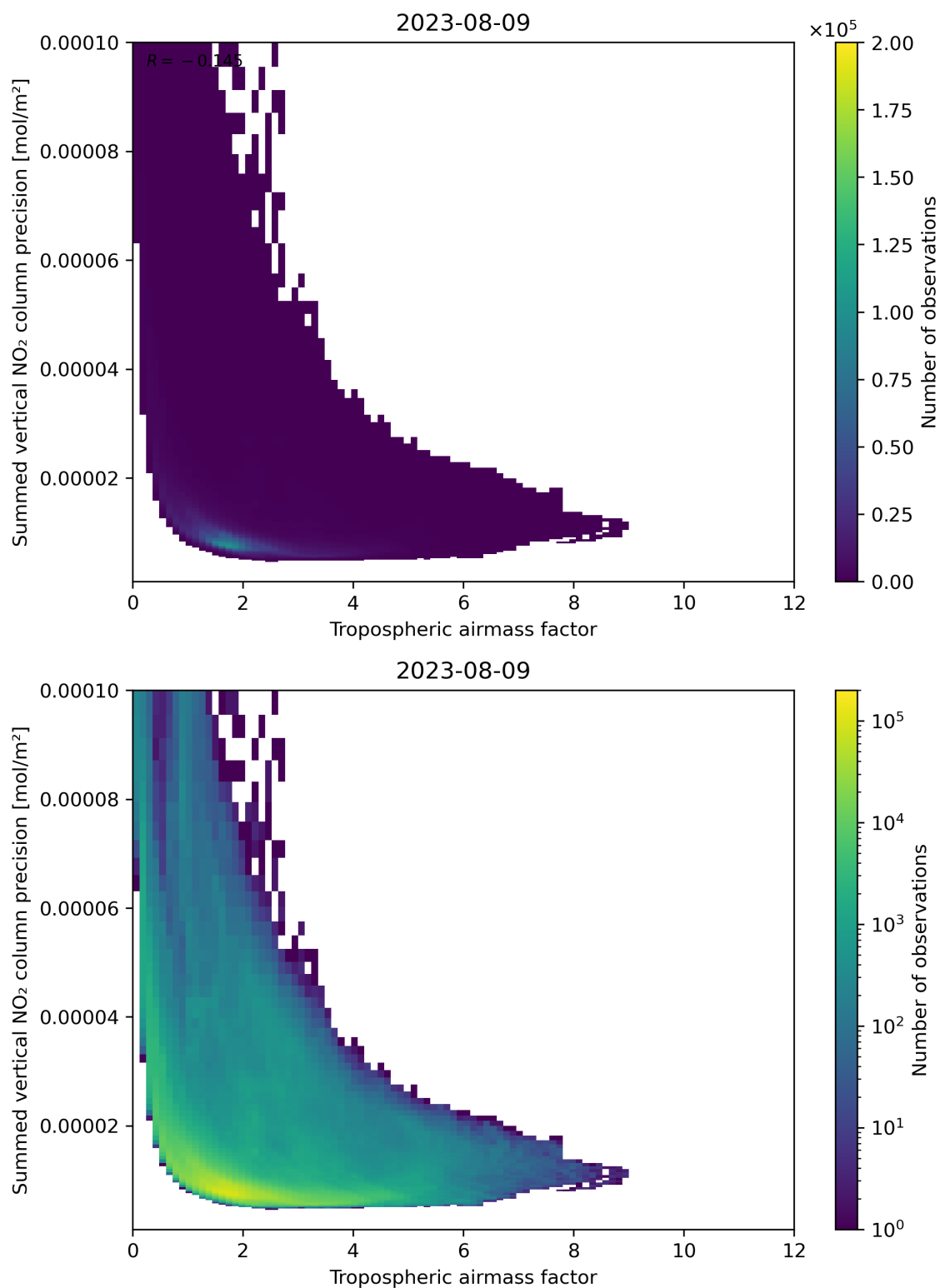
Figure 76: Scatter density plot of “Tropospheric air mass factor” against “Summed vertical NO 2 column precision” for 2023-08-09 to 2023-08-10.
