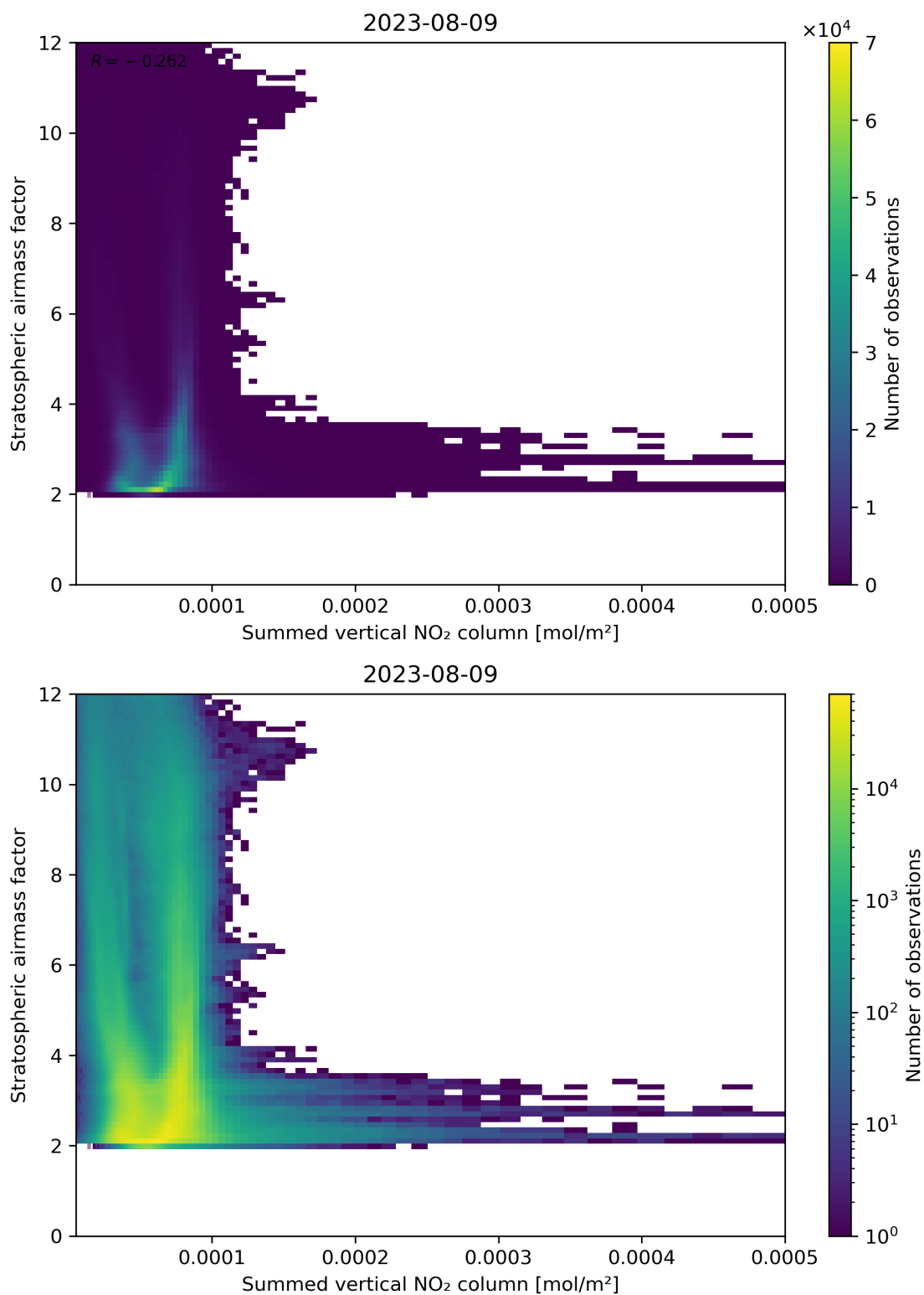
Figure 103: Scatter density plot of “Summed vertical NO 2 column” against “Stratospheric air mass factor” for 2023-08-09 to 2023-08-10.
