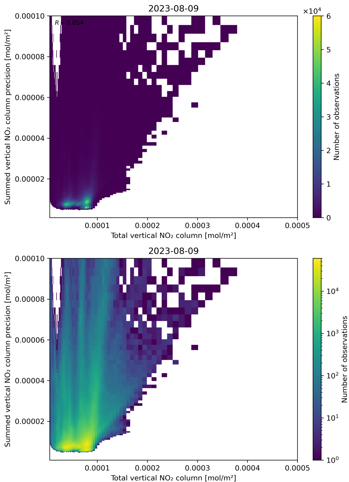
Figure 113: Scatter density plot of “Total vertical NO 2 column” against “Summed vertical NO 2 column precision” for 2023-08-09 to 2023-08-10.
