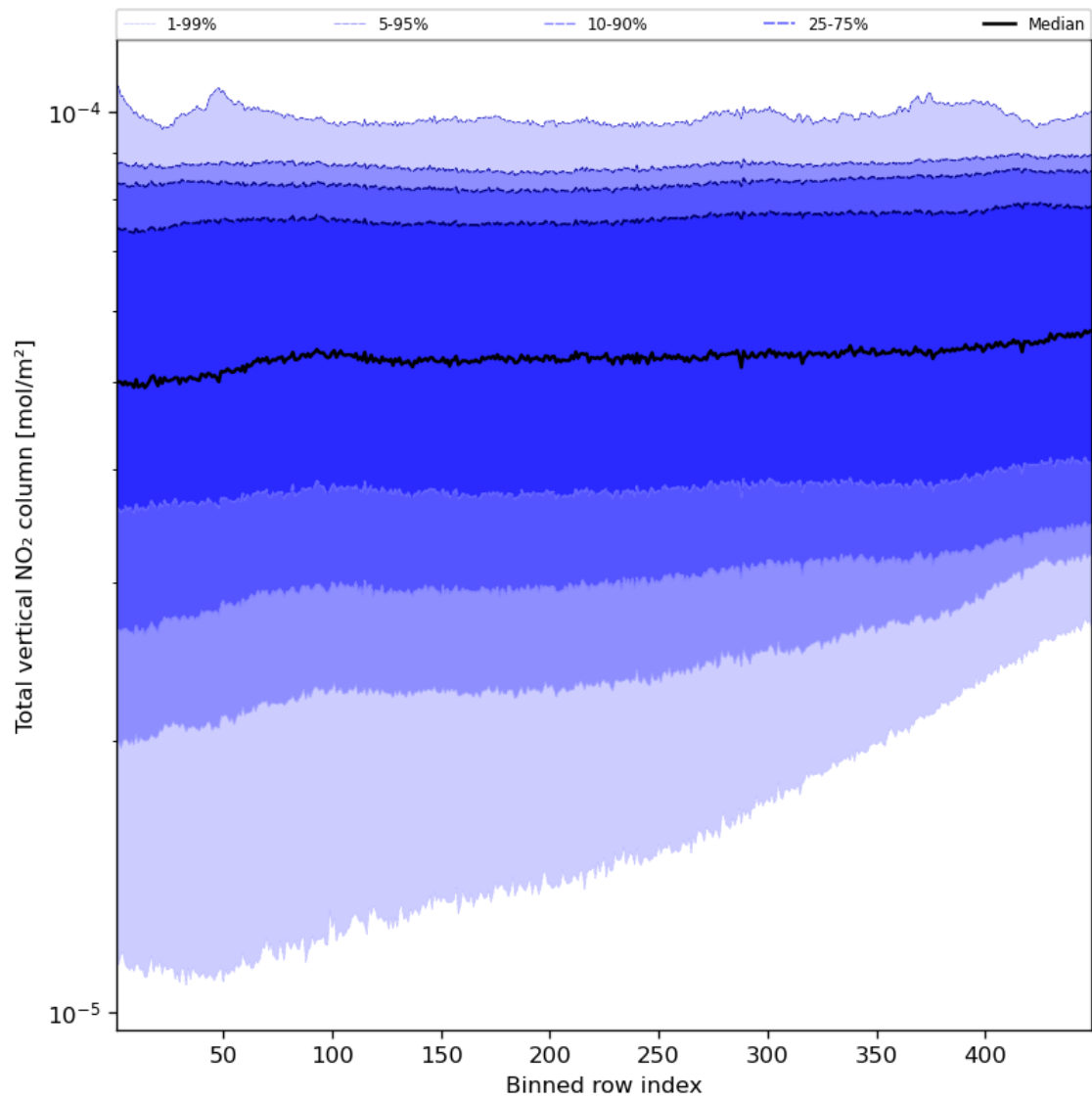
Figure 55: Along track statistics of “Total vertical NO 2 column” for 2023-08-09 to 2023-08-10
