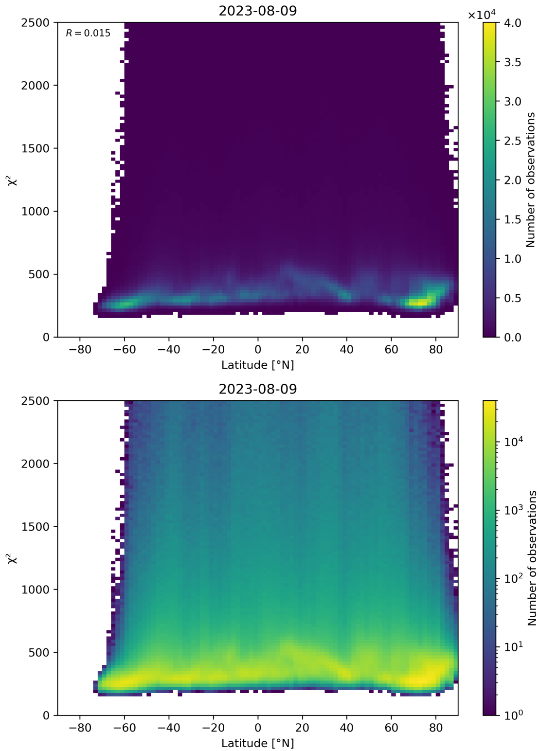
Figure 86: Scatter density plot of “Latitude” against “ \chi^2 ” for 2023-08-09 to 2023-08-10.
