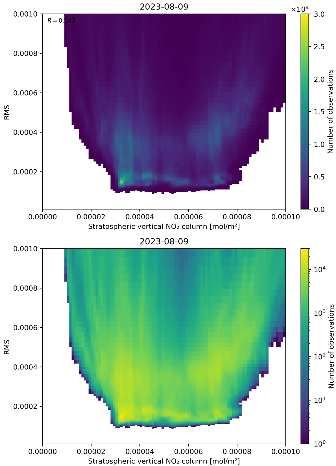
Figure 102: Scatter density plot of “Stratospheric vertical NO 2 column” against “RMS” for 2023-08-09 to 2023-08-10.
