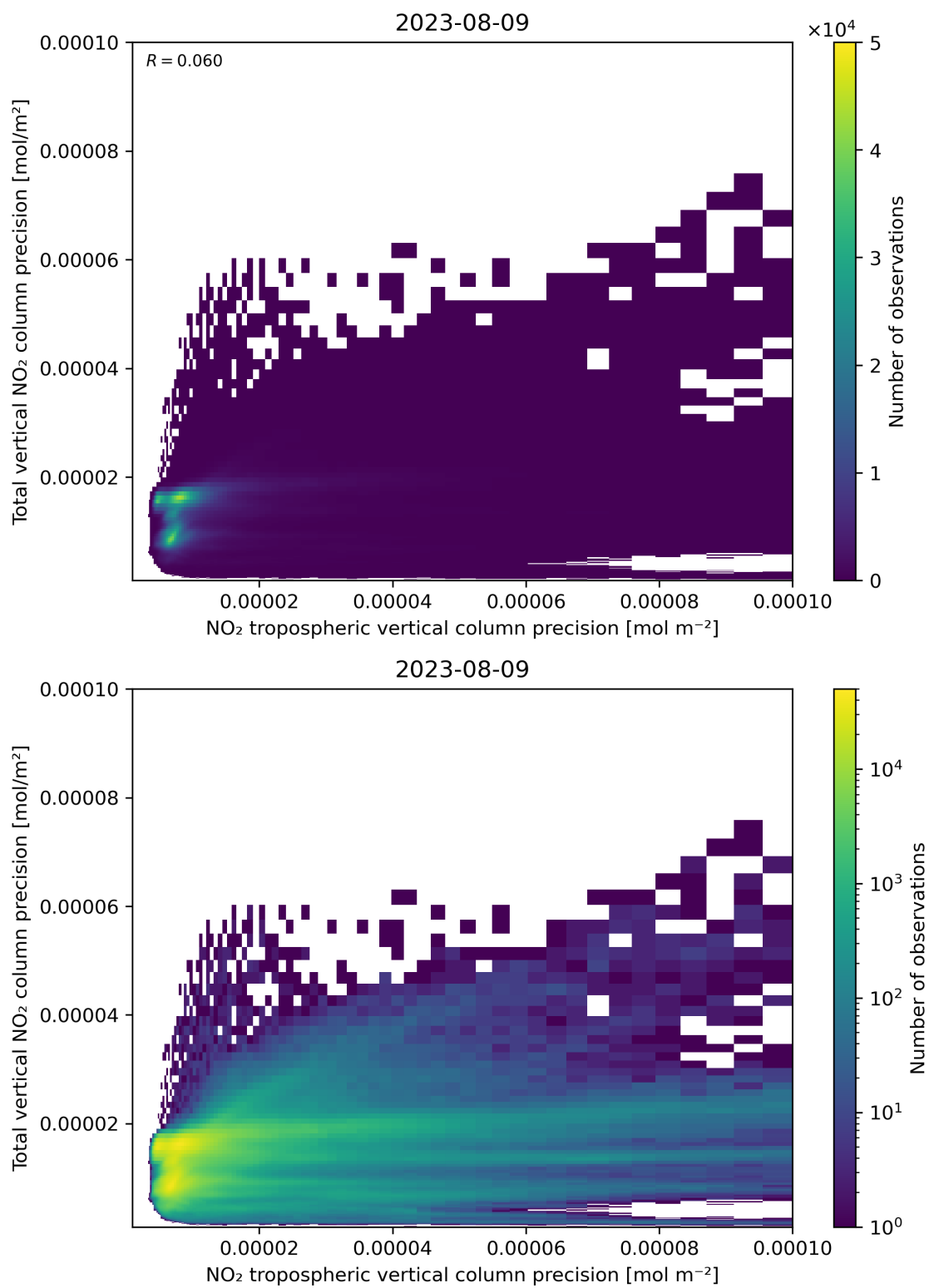
Figure 139: Scatter density plot of “NO 2 tropospheric vertical column precision” against “Total vertical NO 2 column precision” for 2023-08-09 to 2023-08-10.
