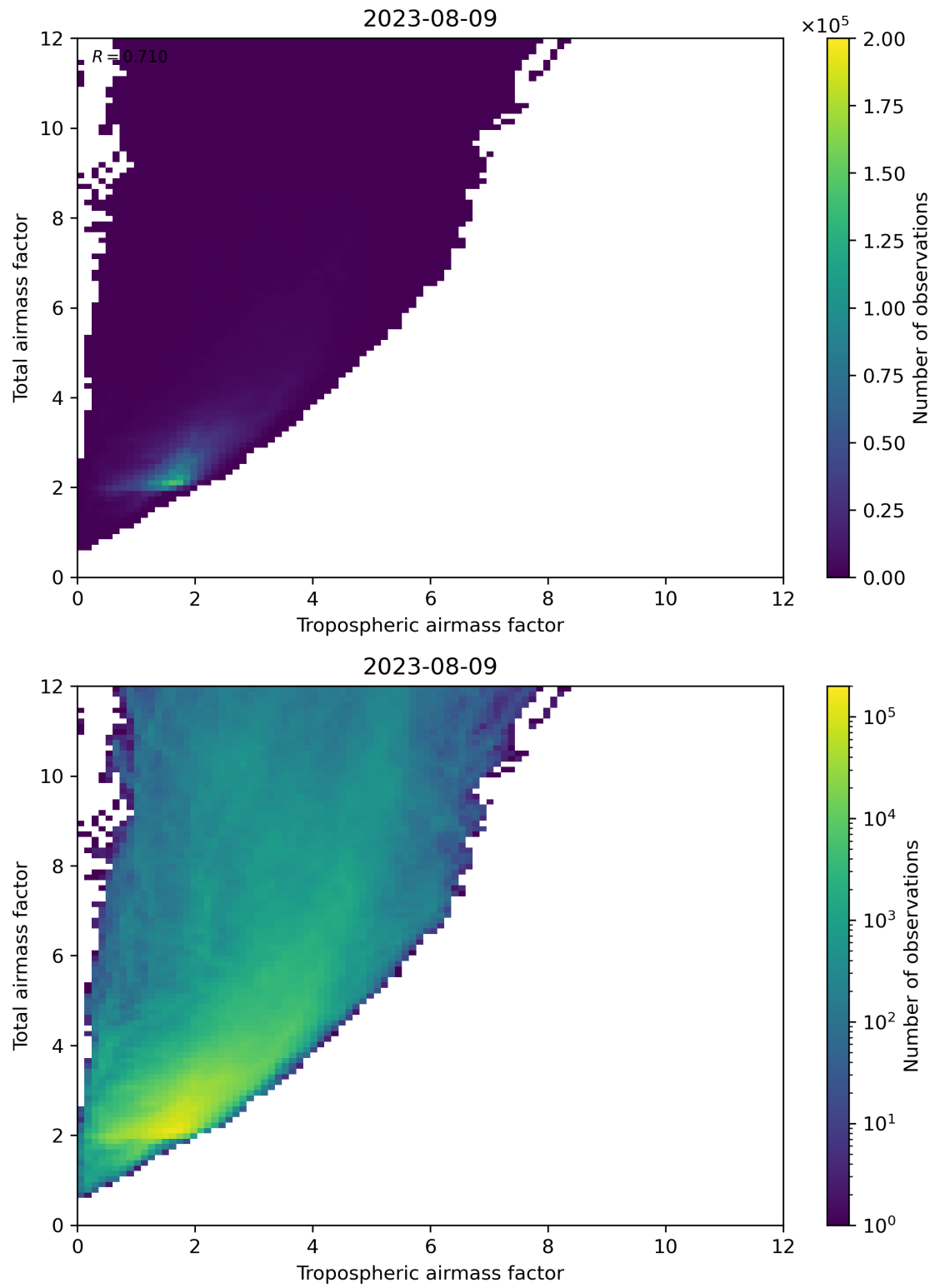
Figure 72: Scatter density plot of “Tropospheric airmass factor” against “Total airmass factor” for 2023-08-09 to 2023-08-10.
