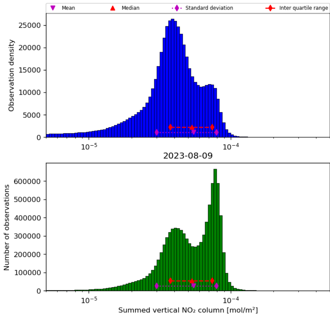
Figure 40: Histogram of “Summed vertical NO 2 column” for 2023-08-09 to 2023-08-10
