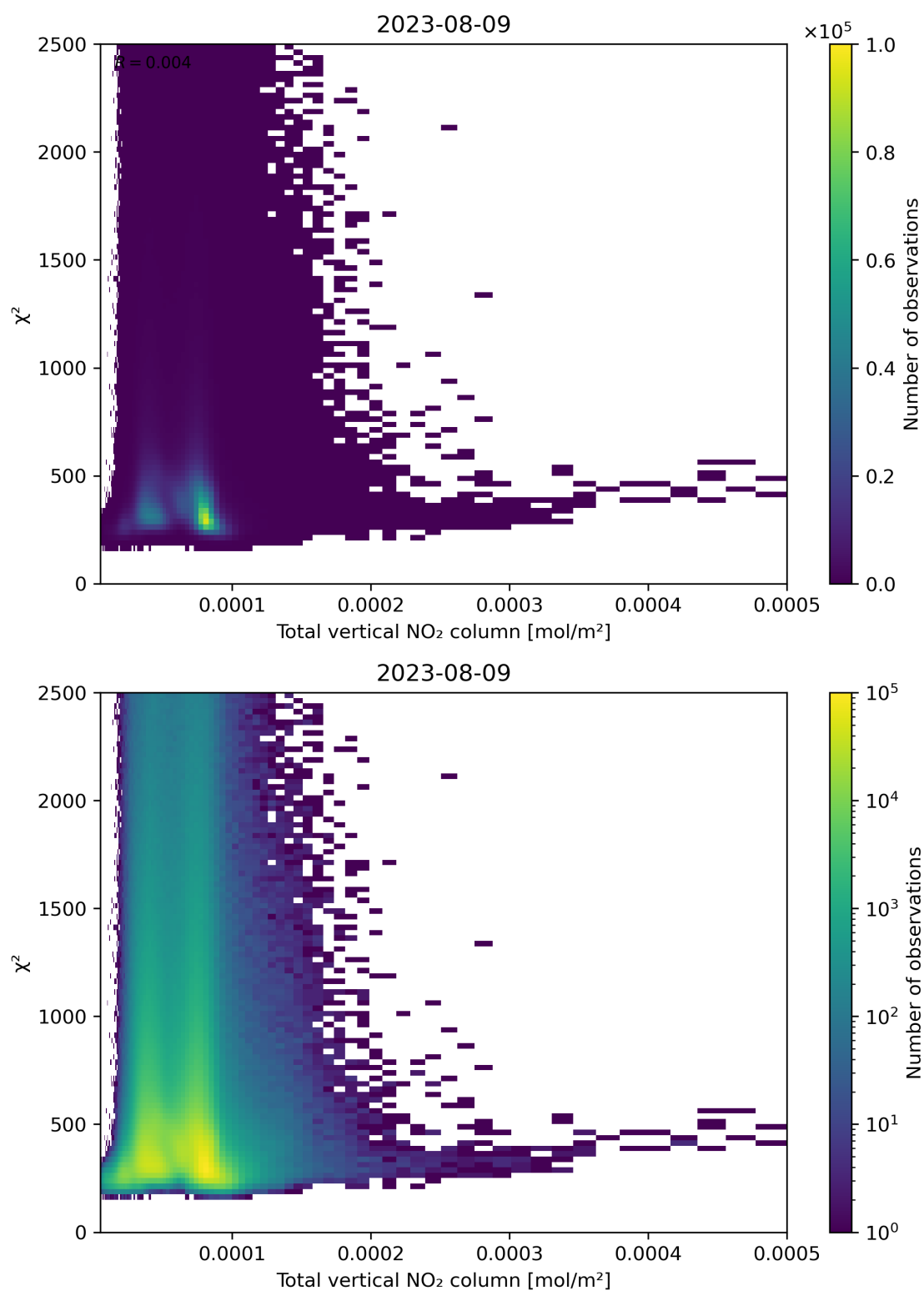
Figure 111: Scatter density plot of “Total vertical NO 2 column” against “ \chi^2 ” for 2023-08-09 to 2023-08-10.
