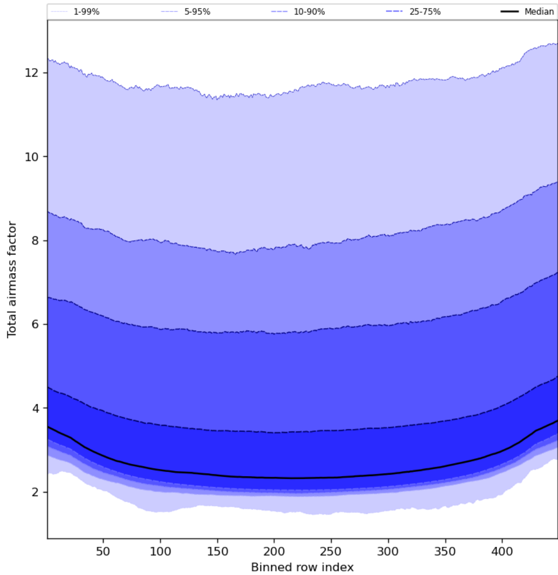
Figure 49: Along track statistics of “Total airmass factor” for 2023-08-09 to 2023-08-10
