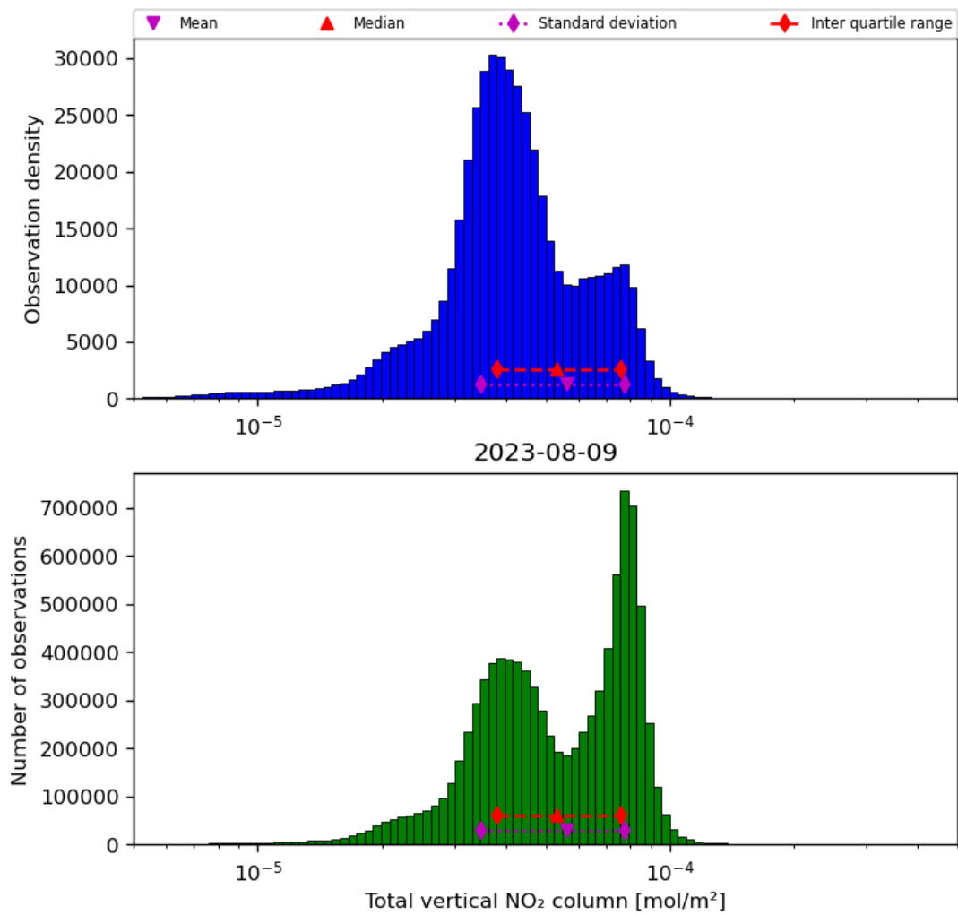
Figure 38: Histogram of “Total vertical NO 2 column” for 2023-08-09 to 2023-08-10
