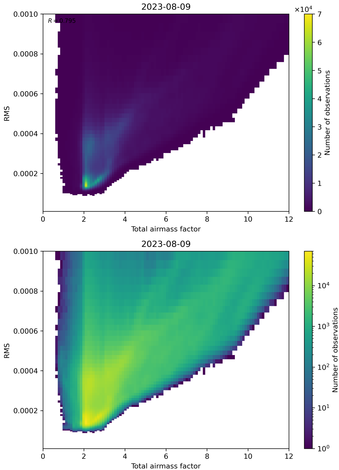
Figure 69: Scatter density plot of “Total airmass factor” against “RMS” for 2023-08-09 to 2023-08-10.
