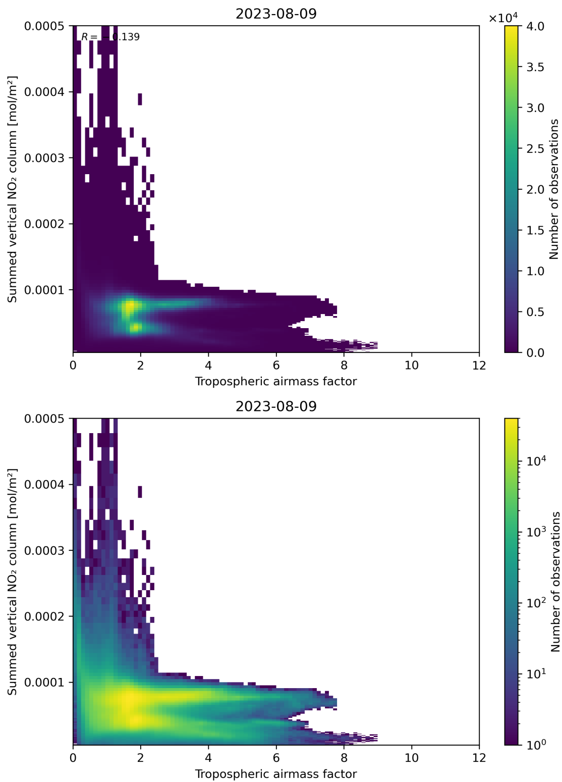
Figure 75: Scatter density plot of “Tropospheric air mass factor” against “Summed vertical NO 2 column” for 2023-08-09 to 2023-08-10.
