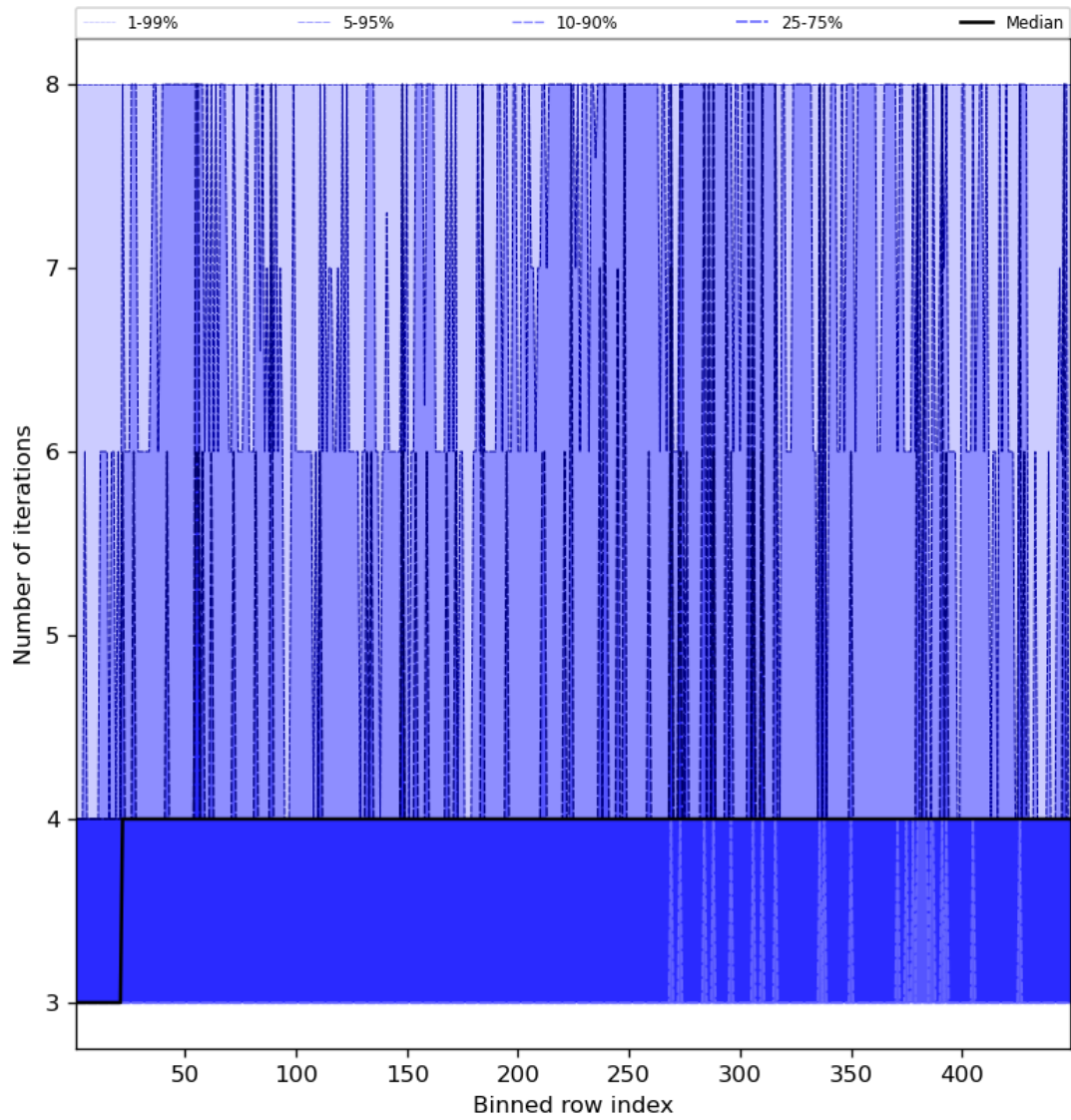
Figure 51: Along track statistics of “Number of iterations” for 2023-08-09 to 2023-08-10
