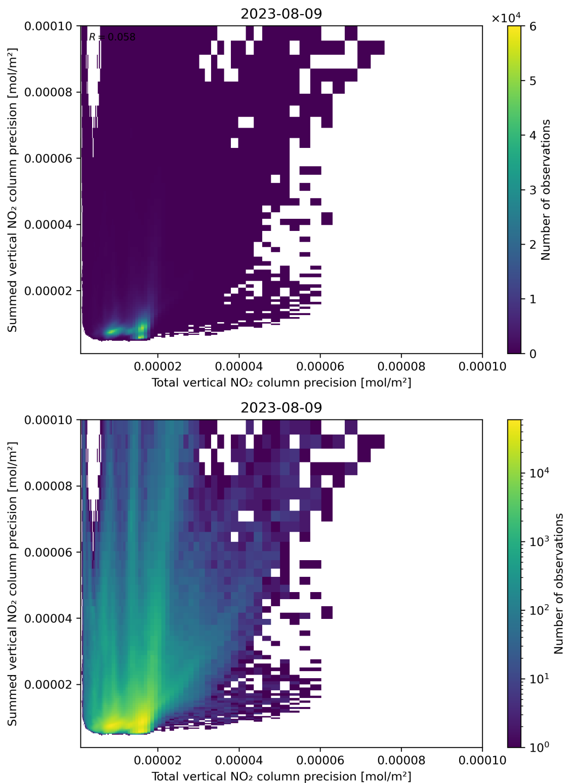
Figure 118: Scatter density plot of “Total vertical NO 2 column precision” against “Summed vertical NO 2 column precision” for 2023-08-09 to 2023-08-10.
