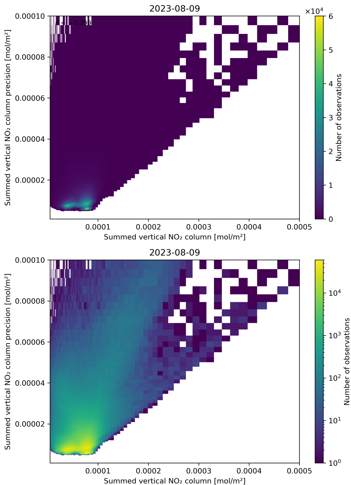
Figure 105: Scatter density plot of “Summed vertical NO 2 column” against “Summed vertical NO 2 column precision” for 2023-08-09 to 2023-08-10.
