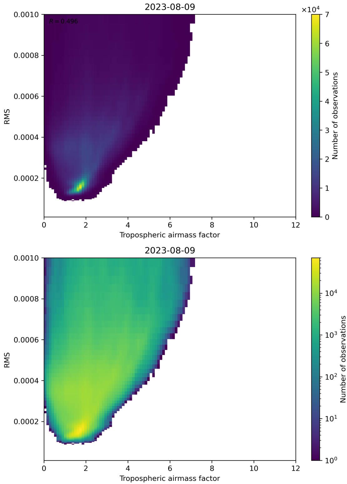
Figure 79: Scatter density plot of “Tropospheric airmass factor” against “RMS” for 2023-08-09 to 2023-08-10.
