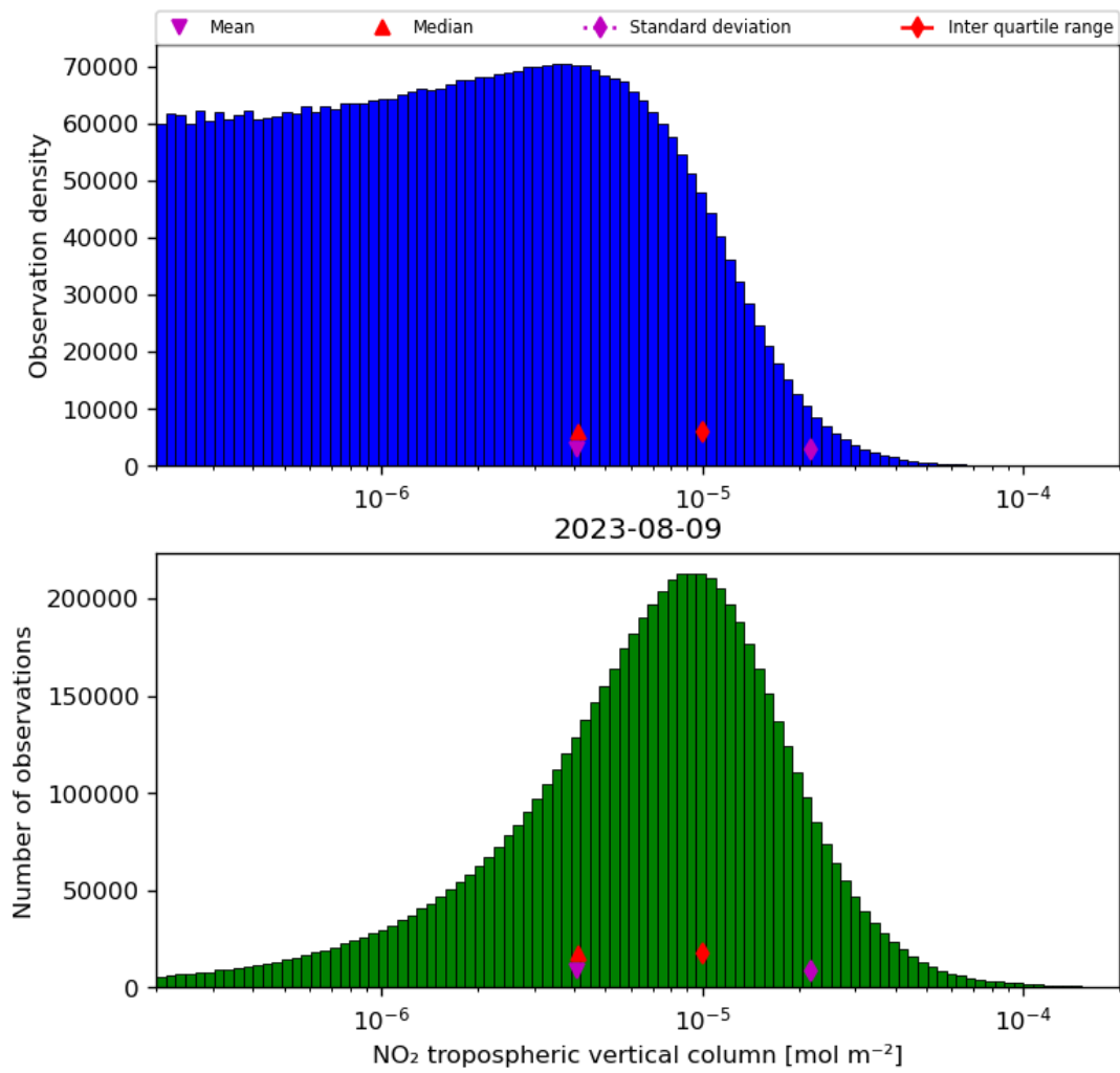
Figure 29: Histogram of “NO 2 tropospheric vertical column” for 2023-08-09 to 2023-08-10
