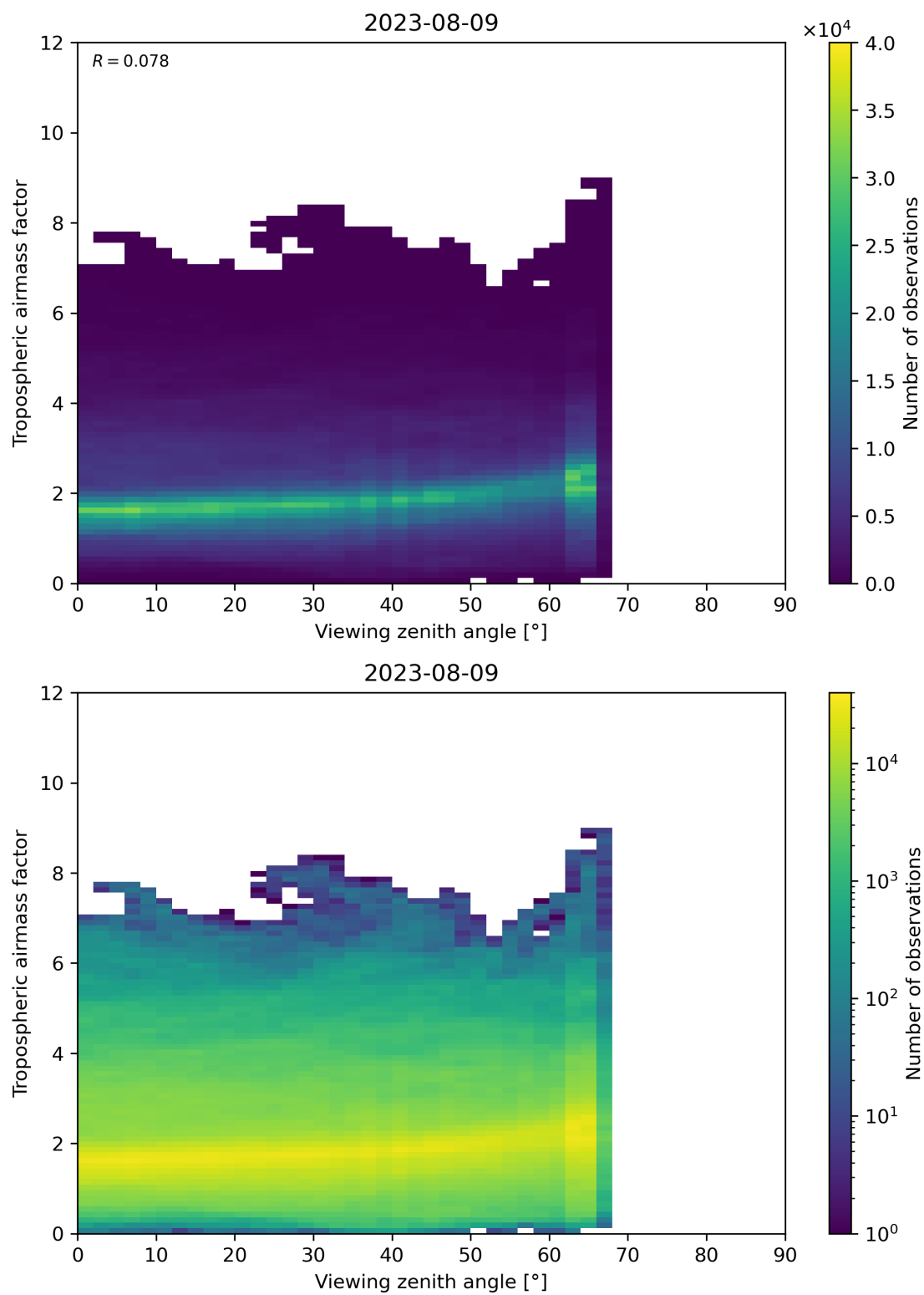
Figure 161: Scatter density plot of “Viewing zenith angle” against “Tropospheric airmass factor” for 2023-08-09 to 2023-08-10.
