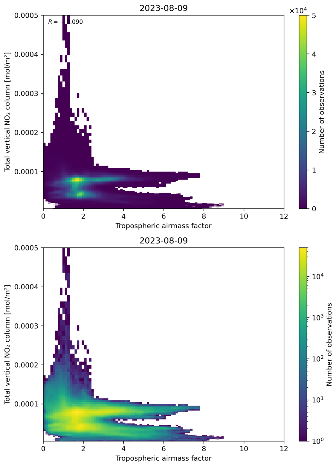
Figure 77: Scatter density plot of “Tropospheric airmass factor” against “Total vertical NO 2 column” for 2023-08-09 to 2023-08-10.
