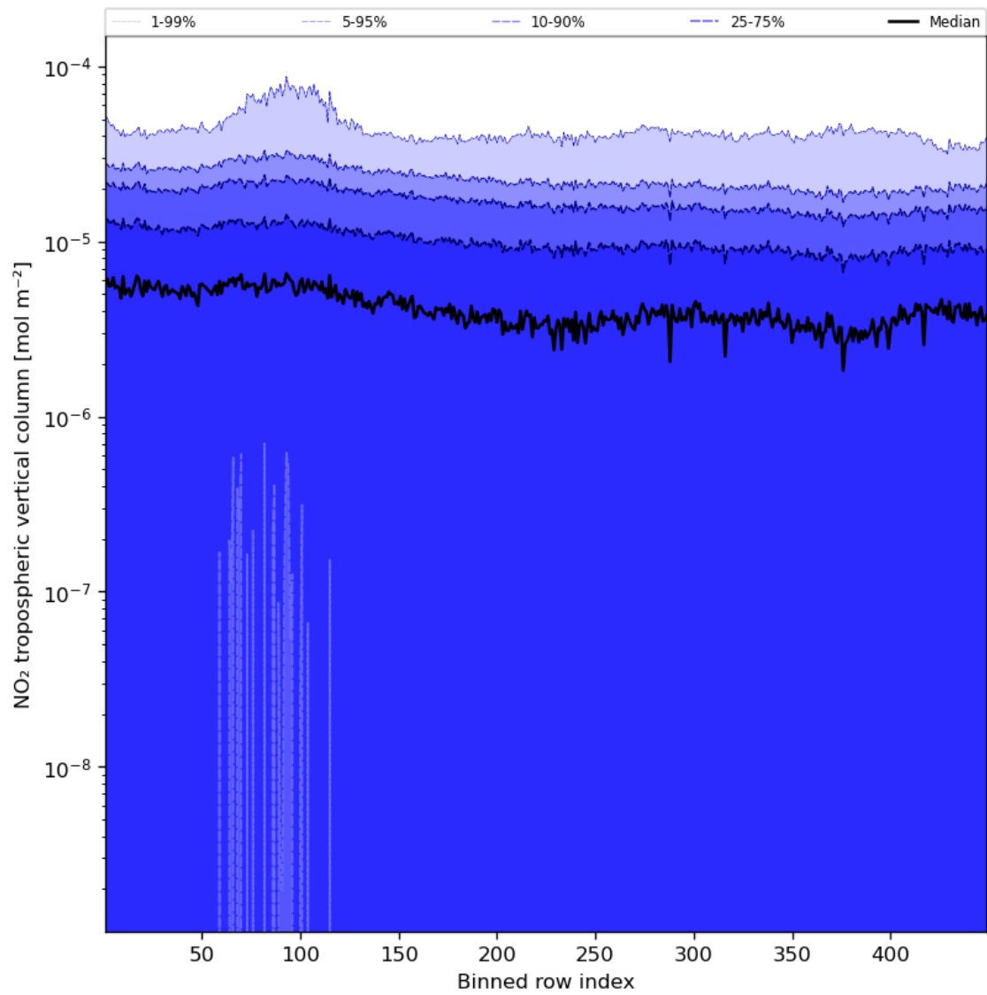
Figure 46: Along track statistics of “ \text{NO}_2 tropospheric vertical column” for 2023-08-09 to 2023-08-10
