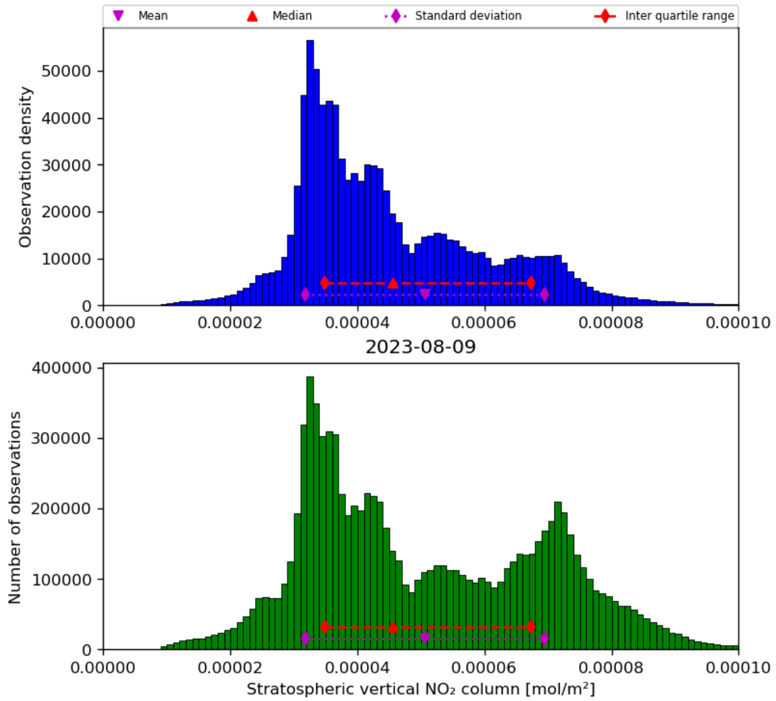
Figure 36: Histogram of “Stratospheric vertical NO 2 column” for 2023-08-09 to 2023-08-10
