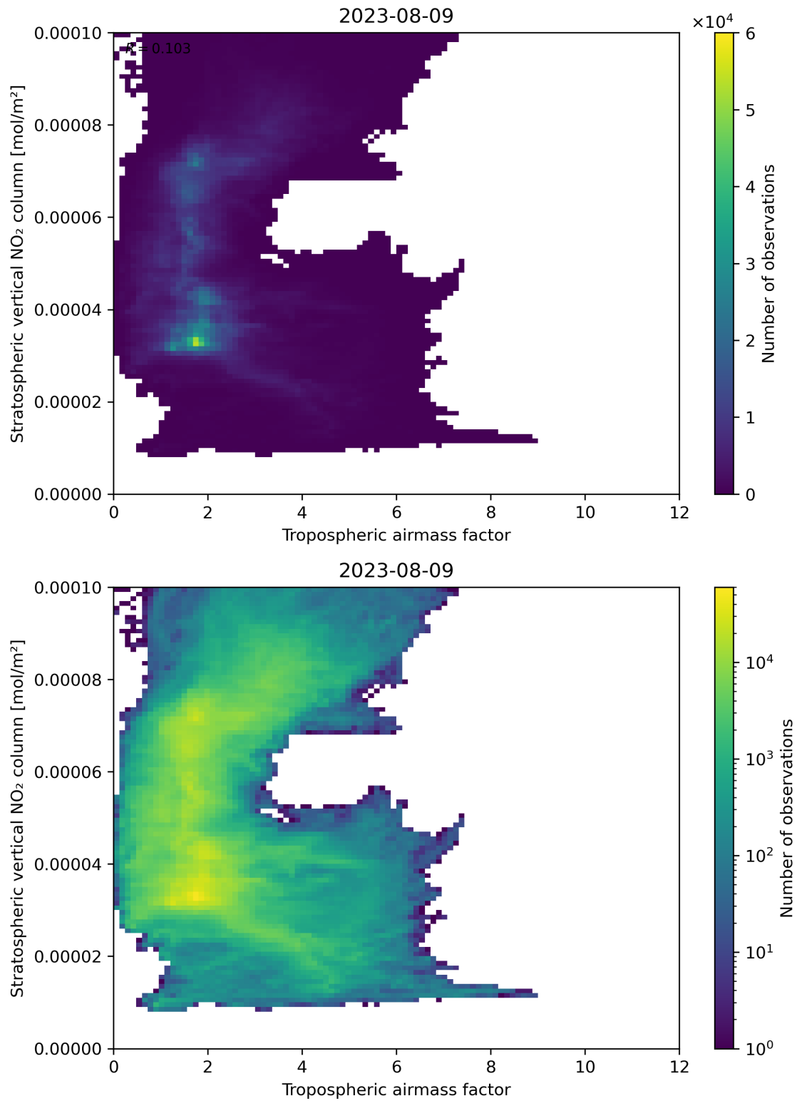
Figure 74: Scatter density plot of “Tropospheric air mass factor” against “Stratospheric vertical NO 2 column” for 2023-08-09 to 2023-08-10.
