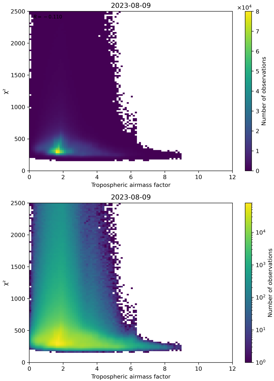
Figure 73: Scatter density plot of “Tropospheric airmass factor” against “ \chi^2 ” for 2023-08-09 to 2023-08-10.
