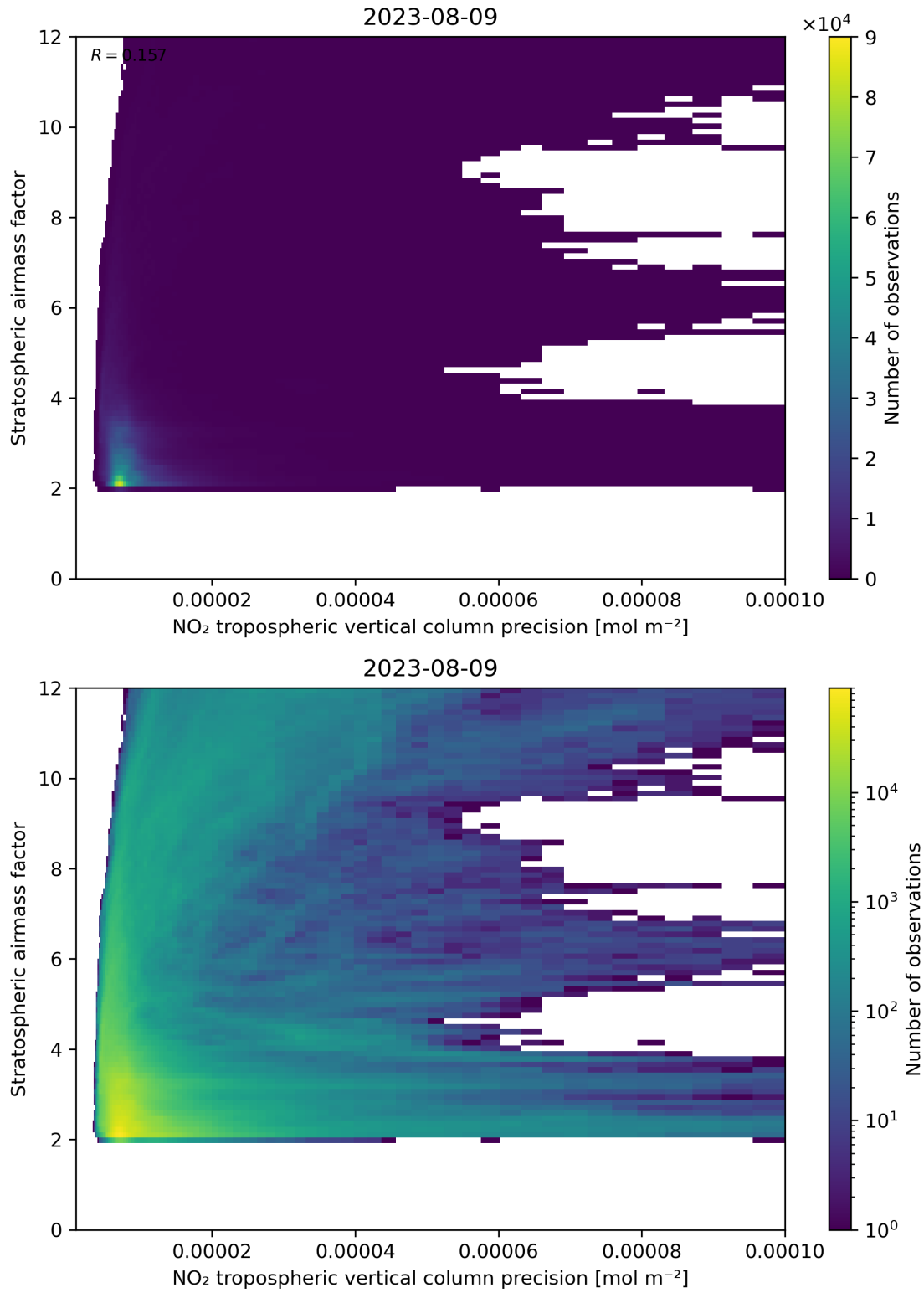
Figure 131: Scatter density plot of “NO 2 tropospheric vertical column precision” against “Stratospheric airmass factor” for 2023-08-09 to 2023-08-10.
