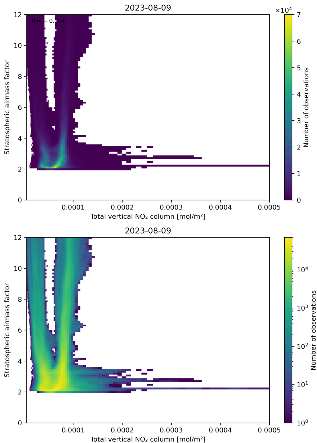
Figure 110: Scatter density plot of “Total vertical NO 2 column” against “Stratospheric air mass factor” for 2023-08-09 to 2023-08-10.
