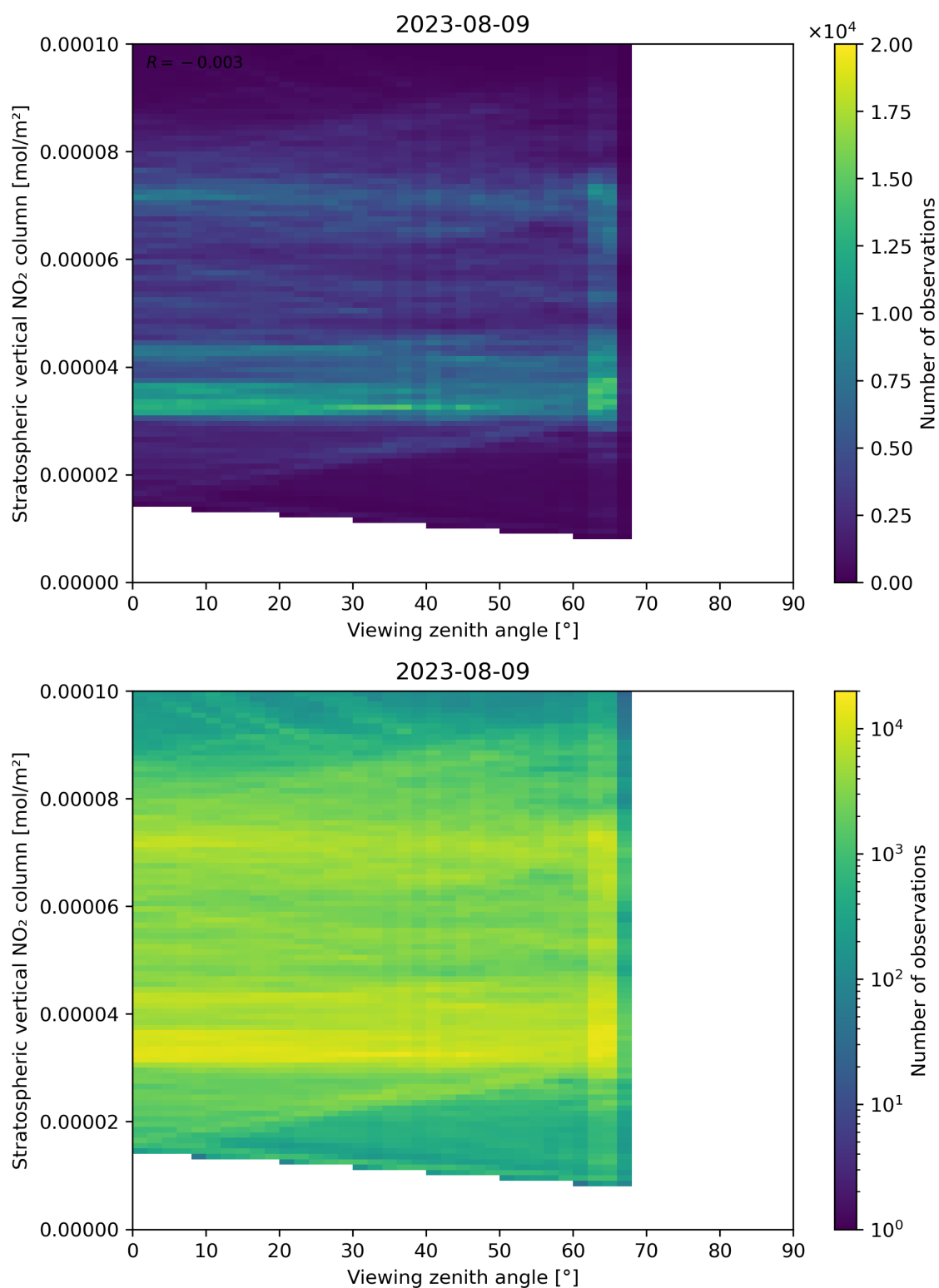
Figure 164: Scatter density plot of “Viewing zenith angle” against “Stratospheric vertical NO 2 column” for 2023-08-09 to 2023-08-10.
