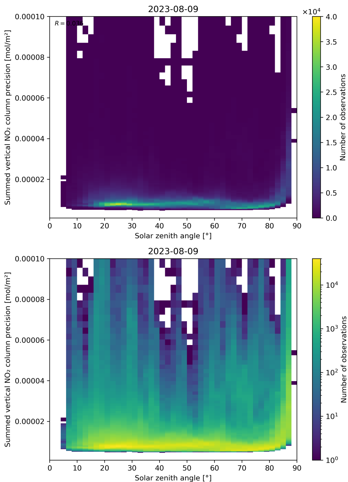
Figure 152: Scatter density plot of “Solar zenith angle” against “Summed vertical NO 2 column precision” for 2023-08-09 to 2023-08-10.
