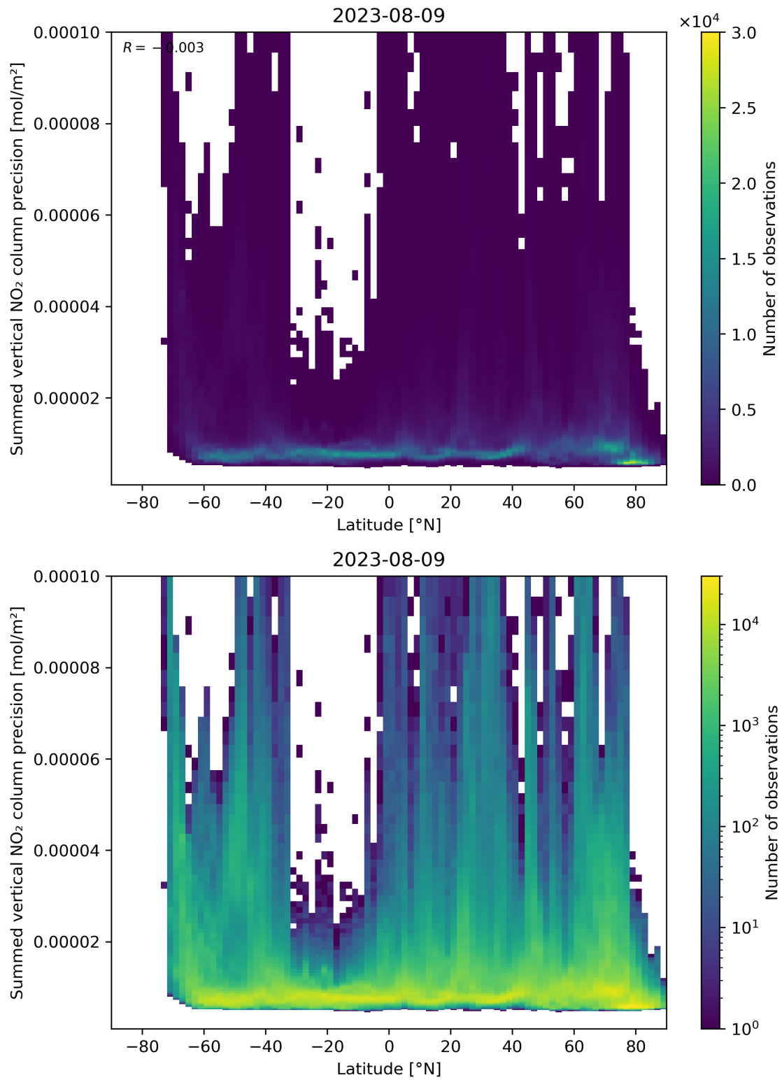
Figure 89: Scatter density plot of “Latitude” against “Summed vertical NO 2 column precision” for 2023-08-09 to 2023-08-10.
