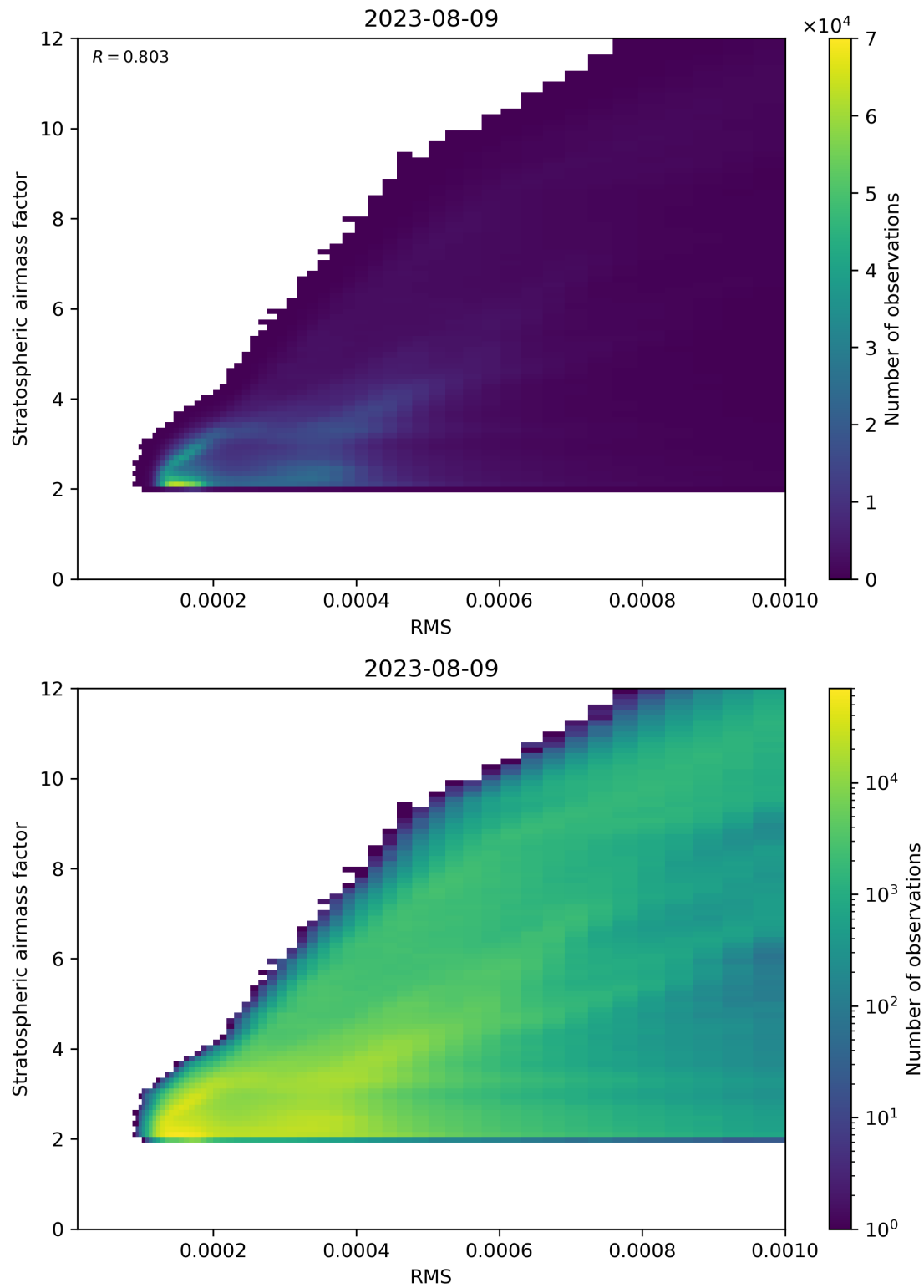
Figure 144: Scatter density plot of “RMS” against “Stratospheric airmass factor” for 2023-08-09 to 2023-08-10.
