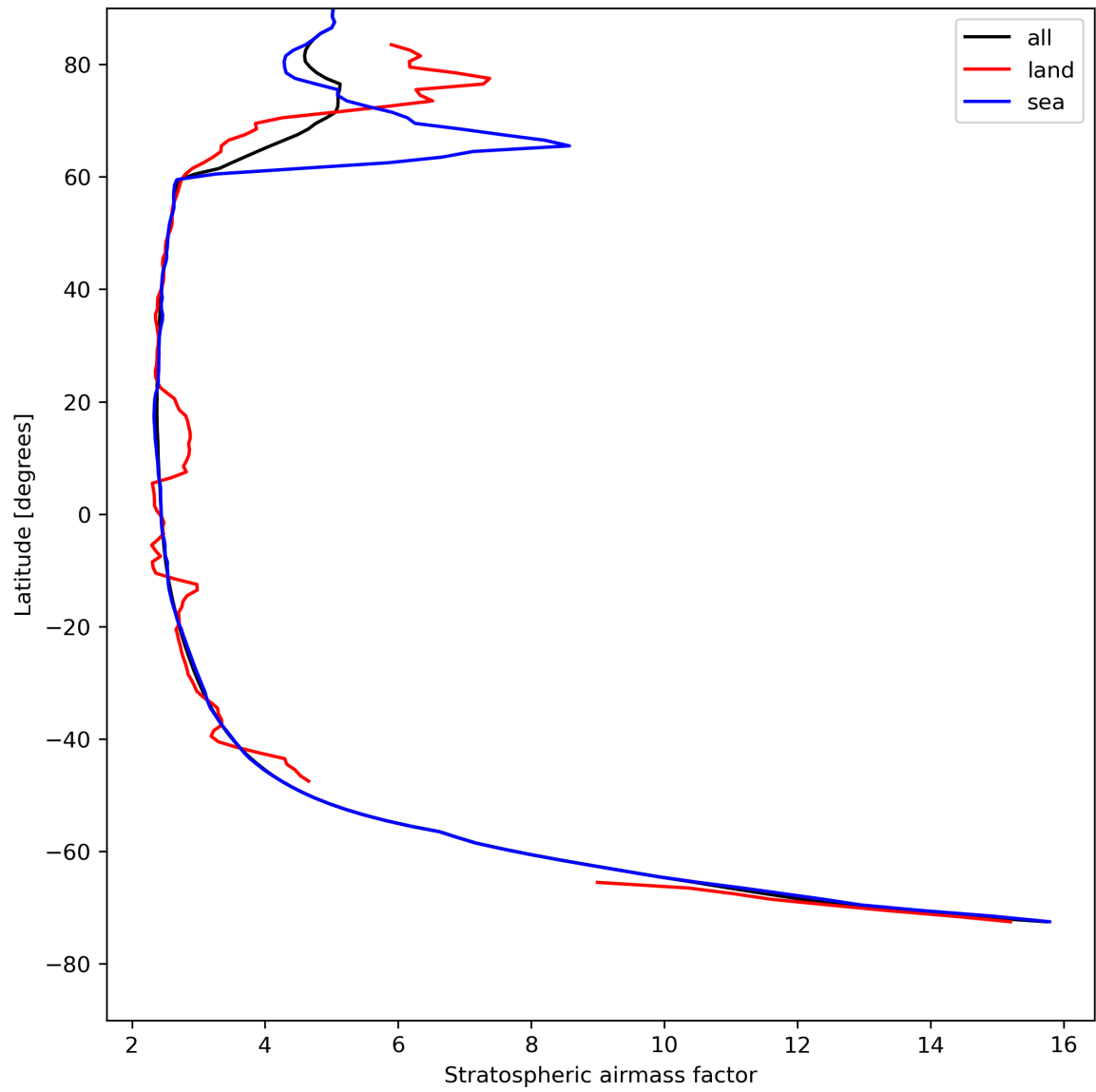
Figure 27: Zonal average of “Stratospheric airmass factor” for 2023-08-09 to 2023-08-10.
