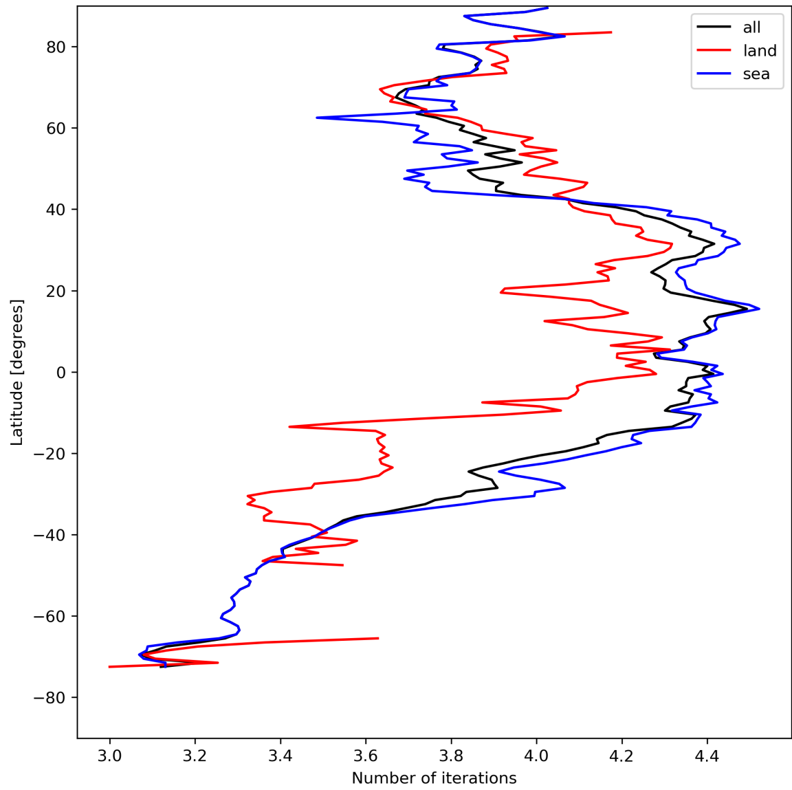
Figure 17: Zonal average of “Number of iterations” for 2023-08-09 to 2023-08-10.
