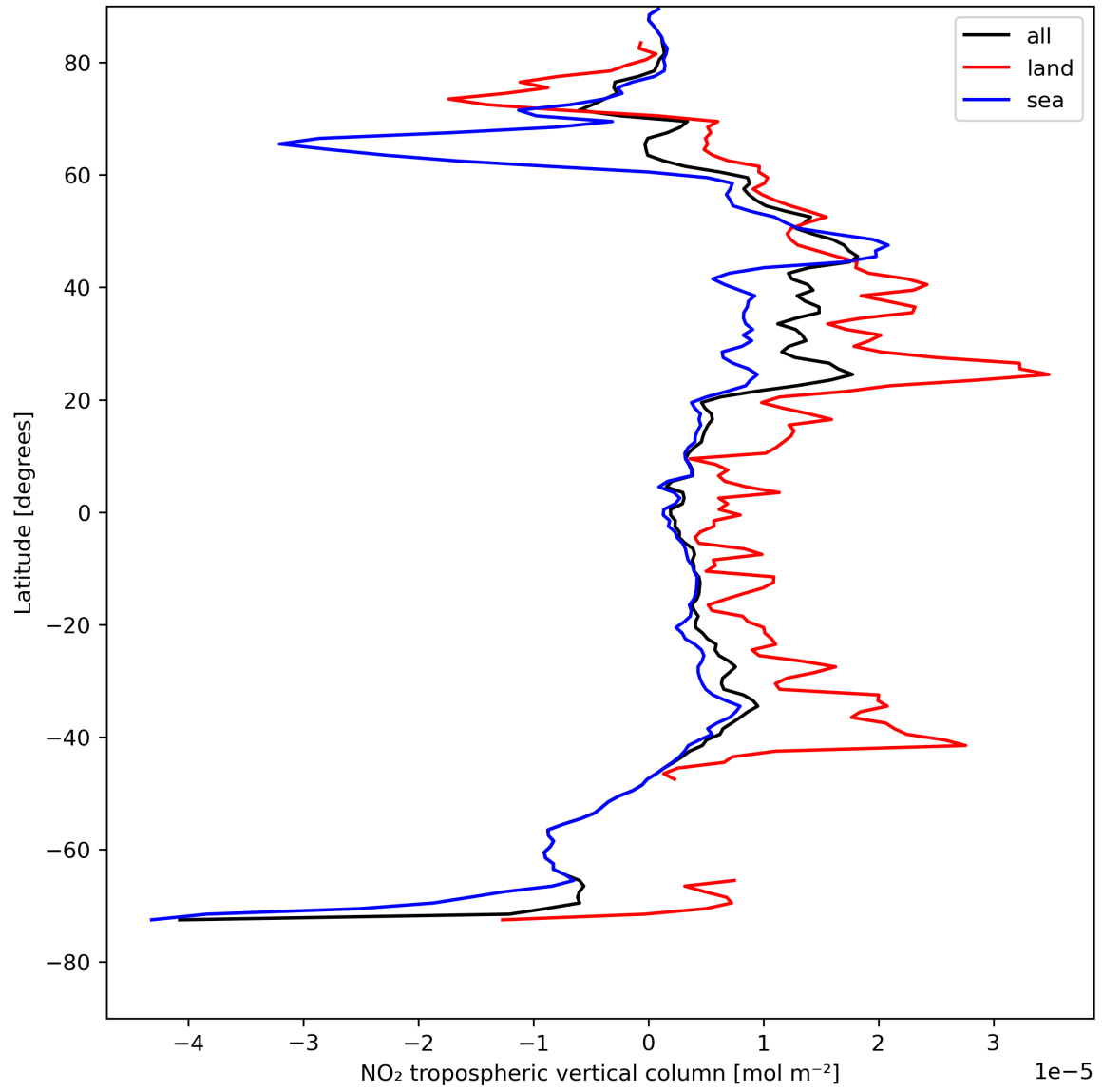
Figure 12: Zonal average of “NO 2 tropospheric vertical column” for 2023-08-09 to 2023-08-10.
