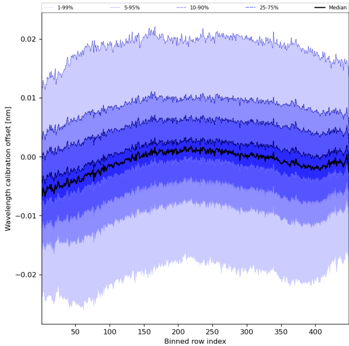
Figure 52: Along track statistics of “Wavelength calibration offset” for 2023-08-09 to 2023-08-10
