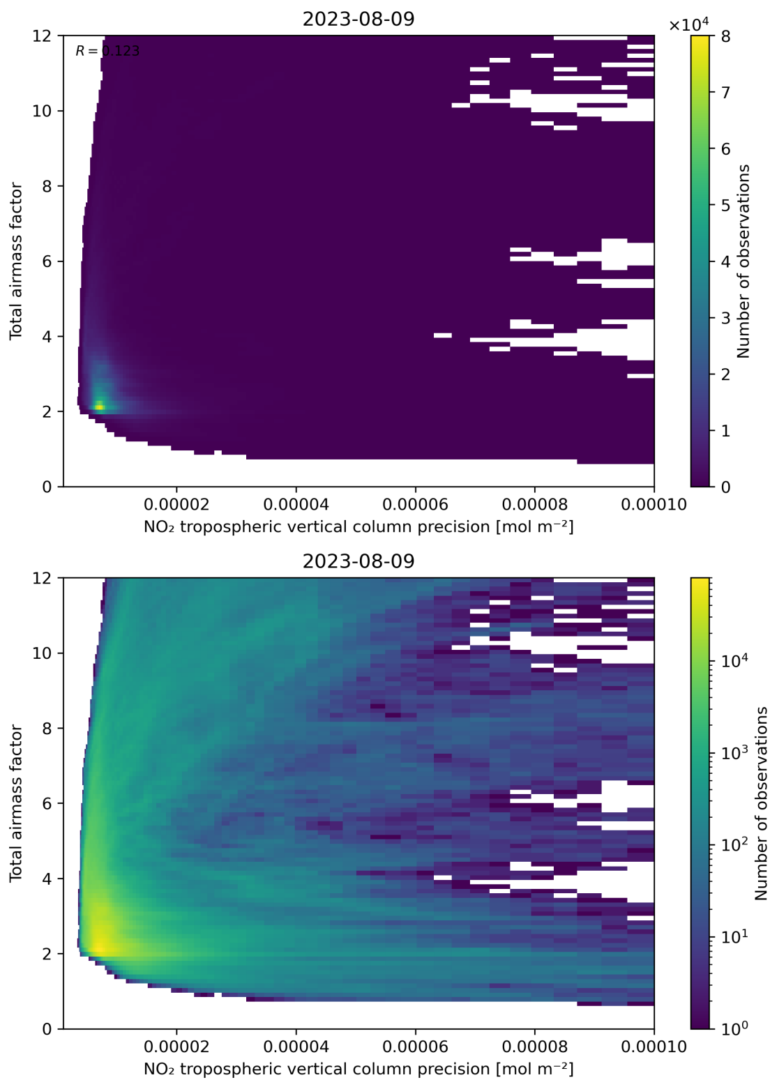
Figure 132: Scatter density plot of “NO 2 tropospheric vertical column precision” against “Total air mass factor” for 2023-08-09 to 2023-08-10.
