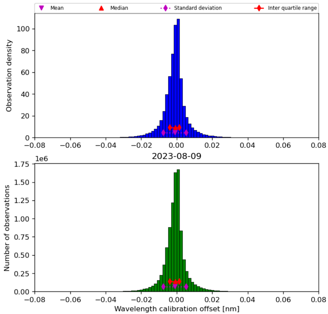
Figure 35: Histogram of “Wavelength calibration offset” for 2023-08-09 to 2023-08-10
