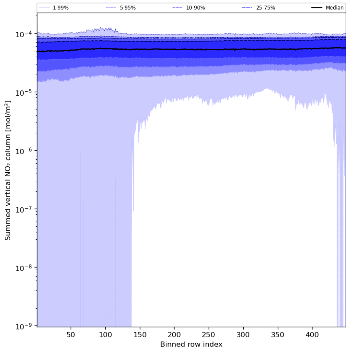
Figure 57: Along track statistics of “Summed vertical NO 2 column” for 2023-08-09 to 2023-08-10
