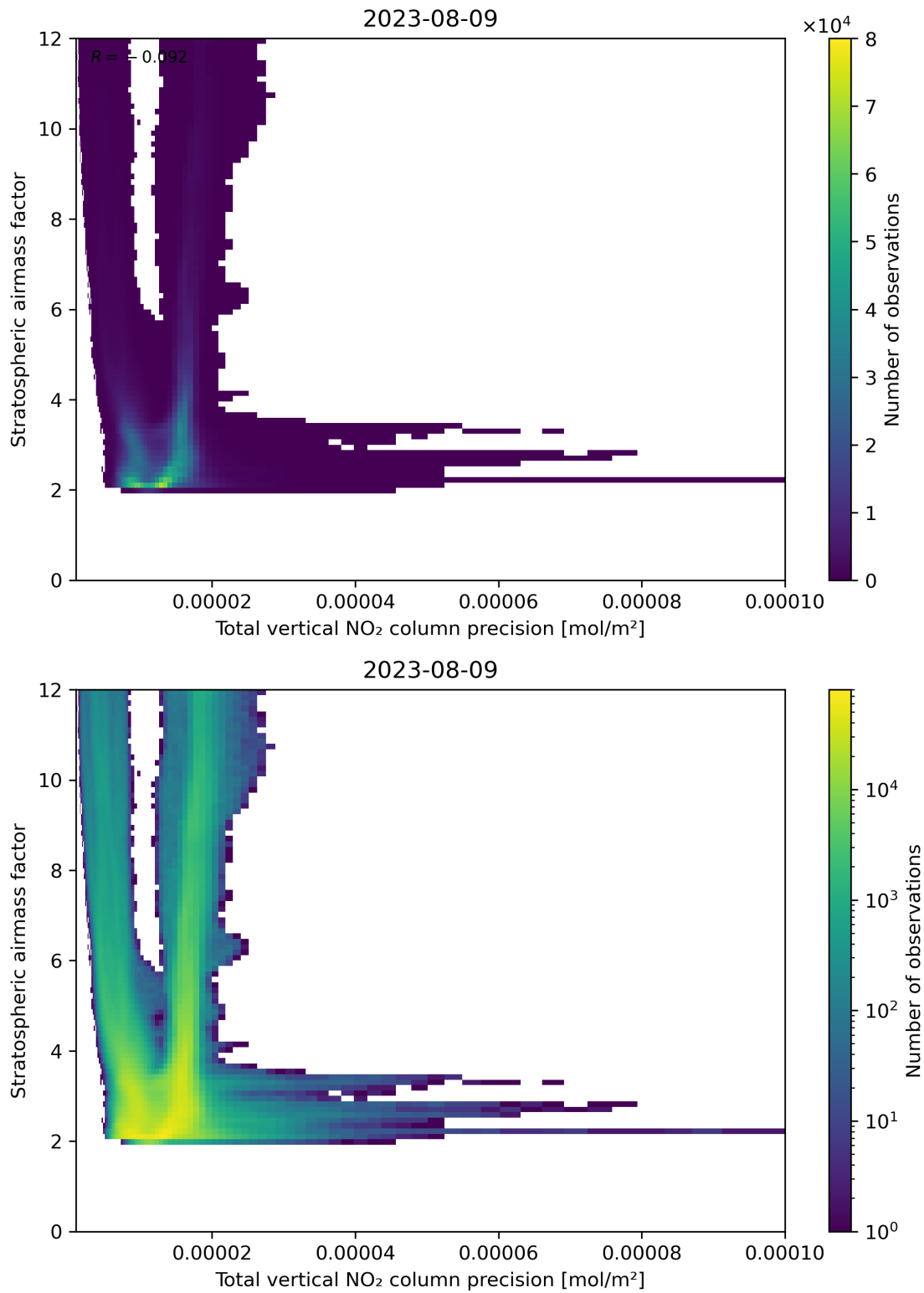
Figure 115: Scatter density plot of “Total vertical NO 2 column precision” against “Stratospheric air mass factor” for 2023-08-09 to 2023-08-10.
