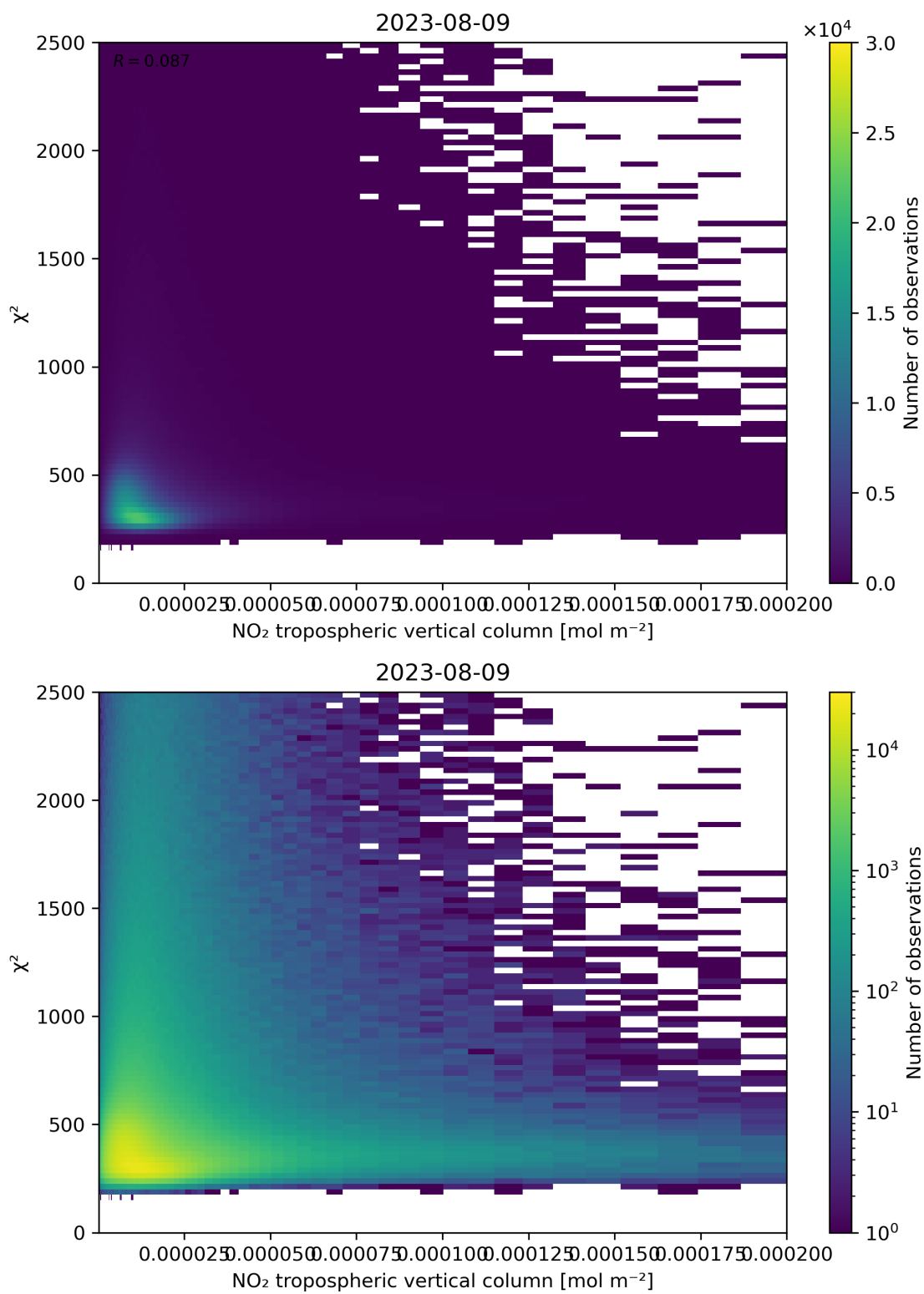
Figure 124: Scatter density plot of “NO 2 tropospheric vertical column” against “ \chi^2 ” for 2023-08-09 to 2023-08-10.
