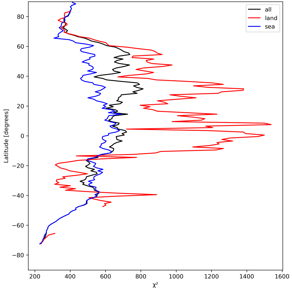
Figure 25: Zonal average of “ \chi^2 ” for 2023-08-09 to 2023-08-10.
