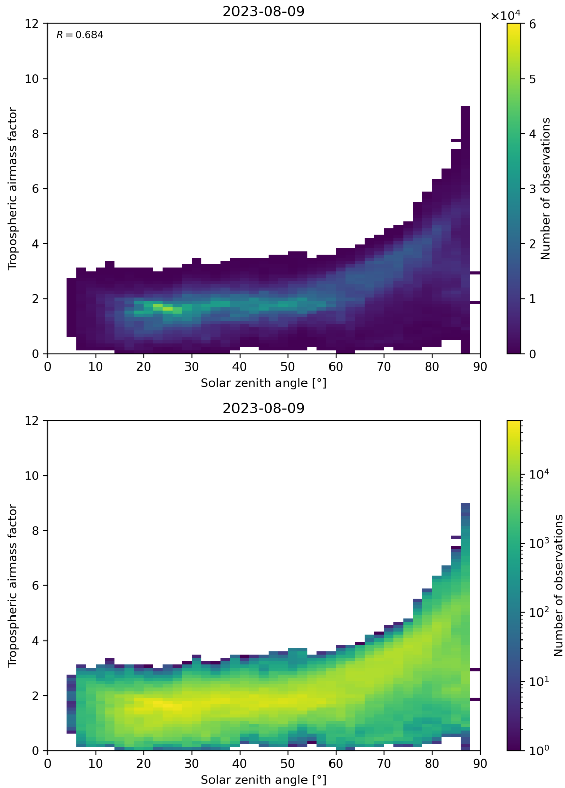
Figure 147: Scatter density plot of “Solar zenith angle” against “Tropospheric airmass factor” for 2023-08-09 to 2023-08-10.
