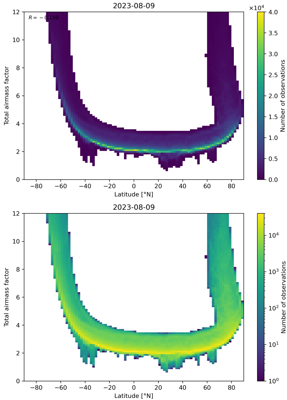
Figure 84: Scatter density plot of “Latitude” against “Total airmass factor” for 2023-08-09 to 2023-08-10.
