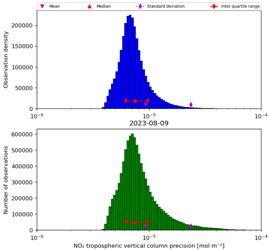
Figure 30: Histogram of “NO 2 tropospheric vertical column precision” for 2023-08-09 to 2023-08-10
