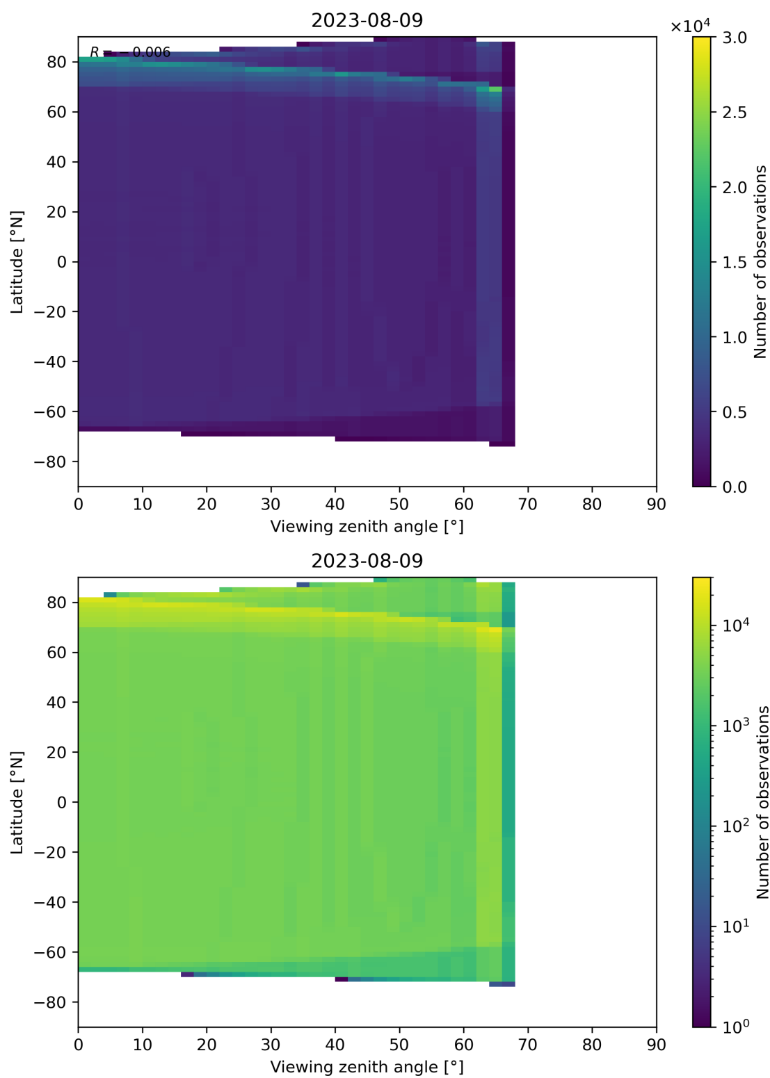
Figure 163: Scatter density plot of “Viewing zenith angle” against “Latitude” for 2023-08-09 to 2023-08-10.
