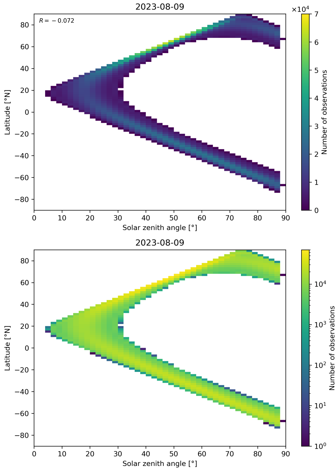
Figure 149: Scatter density plot of “Solar zenith angle” against “Latitude” for 2023-08-09 to 2023-08-10.
