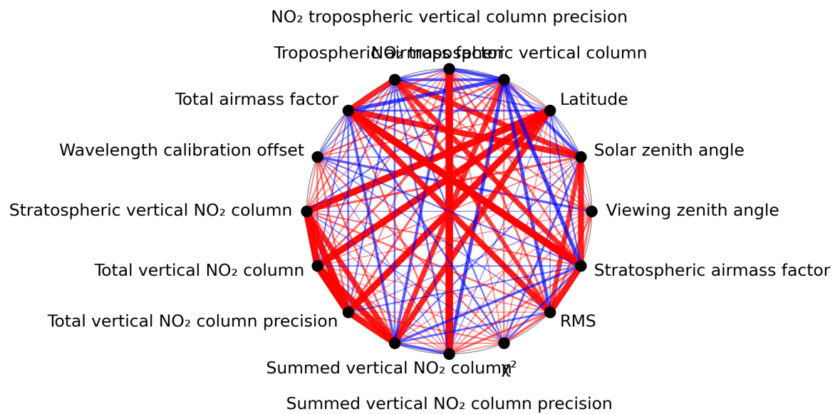
Figure 1: Map of correlation graph for 2023-08-09 to 2023-08-10.
