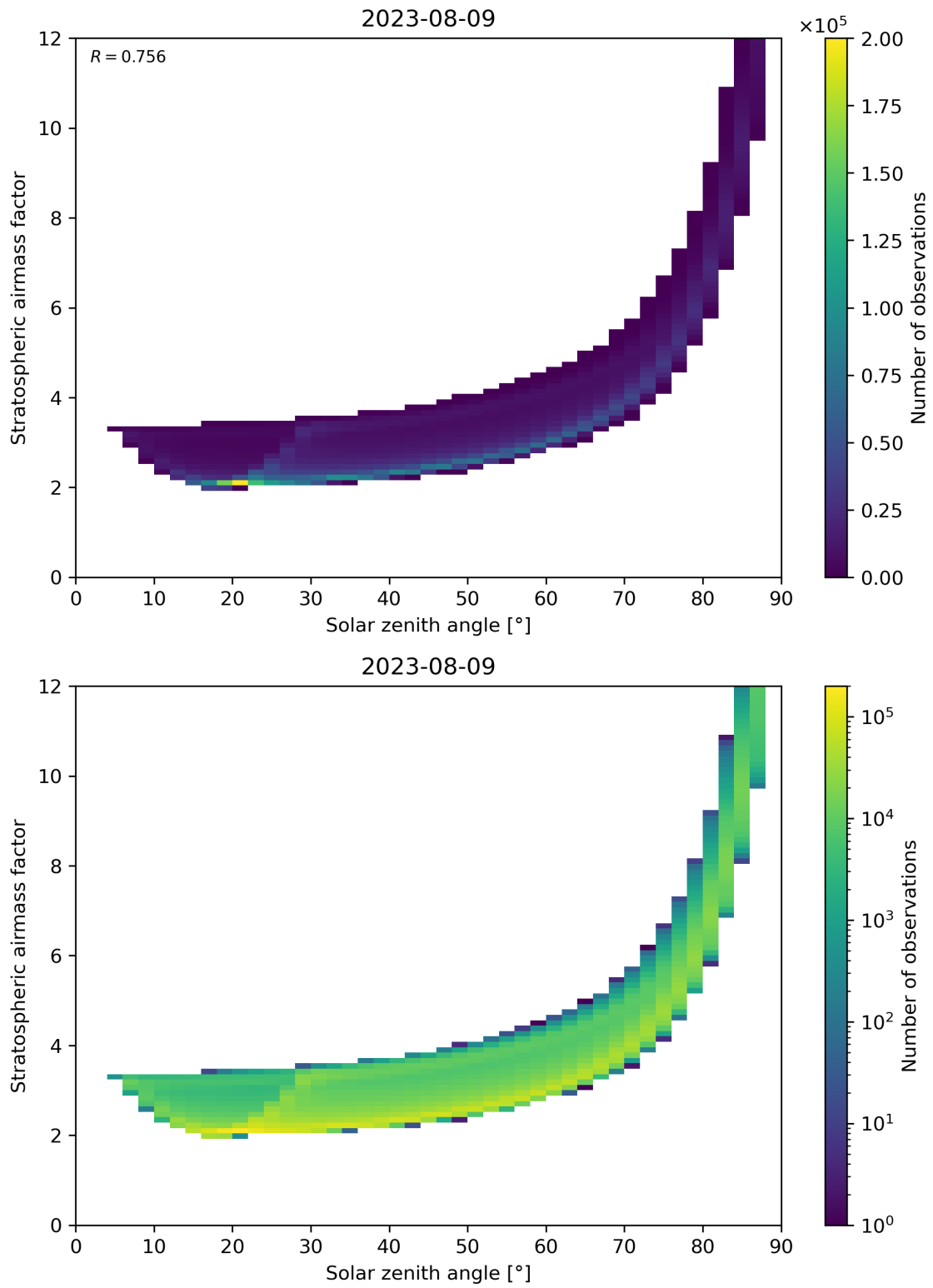
Figure 145: Scatter density plot of “Solar zenith angle” against “Stratospheric airmass factor” for 2023-08-09 to 2023-08-10.
