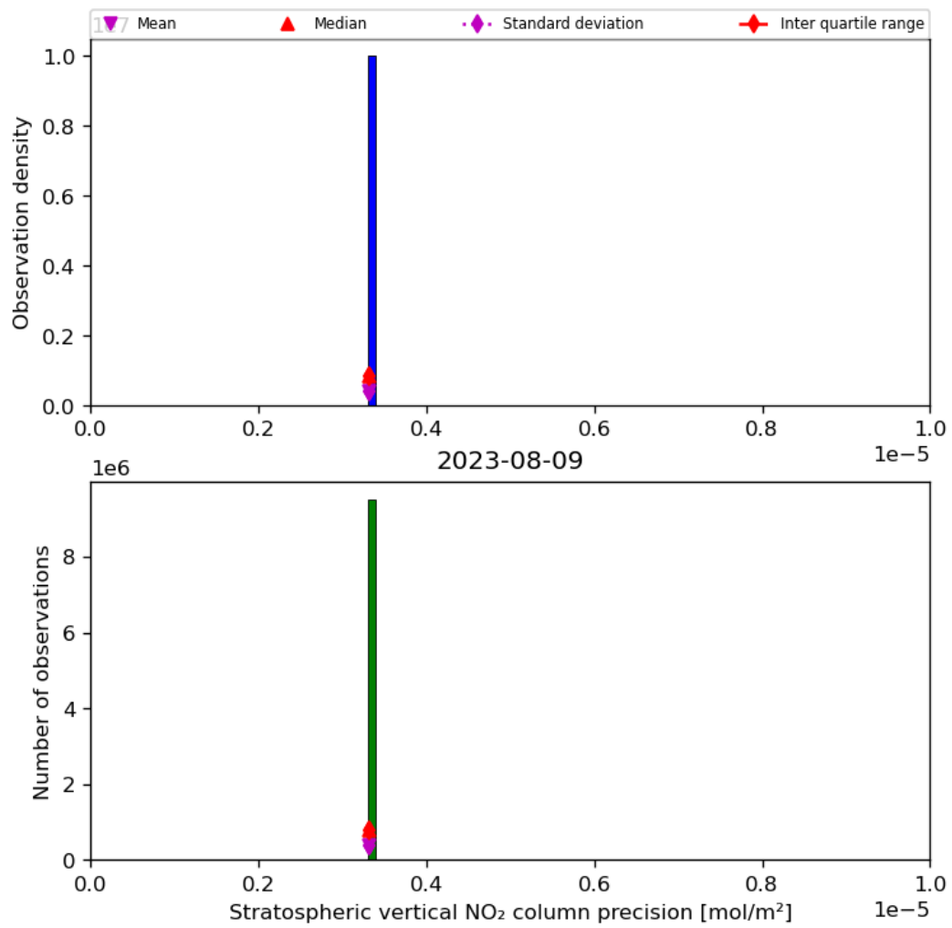
Figure 37: Histogram of “Stratospheric vertical NO 2 column precision” for 2023-08-09 to 2023-08-10
