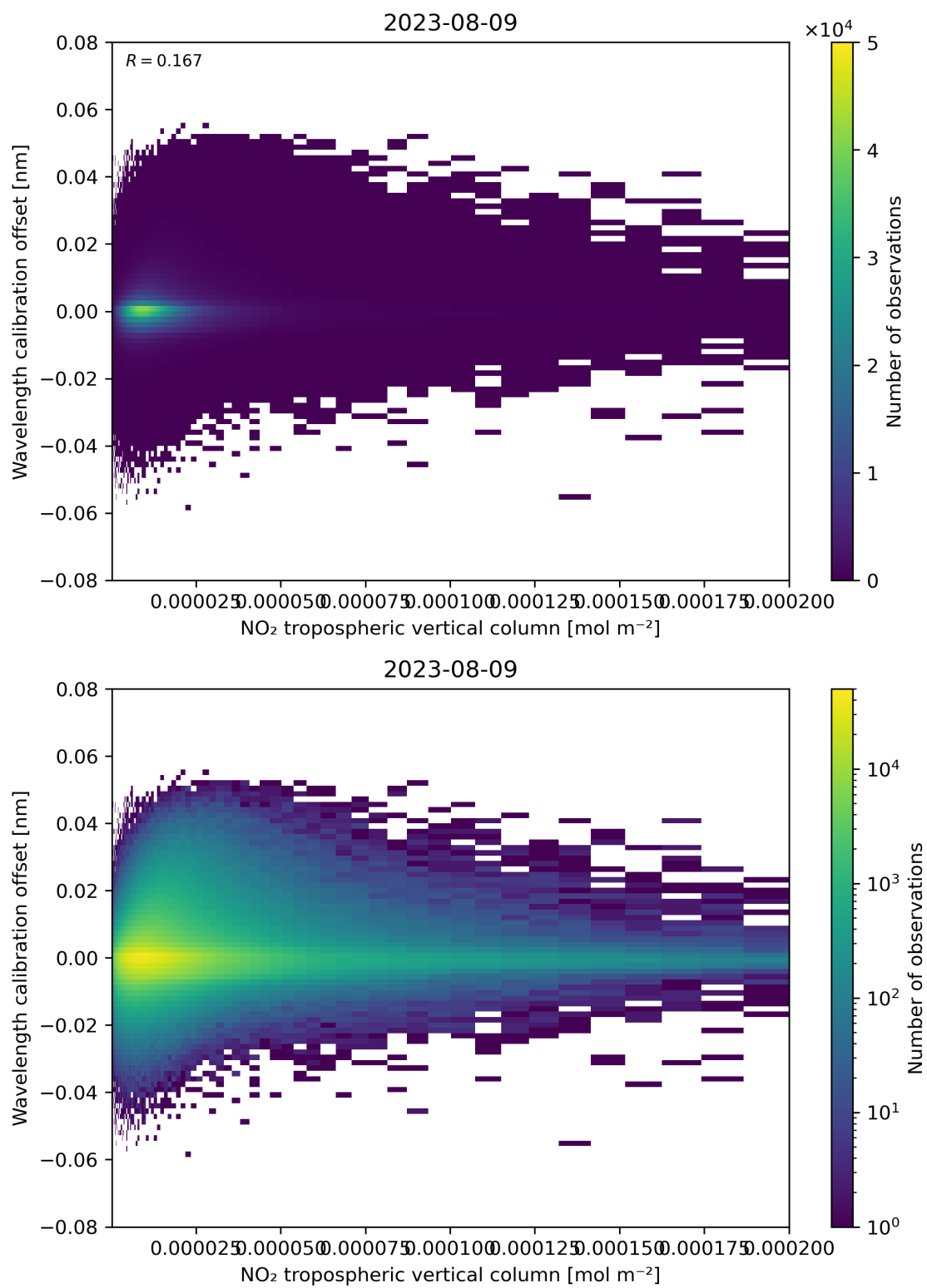
Figure 143: Scatter density plot of “NO 2 tropospheric vertical column” against “Wavelength calibration offset” for 2023-08-09 to 2023-08-10.
