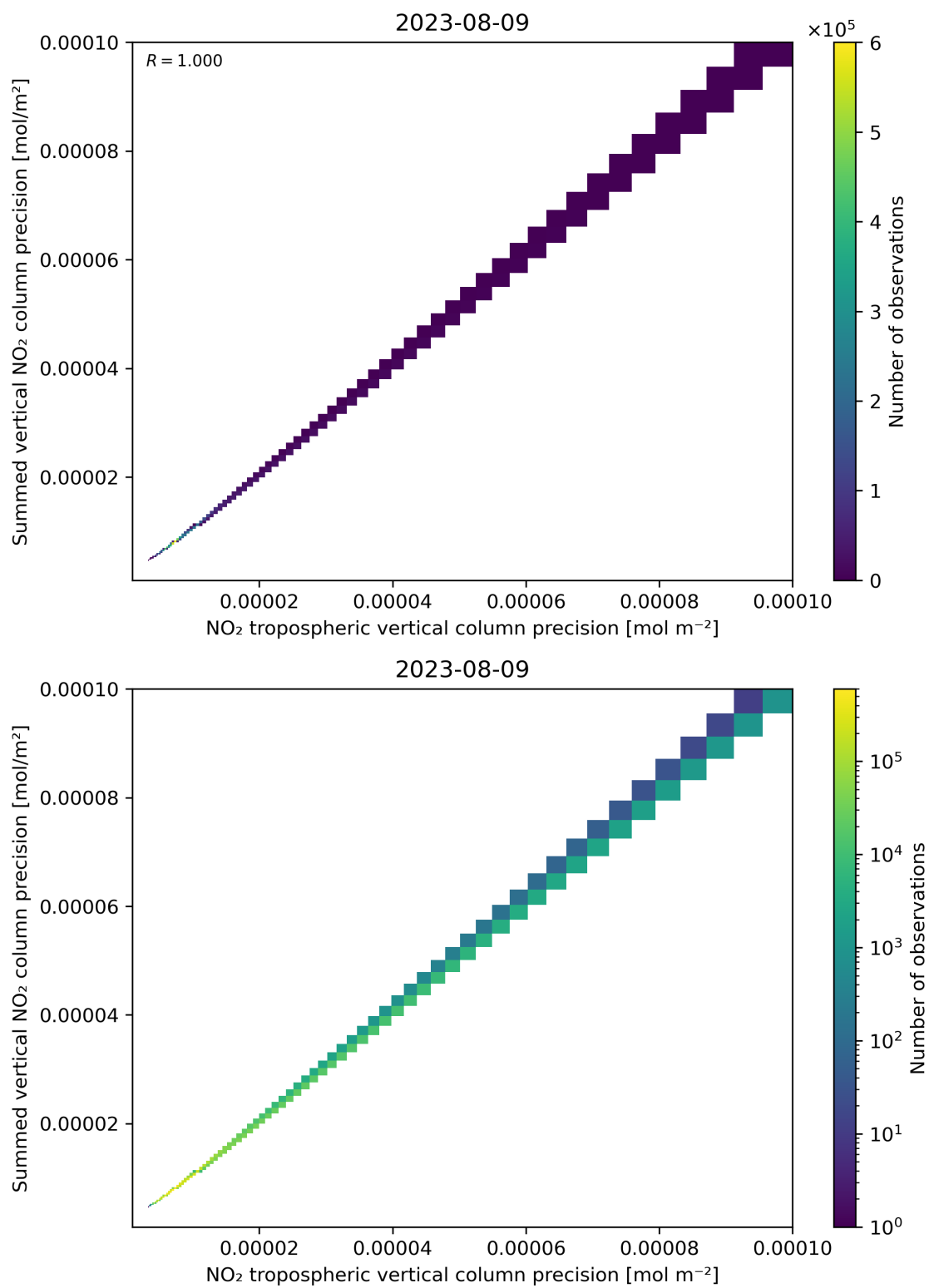
Figure 137: Scatter density plot of “NO 2 tropospheric vertical column precision” against “Summed vertical NO 2 column precision” for 2023-08-09 to 2023-08-10.
