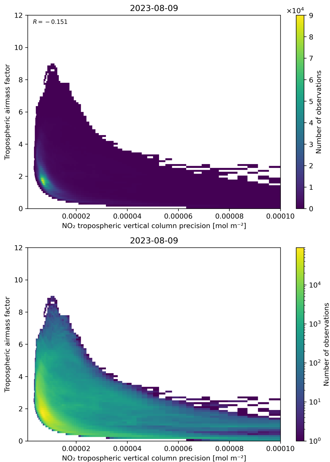
Figure 133: Scatter density plot of “NO 2 tropospheric vertical column precision” against “Tropospheric air mass factor” for 2023-08-09 to 2023-08-10.
