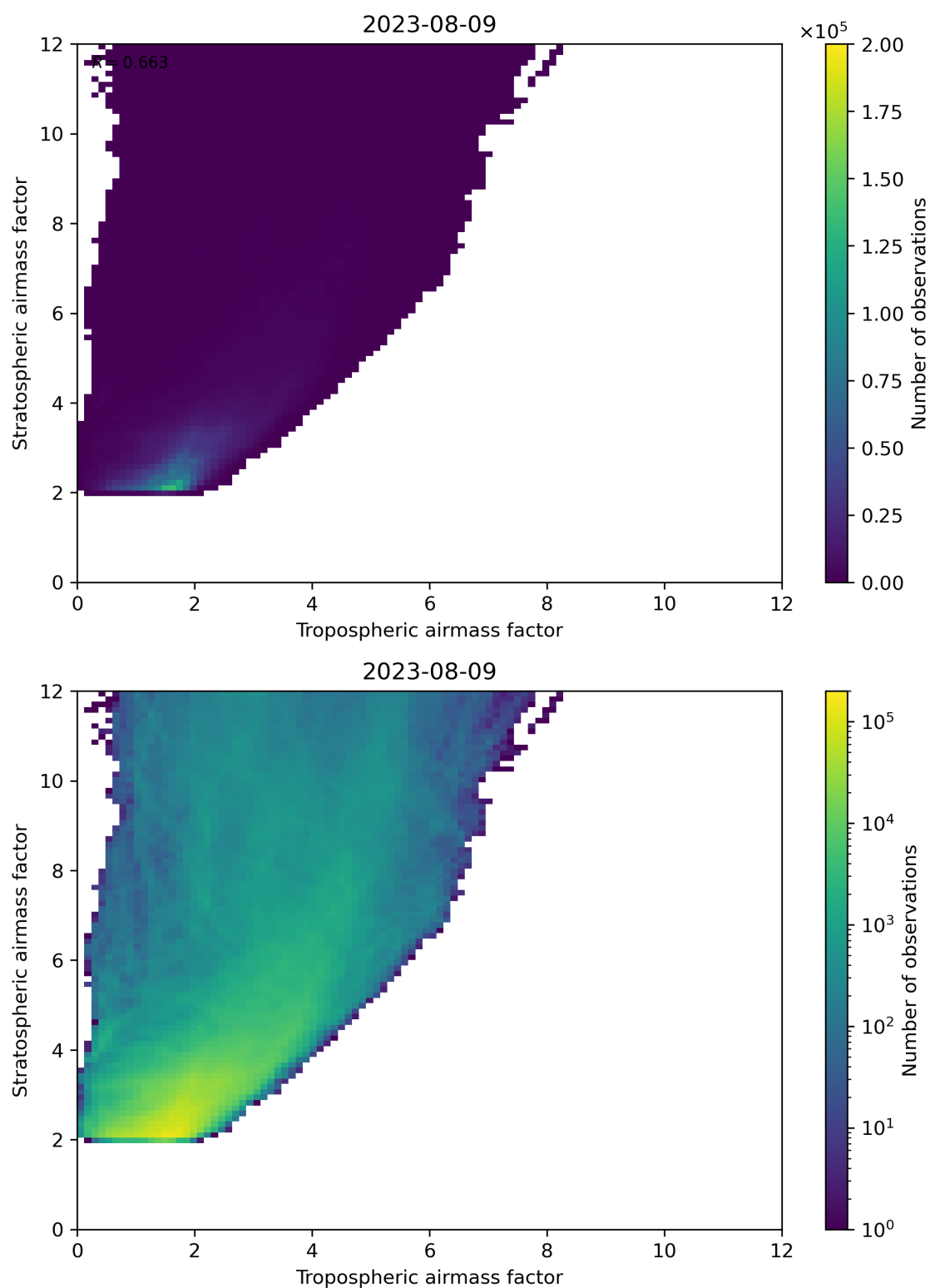
Figure 71: Scatter density plot of “Tropospheric airmass factor” against “Stratospheric airmass factor” for 2023-08-09 to 2023-08-10.
