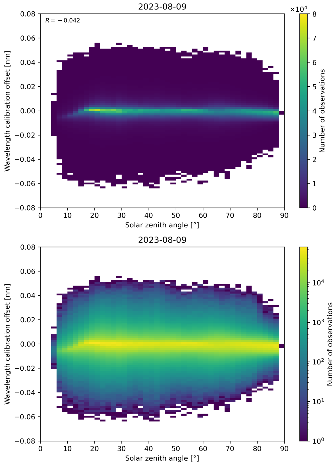
Figure 158: Scatter density plot of “Solar zenith angle” against “Wavelength calibration offset” for 2023-08-09 to 2023-08-10.
