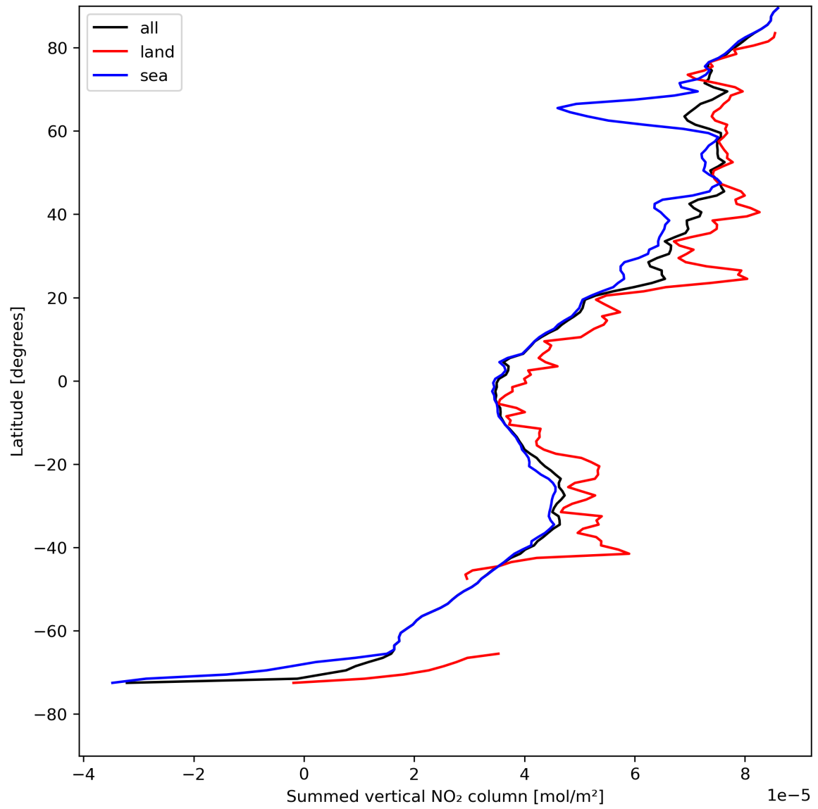
Figure 23: Zonal average of “Summed vertical NO 2 column” for 2023-08-09 to 2023-08-10.
