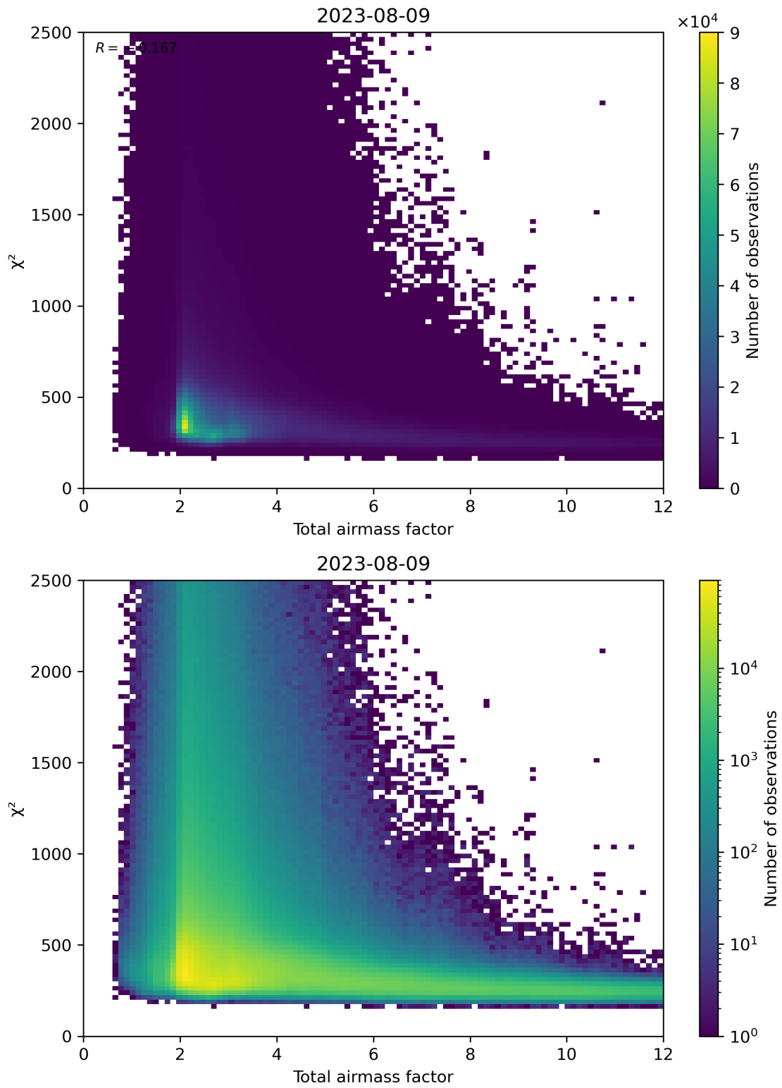
Figure 63: Scatter density plot of “Total airmass factor” against “ \chi^2 ” for 2023-08-09 to 2023-08-10.
