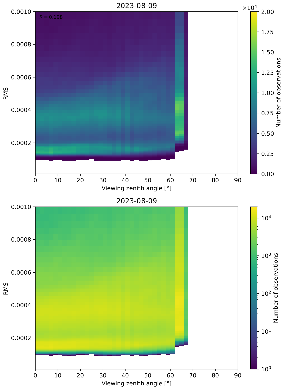
Figure 171: Scatter density plot of “Viewing zenith angle” against “RMS” for 2023-08-09 to 2023-08-10.
