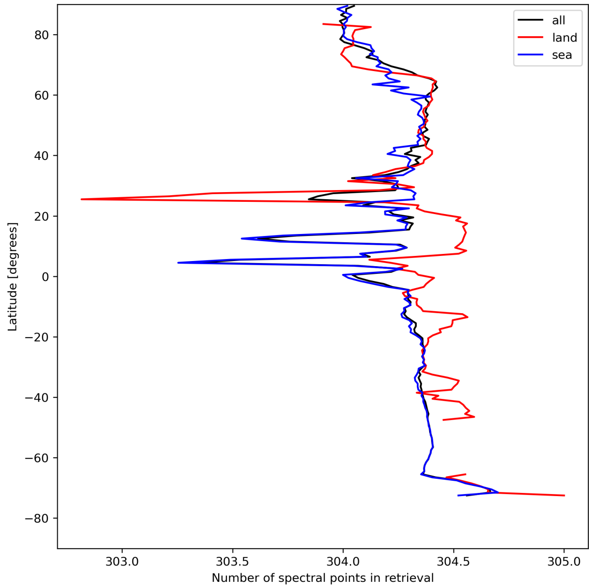
Figure 16: Zonal average of “Number of spectral points in retrieval” for 2023-08-09 to 2023-08-10.
