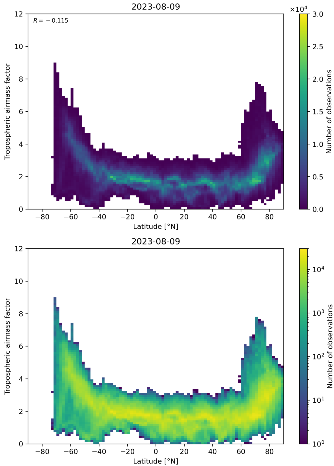
Figure 85: Scatter density plot of “Latitude” against “Tropospheric air mass factor” for 2023-08-09 to 2023-08-10.
