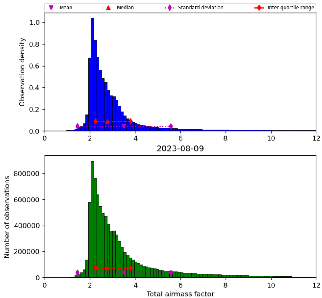
Figure 32: Histogram of “Total airmass factor” for 2023-08-09 to 2023-08-10
