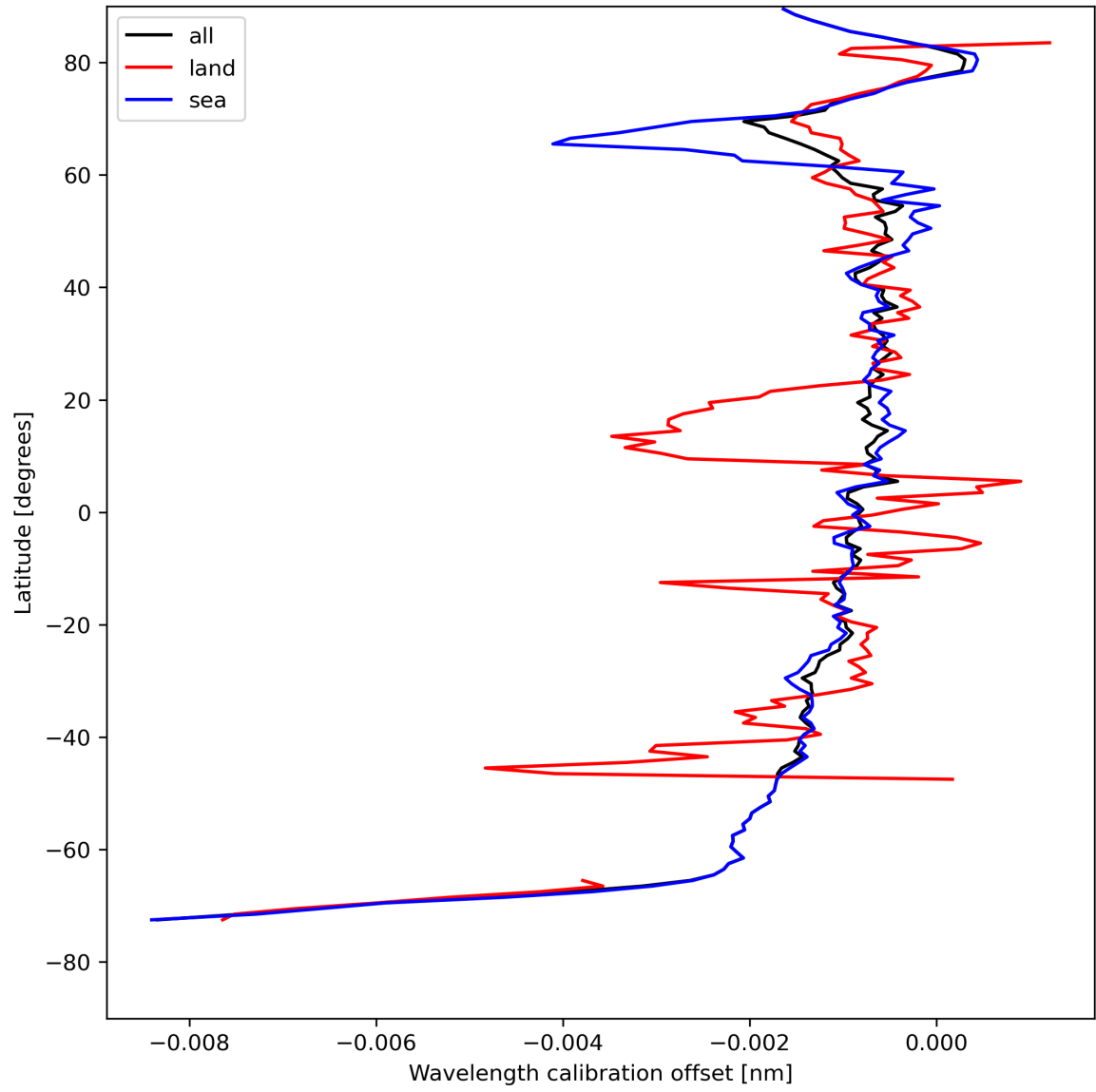
Figure 18: Zonal average of “Wavelength calibration offset” for 2023-08-09 to 2023-08-10.
