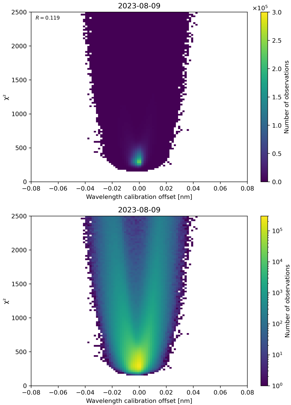
Figure 175: Scatter density plot of “Wavelength calibration offset” against “ \chi^2 ” for 2023-08-09 to 2023-08-10.
