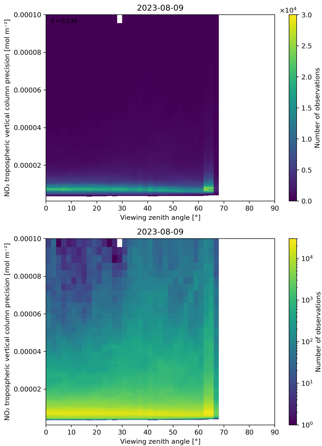
Figure 170: Scatter density plot of “Viewing zenith angle” against “NO 2 tropospheric vertical column precision” for 2023-08-09 to 2023-08-10.
