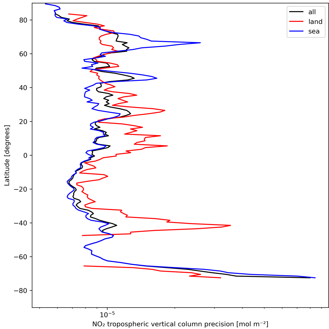
Figure 13: Zonal average of “NO 2 tropospheric vertical column precision” for 2023-08-09 to 2023-08-10.
