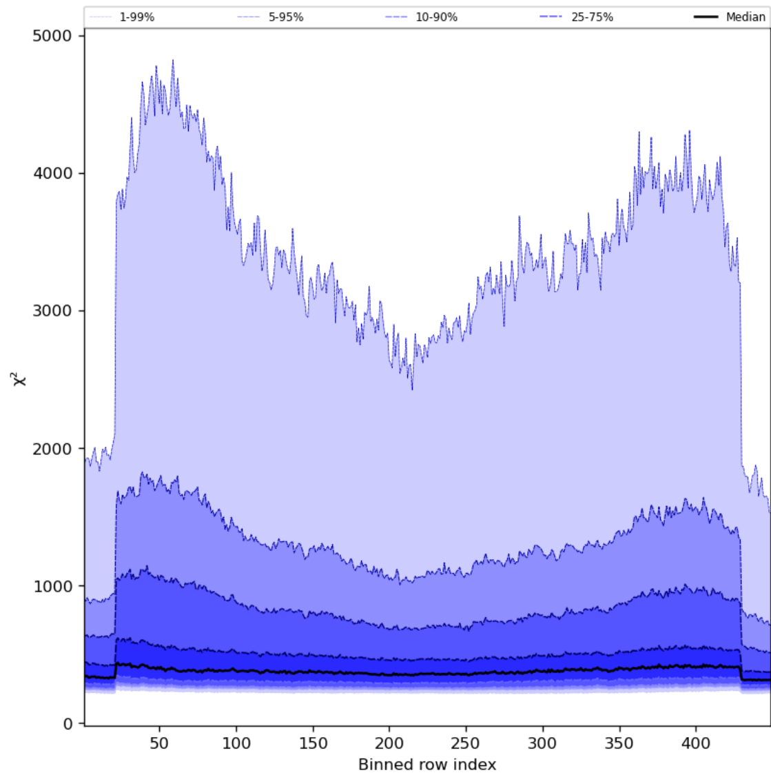
Figure 59: Along track statistics of “ \chi^2 ” for 2023-08-09 to 2023-08-10
