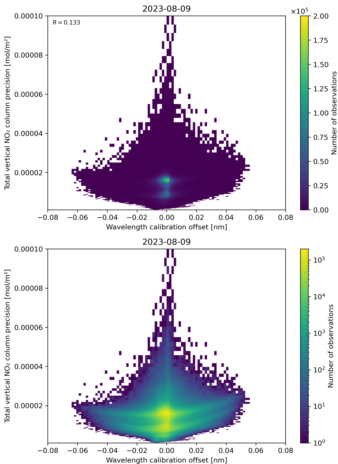
Figure 180: Scatter density plot of “Wavelength calibration offset” against “Total vertical NO 2 column precision” for 2023-08-09 to 2023-08-10.
