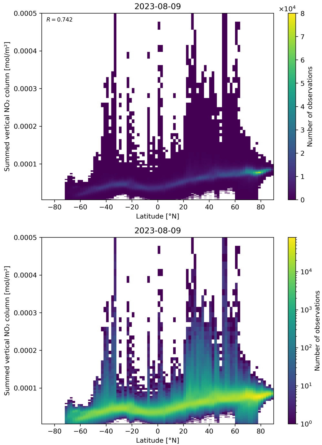
Figure 88: Scatter density plot of “Latitude” against “Summed vertical NO 2 column” for 2023-08-09 to 2023-08-10.
