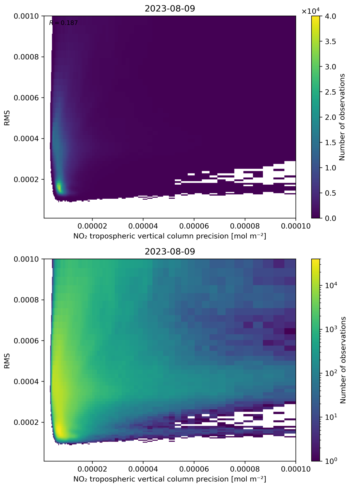
Figure 140: Scatter density plot of “NO 2 tropospheric vertical column precision” against “RMS” for 2023-08-09 to 2023-08-10.
