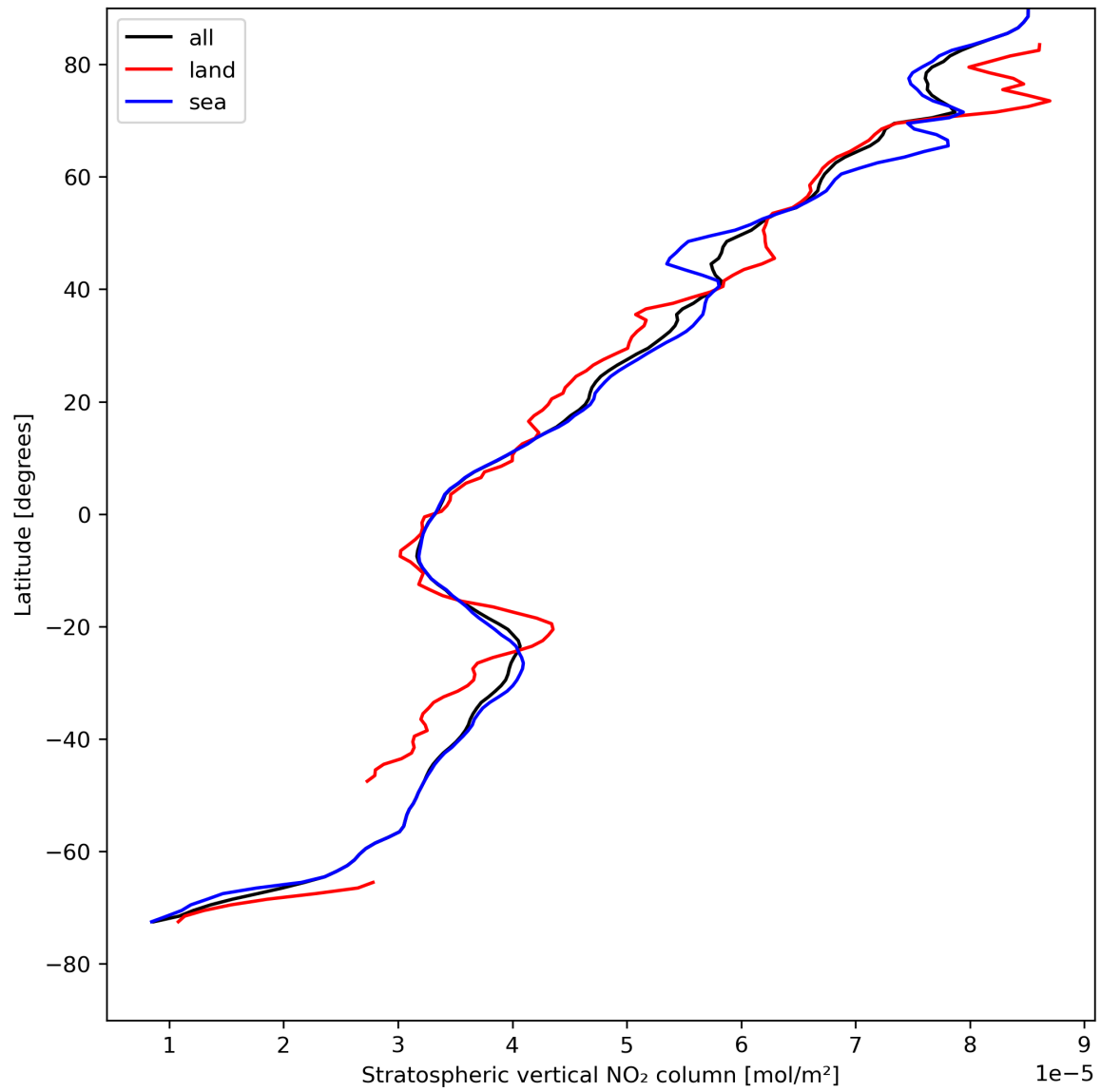
Figure 19: Zonal average of “Stratospheric vertical NO 2 column” for 2023-08-09 to 2023-08-10.
