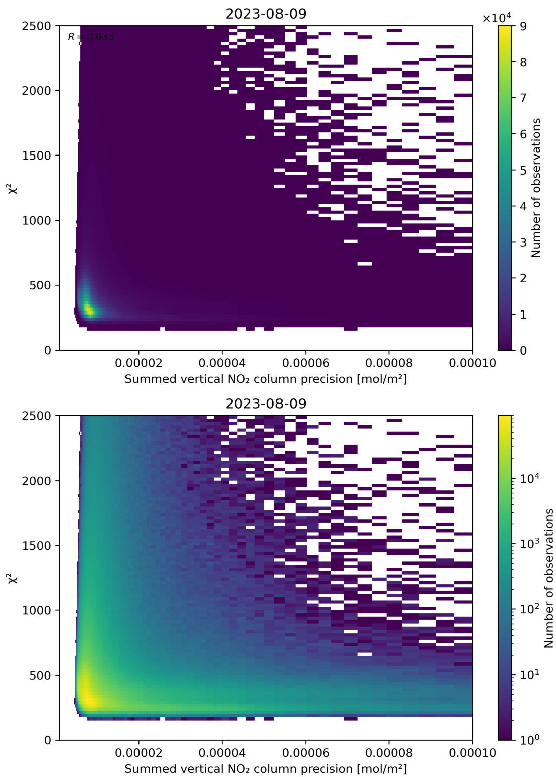
Figure 107: Scatter density plot of “Summed vertical NO 2 column precision” against “ \chi^2 ” for 2023-08-09 to 2023-08-10.
