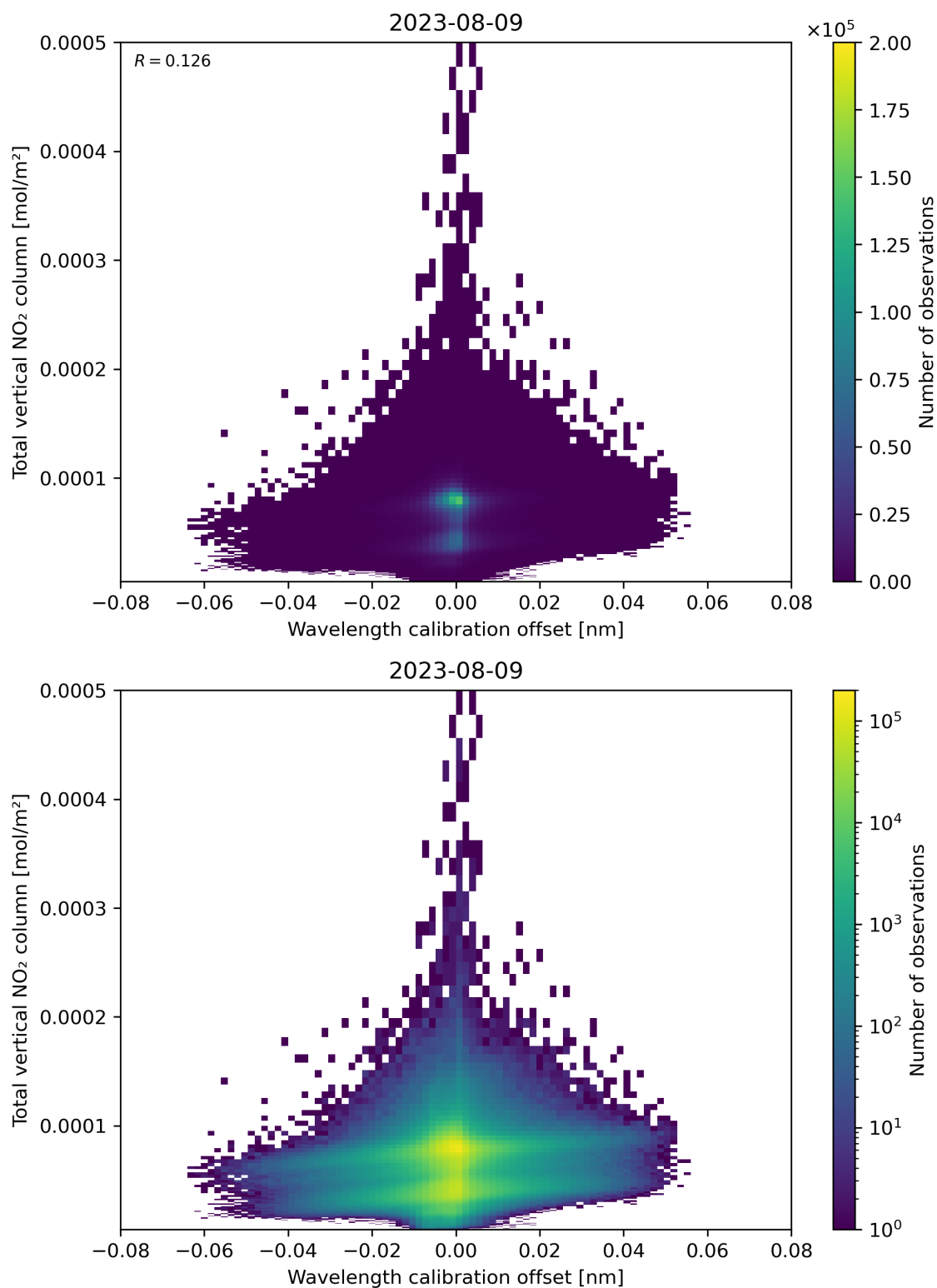
Figure 179: Scatter density plot of “Wavelength calibration offset” against “Total vertical NO 2 column” for 2023-08-09 to 2023-08-10.
