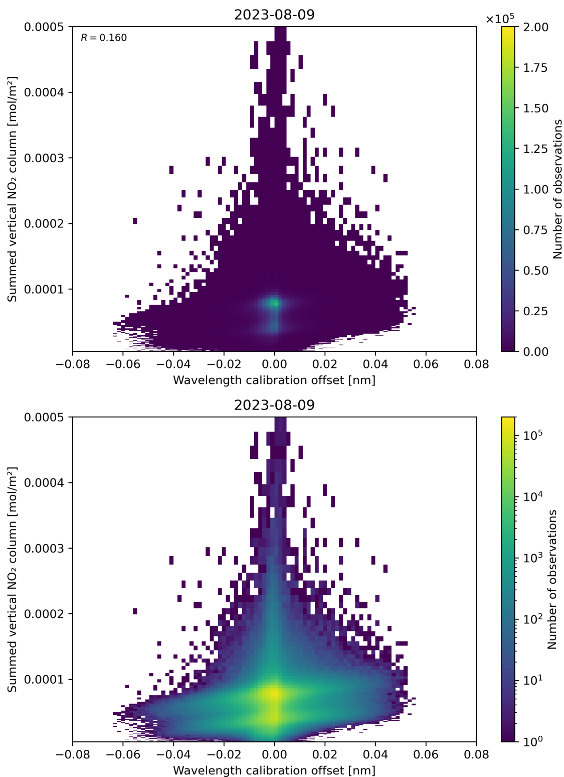
Figure 177: Scatter density plot of “Wavelength calibration offset” against “Summed vertical NO 2 column” for 2023-08-09 to 2023-08-10.
