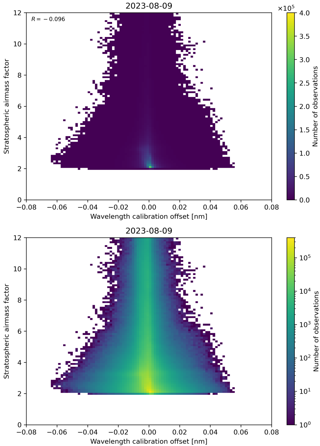
Figure 174: Scatter density plot of “Wavelength calibration offset” against “Stratospheric air mass factor” for 2023-08-09 to 2023-08-10.
