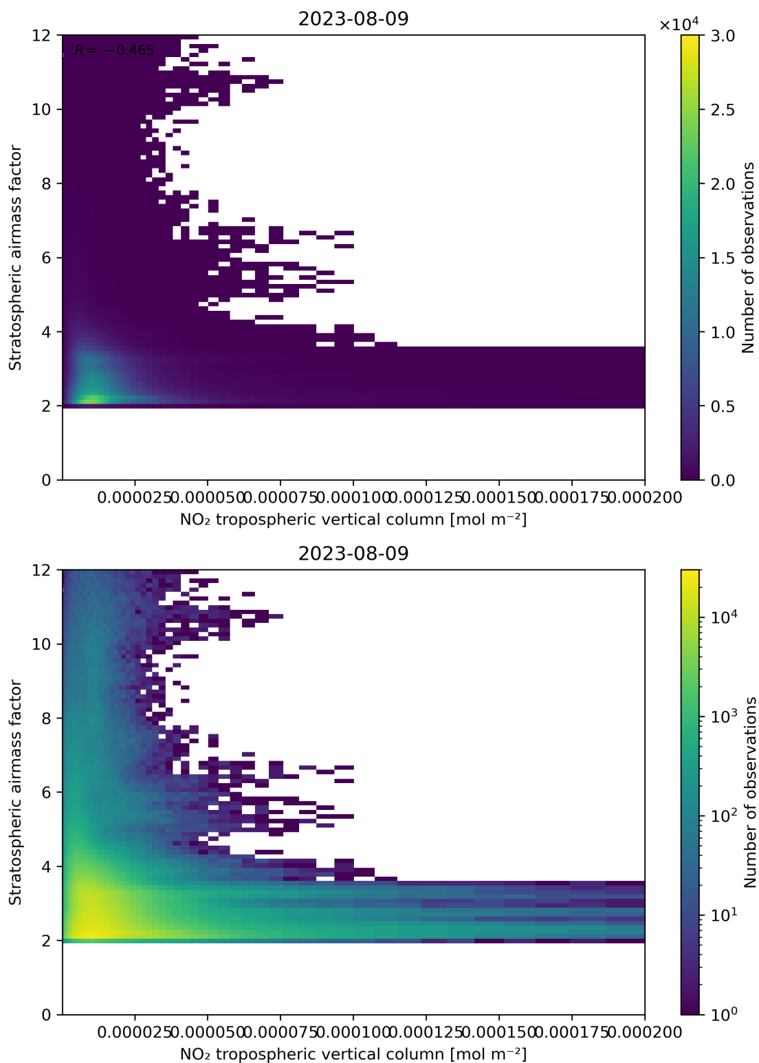
Figure 121: Scatter density plot of “NO 2 tropospheric vertical column” against “Stratospheric airmass factor” for 2023-08-09 to 2023-08-10.
