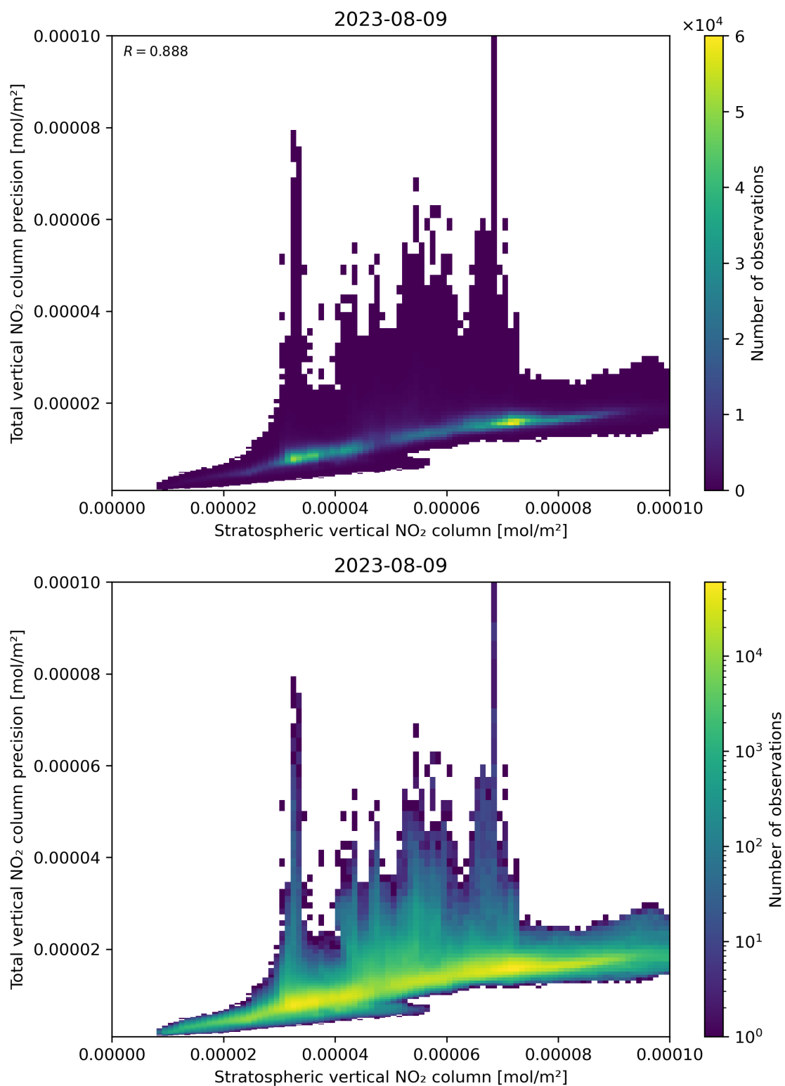
Figure 101: Scatter density plot of “Stratospheric vertical NO 2 column” against “Total vertical NO 2 column precision” for 2023-08-09 to 2023-08-10.
