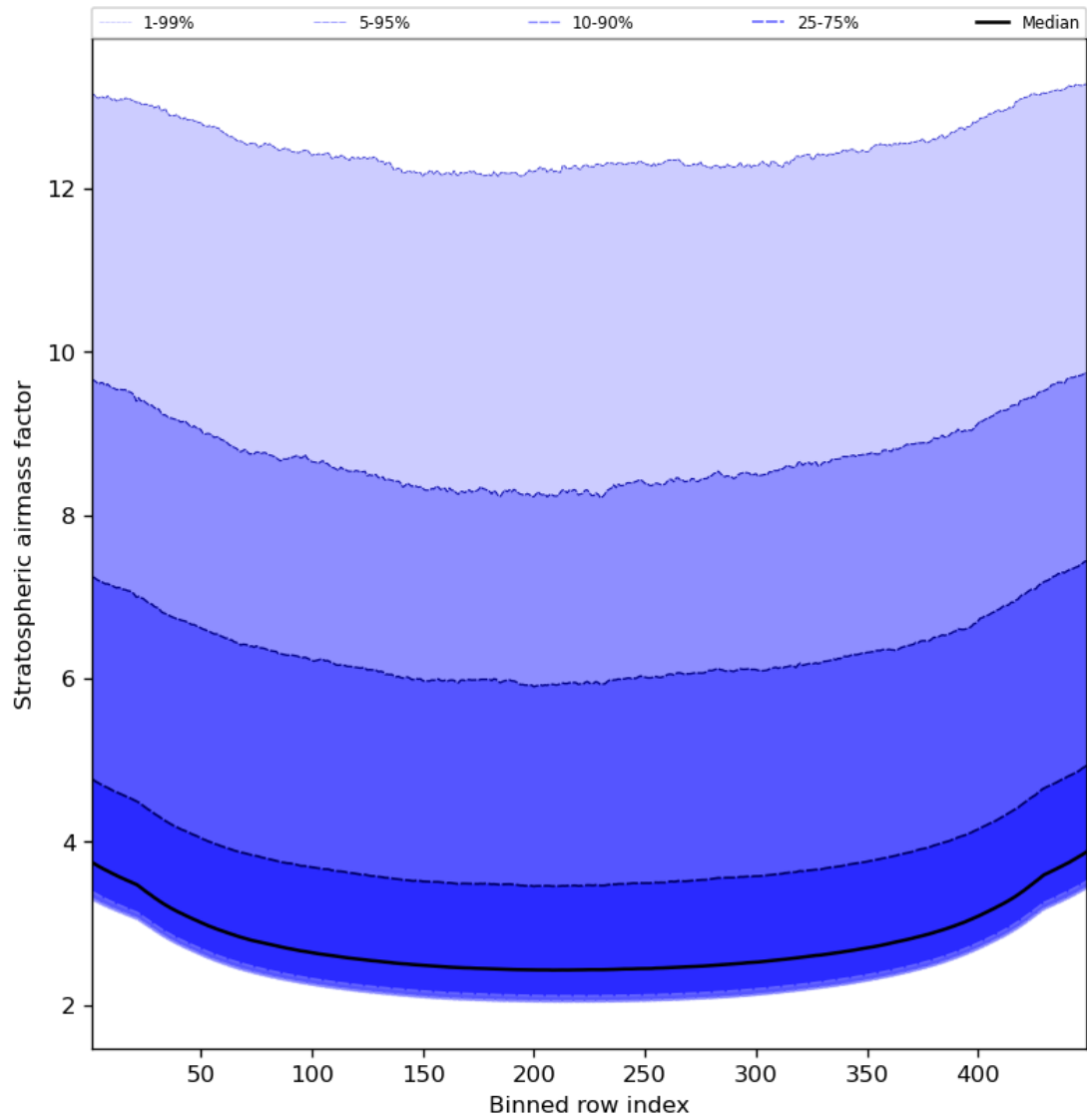
Figure 61: Along track statistics of “Stratospheric airmass factor” for 2023-08-09 to 2023-08-10
