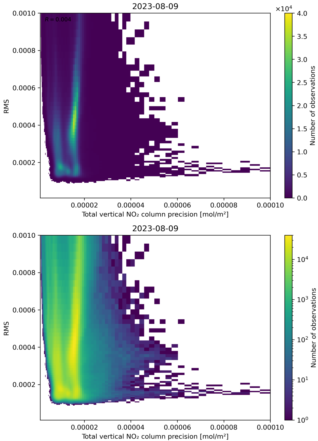
Figure 119: Scatter density plot of “Total vertical NO 2 column precision” against “RMS” for 2023-08-09 to 2023-08-10.
