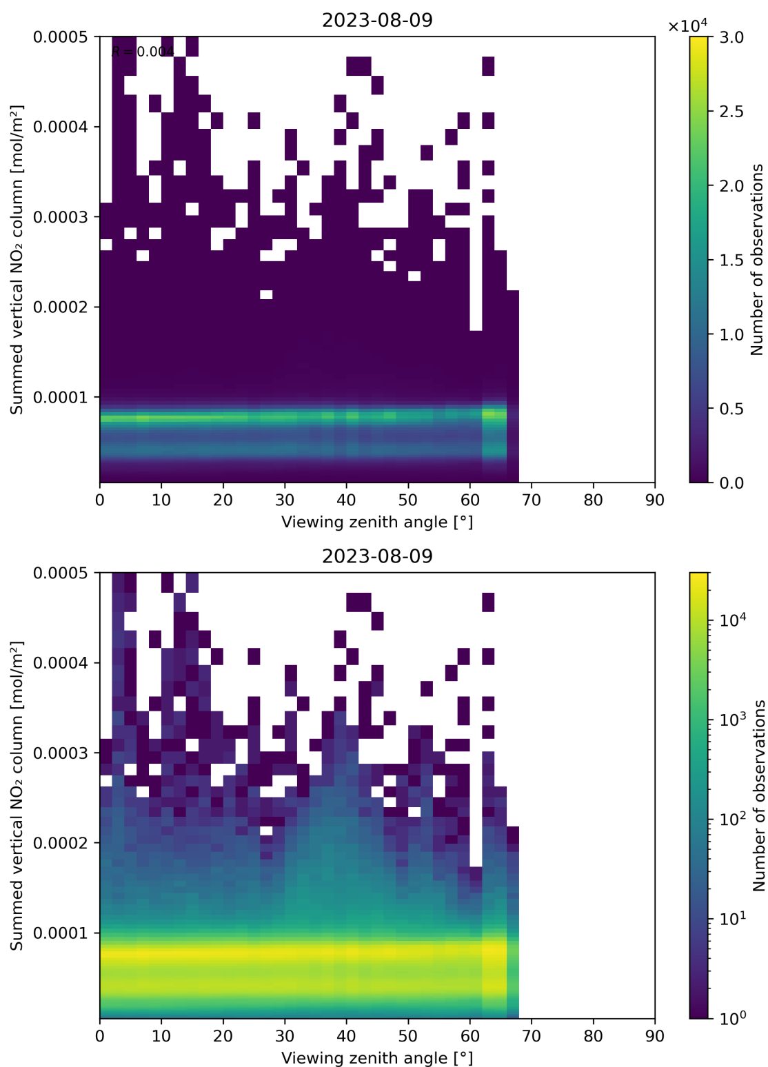
Figure 165: Scatter density plot of “Viewing zenith angle” against “Summed vertical NO 2 column” for 2023-08-09 to 2023-08-10.
