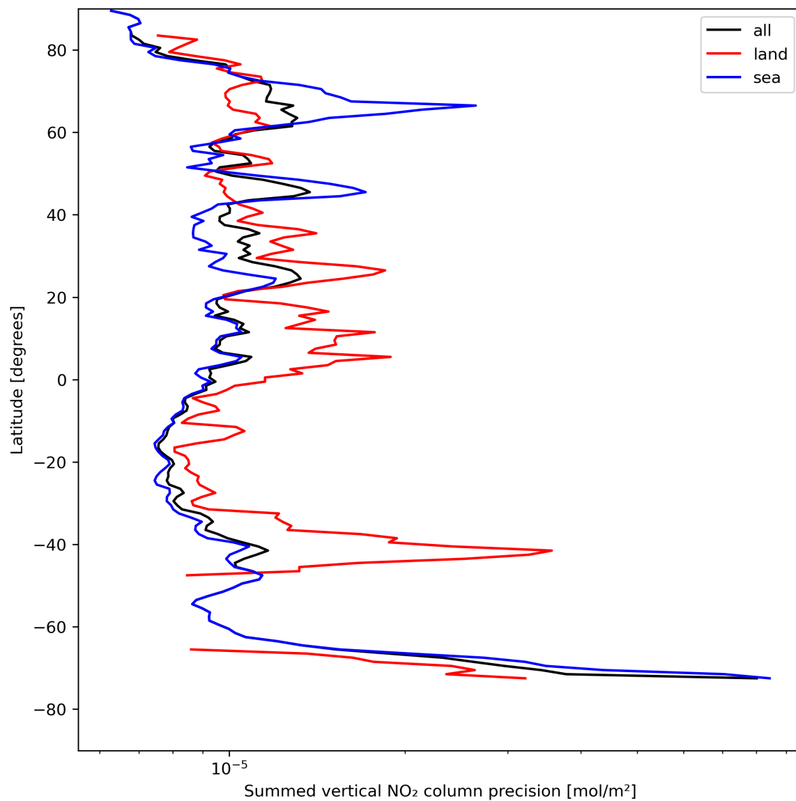
Figure 24: Zonal average of “Summed vertical NO 2 column precision” for 2023-08-09 to 2023-08-10.
