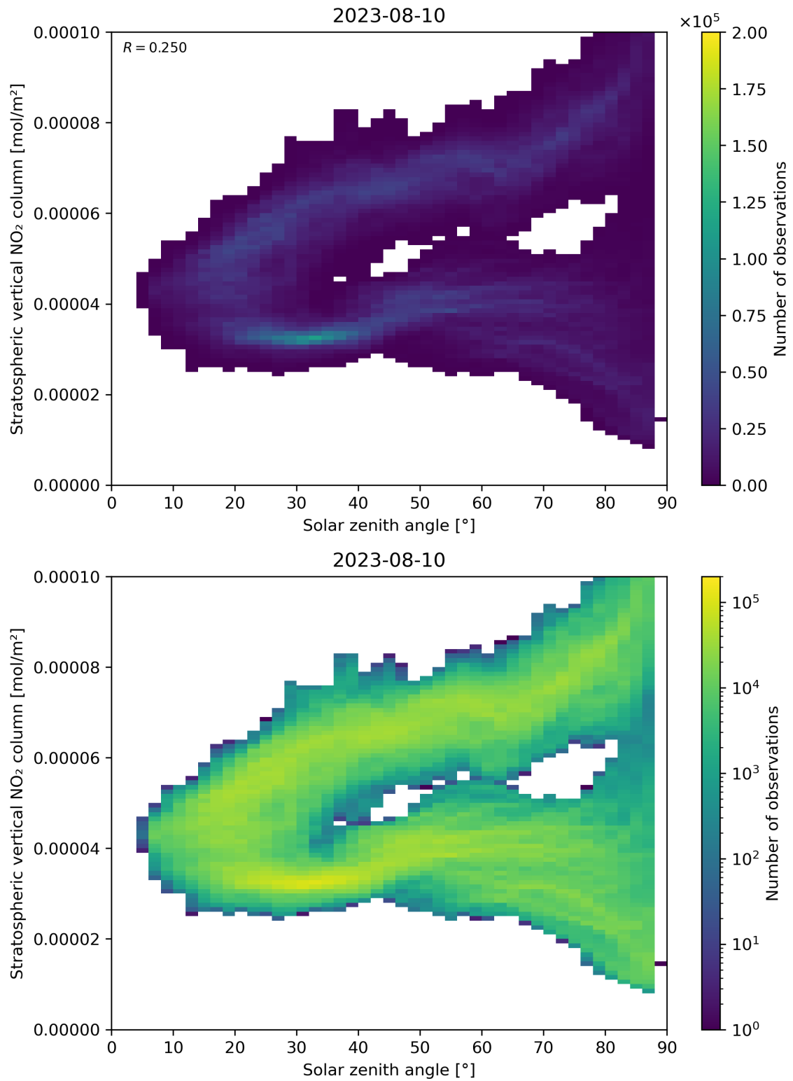
Figure 150: Scatter density plot of “Solar zenith angle” against “Stratospheric vertical NO 2 column” for 2023-08-09 to 2023-08-11.
