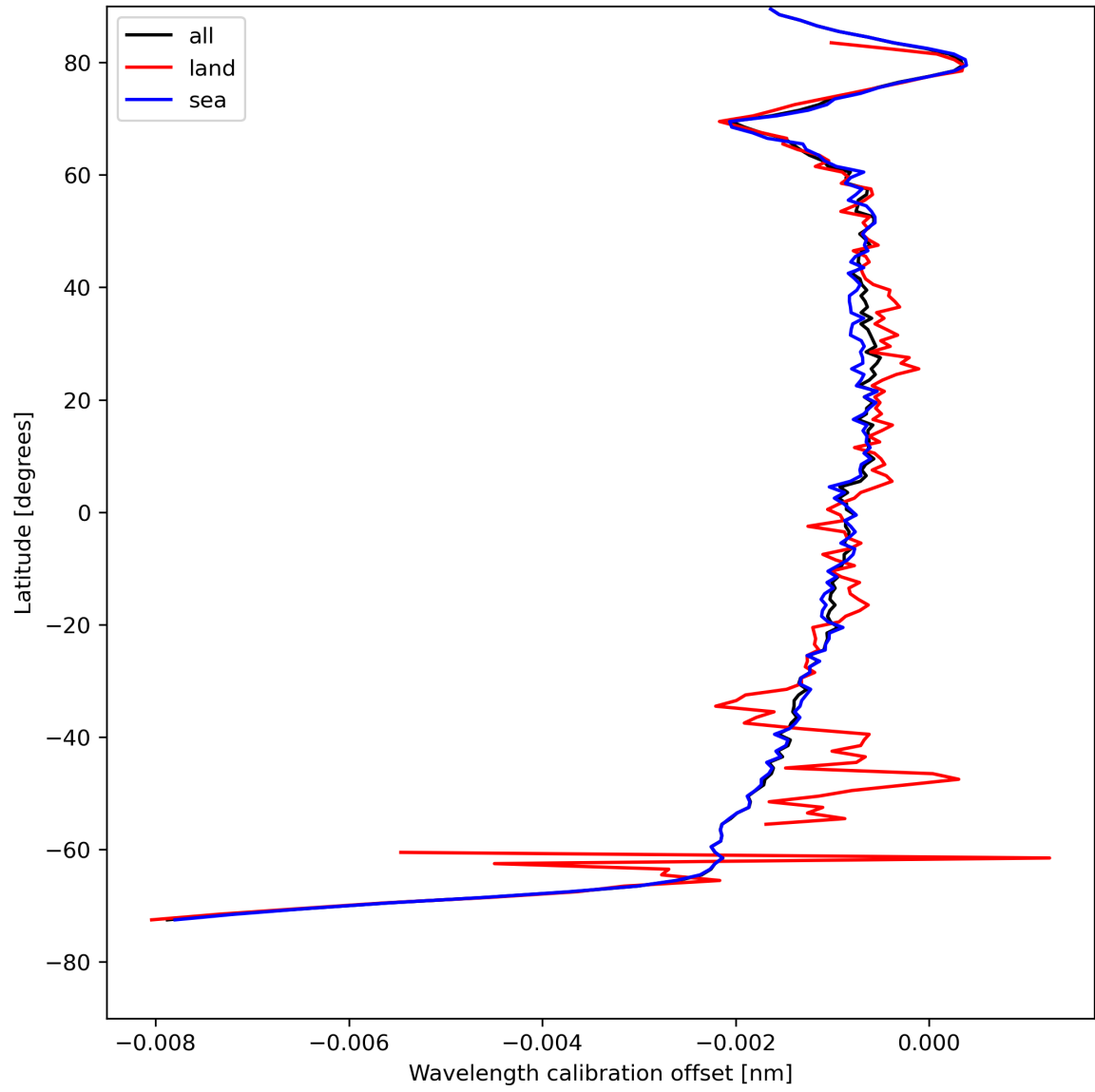
Figure 18: Zonal average of “Wavelength calibration offset” for 2023-08-09 to 2023-08-11.
