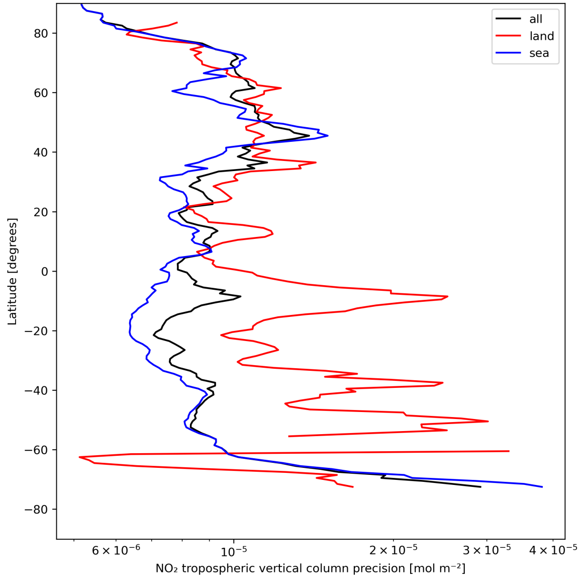
Figure 13: Zonal average of “NO 2 tropospheric vertical column precision” for 2023-08-09 to 2023-08-11.
