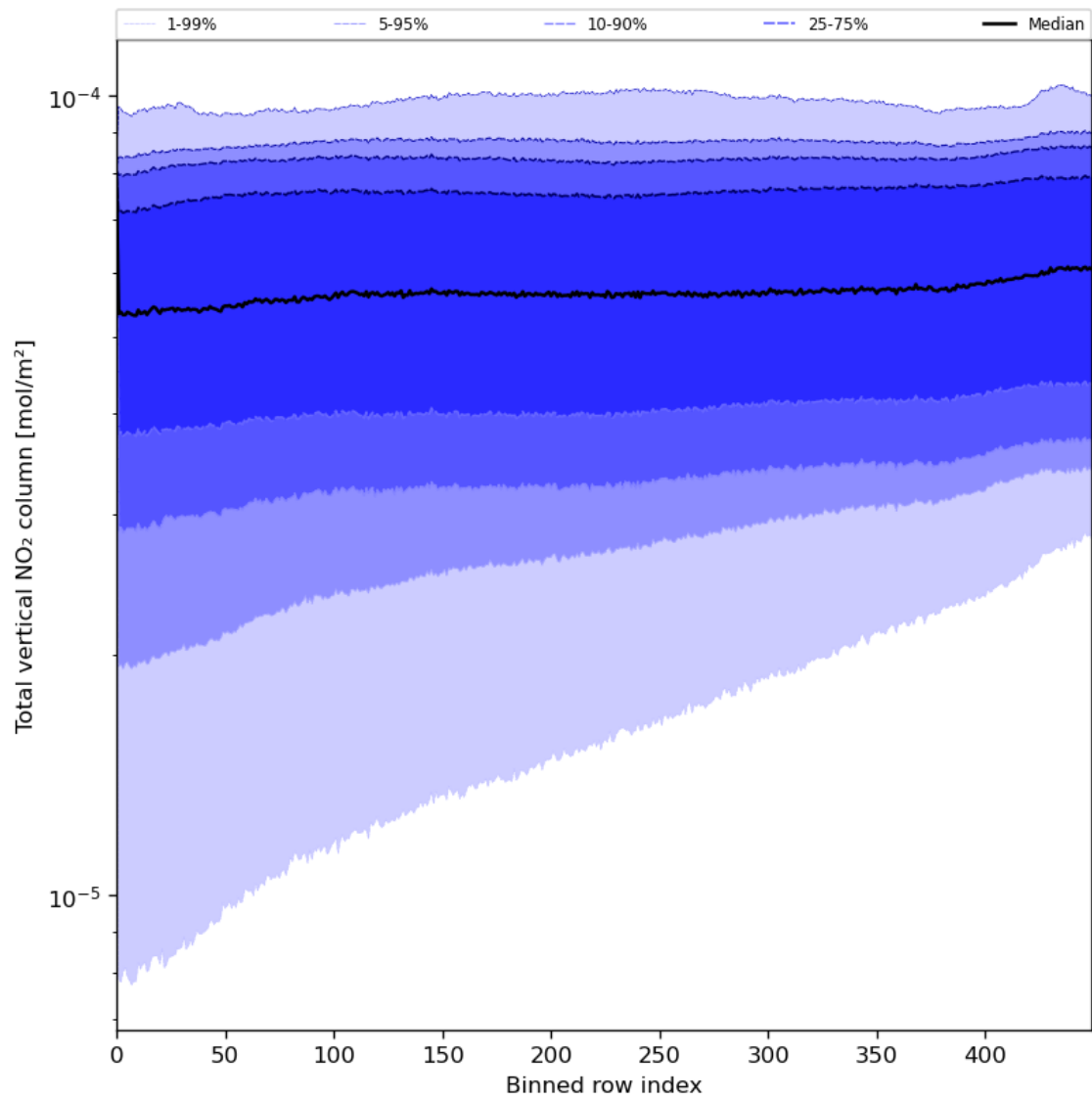
Figure 55: Along track statistics of “Total vertical NO 2 column” for 2023-08-09 to 2023-08-11
