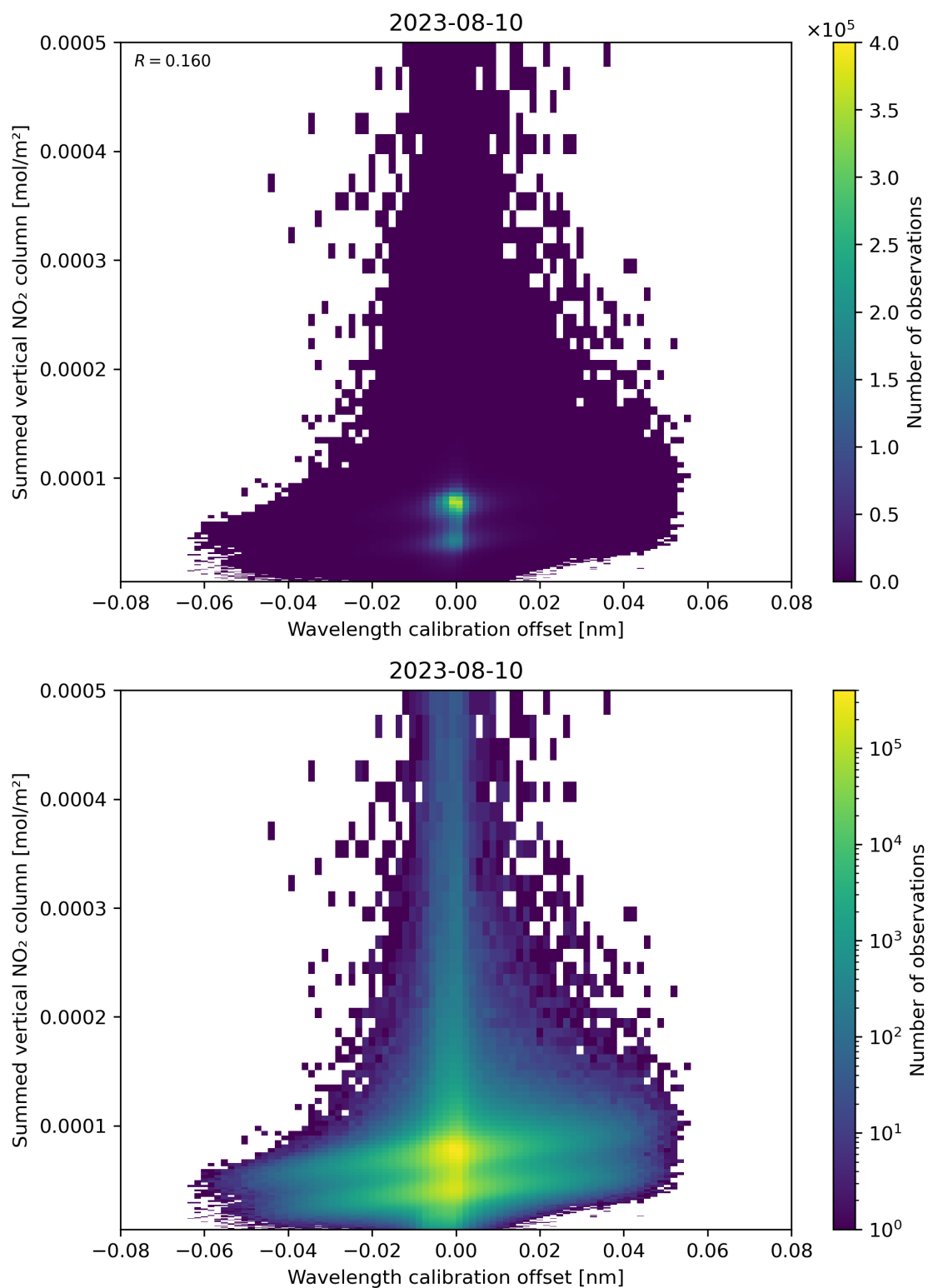
Figure 177: Scatter density plot of “Wavelength calibration offset” against “Summed vertical NO 2 column” for 2023-08-09 to 2023-08-11.
