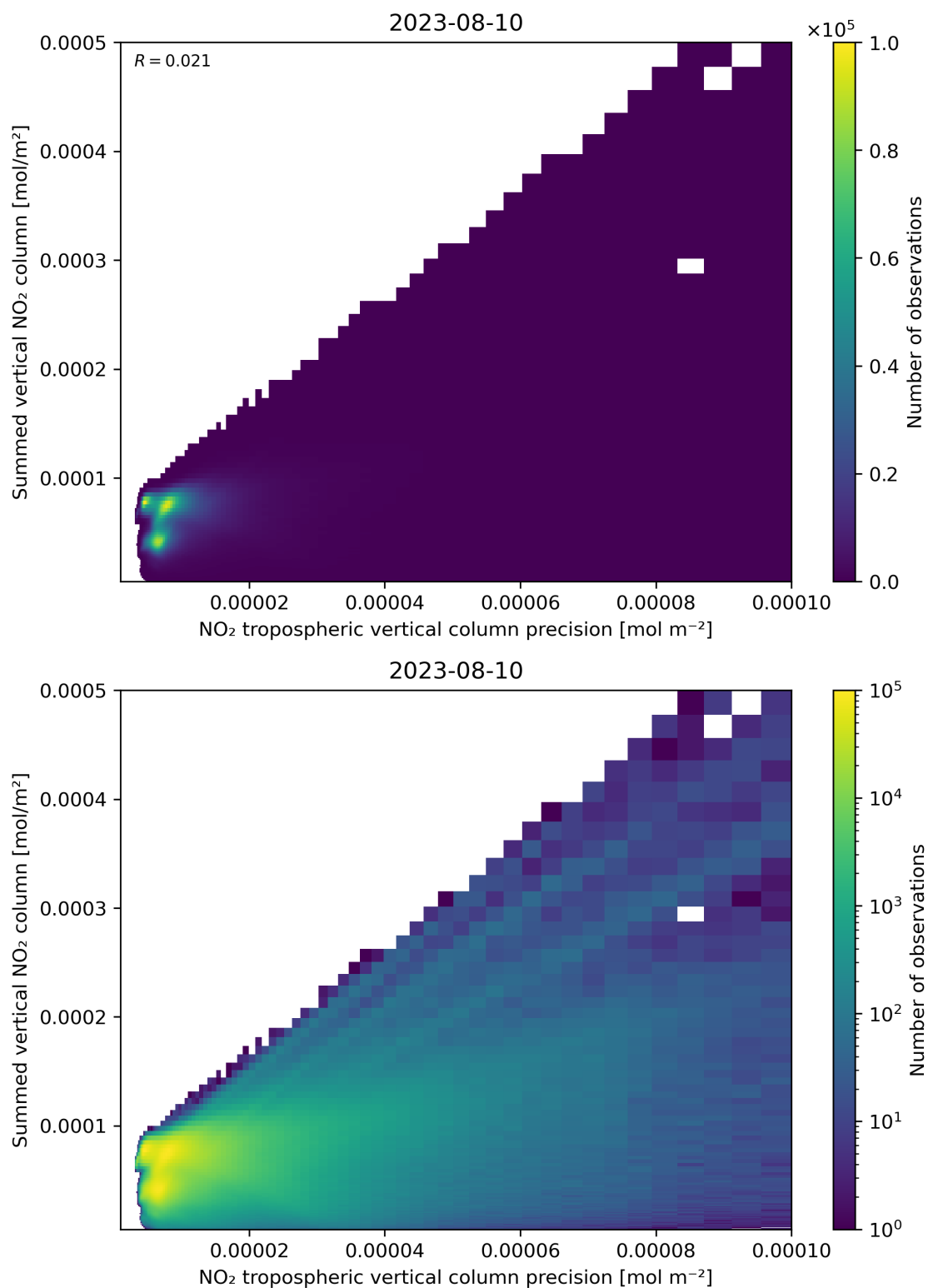
Figure 136: Scatter density plot of “NO 2 tropospheric vertical column precision” against “Summed vertical NO 2 column” for 2023-08-09 to 2023-08-11.
