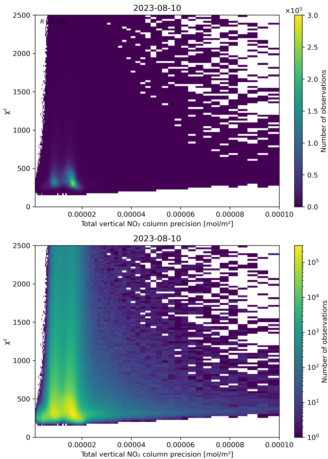
Figure 116: Scatter density plot of “Total vertical NO 2 column precision” against “ \chi^2 ” for 2023-08-09 to 2023-08-11.
