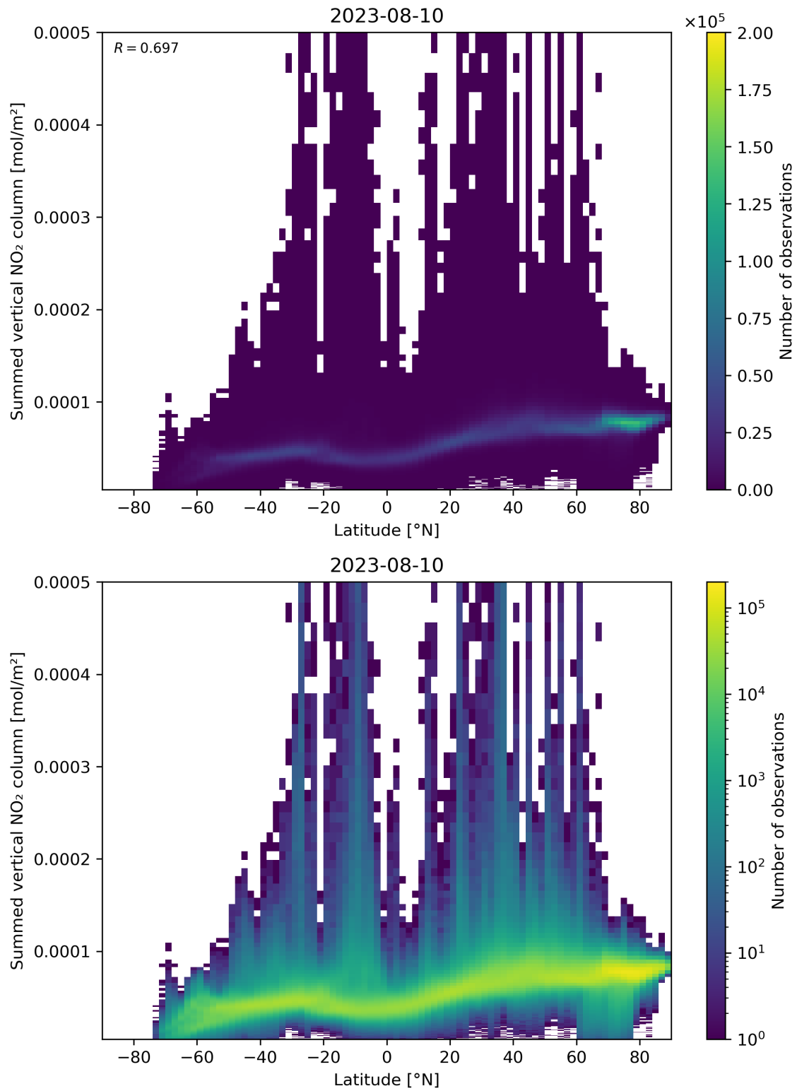
Figure 88: Scatter density plot of “Latitude” against “Summed vertical NO 2 column” for 2023-08-09 to 2023-08-11.
