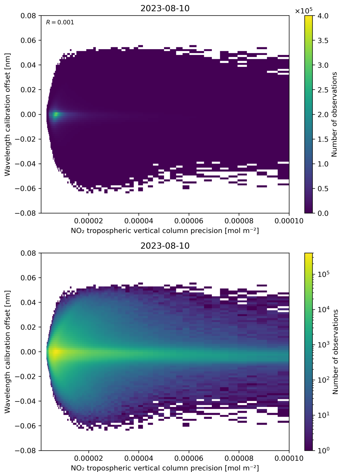
Figure 141: Scatter density plot of “NO 2 tropospheric vertical column precision” against “Wavelength calibration offset” for 2023-08-09 to 2023-08-11.
