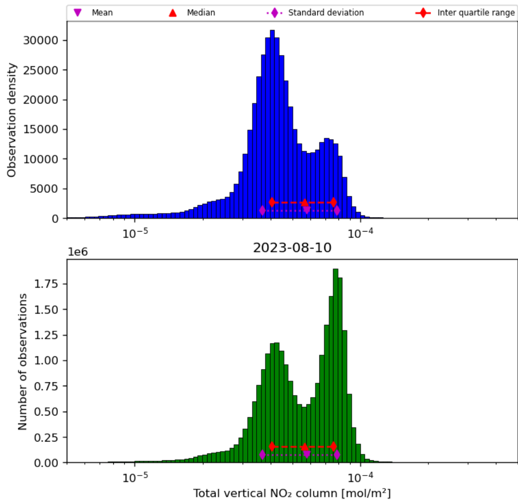
Figure 38: Histogram of “Total vertical NO 2 column” for 2023-08-09 to 2023-08-11
