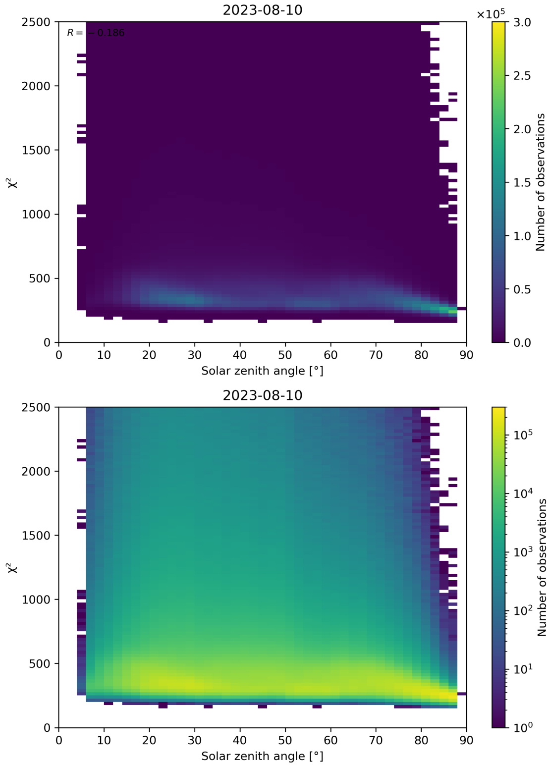
Figure 148: Scatter density plot of “Solar zenith angle” against “ \chi^2 ” for 2023-08-09 to 2023-08-11.
