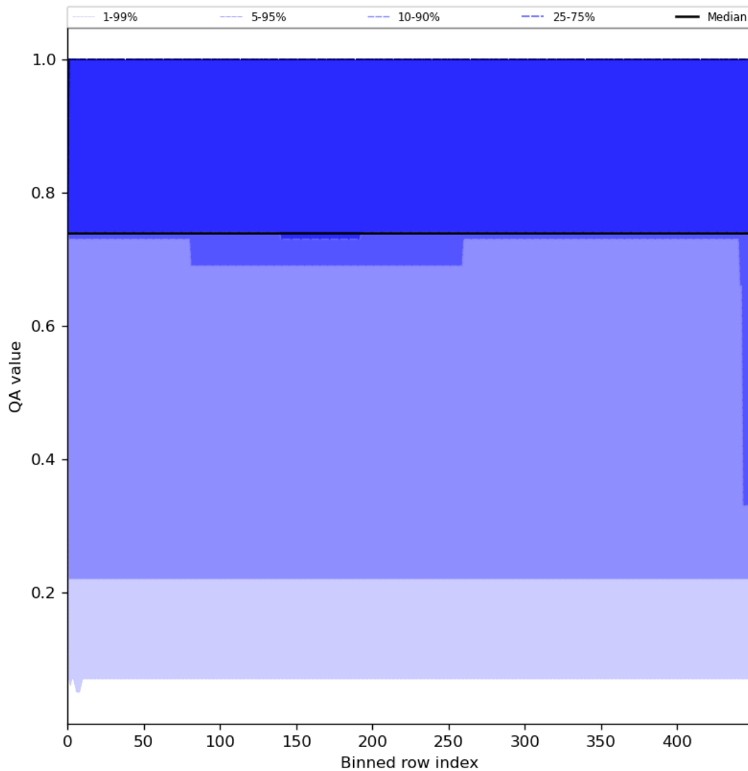
Figure 45: Along track statistics of “QA value” for 2023-08-09 to 2023-08-11
