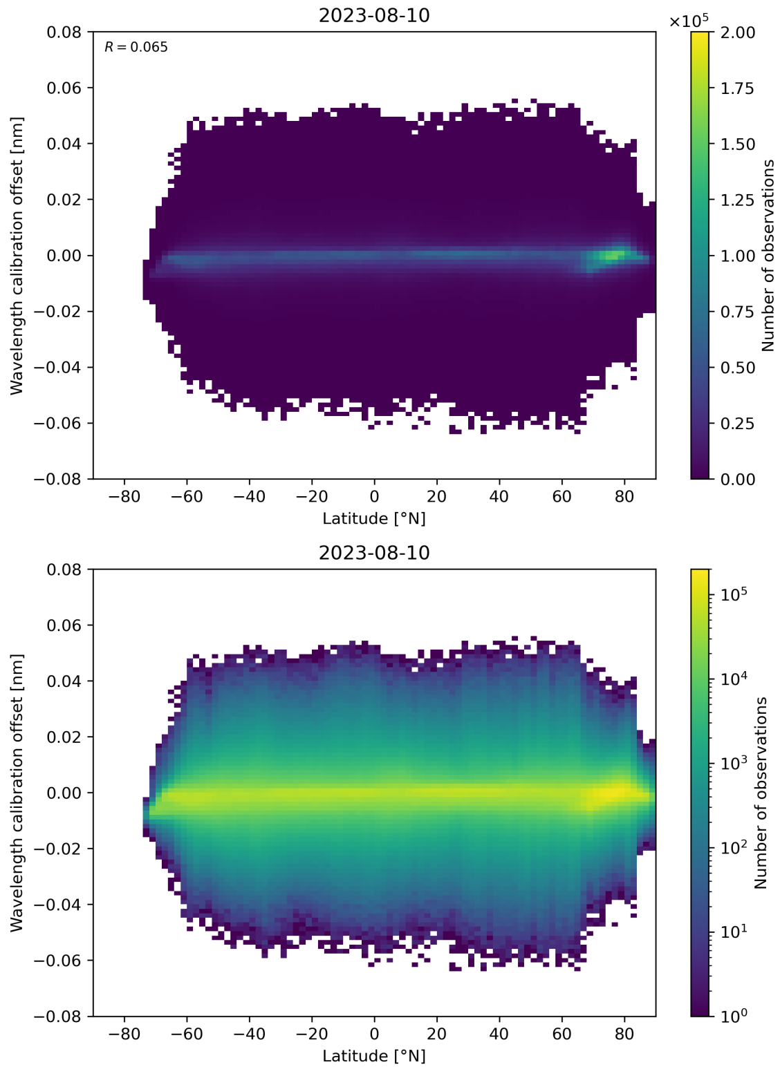
Figure 95: Scatter density plot of “Latitude” against “Wavelength calibration offset” for 2023-08-09 to 2023-08-11.
