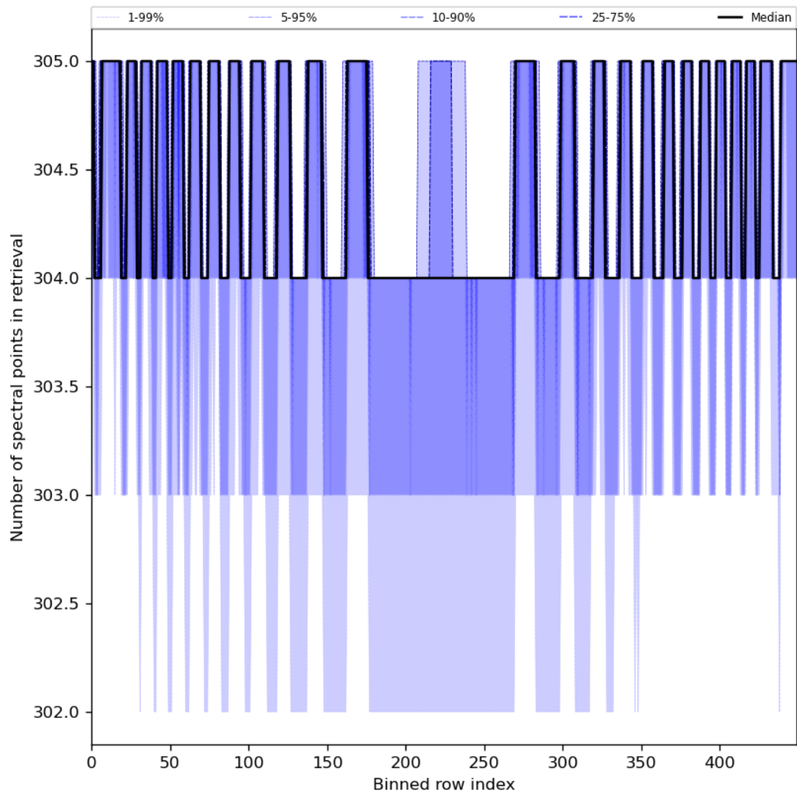
Figure 50: Along track statistics of “Number of spectral points in retrieval” for 2023-08-09 to 2023-08-11
