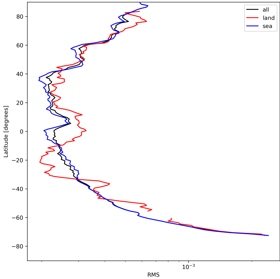
Figure 26: Zonal average of “RMS” for 2023-08-09 to 2023-08-11.
