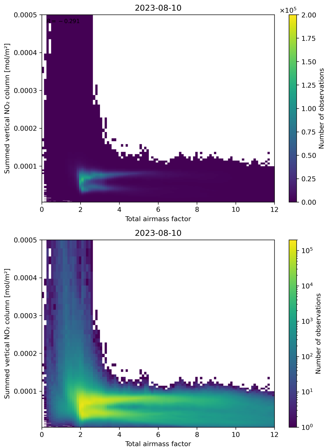
Figure 65: Scatter density plot of “Total airmass factor” against “Summed vertical NO 2 column” for 2023-08-09 to 2023-08-11.
