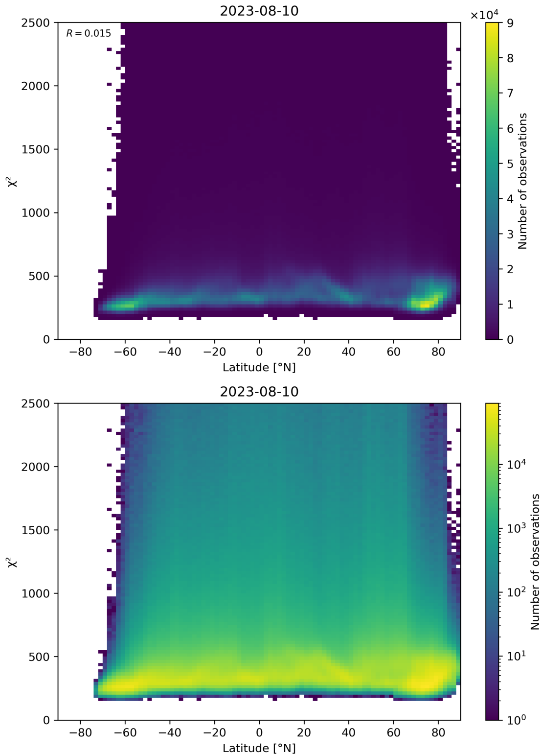
Figure 86: Scatter density plot of “Latitude” against “ \chi^2 ” for 2023-08-09 to 2023-08-11.
