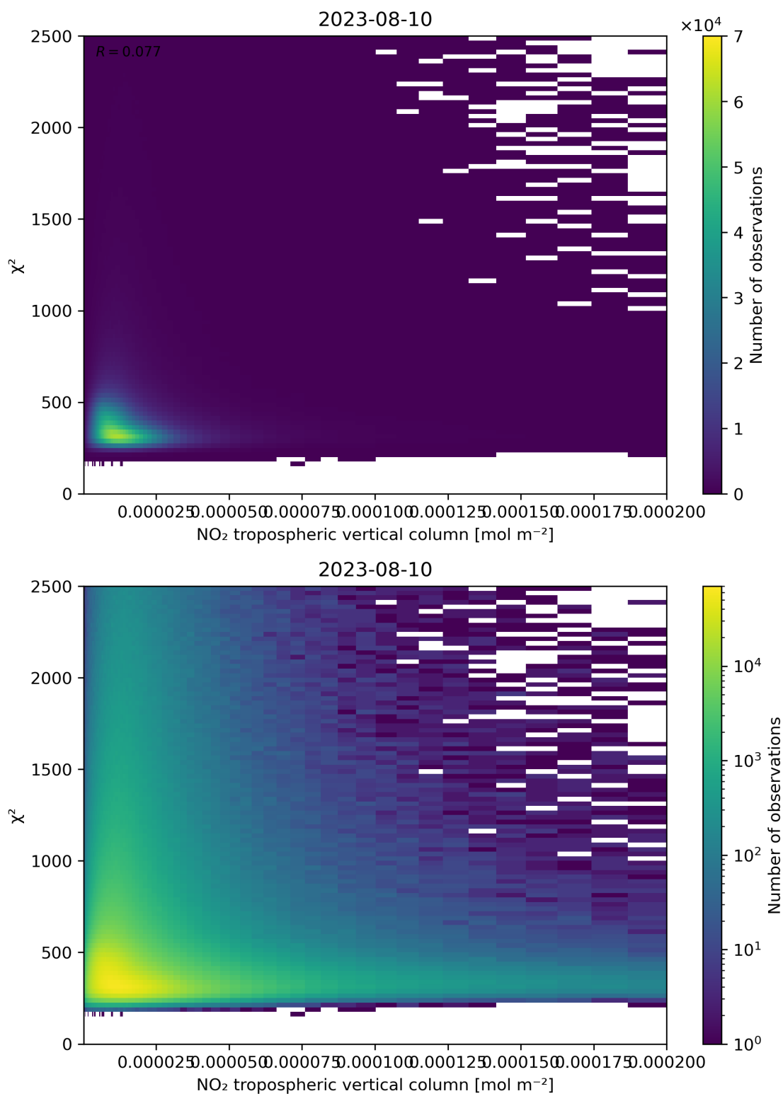
Figure 124: Scatter density plot of “NO 2 tropospheric vertical column” against “ \chi^2 ” for 2023-08-09 to 2023-08-11.
