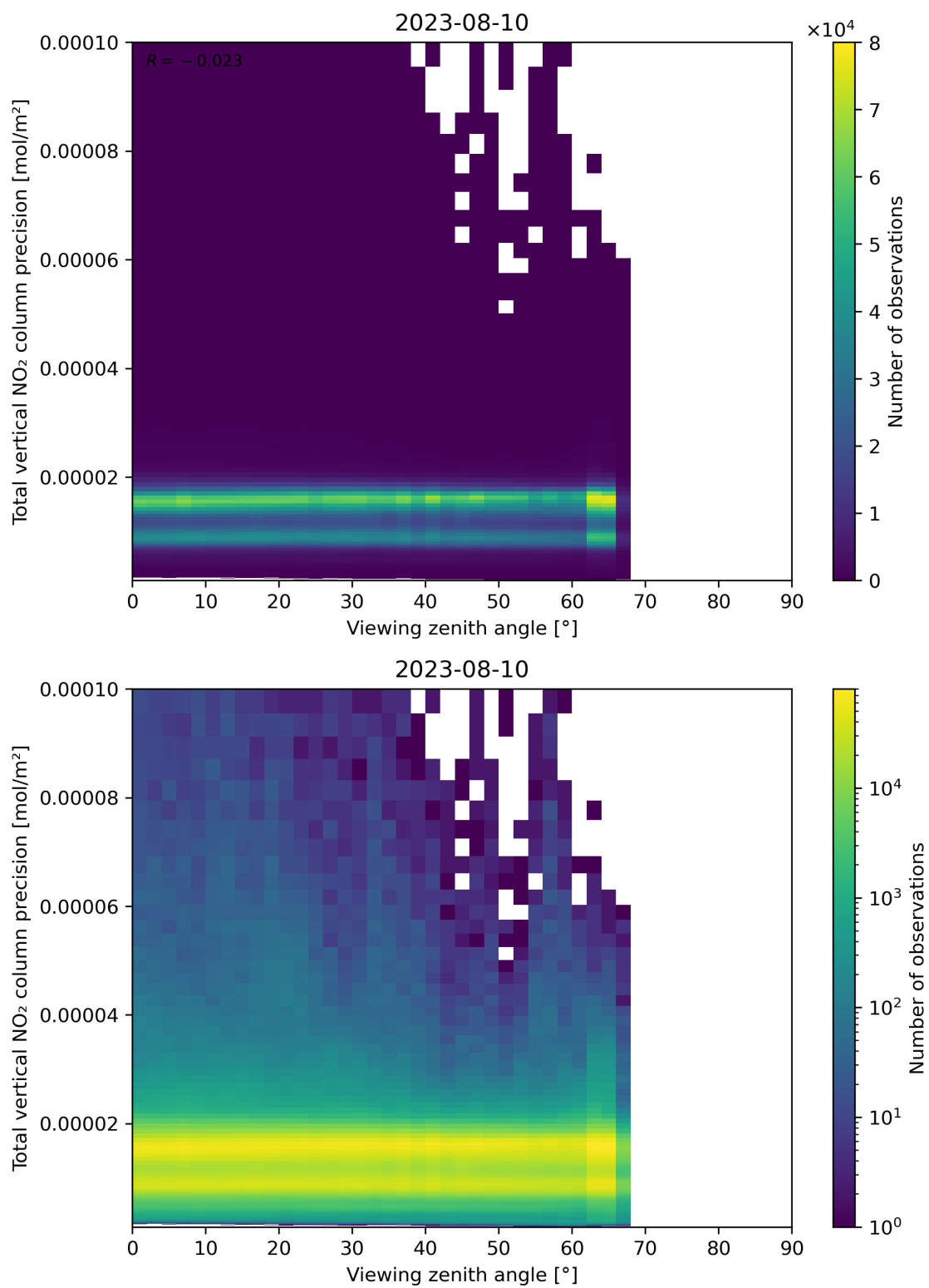
Figure 168: Scatter density plot of “Viewing zenith angle” against “Total vertical NO 2 column precision” for 2023-08-09 to 2023-08-11.
