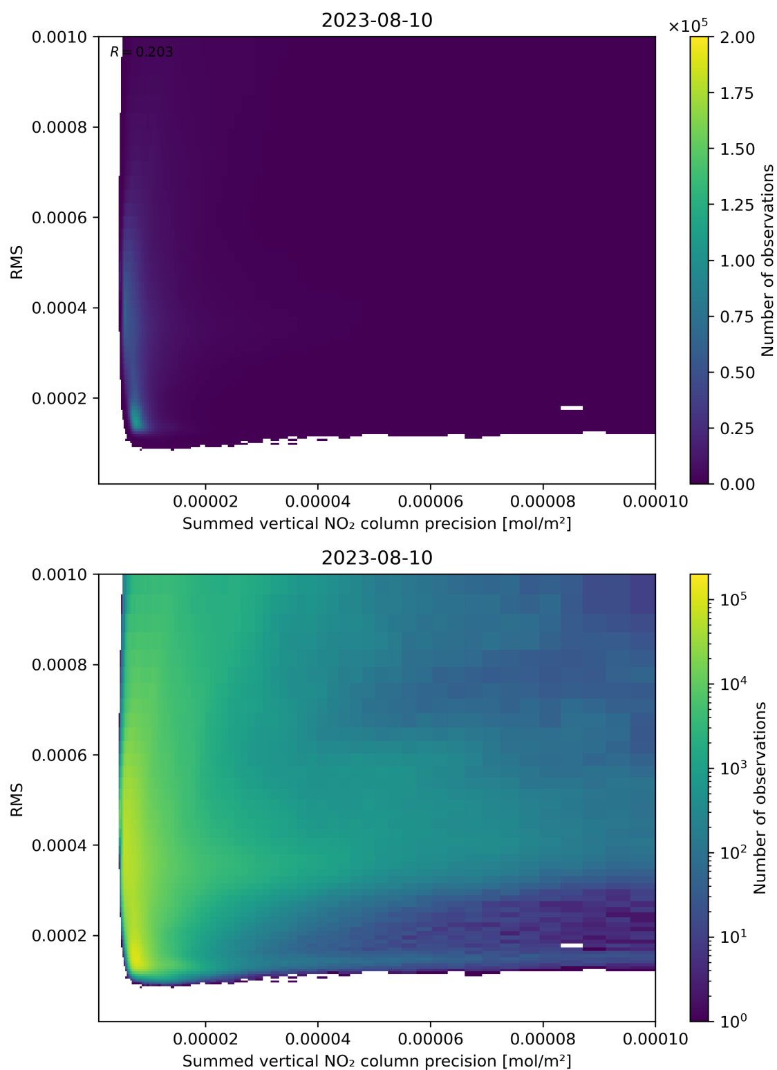
Figure 108: Scatter density plot of “Summed vertical NO 2 column precision” against “RMS” for 2023-08-09 to 2023-08-11.
