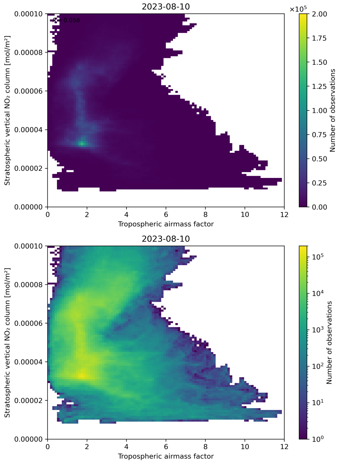
Figure 74: Scatter density plot of “Tropospheric air mass factor” against “Stratospheric vertical NO 2 column” for 2023-08-09 to 2023-08-11.
