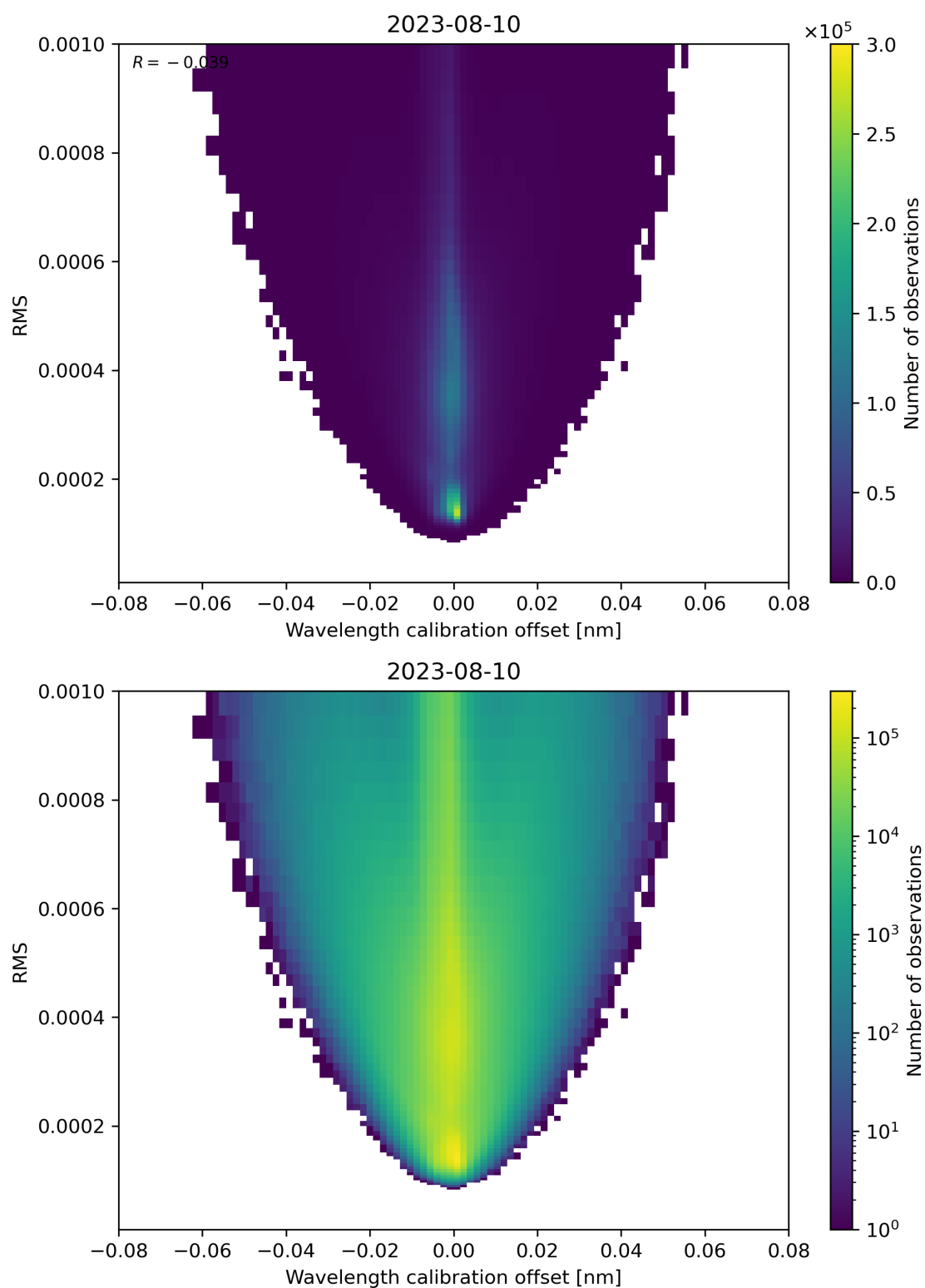
Figure 181: Scatter density plot of “Wavelength calibration offset” against “RMS” for 2023-08-09 to 2023-08-11.
