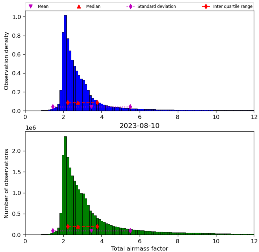
Figure 32: Histogram of “Total airmass factor” for 2023-08-09 to 2023-08-11
