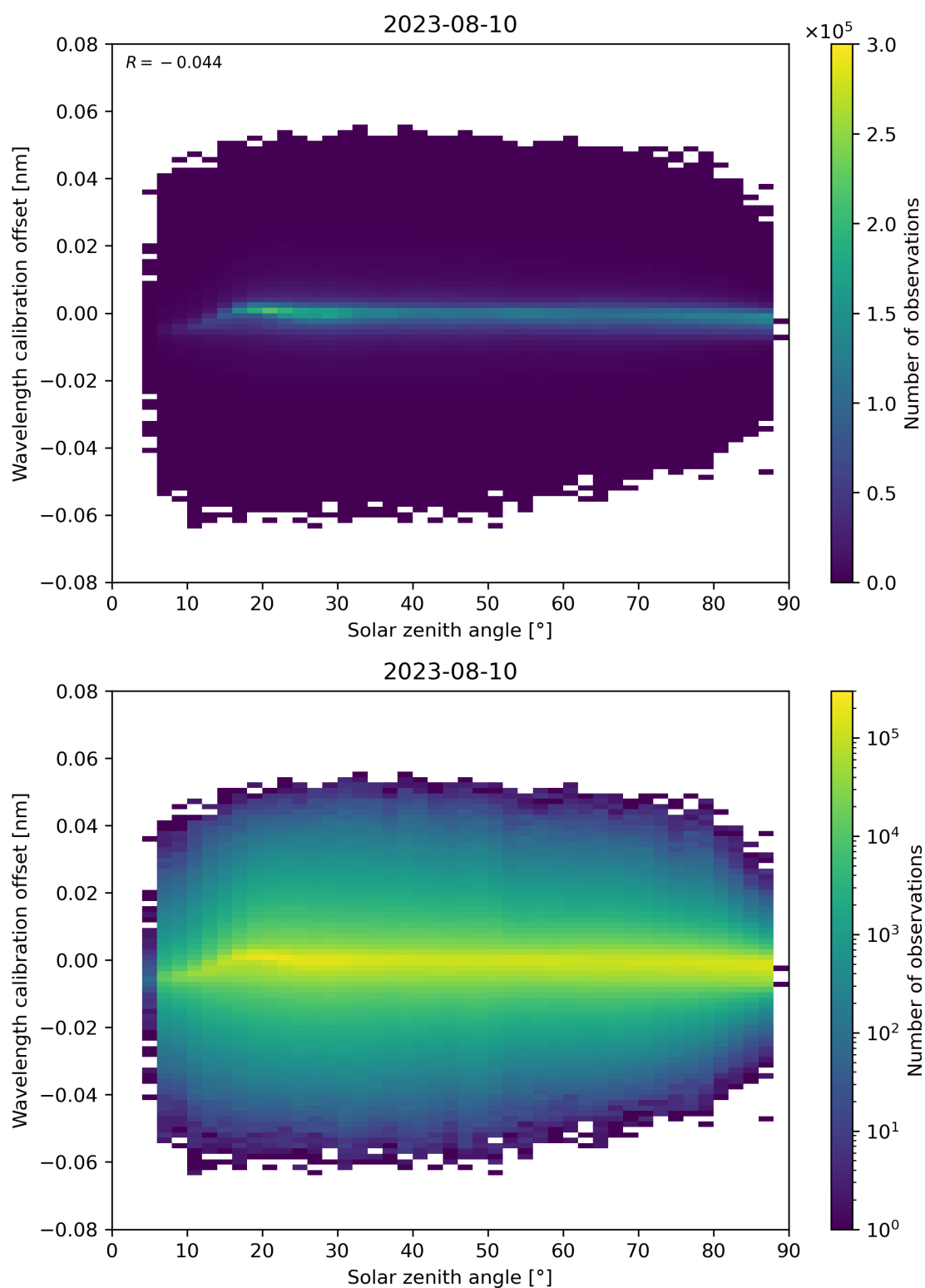
Figure 158: Scatter density plot of “Solar zenith angle” against “Wavelength calibration offset” for 2023-08-09 to 2023-08-11.
