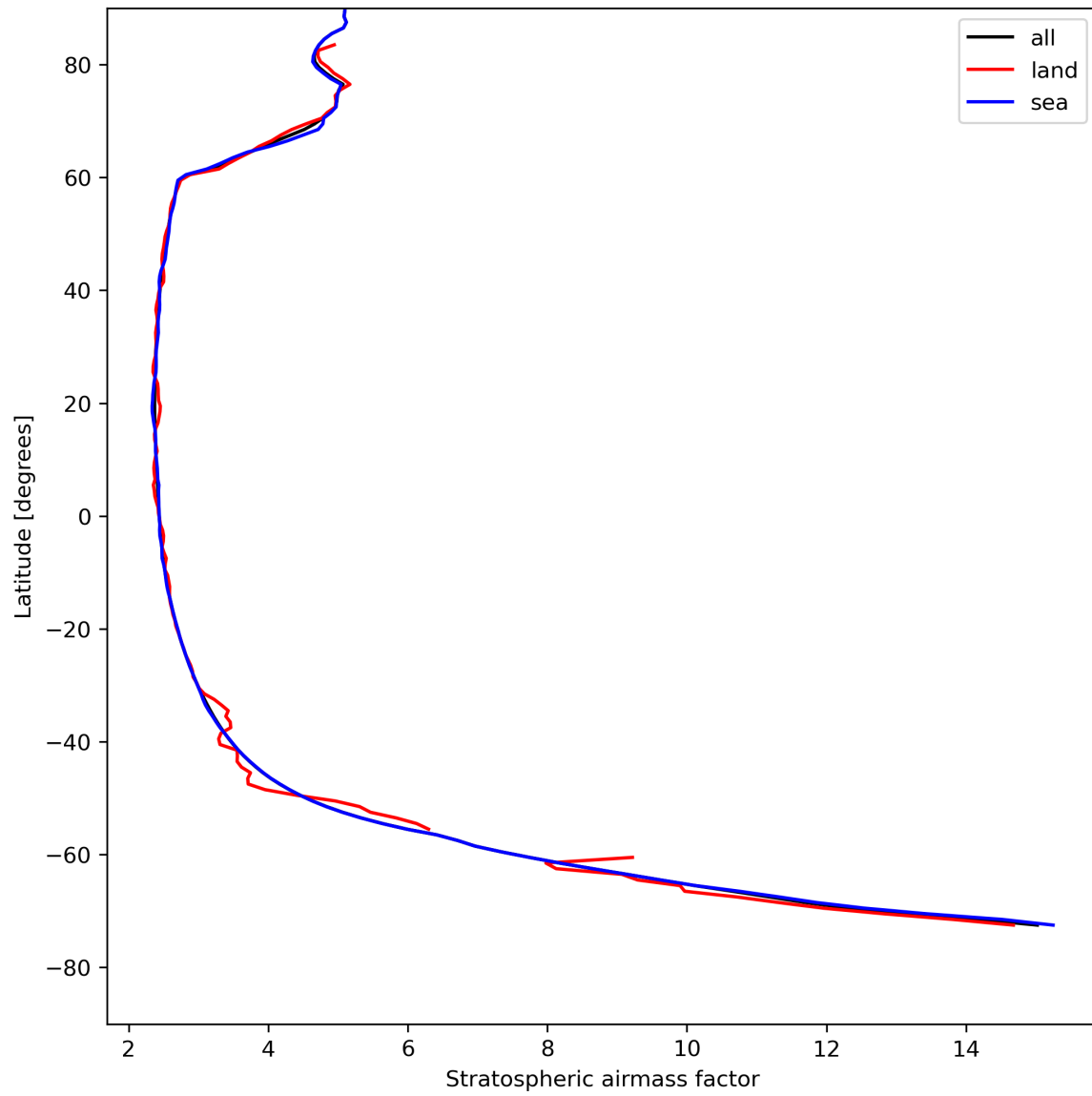
Figure 27: Zonal average of “Stratospheric air mass factor” for 2023-08-09 to 2023-08-11.
