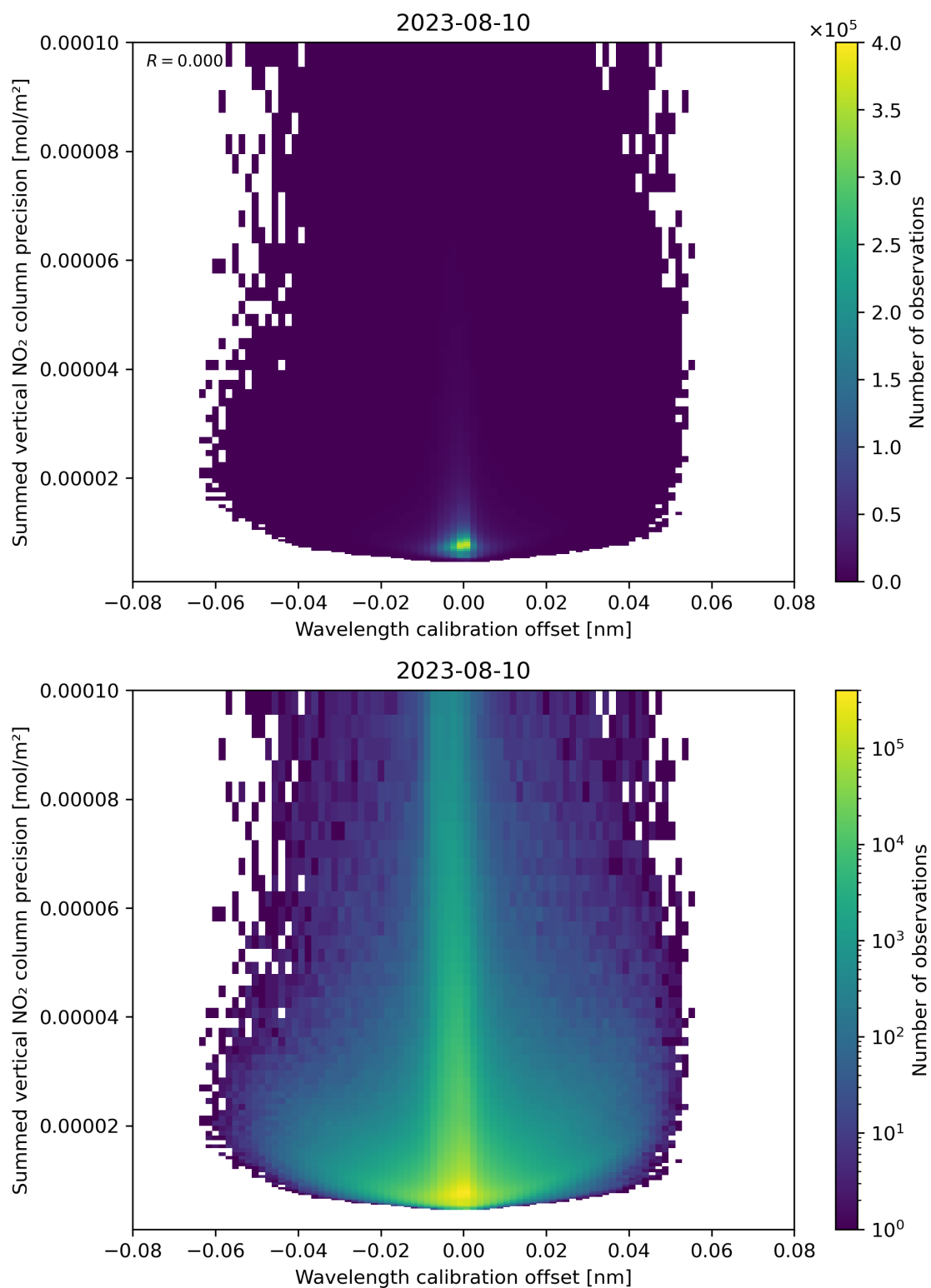
Figure 178: Scatter density plot of “Wavelength calibration offset” against “Summed vertical NO 2 column precision” for 2023-08-09 to 2023-08-11.
