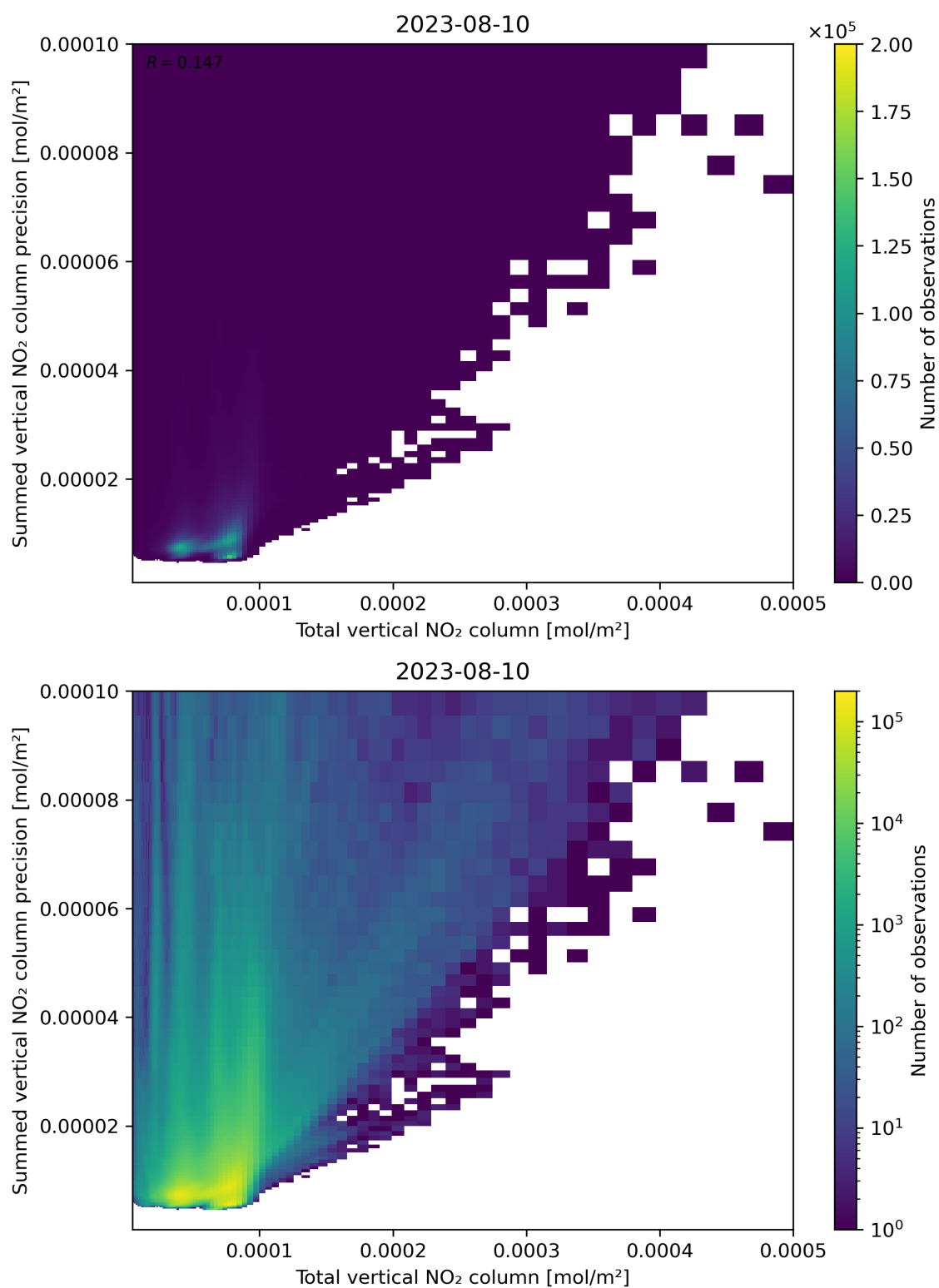
Figure 113: Scatter density plot of “Total vertical NO 2 column” against “Summed vertical NO 2 column precision” for 2023-08-09 to 2023-08-11.
