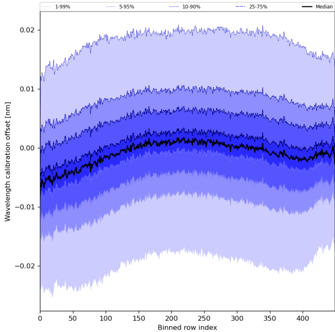
Figure 52: Along track statistics of “Wavelength calibration offset” for 2023-08-09 to 2023-08-11
