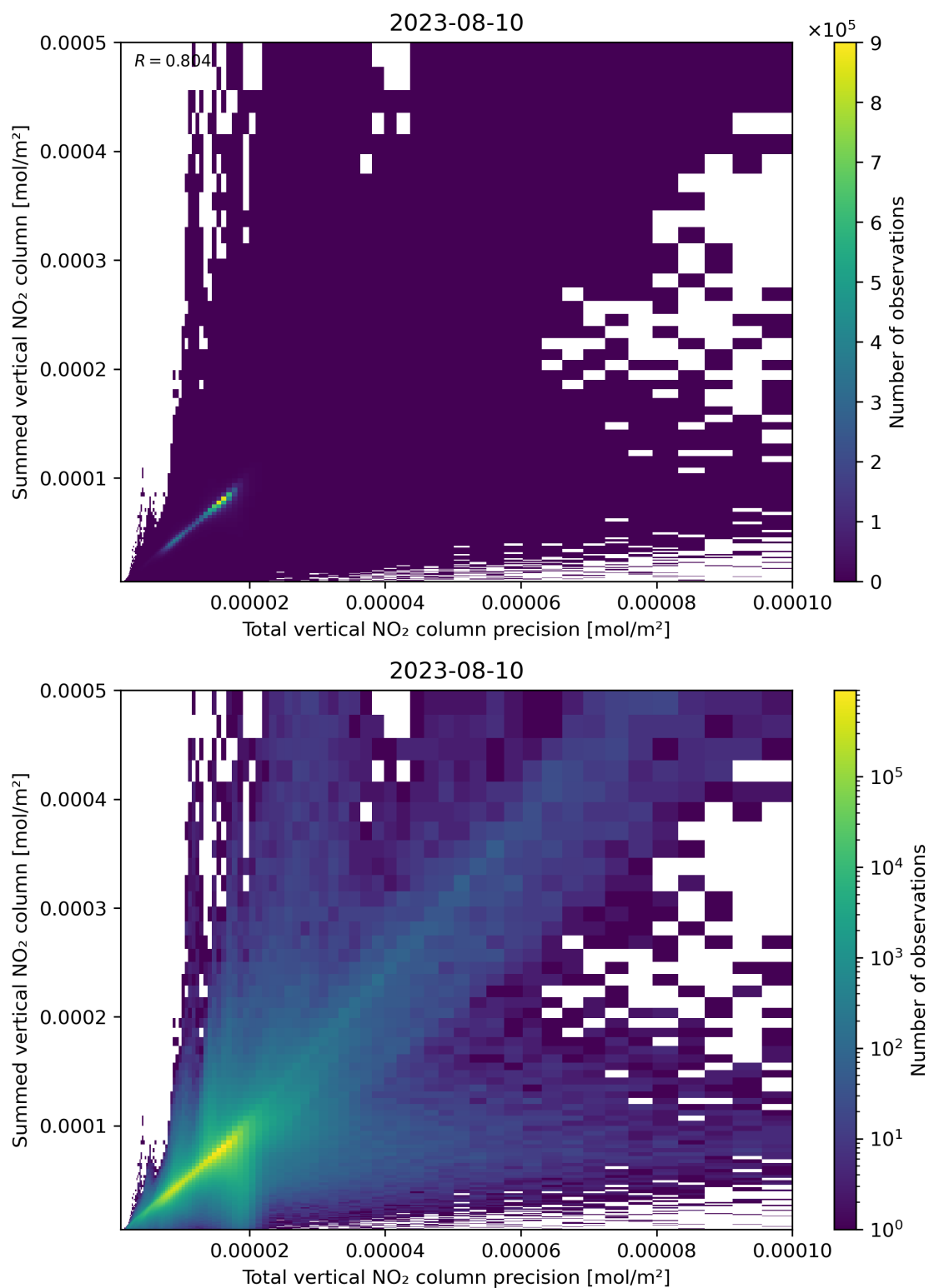
Figure 117: Scatter density plot of “Total vertical NO 2 column precision” against “Summed vertical NO 2 column” for 2023-08-09 to 2023-08-11.
