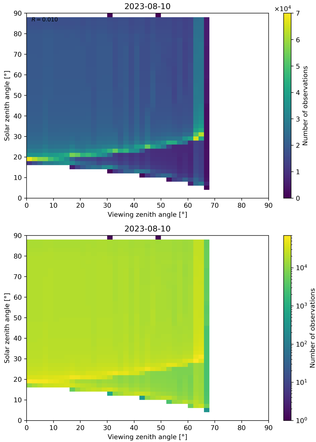
Figure 172: Scatter density plot of “Viewing zenith angle” against “Solar zenith angle” for 2023-08-09 to 2023-08-11.
