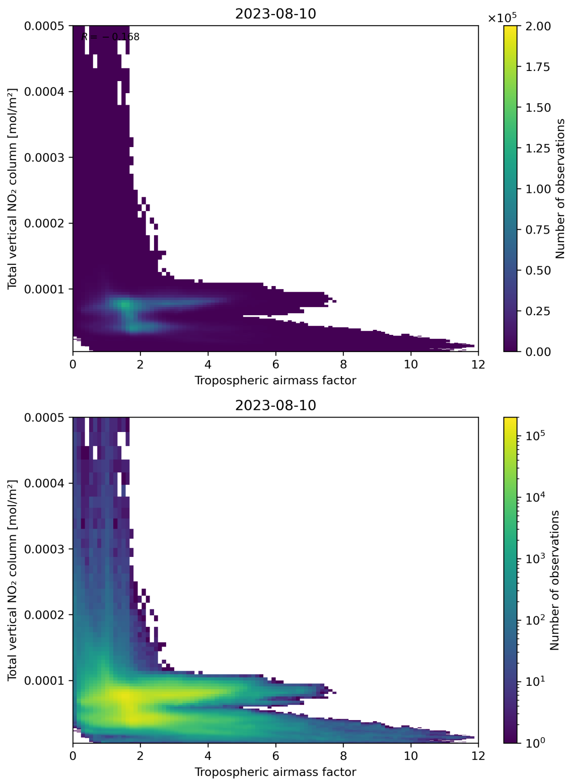
Figure 77: Scatter density plot of “Tropospheric airmass factor” against “Total vertical NO 2 column” for 2023-08-09 to 2023-08-11.
