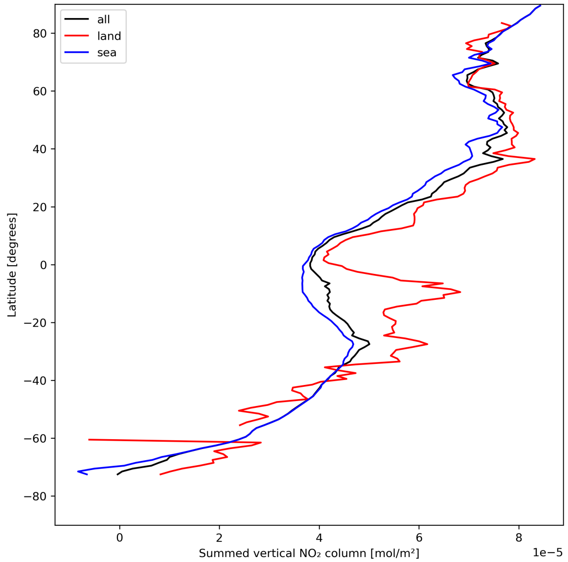
Figure 23: Zonal average of “Summed vertical NO 2 column” for 2023-08-09 to 2023-08-11.
