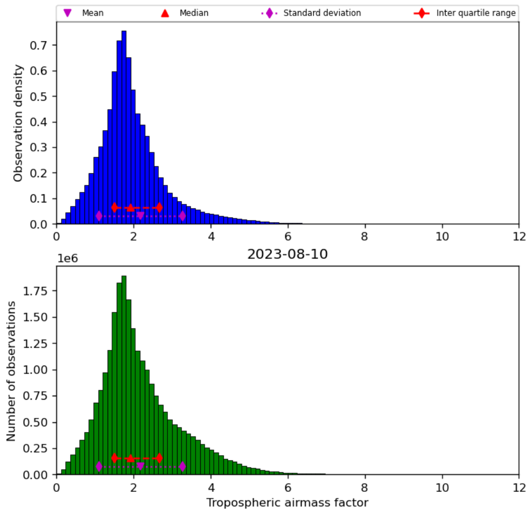
Figure 31: Histogram of “Tropospheric air mass factor” for 2023-08-09 to 2023-08-11
