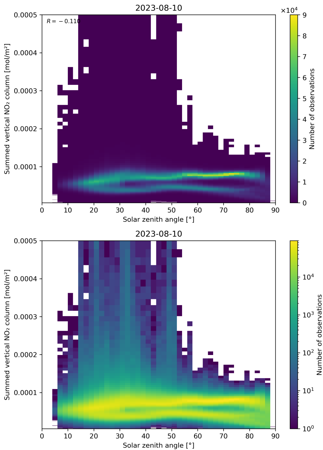
Figure 151: Scatter density plot of “Solar zenith angle” against “Summed vertical NO 2 column” for 2023-08-09 to 2023-08-11.
