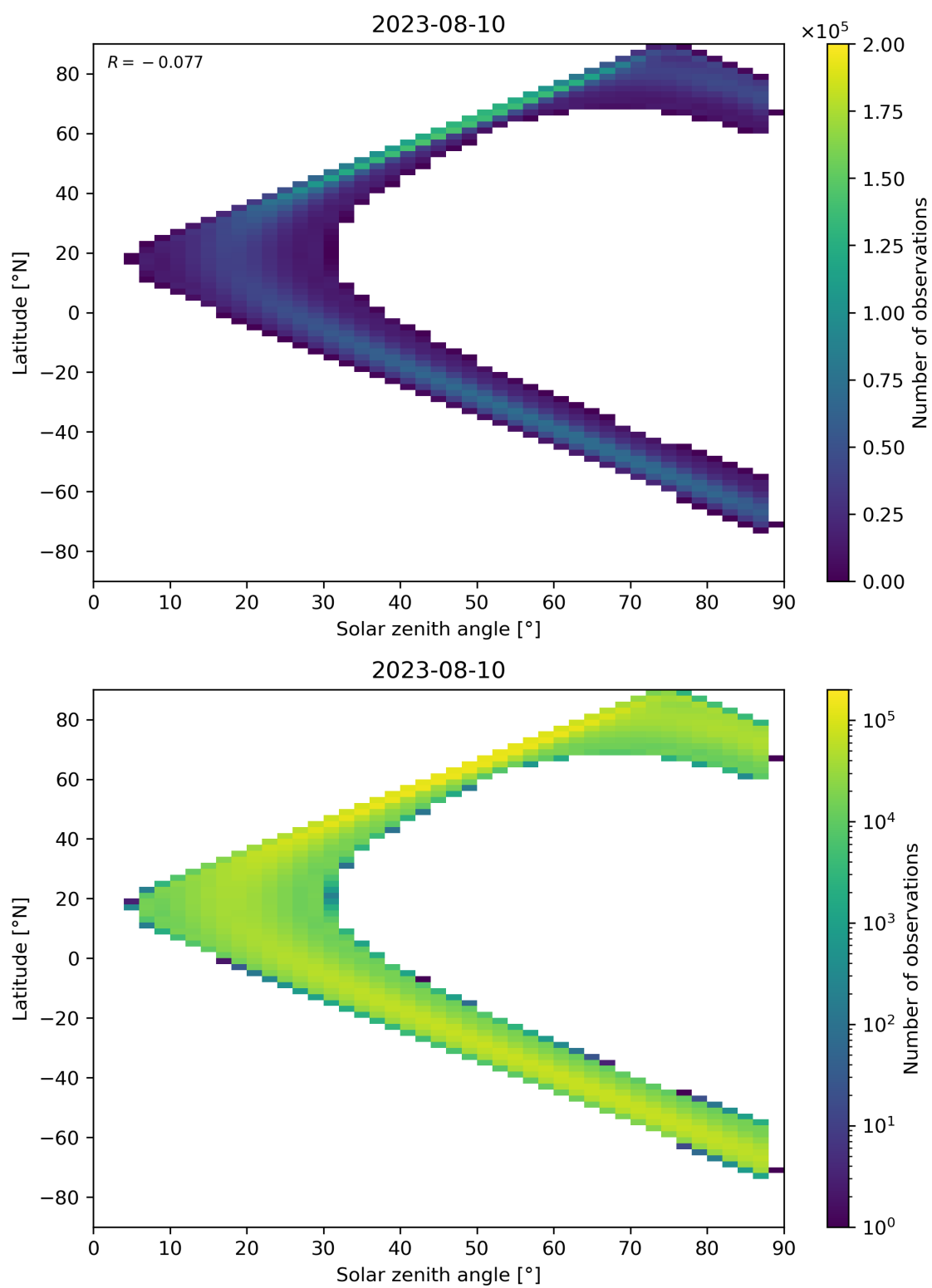
Figure 149: Scatter density plot of “Solar zenith angle” against “Latitude” for 2023-08-09 to 2023-08-11.
