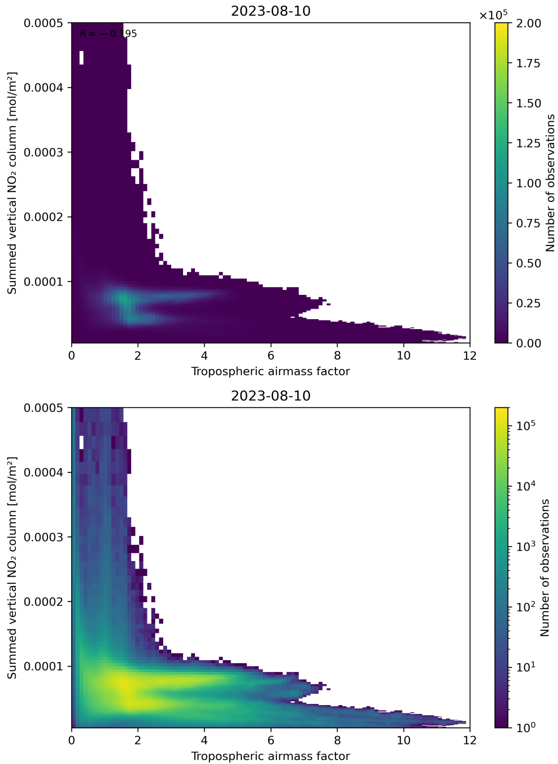
Figure 75: Scatter density plot of “Tropospheric airmass factor” against “Summed vertical NO 2 column” for 2023-08-09 to 2023-08-11.
