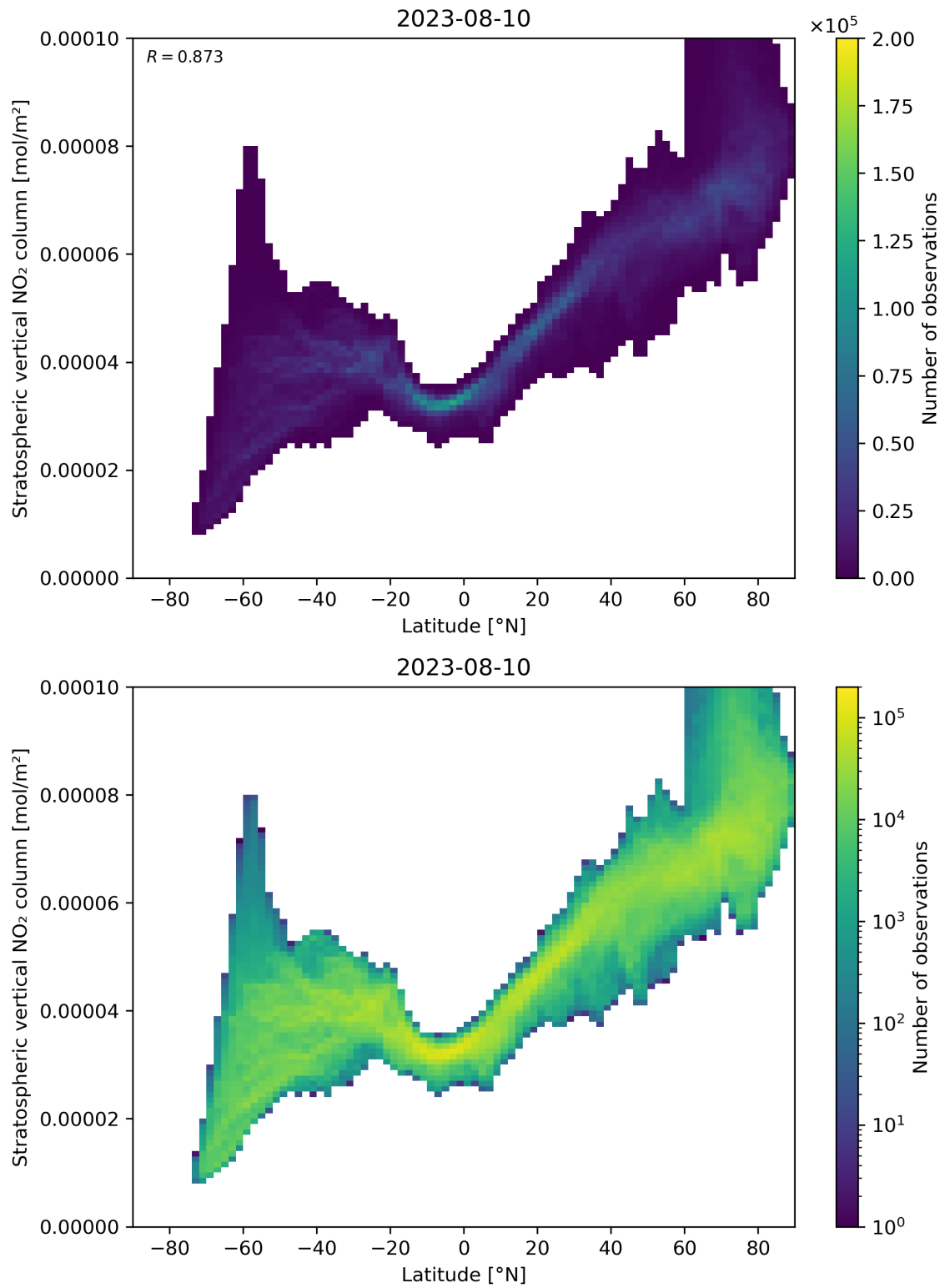
Figure 87: Scatter density plot of “Latitude” against “Stratospheric vertical NO 2 column” for 2023-08-09 to 2023-08-11.
