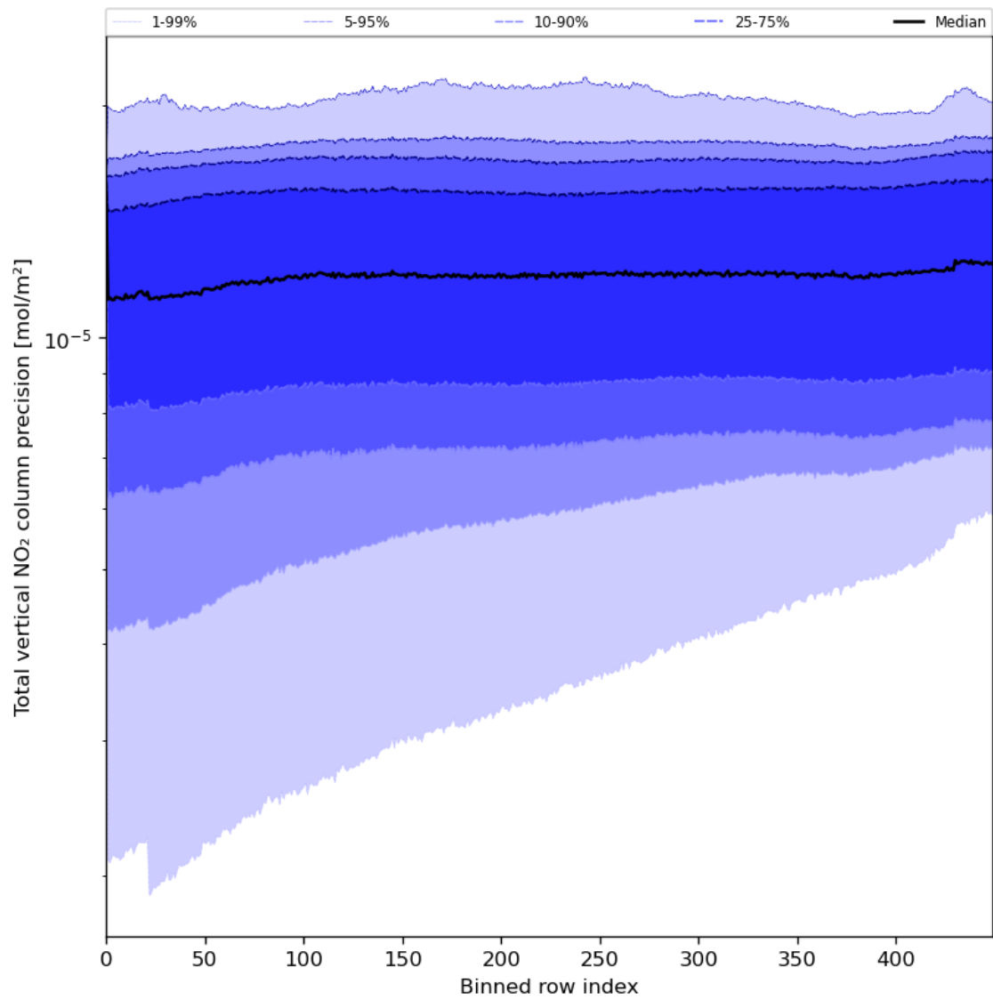
Figure 56: Along track statistics of “Total vertical NO 2 column precision” for 2023-08-09 to 2023-08-11
