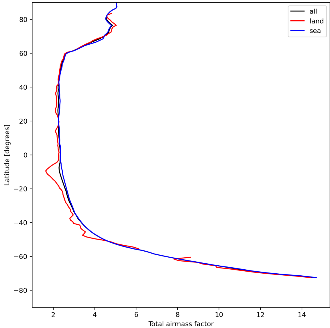
Figure 15: Zonal average of “Total airmass factor” for 2023-08-09 to 2023-08-11.
