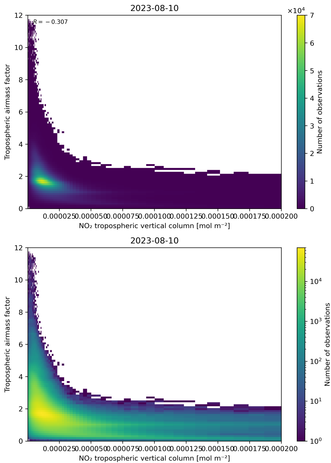
Figure 123: Scatter density plot of “NO 2 tropospheric vertical column” against “Tropospheric air mass factor” for 2023-08-09 to 2023-08-11.
