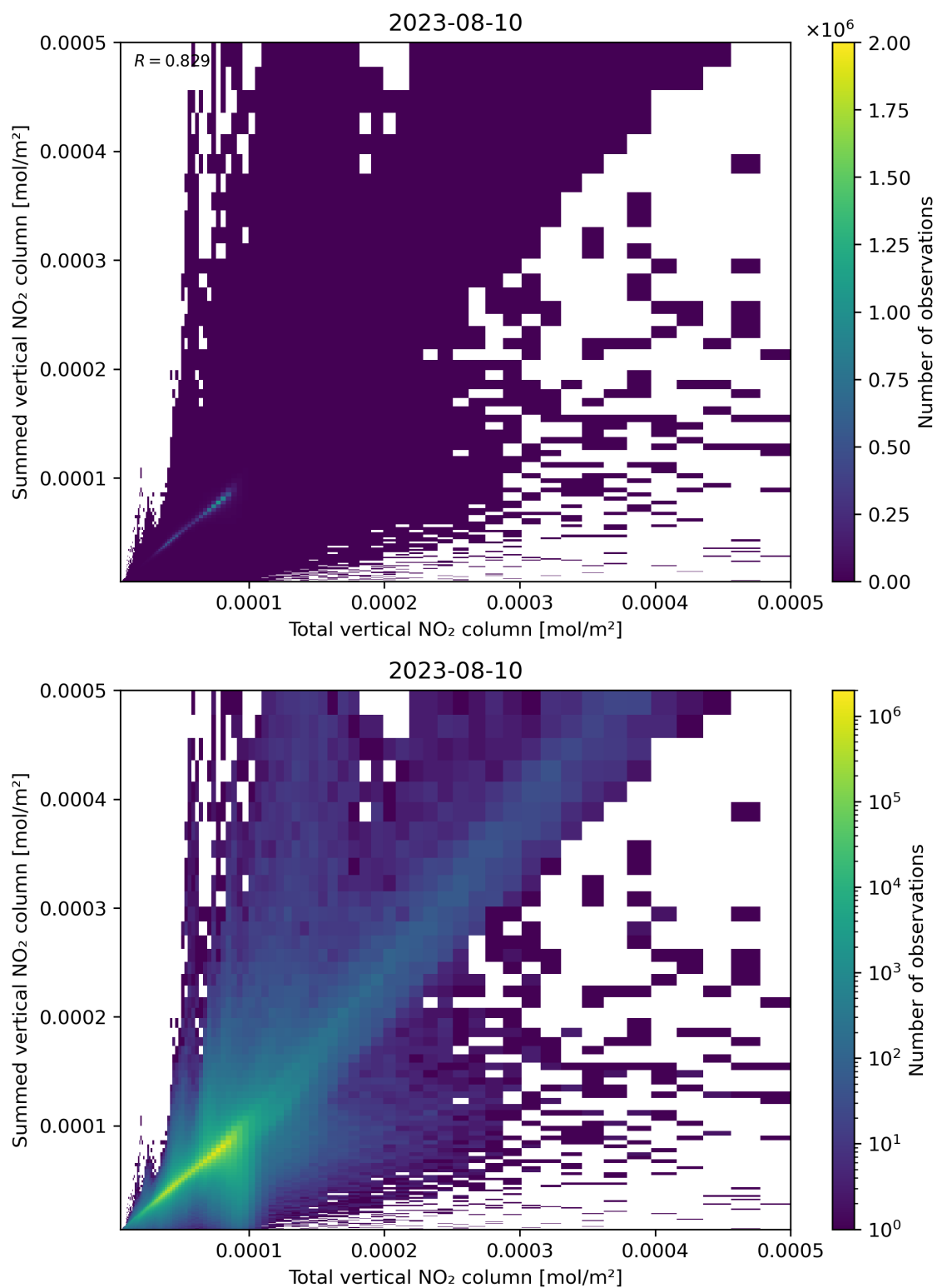
Figure 112: Scatter density plot of “Total vertical NO 2 column” against “Summed vertical NO 2 column” for 2023-08-09 to 2023-08-11.
