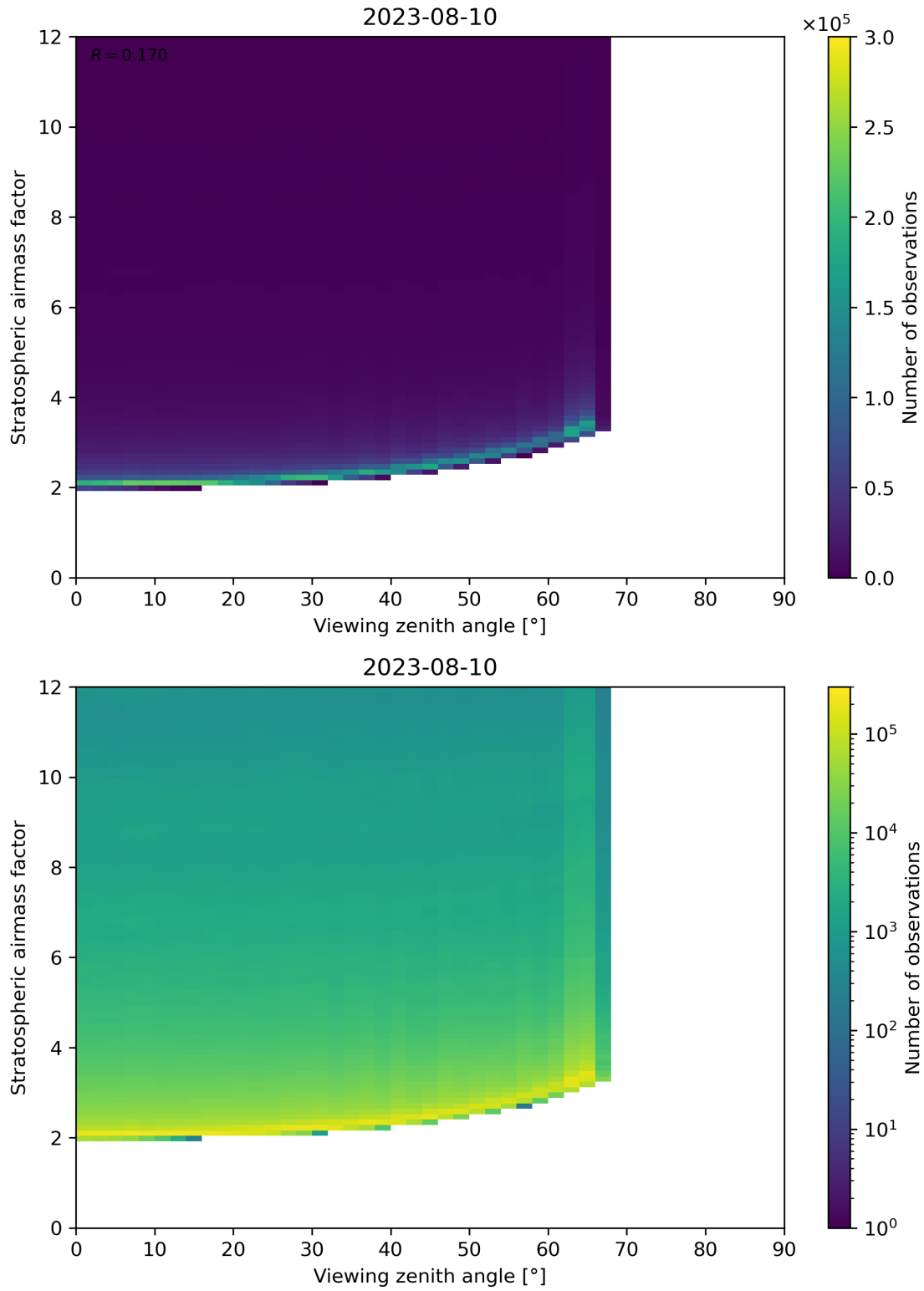
Figure 159: Scatter density plot of “Viewing zenith angle” against “Stratospheric airmass factor” for 2023-08-09 to 2023-08-11.
