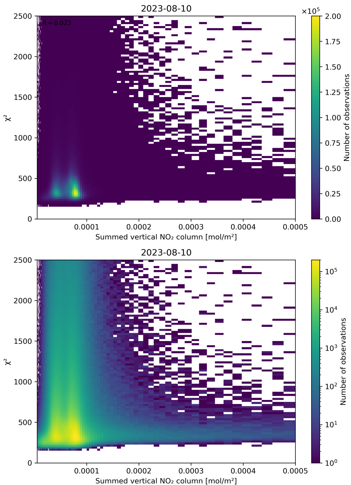
Figure 104: Scatter density plot of “Summed vertical NO 2 column” against “ \chi^2 ” for 2023-08-09 to 2023-08-11.
