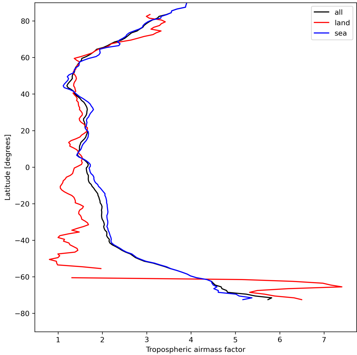
Figure 14: Zonal average of “Tropospheric airmass factor” for 2023-08-09 to 2023-08-11.
