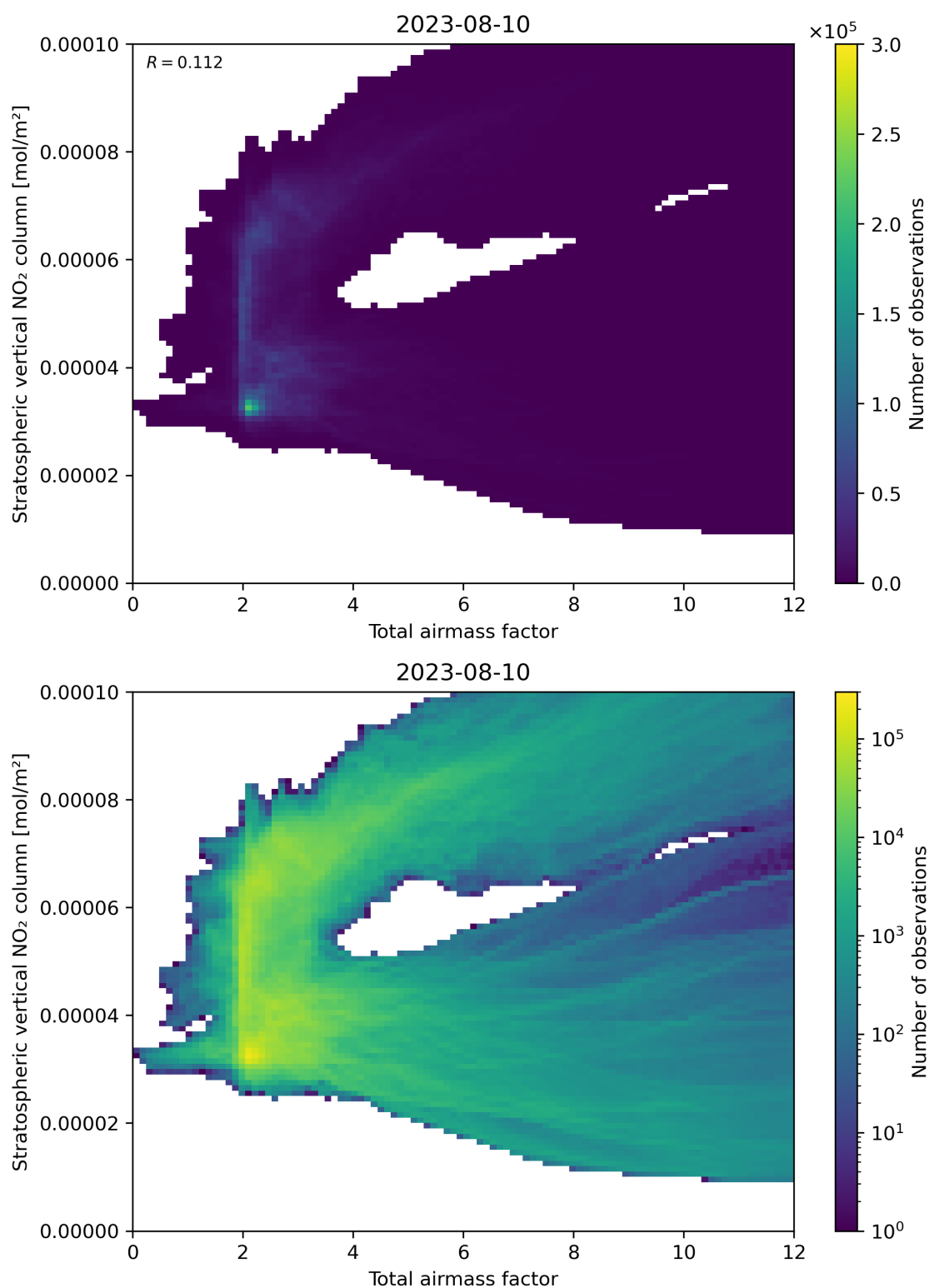
Figure 64: Scatter density plot of “Total airmass factor” against “Stratospheric vertical NO 2 column” for 2023-08-09 to 2023-08-11.
