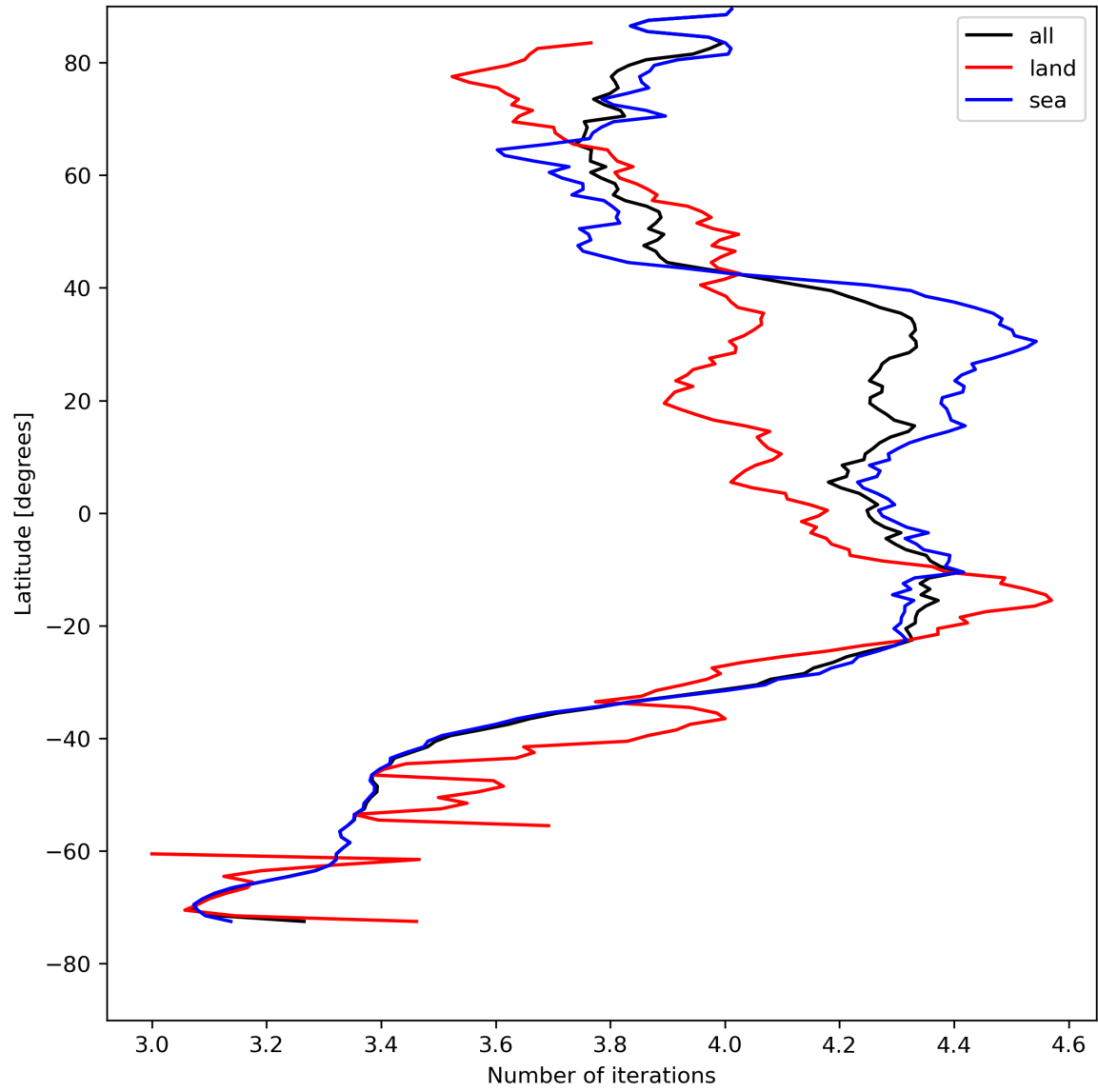
Figure 17: Zonal average of “Number of iterations” for 2023-08-09 to 2023-08-11.
