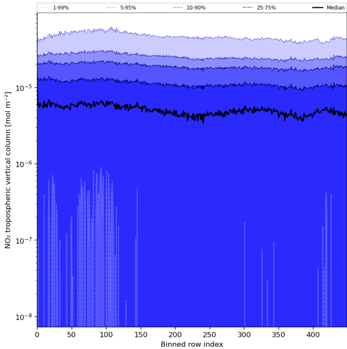
Figure 46: Along track statistics of "NO 2 tropospheric vertical column" for 2023-08-09 to 2023-08-11
