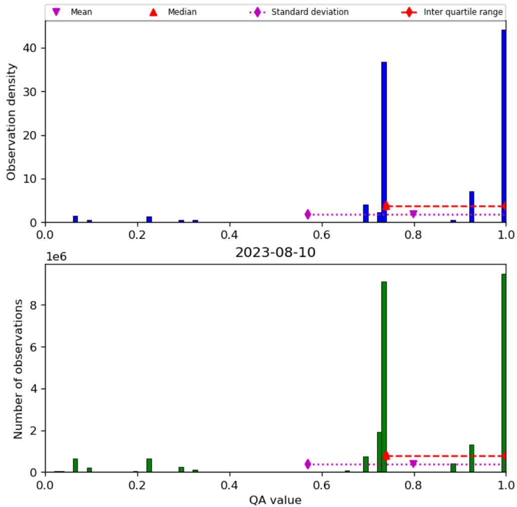
Figure 28: Histogram of “QA value” for 2023-08-09 to 2023-08-11
