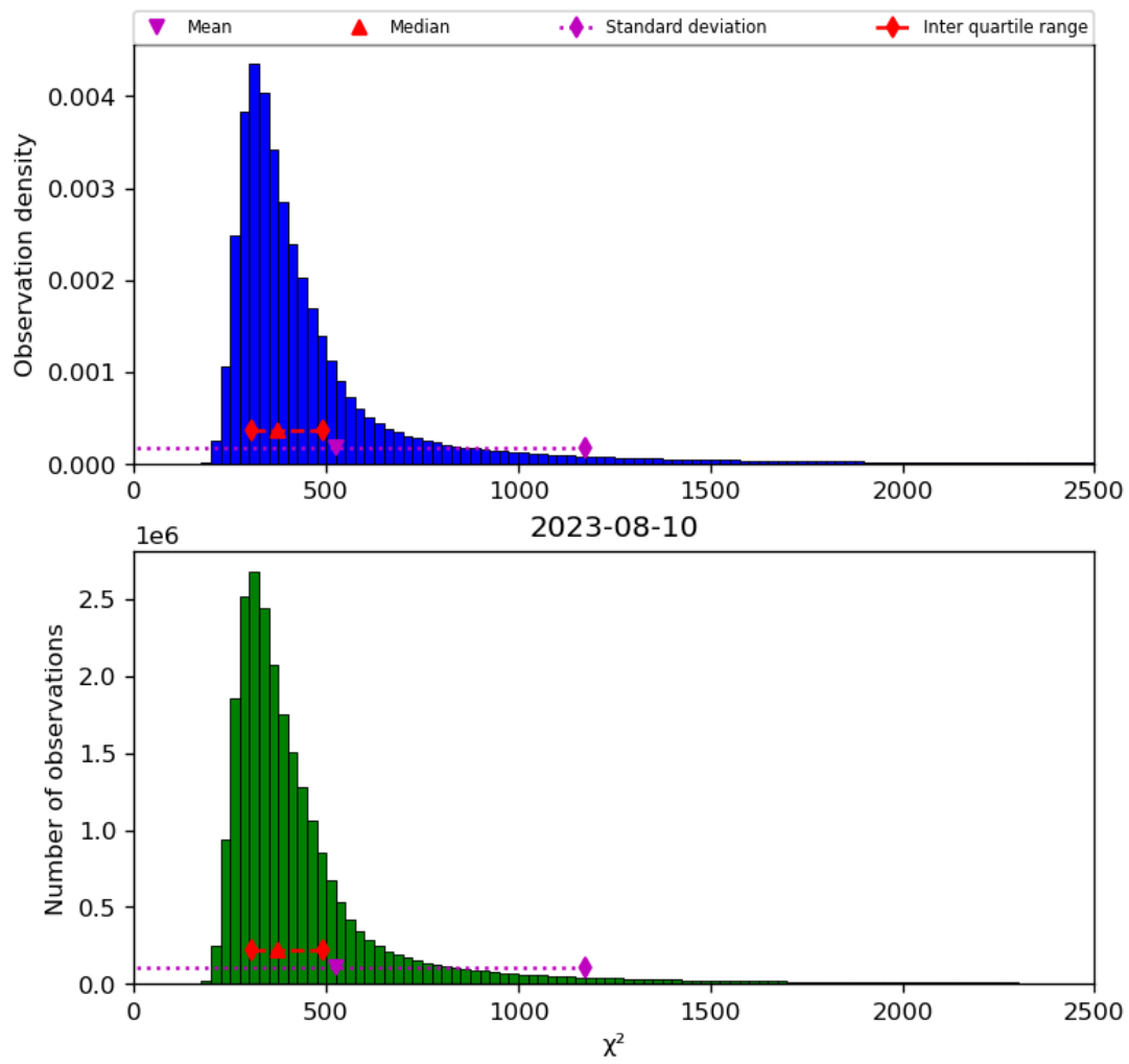
Figure 42: Histogram of “ \chi^2 ” for 2023-08-09 to 2023-08-11
