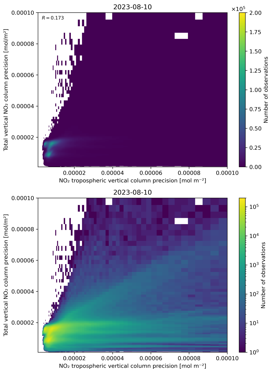
Figure 139: Scatter density plot of “NO 2 tropospheric vertical column precision” against “Total vertical NO 2 column precision” for 2023-08-09 to 2023-08-11.
