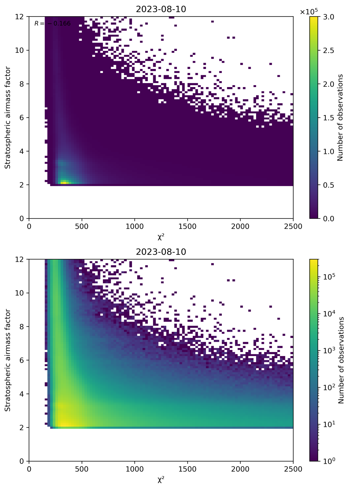
Figure 81: Scatter density plot of “ \chi^2 ” against “Stratospheric airmass factor” for 2023-08-09 to 2023-08-11.
