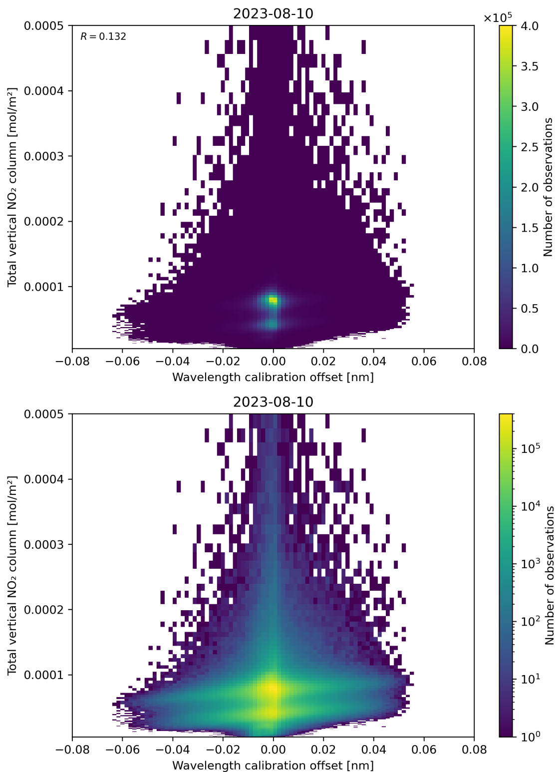
Figure 179: Scatter density plot of “Wavelength calibration offset” against “Total vertical NO 2 column” for 2023-08-09 to 2023-08-11.
