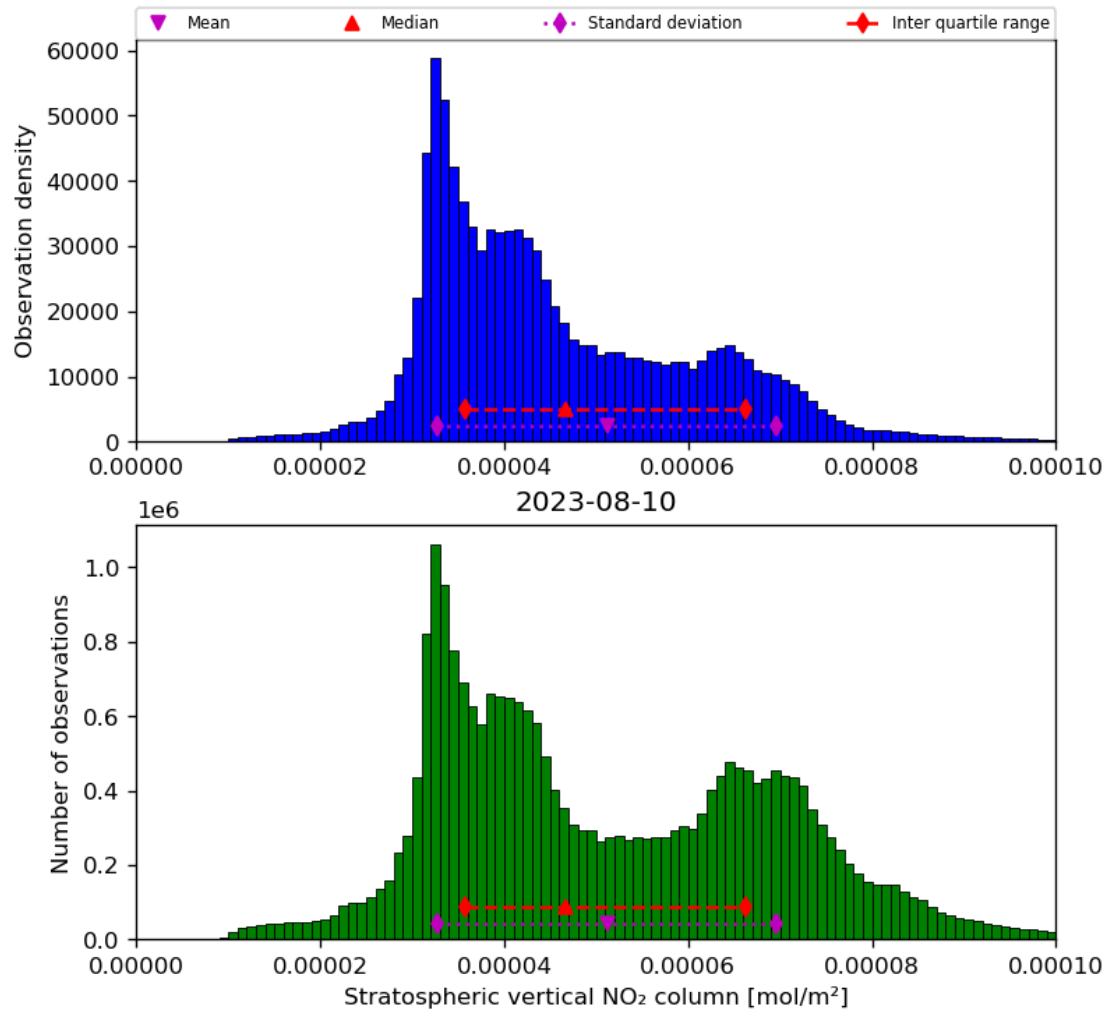
Figure 36: Histogram of “Stratospheric vertical NO 2 column” for 2023-08-09 to 2023-08-11
