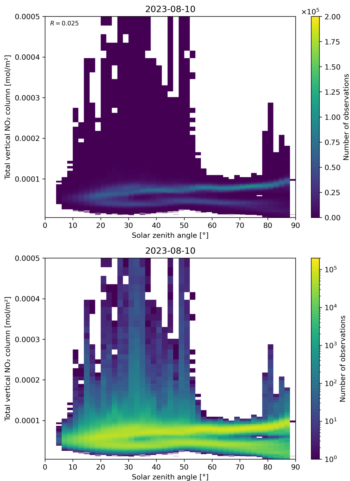
Figure 153: Scatter density plot of “Solar zenith angle” against “Total vertical NO 2 column” for 2023-08-09 to 2023-08-11.
