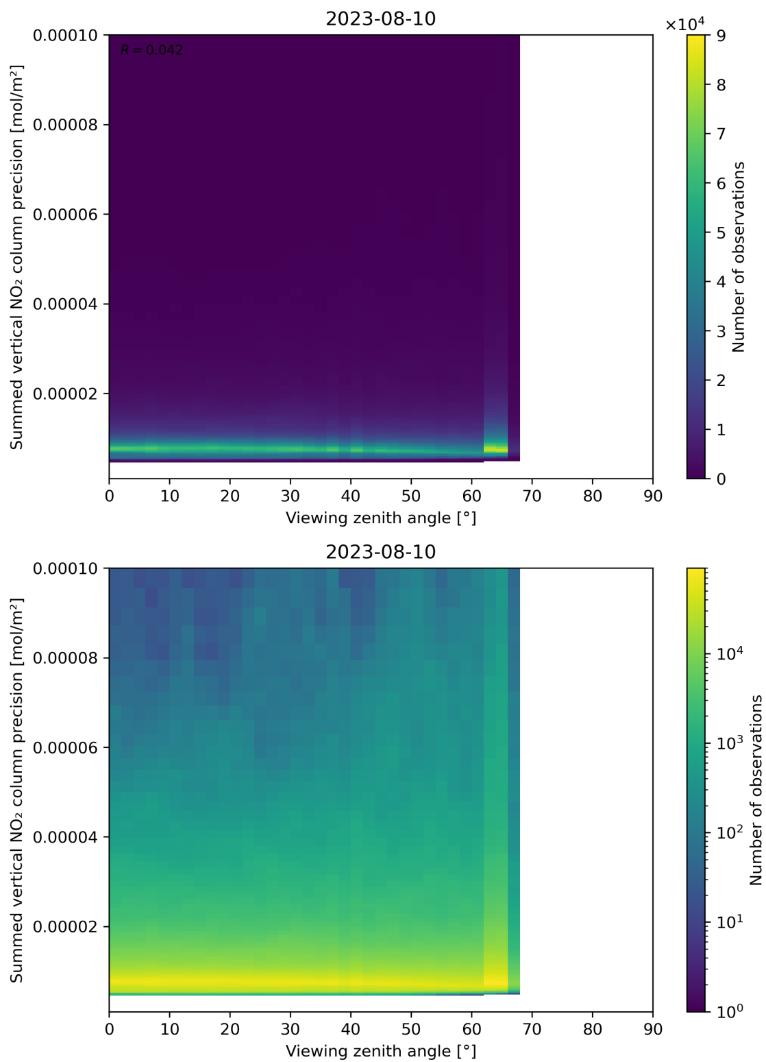
Figure 166: Scatter density plot of “Viewing zenith angle” against “Summed vertical NO 2 column precision” for 2023-08-09 to 2023-08-11.
