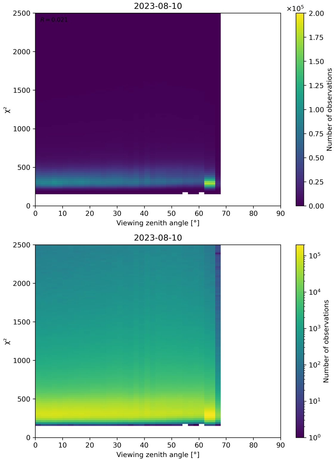
Figure 162: Scatter density plot of “Viewing zenith angle” against “ \chi^2 ” for 2023-08-09 to 2023-08-11.
