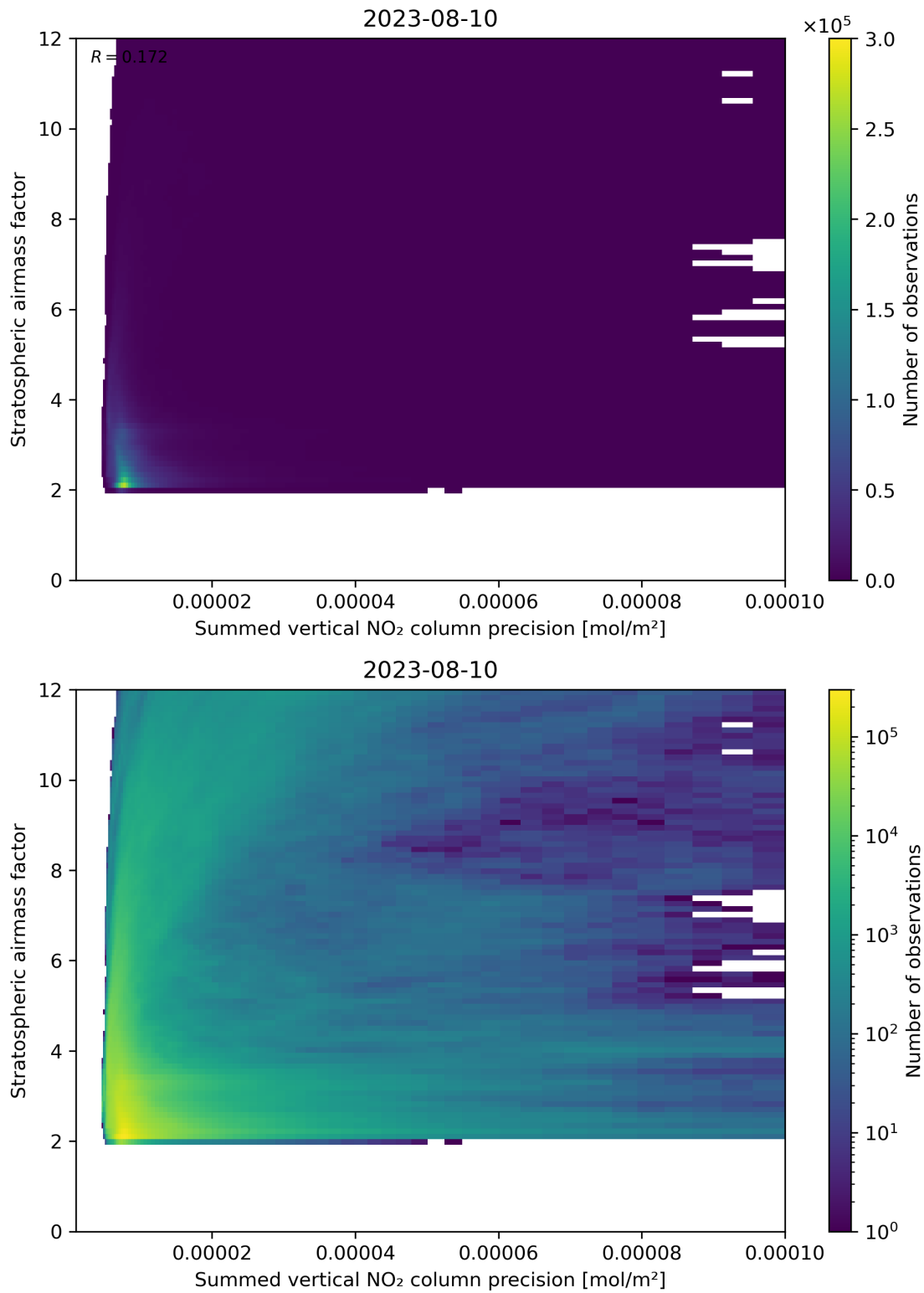
Figure 106: Scatter density plot of “Summed vertical NO 2 column precision” against “Stratospheric airmass factor” for 2023-08-09 to 2023-08-11.
