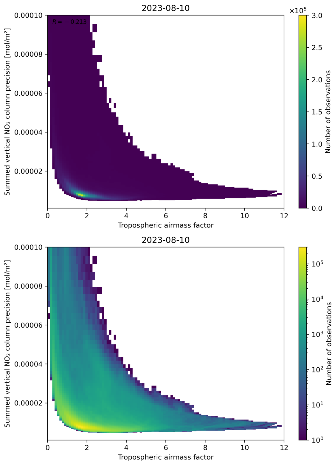
Figure 76: Scatter density plot of “Tropospheric air mass factor” against “Summed vertical NO 2 column precision” for 2023-08-09 to 2023-08-11.
