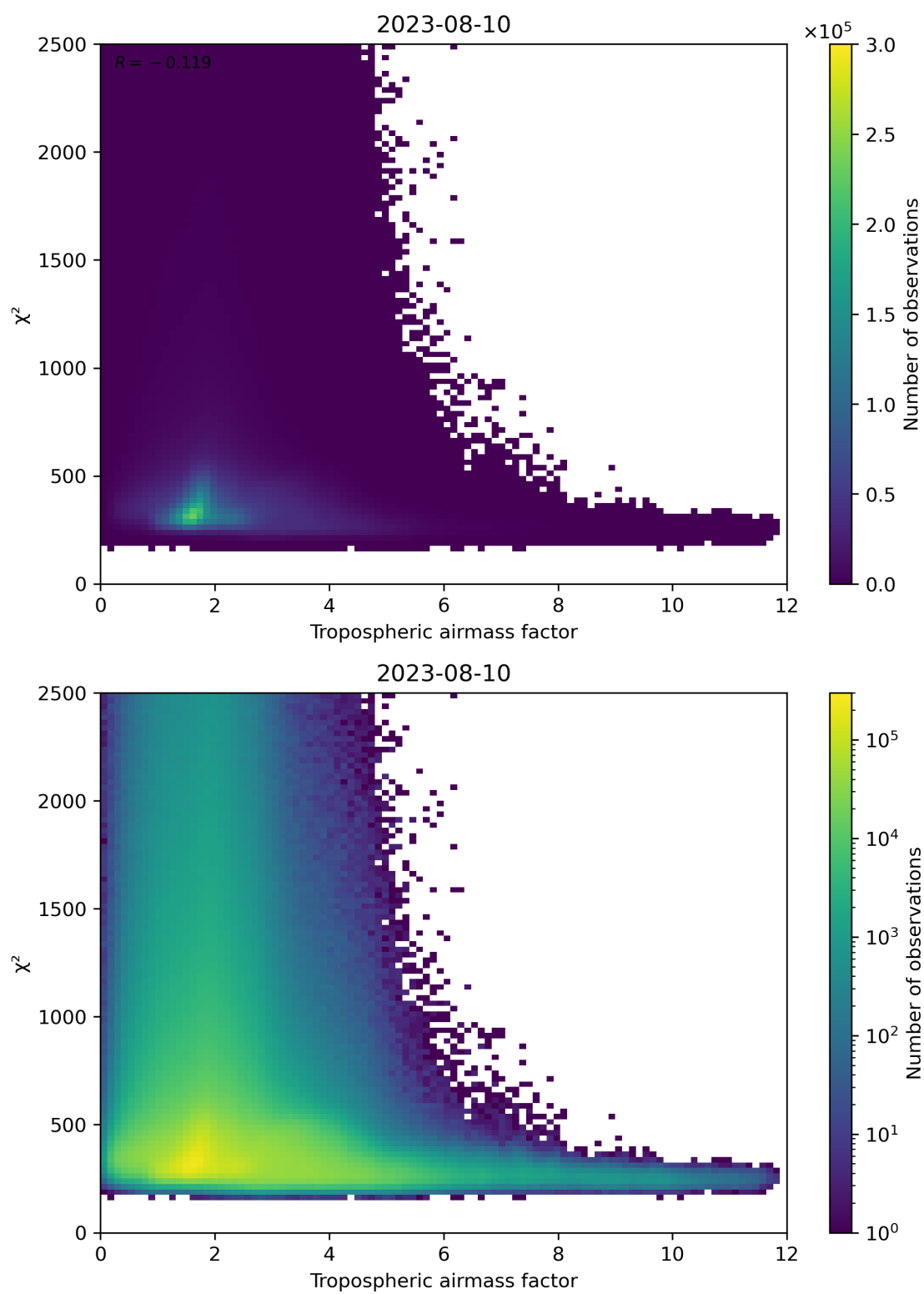
Figure 73: Scatter density plot of “Tropospheric airmass factor” against “ \chi^2 ” for 2023-08-09 to 2023-08-11.
