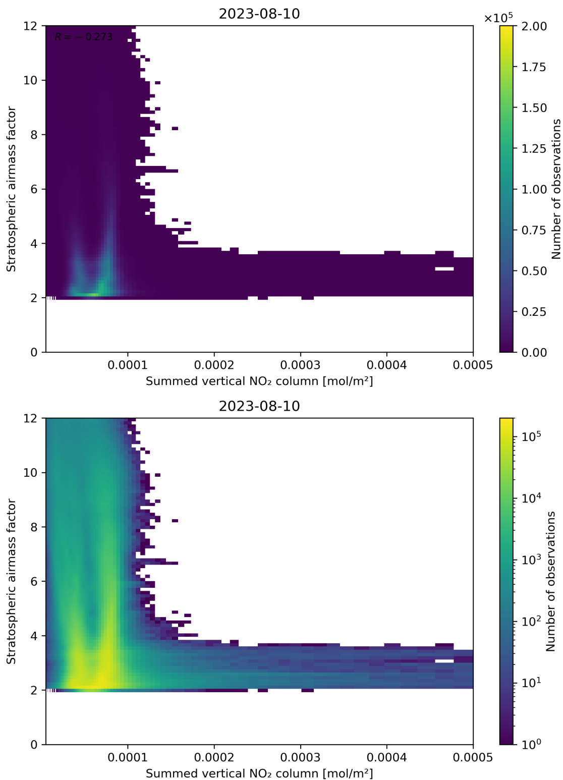
Figure 103: Scatter density plot of “Summed vertical NO 2 column” against “Stratospheric airmass factor” for 2023-08-09 to 2023-08-11.
