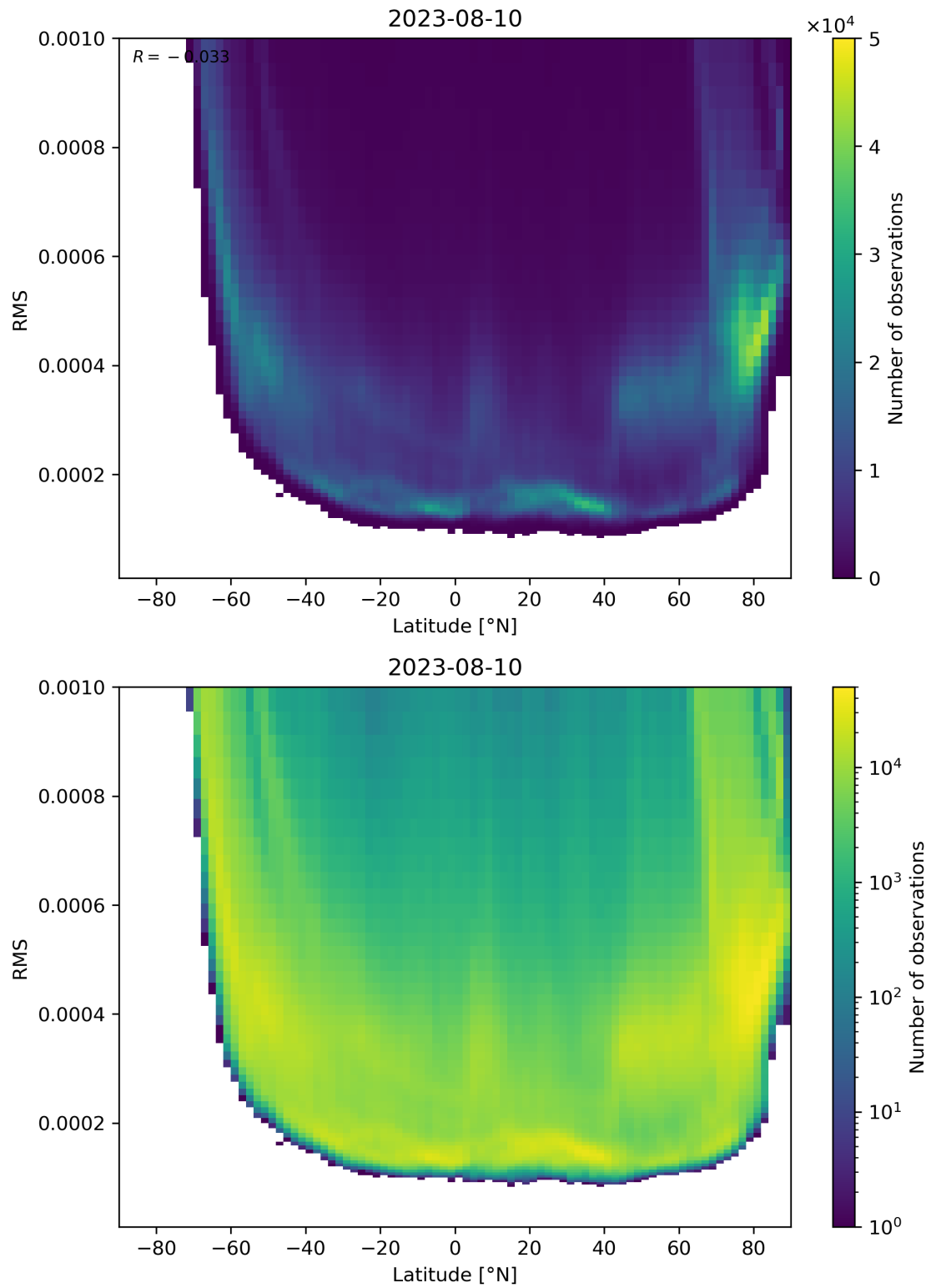
Figure 94: Scatter density plot of “Latitude” against “RMS” for 2023-08-09 to 2023-08-11.
