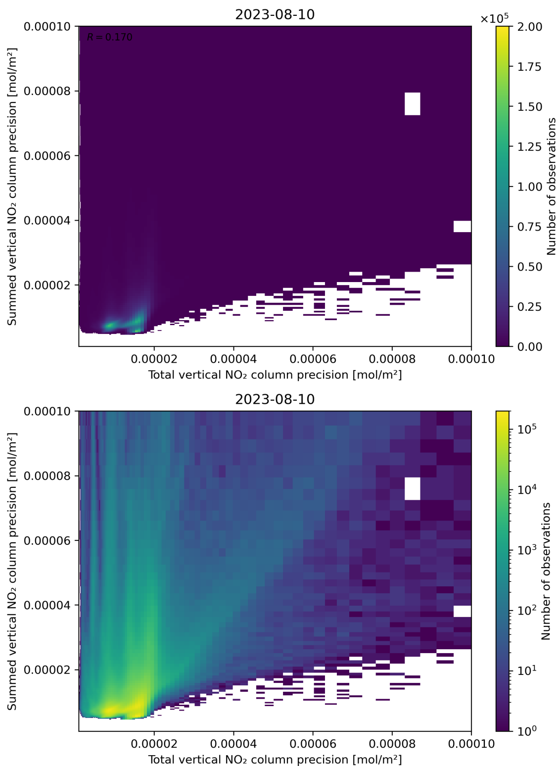
Figure 118: Scatter density plot of “Total vertical NO 2 column precision” against “Summed vertical NO 2 column precision” for 2023-08-09 to 2023-08-11.
