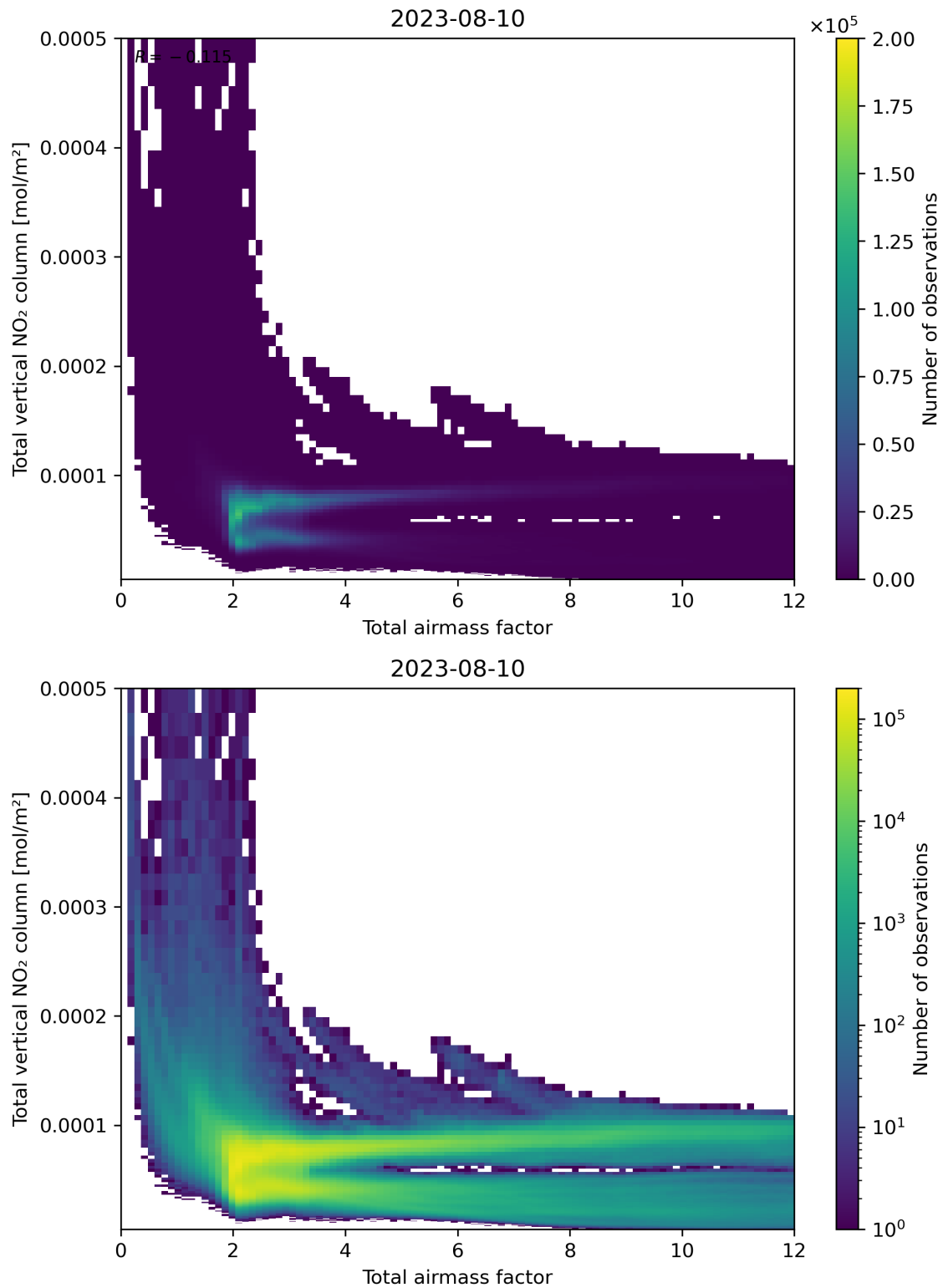
Figure 67: Scatter density plot of “Total airmass factor” against “Total vertical NO 2 column” for 2023-08-09 to 2023-08-11.
