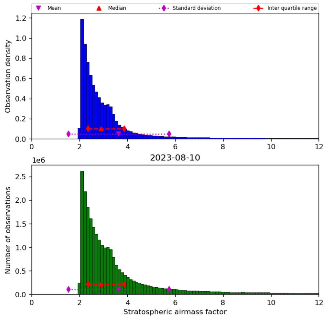
Figure 44: Histogram of “Stratospheric airmass factor” for 2023-08-09 to 2023-08-11
