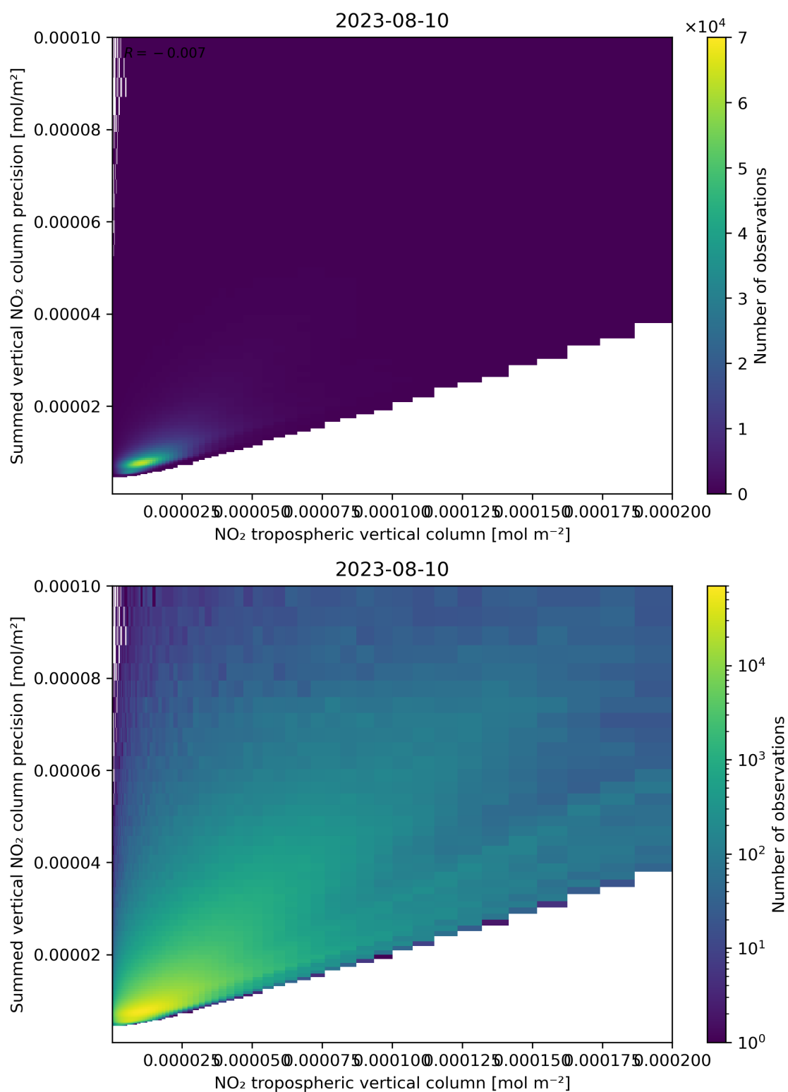
Figure 127: Scatter density plot of “NO 2 tropospheric vertical column” against “Summed vertical NO 2 column precision” for 2023-08-09 to 2023-08-11.
