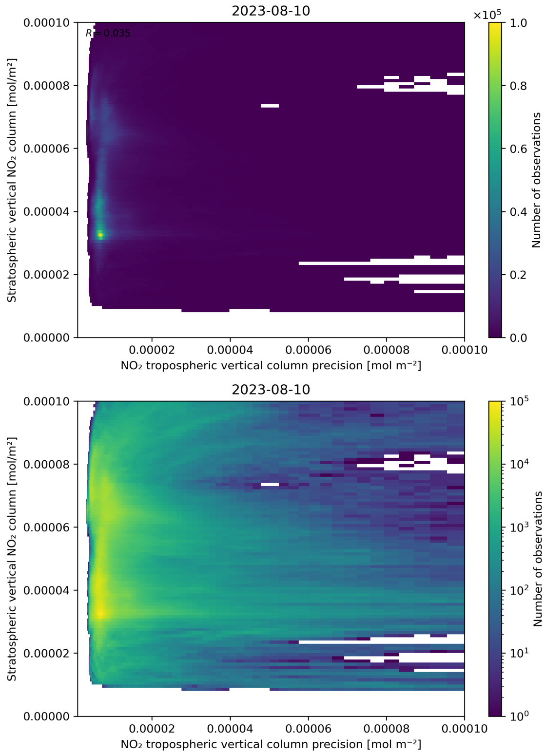
Figure 135: Scatter density plot of “NO 2 tropospheric vertical column precision” against “Stratospheric vertical NO 2 column” for 2023-08-09 to 2023-08-11.
