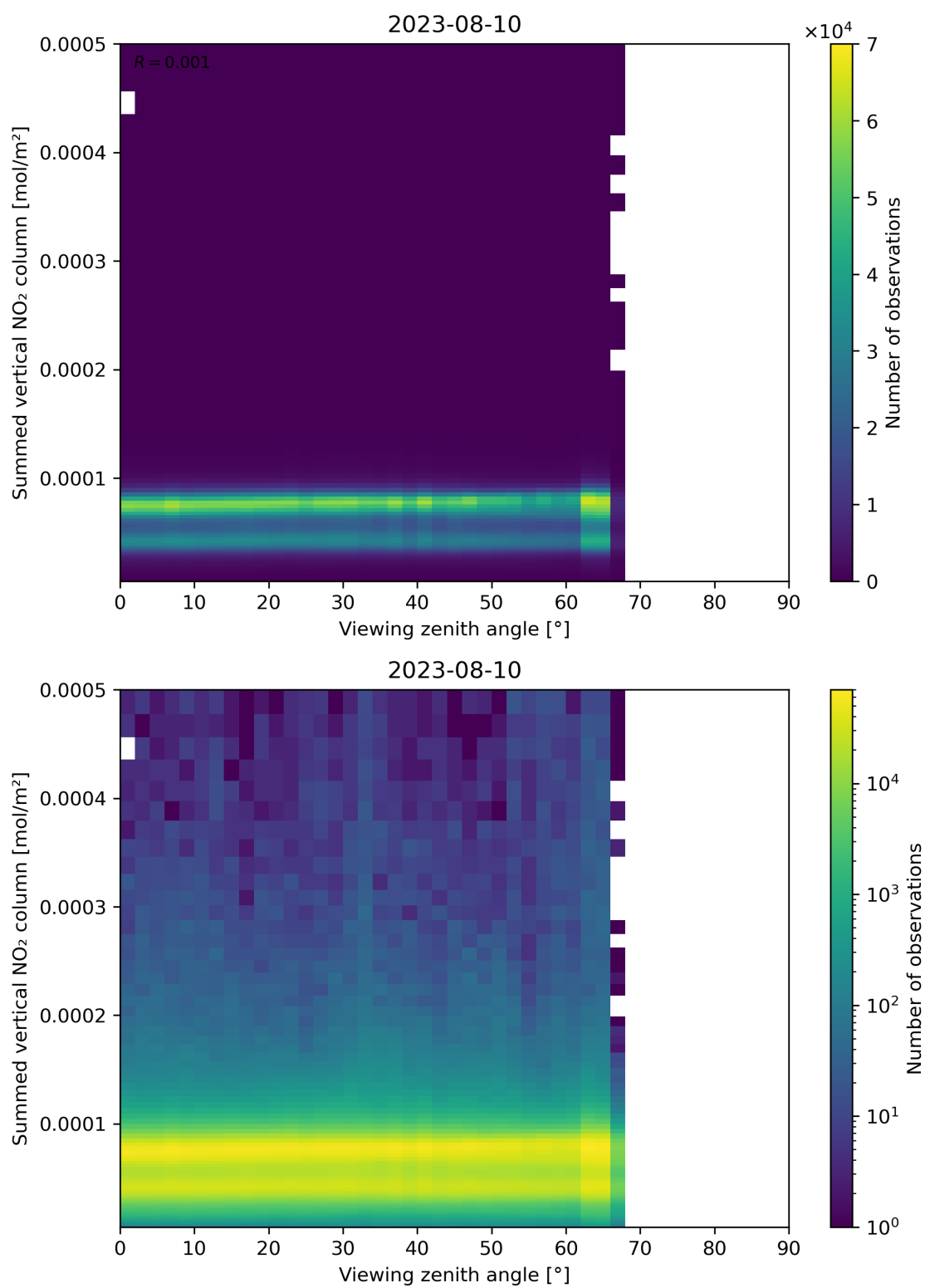
Figure 165: Scatter density plot of “Viewing zenith angle” against “Summed vertical NO 2 column” for 2023-08-09 to 2023-08-11.
