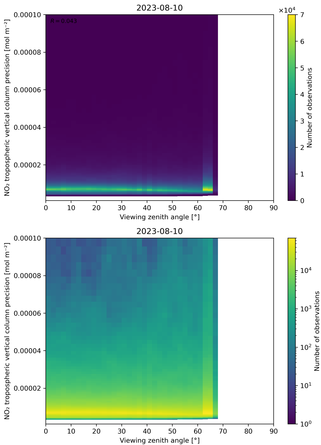
Figure 170: Scatter density plot of “Viewing zenith angle” against “NO 2 tropospheric vertical column precision” for 2023-08-09 to 2023-08-11.
