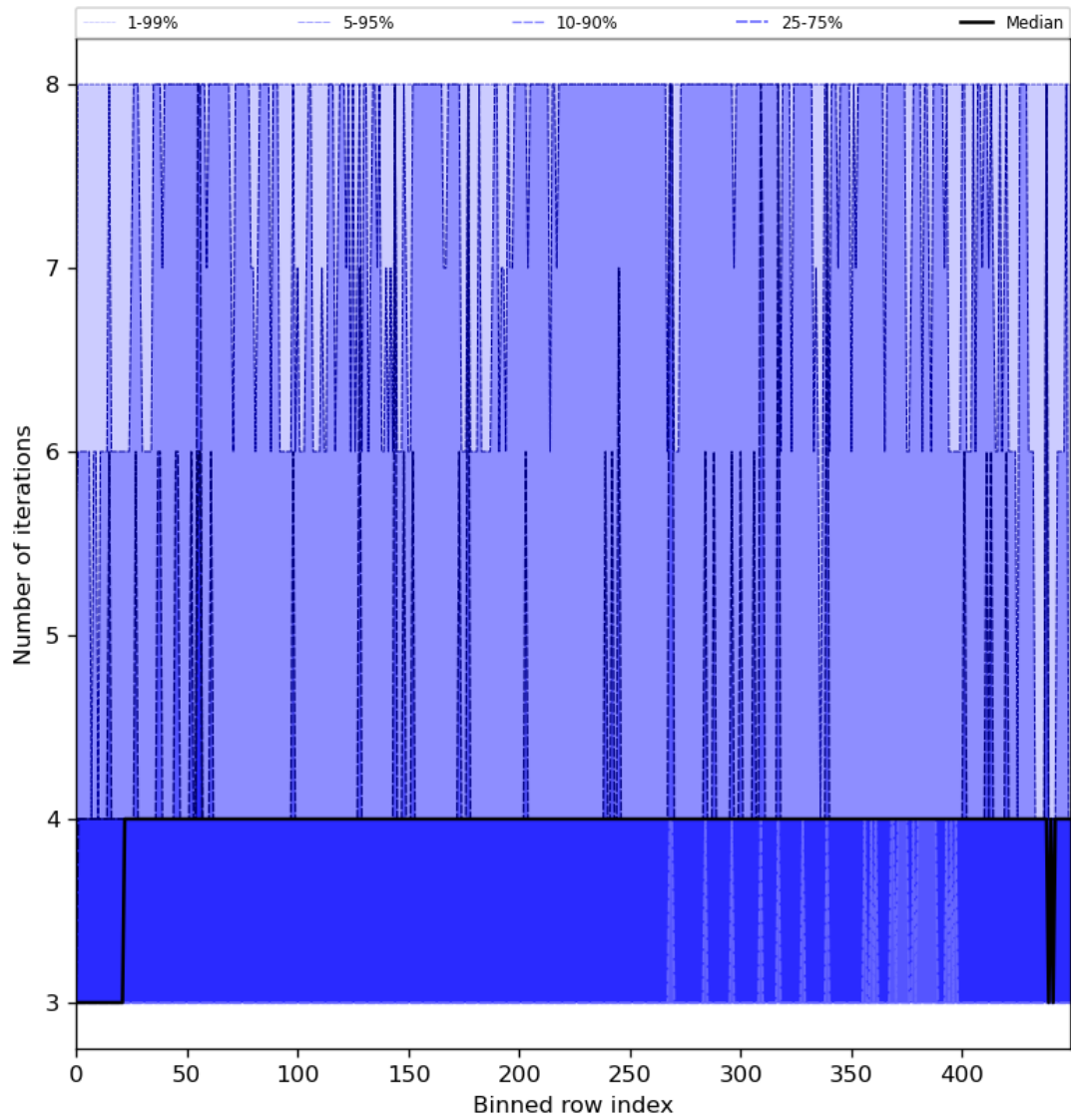
Figure 51: Along track statistics of “Number of iterations” for 2023-08-09 to 2023-08-11
