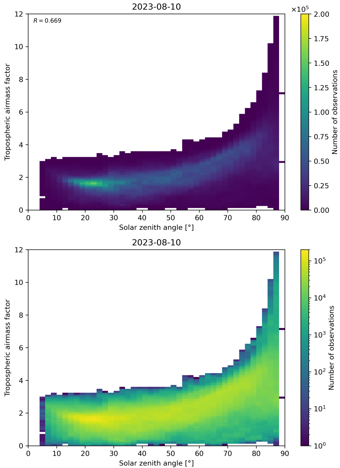
Figure 147: Scatter density plot of “Solar zenith angle” against “Tropospheric airmass factor” for 2023-08-09 to 2023-08-11.
