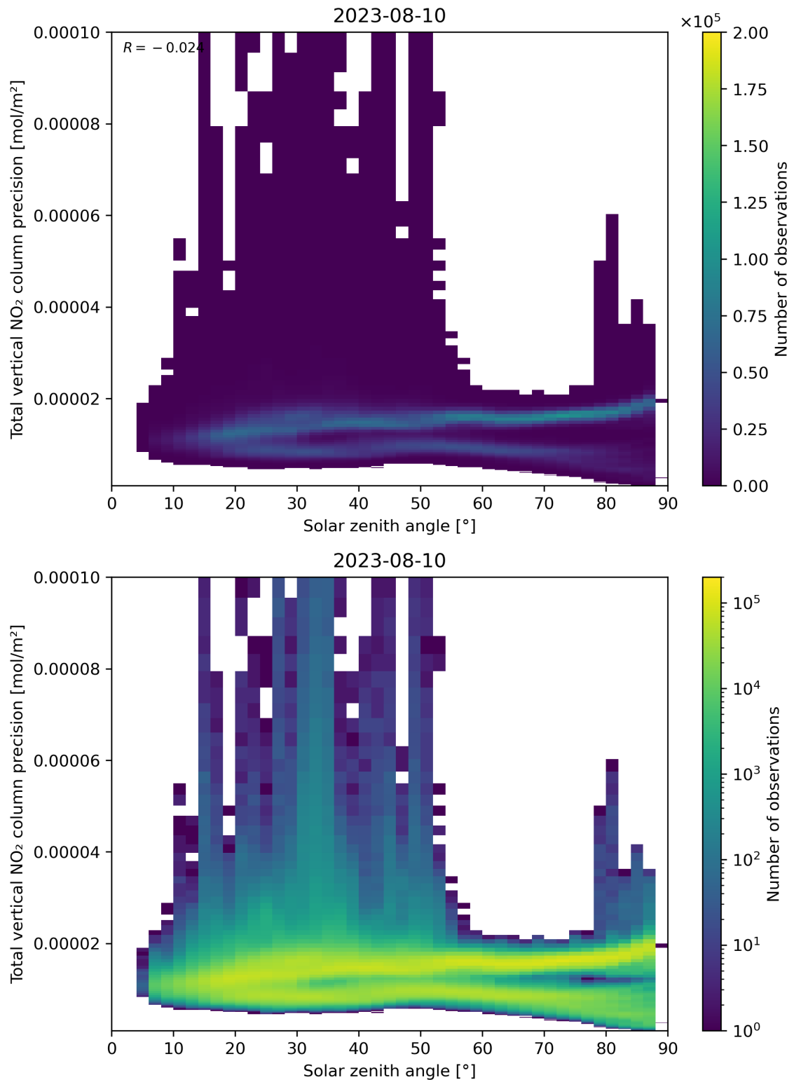
Figure 154: Scatter density plot of “Solar zenith angle” against “Total vertical NO 2 column precision” for 2023-08-09 to 2023-08-11.
