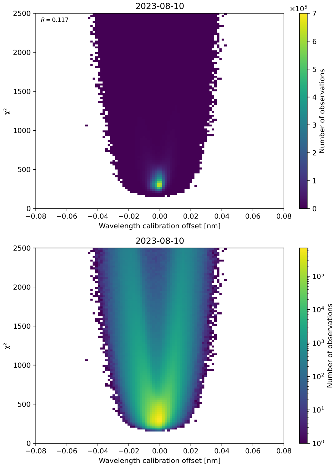
Figure 175: Scatter density plot of “Wavelength calibration offset” against “ \chi^2 ” for 2023-08-09 to 2023-08-11.
