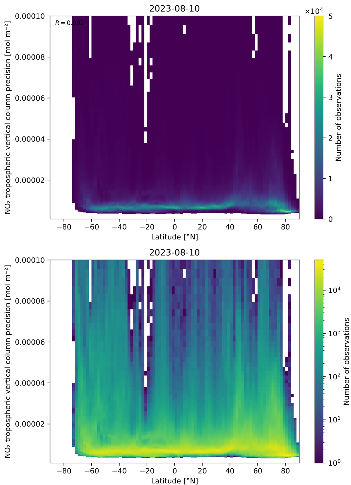
Figure 93: Scatter density plot of “Latitude” against “NO 2 tropospheric vertical column precision” for 2023-08-09 to 2023-08-11.
