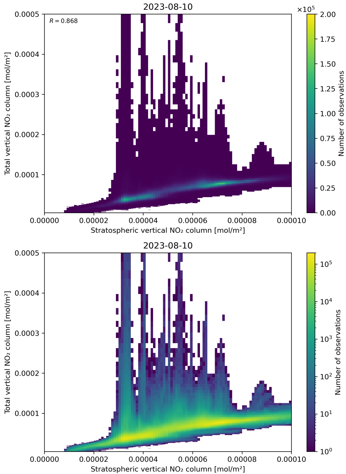
Figure 100: Scatter density plot of “Stratospheric vertical NO 2 column” against “Total vertical NO 2 column” for 2023-08-09 to 2023-08-11.
