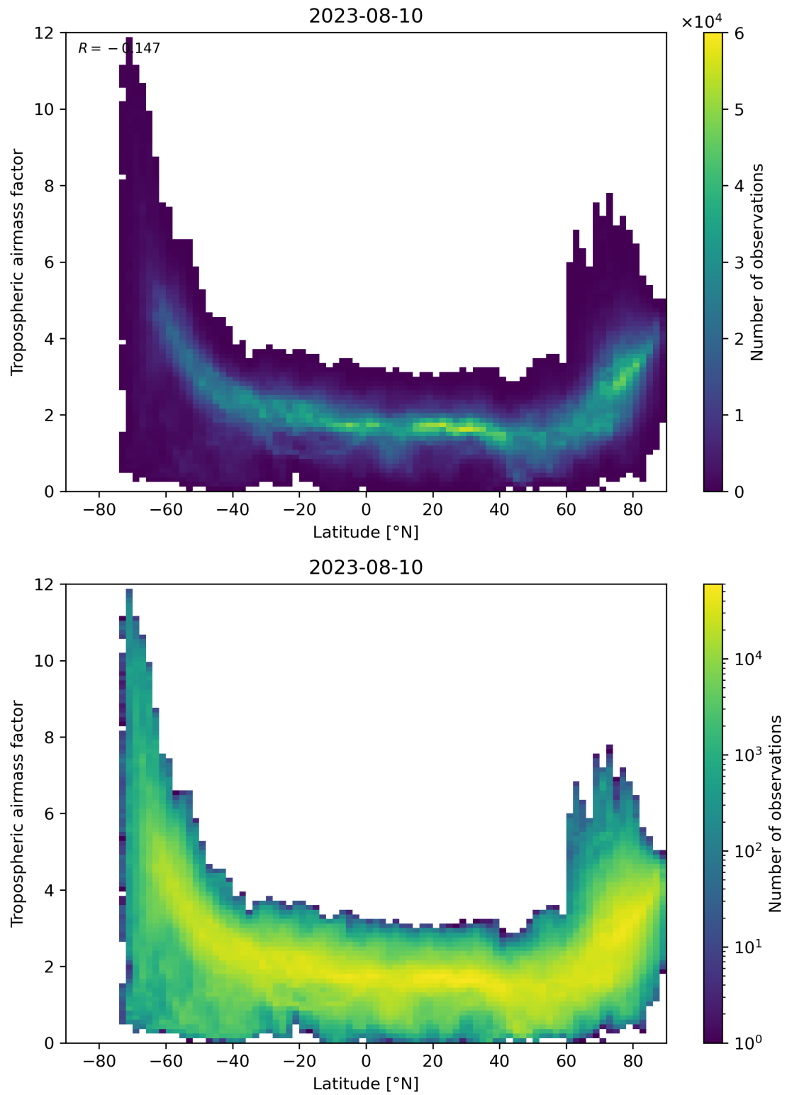
Figure 85: Scatter density plot of “Latitude” against “Tropospheric air mass factor” for 2023-08-09 to 2023-08-11.
