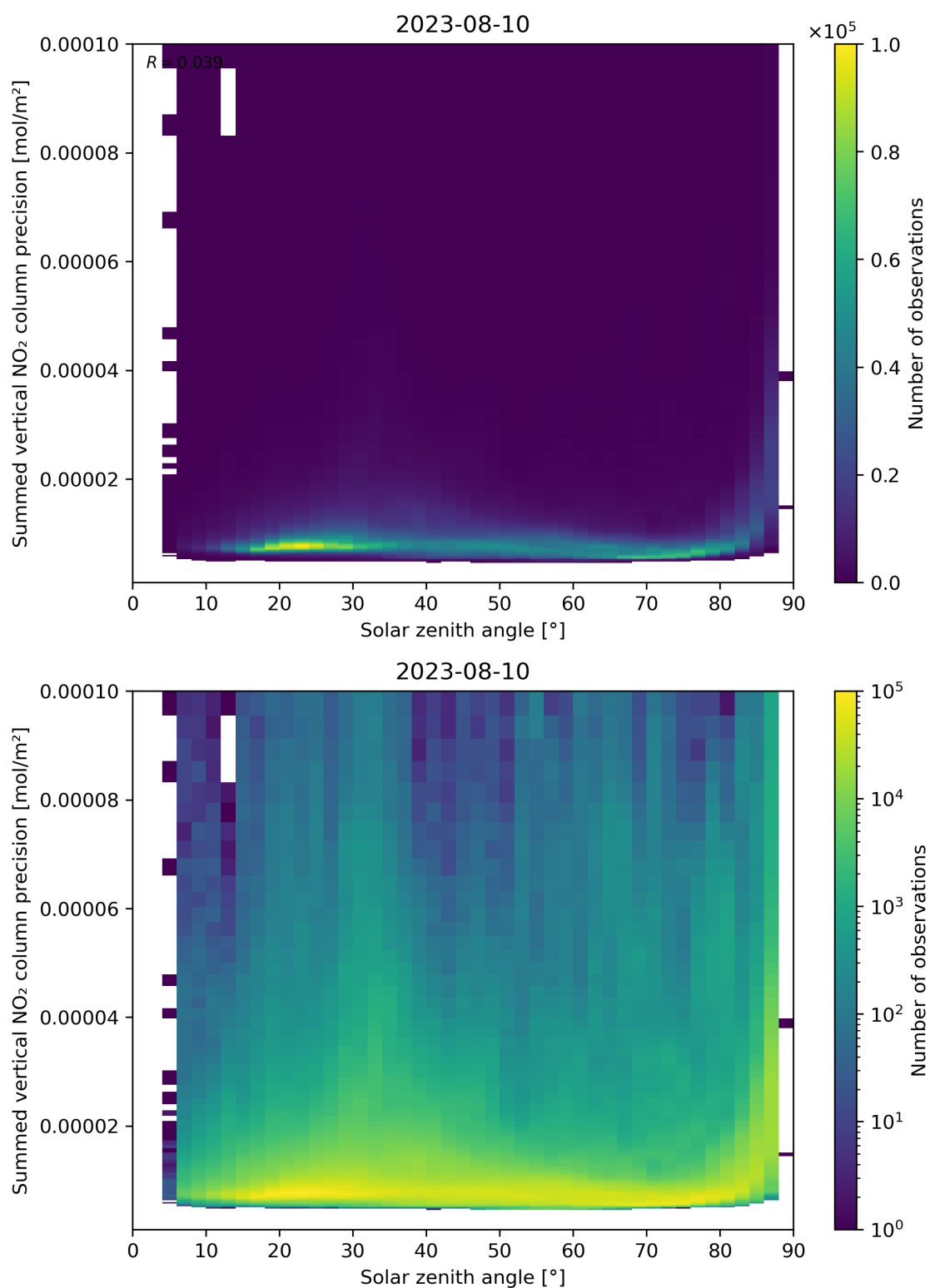
Figure 152: Scatter density plot of “Solar zenith angle” against “Summed vertical NO 2 column precision” for 2023-08-09 to 2023-08-11.
