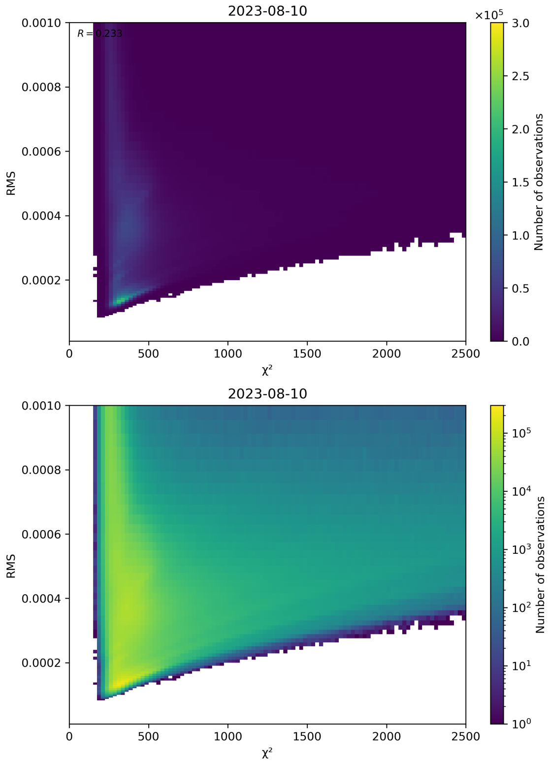
Figure 82: Scatter density plot of “ \chi^2 ” against “RMS” for 2023-08-09 to 2023-08-11.
