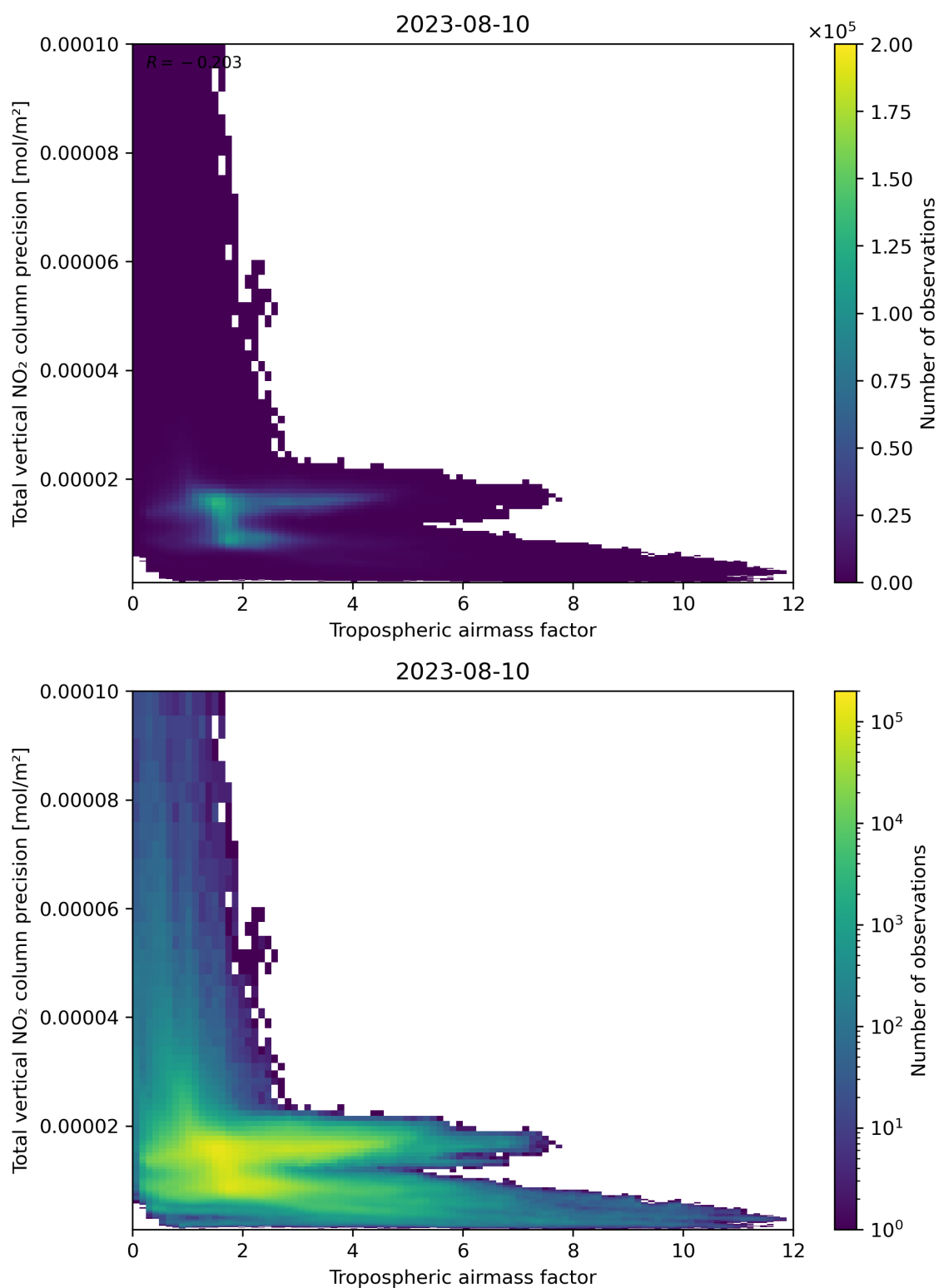
Figure 78: Scatter density plot of “Tropospheric air mass factor” against “Total vertical NO 2 column precision” for 2023-08-09 to 2023-08-11.
