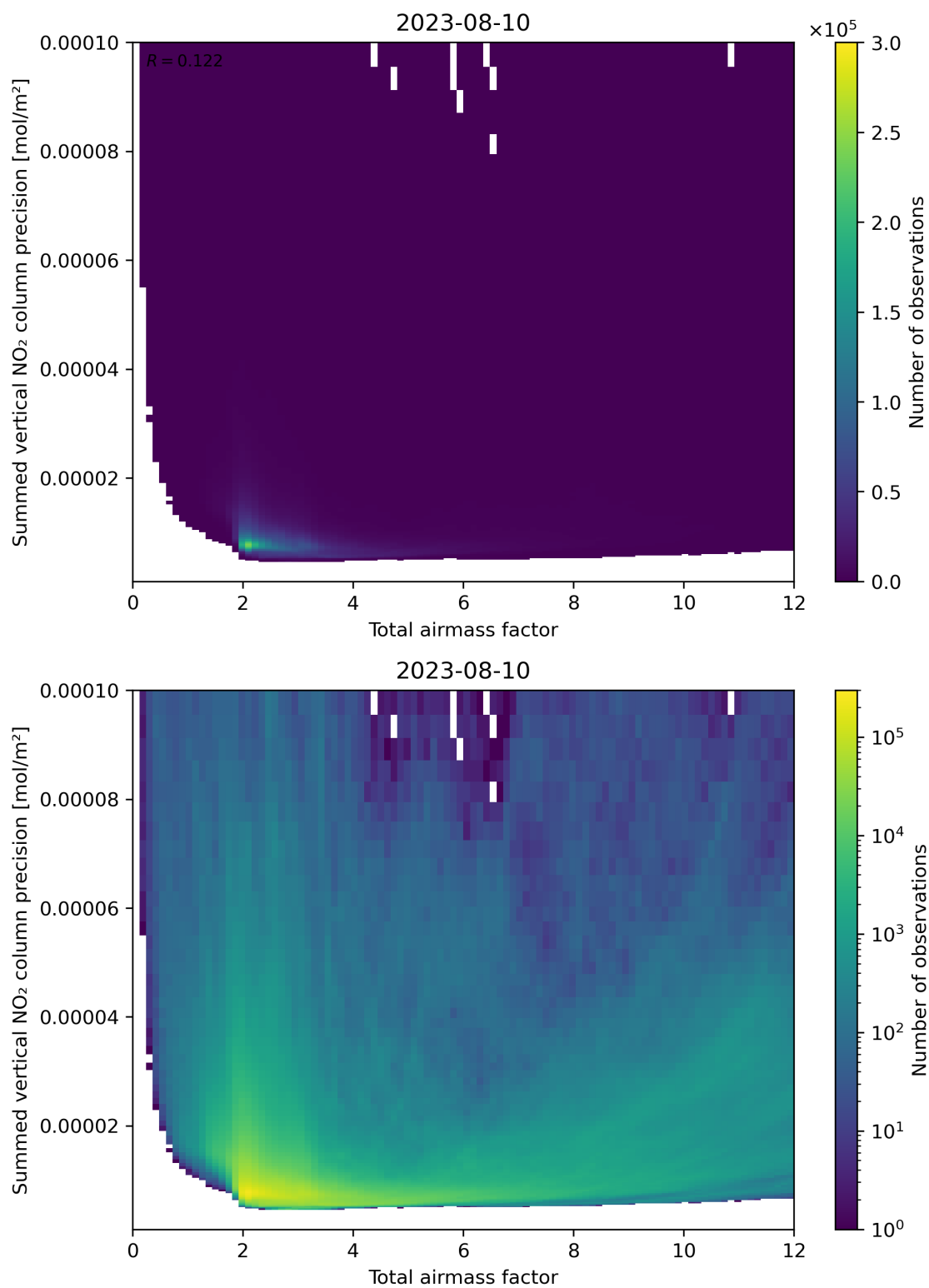
Figure 66: Scatter density plot of “Total airmass factor” against “Summed vertical NO 2 column precision” for 2023-08-09 to 2023-08-11.
