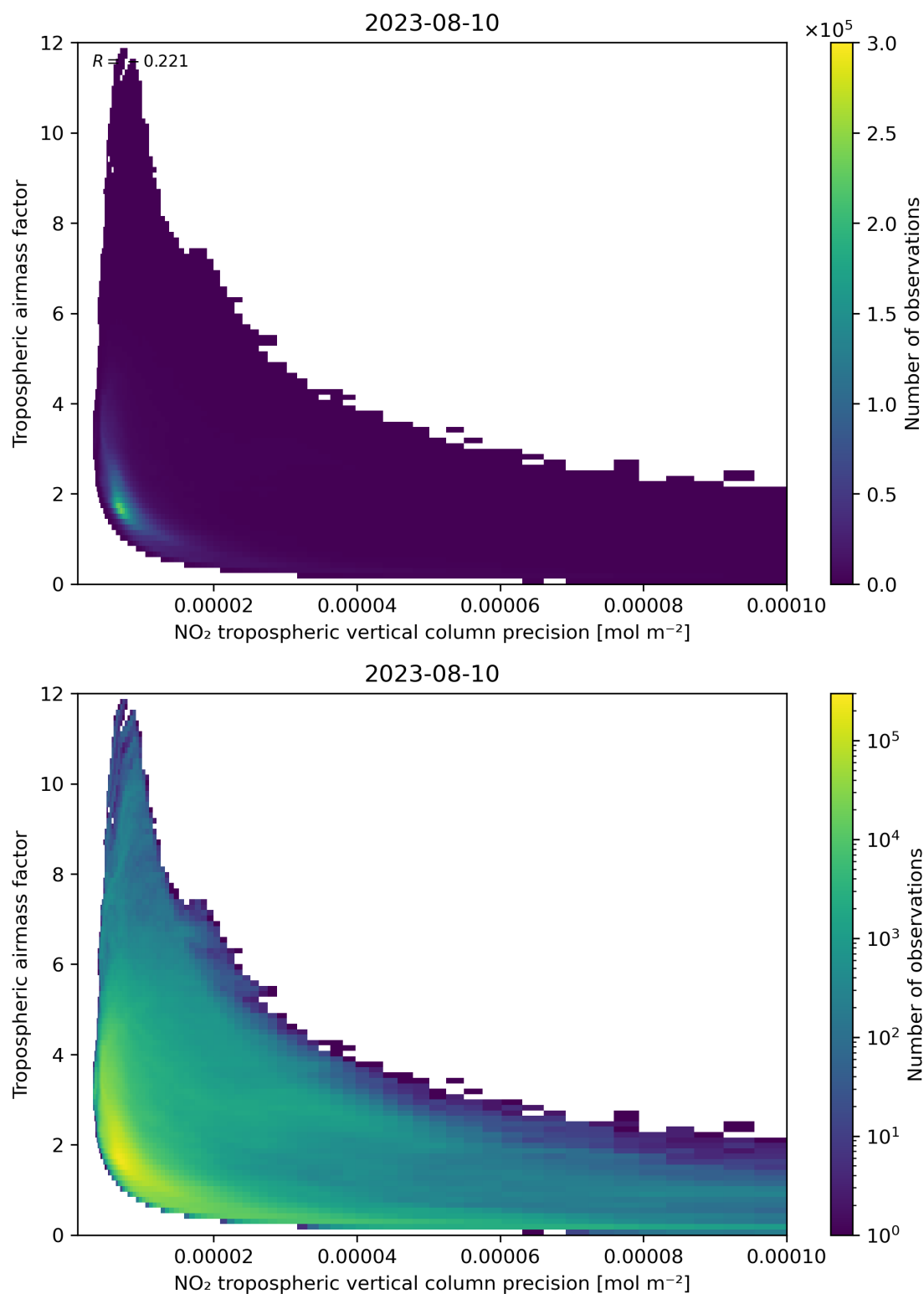
Figure 133: Scatter density plot of “NO 2 tropospheric vertical column precision” against “Tropospheric airmass factor” for 2023-08-09 to 2023-08-11.
