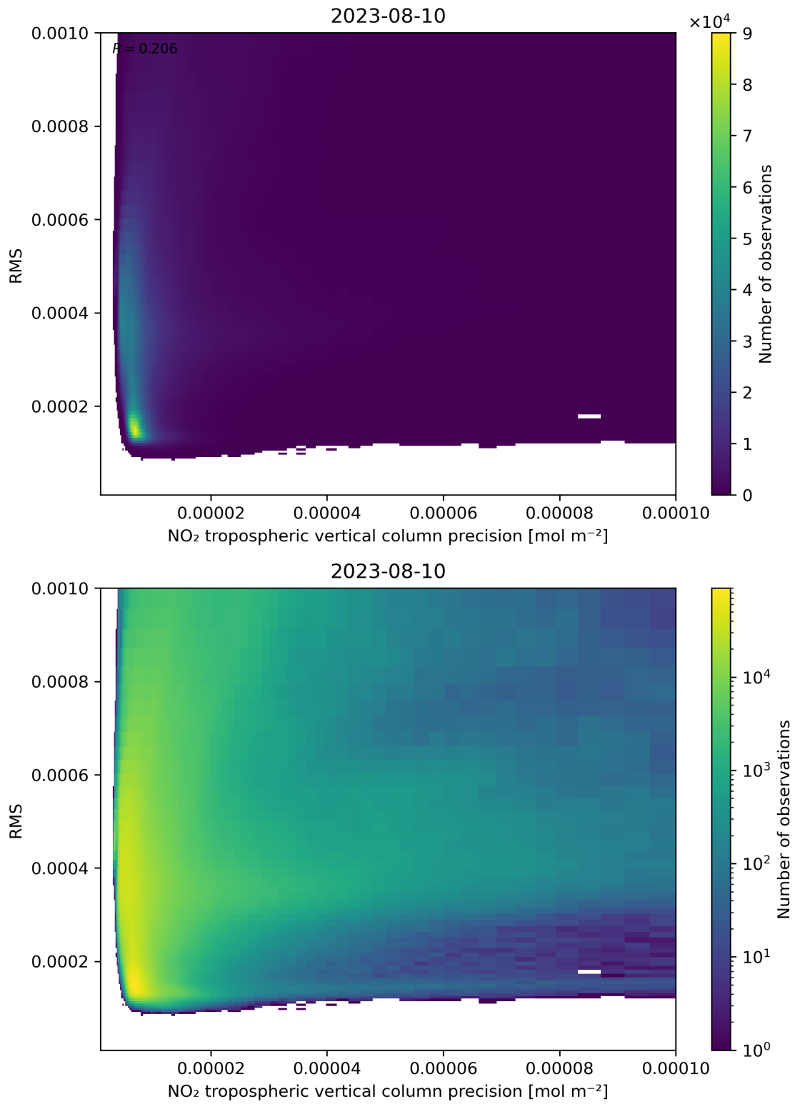
Figure 140: Scatter density plot of “NO 2 tropospheric vertical column precision” against “RMS” for 2023-08-09 to 2023-08-11.
