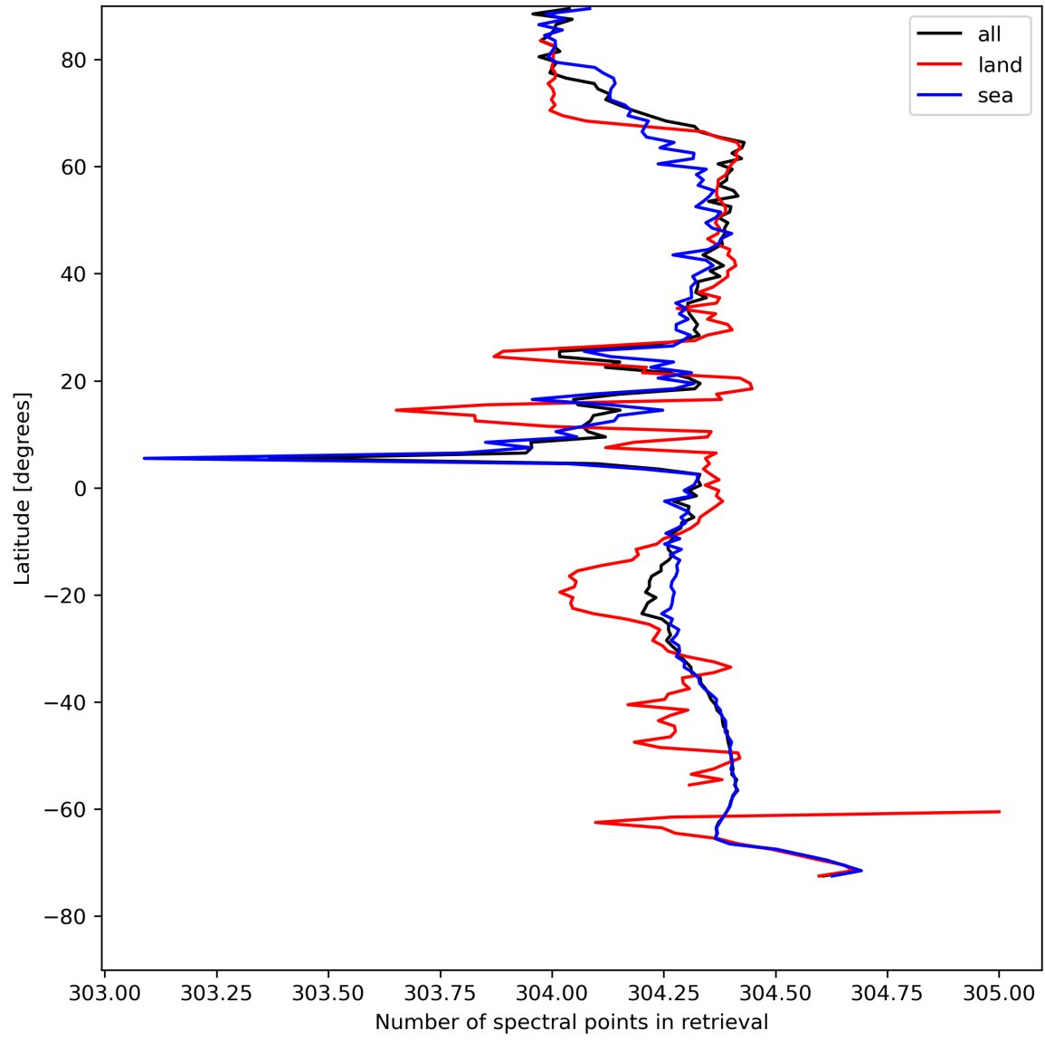
Figure 16: Zonal average of “Number of spectral points in retrieval” for 2023-08-09 to 2023-08-11.
