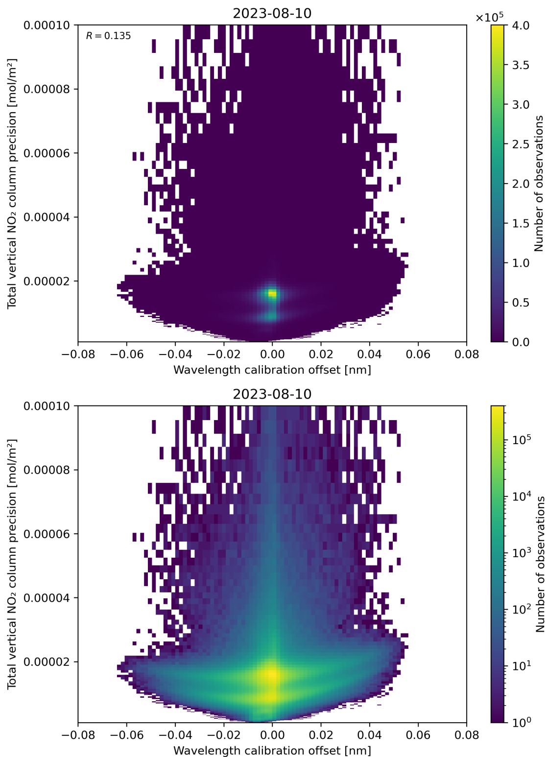
Figure 180: Scatter density plot of “Wavelength calibration offset” against “Total vertical NO 2 column precision” for 2023-08-09 to 2023-08-11.
