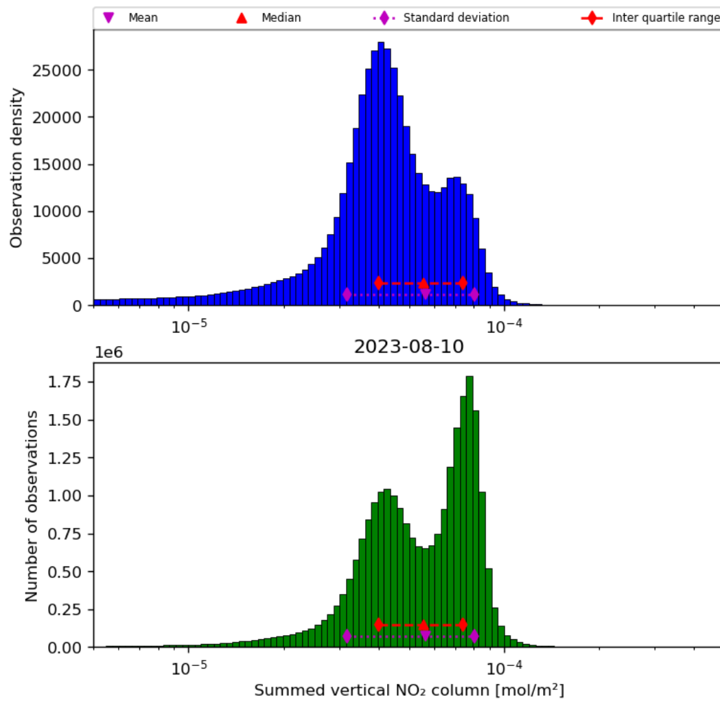
Figure 40: Histogram of “Summed vertical NO 2 column” for 2023-08-09 to 2023-08-11
