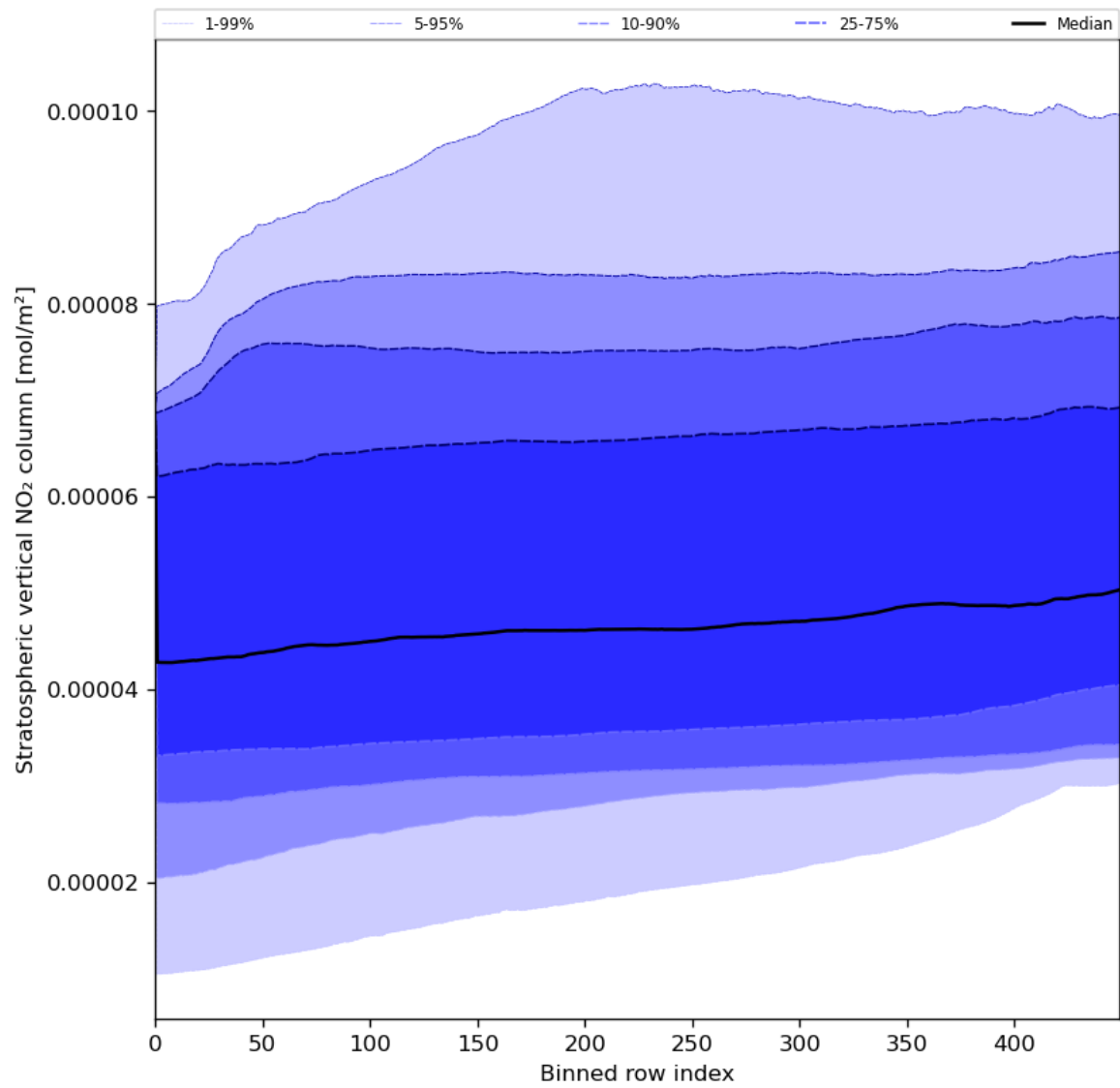
Figure 53: Along track statistics of “Stratospheric vertical NO 2 column” for 2023-08-09 to 2023-08-11
