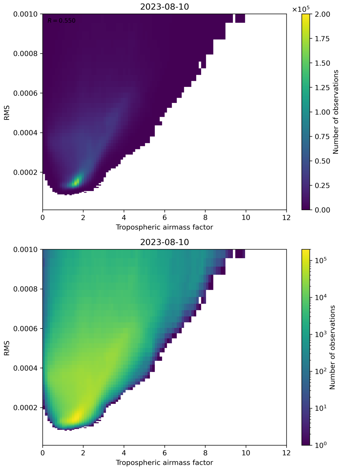
Figure 79: Scatter density plot of “Tropospheric airmass factor” against “RMS” for 2023-08-09 to 2023-08-11.
