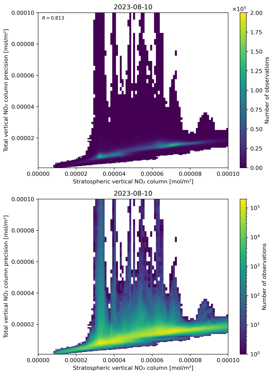
Figure 101: Scatter density plot of “Stratospheric vertical NO 2 column” against “Total vertical NO 2 column precision” for 2023-08-09 to 2023-08-11.
