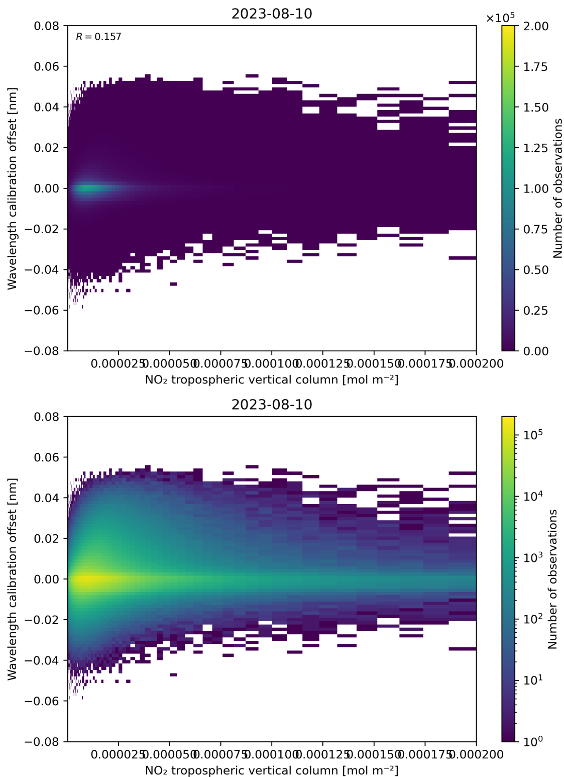
Figure 143: Scatter density plot of “NO 2 tropospheric vertical column” against “Wavelength calibration offset” for 2023-08-09 to 2023-08-11.
