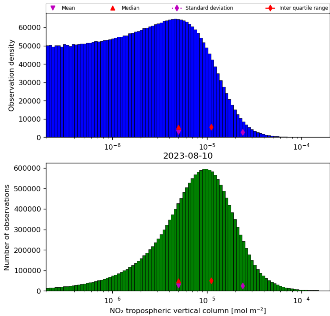
Figure 29: Histogram of “NO 2 tropospheric vertical column” for 2023-08-09 to 2023-08-11
