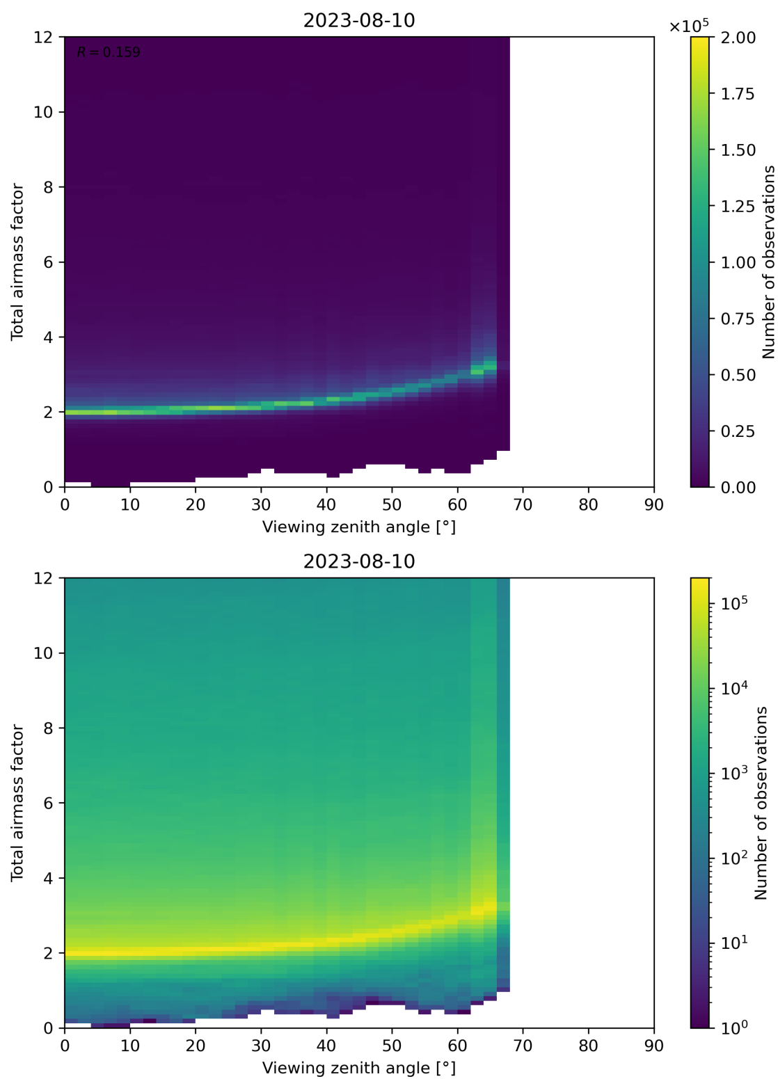
Figure 160: Scatter density plot of “Viewing zenith angle” against “Total airmass factor” for 2023-08-09 to 2023-08-11.
