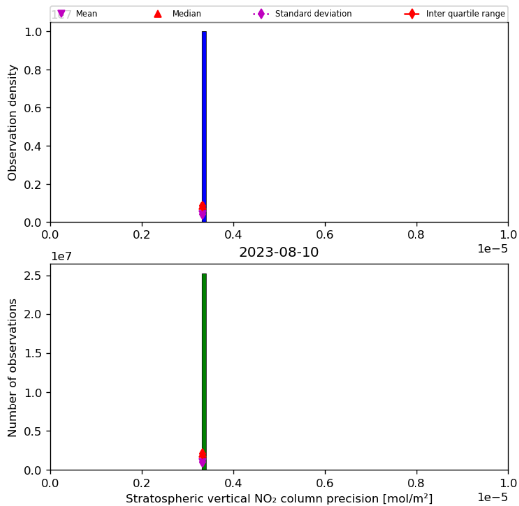
Figure 37: Histogram of “Stratospheric vertical NO 2 column precision” for 2023-08-09 to 2023-08-11
