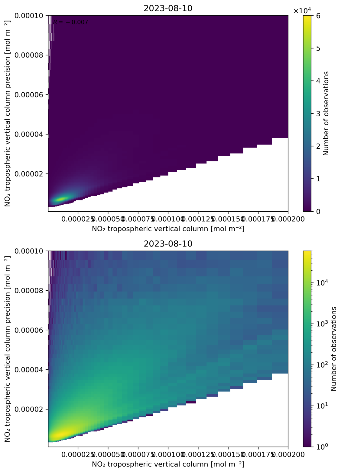
Figure 130: Scatter density plot of “NO 2 tropospheric vertical column” against “NO 2 tropospheric vertical column precision” for 2023-08-09 to 2023-08-11.
