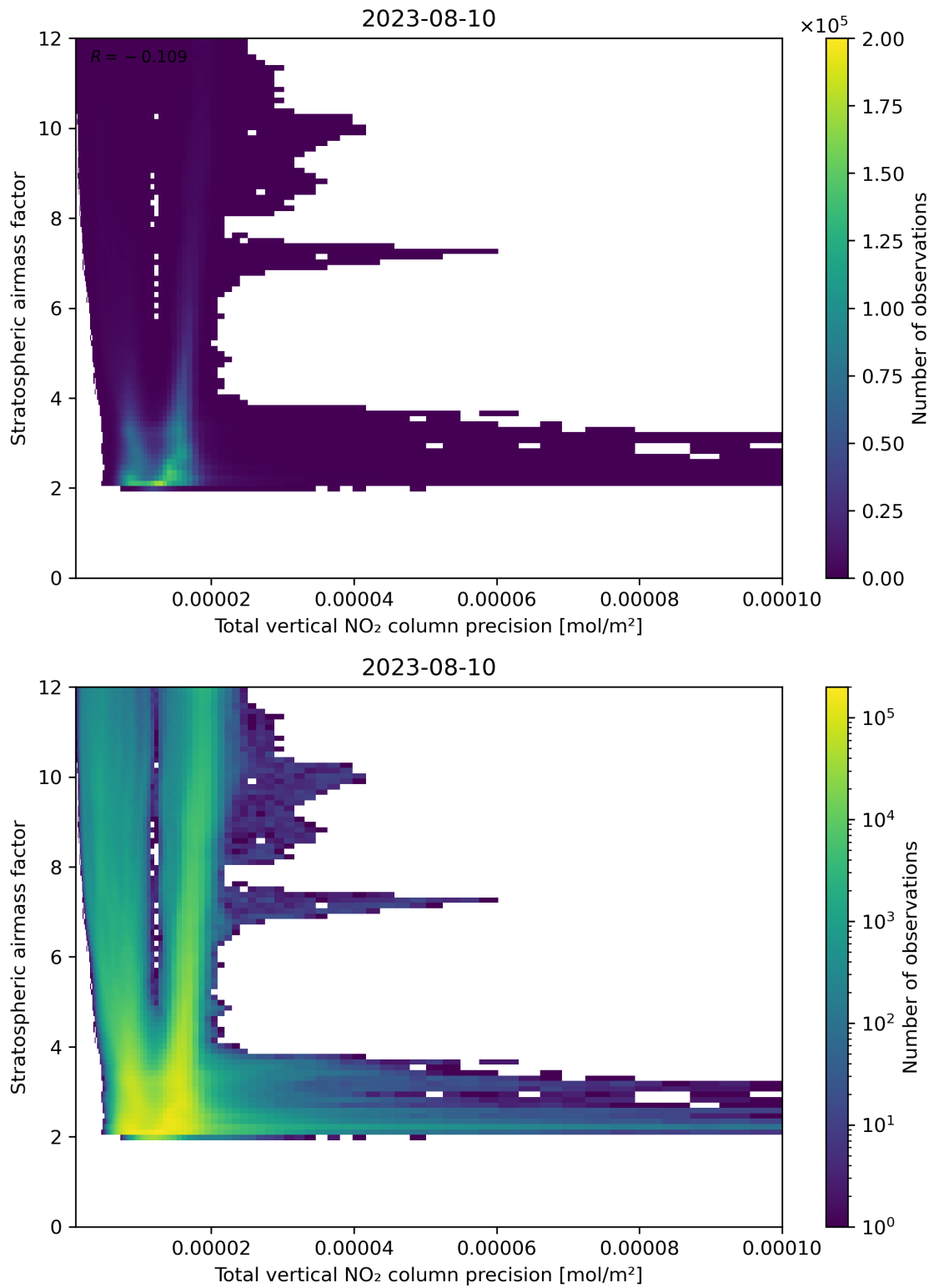
Figure 115: Scatter density plot of “Total vertical NO 2 column precision” against “Stratospheric air mass factor” for 2023-08-09 to 2023-08-11.
