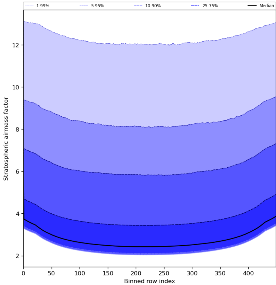
Figure 61: Along track statistics of “Stratospheric airmass factor” for 2023-08-09 to 2023-08-11
