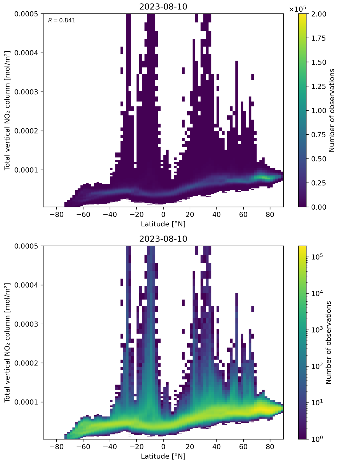
Figure 90: Scatter density plot of “Latitude” against “Total vertical NO 2 column” for 2023-08-09 to 2023-08-11.
