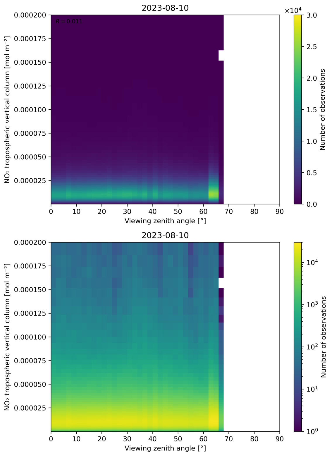
Figure 169: Scatter density plot of “Viewing zenith angle” against “NO 2 tropospheric vertical column” for 2023-08-09 to 2023-08-11.
