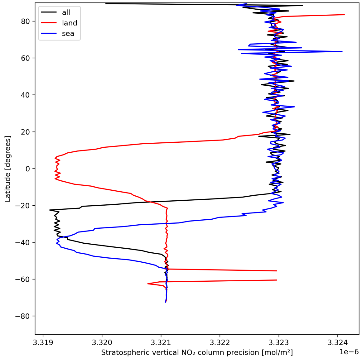
Figure 20: Zonal average of “Stratospheric vertical NO 2 column precision” for 2023-08-09 to 2023-08-11.
