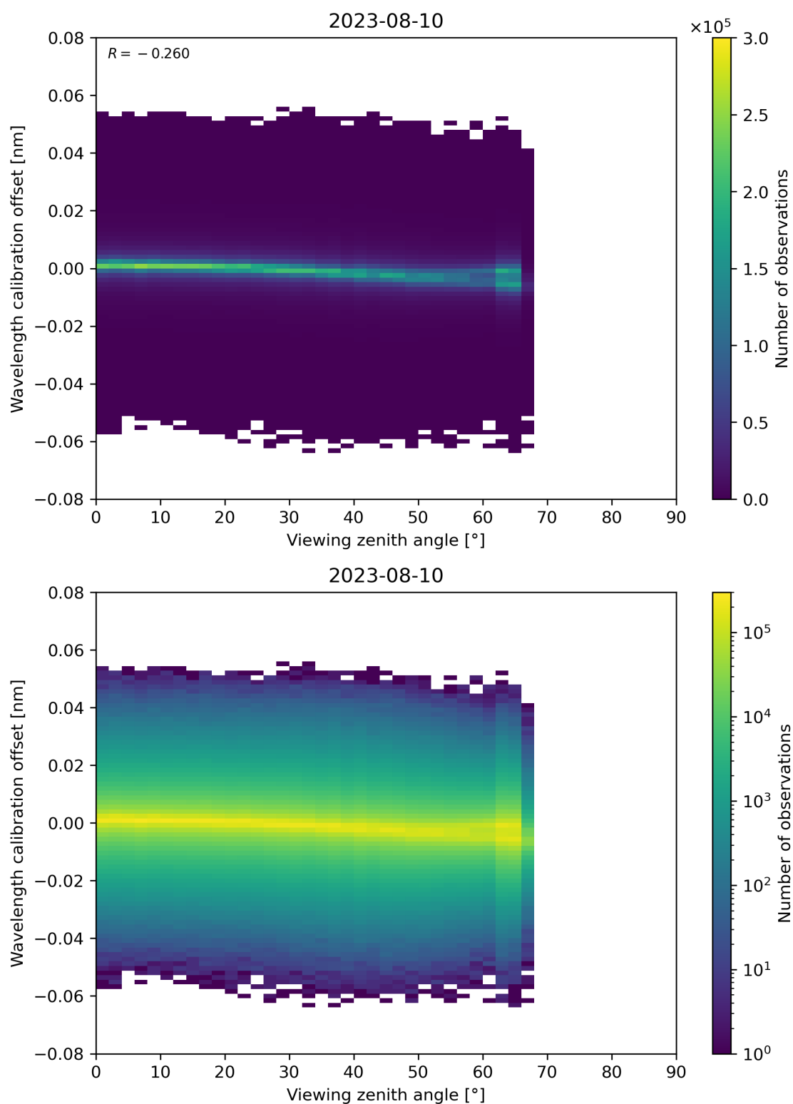
Figure 173: Scatter density plot of “Viewing zenith angle” against “Wavelength calibration offset” for 2023-08-09 to 2023-08-11.
