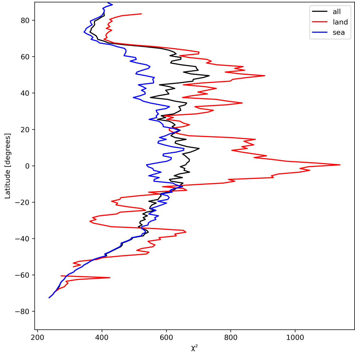
Figure 25: Zonal average of “ \chi^2 ” for 2023-08-09 to 2023-08-11.
