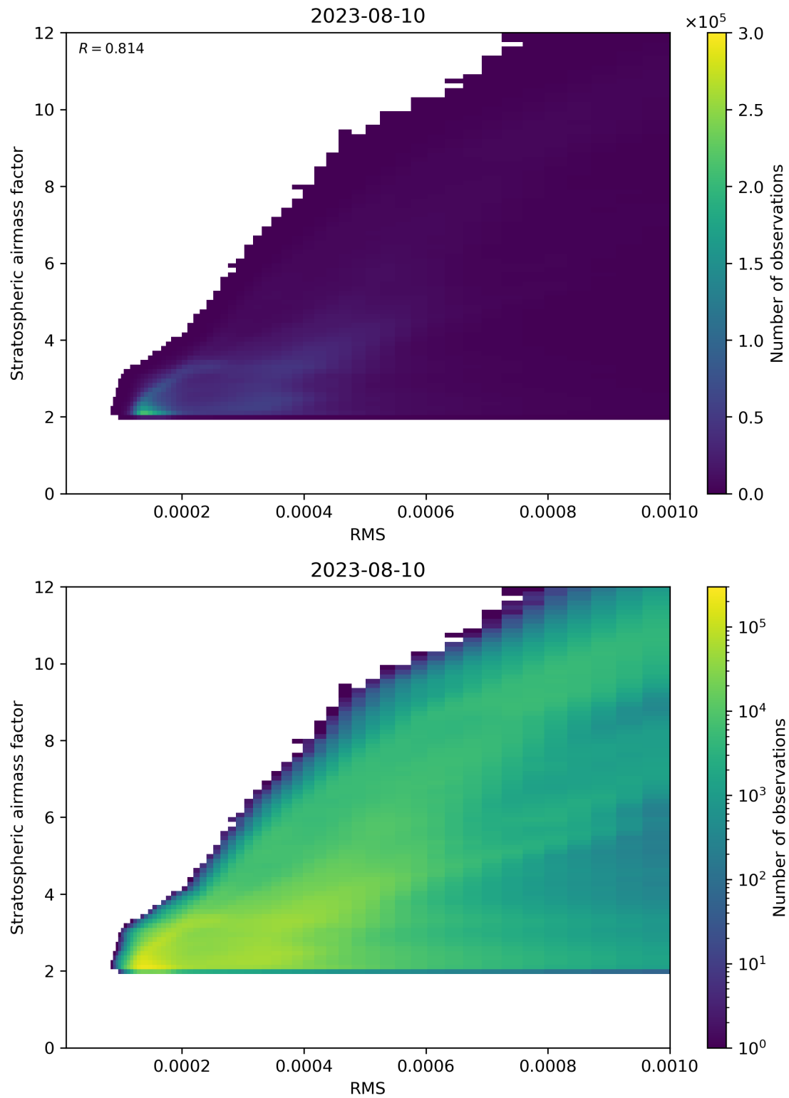
Figure 144: Scatter density plot of “RMS” against “Stratospheric airmass factor” for 2023-08-09 to 2023-08-11.
