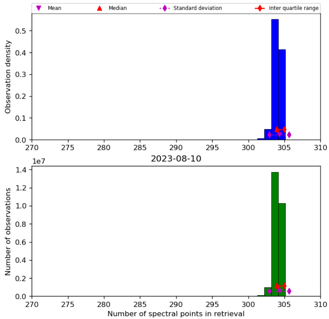
Figure 33: Histogram of “Number of spectral points in retrieval” for 2023-08-09 to 2023-08-11
