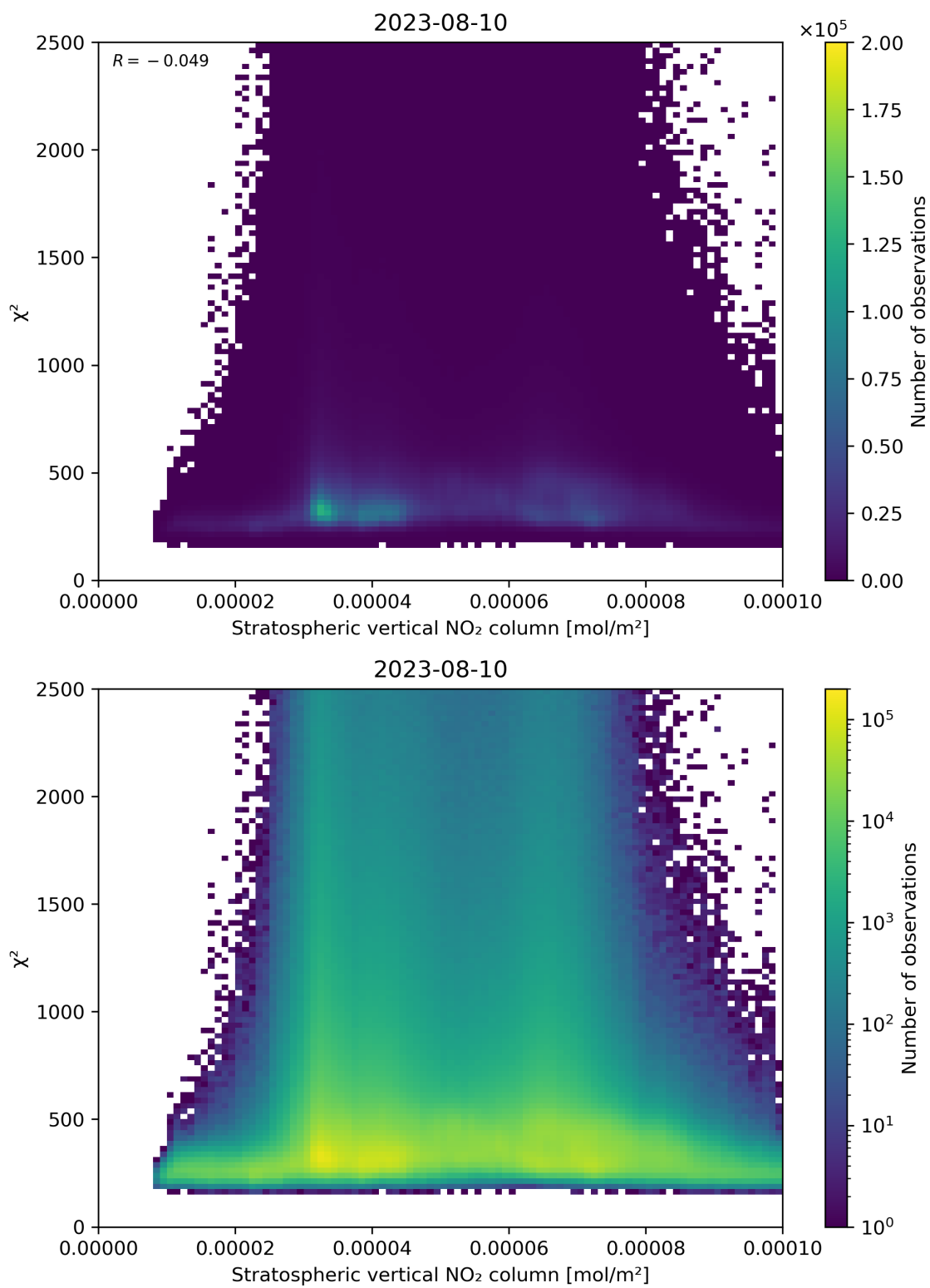
Figure 97: Scatter density plot of “Stratospheric vertical NO 2 column” against “ \chi^2 ” for 2023-08-09 to 2023-08-11.
