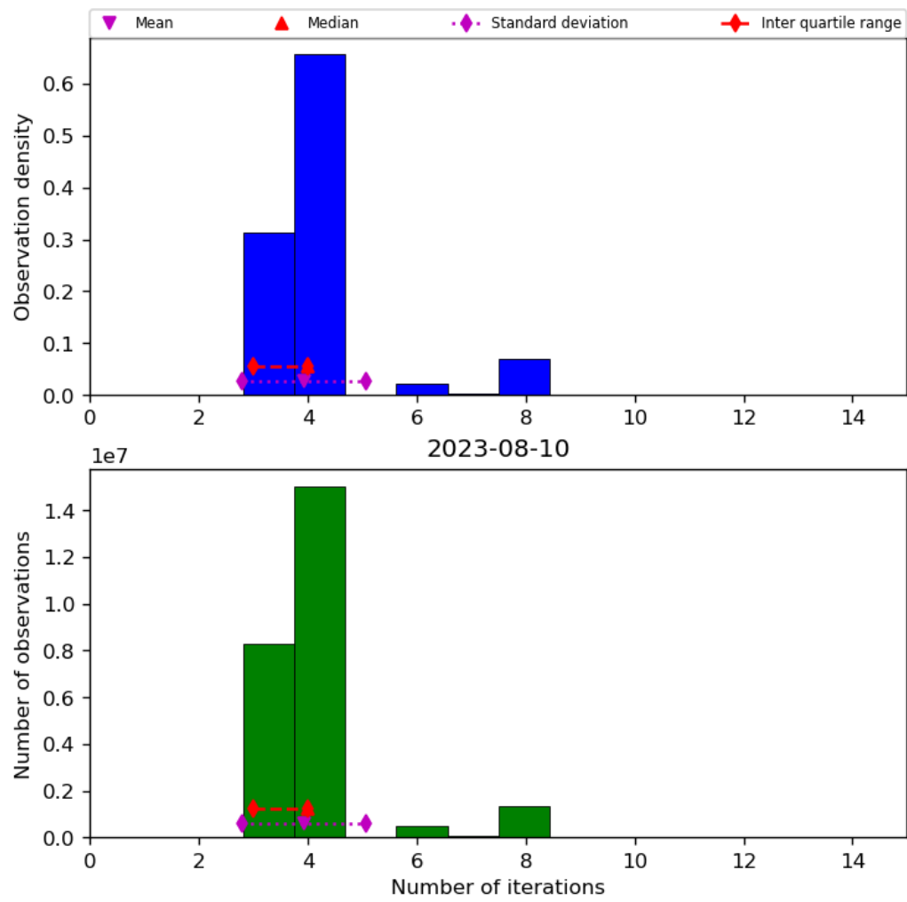
Figure 34: Histogram of “Number of iterations” for 2023-08-09 to 2023-08-11
