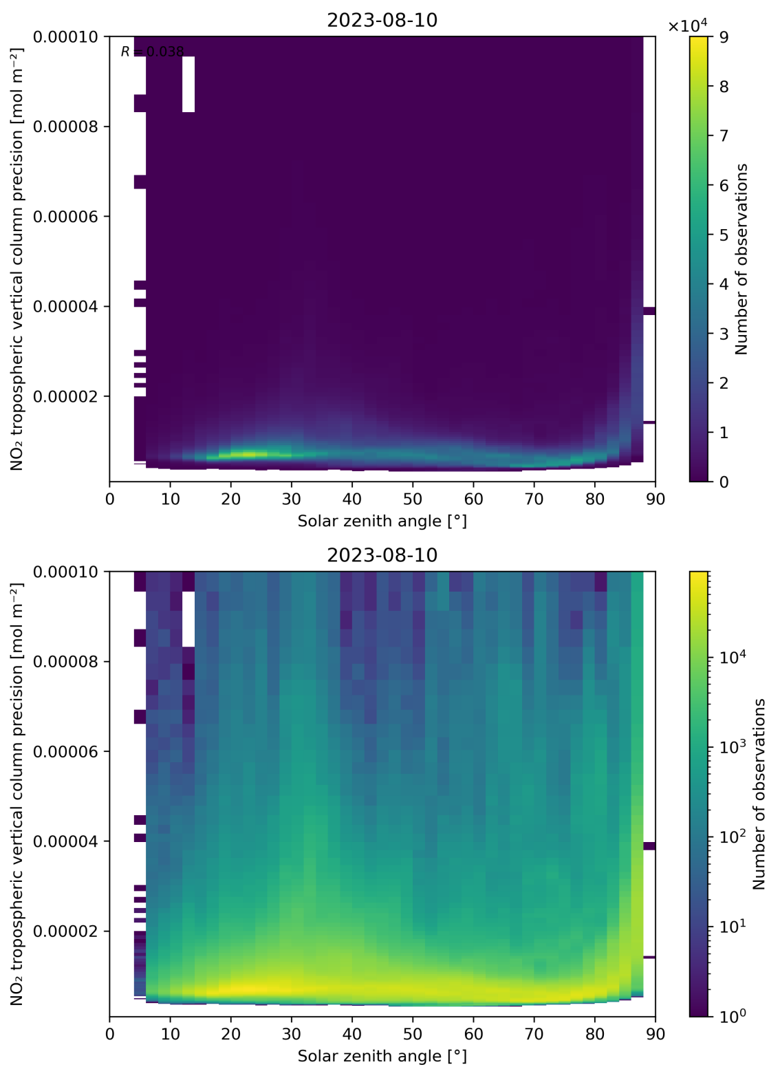
Figure 156: Scatter density plot of “Solar zenith angle” against “NO 2 tropospheric vertical column precision” for 2023-08-09 to 2023-08-11.
