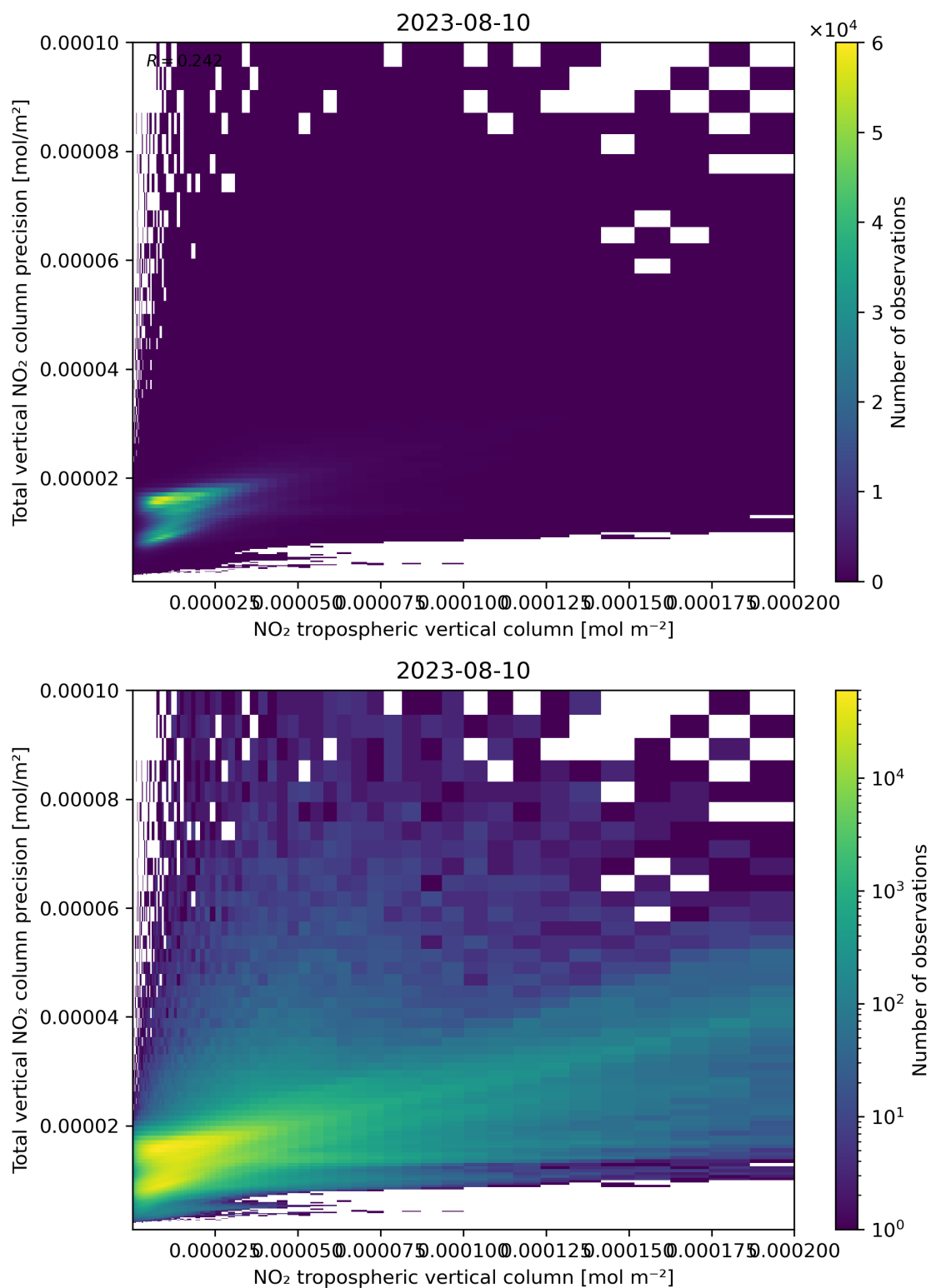
Figure 129: Scatter density plot of “NO 2 tropospheric vertical column” against “Total vertical NO 2 column precision” for 2023-08-09 to 2023-08-11.
