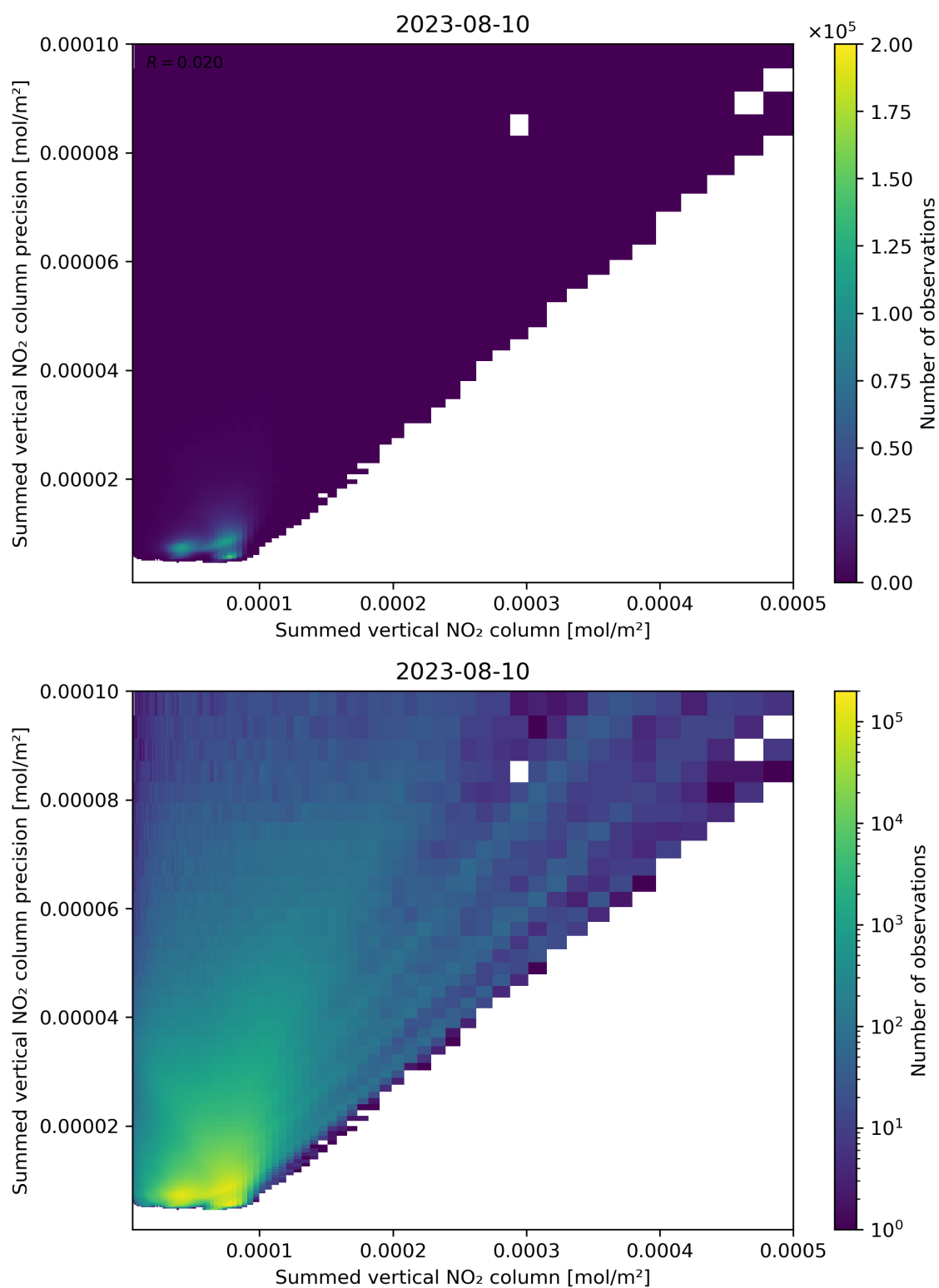
Figure 105: Scatter density plot of “Summed vertical NO 2 column” against “Summed vertical NO 2 column precision” for 2023-08-09 to 2023-08-11.
