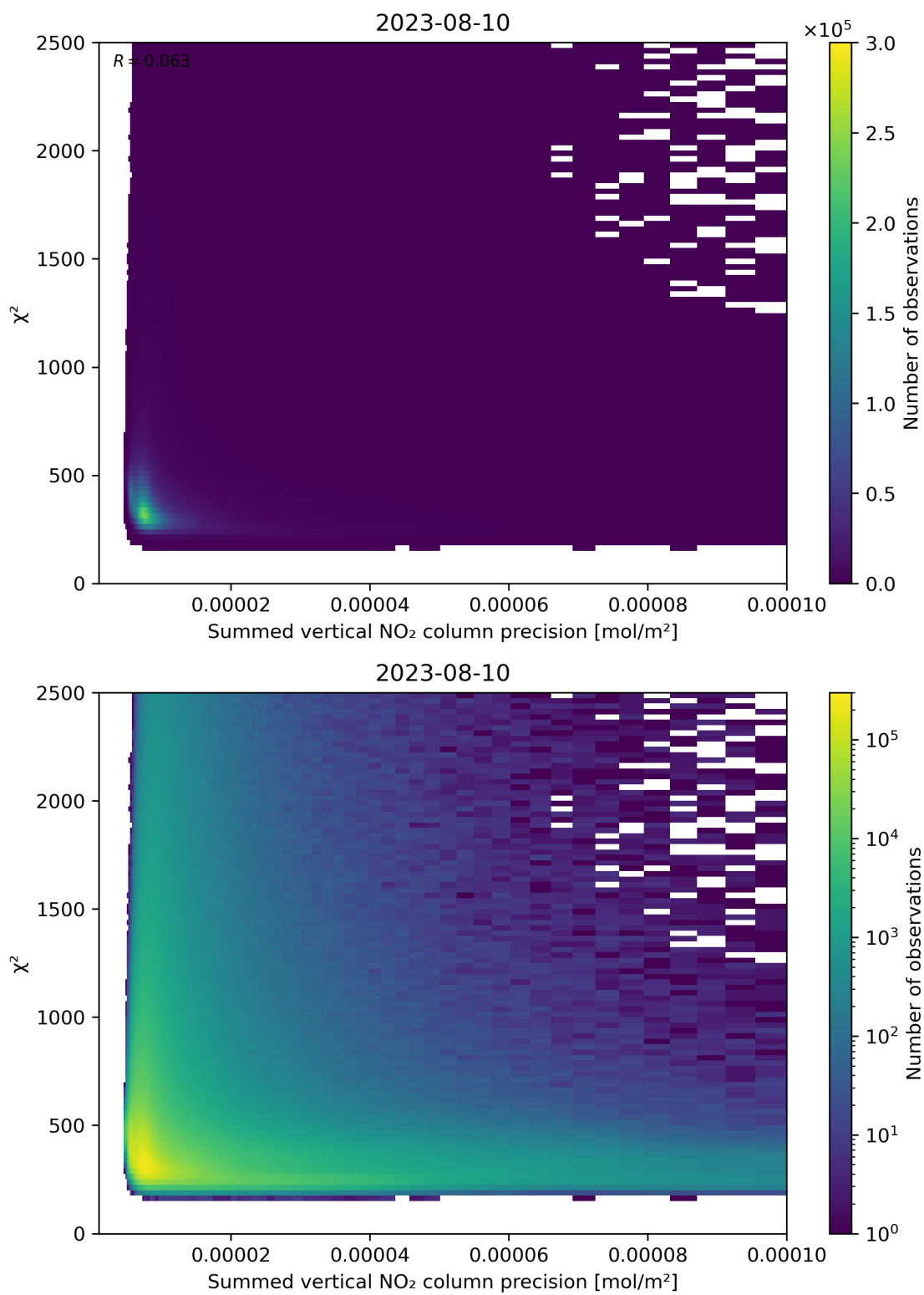
Figure 107: Scatter density plot of “Summed vertical NO 2 column precision” against “ \chi^2 ” for 2023-08-09 to 2023-08-11.
