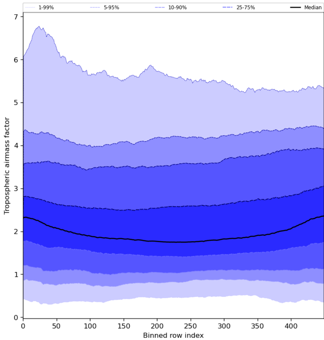
Figure 48: Along track statistics of “Tropospheric air mass factor” for 2023-08-09 to 2023-08-11
