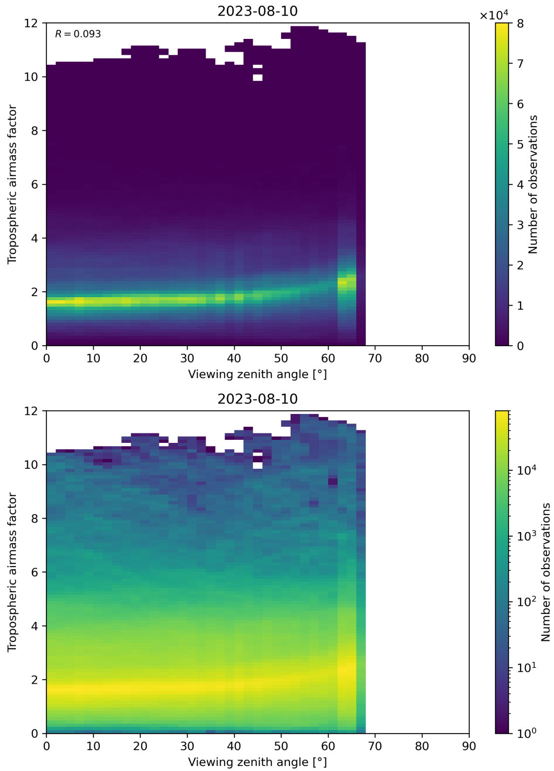
Figure 161: Scatter density plot of “Viewing zenith angle” against “Tropospheric airmass factor” for 2023-08-09 to 2023-08-11.
