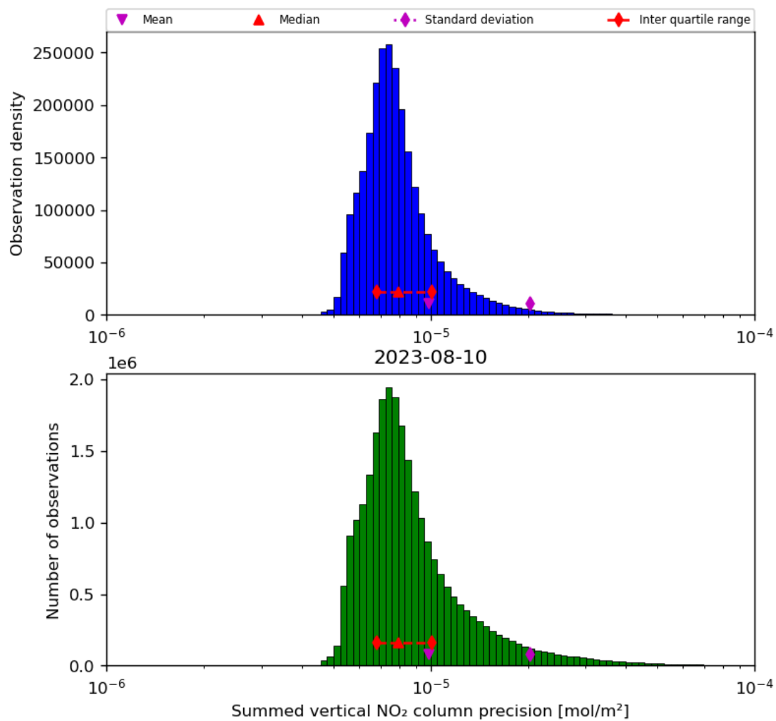
Figure 41: Histogram of “Summed vertical NO 2 column precision” for 2023-08-09 to 2023-08-11
