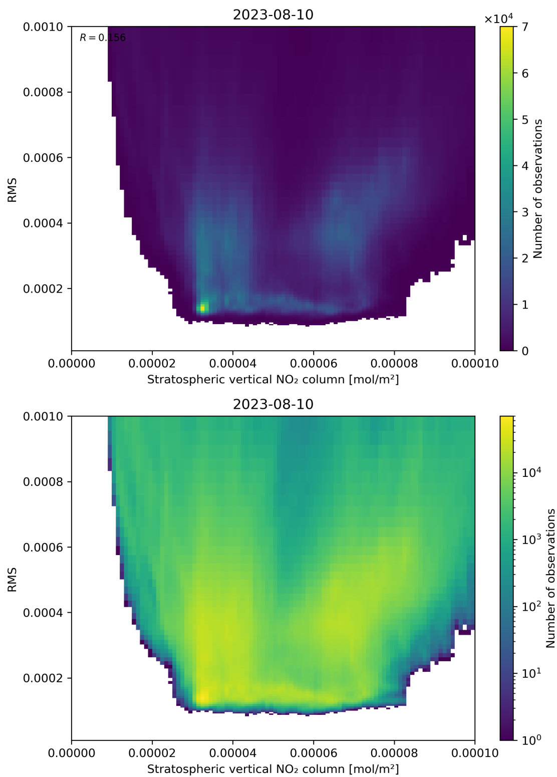
Figure 102: Scatter density plot of “Stratospheric vertical NO 2 column” against “RMS” for 2023-08-09 to 2023-08-11.
