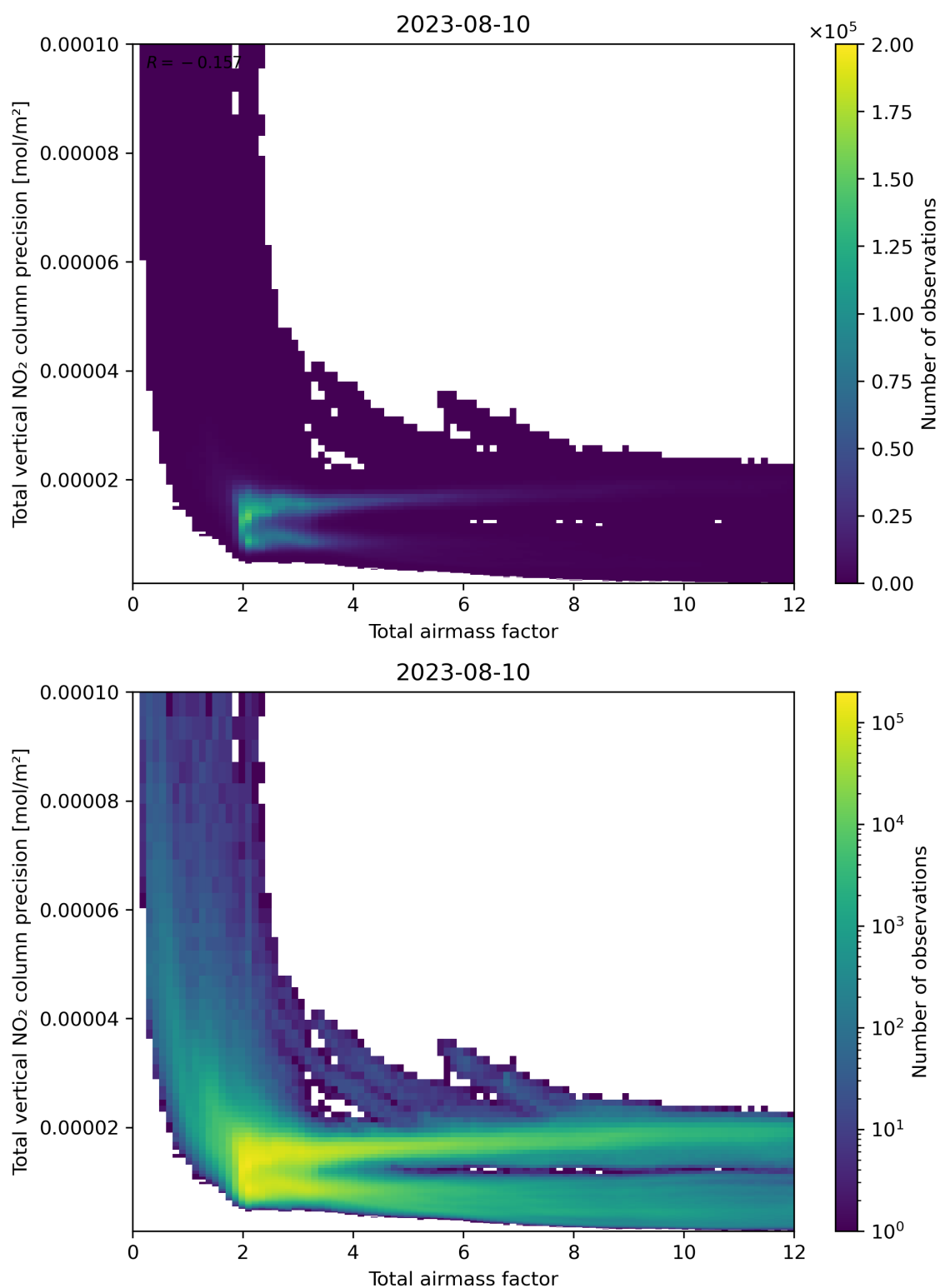
Figure 68: Scatter density plot of “Total airmass factor” against “Total vertical NO 2 column precision” for 2023-08-09 to 2023-08-11.
