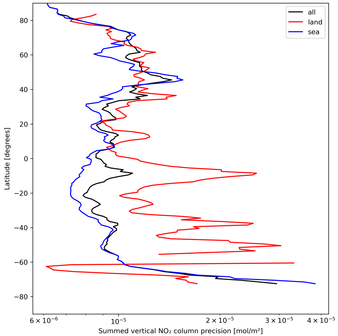
Figure 24: Zonal average of “Summed vertical NO 2 column precision” for 2023-08-09 to 2023-08-11.
