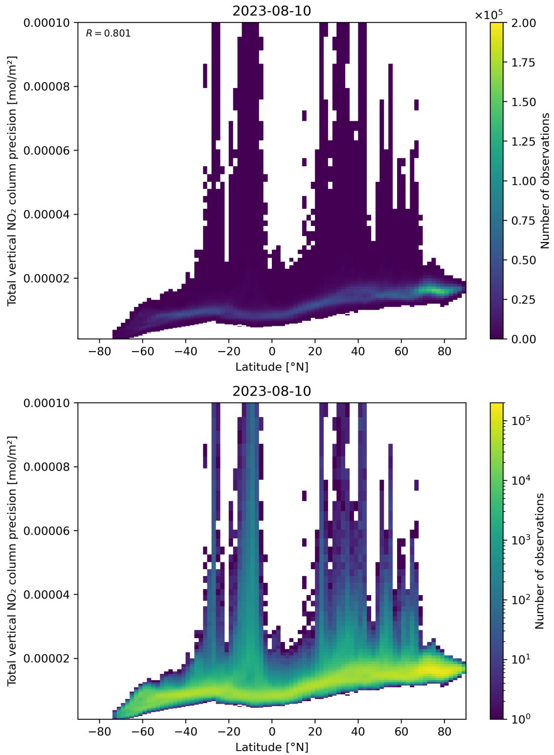
Figure 91: Scatter density plot of “Latitude” against “Total vertical NO 2 column precision” for 2023-08-09 to 2023-08-11.
