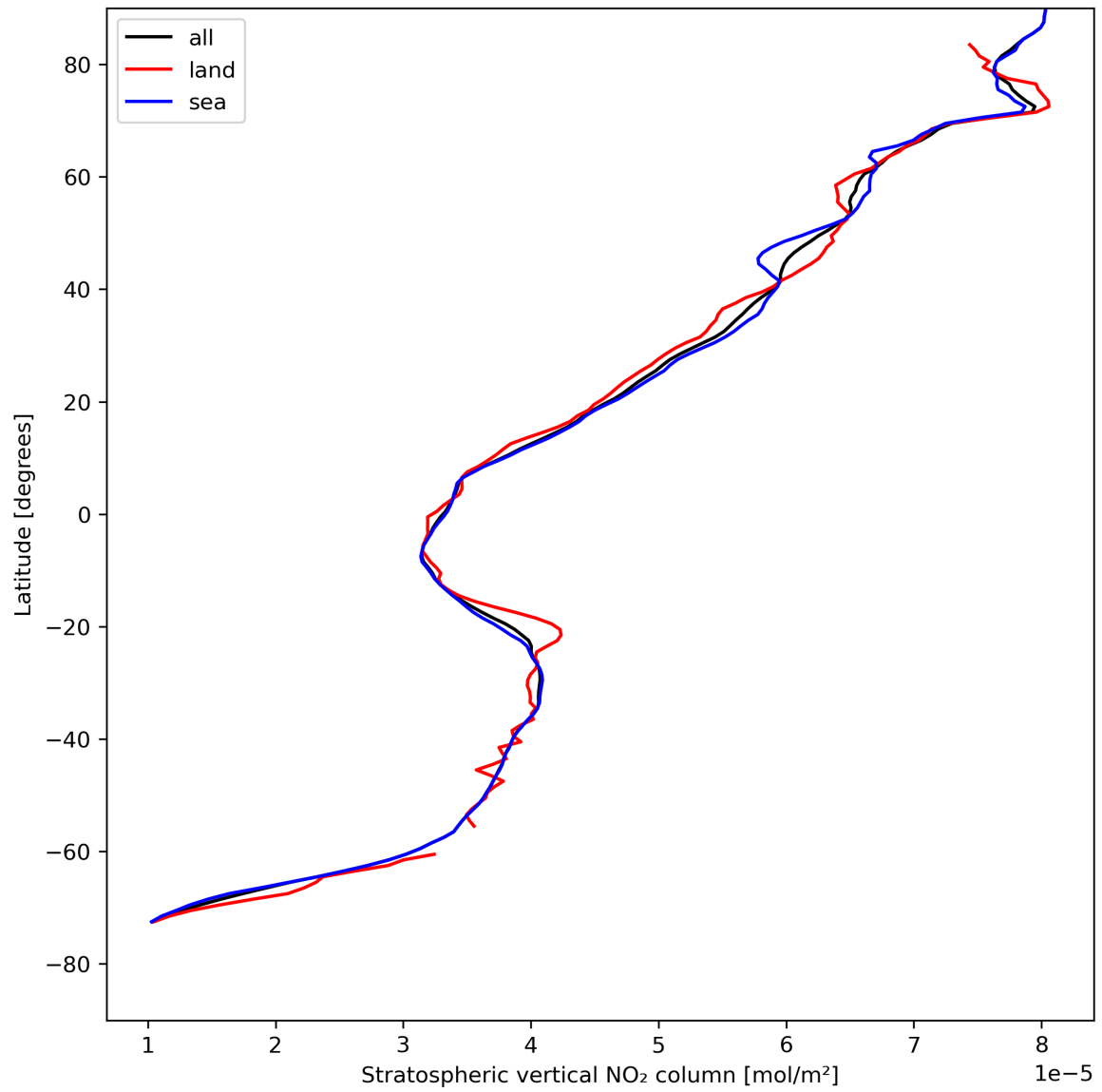
Figure 19: Zonal average of “Stratospheric vertical NO 2 column” for 2023-08-09 to 2023-08-11.
