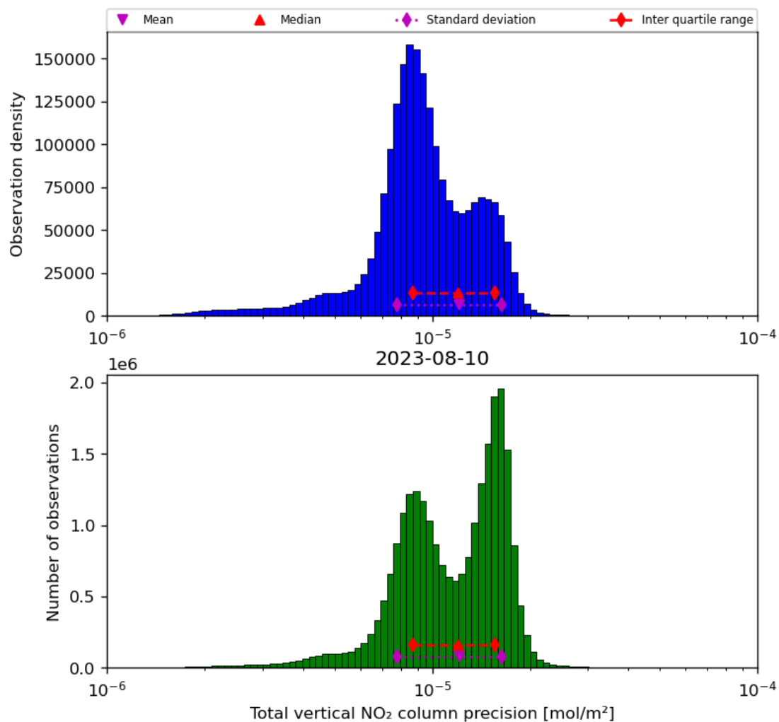
Figure 39: Histogram of “Total vertical NO 2 column precision” for 2023-08-09 to 2023-08-11
