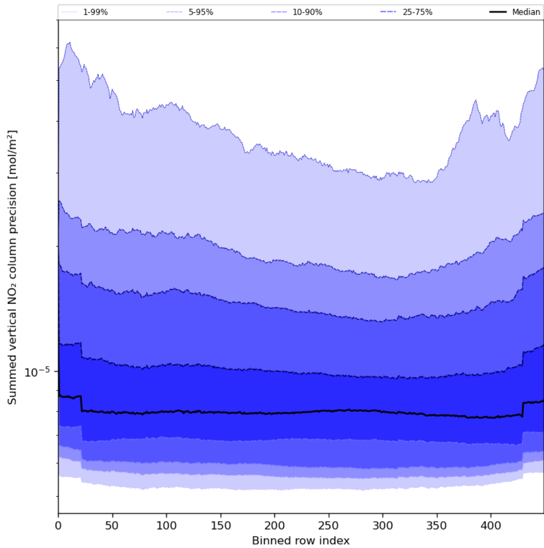
Figure 58: Along track statistics of “Summed vertical NO 2 column precision” for 2023-08-09 to 2023-08-11
