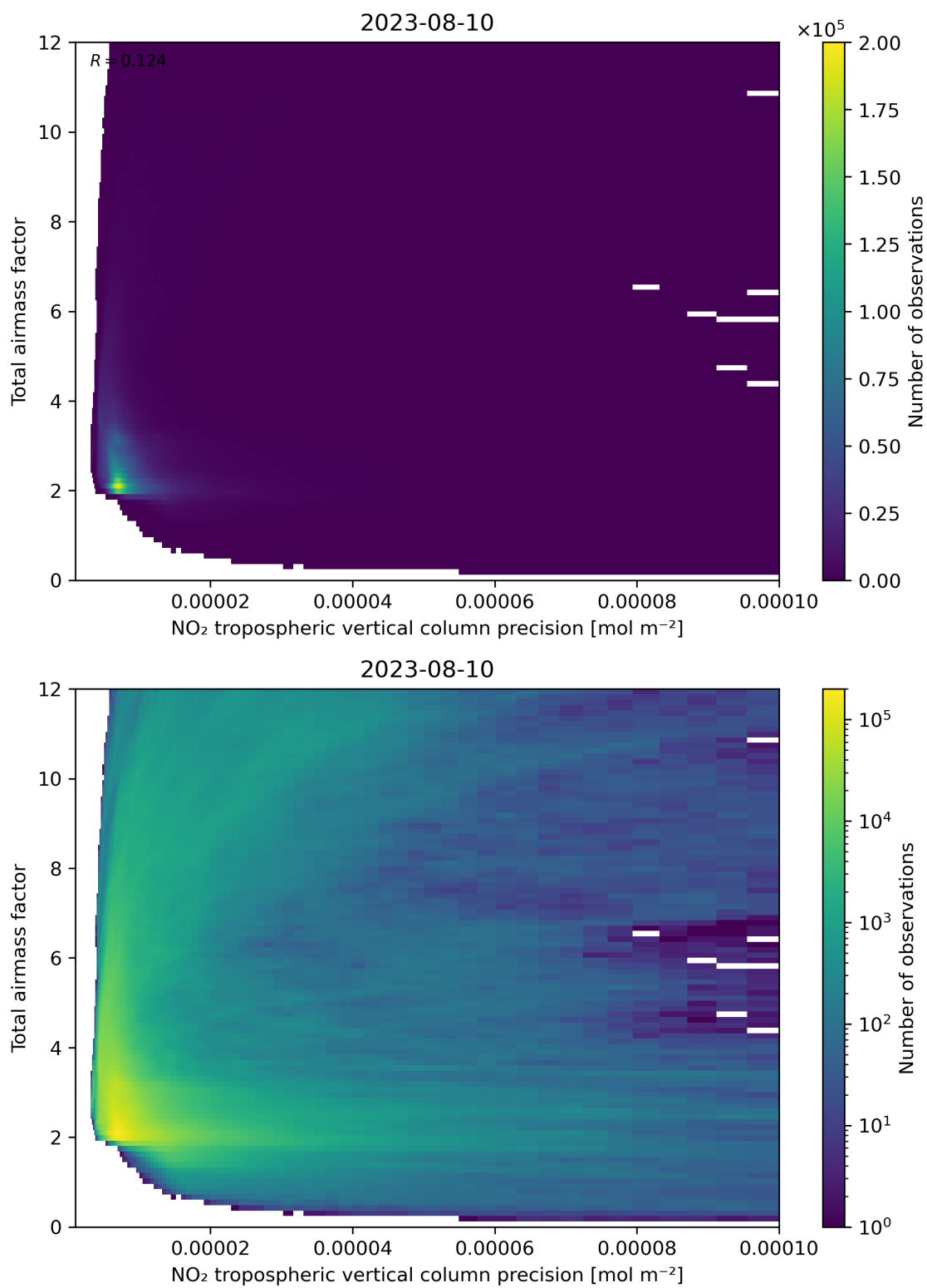
Figure 132: Scatter density plot of “NO 2 tropospheric vertical column precision” against “Total air mass factor” for 2023-08-09 to 2023-08-11.
