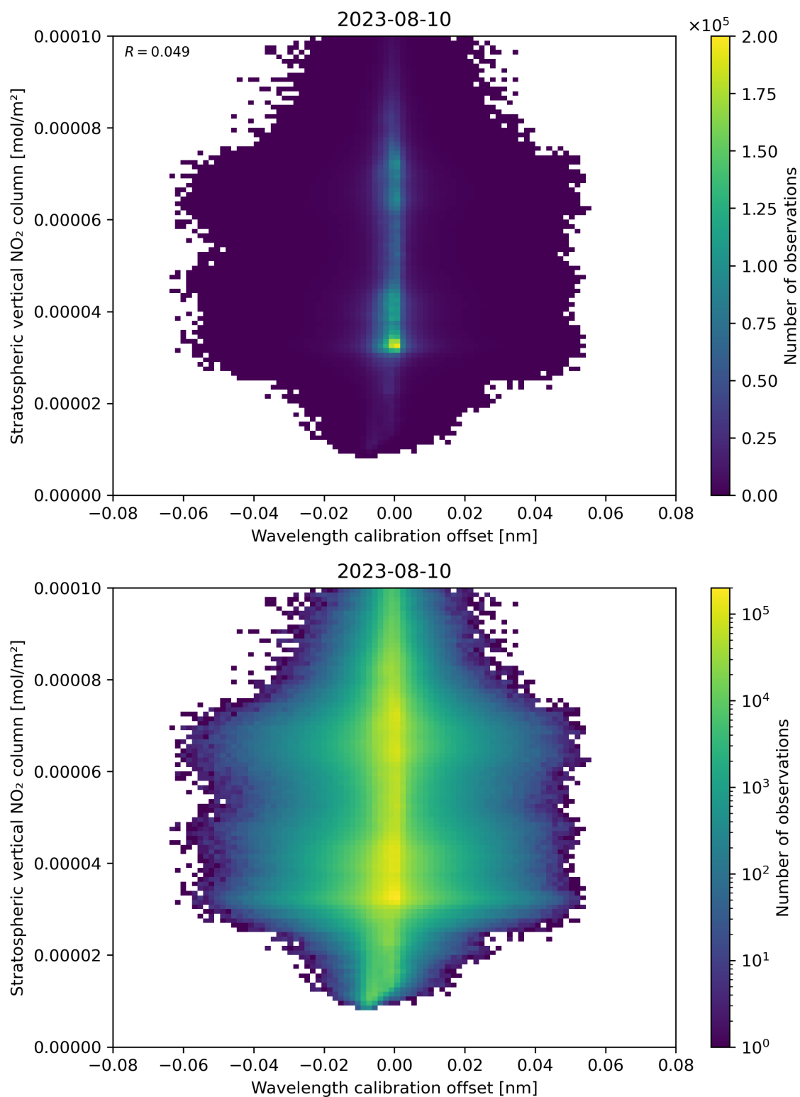
Figure 176: Scatter density plot of “Wavelength calibration offset” against “Stratospheric vertical NO 2 column” for 2023-08-09 to 2023-08-11.
