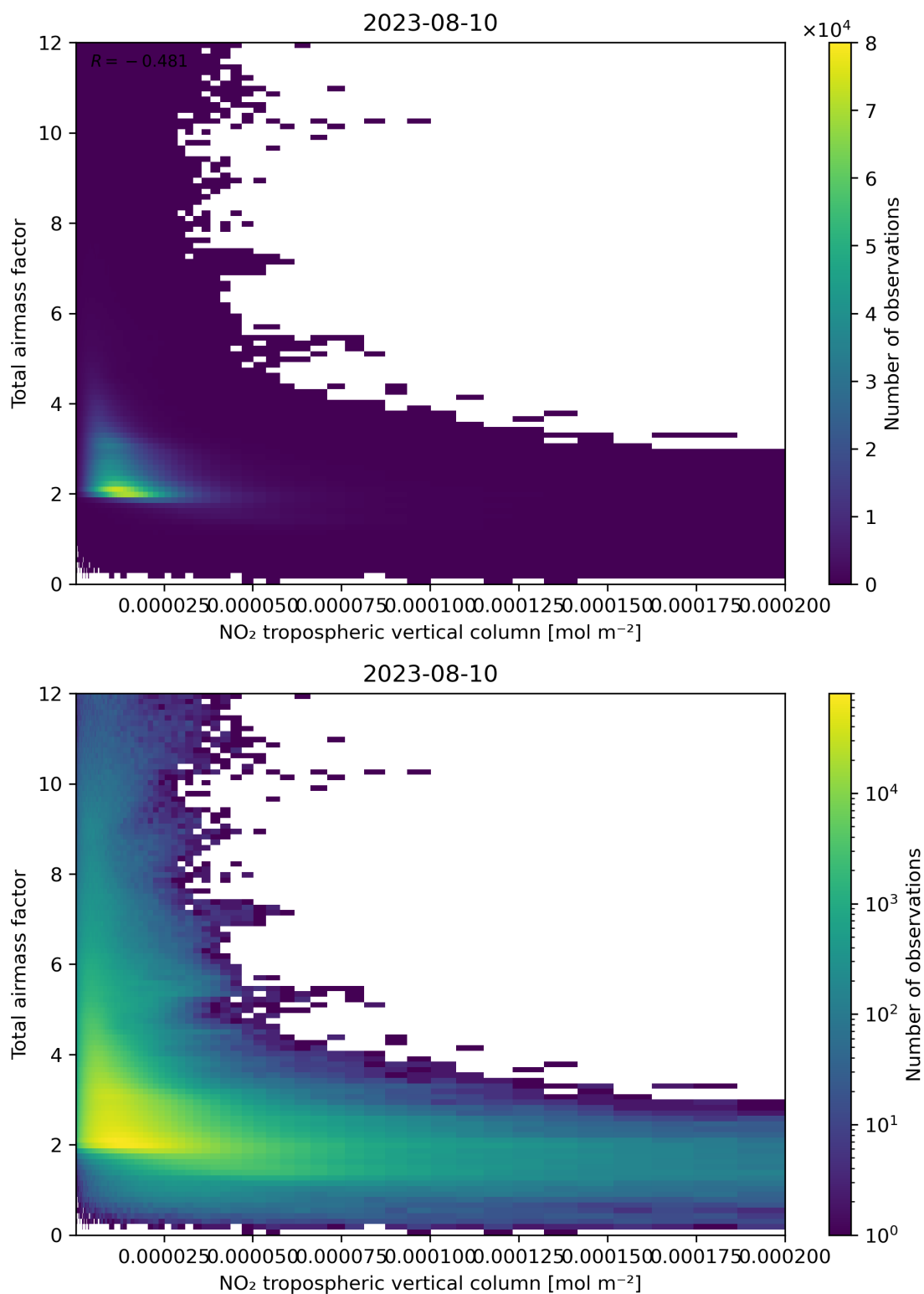
Figure 122: Scatter density plot of “NO 2 tropospheric vertical column” against “Total air mass factor” for 2023-08-09 to 2023-08-11.
