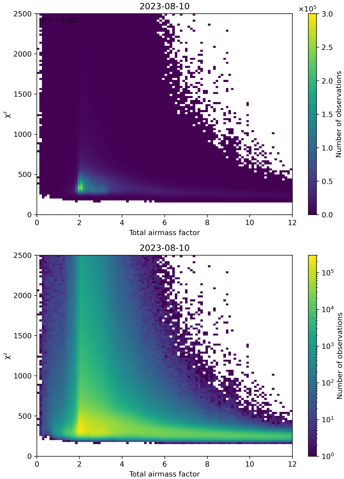
Figure 63: Scatter density plot of “Total airmass factor” against “ \chi^2 ” for 2023-08-09 to 2023-08-11.
