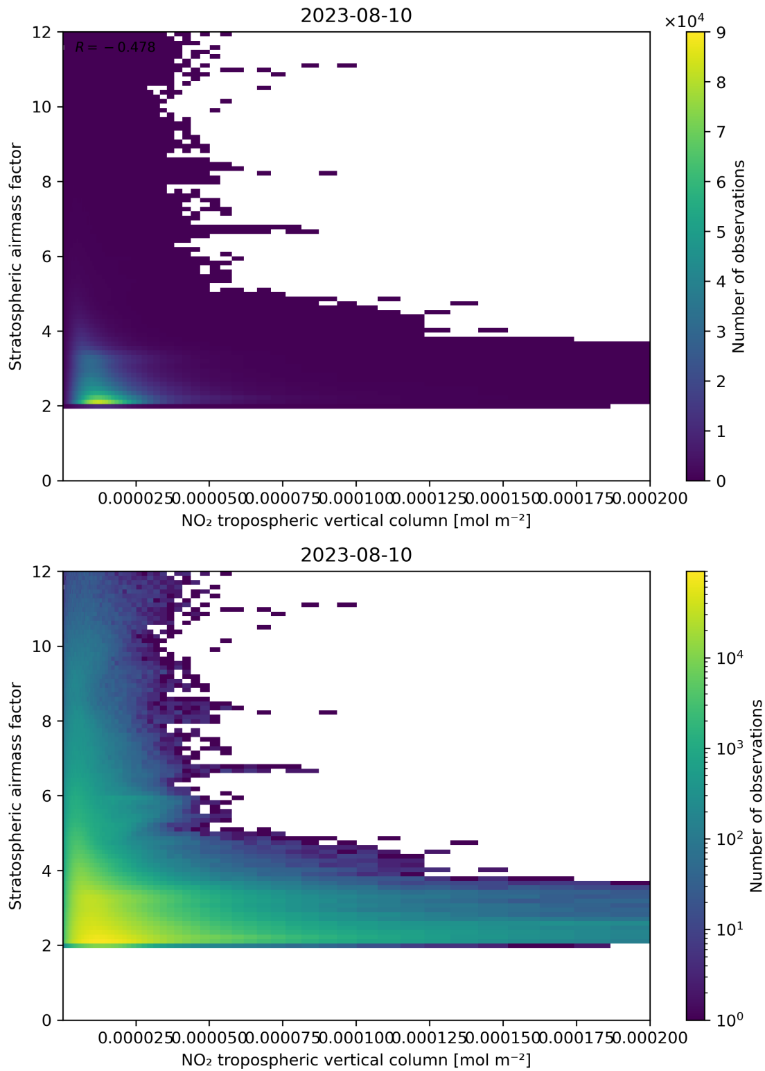
Figure 121: Scatter density plot of “NO 2 tropospheric vertical column” against “Stratospheric air mass factor” for 2023-08-09 to 2023-08-11.
