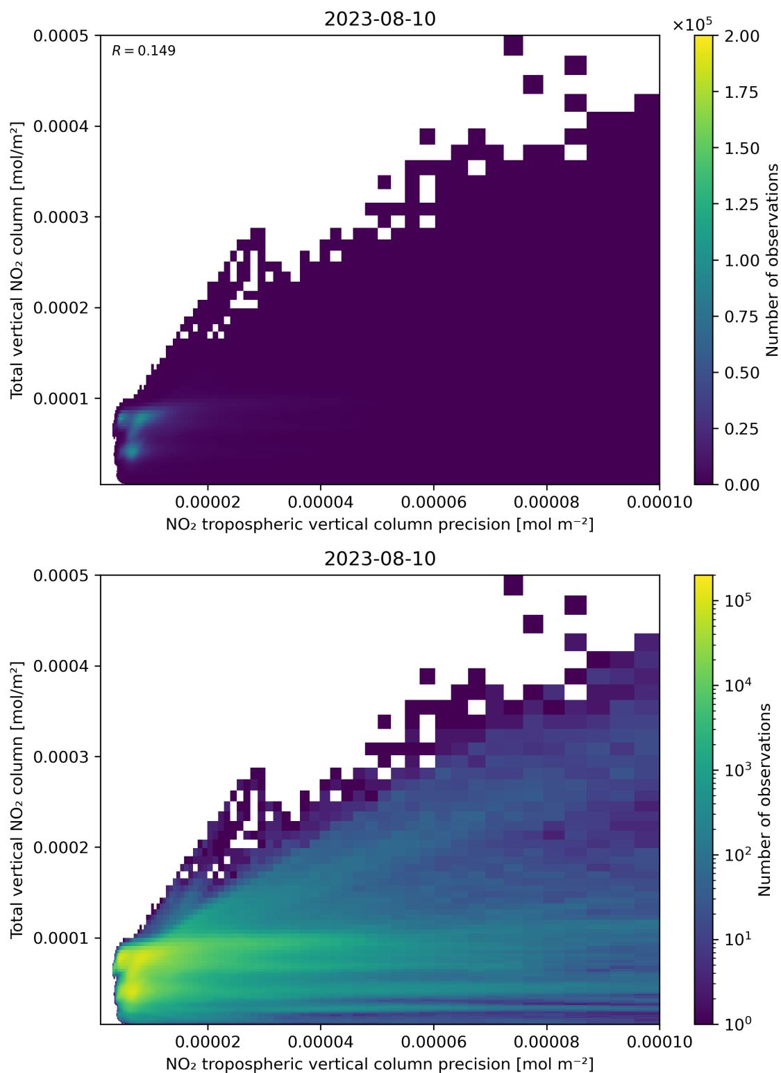
Figure 138: Scatter density plot of “NO 2 tropospheric vertical column precision” against “Total vertical NO 2 column” for 2023-08-09 to 2023-08-11.
