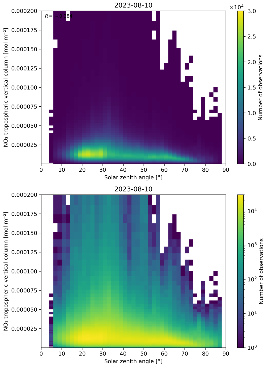
Figure 155: Scatter density plot of “Solar zenith angle” against “NO 2 tropospheric vertical column” for 2023-08-09 to 2023-08-11.
