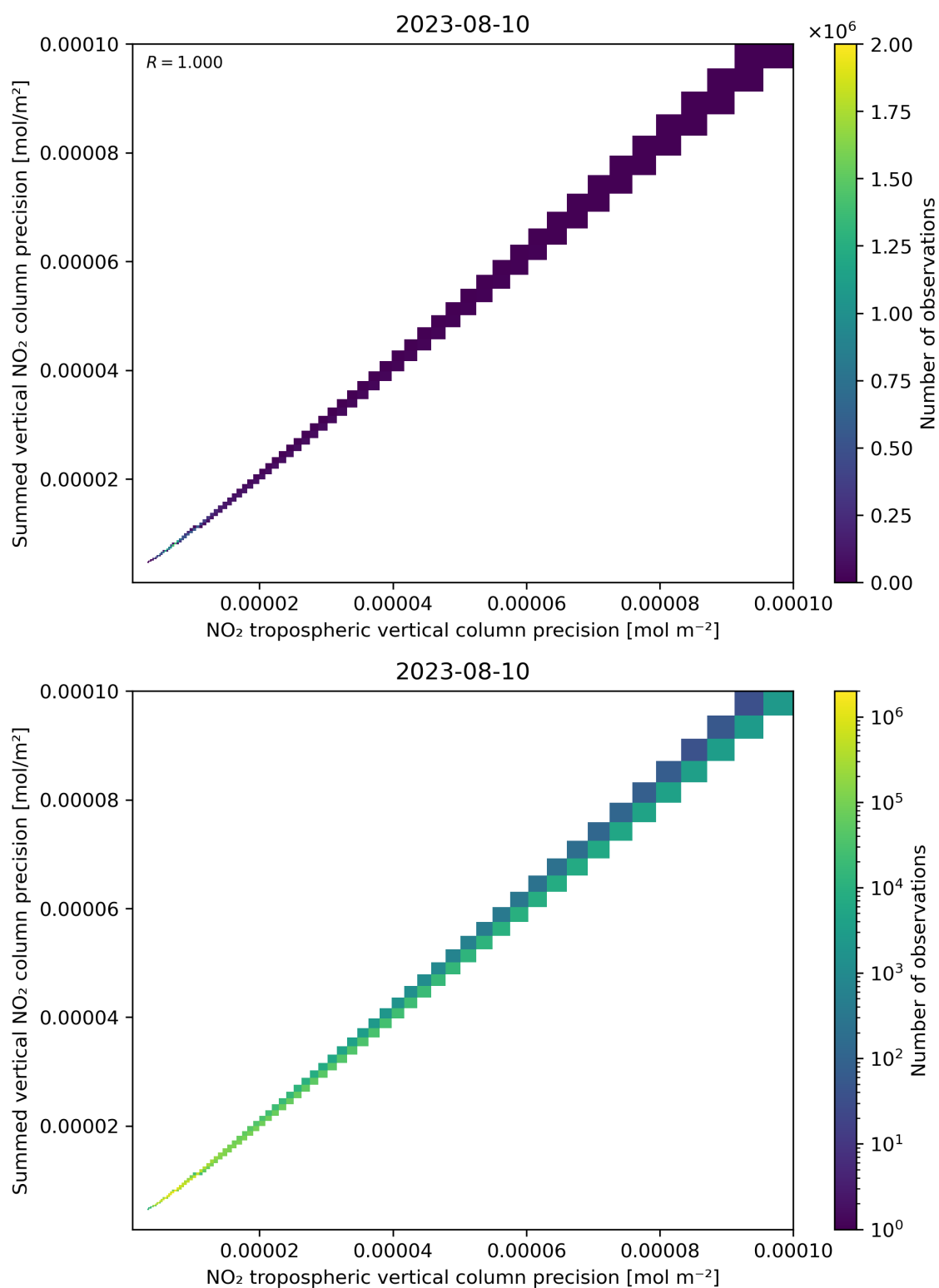
Figure 137: Scatter density plot of “NO 2 tropospheric vertical column precision” against “Summed vertical NO 2 column precision” for 2023-08-09 to 2023-08-11.
