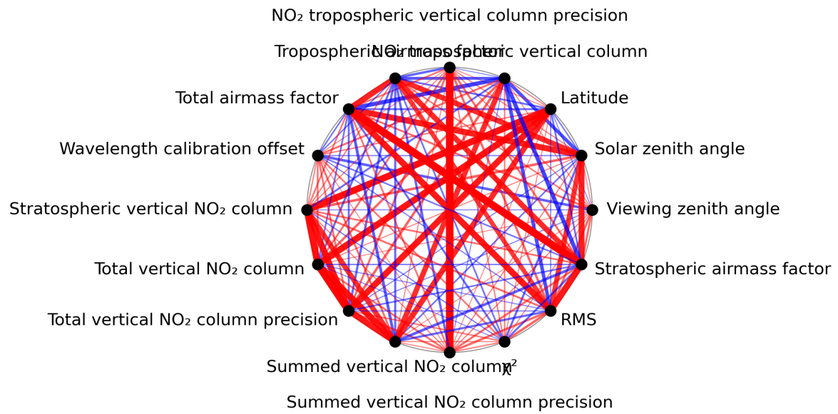
Figure 1: Map of correlation graph for 2023-08-09 to 2023-08-11.
