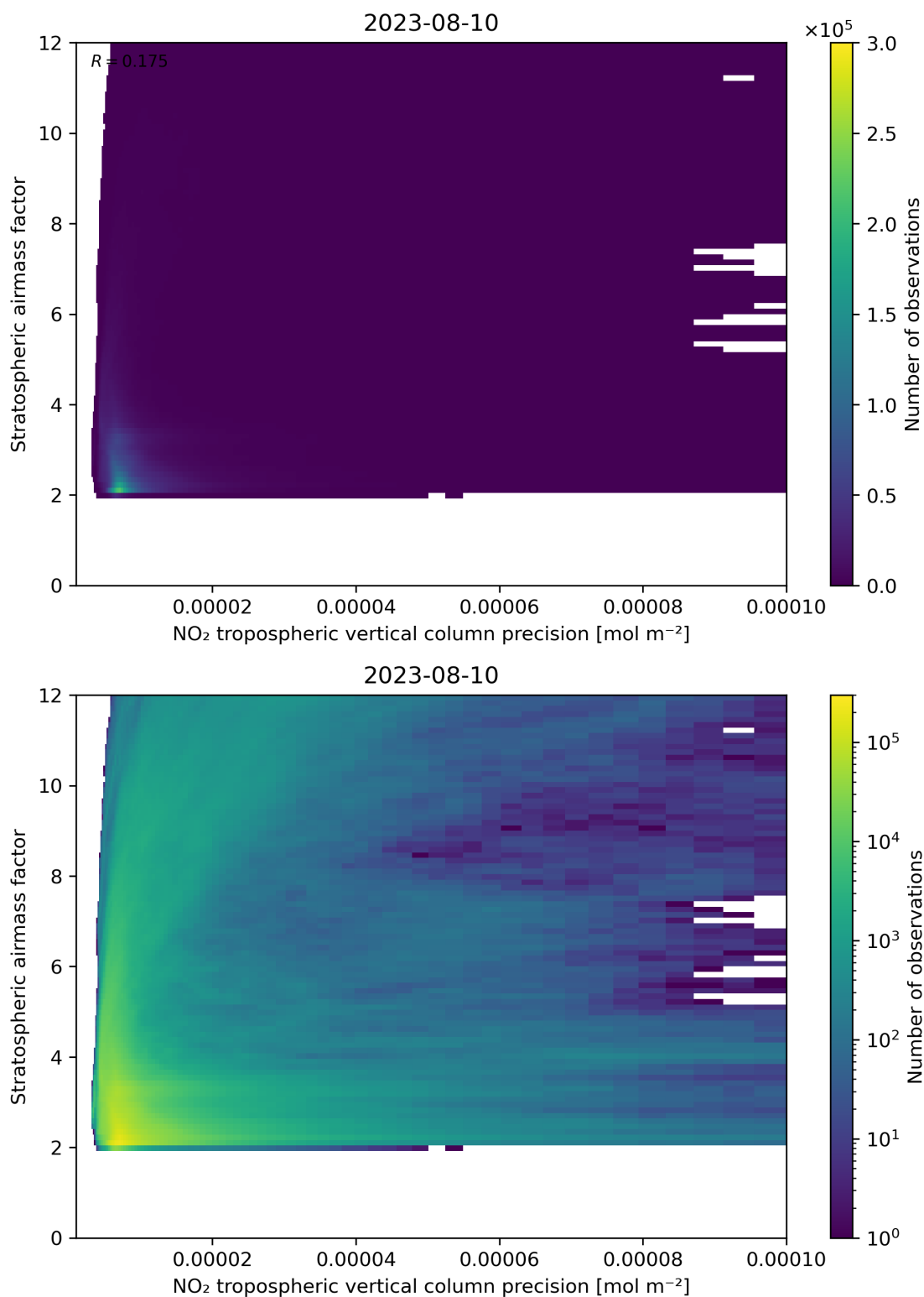
Figure 131: Scatter density plot of “NO 2 tropospheric vertical column precision” against “Stratospheric airmass factor” for 2023-08-09 to 2023-08-11.
