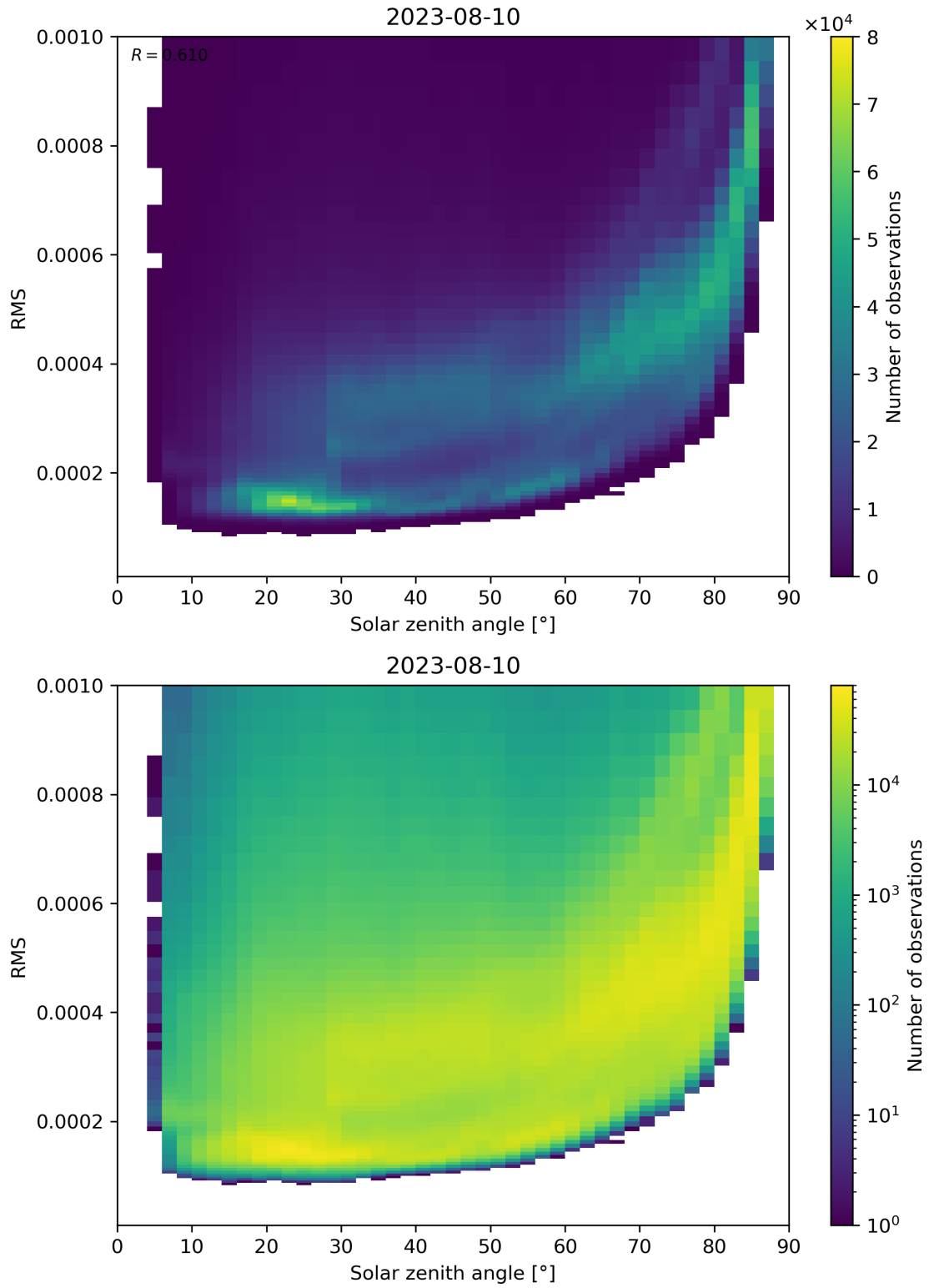
Figure 157: Scatter density plot of “Solar zenith angle” against “RMS” for 2023-08-09 to 2023-08-11.
