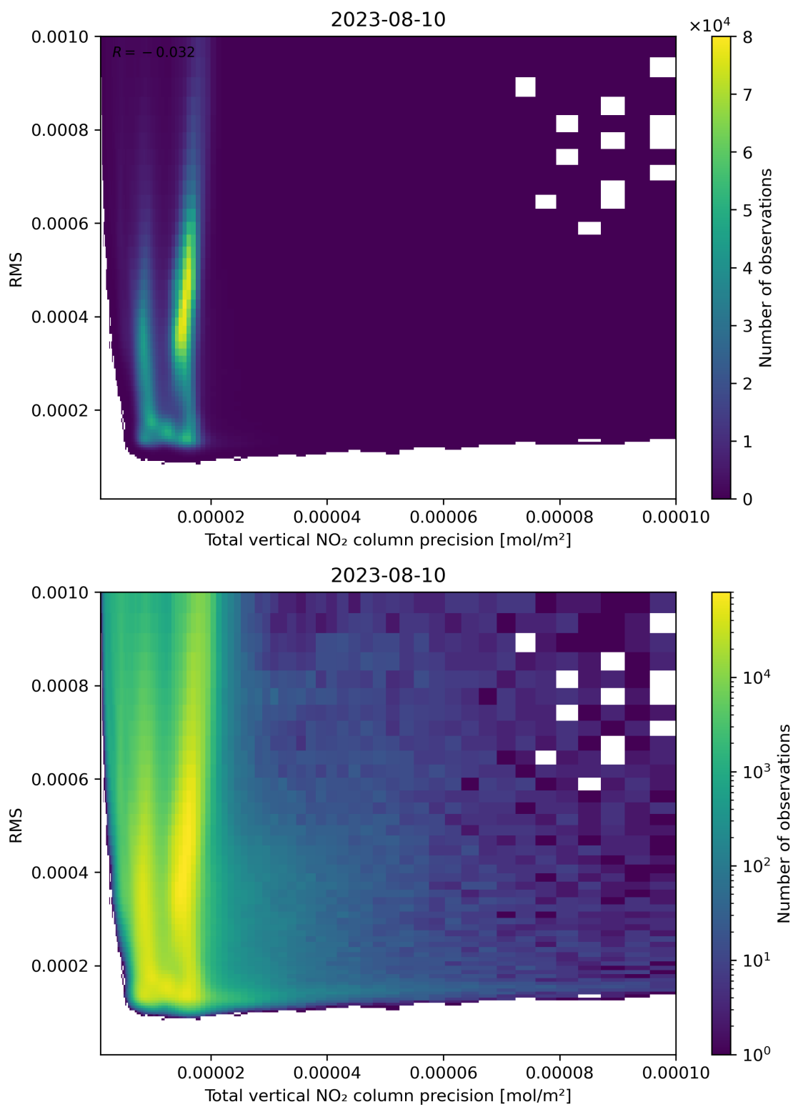
Figure 119: Scatter density plot of “Total vertical NO 2 column precision” against “RMS” for 2023-08-09 to 2023-08-11.
