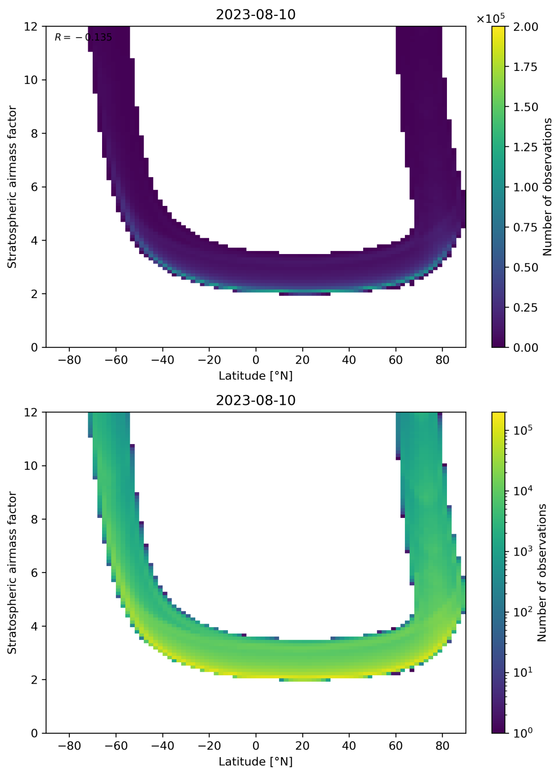
Figure 83: Scatter density plot of “Latitude” against “Stratospheric air mass factor” for 2023-08-09 to 2023-08-11.
