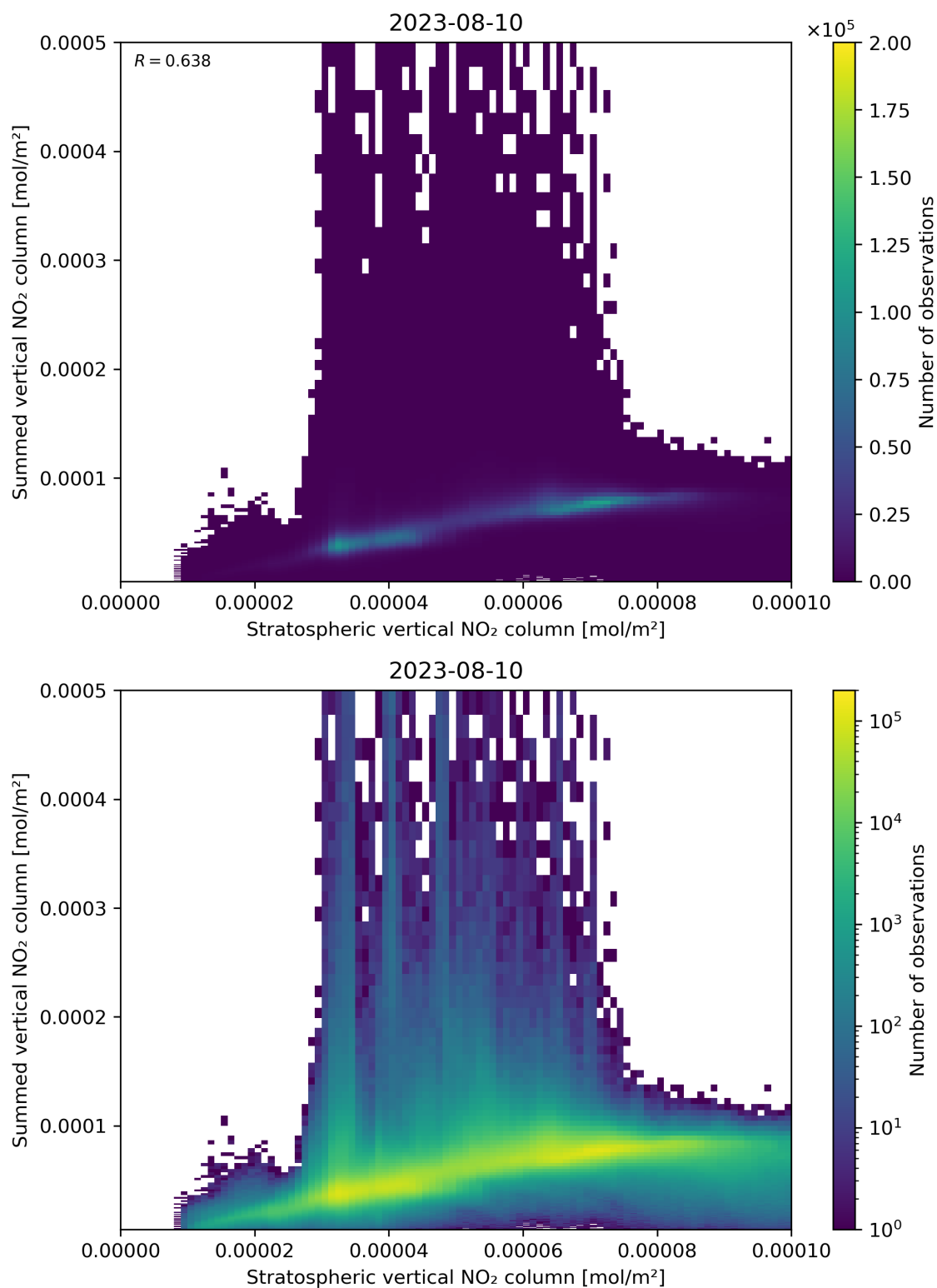
Figure 98: Scatter density plot of “Stratospheric vertical NO 2 column” against “Summed vertical NO 2 column” for 2023-08-09 to 2023-08-11.
