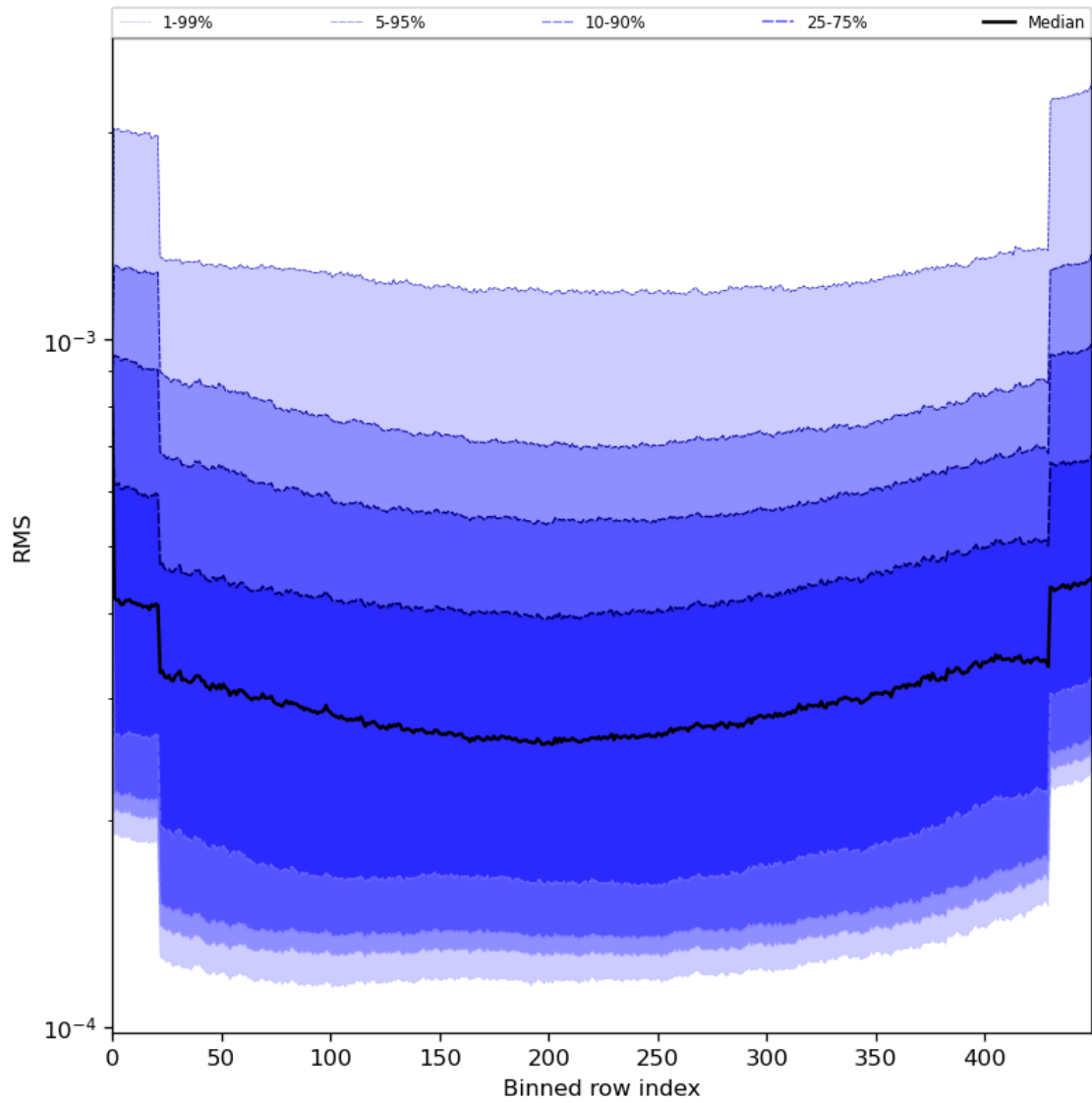
Figure 60: Along track statistics of “RMS” for 2023-08-09 to 2023-08-11
