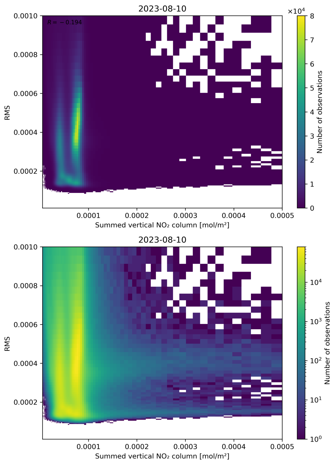
Figure 109: Scatter density plot of “Summed vertical NO 2 column” against “RMS” for 2023-08-09 to 2023-08-11.
