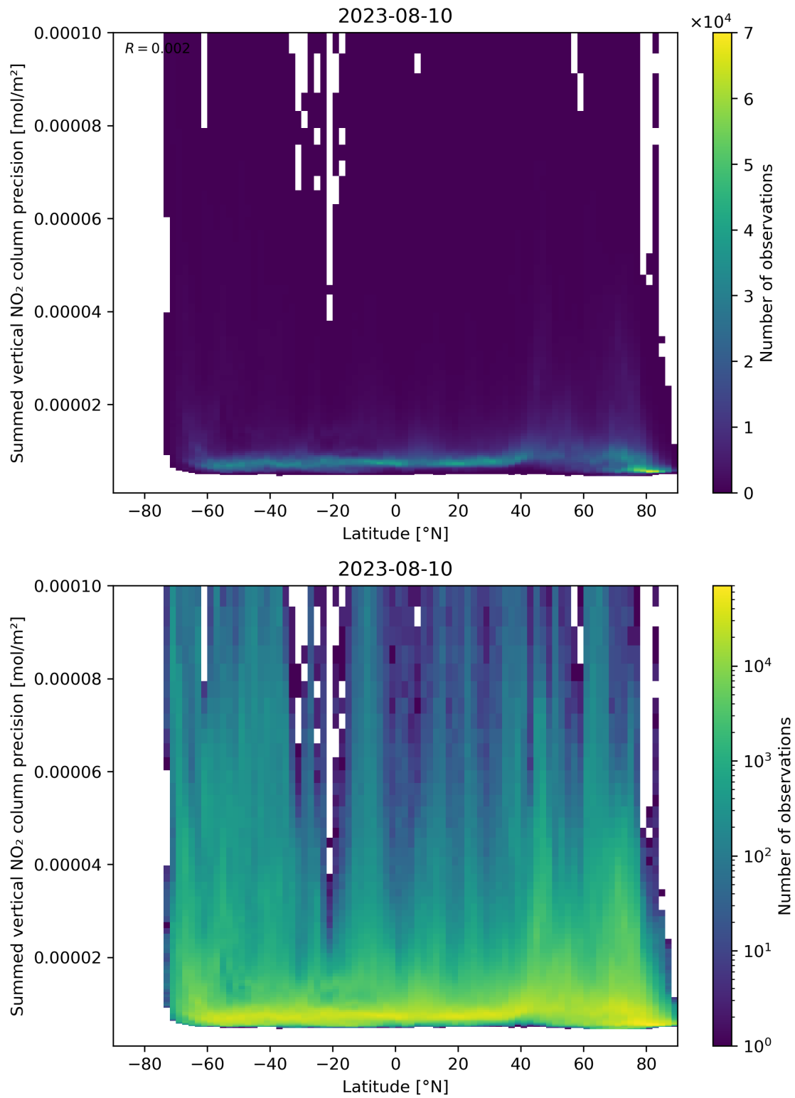
Figure 89: Scatter density plot of “Latitude” against “Summed vertical NO 2 column precision” for 2023-08-09 to 2023-08-11.
