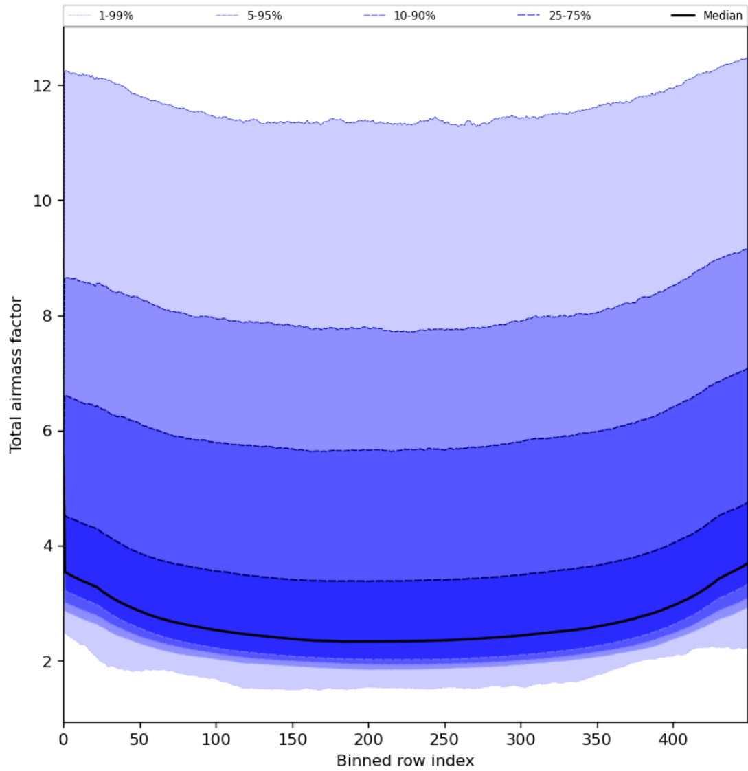
Figure 49: Along track statistics of “Total airmass factor” for 2023-08-09 to 2023-08-11
