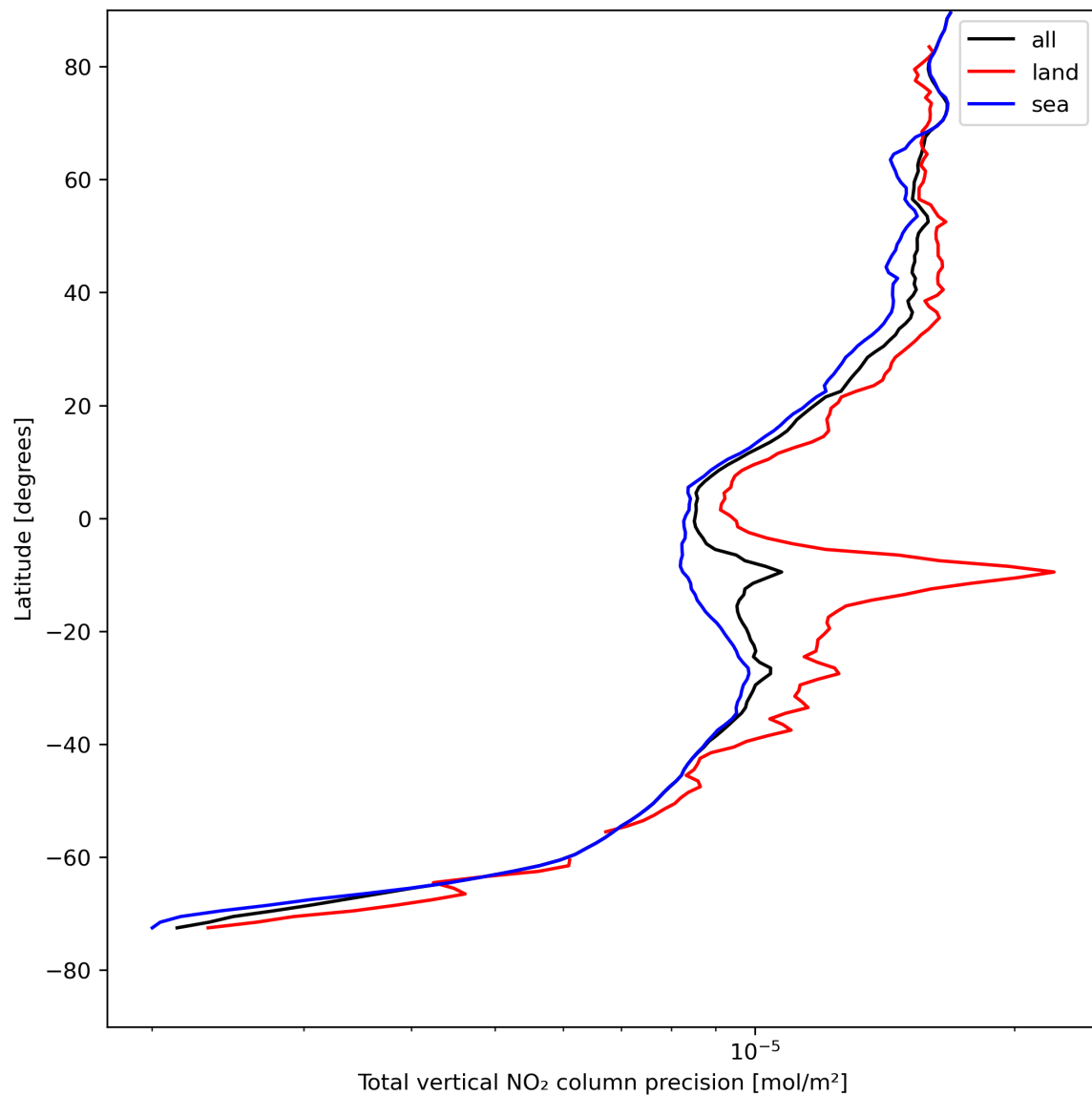
Figure 22: Zonal average of "Total vertical NO 2 column precision" for 2023-08-09 to 2023-08-11.
