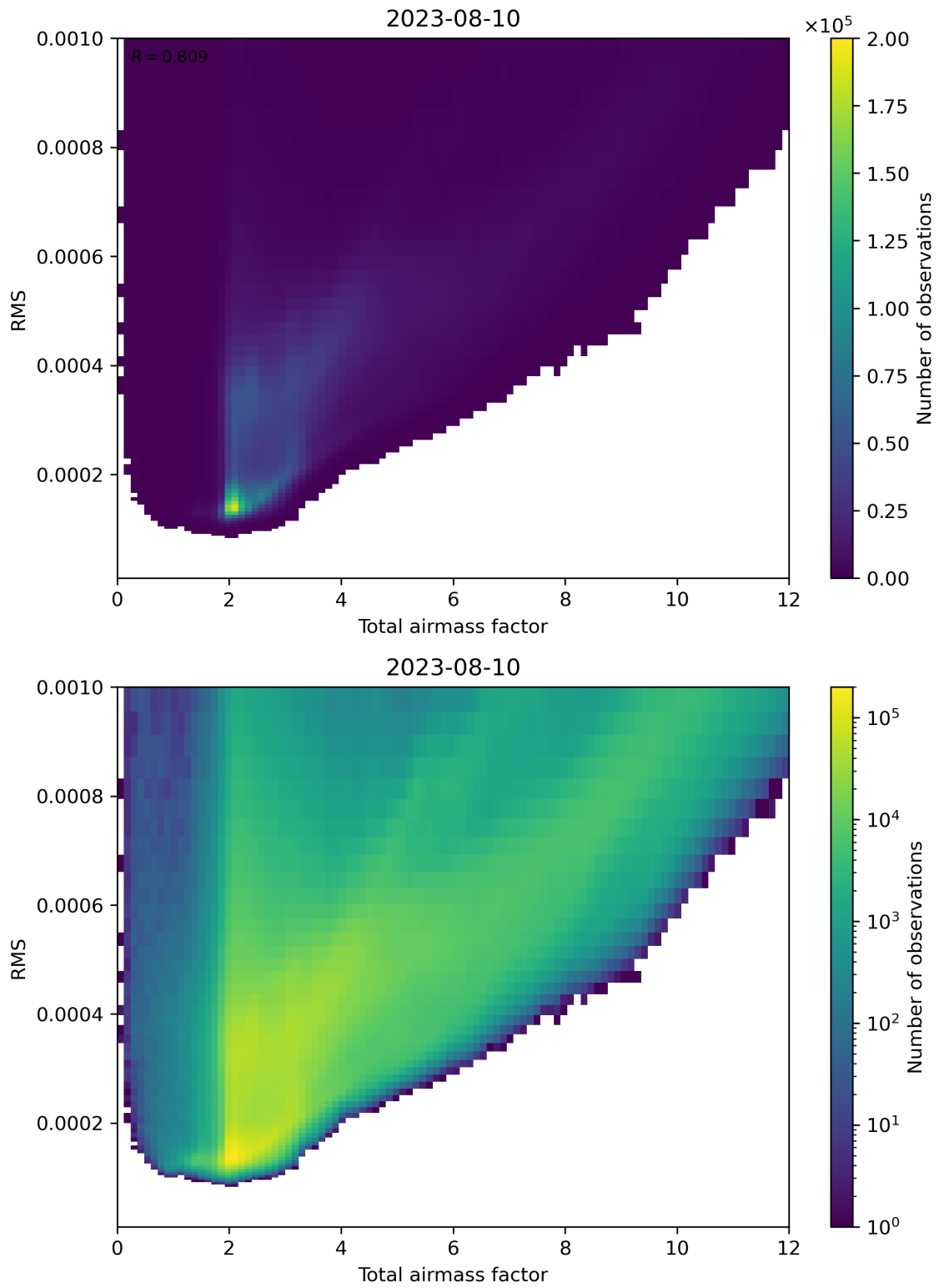
Figure 69: Scatter density plot of “Total airmass factor” against “RMS” for 2023-08-09 to 2023-08-11.
