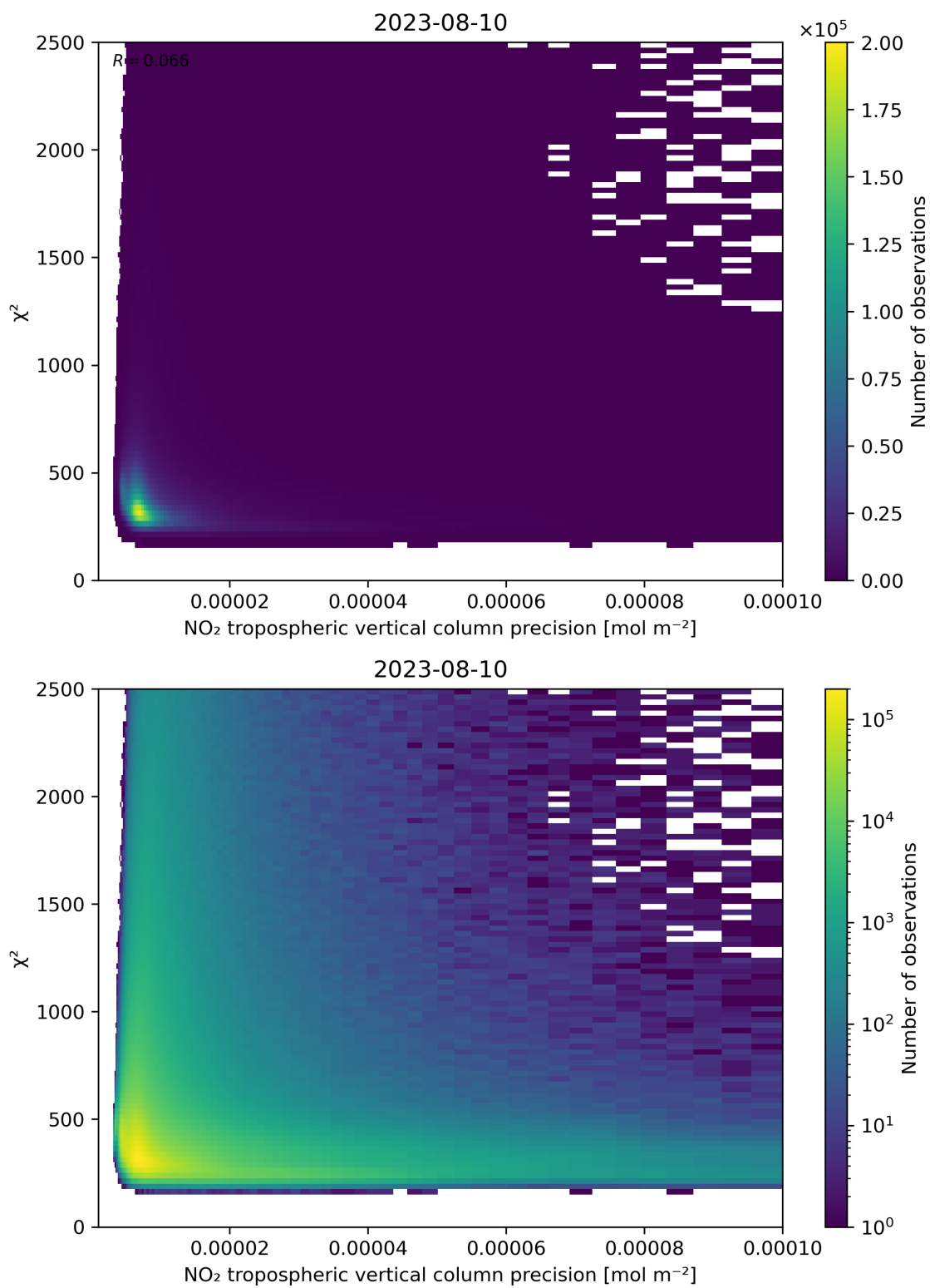
Figure 134: Scatter density plot of “NO 2 tropospheric vertical column precision” against “ \chi^2 ” for 2023-08-09 to 2023-08-11.
