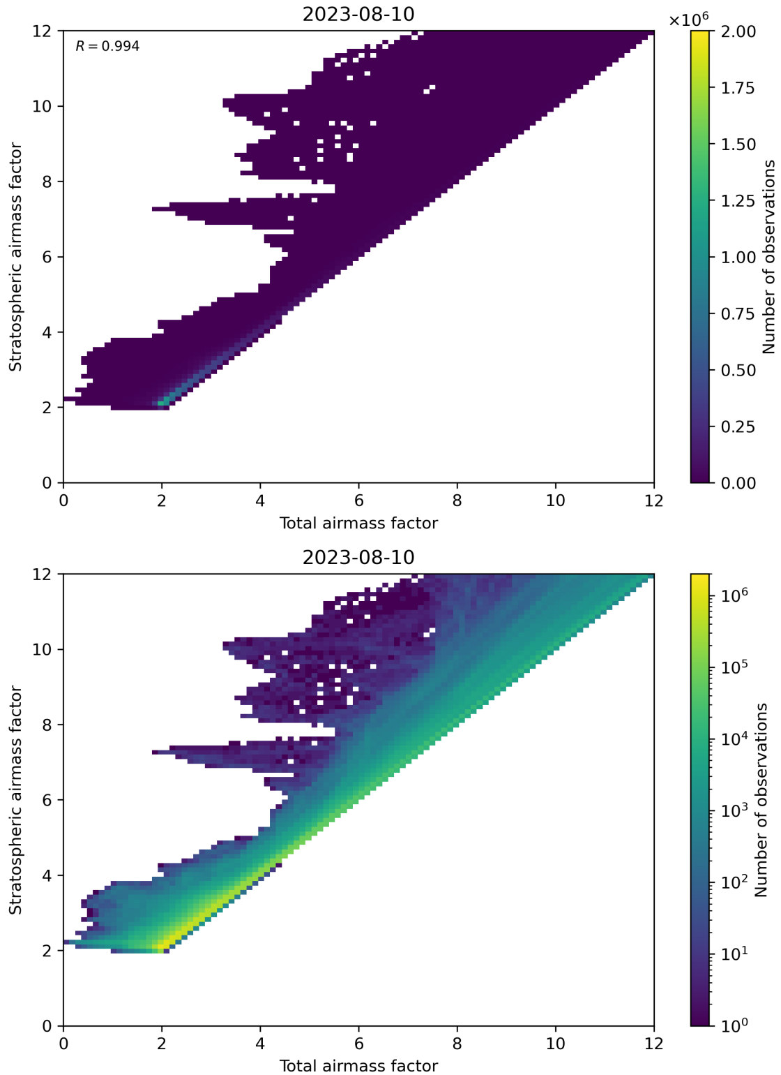
Figure 62: Scatter density plot of “Total airmass factor” against “Stratospheric airmass factor” for 2023-08-09 to 2023-08-11.
