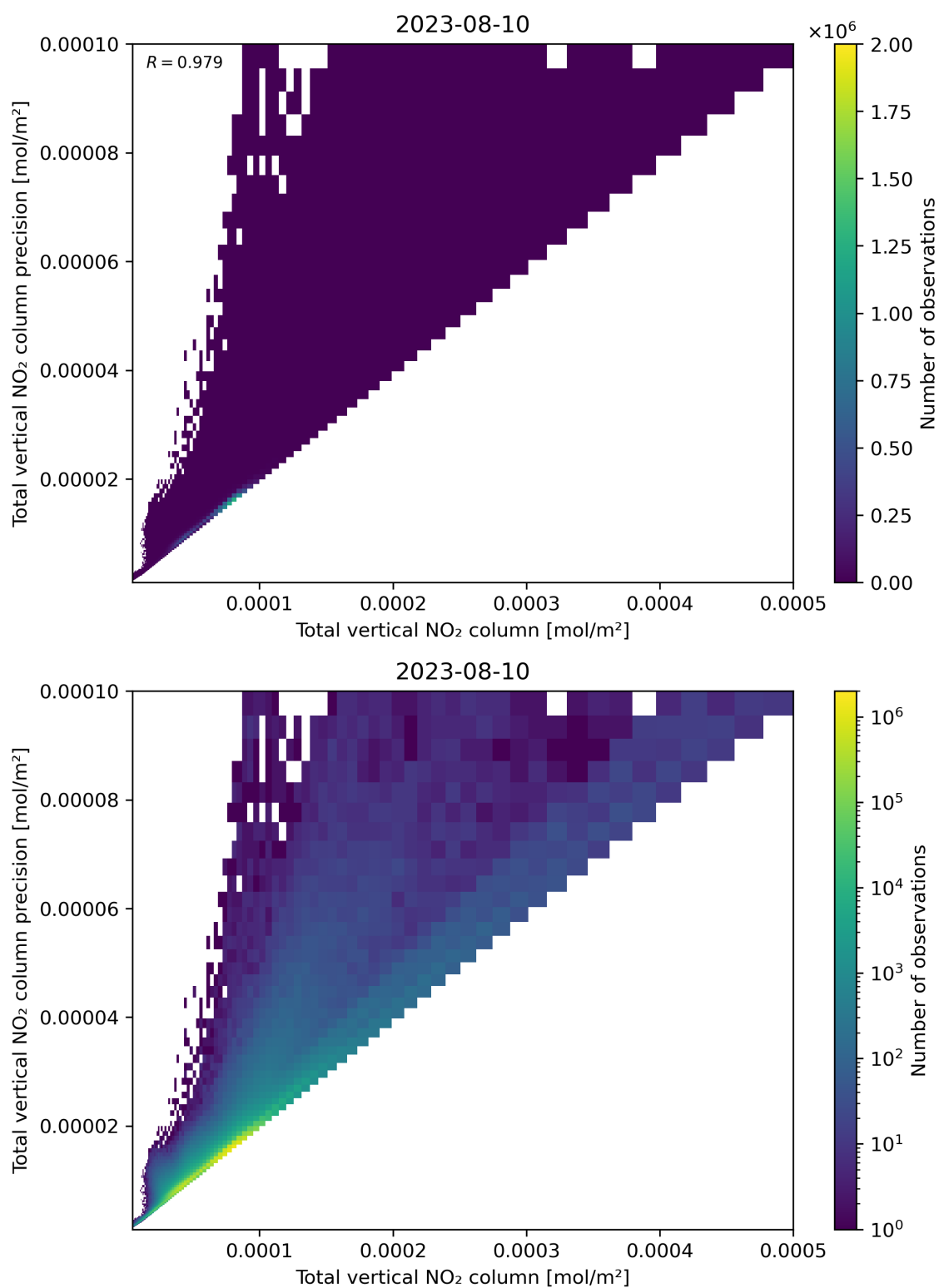
Figure 114: Scatter density plot of “Total vertical NO 2 column” against “Total vertical NO 2 column precision” for 2023-08-09 to 2023-08-11.
