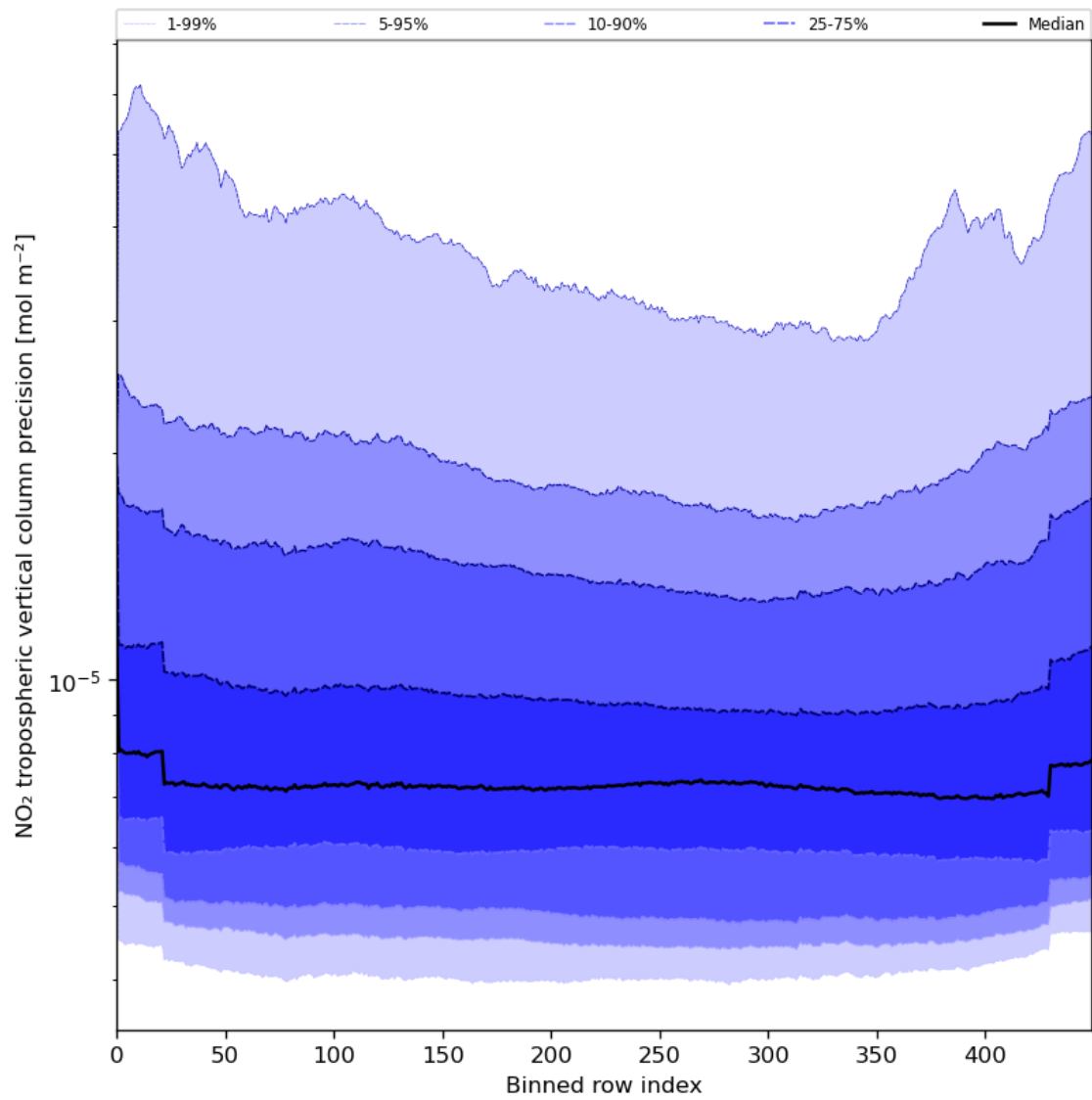
Figure 47: Along track statistics of “NO 2 tropospheric vertical column precision” for 2023-08-09 to 2023-08-11
