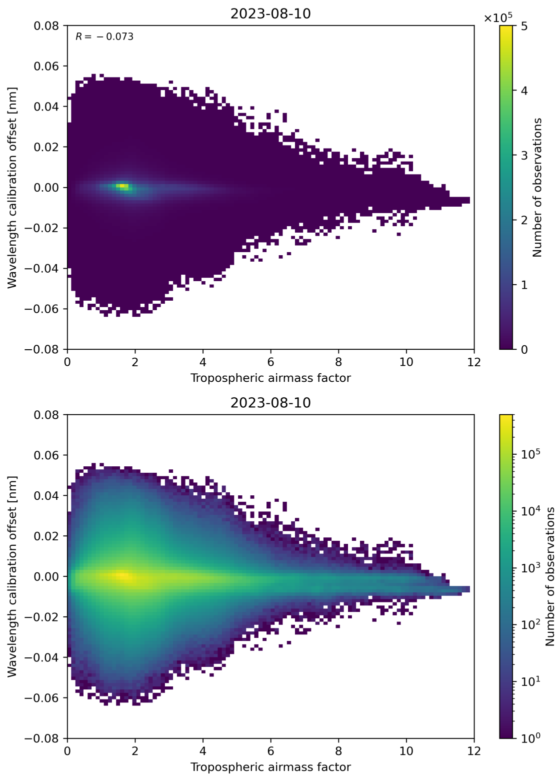
Figure 80: Scatter density plot of “Tropospheric airmass factor” against “Wavelength calibration offset” for 2023-08-09 to 2023-08-11.
