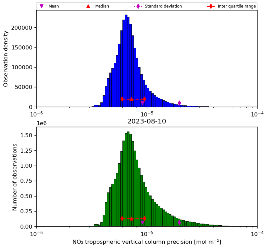
Figure 30: Histogram of “NO 2 tropospheric vertical column precision” for 2023-08-09 to 2023-08-11
