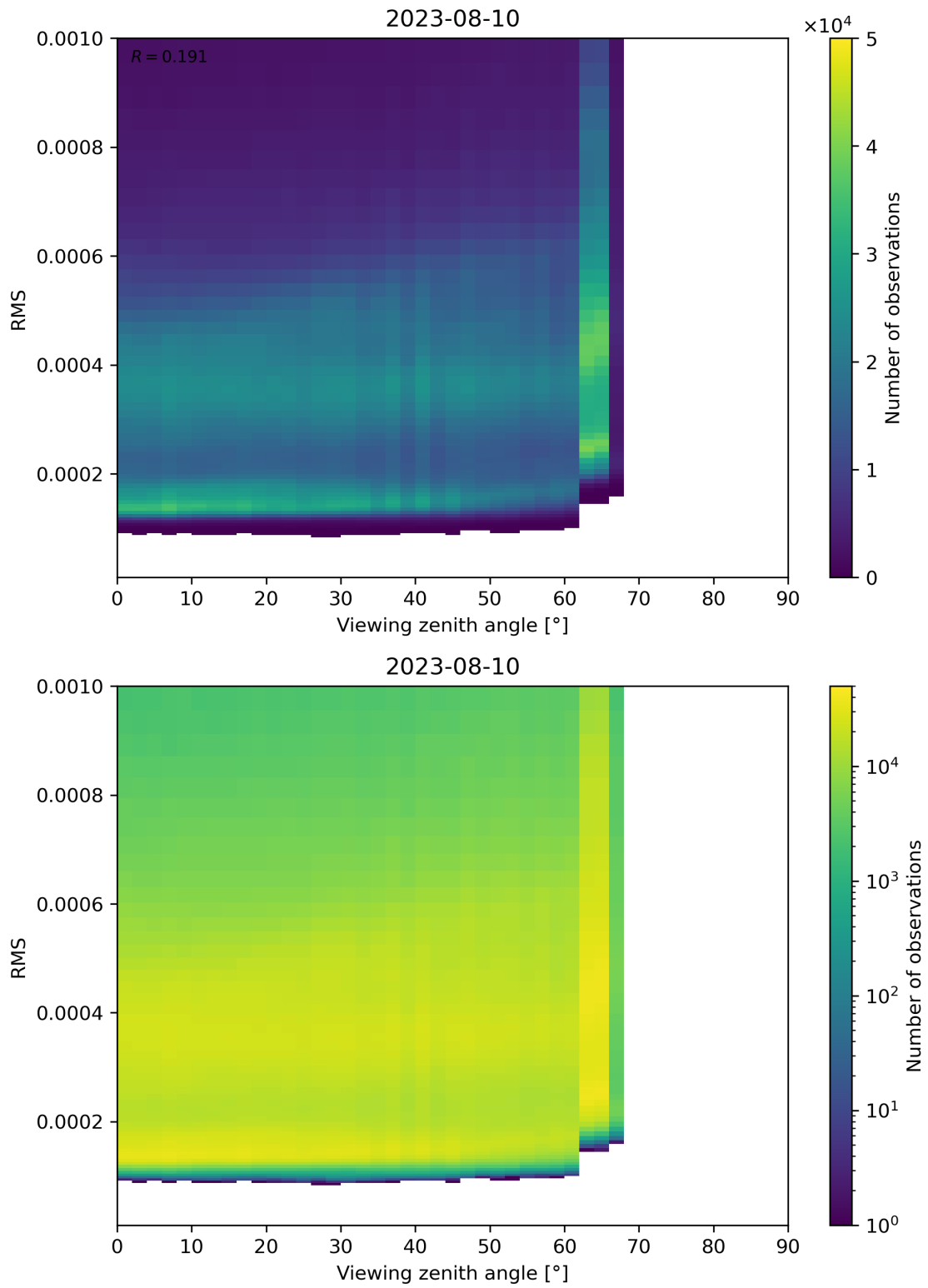
Figure 171: Scatter density plot of “Viewing zenith angle” against “RMS” for 2023-08-09 to 2023-08-11.
