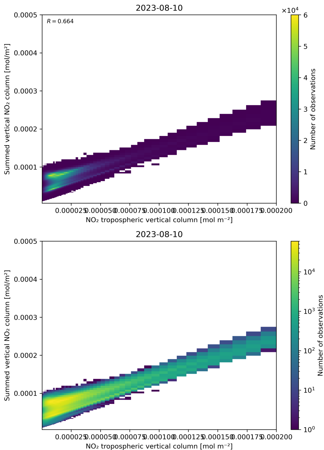
Figure 126: Scatter density plot of “NO 2 tropospheric vertical column” against “Summed vertical NO 2 column” for 2023-08-09 to 2023-08-11.
