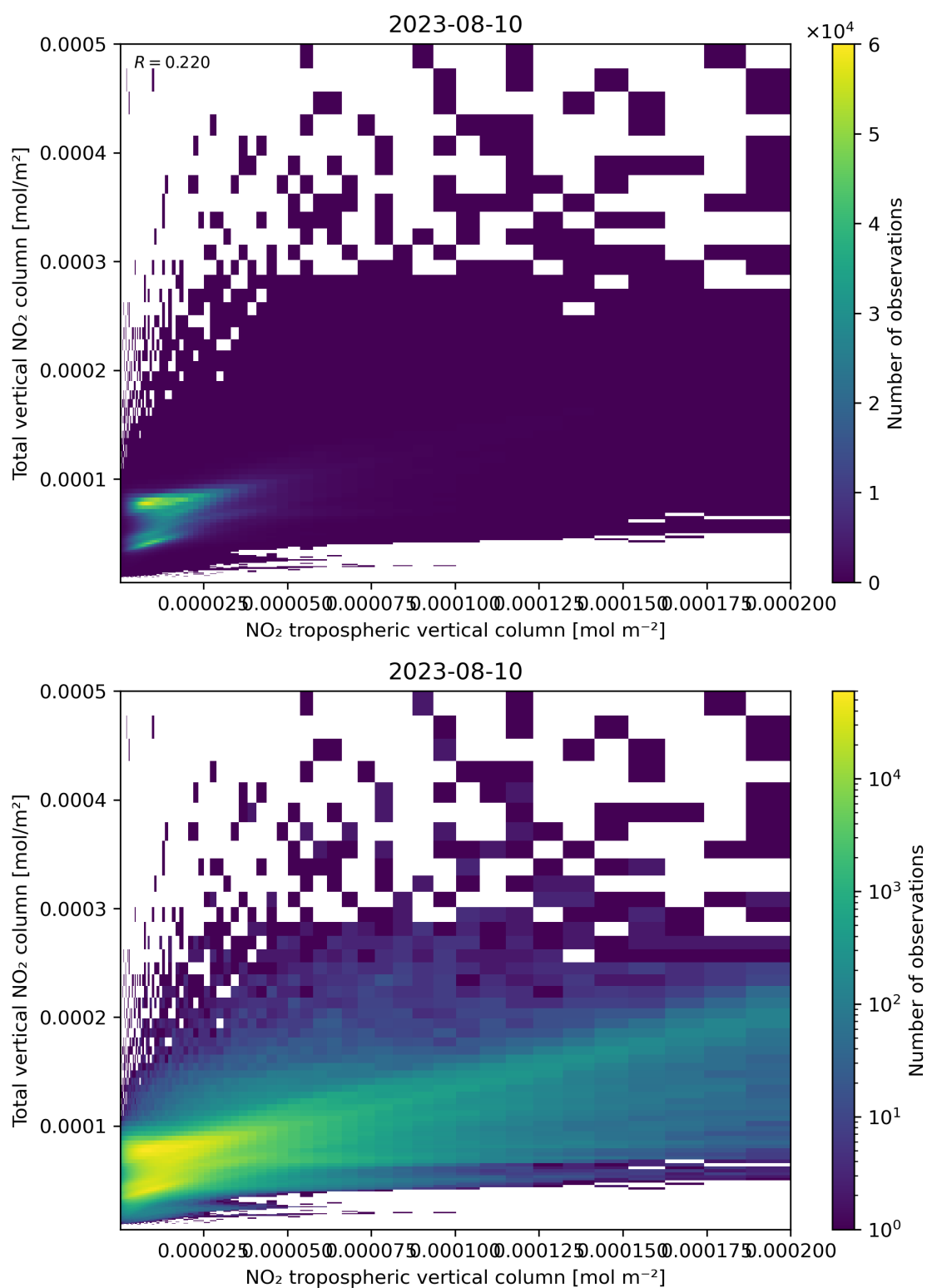
Figure 128: Scatter density plot of “NO 2 tropospheric vertical column” against “Total vertical NO 2 column” for 2023-08-09 to 2023-08-11.
