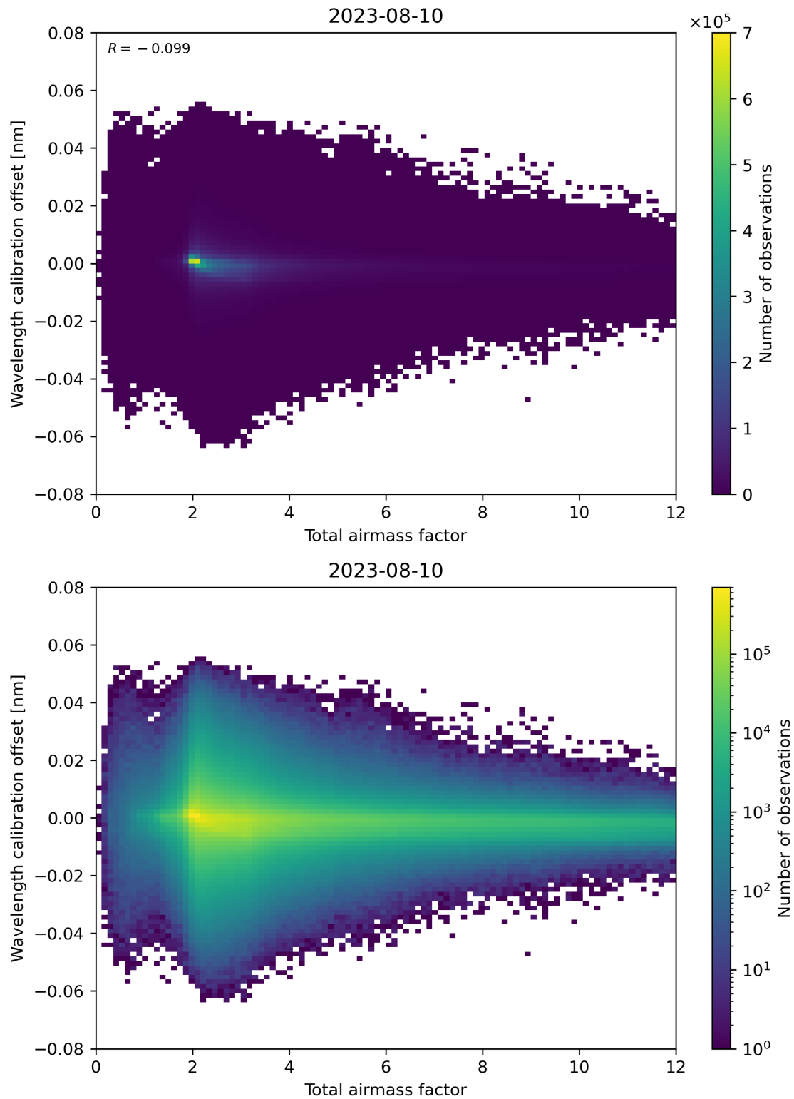
Figure 70: Scatter density plot of “Total airmass factor” against “Wavelength calibration offset” for 2023-08-09 to 2023-08-11.
