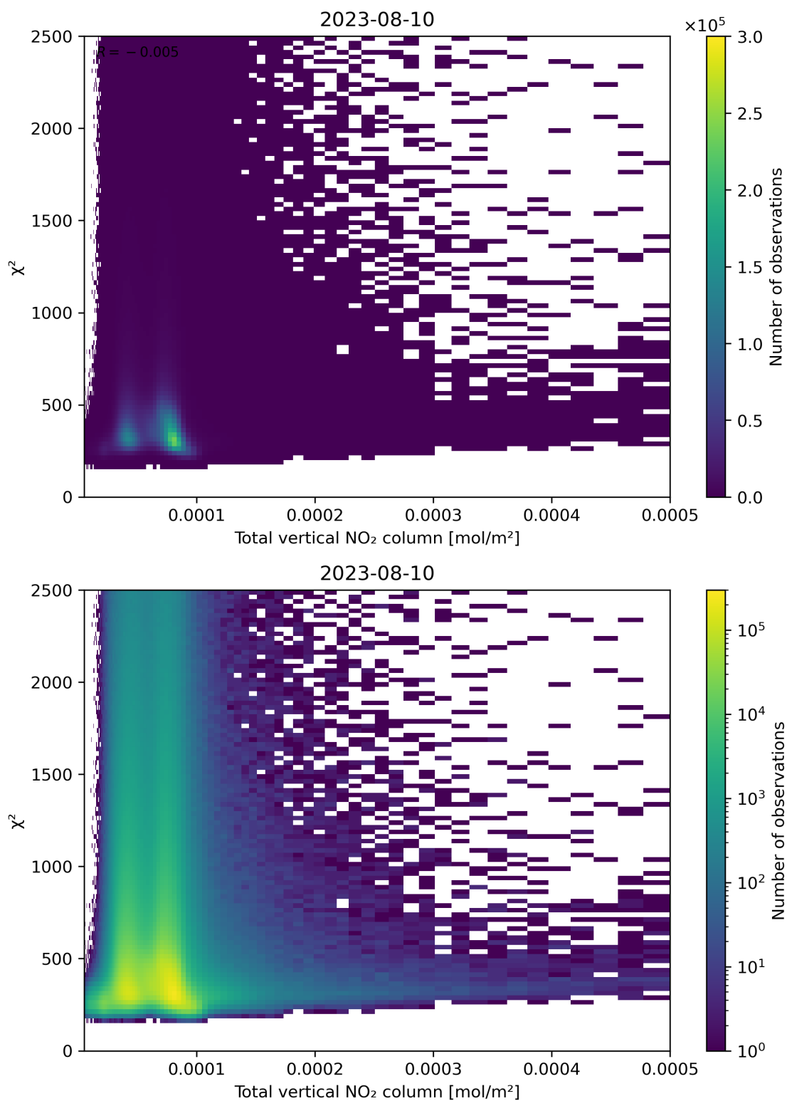
Figure 111: Scatter density plot of “Total vertical NO 2 column” against “ \chi^2 ” for 2023-08-09 to 2023-08-11.
