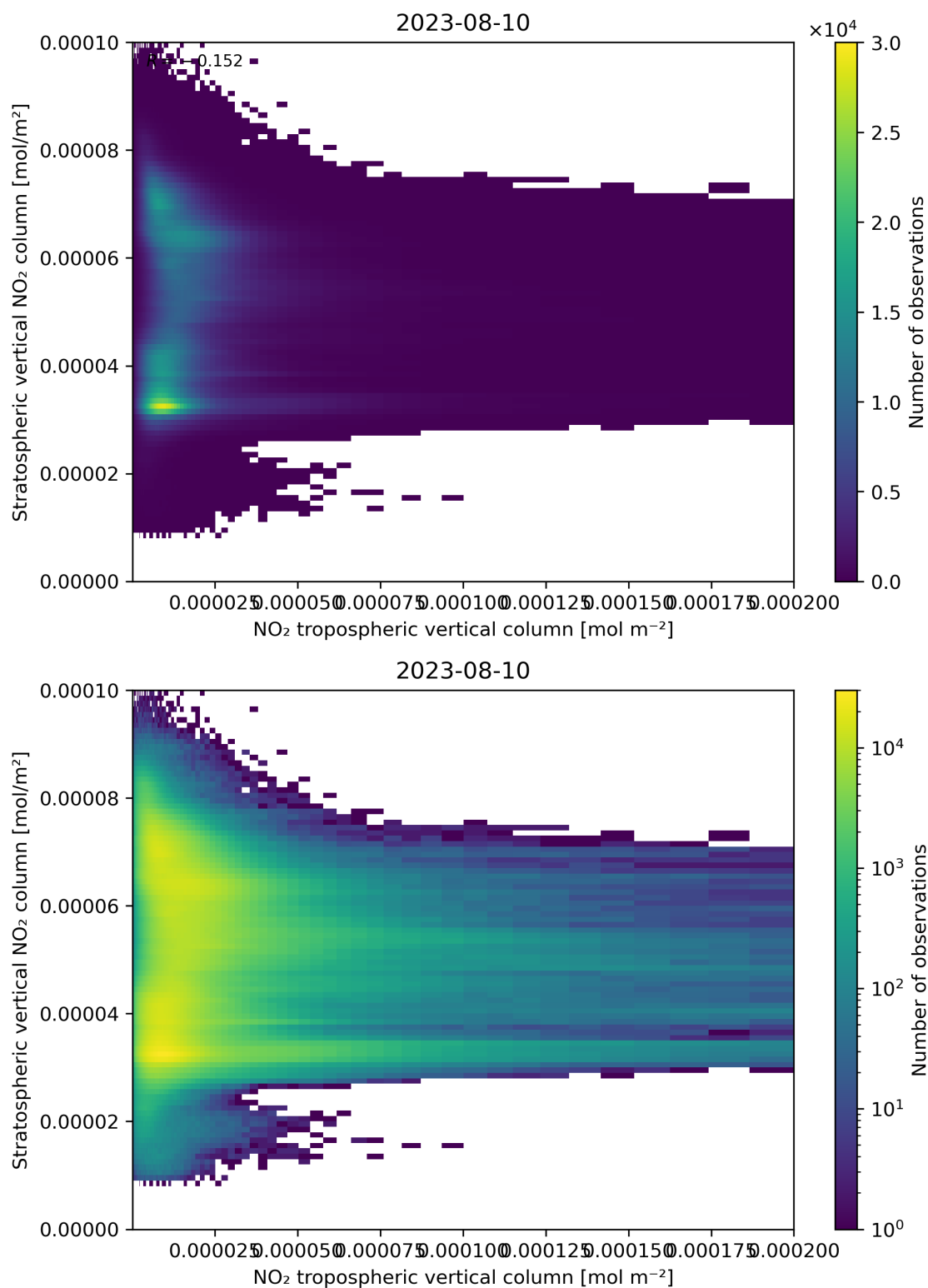
Figure 125: Scatter density plot of “NO 2 tropospheric vertical column” against “Stratospheric vertical NO 2 column” for 2023-08-09 to 2023-08-11.
