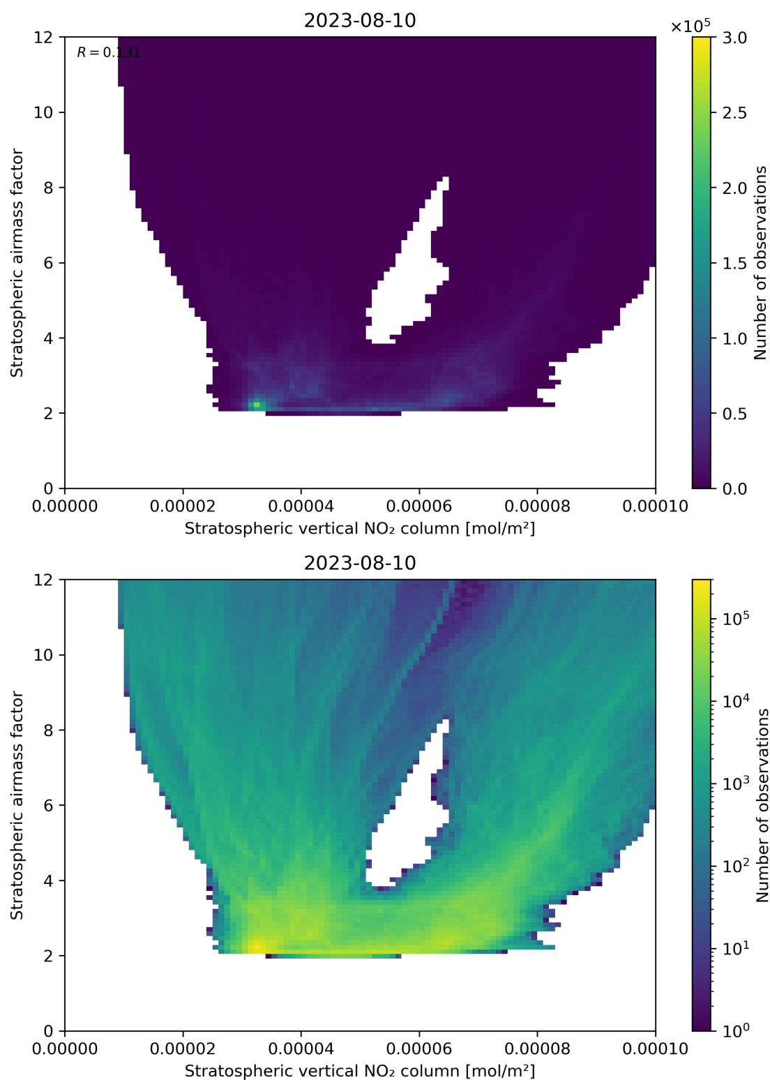
Figure 96: Scatter density plot of “Stratospheric vertical NO 2 column” against “Stratospheric airmass factor” for 2023-08-09 to 2023-08-11.
