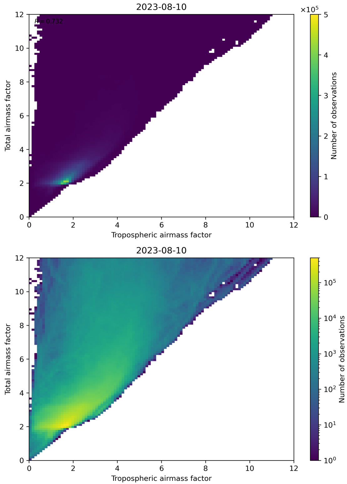
Figure 72: Scatter density plot of “Tropospheric airmass factor” against “Total airmass factor” for 2023-08-09 to 2023-08-11.
