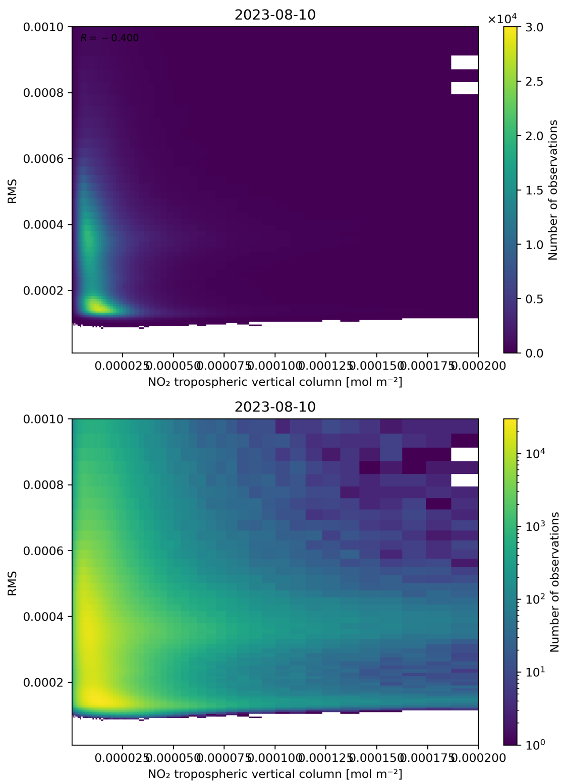
Figure 142: Scatter density plot of “NO 2 tropospheric vertical column” against “RMS” for 2023-08-09 to 2023-08-11.
