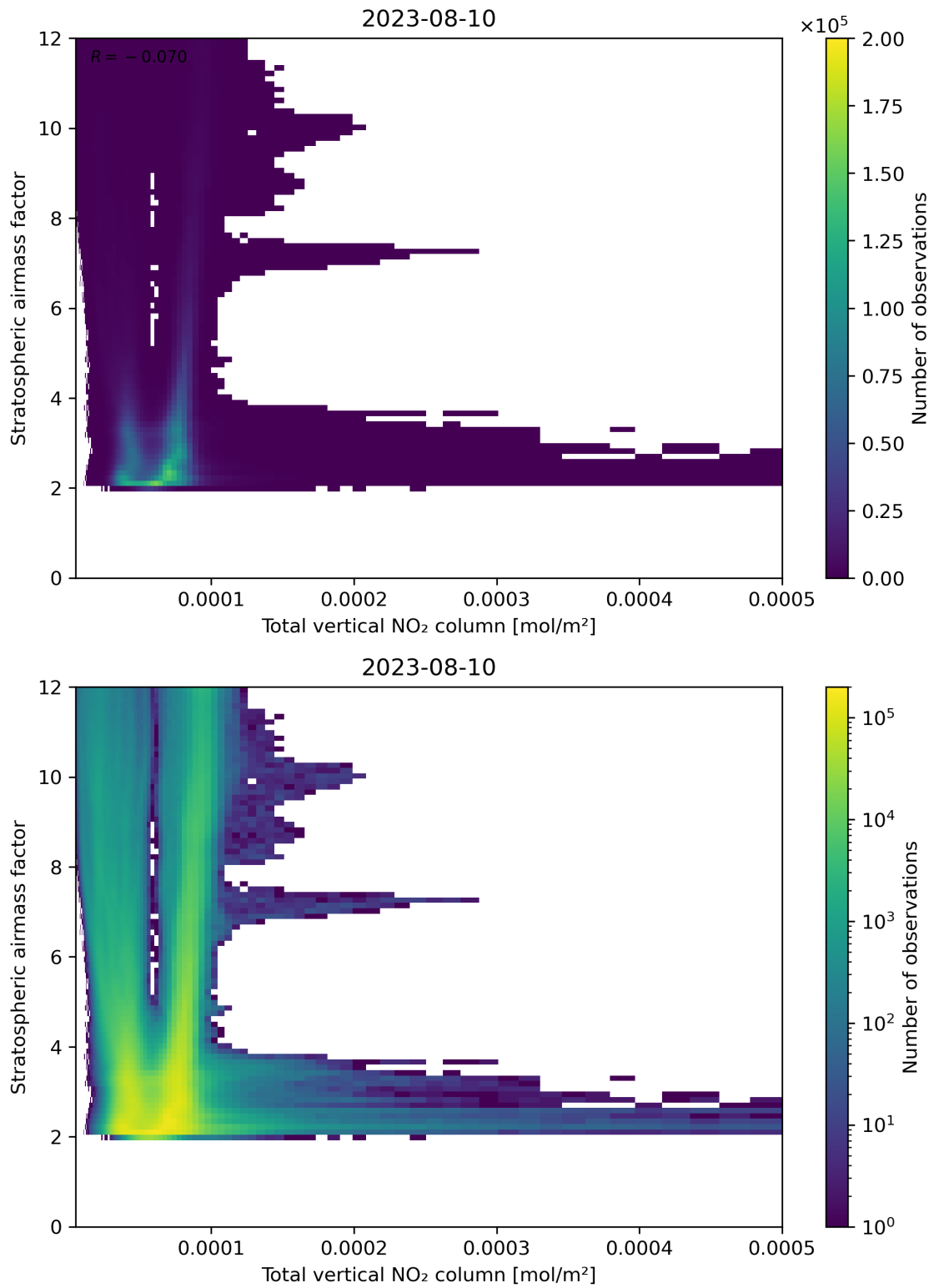
Figure 110: Scatter density plot of “Total vertical NO 2 column” against “Stratospheric airmass factor” for 2023-08-09 to 2023-08-11.
