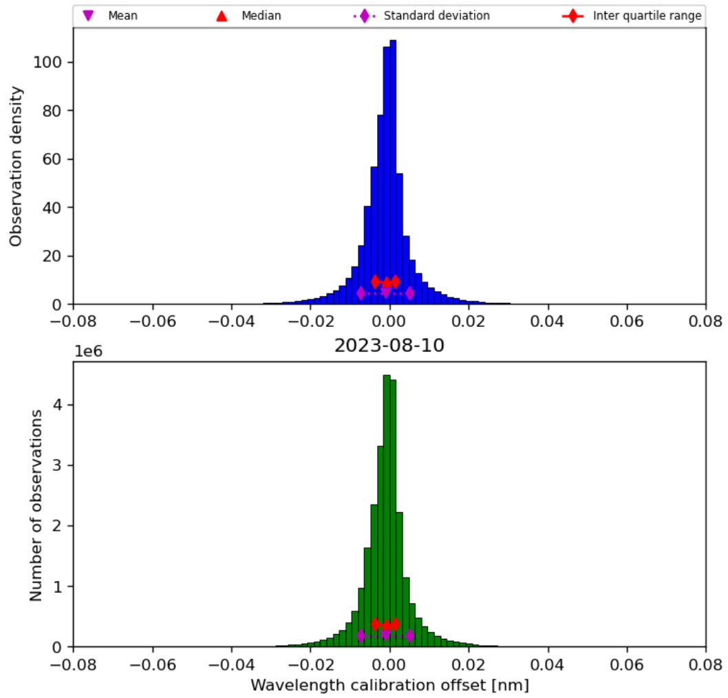
Figure 35: Histogram of “Wavelength calibration offset” for 2023-08-09 to 2023-08-11
