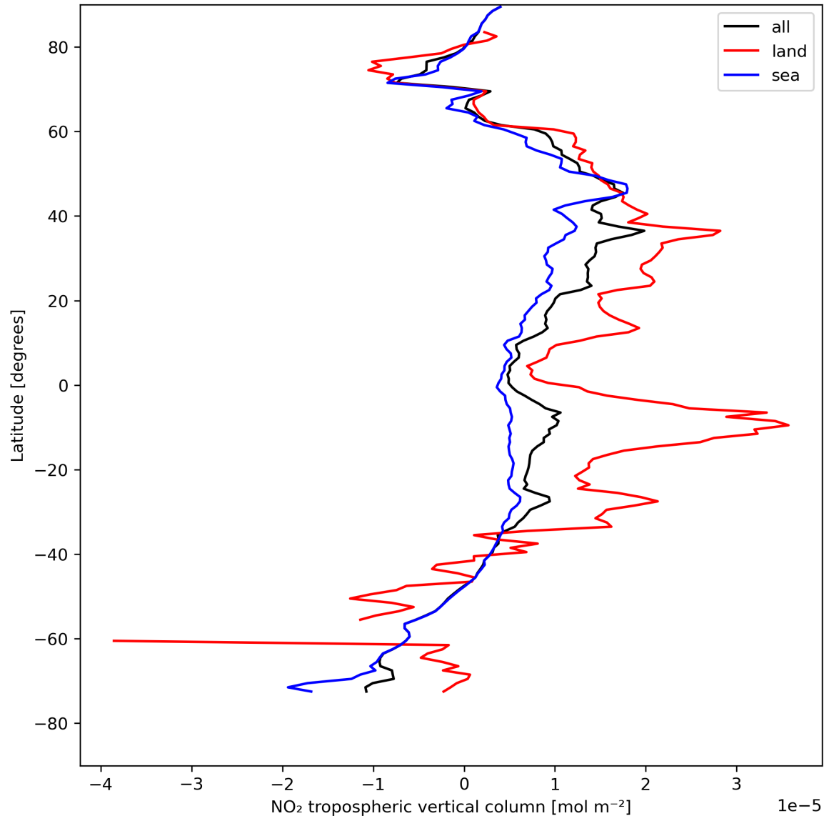
Figure 12: Zonal average of “NO 2 tropospheric vertical column” for 2023-08-09 to 2023-08-11.
