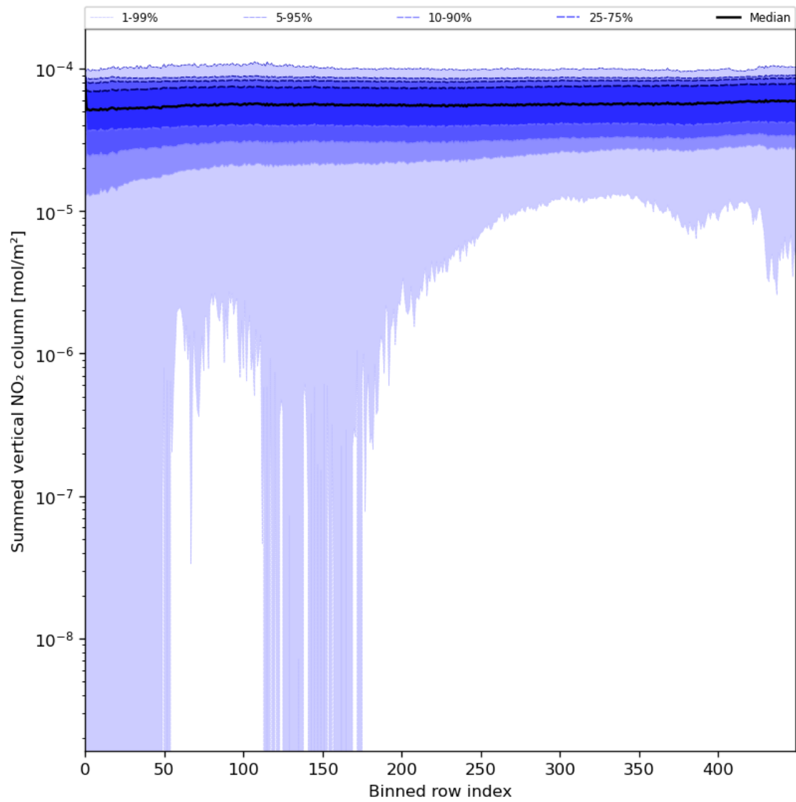
Figure 57: Along track statistics of “Summed vertical NO 2 column” for 2023-08-09 to 2023-08-11
