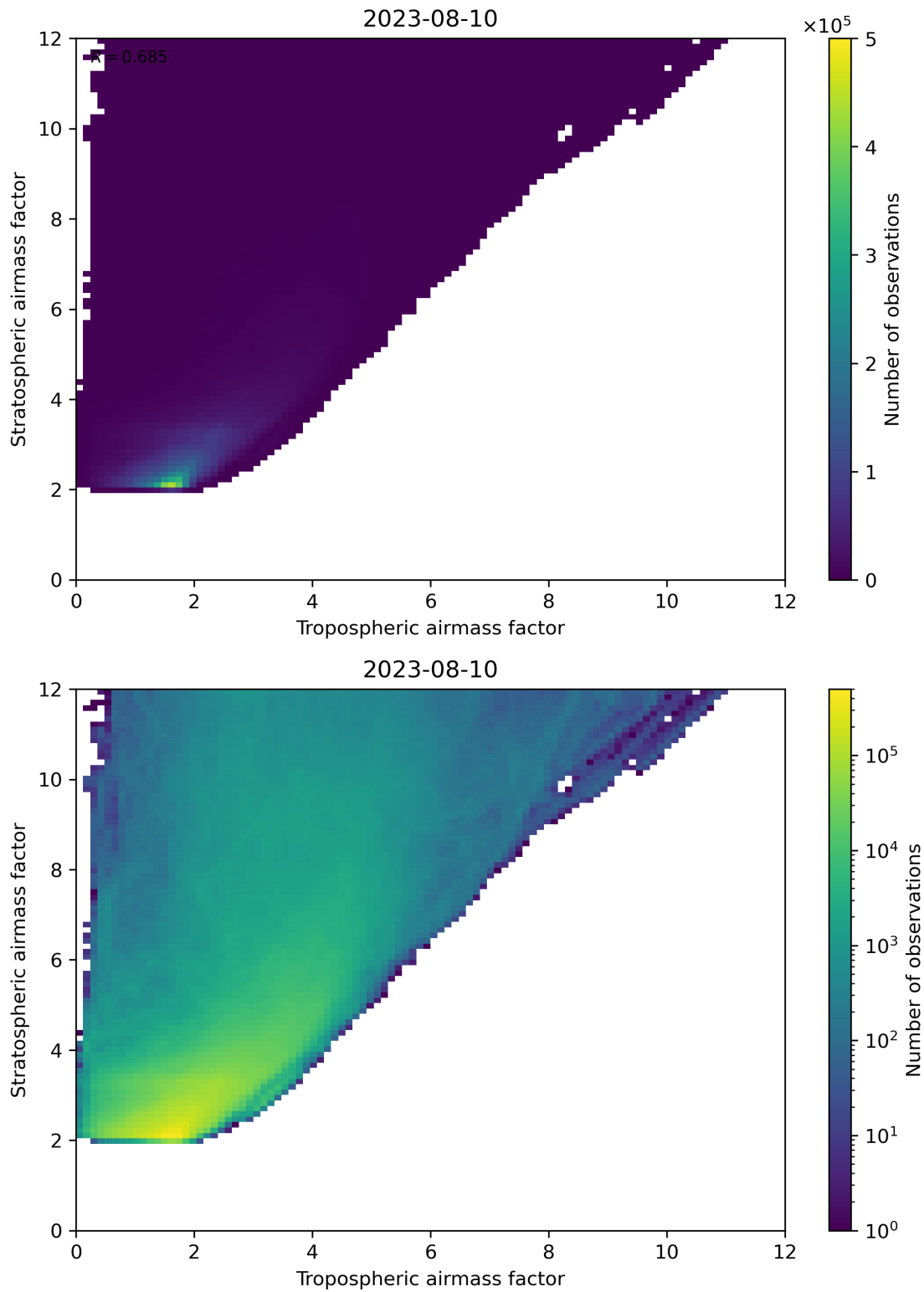
Figure 71: Scatter density plot of “Tropospheric airmass factor” against “Stratospheric airmass factor” for 2023-08-09 to 2023-08-11.
