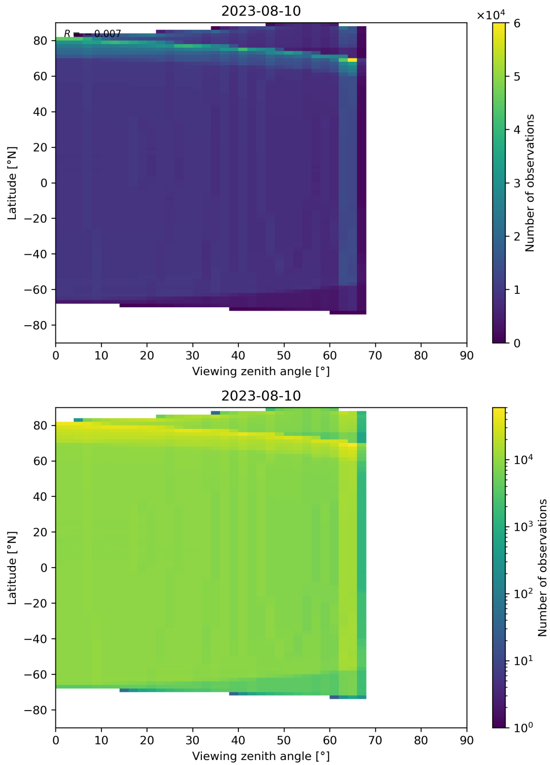
Figure 163: Scatter density plot of “Viewing zenith angle” against “Latitude” for 2023-08-09 to 2023-08-11.
