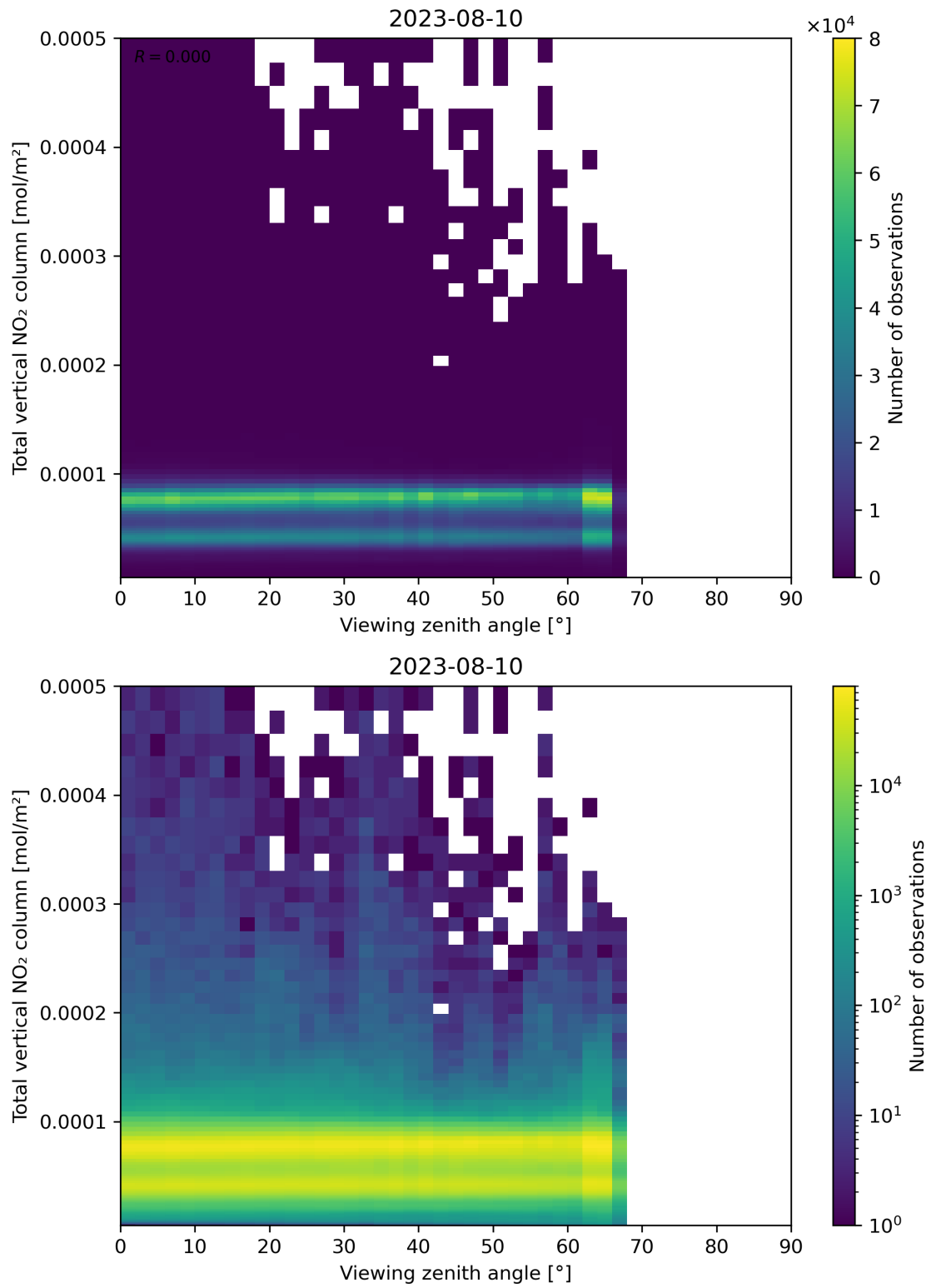
Figure 167: Scatter density plot of “Viewing zenith angle” against “Total vertical NO 2 column” for 2023-08-09 to 2023-08-11.
