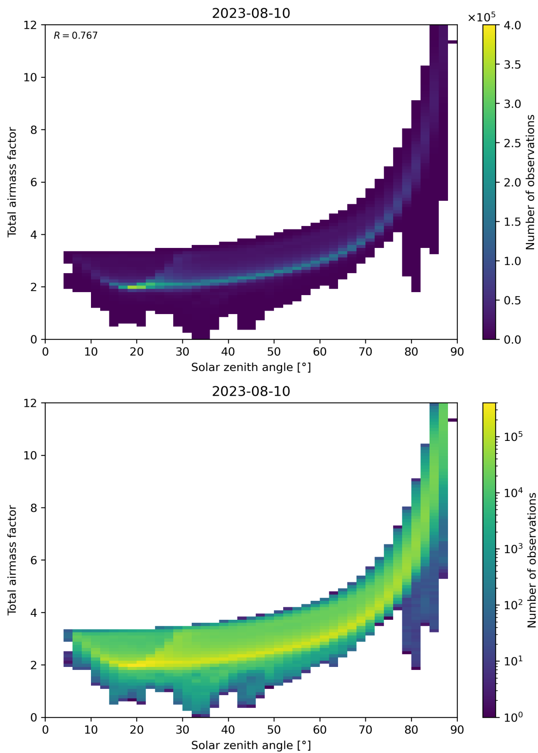
Figure 146: Scatter density plot of “Solar zenith angle” against “Total air mass factor” for 2023-08-09 to 2023-08-11.
