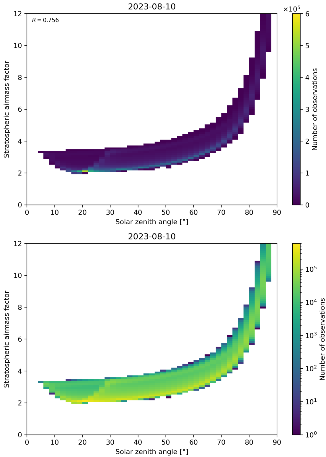
Figure 145: Scatter density plot of “Solar zenith angle” against “Stratospheric airmass factor” for 2023-08-09 to 2023-08-11.
