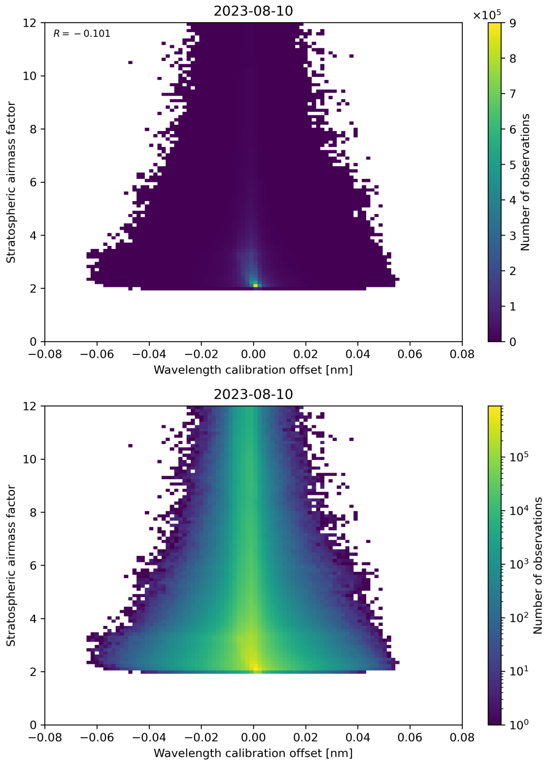
Figure 174: Scatter density plot of “Wavelength calibration offset” against “Stratospheric air mass factor” for 2023-08-09 to 2023-08-11.
