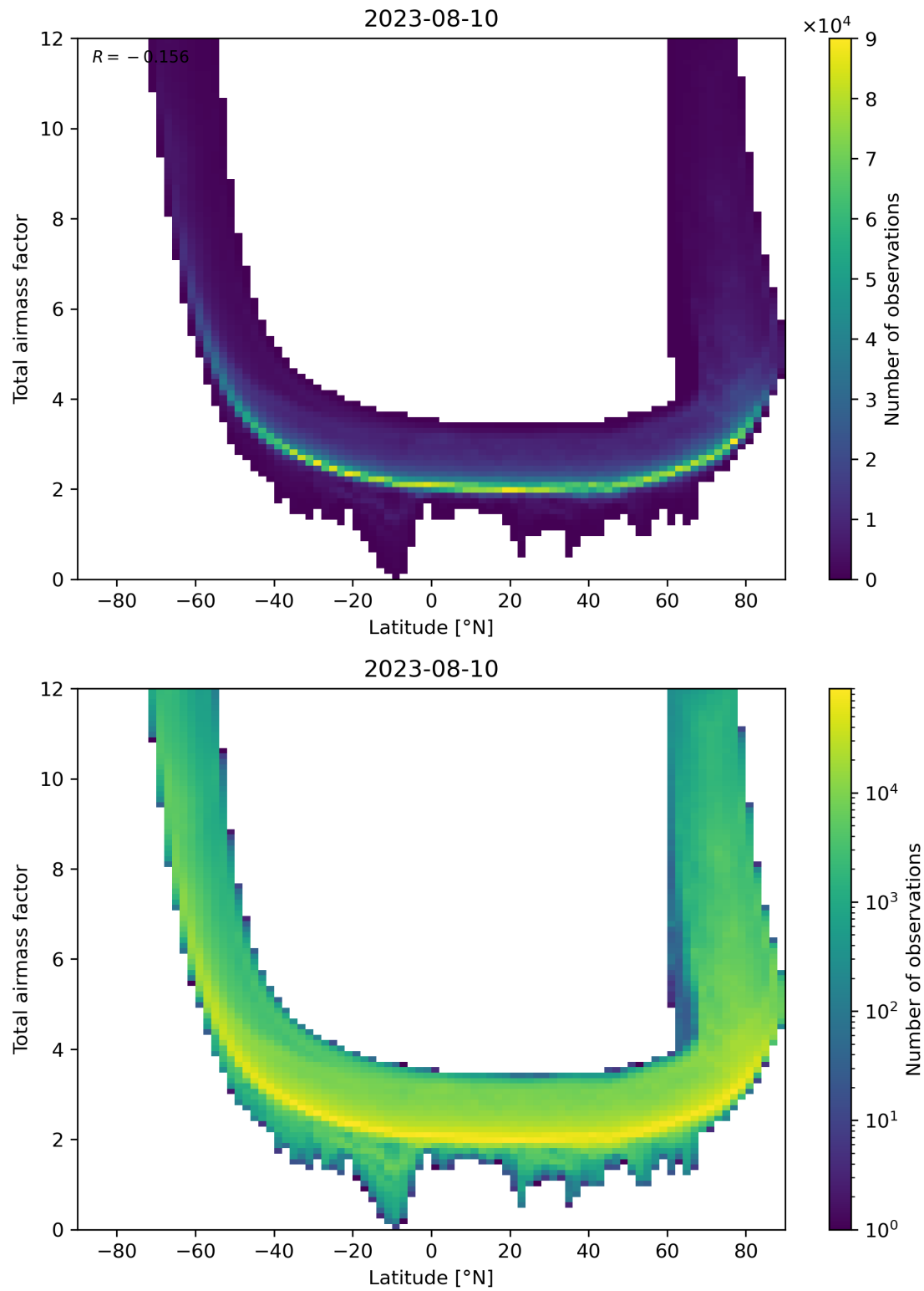
Figure 84: Scatter density plot of “Latitude” against “Total airmass factor” for 2023-08-09 to 2023-08-11.
