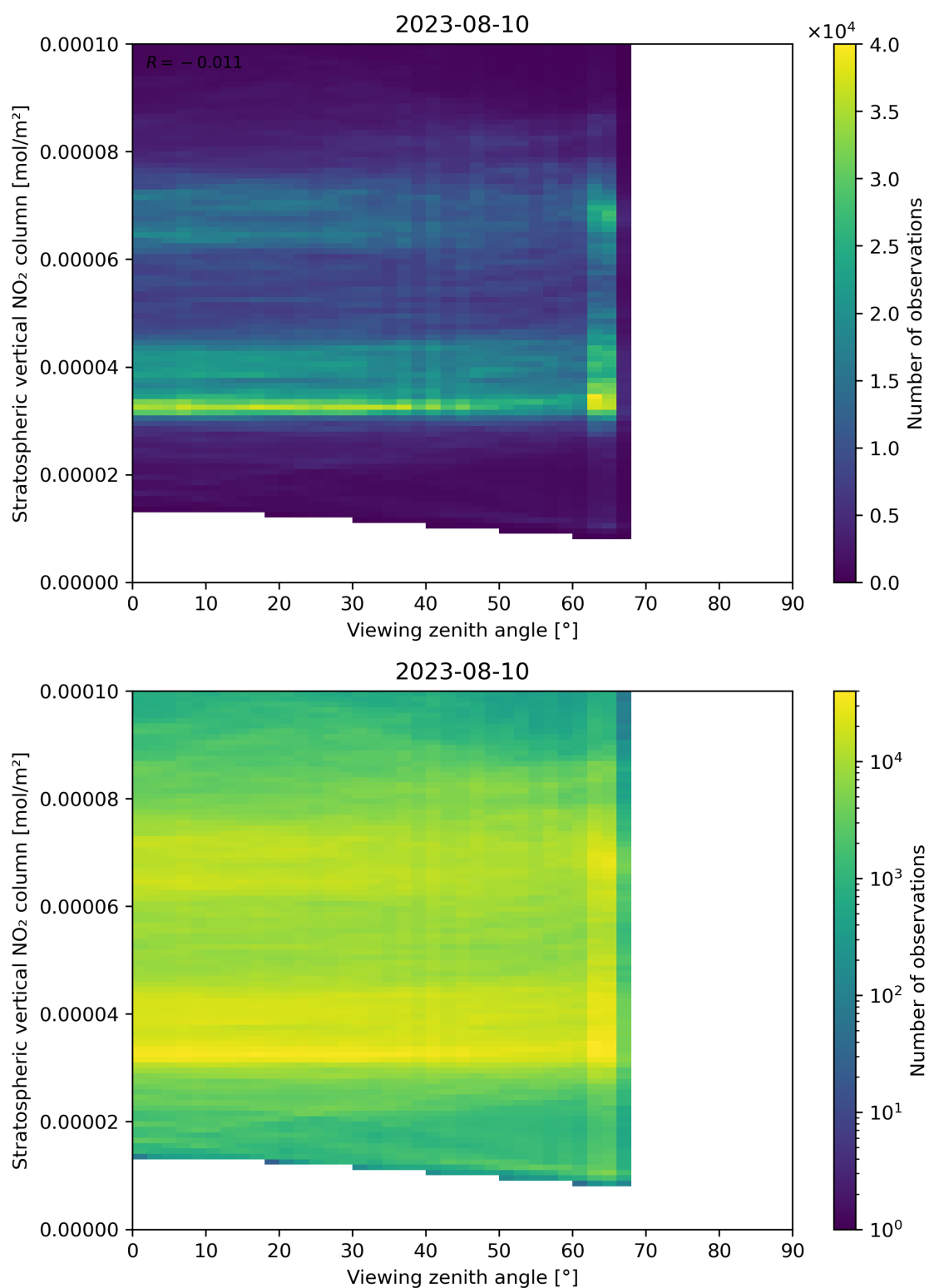
Figure 164: Scatter density plot of “Viewing zenith angle” against “Stratospheric vertical NO 2 column” for 2023-08-09 to 2023-08-11.
