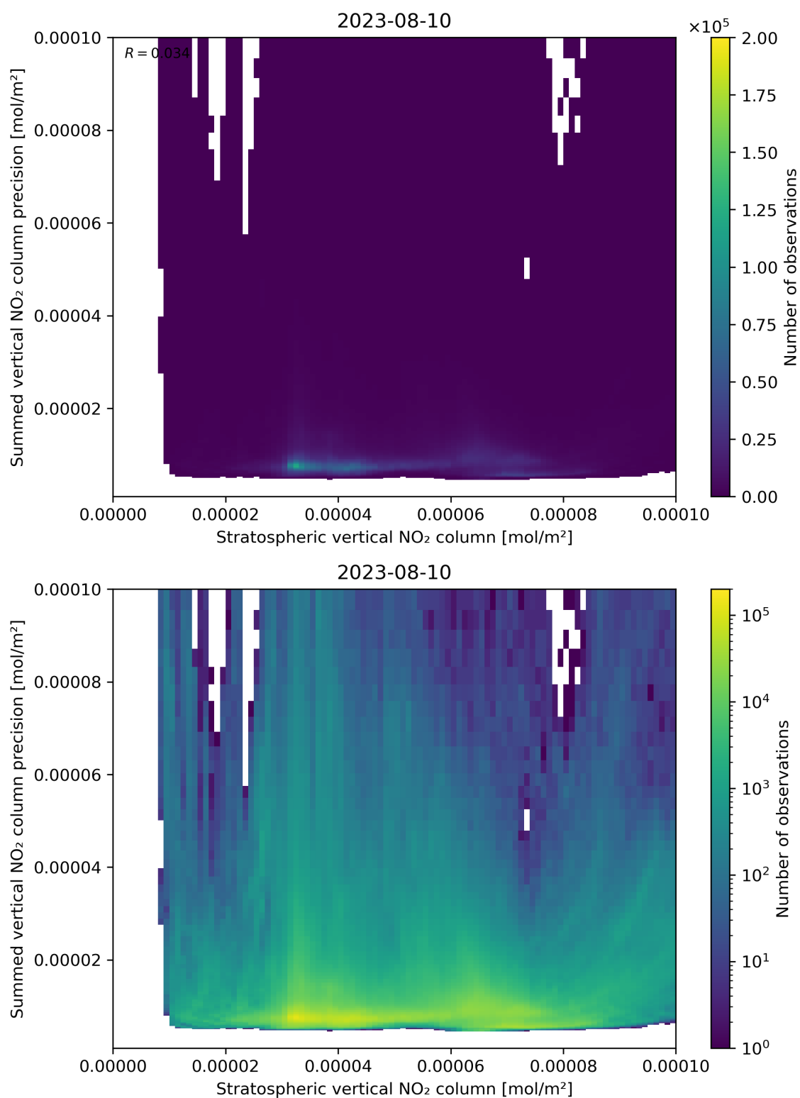
Figure 99: Scatter density plot of “Stratospheric vertical NO 2 column” against “Summed vertical NO 2 column precision” for 2023-08-09 to 2023-08-11.
