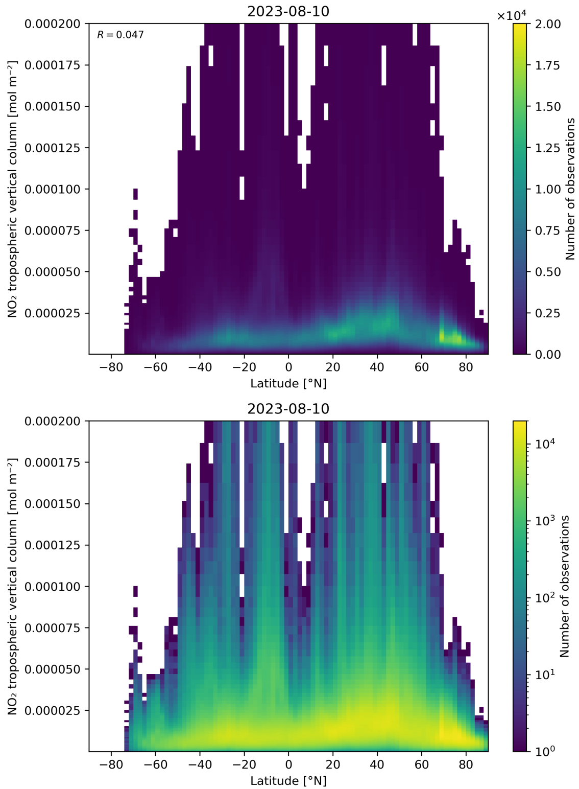
Figure 92: Scatter density plot of “Latitude” against “NO 2 tropospheric vertical column” for 2023-08-09 to 2023-08-11.
