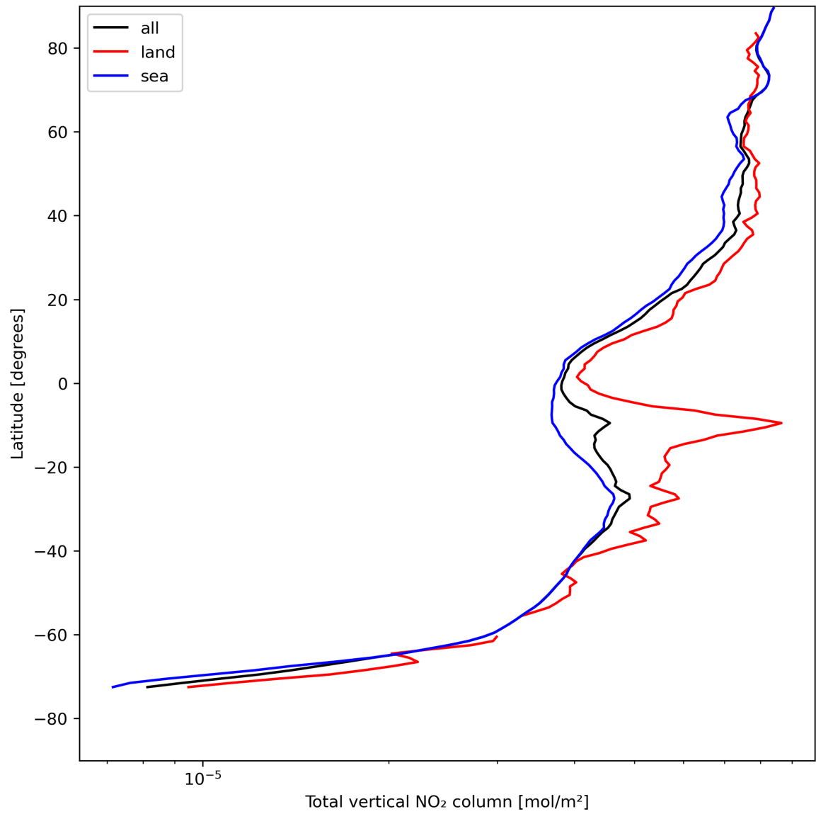
Figure 21: Zonal average of “Total vertical NO 2 column” for 2023-08-09 to 2023-08-11.
