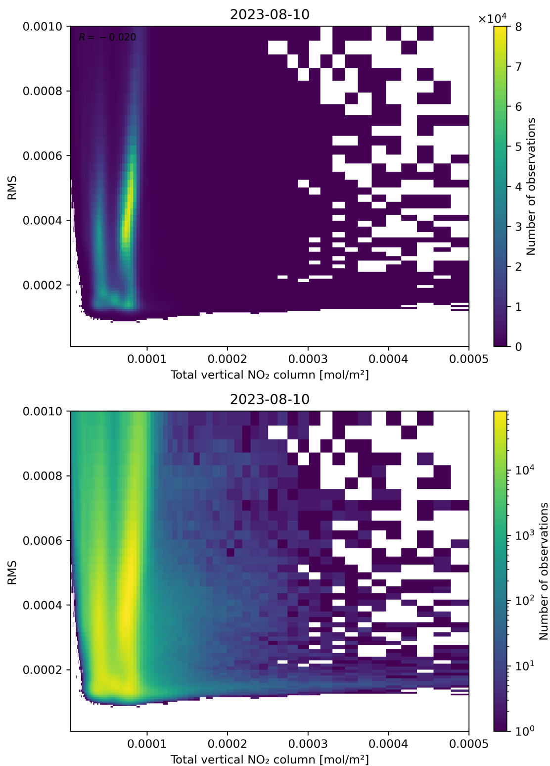
Figure 120: Scatter density plot of “Total vertical NO 2 column” against “RMS” for 2023-08-09 to 2023-08-11.
