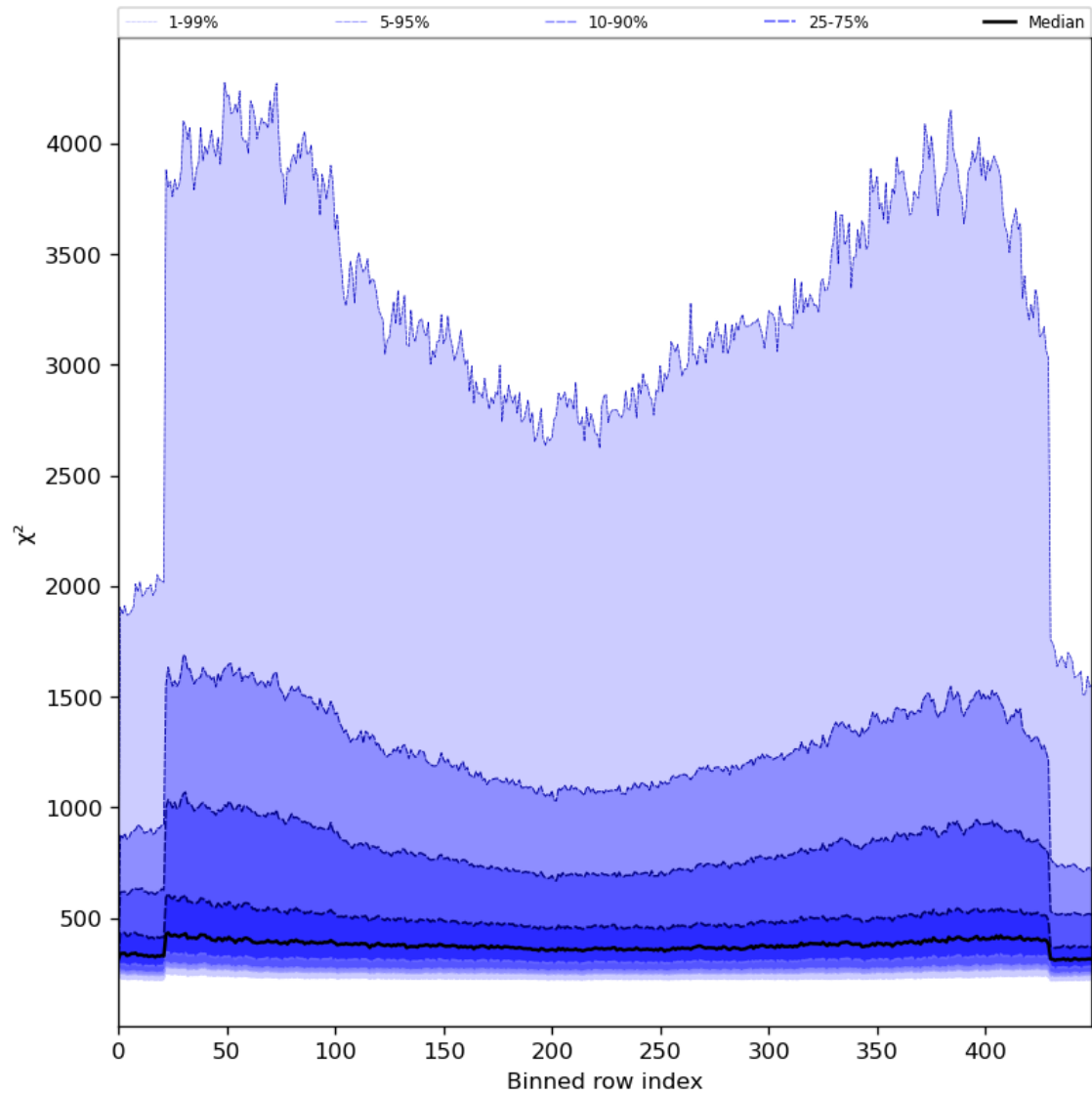
Figure 59: Along track statistics of “ \chi^2 ” for 2023-08-09 to 2023-08-11
