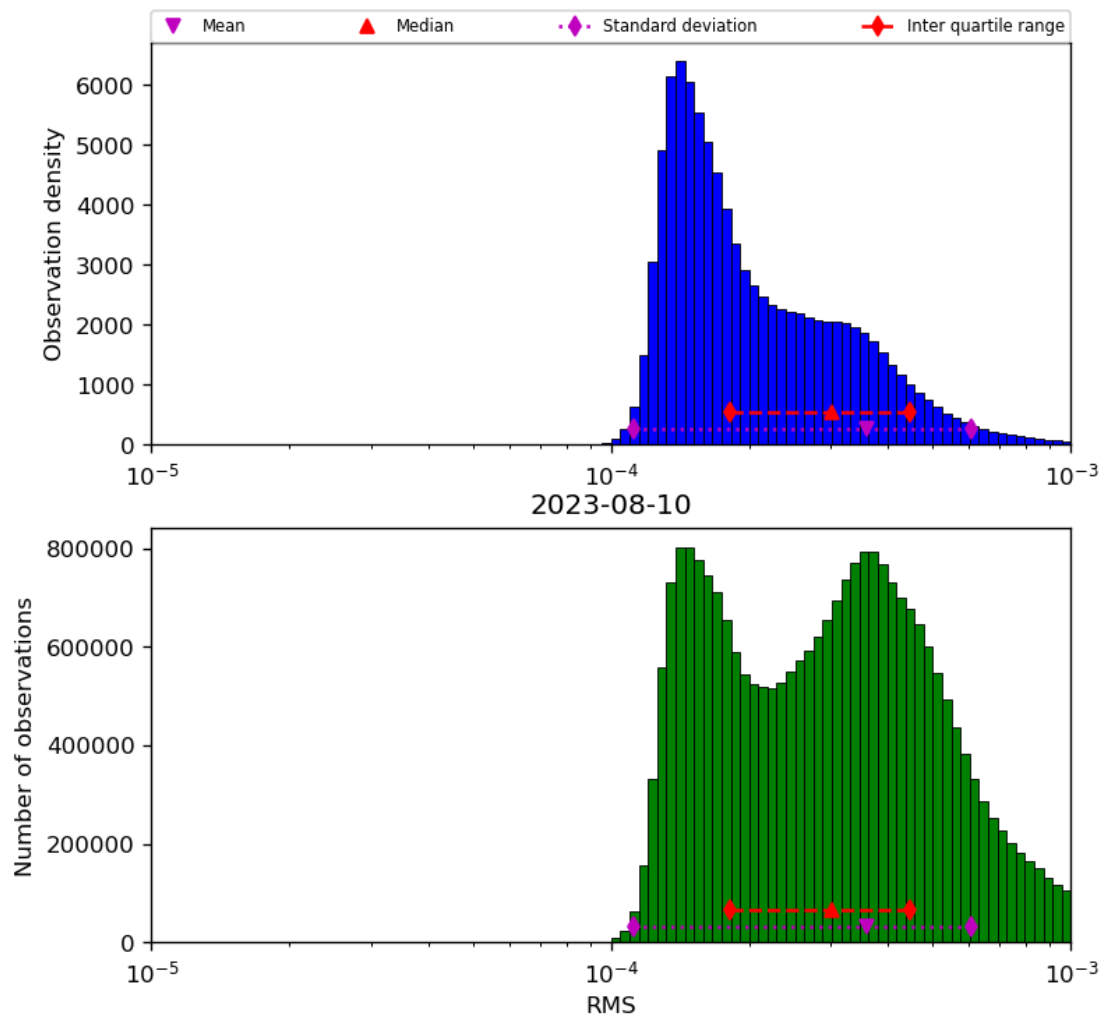
Figure 43: Histogram of “RMS” for 2023-08-09 to 2023-08-11
