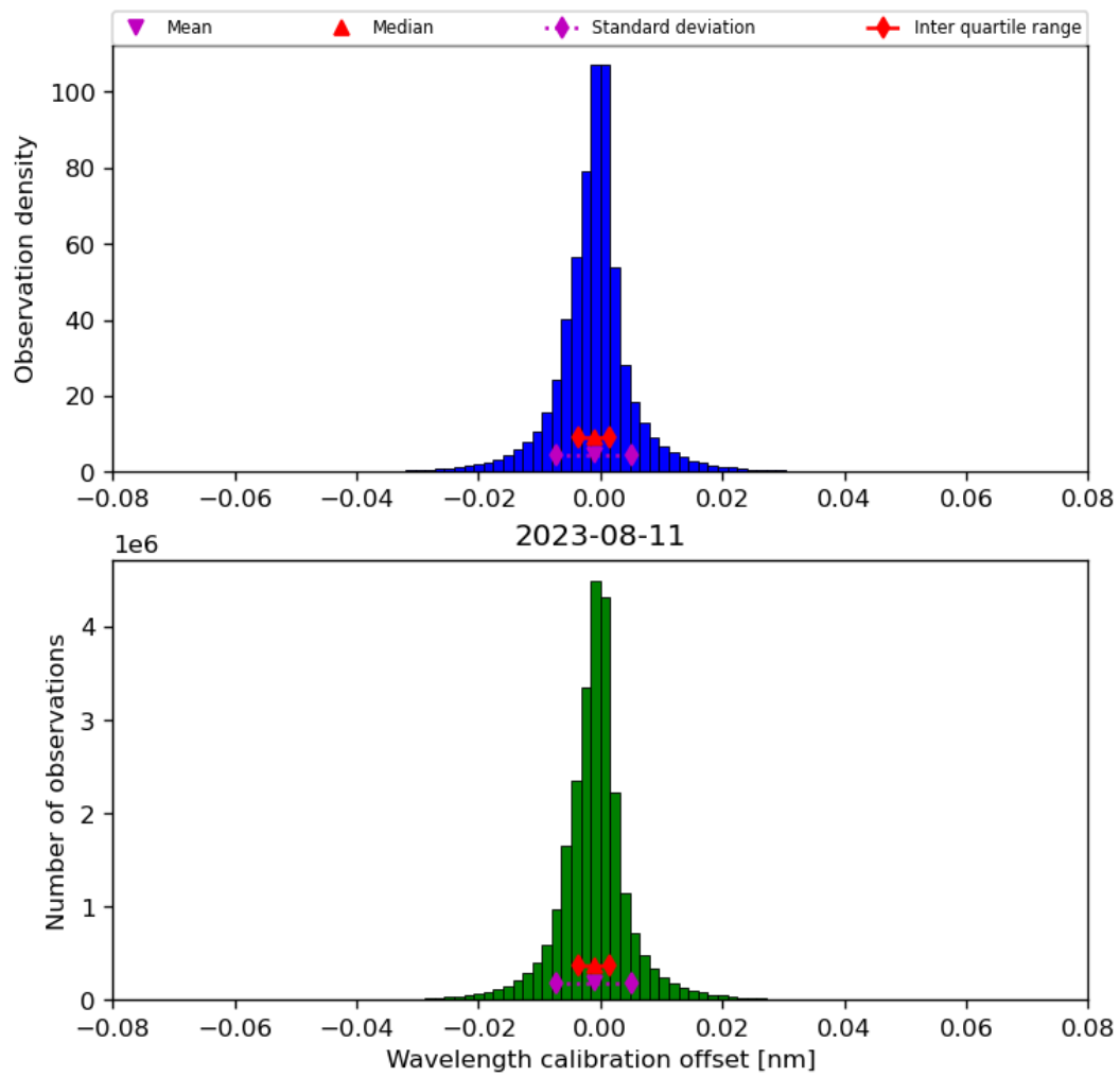
Figure 35: Histogram of “Wavelength calibration offset” for 2023-08-10 to 2023-08-12
