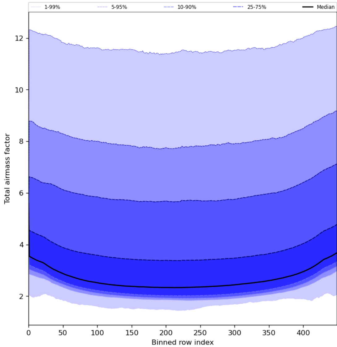
Figure 49: Along track statistics of “Total airmass factor” for 2023-08-10 to 2023-08-12
