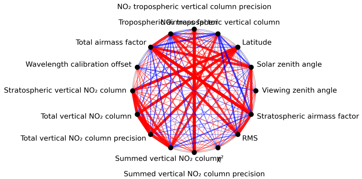
Figure 1: Map of correlation graph for 2023-08-10 to 2023-08-12.
