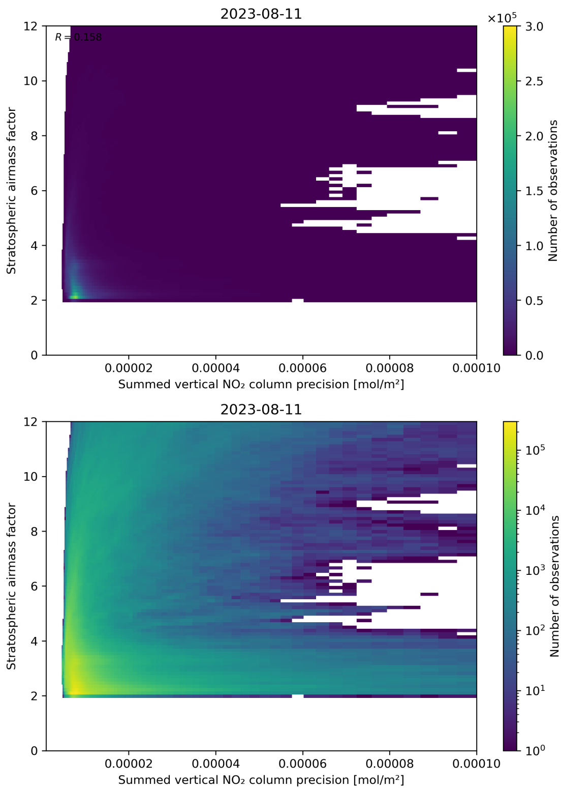
Figure 106: Scatter density plot of “Summed vertical NO 2 column precision” against “Stratospheric airmass factor” for 2023-08-10 to 2023-08-12.
