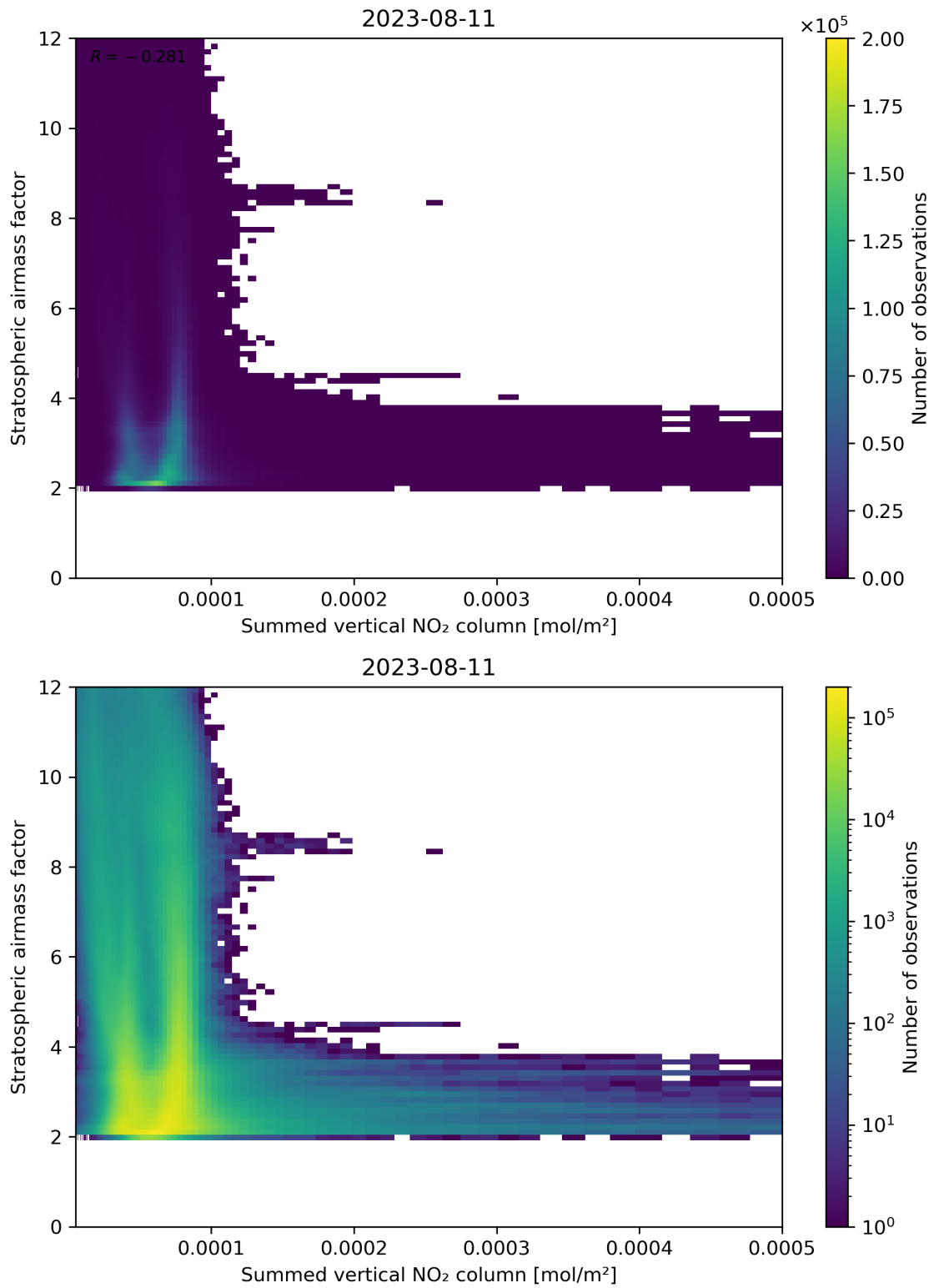
Figure 103: Scatter density plot of “Summed vertical NO 2 column” against “Stratospheric air mass factor” for 2023-08-10 to 2023-08-12.
