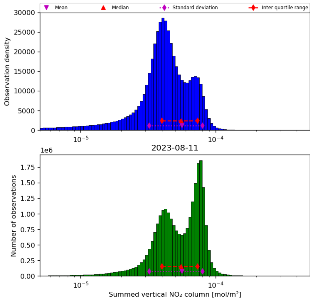
Figure 40: Histogram of “Summed vertical NO 2 column” for 2023-08-10 to 2023-08-12
