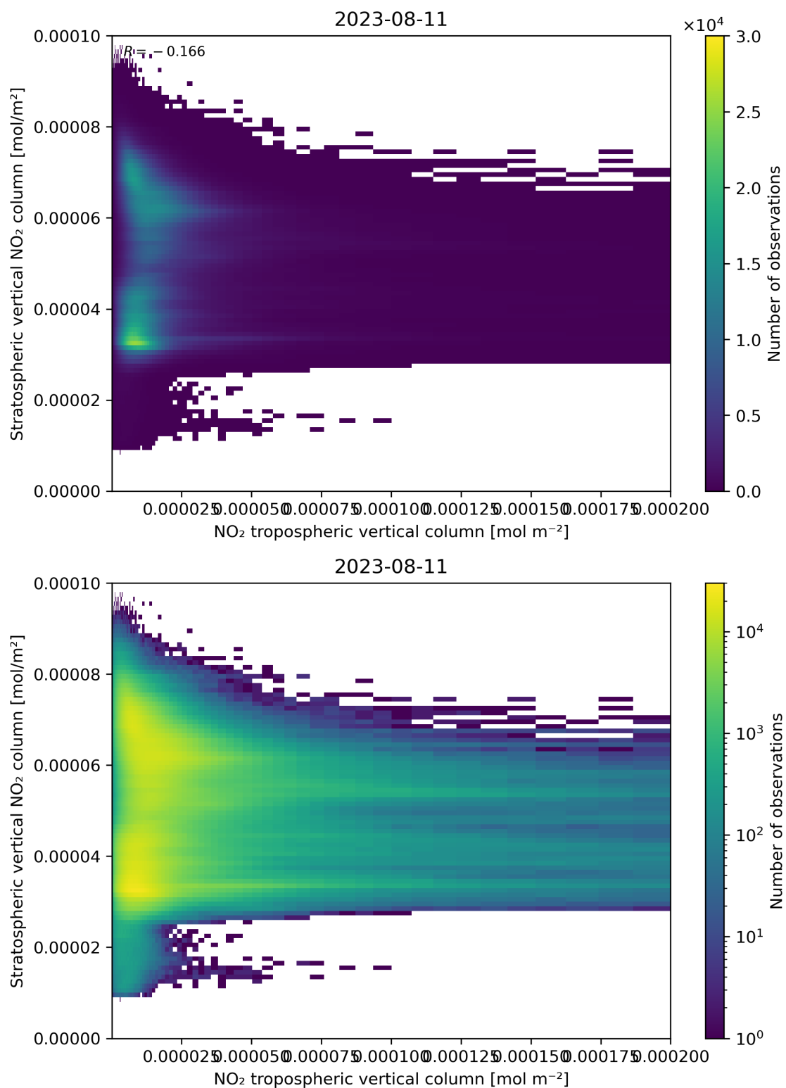
Figure 125: Scatter density plot of “NO 2 tropospheric vertical column” against “Stratospheric vertical NO 2 column” for 2023-08-10 to 2023-08-12.
