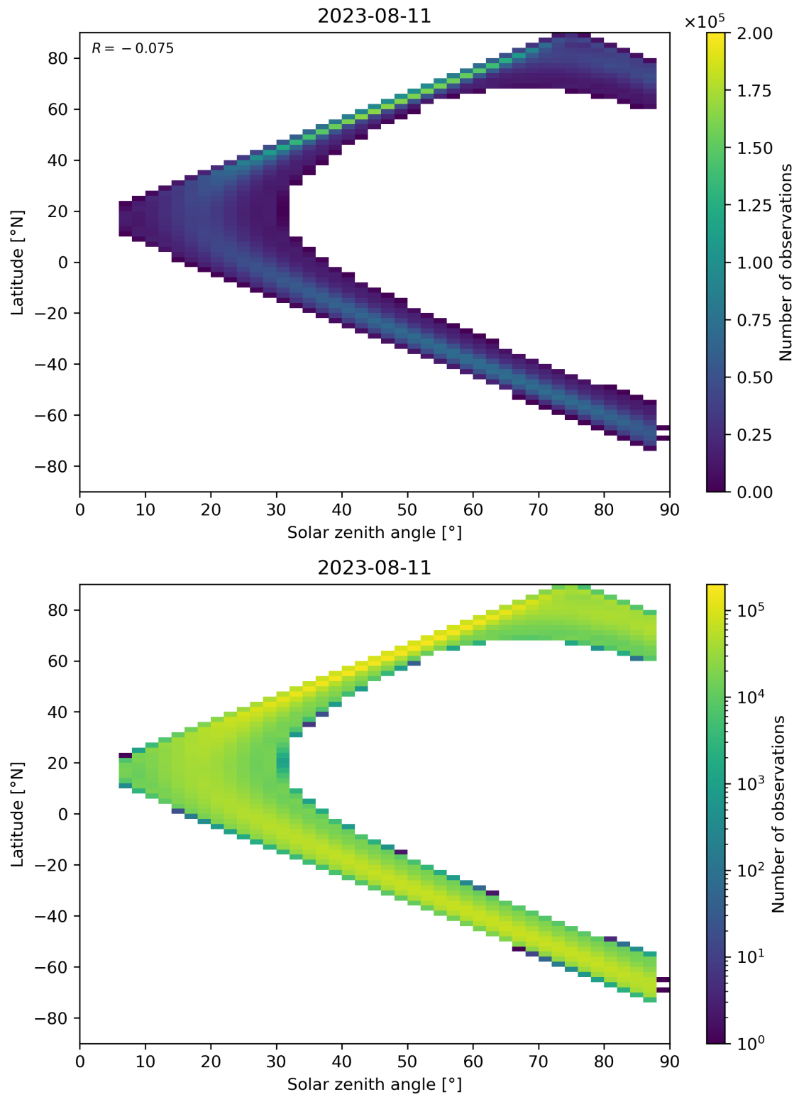
Figure 149: Scatter density plot of “Solar zenith angle” against “Latitude” for 2023-08-10 to 2023-08-12.
