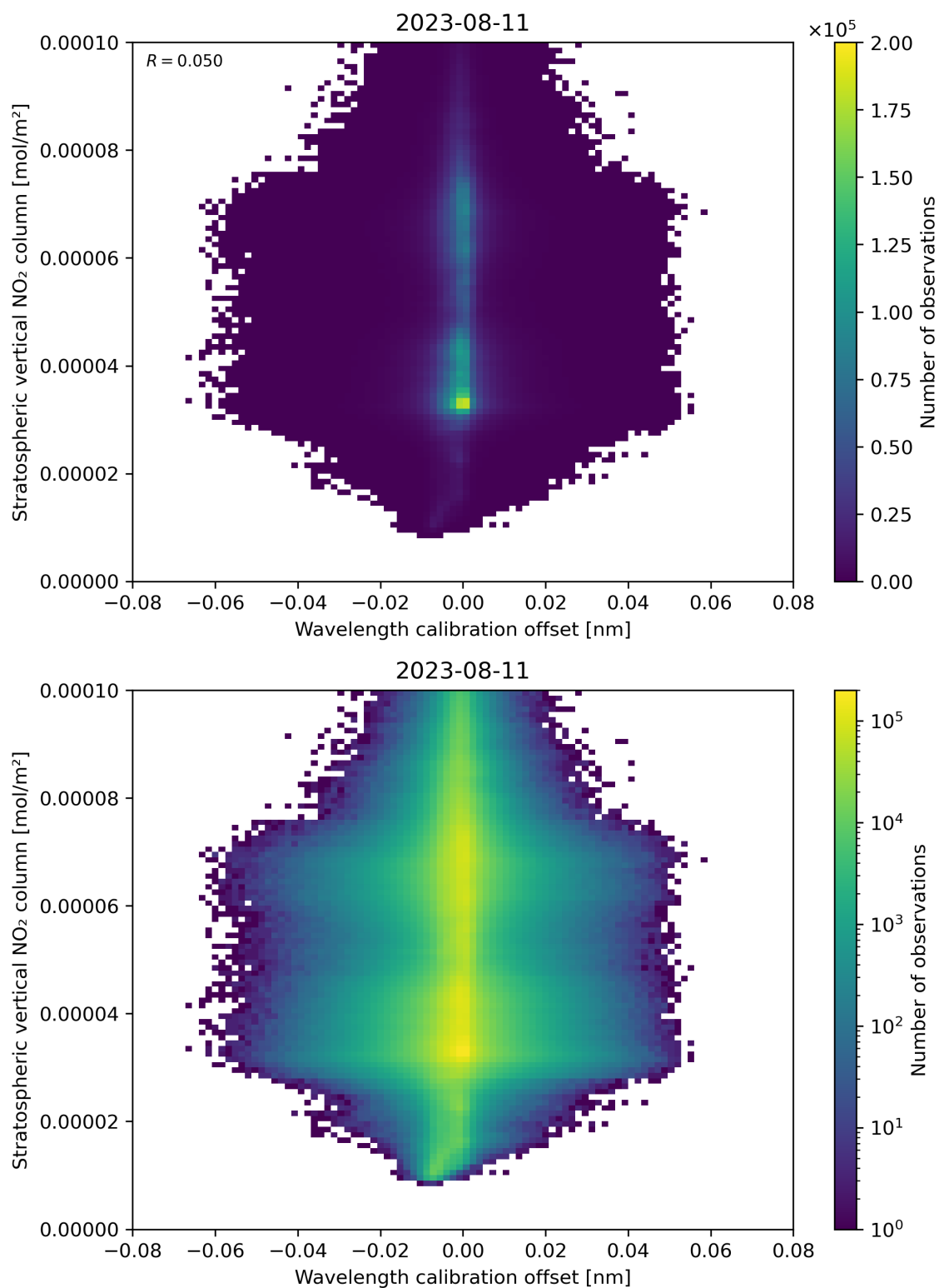
Figure 176: Scatter density plot of “Wavelength calibration offset” against “Stratospheric vertical NO 2 column” for 2023-08-10 to 2023-08-12.
