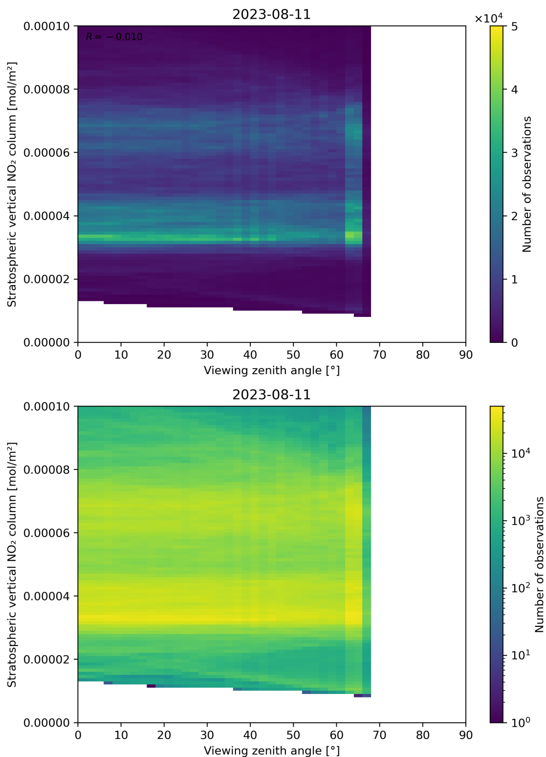
Figure 164: Scatter density plot of “Viewing zenith angle” against “Stratospheric vertical NO 2 column” for 2023-08-10 to 2023-08-12.
