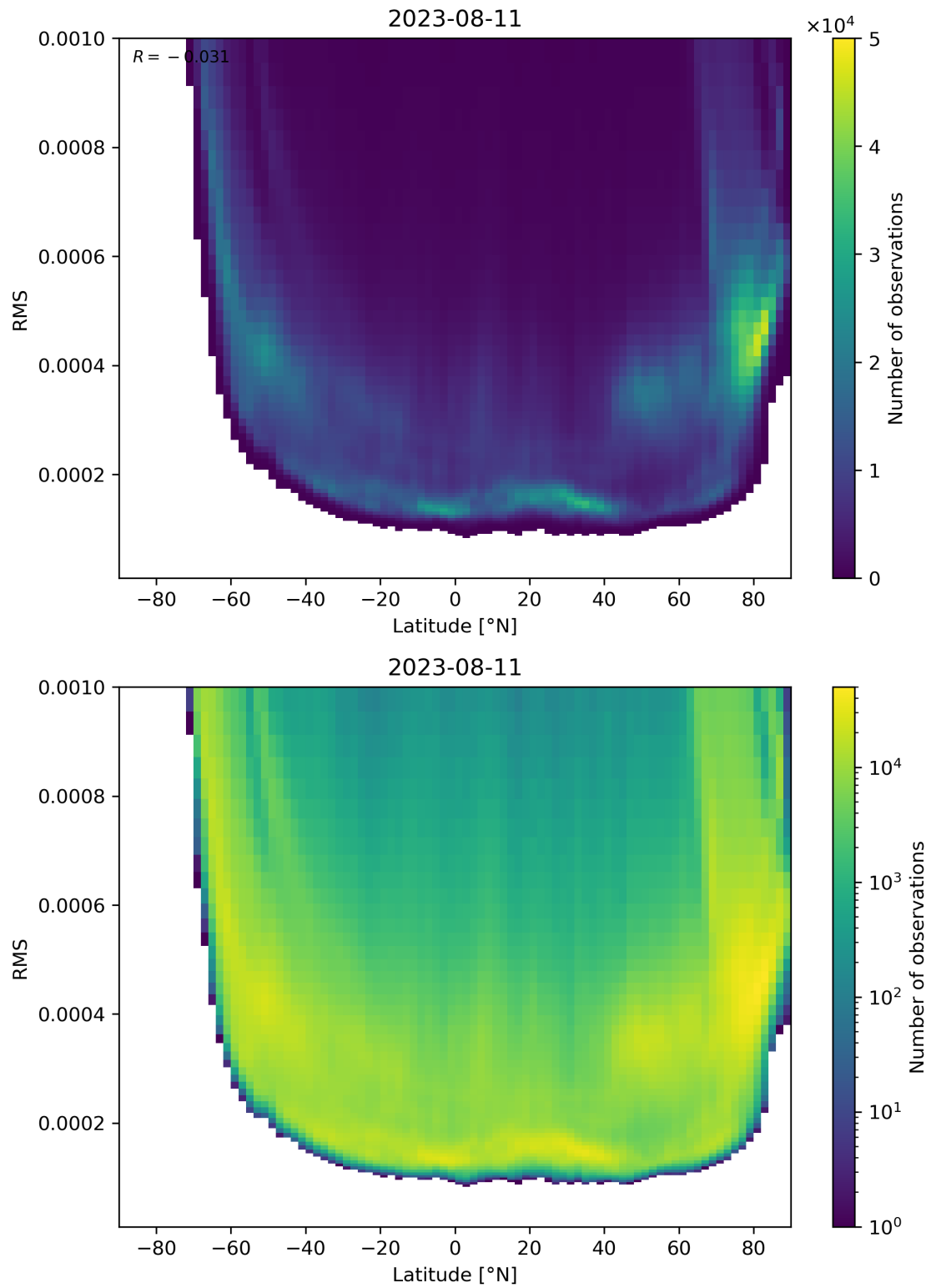
Figure 94: Scatter density plot of “Latitude” against “RMS” for 2023-08-10 to 2023-08-12.
