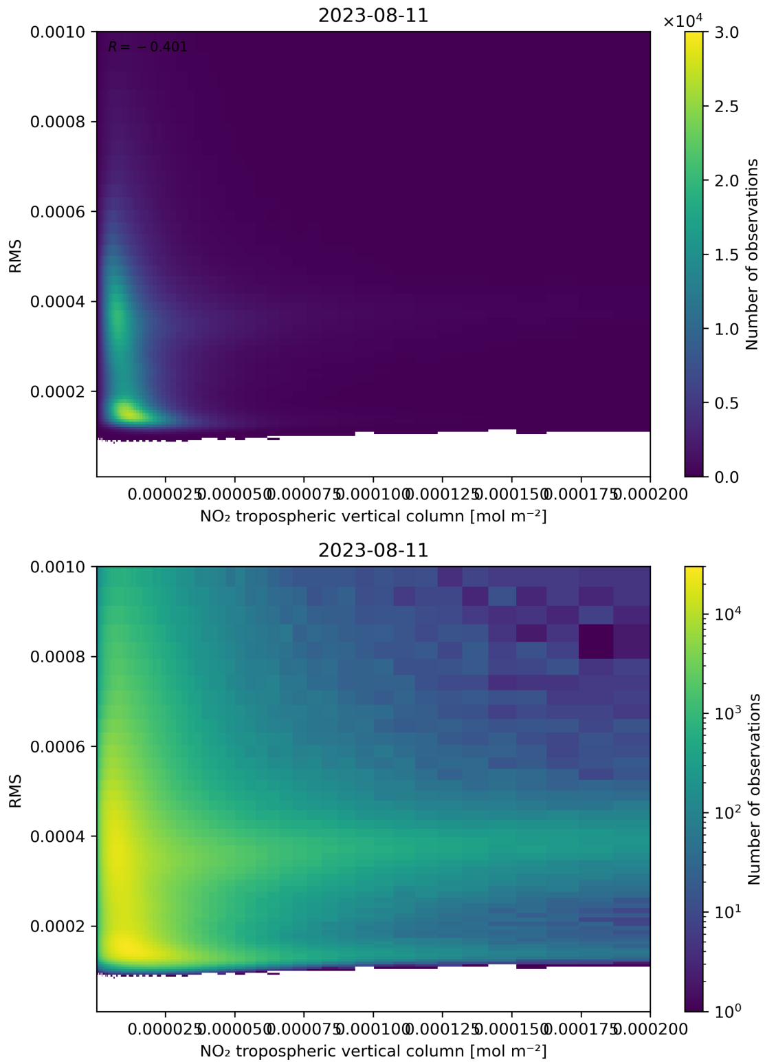
Figure 142: Scatter density plot of “NO 2 tropospheric vertical column” against “RMS” for 2023-08-10 to 2023-08-12.
