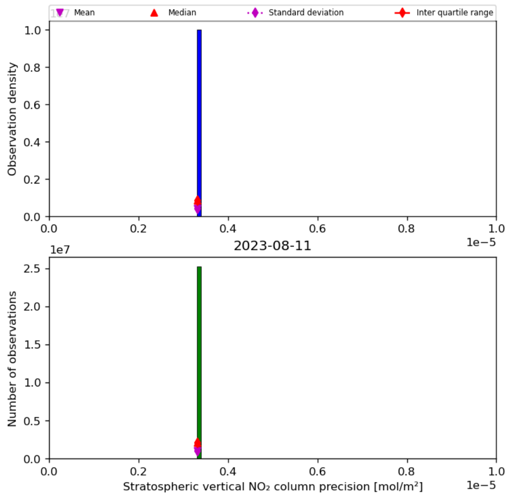
Figure 37: Histogram of “Stratospheric vertical NO 2 column precision” for 2023-08-10 to 2023-08-12
