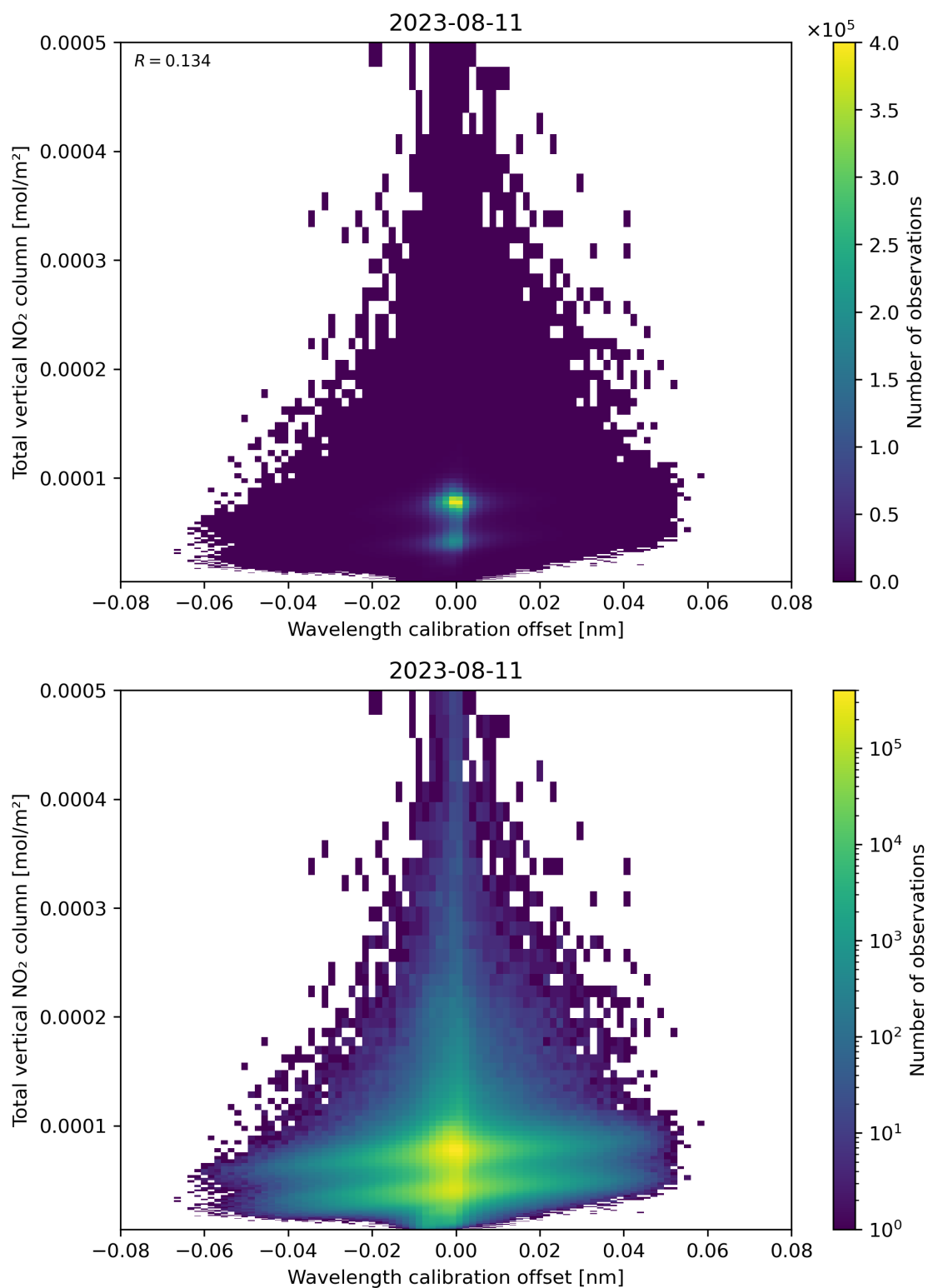
Figure 179: Scatter density plot of “Wavelength calibration offset” against “Total vertical NO 2 column” for 2023-08-10 to 2023-08-12.
