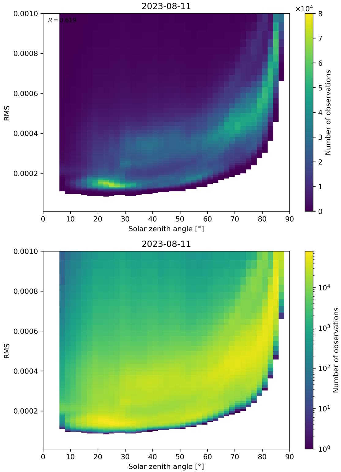
Figure 157: Scatter density plot of “Solar zenith angle” against “RMS” for 2023-08-10 to 2023-08-12.
