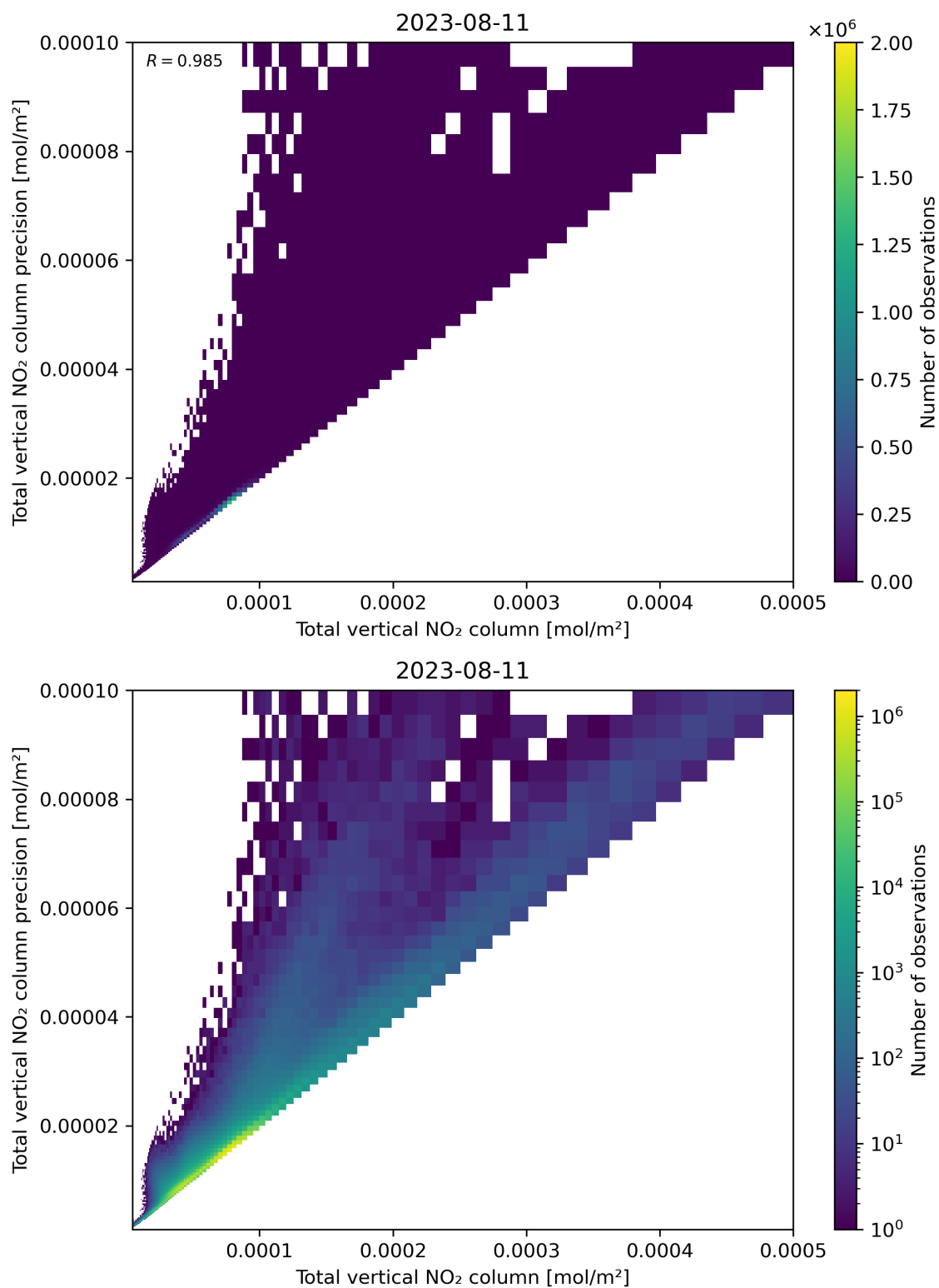
Figure 114: Scatter density plot of “Total vertical NO 2 column” against “Total vertical NO 2 column precision” for 2023-08-10 to 2023-08-12.
