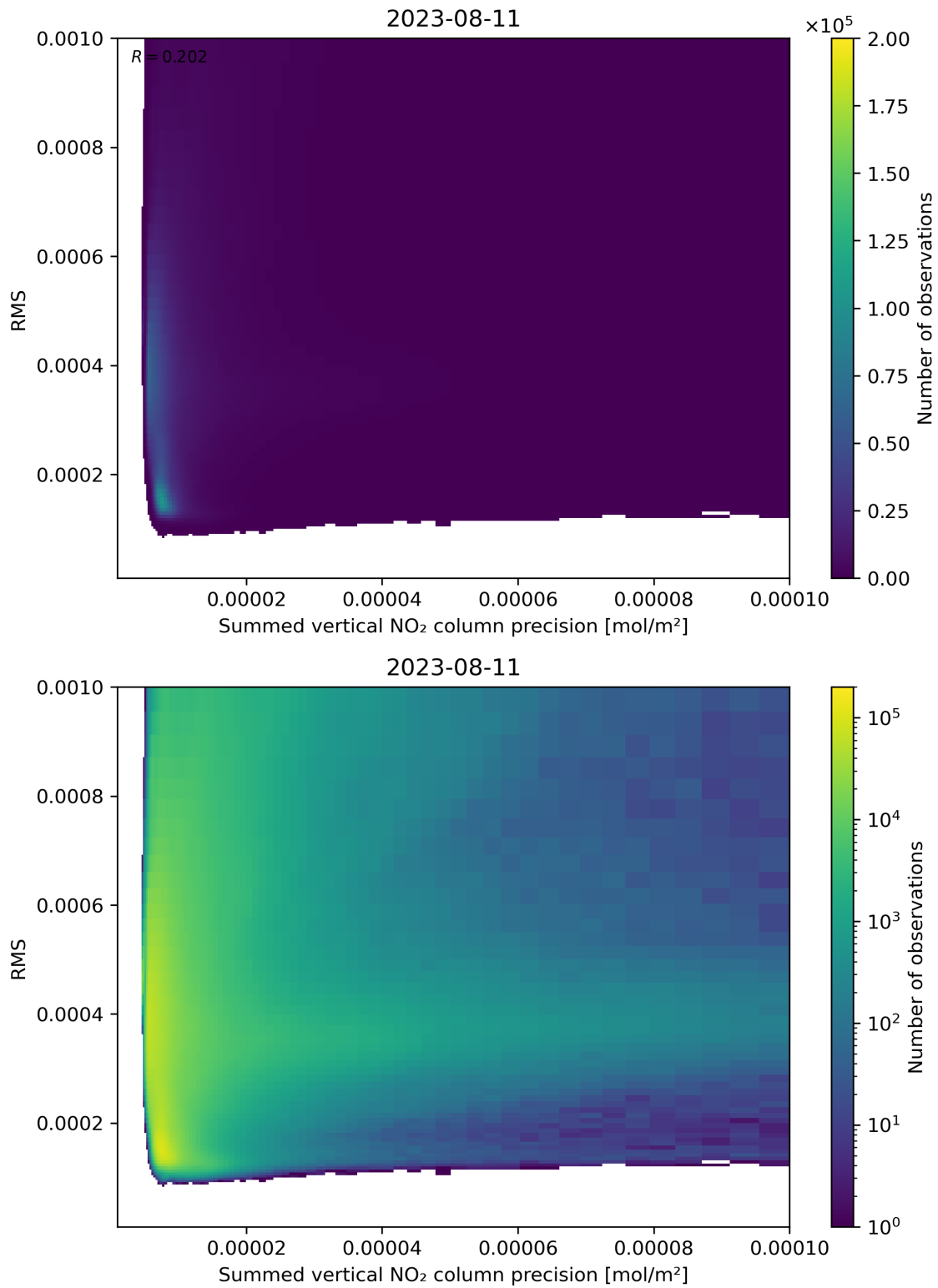
Figure 108: Scatter density plot of “Summed vertical NO 2 column precision” against “RMS” for 2023-08-10 to 2023-08-12.
