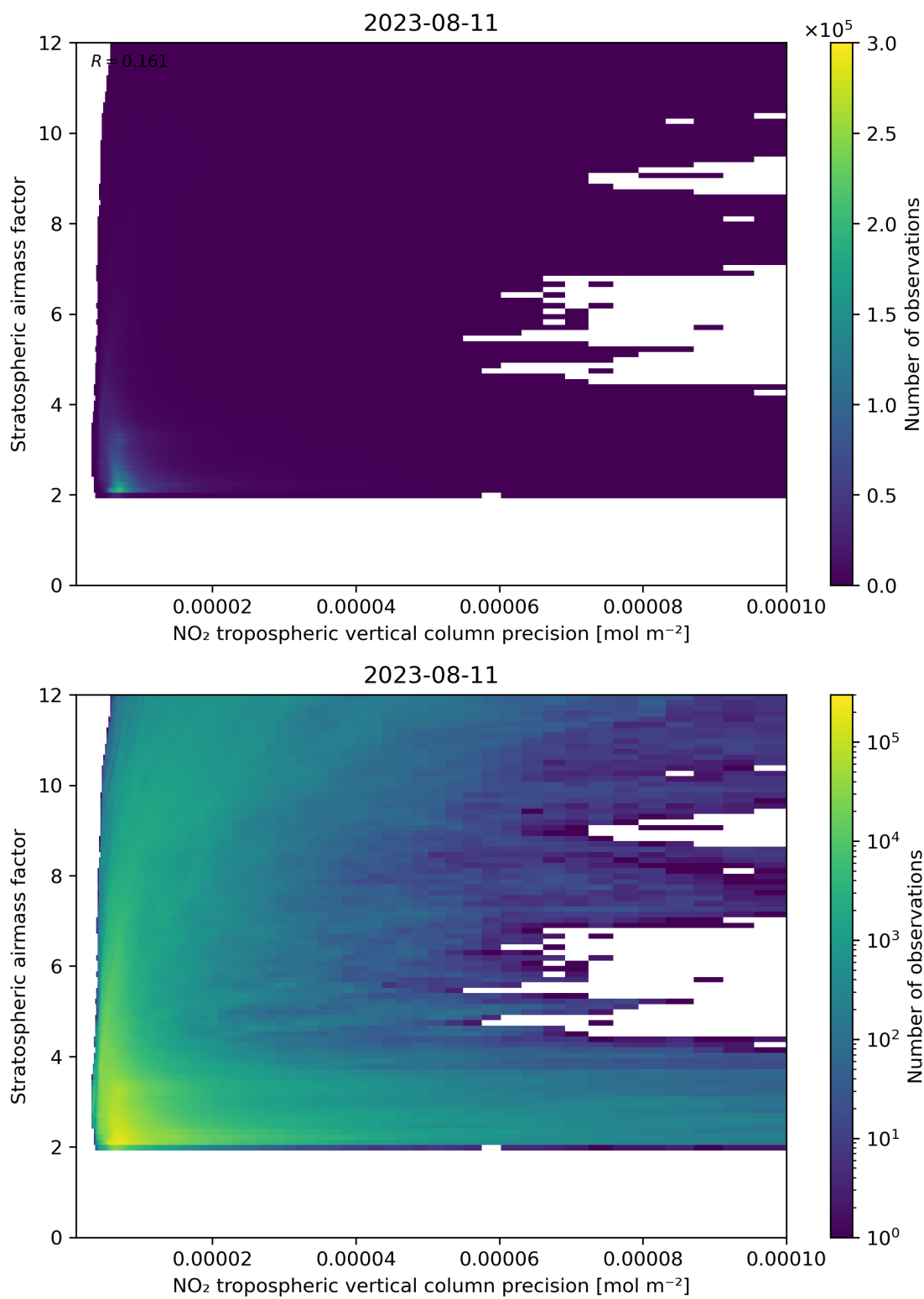
Figure 131: Scatter density plot of “NO 2 tropospheric vertical column precision” against “Stratospheric airmass factor” for 2023-08-10 to 2023-08-12.
