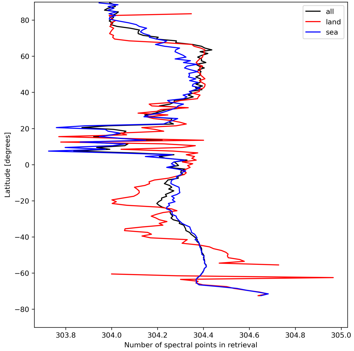
Figure 16: Zonal average of “Number of spectral points in retrieval” for 2023-08-10 to 2023-08-12.
