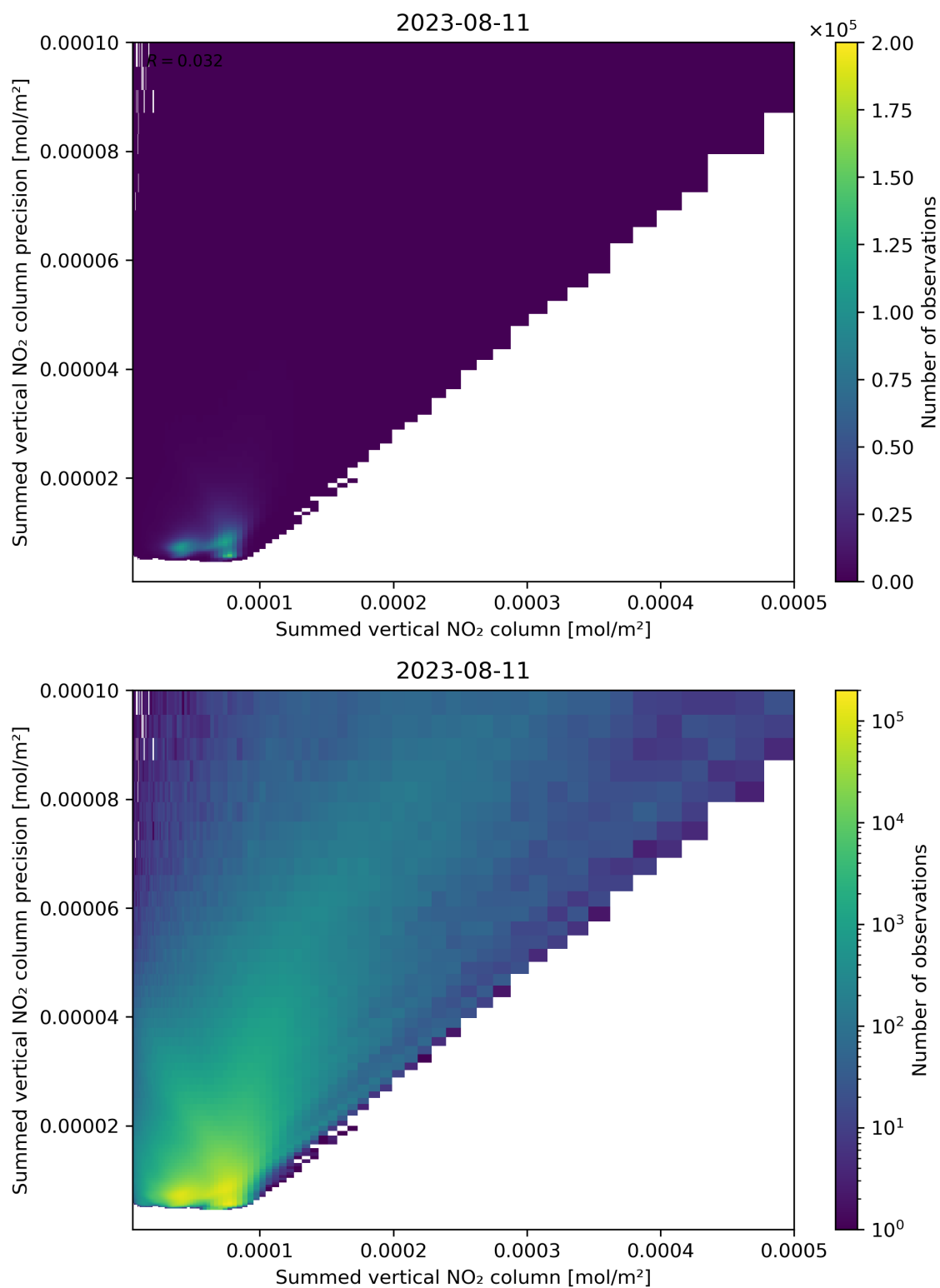
Figure 105: Scatter density plot of “Summed vertical NO 2 column” against “Summed vertical NO 2 column precision” for 2023-08-10 to 2023-08-12.
