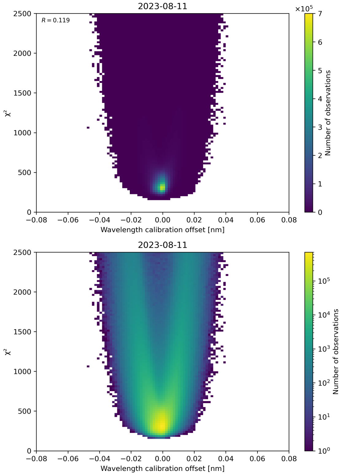
Figure 175: Scatter density plot of “Wavelength calibration offset” against “ \chi^2 ” for 2023-08-10 to 2023-08-12.
