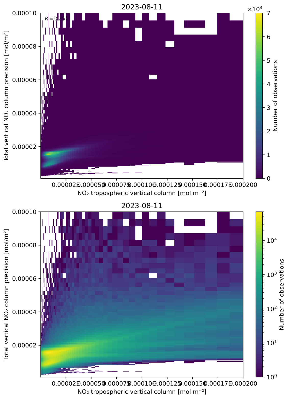
Figure 129: Scatter density plot of “NO 2 tropospheric vertical column” against “Total vertical NO 2 column precision” for 2023-08-10 to 2023-08-12.
