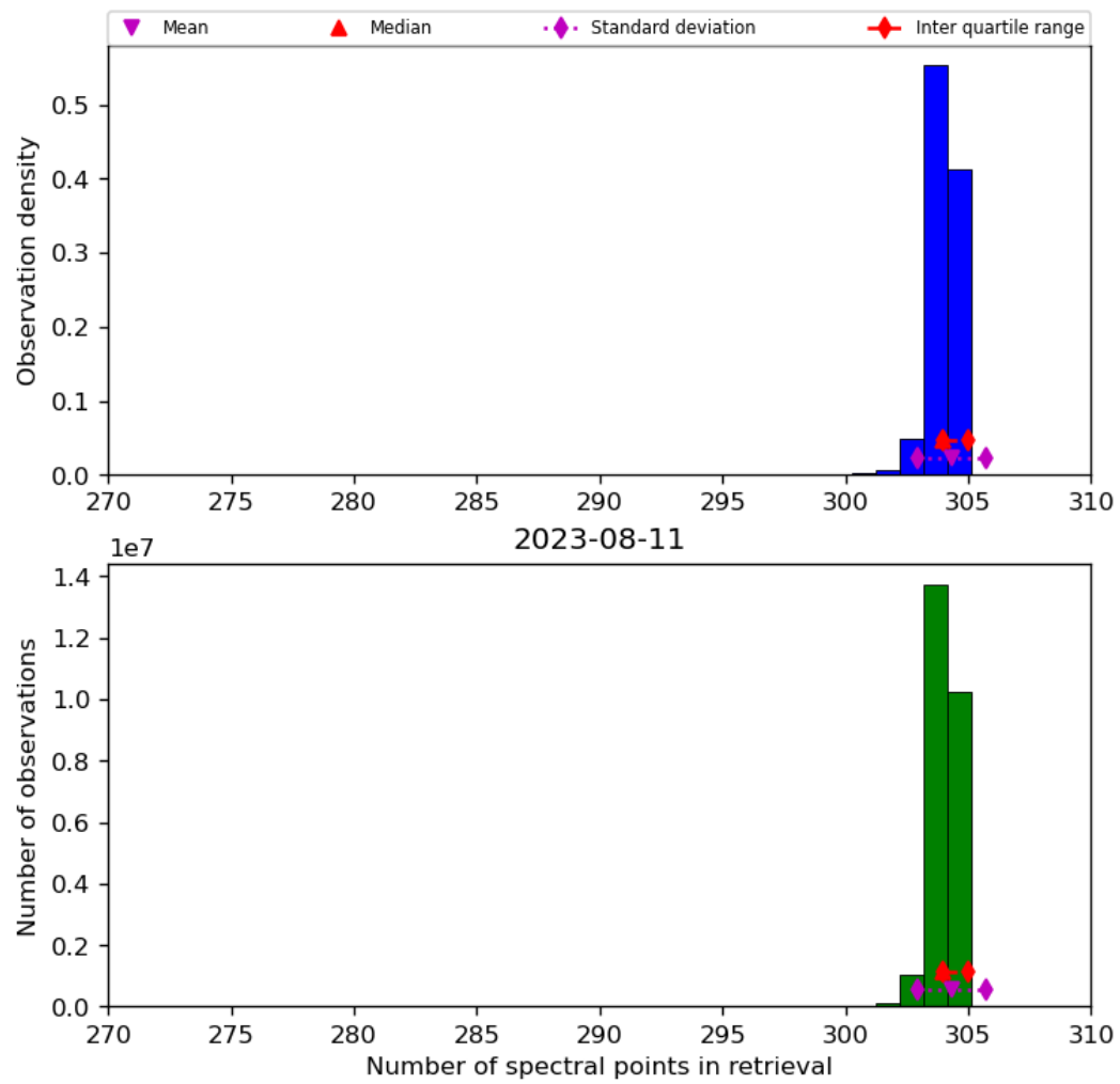
Figure 33: Histogram of “Number of spectral points in retrieval” for 2023-08-10 to 2023-08-12
