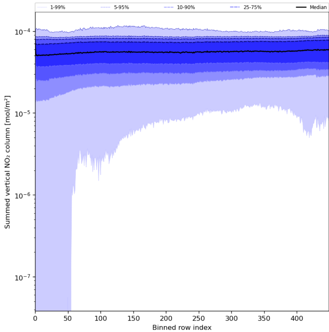
Figure 57: Along track statistics of “Summed vertical NO 2 column” for 2023-08-10 to 2023-08-12
