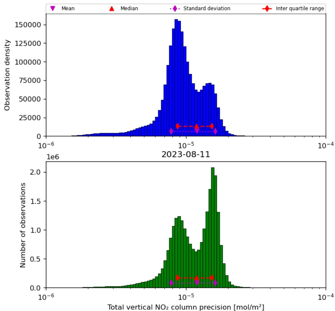
Figure 39: Histogram of "Total vertical NO 2 column precision" for 2023-08-10 to 2023-08-12
