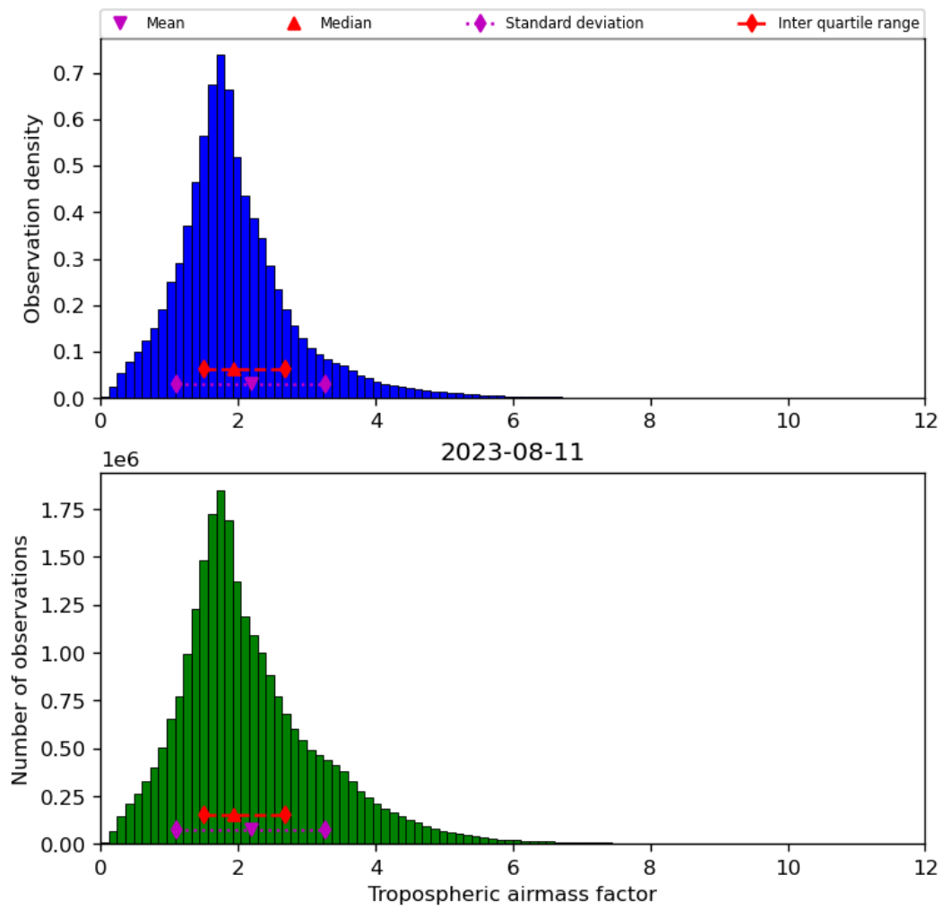
Figure 31: Histogram of “Tropospheric airmass factor” for 2023-08-10 to 2023-08-12
