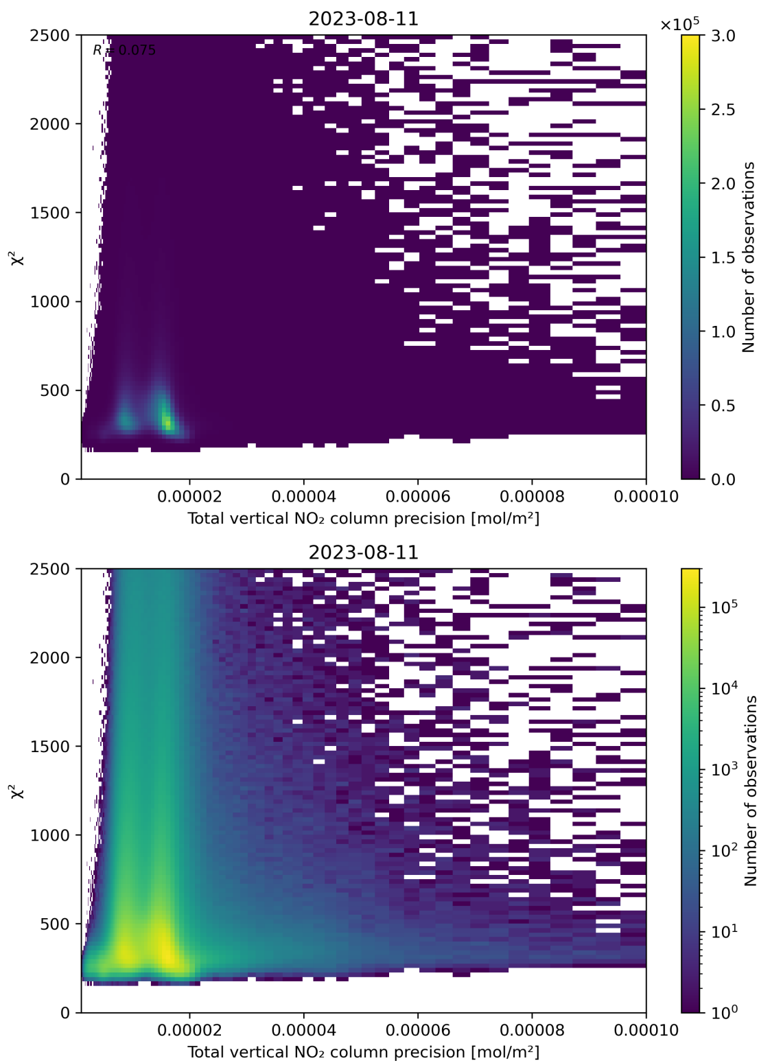
Figure 116: Scatter density plot of “Total vertical NO 2 column precision” against “ \chi^2 ” for 2023-08-10 to 2023-08-12.
