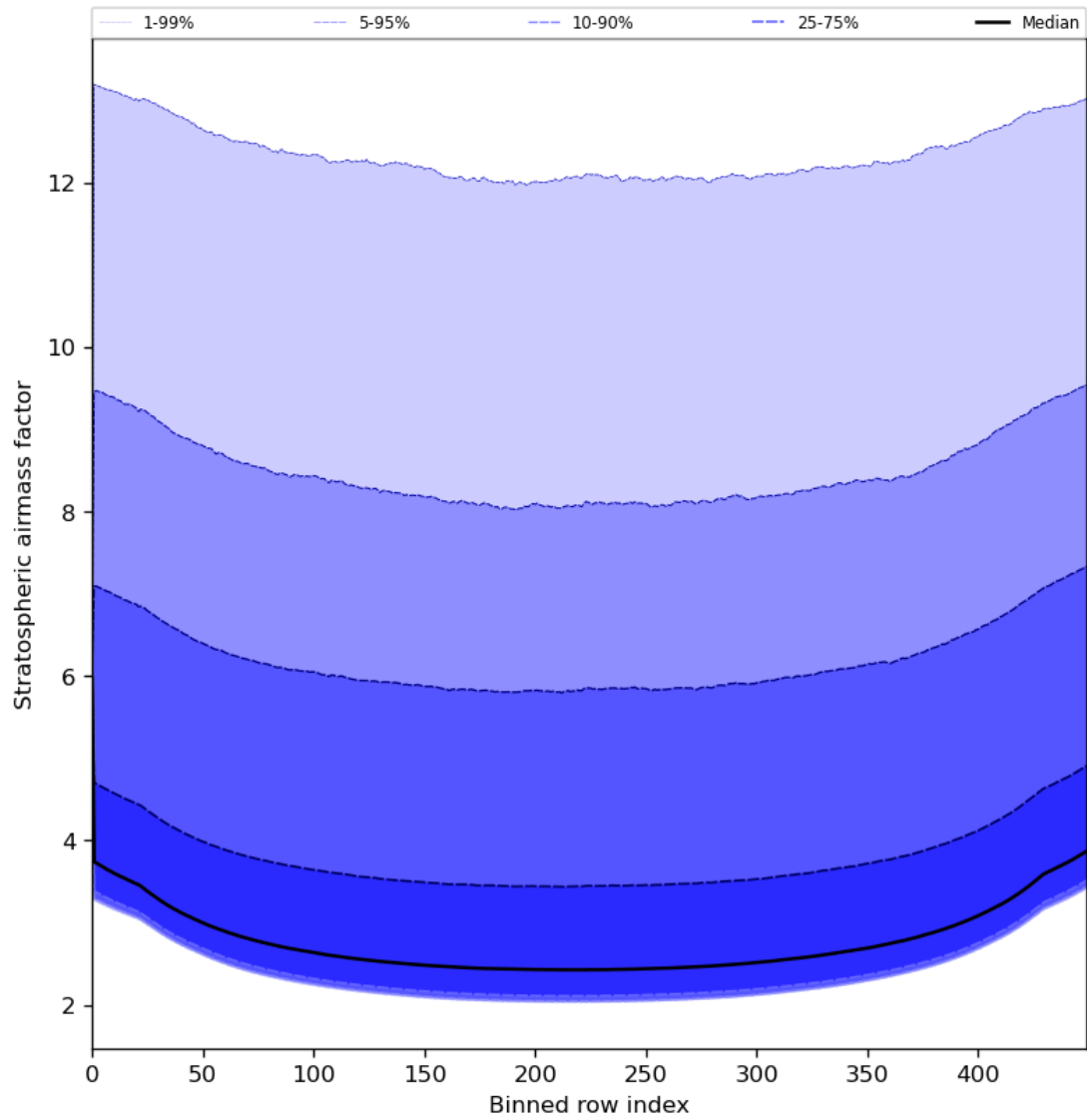
Figure 61: Along track statistics of “Stratospheric airmass factor” for 2023-08-10 to 2023-08-12
