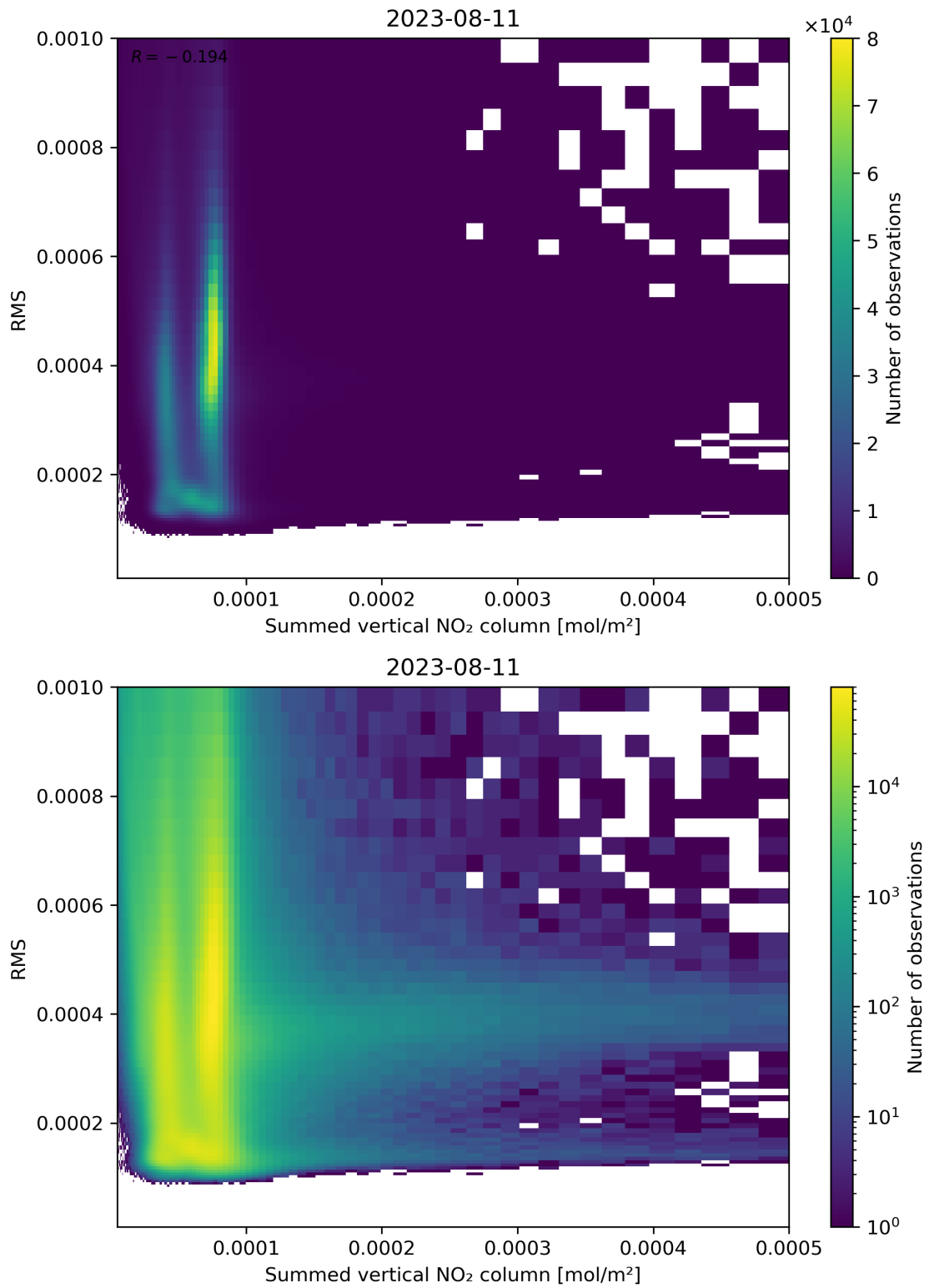
Figure 109: Scatter density plot of “Summed vertical NO 2 column” against “RMS” for 2023-08-10 to 2023-08-12.
