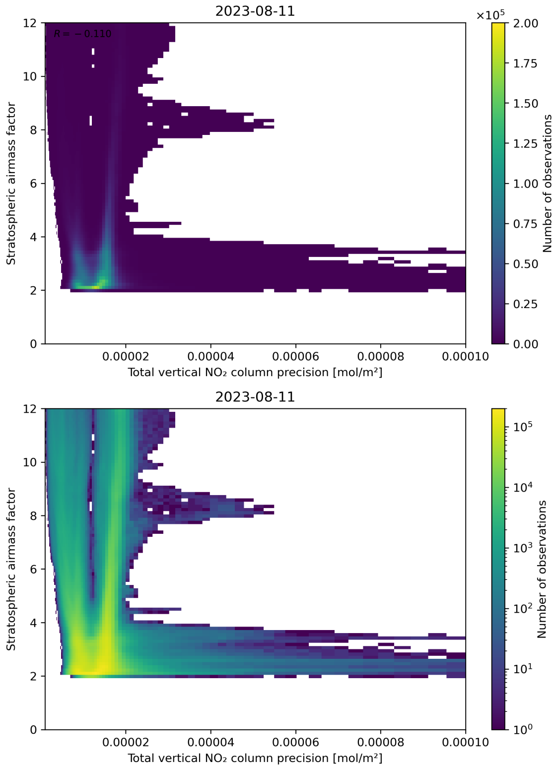
Figure 115: Scatter density plot of “Total vertical NO 2 column precision” against “Stratospheric air mass factor” for 2023-08-10 to 2023-08-12.
