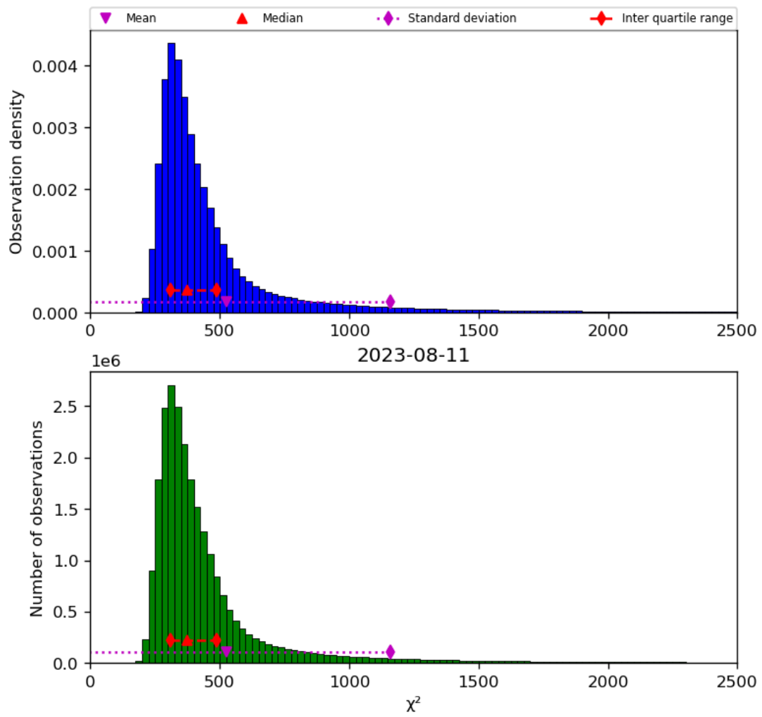
Figure 42: Histogram of “ \chi^2 ” for 2023-08-10 to 2023-08-12
