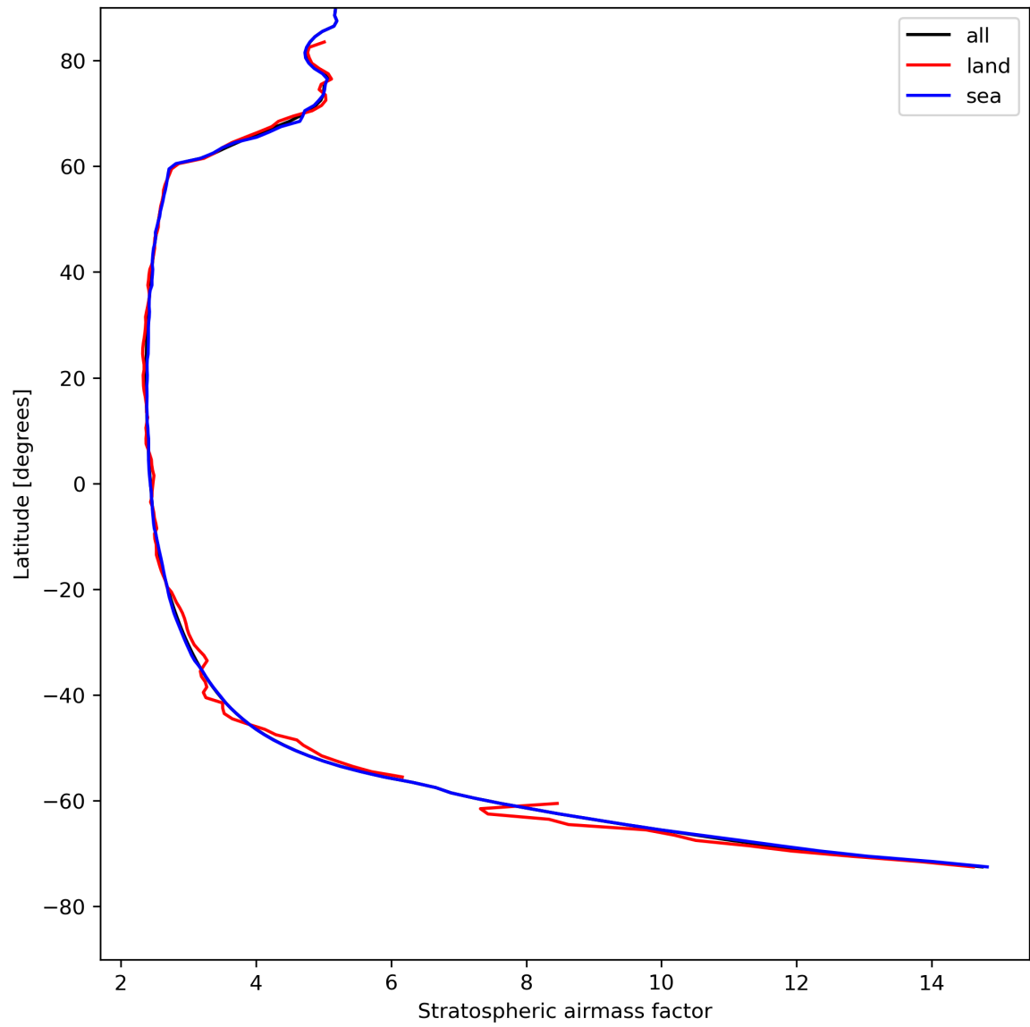
Figure 27: Zonal average of “Stratospheric airmass factor” for 2023-08-10 to 2023-08-12.
