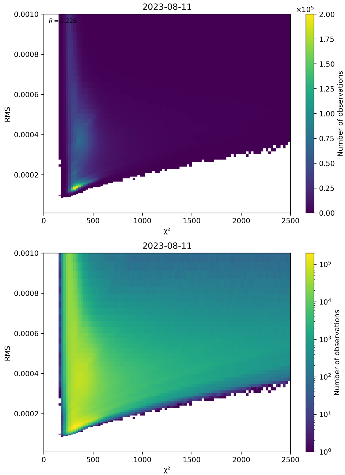
Figure 82: Scatter density plot of “ \chi^2 ” against “RMS” for 2023-08-10 to 2023-08-12.
