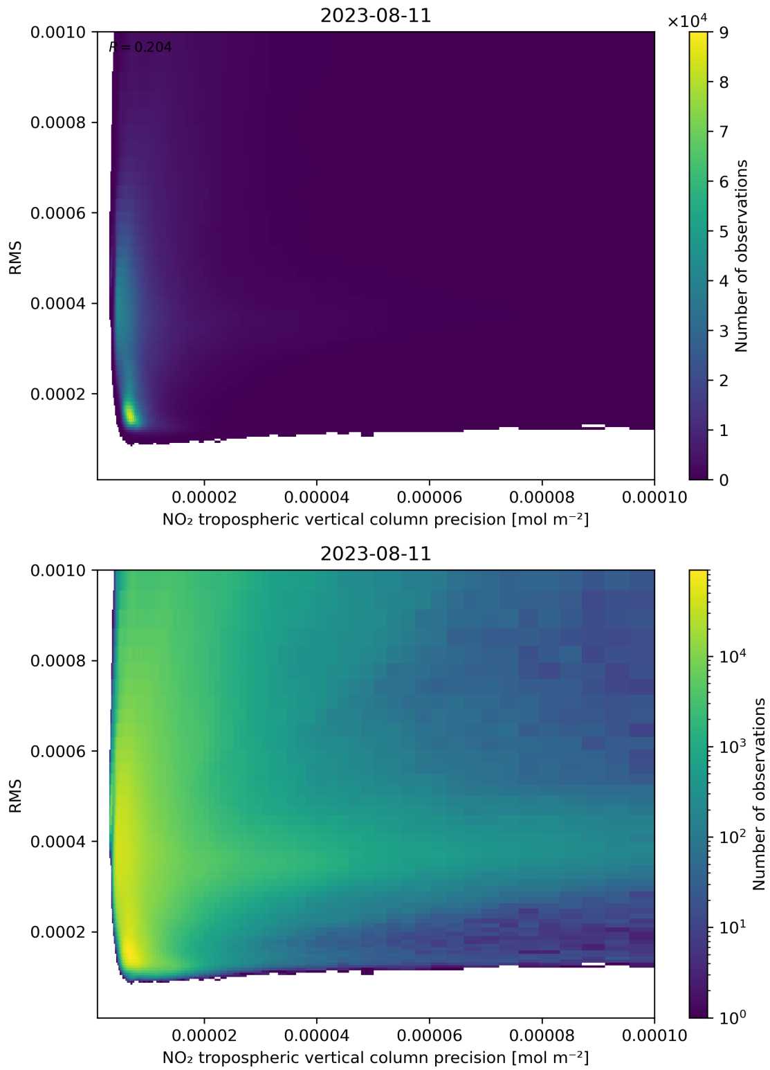
Figure 140: Scatter density plot of “NO 2 tropospheric vertical column precision” against “RMS” for 2023-08-10 to 2023-08-12.
