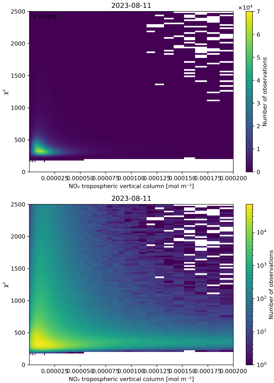
Figure 124: Scatter density plot of “NO 2 tropospheric vertical column” against “ \chi^2 ” for 2023-08-10 to 2023-08-12.
