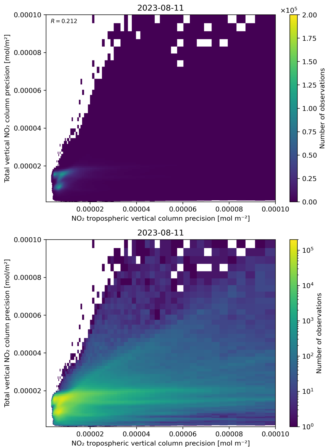
Figure 139: Scatter density plot of “NO 2 tropospheric vertical column precision” against “Total vertical NO 2 column precision” for 2023-08-10 to 2023-08-12.
