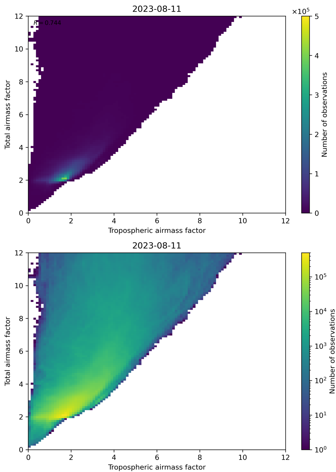
Figure 72: Scatter density plot of “Tropospheric airmass factor” against “Total airmass factor” for 2023-08-10 to 2023-08-12.
