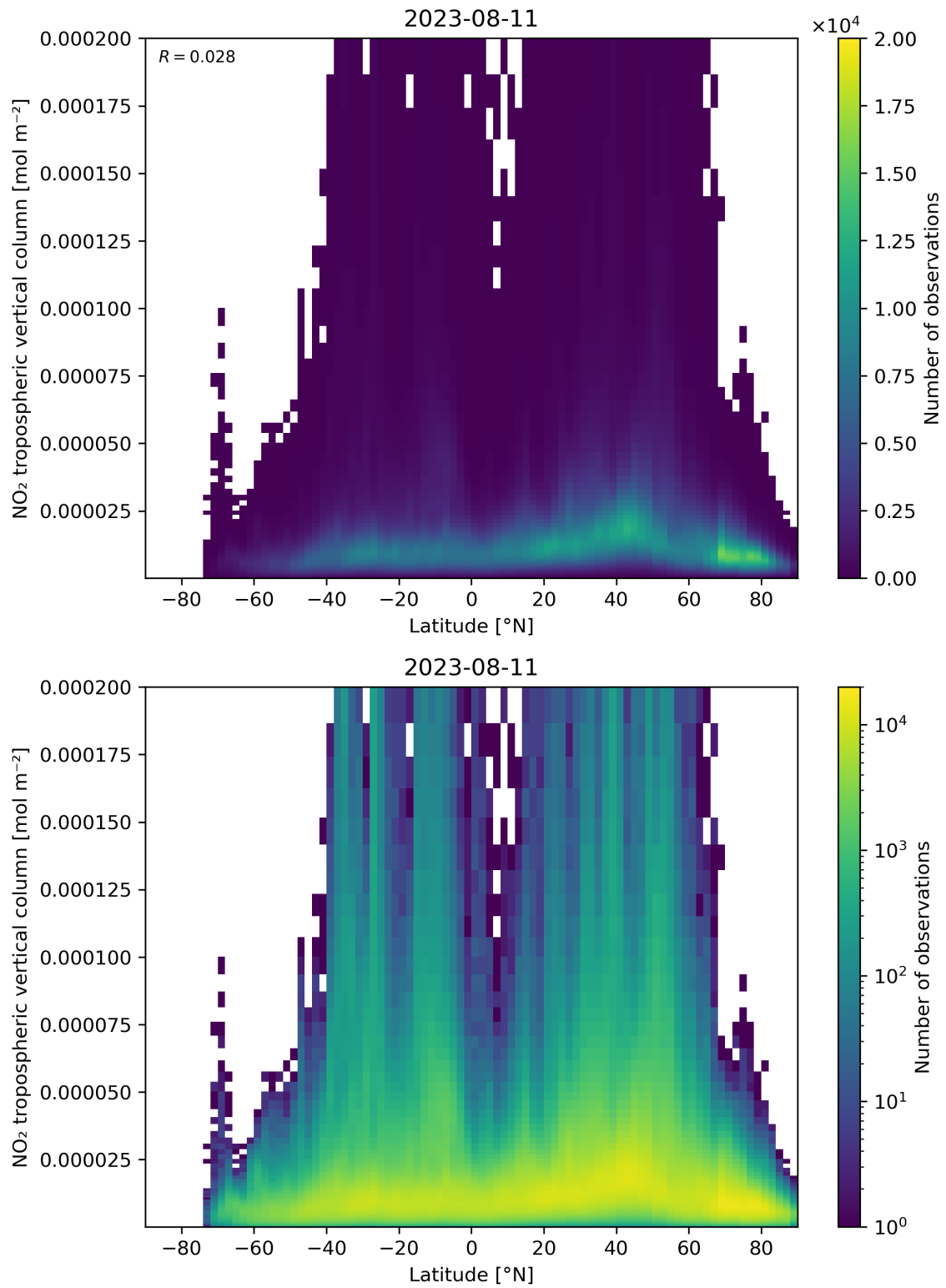
Figure 92: Scatter density plot of “Latitude” against “NO 2 tropospheric vertical column” for 2023-08-10 to 2023-08-12.
