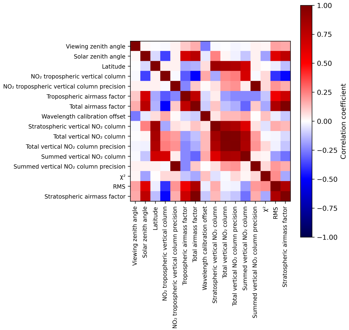
Figure 2: Map of correlation matrix for 2023-08-10 to 2023-08-12.
