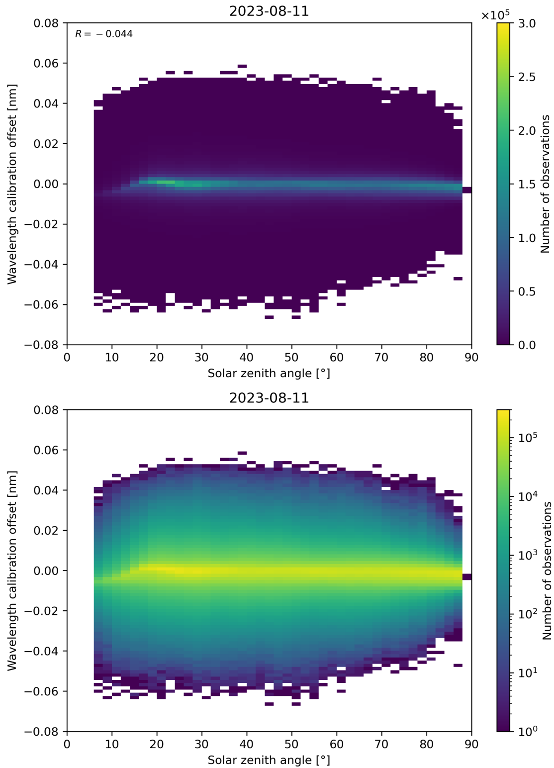
Figure 158: Scatter density plot of “Solar zenith angle” against “Wavelength calibration offset” for 2023-08-10 to 2023-08-12.
