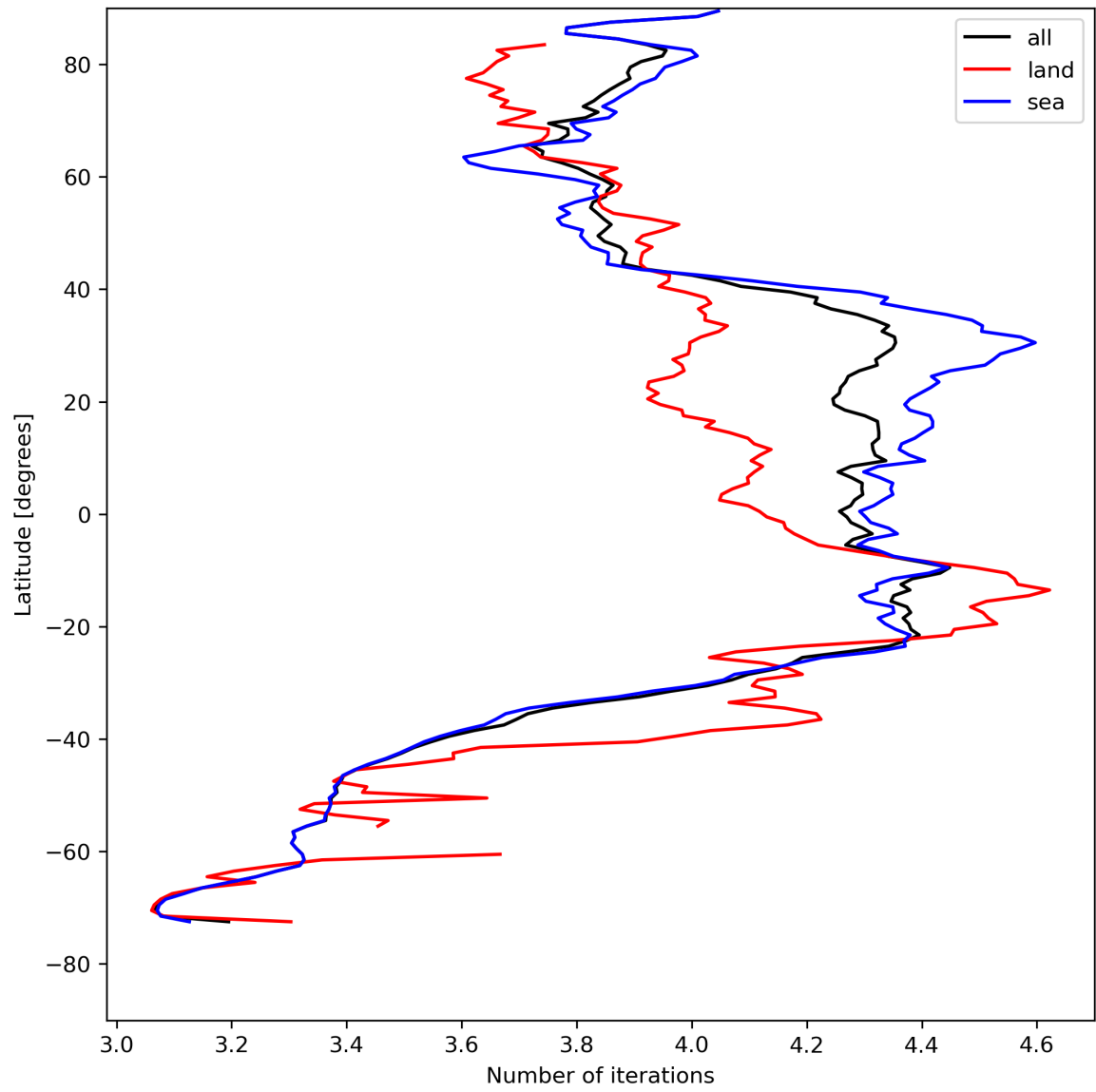
Figure 17: Zonal average of “Number of iterations” for 2023-08-10 to 2023-08-12.
