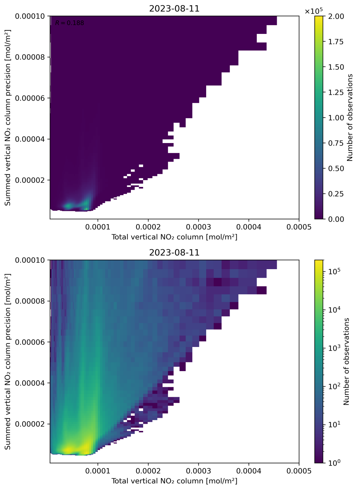
Figure 113: Scatter density plot of “Total vertical NO 2 column” against “Summed vertical NO 2 column precision” for 2023-08-10 to 2023-08-12.
