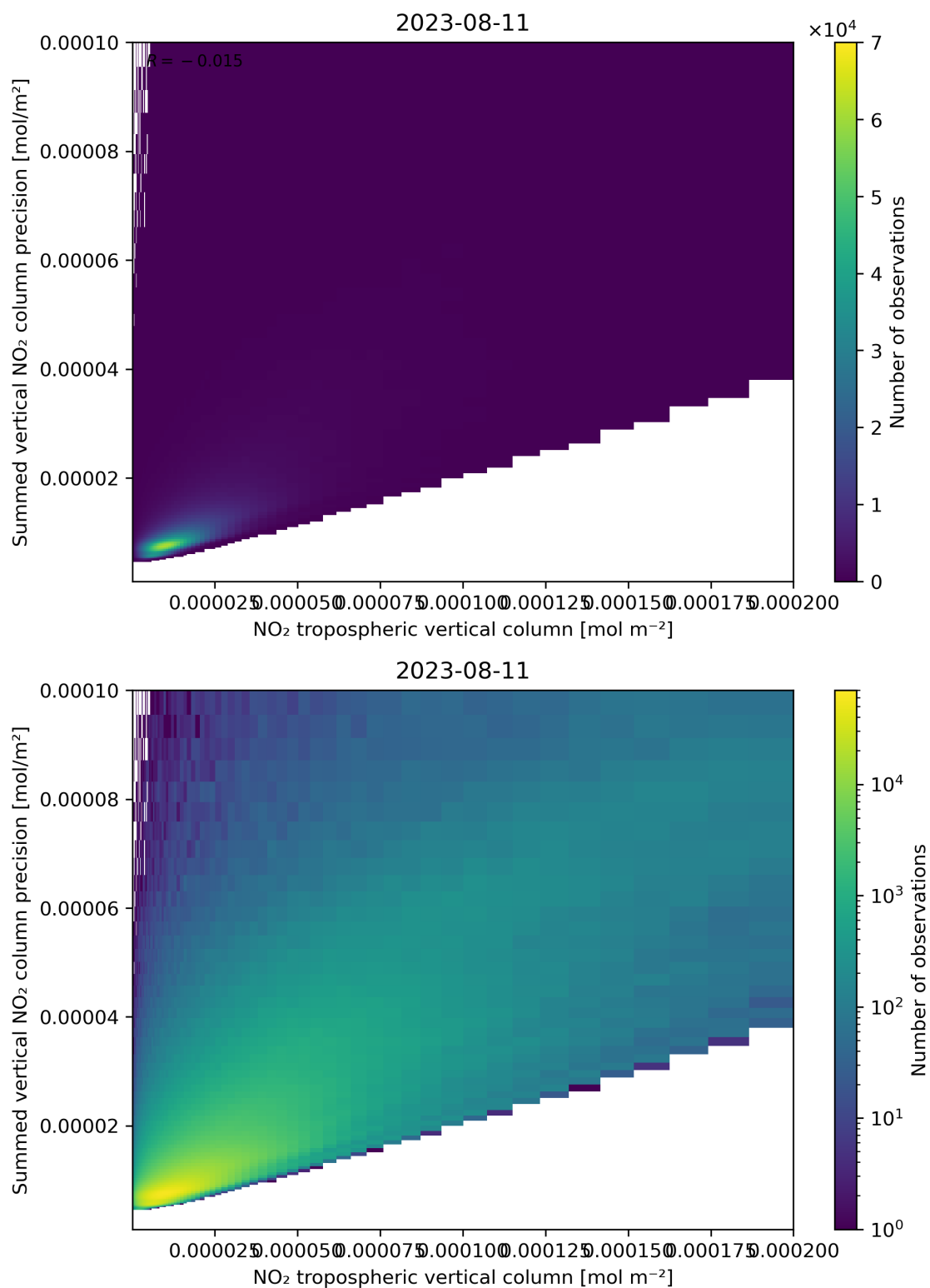
Figure 127: Scatter density plot of “NO 2 tropospheric vertical column” against “Summed vertical NO 2 column precision” for 2023-08-10 to 2023-08-12.
