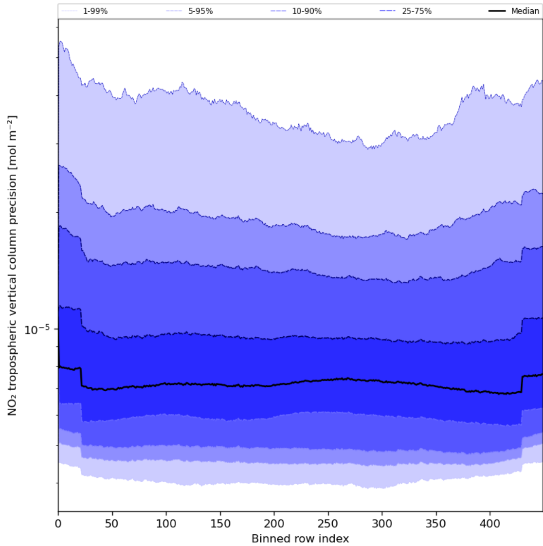
Figure 47: Along track statistics of “NO 2 tropospheric vertical column precision” for 2023-08-10 to 2023-08-12
