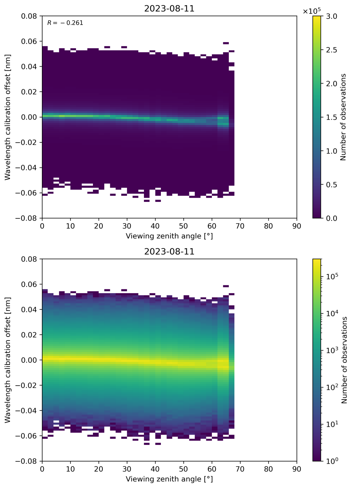
Figure 173: Scatter density plot of “Viewing zenith angle” against “Wavelength calibration offset” for 2023-08-10 to 2023-08-12.
