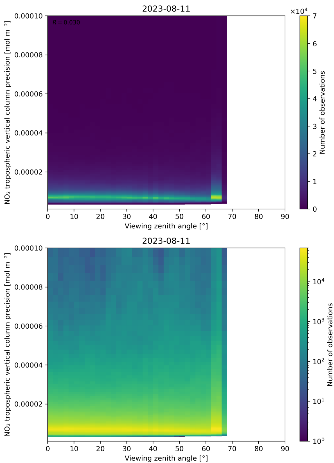
Figure 170: Scatter density plot of “Viewing zenith angle” against “NO 2 tropospheric vertical column precision” for 2023-08-10 to 2023-08-12.
