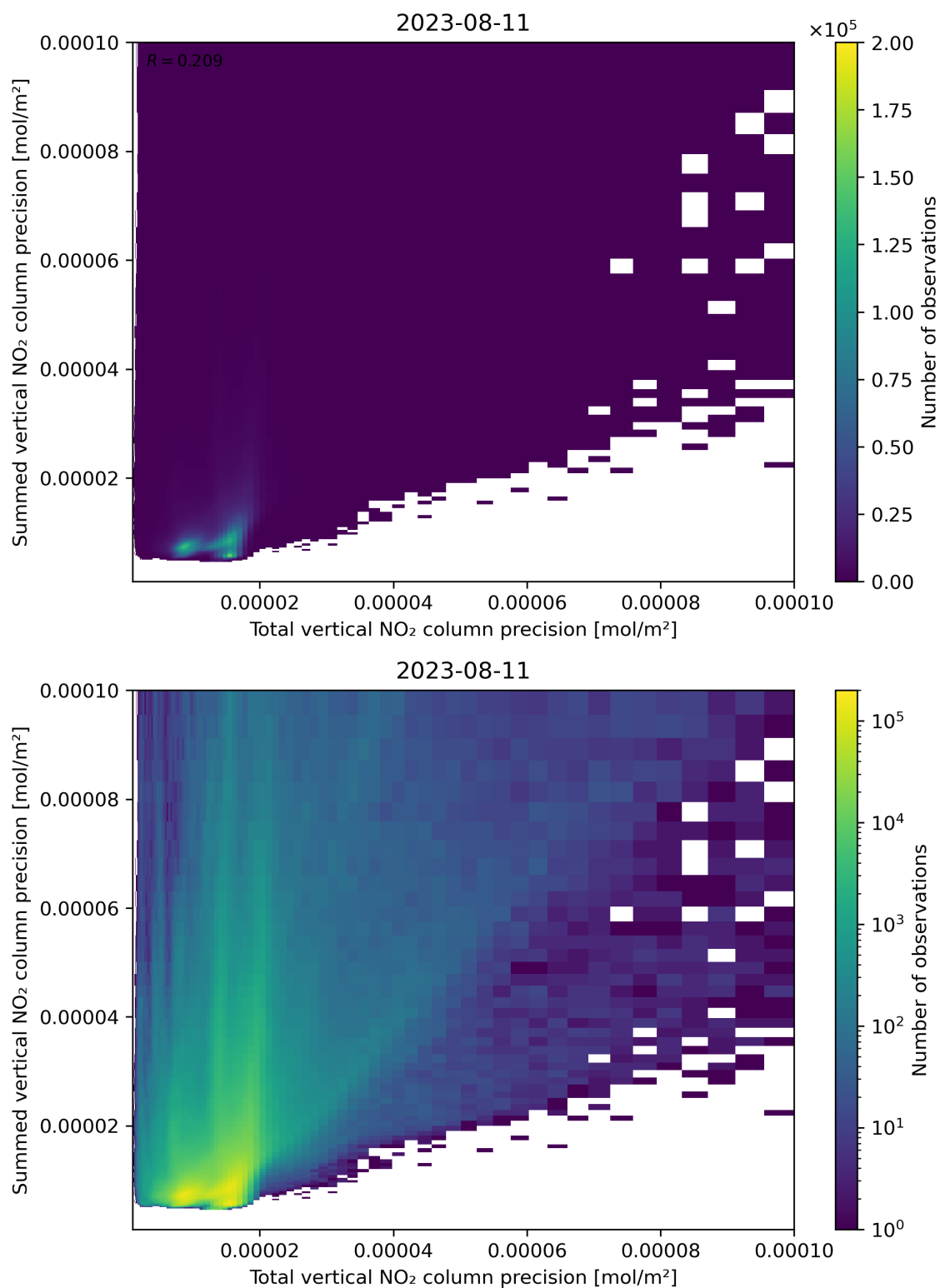
Figure 118: Scatter density plot of “Total vertical NO 2 column precision” against “Summed vertical NO 2 column precision” for 2023-08-10 to 2023-08-12.
