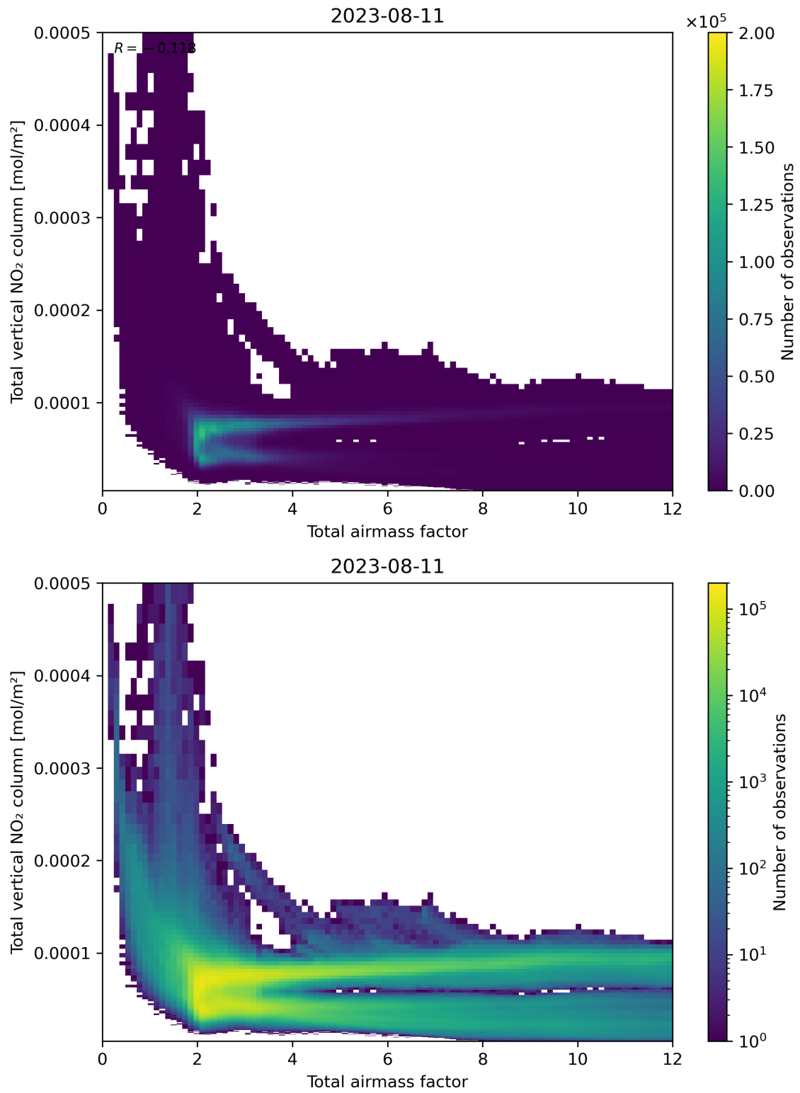
Figure 67: Scatter density plot of “Total airmass factor” against “Total vertical NO 2 column” for 2023-08-10 to 2023-08-12.
