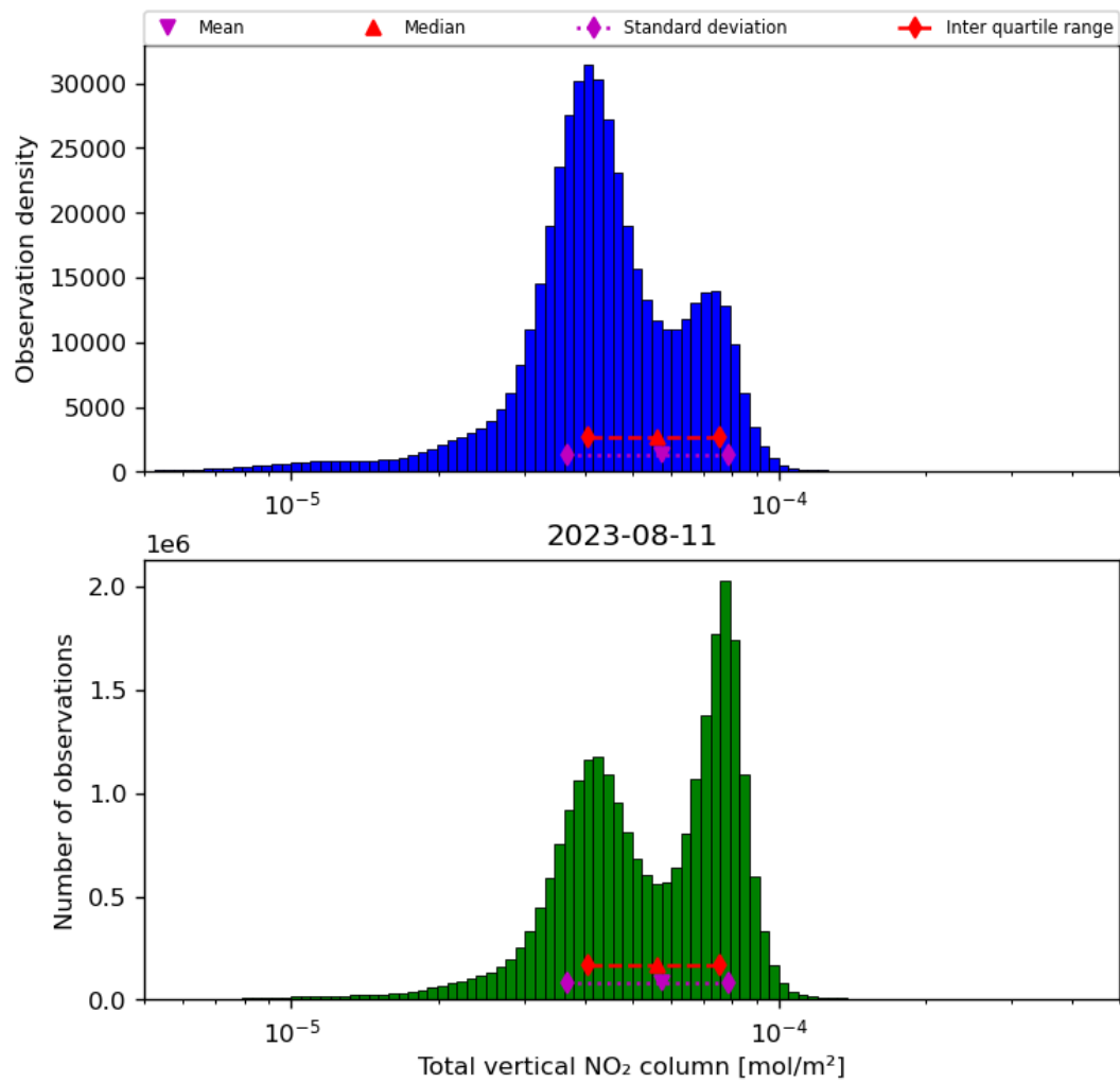
Figure 38: Histogram of “Total vertical NO 2 column” for 2023-08-10 to 2023-08-12
