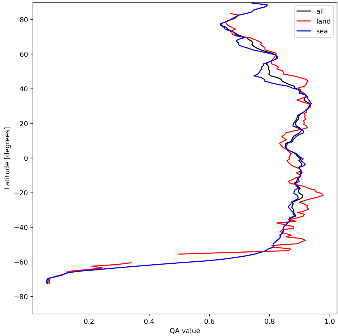
Figure 11: Zonal average of “QA value” for 2023-08-10 to 2023-08-12.
