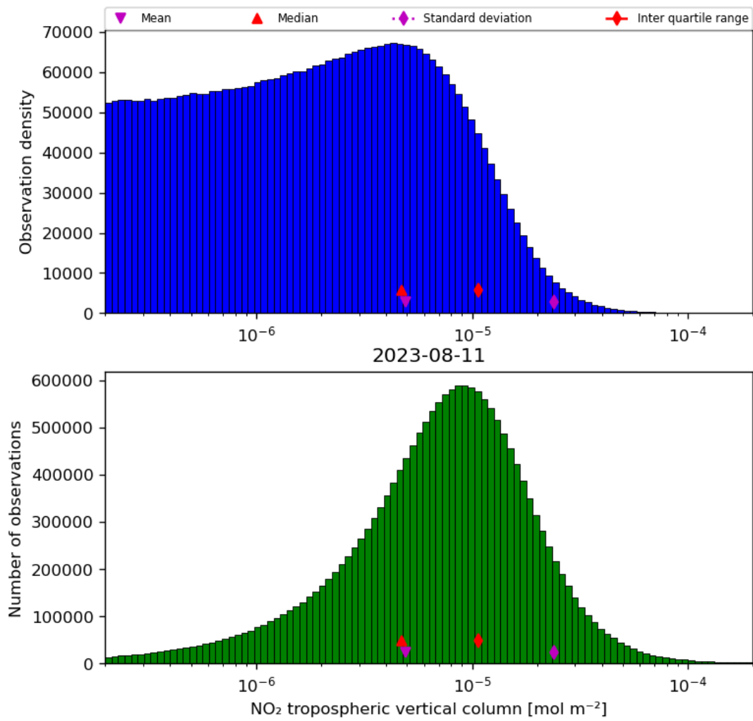
Figure 29: Histogram of “NO 2 tropospheric vertical column” for 2023-08-10 to 2023-08-12
