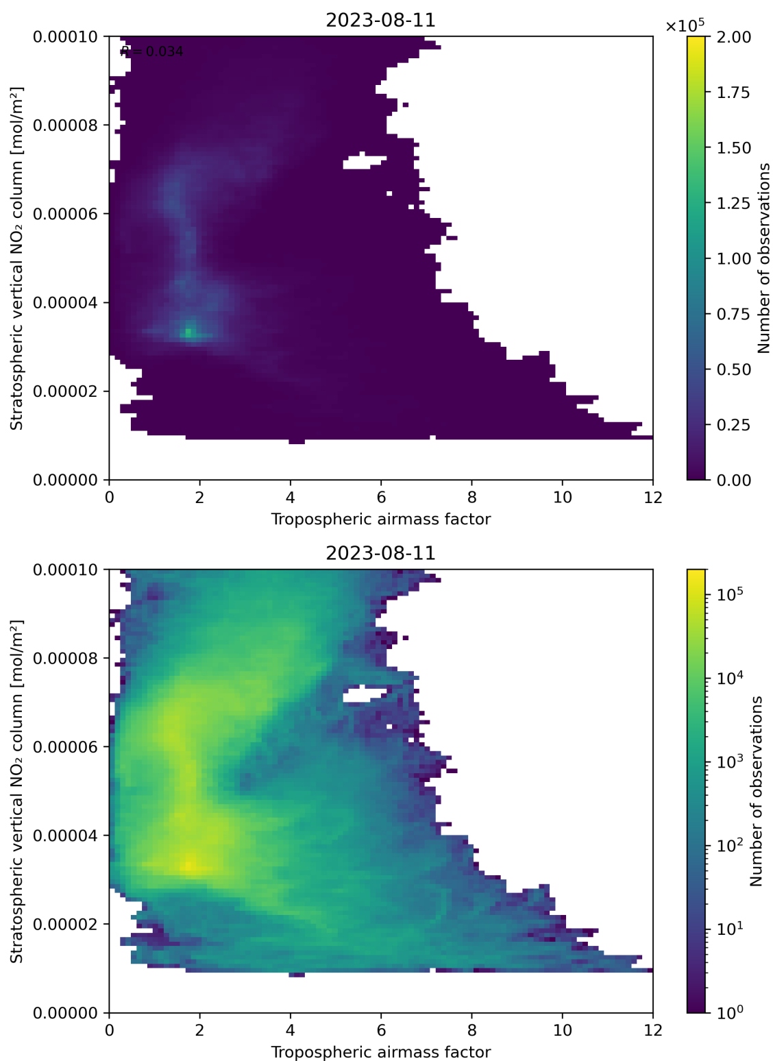
Figure 74: Scatter density plot of “Tropospheric air mass factor” against “Stratospheric vertical NO 2 column” for 2023-08-10 to 2023-08-12.
