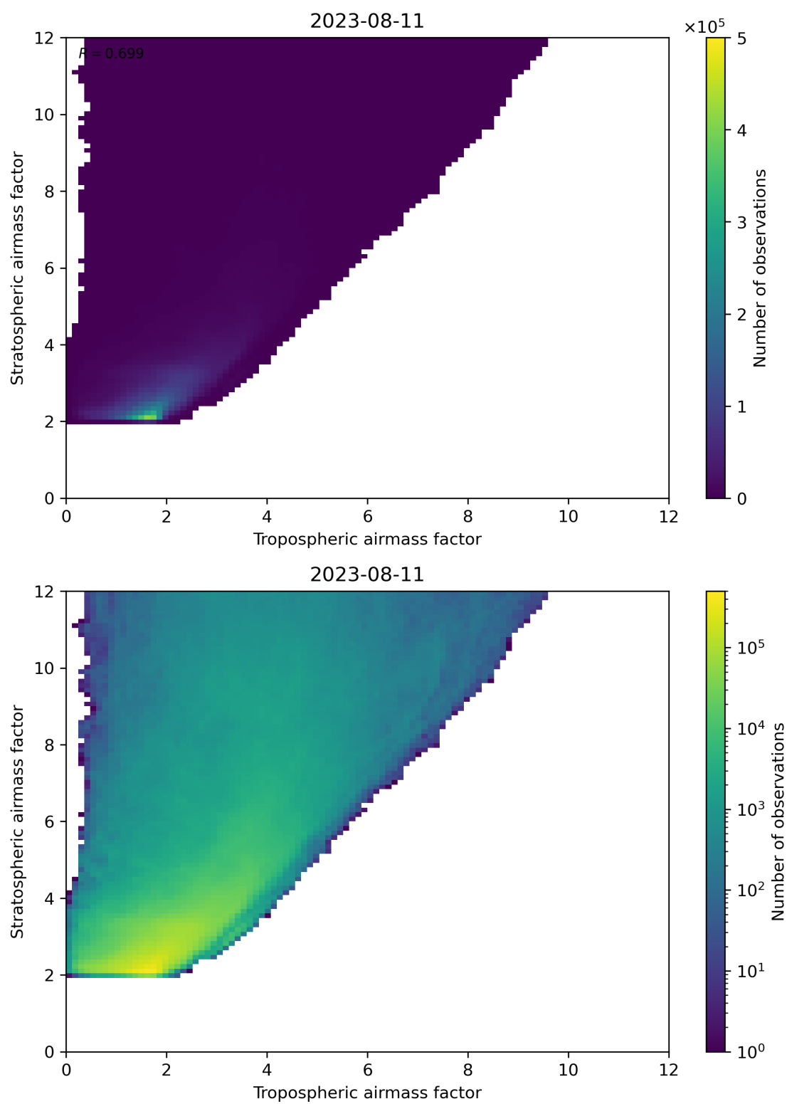
Figure 71: Scatter density plot of “Tropospheric airmass factor” against “Stratospheric airmass factor” for 2023-08-10 to 2023-08-12.
