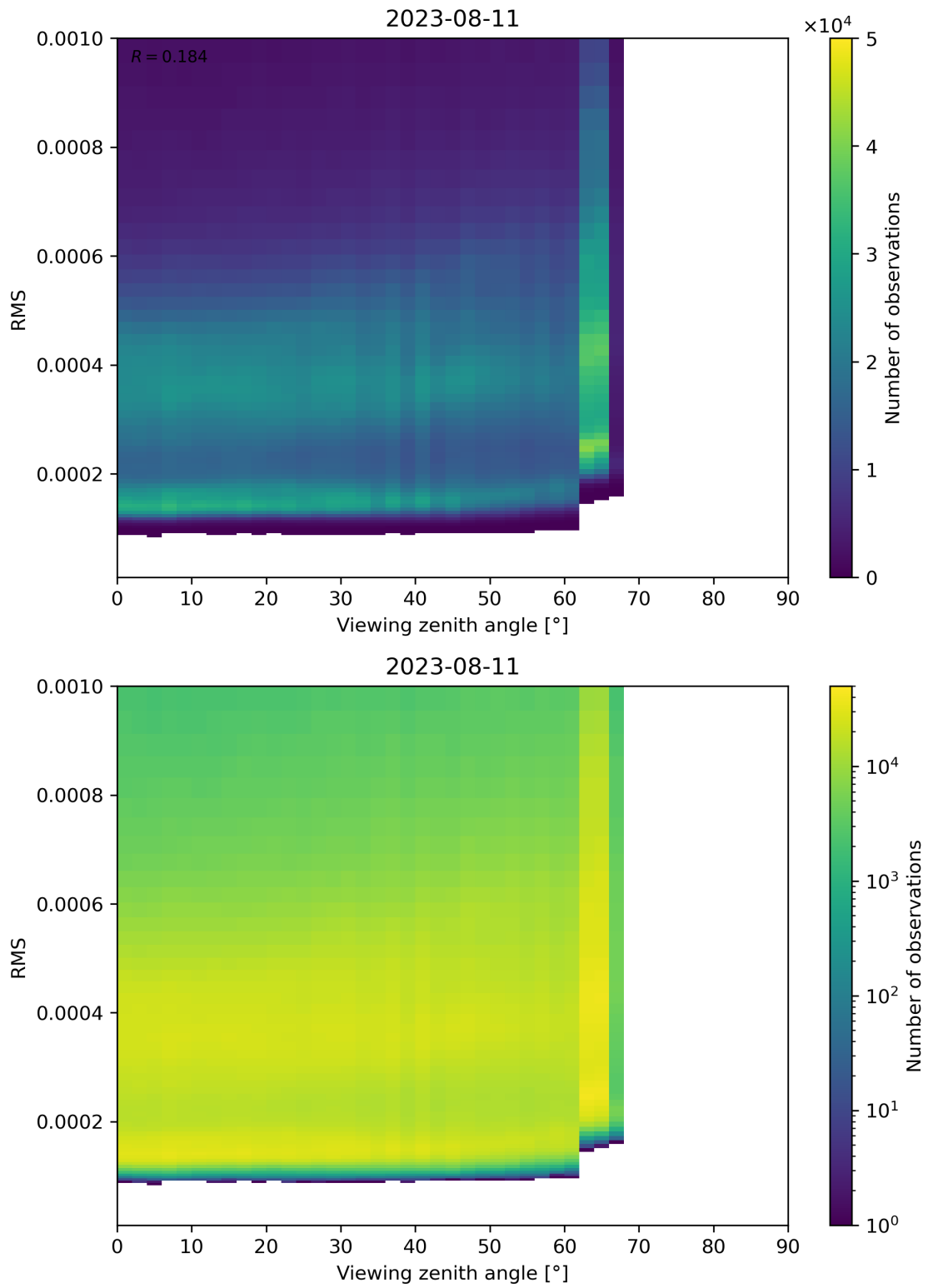
Figure 171: Scatter density plot of “Viewing zenith angle” against “RMS” for 2023-08-10 to 2023-08-12.
