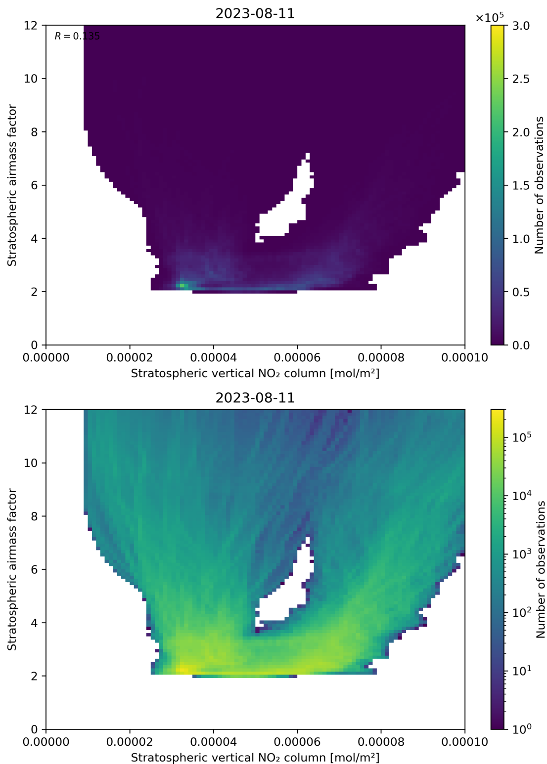
Figure 96: Scatter density plot of “Stratospheric vertical NO 2 column” against “Stratospheric airmass factor” for 2023-08-10 to 2023-08-12.
