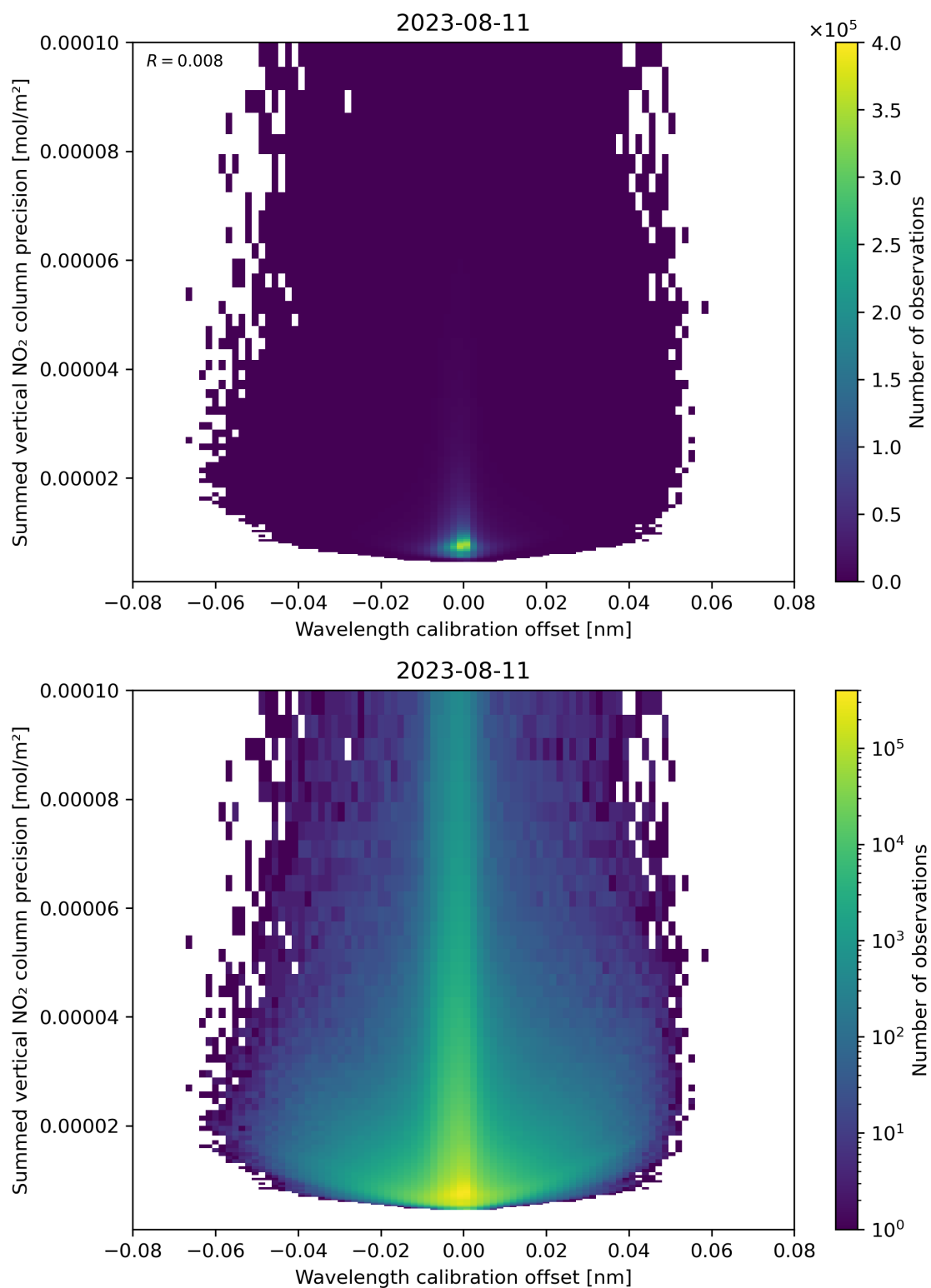
Figure 178: Scatter density plot of “Wavelength calibration offset” against “Summed vertical NO 2 column precision” for 2023-08-10 to 2023-08-12.
