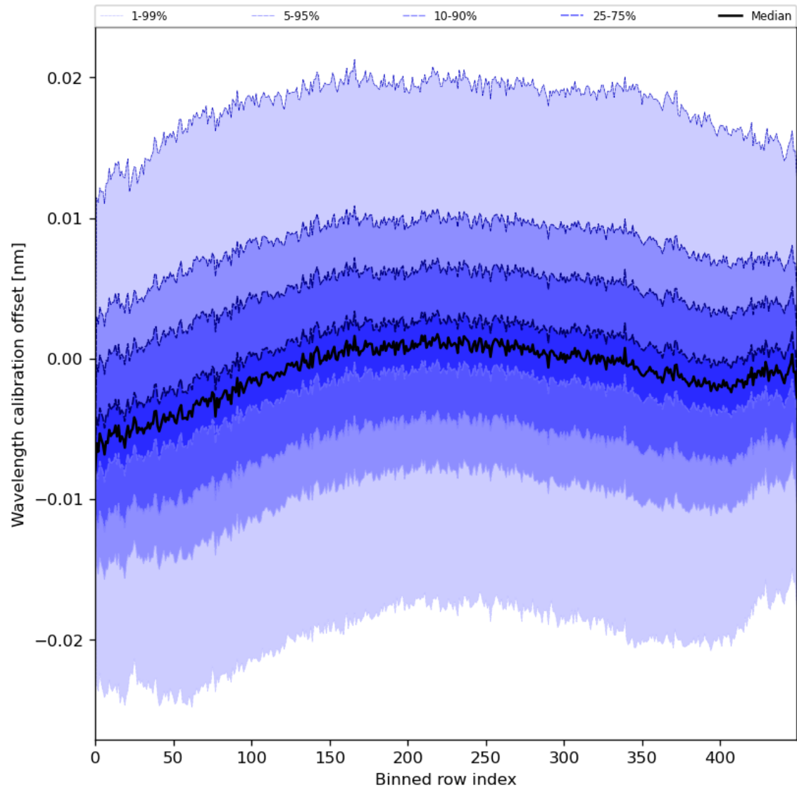
Figure 52: Along track statistics of “Wavelength calibration offset” for 2023-08-10 to 2023-08-12
