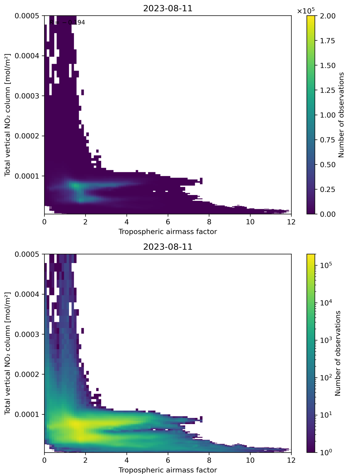
Figure 77: Scatter density plot of “Tropospheric airmass factor” against “Total vertical NO 2 column” for 2023-08-10 to 2023-08-12.
