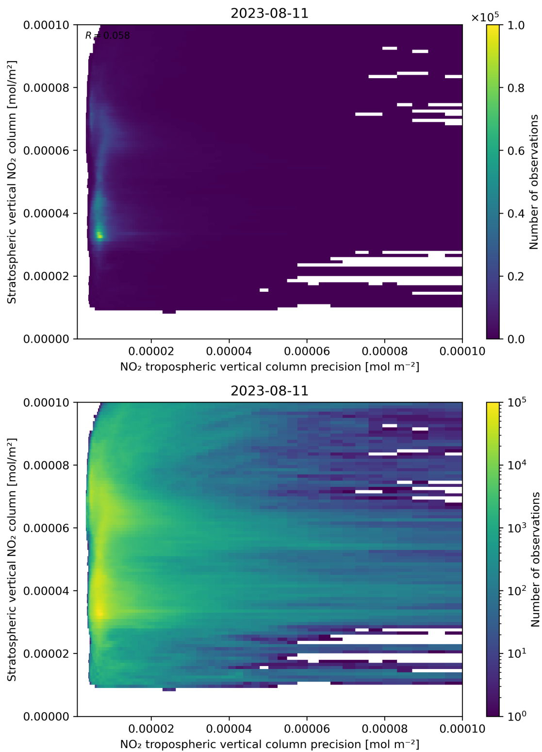
Figure 135: Scatter density plot of “NO 2 tropospheric vertical column precision” against “Stratospheric vertical NO 2 column” for 2023-08-10 to 2023-08-12.
