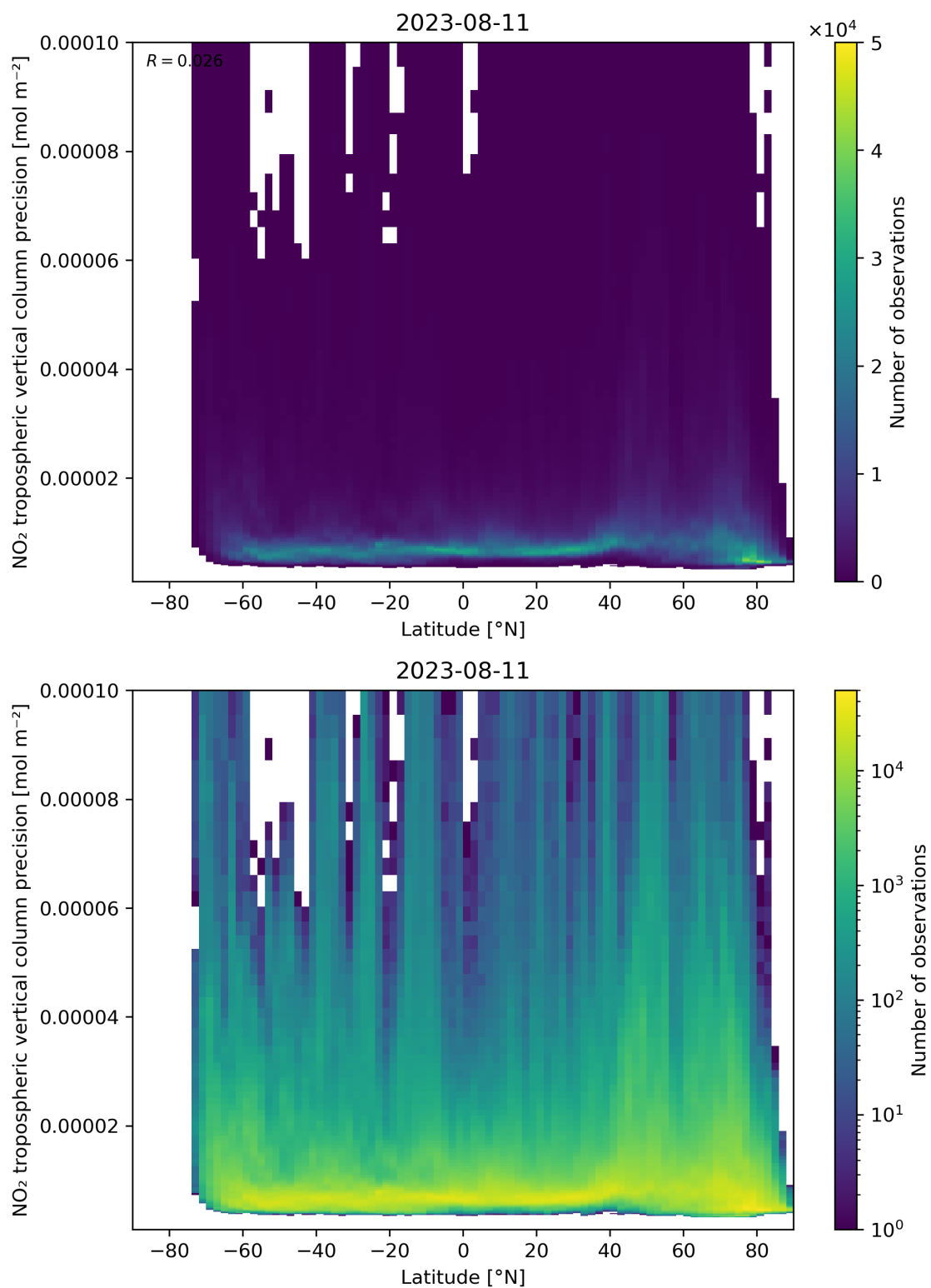
Figure 93: Scatter density plot of “Latitude” against “NO 2 tropospheric vertical column precision” for 2023-08-10 to 2023-08-12.
