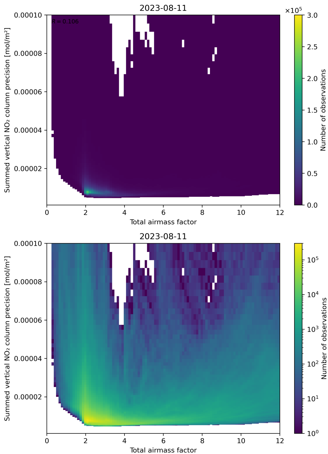
Figure 66: Scatter density plot of “Total airmass factor” against “Summed vertical NO 2 column precision” for 2023-08-10 to 2023-08-12.
