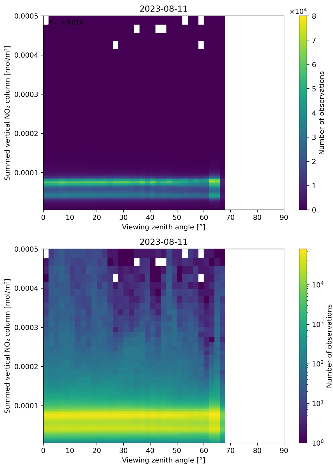
Figure 165: Scatter density plot of “Viewing zenith angle” against “Summed vertical NO 2 column” for 2023-08-10 to 2023-08-12.
