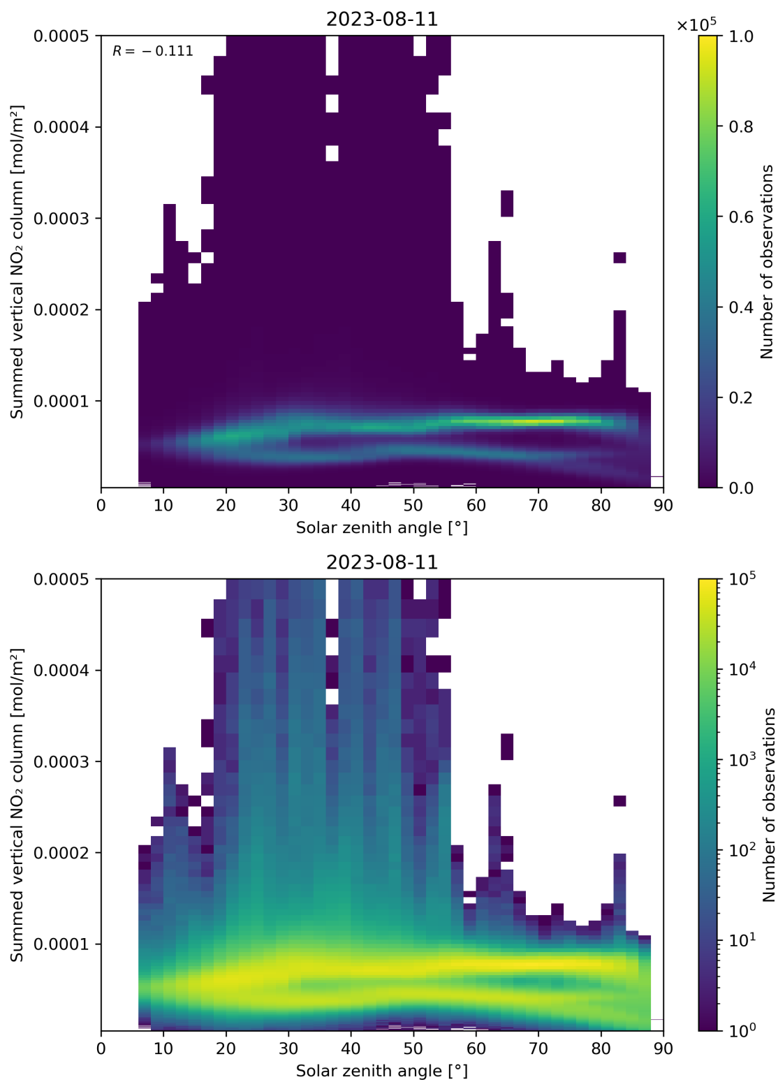
Figure 151: Scatter density plot of “Solar zenith angle” against “Summed vertical NO 2 column” for 2023-08-10 to 2023-08-12.
