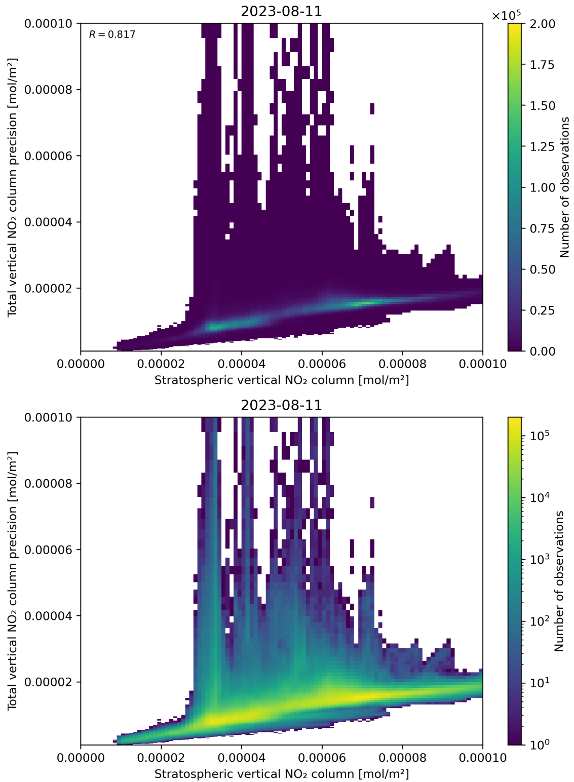
Figure 101: Scatter density plot of “Stratospheric vertical NO 2 column” against “Total vertical NO 2 column precision” for 2023-08-10 to 2023-08-12.
