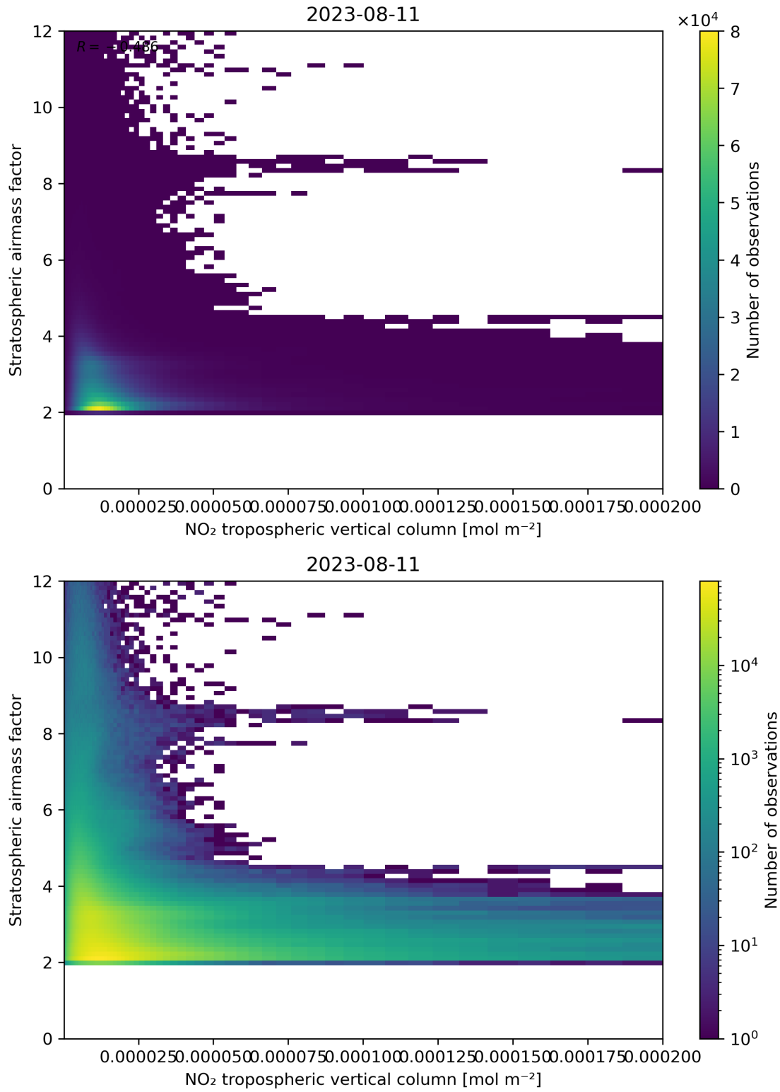
Figure 121: Scatter density plot of “NO 2 tropospheric vertical column” against “Stratospheric air mass factor” for 2023-08-10 to 2023-08-12.
