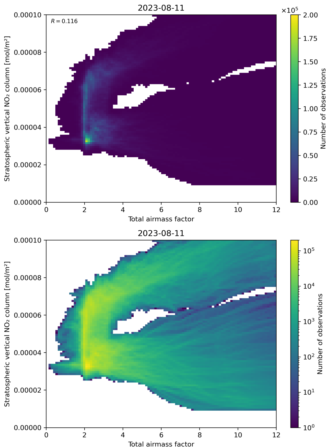
Figure 64: Scatter density plot of “Total airmass factor” against “Stratospheric vertical NO 2 column” for 2023-08-10 to 2023-08-12.
