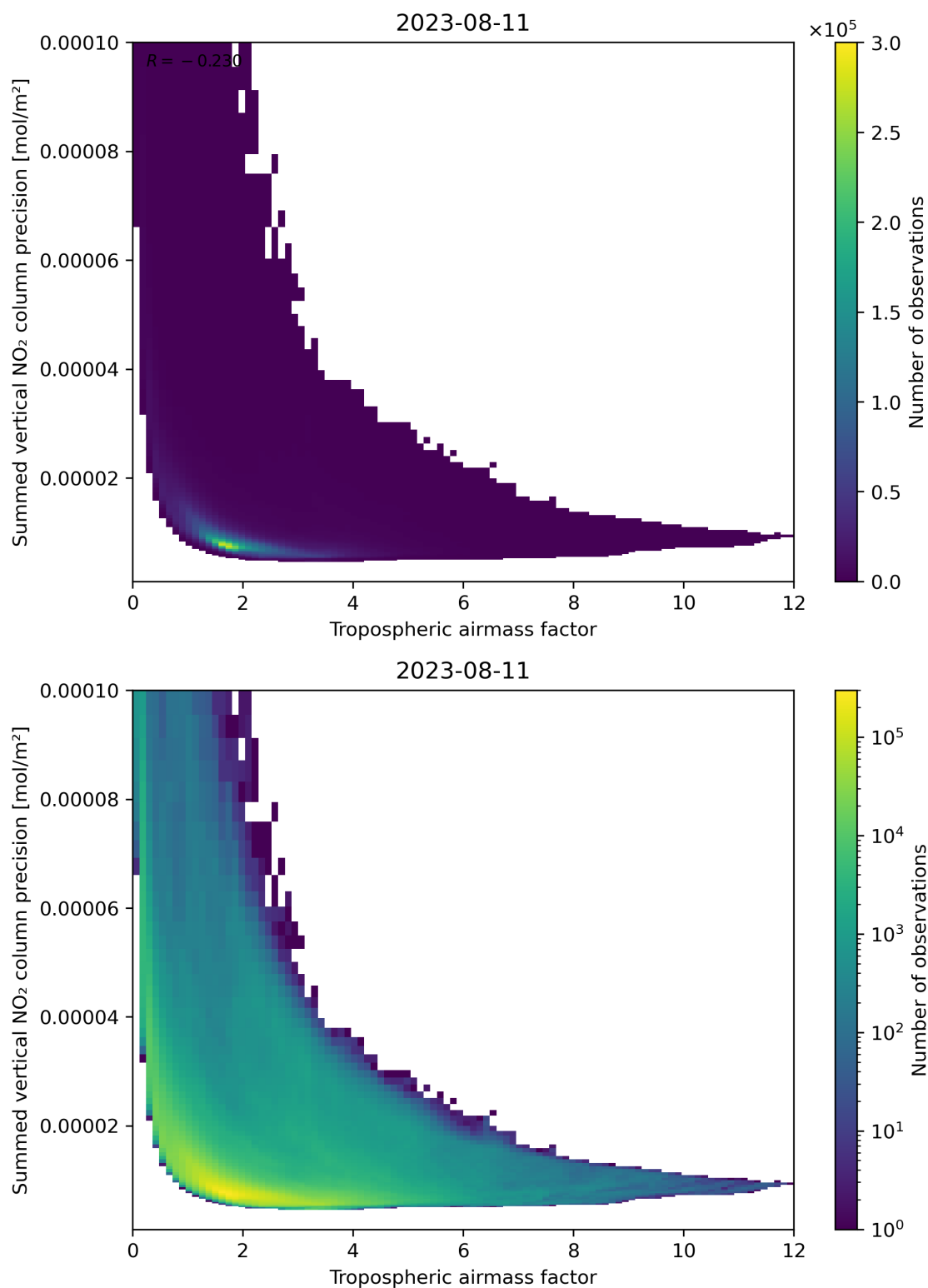
Figure 76: Scatter density plot of “Tropospheric air mass factor” against “Summed vertical NO 2 column precision” for 2023-08-10 to 2023-08-12.
