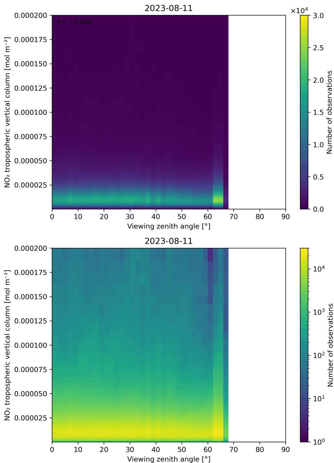
Figure 169: Scatter density plot of “Viewing zenith angle” against “NO 2 tropospheric vertical column” for 2023-08-10 to 2023-08-12.
