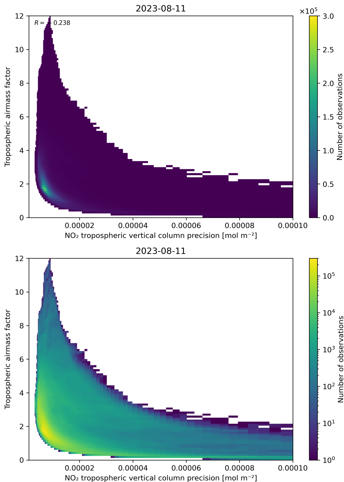
Figure 133: Scatter density plot of “NO 2 tropospheric vertical column precision” against “Tropospheric airmass factor” for 2023-08-10 to 2023-08-12.
