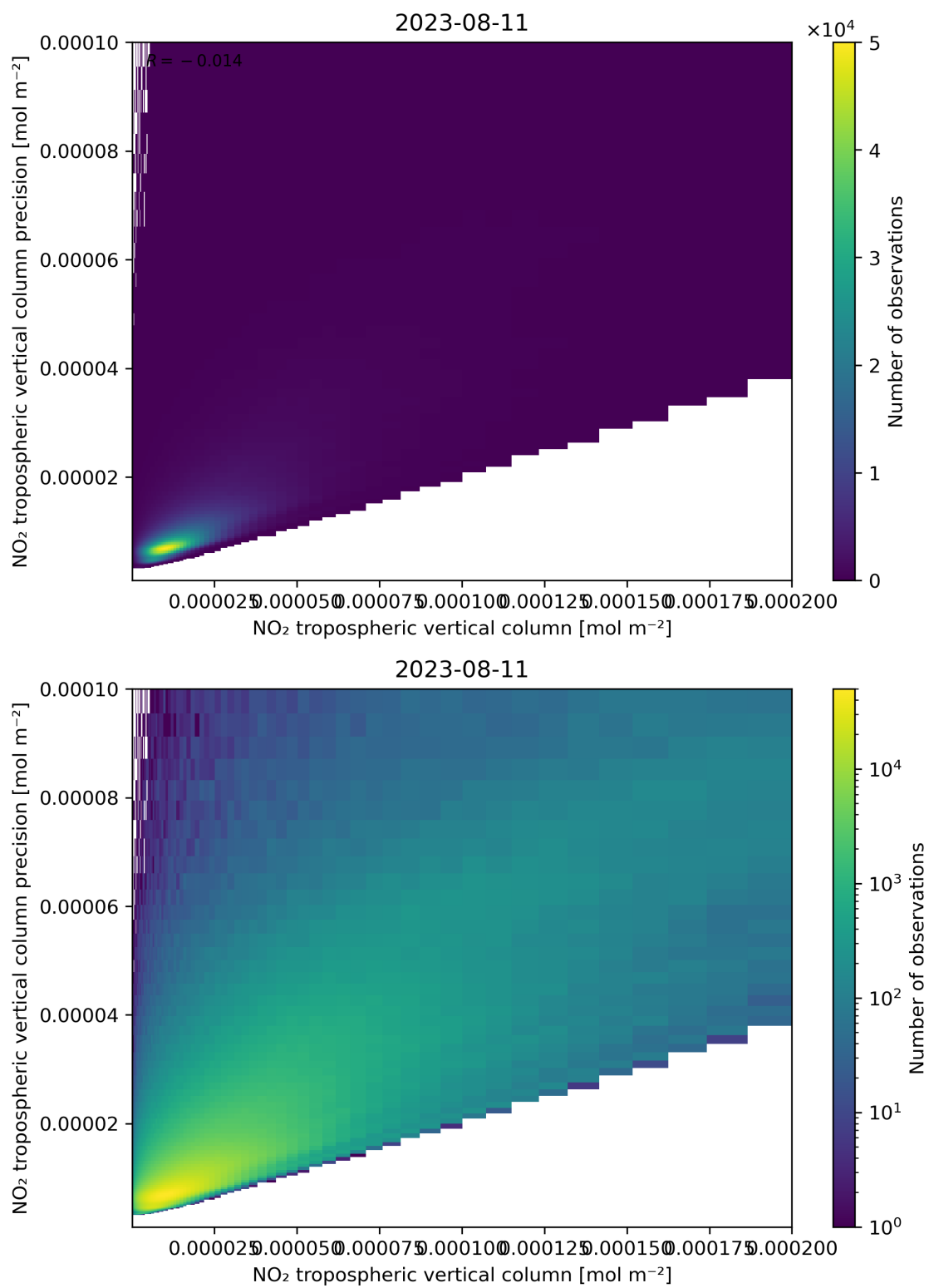
Figure 130: Scatter density plot of “NO 2 tropospheric vertical column” against “NO 2 tropospheric vertical column precision” for 2023-08-10 to 2023-08-12.
