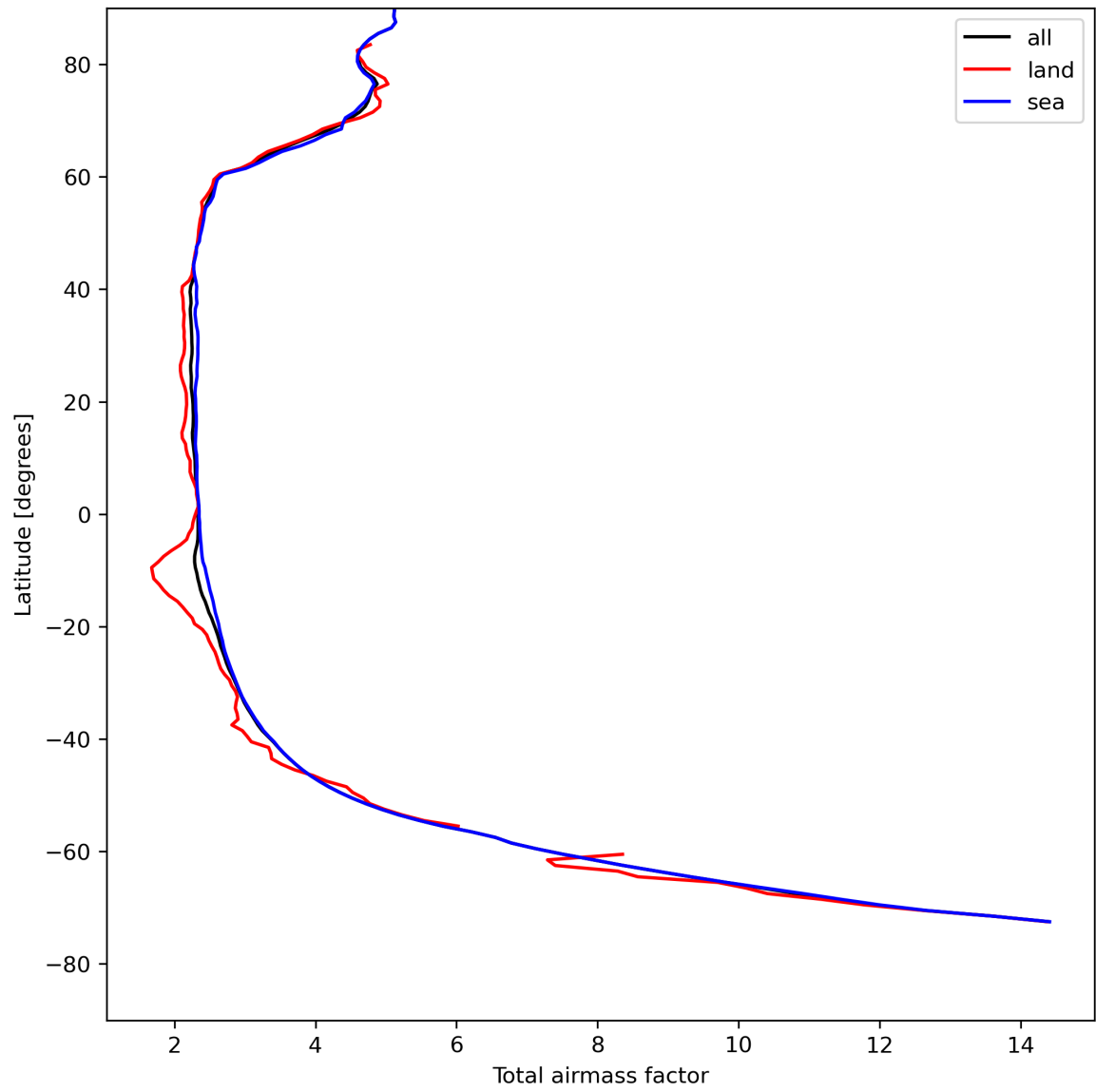
Figure 15: Zonal average of “Total airmass factor” for 2023-08-10 to 2023-08-12.
