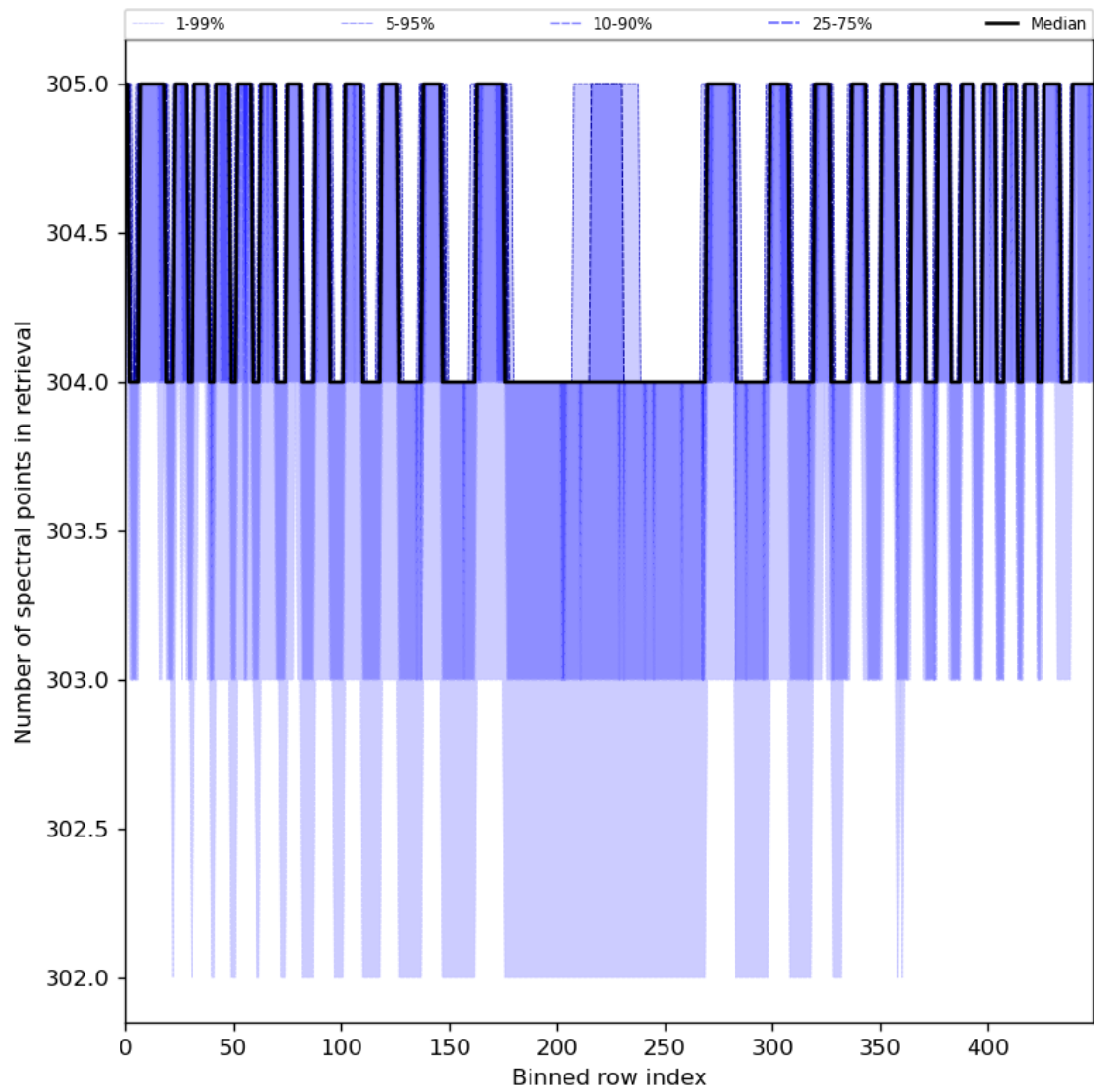
Figure 50: Along track statistics of “Number of spectral points in retrieval” for 2023-08-10 to 2023-08-12
