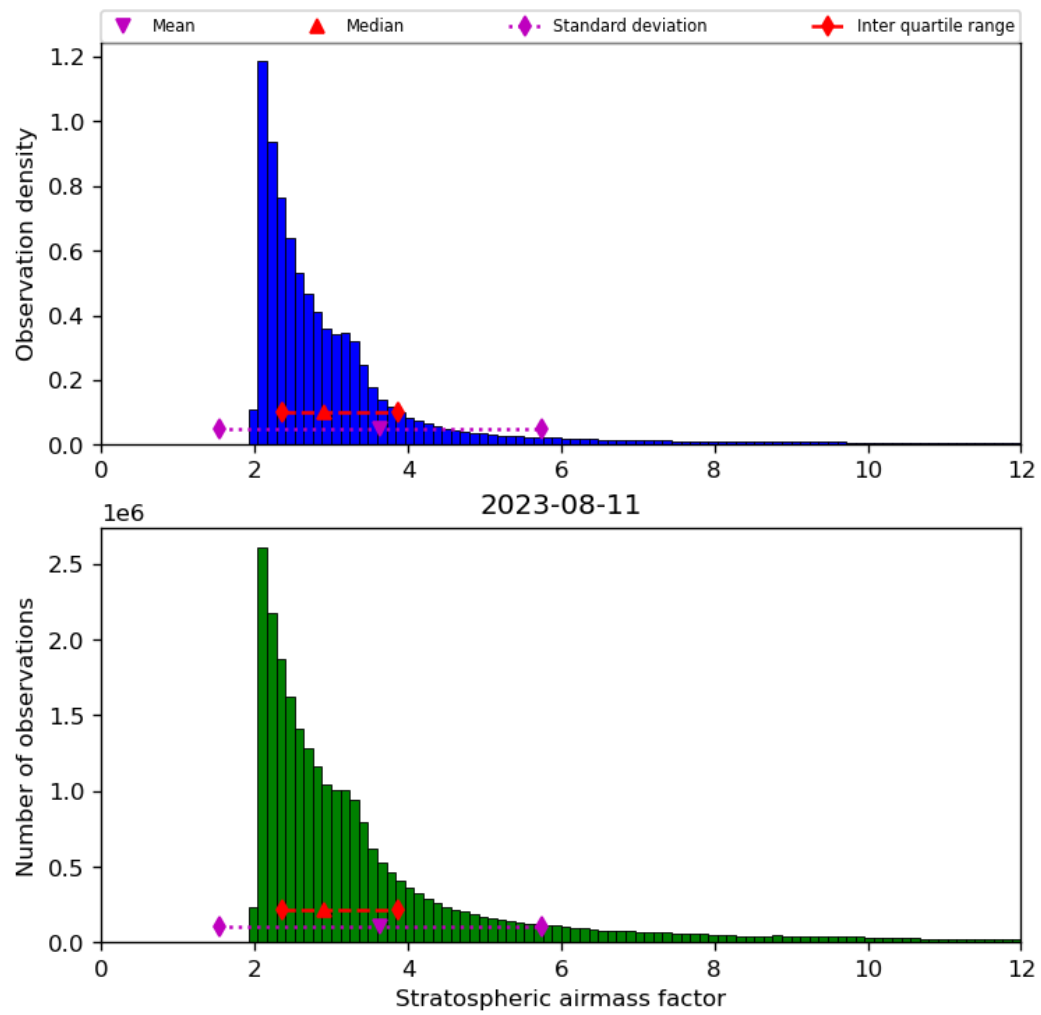
Figure 44: Histogram of “Stratospheric airmass factor” for 2023-08-10 to 2023-08-12
