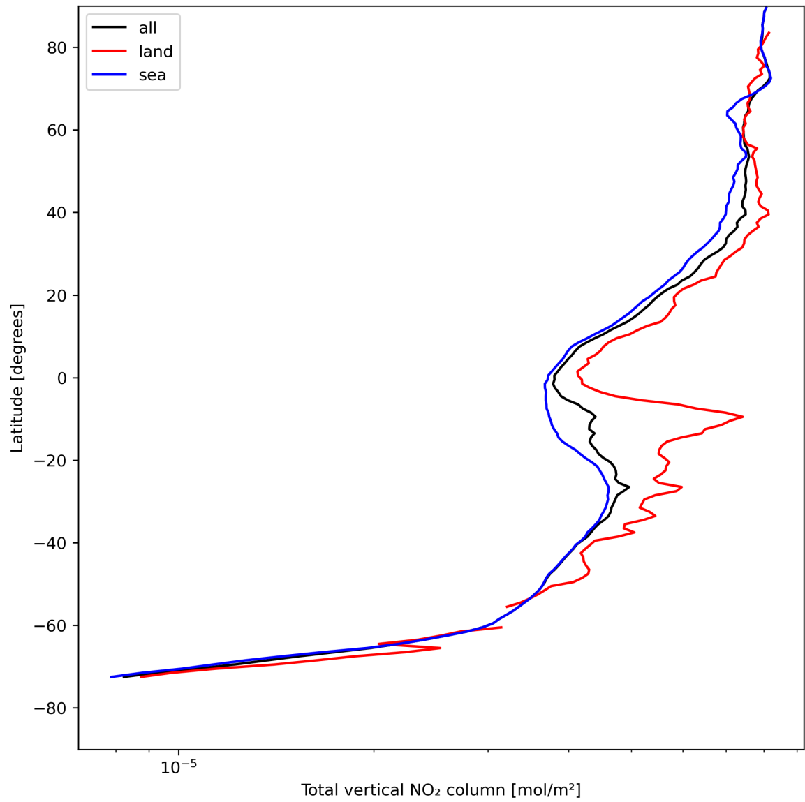
Figure 21: Zonal average of “Total vertical NO 2 column” for 2023-08-10 to 2023-08-12.
