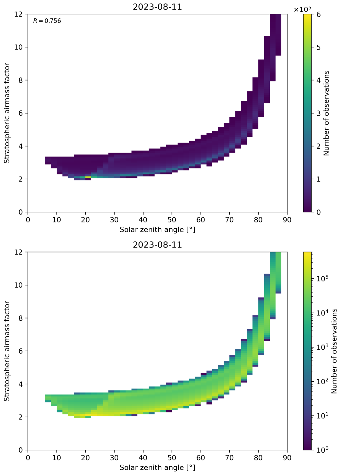
Figure 145: Scatter density plot of “Solar zenith angle” against “Stratospheric airmass factor” for 2023-08-10 to 2023-08-12.
