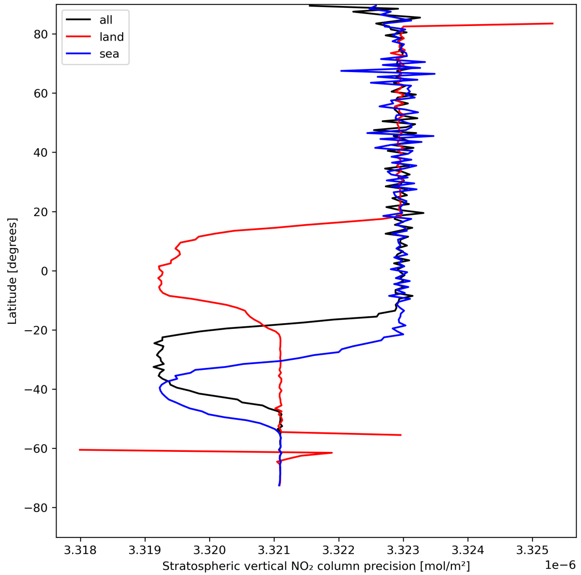
Figure 20: Zonal average of “Stratospheric vertical NO 2 column precision” for 2023-08-10 to 2023-08-12.
