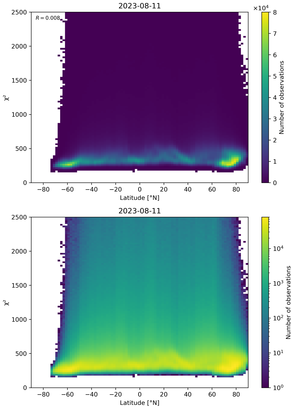
Figure 86: Scatter density plot of “Latitude” against “ \chi^2 ” for 2023-08-10 to 2023-08-12.
