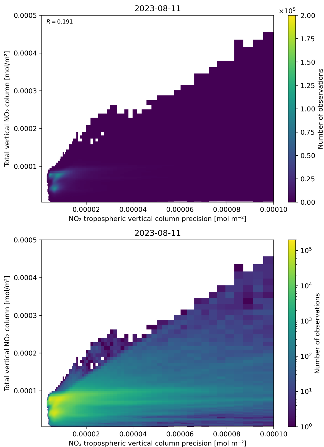
Figure 138: Scatter density plot of “NO 2 tropospheric vertical column precision” against “Total vertical NO 2 column” for 2023-08-10 to 2023-08-12.
