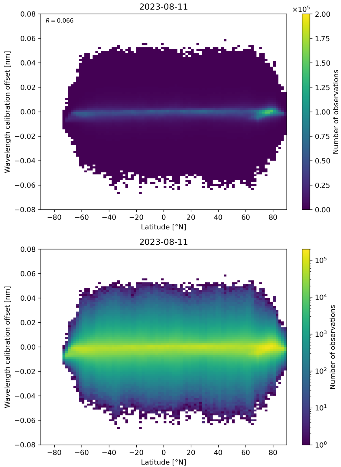
Figure 95: Scatter density plot of “Latitude” against “Wavelength calibration offset” for 2023-08-10 to 2023-08-12.
