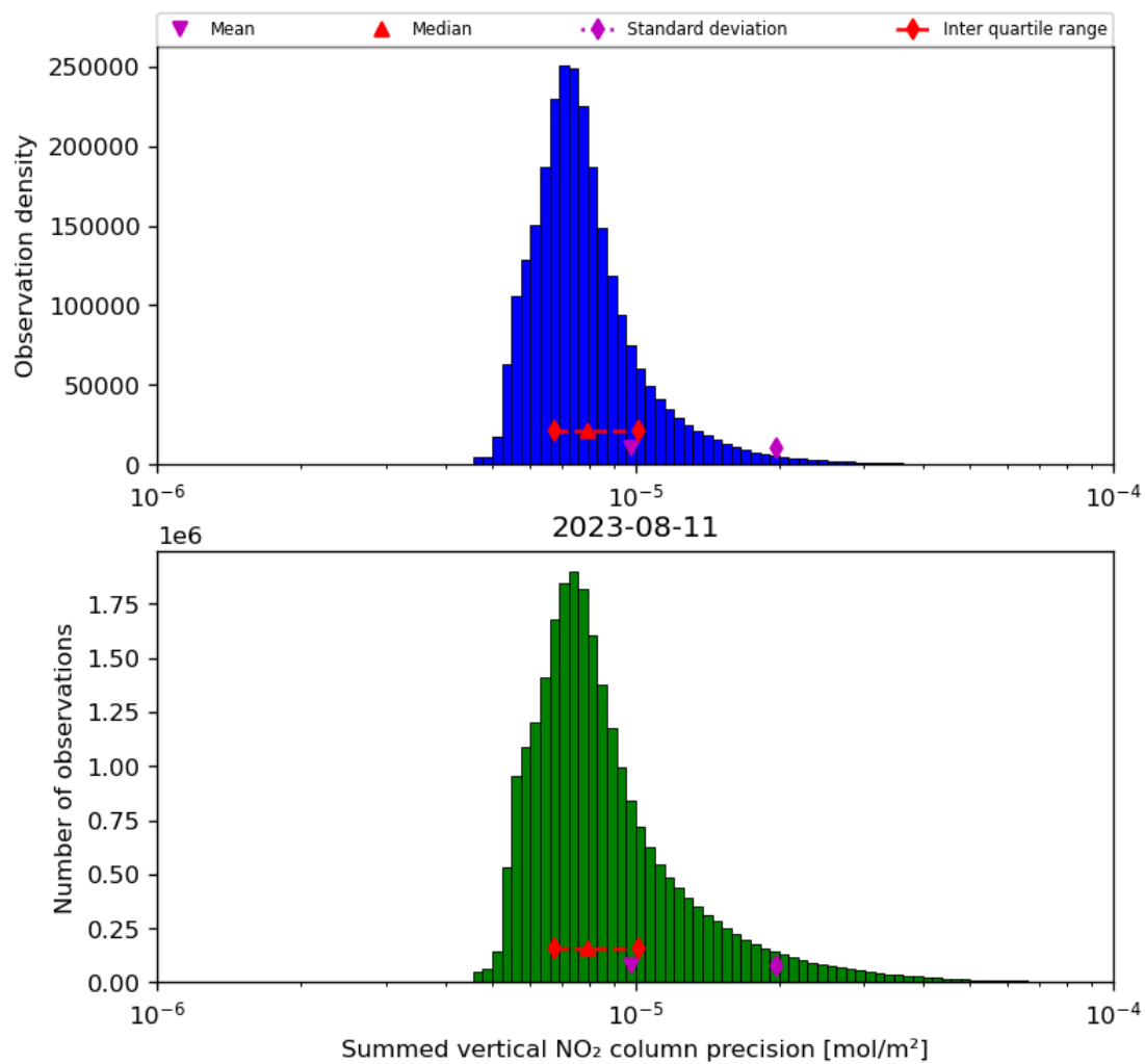
Figure 41: Histogram of “Summed vertical NO 2 column precision” for 2023-08-10 to 2023-08-12
