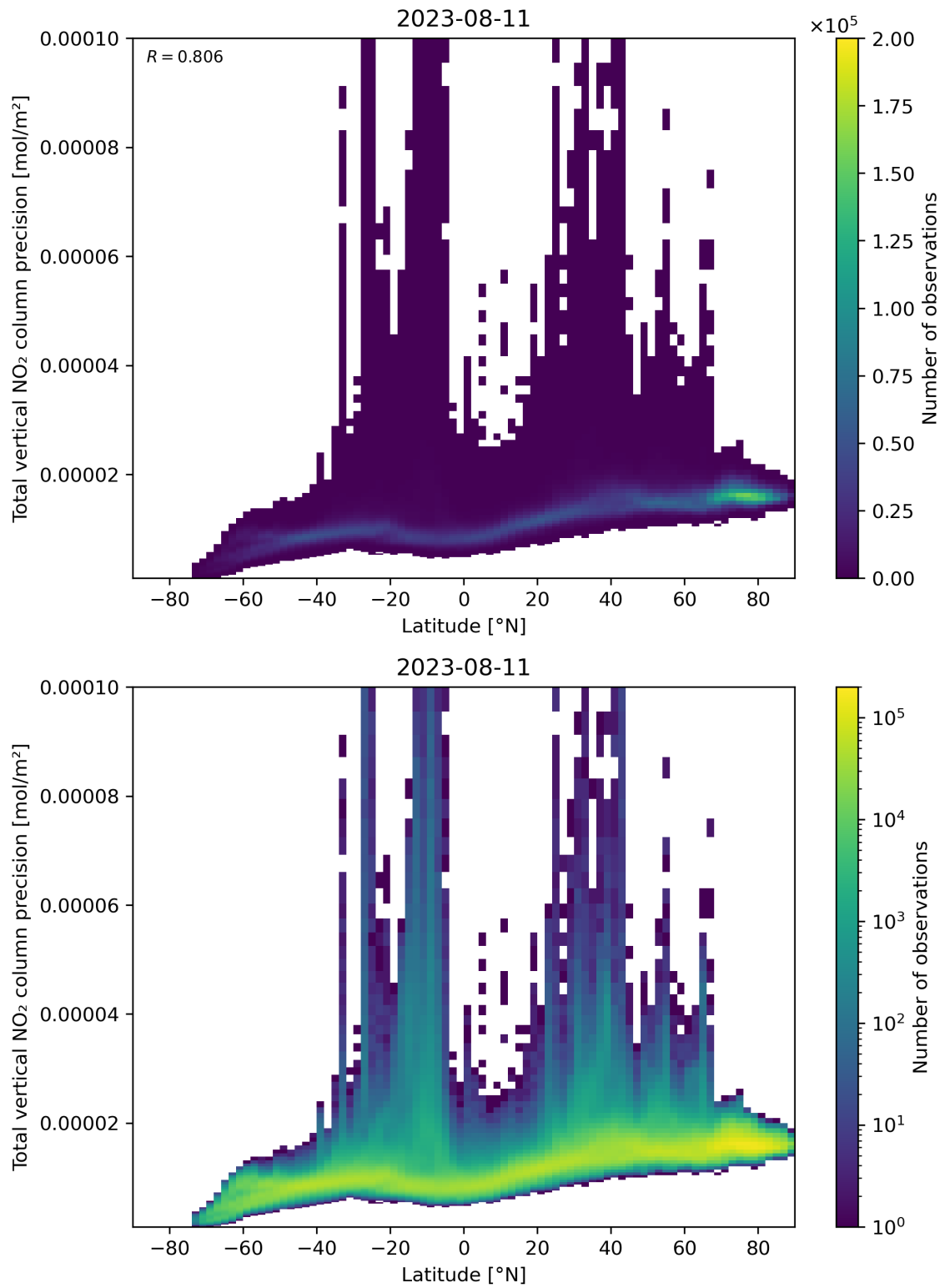
Figure 91: Scatter density plot of “Latitude” against “Total vertical NO 2 column precision” for 2023-08-10 to 2023-08-12.
