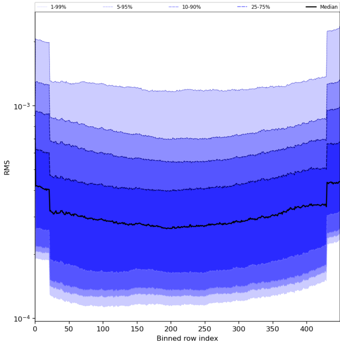
Figure 60: Along track statistics of “RMS” for 2023-08-10 to 2023-08-12
