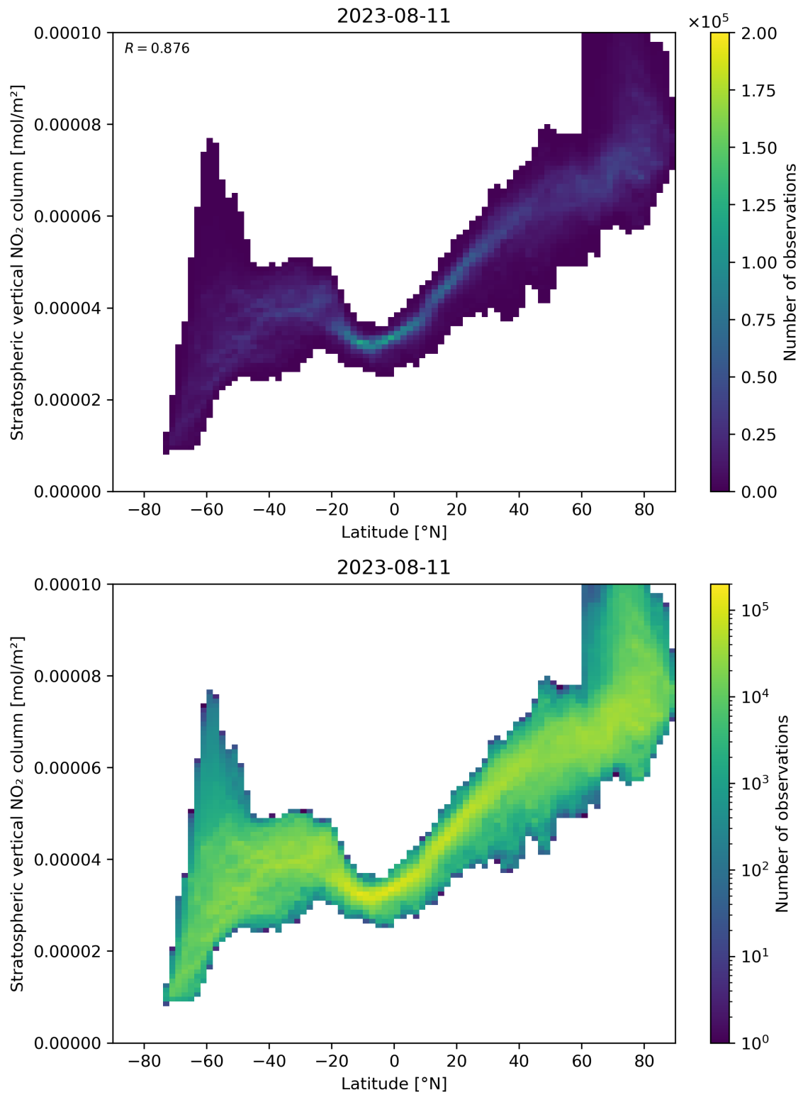
Figure 87: Scatter density plot of “Latitude” against “Stratospheric vertical NO 2 column” for 2023-08-10 to 2023-08-12.
