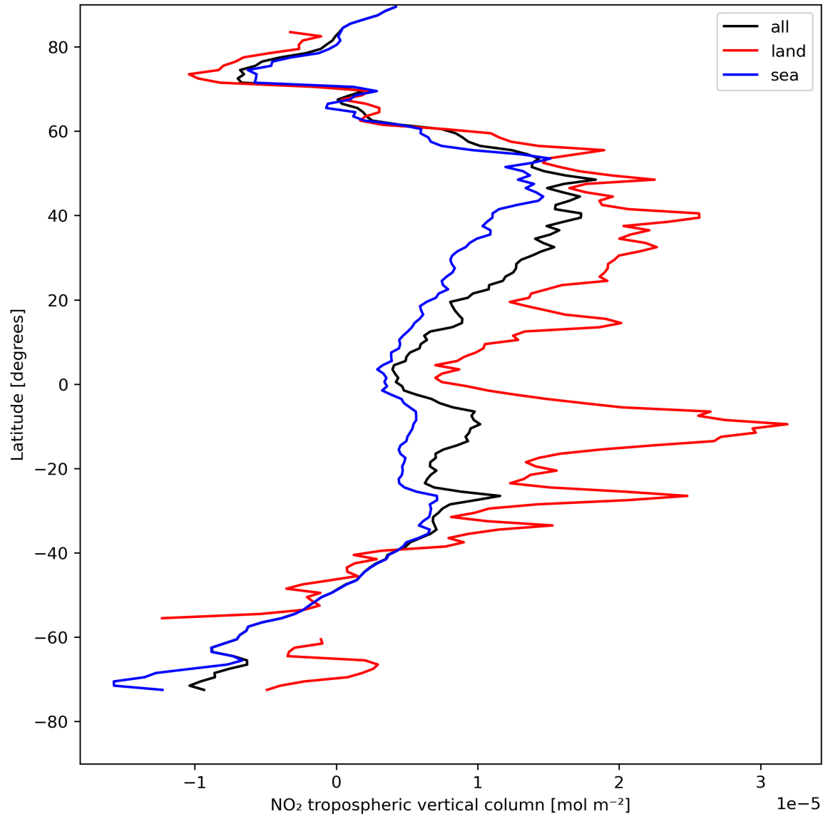
Figure 12: Zonal average of “NO 2 tropospheric vertical column” for 2023-08-10 to 2023-08-12.
