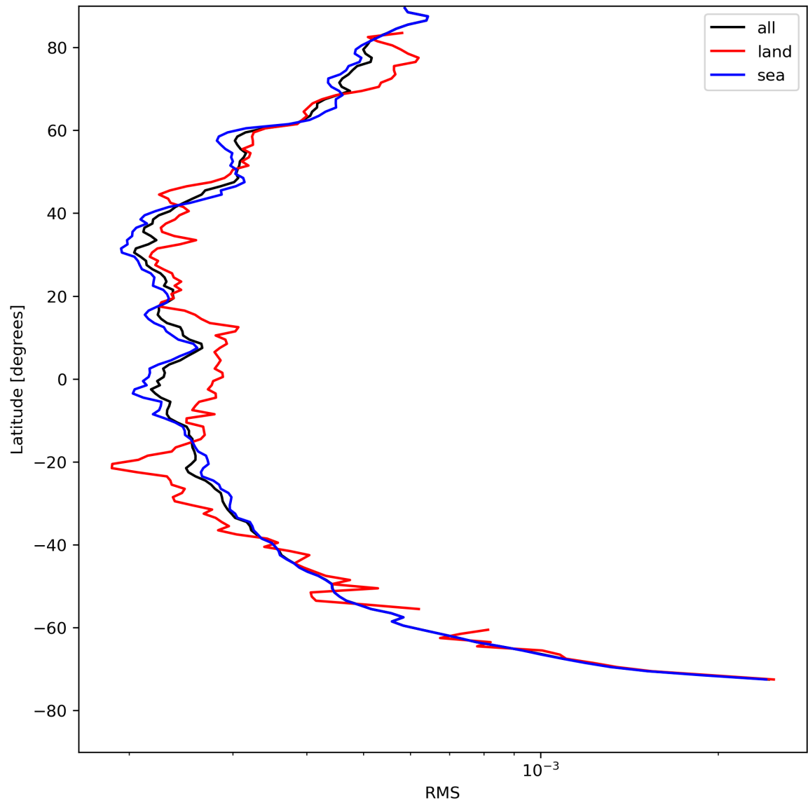
Figure 26: Zonal average of “RMS” for 2023-08-10 to 2023-08-12.
