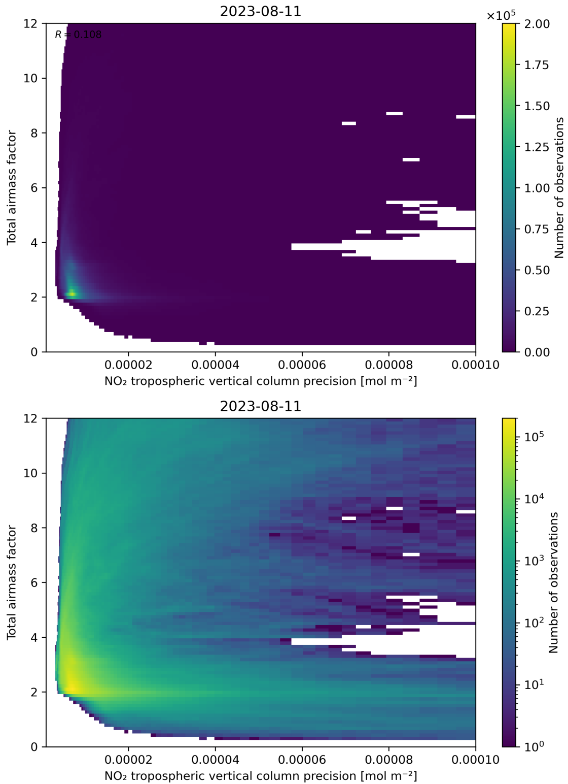
Figure 132: Scatter density plot of “NO 2 tropospheric vertical column precision” against “Total air mass factor” for 2023-08-10 to 2023-08-12.
