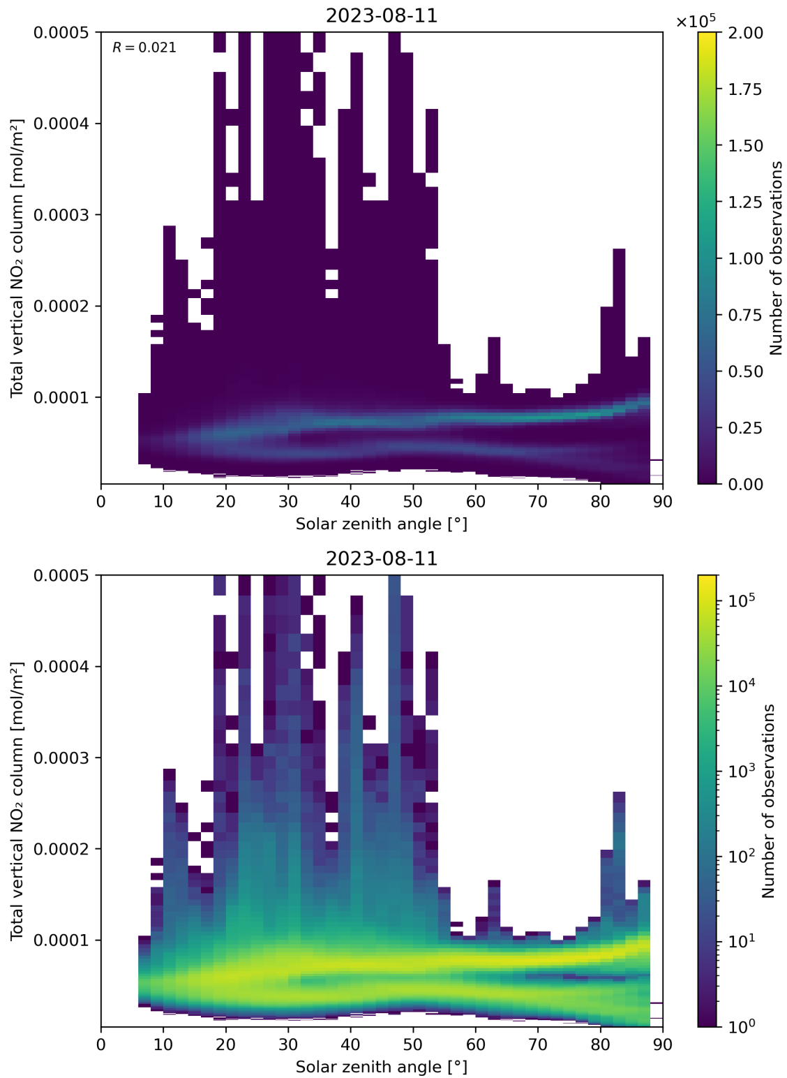
Figure 153: Scatter density plot of “Solar zenith angle” against “Total vertical NO 2 column” for 2023-08-10 to 2023-08-12.
