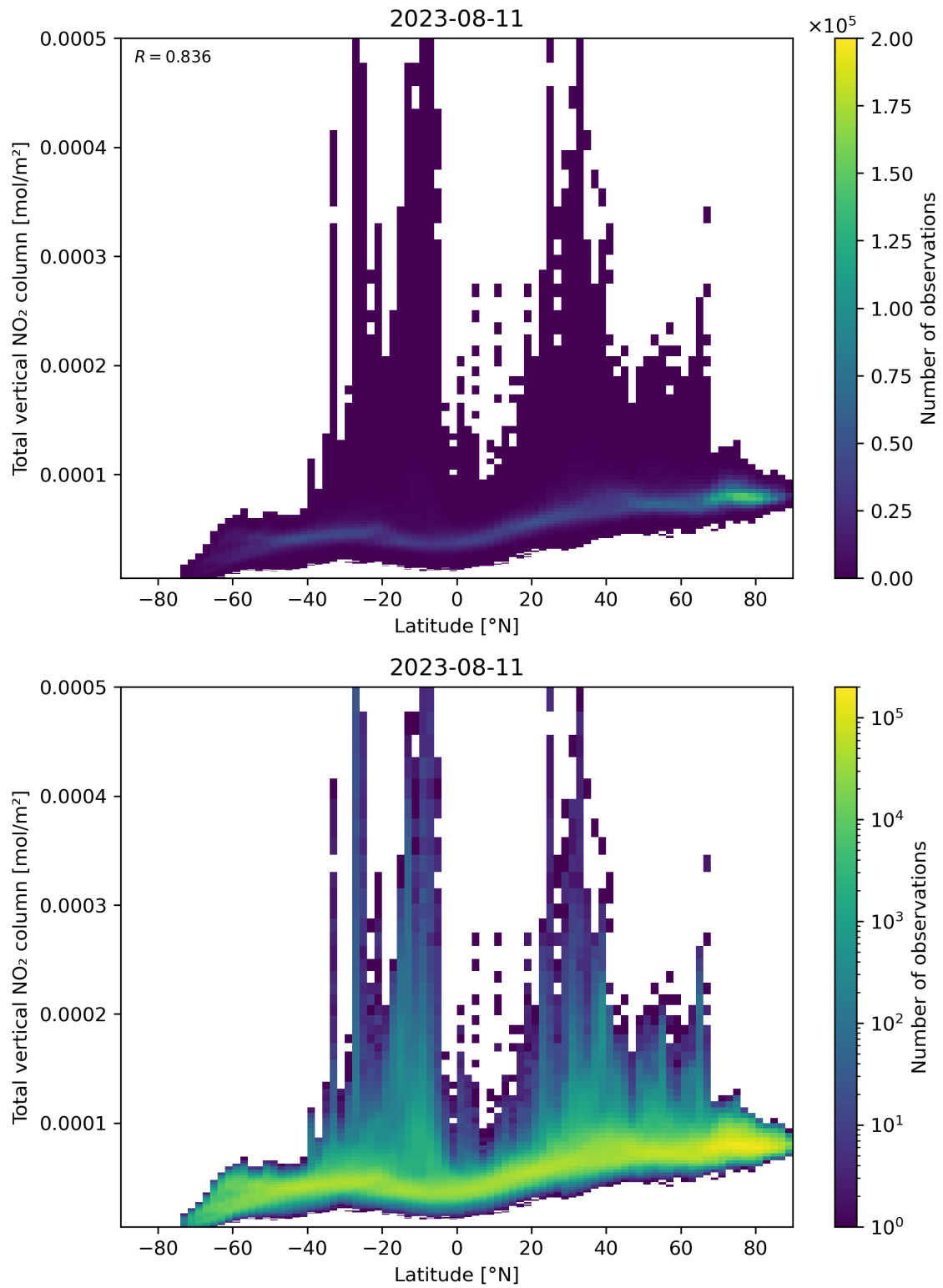
Figure 90: Scatter density plot of “Latitude” against “Total vertical NO 2 column” for 2023-08-10 to 2023-08-12.
