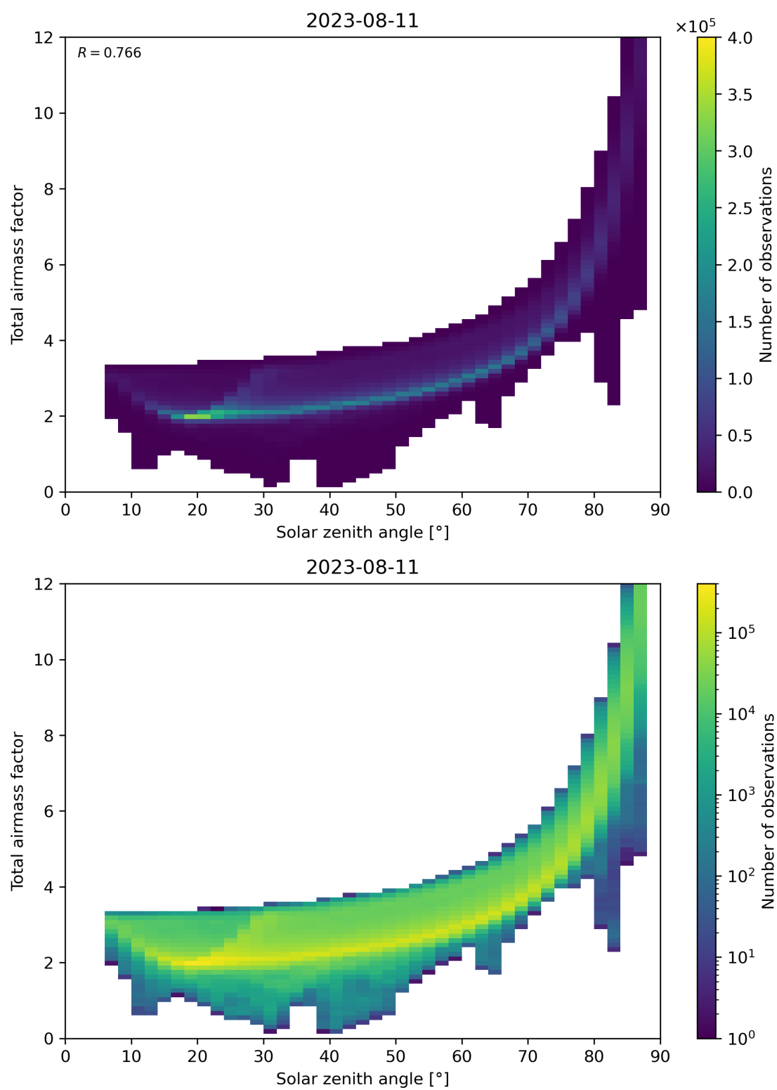
Figure 146: Scatter density plot of “Solar zenith angle” against “Total air mass factor” for 2023-08-10 to 2023-08-12.
