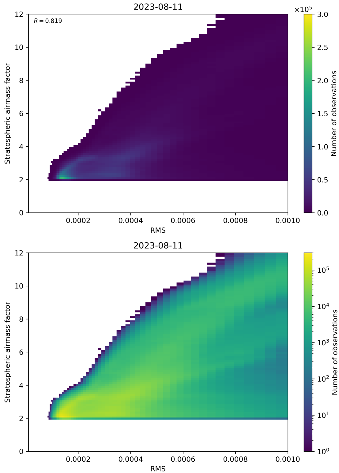
Figure 144: Scatter density plot of “RMS” against “Stratospheric airmass factor” for 2023-08-10 to 2023-08-12.
