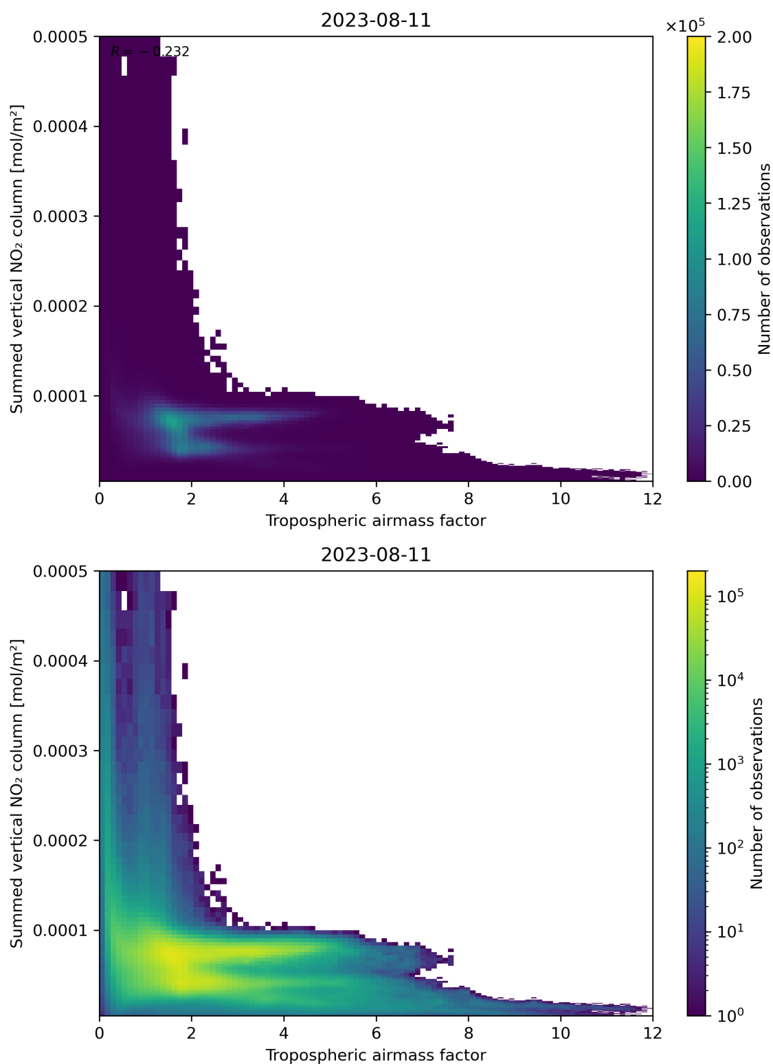
Figure 75: Scatter density plot of “Tropospheric airmass factor” against “Summed vertical NO 2 column” for 2023-08-10 to 2023-08-12.
