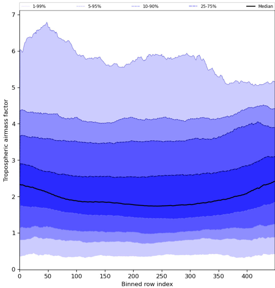
Figure 48: Along track statistics of “Tropospheric airmass factor” for 2023-08-10 to 2023-08-12
