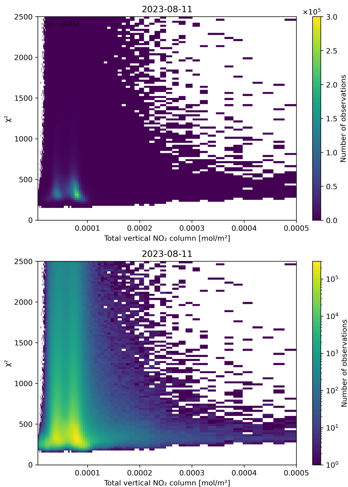
Figure 111: Scatter density plot of “Total vertical NO 2 column” against “ \chi^2 ” for 2023-08-10 to 2023-08-12.
