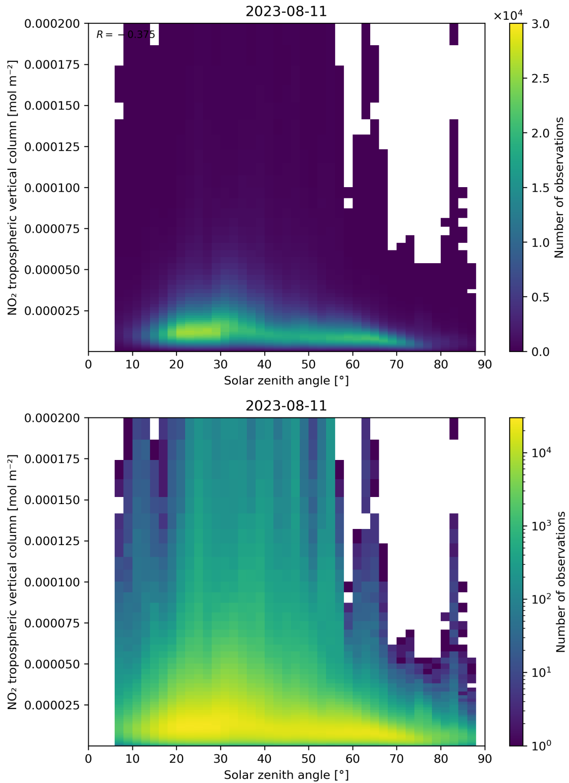
Figure 155: Scatter density plot of “Solar zenith angle” against “NO 2 tropospheric vertical column” for 2023-08-10 to 2023-08-12.
