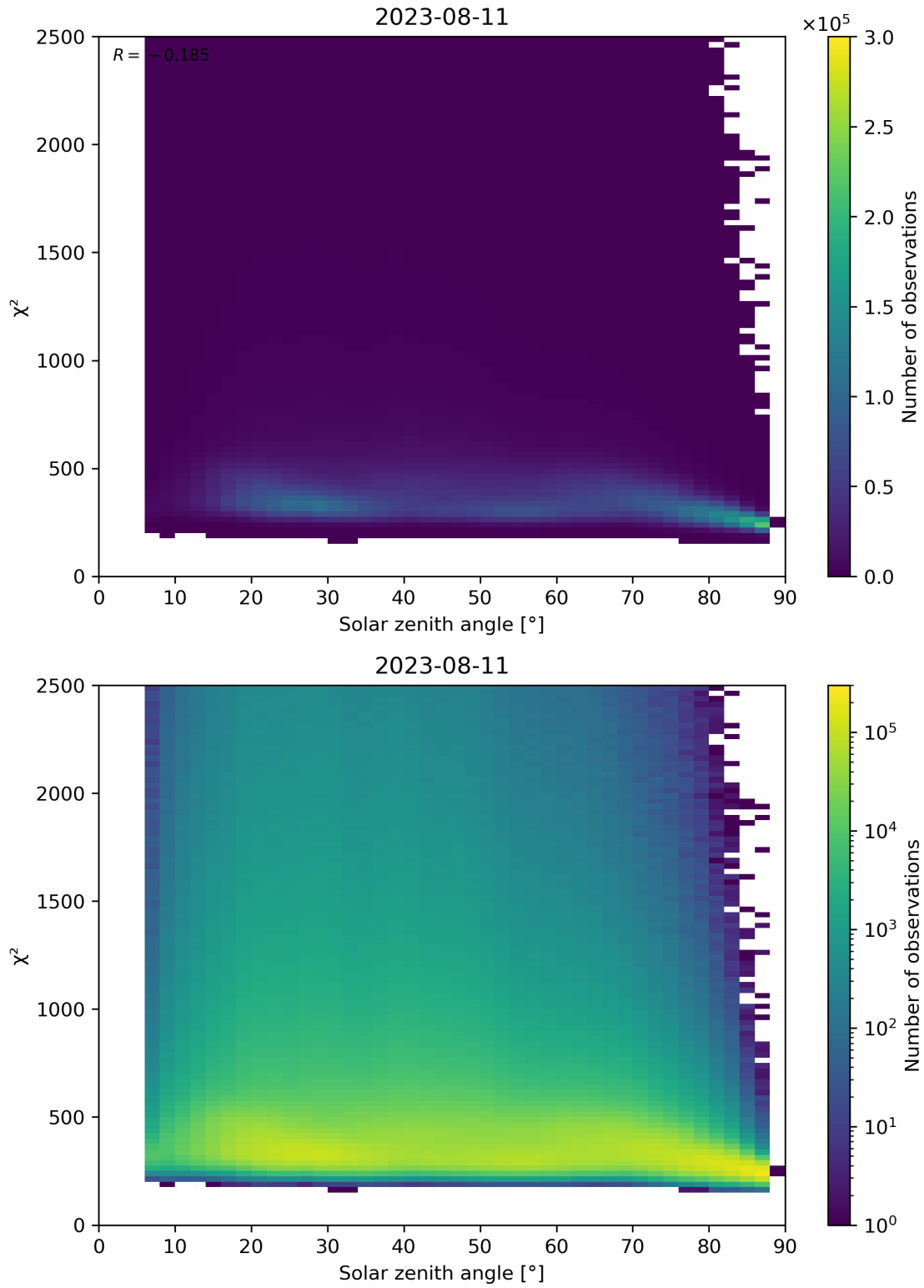
Figure 148: Scatter density plot of “Solar zenith angle” against “ \chi^2 ” for 2023-08-10 to 2023-08-12.
