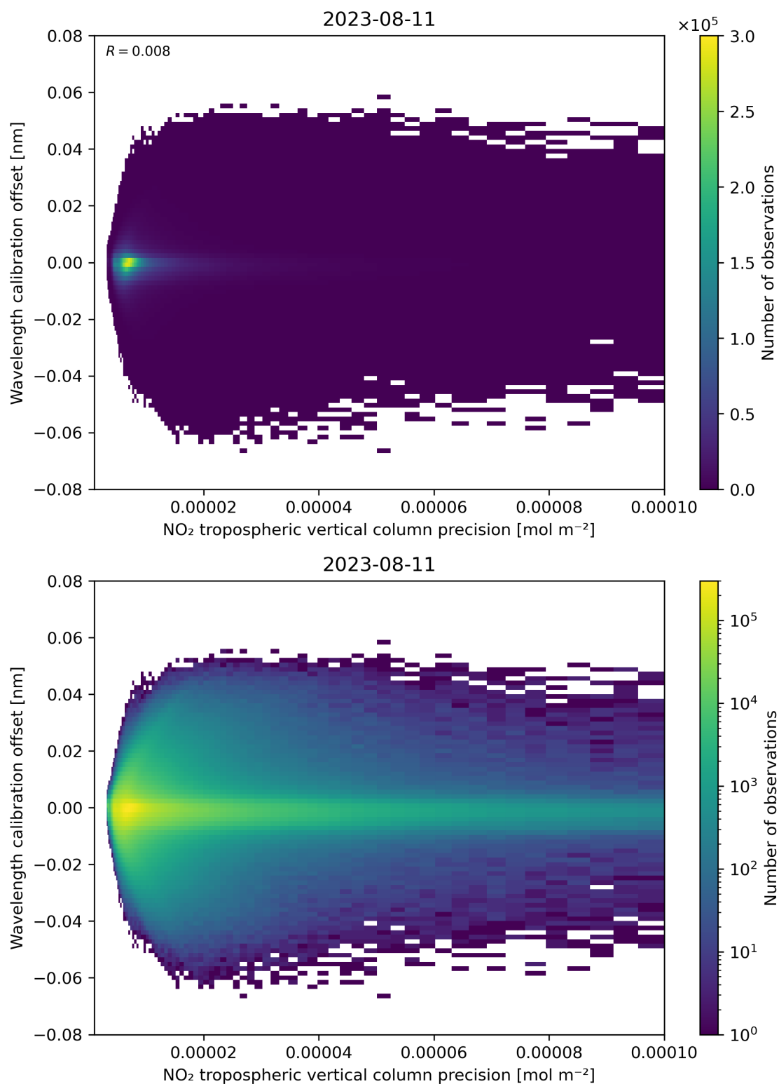
Figure 141: Scatter density plot of “NO 2 tropospheric vertical column precision” against “Wavelength calibration offset” for 2023-08-10 to 2023-08-12.
