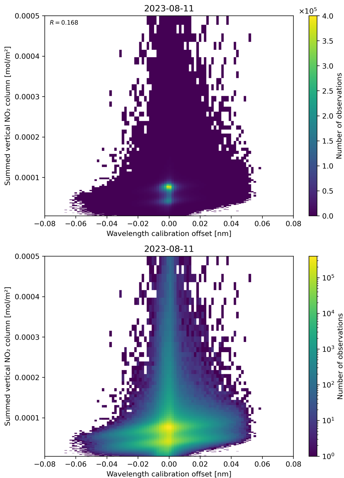
Figure 177: Scatter density plot of “Wavelength calibration offset” against “Summed vertical NO 2 column” for 2023-08-10 to 2023-08-12.
