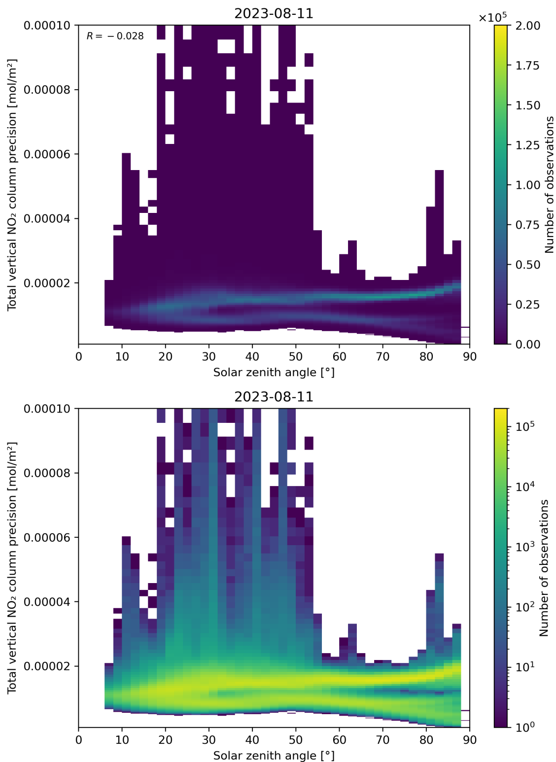
Figure 154: Scatter density plot of “Solar zenith angle” against “Total vertical NO 2 column precision” for 2023-08-10 to 2023-08-12.
