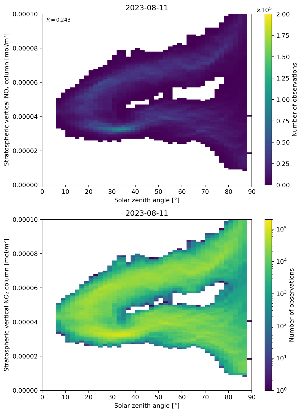
Figure 150: Scatter density plot of “Solar zenith angle” against “Stratospheric vertical NO 2 column” for 2023-08-10 to 2023-08-12.
