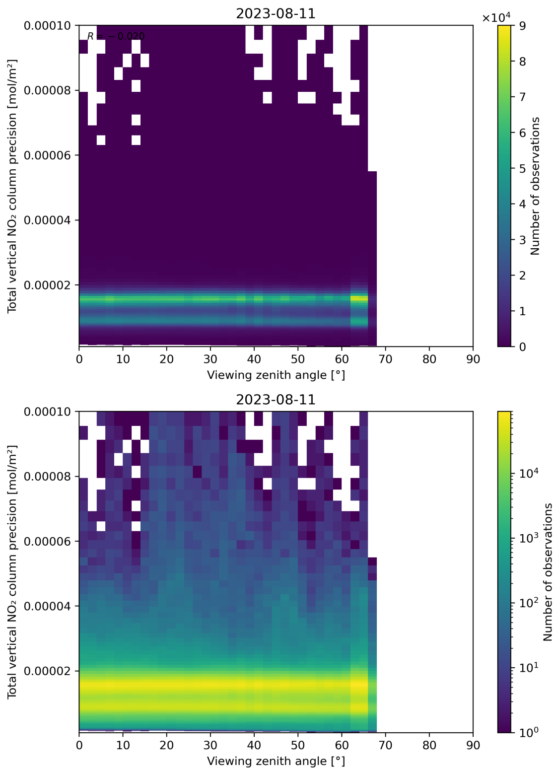
Figure 168: Scatter density plot of “Viewing zenith angle” against “Total vertical NO 2 column precision” for 2023-08-10 to 2023-08-12.
