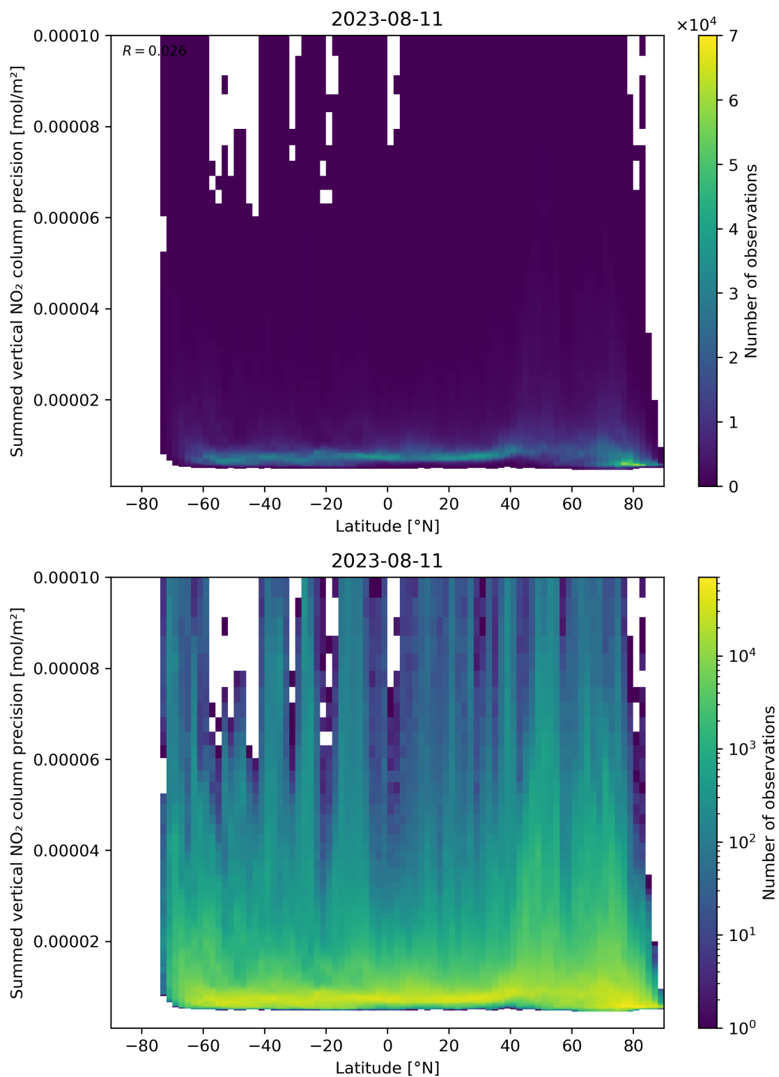
Figure 89: Scatter density plot of “Latitude” against “Summed vertical NO 2 column precision” for 2023-08-10 to 2023-08-12.
