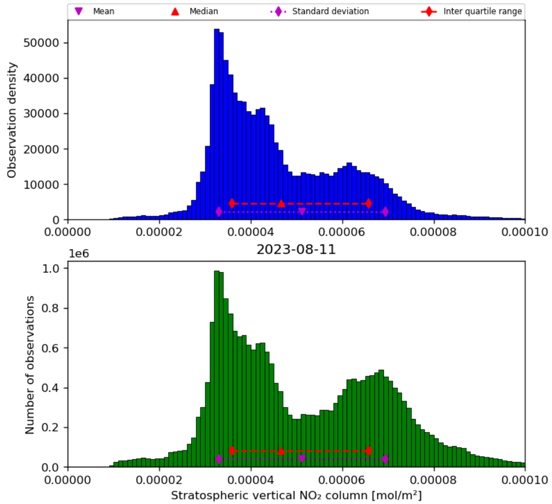
Figure 36: Histogram of “Stratospheric vertical NO 2 column” for 2023-08-10 to 2023-08-12
