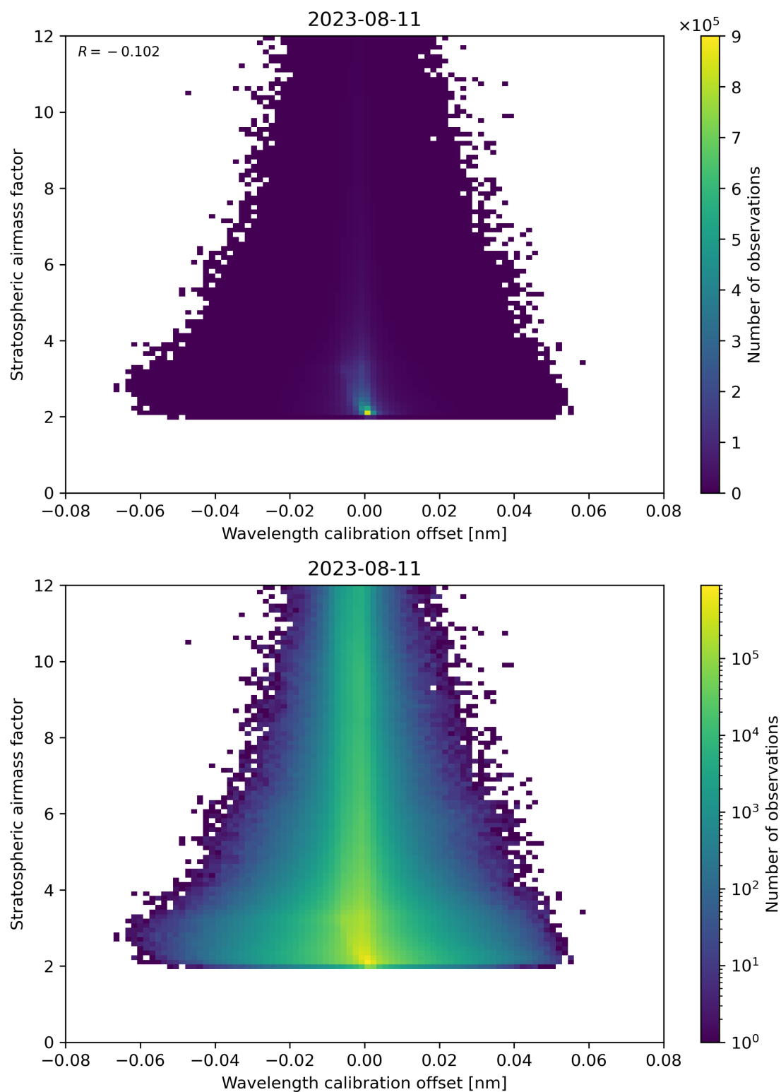
Figure 174: Scatter density plot of “Wavelength calibration offset” against “Stratospheric airmass factor” for 2023-08-10 to 2023-08-12.
