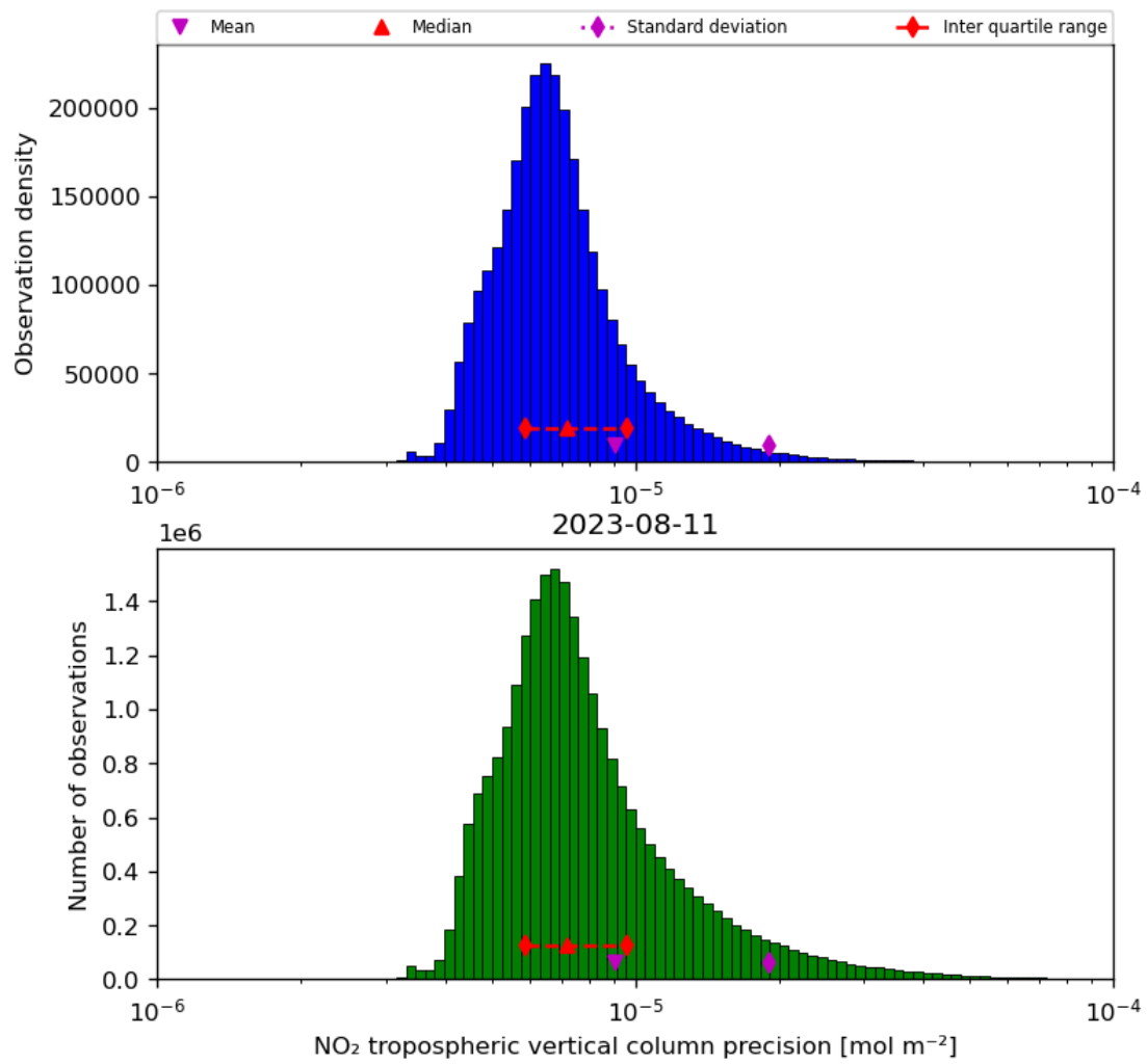
Figure 30: Histogram of “NO 2 tropospheric vertical column precision” for 2023-08-10 to 2023-08-12
