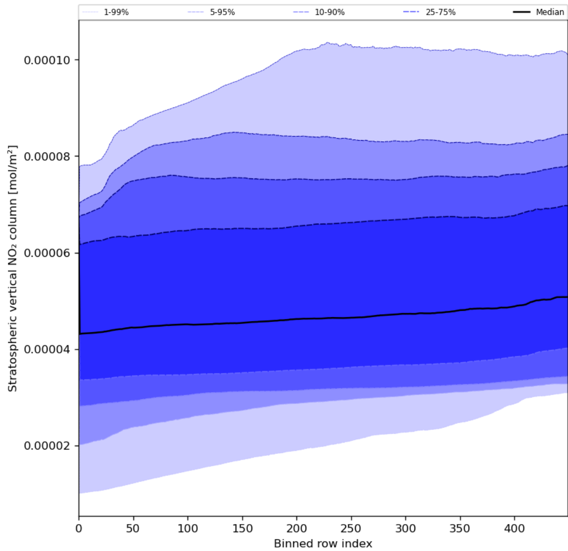
Figure 53: Along track statistics of “Stratospheric vertical NO 2 column” for 2023-08-10 to 2023-08-12
