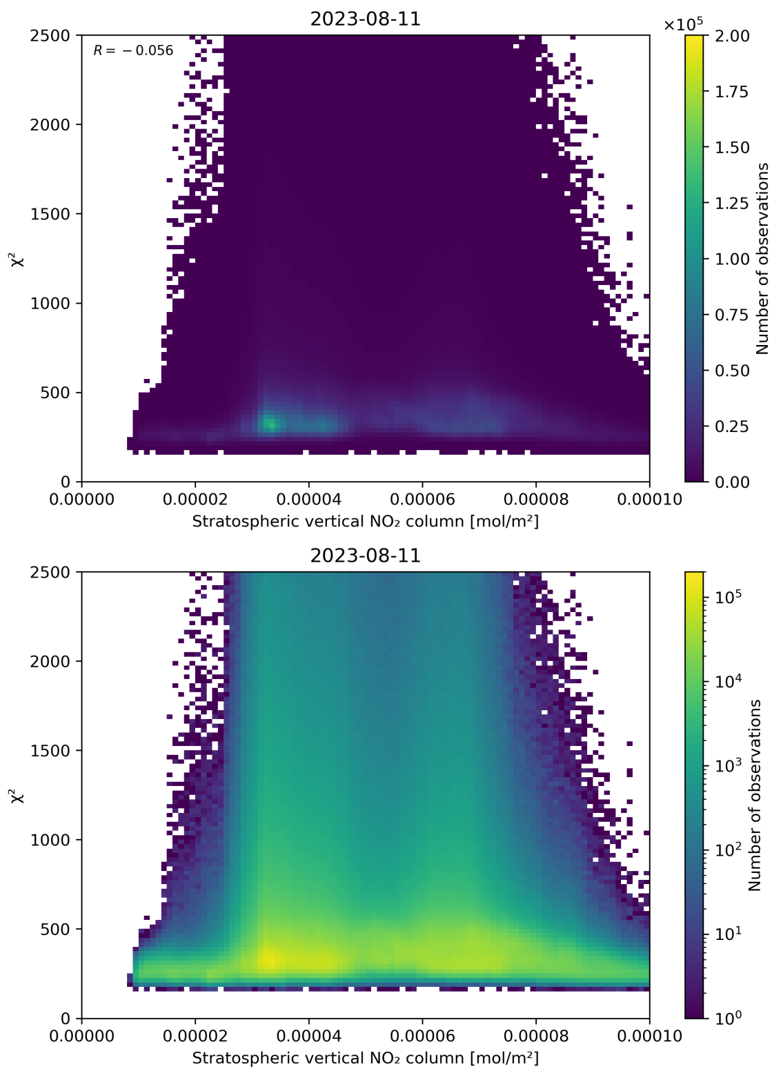
Figure 97: Scatter density plot of “Stratospheric vertical NO 2 column” against “ \chi^2 ” for 2023-08-10 to 2023-08-12.
