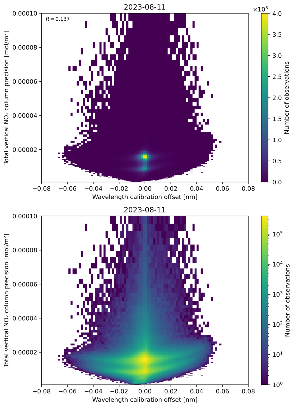
Figure 180: Scatter density plot of “Wavelength calibration offset” against “Total vertical NO 2 column precision” for 2023-08-10 to 2023-08-12.
