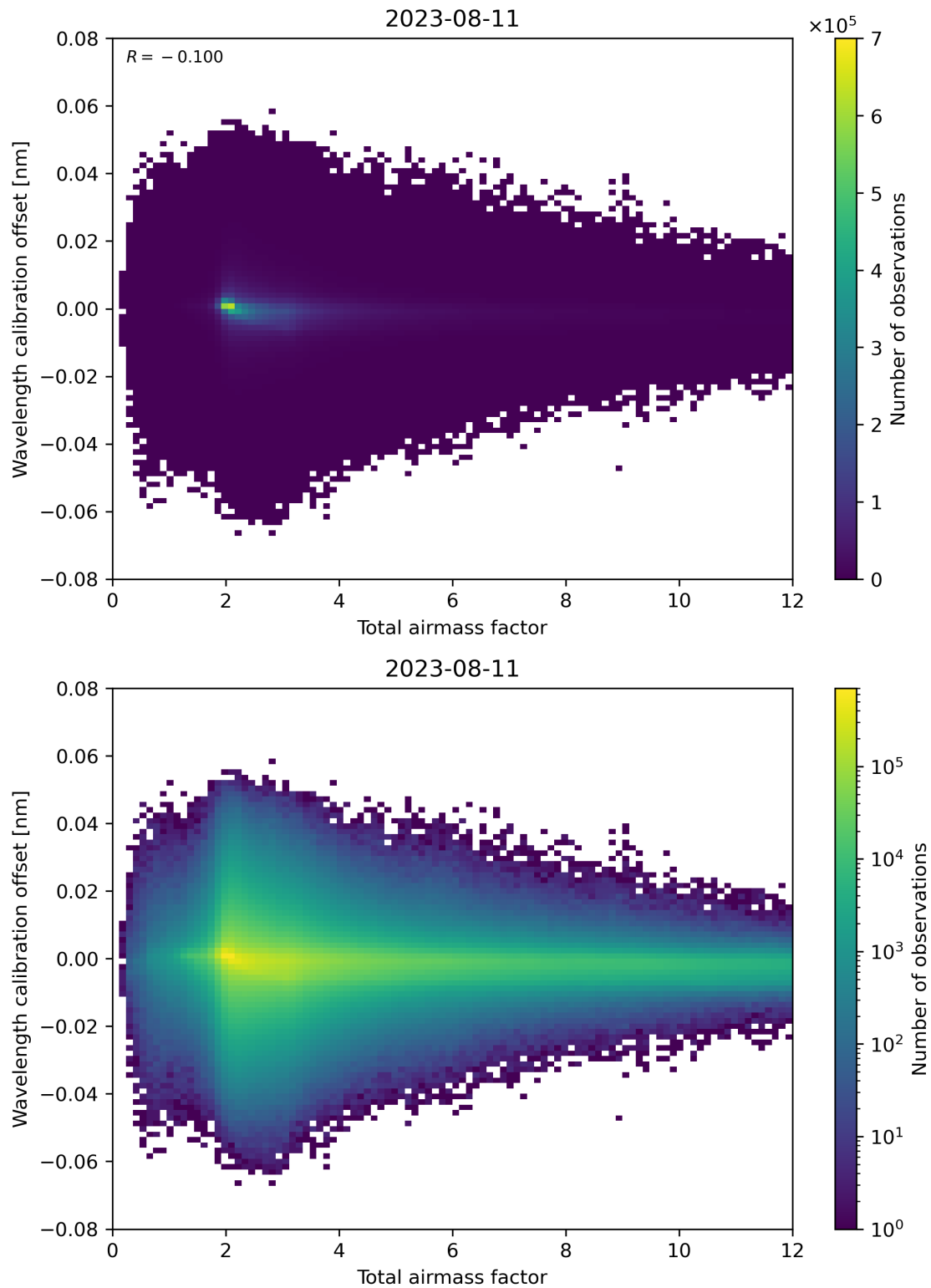
Figure 70: Scatter density plot of “Total airmass factor” against “Wavelength calibration offset” for 2023-08-10 to 2023-08-12.
