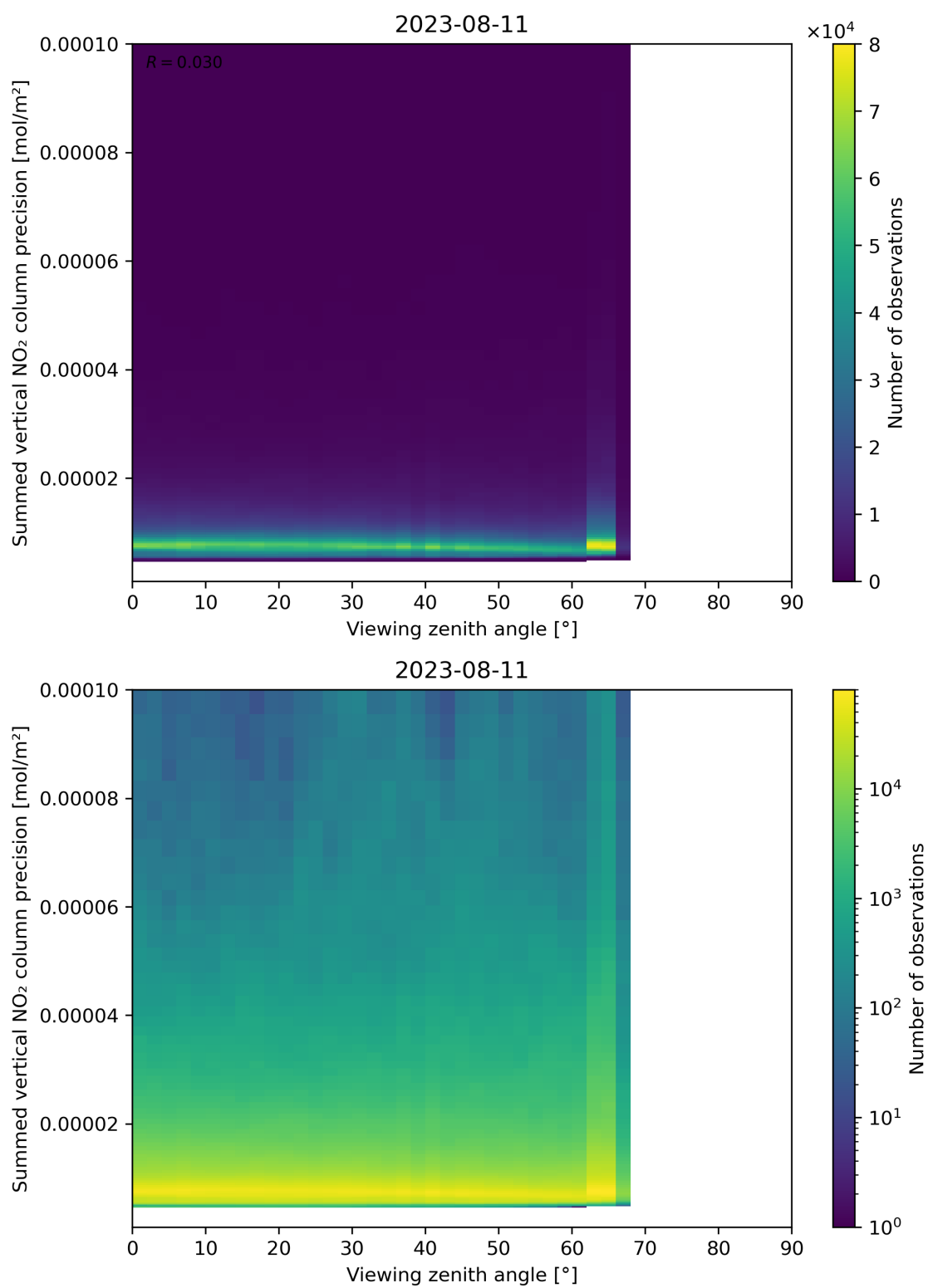
Figure 166: Scatter density plot of “Viewing zenith angle” against “Summed vertical NO 2 column precision” for 2023-08-10 to 2023-08-12.
