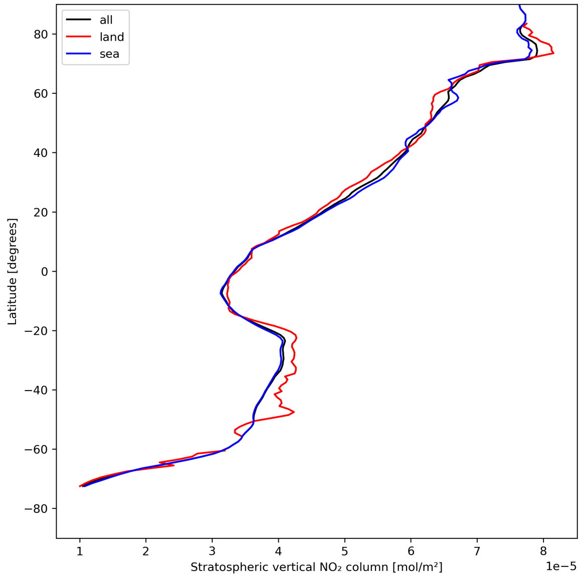
Figure 19: Zonal average of “Stratospheric vertical NO 2 column” for 2023-08-10 to 2023-08-12.
