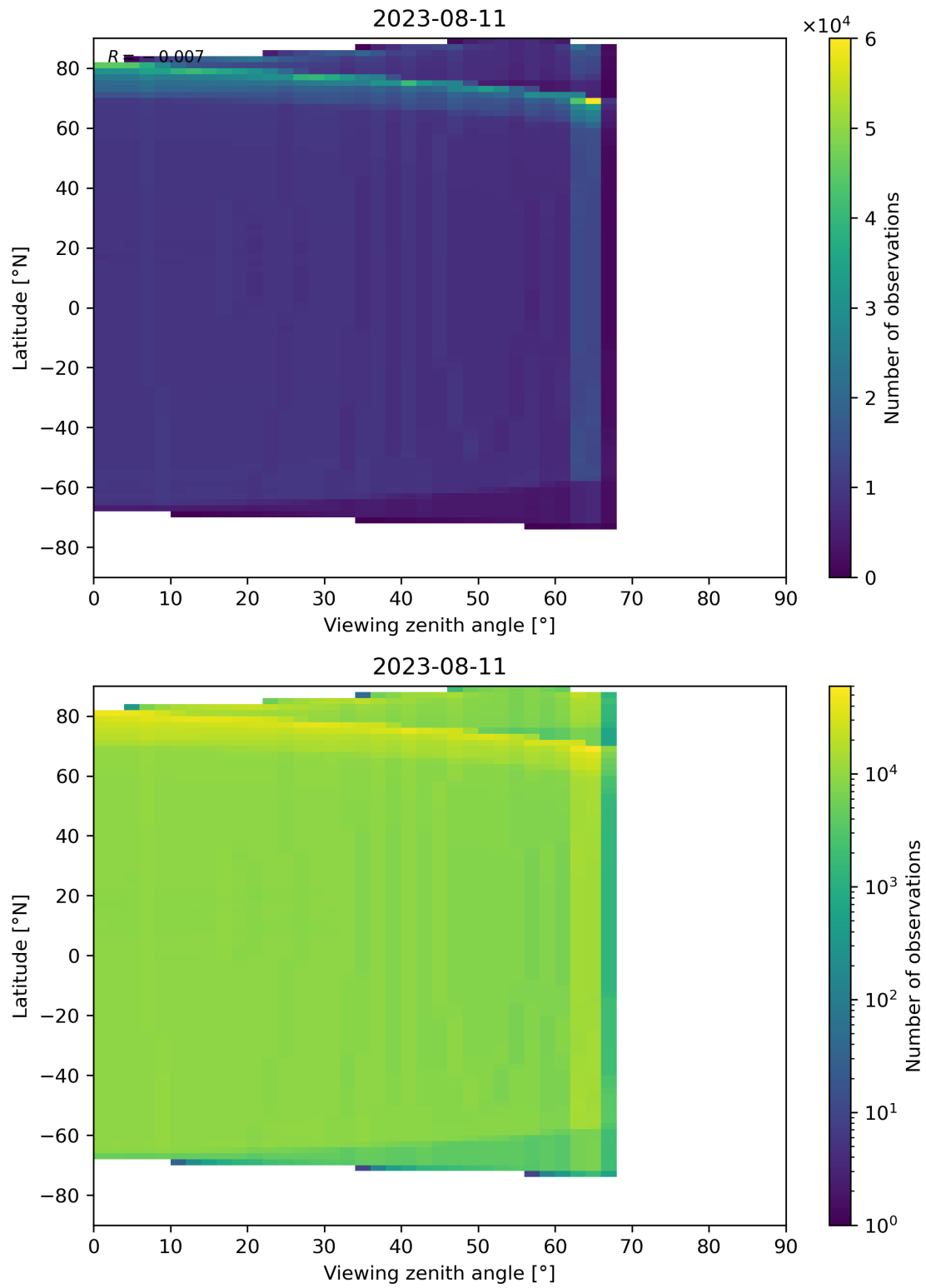
Figure 163: Scatter density plot of “Viewing zenith angle” against “Latitude” for 2023-08-10 to 2023-08-12.
