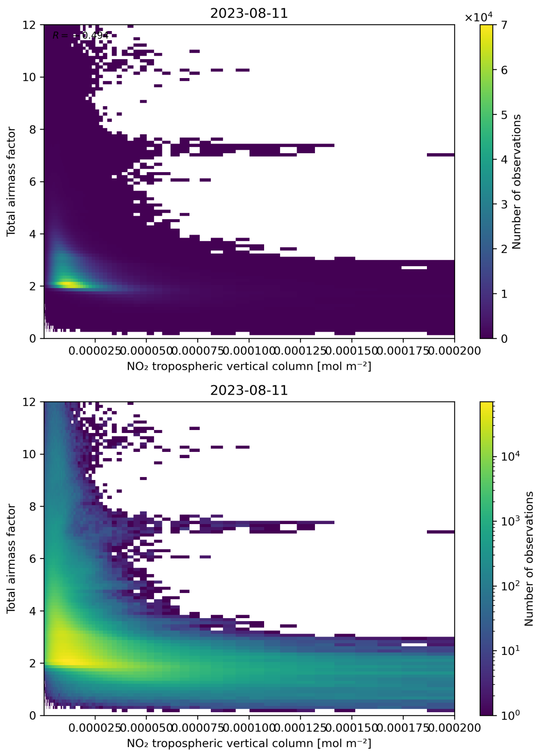
Figure 122: Scatter density plot of “NO 2 tropospheric vertical column” against “Total air mass factor” for 2023-08-10 to 2023-08-12.
