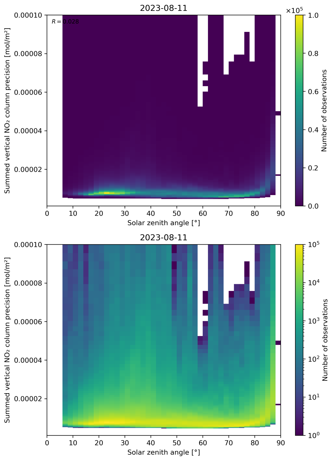
Figure 152: Scatter density plot of “Solar zenith angle” against “Summed vertical NO 2 column precision” for 2023-08-10 to 2023-08-12.
