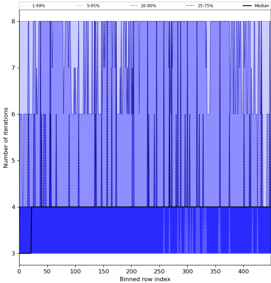
Figure 51: Along track statistics of “Number of iterations” for 2023-08-10 to 2023-08-12
