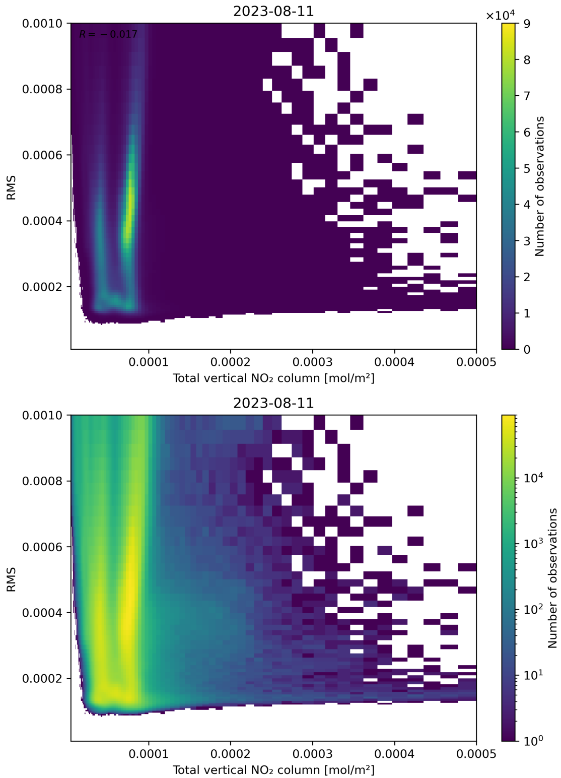
Figure 120: Scatter density plot of “Total vertical NO 2 column” against “RMS” for 2023-08-10 to 2023-08-12.
