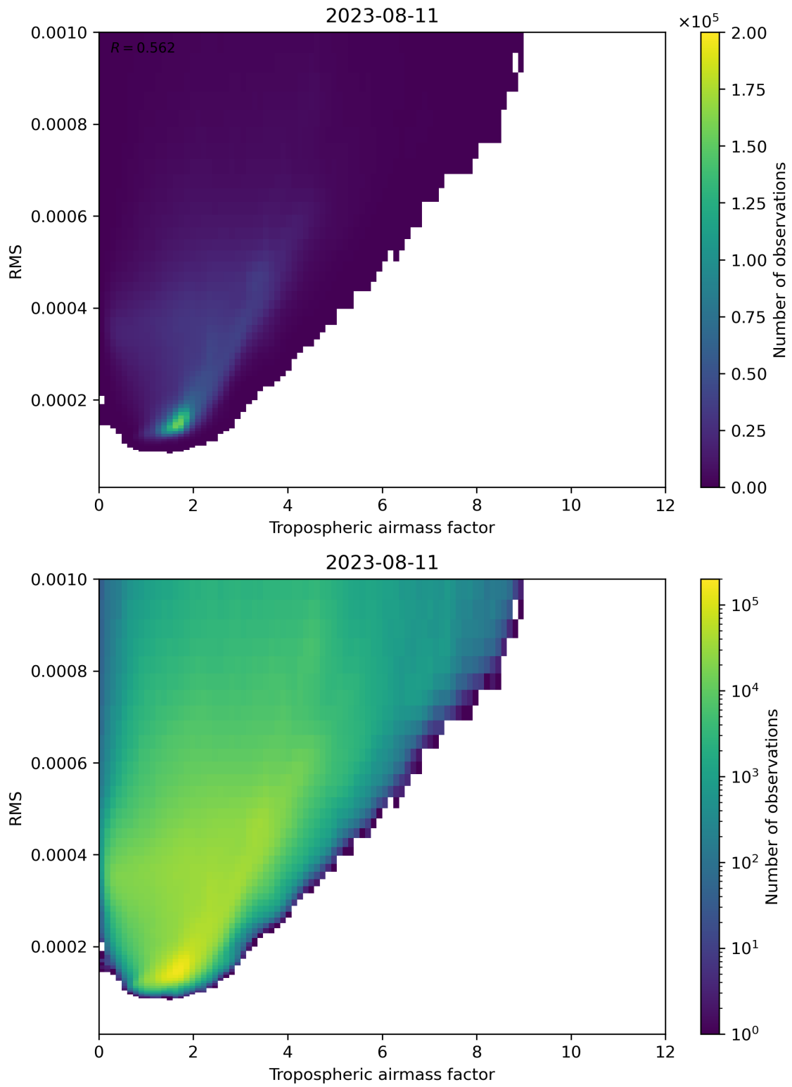
Figure 79: Scatter density plot of “Tropospheric airmass factor” against “RMS” for 2023-08-10 to 2023-08-12.
