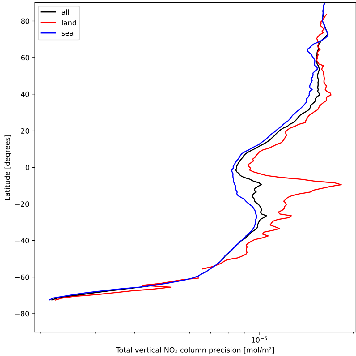
Figure 22: Zonal average of “Total vertical NO 2 column precision” for 2023-08-10 to 2023-08-12.
