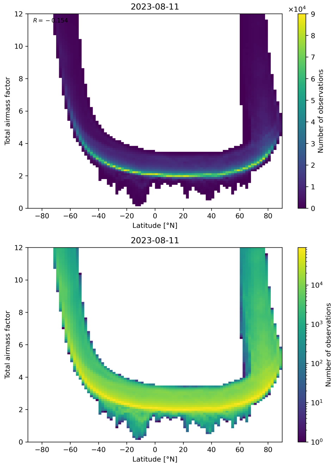
Figure 84: Scatter density plot of “Latitude” against “Total airmass factor” for 2023-08-10 to 2023-08-12.
