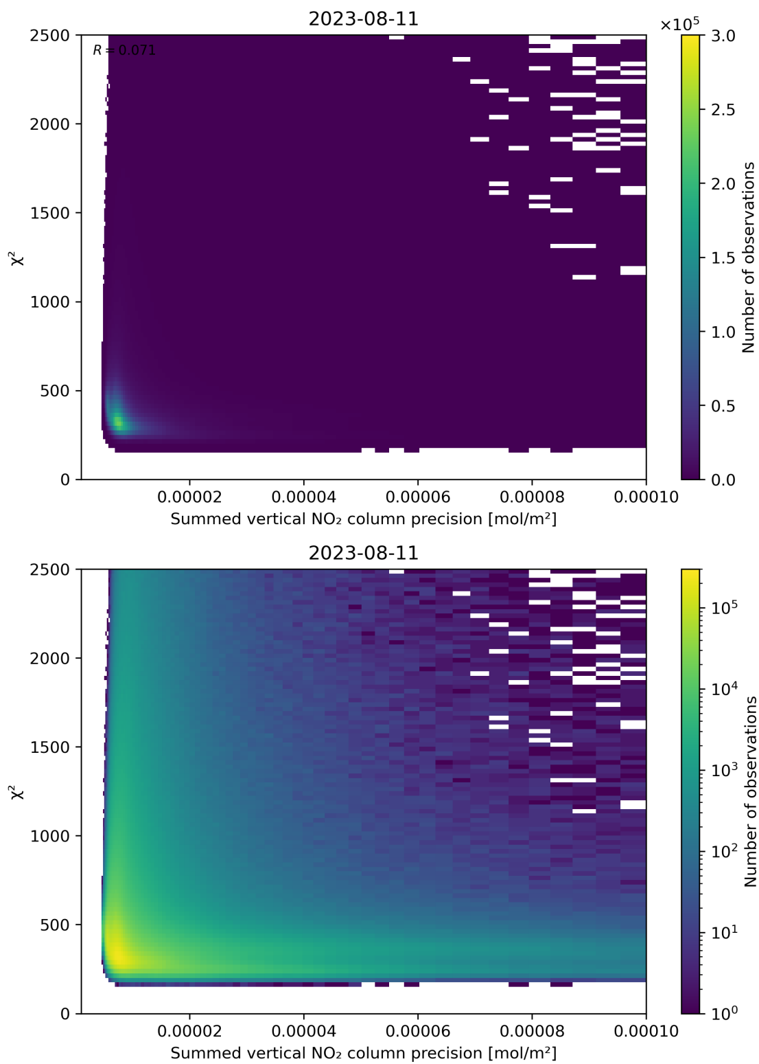
Figure 107: Scatter density plot of “Summed vertical NO 2 column precision” against “ \chi^2 ” for 2023-08-10 to 2023-08-12.
