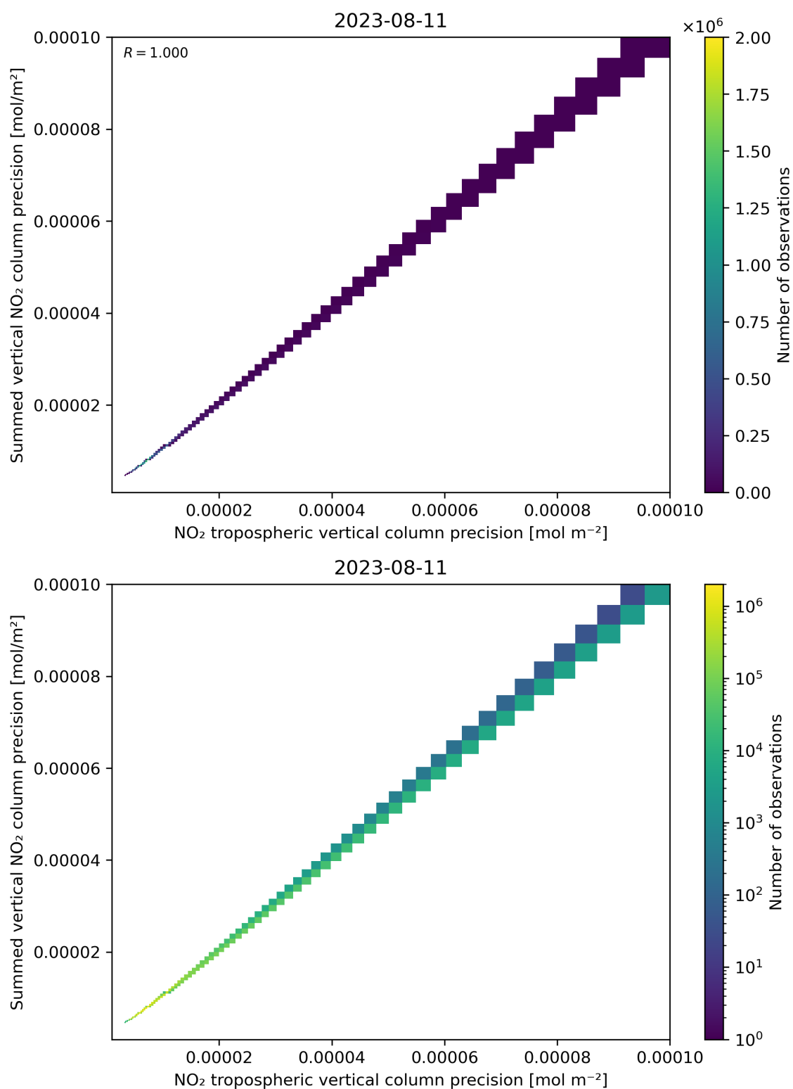
Figure 137: Scatter density plot of “NO 2 tropospheric vertical column precision” against “Summed vertical NO 2 column precision” for 2023-08-10 to 2023-08-12.
