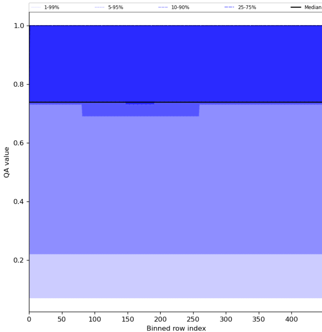
Figure 45: Along track statistics of “QA value” for 2023-08-10 to 2023-08-12
