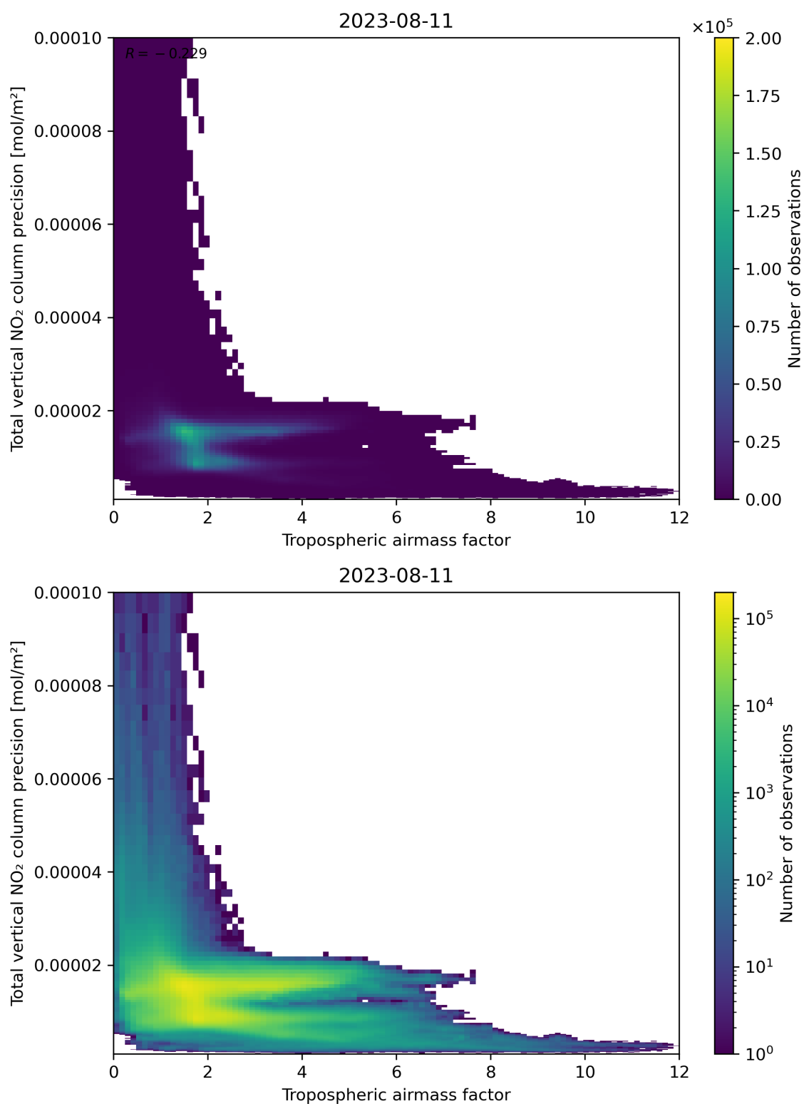
Figure 78: Scatter density plot of “Tropospheric air mass factor” against “Total vertical NO 2 column precision” for 2023-08-10 to 2023-08-12.
