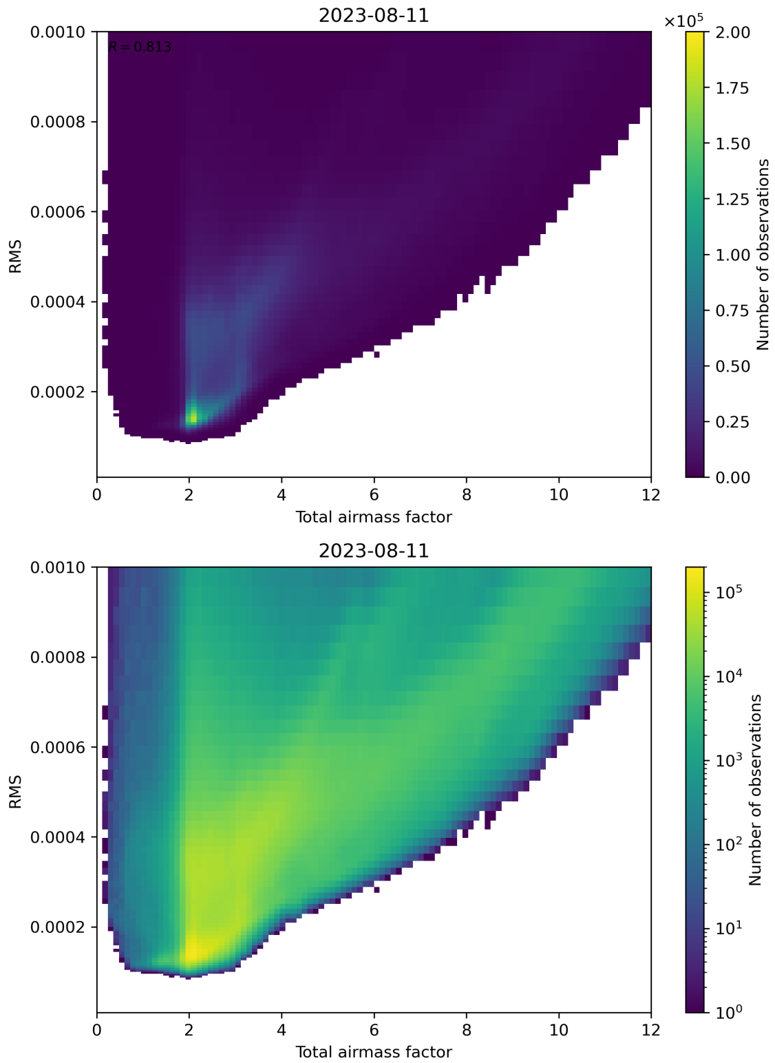
Figure 69: Scatter density plot of “Total airmass factor” against “RMS” for 2023-08-10 to 2023-08-12.
