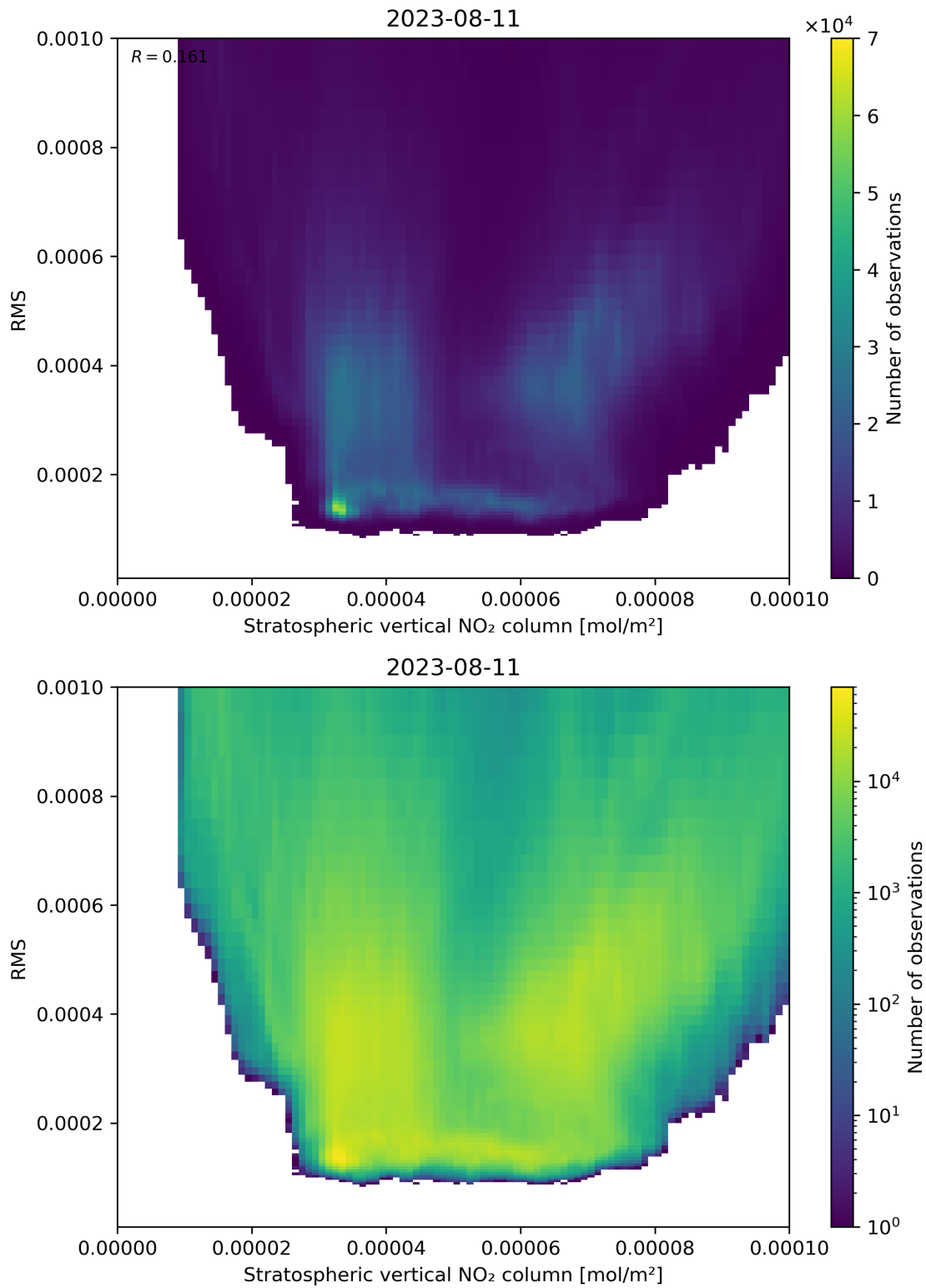
Figure 102: Scatter density plot of “Stratospheric vertical NO 2 column” against “RMS” for 2023-08-10 to 2023-08-12.
