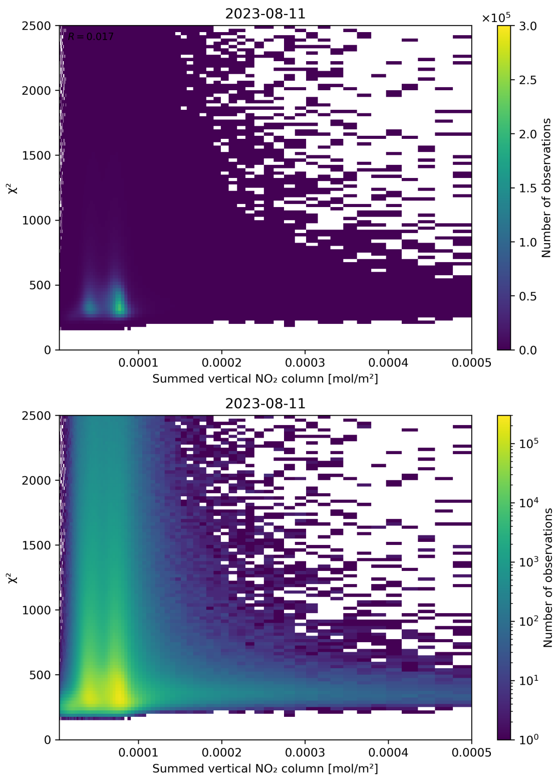
Figure 104: Scatter density plot of “Summed vertical NO 2 column” against “ \chi^2 ” for 2023-08-10 to 2023-08-12.
