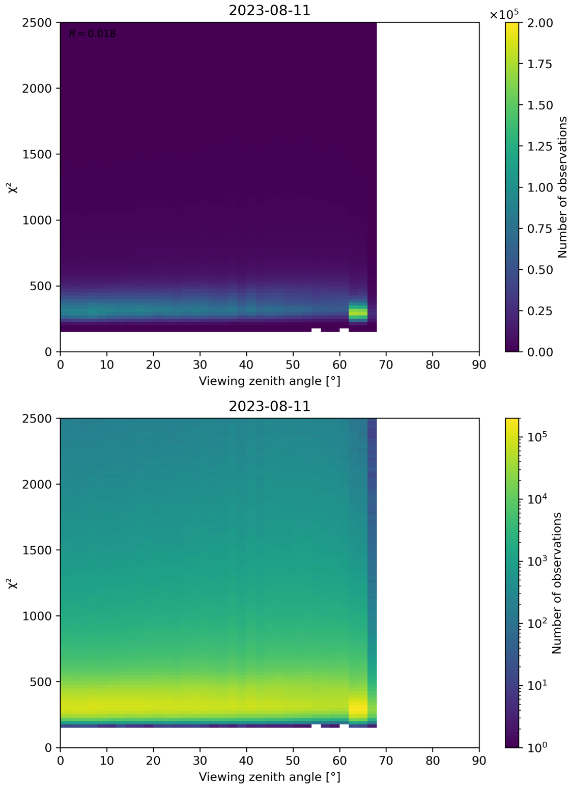
Figure 162: Scatter density plot of “Viewing zenith angle” against “ \chi^2 ” for 2023-08-10 to 2023-08-12.
