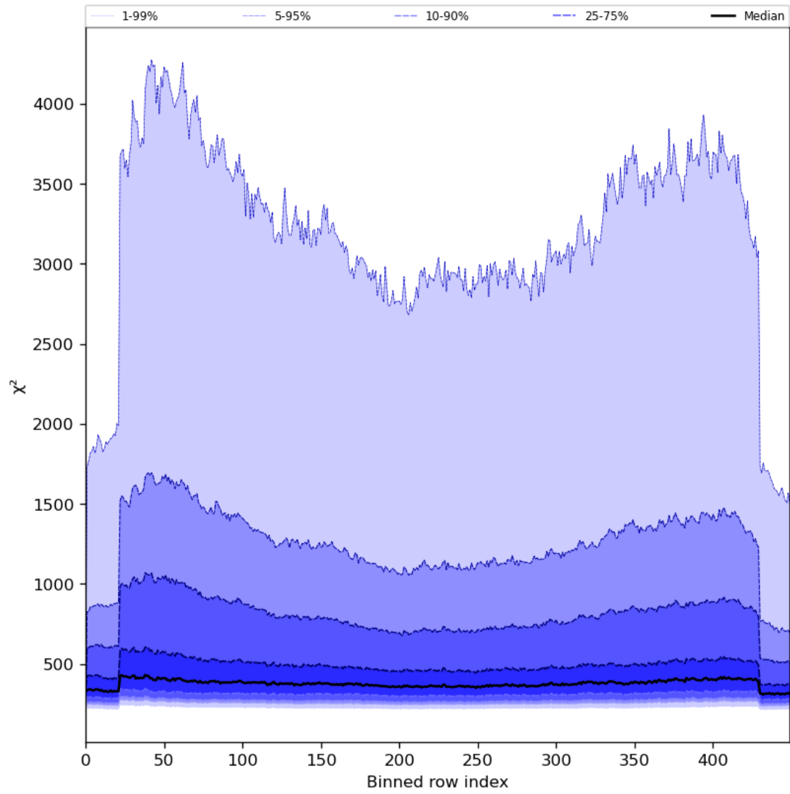
Figure 59: Along track statistics of “ \chi^2 ” for 2023-08-10 to 2023-08-12
