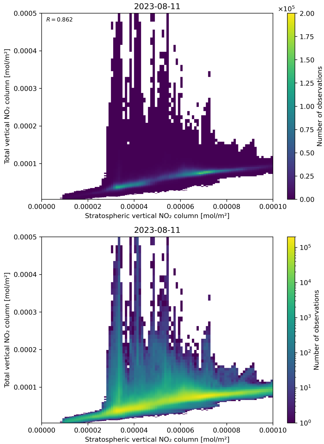
Figure 100: Scatter density plot of “Stratospheric vertical NO 2 column” against “Total vertical NO 2 column” for 2023-08-10 to 2023-08-12.
