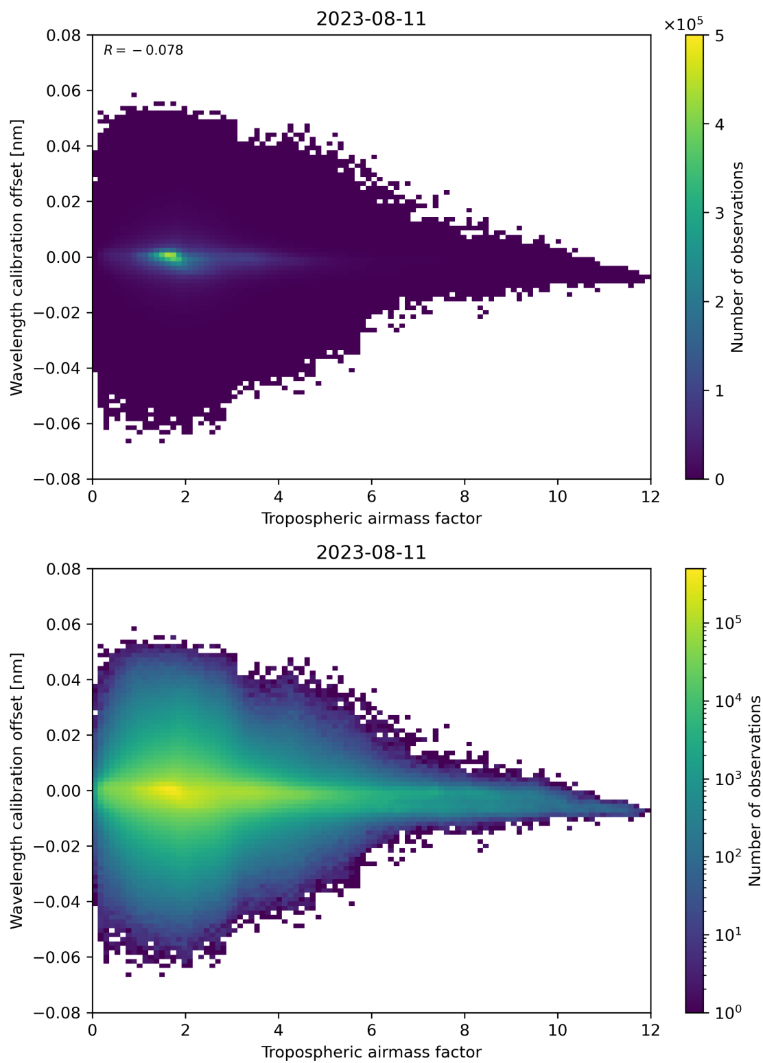
Figure 80: Scatter density plot of “Tropospheric airmass factor” against “Wavelength calibration offset” for 2023-08-10 to 2023-08-12.
