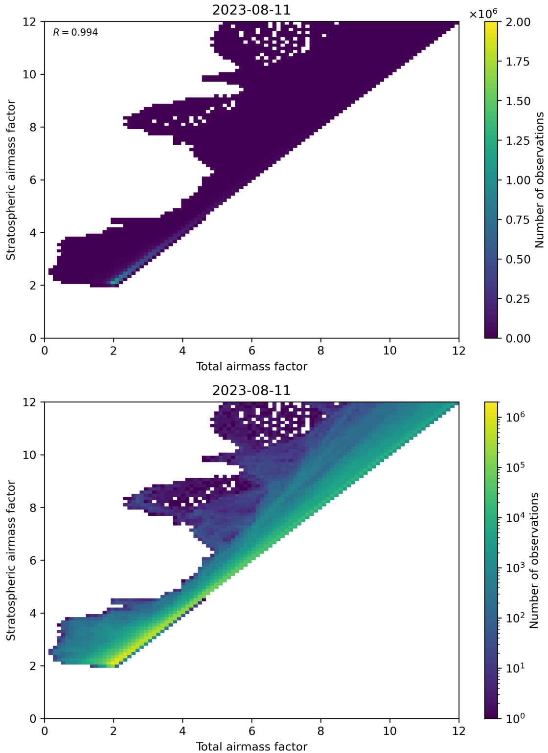
Figure 62: Scatter density plot of “Total air mass factor” against “Stratospheric air mass factor” for 2023-08-10 to 2023-08-12.
