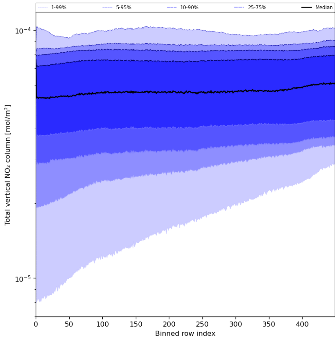
Figure 55: Along track statistics of “Total vertical NO 2 column” for 2023-08-10 to 2023-08-12
