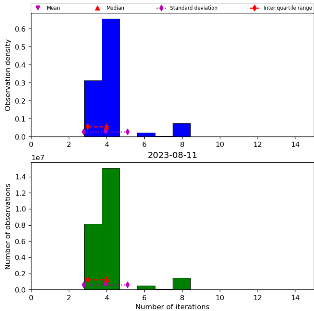
Figure 34: Histogram of “Number of iterations” for 2023-08-10 to 2023-08-12
