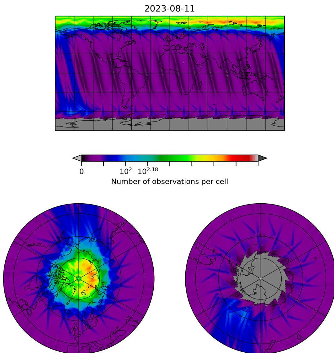
Figure 10: Map of the number of observations for 2023-08-10 to 2023-08-12
