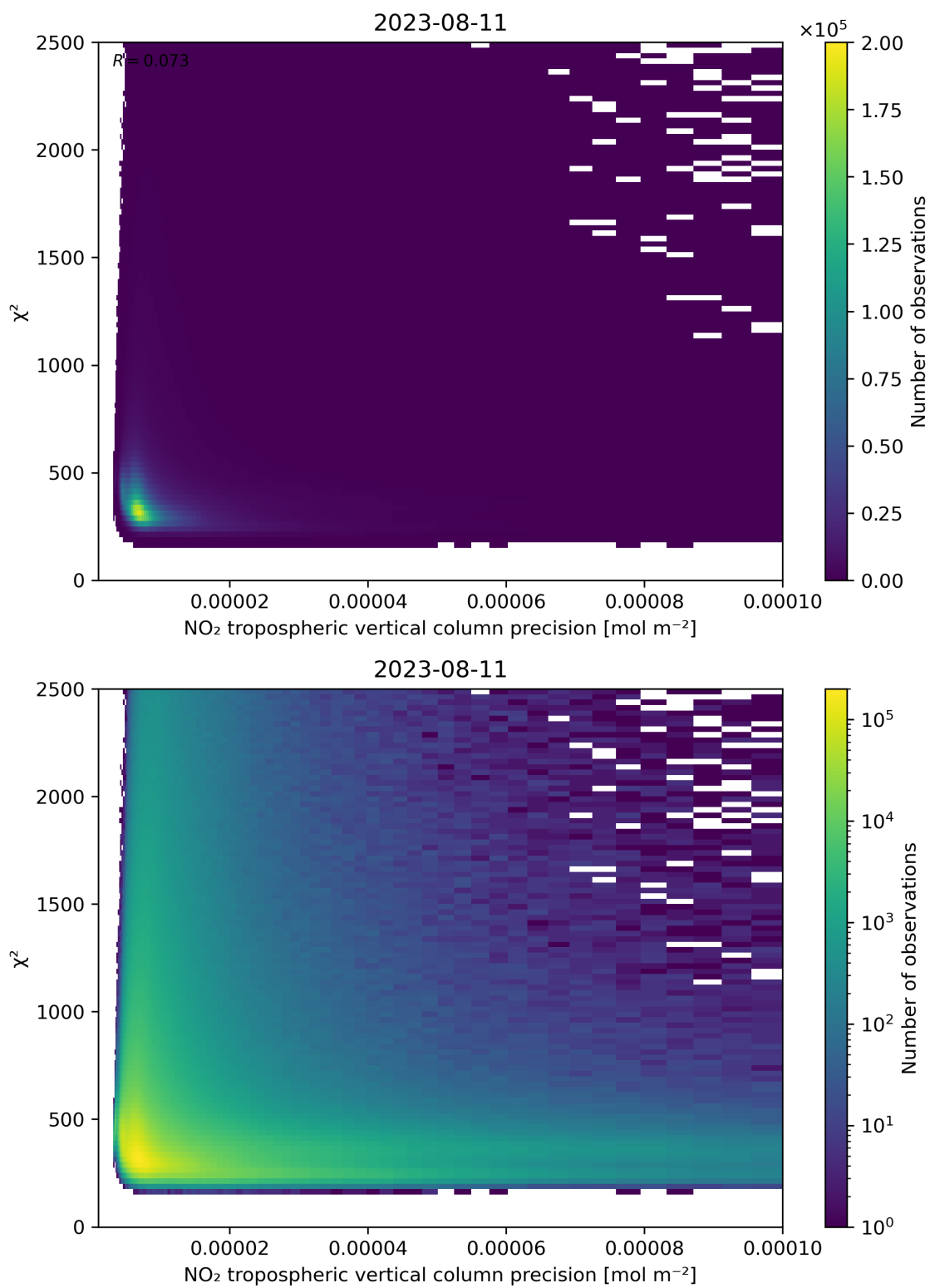
Figure 134: Scatter density plot of “NO 2 tropospheric vertical column precision” against “ \chi^2 ” for 2023-08-10 to 2023-08-12.
