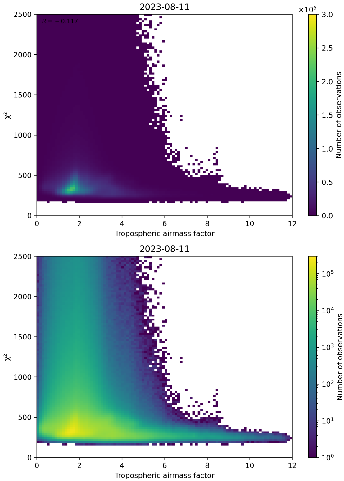
Figure 73: Scatter density plot of “Tropospheric airmass factor” against “ \chi^2 ” for 2023-08-10 to 2023-08-12.
