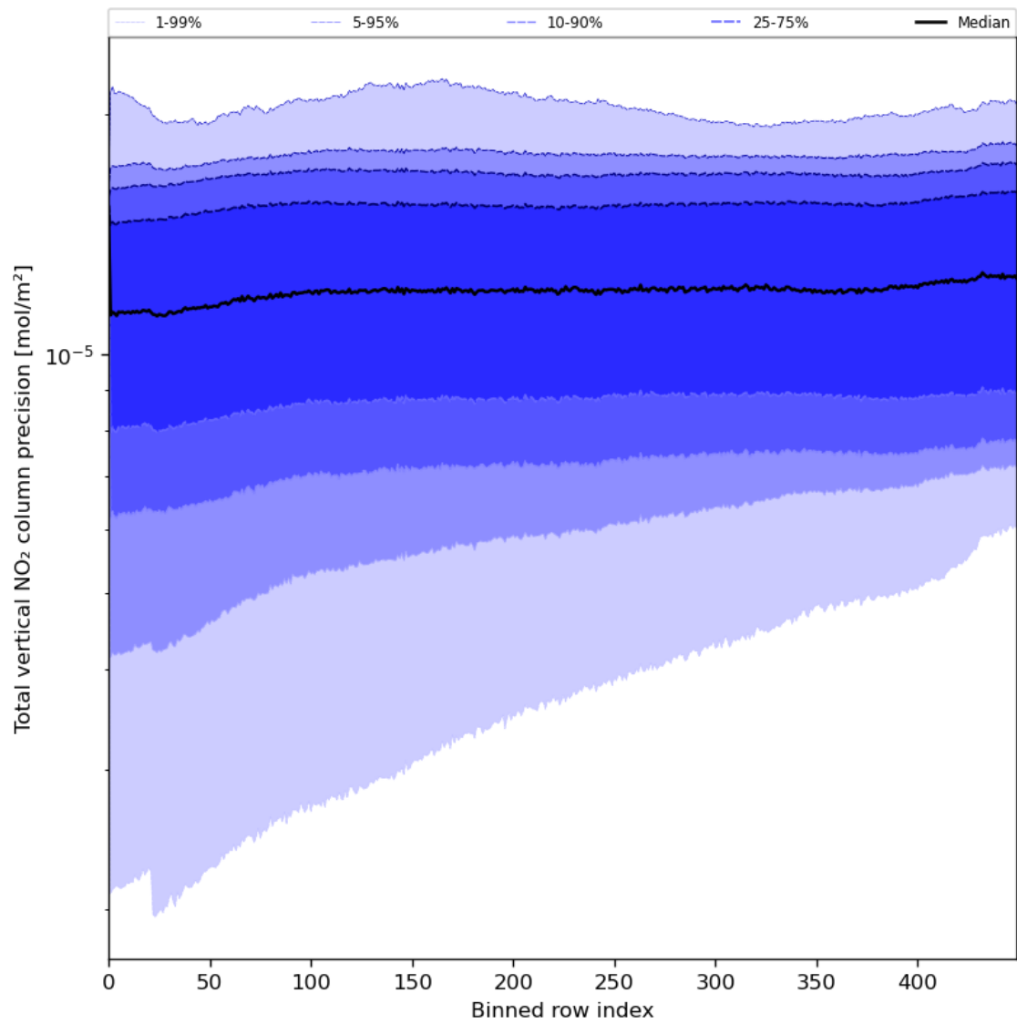
Figure 56: Along track statistics of “Total vertical NO 2 column precision” for 2023-08-10 to 2023-08-12
