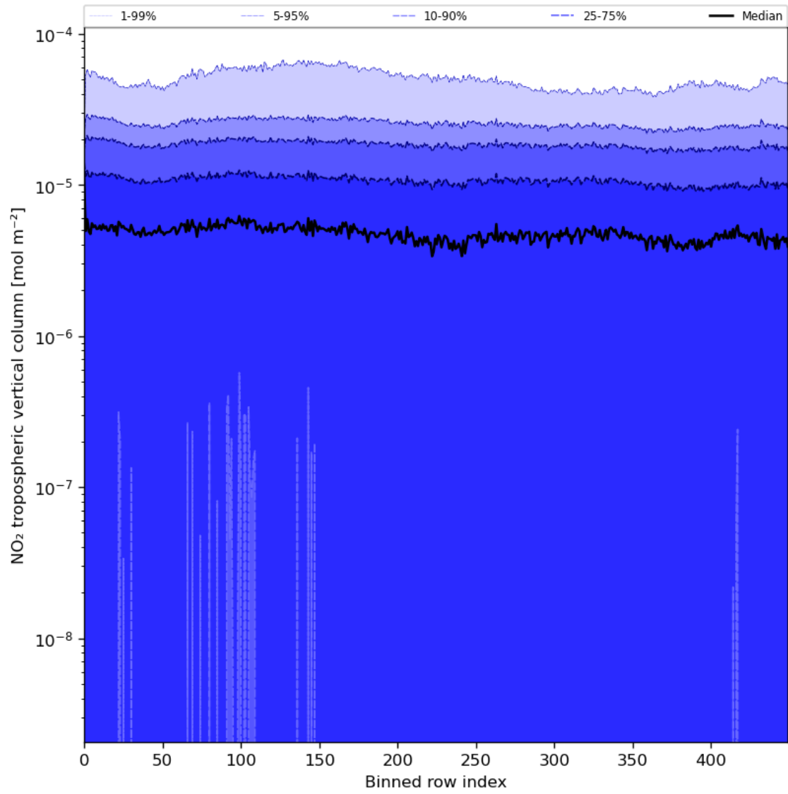
Figure 46: Along track statistics of “NO 2 tropospheric vertical column” for 2023-08-10 to 2023-08-12
