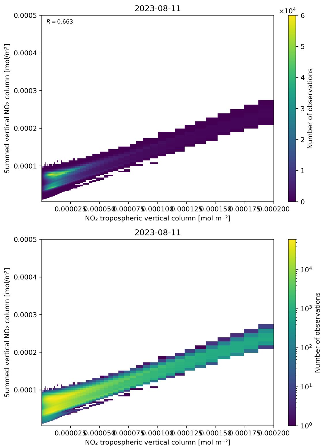
Figure 126: Scatter density plot of “NO 2 tropospheric vertical column” against “Summed vertical NO 2 column” for 2023-08-10 to 2023-08-12.
