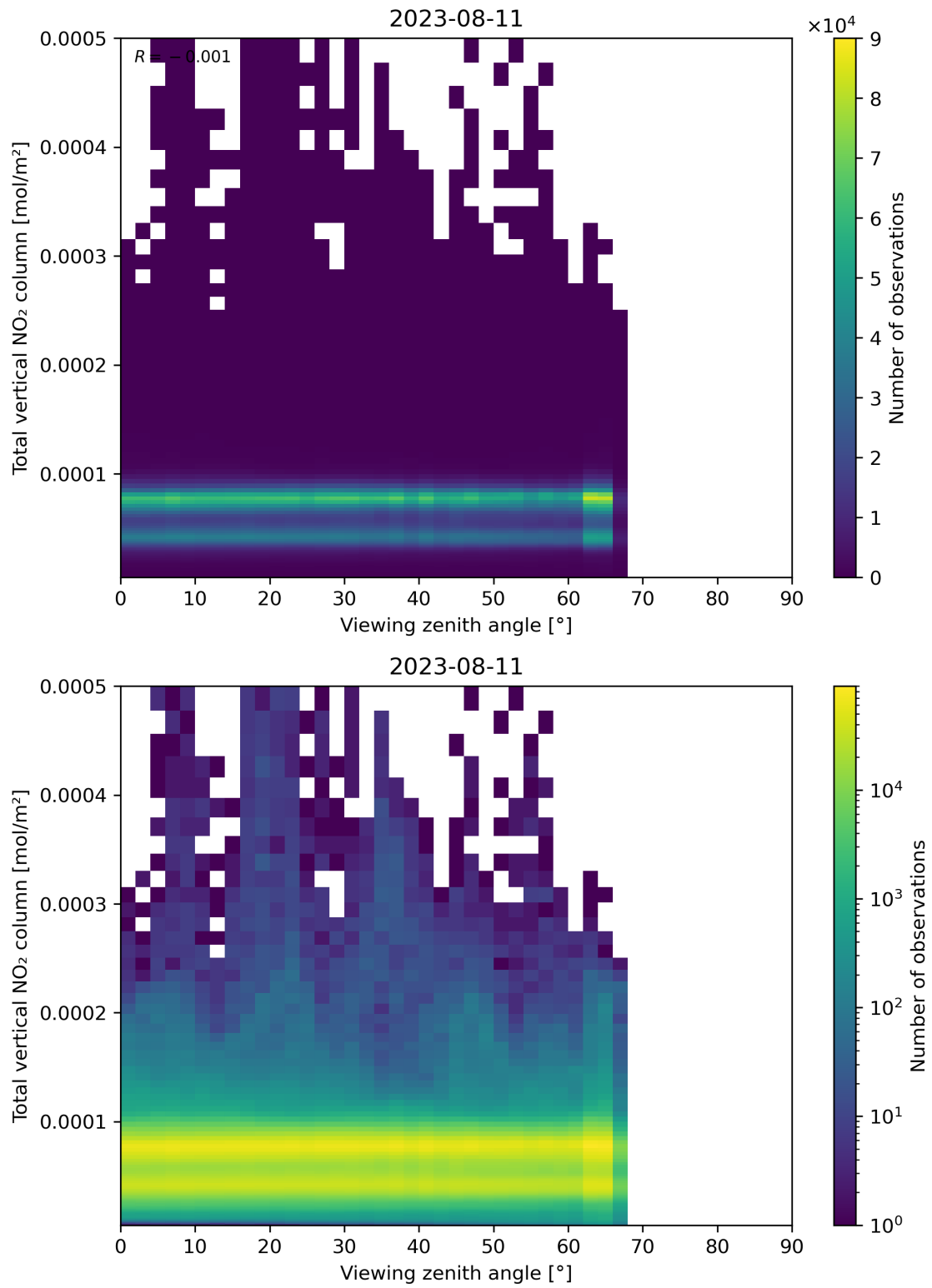
Figure 167: Scatter density plot of “Viewing zenith angle” against “Total vertical NO 2 column” for 2023-08-10 to 2023-08-12.
