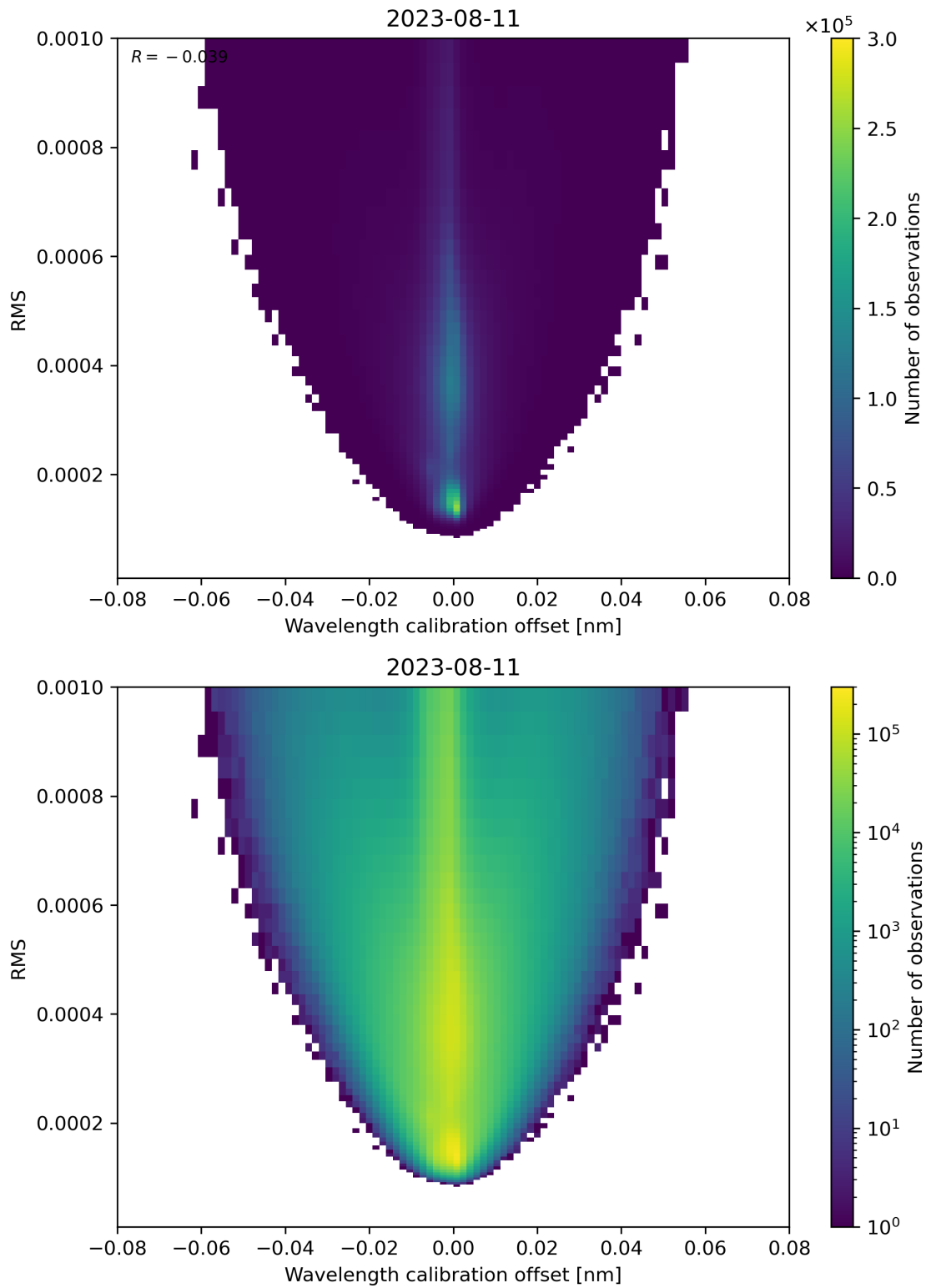
Figure 181: Scatter density plot of “Wavelength calibration offset” against “RMS” for 2023-08-10 to 2023-08-12.
