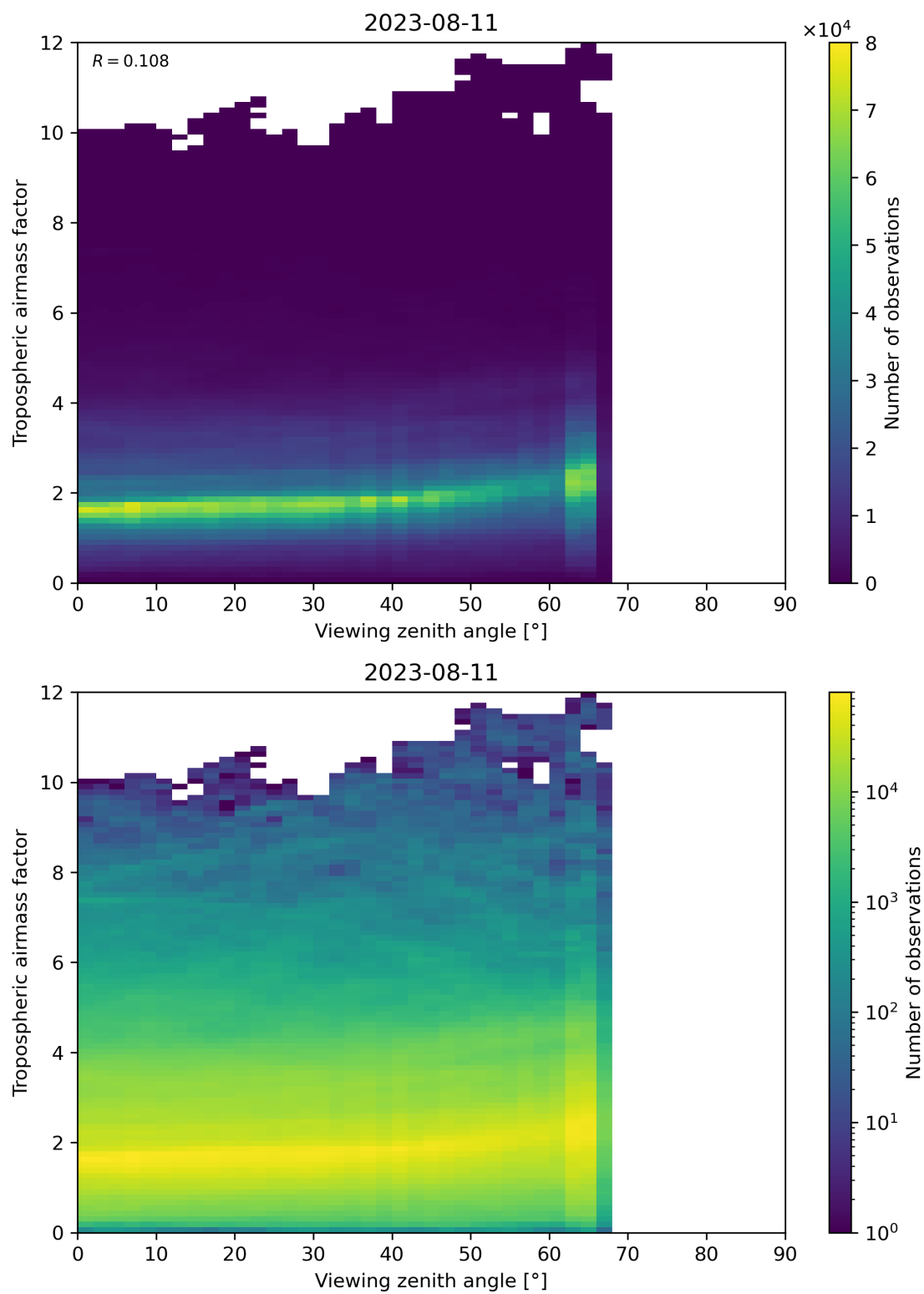
Figure 161: Scatter density plot of “Viewing zenith angle” against “Tropospheric airmass factor” for 2023-08-10 to 2023-08-12.
