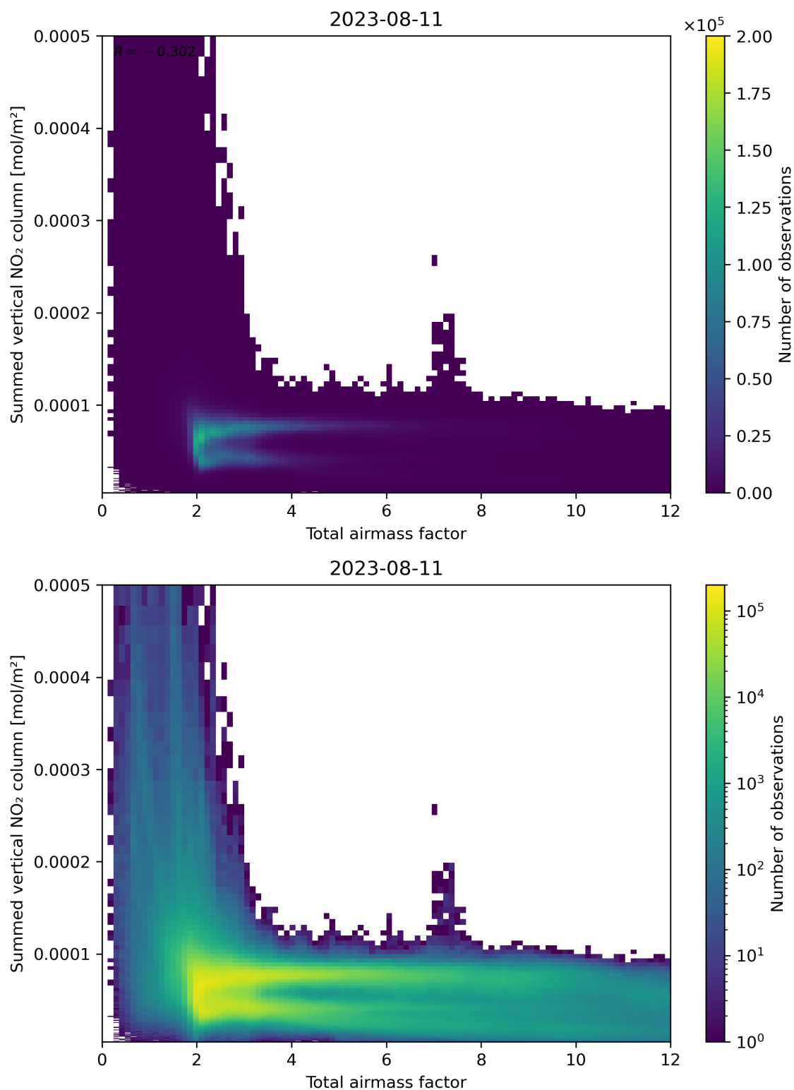
Figure 65: Scatter density plot of “Total airmass factor” against “Summed vertical NO 2 column” for 2023-08-10 to 2023-08-12.
