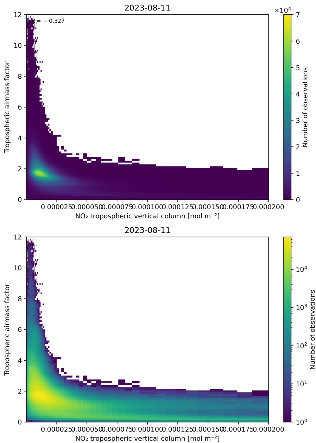
Figure 123: Scatter density plot of “NO 2 tropospheric vertical column” against “Tropospheric air mass factor” for 2023-08-10 to 2023-08-12.
