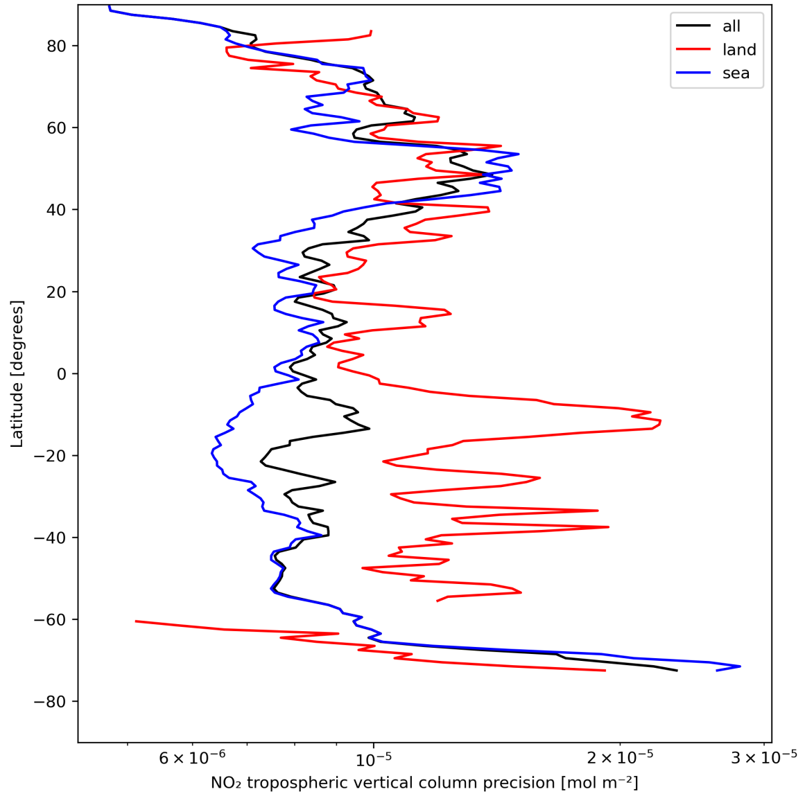
Figure 13: Zonal average of “NO 2 tropospheric vertical column precision” for 2023-08-10 to 2023-08-12.
