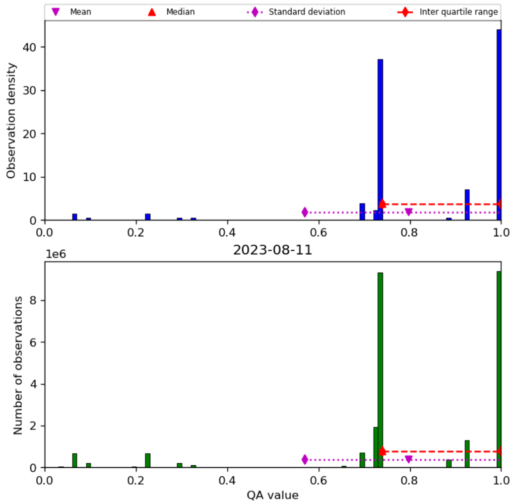
Figure 28: Histogram of “QA value” for 2023-08-10 to 2023-08-12
