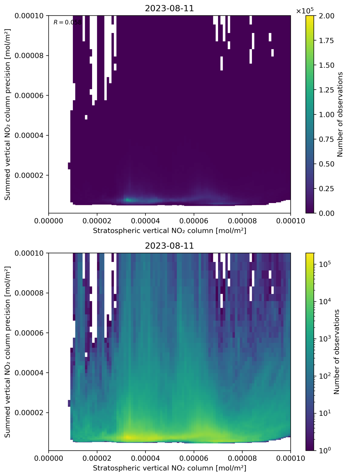
Figure 99: Scatter density plot of “Stratospheric vertical NO 2 column” against “Summed vertical NO 2 column precision” for 2023-08-10 to 2023-08-12.
