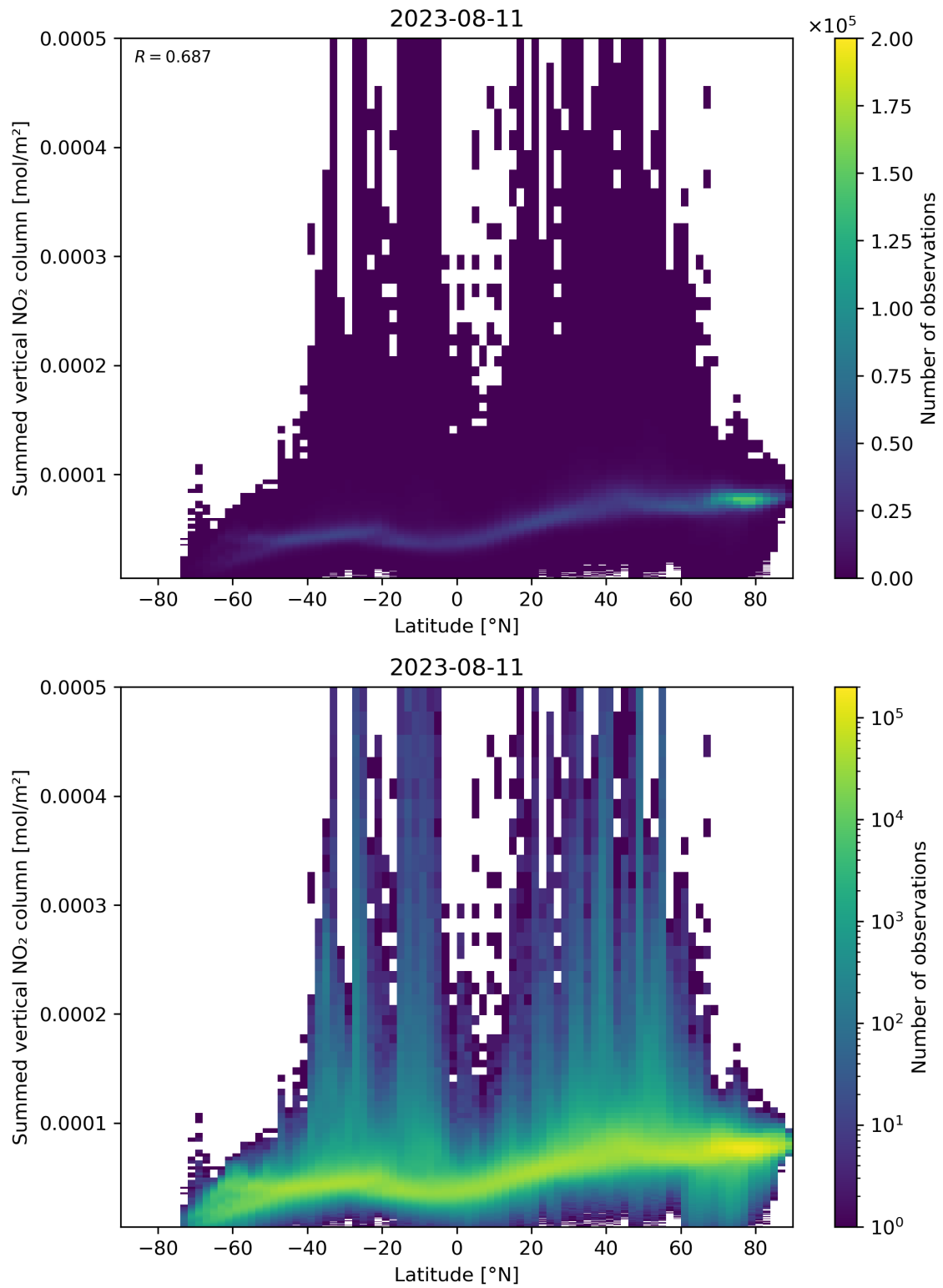
Figure 88: Scatter density plot of “Latitude” against “Summed vertical NO 2 column” for 2023-08-10 to 2023-08-12.
