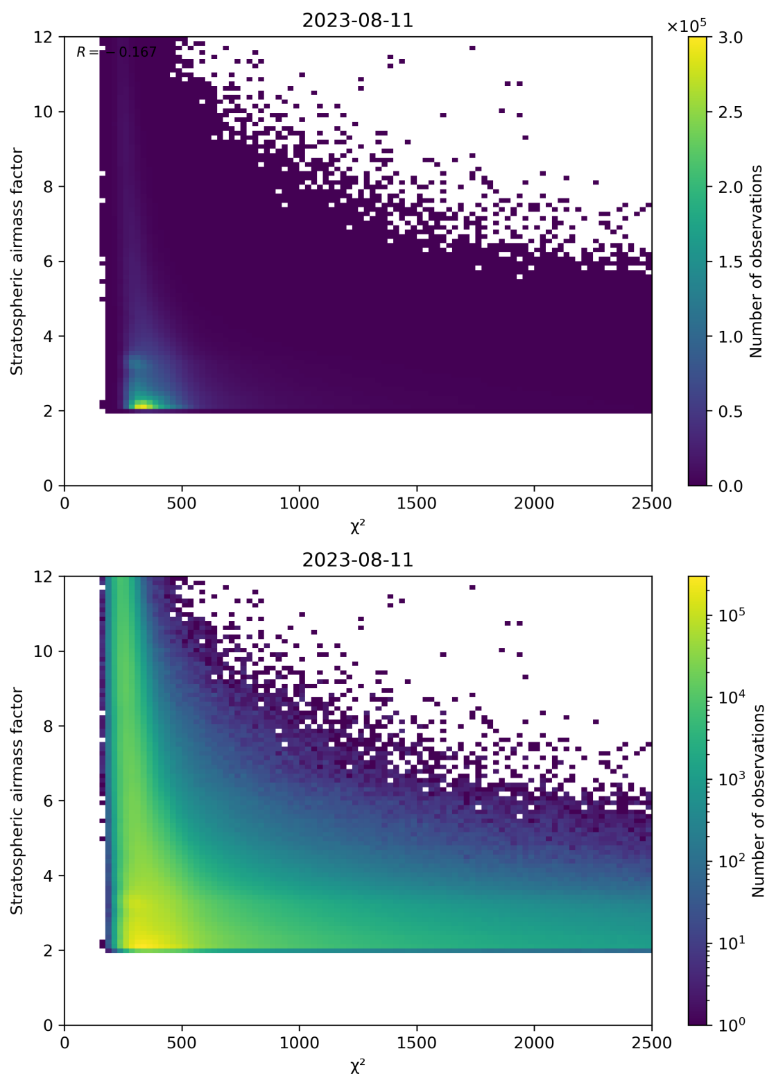
Figure 81: Scatter density plot of “ \chi^2 ” against “Stratospheric airmass factor” for 2023-08-10 to 2023-08-12.
