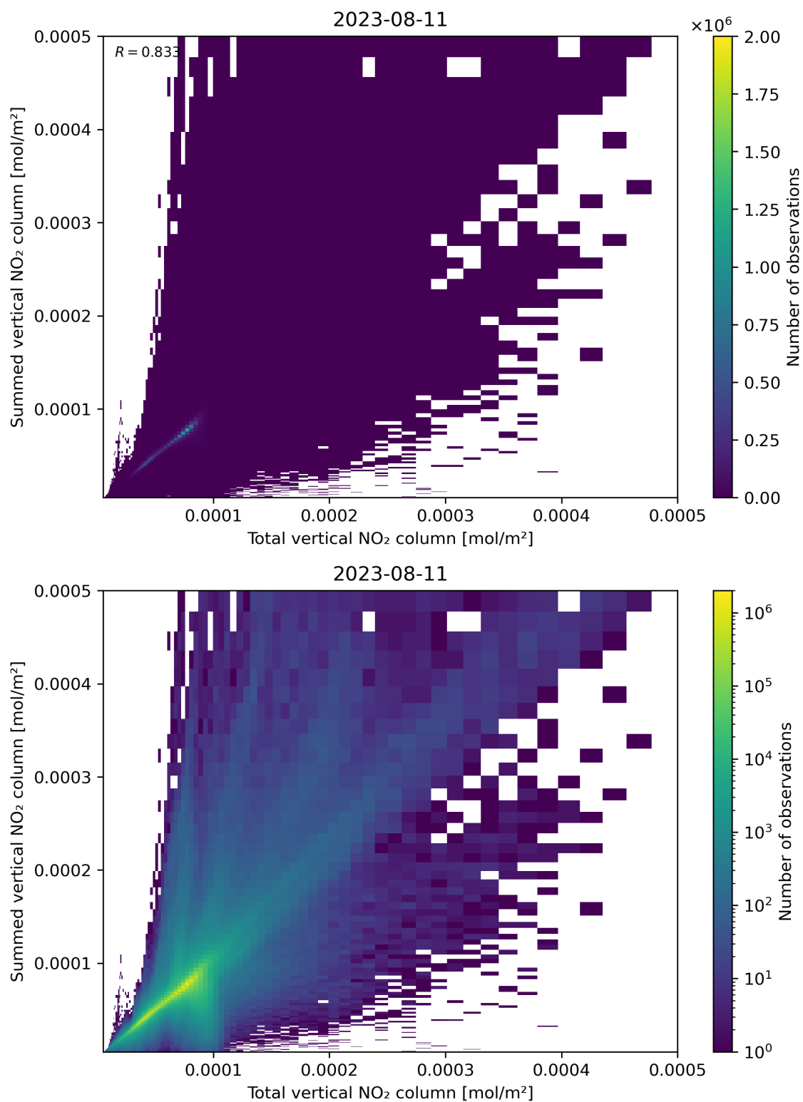
Figure 112: Scatter density plot of “Total vertical NO 2 column” against “Summed vertical NO 2 column” for 2023-08-10 to 2023-08-12.
