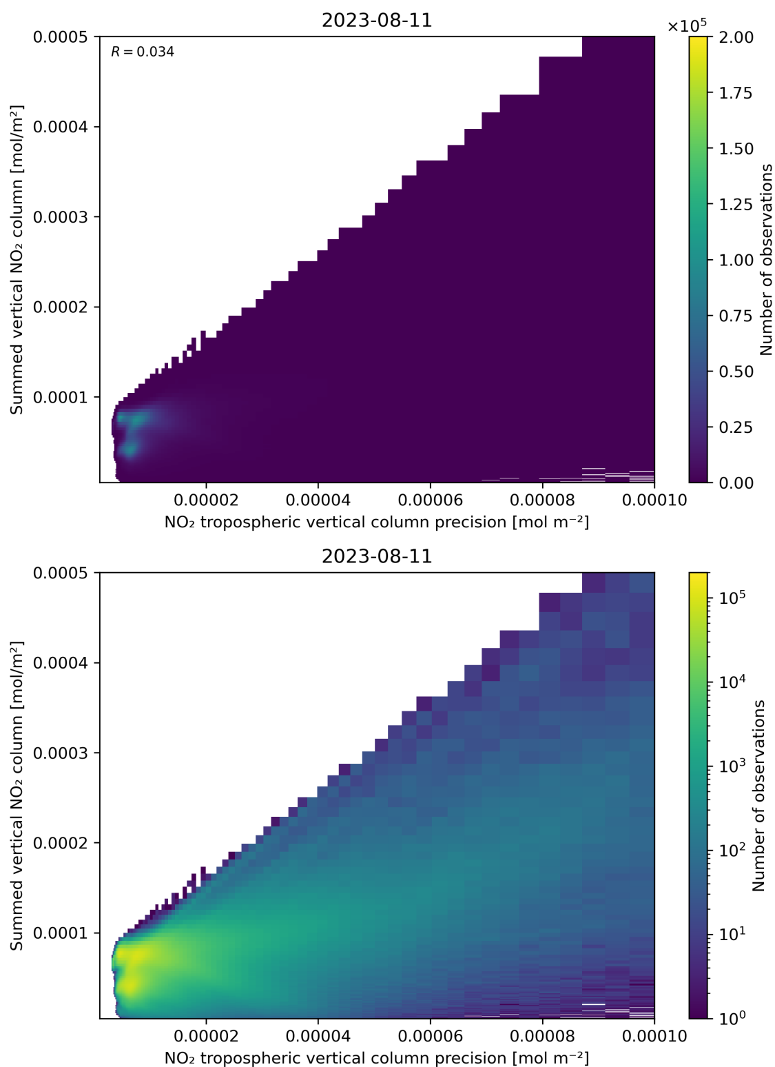
Figure 136: Scatter density plot of “NO 2 tropospheric vertical column precision” against “Summed vertical NO 2 column” for 2023-08-10 to 2023-08-12.
