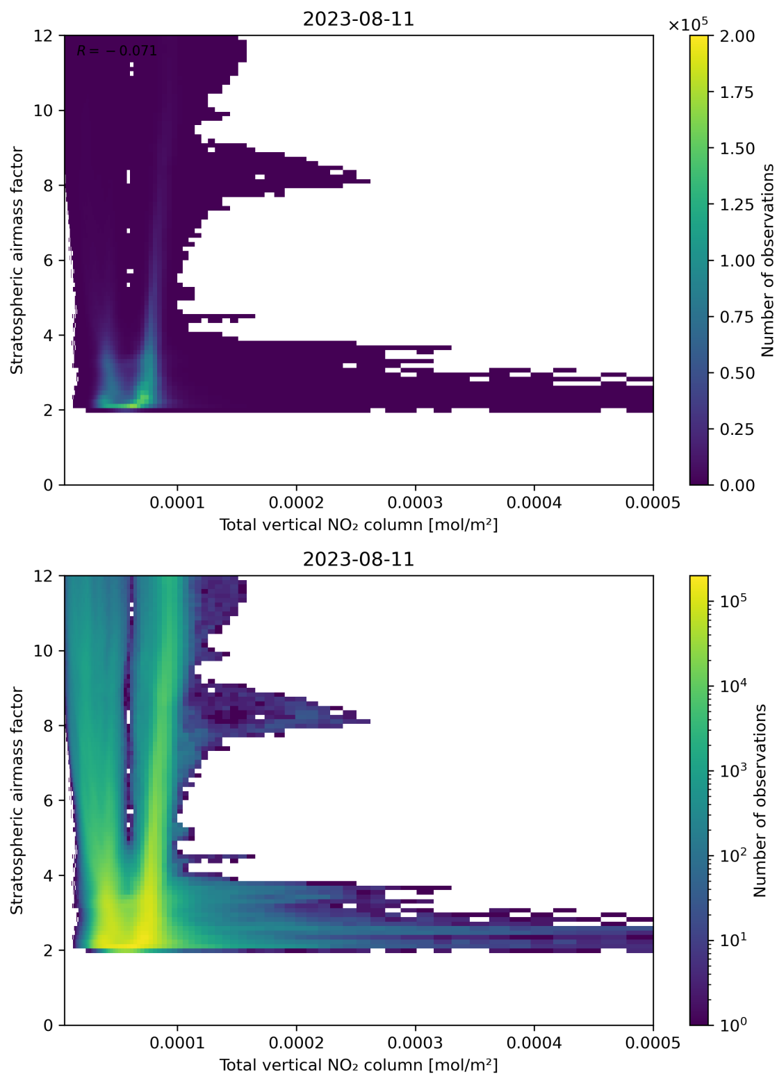
Figure 110: Scatter density plot of “Total vertical NO 2 column” against “Stratospheric airmass factor” for 2023-08-10 to 2023-08-12.
