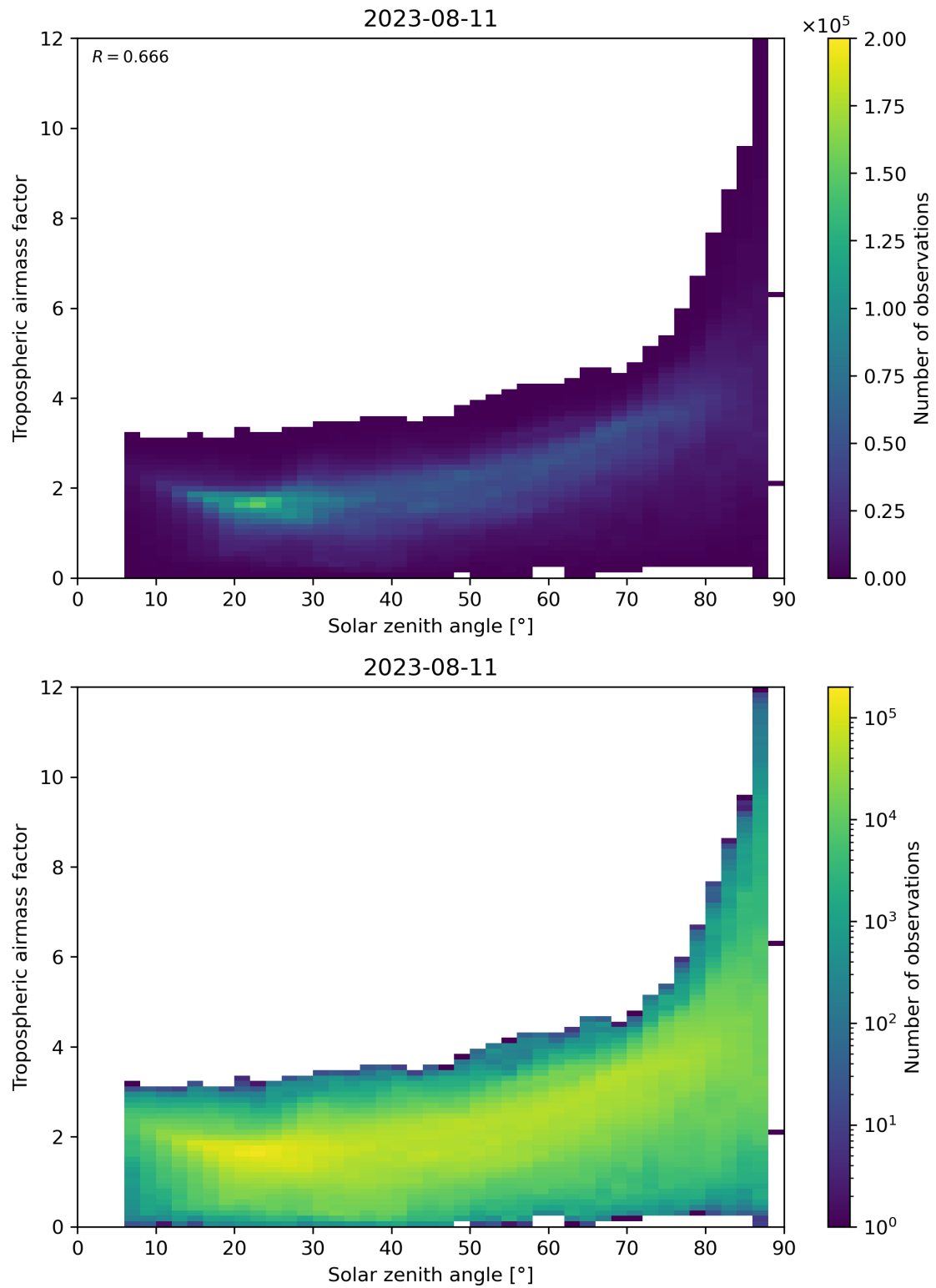
Figure 147: Scatter density plot of “Solar zenith angle” against “Tropospheric airmass factor” for 2023-08-10 to 2023-08-12.
