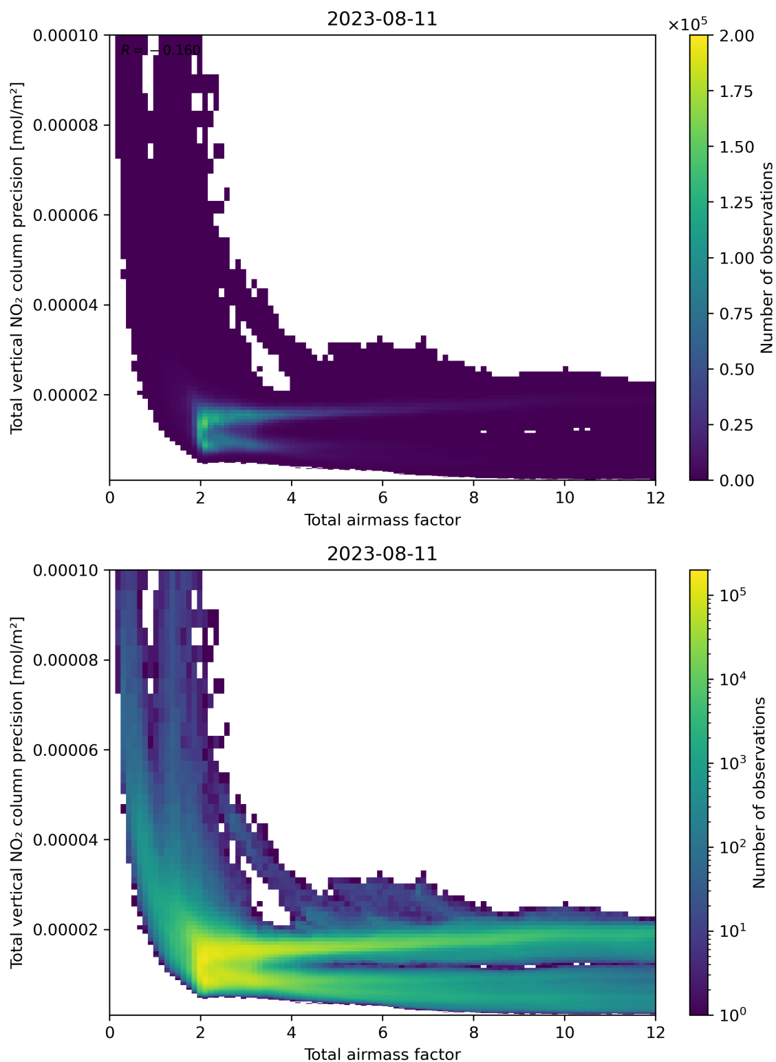
Figure 68: Scatter density plot of “Total airmass factor” against “Total vertical NO 2 column precision” for 2023-08-10 to 2023-08-12.
