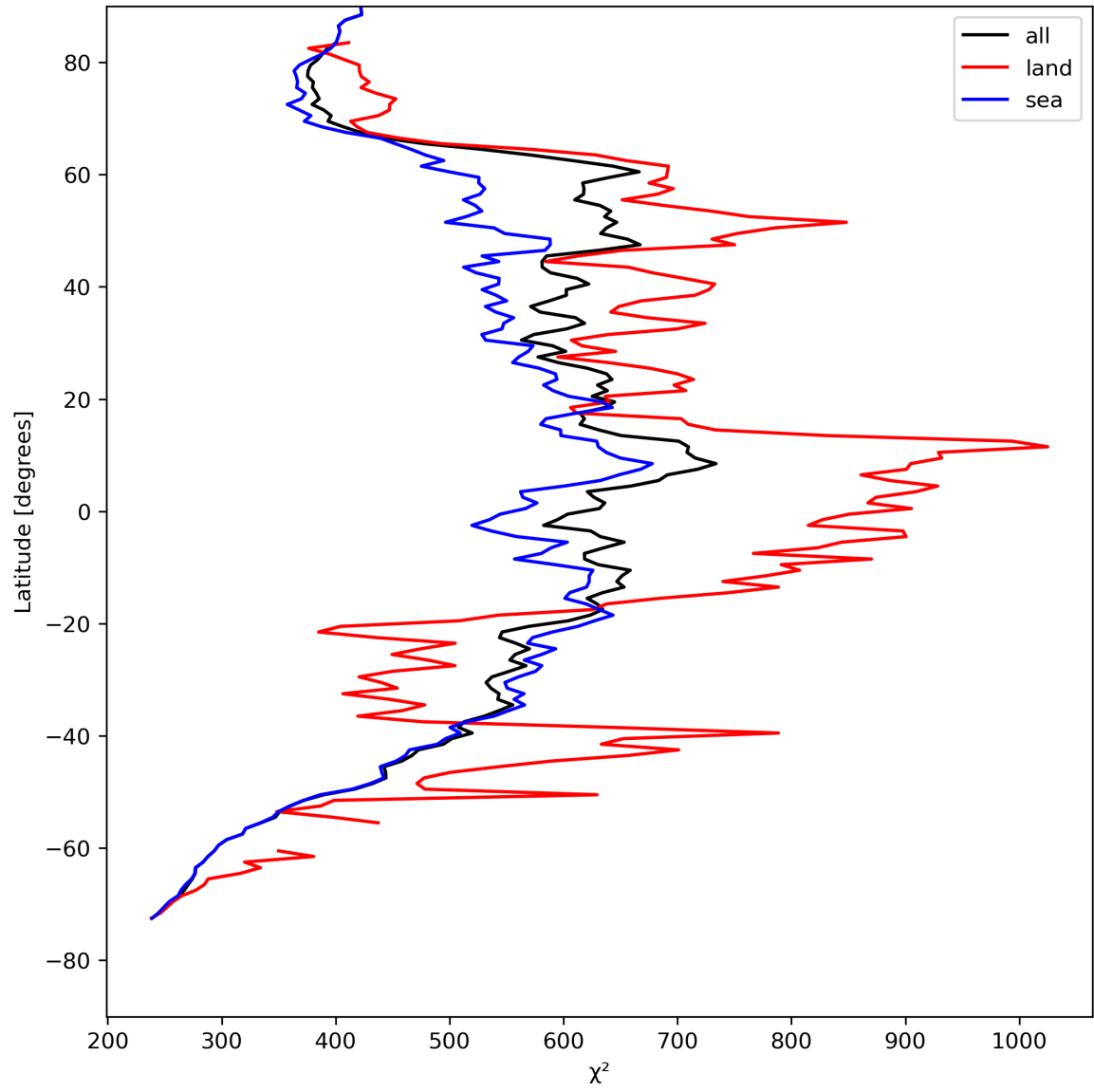
Figure 25: Zonal average of “ \chi^2 ” for 2023-08-10 to 2023-08-12.
