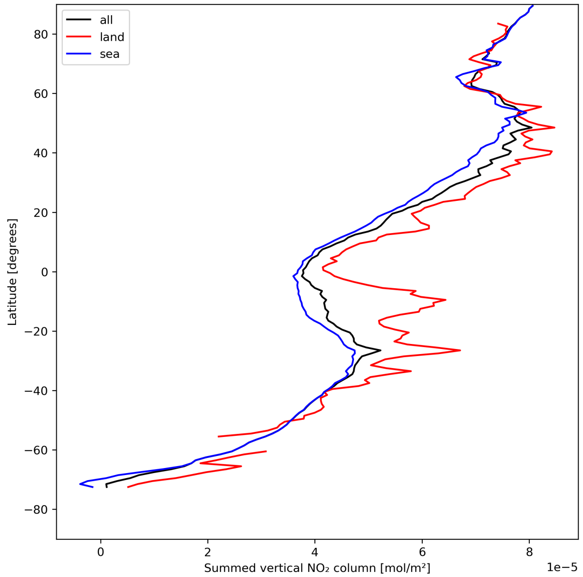
Figure 23: Zonal average of “Summed vertical NO 2 column” for 2023-08-10 to 2023-08-12.
