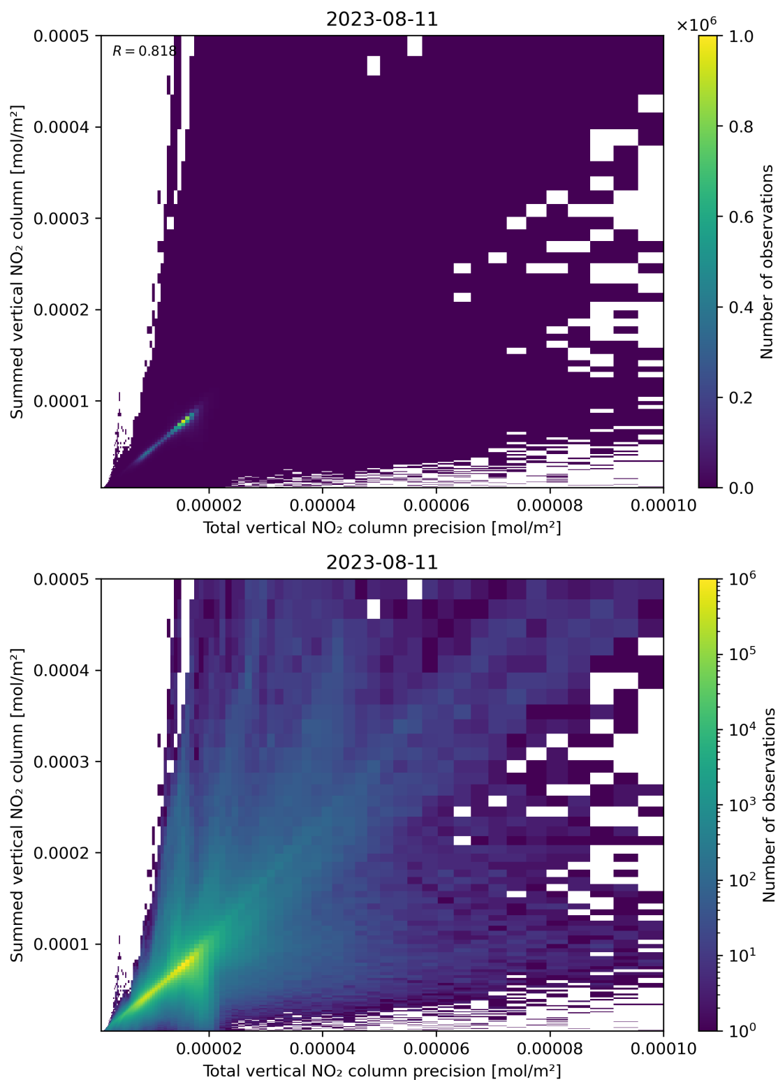
Figure 117: Scatter density plot of “Total vertical NO 2 column precision” against “Summed vertical NO 2 column” for 2023-08-10 to 2023-08-12.
