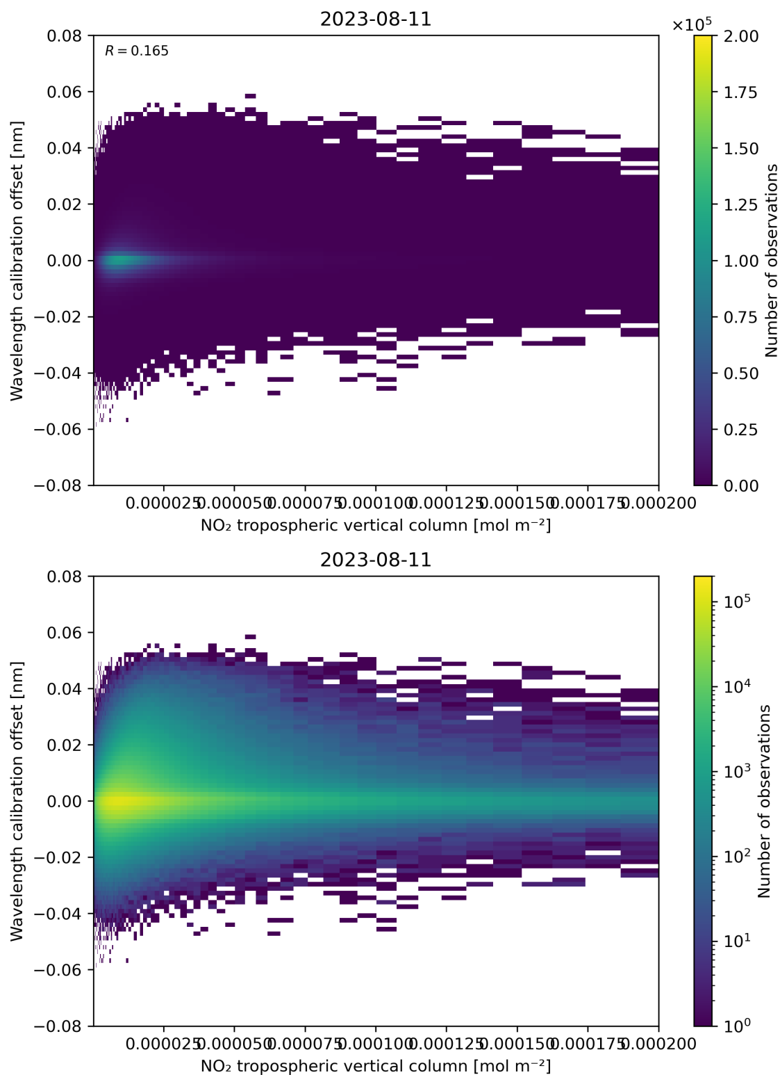
Figure 143: Scatter density plot of “NO 2 tropospheric vertical column” against “Wavelength calibration offset” for 2023-08-10 to 2023-08-12.
