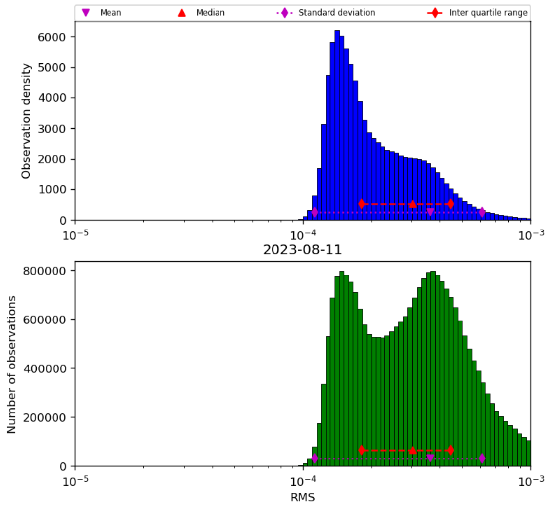
Figure 43: Histogram of “RMS” for 2023-08-10 to 2023-08-12
