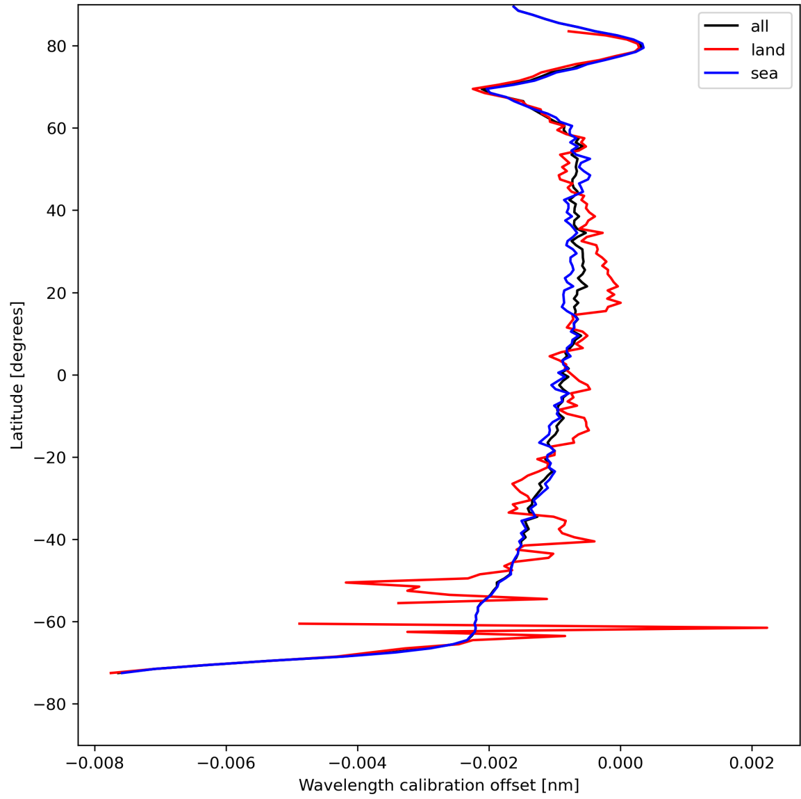
Figure 18: Zonal average of “Wavelength calibration offset” for 2023-08-10 to 2023-08-12.
