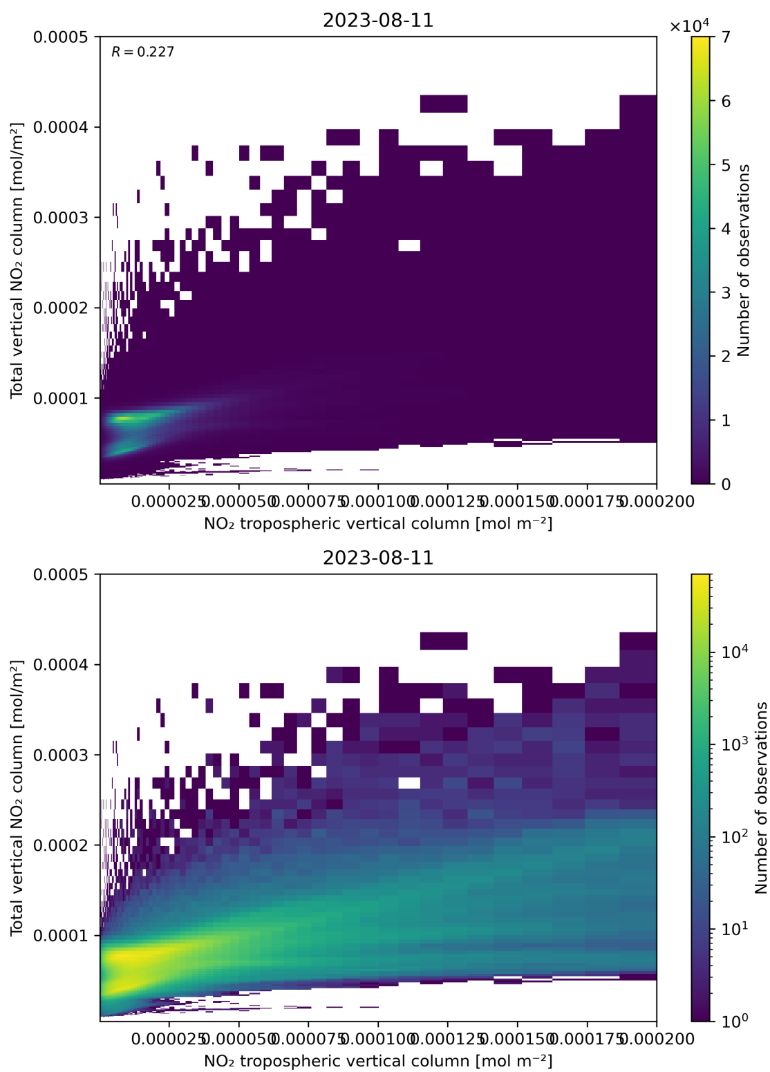
Figure 128: Scatter density plot of “NO 2 tropospheric vertical column” against “Total vertical NO 2 column” for 2023-08-10 to 2023-08-12.
