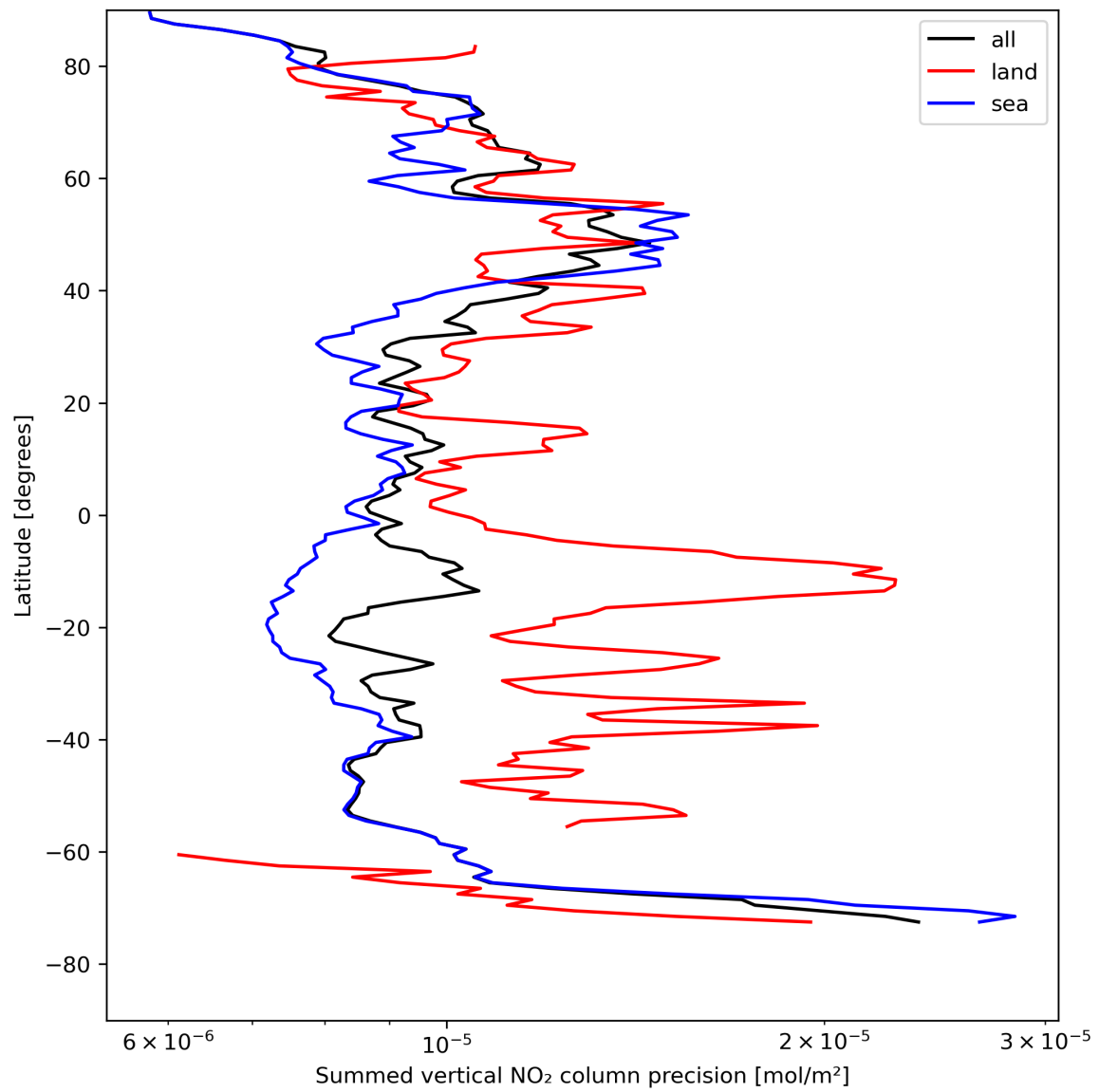
Figure 24: Zonal average of “Summed vertical NO 2 column precision” for 2023-08-10 to 2023-08-12.
