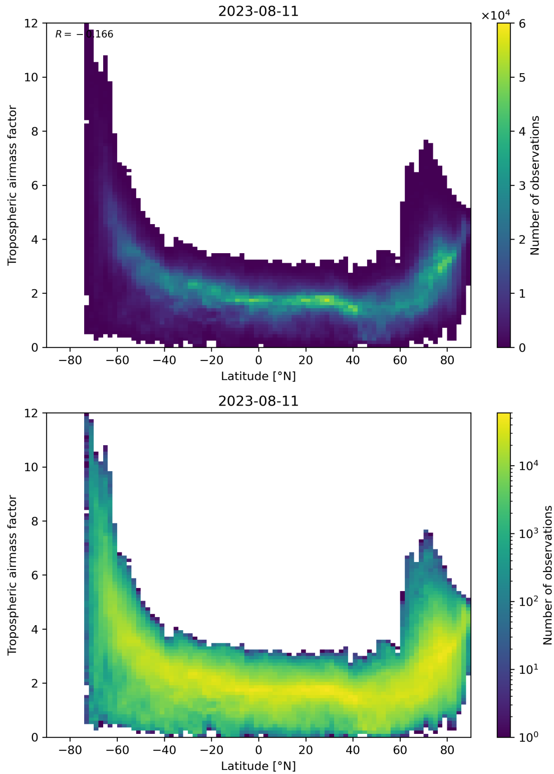
Figure 85: Scatter density plot of “Latitude” against “Tropospheric air mass factor” for 2023-08-10 to 2023-08-12.
