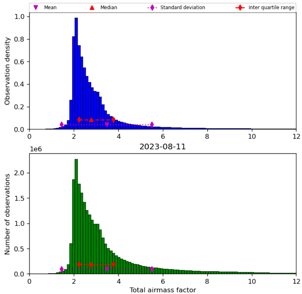
Figure 32: Histogram of “Total airmass factor” for 2023-08-10 to 2023-08-12
