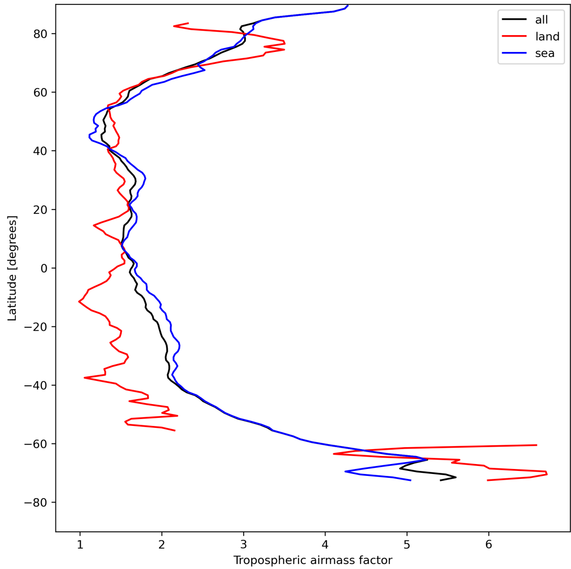
Figure 14: Zonal average of “Tropospheric airmass factor” for 2023-08-10 to 2023-08-12.
