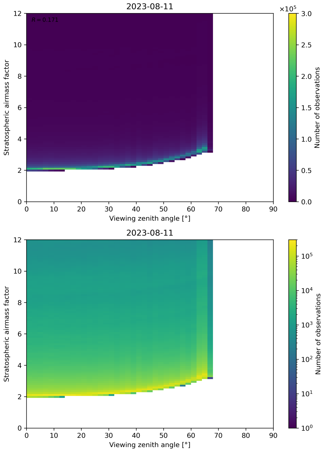
Figure 159: Scatter density plot of “Viewing zenith angle” against “Stratospheric airmass factor” for 2023-08-10 to 2023-08-12.
