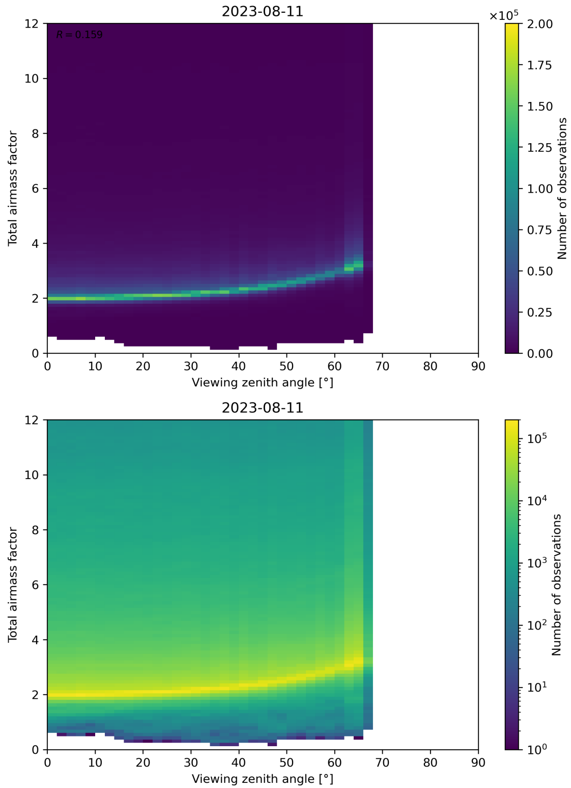
Figure 160: Scatter density plot of “Viewing zenith angle” against “Total airmass factor” for 2023-08-10 to 2023-08-12.
