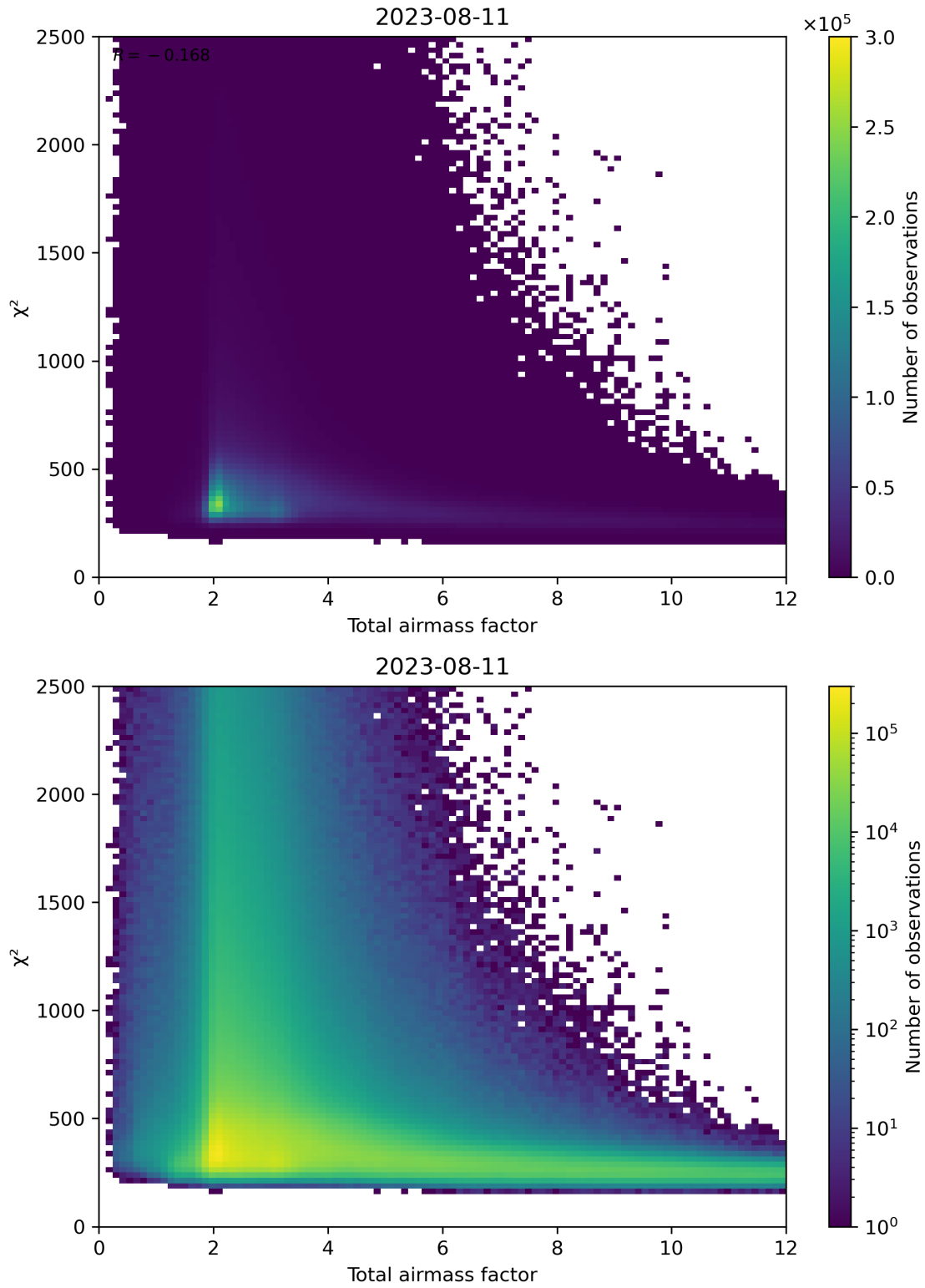
Figure 63: Scatter density plot of “Total airmass factor” against “ \chi^2 ” for 2023-08-10 to 2023-08-12.
