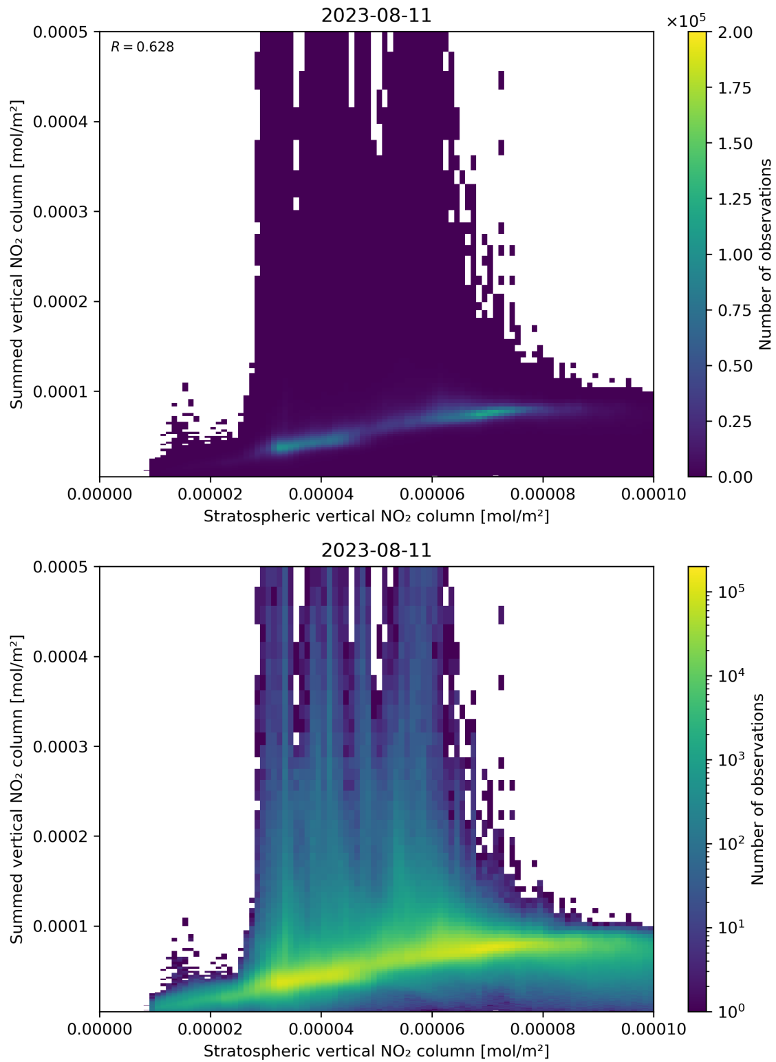
Figure 98: Scatter density plot of “Stratospheric vertical NO 2 column” against “Summed vertical NO 2 column” for 2023-08-10 to 2023-08-12.
