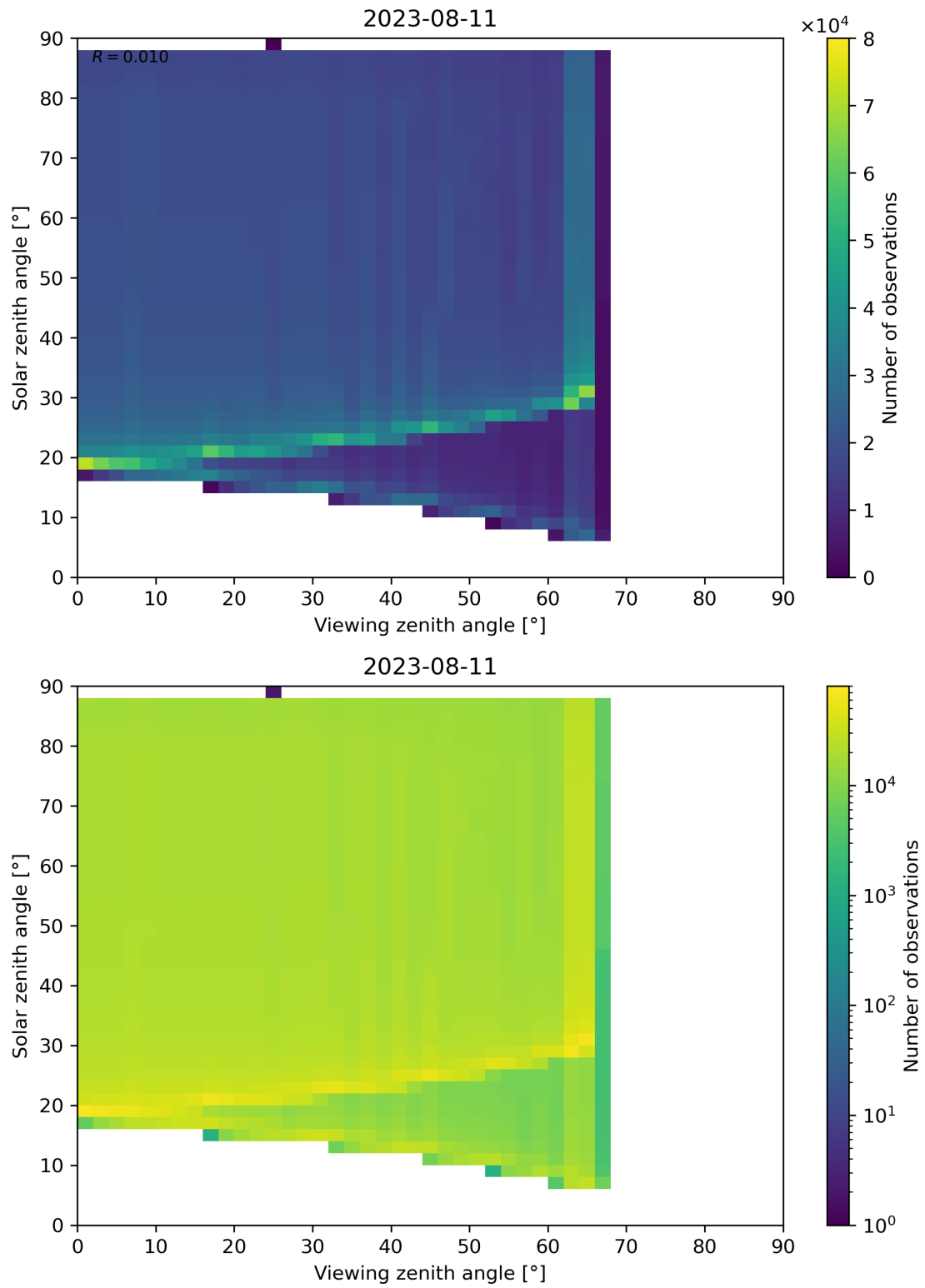
Figure 172: Scatter density plot of “Viewing zenith angle” against “Solar zenith angle” for 2023-08-10 to 2023-08-12.
