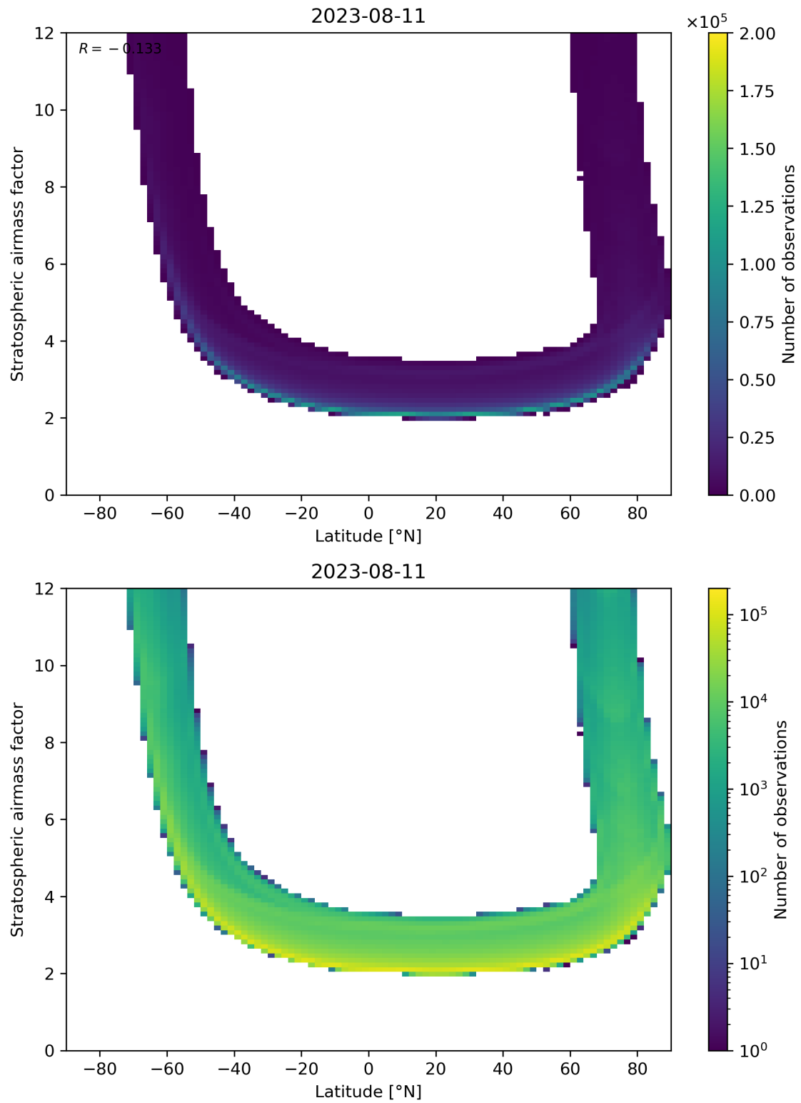
Figure 83: Scatter density plot of “Latitude” against “Stratospheric air mass factor” for 2023-08-10 to 2023-08-12.
