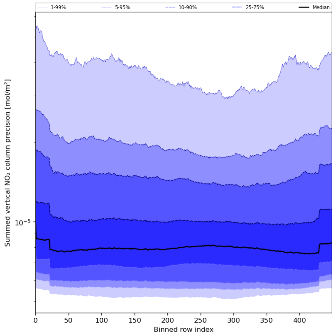
Figure 58: Along track statistics of “Summed vertical NO 2 column precision” for 2023-08-10 to 2023-08-12
