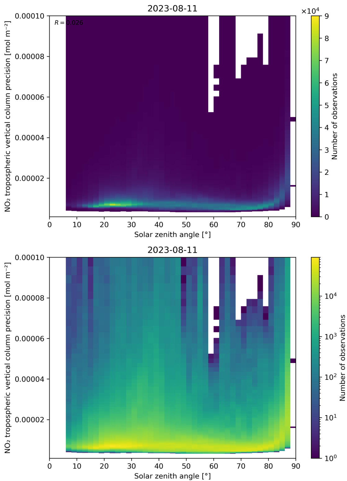
Figure 156: Scatter density plot of “Solar zenith angle” against “NO 2 tropospheric vertical column precision” for 2023-08-10 to 2023-08-12.
