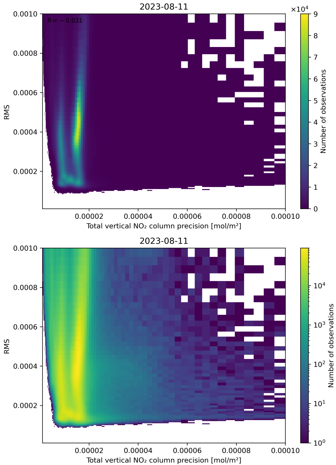
Figure 119: Scatter density plot of “Total vertical NO 2 column precision” against “RMS” for 2023-08-10 to 2023-08-12.
