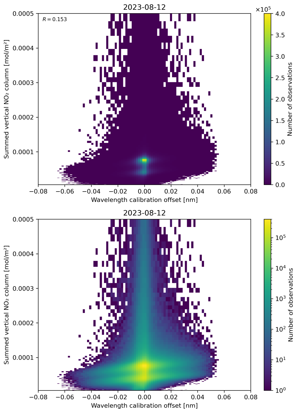
Figure 177: Scatter density plot of “Wavelength calibration offset” against “Summed vertical NO 2 column” for 2023-08-11 to 2023-08-13.
