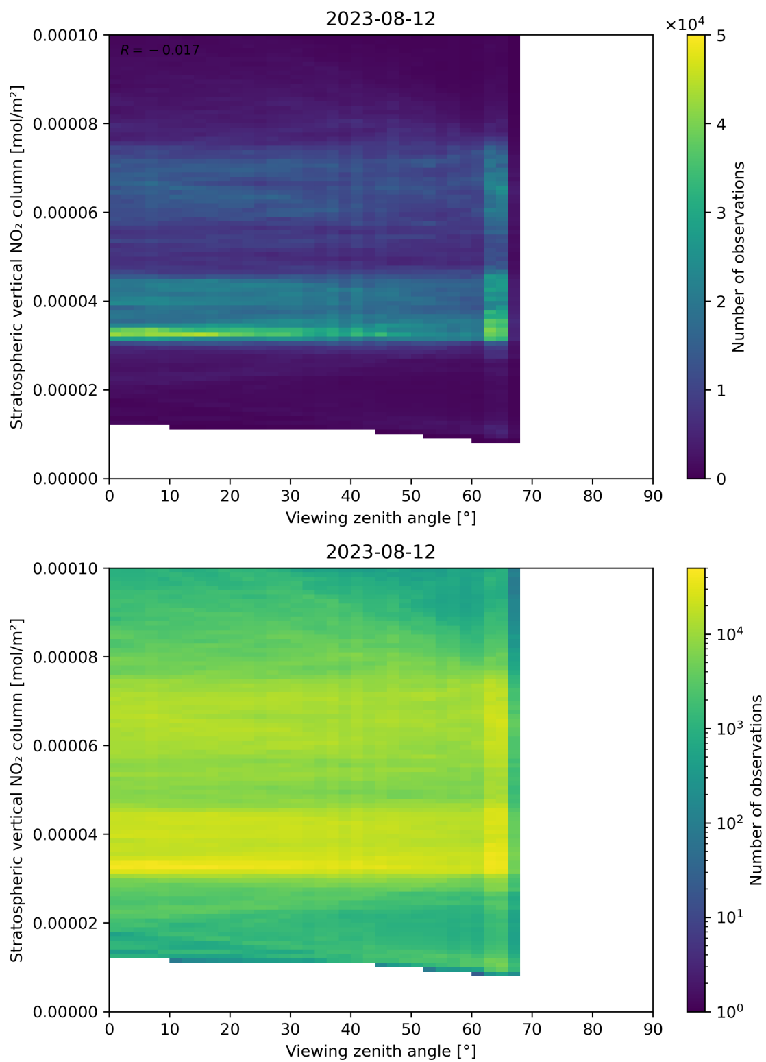
Figure 164: Scatter density plot of “Viewing zenith angle” against “Stratospheric vertical NO 2 column” for 2023-08-11 to 2023-08-13.
