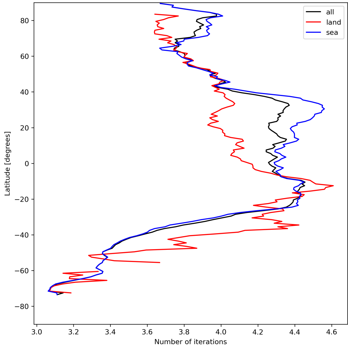
Figure 17: Zonal average of “Number of iterations” for 2023-08-11 to 2023-08-13.
