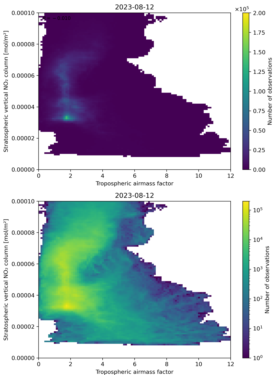
Figure 74: Scatter density plot of “Tropospheric air mass factor” against “Stratospheric vertical NO 2 column” for 2023-08-11 to 2023-08-13.
