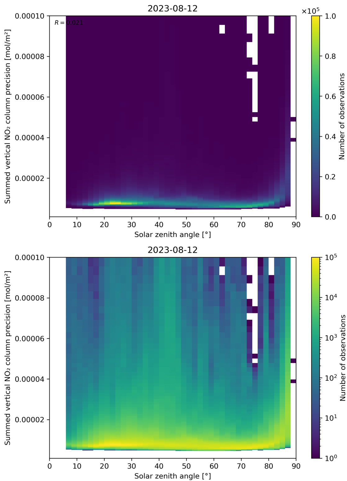
Figure 152: Scatter density plot of “Solar zenith angle” against “Summed vertical NO 2 column precision” for 2023-08-11 to 2023-08-13.
