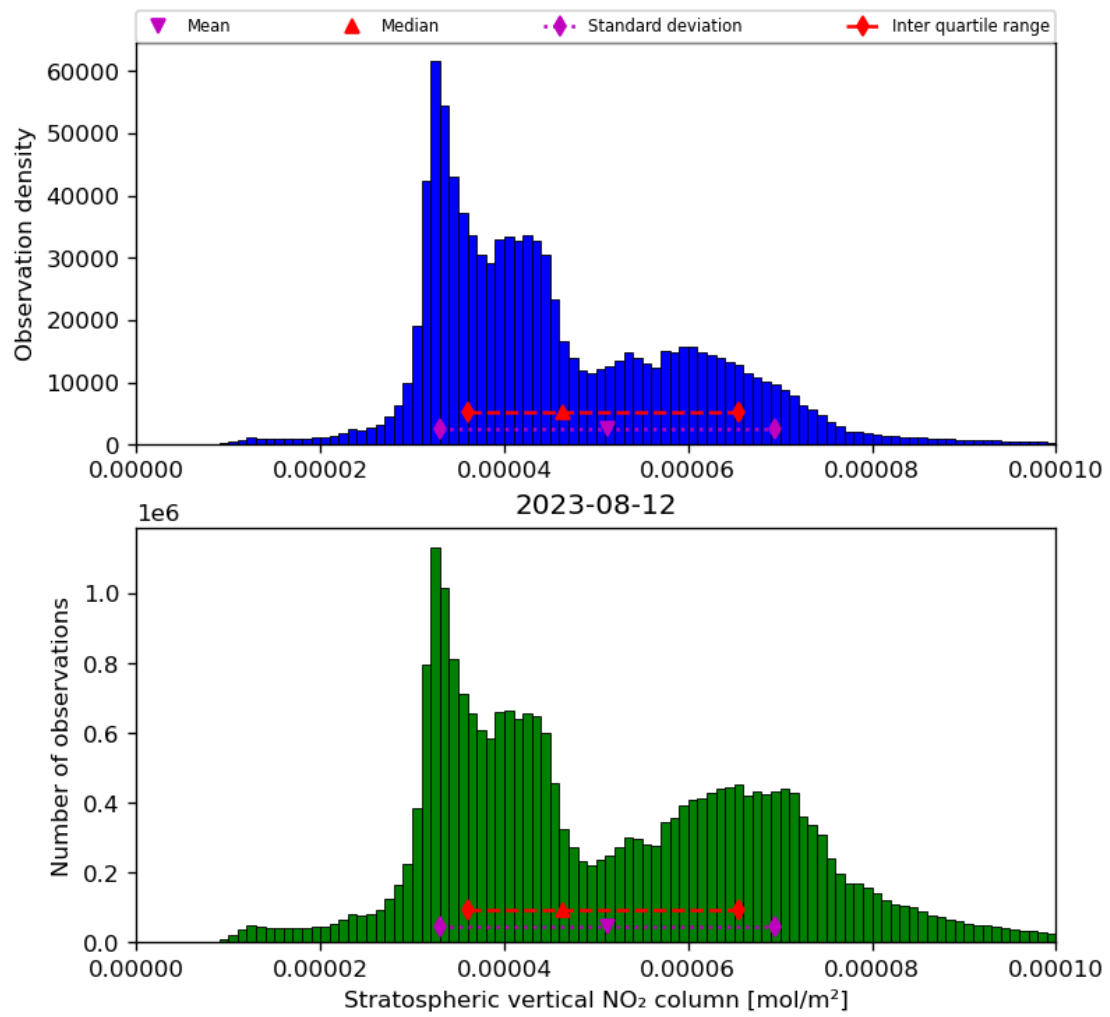
Figure 36: Histogram of “Stratospheric vertical NO 2 column” for 2023-08-11 to 2023-08-13
