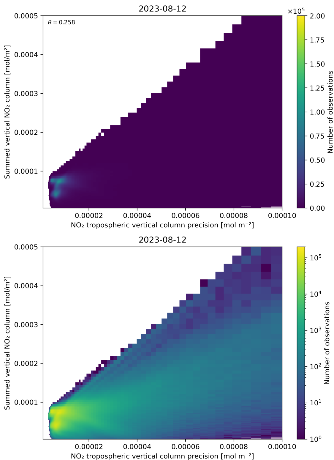
Figure 136: Scatter density plot of “NO 2 tropospheric vertical column precision” against “Summed vertical NO 2 column” for 2023-08-11 to 2023-08-13.
