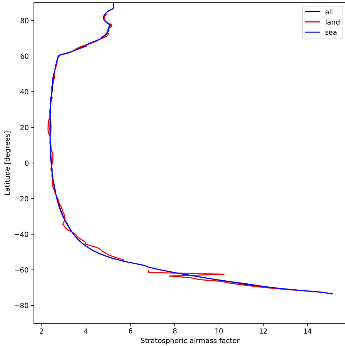
Figure 27: Zonal average of “Stratospheric air mass factor” for 2023-08-11 to 2023-08-13.
