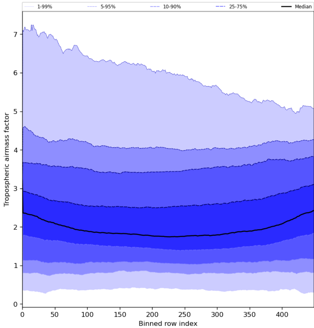
Figure 48: Along track statistics of “Tropospheric airmass factor” for 2023-08-11 to 2023-08-13
