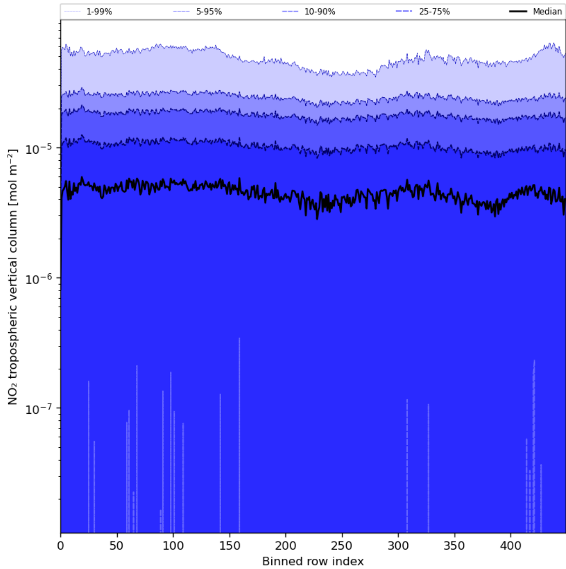
Figure 46: Along track statistics of “NO 2 tropospheric vertical column” for 2023-08-11 to 2023-08-13
