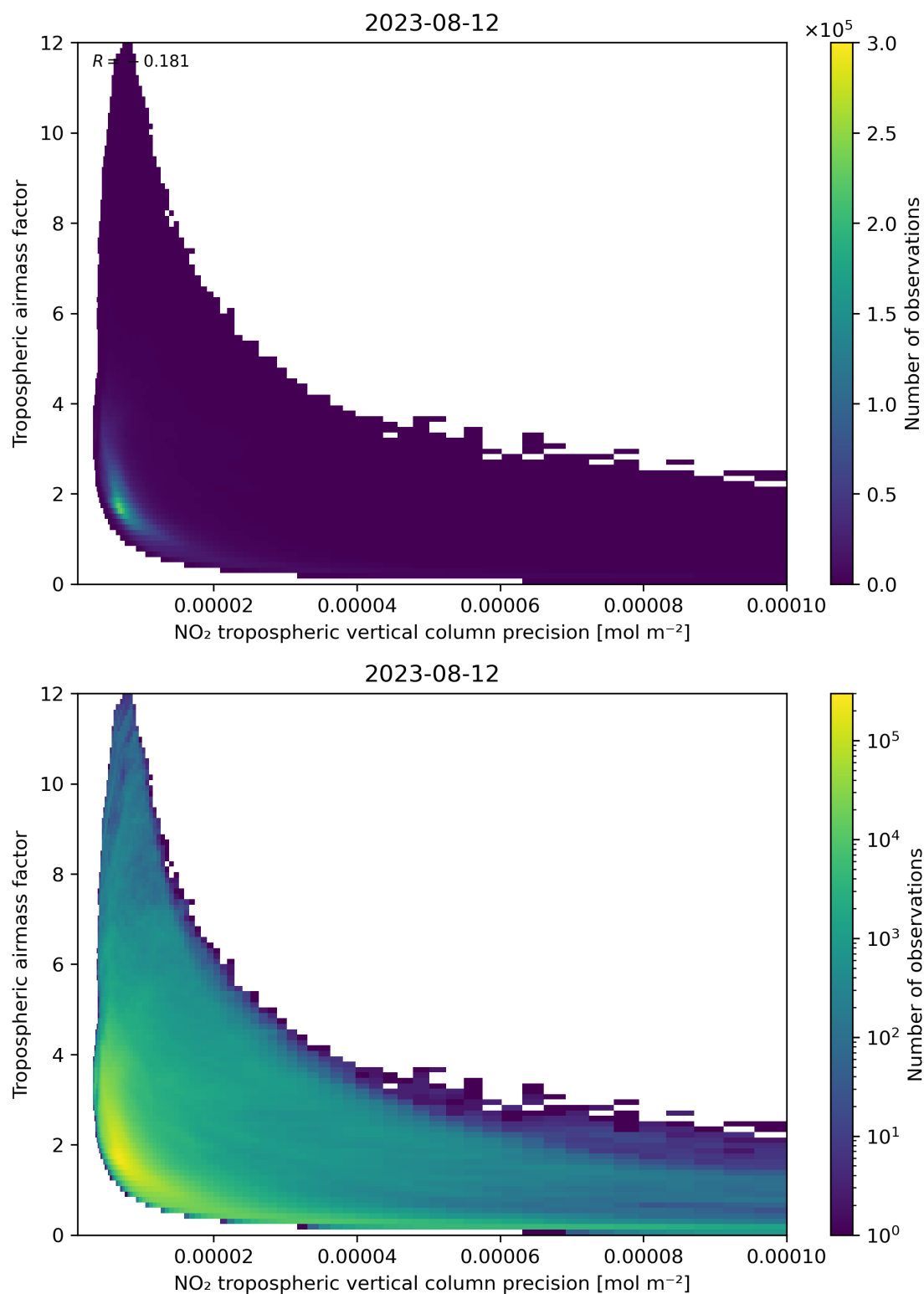
Figure 133: Scatter density plot of “NO 2 tropospheric vertical column precision” against “Tropospheric air mass factor” for 2023-08-11 to 2023-08-13.
