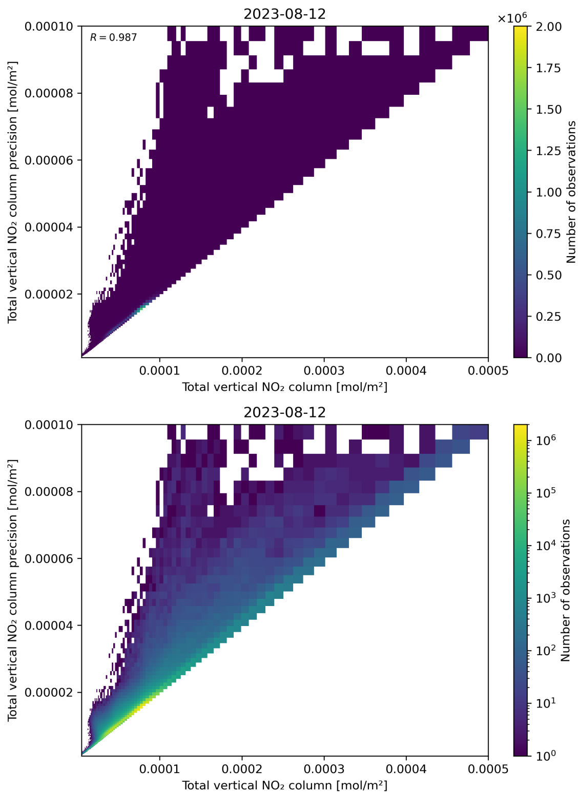
Figure 114: Scatter density plot of “Total vertical NO 2 column” against “Total vertical NO 2 column precision” for 2023-08-11 to 2023-08-13.
