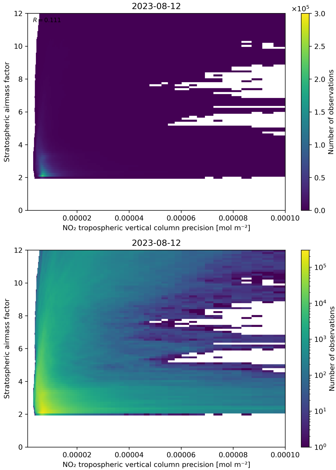
Figure 131: Scatter density plot of “NO 2 tropospheric vertical column precision” against “Stratospheric airmass factor” for 2023-08-11 to 2023-08-13.
