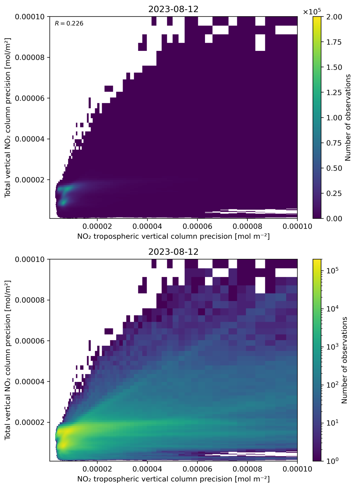
Figure 139: Scatter density plot of “NO 2 tropospheric vertical column precision” against “Total vertical NO 2 column precision” for 2023-08-11 to 2023-08-13.
