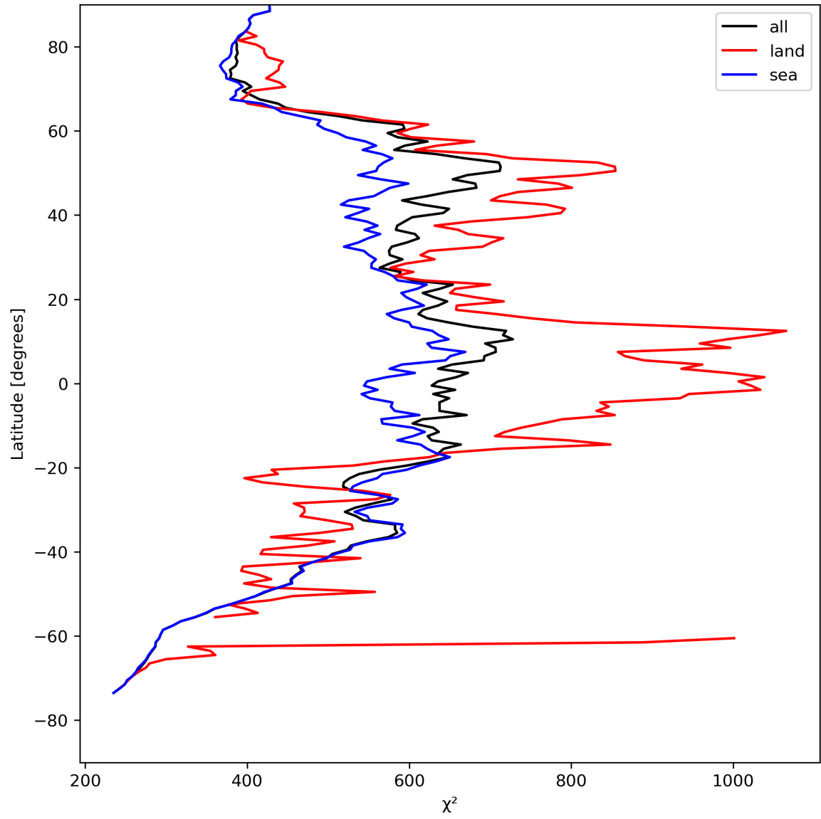
Figure 25: Zonal average of “ \chi^2 ” for 2023-08-11 to 2023-08-13.
