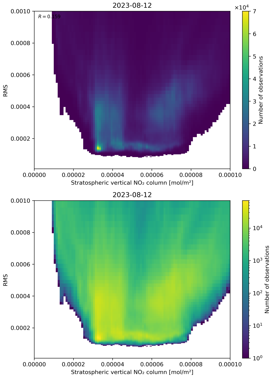
Figure 102: Scatter density plot of “Stratospheric vertical NO 2 column” against “RMS” for 2023-08-11 to 2023-08-13.
