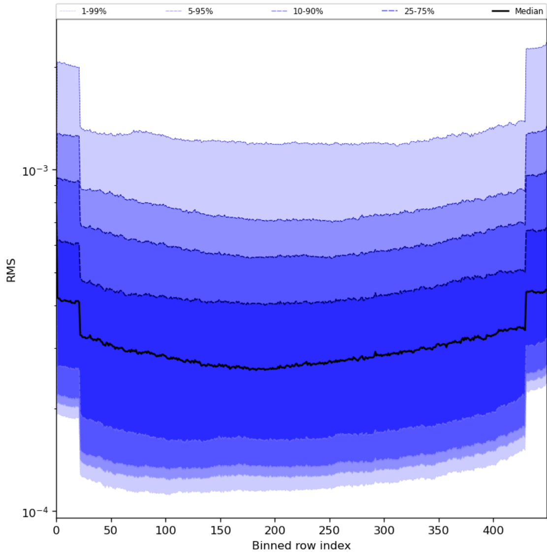
Figure 60: Along track statistics of “RMS” for 2023-08-11 to 2023-08-13
