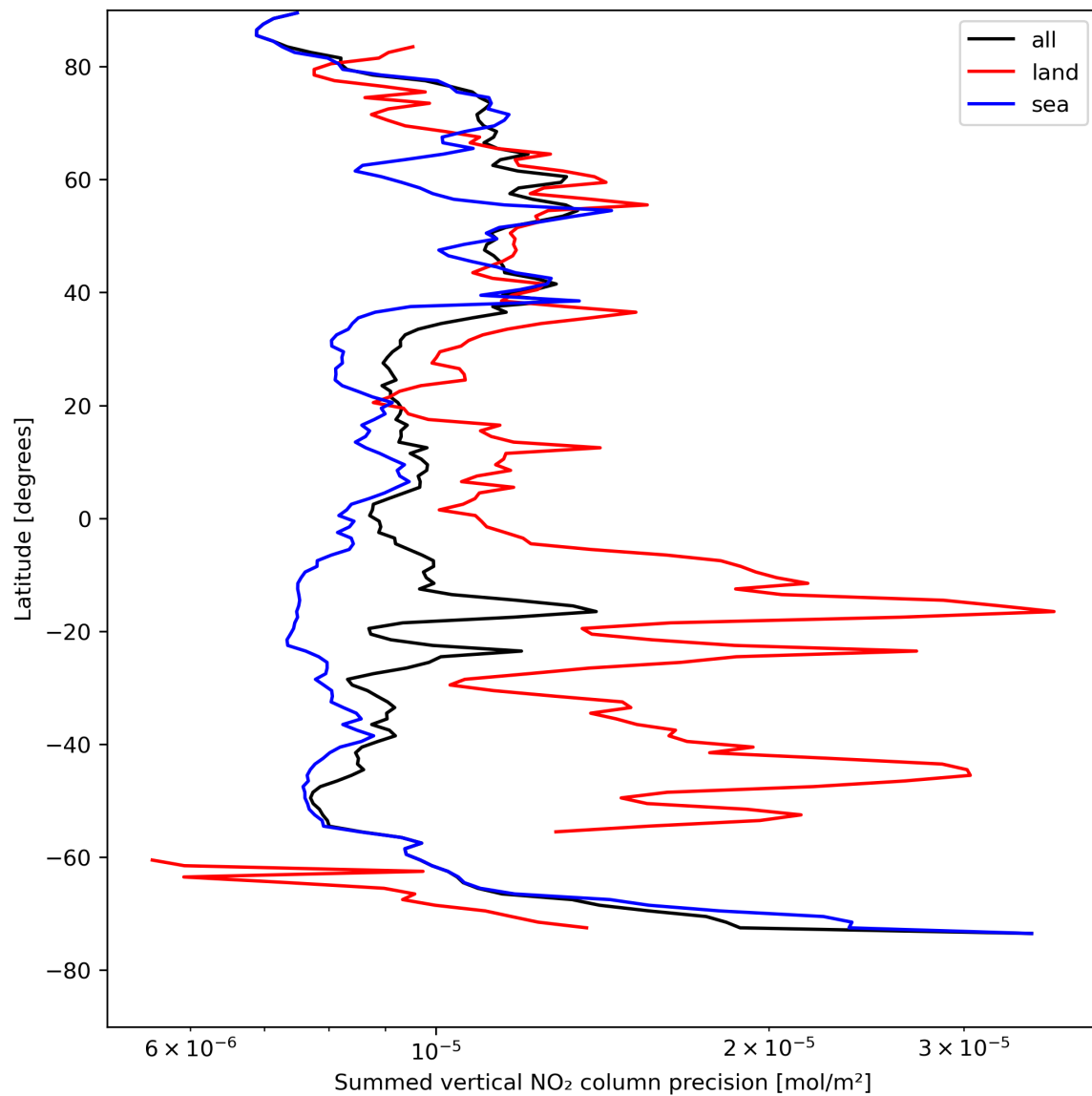
Figure 24: Zonal average of “Summed vertical NO 2 column precision” for 2023-08-11 to 2023-08-13.
