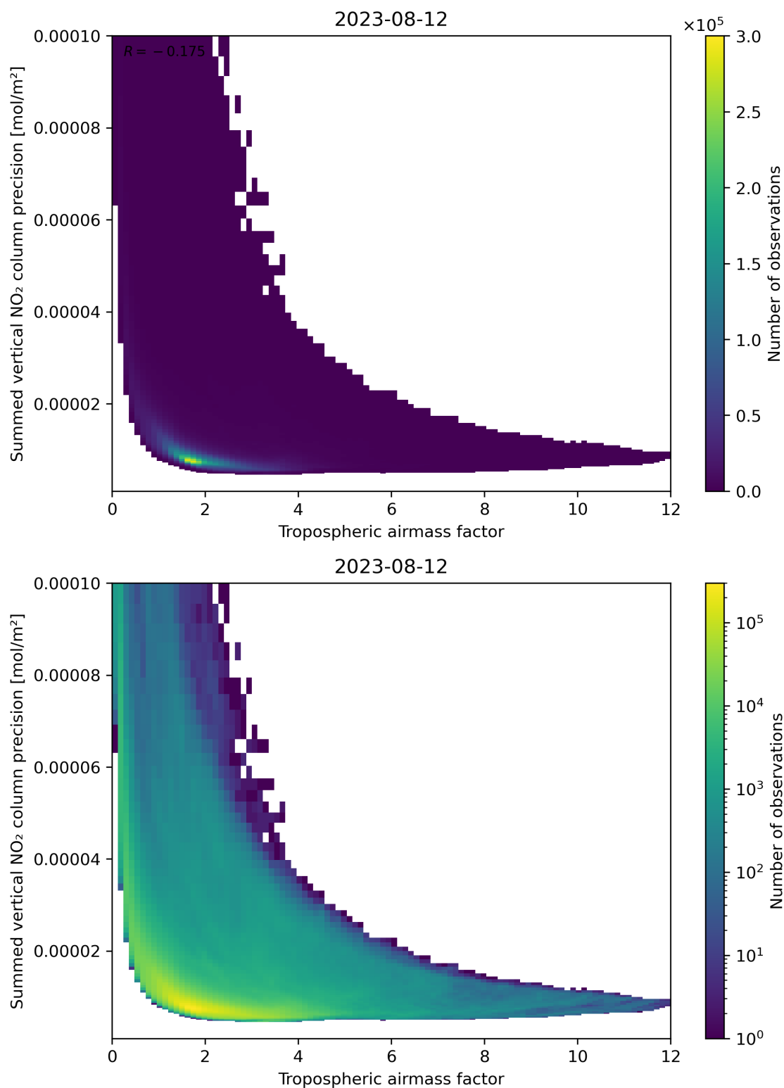
Figure 76: Scatter density plot of “Tropospheric air mass factor” against “Summed vertical NO 2 column precision” for 2023-08-11 to 2023-08-13.
