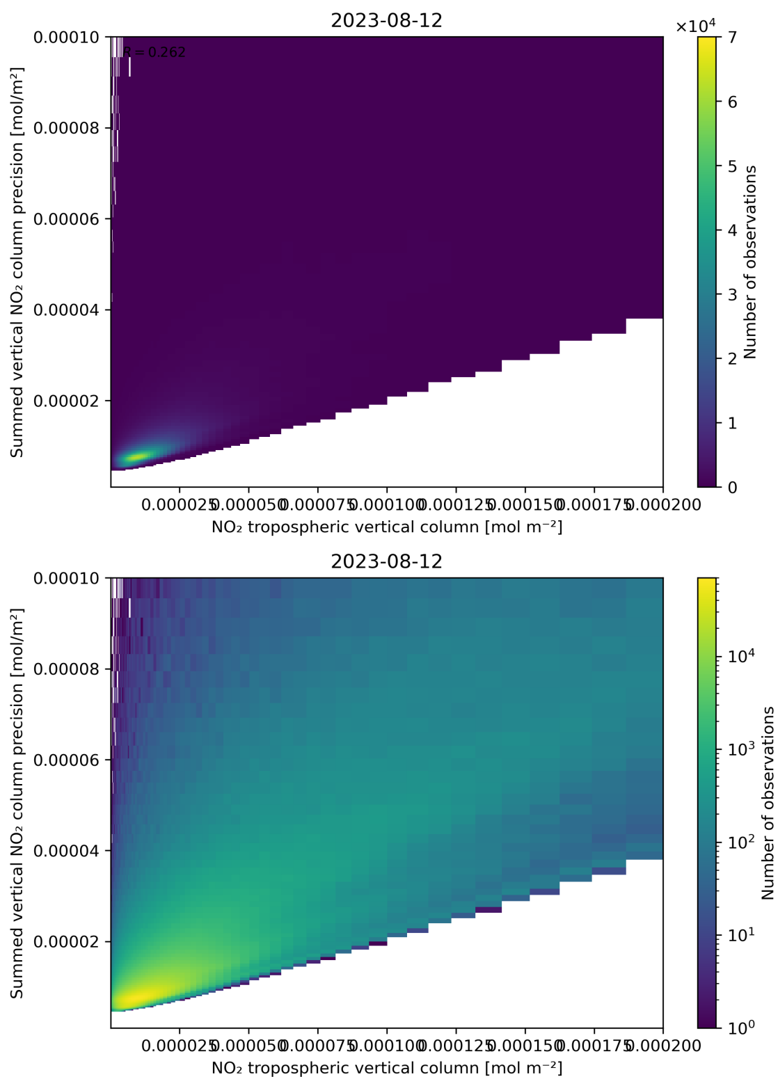
Figure 127: Scatter density plot of “NO 2 tropospheric vertical column” against “Summed vertical NO 2 column precision” for 2023-08-11 to 2023-08-13.
