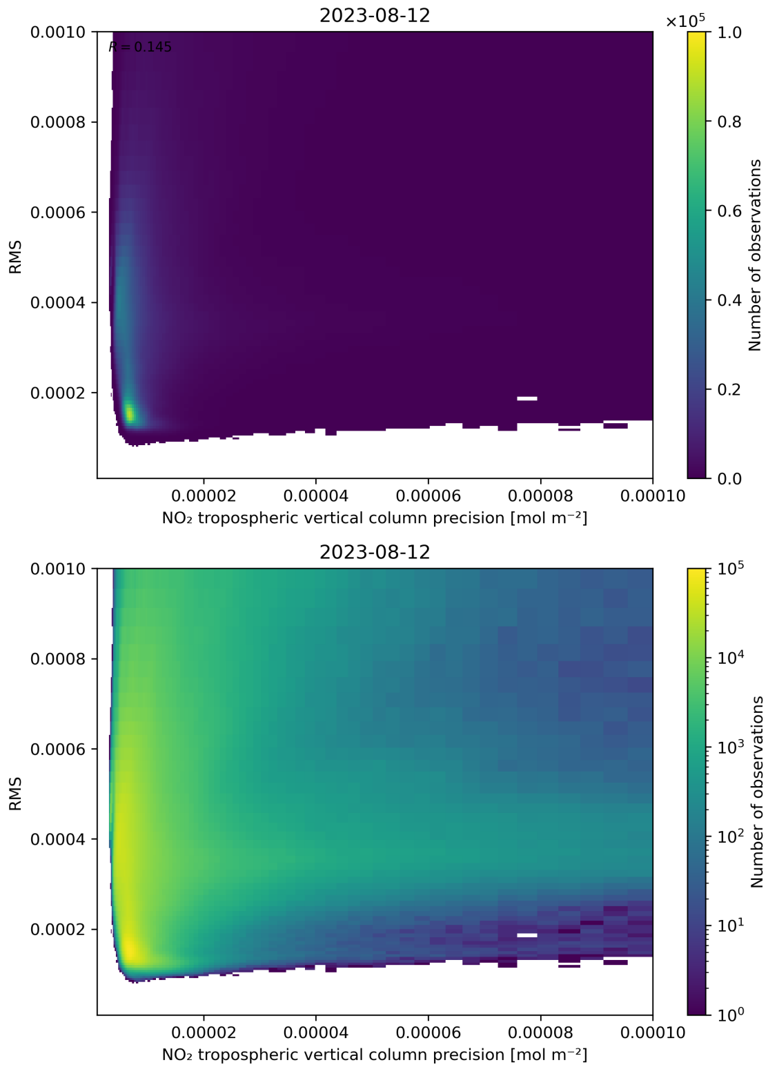
Figure 140: Scatter density plot of “NO 2 tropospheric vertical column precision” against “RMS” for 2023-08-11 to 2023-08-13.
