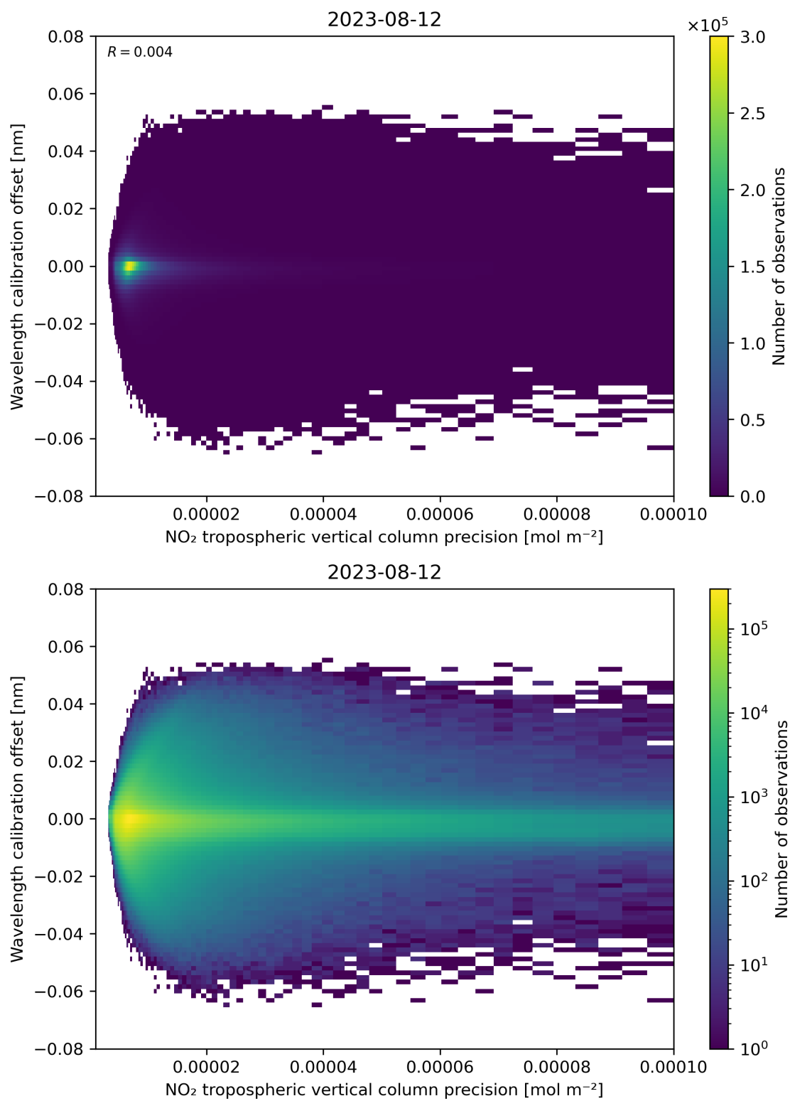
Figure 141: Scatter density plot of “NO 2 tropospheric vertical column precision” against “Wavelength calibration offset” for 2023-08-11 to 2023-08-13.
