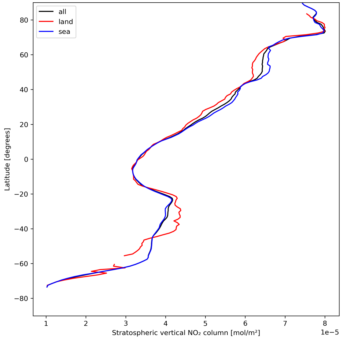
Figure 19: Zonal average of “Stratospheric vertical NO 2 column” for 2023-08-11 to 2023-08-13.
