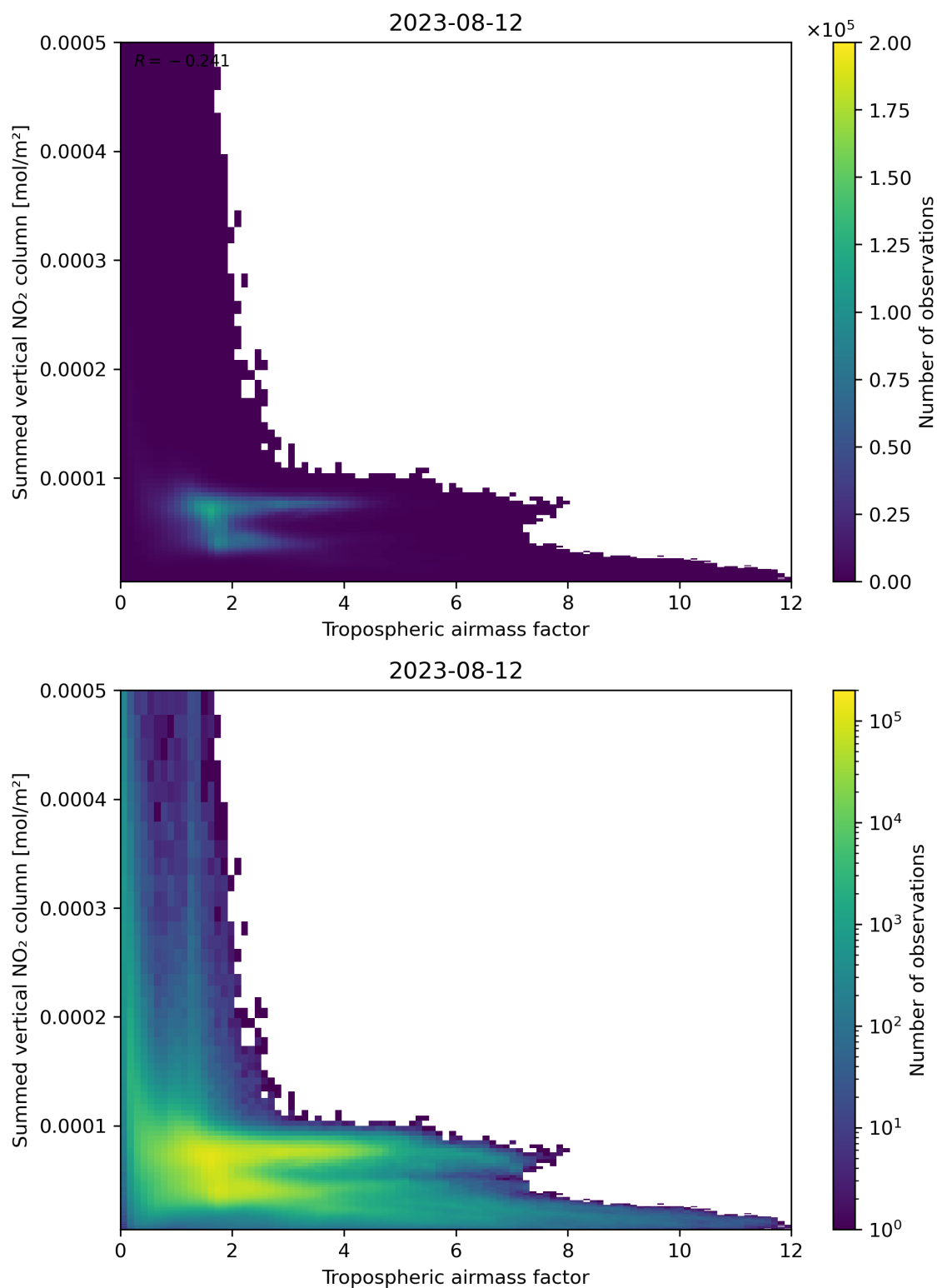
Figure 75: Scatter density plot of “Tropospheric airmass factor” against “Summed vertical NO 2 column” for 2023-08-11 to 2023-08-13.
