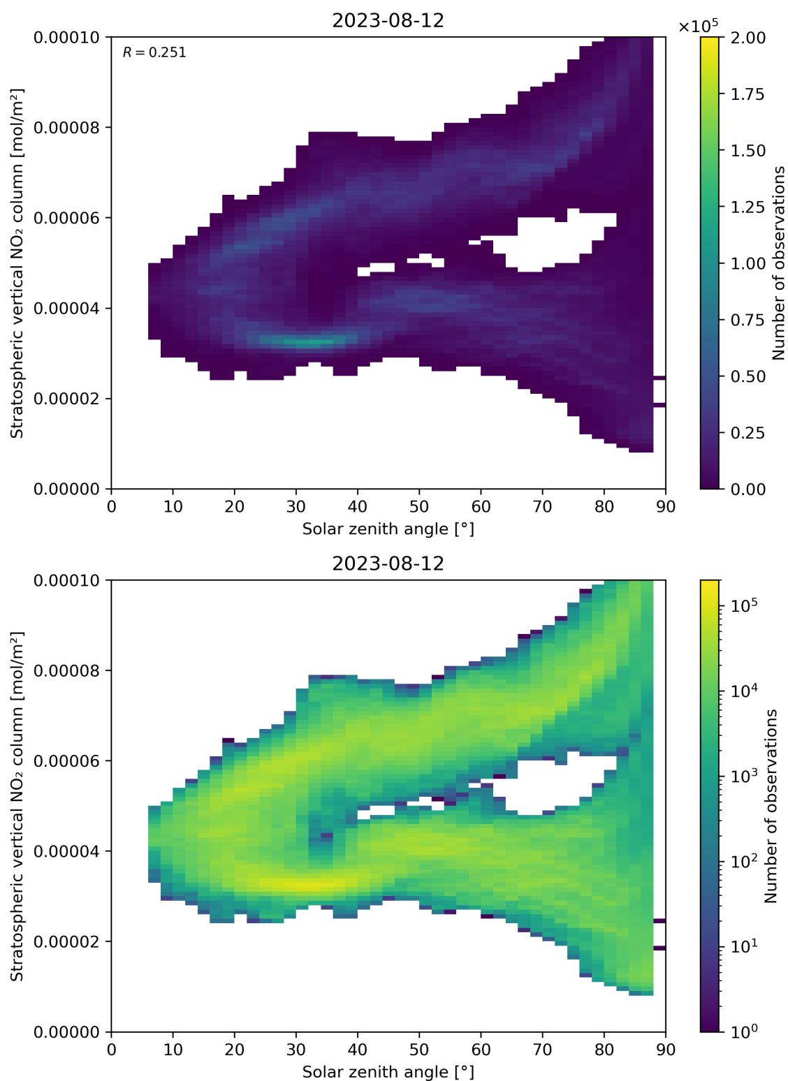
Figure 150: Scatter density plot of “Solar zenith angle” against “Stratospheric vertical NO 2 column” for 2023-08-11 to 2023-08-13.
