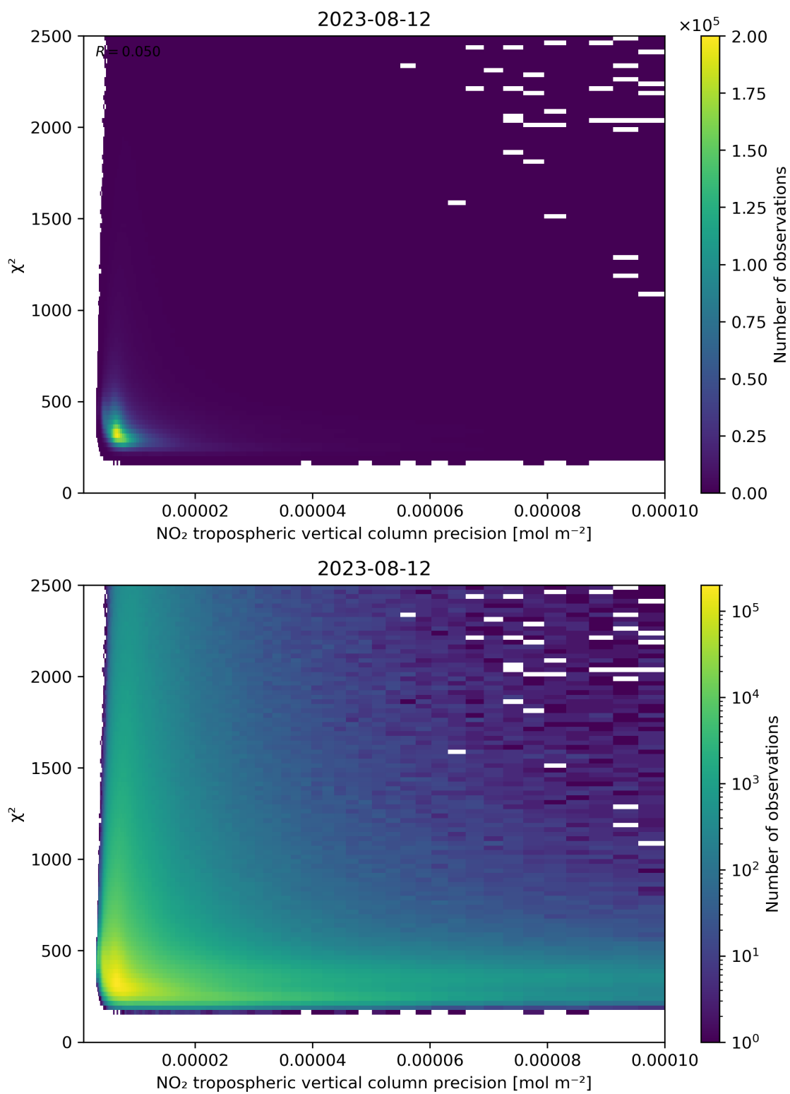
Figure 134: Scatter density plot of “NO 2 tropospheric vertical column precision” against “ \chi^2 ” for 2023-08-11 to 2023-08-13.
