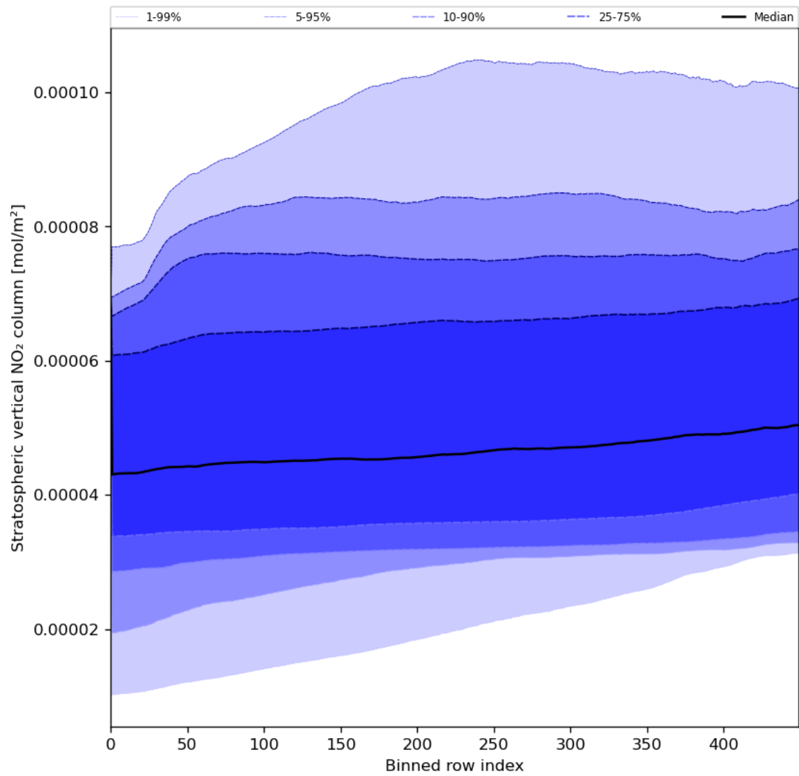
Figure 53: Along track statistics of “Stratospheric vertical NO 2 column” for 2023-08-11 to 2023-08-13
