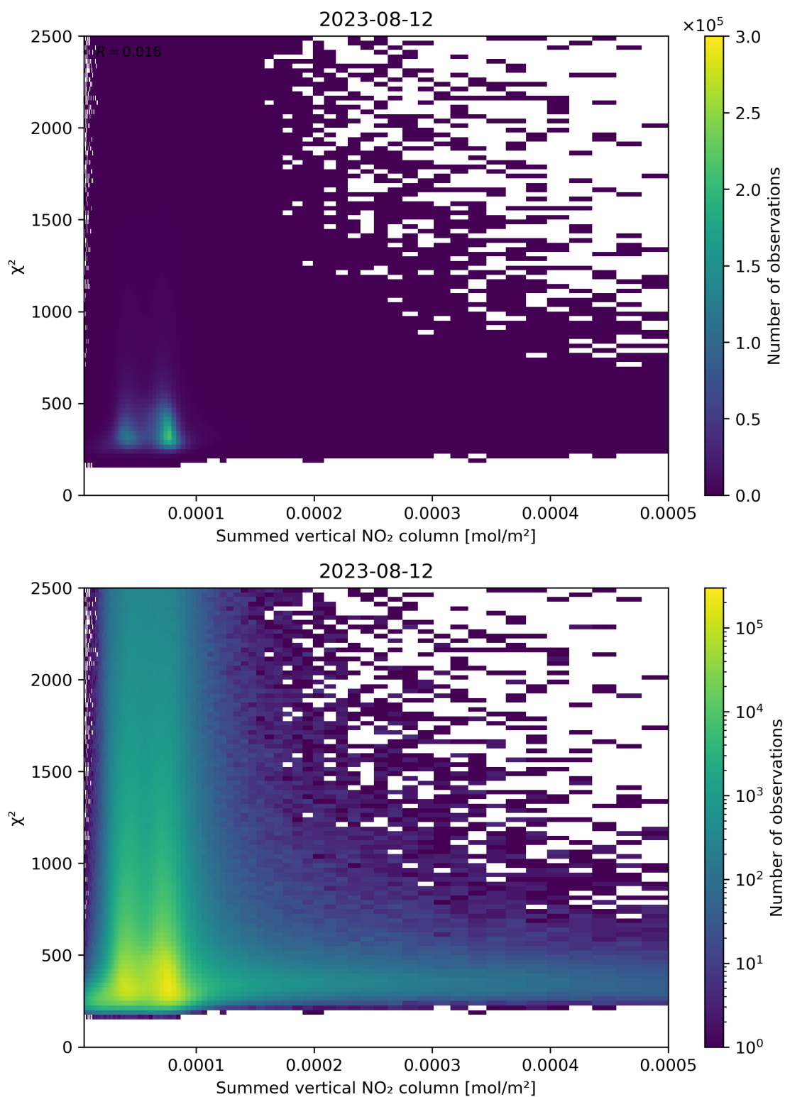
Figure 104: Scatter density plot of “Summed vertical NO 2 column” against “ \chi^2 ” for 2023-08-11 to 2023-08-13.
