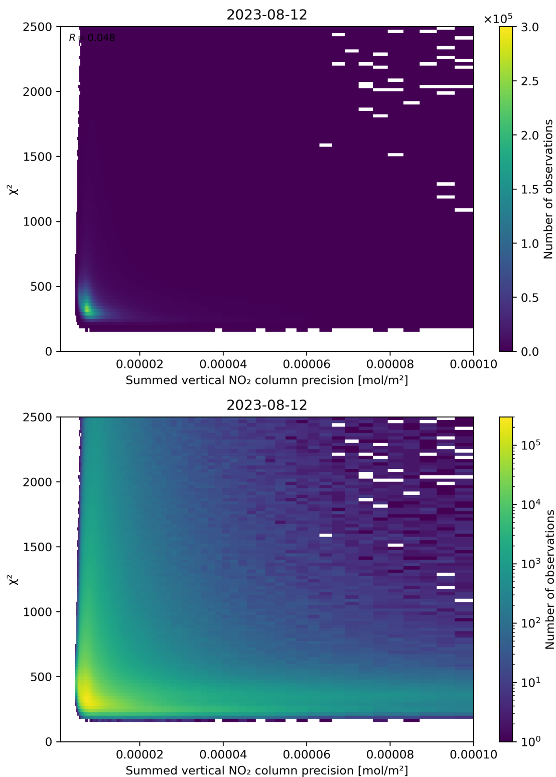
Figure 107: Scatter density plot of “Summed vertical NO 2 column precision” against “ \chi^2 ” for 2023-08-11 to 2023-08-13.
