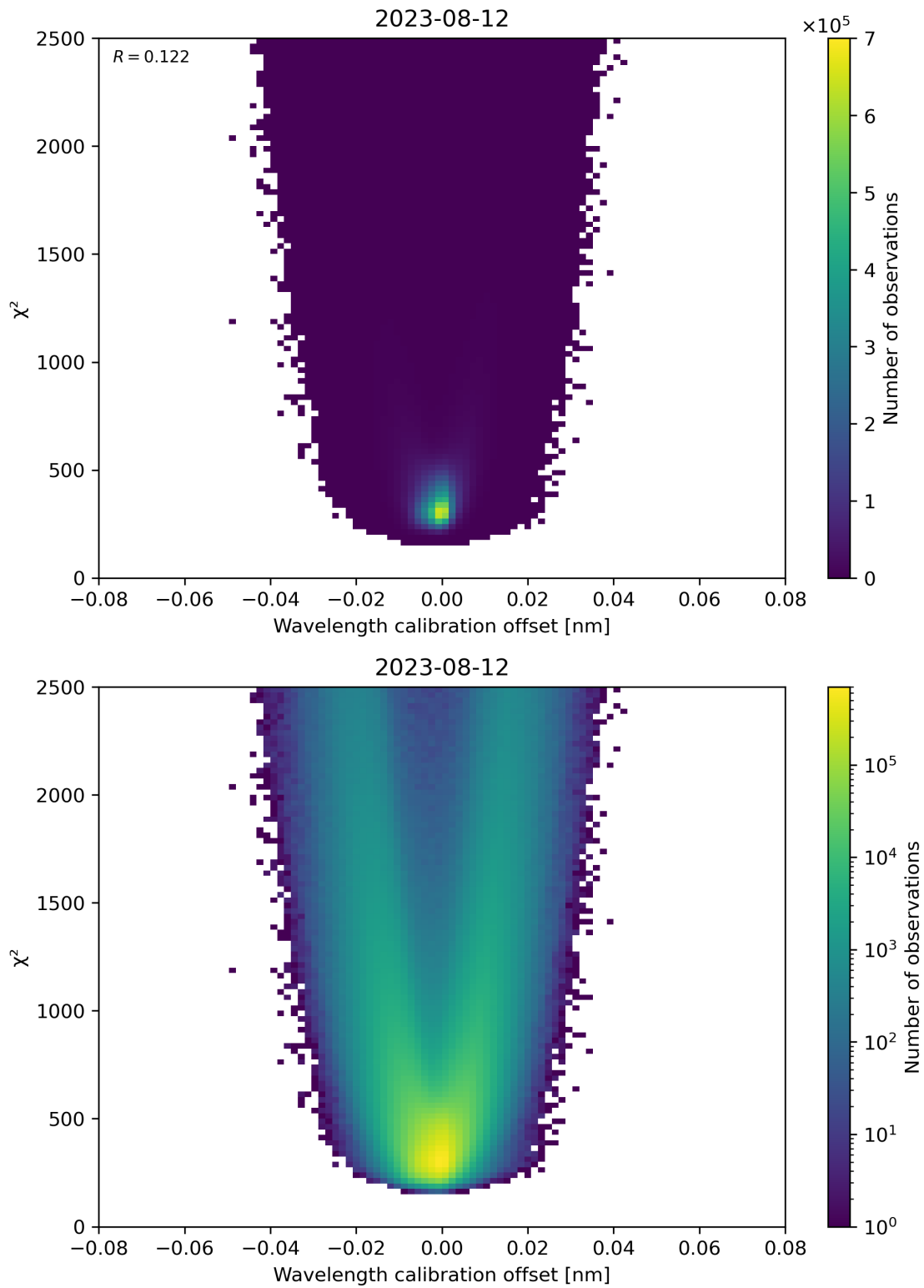
Figure 175: Scatter density plot of “Wavelength calibration offset” against “ \chi^2 ” for 2023-08-11 to 2023-08-13.
