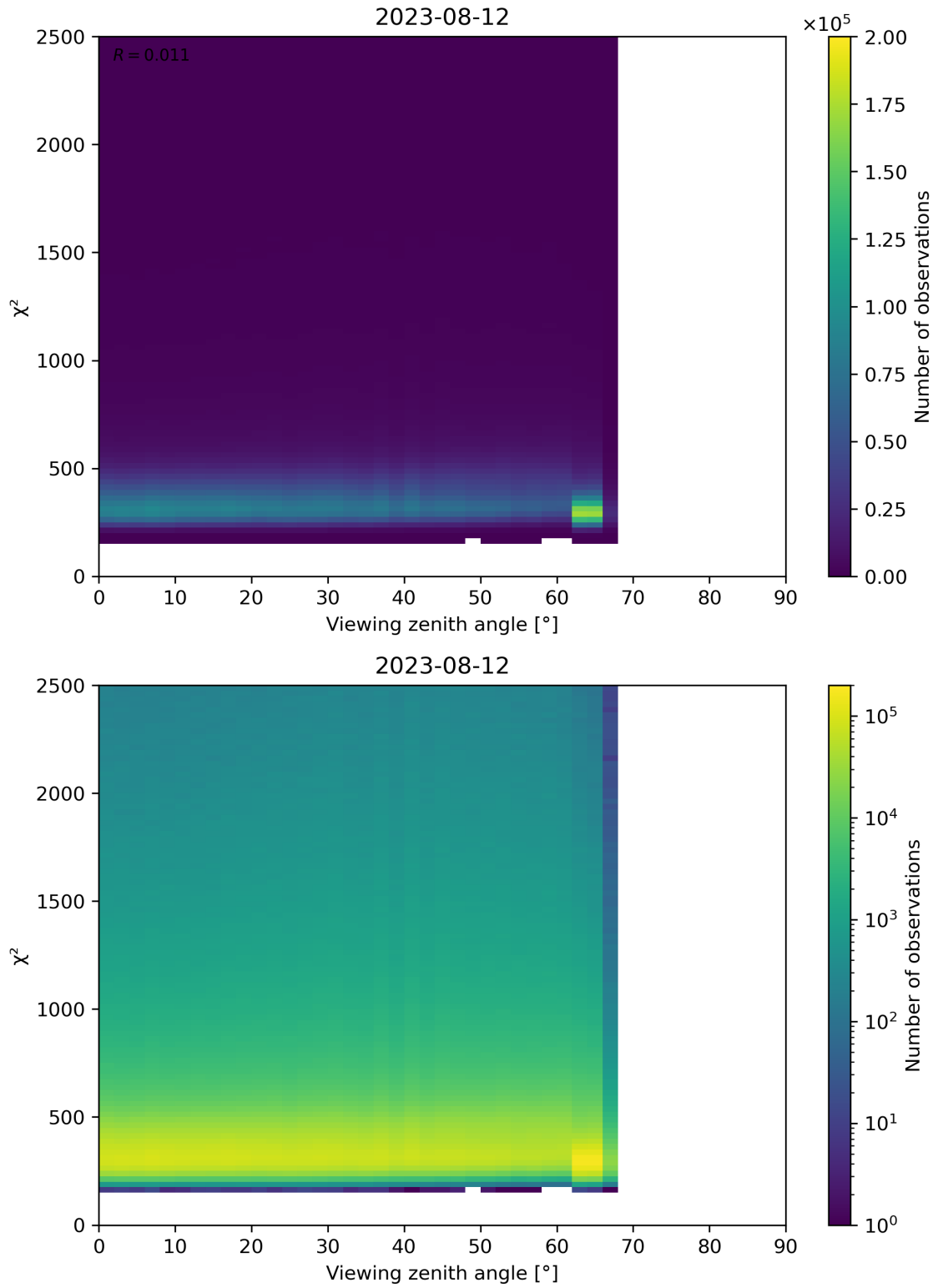
Figure 162: Scatter density plot of “Viewing zenith angle” against “ \chi^2 ” for 2023-08-11 to 2023-08-13.
