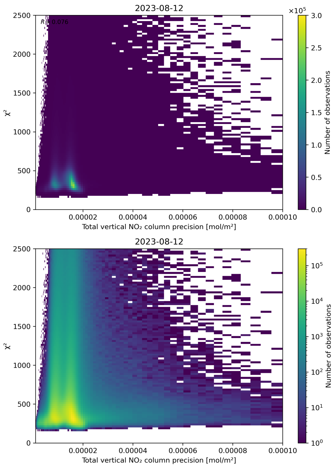
Figure 116: Scatter density plot of “Total vertical NO 2 column precision” against “ \chi^2 ” for 2023-08-11 to 2023-08-13.
