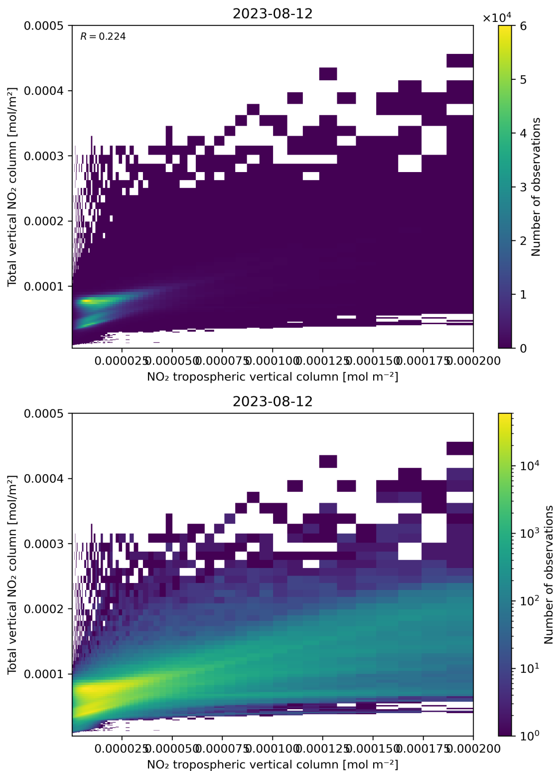
Figure 128: Scatter density plot of “NO 2 tropospheric vertical column” against “Total vertical NO 2 column” for 2023-08-11 to 2023-08-13.
