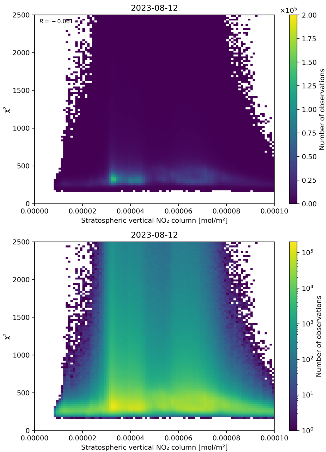
Figure 97: Scatter density plot of “Stratospheric vertical NO 2 column” against “ \chi^2 ” for 2023-08-11 to 2023-08-13.
