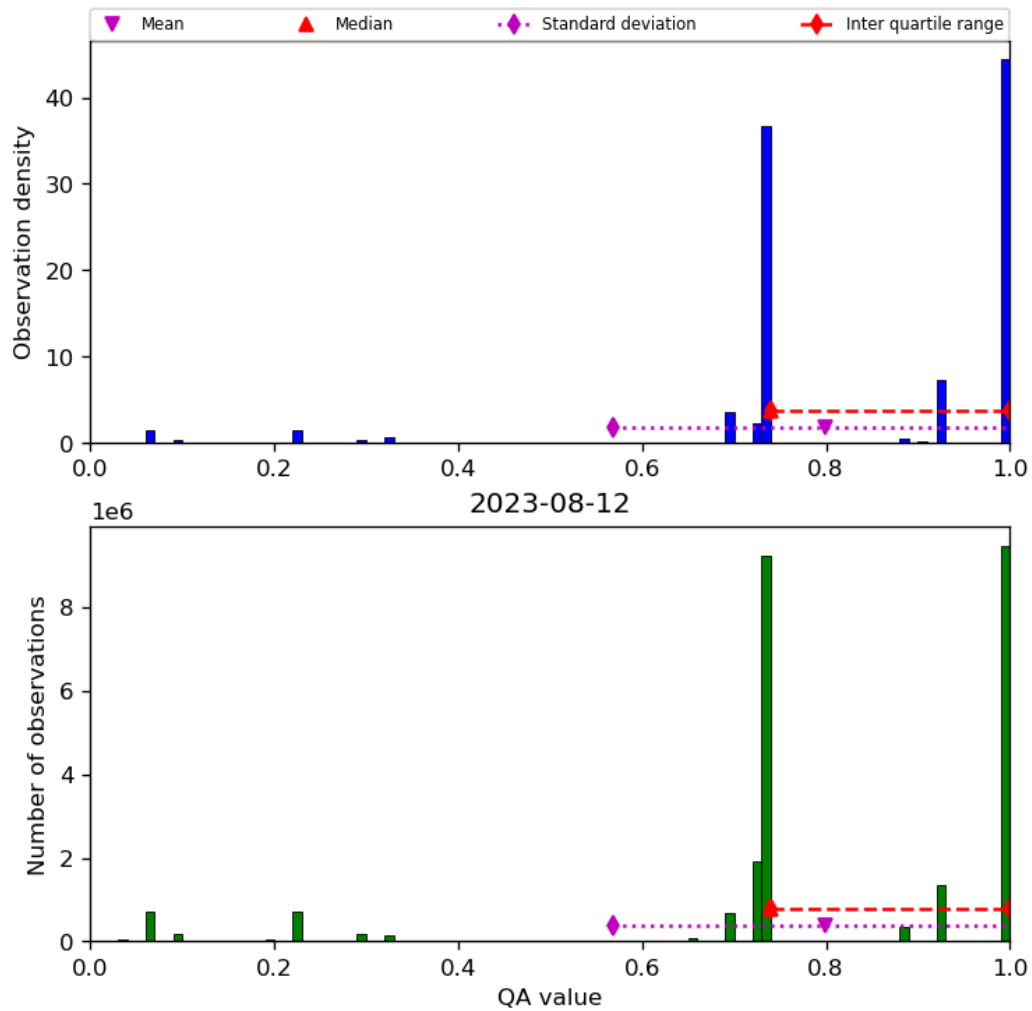
Figure 28: Histogram of “QA value” for 2023-08-11 to 2023-08-13
