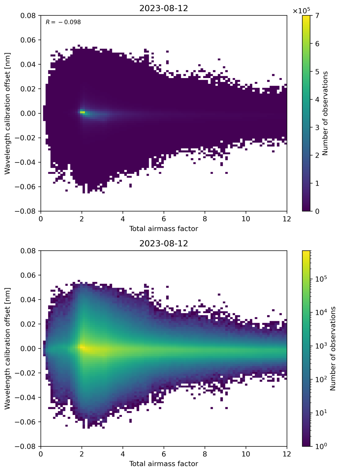
Figure 70: Scatter density plot of “Total airmass factor” against “Wavelength calibration offset” for 2023-08-11 to 2023-08-13.
