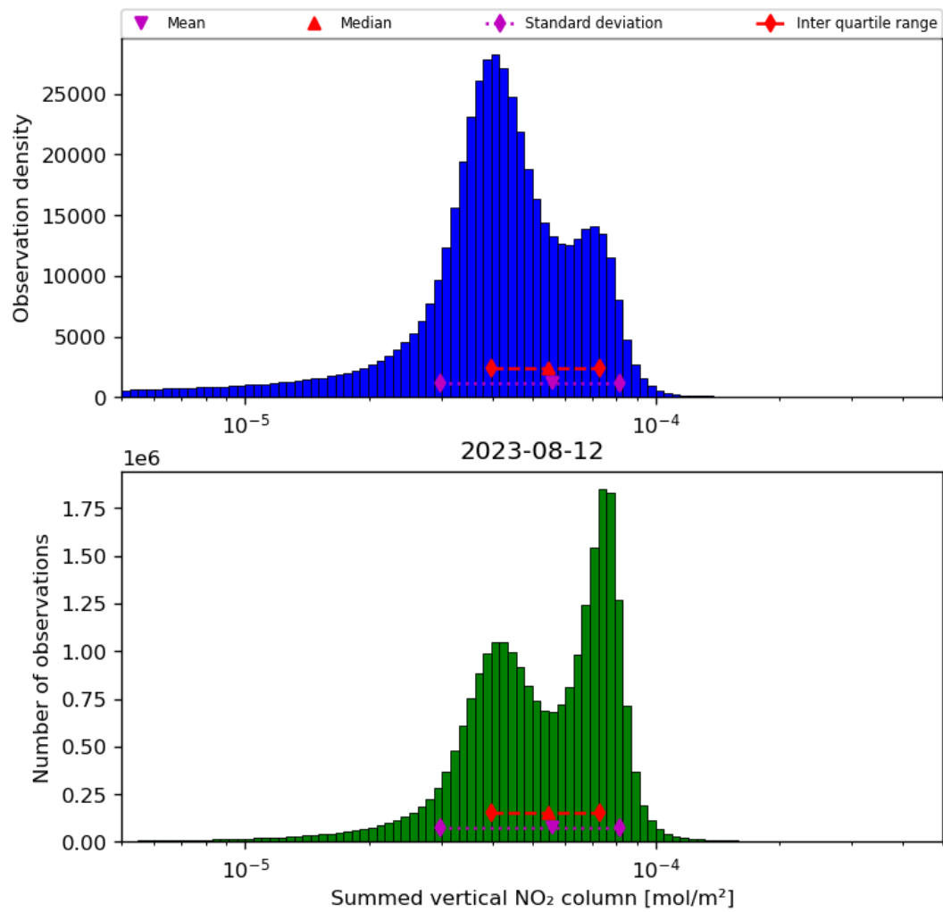
Figure 40: Histogram of “Summed vertical NO 2 column” for 2023-08-11 to 2023-08-13
