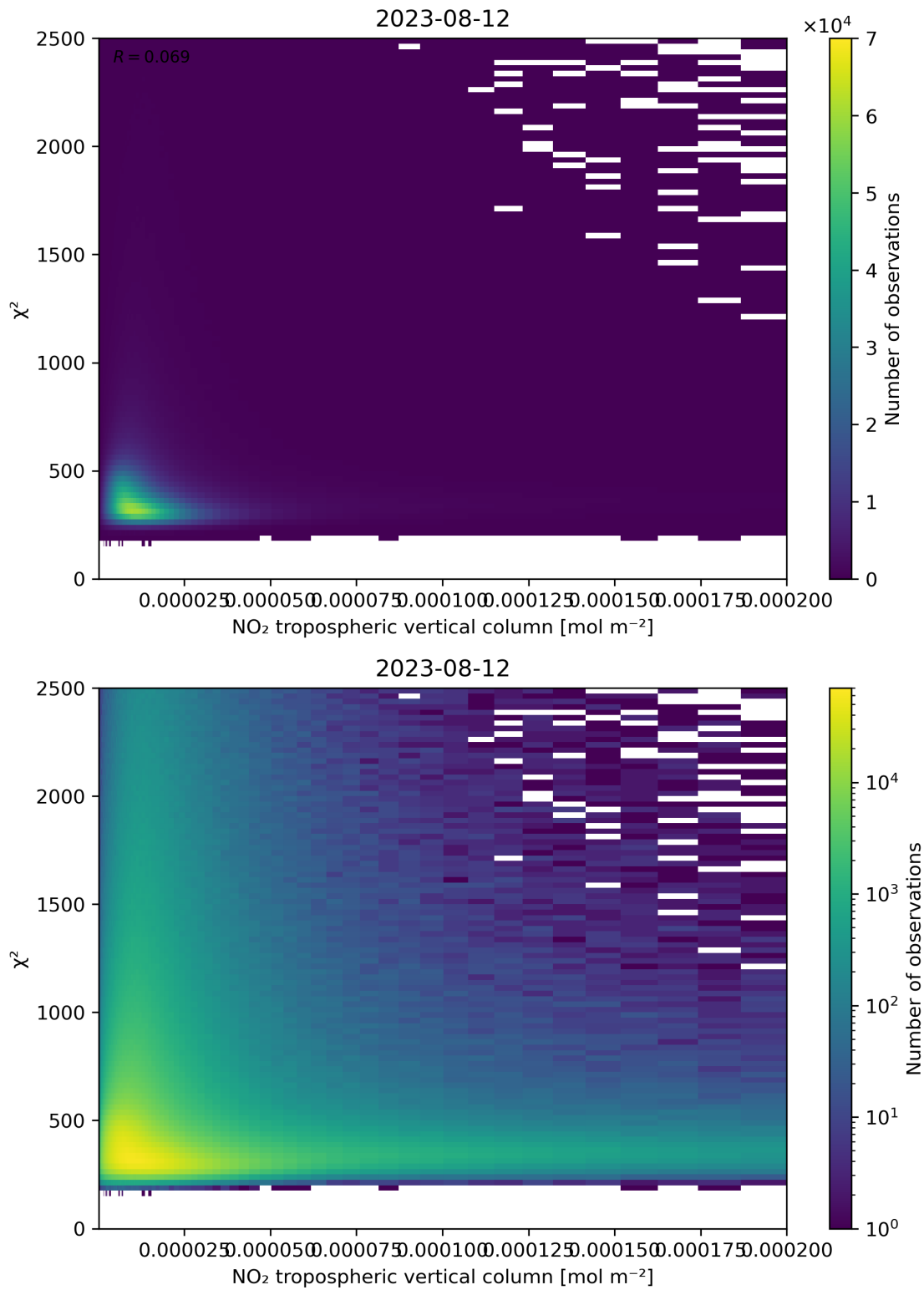
Figure 124: Scatter density plot of “NO 2 tropospheric vertical column” against “ \chi^2 ” for 2023-08-11 to 2023-08-13.
