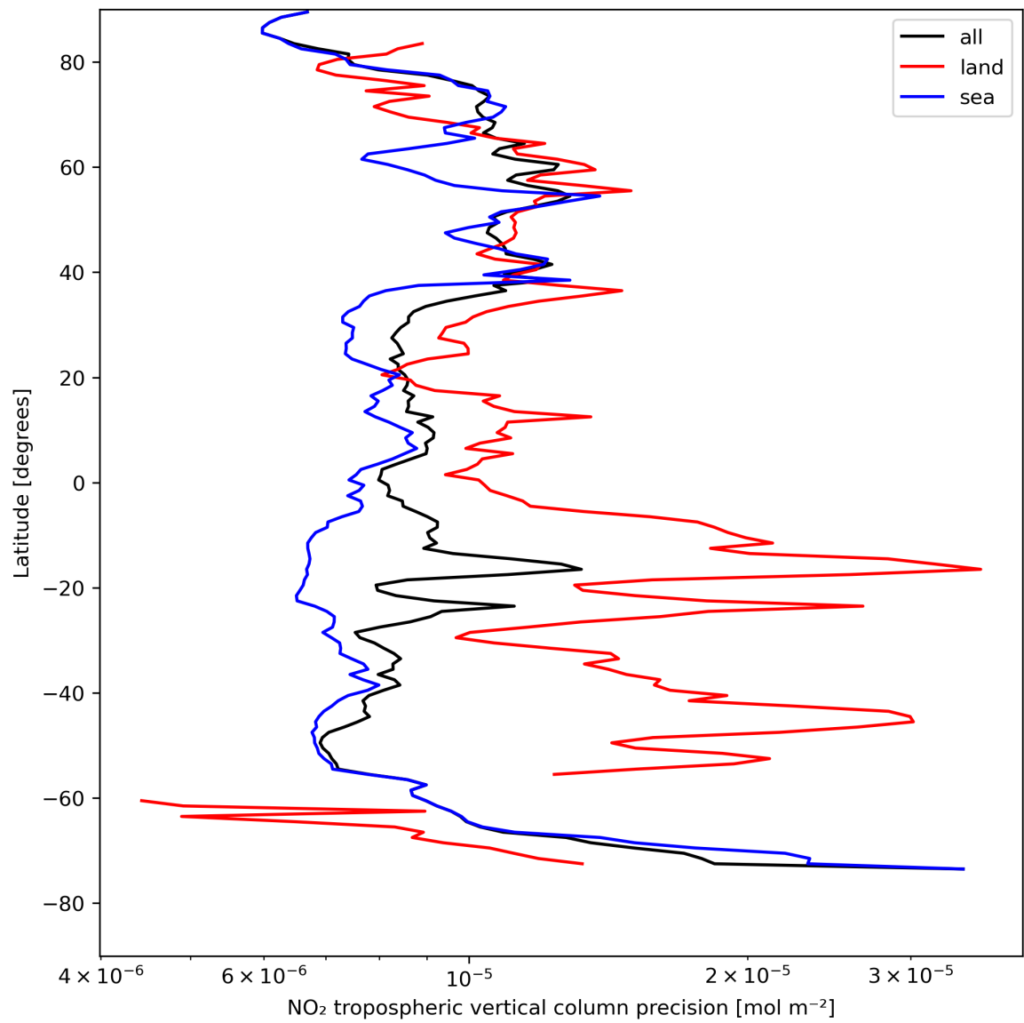
Figure 13: Zonal average of “NO 2 tropospheric vertical column precision” for 2023-08-11 to 2023-08-13.
