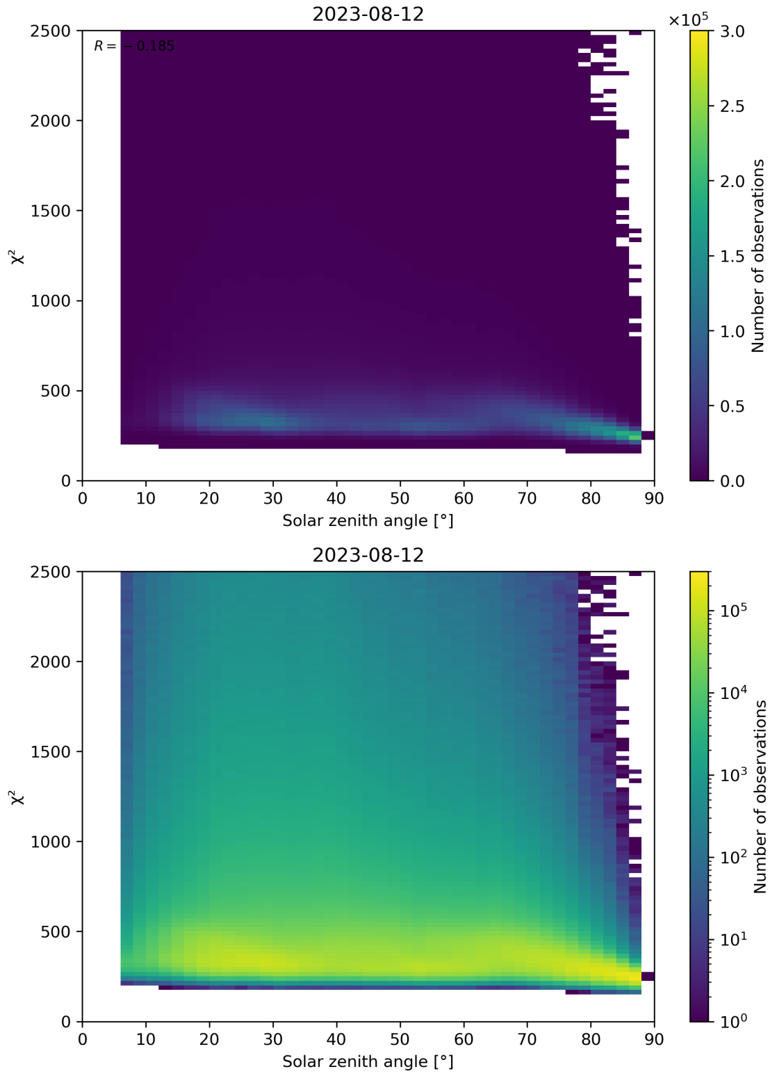
Figure 148: Scatter density plot of “Solar zenith angle” against “ \chi^2 ” for 2023-08-11 to 2023-08-13.
