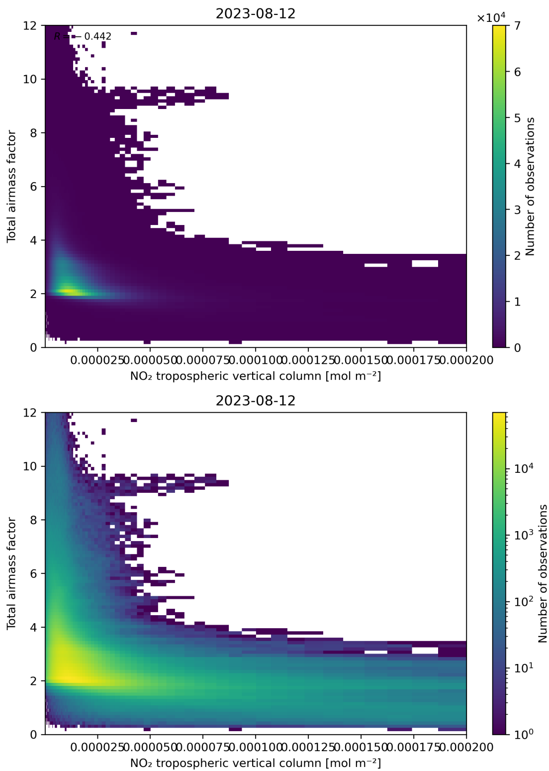
Figure 122: Scatter density plot of “NO 2 tropospheric vertical column” against “Total airmass factor” for 2023-08-11 to 2023-08-13.
