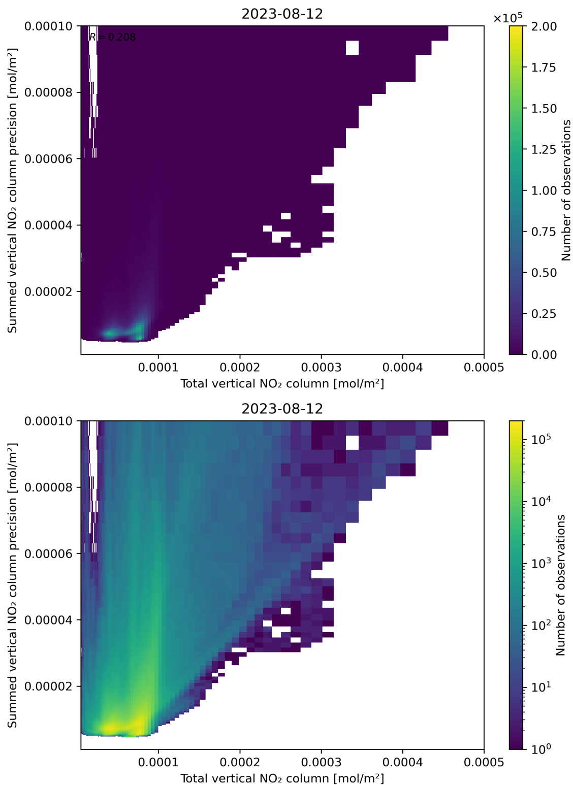
Figure 113: Scatter density plot of “Total vertical NO 2 column” against “Summed vertical NO 2 column precision” for 2023-08-11 to 2023-08-13.
