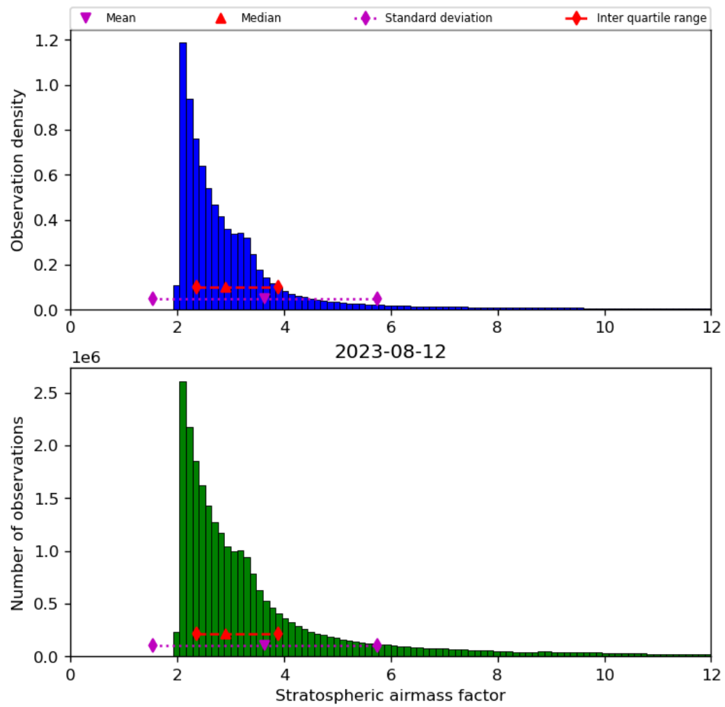
Figure 44: Histogram of “Stratospheric airmass factor” for 2023-08-11 to 2023-08-13
