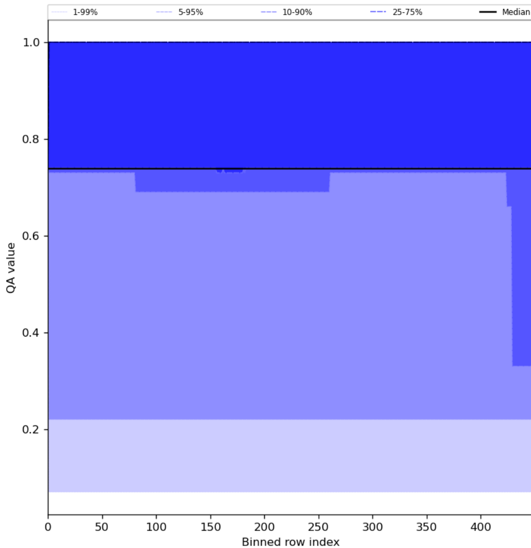
Figure 45: Along track statistics of "QA value" for 2023-08-11 to 2023-08-13
