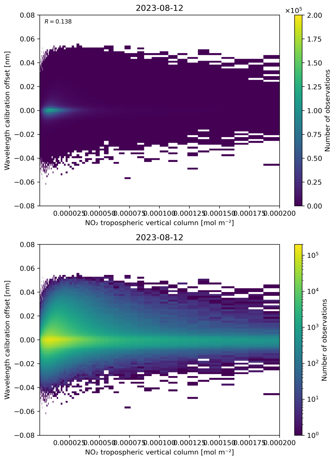
Figure 143: Scatter density plot of “NO 2 tropospheric vertical column” against “Wavelength calibration offset” for 2023-08-11 to 2023-08-13.
