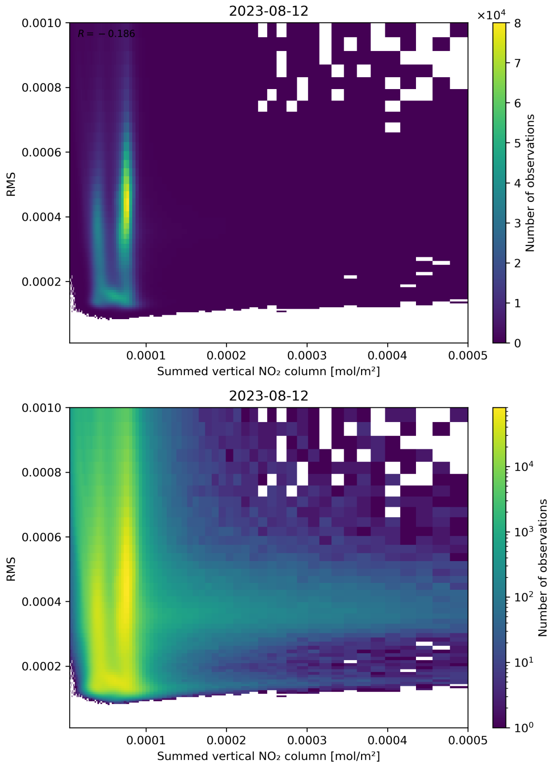
Figure 109: Scatter density plot of “Summed vertical NO 2 column” against “RMS” for 2023-08-11 to 2023-08-13.
