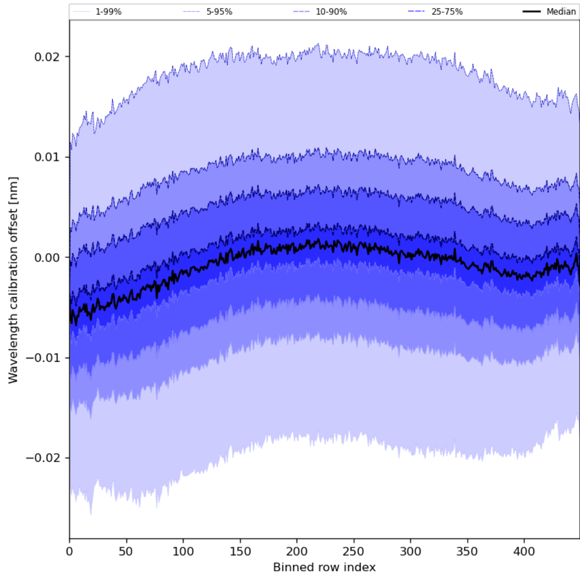
Figure 52: Along track statistics of “Wavelength calibration offset” for 2023-08-11 to 2023-08-13
