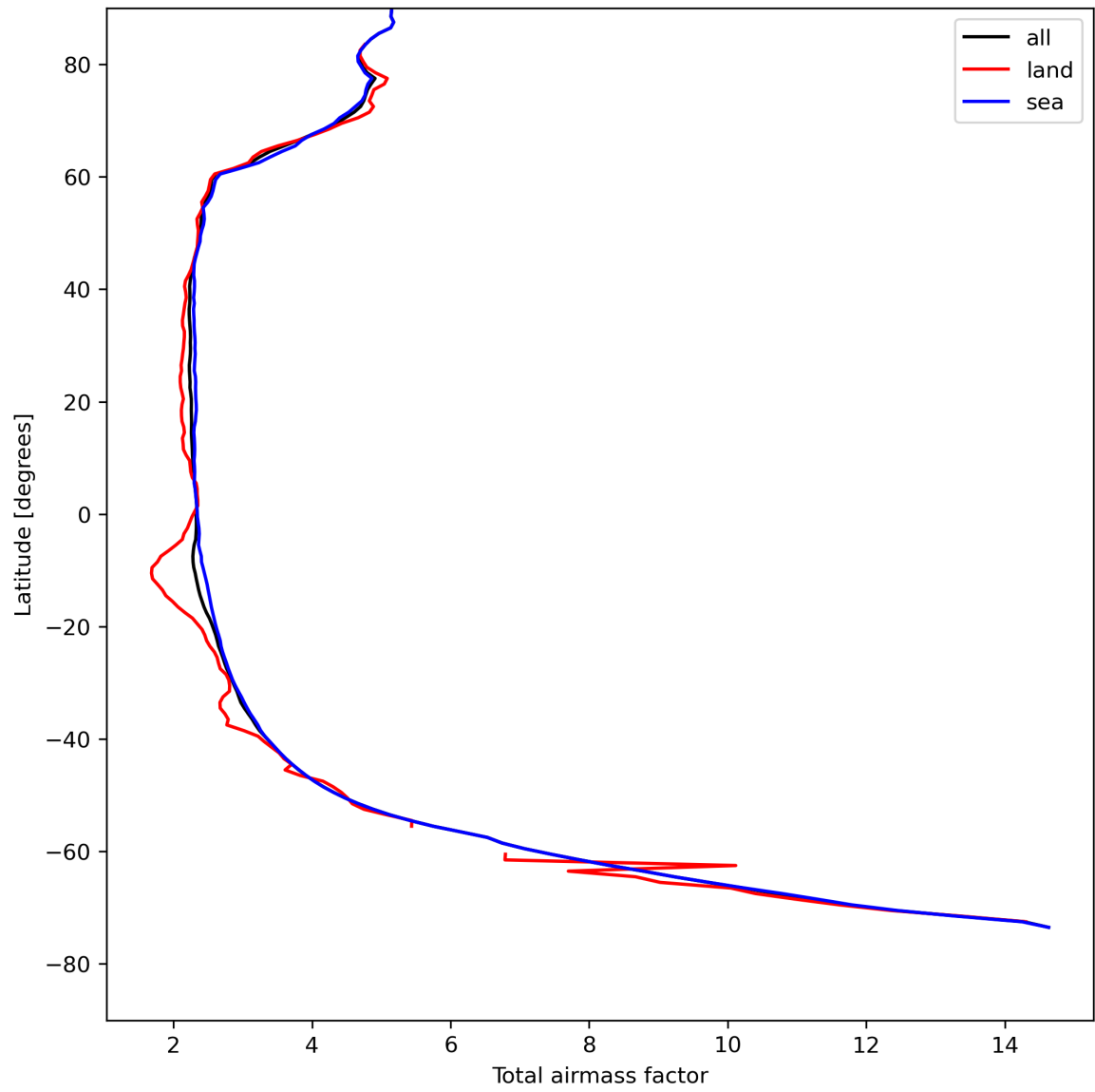
Figure 15: Zonal average of “Total airmass factor” for 2023-08-11 to 2023-08-13.
