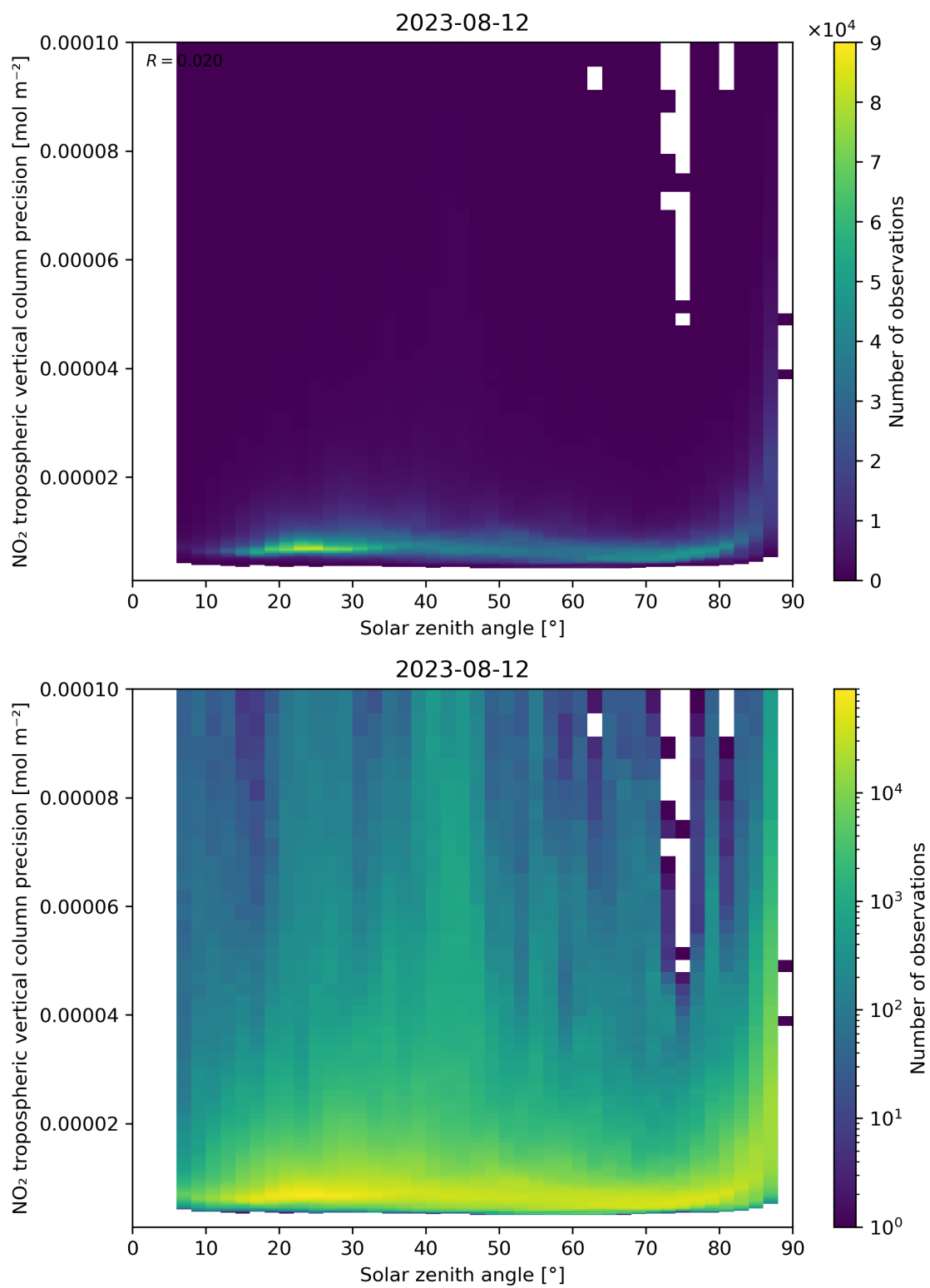
Figure 156: Scatter density plot of “Solar zenith angle” against “NO 2 tropospheric vertical column precision” for 2023-08-11 to 2023-08-13.
