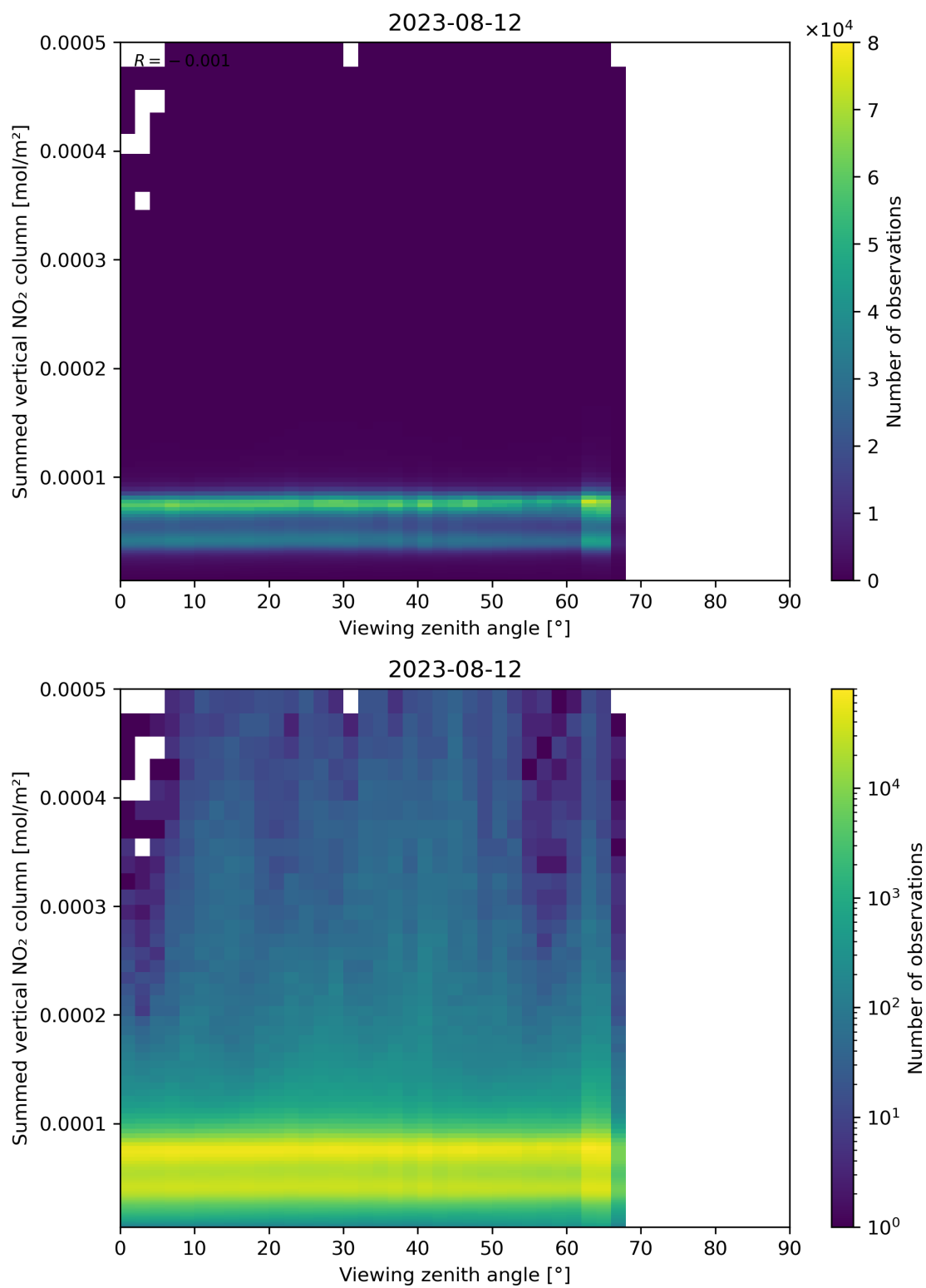
Figure 165: Scatter density plot of “Viewing zenith angle” against “Summed vertical NO 2 column” for 2023-08-11 to 2023-08-13.
