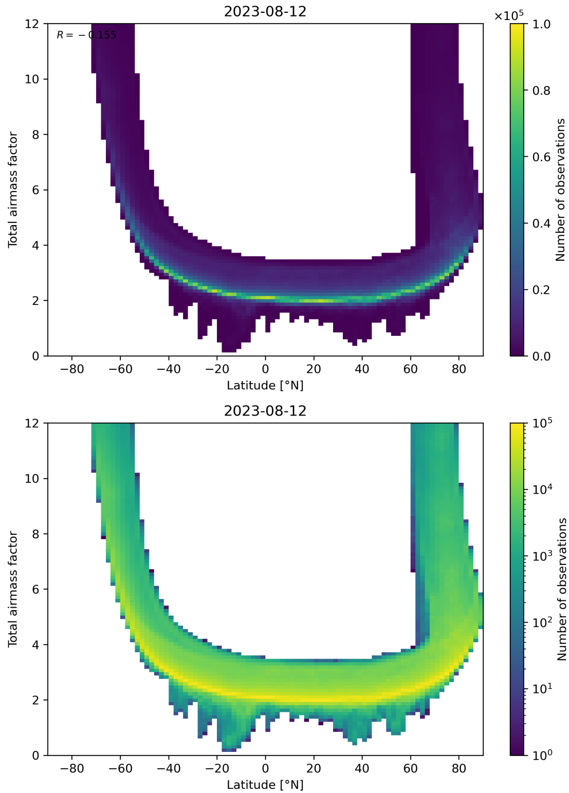
Figure 84: Scatter density plot of “Latitude” against “Total airmass factor” for 2023-08-11 to 2023-08-13.
