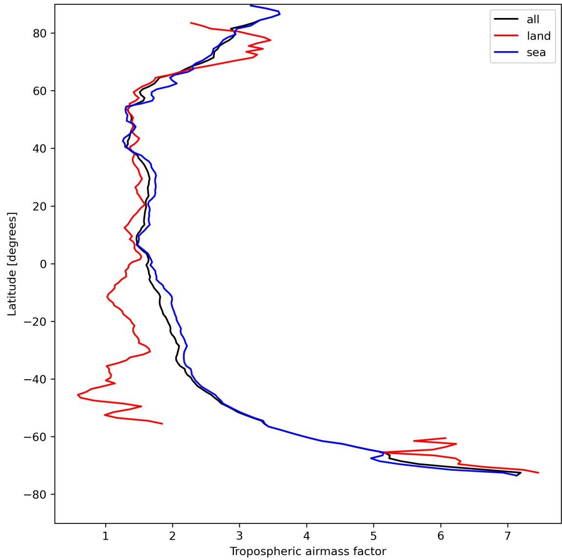
Figure 14: Zonal average of “Tropospheric airmass factor” for 2023-08-11 to 2023-08-13.
