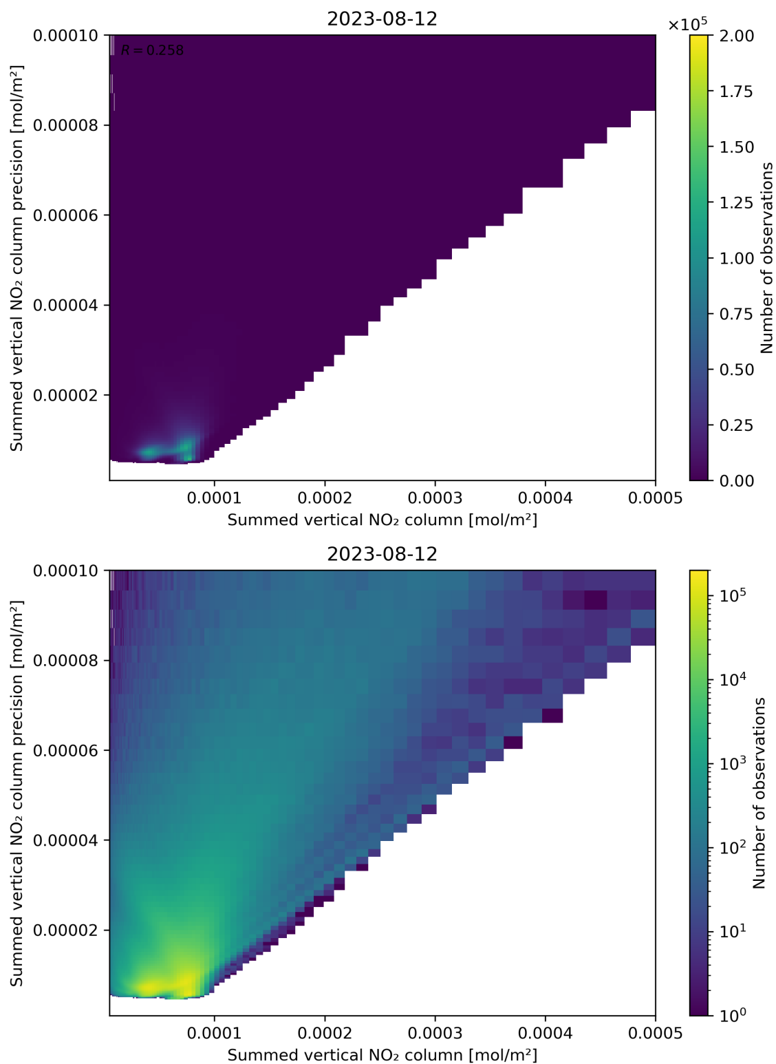
Figure 105: Scatter density plot of “Summed vertical NO 2 column” against “Summed vertical NO 2 column precision” for 2023-08-11 to 2023-08-13.
