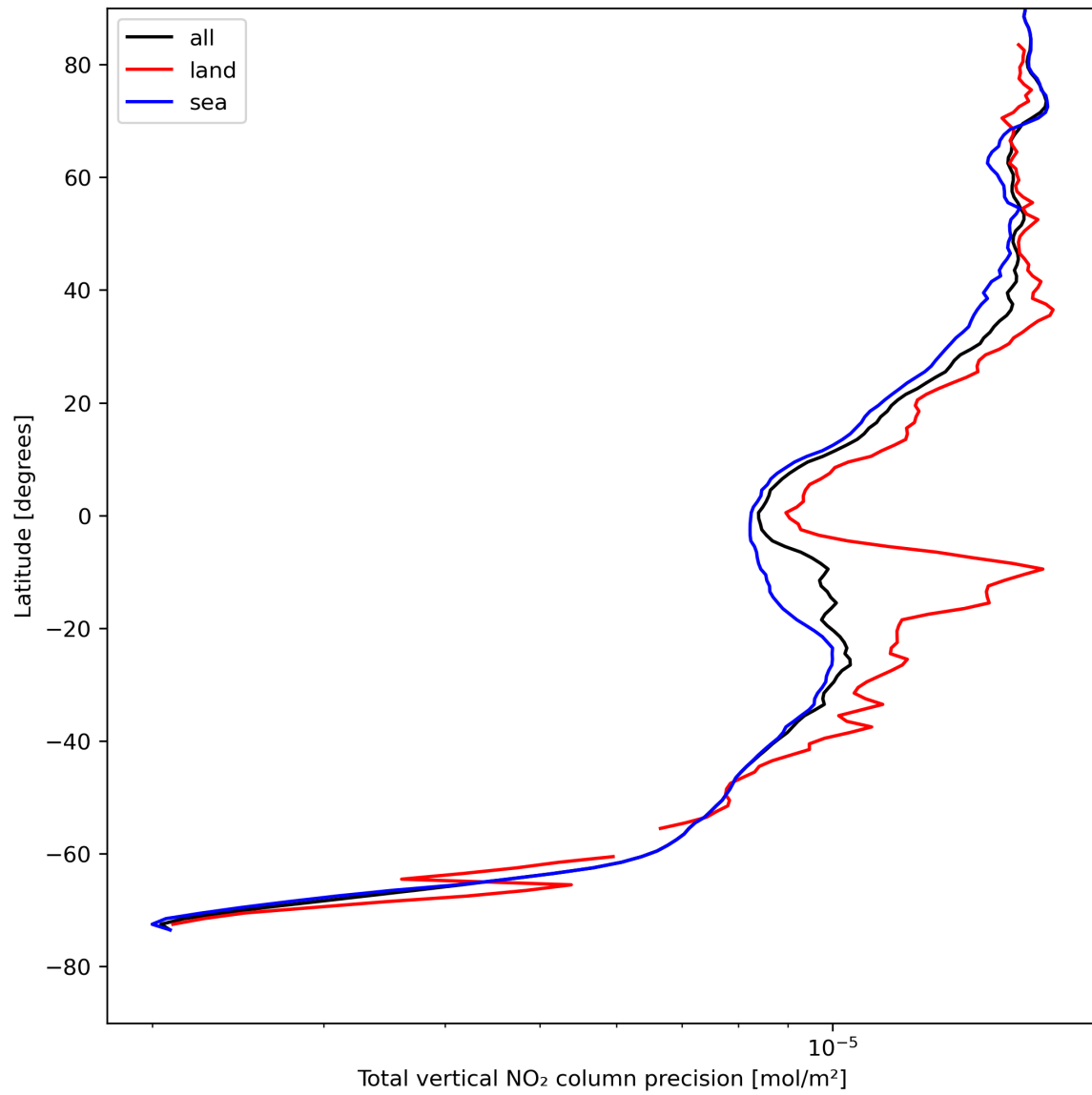
Figure 22: Zonal average of “Total vertical NO 2 column precision” for 2023-08-11 to 2023-08-13.
