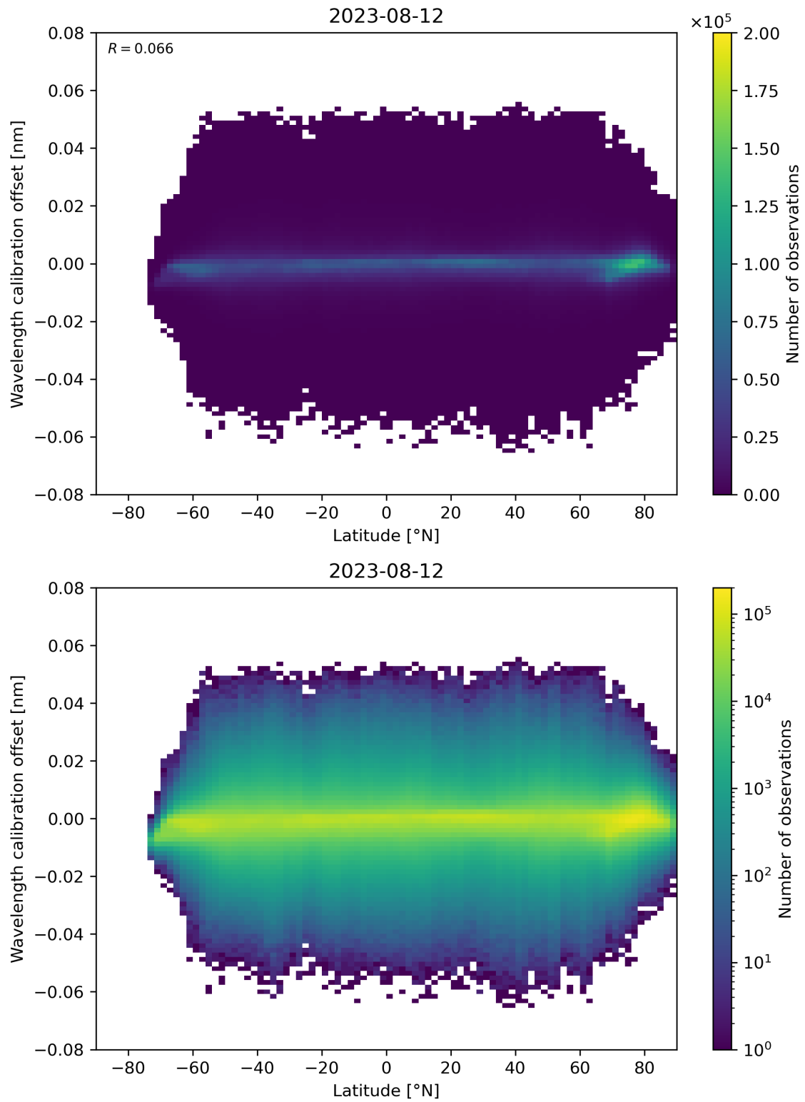
Figure 95: Scatter density plot of “Latitude” against “Wavelength calibration offset” for 2023-08-11 to 2023-08-13.
