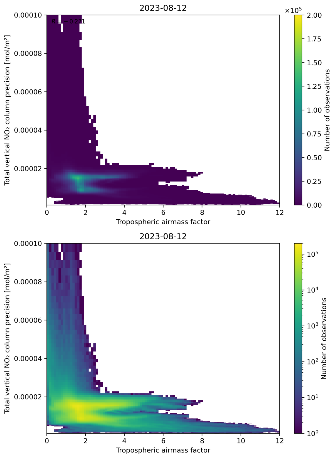
Figure 78: Scatter density plot of “Tropospheric air mass factor” against “Total vertical NO 2 column precision” for 2023-08-11 to 2023-08-13.
