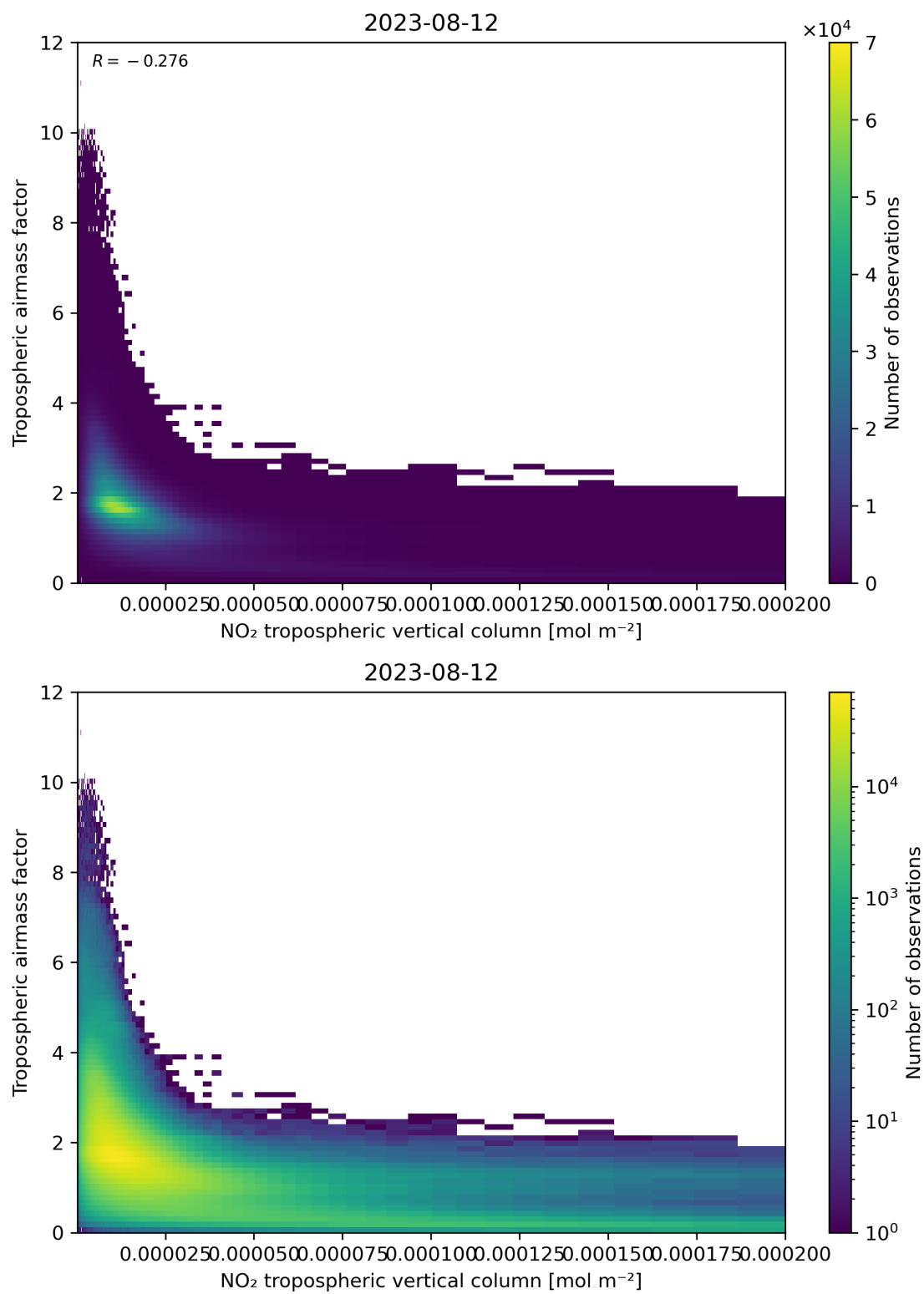
Figure 123: Scatter density plot of “NO 2 tropospheric vertical column” against “Tropospheric air mass factor” for 2023-08-11 to 2023-08-13.
