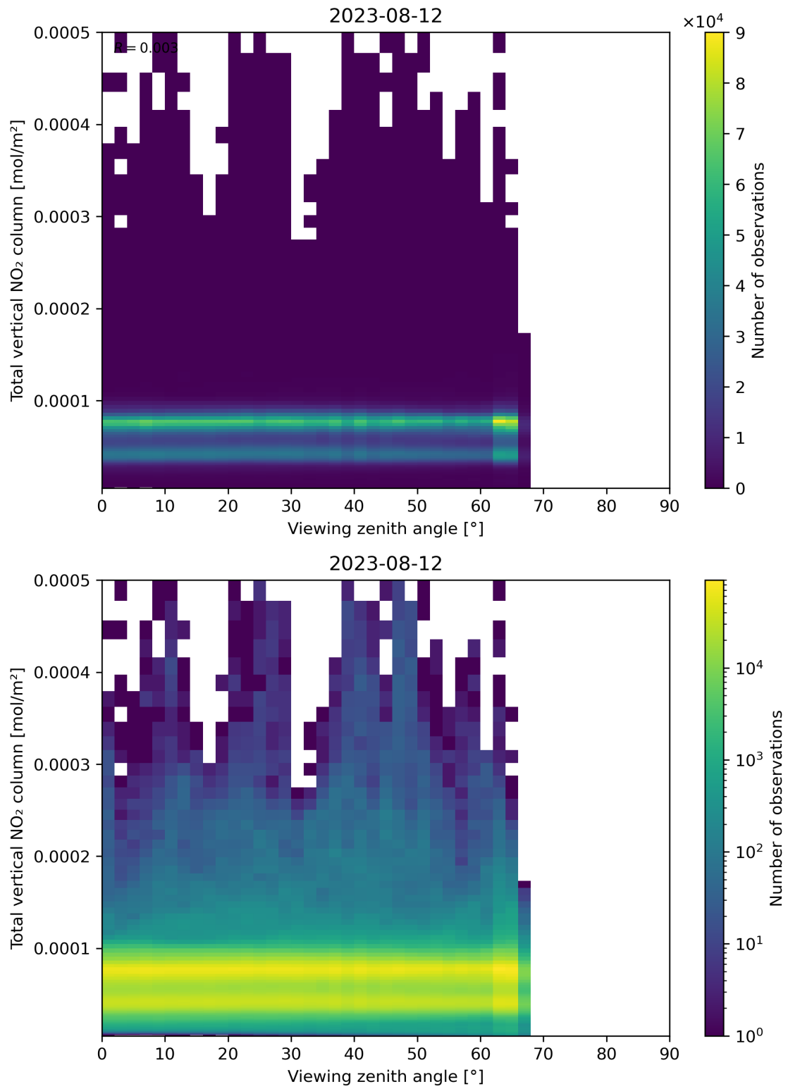
Figure 167: Scatter density plot of “Viewing zenith angle” against “Total vertical NO 2 column” for 2023-08-11 to 2023-08-13.
