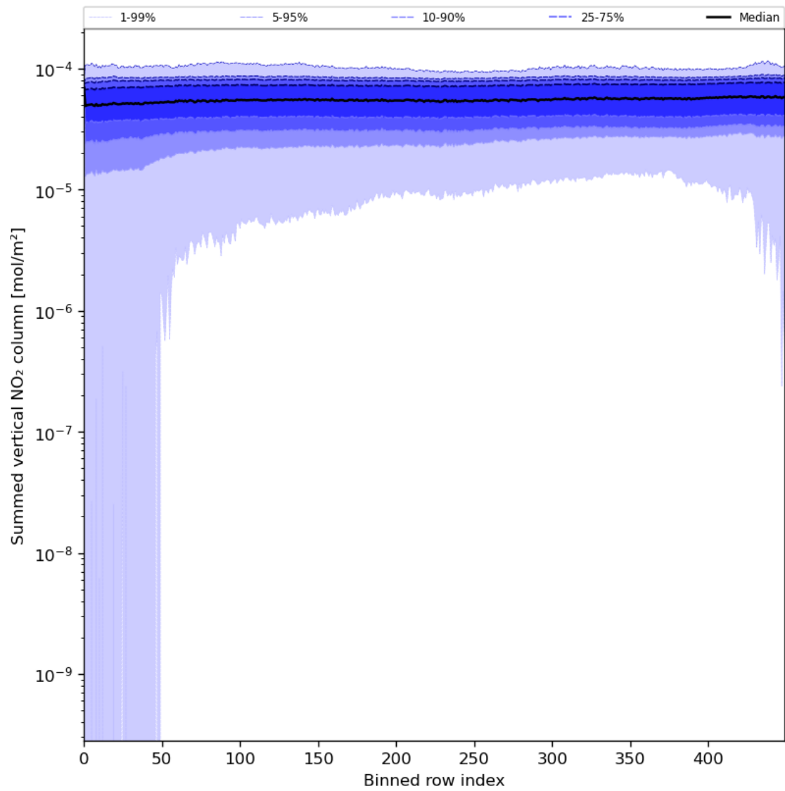
Figure 57: Along track statistics of “Summed vertical NO 2 column” for 2023-08-11 to 2023-08-13
