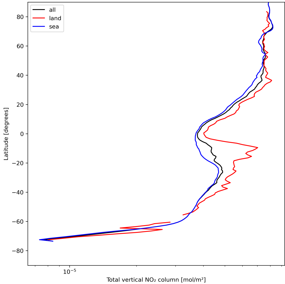
Figure 21: Zonal average of “Total vertical NO 2 column” for 2023-08-11 to 2023-08-13.
