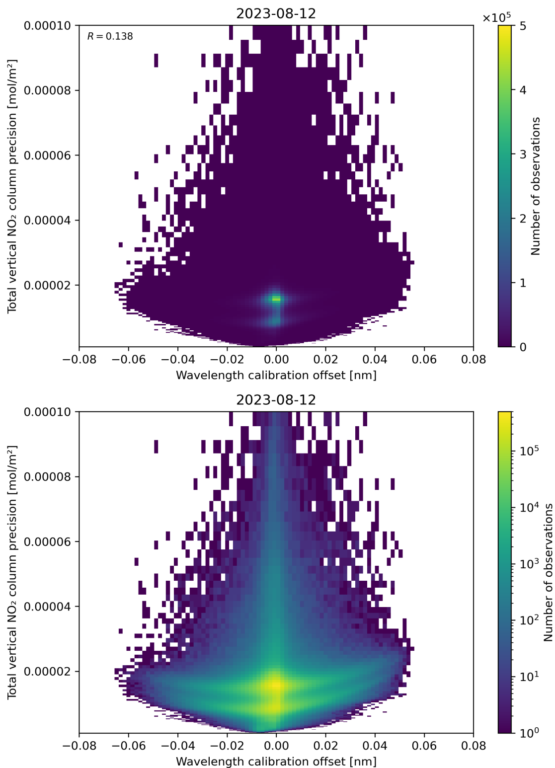
Figure 180: Scatter density plot of “Wavelength calibration offset” against “Total vertical NO 2 column precision” for 2023-08-11 to 2023-08-13.
