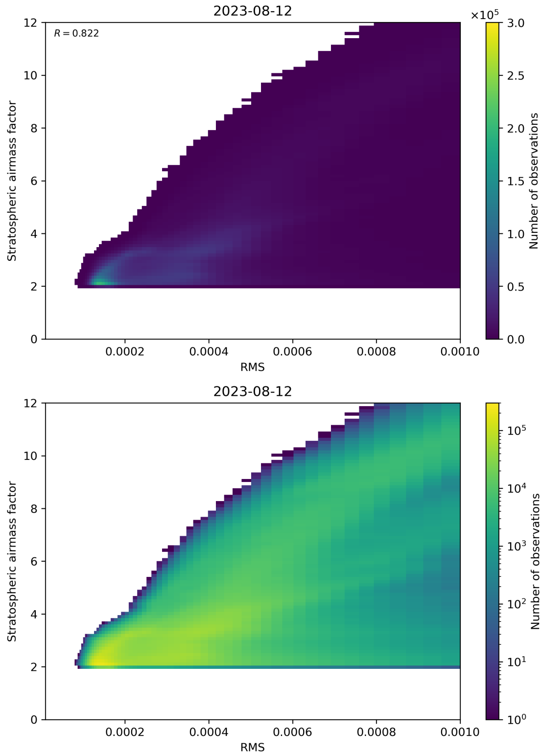
Figure 144: Scatter density plot of “RMS” against “Stratospheric airmass factor” for 2023-08-11 to 2023-08-13.
