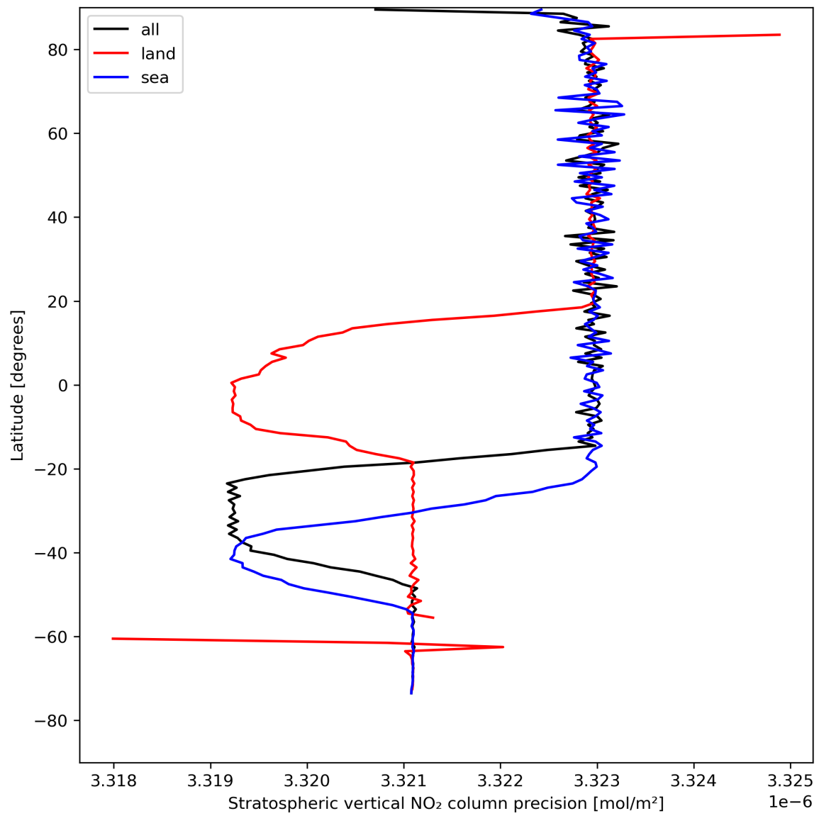
Figure 20: Zonal average of “Stratospheric vertical NO 2 column precision” for 2023-08-11 to 2023-08-13.
