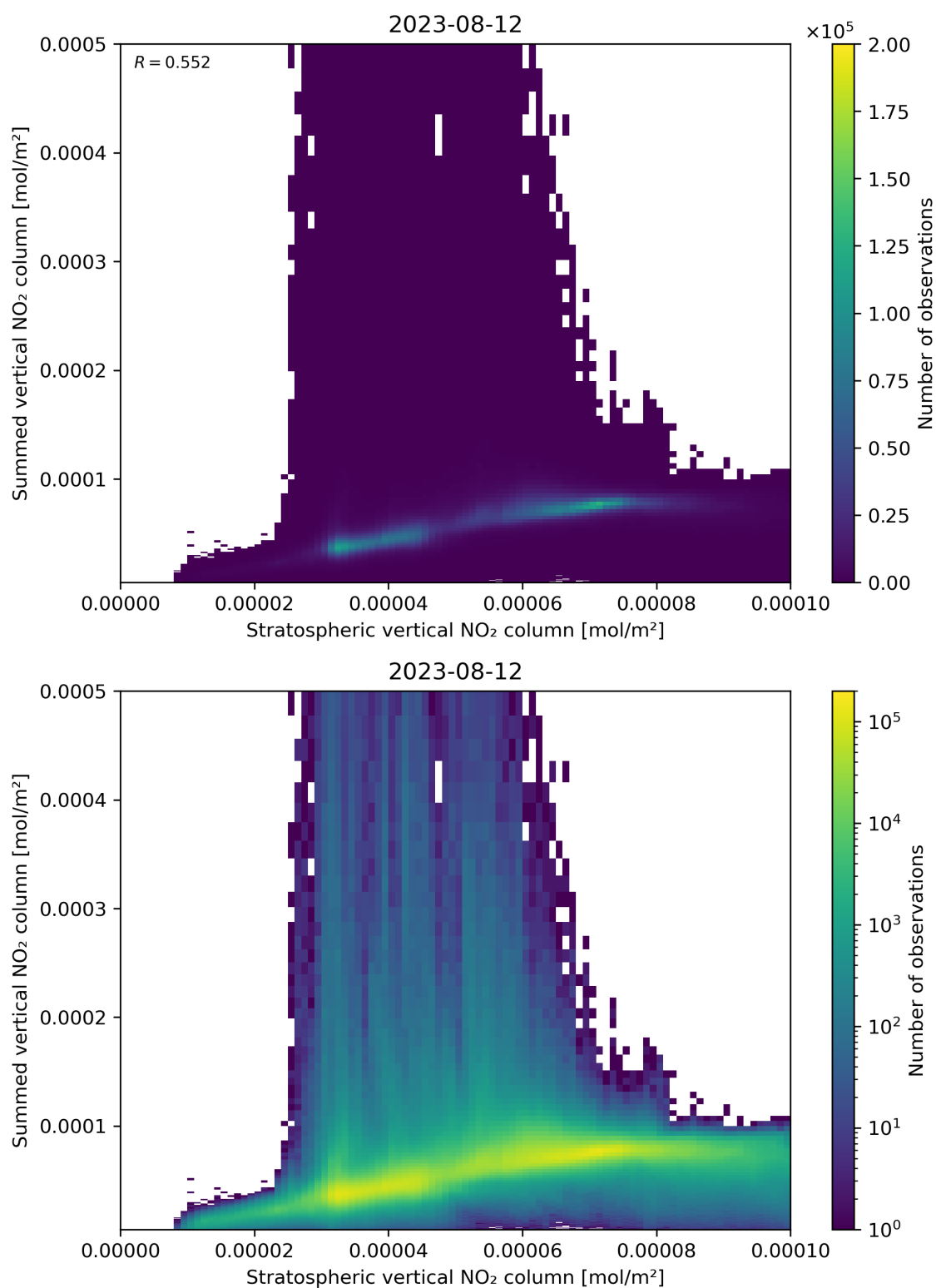
Figure 98: Scatter density plot of “Stratospheric vertical NO 2 column” against “Summed vertical NO 2 column” for 2023-08-11 to 2023-08-13.
