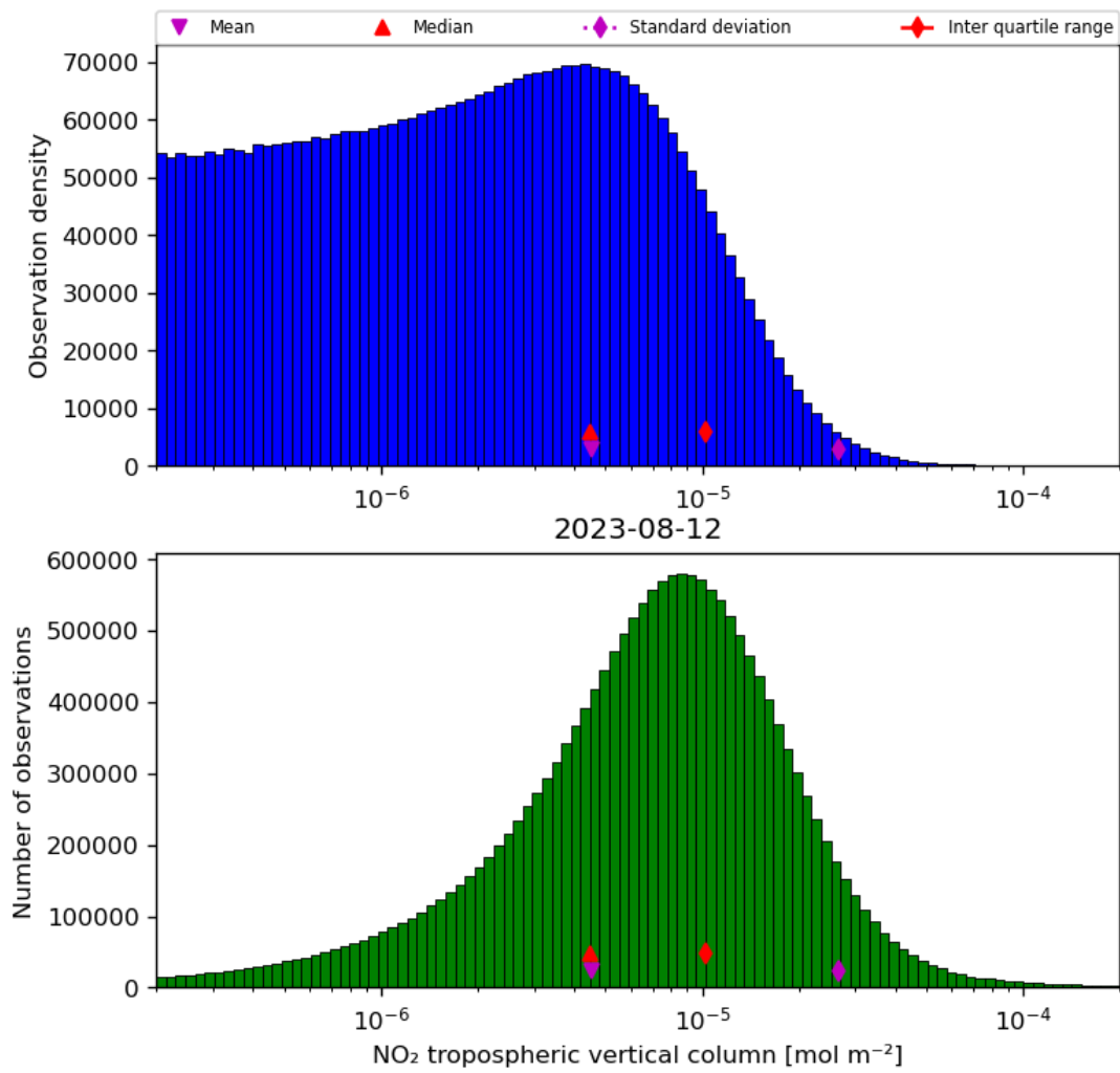
Figure 29: Histogram of “NO 2 tropospheric vertical column” for 2023-08-11 to 2023-08-13
