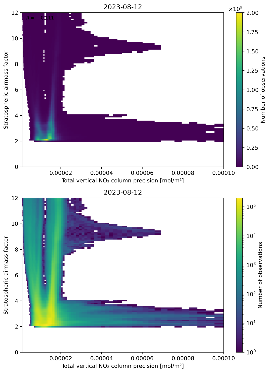
Figure 115: Scatter density plot of “Total vertical NO 2 column precision” against “Stratospheric air mass factor” for 2023-08-11 to 2023-08-13.
