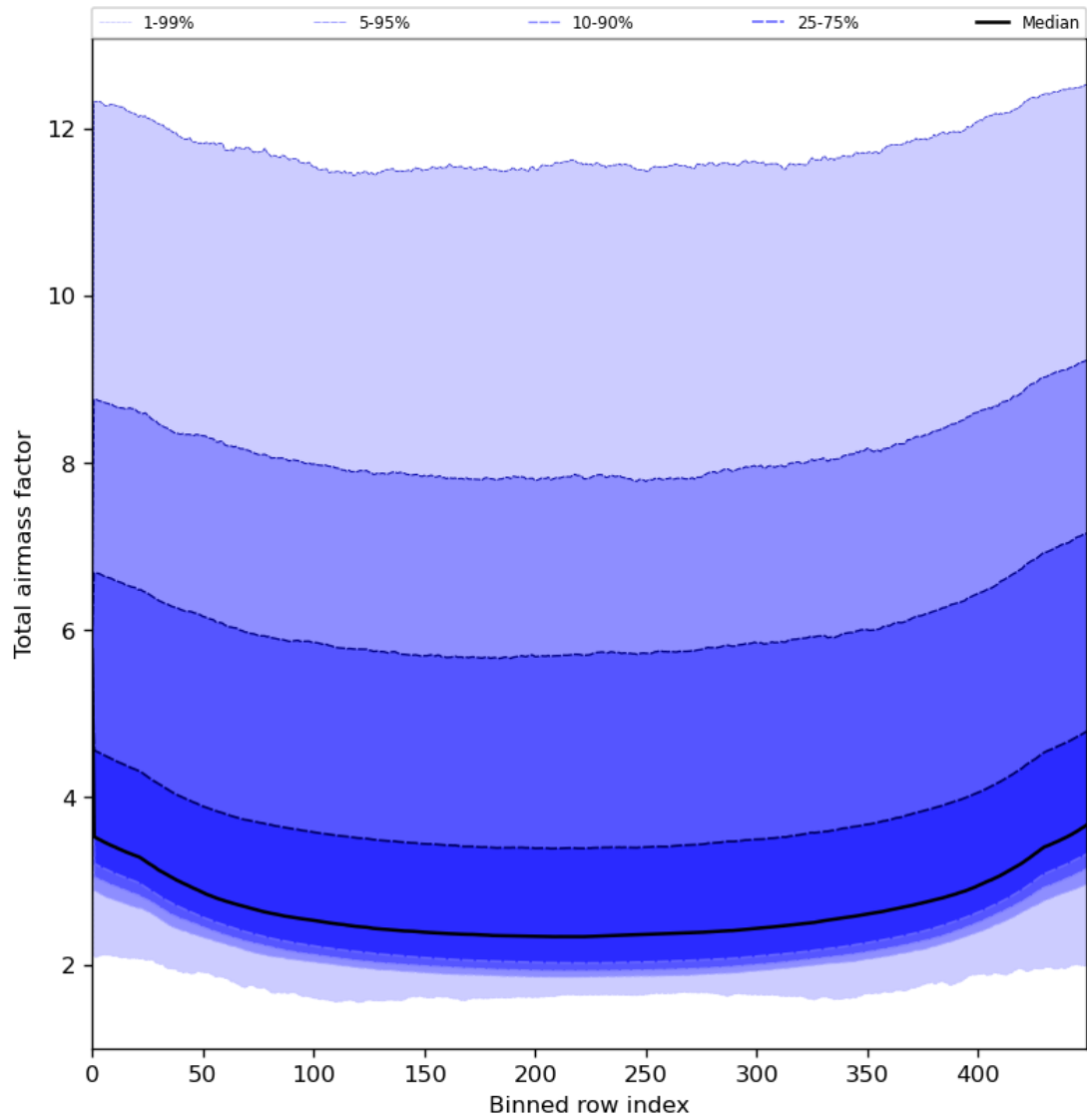
Figure 49: Along track statistics of “Total airmass factor” for 2023-08-11 to 2023-08-13
