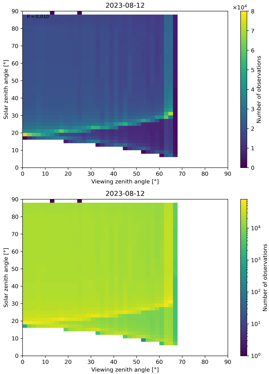
Figure 172: Scatter density plot of “Viewing zenith angle” against “Solar zenith angle” for 2023-08-11 to 2023-08-13.
