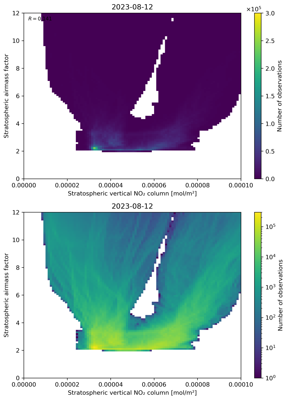
Figure 96: Scatter density plot of “Stratospheric vertical NO 2 column” against “Stratospheric airmass factor” for 2023-08-11 to 2023-08-13.
