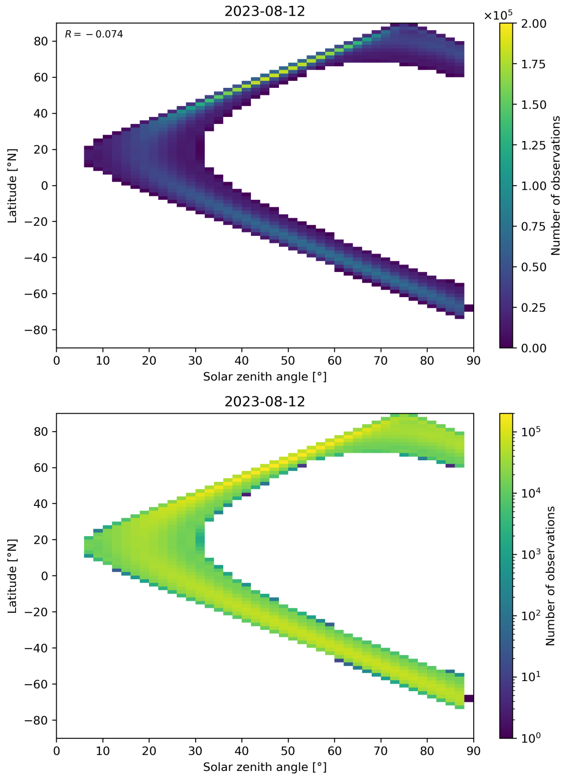
Figure 149: Scatter density plot of “Solar zenith angle” against “Latitude” for 2023-08-11 to 2023-08-13.
