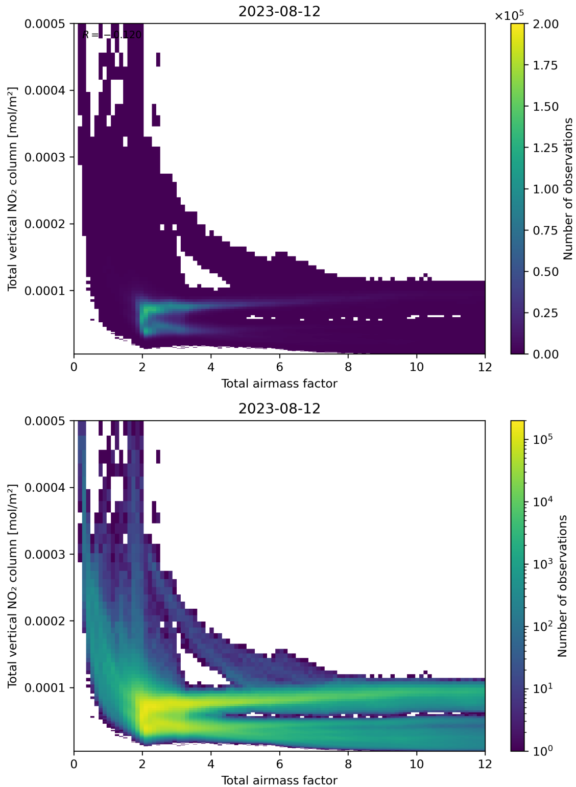
Figure 67: Scatter density plot of “Total airmass factor” against “Total vertical NO 2 column” for 2023-08-11 to 2023-08-13.
