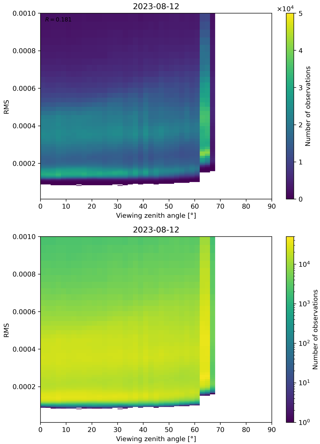
Figure 171: Scatter density plot of “Viewing zenith angle” against “RMS” for 2023-08-11 to 2023-08-13.
