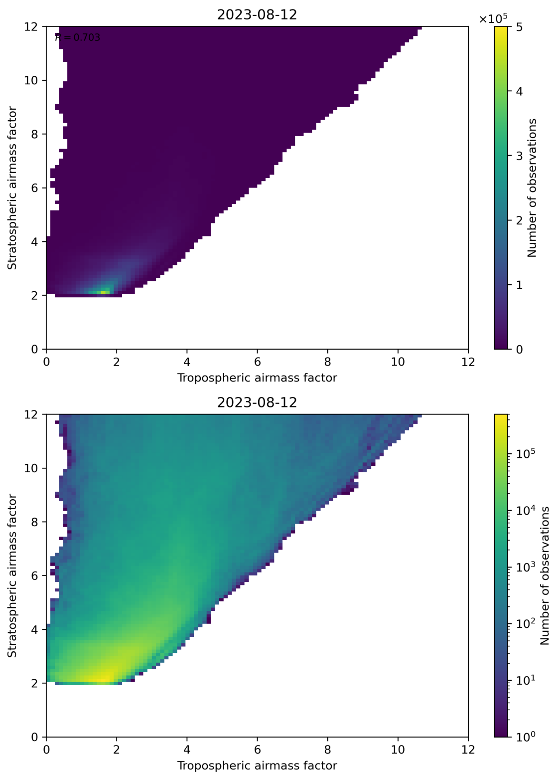
Figure 71: Scatter density plot of “Tropospheric airmass factor” against “Stratospheric airmass factor” for 2023-08-11 to 2023-08-13.
