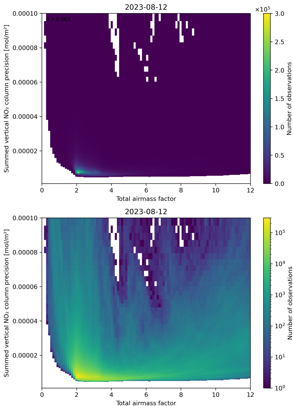
Figure 66: Scatter density plot of “Total airmass factor” against “Summed vertical NO 2 column precision” for 2023-08-11 to 2023-08-13.
