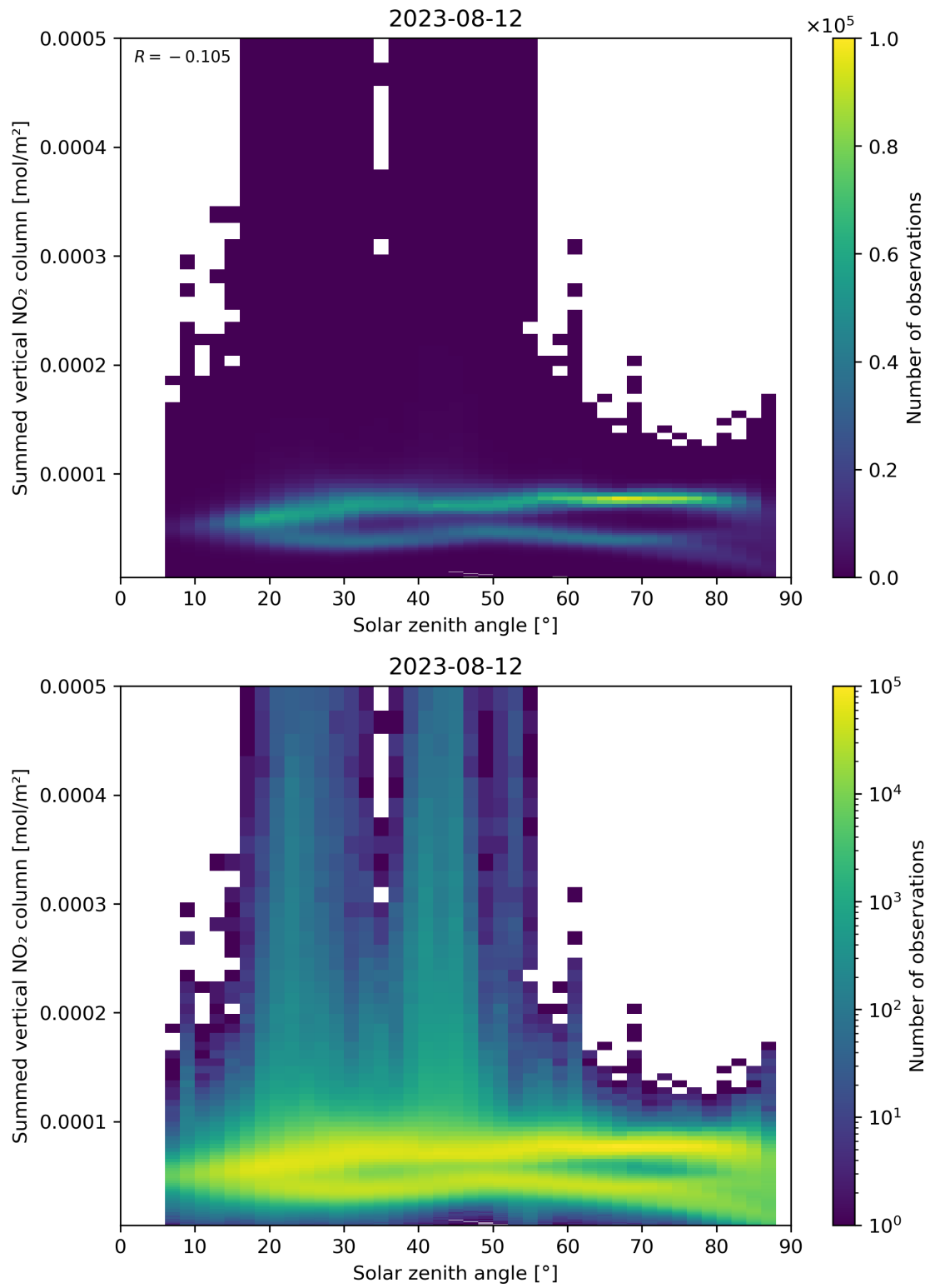
Figure 151: Scatter density plot of “Solar zenith angle” against “Summed vertical NO 2 column” for 2023-08-11 to 2023-08-13.
