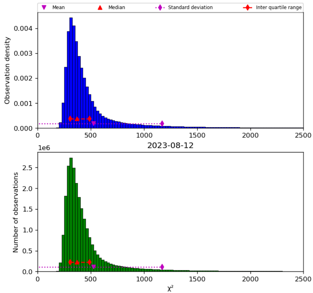
Figure 42: Histogram of “ \chi^2 ” for 2023-08-11 to 2023-08-13
