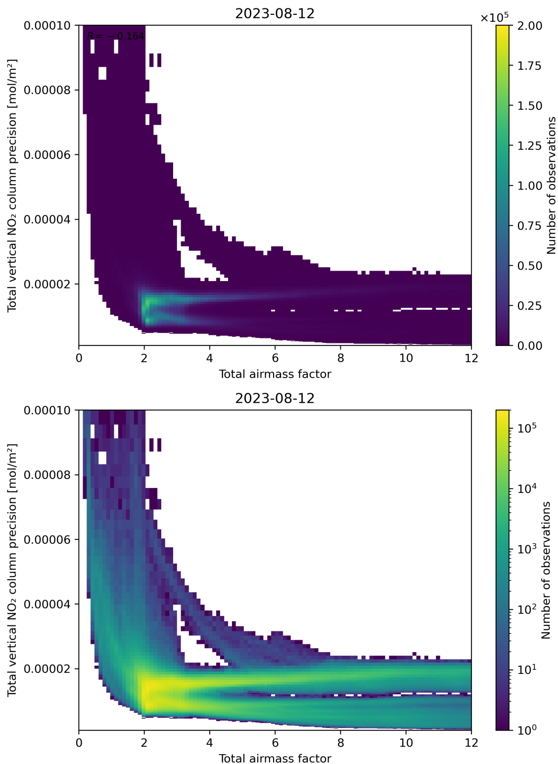
Figure 68: Scatter density plot of “Total airmass factor” against “Total vertical NO 2 column precision” for 2023-08-11 to 2023-08-13.
