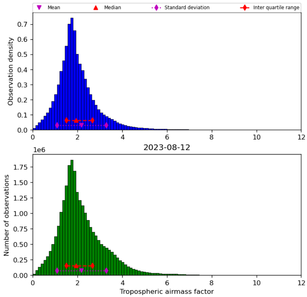
Figure 31: Histogram of “Tropospheric airmass factor” for 2023-08-11 to 2023-08-13
