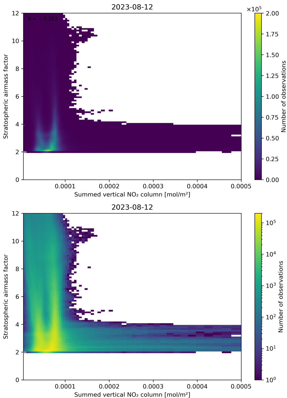
Figure 103: Scatter density plot of “Summed vertical NO 2 column” against “Stratospheric airmass factor” for 2023-08-11 to 2023-08-13.
