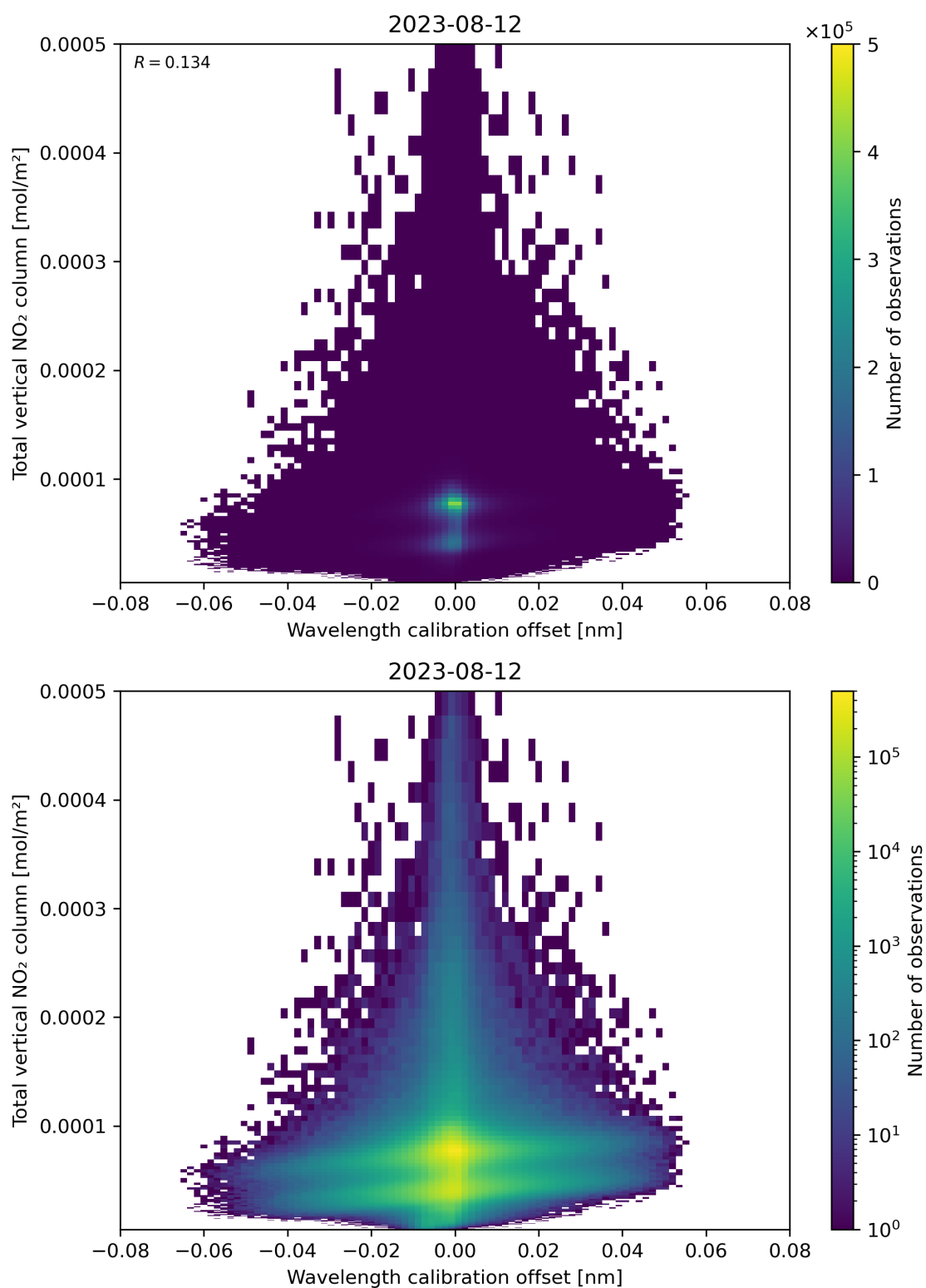
Figure 179: Scatter density plot of “Wavelength calibration offset” against “Total vertical NO 2 column” for 2023-08-11 to 2023-08-13.
