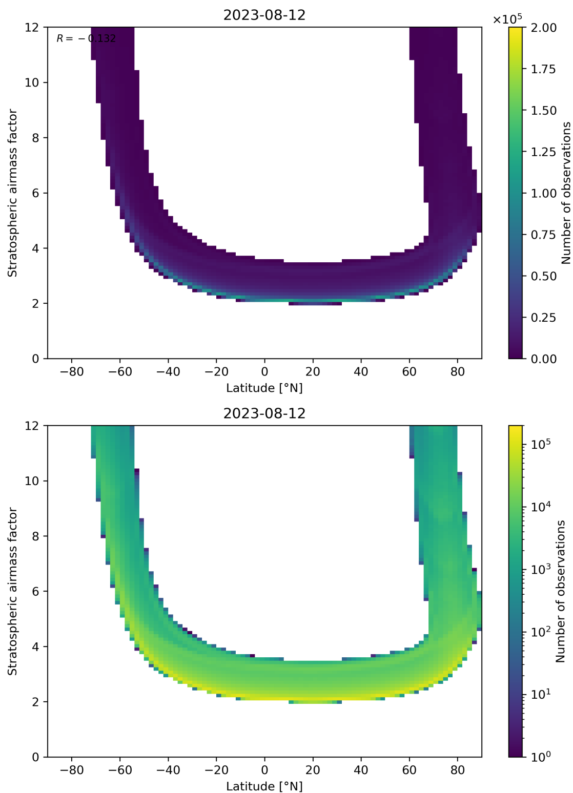
Figure 83: Scatter density plot of “Latitude” against “Stratospheric airmass factor” for 2023-08-11 to 2023-08-13.
