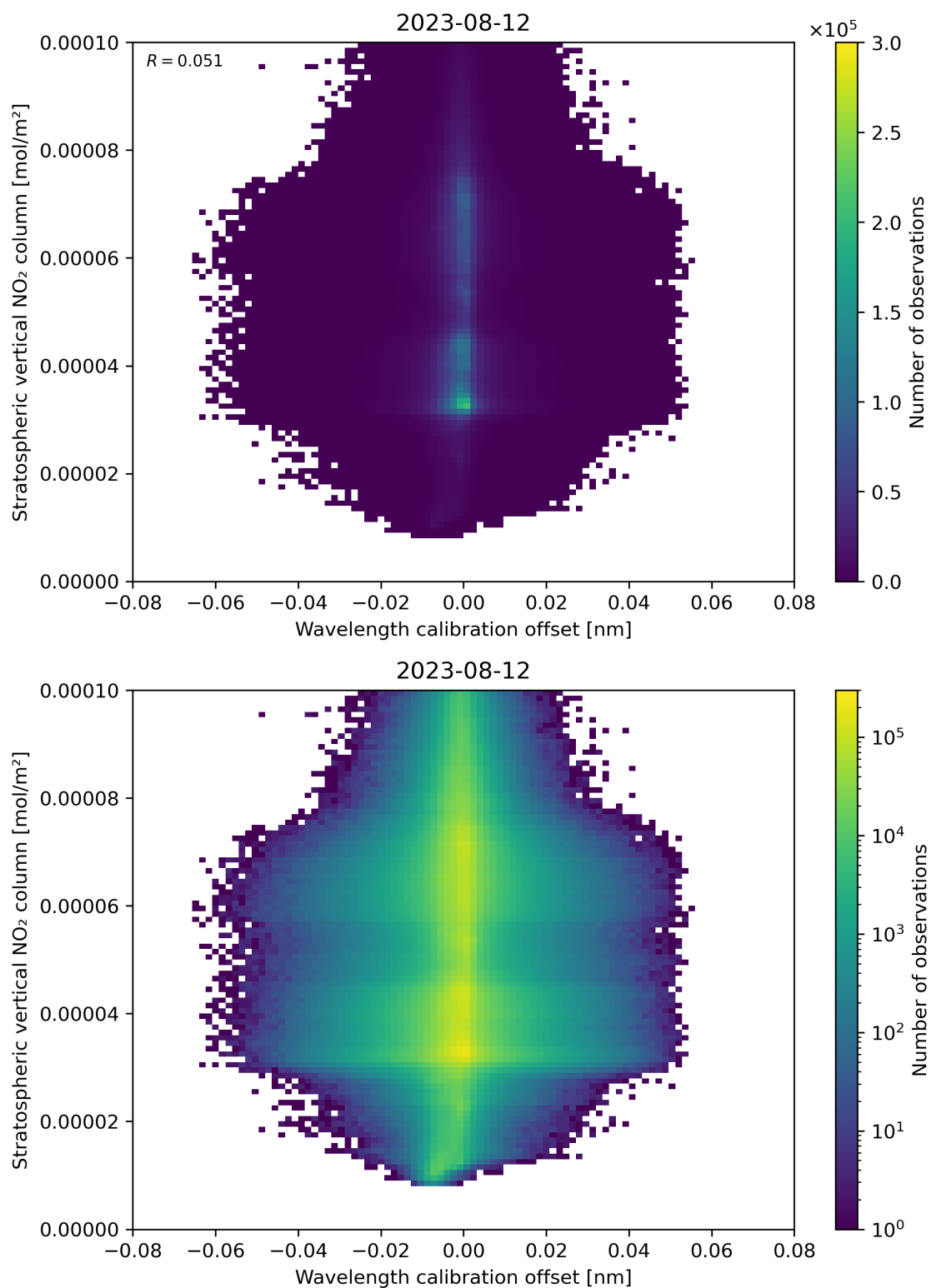
Figure 176: Scatter density plot of “Wavelength calibration offset” against “Stratospheric vertical NO 2 column” for 2023-08-11 to 2023-08-13.
