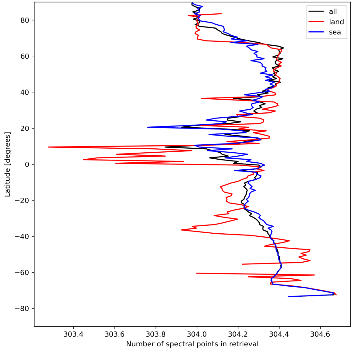
Figure 16: Zonal average of “Number of spectral points in retrieval” for 2023-08-11 to 2023-08-13.
