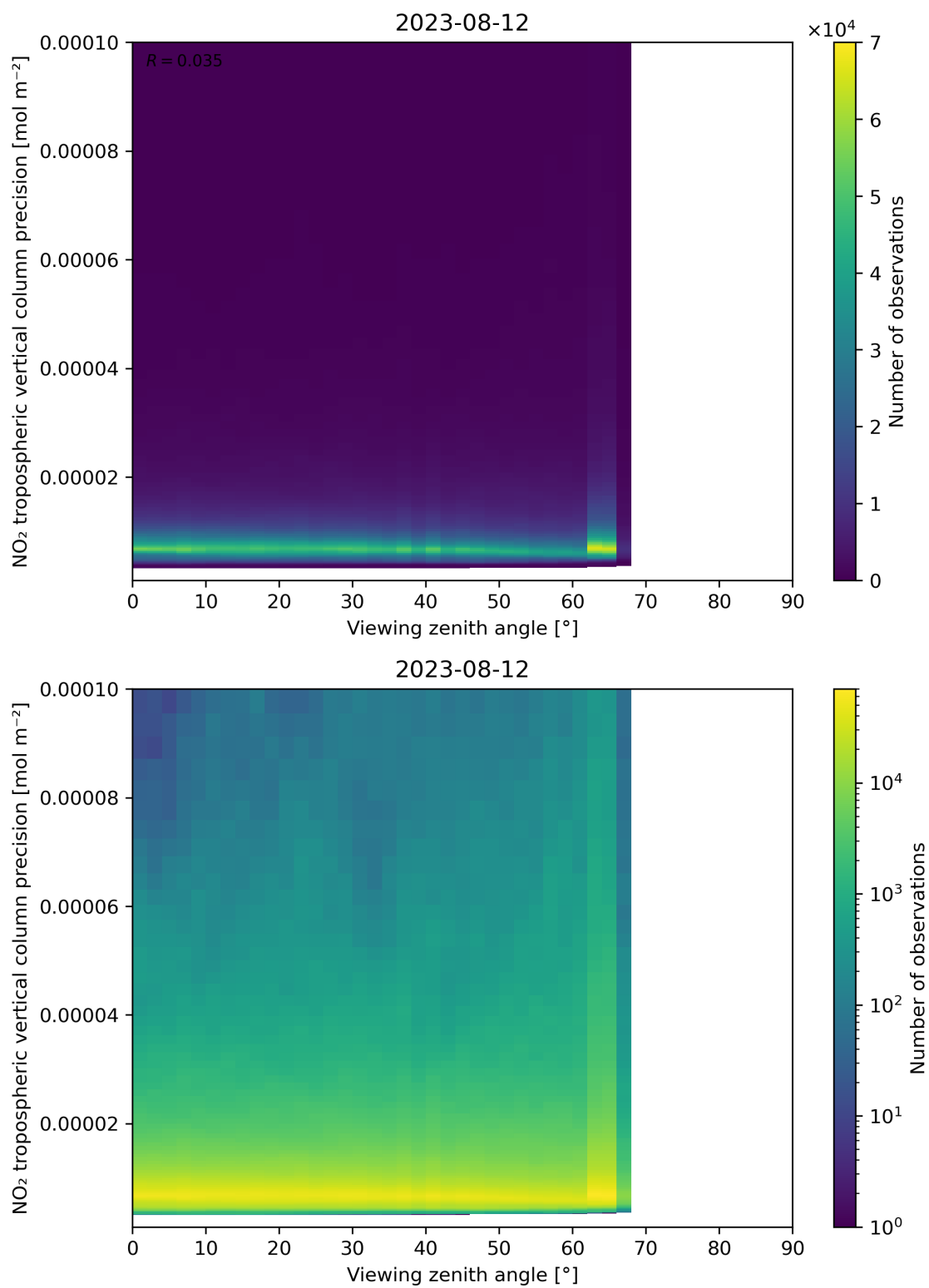
Figure 170: Scatter density plot of “Viewing zenith angle” against “NO 2 tropospheric vertical column precision” for 2023-08-11 to 2023-08-13.
