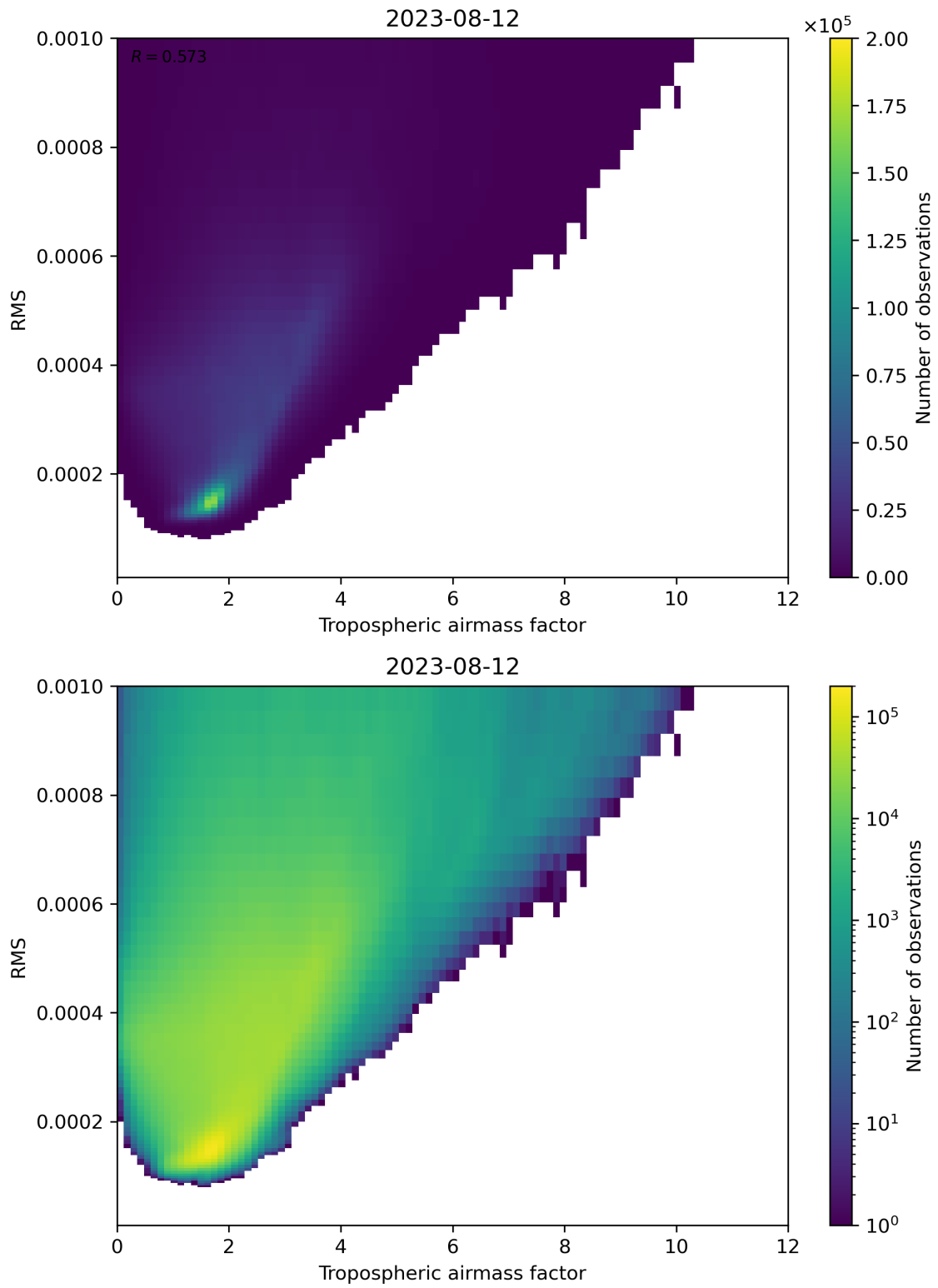
Figure 79: Scatter density plot of “Tropospheric airmass factor” against “RMS” for 2023-08-11 to 2023-08-13.
