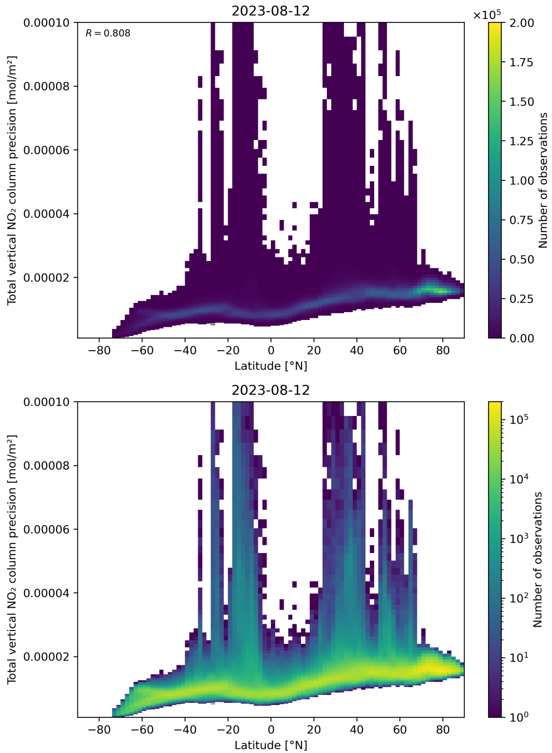
Figure 91: Scatter density plot of “Latitude” against “Total vertical NO 2 column precision” for 2023-08-11 to 2023-08-13.
