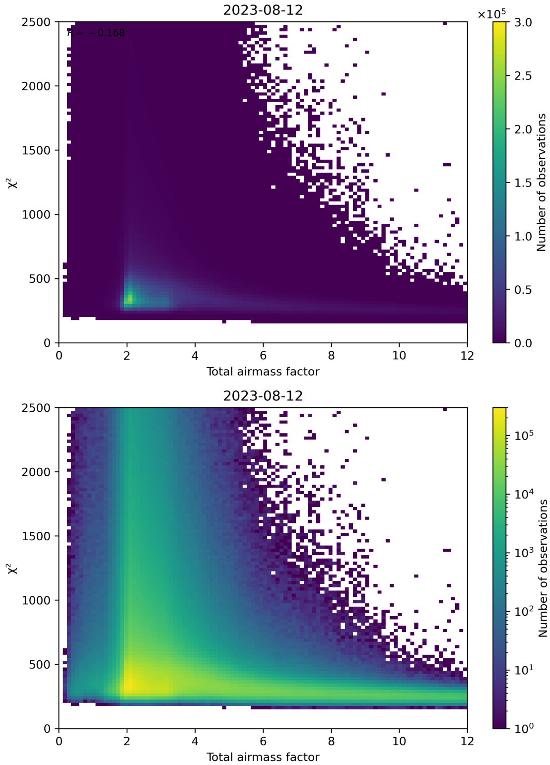
Figure 63: Scatter density plot of “Total airmass factor” against “ \chi^2 ” for 2023-08-11 to 2023-08-13.
