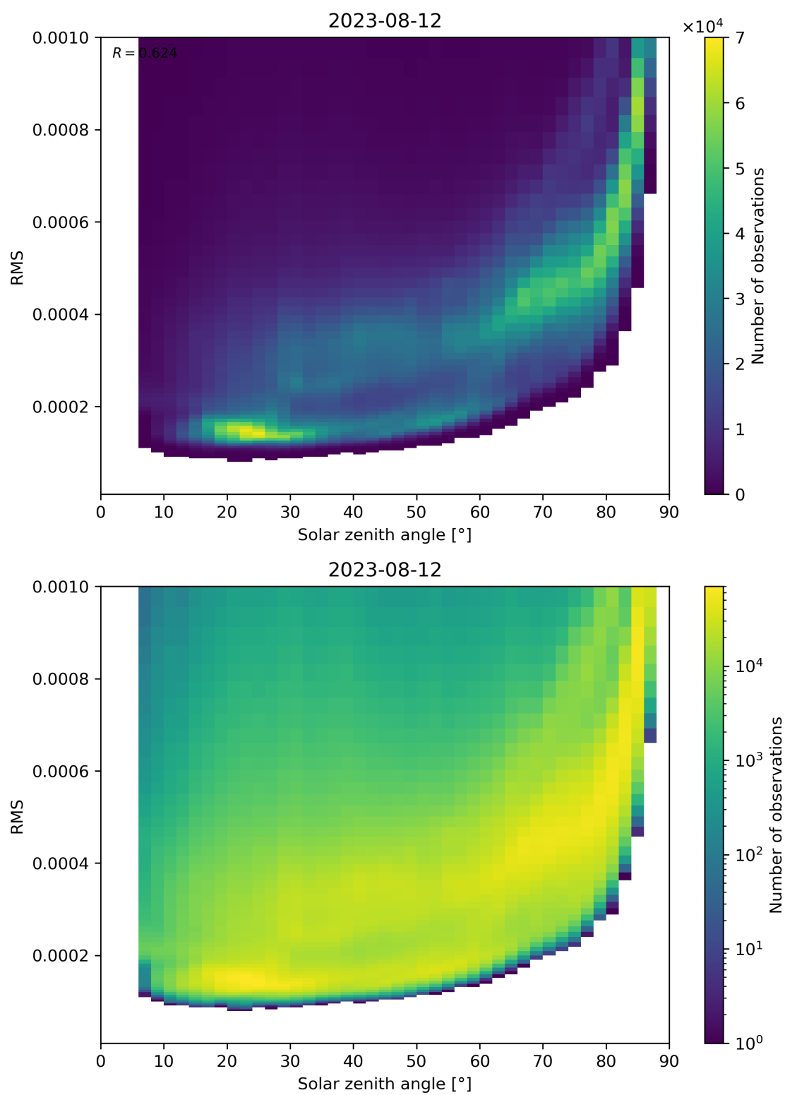
Figure 157: Scatter density plot of “Solar zenith angle” against “RMS” for 2023-08-11 to 2023-08-13.
