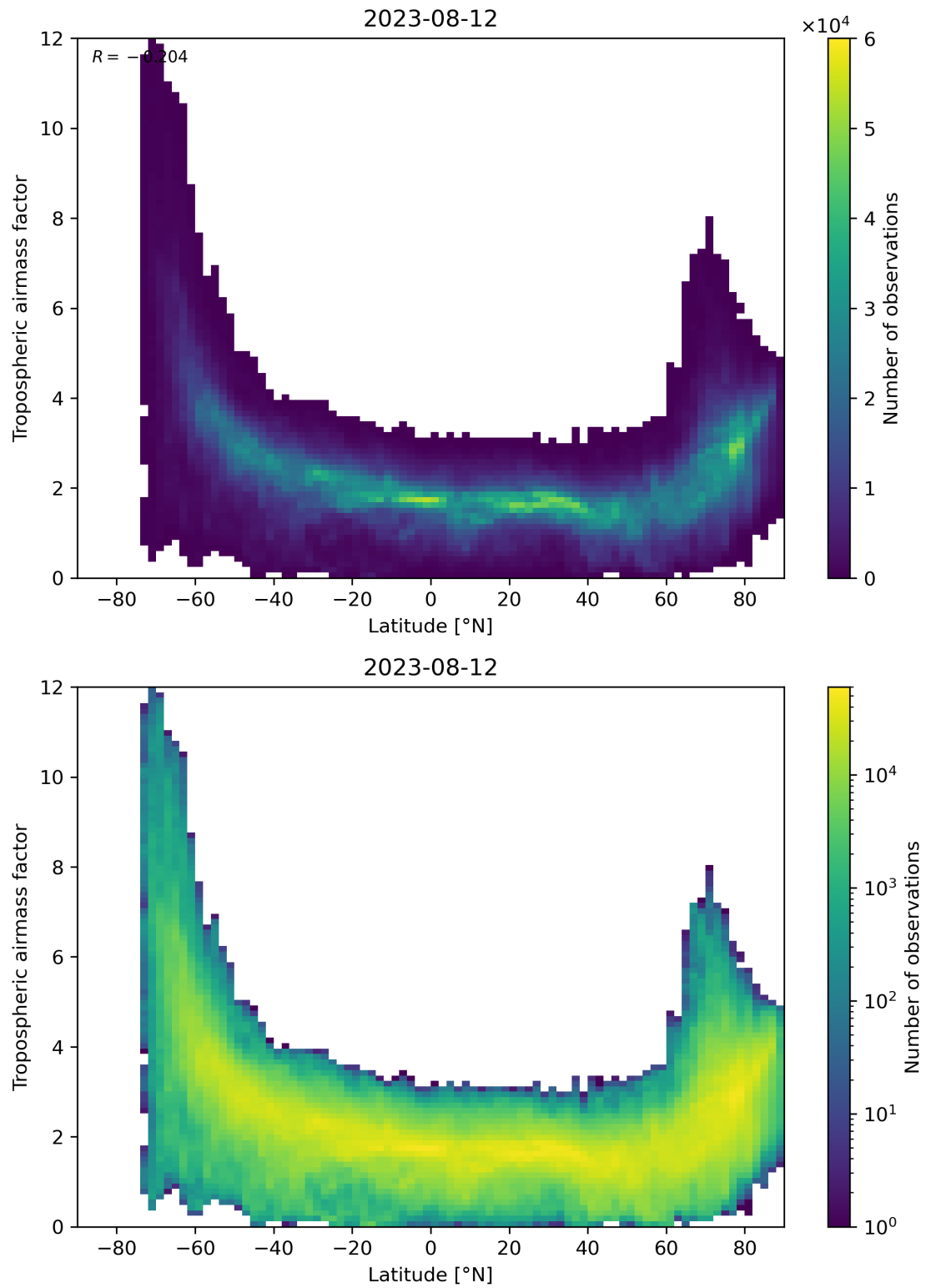
Figure 85: Scatter density plot of “Latitude” against “Tropospheric air mass factor” for 2023-08-11 to 2023-08-13.
