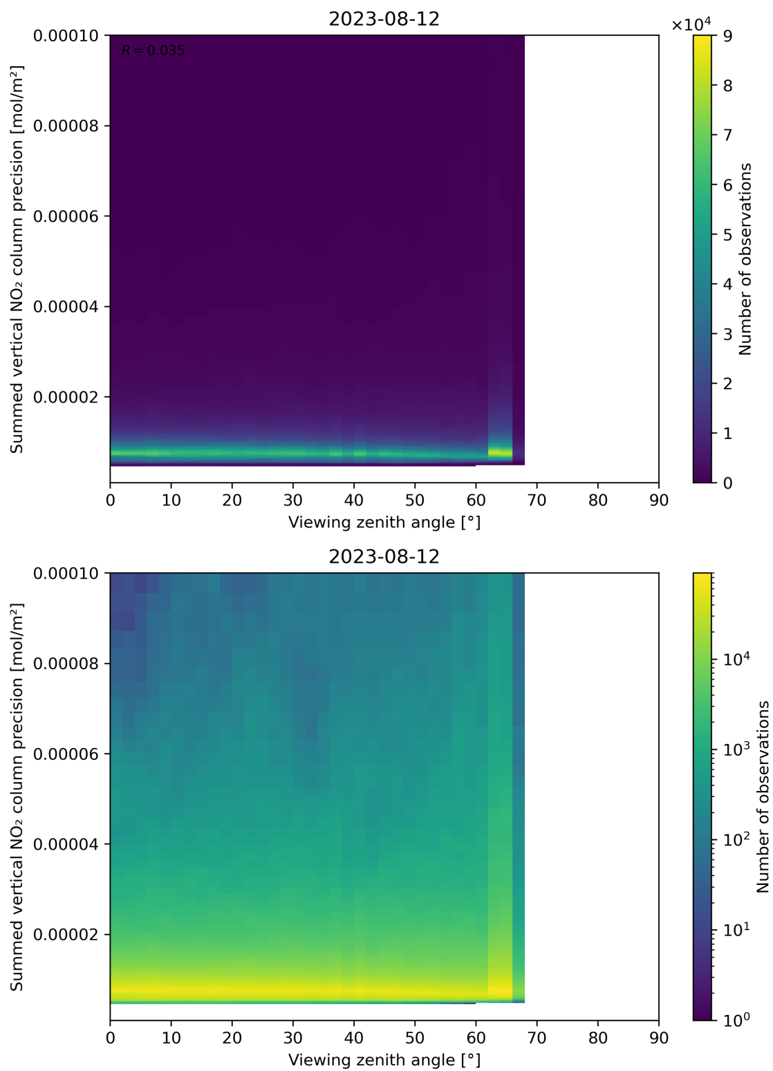
Figure 166: Scatter density plot of “Viewing zenith angle” against “Summed vertical NO 2 column precision” for 2023-08-11 to 2023-08-13.
