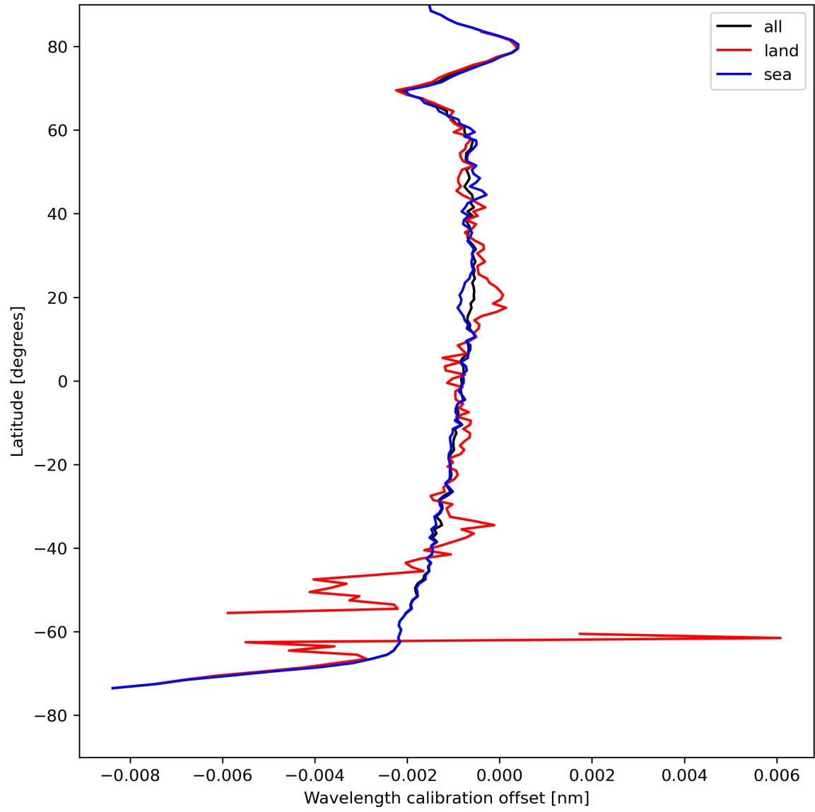
Figure 18: Zonal average of “Wavelength calibration offset” for 2023-08-11 to 2023-08-13.
