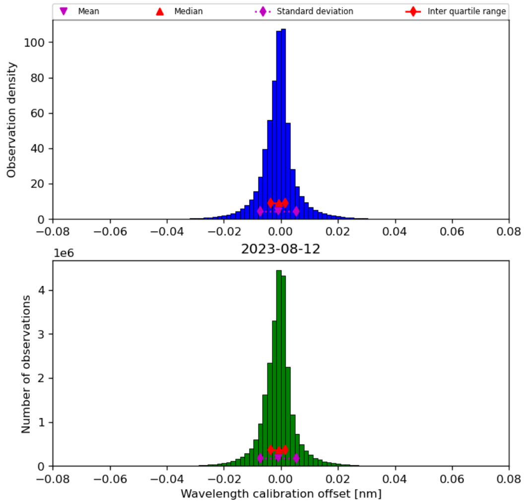
Figure 35: Histogram of “Wavelength calibration offset” for 2023-08-11 to 2023-08-13
