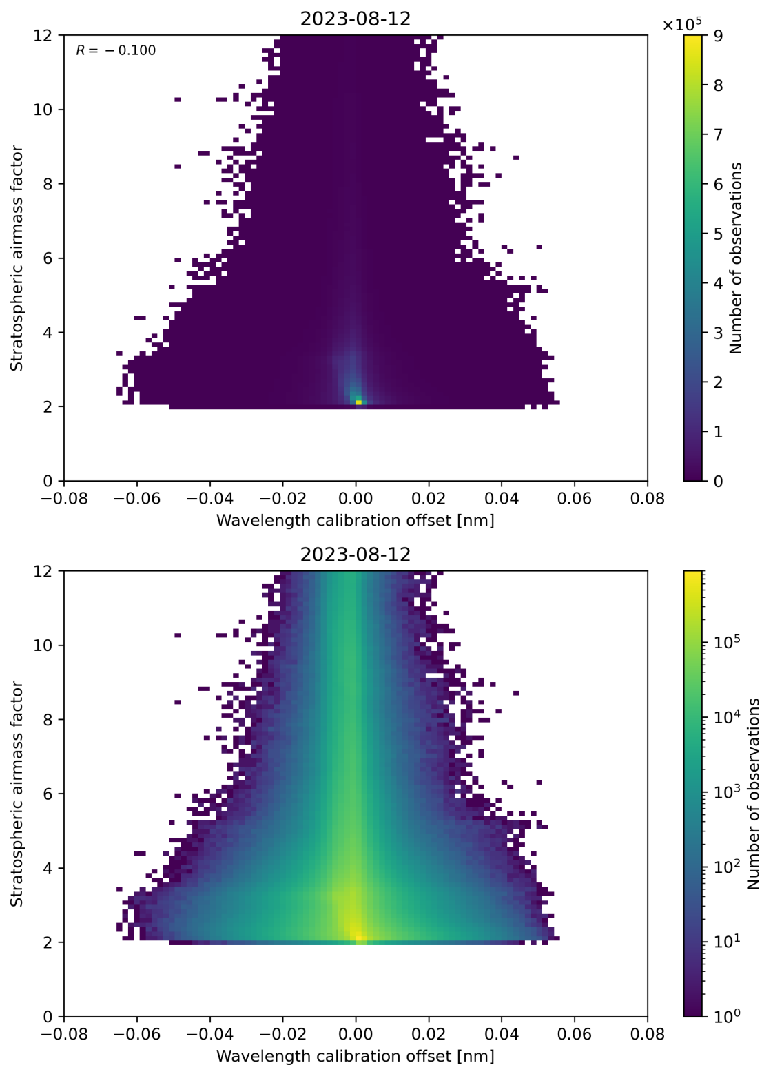
Figure 174: Scatter density plot of “Wavelength calibration offset” against “Stratospheric airmass factor” for 2023-08-11 to 2023-08-13.
