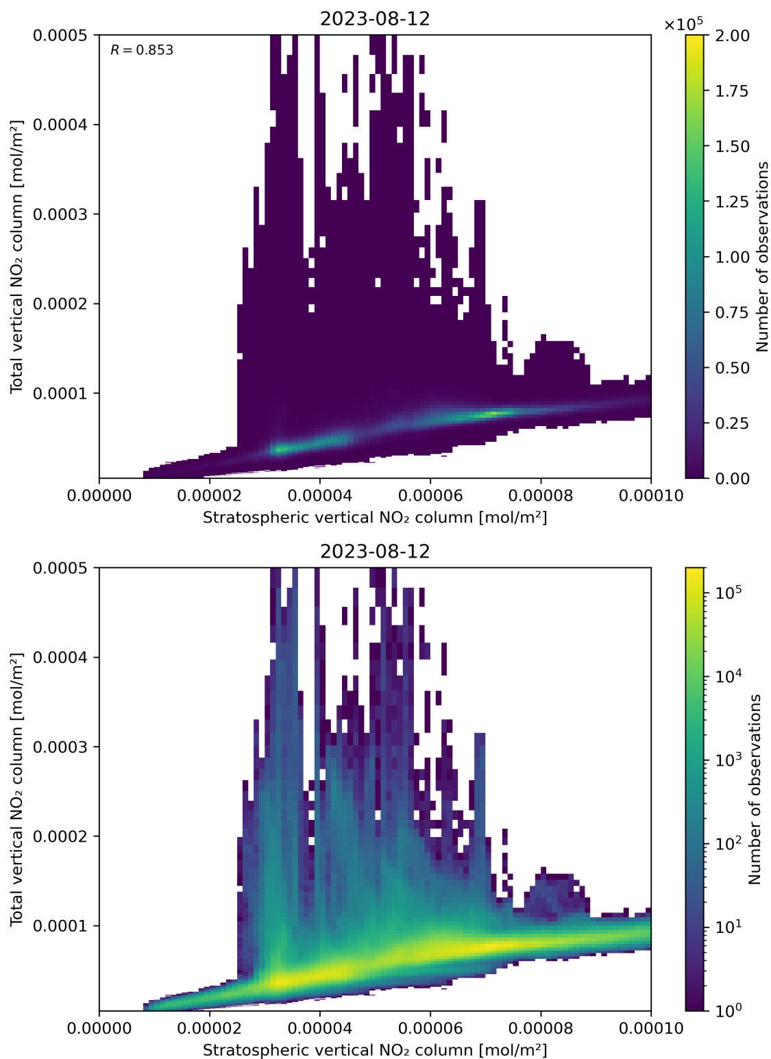
Figure 100: Scatter density plot of “Stratospheric vertical NO 2 column” against “Total vertical NO 2 column” for 2023-08-11 to 2023-08-13.
