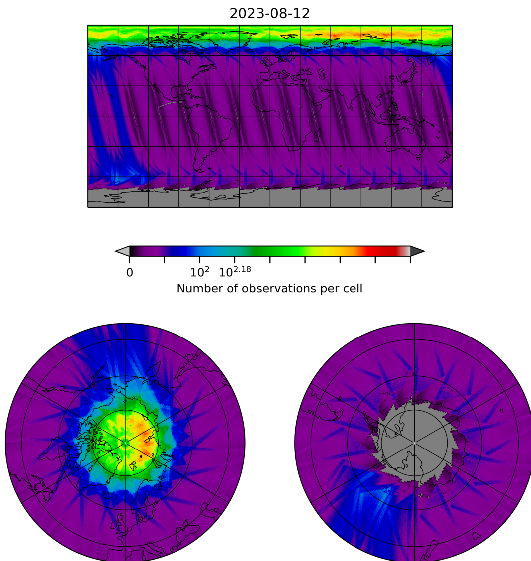
Figure 10: Map of the number of observations for 2023-08-11 to 2023-08-13
