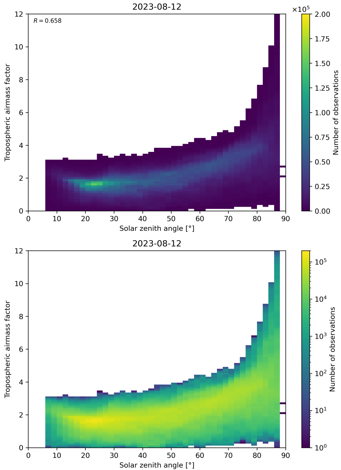
Figure 147: Scatter density plot of “Solar zenith angle” against “Tropospheric airmass factor” for 2023-08-11 to 2023-08-13.
