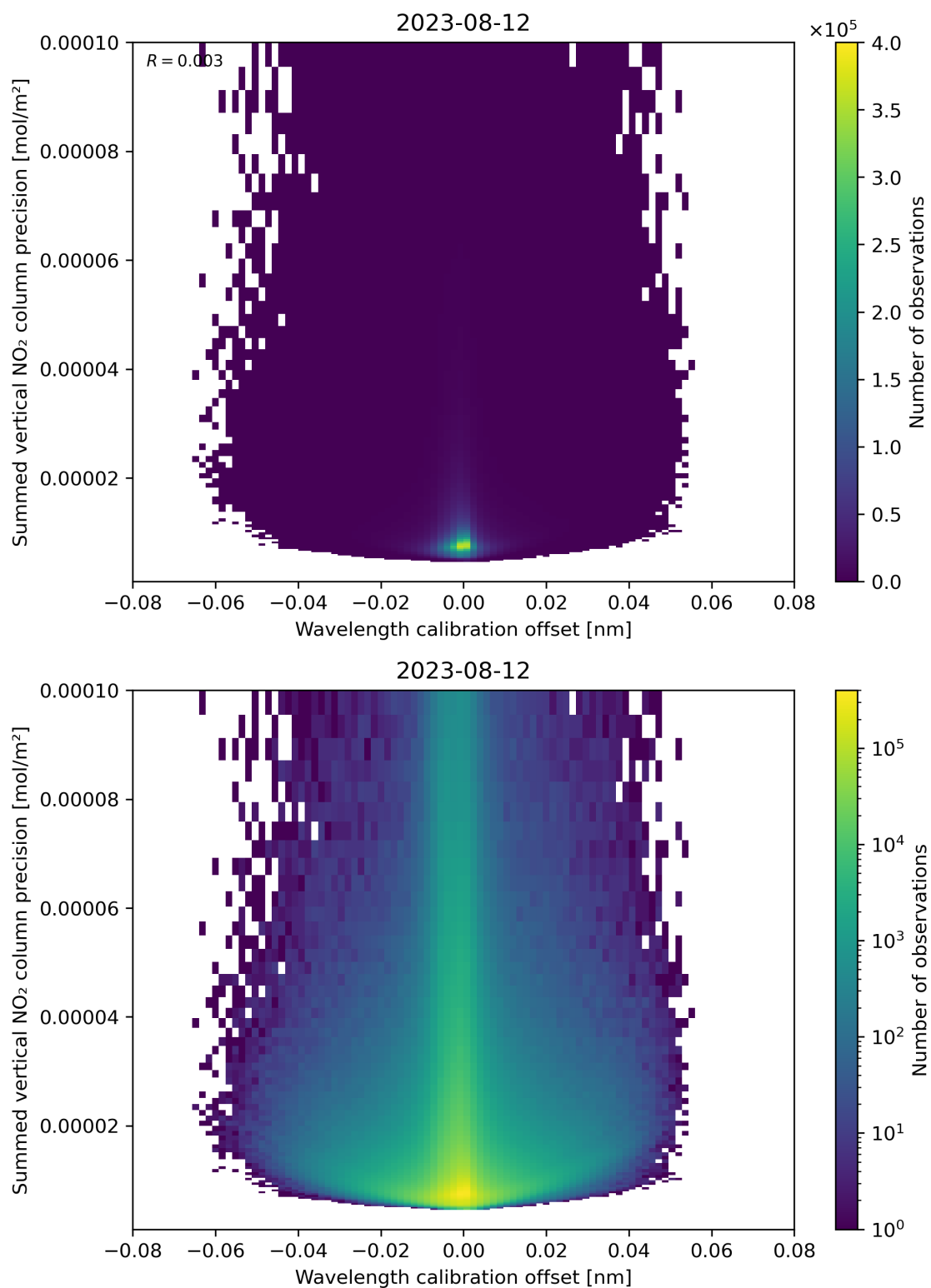
Figure 178: Scatter density plot of “Wavelength calibration offset” against “Summed vertical NO 2 column precision” for 2023-08-11 to 2023-08-13.
