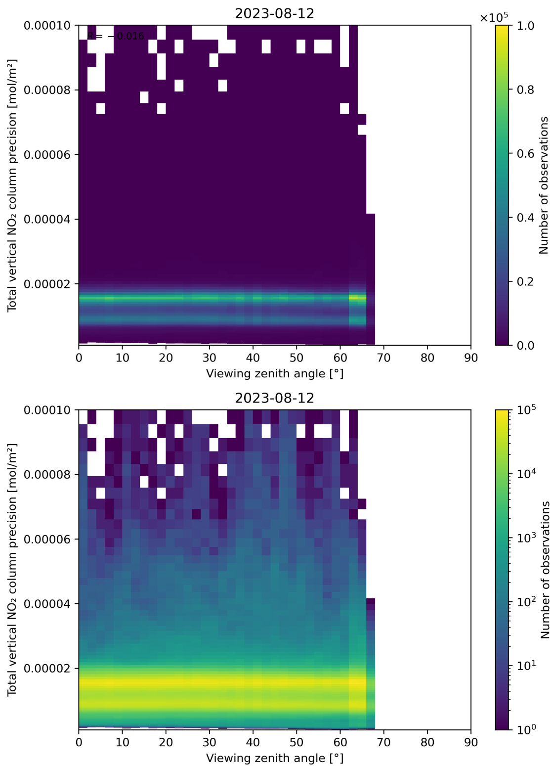
Figure 168: Scatter density plot of “Viewing zenith angle” against “Total vertical NO 2 column precision” for 2023-08-11 to 2023-08-13.
