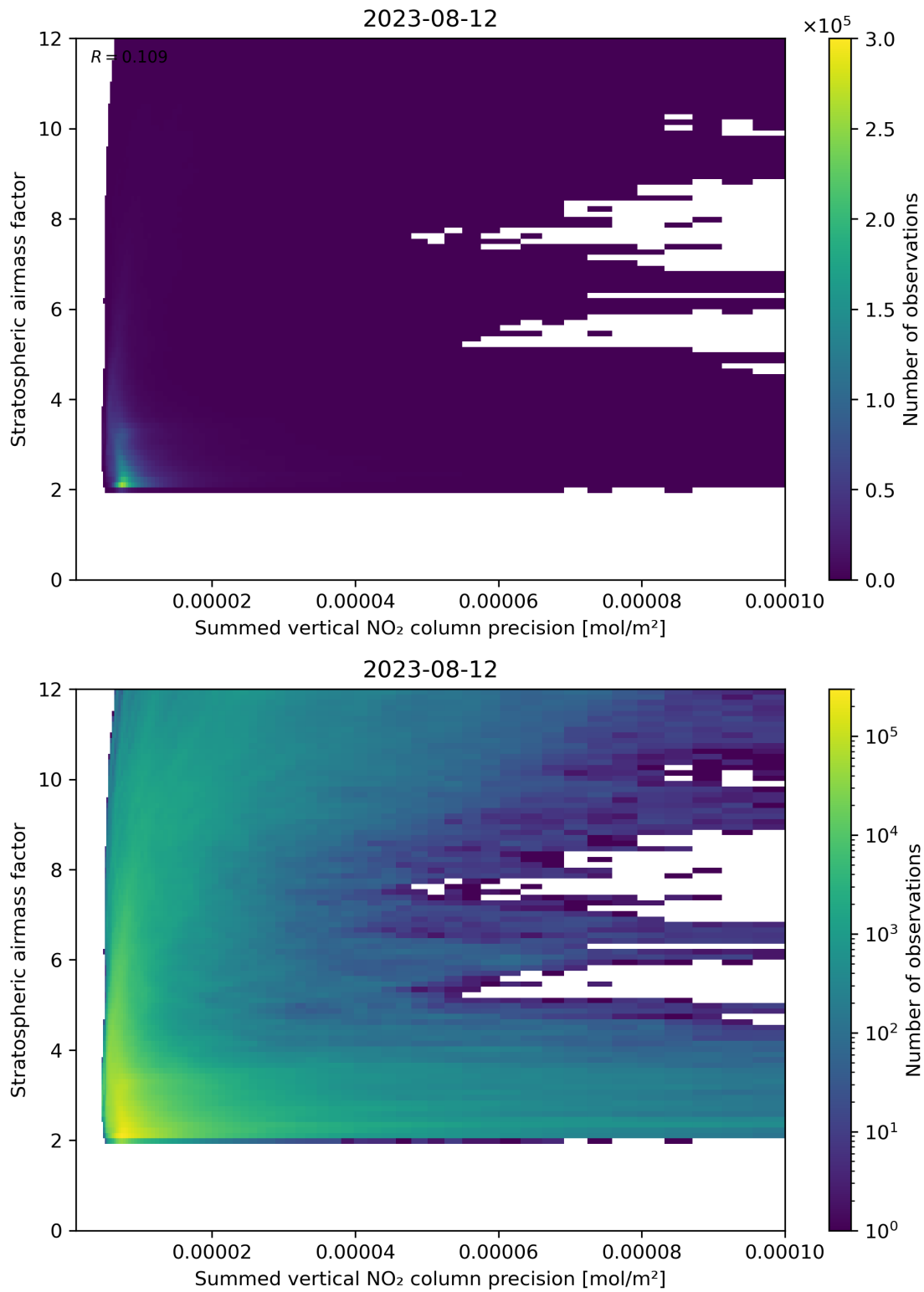
Figure 106: Scatter density plot of “Summed vertical NO 2 column precision” against “Stratospheric airmass factor” for 2023-08-11 to 2023-08-13.
