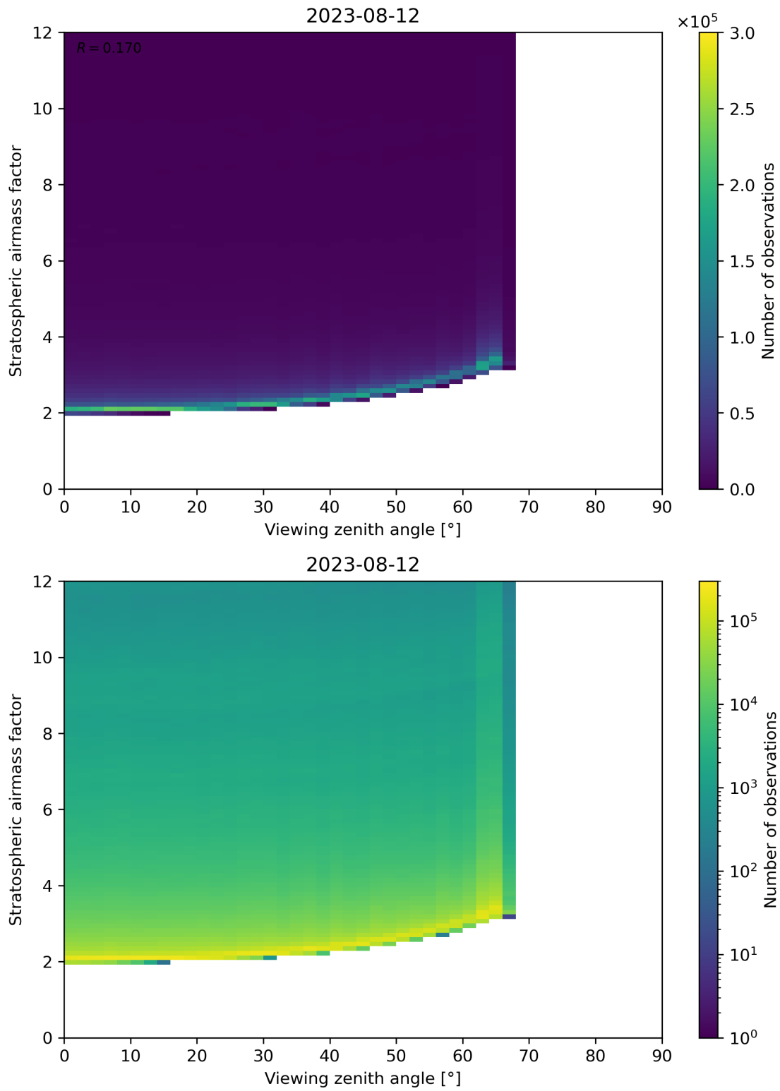
Figure 159: Scatter density plot of “Viewing zenith angle” against “Stratospheric airmass factor” for 2023-08-11 to 2023-08-13.
