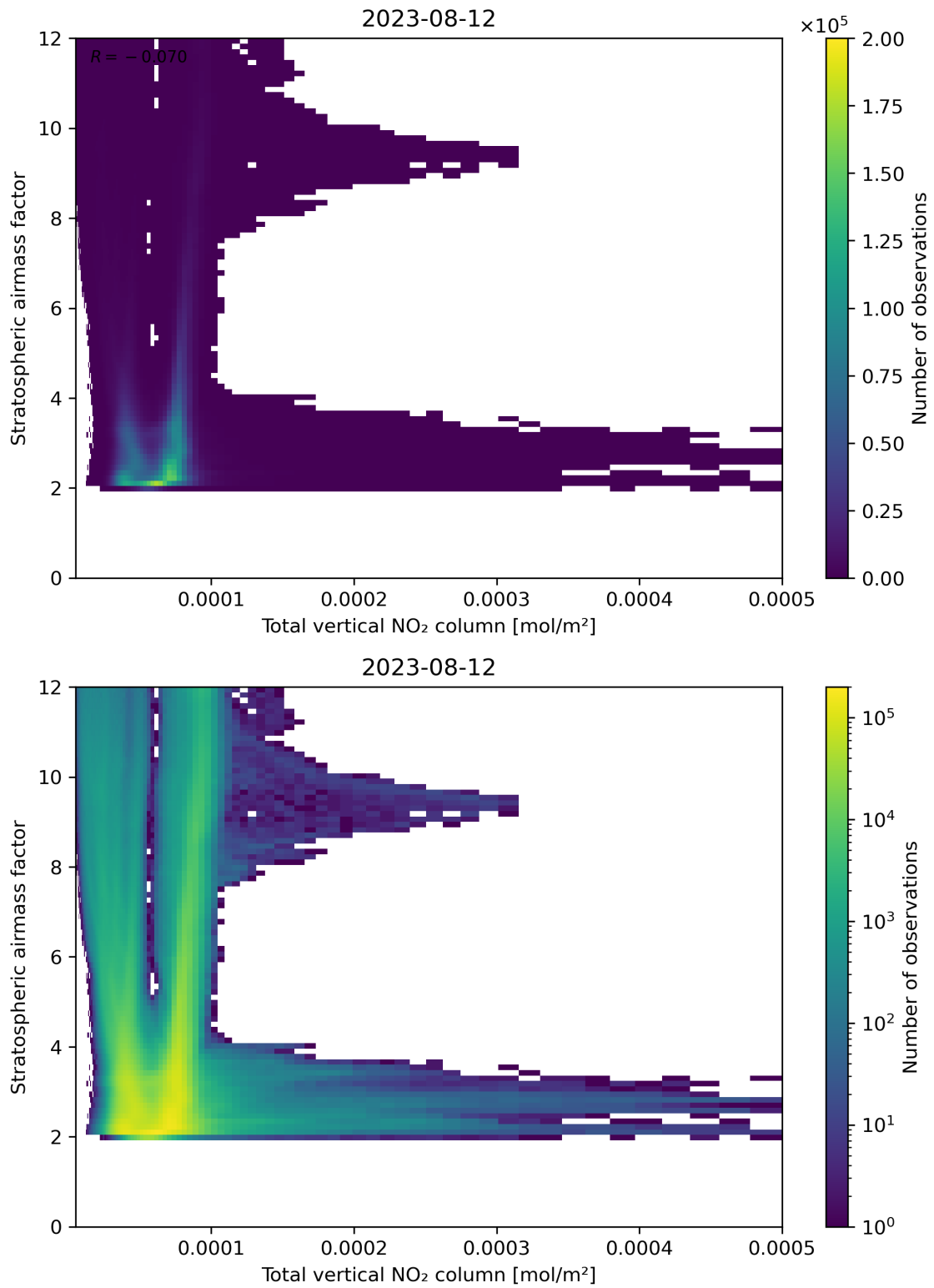
Figure 110: Scatter density plot of “Total vertical NO 2 column” against “Stratospheric airmass factor” for 2023-08-11 to 2023-08-13.
