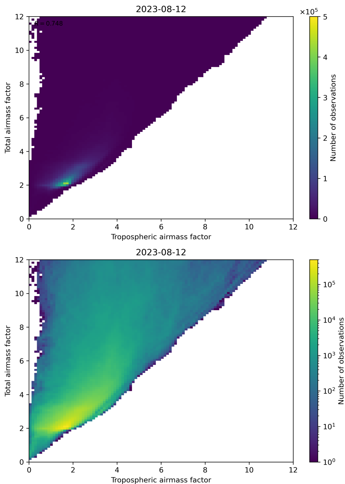
Figure 72: Scatter density plot of “Tropospheric airmass factor” against “Total airmass factor” for 2023-08-11 to 2023-08-13.
