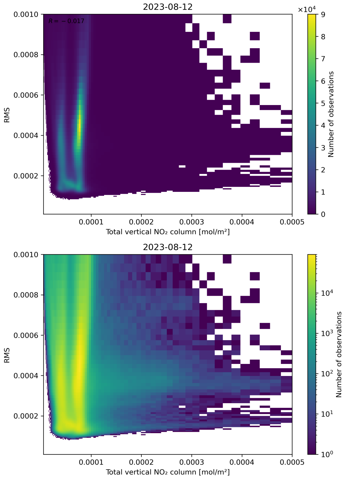
Figure 120: Scatter density plot of “Total vertical NO 2 column” against “RMS” for 2023-08-11 to 2023-08-13.
