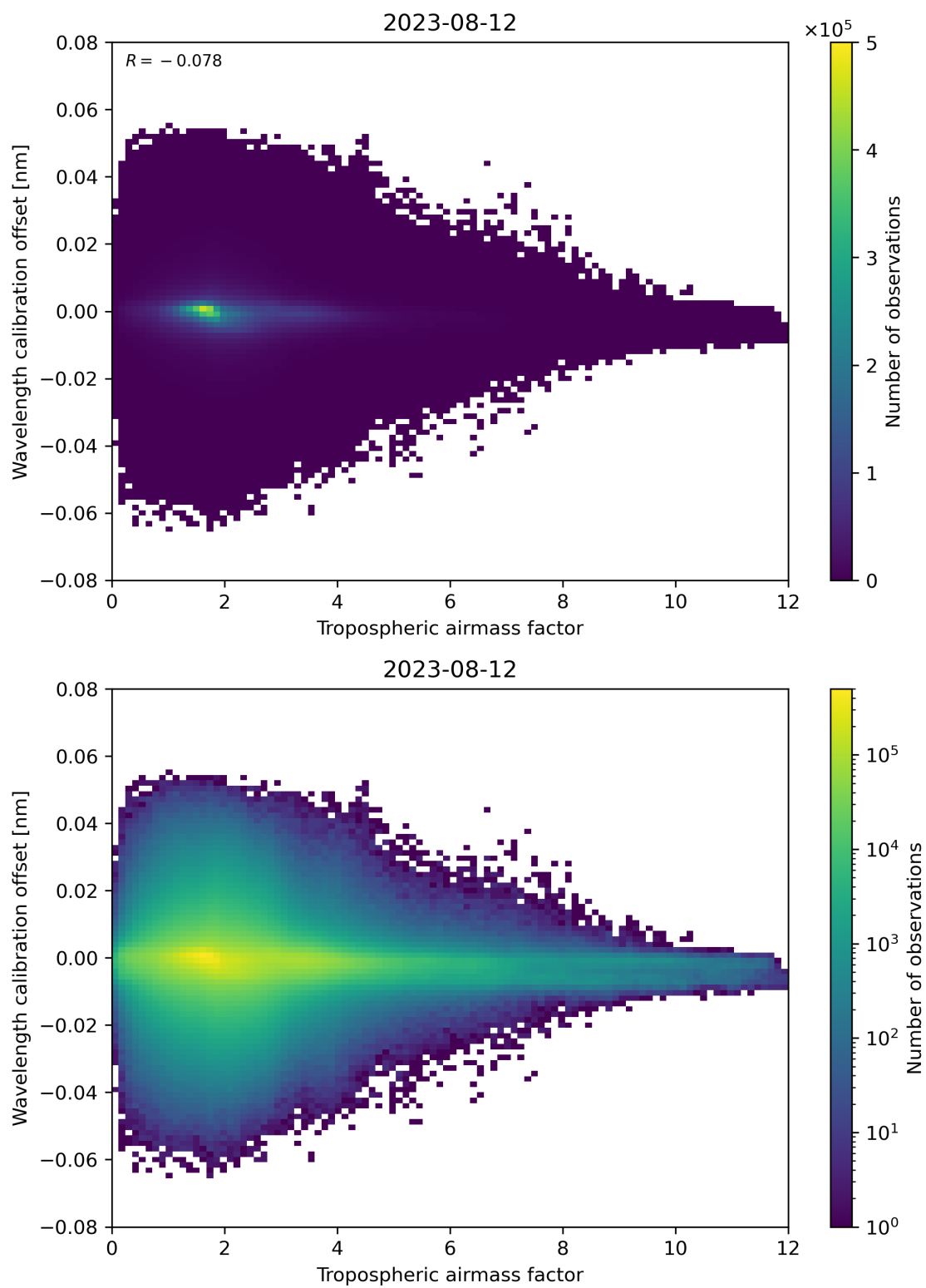
Figure 80: Scatter density plot of “Tropospheric air mass factor” against “Wavelength calibration offset” for 2023-08-11 to 2023-08-13.
