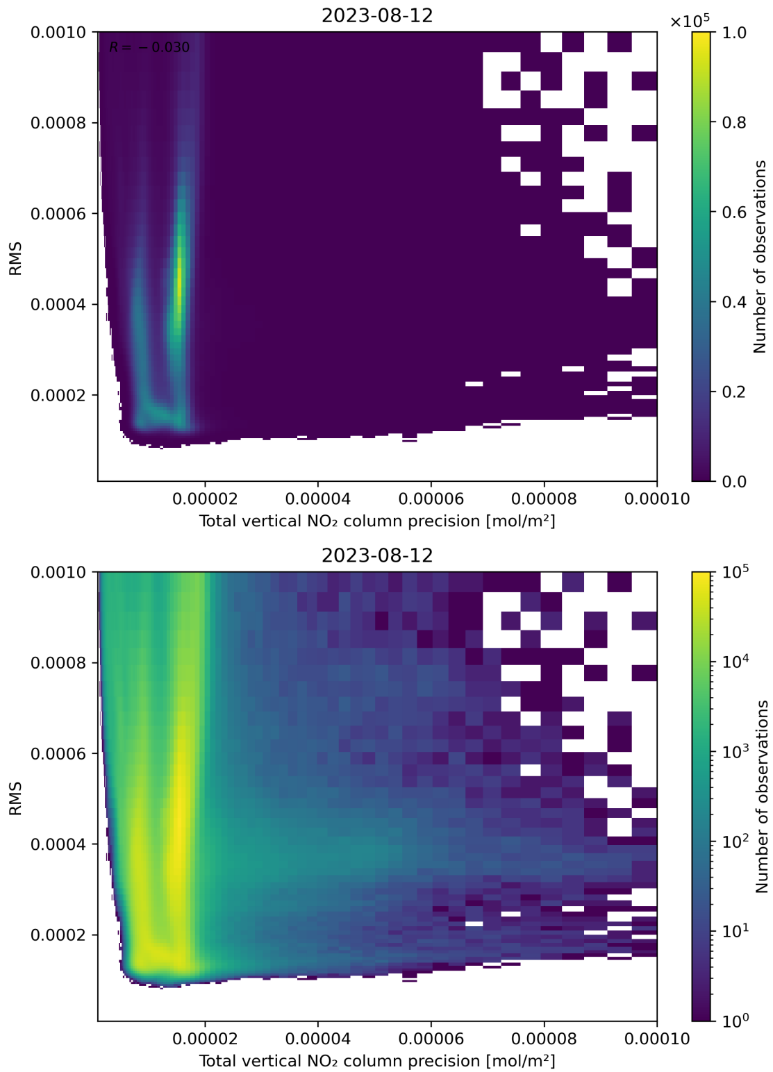
Figure 119: Scatter density plot of “Total vertical NO 2 column precision” against “RMS” for 2023-08-11 to 2023-08-13.
