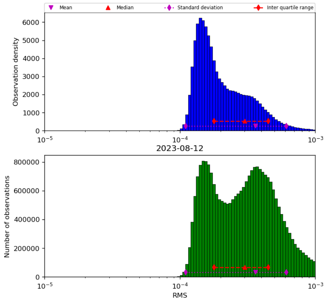
Figure 43: Histogram of “RMS” for 2023-08-11 to 2023-08-13
