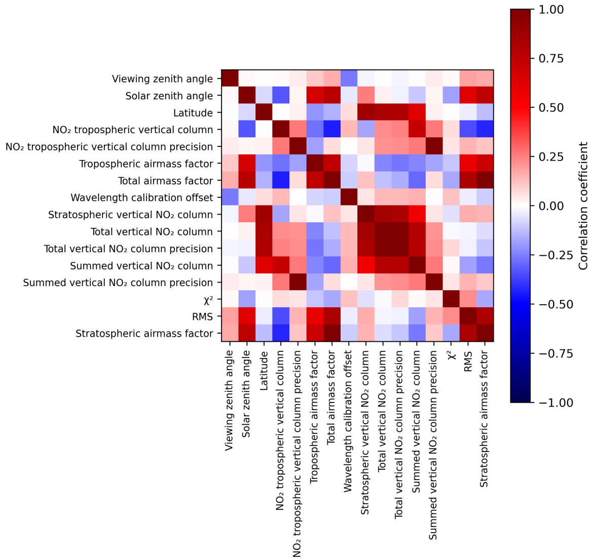
Figure 2: Map of correlation matrix for 2023-08-11 to 2023-08-13.
