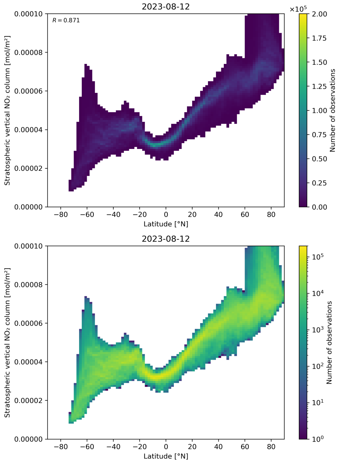
Figure 87: Scatter density plot of “Latitude” against “Stratospheric vertical NO 2 column” for 2023-08-11 to 2023-08-13.
