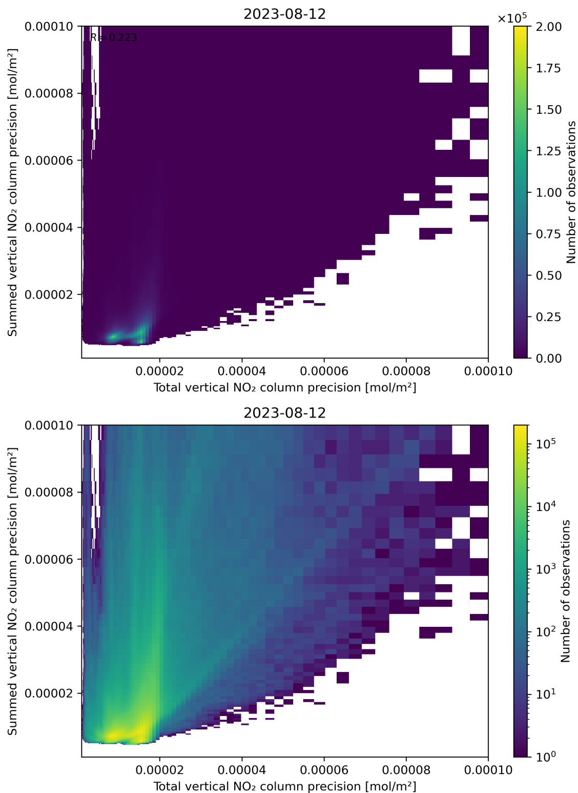
Figure 118: Scatter density plot of “Total vertical NO 2 column precision” against “Summed vertical NO 2 column precision” for 2023-08-11 to 2023-08-13.
