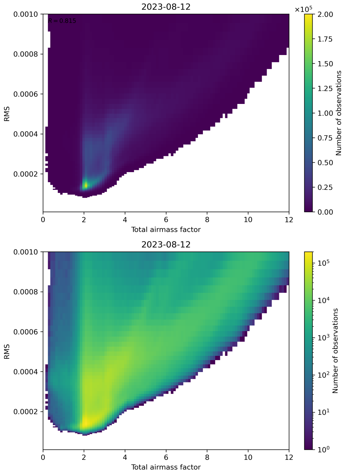
Figure 69: Scatter density plot of “Total airmass factor” against “RMS” for 2023-08-11 to 2023-08-13.
