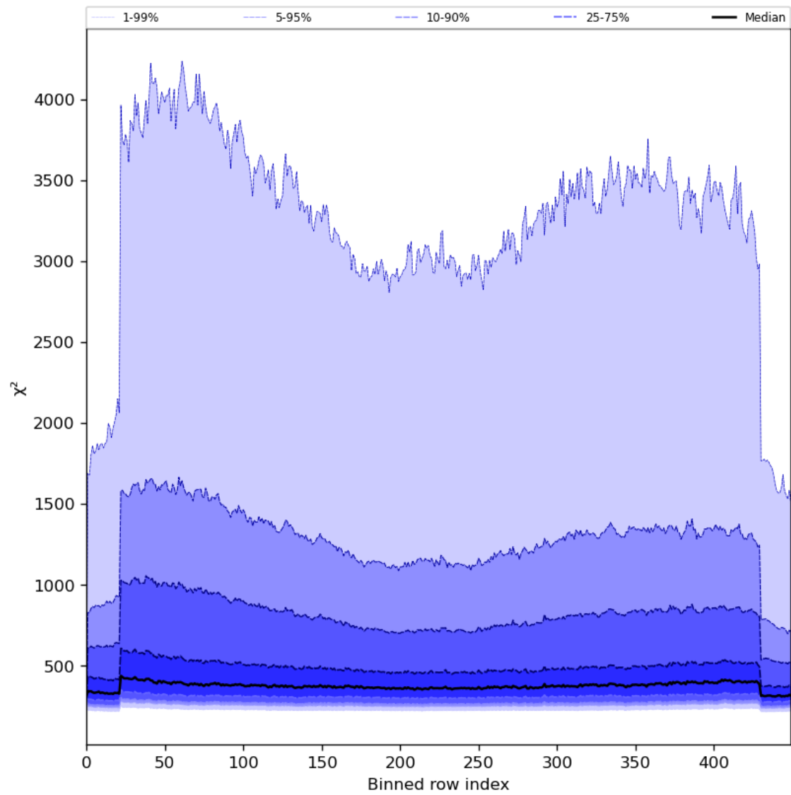
Figure 59: Along track statistics of “ \chi^2 ” for 2023-08-11 to 2023-08-13
