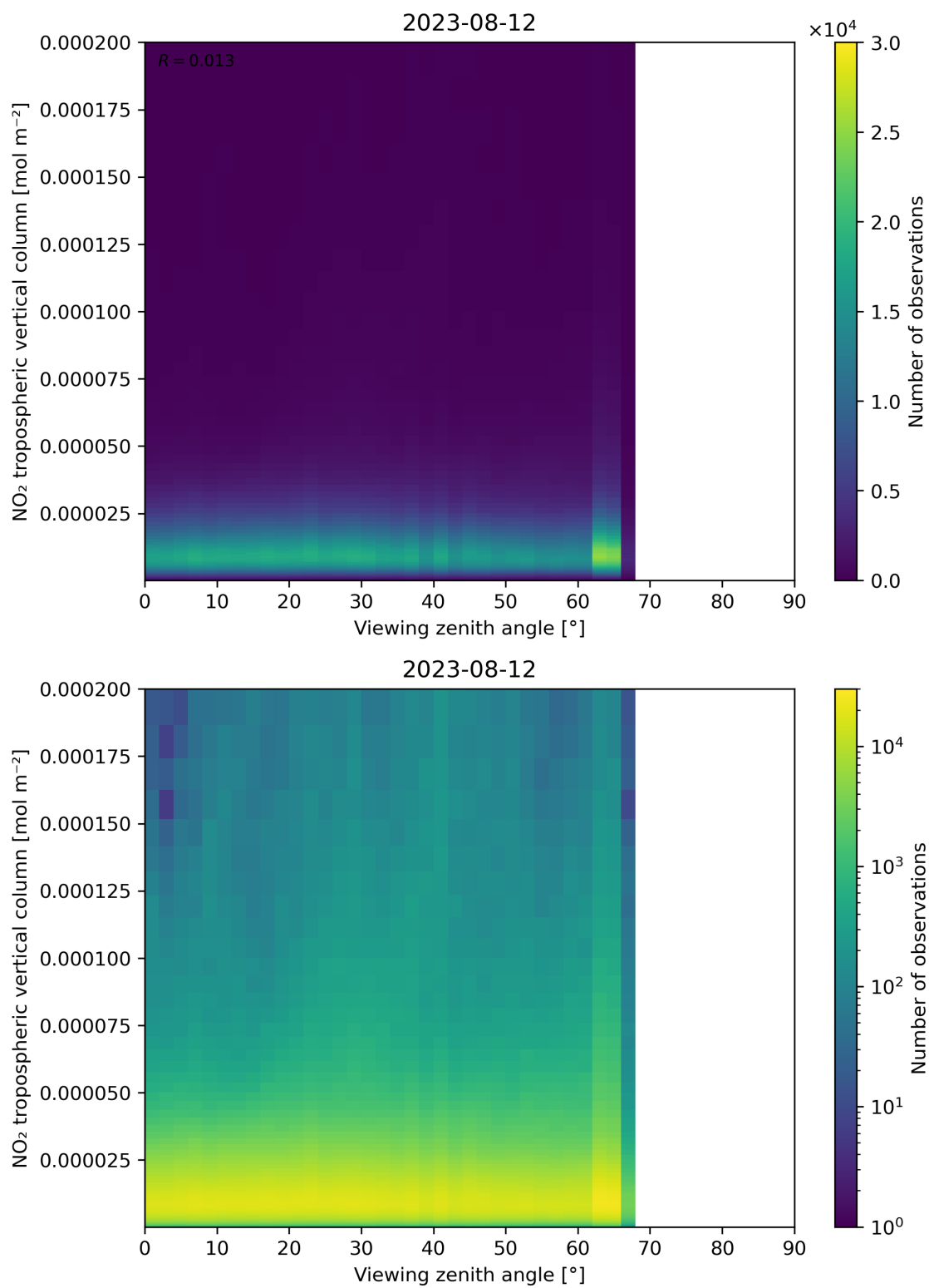
Figure 169: Scatter density plot of “Viewing zenith angle” against “NO 2 tropospheric vertical column” for 2023-08-11 to 2023-08-13.
