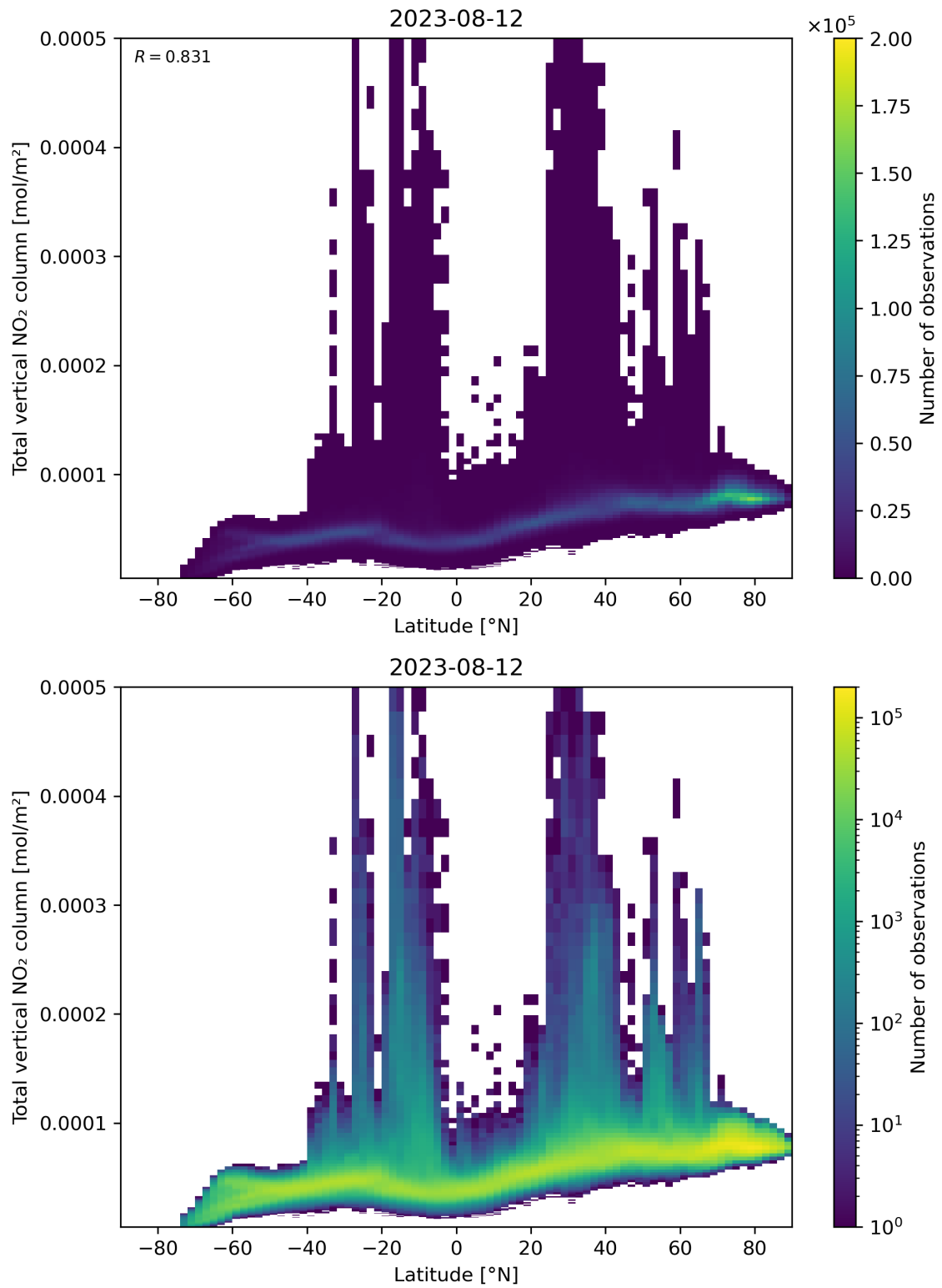
Figure 90: Scatter density plot of “Latitude” against “Total vertical NO 2 column” for 2023-08-11 to 2023-08-13.
