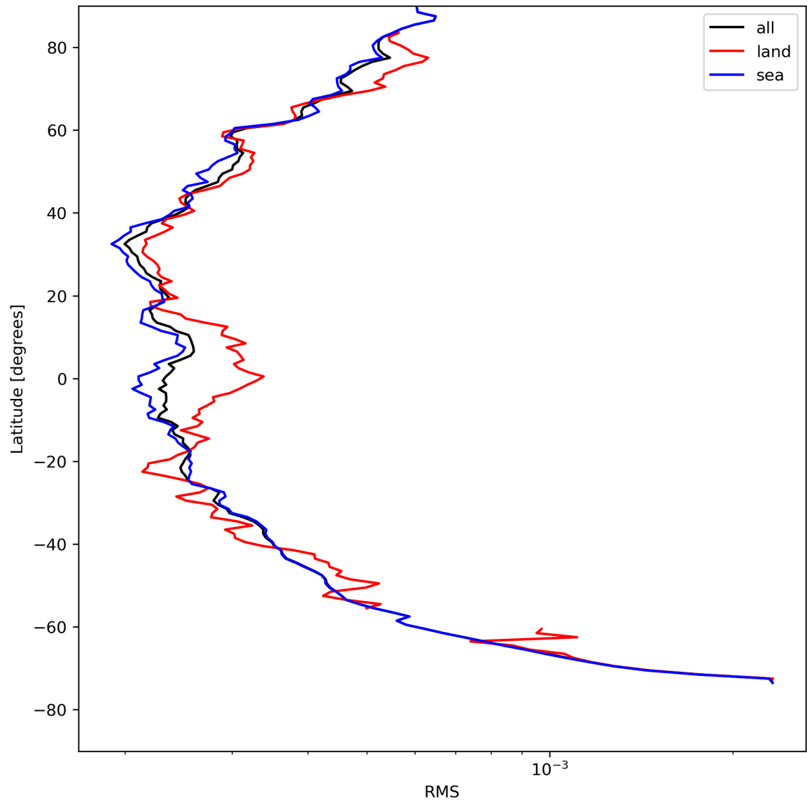
Figure 26: Zonal average of “RMS” for 2023-08-11 to 2023-08-13.
