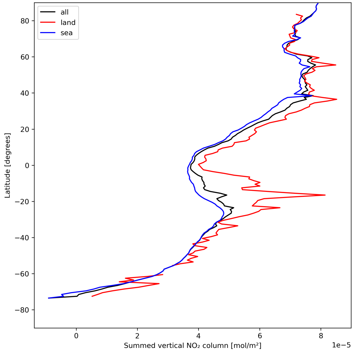
Figure 23: Zonal average of “Summed vertical NO 2 column” for 2023-08-11 to 2023-08-13.
