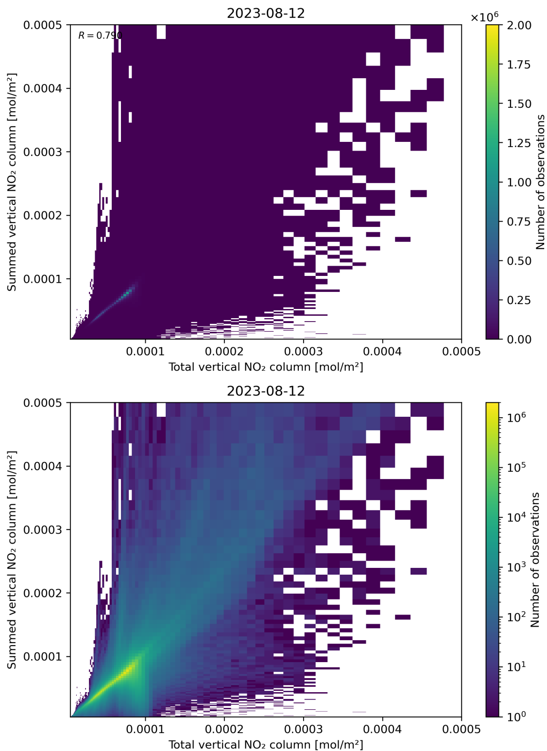
Figure 112: Scatter density plot of “Total vertical NO 2 column” against “Summed vertical NO 2 column” for 2023-08-11 to 2023-08-13.
