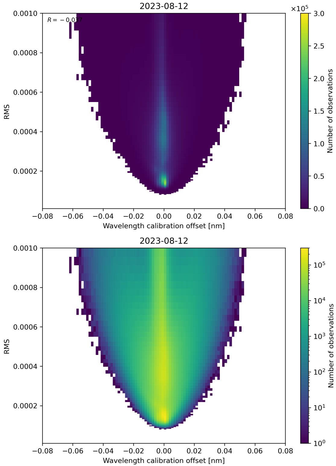
Figure 181: Scatter density plot of “Wavelength calibration offset” against “RMS” for 2023-08-11 to 2023-08-13.
