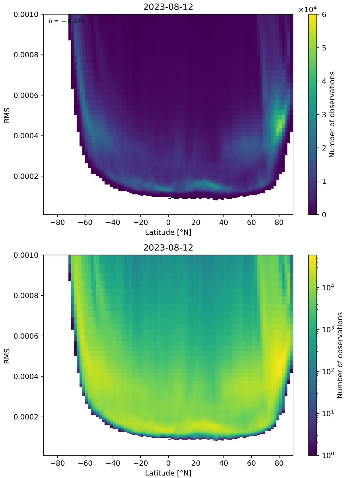
Figure 94: Scatter density plot of “Latitude” against “RMS” for 2023-08-11 to 2023-08-13.
