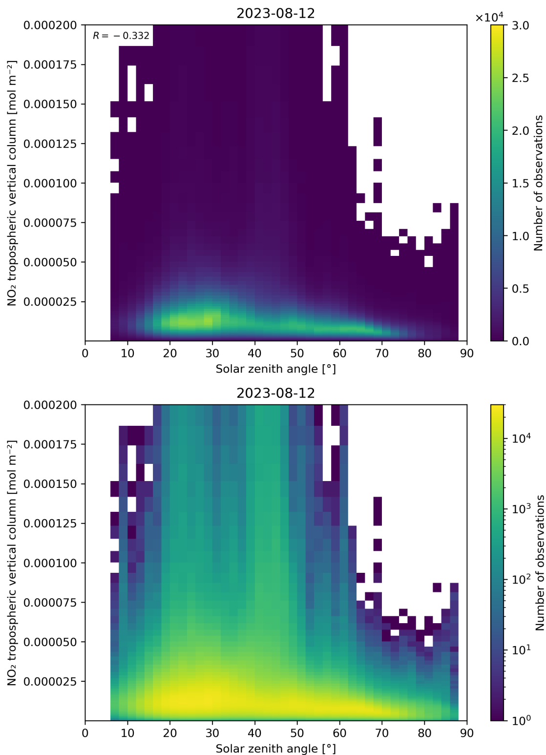
Figure 155: Scatter density plot of “Solar zenith angle” against “NO 2 tropospheric vertical column” for 2023-08-11 to 2023-08-13.
