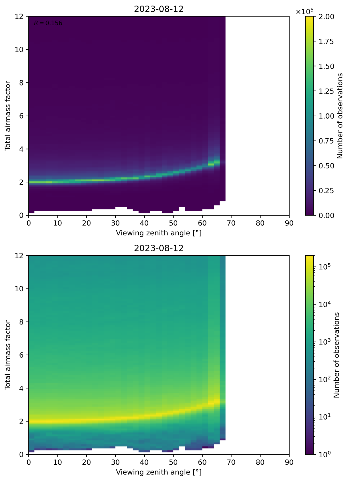
Figure 160: Scatter density plot of “Viewing zenith angle” against “Total airmass factor” for 2023-08-11 to 2023-08-13.
