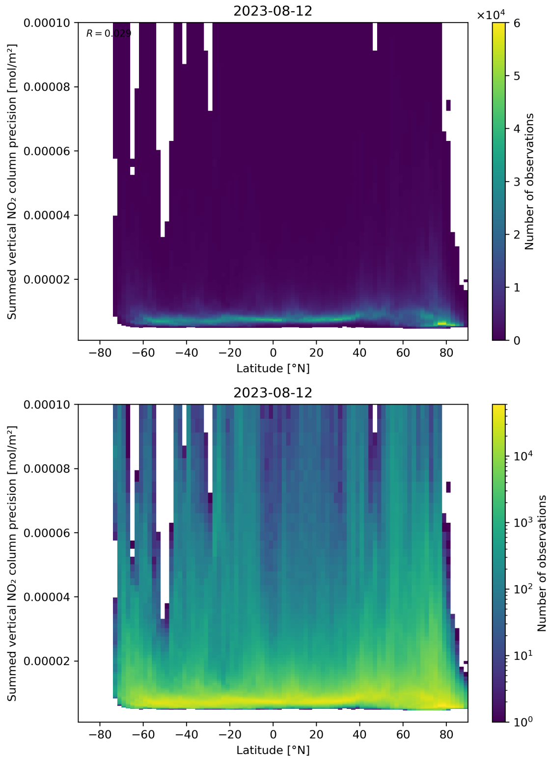
Figure 89: Scatter density plot of “Latitude” against “Summed vertical NO 2 column precision” for 2023-08-11 to 2023-08-13.
