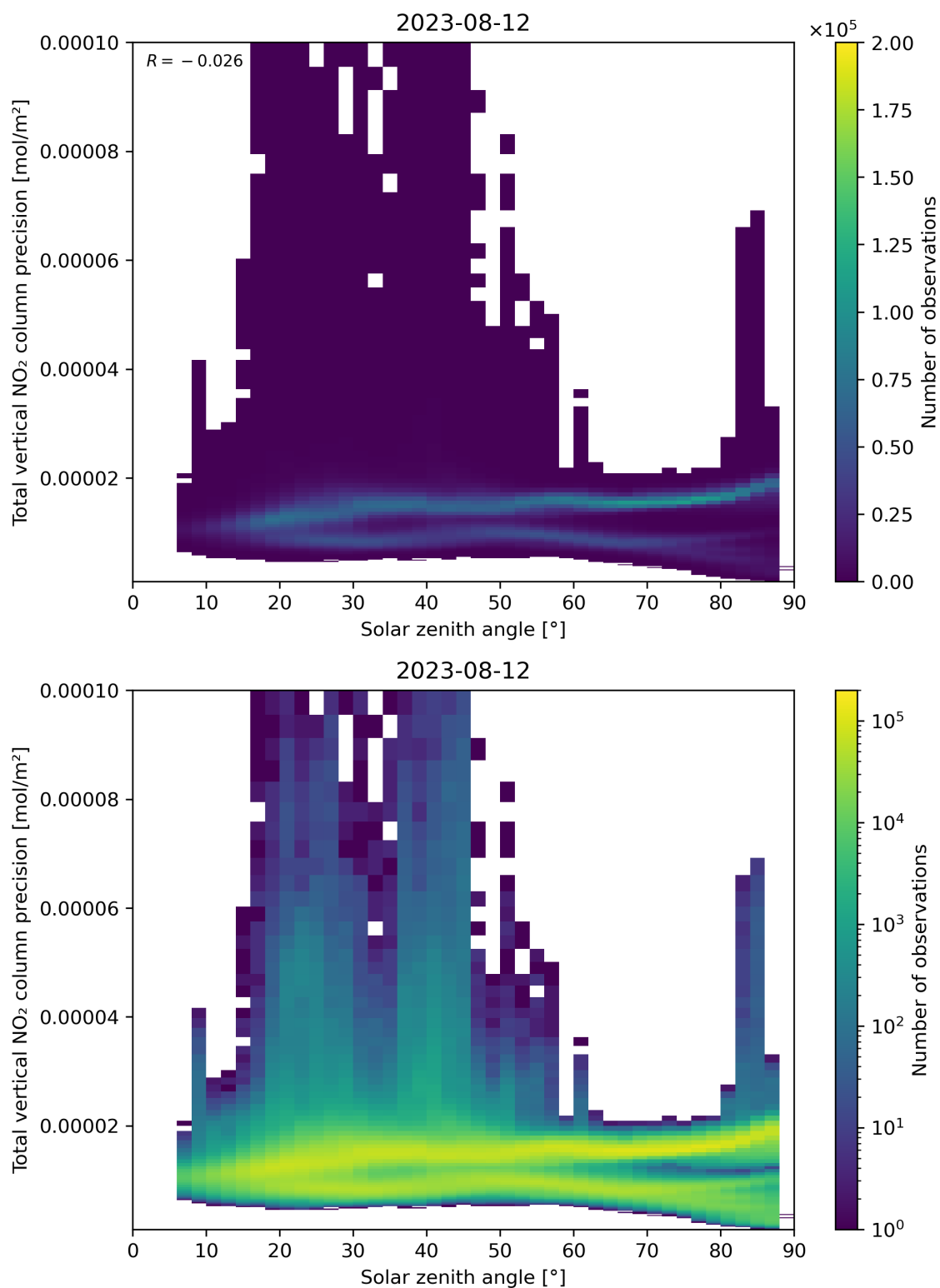
Figure 154: Scatter density plot of “Solar zenith angle” against “Total vertical NO 2 column precision” for 2023-08-11 to 2023-08-13.
