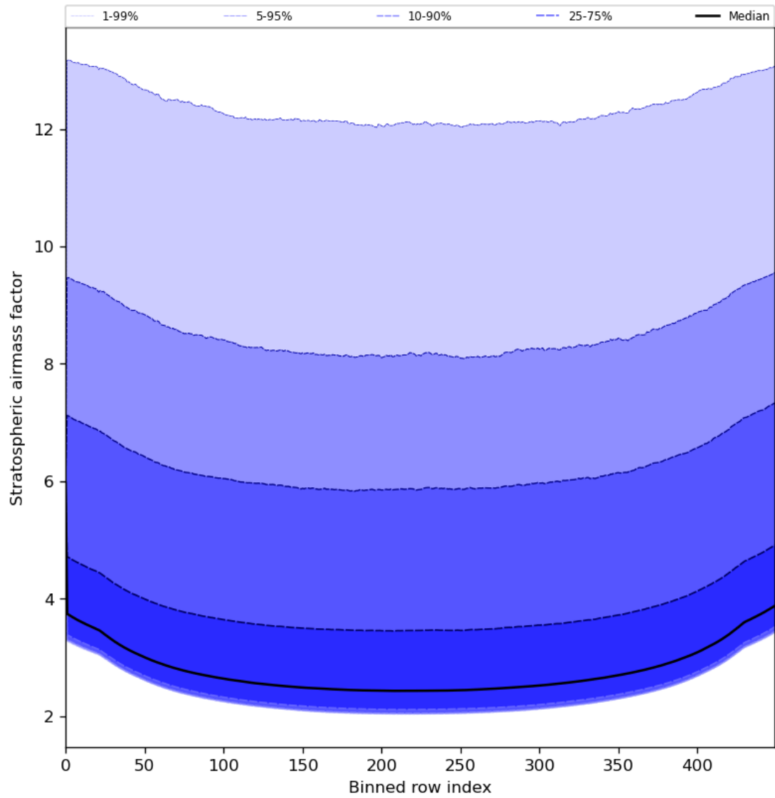
Figure 61: Along track statistics of “Stratospheric air mass factor” for 2023-08-11 to 2023-08-13
