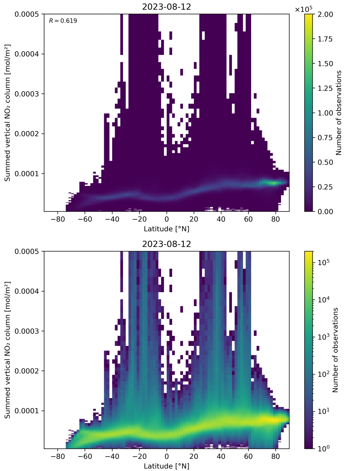
Figure 88: Scatter density plot of “Latitude” against “Summed vertical NO 2 column” for 2023-08-11 to 2023-08-13.
