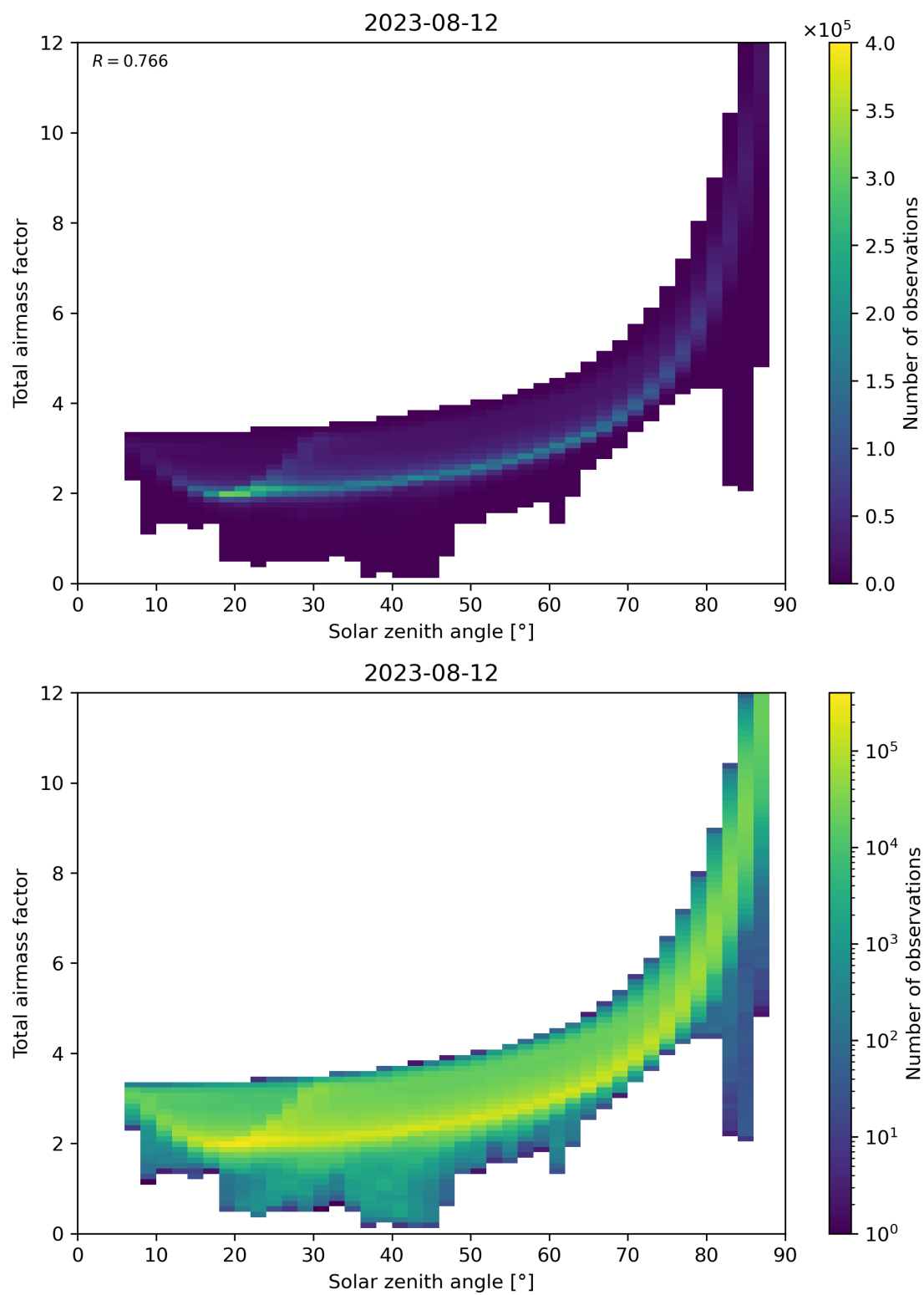
Figure 146: Scatter density plot of “Solar zenith angle” against “Total air mass factor” for 2023-08-11 to 2023-08-13.
