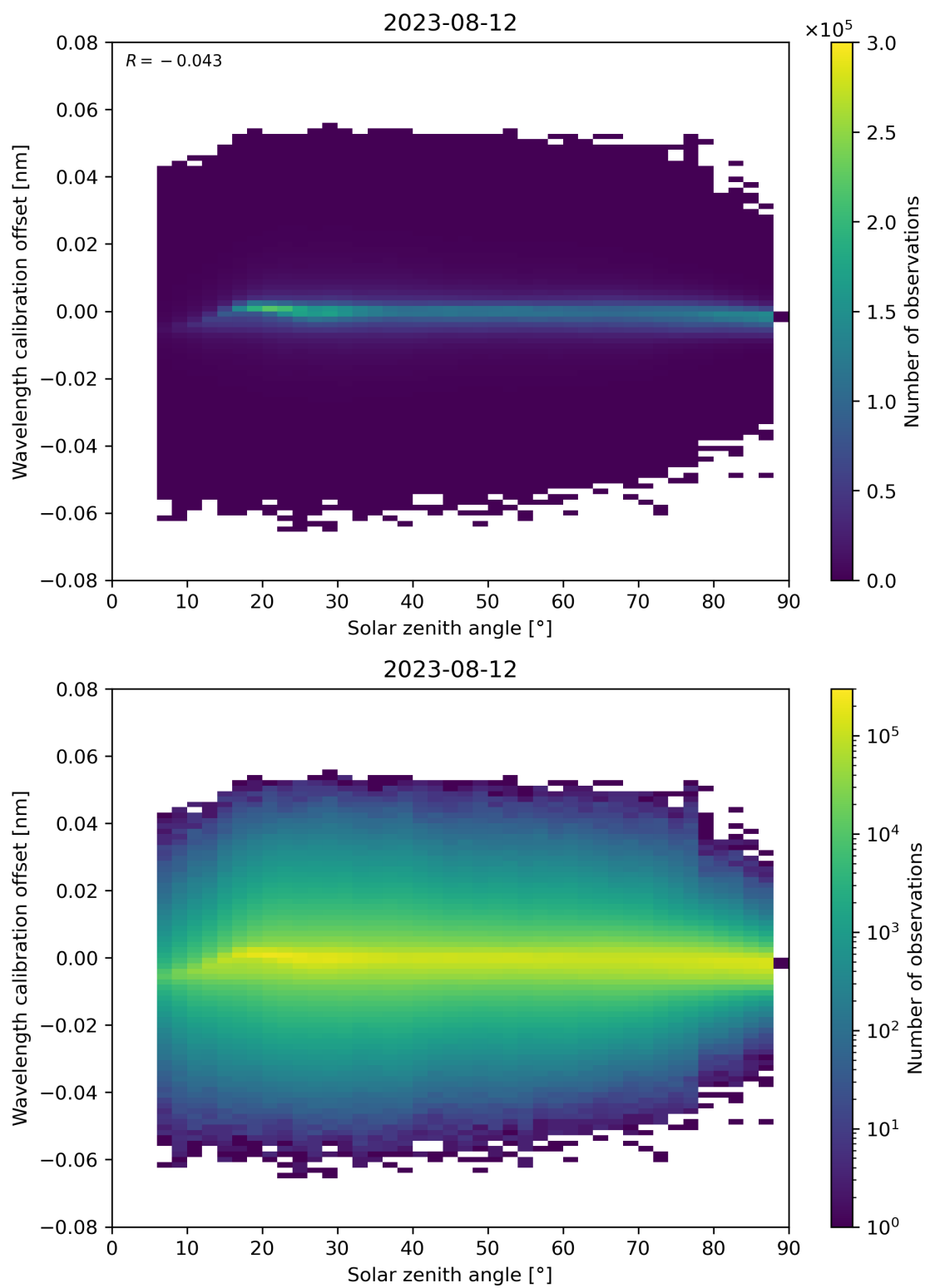
Figure 158: Scatter density plot of “Solar zenith angle” against “Wavelength calibration offset” for 2023-08-11 to 2023-08-13.
