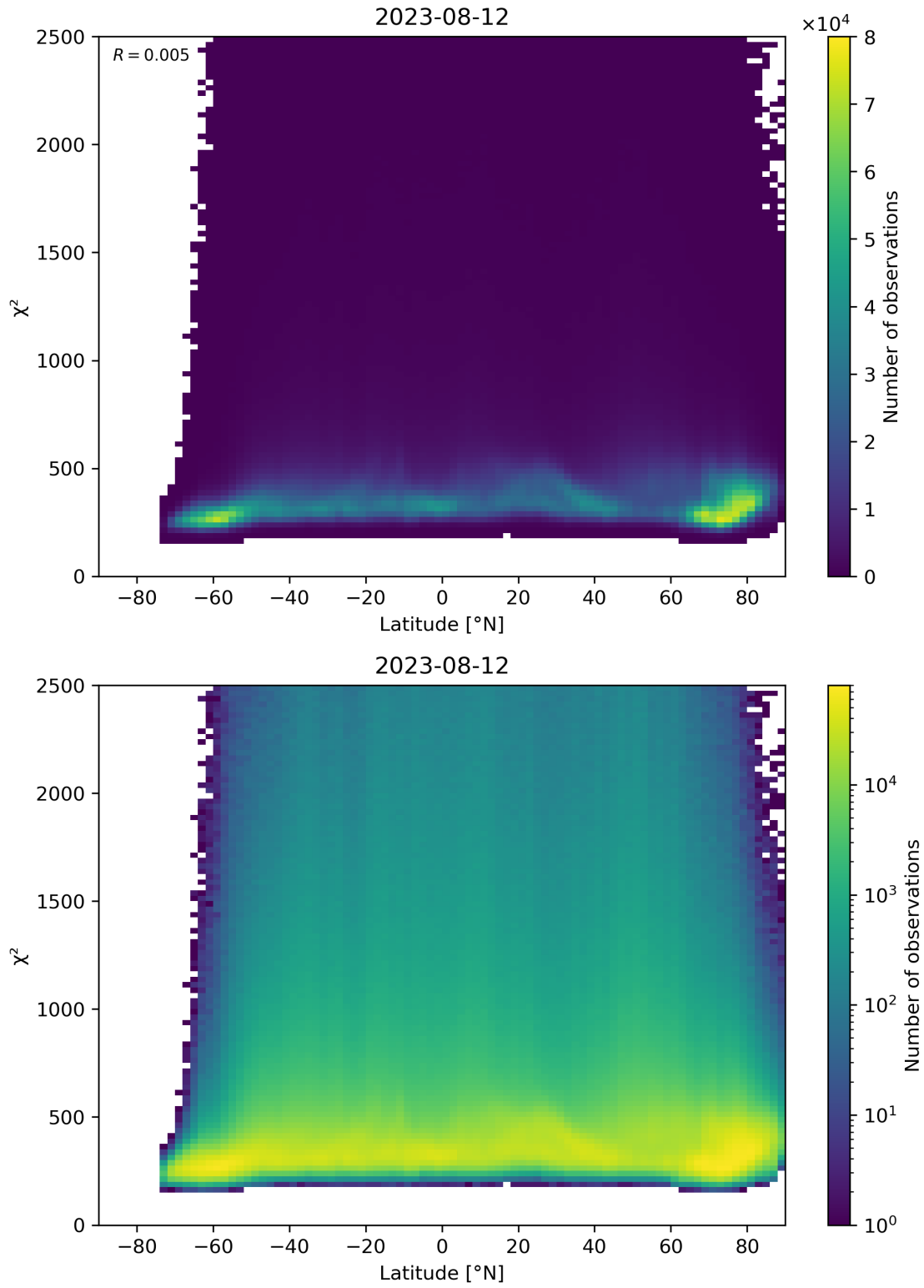
Figure 86: Scatter density plot of “Latitude” against “ \chi^2 ” for 2023-08-11 to 2023-08-13.
