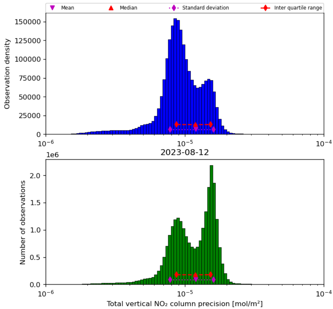
Figure 39: Histogram of "Total vertical NO 2 column precision" for 2023-08-11 to 2023-08-13
