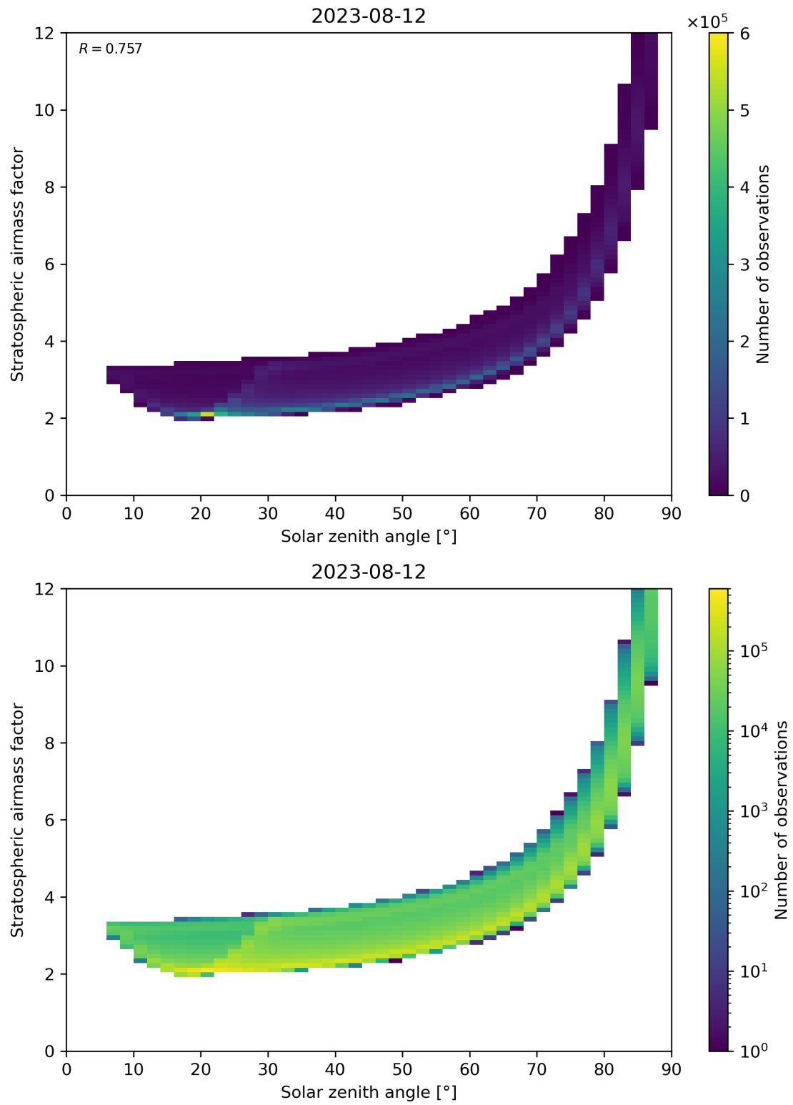
Figure 145: Scatter density plot of “Solar zenith angle” against “Stratospheric airmass factor” for 2023-08-11 to 2023-08-13.
