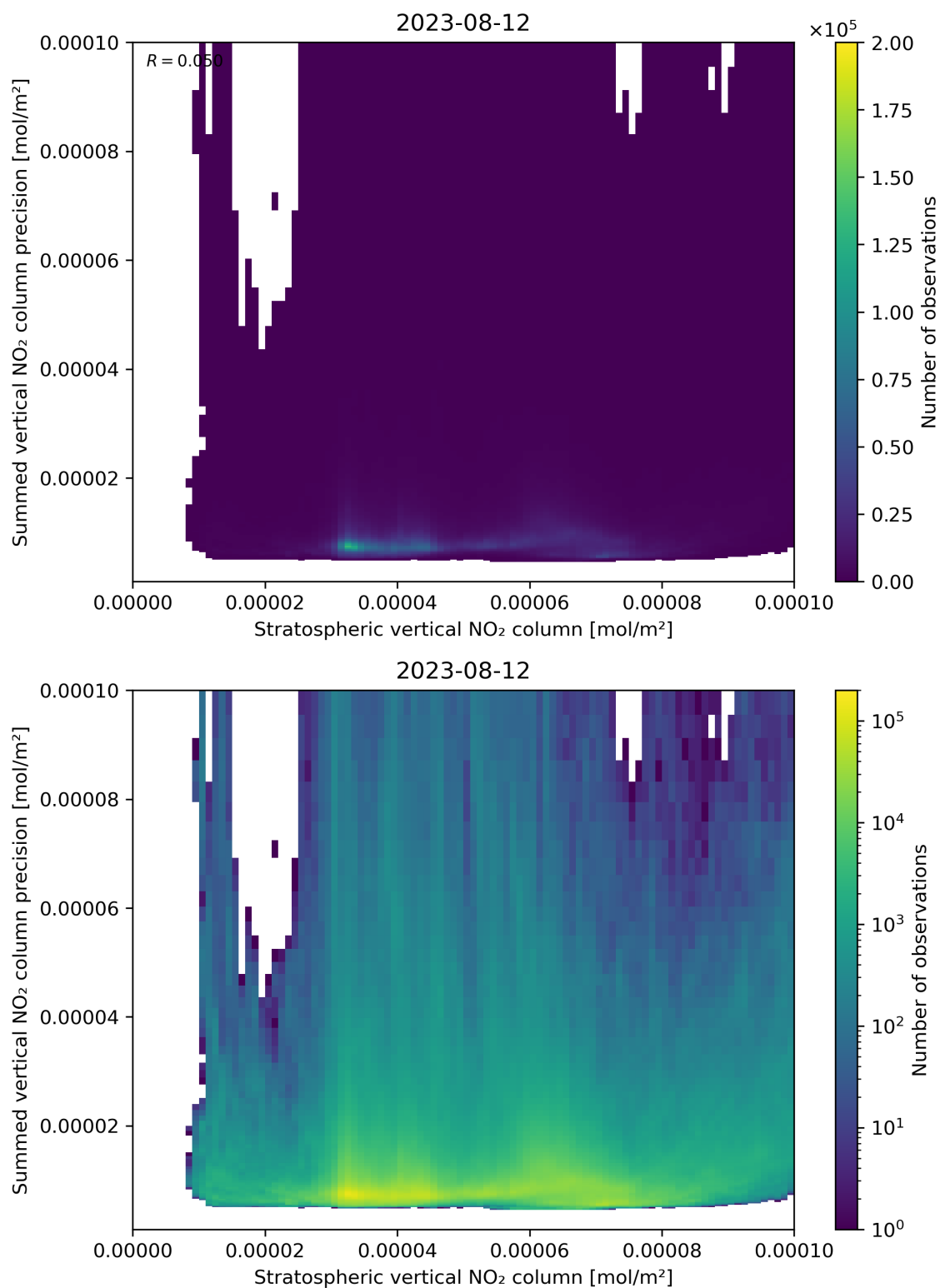
Figure 99: Scatter density plot of “Stratospheric vertical NO 2 column” against “Summed vertical NO 2 column precision” for 2023-08-11 to 2023-08-13.
