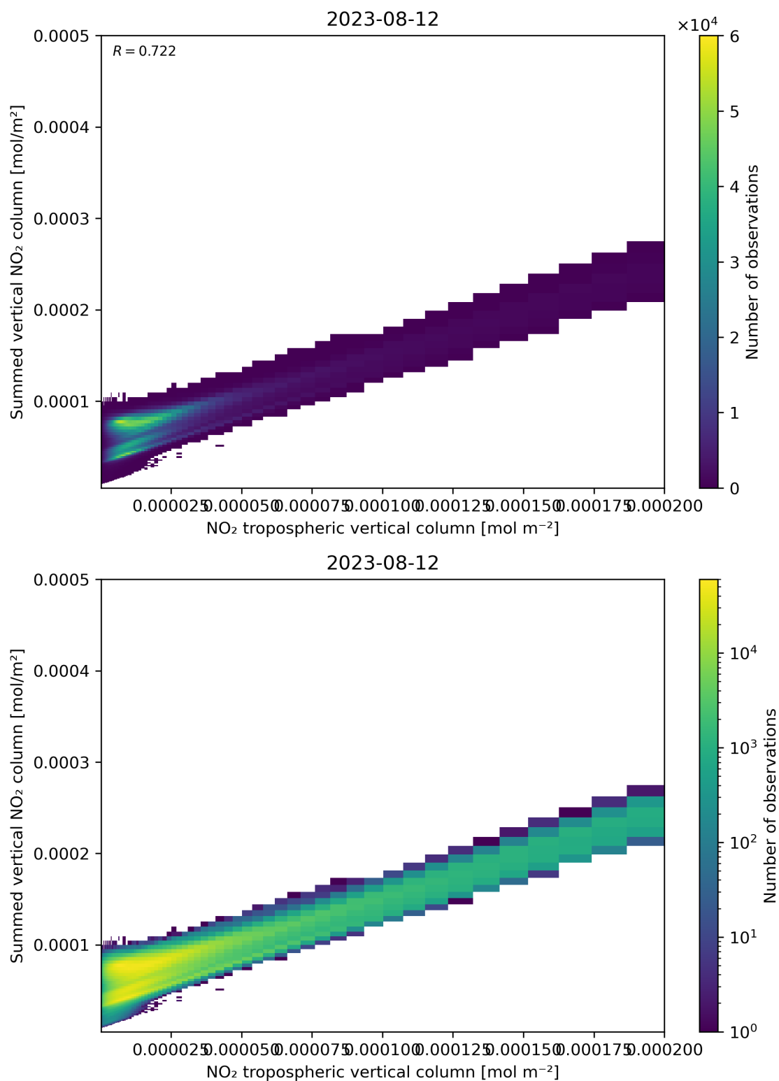
Figure 126: Scatter density plot of “NO 2 tropospheric vertical column” against “Summed vertical NO 2 column” for 2023-08-11 to 2023-08-13.
