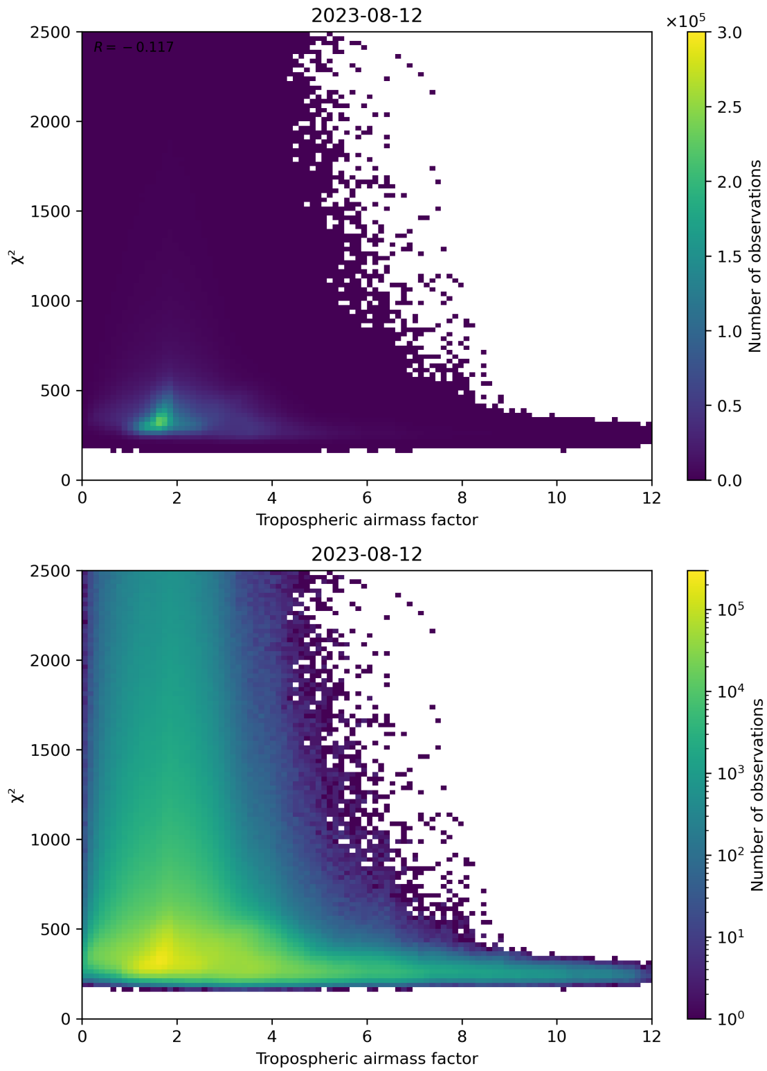
Figure 73: Scatter density plot of “Tropospheric airmass factor” against “ \chi^2 ” for 2023-08-11 to 2023-08-13.
