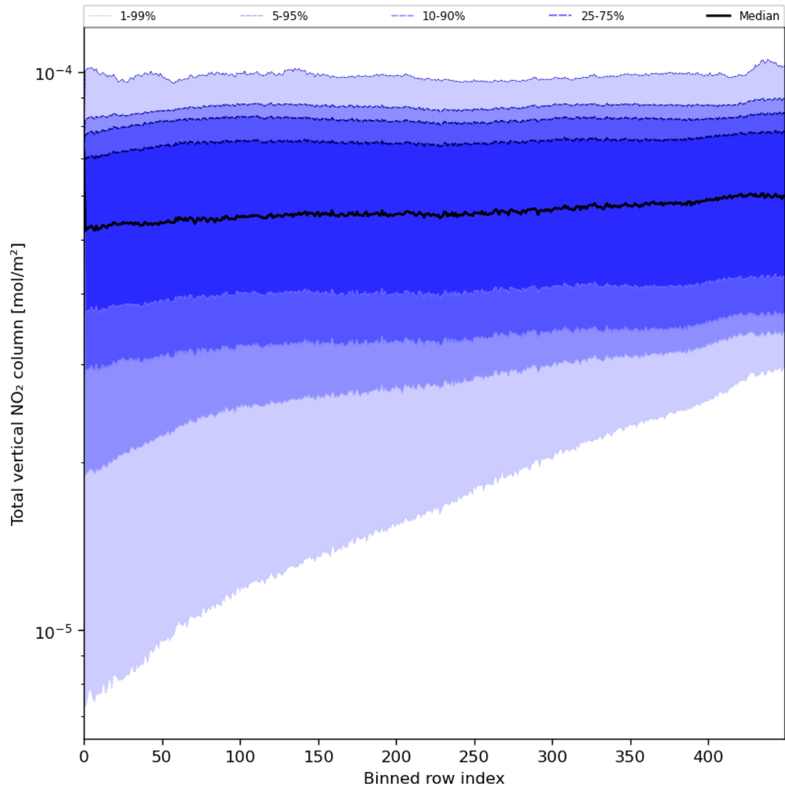
Figure 55: Along track statistics of “Total vertical NO 2 column” for 2023-08-11 to 2023-08-13
