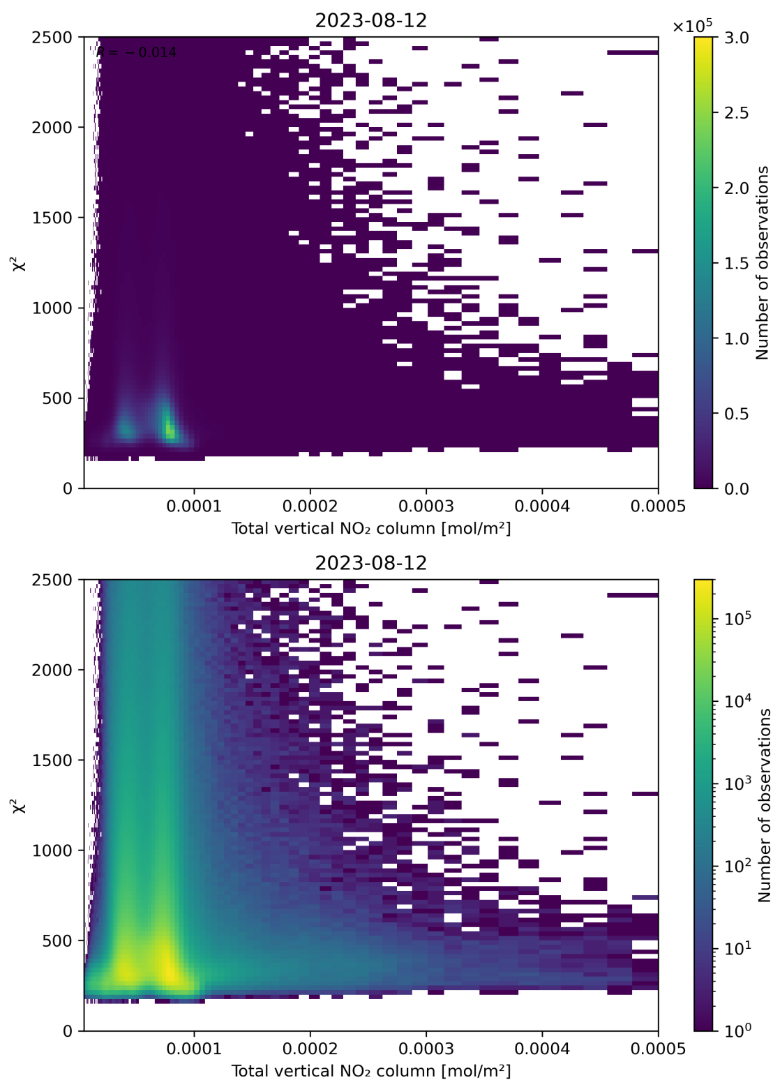
Figure 111: Scatter density plot of “Total vertical NO 2 column” against “ \chi^2 ” for 2023-08-11 to 2023-08-13.
