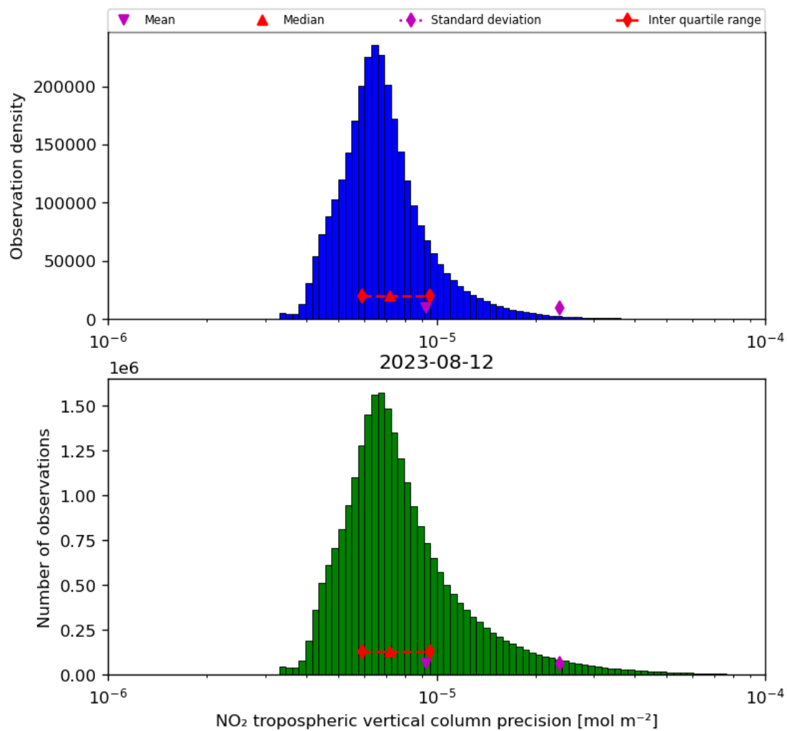
Figure 30: Histogram of “NO 2 tropospheric vertical column precision” for 2023-08-11 to 2023-08-13
