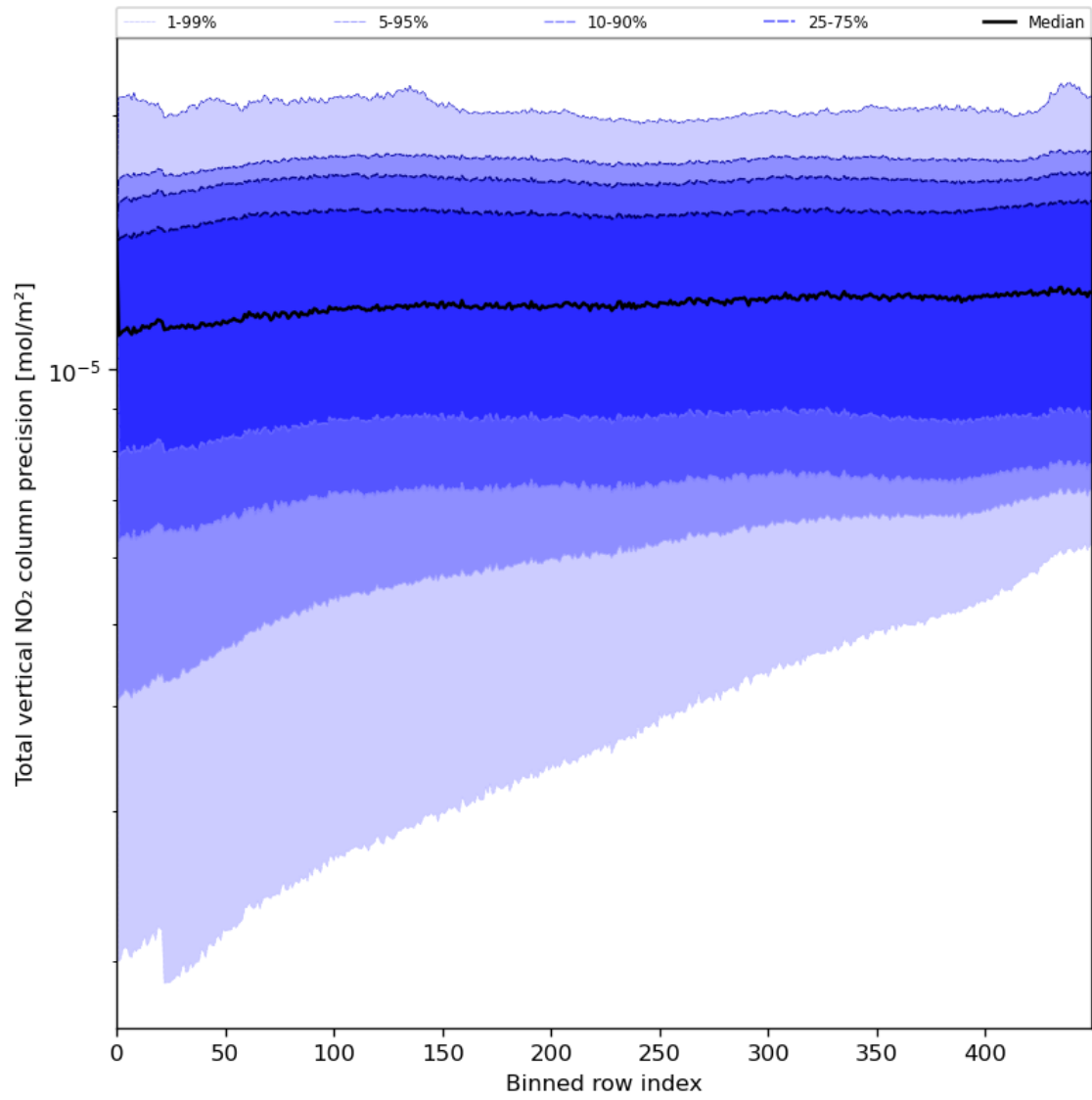
Figure 56: Along track statistics of “Total vertical NO 2 column precision” for 2023-08-11 to 2023-08-13
