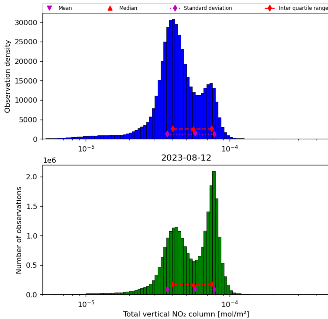
Figure 38: Histogram of "Total vertical NO 2 column" for 2023-08-11 to 2023-08-13
