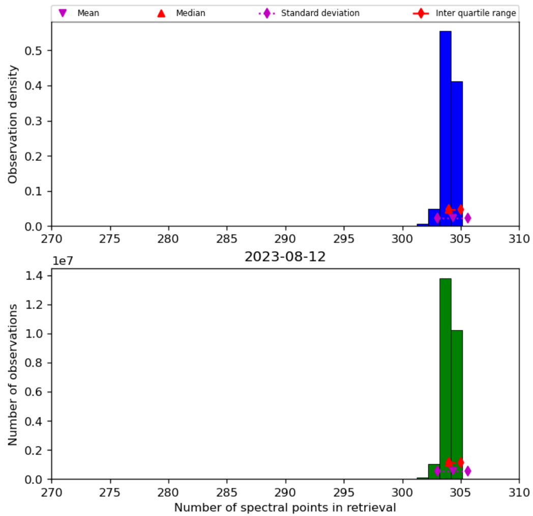
Figure 33: Histogram of “Number of spectral points in retrieval” for 2023-08-11 to 2023-08-13
