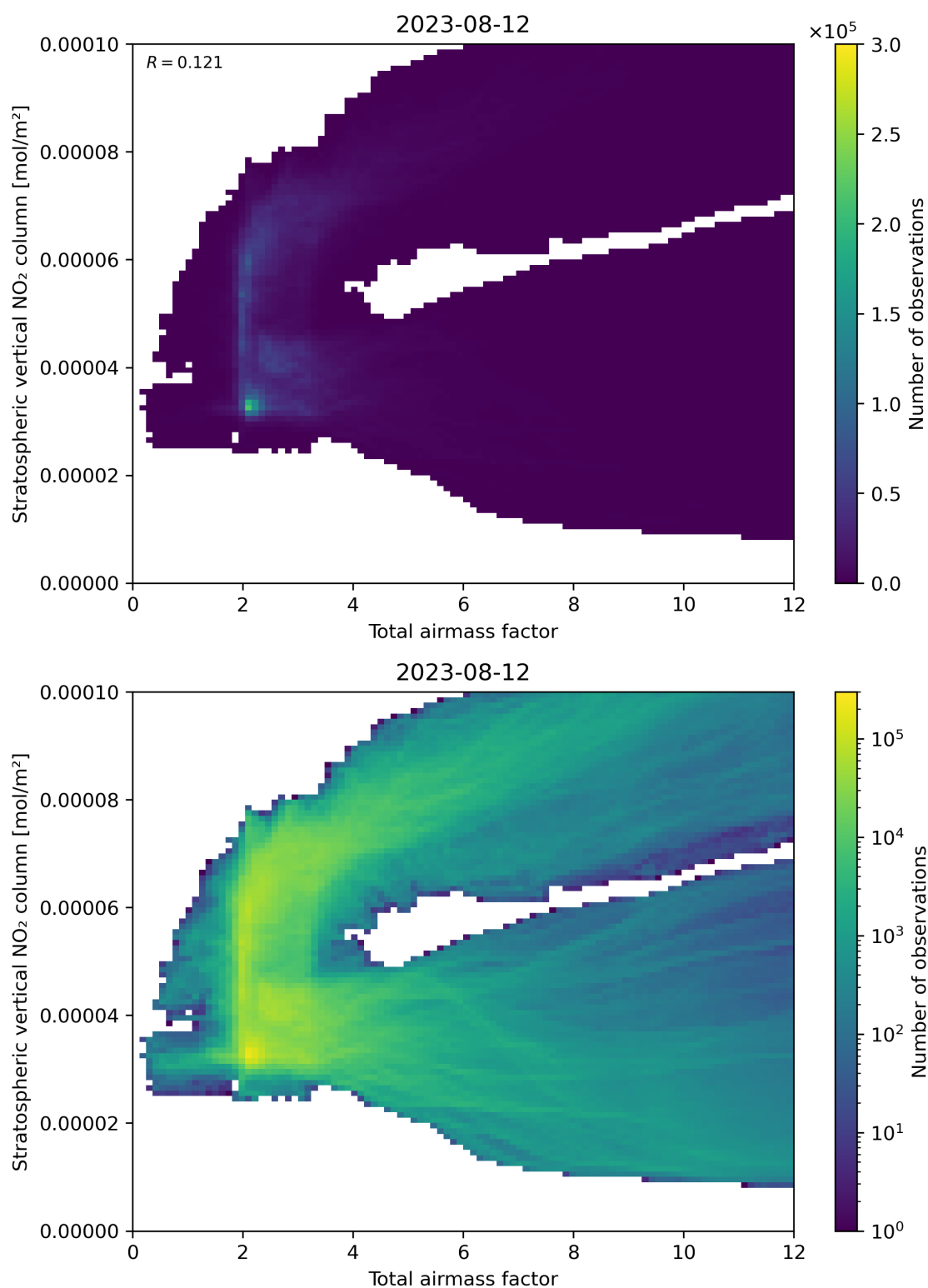
Figure 64: Scatter density plot of “Total airmass factor” against “Stratospheric vertical \text{NO}_2 column” for 2023-08-11 to 2023-08-13.
