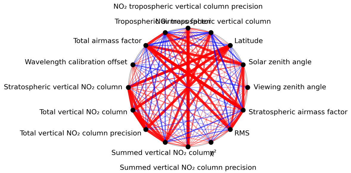
Figure 1: Map of correlation graph for 2023-08-11 to 2023-08-13.
