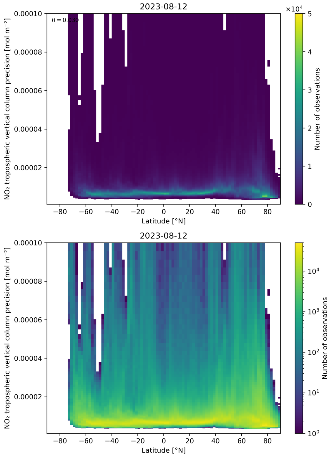
Figure 93: Scatter density plot of “Latitude” against “NO 2 tropospheric vertical column precision” for 2023-08-11 to 2023-08-13.
