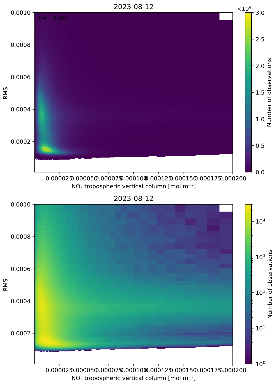
Figure 142: Scatter density plot of “NO 2 tropospheric vertical column” against “RMS” for 2023-08-11 to 2023-08-13.
