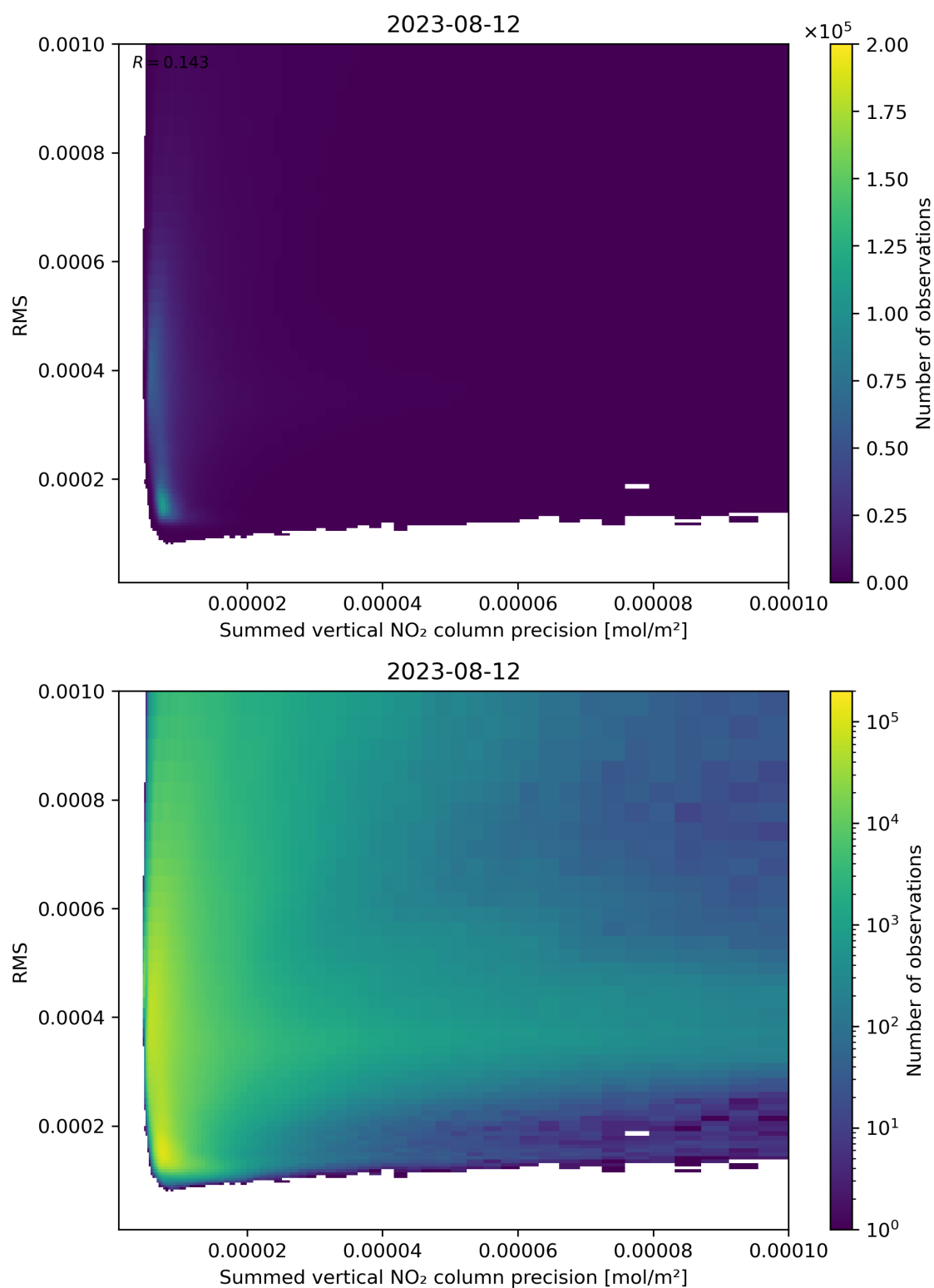
Figure 108: Scatter density plot of “Summed vertical NO 2 column precision” against “RMS” for 2023-08-11 to 2023-08-13.
