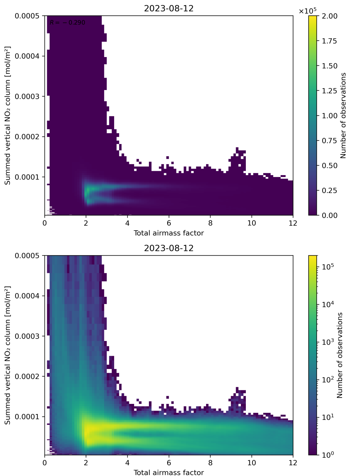
Figure 65: Scatter density plot of “Total airmass factor” against “Summed vertical NO 2 column” for 2023-08-11 to 2023-08-13.
