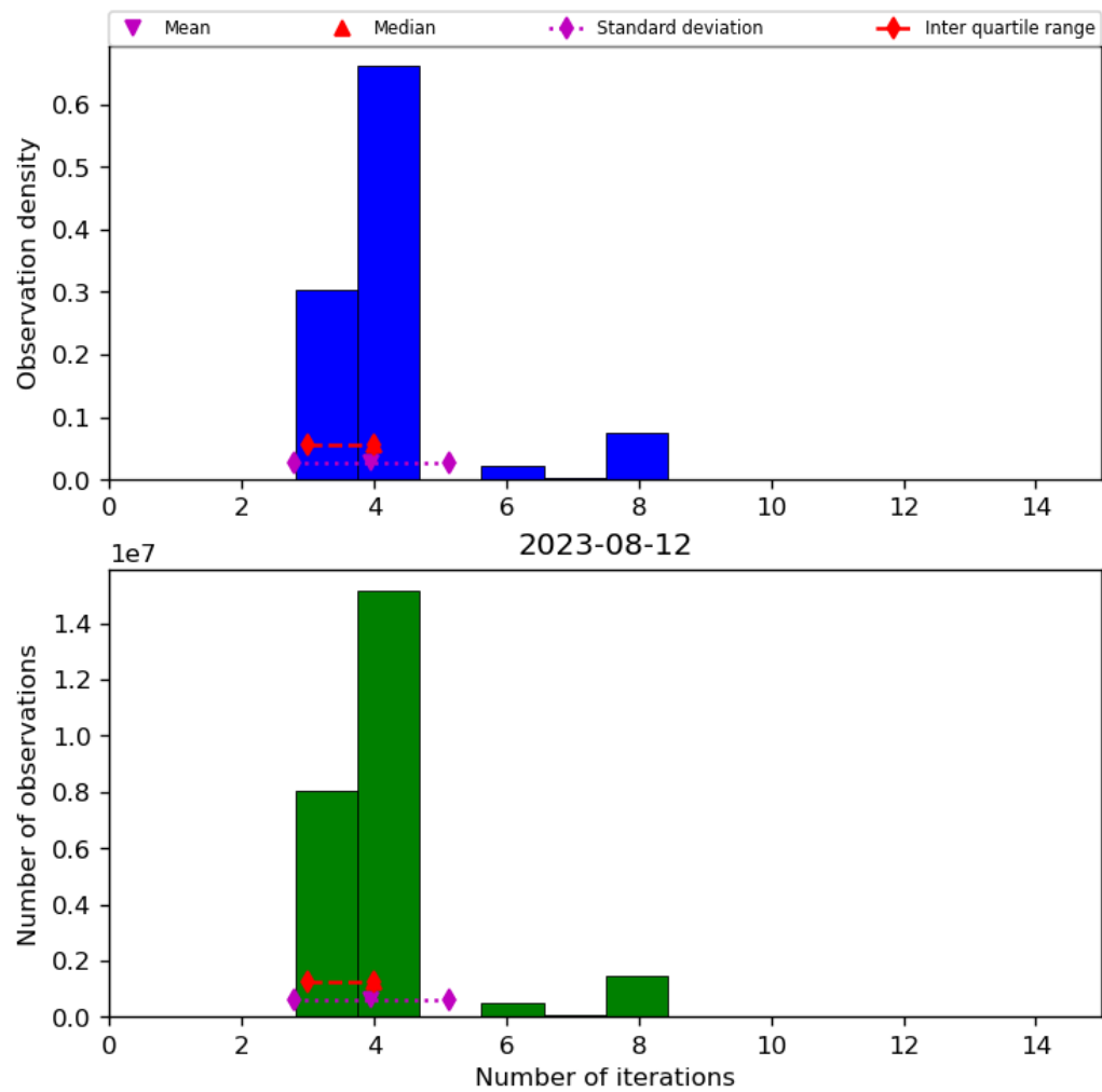
Figure 34: Histogram of “Number of iterations” for 2023-08-11 to 2023-08-13
