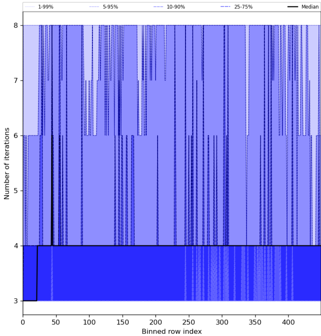
Figure 51: Along track statistics of “Number of iterations” for 2023-08-11 to 2023-08-13
