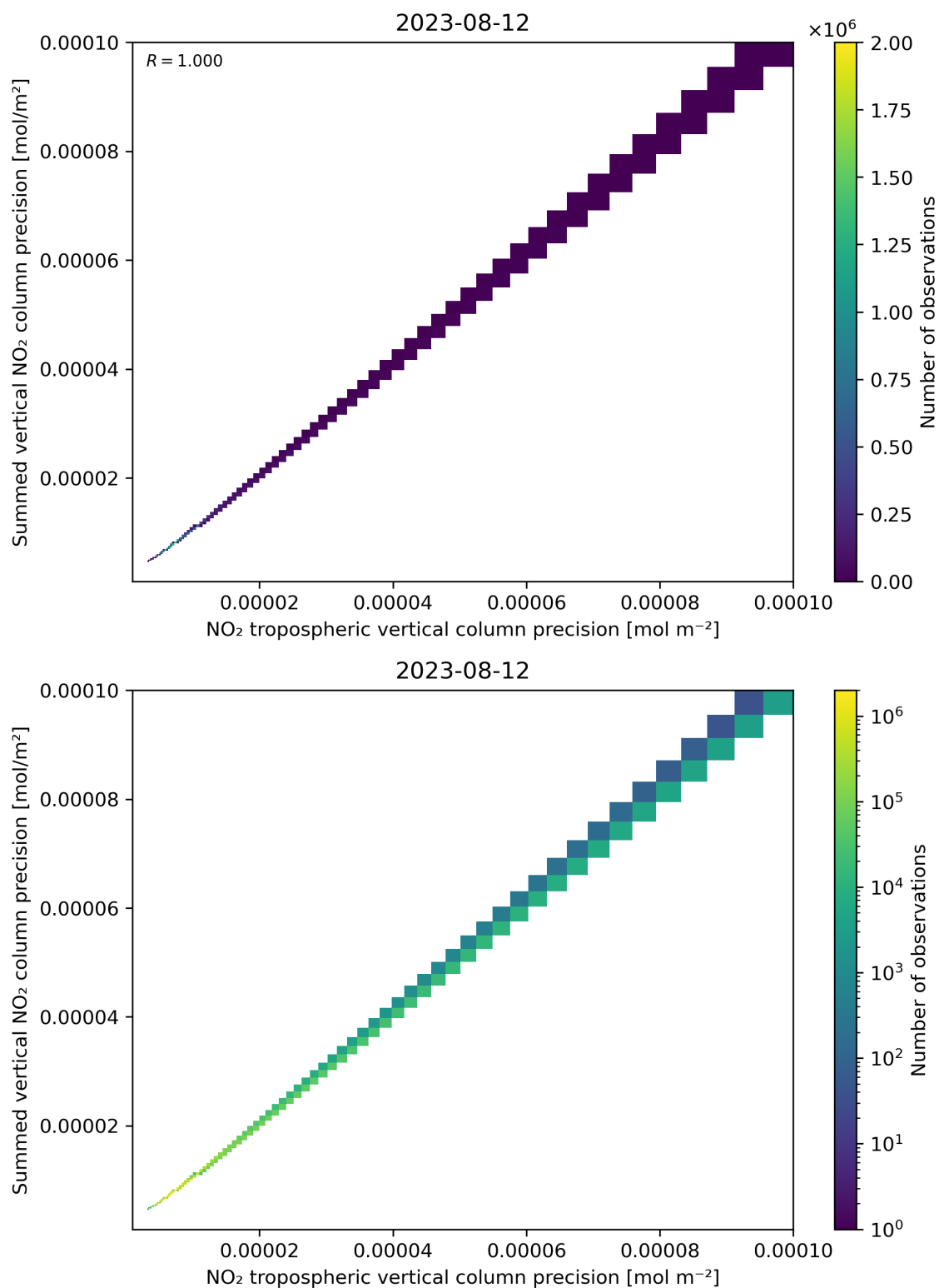
Figure 137: Scatter density plot of “NO 2 tropospheric vertical column precision” against “Summed vertical NO 2 column precision” for 2023-08-11 to 2023-08-13.
