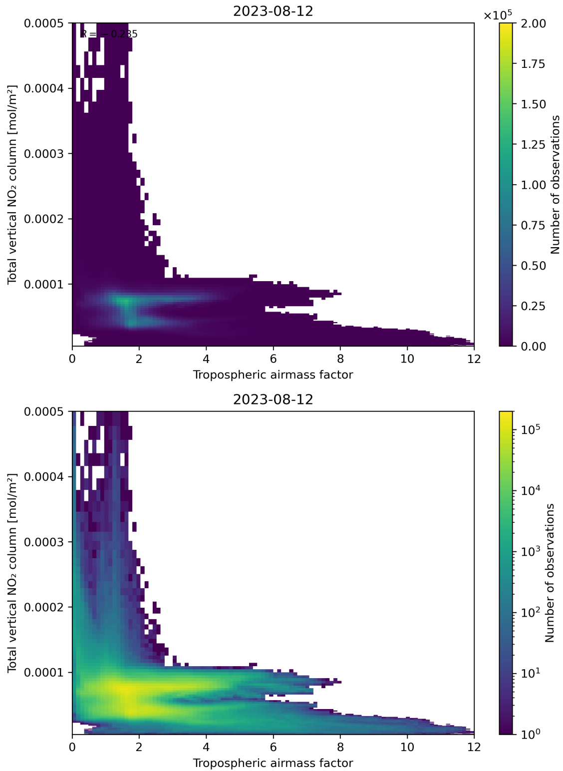
Figure 77: Scatter density plot of “Tropospheric airmass factor” against “Total vertical NO 2 column” for 2023-08-11 to 2023-08-13.
