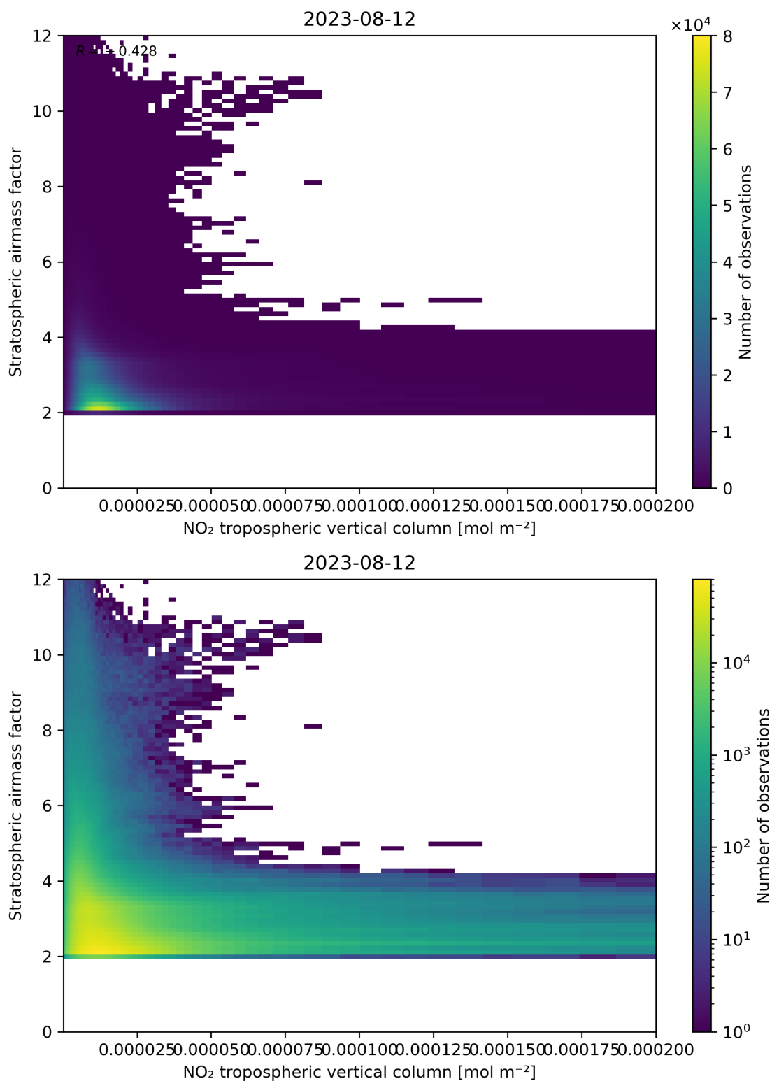
Figure 121: Scatter density plot of “NO 2 tropospheric vertical column” against “Stratospheric air mass factor” for 2023-08-11 to 2023-08-13.
