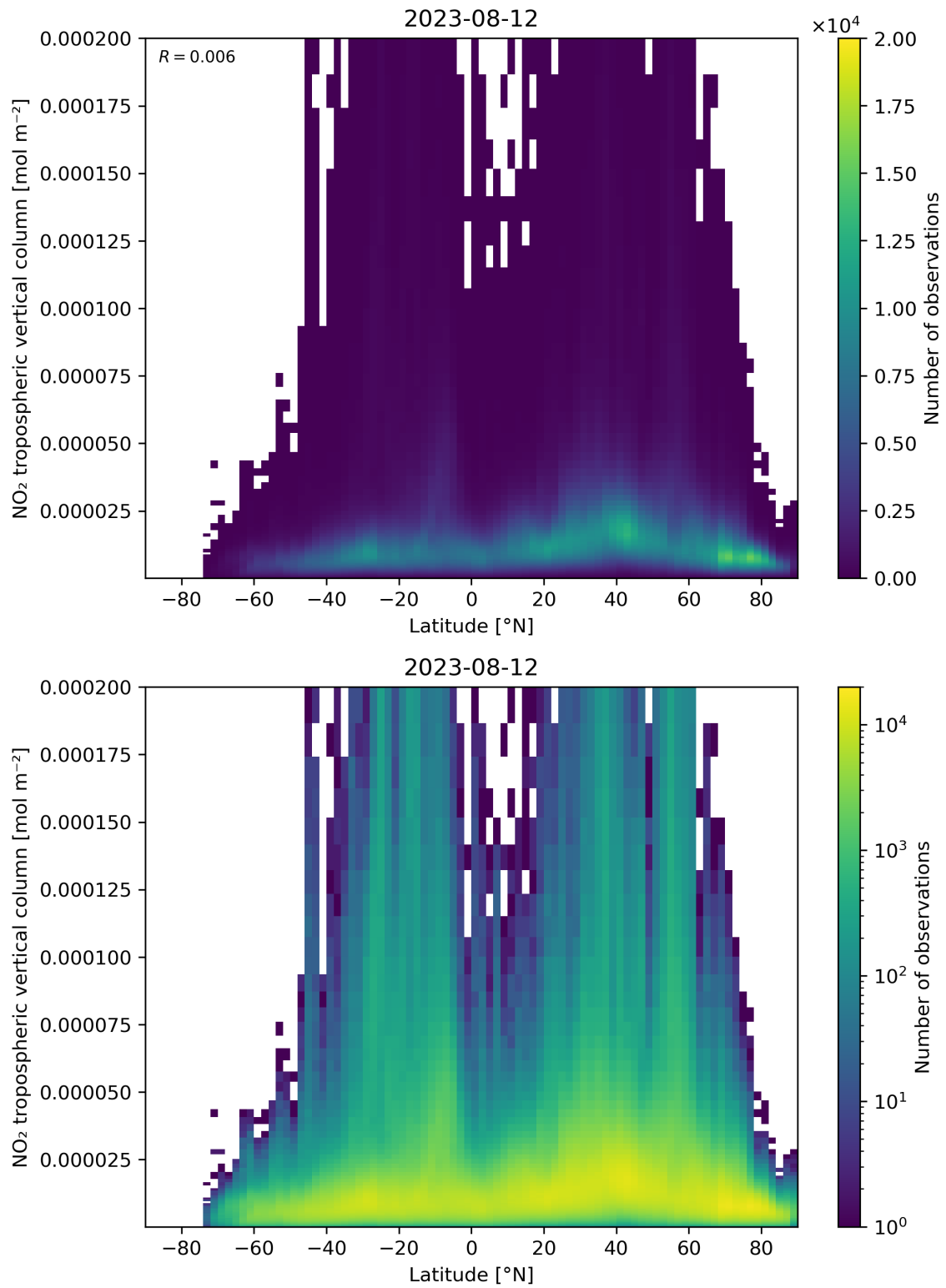
Figure 92: Scatter density plot of “Latitude” against “NO 2 tropospheric vertical column” for 2023-08-11 to 2023-08-13.
