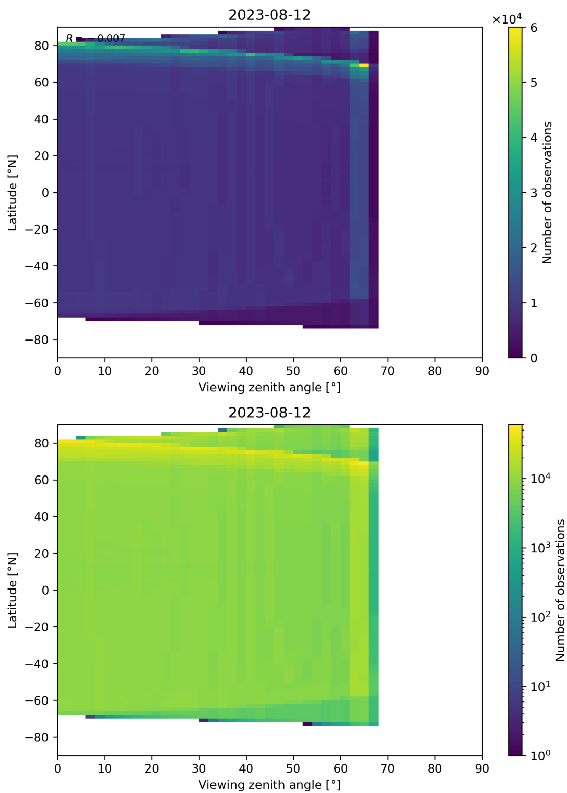
Figure 163: Scatter density plot of “Viewing zenith angle” against “Latitude” for 2023-08-11 to 2023-08-13.
