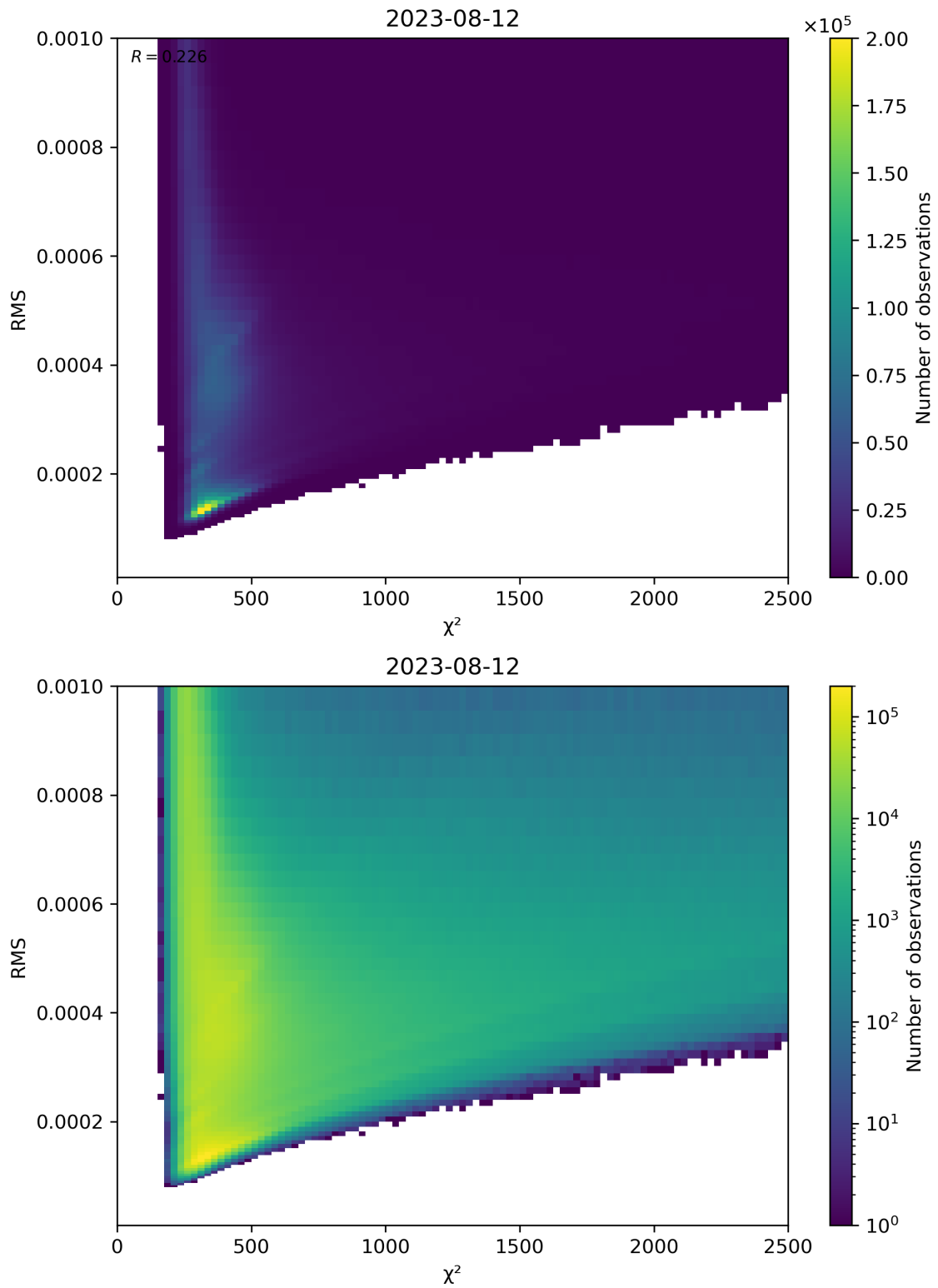
Figure 82: Scatter density plot of “ \chi^2 ” against “RMS” for 2023-08-11 to 2023-08-13.
