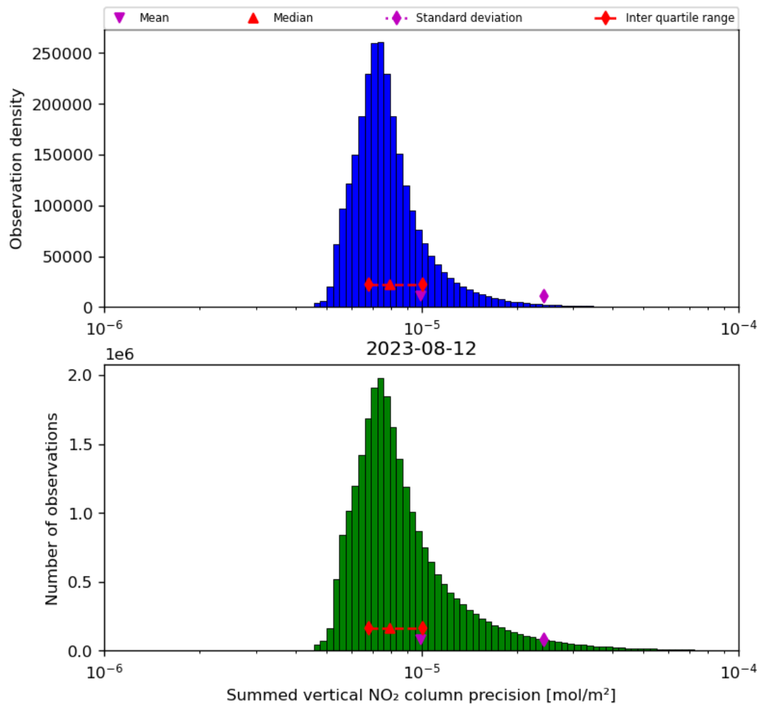
Figure 41: Histogram of "Summed vertical NO 2 column precision" for 2023-08-11 to 2023-08-13
