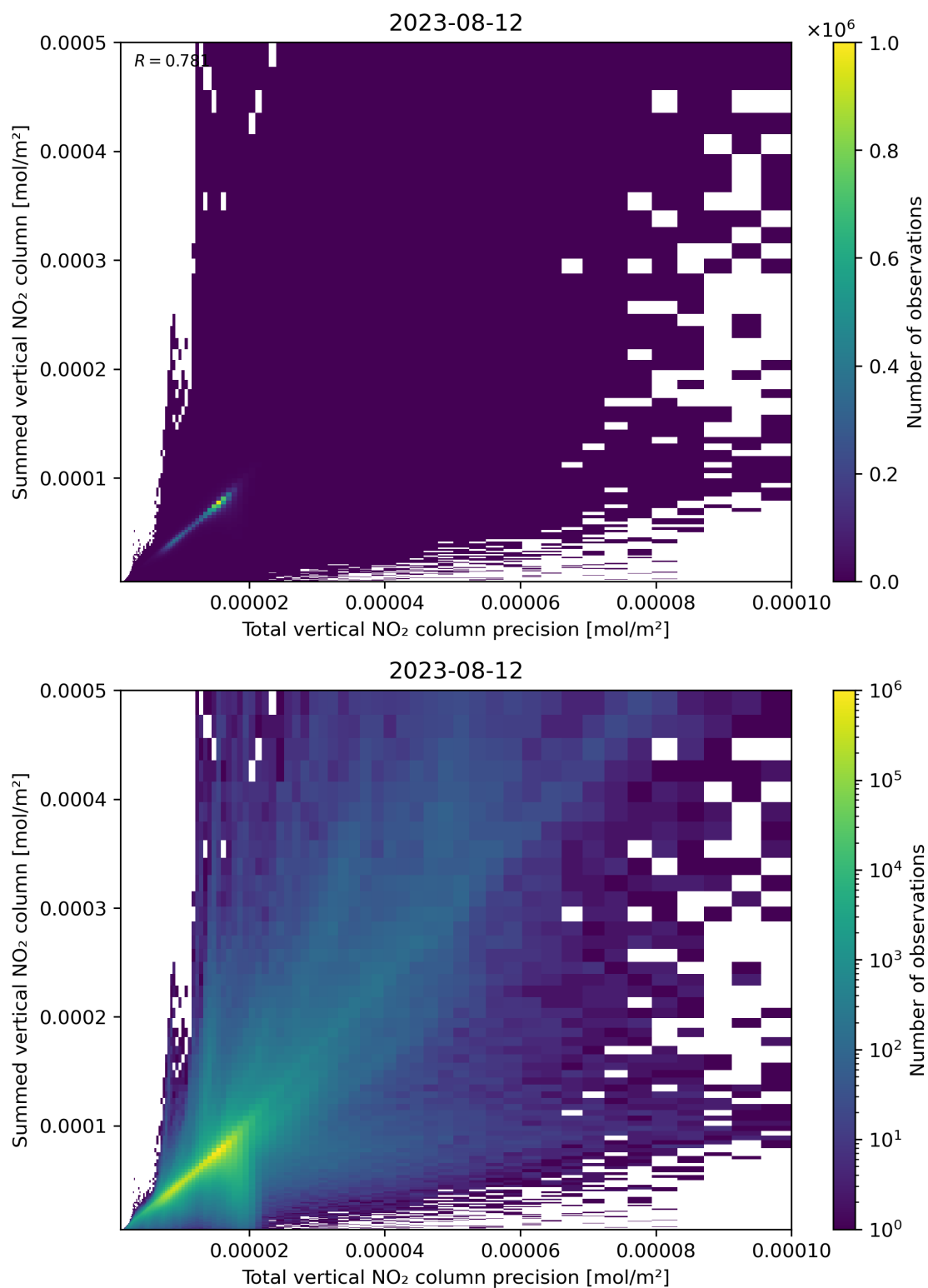
Figure 117: Scatter density plot of “Total vertical NO 2 column precision” against “Summed vertical NO 2 column” for 2023-08-11 to 2023-08-13.
