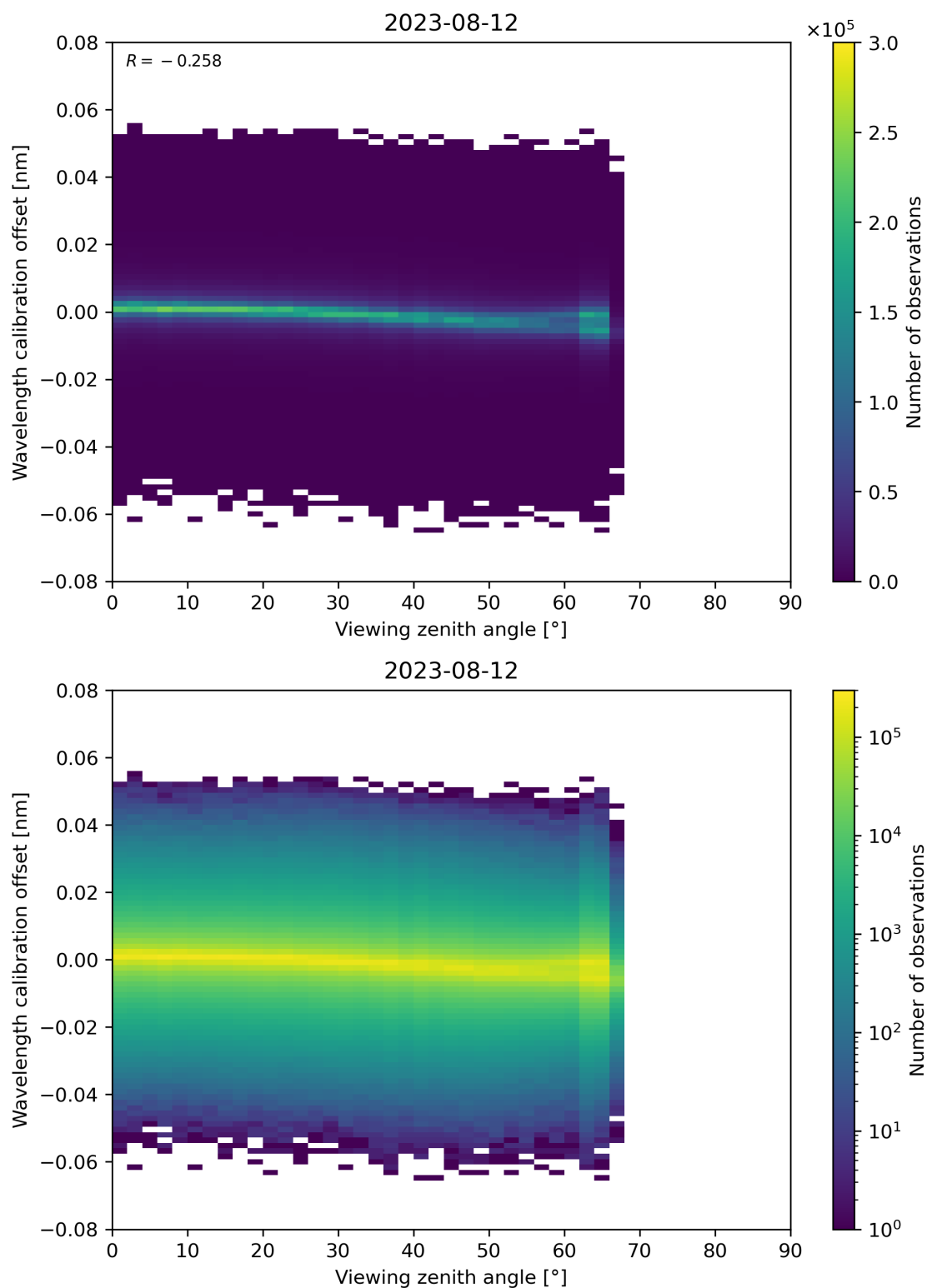
Figure 173: Scatter density plot of “Viewing zenith angle” against “Wavelength calibration offset” for 2023-08-11 to 2023-08-13.
