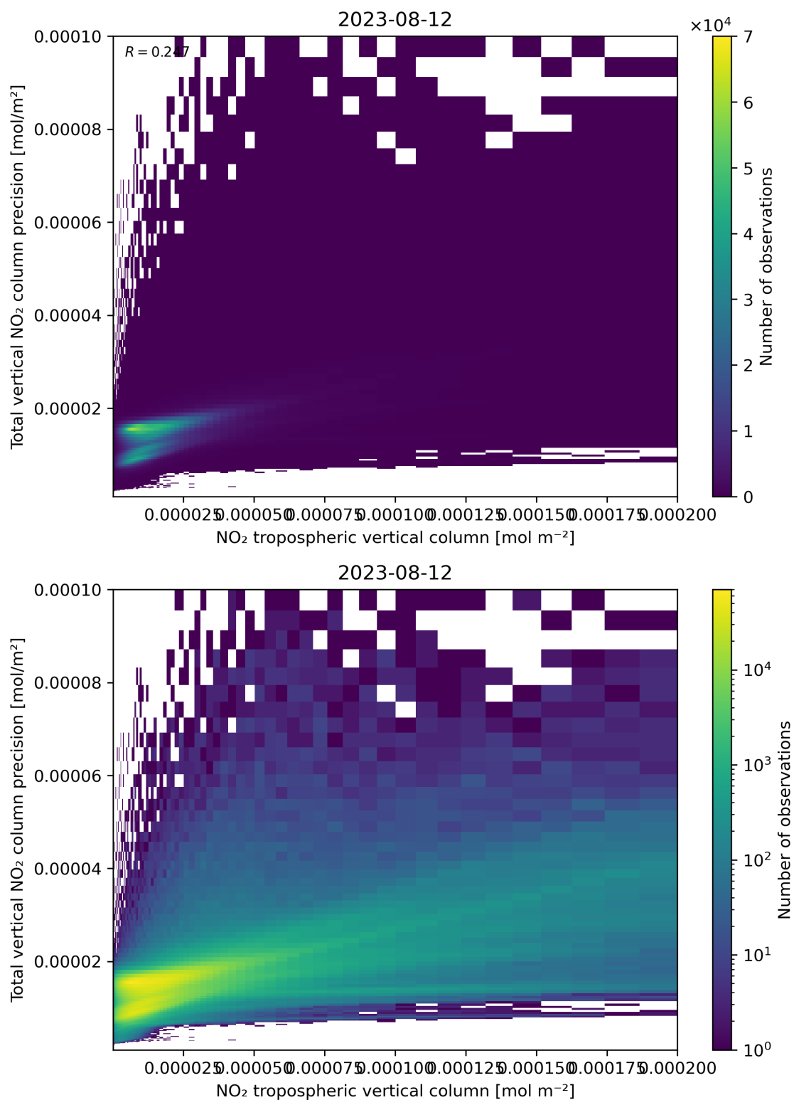
Figure 129: Scatter density plot of “NO 2 tropospheric vertical column” against “Total vertical NO 2 column precision” for 2023-08-11 to 2023-08-13.
