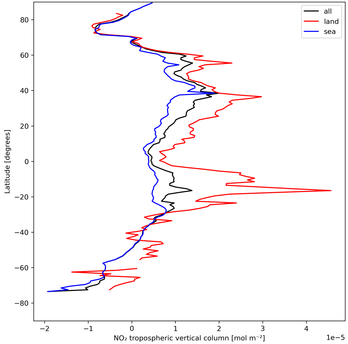
Figure 12: Zonal average of “NO 2 tropospheric vertical column” for 2023-08-11 to 2023-08-13.
