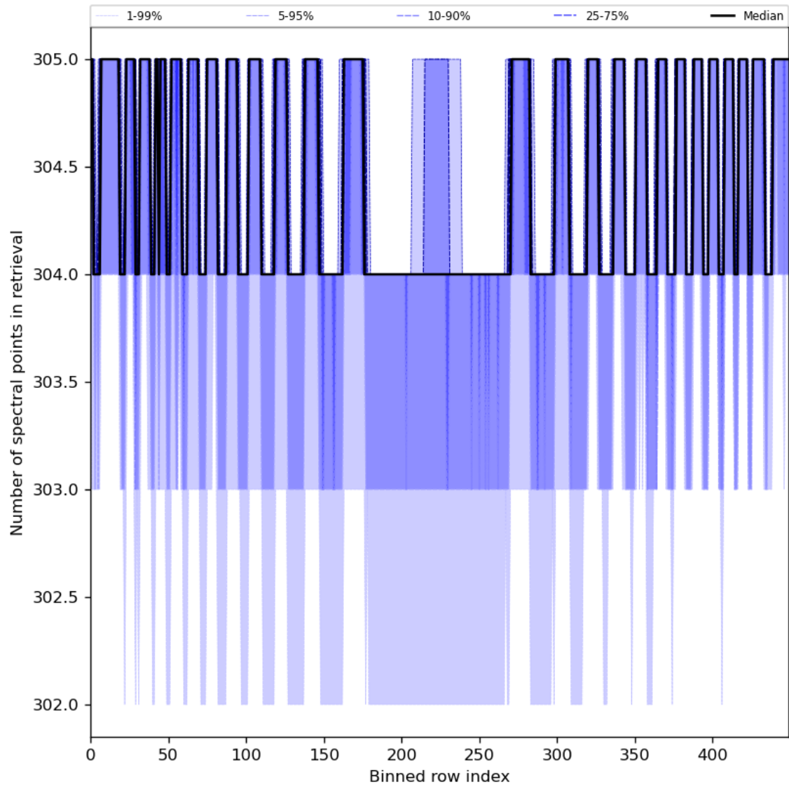
Figure 50: Along track statistics of “Number of spectral points in retrieval” for 2023-08-11 to 2023-08-13
