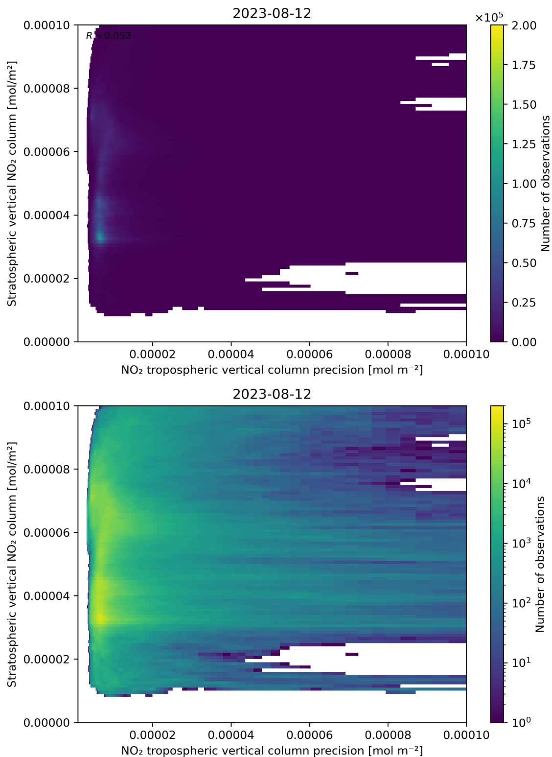
Figure 135: Scatter density plot of “NO 2 tropospheric vertical column precision” against “Stratospheric vertical NO 2 column” for 2023-08-11 to 2023-08-13.
