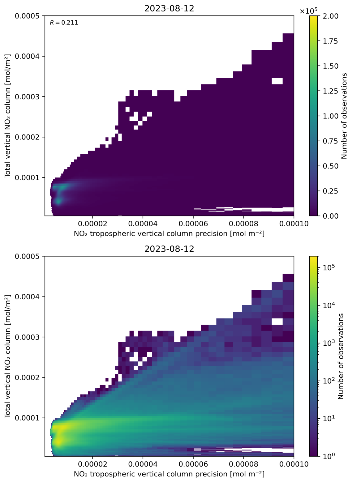
Figure 138: Scatter density plot of “NO 2 tropospheric vertical column precision” against “Total vertical NO 2 column” for 2023-08-11 to 2023-08-13.
