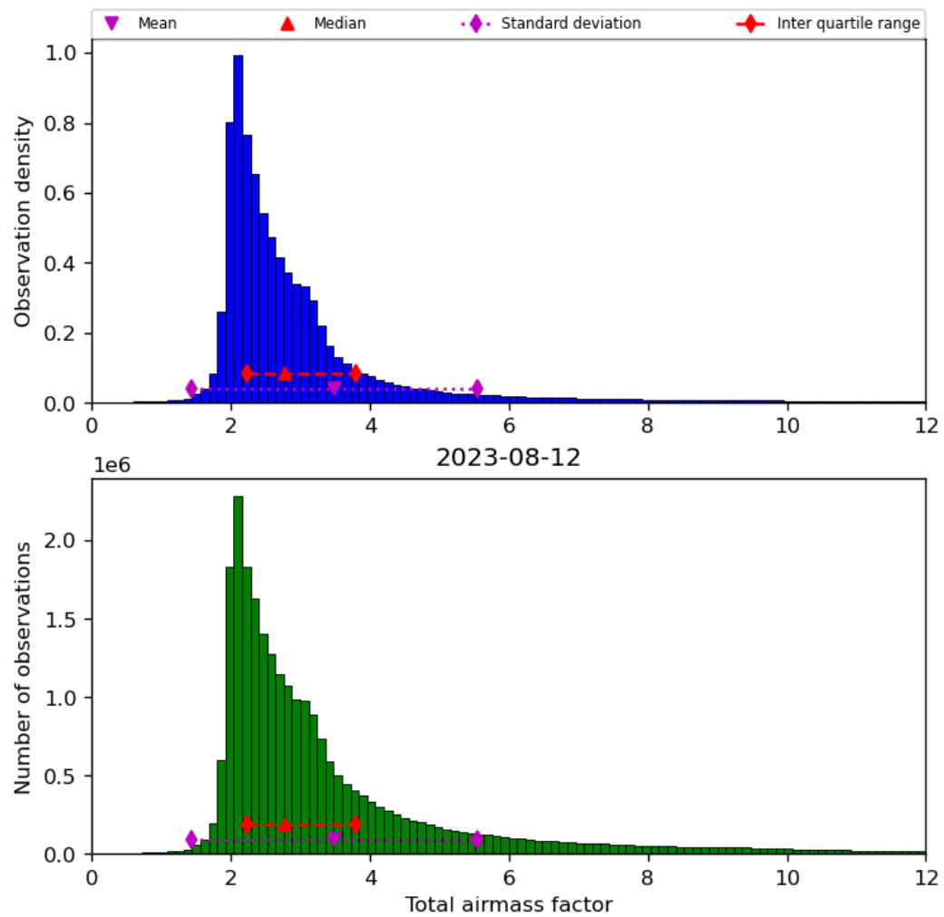
Figure 32: Histogram of “Total airmass factor” for 2023-08-11 to 2023-08-13
