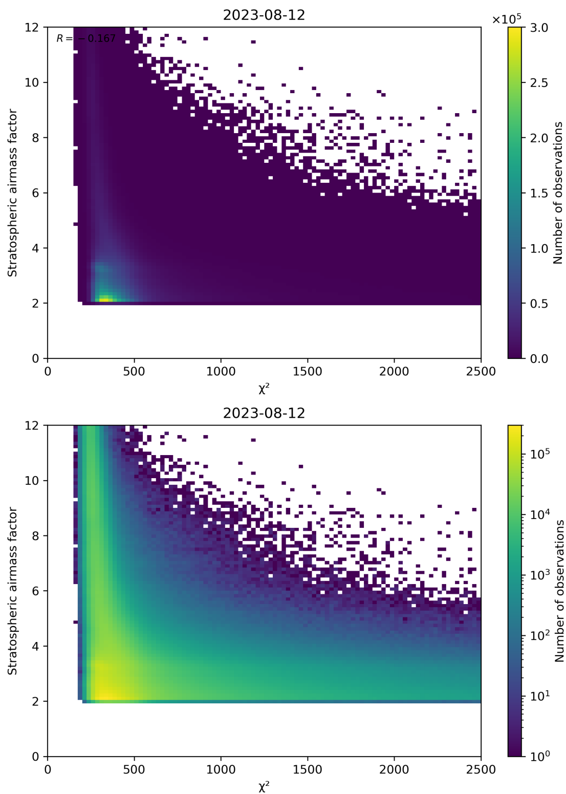
Figure 81: Scatter density plot of “ \chi^2 ” against “Stratospheric air mass factor” for 2023-08-11 to 2023-08-13.
