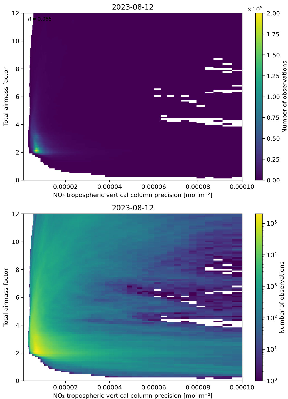
Figure 132: Scatter density plot of “NO 2 tropospheric vertical column precision” against “Total air mass factor” for 2023-08-11 to 2023-08-13.
