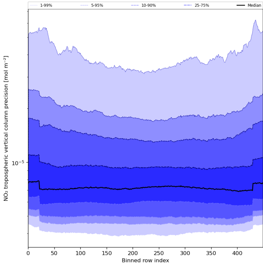
Figure 47: Along track statistics of “NO 2 tropospheric vertical column precision” for 2023-08-11 to 2023-08-13
