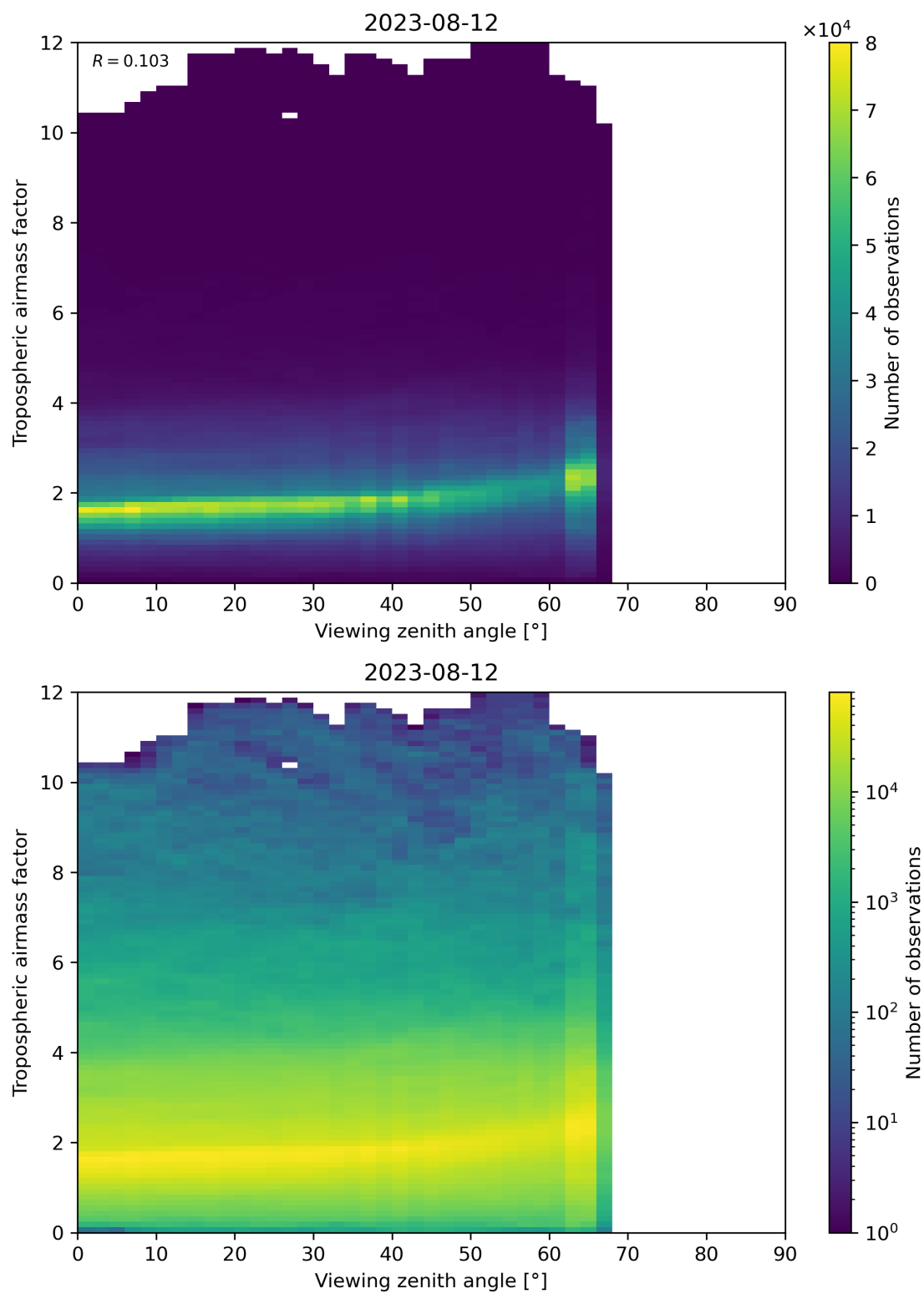
Figure 161: Scatter density plot of “Viewing zenith angle” against “Tropospheric airmass factor” for 2023-08-11 to 2023-08-13.
