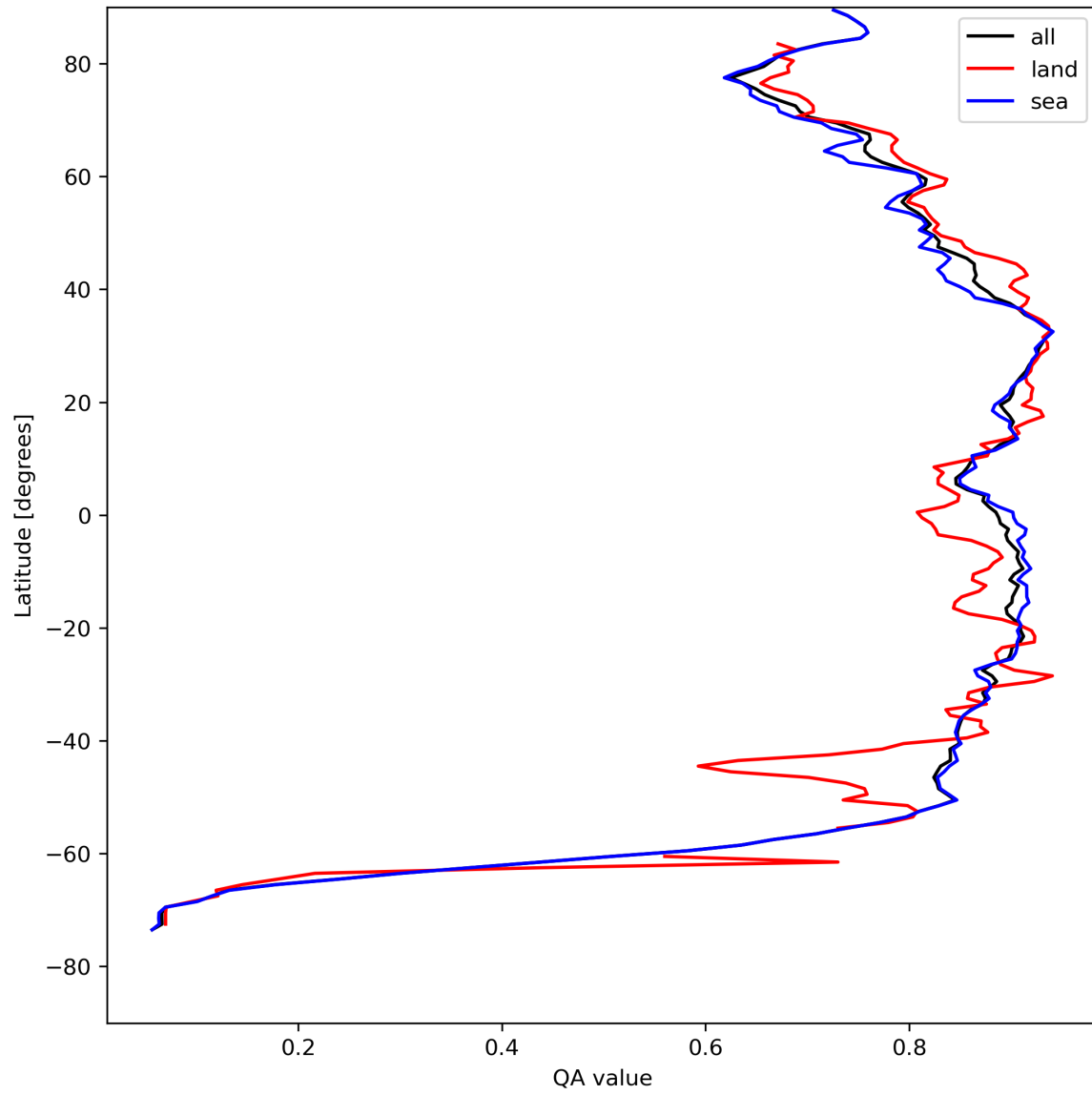
Figure 11: Zonal average of “QA value” for 2023-08-11 to 2023-08-13.
