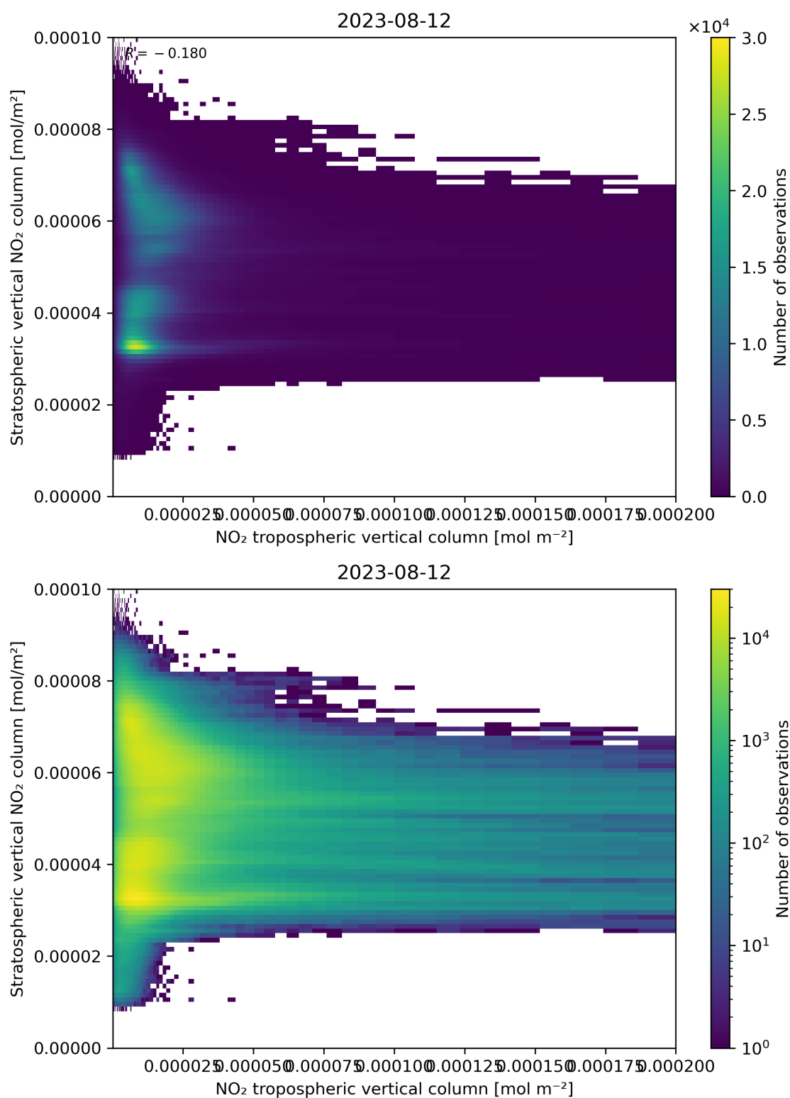
Figure 125: Scatter density plot of “NO 2 tropospheric vertical column” against “Stratospheric vertical NO 2 column” for 2023-08-11 to 2023-08-13.
