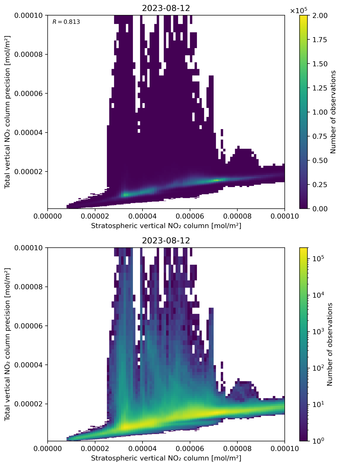
Figure 101: Scatter density plot of “Stratospheric vertical NO 2 column” against “Total vertical NO 2 column precision” for 2023-08-11 to 2023-08-13.
