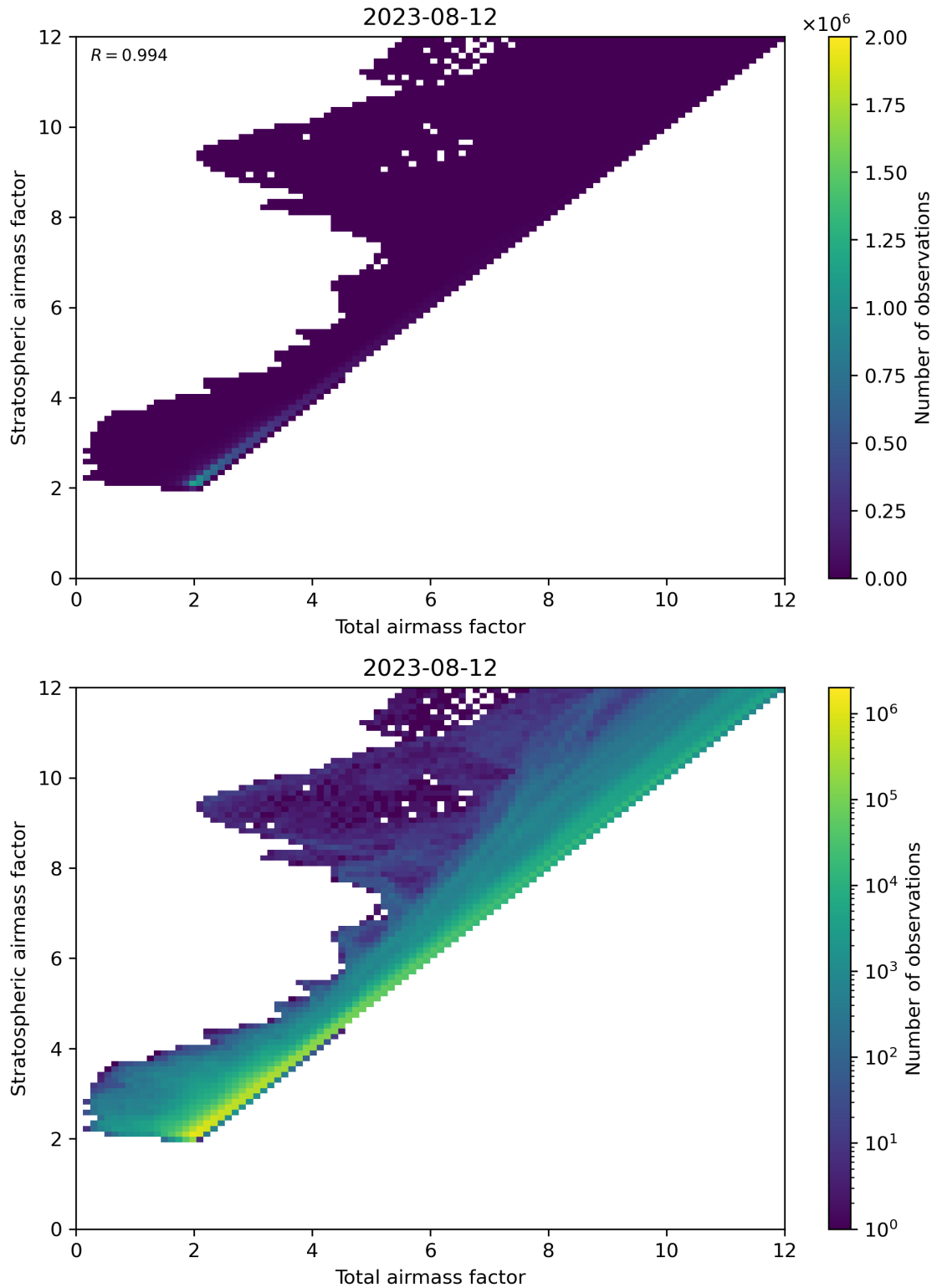
Figure 62: Scatter density plot of “Total airmass factor” against “Stratospheric airmass factor” for 2023-08-11 to 2023-08-13.
