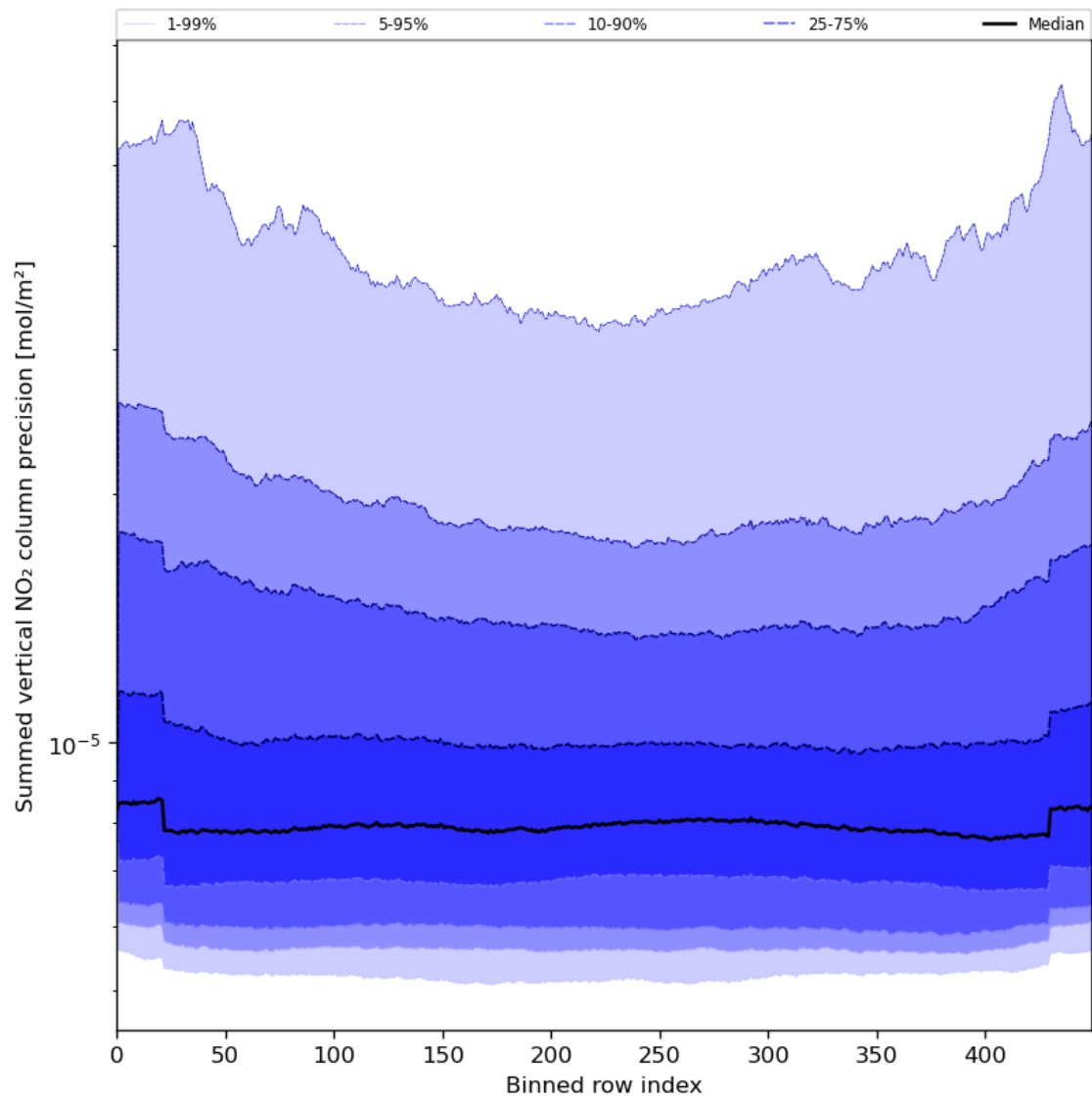
Figure 58: Along track statistics of “Summed vertical NO 2 column precision” for 2023-08-11 to 2023-08-13
