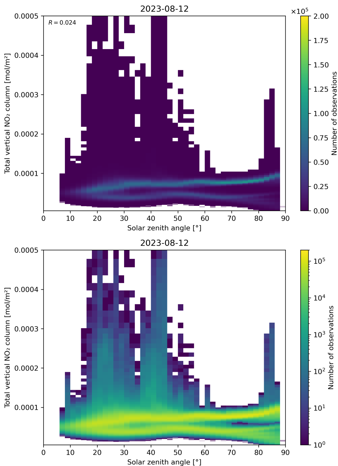
Figure 153: Scatter density plot of “Solar zenith angle” against “Total vertical NO 2 column” for 2023-08-11 to 2023-08-13.
