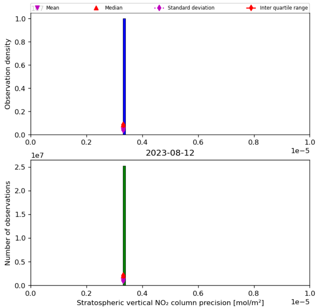
Figure 37: Histogram of “Stratospheric vertical NO 2 column precision” for 2023-08-11 to 2023-08-13
