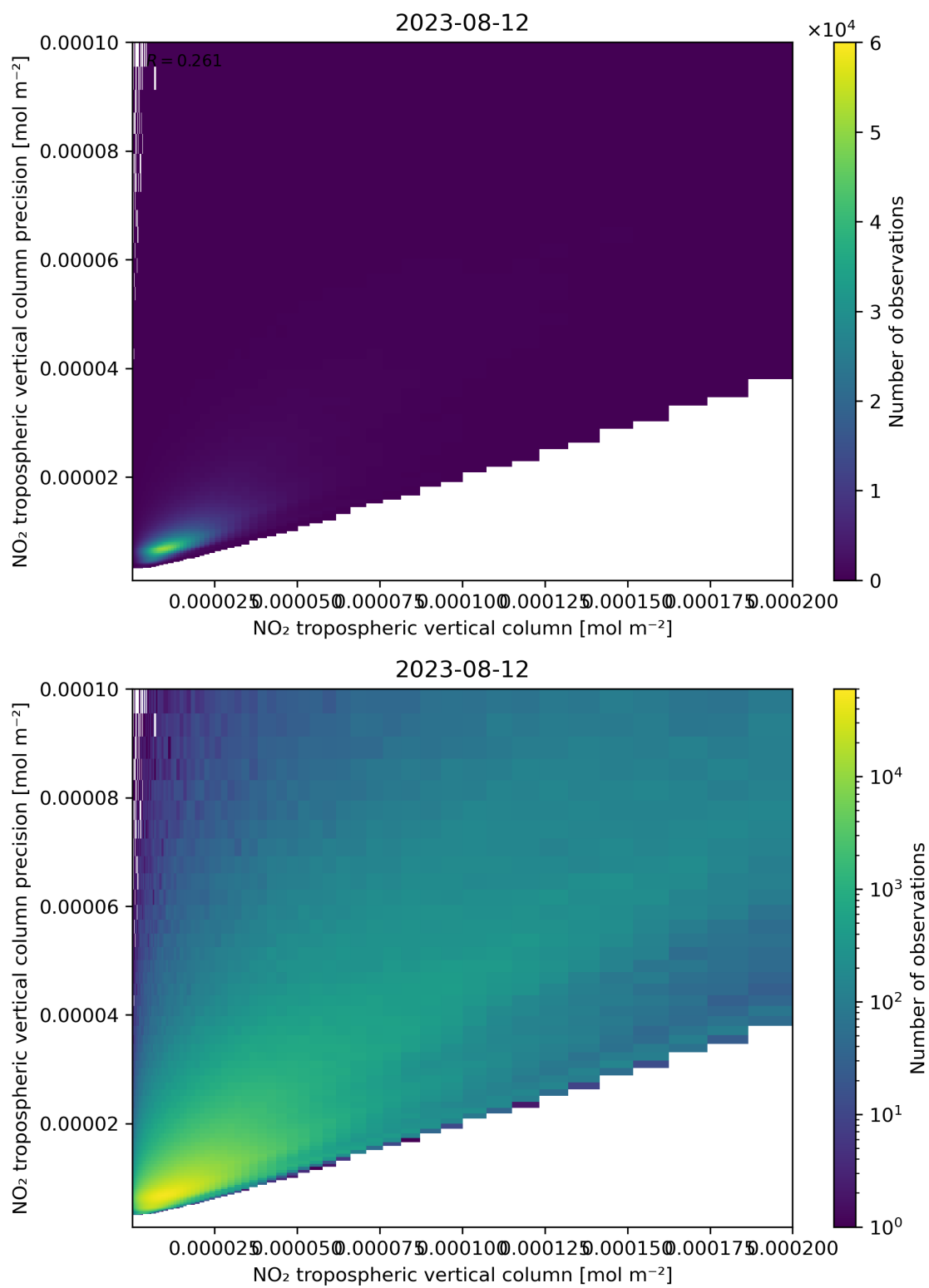
Figure 130: Scatter density plot of “NO 2 tropospheric vertical column” against “NO 2 tropospheric vertical column precision” for 2023-08-11 to 2023-08-13.
