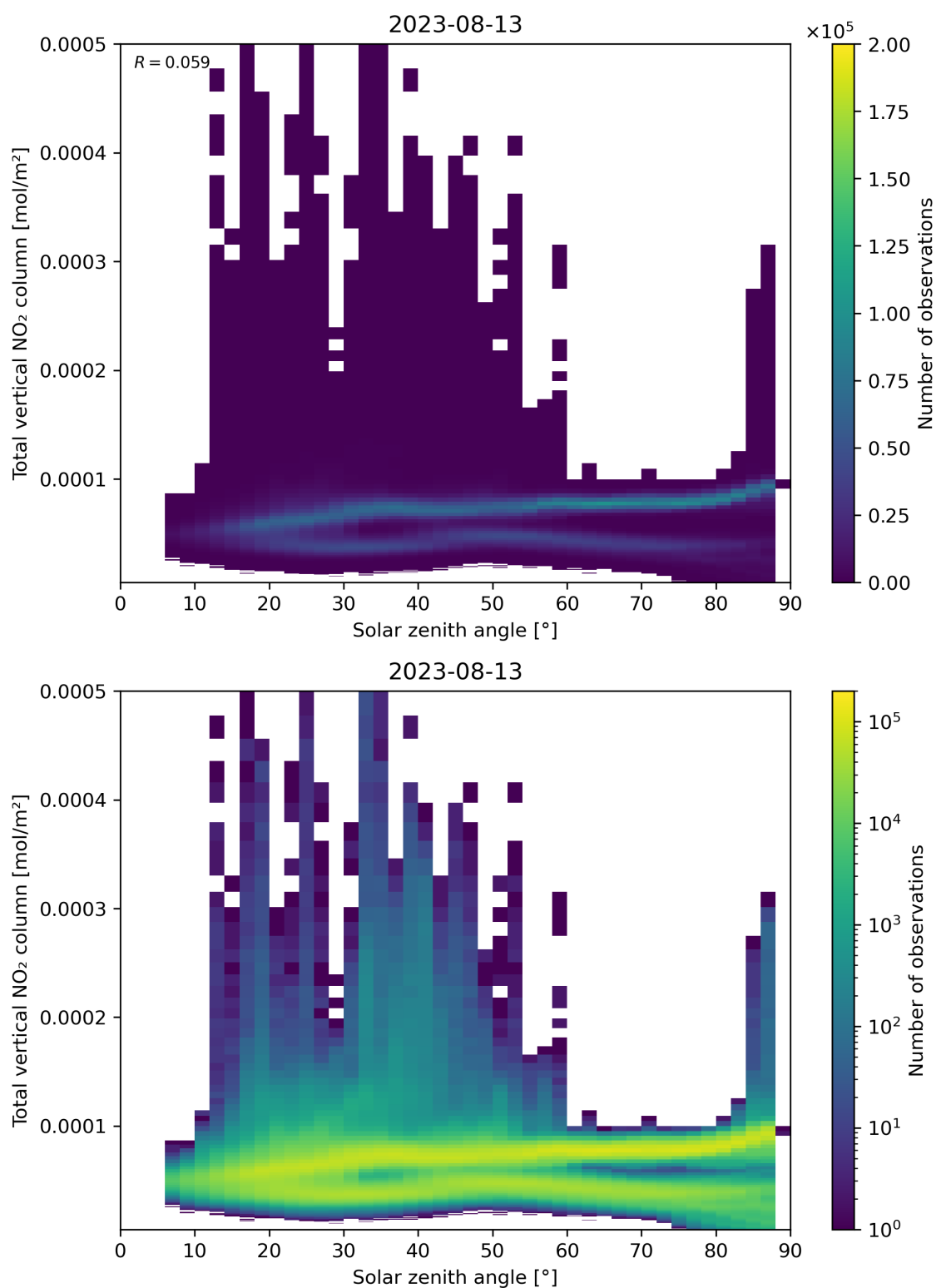
Figure 153: Scatter density plot of “Solar zenith angle” against “Total vertical NO 2 column” for 2023-08-12 to 2023-08-14.
