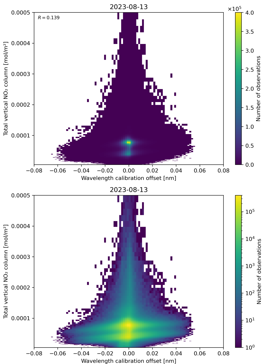
Figure 179: Scatter density plot of “Wavelength calibration offset” against “Total vertical NO 2 column” for 2023-08-12 to 2023-08-14.
