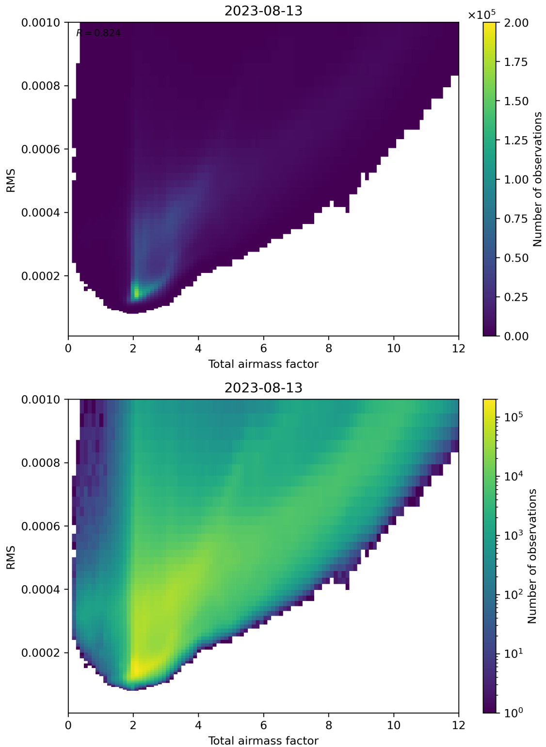
Figure 69: Scatter density plot of “Total airmass factor” against “RMS” for 2023-08-12 to 2023-08-14.
