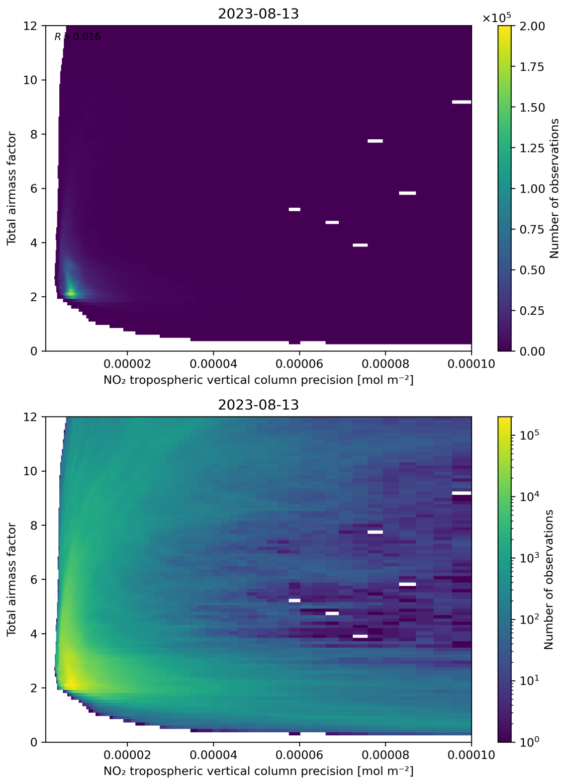
Figure 132: Scatter density plot of “NO 2 tropospheric vertical column precision” against “Total air mass factor” for 2023-08-12 to 2023-08-14.
