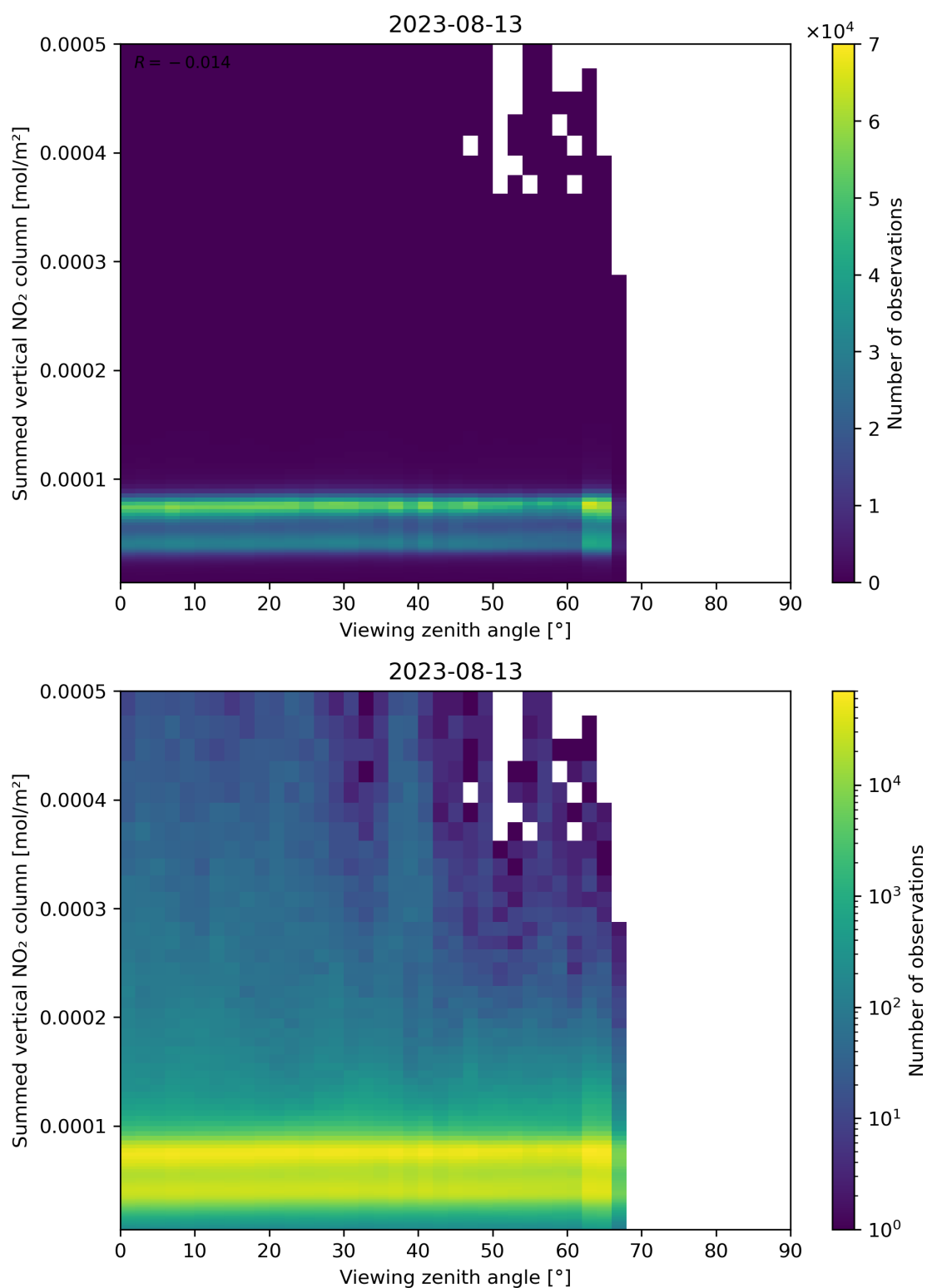
Figure 165: Scatter density plot of “Viewing zenith angle” against “Summed vertical NO 2 column” for 2023-08-12 to 2023-08-14.
