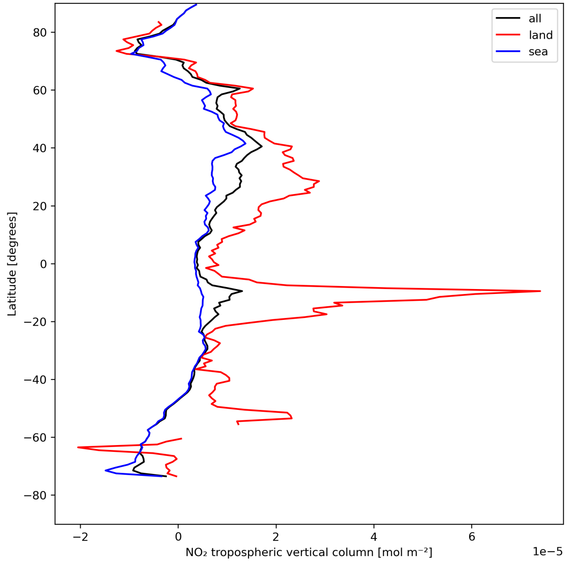
Figure 12: Zonal average of “NO 2 tropospheric vertical column” for 2023-08-12 to 2023-08-14.
