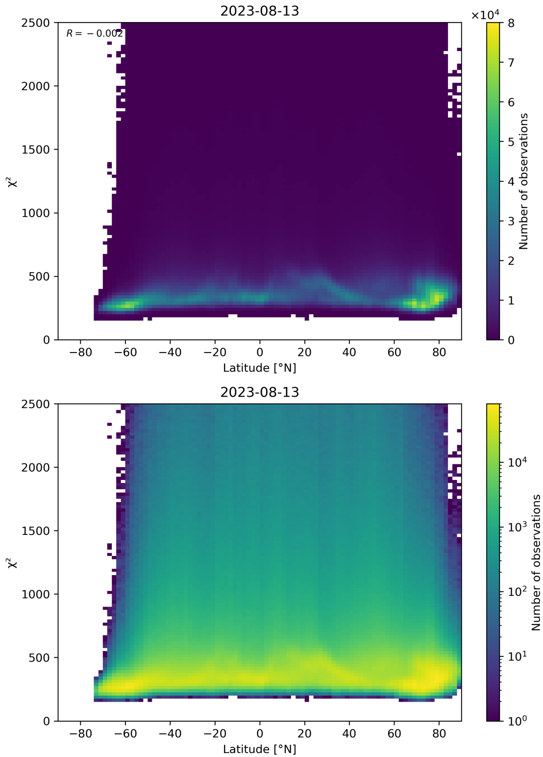
Figure 86: Scatter density plot of “Latitude” against “ \chi^2 ” for 2023-08-12 to 2023-08-14.
