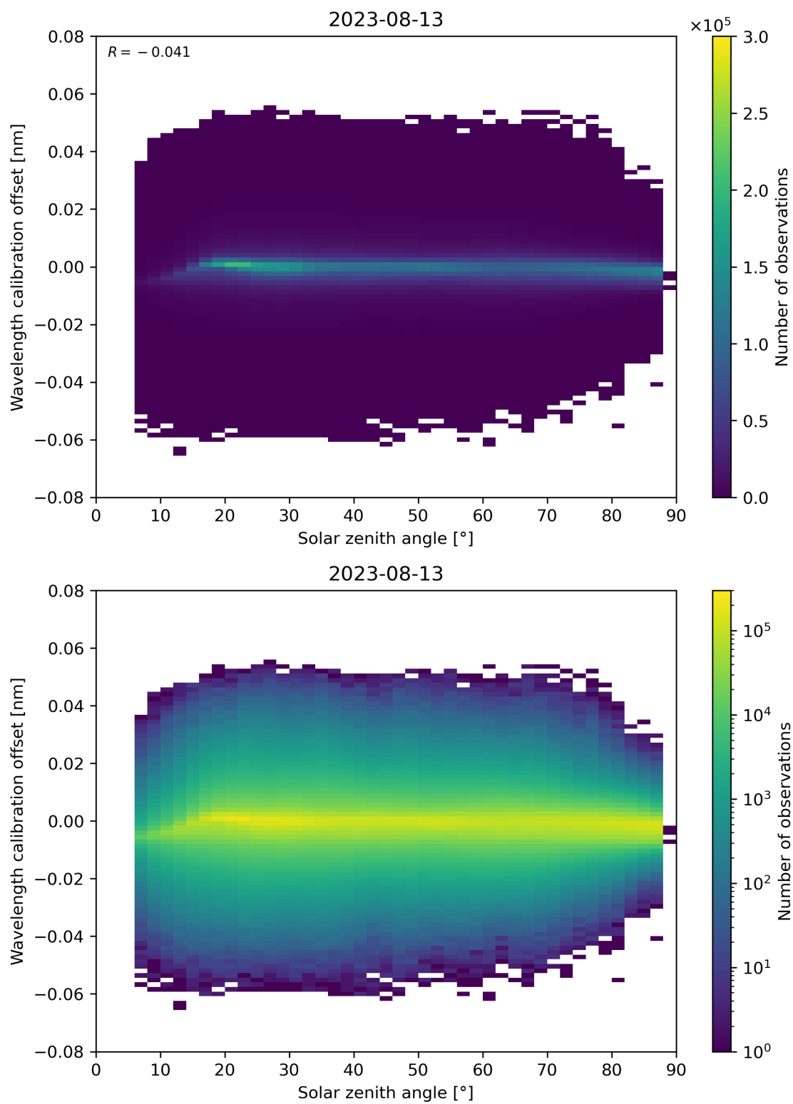
Figure 158: Scatter density plot of “Solar zenith angle” against “Wavelength calibration offset” for 2023-08-12 to 2023-08-14.
