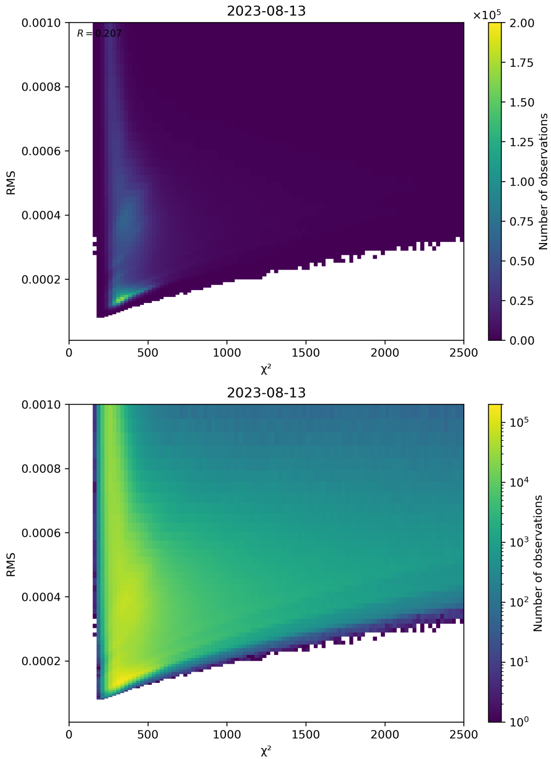
Figure 82: Scatter density plot of “ \chi^2 ” against “RMS” for 2023-08-12 to 2023-08-14.
