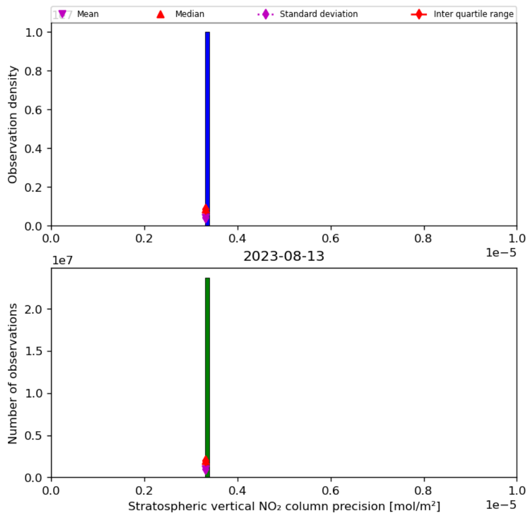
Figure 37: Histogram of “Stratospheric vertical NO 2 column precision” for 2023-08-12 to 2023-08-14
