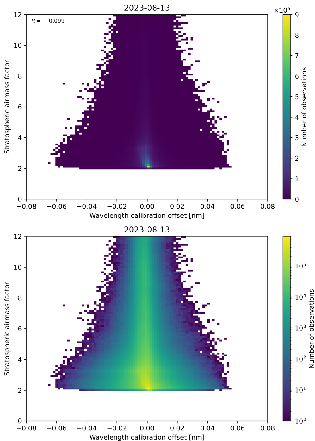
Figure 174: Scatter density plot of “Wavelength calibration offset” against “Stratospheric airmass factor” for 2023-08-12 to 2023-08-14.
