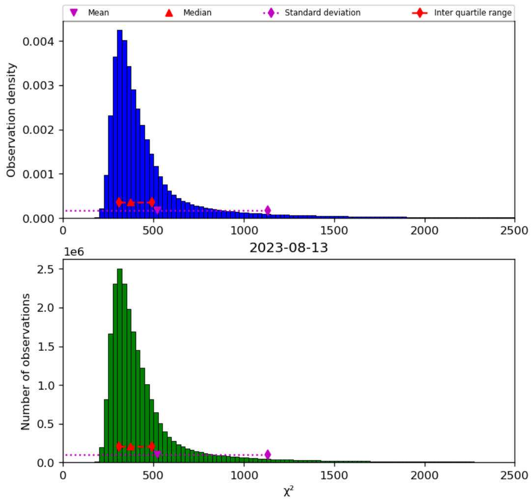
Figure 42: Histogram of “ \chi^2 ” for 2023-08-12 to 2023-08-14
