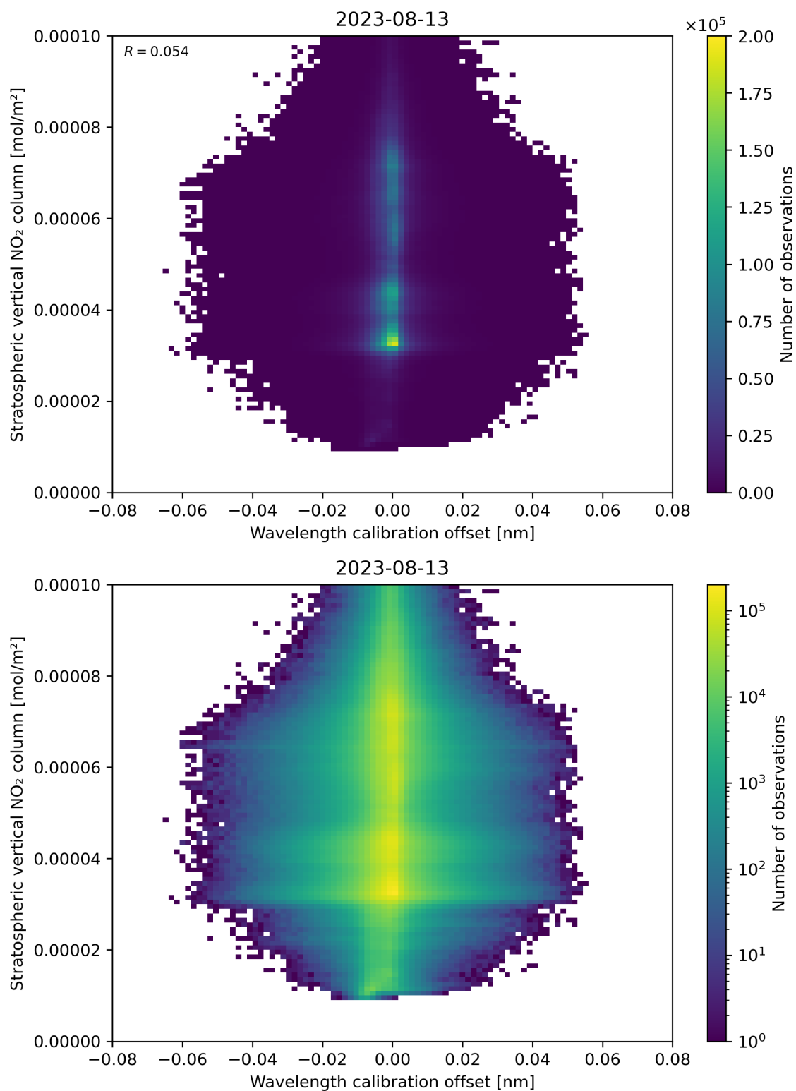
Figure 176: Scatter density plot of “Wavelength calibration offset” against “Stratospheric vertical NO 2 column” for 2023-08-12 to 2023-08-14.
