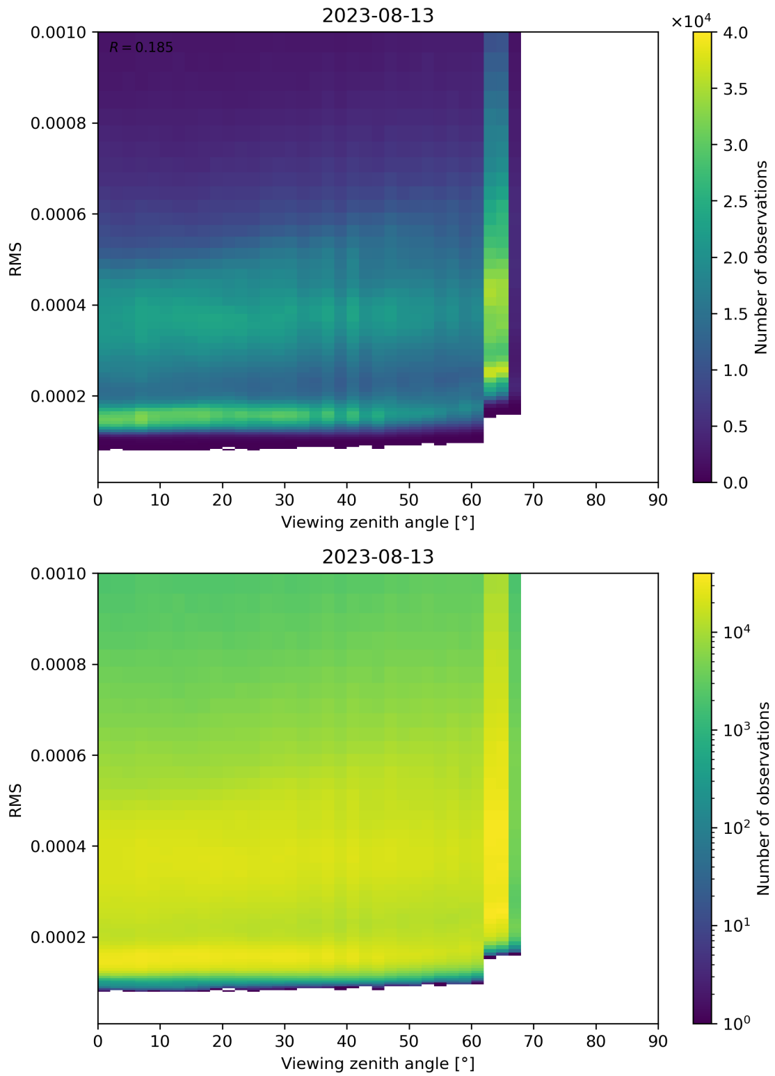
Figure 171: Scatter density plot of “Viewing zenith angle” against “RMS” for 2023-08-12 to 2023-08-14.
