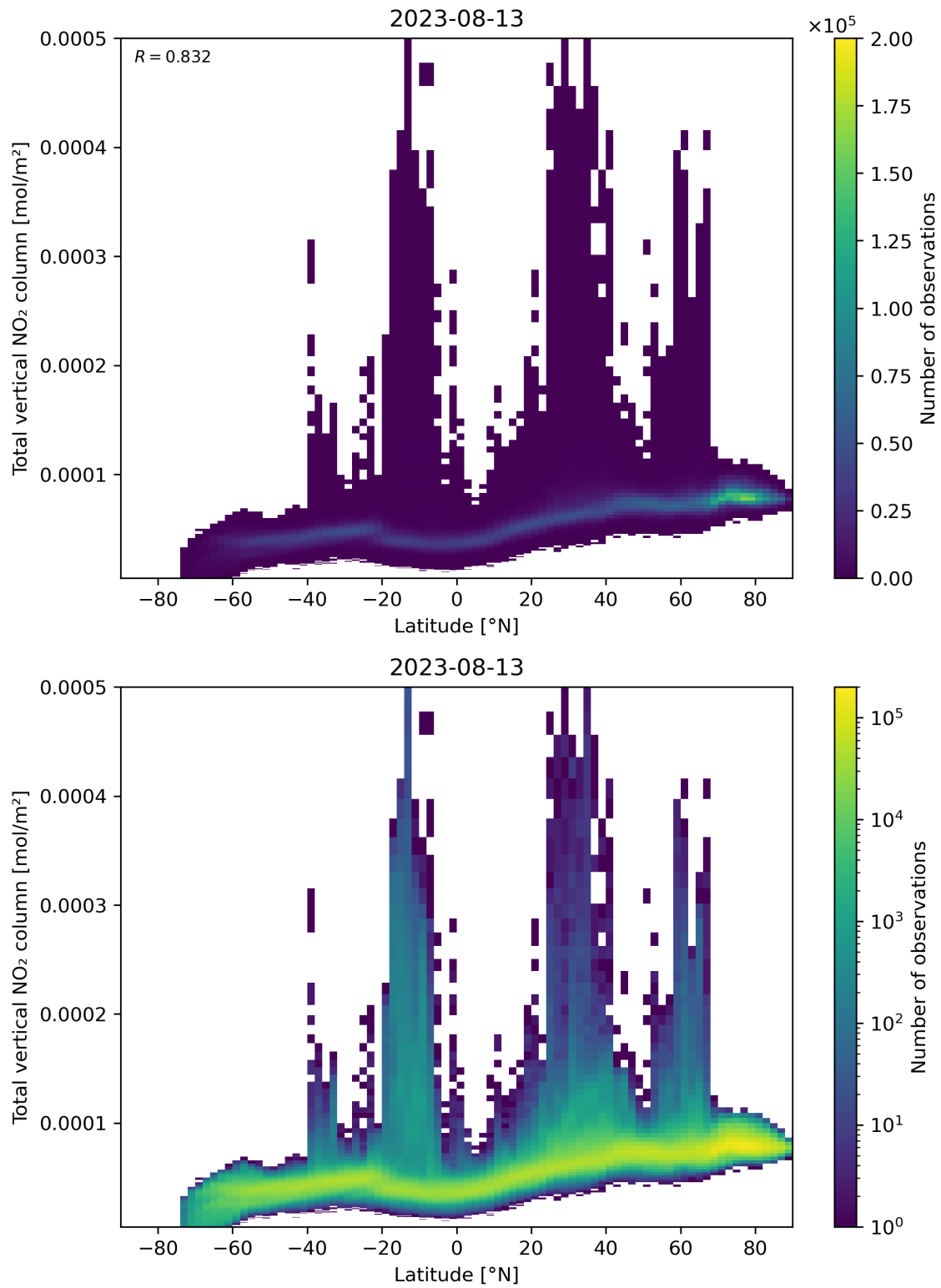
Figure 90: Scatter density plot of “Latitude” against “Total vertical NO 2 column” for 2023-08-12 to 2023-08-14.
