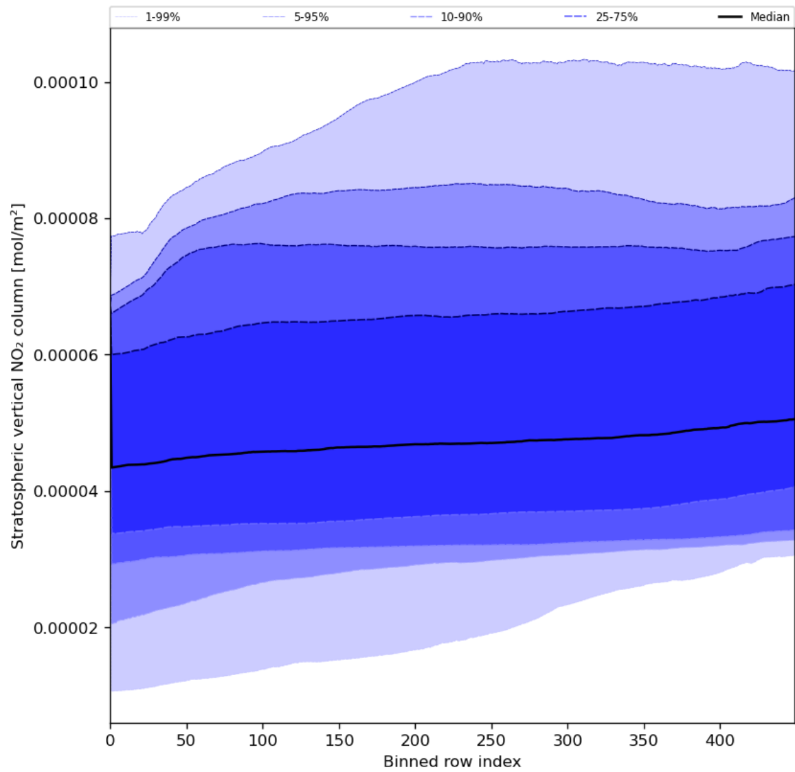
Figure 53: Along track statistics of “Stratospheric vertical NO 2 column” for 2023-08-12 to 2023-08-14
