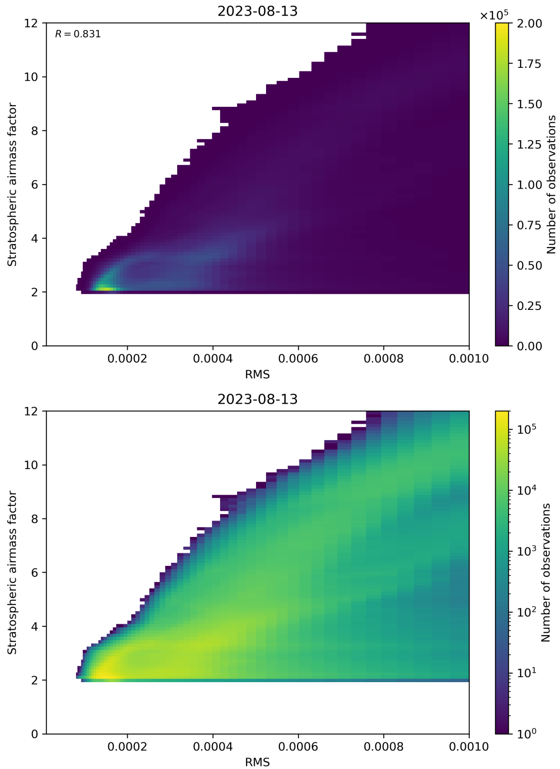
Figure 144: Scatter density plot of “RMS” against “Stratospheric airmass factor” for 2023-08-12 to 2023-08-14.
