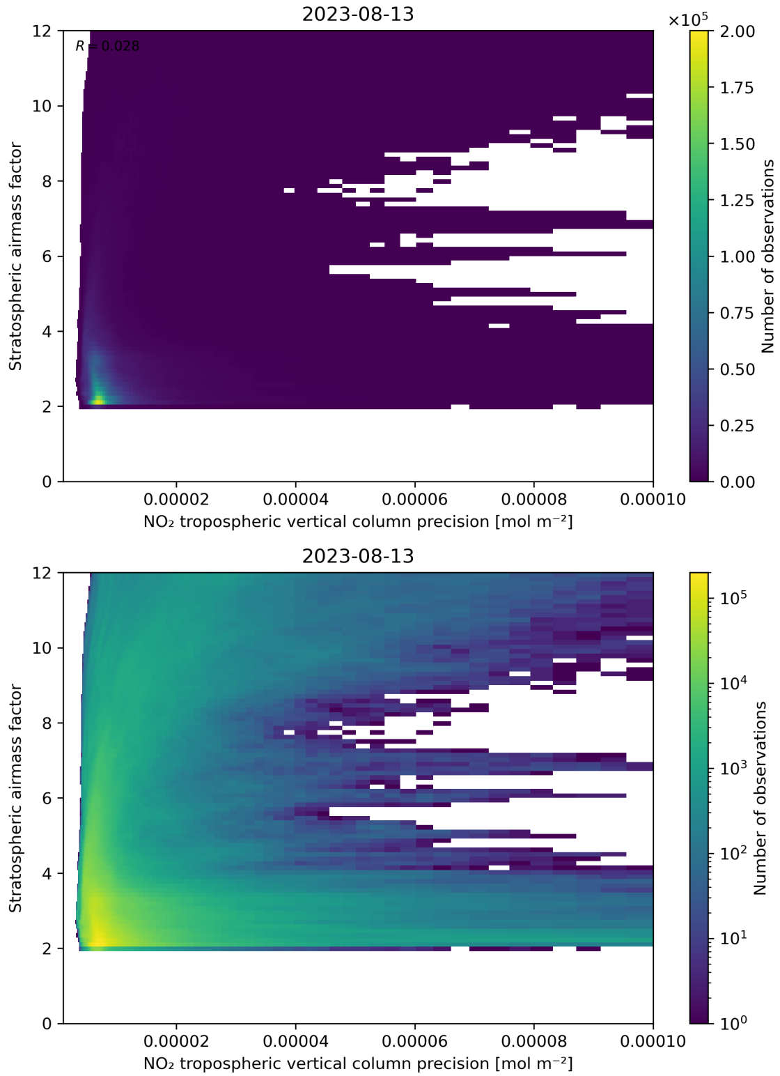
Figure 131: Scatter density plot of “NO 2 tropospheric vertical column precision” against “Stratospheric airmass factor” for 2023-08-12 to 2023-08-14.
