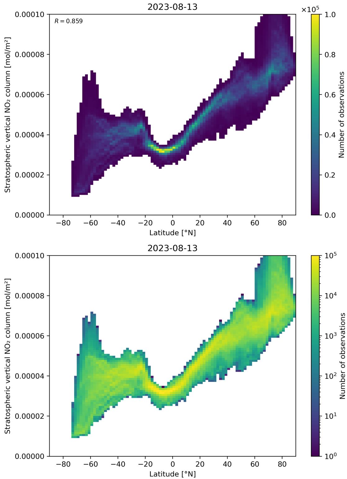
Figure 87: Scatter density plot of “Latitude” against “Stratospheric vertical NO 2 column” for 2023-08-12 to 2023-08-14.
