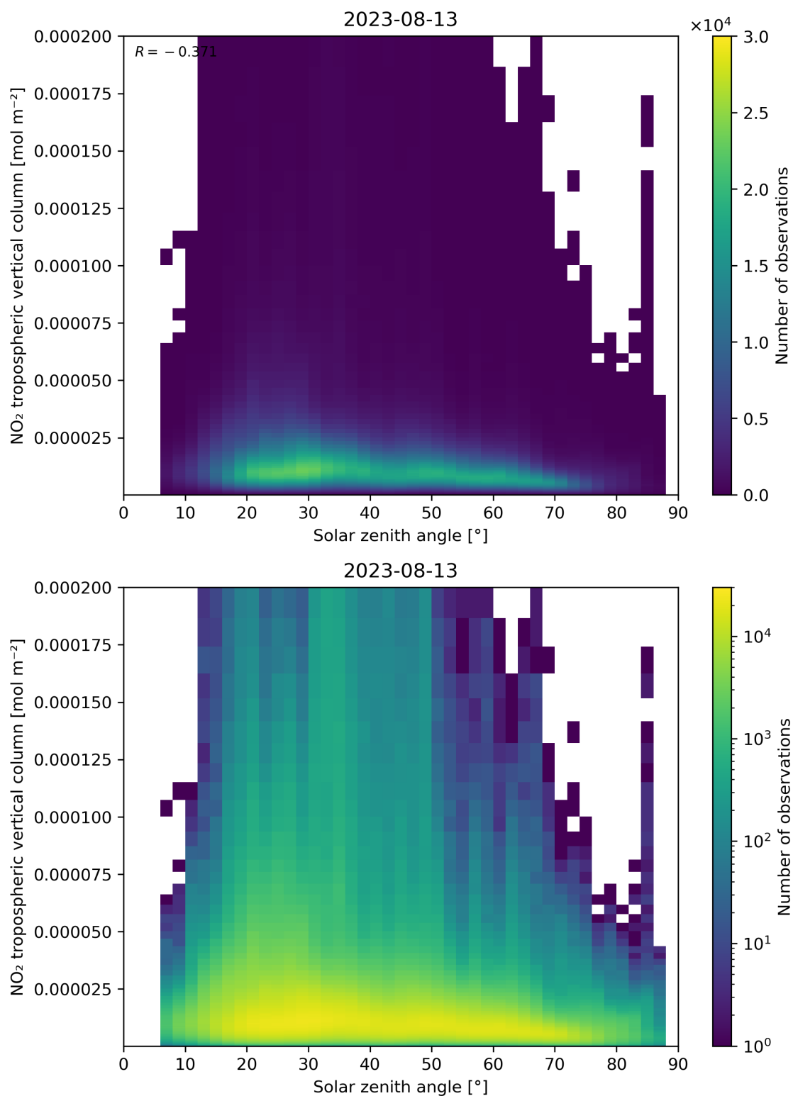
Figure 155: Scatter density plot of “Solar zenith angle” against “NO 2 tropospheric vertical column” for 2023-08-12 to 2023-08-14.
