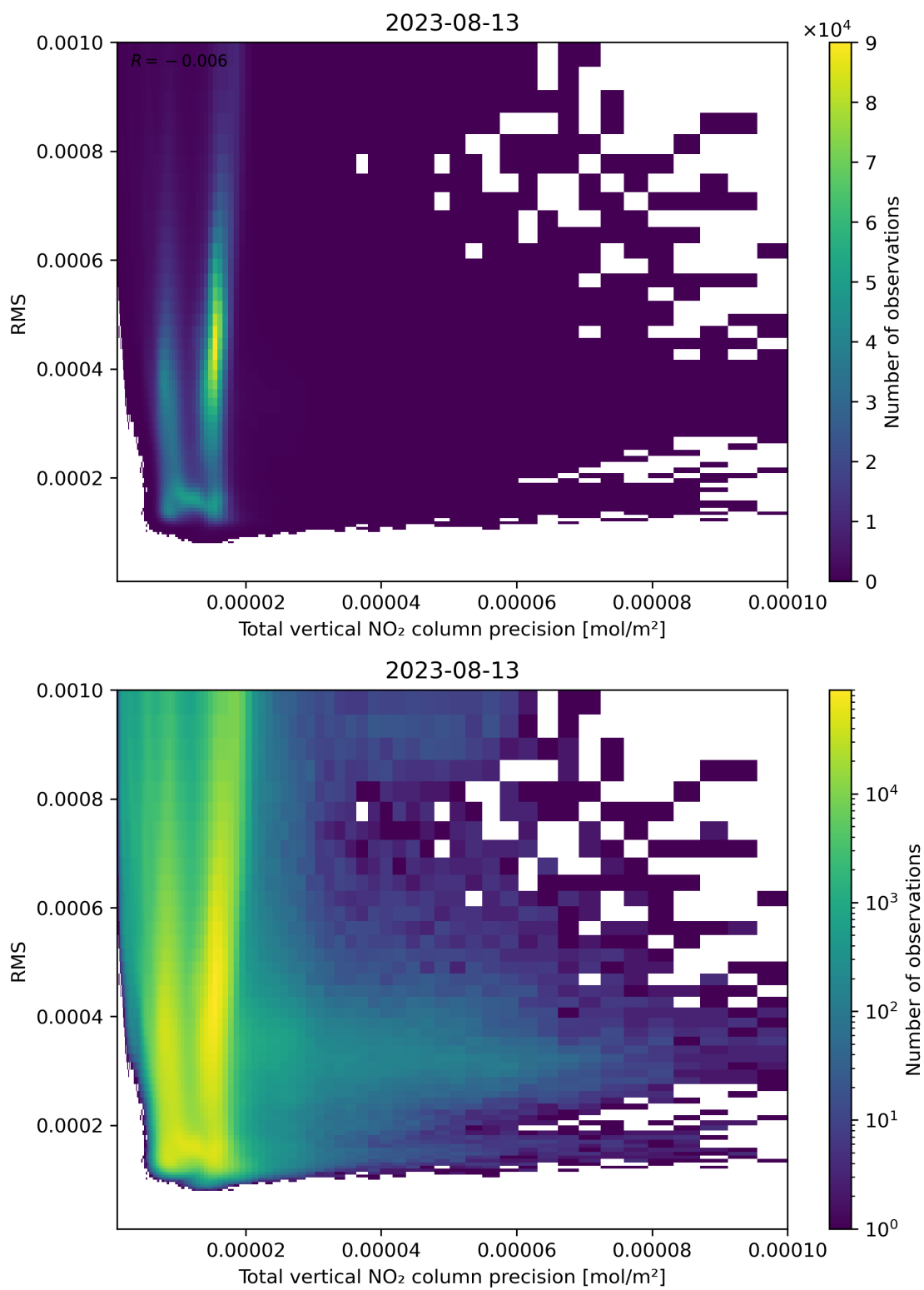
Figure 119: Scatter density plot of “Total vertical NO 2 column precision” against “RMS” for 2023-08-12 to 2023-08-14.
