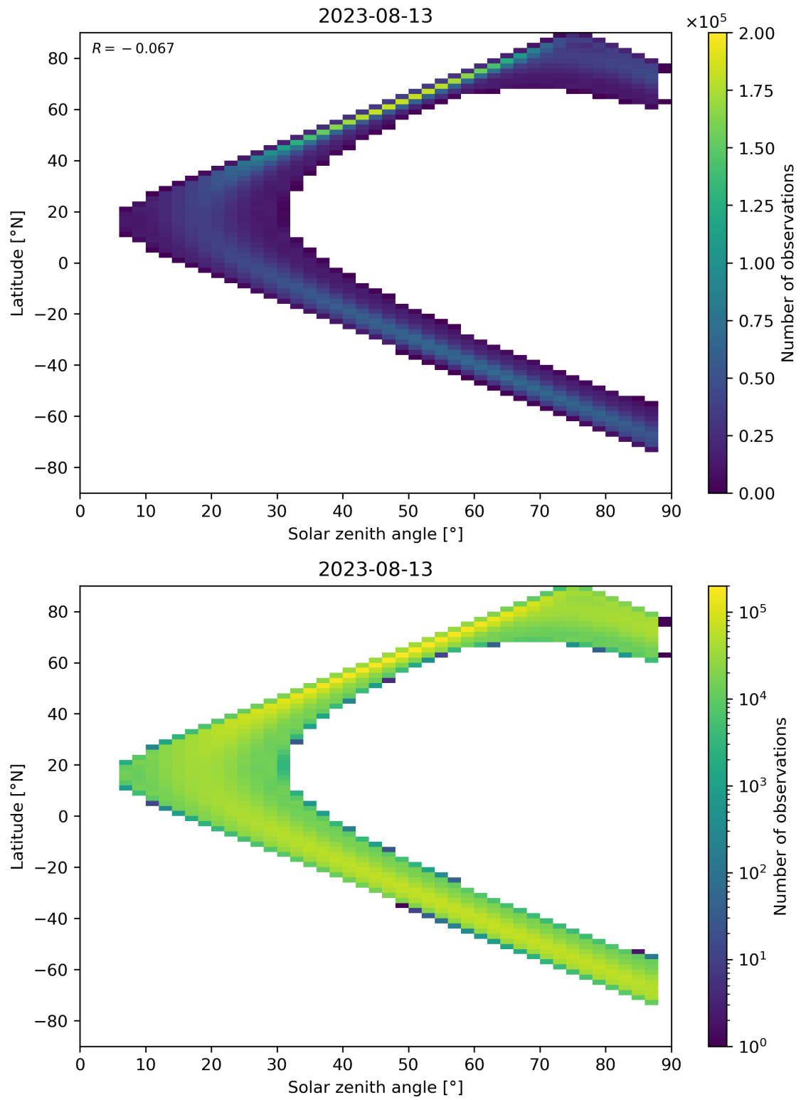
Figure 149: Scatter density plot of “Solar zenith angle” against “Latitude” for 2023-08-12 to 2023-08-14.
