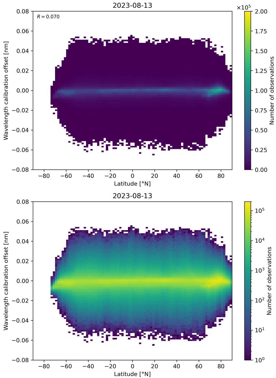
Figure 95: Scatter density plot of “Latitude” against “Wavelength calibration offset” for 2023-08-12 to 2023-08-14.
