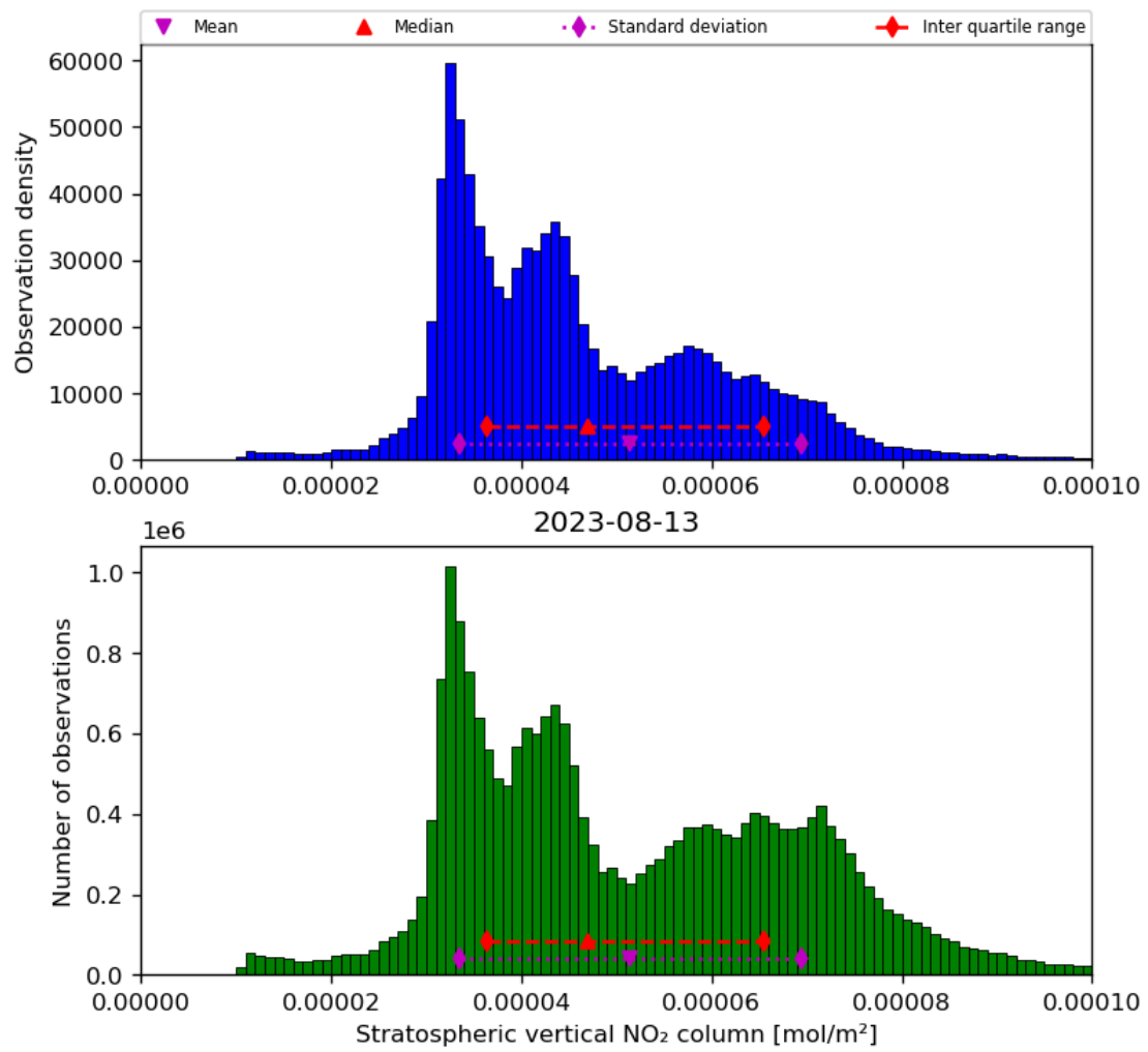
Figure 36: Histogram of “Stratospheric vertical NO 2 column” for 2023-08-12 to 2023-08-14
