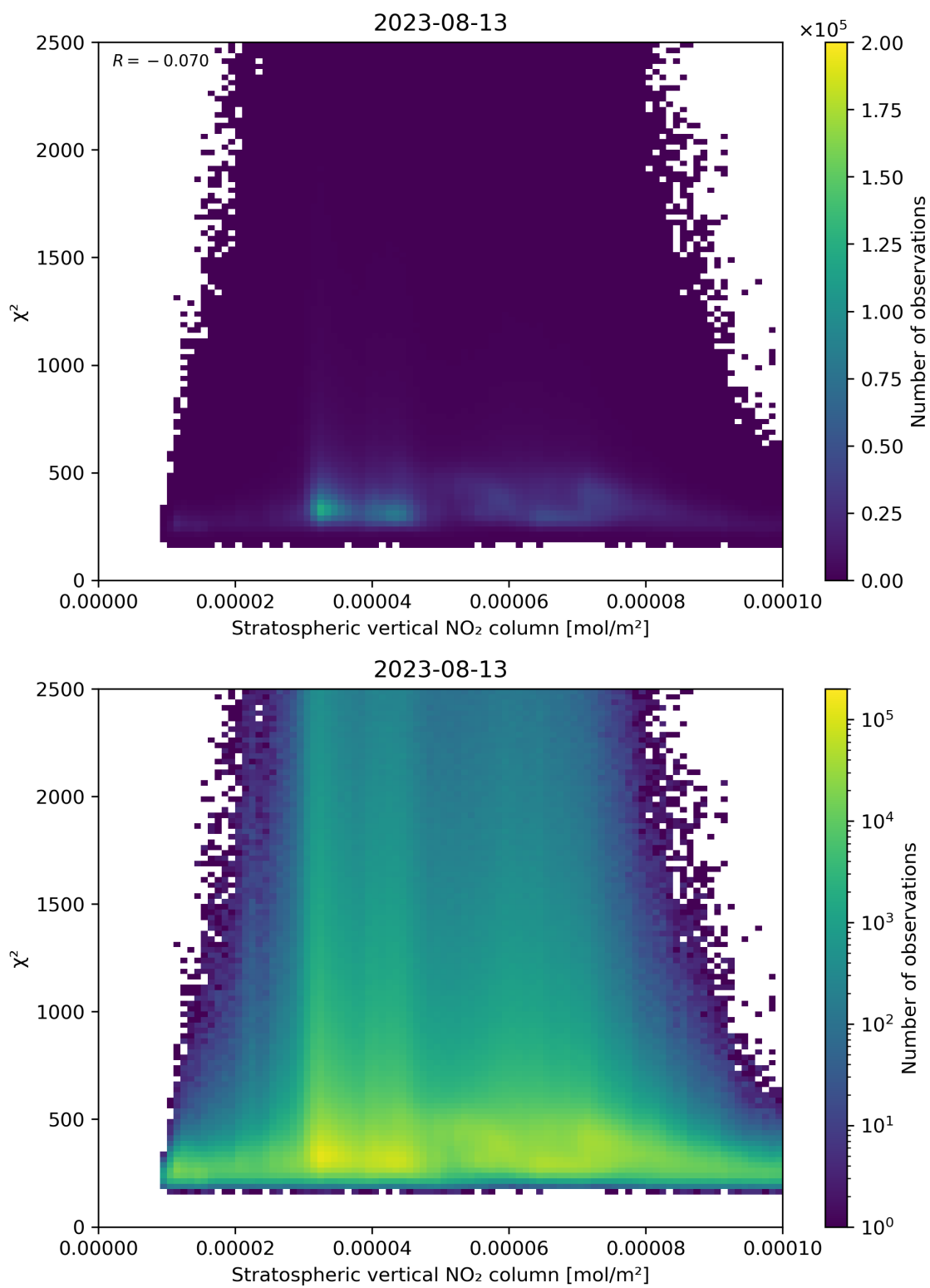
Figure 97: Scatter density plot of “Stratospheric vertical NO 2 column” against “ \chi^2 ” for 2023-08-12 to 2023-08-14.
