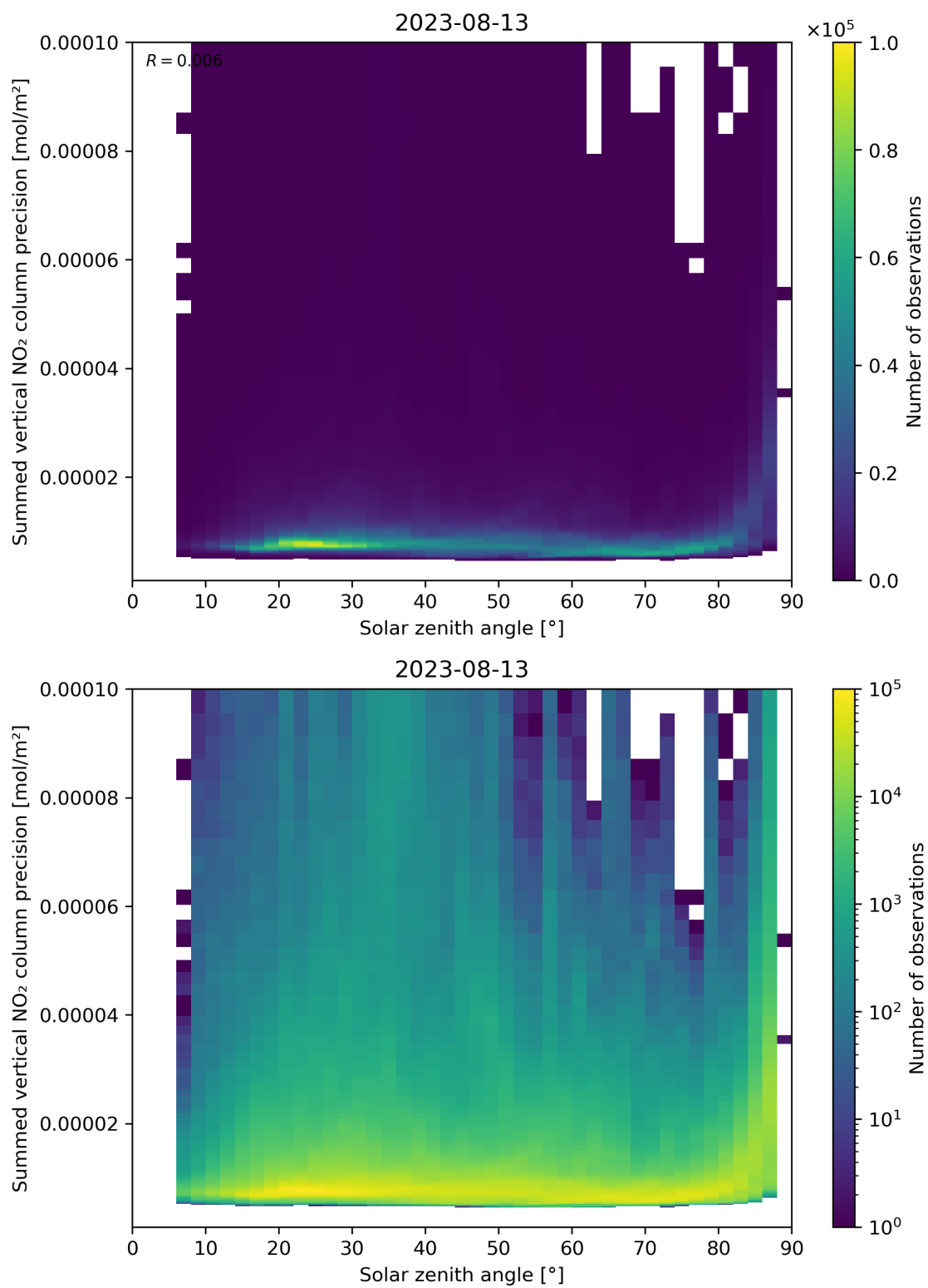
Figure 152: Scatter density plot of “Solar zenith angle” against “Summed vertical NO 2 column precision” for 2023-08-12 to 2023-08-14.
