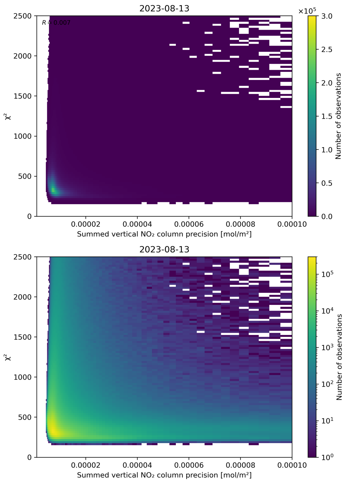
Figure 107: Scatter density plot of “Summed vertical NO 2 column precision” against “ \chi^2 ” for 2023-08-12 to 2023-08-14.
