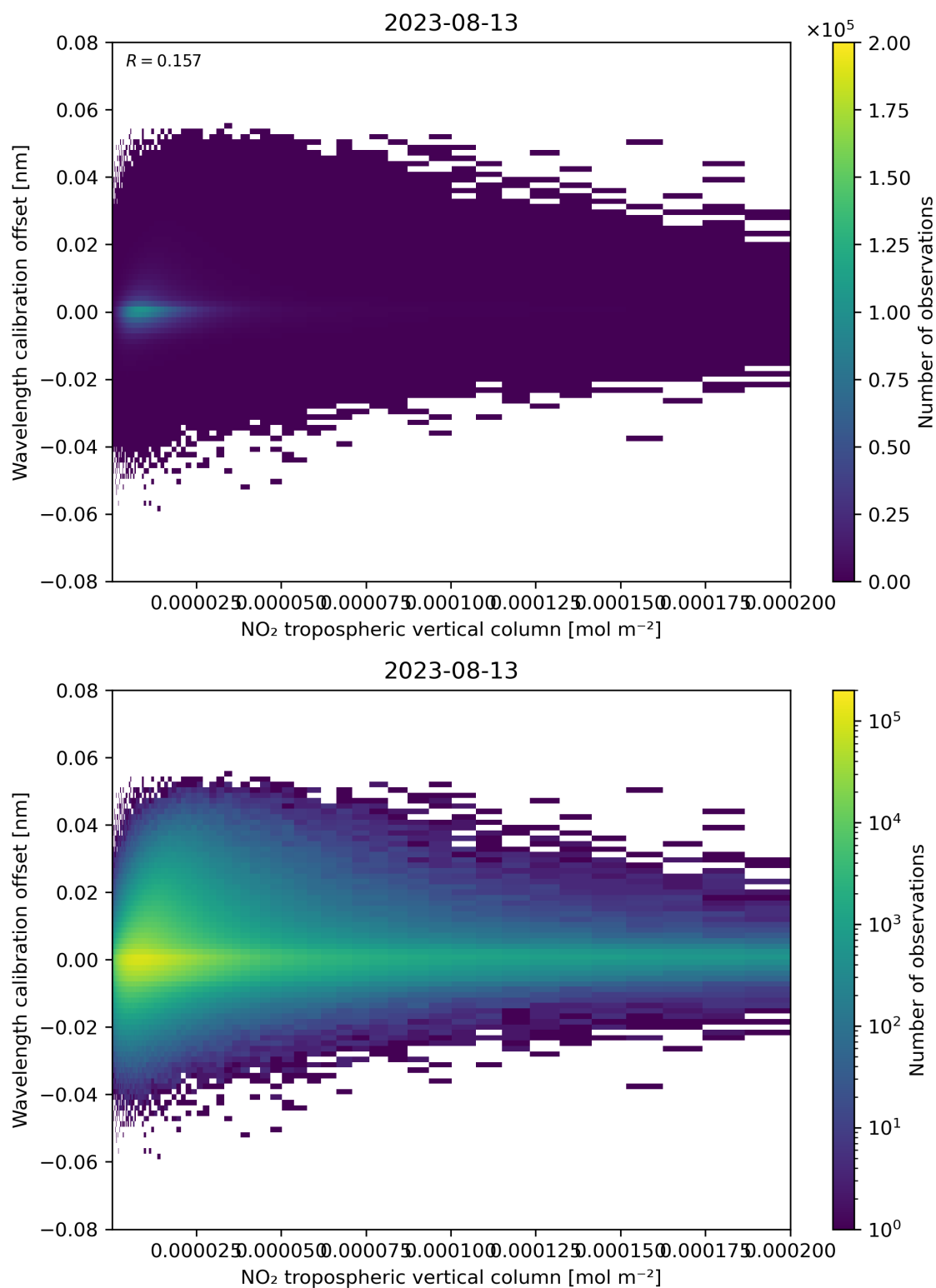
Figure 143: Scatter density plot of “NO 2 tropospheric vertical column” against “Wavelength calibration offset” for 2023-08-12 to 2023-08-14.
