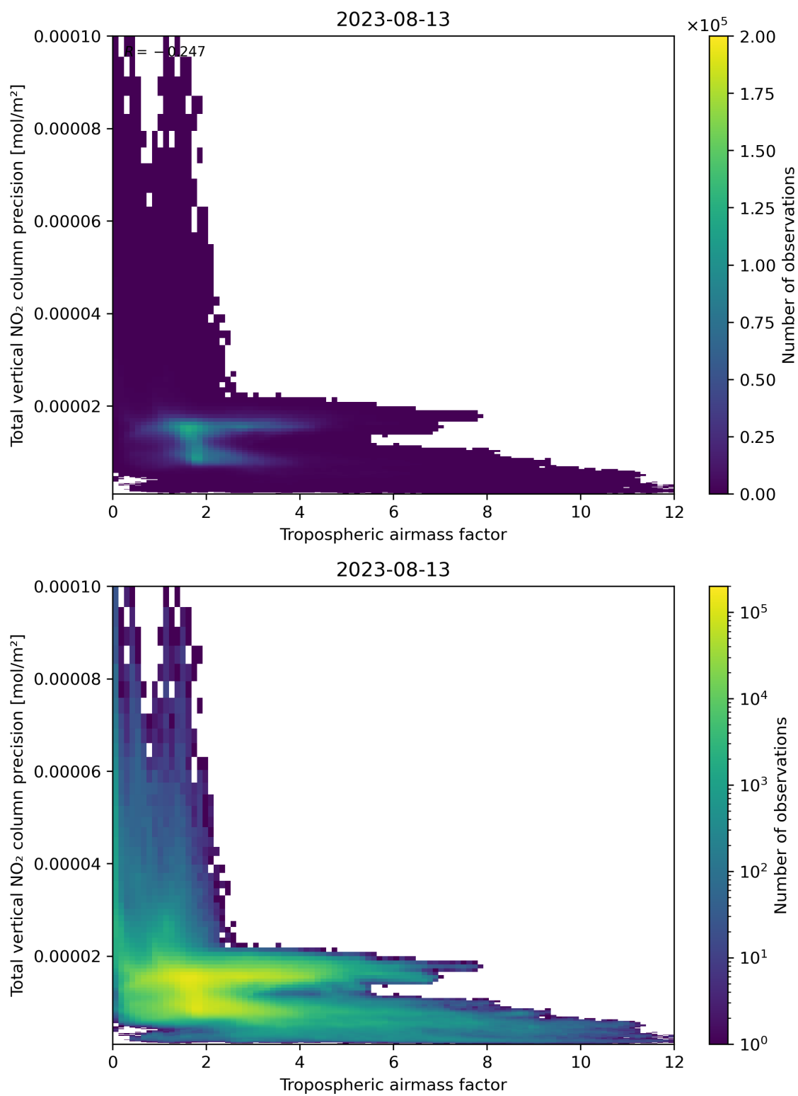
Figure 78: Scatter density plot of “Tropospheric air mass factor” against “Total vertical NO 2 column precision” for 2023-08-12 to 2023-08-14.
