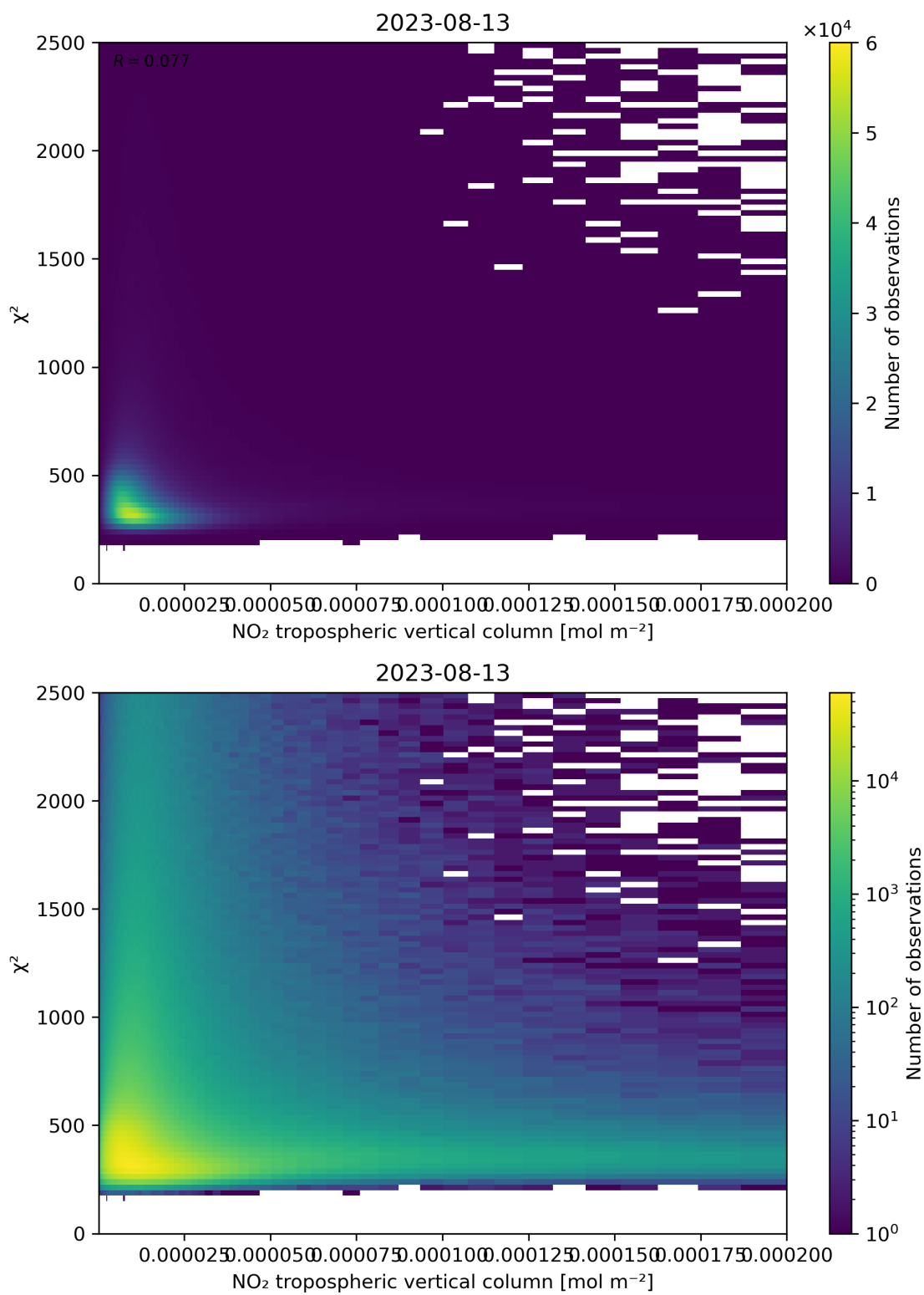
Figure 124: Scatter density plot of “NO 2 tropospheric vertical column” against “ \chi^2 ” for 2023-08-12 to 2023-08-14.
