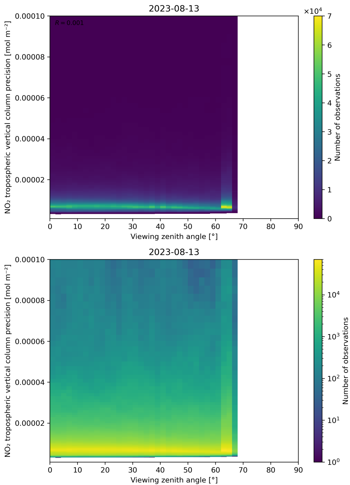
Figure 170: Scatter density plot of “Viewing zenith angle” against “NO 2 tropospheric vertical column precision” for 2023-08-12 to 2023-08-14.
