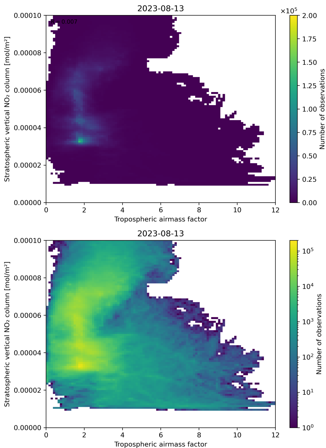
Figure 74: Scatter density plot of “Tropospheric air mass factor” against “Stratospheric vertical NO 2 column” for 2023-08-12 to 2023-08-14.
