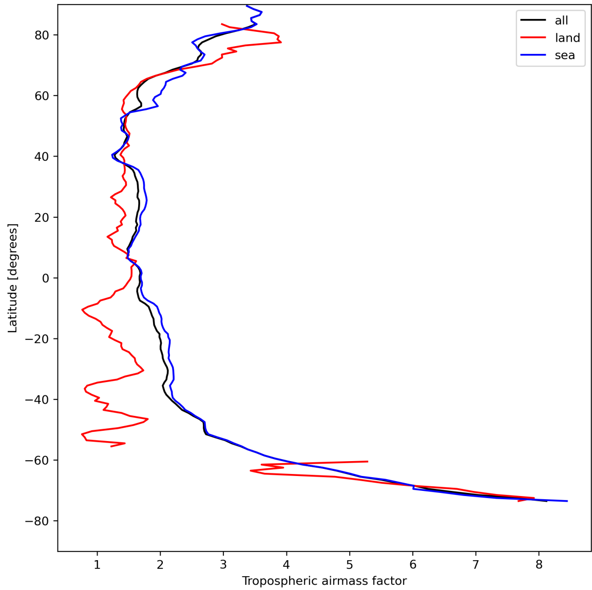
Figure 14: Zonal average of “Tropospheric airmass factor” for 2023-08-12 to 2023-08-14.
