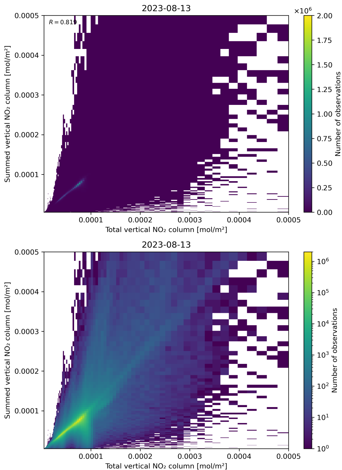
Figure 112: Scatter density plot of “Total vertical NO 2 column” against “Summed vertical NO 2 column” for 2023-08-12 to 2023-08-14.
