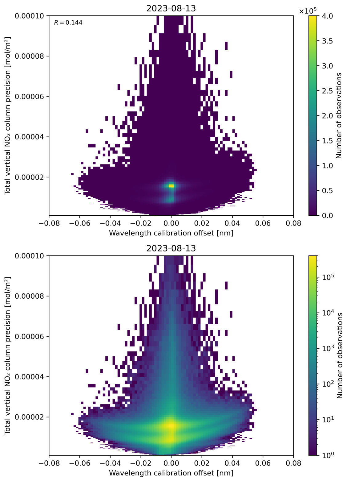
Figure 180: Scatter density plot of “Wavelength calibration offset” against “Total vertical NO 2 column precision” for 2023-08-12 to 2023-08-14.
