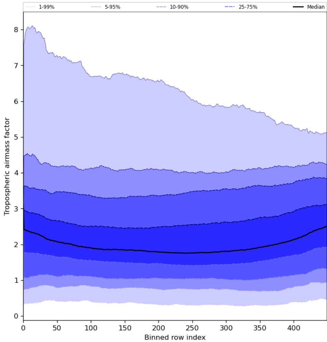
Figure 48: Along track statistics of “Tropospheric airmass factor” for 2023-08-12 to 2023-08-14
