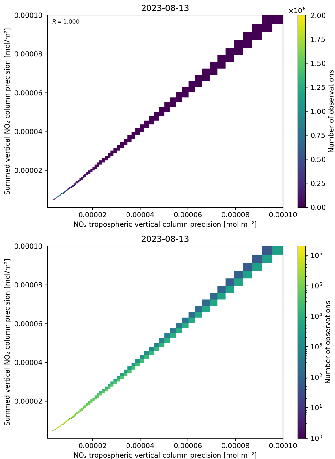
Figure 137: Scatter density plot of “NO 2 tropospheric vertical column precision” against “Summed vertical NO 2 column precision” for 2023-08-12 to 2023-08-14.
