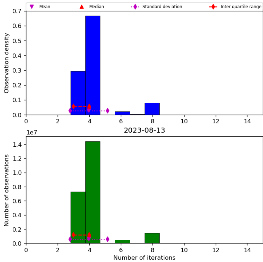
Figure 34: Histogram of “Number of iterations” for 2023-08-12 to 2023-08-14
