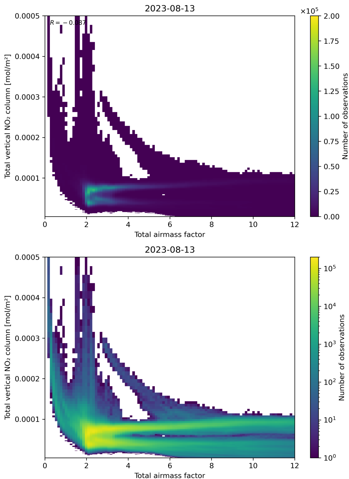
Figure 67: Scatter density plot of “Total airmass factor” against “Total vertical NO 2 column” for 2023-08-12 to 2023-08-14.
