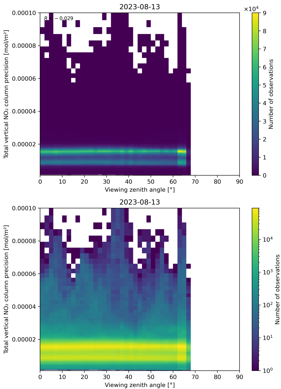
Figure 168: Scatter density plot of “Viewing zenith angle” against “Total vertical NO 2 column precision” for 2023-08-12 to 2023-08-14.
