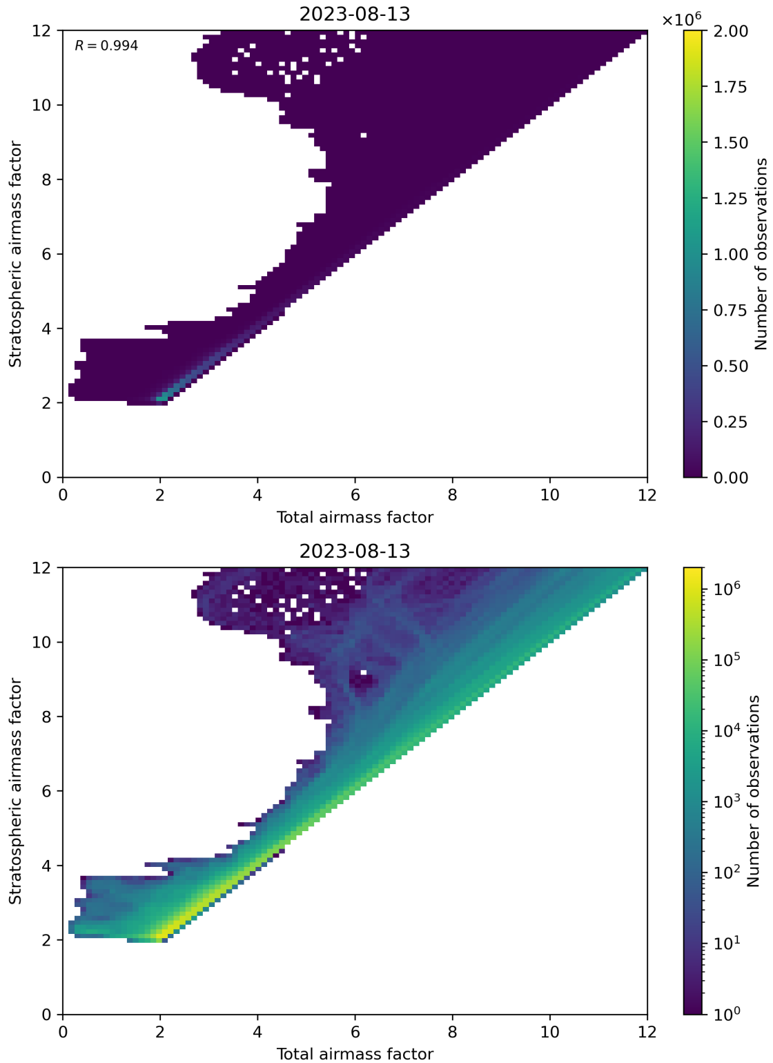
Figure 62: Scatter density plot of “Total airmass factor” against “Stratospheric airmass factor” for 2023-08-12 to 2023-08-14.
