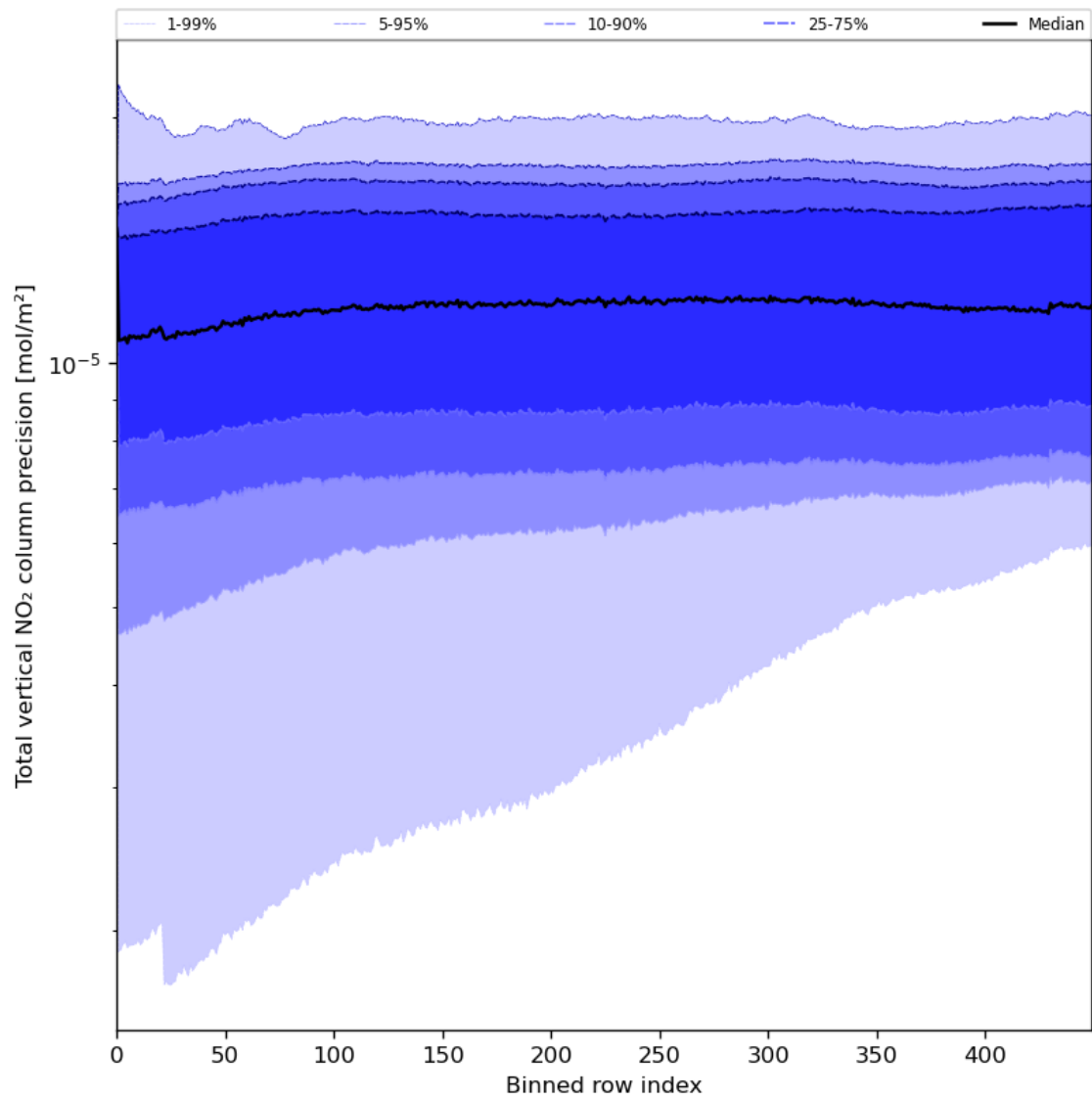
Figure 56: Along track statistics of “Total vertical NO 2 column precision” for 2023-08-12 to 2023-08-14
