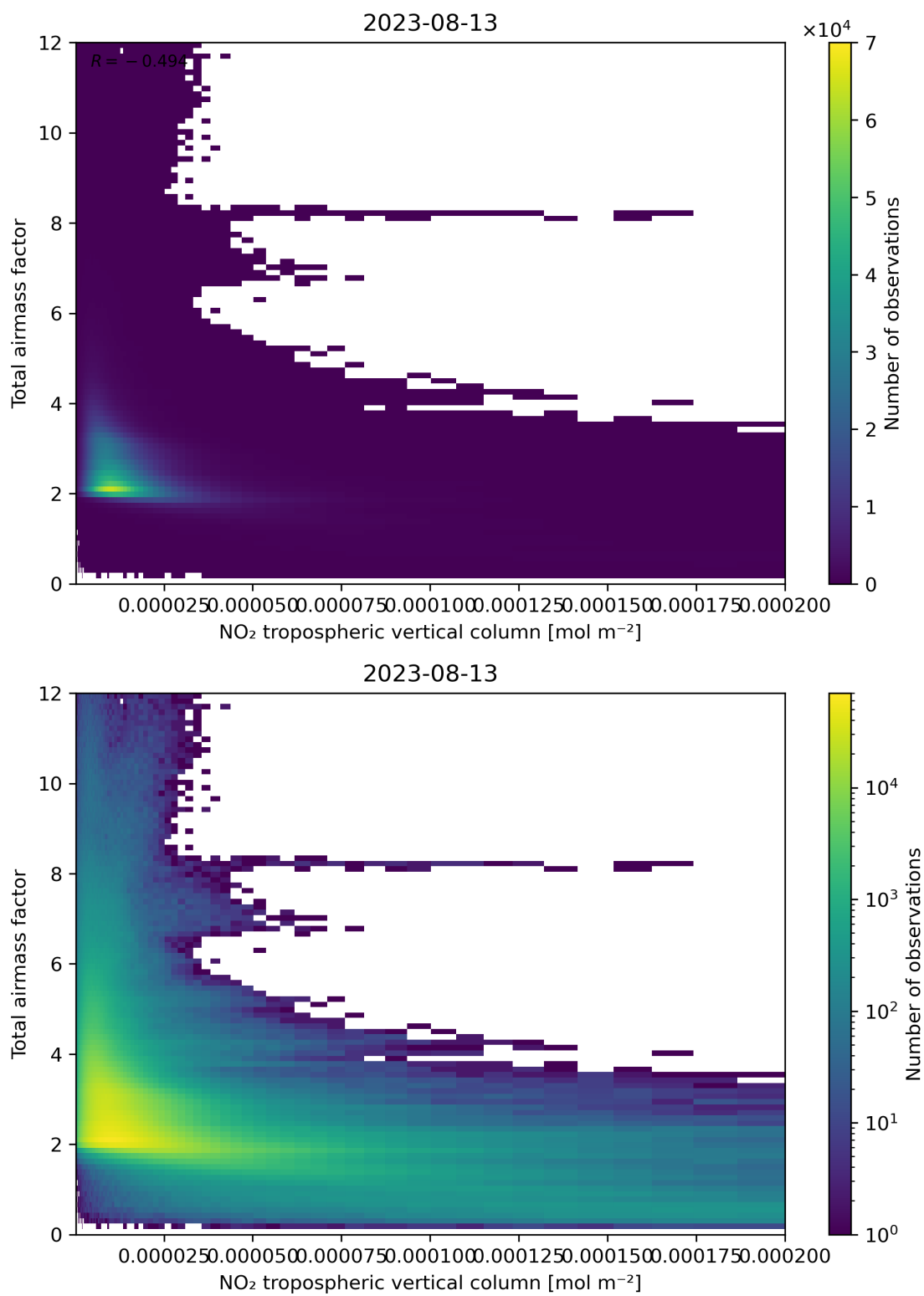
Figure 122: Scatter density plot of “NO 2 tropospheric vertical column” against “Total air mass factor” for 2023-08-12 to 2023-08-14.
