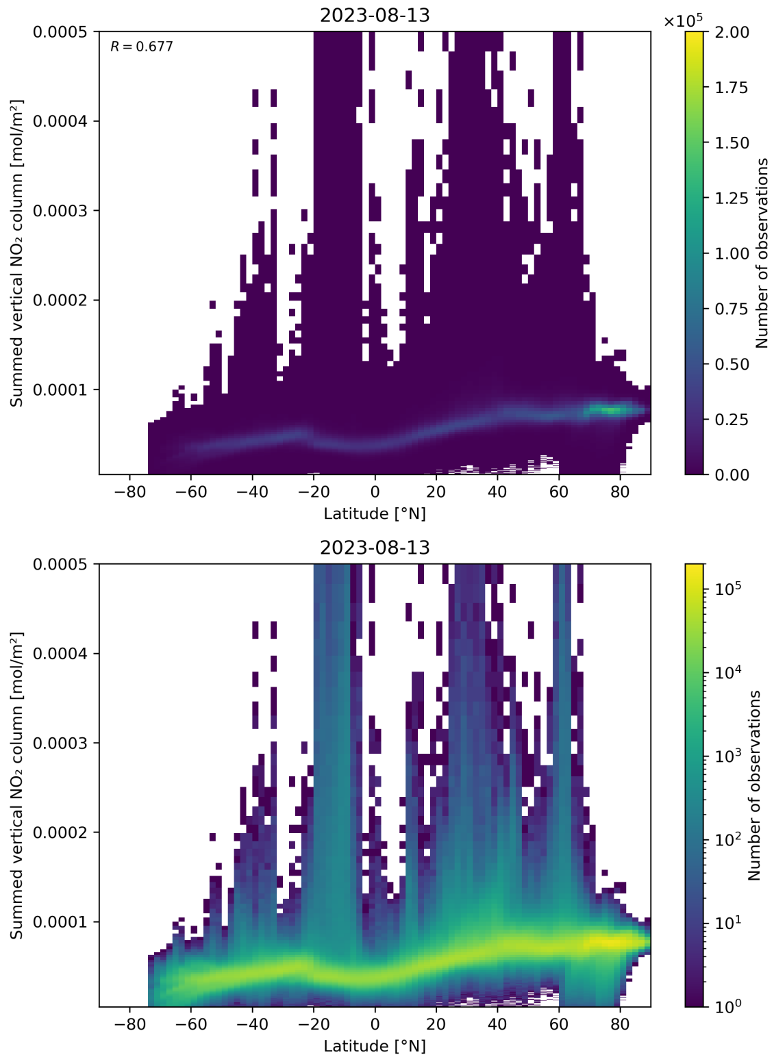
Figure 88: Scatter density plot of “Latitude” against “Summed vertical NO 2 column” for 2023-08-12 to 2023-08-14.
