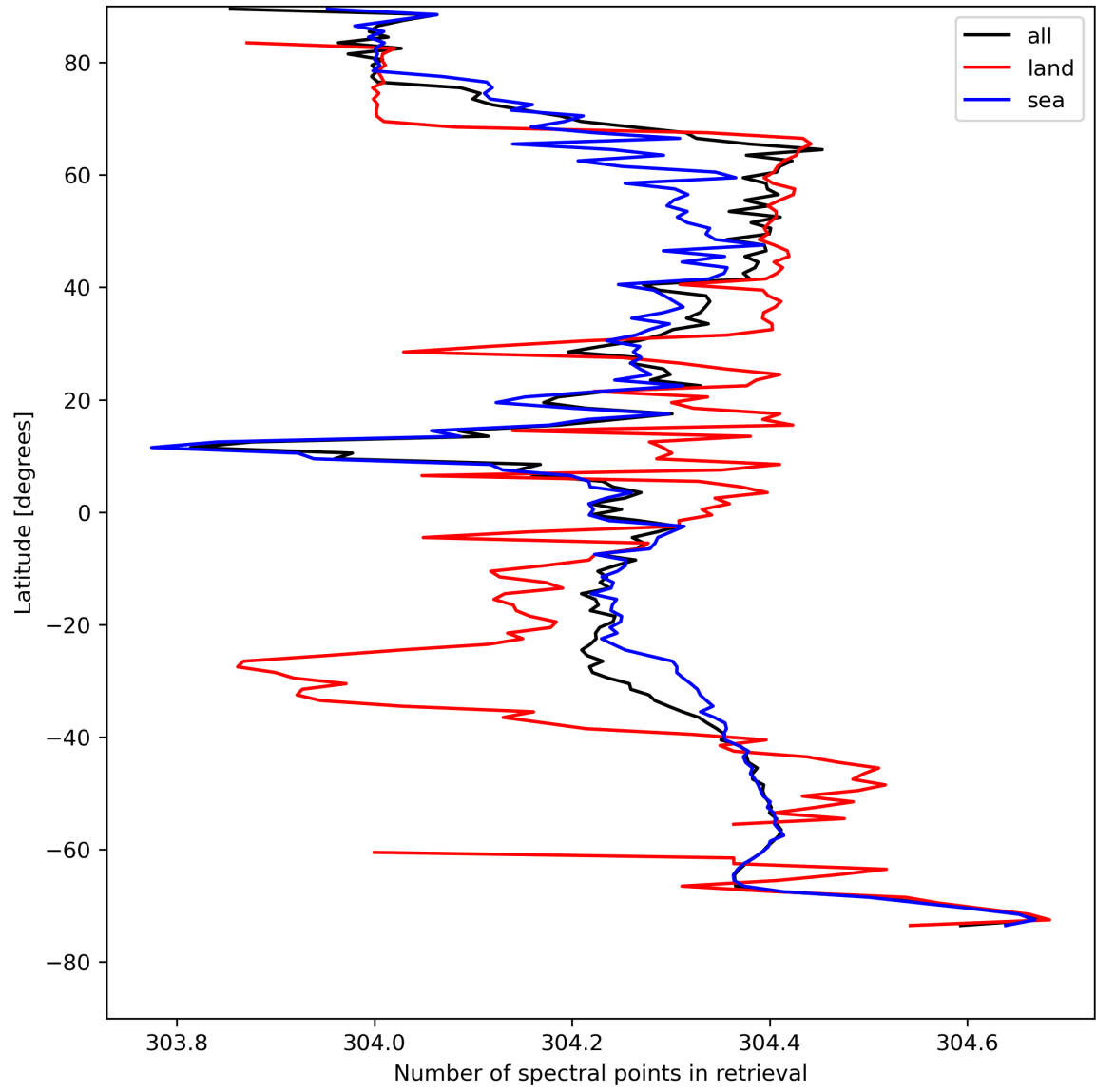
Figure 16: Zonal average of “Number of spectral points in retrieval” for 2023-08-12 to 2023-08-14.
