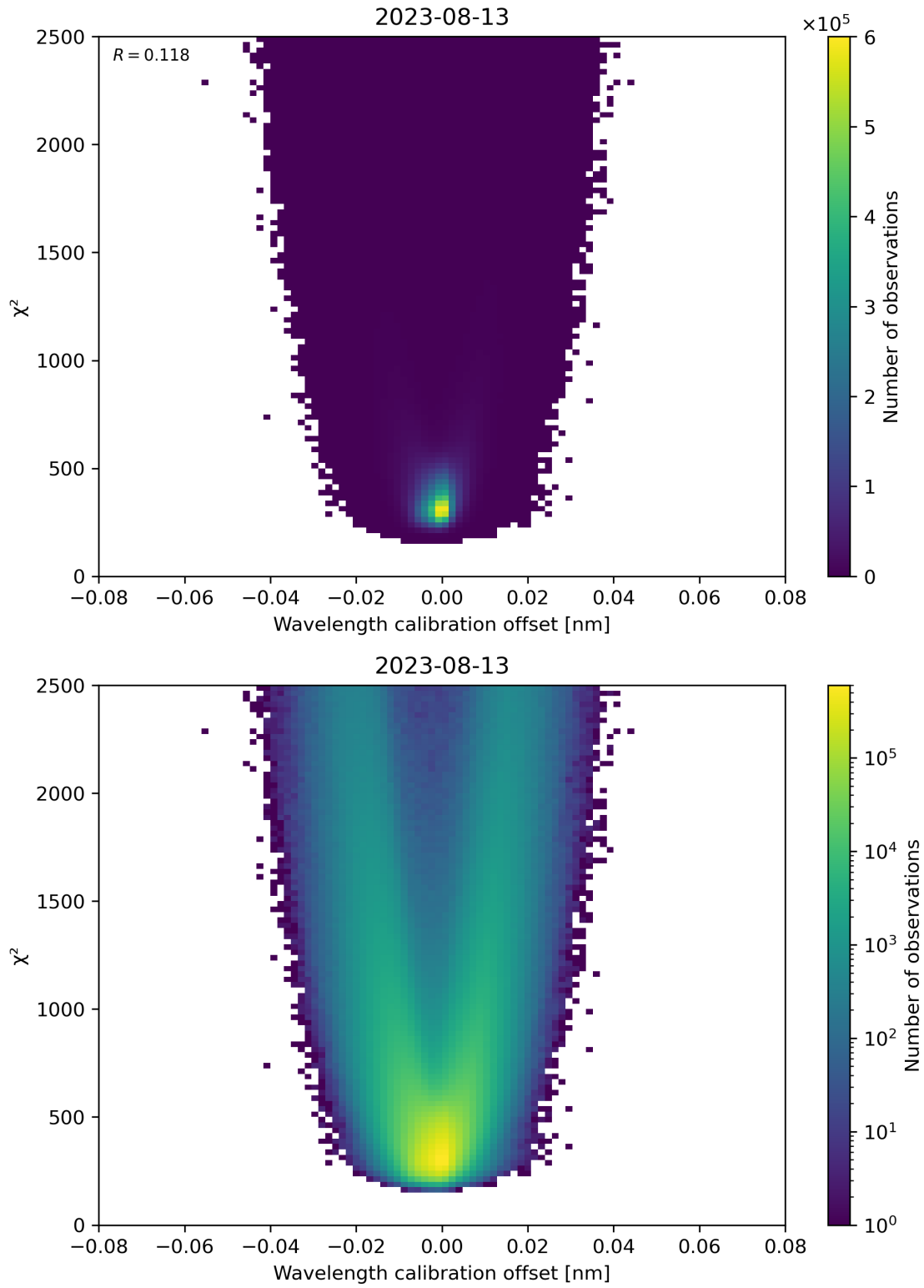
Figure 175: Scatter density plot of “Wavelength calibration offset” against “ \chi^2 ” for 2023-08-12 to 2023-08-14.
