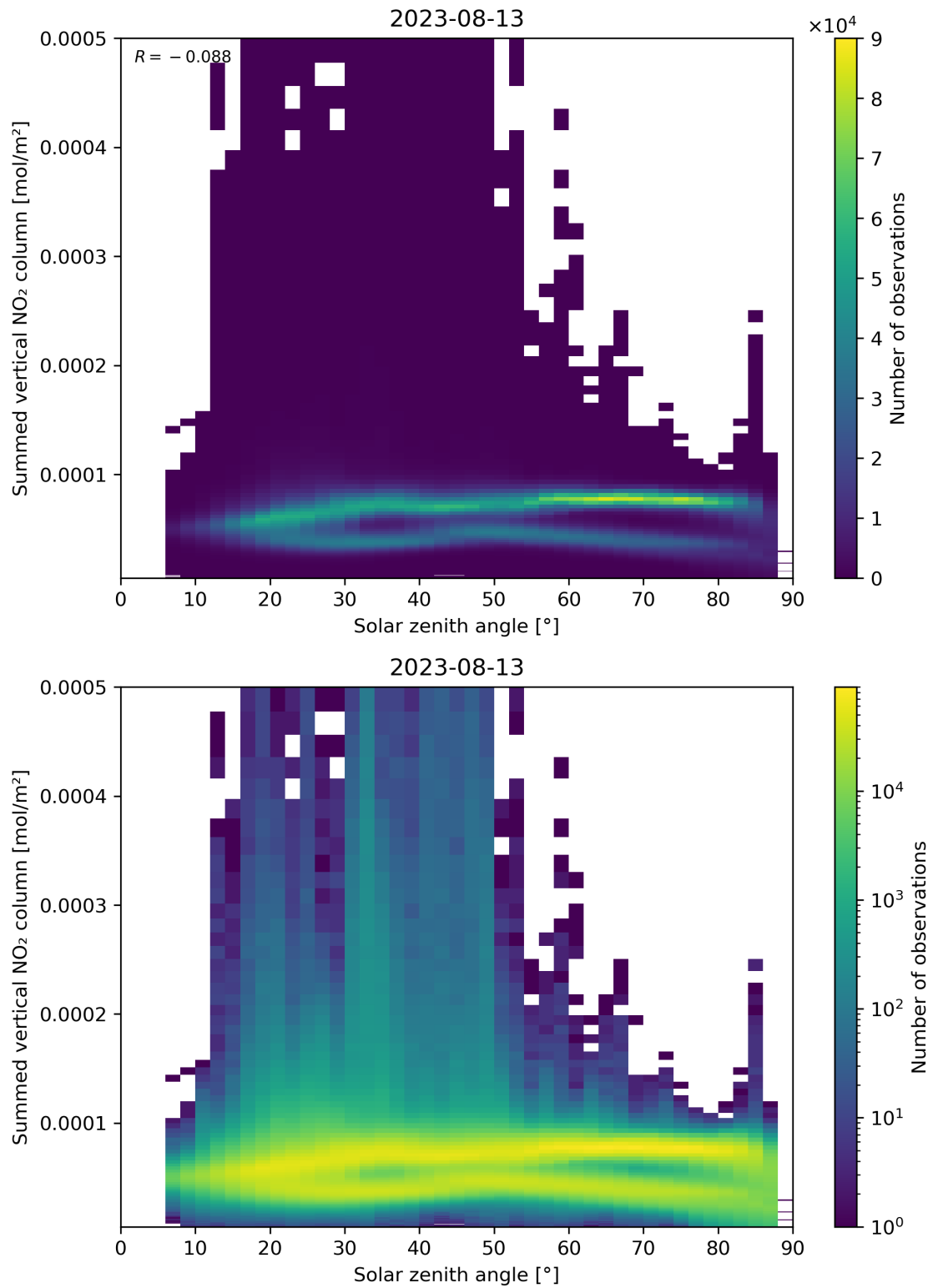
Figure 151: Scatter density plot of “Solar zenith angle” against “Summed vertical NO 2 column” for 2023-08-12 to 2023-08-14.
