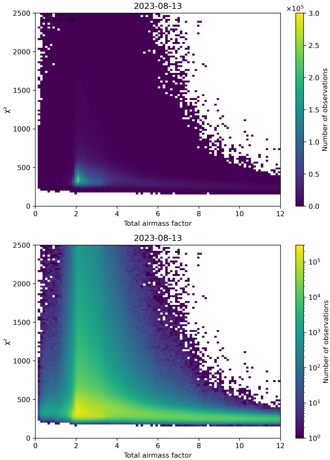
Figure 63: Scatter density plot of “Total airmass factor” against “ \chi^2 ” for 2023-08-12 to 2023-08-14.
