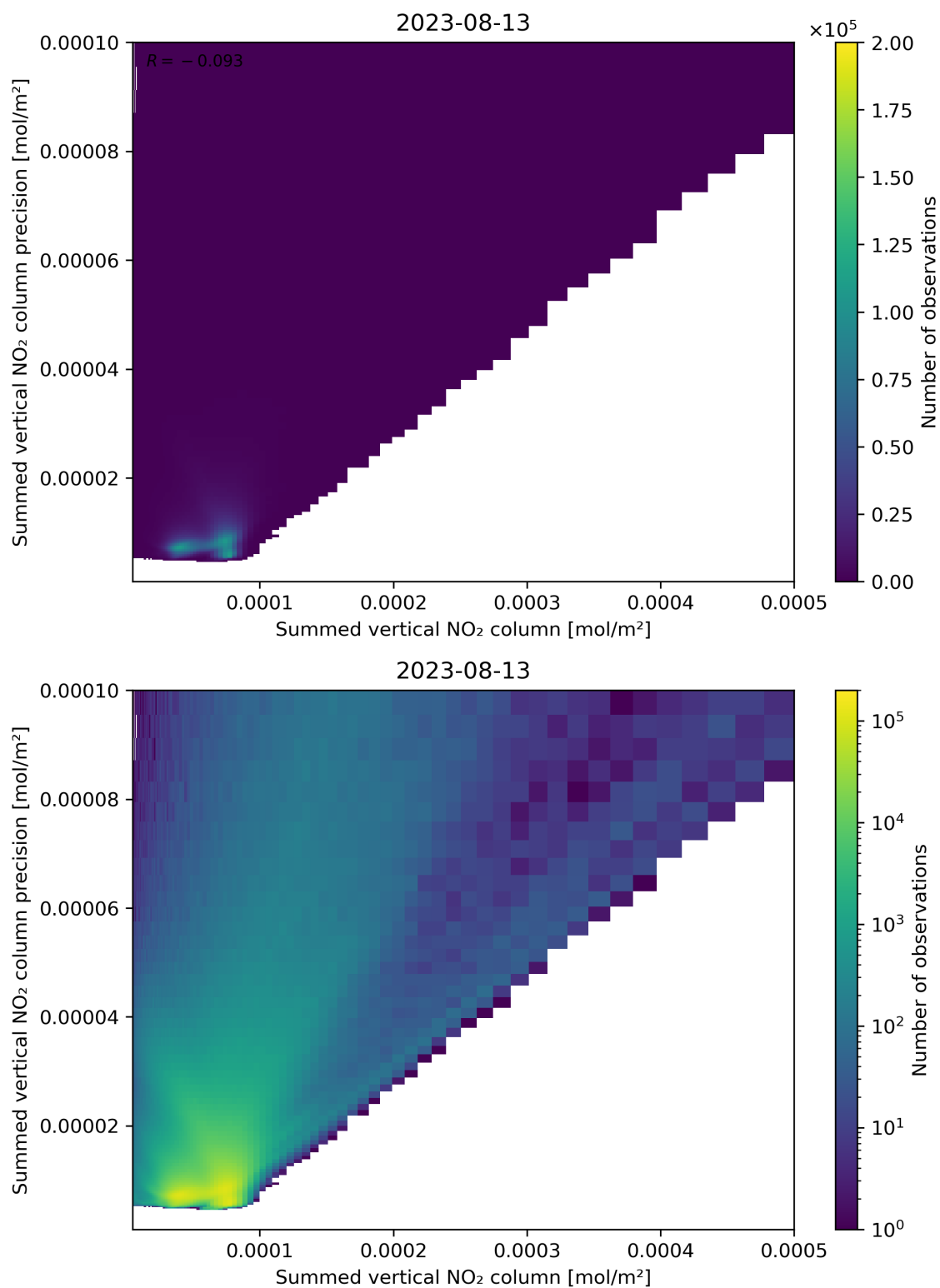
Figure 105: Scatter density plot of “Summed vertical NO 2 column” against “Summed vertical NO 2 column precision” for 2023-08-12 to 2023-08-14.
