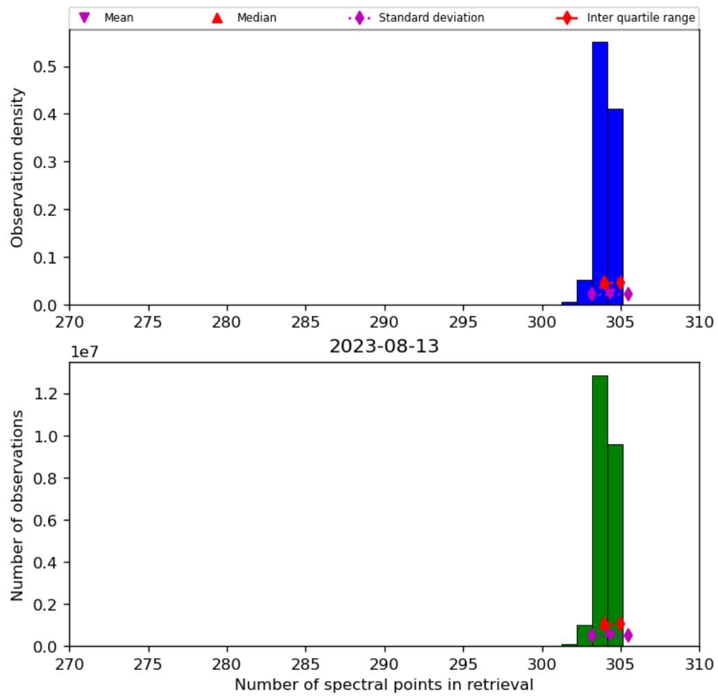
Figure 33: Histogram of “Number of spectral points in retrieval” for 2023-08-12 to 2023-08-14
