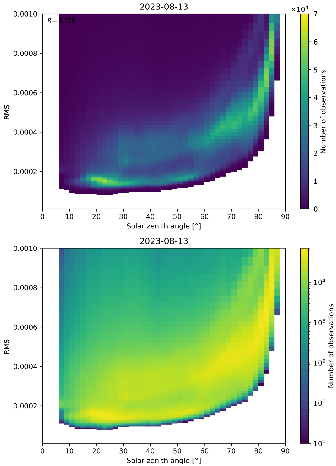
Figure 157: Scatter density plot of “Solar zenith angle” against “RMS” for 2023-08-12 to 2023-08-14.
