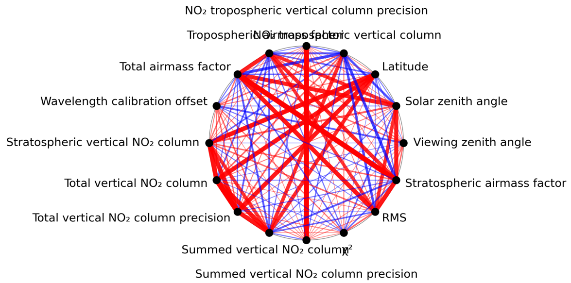
Figure 1: Map of correlation graph for 2023-08-12 to 2023-08-14.
