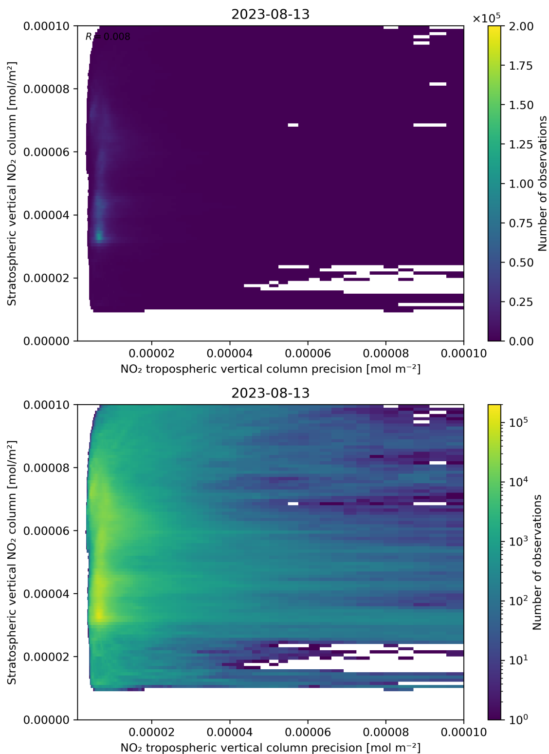
Figure 135: Scatter density plot of “NO 2 tropospheric vertical column precision” against “Stratospheric vertical NO 2 column” for 2023-08-12 to 2023-08-14.
