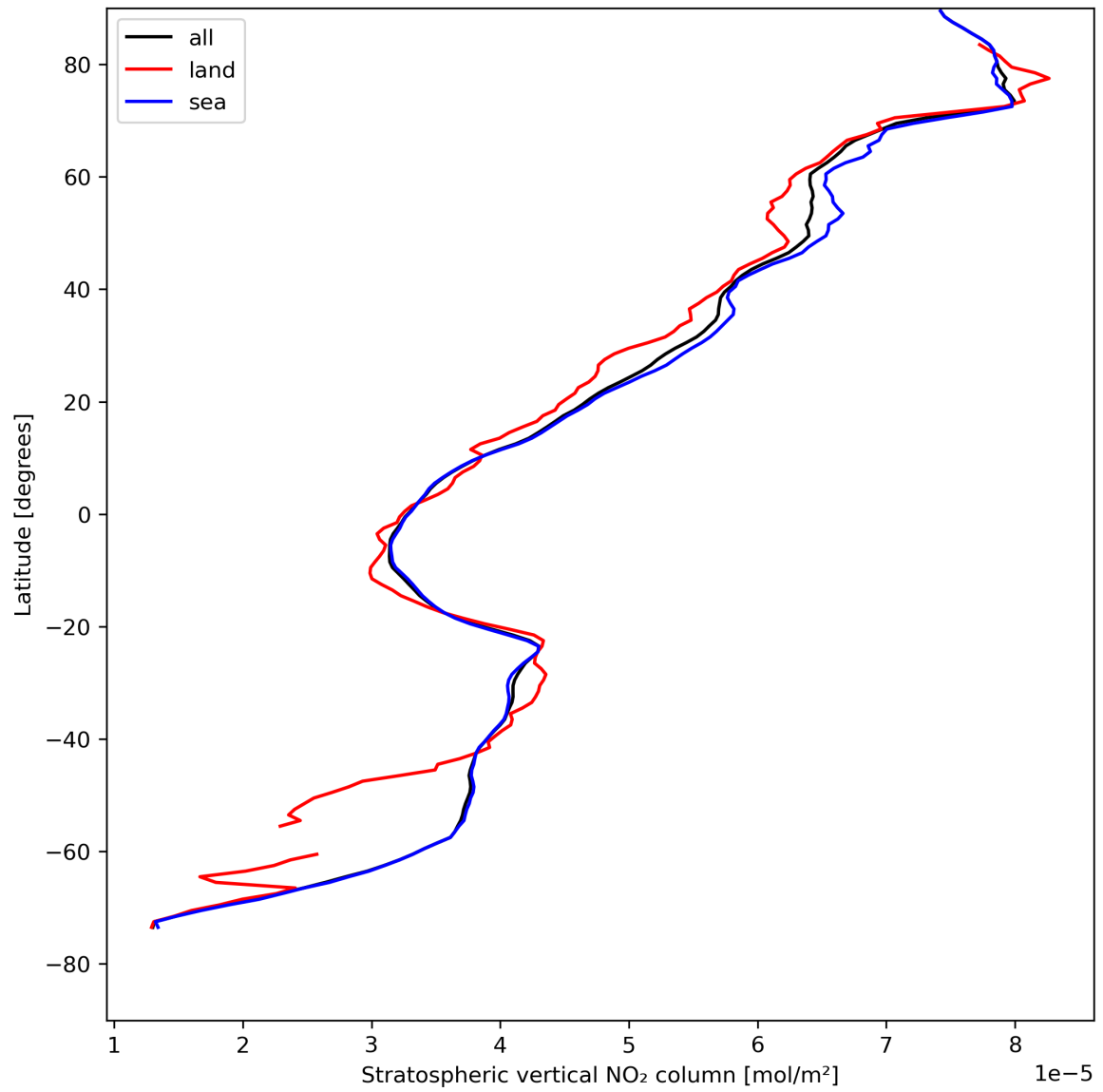
Figure 19: Zonal average of “Stratospheric vertical NO 2 column” for 2023-08-12 to 2023-08-14.
