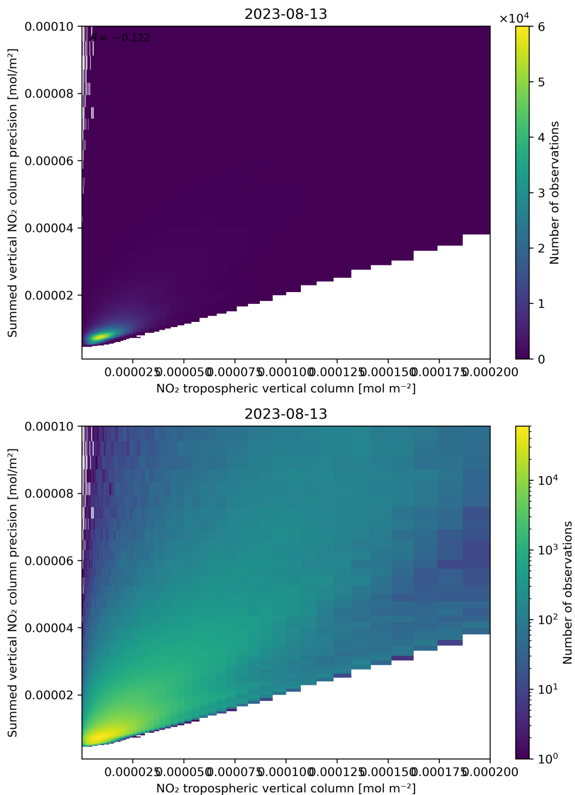
Figure 127: Scatter density plot of “NO 2 tropospheric vertical column” against “Summed vertical NO 2 column precision” for 2023-08-12 to 2023-08-14.
