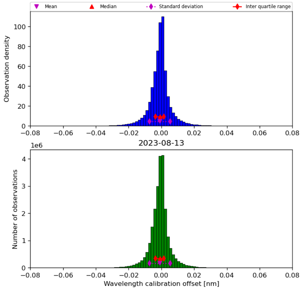
Figure 35: Histogram of “Wavelength calibration offset” for 2023-08-12 to 2023-08-14
