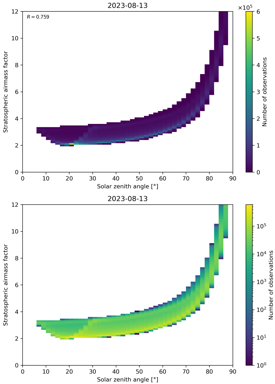
Figure 145: Scatter density plot of “Solar zenith angle” against “Stratospheric airmass factor” for 2023-08-12 to 2023-08-14.
