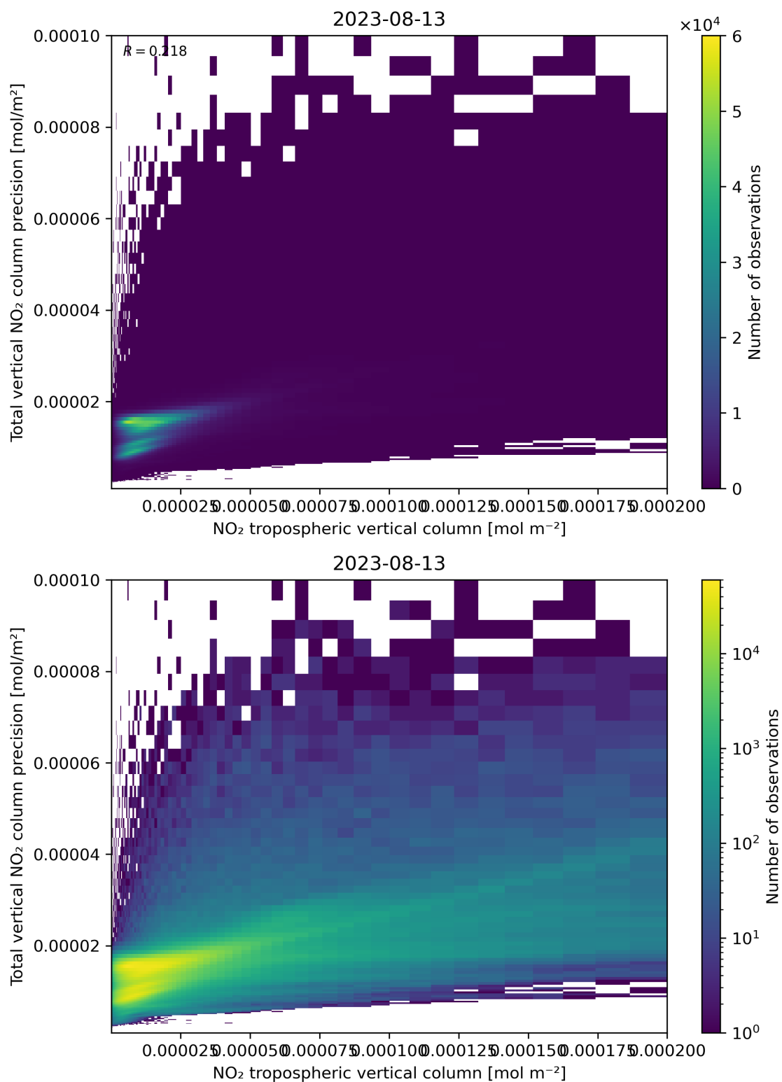
Figure 129: Scatter density plot of “NO 2 tropospheric vertical column” against “Total vertical NO 2 column precision” for 2023-08-12 to 2023-08-14.
