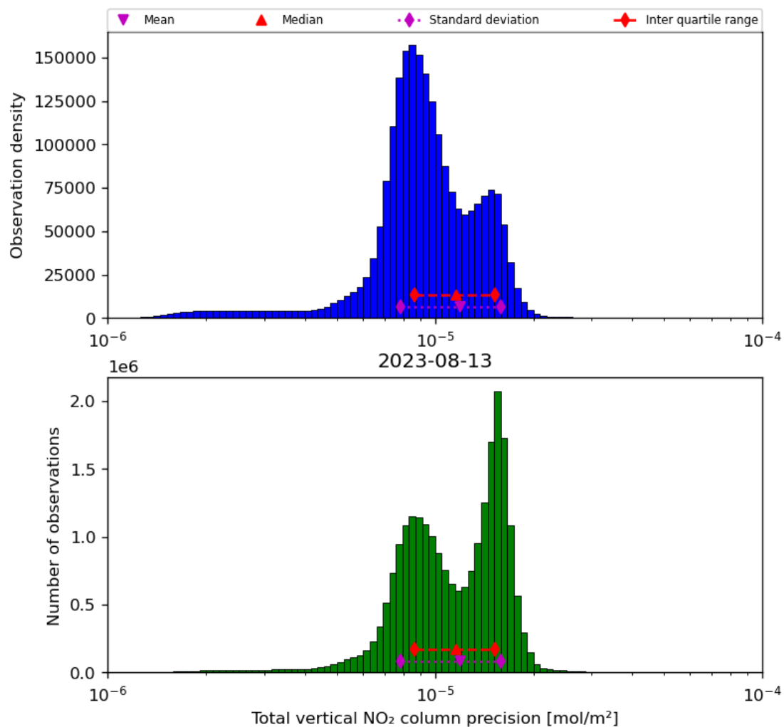
Figure 39: Histogram of “Total vertical NO 2 column precision” for 2023-08-12 to 2023-08-14
