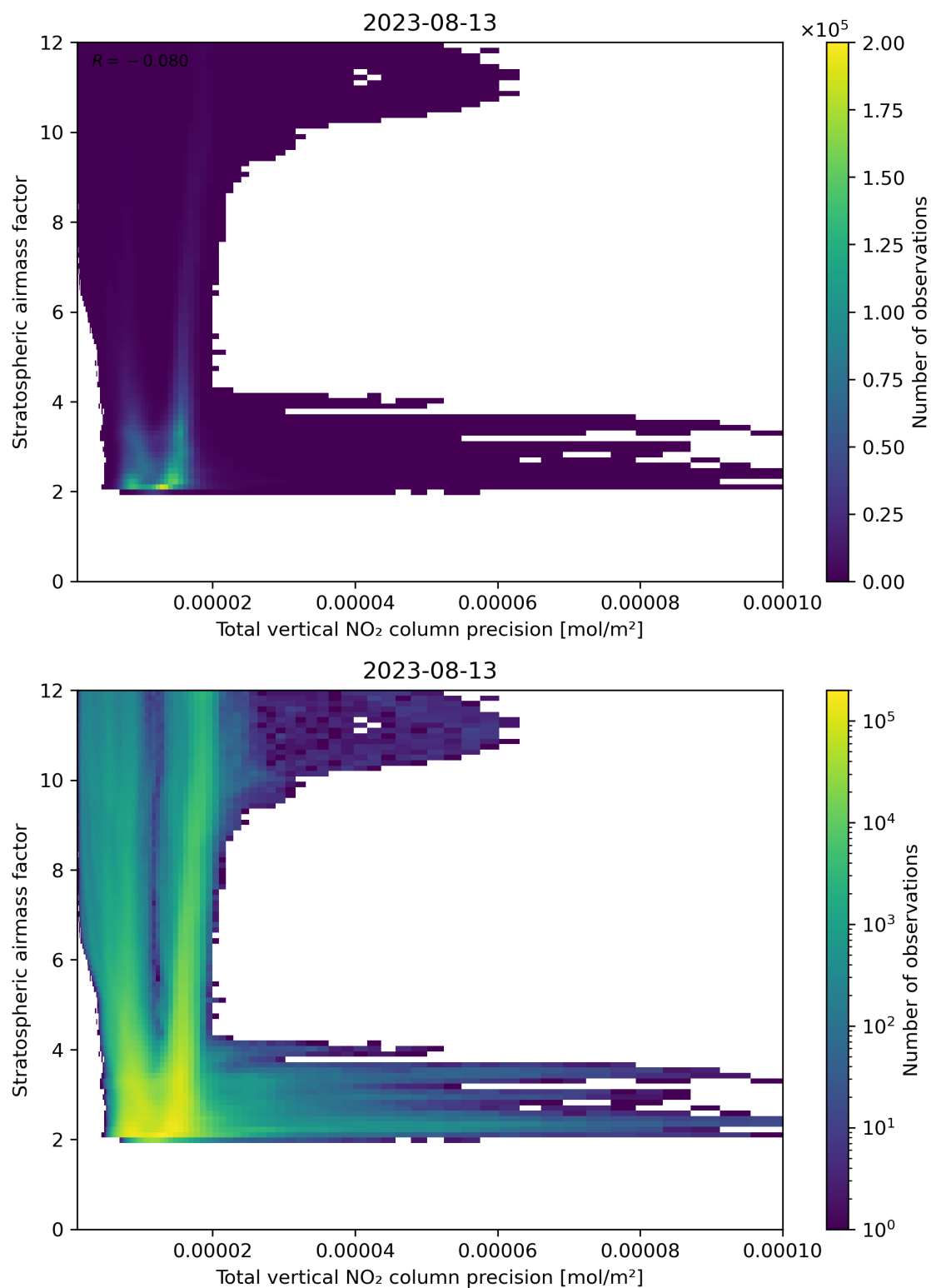
Figure 115: Scatter density plot of “Total vertical NO 2 column precision” against “Stratospheric air mass factor” for 2023-08-12 to 2023-08-14.
