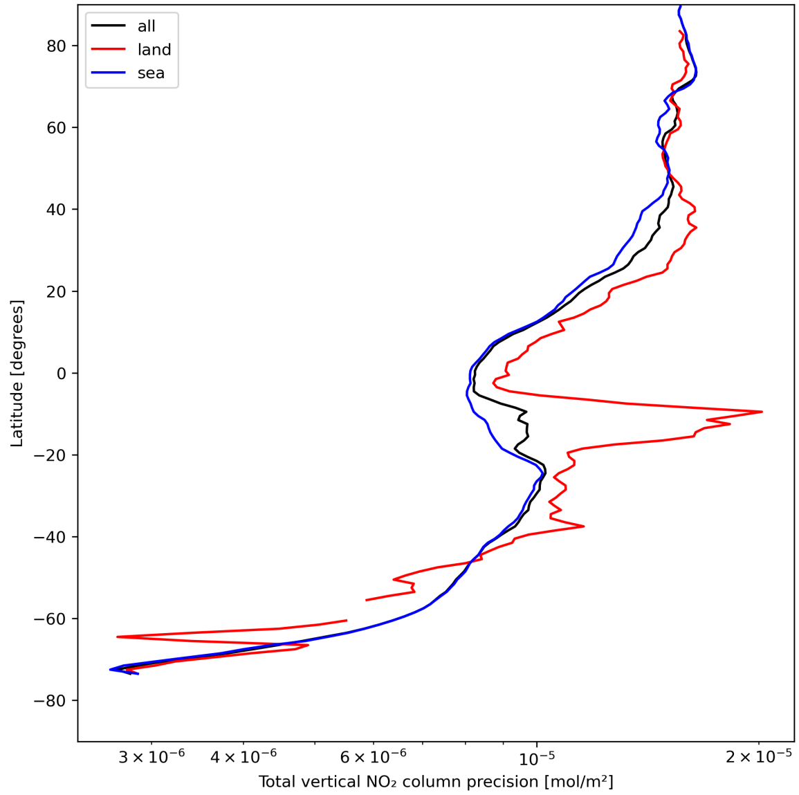
Figure 22: Zonal average of “Total vertical NO 2 column precision” for 2023-08-12 to 2023-08-14.
