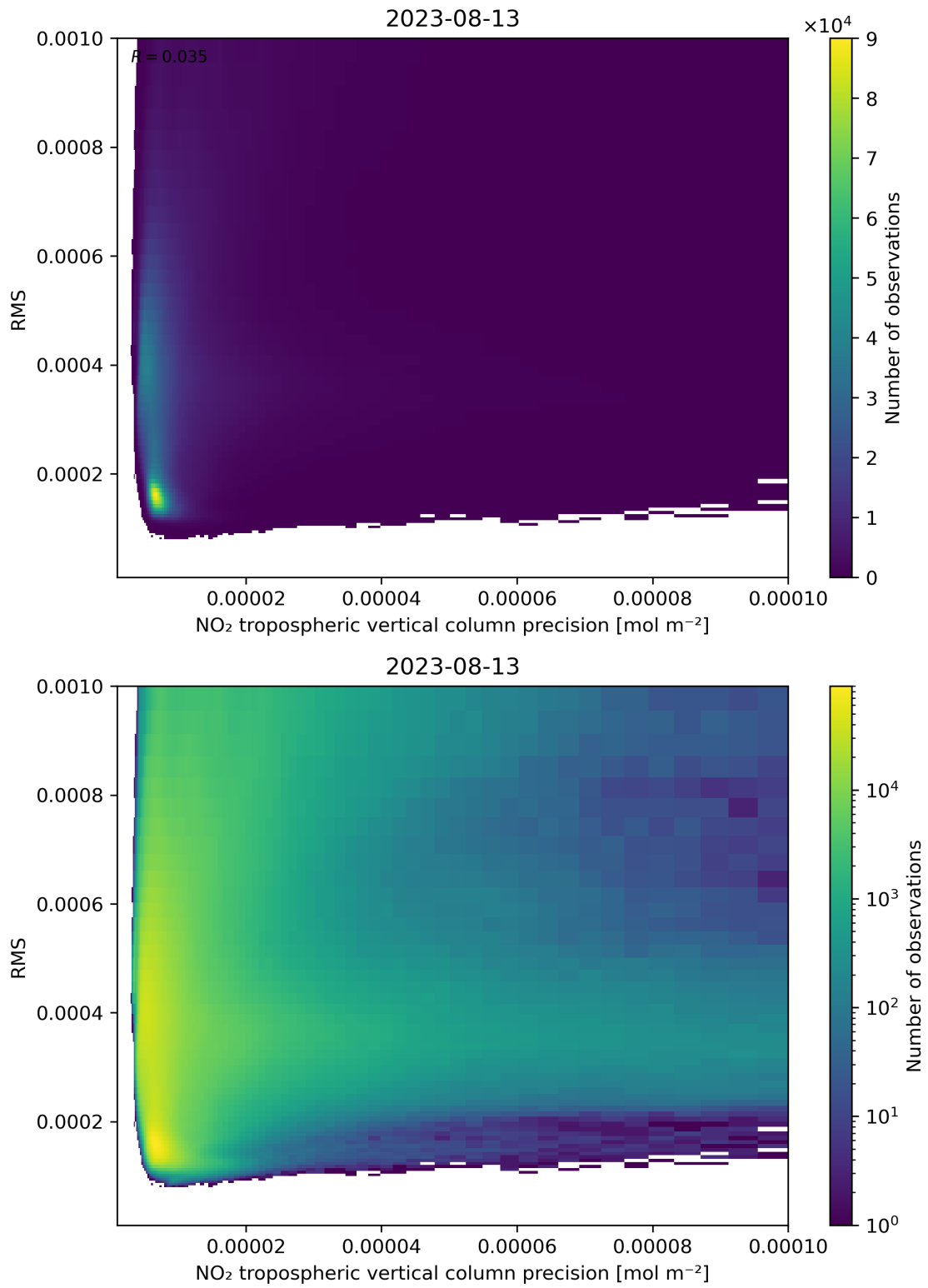
Figure 140: Scatter density plot of “NO 2 tropospheric vertical column precision” against “RMS” for 2023-08-12 to 2023-08-14.
