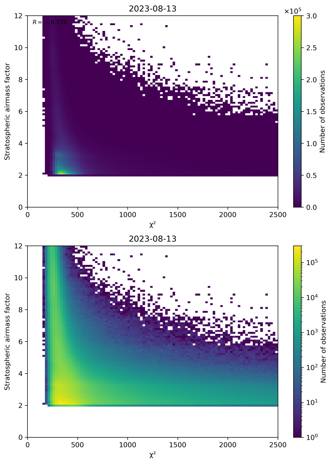
Figure 81: Scatter density plot of “ \chi^2 ” against “Stratospheric airmass factor” for 2023-08-12 to 2023-08-14.
