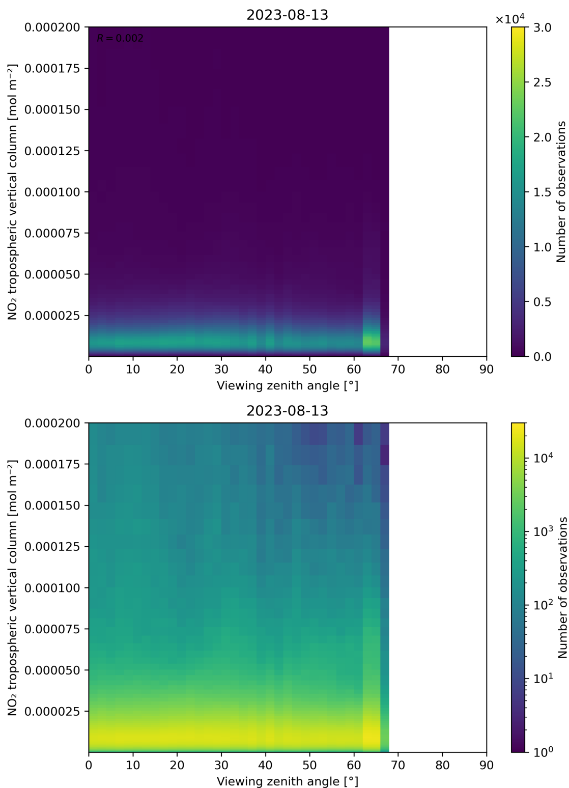
Figure 169: Scatter density plot of “Viewing zenith angle” against “NO 2 tropospheric vertical column” for 2023-08-12 to 2023-08-14.
