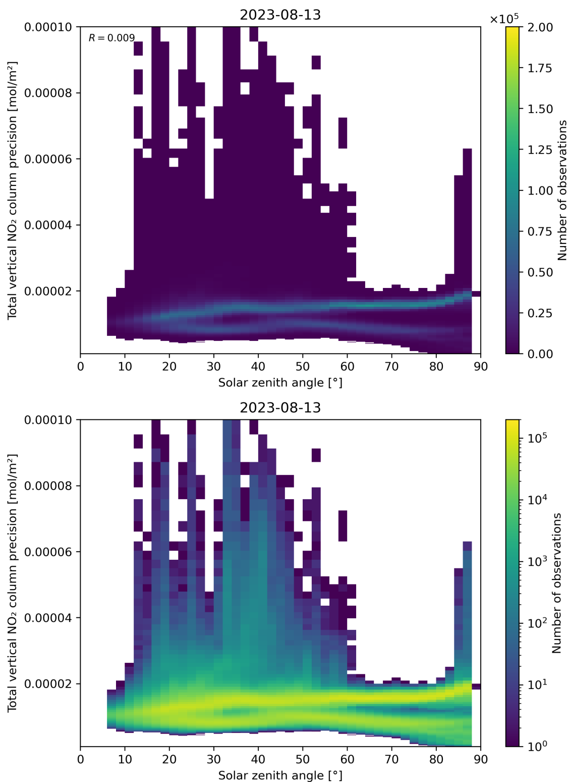
Figure 154: Scatter density plot of “Solar zenith angle” against “Total vertical NO 2 column precision” for 2023-08-12 to 2023-08-14.
