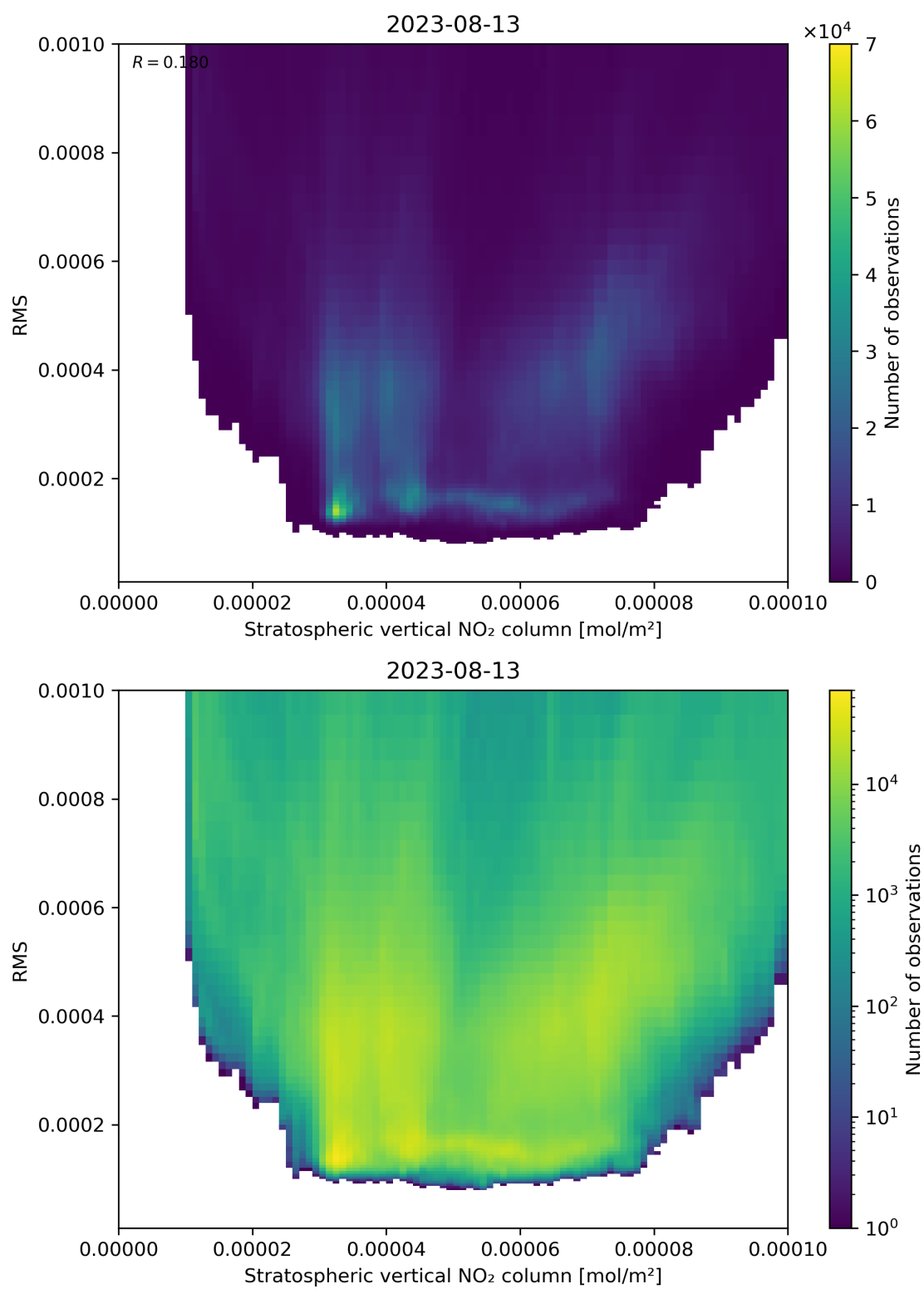
Figure 102: Scatter density plot of “Stratospheric vertical NO 2 column” against “RMS” for 2023-08-12 to 2023-08-14.
