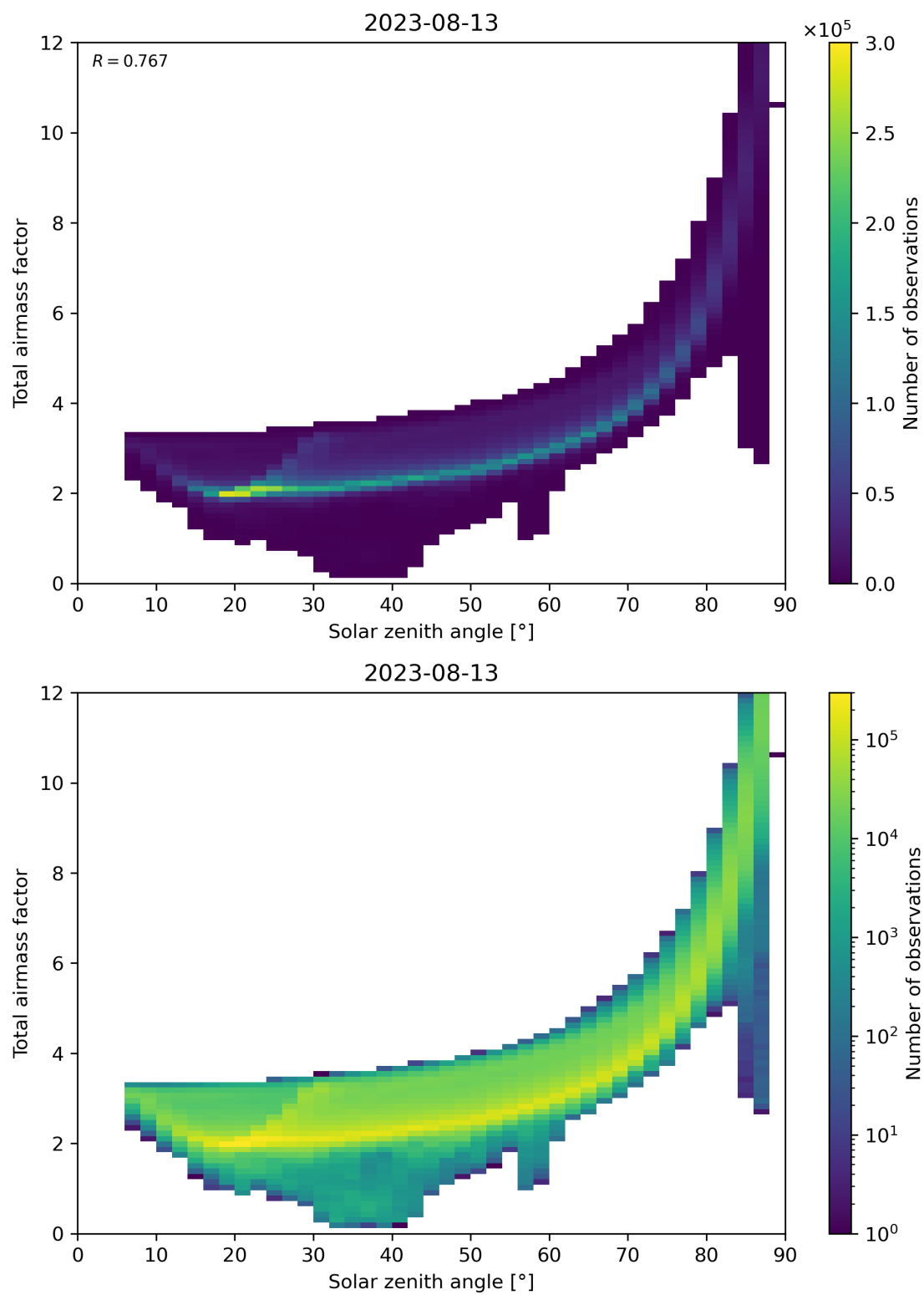
Figure 146: Scatter density plot of “Solar zenith angle” against “Total air mass factor” for 2023-08-12 to 2023-08-14.
