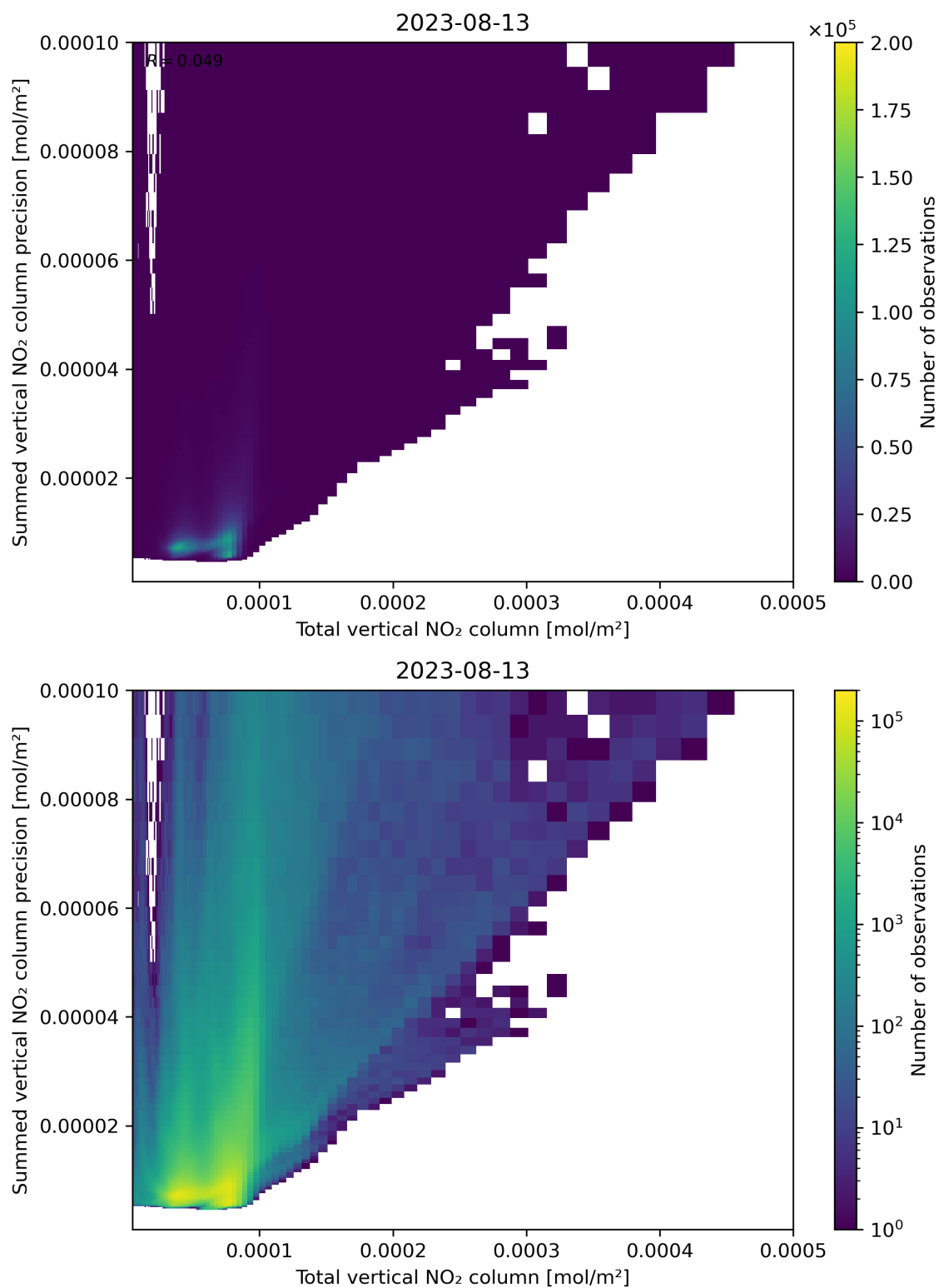
Figure 113: Scatter density plot of “Total vertical NO 2 column” against “Summed vertical NO 2 column precision” for 2023-08-12 to 2023-08-14.
