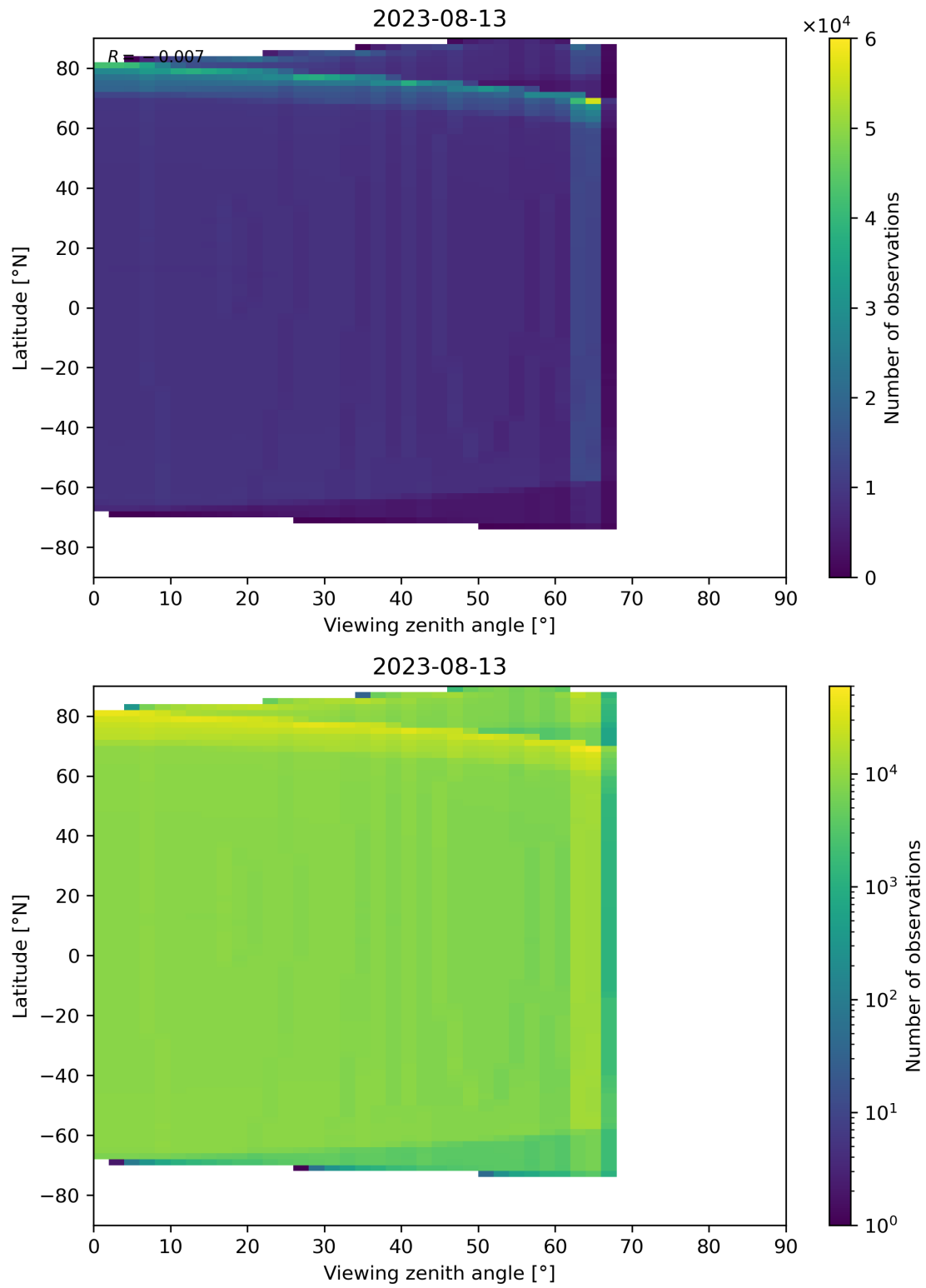
Figure 163: Scatter density plot of “Viewing zenith angle” against “Latitude” for 2023-08-12 to 2023-08-14.
