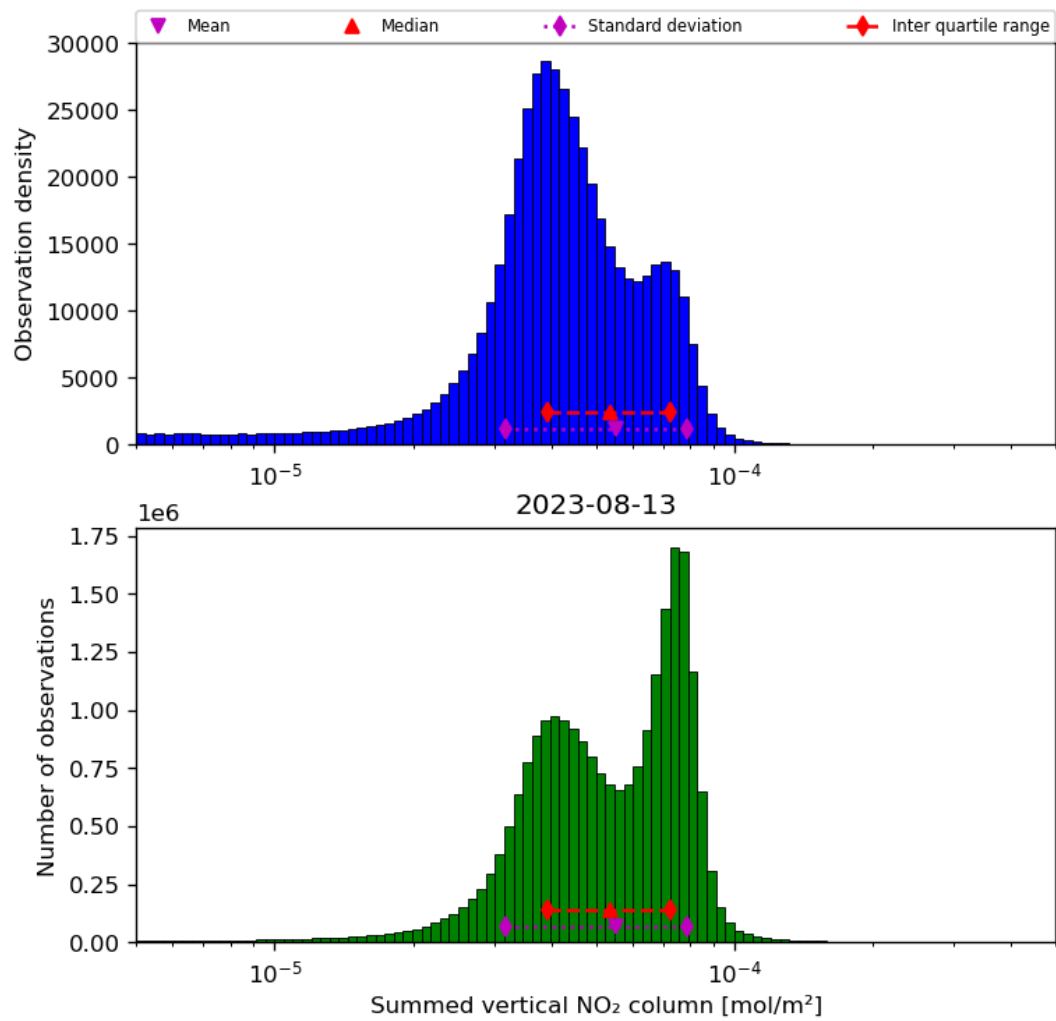
Figure 40: Histogram of “Summed vertical NO 2 column” for 2023-08-12 to 2023-08-14
