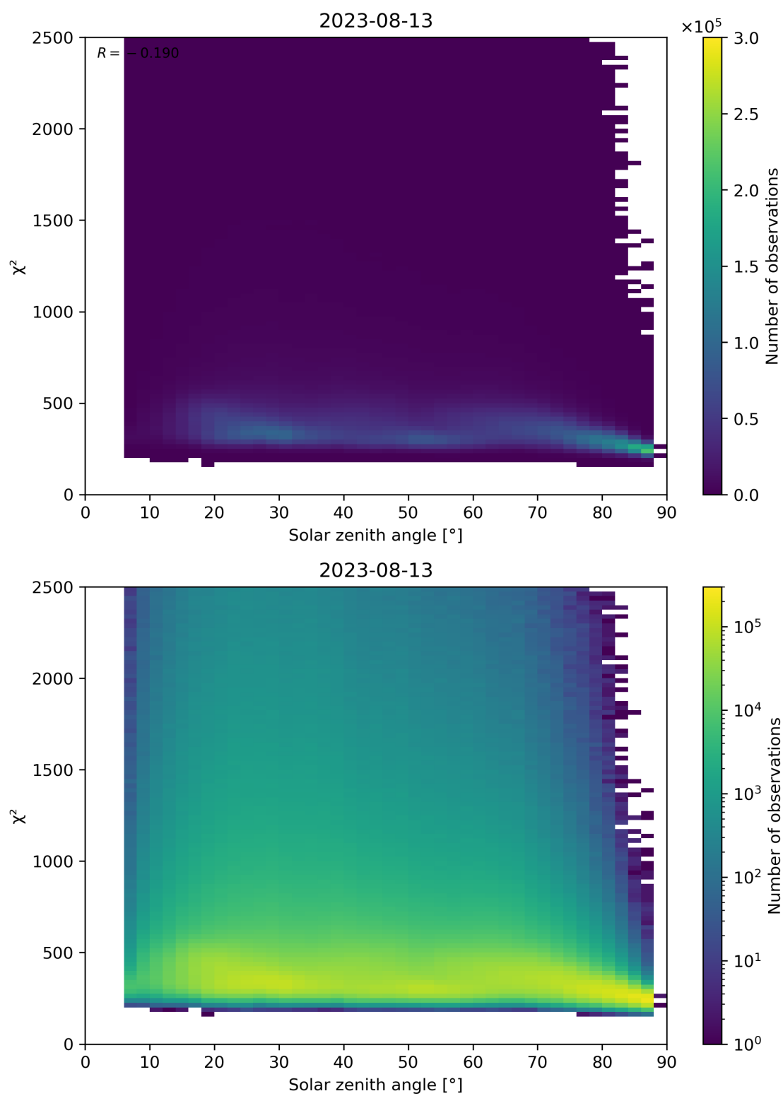
Figure 148: Scatter density plot of “Solar zenith angle” against “ \chi^2 ” for 2023-08-12 to 2023-08-14.
