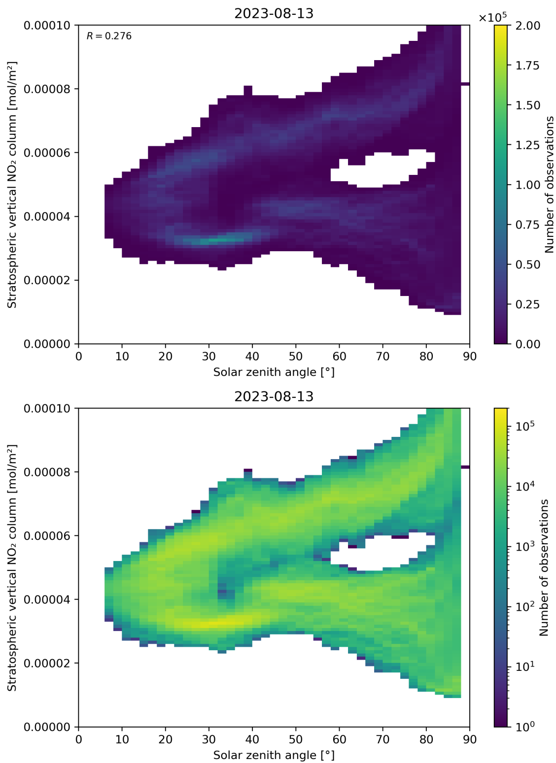
Figure 150: Scatter density plot of “Solar zenith angle” against “Stratospheric vertical \text{NO}_2 column” for 2023-08-12 to 2023-08-14.
