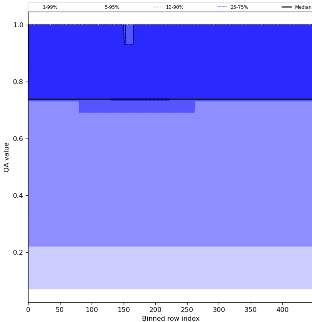
Figure 45: Along track statistics of “QA value” for 2023-08-12 to 2023-08-14
