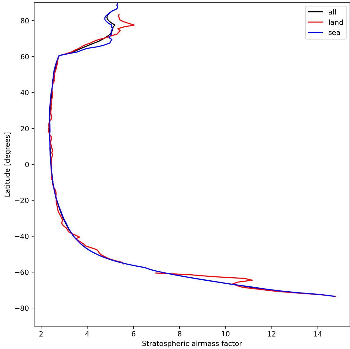
Figure 27: Zonal average of “Stratospheric air mass factor” for 2023-08-12 to 2023-08-14.
