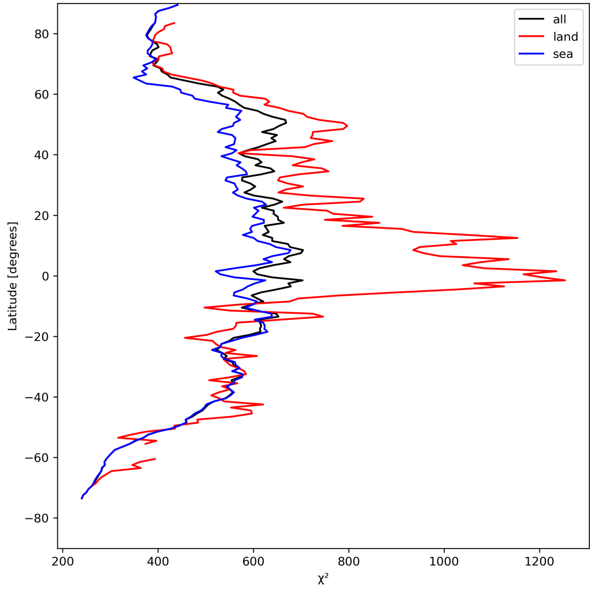
Figure 25: Zonal average of “ \chi^2 ” for 2023-08-12 to 2023-08-14.
