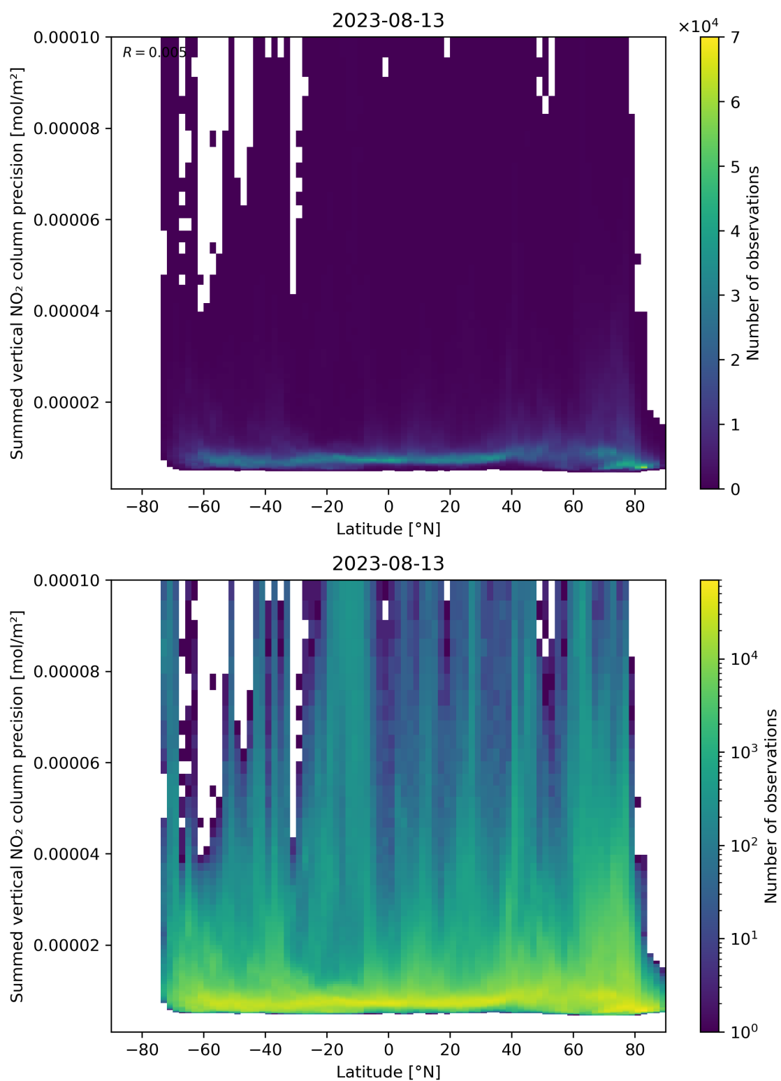
Figure 89: Scatter density plot of “Latitude” against “Summed vertical NO 2 column precision” for 2023-08-12 to 2023-08-14.
