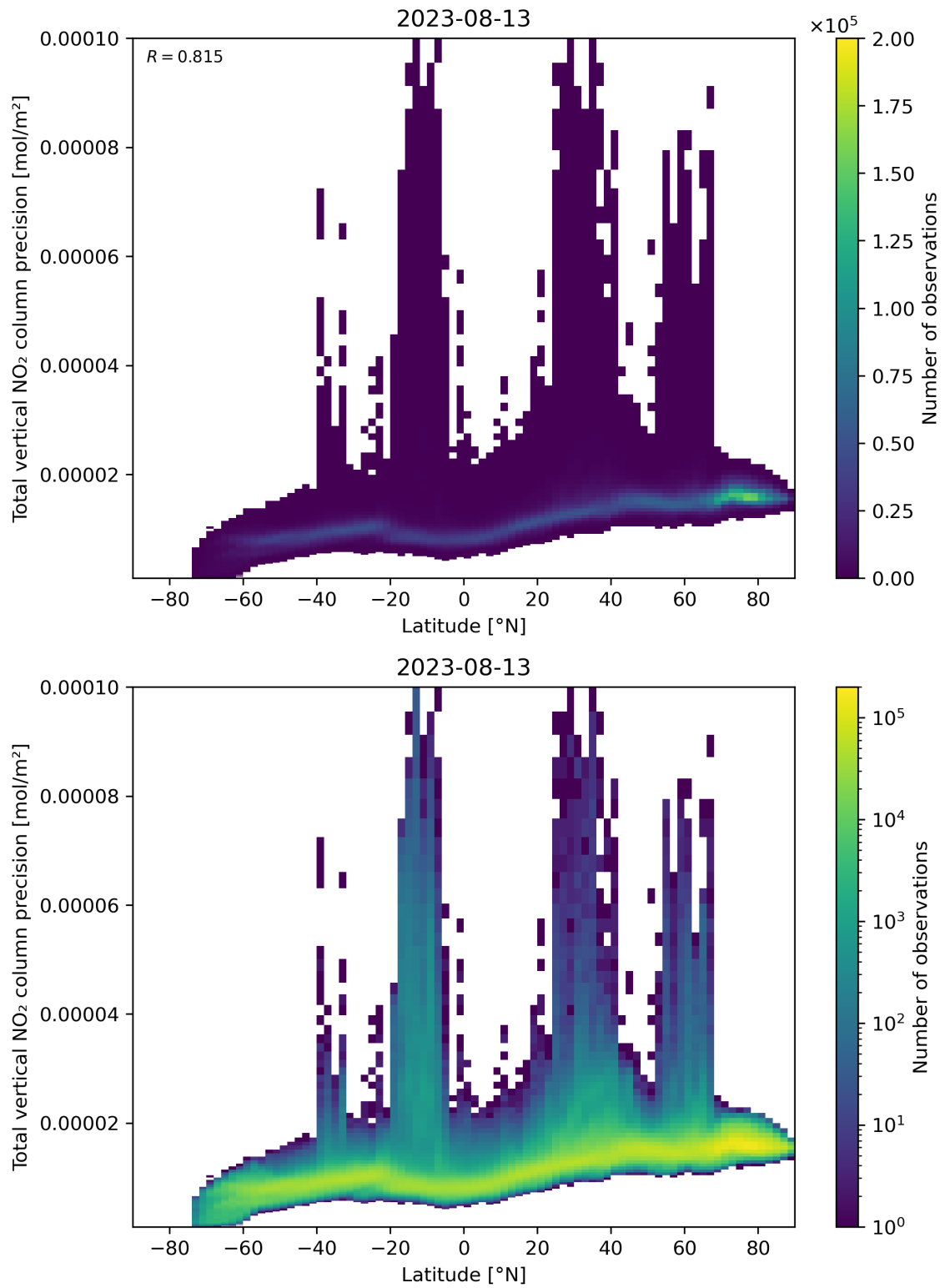
Figure 91: Scatter density plot of “Latitude” against “Total vertical NO 2 column precision” for 2023-08-12 to 2023-08-14.
