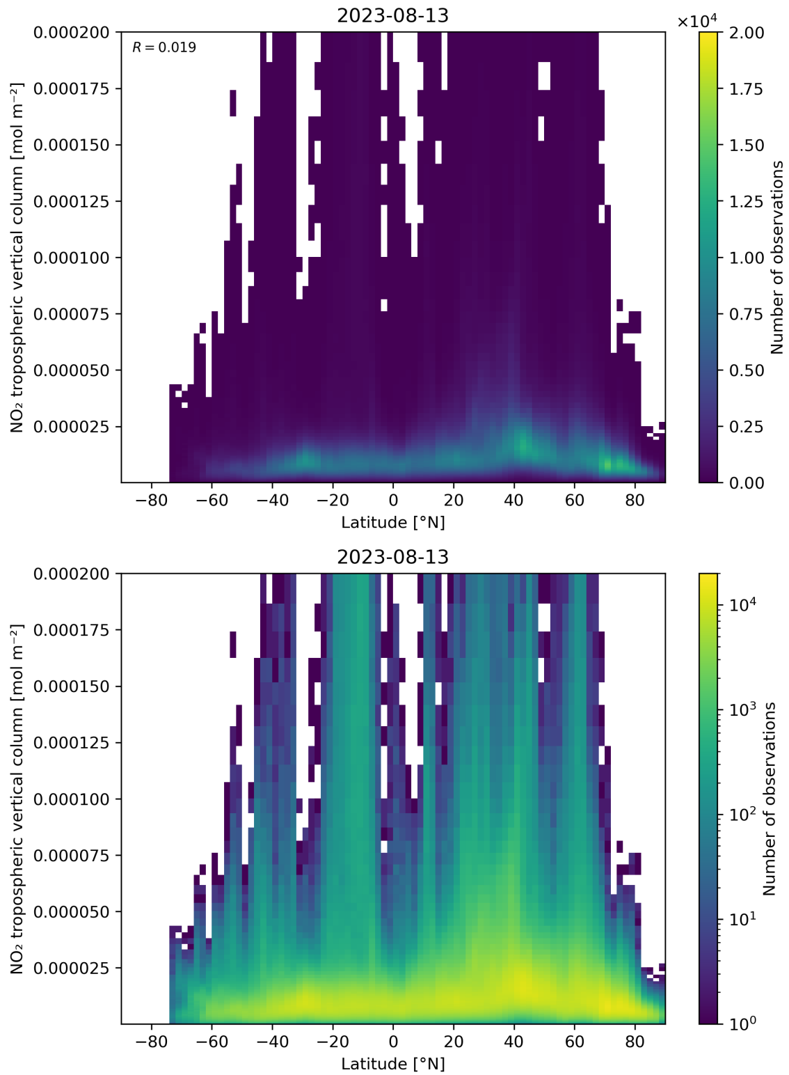
Figure 92: Scatter density plot of “Latitude” against “NO 2 tropospheric vertical column” for 2023-08-12 to 2023-08-14.
