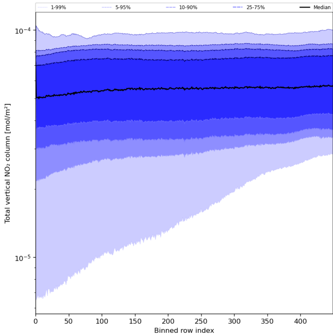
Figure 55: Along track statistics of “Total vertical NO 2 column” for 2023-08-12 to 2023-08-14
