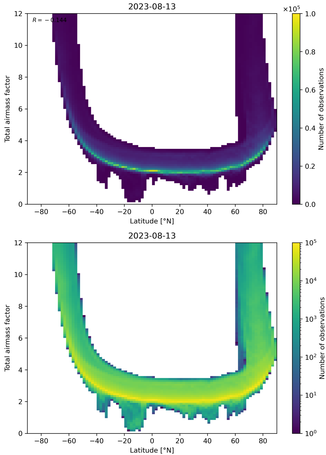
Figure 84: Scatter density plot of “Latitude” against “Total airmass factor” for 2023-08-12 to 2023-08-14.
