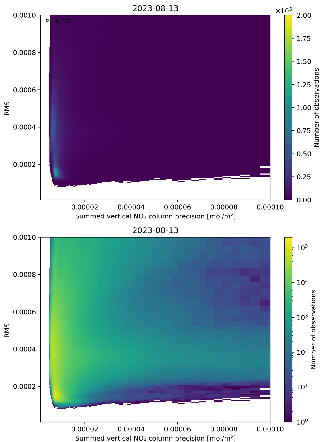
Figure 108: Scatter density plot of “Summed vertical NO 2 column precision” against “RMS” for 2023-08-12 to 2023-08-14.
