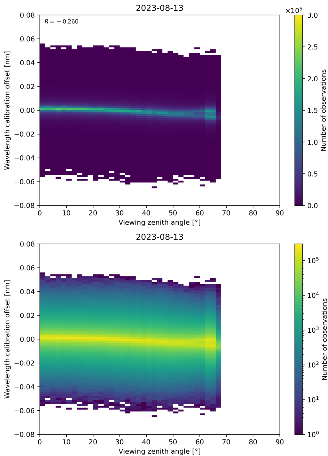
Figure 173: Scatter density plot of “Viewing zenith angle” against “Wavelength calibration offset” for 2023-08-12 to 2023-08-14.
