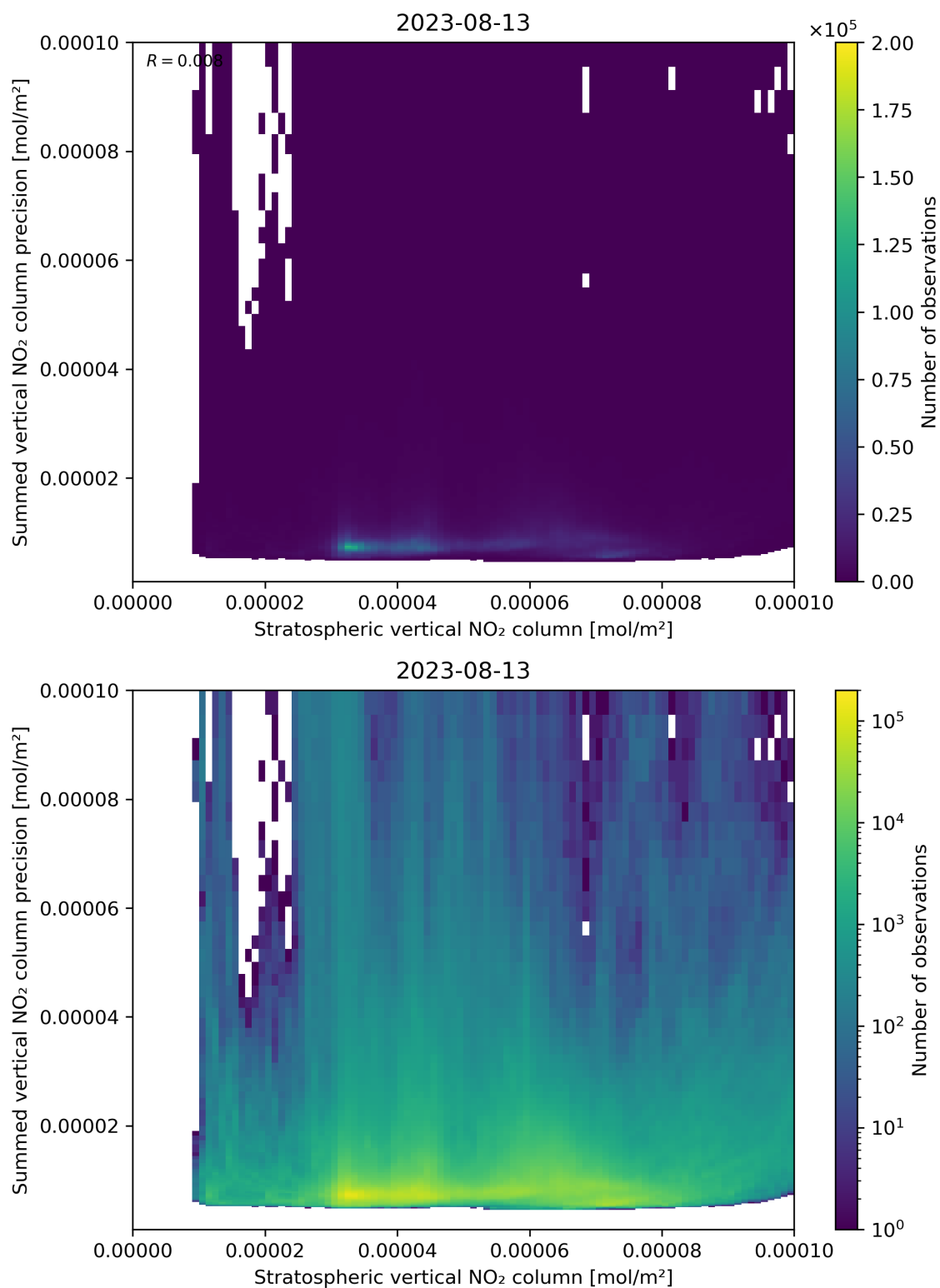
Figure 99: Scatter density plot of “Stratospheric vertical NO 2 column” against “Summed vertical NO 2 column precision” for 2023-08-12 to 2023-08-14.
