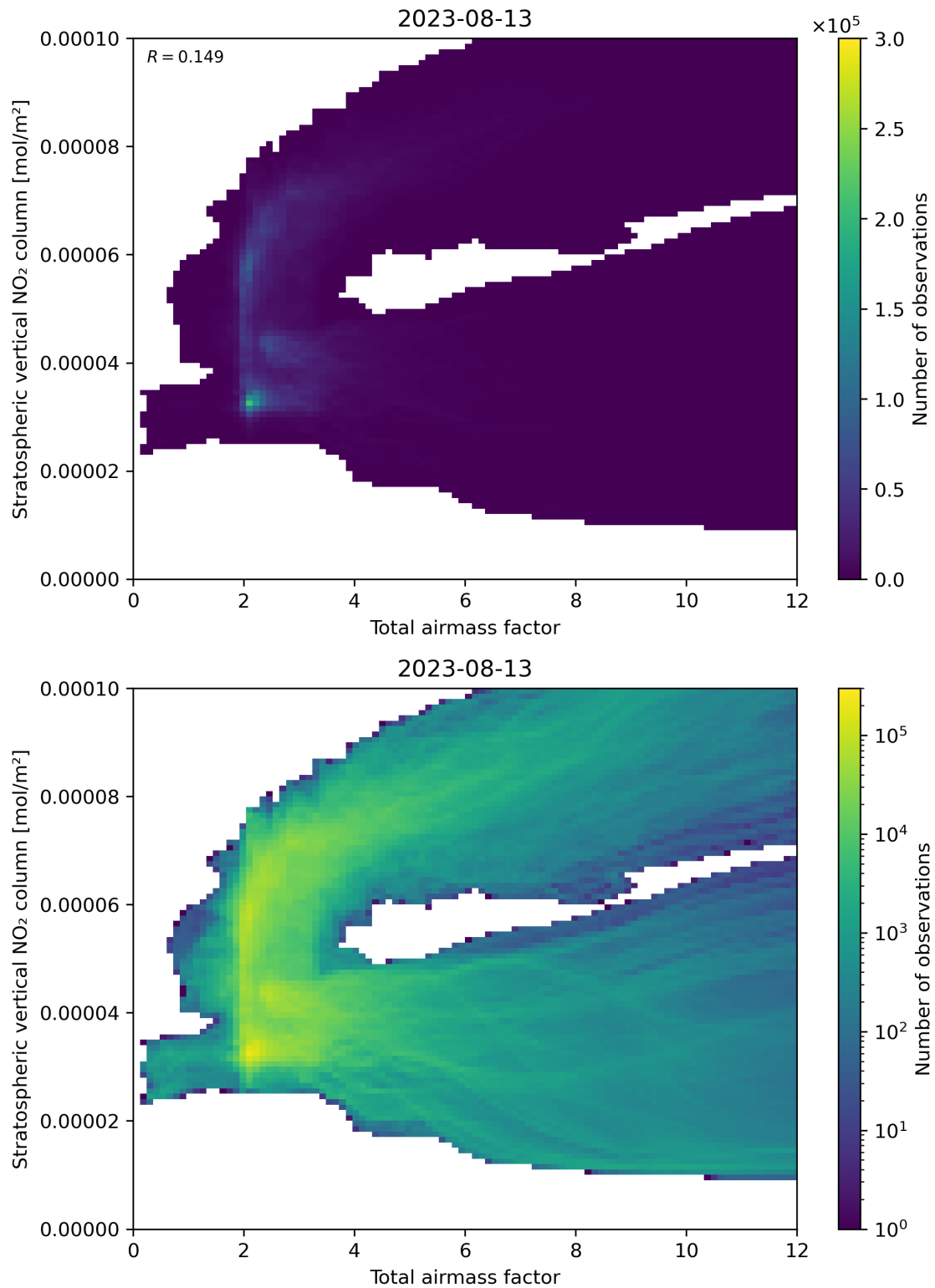
Figure 64: Scatter density plot of “Total airmass factor” against “Stratospheric vertical \text{NO}_2 column” for 2023-08-12 to 2023-08-14.
