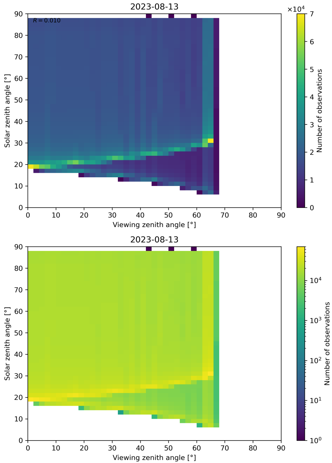
Figure 172: Scatter density plot of “Viewing zenith angle” against “Solar zenith angle” for 2023-08-12 to 2023-08-14.
