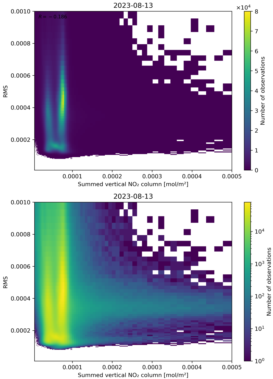
Figure 109: Scatter density plot of “Summed vertical NO 2 column” against “RMS” for 2023-08-12 to 2023-08-14.
