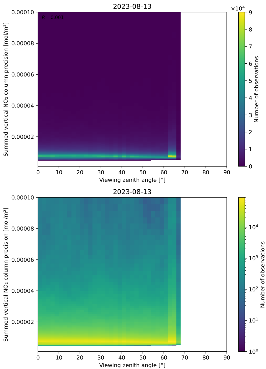
Figure 166: Scatter density plot of “Viewing zenith angle” against “Summed vertical NO 2 column precision” for 2023-08-12 to 2023-08-14.
