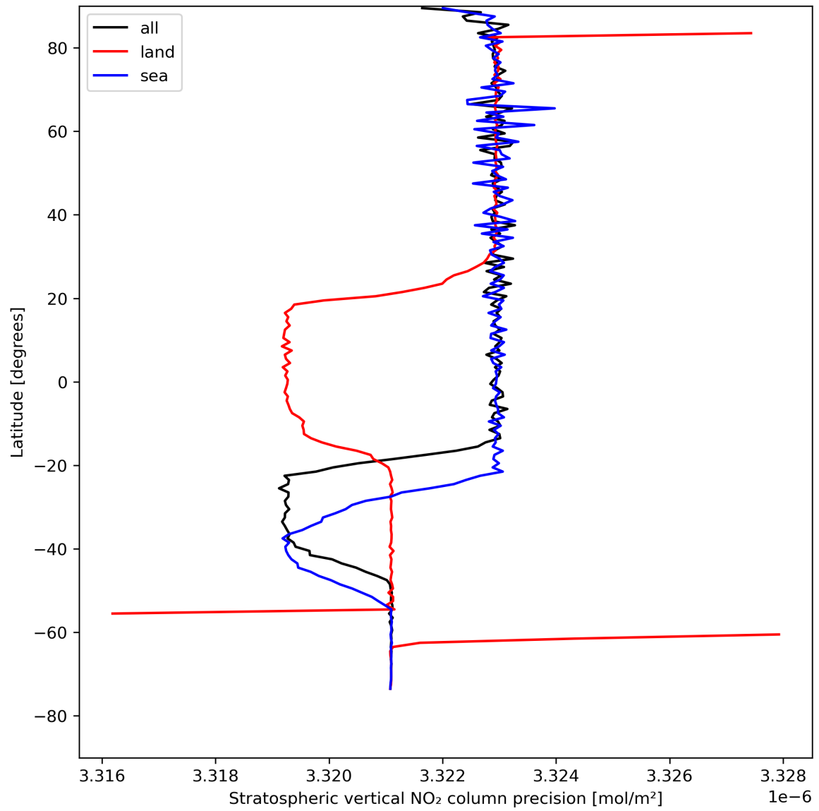
Figure 20: Zonal average of “Stratospheric vertical NO 2 column precision” for 2023-08-12 to 2023-08-14.
