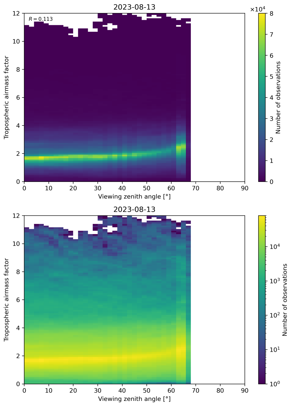
Figure 161: Scatter density plot of “Viewing zenith angle” against “Tropospheric airmass factor” for 2023-08-12 to 2023-08-14.
