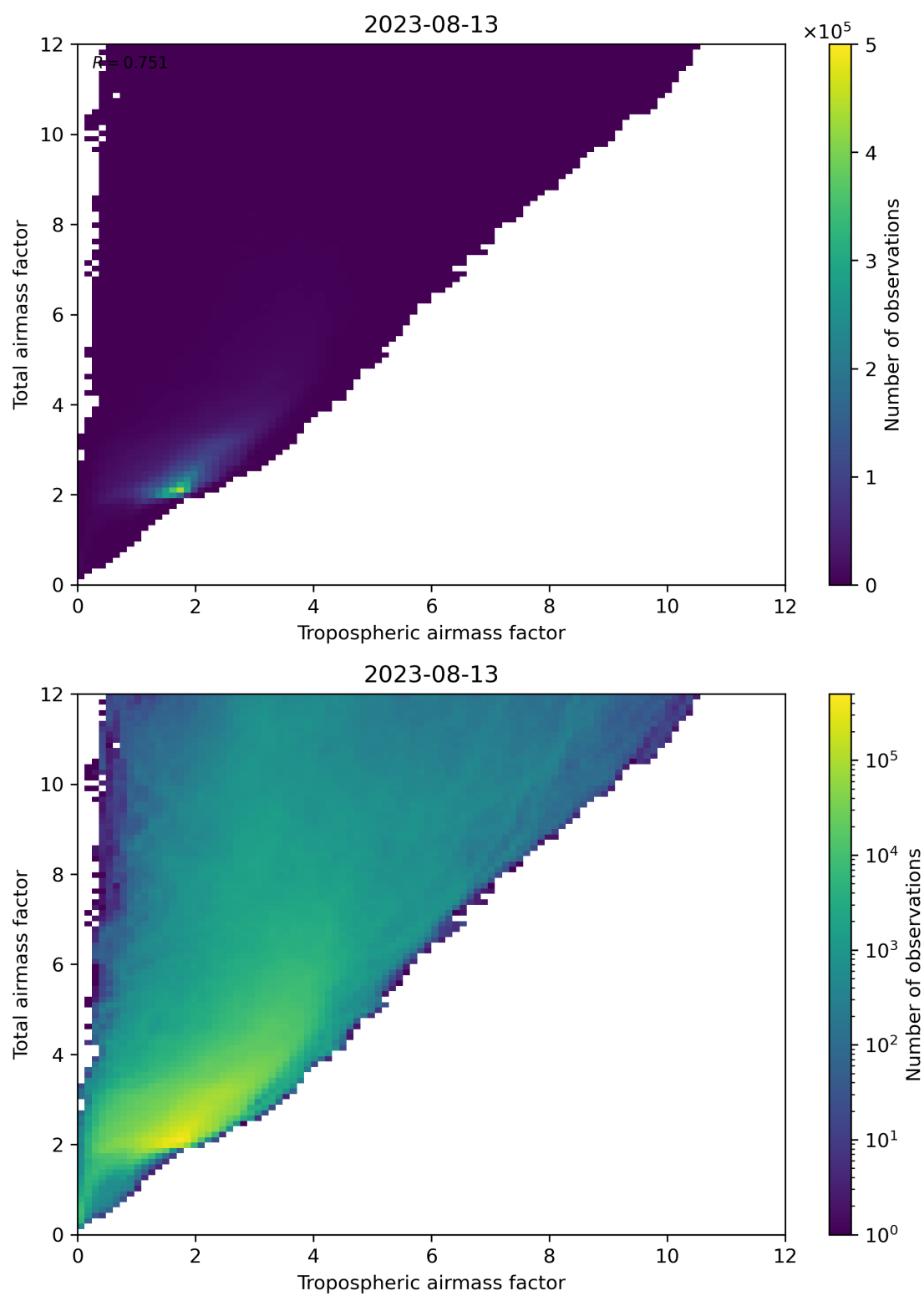
Figure 72: Scatter density plot of “Tropospheric airmass factor” against “Total airmass factor” for 2023-08-12 to 2023-08-14.
