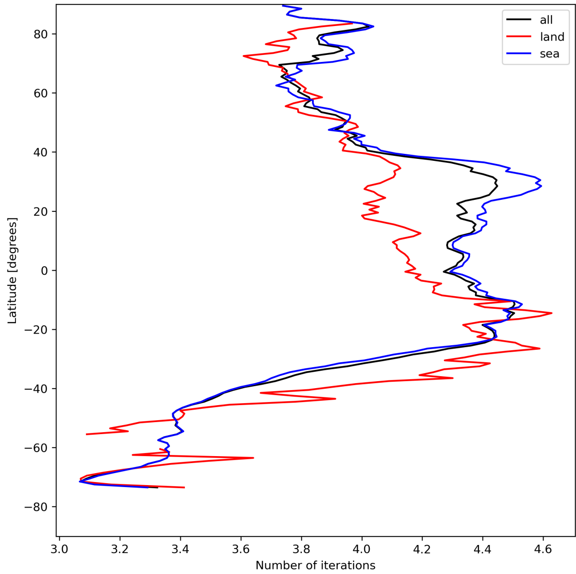
Figure 17: Zonal average of “Number of iterations” for 2023-08-12 to 2023-08-14.
