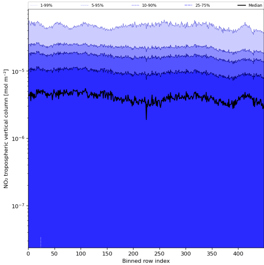
Figure 46: Along track statistics of “NO 2 tropospheric vertical column” for 2023-08-12 to 2023-08-14
