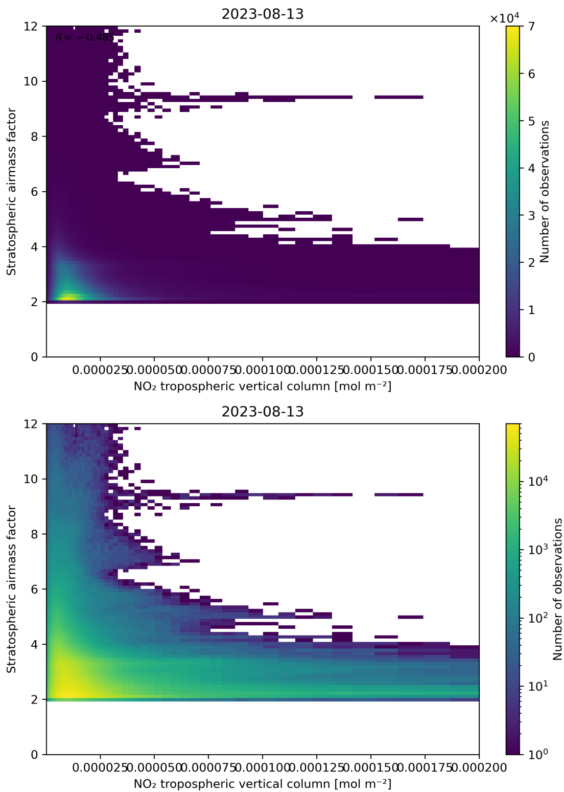
Figure 121: Scatter density plot of “NO 2 tropospheric vertical column” against “Stratospheric air mass factor” for 2023-08-12 to 2023-08-14.
