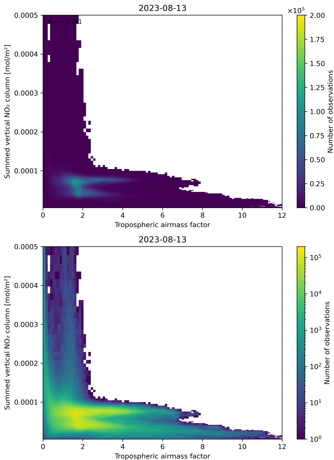
Figure 75: Scatter density plot of “Tropospheric airmass factor” against “Summed vertical NO 2 column” for 2023-08-12 to 2023-08-14.
