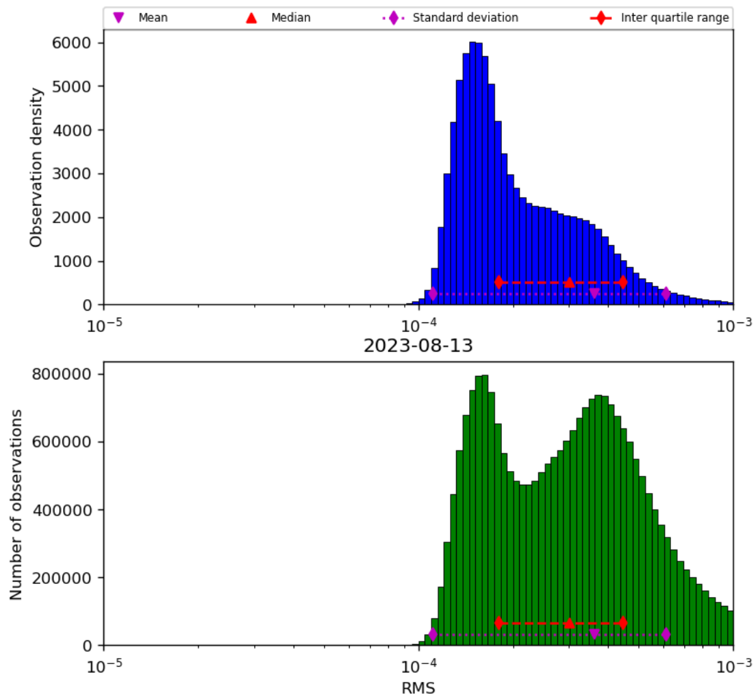
Figure 43: Histogram of “RMS” for 2023-08-12 to 2023-08-14
