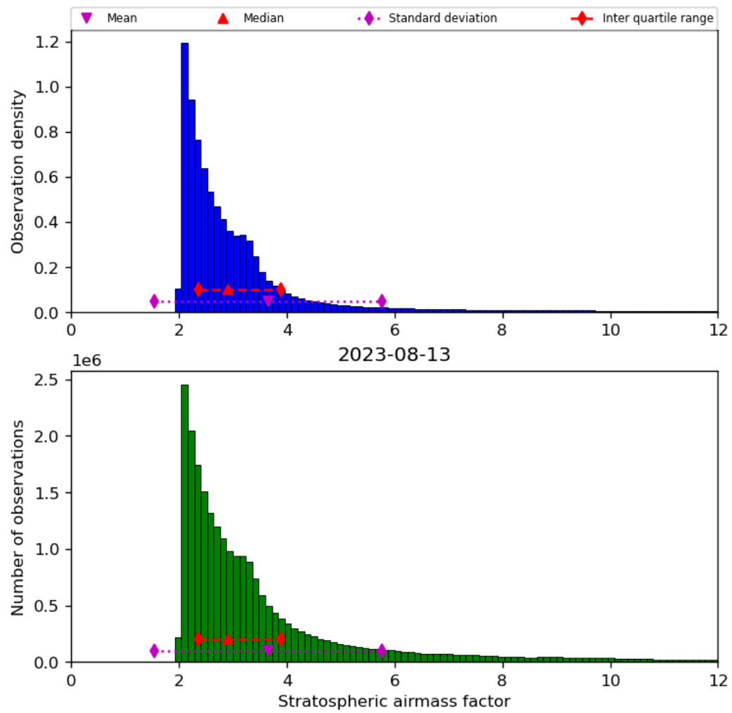
Figure 44: Histogram of “Stratospheric airmass factor” for 2023-08-12 to 2023-08-14
