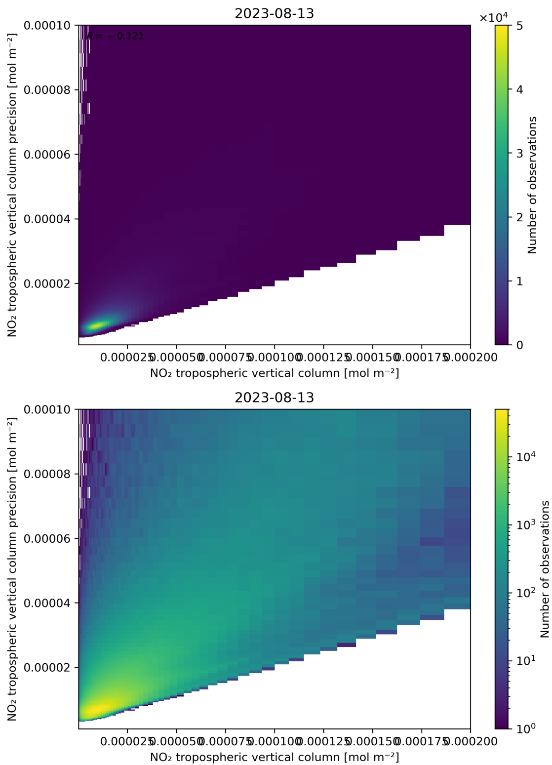
Figure 130: Scatter density plot of “NO 2 tropospheric vertical column” against “NO 2 tropospheric vertical column precision” for 2023-08-12 to 2023-08-14.
