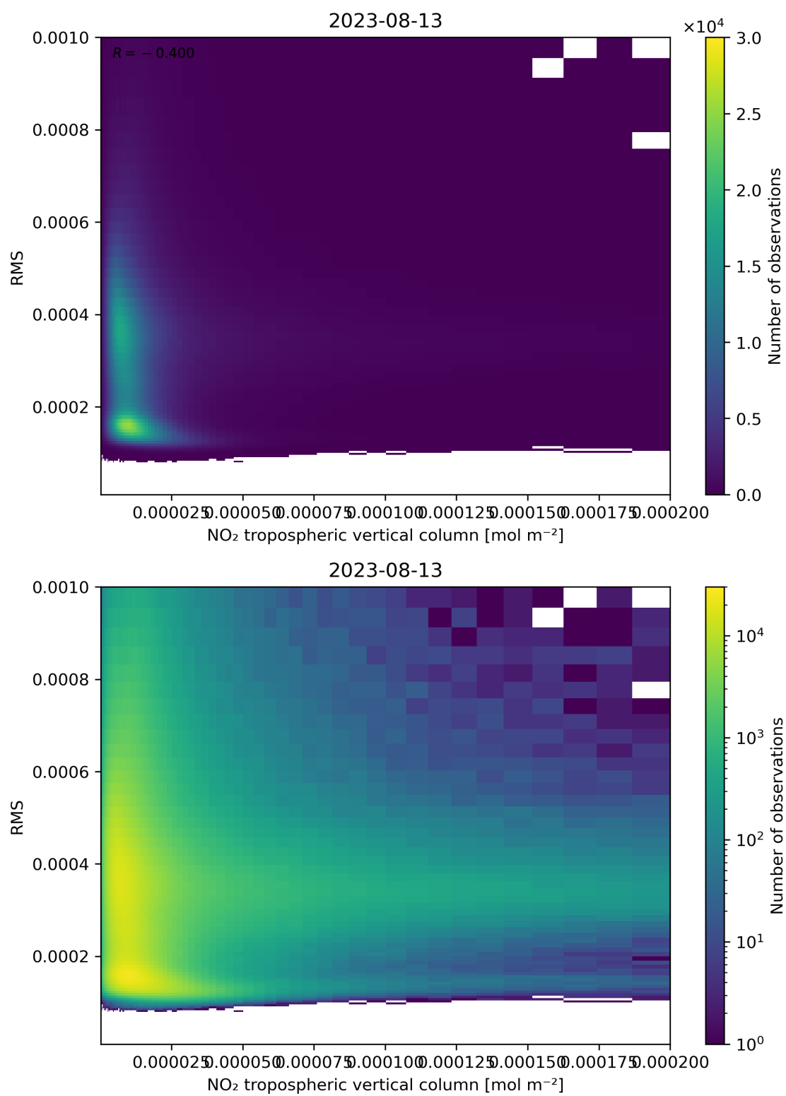
Figure 142: Scatter density plot of “NO 2 tropospheric vertical column” against “RMS” for 2023-08-12 to 2023-08-14.
