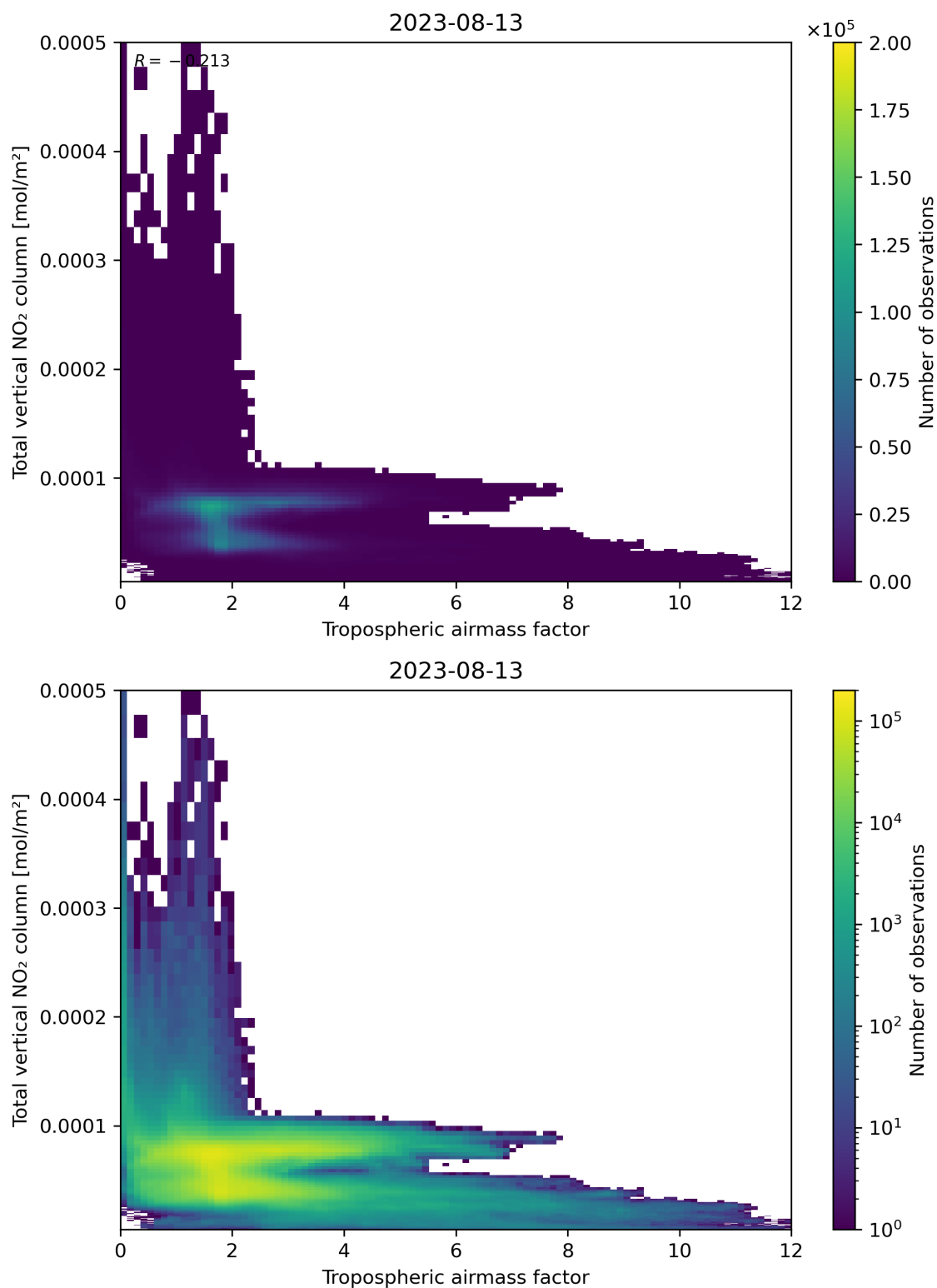
Figure 77: Scatter density plot of “Tropospheric airmass factor” against “Total vertical NO 2 column” for 2023-08-12 to 2023-08-14.
