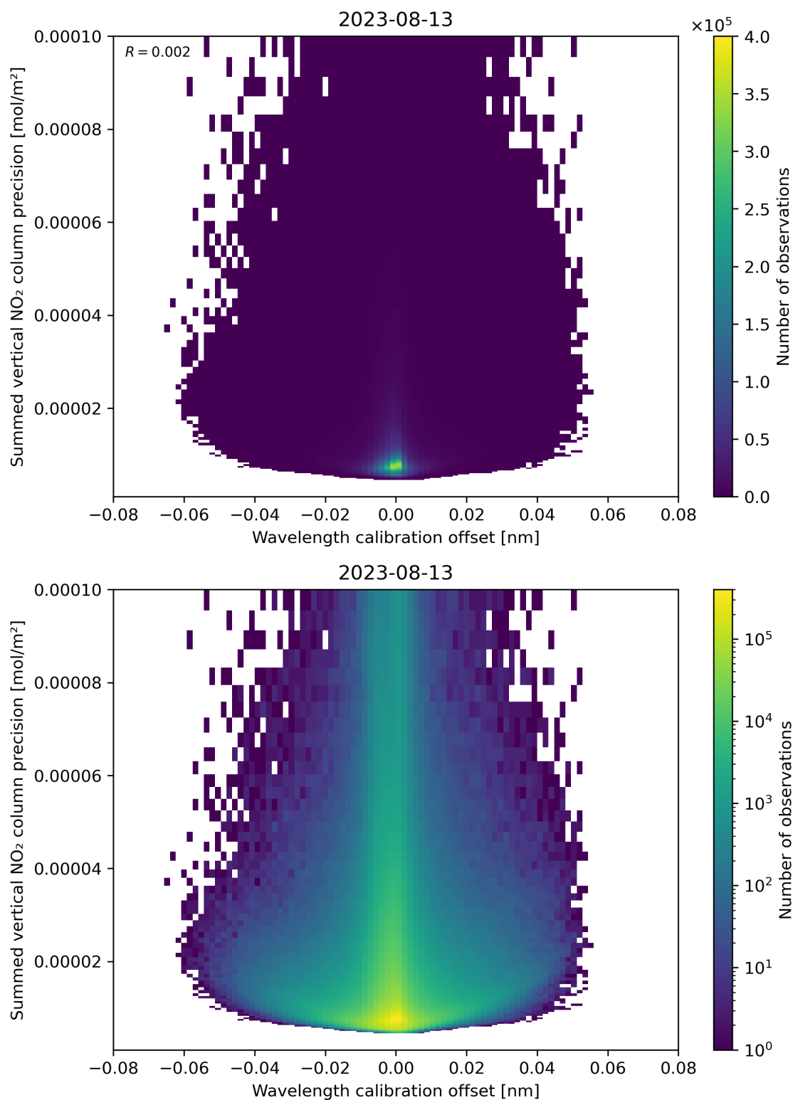
Figure 178: Scatter density plot of “Wavelength calibration offset” against “Summed vertical NO 2 column precision” for 2023-08-12 to 2023-08-14.
