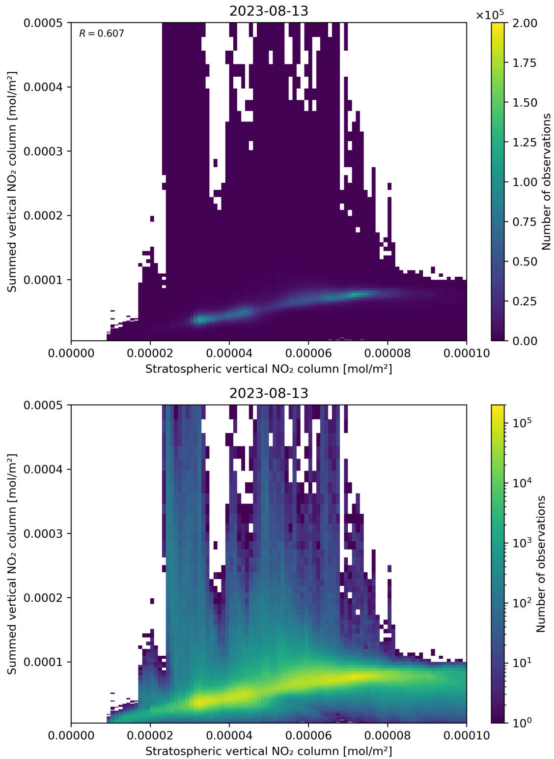
Figure 98: Scatter density plot of “Stratospheric vertical NO 2 column” against “Summed vertical NO 2 column” for 2023-08-12 to 2023-08-14.
