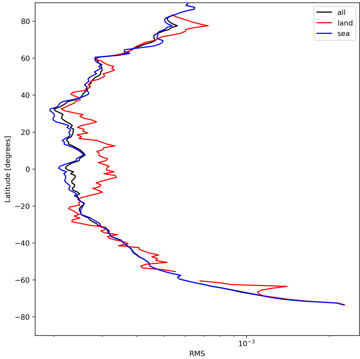
Figure 26: Zonal average of “RMS” for 2023-08-12 to 2023-08-14.
