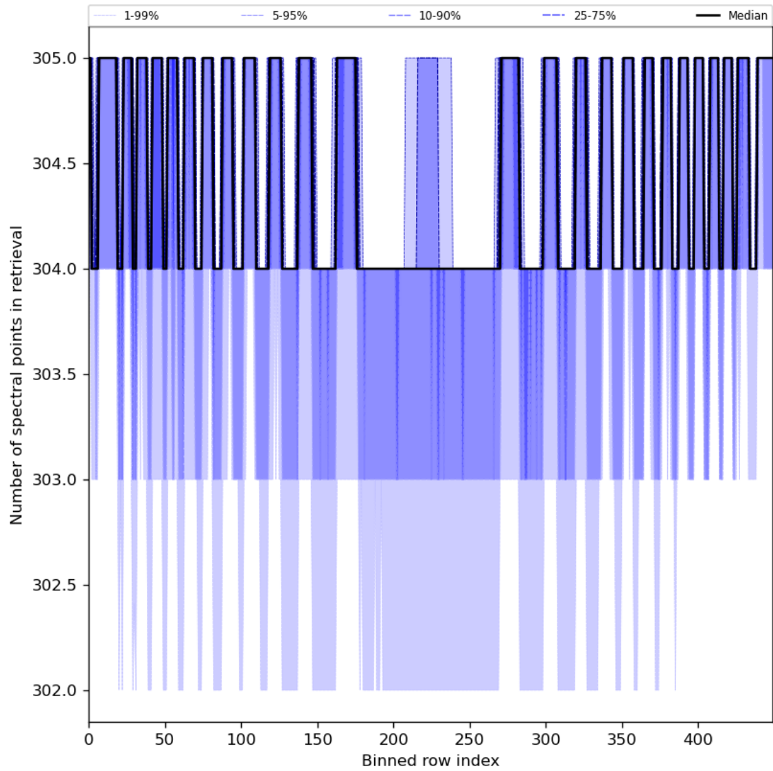
Figure 50: Along track statistics of “Number of spectral points in retrieval” for 2023-08-12 to 2023-08-14
