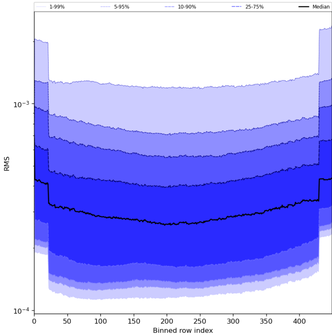
Figure 60: Along track statistics of “RMS” for 2023-08-12 to 2023-08-14
