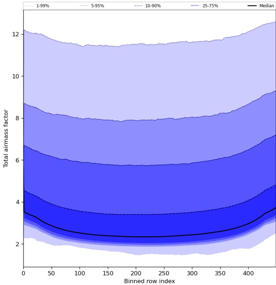
Figure 49: Along track statistics of “Total airmass factor” for 2023-08-12 to 2023-08-14
