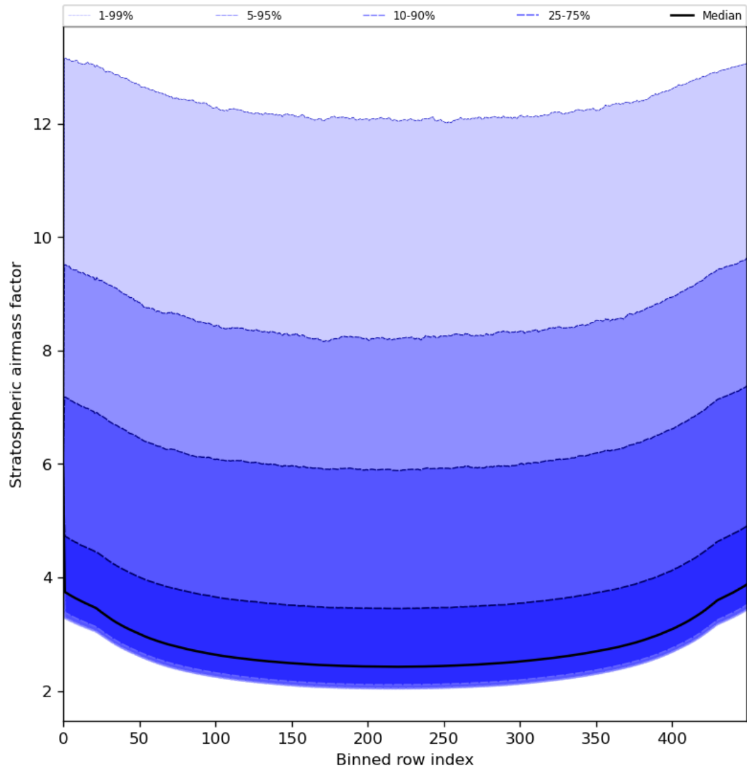
Figure 61: Along track statistics of “Stratospheric airmass factor” for 2023-08-12 to 2023-08-14
