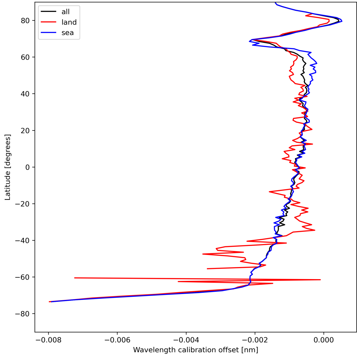
Figure 18: Zonal average of “Wavelength calibration offset” for 2023-08-12 to 2023-08-14.
