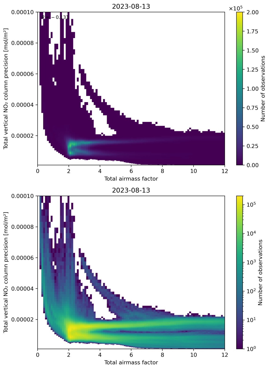
Figure 68: Scatter density plot of “Total airmass factor” against “Total vertical NO 2 column precision” for 2023-08-12 to 2023-08-14.
