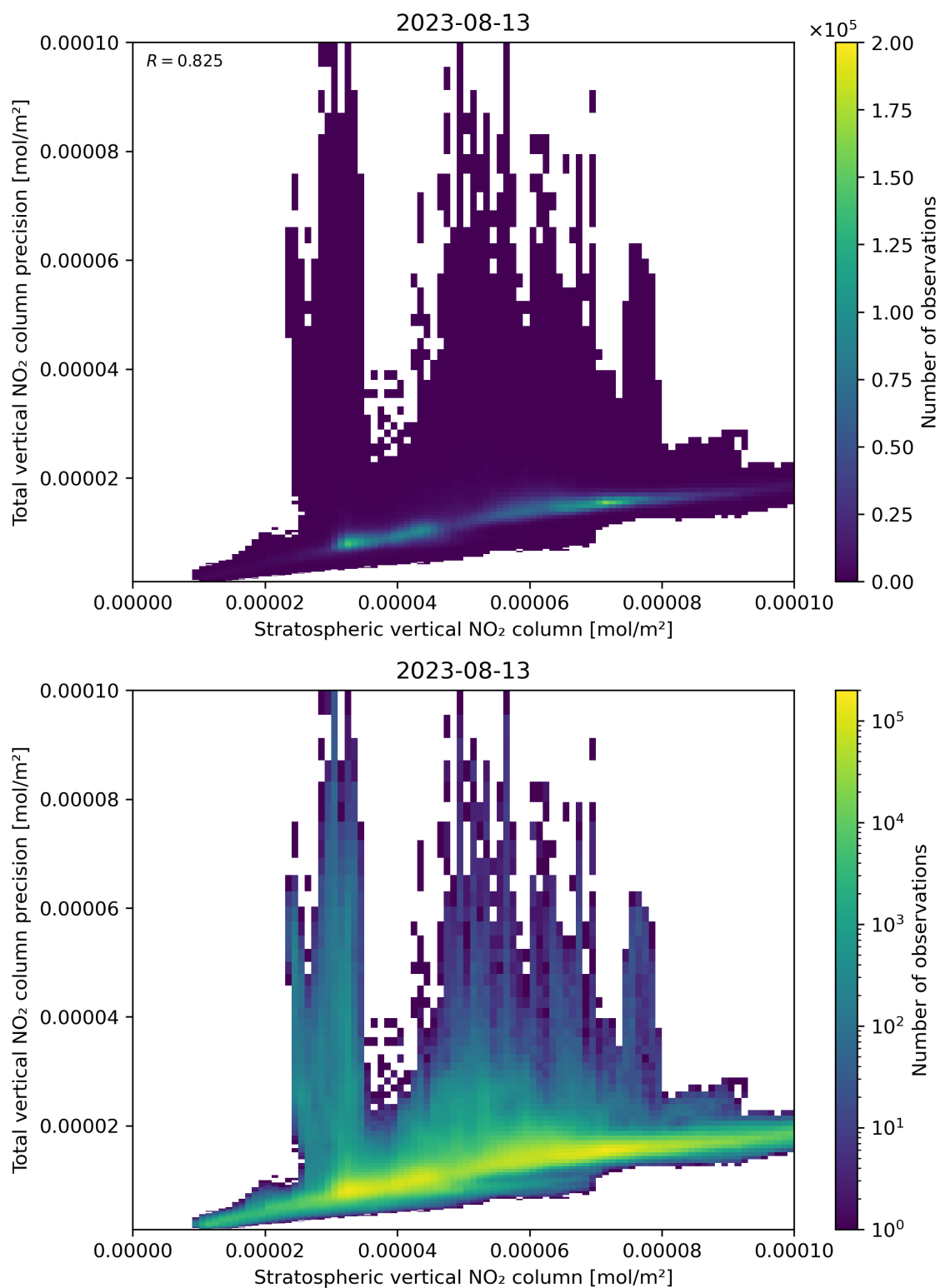
Figure 101: Scatter density plot of “Stratospheric vertical NO 2 column” against “Total vertical NO 2 column precision” for 2023-08-12 to 2023-08-14.
