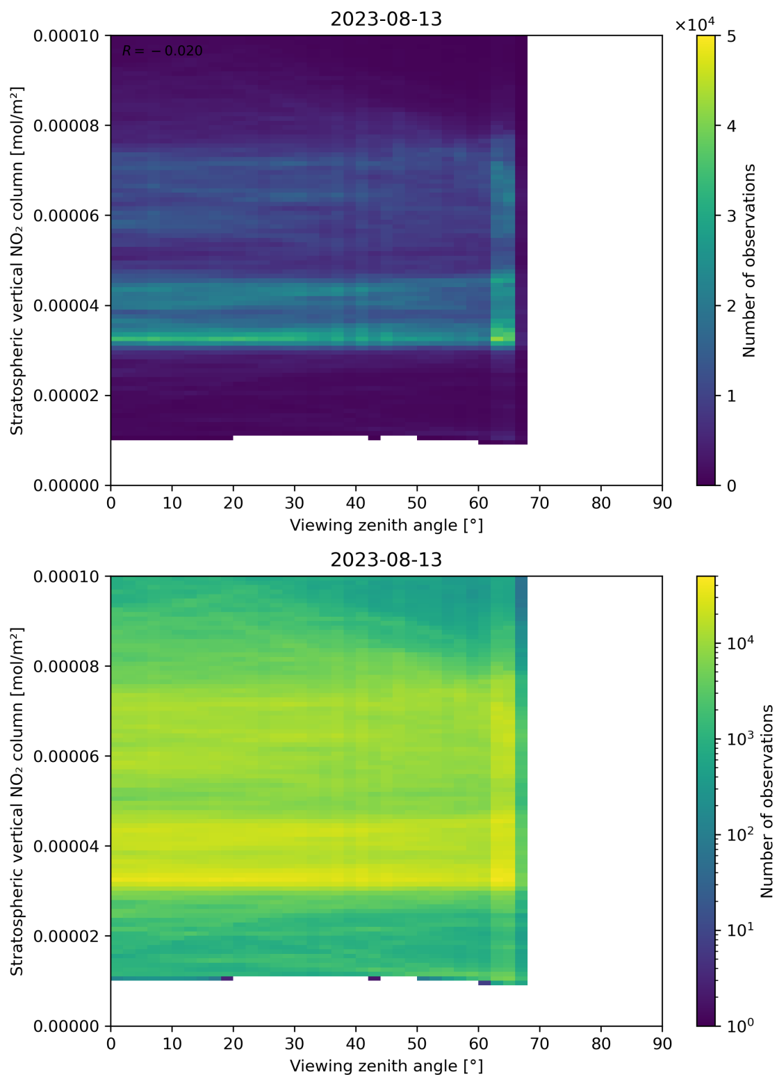
Figure 164: Scatter density plot of “Viewing zenith angle” against “Stratospheric vertical NO 2 column” for 2023-08-12 to 2023-08-14.
