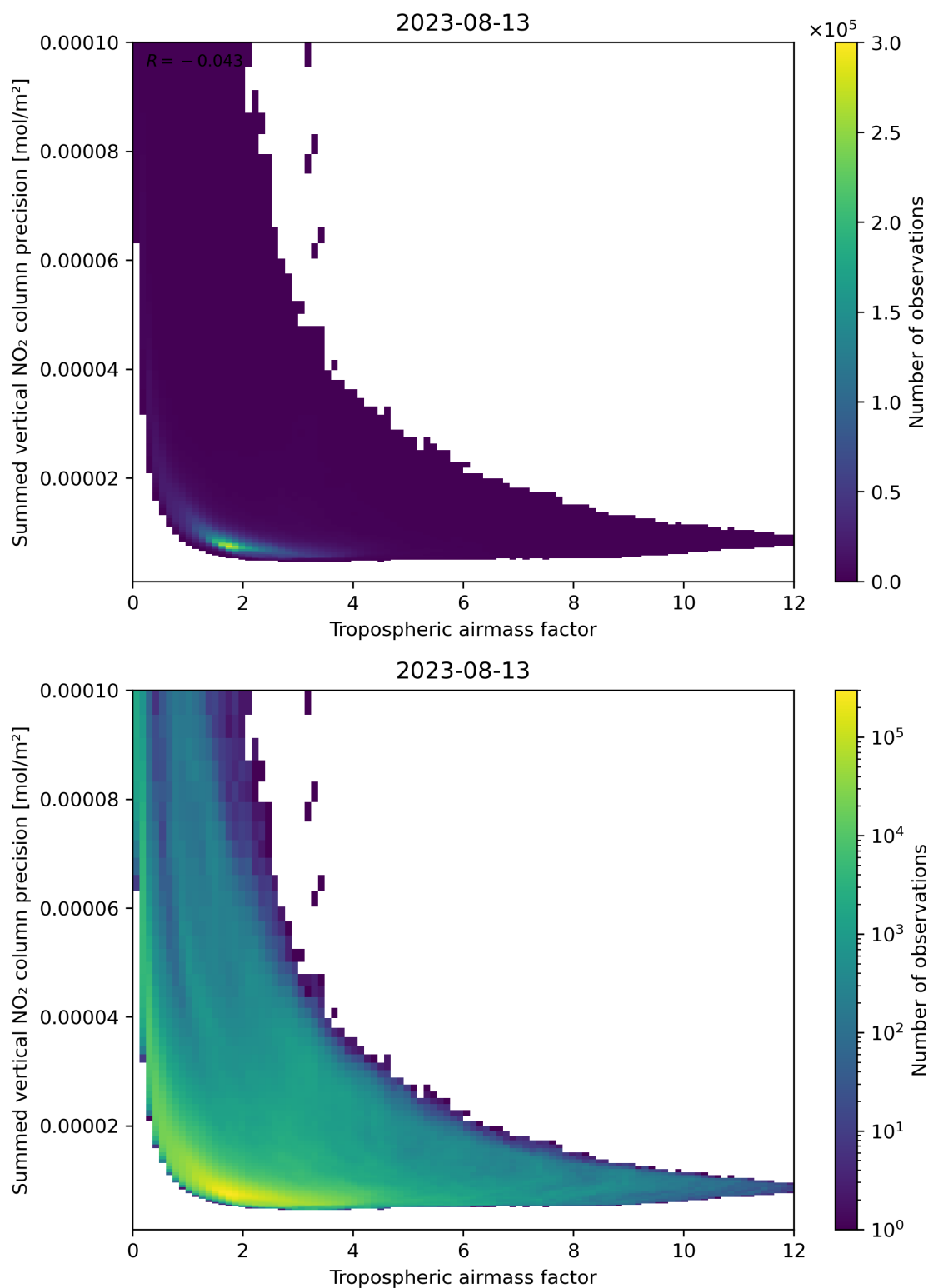
Figure 76: Scatter density plot of “Tropospheric air mass factor” against “Summed vertical NO 2 column precision” for 2023-08-12 to 2023-08-14.
