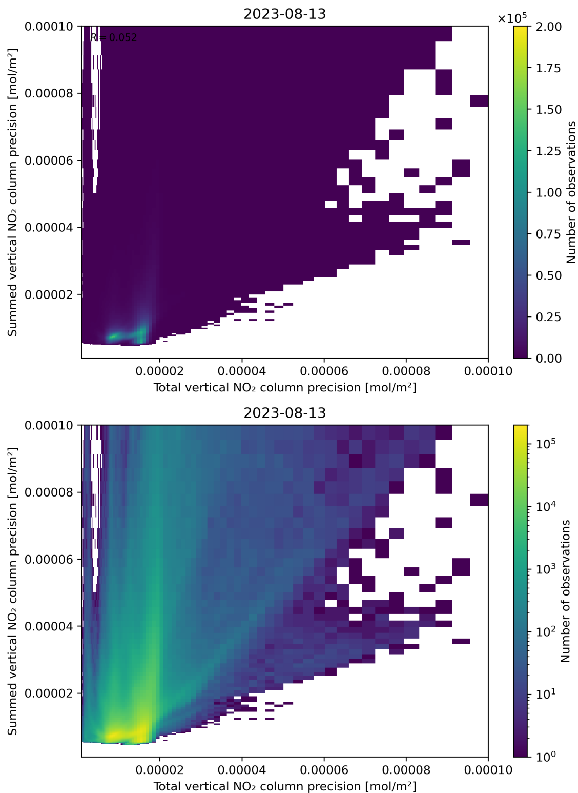
Figure 118: Scatter density plot of “Total vertical NO 2 column precision” against “Summed vertical NO 2 column precision” for 2023-08-12 to 2023-08-14.
