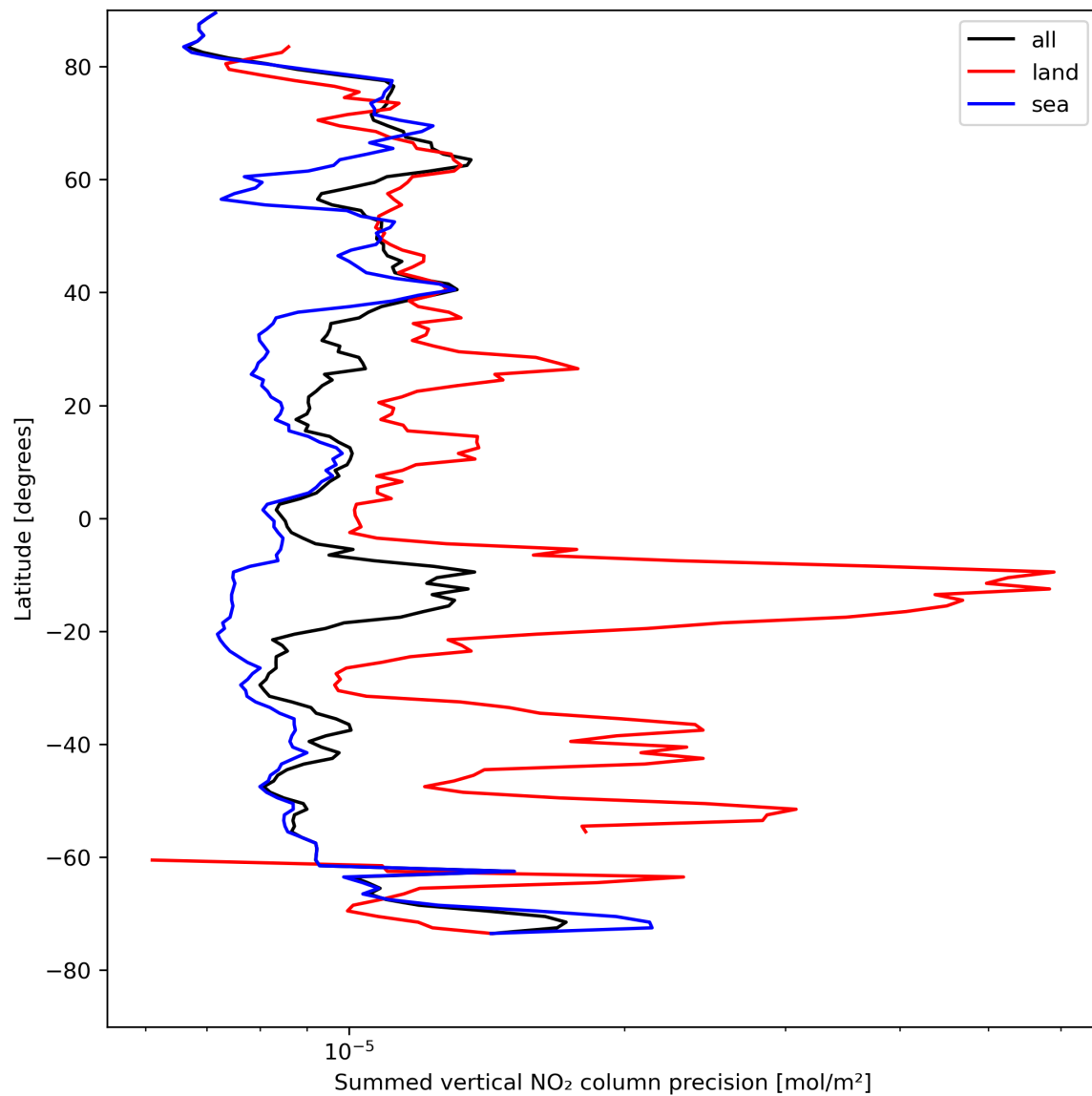
Figure 24: Zonal average of “Summed vertical NO 2 column precision” for 2023-08-12 to 2023-08-14.
