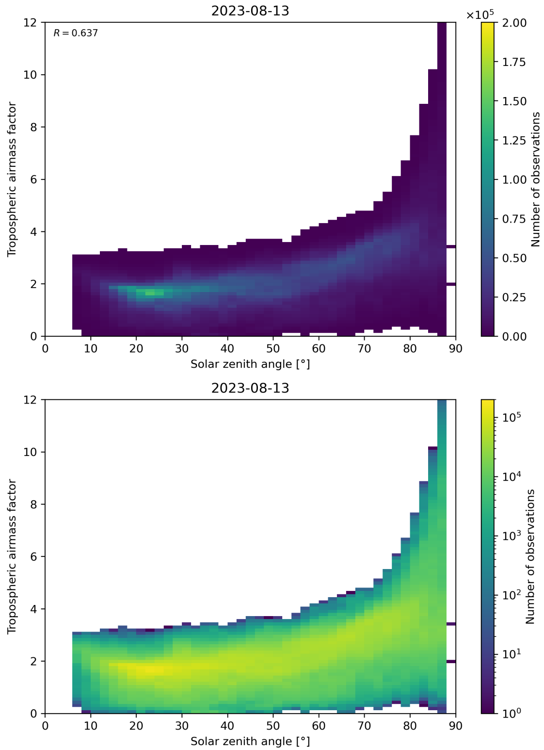
Figure 147: Scatter density plot of “Solar zenith angle” against “Tropospheric airmass factor” for 2023-08-12 to 2023-08-14.
