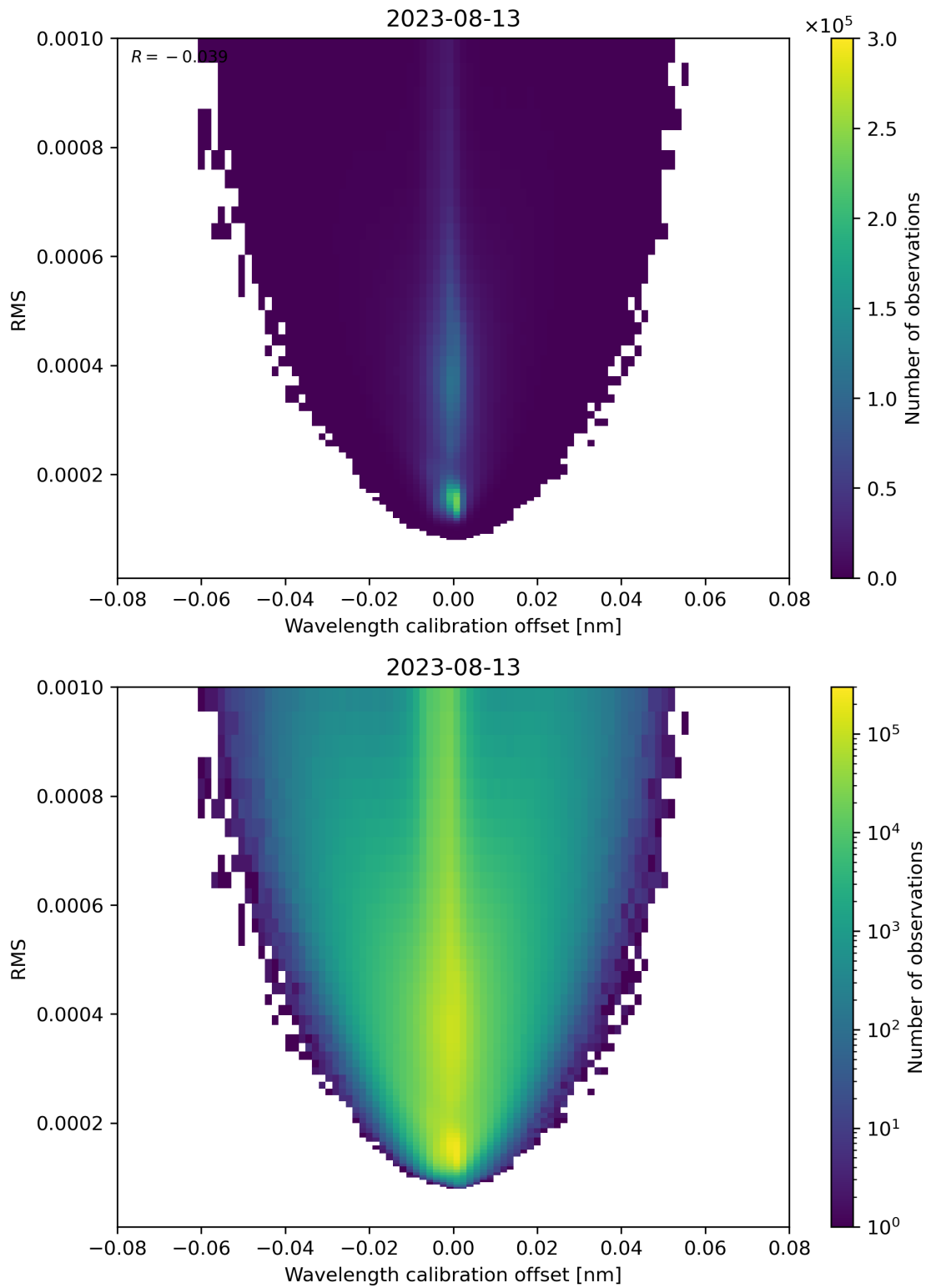
Figure 181: Scatter density plot of “Wavelength calibration offset” against “RMS” for 2023-08-12 to 2023-08-14.
