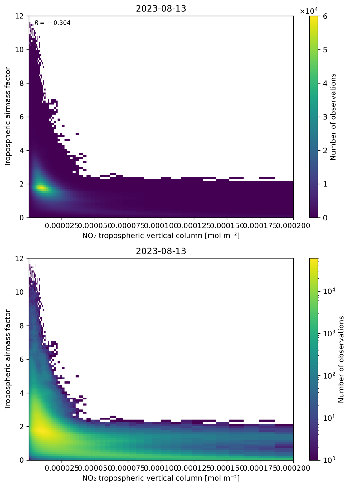
Figure 123: Scatter density plot of “NO 2 tropospheric vertical column” against “Tropospheric air mass factor” for 2023-08-12 to 2023-08-14.
