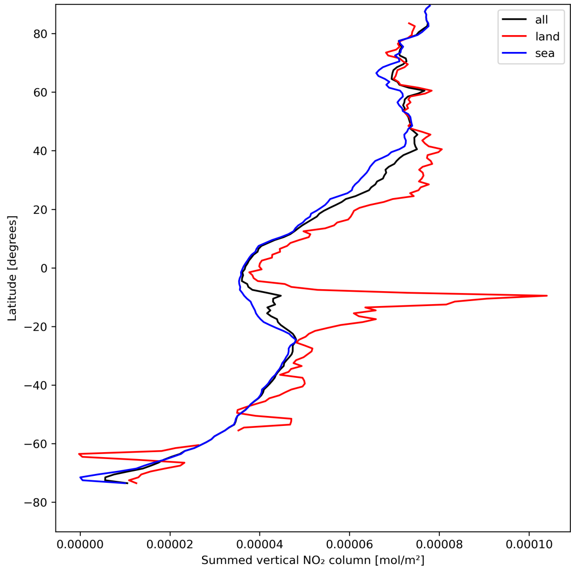
Figure 23: Zonal average of “Summed vertical NO 2 column” for 2023-08-12 to 2023-08-14.
