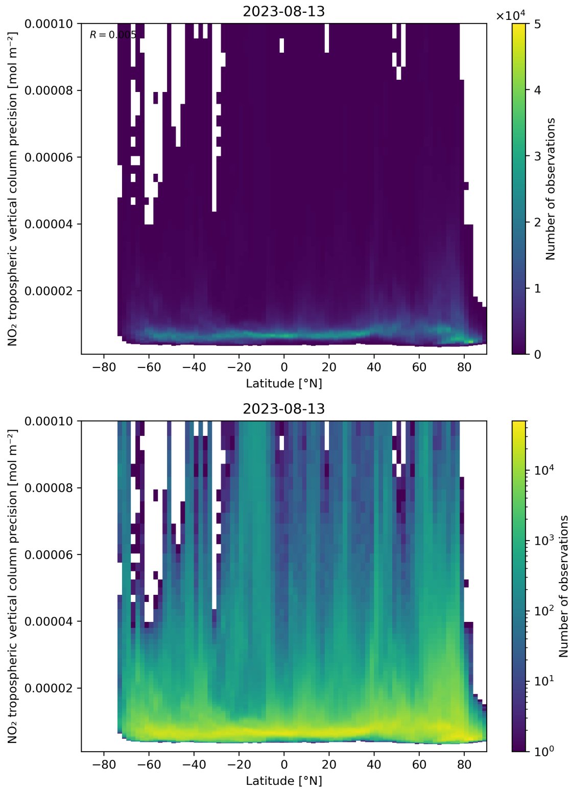
Figure 93: Scatter density plot of “Latitude” against “NO 2 tropospheric vertical column precision” for 2023-08-12 to 2023-08-14.
