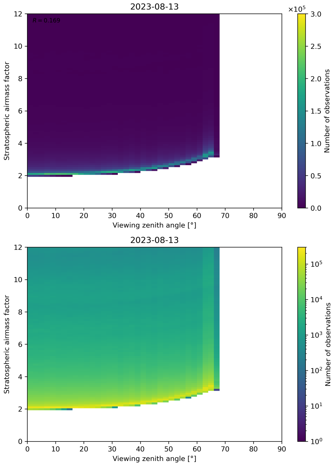
Figure 159: Scatter density plot of “Viewing zenith angle” against “Stratospheric airmass factor” for 2023-08-12 to 2023-08-14.
