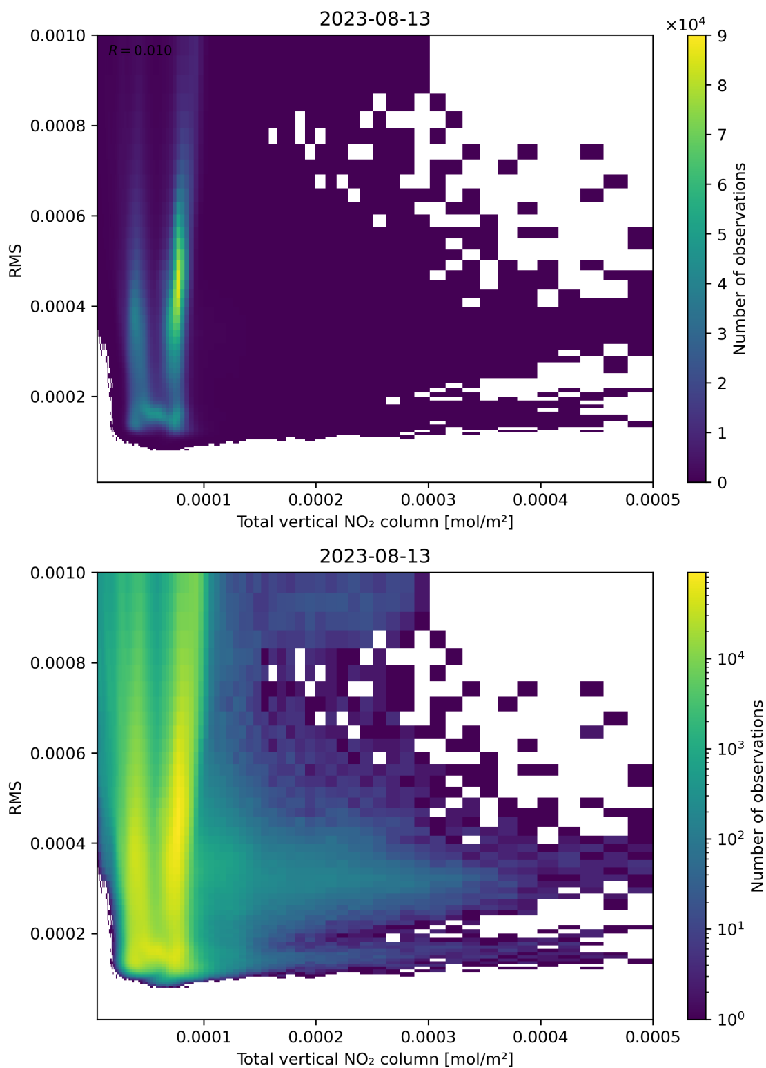
Figure 120: Scatter density plot of “Total vertical NO 2 column” against “RMS” for 2023-08-12 to 2023-08-14.
