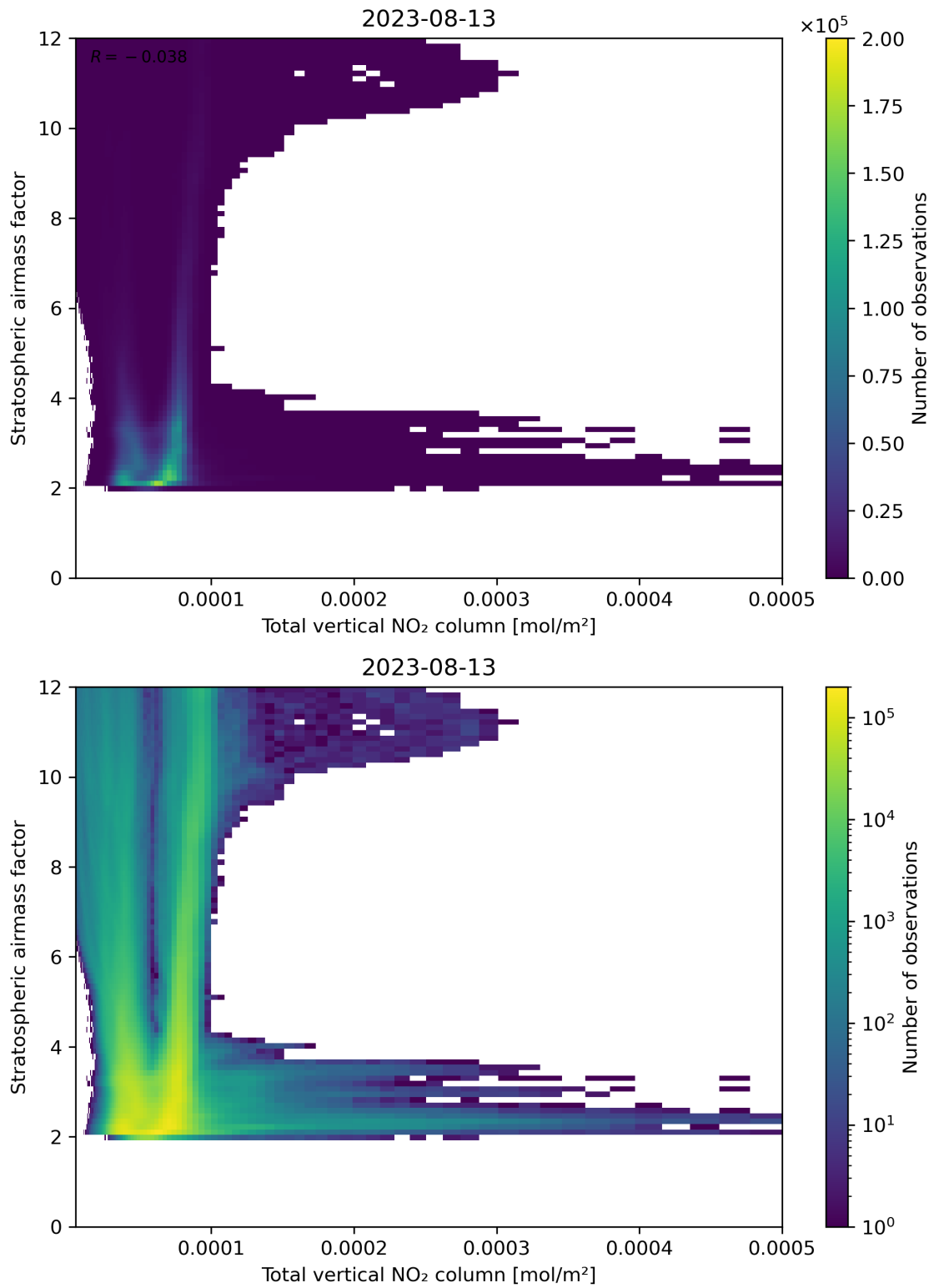
Figure 110: Scatter density plot of “Total vertical NO 2 column” against “Stratospheric airmass factor” for 2023-08-12 to 2023-08-14.
