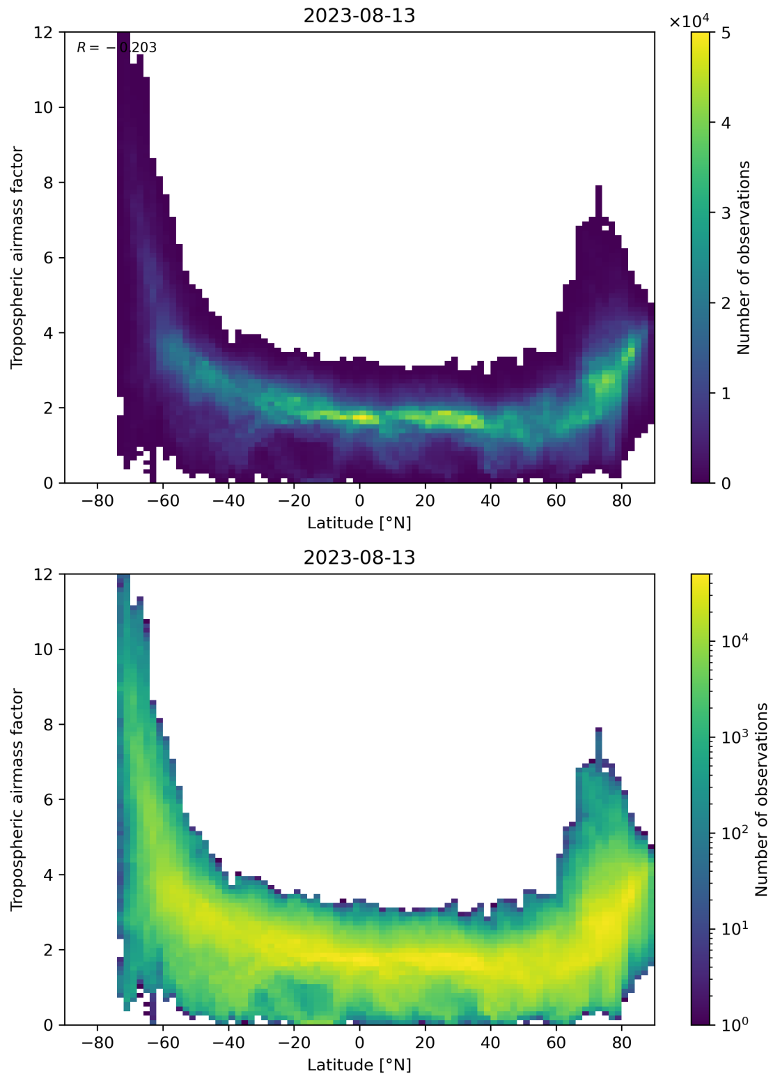
Figure 85: Scatter density plot of “Latitude” against “Tropospheric airmass factor” for 2023-08-12 to 2023-08-14.
