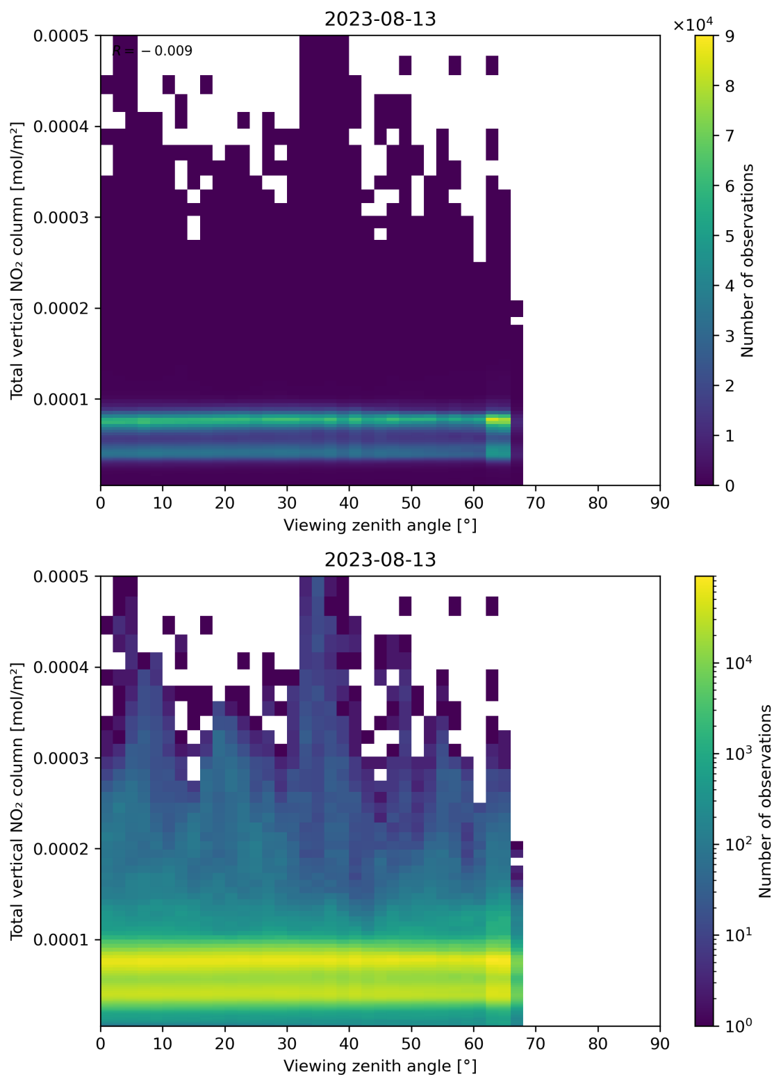
Figure 167: Scatter density plot of “Viewing zenith angle” against “Total vertical NO 2 column” for 2023-08-12 to 2023-08-14.
