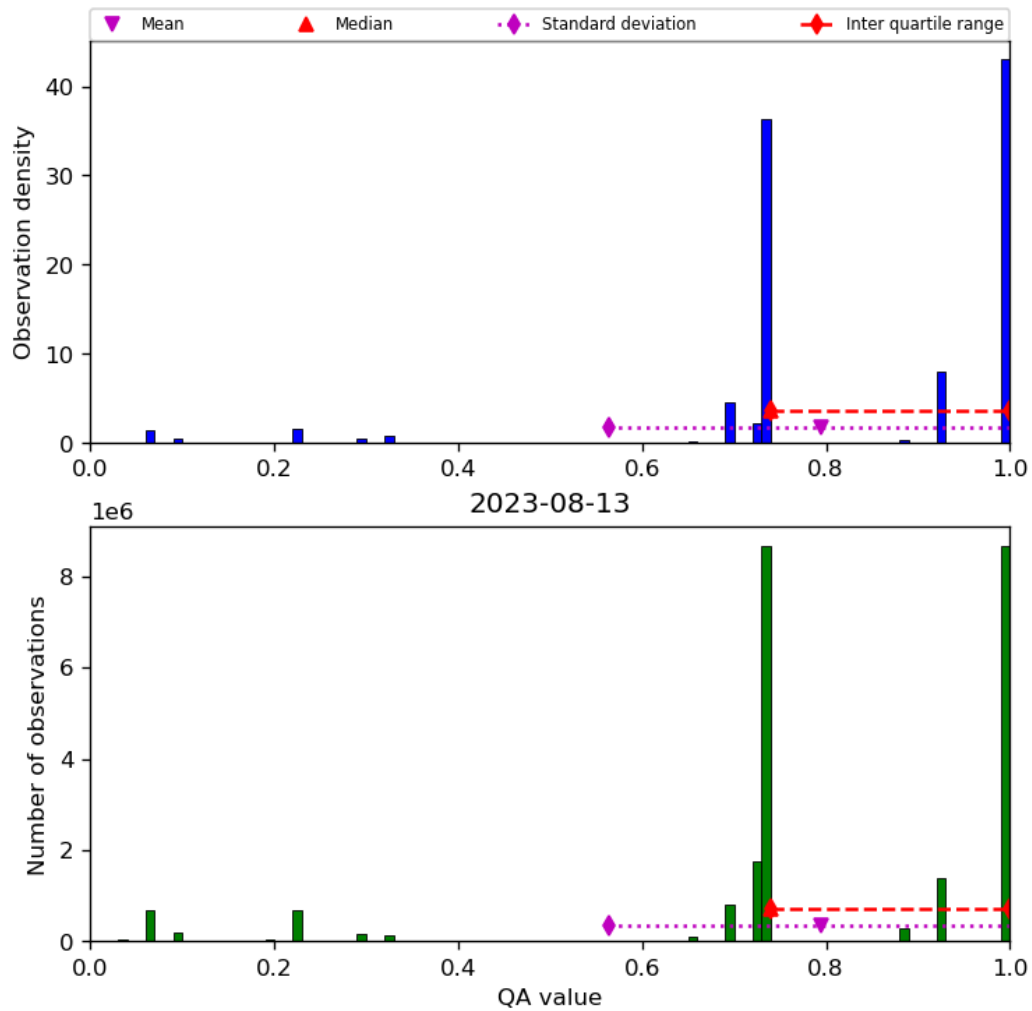
Figure 28: Histogram of “QA value” for 2023-08-12 to 2023-08-14
