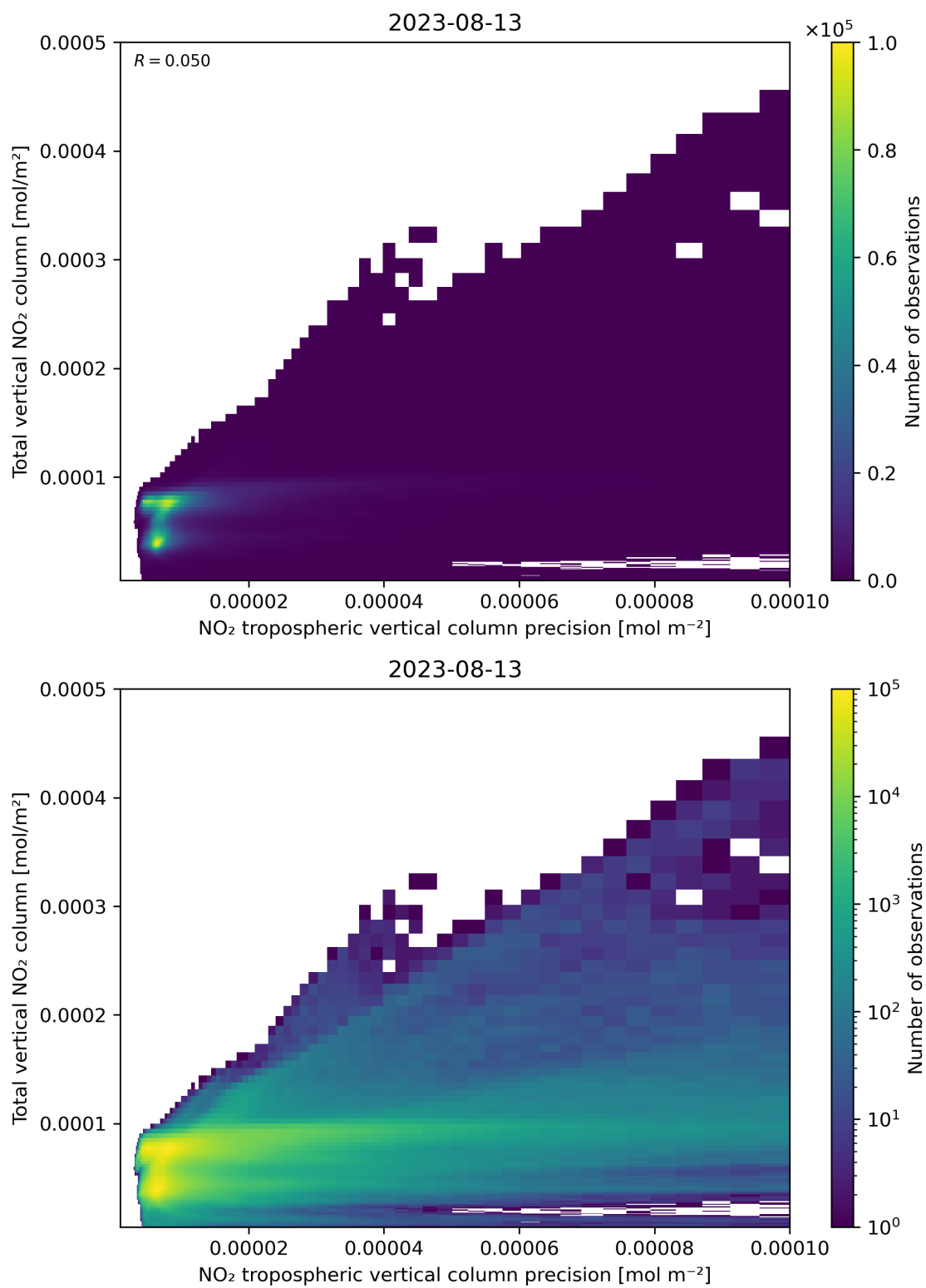
Figure 138: Scatter density plot of “NO 2 tropospheric vertical column precision” against “Total vertical NO 2 column” for 2023-08-12 to 2023-08-14.
