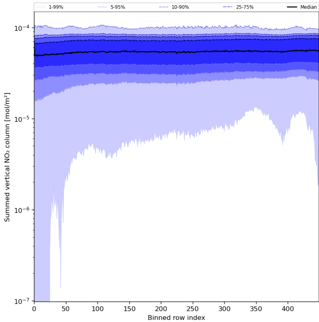
Figure 57: Along track statistics of “Summed vertical NO 2 column” for 2023-08-12 to 2023-08-14
