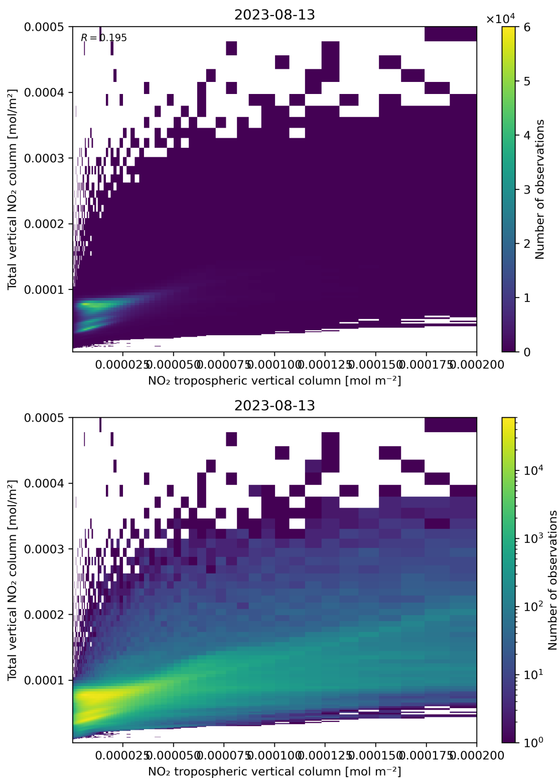
Figure 128: Scatter density plot of “NO 2 tropospheric vertical column” against “Total vertical NO 2 column” for 2023-08-12 to 2023-08-14.
