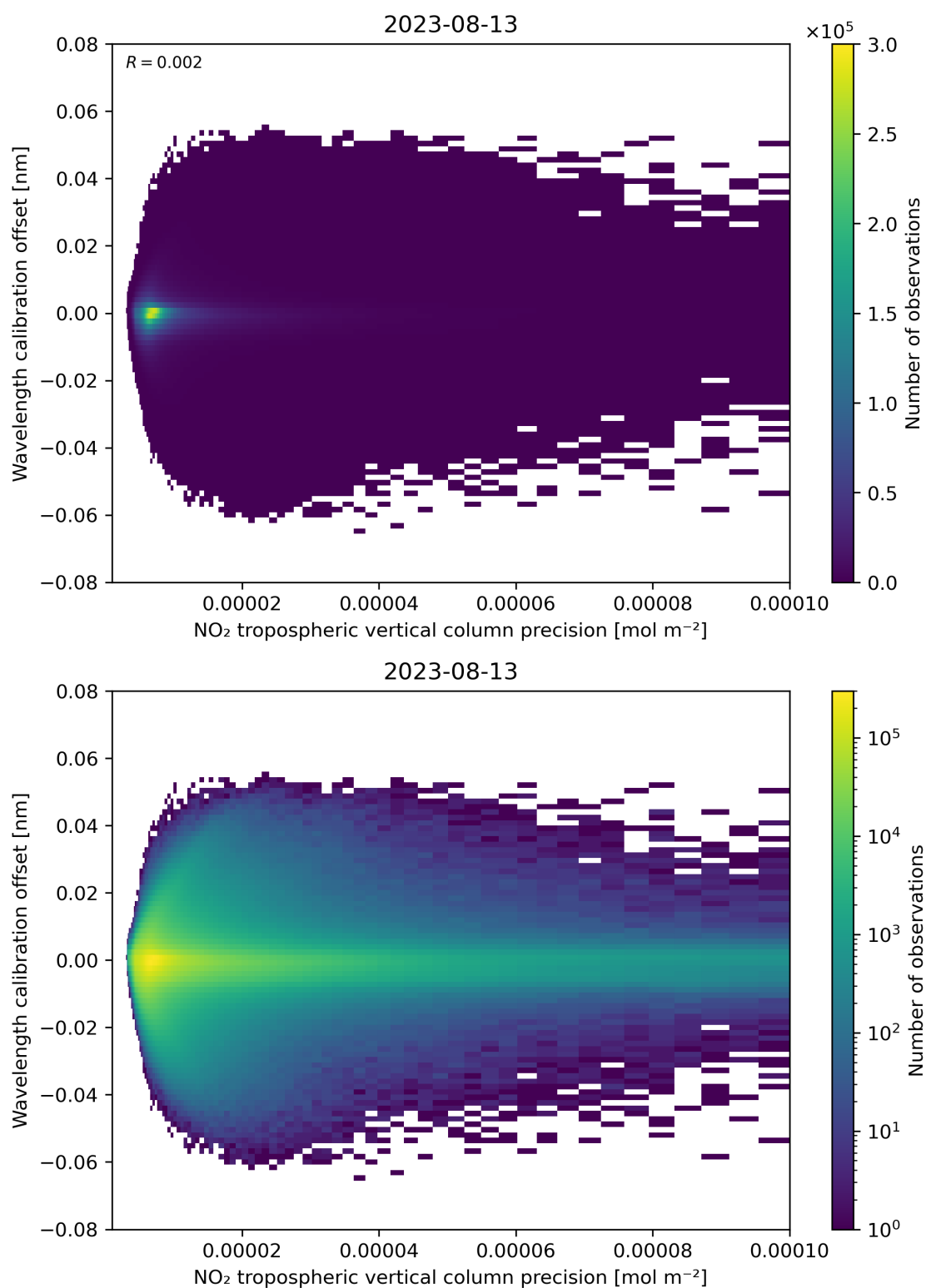
Figure 141: Scatter density plot of “NO 2 tropospheric vertical column precision” against “Wavelength calibration offset” for 2023-08-12 to 2023-08-14.
