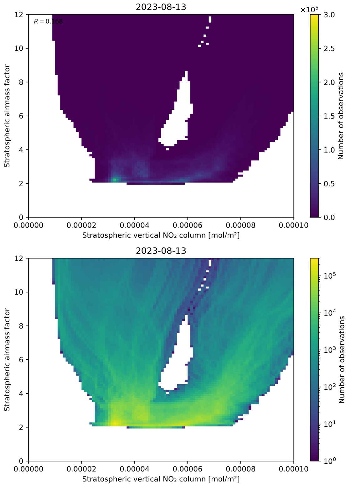
Figure 96: Scatter density plot of “Stratospheric vertical NO 2 column” against “Stratospheric airmass factor” for 2023-08-12 to 2023-08-14.
