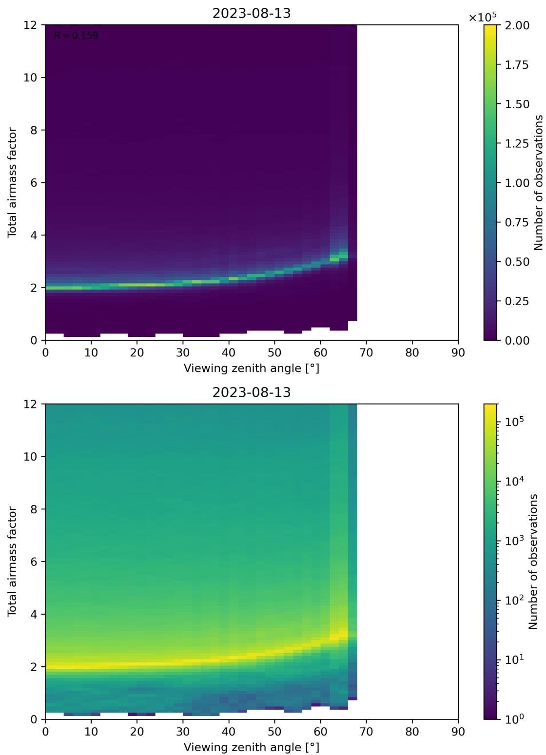
Figure 160: Scatter density plot of “Viewing zenith angle” against “Total airmass factor” for 2023-08-12 to 2023-08-14.
