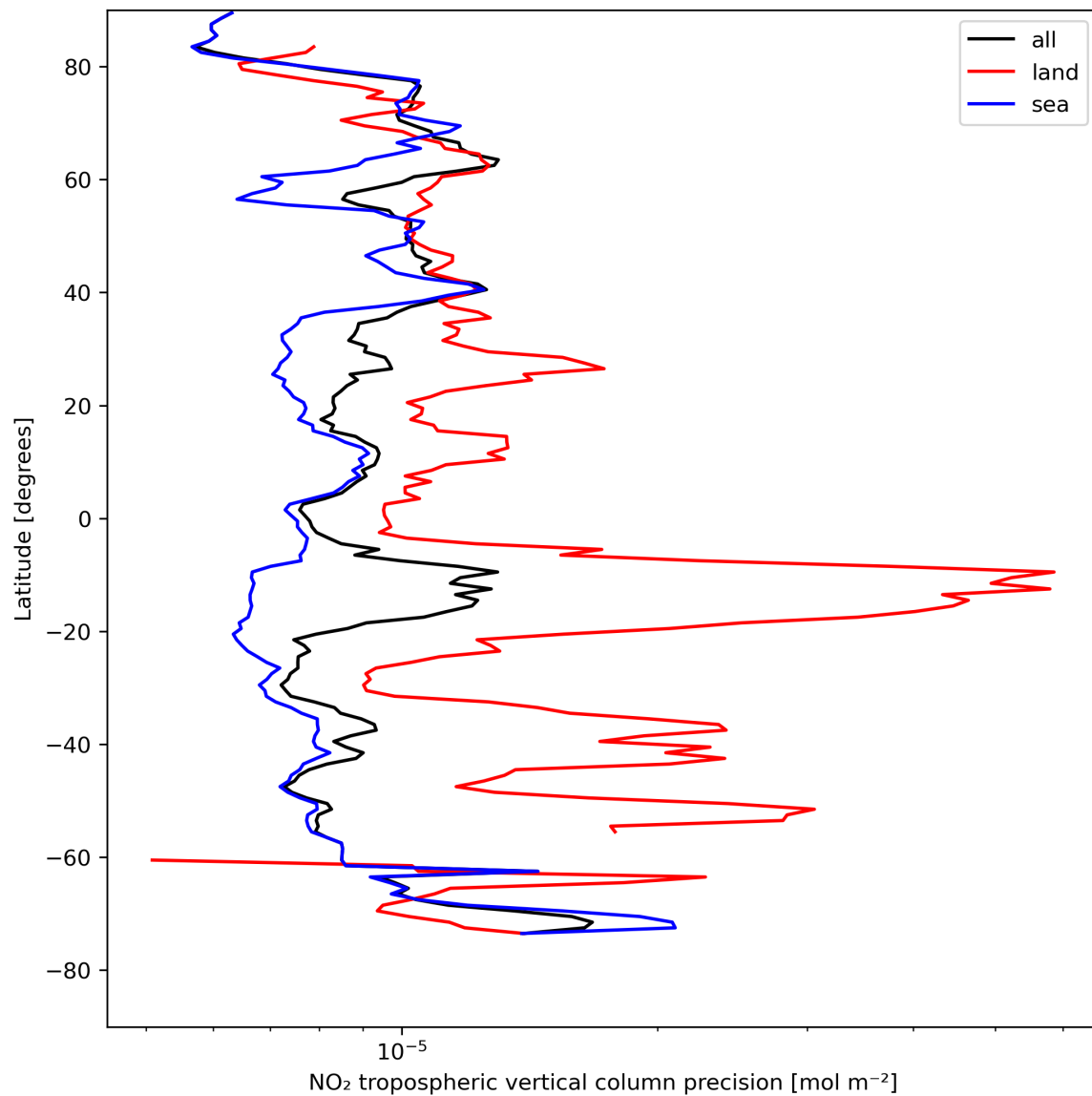
Figure 13: Zonal average of “NO 2 tropospheric vertical column precision” for 2023-08-12 to 2023-08-14.
