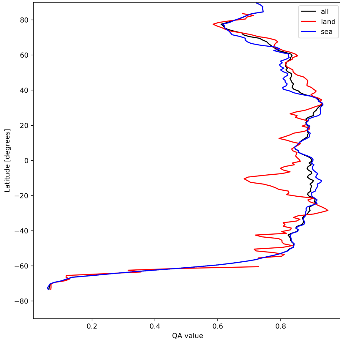
Figure 11: Zonal average of “QA value” for 2023-08-12 to 2023-08-14.
