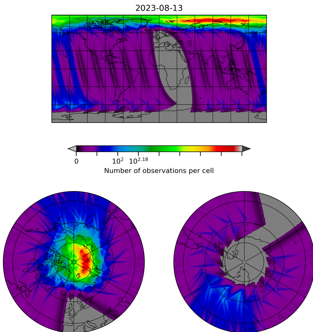
Figure 10: Map of the number of observations for 2023-08-12 to 2023-08-14
