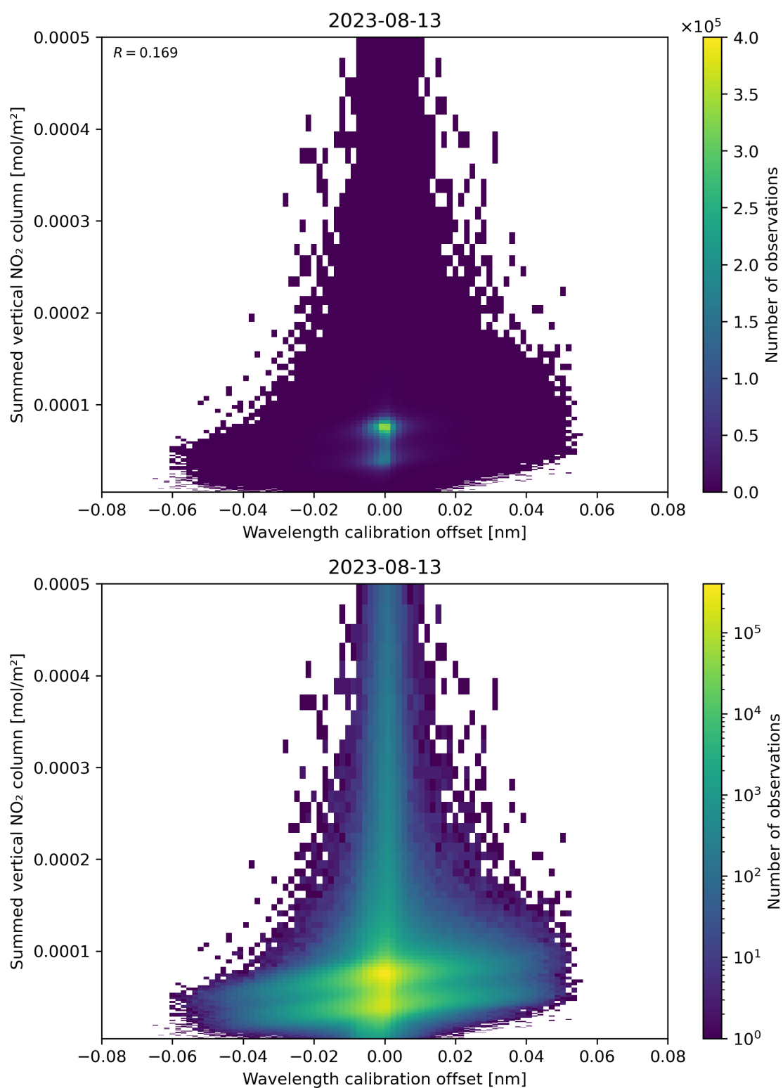
Figure 177: Scatter density plot of “Wavelength calibration offset” against “Summed vertical NO 2 column” for 2023-08-12 to 2023-08-14.
