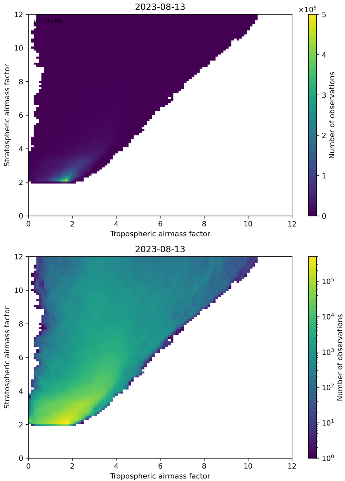
Figure 71: Scatter density plot of “Tropospheric airmass factor” against “Stratospheric airmass factor” for 2023-08-12 to 2023-08-14.
