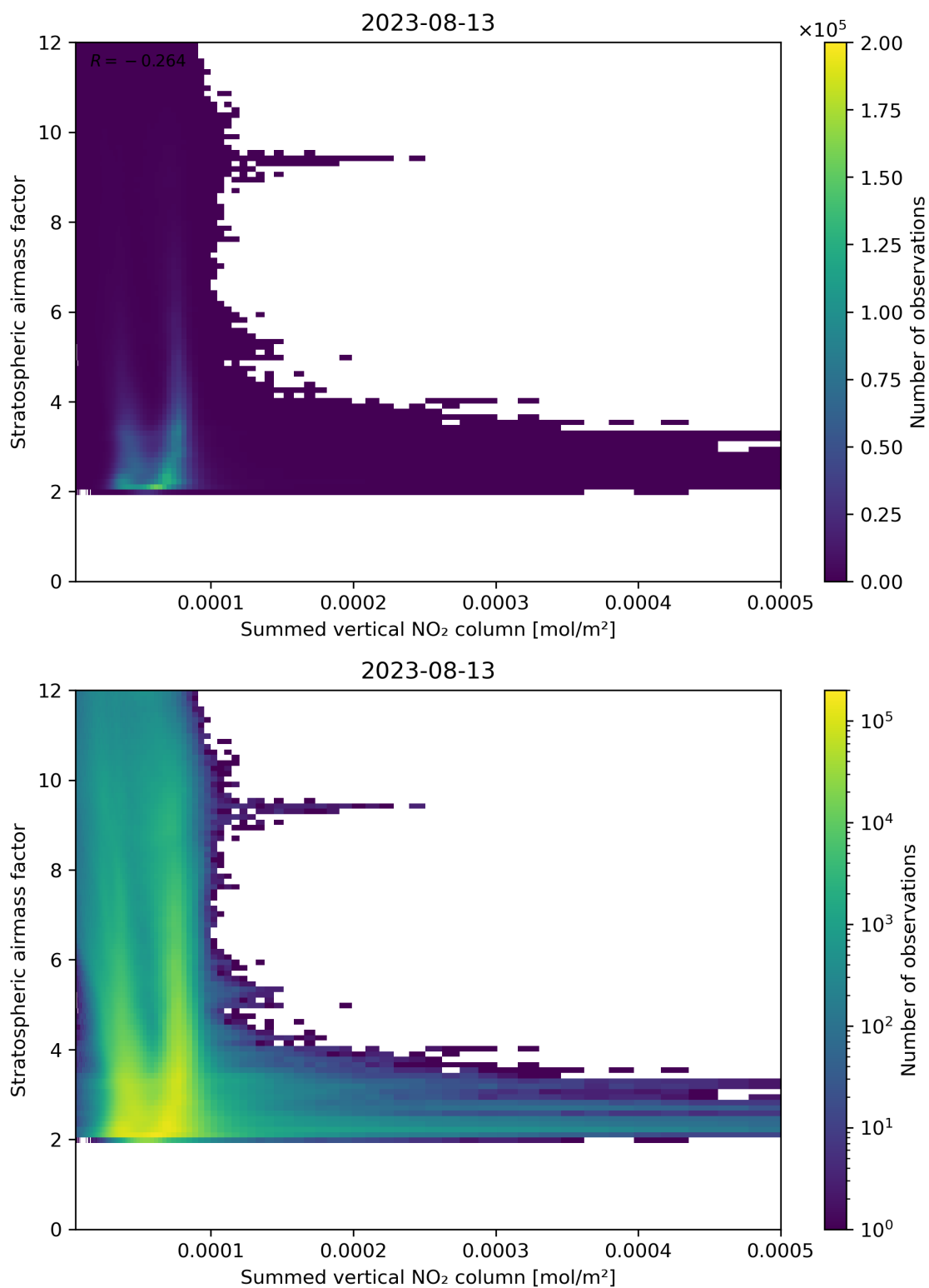
Figure 103: Scatter density plot of “Summed vertical NO 2 column” against “Stratospheric airmass factor” for 2023-08-12 to 2023-08-14.
