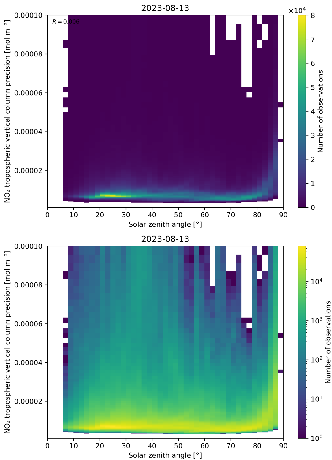
Figure 156: Scatter density plot of “Solar zenith angle” against “NO 2 tropospheric vertical column precision” for 2023-08-12 to 2023-08-14.
