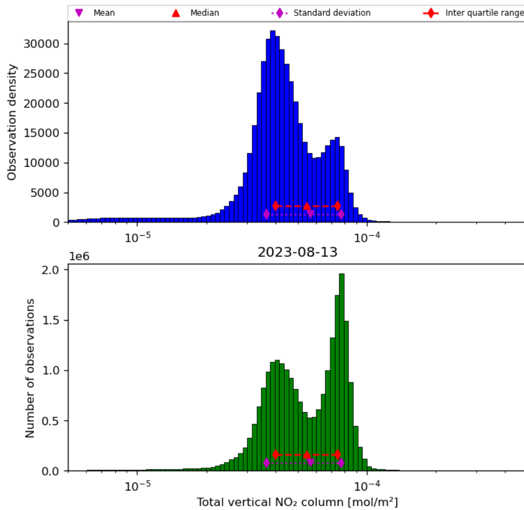
Figure 38: Histogram of "Total vertical NO 2 column" for 2023-08-12 to 2023-08-14
