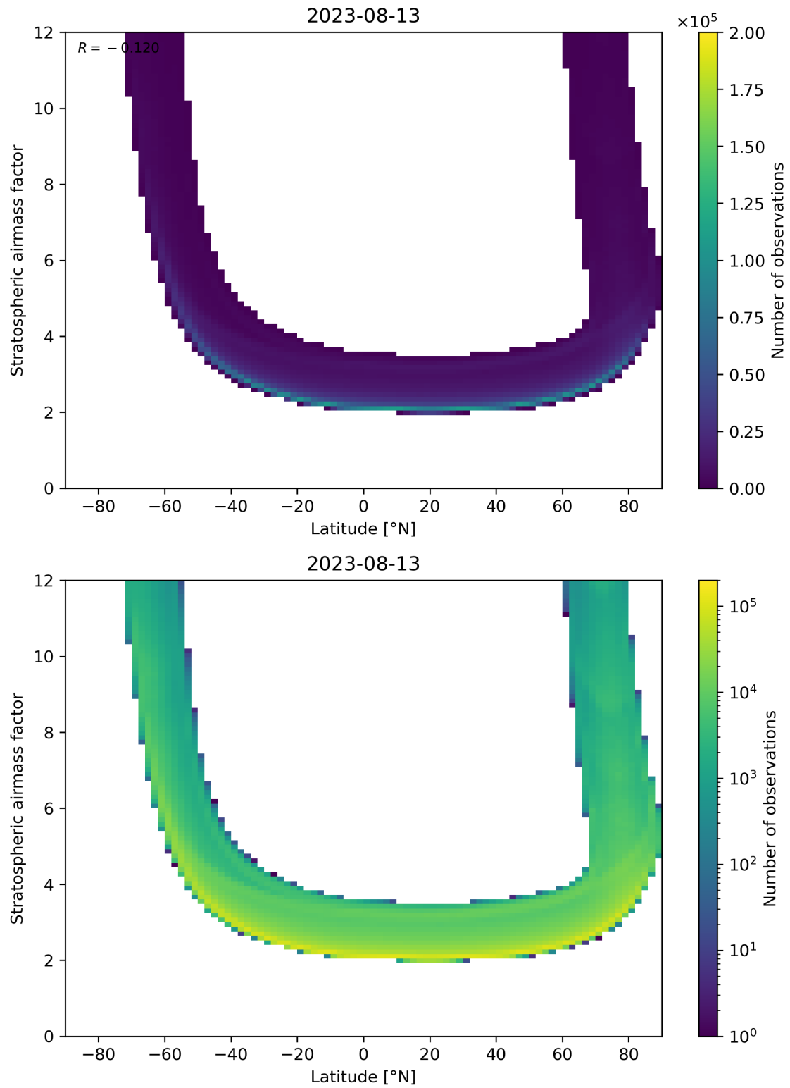
Figure 83: Scatter density plot of “Latitude” against “Stratospheric air mass factor” for 2023-08-12 to 2023-08-14.
