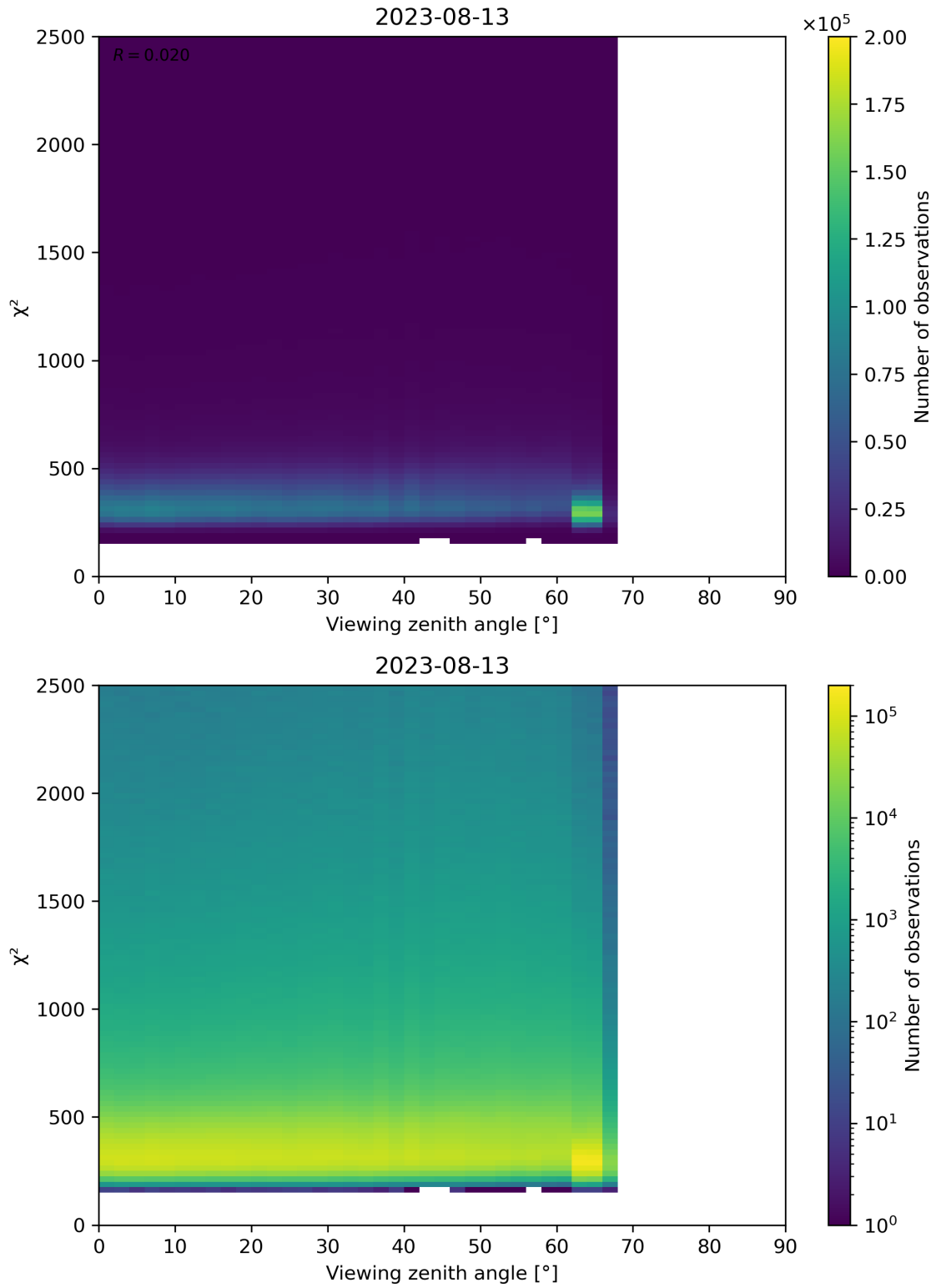
Figure 162: Scatter density plot of “Viewing zenith angle” against “ \chi^2 ” for 2023-08-12 to 2023-08-14.
