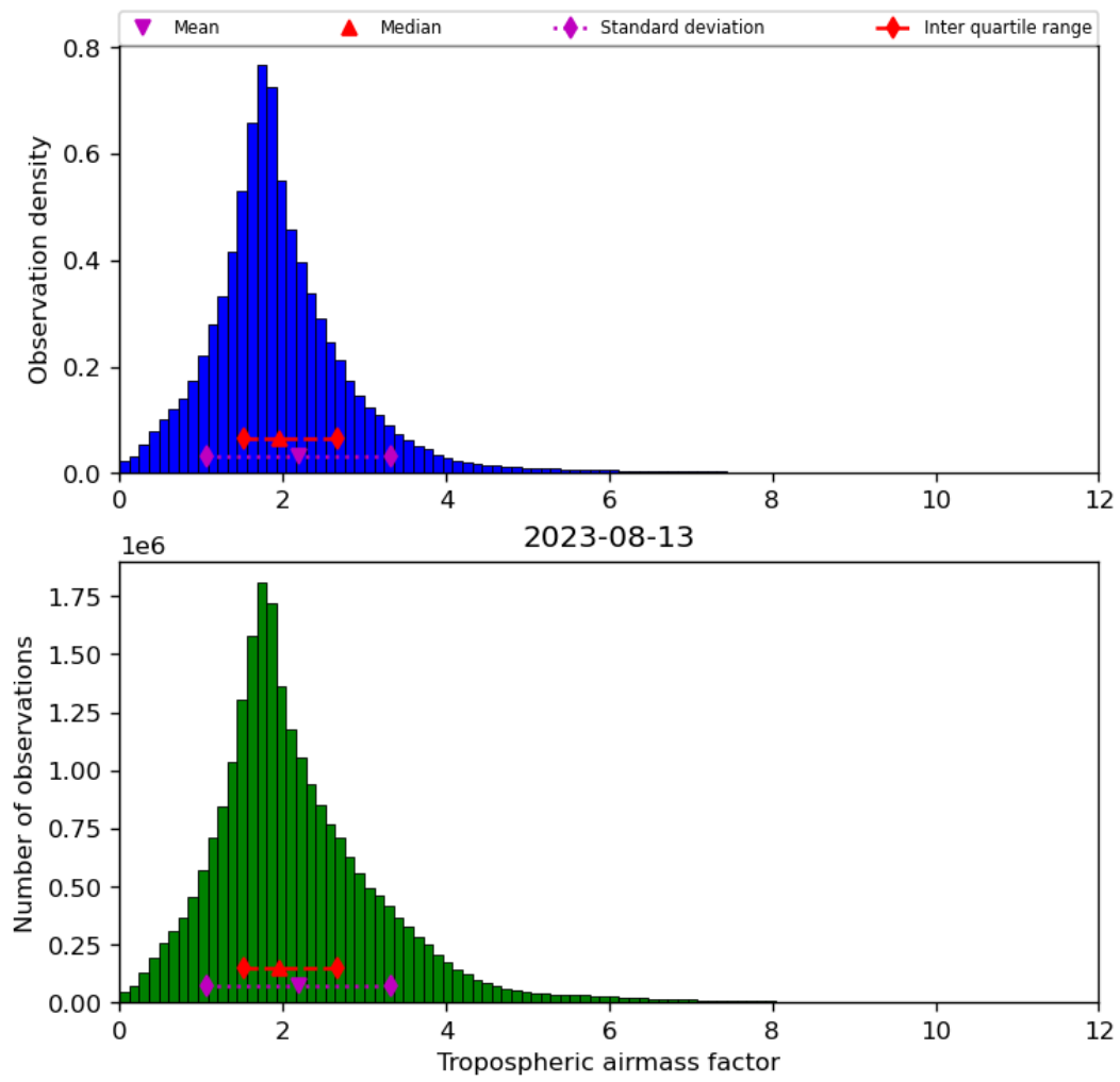
Figure 31: Histogram of “Tropospheric airmass factor” for 2023-08-12 to 2023-08-14
