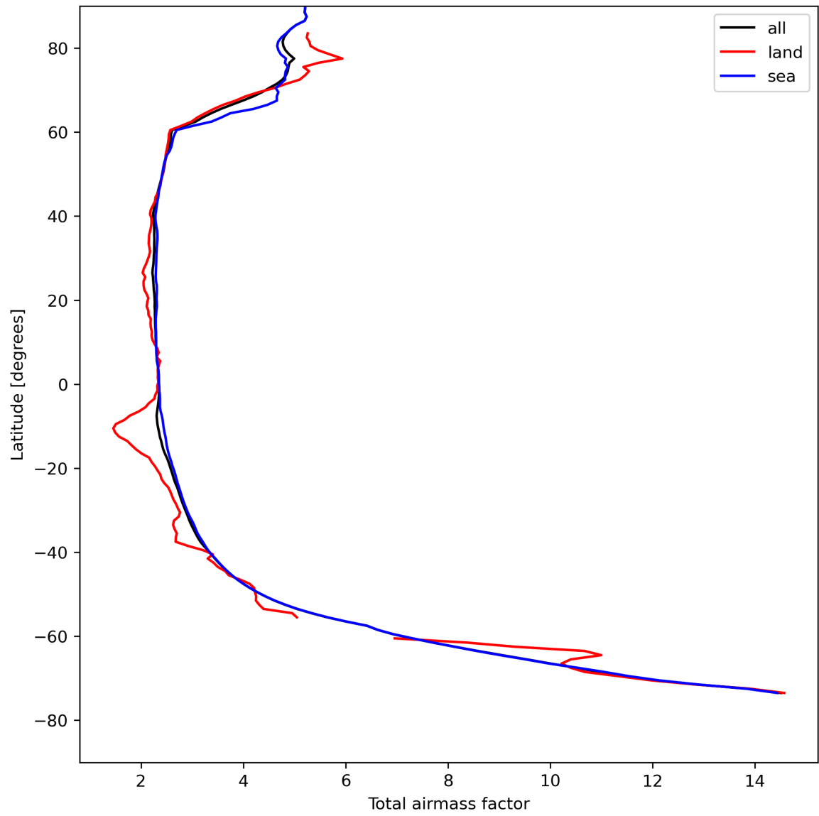
Figure 15: Zonal average of “Total airmass factor” for 2023-08-12 to 2023-08-14.
