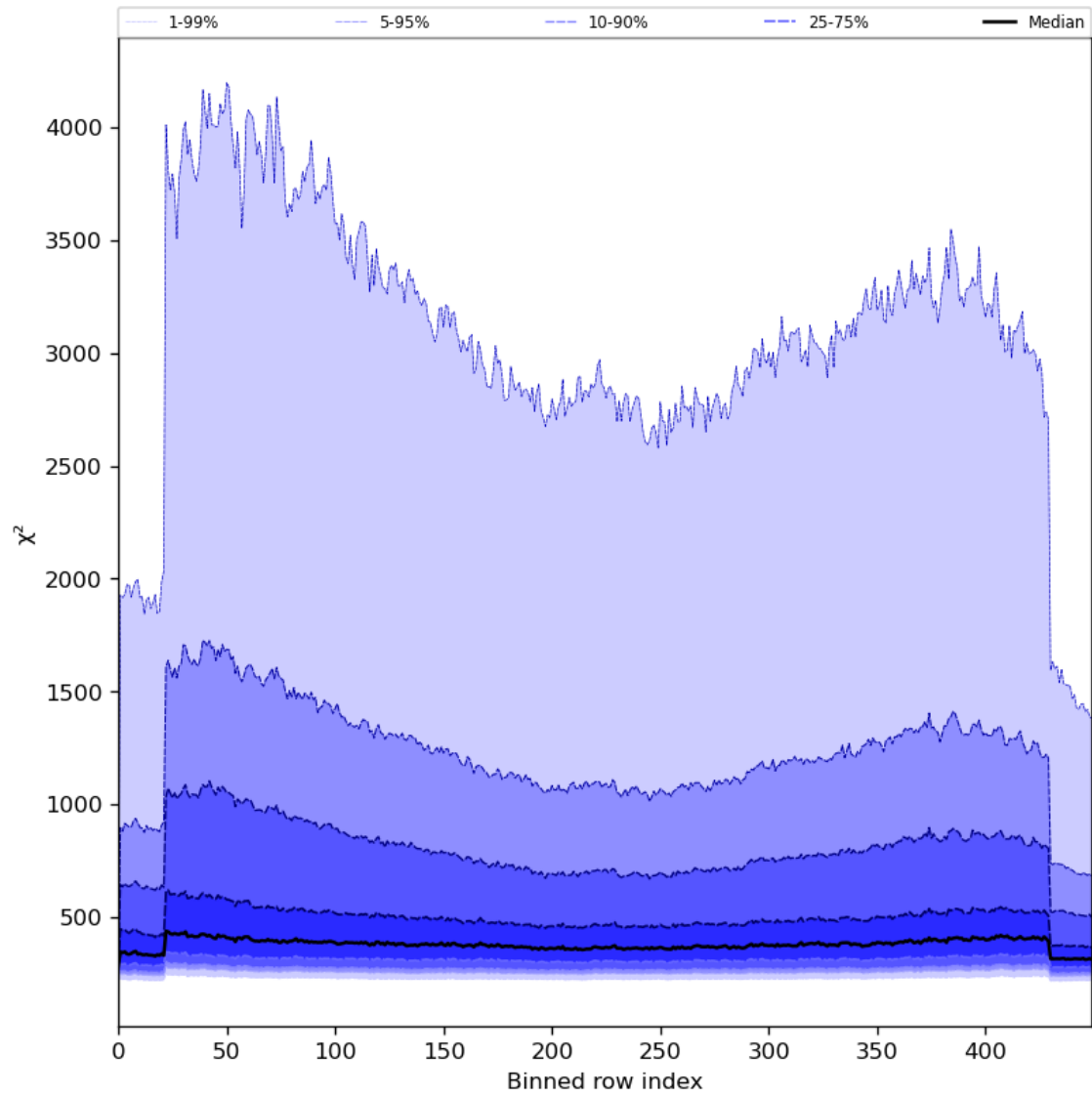
Figure 59: Along track statistics of “ \chi^2 ” for 2023-08-12 to 2023-08-14
