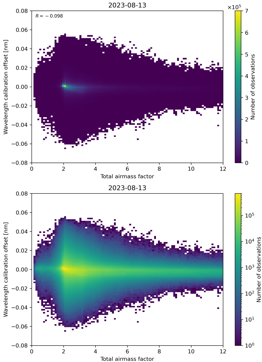
Figure 70: Scatter density plot of “Total airmass factor” against “Wavelength calibration offset” for 2023-08-12 to 2023-08-14.
