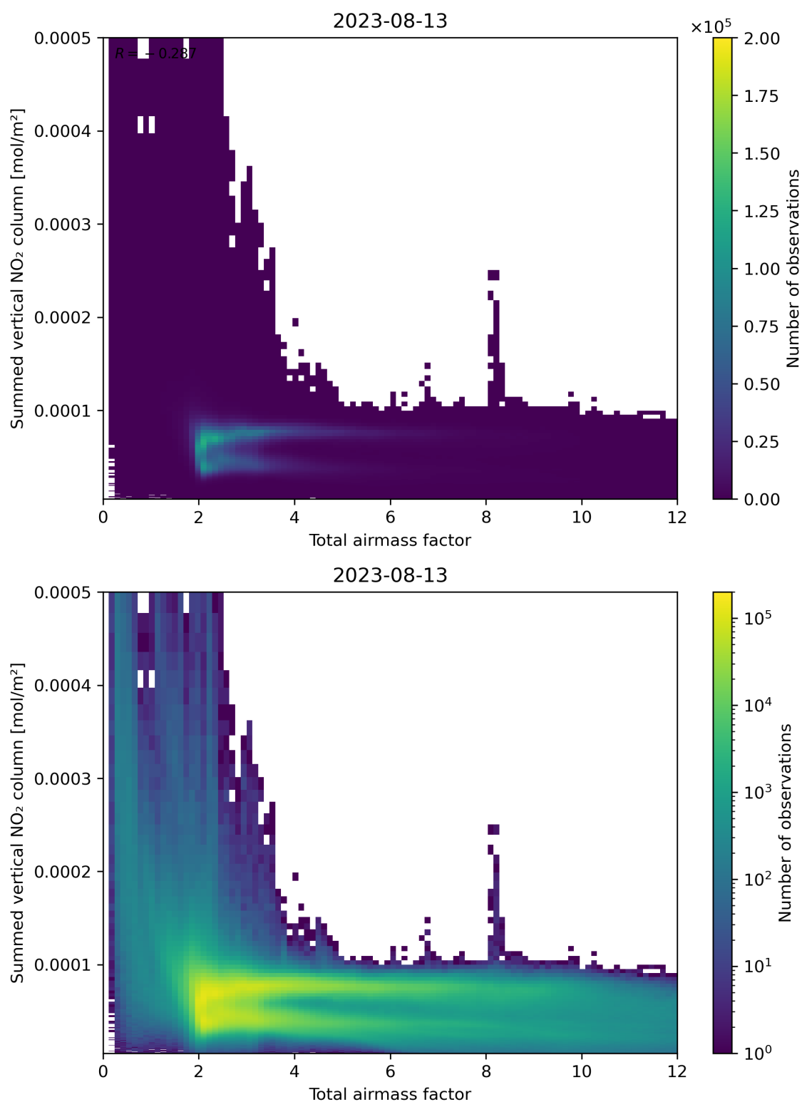
Figure 65: Scatter density plot of “Total airmass factor” against “Summed vertical NO 2 column” for 2023-08-12 to 2023-08-14.
