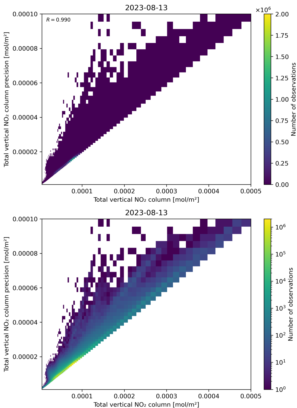
Figure 114: Scatter density plot of “Total vertical NO 2 column” against “Total vertical NO 2 column precision” for 2023-08-12 to 2023-08-14.
