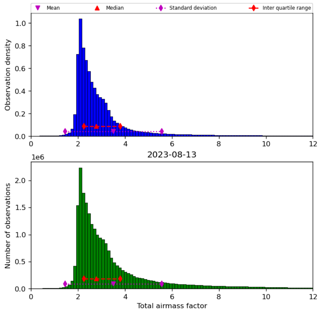
Figure 32: Histogram of “Total airmass factor” for 2023-08-12 to 2023-08-14
