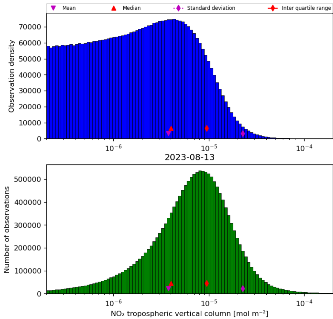
Figure 29: Histogram of “NO 2 tropospheric vertical column” for 2023-08-12 to 2023-08-14
