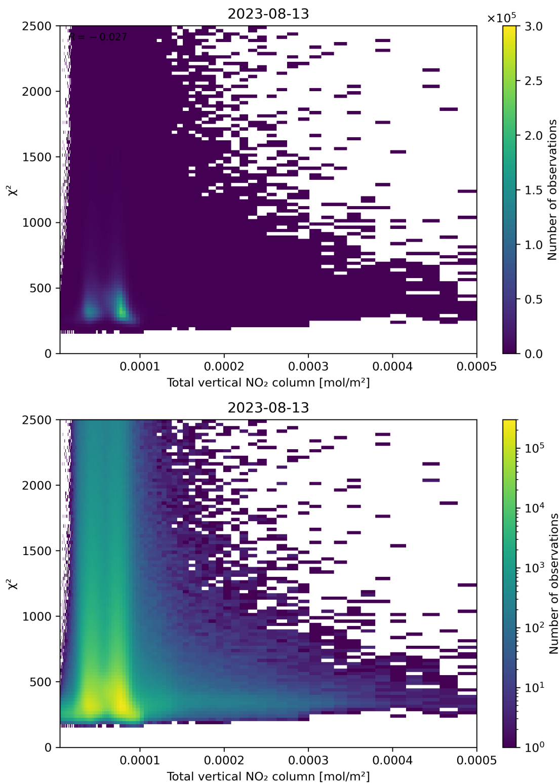
Figure 111: Scatter density plot of “Total vertical NO 2 column” against “ \chi^2 ” for 2023-08-12 to 2023-08-14.
