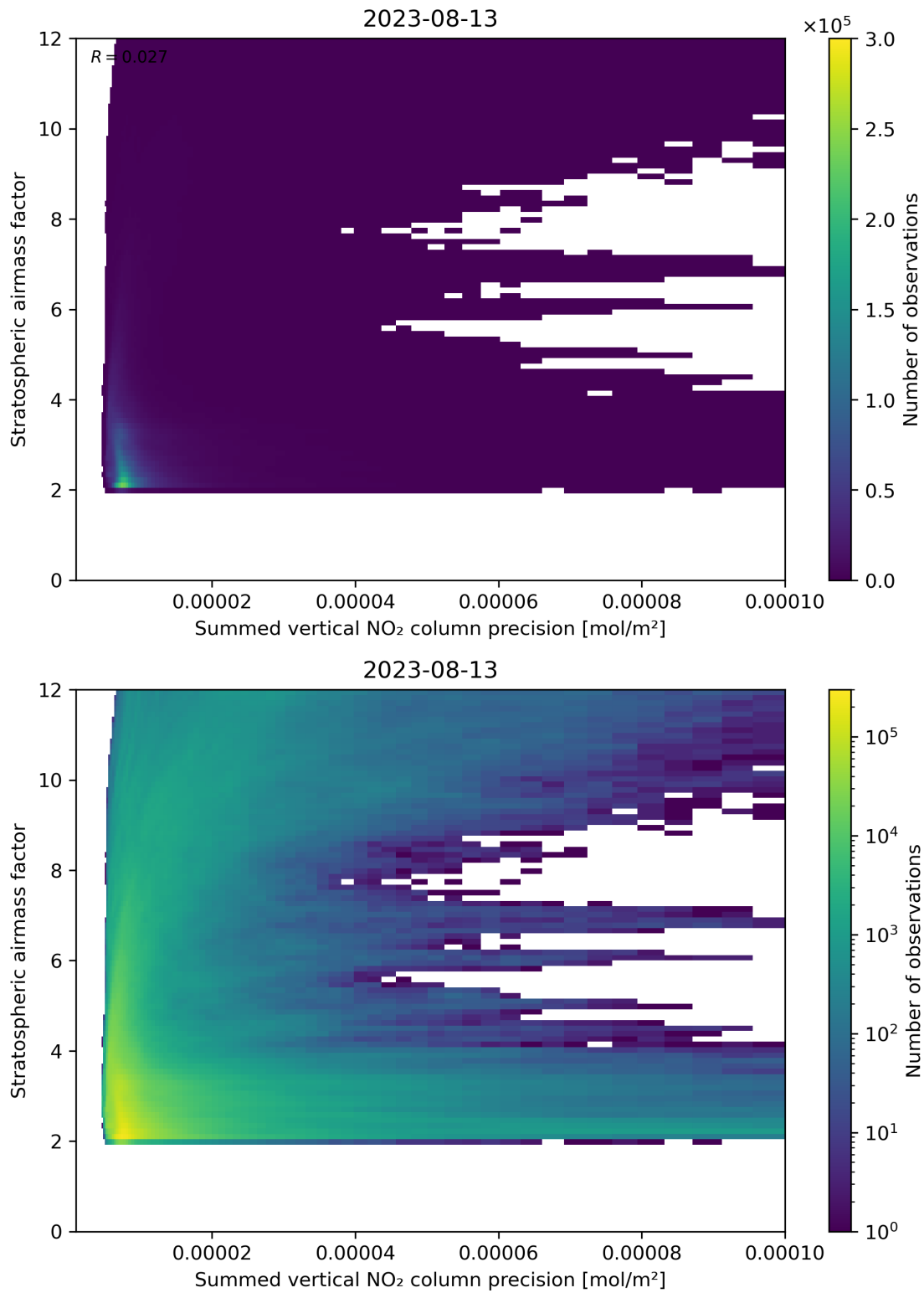
Figure 106: Scatter density plot of “Summed vertical NO 2 column precision” against “Stratospheric airmass factor” for 2023-08-12 to 2023-08-14.
