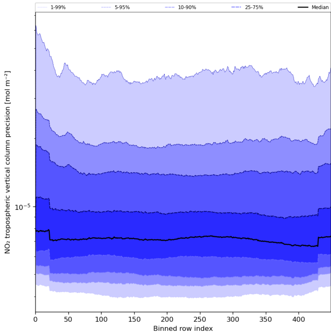
Figure 47: Along track statistics of “NO 2 tropospheric vertical column precision” for 2023-08-12 to 2023-08-14
