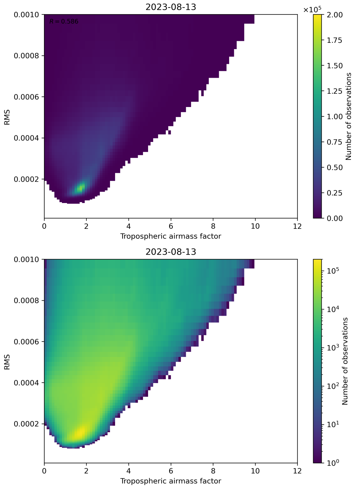
Figure 79: Scatter density plot of “Tropospheric airmass factor” against “RMS” for 2023-08-12 to 2023-08-14.
