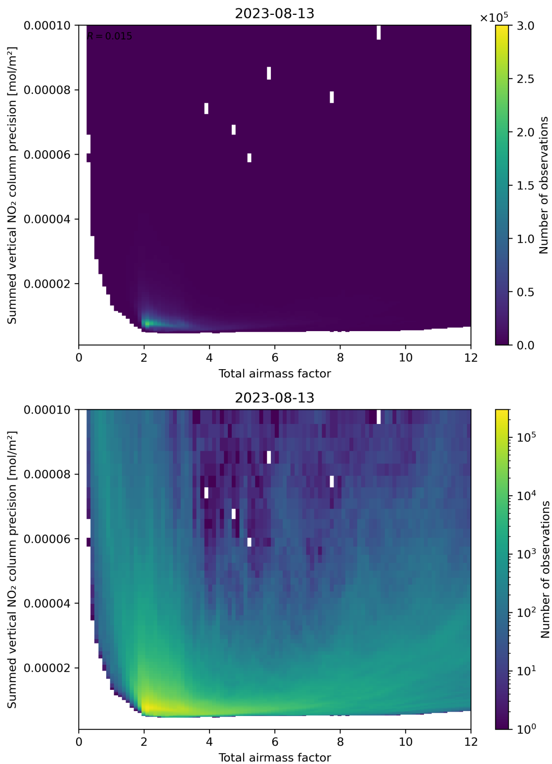
Figure 66: Scatter density plot of “Total airmass factor” against “Summed vertical NO 2 column precision” for 2023-08-12 to 2023-08-14.
