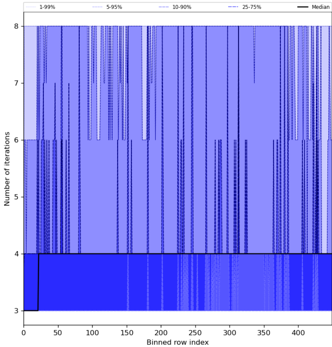
Figure 51: Along track statistics of “Number of iterations” for 2023-08-12 to 2023-08-14
