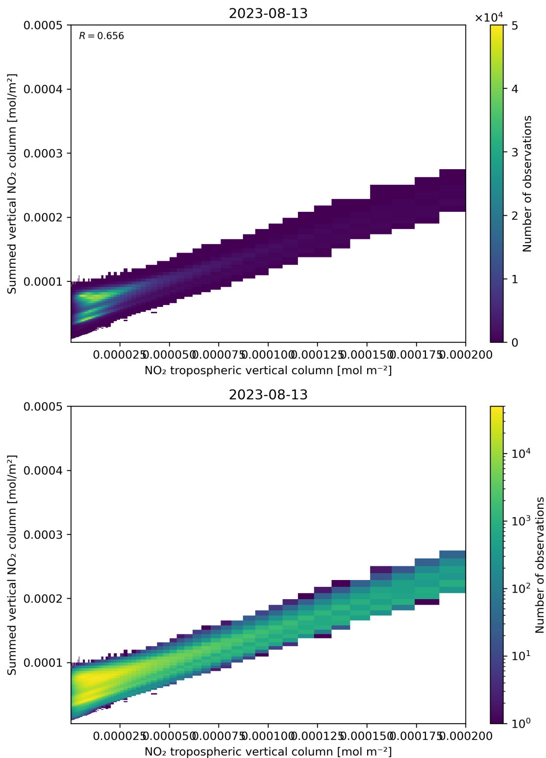
Figure 126: Scatter density plot of “NO 2 tropospheric vertical column” against “Summed vertical NO 2 column” for 2023-08-12 to 2023-08-14.
