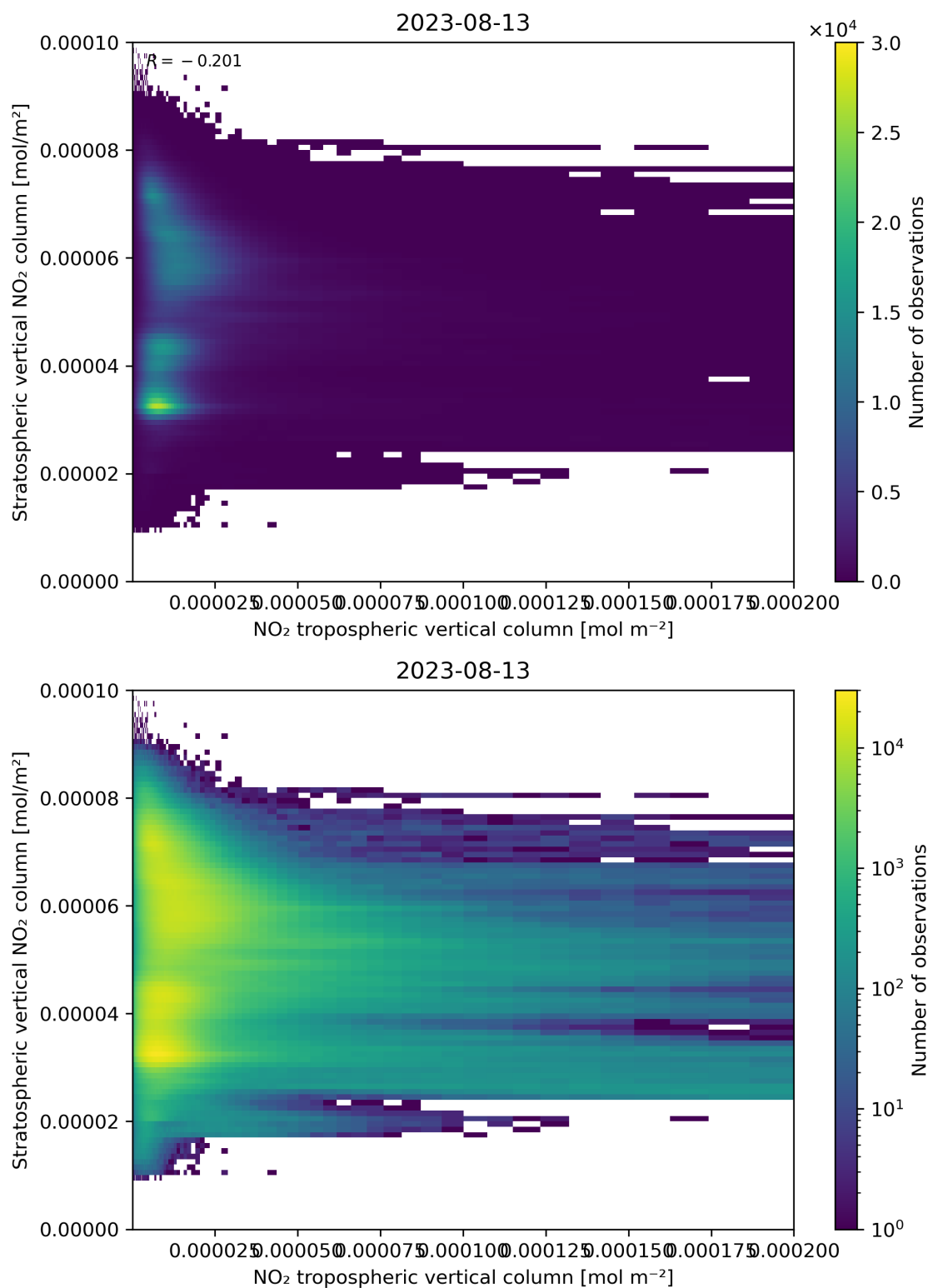
Figure 125: Scatter density plot of “NO 2 tropospheric vertical column” against “Stratospheric vertical NO 2 column” for 2023-08-12 to 2023-08-14.
