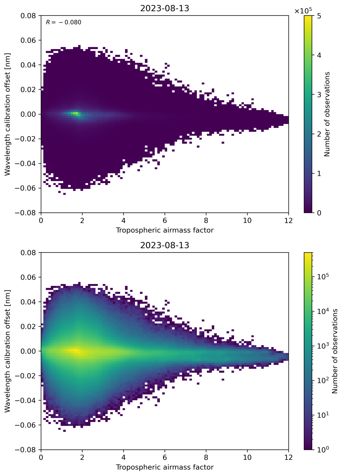
Figure 80: Scatter density plot of “Tropospheric airmass factor” against “Wavelength calibration offset” for 2023-08-12 to 2023-08-14.
