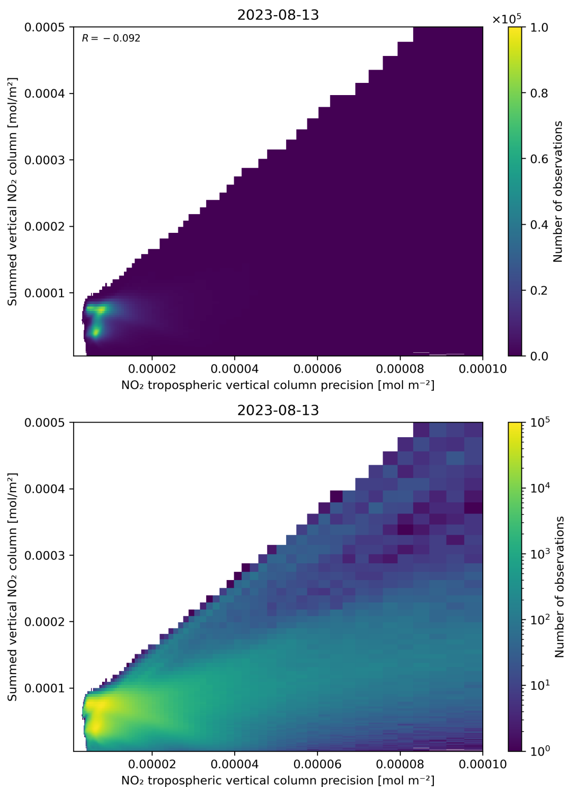
Figure 136: Scatter density plot of “NO 2 tropospheric vertical column precision” against “Summed vertical NO 2 column” for 2023-08-12 to 2023-08-14.
