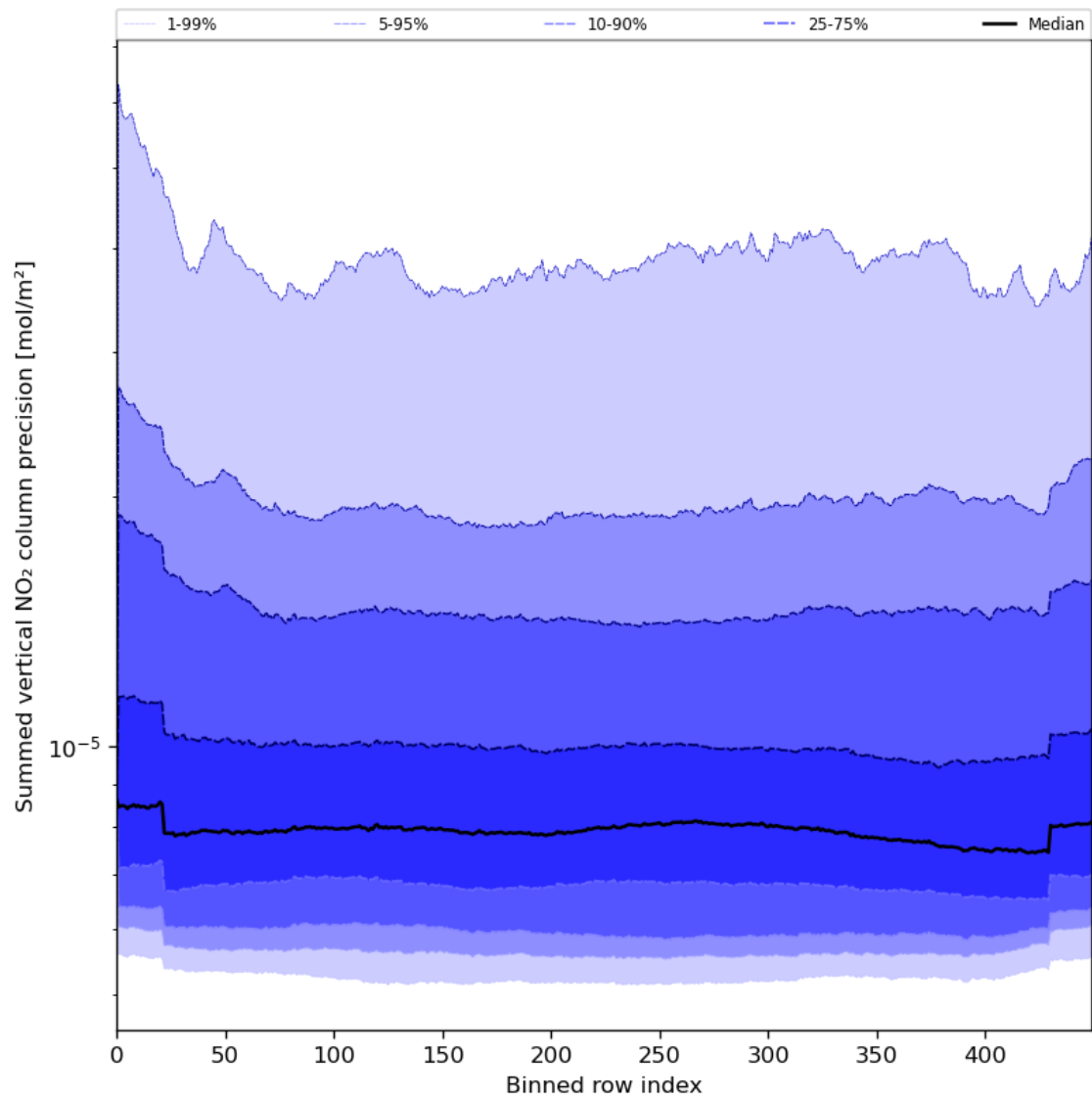
Figure 58: Along track statistics of “Summed vertical NO 2 column precision” for 2023-08-12 to 2023-08-14
