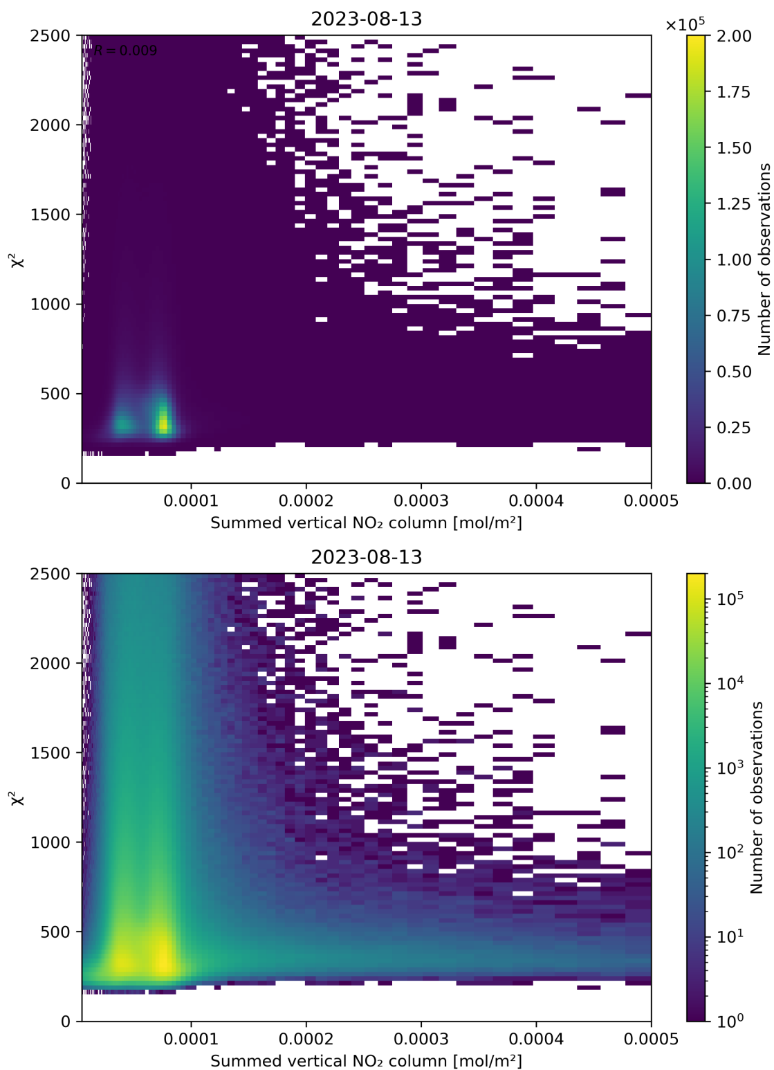
Figure 104: Scatter density plot of “Summed vertical NO 2 column” against “ \chi^2 ” for 2023-08-12 to 2023-08-14.
