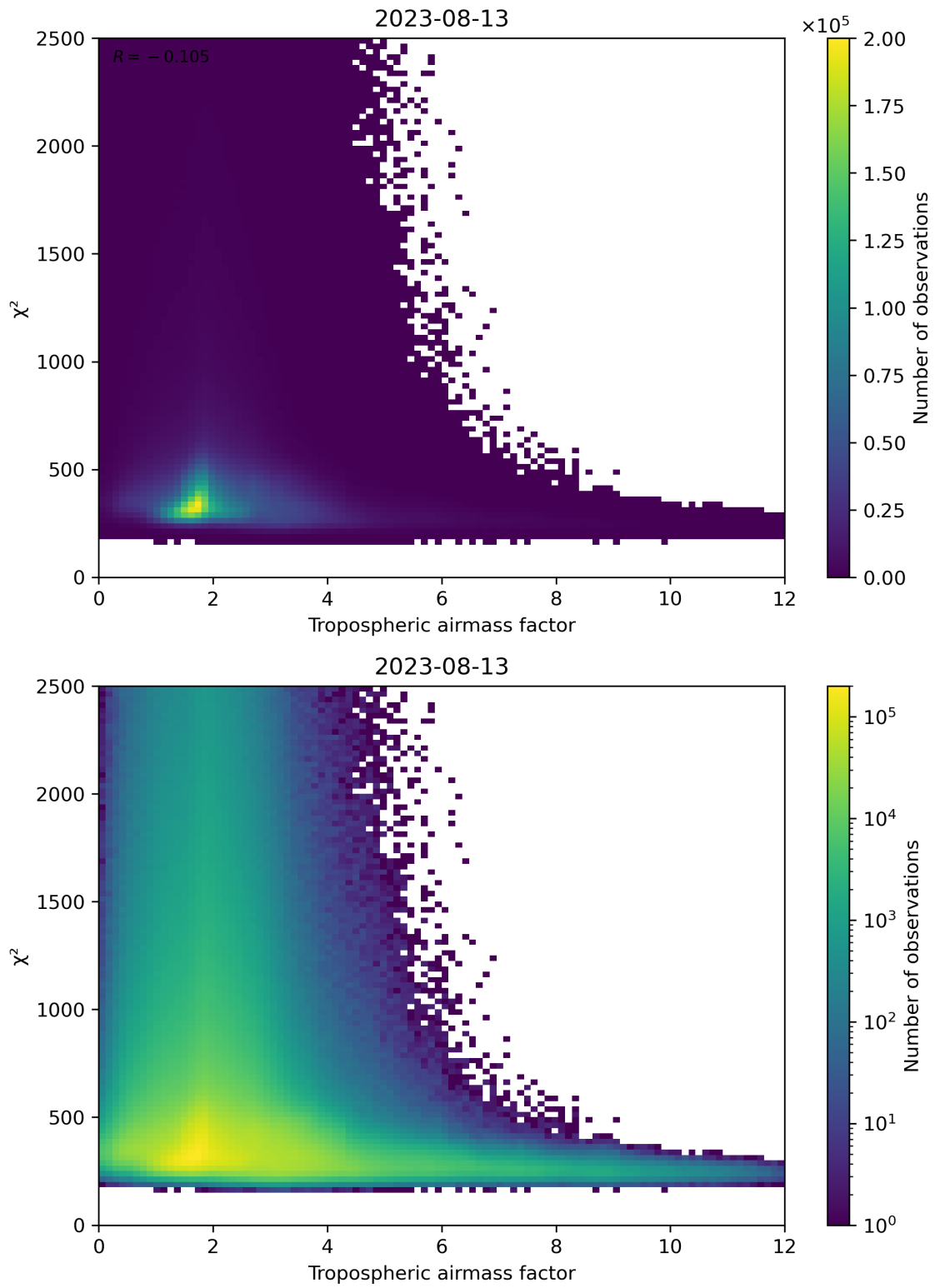
Figure 73: Scatter density plot of “Tropospheric airmass factor” against “ \chi^2 ” for 2023-08-12 to 2023-08-14.
