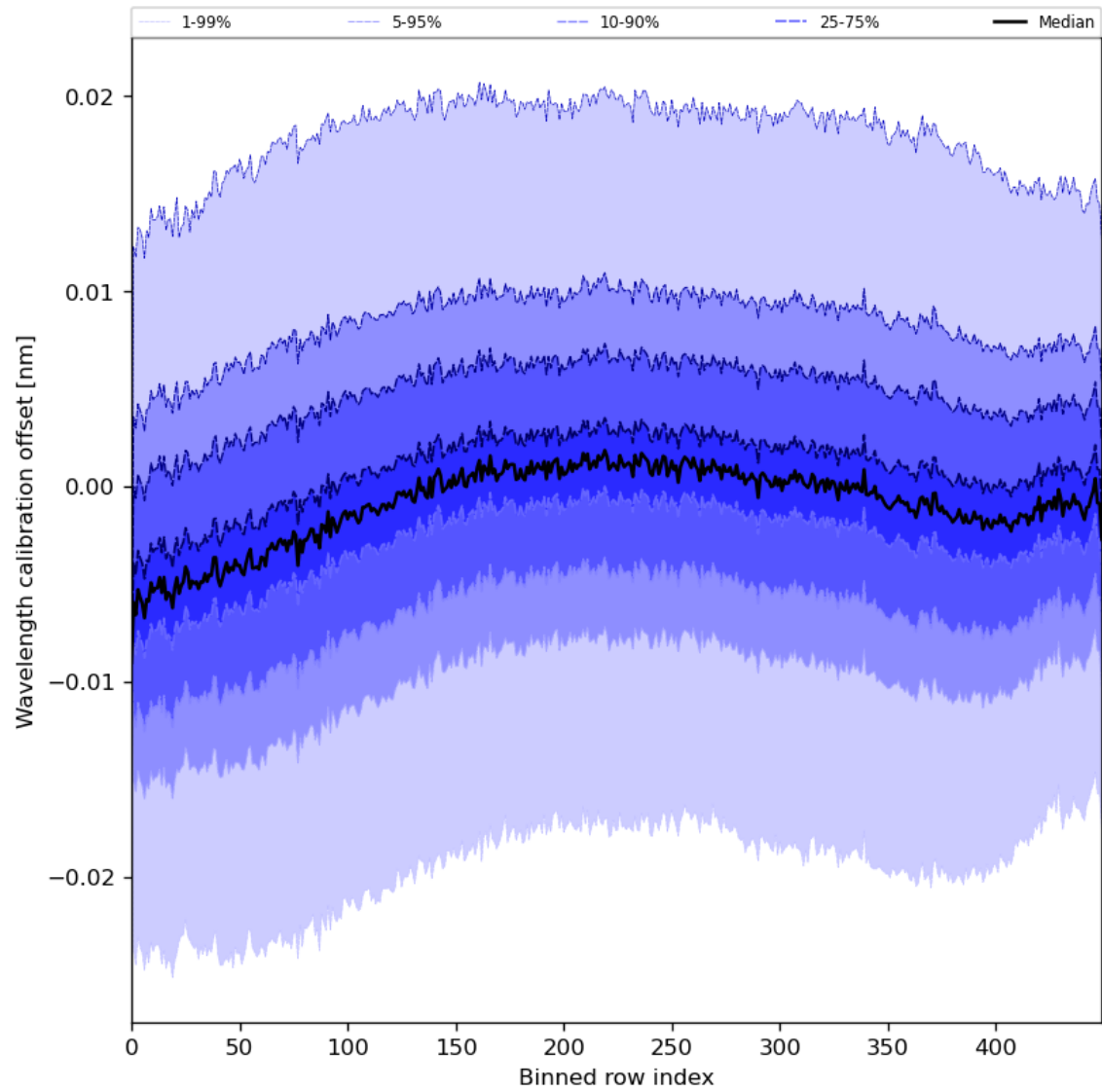
Figure 52: Along track statistics of “Wavelength calibration offset” for 2023-08-12 to 2023-08-14
