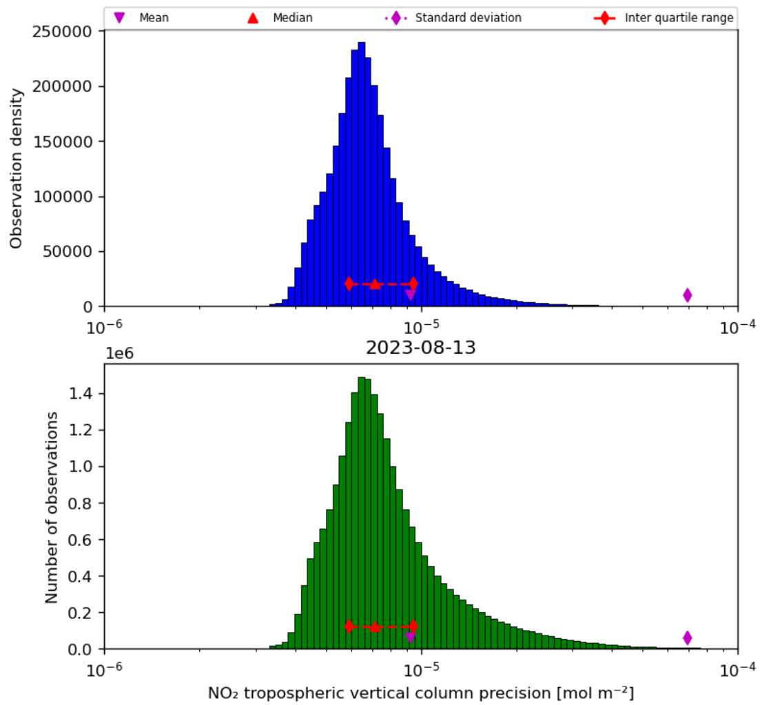
Figure 30: Histogram of “NO 2 tropospheric vertical column precision” for 2023-08-12 to 2023-08-14
