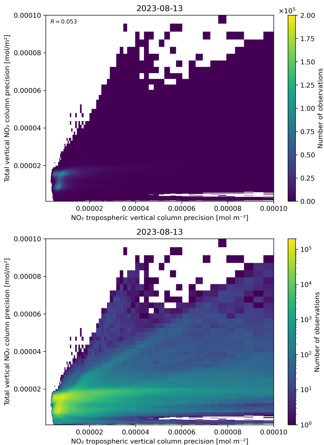
Figure 139: Scatter density plot of “NO 2 tropospheric vertical column precision” against “Total vertical NO 2 column precision” for 2023-08-12 to 2023-08-14.
