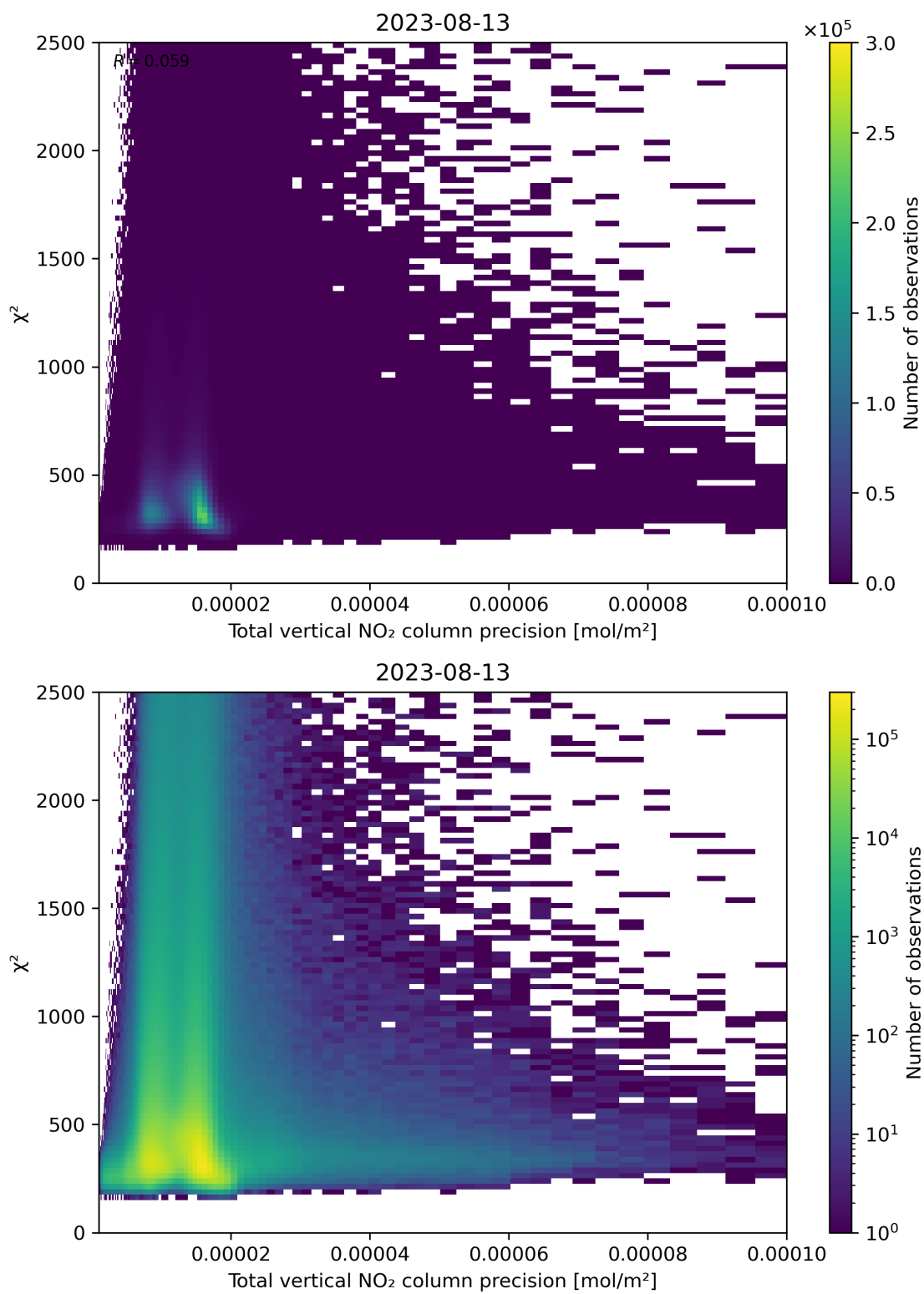
Figure 116: Scatter density plot of “Total vertical NO 2 column precision” against “ \chi^2 ” for 2023-08-12 to 2023-08-14.
