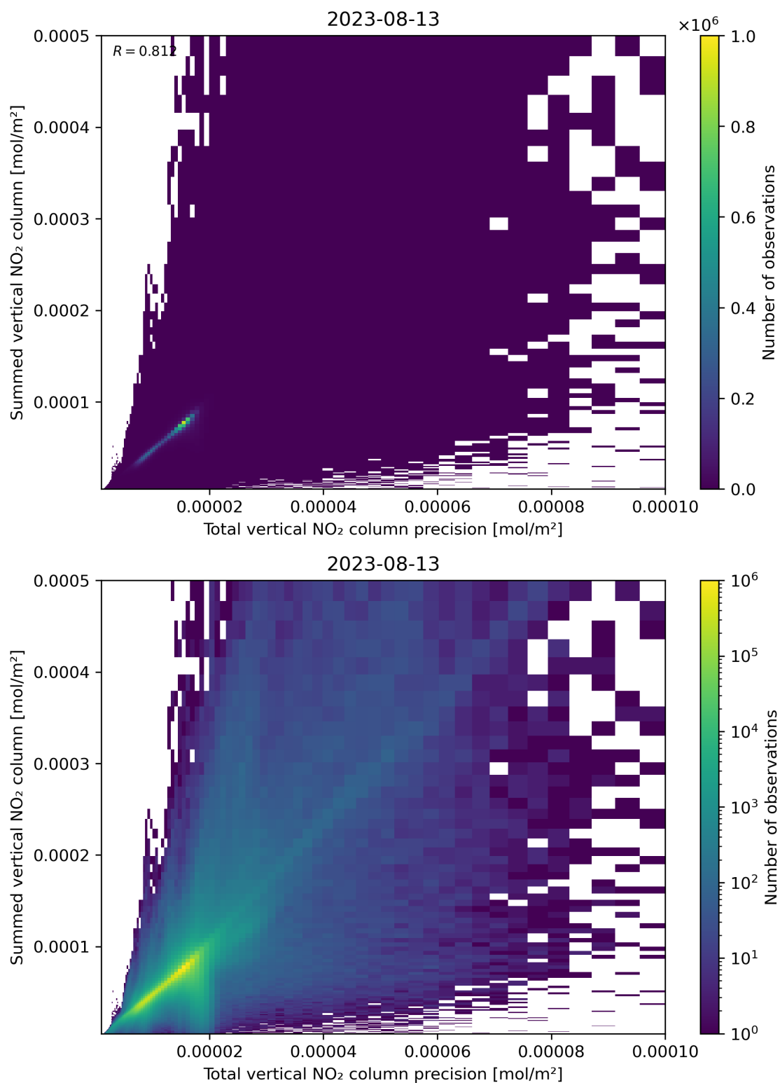
Figure 117: Scatter density plot of “Total vertical NO 2 column precision” against “Summed vertical NO 2 column” for 2023-08-12 to 2023-08-14.
