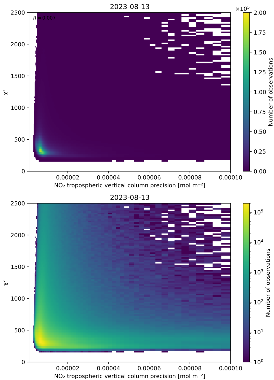
Figure 134: Scatter density plot of “NO 2 tropospheric vertical column precision” against “ \chi^2 ” for 2023-08-12 to 2023-08-14.
