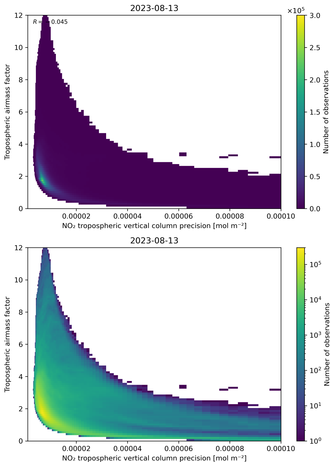
Figure 133: Scatter density plot of “NO 2 tropospheric vertical column precision” against “Tropospheric air mass factor” for 2023-08-12 to 2023-08-14.
