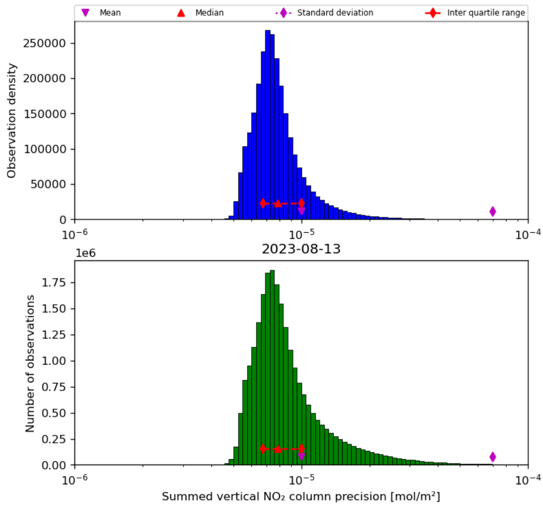
Figure 41: Histogram of “Summed vertical NO 2 column precision” for 2023-08-12 to 2023-08-14
