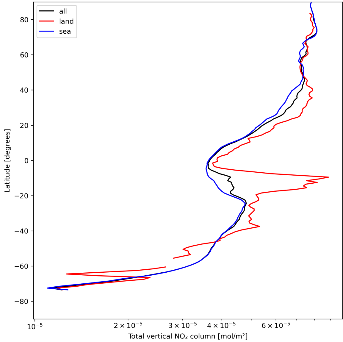
Figure 21: Zonal average of “Total vertical NO 2 column” for 2023-08-12 to 2023-08-14.
