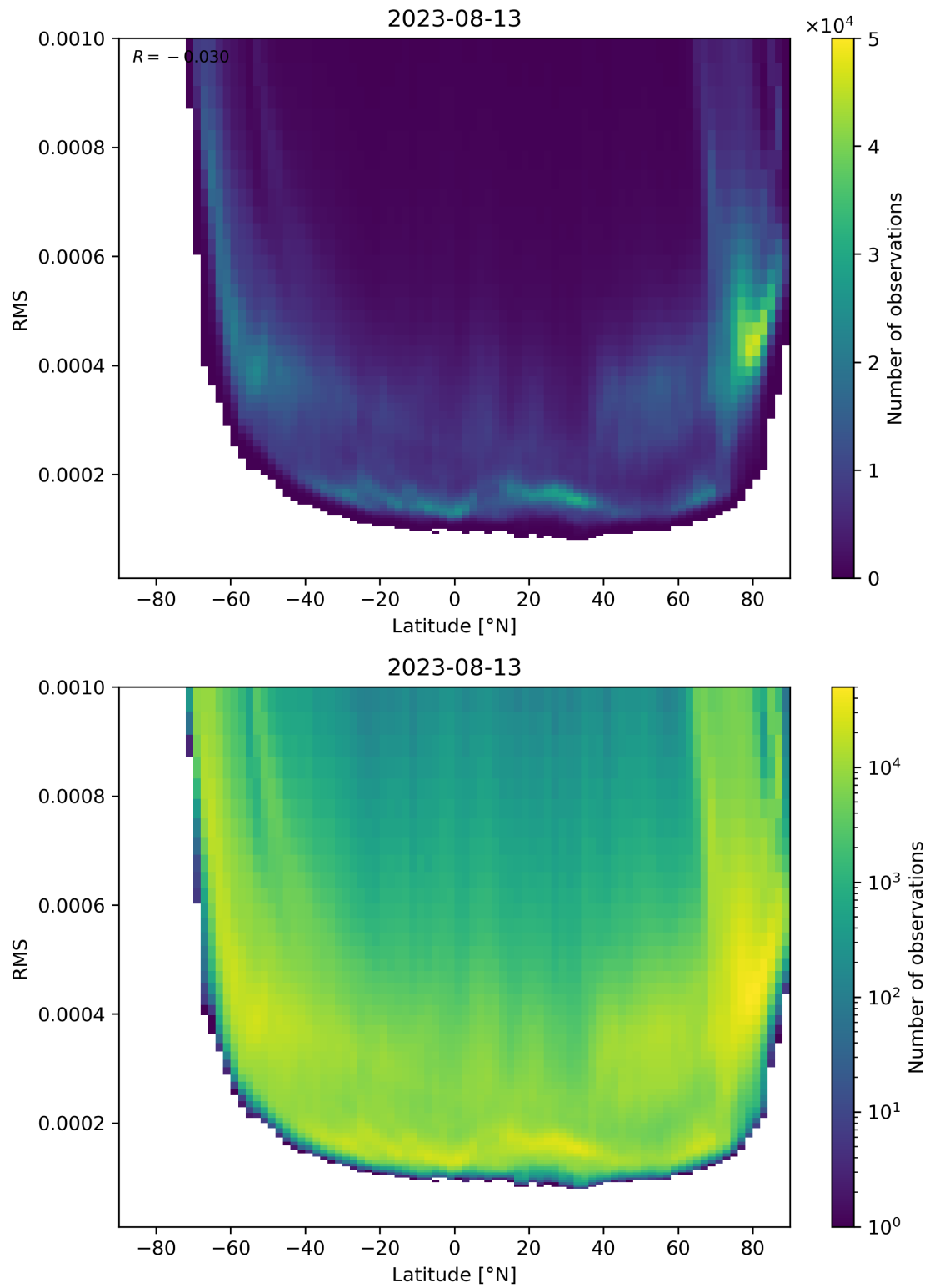
Figure 94: Scatter density plot of “Latitude” against “RMS” for 2023-08-12 to 2023-08-14.
