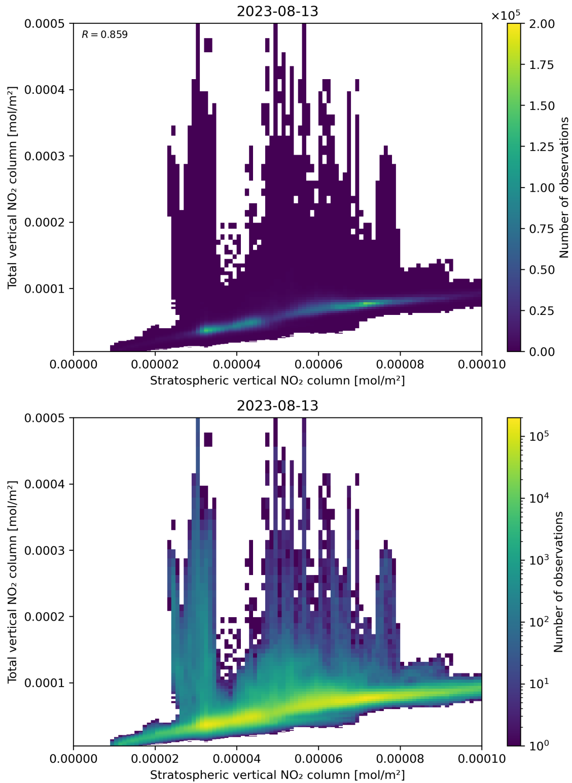
Figure 100: Scatter density plot of “Stratospheric vertical NO 2 column” against “Total vertical NO 2 column” for 2023-08-12 to 2023-08-14.
