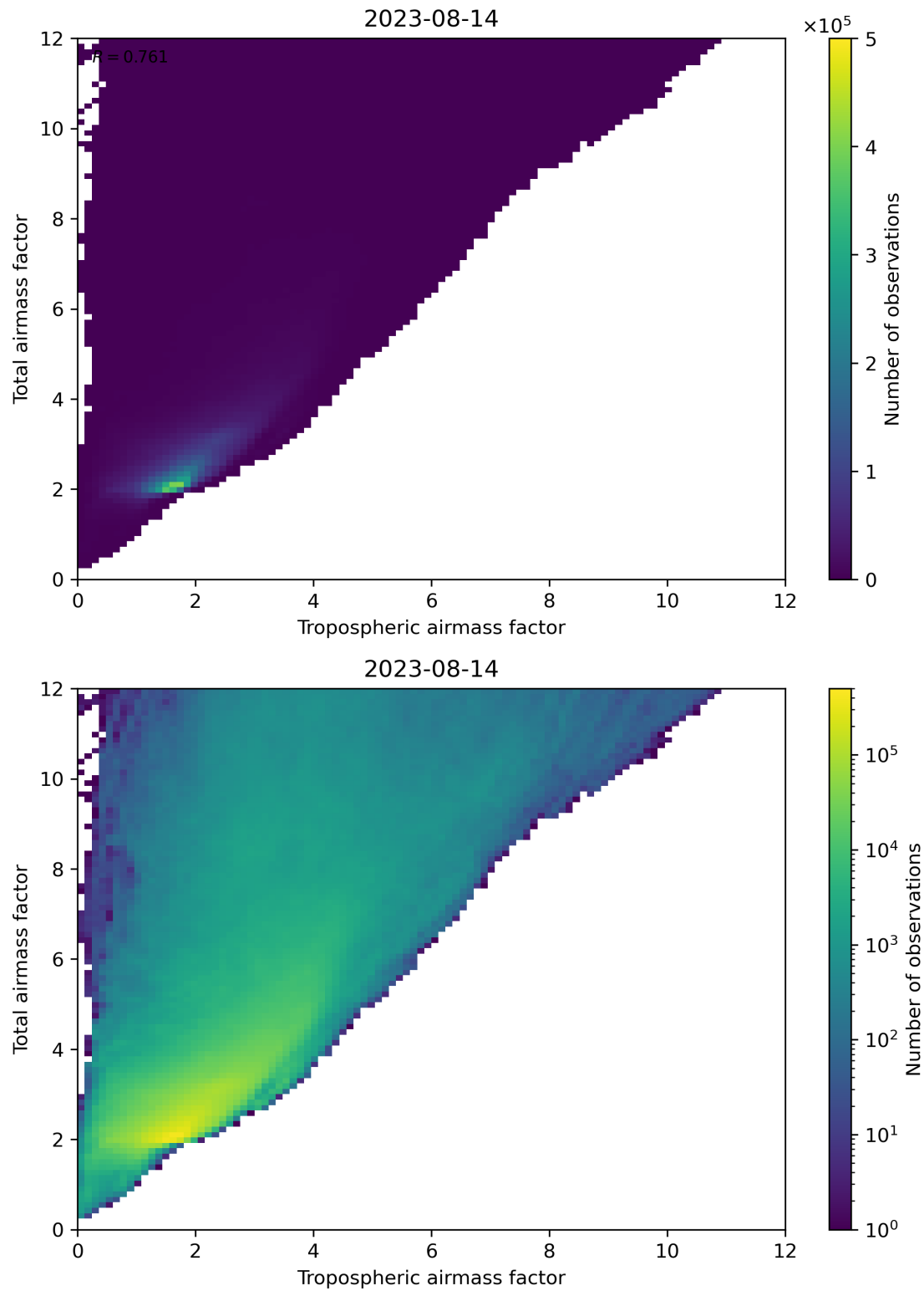
Figure 72: Scatter density plot of “Tropospheric airmass factor” against “Total airmass factor” for 2023-08-14 to 2023-08-15.
