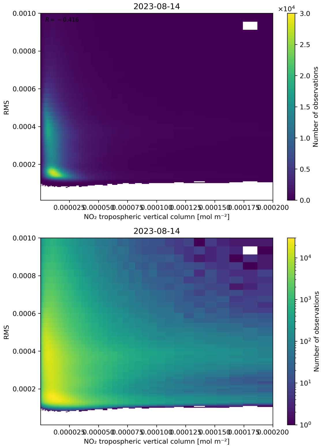
Figure 142: Scatter density plot of “NO 2 tropospheric vertical column” against “RMS” for 2023-08-14 to 2023-08-15.
