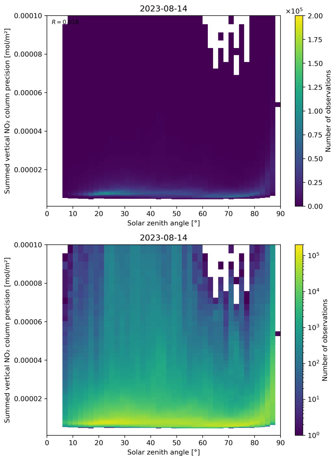
Figure 152: Scatter density plot of “Solar zenith angle” against “Summed vertical NO 2 column precision” for 2023-08-14 to 2023-08-15.
