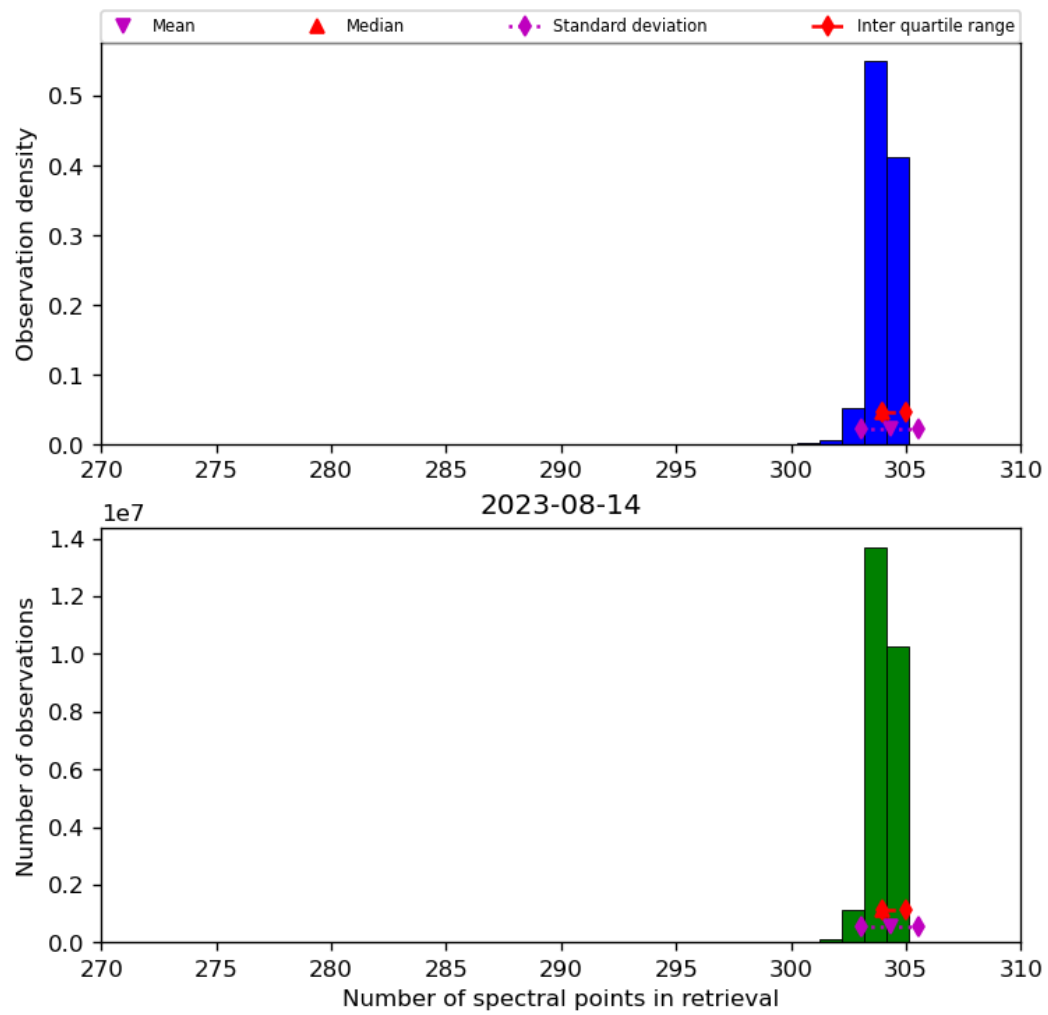
Figure 33: Histogram of “Number of spectral points in retrieval” for 2023-08-14 to 2023-08-15
