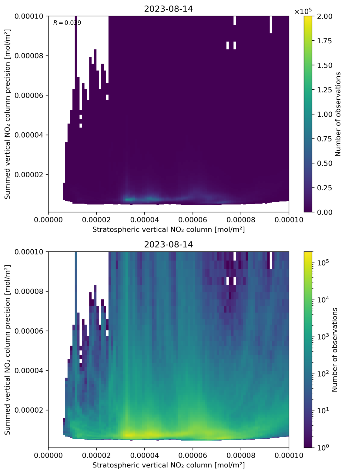
Figure 99: Scatter density plot of “Stratospheric vertical NO 2 column” against “Summed vertical NO 2 column precision” for 2023-08-14 to 2023-08-15.
