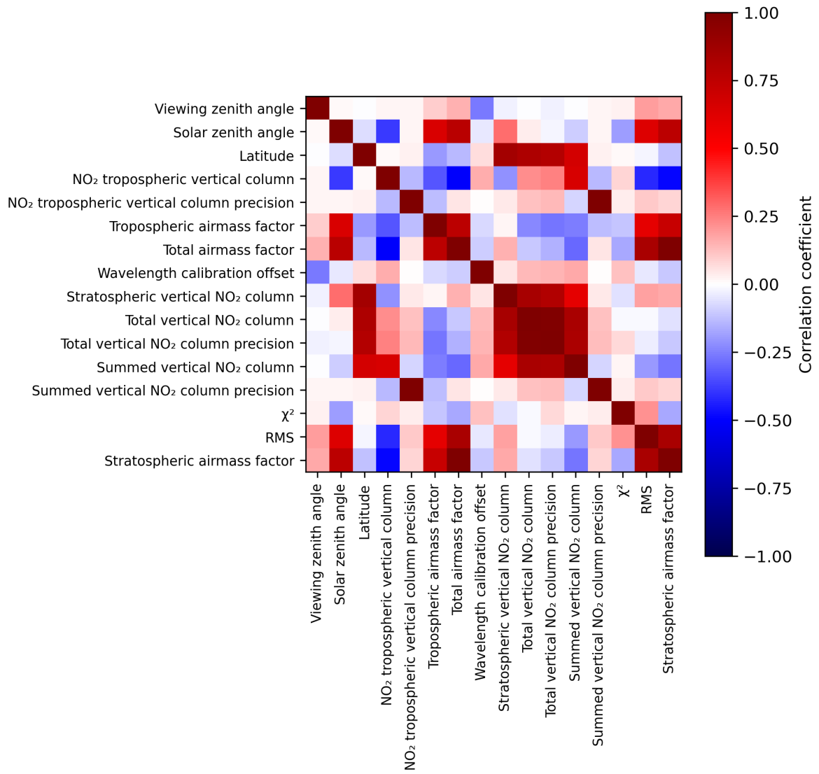
Figure 2: Map of correlation matrix for 2023-08-14 to 2023-08-15.
