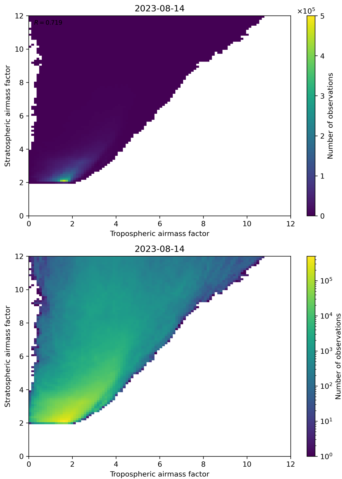
Figure 71: Scatter density plot of “Tropospheric airmass factor” against “Stratospheric airmass factor” for 2023-08-14 to 2023-08-15.
