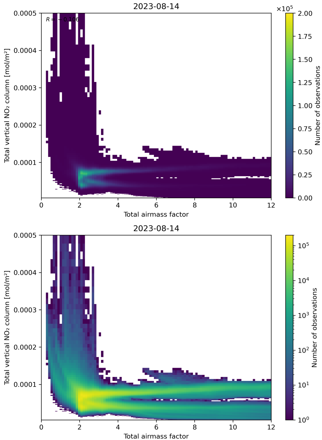
Figure 67: Scatter density plot of “Total airmass factor” against “Total vertical NO 2 column” for 2023-08-14 to 2023-08-15.
