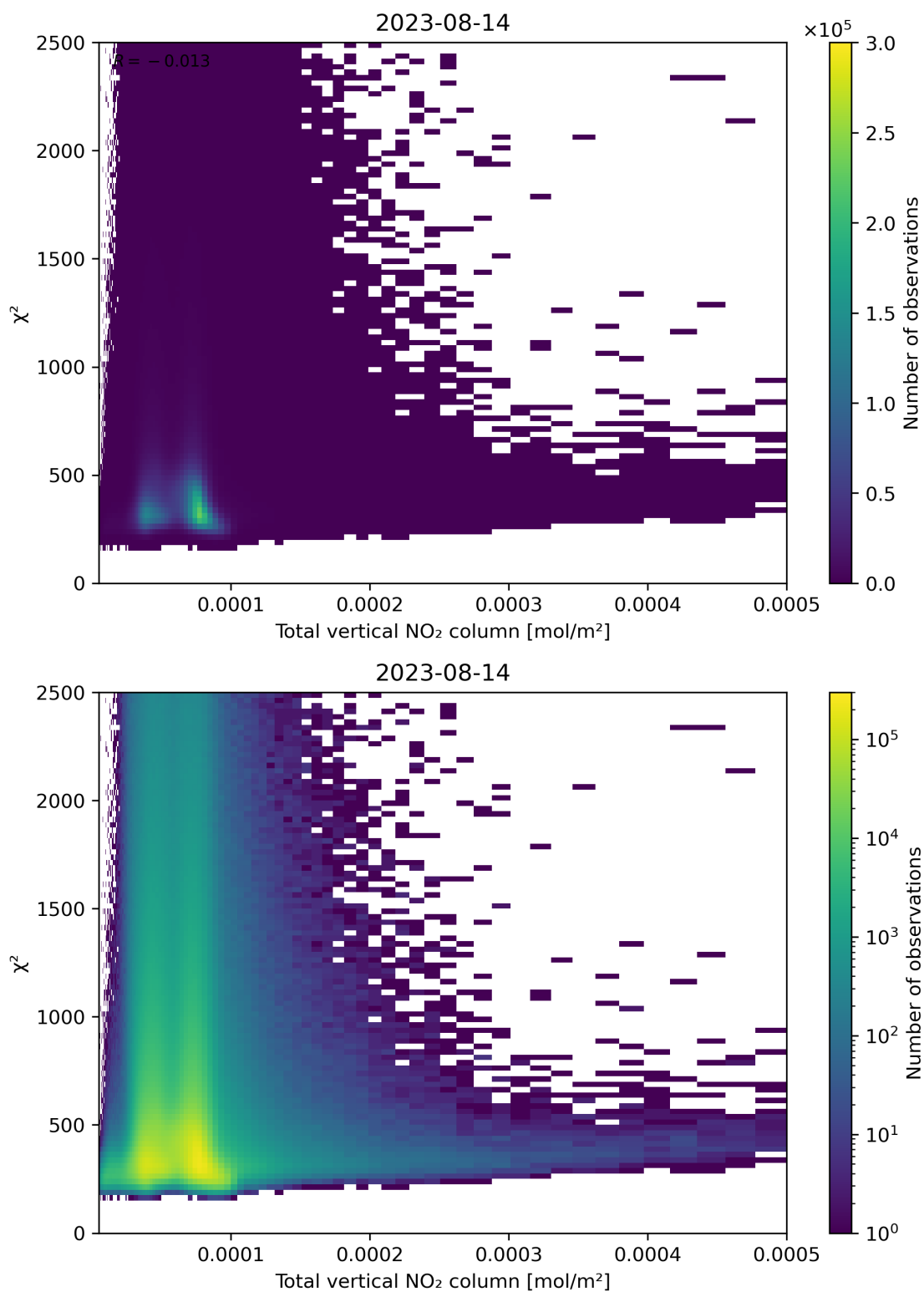
Figure 111: Scatter density plot of “Total vertical NO 2 column” against “ \chi^2 ” for 2023-08-14 to 2023-08-15.
