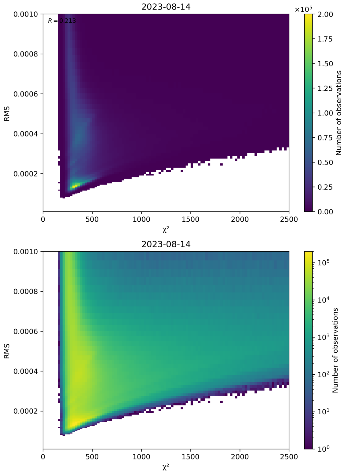
Figure 82: Scatter density plot of “ \chi^2 ” against “RMS” for 2023-08-14 to 2023-08-15.
