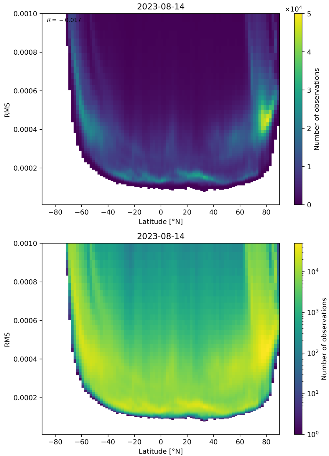
Figure 94: Scatter density plot of “Latitude” against “RMS” for 2023-08-14 to 2023-08-15.
