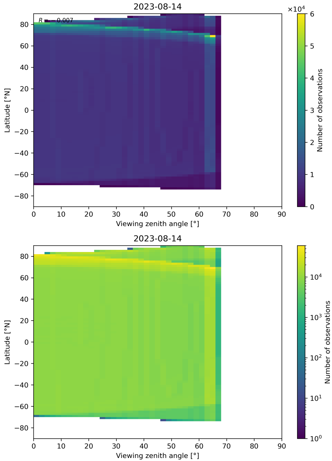
Figure 163: Scatter density plot of “Viewing zenith angle” against “Latitude” for 2023-08-14 to 2023-08-15.
