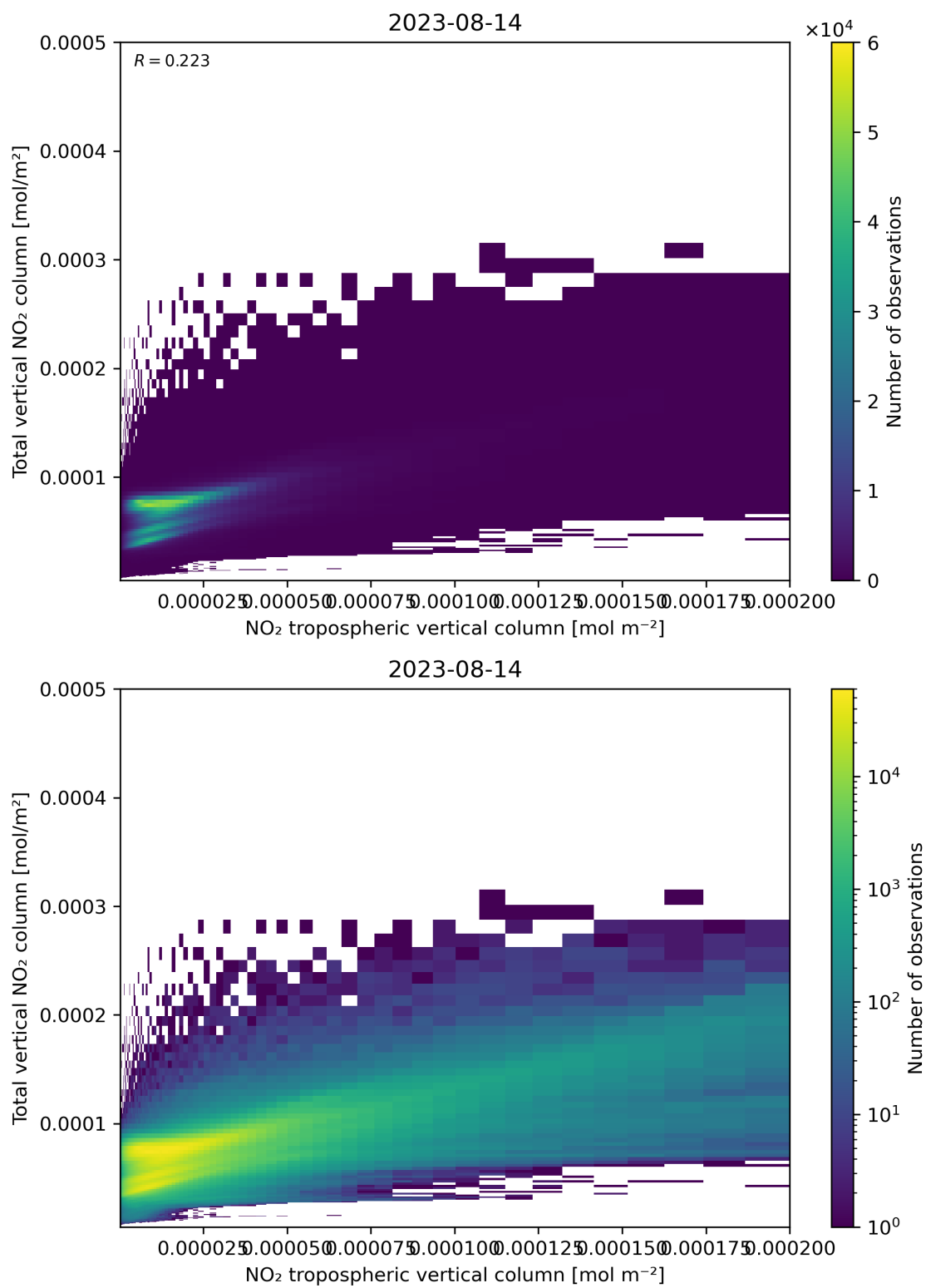
Figure 128: Scatter density plot of “NO 2 tropospheric vertical column” against “Total vertical NO 2 column” for 2023-08-14 to 2023-08-15.
