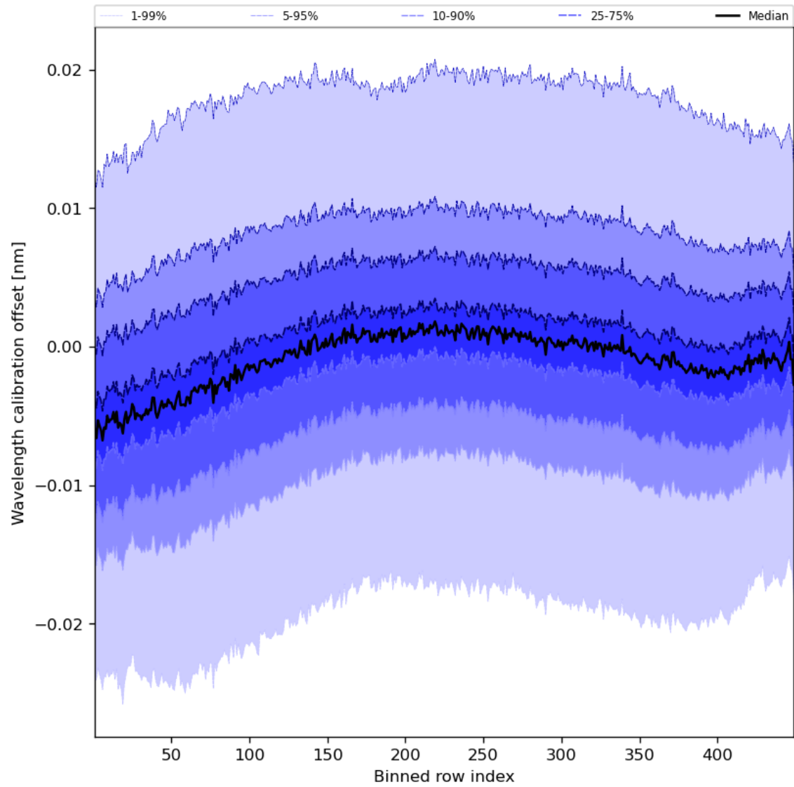
Figure 52: Along track statistics of “Wavelength calibration offset” for 2023-08-14 to 2023-08-15
