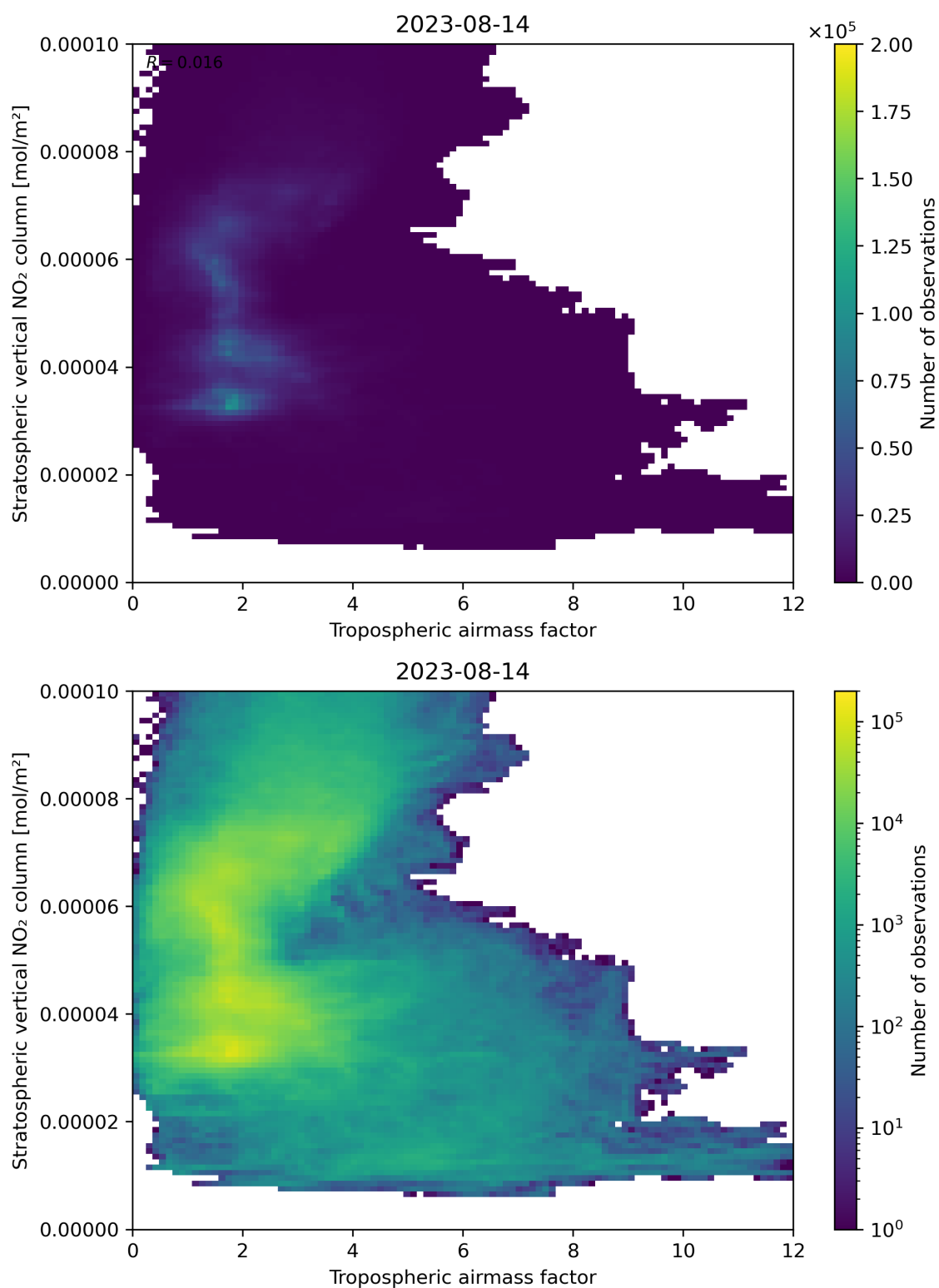
Figure 74: Scatter density plot of “Tropospheric air mass factor” against “Stratospheric vertical NO 2 column” for 2023-08-14 to 2023-08-15.
