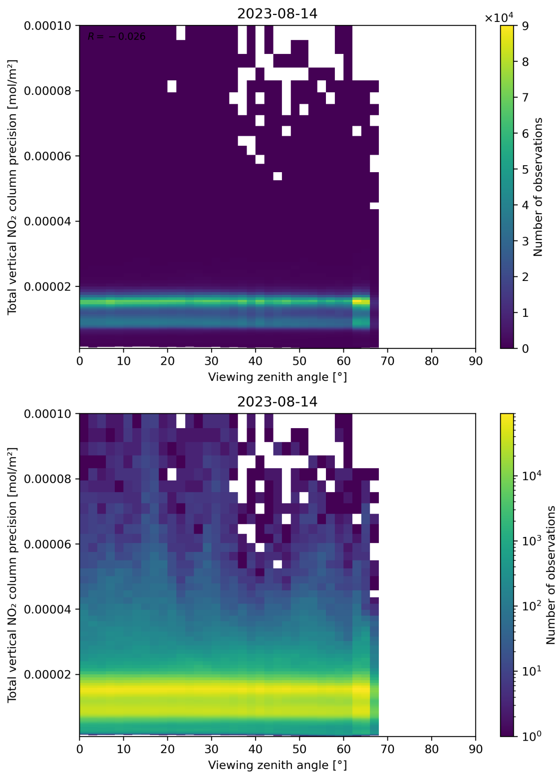
Figure 168: Scatter density plot of “Viewing zenith angle” against “Total vertical NO 2 column precision” for 2023-08-14 to 2023-08-15.
