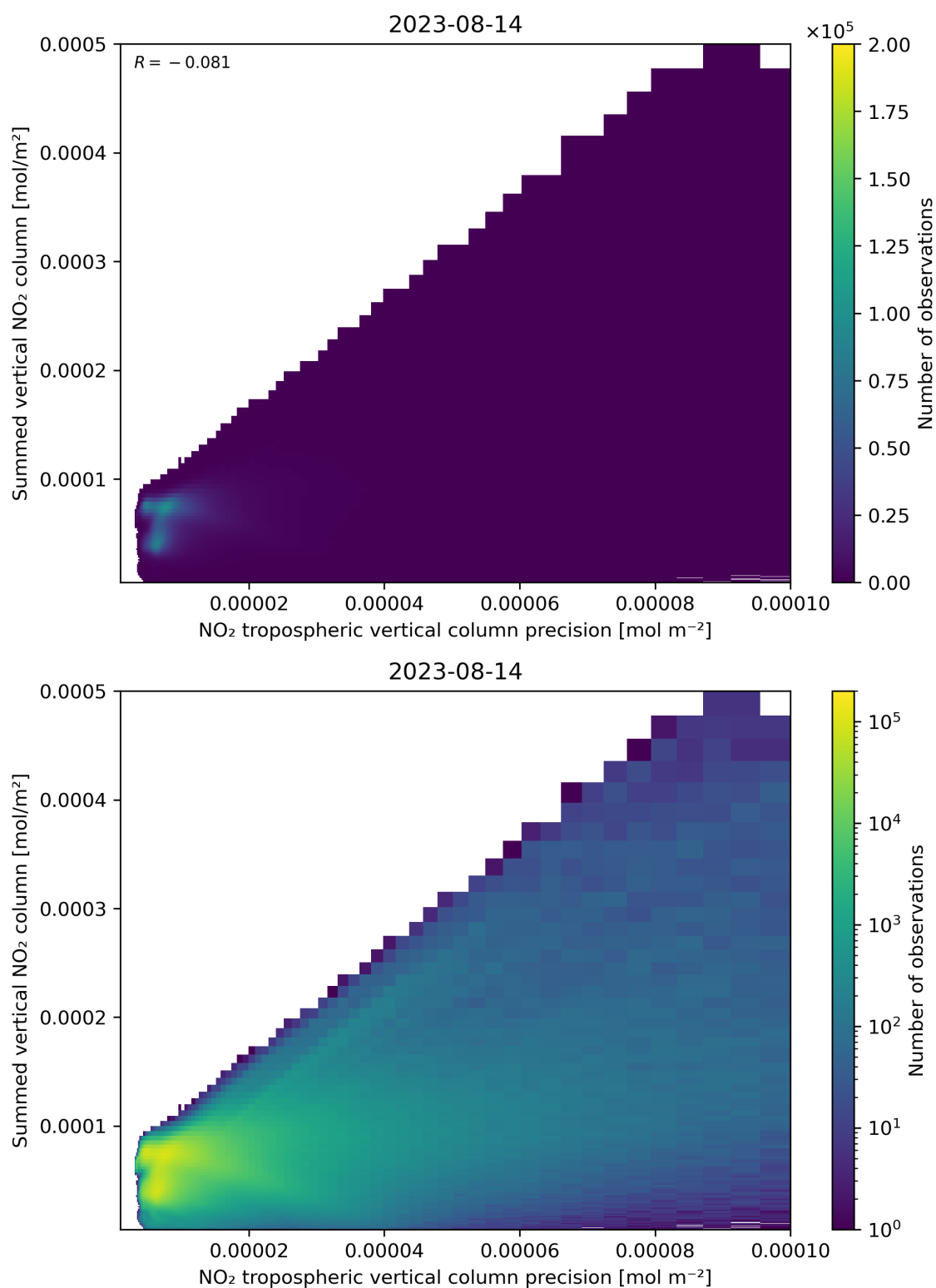
Figure 136: Scatter density plot of “NO 2 tropospheric vertical column precision” against “Summed vertical NO 2 column” for 2023-08-14 to 2023-08-15.
