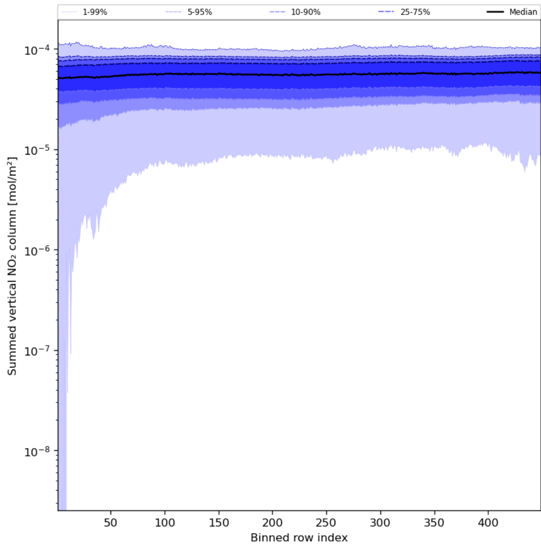
Figure 57: Along track statistics of “Summed vertical NO 2 column” for 2023-08-14 to 2023-08-15
