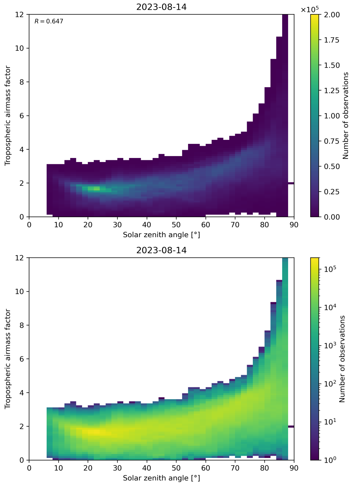
Figure 147: Scatter density plot of “Solar zenith angle” against “Tropospheric airmass factor” for 2023-08-14 to 2023-08-15.
