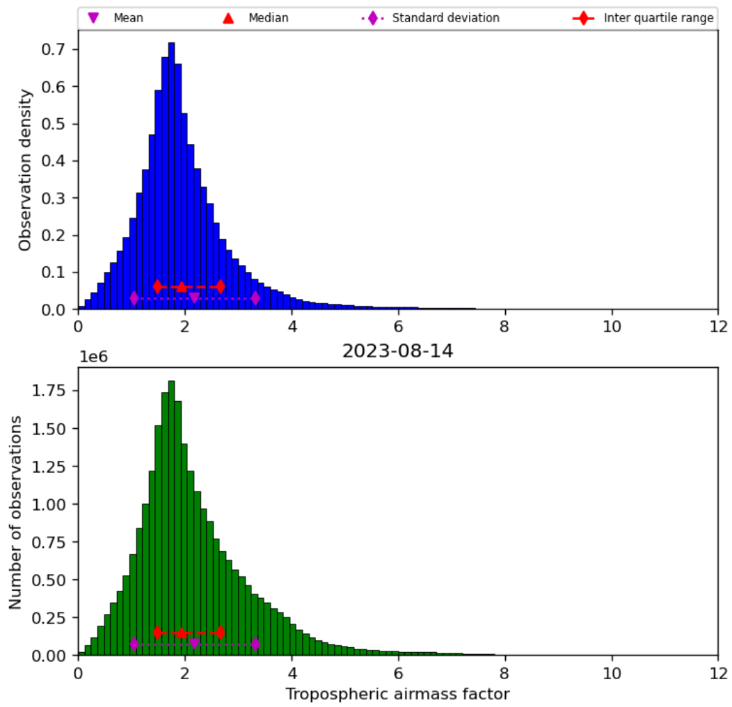
Figure 31: Histogram of “Tropospheric airmass factor” for 2023-08-14 to 2023-08-15
