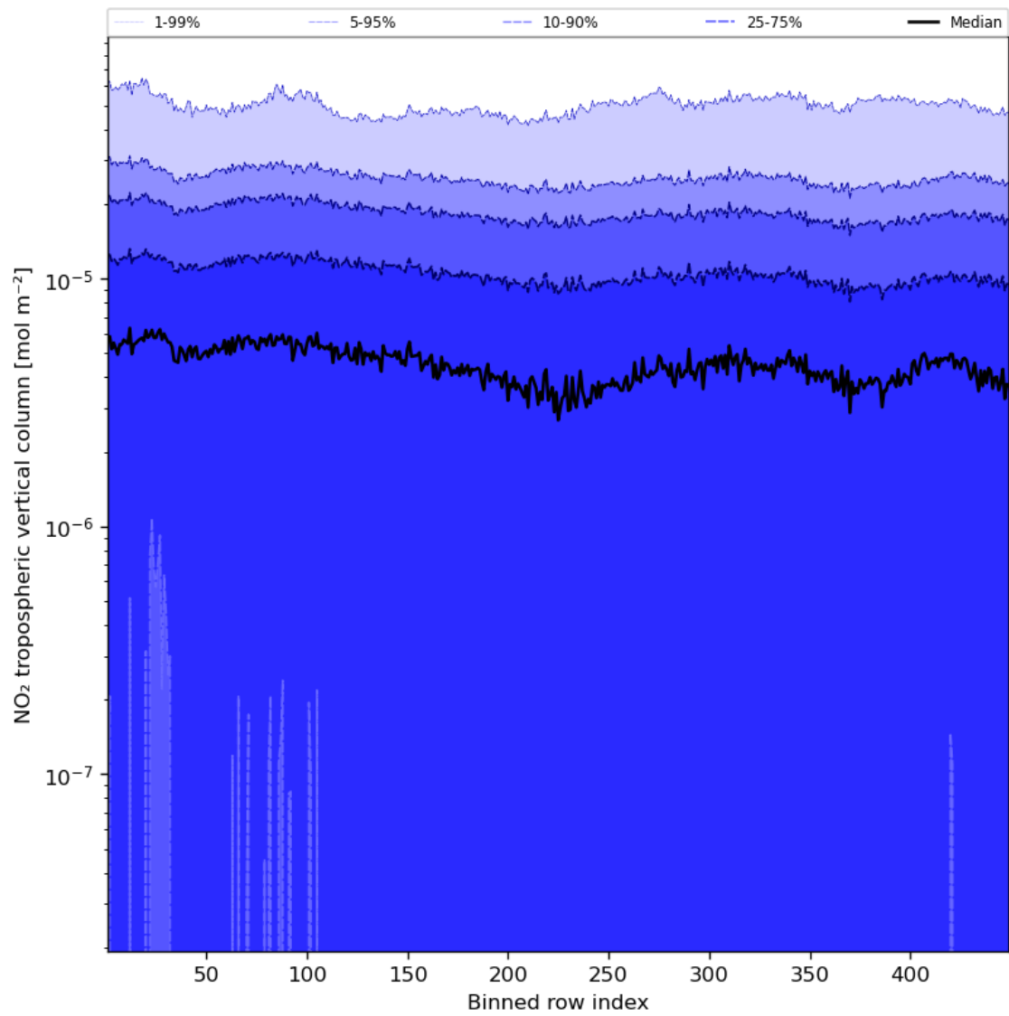
Figure 46: Along track statistics of “NO 2 tropospheric vertical column” for 2023-08-14 to 2023-08-15
