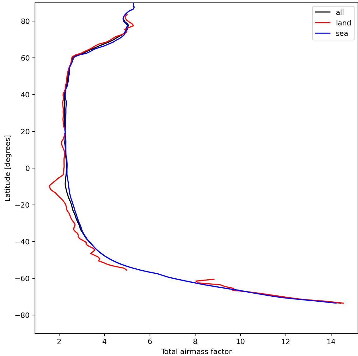
Figure 15: Zonal average of “Total airmass factor” for 2023-08-14 to 2023-08-15.
