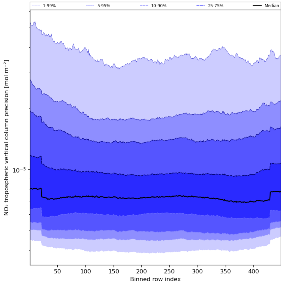
Figure 47: Along track statistics of “NO 2 tropospheric vertical column precision” for 2023-08-14 to 2023-08-15
