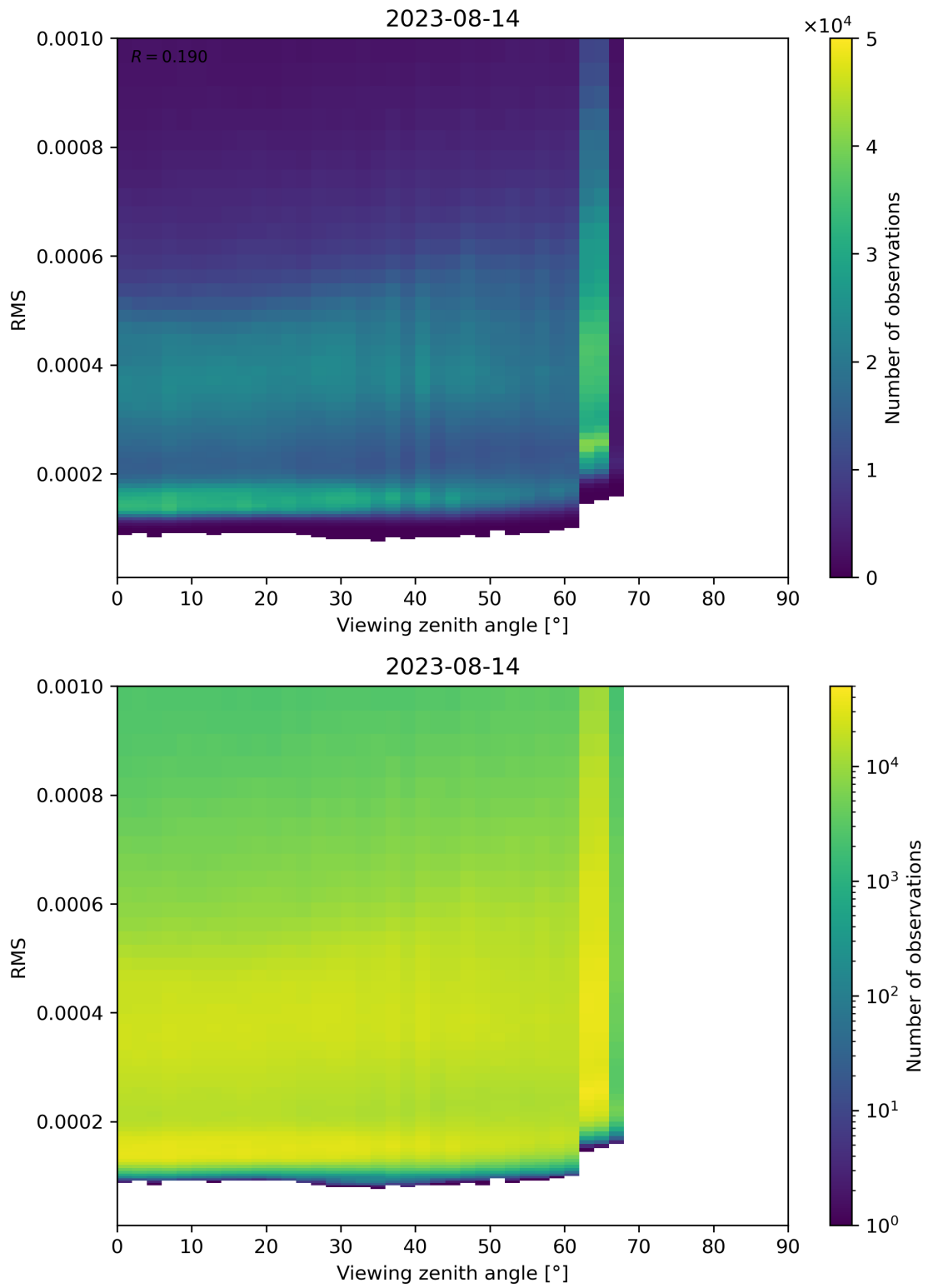
Figure 171: Scatter density plot of “Viewing zenith angle” against “RMS” for 2023-08-14 to 2023-08-15.
