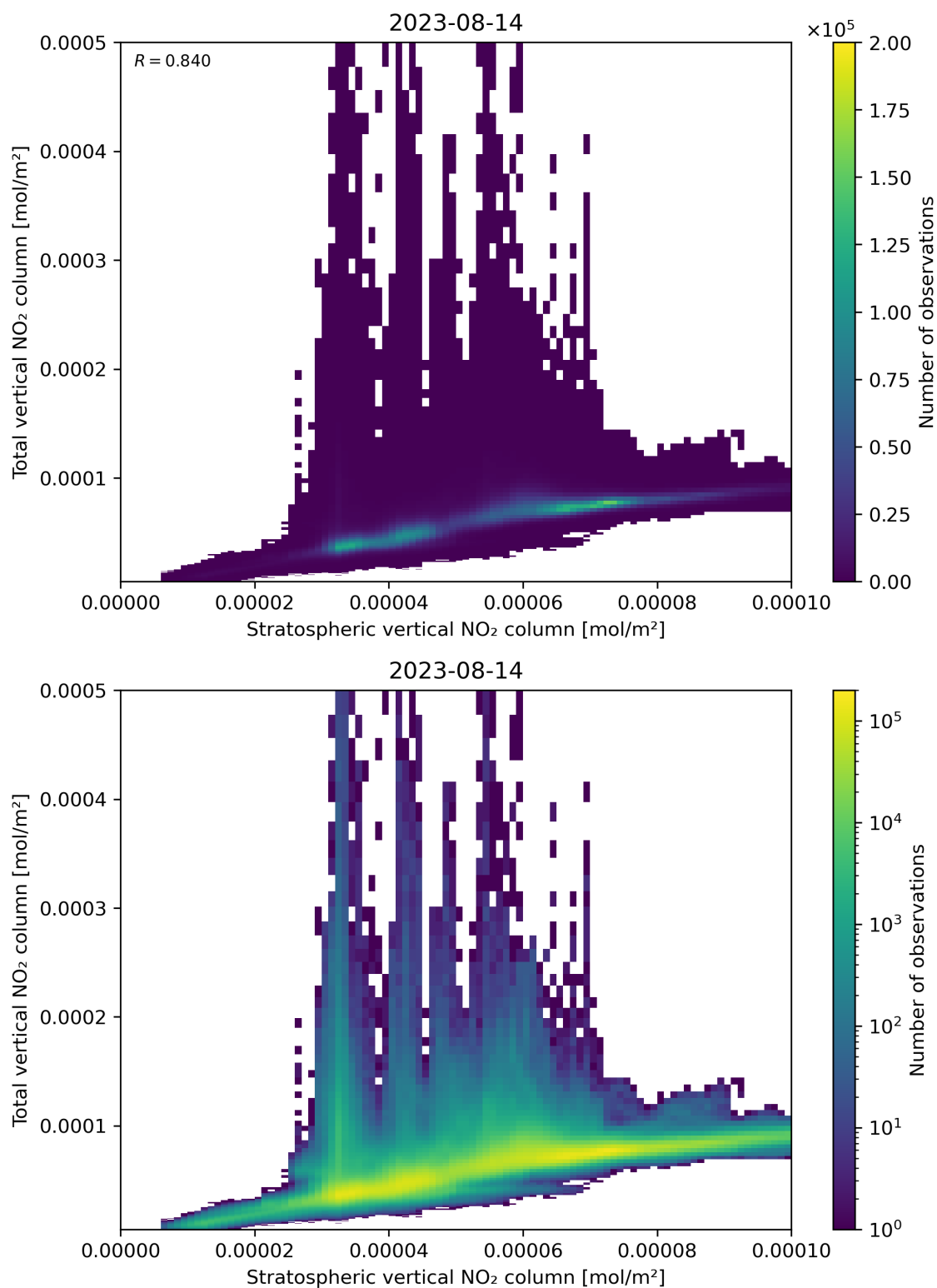
Figure 100: Scatter density plot of “Stratospheric vertical NO 2 column” against “Total vertical NO 2 column” for 2023-08-14 to 2023-08-15.
