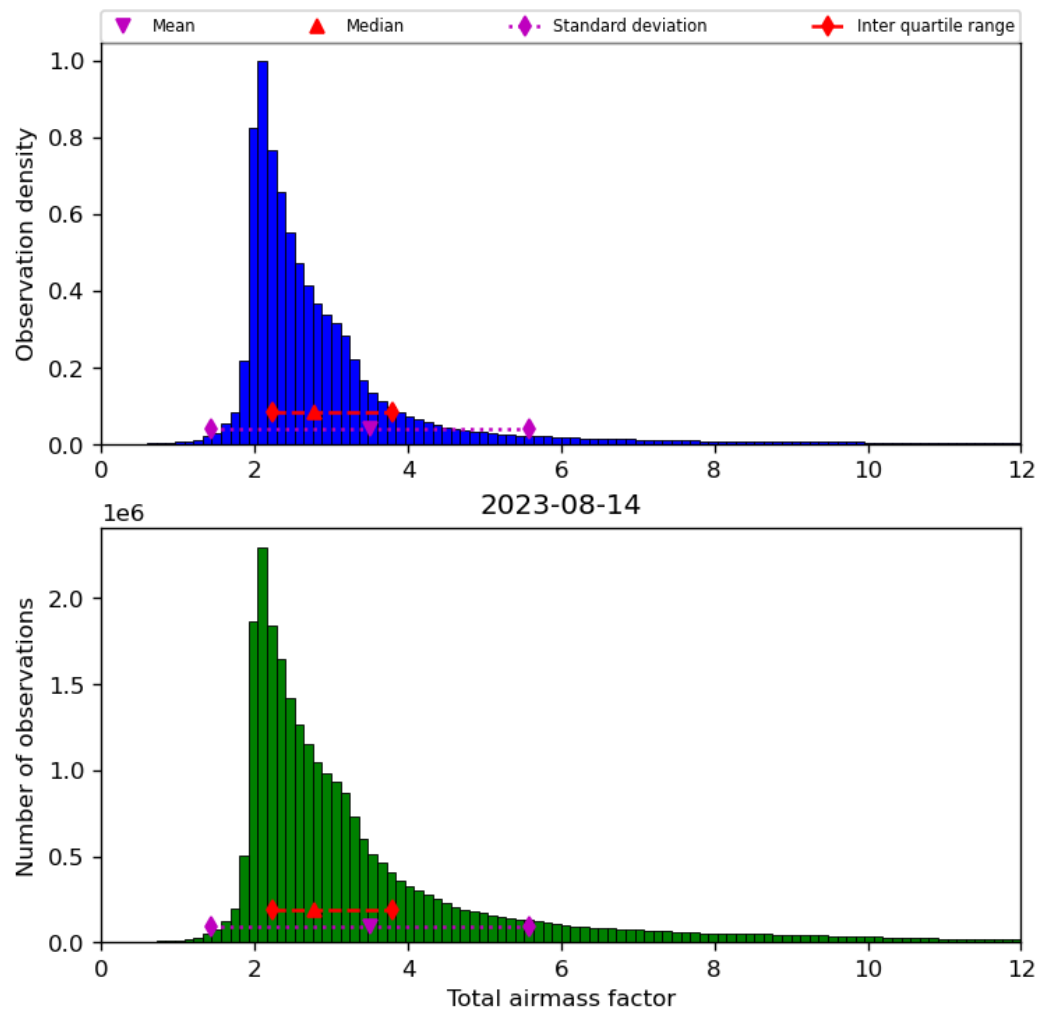
Figure 32: Histogram of “Total airmass factor” for 2023-08-14 to 2023-08-15
