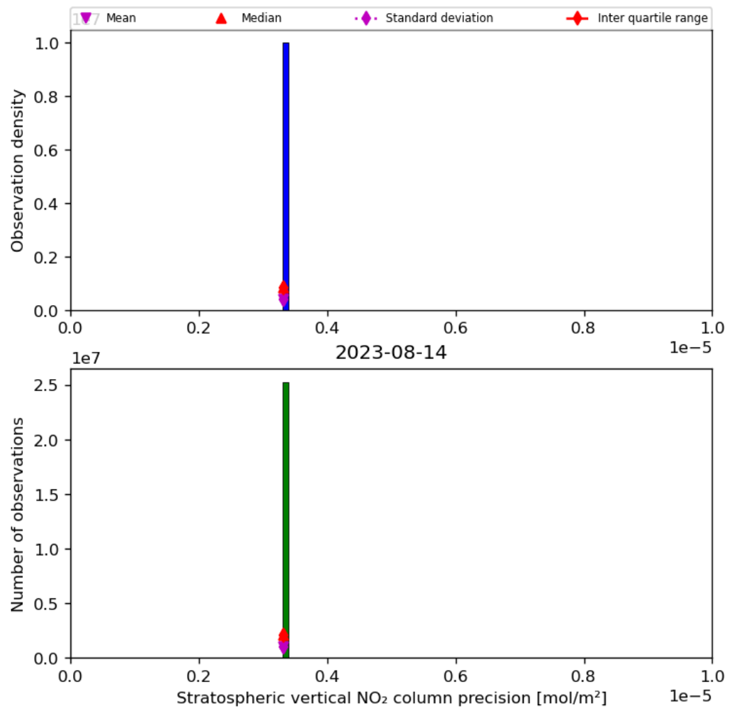
Figure 37: Histogram of “Stratospheric vertical NO 2 column precision” for 2023-08-14 to 2023-08-15
