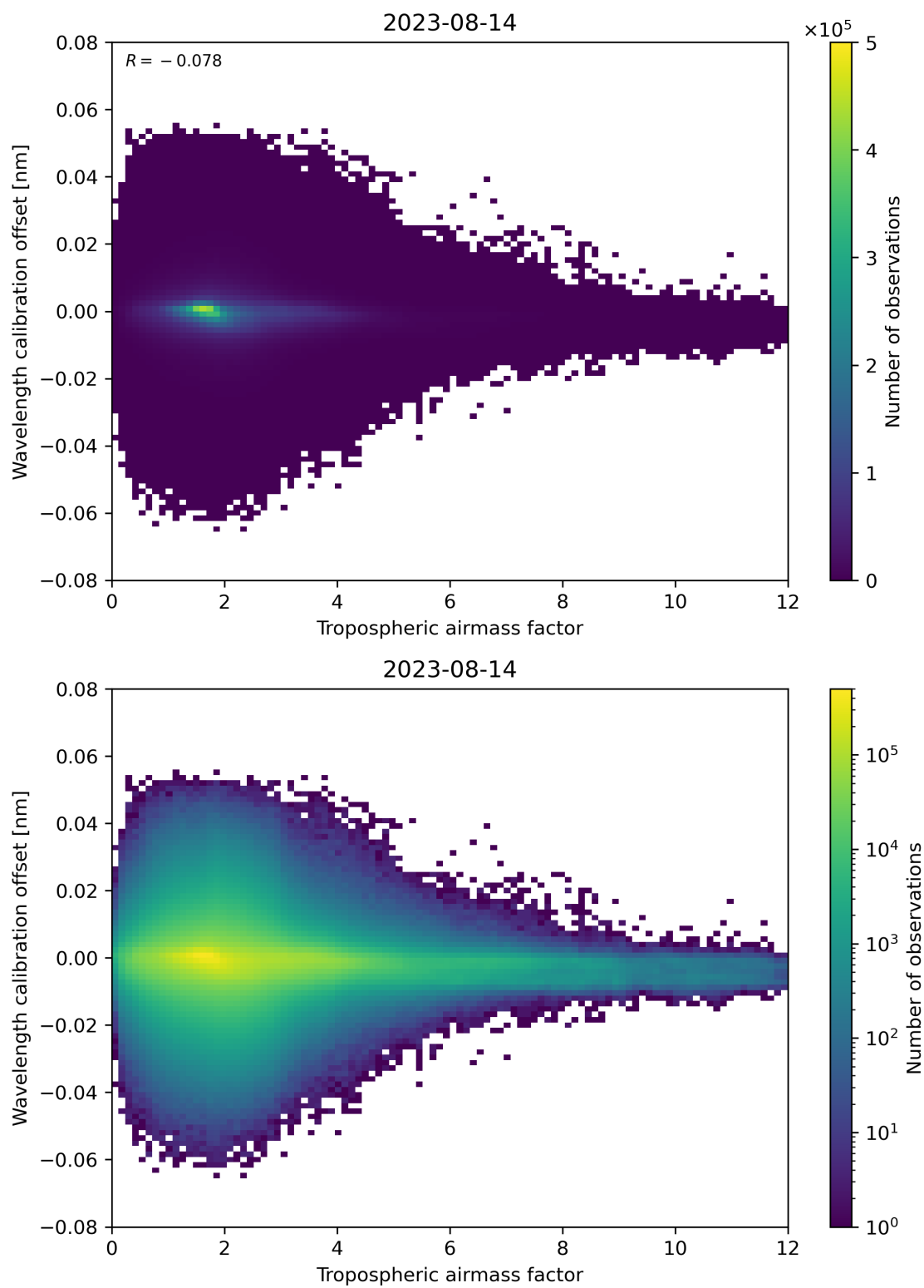
Figure 80: Scatter density plot of “Tropospheric air mass factor” against “Wavelength calibration offset” for 2023-08-14 to 2023-08-15.
