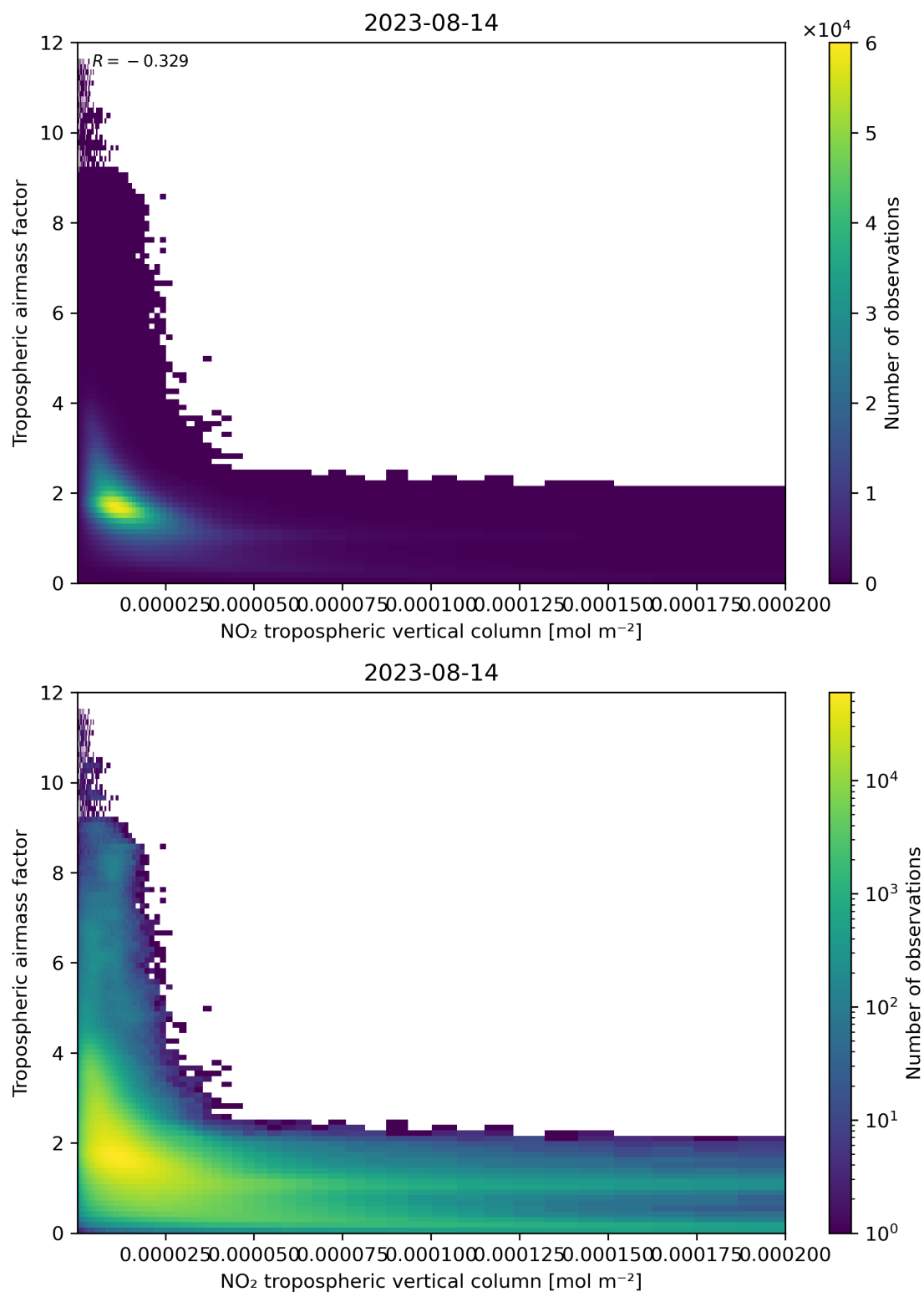
Figure 123: Scatter density plot of “NO 2 tropospheric vertical column” against “Tropospheric air mass factor” for 2023-08-14 to 2023-08-15.
