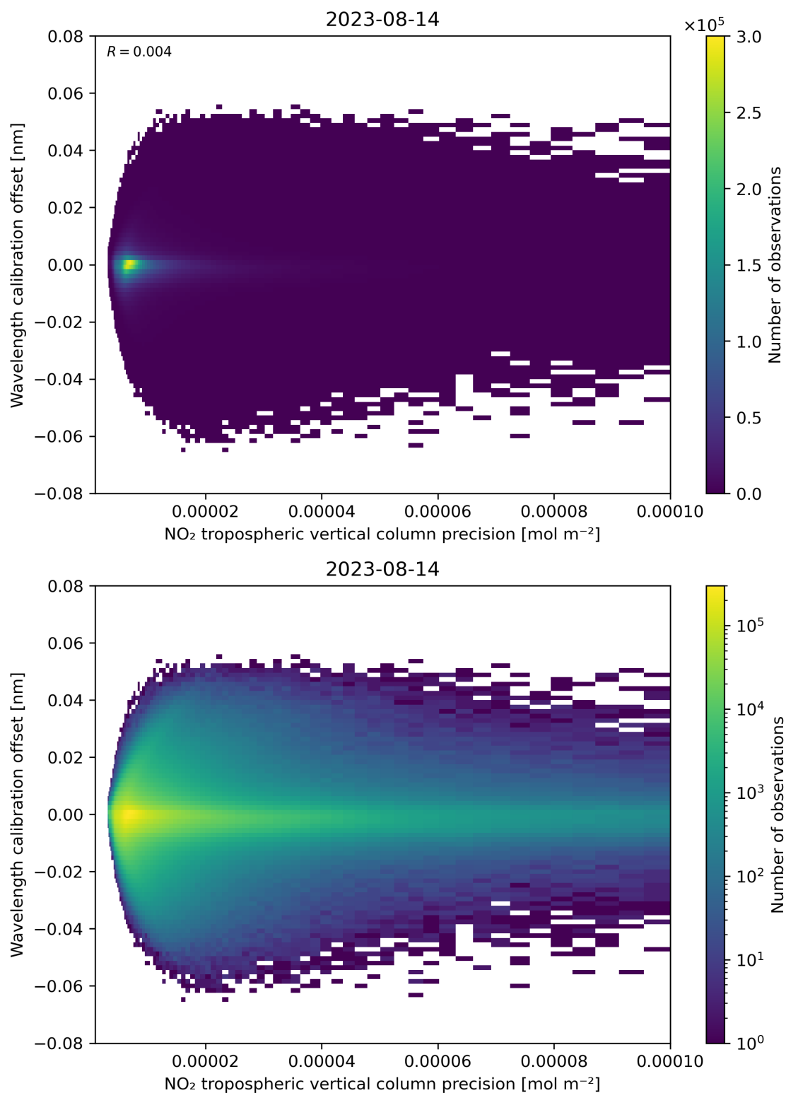
Figure 141: Scatter density plot of “NO 2 tropospheric vertical column precision” against “Wavelength calibration offset” for 2023-08-14 to 2023-08-15.
