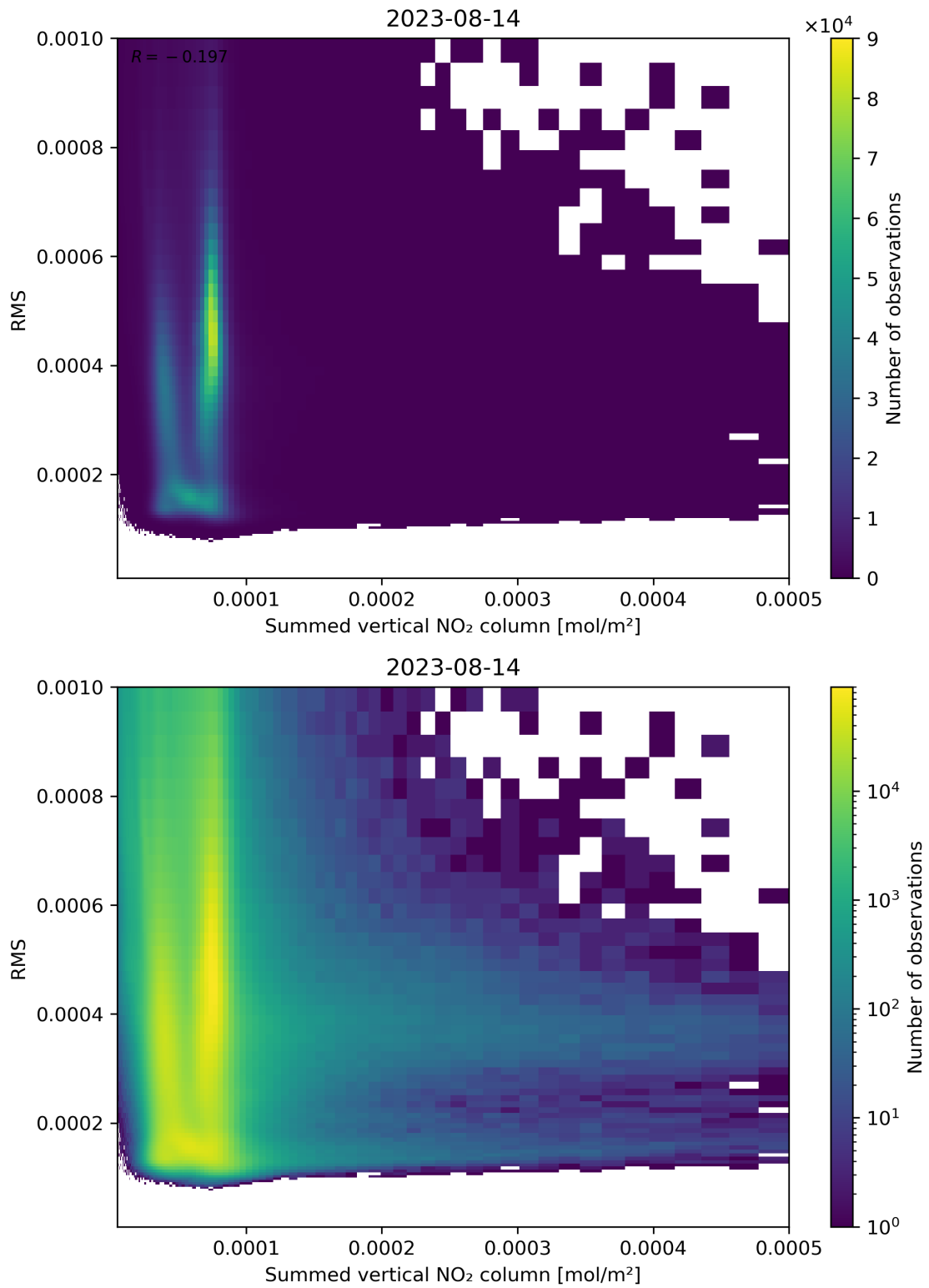
Figure 109: Scatter density plot of “Summed vertical NO 2 column” against “RMS” for 2023-08-14 to 2023-08-15.
