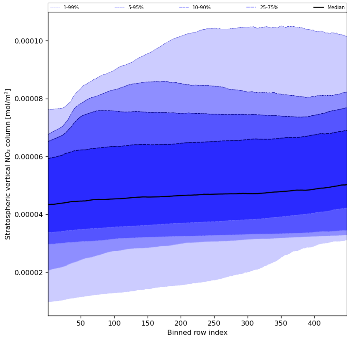
Figure 53: Along track statistics of “Stratospheric vertical NO 2 column” for 2023-08-14 to 2023-08-15
