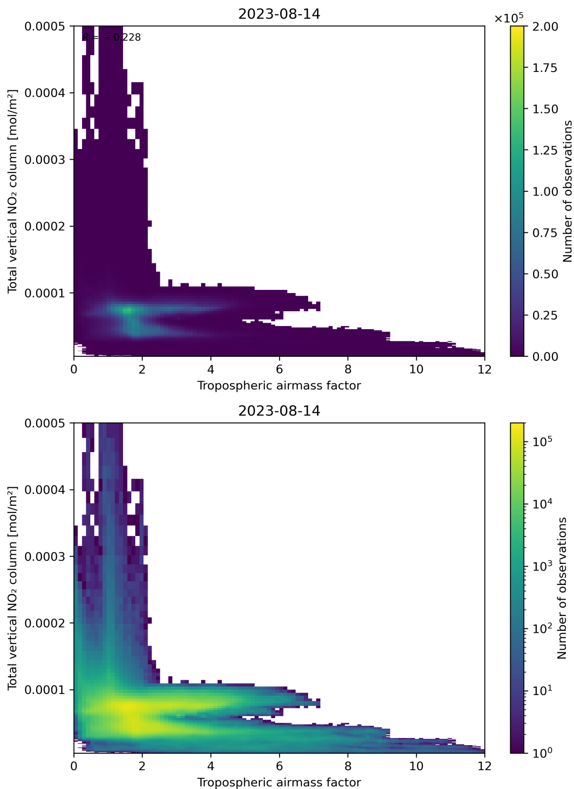
Figure 77: Scatter density plot of “Tropospheric airmass factor” against “Total vertical NO 2 column” for 2023-08-14 to 2023-08-15.
