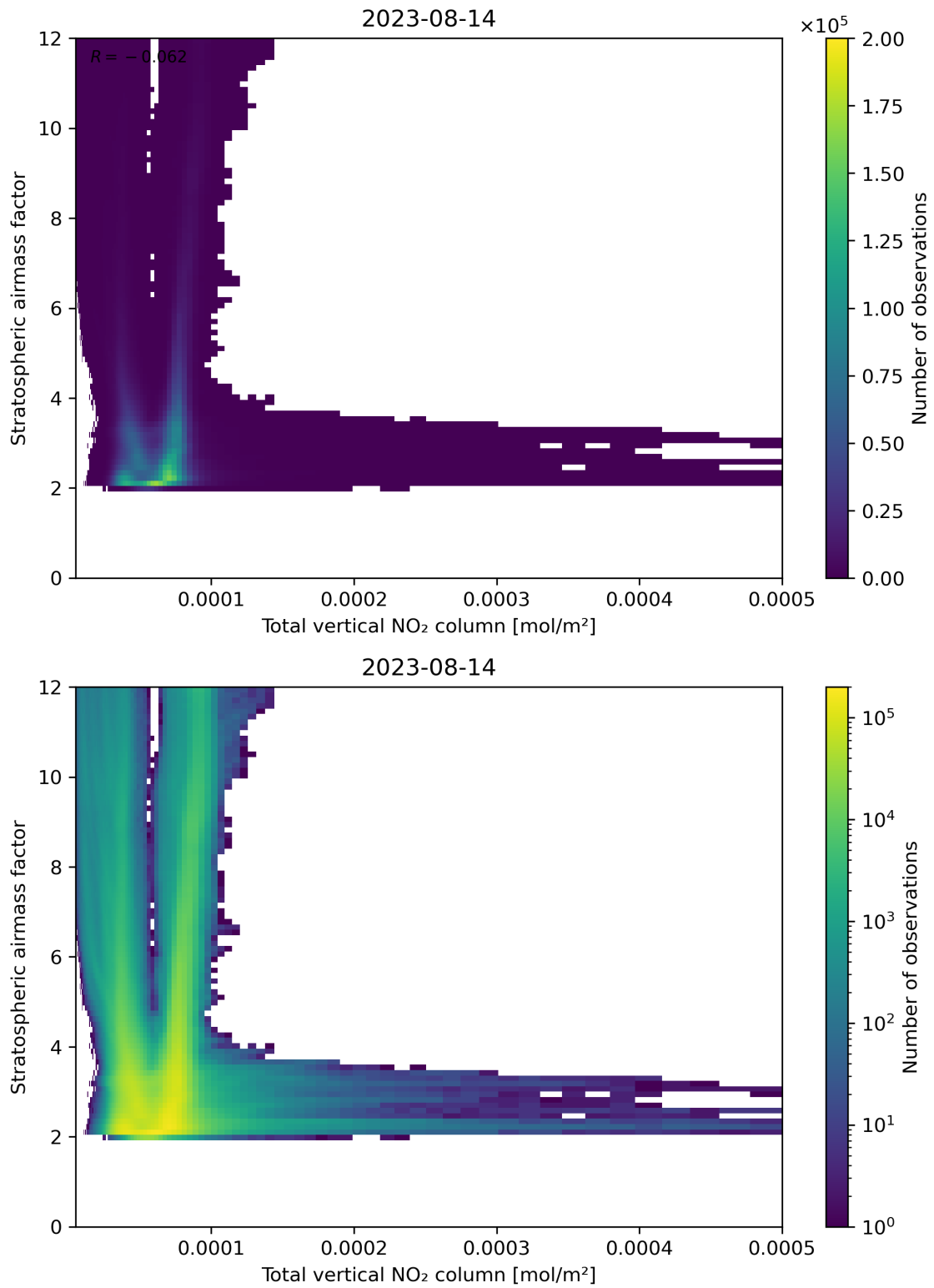
Figure 110: Scatter density plot of “Total vertical NO 2 column” against “Stratospheric airmass factor” for 2023-08-14 to 2023-08-15.
