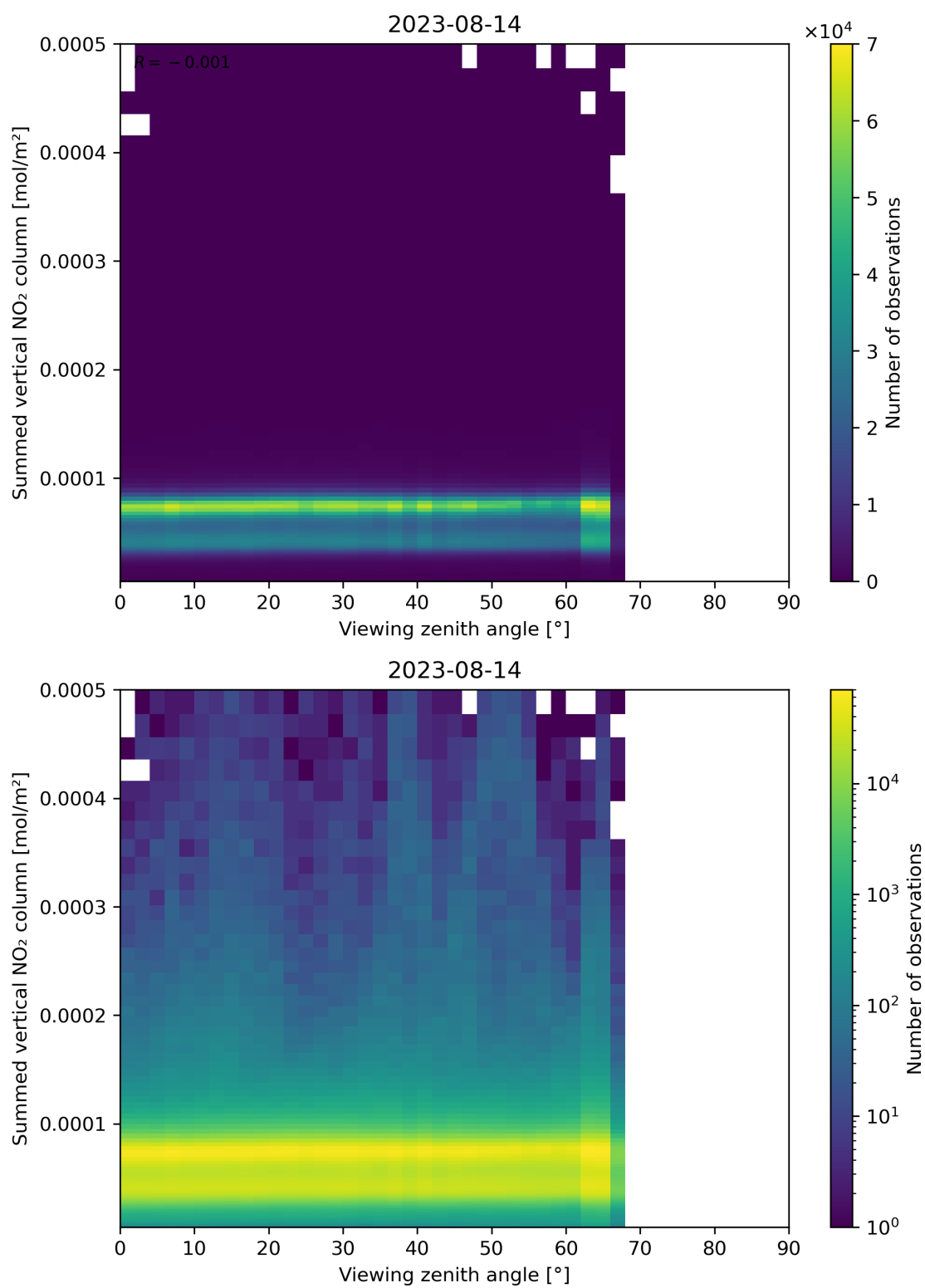
Figure 165: Scatter density plot of “Viewing zenith angle” against “Summed vertical NO 2 column” for 2023-08-14 to 2023-08-15.
