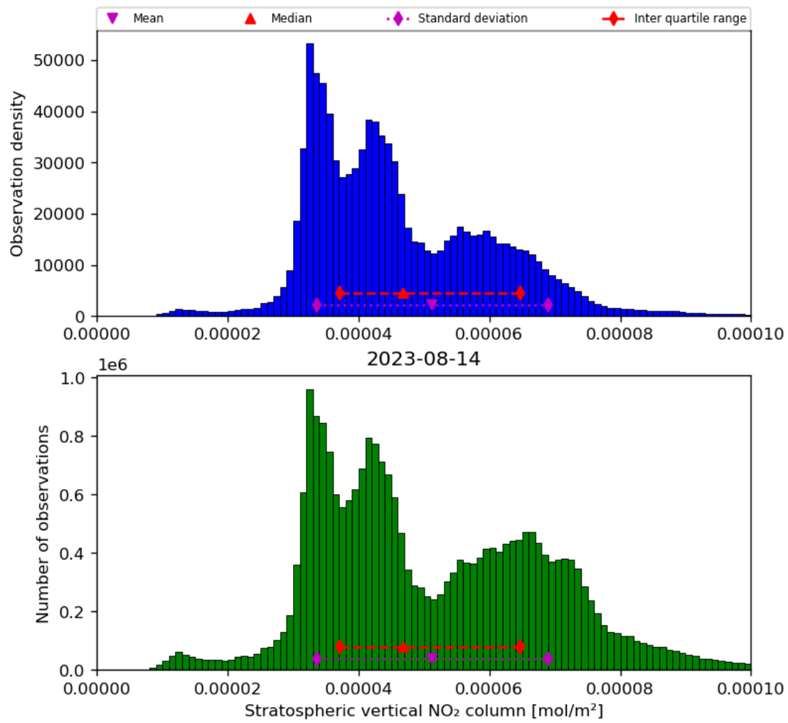
Figure 36: Histogram of “Stratospheric vertical NO 2 column” for 2023-08-14 to 2023-08-15
