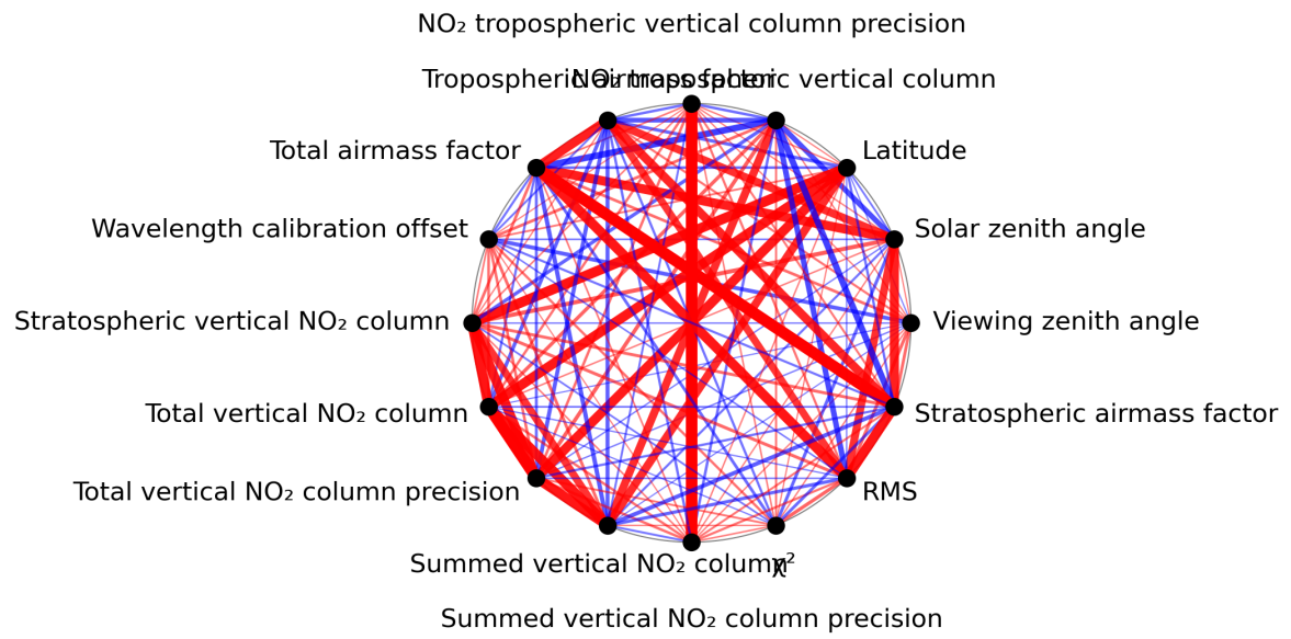
Figure 1: Map of correlation graph for 2023-08-14 to 2023-08-15.
