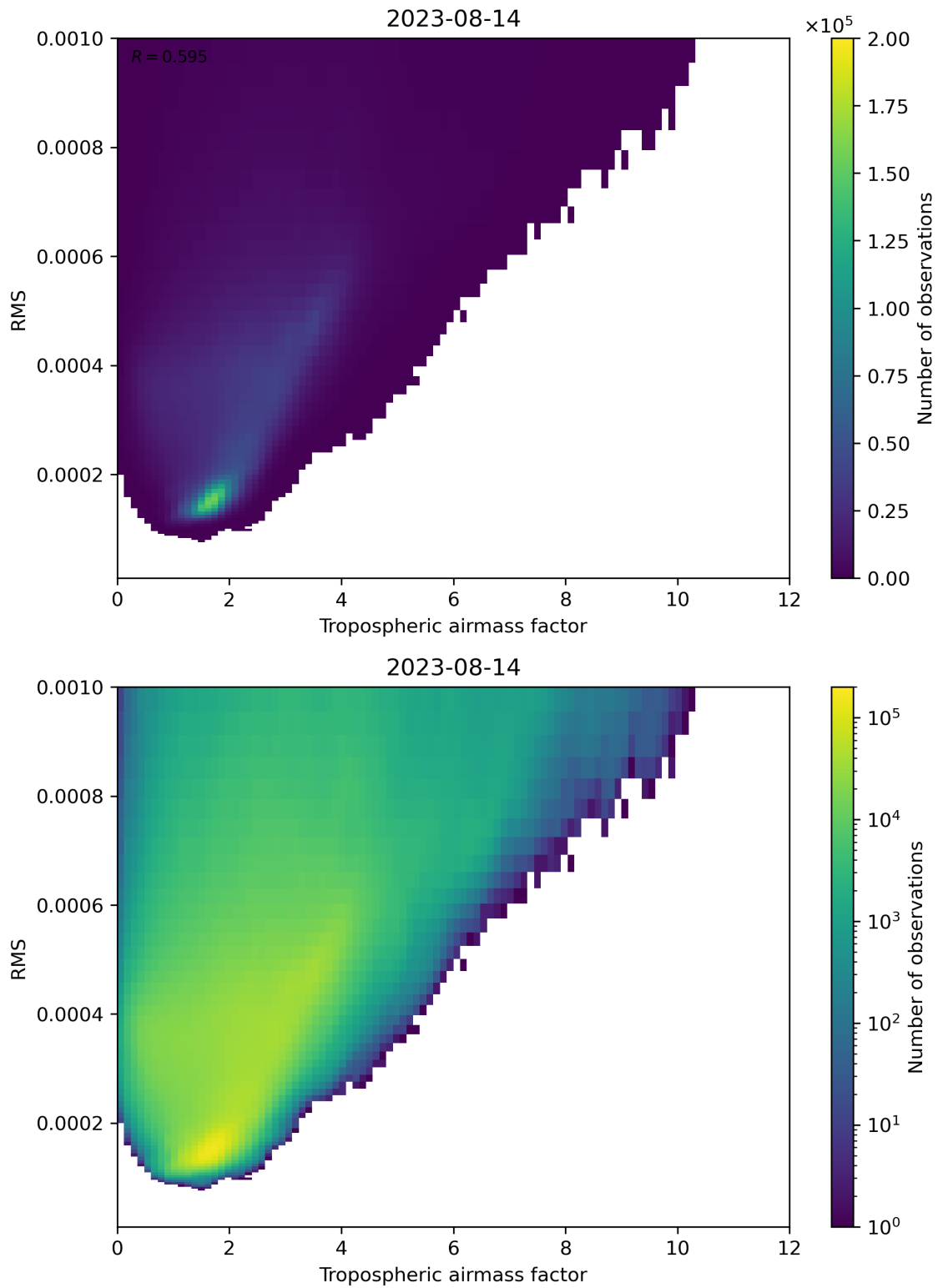
Figure 79: Scatter density plot of “Tropospheric airmass factor” against “RMS” for 2023-08-14 to 2023-08-15.
