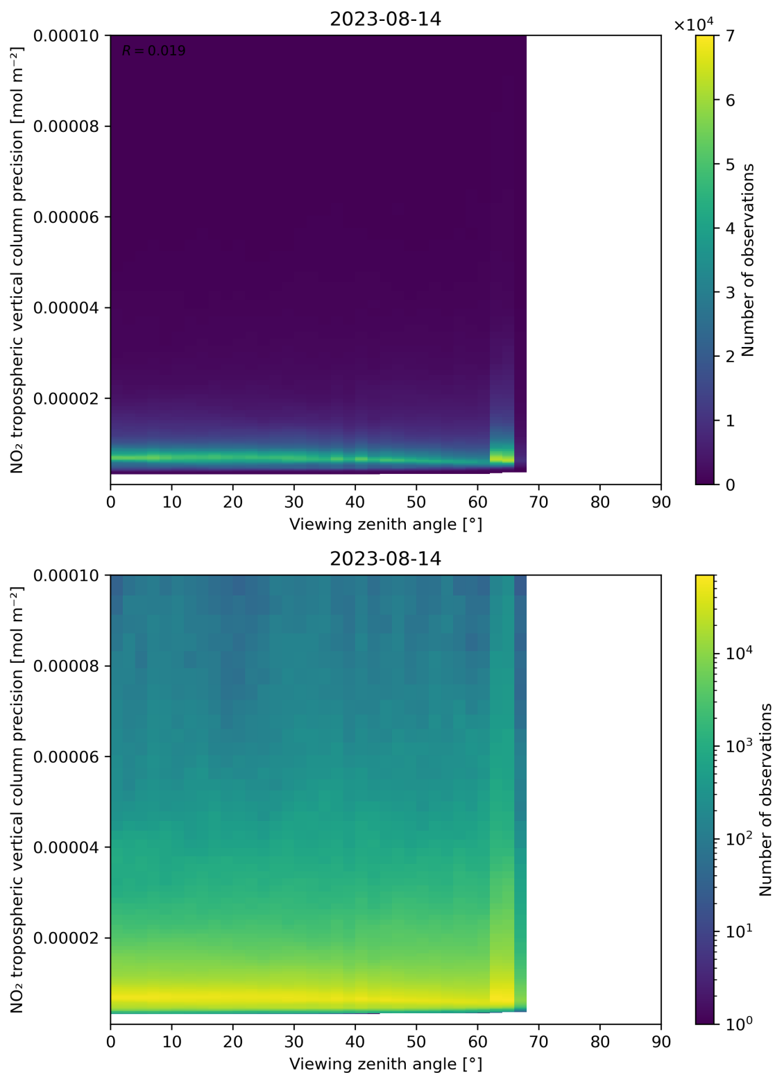
Figure 170: Scatter density plot of “Viewing zenith angle” against “NO 2 tropospheric vertical column precision” for 2023-08-14 to 2023-08-15.
