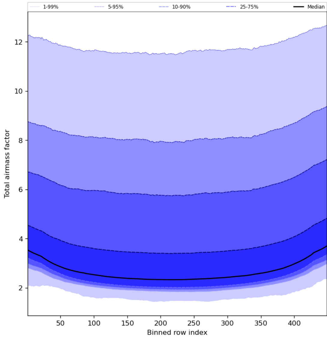
Figure 49: Along track statistics of “Total airmass factor” for 2023-08-14 to 2023-08-15
