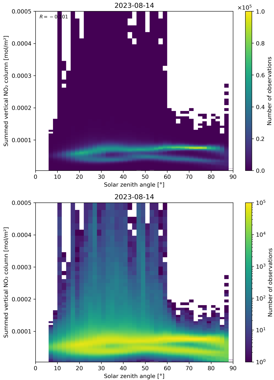
Figure 151: Scatter density plot of “Solar zenith angle” against “Summed vertical NO 2 column” for 2023-08-14 to 2023-08-15.
