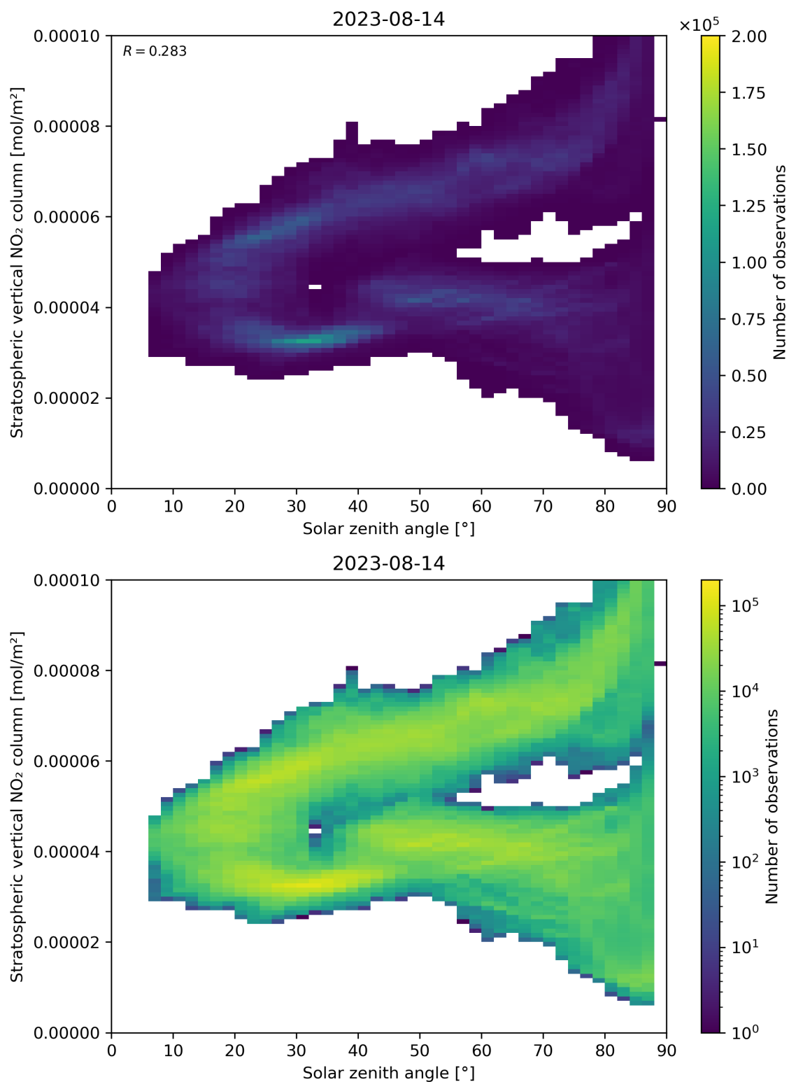
Figure 150: Scatter density plot of “Solar zenith angle” against “Stratospheric vertical NO 2 column” for 2023-08-14 to 2023-08-15.
