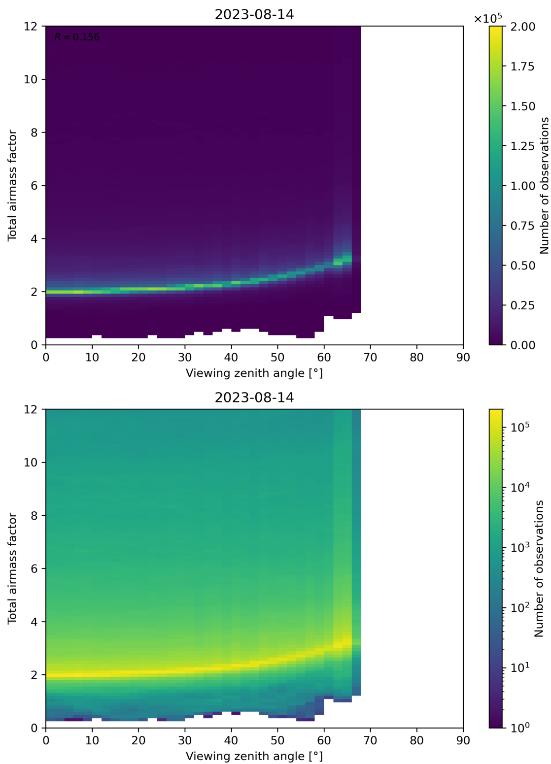
Figure 160: Scatter density plot of “Viewing zenith angle” against “Total airmass factor” for 2023-08-14 to 2023-08-15.
