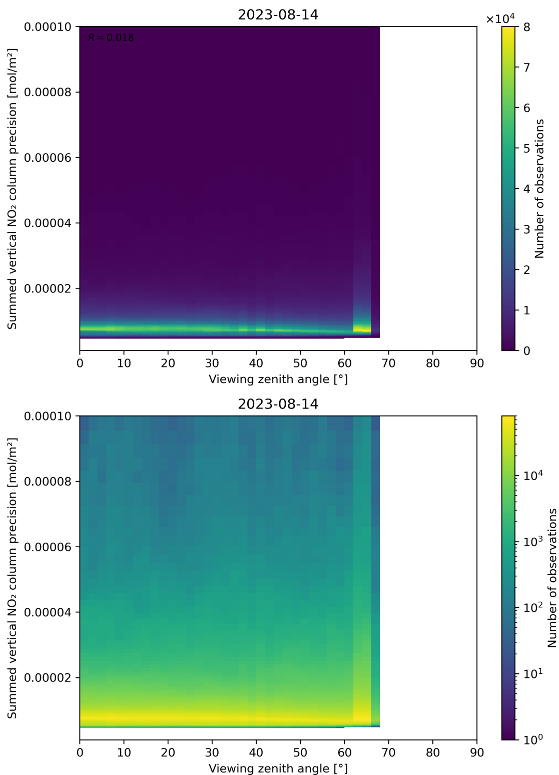
Figure 166: Scatter density plot of “Viewing zenith angle” against “Summed vertical NO 2 column precision” for 2023-08-14 to 2023-08-15.
