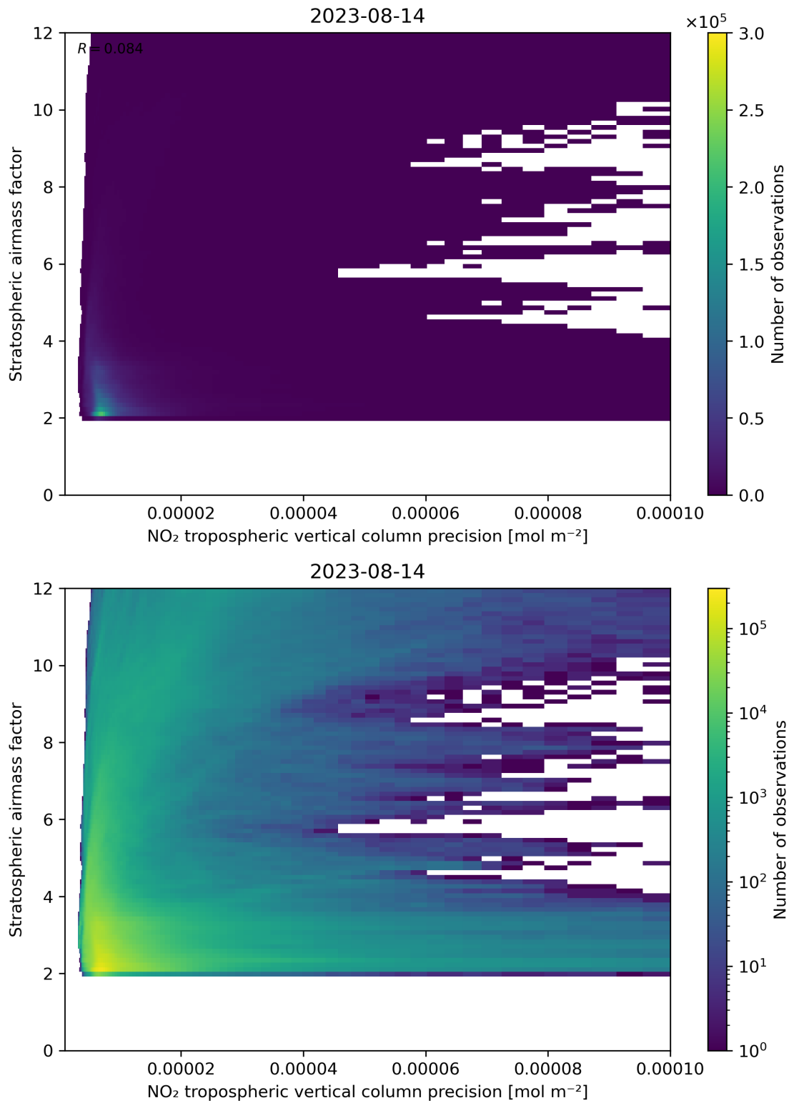
Figure 131: Scatter density plot of “NO 2 tropospheric vertical column precision” against “Stratospheric airmass factor” for 2023-08-14 to 2023-08-15.
