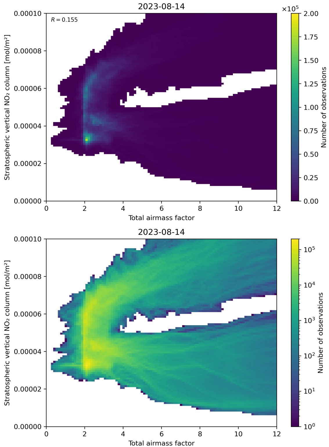
Figure 64: Scatter density plot of “Total airmass factor” against “Stratospheric vertical NO 2 column” for 2023-08-14 to 2023-08-15.
