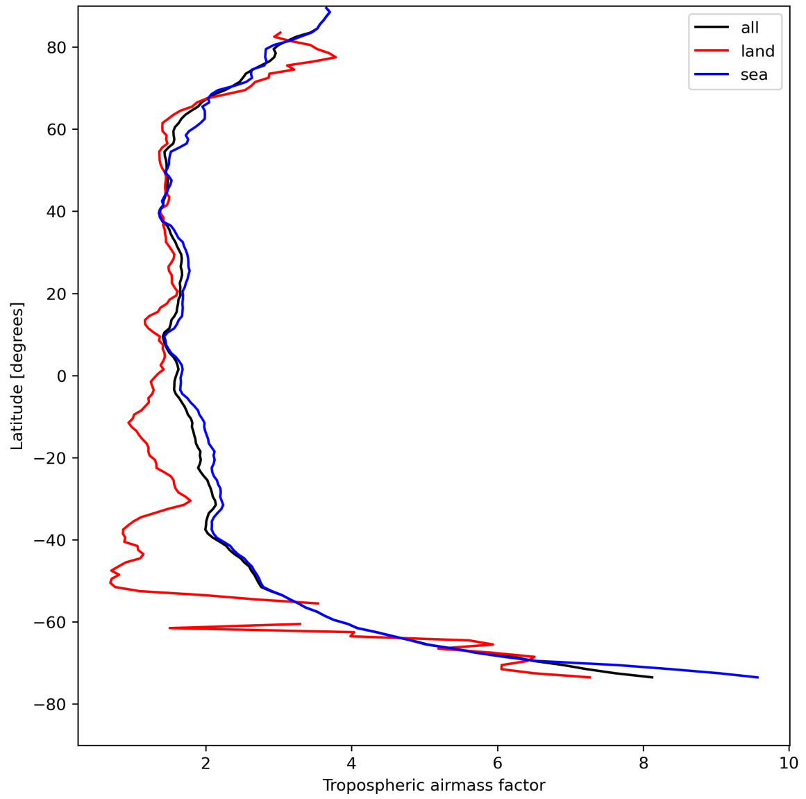
Figure 14: Zonal average of “Tropospheric airmass factor” for 2023-08-14 to 2023-08-15.
