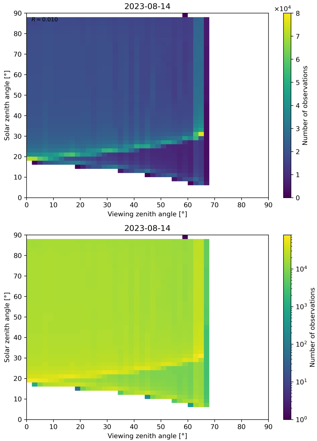
Figure 172: Scatter density plot of “Viewing zenith angle” against “Solar zenith angle” for 2023-08-14 to 2023-08-15.
