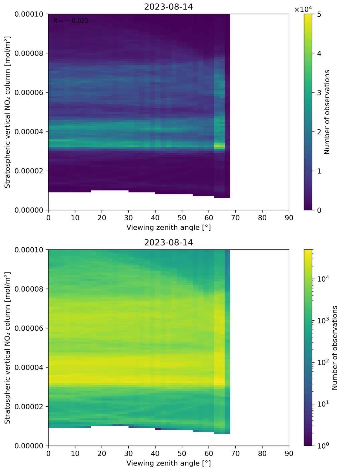
Figure 164: Scatter density plot of “Viewing zenith angle” against “Stratospheric vertical NO 2 column” for 2023-08-14 to 2023-08-15.
