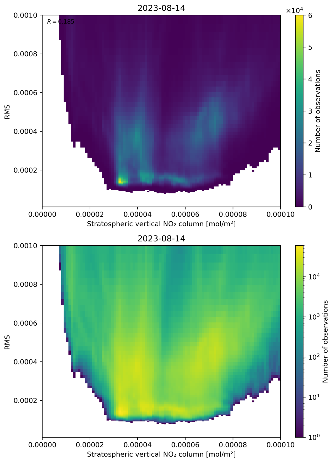
Figure 102: Scatter density plot of “Stratospheric vertical NO 2 column” against “RMS” for 2023-08-14 to 2023-08-15.
