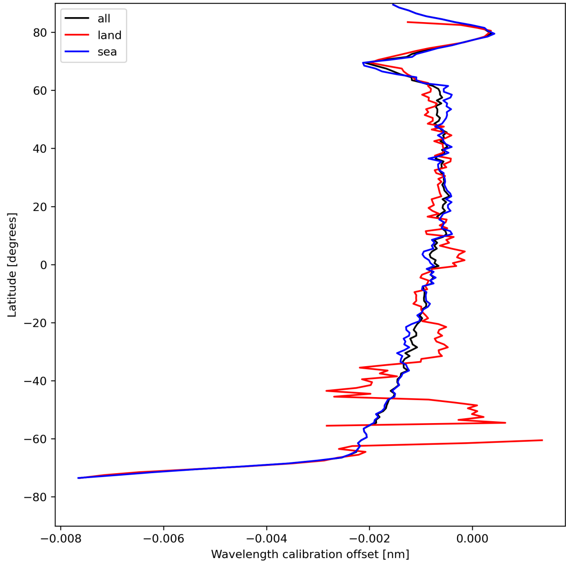
Figure 18: Zonal average of “Wavelength calibration offset” for 2023-08-14 to 2023-08-15.
