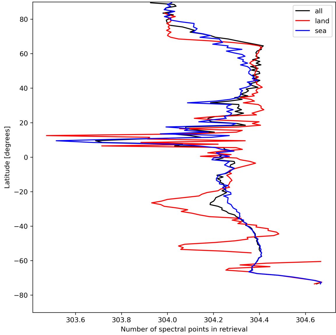
Figure 16: Zonal average of “Number of spectral points in retrieval” for 2023-08-14 to 2023-08-15.
