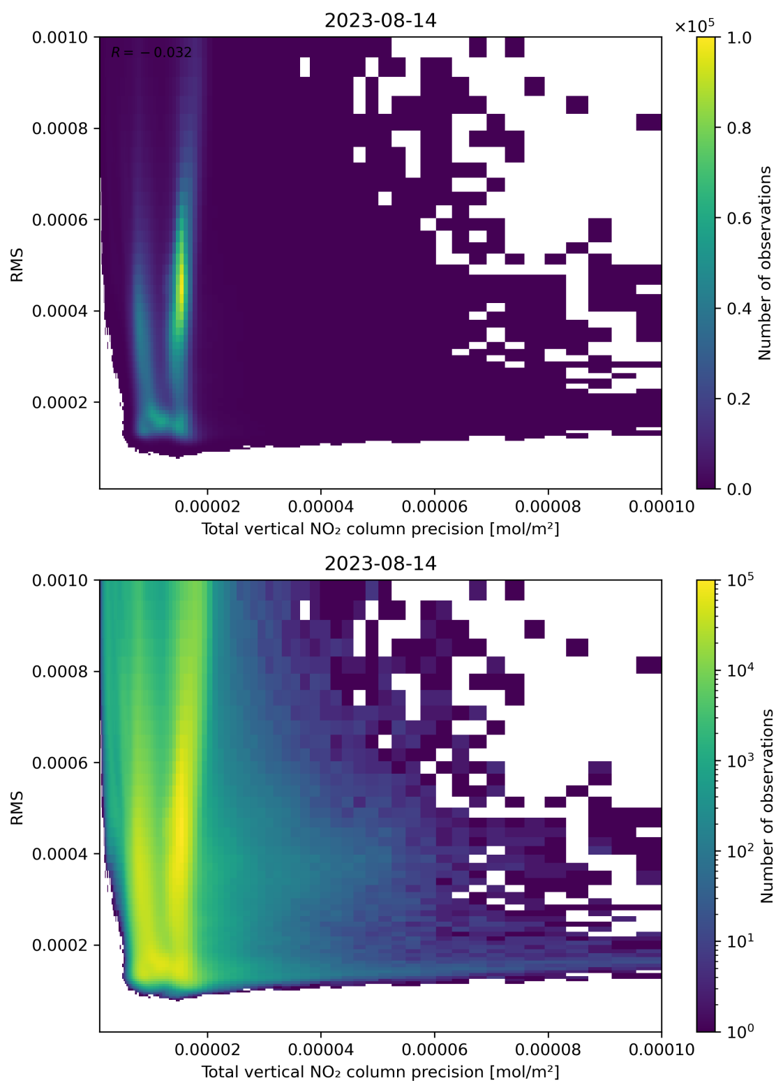
Figure 119: Scatter density plot of “Total vertical NO 2 column precision” against “RMS” for 2023-08-14 to 2023-08-15.
