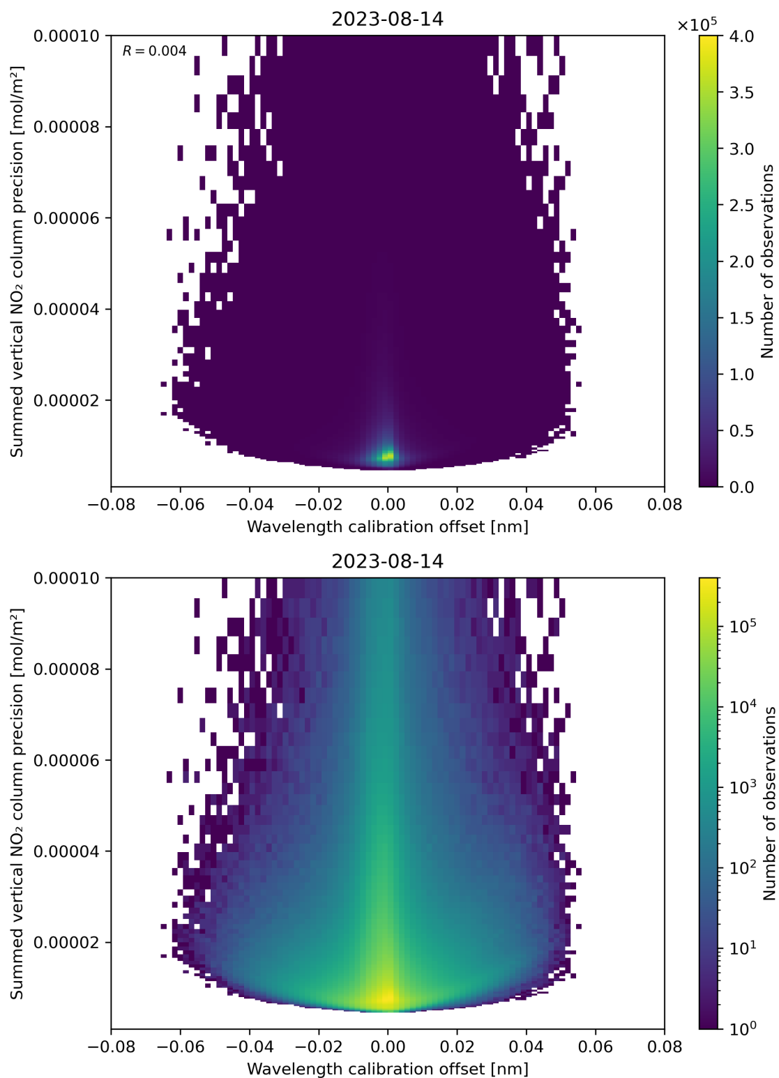
Figure 178: Scatter density plot of “Wavelength calibration offset” against “Summed vertical NO 2 column precision” for 2023-08-14 to 2023-08-15.
