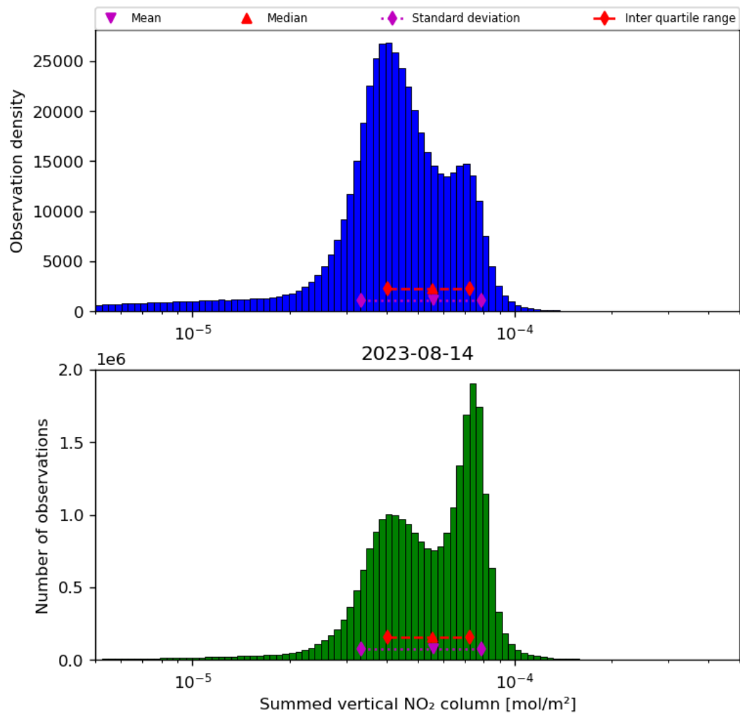
Figure 40: Histogram of “Summed vertical NO 2 column” for 2023-08-14 to 2023-08-15
