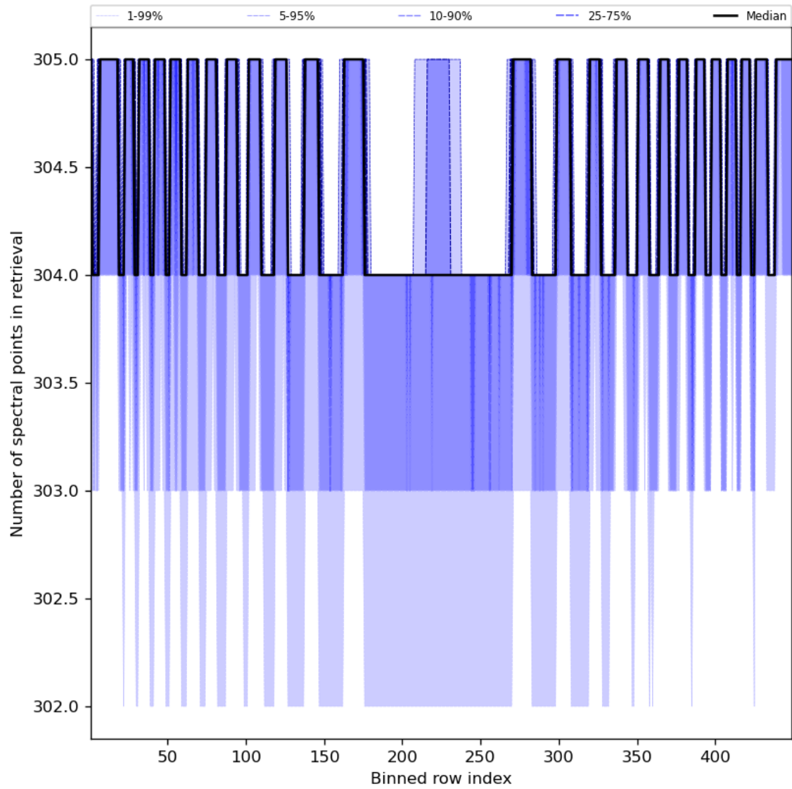
Figure 50: Along track statistics of “Number of spectral points in retrieval” for 2023-08-14 to 2023-08-15
