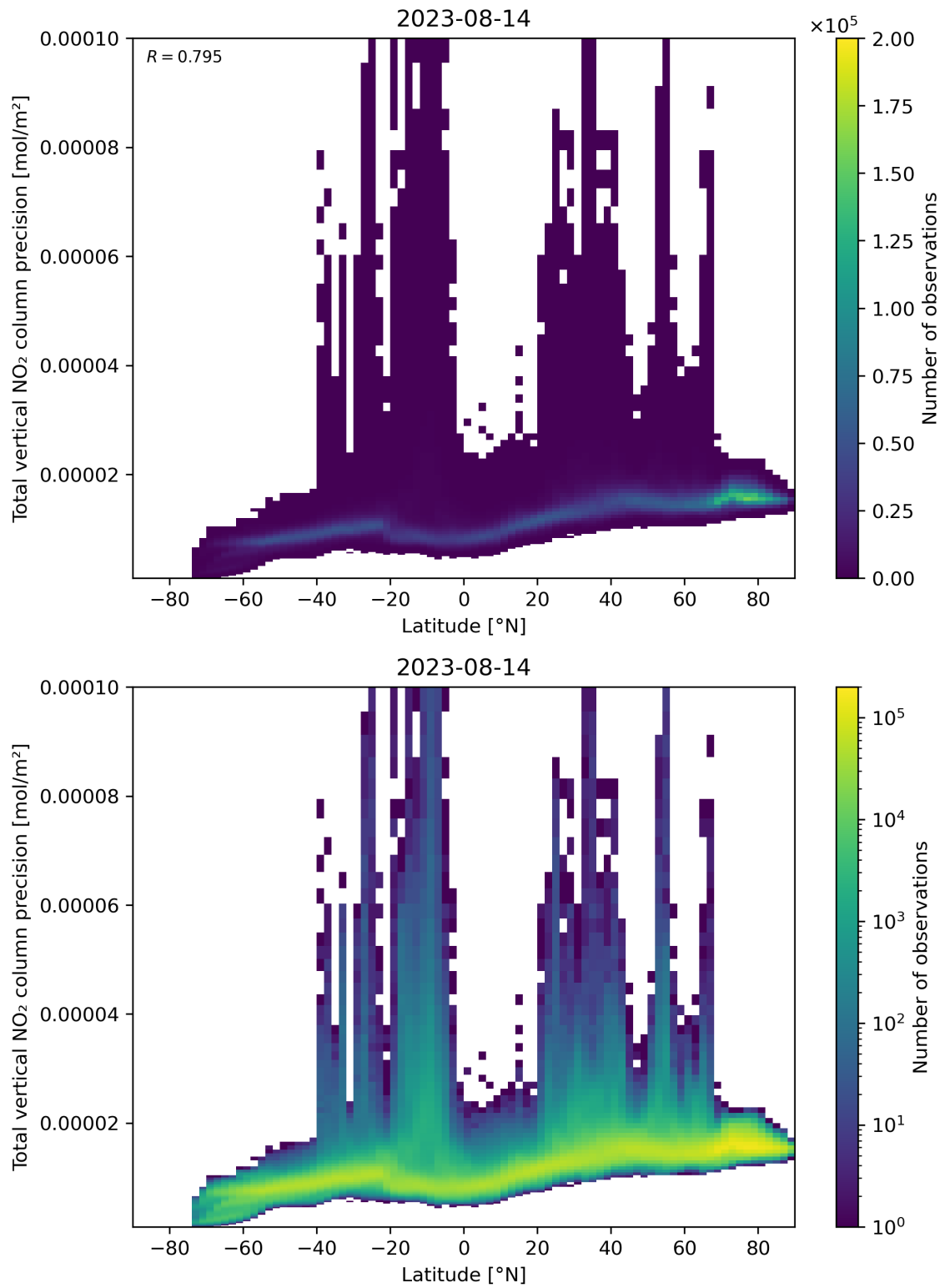
Figure 91: Scatter density plot of “Latitude” against “Total vertical NO 2 column precision” for 2023-08-14 to 2023-08-15.
