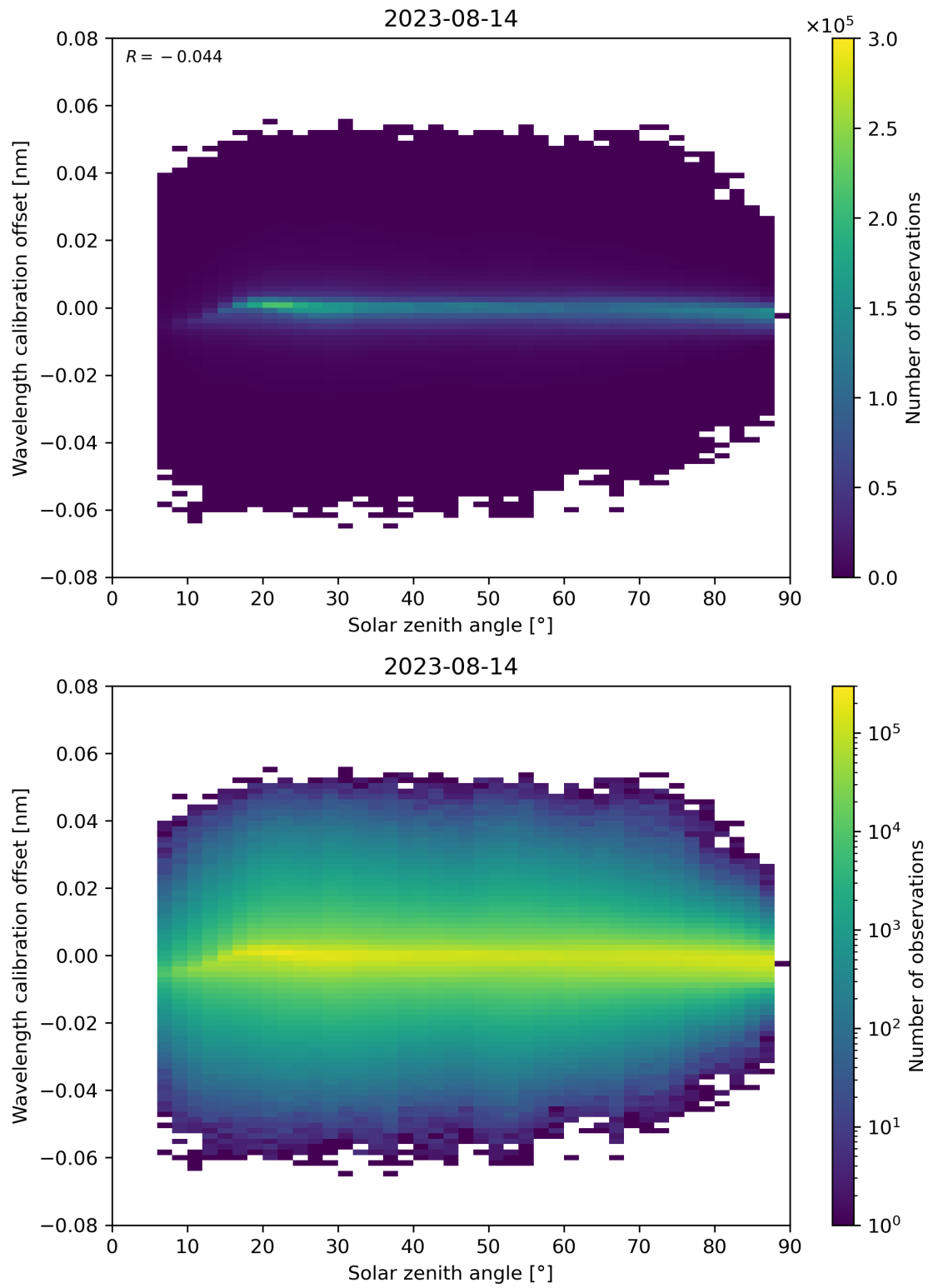
Figure 158: Scatter density plot of “Solar zenith angle” against “Wavelength calibration offset” for 2023-08-14 to 2023-08-15.
