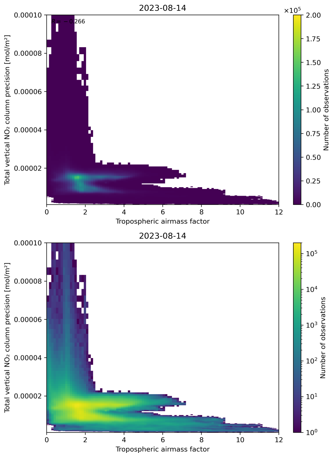
Figure 78: Scatter density plot of “Tropospheric air mass factor” against “Total vertical NO 2 column precision” for 2023-08-14 to 2023-08-15.
