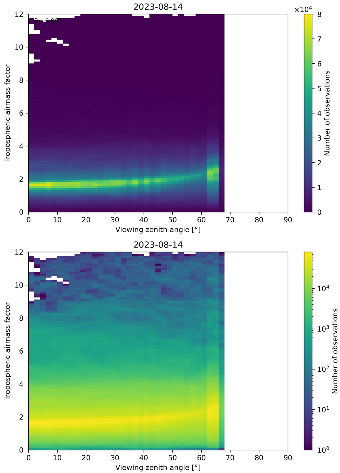
Figure 161: Scatter density plot of “Viewing zenith angle” against “Tropospheric airmass factor” for 2023-08-14 to 2023-08-15.
