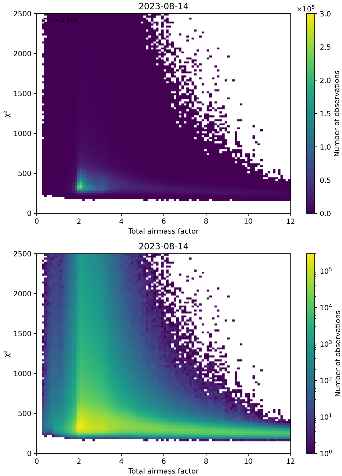
Figure 63: Scatter density plot of “Total airmass factor” against “ \chi^2 ” for 2023-08-14 to 2023-08-15.
