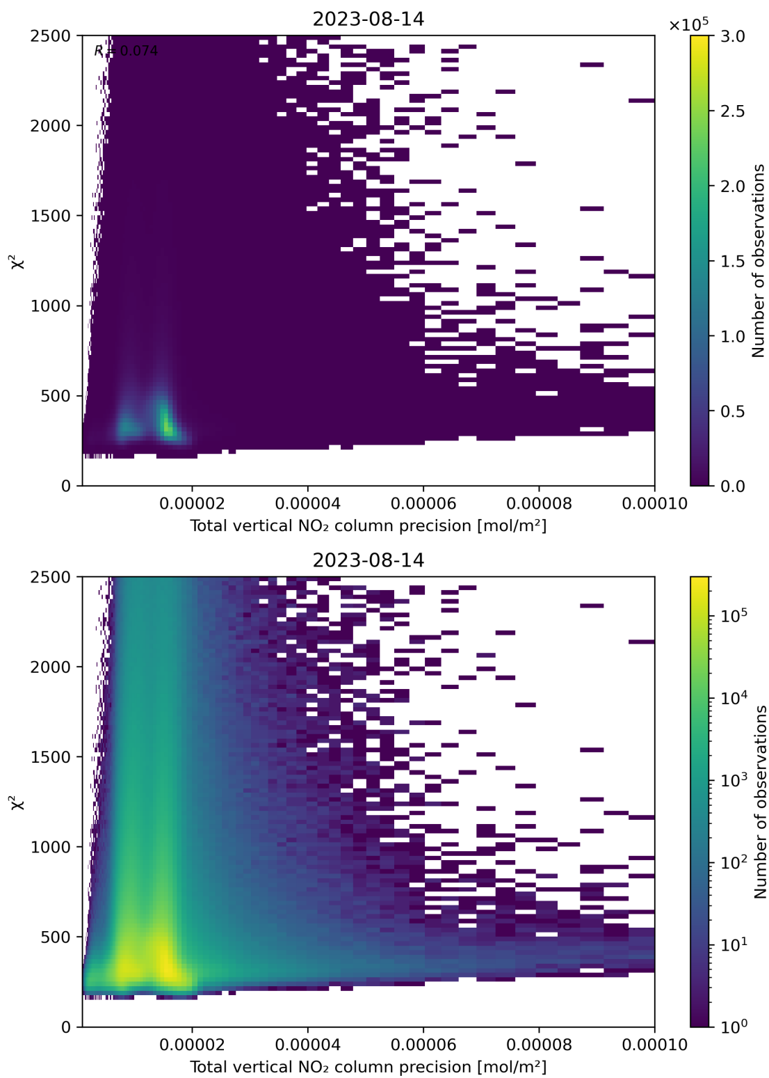
Figure 116: Scatter density plot of “Total vertical NO 2 column precision” against “ \chi^2 ” for 2023-08-14 to 2023-08-15.
