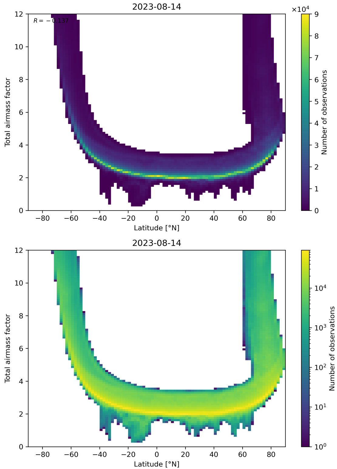
Figure 84: Scatter density plot of “Latitude” against “Total airmass factor” for 2023-08-14 to 2023-08-15.
