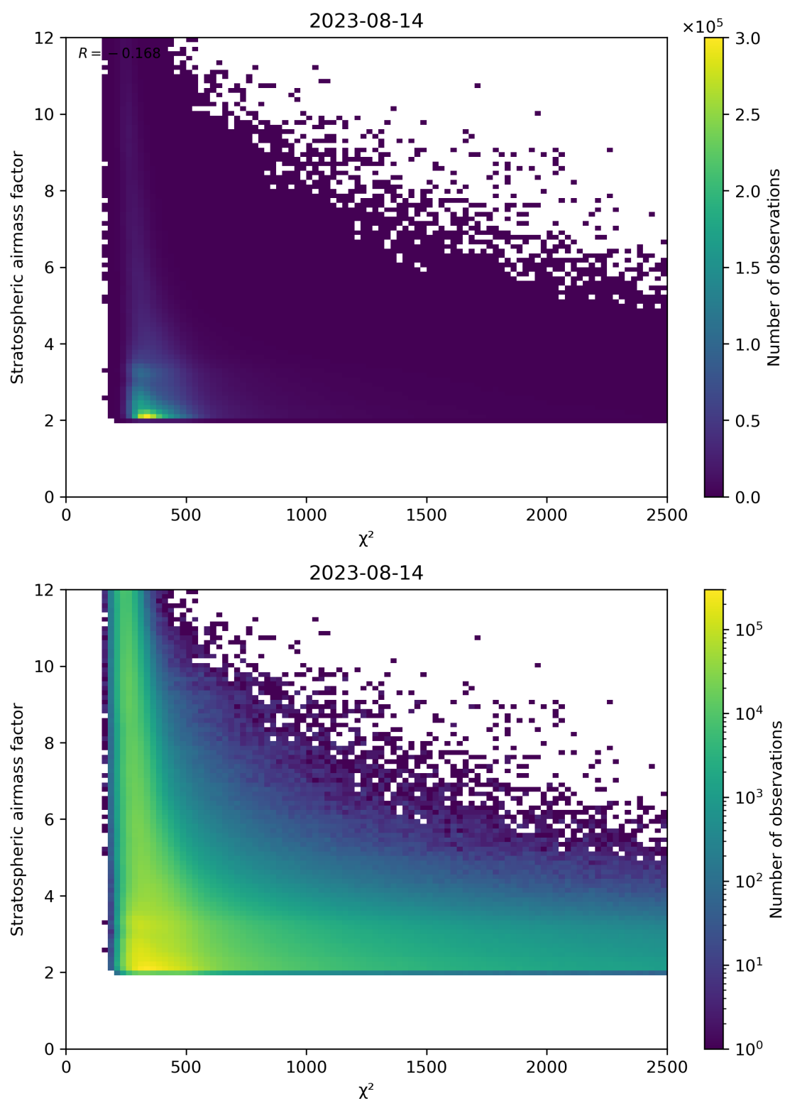
Figure 81: Scatter density plot of " \chi^2 " against "Stratospheric air mass factor" for 2023-08-14 to 2023-08-15.
