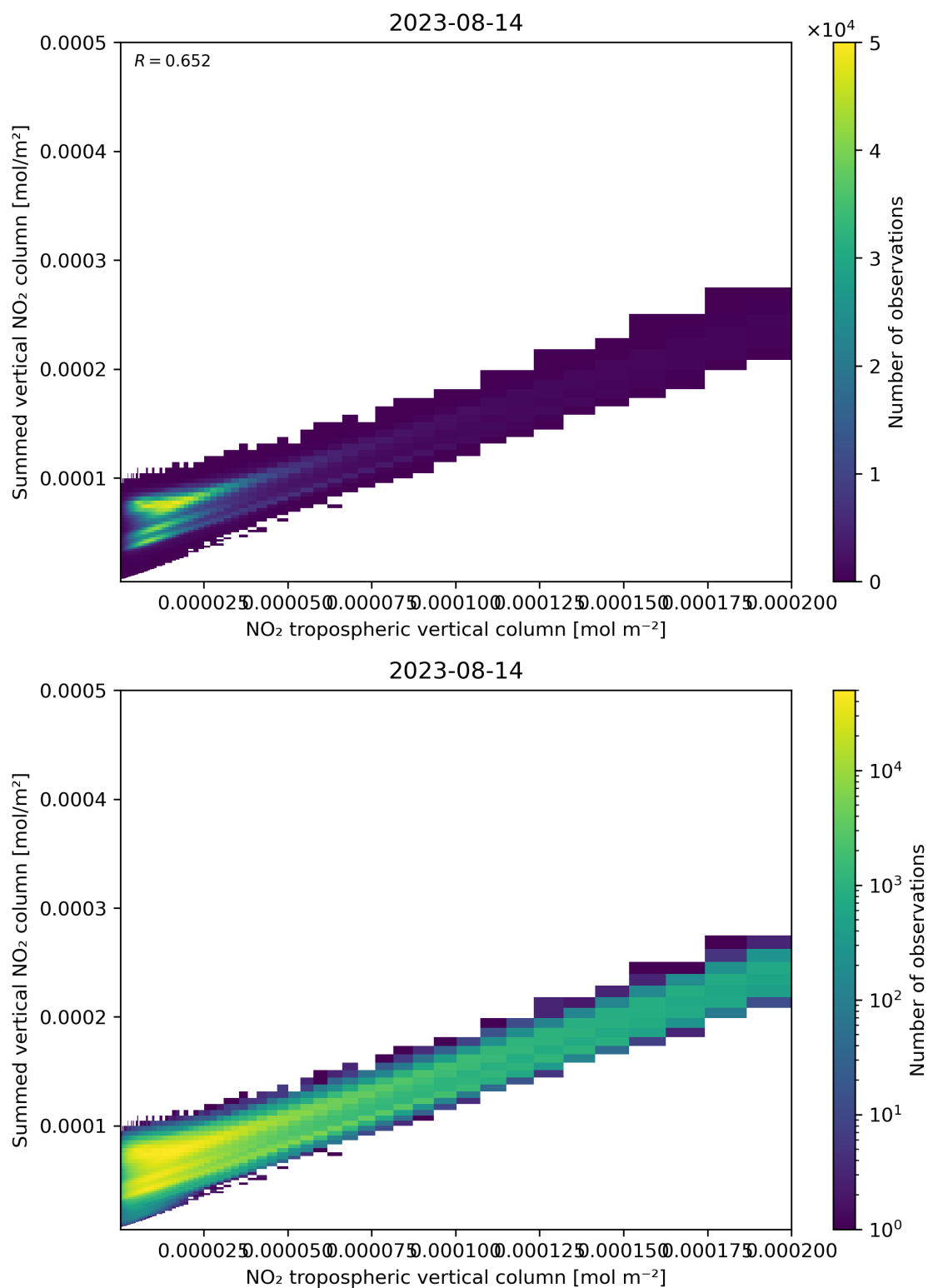
Figure 126: Scatter density plot of “NO 2 tropospheric vertical column” against “Summed vertical NO 2 column” for 2023-08-14 to 2023-08-15.
