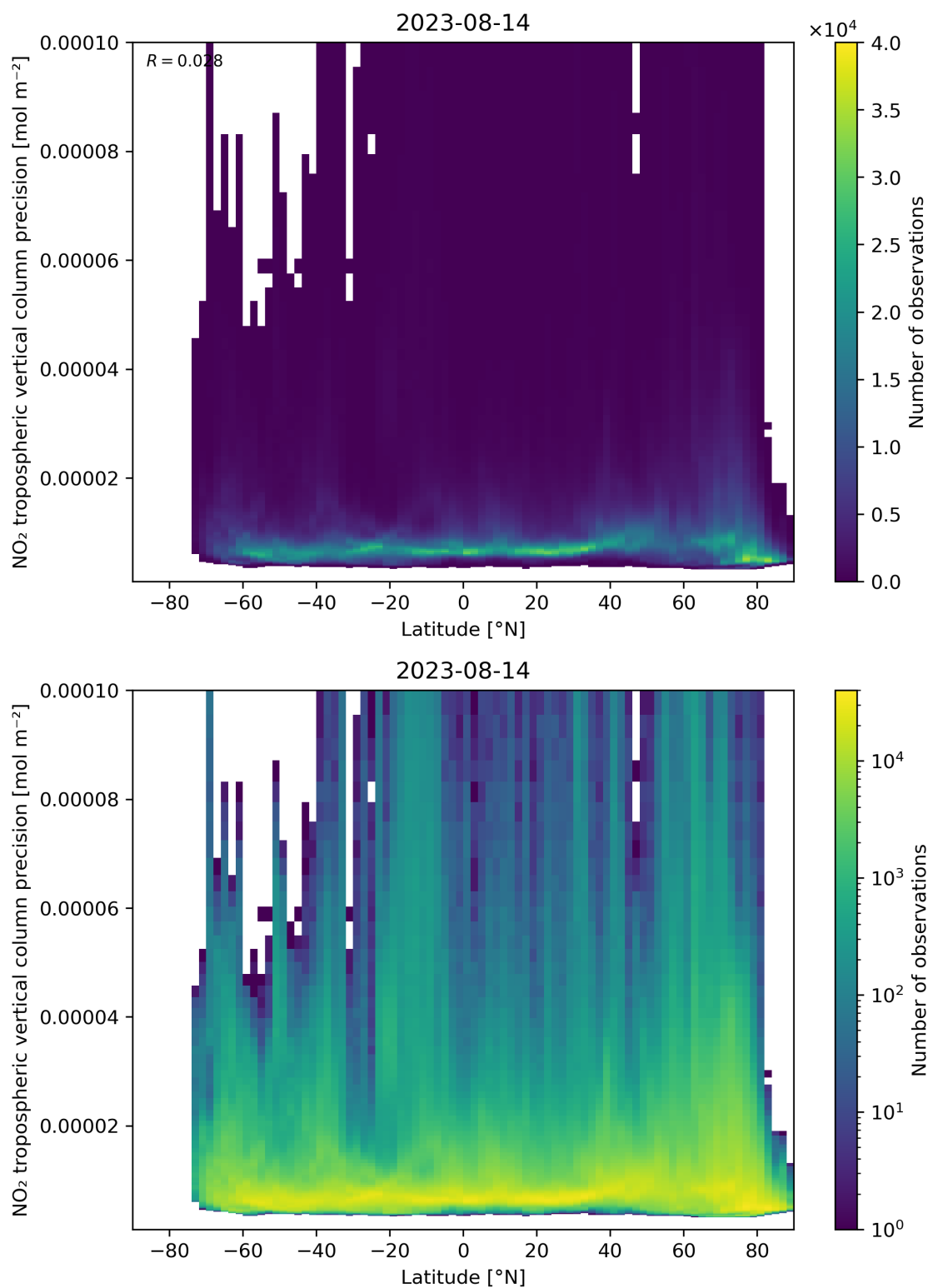
Figure 93: Scatter density plot of “Latitude” against “NO 2 tropospheric vertical column precision” for 2023-08-14 to 2023-08-15.
