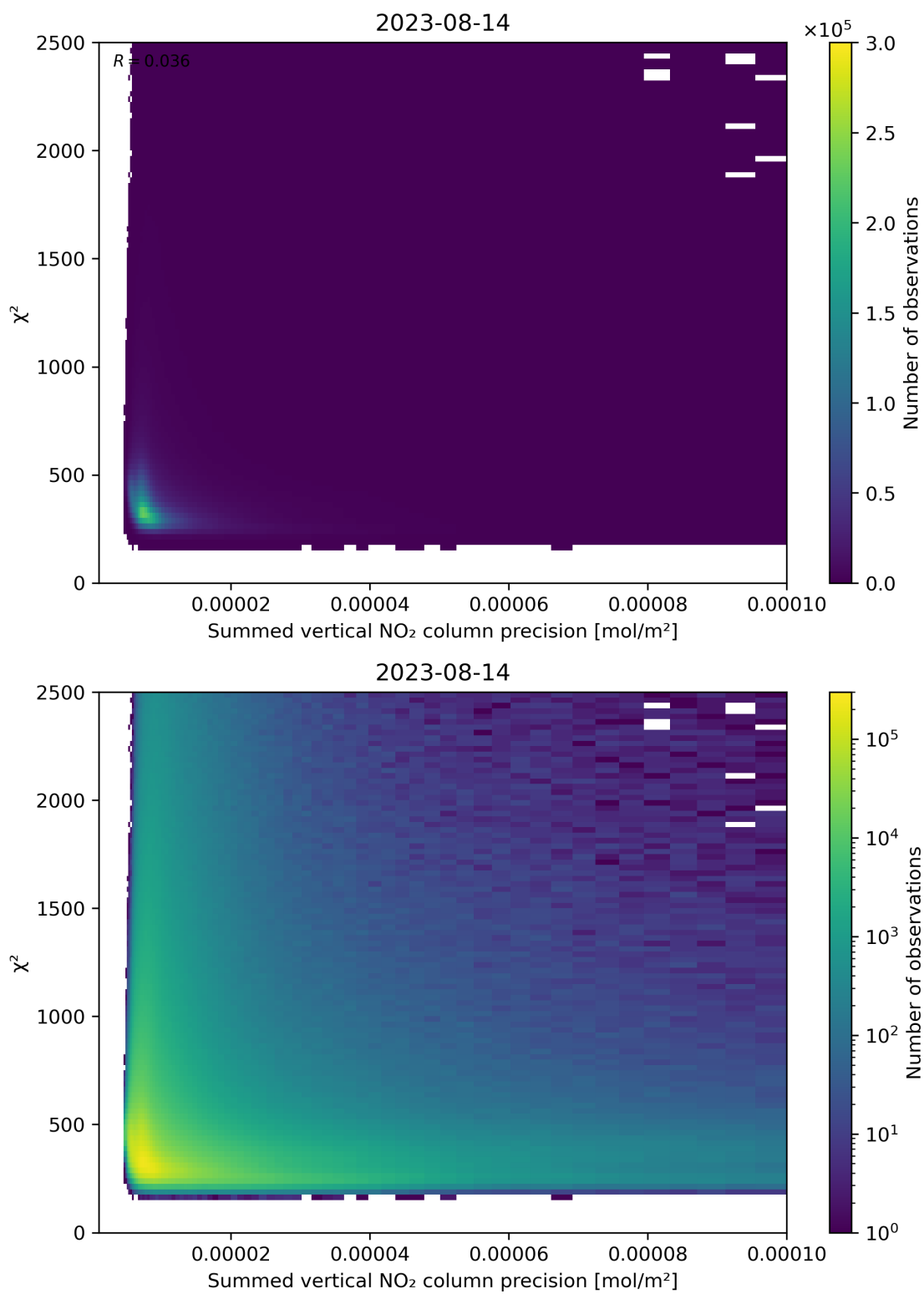
Figure 107: Scatter density plot of “Summed vertical NO 2 column precision” against “ \chi^2 ” for 2023-08-14 to 2023-08-15.
