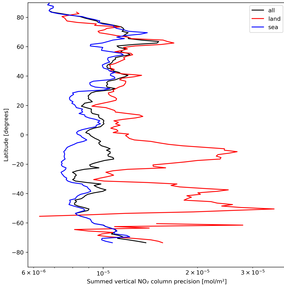
Figure 24: Zonal average of “Summed vertical NO 2 column precision” for 2023-08-14 to 2023-08-15.
