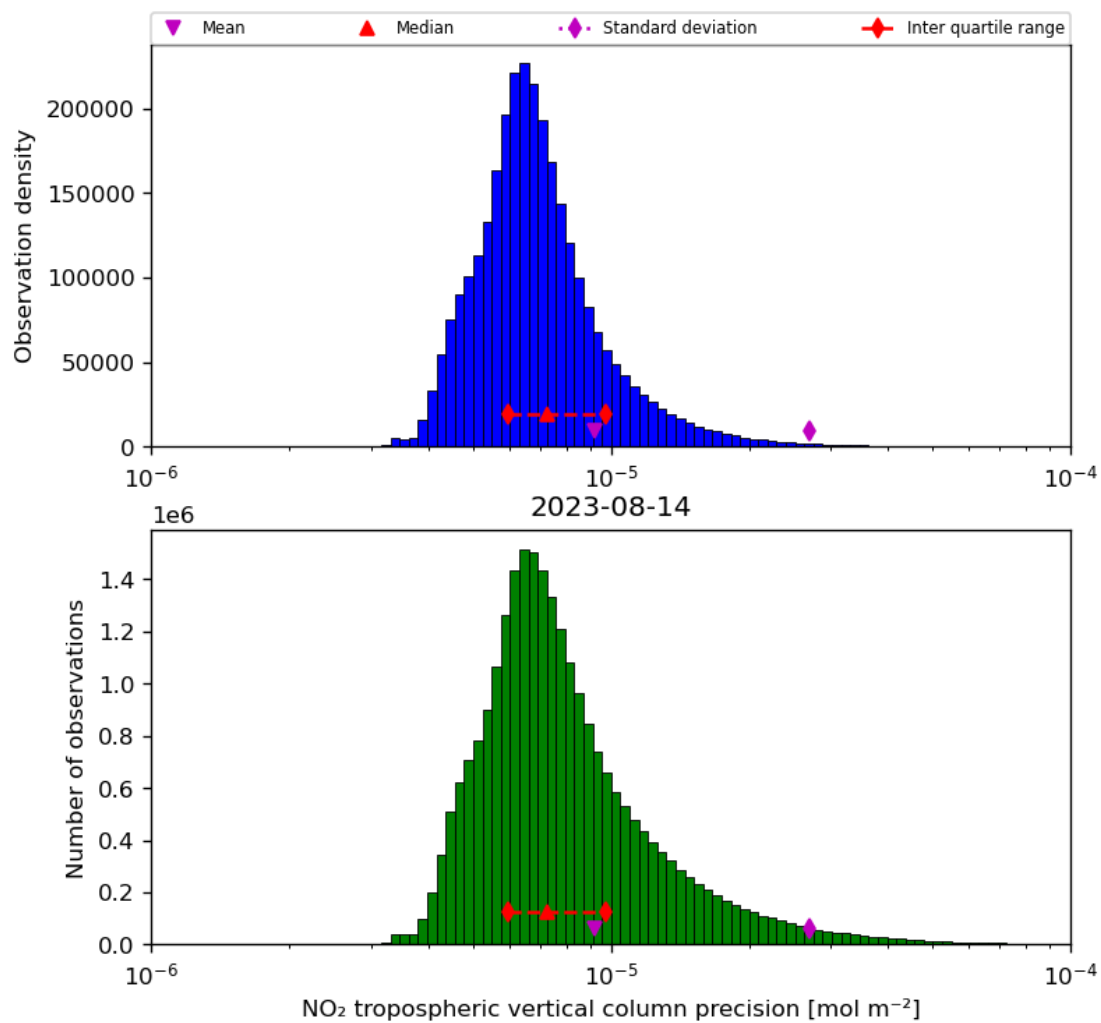
Figure 30: Histogram of “NO 2 tropospheric vertical column precision” for 2023-08-14 to 2023-08-15
