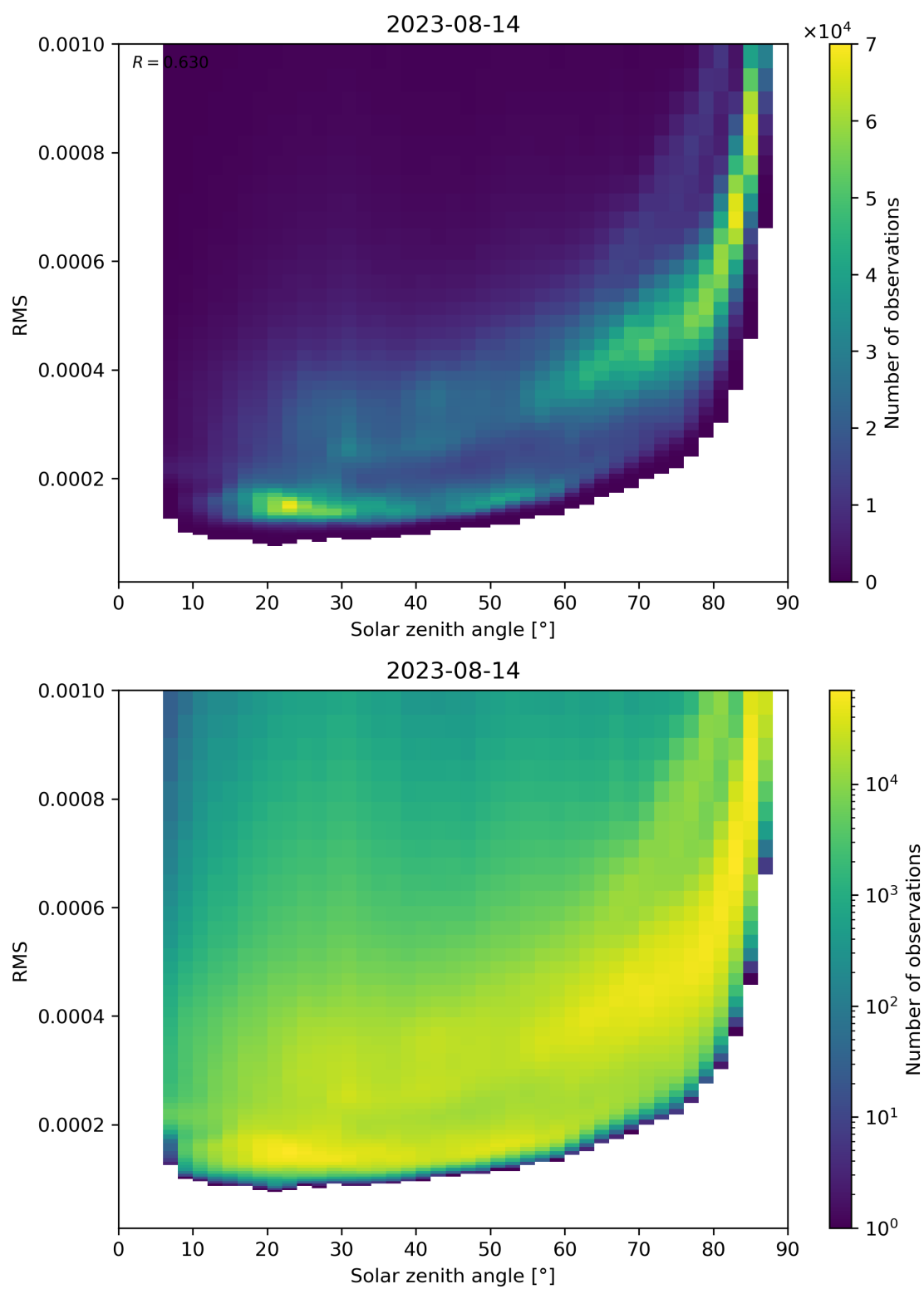
Figure 157: Scatter density plot of “Solar zenith angle” against “RMS” for 2023-08-14 to 2023-08-15.
