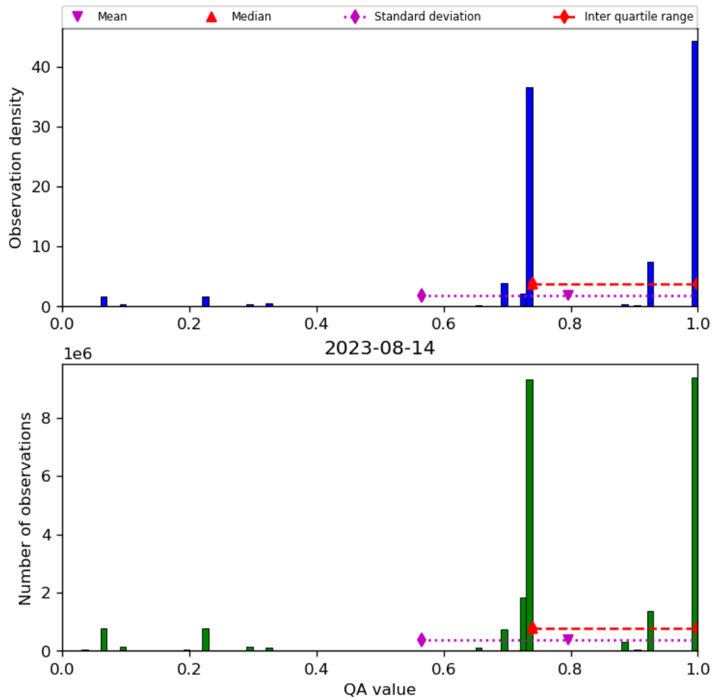
Figure 28: Histogram of “QA value” for 2023-08-14 to 2023-08-15
