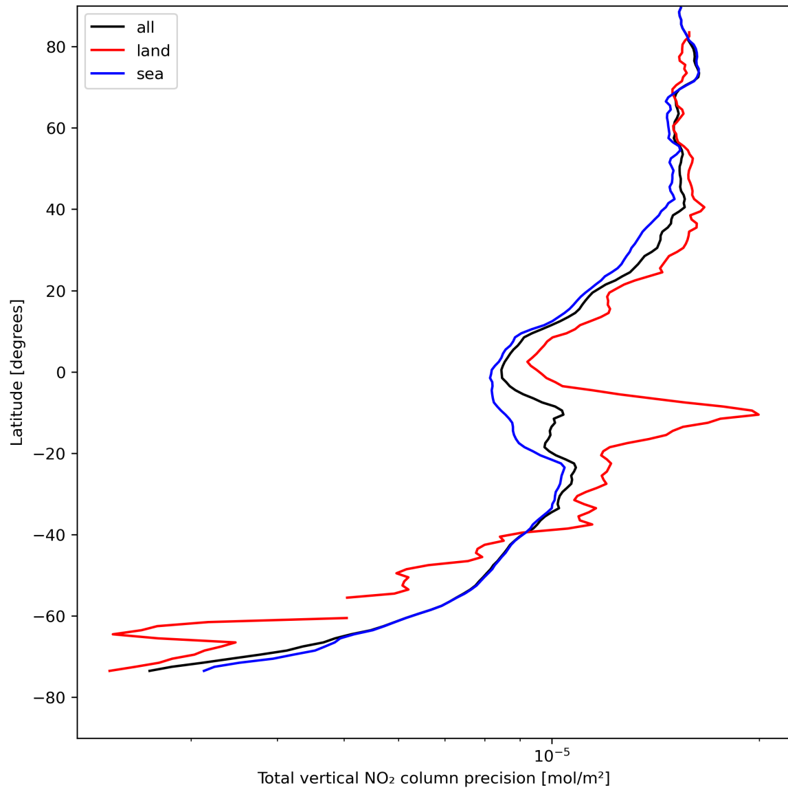
Figure 22: Zonal average of “Total vertical NO 2 column precision” for 2023-08-14 to 2023-08-15.
