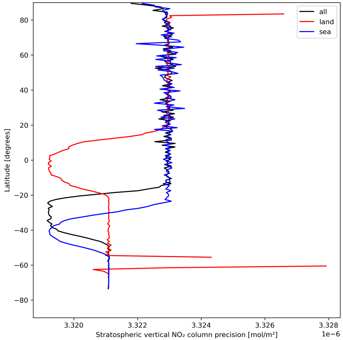
Figure 20: Zonal average of “Stratospheric vertical NO 2 column precision” for 2023-08-14 to 2023-08-15.
