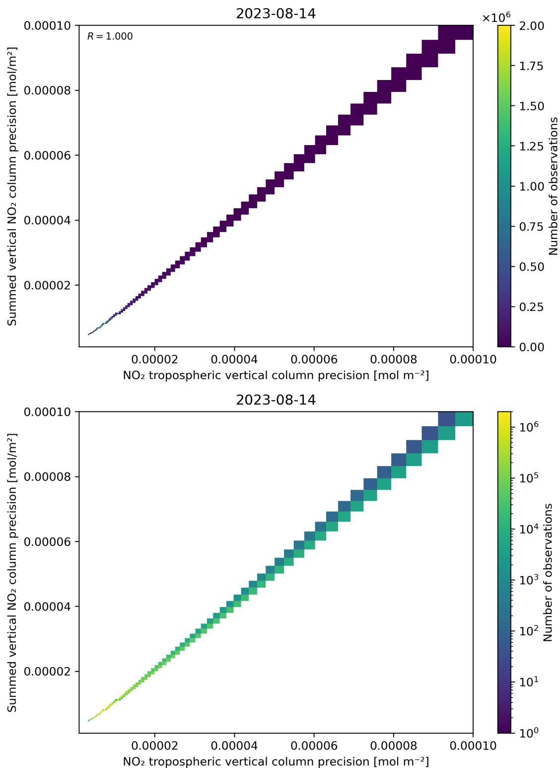
Figure 137: Scatter density plot of “NO 2 tropospheric vertical column precision” against “Summed vertical NO 2 column precision” for 2023-08-14 to 2023-08-15.
