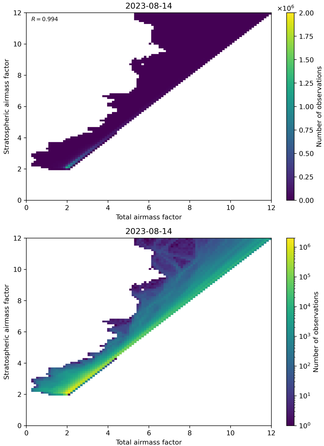
Figure 62: Scatter density plot of “Total airmass factor” against “Stratospheric airmass factor” for 2023-08-14 to 2023-08-15.
