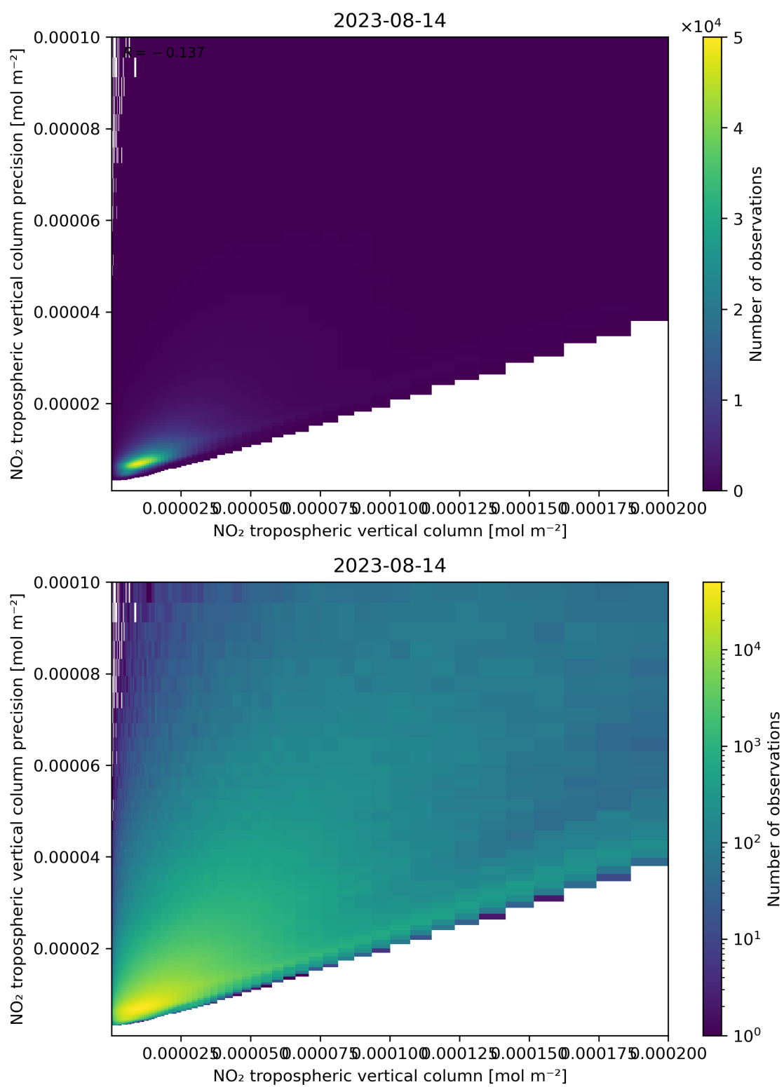
Figure 130: Scatter density plot of “NO 2 tropospheric vertical column” against “NO 2 tropospheric vertical column precision” for 2023-08-14 to 2023-08-15.
