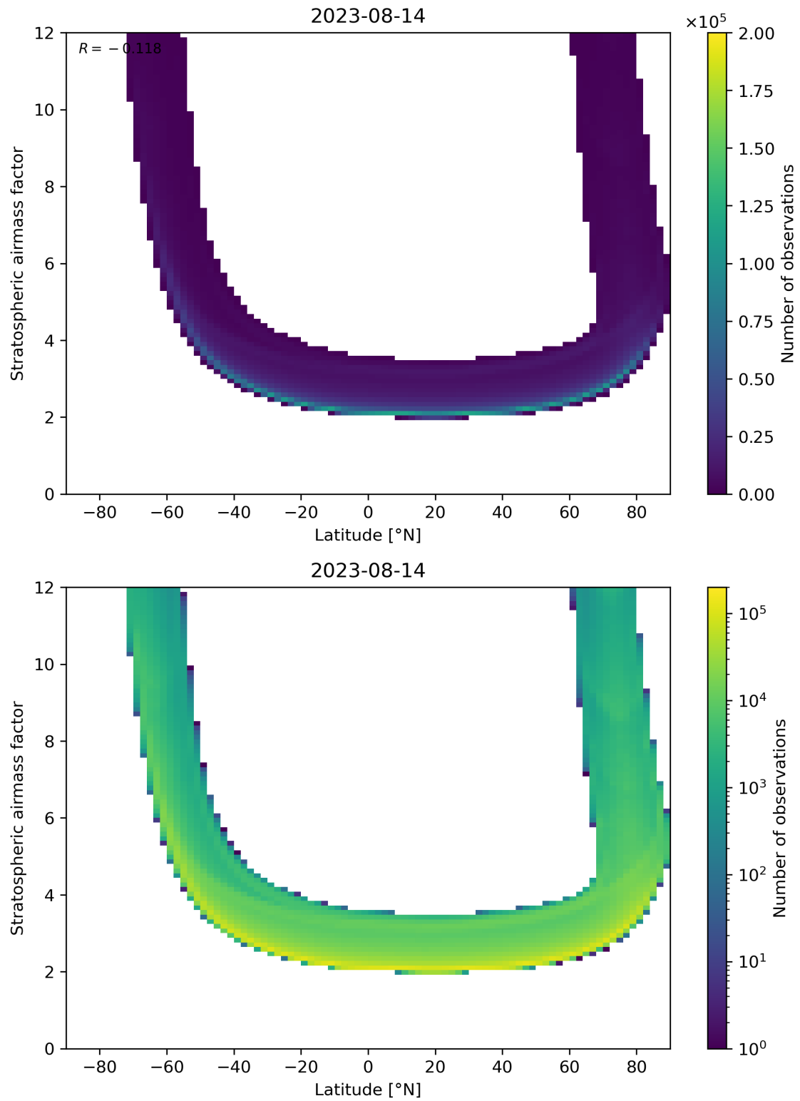
Figure 83: Scatter density plot of “Latitude” against “Stratospheric air mass factor” for 2023-08-14 to 2023-08-15.
