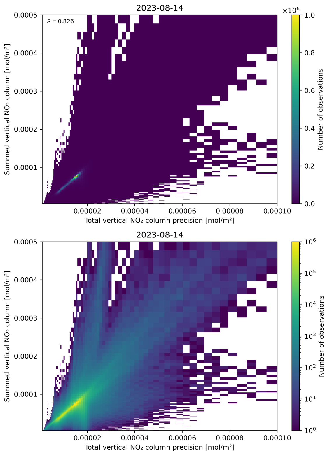
Figure 117: Scatter density plot of “Total vertical NO 2 column precision” against “Summed vertical NO 2 column” for 2023-08-14 to 2023-08-15.
