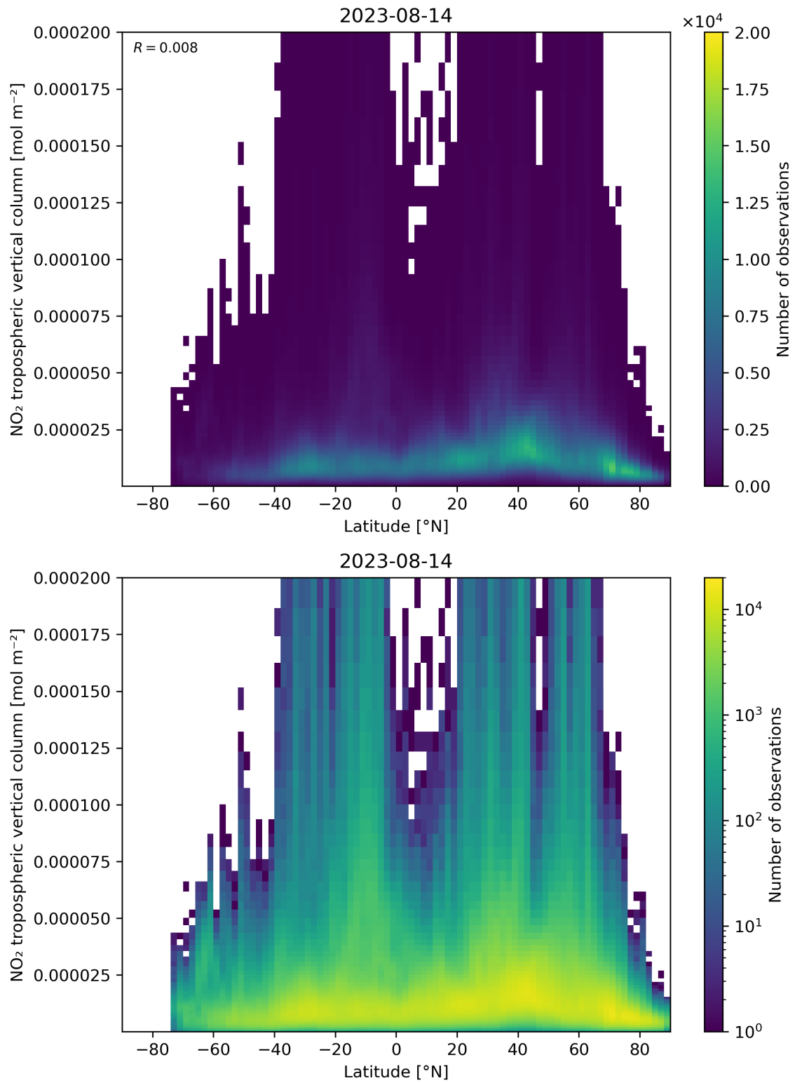
Figure 92: Scatter density plot of “Latitude” against “NO 2 tropospheric vertical column” for 2023-08-14 to 2023-08-15.
