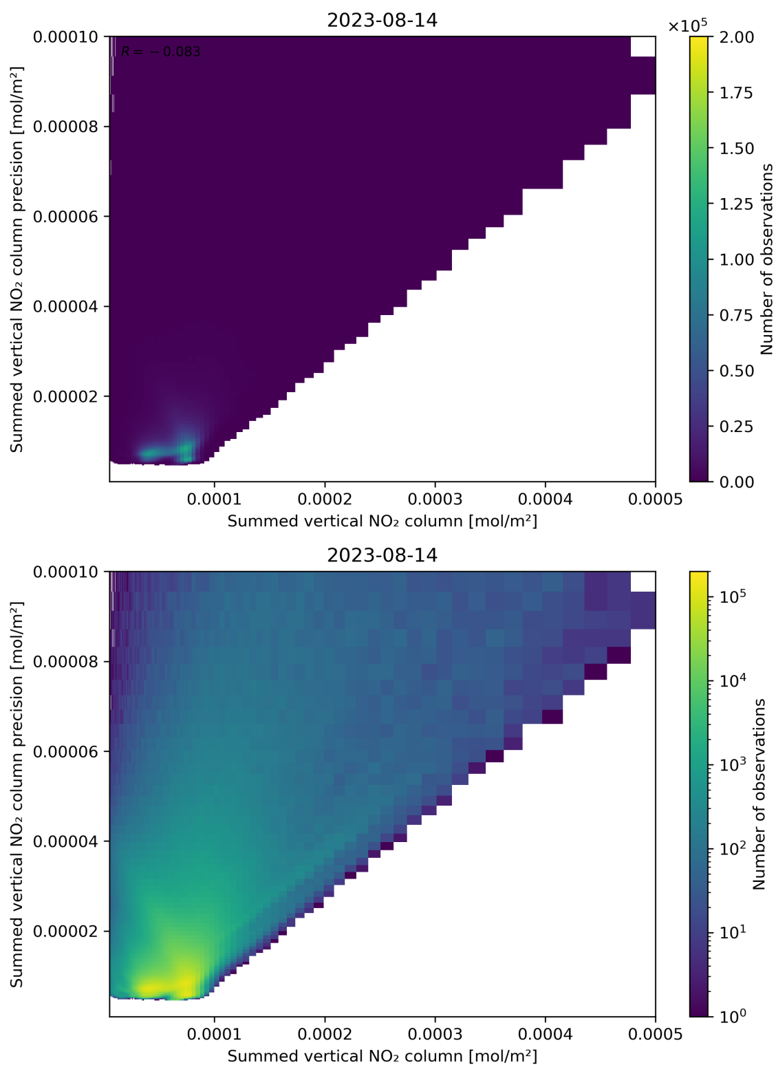
Figure 105: Scatter density plot of “Summed vertical NO 2 column” against “Summed vertical NO 2 column precision” for 2023-08-14 to 2023-08-15.
