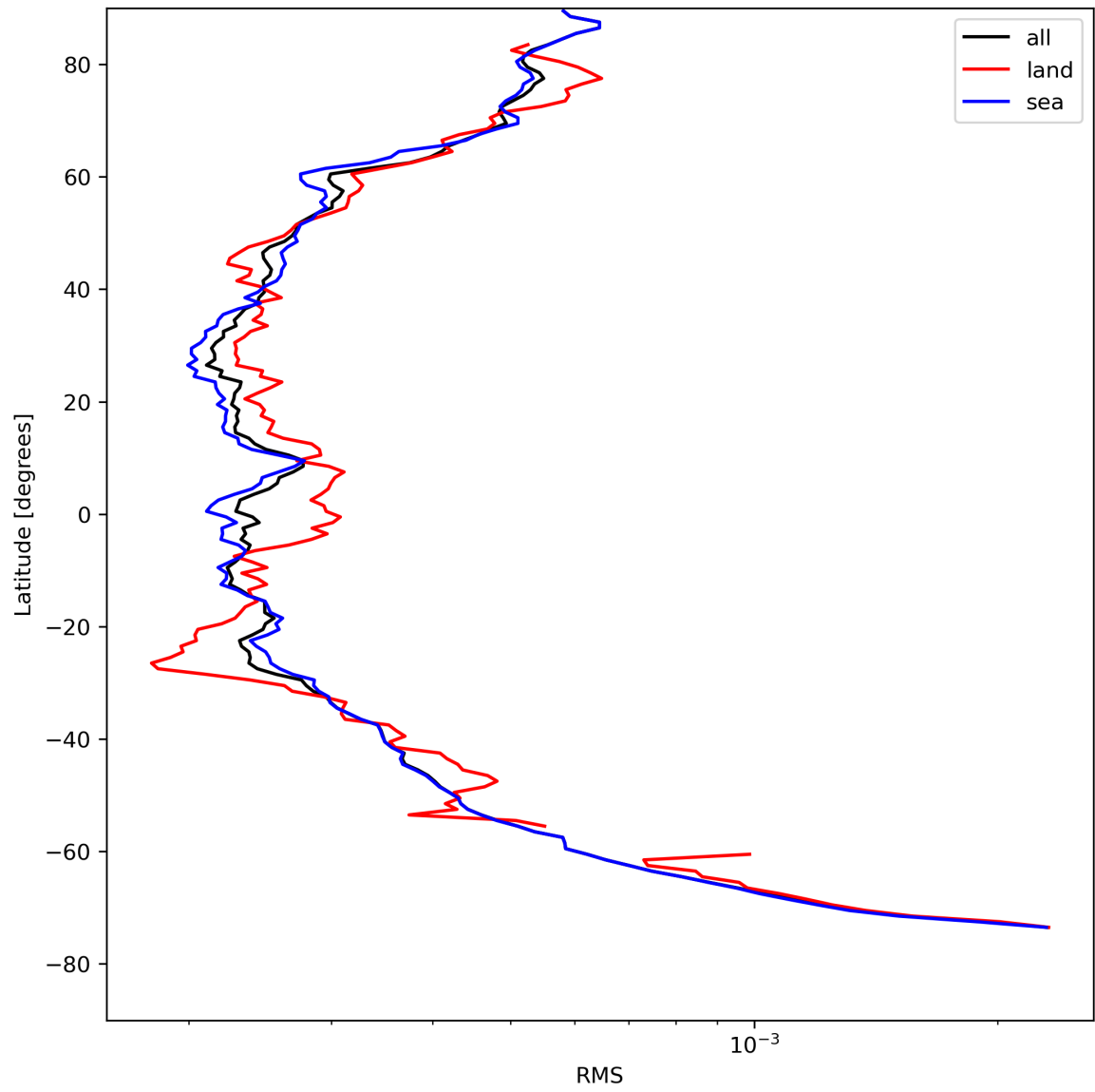
Figure 26: Zonal average of “RMS” for 2023-08-14 to 2023-08-15.
