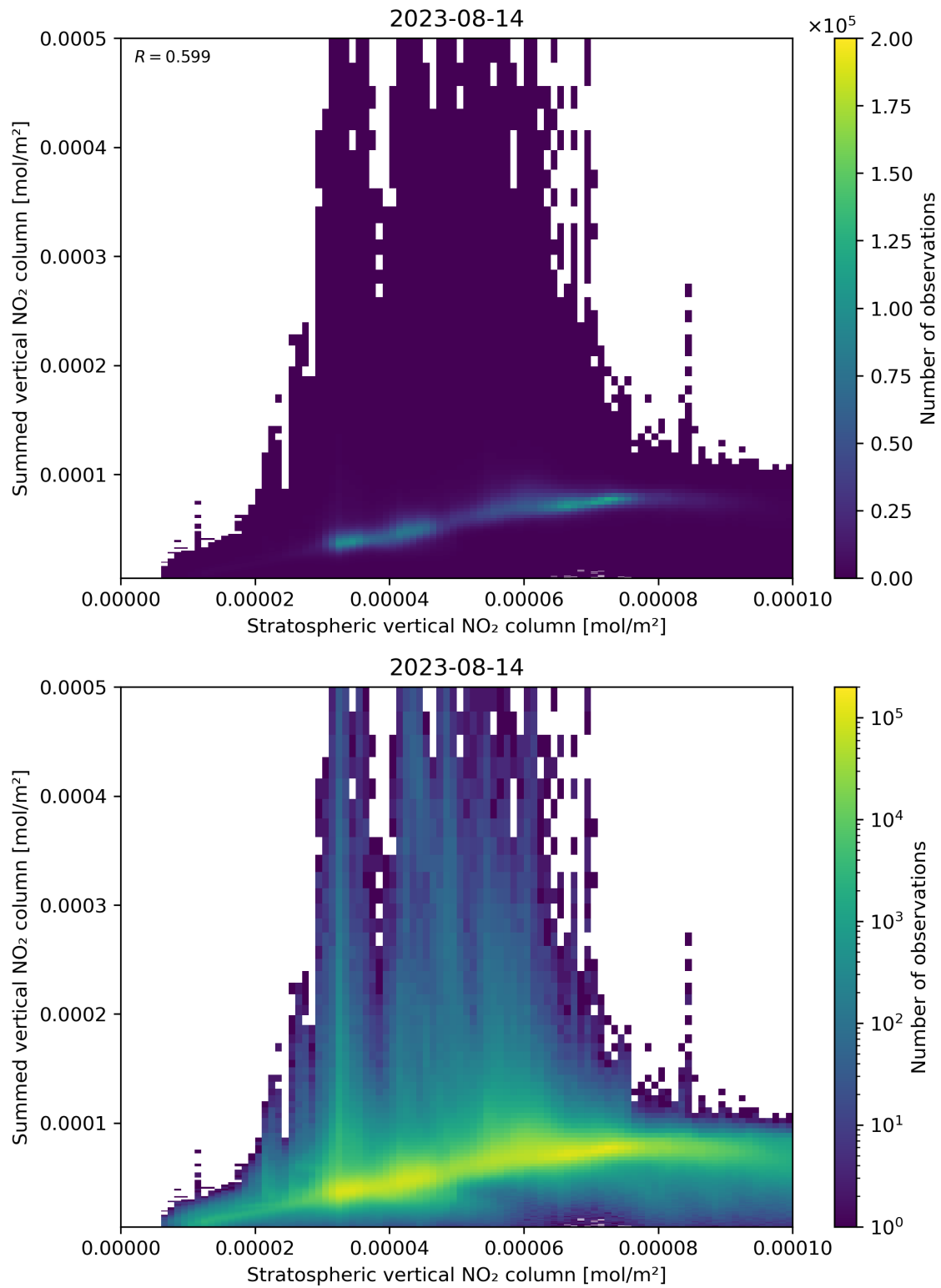
Figure 98: Scatter density plot of “Stratospheric vertical NO 2 column” against “Summed vertical NO 2 column” for 2023-08-14 to 2023-08-15.
