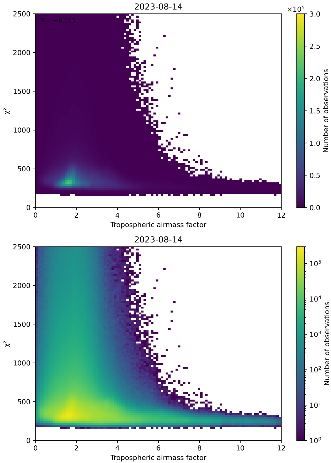
Figure 73: Scatter density plot of “Tropospheric airmass factor” against “ \chi^2 ” for 2023-08-14 to 2023-08-15.
