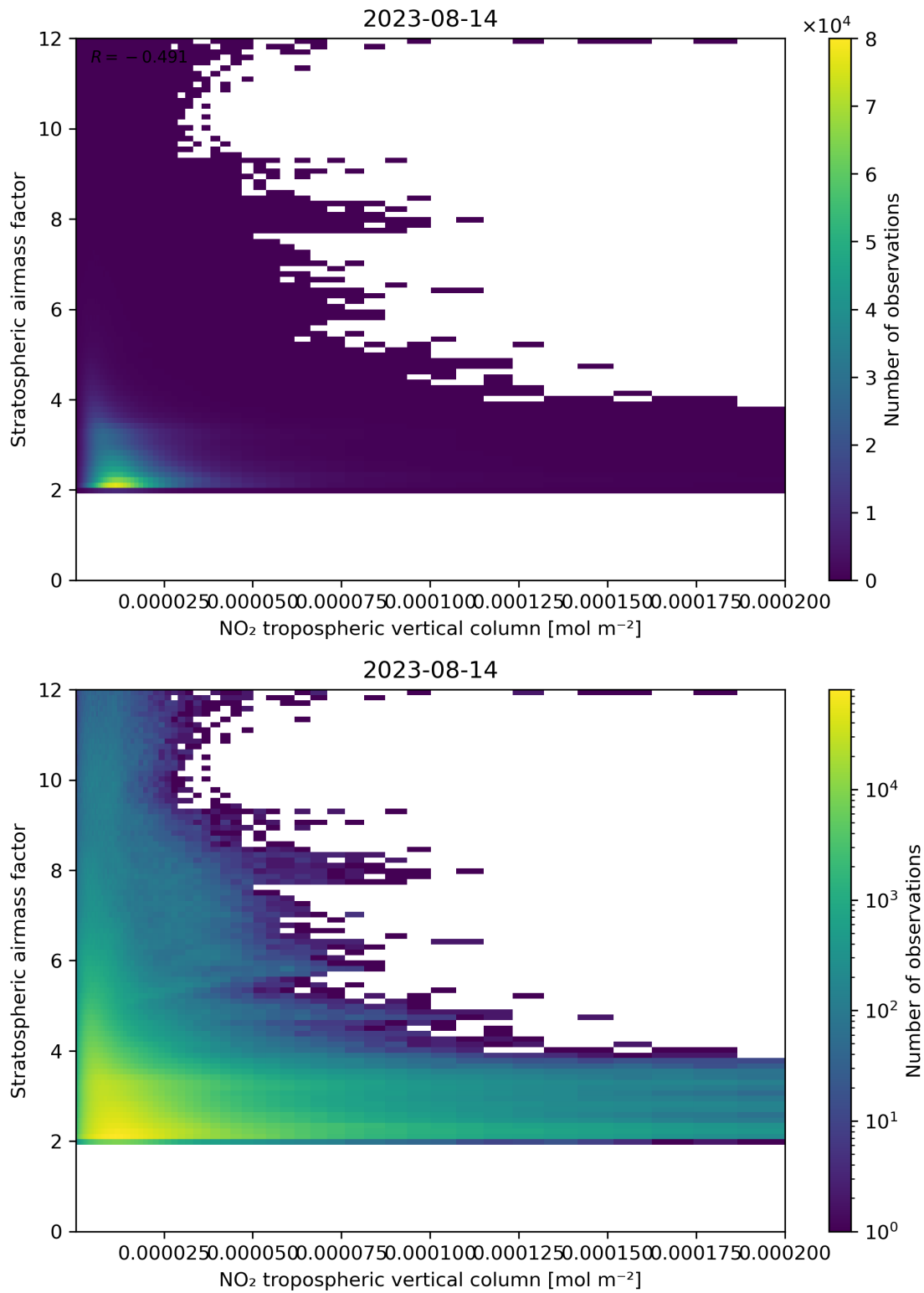
Figure 121: Scatter density plot of “NO 2 tropospheric vertical column” against “Stratospheric air mass factor” for 2023-08-14 to 2023-08-15.
