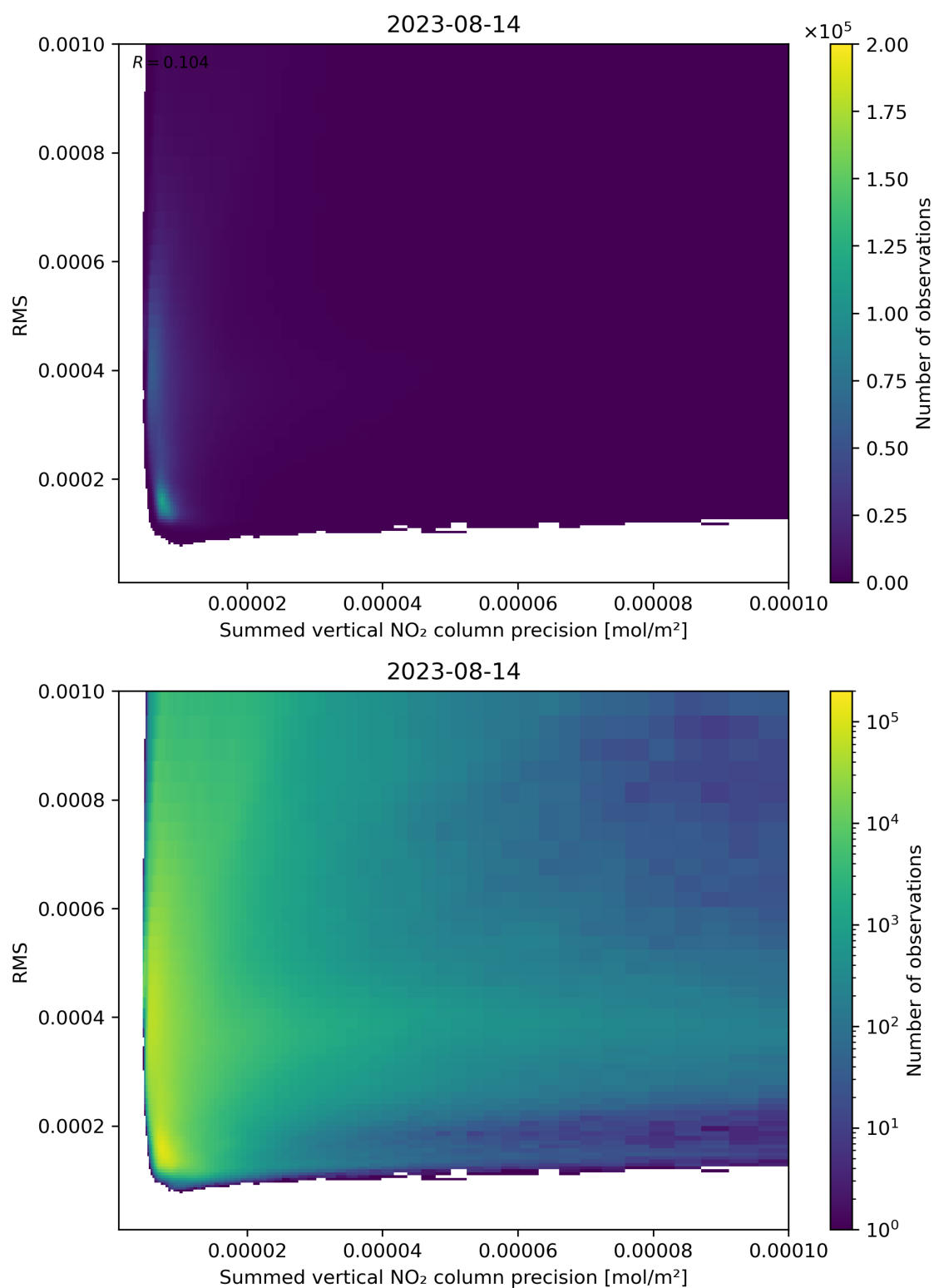
Figure 108: Scatter density plot of “Summed vertical NO 2 column precision” against “RMS” for 2023-08-14 to 2023-08-15.
