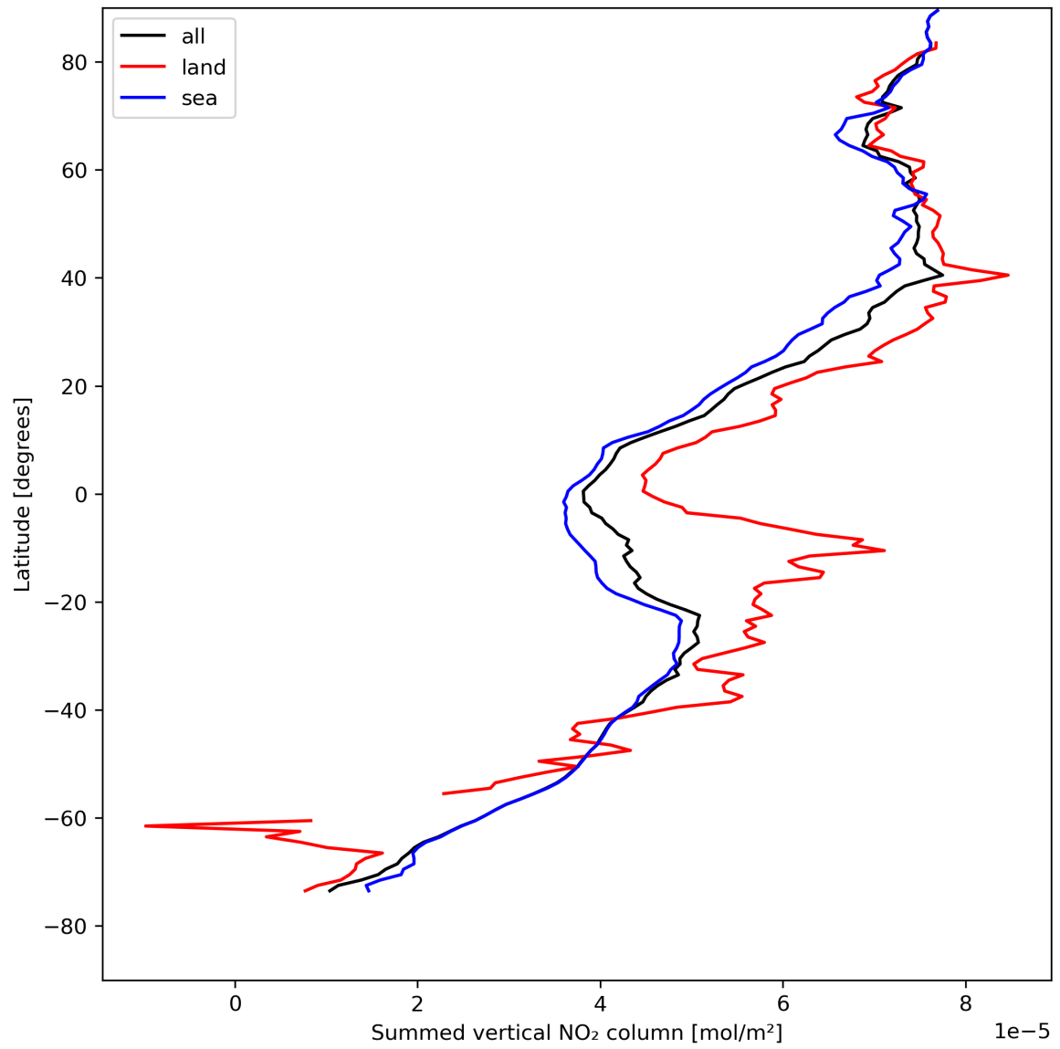
Figure 23: Zonal average of “Summed vertical NO 2 column” for 2023-08-14 to 2023-08-15.
