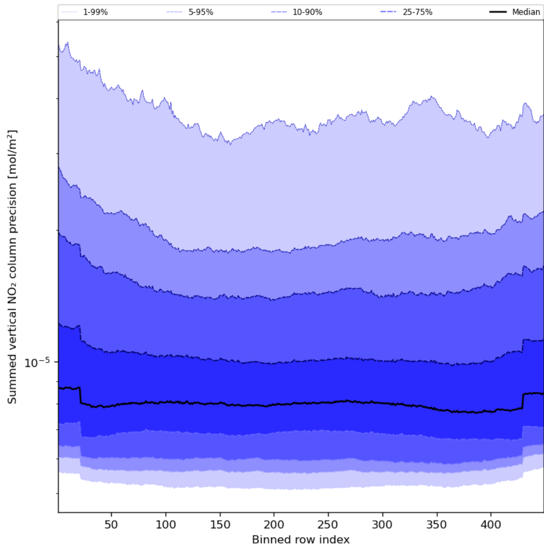
Figure 58: Along track statistics of “Summed vertical NO 2 column precision” for 2023-08-14 to 2023-08-15
