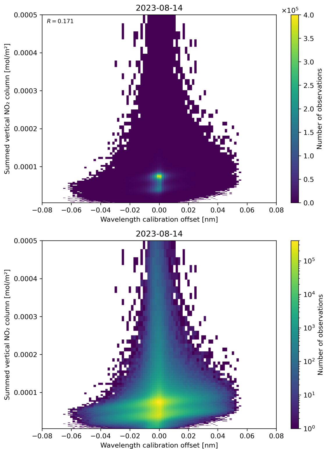
Figure 177: Scatter density plot of “Wavelength calibration offset” against “Summed vertical NO 2 column” for 2023-08-14 to 2023-08-15.
