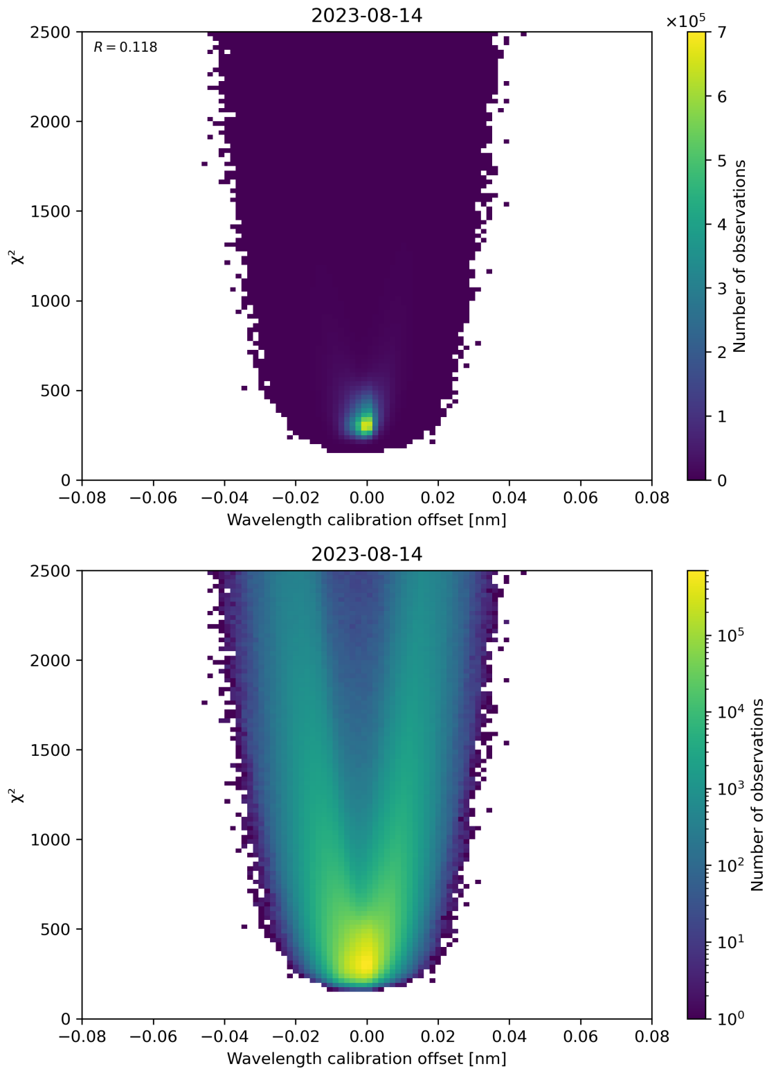
Figure 175: Scatter density plot of “Wavelength calibration offset” against “ \chi^2 ” for 2023-08-14 to 2023-08-15.
