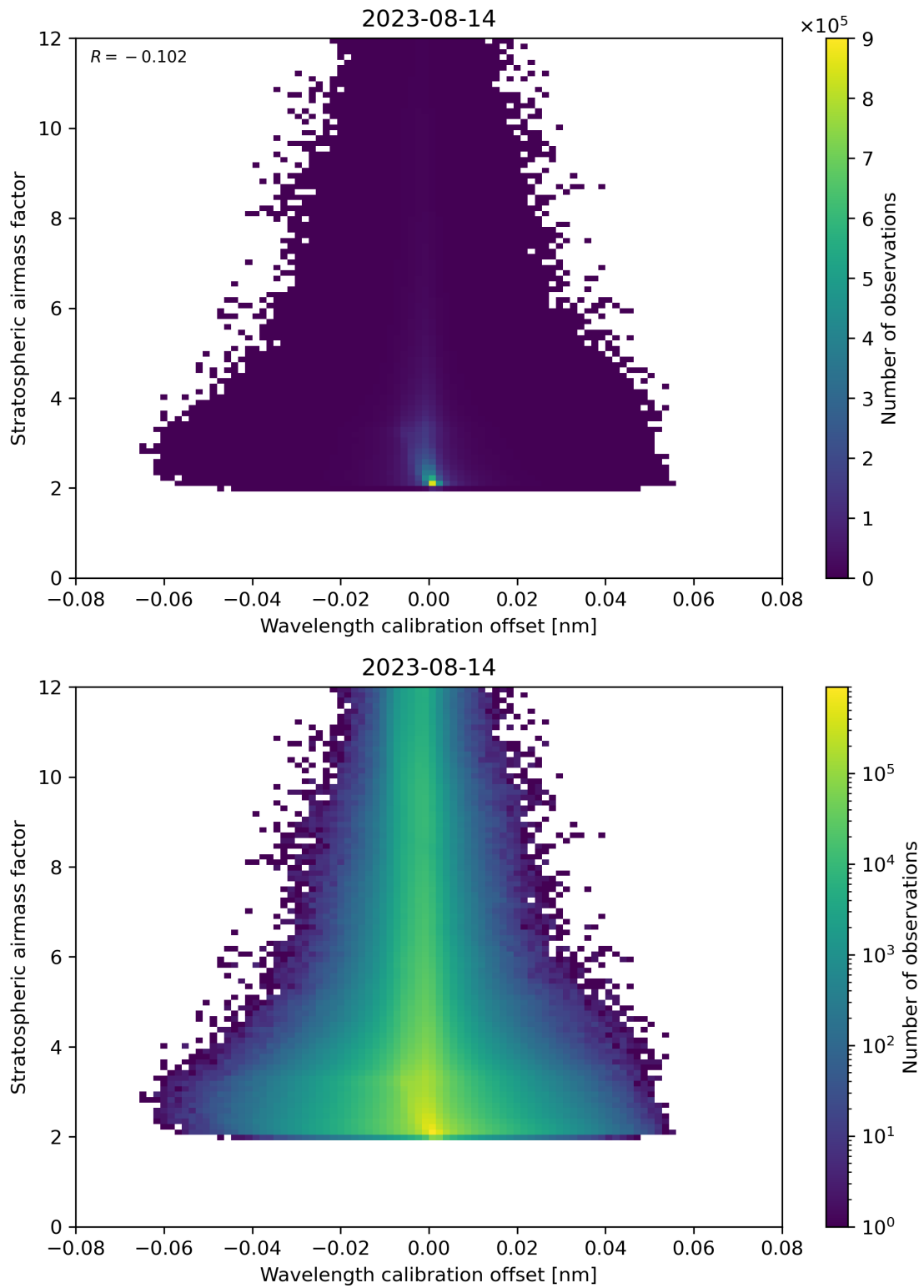
Figure 174: Scatter density plot of “Wavelength calibration offset” against “Stratospheric airmass factor” for 2023-08-14 to 2023-08-15.
