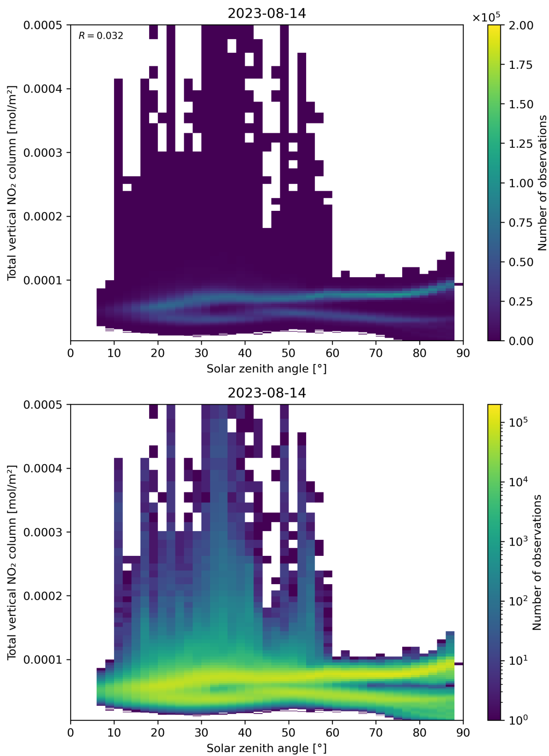
Figure 153: Scatter density plot of “Solar zenith angle” against “Total vertical \text{NO}_2 column” for 2023-08-14 to 2023-08-15.
