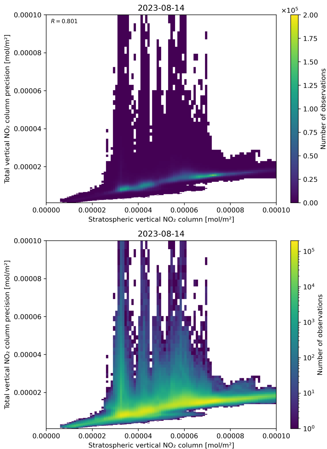
Figure 101: Scatter density plot of “Stratospheric vertical NO 2 column” against “Total vertical NO 2 column precision” for 2023-08-14 to 2023-08-15.
