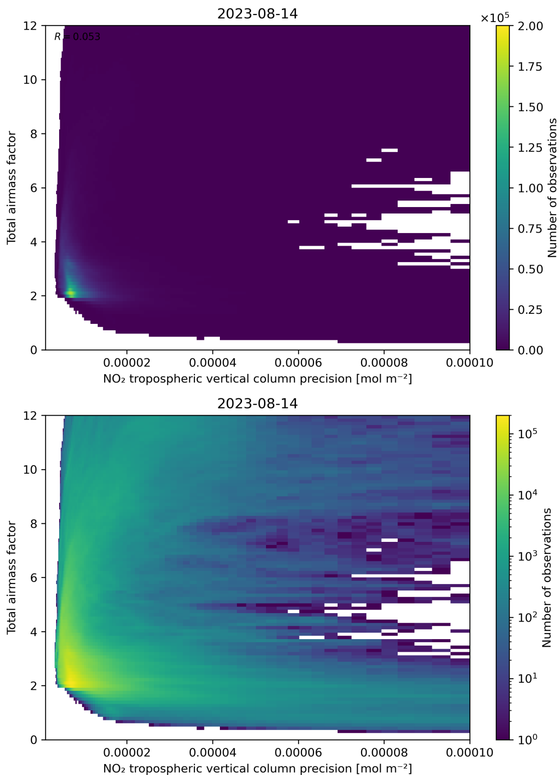
Figure 132: Scatter density plot of “NO 2 tropospheric vertical column precision” against “Total air mass factor” for 2023-08-14 to 2023-08-15.
