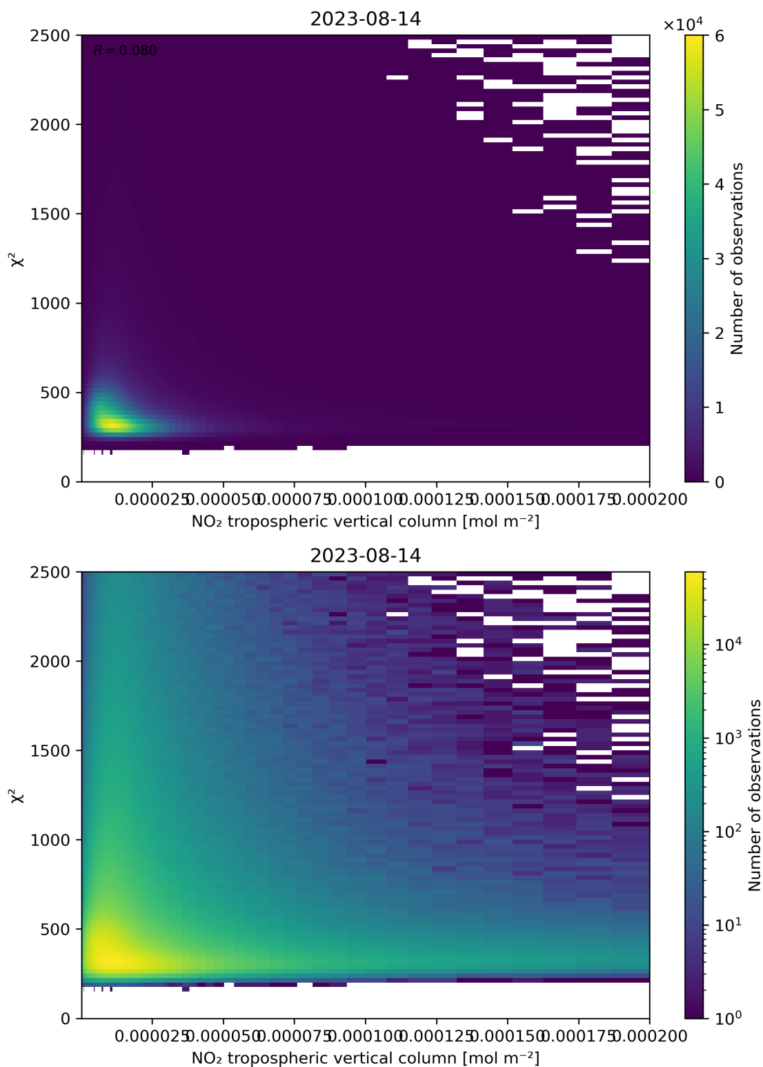
Figure 124: Scatter density plot of “NO 2 tropospheric vertical column” against “ \chi^2 ” for 2023-08-14 to 2023-08-15.
