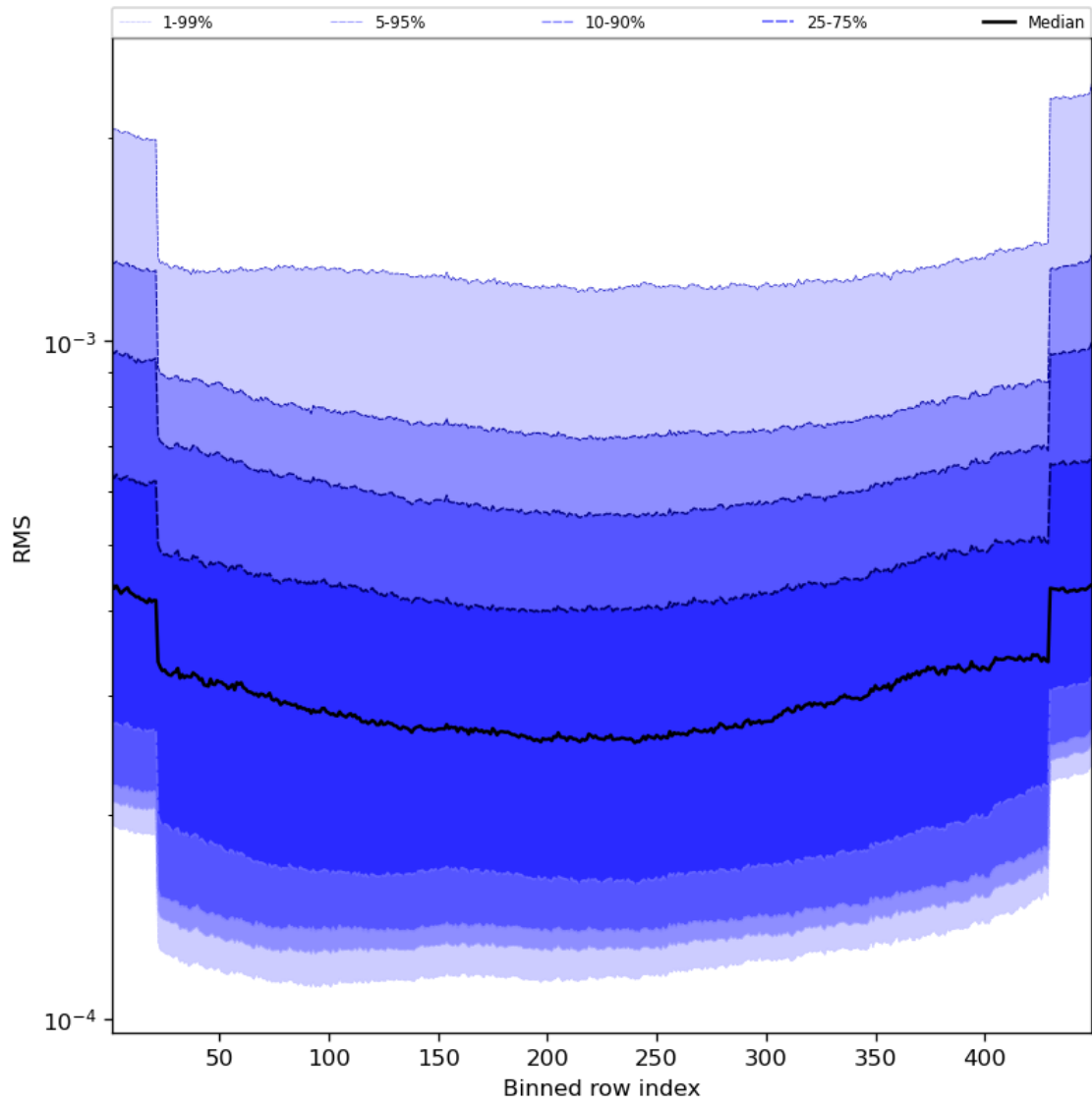
Figure 60: Along track statistics of “RMS” for 2023-08-14 to 2023-08-15
