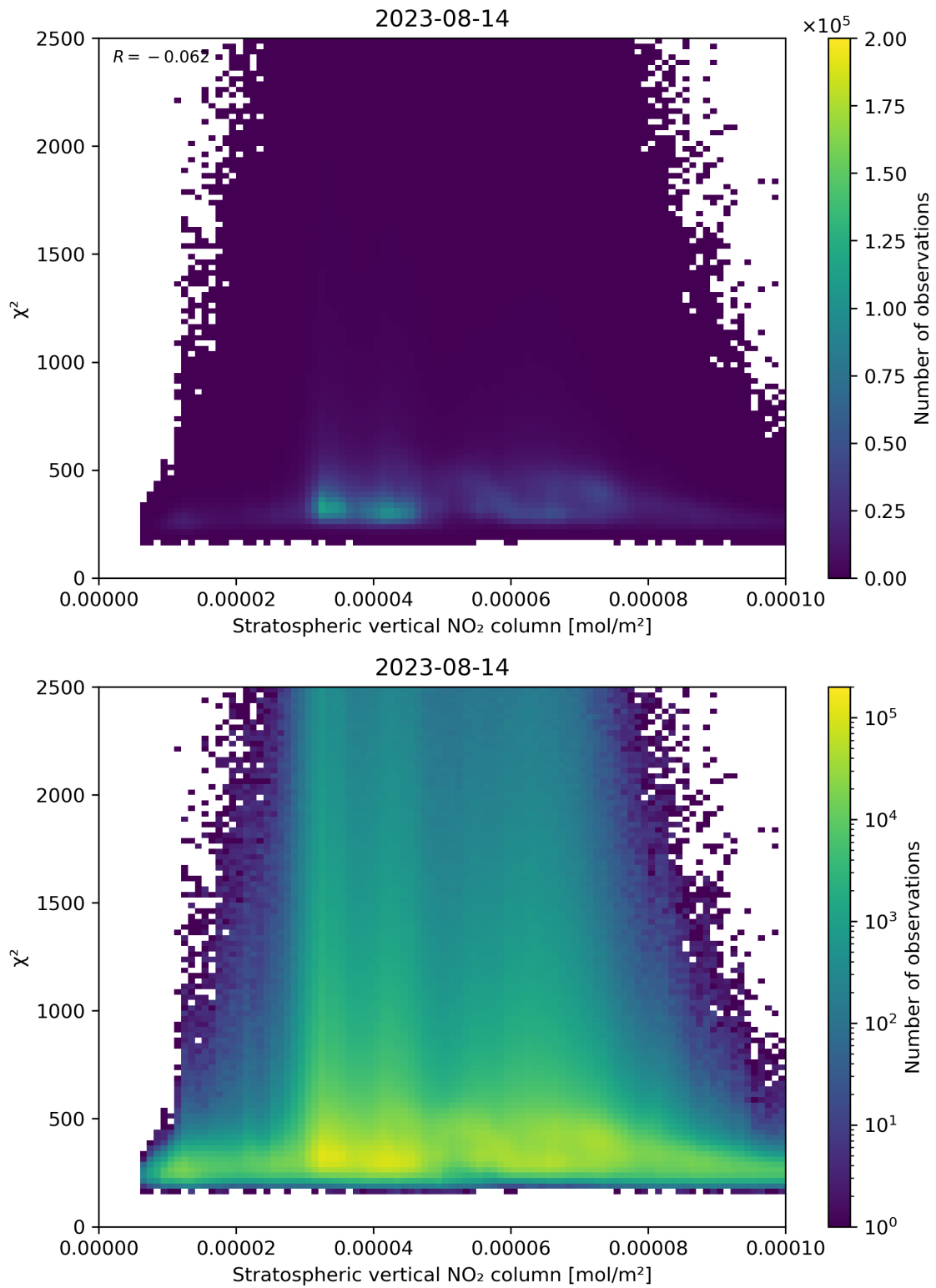
Figure 97: Scatter density plot of “Stratospheric vertical NO 2 column” against “ \chi^2 ” for 2023-08-14 to 2023-08-15.
