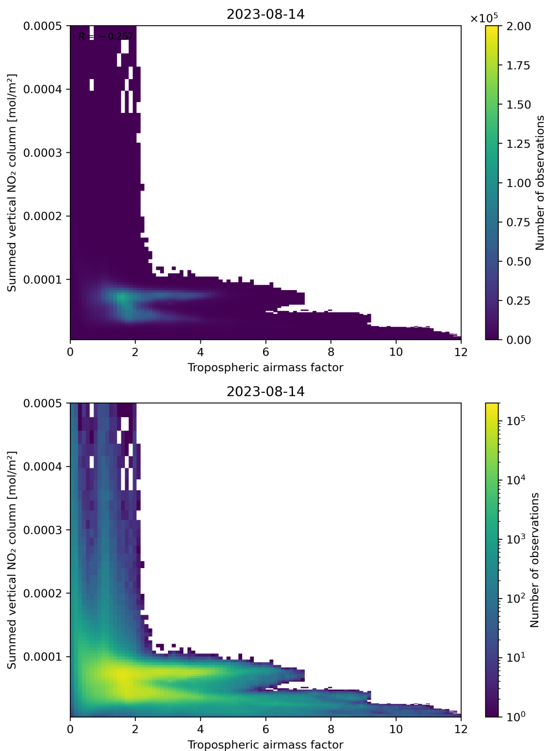
Figure 75: Scatter density plot of “Tropospheric airmass factor” against “Summed vertical NO 2 column” for 2023-08-14 to 2023-08-15.
