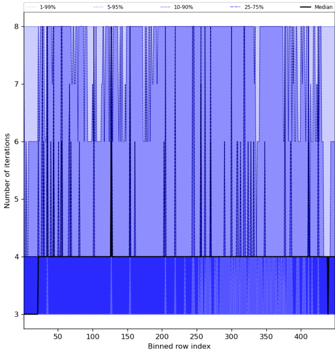
Figure 51: Along track statistics of “Number of iterations” for 2023-08-14 to 2023-08-15
