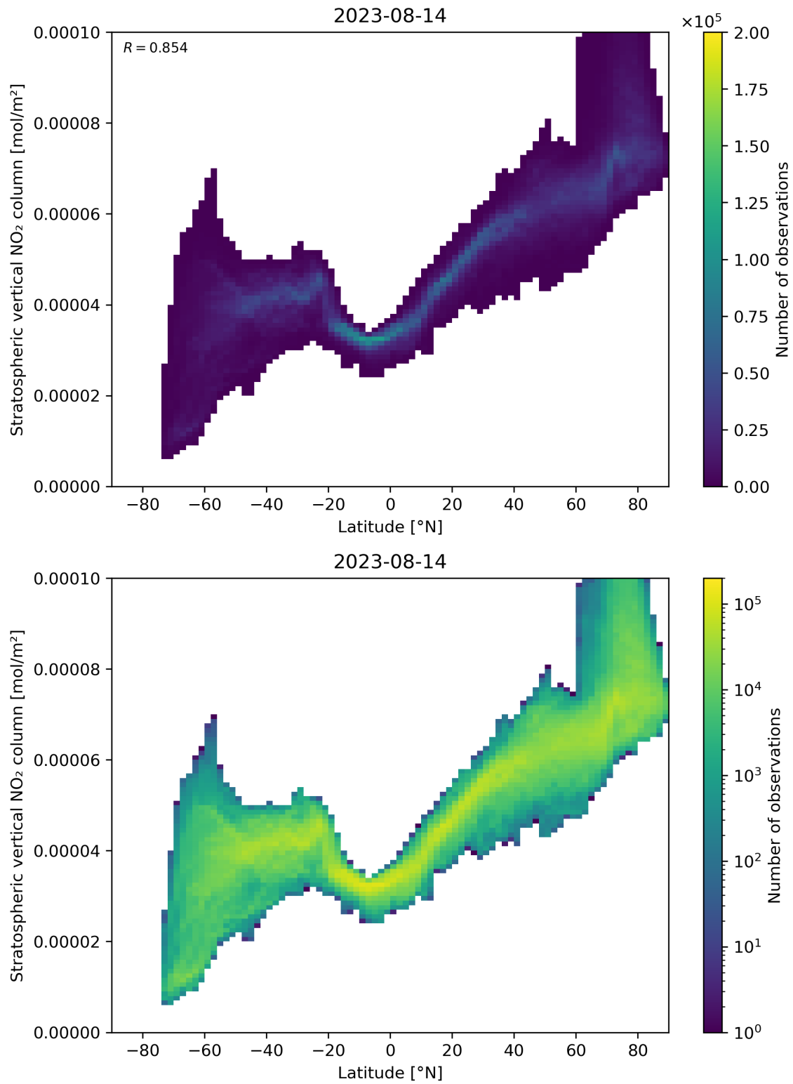
Figure 87: Scatter density plot of “Latitude” against “Stratospheric vertical \text{NO}_2 column” for 2023-08-14 to 2023-08-15.
