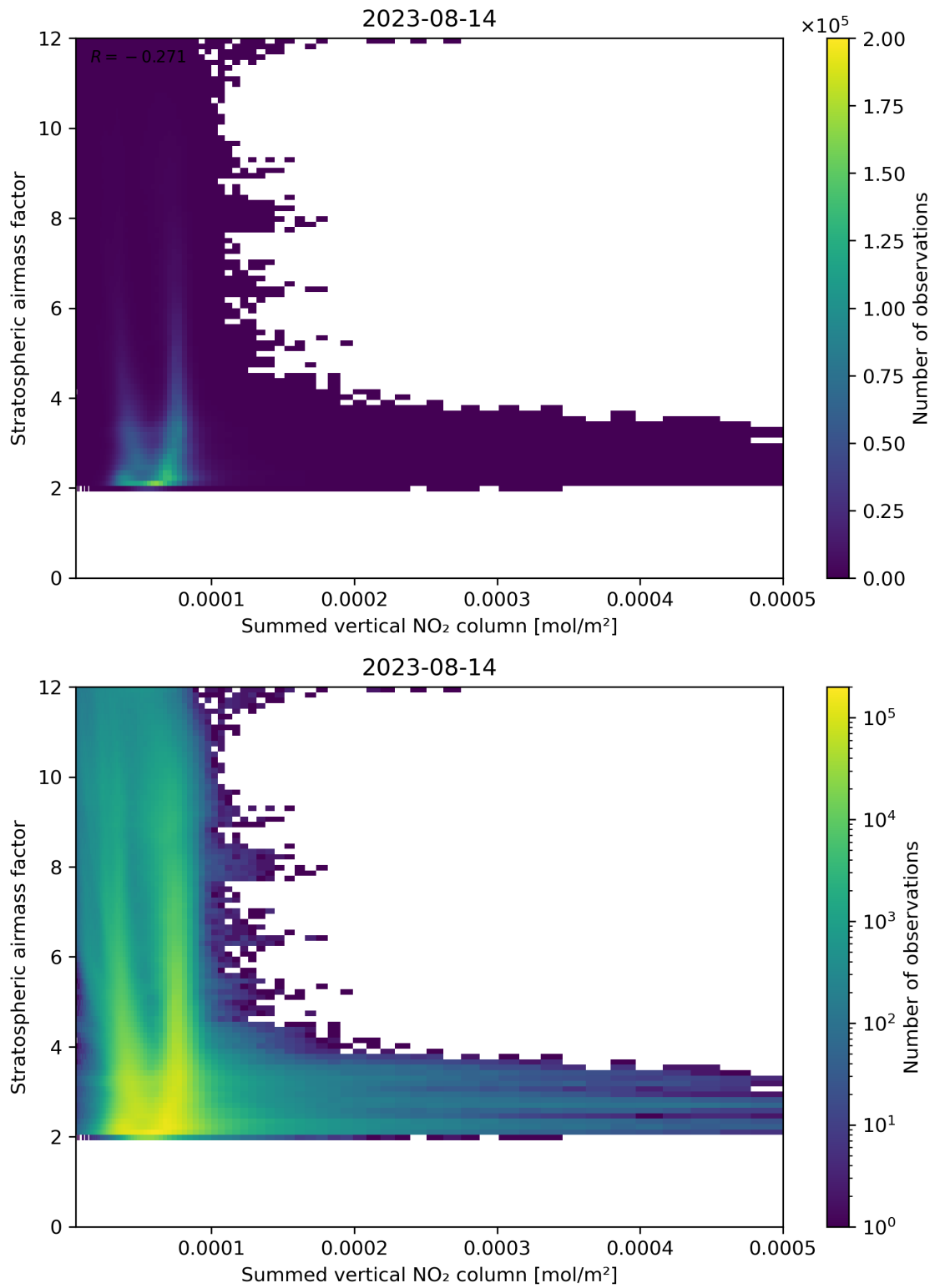
Figure 103: Scatter density plot of “Summed vertical NO 2 column” against “Stratospheric airmass factor” for 2023-08-14 to 2023-08-15.
