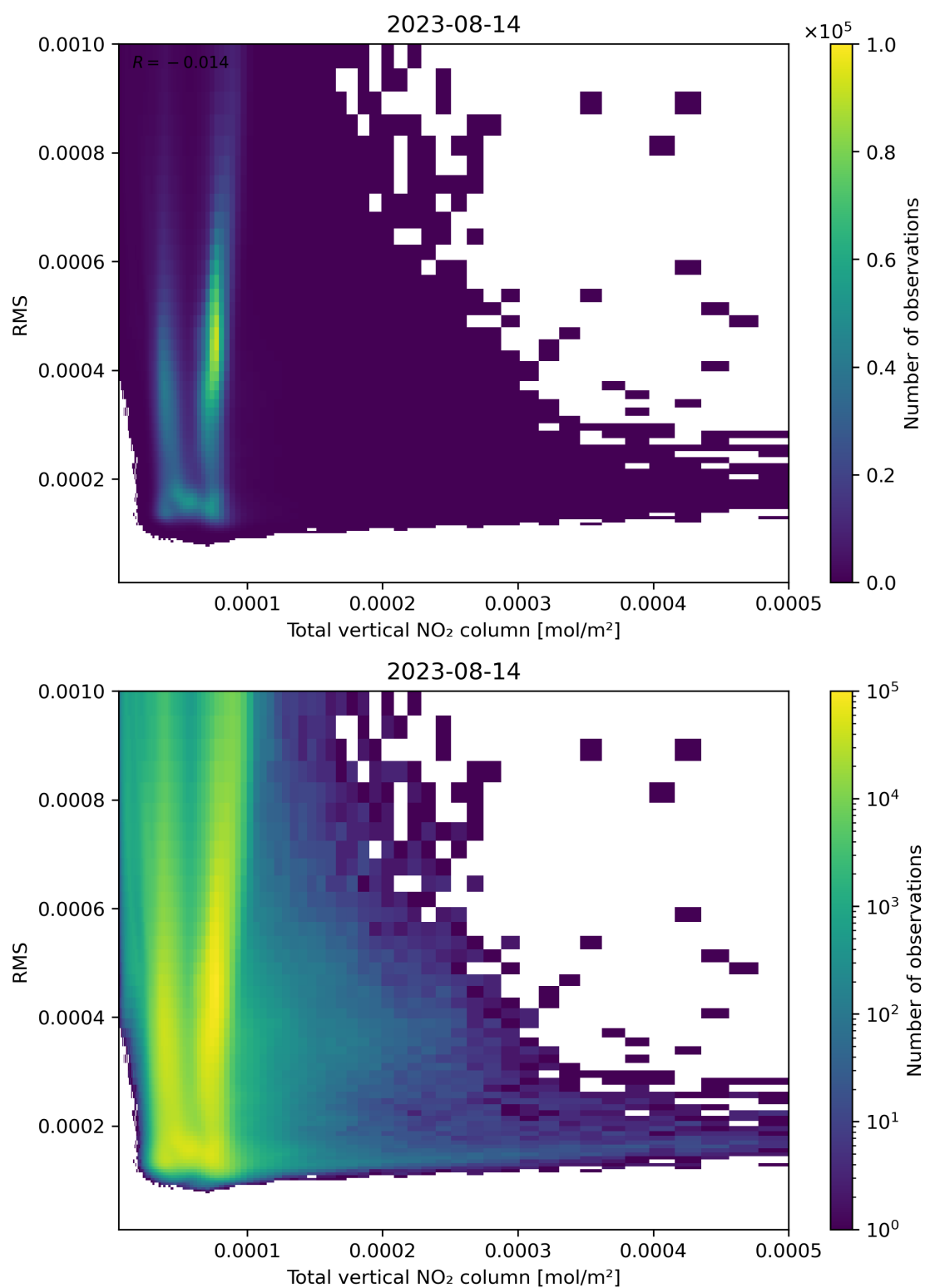
Figure 120: Scatter density plot of “Total vertical NO 2 column” against “RMS” for 2023-08-14 to 2023-08-15.
