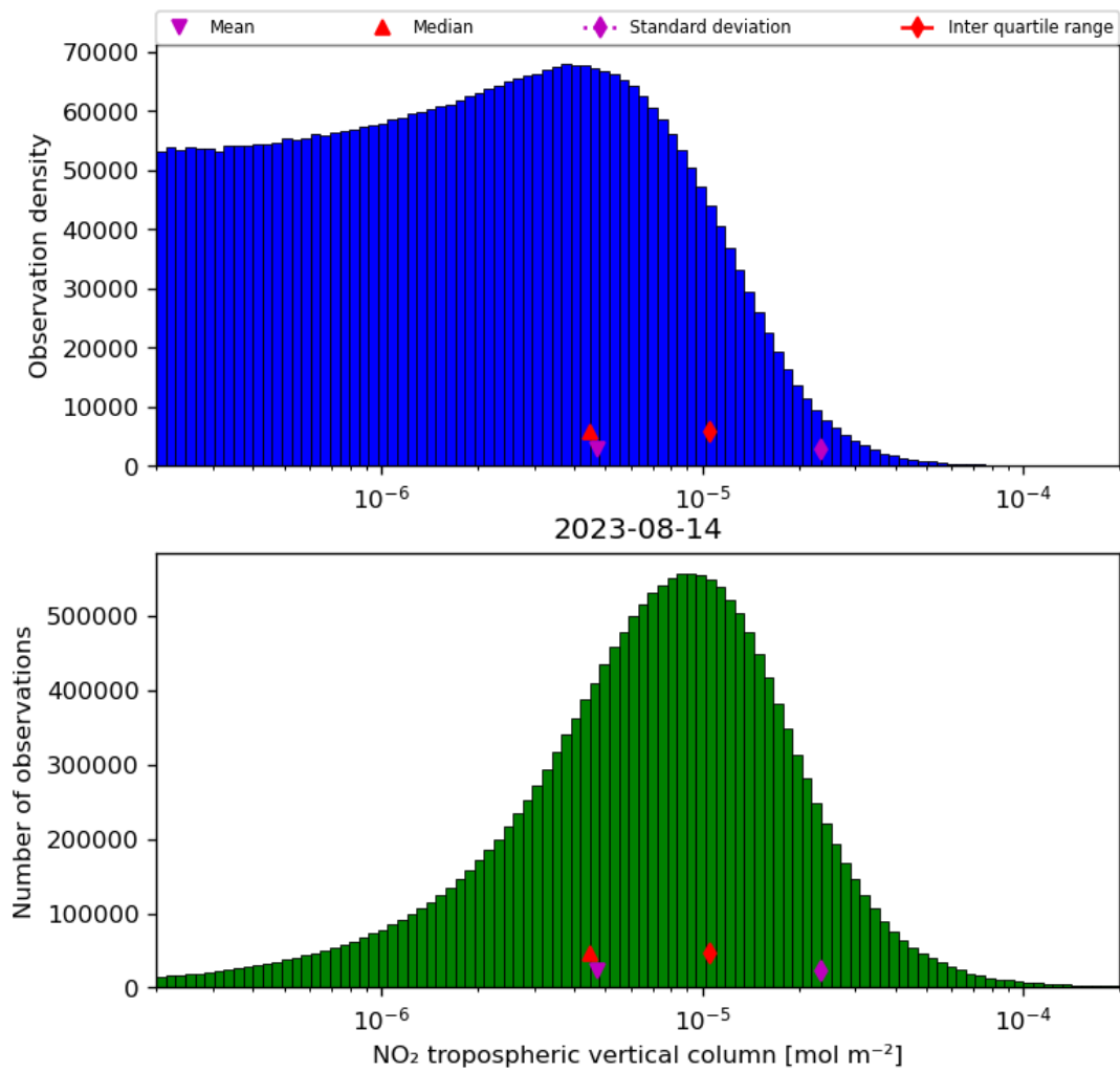
Figure 29: Histogram of “NO 2 tropospheric vertical column” for 2023-08-14 to 2023-08-15
