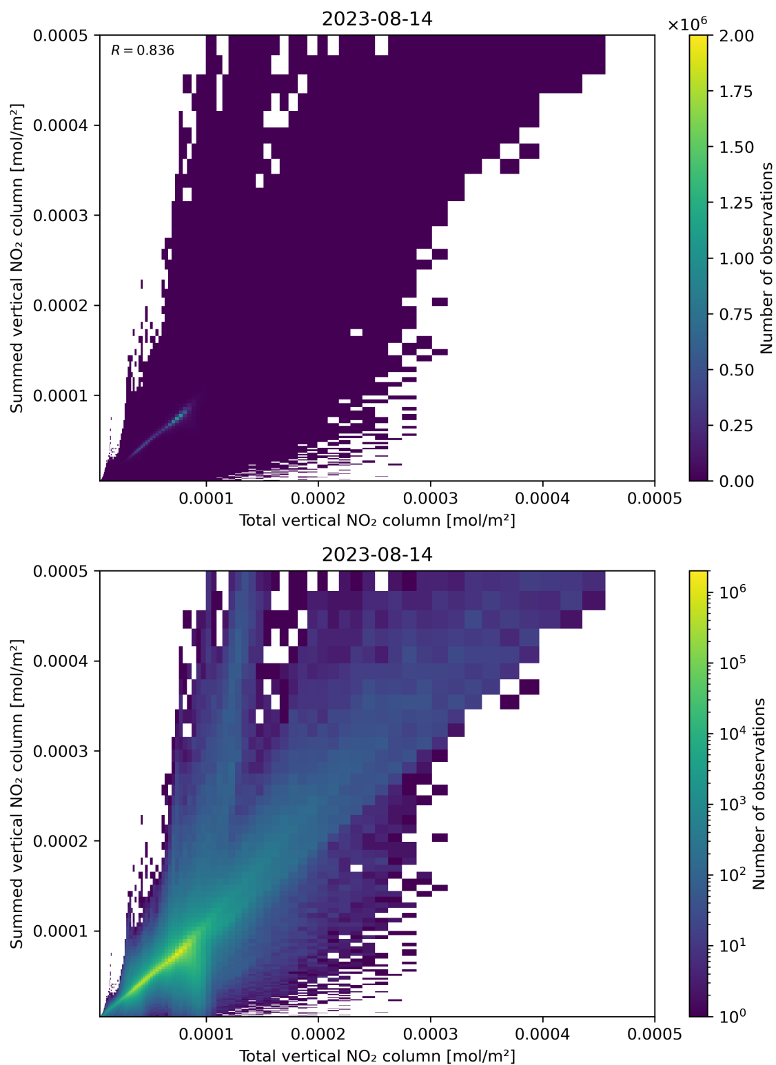
Figure 112: Scatter density plot of “Total vertical NO 2 column” against “Summed vertical NO 2 column” for 2023-08-14 to 2023-08-15.
