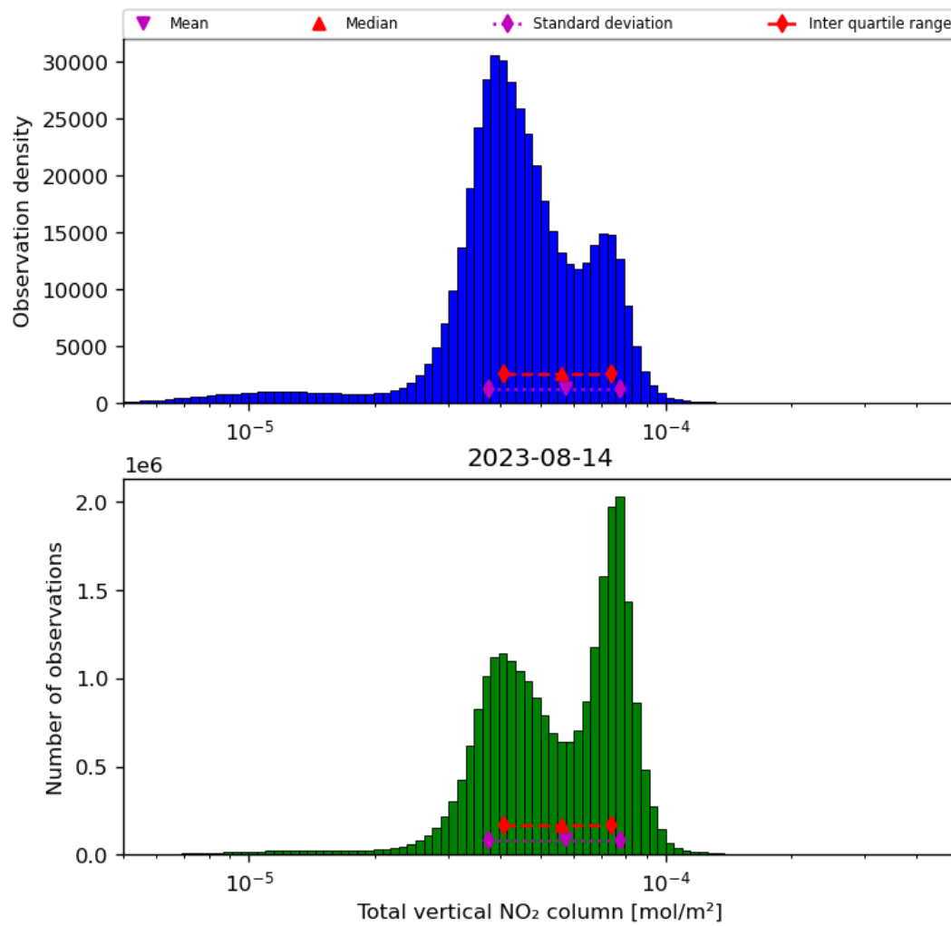
Figure 38: Histogram of “Total vertical NO 2 column” for 2023-08-14 to 2023-08-15
