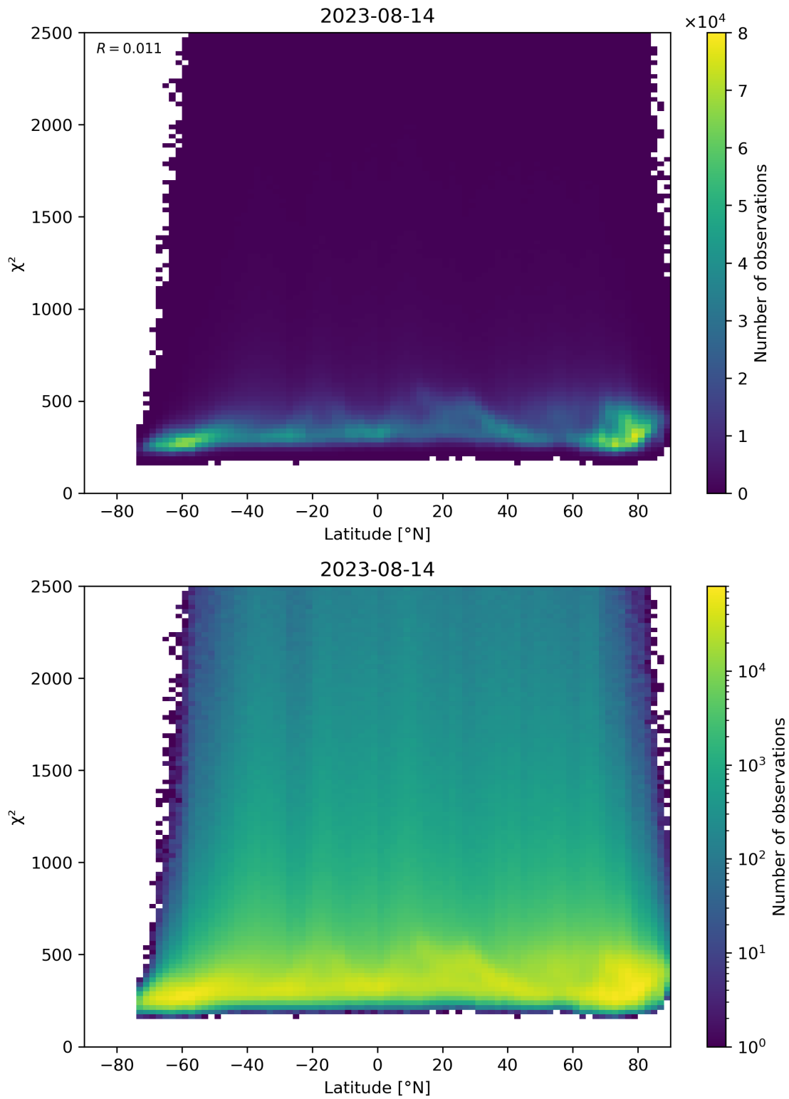
Figure 86: Scatter density plot of “Latitude” against “ \chi^2 ” for 2023-08-14 to 2023-08-15.
