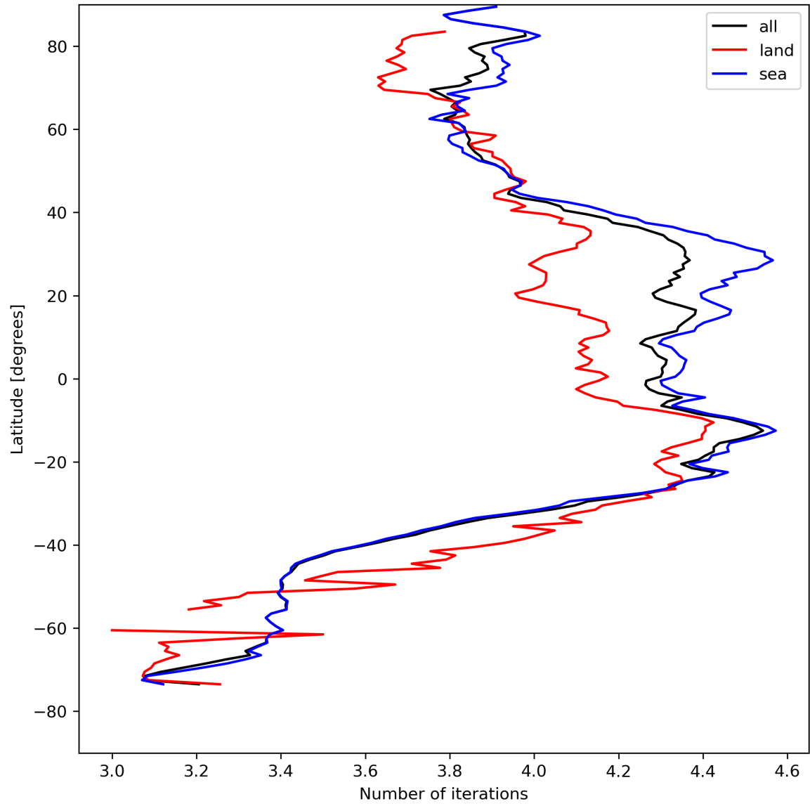
Figure 17: Zonal average of “Number of iterations” for 2023-08-14 to 2023-08-15.
