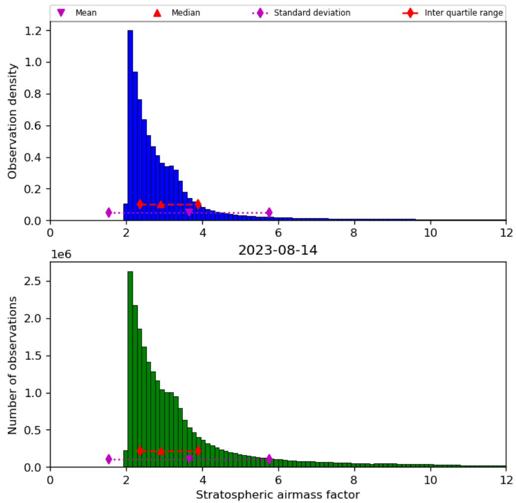
Figure 44: Histogram of “Stratospheric airmass factor” for 2023-08-14 to 2023-08-15
