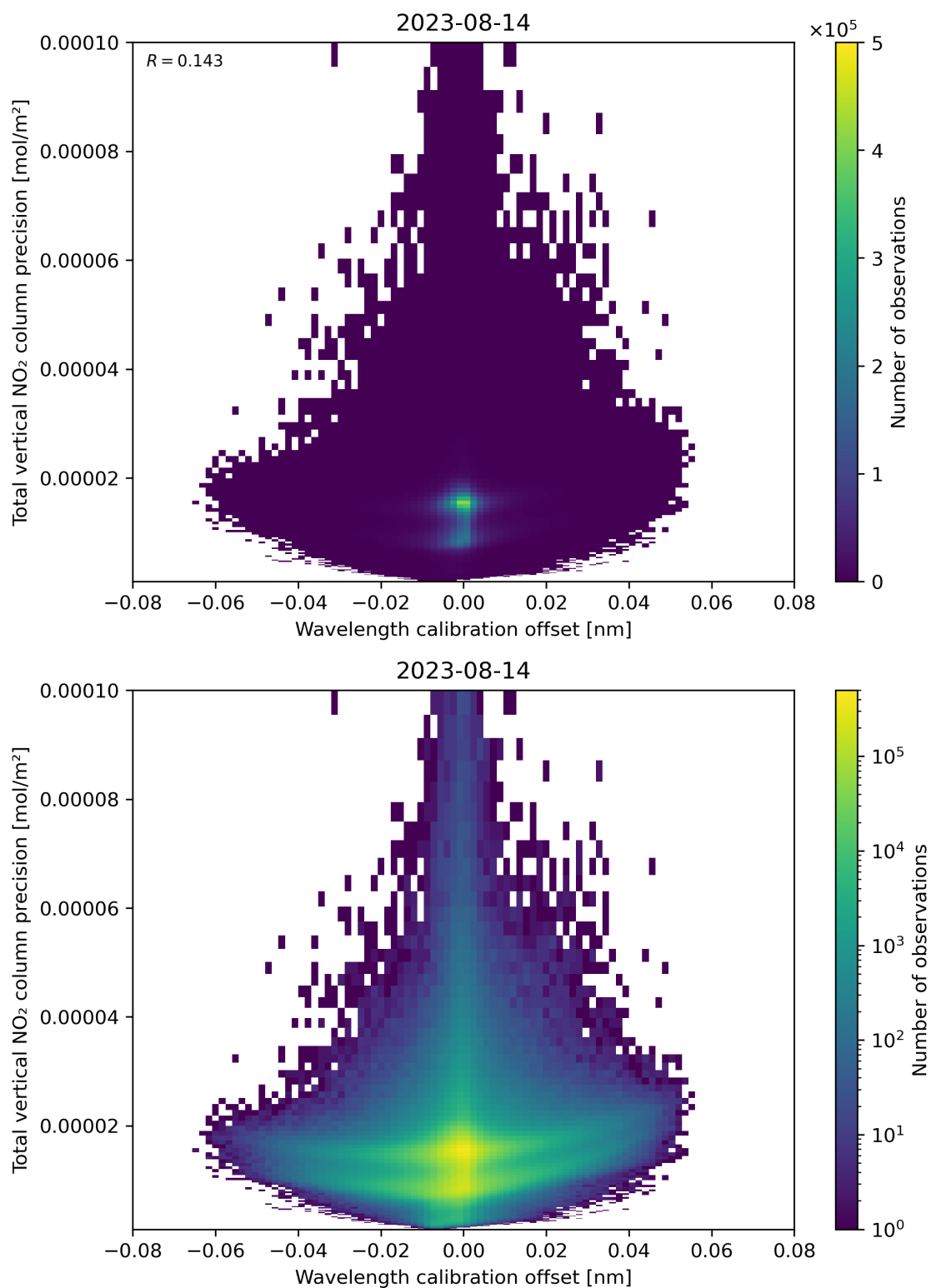
Figure 180: Scatter density plot of “Wavelength calibration offset” against “Total vertical NO 2 column precision” for 2023-08-14 to 2023-08-15.
