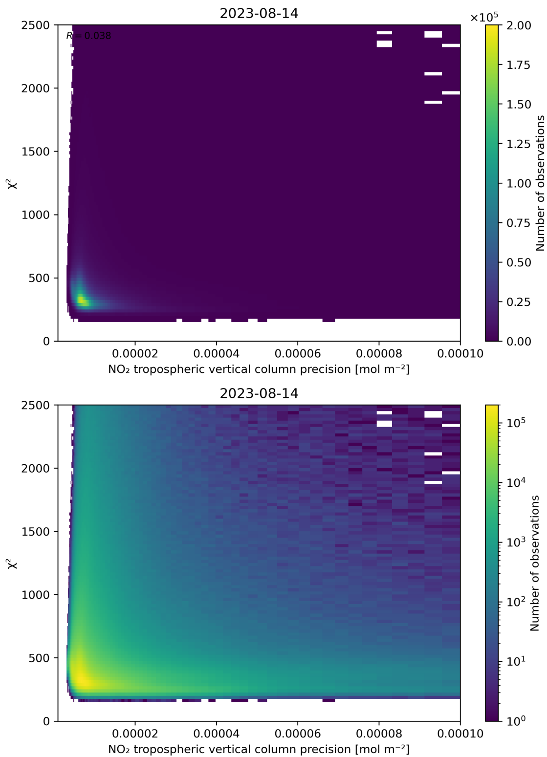
Figure 134: Scatter density plot of “NO 2 tropospheric vertical column precision” against “ \chi^2 ” for 2023-08-14 to 2023-08-15.
