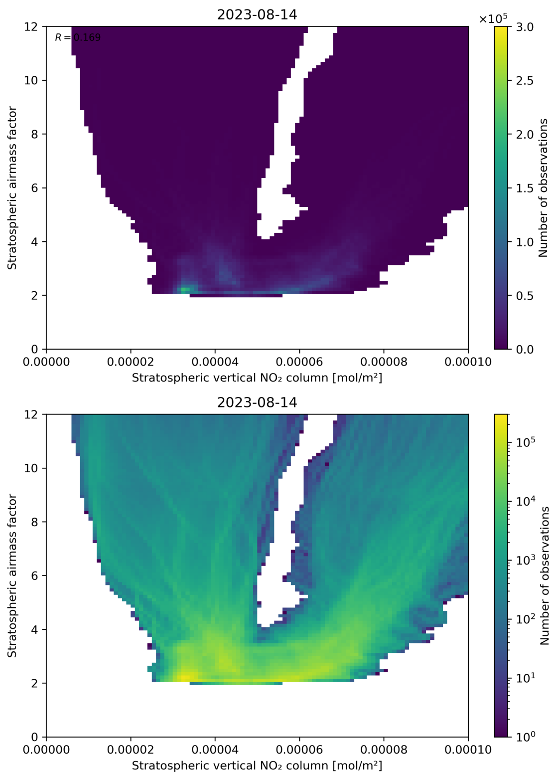
Figure 96: Scatter density plot of “Stratospheric vertical NO 2 column” against “Stratospheric airmass factor” for 2023-08-14 to 2023-08-15.
