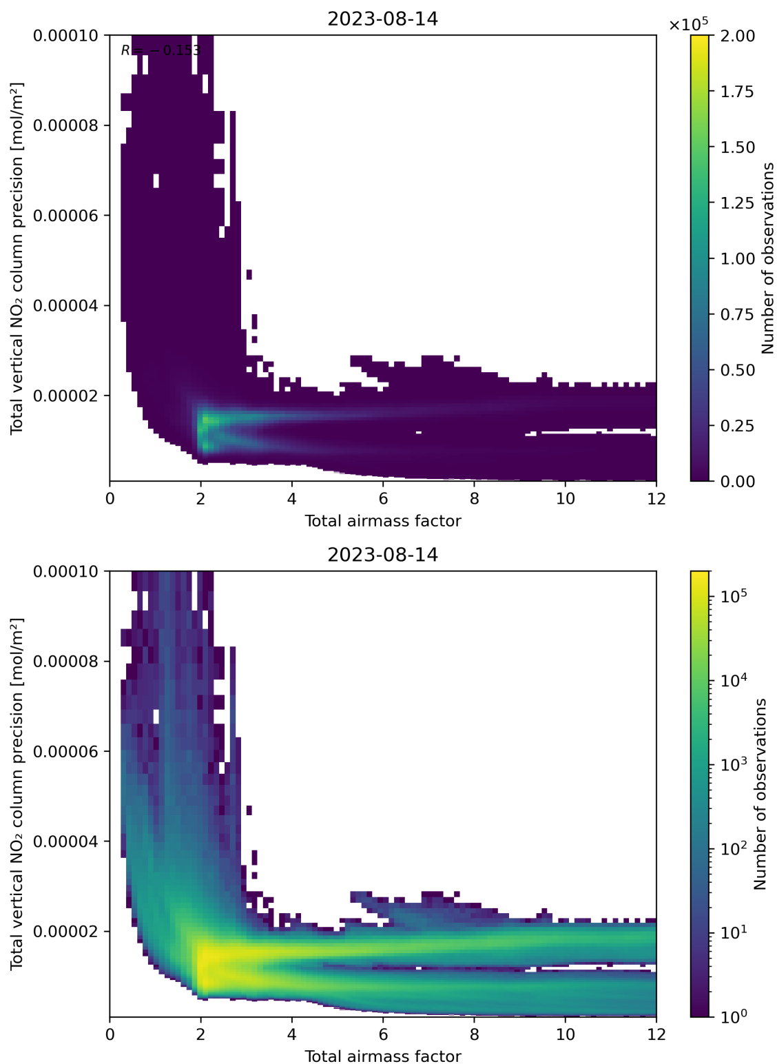
Figure 68: Scatter density plot of “Total airmass factor” against “Total vertical NO 2 column precision” for 2023-08-14 to 2023-08-15.
