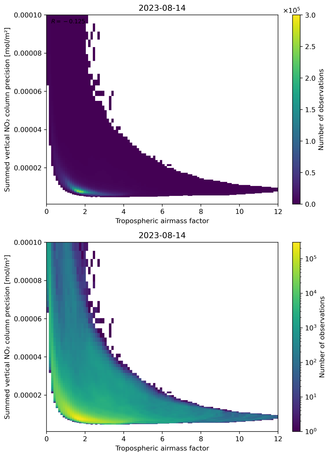
Figure 76: Scatter density plot of “Tropospheric air mass factor” against “Summed vertical NO 2 column precision” for 2023-08-14 to 2023-08-15.
