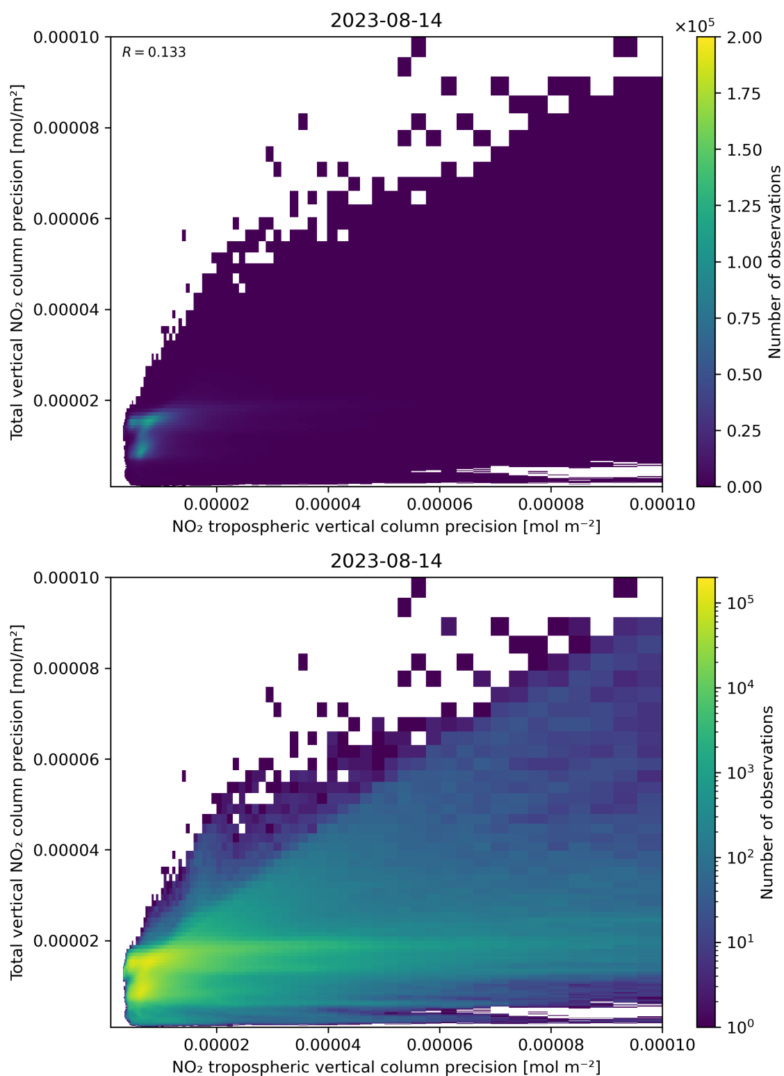
Figure 139: Scatter density plot of “NO 2 tropospheric vertical column precision” against “Total vertical NO 2 column precision” for 2023-08-14 to 2023-08-15.
