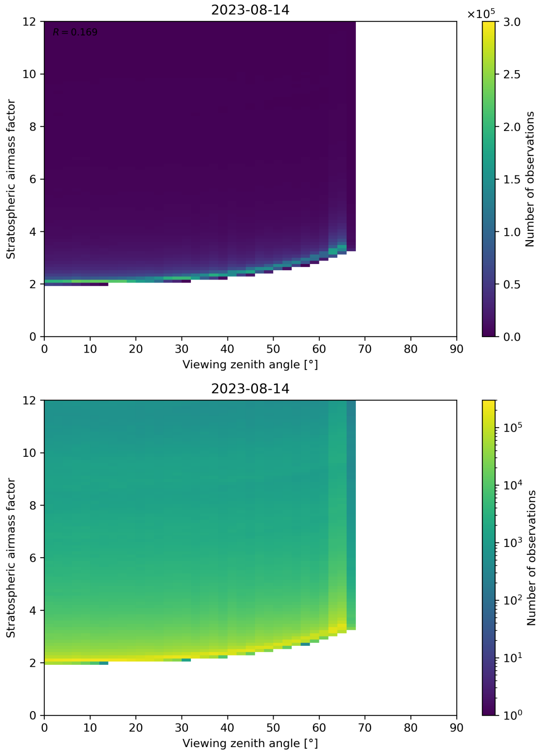
Figure 159: Scatter density plot of “Viewing zenith angle” against “Stratospheric airmass factor” for 2023-08-14 to 2023-08-15.
