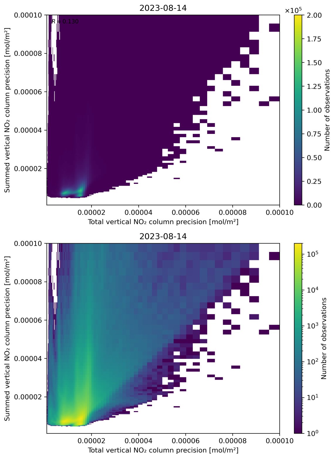
Figure 118: Scatter density plot of “Total vertical NO 2 column precision” against “Summed vertical NO 2 column precision” for 2023-08-14 to 2023-08-15.
