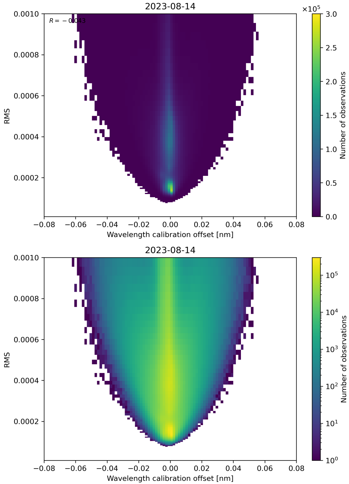
Figure 181: Scatter density plot of “Wavelength calibration offset” against “RMS” for 2023-08-14 to 2023-08-15.
