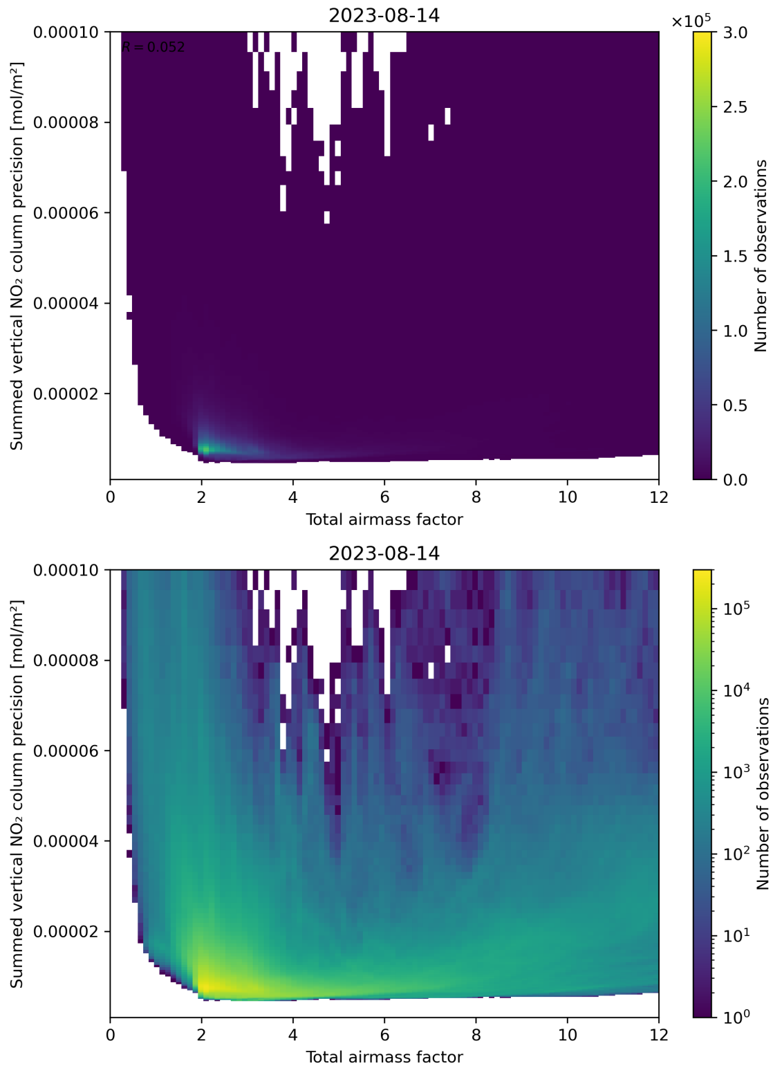
Figure 66: Scatter density plot of “Total airmass factor” against “Summed vertical NO 2 column precision” for 2023-08-14 to 2023-08-15.
