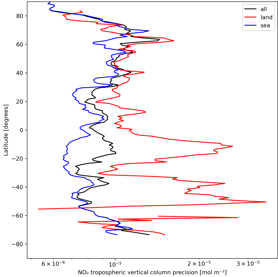
Figure 13: Zonal average of “NO 2 tropospheric vertical column precision” for 2023-08-14 to 2023-08-15.
