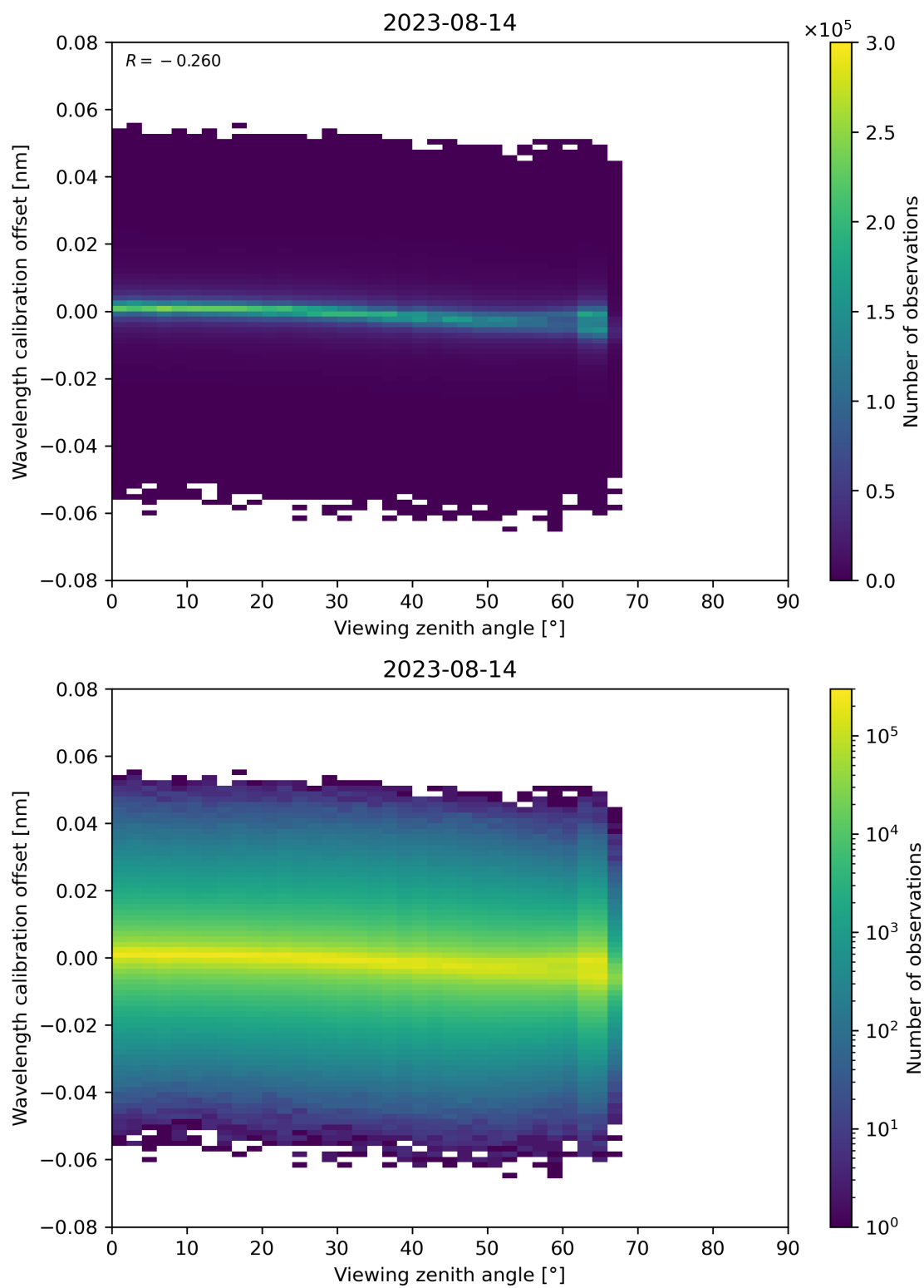
Figure 173: Scatter density plot of “Viewing zenith angle” against “Wavelength calibration offset” for 2023-08-14 to 2023-08-15.
