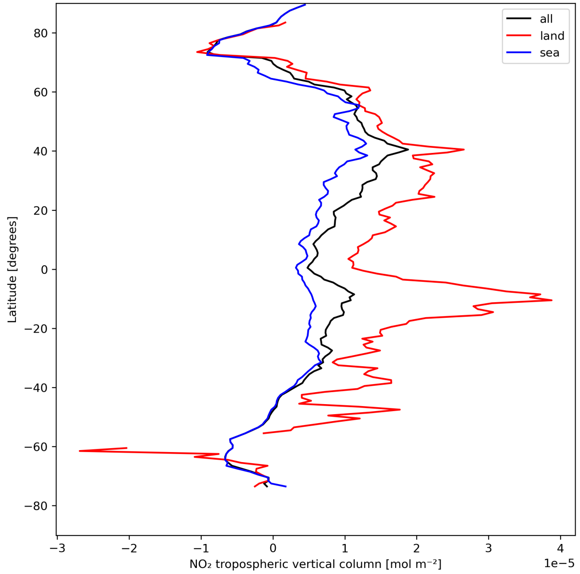
Figure 12: Zonal average of “NO 2 tropospheric vertical column” for 2023-08-14 to 2023-08-15.
