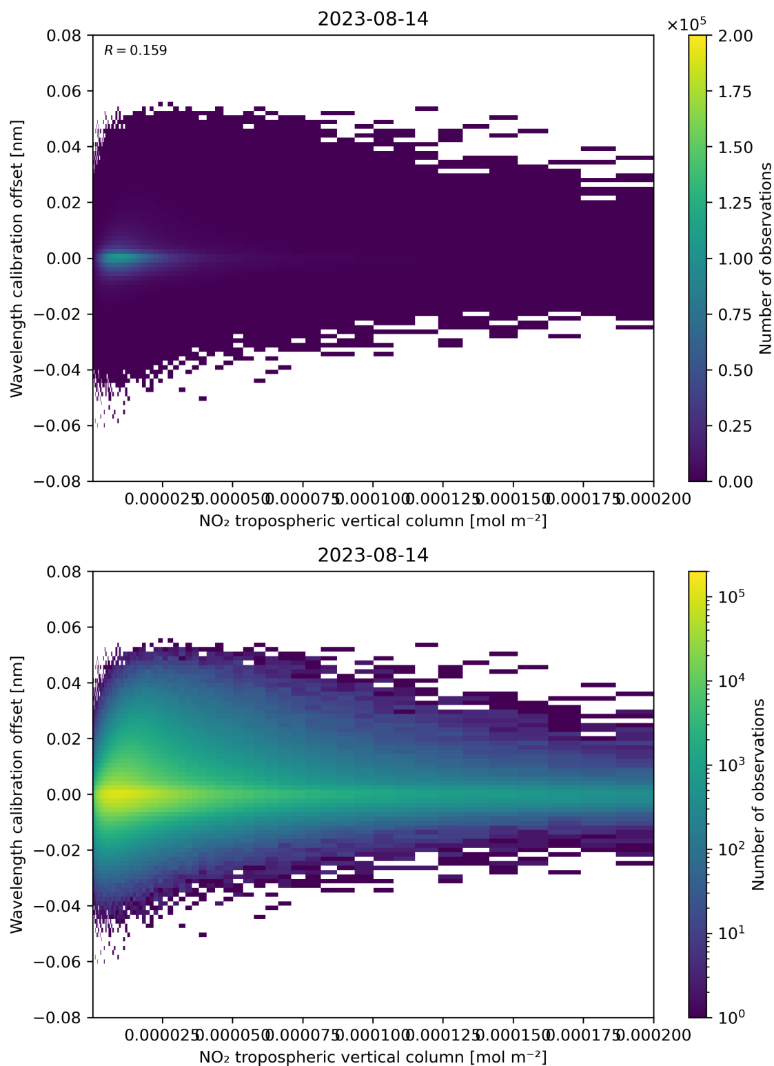
Figure 143: Scatter density plot of “NO 2 tropospheric vertical column” against “Wavelength calibration offset” for 2023-08-14 to 2023-08-15.
