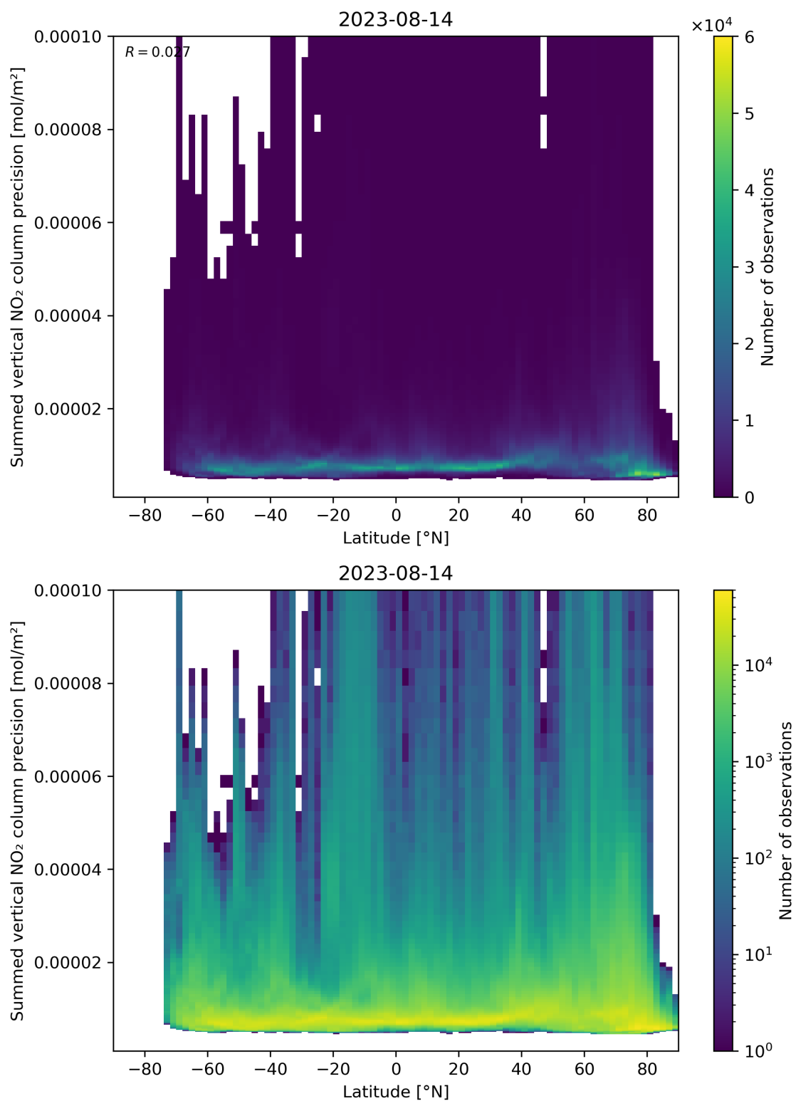
Figure 89: Scatter density plot of “Latitude” against “Summed vertical NO 2 column precision” for 2023-08-14 to 2023-08-15.
