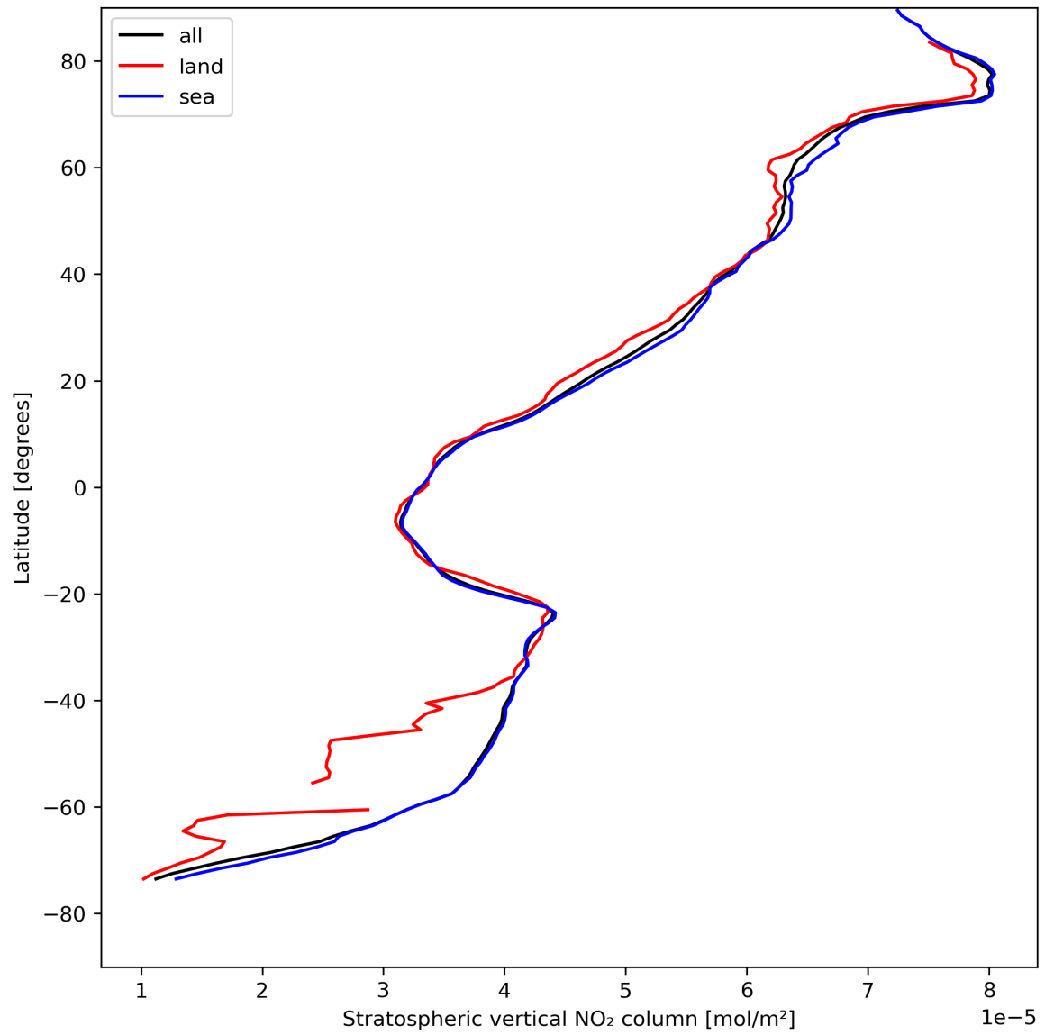
Figure 19: Zonal average of “Stratospheric vertical NO 2 column” for 2023-08-14 to 2023-08-15.
