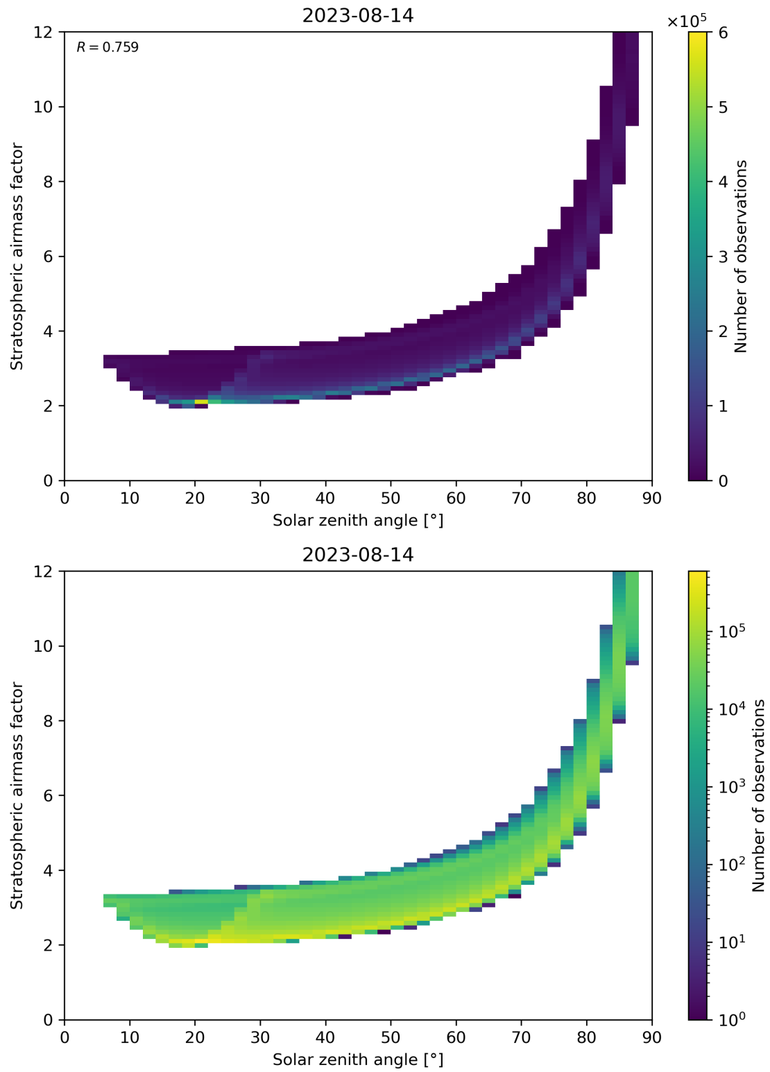
Figure 145: Scatter density plot of “Solar zenith angle” against “Stratospheric airmass factor” for 2023-08-14 to 2023-08-15.
