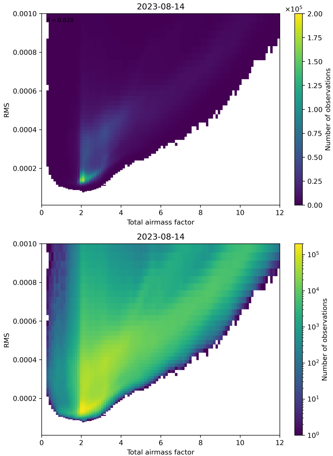
Figure 69: Scatter density plot of “Total airmass factor” against “RMS” for 2023-08-14 to 2023-08-15.
