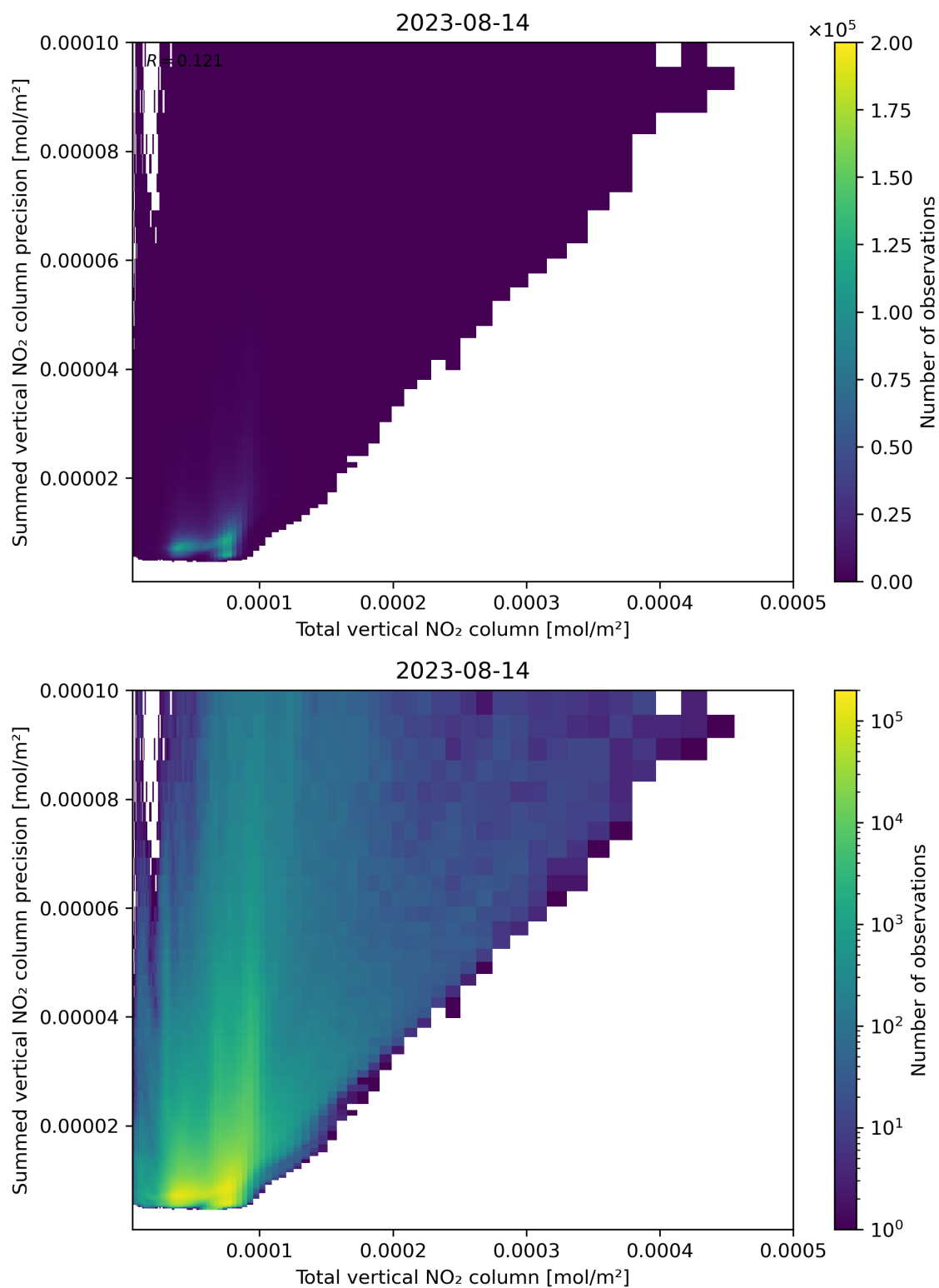
Figure 113: Scatter density plot of “Total vertical NO 2 column” against “Summed vertical NO 2 column precision” for 2023-08-14 to 2023-08-15.
