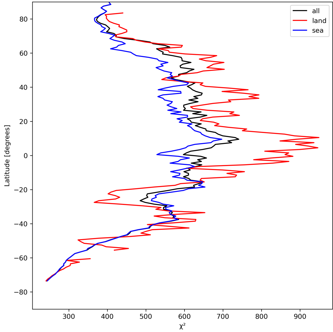
Figure 25: Zonal average of “ \chi^2 ” for 2023-08-14 to 2023-08-15.
