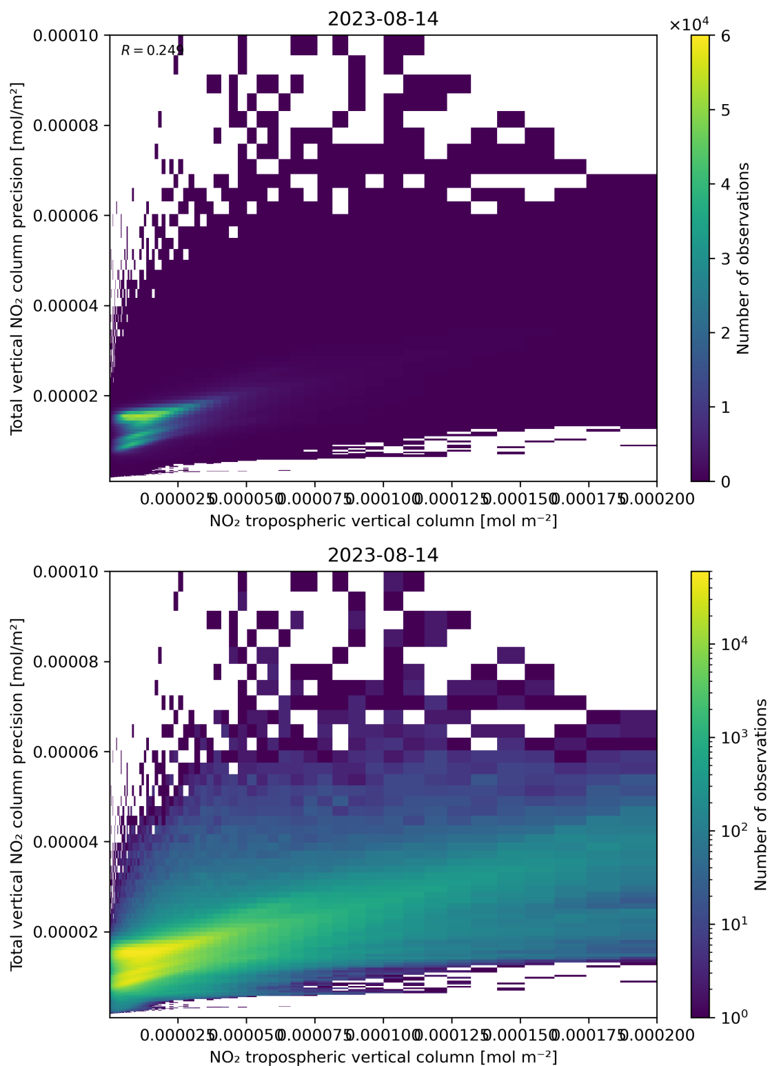
Figure 129: Scatter density plot of “NO 2 tropospheric vertical column” against “Total vertical NO 2 column precision” for 2023-08-14 to 2023-08-15.
