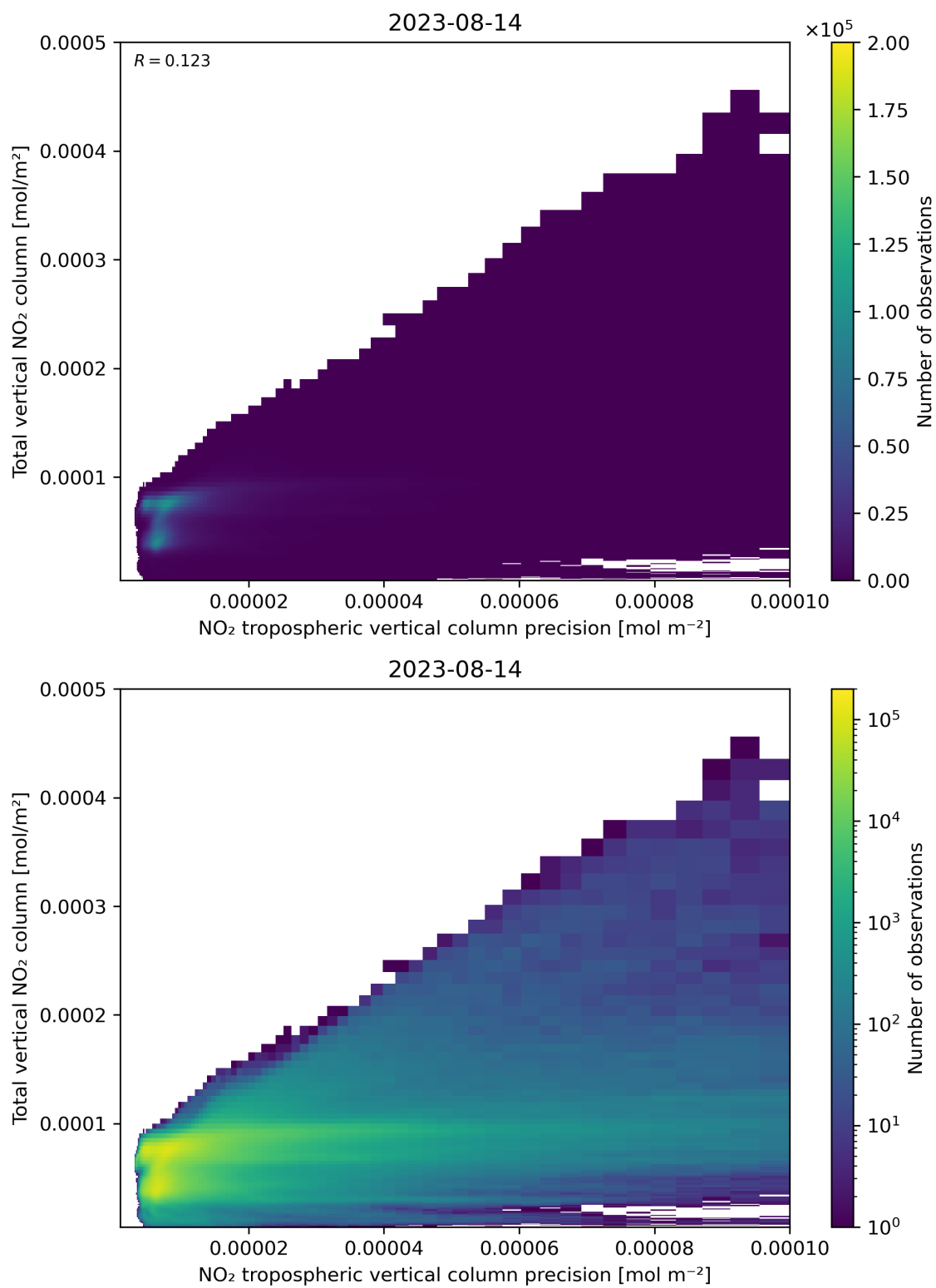
Figure 138: Scatter density plot of “NO 2 tropospheric vertical column precision” against “Total vertical NO 2 column” for 2023-08-14 to 2023-08-15.
