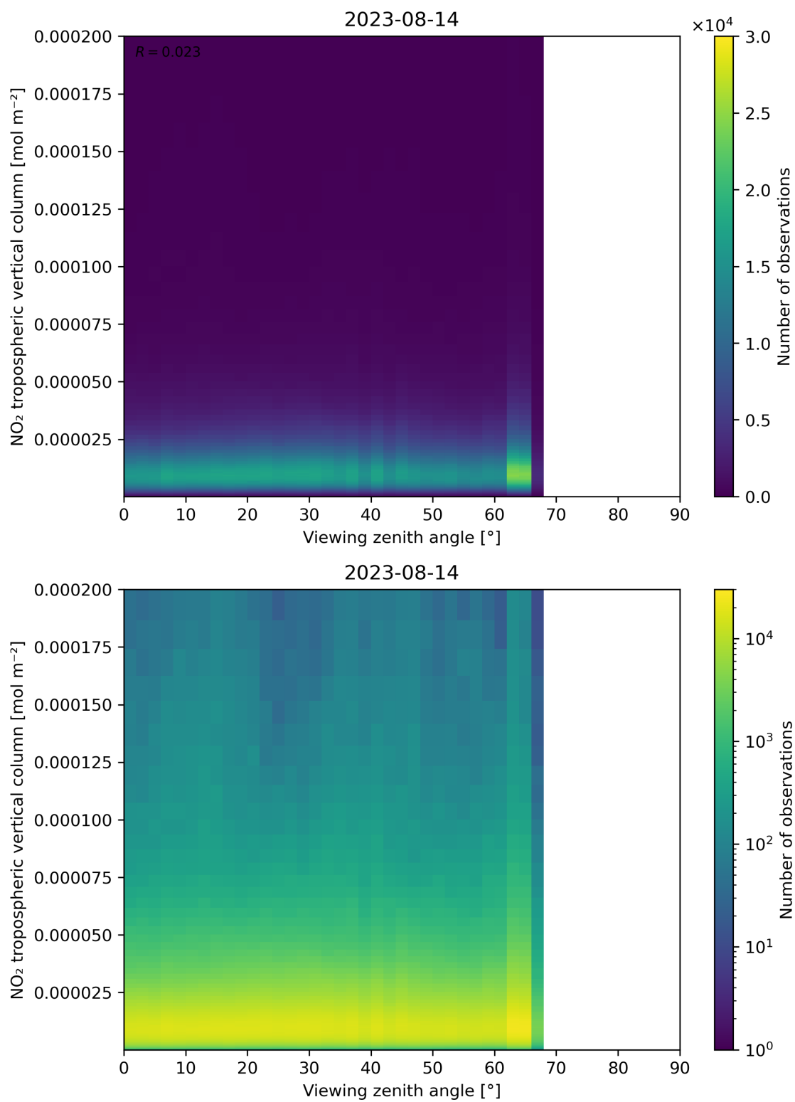
Figure 169: Scatter density plot of “Viewing zenith angle” against “NO 2 tropospheric vertical column” for 2023-08-14 to 2023-08-15.
