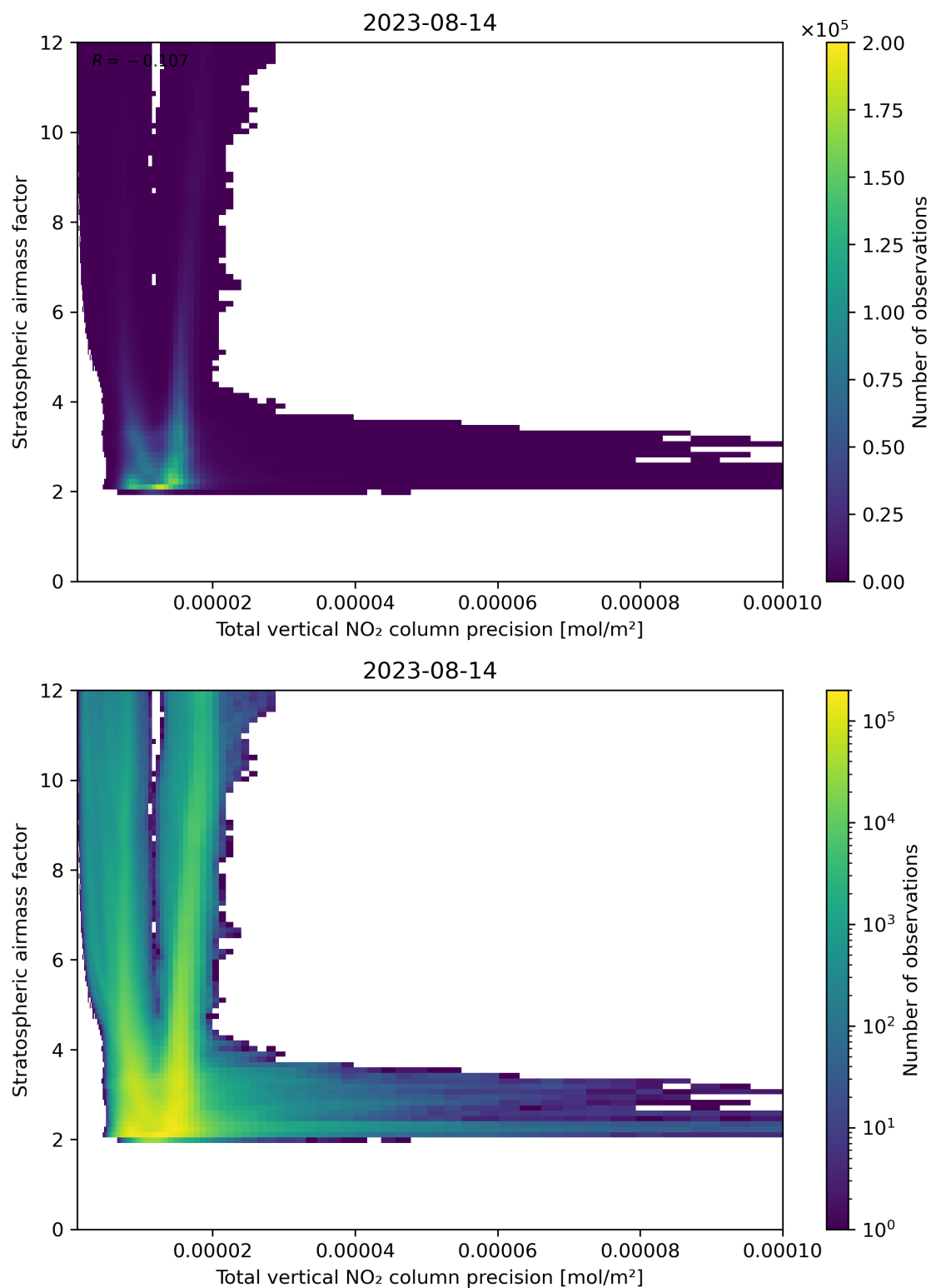
Figure 115: Scatter density plot of “Total vertical NO 2 column precision” against “Stratospheric air mass factor” for 2023-08-14 to 2023-08-15.
