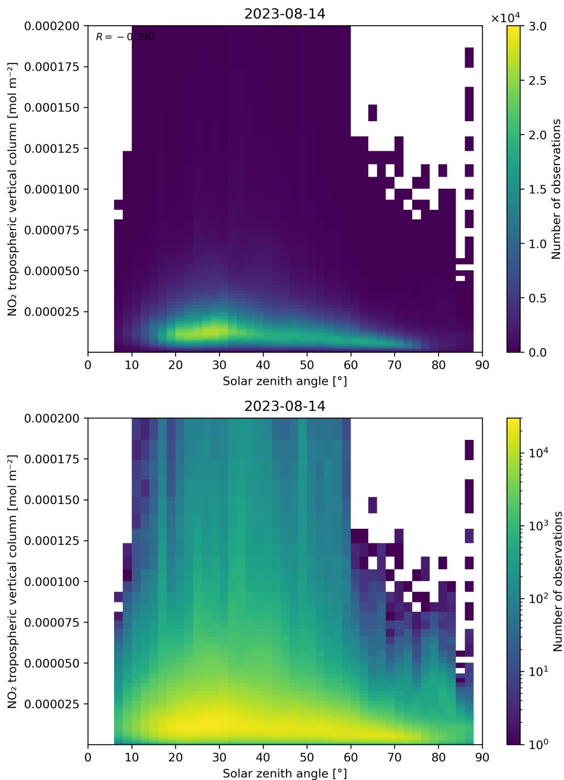
Figure 155: Scatter density plot of “Solar zenith angle” against “NO 2 tropospheric vertical column” for 2023-08-14 to 2023-08-15.
