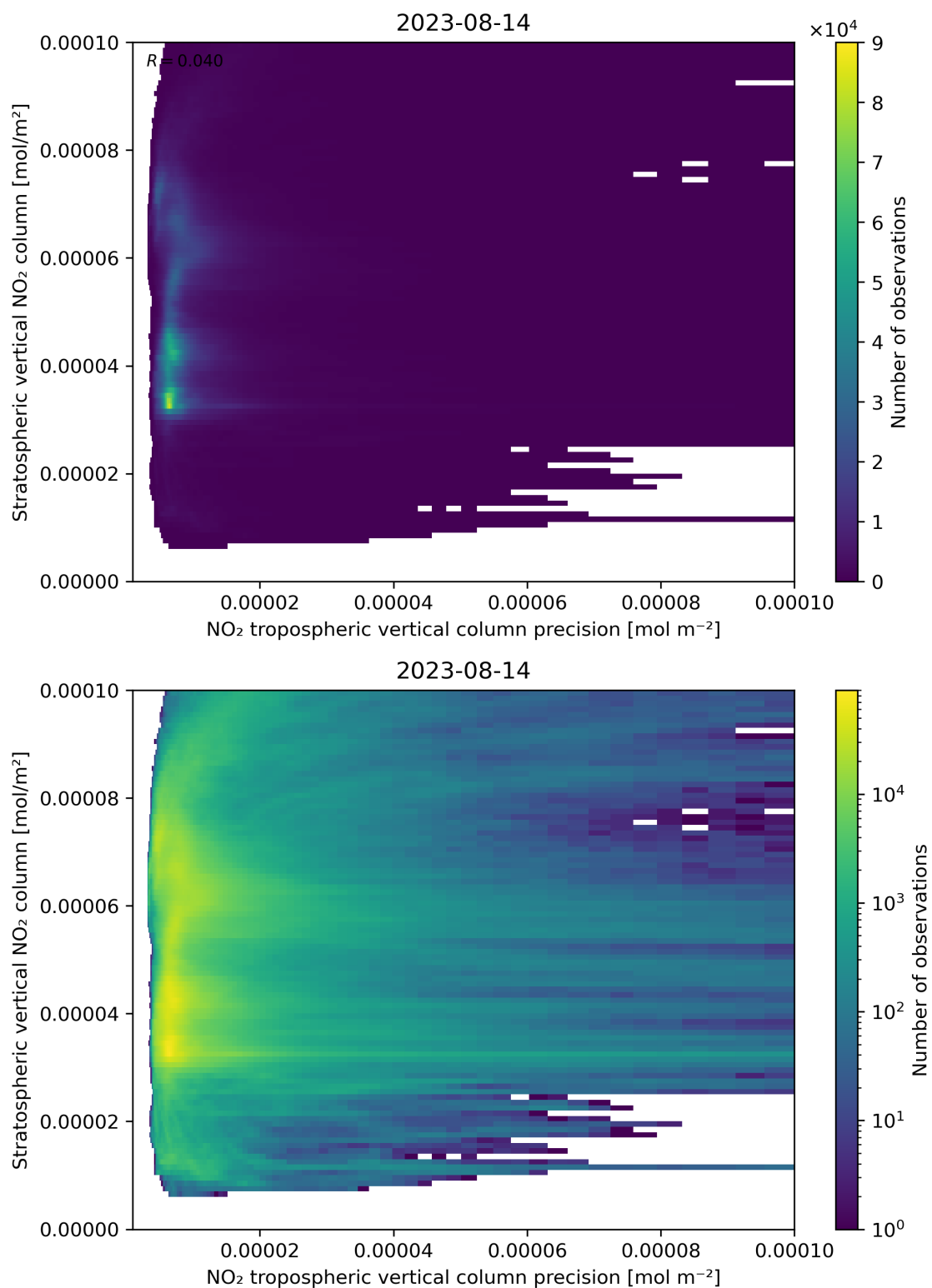
Figure 135: Scatter density plot of “NO 2 tropospheric vertical column precision” against “Stratospheric vertical NO 2 column” for 2023-08-14 to 2023-08-15.
