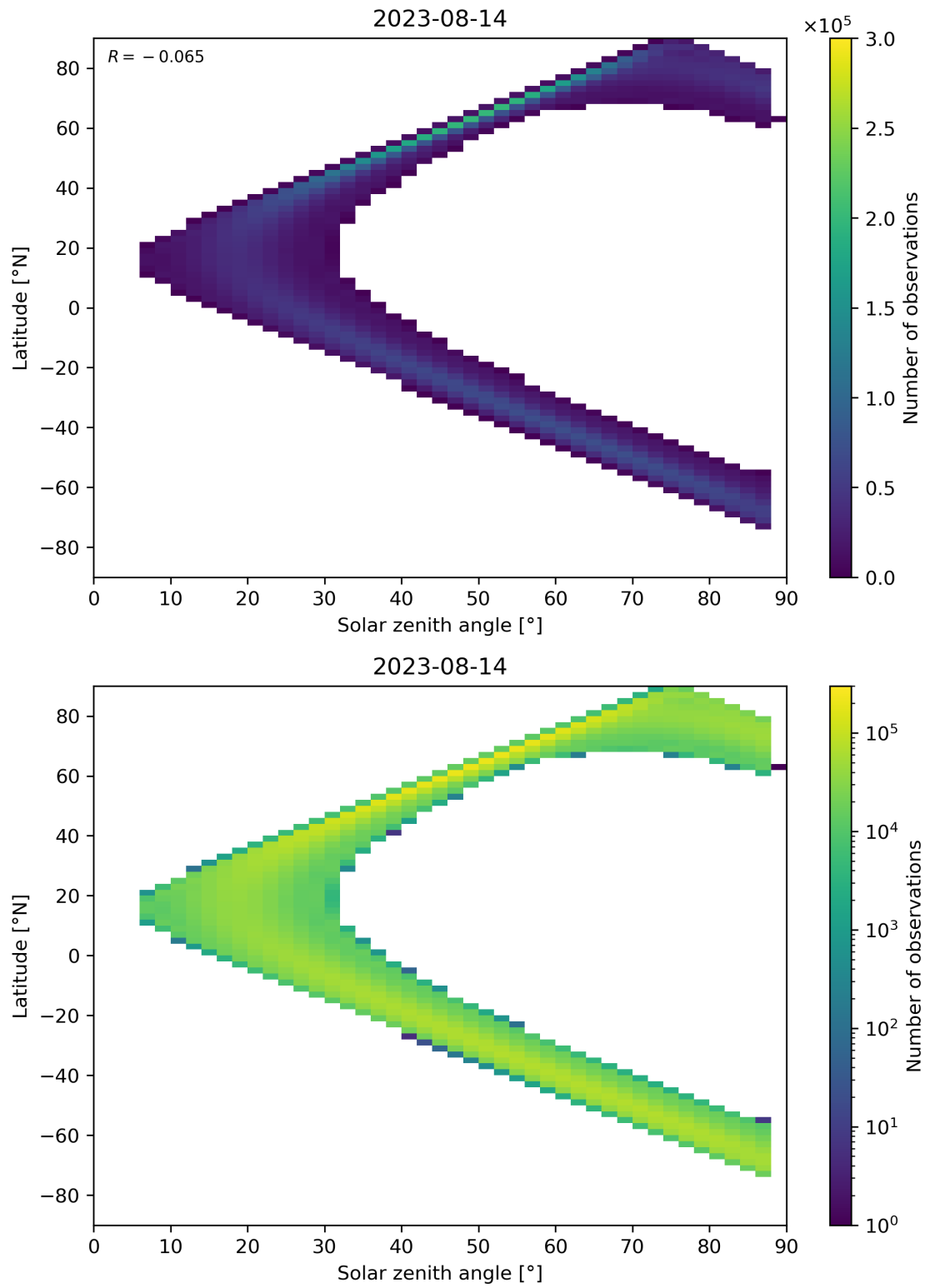
Figure 149: Scatter density plot of “Solar zenith angle” against “Latitude” for 2023-08-14 to 2023-08-15.
