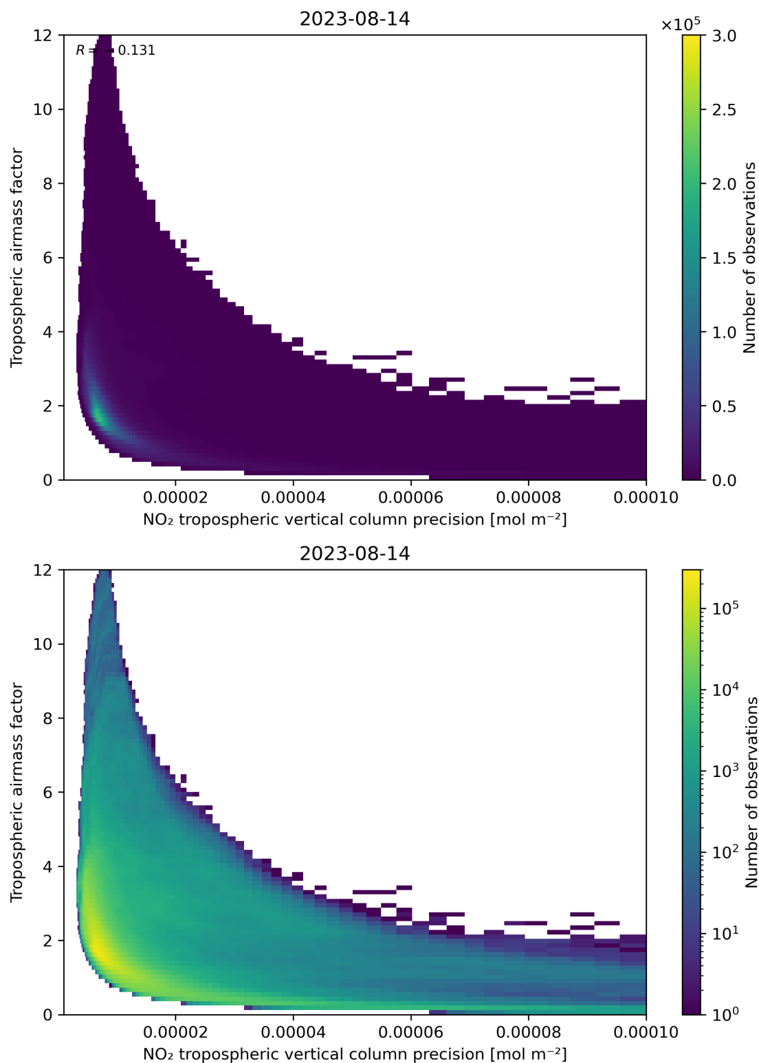
Figure 133: Scatter density plot of “NO 2 tropospheric vertical column precision” against “Tropospheric airmass factor” for 2023-08-14 to 2023-08-15.
