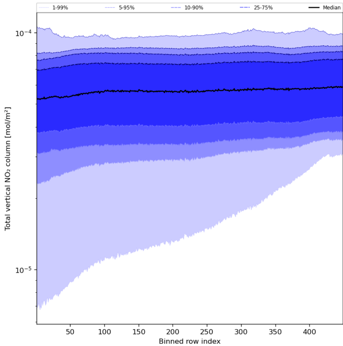
Figure 55: Along track statistics of “Total vertical NO 2 column” for 2023-08-14 to 2023-08-15
