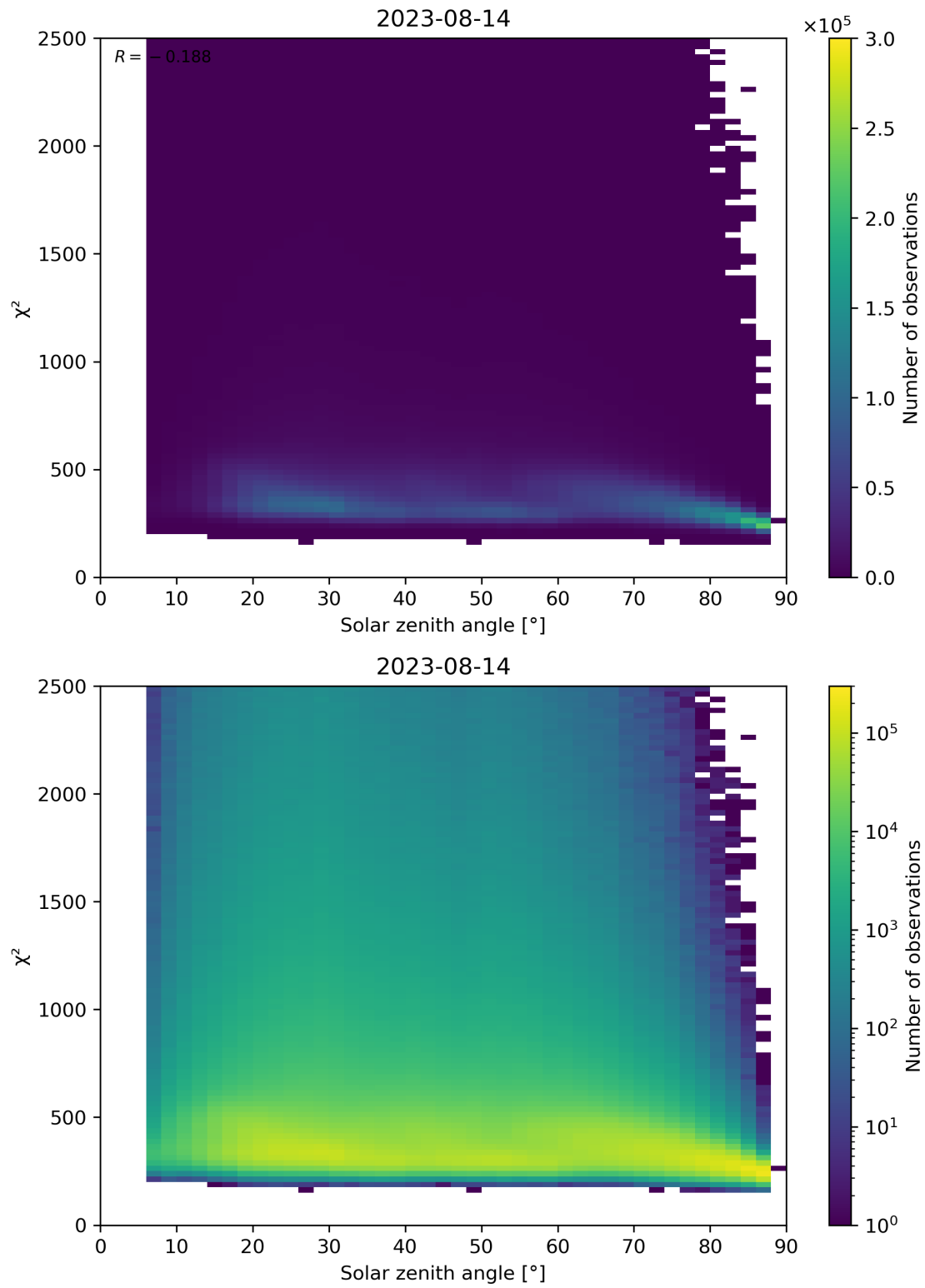
Figure 148: Scatter density plot of “Solar zenith angle” against “ \chi^2 ” for 2023-08-14 to 2023-08-15.
