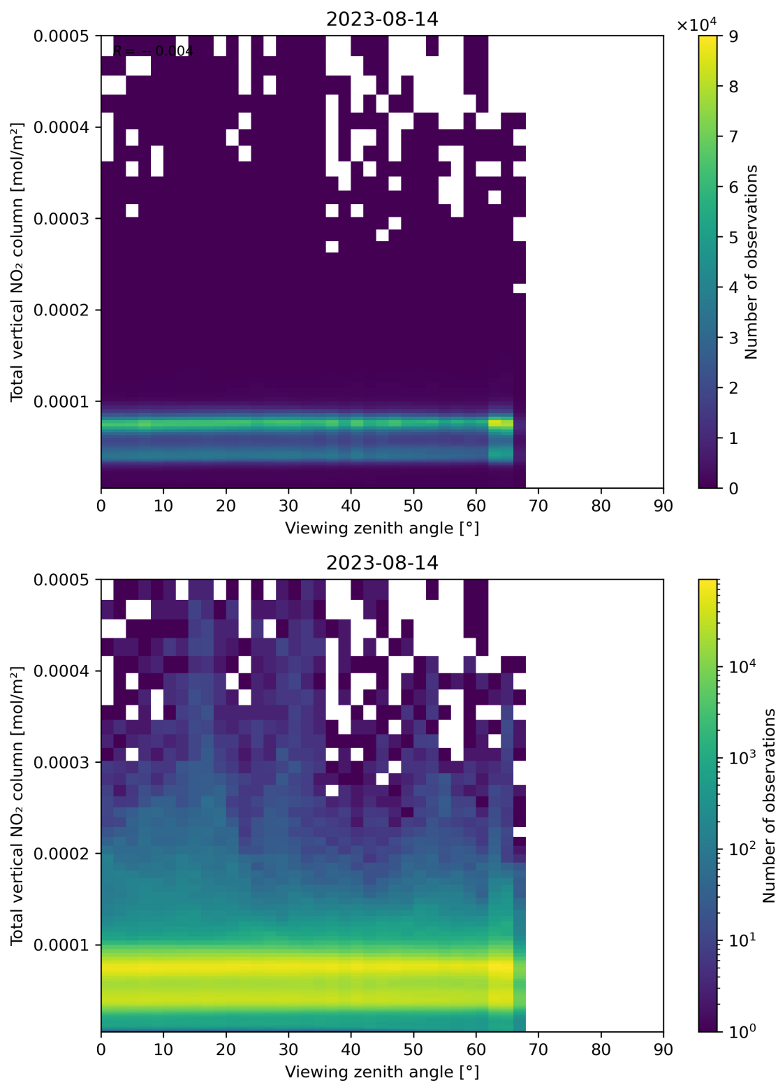
Figure 167: Scatter density plot of “Viewing zenith angle” against “Total vertical NO 2 column” for 2023-08-14 to 2023-08-15.
