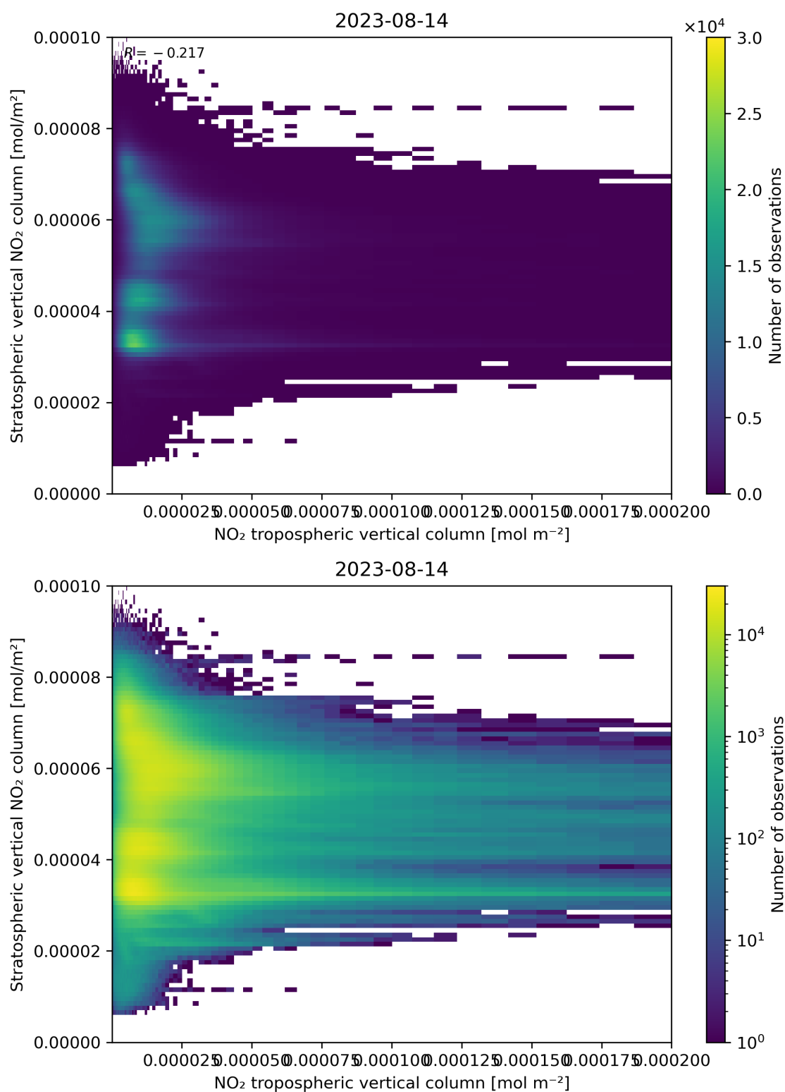
Figure 125: Scatter density plot of “NO 2 tropospheric vertical column” against “Stratospheric vertical NO 2 column” for 2023-08-14 to 2023-08-15.
