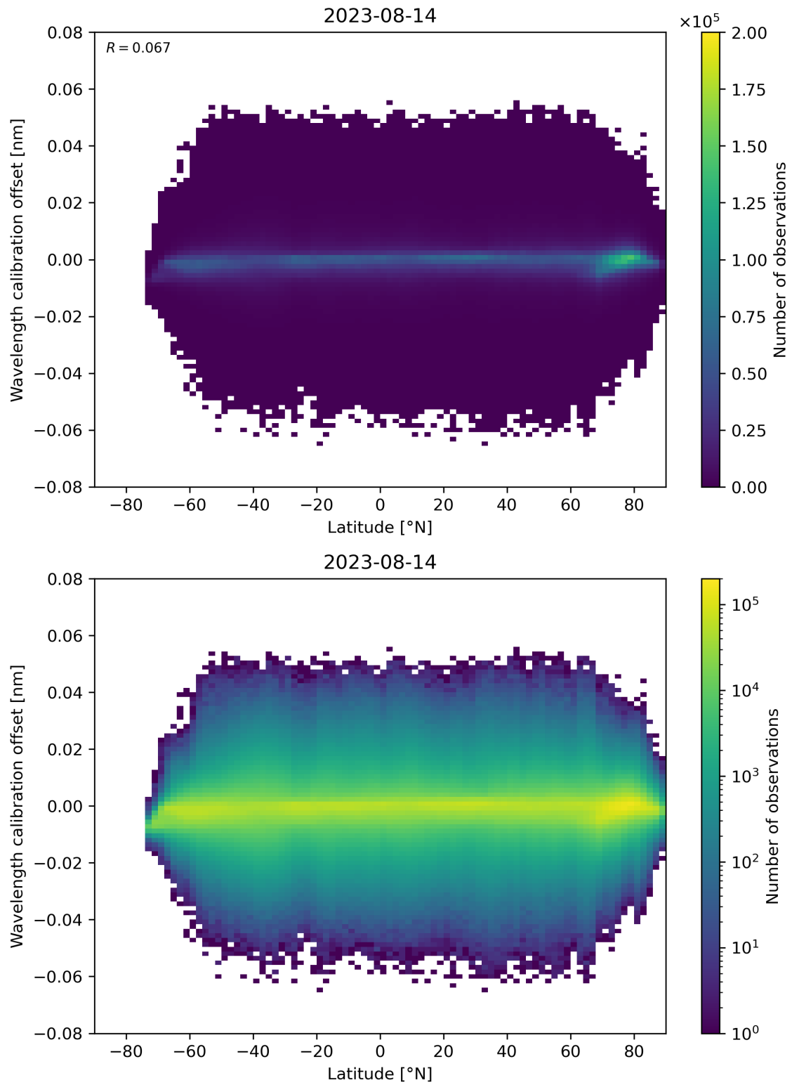
Figure 95: Scatter density plot of “Latitude” against “Wavelength calibration offset” for 2023-08-14 to 2023-08-15.
