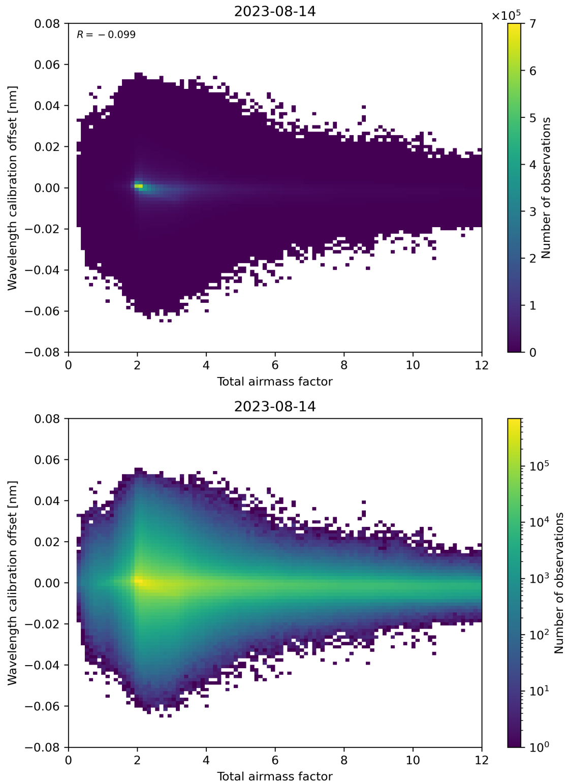
Figure 70: Scatter density plot of “Total airmass factor” against “Wavelength calibration offset” for 2023-08-14 to 2023-08-15.
