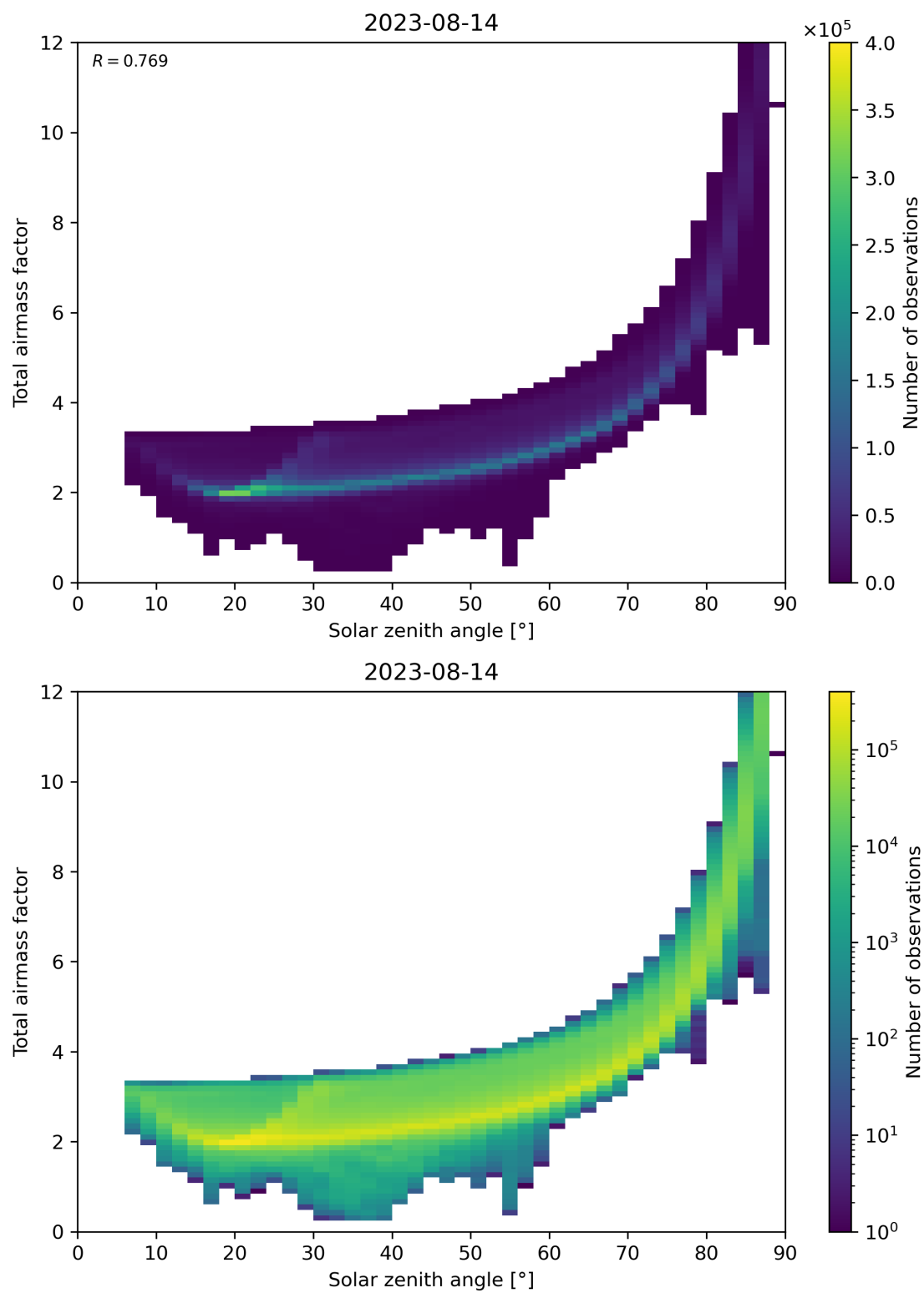
Figure 146: Scatter density plot of “Solar zenith angle” against “Total air mass factor” for 2023-08-14 to 2023-08-15.
