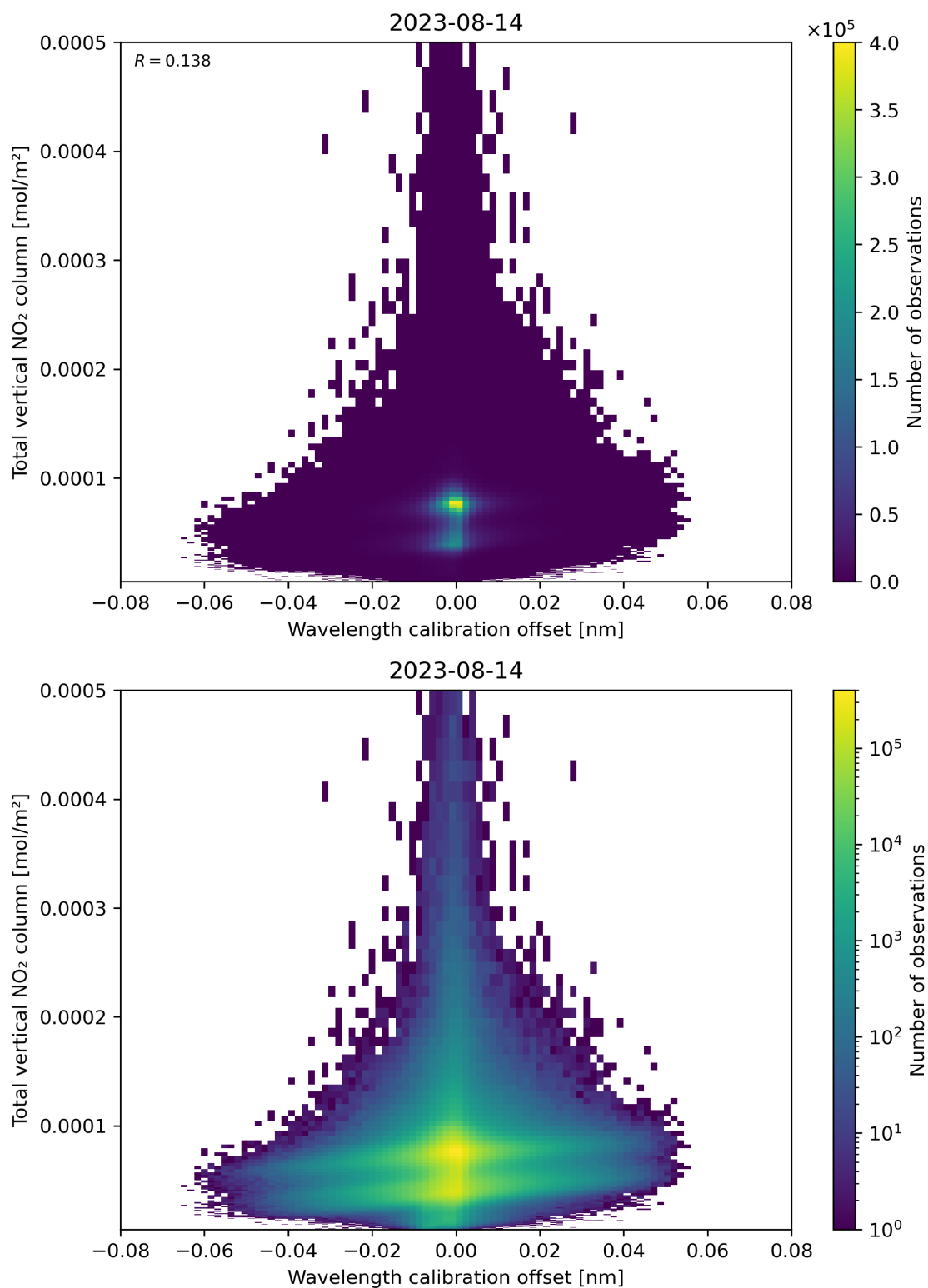
Figure 179: Scatter density plot of “Wavelength calibration offset” against “Total vertical NO 2 column” for 2023-08-14 to 2023-08-15.
