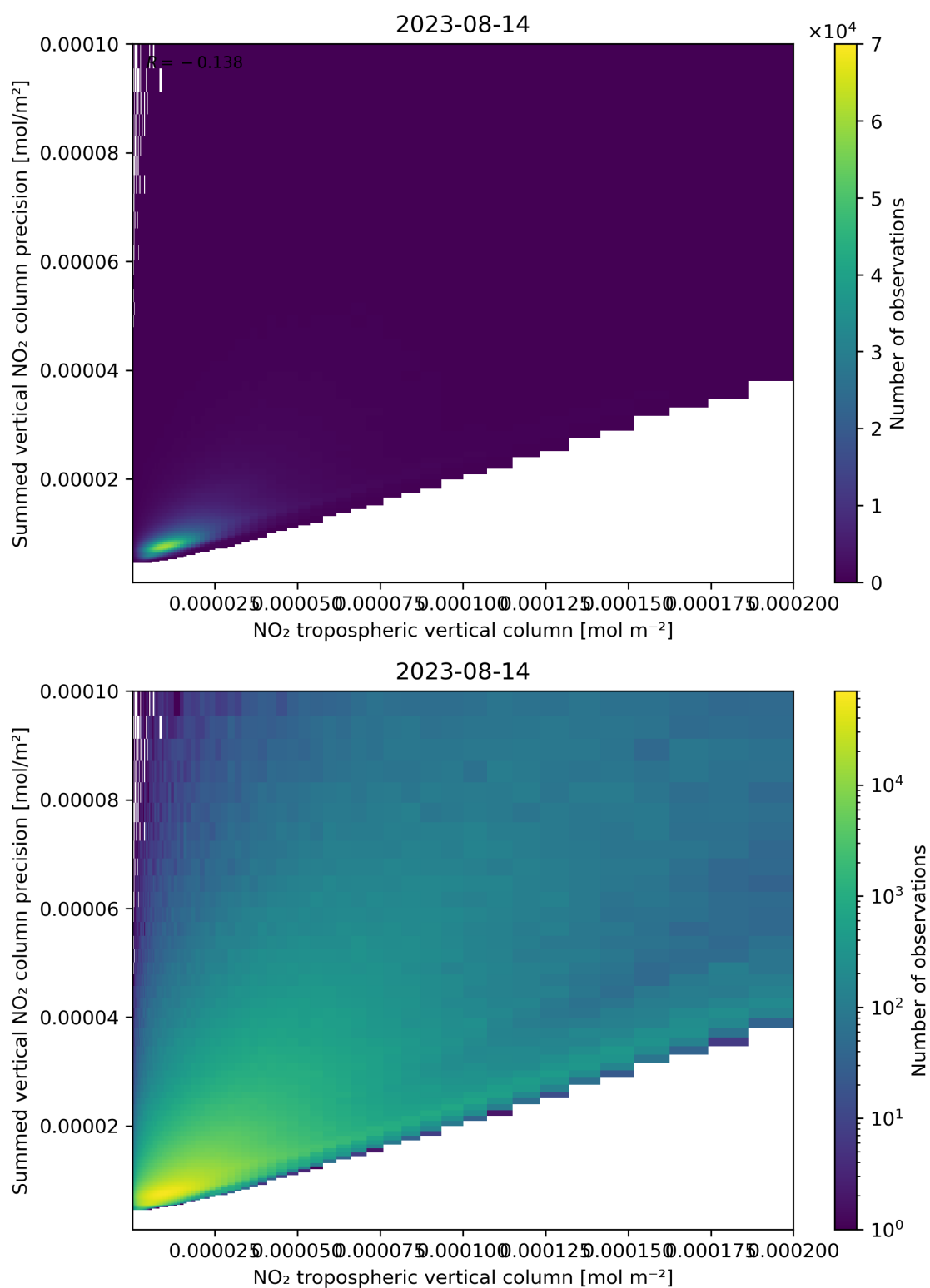
Figure 127: Scatter density plot of “NO 2 tropospheric vertical column” against “Summed vertical NO 2 column precision” for 2023-08-14 to 2023-08-15.
