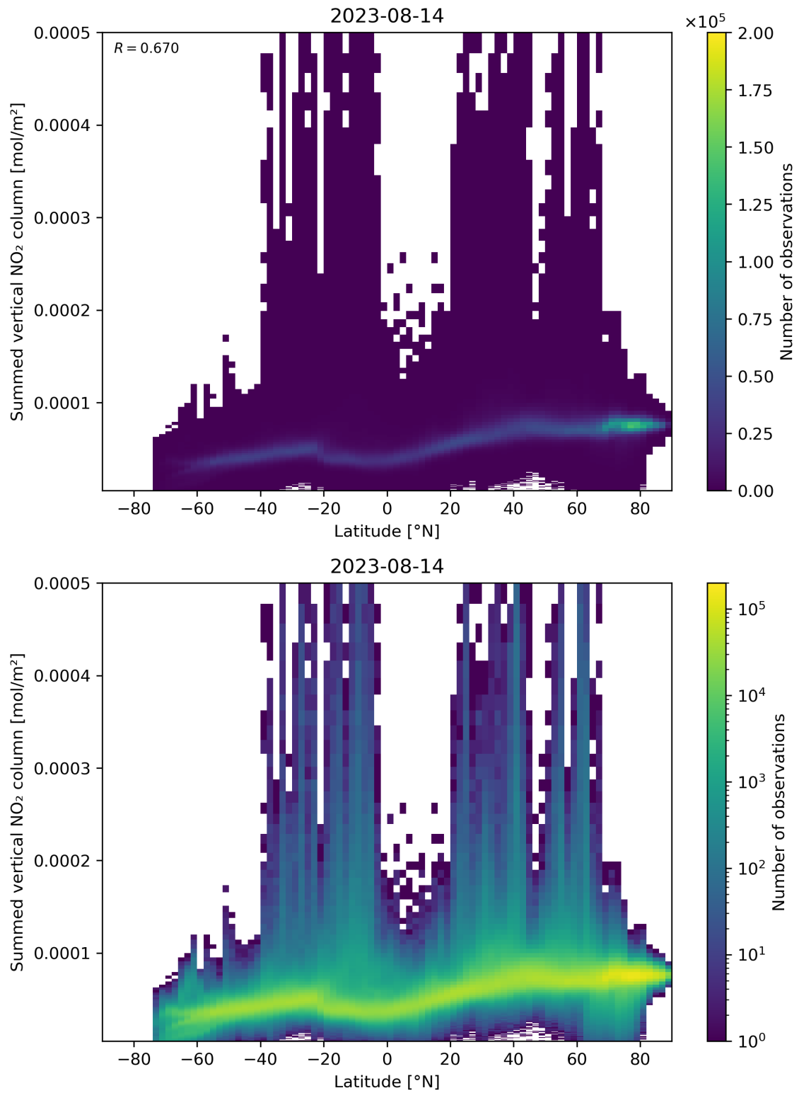
Figure 88: Scatter density plot of “Latitude” against “Summed vertical NO 2 column” for 2023-08-14 to 2023-08-15.
