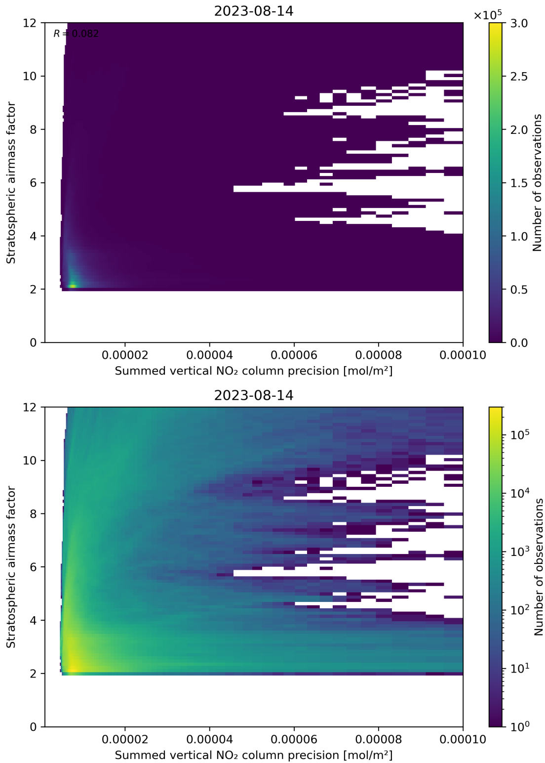
Figure 106: Scatter density plot of “Summed vertical NO 2 column precision” against “Stratospheric airmass factor” for 2023-08-14 to 2023-08-15.
