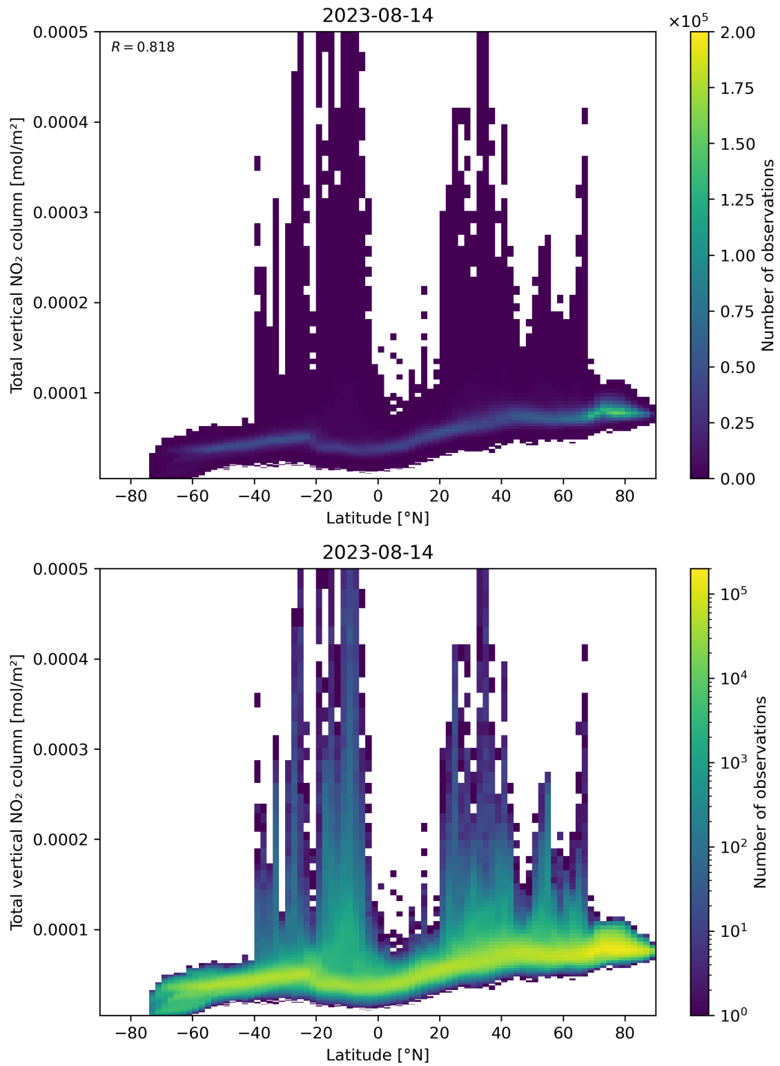
Figure 90: Scatter density plot of “Latitude” against “Total vertical NO 2 column” for 2023-08-14 to 2023-08-15.
