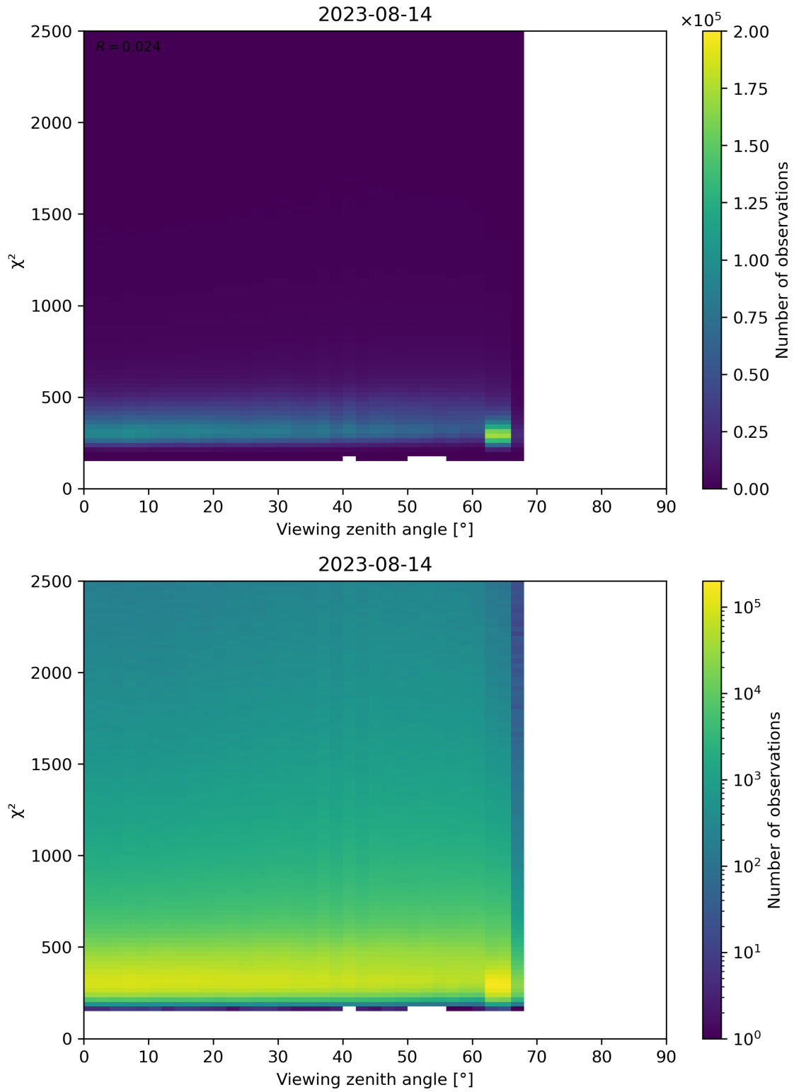
Figure 162: Scatter density plot of “Viewing zenith angle” against “ \chi^2 ” for 2023-08-14 to 2023-08-15.
