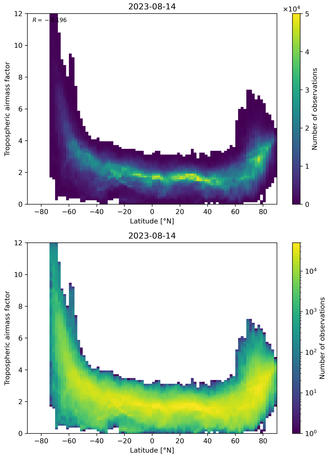
Figure 85: Scatter density plot of “Latitude” against “Tropospheric airmass factor” for 2023-08-14 to 2023-08-15.
