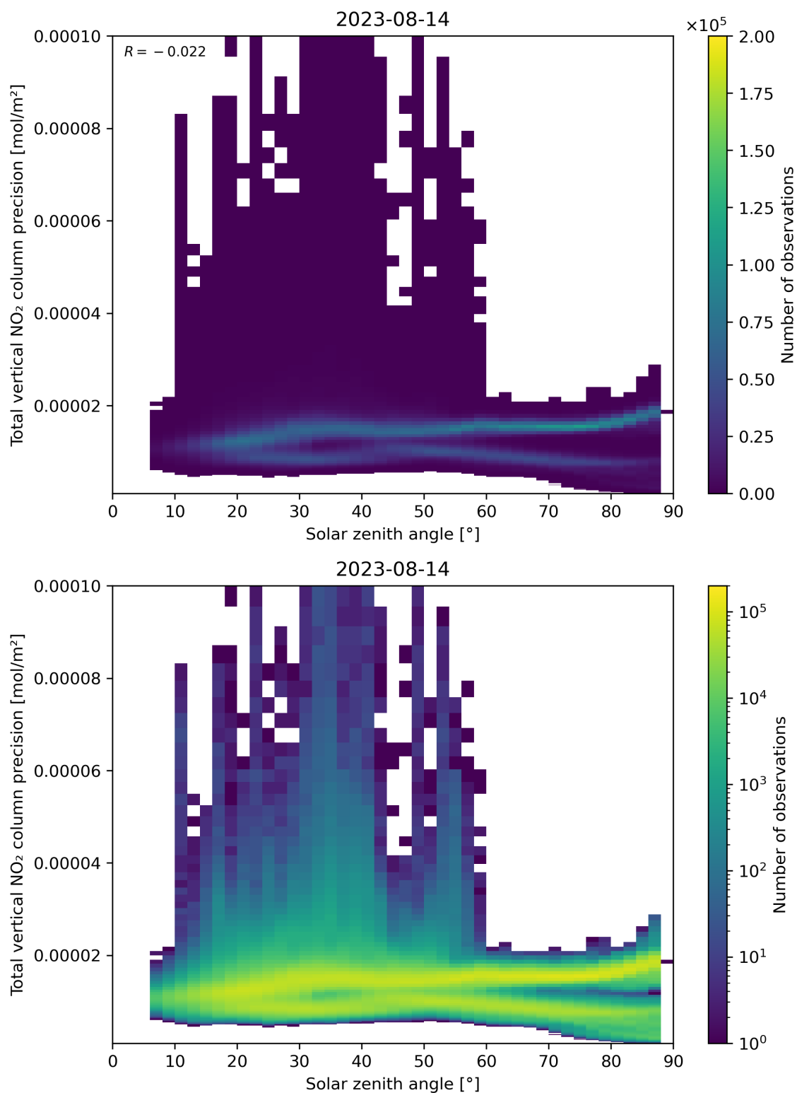
Figure 154: Scatter density plot of “Solar zenith angle” against “Total vertical NO 2 column precision” for 2023-08-14 to 2023-08-15.
