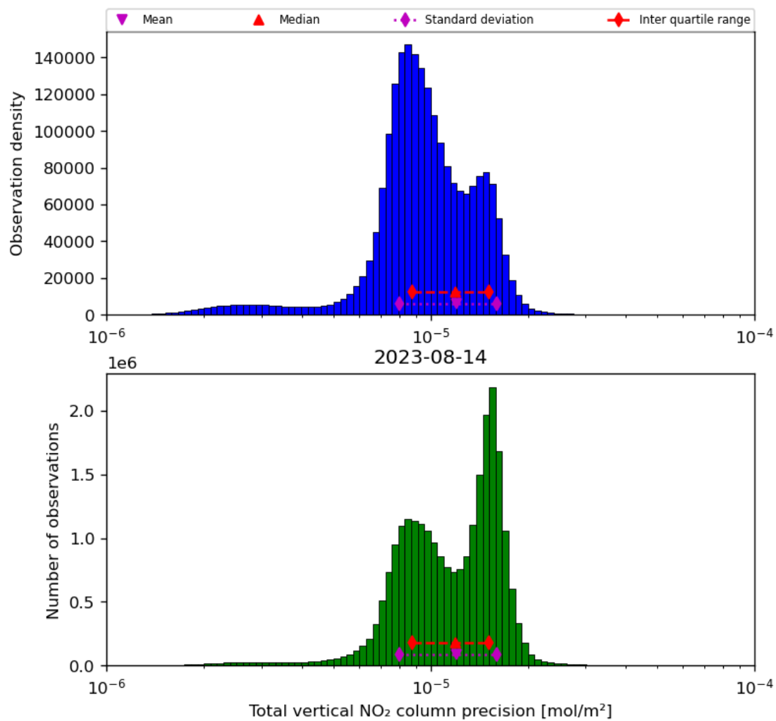
Figure 39: Histogram of “Total vertical NO 2 column precision” for 2023-08-14 to 2023-08-15
