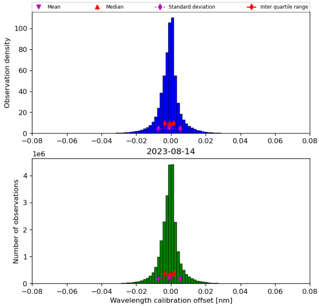
Figure 35: Histogram of “Wavelength calibration offset” for 2023-08-14 to 2023-08-15
