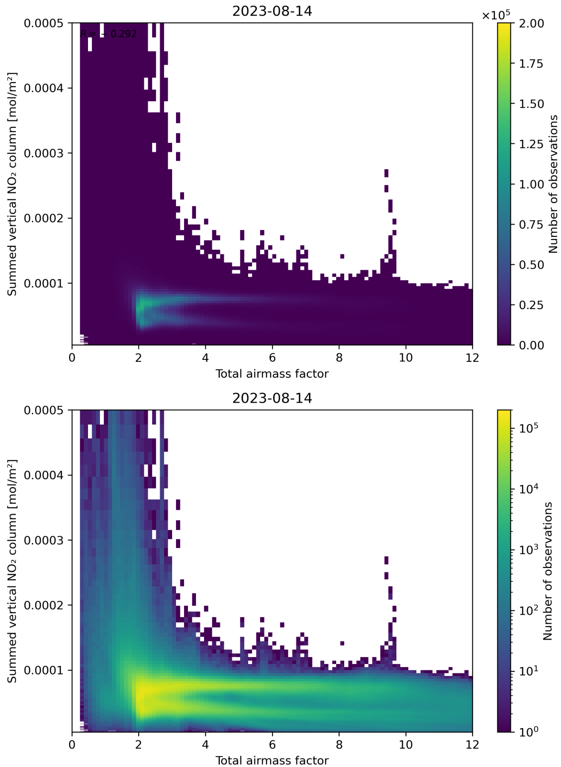
Figure 65: Scatter density plot of “Total airmass factor” against “Summed vertical NO 2 column” for 2023-08-14 to 2023-08-15.
