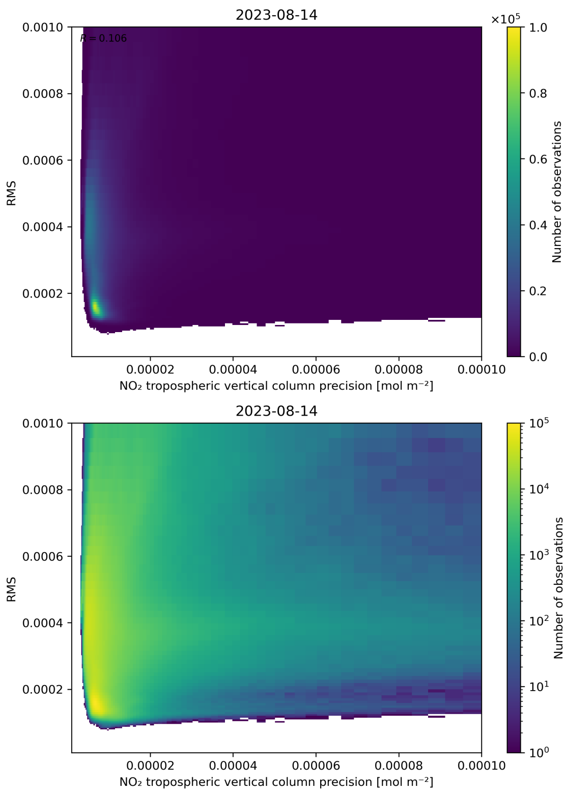
Figure 140: Scatter density plot of “NO 2 tropospheric vertical column precision” against “RMS” for 2023-08-14 to 2023-08-15.
