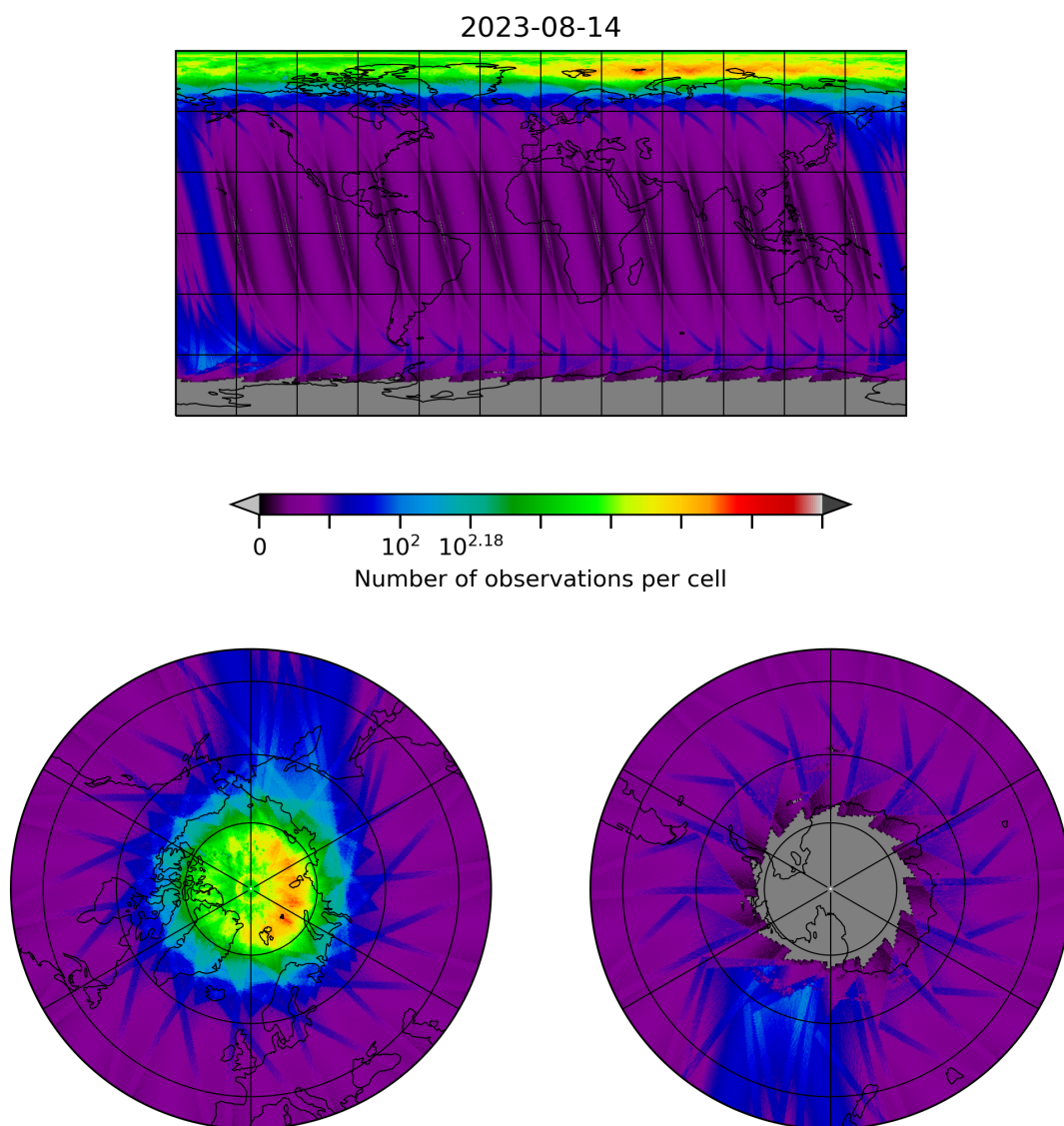
Figure 10: Map of the number of observations for 2023-08-14 to 2023-08-15
