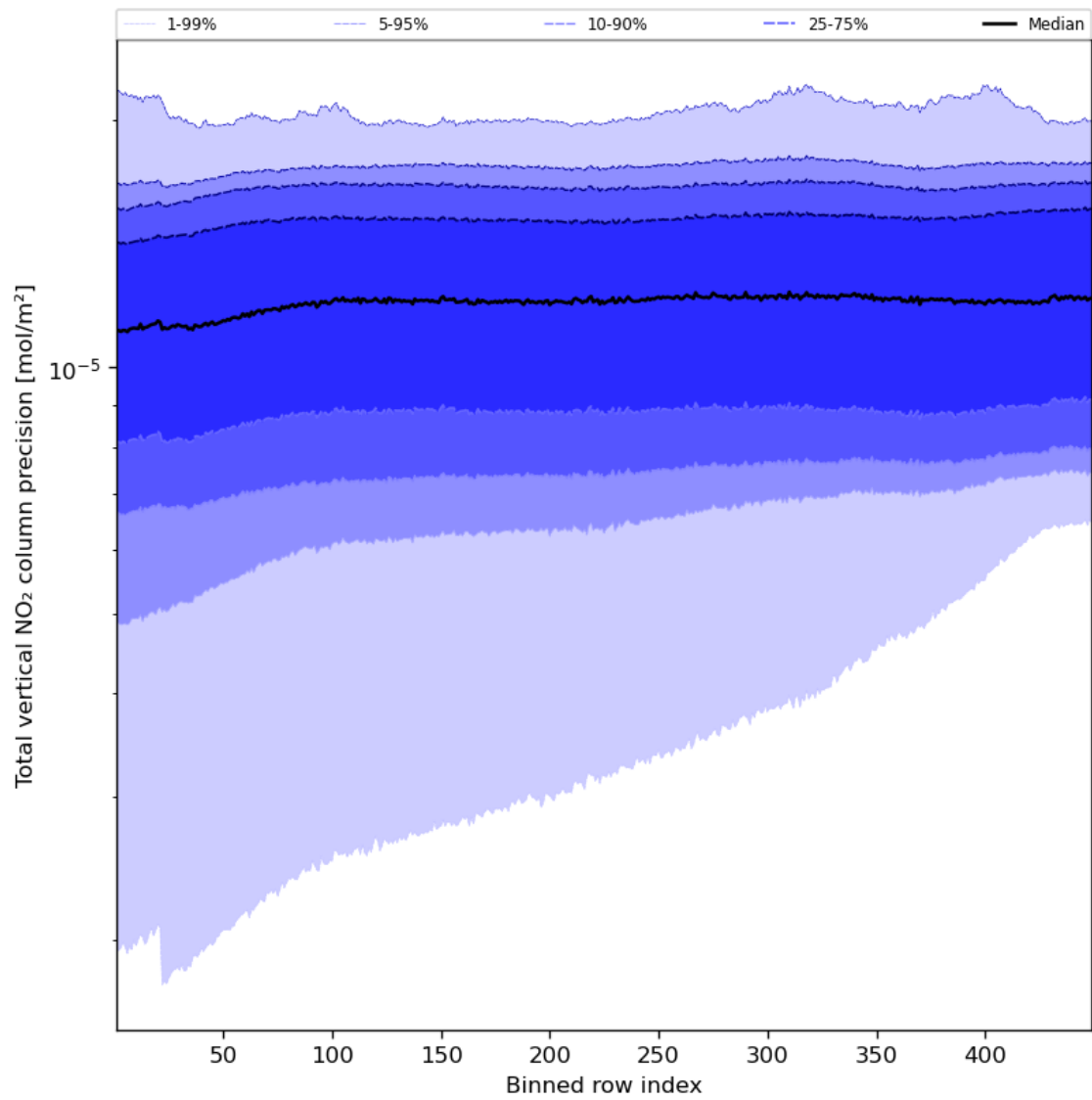
Figure 56: Along track statistics of “Total vertical NO 2 column precision” for 2023-08-14 to 2023-08-15
