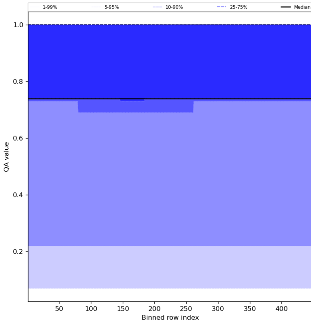
Figure 45: Along track statistics of “QA value” for 2023-08-14 to 2023-08-15
