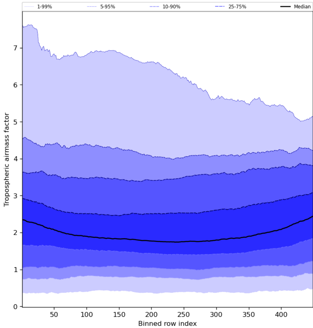
Figure 48: Along track statistics of “Tropospheric airmass factor” for 2023-08-14 to 2023-08-15
