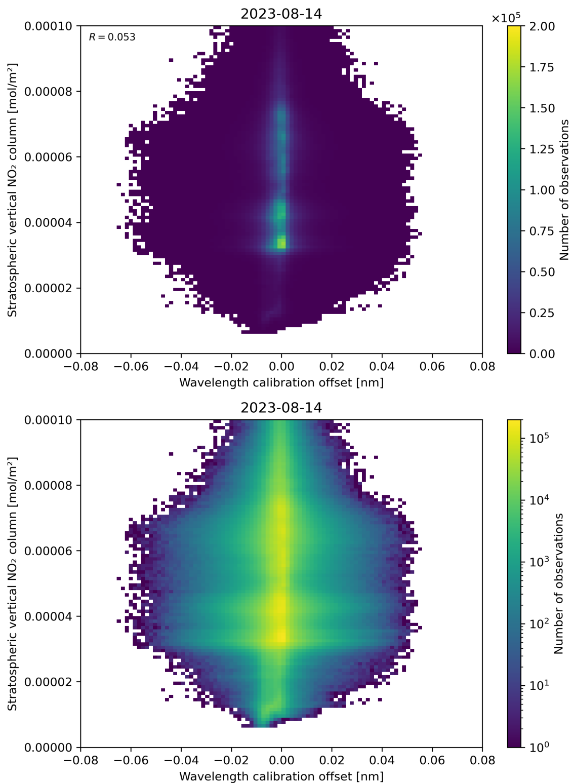
Figure 176: Scatter density plot of “Wavelength calibration offset” against “Stratospheric vertical NO 2 column” for 2023-08-14 to 2023-08-15.
