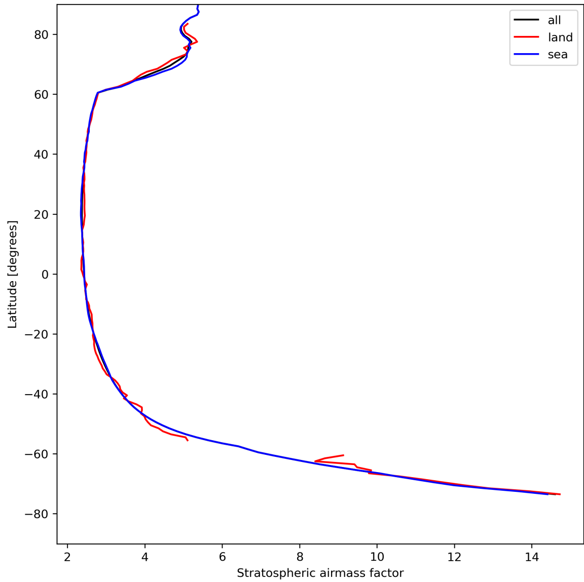
Figure 27: Zonal average of “Stratospheric air mass factor” for 2023-08-14 to 2023-08-15.
