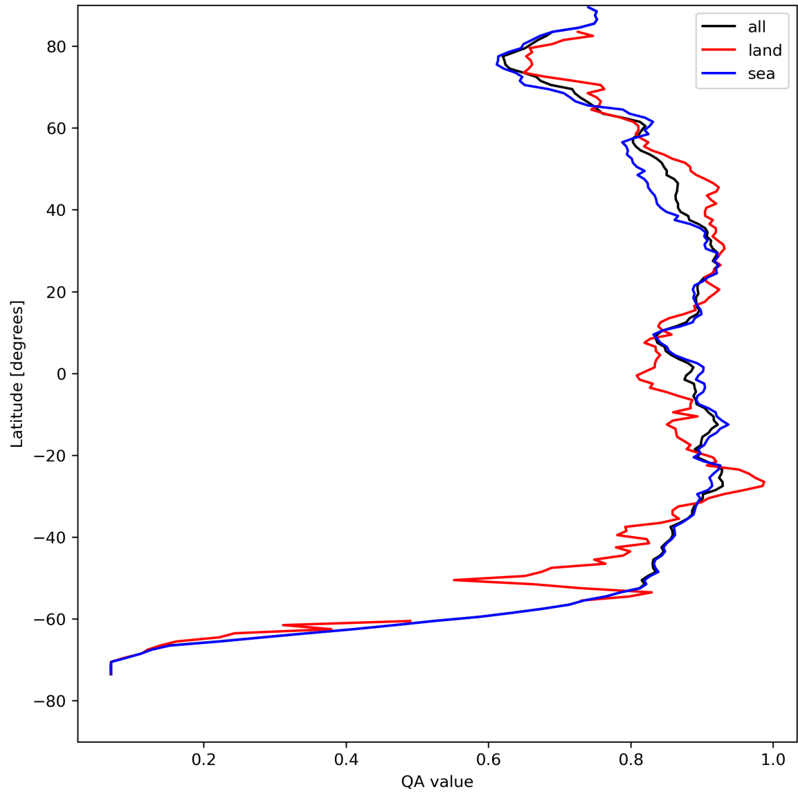
Figure 11: Zonal average of “QA value” for 2023-08-14 to 2023-08-15.
