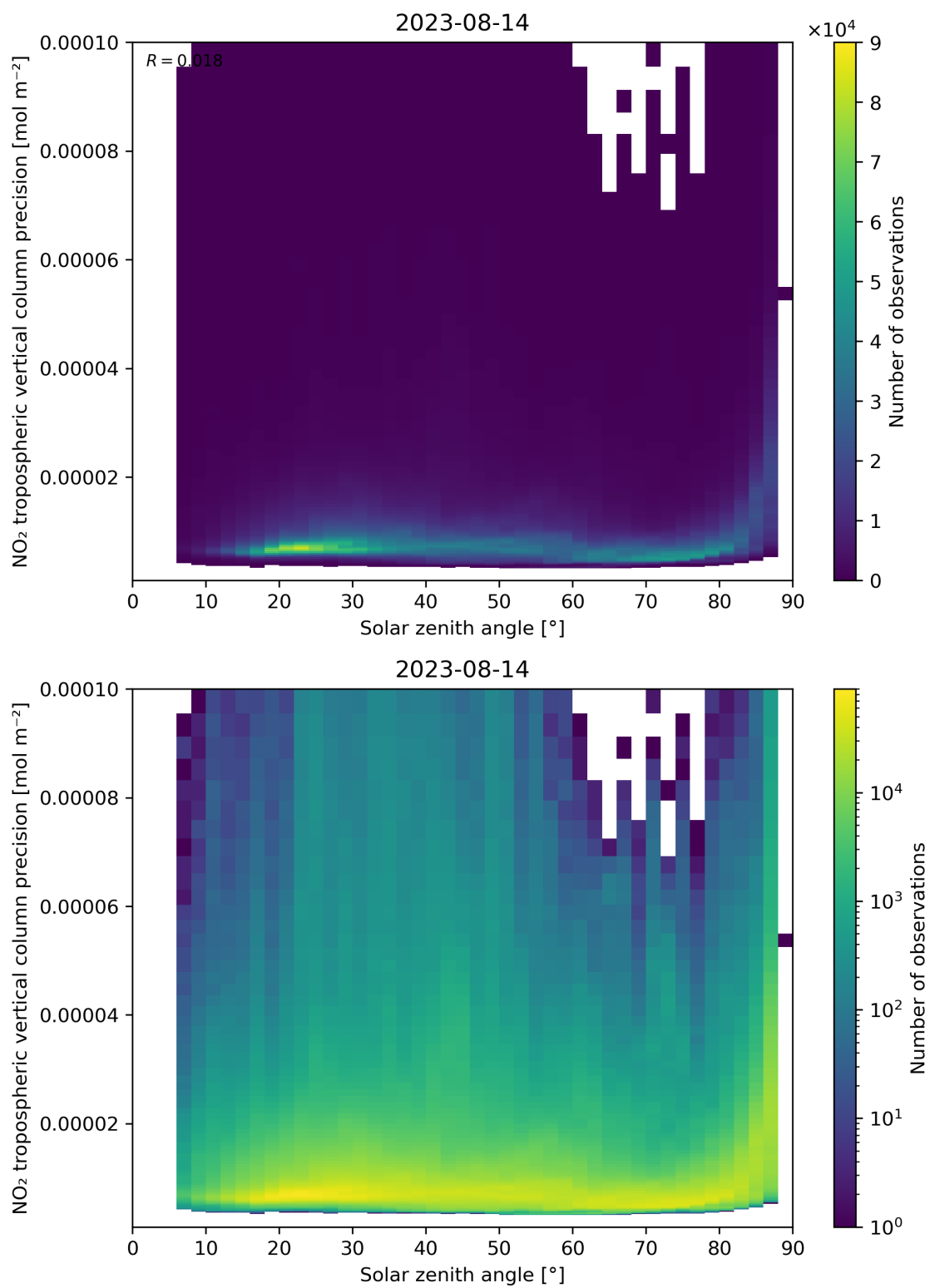
Figure 156: Scatter density plot of “Solar zenith angle” against “NO 2 tropospheric vertical column precision” for 2023-08-14 to 2023-08-15.
