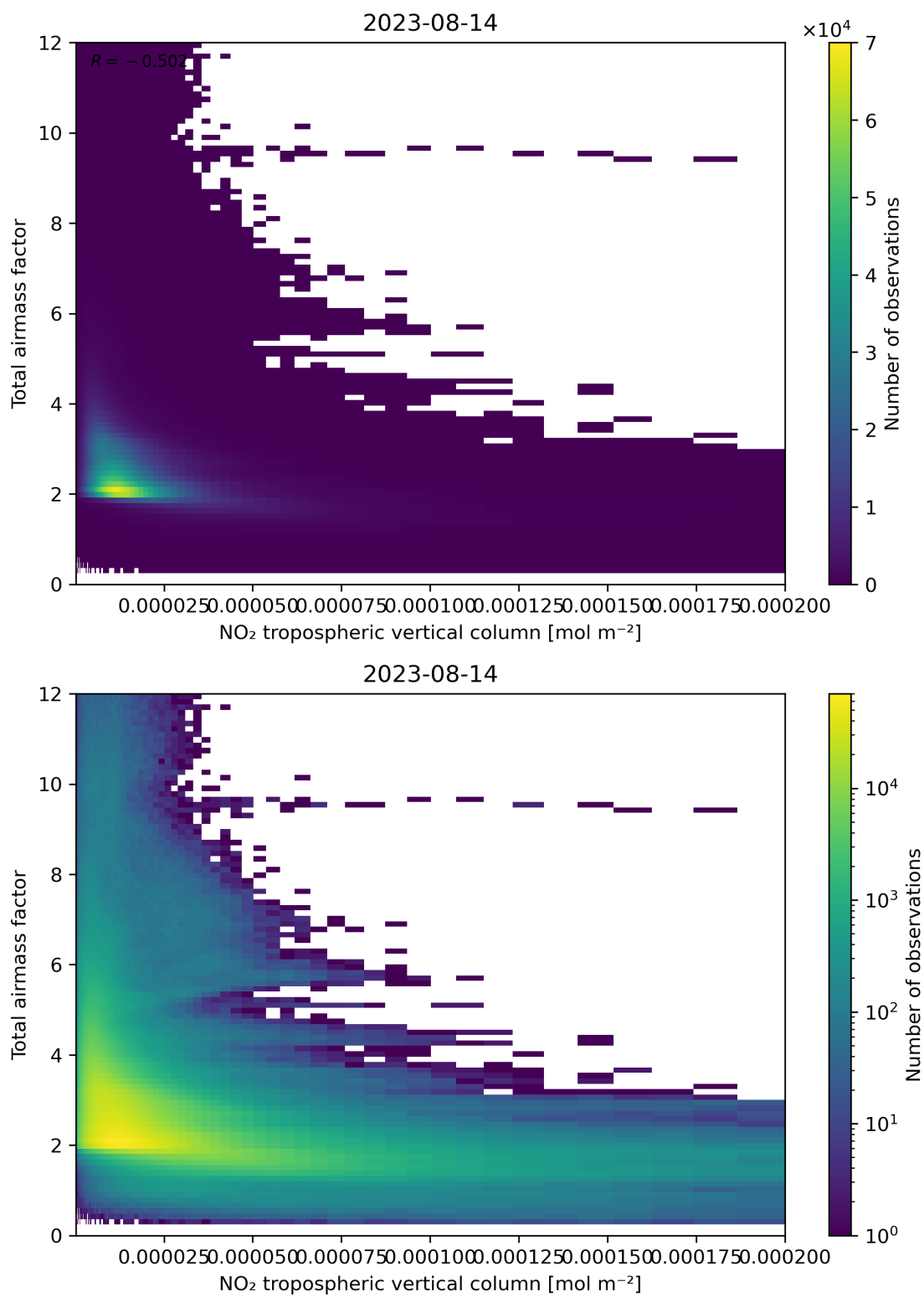
Figure 122: Scatter density plot of “NO 2 tropospheric vertical column” against “Total air mass factor” for 2023-08-14 to 2023-08-15.
