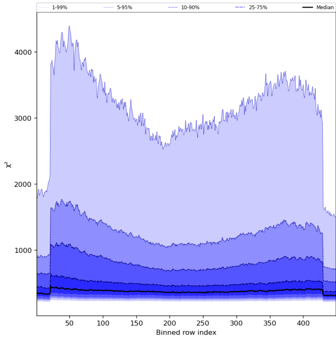
Figure 59: Along track statistics of “ \chi^2 ” for 2023-08-14 to 2023-08-15
