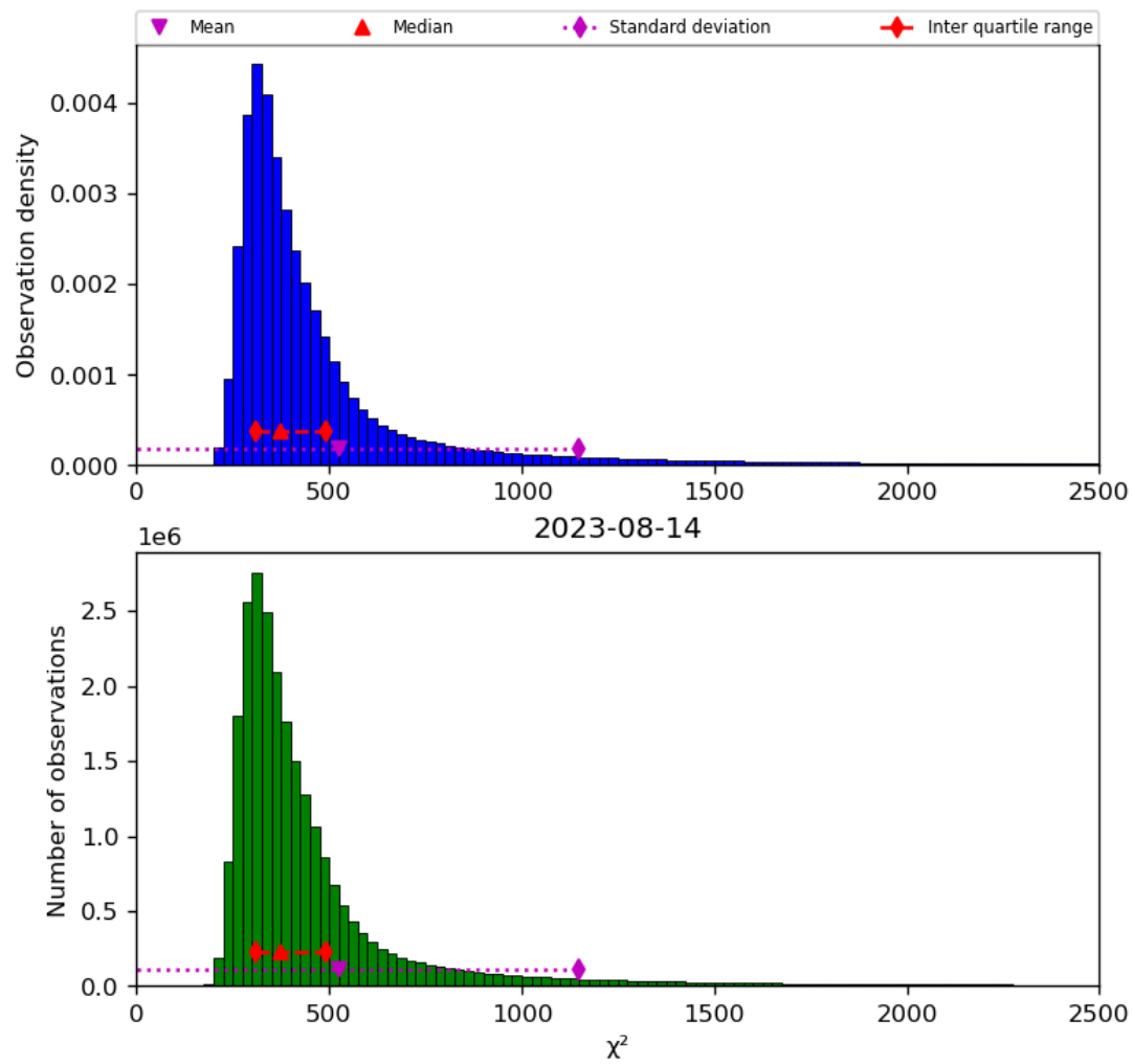
Figure 42: Histogram of “ \chi^2 ” for 2023-08-14 to 2023-08-15
