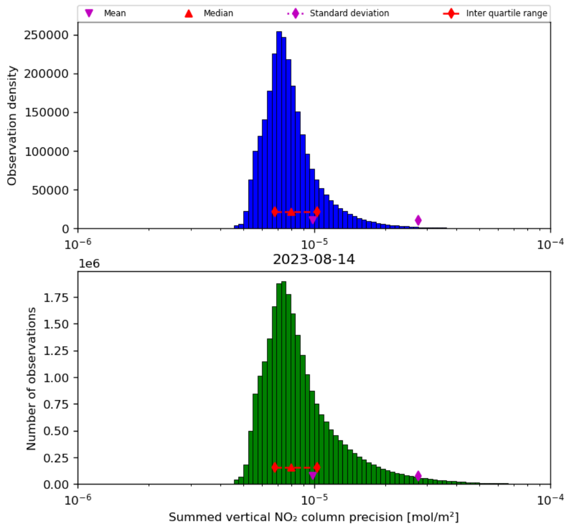
Figure 41: Histogram of “Summed vertical NO 2 column precision” for 2023-08-14 to 2023-08-15
