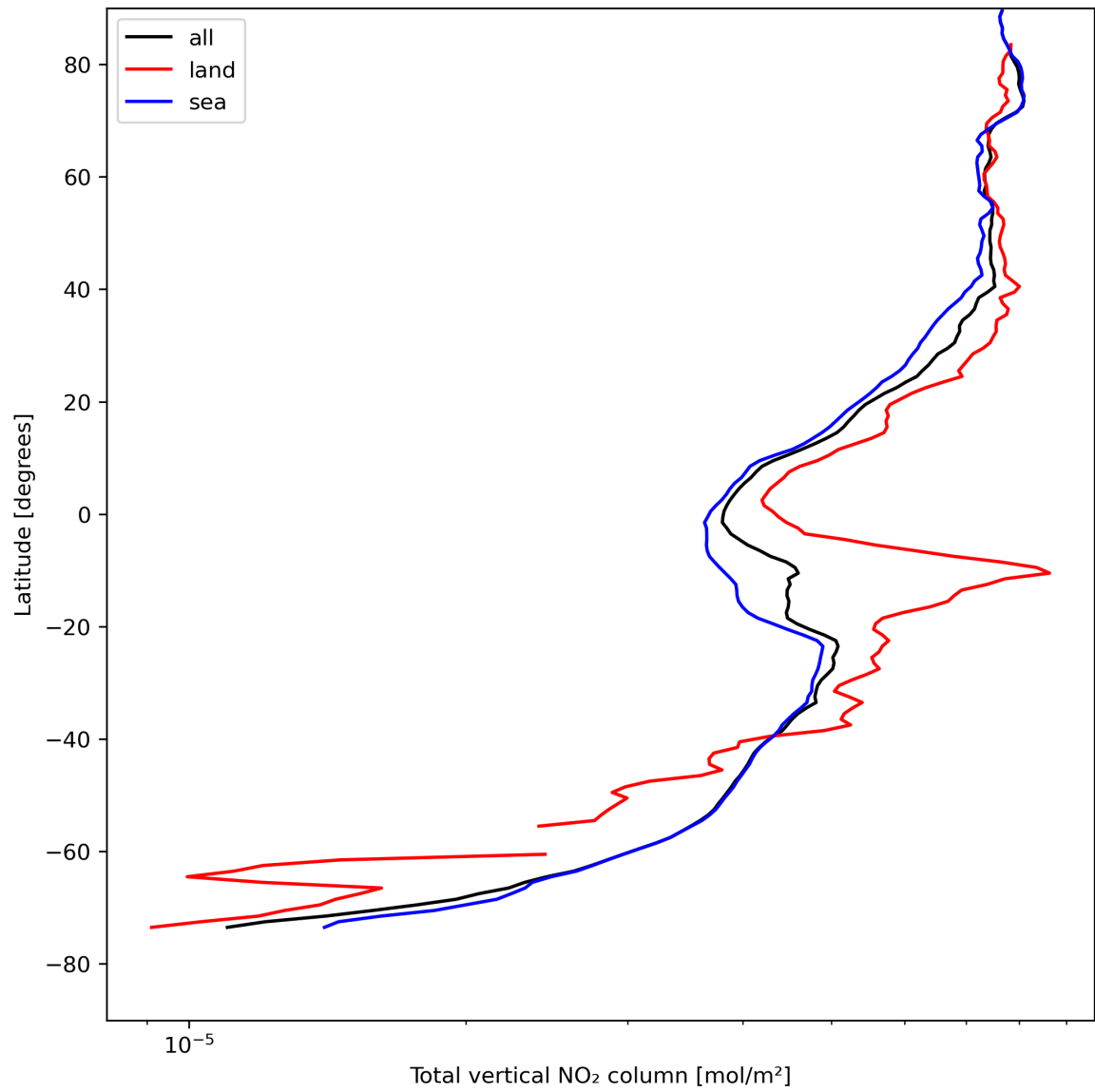
Figure 21: Zonal average of “Total vertical NO 2 column” for 2023-08-14 to 2023-08-15.
