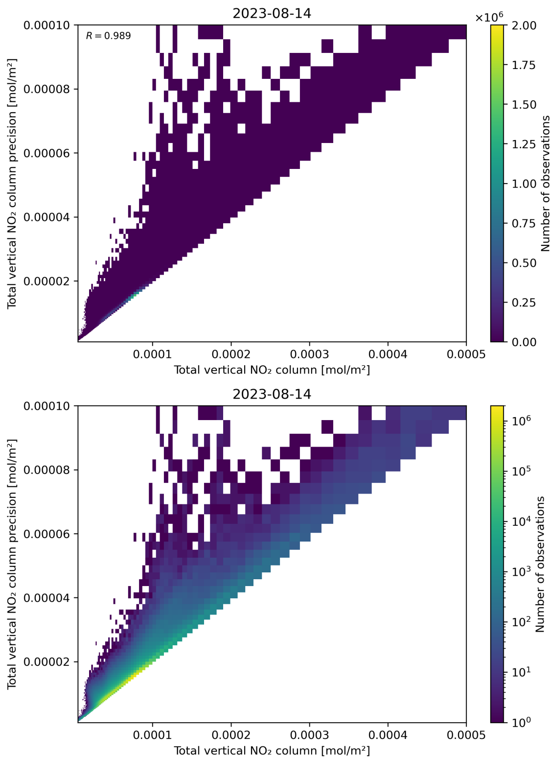
Figure 114: Scatter density plot of “Total vertical NO 2 column” against “Total vertical NO 2 column precision” for 2023-08-14 to 2023-08-15.
