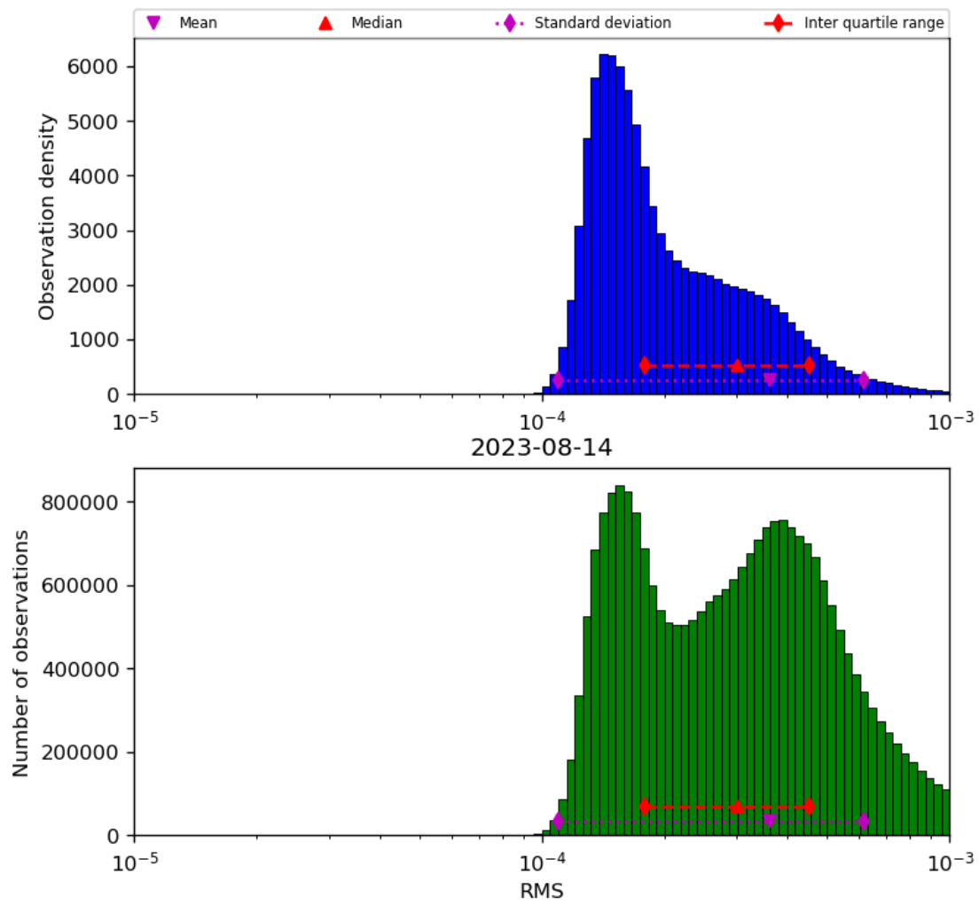
Figure 43: Histogram of “RMS” for 2023-08-14 to 2023-08-15
