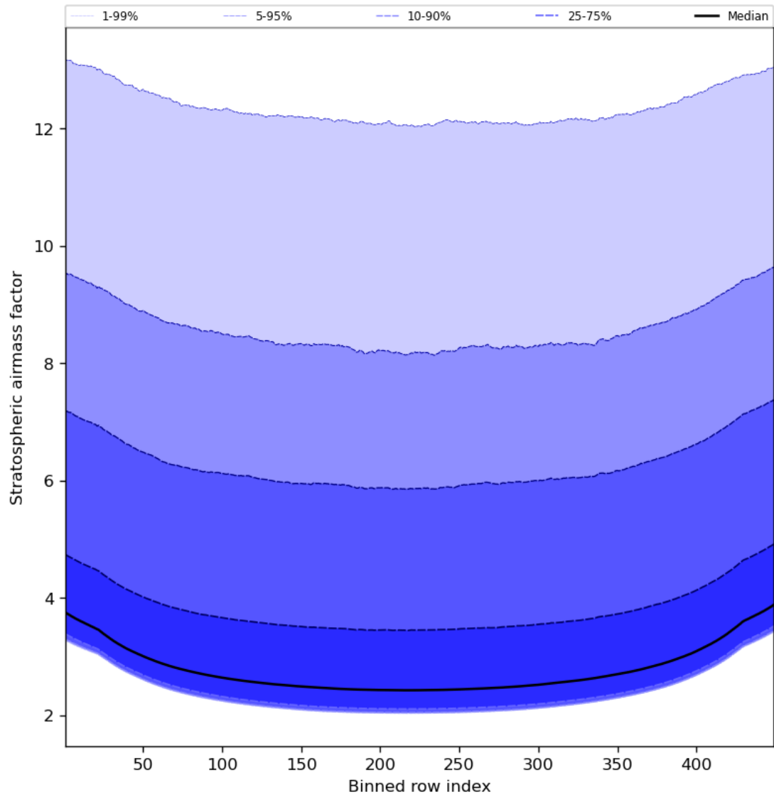
Figure 61: Along track statistics of “Stratospheric airmass factor” for 2023-08-14 to 2023-08-15
