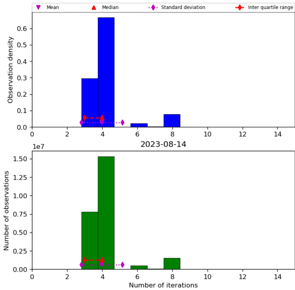
Figure 34: Histogram of “Number of iterations” for 2023-08-14 to 2023-08-15
