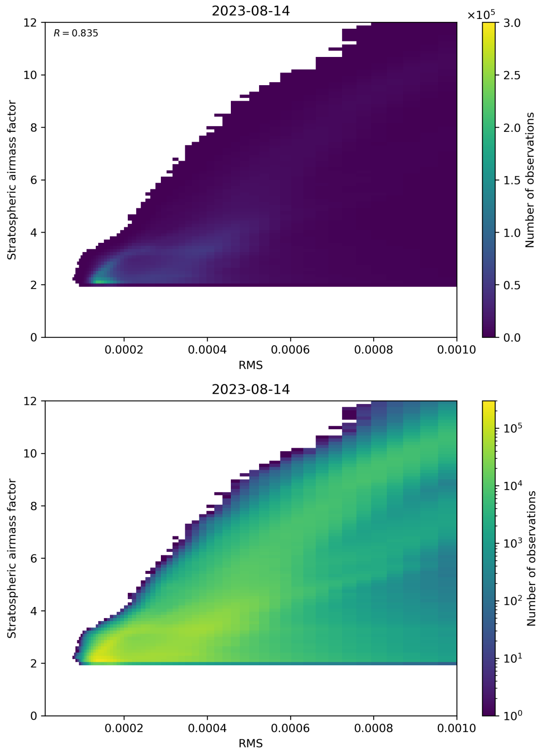
Figure 144: Scatter density plot of “RMS” against “Stratospheric airmass factor” for 2023-08-14 to 2023-08-15.
