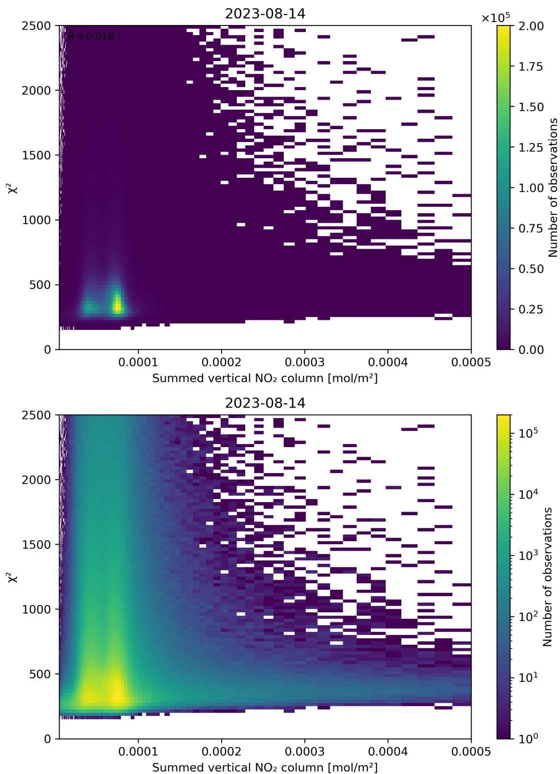
Figure 104: Scatter density plot of “Summed vertical NO 2 column” against “ \chi^2 ” for 2023-08-14 to 2023-08-15.
