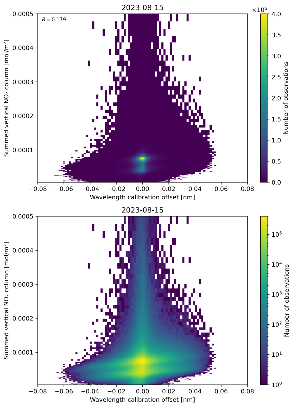
Figure 177: Scatter density plot of “Wavelength calibration offset” against “Summed vertical NO 2 column” for 2023-08-14 to 2023-08-16.
