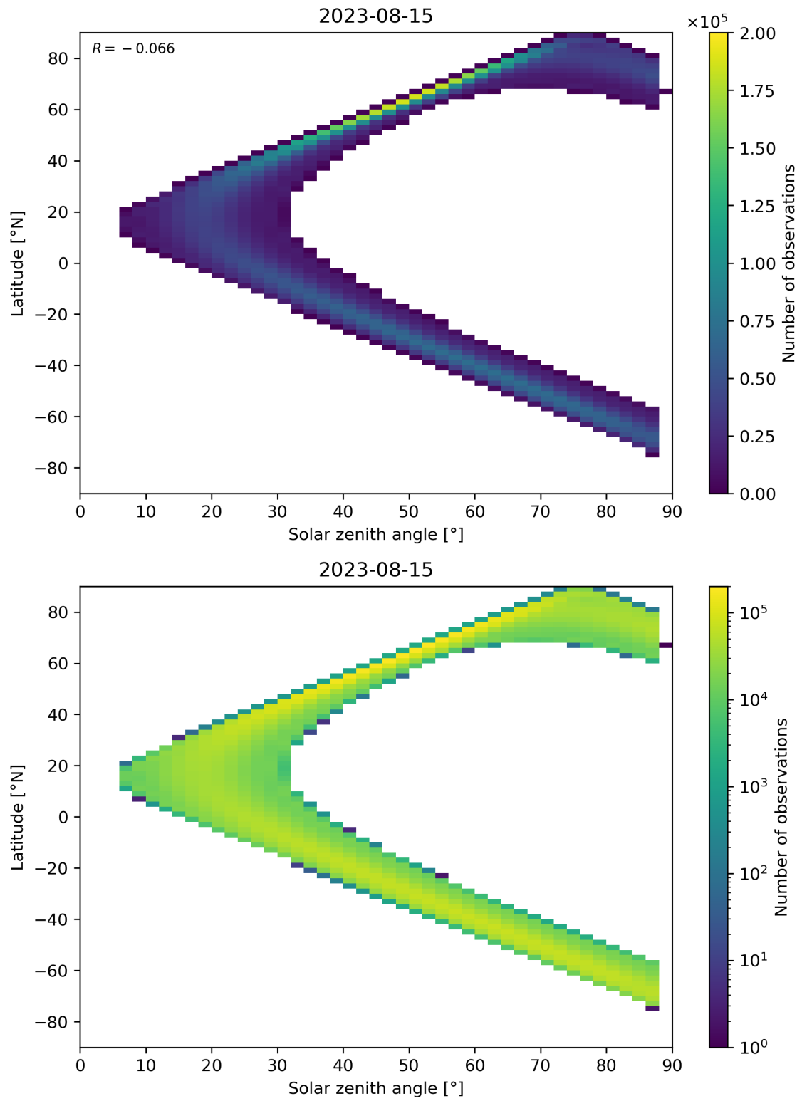
Figure 149: Scatter density plot of “Solar zenith angle” against “Latitude” for 2023-08-14 to 2023-08-16.
