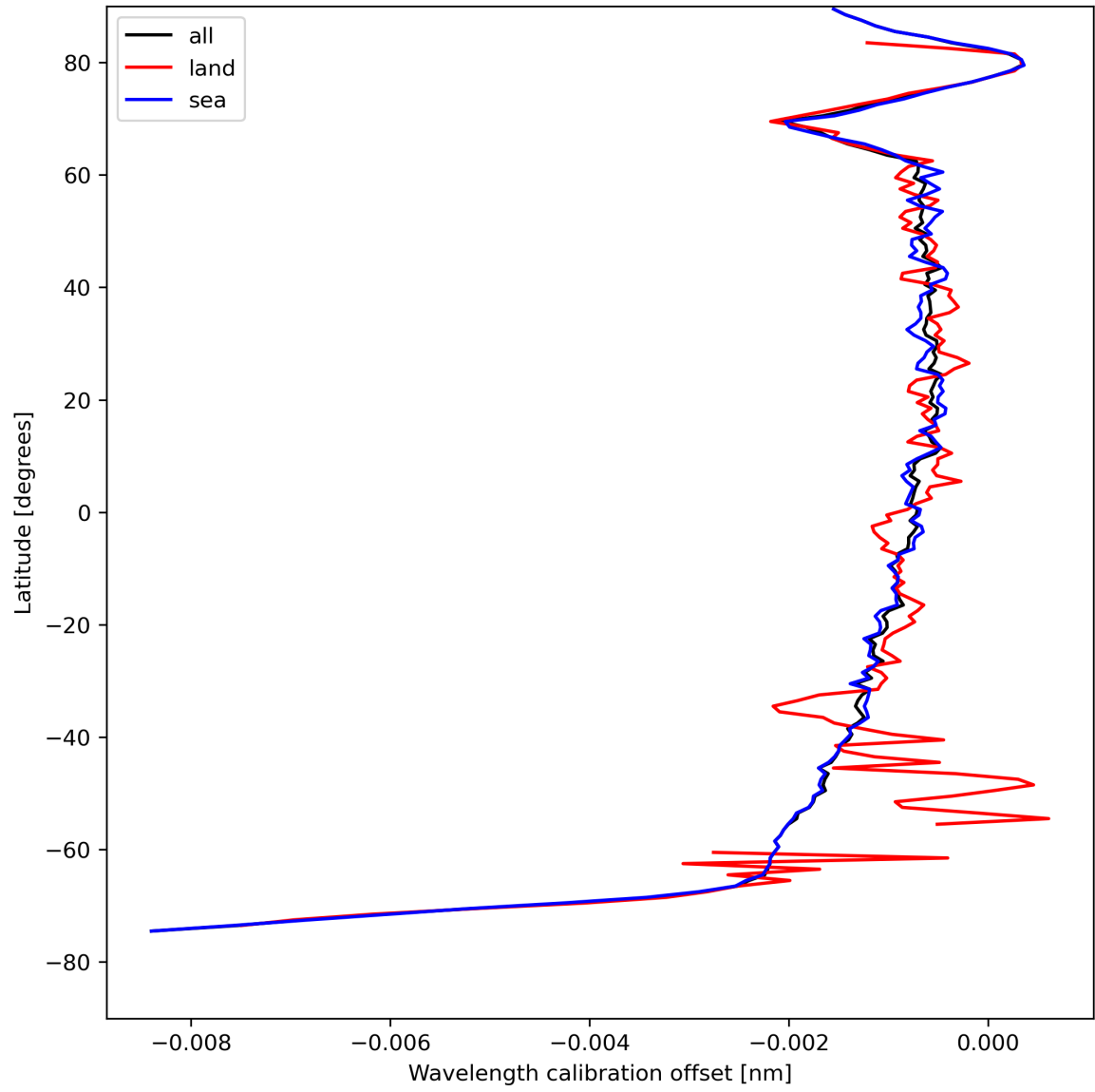
Figure 18: Zonal average of “Wavelength calibration offset” for 2023-08-14 to 2023-08-16.
