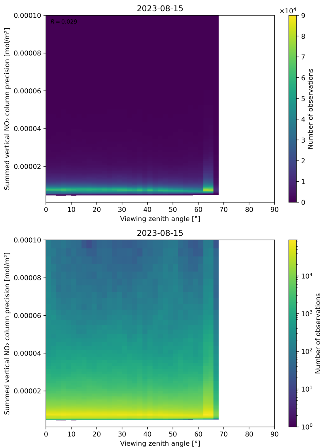
Figure 166: Scatter density plot of “Viewing zenith angle” against “Summed vertical NO 2 column precision” for 2023-08-14 to 2023-08-16.
