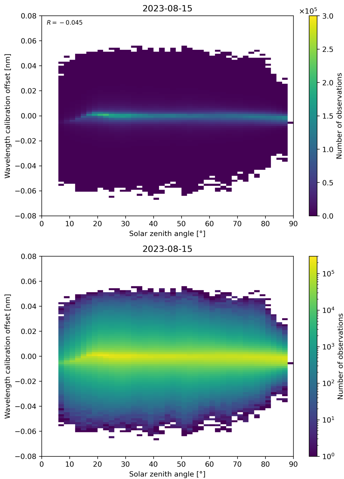
Figure 158: Scatter density plot of “Solar zenith angle” against “Wavelength calibration offset” for 2023-08-14 to 2023-08-16.
