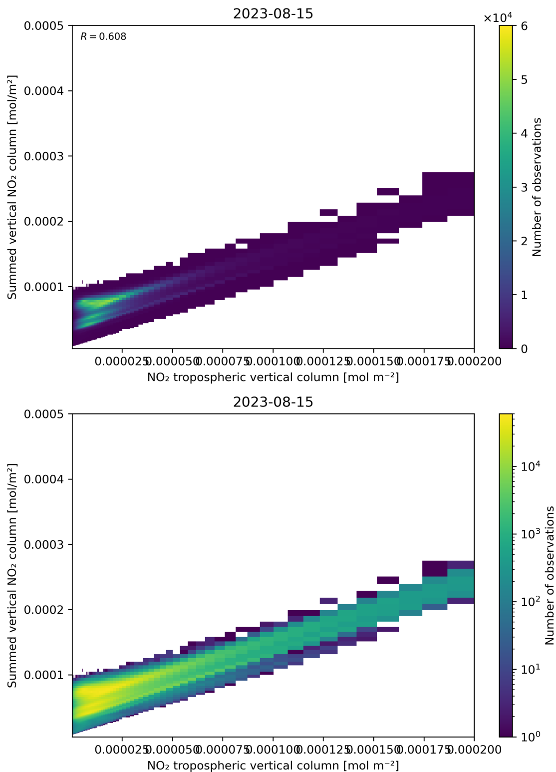
Figure 126: Scatter density plot of “NO 2 tropospheric vertical column” against “Summed vertical NO 2 column” for 2023-08-14 to 2023-08-16.
