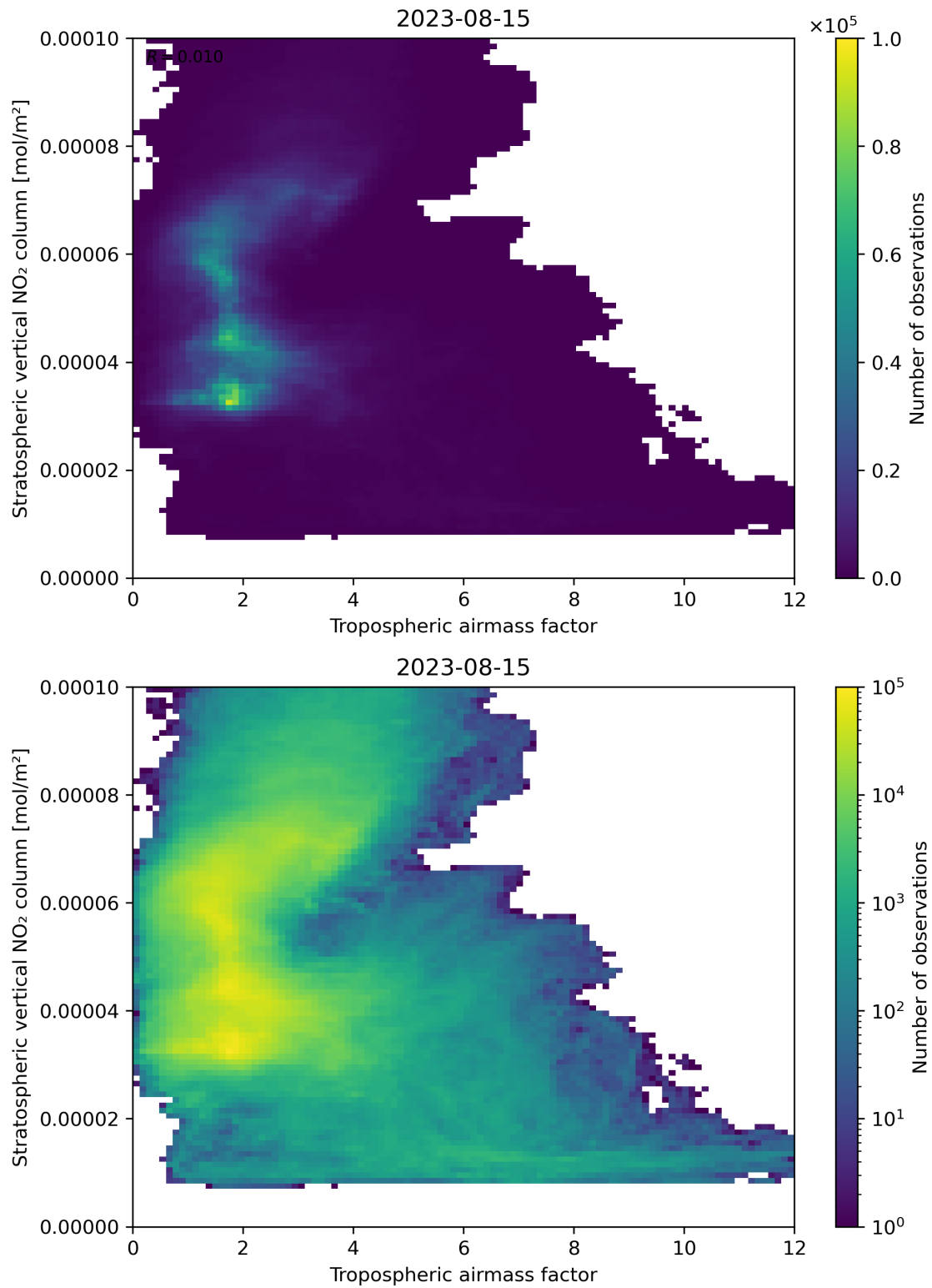
Figure 74: Scatter density plot of “Tropospheric air mass factor” against “Stratospheric vertical NO 2 column” for 2023-08-14 to 2023-08-16.
