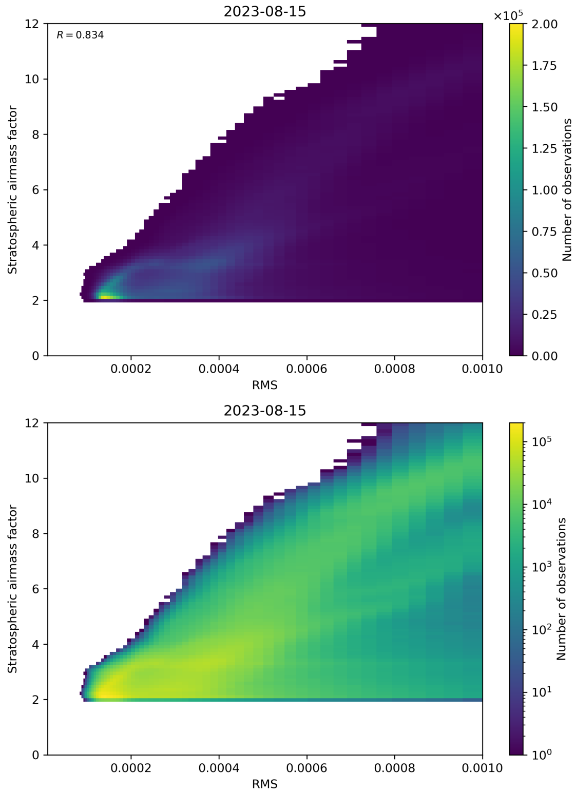
Figure 144: Scatter density plot of “RMS” against “Stratospheric airmass factor” for 2023-08-14 to 2023-08-16.
