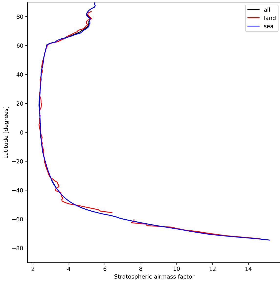
Figure 27: Zonal average of “Stratospheric airmass factor” for 2023-08-14 to 2023-08-16.
