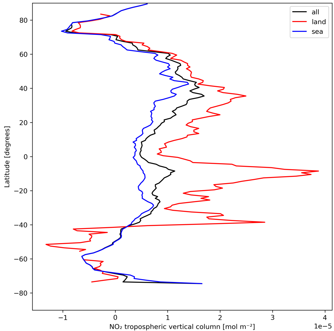
Figure 12: Zonal average of “NO 2 tropospheric vertical column” for 2023-08-14 to 2023-08-16.
