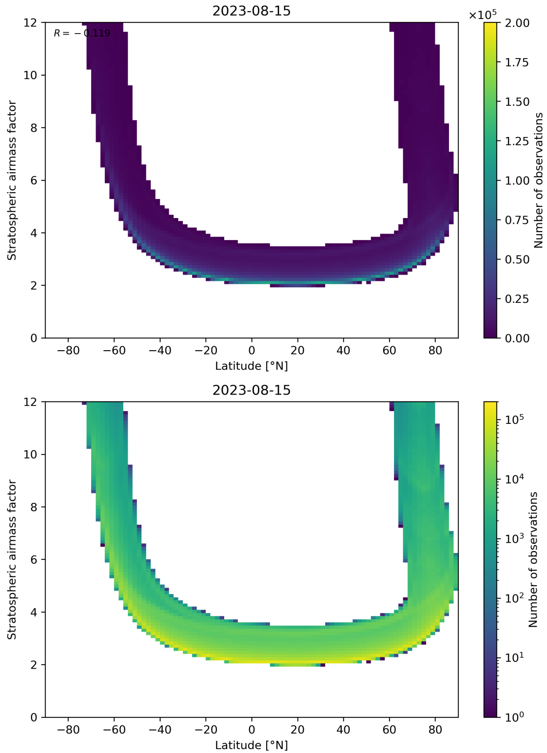
Figure 83: Scatter density plot of “Latitude” against “Stratospheric air mass factor” for 2023-08-14 to 2023-08-16.
