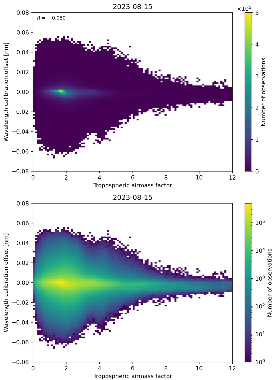
Figure 80: Scatter density plot of “Tropospheric airmass factor” against “Wavelength calibration offset” for 2023-08-14 to 2023-08-16.
