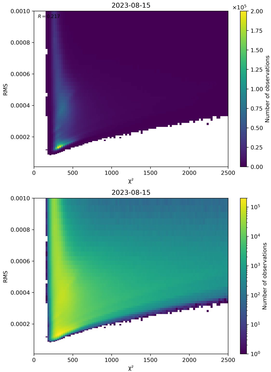
Figure 82: Scatter density plot of “ \chi^2 ” against “RMS” for 2023-08-14 to 2023-08-16.
