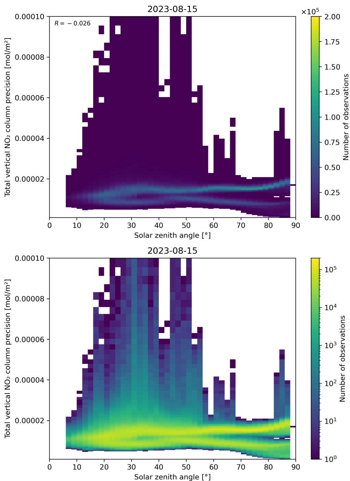
Figure 154: Scatter density plot of “Solar zenith angle” against “Total vertical NO 2 column precision” for 2023-08-14 to 2023-08-16.
