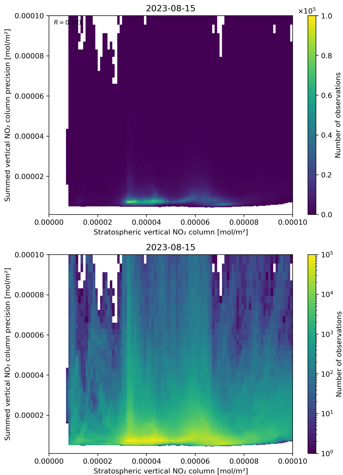
Figure 99: Scatter density plot of “Stratospheric vertical NO 2 column” against “Summed vertical NO 2 column precision” for 2023-08-14 to 2023-08-16.
