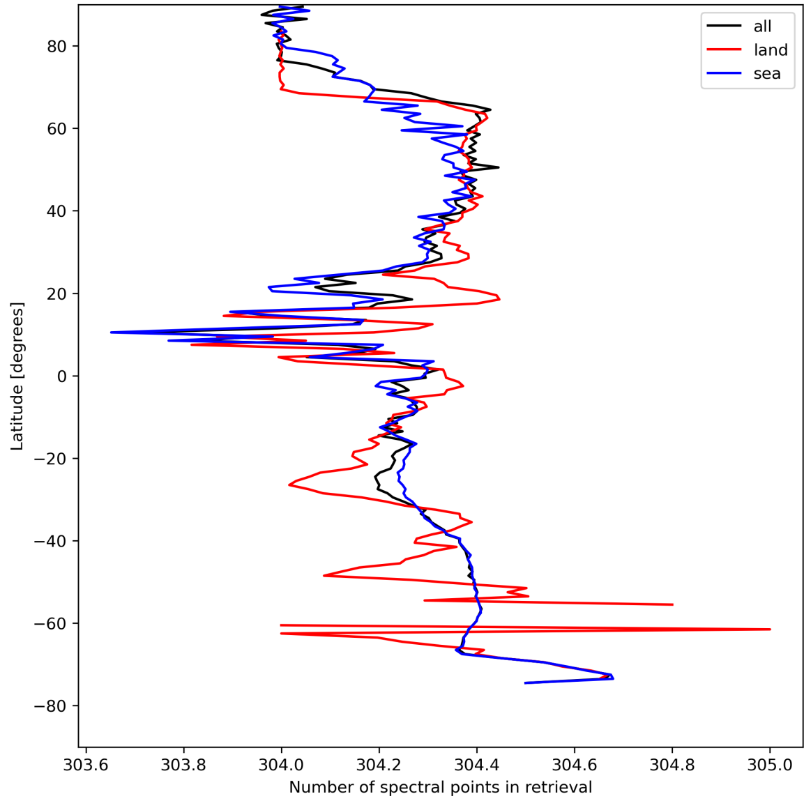
Figure 16: Zonal average of “Number of spectral points in retrieval” for 2023-08-14 to 2023-08-16.
