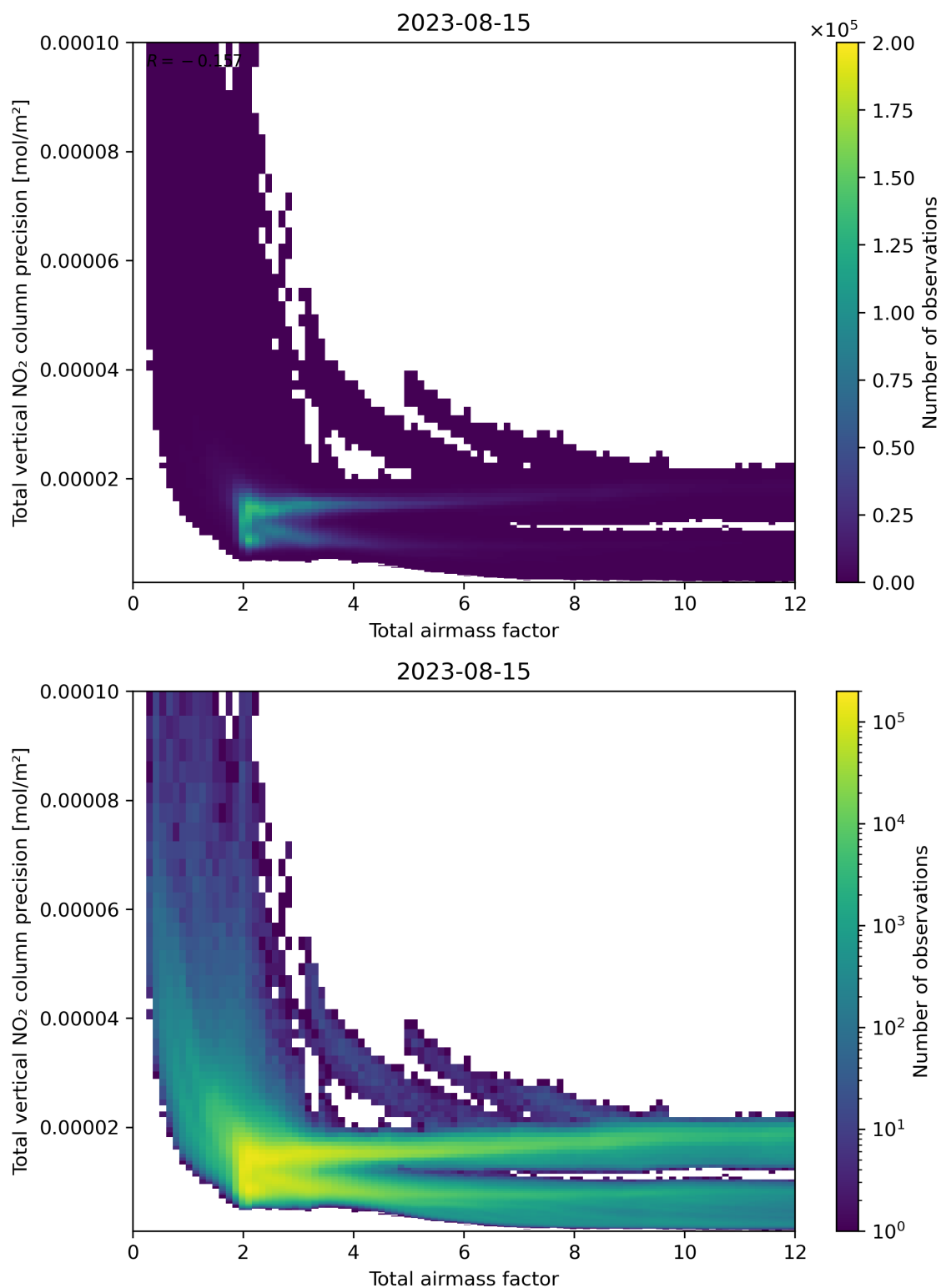
Figure 68: Scatter density plot of “Total airmass factor” against “Total vertical NO 2 column precision” for 2023-08-14 to 2023-08-16.
