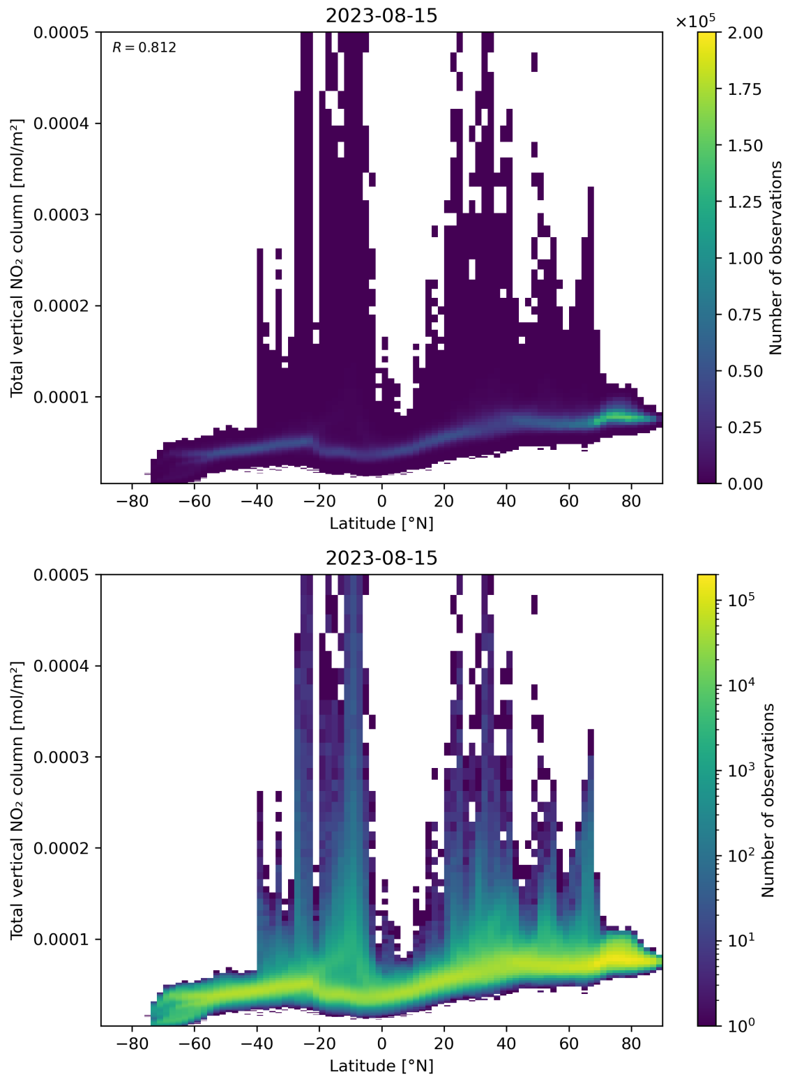
Figure 90: Scatter density plot of “Latitude” against “Total vertical NO 2 column” for 2023-08-14 to 2023-08-16.
