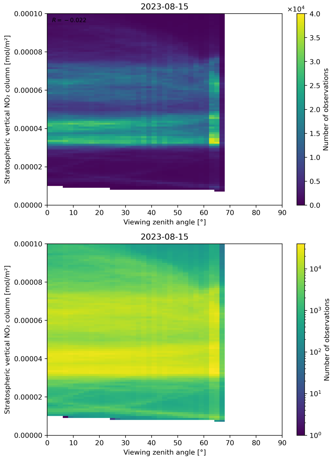
Figure 164: Scatter density plot of “Viewing zenith angle” against “Stratospheric vertical NO 2 column” for 2023-08-14 to 2023-08-16.
