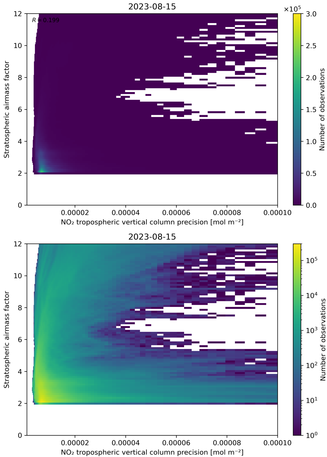
Figure 131: Scatter density plot of “NO 2 tropospheric vertical column precision” against “Stratospheric airmass factor” for 2023-08-14 to 2023-08-16.
