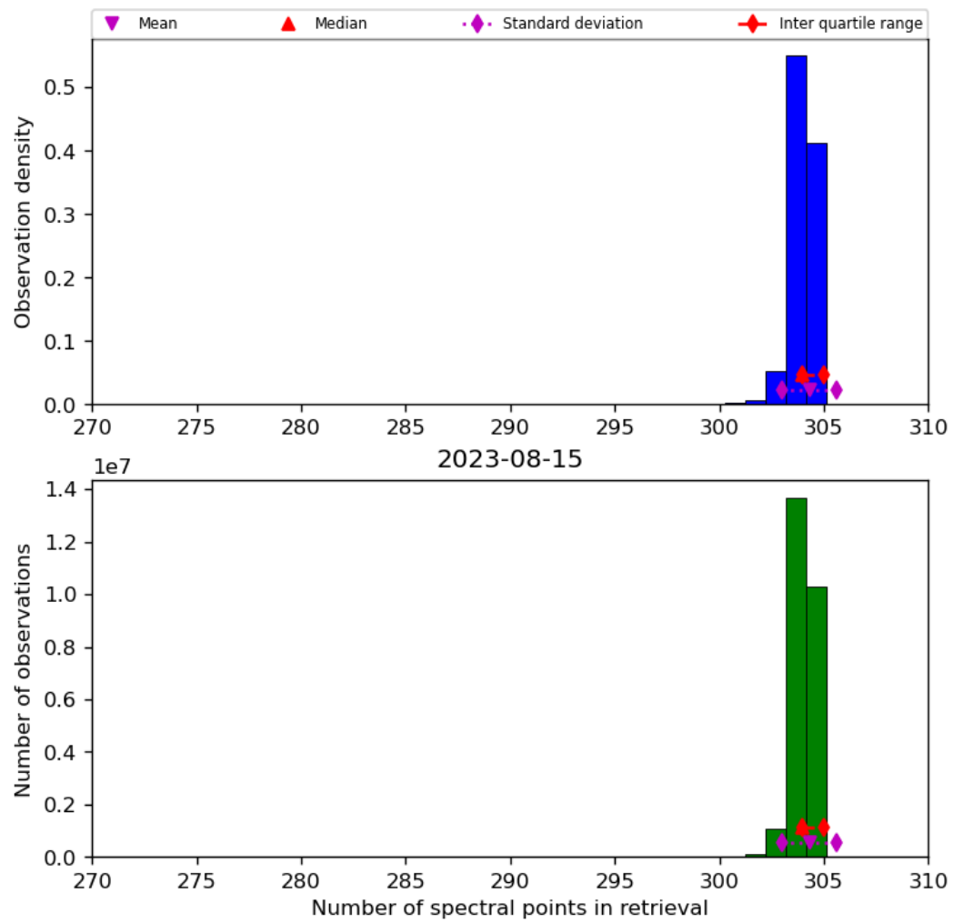
Figure 33: Histogram of “Number of spectral points in retrieval” for 2023-08-14 to 2023-08-16
