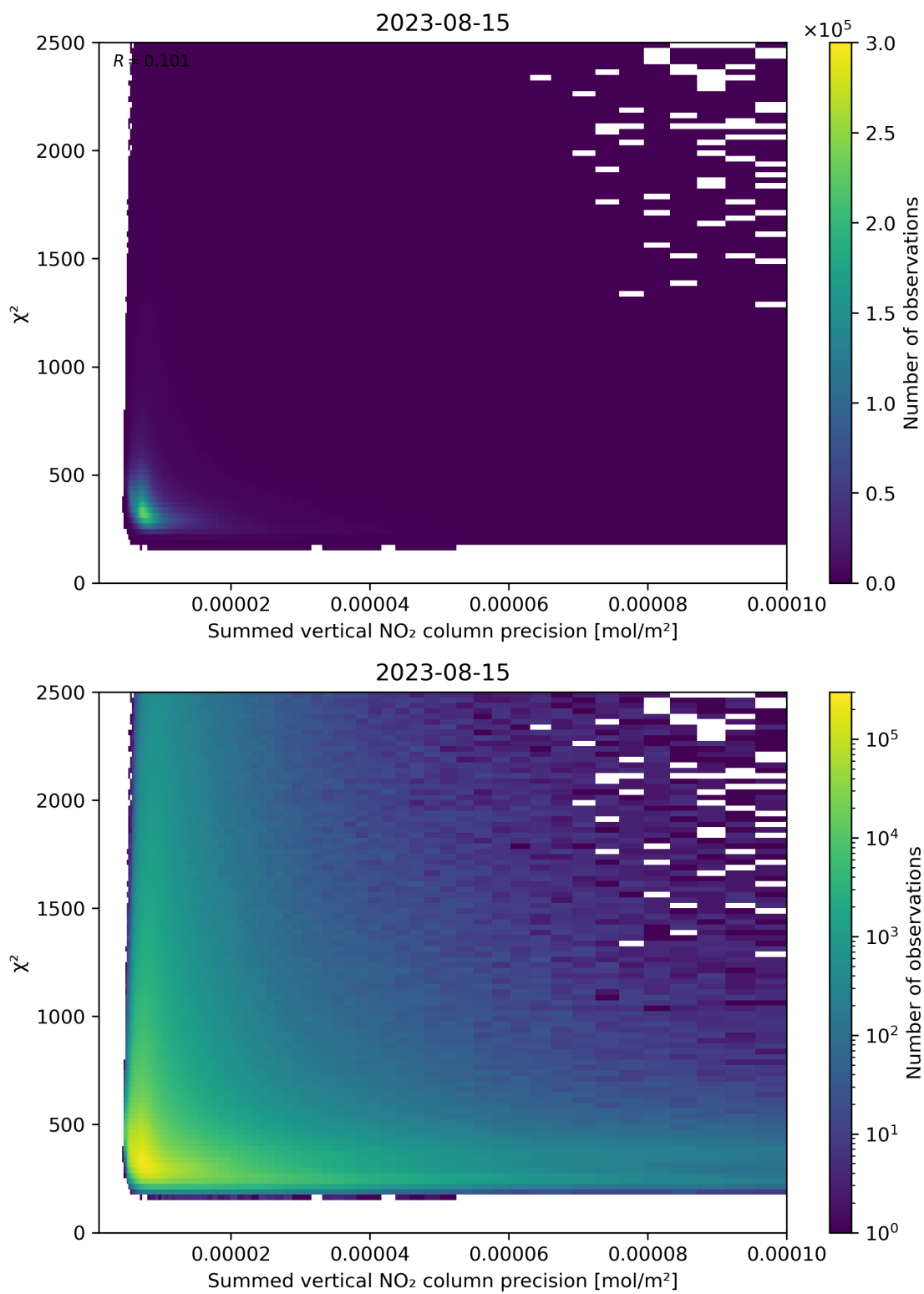
Figure 107: Scatter density plot of “Summed vertical NO 2 column precision” against “ \chi^2 ” for 2023-08-14 to 2023-08-16.
