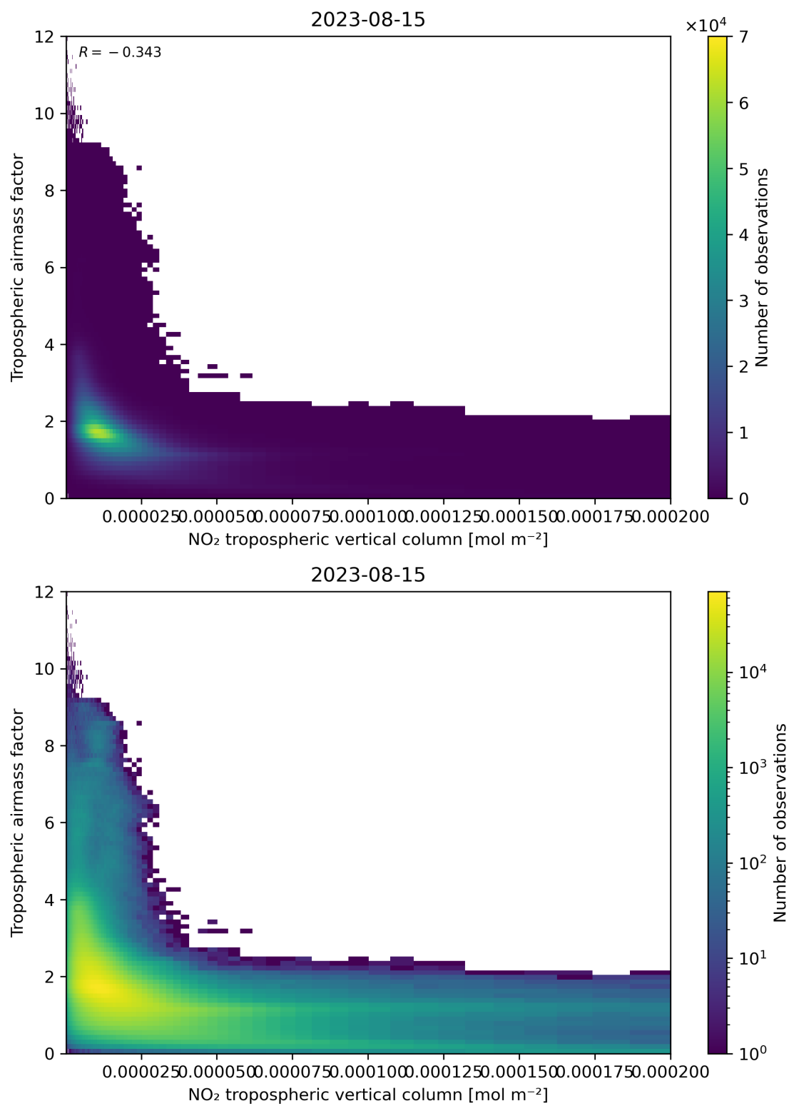
Figure 123: Scatter density plot of “NO 2 tropospheric vertical column” against “Tropospheric air mass factor” for 2023-08-14 to 2023-08-16.
