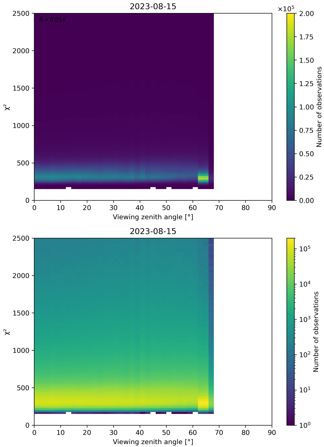
Figure 162: Scatter density plot of “Viewing zenith angle” against “ \chi^2 ” for 2023-08-14 to 2023-08-16.
