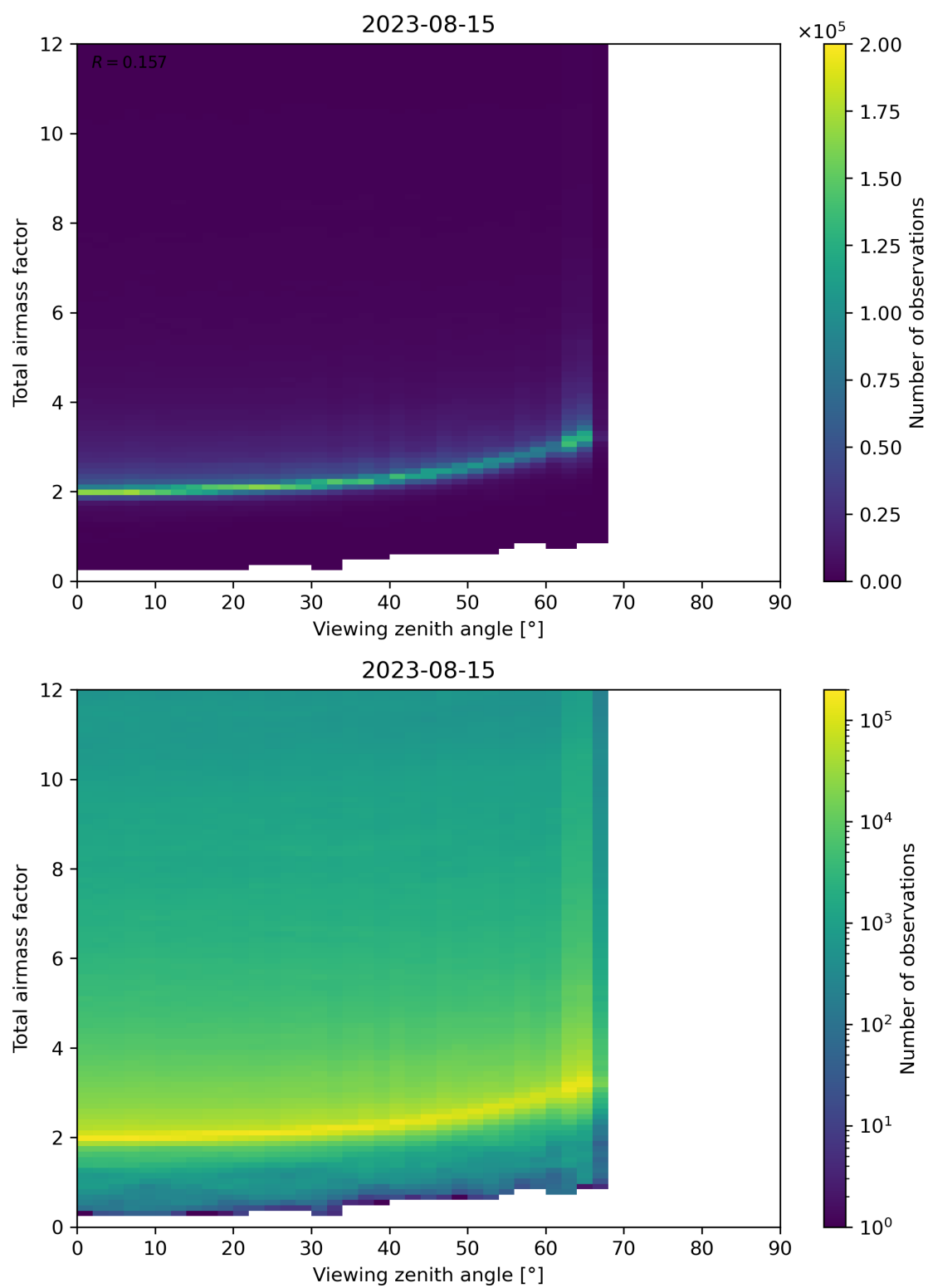
Figure 160: Scatter density plot of “Viewing zenith angle” against “Total airmass factor” for 2023-08-14 to 2023-08-16.
