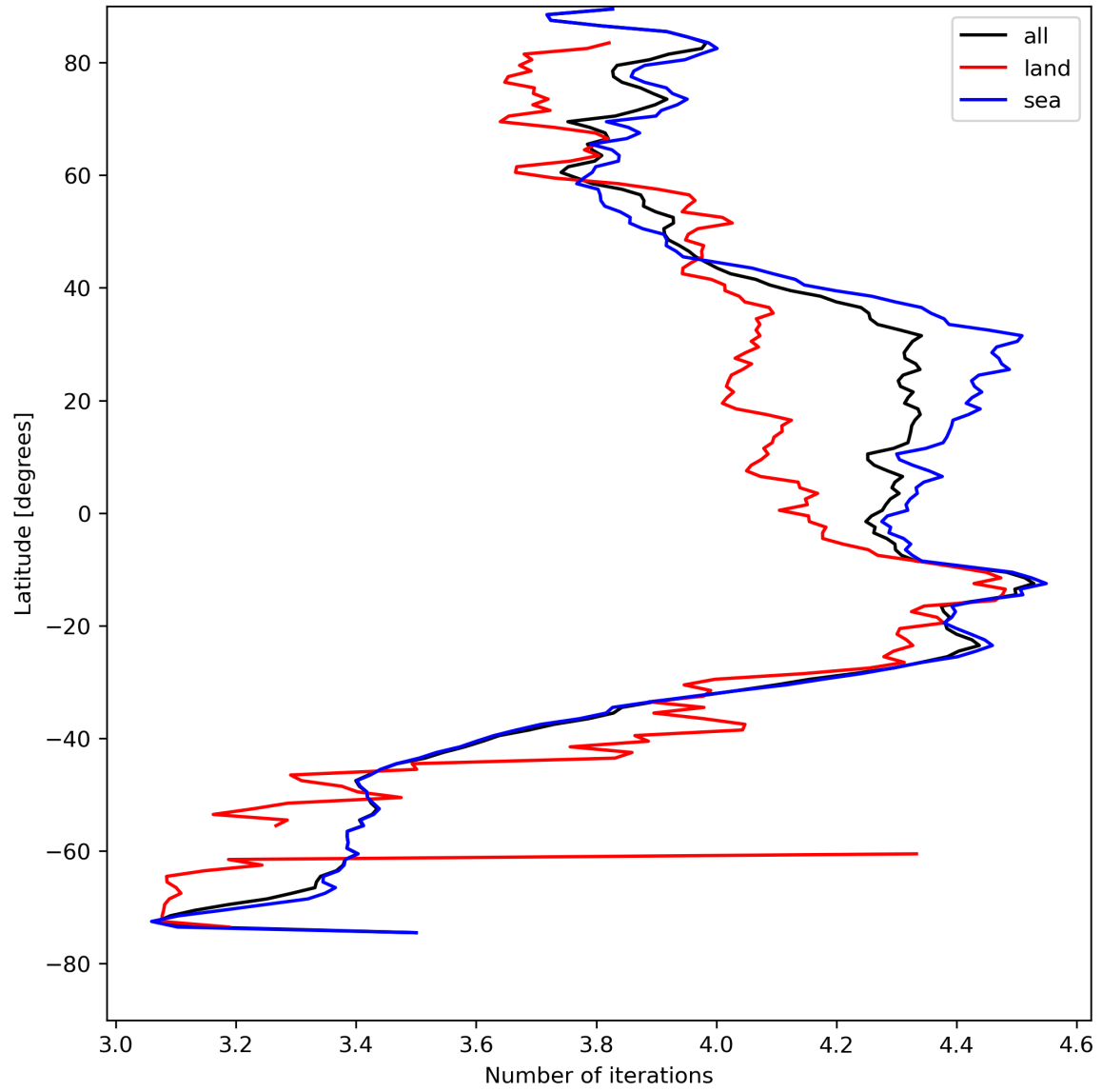
Figure 17: Zonal average of “Number of iterations” for 2023-08-14 to 2023-08-16.
