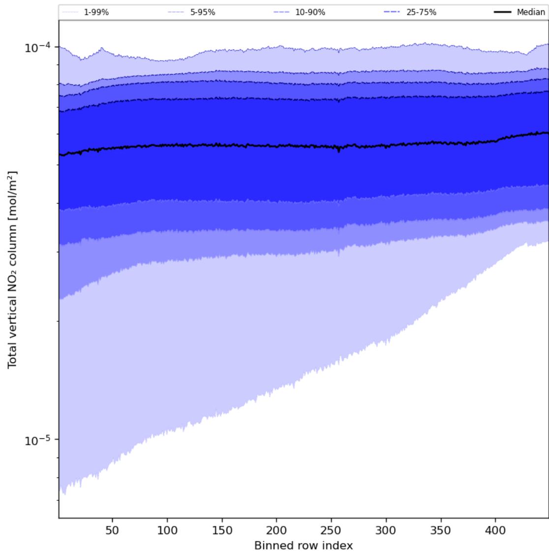
Figure 55: Along track statistics of “Total vertical NO 2 column” for 2023-08-14 to 2023-08-16
