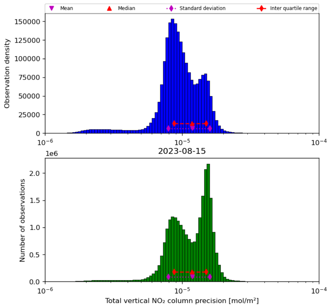
Figure 39: Histogram of “Total vertical NO 2 column precision” for 2023-08-14 to 2023-08-16
