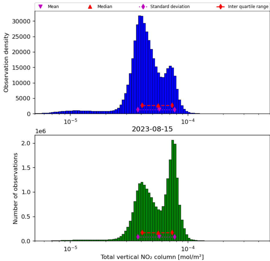
Figure 38: Histogram of “Total vertical NO 2 column” for 2023-08-14 to 2023-08-16
