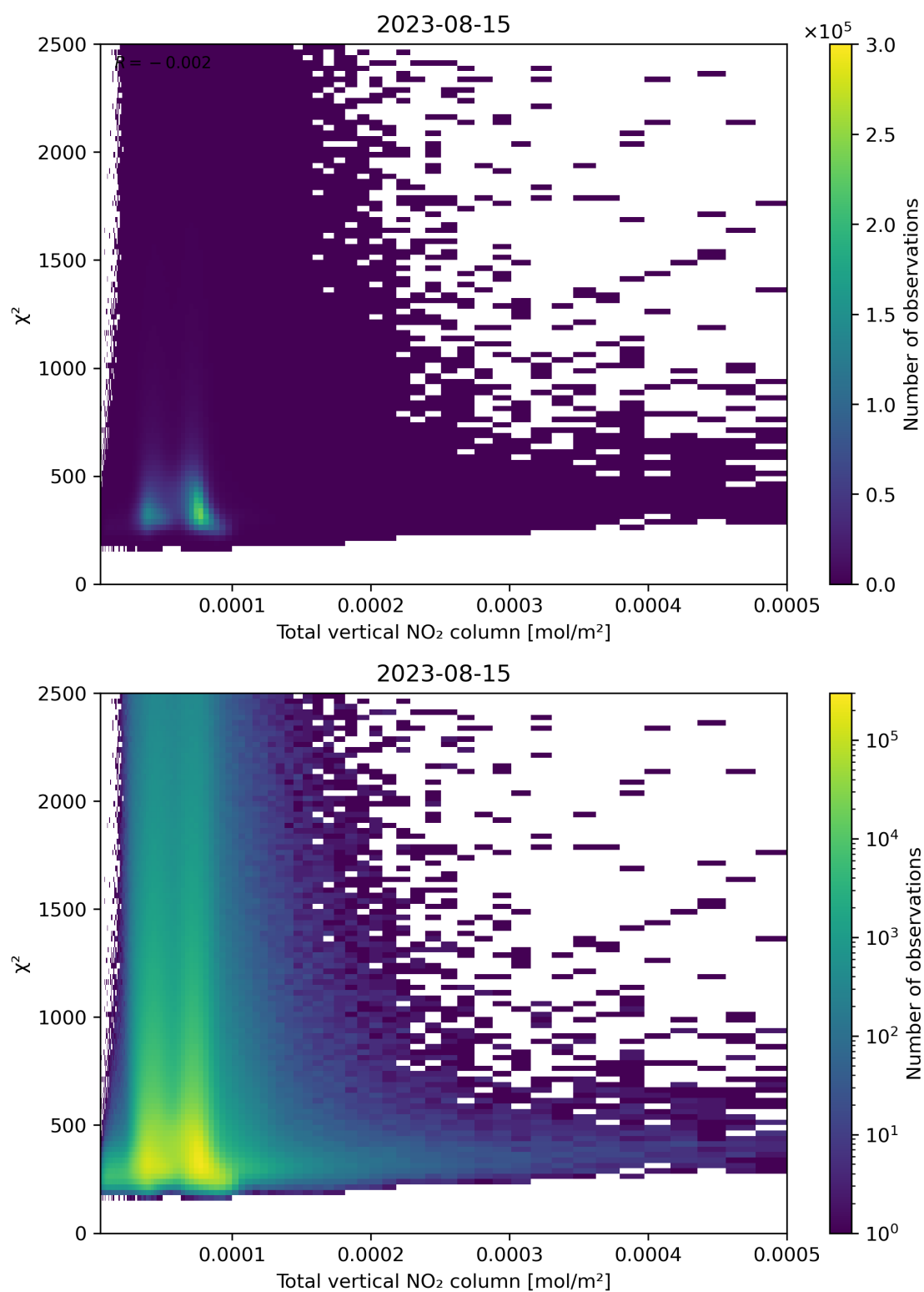
Figure 111: Scatter density plot of “Total vertical NO 2 column” against “ \chi^2 ” for 2023-08-14 to 2023-08-16.
