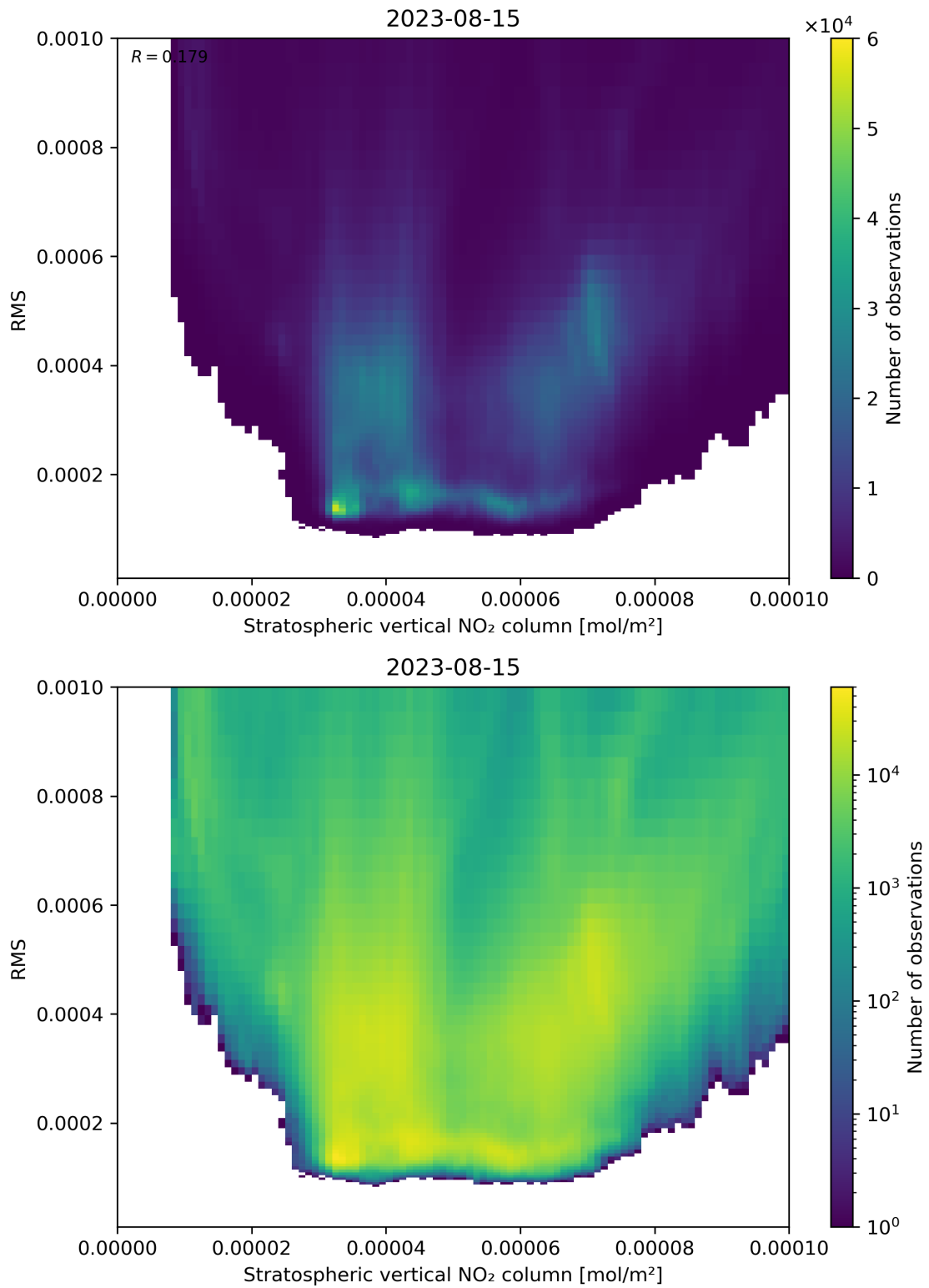
Figure 102: Scatter density plot of “Stratospheric vertical NO 2 column” against “RMS” for 2023-08-14 to 2023-08-16.
