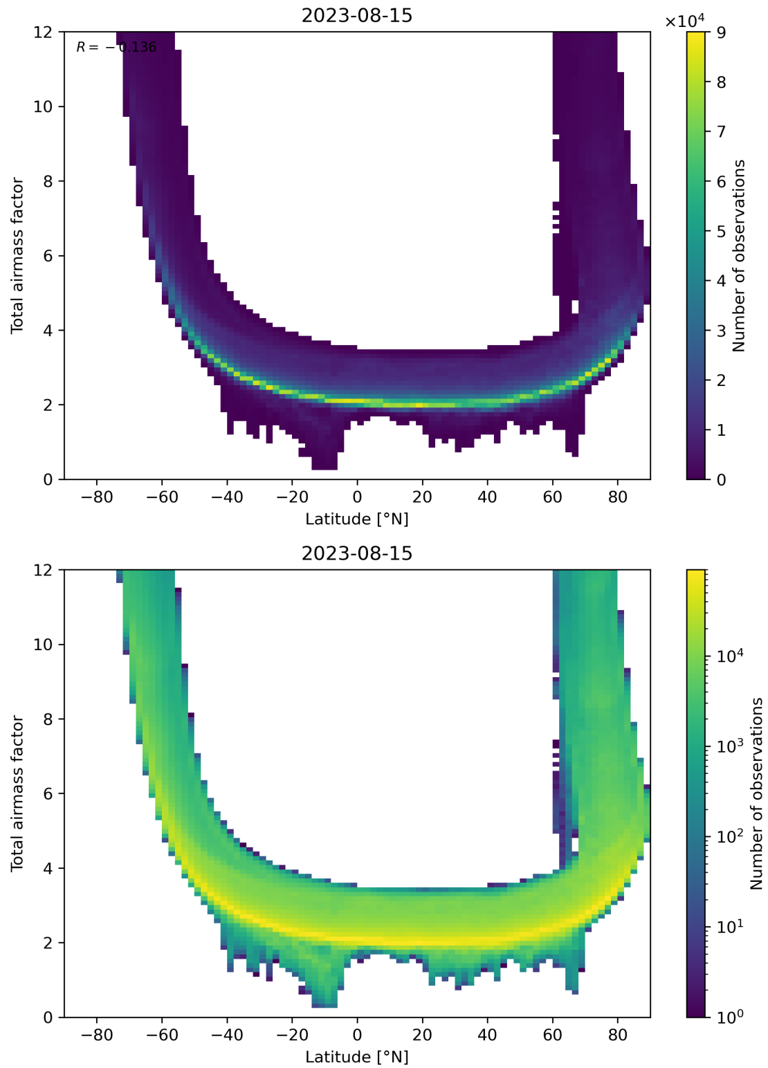
Figure 84: Scatter density plot of “Latitude” against “Total airmass factor” for 2023-08-14 to 2023-08-16.
