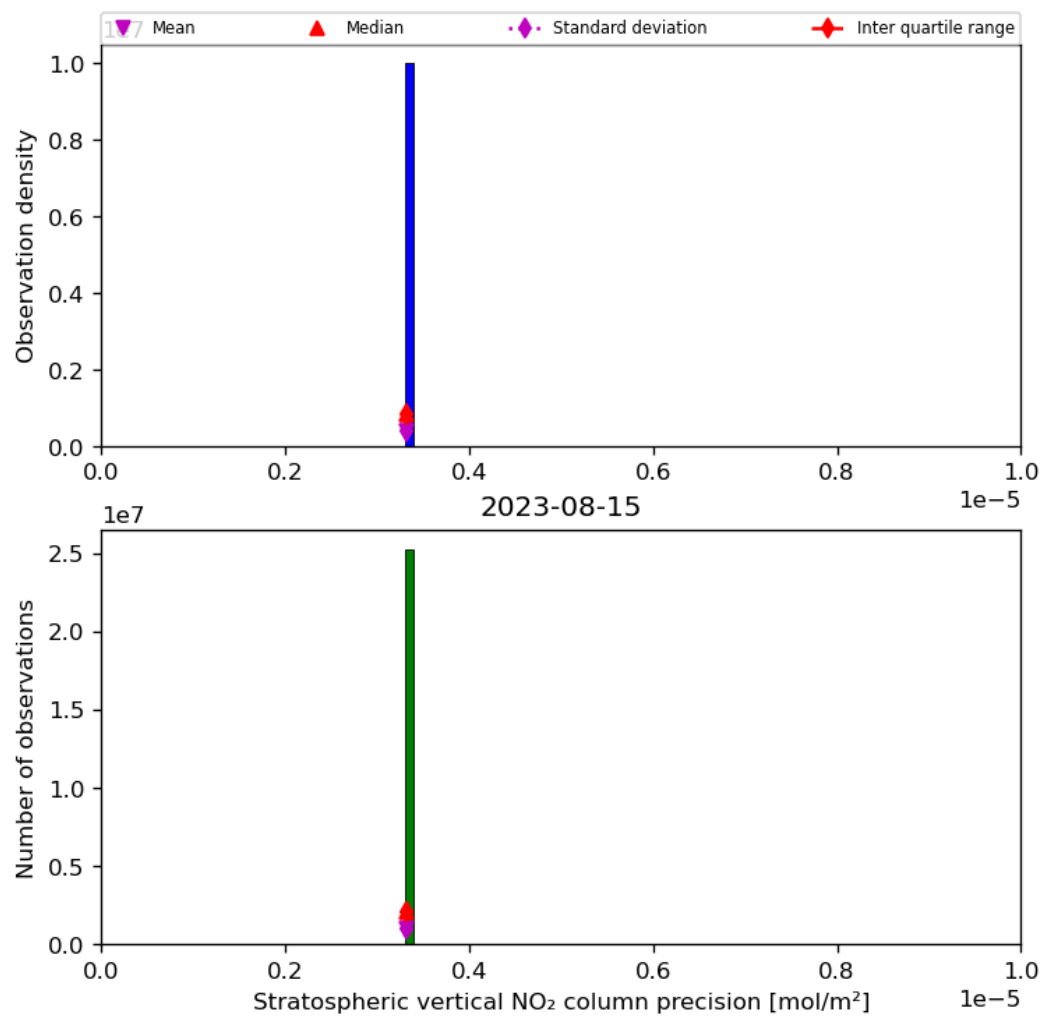
Figure 37: Histogram of “Stratospheric vertical NO 2 column precision” for 2023-08-14 to 2023-08-16
