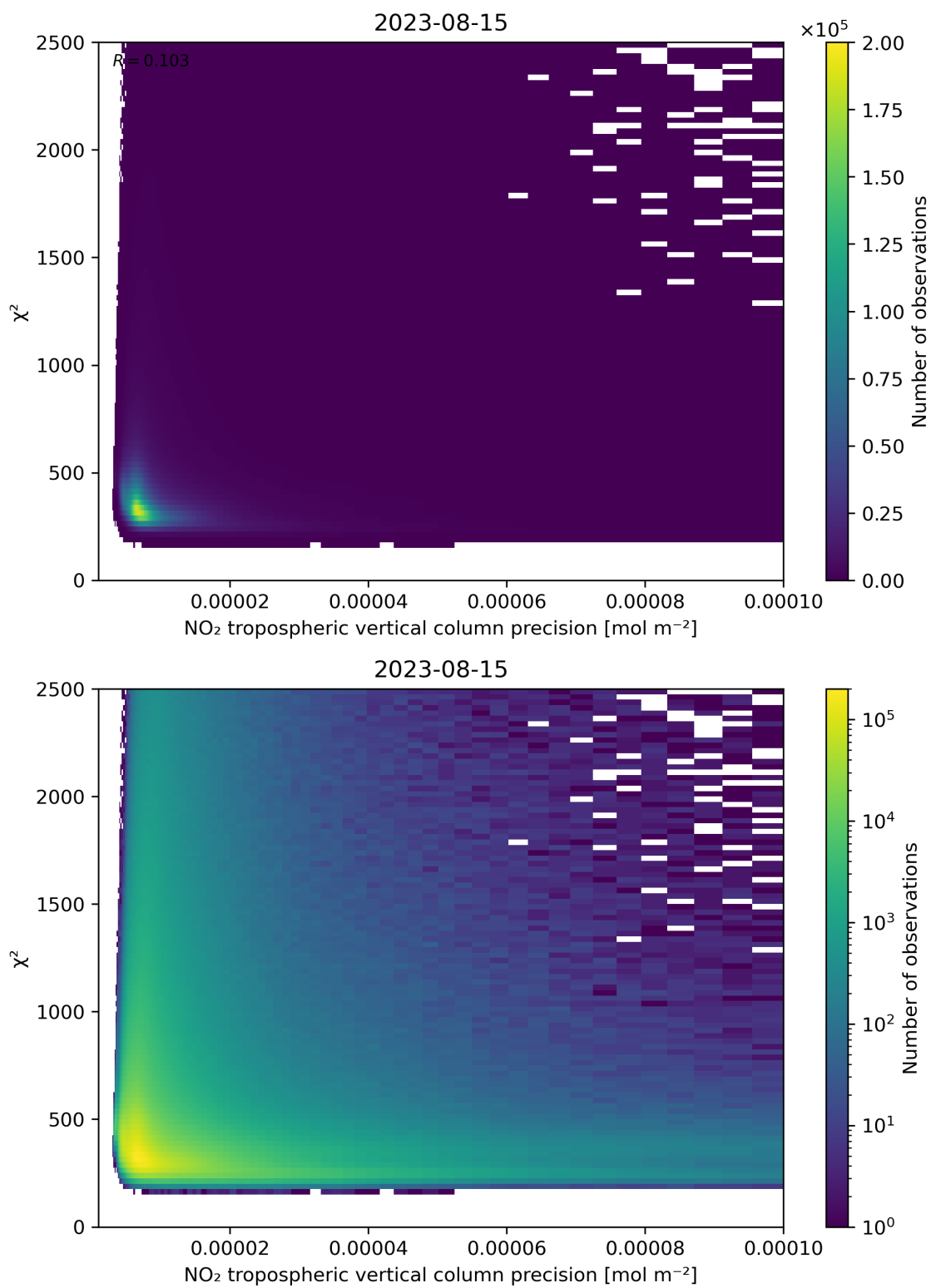
Figure 134: Scatter density plot of “NO 2 tropospheric vertical column precision” against “ \chi^2 ” for 2023-08-14 to 2023-08-16.
