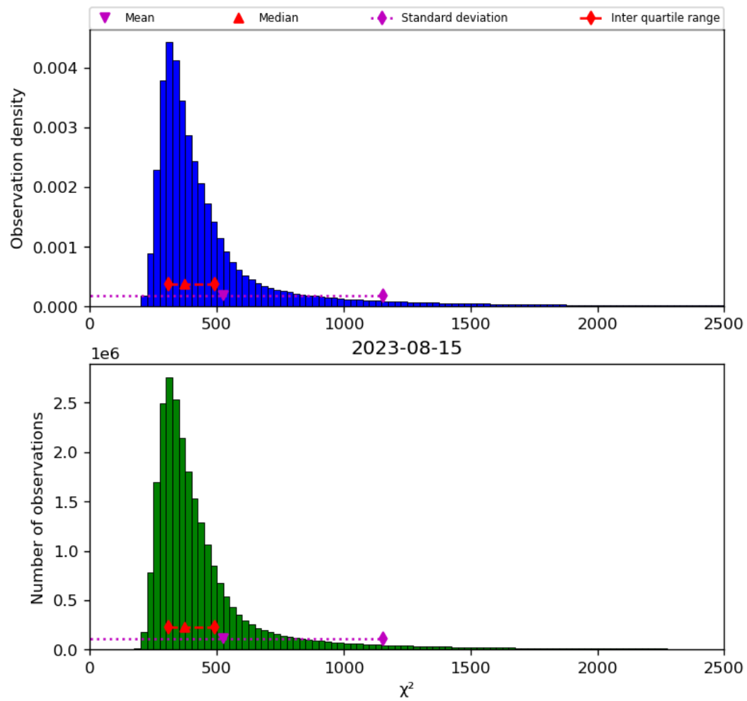
Figure 42: Histogram of “ \chi^2 ” for 2023-08-14 to 2023-08-16
