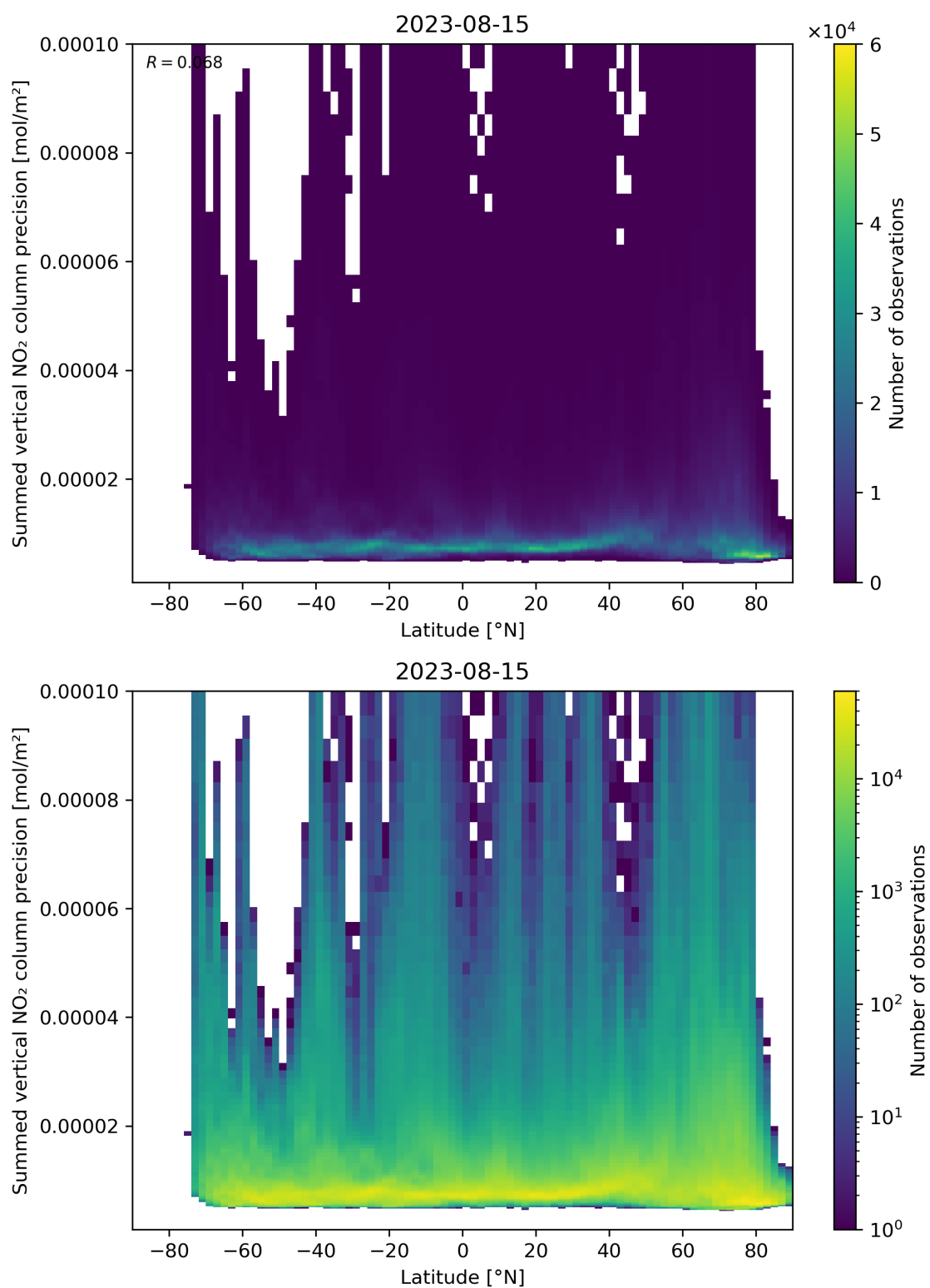
Figure 89: Scatter density plot of “Latitude” against “Summed vertical NO 2 column precision” for 2023-08-14 to 2023-08-16.
