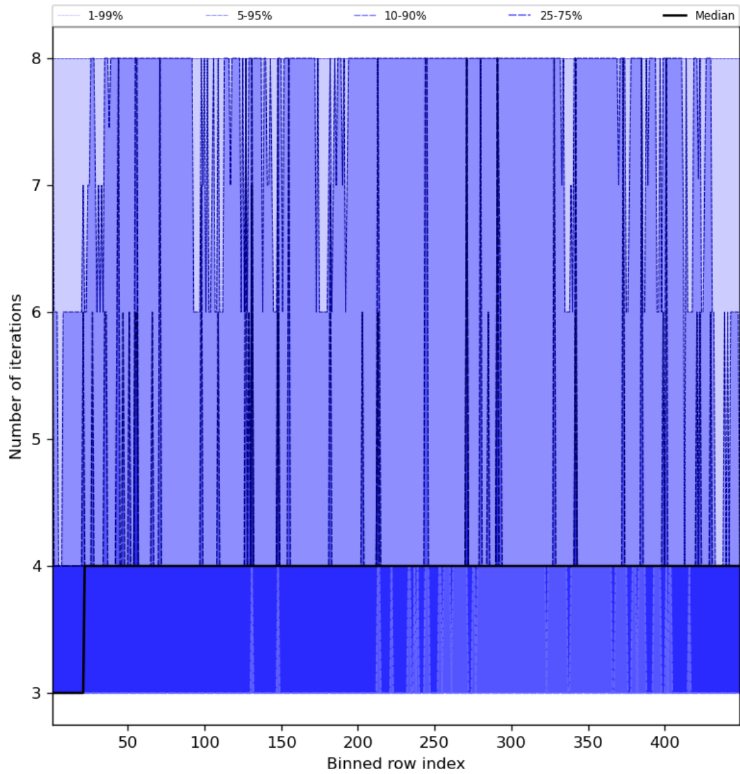
Figure 51: Along track statistics of “Number of iterations” for 2023-08-14 to 2023-08-16
