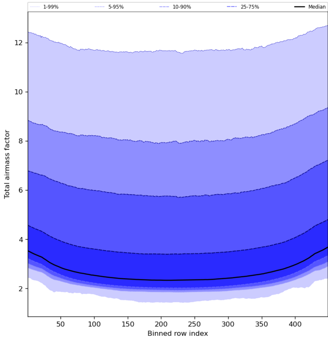
Figure 49: Along track statistics of “Total airmass factor” for 2023-08-14 to 2023-08-16
