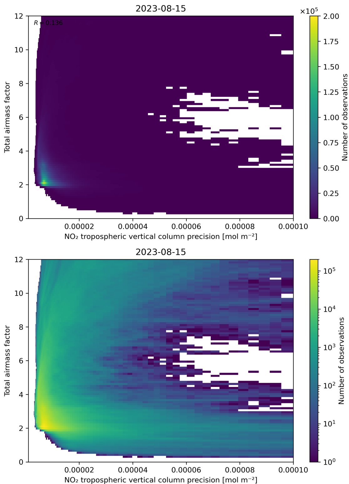
Figure 132: Scatter density plot of “NO 2 tropospheric vertical column precision” against “Total air mass factor” for 2023-08-14 to 2023-08-16.
