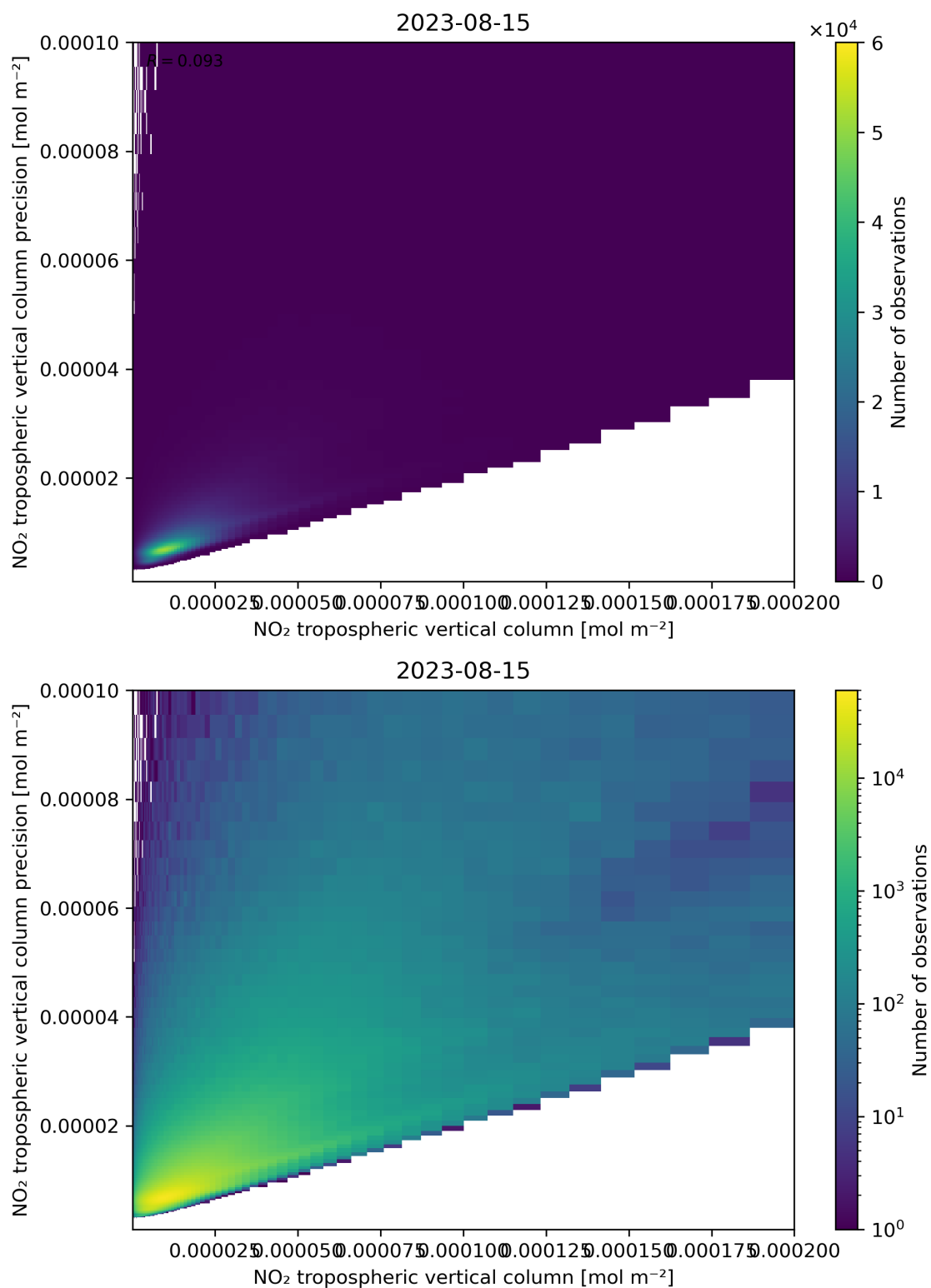
Figure 130: Scatter density plot of “NO 2 tropospheric vertical column” against “NO 2 tropospheric vertical column precision” for 2023-08-14 to 2023-08-16.
