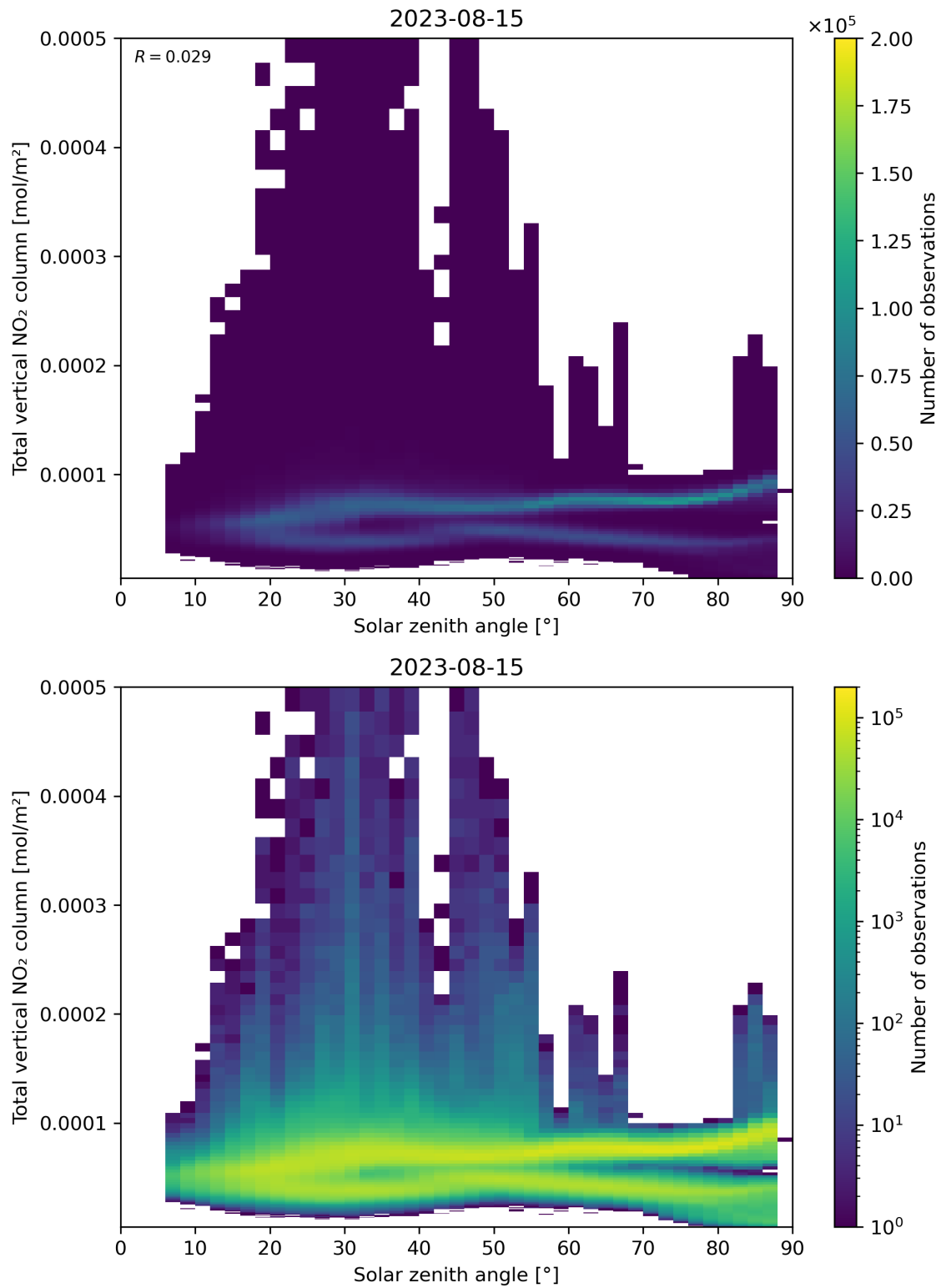
Figure 153: Scatter density plot of “Solar zenith angle” against “Total vertical NO 2 column” for 2023-08-14 to 2023-08-16.
