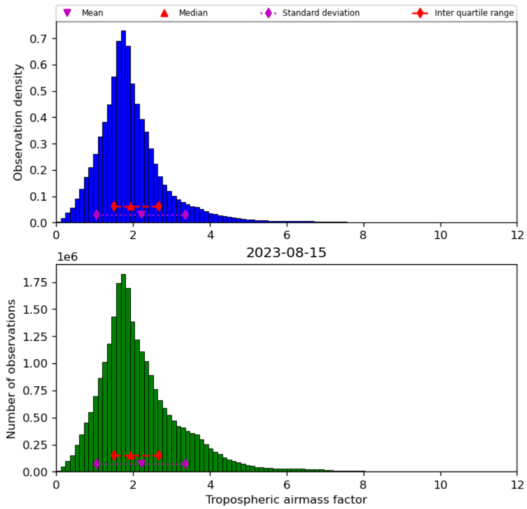
Figure 31: Histogram of “Tropospheric airmass factor” for 2023-08-14 to 2023-08-16
