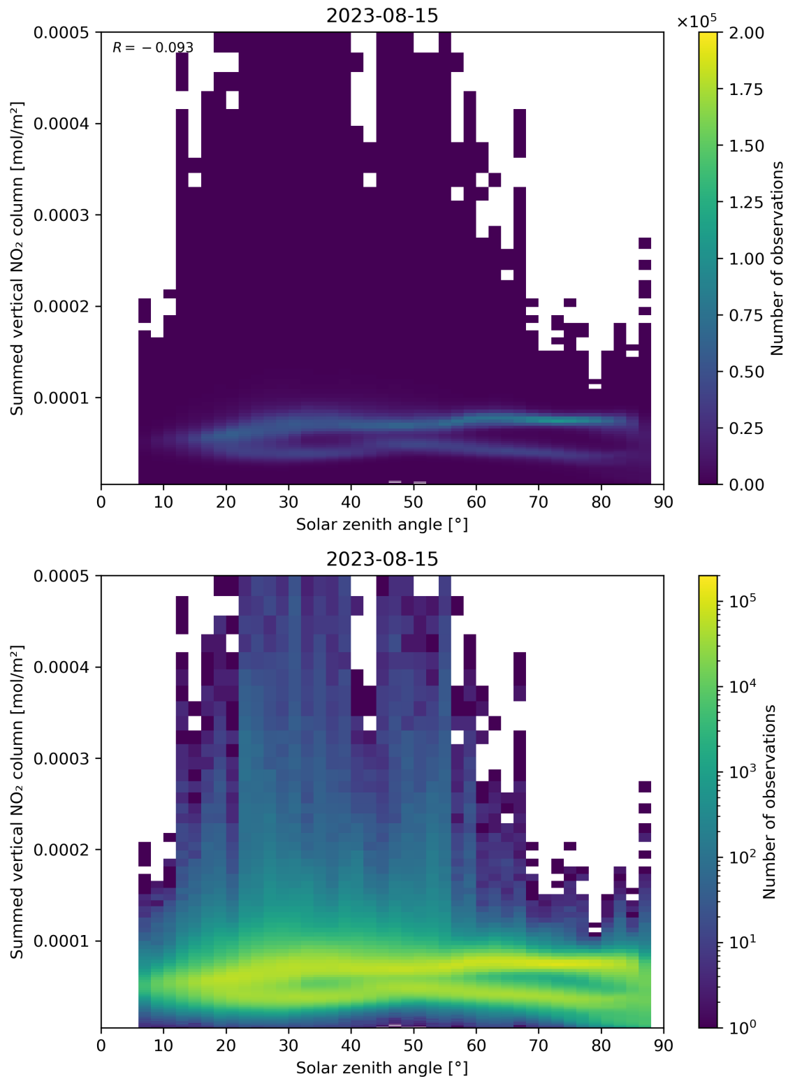
Figure 151: Scatter density plot of “Solar zenith angle” against “Summed vertical NO 2 column” for 2023-08-14 to 2023-08-16.
