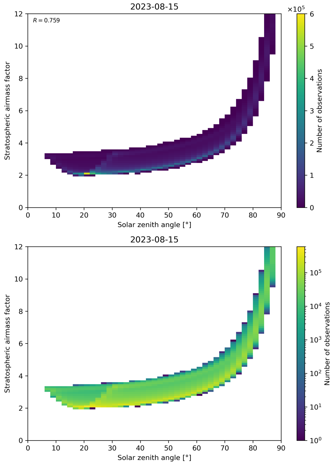
Figure 145: Scatter density plot of “Solar zenith angle” against “Stratospheric airmass factor” for 2023-08-14 to 2023-08-16.
