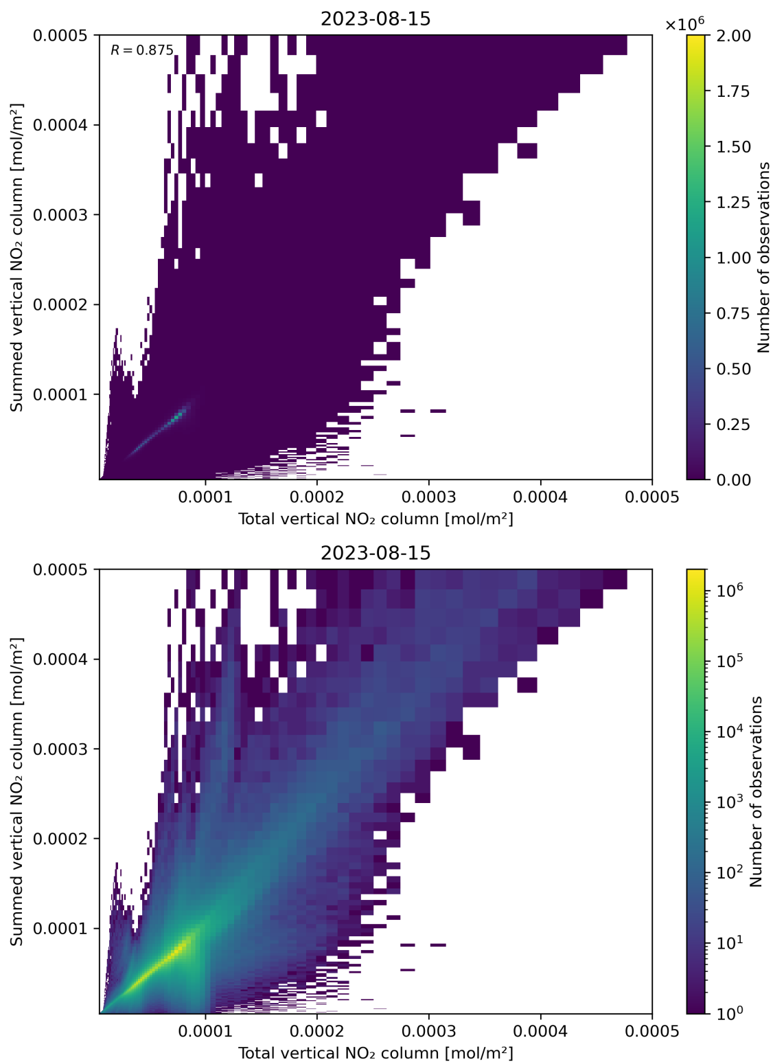
Figure 112: Scatter density plot of “Total vertical NO 2 column” against “Summed vertical NO 2 column” for 2023-08-14 to 2023-08-16.
