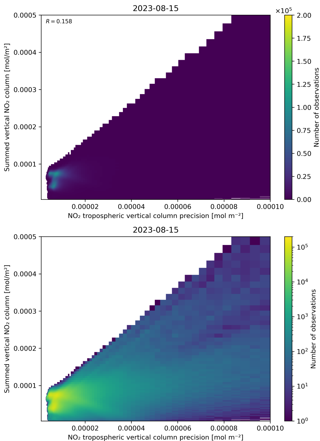
Figure 136: Scatter density plot of “NO 2 tropospheric vertical column precision” against “Summed vertical NO 2 column” for 2023-08-14 to 2023-08-16.
