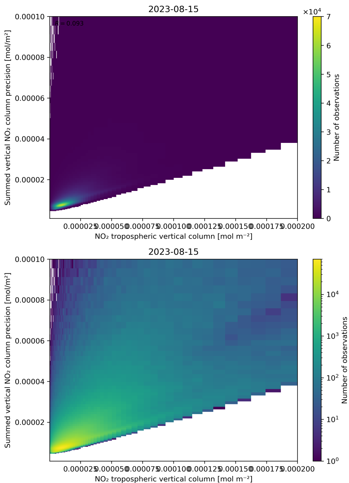
Figure 127: Scatter density plot of “NO 2 tropospheric vertical column” against “Summed vertical NO 2 column precision” for 2023-08-14 to 2023-08-16.
