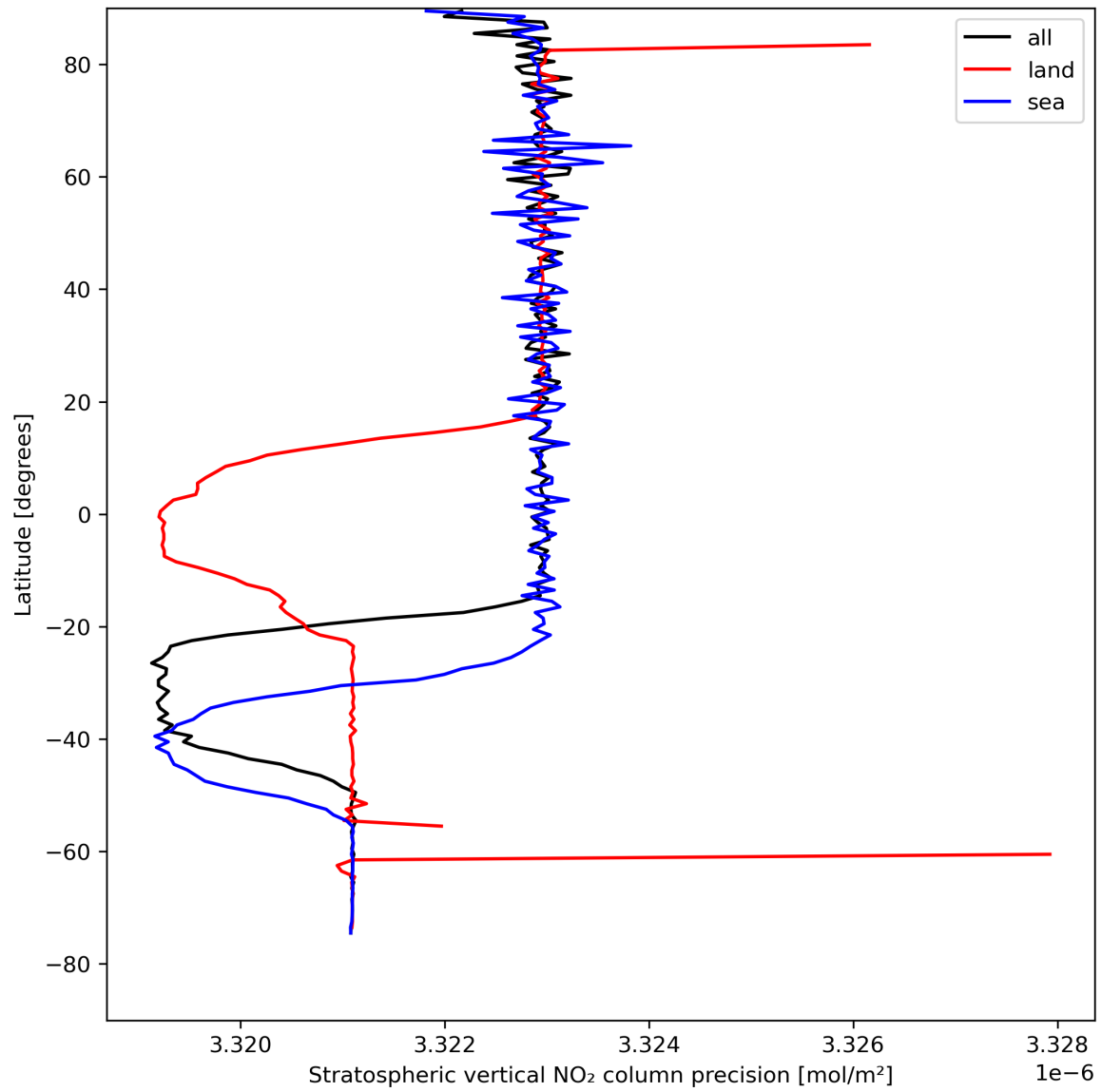
Figure 20: Zonal average of “Stratospheric vertical NO 2 column precision” for 2023-08-14 to 2023-08-16.
