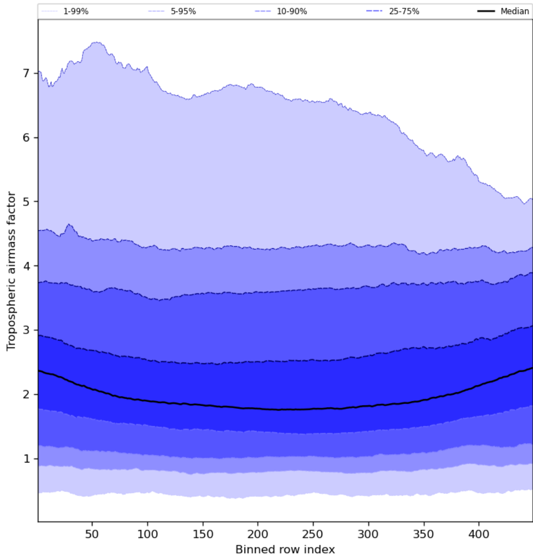
Figure 48: Along track statistics of “Tropospheric airmass factor” for 2023-08-14 to 2023-08-16
