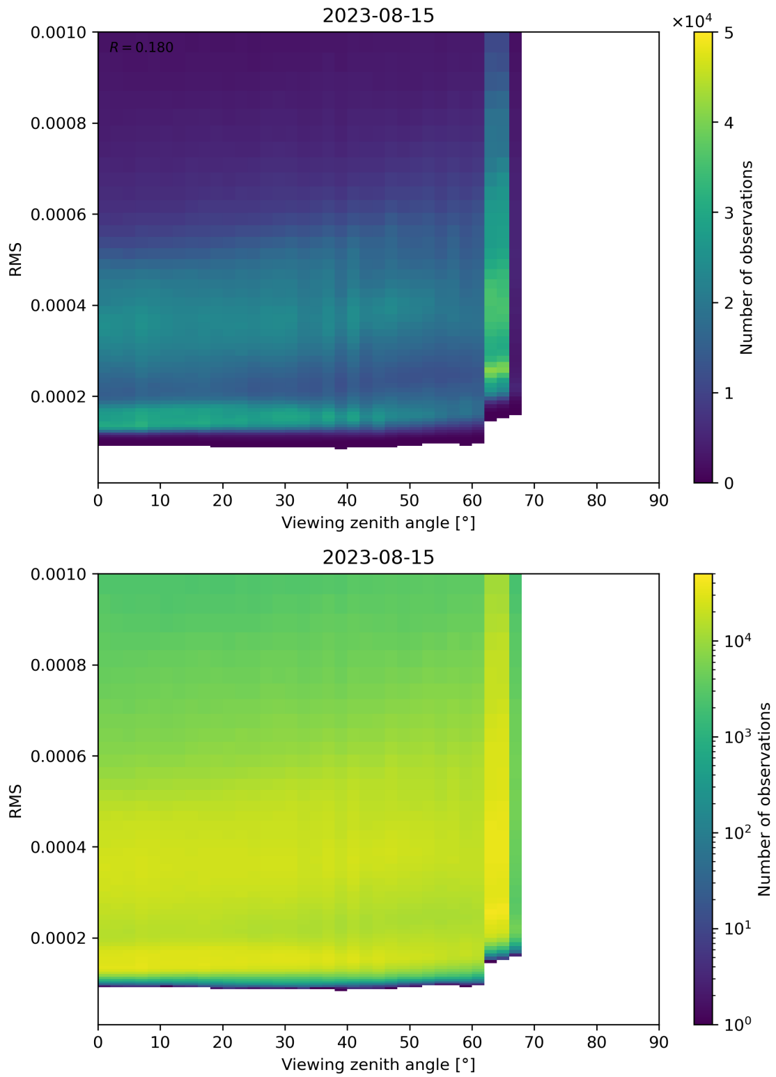
Figure 171: Scatter density plot of “Viewing zenith angle” against “RMS” for 2023-08-14 to 2023-08-16.
