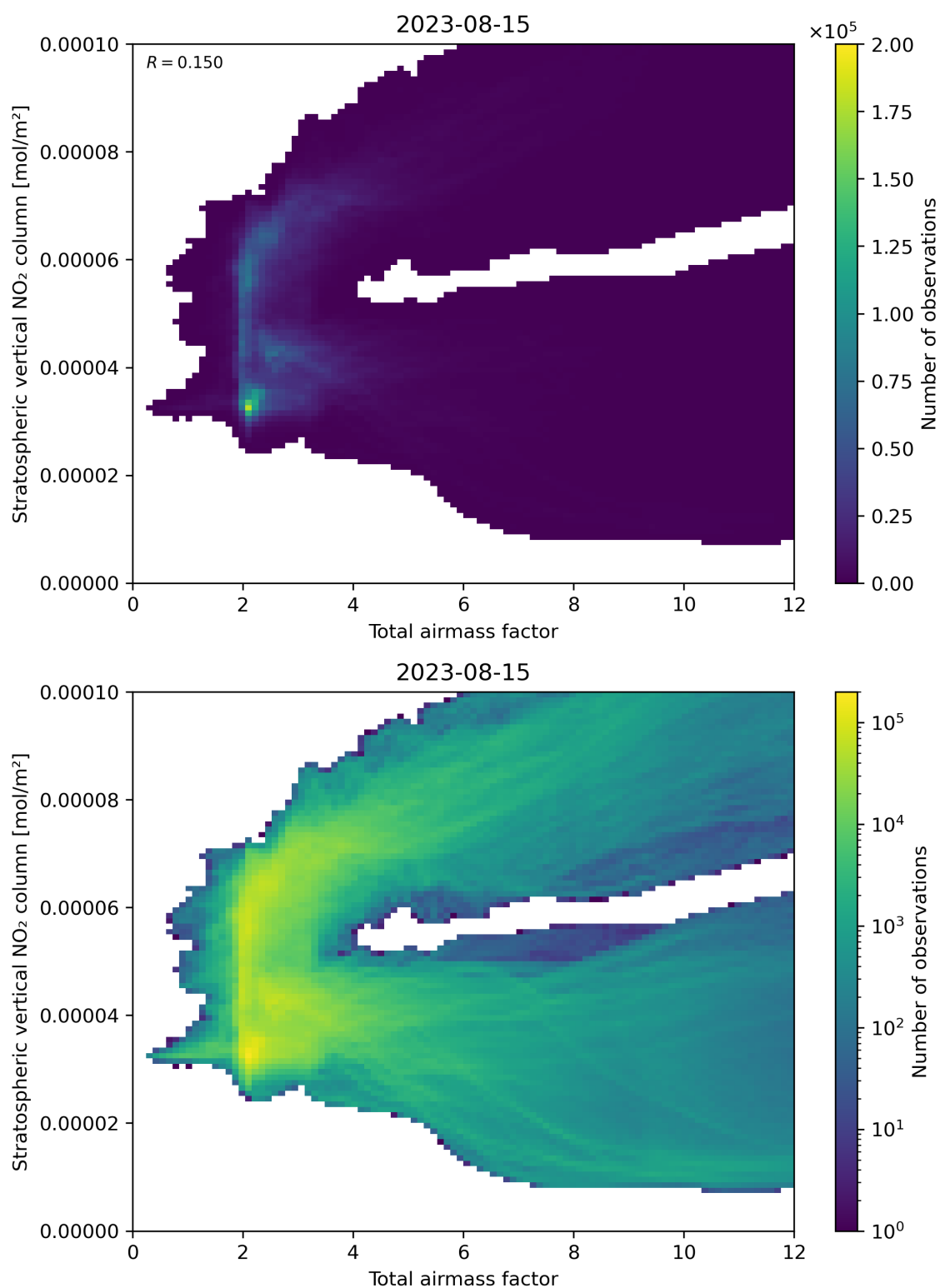
Figure 64: Scatter density plot of “Total airmass factor” against “Stratospheric vertical NO 2 column” for 2023-08-14 to 2023-08-16.
