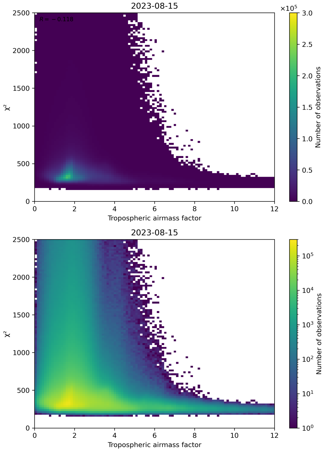
Figure 73: Scatter density plot of “Tropospheric airmass factor” against “ \chi^2 ” for 2023-08-14 to 2023-08-16.
