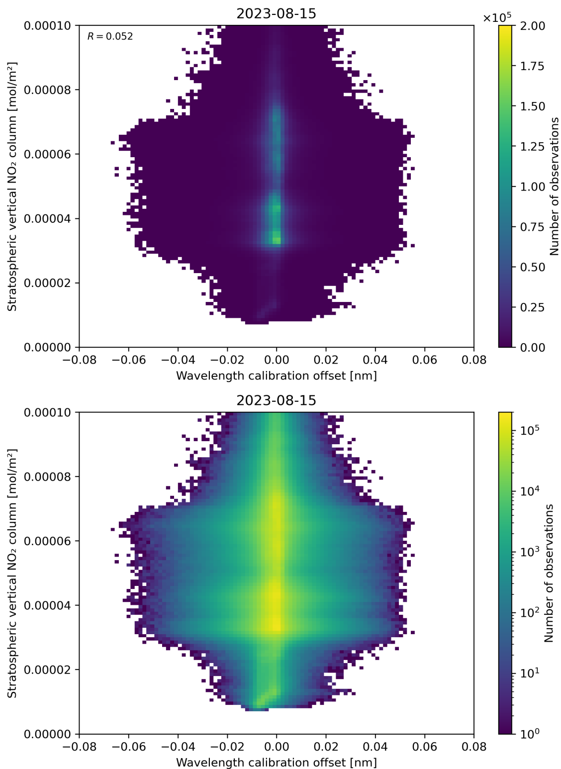
Figure 176: Scatter density plot of “Wavelength calibration offset” against “Stratospheric vertical NO 2 column” for 2023-08-14 to 2023-08-16.
