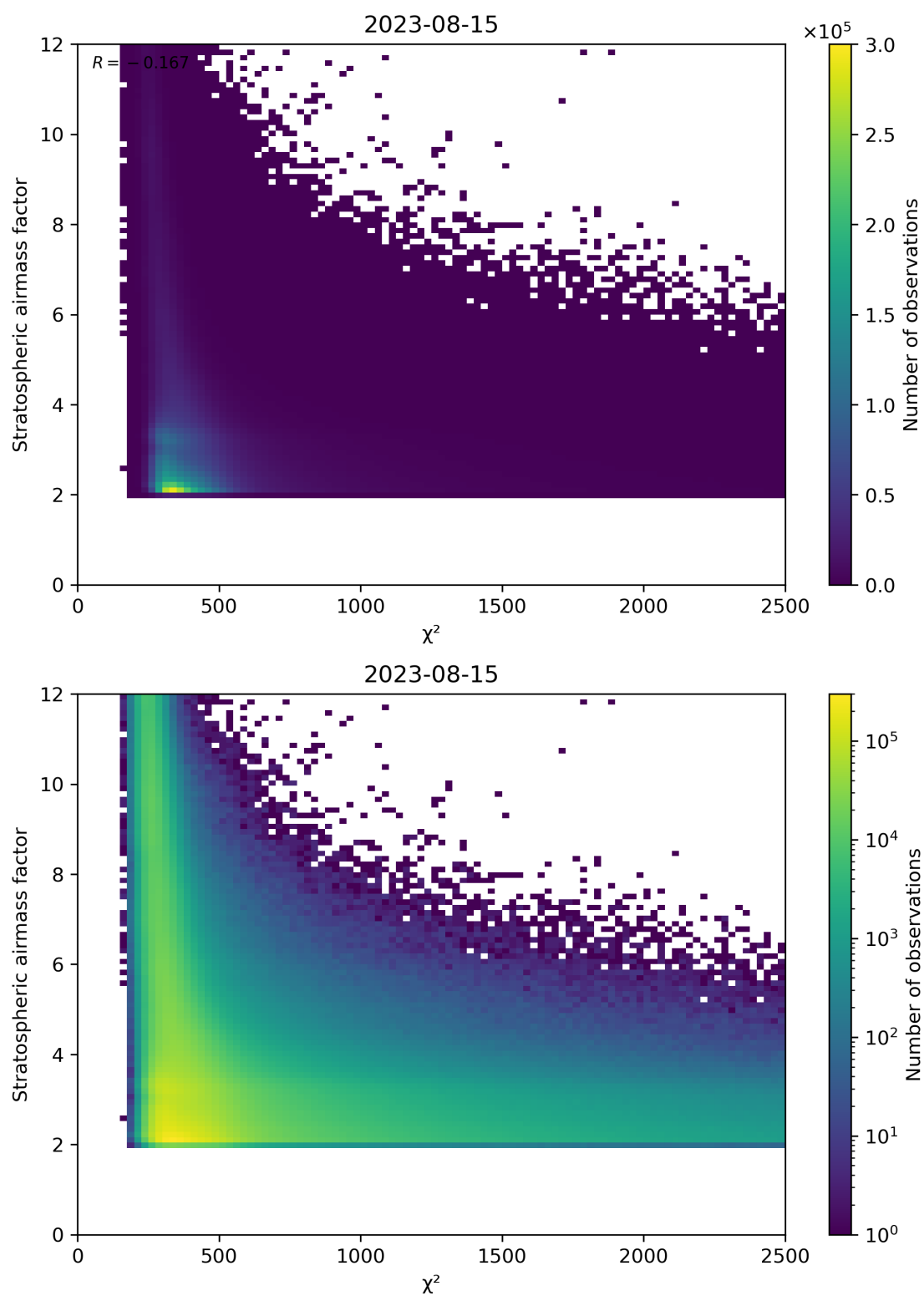
Figure 81: Scatter density plot of “ \chi^2 ” against “Stratospheric airmass factor” for 2023-08-14 to 2023-08-16.
