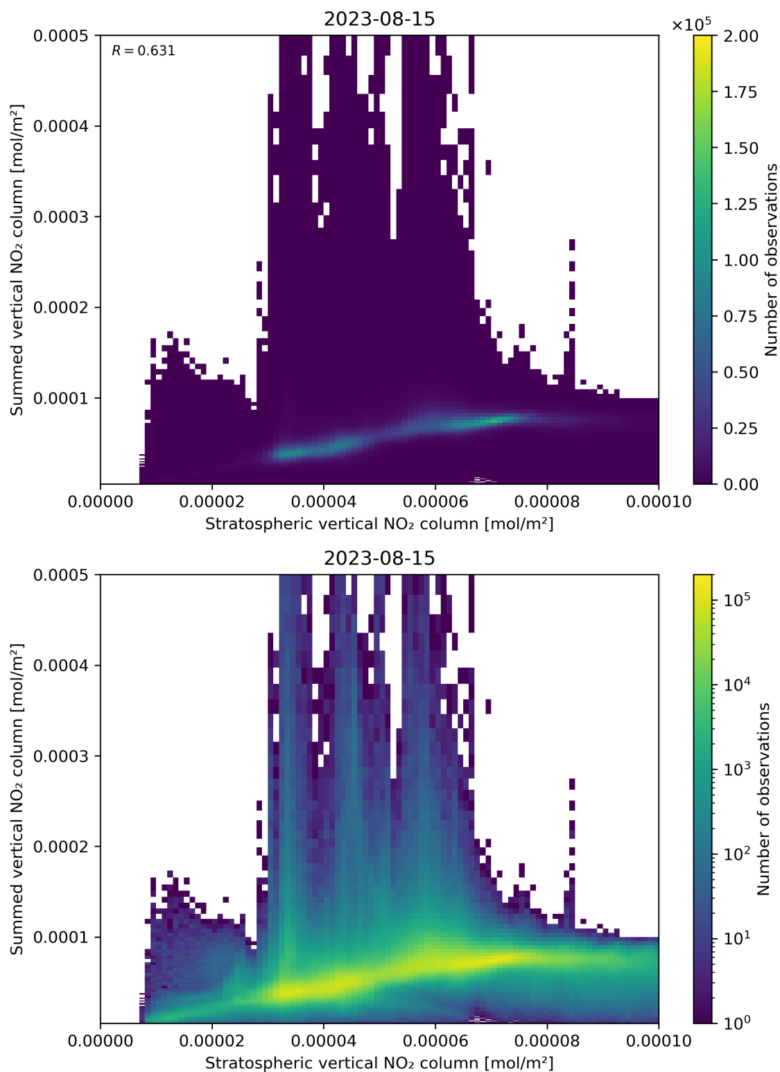
Figure 98: Scatter density plot of “Stratospheric vertical NO 2 column” against “Summed vertical NO 2 column” for 2023-08-14 to 2023-08-16.
