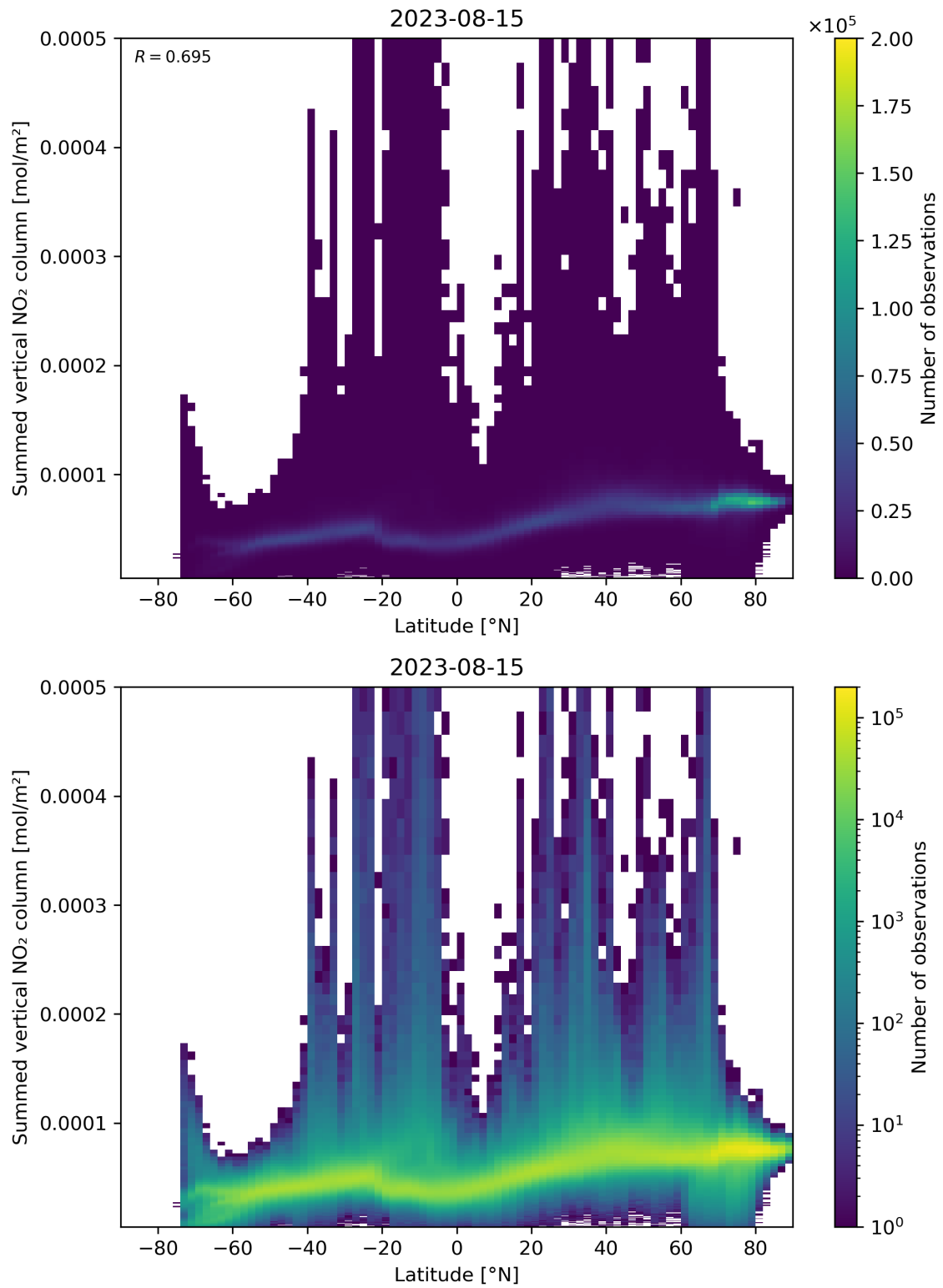
Figure 88: Scatter density plot of “Latitude” against “Summed vertical NO 2 column” for 2023-08-14 to 2023-08-16.
