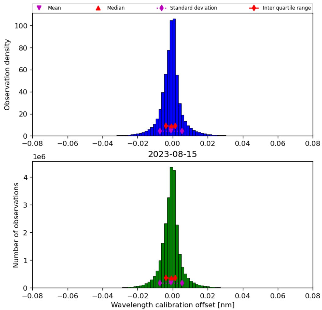
Figure 35: Histogram of “Wavelength calibration offset” for 2023-08-14 to 2023-08-16
