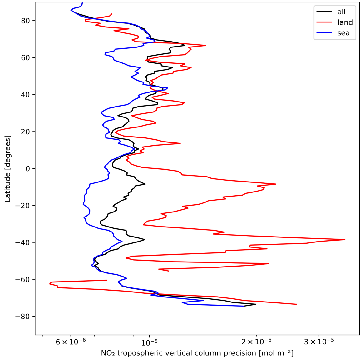
Figure 13: Zonal average of “NO 2 tropospheric vertical column precision” for 2023-08-14 to 2023-08-16.
