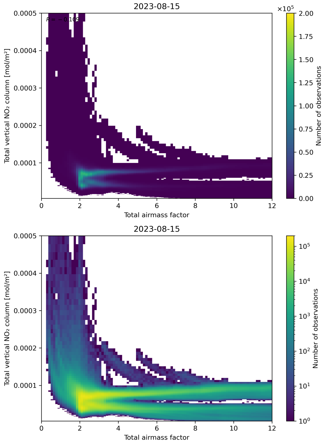
Figure 67: Scatter density plot of “Total airmass factor” against “Total vertical NO 2 column” for 2023-08-14 to 2023-08-16.
