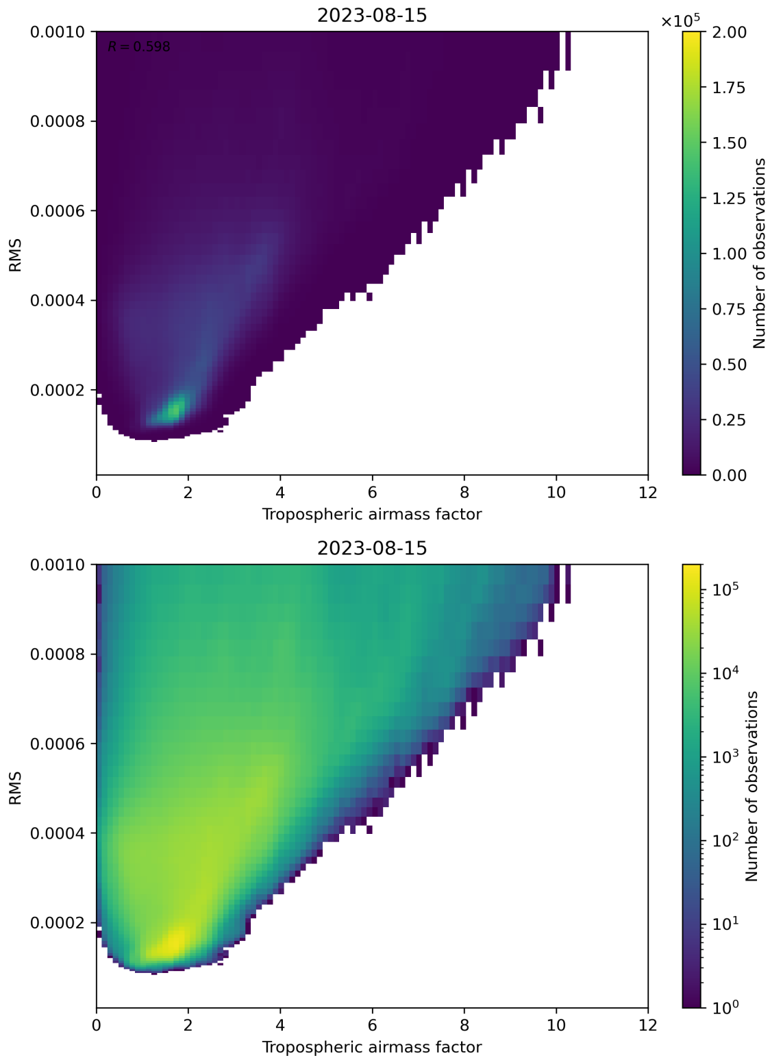
Figure 79: Scatter density plot of “Tropospheric airmass factor” against “RMS” for 2023-08-14 to 2023-08-16.
