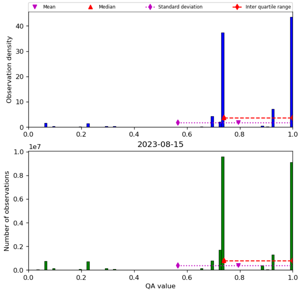
Figure 28: Histogram of “QA value” for 2023-08-14 to 2023-08-16
