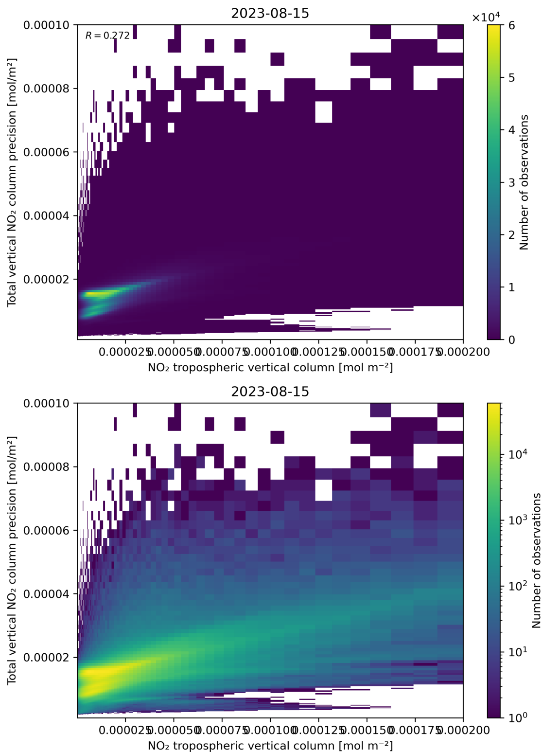
Figure 129: Scatter density plot of “NO 2 tropospheric vertical column” against “Total vertical NO 2 column precision” for 2023-08-14 to 2023-08-16.
