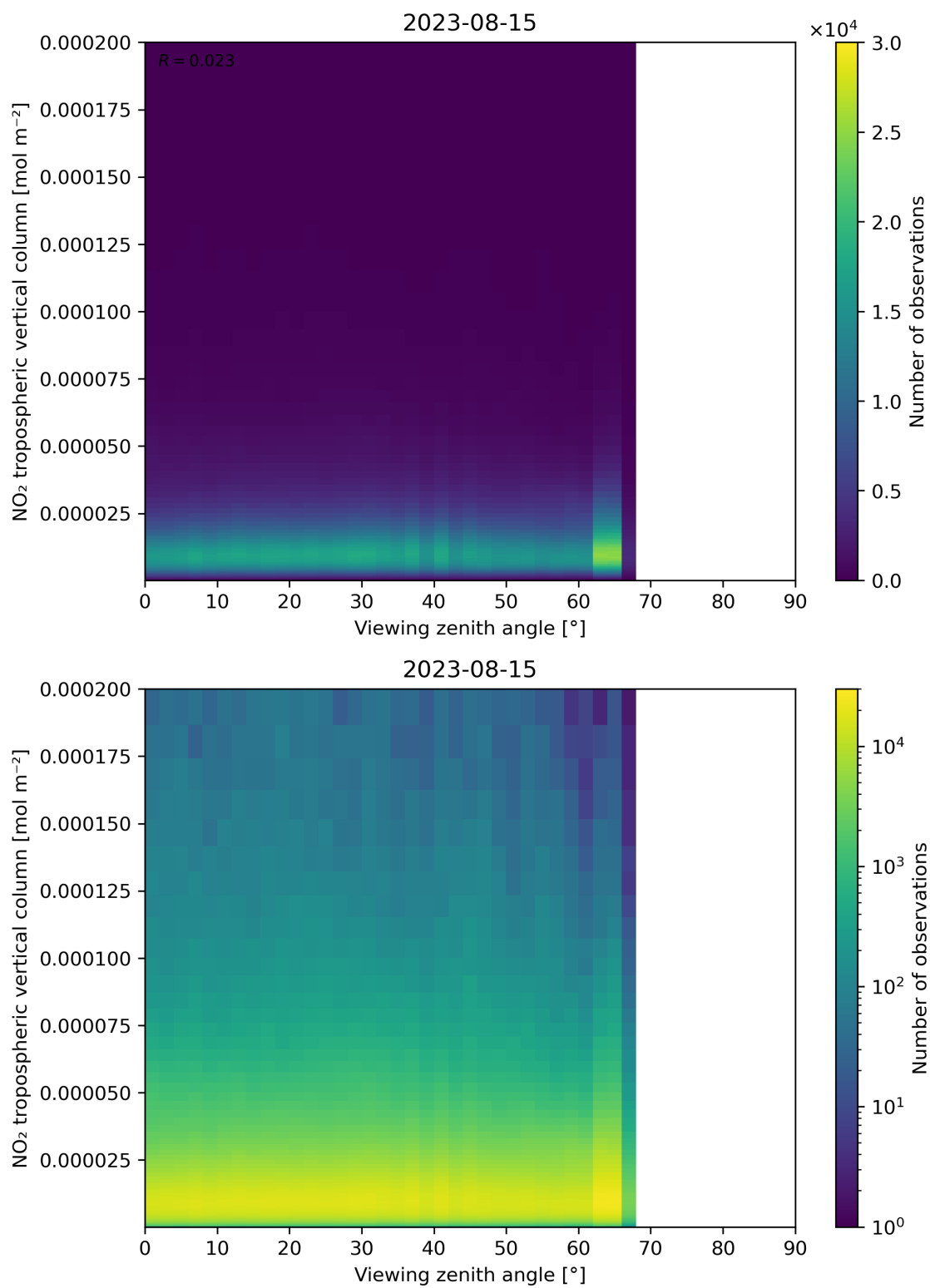
Figure 169: Scatter density plot of “Viewing zenith angle” against “NO 2 tropospheric vertical column” for 2023-08-14 to 2023-08-16.
