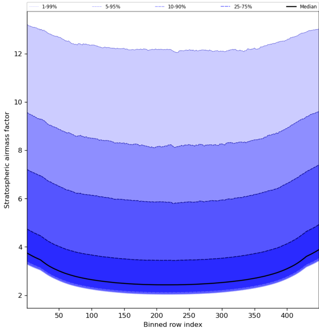
Figure 61: Along track statistics of “Stratospheric airmass factor” for 2023-08-14 to 2023-08-16
