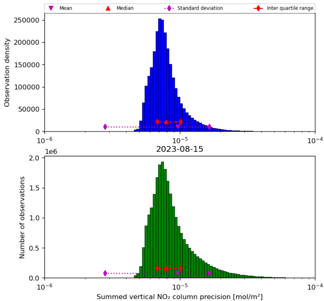
Figure 41: Histogram of “Summed vertical NO 2 column precision” for 2023-08-14 to 2023-08-16
