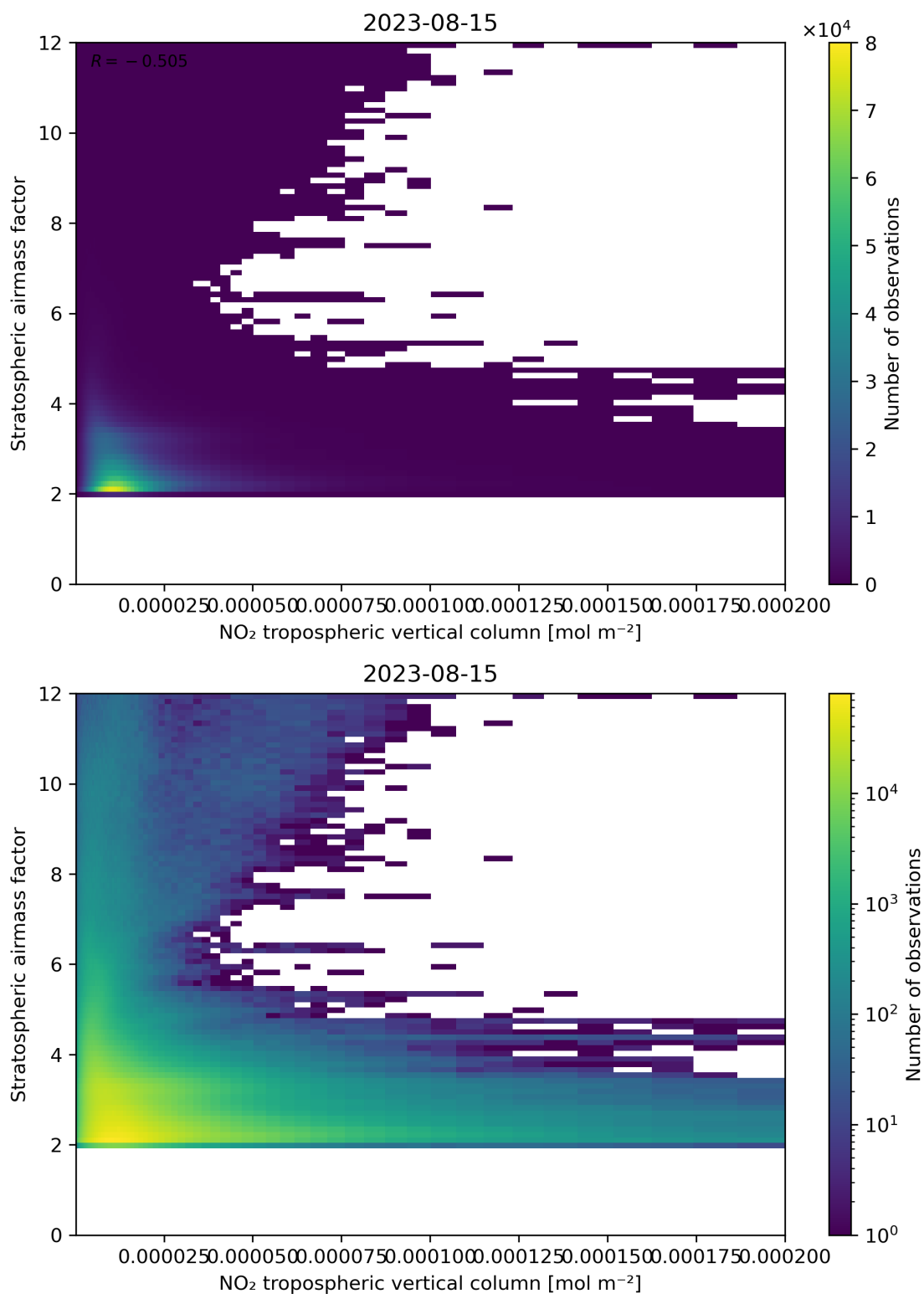
Figure 121: Scatter density plot of “NO 2 tropospheric vertical column” against “Stratospheric air mass factor” for 2023-08-14 to 2023-08-16.
