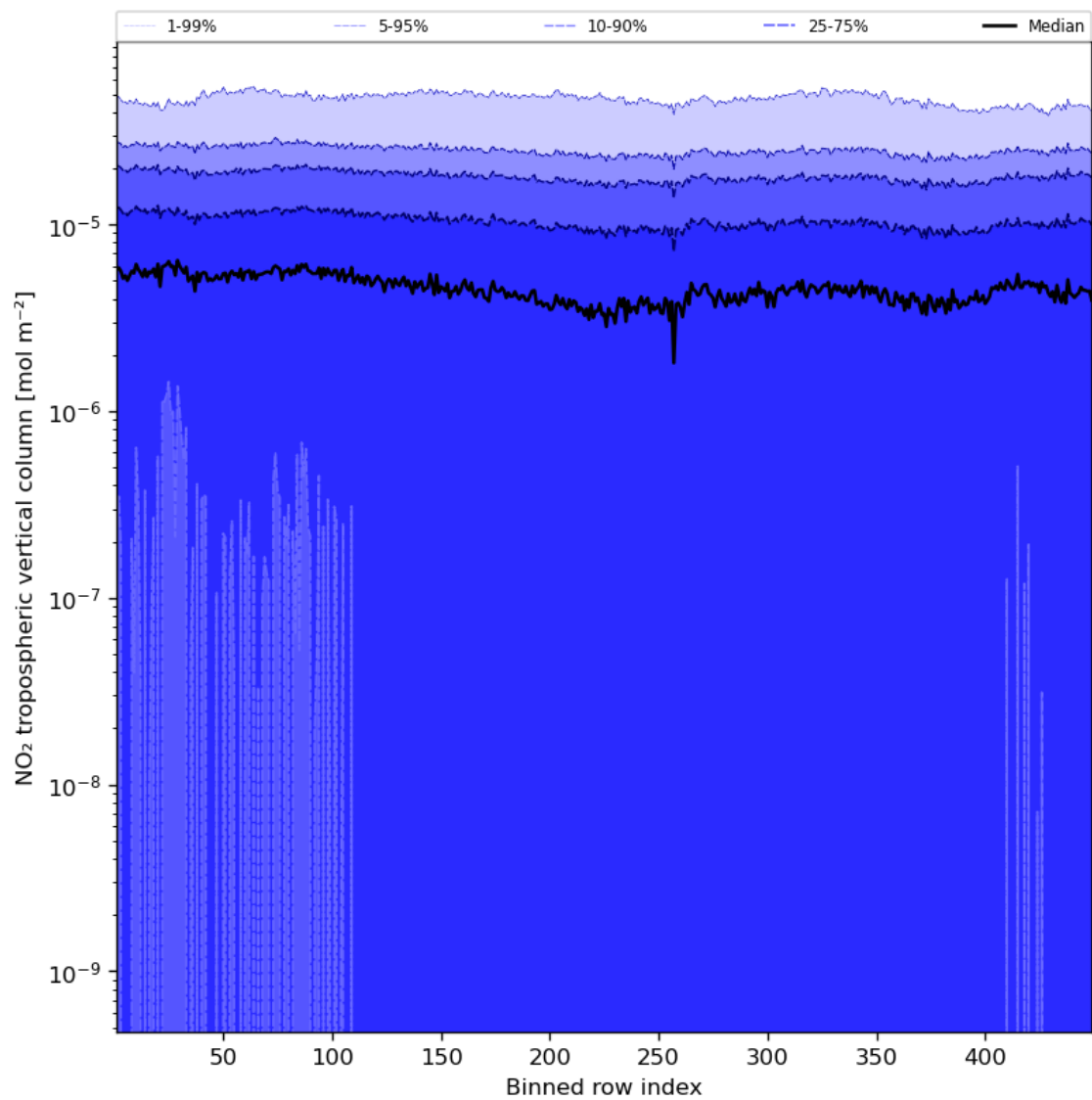
Figure 46: Along track statistics of “NO 2 tropospheric vertical column” for 2023-08-14 to 2023-08-16
