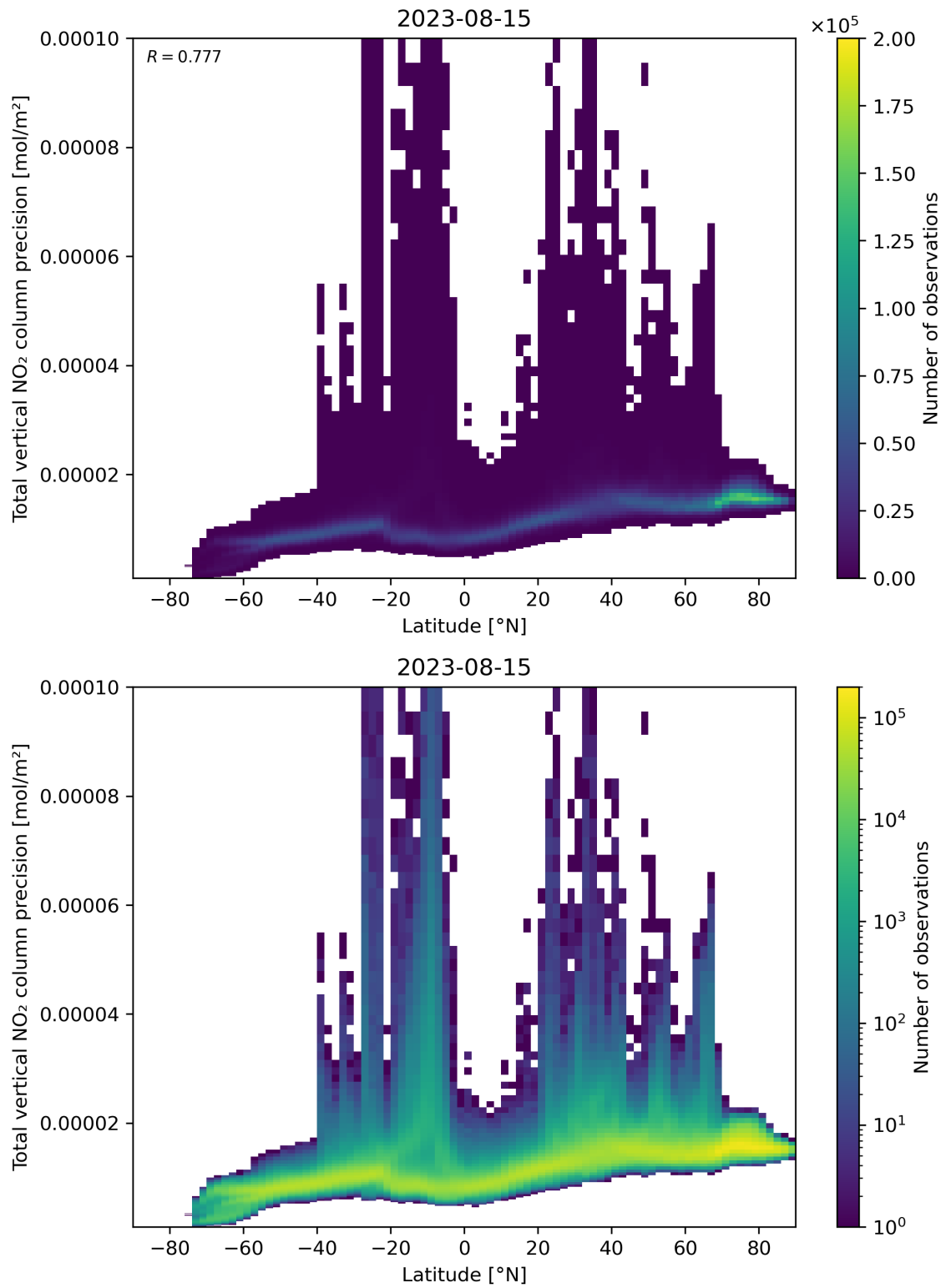
Figure 91: Scatter density plot of “Latitude” against “Total vertical NO 2 column precision” for 2023-08-14 to 2023-08-16.
