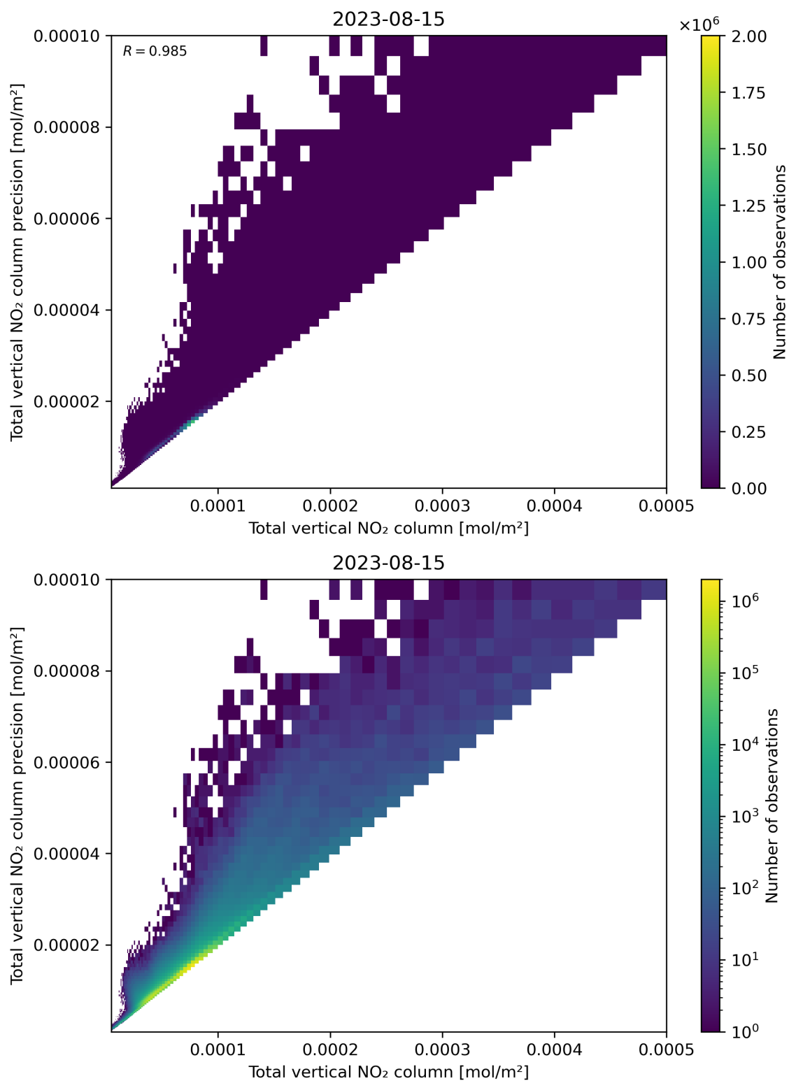
Figure 114: Scatter density plot of “Total vertical NO 2 column” against “Total vertical NO 2 column precision” for 2023-08-14 to 2023-08-16.
