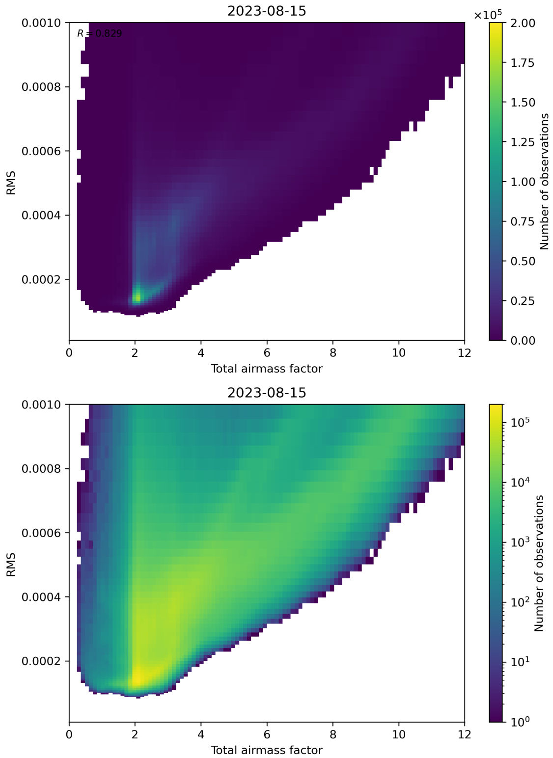
Figure 69: Scatter density plot of “Total airmass factor” against “RMS” for 2023-08-14 to 2023-08-16.
