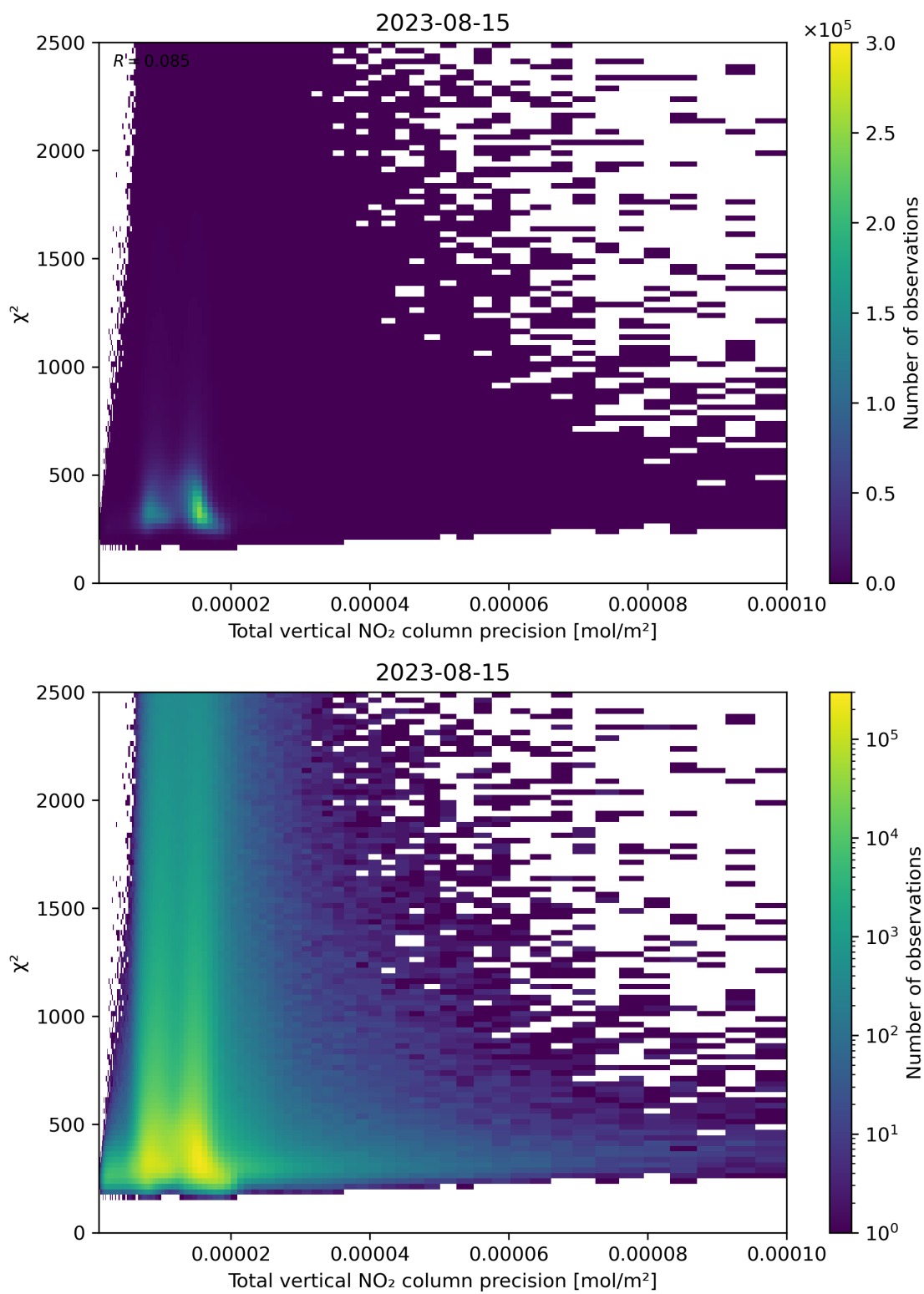
Figure 116: Scatter density plot of “Total vertical NO 2 column precision” against “ \chi^2 ” for 2023-08-14 to 2023-08-16.
