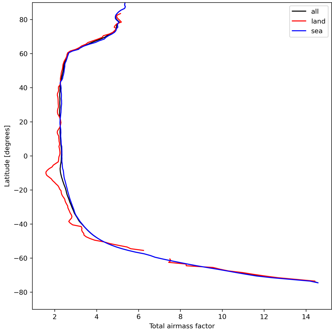
Figure 15: Zonal average of “Total airmass factor” for 2023-08-14 to 2023-08-16.
