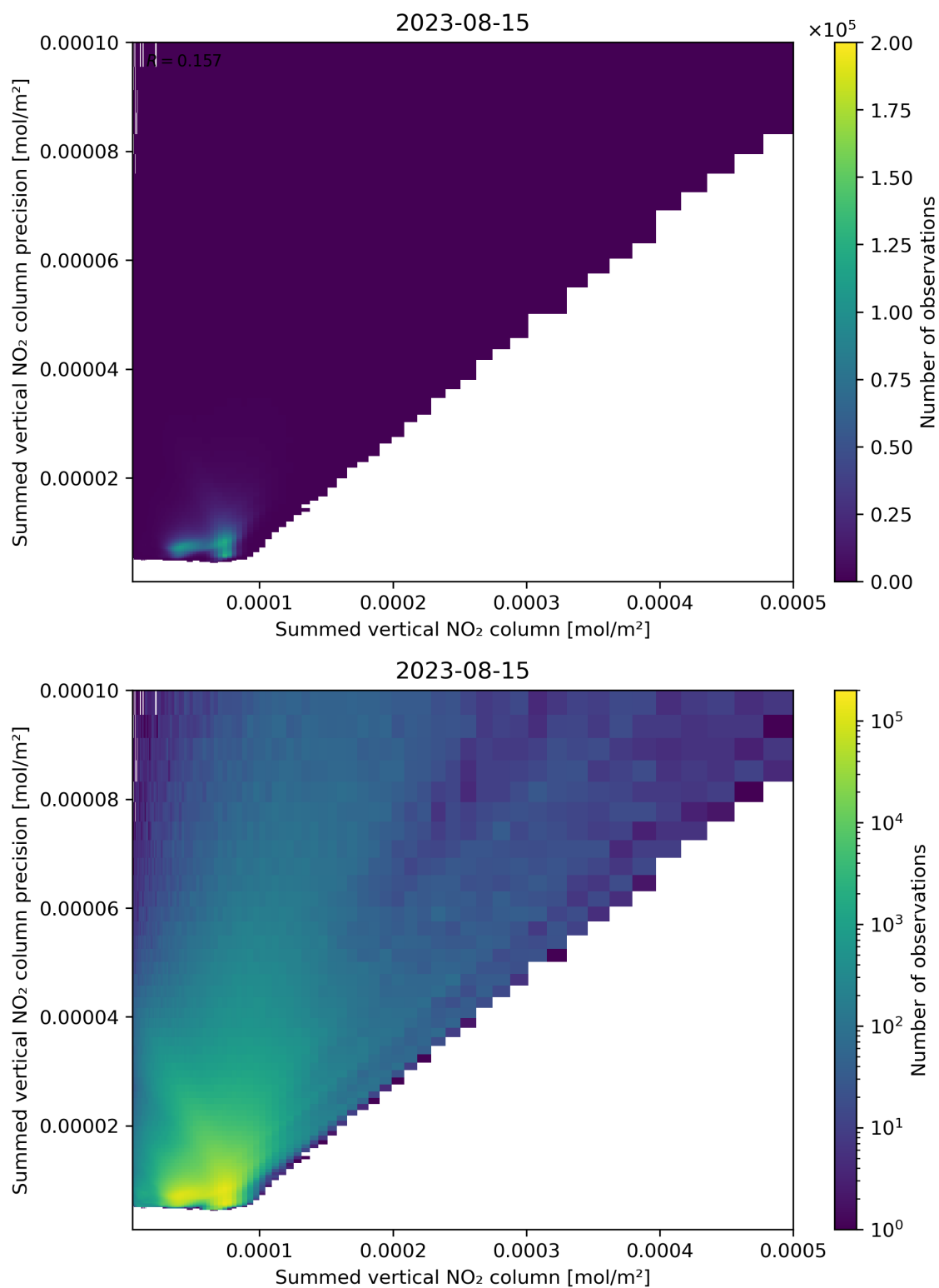
Figure 105: Scatter density plot of “Summed vertical NO 2 column” against “Summed vertical NO 2 column precision” for 2023-08-14 to 2023-08-16.
