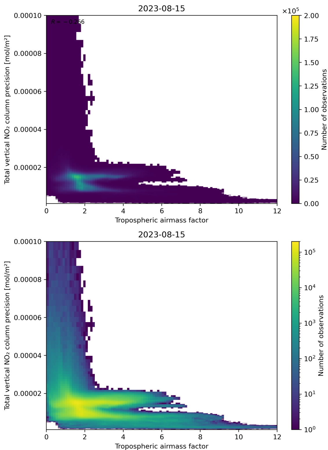
Figure 78: Scatter density plot of “Tropospheric air mass factor” against “Total vertical NO 2 column precision” for 2023-08-14 to 2023-08-16.
