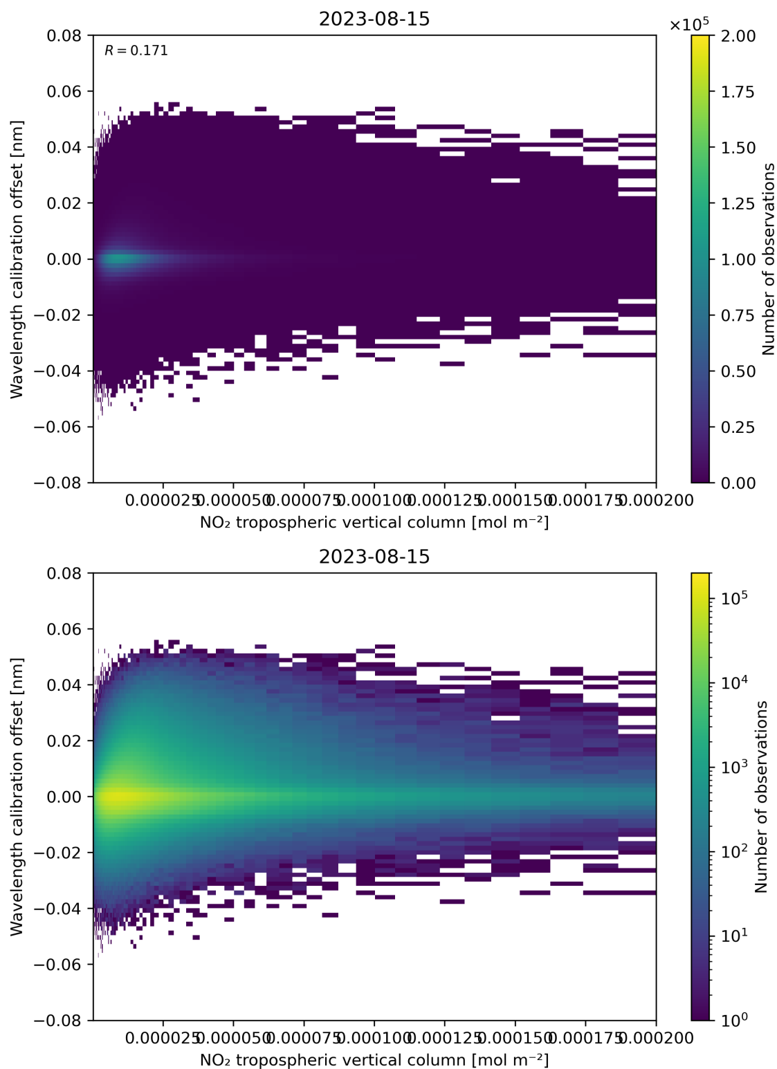
Figure 143: Scatter density plot of “NO 2 tropospheric vertical column” against “Wavelength calibration offset” for 2023-08-14 to 2023-08-16.
