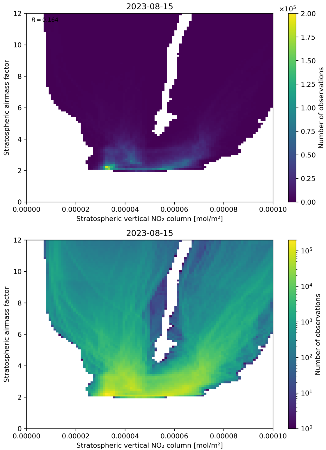
Figure 96: Scatter density plot of “Stratospheric vertical NO 2 column” against “Stratospheric airmass factor” for 2023-08-14 to 2023-08-16.
