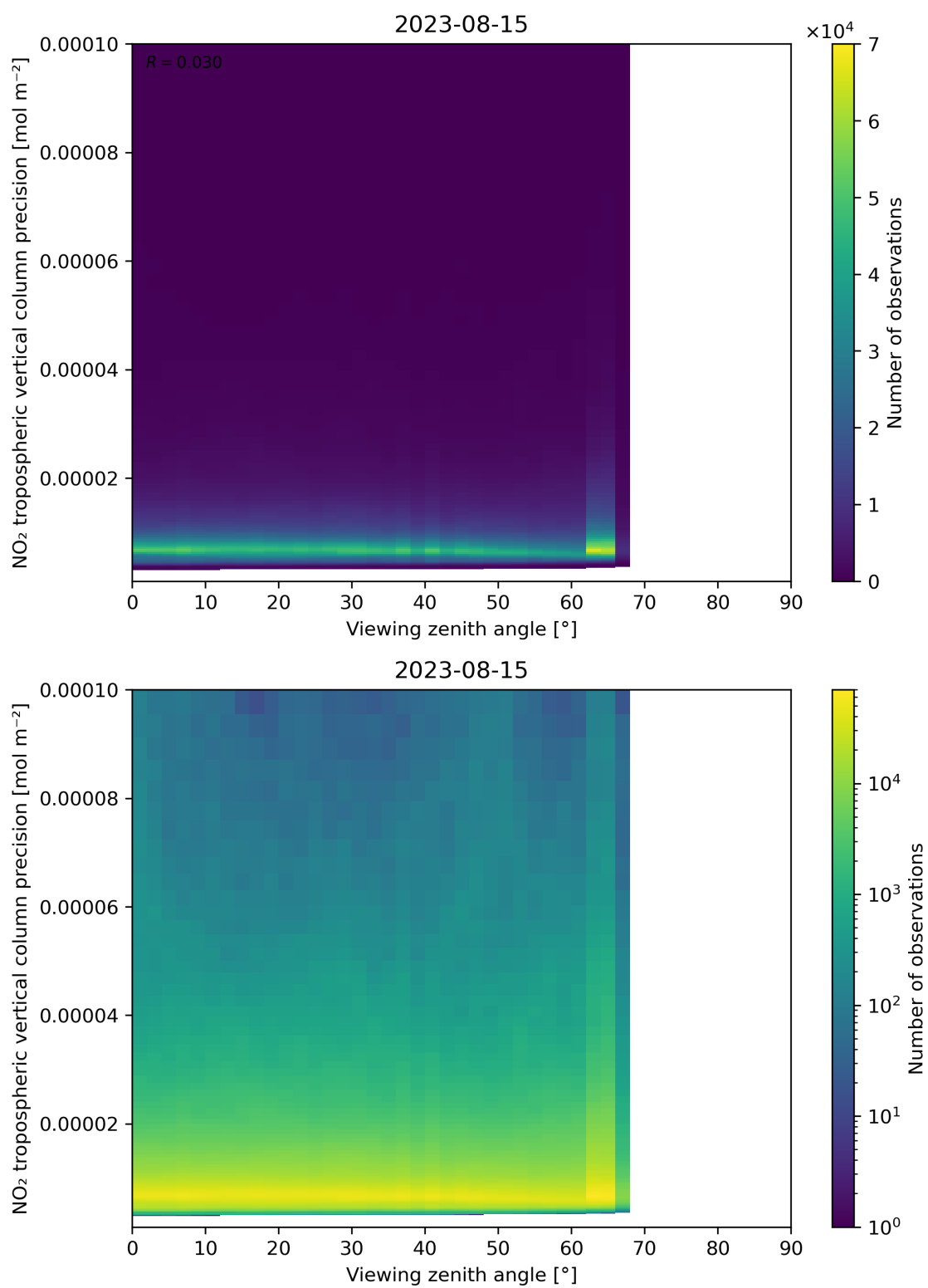
Figure 170: Scatter density plot of “Viewing zenith angle” against “NO 2 tropospheric vertical column precision” for 2023-08-14 to 2023-08-16.
