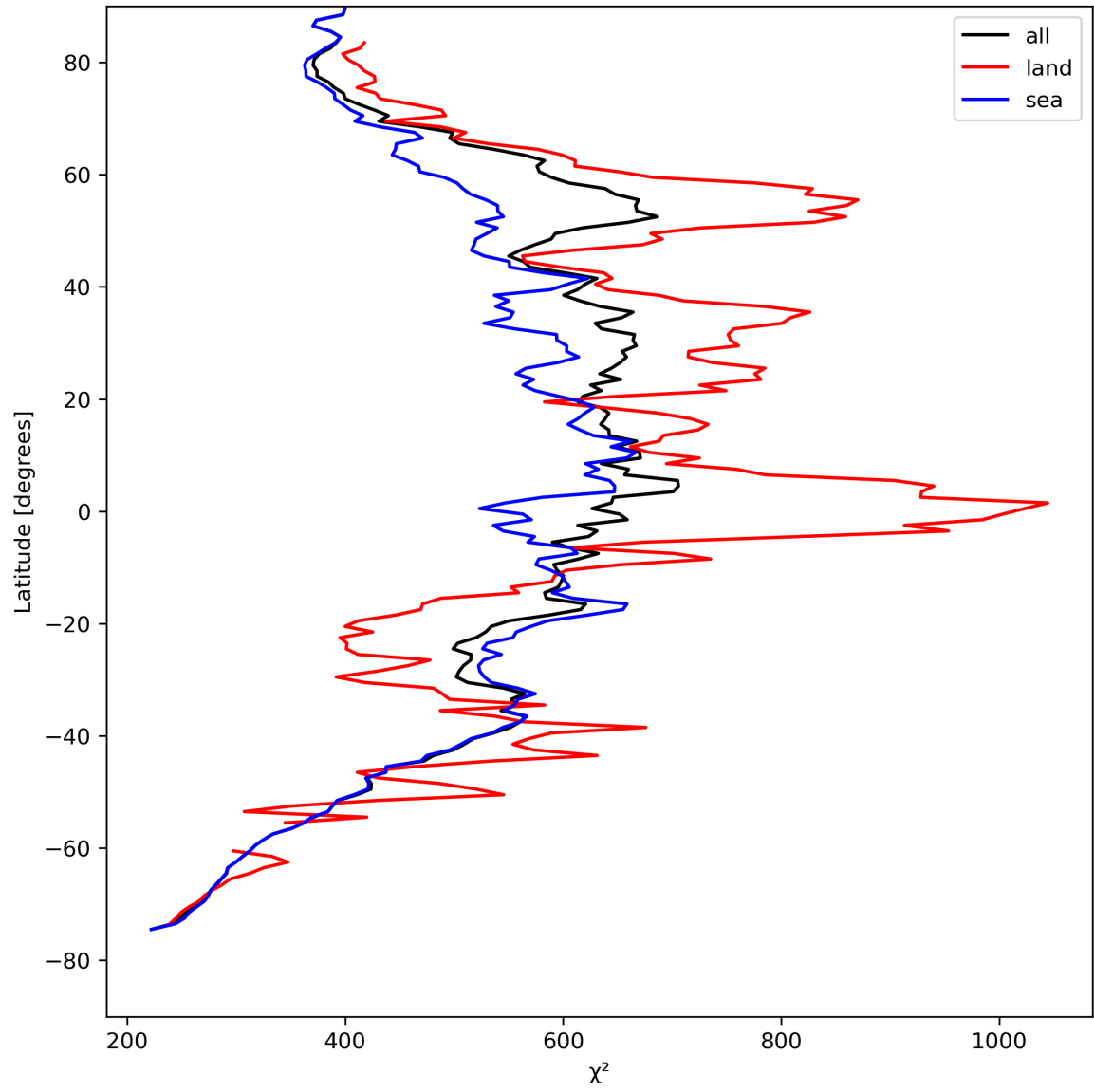
Figure 25: Zonal average of “ \chi^2 ” for 2023-08-14 to 2023-08-16.
