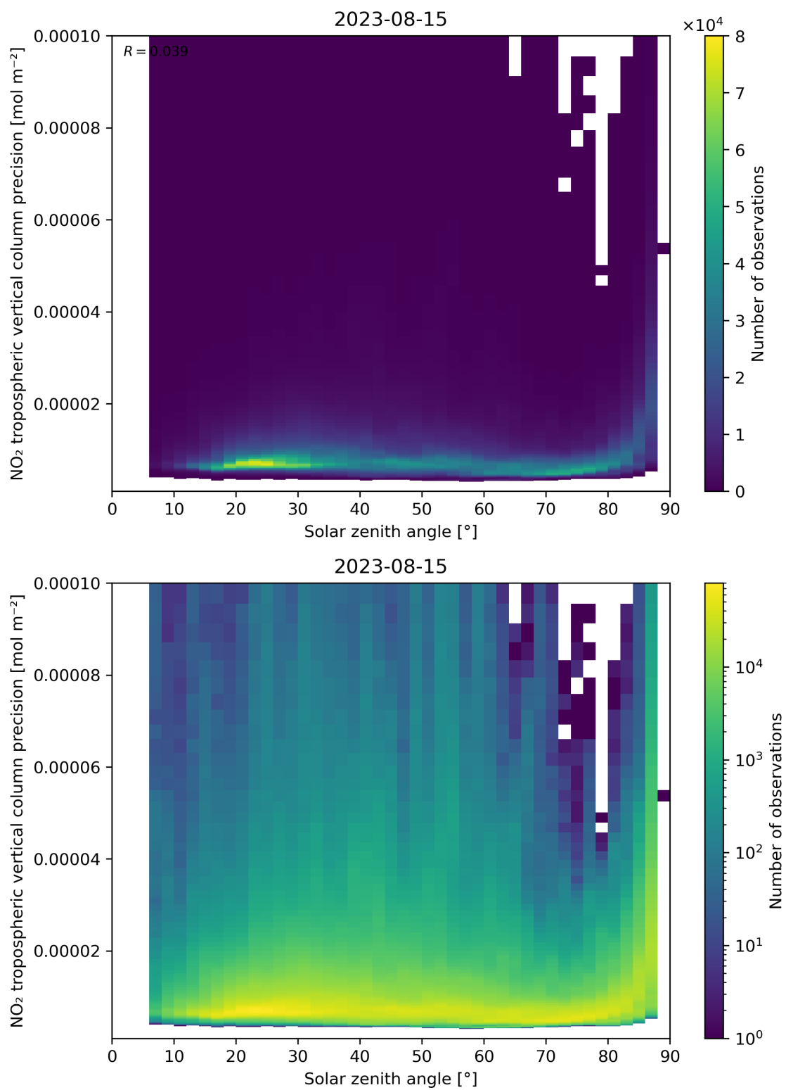
Figure 156: Scatter density plot of “Solar zenith angle” against “NO 2 tropospheric vertical column precision” for 2023-08-14 to 2023-08-16.
