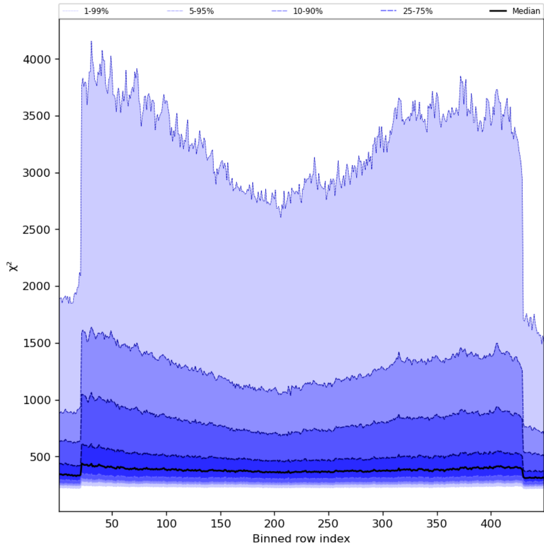
Figure 59: Along track statistics of “ \chi^2 ” for 2023-08-14 to 2023-08-16
