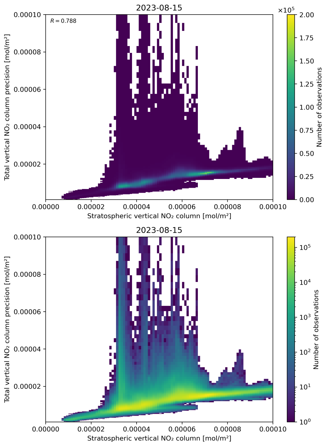
Figure 101: Scatter density plot of “Stratospheric vertical NO 2 column” against “Total vertical NO 2 column precision” for 2023-08-14 to 2023-08-16.
