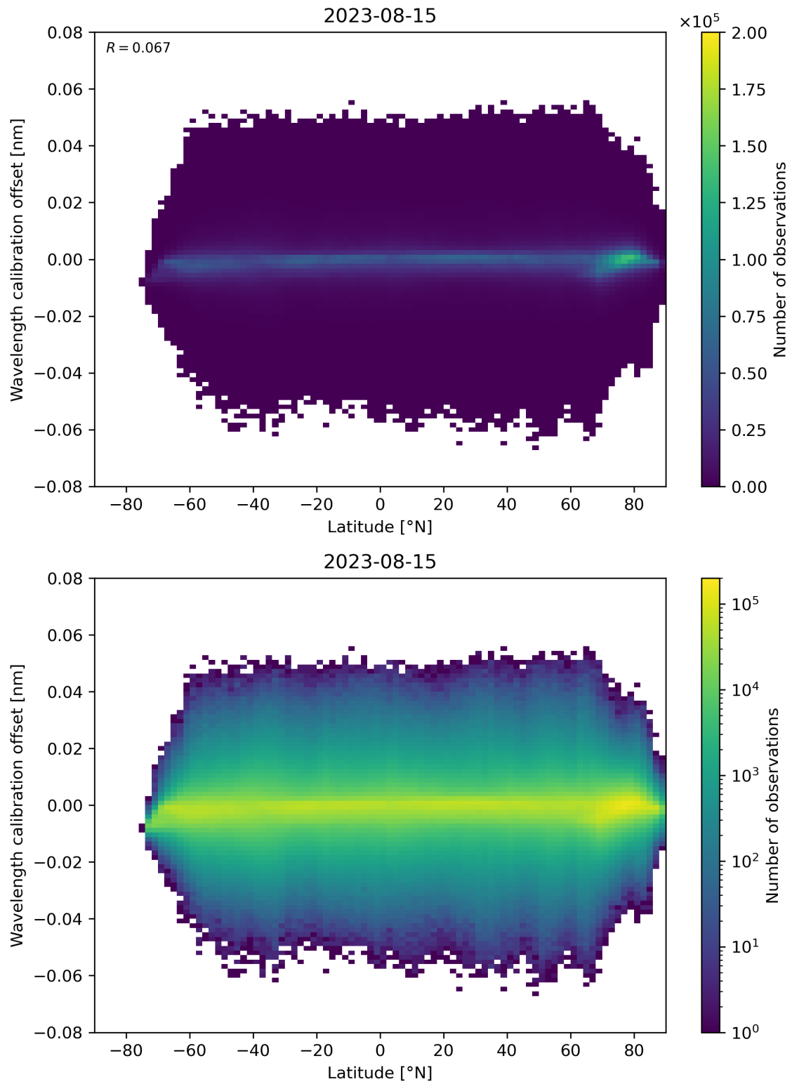
Figure 95: Scatter density plot of “Latitude” against “Wavelength calibration offset” for 2023-08-14 to 2023-08-16.
