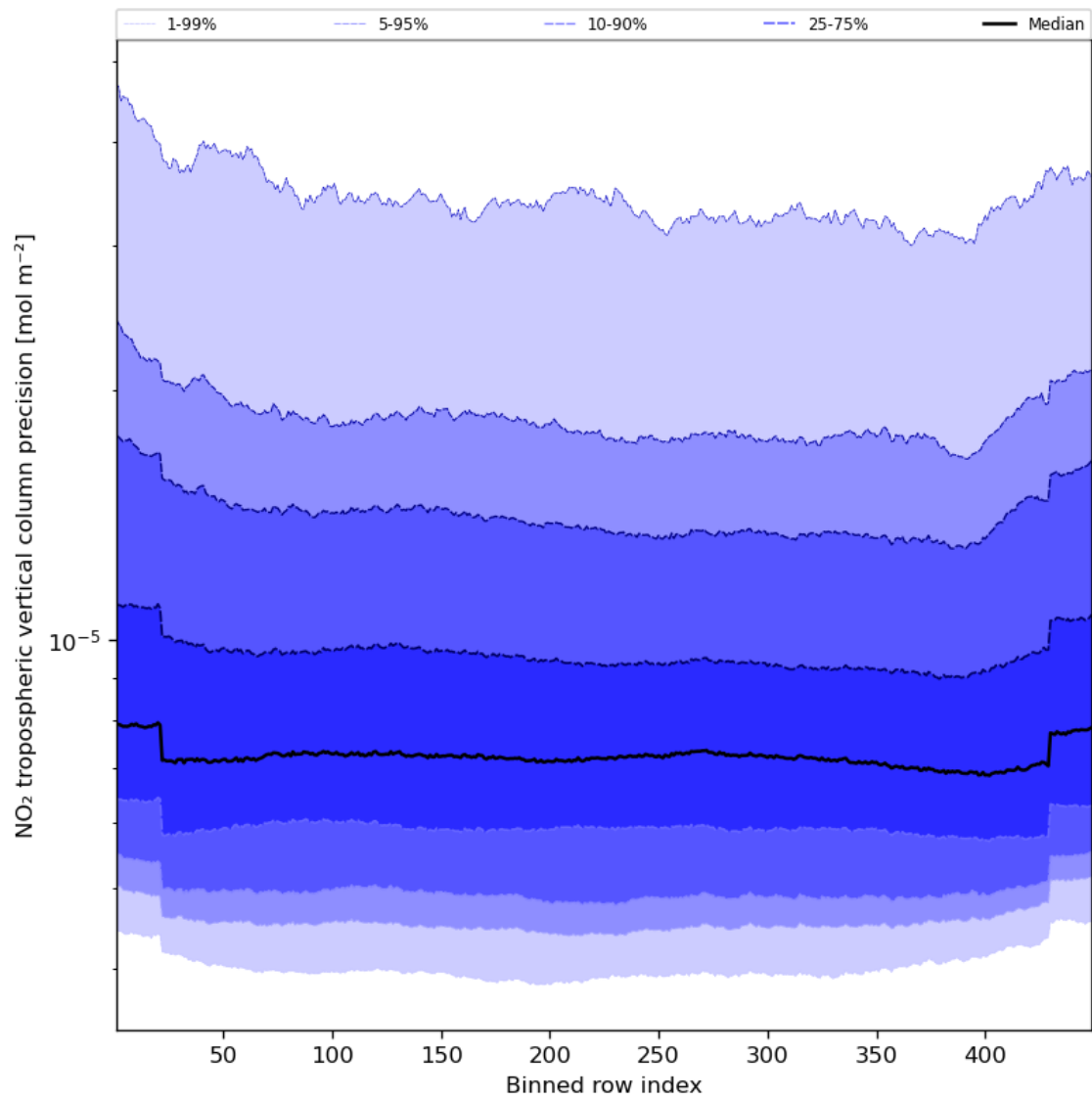
Figure 47: Along track statistics of “NO 2 tropospheric vertical column precision” for 2023-08-14 to 2023-08-16
