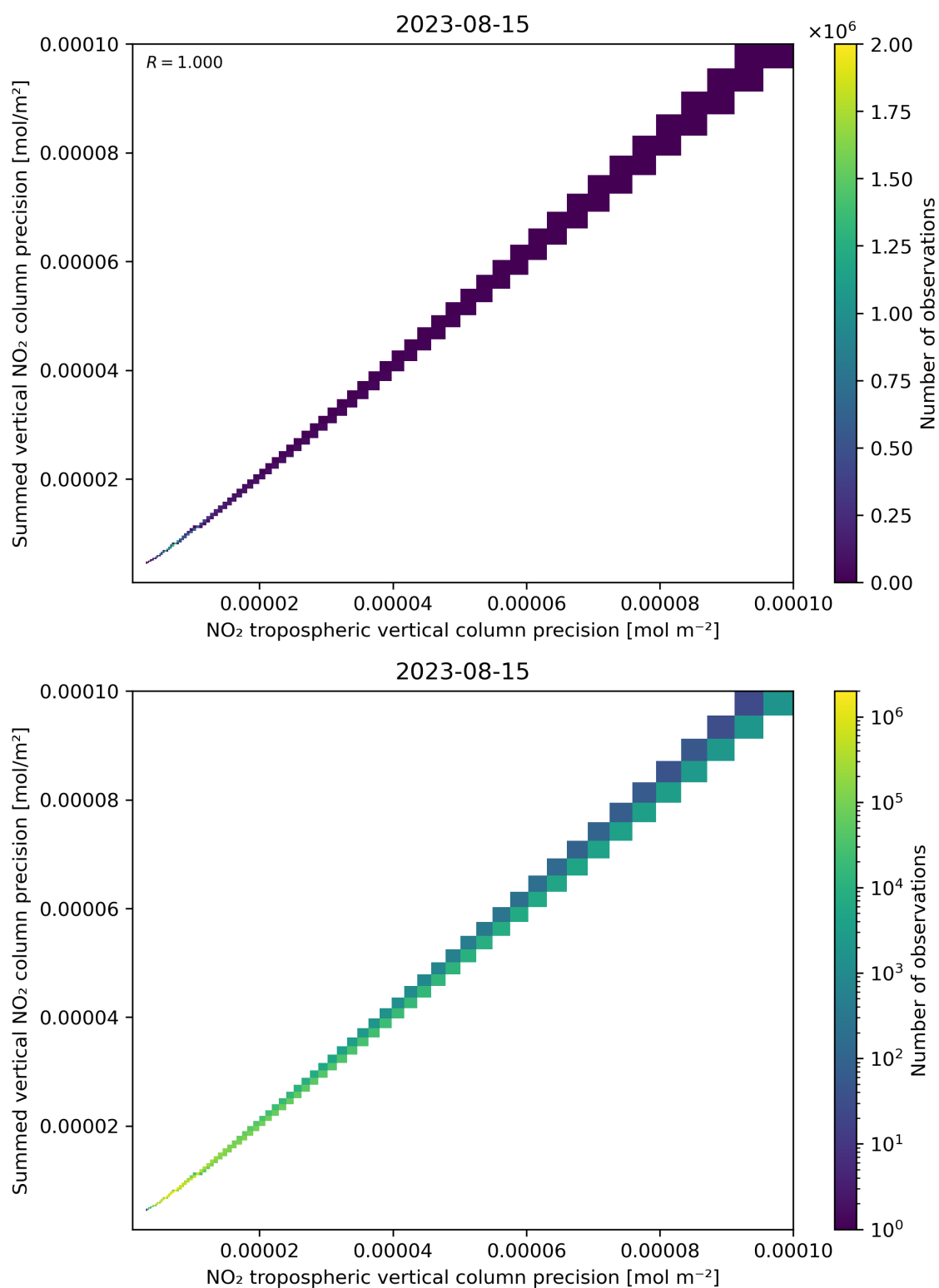
Figure 137: Scatter density plot of “NO 2 tropospheric vertical column precision” against “Summed vertical NO 2 column precision” for 2023-08-14 to 2023-08-16.
