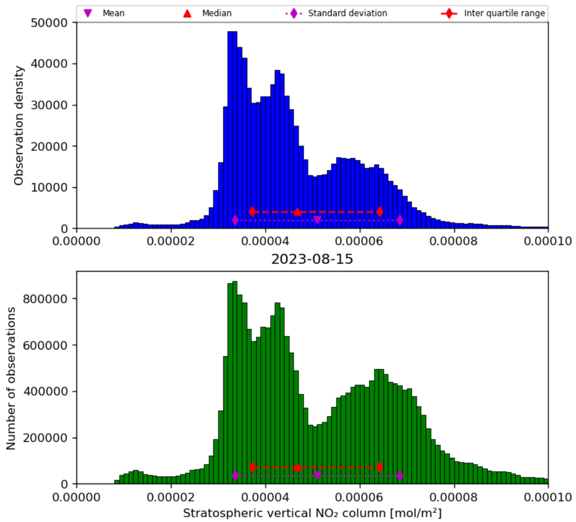
Figure 36: Histogram of “Stratospheric vertical NO 2 column” for 2023-08-14 to 2023-08-16
