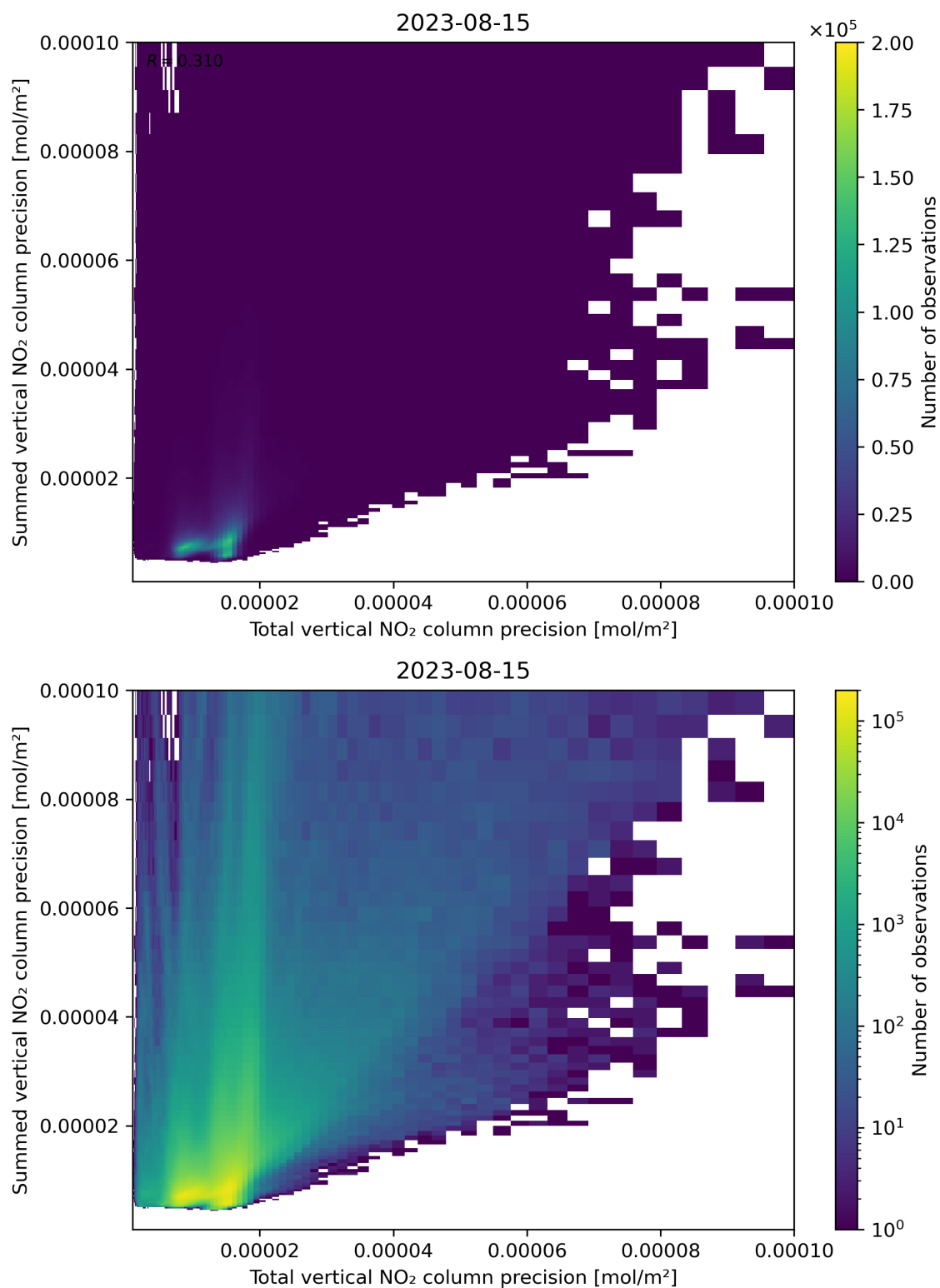
Figure 118: Scatter density plot of “Total vertical NO 2 column precision” against “Summed vertical NO 2 column precision” for 2023-08-14 to 2023-08-16.
