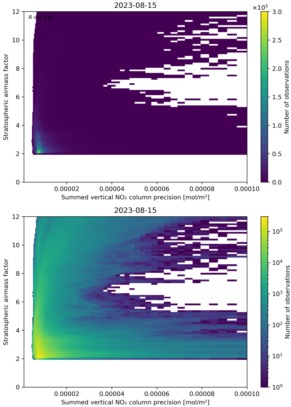
Figure 106: Scatter density plot of “Summed vertical NO 2 column precision” against “Stratospheric airmass factor” for 2023-08-14 to 2023-08-16.
