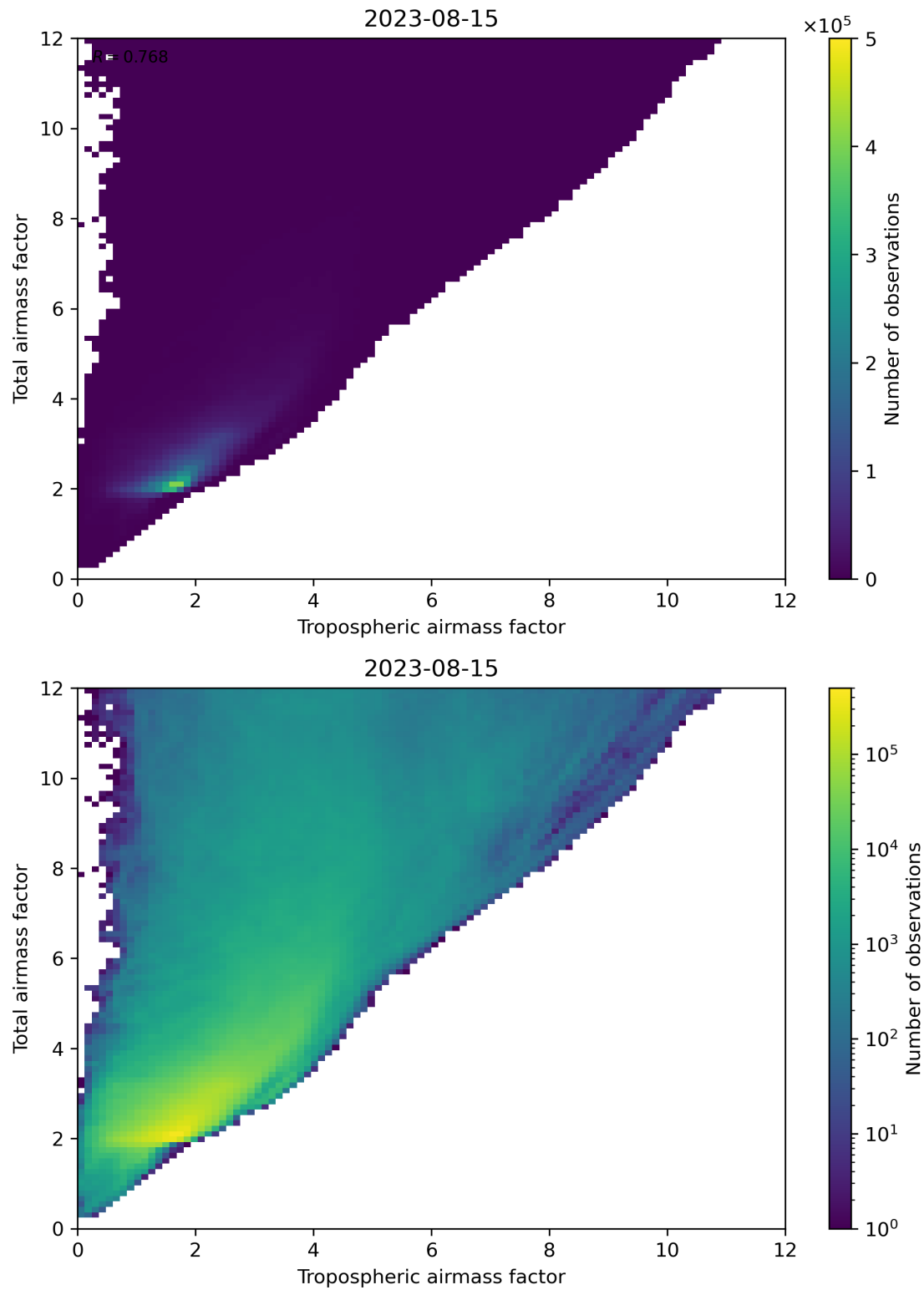
Figure 72: Scatter density plot of “Tropospheric airmass factor” against “Total airmass factor” for 2023-08-14 to 2023-08-16.
