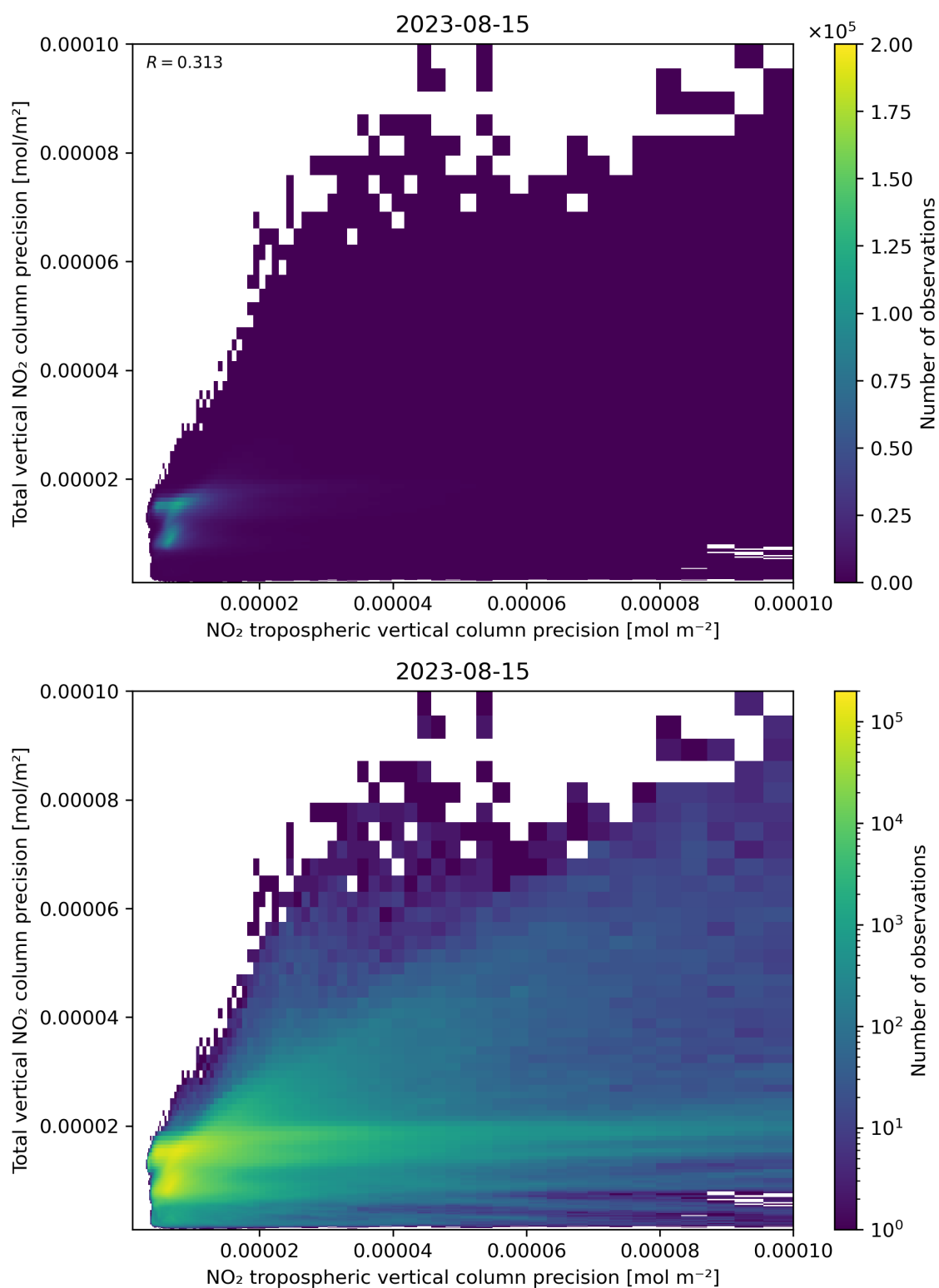
Figure 139: Scatter density plot of “NO 2 tropospheric vertical column precision” against “Total vertical NO 2 column precision” for 2023-08-14 to 2023-08-16.
