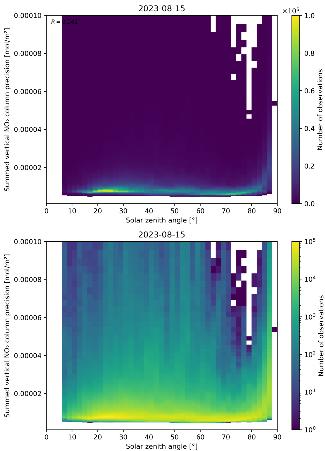
Figure 152: Scatter density plot of “Solar zenith angle” against “Summed vertical NO 2 column precision” for 2023-08-14 to 2023-08-16.
