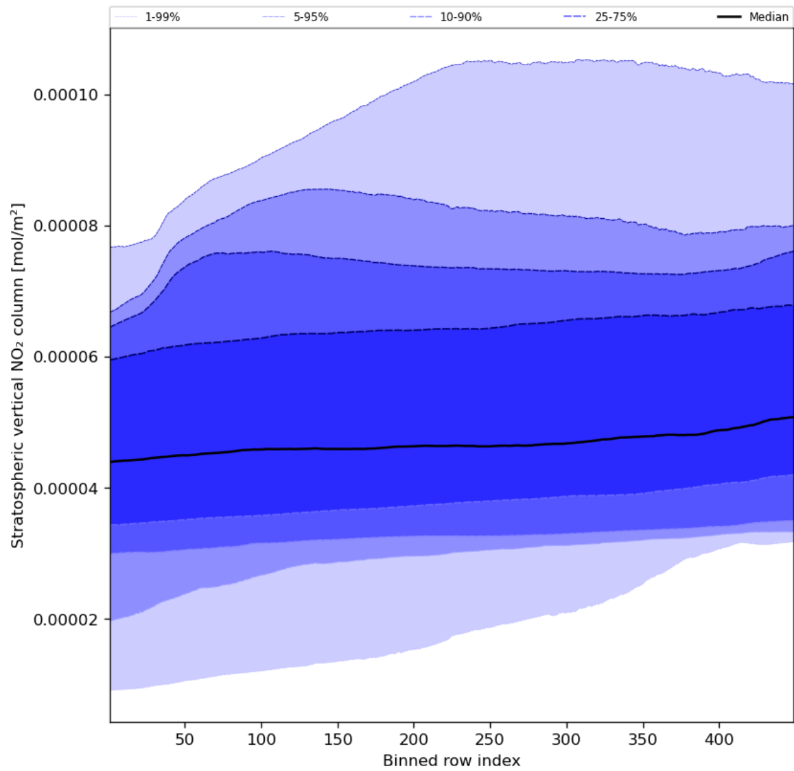
Figure 53: Along track statistics of “Stratospheric vertical NO 2 column” for 2023-08-14 to 2023-08-16
