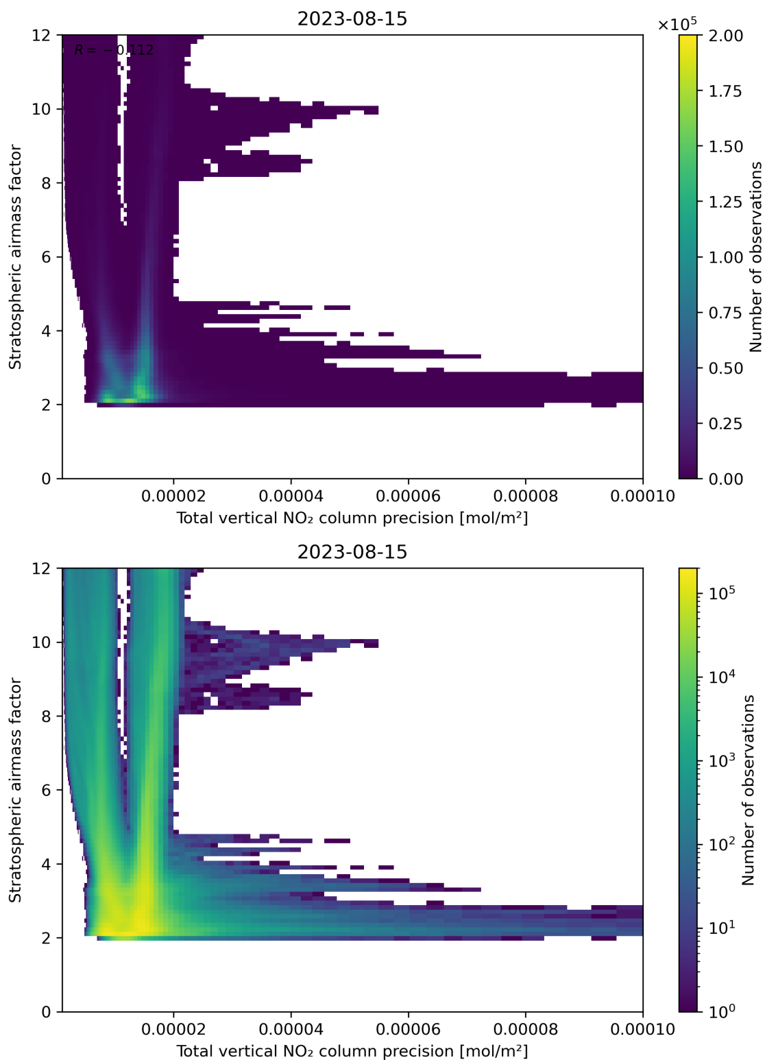
Figure 115: Scatter density plot of “Total vertical NO 2 column precision” against “Stratospheric airmass factor” for 2023-08-14 to 2023-08-16.
