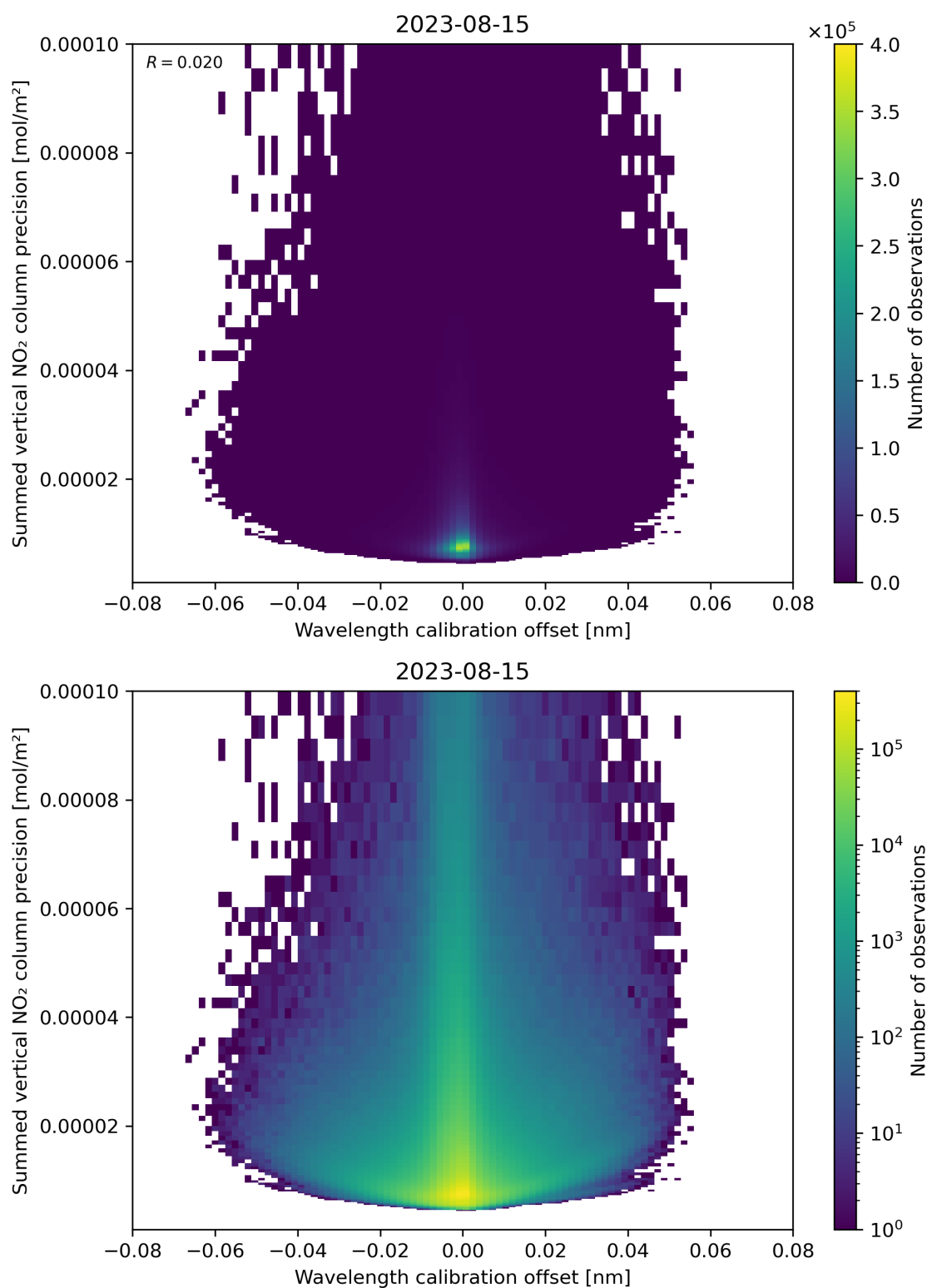
Figure 178: Scatter density plot of “Wavelength calibration offset” against “Summed vertical NO 2 column precision” for 2023-08-14 to 2023-08-16.
