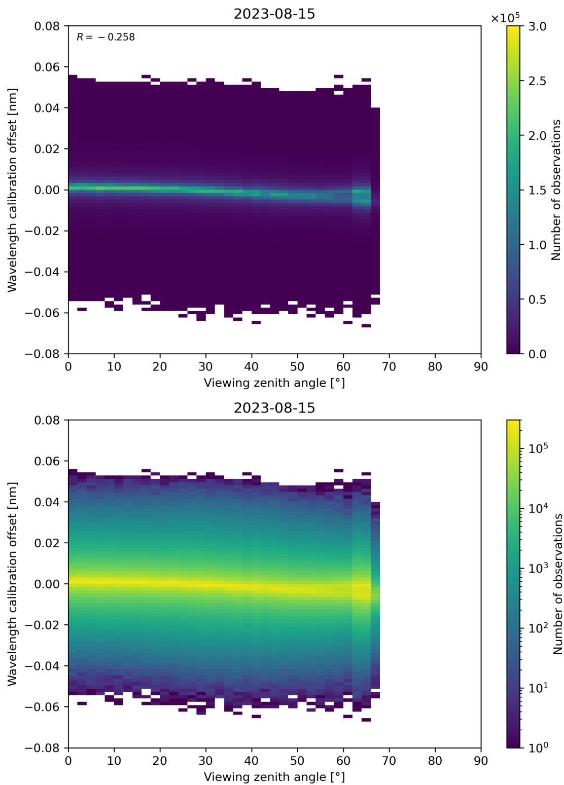
Figure 173: Scatter density plot of “Viewing zenith angle” against “Wavelength calibration offset” for 2023-08-14 to 2023-08-16.
