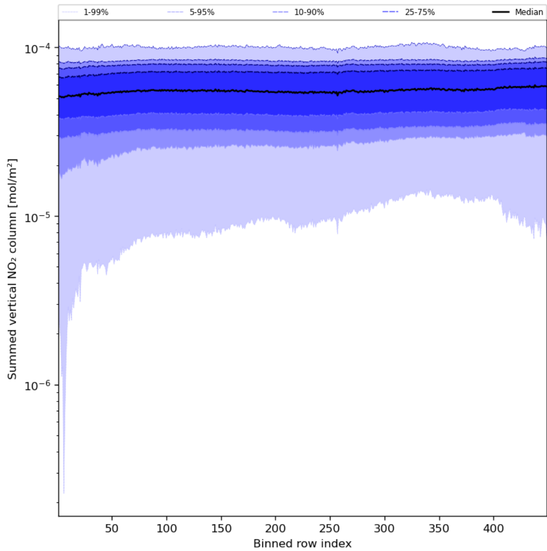
Figure 57: Along track statistics of “Summed vertical NO 2 column” for 2023-08-14 to 2023-08-16
