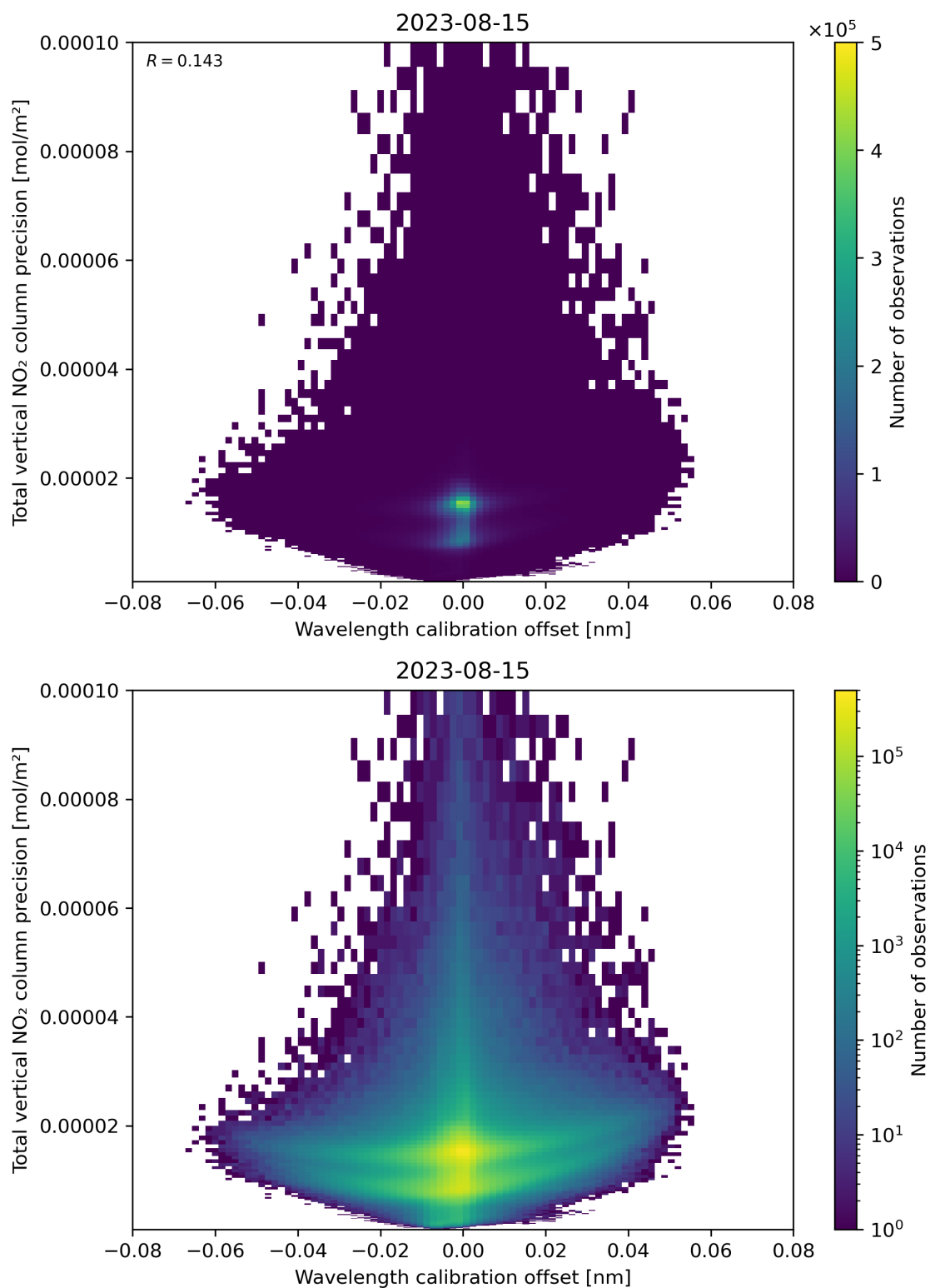
Figure 180: Scatter density plot of “Wavelength calibration offset” against “Total vertical NO 2 column precision” for 2023-08-14 to 2023-08-16.
