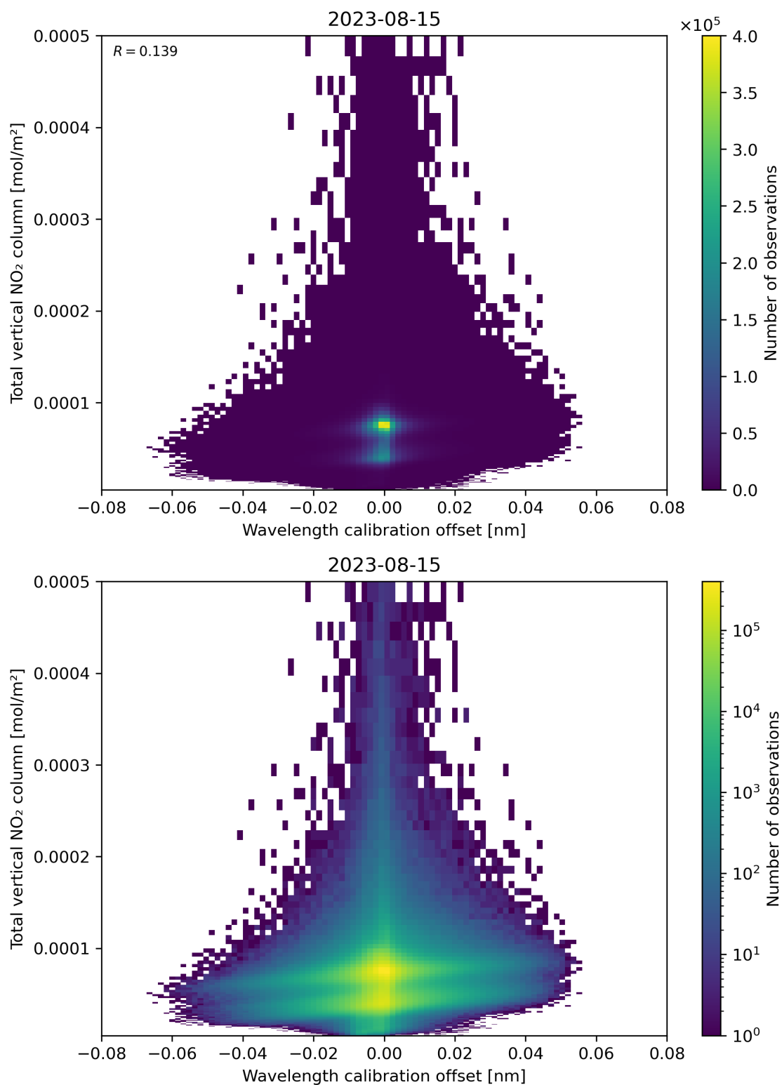
Figure 179: Scatter density plot of “Wavelength calibration offset” against “Total vertical NO 2 column” for 2023-08-14 to 2023-08-16.
