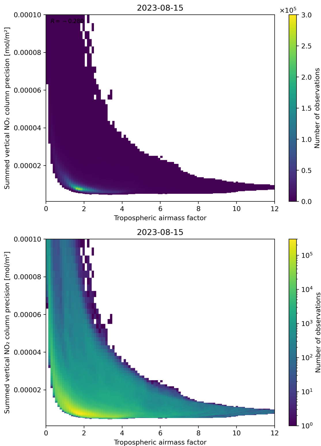
Figure 76: Scatter density plot of “Tropospheric air mass factor” against “Summed vertical NO 2 column precision” for 2023-08-14 to 2023-08-16.
