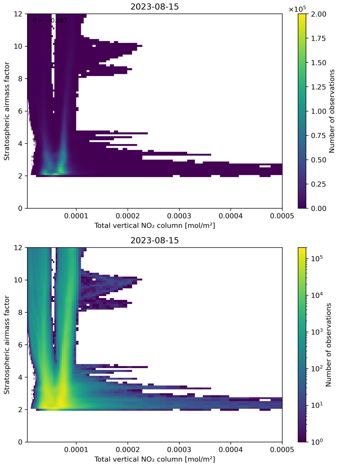
Figure 110: Scatter density plot of “Total vertical NO 2 column” against “Stratospheric airmass factor” for 2023-08-14 to 2023-08-16.
