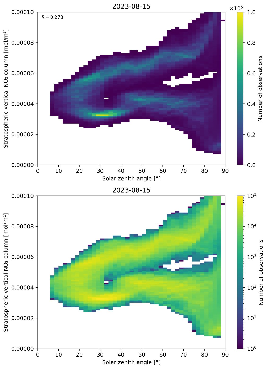
Figure 150: Scatter density plot of “Solar zenith angle” against “Stratospheric vertical NO 2 column” for 2023-08-14 to 2023-08-16.
