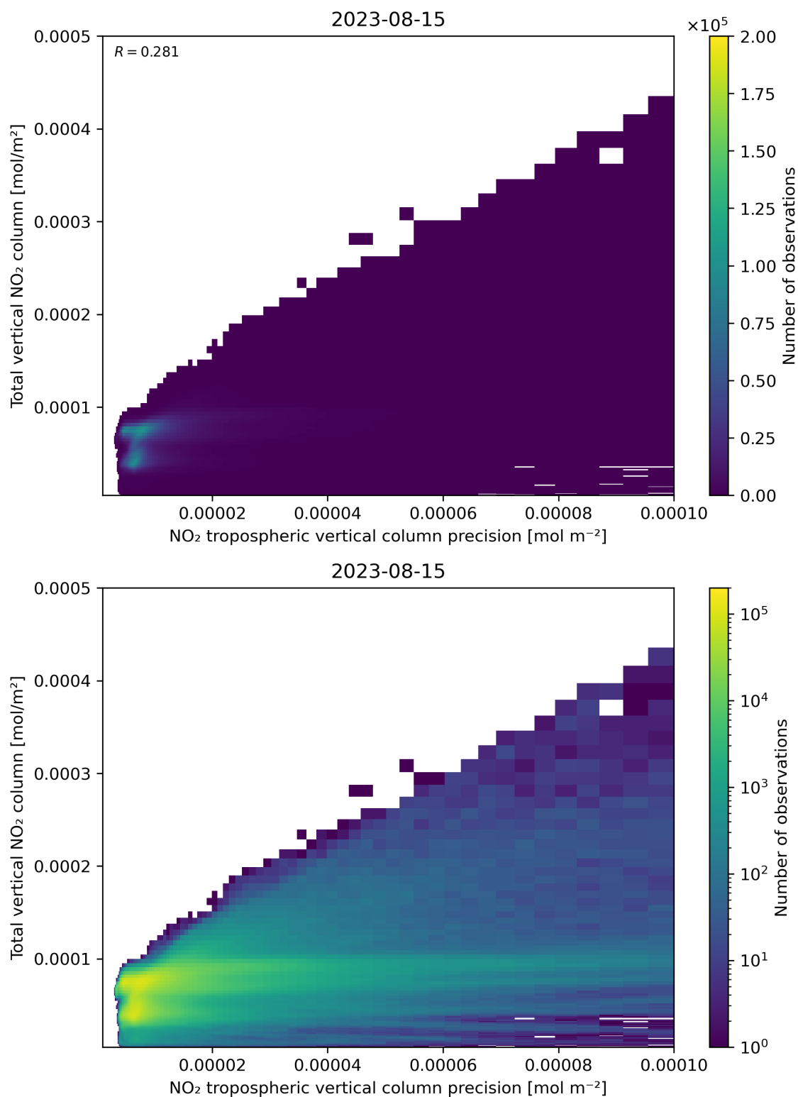
Figure 138: Scatter density plot of “NO 2 tropospheric vertical column precision” against “Total vertical NO 2 column” for 2023-08-14 to 2023-08-16.
