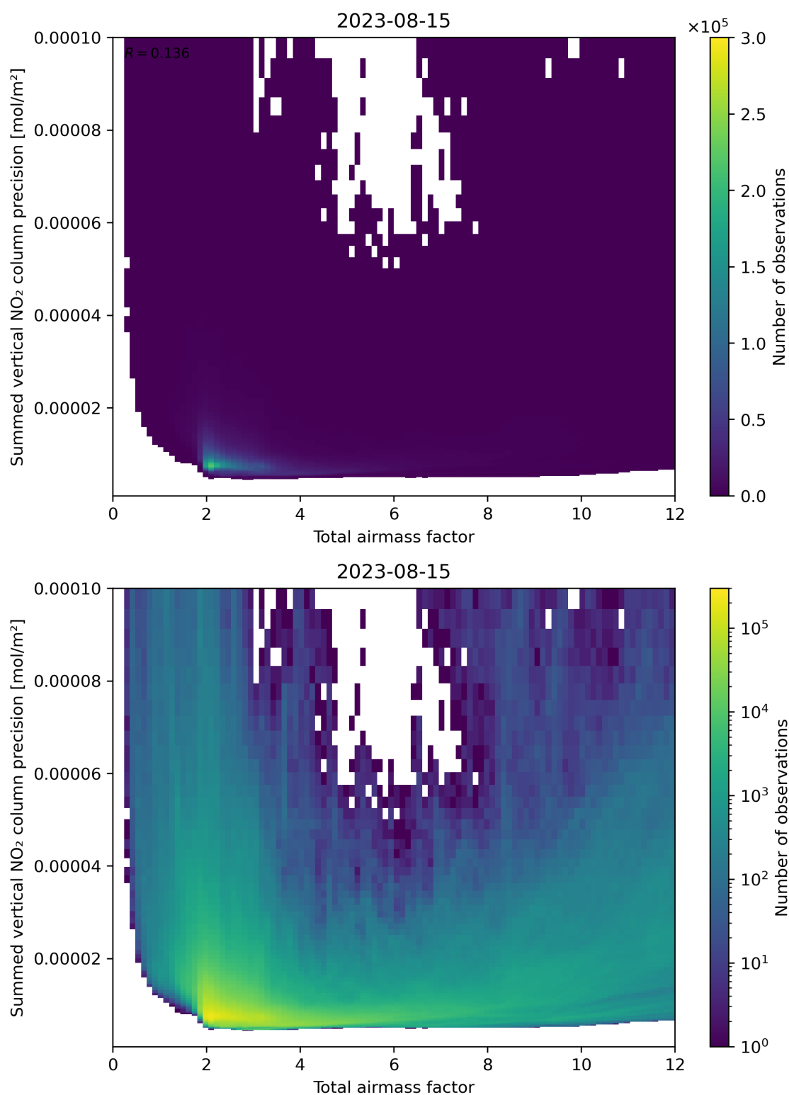
Figure 66: Scatter density plot of “Total airmass factor” against “Summed vertical NO 2 column precision” for 2023-08-14 to 2023-08-16.
