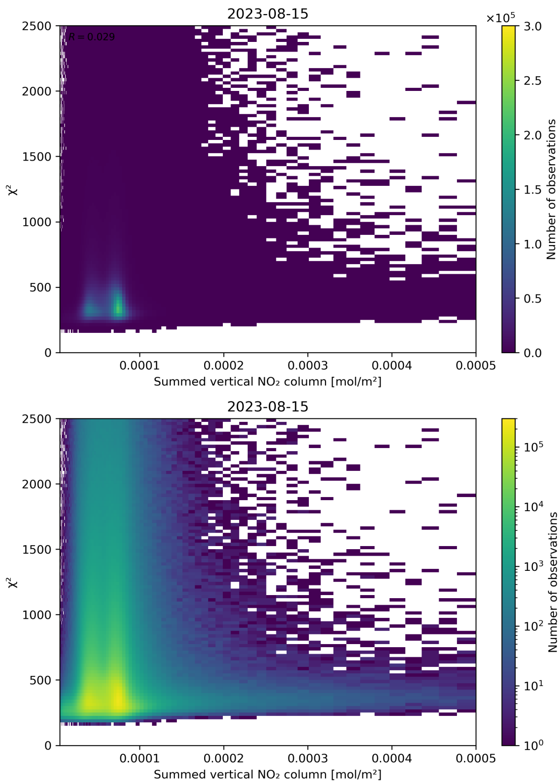
Figure 104: Scatter density plot of “Summed vertical NO 2 column” against “ \chi^2 ” for 2023-08-14 to 2023-08-16.
