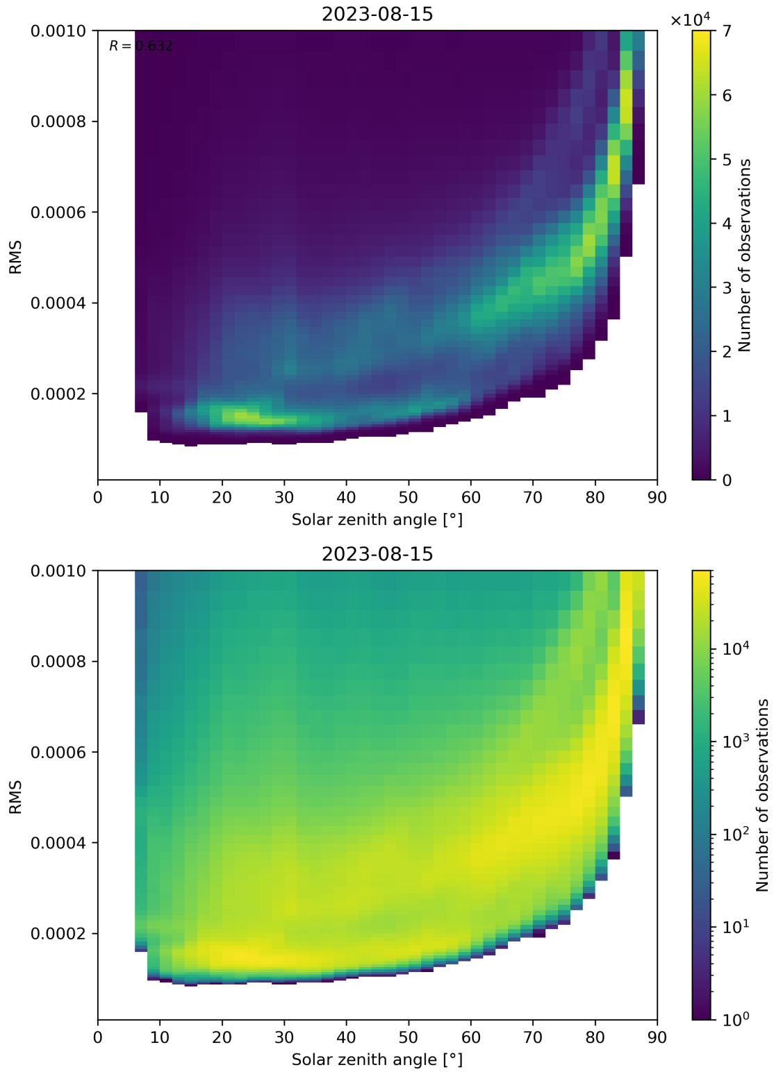
Figure 157: Scatter density plot of “Solar zenith angle” against “RMS” for 2023-08-14 to 2023-08-16.
