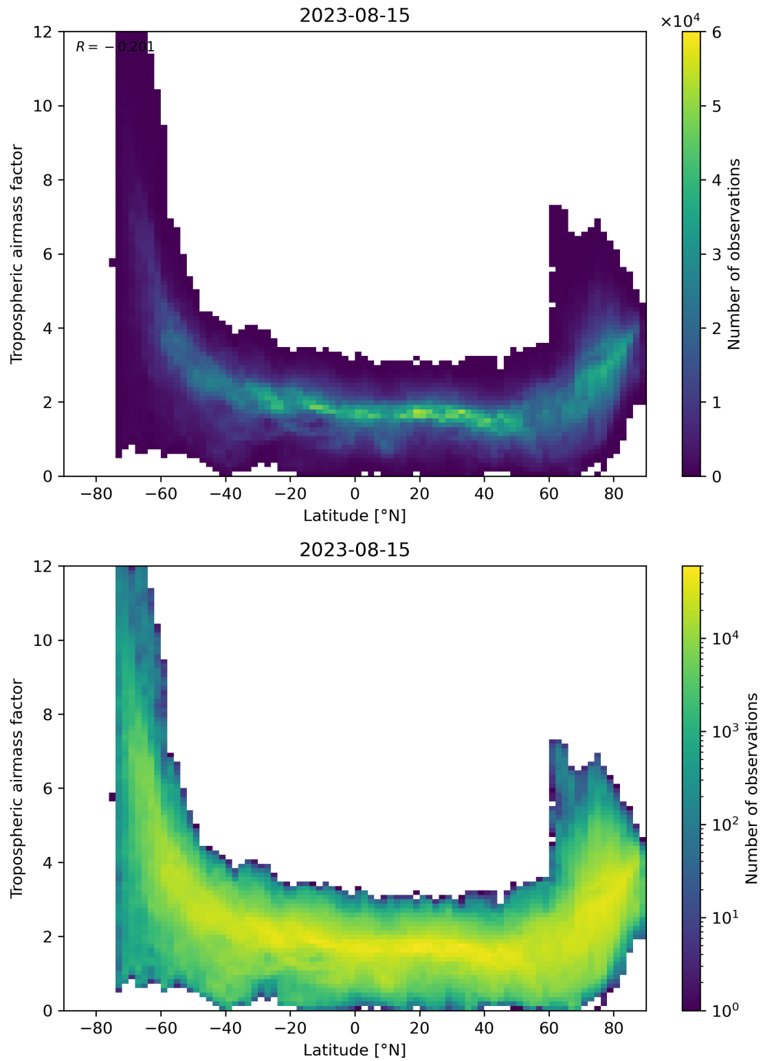
Figure 85: Scatter density plot of “Latitude” against “Tropospheric airmass factor” for 2023-08-14 to 2023-08-16.
