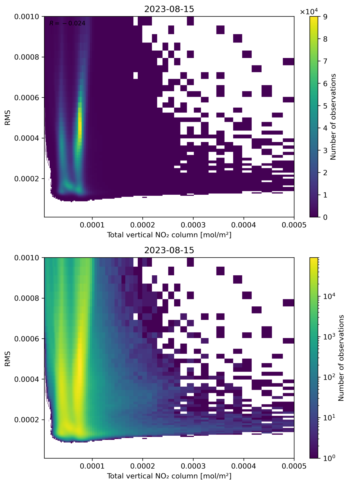
Figure 120: Scatter density plot of “Total vertical NO 2 column” against “RMS” for 2023-08-14 to 2023-08-16.
