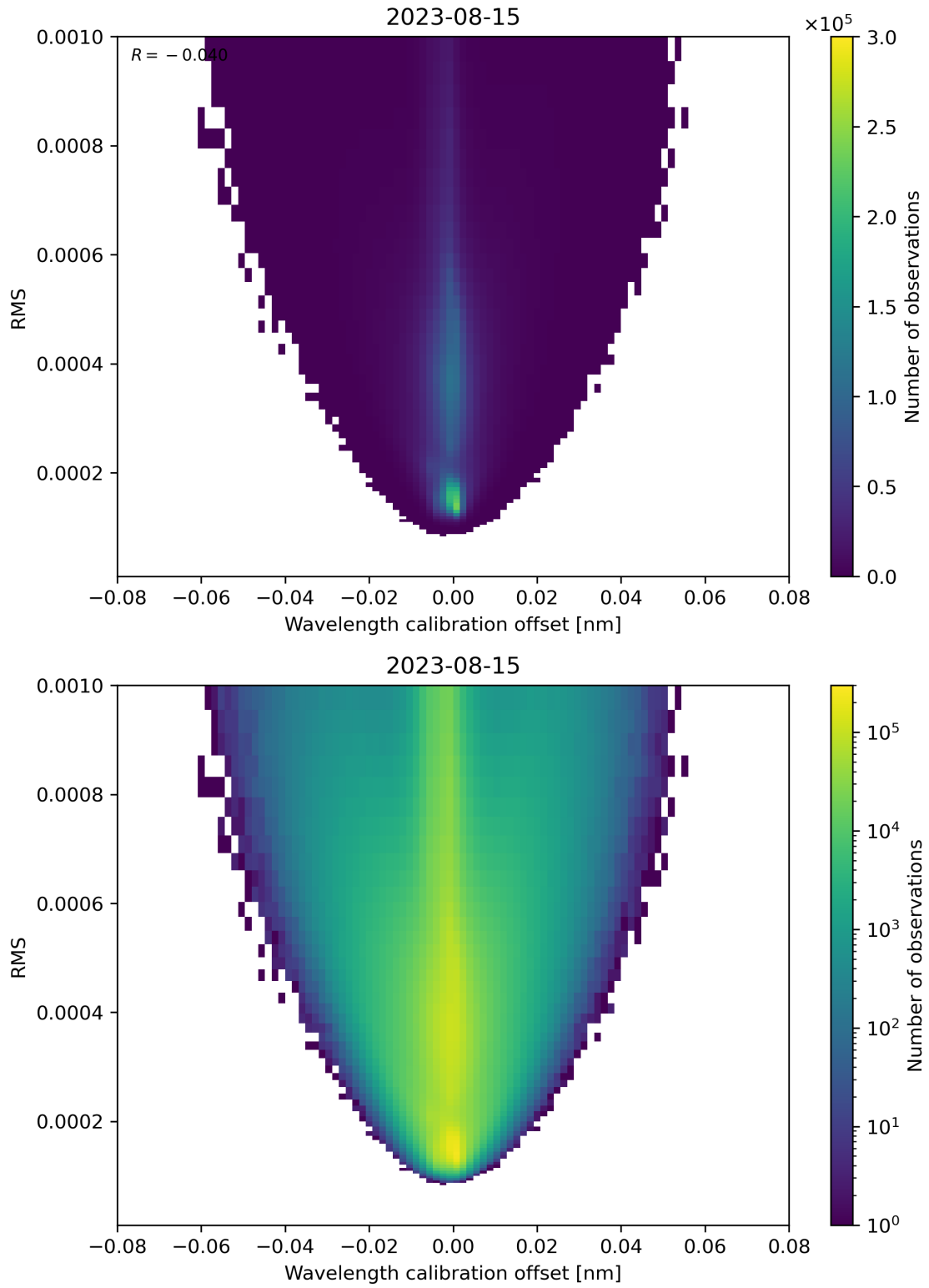
Figure 181: Scatter density plot of “Wavelength calibration offset” against “RMS” for 2023-08-14 to 2023-08-16.
