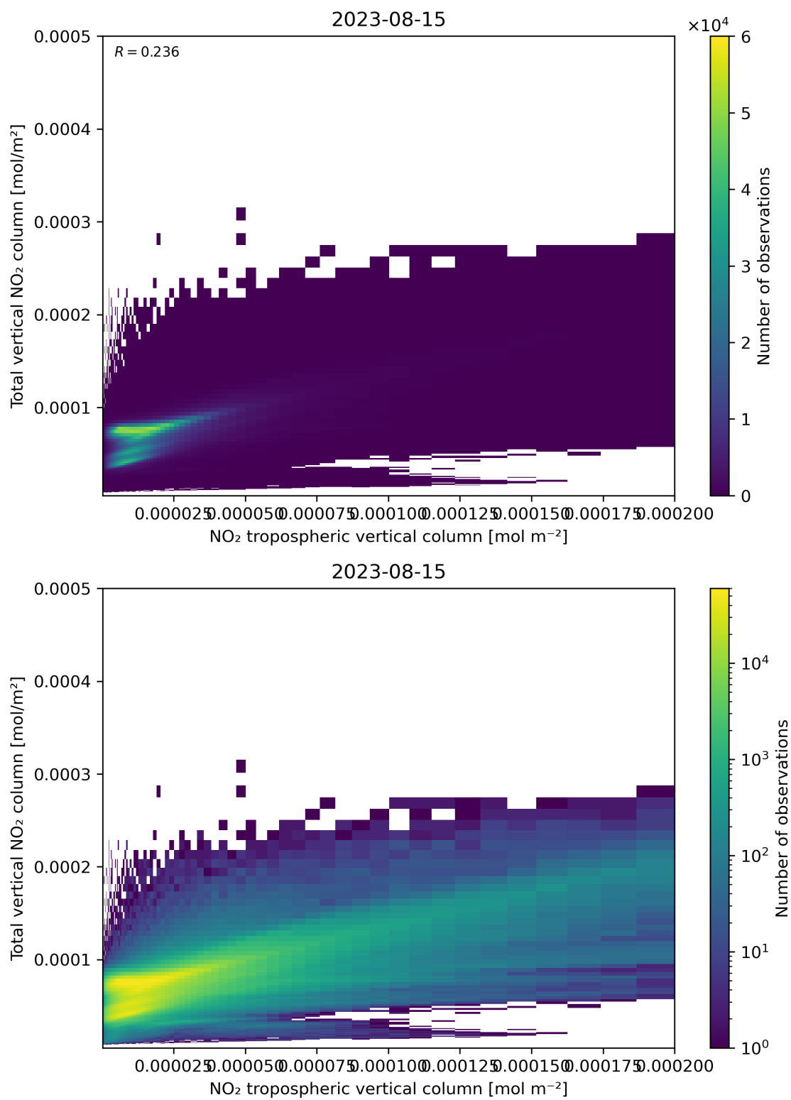
Figure 128: Scatter density plot of “NO 2 tropospheric vertical column” against “Total vertical NO 2 column” for 2023-08-14 to 2023-08-16.
