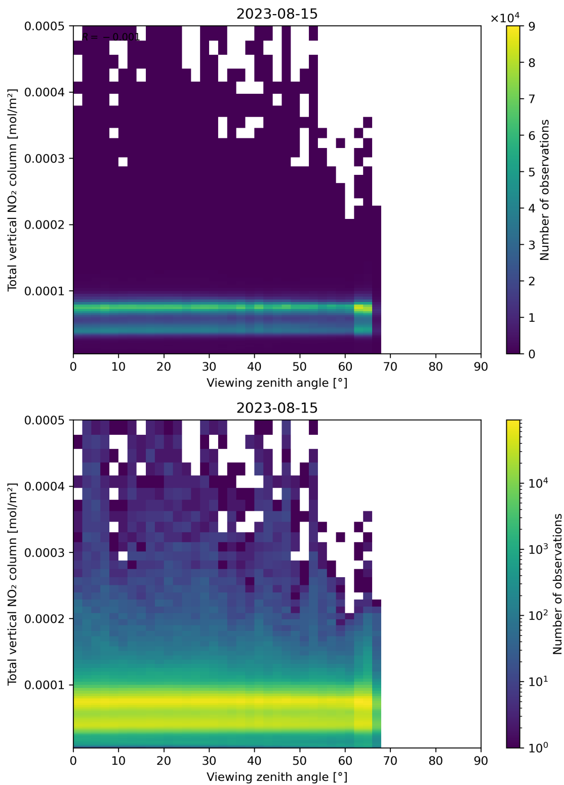
Figure 167: Scatter density plot of “Viewing zenith angle” against “Total vertical NO 2 column” for 2023-08-14 to 2023-08-16.
