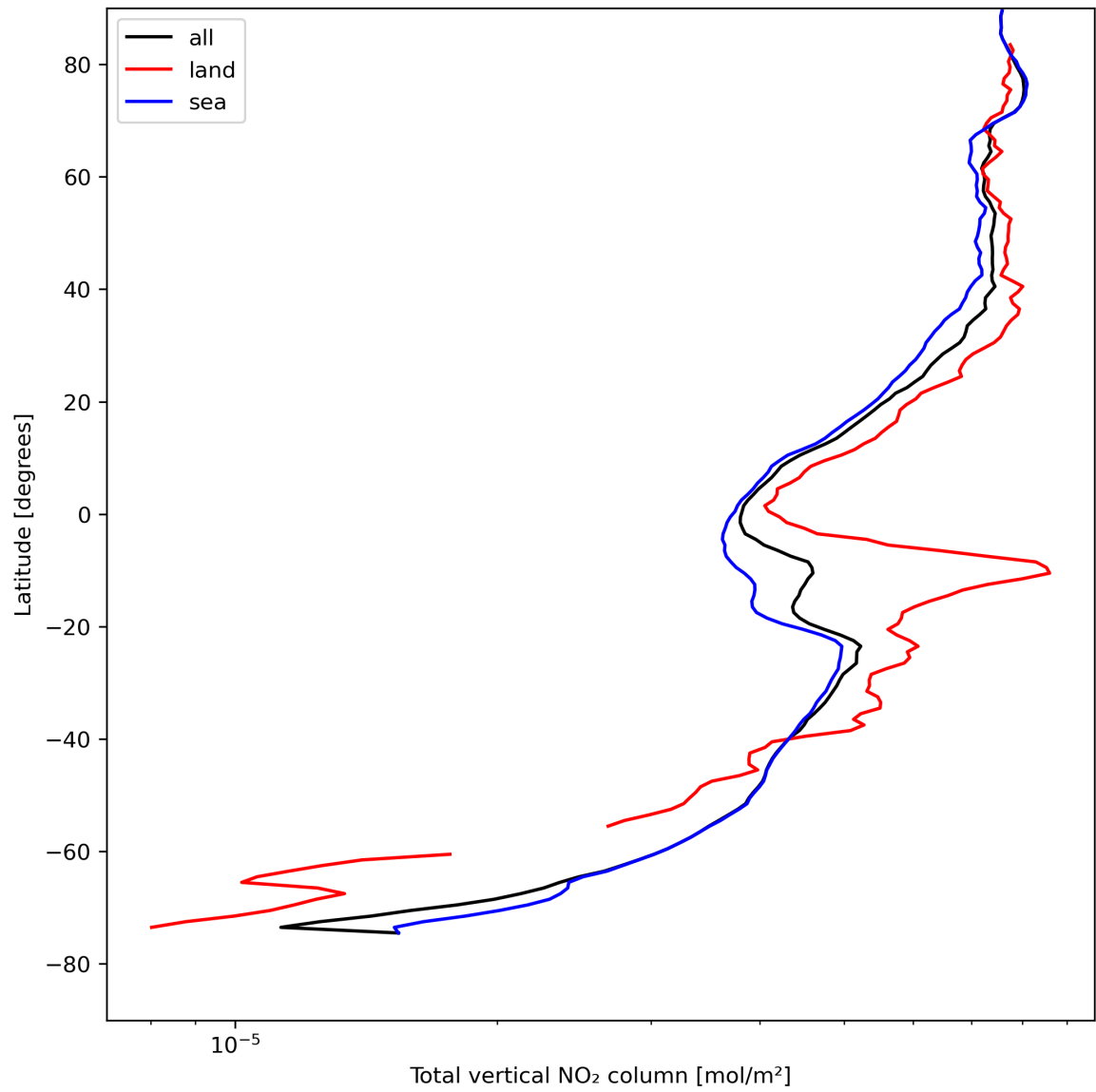
Figure 21: Zonal average of “Total vertical NO 2 column” for 2023-08-14 to 2023-08-16.
