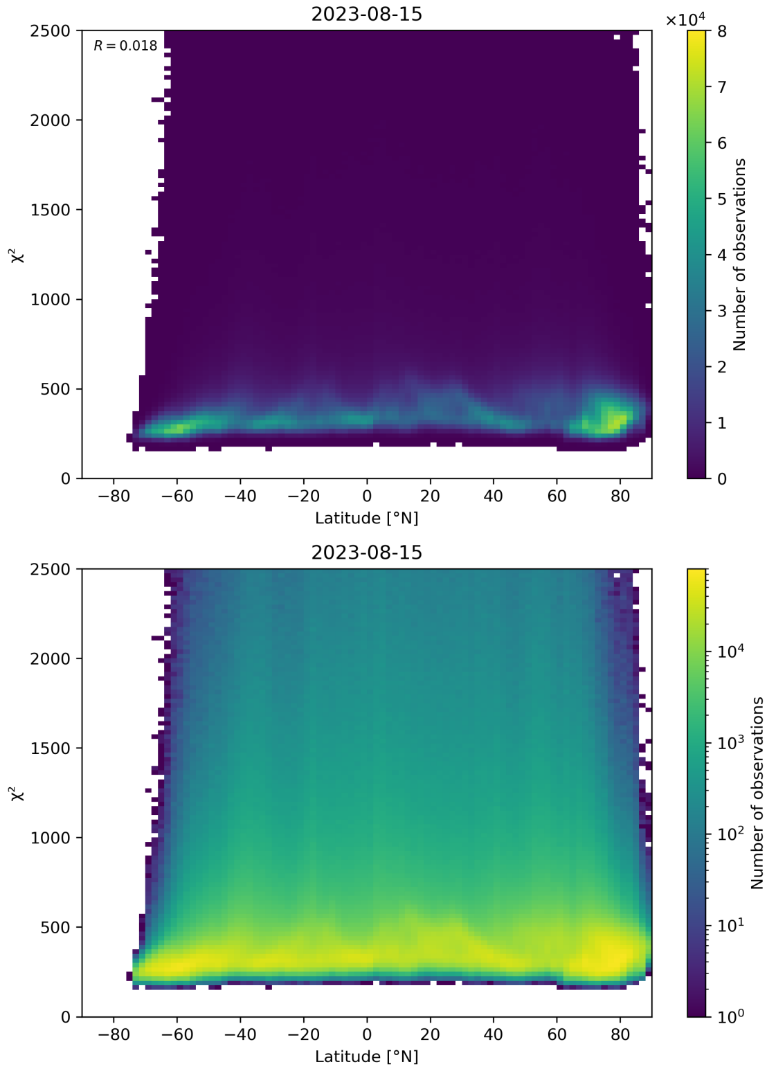
Figure 86: Scatter density plot of “Latitude” against “ \chi^2 ” for 2023-08-14 to 2023-08-16.
