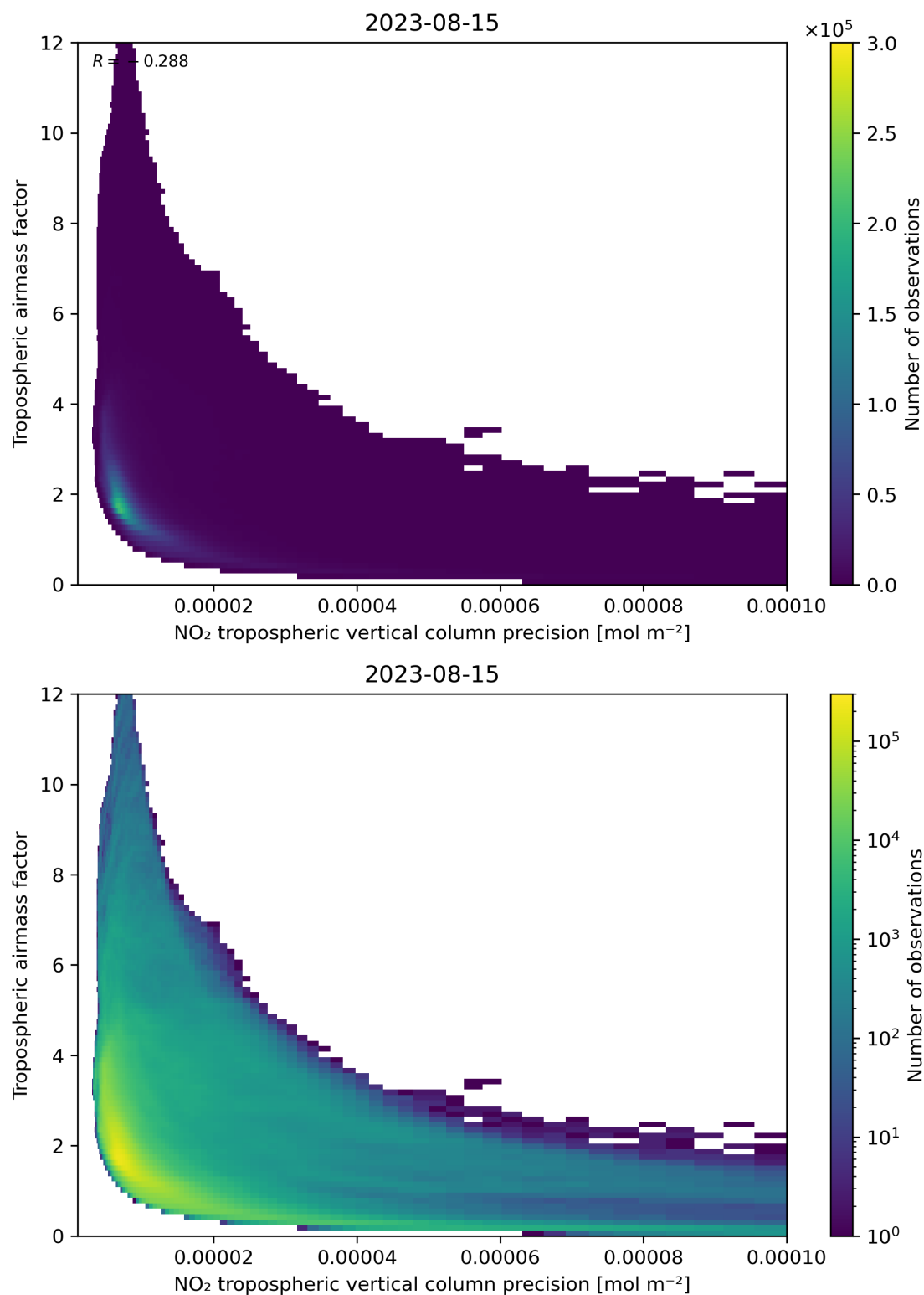
Figure 133: Scatter density plot of “NO 2 tropospheric vertical column precision” against “Tropospheric airmass factor” for 2023-08-14 to 2023-08-16.
