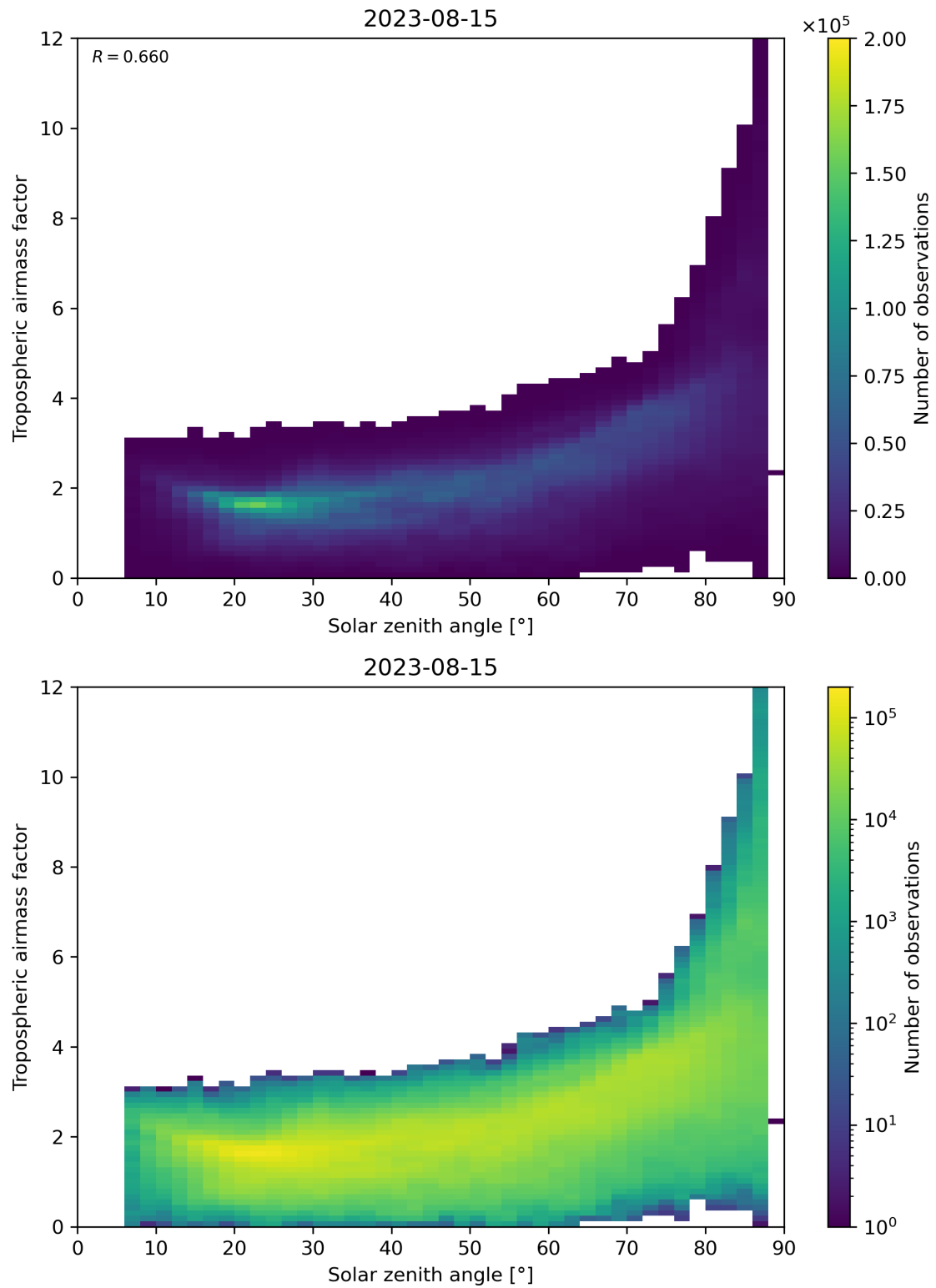
Figure 147: Scatter density plot of “Solar zenith angle” against “Tropospheric airmass factor” for 2023-08-14 to 2023-08-16.
