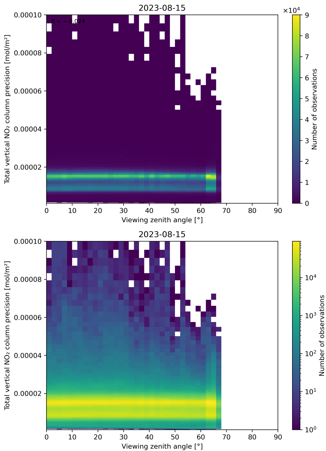
Figure 168: Scatter density plot of “Viewing zenith angle” against “Total vertical NO 2 column precision” for 2023-08-14 to 2023-08-16.
