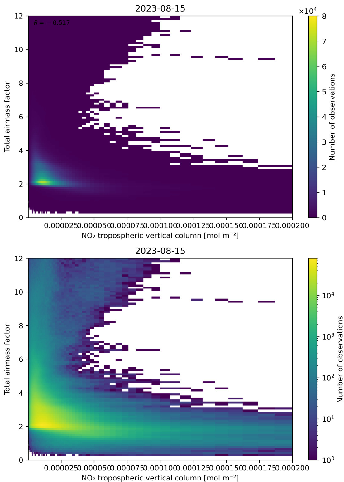
Figure 122: Scatter density plot of “NO 2 tropospheric vertical column” against “Total air mass factor” for 2023-08-14 to 2023-08-16.
