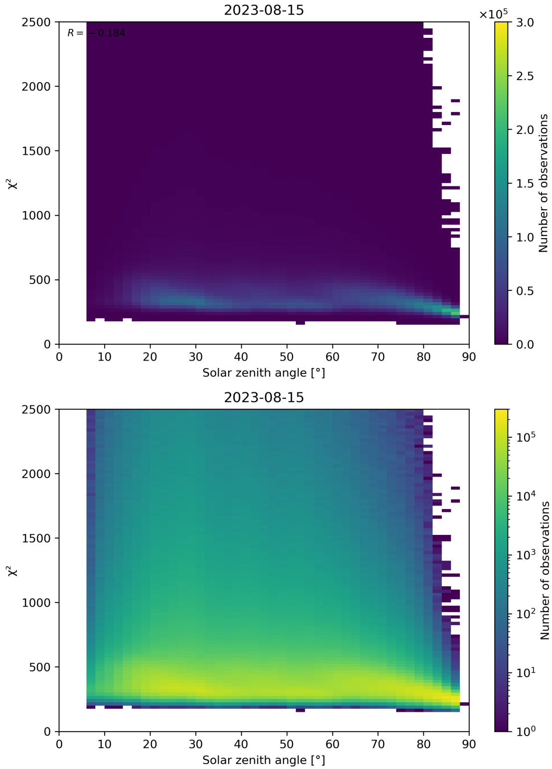
Figure 148: Scatter density plot of “Solar zenith angle” against “ \chi^2 ” for 2023-08-14 to 2023-08-16.
