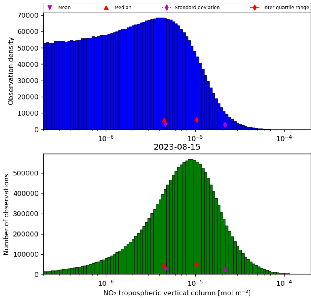
Figure 29: Histogram of “NO 2 tropospheric vertical column” for 2023-08-14 to 2023-08-16
