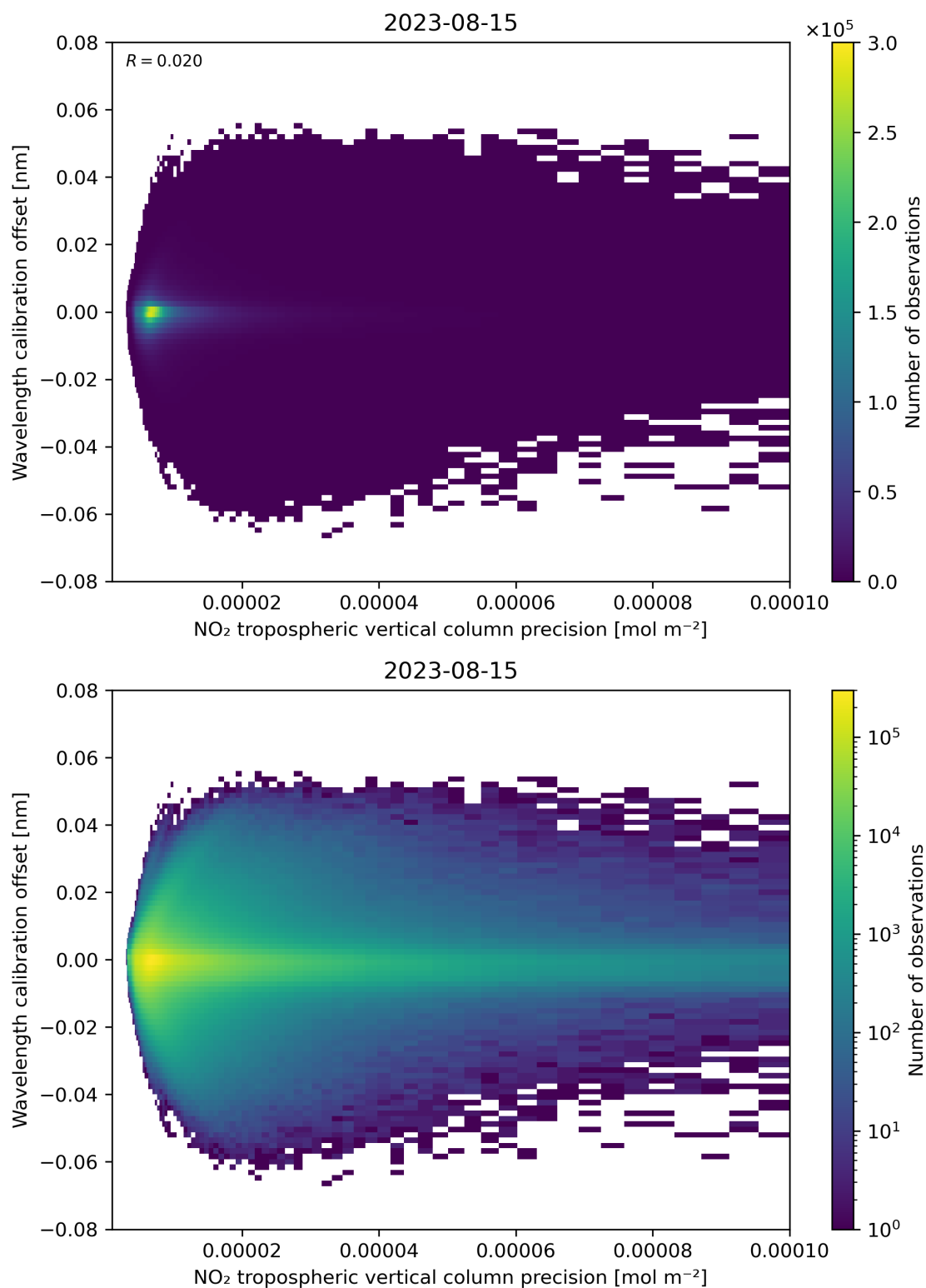
Figure 141: Scatter density plot of “NO 2 tropospheric vertical column precision” against “Wavelength calibration offset” for 2023-08-14 to 2023-08-16.
