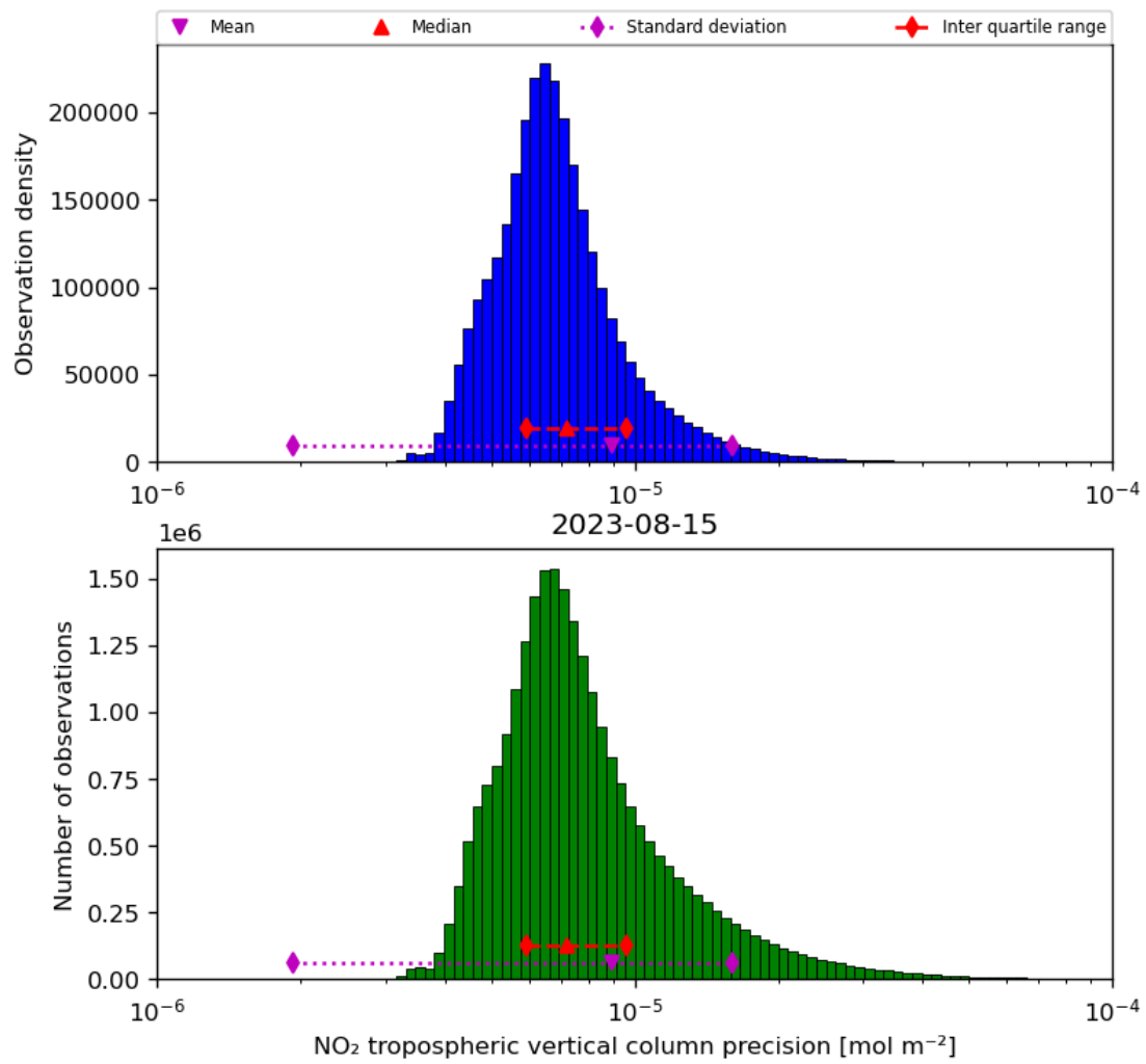
Figure 30: Histogram of “NO 2 tropospheric vertical column precision” for 2023-08-14 to 2023-08-16
