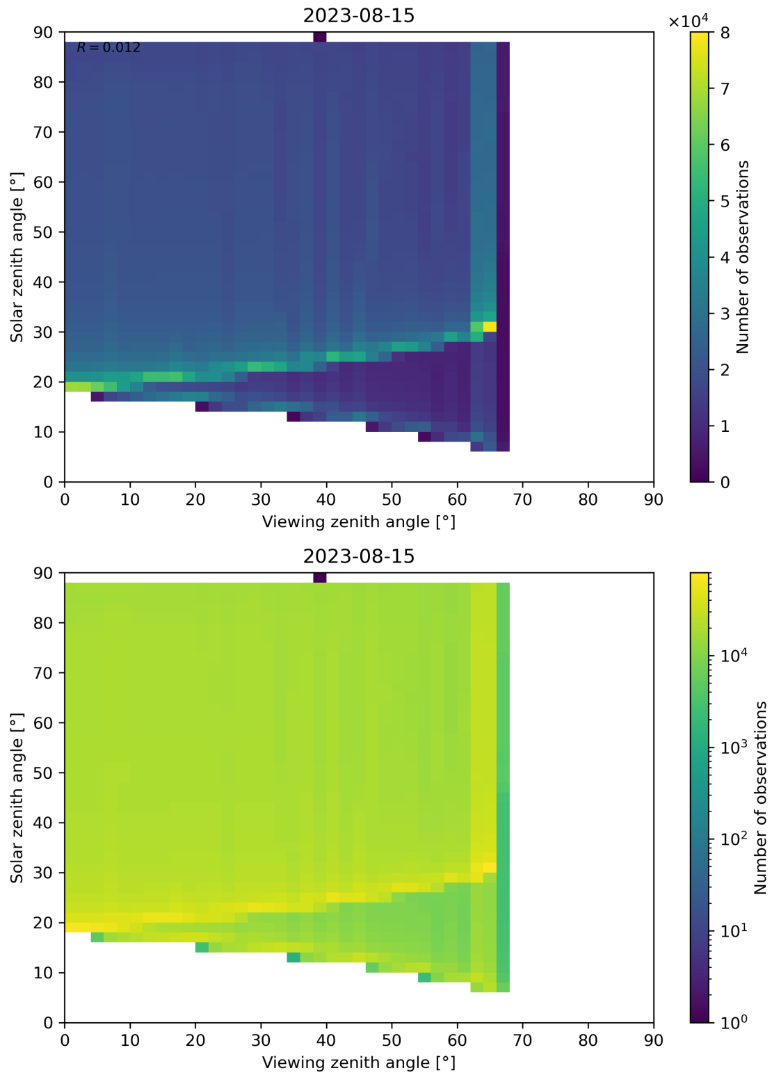
Figure 172: Scatter density plot of “Viewing zenith angle” against “Solar zenith angle” for 2023-08-14 to 2023-08-16.
