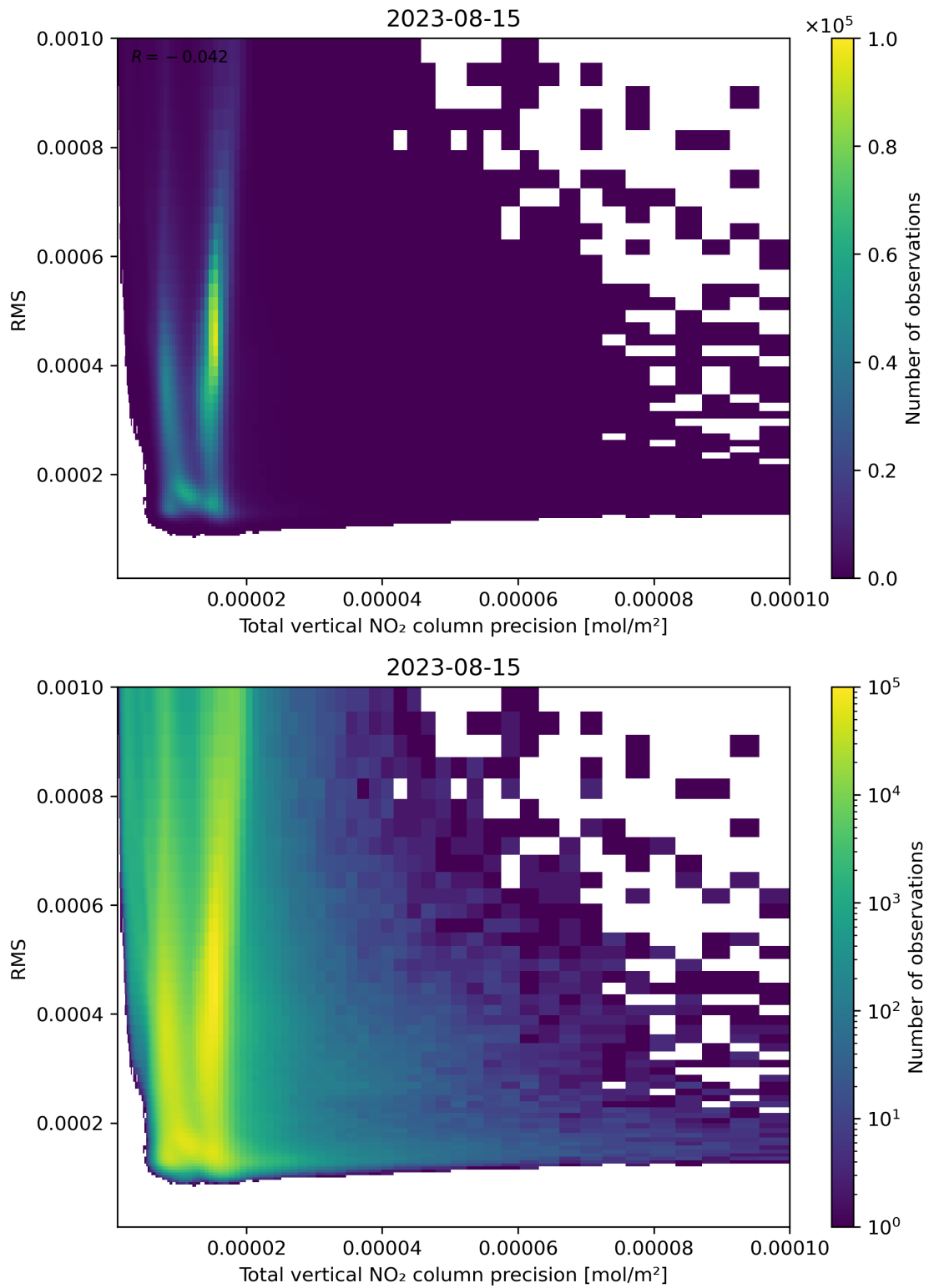
Figure 119: Scatter density plot of “Total vertical NO 2 column precision” against “RMS” for 2023-08-14 to 2023-08-16.
