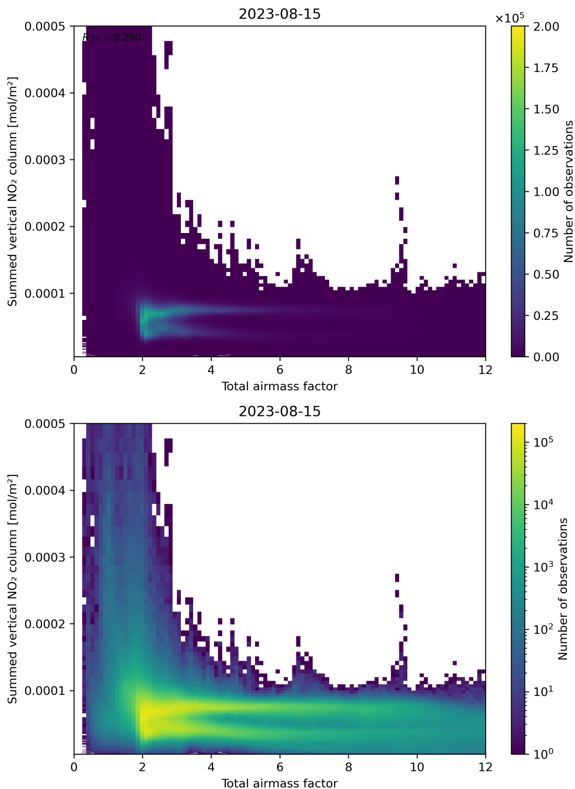
Figure 65: Scatter density plot of “Total airmass factor” against “Summed vertical NO 2 column” for 2023-08-14 to 2023-08-16.
