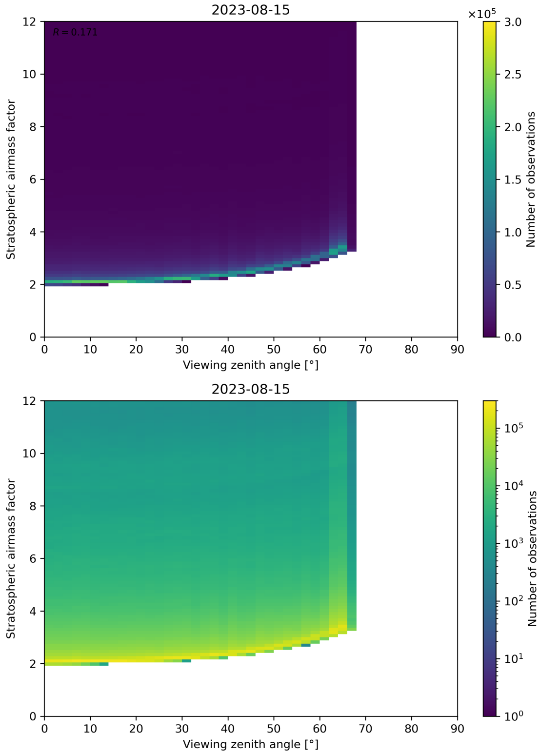
Figure 159: Scatter density plot of “Viewing zenith angle” against “Stratospheric airmass factor” for 2023-08-14 to 2023-08-16.
