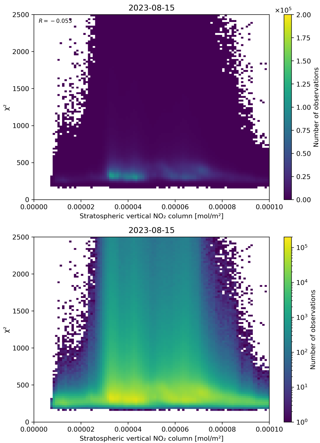
Figure 97: Scatter density plot of “Stratospheric vertical NO 2 column” against “ \chi^2 ” for 2023-08-14 to 2023-08-16.
