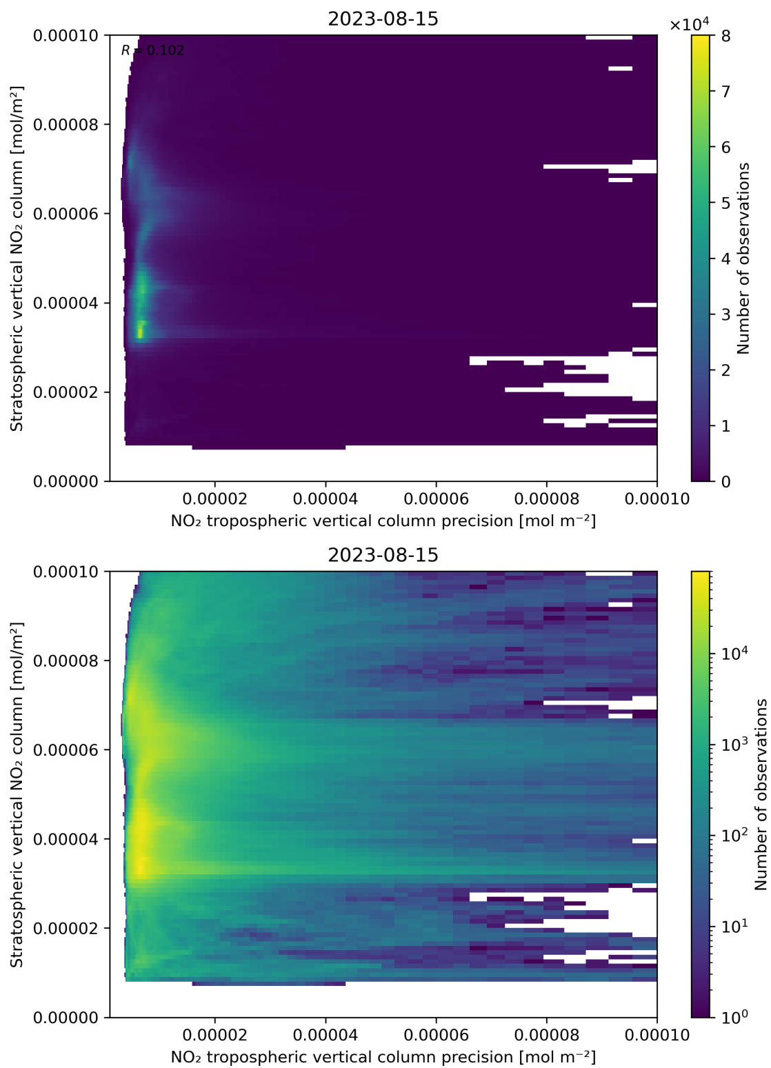
Figure 135: Scatter density plot of “NO 2 tropospheric vertical column precision” against “Stratospheric vertical NO 2 column” for 2023-08-14 to 2023-08-16.
