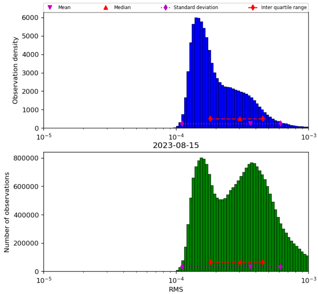
Figure 43: Histogram of “RMS” for 2023-08-14 to 2023-08-16
