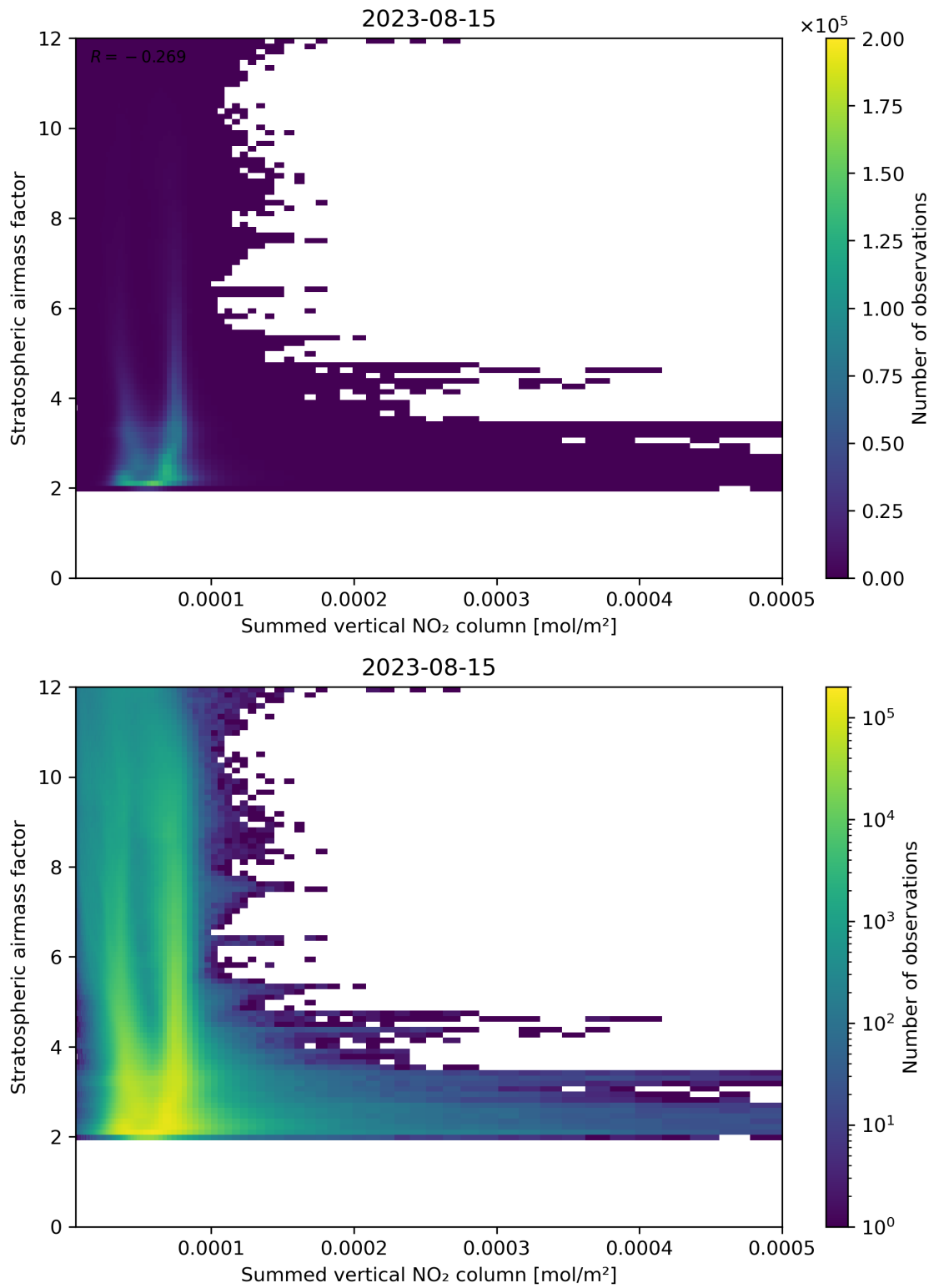
Figure 103: Scatter density plot of “Summed vertical NO 2 column” against “Stratospheric airmass factor” for 2023-08-14 to 2023-08-16.
