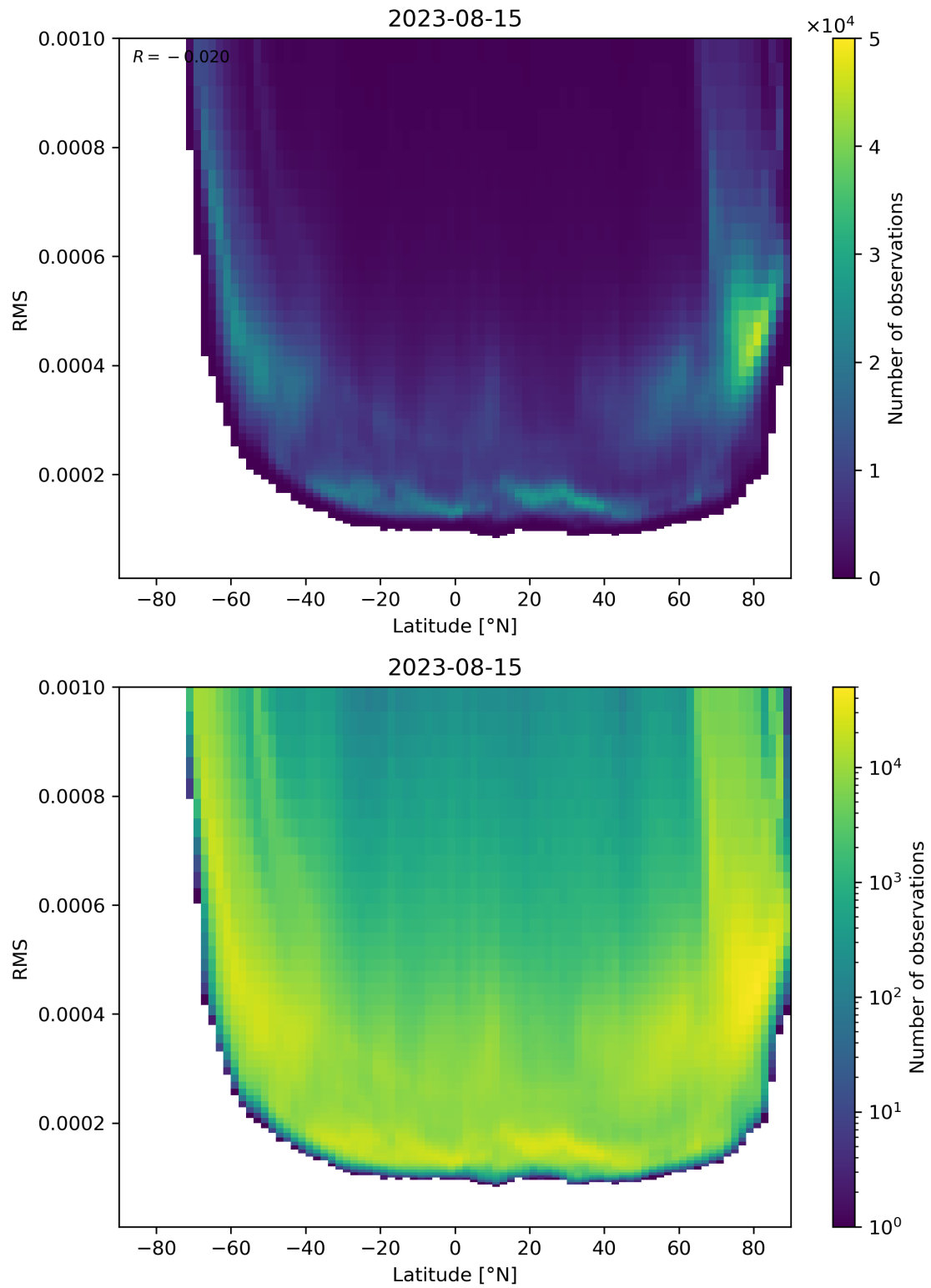
Figure 94: Scatter density plot of “Latitude” against “RMS” for 2023-08-14 to 2023-08-16.
