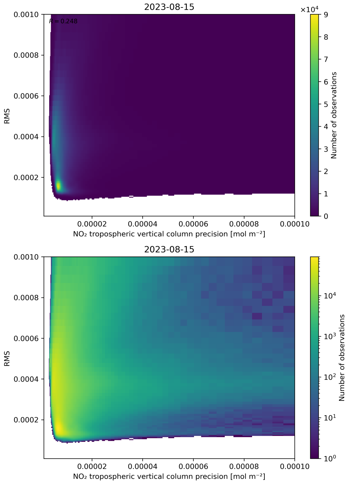
Figure 140: Scatter density plot of “NO 2 tropospheric vertical column precision” against “RMS” for 2023-08-14 to 2023-08-16.
