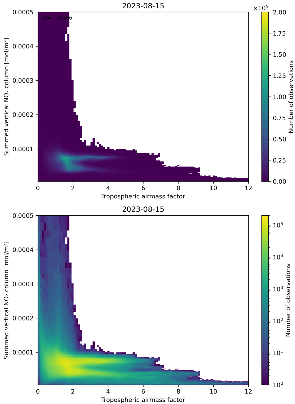
Figure 75: Scatter density plot of “Tropospheric airmass factor” against “Summed vertical NO 2 column” for 2023-08-14 to 2023-08-16.
