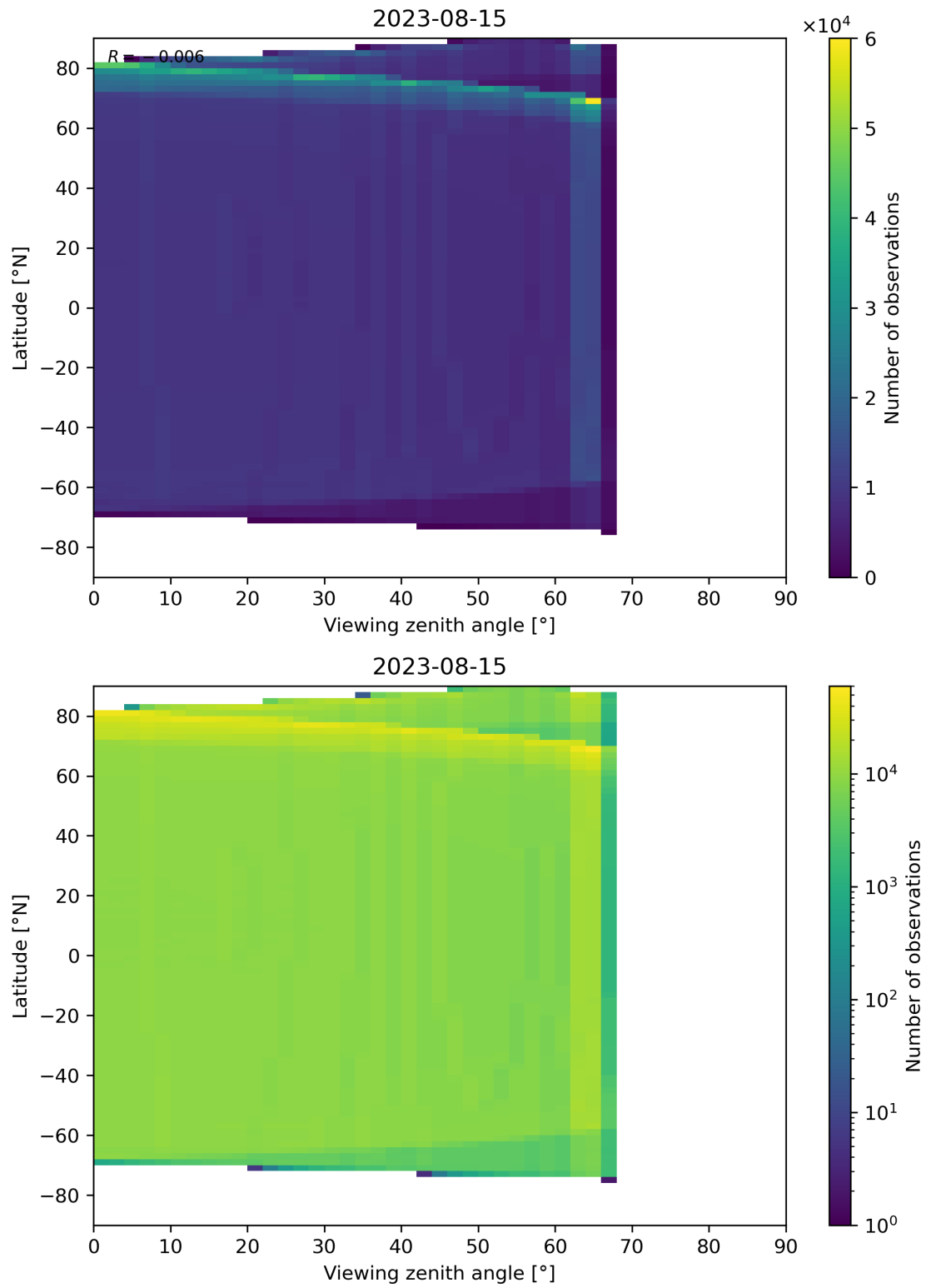
Figure 163: Scatter density plot of “Viewing zenith angle” against “Latitude” for 2023-08-14 to 2023-08-16.
