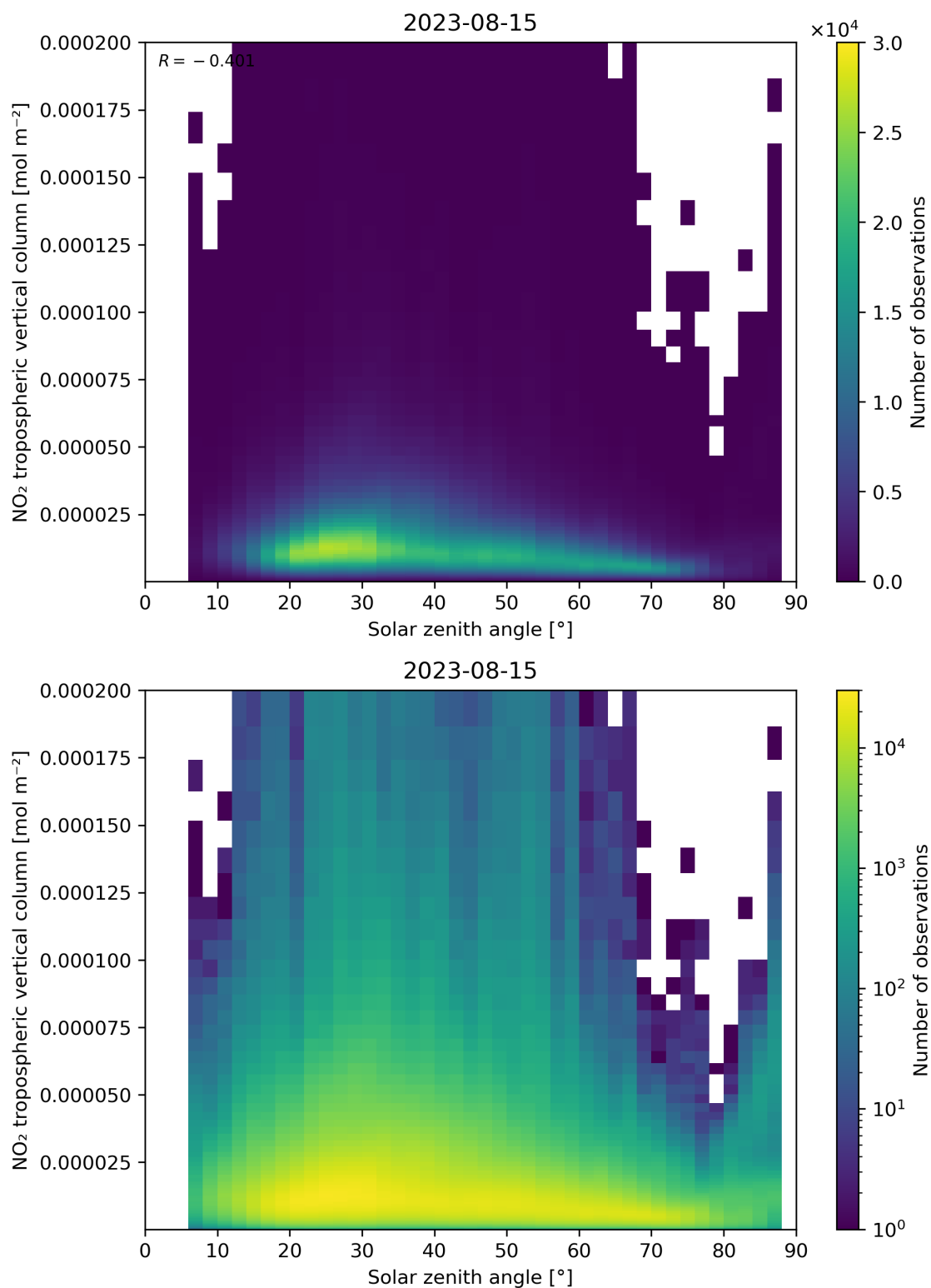
Figure 155: Scatter density plot of “Solar zenith angle” against “NO 2 tropospheric vertical column” for 2023-08-14 to 2023-08-16.
