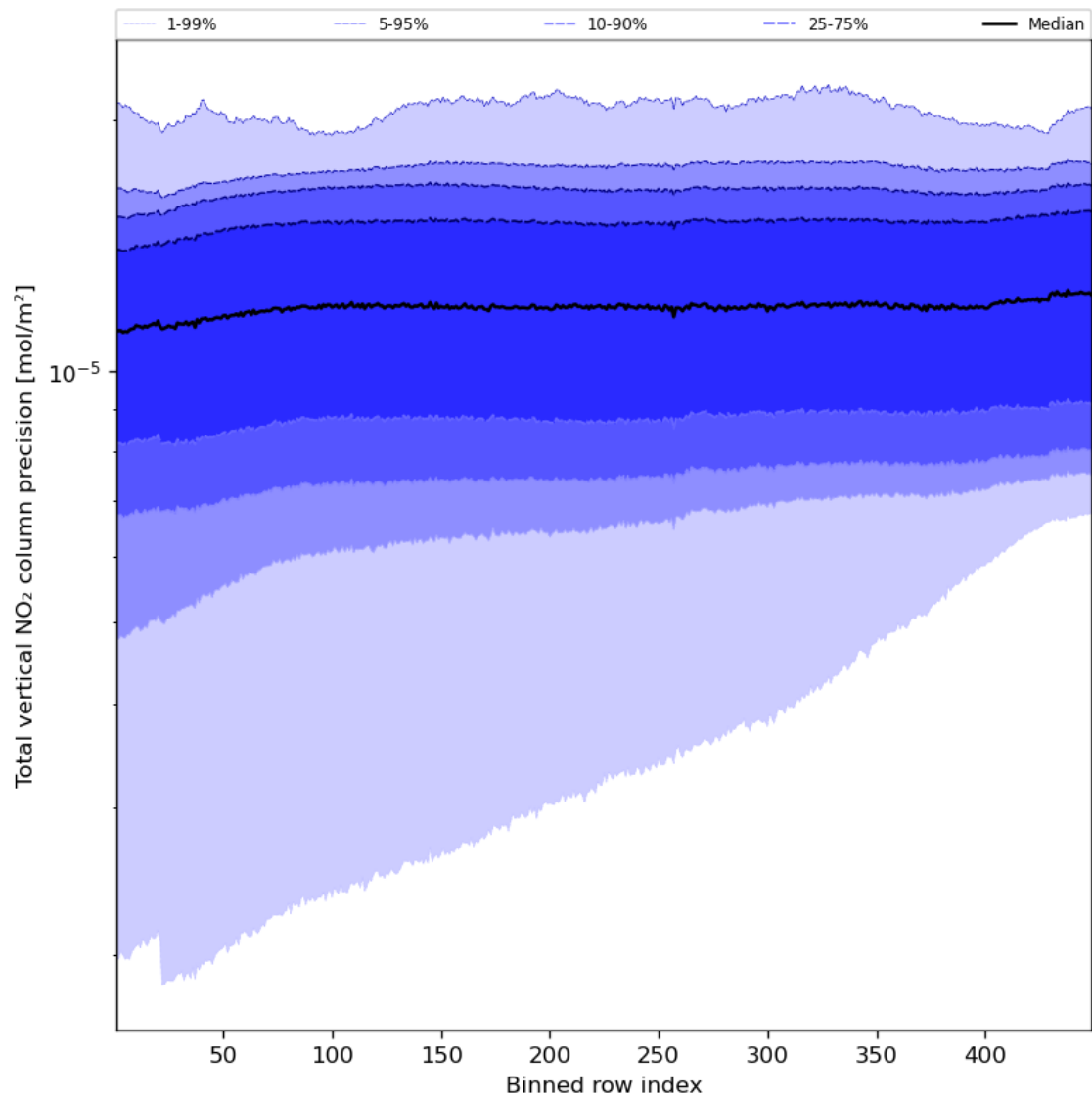
Figure 56: Along track statistics of “Total vertical NO 2 column precision” for 2023-08-14 to 2023-08-16
