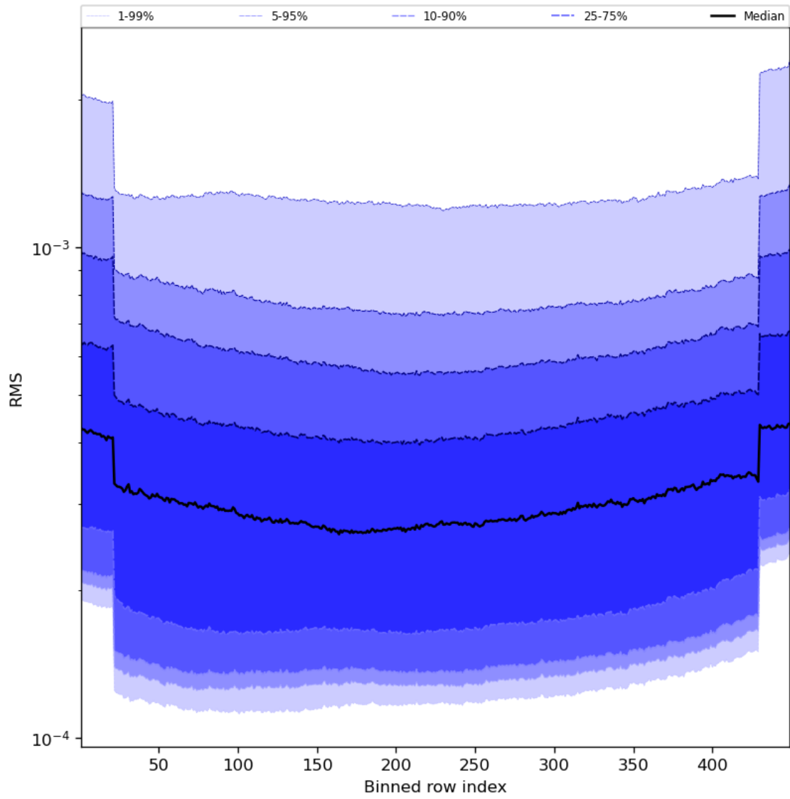
Figure 60: Along track statistics of “RMS” for 2023-08-14 to 2023-08-16
