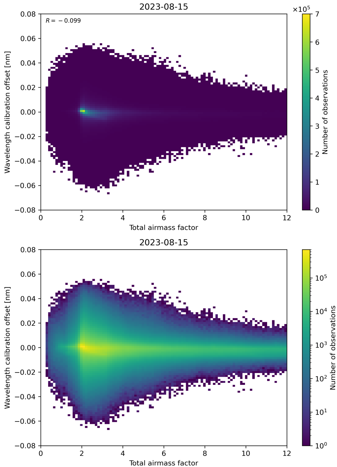
Figure 70: Scatter density plot of “Total airmass factor” against “Wavelength calibration offset” for 2023-08-14 to 2023-08-16.
