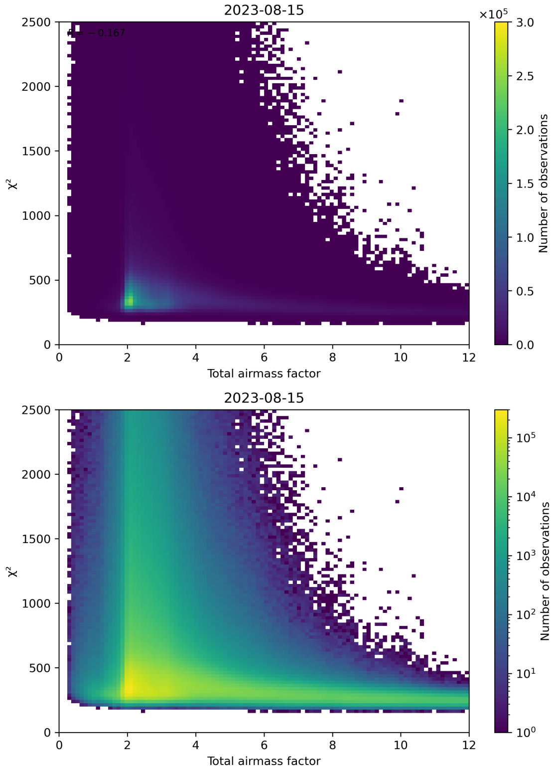
Figure 63: Scatter density plot of “Total airmass factor” against “ \chi^2 ” for 2023-08-14 to 2023-08-16.
