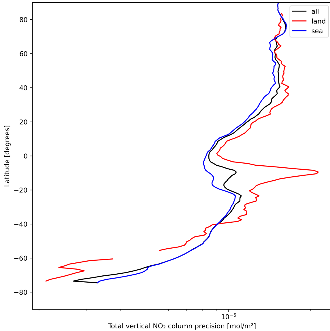
Figure 22: Zonal average of “Total vertical NO 2 column precision” for 2023-08-14 to 2023-08-16.
