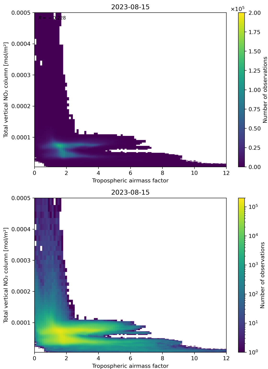
Figure 77: Scatter density plot of “Tropospheric airmass factor” against “Total vertical NO 2 column” for 2023-08-14 to 2023-08-16.
