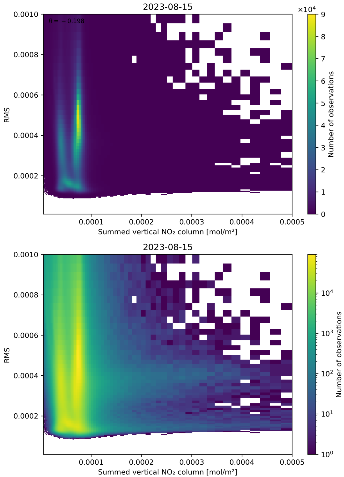
Figure 109: Scatter density plot of “Summed vertical NO 2 column” against “RMS” for 2023-08-14 to 2023-08-16.
