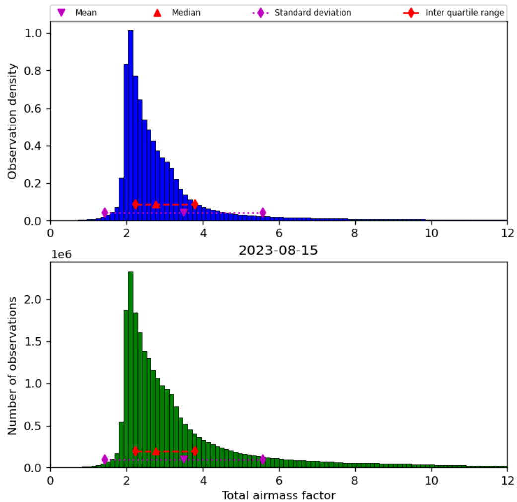
Figure 32: Histogram of “Total airmass factor” for 2023-08-14 to 2023-08-16
