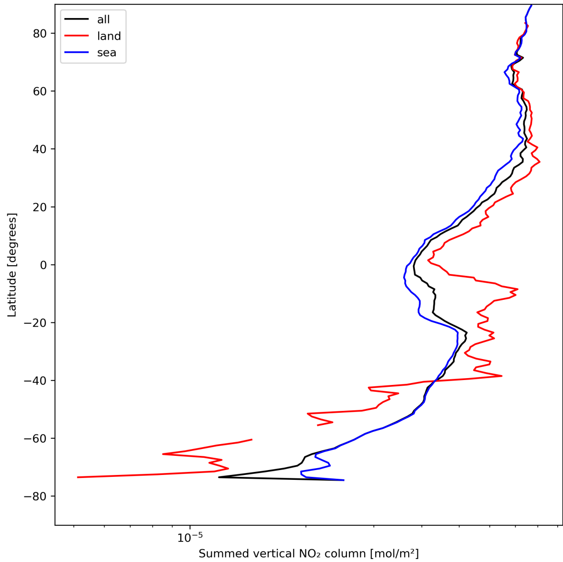
Figure 23: Zonal average of “Summed vertical NO 2 column” for 2023-08-14 to 2023-08-16.
