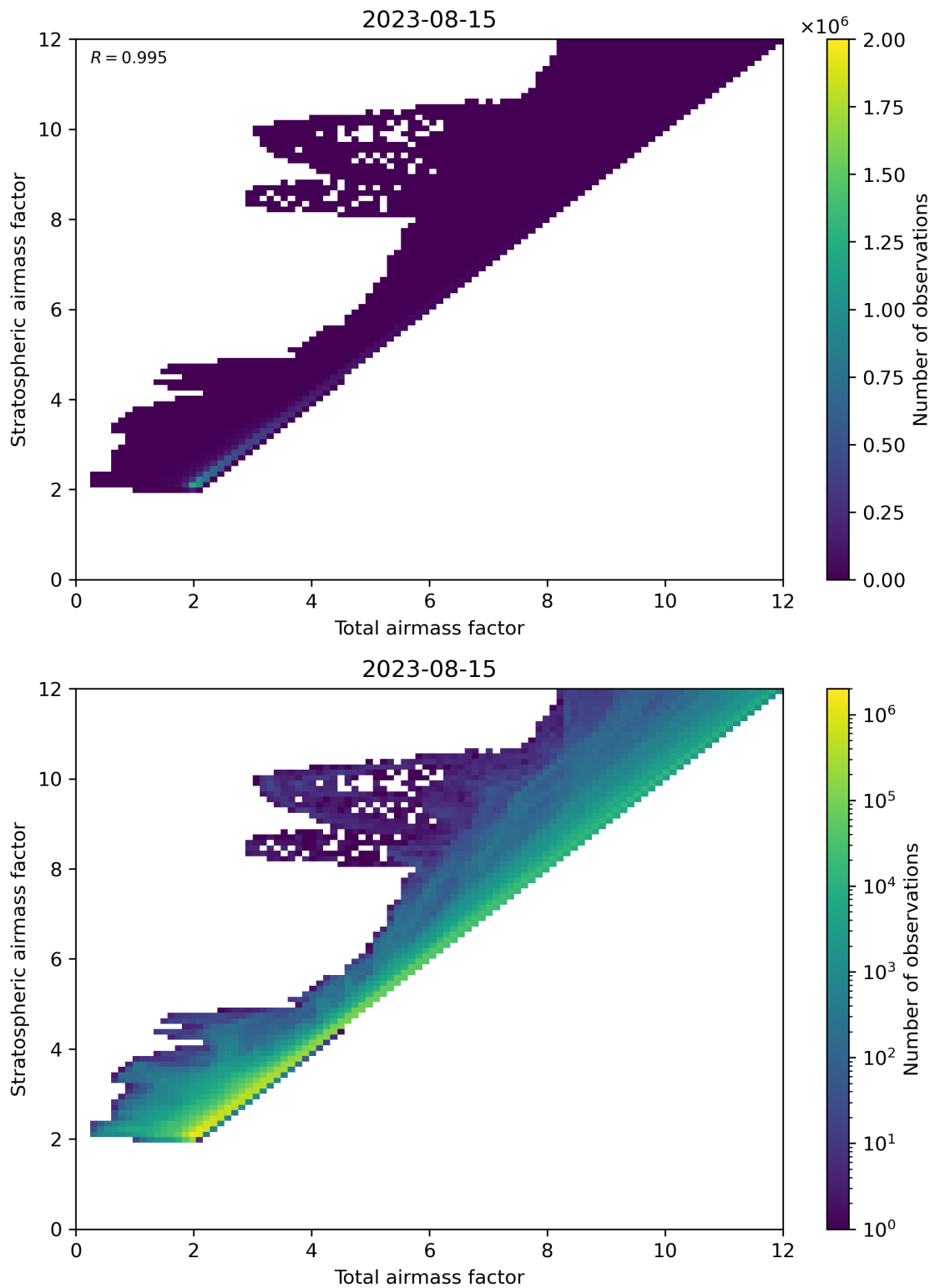
Figure 62: Scatter density plot of “Total air mass factor” against “Stratospheric air mass factor” for 2023-08-14 to 2023-08-16.
