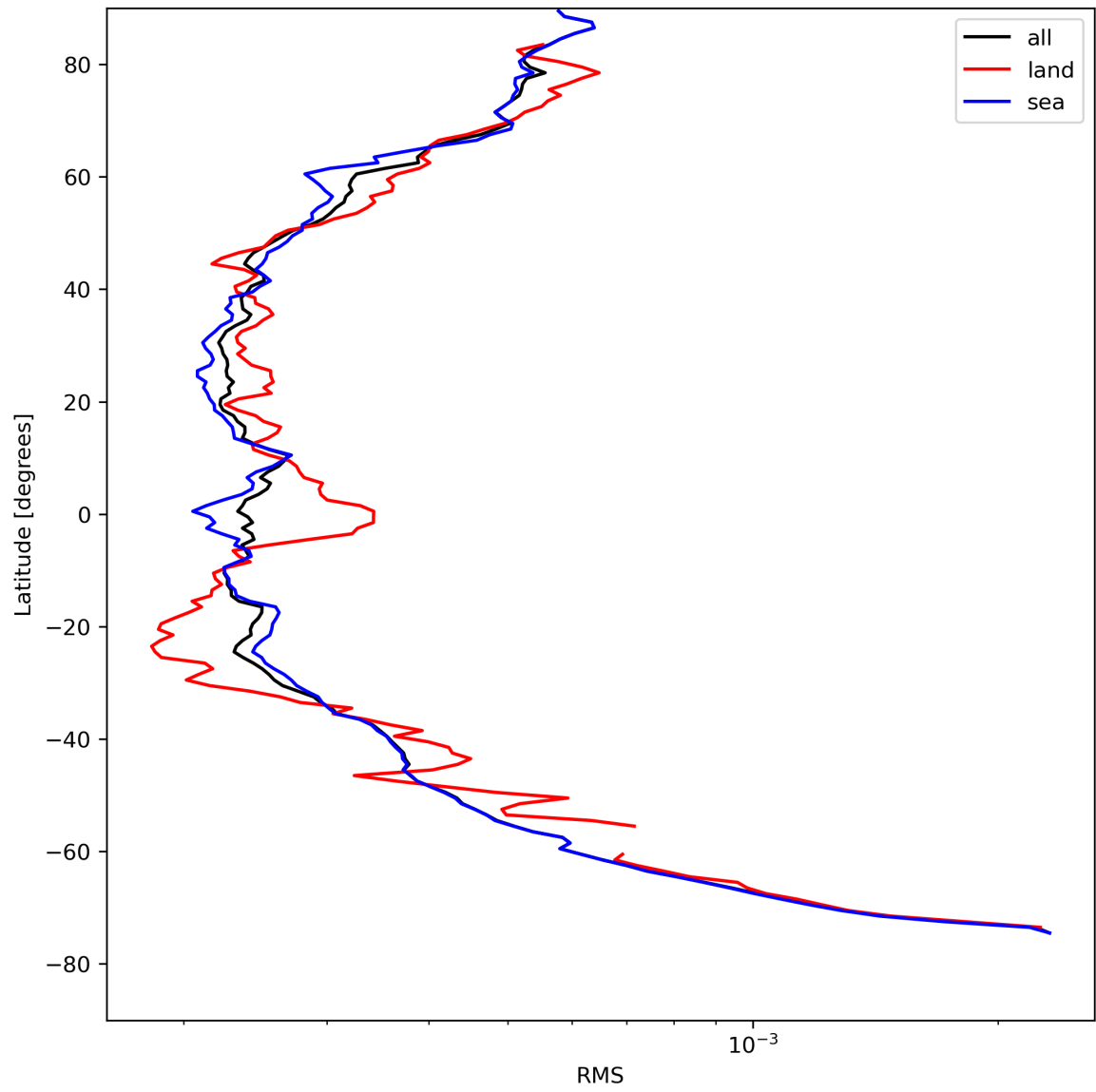
Figure 26: Zonal average of “RMS” for 2023-08-14 to 2023-08-16.
