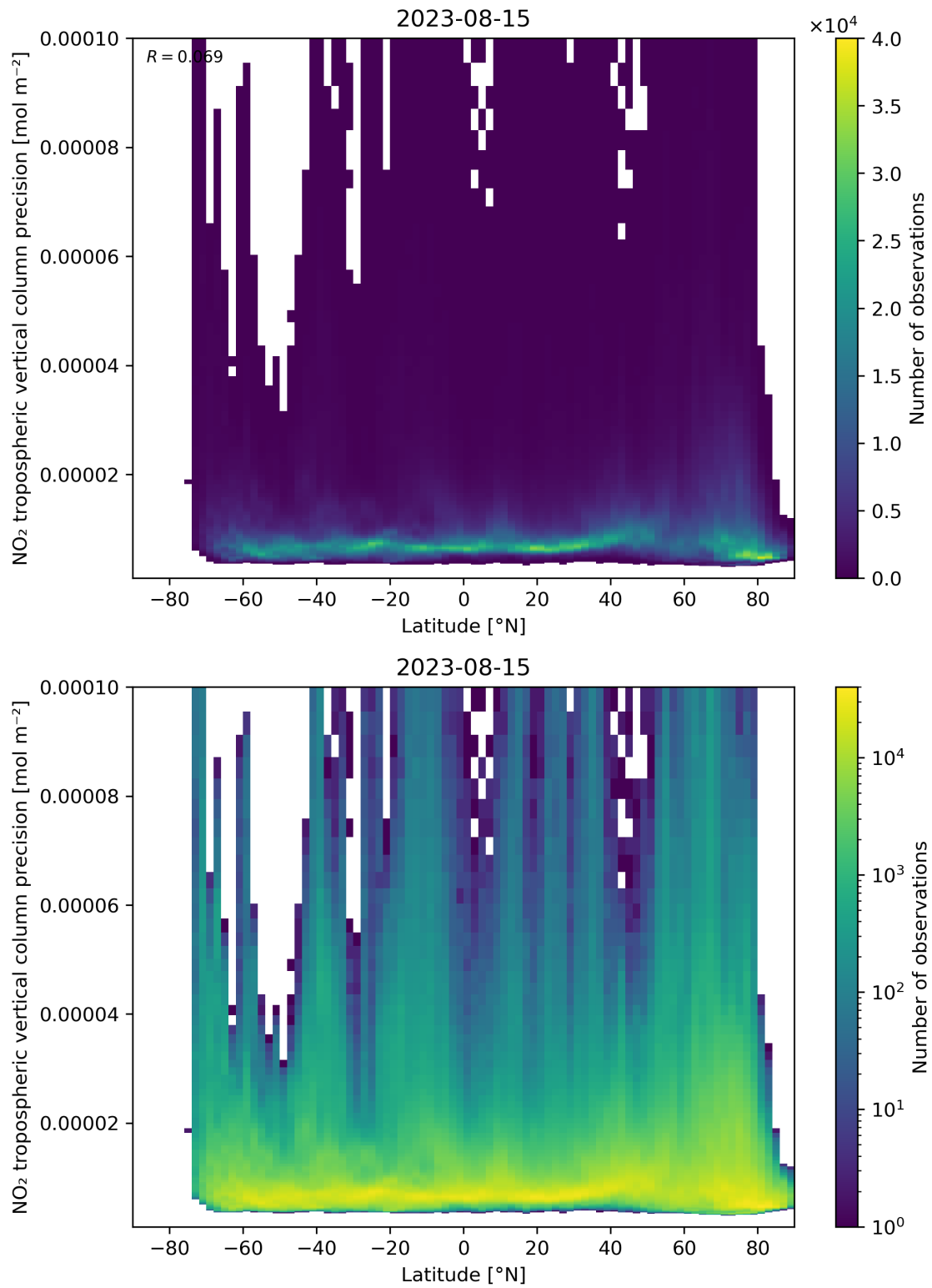
Figure 93: Scatter density plot of “Latitude” against “NO 2 tropospheric vertical column precision” for 2023-08-14 to 2023-08-16.
