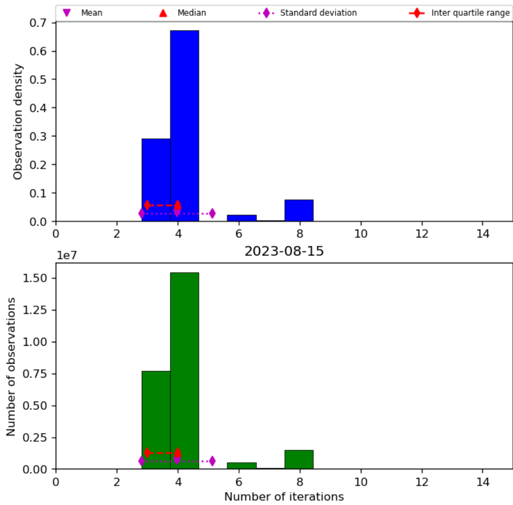
Figure 34: Histogram of “Number of iterations” for 2023-08-14 to 2023-08-16
