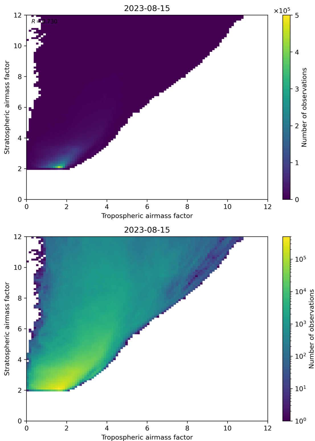
Figure 71: Scatter density plot of “Tropospheric airmass factor” against “Stratospheric airmass factor” for 2023-08-14 to 2023-08-16.
