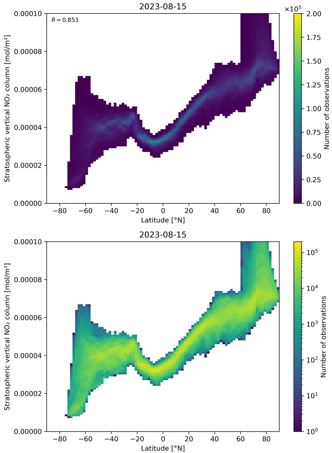
Figure 87: Scatter density plot of “Latitude” against “Stratospheric vertical NO 2 column” for 2023-08-14 to 2023-08-16.
