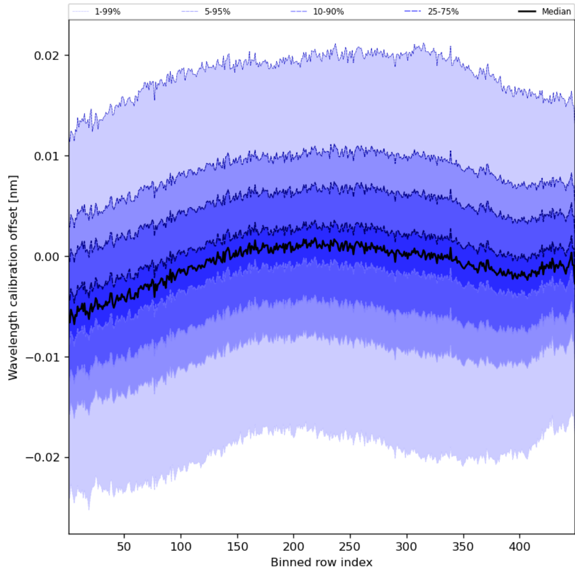
Figure 52: Along track statistics of “Wavelength calibration offset” for 2023-08-14 to 2023-08-16
