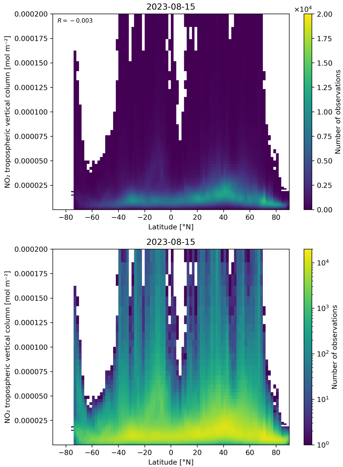
Figure 92: Scatter density plot of “Latitude” against “NO 2 tropospheric vertical column” for 2023-08-14 to 2023-08-16.
