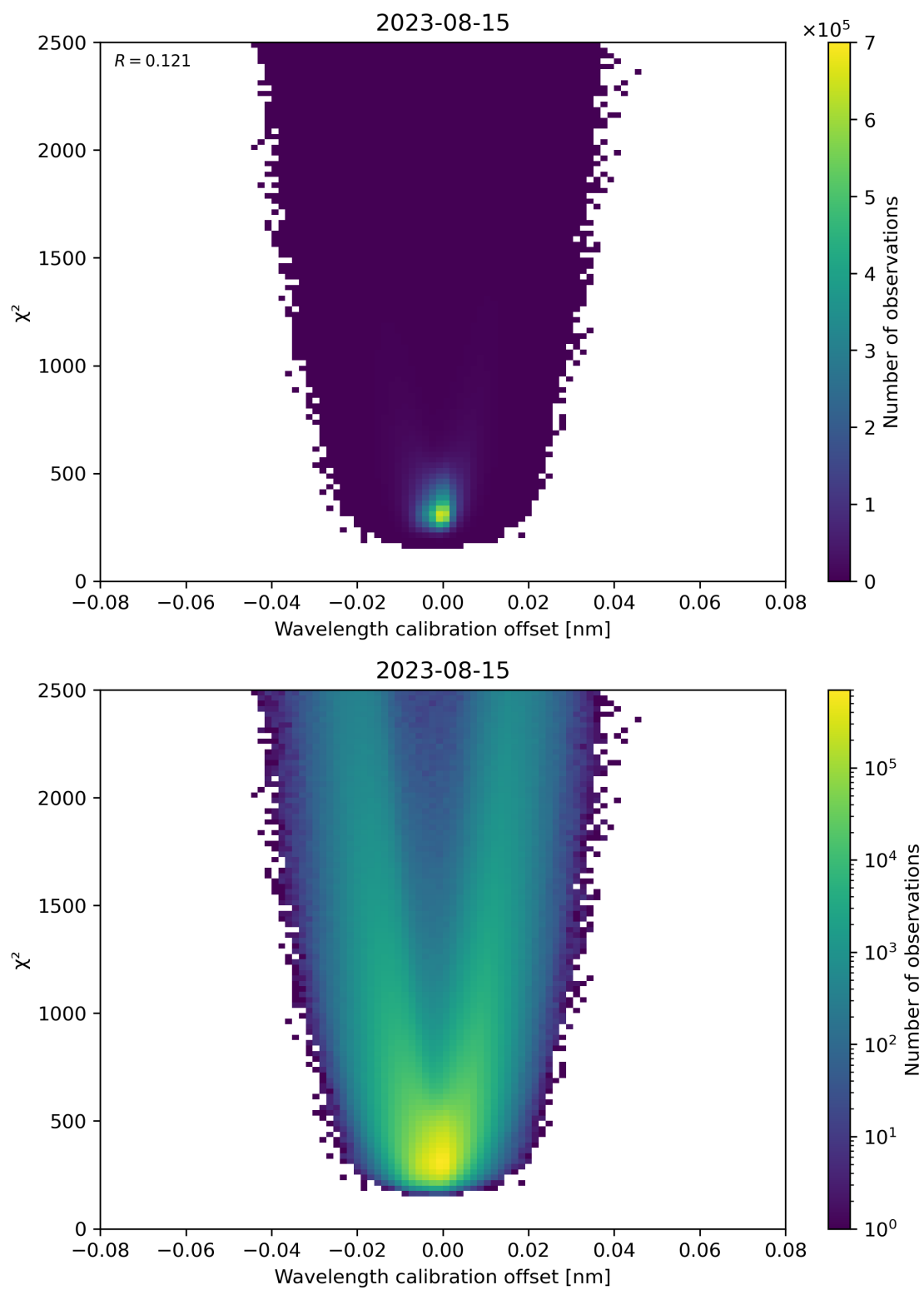
Figure 175: Scatter density plot of “Wavelength calibration offset” against “ \chi^2 ” for 2023-08-14 to 2023-08-16.
