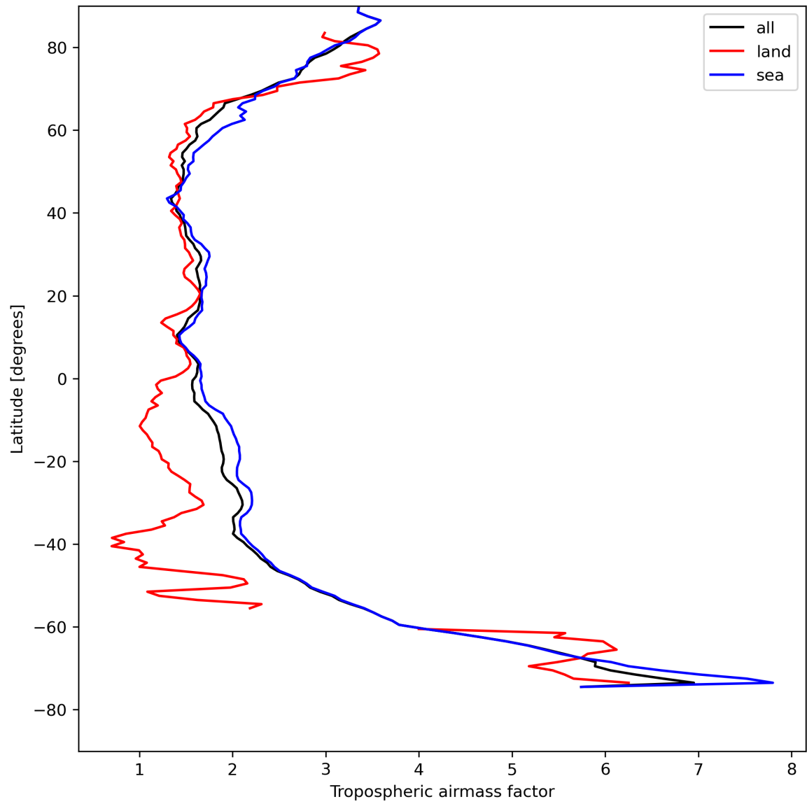
Figure 14: Zonal average of “Tropospheric airmass factor” for 2023-08-14 to 2023-08-16.
