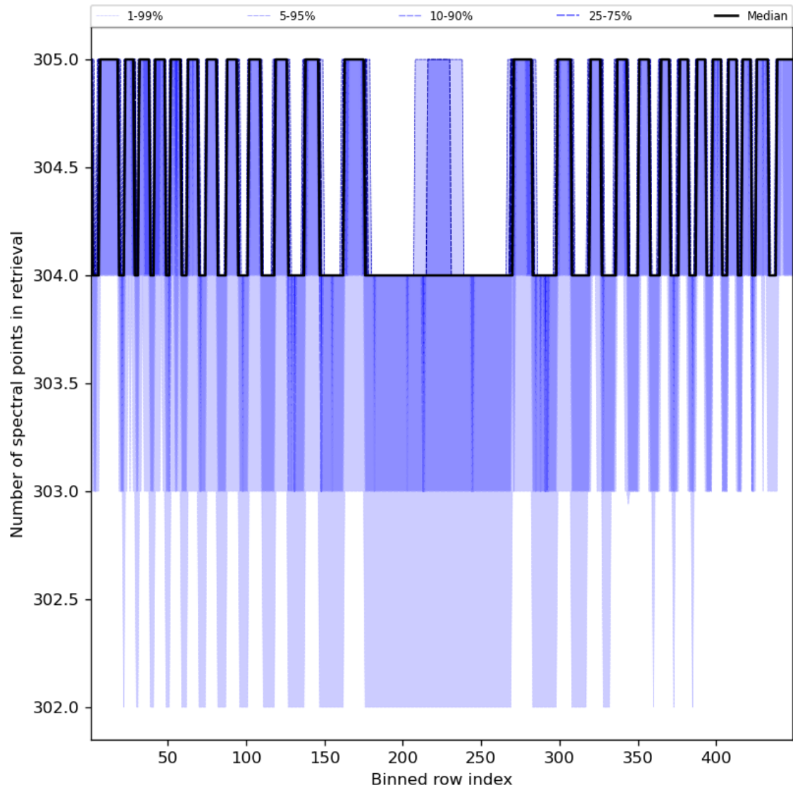
Figure 50: Along track statistics of “Number of spectral points in retrieval” for 2023-08-14 to 2023-08-16
