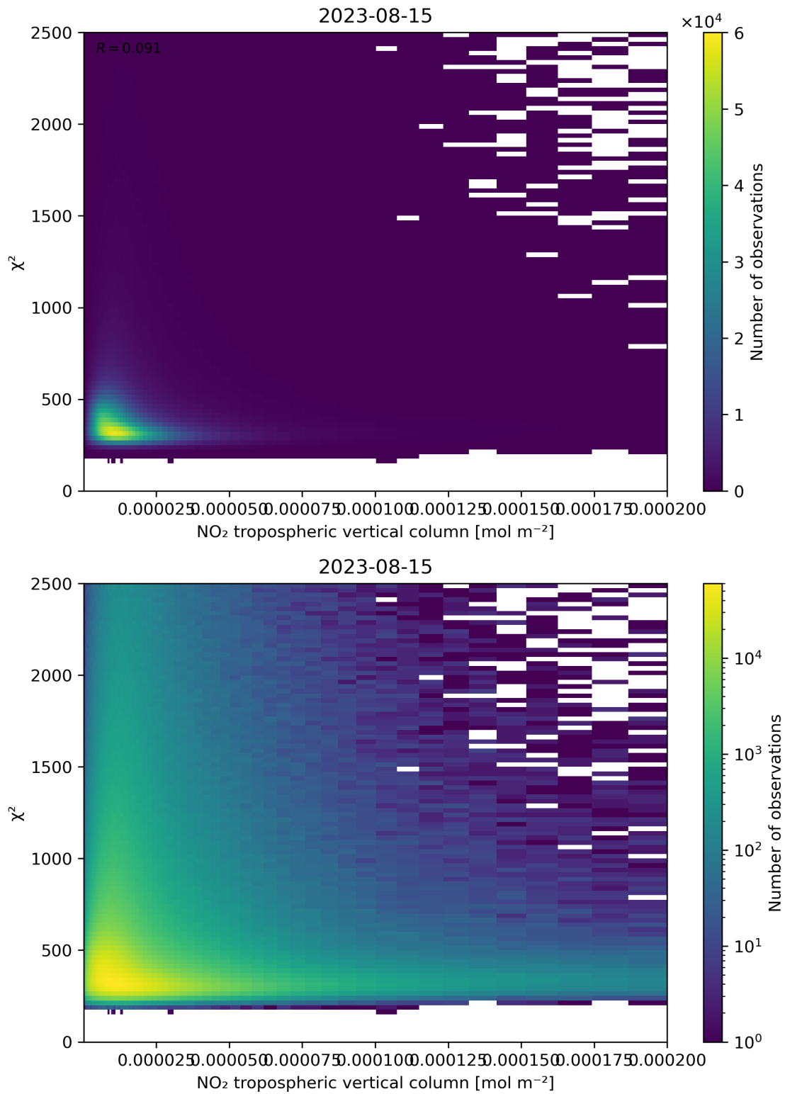
Figure 124: Scatter density plot of “NO 2 tropospheric vertical column” against “ \chi^2 ” for 2023-08-14 to 2023-08-16.
