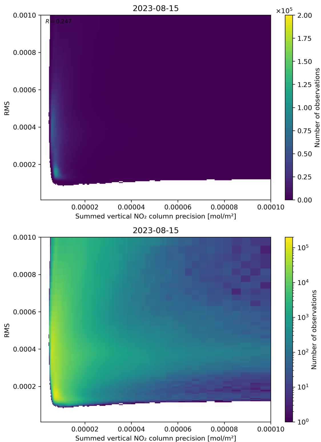
Figure 108: Scatter density plot of “Summed vertical NO 2 column precision” against “RMS” for 2023-08-14 to 2023-08-16.
