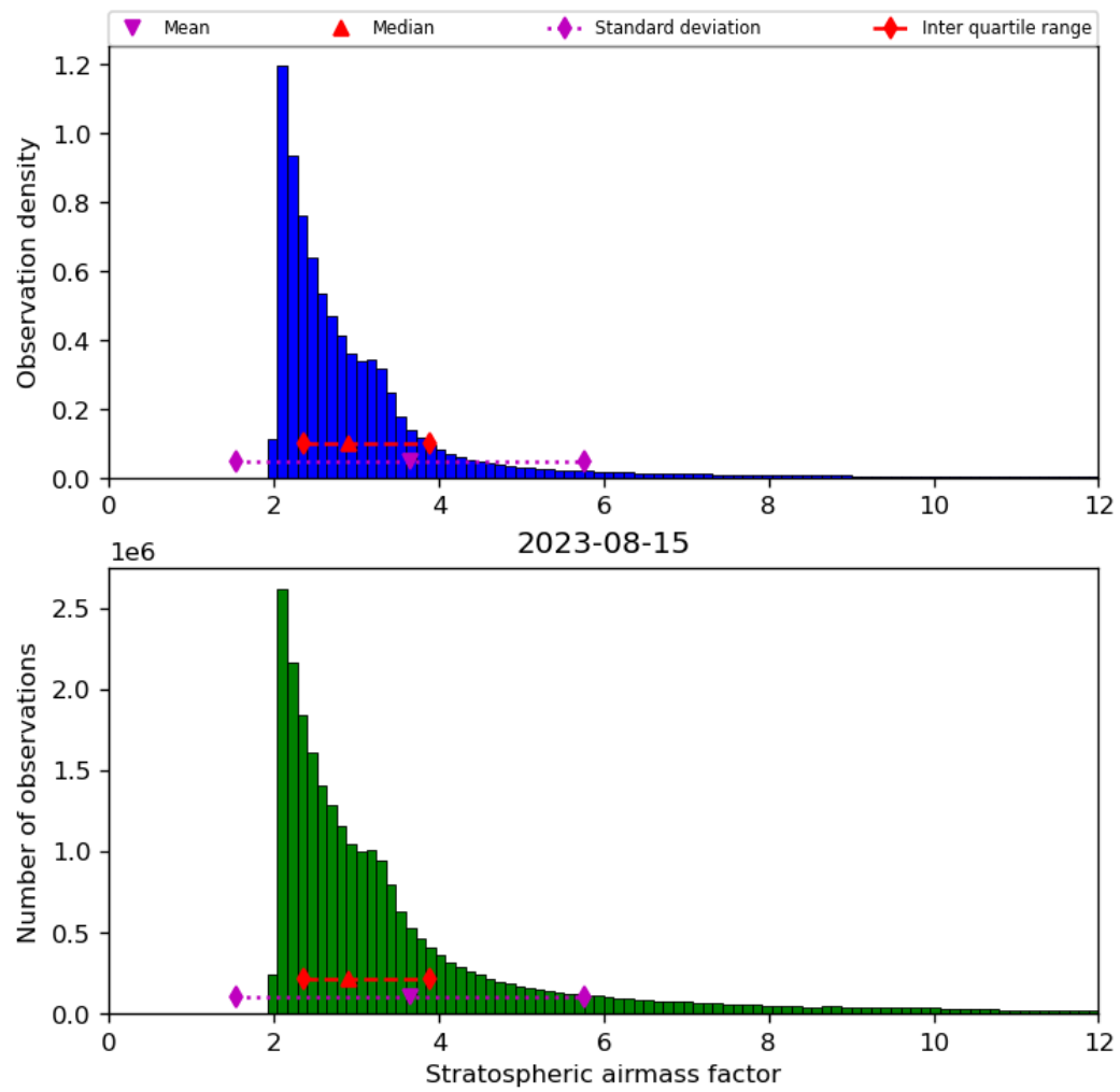
Figure 44: Histogram of “Stratospheric airmass factor” for 2023-08-14 to 2023-08-16
