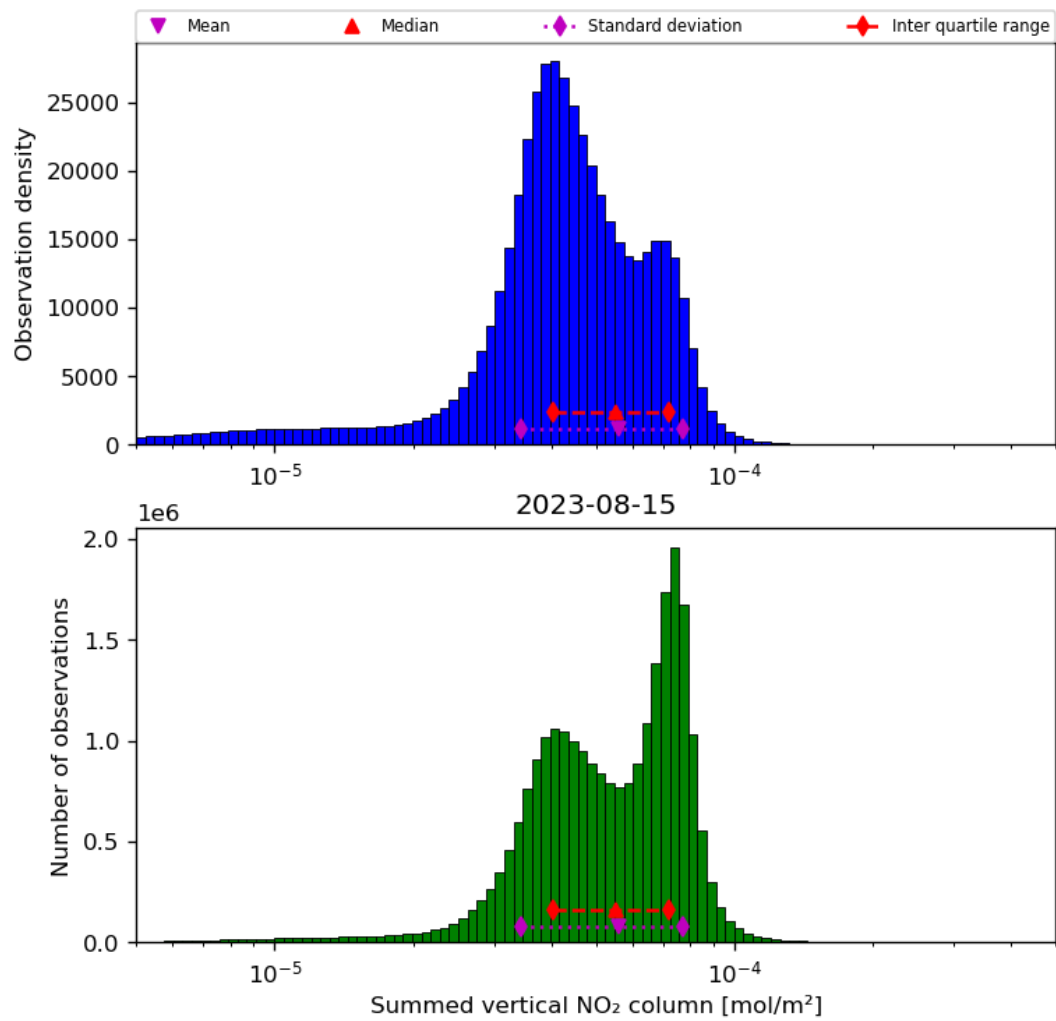
Figure 40: Histogram of “Summed vertical NO 2 column” for 2023-08-14 to 2023-08-16
