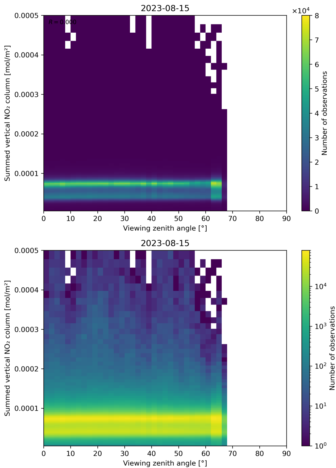
Figure 165: Scatter density plot of “Viewing zenith angle” against “Summed vertical NO 2 column” for 2023-08-14 to 2023-08-16.
