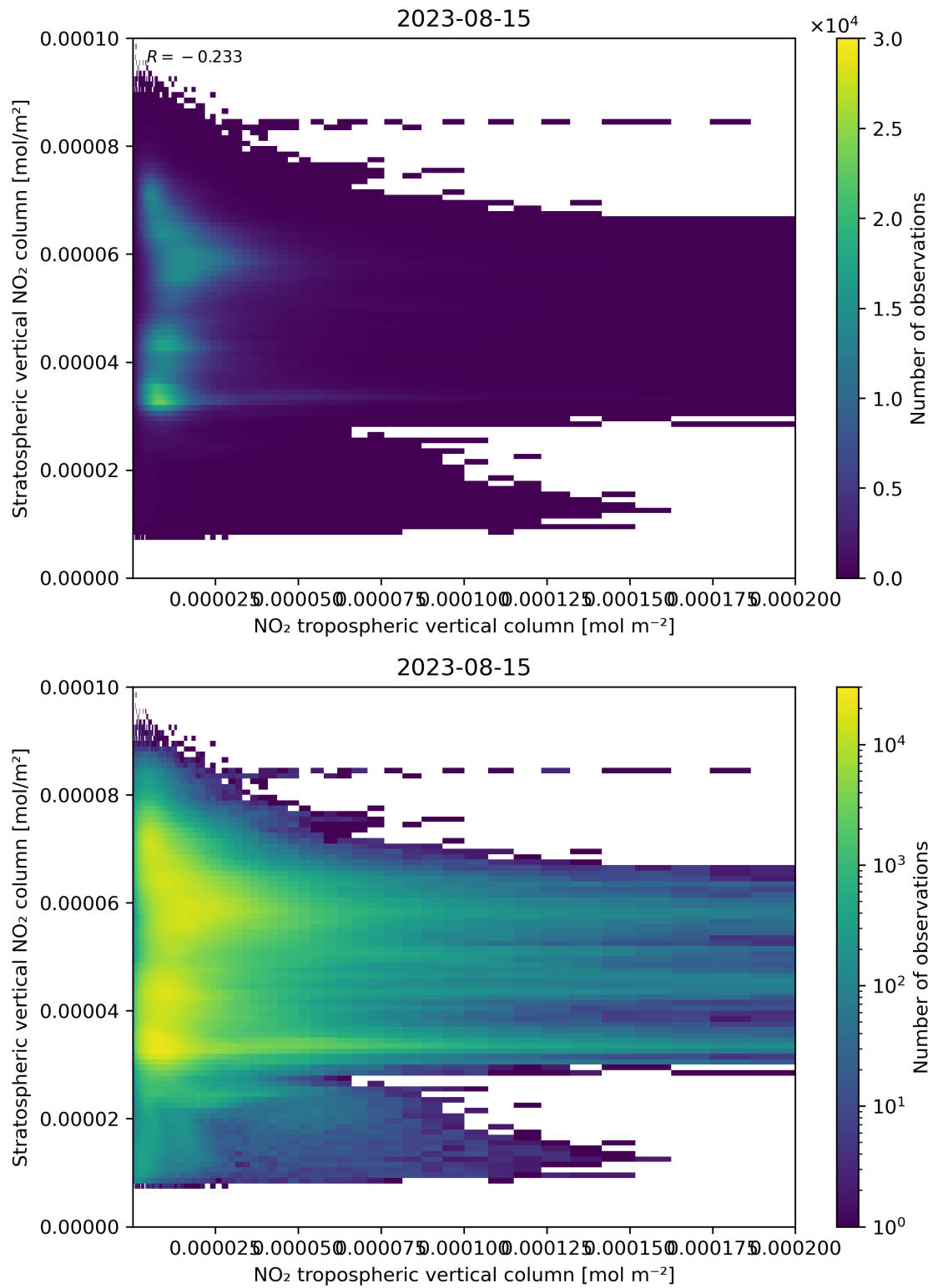
Figure 125: Scatter density plot of “NO 2 tropospheric vertical column” against “Stratospheric vertical NO 2 column” for 2023-08-14 to 2023-08-16.
