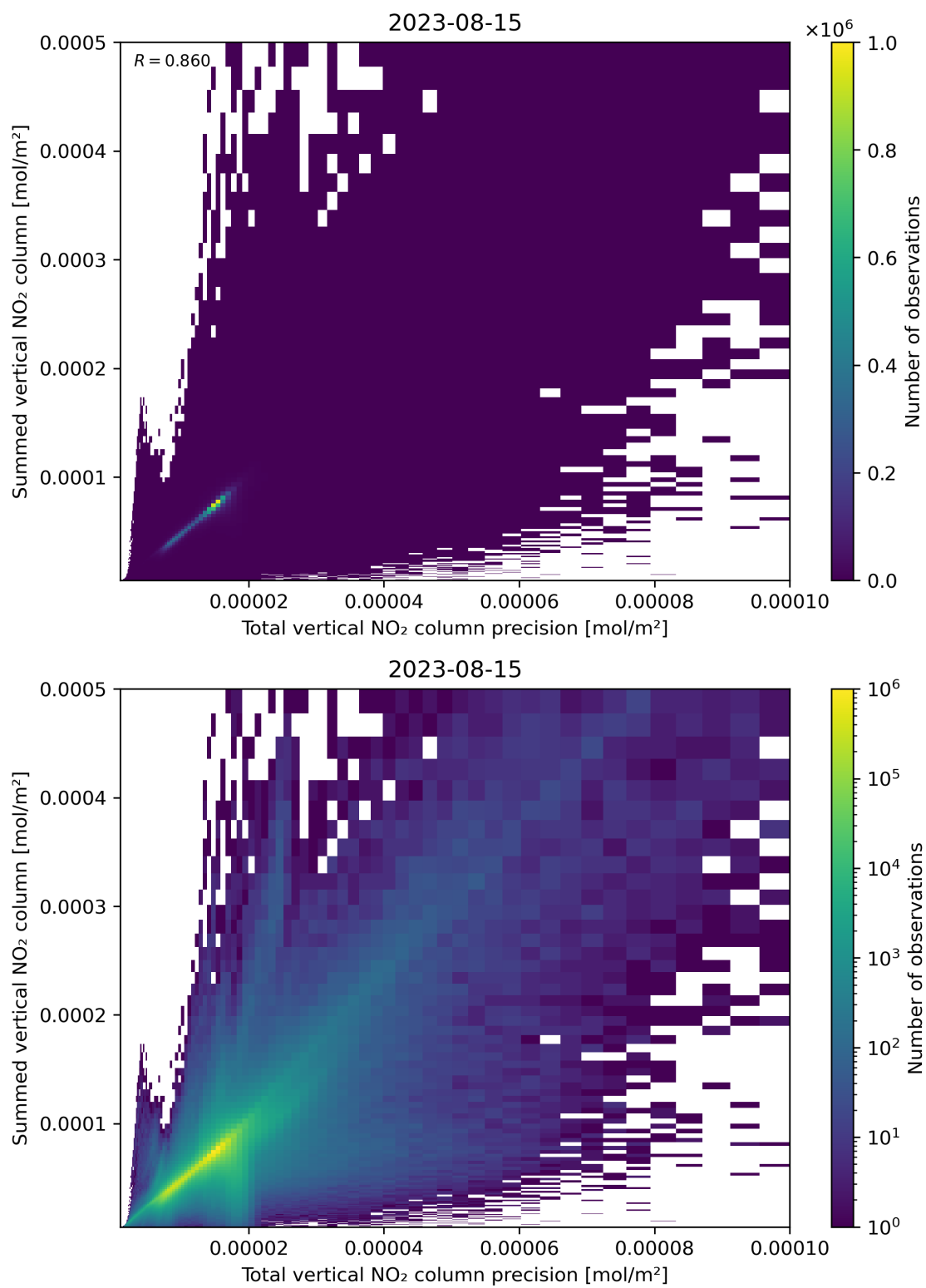
Figure 117: Scatter density plot of “Total vertical NO 2 column precision” against “Summed vertical NO 2 column” for 2023-08-14 to 2023-08-16.
