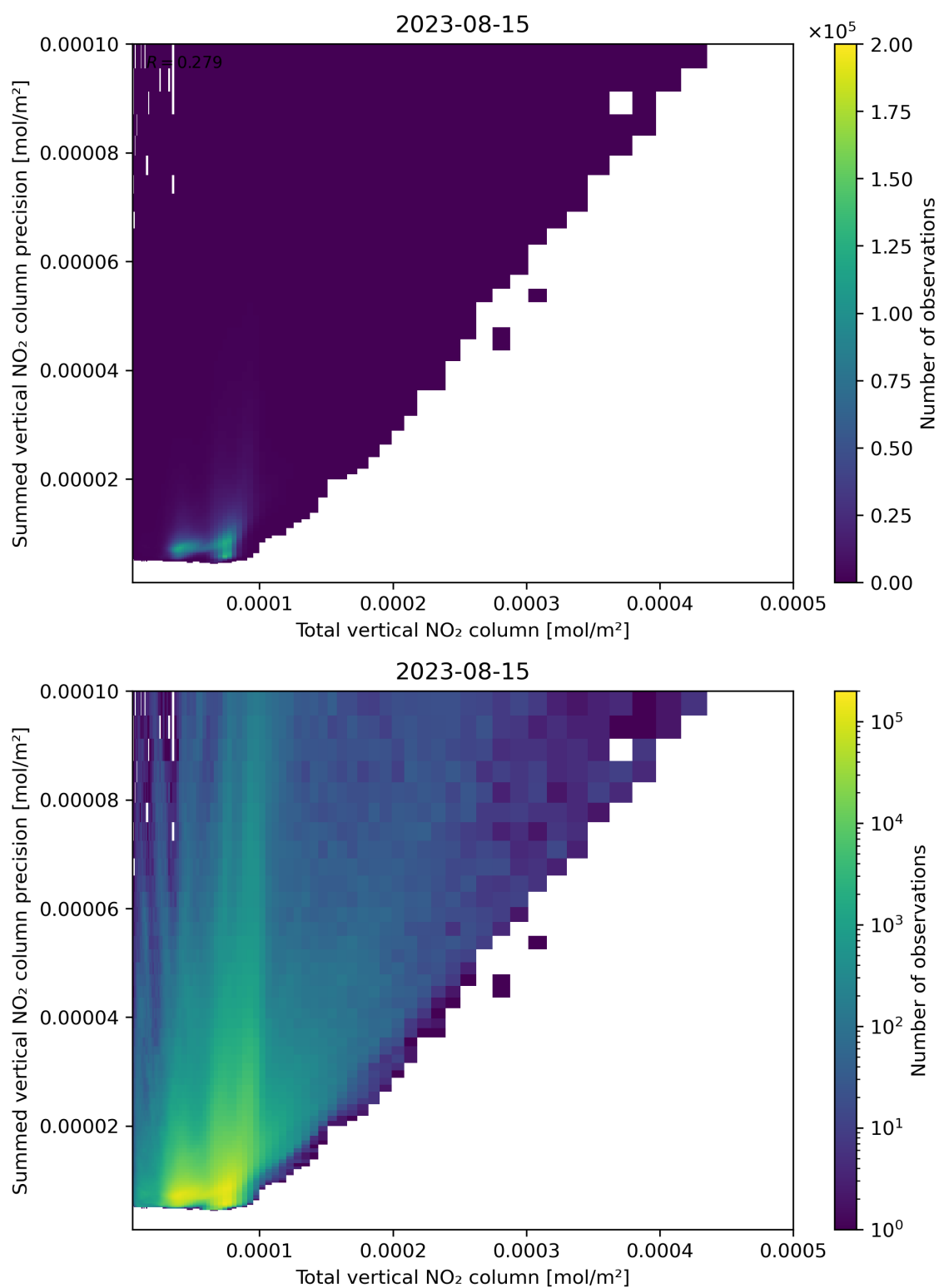
Figure 113: Scatter density plot of “Total vertical NO 2 column” against “Summed vertical NO 2 column precision” for 2023-08-14 to 2023-08-16.
