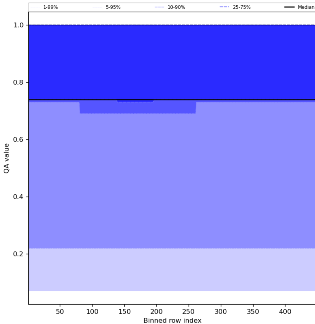
Figure 45: Along track statistics of “QA value” for 2023-08-14 to 2023-08-16
