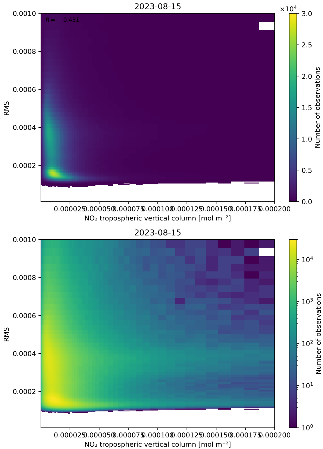
Figure 142: Scatter density plot of “NO 2 tropospheric vertical column” against “RMS” for 2023-08-14 to 2023-08-16.
