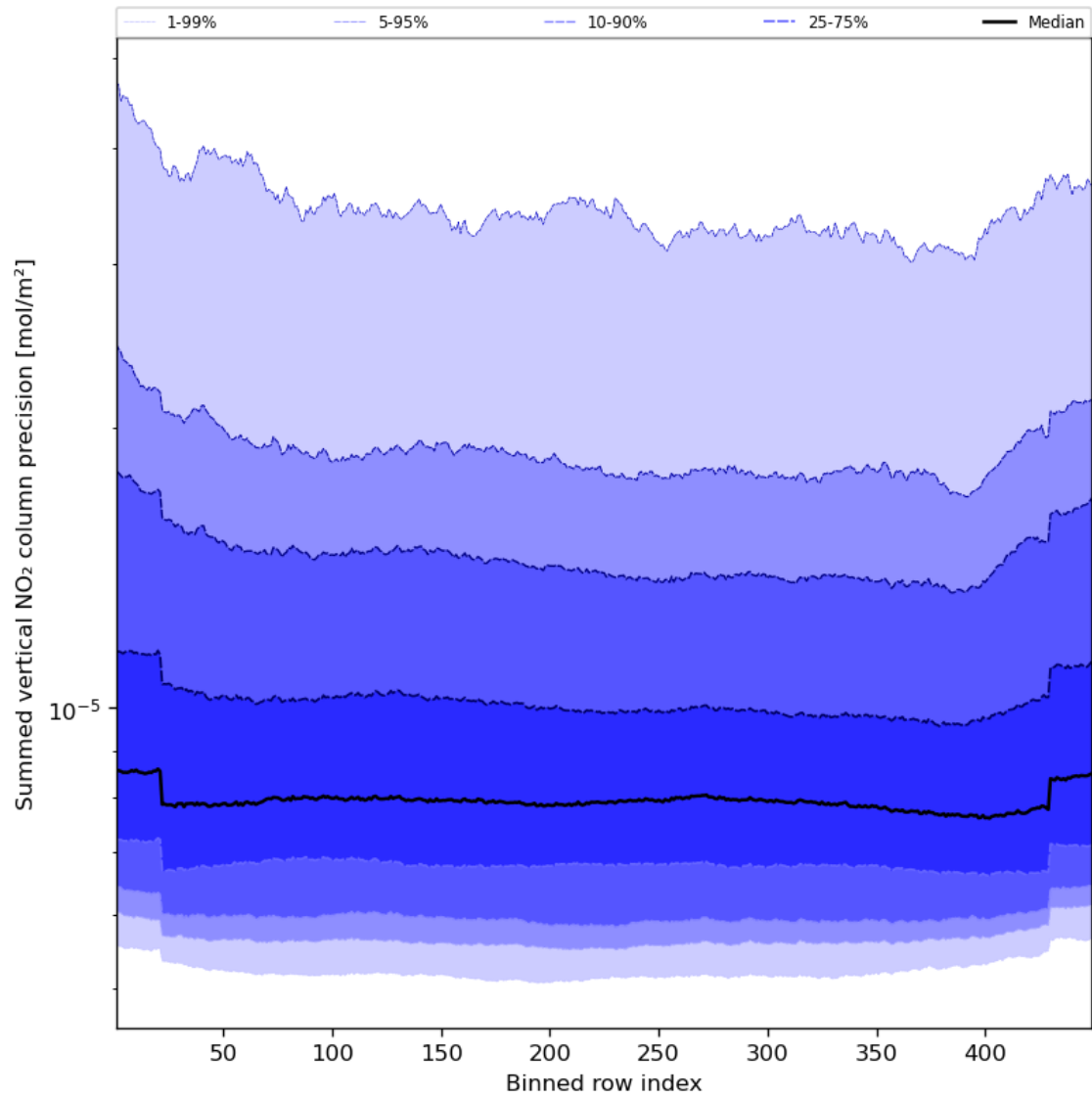
Figure 58: Along track statistics of “Summed vertical NO 2 column precision” for 2023-08-14 to 2023-08-16
