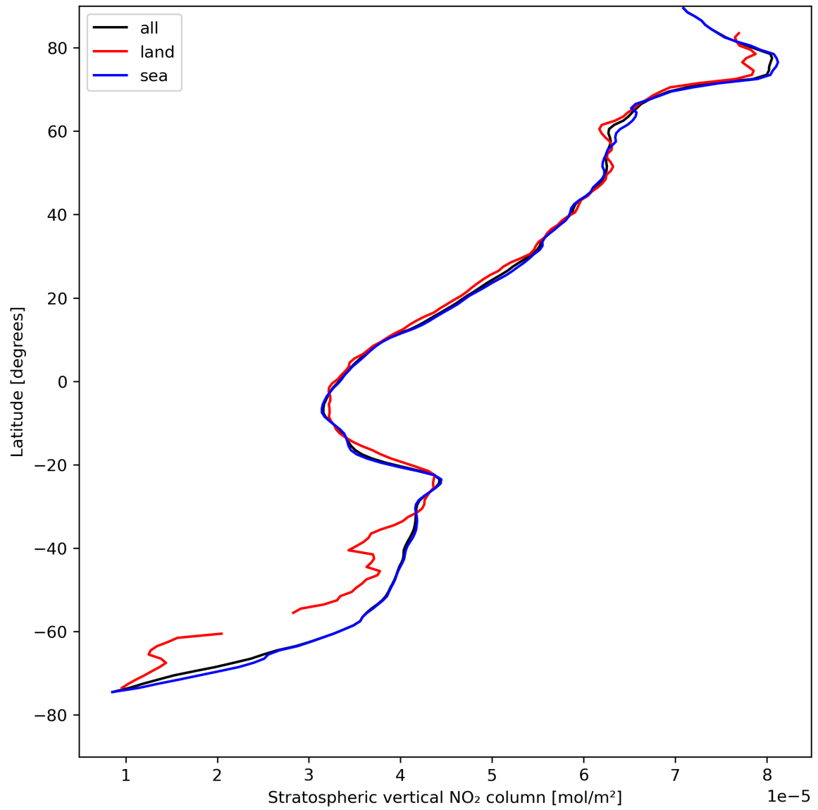
Figure 19: Zonal average of “Stratospheric vertical NO 2 column” for 2023-08-14 to 2023-08-16.
