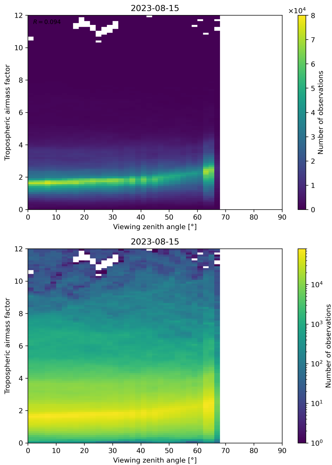
Figure 161: Scatter density plot of “Viewing zenith angle” against “Tropospheric airmass factor” for 2023-08-14 to 2023-08-16.
