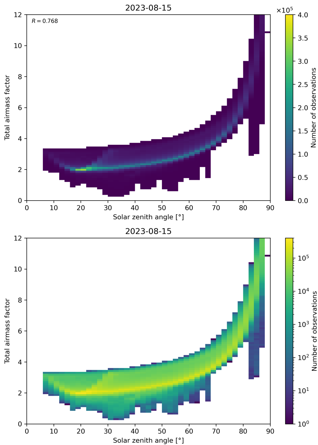
Figure 146: Scatter density plot of “Solar zenith angle” against “Total air mass factor” for 2023-08-14 to 2023-08-16.
