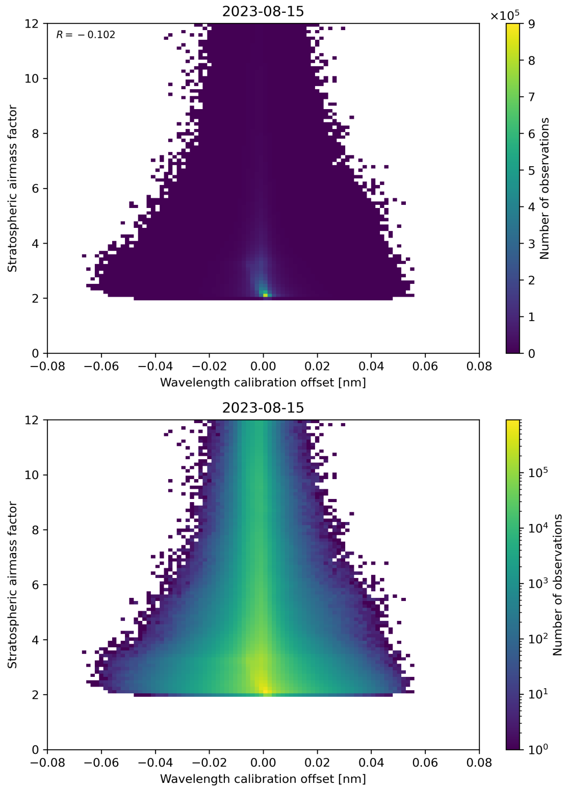
Figure 174: Scatter density plot of “Wavelength calibration offset” against “Stratospheric airmass factor” for 2023-08-14 to 2023-08-16.
