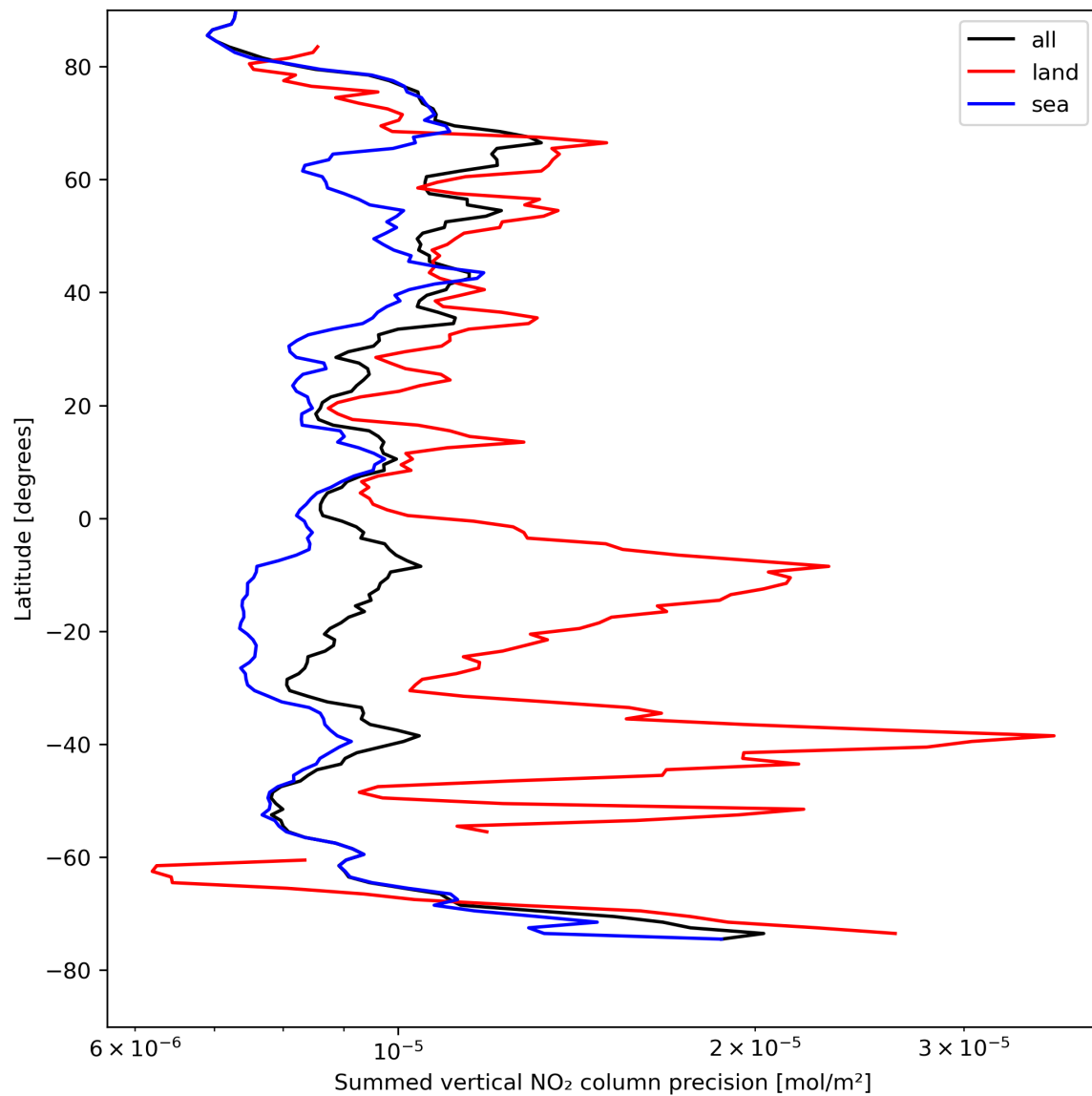
Figure 24: Zonal average of “Summed vertical NO 2 column precision” for 2023-08-14 to 2023-08-16.
