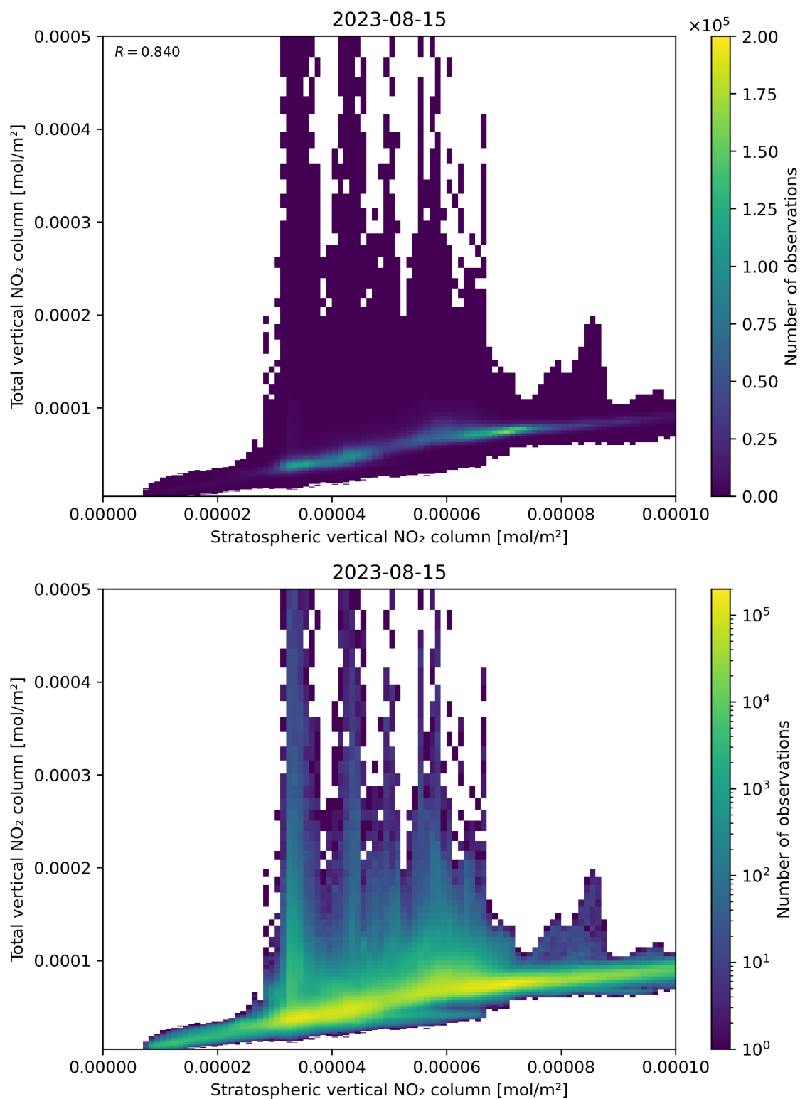
Figure 100: Scatter density plot of “Stratospheric vertical NO 2 column” against “Total vertical NO 2 column” for 2023-08-14 to 2023-08-16.
