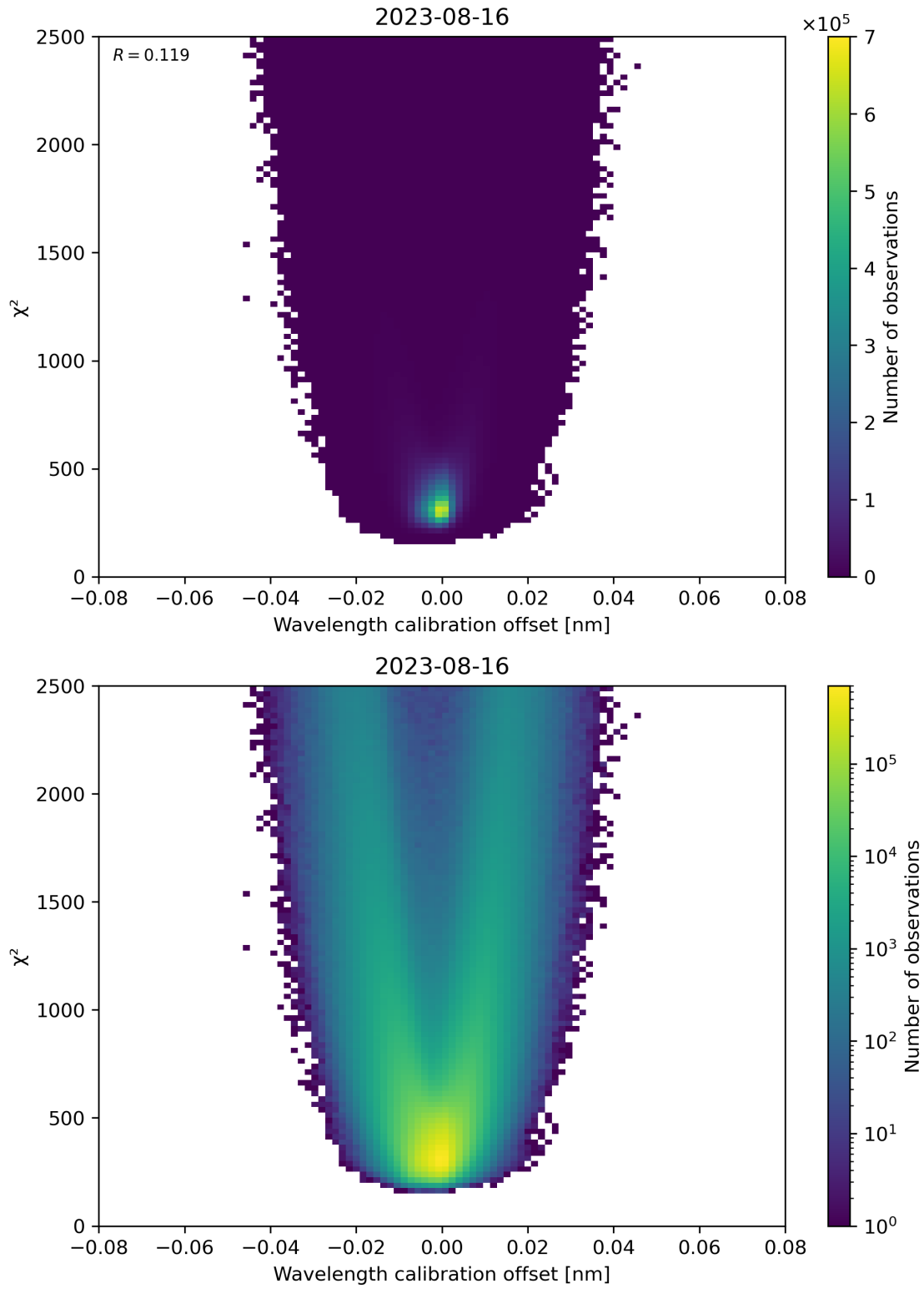
Figure 175: Scatter density plot of “Wavelength calibration offset” against “ \chi^2 ” for 2023-08-15 to 2023-08-17.
