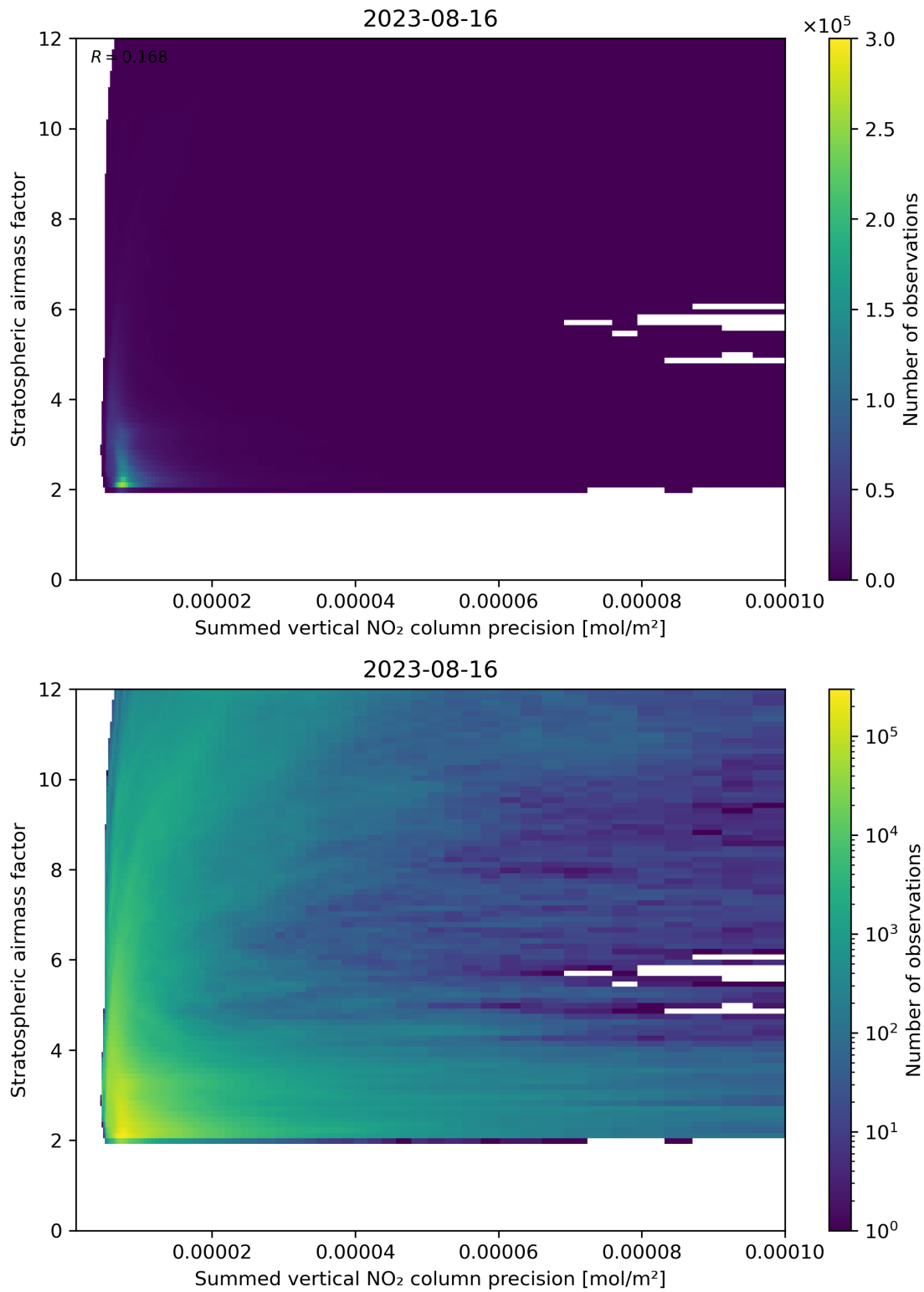
Figure 106: Scatter density plot of “Summed vertical NO 2 column precision” against “Stratospheric airmass factor” for 2023-08-15 to 2023-08-17.
