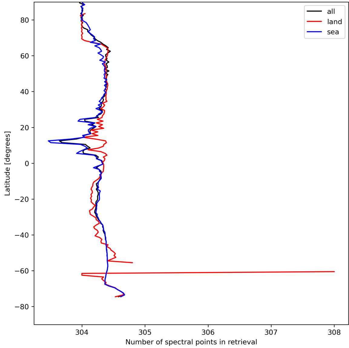
Figure 16: Zonal average of “Number of spectral points in retrieval” for 2023-08-15 to 2023-08-17.
