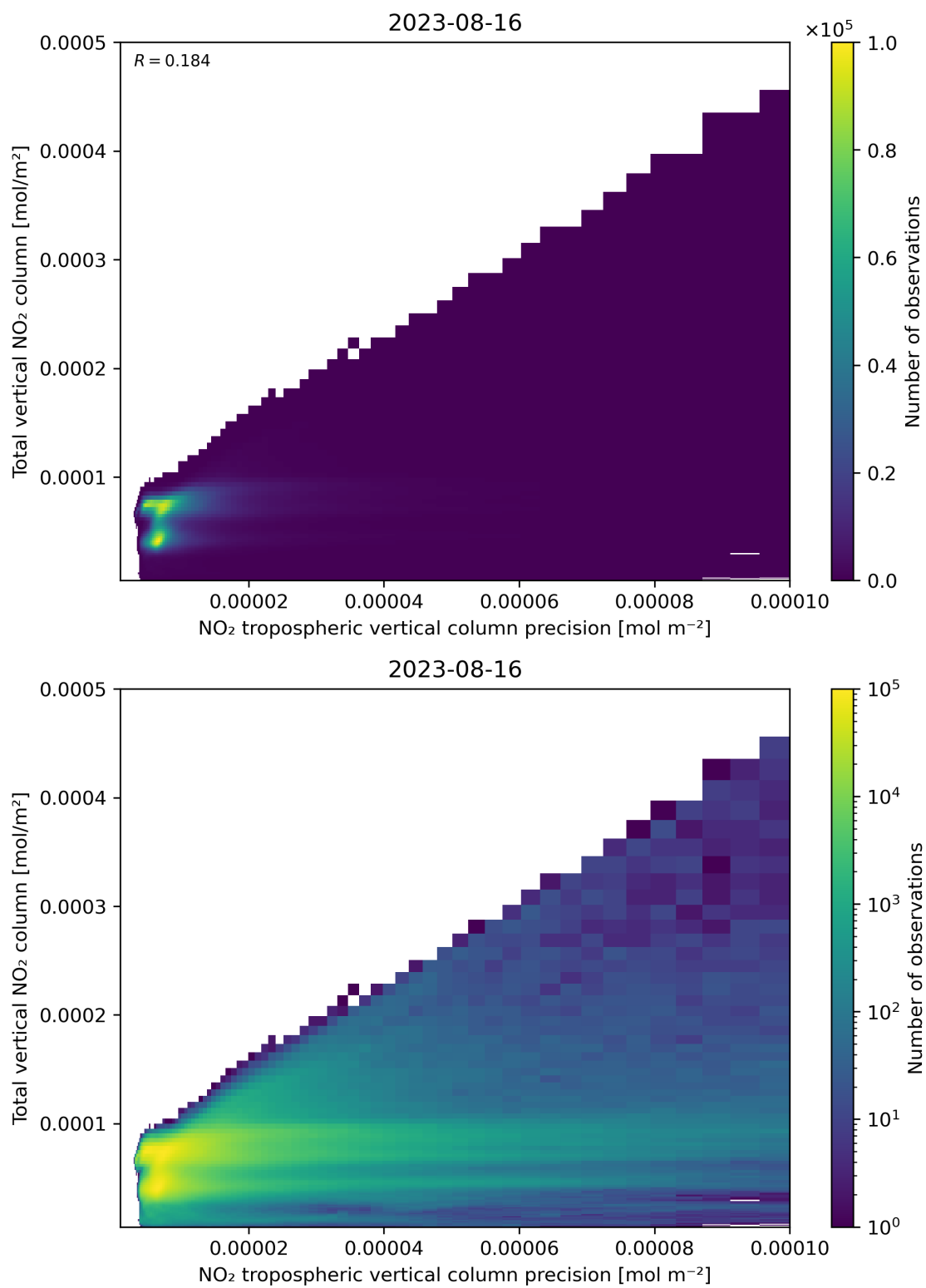
Figure 138: Scatter density plot of “NO 2 tropospheric vertical column precision” against “Total vertical NO 2 column” for 2023-08-15 to 2023-08-17.
