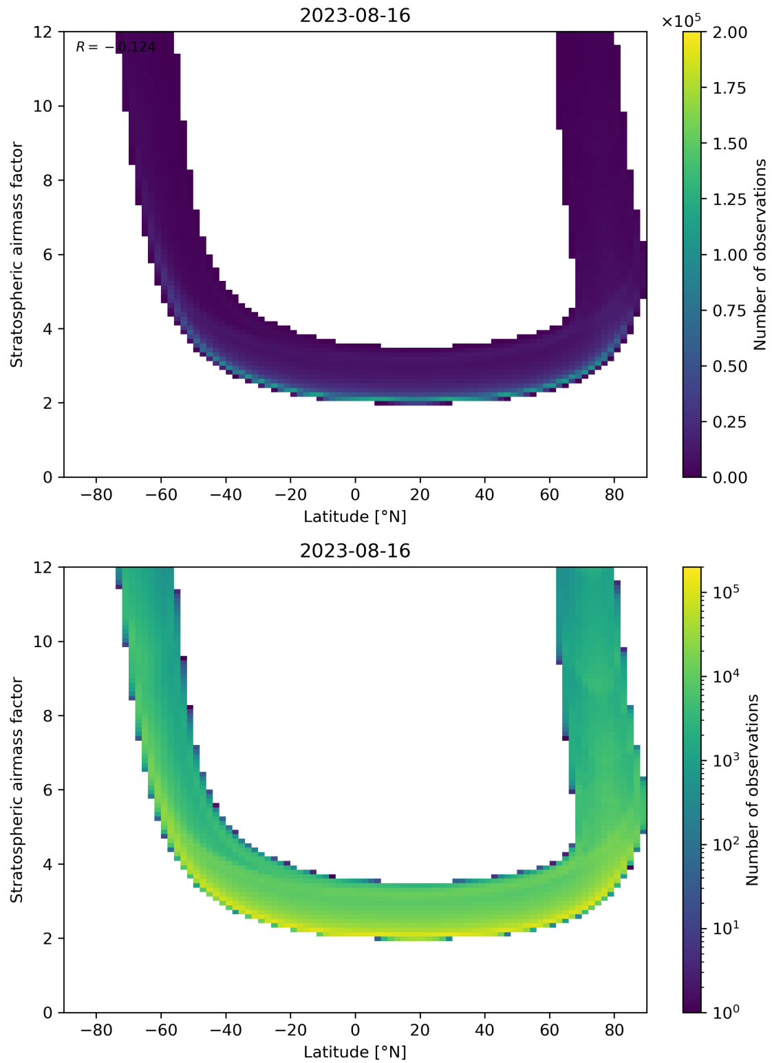
Figure 83: Scatter density plot of “Latitude” against “Stratospheric air mass factor” for 2023-08-15 to 2023-08-17.
