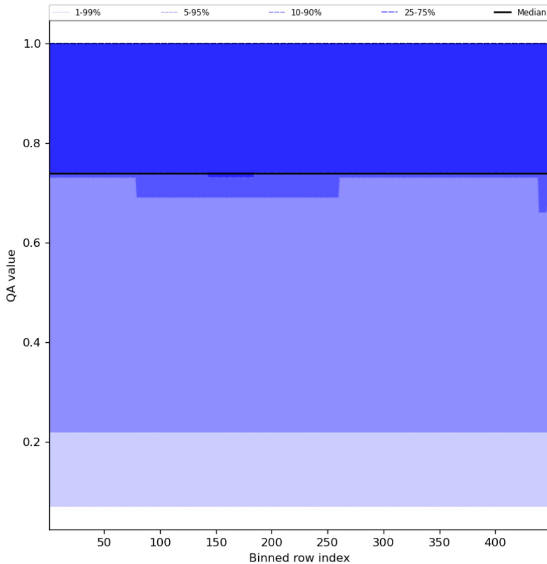
Figure 45: Along track statistics of “QA value” for 2023-08-15 to 2023-08-17
