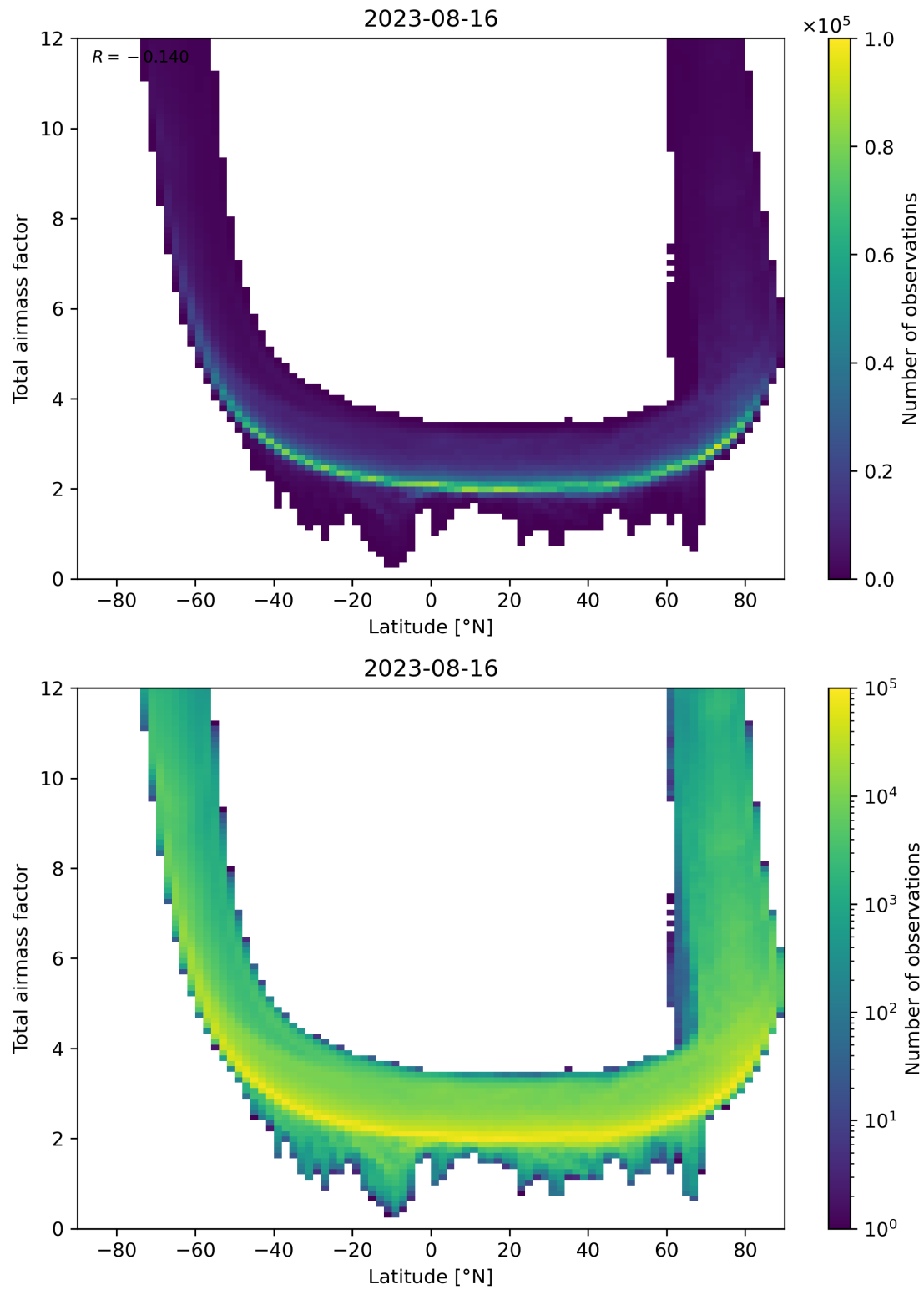
Figure 84: Scatter density plot of “Latitude” against “Total airmass factor” for 2023-08-15 to 2023-08-17.
