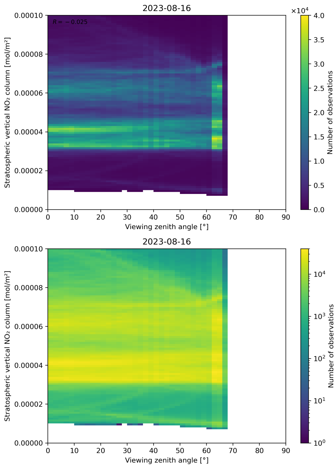
Figure 164: Scatter density plot of “Viewing zenith angle” against “Stratospheric vertical NO 2 column” for 2023-08-15 to 2023-08-17.
