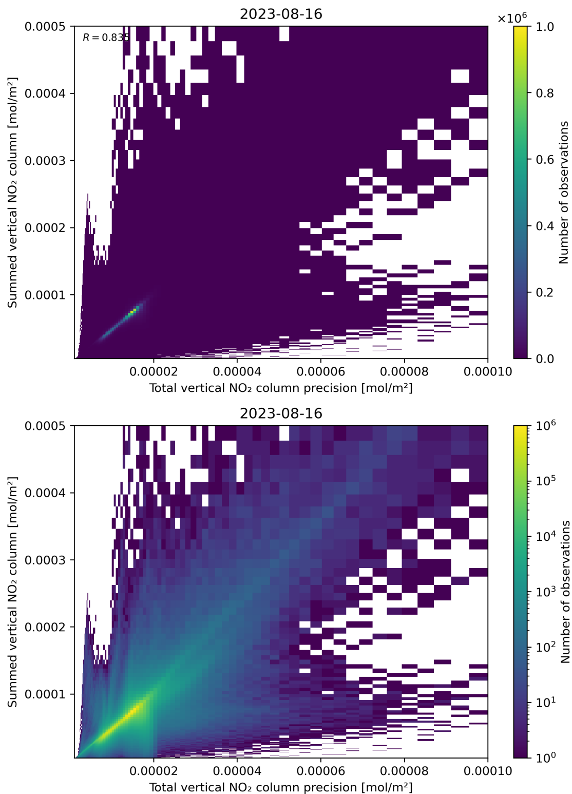
Figure 117: Scatter density plot of “Total vertical NO 2 column precision” against “Summed vertical NO 2 column” for 2023-08-15 to 2023-08-17.
