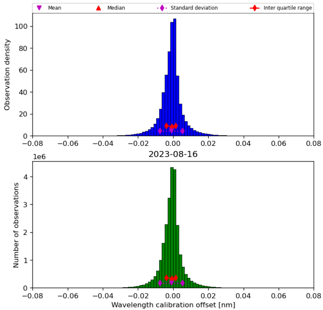
Figure 35: Histogram of “Wavelength calibration offset” for 2023-08-15 to 2023-08-17
