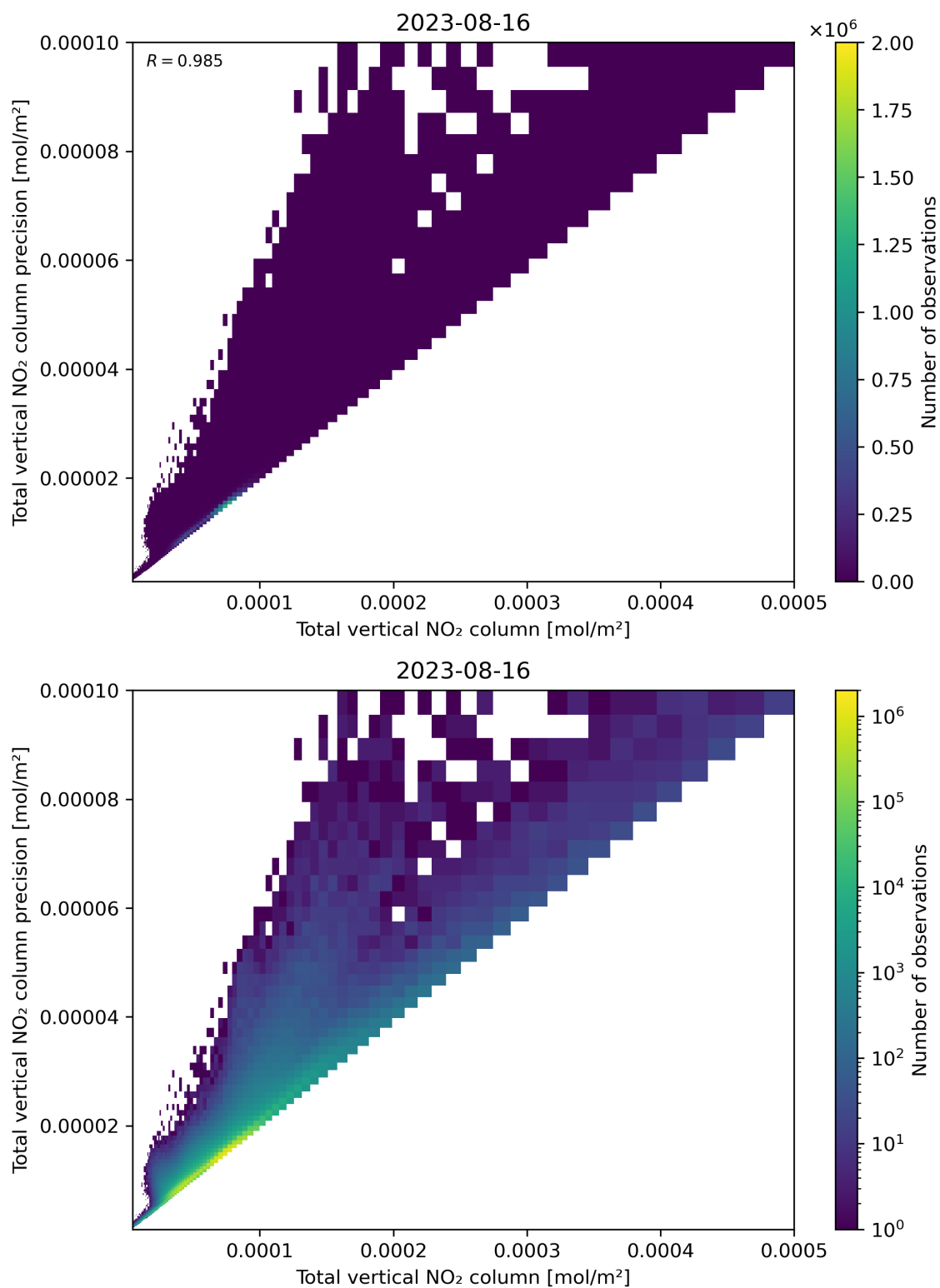
Figure 114: Scatter density plot of “Total vertical NO 2 column” against “Total vertical NO 2 column precision” for 2023-08-15 to 2023-08-17.
