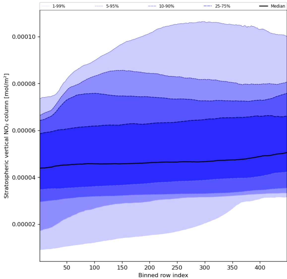
Figure 53: Along track statistics of “Stratospheric vertical NO 2 column” for 2023-08-15 to 2023-08-17
