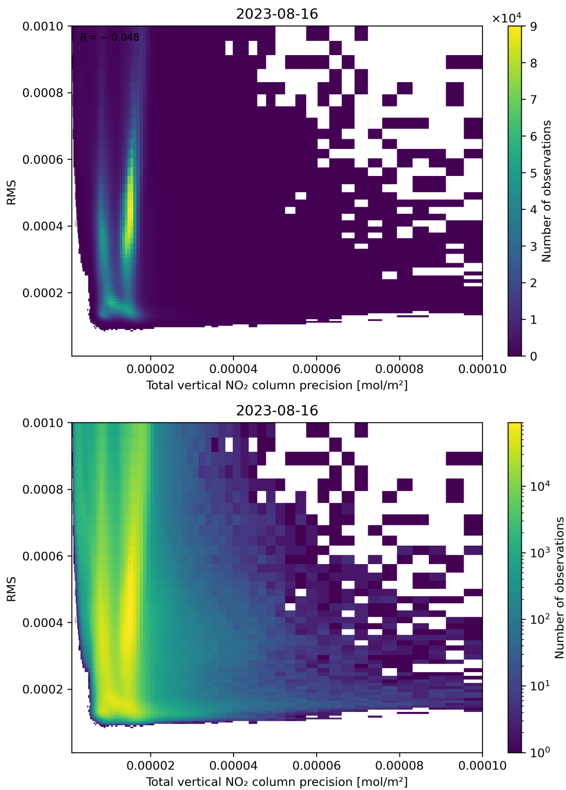
Figure 119: Scatter density plot of “Total vertical NO 2 column precision” against “RMS” for 2023-08-15 to 2023-08-17.
