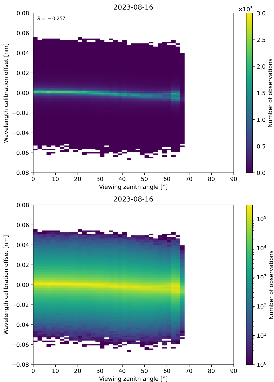
Figure 173: Scatter density plot of “Viewing zenith angle” against “Wavelength calibration offset” for 2023-08-15 to 2023-08-17.
