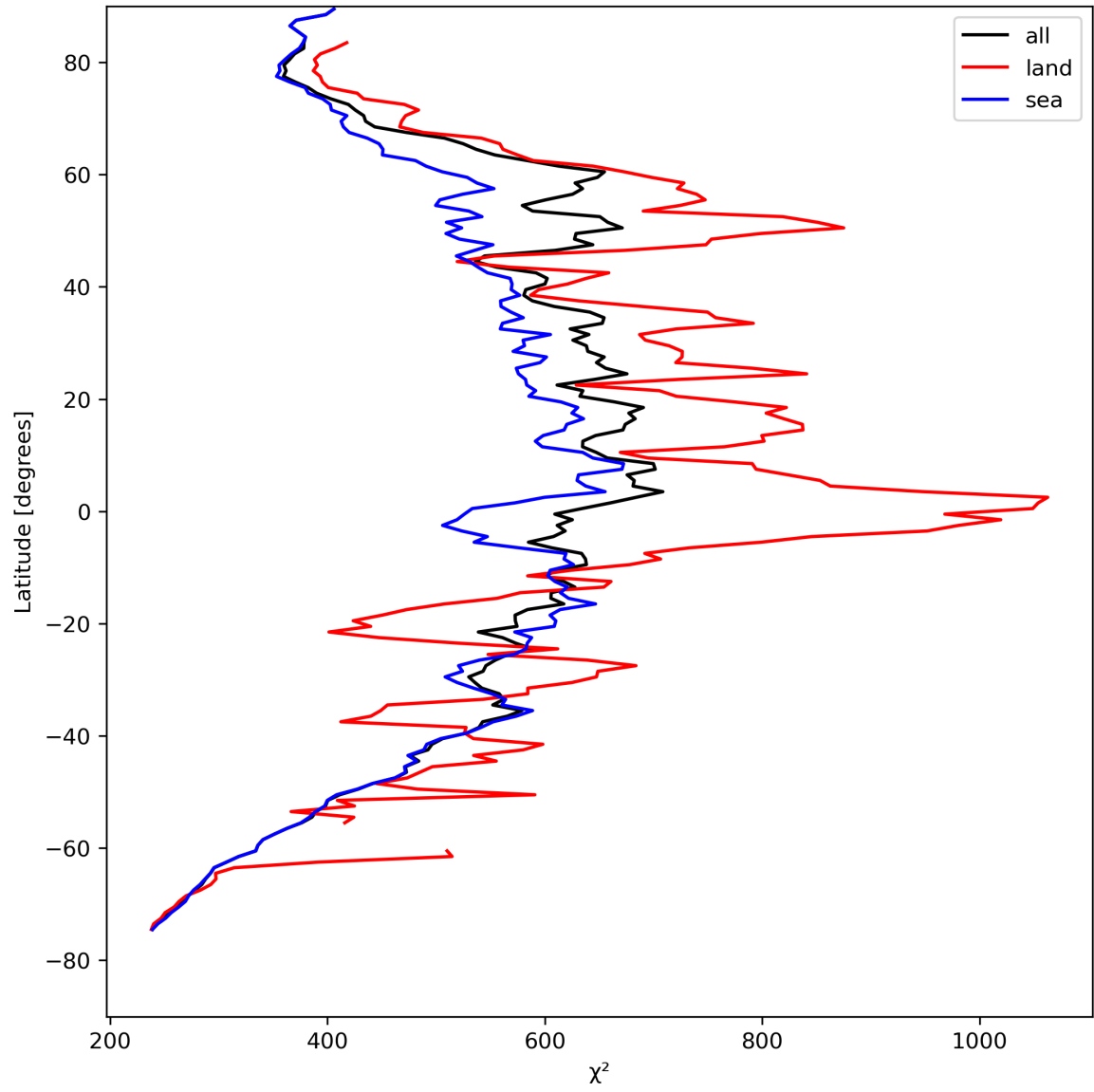
Figure 25: Zonal average of “ \chi^2 ” for 2023-08-15 to 2023-08-17.
