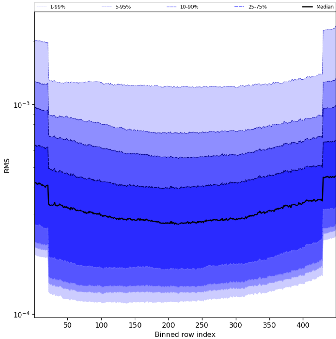
Figure 60: Along track statistics of “RMS” for 2023-08-15 to 2023-08-17
