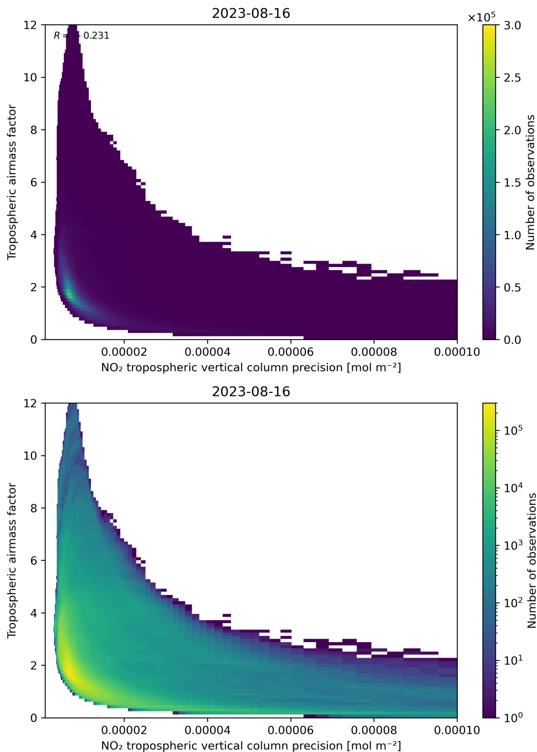
Figure 133: Scatter density plot of “NO 2 tropospheric vertical column precision” against “Tropospheric air mass factor” for 2023-08-15 to 2023-08-17.
