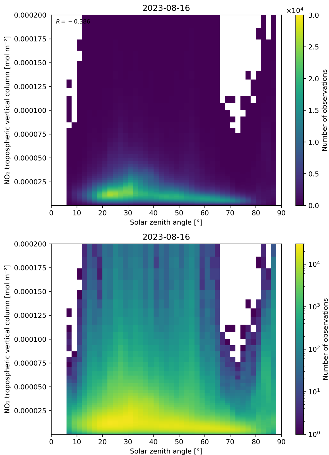
Figure 155: Scatter density plot of “Solar zenith angle” against “NO 2 tropospheric vertical column” for 2023-08-15 to 2023-08-17.
