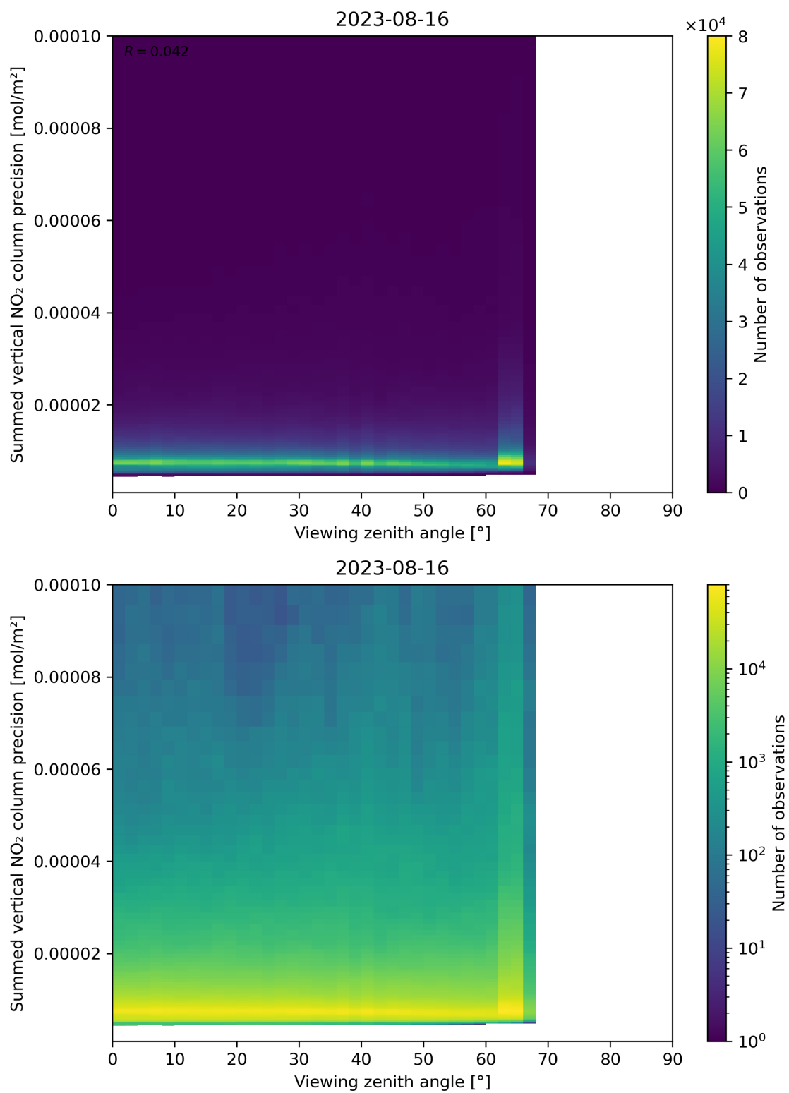
Figure 166: Scatter density plot of “Viewing zenith angle” against “Summed vertical NO 2 column precision” for 2023-08-15 to 2023-08-17.
