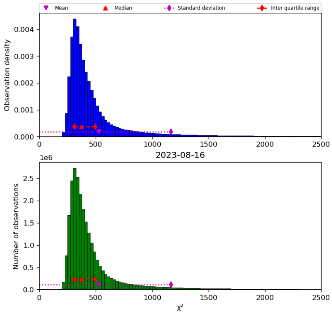
Figure 42: Histogram of “ \chi^2 ” for 2023-08-15 to 2023-08-17
