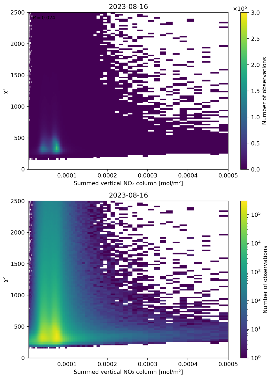
Figure 104: Scatter density plot of “Summed vertical NO 2 column” against “ \chi^2 ” for 2023-08-15 to 2023-08-17.
