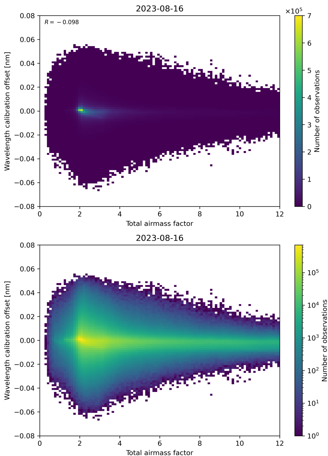
Figure 70: Scatter density plot of “Total airmass factor” against “Wavelength calibration offset” for 2023-08-15 to 2023-08-17.
