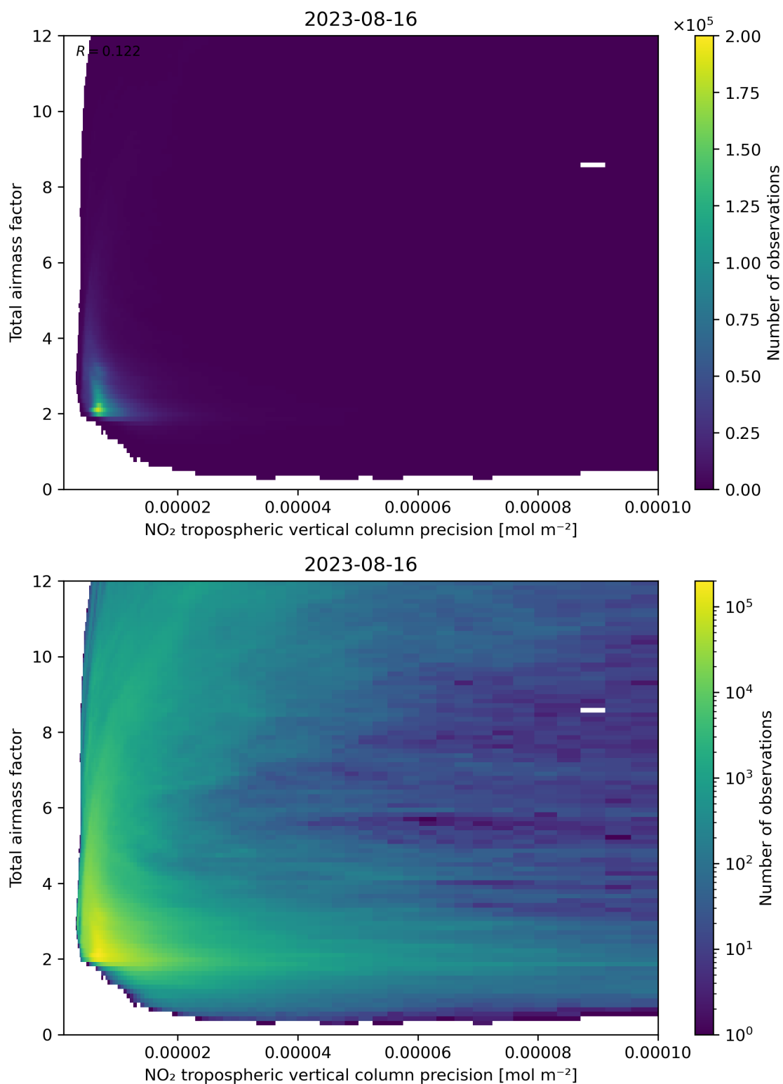
Figure 132: Scatter density plot of “NO 2 tropospheric vertical column precision” against “Total air mass factor” for 2023-08-15 to 2023-08-17.
