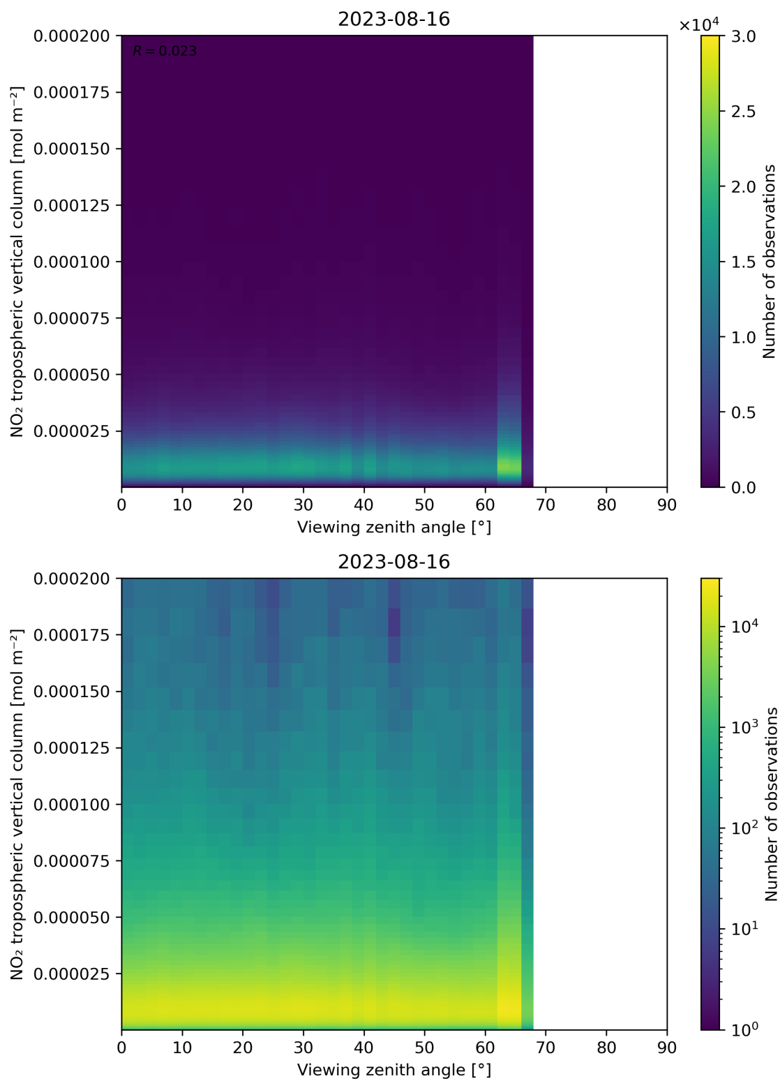
Figure 169: Scatter density plot of “Viewing zenith angle” against “NO 2 tropospheric vertical column” for 2023-08-15 to 2023-08-17.
