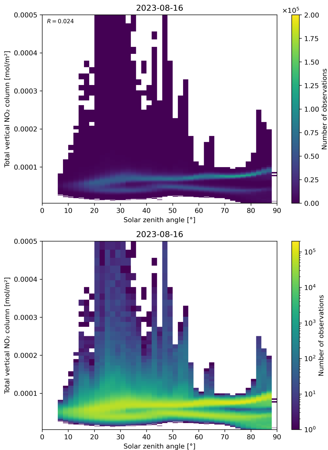
Figure 153: Scatter density plot of “Solar zenith angle” against “Total vertical NO 2 column” for 2023-08-15 to 2023-08-17.
