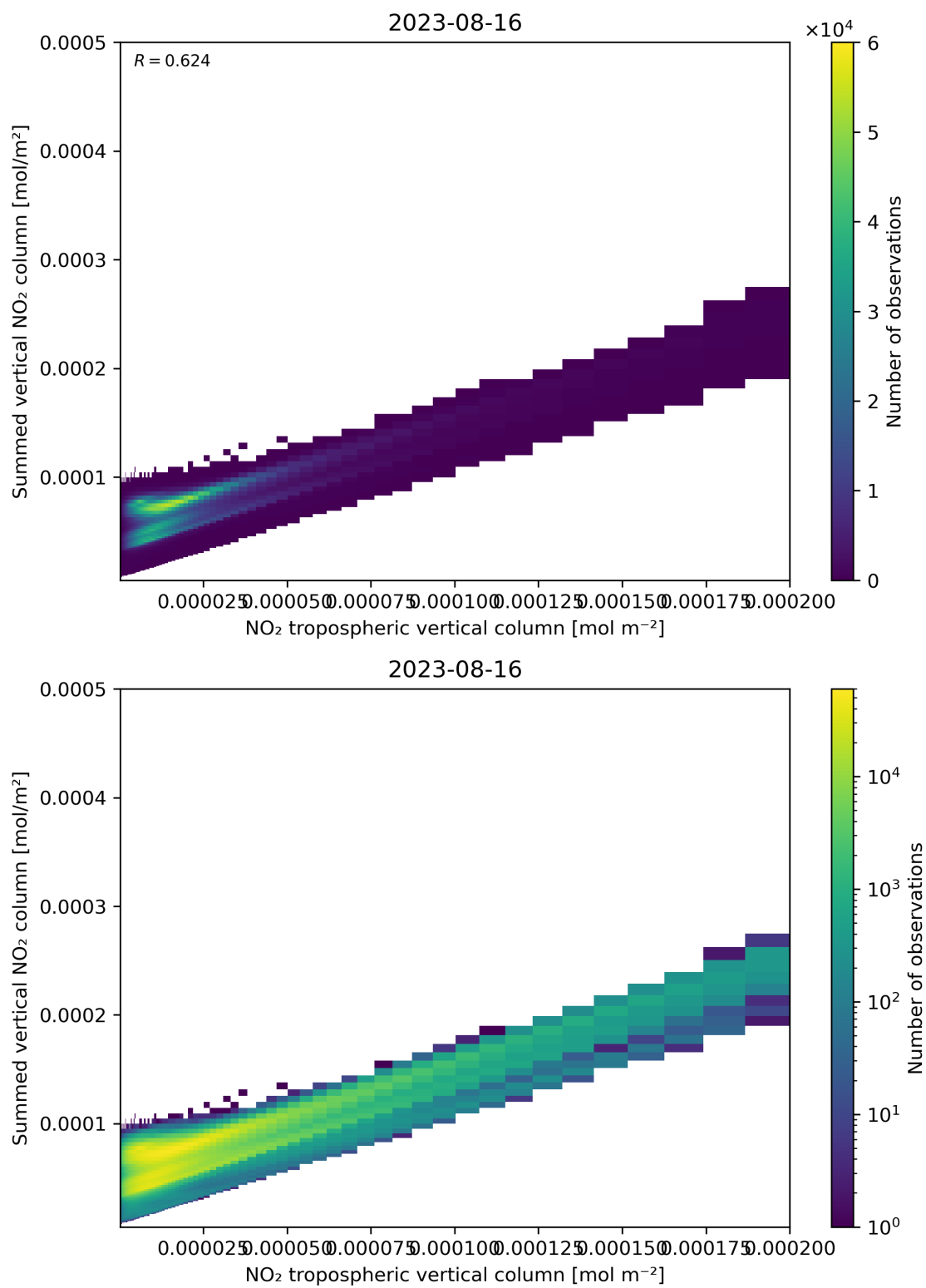
Figure 126: Scatter density plot of “NO 2 tropospheric vertical column” against “Summed vertical NO 2 column” for 2023-08-15 to 2023-08-17.
