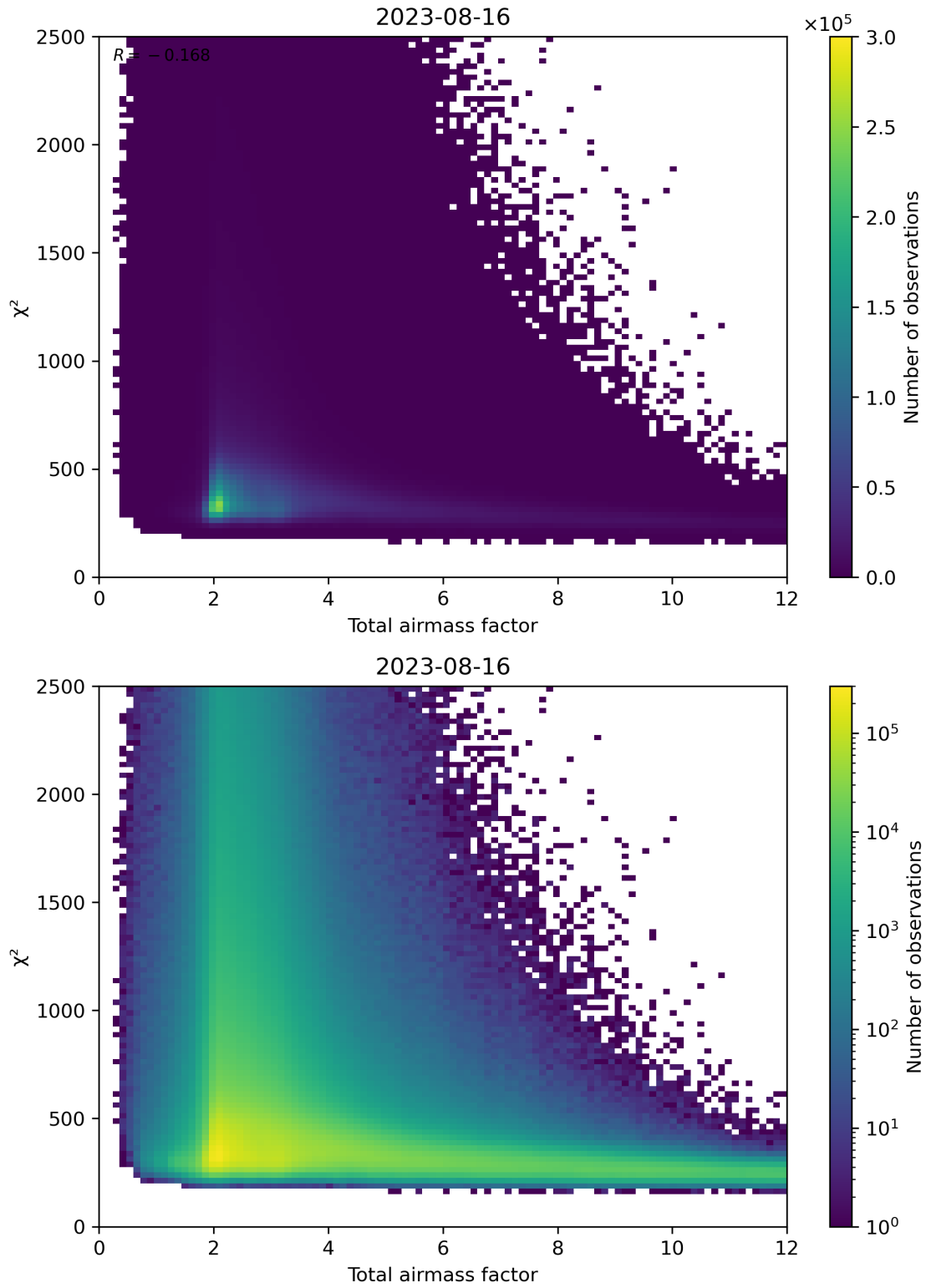
Figure 63: Scatter density plot of “Total airmass factor” against “ \chi^2 ” for 2023-08-15 to 2023-08-17.
