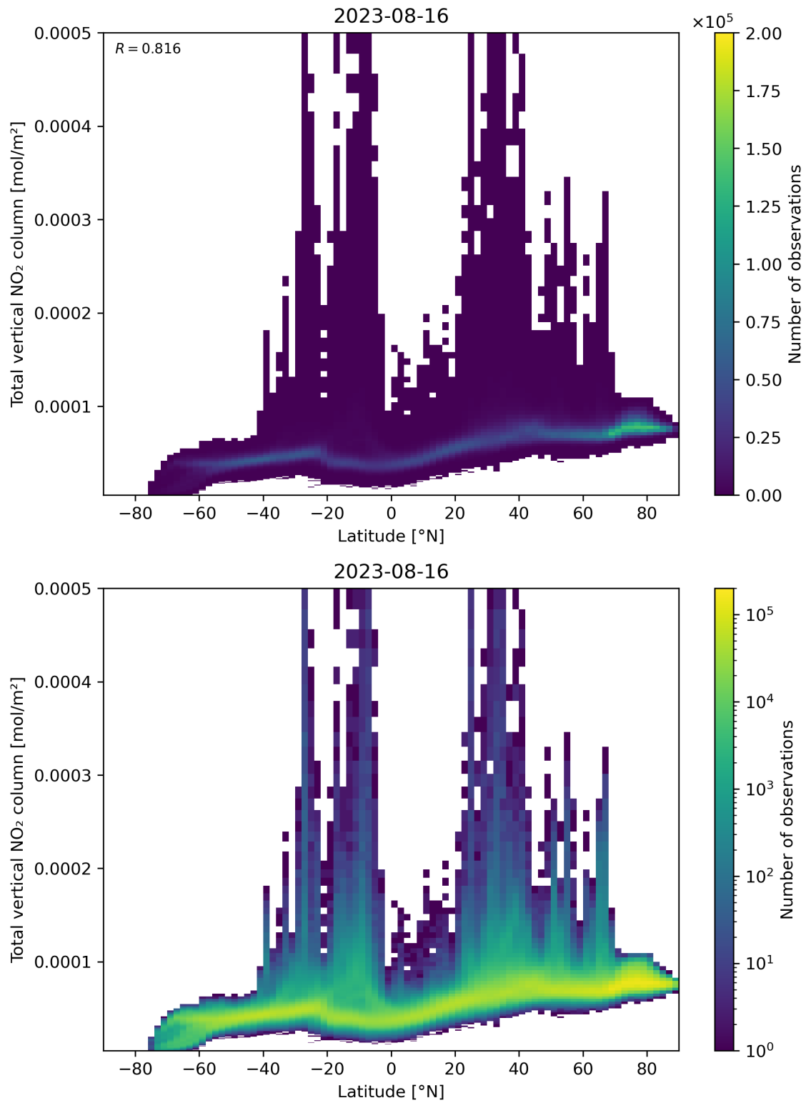
Figure 90: Scatter density plot of “Latitude” against “Total vertical NO 2 column” for 2023-08-15 to 2023-08-17.
