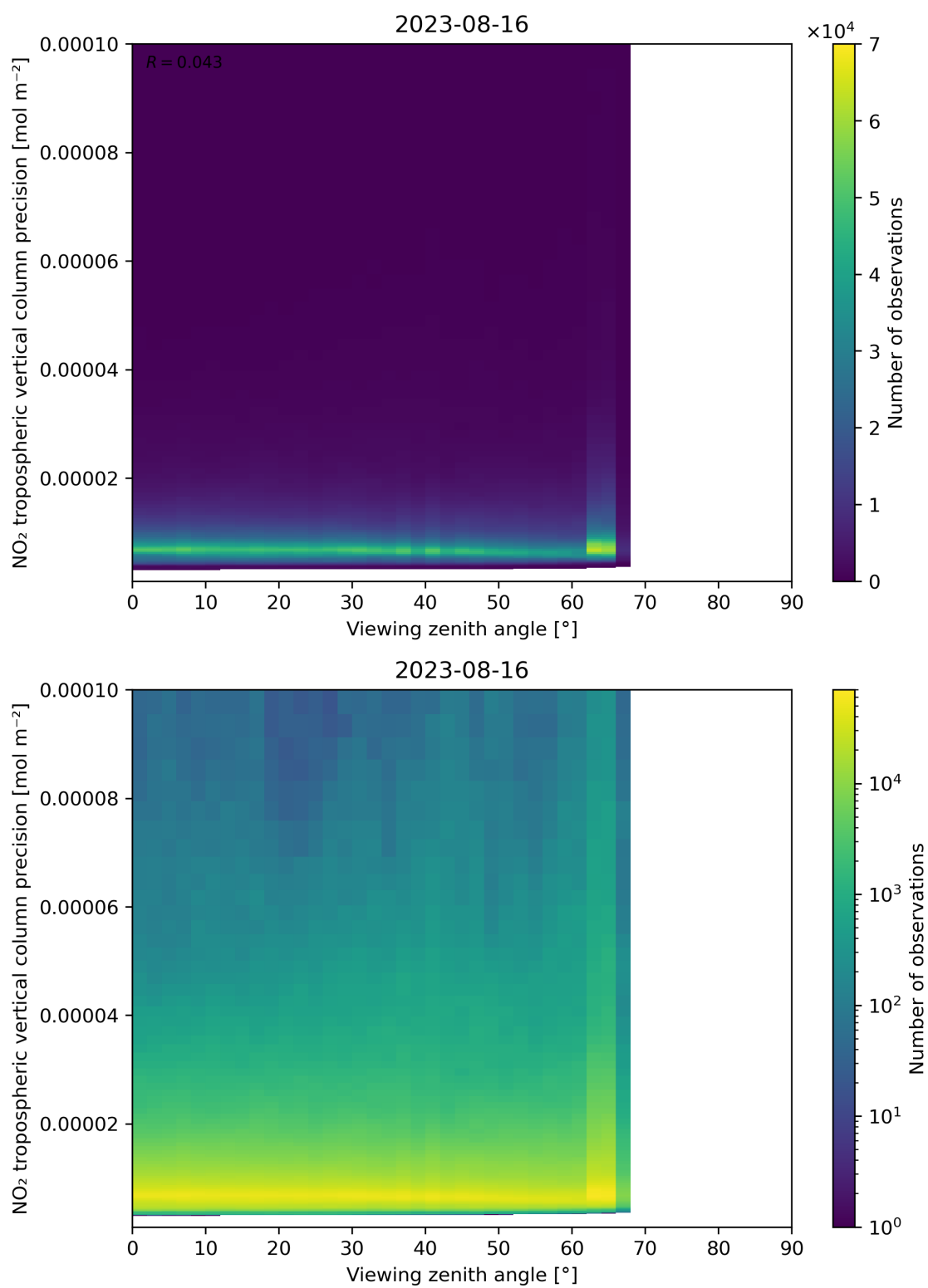
Figure 170: Scatter density plot of “Viewing zenith angle” against “NO 2 tropospheric vertical column precision” for 2023-08-15 to 2023-08-17.
