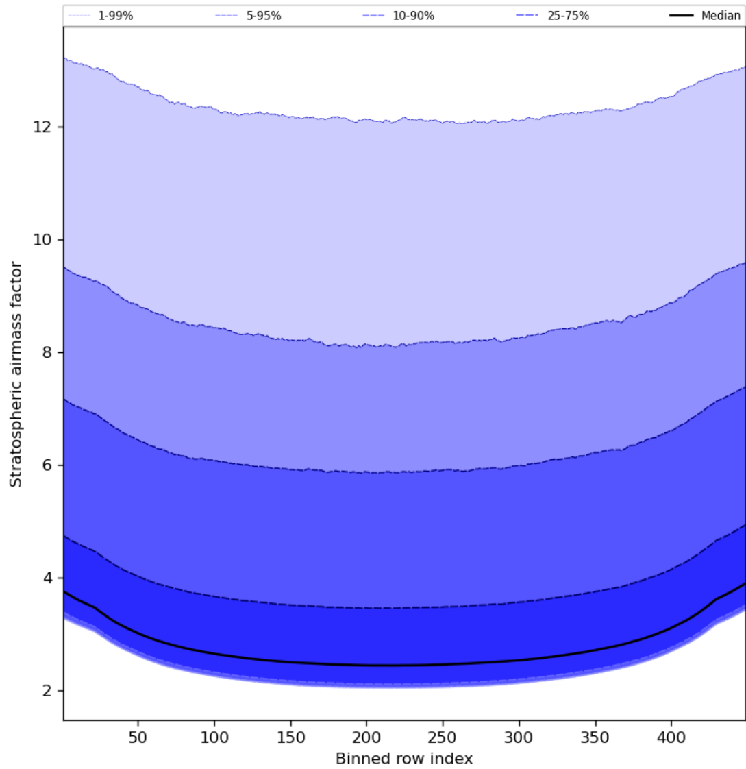
Figure 61: Along track statistics of “Stratospheric airmass factor” for 2023-08-15 to 2023-08-17
