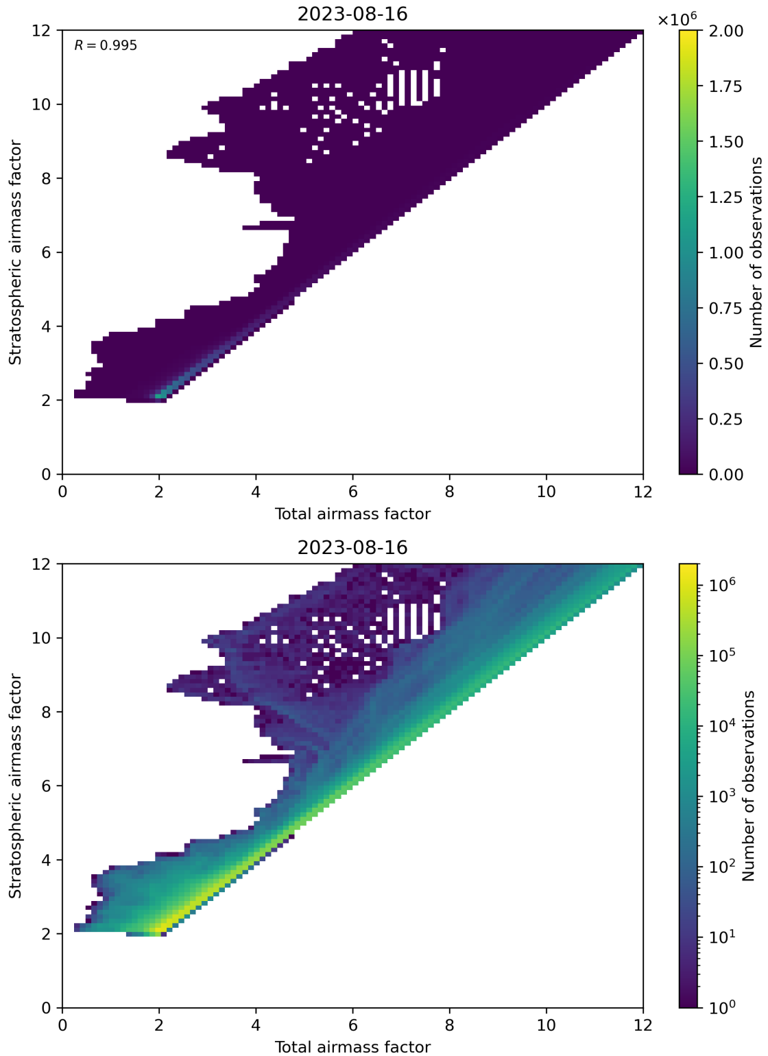
Figure 62: Scatter density plot of “Total airmass factor” against “Stratospheric airmass factor” for 2023-08-15 to 2023-08-17.
