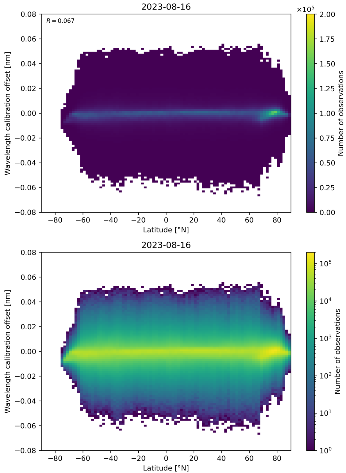
Figure 95: Scatter density plot of “Latitude” against “Wavelength calibration offset” for 2023-08-15 to 2023-08-17.
