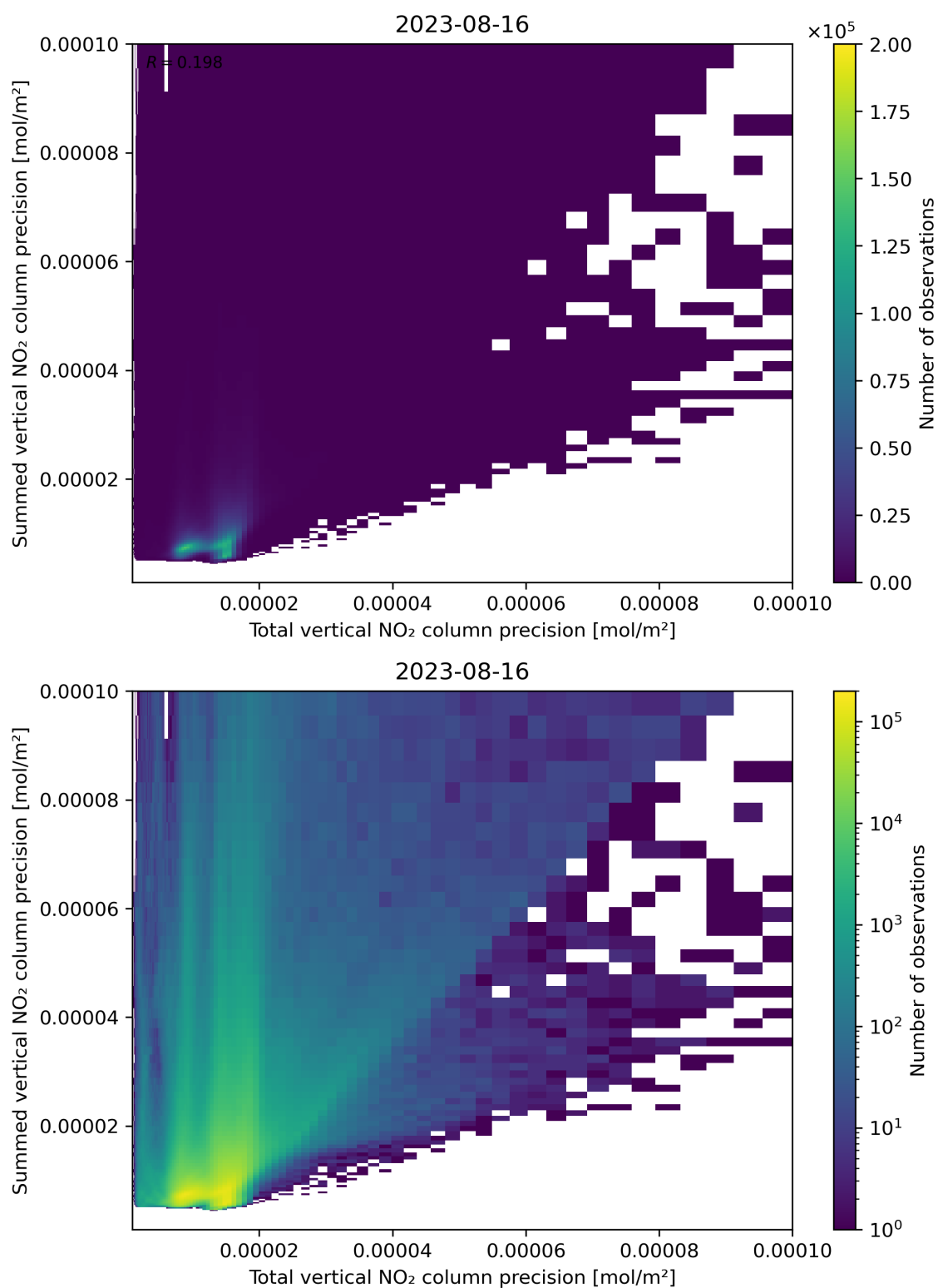
Figure 118: Scatter density plot of “Total vertical NO 2 column precision” against “Summed vertical NO 2 column precision” for 2023-08-15 to 2023-08-17.
