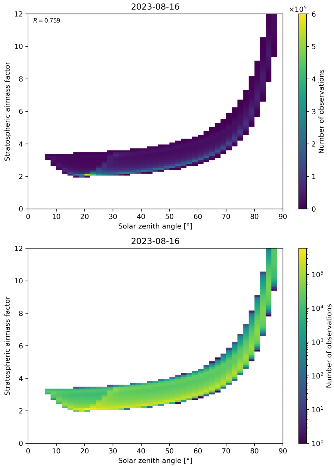
Figure 145: Scatter density plot of “Solar zenith angle” against “Stratospheric airmass factor” for 2023-08-15 to 2023-08-17.
