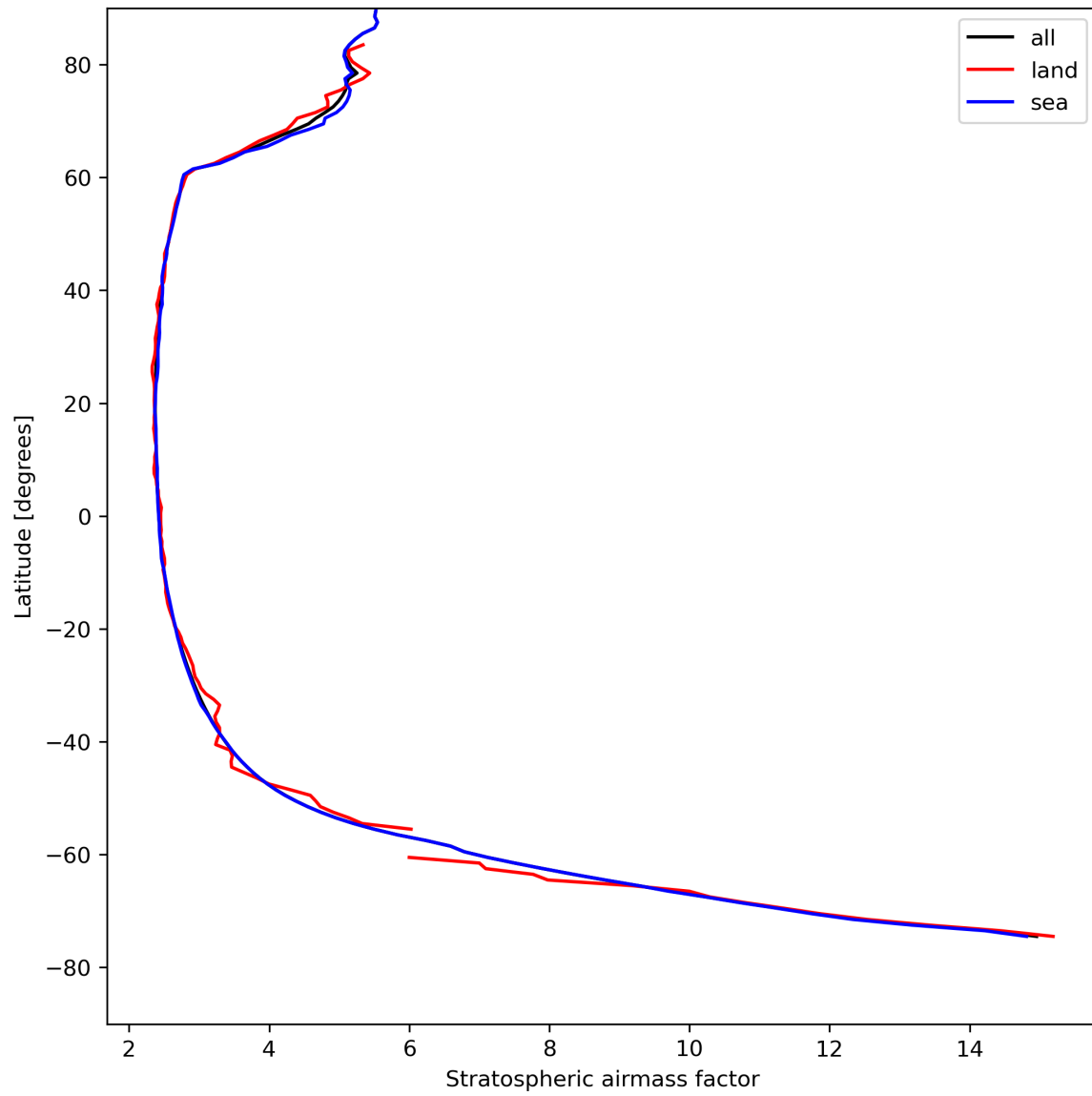
Figure 27: Zonal average of “Stratospheric airmass factor” for 2023-08-15 to 2023-08-17.
