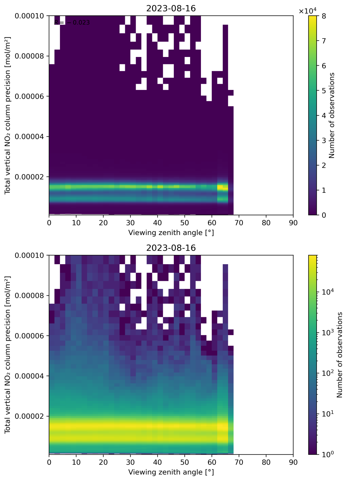
Figure 168: Scatter density plot of “Viewing zenith angle” against “Total vertical NO 2 column precision” for 2023-08-15 to 2023-08-17.
