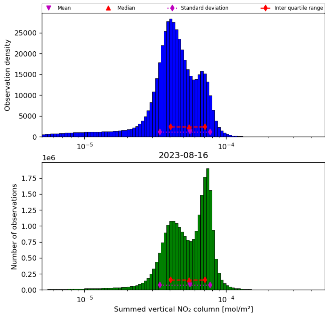
Figure 40: Histogram of “Summed vertical NO 2 column” for 2023-08-15 to 2023-08-17
