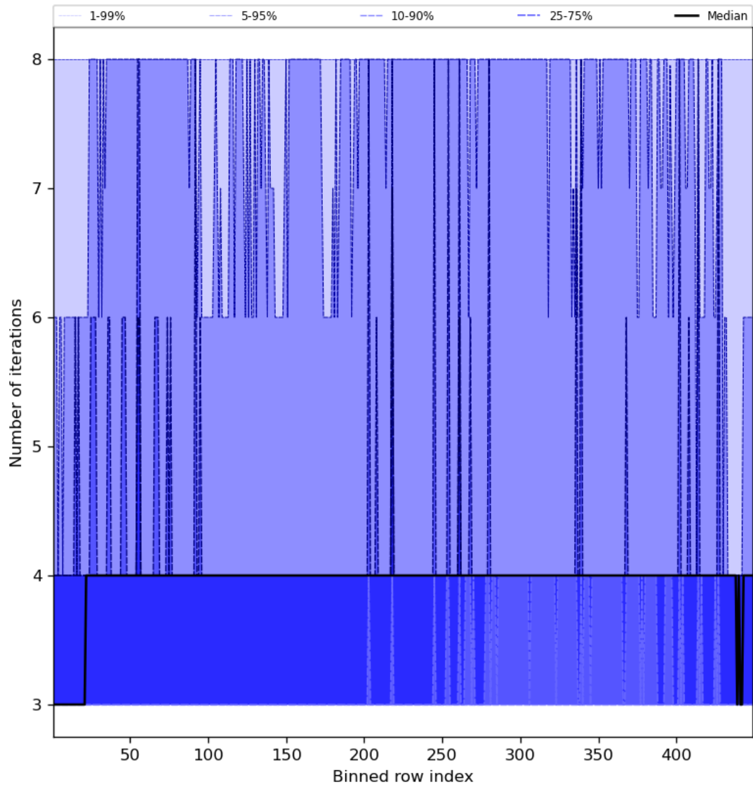
Figure 51: Along track statistics of “Number of iterations” for 2023-08-15 to 2023-08-17
