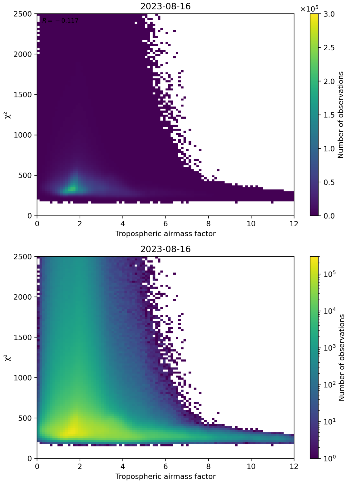
Figure 73: Scatter density plot of “Tropospheric airmass factor” against “ \chi^2 ” for 2023-08-15 to 2023-08-17.
