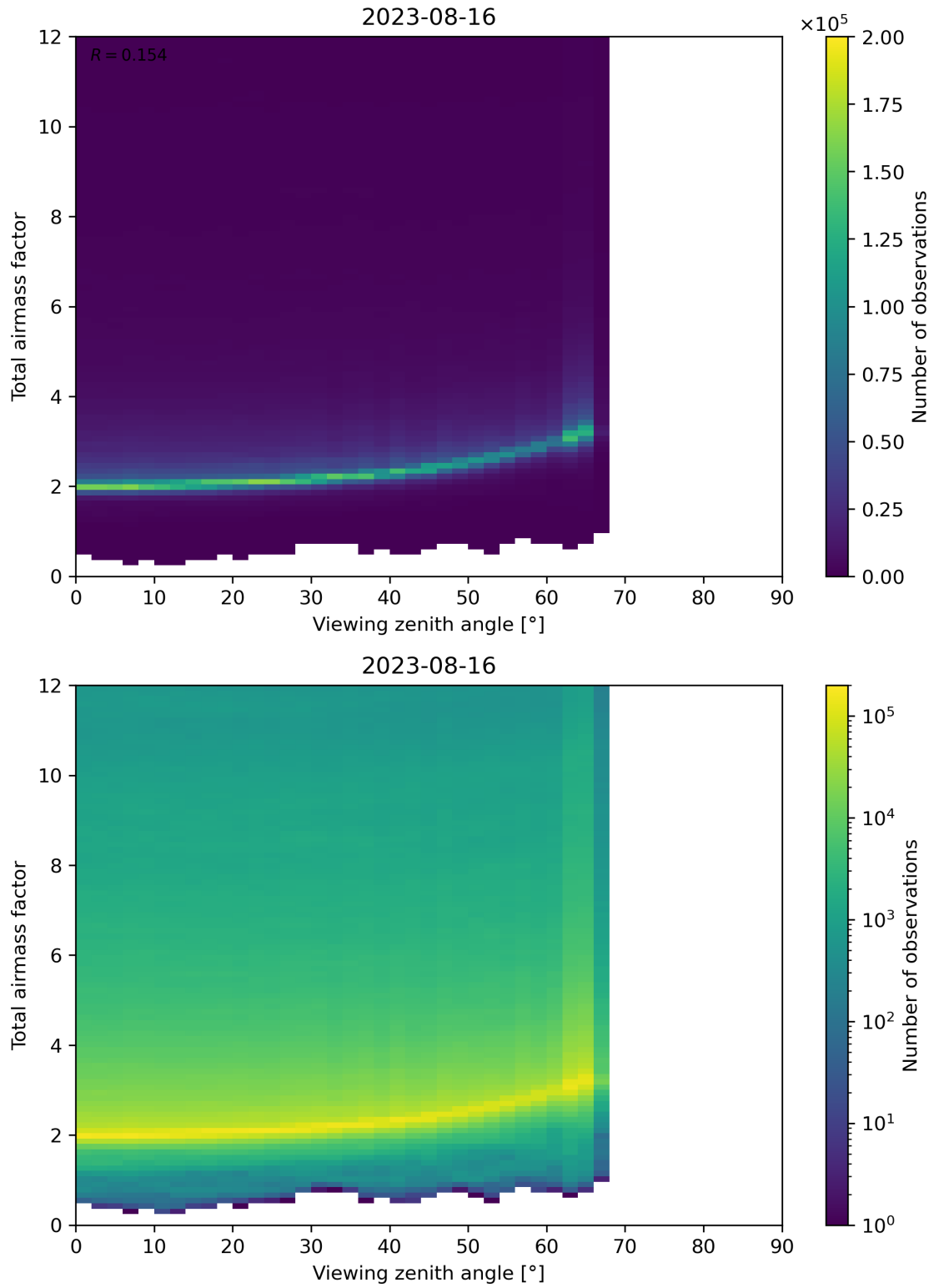
Figure 160: Scatter density plot of “Viewing zenith angle” against “Total airmass factor” for 2023-08-15 to 2023-08-17.
