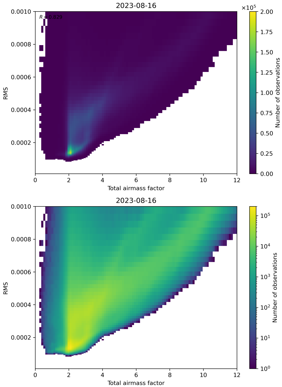
Figure 69: Scatter density plot of “Total airmass factor” against “RMS” for 2023-08-15 to 2023-08-17.
