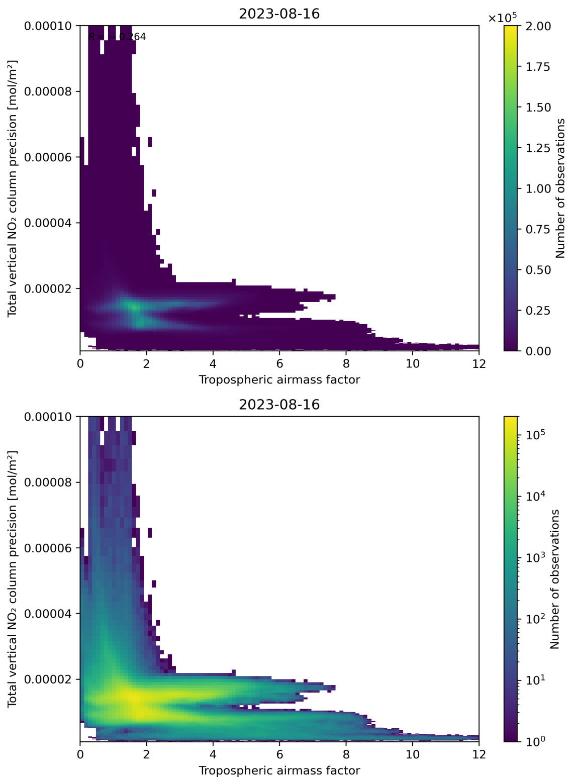
Figure 78: Scatter density plot of “Tropospheric air mass factor” against “Total vertical NO 2 column precision” for 2023-08-15 to 2023-08-17.
