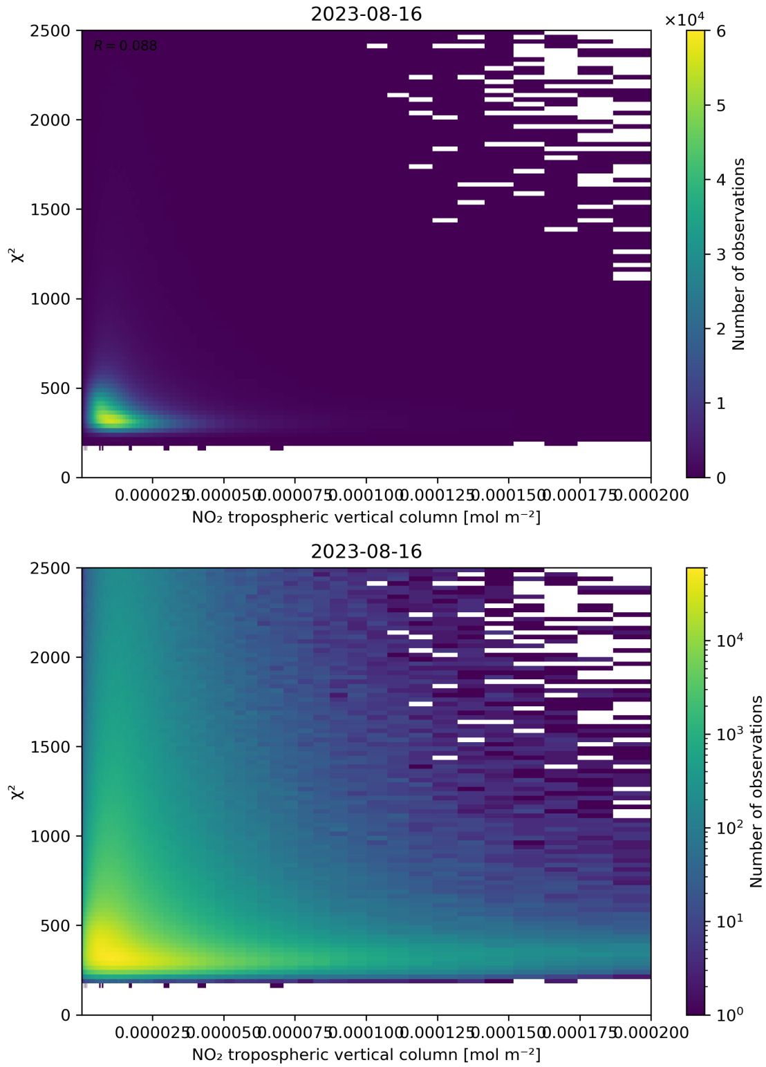
Figure 124: Scatter density plot of “NO 2 tropospheric vertical column” against “ \chi^2 ” for 2023-08-15 to 2023-08-17.
