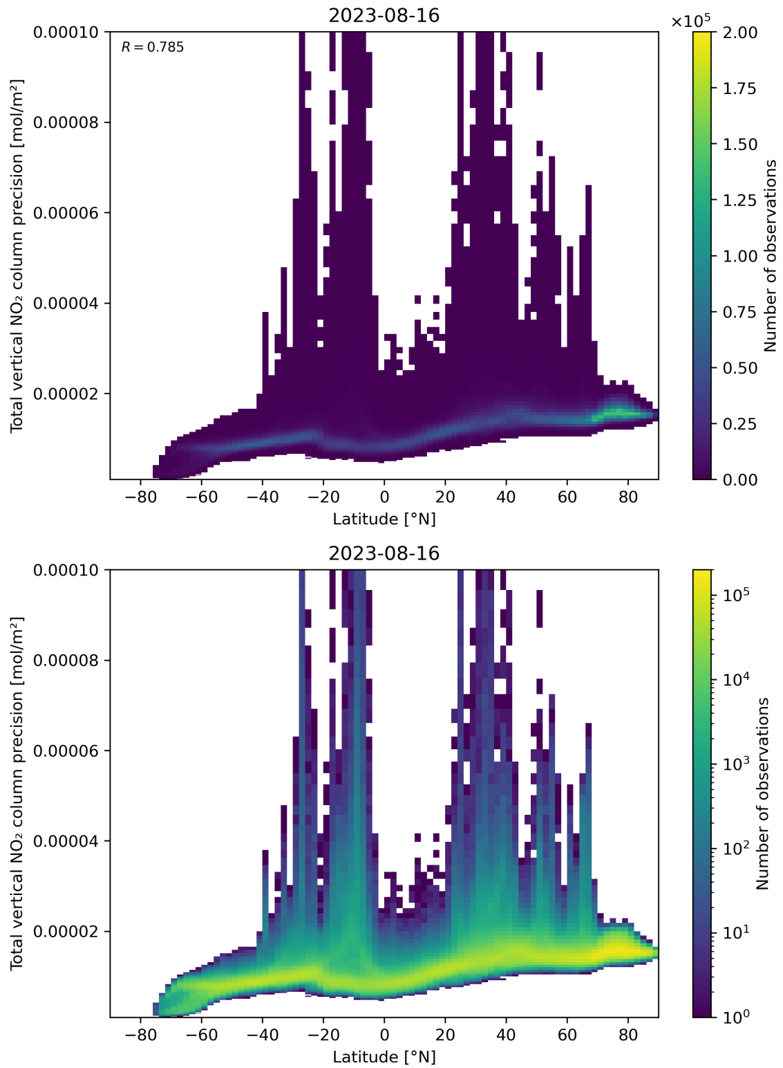
Figure 91: Scatter density plot of “Latitude” against “Total vertical NO 2 column precision” for 2023-08-15 to 2023-08-17.
