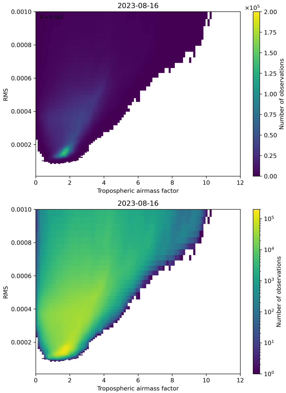
Figure 79: Scatter density plot of “Tropospheric airmass factor” against “RMS” for 2023-08-15 to 2023-08-17.
