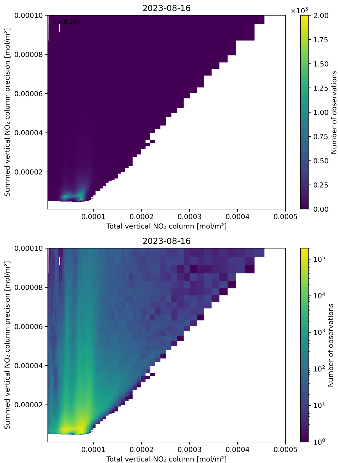
Figure 113: Scatter density plot of “Total vertical NO 2 column” against “Summed vertical NO 2 column precision” for 2023-08-15 to 2023-08-17.
