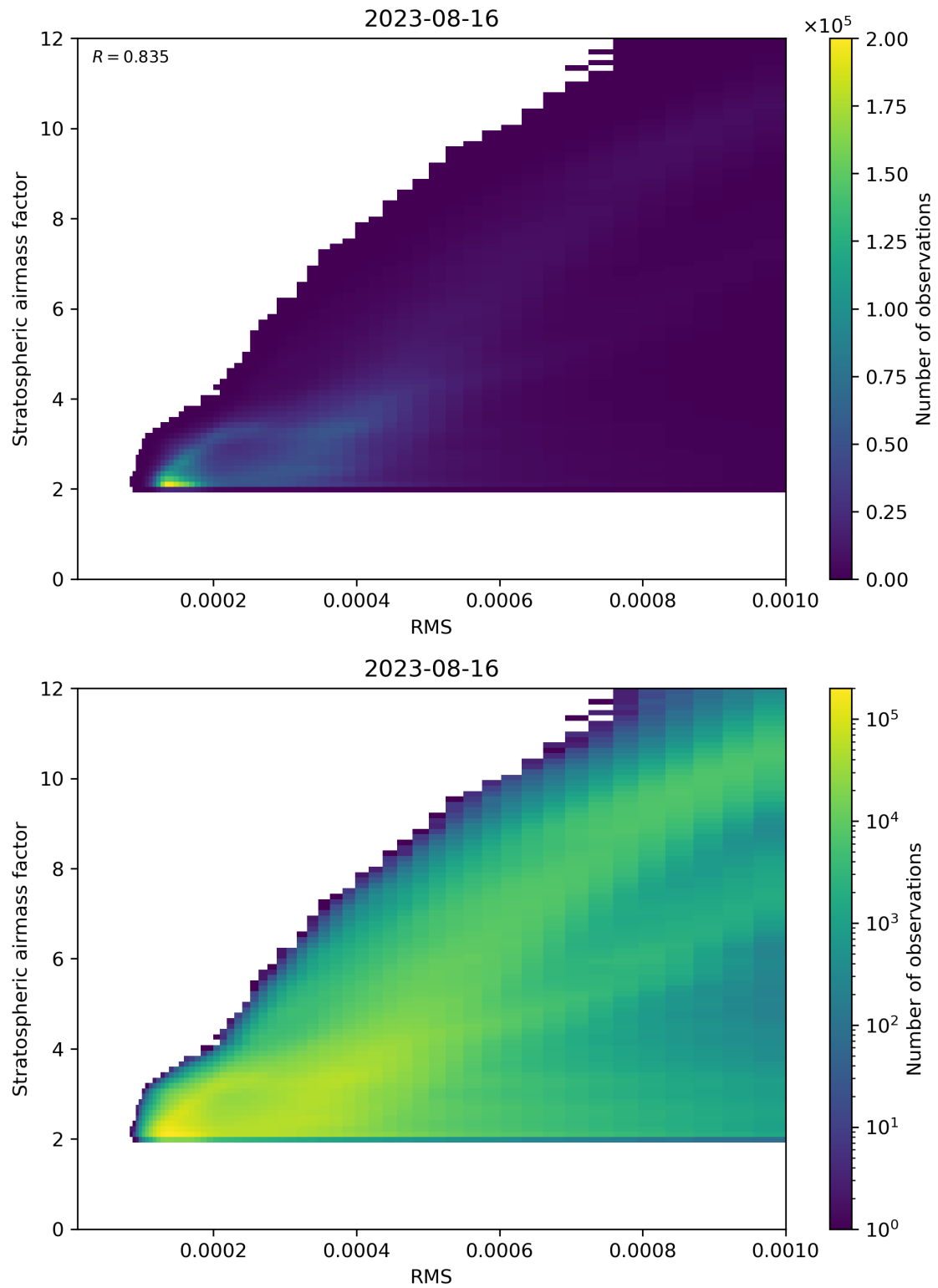
Figure 144: Scatter density plot of “RMS” against “Stratospheric airmass factor” for 2023-08-15 to 2023-08-17.
