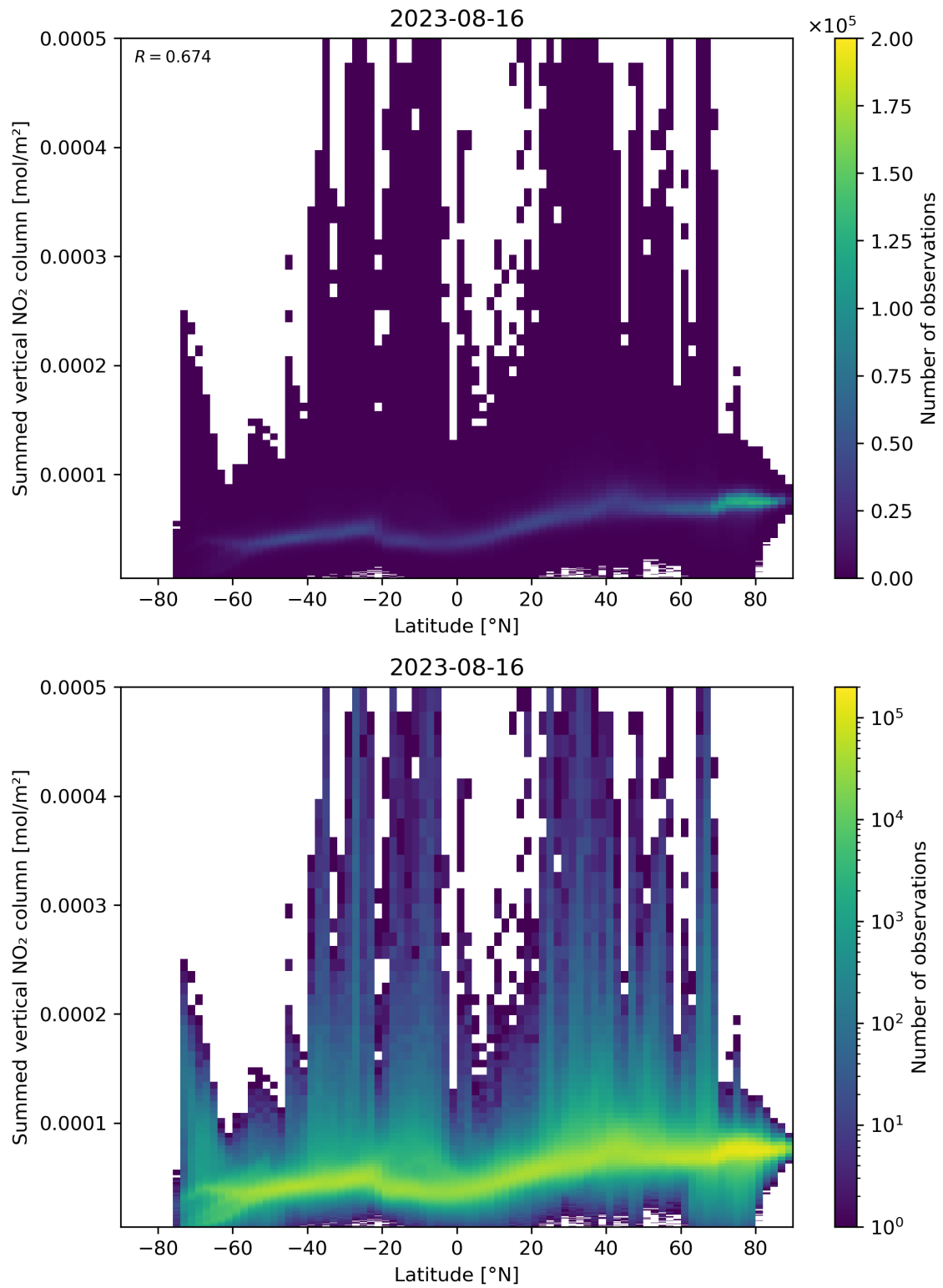
Figure 88: Scatter density plot of “Latitude” against “Summed vertical NO 2 column” for 2023-08-15 to 2023-08-17.
