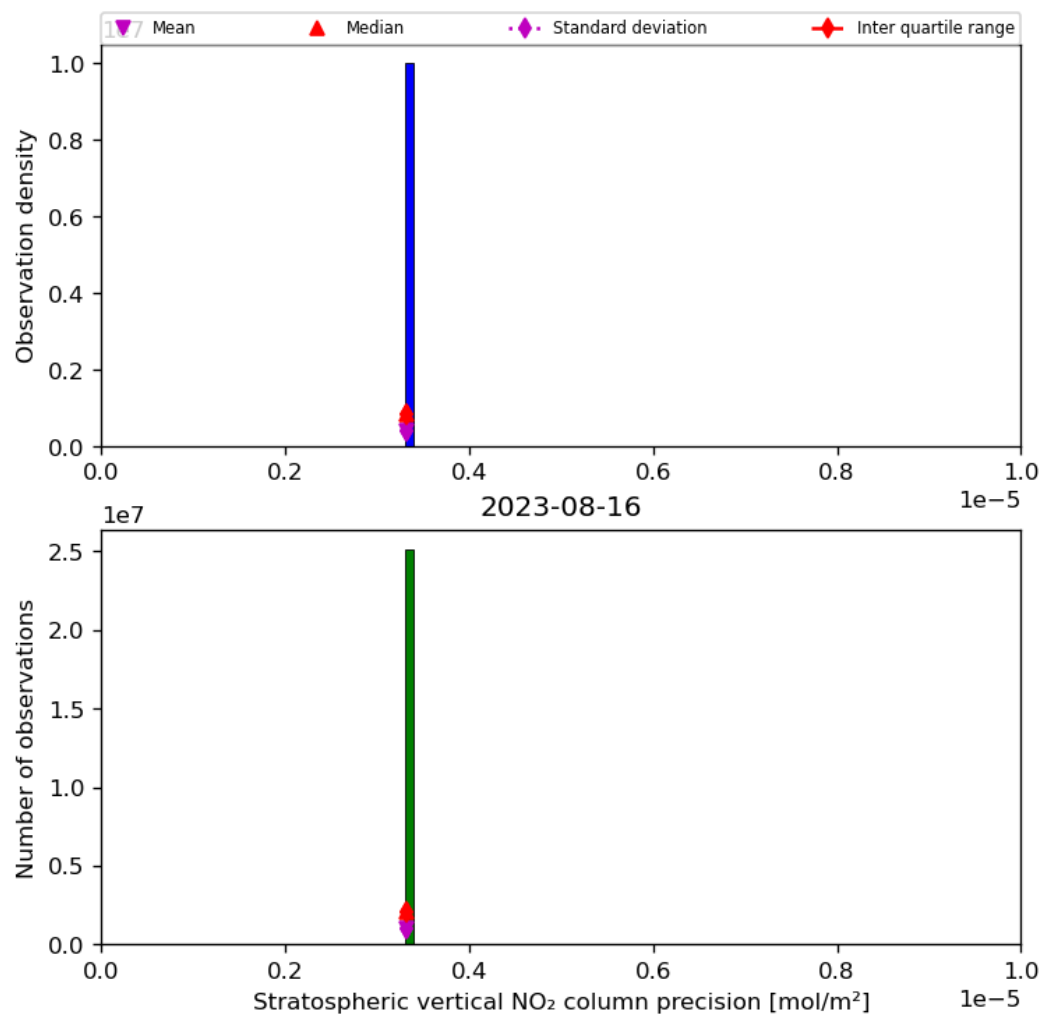
Figure 37: Histogram of “Stratospheric vertical NO 2 column precision” for 2023-08-15 to 2023-08-17
