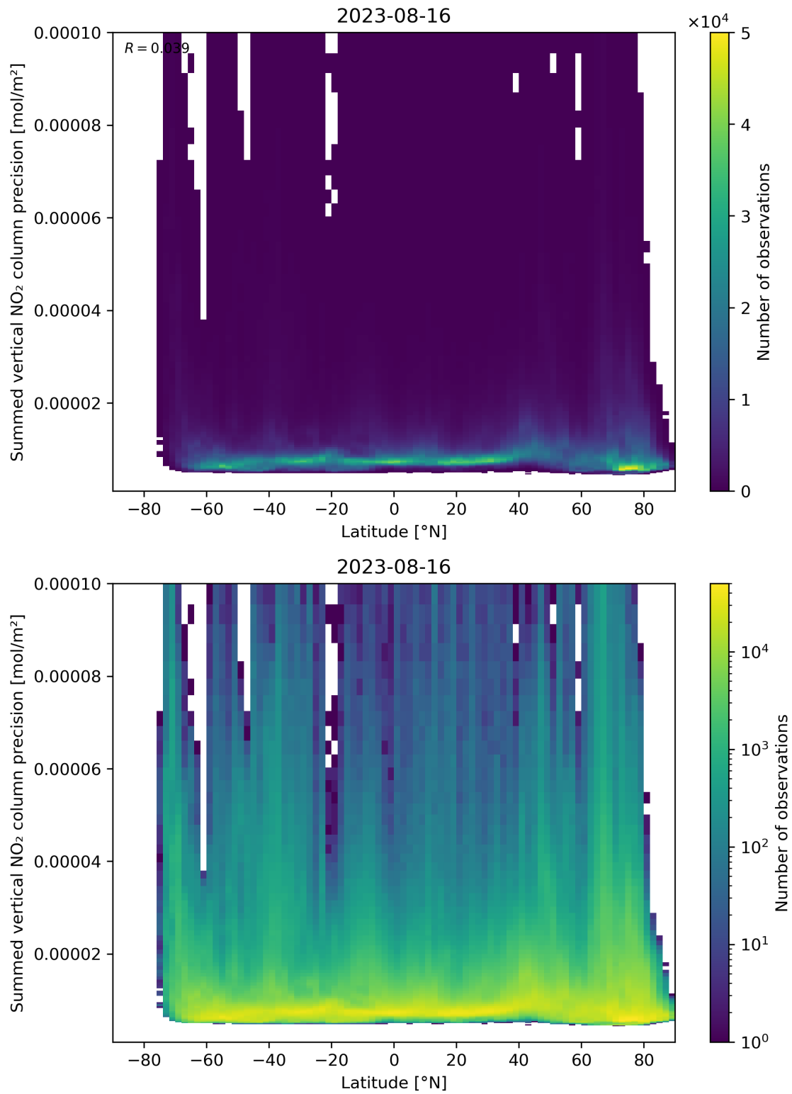
Figure 89: Scatter density plot of “Latitude” against “Summed vertical NO 2 column precision” for 2023-08-15 to 2023-08-17.
