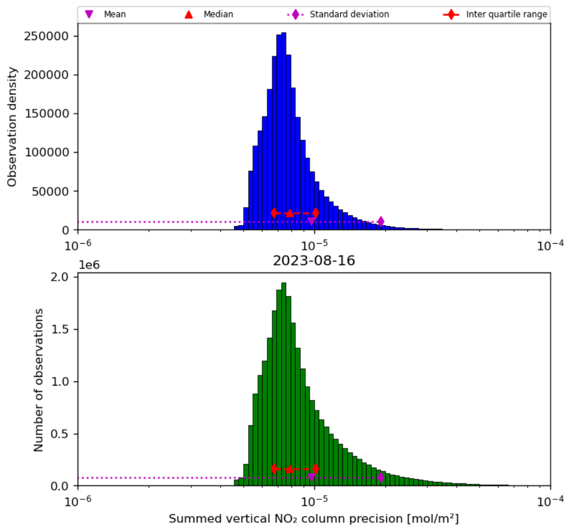
Figure 41: Histogram of "Summed vertical NO 2 column precision" for 2023-08-15 to 2023-08-17
