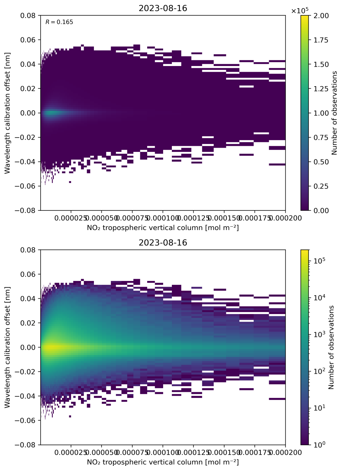
Figure 143: Scatter density plot of “NO 2 tropospheric vertical column” against “Wavelength calibration offset” for 2023-08-15 to 2023-08-17.
