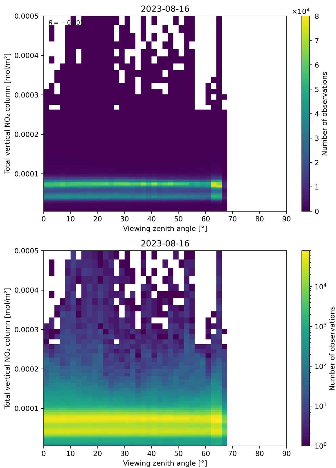
Figure 167: Scatter density plot of “Viewing zenith angle” against “Total vertical NO 2 column” for 2023-08-15 to 2023-08-17.
