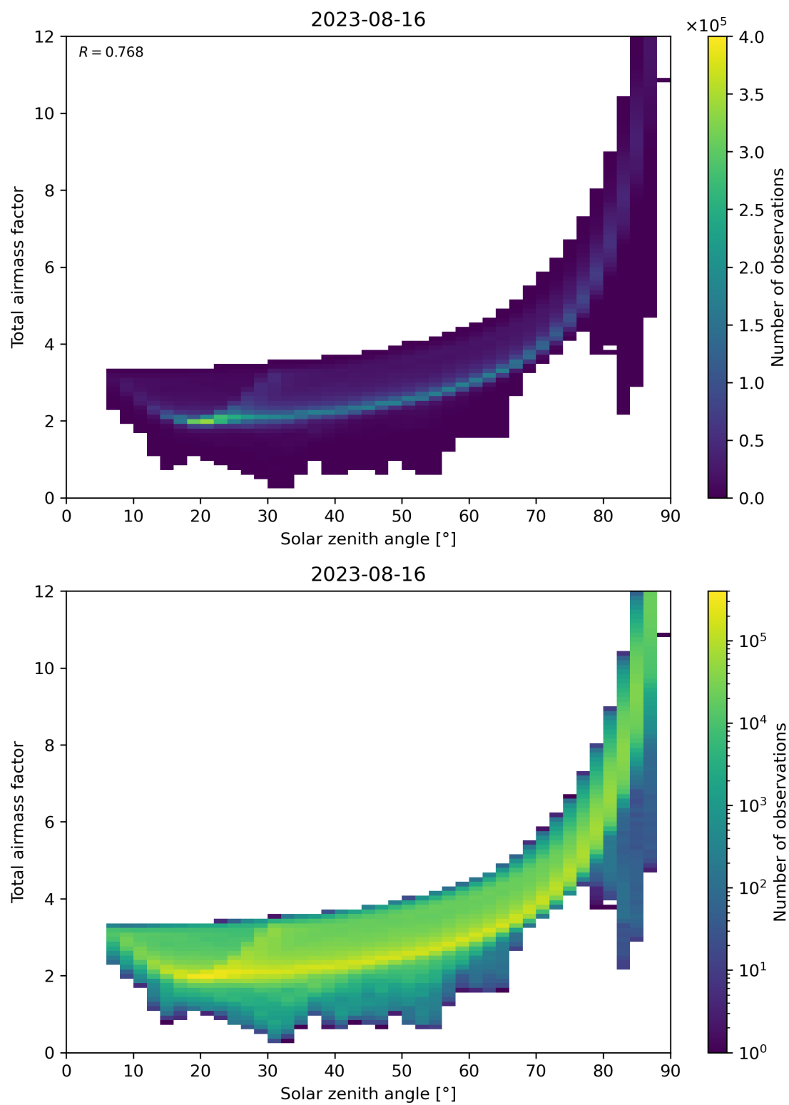
Figure 146: Scatter density plot of “Solar zenith angle” against “Total air mass factor” for 2023-08-15 to 2023-08-17.
