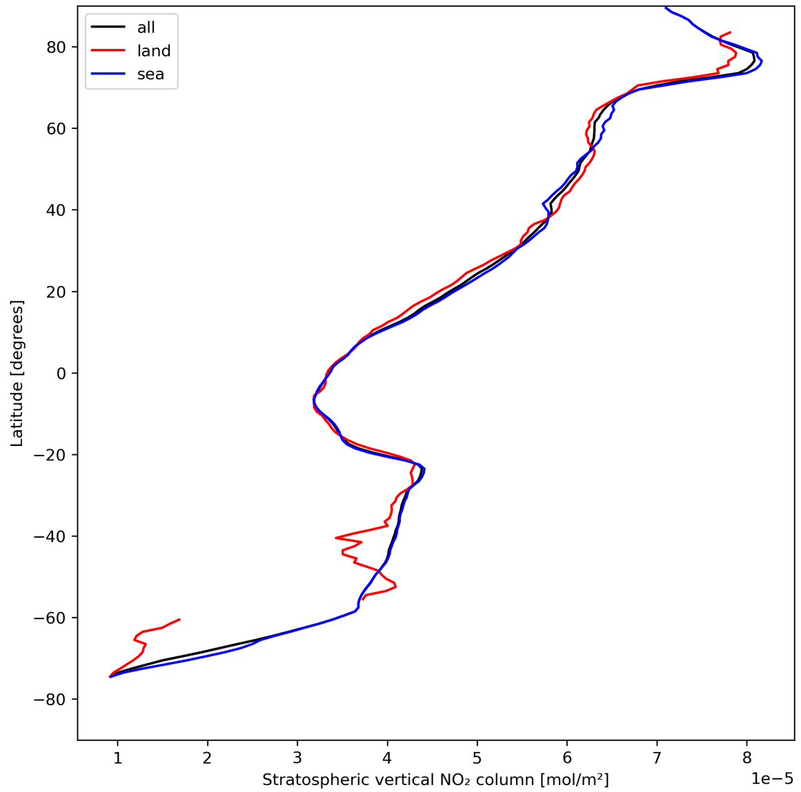
Figure 19: Zonal average of “Stratospheric vertical NO 2 column” for 2023-08-15 to 2023-08-17.
