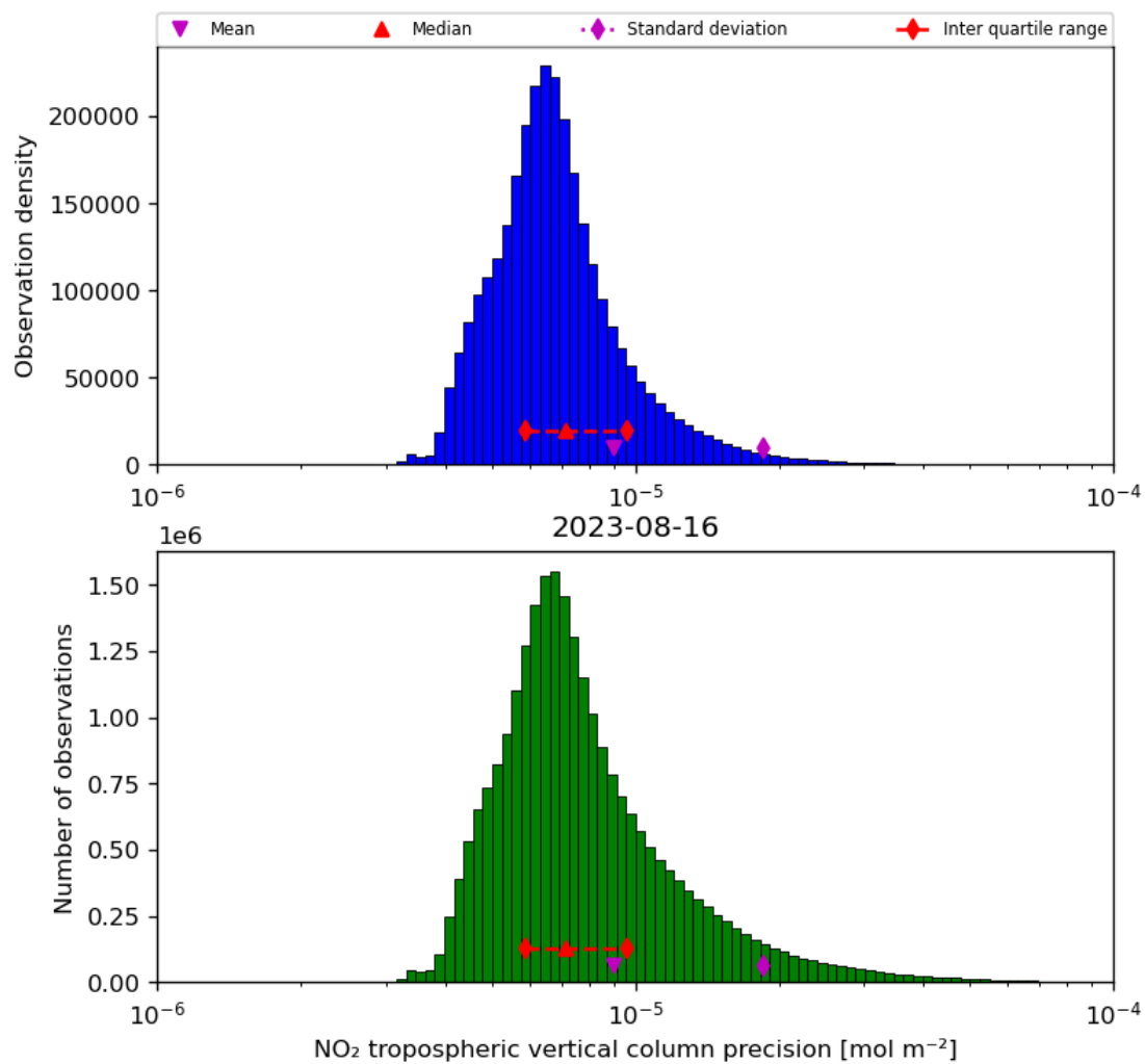
Figure 30: Histogram of “NO 2 tropospheric vertical column precision” for 2023-08-15 to 2023-08-17
