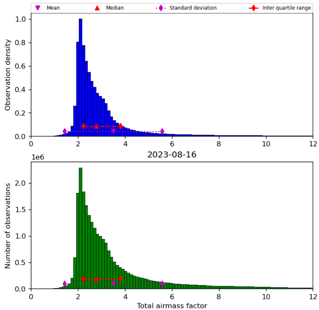
Figure 32: Histogram of “Total airmass factor” for 2023-08-15 to 2023-08-17
