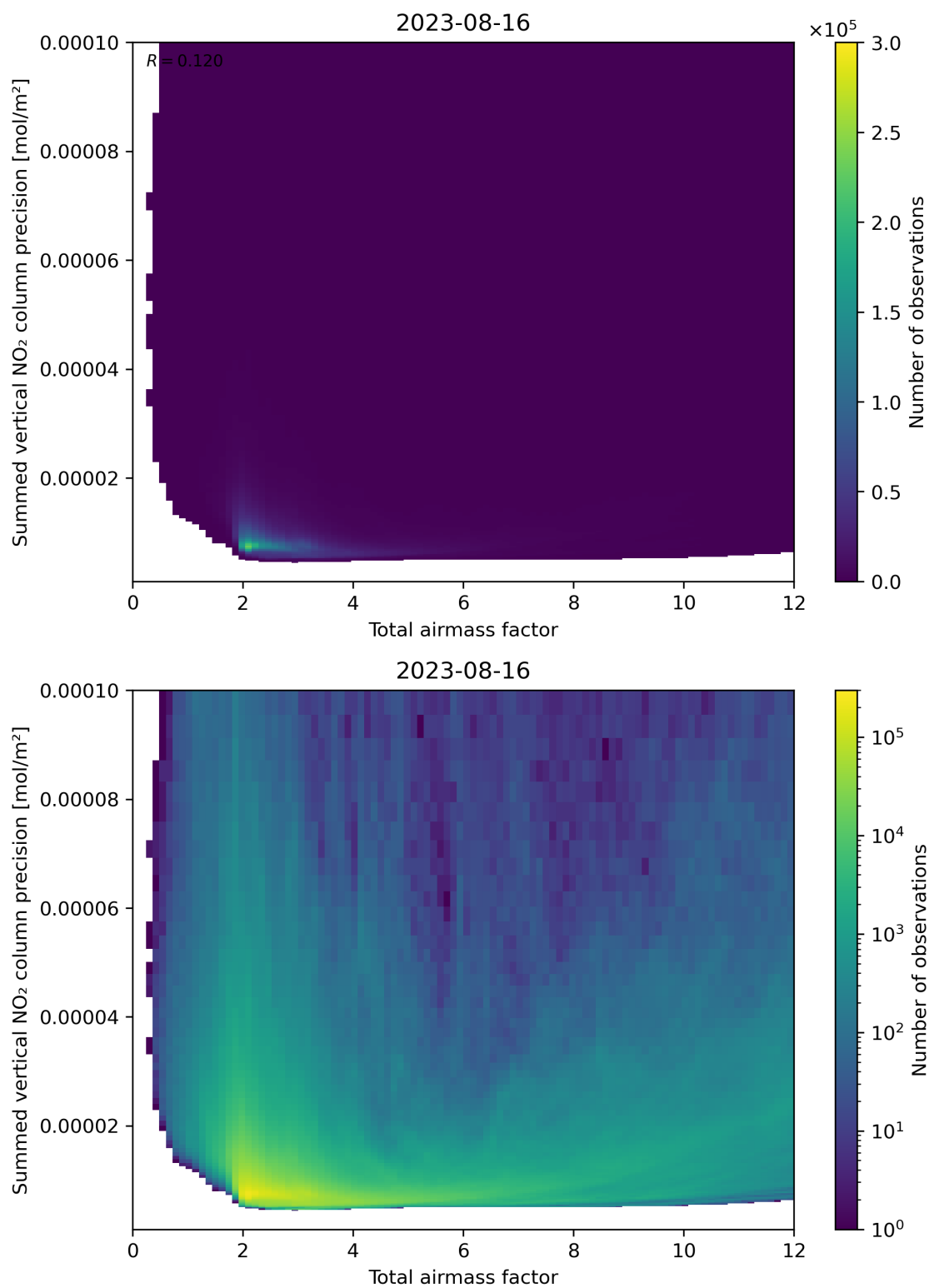
Figure 66: Scatter density plot of “Total airmass factor” against “Summed vertical NO 2 column precision” for 2023-08-15 to 2023-08-17.
