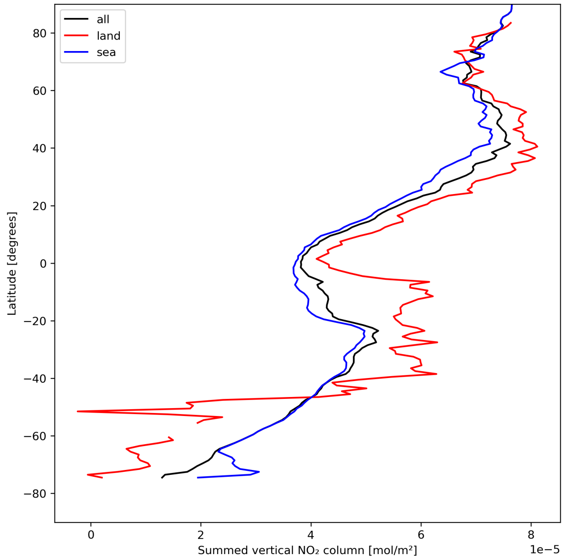
Figure 23: Zonal average of “Summed vertical NO 2 column” for 2023-08-15 to 2023-08-17.
