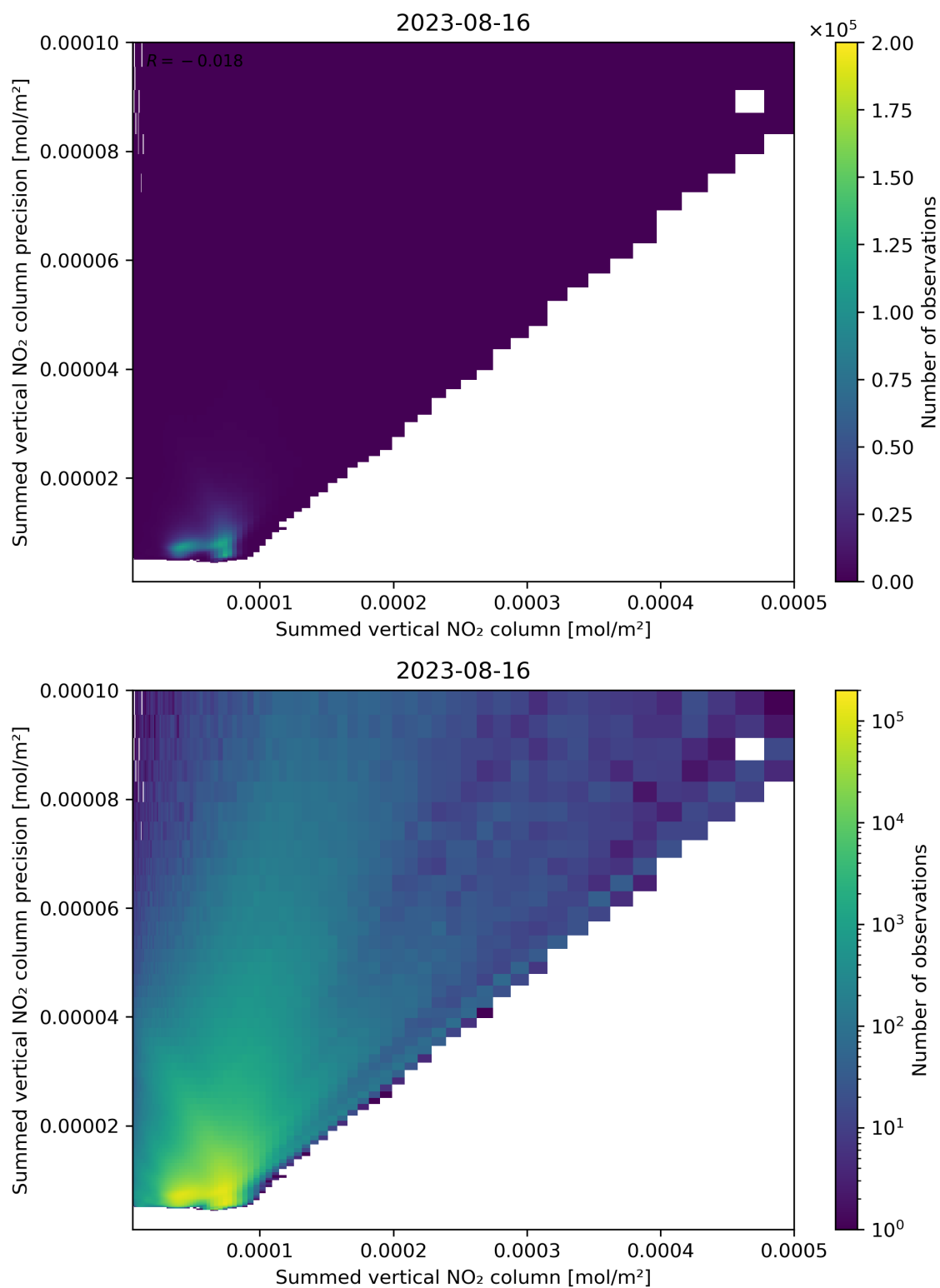
Figure 105: Scatter density plot of “Summed vertical NO 2 column” against “Summed vertical NO 2 column precision” for 2023-08-15 to 2023-08-17.
