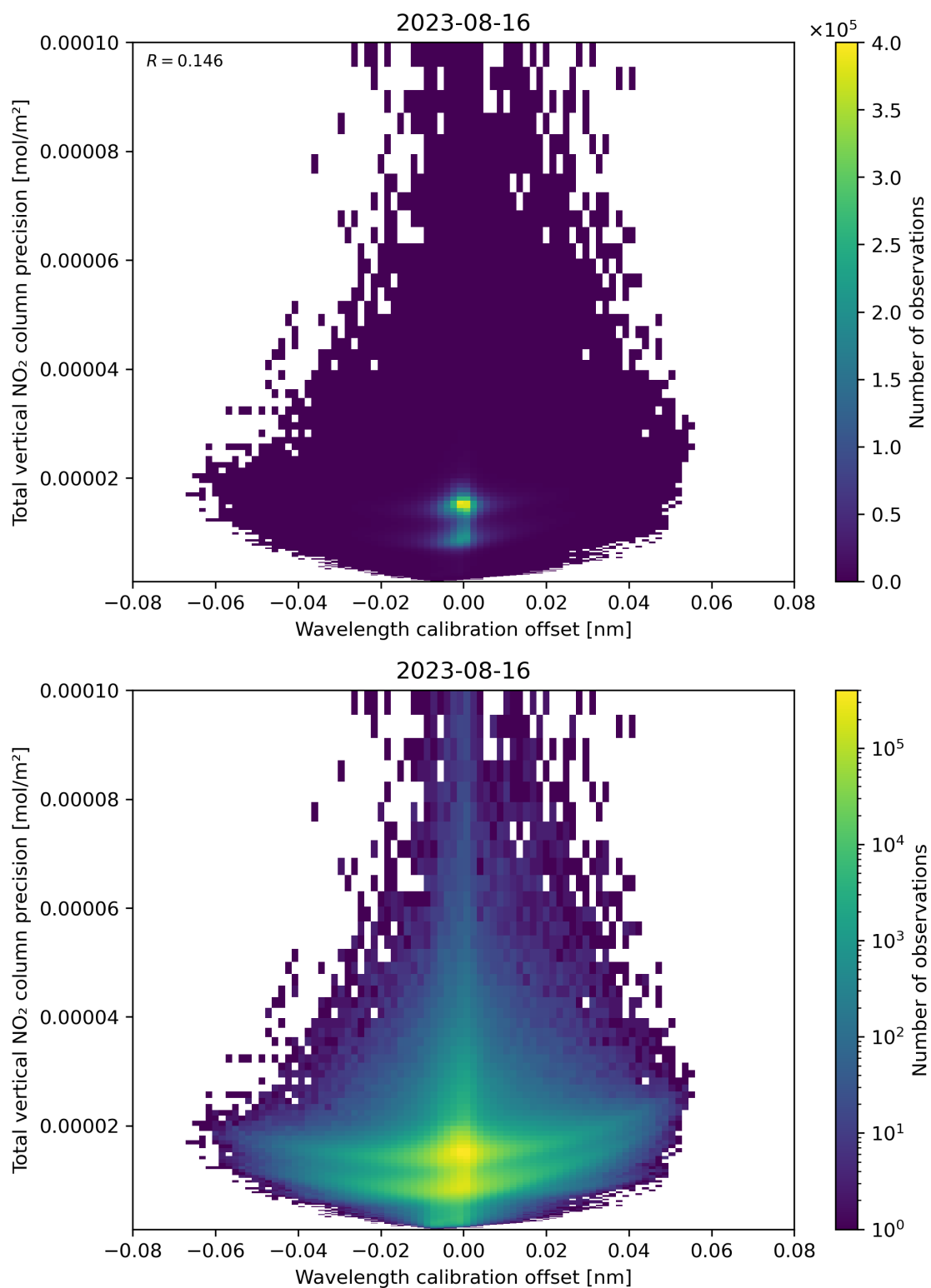
Figure 180: Scatter density plot of “Wavelength calibration offset” against “Total vertical NO 2 column precision” for 2023-08-15 to 2023-08-17.
