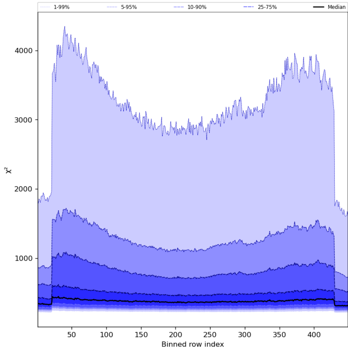
Figure 59: Along track statistics of “ \chi^2 ” for 2023-08-15 to 2023-08-17
