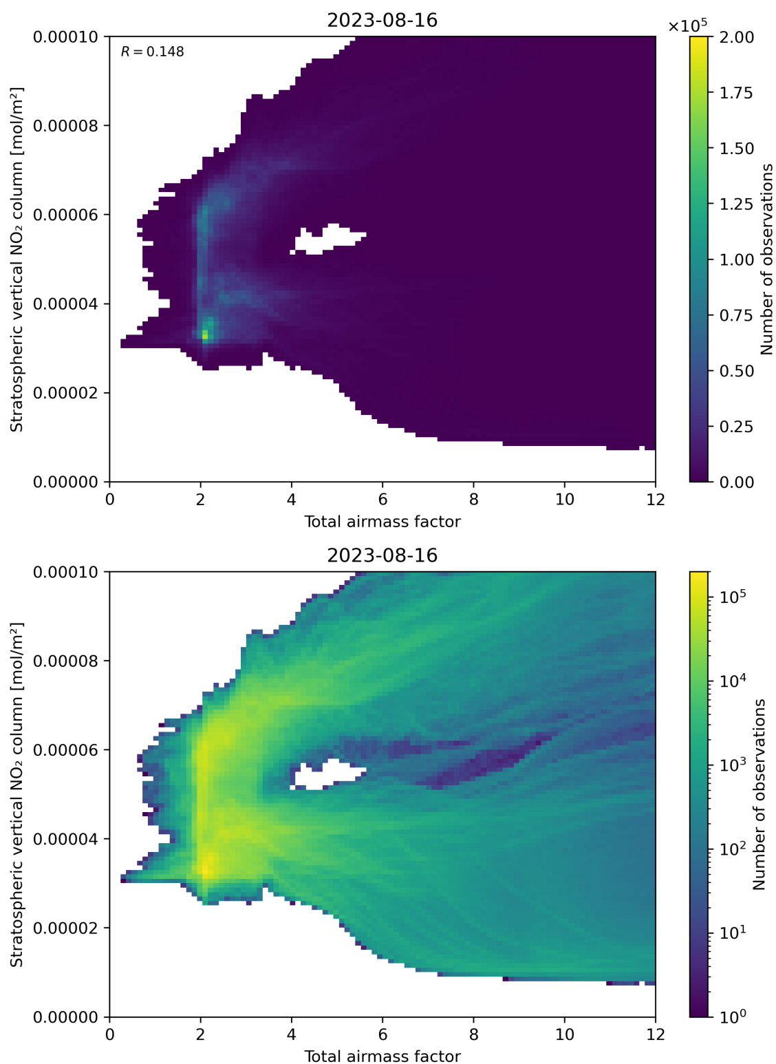
Figure 64: Scatter density plot of “Total airmass factor” against “Stratospheric vertical \text{NO}_2 column” for 2023-08-15 to 2023-08-17.
