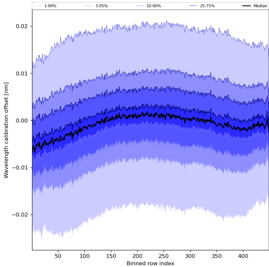
Figure 52: Along track statistics of “Wavelength calibration offset” for 2023-08-15 to 2023-08-17
