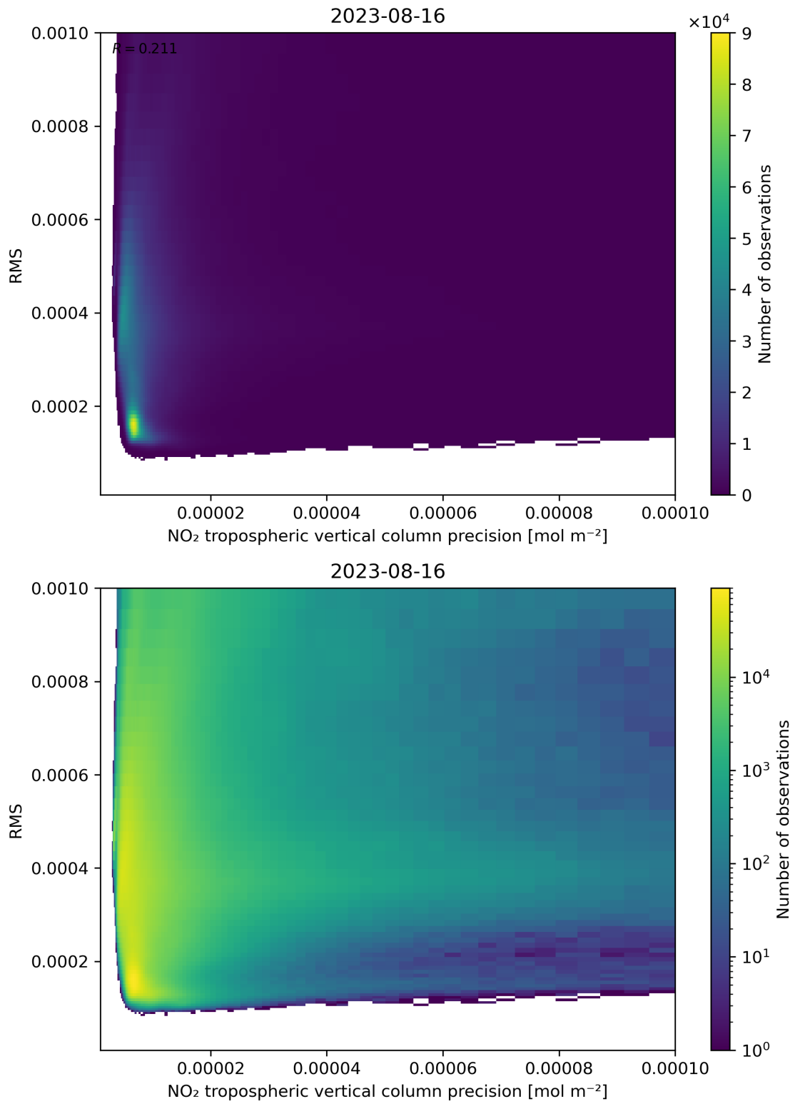
Figure 140: Scatter density plot of “NO 2 tropospheric vertical column precision” against “RMS” for 2023-08-15 to 2023-08-17.
