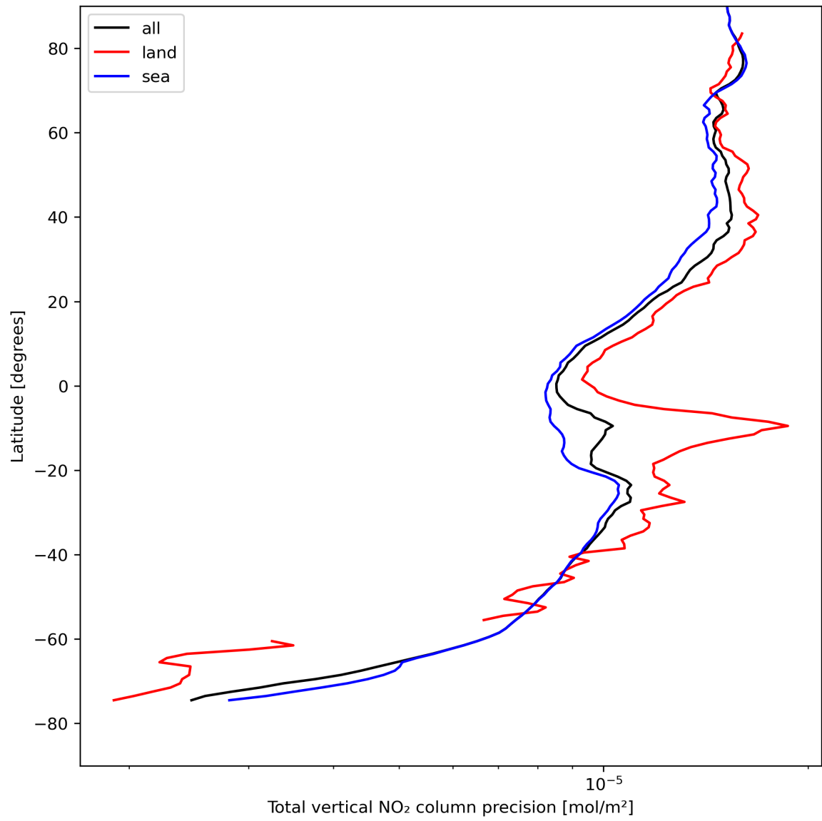
Figure 22: Zonal average of “Total vertical NO 2 column precision” for 2023-08-15 to 2023-08-17.
