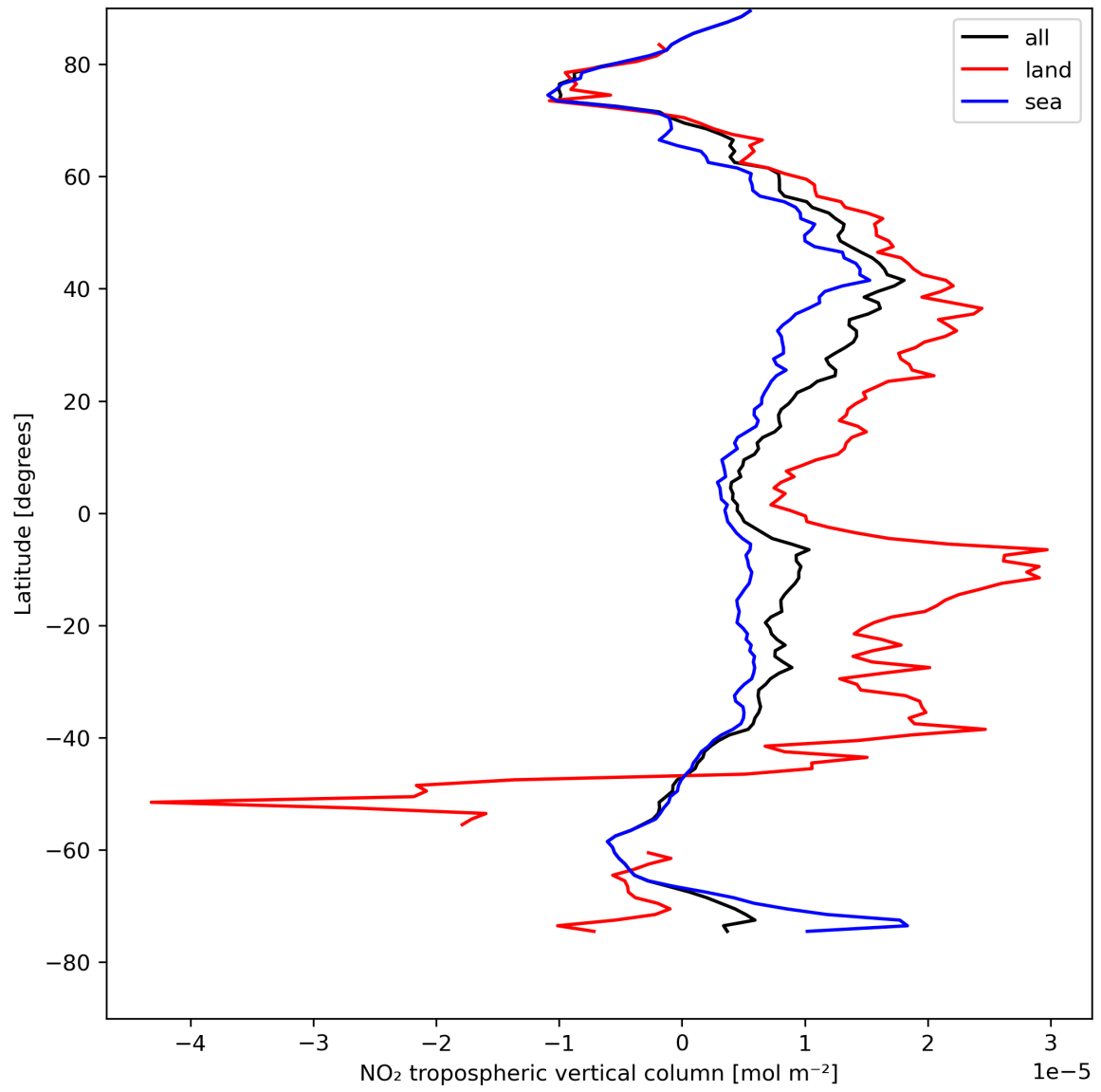
Figure 12: Zonal average of “NO 2 tropospheric vertical column” for 2023-08-15 to 2023-08-17.
