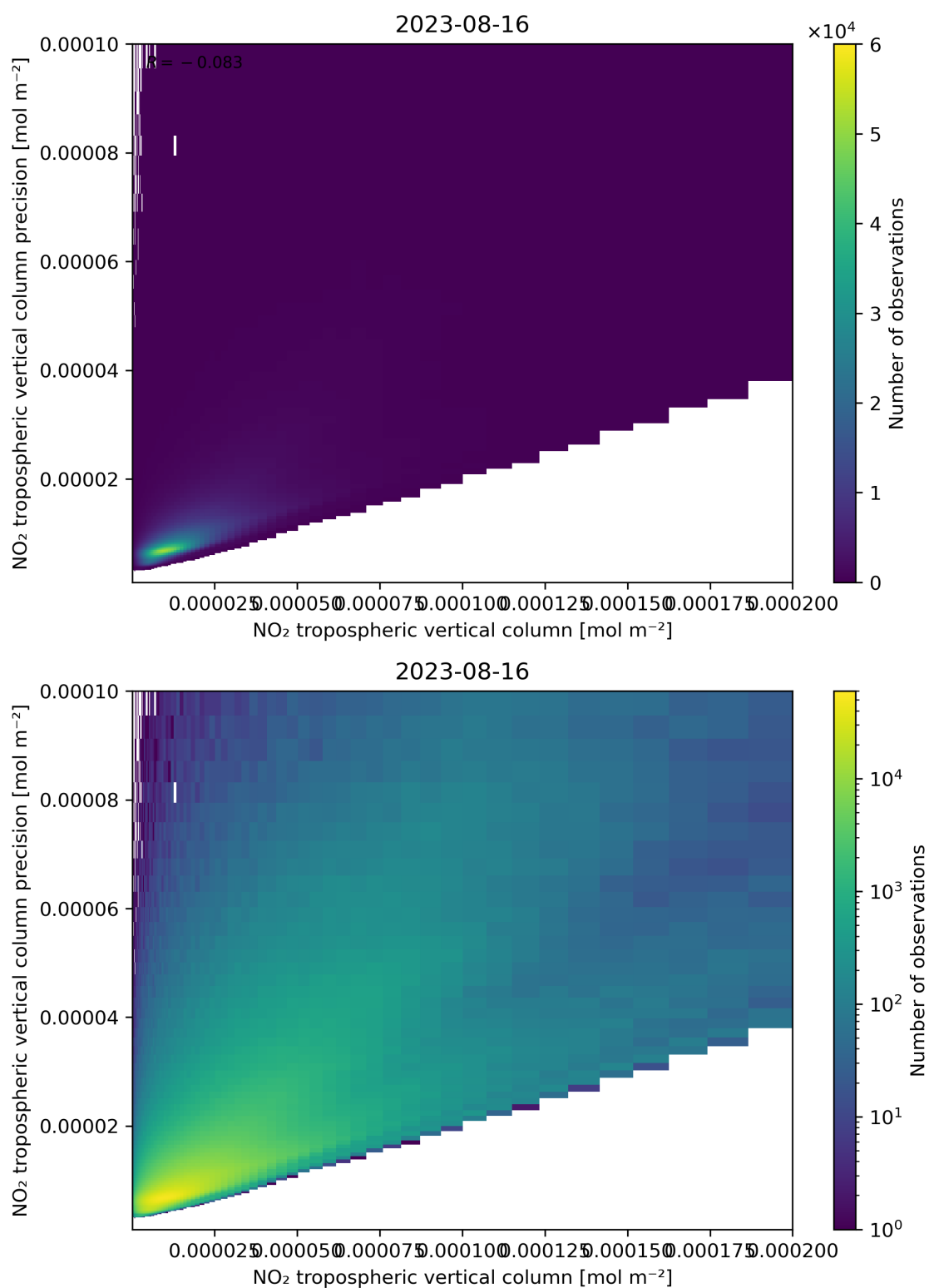
Figure 130: Scatter density plot of “NO 2 tropospheric vertical column” against “NO 2 tropospheric vertical column precision” for 2023-08-15 to 2023-08-17.
