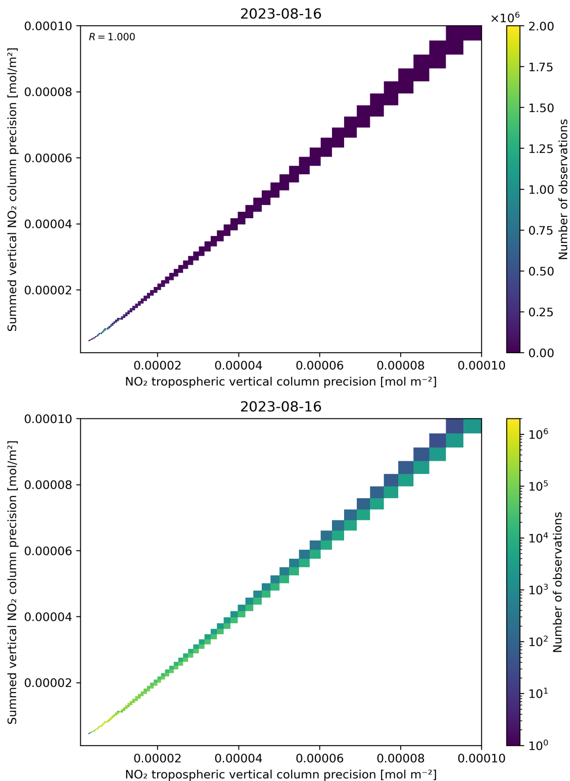
Figure 137: Scatter density plot of “NO 2 tropospheric vertical column precision” against “Summed vertical NO 2 column precision” for 2023-08-15 to 2023-08-17.
