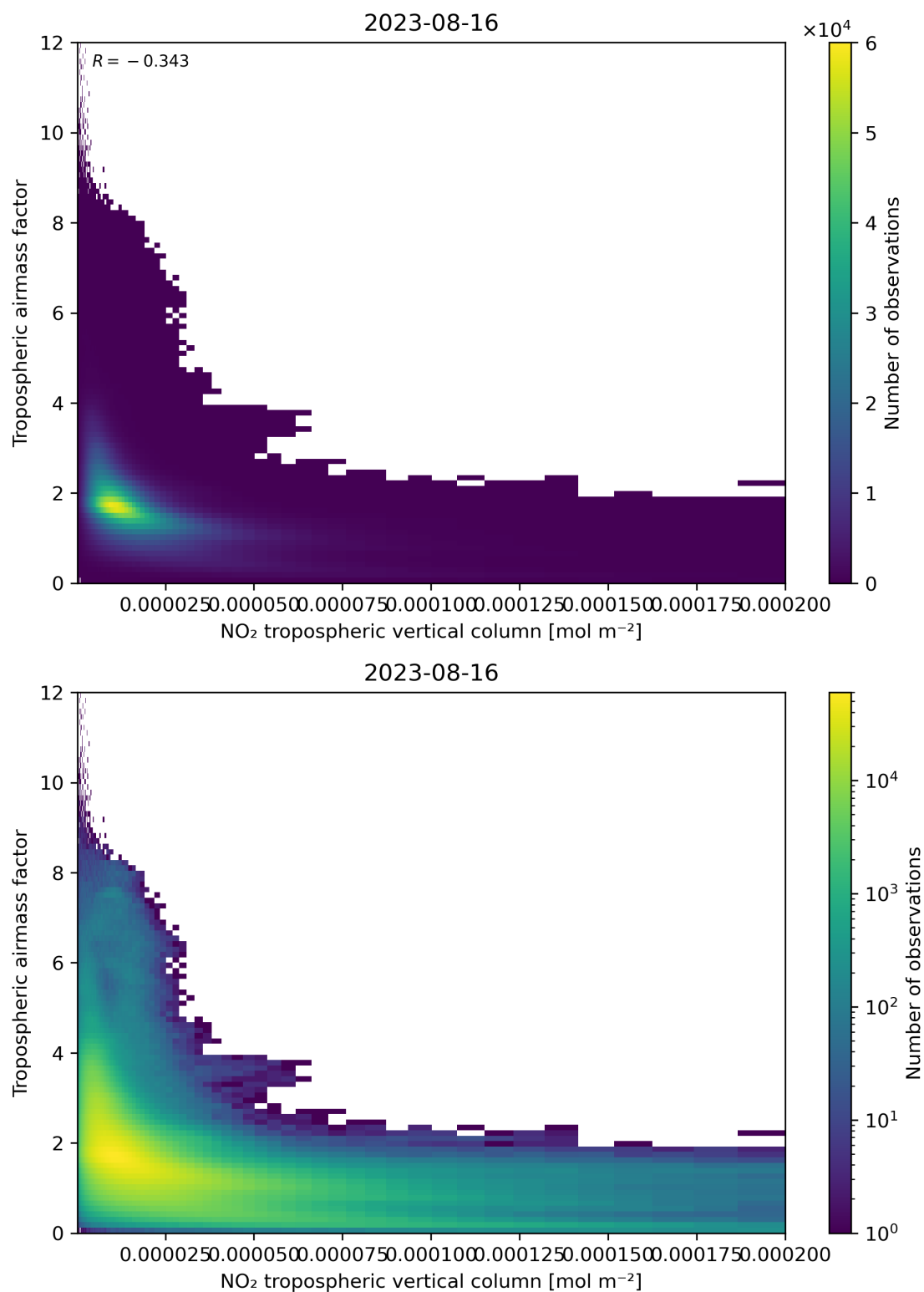
Figure 123: Scatter density plot of “NO 2 tropospheric vertical column” against “Tropospheric airmass factor” for 2023-08-15 to 2023-08-17.
