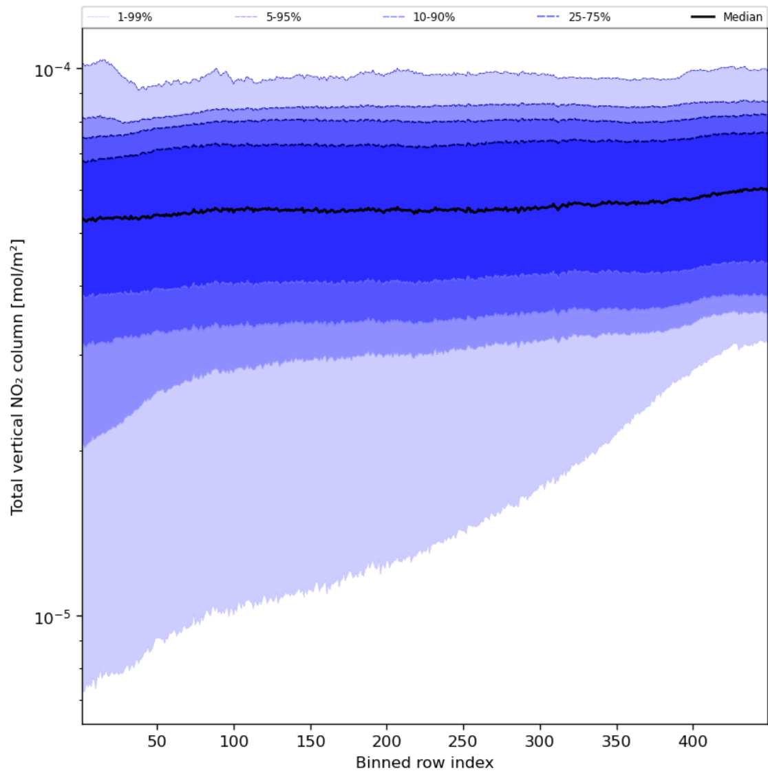
Figure 55: Along track statistics of “Total vertical NO 2 column” for 2023-08-15 to 2023-08-17
