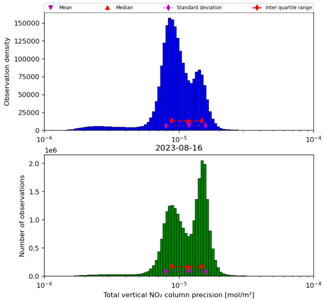
Figure 39: Histogram of "Total vertical NO 2 column precision" for 2023-08-15 to 2023-08-17
