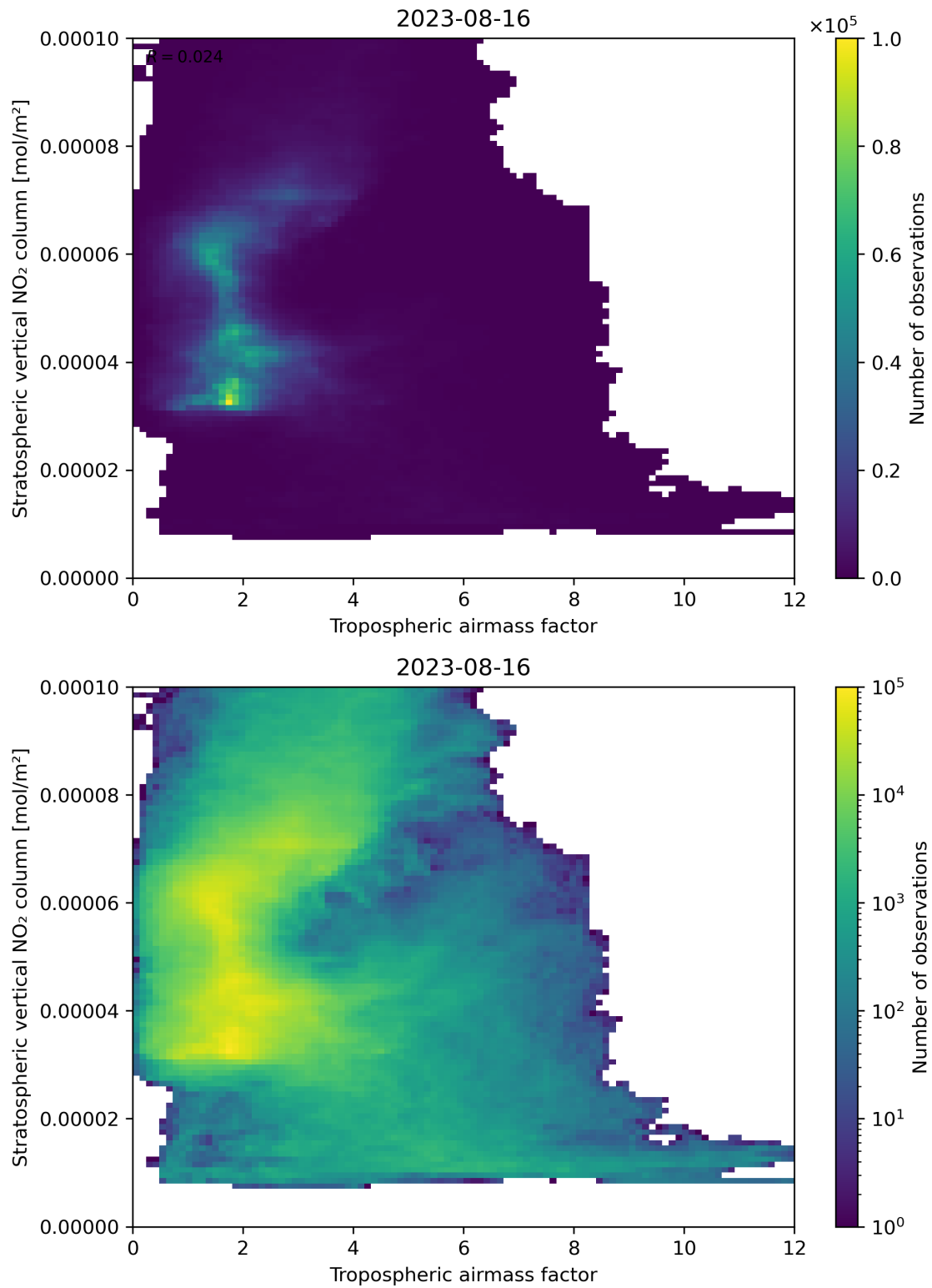
Figure 74: Scatter density plot of “Tropospheric air mass factor” against “Stratospheric vertical NO 2 column” for 2023-08-15 to 2023-08-17.
