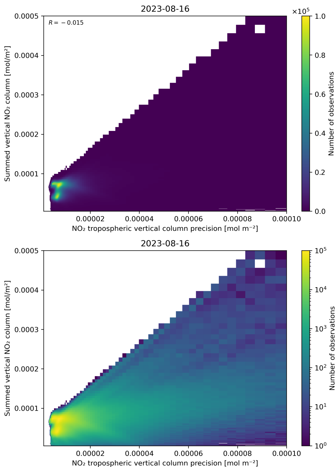
Figure 136: Scatter density plot of “NO 2 tropospheric vertical column precision” against “Summed vertical NO 2 column” for 2023-08-15 to 2023-08-17.
