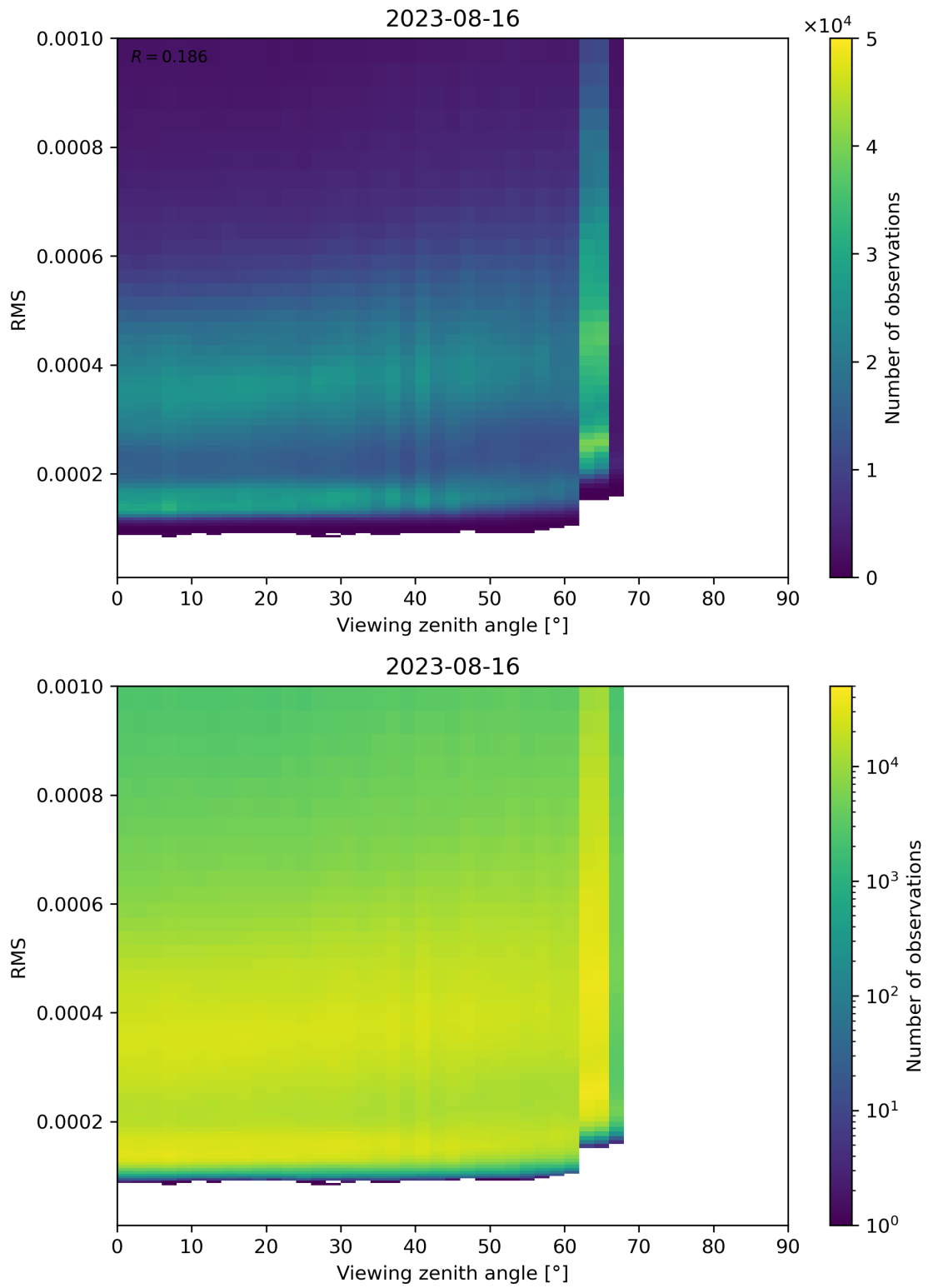
Figure 171: Scatter density plot of “Viewing zenith angle” against “RMS” for 2023-08-15 to 2023-08-17.
