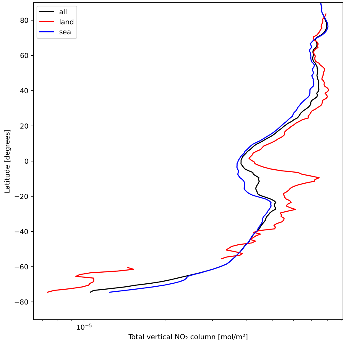
Figure 21: Zonal average of “Total vertical NO 2 column” for 2023-08-15 to 2023-08-17.
