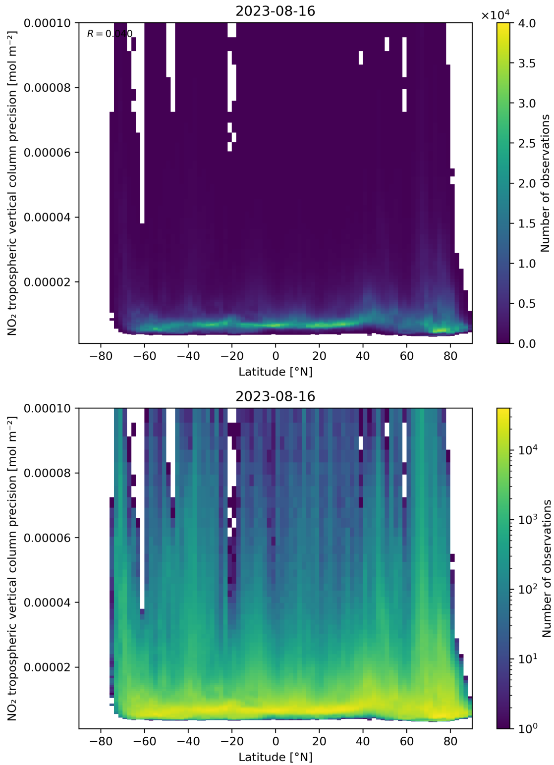
Figure 93: Scatter density plot of “Latitude” against “NO 2 tropospheric vertical column precision” for 2023-08-15 to 2023-08-17.
