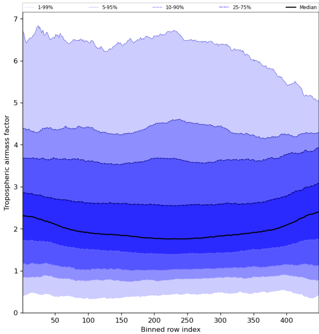
Figure 48: Along track statistics of “Tropospheric air mass factor” for 2023-08-15 to 2023-08-17
