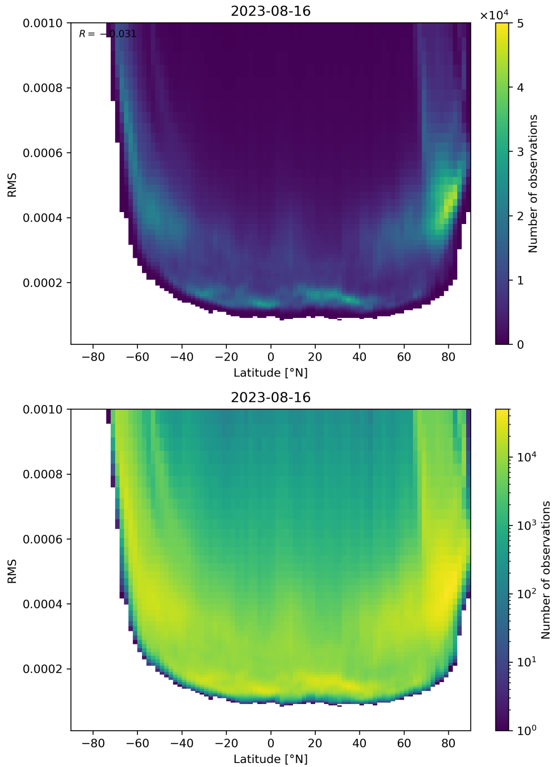
Figure 94: Scatter density plot of “Latitude” against “RMS” for 2023-08-15 to 2023-08-17.
