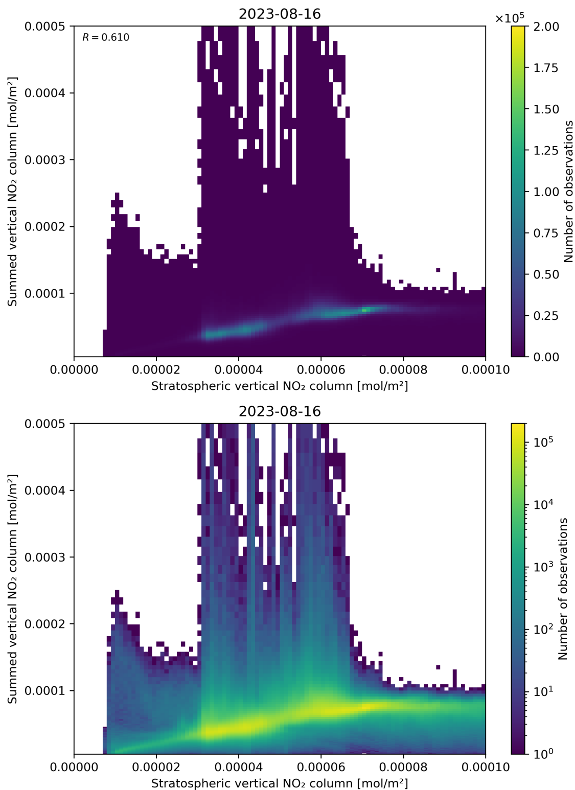
Figure 98: Scatter density plot of “Stratospheric vertical NO 2 column” against “Summed vertical NO 2 column” for 2023-08-15 to 2023-08-17.
