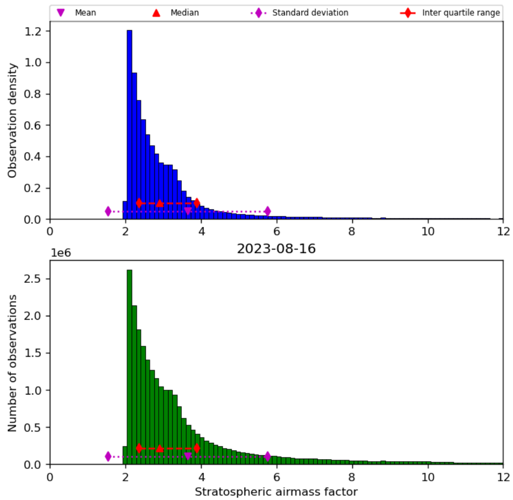
Figure 44: Histogram of “Stratospheric airmass factor” for 2023-08-15 to 2023-08-17
