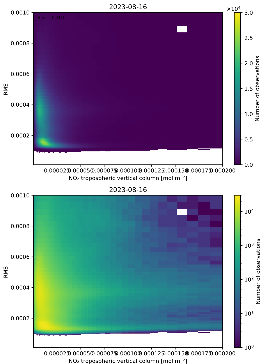
Figure 142: Scatter density plot of “NO 2 tropospheric vertical column” against “RMS” for 2023-08-15 to 2023-08-17.
