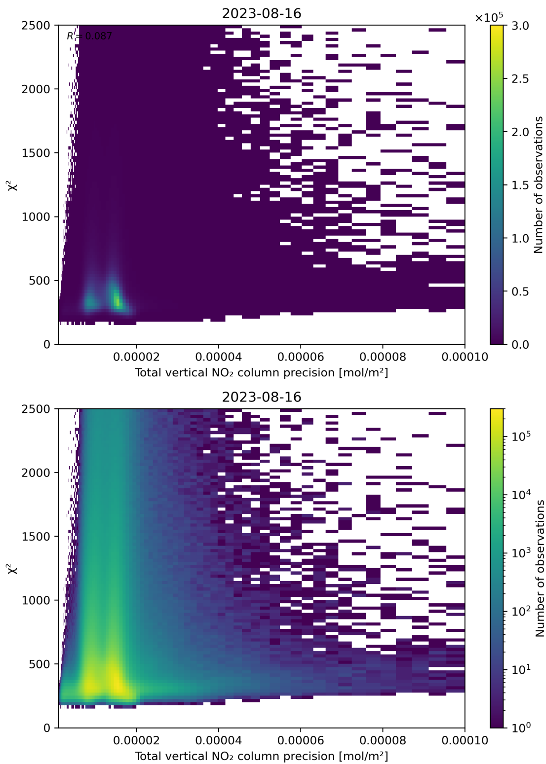
Figure 116: Scatter density plot of “Total vertical NO 2 column precision” against “ \chi^2 ” for 2023-08-15 to 2023-08-17.
