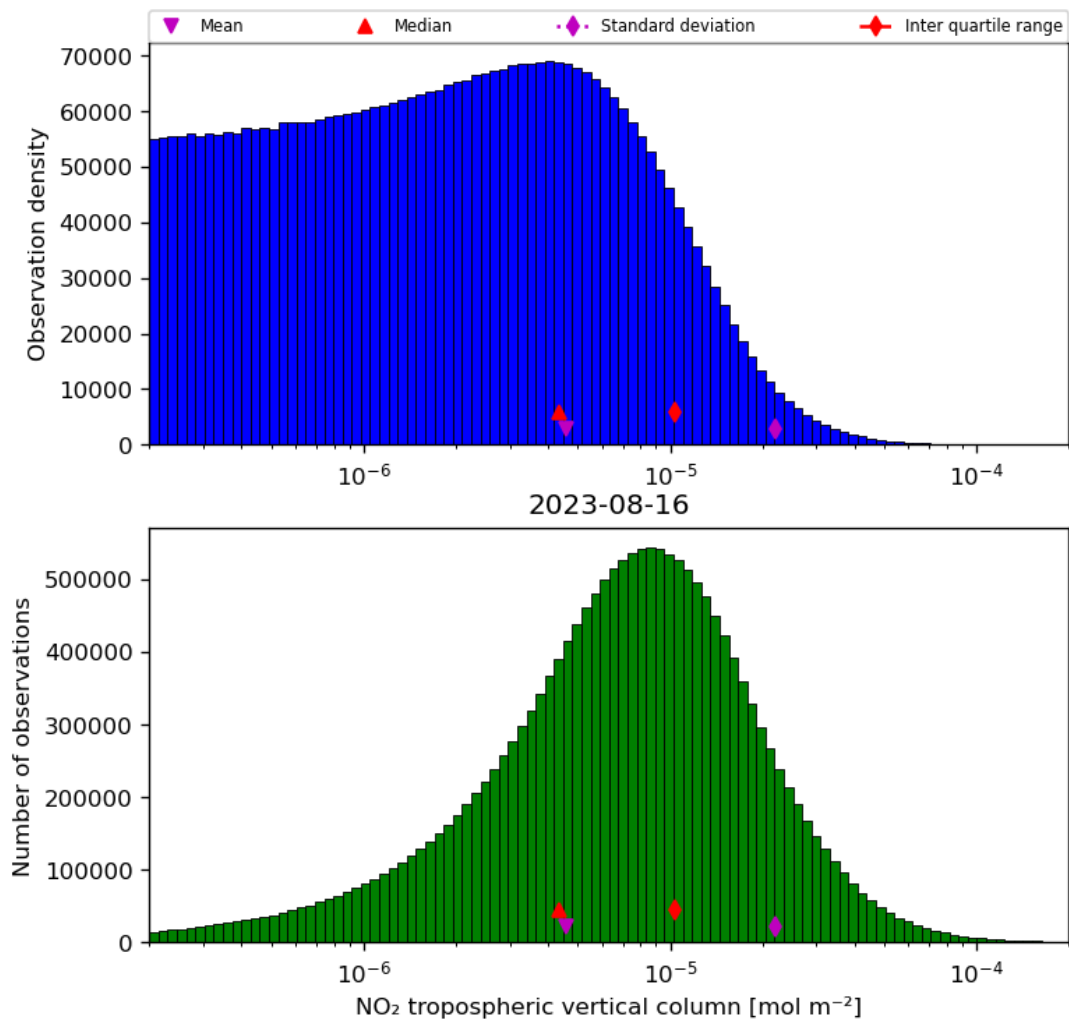
Figure 29: Histogram of “NO 2 tropospheric vertical column” for 2023-08-15 to 2023-08-17
