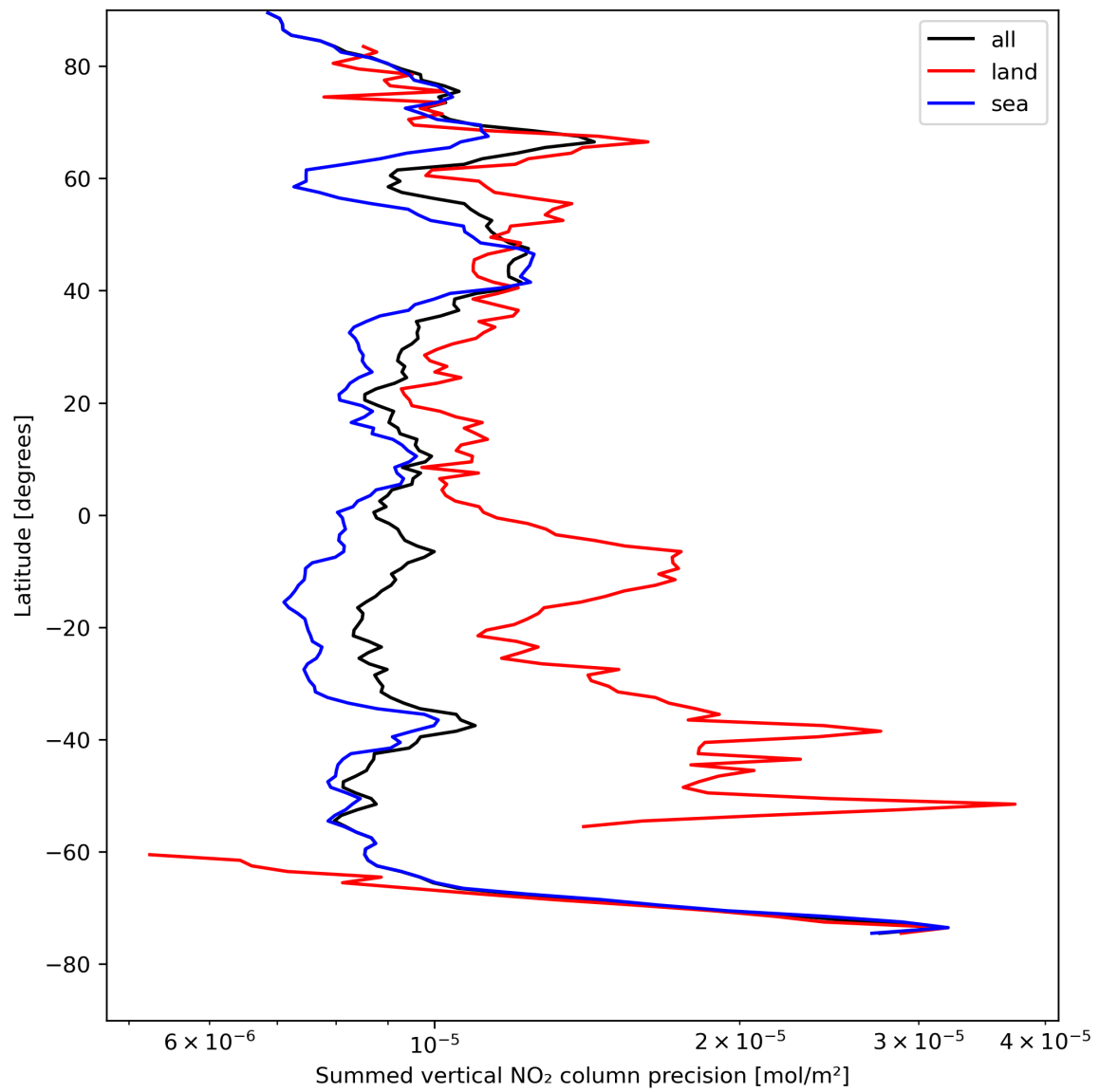
Figure 24: Zonal average of “Summed vertical NO 2 column precision” for 2023-08-15 to 2023-08-17.
