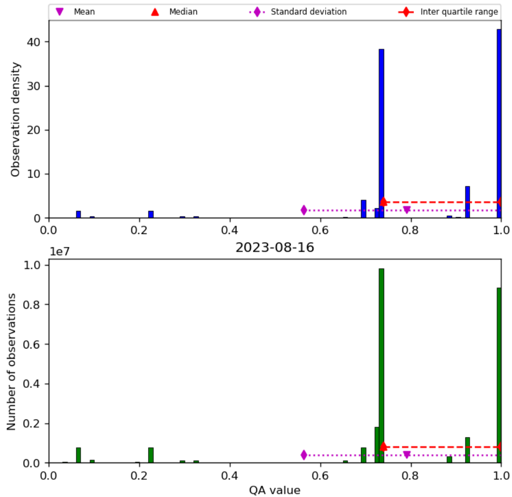
Figure 28: Histogram of “QA value” for 2023-08-15 to 2023-08-17
