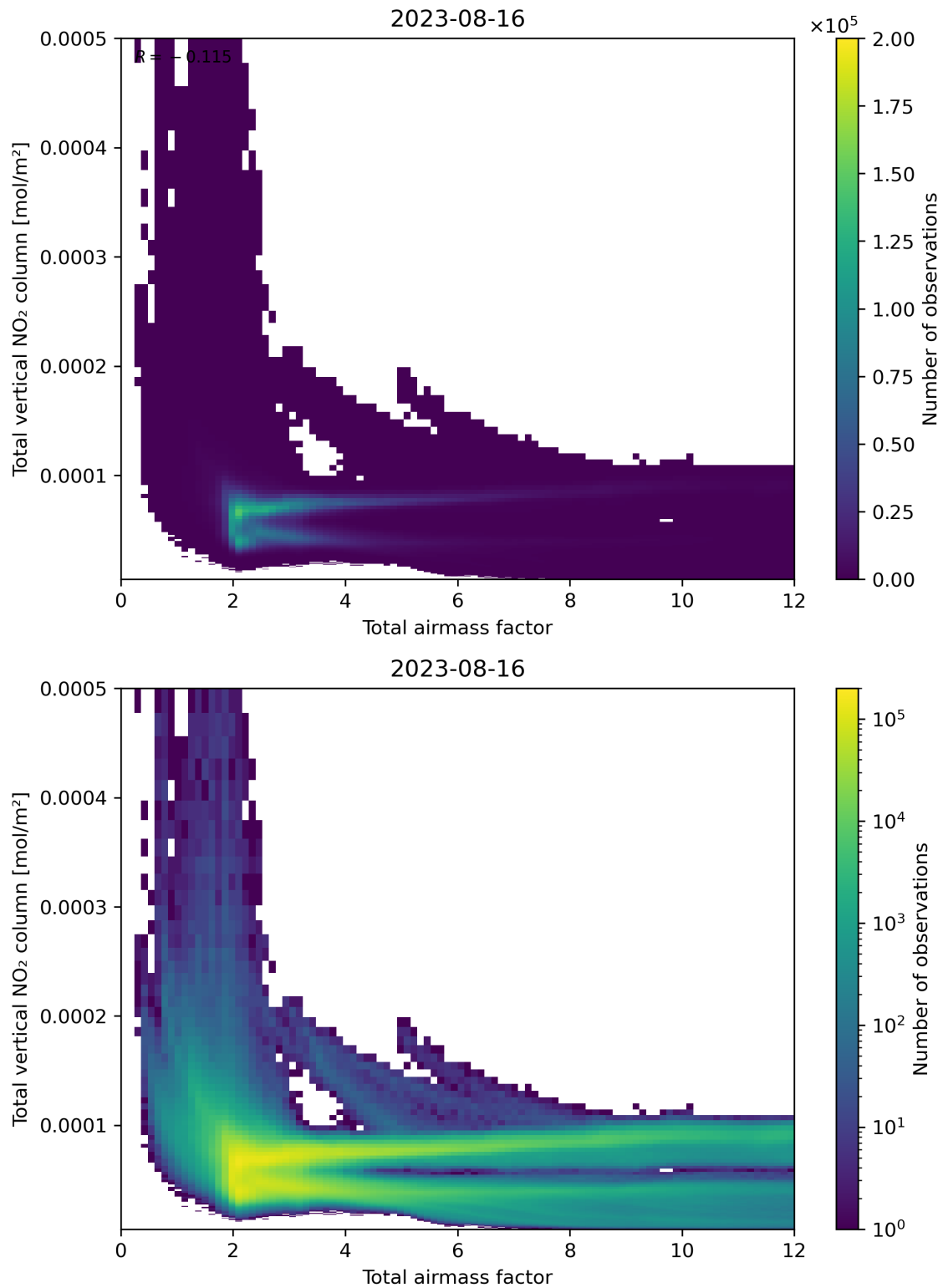
Figure 67: Scatter density plot of “Total airmass factor” against “Total vertical NO 2 column” for 2023-08-15 to 2023-08-17.
