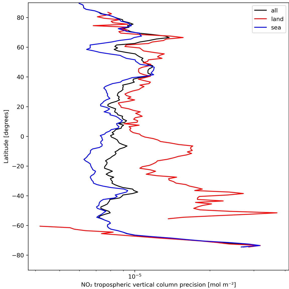
Figure 13: Zonal average of “NO 2 tropospheric vertical column precision” for 2023-08-15 to 2023-08-17.
