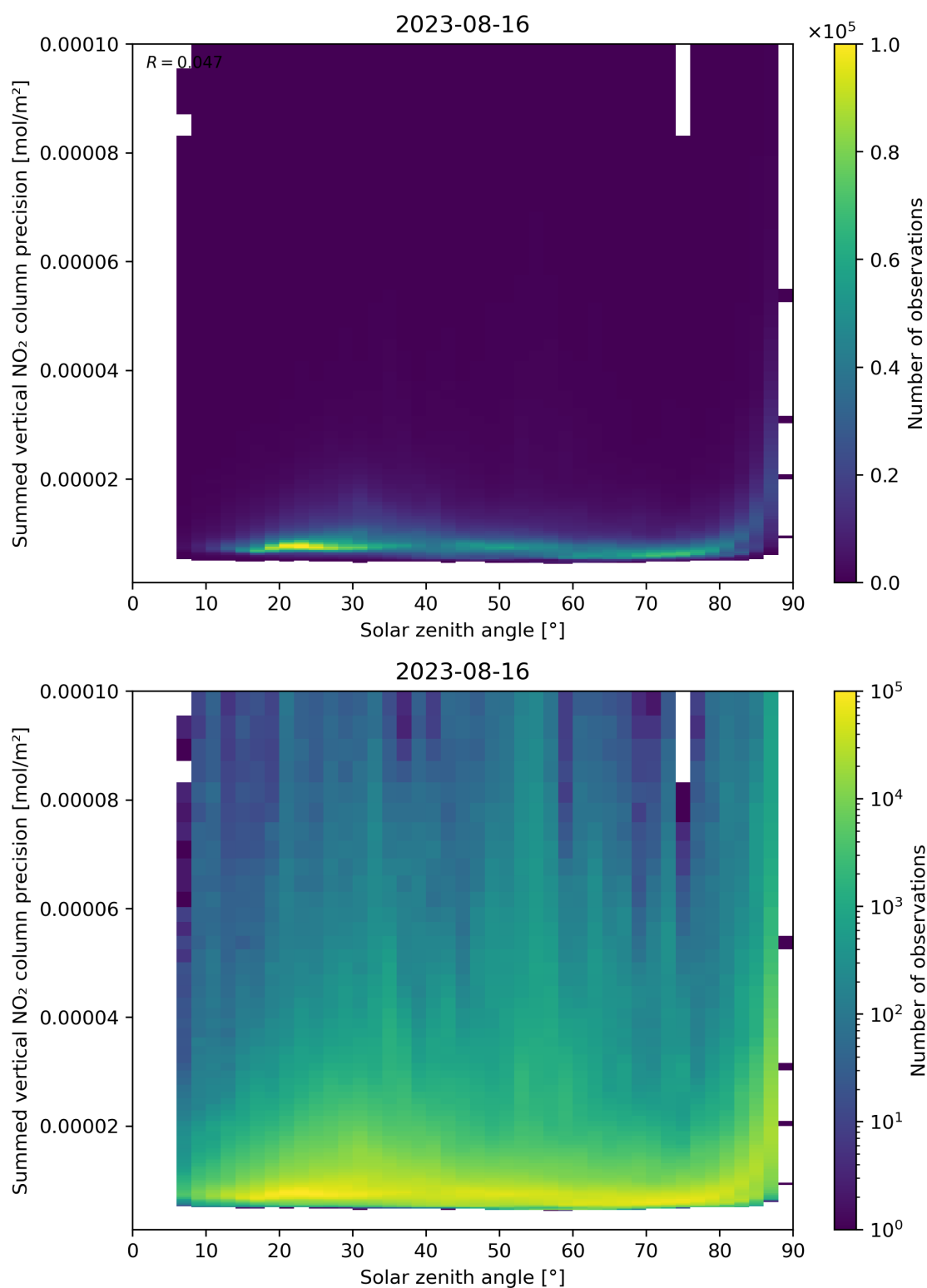
Figure 152: Scatter density plot of “Solar zenith angle” against “Summed vertical NO 2 column precision” for 2023-08-15 to 2023-08-17.
