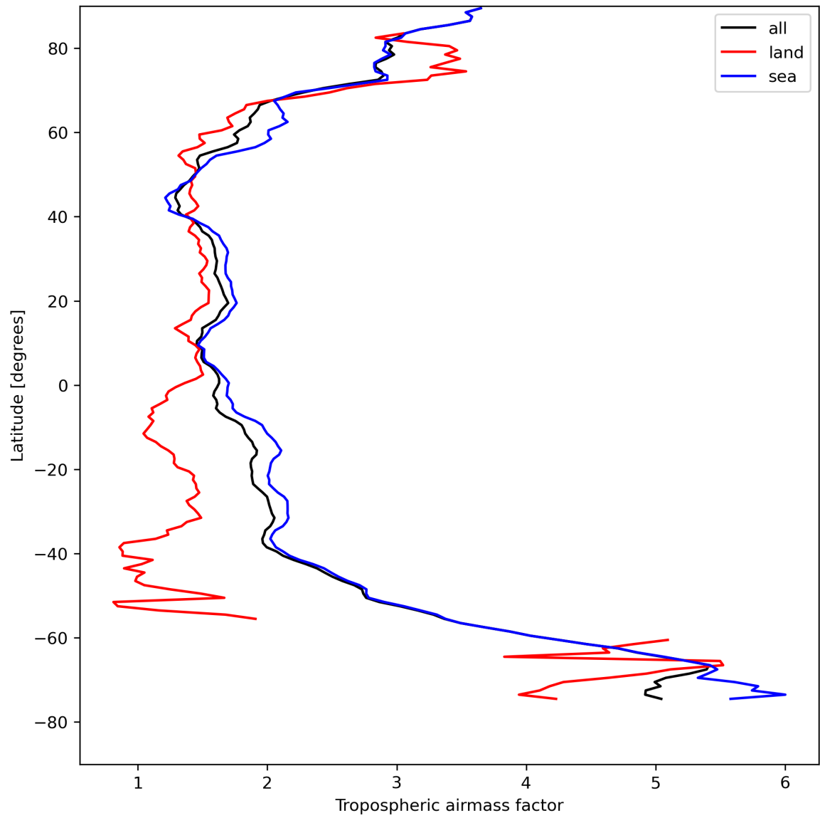
Figure 14: Zonal average of “Tropospheric airmass factor” for 2023-08-15 to 2023-08-17.
