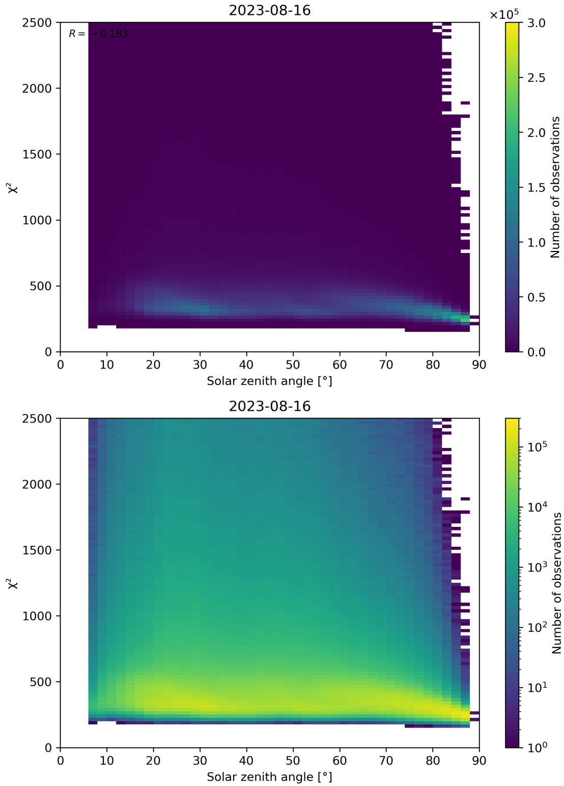
Figure 148: Scatter density plot of “Solar zenith angle” against “ \chi^2 ” for 2023-08-15 to 2023-08-17.
