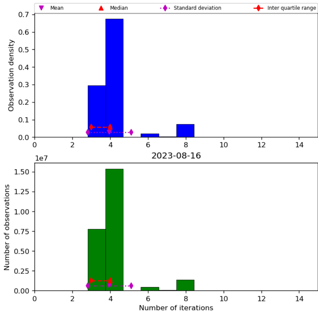
Figure 34: Histogram of “Number of iterations” for 2023-08-15 to 2023-08-17
