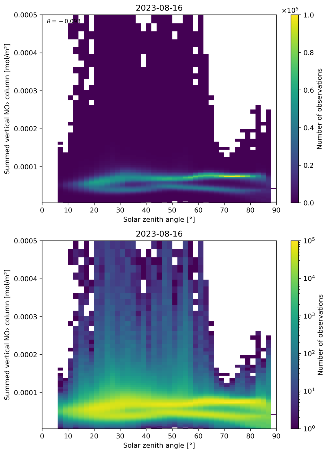
Figure 151: Scatter density plot of “Solar zenith angle” against “Summed vertical NO 2 column” for 2023-08-15 to 2023-08-17.
