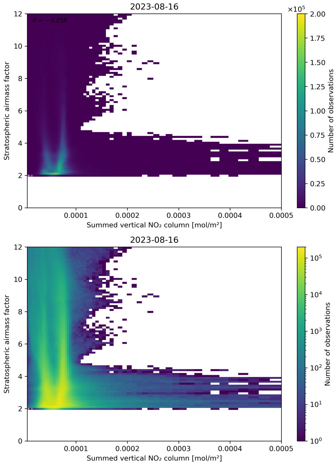
Figure 103: Scatter density plot of “Summed vertical NO 2 column” against “Stratospheric air mass factor” for 2023-08-15 to 2023-08-17.
