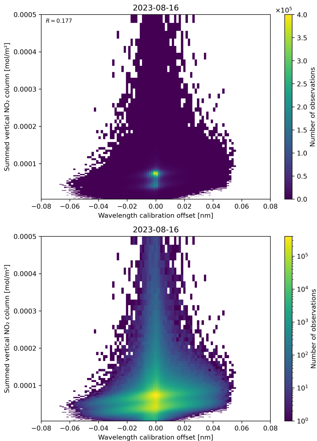
Figure 177: Scatter density plot of “Wavelength calibration offset” against “Summed vertical NO 2 column” for 2023-08-15 to 2023-08-17.
