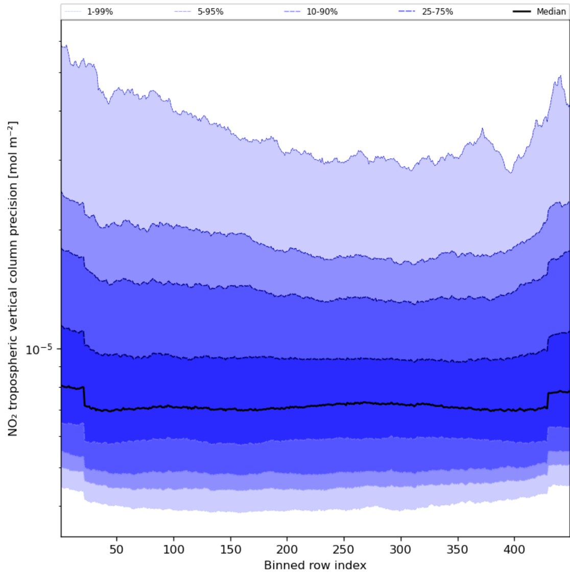
Figure 47: Along track statistics of “NO 2 tropospheric vertical column precision” for 2023-08-15 to 2023-08-17
