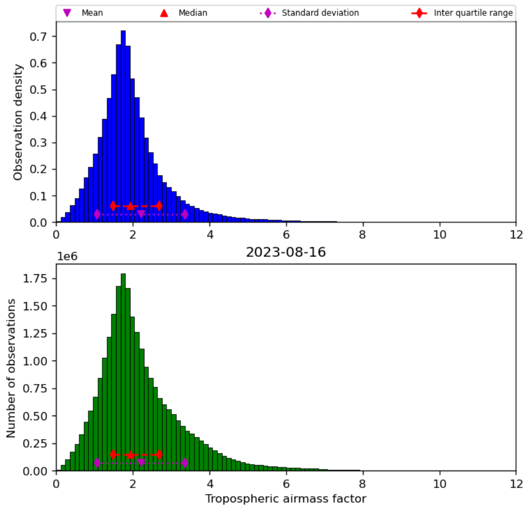
Figure 31: Histogram of “Tropospheric airmass factor” for 2023-08-15 to 2023-08-17
