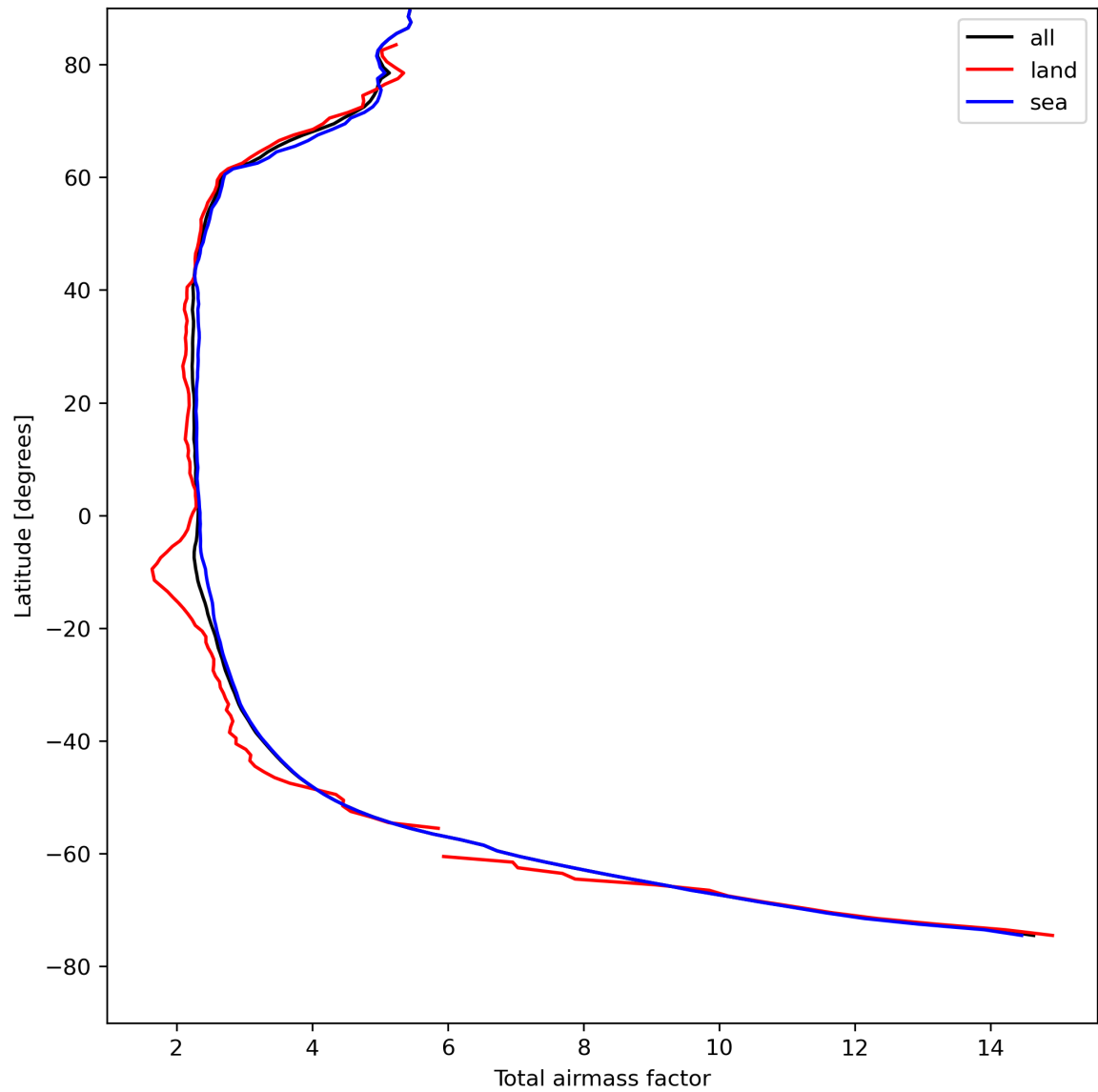
Figure 15: Zonal average of “Total airmass factor” for 2023-08-15 to 2023-08-17.
