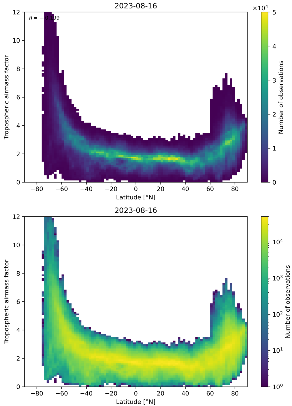
Figure 85: Scatter density plot of “Latitude” against “Tropospheric airmass factor” for 2023-08-15 to 2023-08-17.
