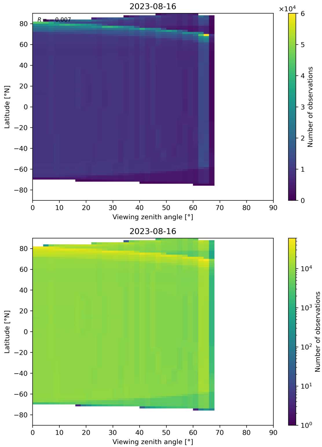
Figure 163: Scatter density plot of “Viewing zenith angle” against “Latitude” for 2023-08-15 to 2023-08-17.
