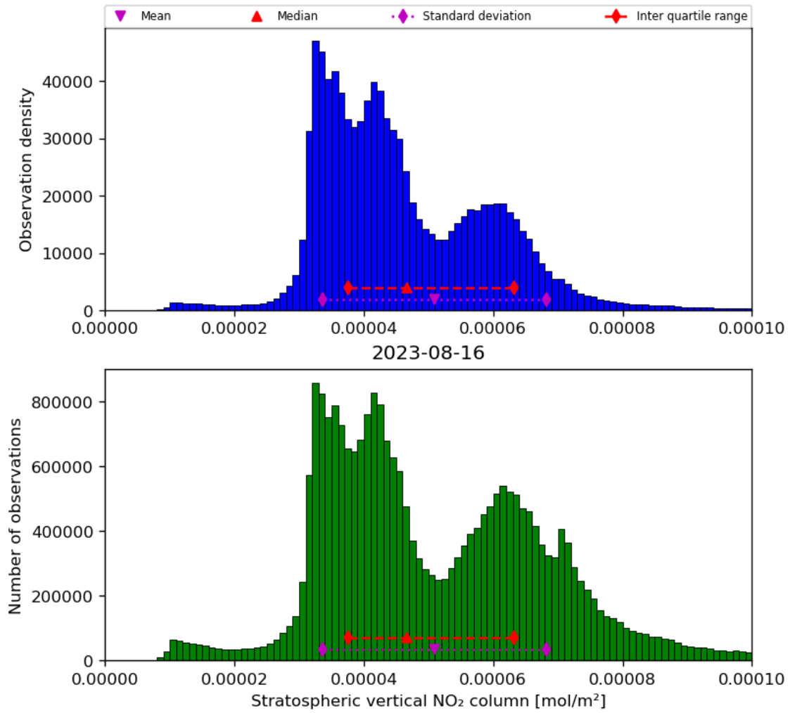
Figure 36: Histogram of “Stratospheric vertical NO 2 column” for 2023-08-15 to 2023-08-17
