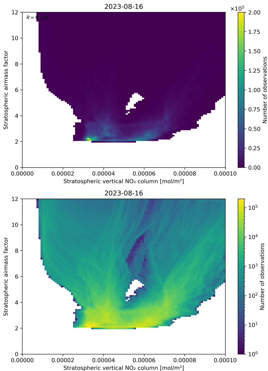
Figure 96: Scatter density plot of “Stratospheric vertical NO 2 column” against “Stratospheric airmass factor” for 2023-08-15 to 2023-08-17.
