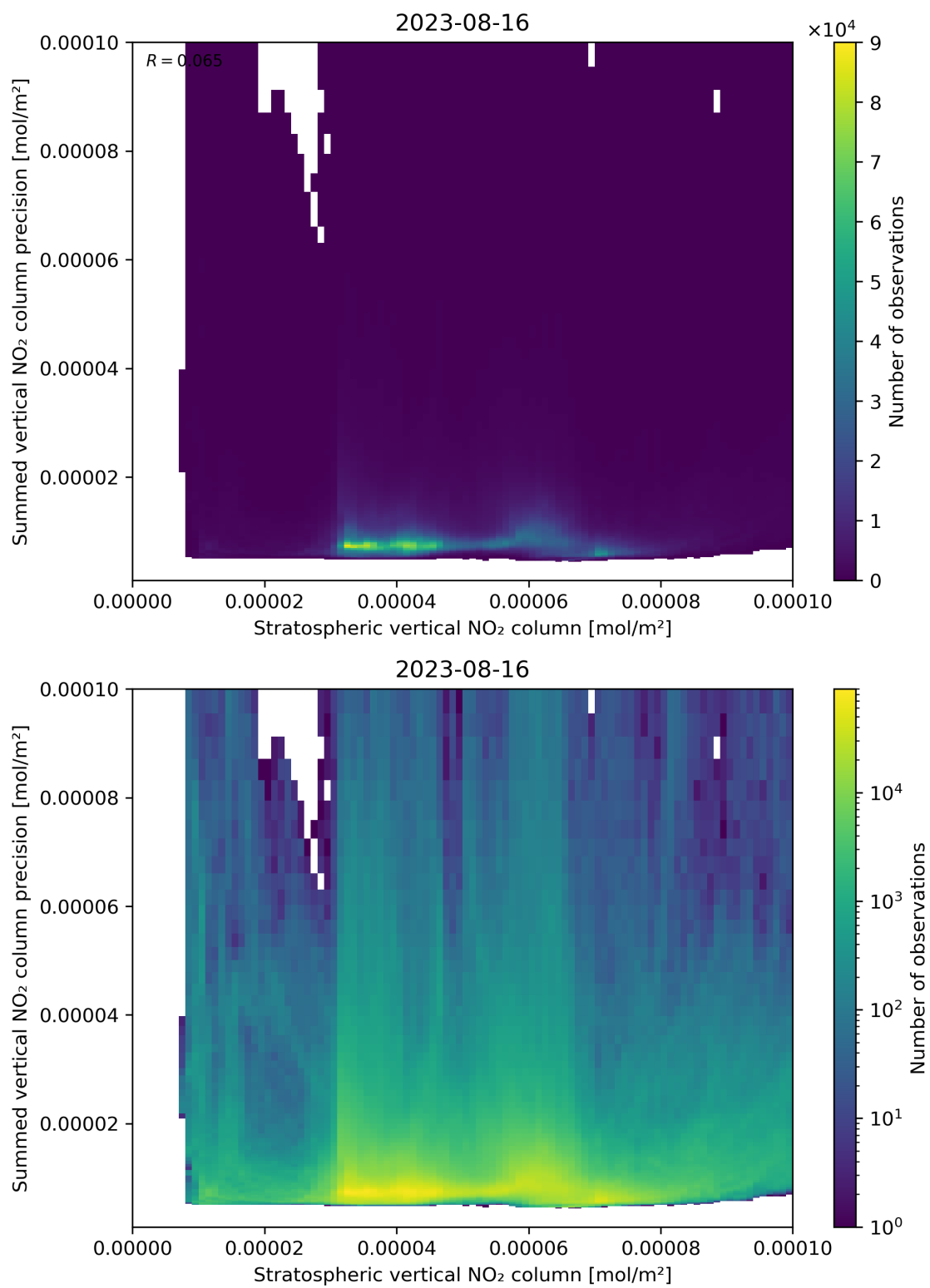
Figure 99: Scatter density plot of “Stratospheric vertical NO 2 column” against “Summed vertical NO 2 column precision” for 2023-08-15 to 2023-08-17.
