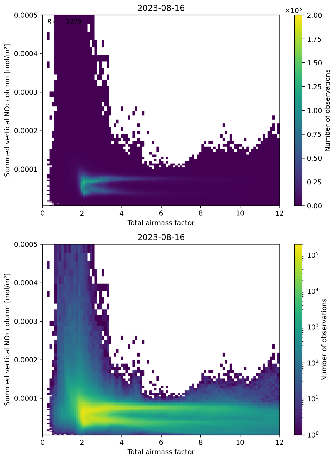
Figure 65: Scatter density plot of “Total airmass factor” against “Summed vertical NO 2 column” for 2023-08-15 to 2023-08-17.
