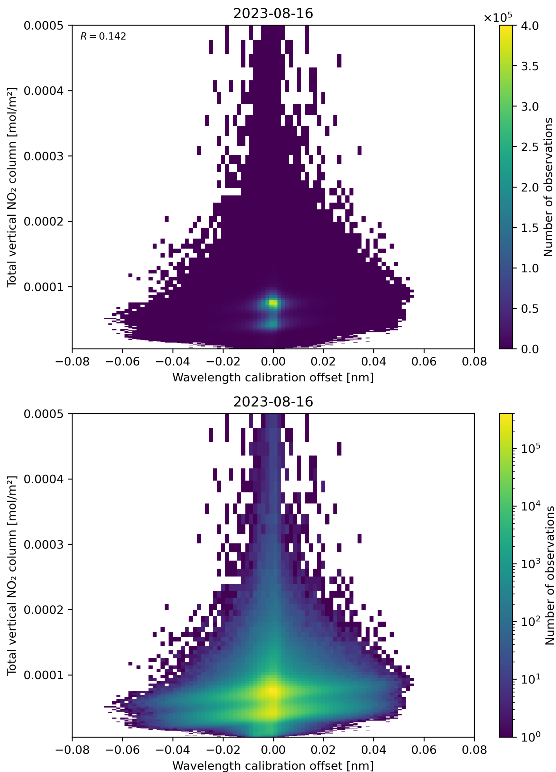
Figure 179: Scatter density plot of “Wavelength calibration offset” against “Total vertical NO 2 column” for 2023-08-15 to 2023-08-17.
