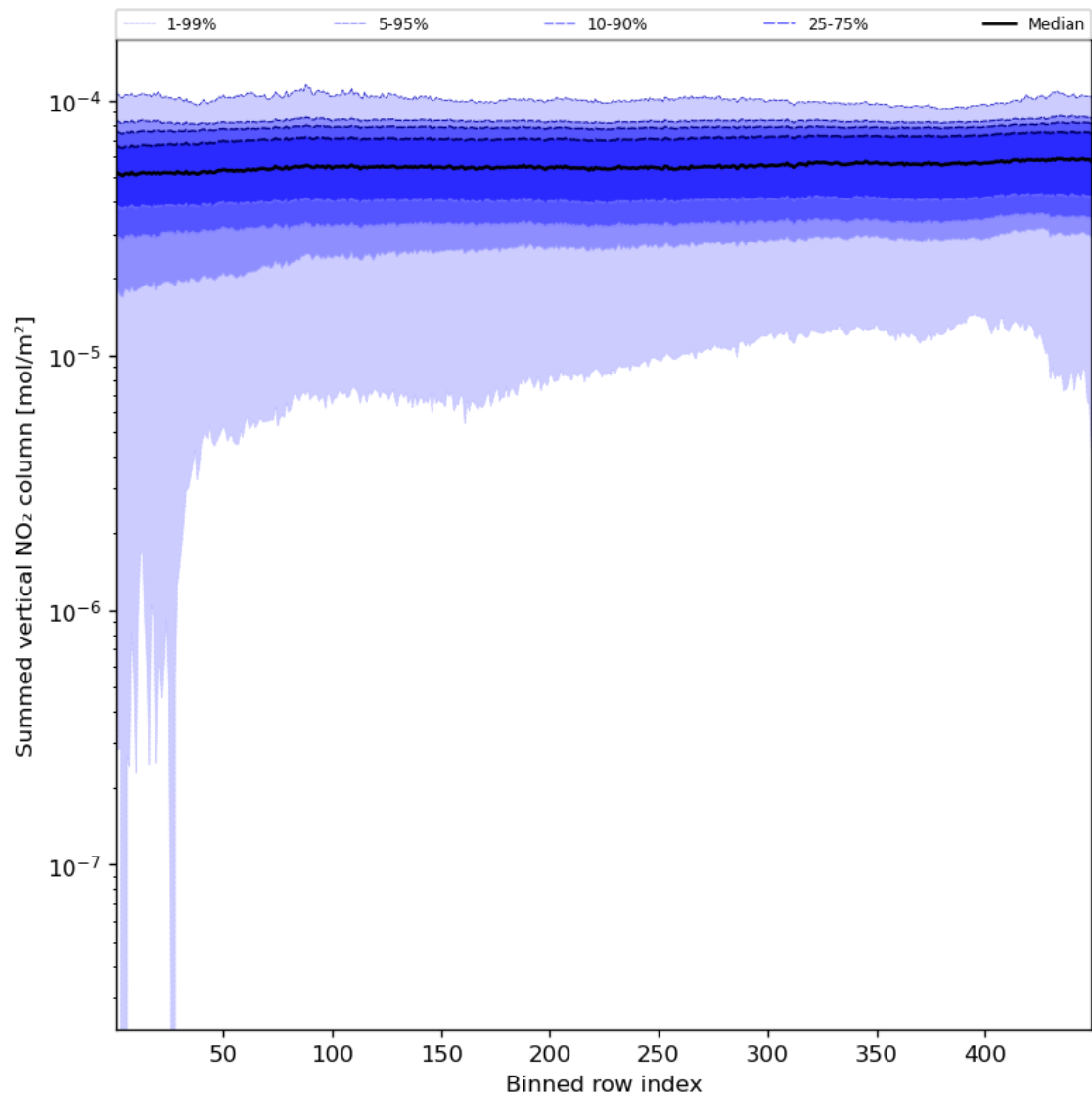
Figure 57: Along track statistics of “Summed vertical NO 2 column” for 2023-08-15 to 2023-08-17
