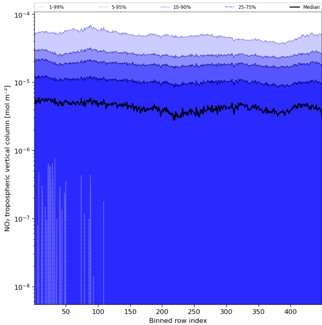
Figure 46: Along track statistics of “NO 2 tropospheric vertical column” for 2023-08-15 to 2023-08-17
