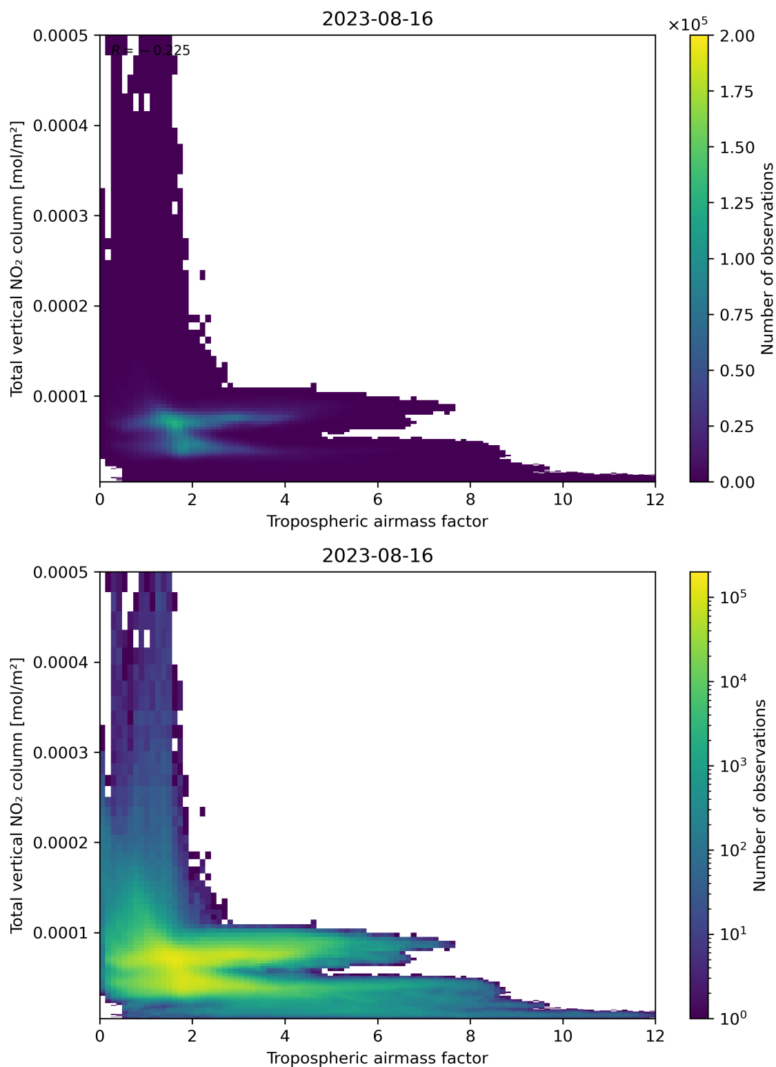
Figure 77: Scatter density plot of “Tropospheric airmass factor” against “Total vertical NO 2 column” for 2023-08-15 to 2023-08-17.
