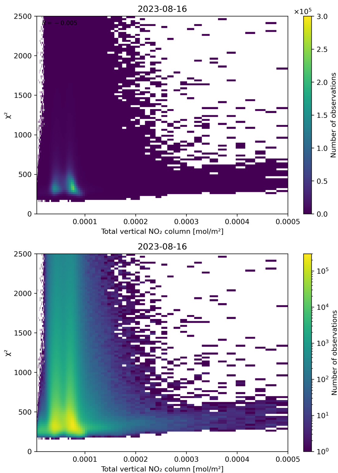
Figure 111: Scatter density plot of “Total vertical NO 2 column” against “ \chi^2 ” for 2023-08-15 to 2023-08-17.
