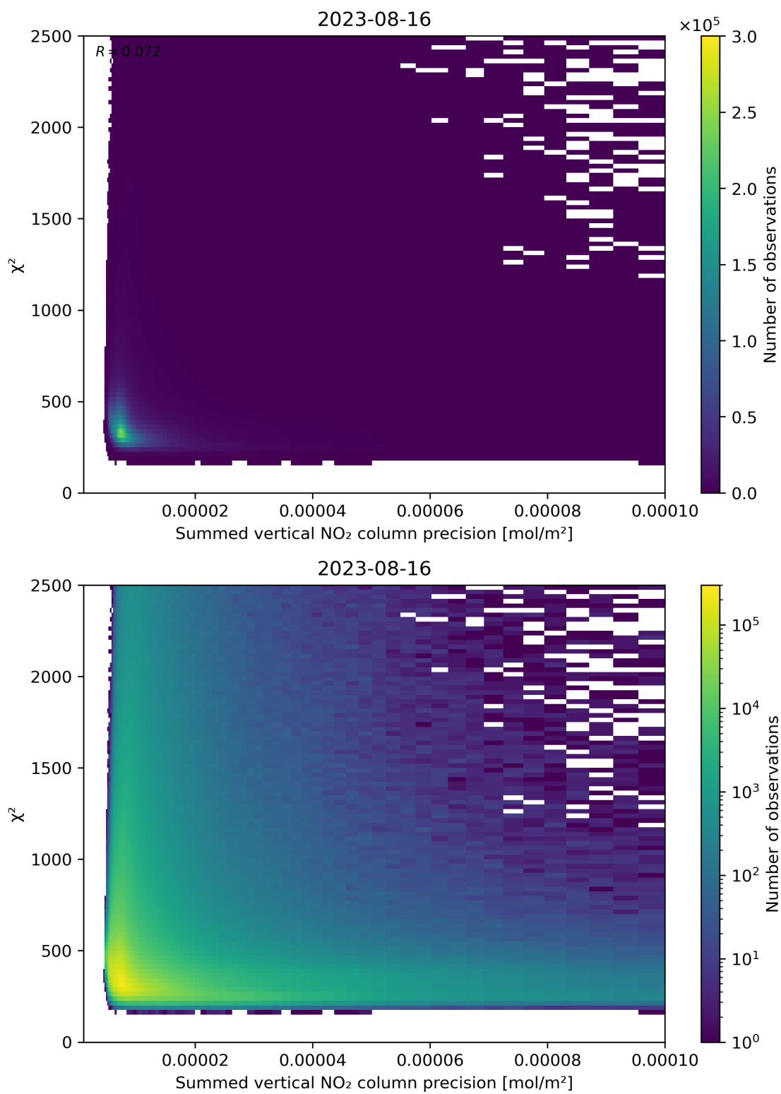
Figure 107: Scatter density plot of “Summed vertical NO 2 column precision” against “ \chi^2 ” for 2023-08-15 to 2023-08-17.
