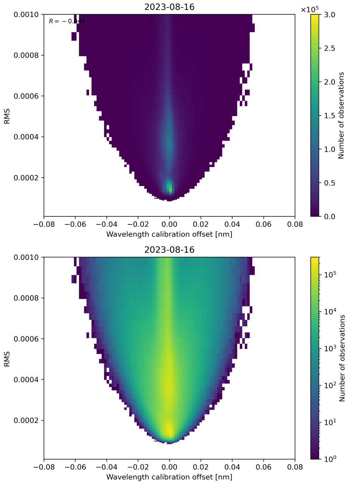
Figure 181: Scatter density plot of “Wavelength calibration offset” against “RMS” for 2023-08-15 to 2023-08-17.
