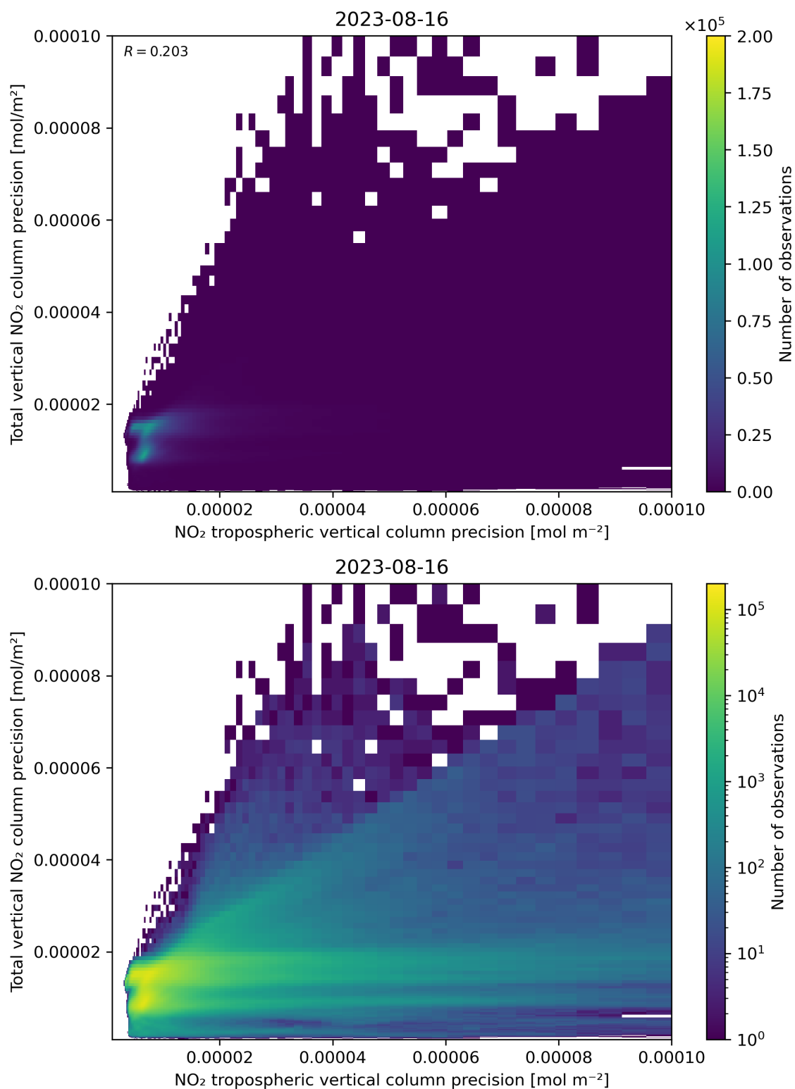
Figure 139: Scatter density plot of “NO 2 tropospheric vertical column precision” against “Total vertical NO 2 column precision” for 2023-08-15 to 2023-08-17.
