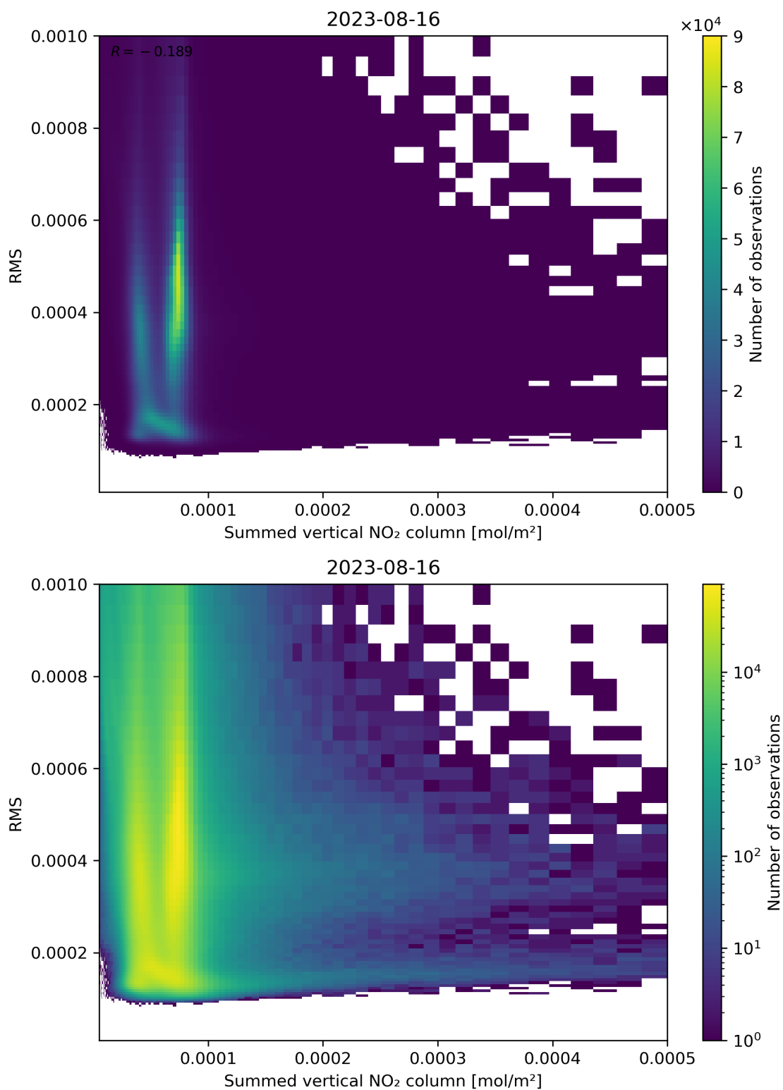
Figure 109: Scatter density plot of “Summed vertical NO 2 column” against “RMS” for 2023-08-15 to 2023-08-17.
