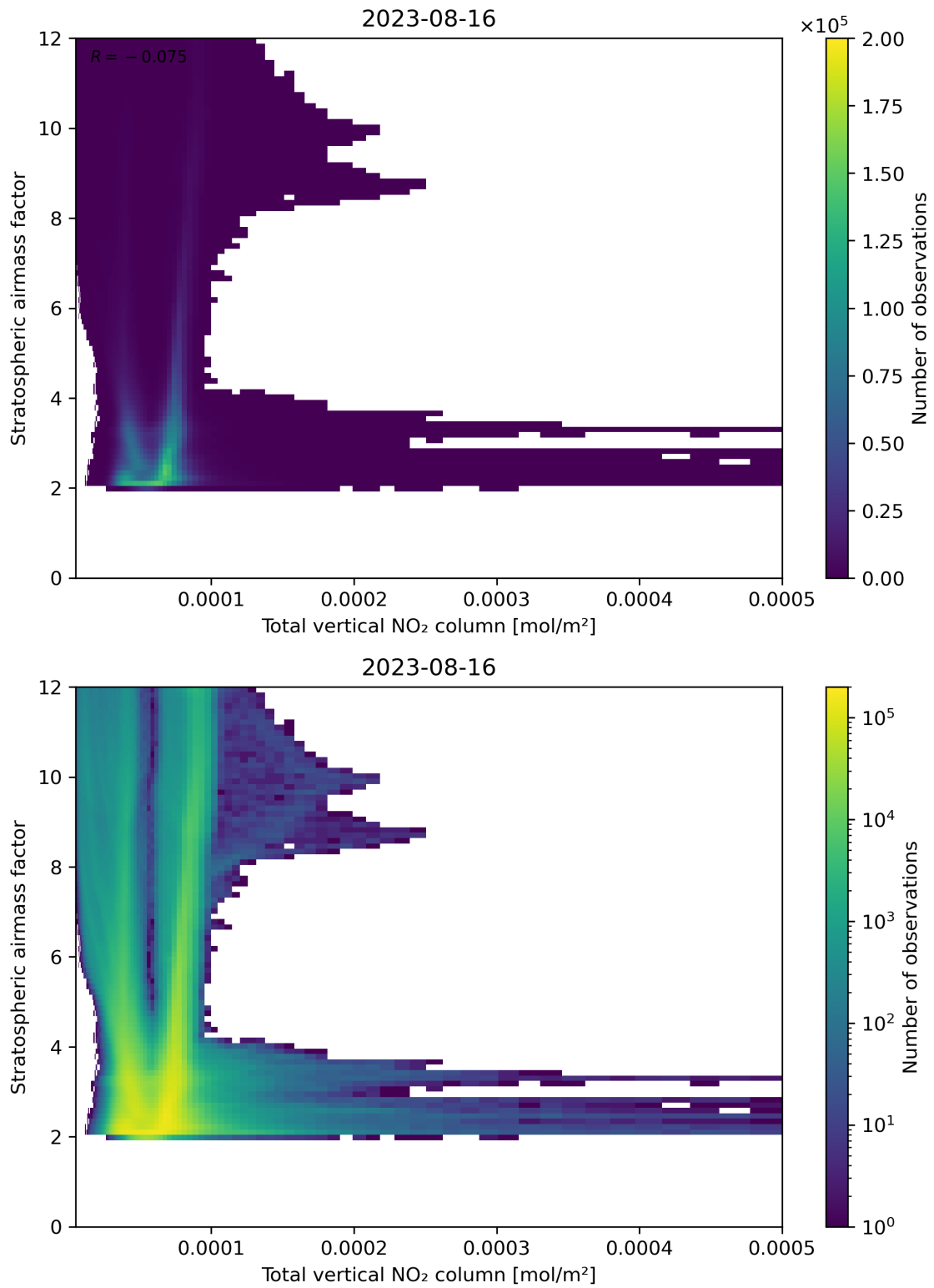
Figure 110: Scatter density plot of “Total vertical NO 2 column” against “Stratospheric air mass factor” for 2023-08-15 to 2023-08-17.
