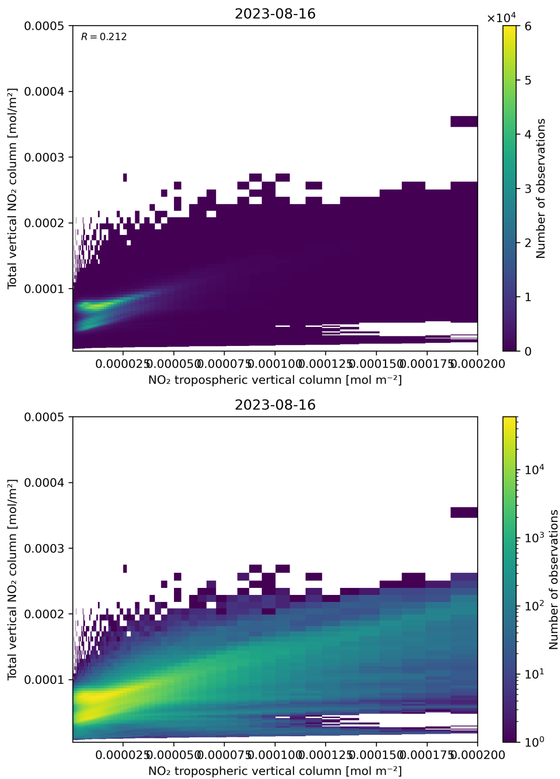
Figure 128: Scatter density plot of “NO 2 tropospheric vertical column” against “Total vertical NO 2 column” for 2023-08-15 to 2023-08-17.
