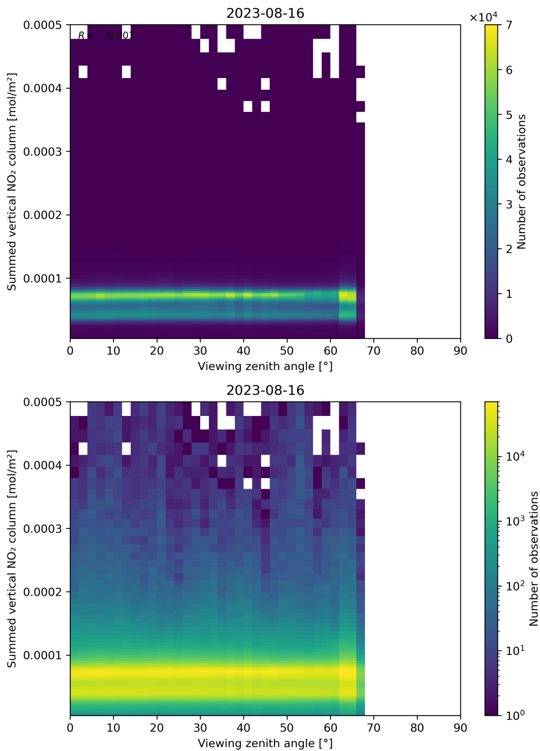
Figure 165: Scatter density plot of “Viewing zenith angle” against “Summed vertical NO 2 column” for 2023-08-15 to 2023-08-17.
