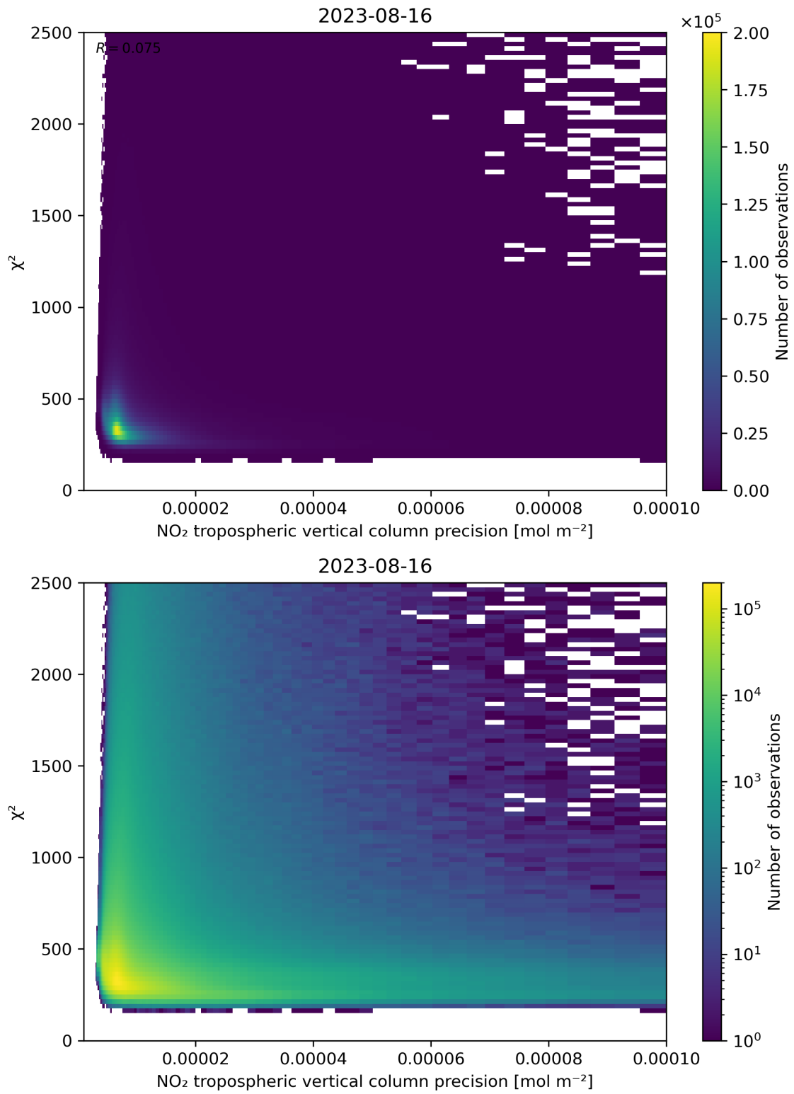
Figure 134: Scatter density plot of “NO 2 tropospheric vertical column precision” against “ \chi^2 ” for 2023-08-15 to 2023-08-17.
