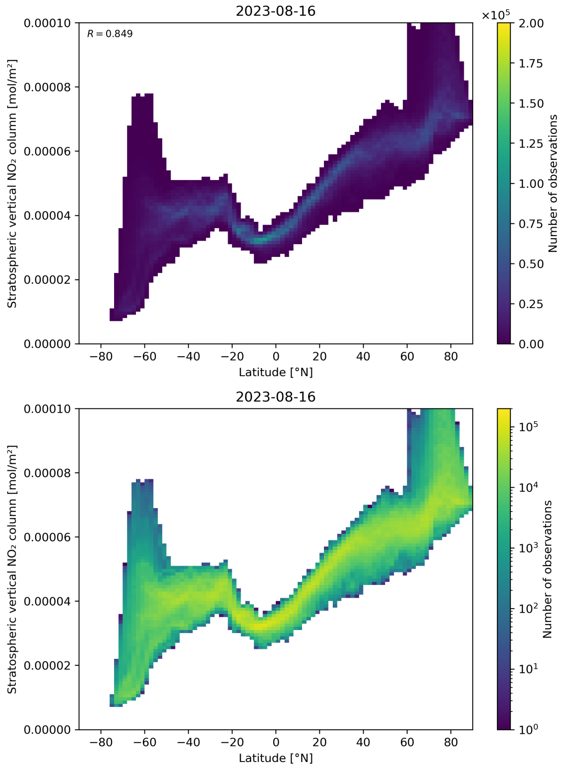
Figure 87: Scatter density plot of “Latitude” against “Stratospheric vertical NO 2 column” for 2023-08-15 to 2023-08-17.
