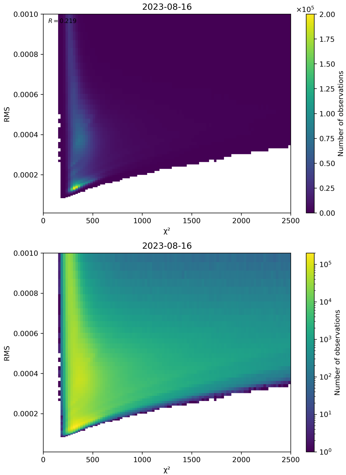
Figure 82: Scatter density plot of “ \chi^2 ” against “RMS” for 2023-08-15 to 2023-08-17.
