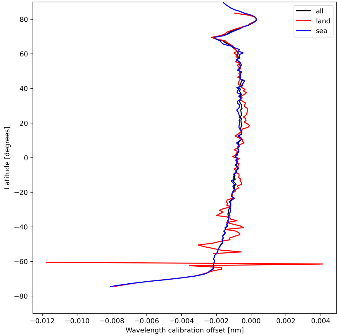
Figure 18: Zonal average of “Wavelength calibration offset” for 2023-08-15 to 2023-08-17.
