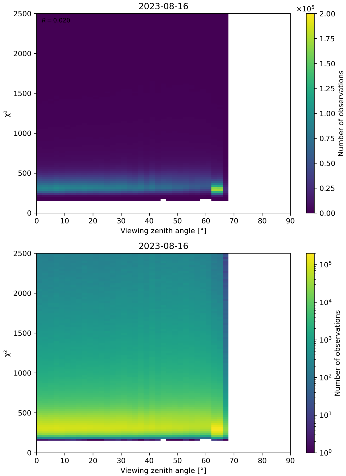
Figure 162: Scatter density plot of “Viewing zenith angle” against “ \chi^2 ” for 2023-08-15 to 2023-08-17.
