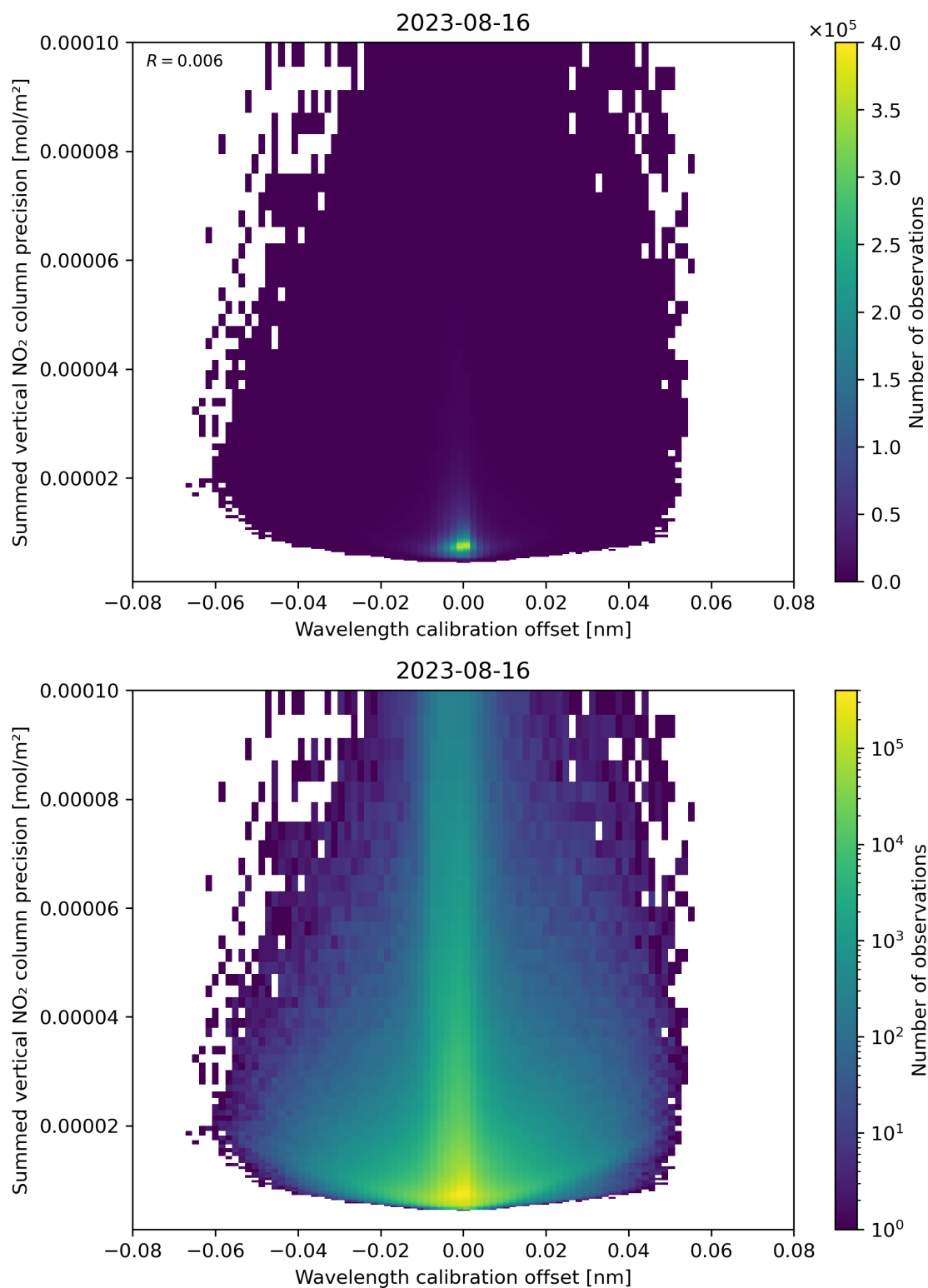
Figure 178: Scatter density plot of “Wavelength calibration offset” against “Summed vertical NO 2 column precision” for 2023-08-15 to 2023-08-17.
