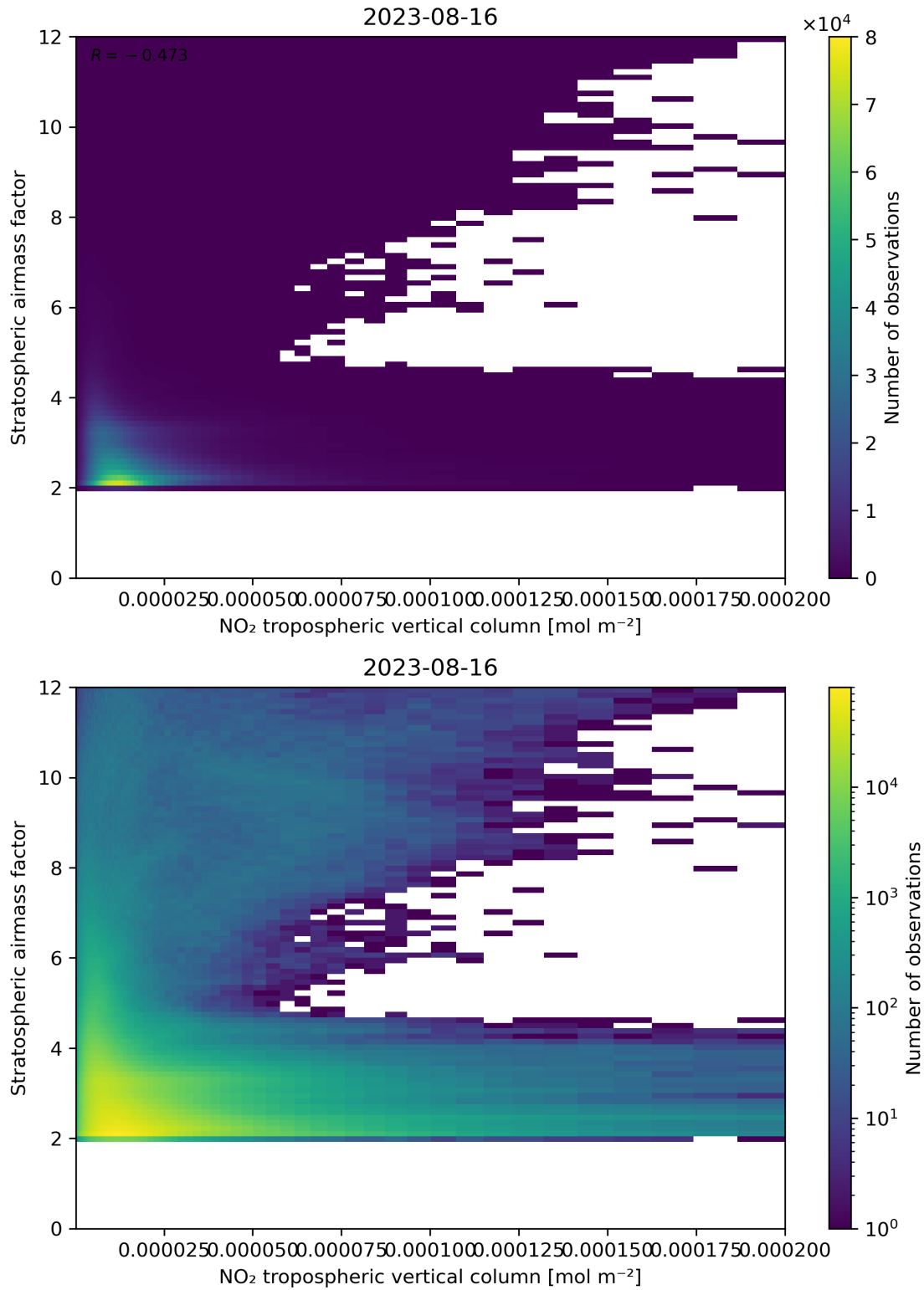
Figure 121: Scatter density plot of “NO 2 tropospheric vertical column” against “Stratospheric air mass factor” for 2023-08-15 to 2023-08-17.
