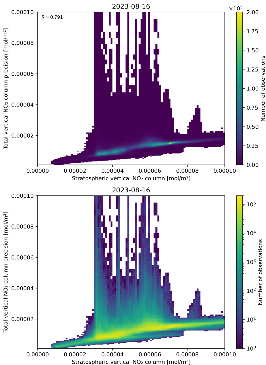
Figure 101: Scatter density plot of “Stratospheric vertical NO 2 column” against “Total vertical NO 2 column precision” for 2023-08-15 to 2023-08-17.
