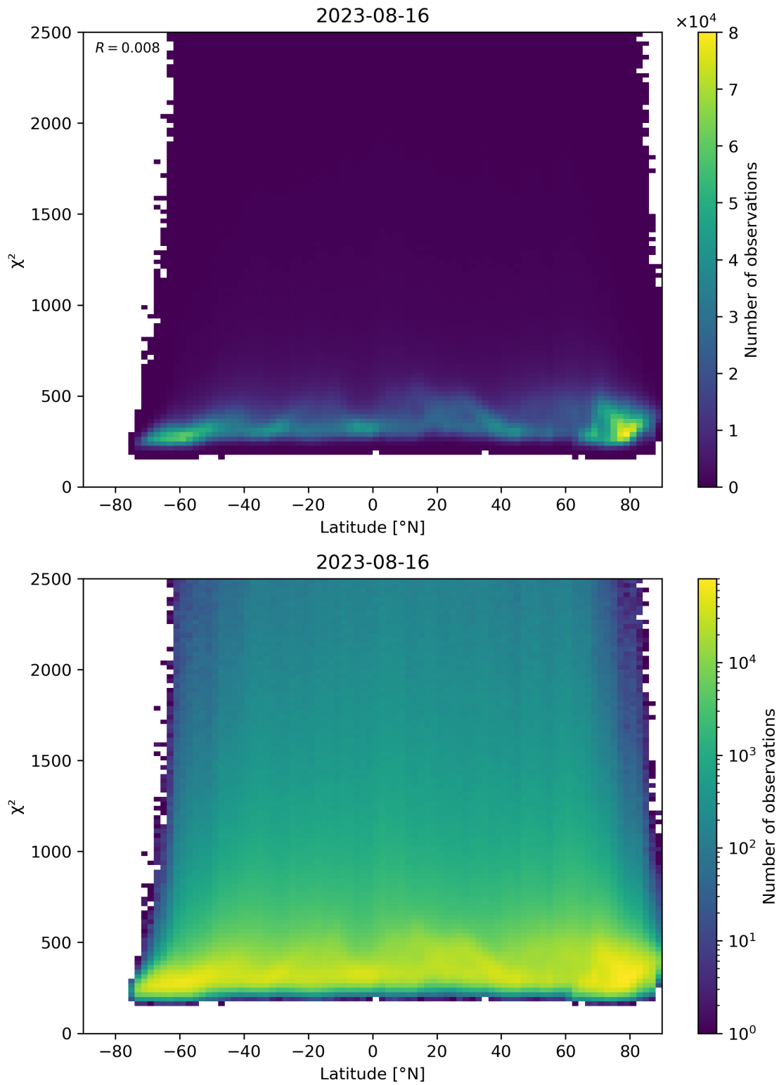
Figure 86: Scatter density plot of “Latitude” against “ \chi^2 ” for 2023-08-15 to 2023-08-17.
