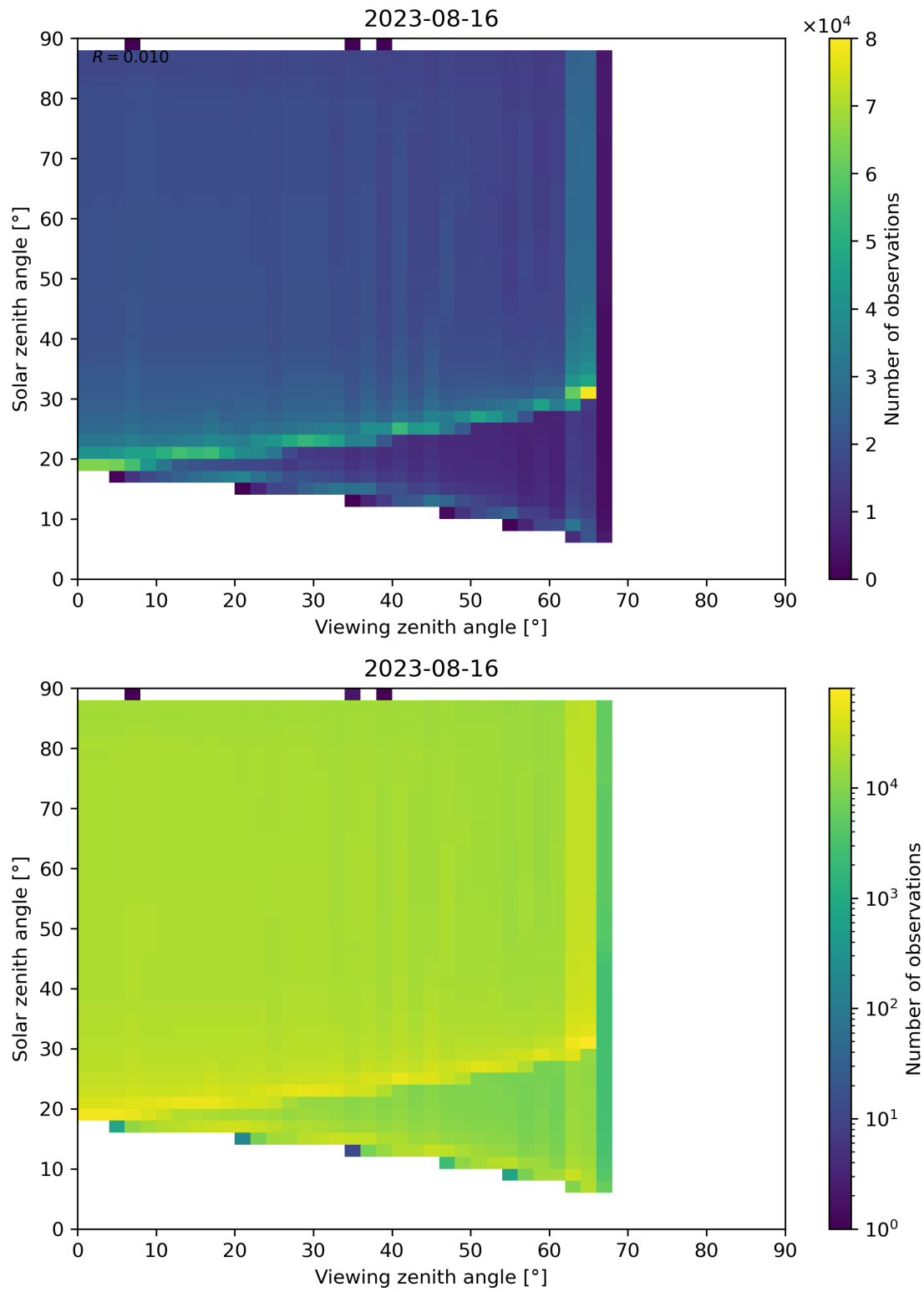
Figure 172: Scatter density plot of “Viewing zenith angle” against “Solar zenith angle” for 2023-08-15 to 2023-08-17.
