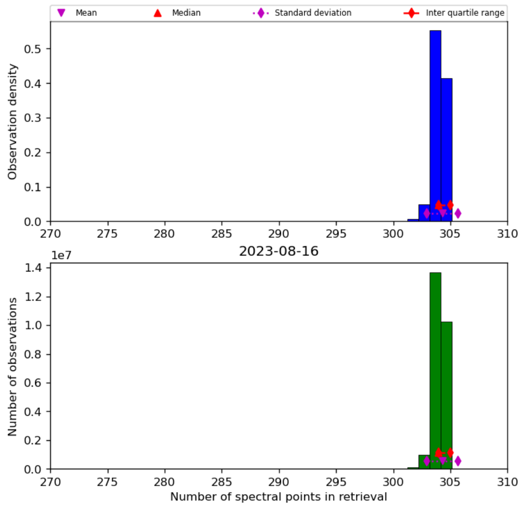
Figure 33: Histogram of “Number of spectral points in retrieval” for 2023-08-15 to 2023-08-17
