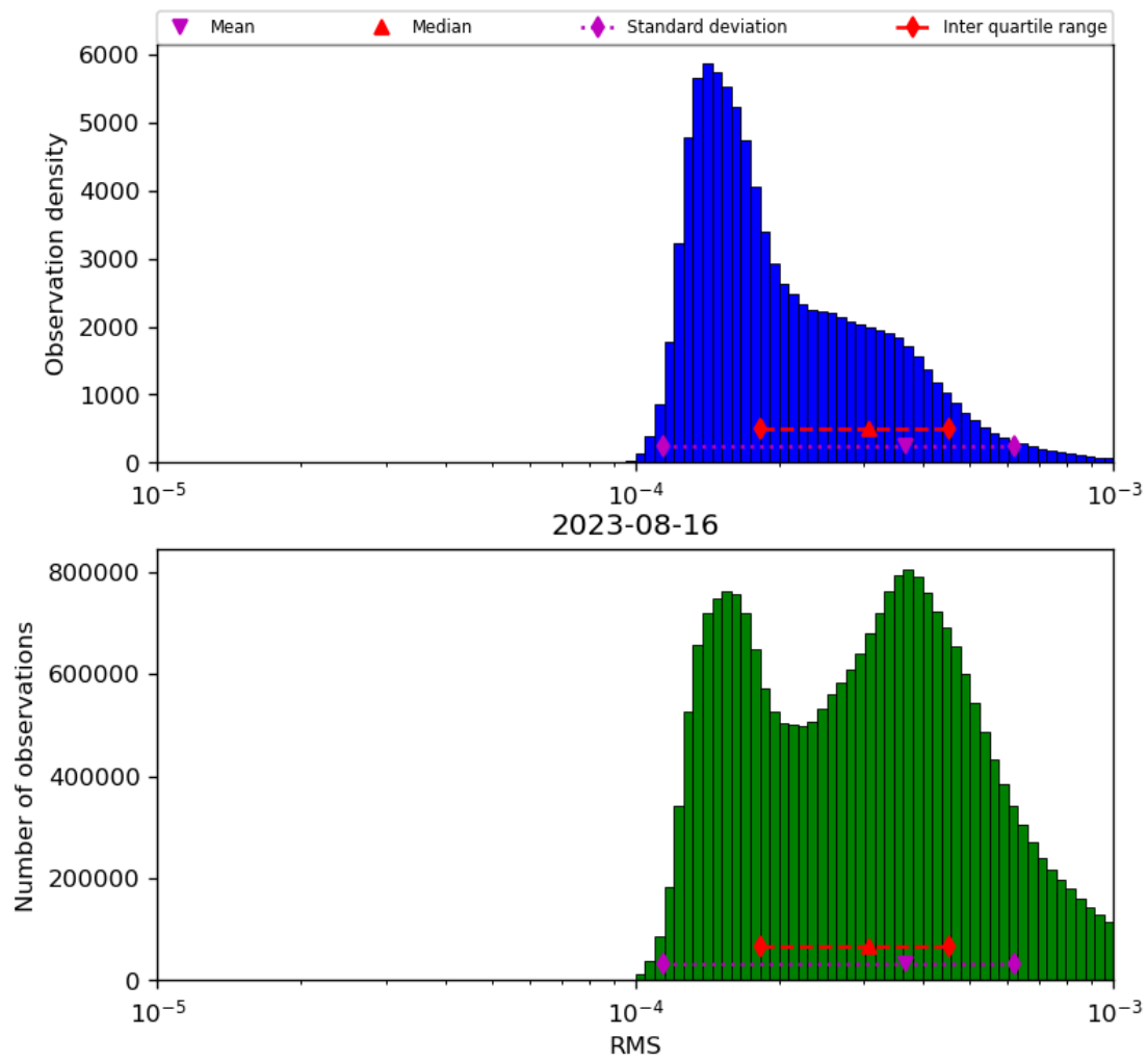
Figure 43: Histogram of “RMS” for 2023-08-15 to 2023-08-17
