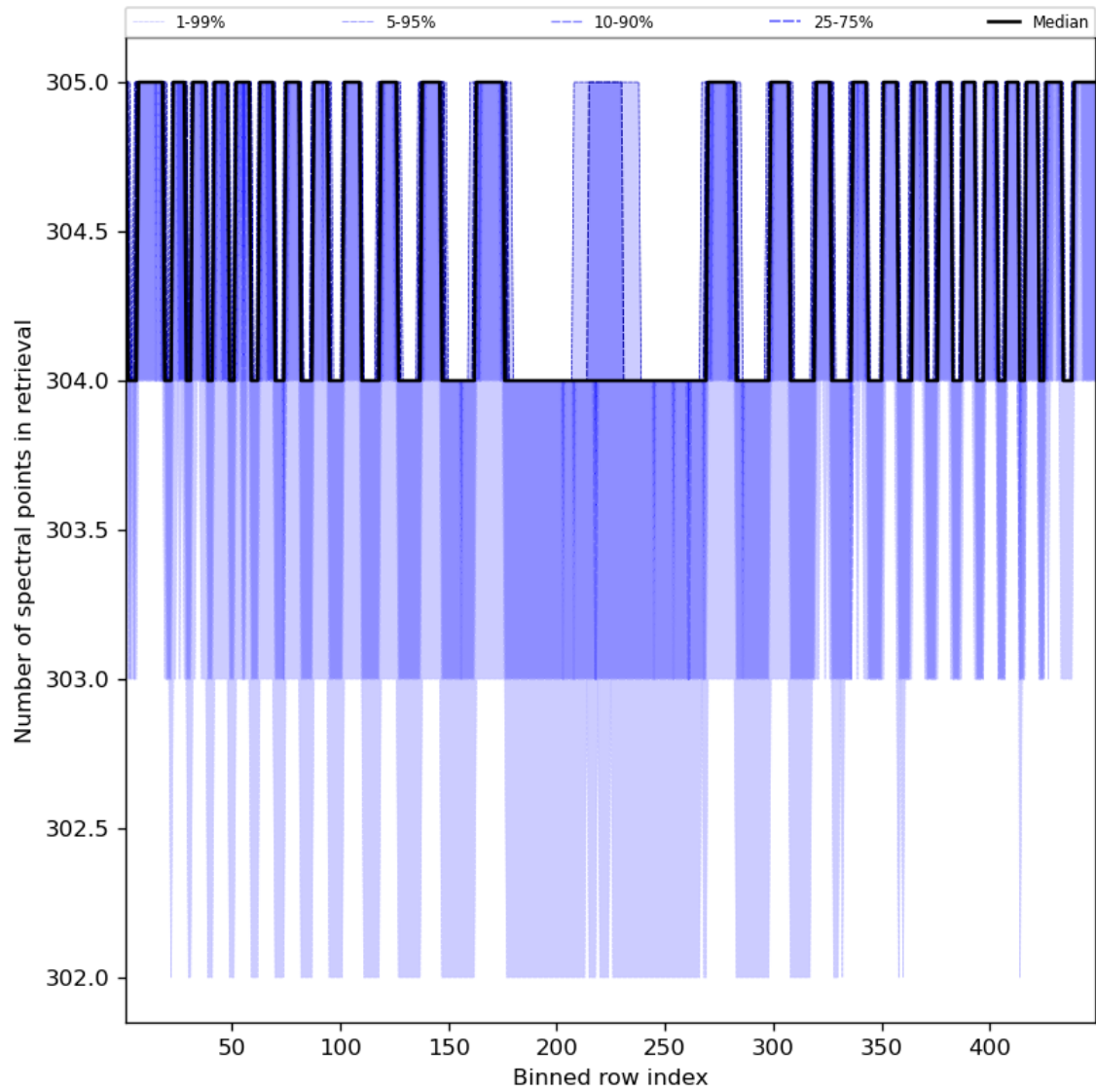
Figure 50: Along track statistics of “Number of spectral points in retrieval” for 2023-08-15 to 2023-08-17
