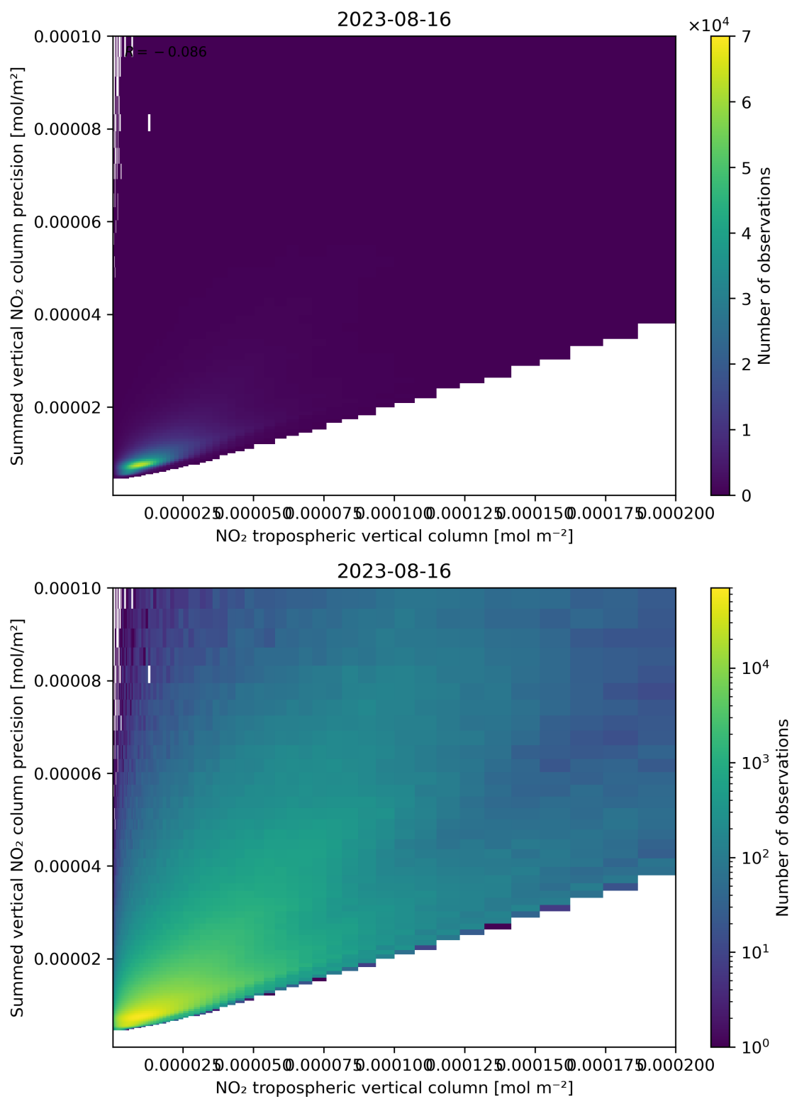
Figure 127: Scatter density plot of “NO 2 tropospheric vertical column” against “Summed vertical NO 2 column precision” for 2023-08-15 to 2023-08-17.
