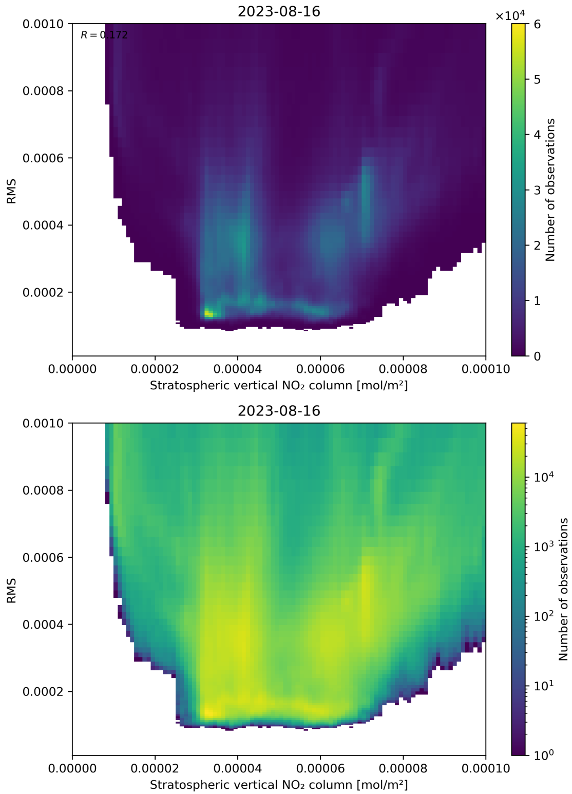
Figure 102: Scatter density plot of “Stratospheric vertical NO 2 column” against “RMS” for 2023-08-15 to 2023-08-17.
