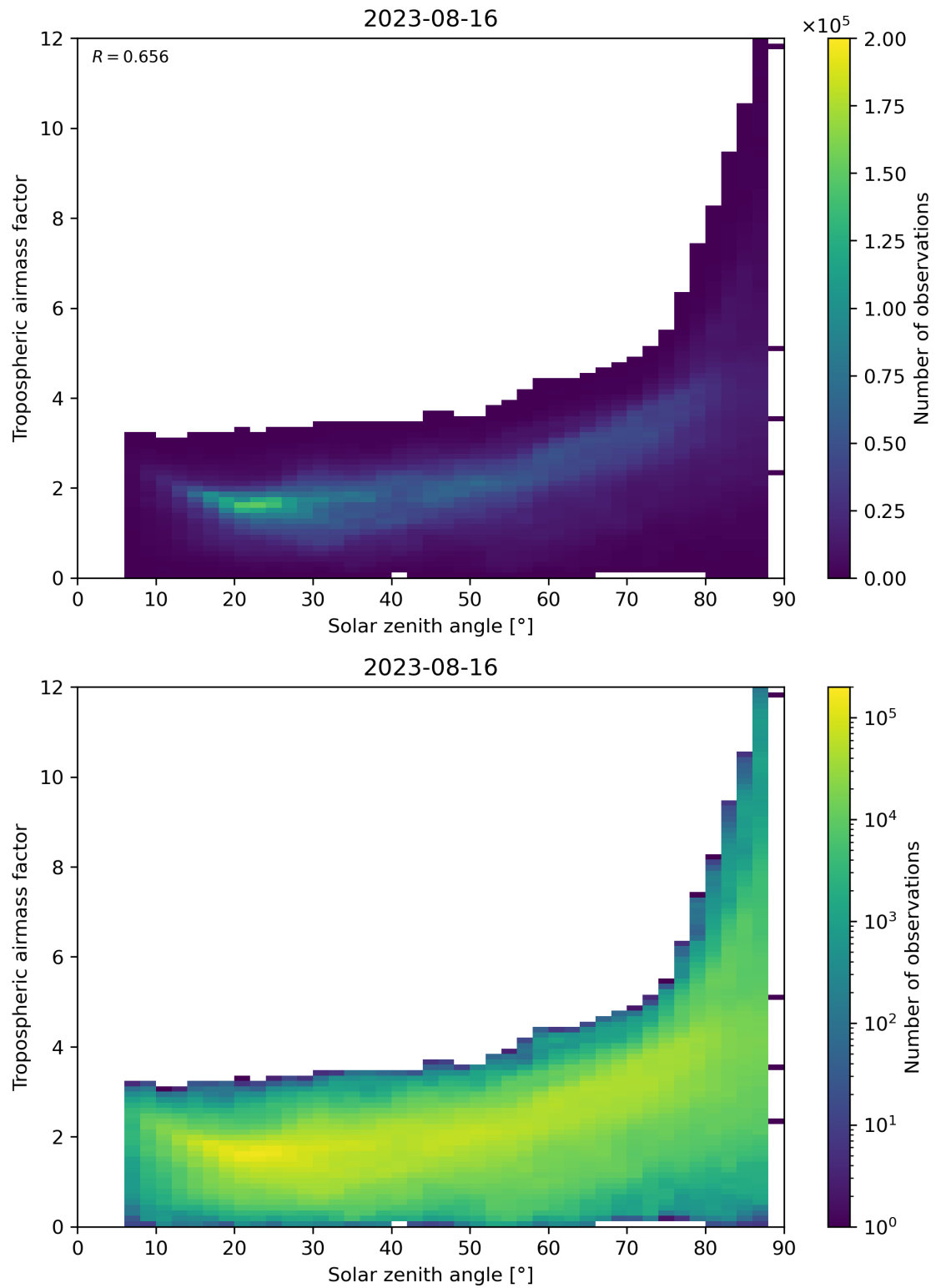
Figure 147: Scatter density plot of “Solar zenith angle” against “Tropospheric airmass factor” for 2023-08-15 to 2023-08-17.
