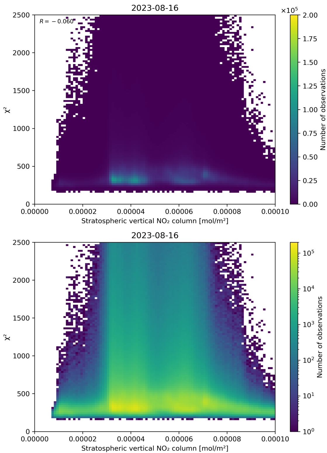
Figure 97: Scatter density plot of “Stratospheric vertical NO 2 column” against “ \chi^2 ” for 2023-08-15 to 2023-08-17.
