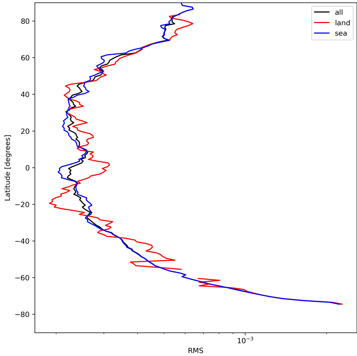
Figure 26: Zonal average of “RMS” for 2023-08-15 to 2023-08-17.
