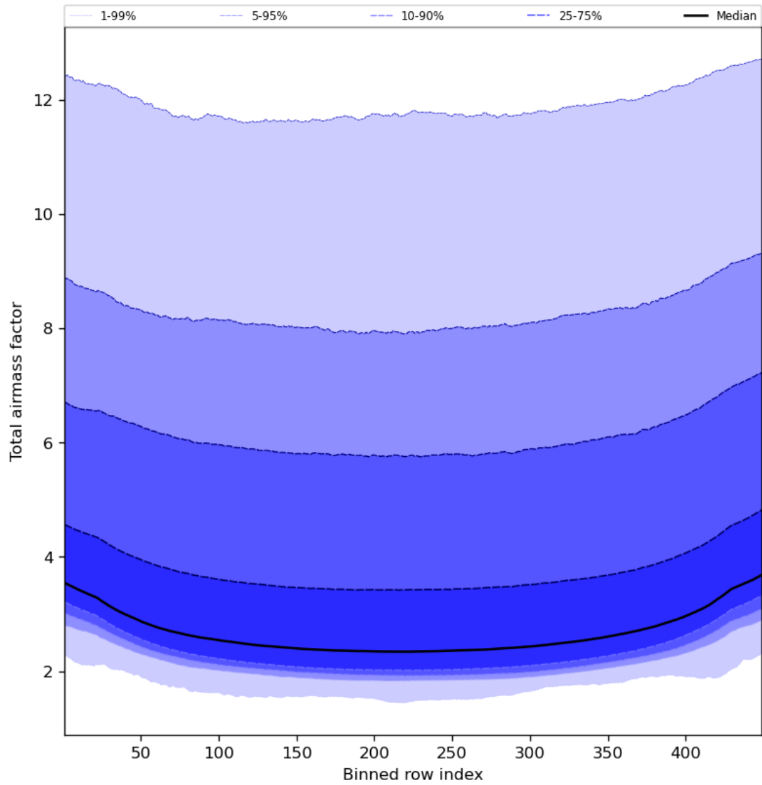
Figure 49: Along track statistics of “Total airmass factor” for 2023-08-15 to 2023-08-17
