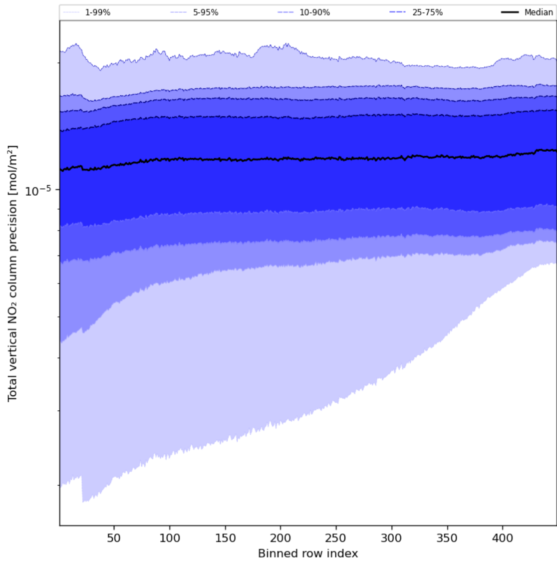
Figure 56: Along track statistics of “Total vertical NO 2 column precision” for 2023-08-15 to 2023-08-17
