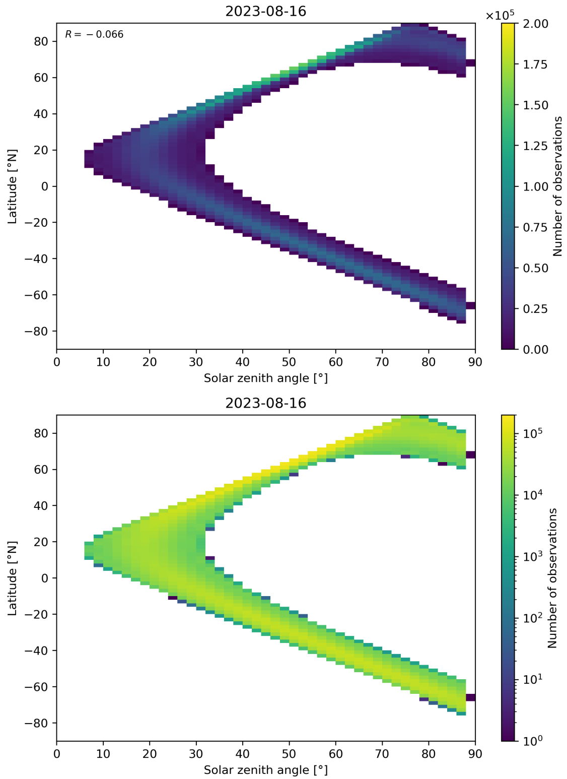
Figure 149: Scatter density plot of “Solar zenith angle” against “Latitude” for 2023-08-15 to 2023-08-17.
