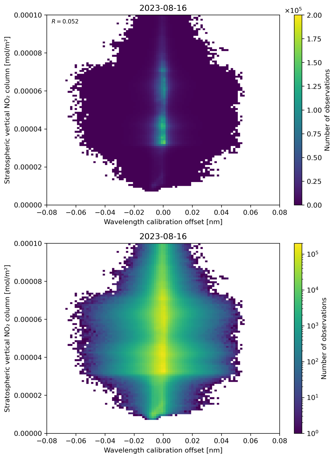
Figure 176: Scatter density plot of “Wavelength calibration offset” against “Stratospheric vertical NO 2 column” for 2023-08-15 to 2023-08-17.
