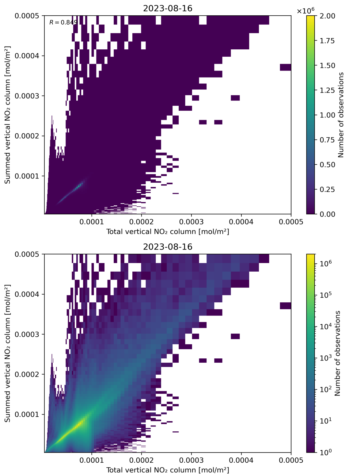
Figure 112: Scatter density plot of “Total vertical NO 2 column” against “Summed vertical NO 2 column” for 2023-08-15 to 2023-08-17.
