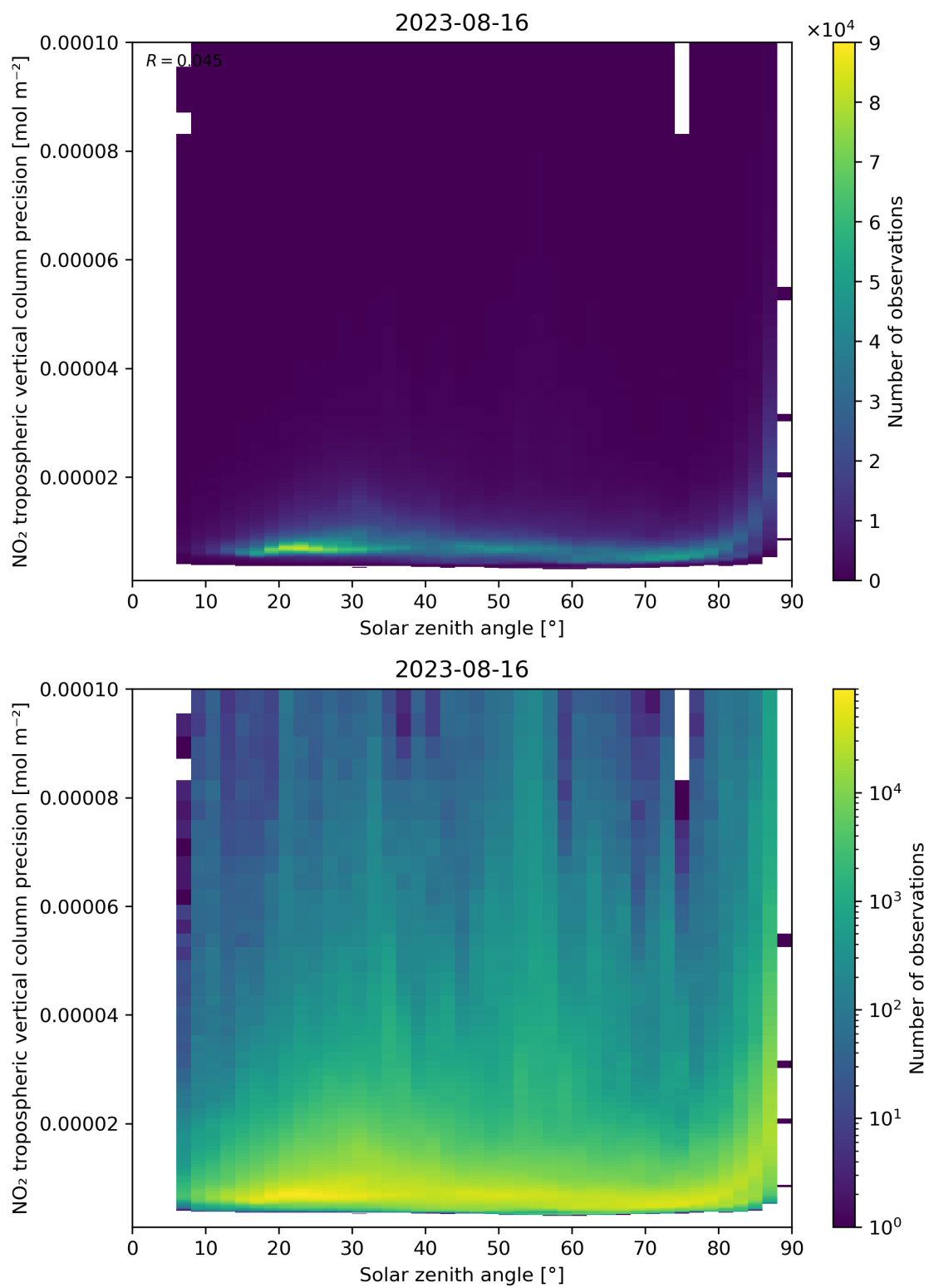
Figure 156: Scatter density plot of “Solar zenith angle” against “NO 2 tropospheric vertical column precision” for 2023-08-15 to 2023-08-17.
