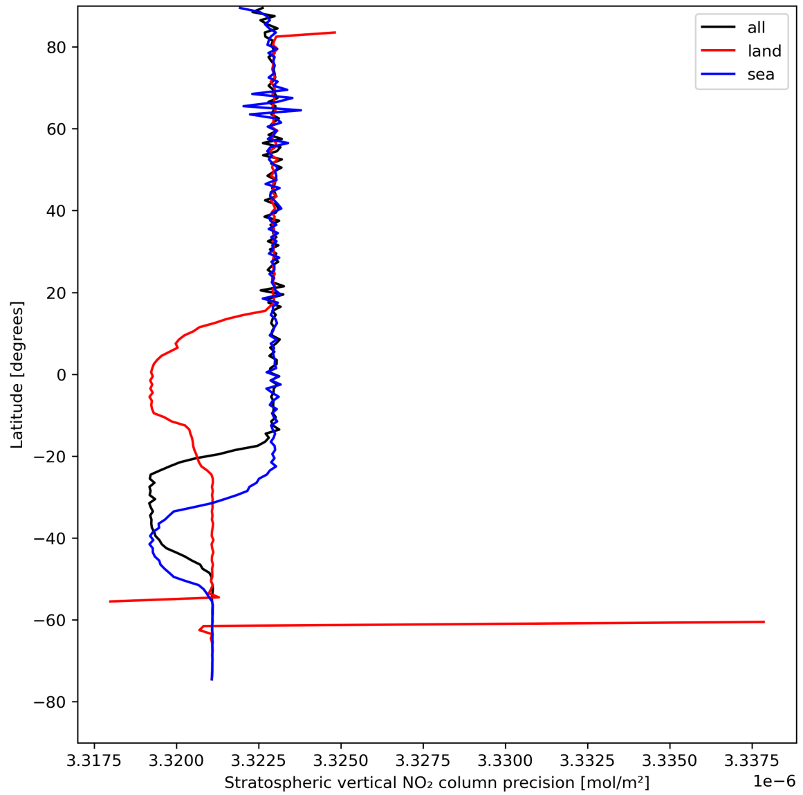
Figure 20: Zonal average of “Stratospheric vertical NO 2 column precision” for 2023-08-15 to 2023-08-17.
