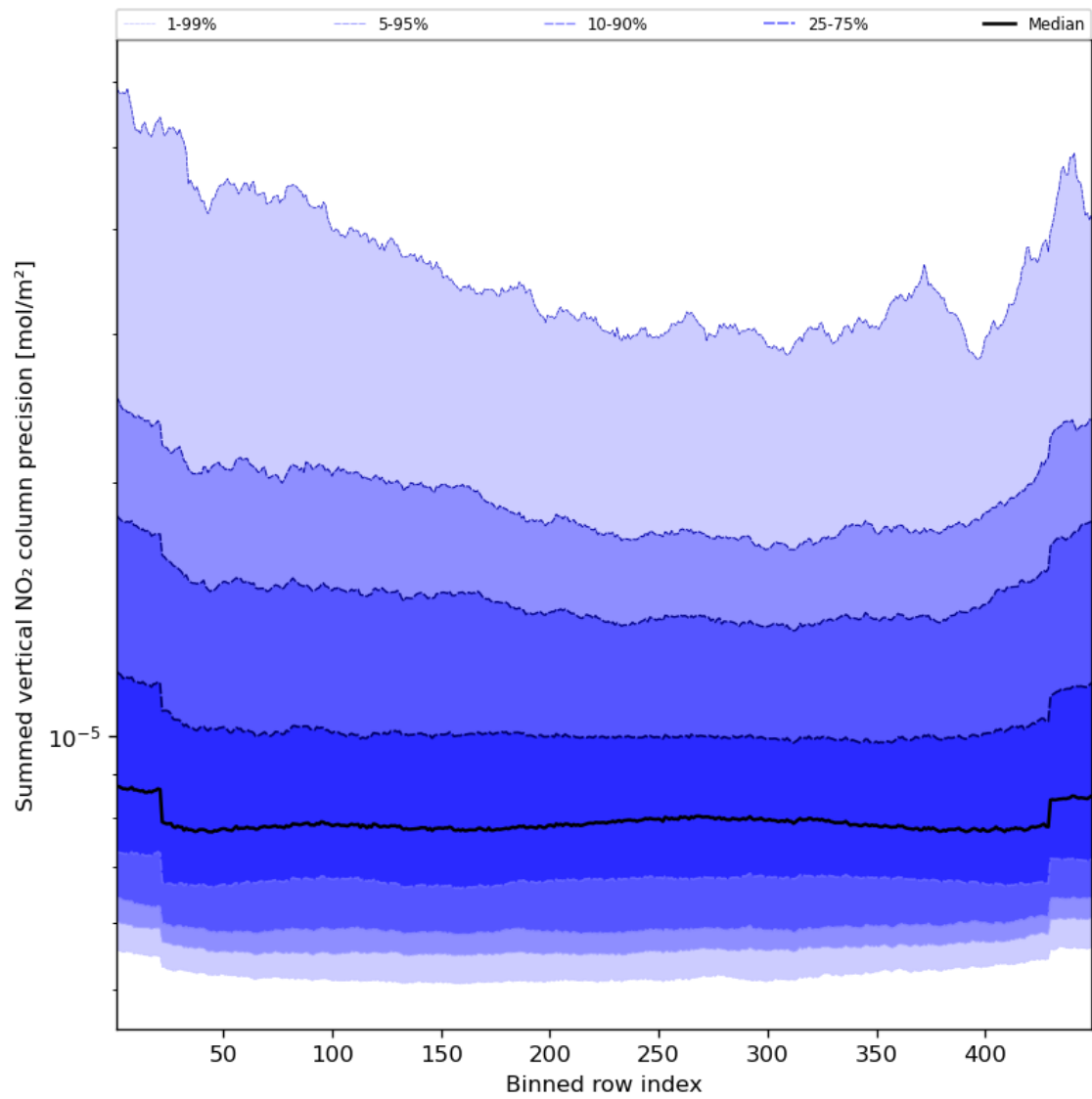
Figure 58: Along track statistics of “Summed vertical NO 2 column precision” for 2023-08-15 to 2023-08-17
