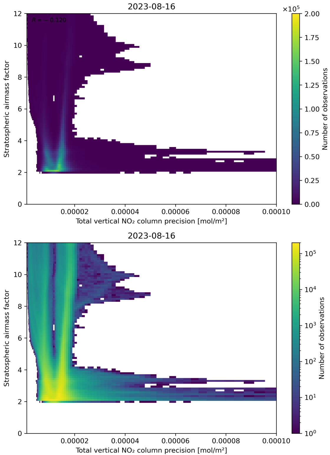
Figure 115: Scatter density plot of “Total vertical NO 2 column precision” against “Stratospheric air mass factor” for 2023-08-15 to 2023-08-17.
