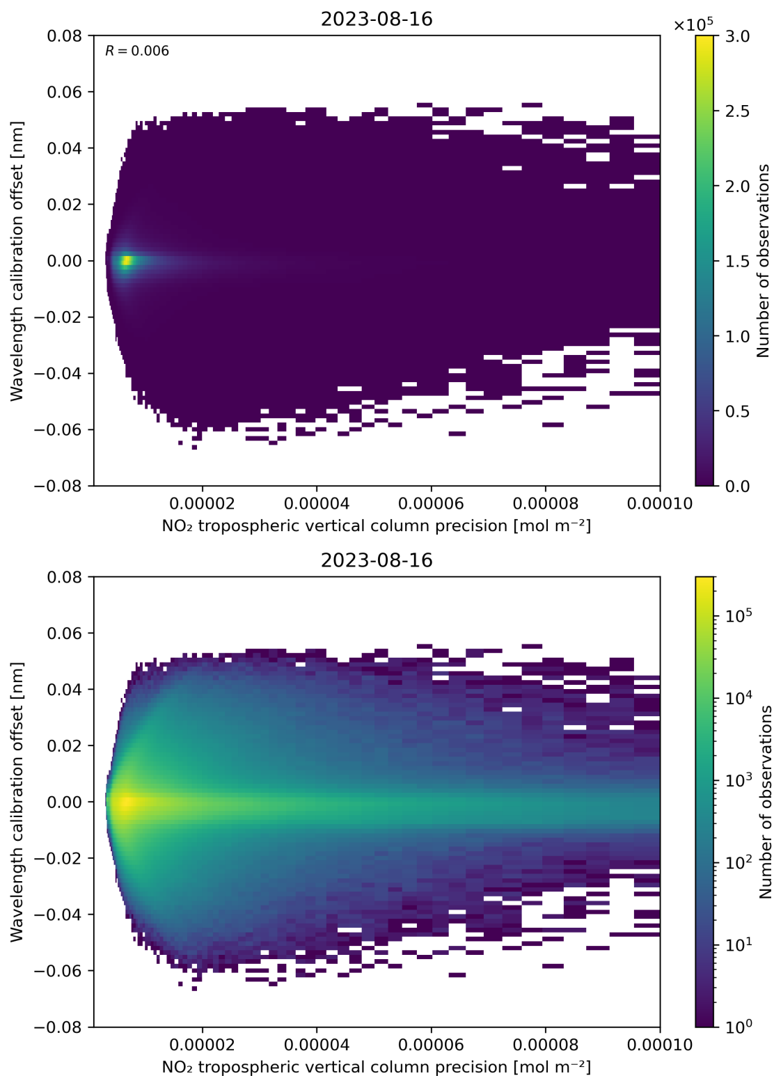
Figure 141: Scatter density plot of “NO 2 tropospheric vertical column precision” against “Wavelength calibration offset” for 2023-08-15 to 2023-08-17.
