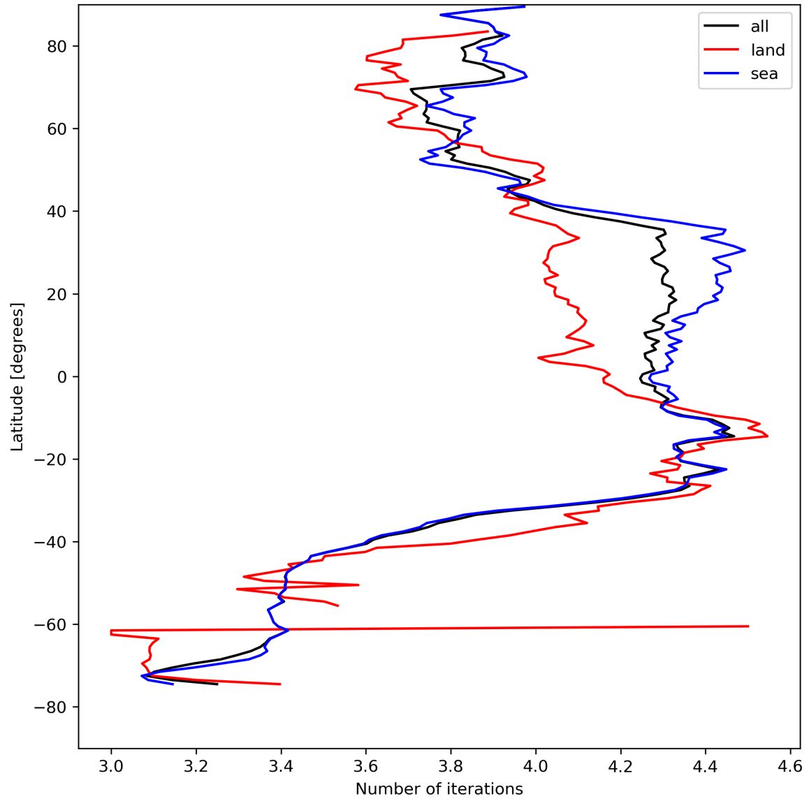
Figure 17: Zonal average of “Number of iterations” for 2023-08-15 to 2023-08-17.
