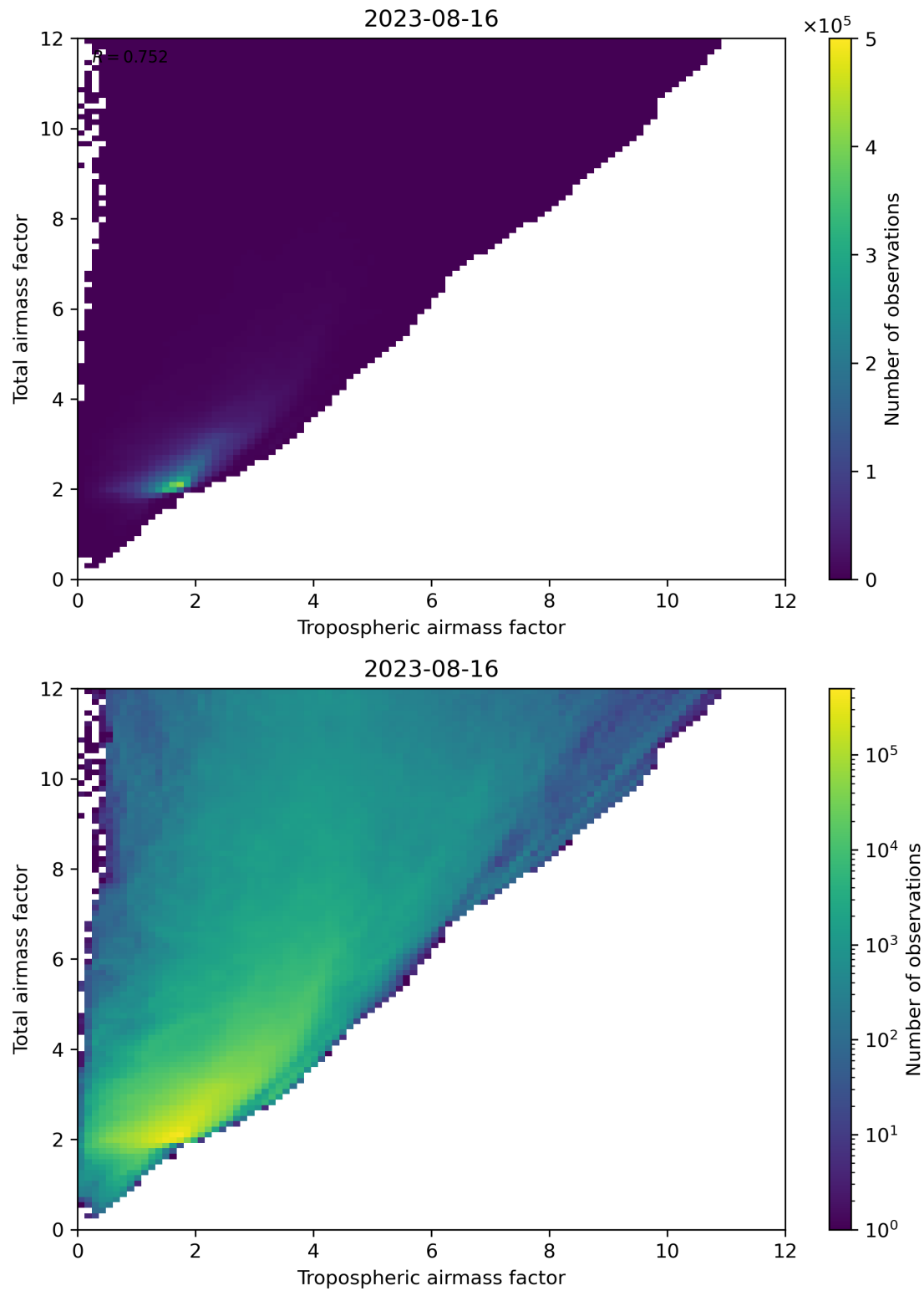
Figure 72: Scatter density plot of “Tropospheric airmass factor” against “Total airmass factor” for 2023-08-15 to 2023-08-17.
