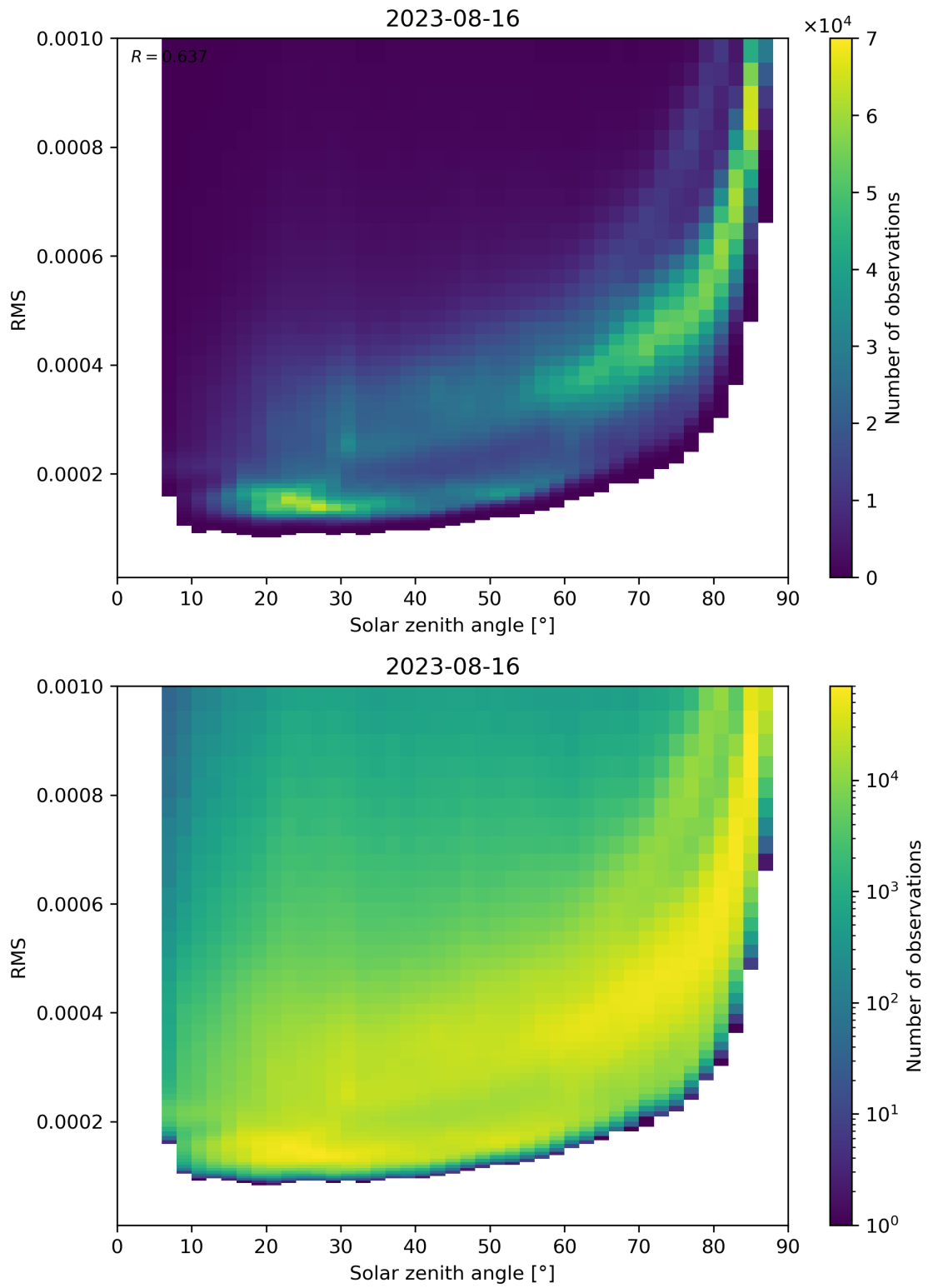
Figure 157: Scatter density plot of “Solar zenith angle” against “RMS” for 2023-08-15 to 2023-08-17.
