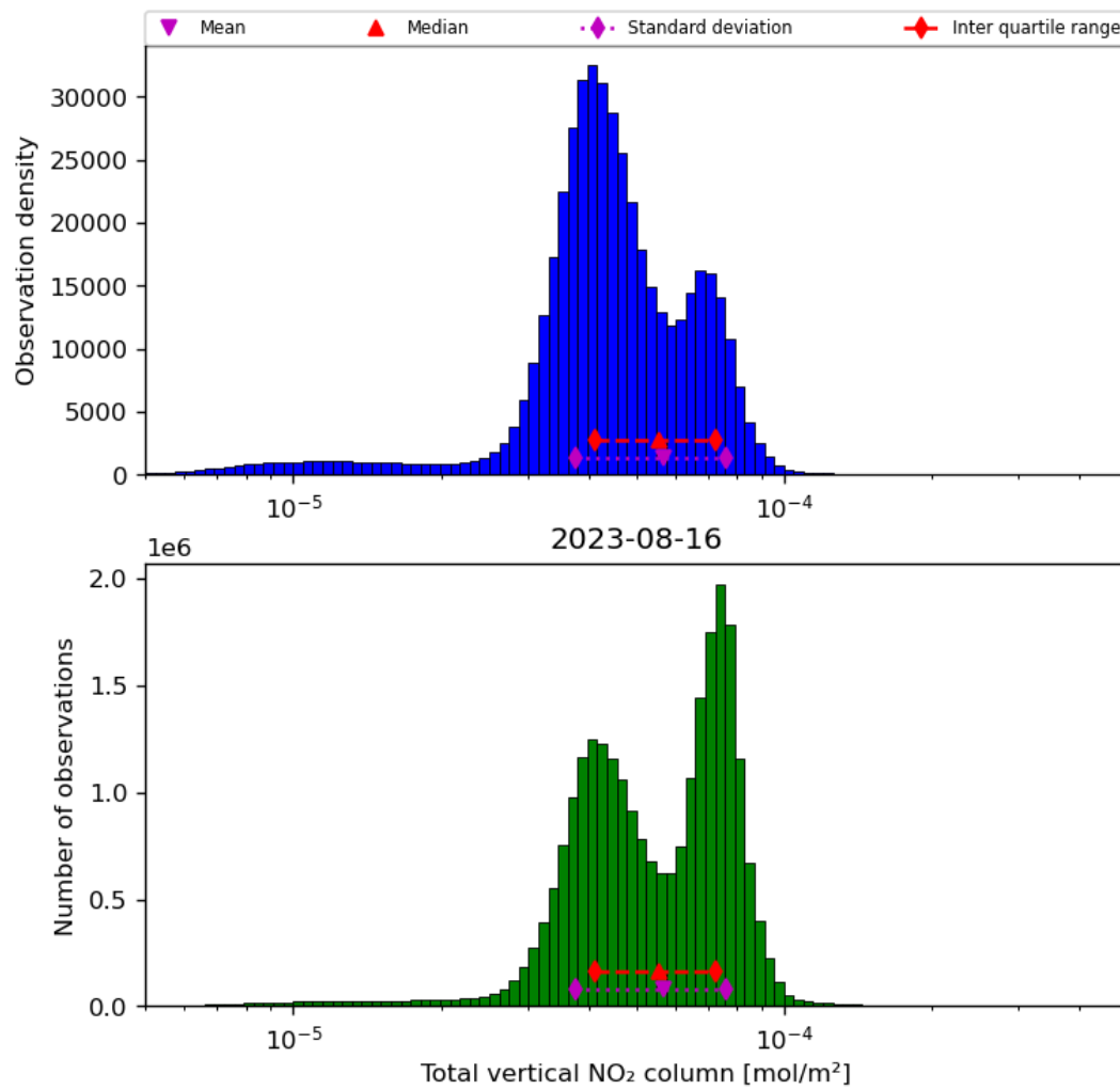
Figure 38: Histogram of “Total vertical NO 2 column” for 2023-08-15 to 2023-08-17
