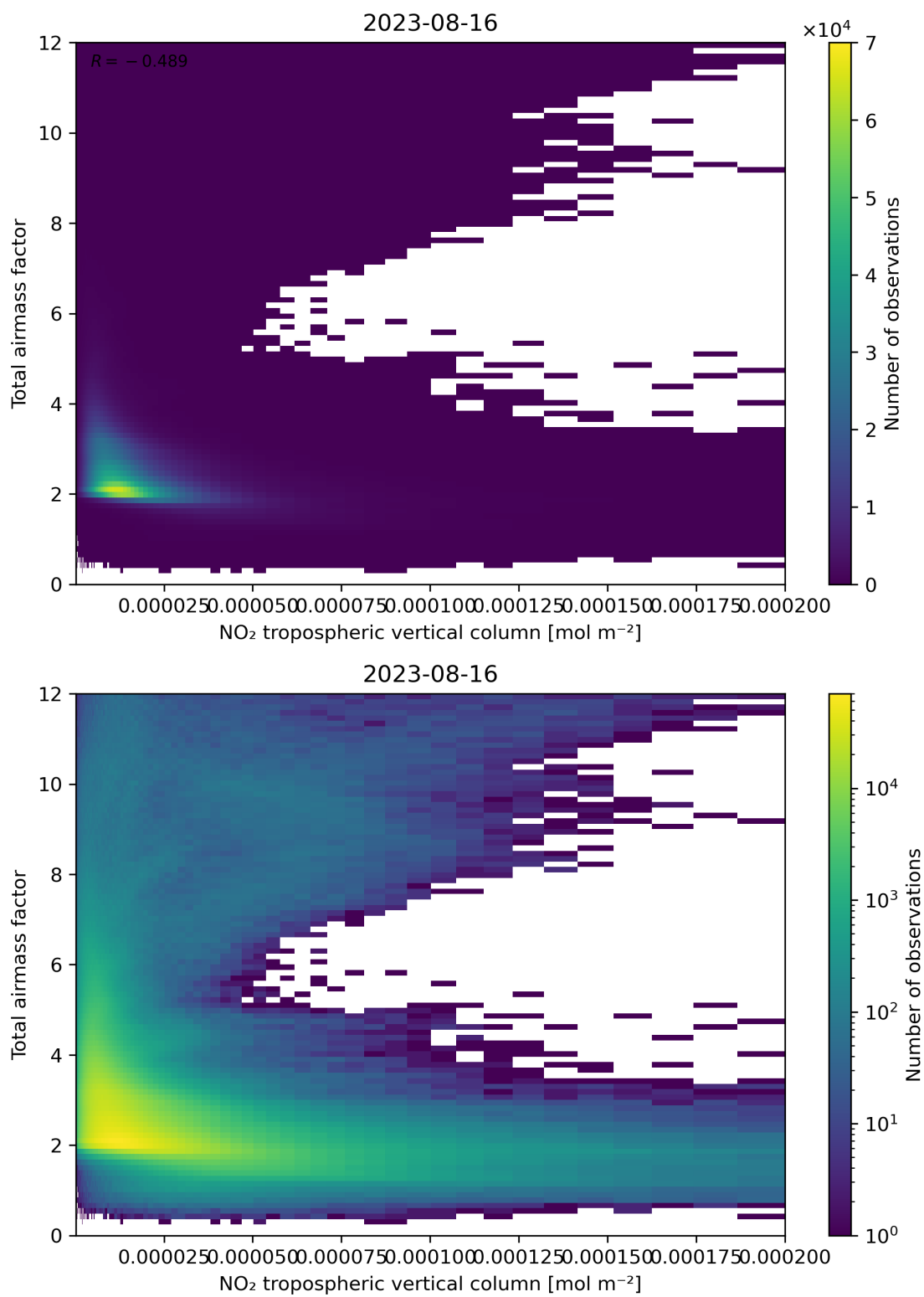
Figure 122: Scatter density plot of “NO 2 tropospheric vertical column” against “Total air mass factor” for 2023-08-15 to 2023-08-17.
