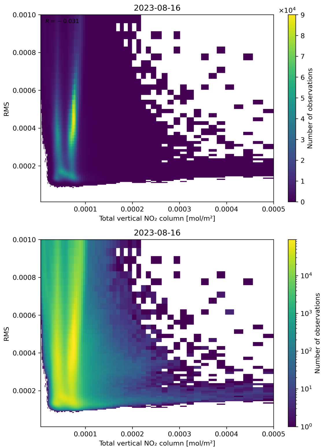
Figure 120: Scatter density plot of “Total vertical NO 2 column” against “RMS” for 2023-08-15 to 2023-08-17.
