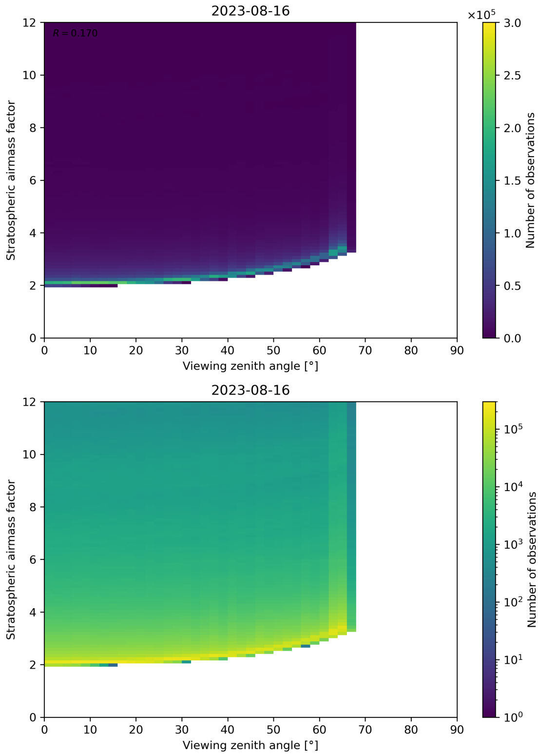
Figure 159: Scatter density plot of “Viewing zenith angle” against “Stratospheric airmass factor” for 2023-08-15 to 2023-08-17.
