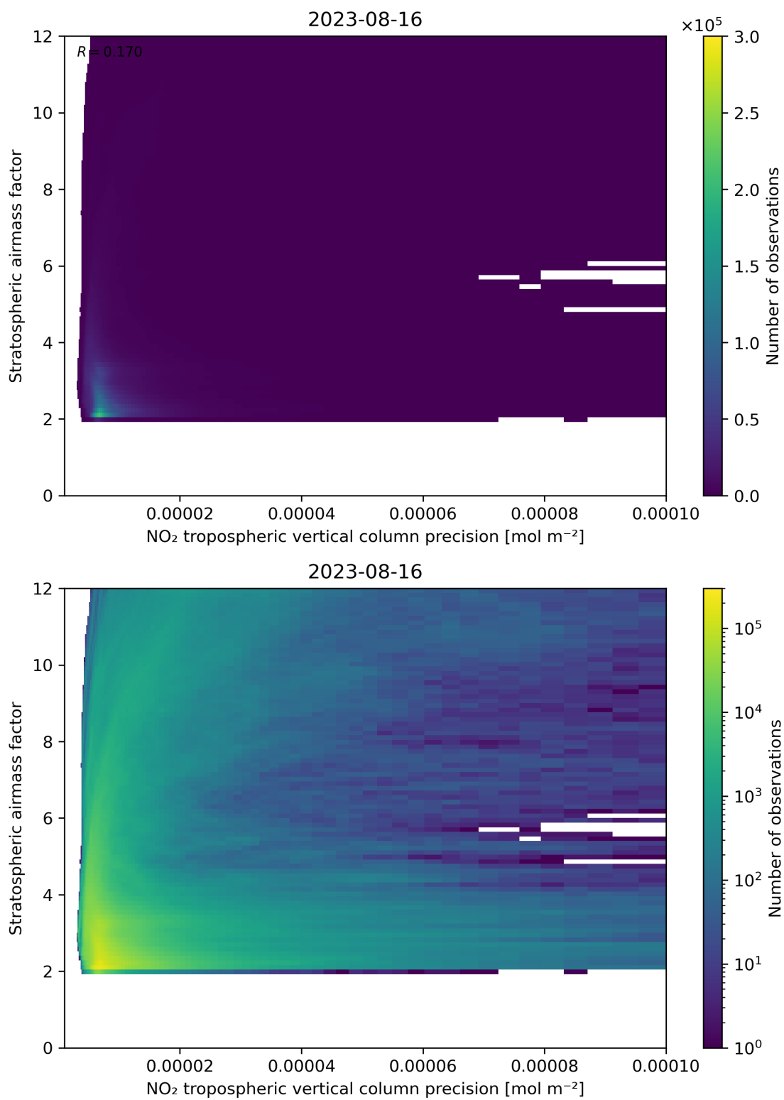
Figure 131: Scatter density plot of “NO 2 tropospheric vertical column precision” against “Stratospheric airmass factor” for 2023-08-15 to 2023-08-17.
