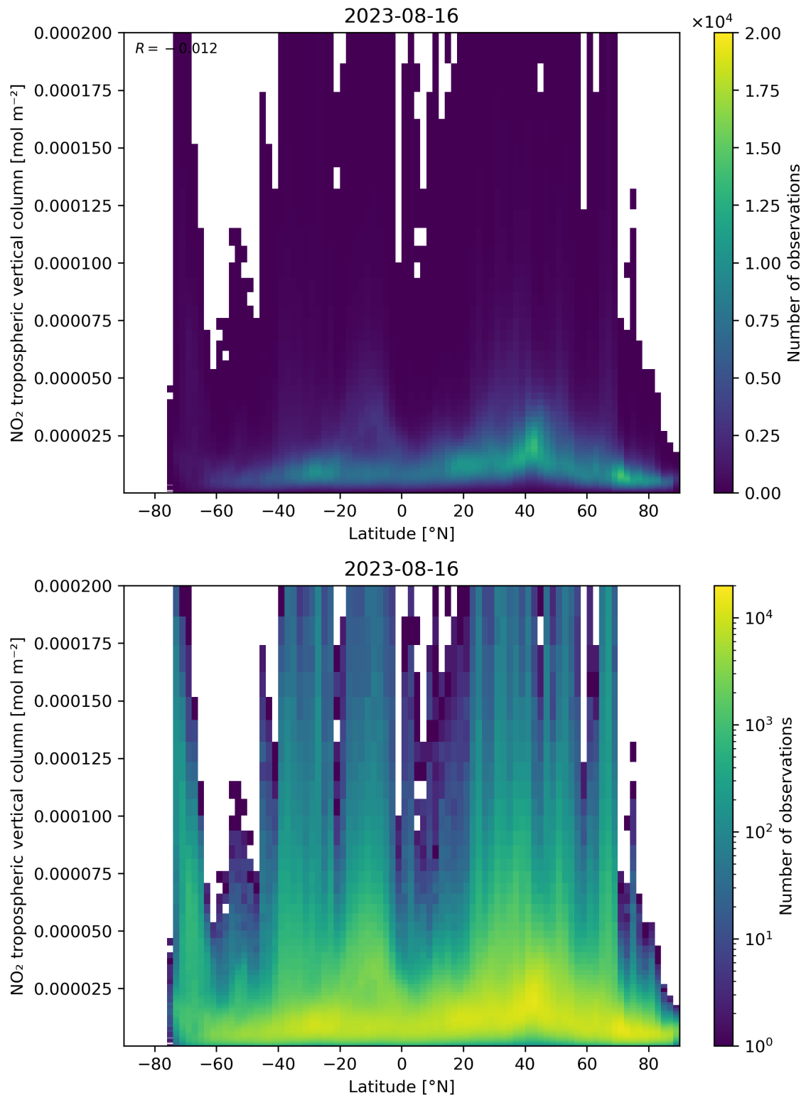
Figure 92: Scatter density plot of “Latitude” against “NO 2 tropospheric vertical column” for 2023-08-15 to 2023-08-17.
