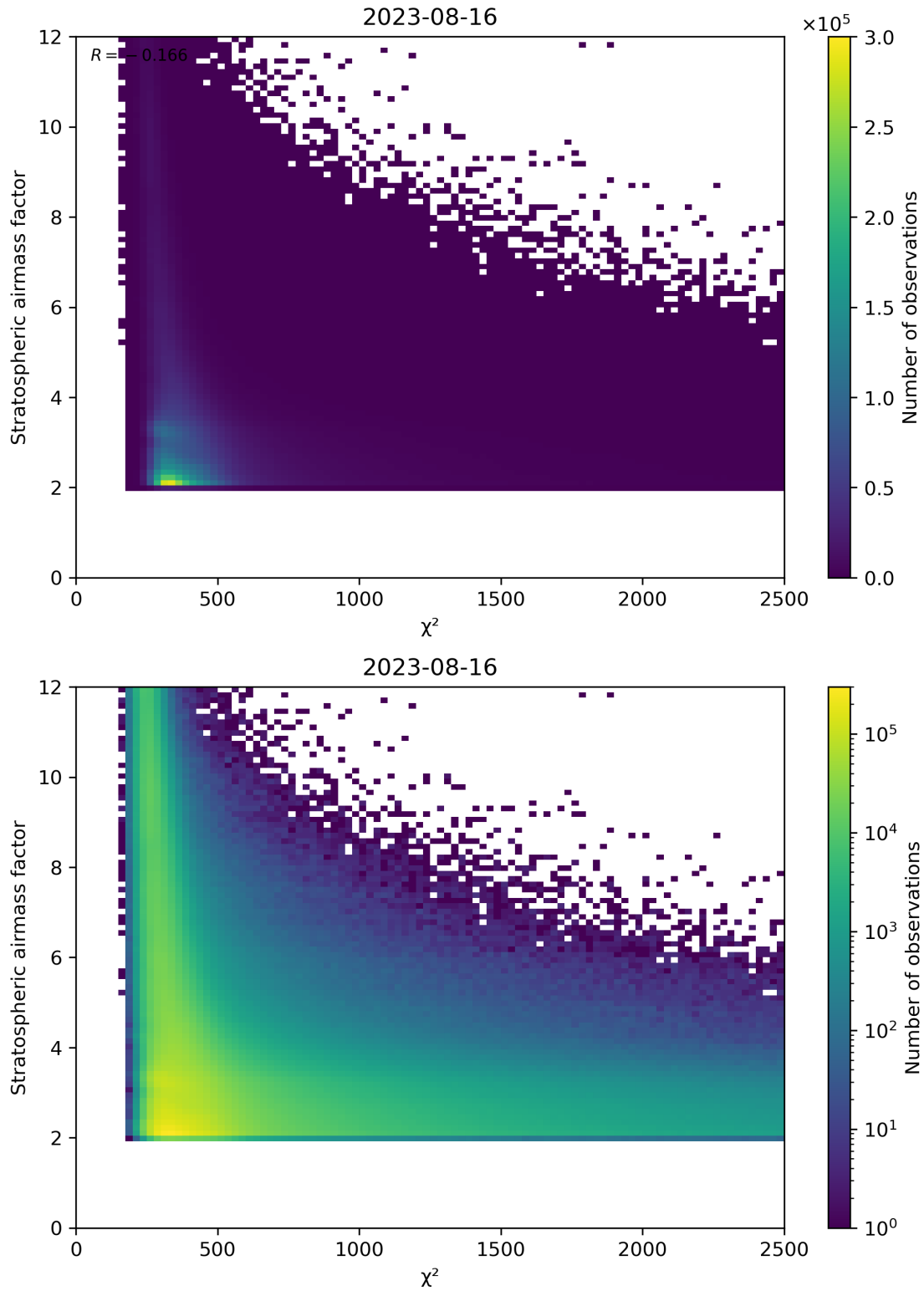
Figure 81: Scatter density plot of “ \chi^2 ” against “Stratospheric airmass factor” for 2023-08-15 to 2023-08-17.
