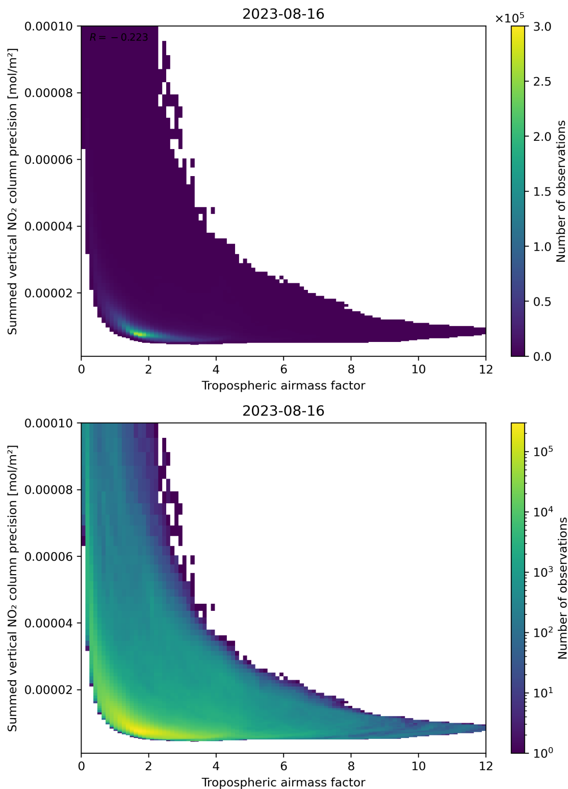
Figure 76: Scatter density plot of “Tropospheric air mass factor” against “Summed vertical NO 2 column precision” for 2023-08-15 to 2023-08-17.
