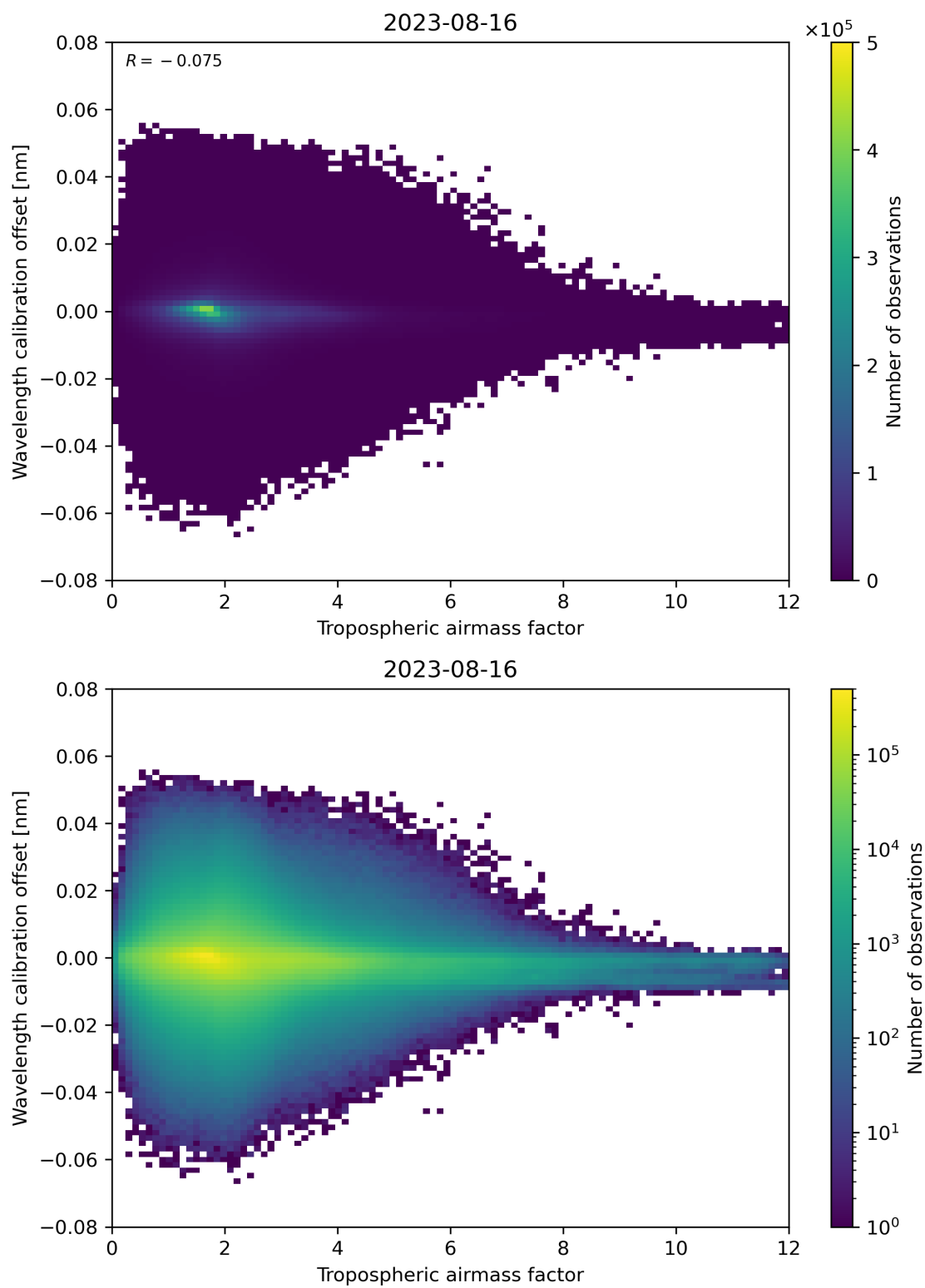
Figure 80: Scatter density plot of “Tropospheric airmass factor” against “Wavelength calibration offset” for 2023-08-15 to 2023-08-17.
