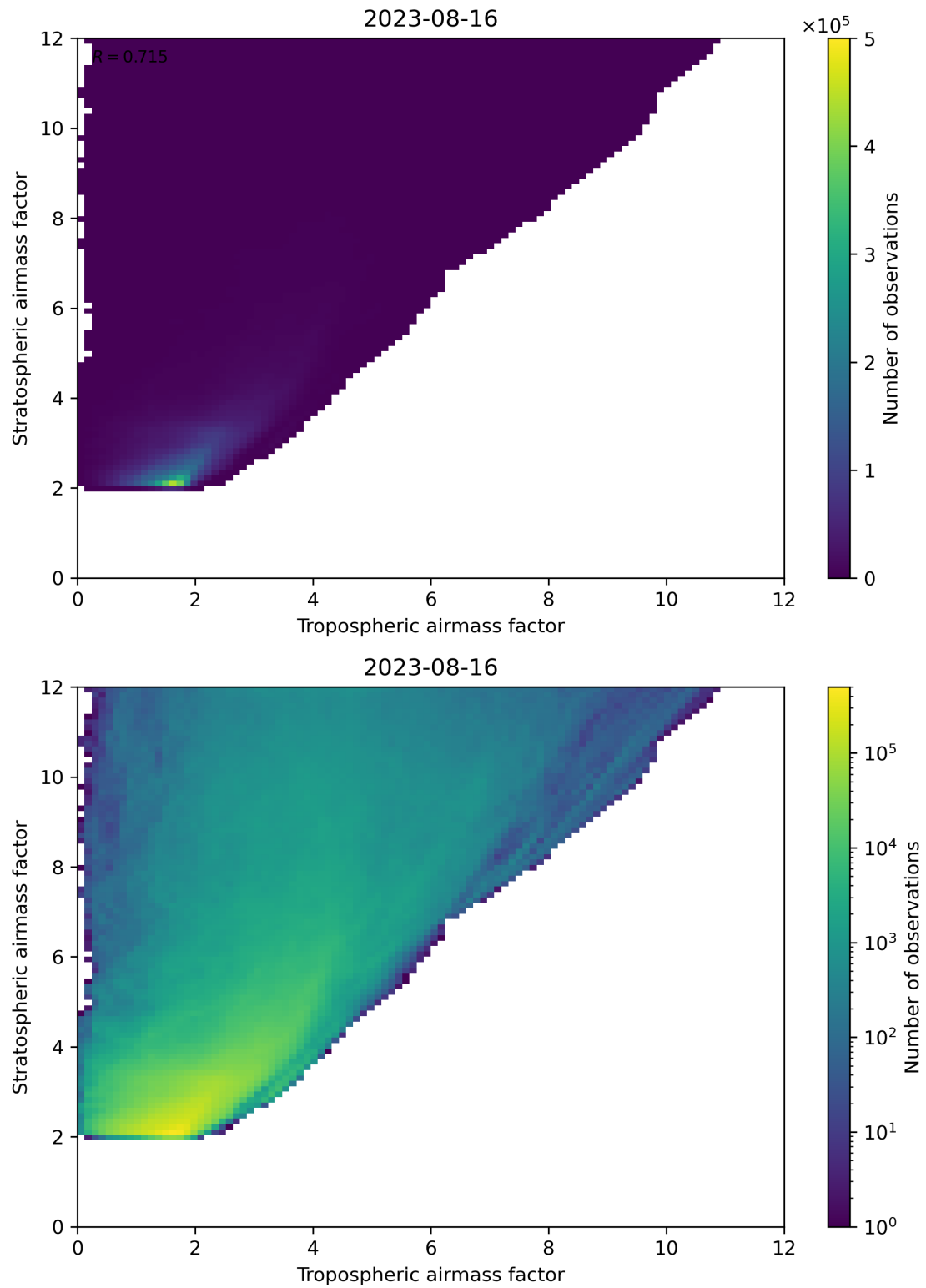
Figure 71: Scatter density plot of “Tropospheric airmass factor” against “Stratospheric airmass factor” for 2023-08-15 to 2023-08-17.
