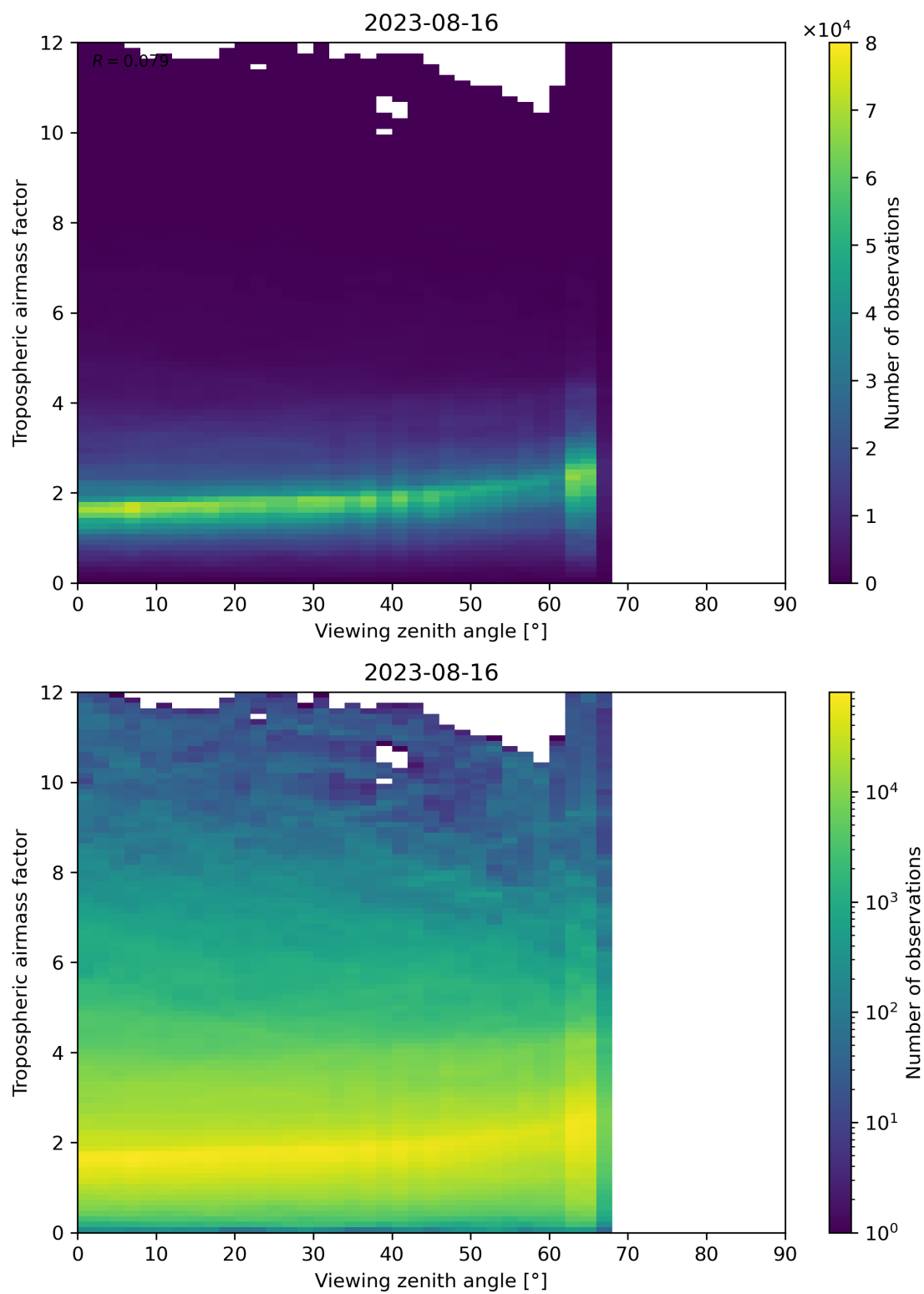
Figure 161: Scatter density plot of “Viewing zenith angle” against “Tropospheric airmass factor” for 2023-08-15 to 2023-08-17.
