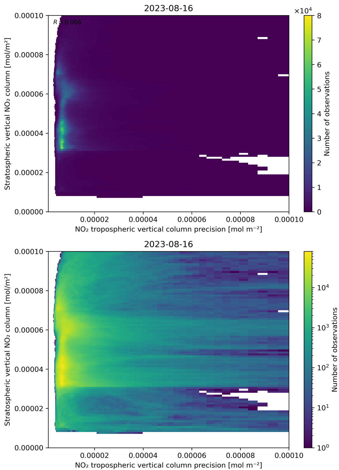
Figure 135: Scatter density plot of “NO 2 tropospheric vertical column precision” against “Stratospheric vertical NO 2 column” for 2023-08-15 to 2023-08-17.
