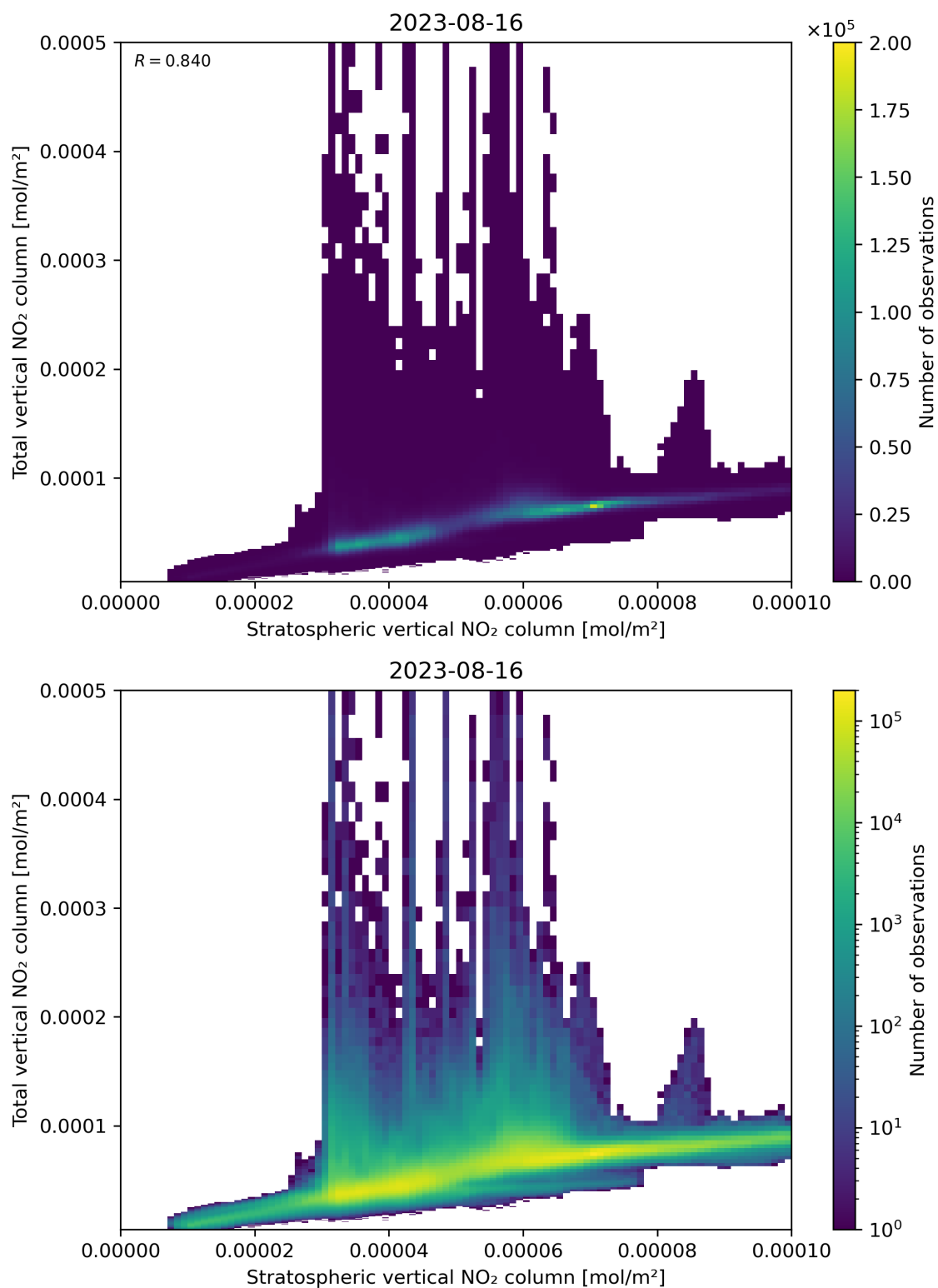
Figure 100: Scatter density plot of “Stratospheric vertical NO 2 column” against “Total vertical NO 2 column” for 2023-08-15 to 2023-08-17.
