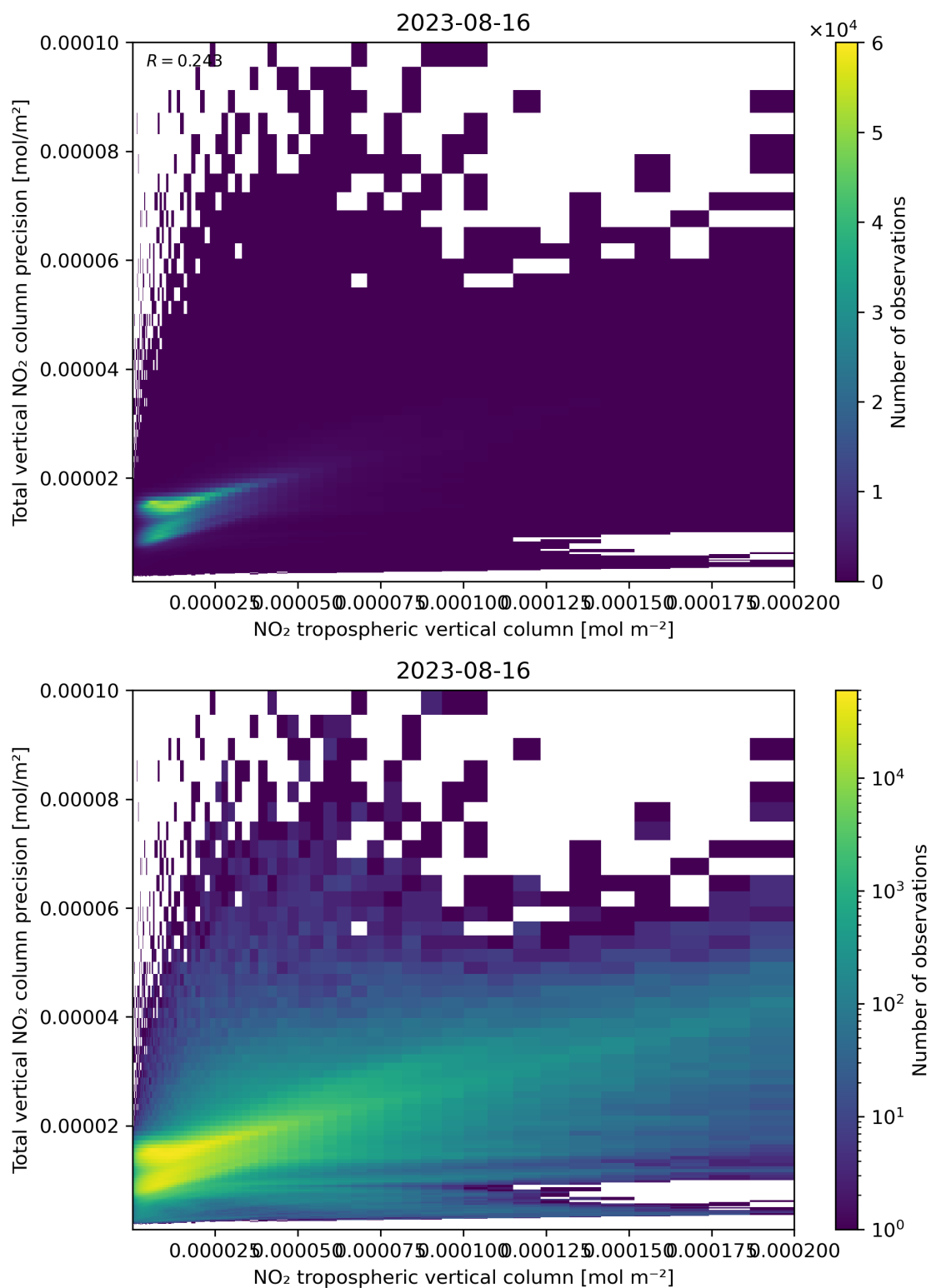
Figure 129: Scatter density plot of “NO 2 tropospheric vertical column” against “Total vertical NO 2 column precision” for 2023-08-15 to 2023-08-17.
