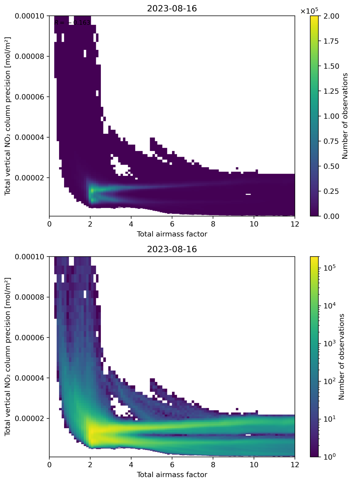
Figure 68: Scatter density plot of “Total airmass factor” against “Total vertical NO 2 column precision” for 2023-08-15 to 2023-08-17.
