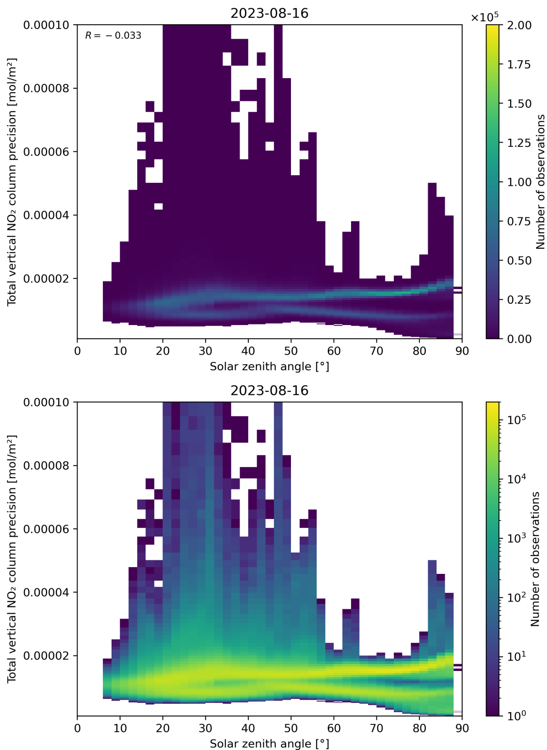
Figure 154: Scatter density plot of “Solar zenith angle” against “Total vertical NO 2 column precision” for 2023-08-15 to 2023-08-17.
