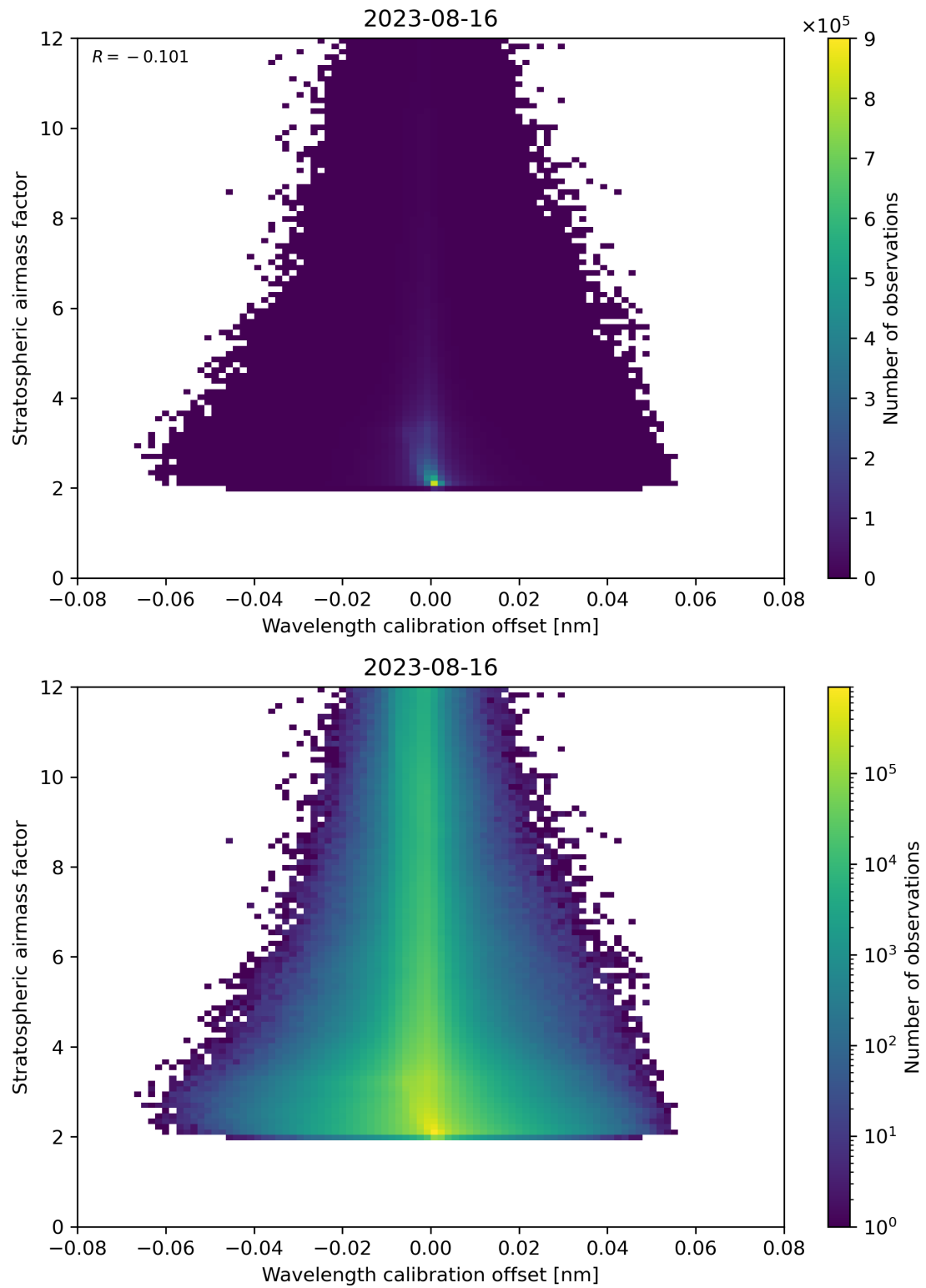
Figure 174: Scatter density plot of “Wavelength calibration offset” against “Stratospheric airmass factor” for 2023-08-15 to 2023-08-17.
