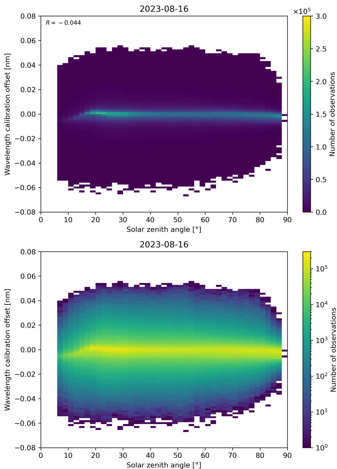
Figure 158: Scatter density plot of “Solar zenith angle” against “Wavelength calibration offset” for 2023-08-15 to 2023-08-17.
