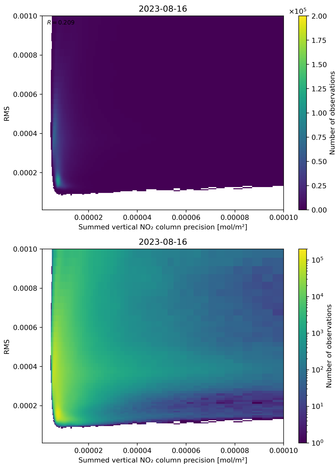
Figure 108: Scatter density plot of “Summed vertical NO 2 column precision” against “RMS” for 2023-08-15 to 2023-08-17.
