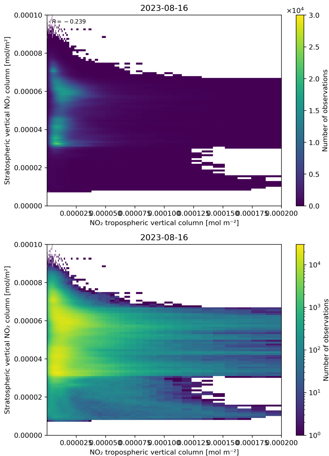
Figure 125: Scatter density plot of “NO 2 tropospheric vertical column” against “Stratospheric vertical NO 2 column” for 2023-08-15 to 2023-08-17.
