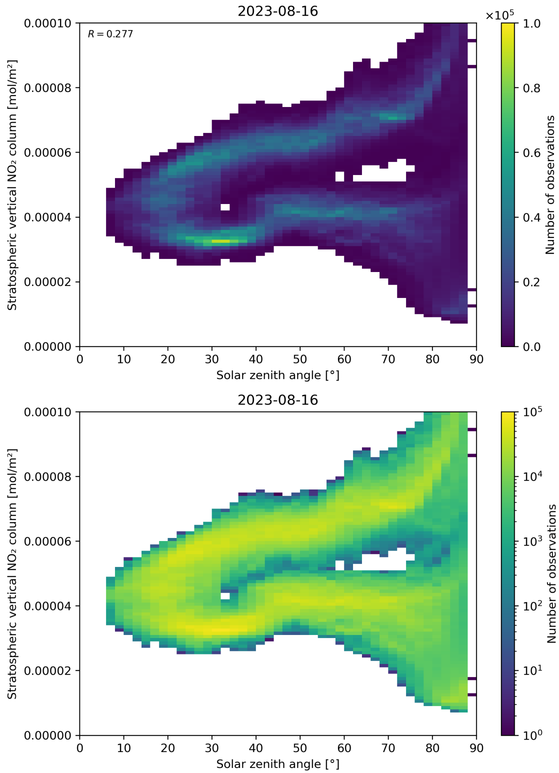
Figure 150: Scatter density plot of “Solar zenith angle” against “Stratospheric vertical NO 2 column” for 2023-08-15 to 2023-08-17.
