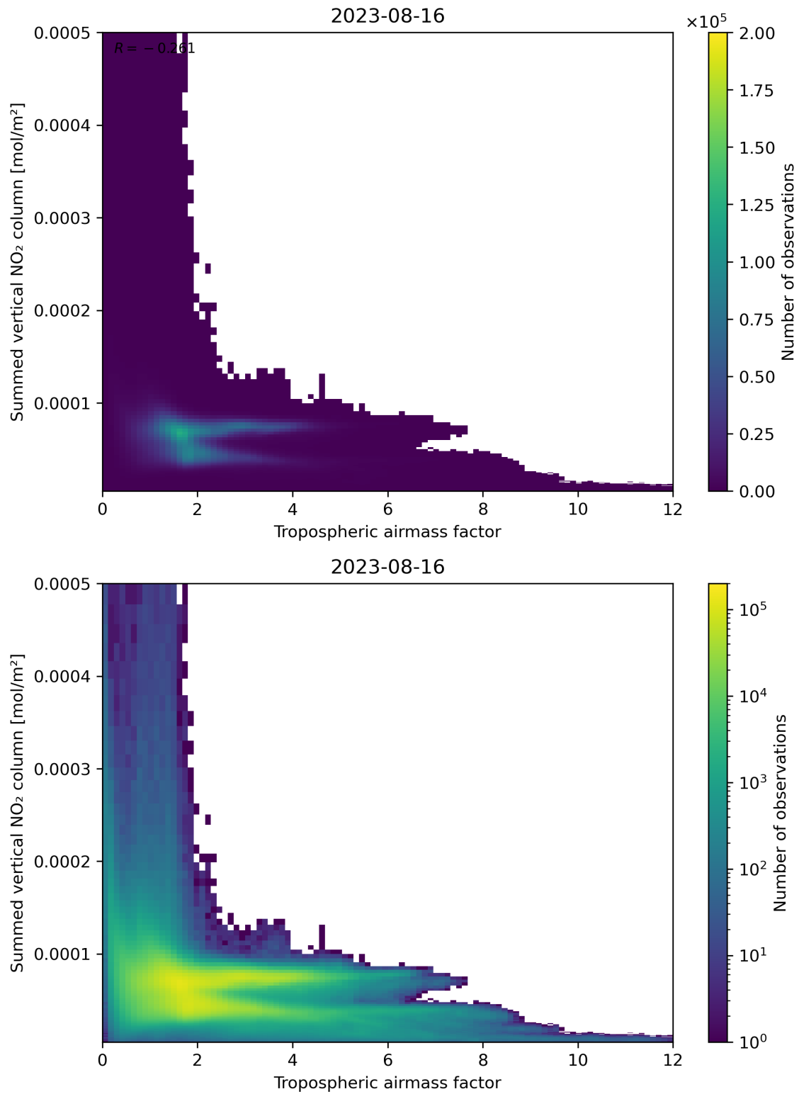
Figure 75: Scatter density plot of “Tropospheric airmass factor” against “Summed vertical NO 2 column” for 2023-08-15 to 2023-08-17.
