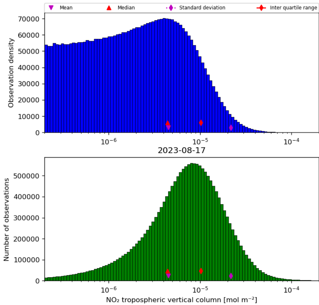
Figure 29: Histogram of “NO 2 tropospheric vertical column” for 2023-08-16 to 2023-08-18
