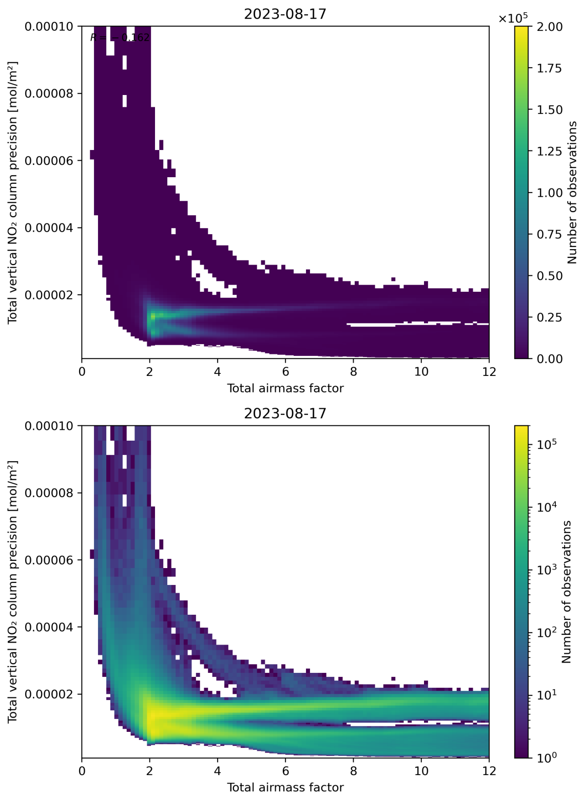
Figure 68: Scatter density plot of “Total airmass factor” against “Total vertical NO 2 column precision” for 2023-08-16 to 2023-08-18.
