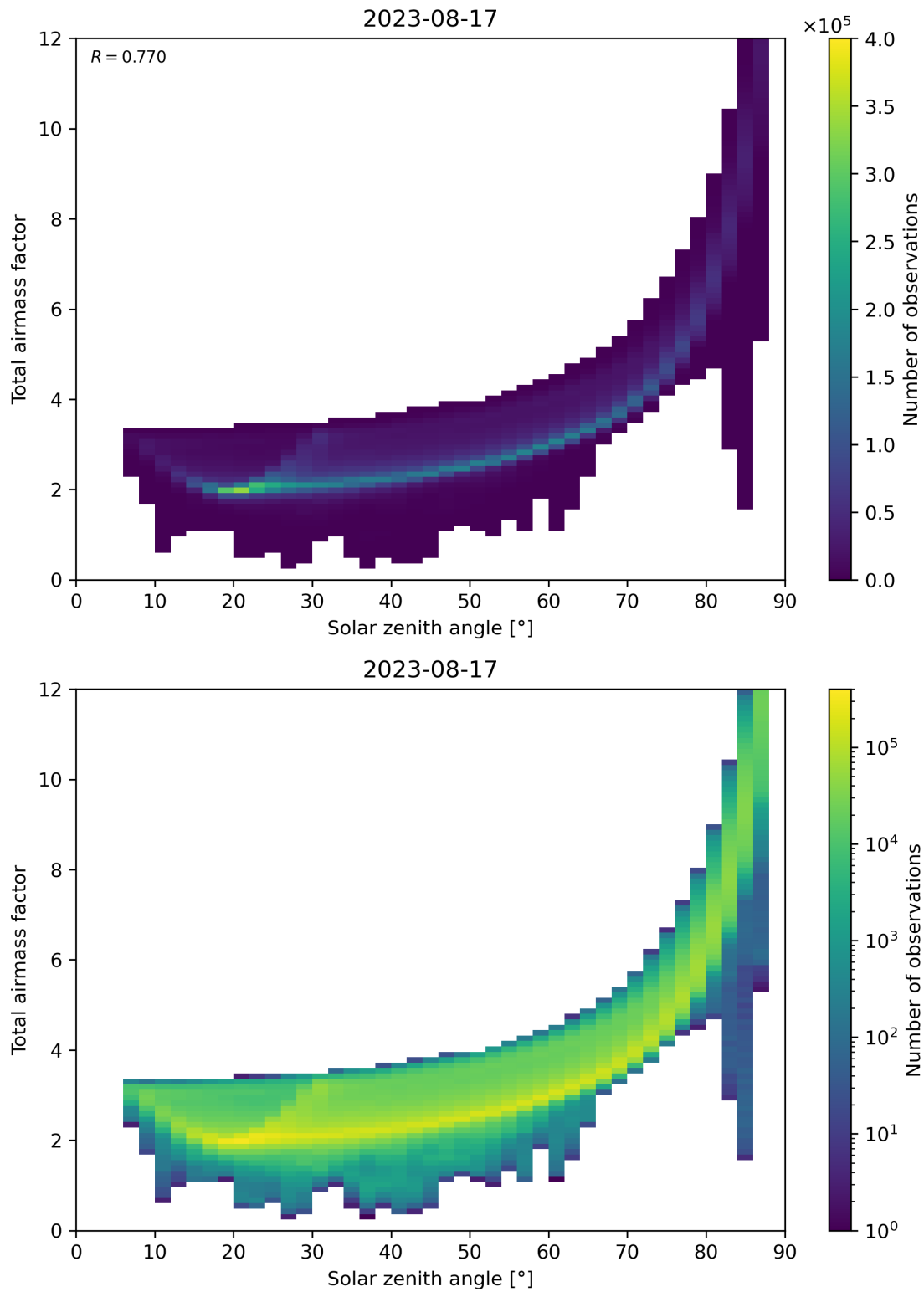
Figure 146: Scatter density plot of “Solar zenith angle” against “Total air mass factor” for 2023-08-16 to 2023-08-18.
