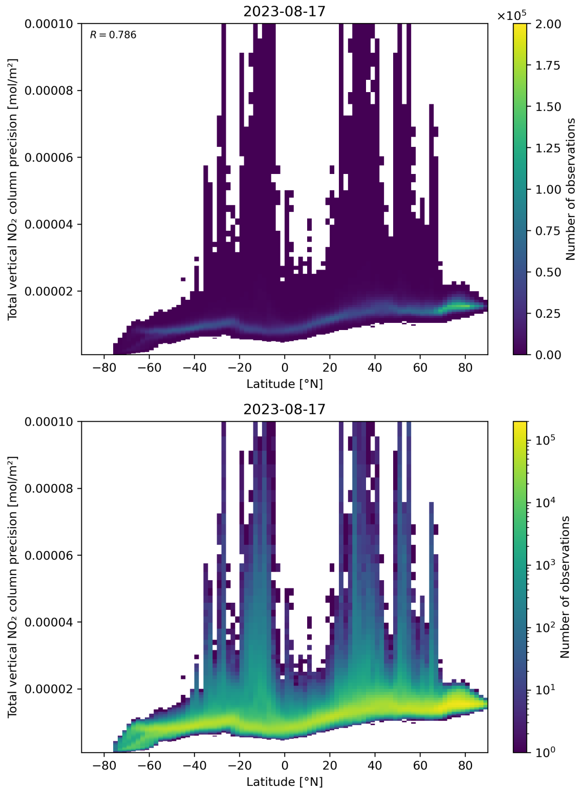
Figure 91: Scatter density plot of “Latitude” against “Total vertical NO 2 column precision” for 2023-08-16 to 2023-08-18.
