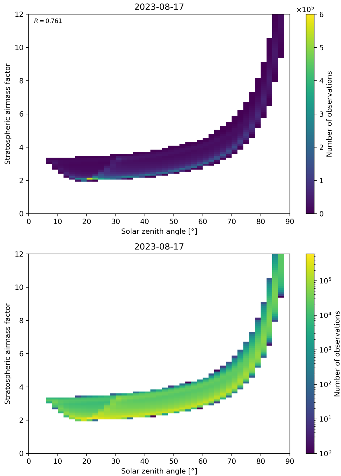
Figure 145: Scatter density plot of “Solar zenith angle” against “Stratospheric airmass factor” for 2023-08-16 to 2023-08-18.
