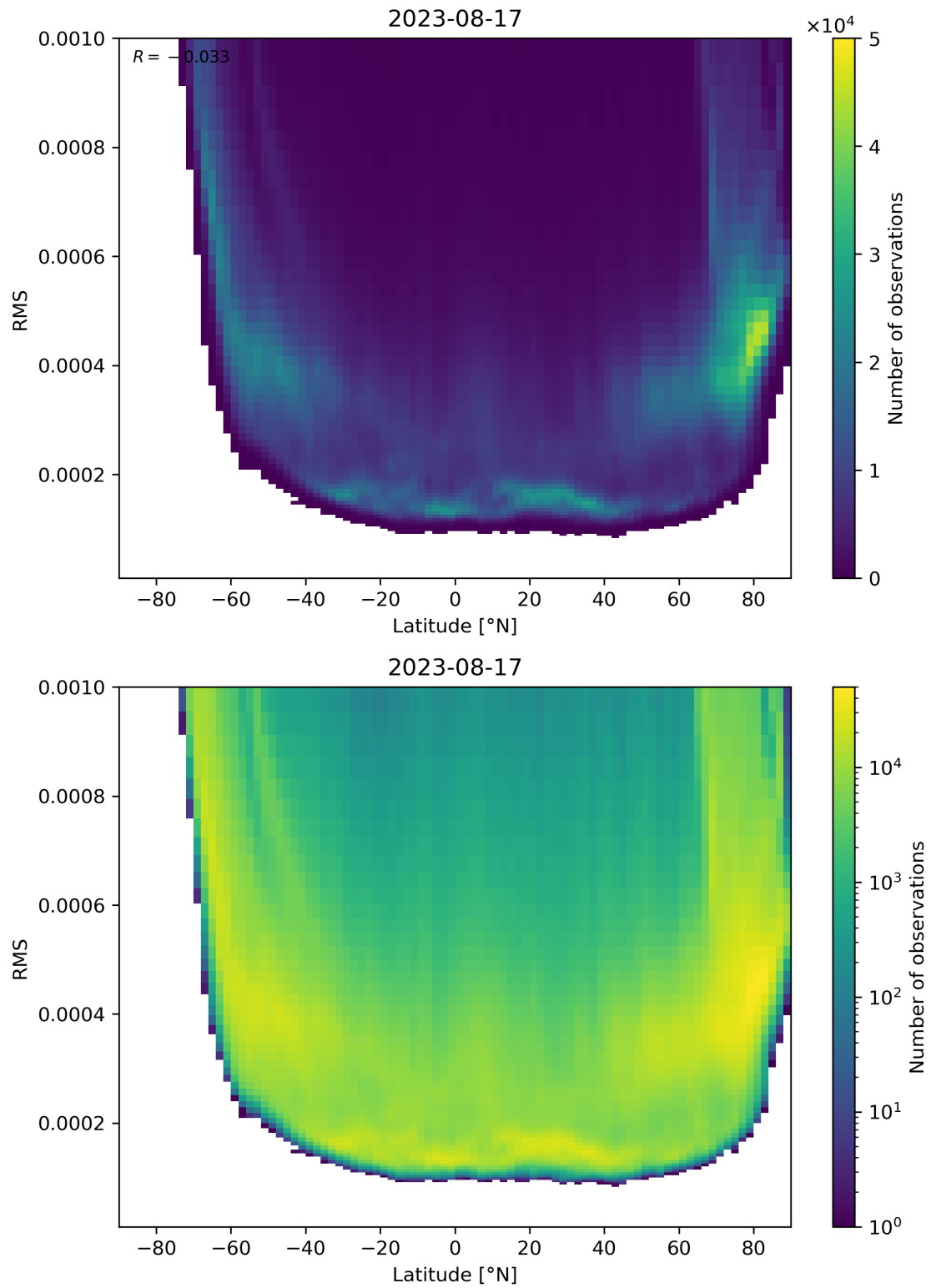
Figure 94: Scatter density plot of “Latitude” against “RMS” for 2023-08-16 to 2023-08-18.
