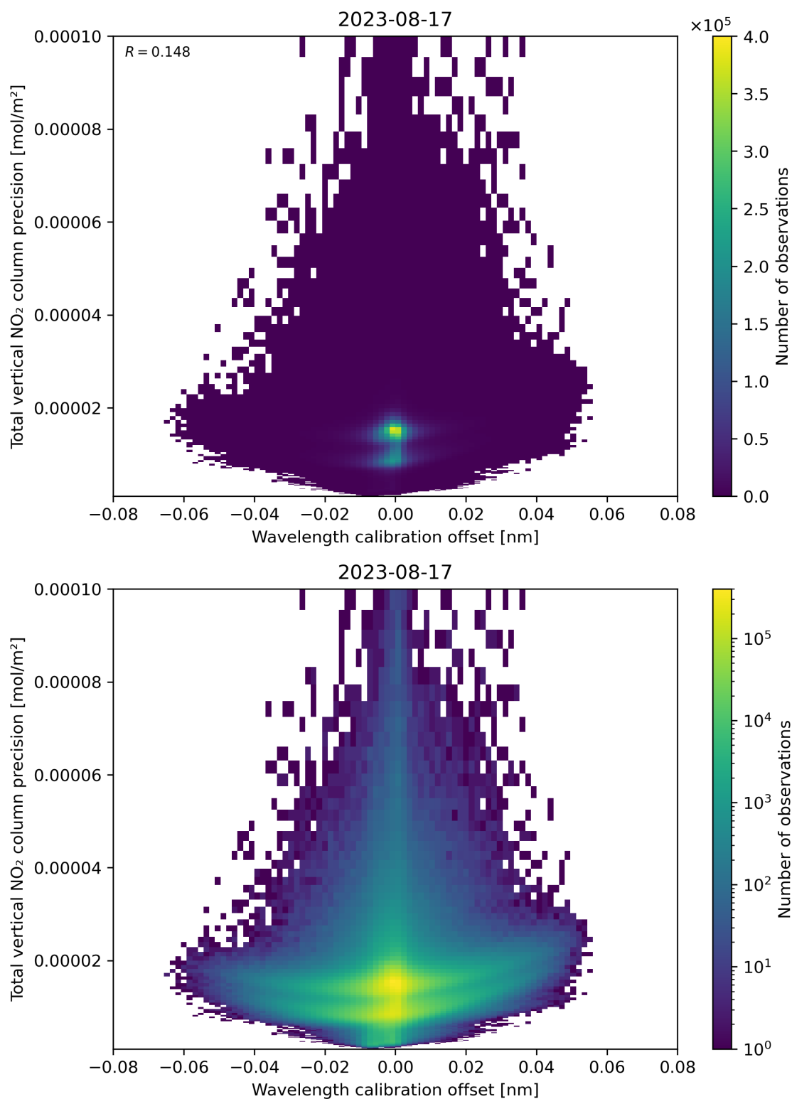
Figure 180: Scatter density plot of “Wavelength calibration offset” against “Total vertical NO 2 column precision” for 2023-08-16 to 2023-08-18.
