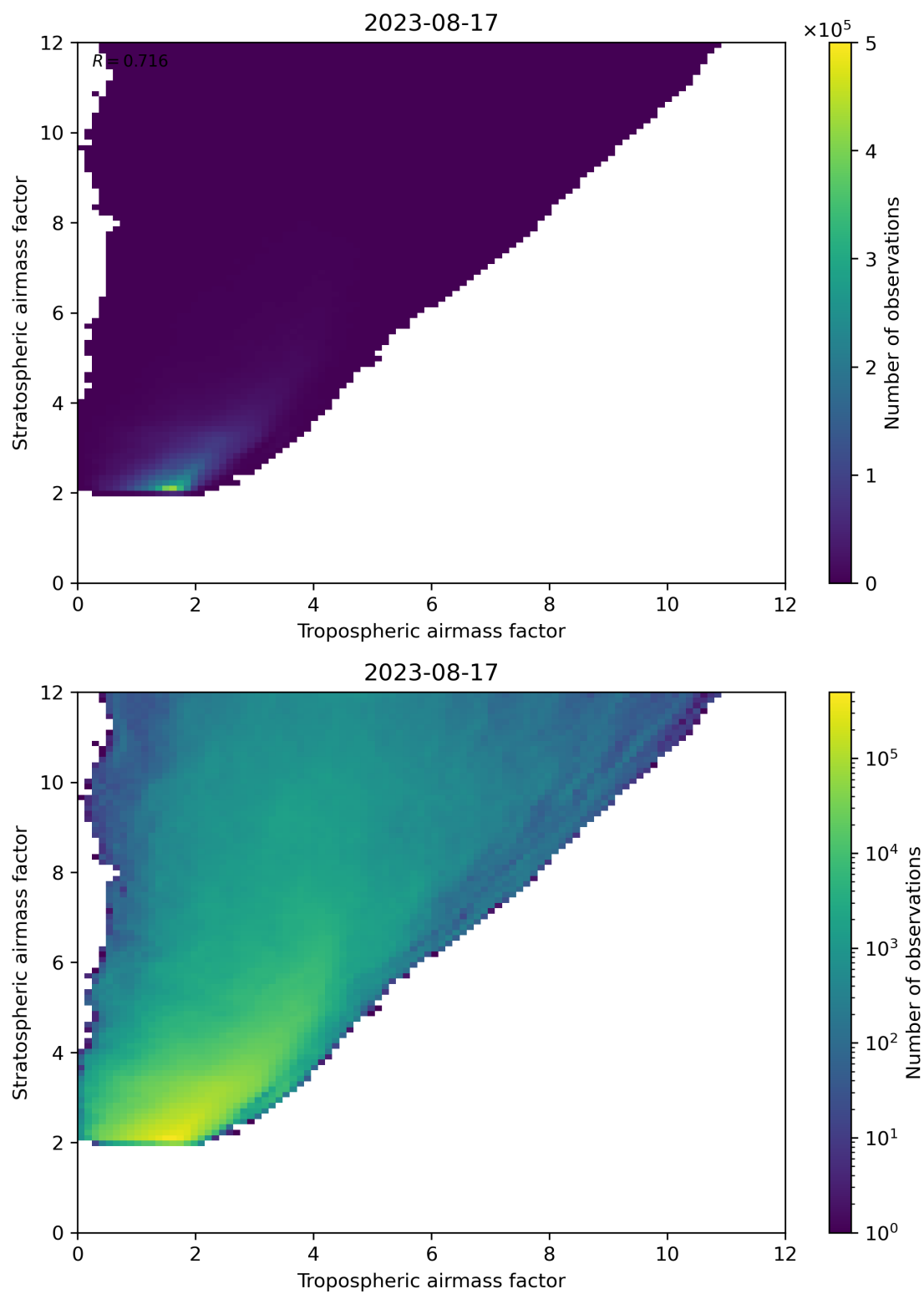
Figure 71: Scatter density plot of “Tropospheric airmass factor” against “Stratospheric airmass factor” for 2023-08-16 to 2023-08-18.
