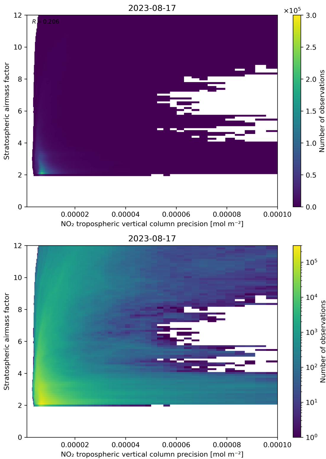
Figure 131: Scatter density plot of “NO 2 tropospheric vertical column precision” against “Stratospheric airmass factor” for 2023-08-16 to 2023-08-18.
