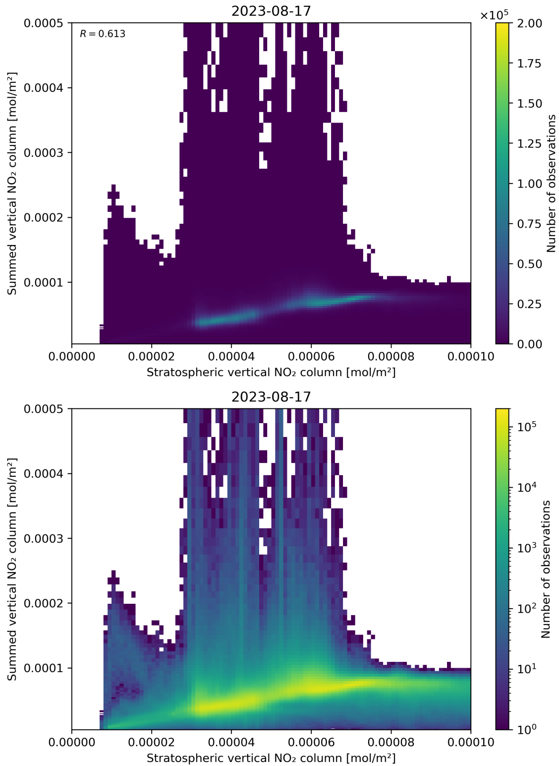
Figure 98: Scatter density plot of “Stratospheric vertical NO 2 column” against “Summed vertical NO 2 column” for 2023-08-16 to 2023-08-18.
