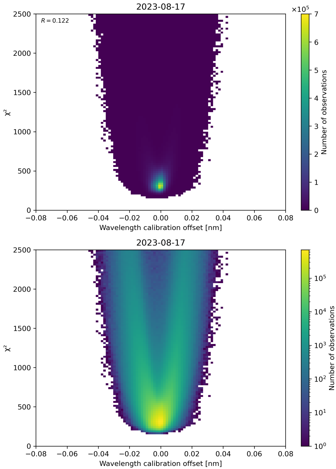
Figure 175: Scatter density plot of “Wavelength calibration offset” against “ \chi^2 ” for 2023-08-16 to 2023-08-18.
