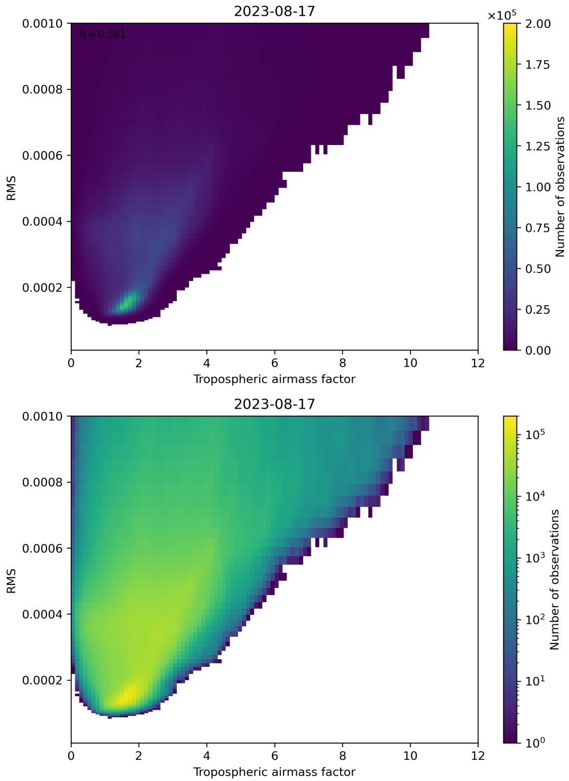
Figure 79: Scatter density plot of “Tropospheric airmass factor” against “RMS” for 2023-08-16 to 2023-08-18.
