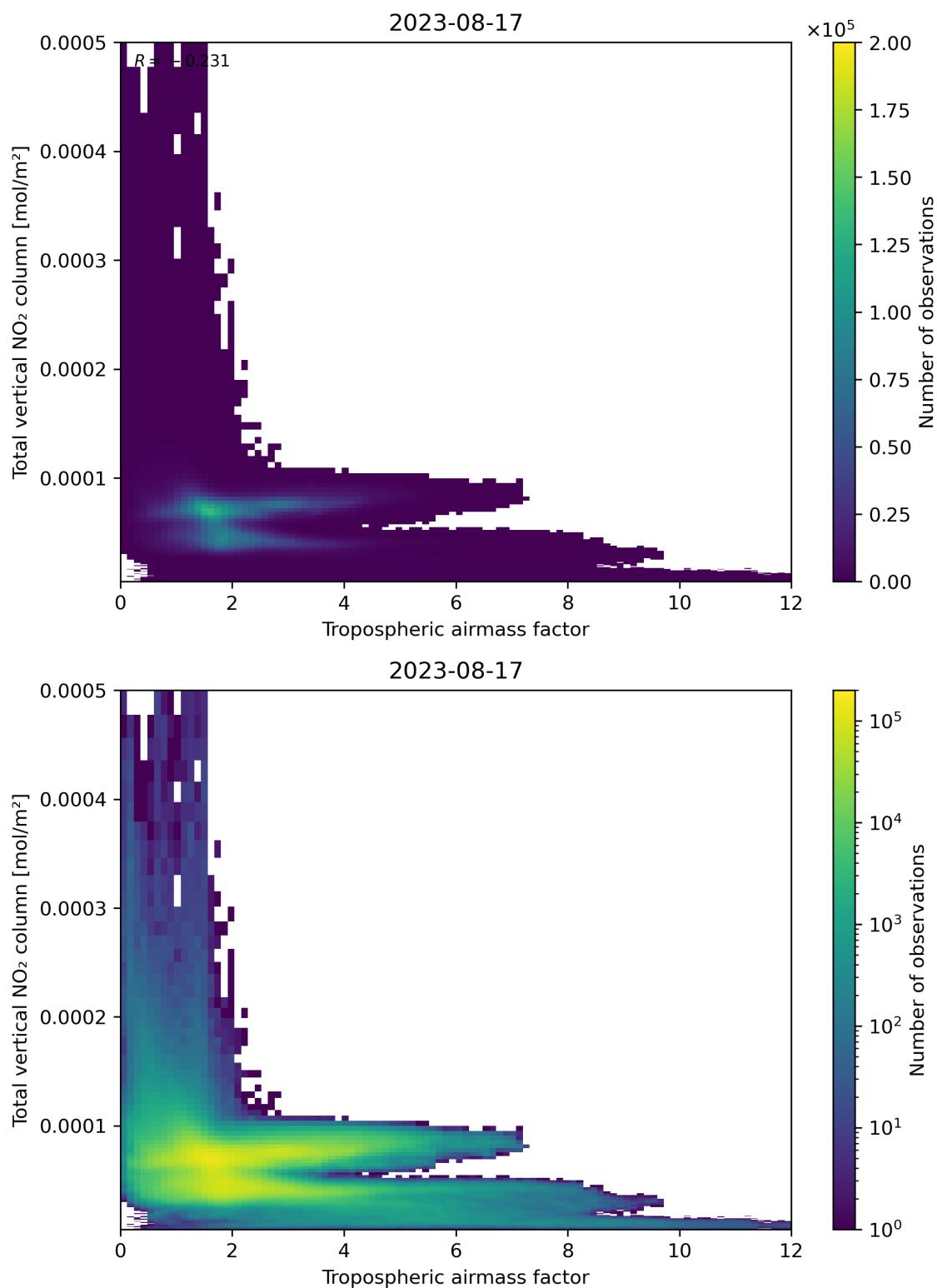
Figure 77: Scatter density plot of “Tropospheric airmass factor” against “Total vertical NO 2 column” for 2023-08-16 to 2023-08-18.
