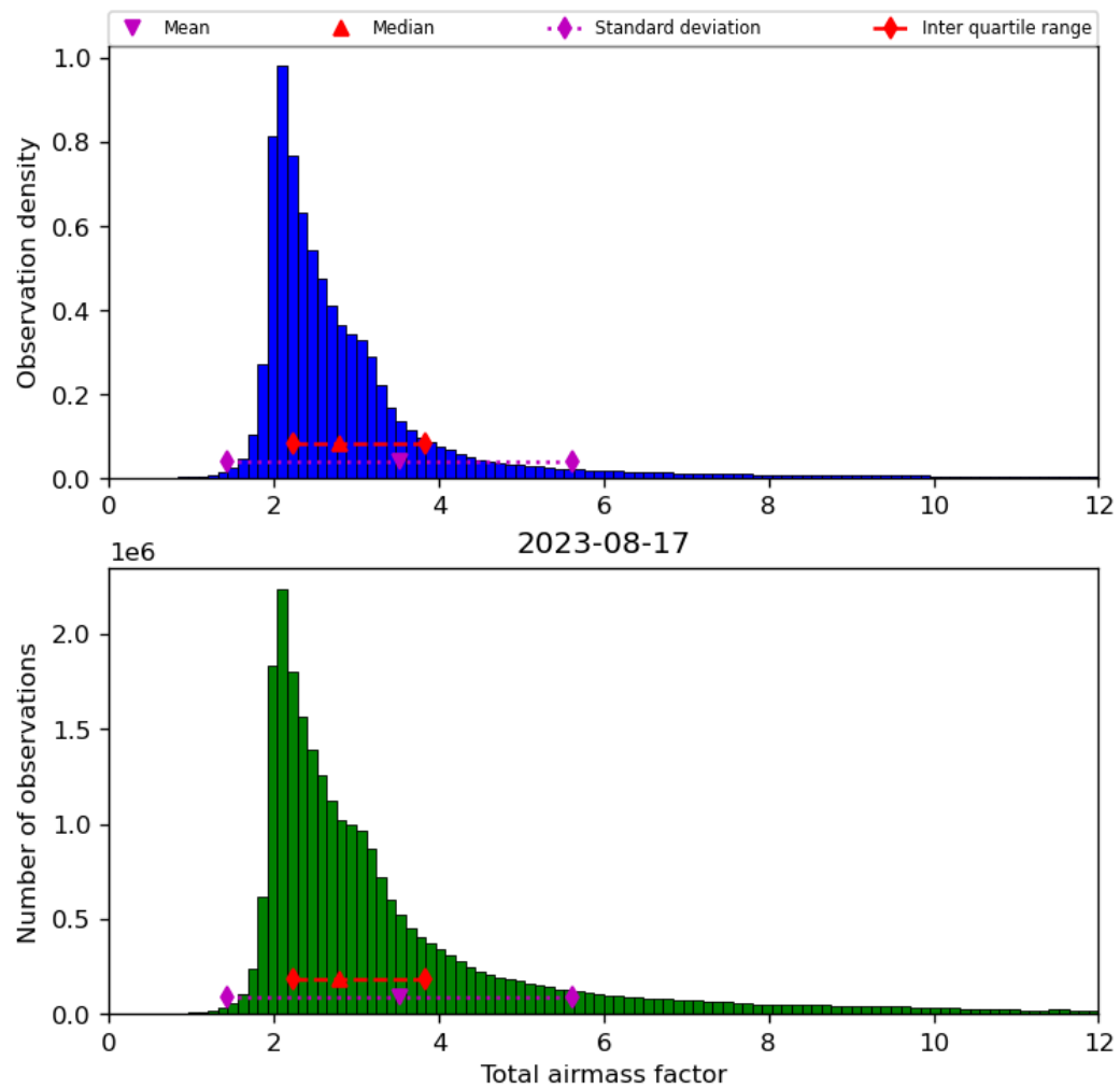
Figure 32: Histogram of “Total airmass factor” for 2023-08-16 to 2023-08-18
