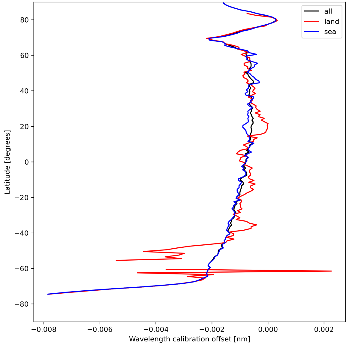
Figure 18: Zonal average of “Wavelength calibration offset” for 2023-08-16 to 2023-08-18.
