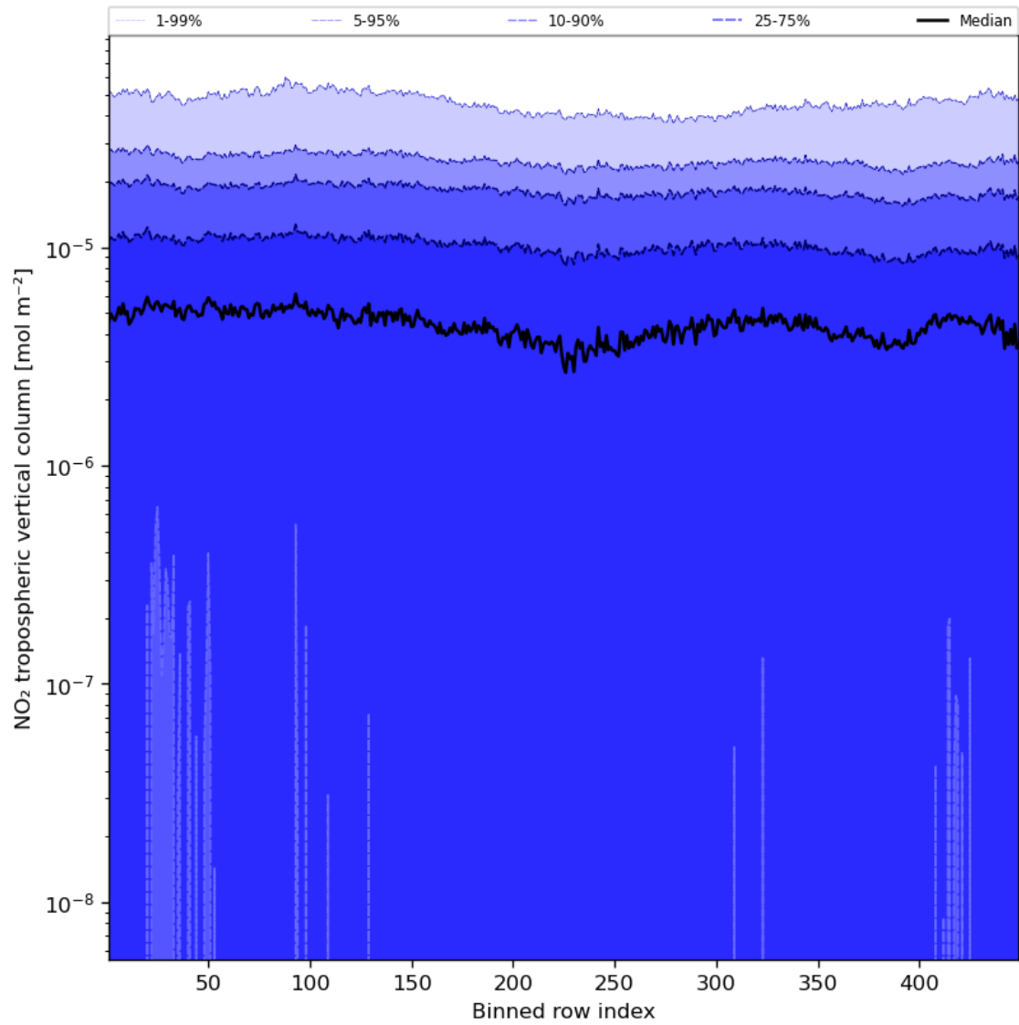
Figure 46: Along track statistics of “NO 2 tropospheric vertical column” for 2023-08-16 to 2023-08-18
