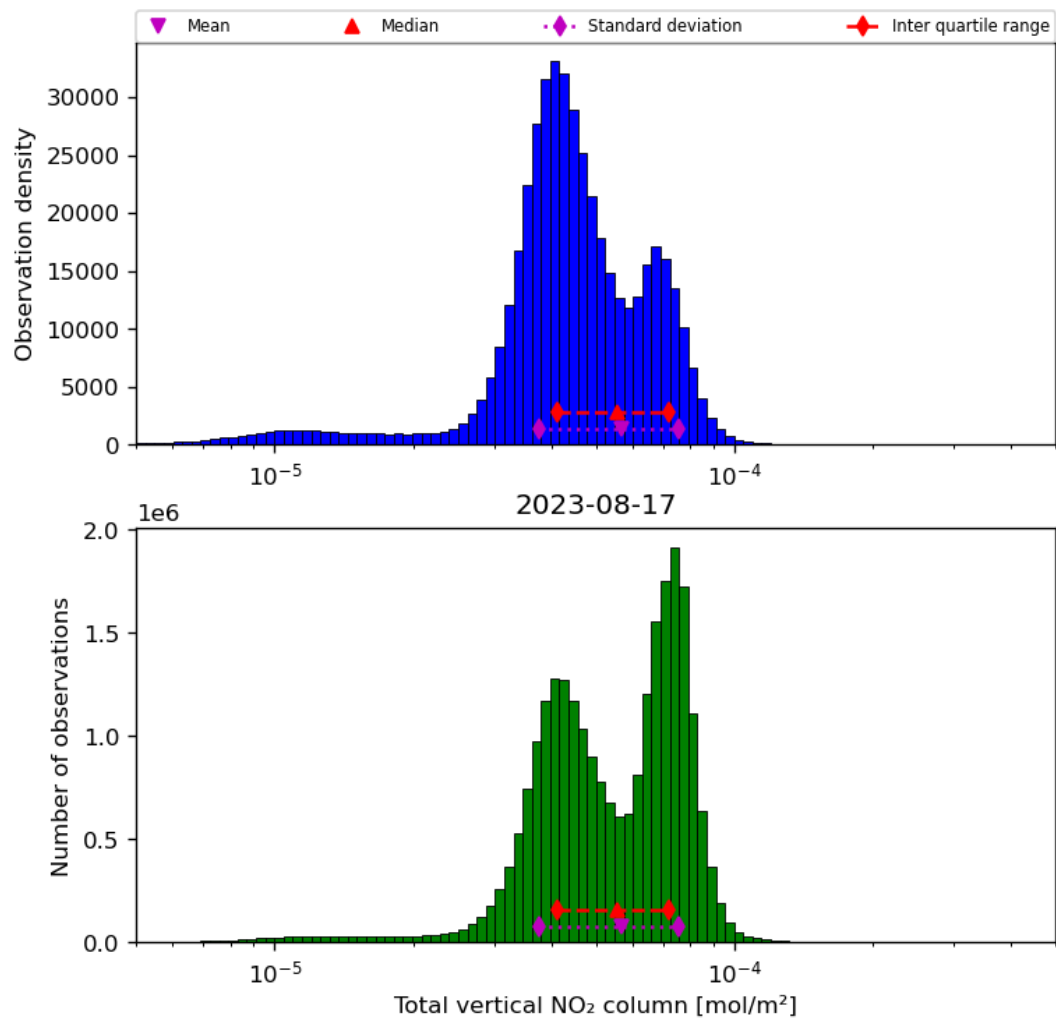
Figure 38: Histogram of "Total vertical NO 2 column" for 2023-08-16 to 2023-08-18
