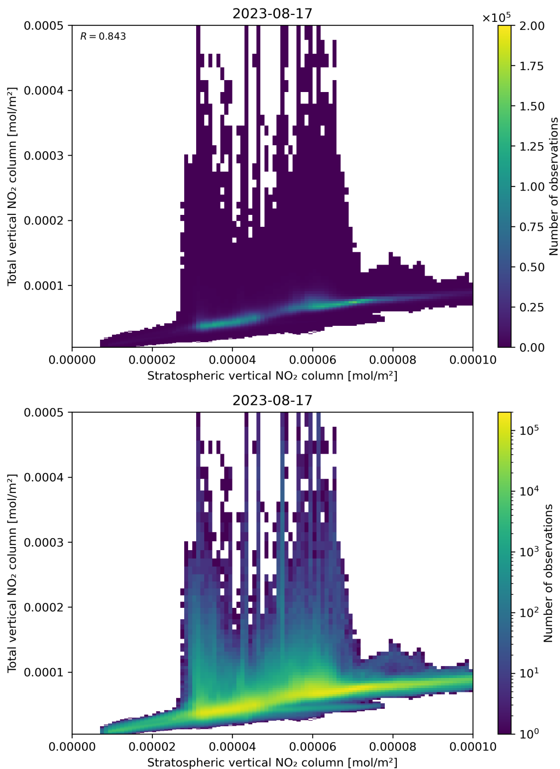
Figure 100: Scatter density plot of “Stratospheric vertical NO 2 column” against “Total vertical NO 2 column” for 2023-08-16 to 2023-08-18.
