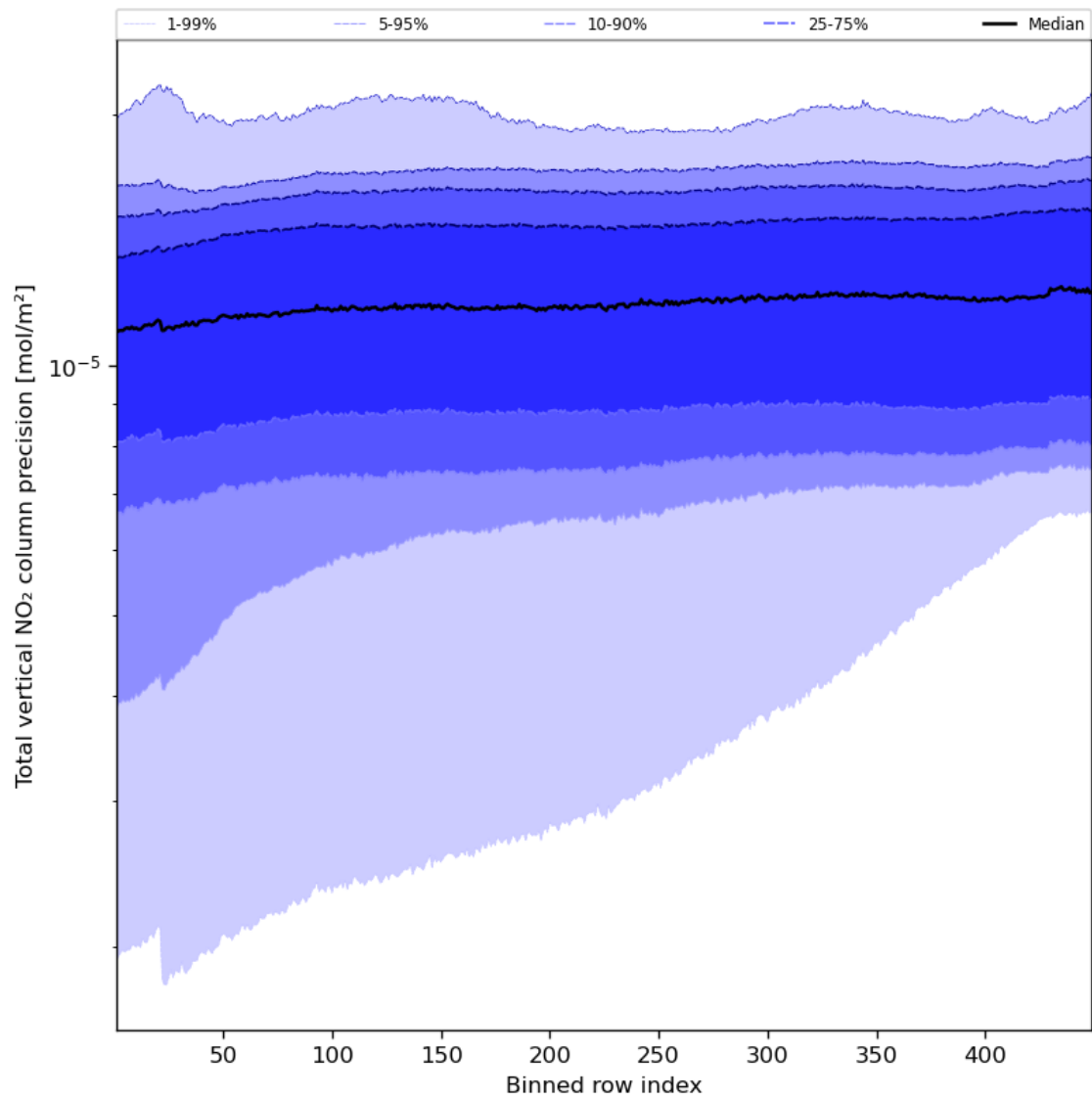
Figure 56: Along track statistics of “Total vertical NO 2 column precision” for 2023-08-16 to 2023-08-18
