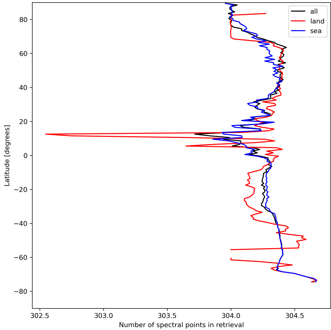
Figure 16: Zonal average of “Number of spectral points in retrieval” for 2023-08-16 to 2023-08-18.
