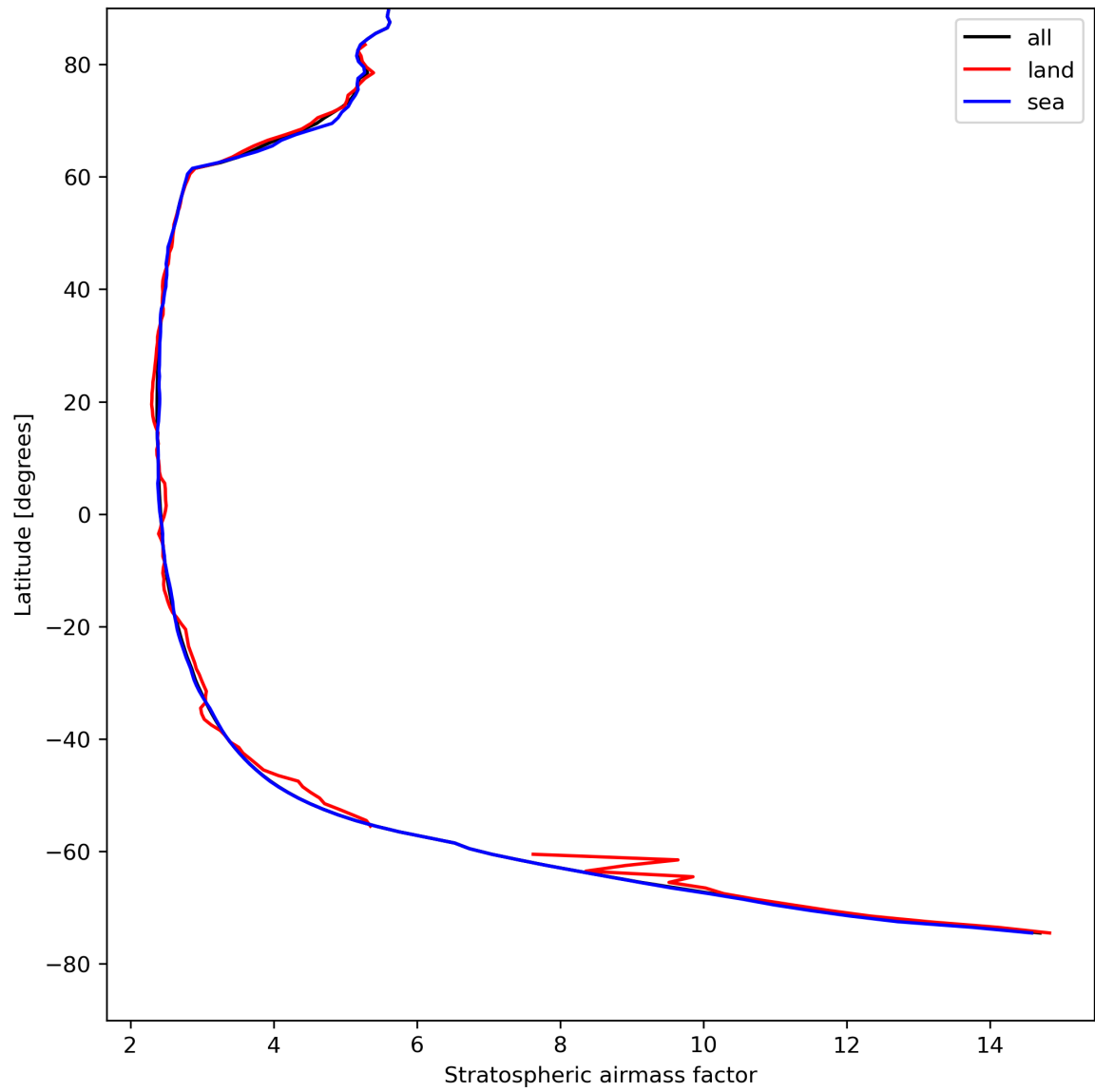
Figure 27: Zonal average of “Stratospheric airmass factor” for 2023-08-16 to 2023-08-18.
