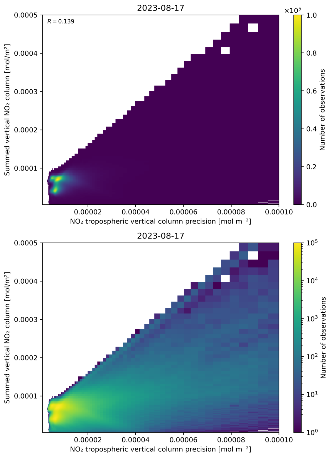
Figure 136: Scatter density plot of “NO 2 tropospheric vertical column precision” against “Summed vertical NO 2 column” for 2023-08-16 to 2023-08-18.
