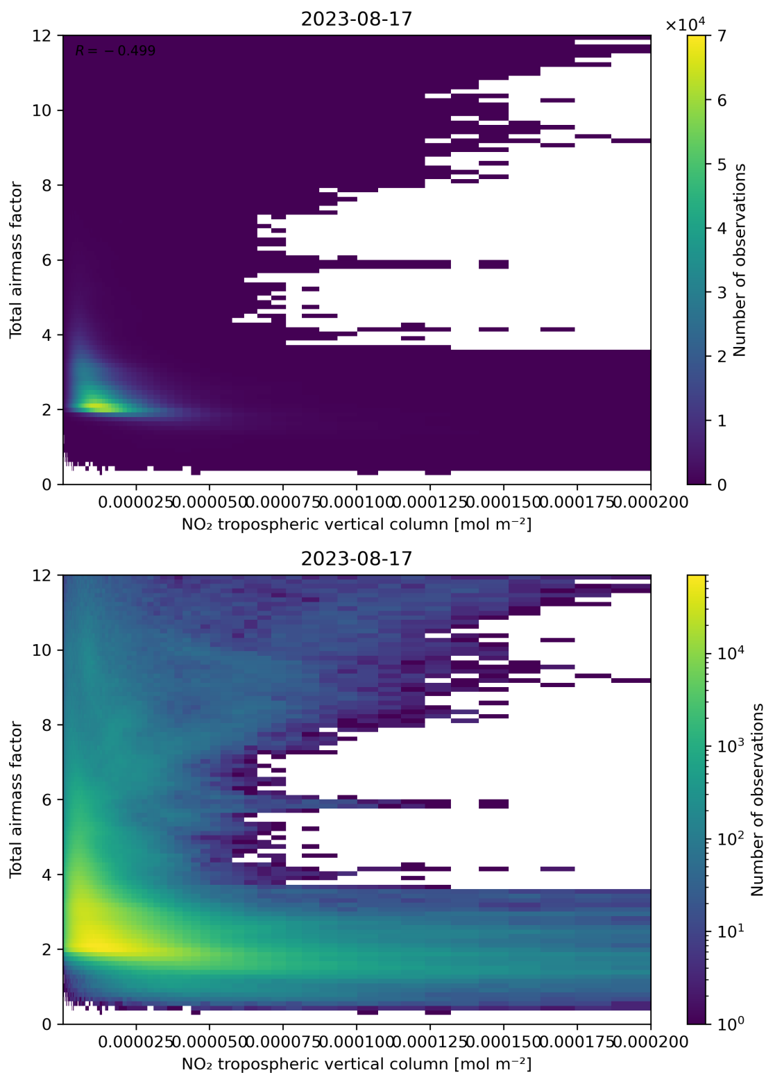
Figure 122: Scatter density plot of “NO 2 tropospheric vertical column” against “Total air mass factor” for 2023-08-16 to 2023-08-18.
