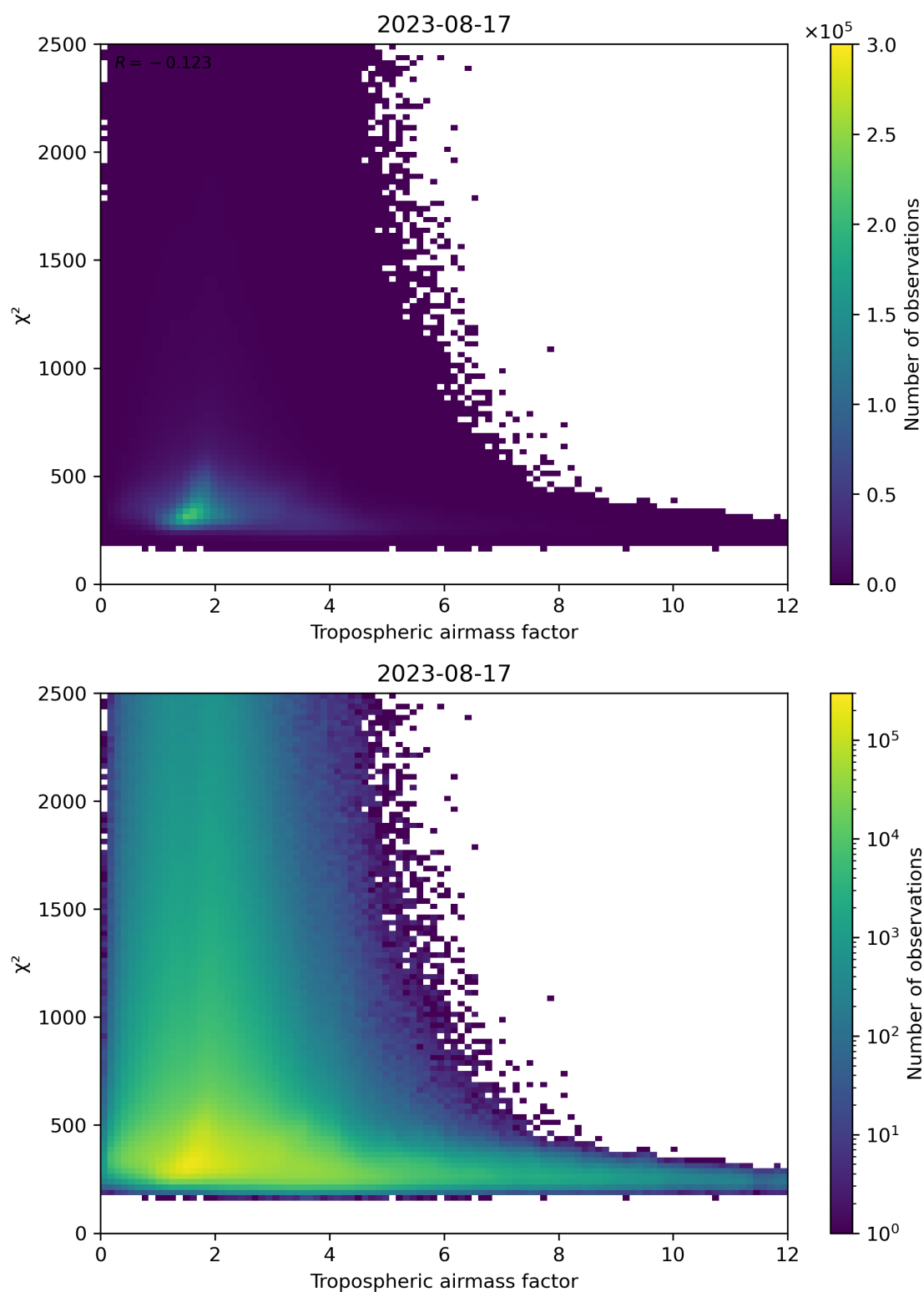
Figure 73: Scatter density plot of “Tropospheric airmass factor” against “ \chi^2 ” for 2023-08-16 to 2023-08-18.
