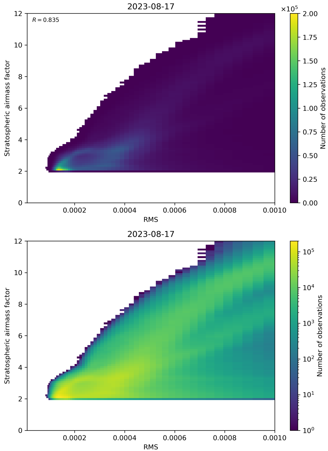
Figure 144: Scatter density plot of “RMS” against “Stratospheric airmass factor” for 2023-08-16 to 2023-08-18.
