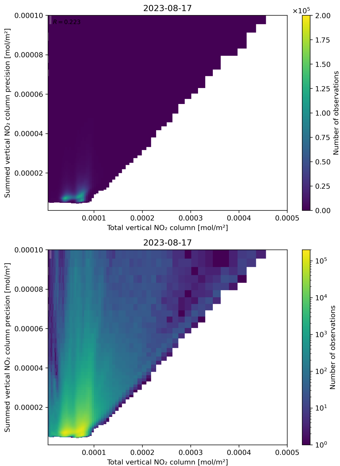
Figure 113: Scatter density plot of “Total vertical NO 2 column” against “Summed vertical NO 2 column precision” for 2023-08-16 to 2023-08-18.
