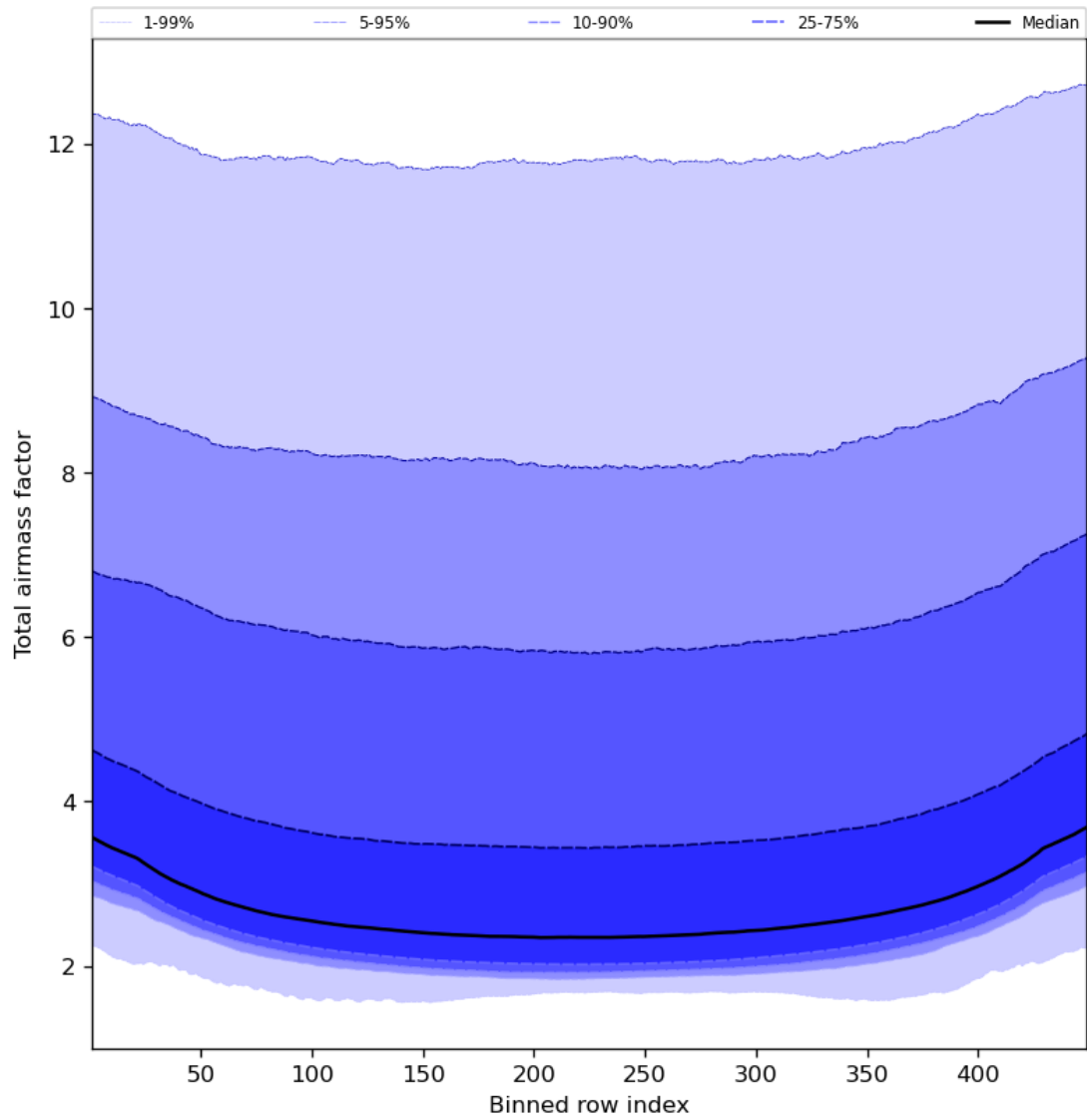
Figure 49: Along track statistics of “Total airmass factor” for 2023-08-16 to 2023-08-18
