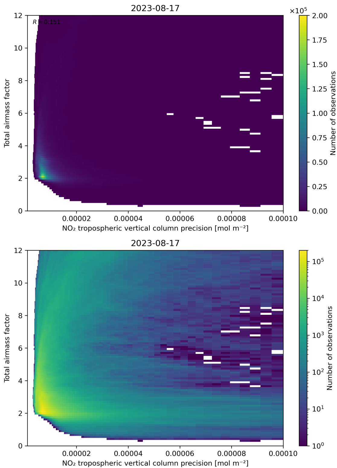
Figure 132: Scatter density plot of “NO 2 tropospheric vertical column precision” against “Total air mass factor” for 2023-08-16 to 2023-08-18.
