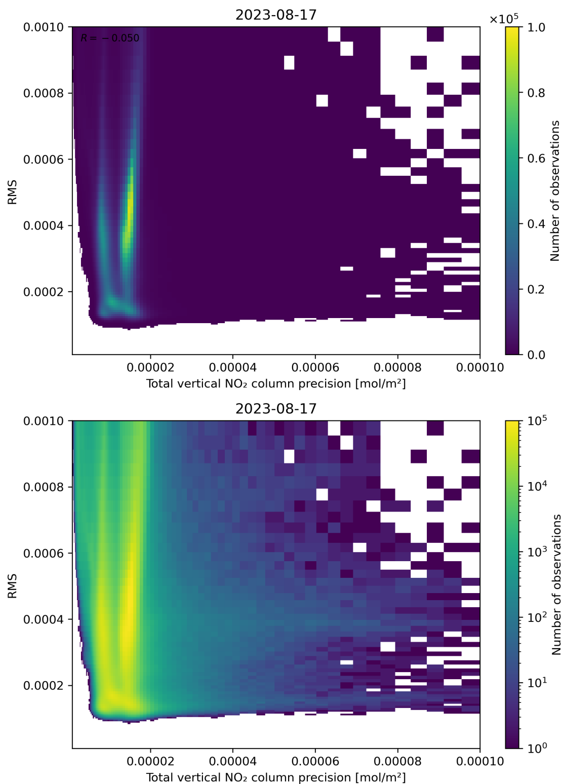
Figure 119: Scatter density plot of “Total vertical NO 2 column precision” against “RMS” for 2023-08-16 to 2023-08-18.
