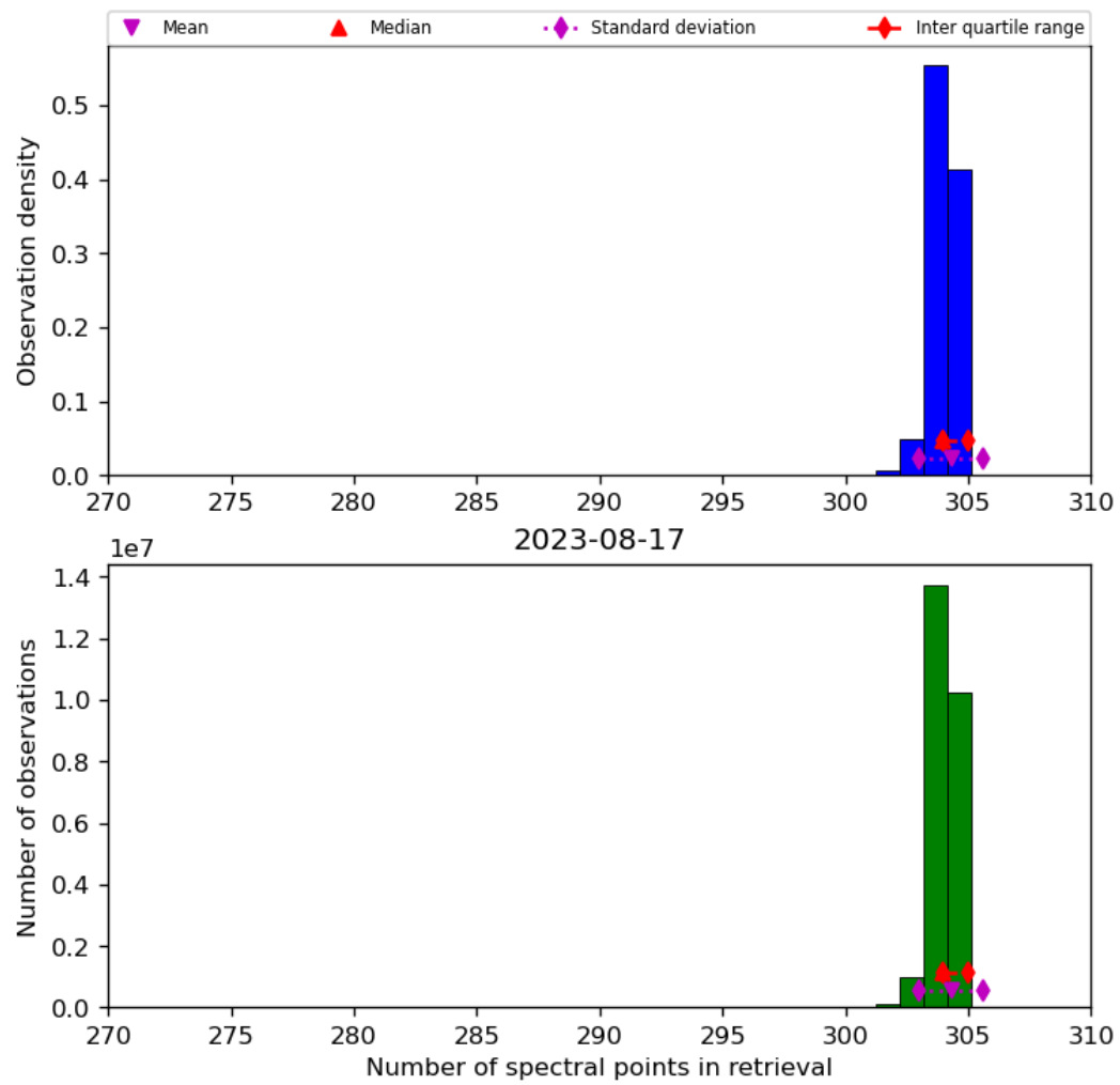
Figure 33: Histogram of “Number of spectral points in retrieval” for 2023-08-16 to 2023-08-18
