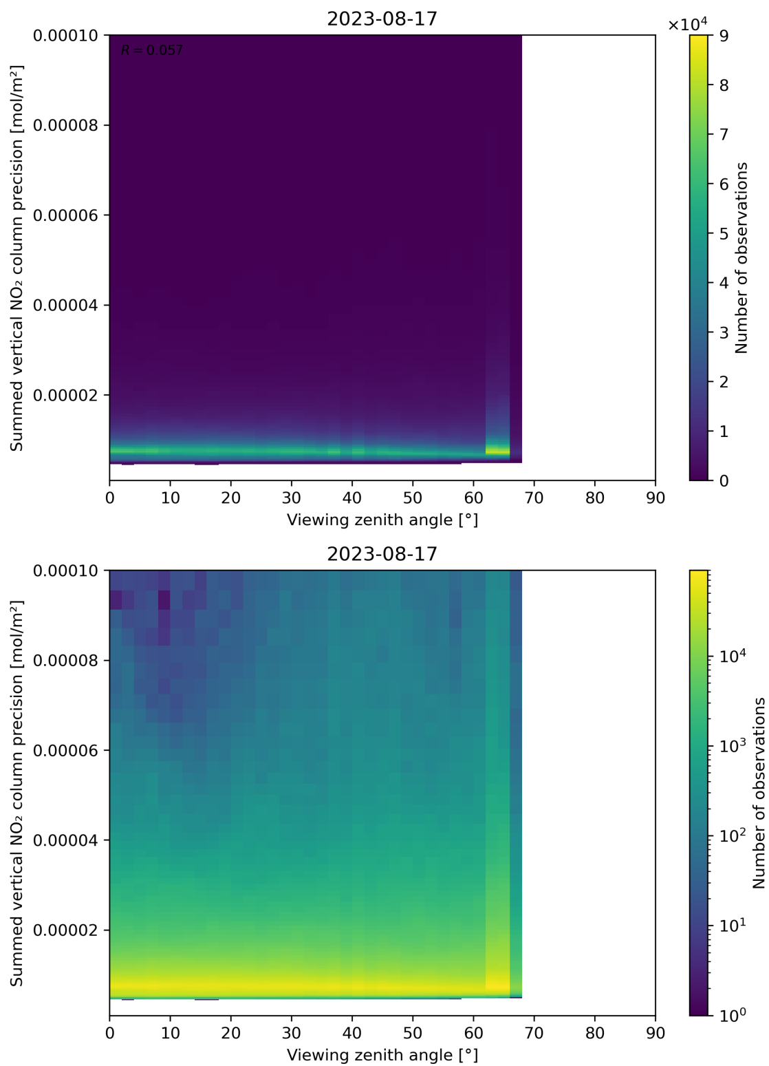
Figure 166: Scatter density plot of “Viewing zenith angle” against “Summed vertical NO 2 column precision” for 2023-08-16 to 2023-08-18.
