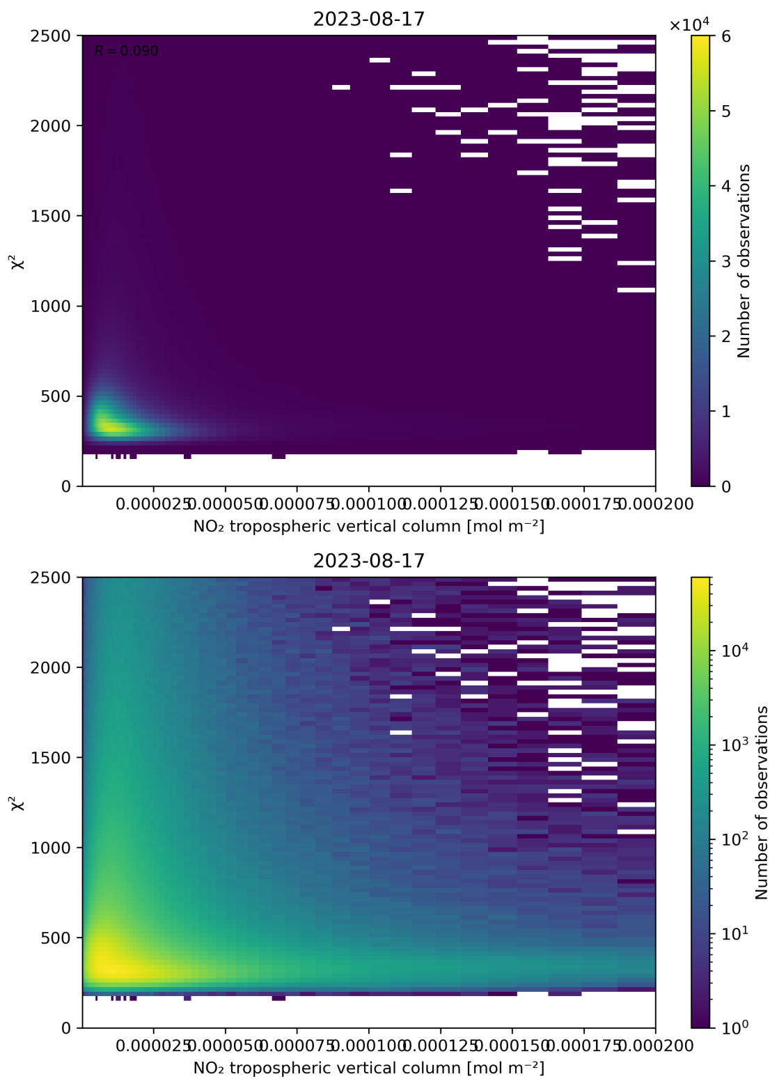
Figure 124: Scatter density plot of “NO 2 tropospheric vertical column” against “ \chi^2 ” for 2023-08-16 to 2023-08-18.
