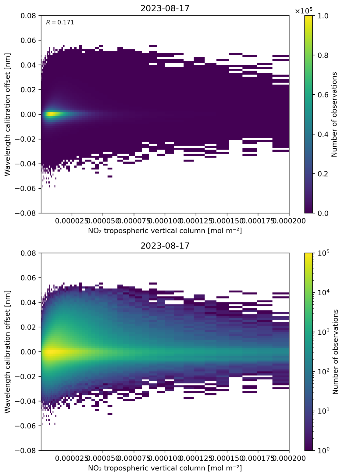
Figure 143: Scatter density plot of “NO 2 tropospheric vertical column” against “Wavelength calibration offset” for 2023-08-16 to 2023-08-18.
