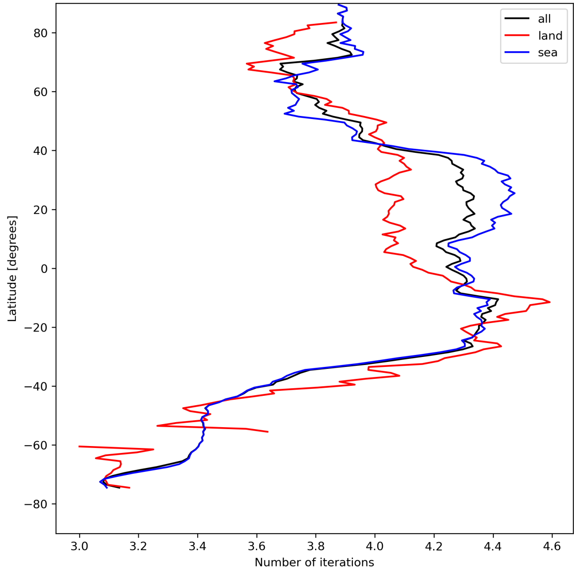
Figure 17: Zonal average of “Number of iterations” for 2023-08-16 to 2023-08-18.
