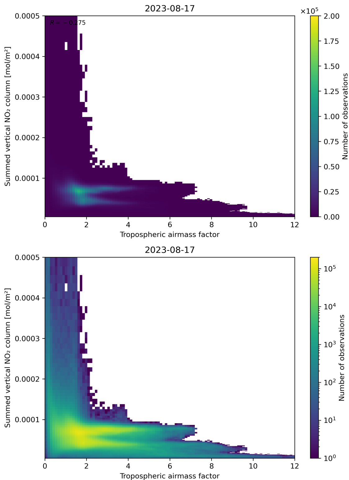
Figure 75: Scatter density plot of “Tropospheric airmass factor” against “Summed vertical NO 2 column” for 2023-08-16 to 2023-08-18.
