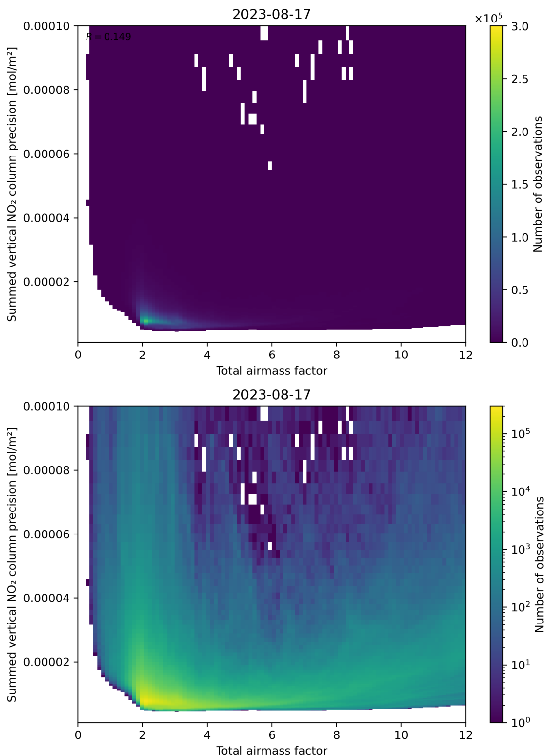
Figure 66: Scatter density plot of “Total airmass factor” against “Summed vertical NO 2 column precision” for 2023-08-16 to 2023-08-18.
