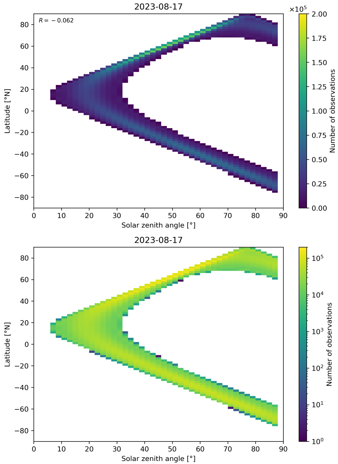
Figure 149: Scatter density plot of “Solar zenith angle” against “Latitude” for 2023-08-16 to 2023-08-18.
