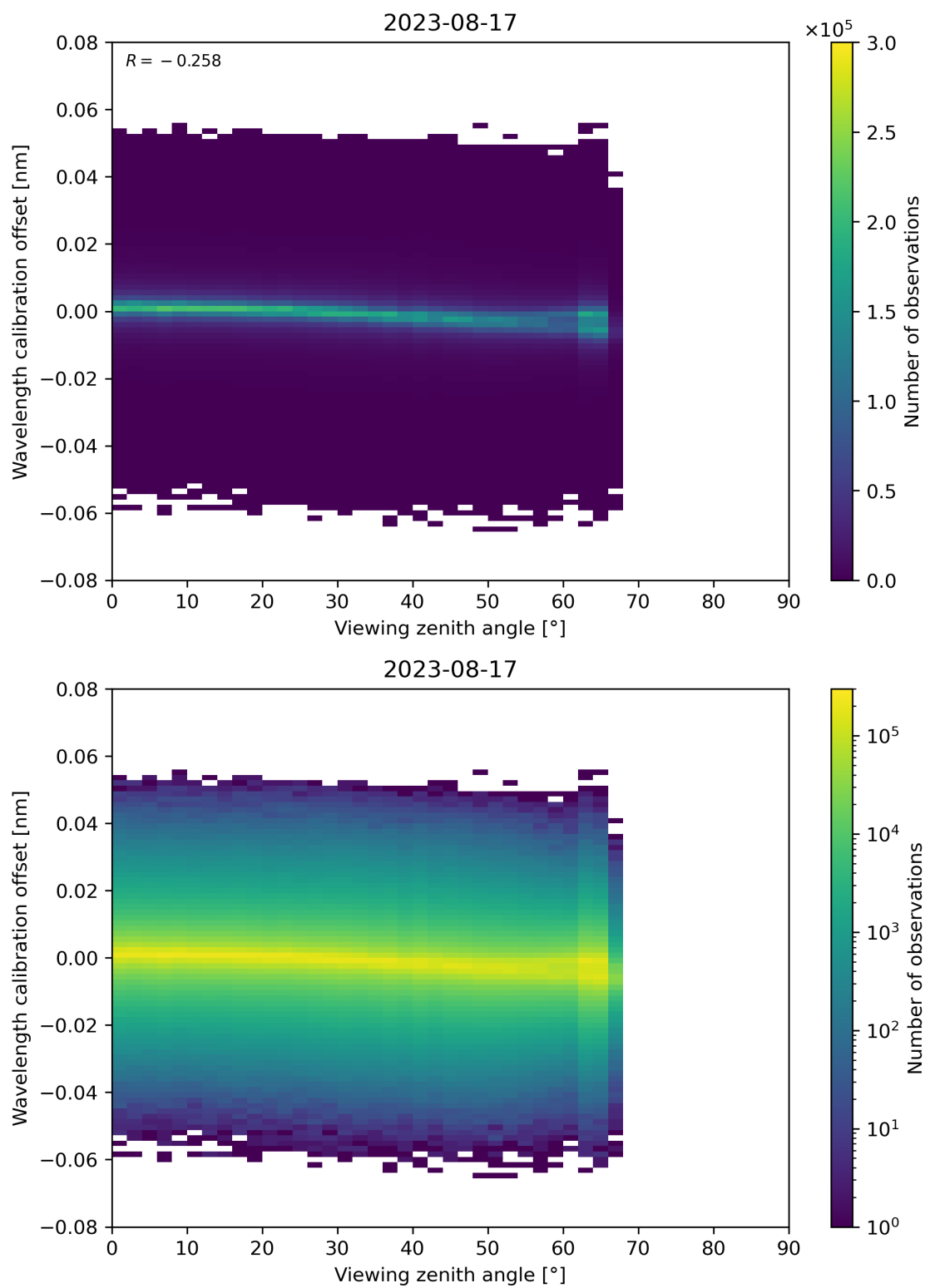
Figure 173: Scatter density plot of “Viewing zenith angle” against “Wavelength calibration offset” for 2023-08-16 to 2023-08-18.
