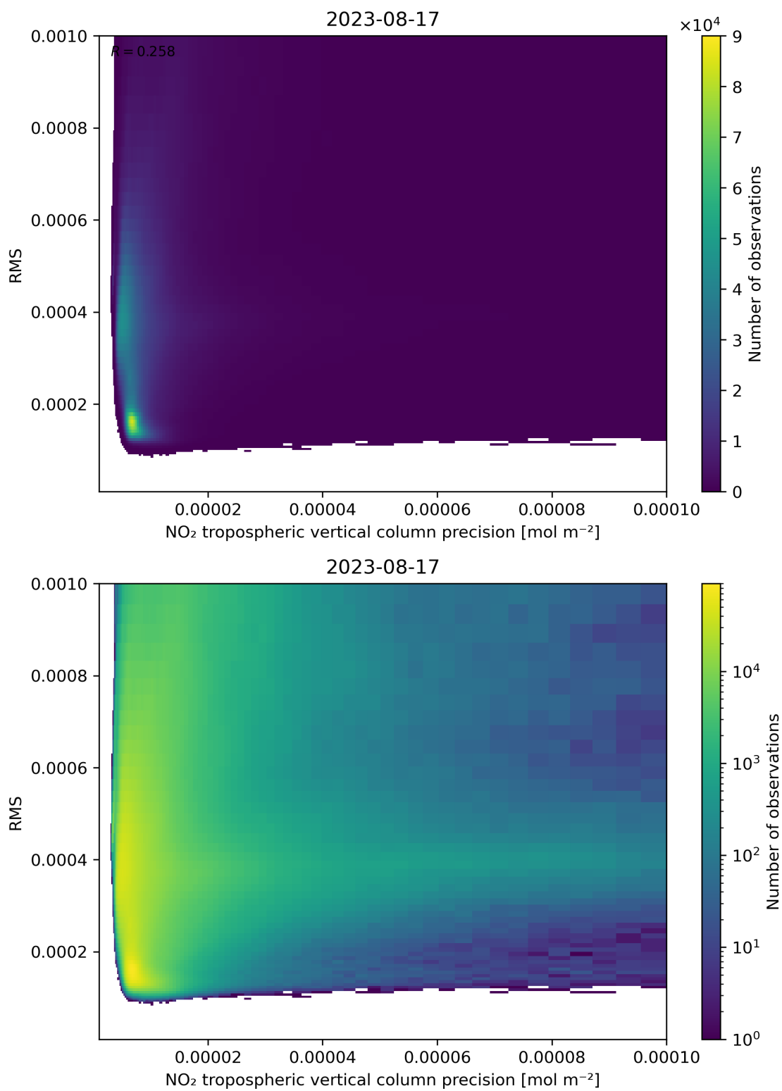
Figure 140: Scatter density plot of “NO 2 tropospheric vertical column precision” against “RMS” for 2023-08-16 to 2023-08-18.
