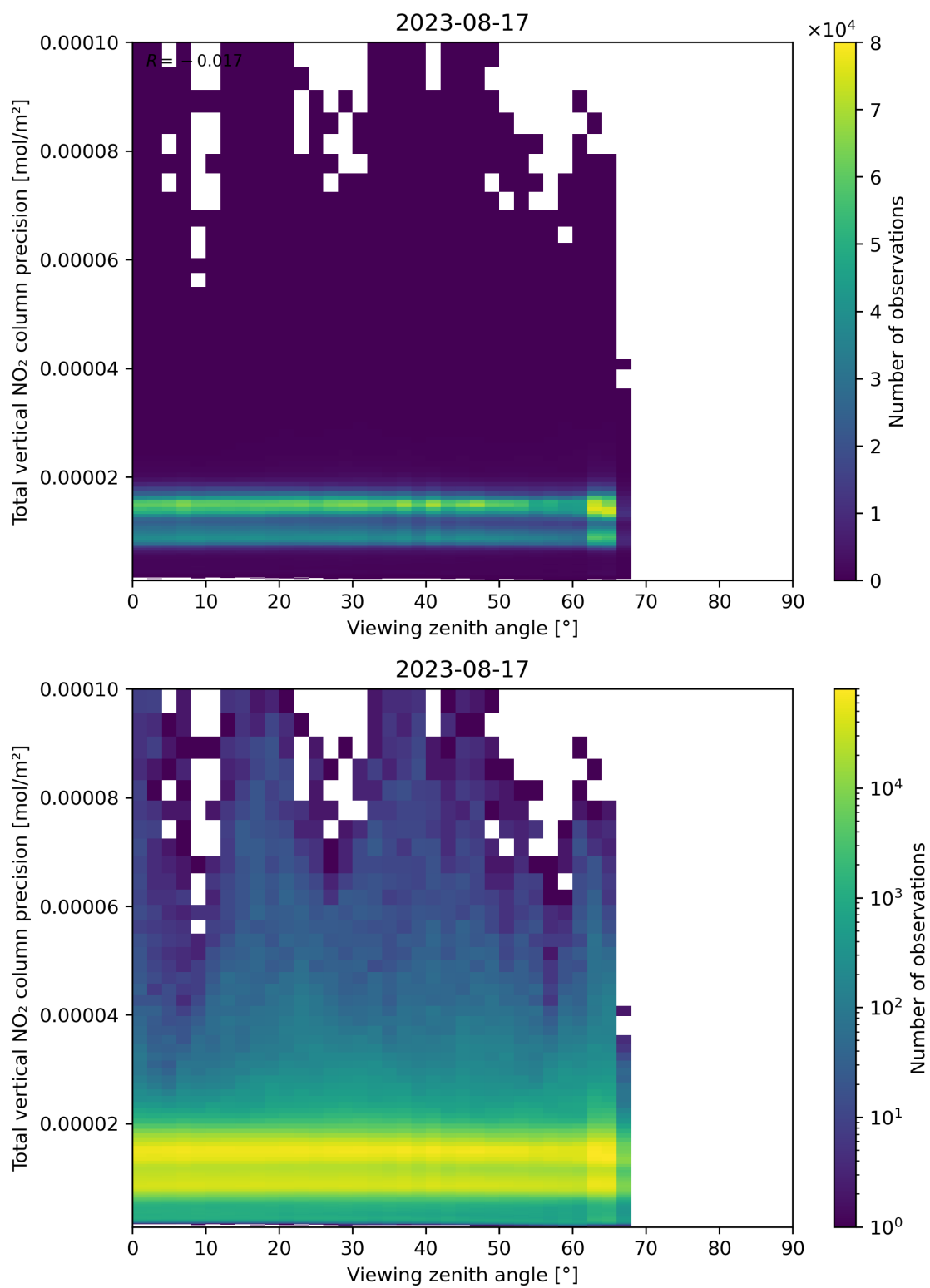
Figure 168: Scatter density plot of “Viewing zenith angle” against “Total vertical NO 2 column precision” for 2023-08-16 to 2023-08-18.
