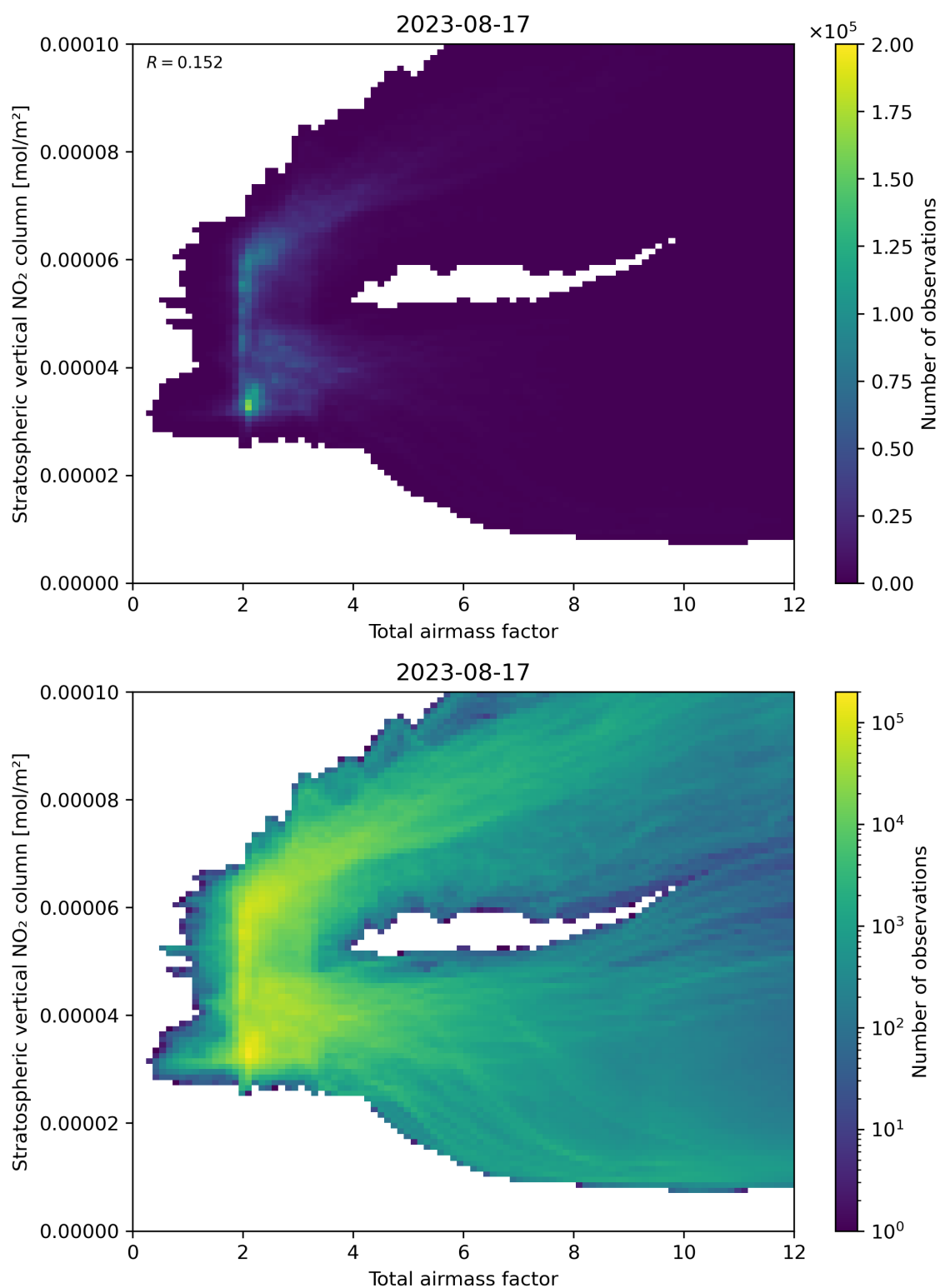
Figure 64: Scatter density plot of “Total airmass factor” against “Stratospheric vertical NO 2 column” for 2023-08-16 to 2023-08-18.
