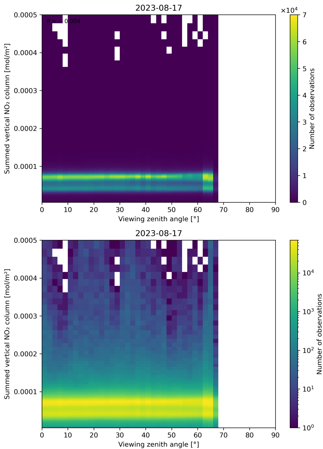
Figure 165: Scatter density plot of “Viewing zenith angle” against “Summed vertical NO 2 column” for 2023-08-16 to 2023-08-18.
