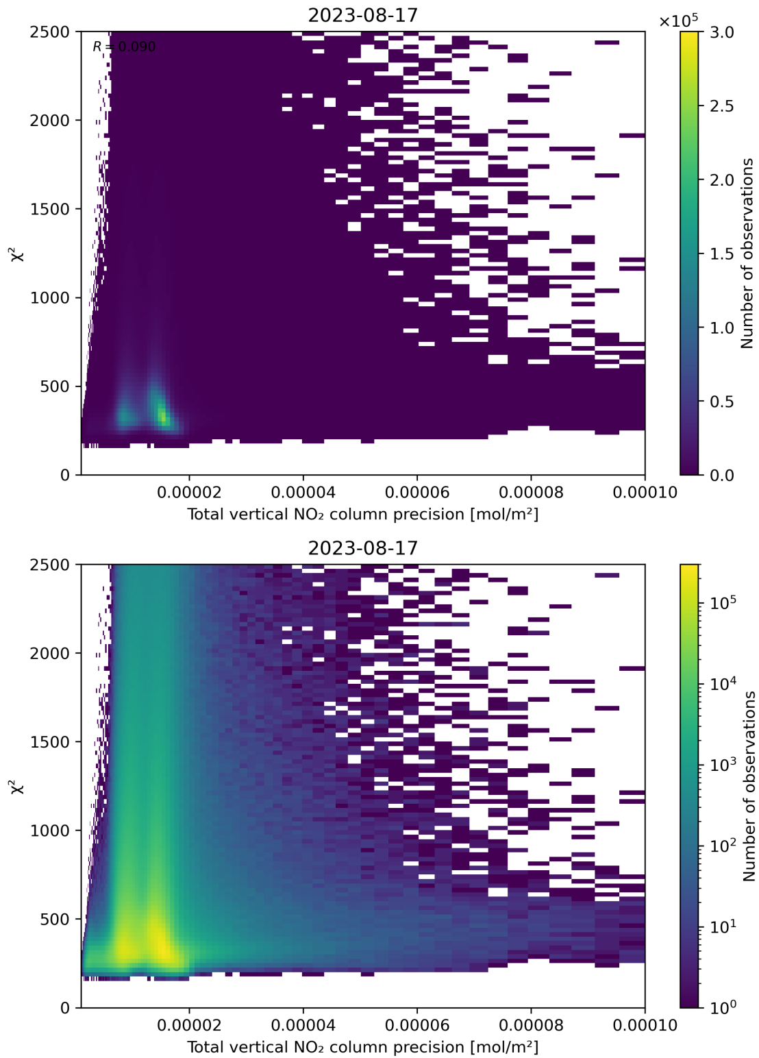
Figure 116: Scatter density plot of “Total vertical NO 2 column precision” against “ \chi^2 ” for 2023-08-16 to 2023-08-18.
