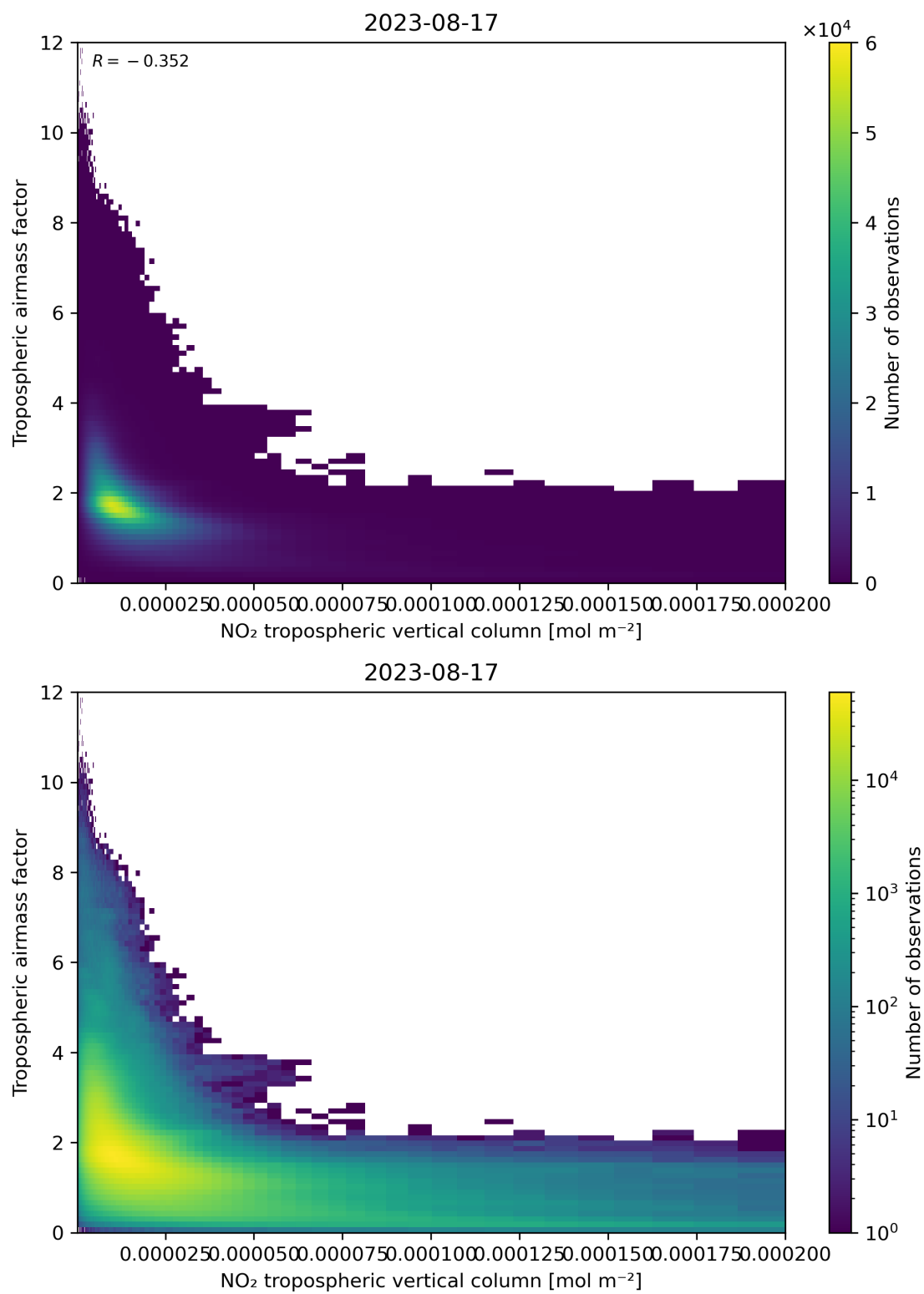
Figure 123: Scatter density plot of “NO 2 tropospheric vertical column” against “Tropospheric air mass factor” for 2023-08-16 to 2023-08-18.
