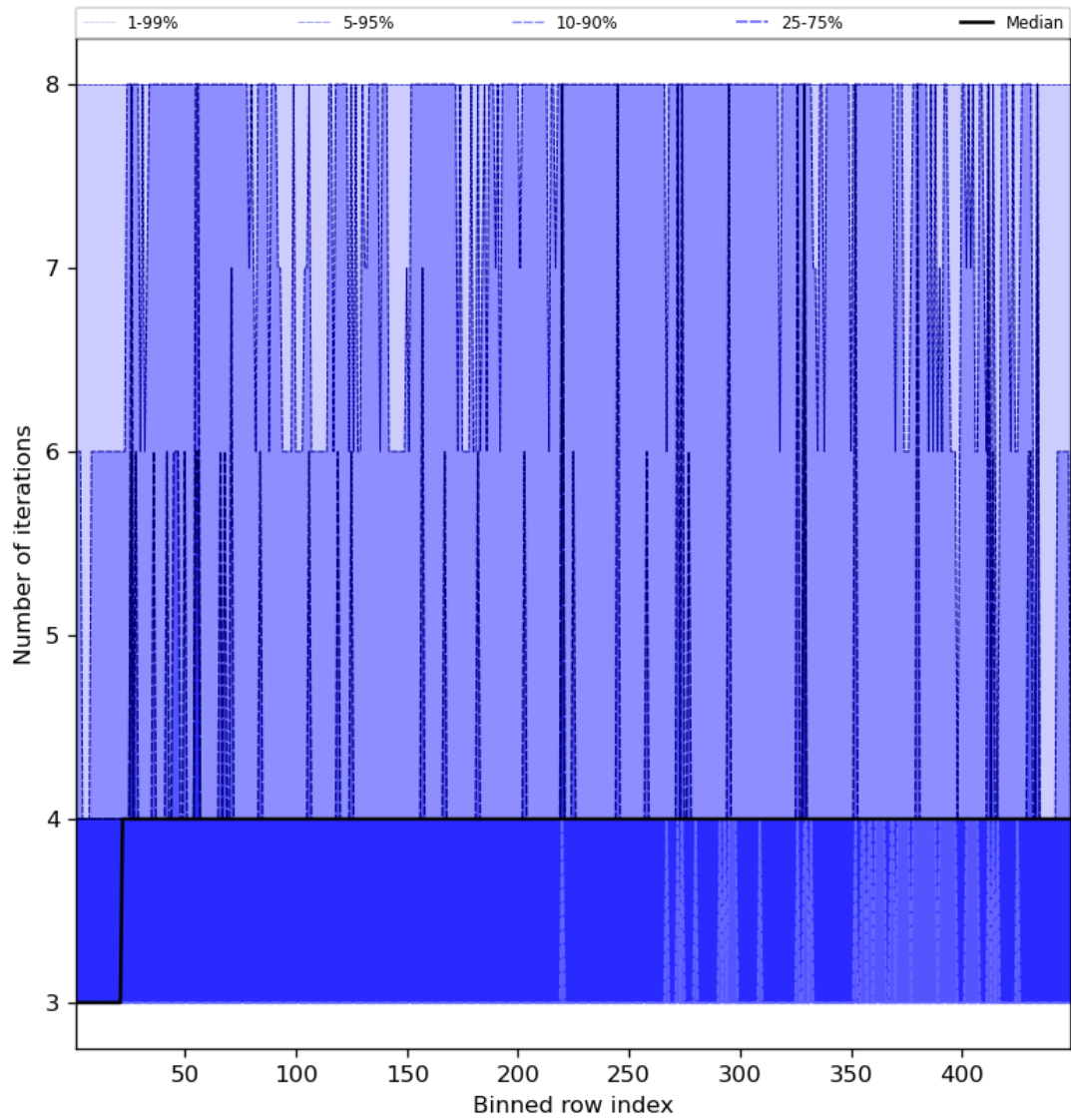
Figure 51: Along track statistics of “Number of iterations” for 2023-08-16 to 2023-08-18
