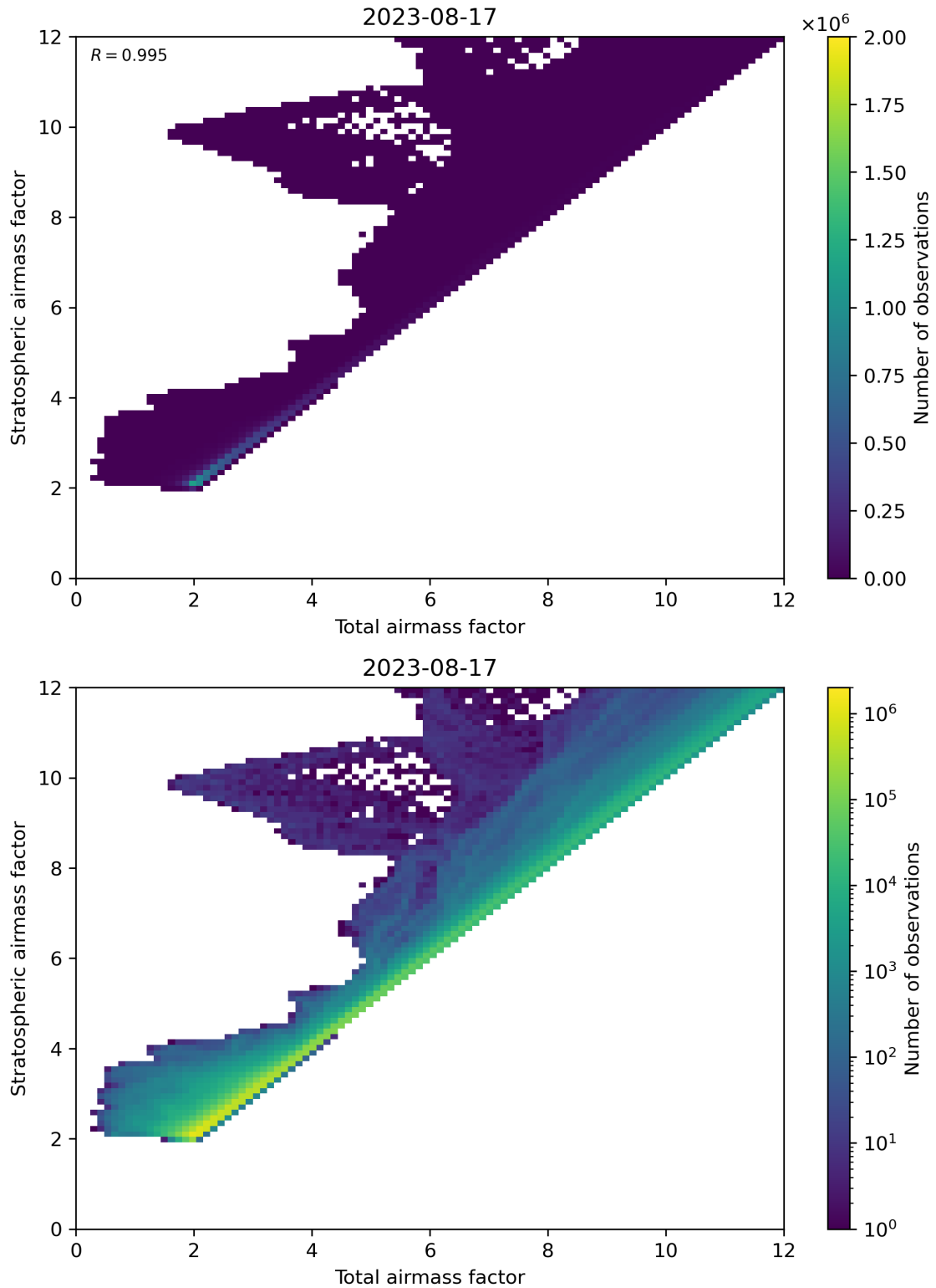
Figure 62: Scatter density plot of “Total airmass factor” against “Stratospheric airmass factor” for 2023-08-16 to 2023-08-18.
