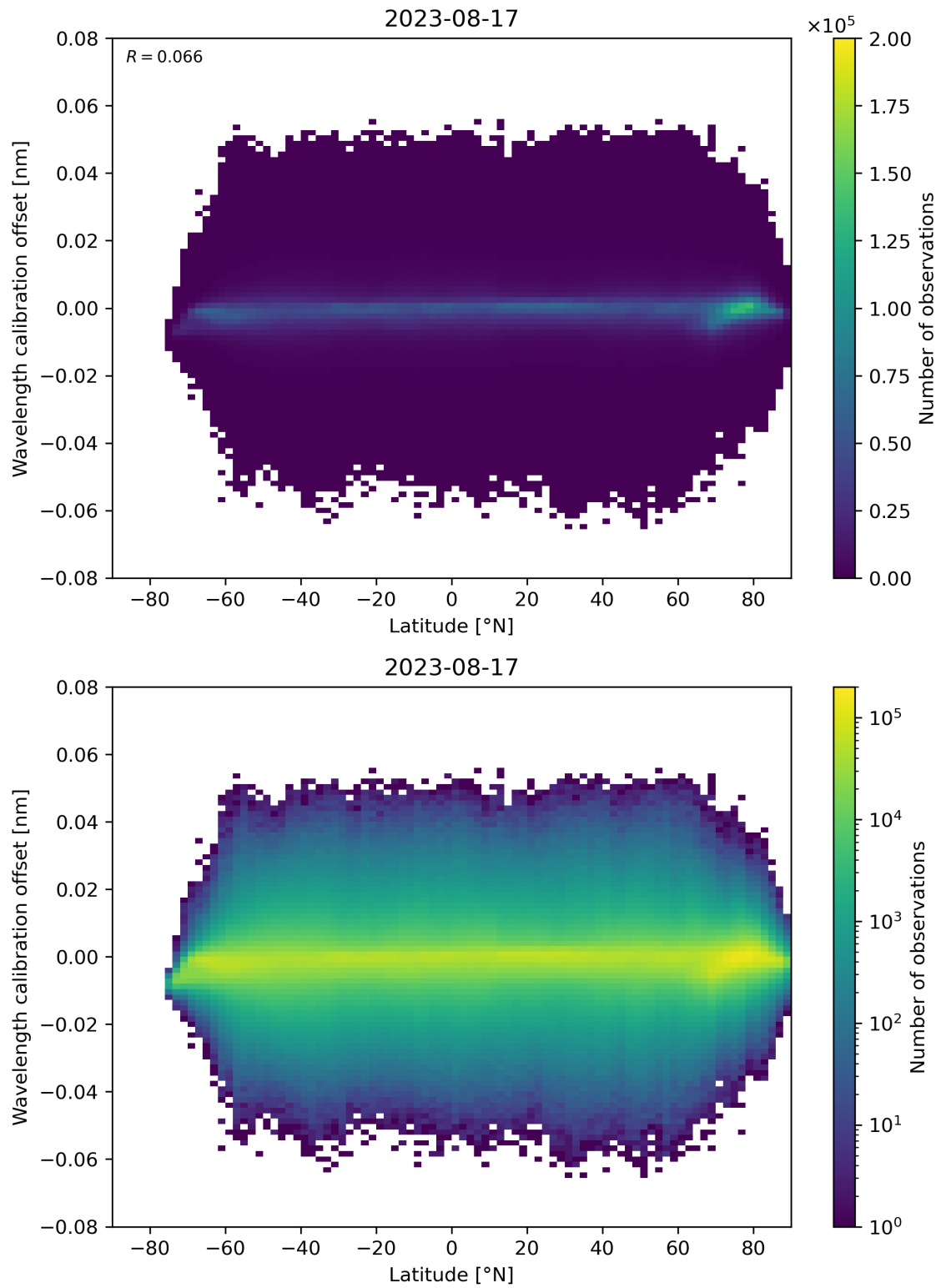
Figure 95: Scatter density plot of “Latitude” against “Wavelength calibration offset” for 2023-08-16 to 2023-08-18.
