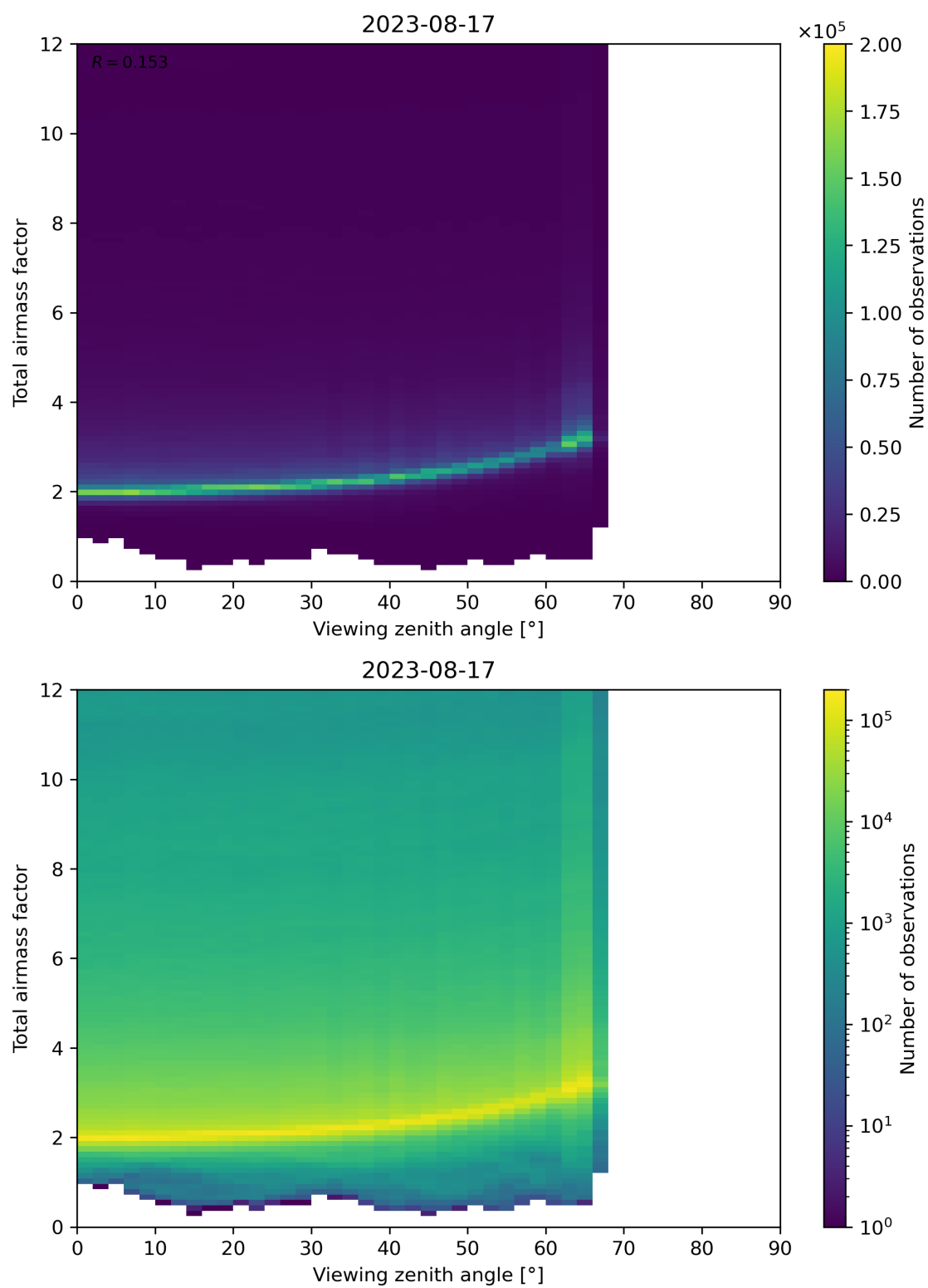
Figure 160: Scatter density plot of “Viewing zenith angle” against “Total airmass factor” for 2023-08-16 to 2023-08-18.
