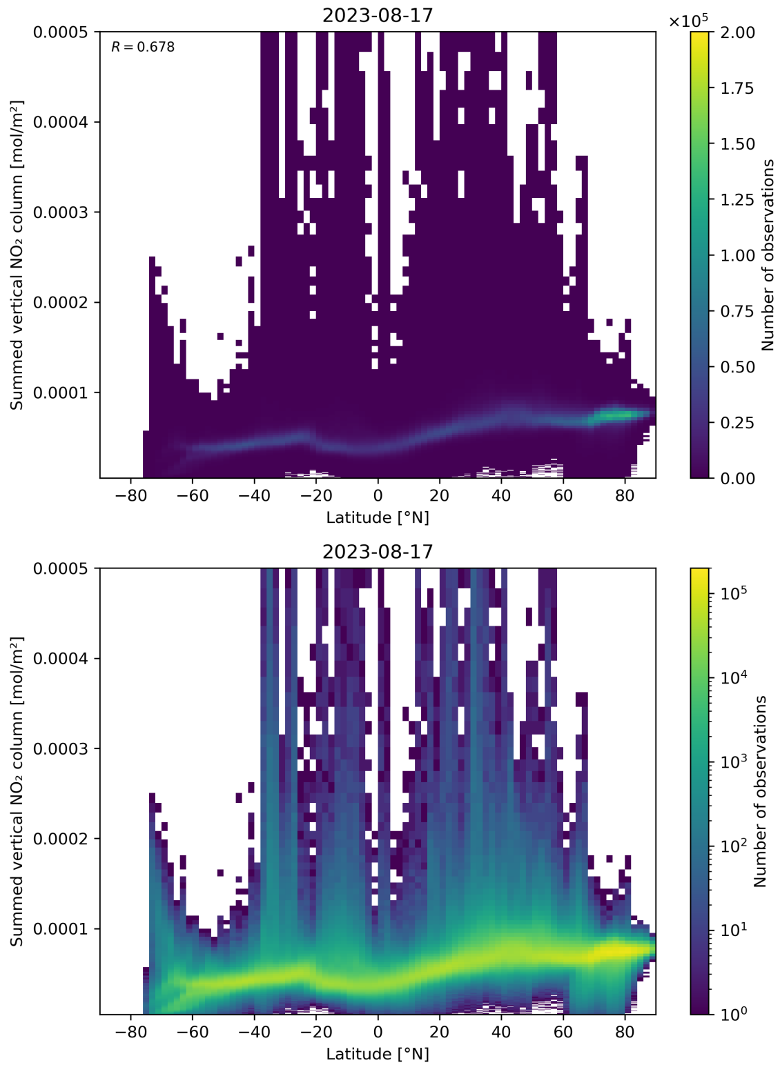
Figure 88: Scatter density plot of “Latitude” against “Summed vertical NO 2 column” for 2023-08-16 to 2023-08-18.
