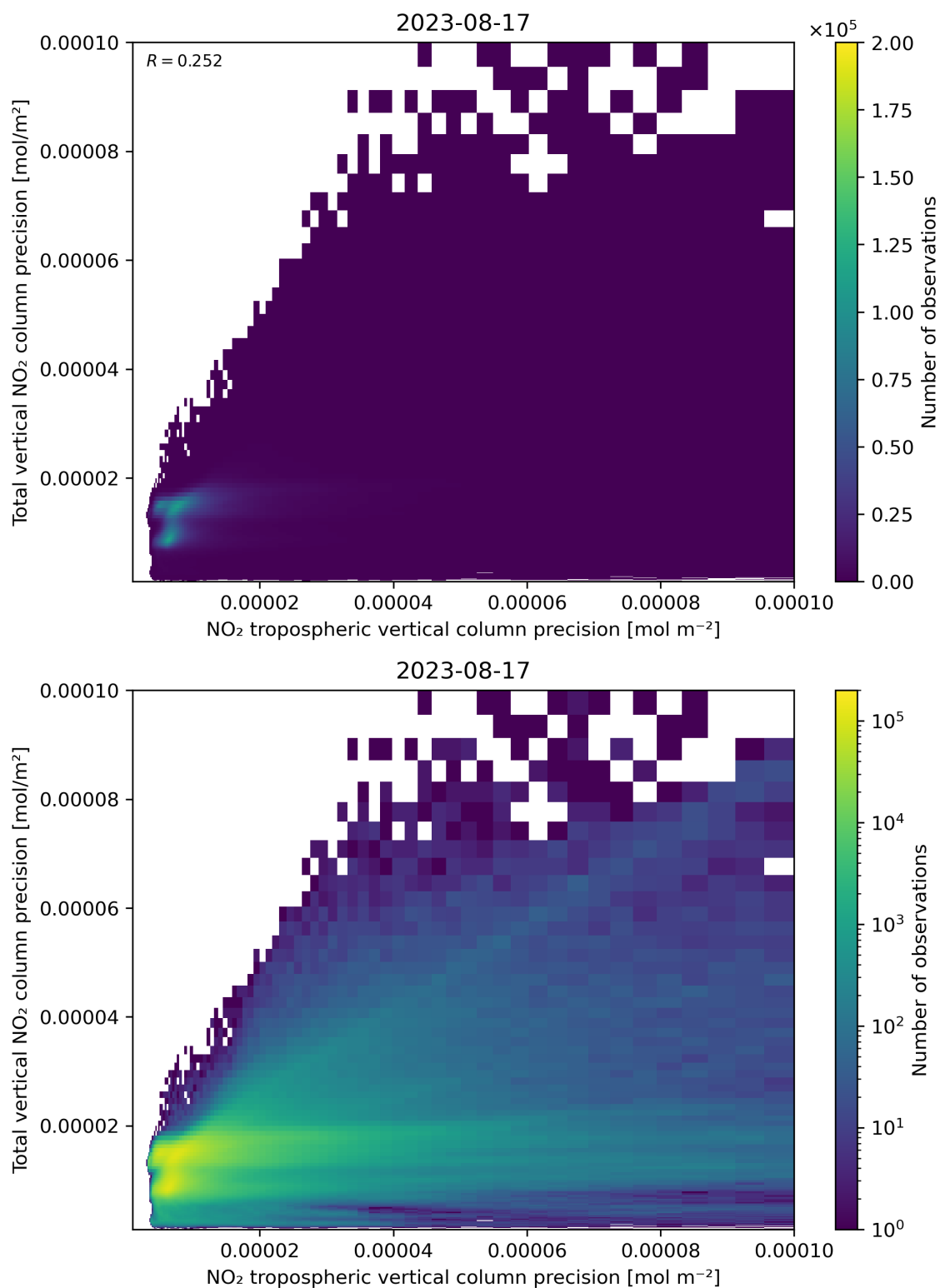
Figure 139: Scatter density plot of “NO 2 tropospheric vertical column precision” against “Total vertical NO 2 column precision” for 2023-08-16 to 2023-08-18.
