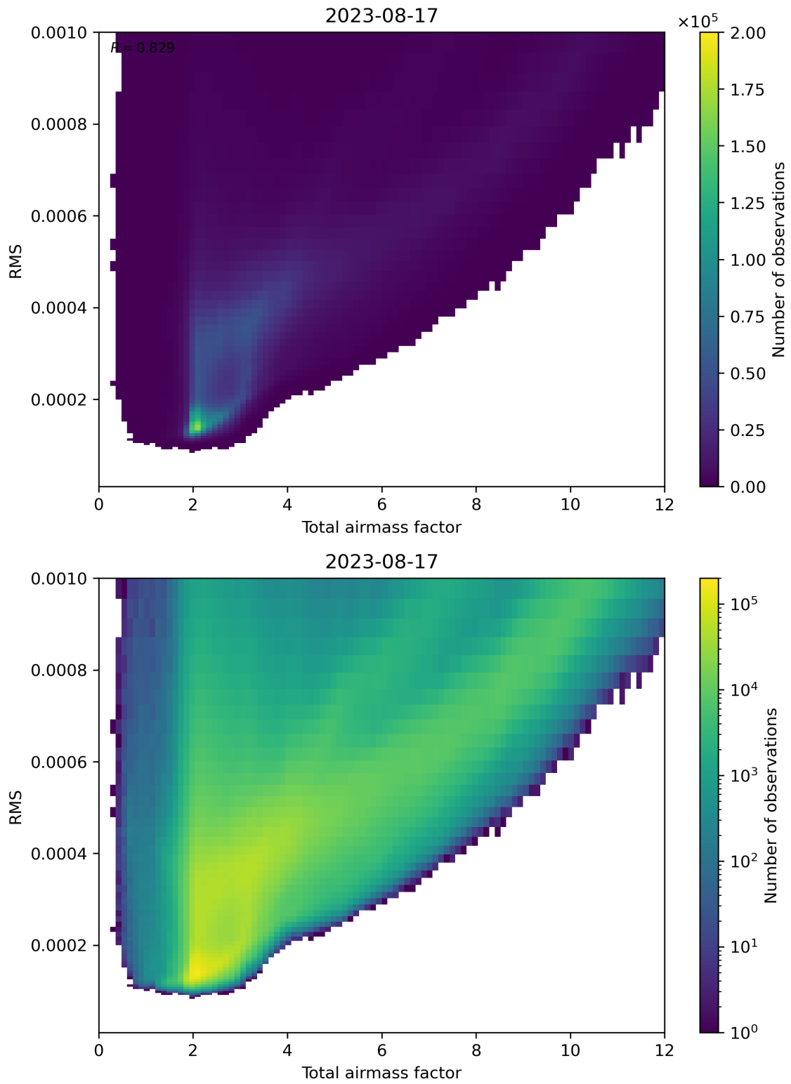
Figure 69: Scatter density plot of “Total airmass factor” against “RMS” for 2023-08-16 to 2023-08-18.
