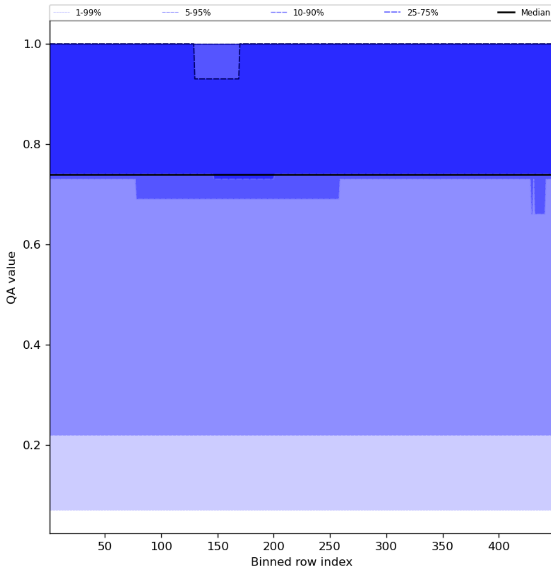
Figure 45: Along track statistics of “QA value” for 2023-08-16 to 2023-08-18
