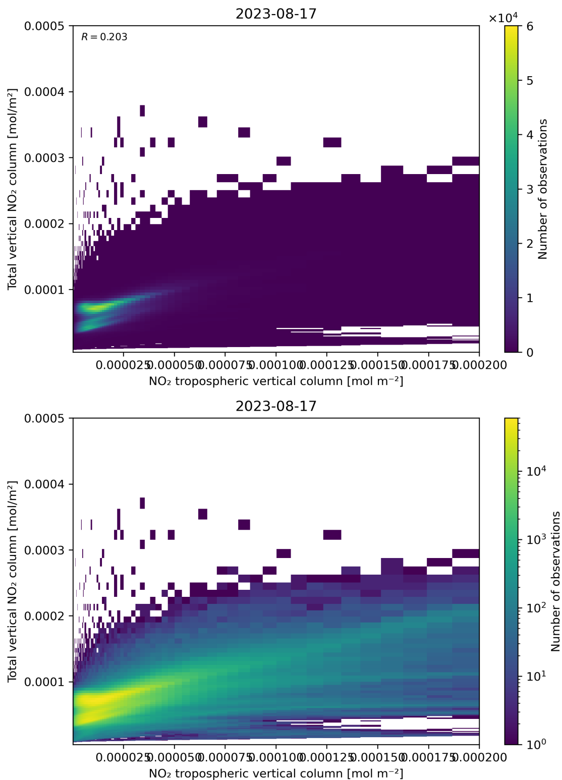
Figure 128: Scatter density plot of “NO 2 tropospheric vertical column” against “Total vertical NO 2 column” for 2023-08-16 to 2023-08-18.
