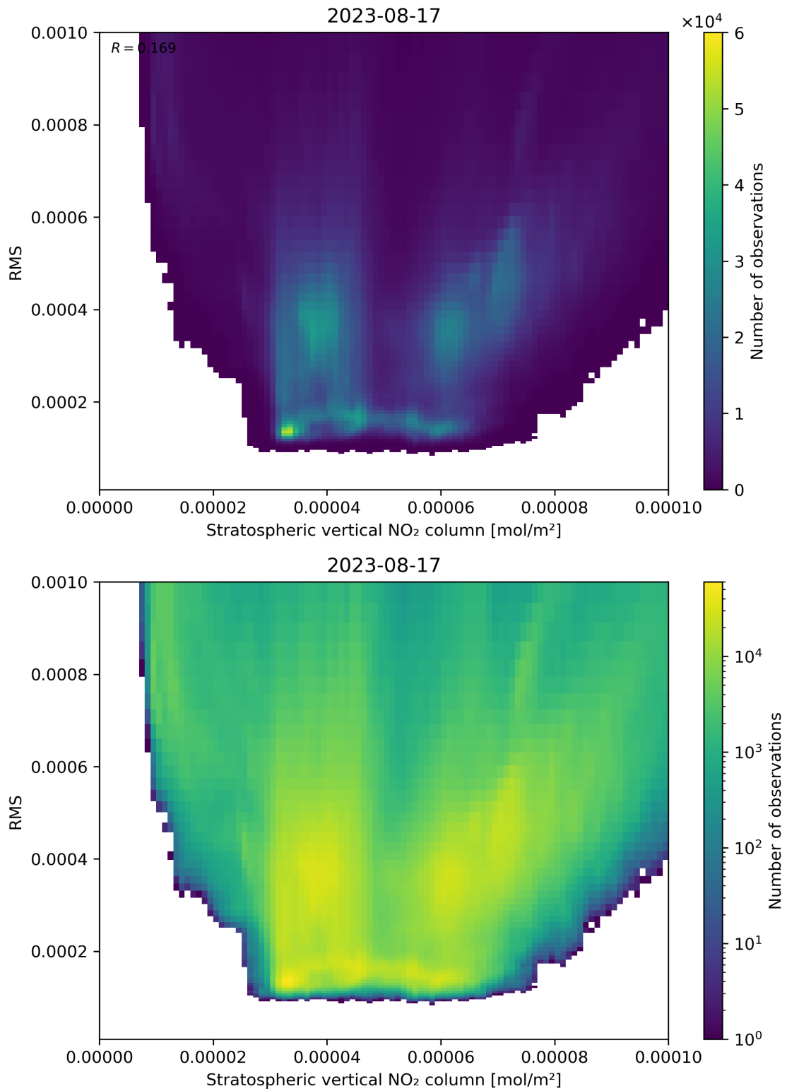
Figure 102: Scatter density plot of “Stratospheric vertical NO 2 column” against “RMS” for 2023-08-16 to 2023-08-18.
