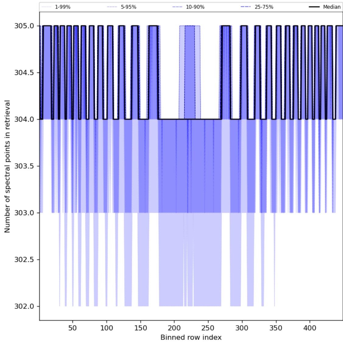
Figure 50: Along track statistics of “Number of spectral points in retrieval” for 2023-08-16 to 2023-08-18
