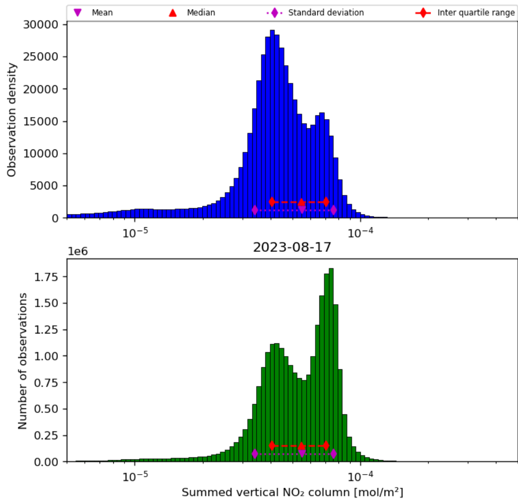
Figure 40: Histogram of “Summed vertical NO 2 column” for 2023-08-16 to 2023-08-18
