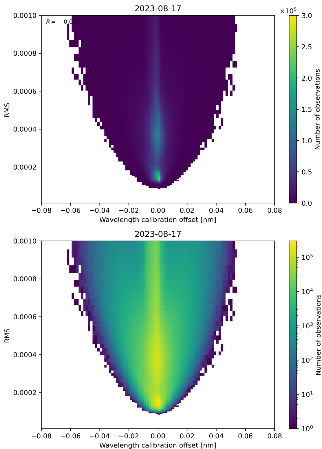
Figure 181: Scatter density plot of “Wavelength calibration offset” against “RMS” for 2023-08-16 to 2023-08-18.
