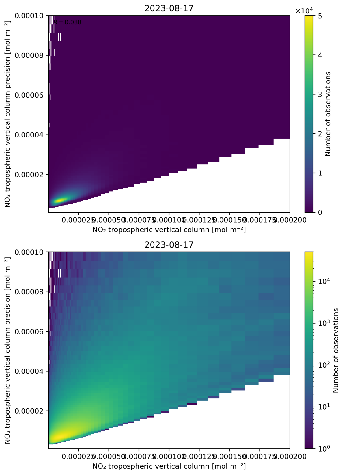
Figure 130: Scatter density plot of “NO 2 tropospheric vertical column” against “NO 2 tropospheric vertical column precision” for 2023-08-16 to 2023-08-18.
