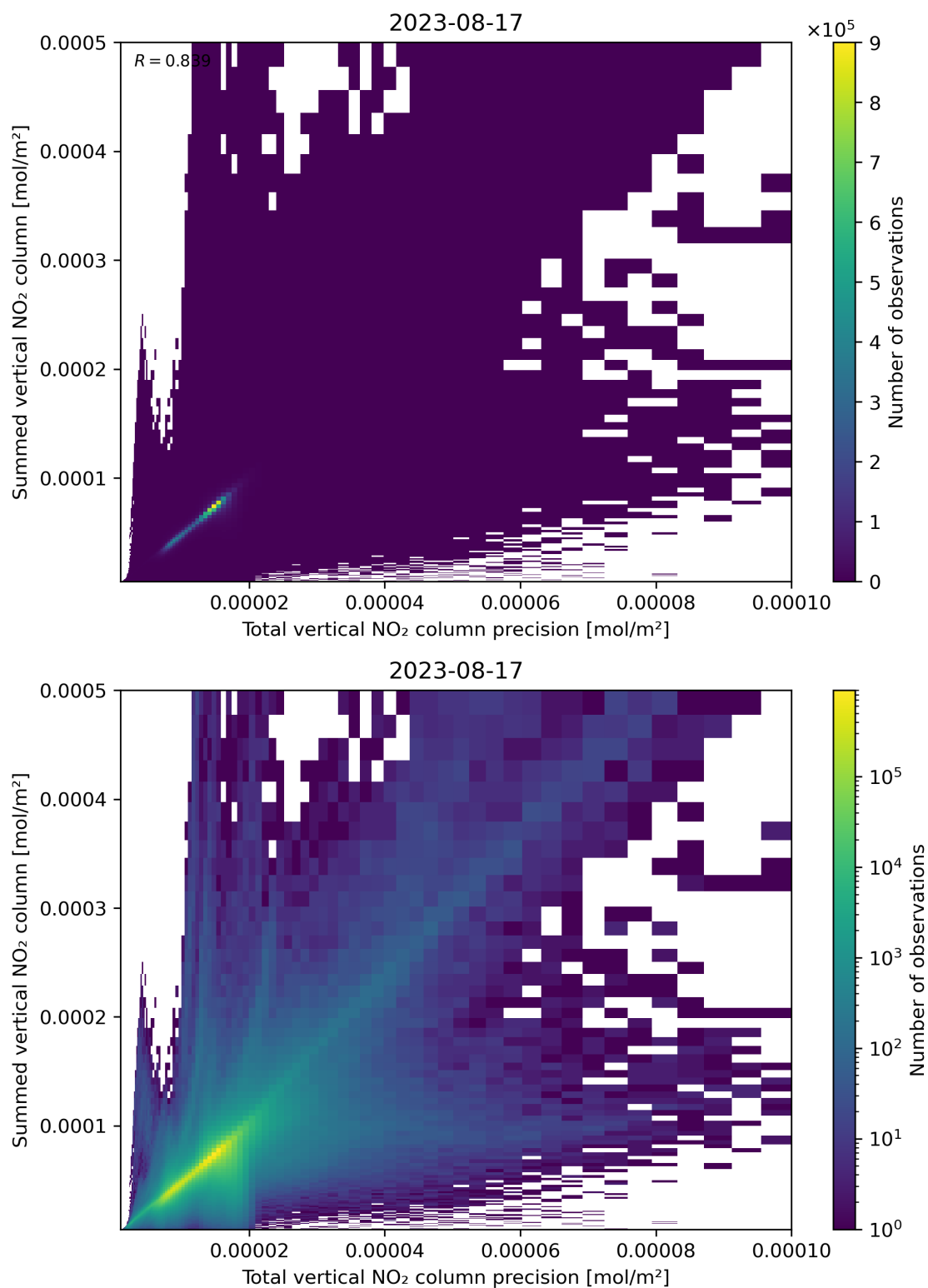
Figure 117: Scatter density plot of “Total vertical NO 2 column precision” against “Summed vertical NO 2 column” for 2023-08-16 to 2023-08-18.
