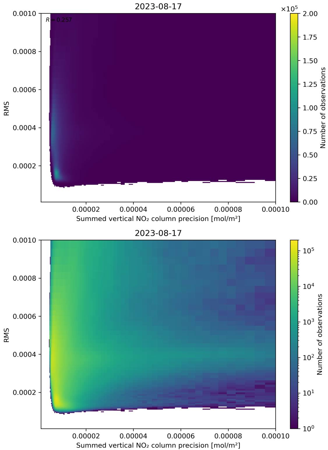
Figure 108: Scatter density plot of “Summed vertical NO 2 column precision” against “RMS” for 2023-08-16 to 2023-08-18.
