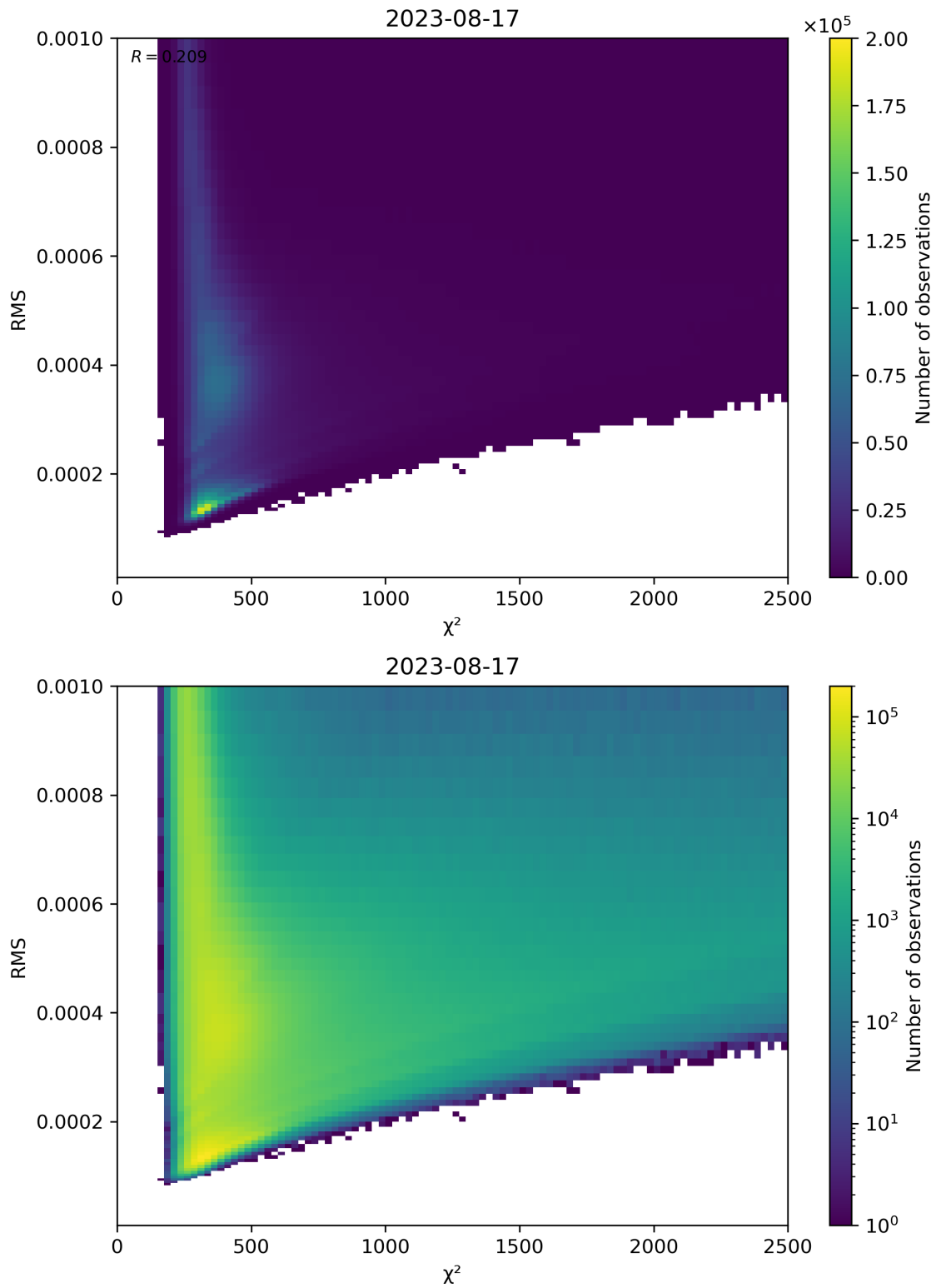
Figure 82: Scatter density plot of “ \chi^2 ” against “RMS” for 2023-08-16 to 2023-08-18.
