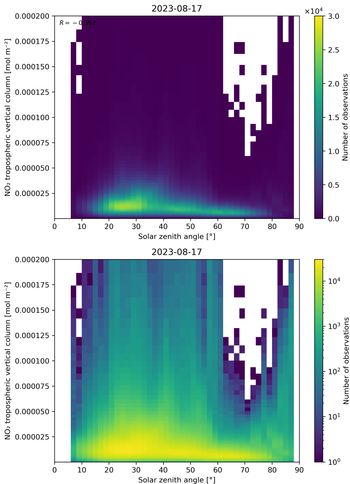
Figure 155: Scatter density plot of “Solar zenith angle” against “NO 2 tropospheric vertical column” for 2023-08-16 to 2023-08-18.
