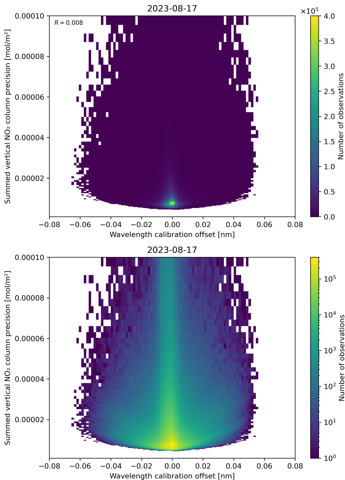
Figure 178: Scatter density plot of “Wavelength calibration offset” against “Summed vertical NO 2 column precision” for 2023-08-16 to 2023-08-18.
