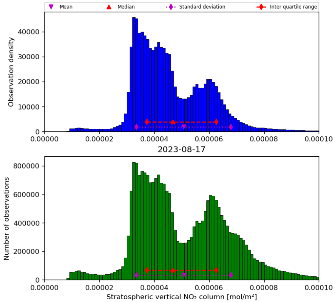
Figure 36: Histogram of “Stratospheric vertical NO 2 column” for 2023-08-16 to 2023-08-18
