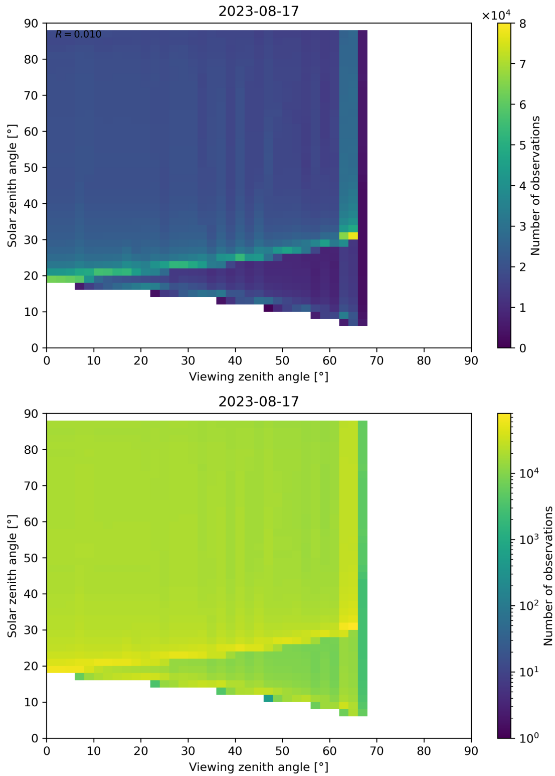
Figure 172: Scatter density plot of “Viewing zenith angle” against “Solar zenith angle” for 2023-08-16 to 2023-08-18.
