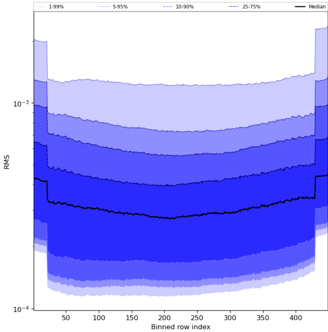
Figure 60: Along track statistics of “RMS” for 2023-08-16 to 2023-08-18
