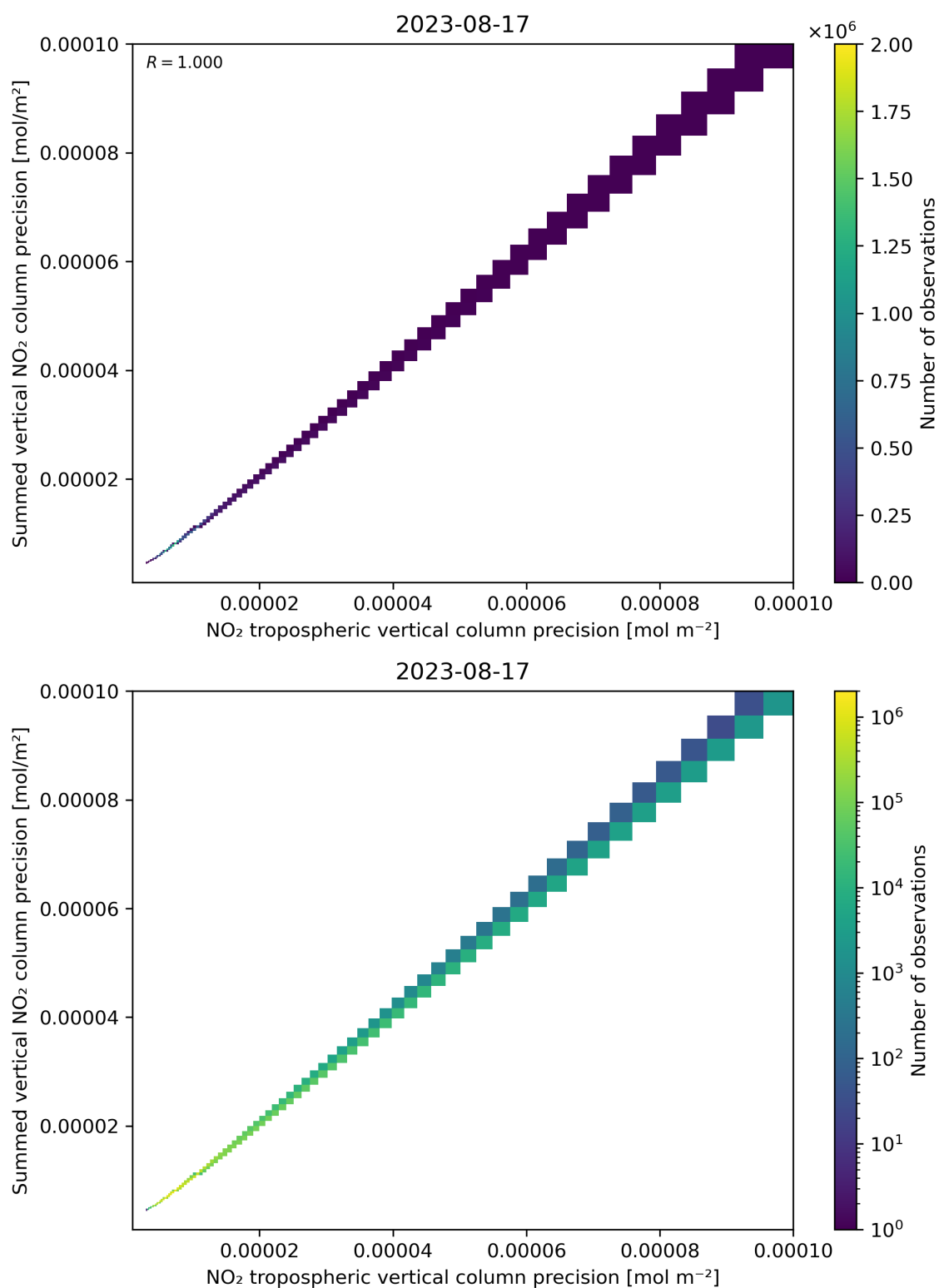
Figure 137: Scatter density plot of “NO 2 tropospheric vertical column precision” against “Summed vertical NO 2 column precision” for 2023-08-16 to 2023-08-18.
