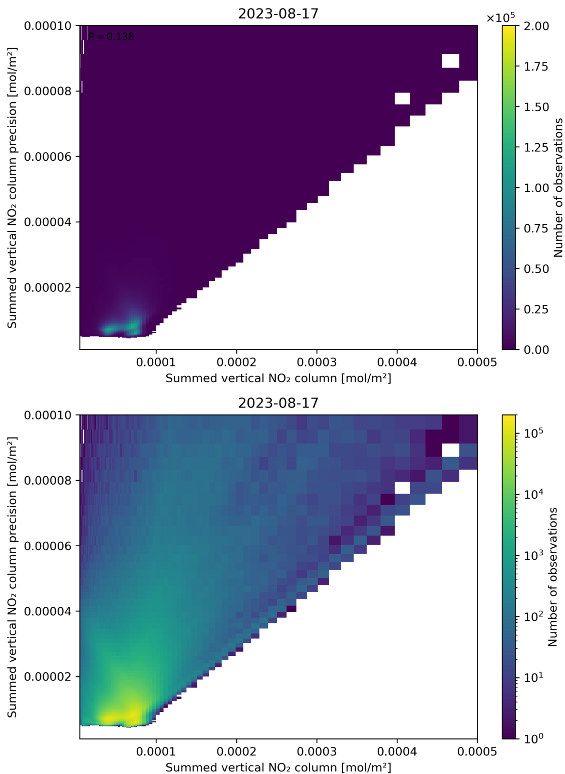
Figure 105: Scatter density plot of “Summed vertical NO 2 column” against “Summed vertical NO 2 column precision” for 2023-08-16 to 2023-08-18.
