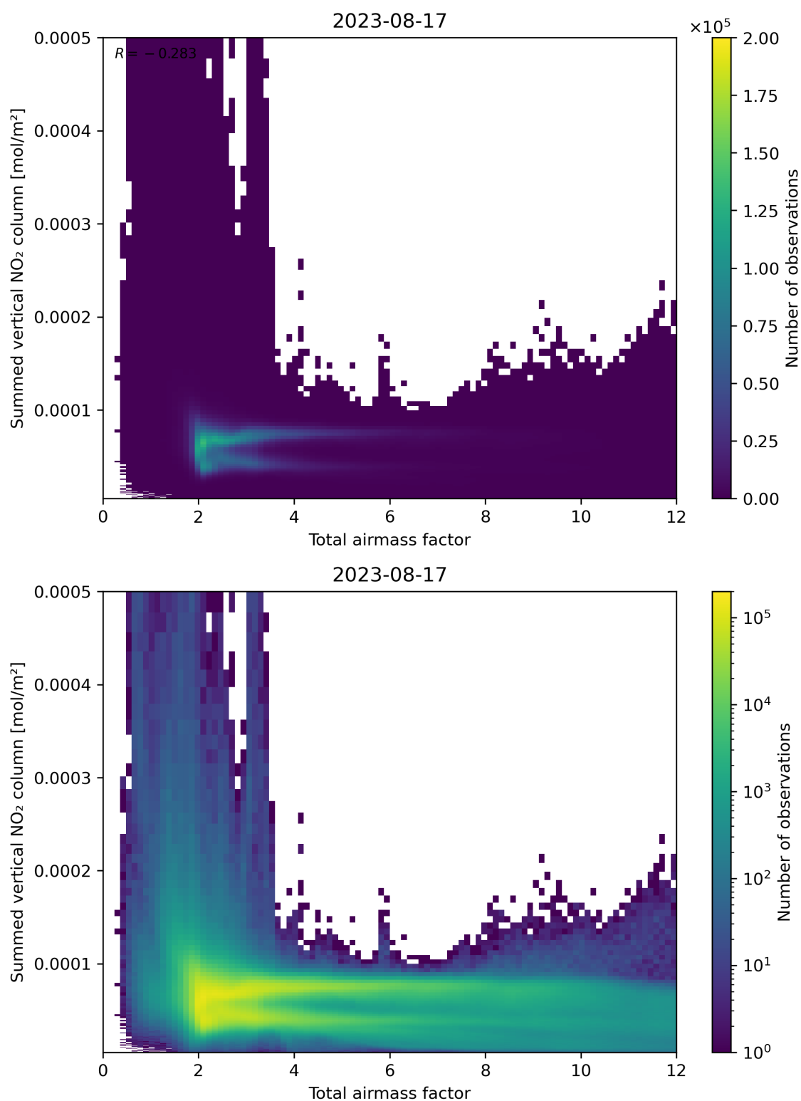
Figure 65: Scatter density plot of “Total airmass factor” against “Summed vertical NO 2 column” for 2023-08-16 to 2023-08-18.
