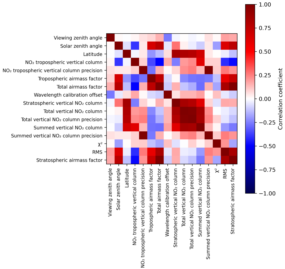
Figure 2: Map of correlation matrix for 2023-08-16 to 2023-08-18.
