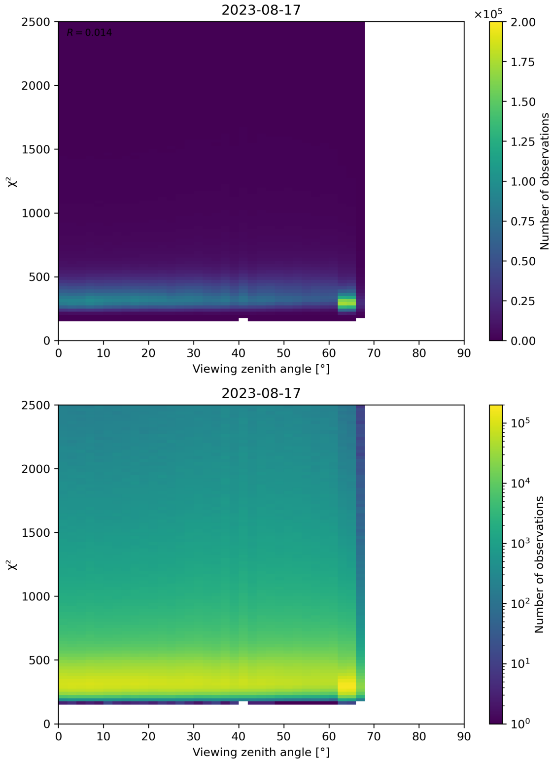
Figure 162: Scatter density plot of “Viewing zenith angle” against “ \chi^2 ” for 2023-08-16 to 2023-08-18.
