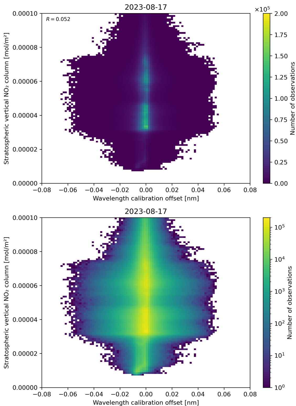
Figure 176: Scatter density plot of “Wavelength calibration offset” against “Stratospheric vertical NO 2 column” for 2023-08-16 to 2023-08-18.
