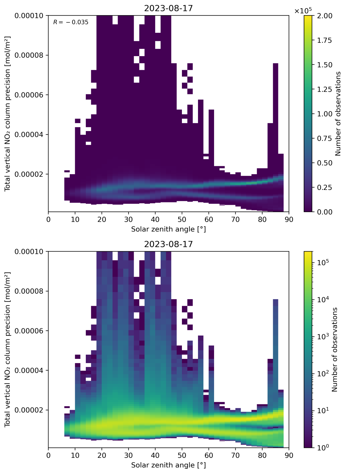
Figure 154: Scatter density plot of “Solar zenith angle” against “Total vertical NO 2 column precision” for 2023-08-16 to 2023-08-18.
