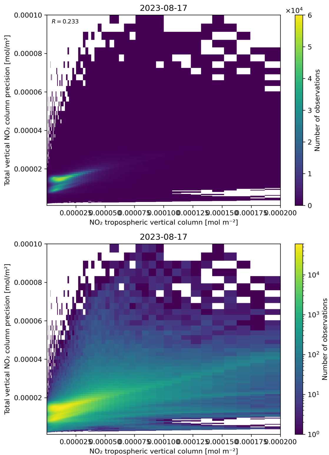
Figure 129: Scatter density plot of “NO 2 tropospheric vertical column” against “Total vertical NO 2 column precision” for 2023-08-16 to 2023-08-18.
