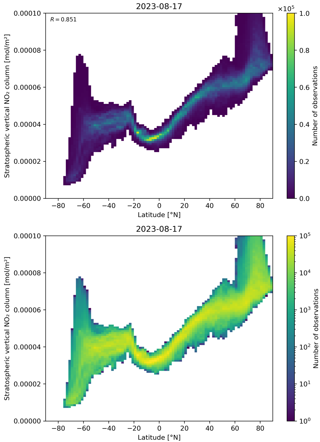
Figure 87: Scatter density plot of “Latitude” against “Stratospheric vertical NO 2 column” for 2023-08-16 to 2023-08-18.
