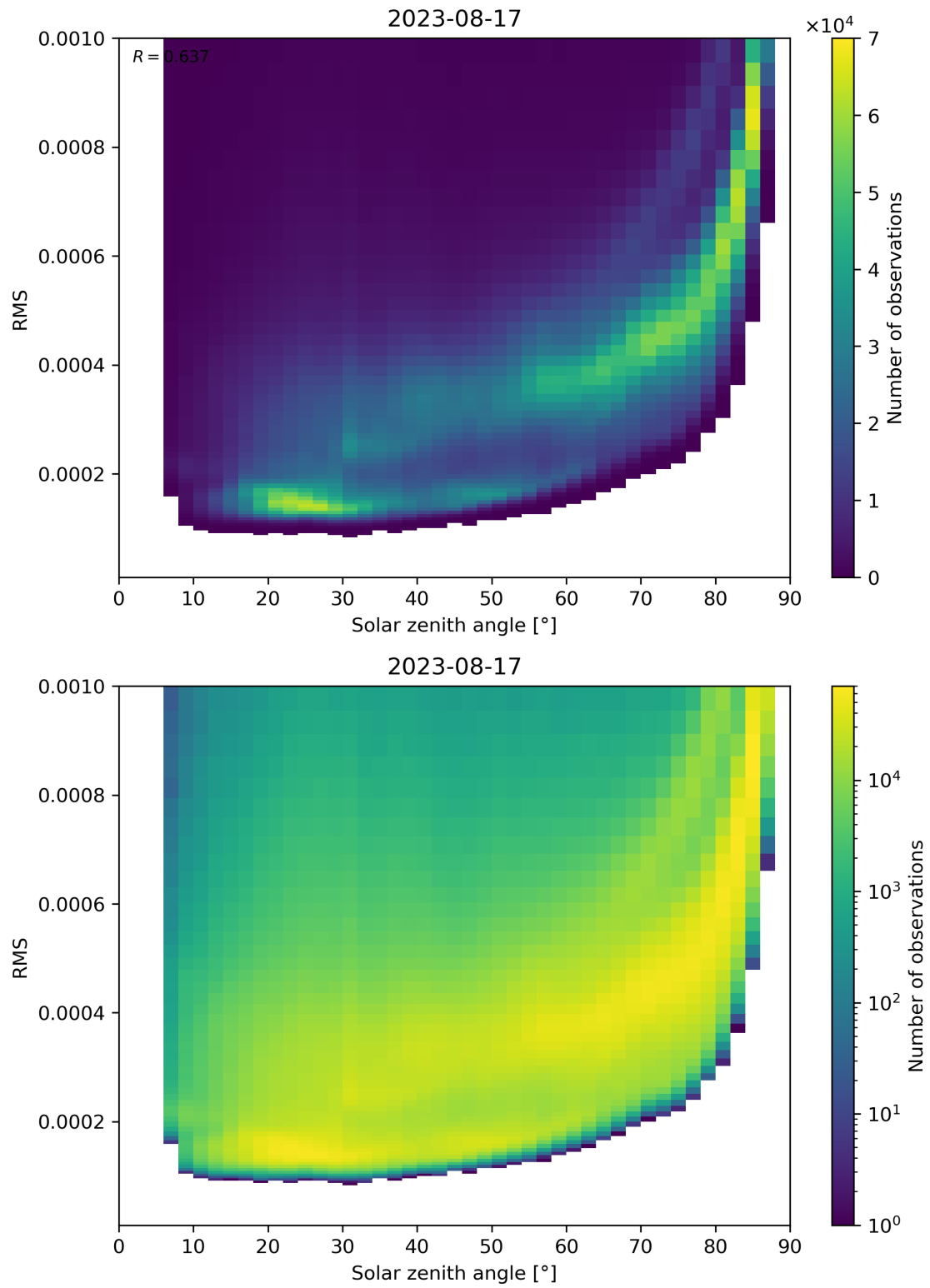
Figure 157: Scatter density plot of “Solar zenith angle” against “RMS” for 2023-08-16 to 2023-08-18.
