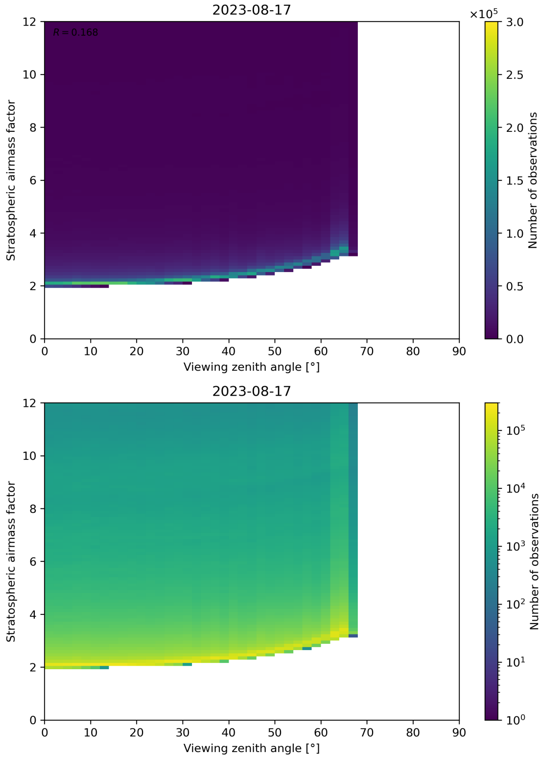
Figure 159: Scatter density plot of “Viewing zenith angle” against “Stratospheric airmass factor” for 2023-08-16 to 2023-08-18.
