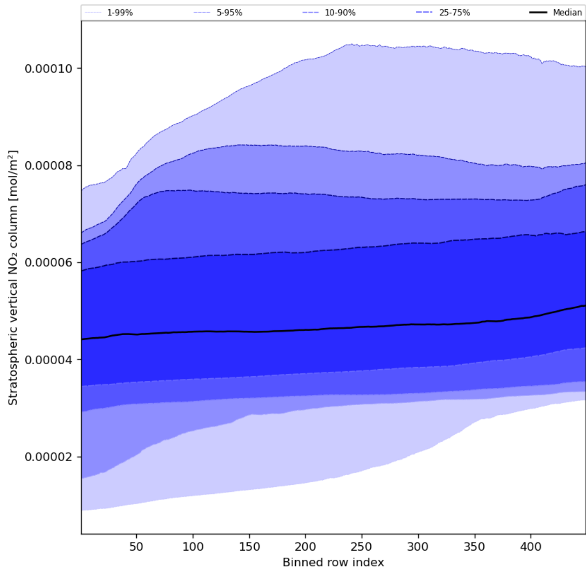
Figure 53: Along track statistics of “Stratospheric vertical NO 2 column” for 2023-08-16 to 2023-08-18
