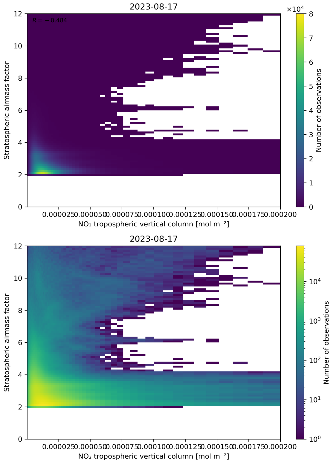
Figure 121: Scatter density plot of “NO 2 tropospheric vertical column” against “Stratospheric air mass factor” for 2023-08-16 to 2023-08-18.
