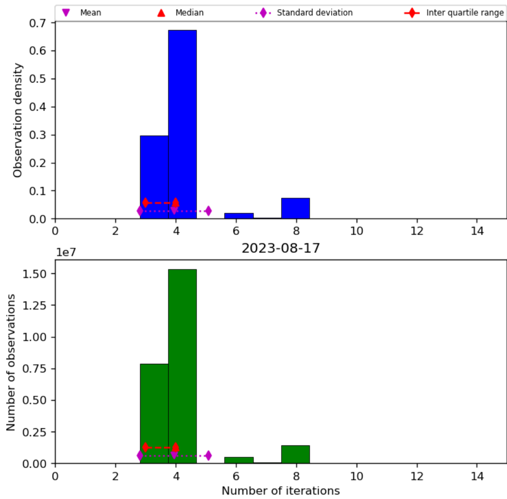
Figure 34: Histogram of “Number of iterations” for 2023-08-16 to 2023-08-18
