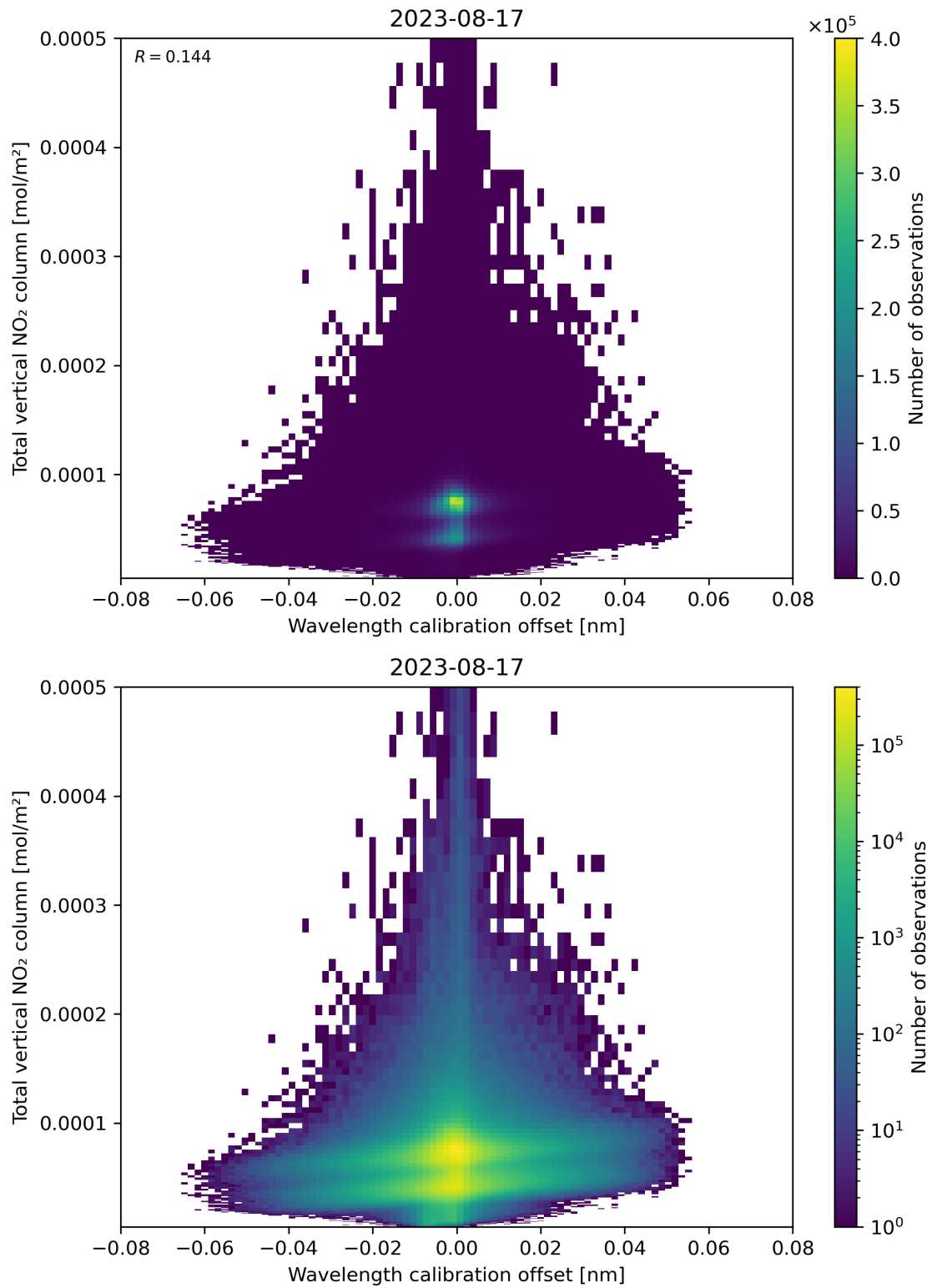
Figure 179: Scatter density plot of “Wavelength calibration offset” against “Total vertical NO 2 column” for 2023-08-16 to 2023-08-18.
