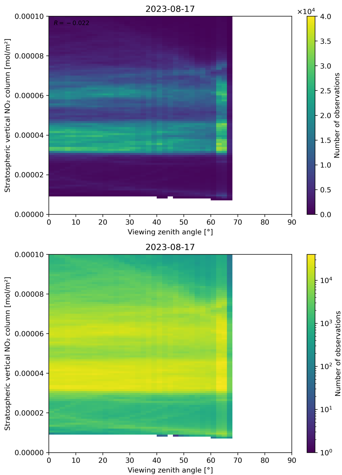
Figure 164: Scatter density plot of “Viewing zenith angle” against “Stratospheric vertical NO 2 column” for 2023-08-16 to 2023-08-18.
