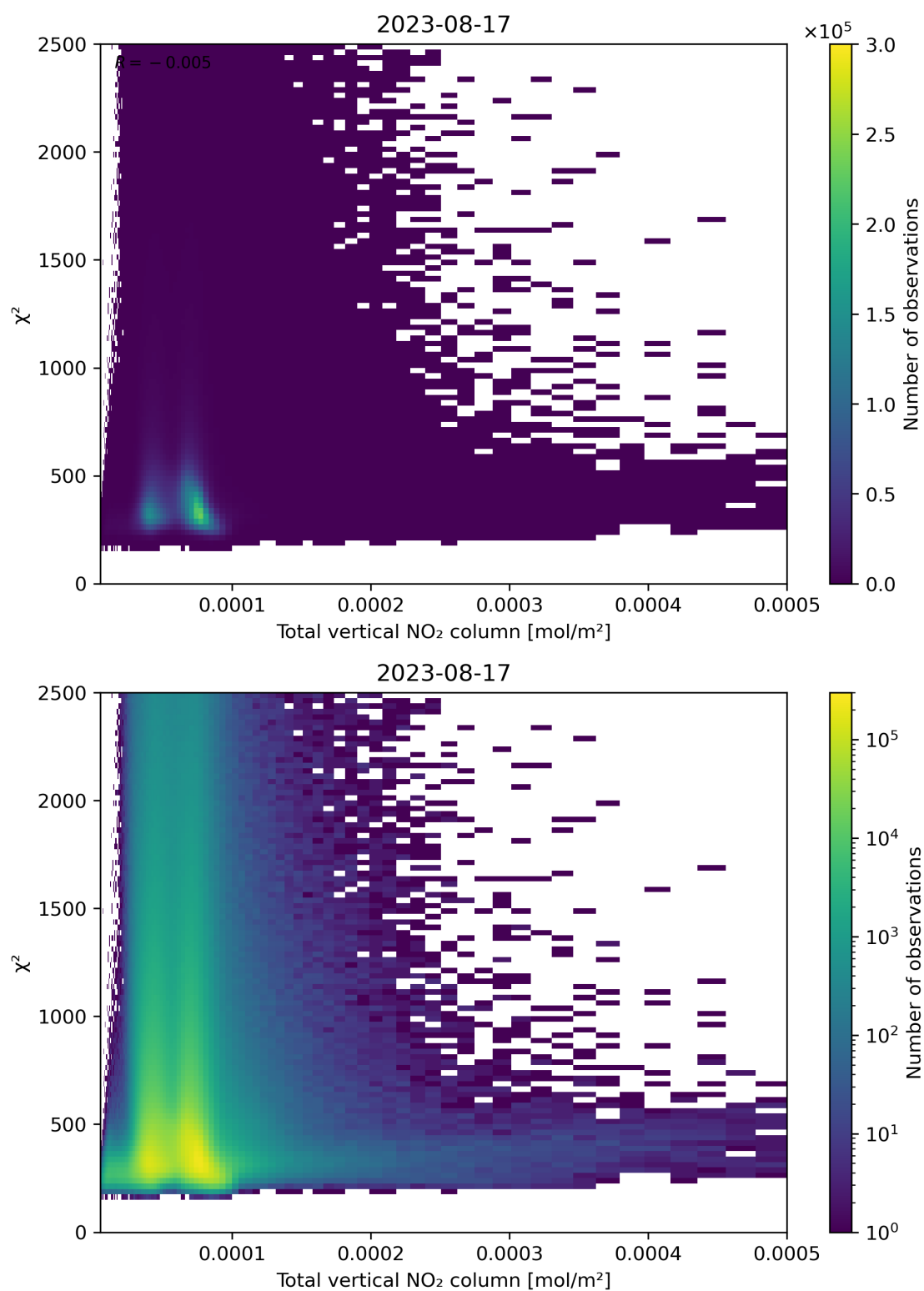
Figure 111: Scatter density plot of “Total vertical NO 2 column” against “ \chi^2 ” for 2023-08-16 to 2023-08-18.
