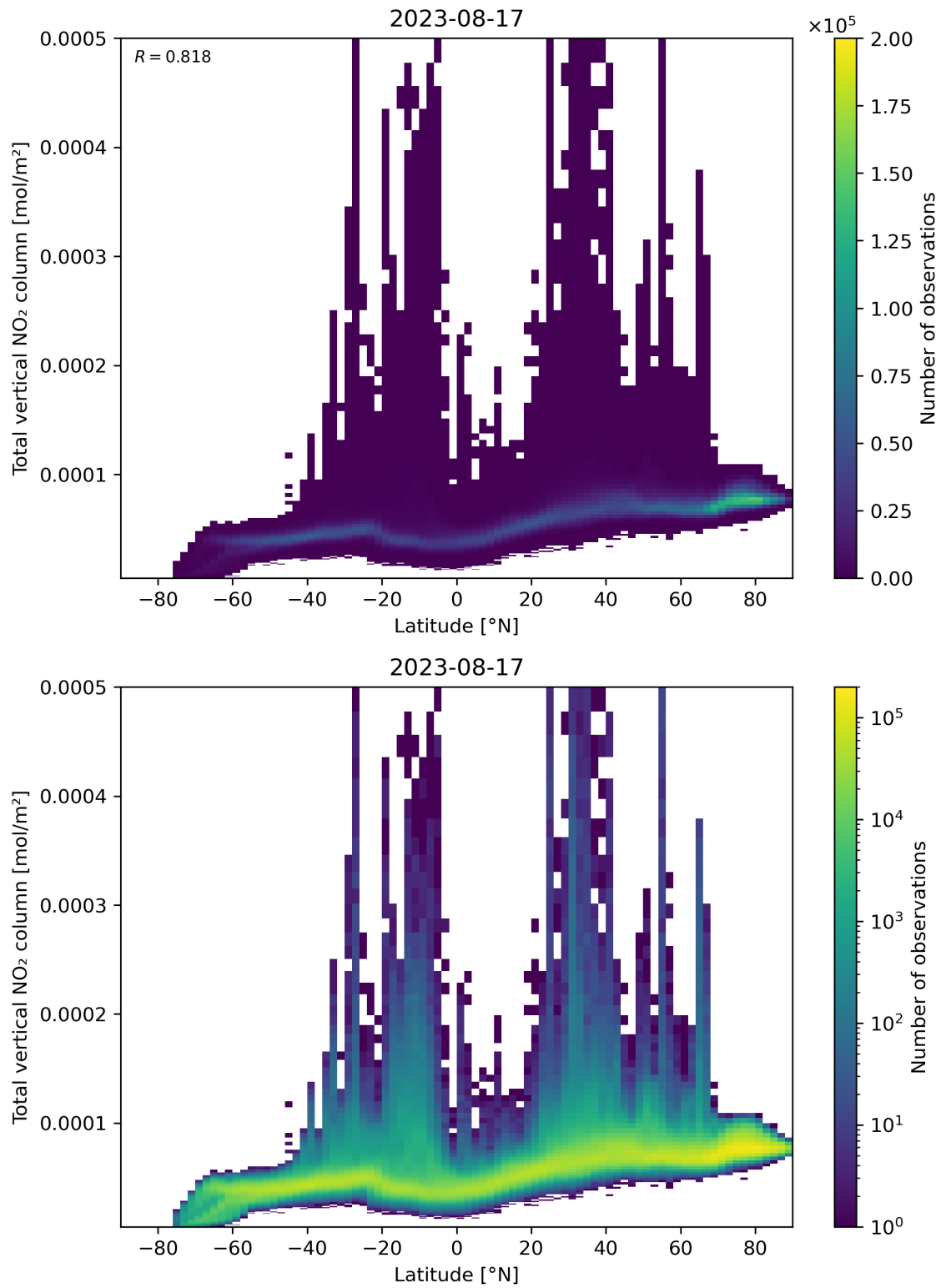
Figure 90: Scatter density plot of “Latitude” against “Total vertical NO 2 column” for 2023-08-16 to 2023-08-18.
