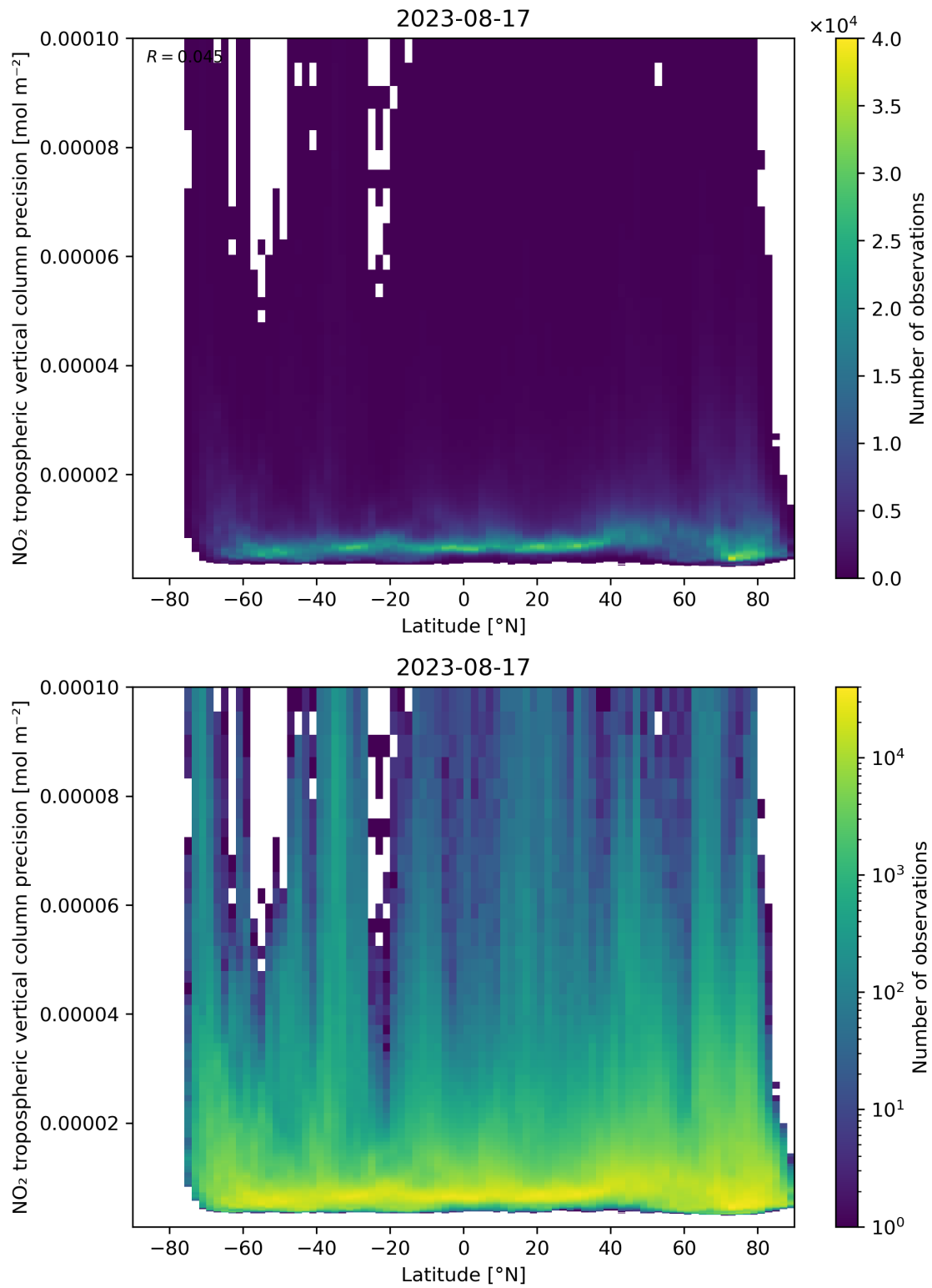
Figure 93: Scatter density plot of “Latitude” against “NO 2 tropospheric vertical column precision” for 2023-08-16 to 2023-08-18.
