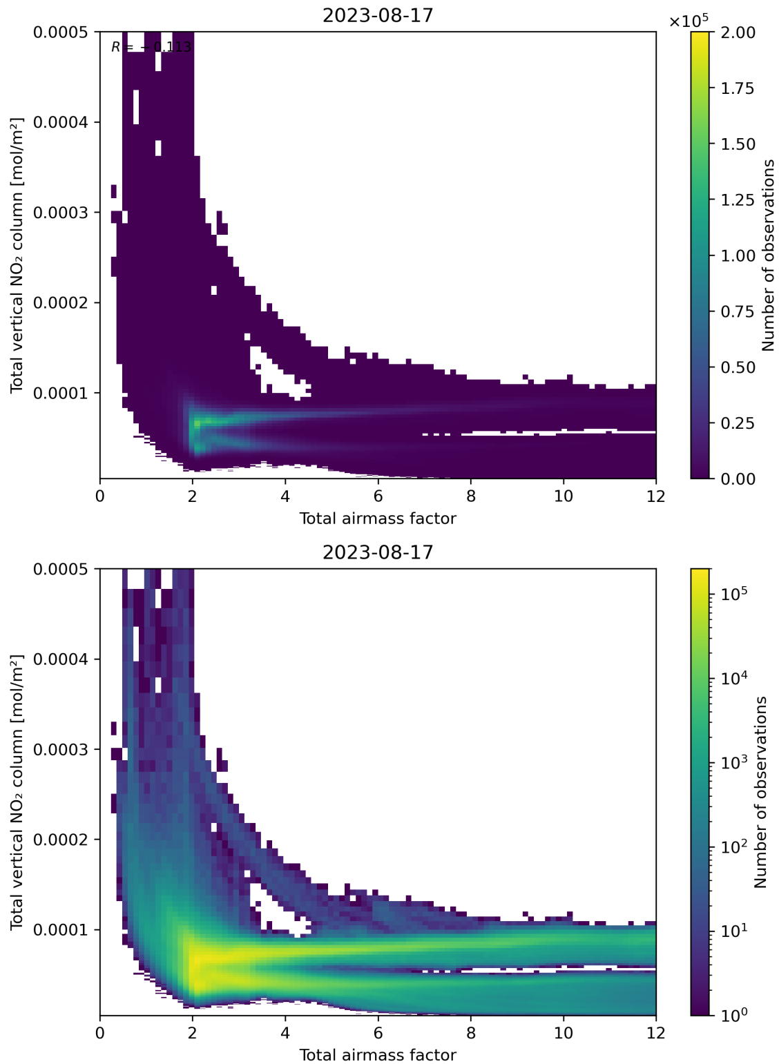
Figure 67: Scatter density plot of “Total airmass factor” against “Total vertical NO 2 column” for 2023-08-16 to 2023-08-18.
