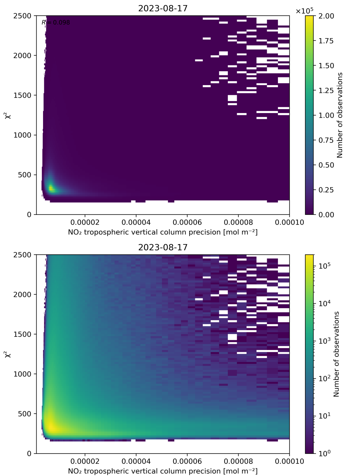
Figure 134: Scatter density plot of “NO 2 tropospheric vertical column precision” against “ \chi^2 ” for 2023-08-16 to 2023-08-18.
