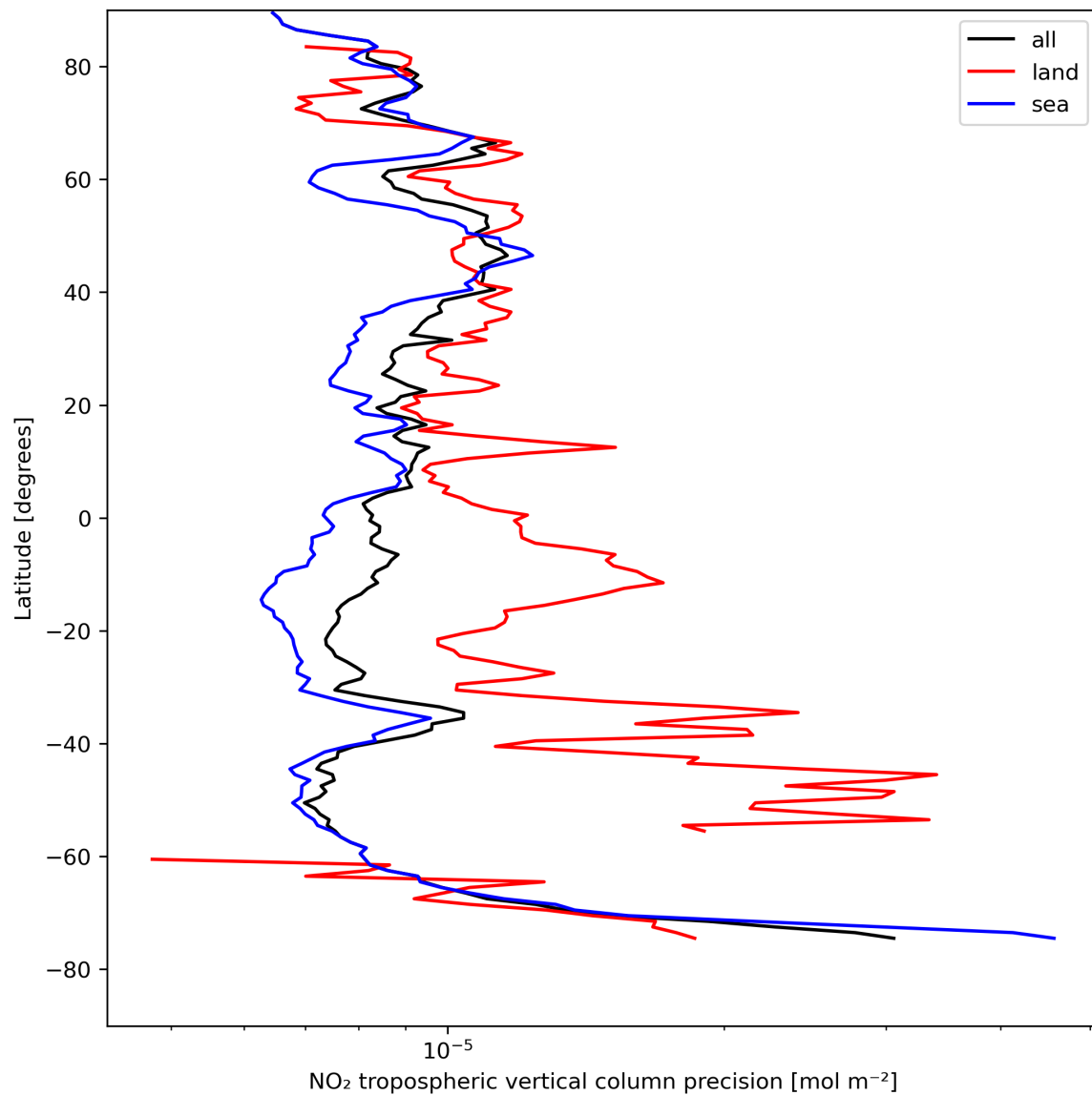
Figure 13: Zonal average of “NO 2 tropospheric vertical column precision” for 2023-08-16 to 2023-08-18.
