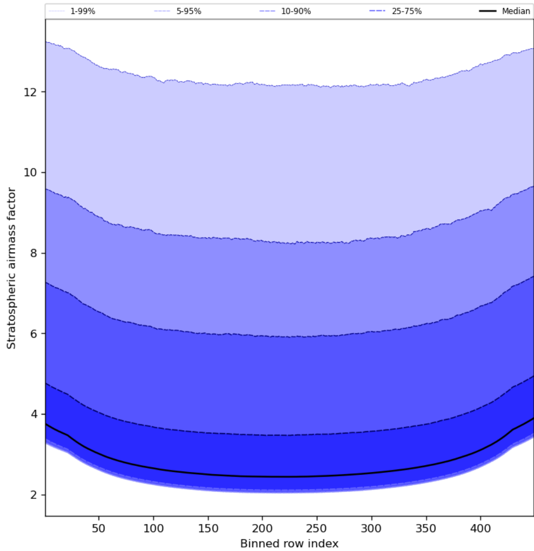
Figure 61: Along track statistics of “Stratospheric airmass factor” for 2023-08-16 to 2023-08-18
