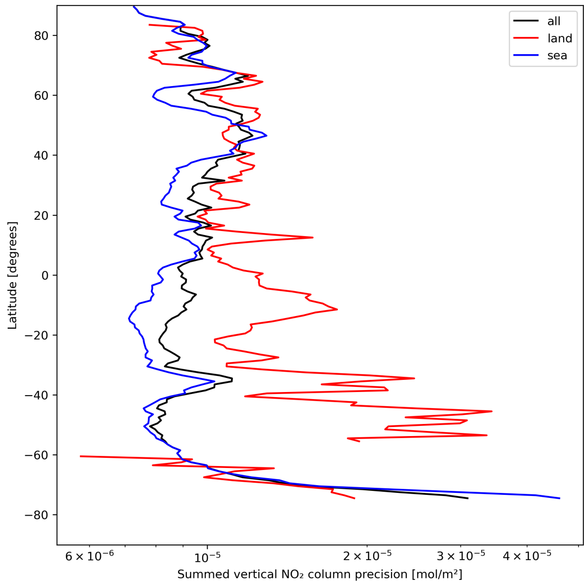
Figure 24: Zonal average of “Summed vertical NO 2 column precision” for 2023-08-16 to 2023-08-18.
