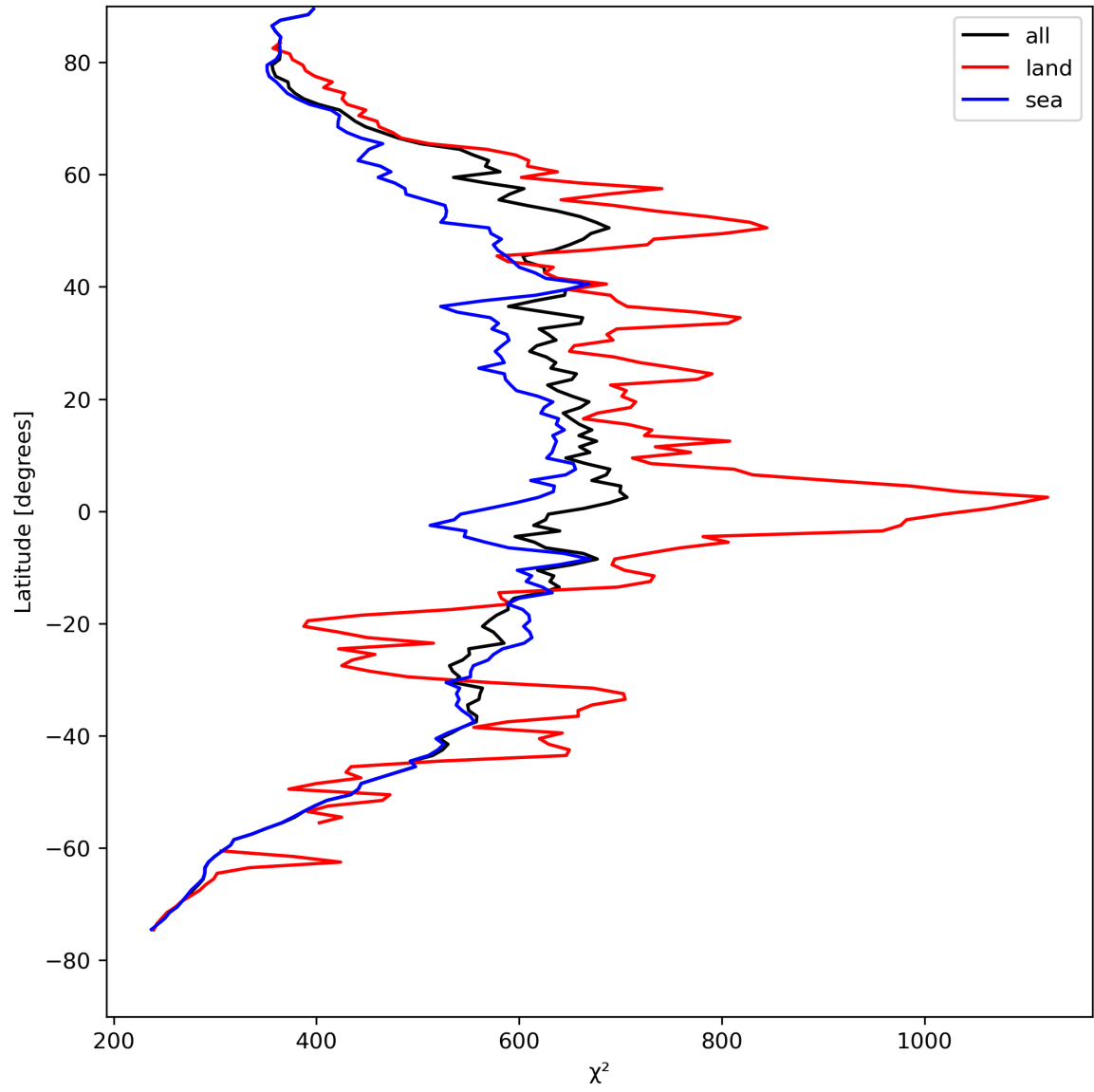
Figure 25: Zonal average of “ \chi^2 ” for 2023-08-16 to 2023-08-18.
