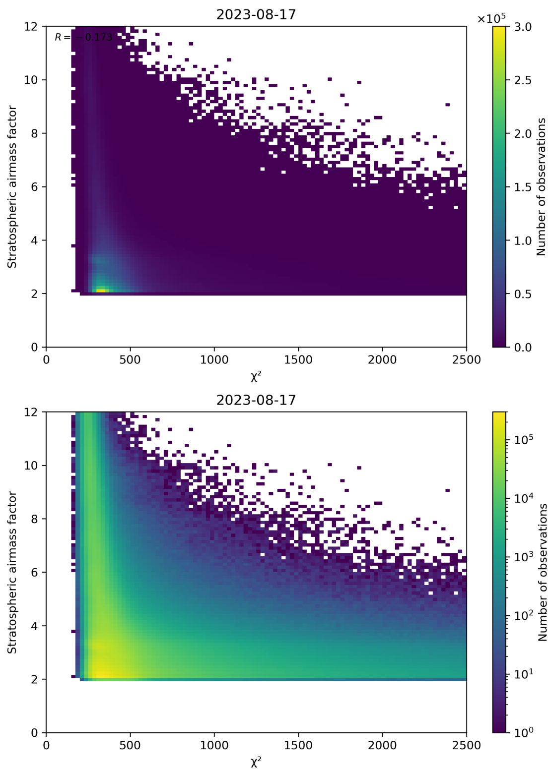
Figure 81: Scatter density plot of “ \chi^2 ” against “Stratospheric airmass factor” for 2023-08-16 to 2023-08-18.
