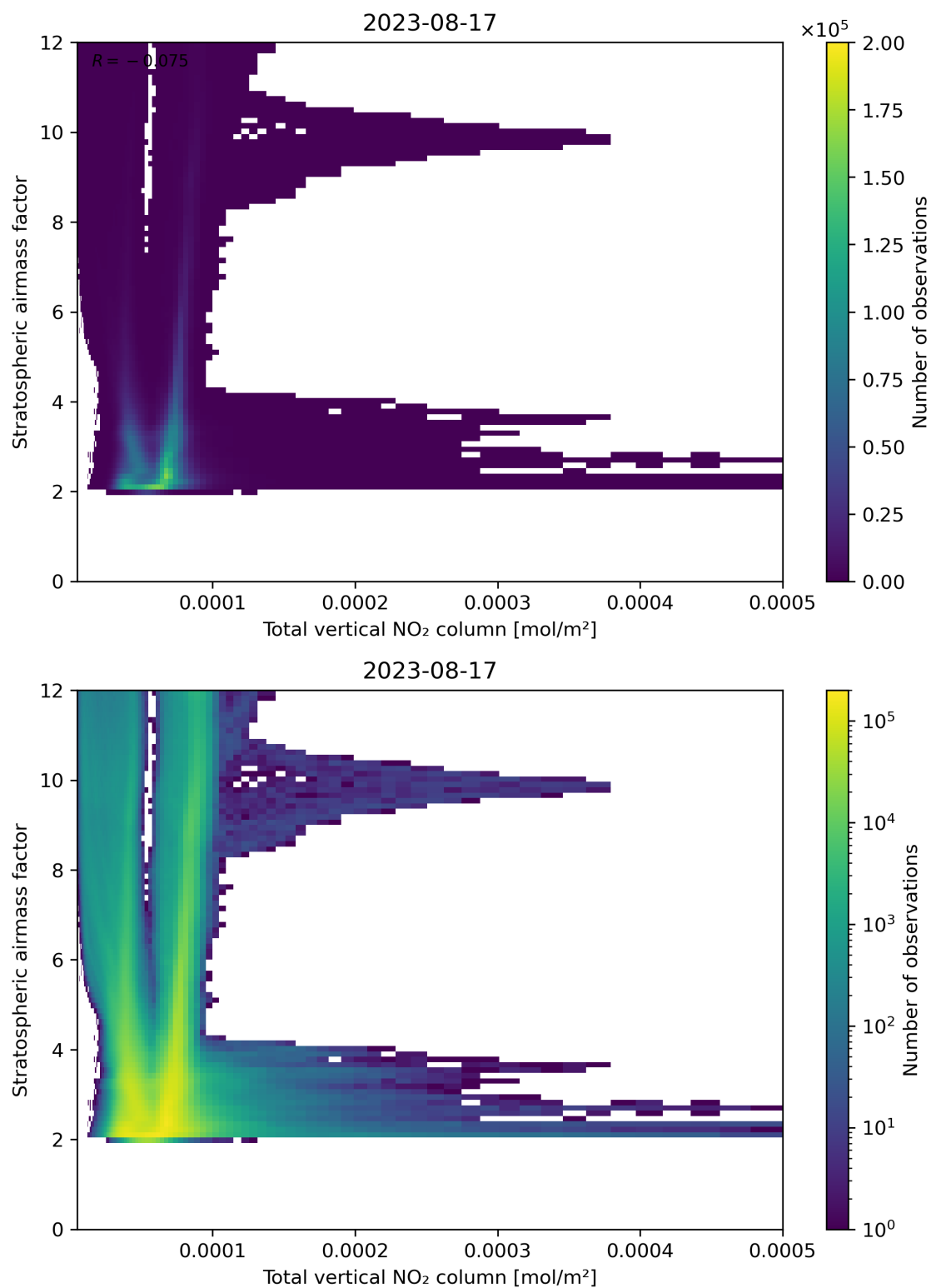
Figure 110: Scatter density plot of “Total vertical NO 2 column” against “Stratospheric airmass factor” for 2023-08-16 to 2023-08-18.
