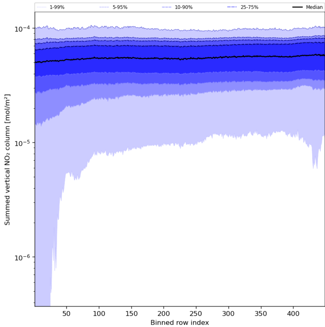
Figure 57: Along track statistics of “Summed vertical NO 2 column” for 2023-08-16 to 2023-08-18
