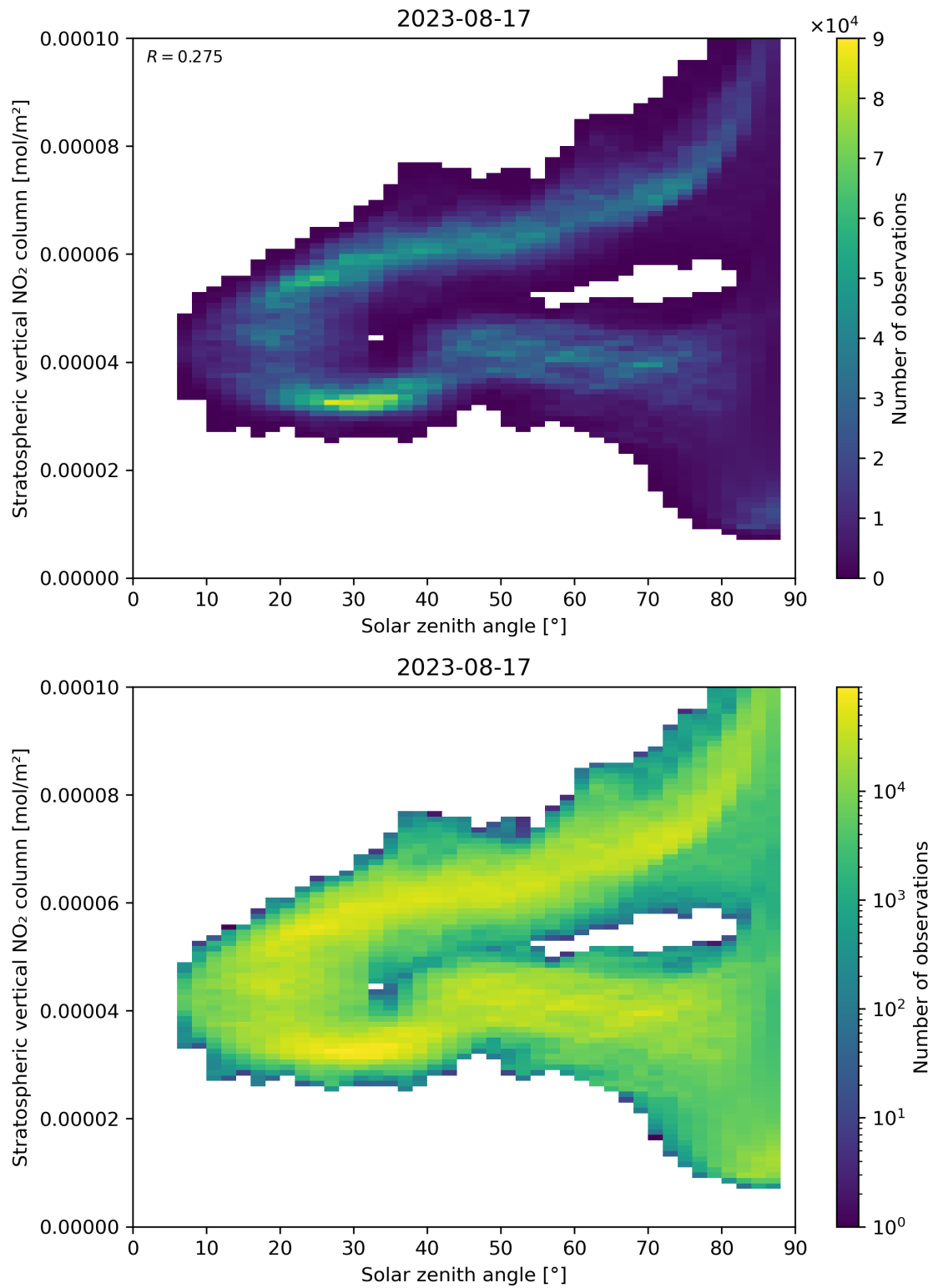
Figure 150: Scatter density plot of “Solar zenith angle” against “Stratospheric vertical NO 2 column” for 2023-08-16 to 2023-08-18.
