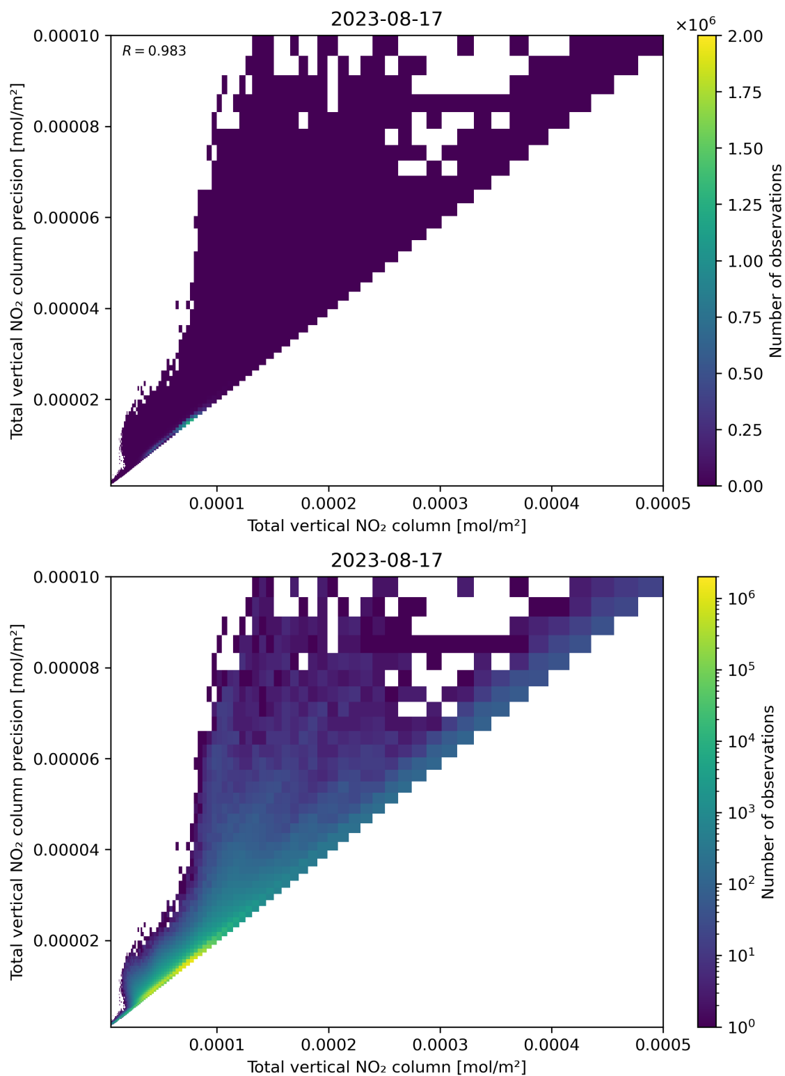
Figure 114: Scatter density plot of “Total vertical NO 2 column” against “Total vertical NO 2 column precision” for 2023-08-16 to 2023-08-18.
