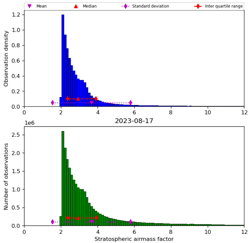
Figure 44: Histogram of “Stratospheric airmass factor” for 2023-08-16 to 2023-08-18
