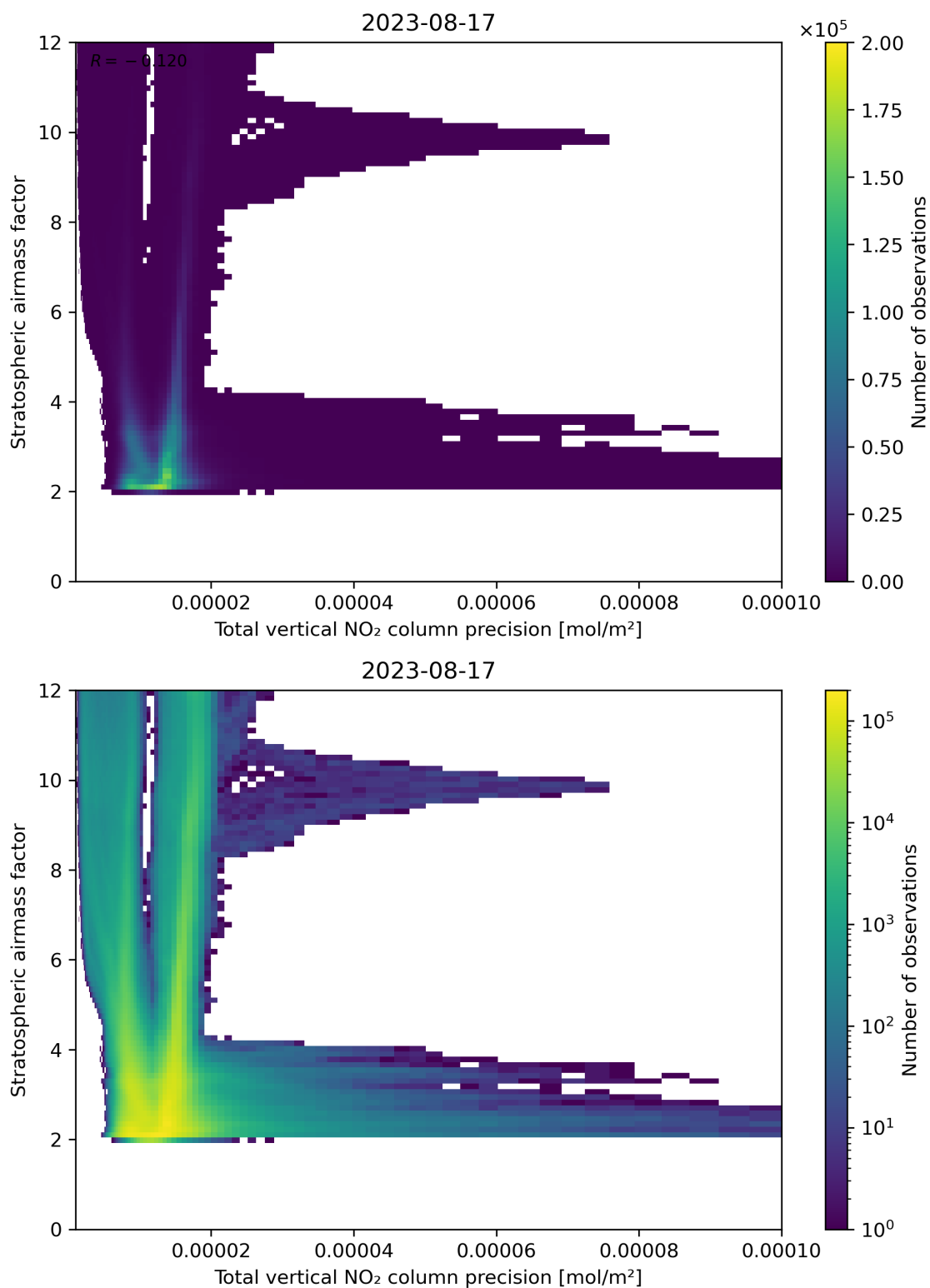
Figure 115: Scatter density plot of “Total vertical NO 2 column precision” against “Stratospheric air mass factor” for 2023-08-16 to 2023-08-18.
