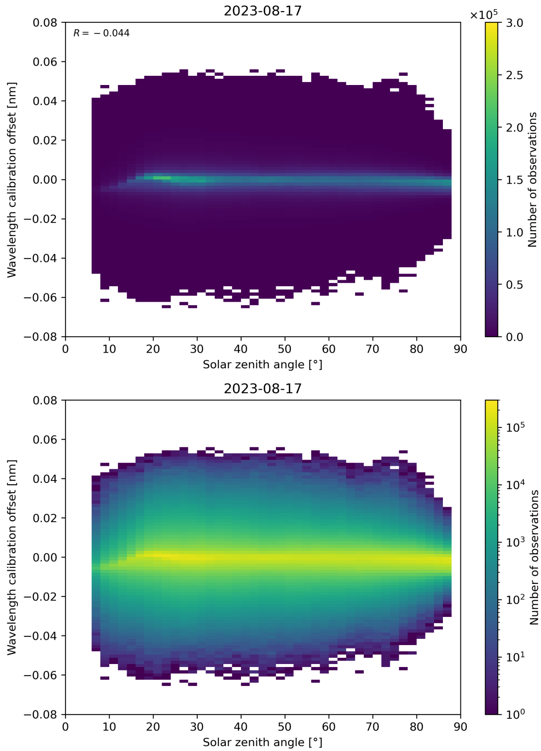
Figure 158: Scatter density plot of “Solar zenith angle” against “Wavelength calibration offset” for 2023-08-16 to 2023-08-18.
