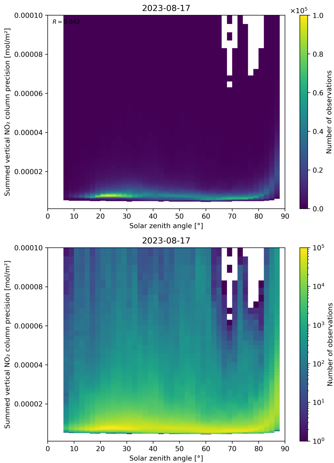
Figure 152: Scatter density plot of “Solar zenith angle” against “Summed vertical NO 2 column precision” for 2023-08-16 to 2023-08-18.
