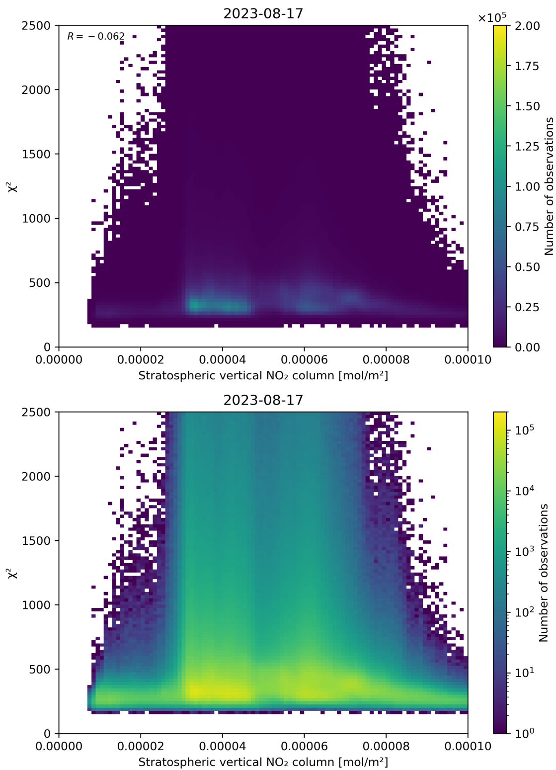
Figure 97: Scatter density plot of “Stratospheric vertical NO 2 column” against “ \chi^2 ” for 2023-08-16 to 2023-08-18.
