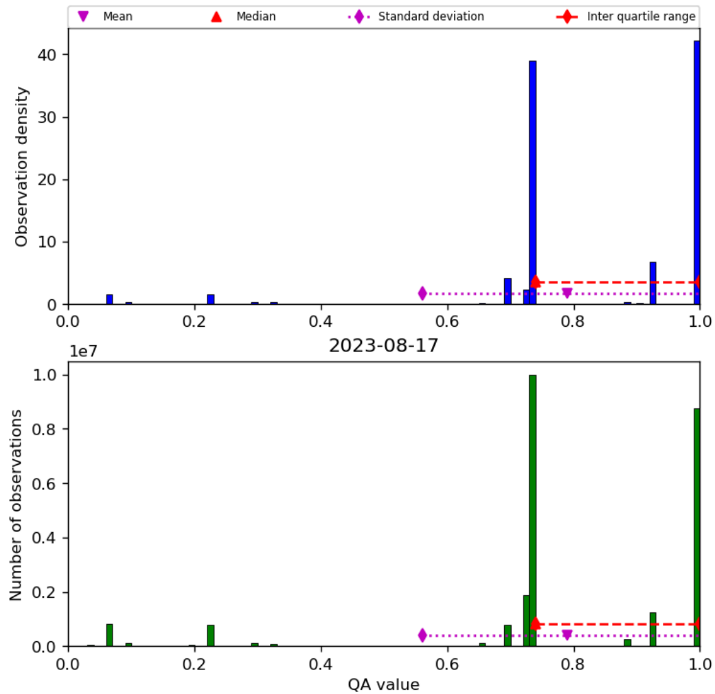
Figure 28: Histogram of “QA value” for 2023-08-16 to 2023-08-18
