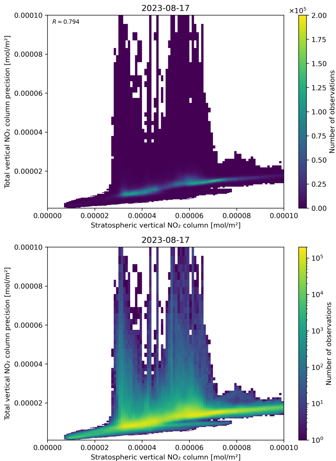
Figure 101: Scatter density plot of “Stratospheric vertical NO 2 column” against “Total vertical NO 2 column precision” for 2023-08-16 to 2023-08-18.
