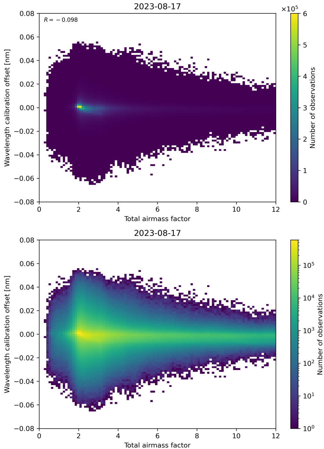
Figure 70: Scatter density plot of “Total airmass factor” against “Wavelength calibration offset” for 2023-08-16 to 2023-08-18.
