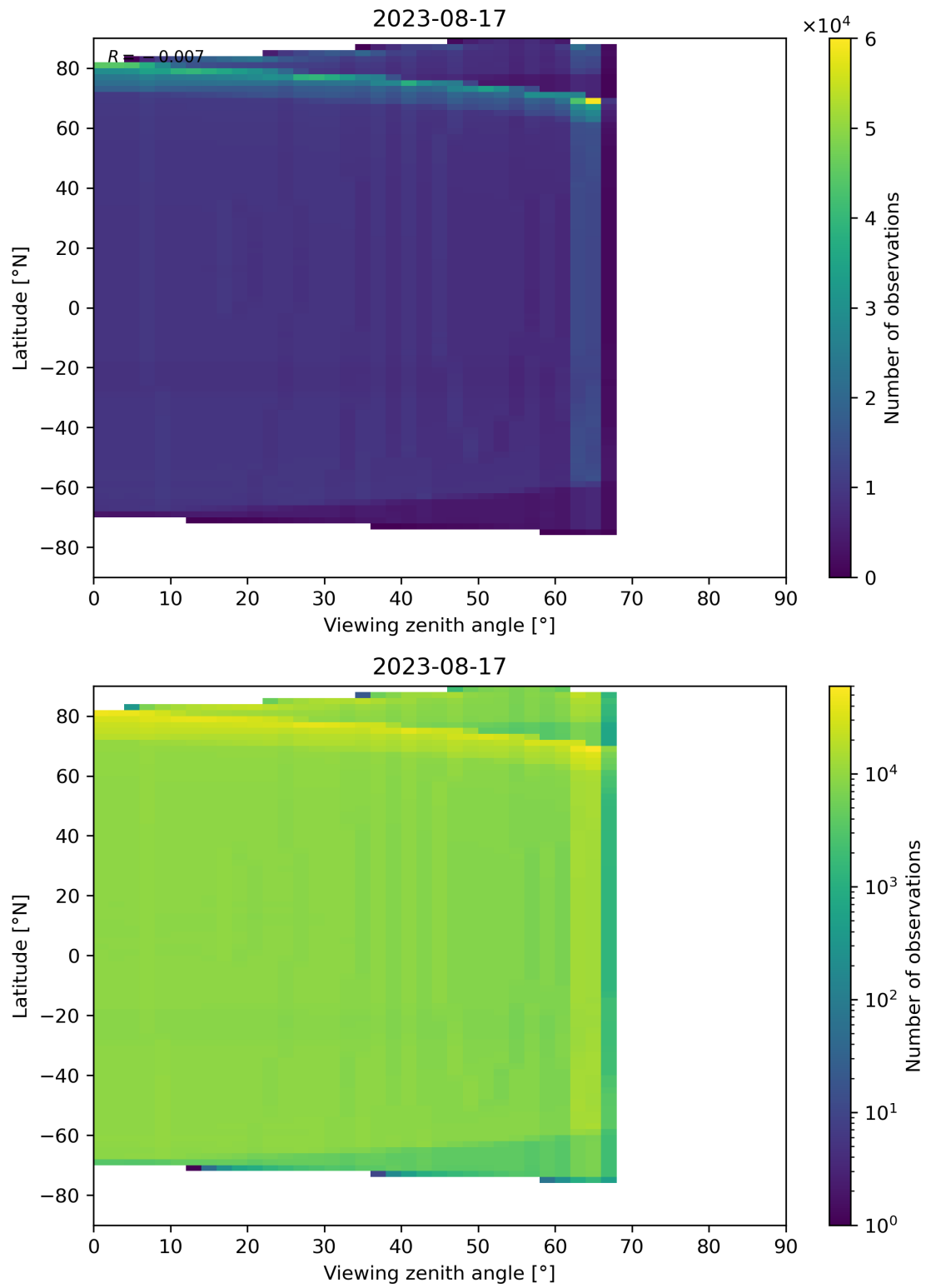
Figure 163: Scatter density plot of “Viewing zenith angle” against “Latitude” for 2023-08-16 to 2023-08-18.
