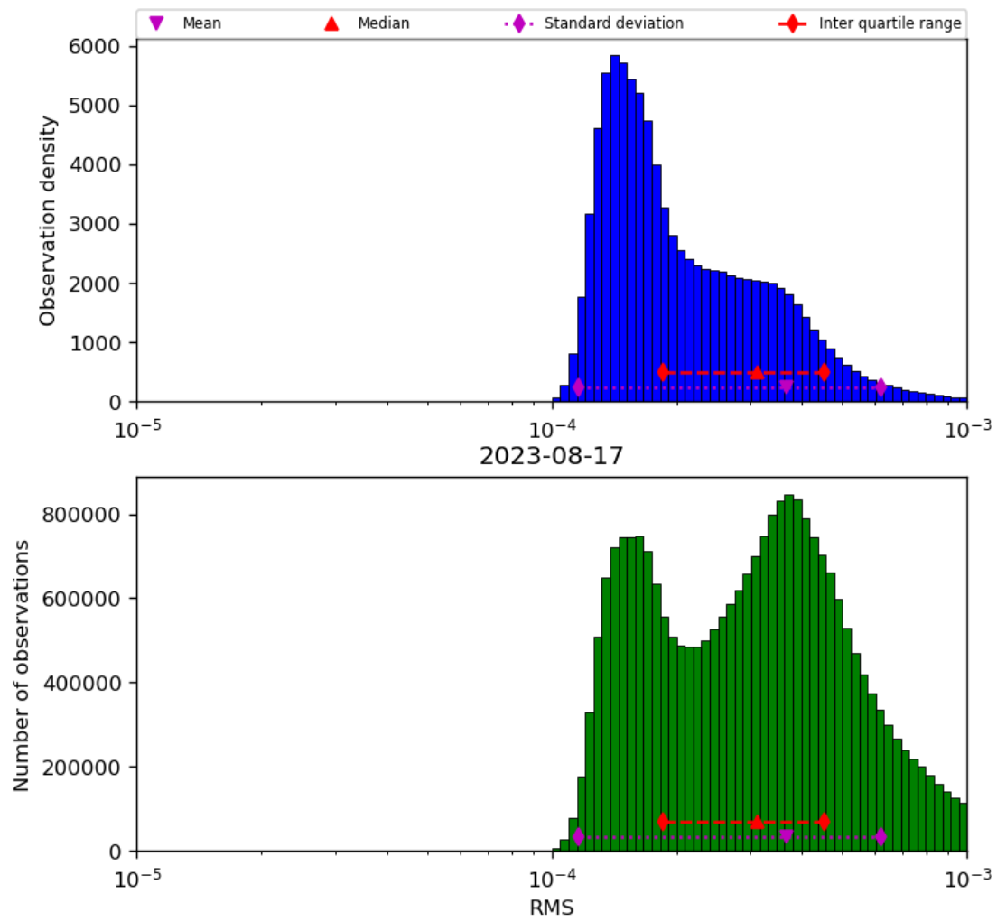
Figure 43: Histogram of “RMS” for 2023-08-16 to 2023-08-18
