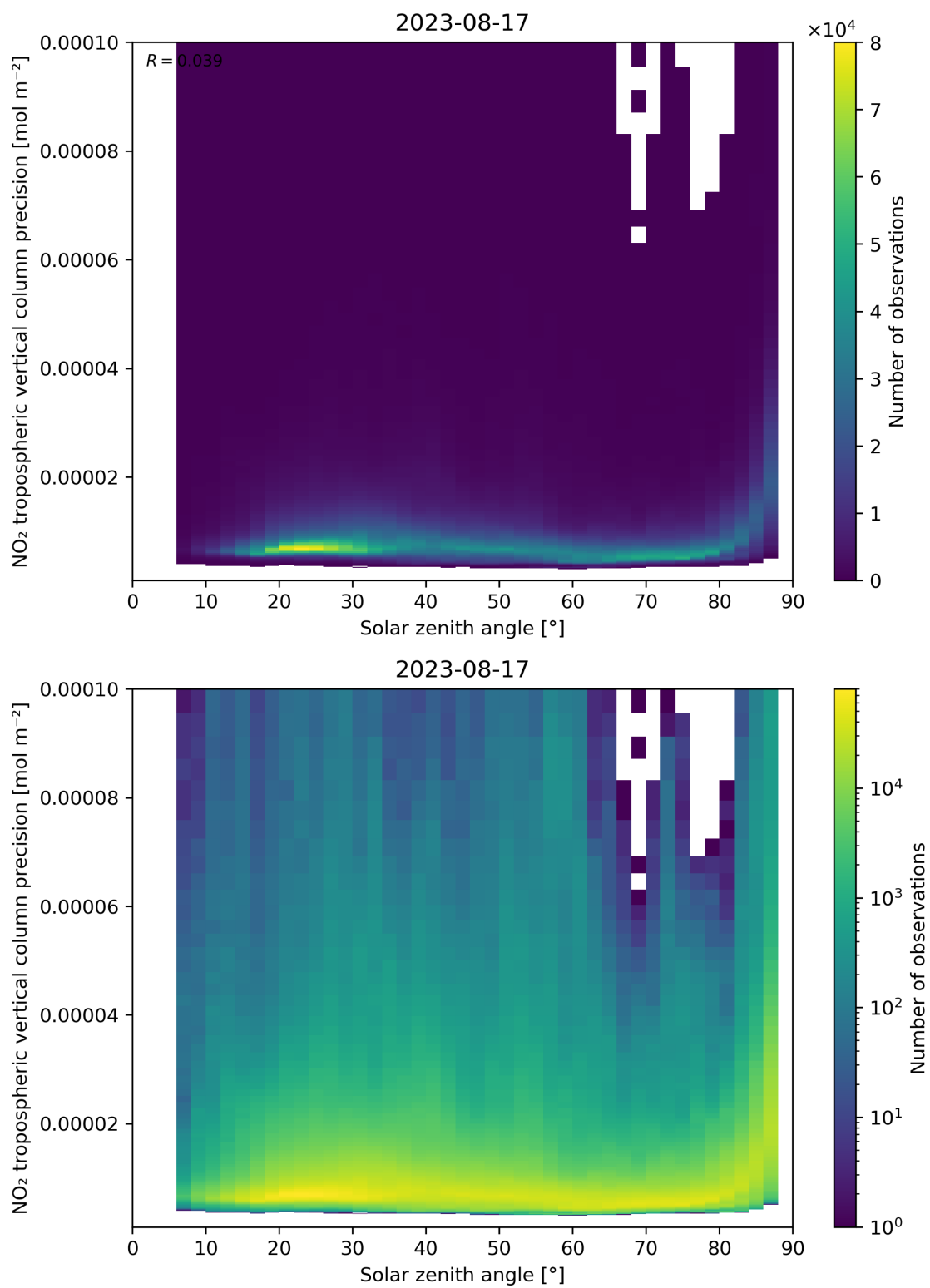
Figure 156: Scatter density plot of “Solar zenith angle” against “NO 2 tropospheric vertical column precision” for 2023-08-16 to 2023-08-18.
