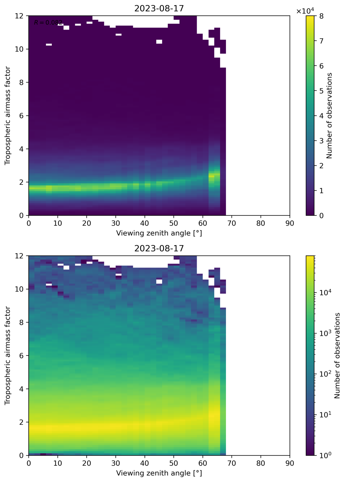
Figure 161: Scatter density plot of “Viewing zenith angle” against “Tropospheric airmass factor” for 2023-08-16 to 2023-08-18.
