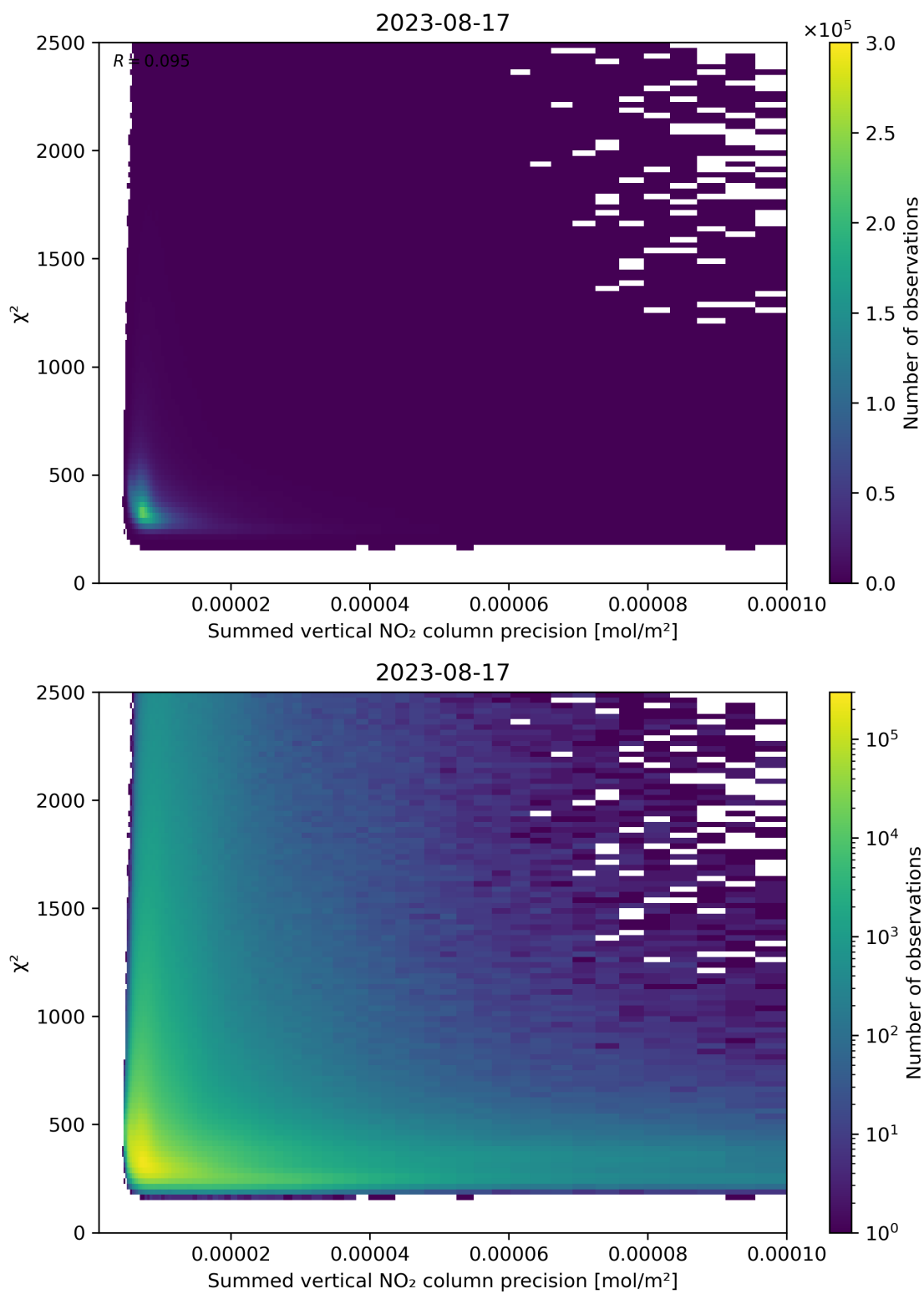
Figure 107: Scatter density plot of “Summed vertical NO 2 column precision” against “ \chi^2 ” for 2023-08-16 to 2023-08-18.
