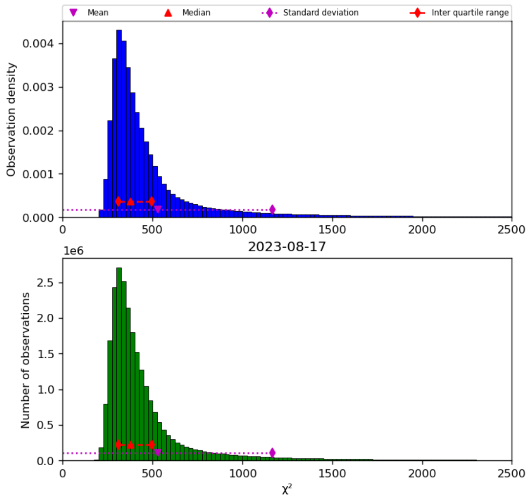
Figure 42: Histogram of “ \chi^2 ” for 2023-08-16 to 2023-08-18
