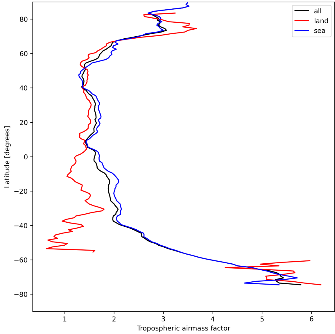
Figure 14: Zonal average of “Tropospheric air mass factor” for 2023-08-16 to 2023-08-18.
