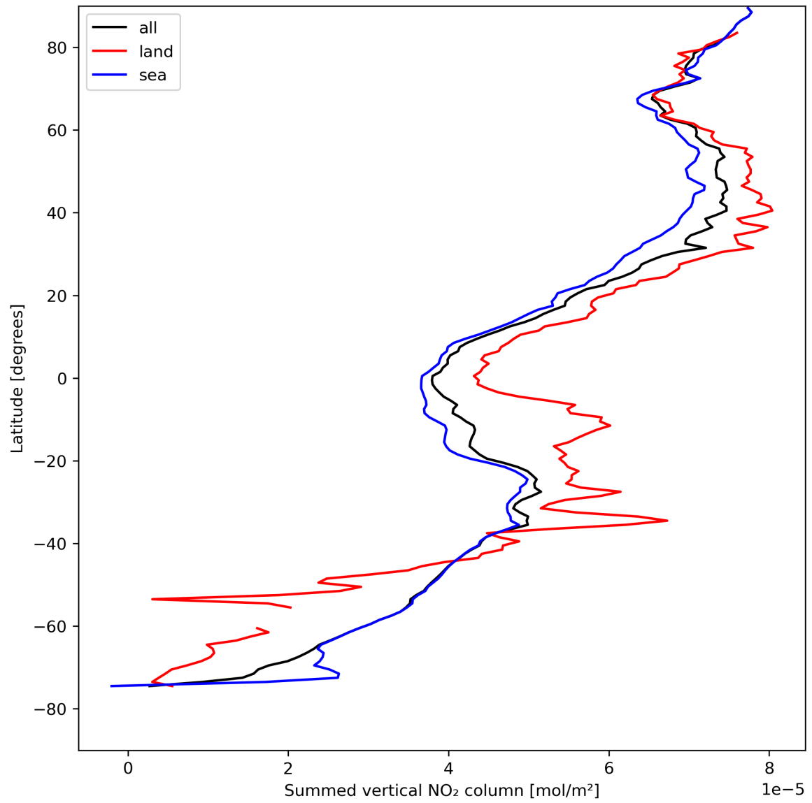
Figure 23: Zonal average of “Summed vertical NO 2 column” for 2023-08-16 to 2023-08-18.
