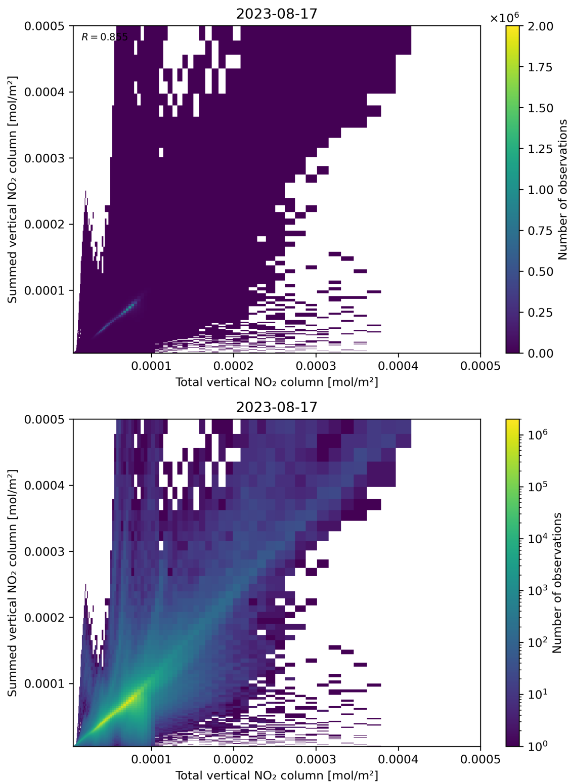
Figure 112: Scatter density plot of “Total vertical NO 2 column” against “Summed vertical NO 2 column” for 2023-08-16 to 2023-08-18.
