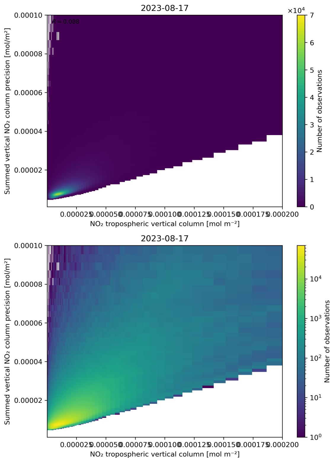
Figure 127: Scatter density plot of “NO 2 tropospheric vertical column” against “Summed vertical NO 2 column precision” for 2023-08-16 to 2023-08-18.
