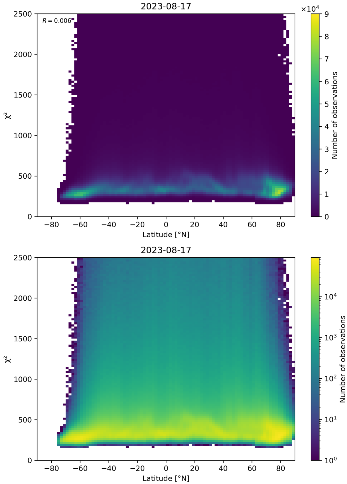
Figure 86: Scatter density plot of “Latitude” against “ \chi^2 ” for 2023-08-16 to 2023-08-18.
