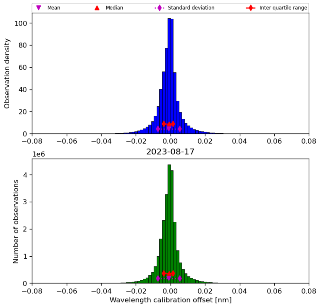
Figure 35: Histogram of “Wavelength calibration offset” for 2023-08-16 to 2023-08-18
