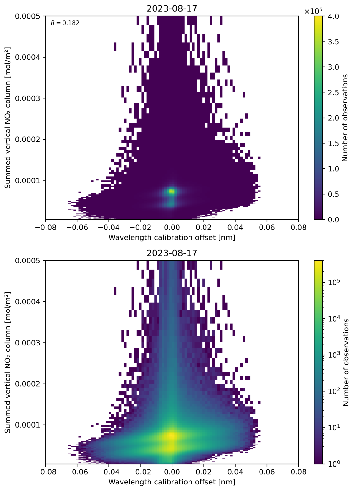
Figure 177: Scatter density plot of “Wavelength calibration offset” against “Summed vertical NO 2 column” for 2023-08-16 to 2023-08-18.
