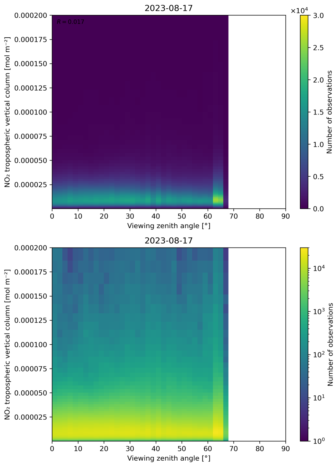
Figure 169: Scatter density plot of “Viewing zenith angle” against “NO 2 tropospheric vertical column” for 2023-08-16 to 2023-08-18.
