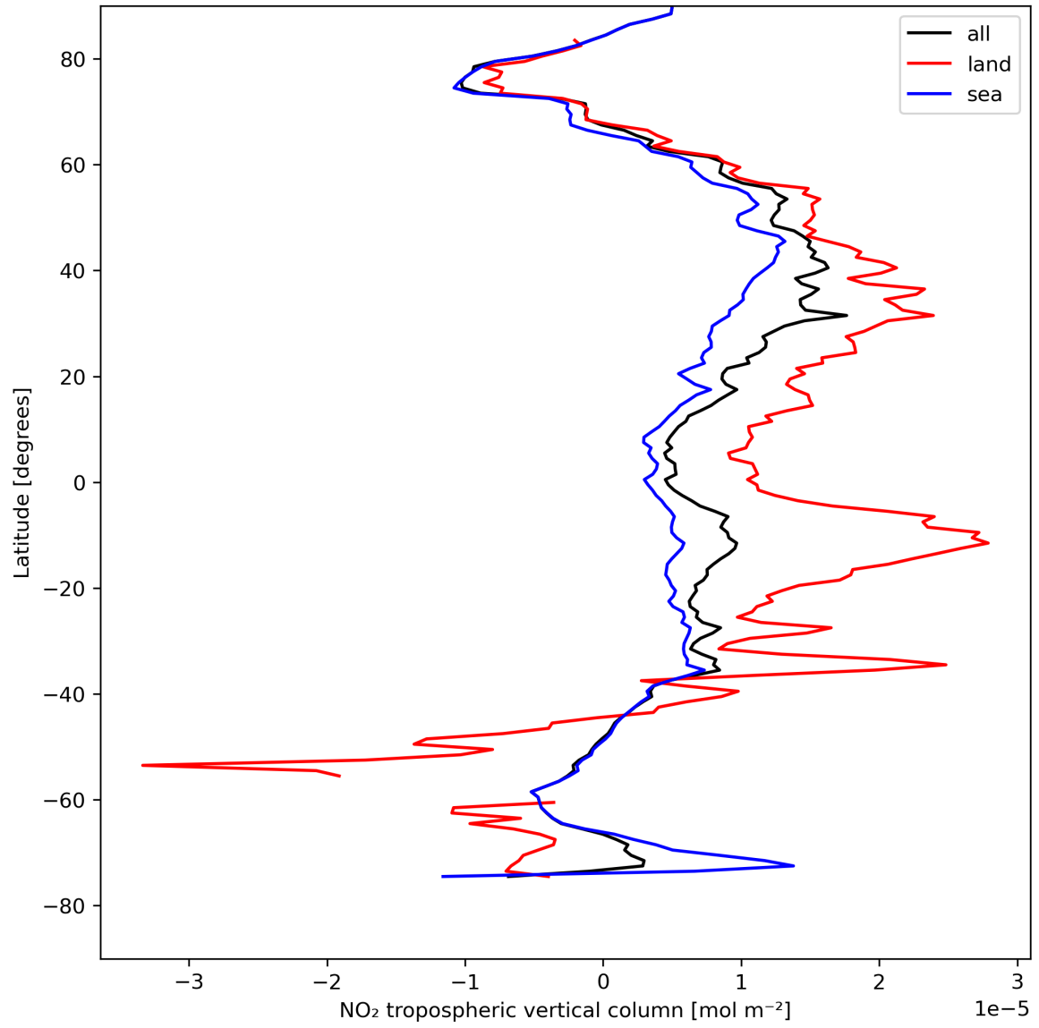
Figure 12: Zonal average of “NO 2 tropospheric vertical column” for 2023-08-16 to 2023-08-18.
