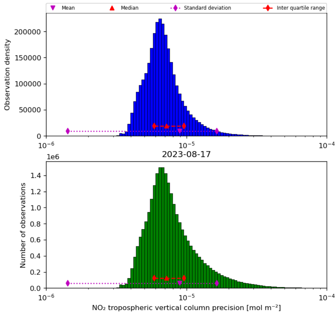
Figure 30: Histogram of “NO 2 tropospheric vertical column precision” for 2023-08-16 to 2023-08-18
