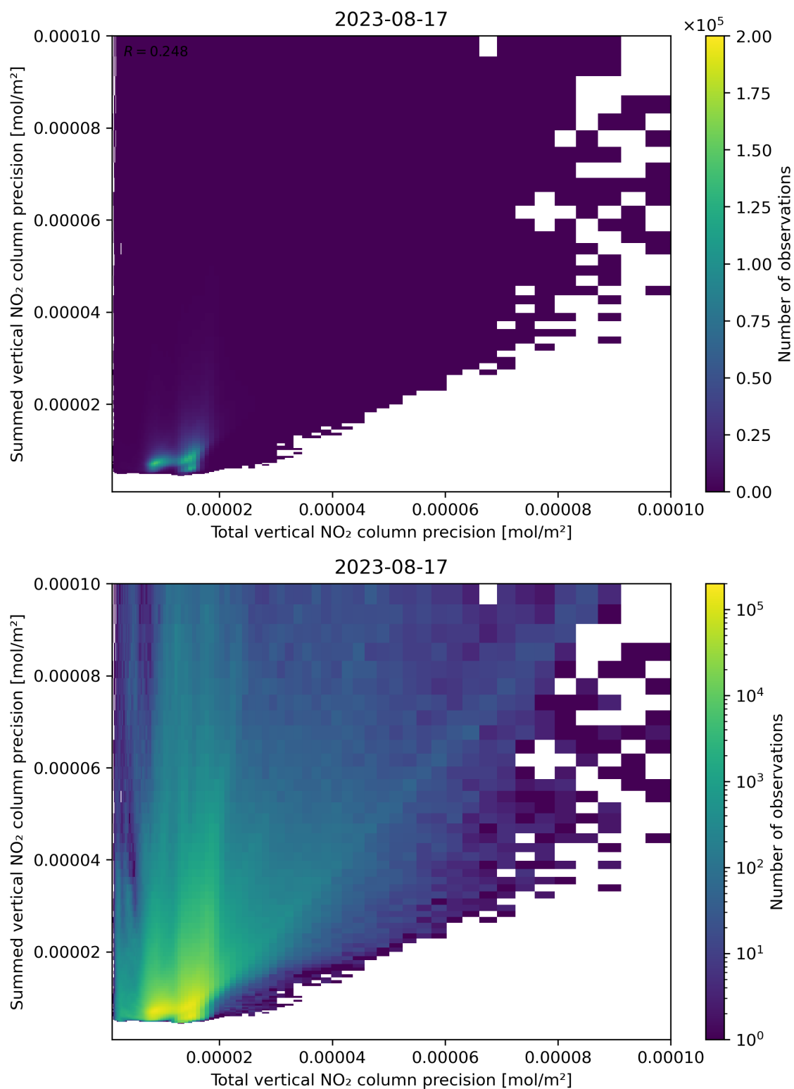
Figure 118: Scatter density plot of “Total vertical NO 2 column precision” against “Summed vertical NO 2 column precision” for 2023-08-16 to 2023-08-18.
