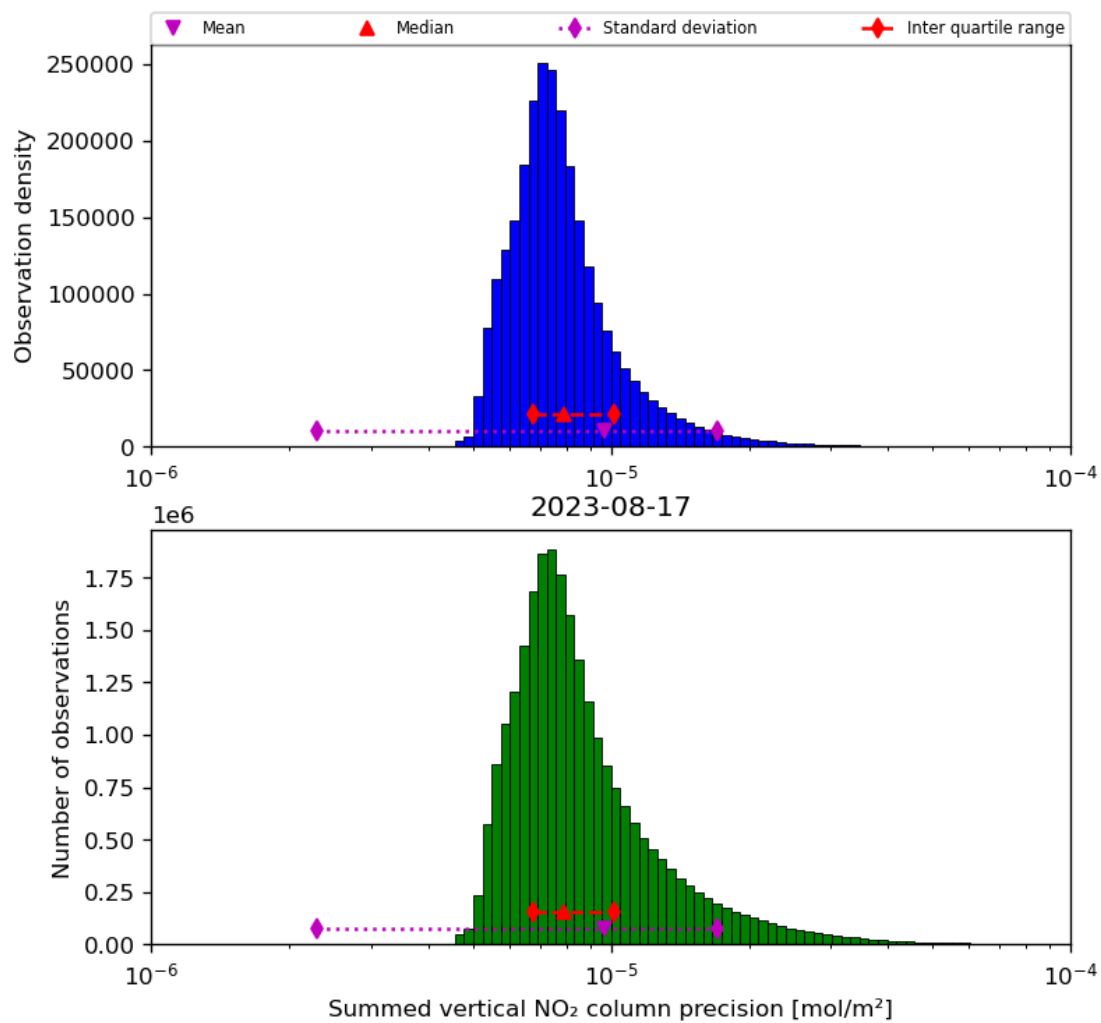
Figure 41: Histogram of “Summed vertical NO 2 column precision” for 2023-08-16 to 2023-08-18
