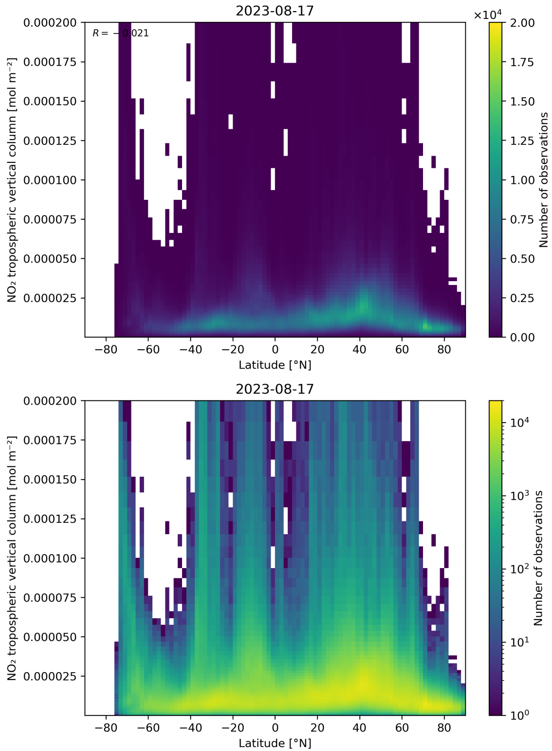
Figure 92: Scatter density plot of “Latitude” against “NO 2 tropospheric vertical column” for 2023-08-16 to 2023-08-18.
