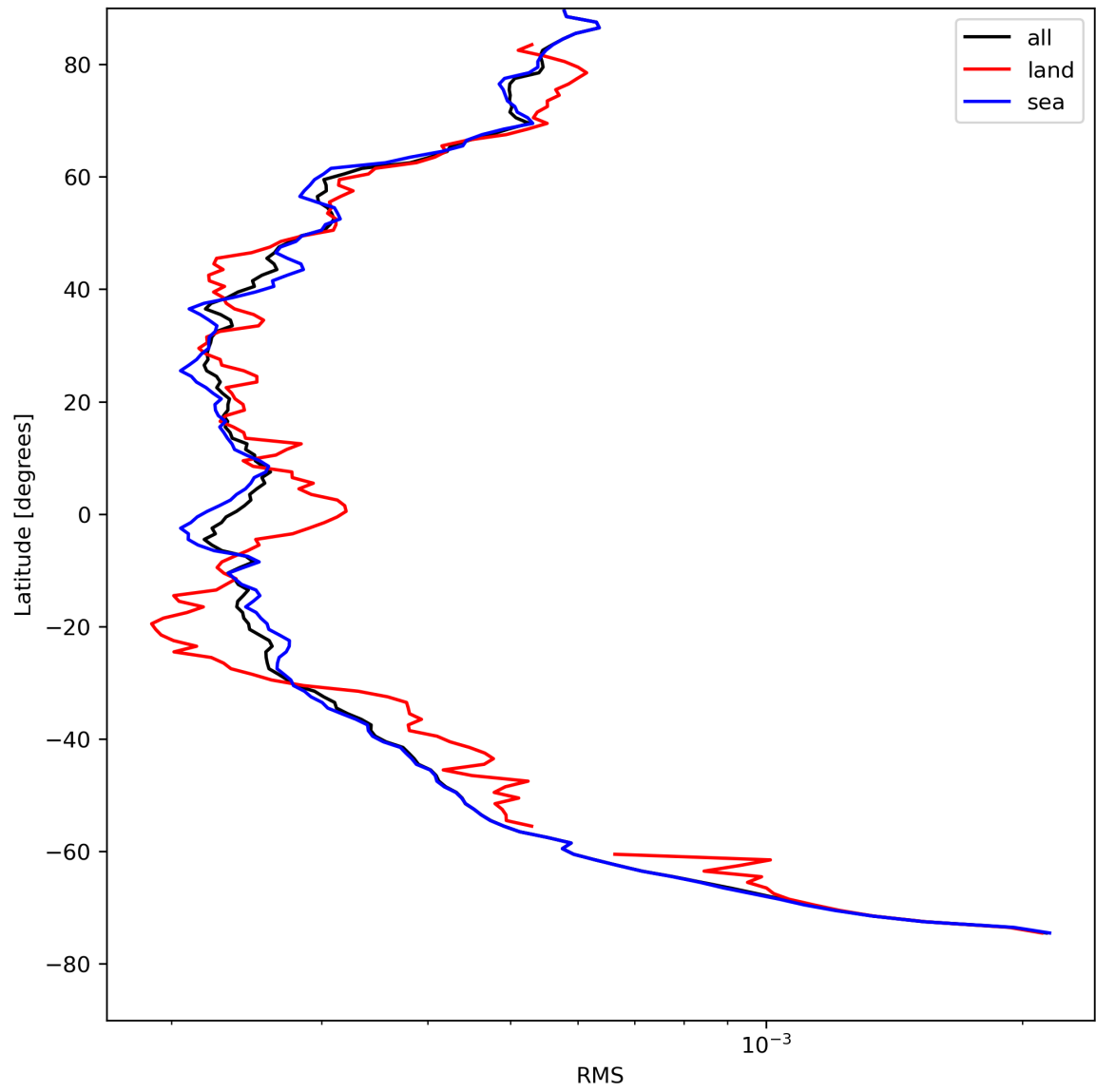
Figure 26: Zonal average of “RMS” for 2023-08-16 to 2023-08-18.
