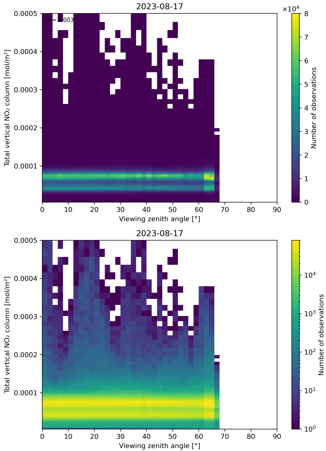
Figure 167: Scatter density plot of “Viewing zenith angle” against “Total vertical NO 2 column” for 2023-08-16 to 2023-08-18.
