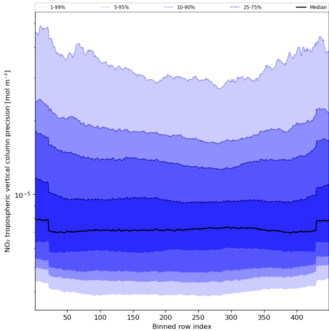
Figure 47: Along track statistics of “NO 2 tropospheric vertical column precision” for 2023-08-16 to 2023-08-18
