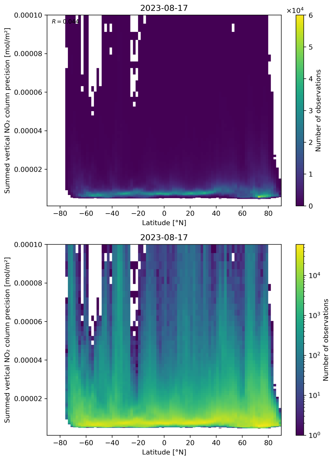
Figure 89: Scatter density plot of “Latitude” against “Summed vertical NO 2 column precision” for 2023-08-16 to 2023-08-18.
