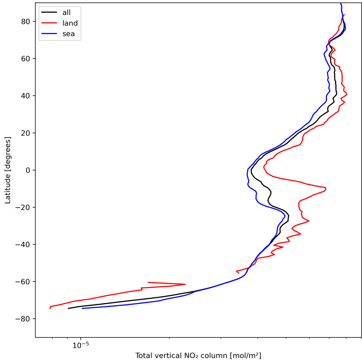
Figure 21: Zonal average of “Total vertical NO 2 column” for 2023-08-16 to 2023-08-18.
