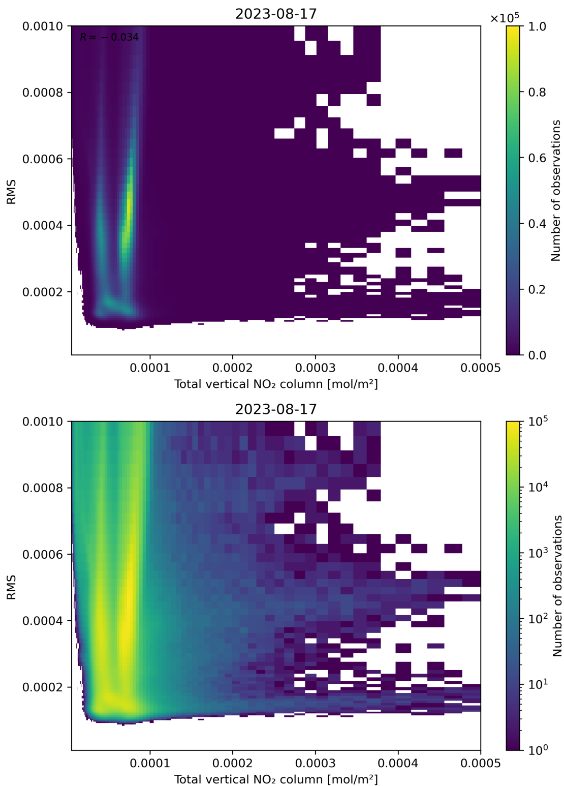
Figure 120: Scatter density plot of “Total vertical NO 2 column” against “RMS” for 2023-08-16 to 2023-08-18.
