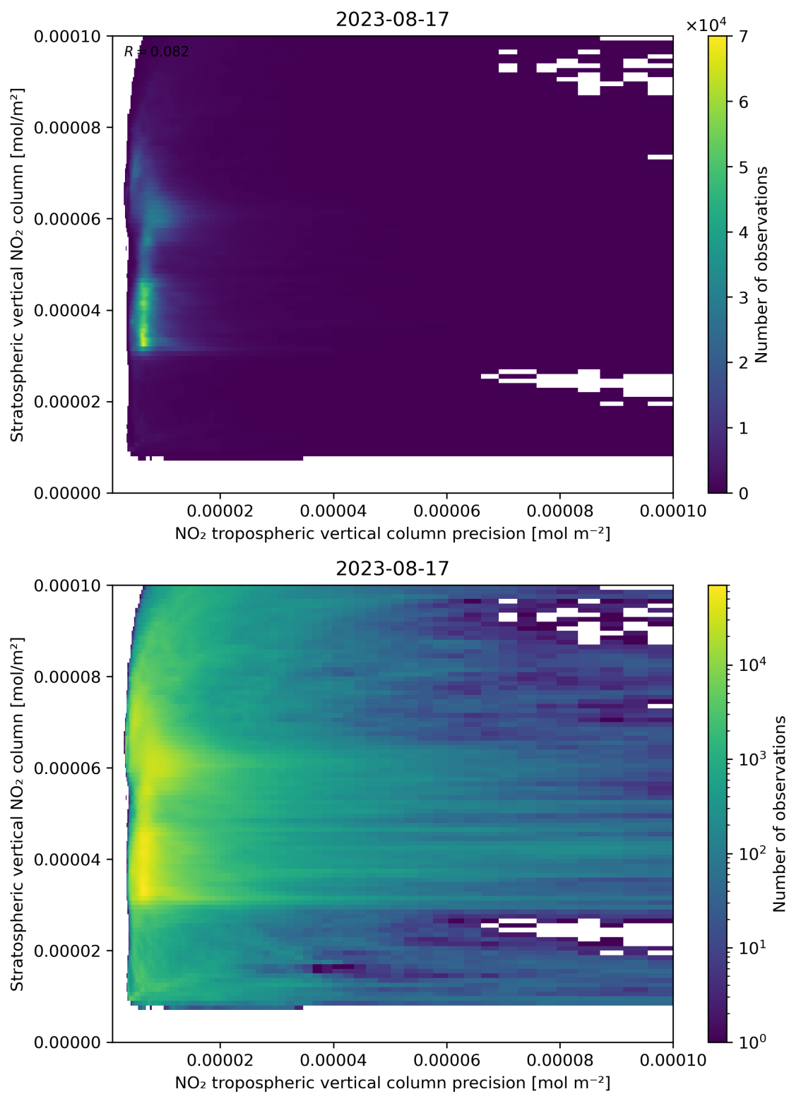
Figure 135: Scatter density plot of “NO 2 tropospheric vertical column precision” against “Stratospheric vertical NO 2 column” for 2023-08-16 to 2023-08-18.
