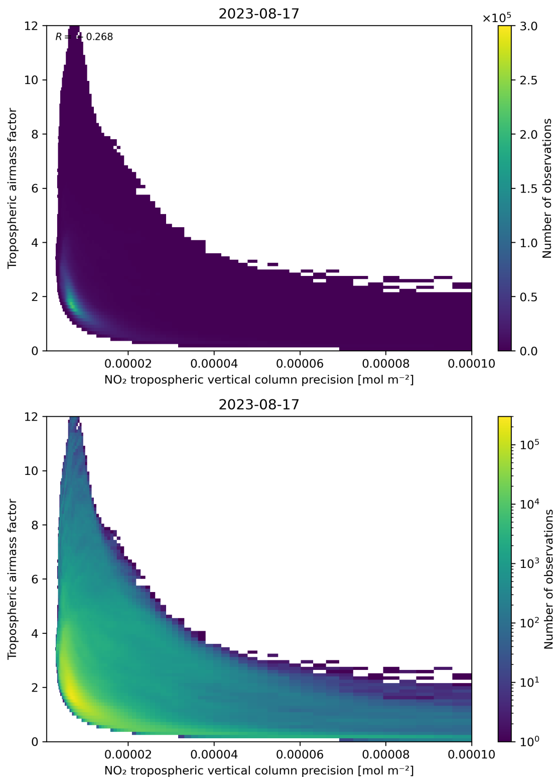
Figure 133: Scatter density plot of “NO 2 tropospheric vertical column precision” against “Tropospheric airmass factor” for 2023-08-16 to 2023-08-18.
