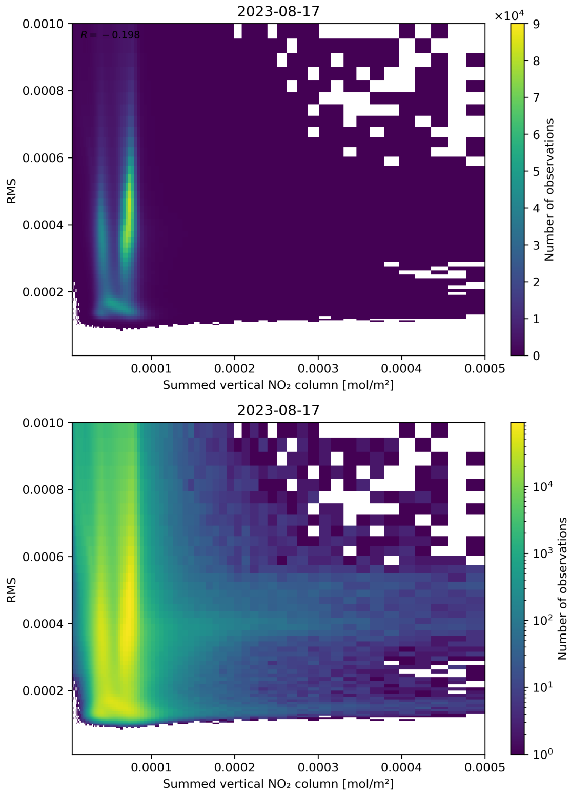
Figure 109: Scatter density plot of “Summed vertical NO 2 column” against “RMS” for 2023-08-16 to 2023-08-18.
