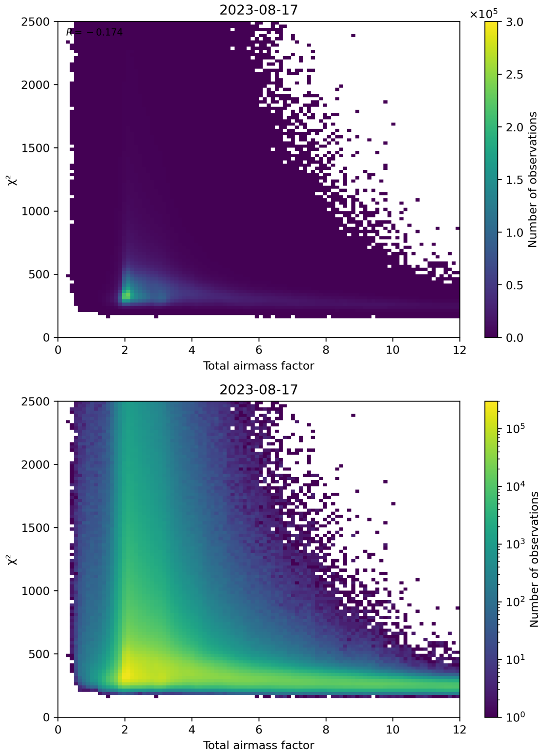
Figure 63: Scatter density plot of “Total airmass factor” against “ \chi^2 ” for 2023-08-16 to 2023-08-18.
