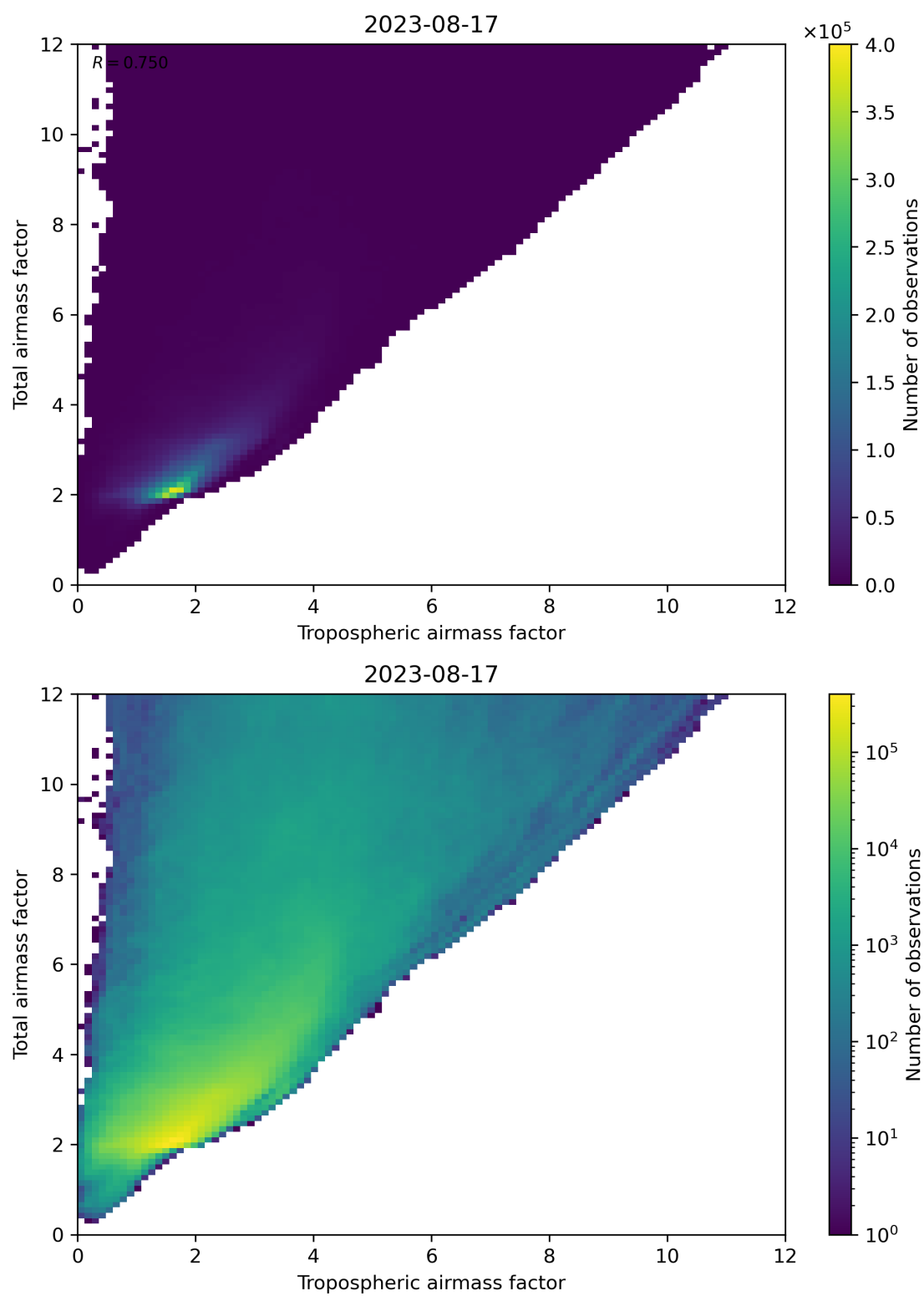
Figure 72: Scatter density plot of “Tropospheric airmass factor” against “Total airmass factor” for 2023-08-16 to 2023-08-18.
