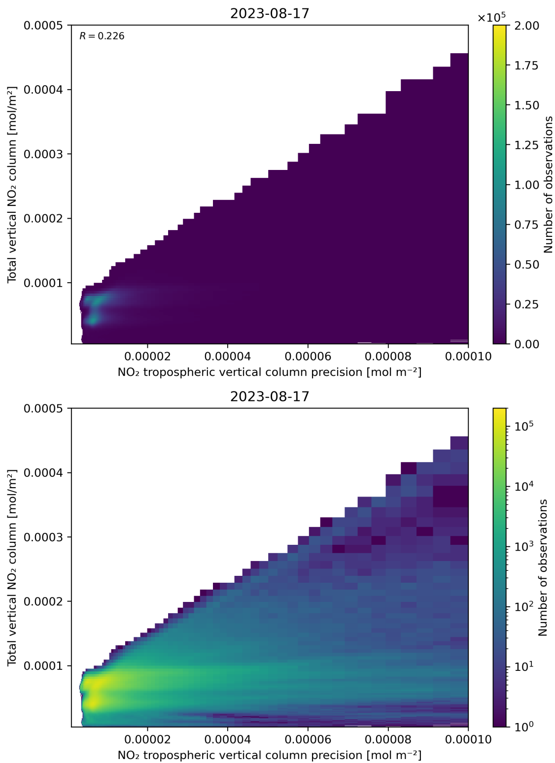
Figure 138: Scatter density plot of “NO 2 tropospheric vertical column precision” against “Total vertical NO 2 column” for 2023-08-16 to 2023-08-18.
