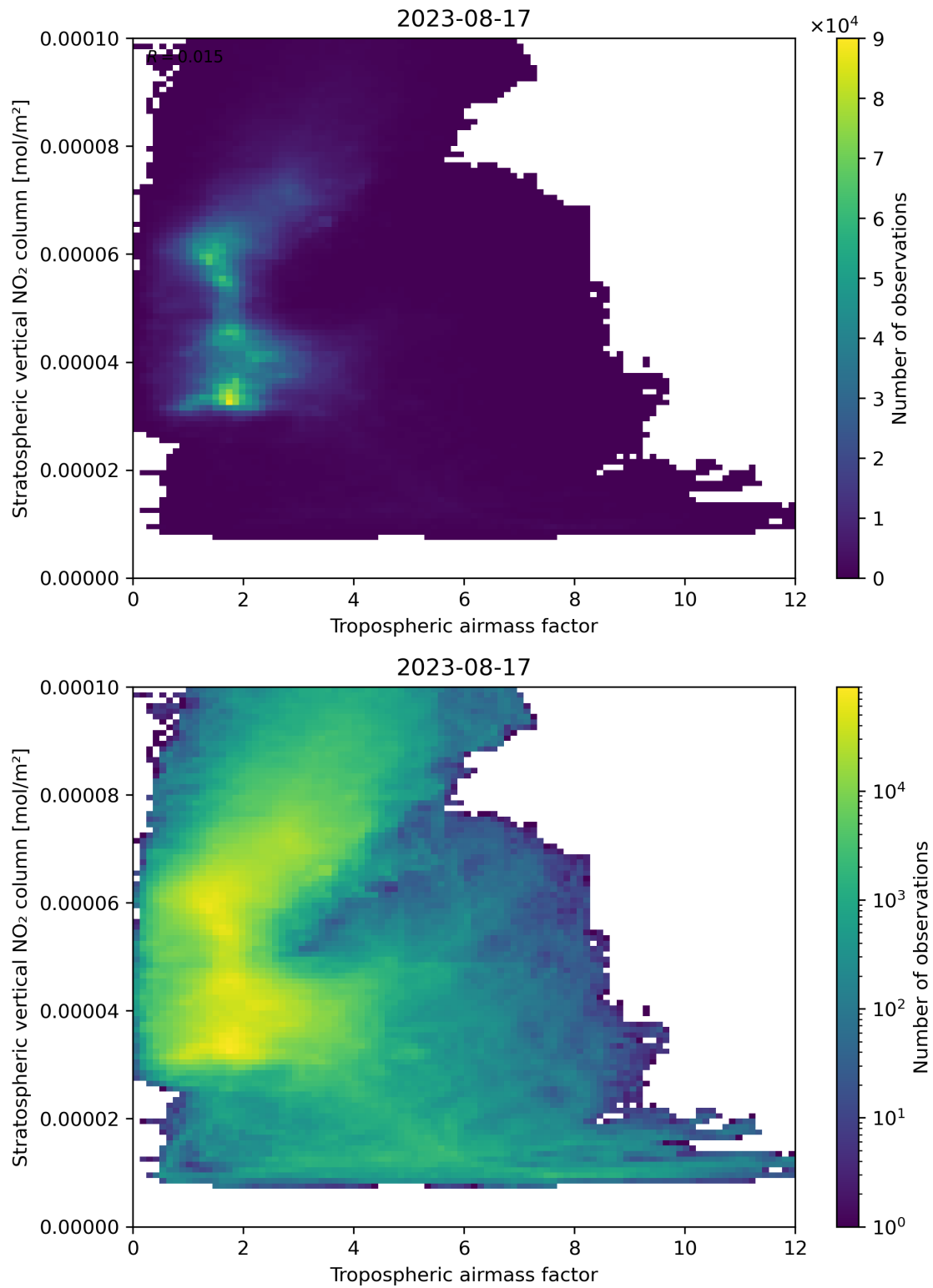
Figure 74: Scatter density plot of “Tropospheric air mass factor” against “Stratospheric vertical NO 2 column” for 2023-08-16 to 2023-08-18.
