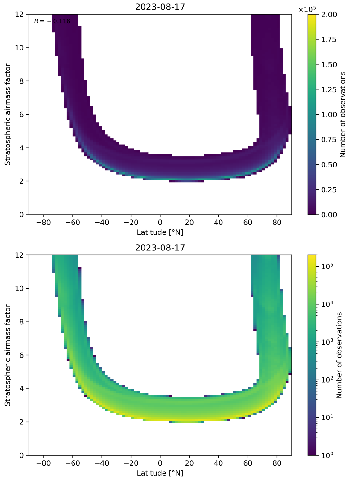
Figure 83: Scatter density plot of “Latitude” against “Stratospheric air mass factor” for 2023-08-16 to 2023-08-18.
