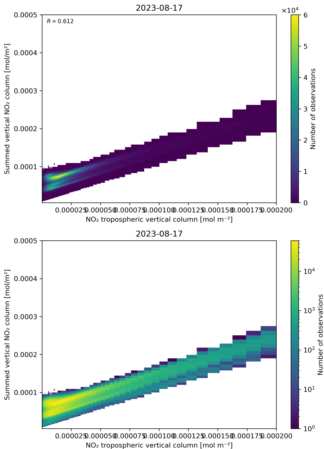
Figure 126: Scatter density plot of “NO 2 tropospheric vertical column” against “Summed vertical NO 2 column” for 2023-08-16 to 2023-08-18.
