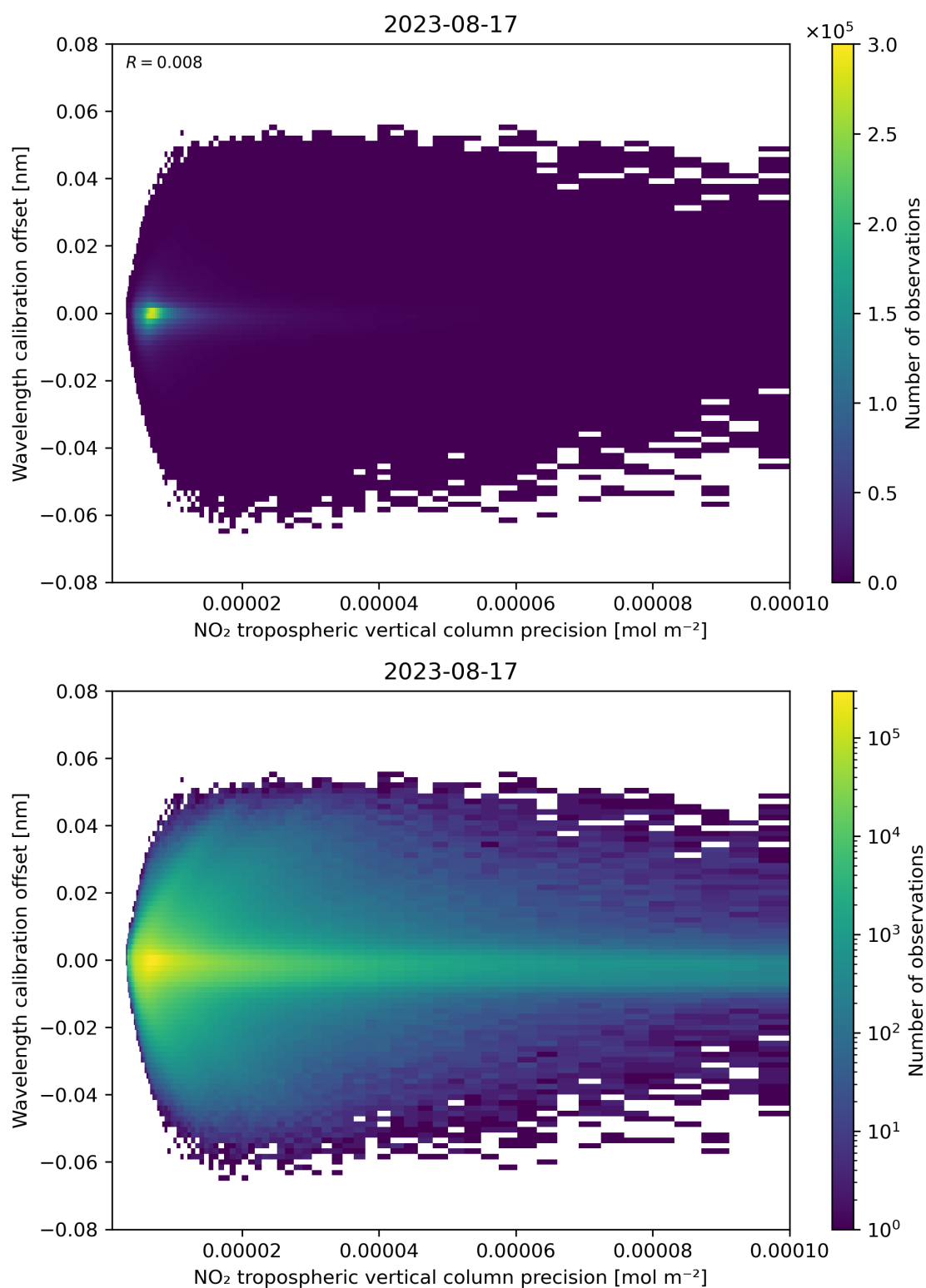
Figure 141: Scatter density plot of “NO 2 tropospheric vertical column precision” against “Wavelength calibration offset” for 2023-08-16 to 2023-08-18.
