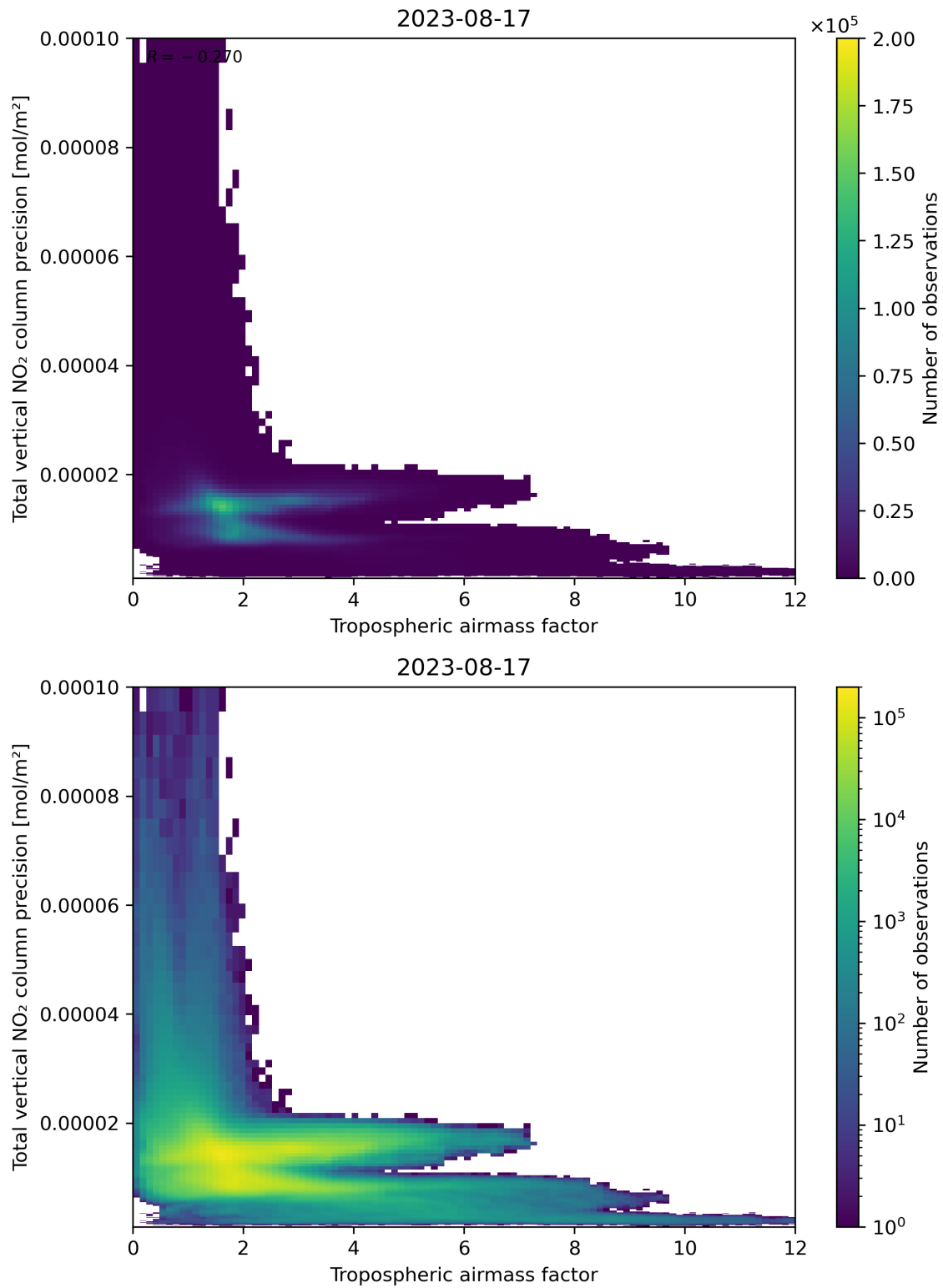
Figure 78: Scatter density plot of “Tropospheric air mass factor” against “Total vertical NO 2 column precision” for 2023-08-16 to 2023-08-18.
