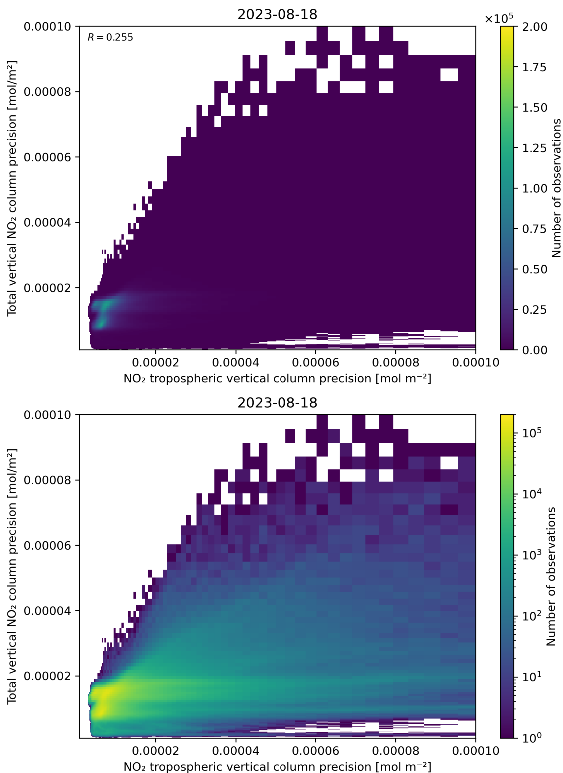
Figure 139: Scatter density plot of “NO 2 tropospheric vertical column precision” against “Total vertical NO 2 column precision” for 2023-08-17 to 2023-08-19.
