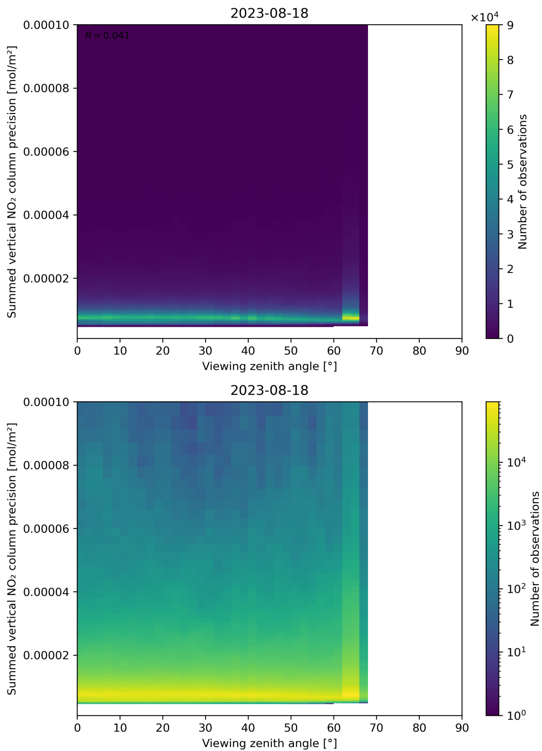
Figure 166: Scatter density plot of “Viewing zenith angle” against “Summed vertical NO 2 column precision” for 2023-08-17 to 2023-08-19.
