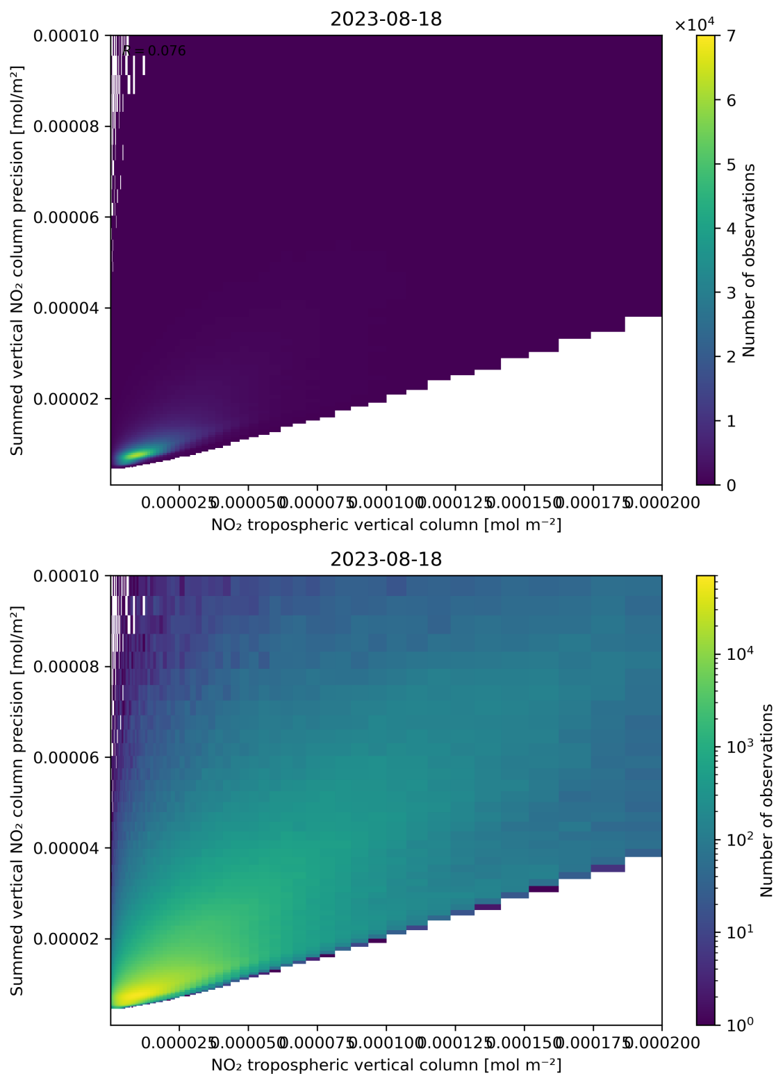
Figure 127: Scatter density plot of “NO 2 tropospheric vertical column” against “Summed vertical NO 2 column precision” for 2023-08-17 to 2023-08-19.
