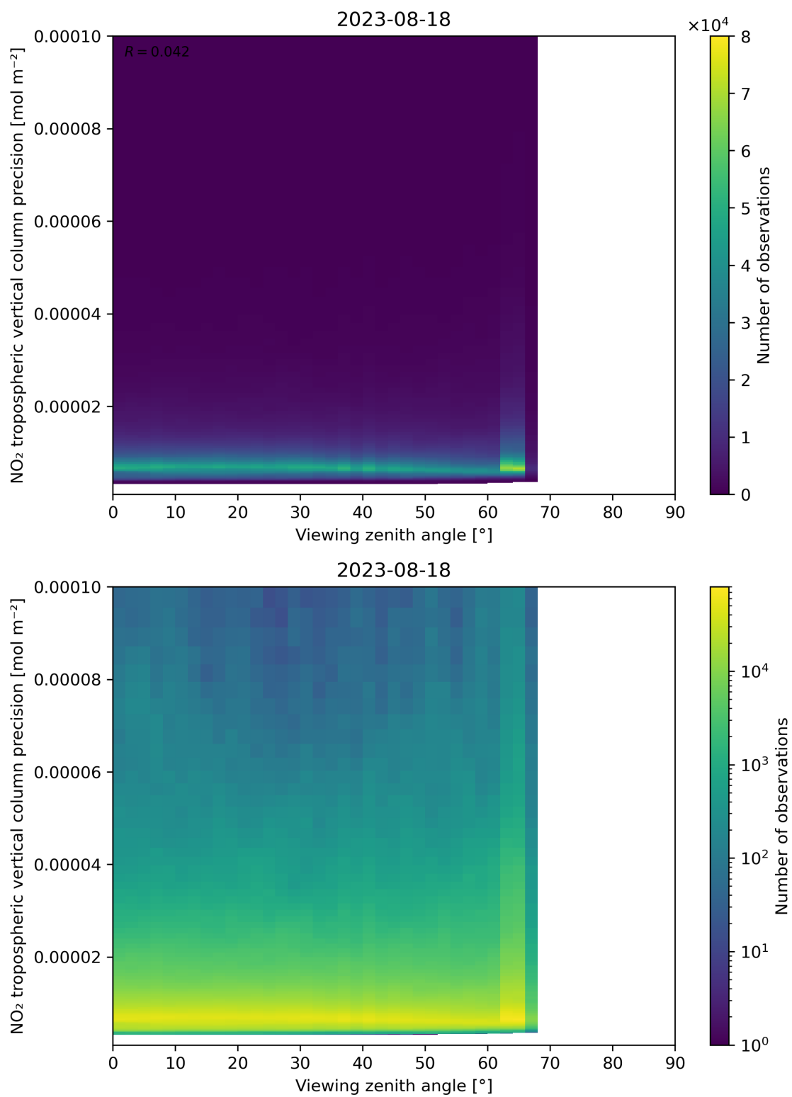
Figure 170: Scatter density plot of “Viewing zenith angle” against “NO 2 tropospheric vertical column precision” for 2023-08-17 to 2023-08-19.
