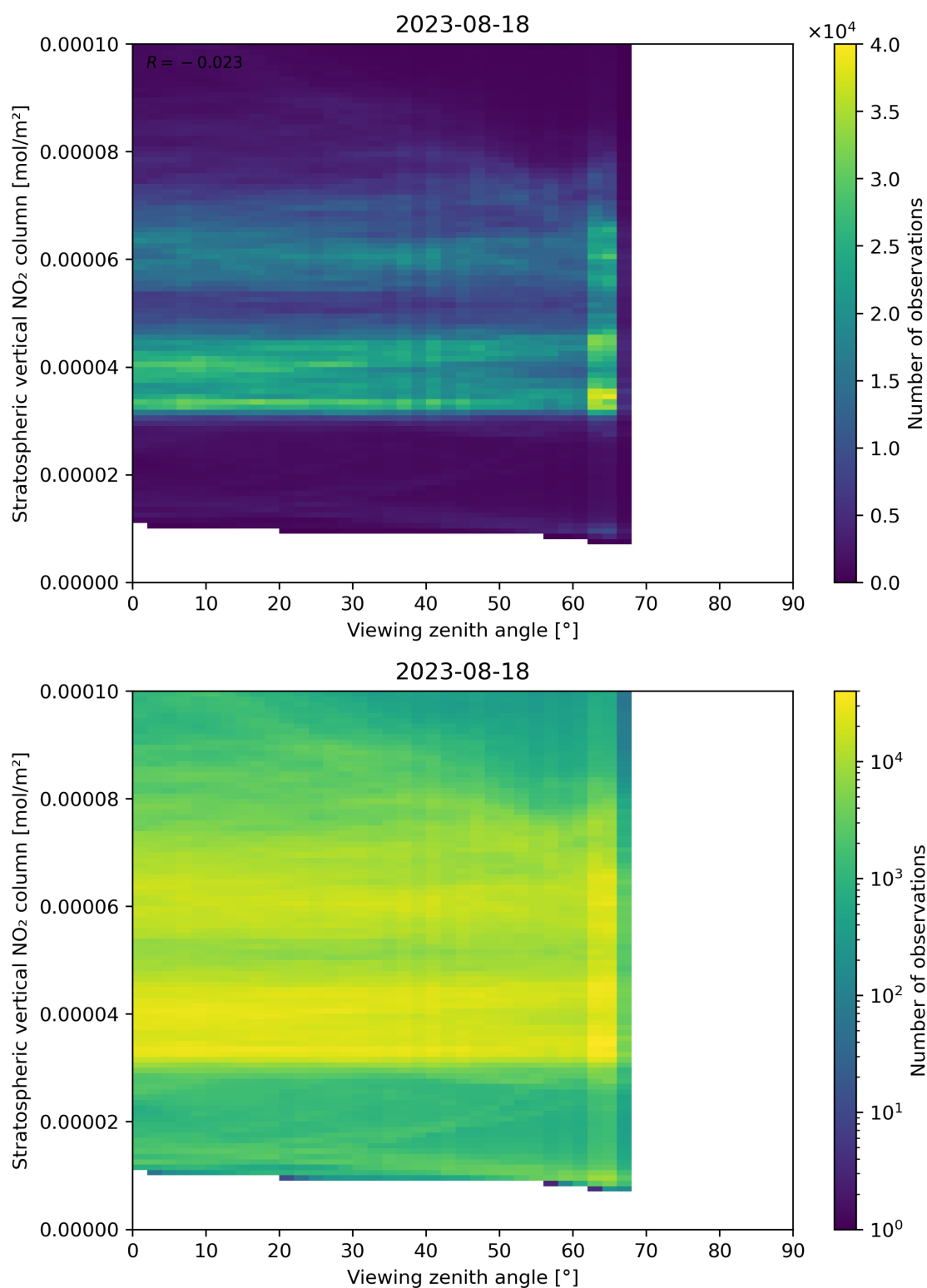
Figure 164: Scatter density plot of “Viewing zenith angle” against “Stratospheric vertical NO 2 column” for 2023-08-17 to 2023-08-19.
