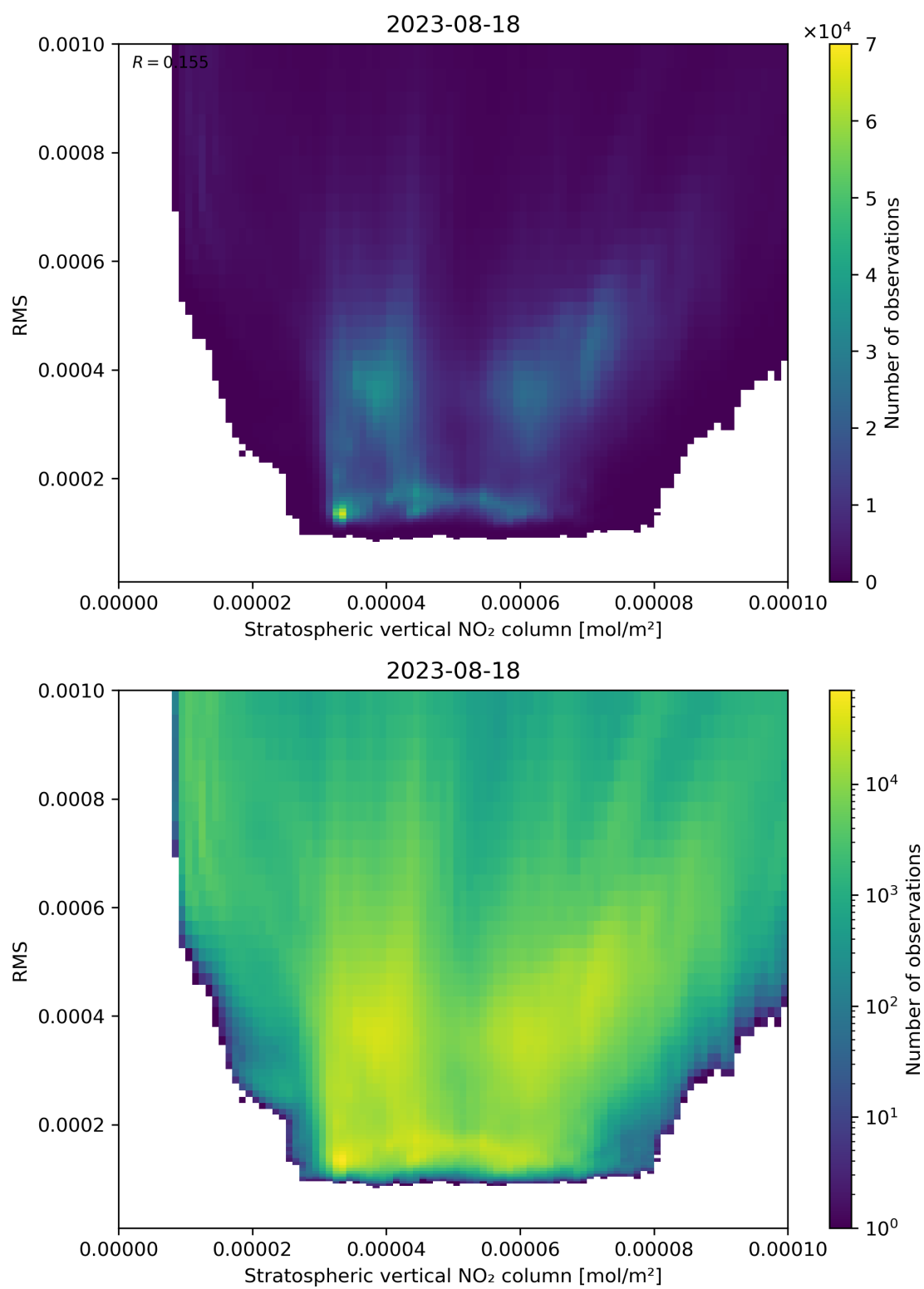
Figure 102: Scatter density plot of “Stratospheric vertical NO 2 column” against “RMS” for 2023-08-17 to 2023-08-19.
