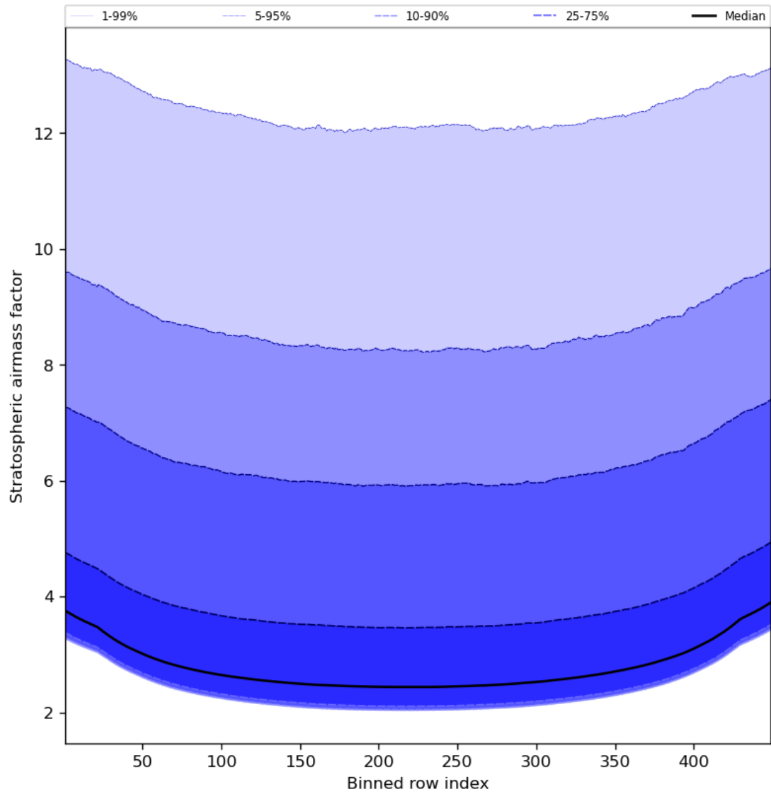
Figure 61: Along track statistics of “Stratospheric airmass factor” for 2023-08-17 to 2023-08-19
