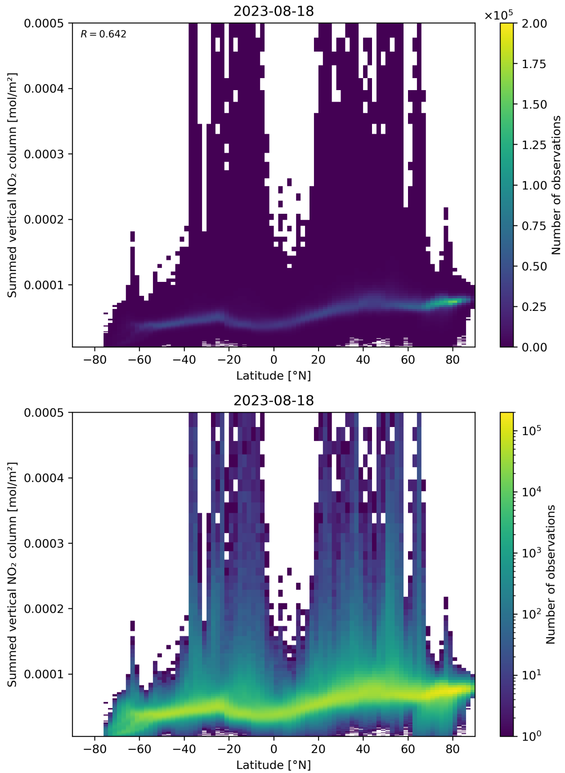
Figure 88: Scatter density plot of “Latitude” against “Summed vertical NO 2 column” for 2023-08-17 to 2023-08-19.
