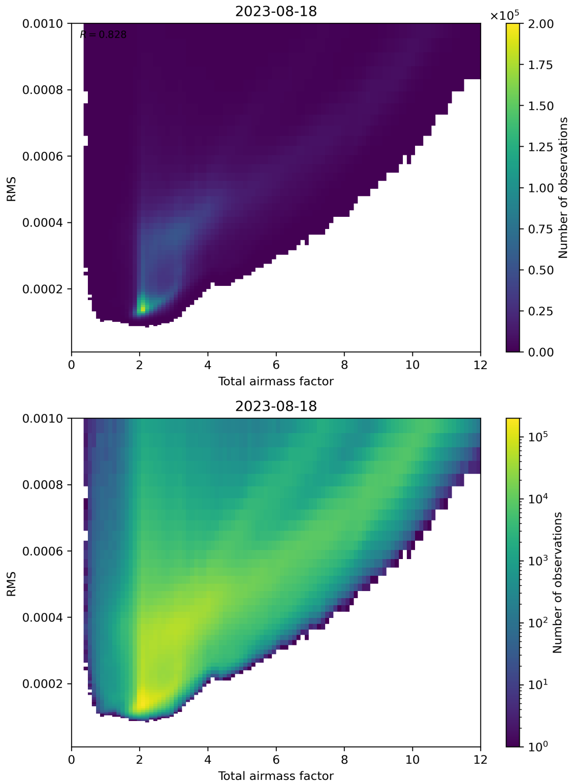
Figure 69: Scatter density plot of “Total airmass factor” against “RMS” for 2023-08-17 to 2023-08-19.
