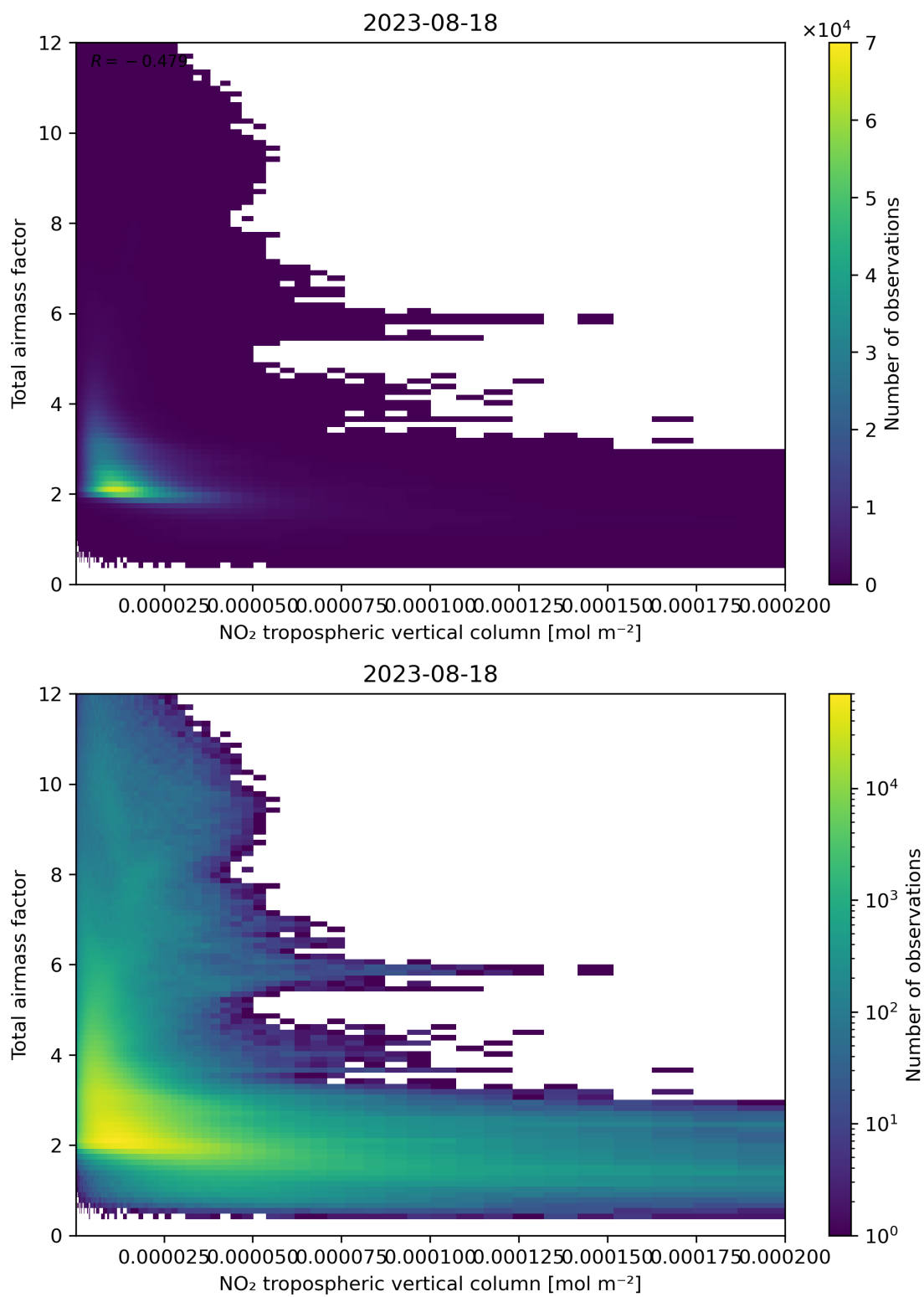
Figure 122: Scatter density plot of “NO 2 tropospheric vertical column” against “Total air mass factor” for 2023-08-17 to 2023-08-19.
