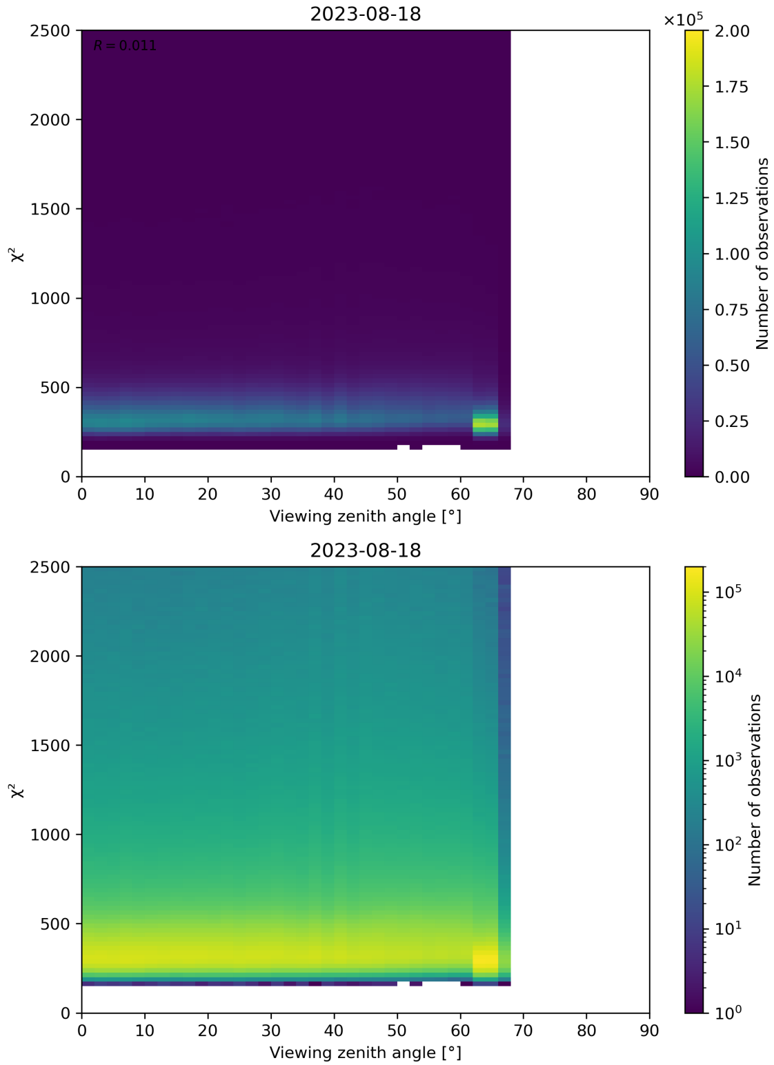
Figure 162: Scatter density plot of “Viewing zenith angle” against “ \chi^2 ” for 2023-08-17 to 2023-08-19.
