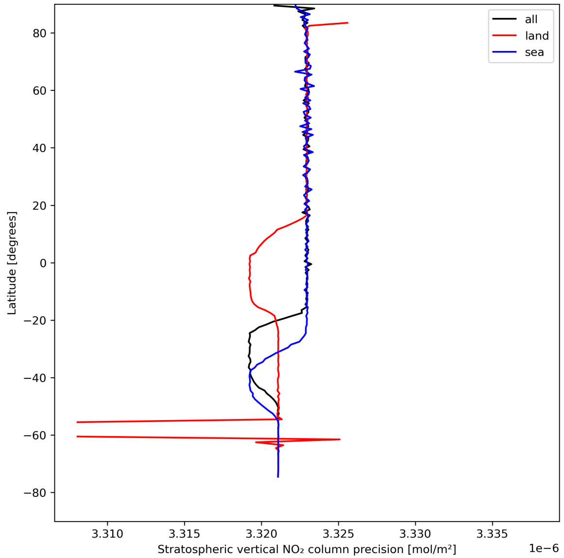
Figure 20: Zonal average of “Stratospheric vertical NO 2 column precision” for 2023-08-17 to 2023-08-19.
