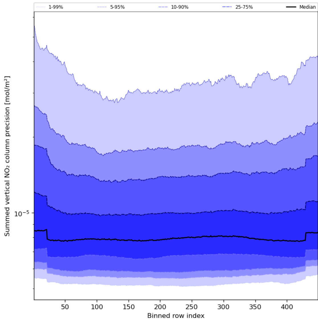
Figure 58: Along track statistics of “Summed vertical NO 2 column precision” for 2023-08-17 to 2023-08-19
