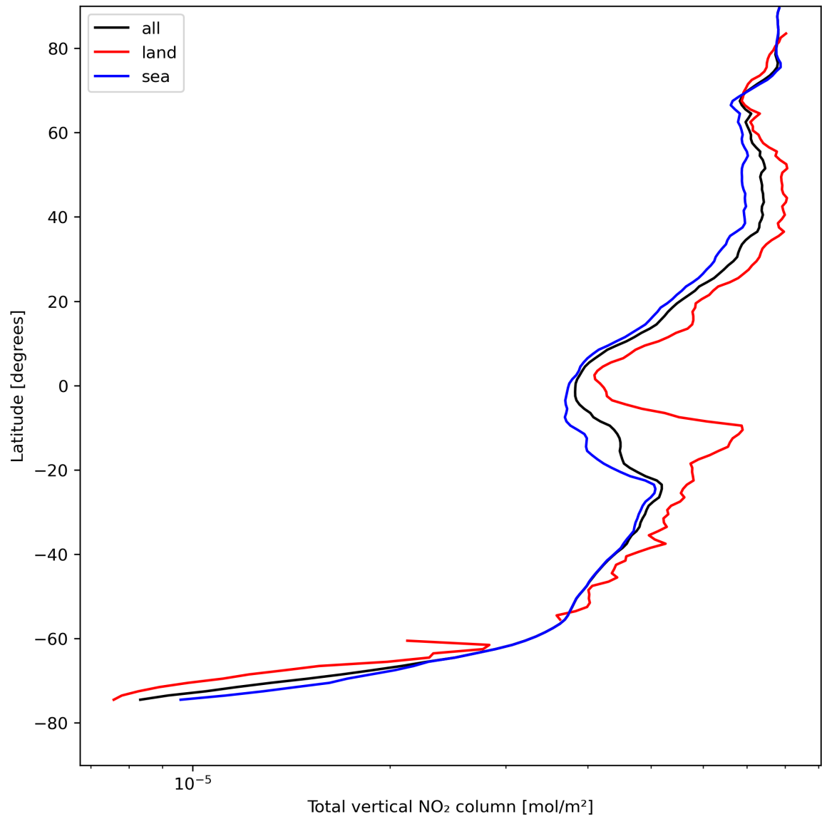
Figure 21: Zonal average of “Total vertical NO 2 column” for 2023-08-17 to 2023-08-19.
