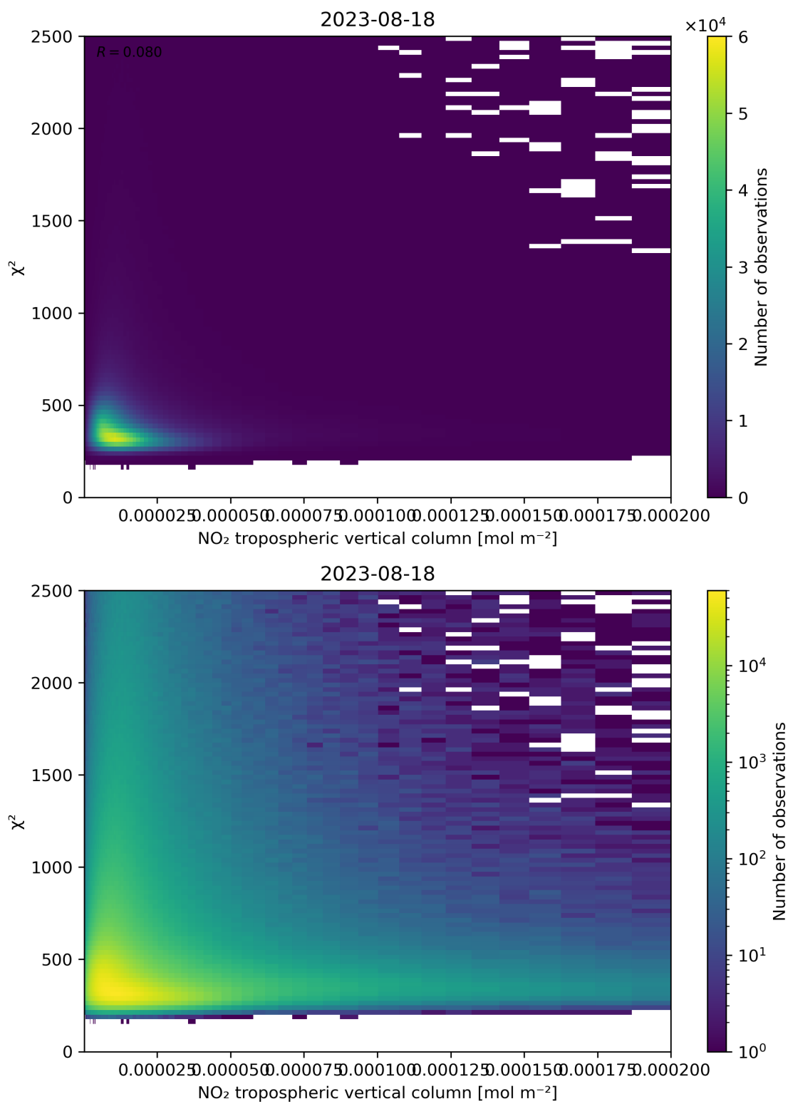
Figure 124: Scatter density plot of “NO 2 tropospheric vertical column” against “ \chi^2 ” for 2023-08-17 to 2023-08-19.
