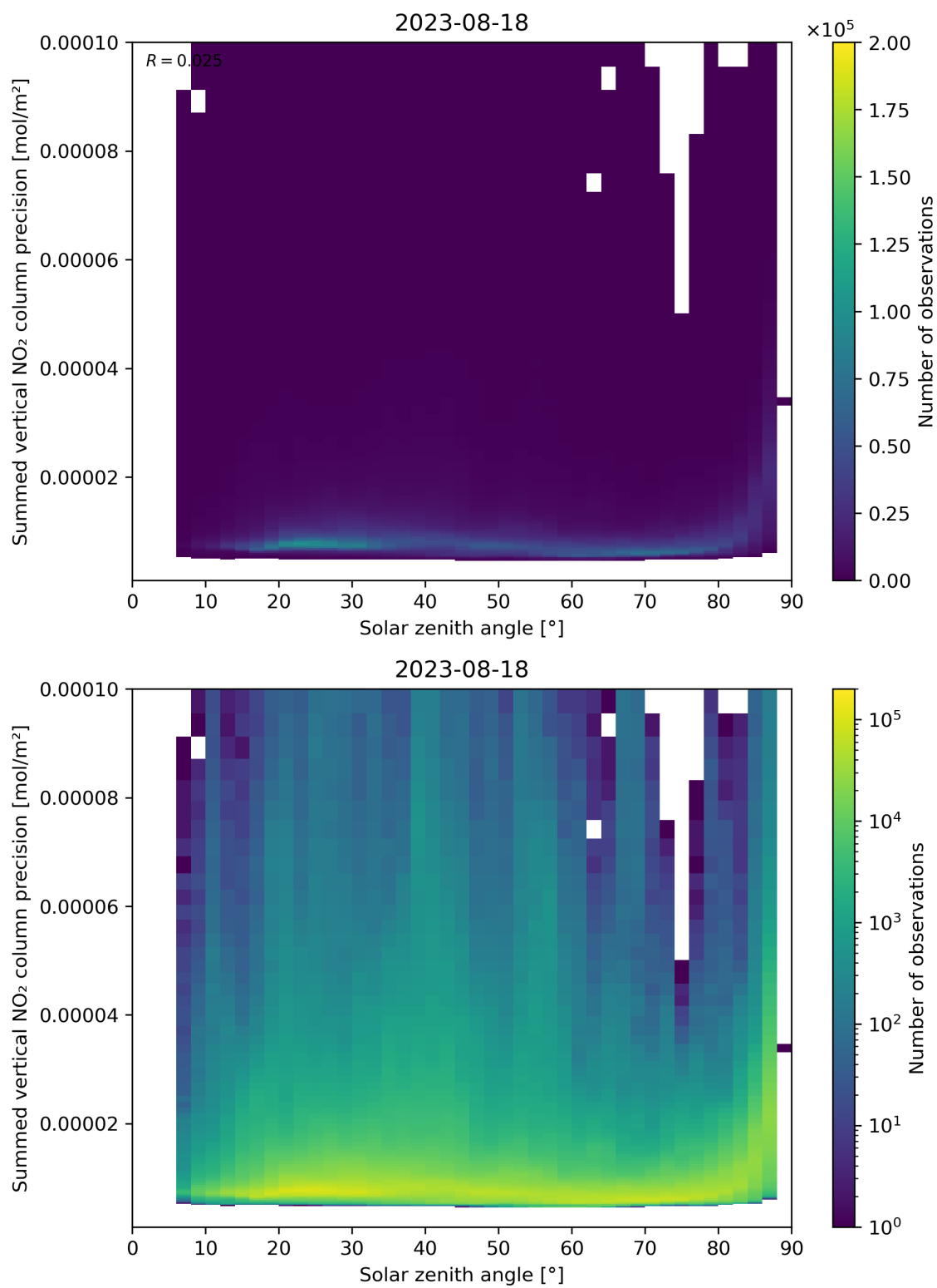
Figure 152: Scatter density plot of “Solar zenith angle” against “Summed vertical NO 2 column precision” for 2023-08-17 to 2023-08-19.
