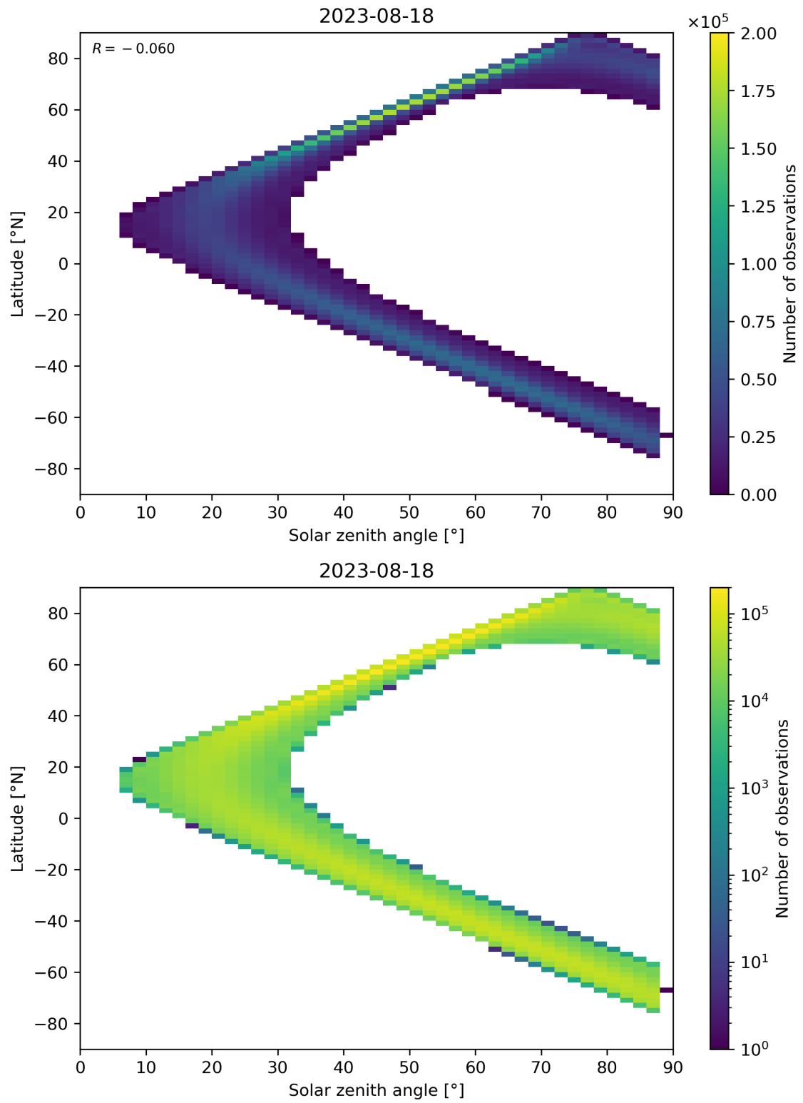
Figure 149: Scatter density plot of “Solar zenith angle” against “Latitude” for 2023-08-17 to 2023-08-19.
