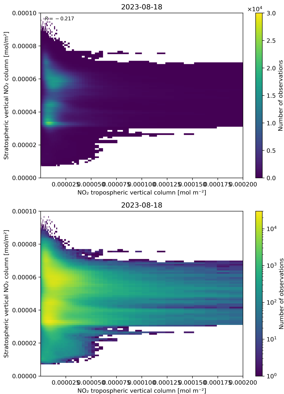
Figure 125: Scatter density plot of “NO 2 tropospheric vertical column” against “Stratospheric vertical NO 2 column” for 2023-08-17 to 2023-08-19.
