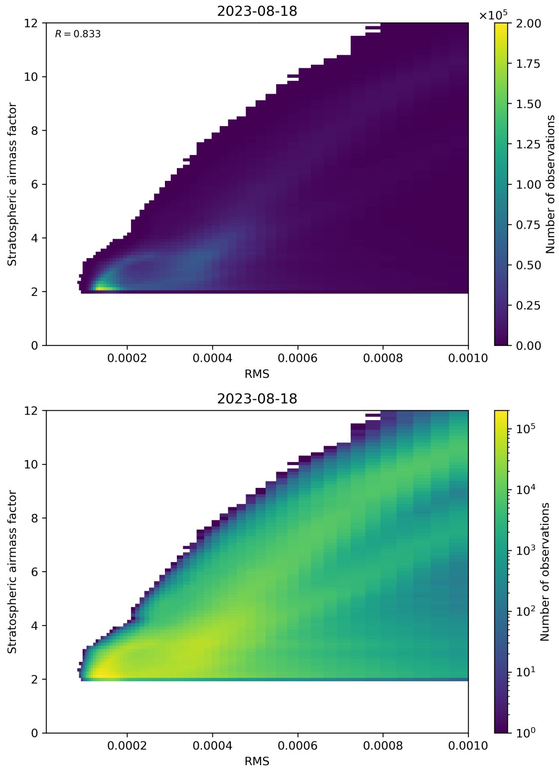
Figure 144: Scatter density plot of “RMS” against “Stratospheric airmass factor” for 2023-08-17 to 2023-08-19.
