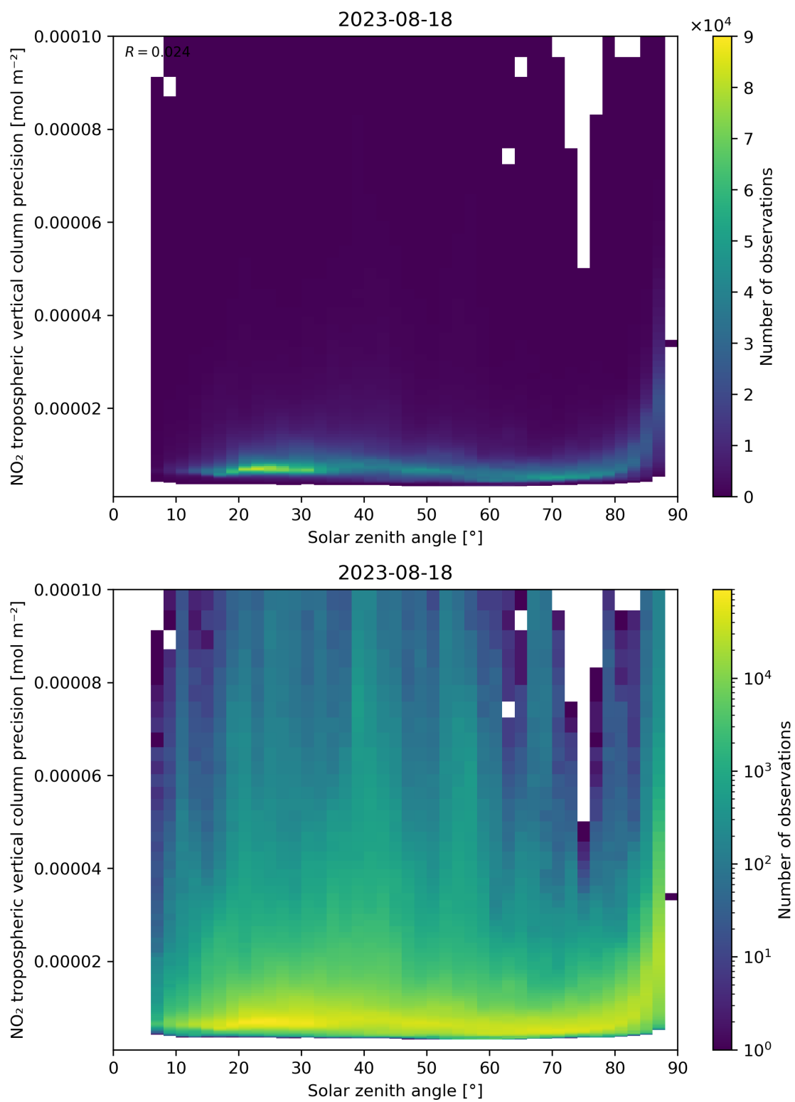
Figure 156: Scatter density plot of “Solar zenith angle” against “NO 2 tropospheric vertical column precision” for 2023-08-17 to 2023-08-19.
