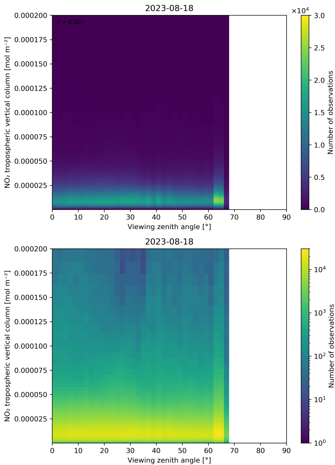
Figure 169: Scatter density plot of “Viewing zenith angle” against “NO 2 tropospheric vertical column” for 2023-08-17 to 2023-08-19.
