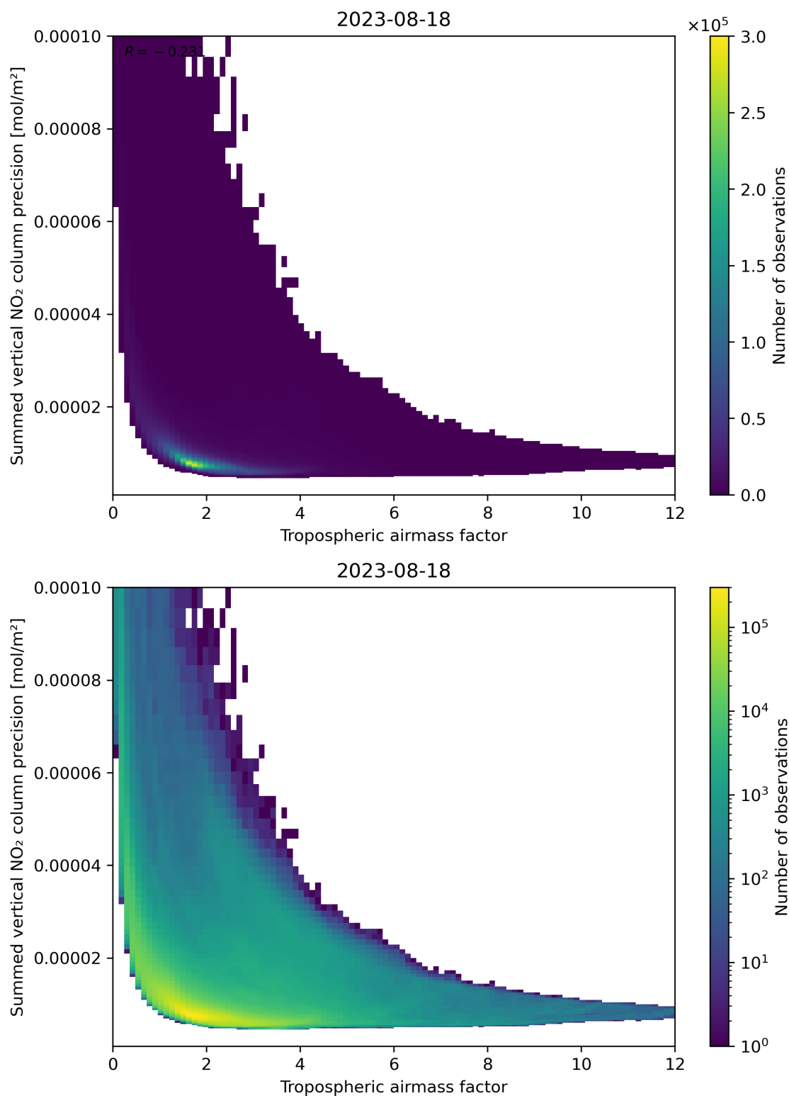
Figure 76: Scatter density plot of “Tropospheric air mass factor” against “Summed vertical NO 2 column precision” for 2023-08-17 to 2023-08-19.
