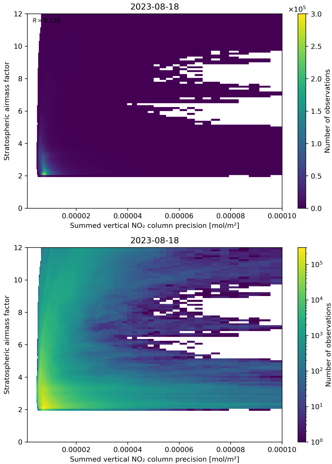
Figure 106: Scatter density plot of “Summed vertical NO 2 column precision” against “Stratospheric airmass factor” for 2023-08-17 to 2023-08-19.
