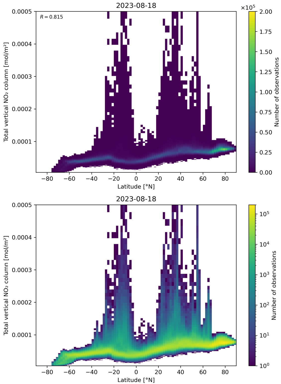
Figure 90: Scatter density plot of “Latitude” against “Total vertical NO 2 column” for 2023-08-17 to 2023-08-19.
