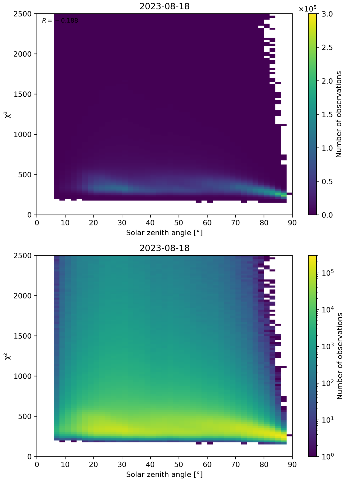
Figure 148: Scatter density plot of “Solar zenith angle” against “ \chi^2 ” for 2023-08-17 to 2023-08-19.
