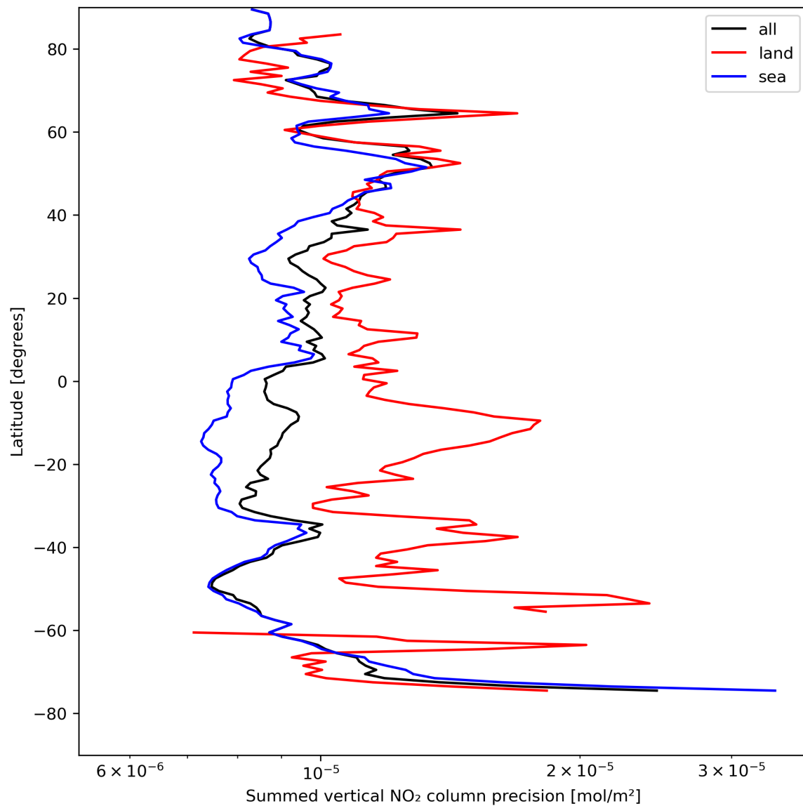
Figure 24: Zonal average of “Summed vertical NO 2 column precision” for 2023-08-17 to 2023-08-19.
