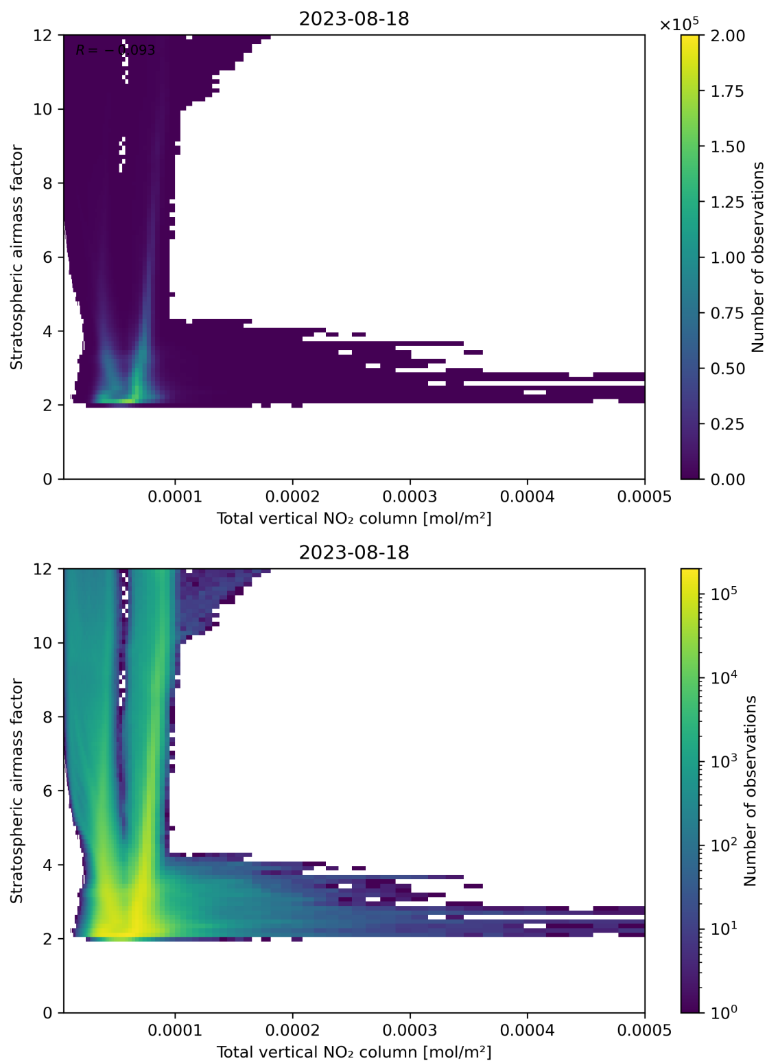
Figure 110: Scatter density plot of “Total vertical NO 2 column” against “Stratospheric airmass factor” for 2023-08-17 to 2023-08-19.
