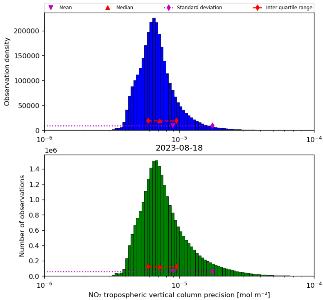
Figure 30: Histogram of “NO 2 tropospheric vertical column precision” for 2023-08-17 to 2023-08-19
