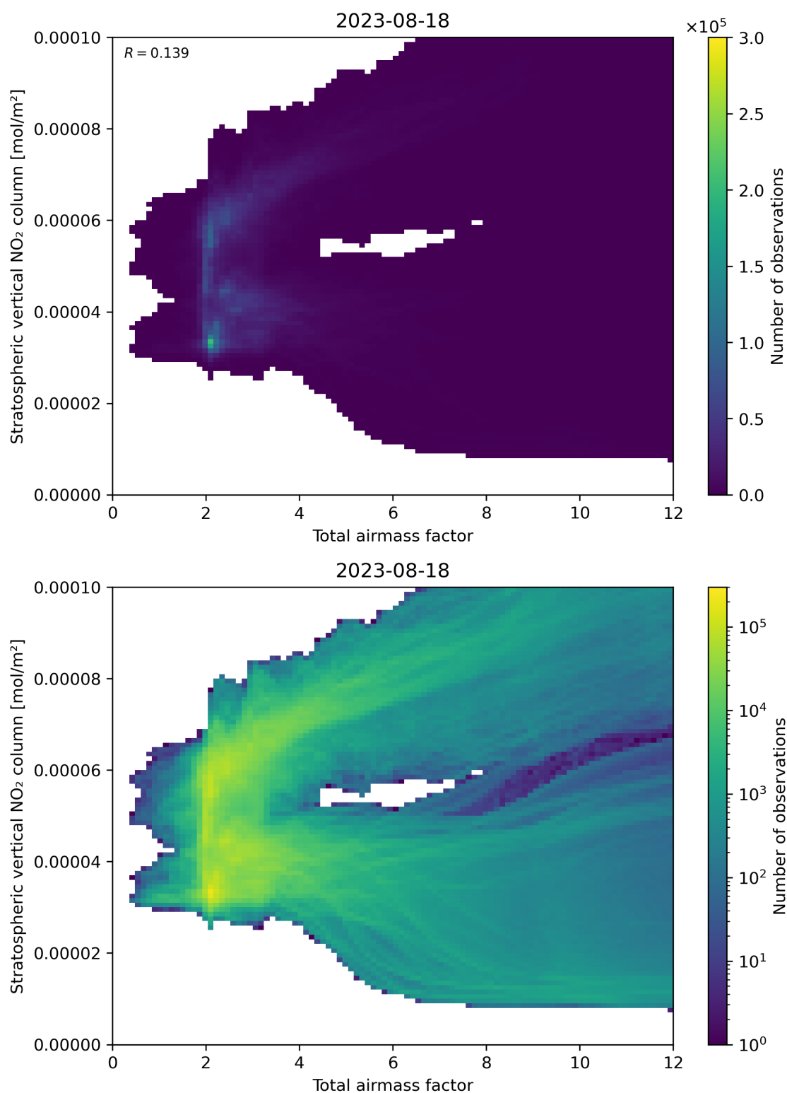
Figure 64: Scatter density plot of “Total airmass factor” against “Stratospheric vertical \text{NO}_2 column” for 2023-08-17 to 2023-08-19.
