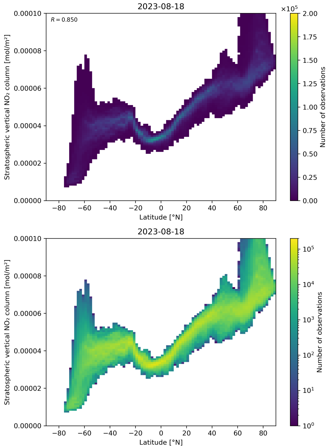
Figure 87: Scatter density plot of “Latitude” against “Stratospheric vertical \text{NO}_2 column” for 2023-08-17 to 2023-08-19.
