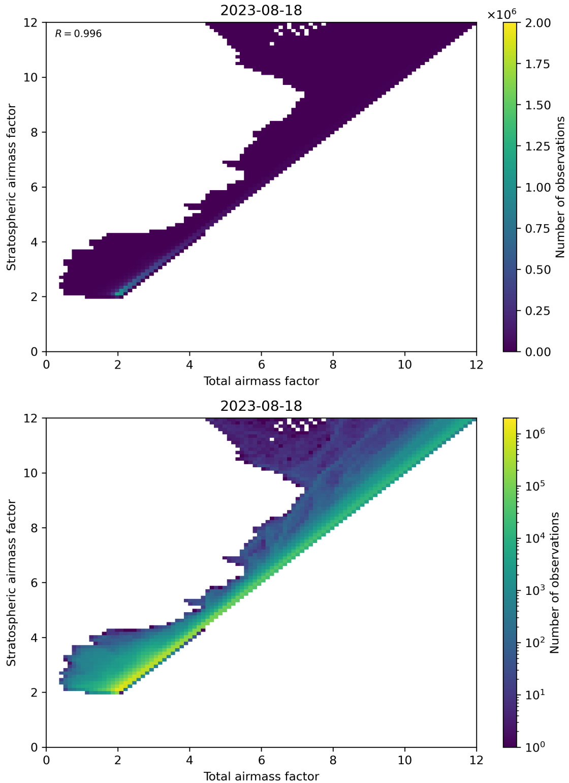
Figure 62: Scatter density plot of “Total airmass factor” against “Stratospheric airmass factor” for 2023-08-17 to 2023-08-19.
