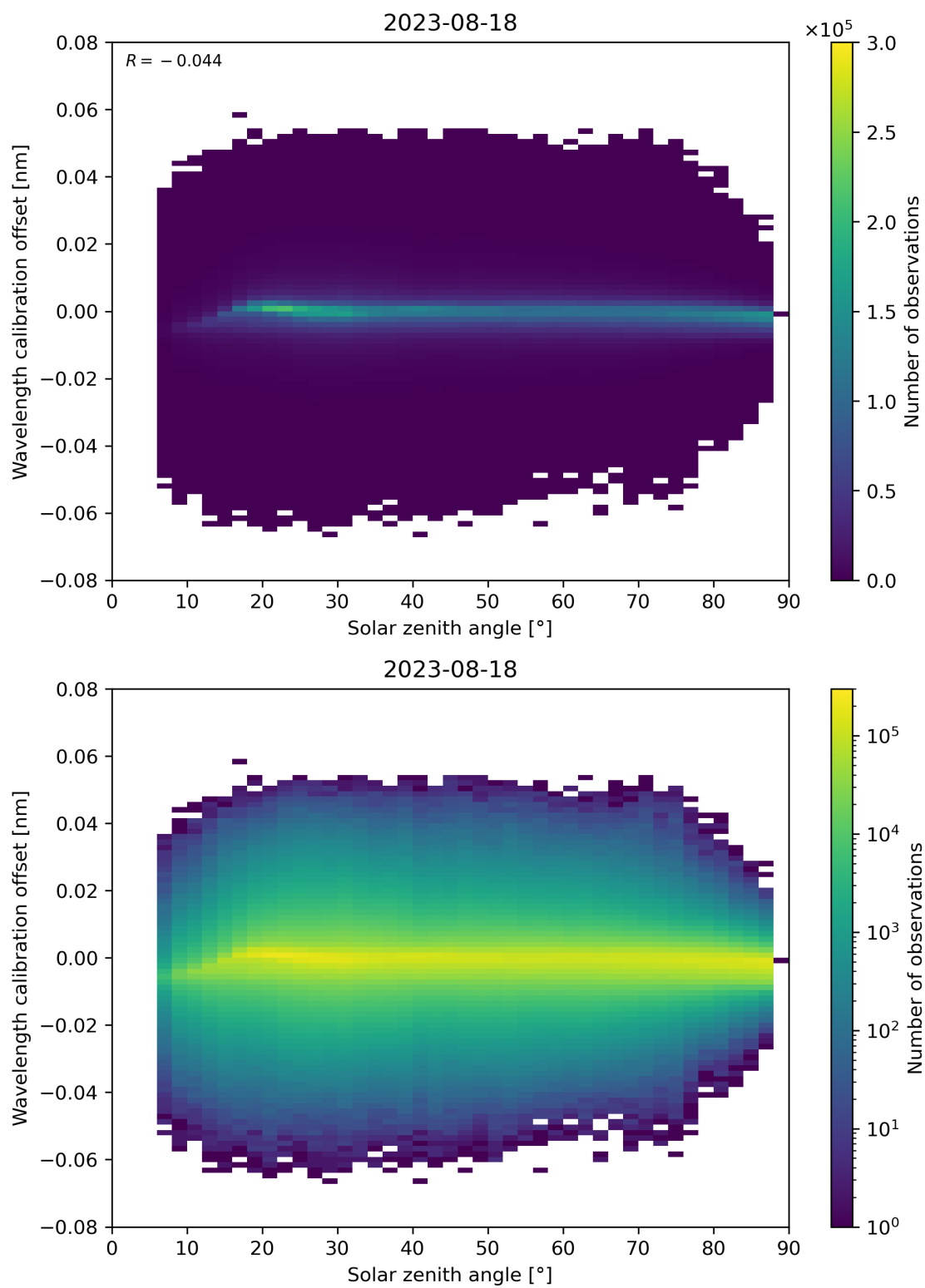
Figure 158: Scatter density plot of “Solar zenith angle” against “Wavelength calibration offset” for 2023-08-17 to 2023-08-19.
