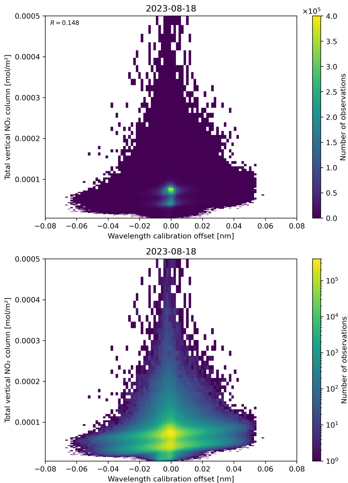
Figure 179: Scatter density plot of “Wavelength calibration offset” against “Total vertical NO 2 column” for 2023-08-17 to 2023-08-19.
