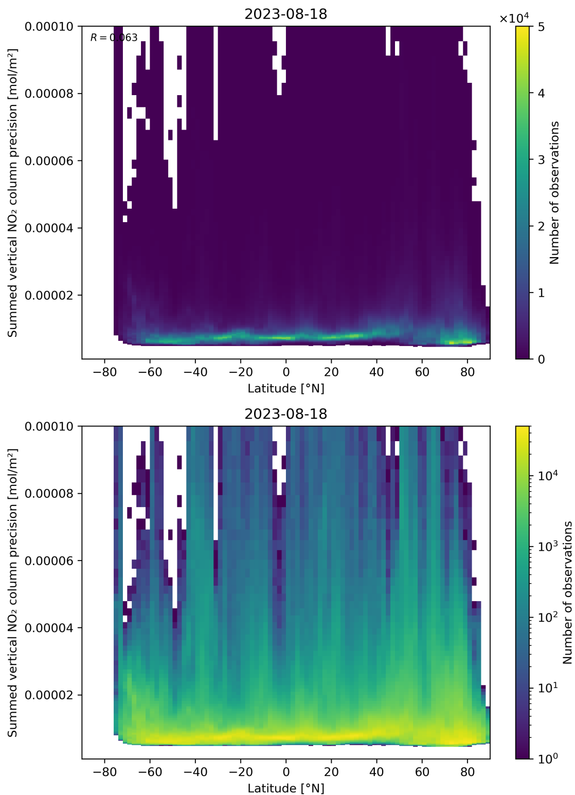
Figure 89: Scatter density plot of “Latitude” against “Summed vertical NO 2 column precision” for 2023-08-17 to 2023-08-19.
