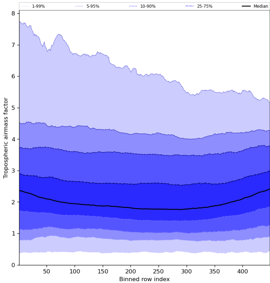
Figure 48: Along track statistics of “Tropospheric airmass factor” for 2023-08-17 to 2023-08-19
