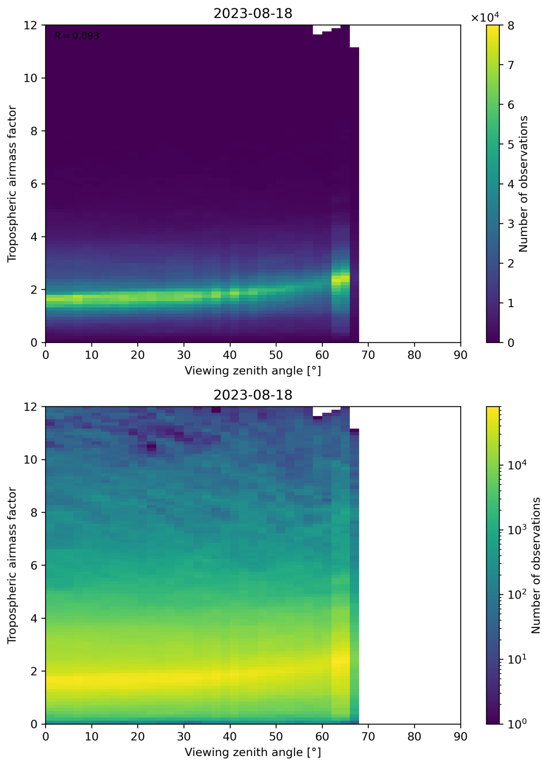
Figure 161: Scatter density plot of “Viewing zenith angle” against “Tropospheric airmass factor” for 2023-08-17 to 2023-08-19.
