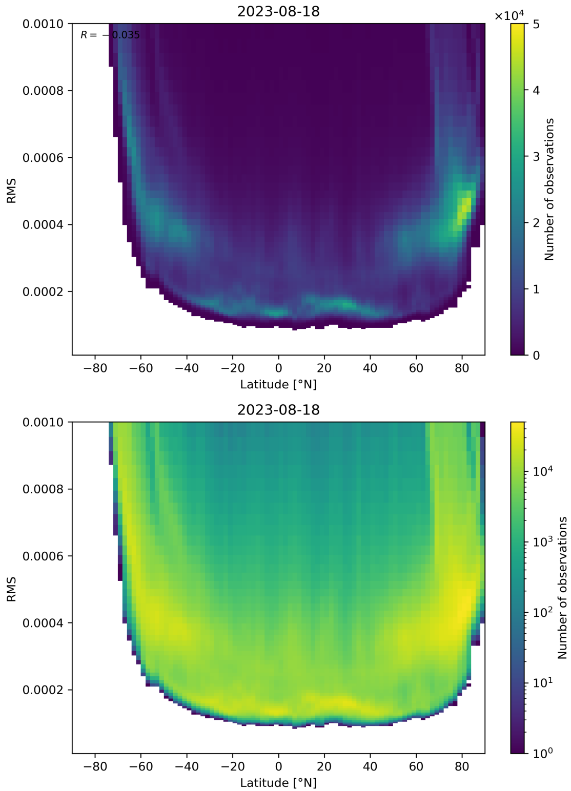
Figure 94: Scatter density plot of “Latitude” against “RMS” for 2023-08-17 to 2023-08-19.
