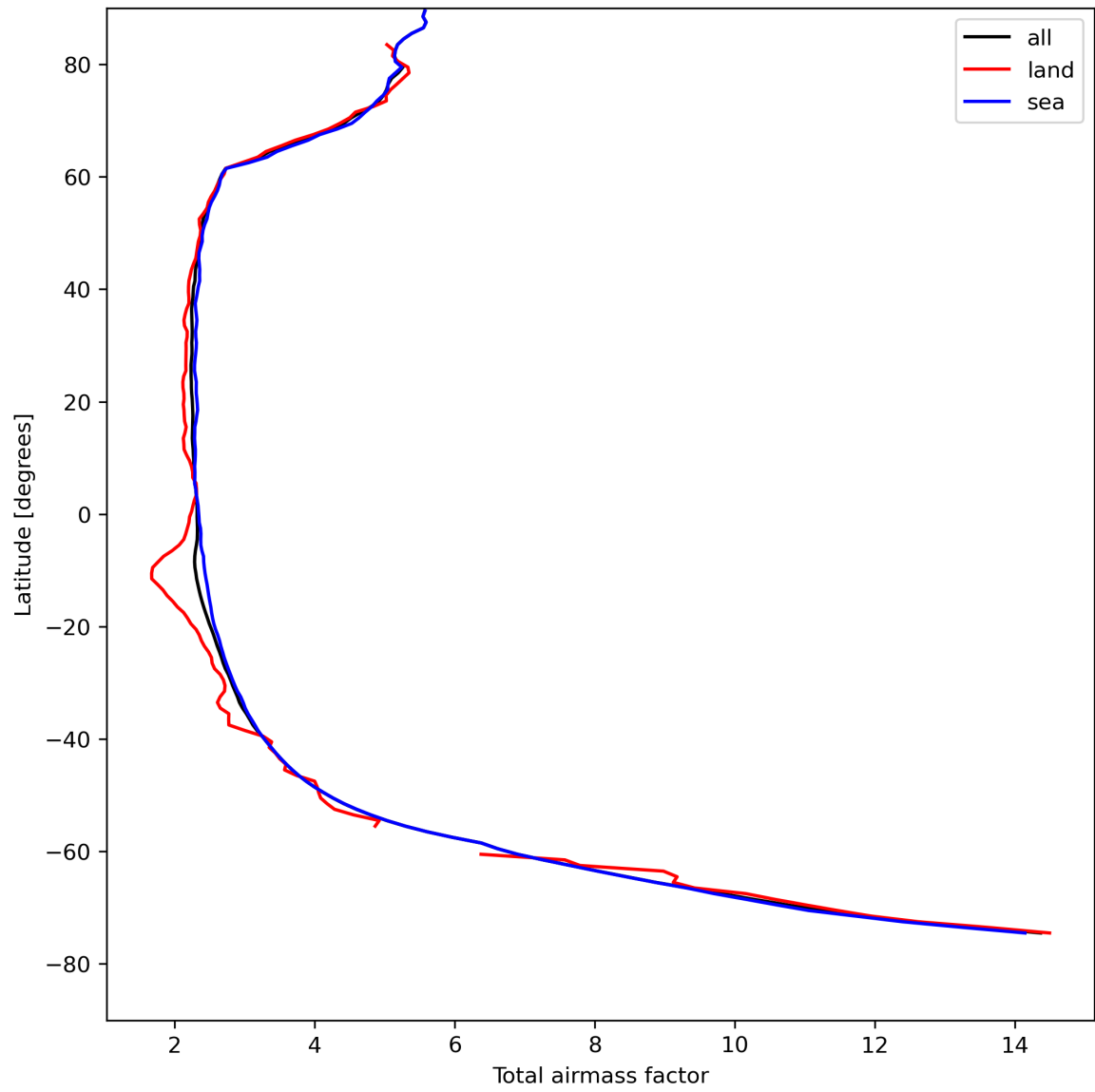
Figure 15: Zonal average of “Total airmass factor” for 2023-08-17 to 2023-08-19.
