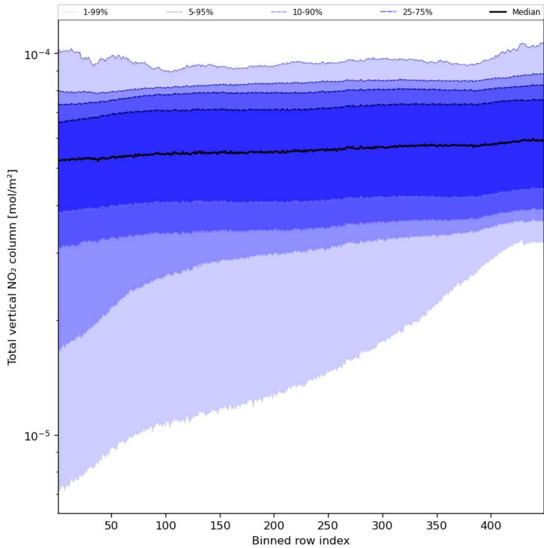
Figure 55: Along track statistics of “Total vertical NO 2 column” for 2023-08-17 to 2023-08-19
