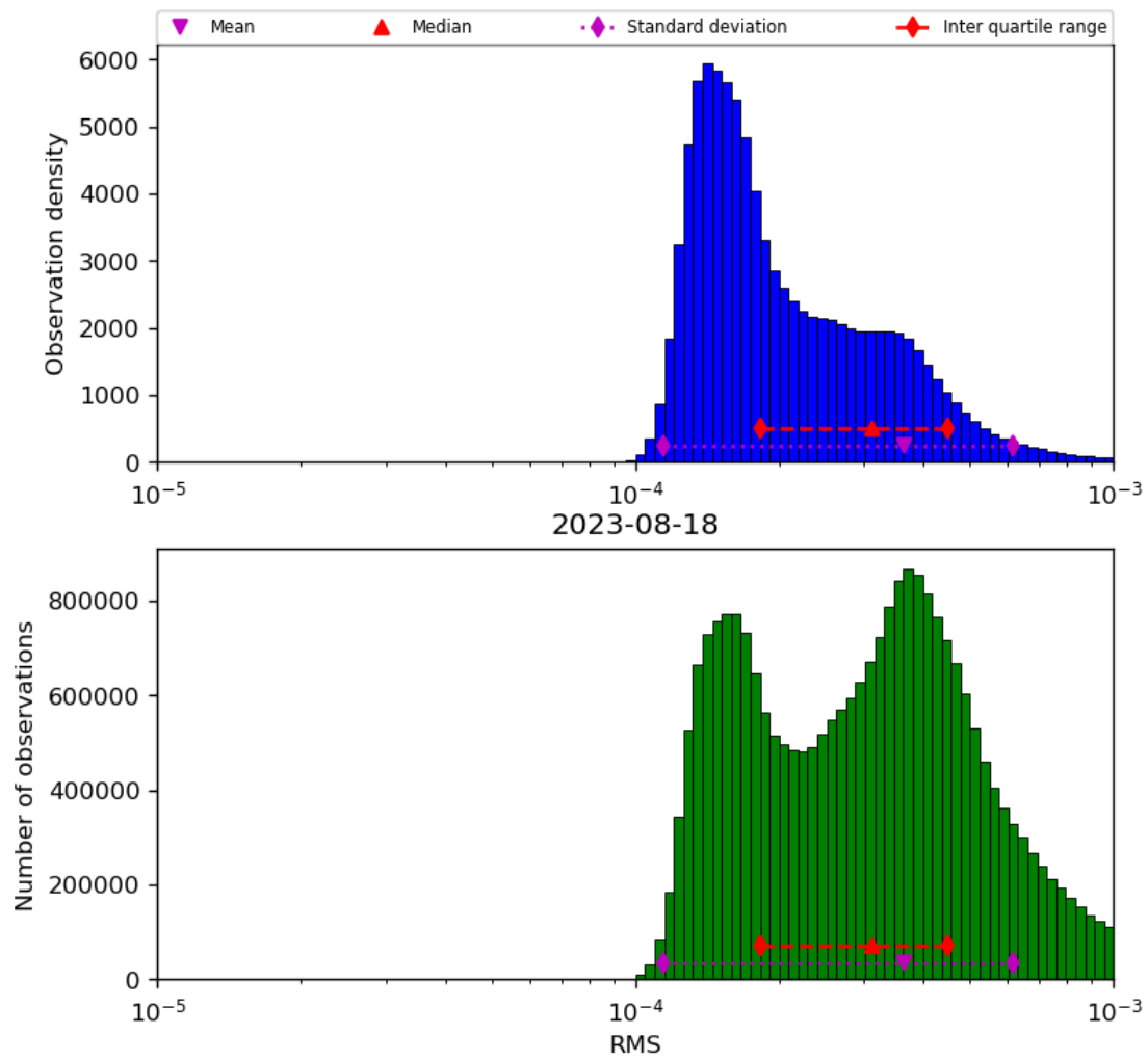
Figure 43: Histogram of “RMS” for 2023-08-17 to 2023-08-19
