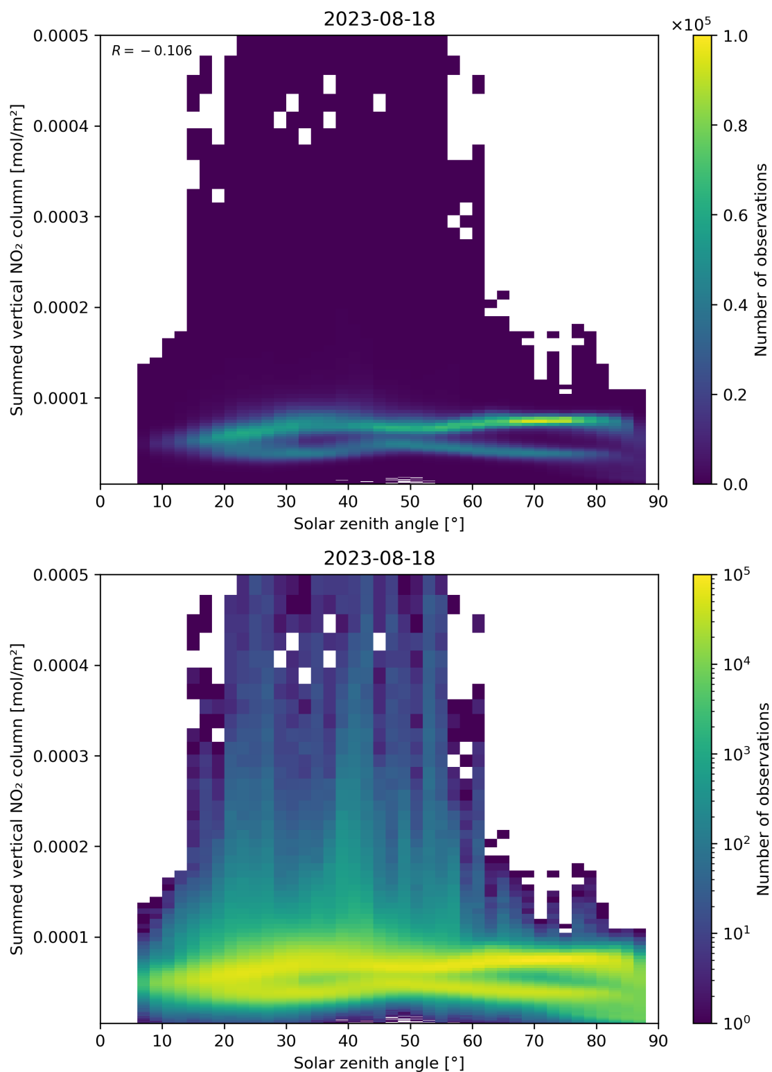
Figure 151: Scatter density plot of “Solar zenith angle” against “Summed vertical NO 2 column” for 2023-08-17 to 2023-08-19.
