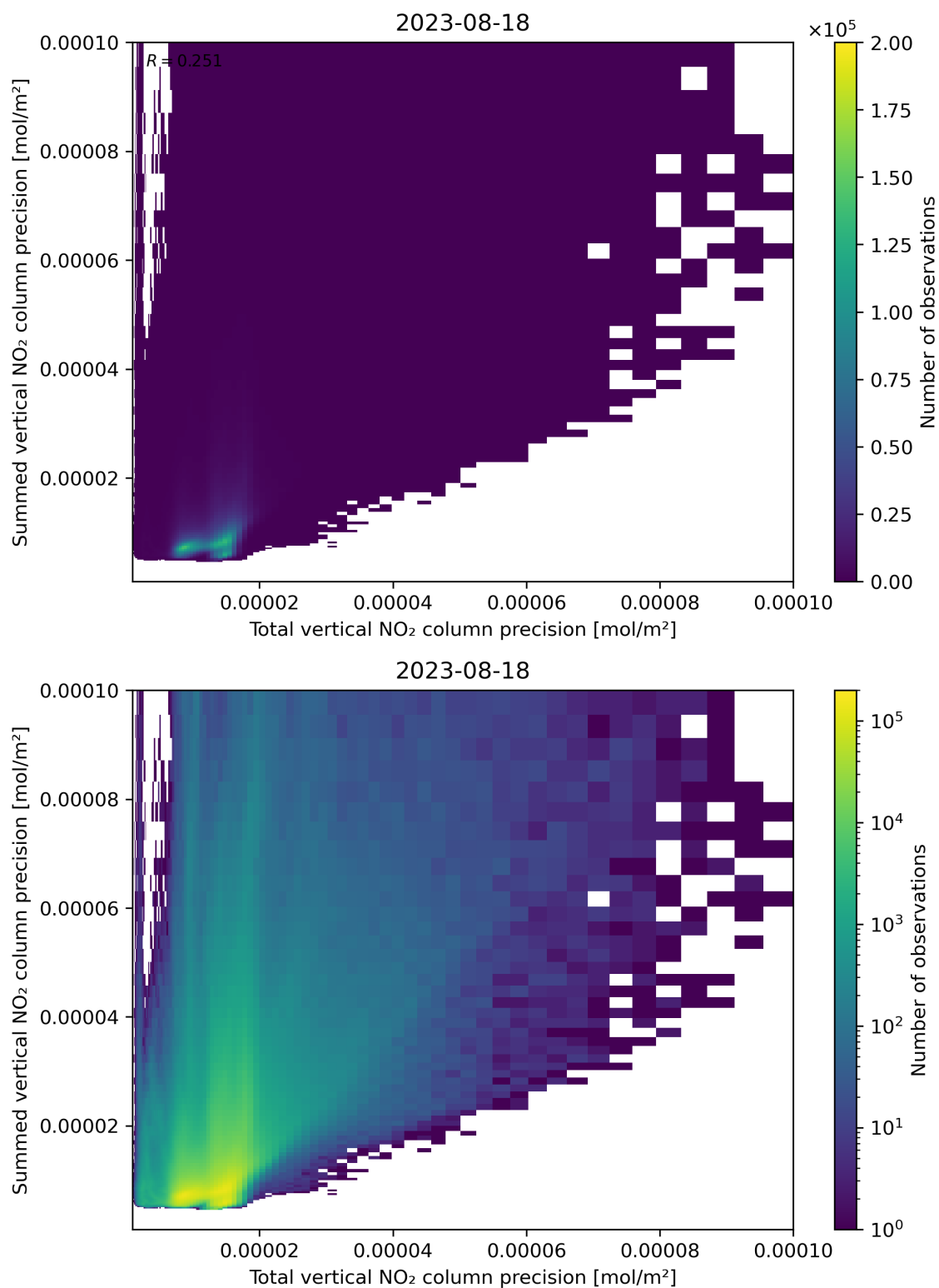
Figure 118: Scatter density plot of “Total vertical NO 2 column precision” against “Summed vertical NO 2 column precision” for 2023-08-17 to 2023-08-19.
