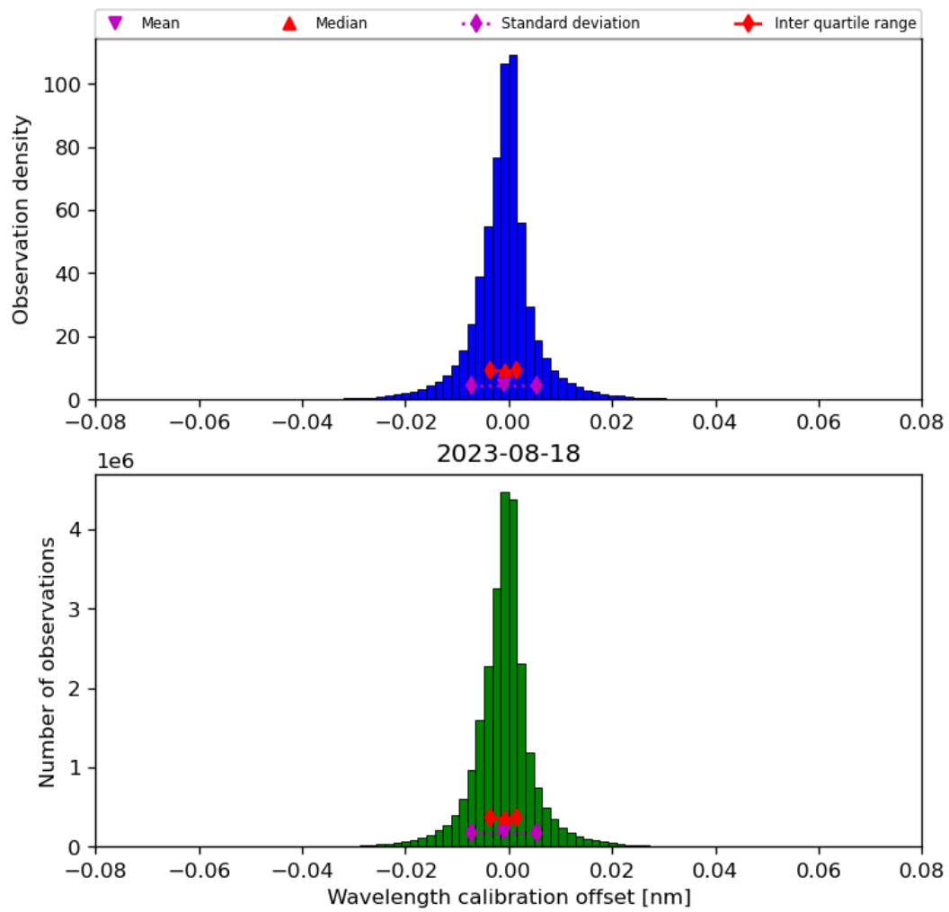
Figure 35: Histogram of “Wavelength calibration offset” for 2023-08-17 to 2023-08-19
