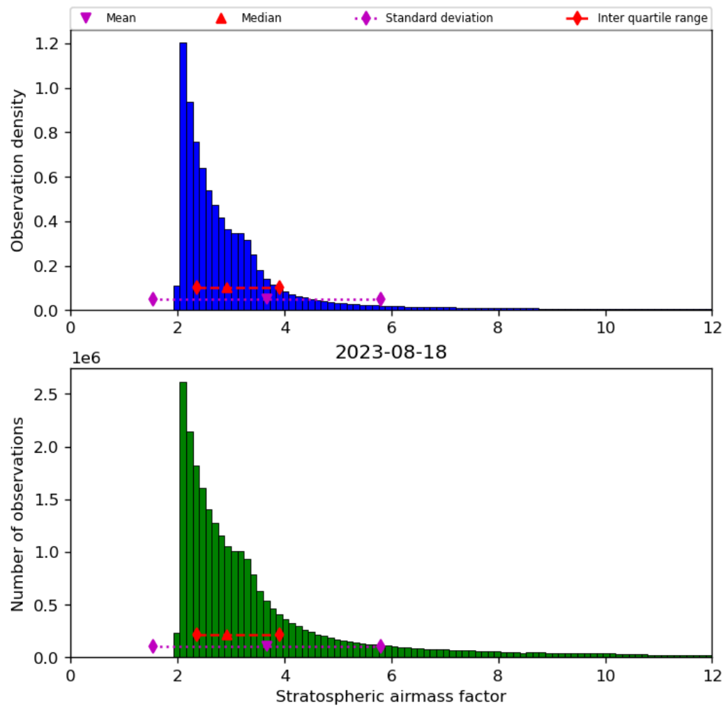
Figure 44: Histogram of “Stratospheric airmass factor” for 2023-08-17 to 2023-08-19
