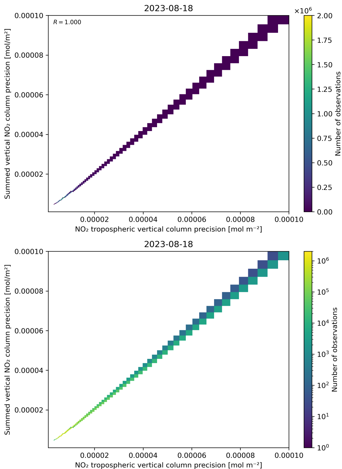
Figure 137: Scatter density plot of “NO 2 tropospheric vertical column precision” against “Summed vertical NO 2 column precision” for 2023-08-17 to 2023-08-19.
