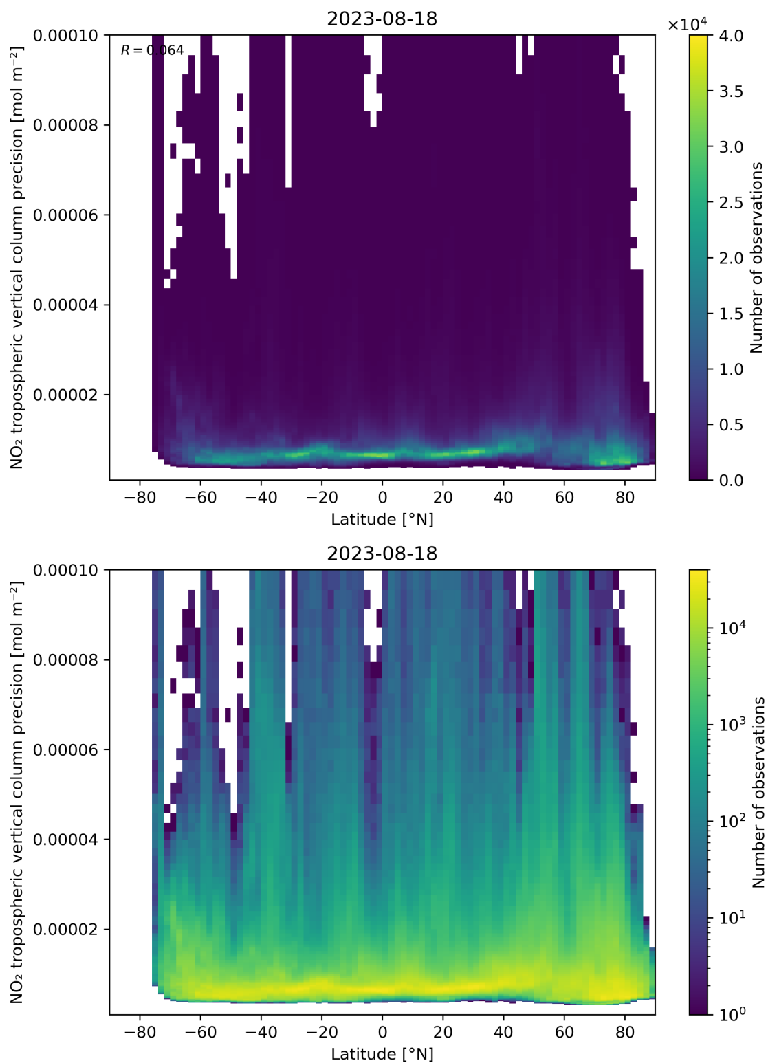
Figure 93: Scatter density plot of “Latitude” against “NO 2 tropospheric vertical column precision” for 2023-08-17 to 2023-08-19.
