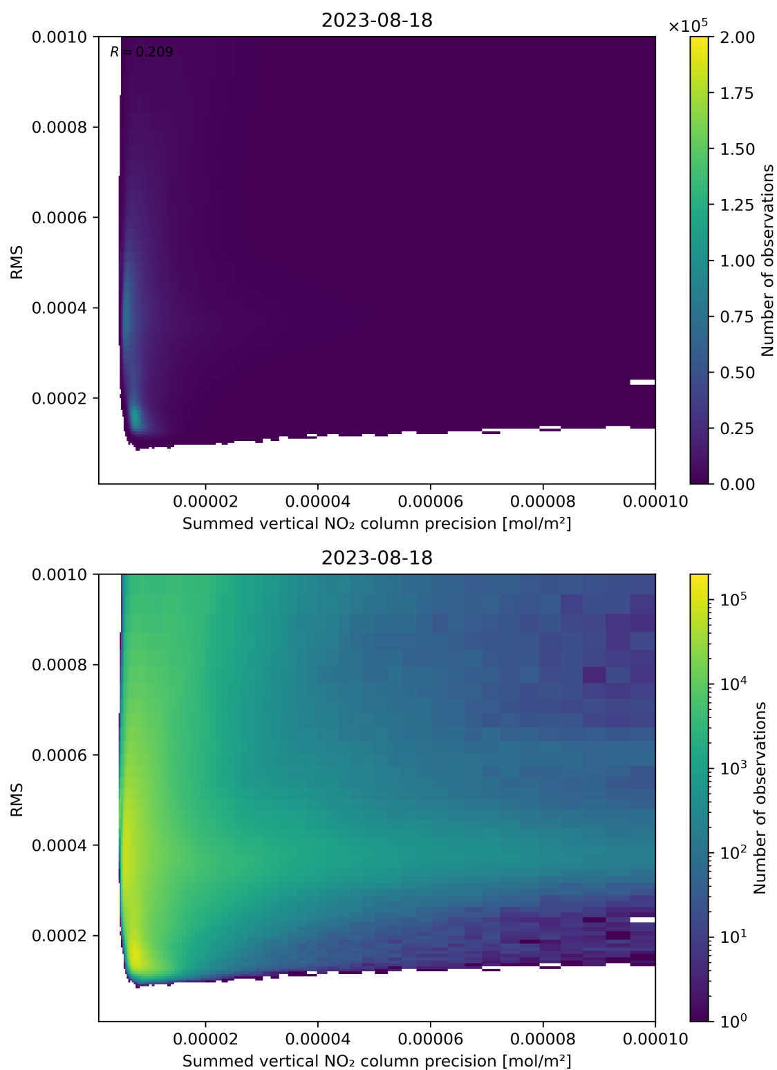
Figure 108: Scatter density plot of “Summed vertical NO 2 column precision” against “RMS” for 2023-08-17 to 2023-08-19.
