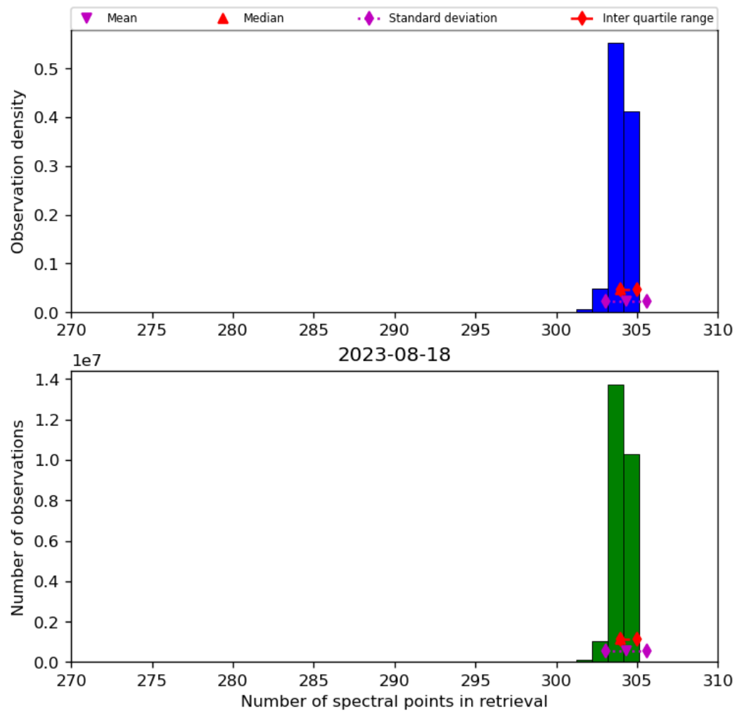
Figure 33: Histogram of “Number of spectral points in retrieval” for 2023-08-17 to 2023-08-19
