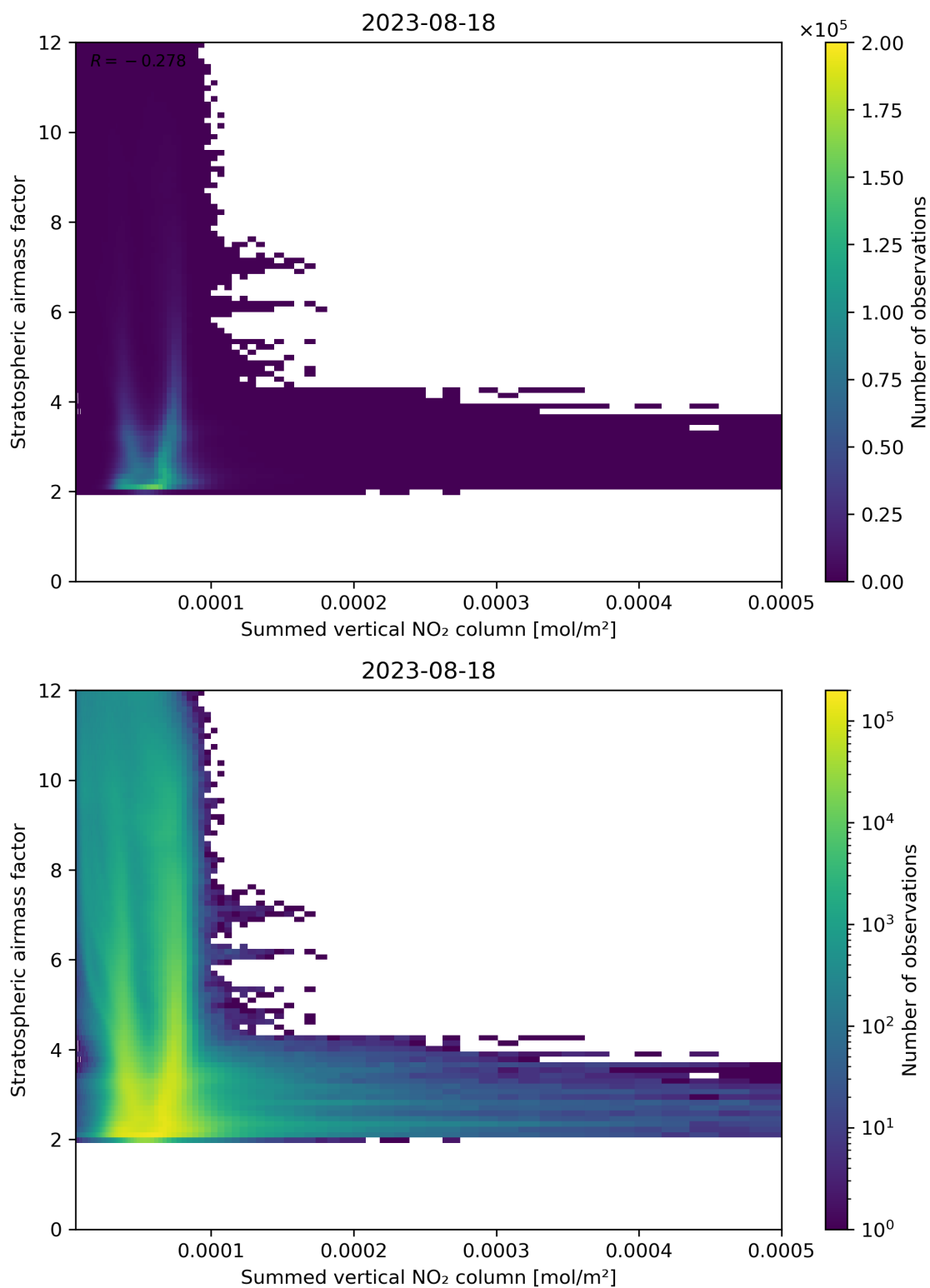
Figure 103: Scatter density plot of “Summed vertical NO 2 column” against “Stratospheric airmass factor” for 2023-08-17 to 2023-08-19.
