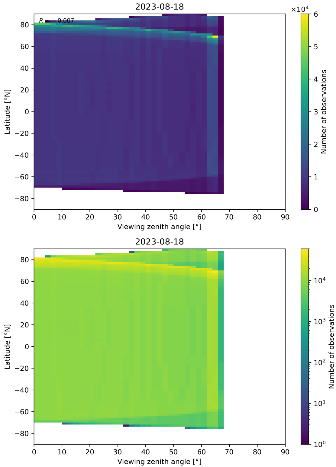
Figure 163: Scatter density plot of “Viewing zenith angle” against “Latitude” for 2023-08-17 to 2023-08-19.
