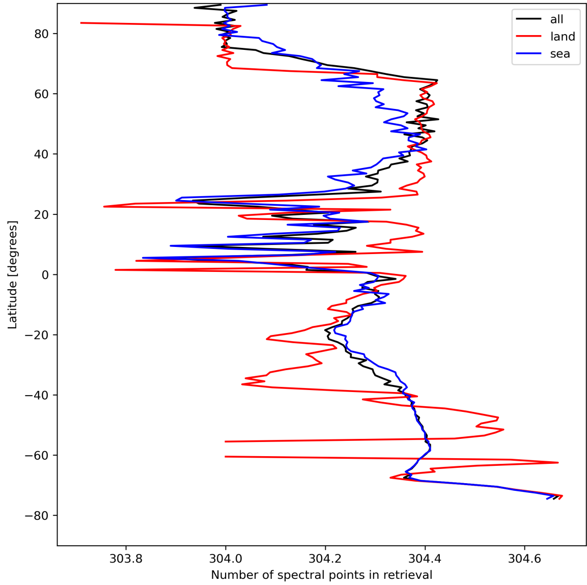
Figure 16: Zonal average of “Number of spectral points in retrieval” for 2023-08-17 to 2023-08-19.
