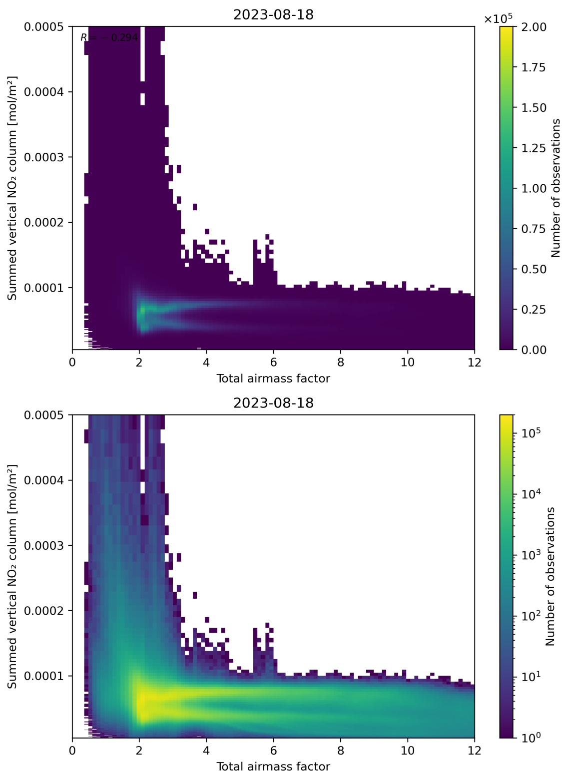
Figure 65: Scatter density plot of “Total airmass factor” against “Summed vertical NO 2 column” for 2023-08-17 to 2023-08-19.
