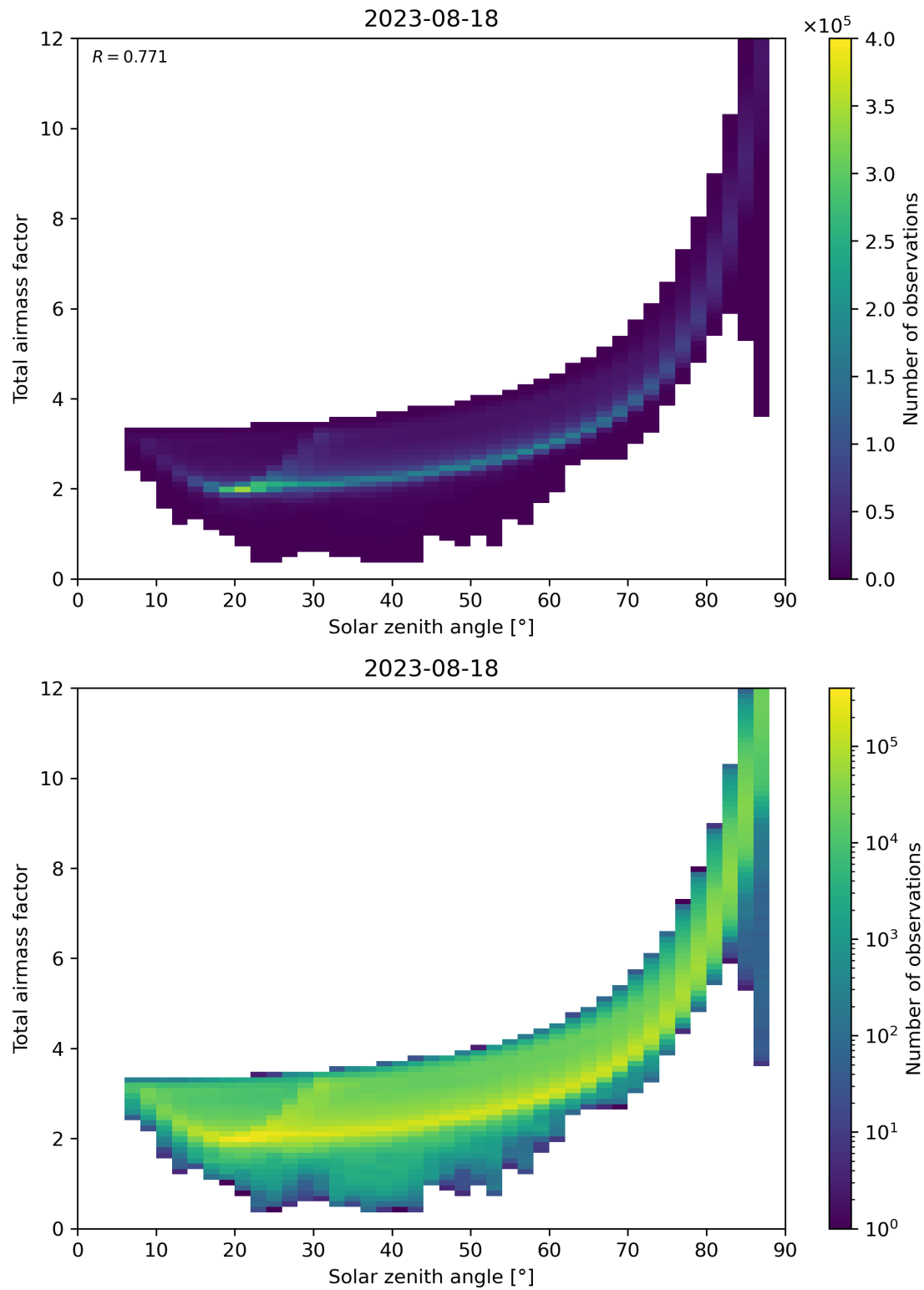
Figure 146: Scatter density plot of “Solar zenith angle” against “Total air mass factor” for 2023-08-17 to 2023-08-19.
