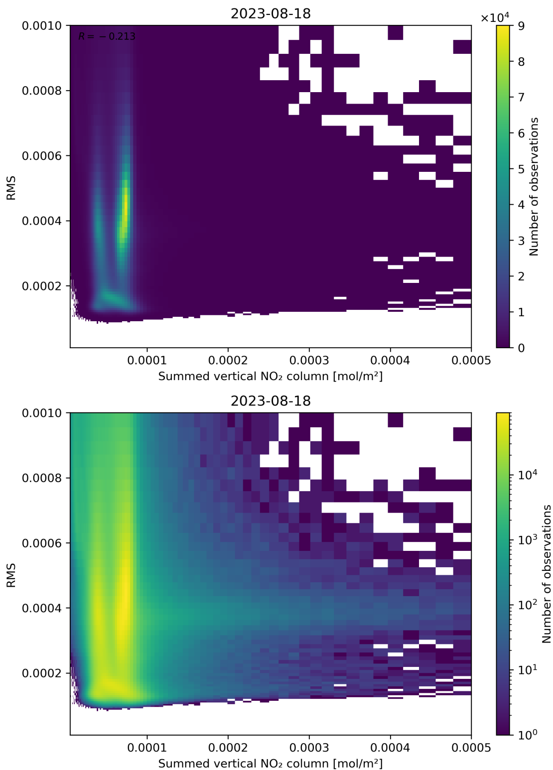
Figure 109: Scatter density plot of “Summed vertical NO 2 column” against “RMS” for 2023-08-17 to 2023-08-19.
