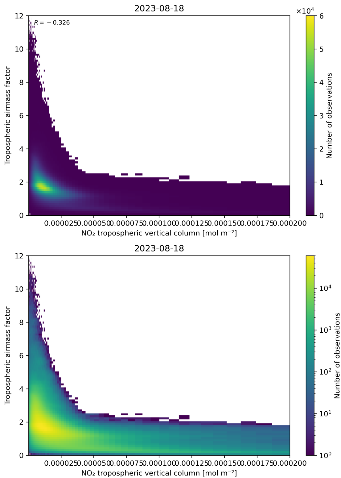
Figure 123: Scatter density plot of “NO 2 tropospheric vertical column” against “Tropospheric airmass factor” for 2023-08-17 to 2023-08-19.
