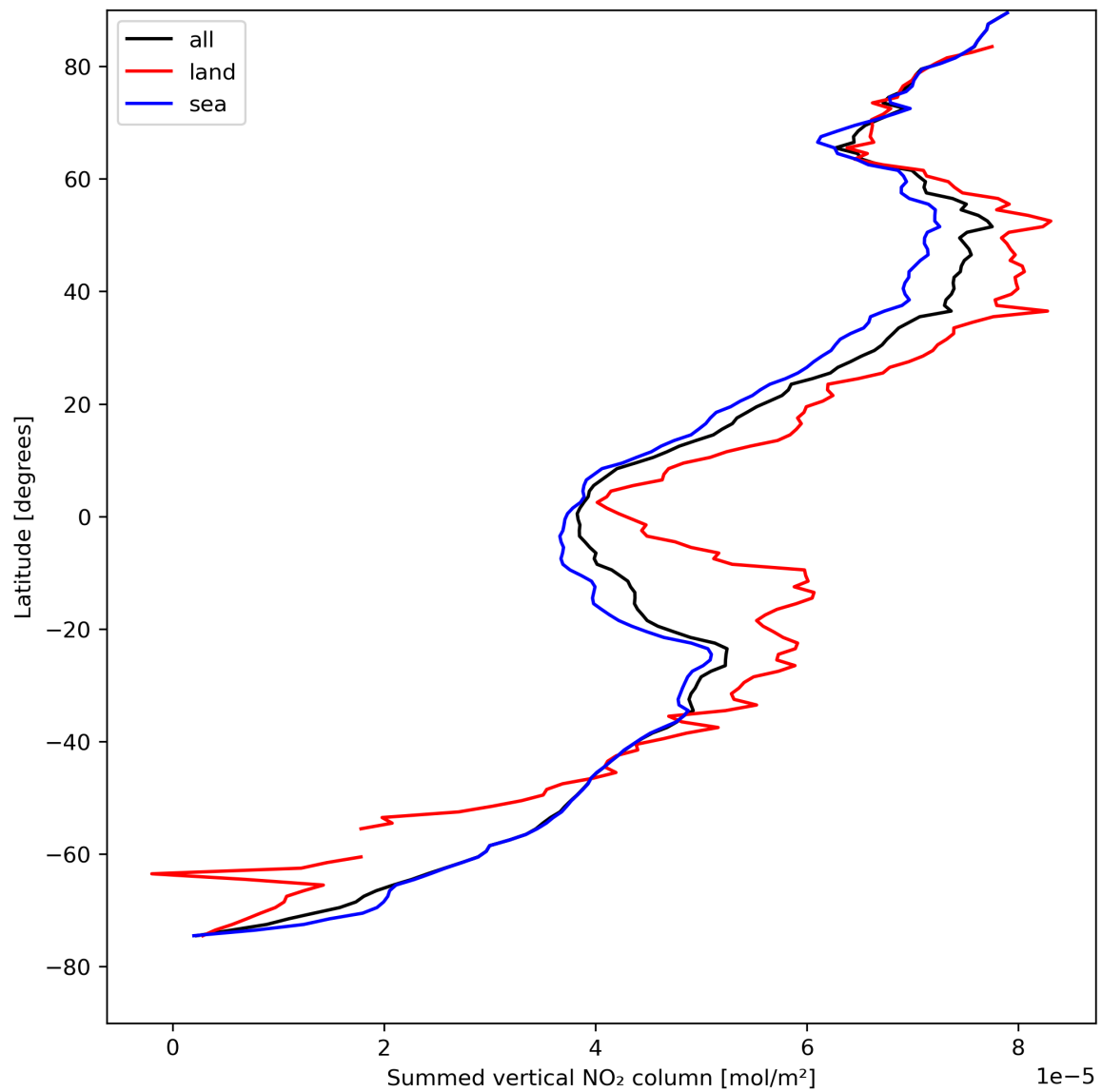
Figure 23: Zonal average of “Summed vertical NO 2 column” for 2023-08-17 to 2023-08-19.
