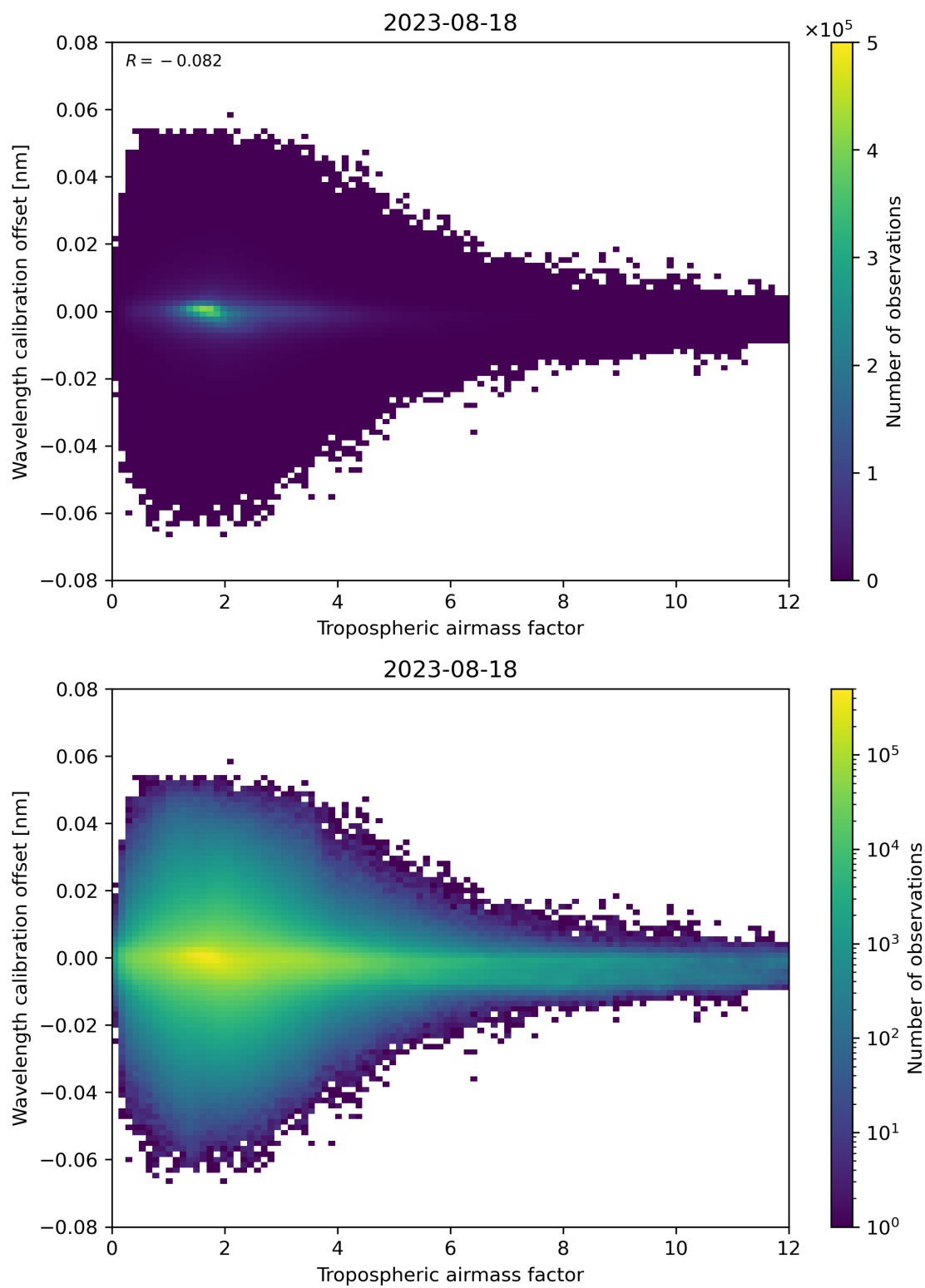
Figure 80: Scatter density plot of “Tropospheric airmass factor” against “Wavelength calibration offset” for 2023-08-17 to 2023-08-19.
