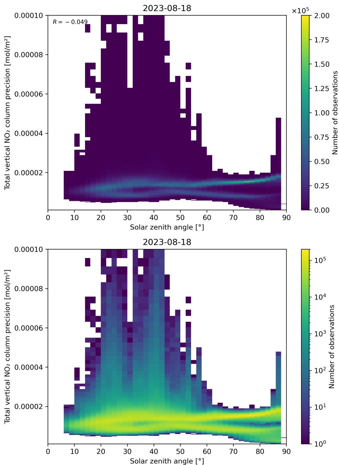
Figure 154: Scatter density plot of “Solar zenith angle” against “Total vertical NO 2 column precision” for 2023-08-17 to 2023-08-19.
