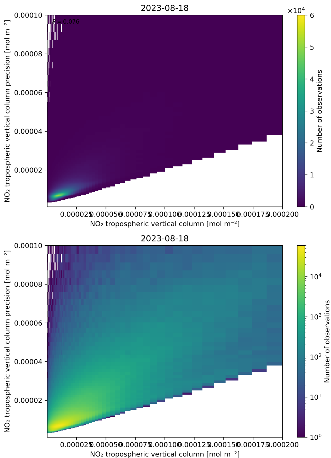
Figure 130: Scatter density plot of “NO 2 tropospheric vertical column” against “NO 2 tropospheric vertical column precision” for 2023-08-17 to 2023-08-19.
