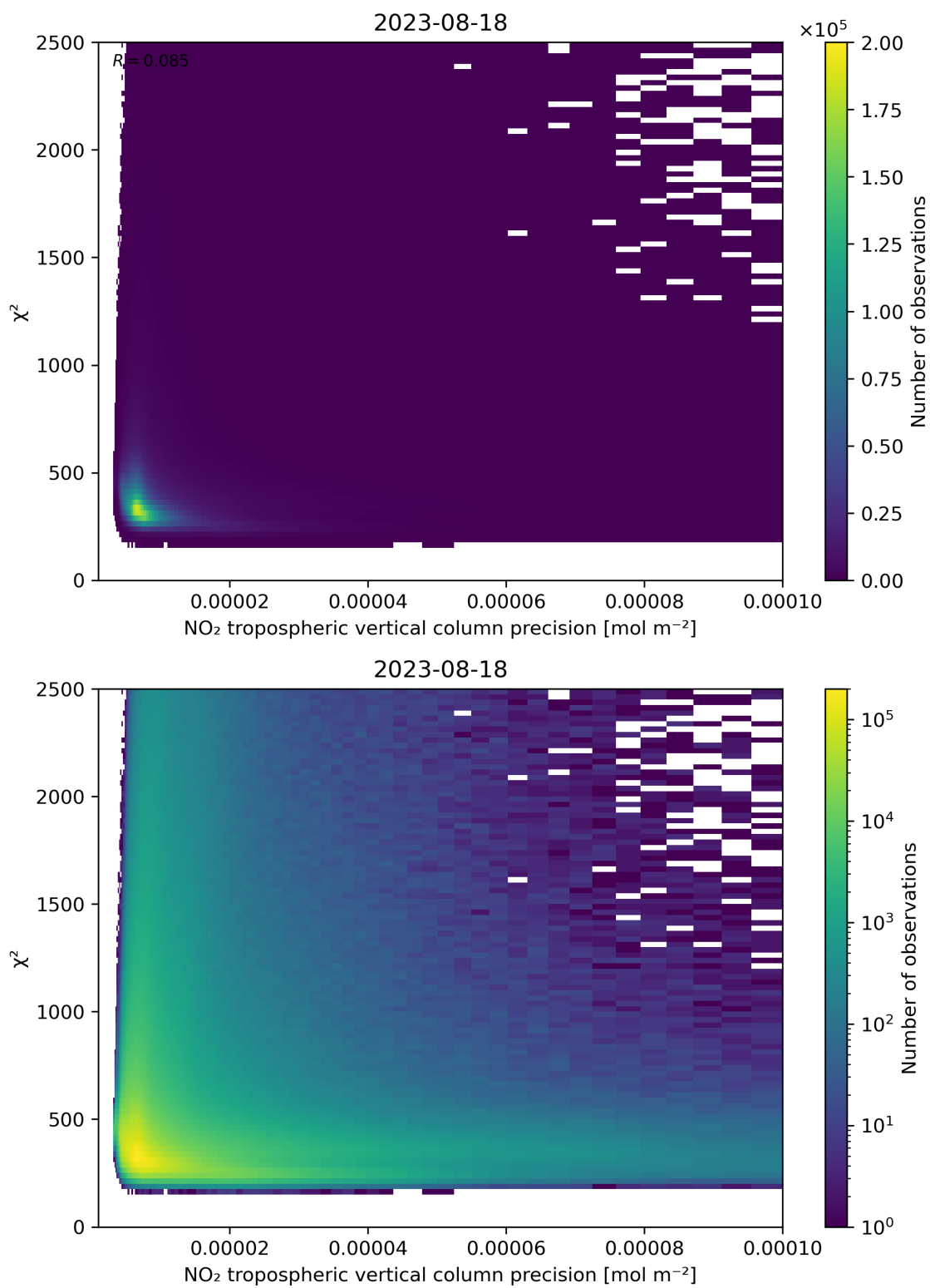
Figure 134: Scatter density plot of “NO 2 tropospheric vertical column precision” against “ \chi^2 ” for 2023-08-17 to 2023-08-19.
