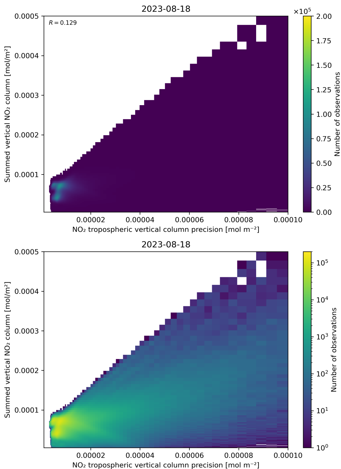
Figure 136: Scatter density plot of “NO 2 tropospheric vertical column precision” against “Summed vertical NO 2 column” for 2023-08-17 to 2023-08-19.
