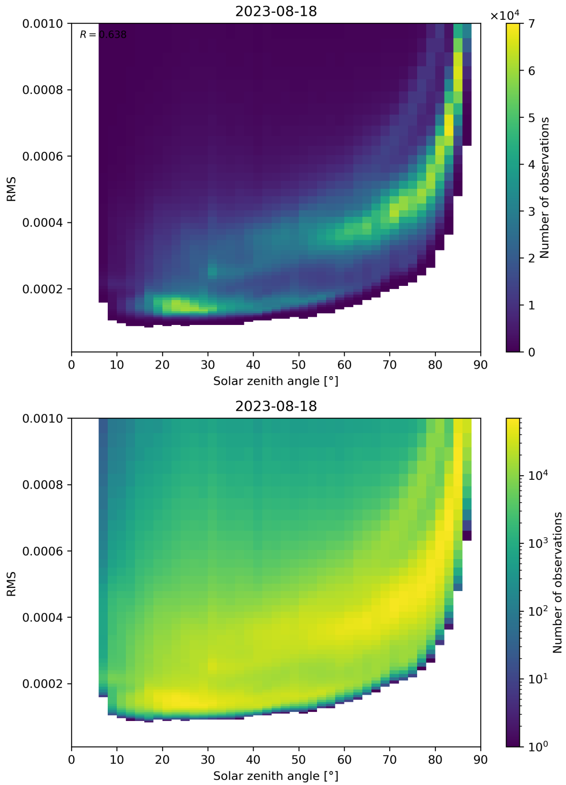
Figure 157: Scatter density plot of “Solar zenith angle” against “RMS” for 2023-08-17 to 2023-08-19.
