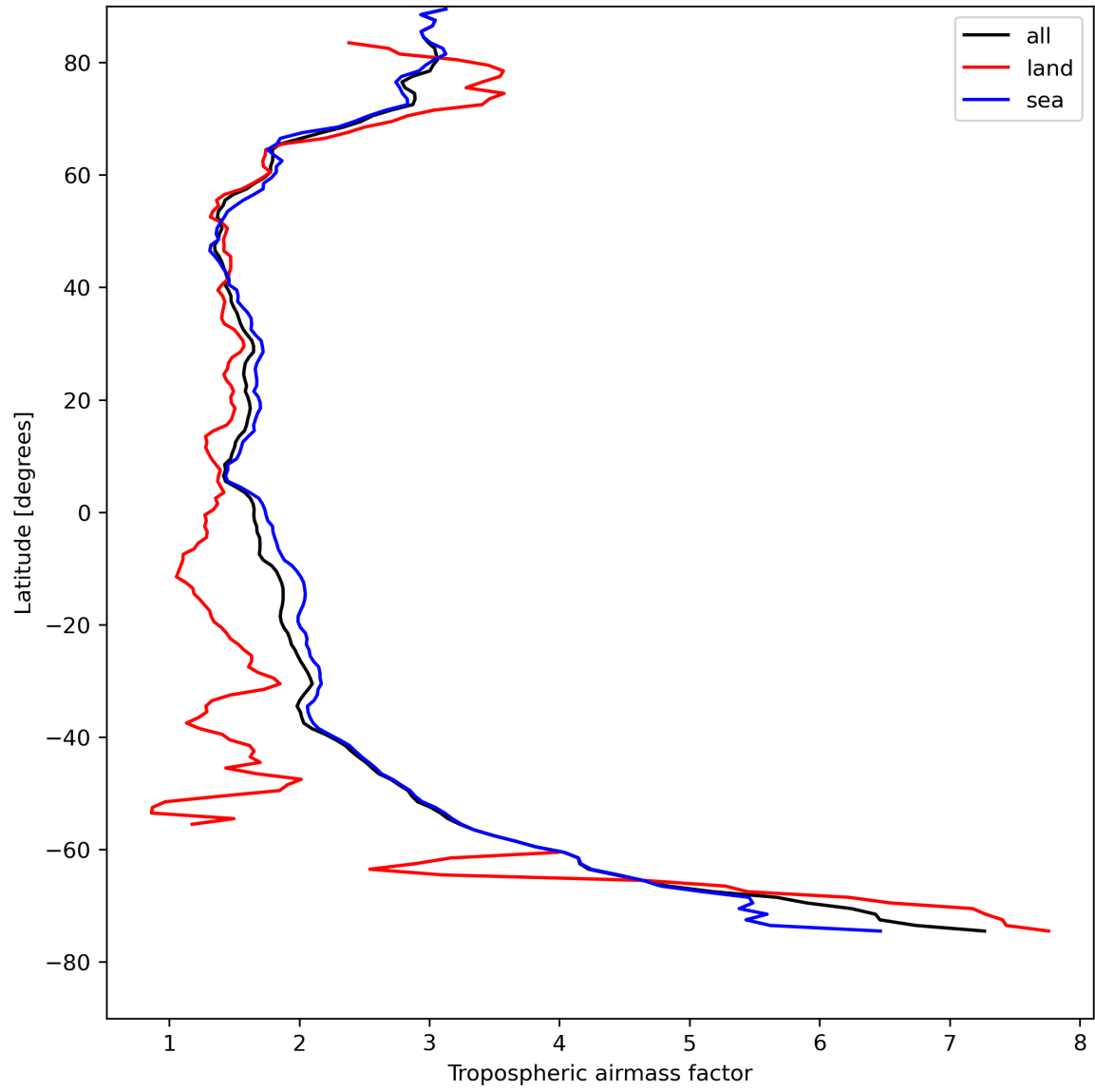
Figure 14: Zonal average of “Tropospheric airmass factor” for 2023-08-17 to 2023-08-19.
