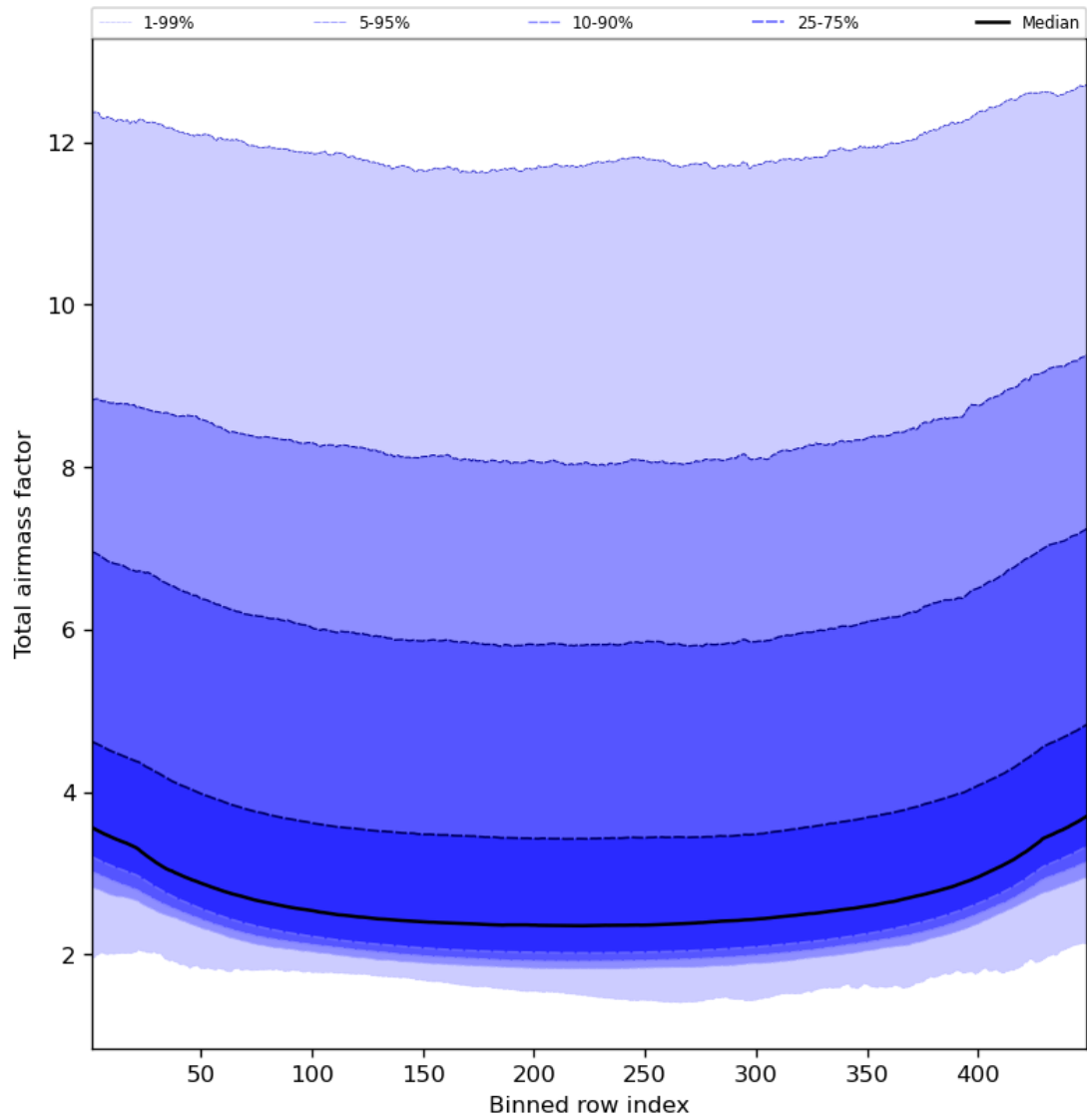
Figure 49: Along track statistics of “Total airmass factor” for 2023-08-17 to 2023-08-19
