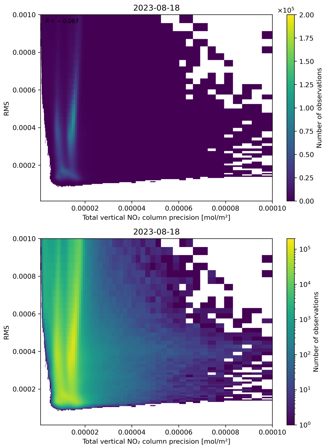
Figure 119: Scatter density plot of “Total vertical NO 2 column precision” against “RMS” for 2023-08-17 to 2023-08-19.
