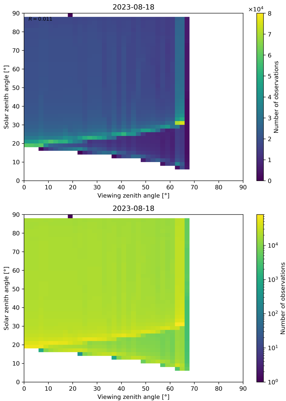
Figure 172: Scatter density plot of “Viewing zenith angle” against “Solar zenith angle” for 2023-08-17 to 2023-08-19.
