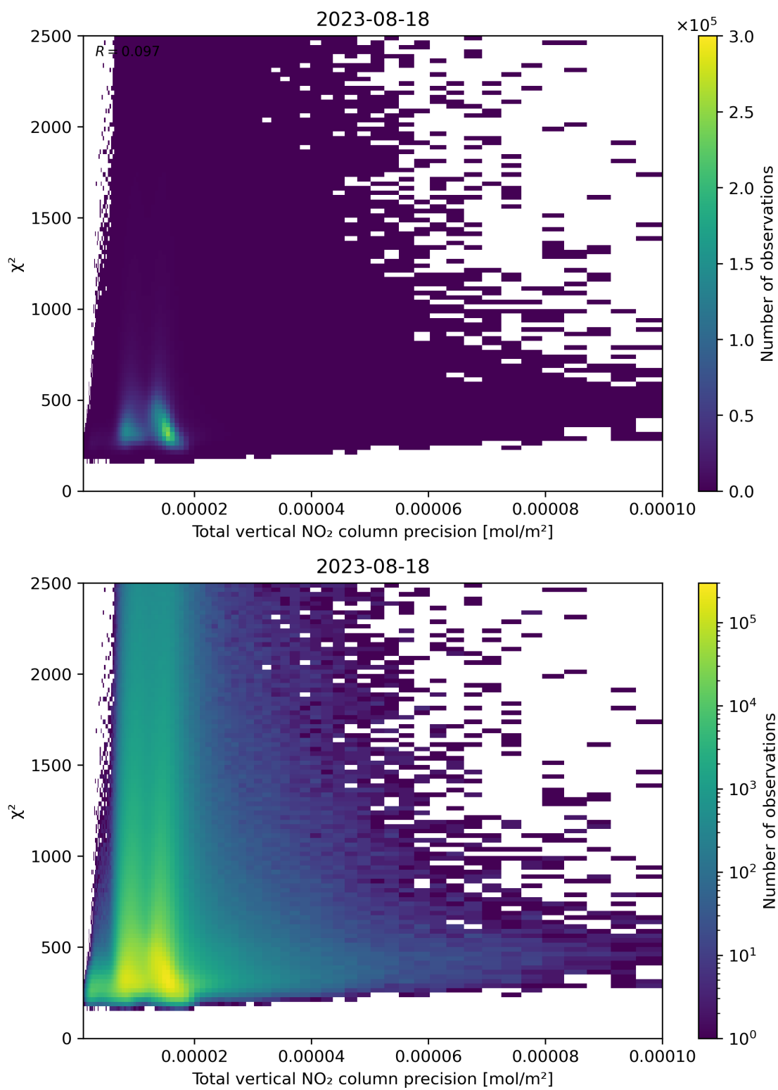
Figure 116: Scatter density plot of “Total vertical NO 2 column precision” against “ \chi^2 ” for 2023-08-17 to 2023-08-19.
