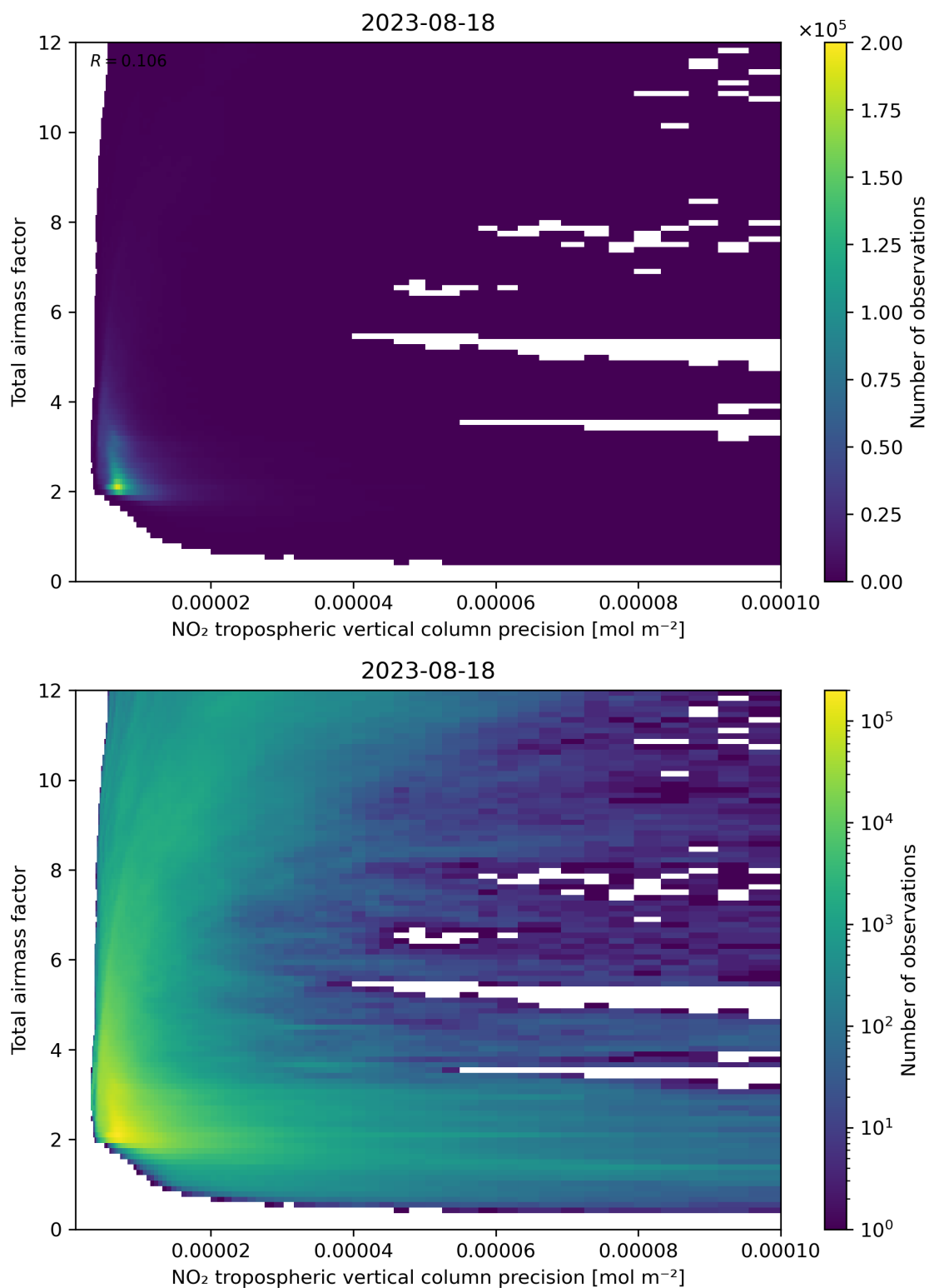
Figure 132: Scatter density plot of “NO 2 tropospheric vertical column precision” against “Total air mass factor” for 2023-08-17 to 2023-08-19.
