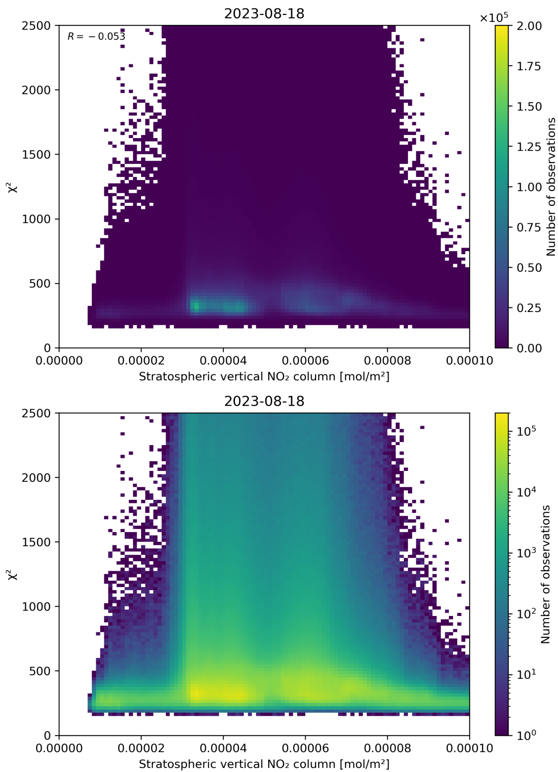
Figure 97: Scatter density plot of “Stratospheric vertical NO 2 column” against “ \chi^2 ” for 2023-08-17 to 2023-08-19.
