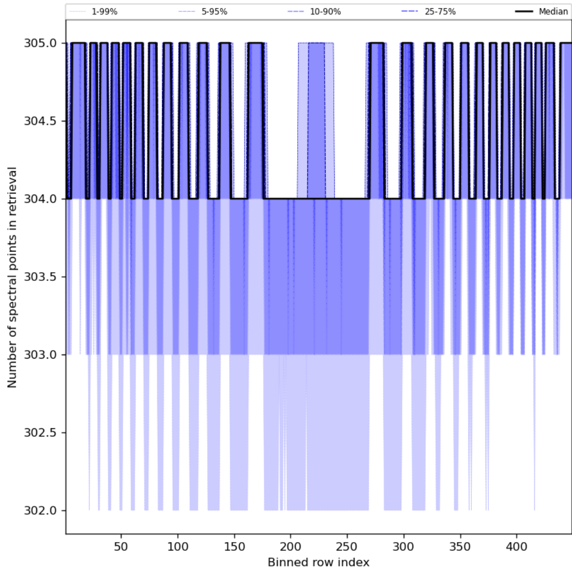
Figure 50: Along track statistics of “Number of spectral points in retrieval” for 2023-08-17 to 2023-08-19
