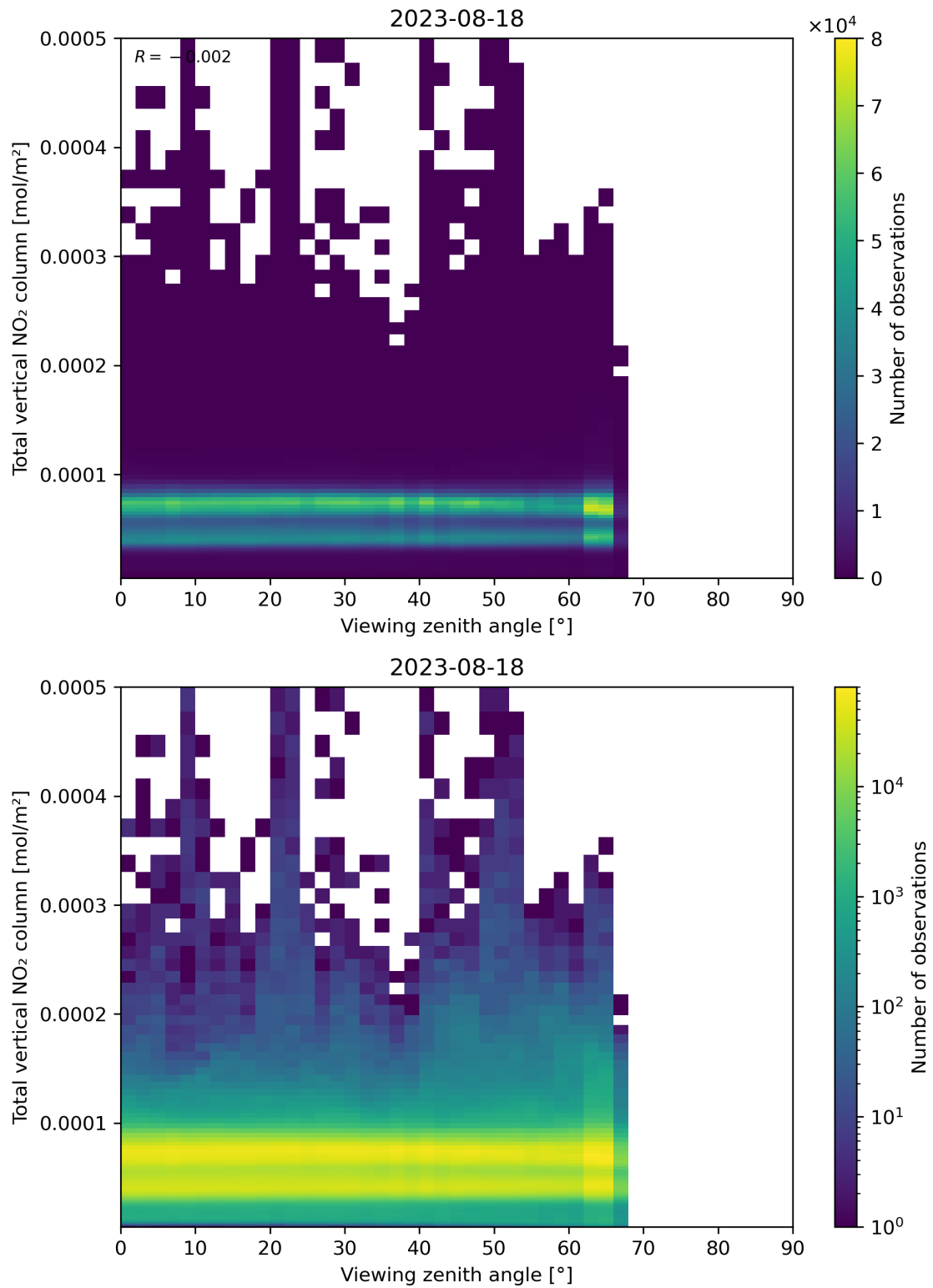
Figure 167: Scatter density plot of “Viewing zenith angle” against “Total vertical NO 2 column” for 2023-08-17 to 2023-08-19.
