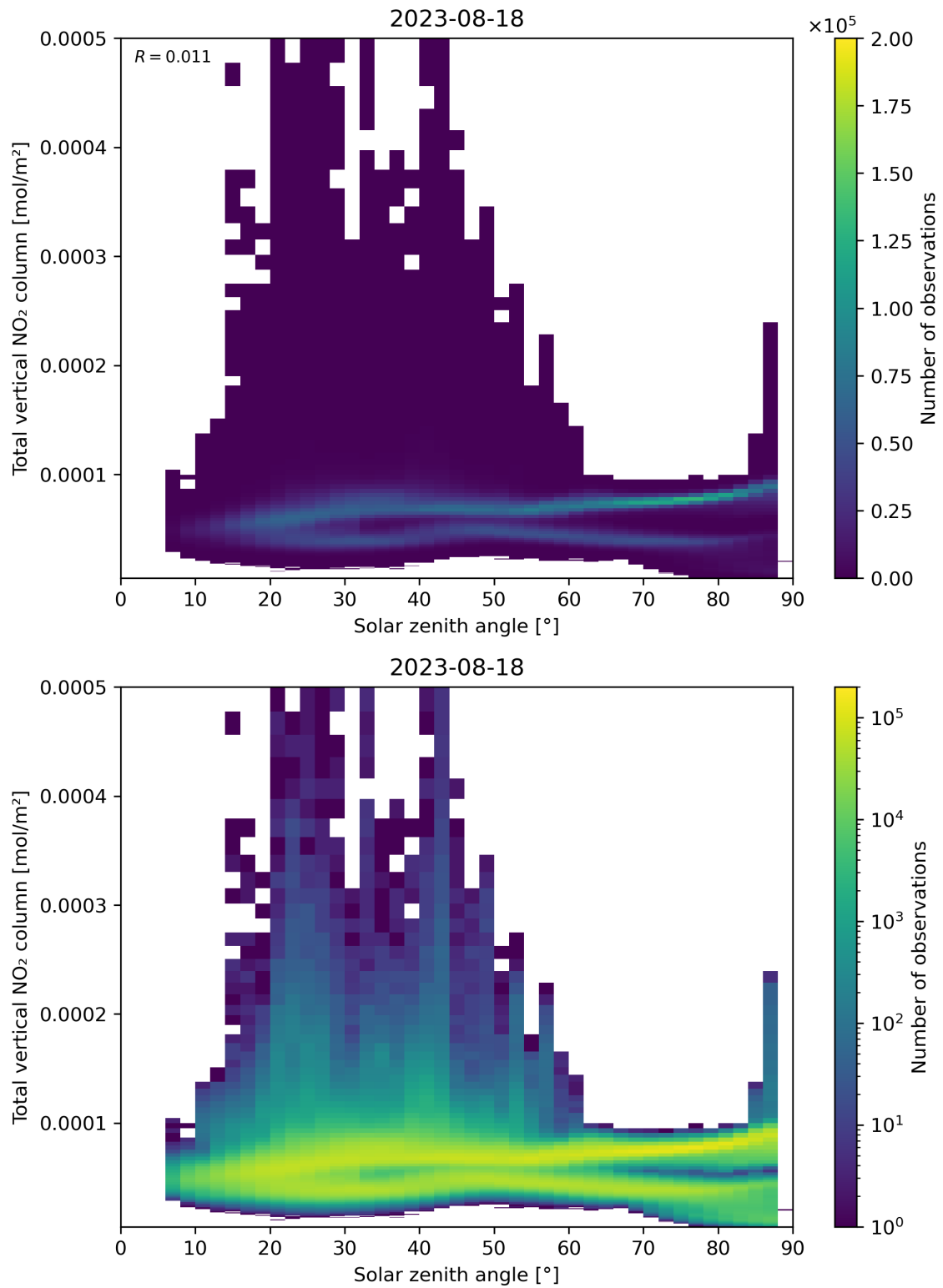
Figure 153: Scatter density plot of “Solar zenith angle” against “Total vertical NO 2 column” for 2023-08-17 to 2023-08-19.
