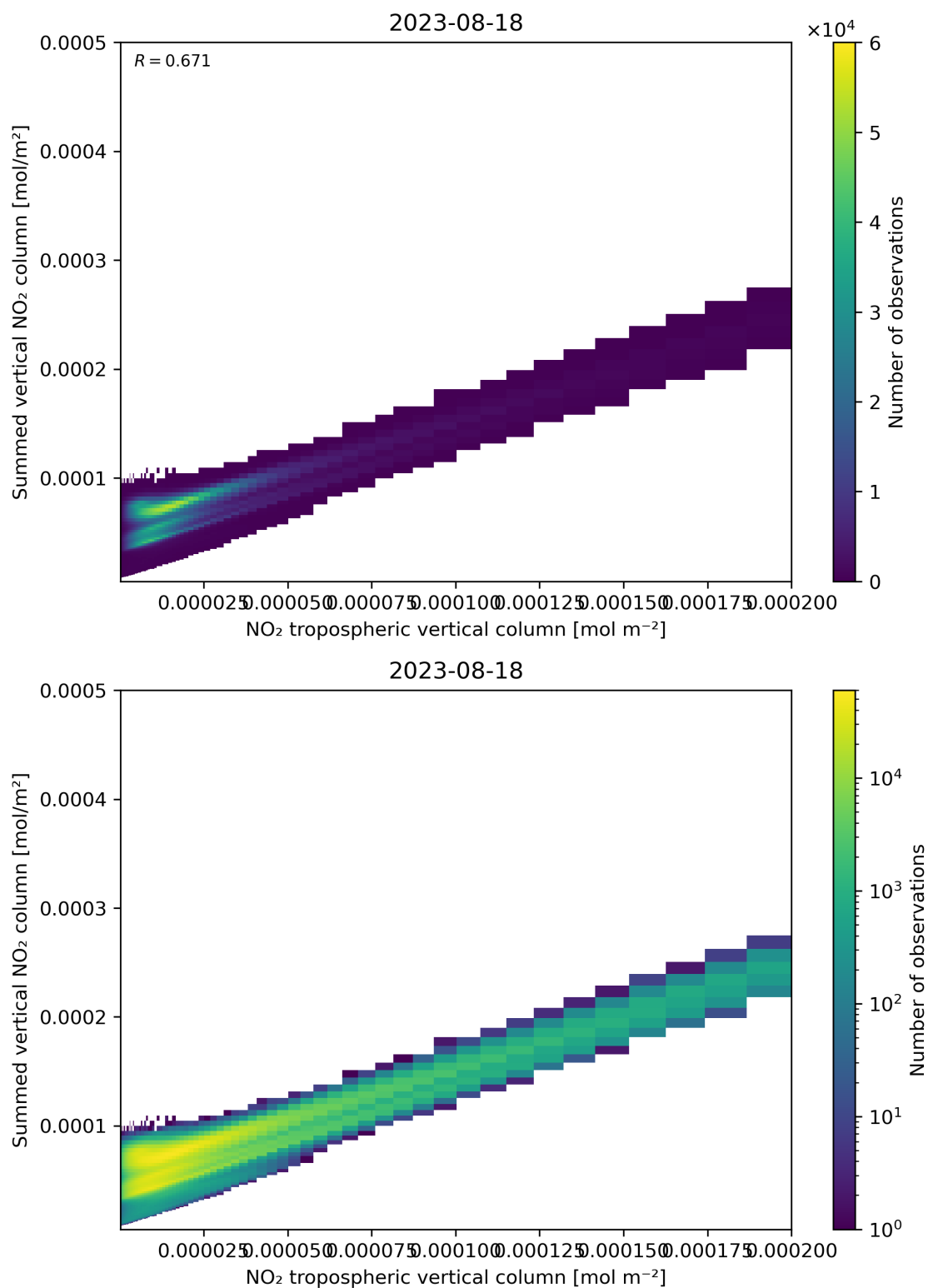
Figure 126: Scatter density plot of “NO 2 tropospheric vertical column” against “Summed vertical NO 2 column” for 2023-08-17 to 2023-08-19.
