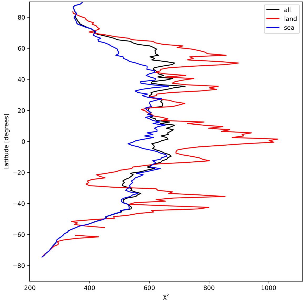
Figure 25: Zonal average of “ \chi^2 ” for 2023-08-17 to 2023-08-19.
