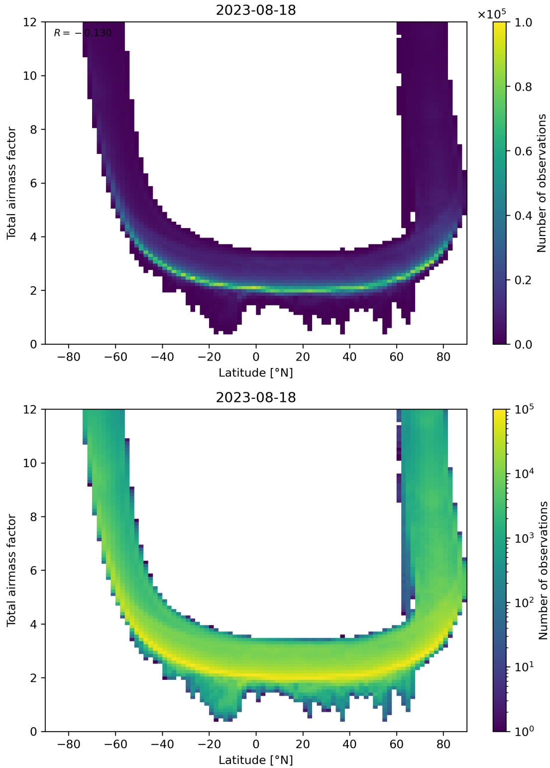
Figure 84: Scatter density plot of “Latitude” against “Total airmass factor” for 2023-08-17 to 2023-08-19.
