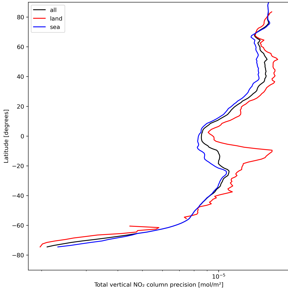
Figure 22: Zonal average of “Total vertical NO 2 column precision” for 2023-08-17 to 2023-08-19.
