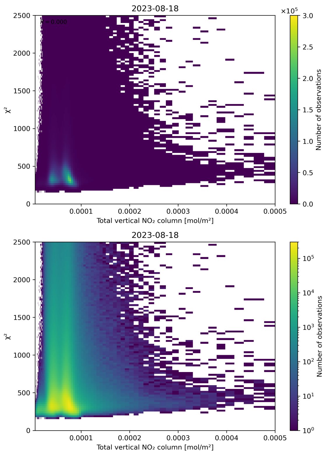
Figure 111: Scatter density plot of “Total vertical NO 2 column” against “ \chi^2 ” for 2023-08-17 to 2023-08-19.
