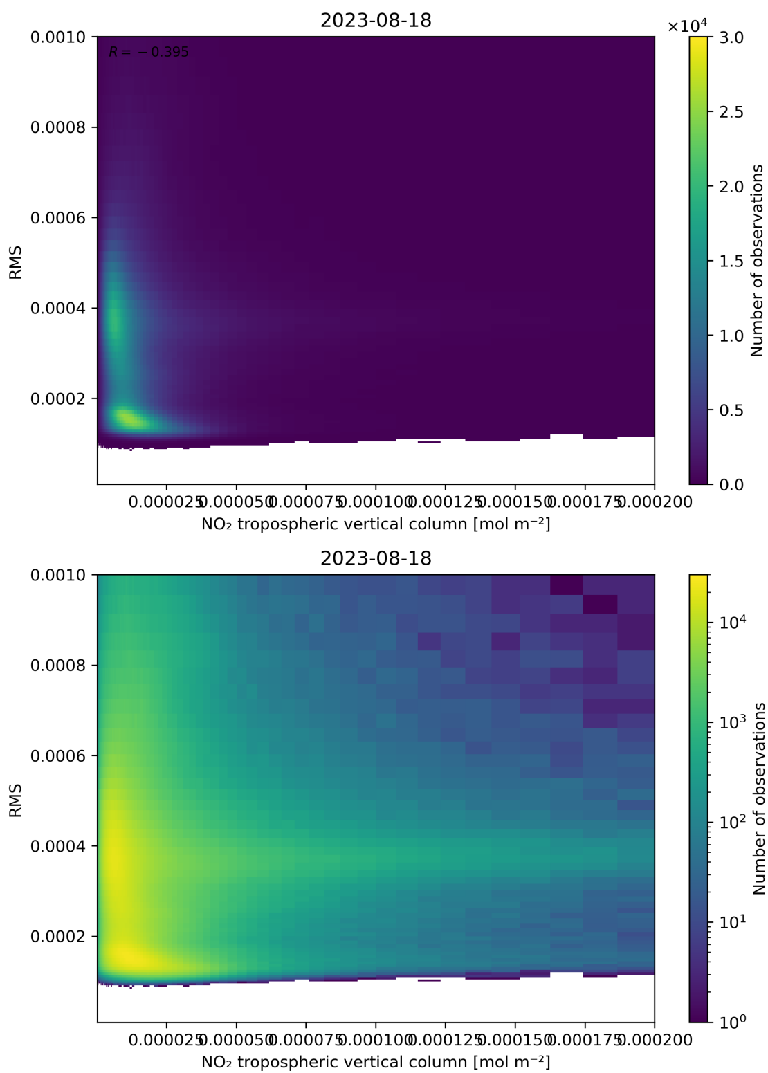
Figure 142: Scatter density plot of “NO 2 tropospheric vertical column” against “RMS” for 2023-08-17 to 2023-08-19.
