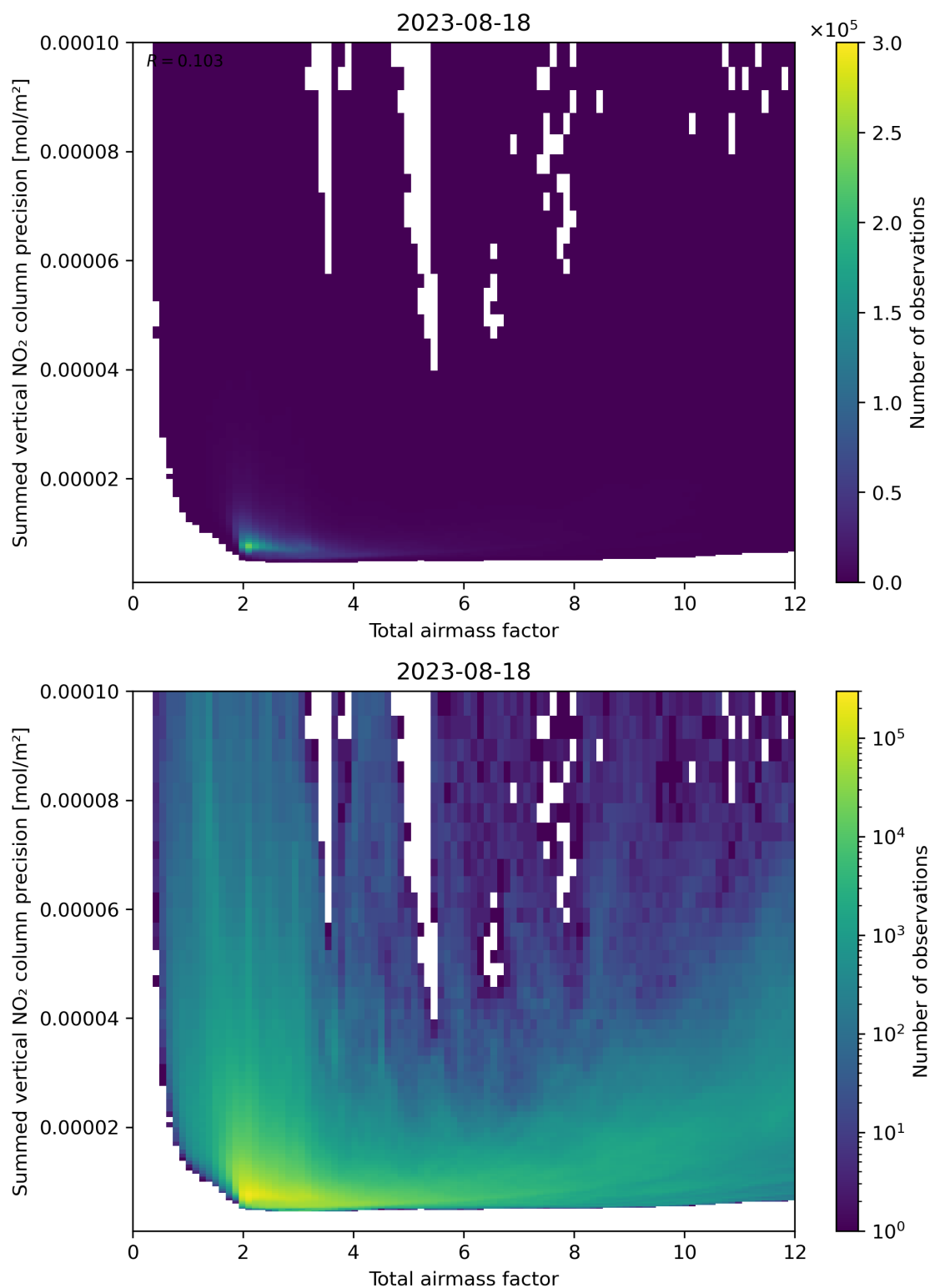
Figure 66: Scatter density plot of “Total airmass factor” against “Summed vertical NO 2 column precision” for 2023-08-17 to 2023-08-19.
