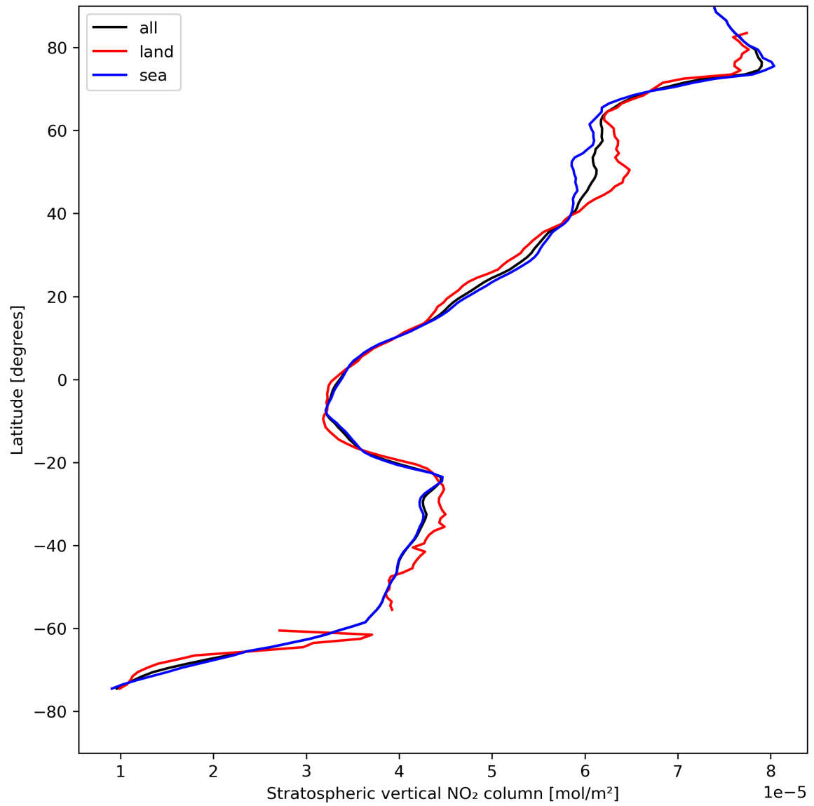
Figure 19: Zonal average of “Stratospheric vertical NO 2 column” for 2023-08-17 to 2023-08-19.
