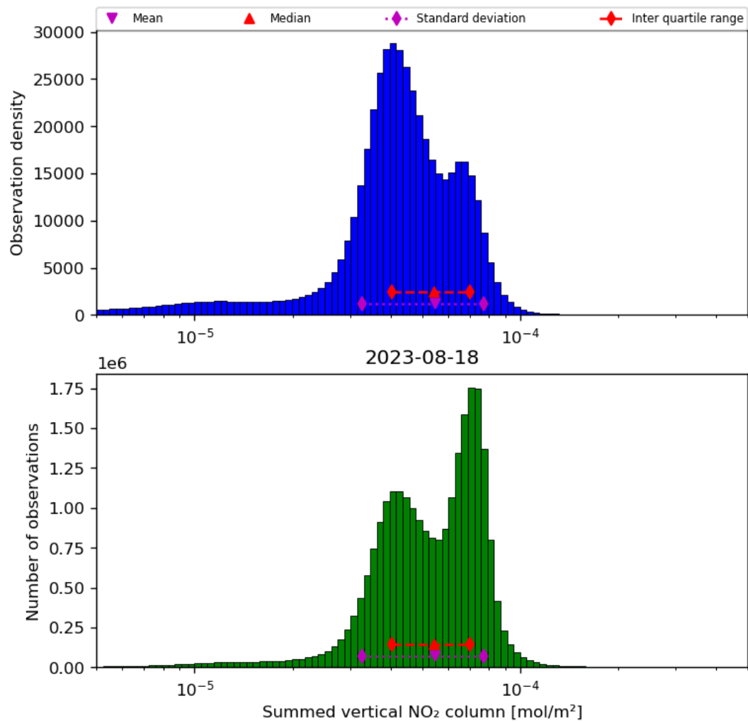
Figure 40: Histogram of "Summed vertical NO 2 column" for 2023-08-17 to 2023-08-19
