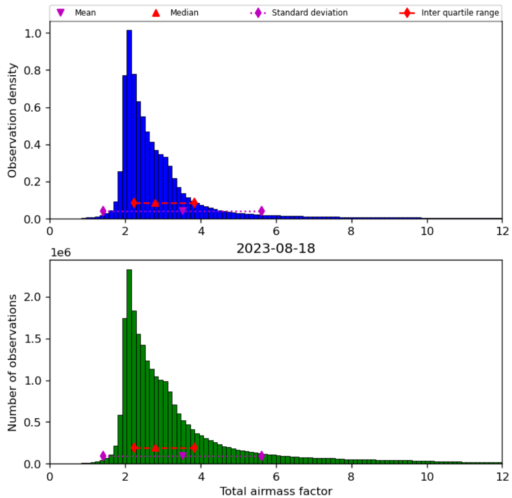
Figure 32: Histogram of “Total airmass factor” for 2023-08-17 to 2023-08-19
