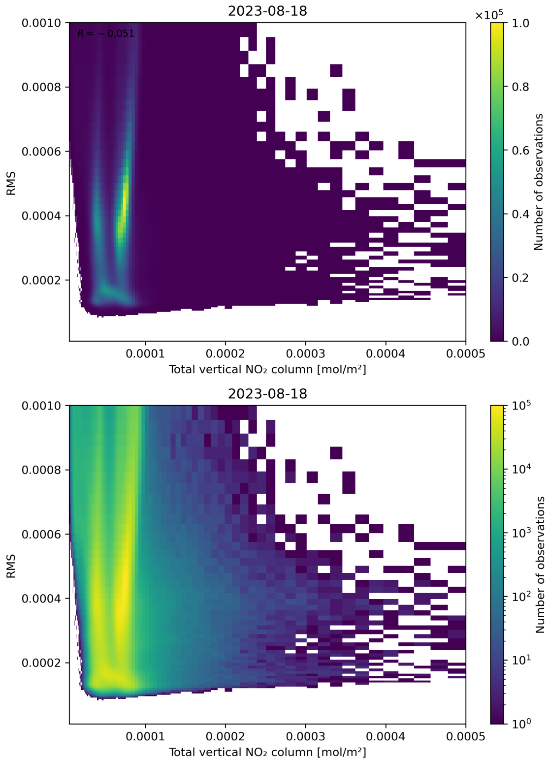
Figure 120: Scatter density plot of “Total vertical NO 2 column” against “RMS” for 2023-08-17 to 2023-08-19.
