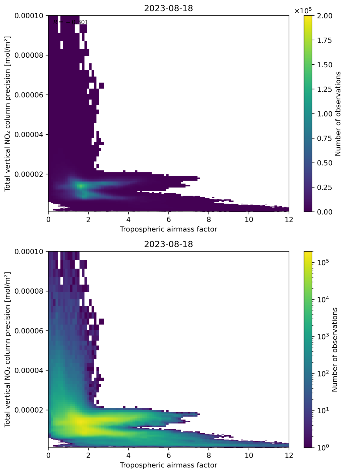
Figure 78: Scatter density plot of “Tropospheric air mass factor” against “Total vertical NO 2 column precision” for 2023-08-17 to 2023-08-19.
