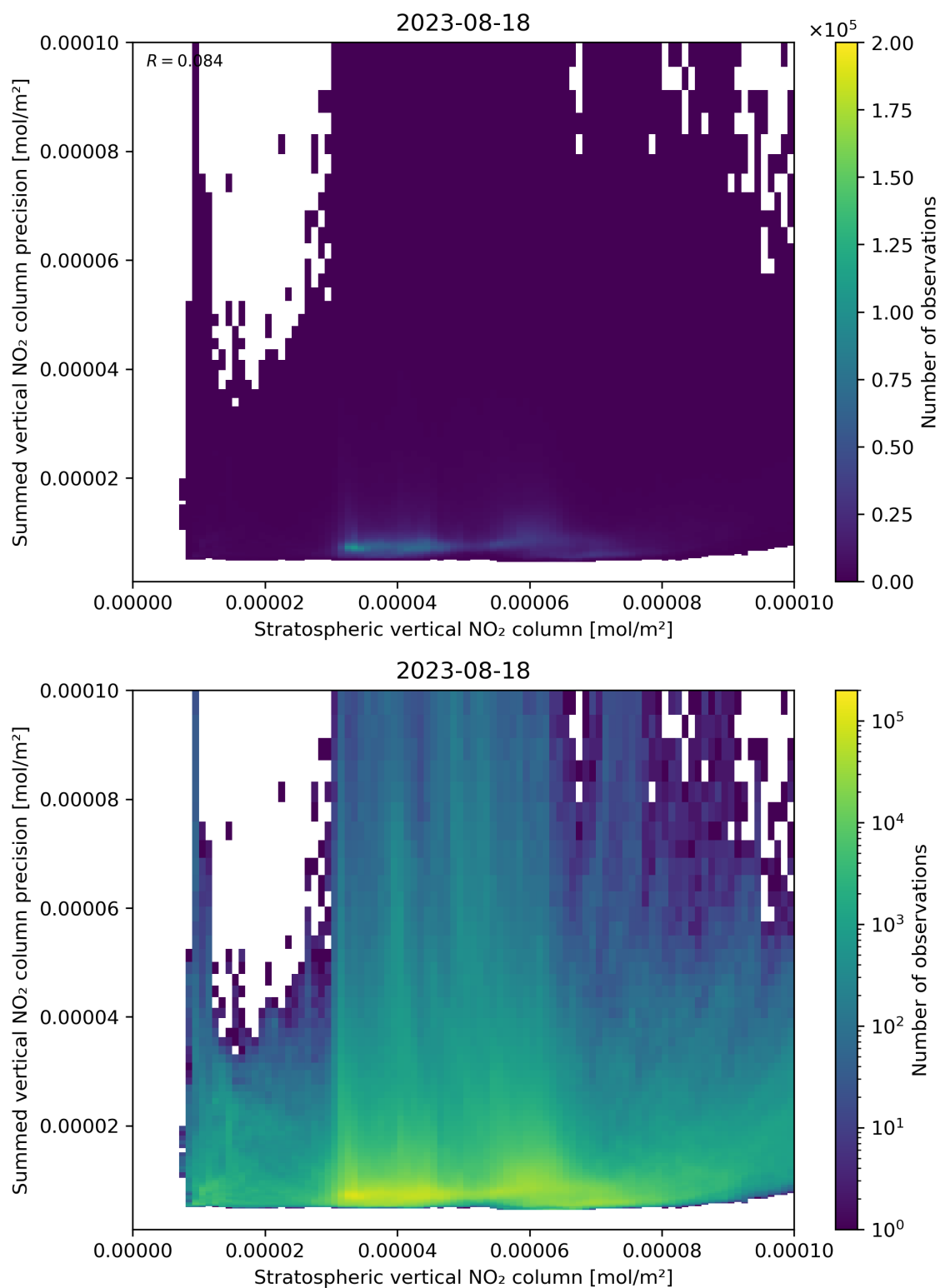
Figure 99: Scatter density plot of “Stratospheric vertical NO 2 column” against “Summed vertical NO 2 column precision” for 2023-08-17 to 2023-08-19.
