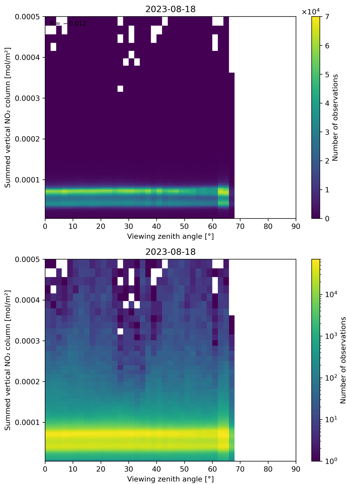
Figure 165: Scatter density plot of “Viewing zenith angle” against “Summed vertical NO 2 column” for 2023-08-17 to 2023-08-19.
