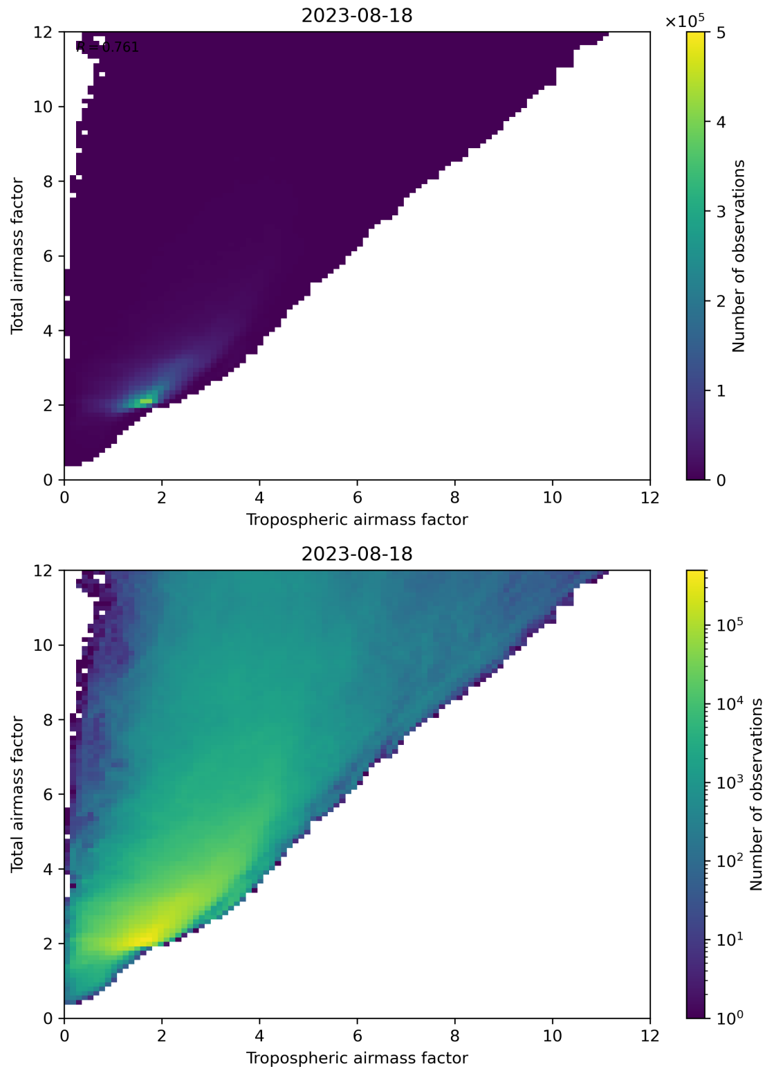
Figure 72: Scatter density plot of “Tropospheric airmass factor” against “Total airmass factor” for 2023-08-17 to 2023-08-19.
