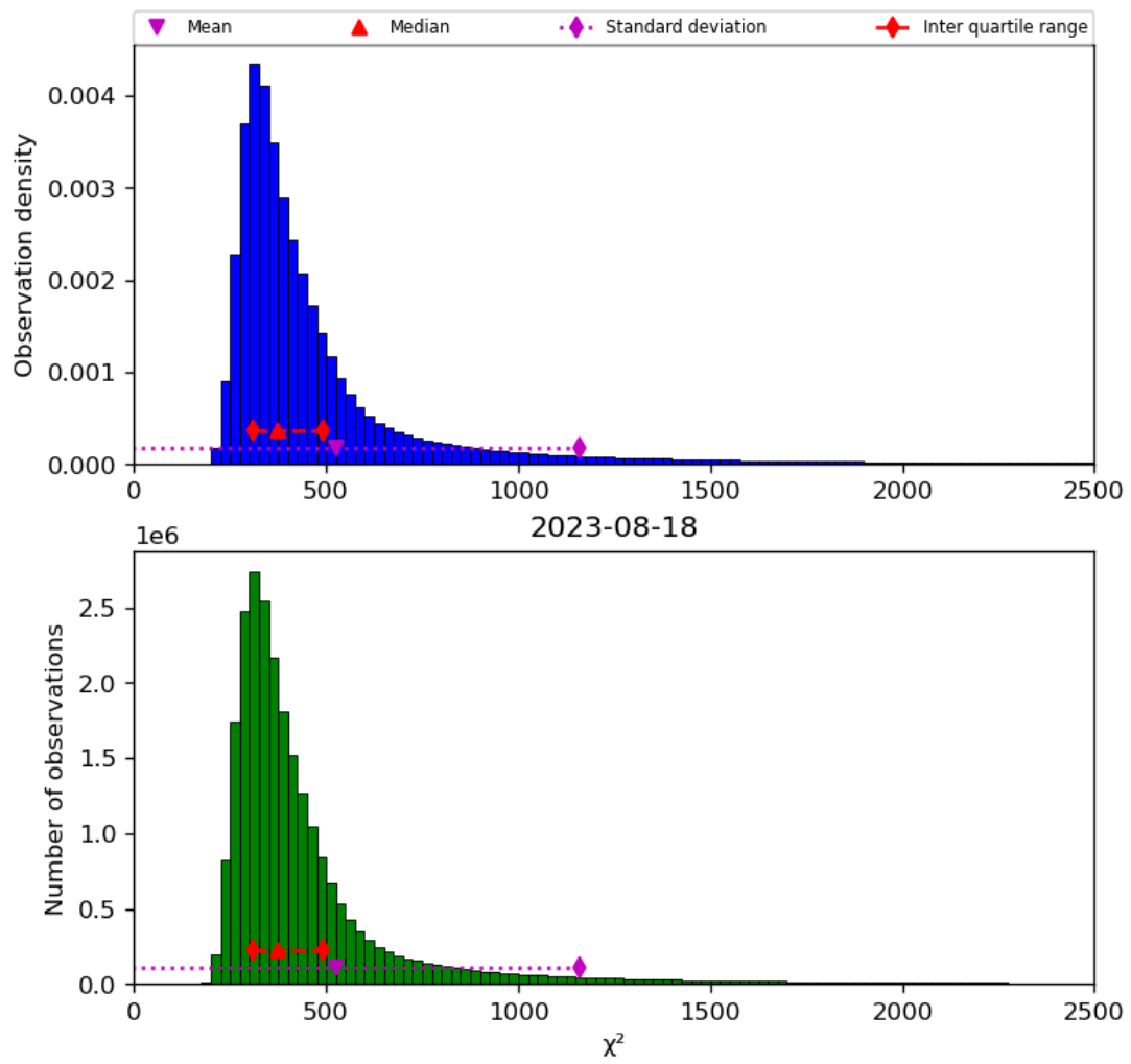
Figure 42: Histogram of “ \chi^2 ” for 2023-08-17 to 2023-08-19
