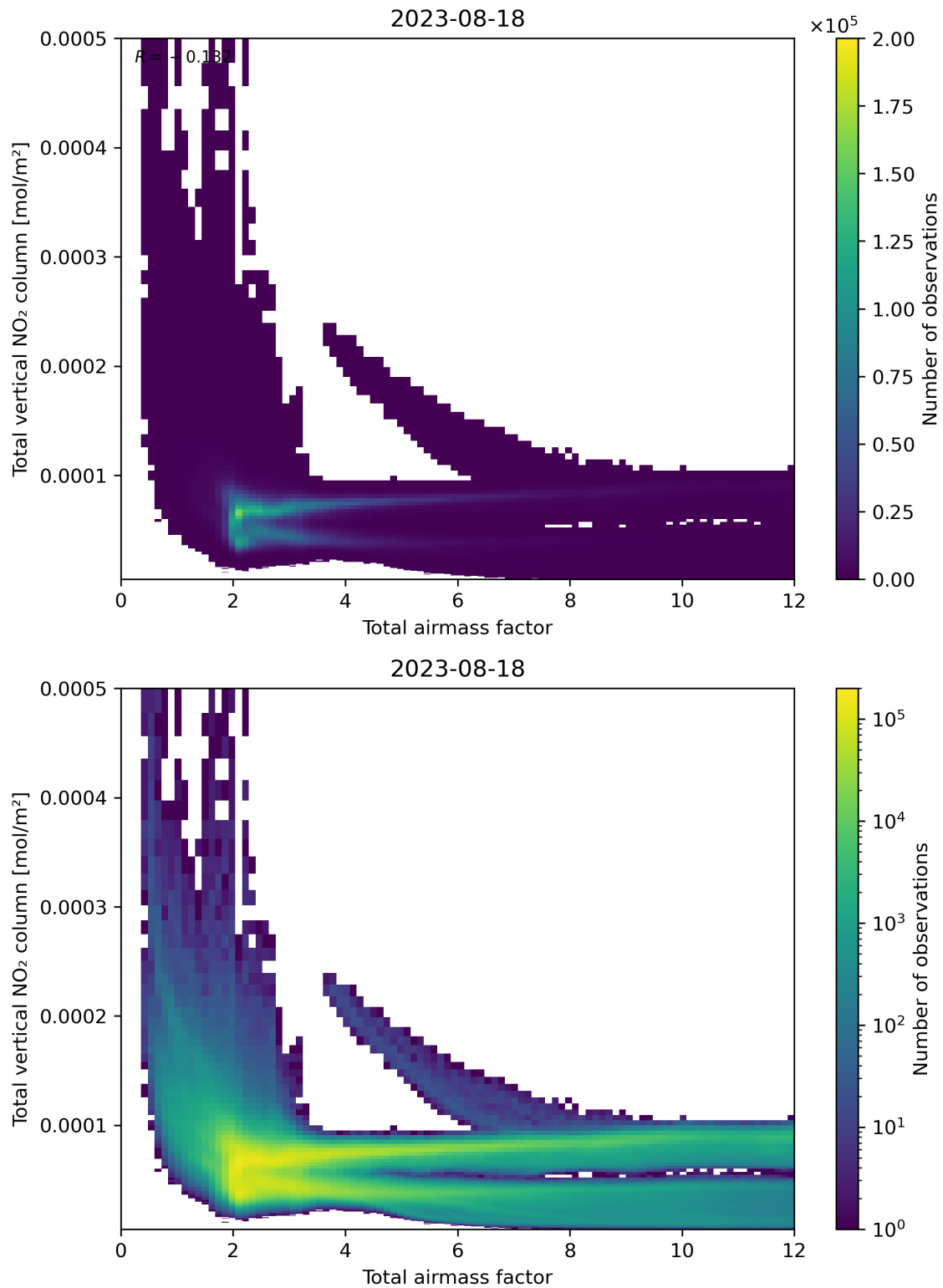
Figure 67: Scatter density plot of “Total airmass factor” against “Total vertical NO 2 column” for 2023-08-17 to 2023-08-19.
