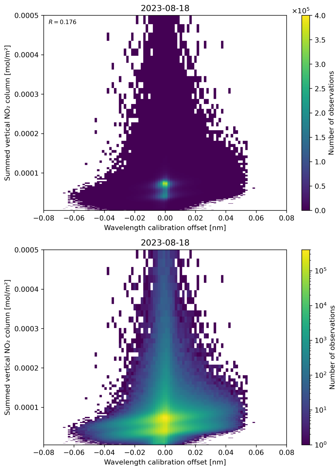
Figure 177: Scatter density plot of “Wavelength calibration offset” against “Summed vertical NO 2 column” for 2023-08-17 to 2023-08-19.
