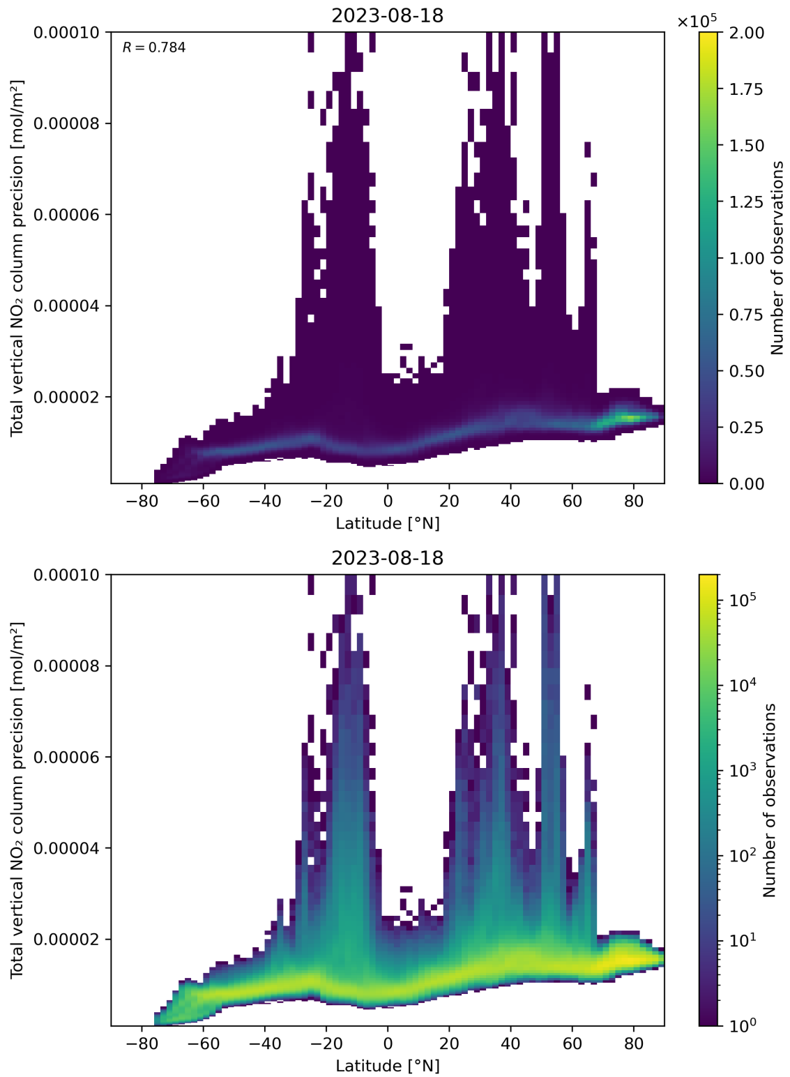
Figure 91: Scatter density plot of “Latitude” against “Total vertical NO 2 column precision” for 2023-08-17 to 2023-08-19.
