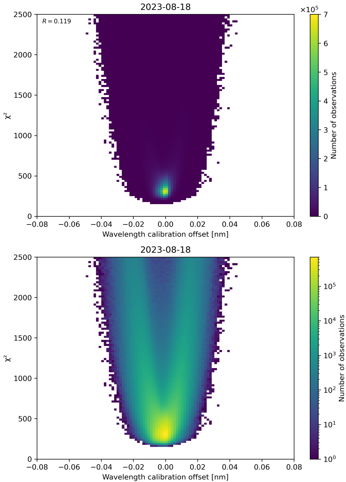
Figure 175: Scatter density plot of “Wavelength calibration offset” against “ \chi^2 ” for 2023-08-17 to 2023-08-19.
