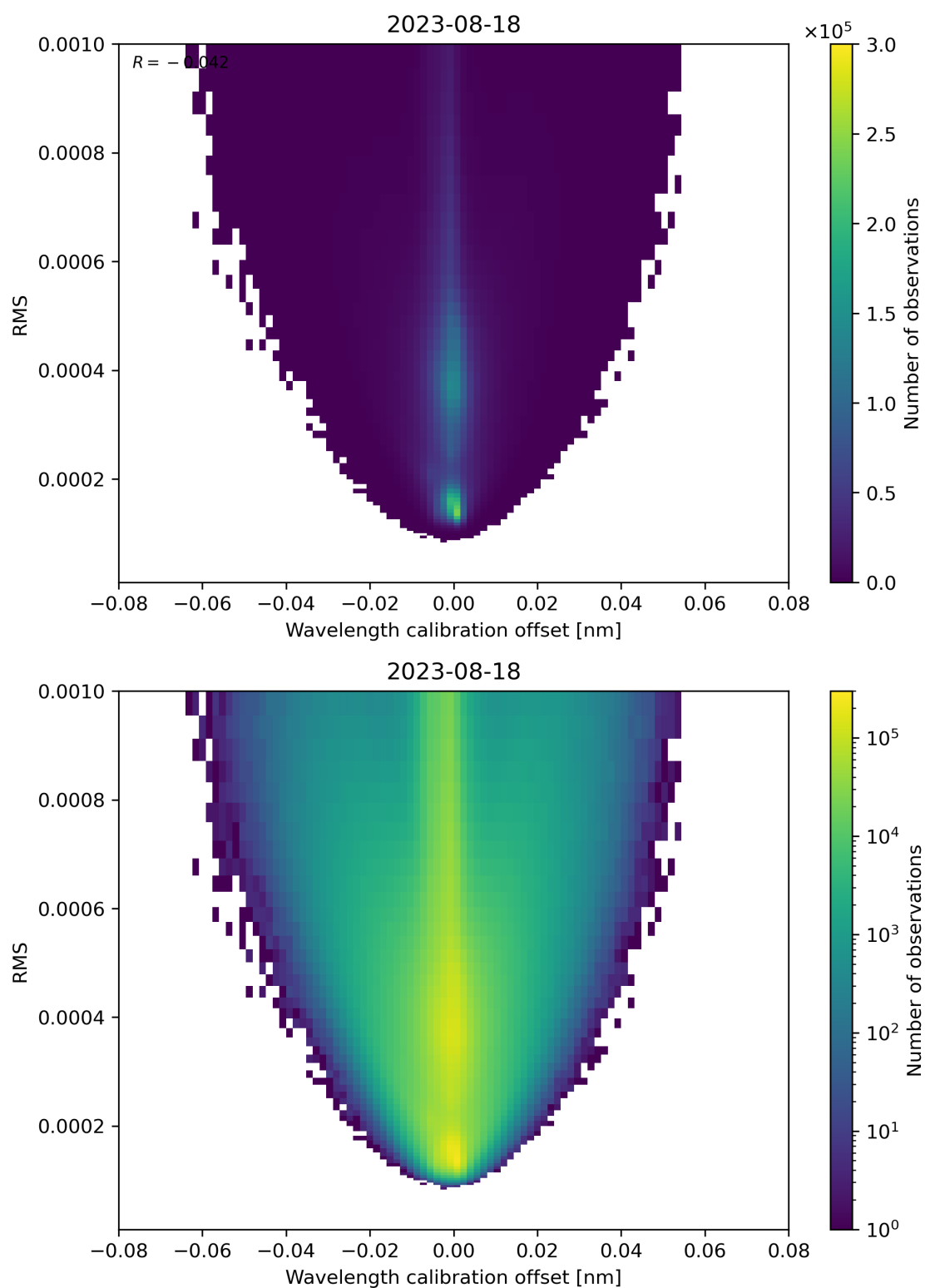
Figure 181: Scatter density plot of “Wavelength calibration offset” against “RMS” for 2023-08-17 to 2023-08-19.
