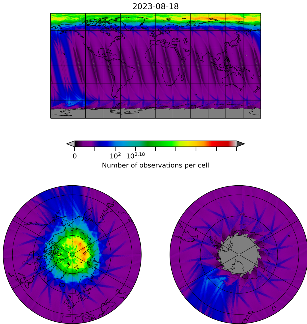
Figure 10: Map of the number of observations for 2023-08-17 to 2023-08-19
