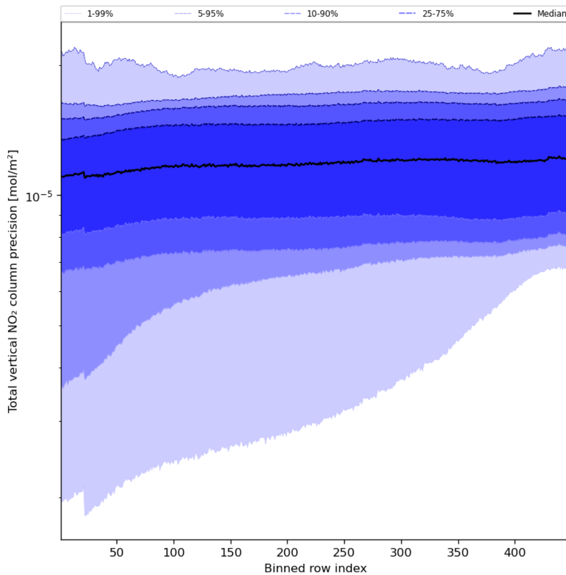
Figure 56: Along track statistics of “Total vertical NO 2 column precision” for 2023-08-17 to 2023-08-19
