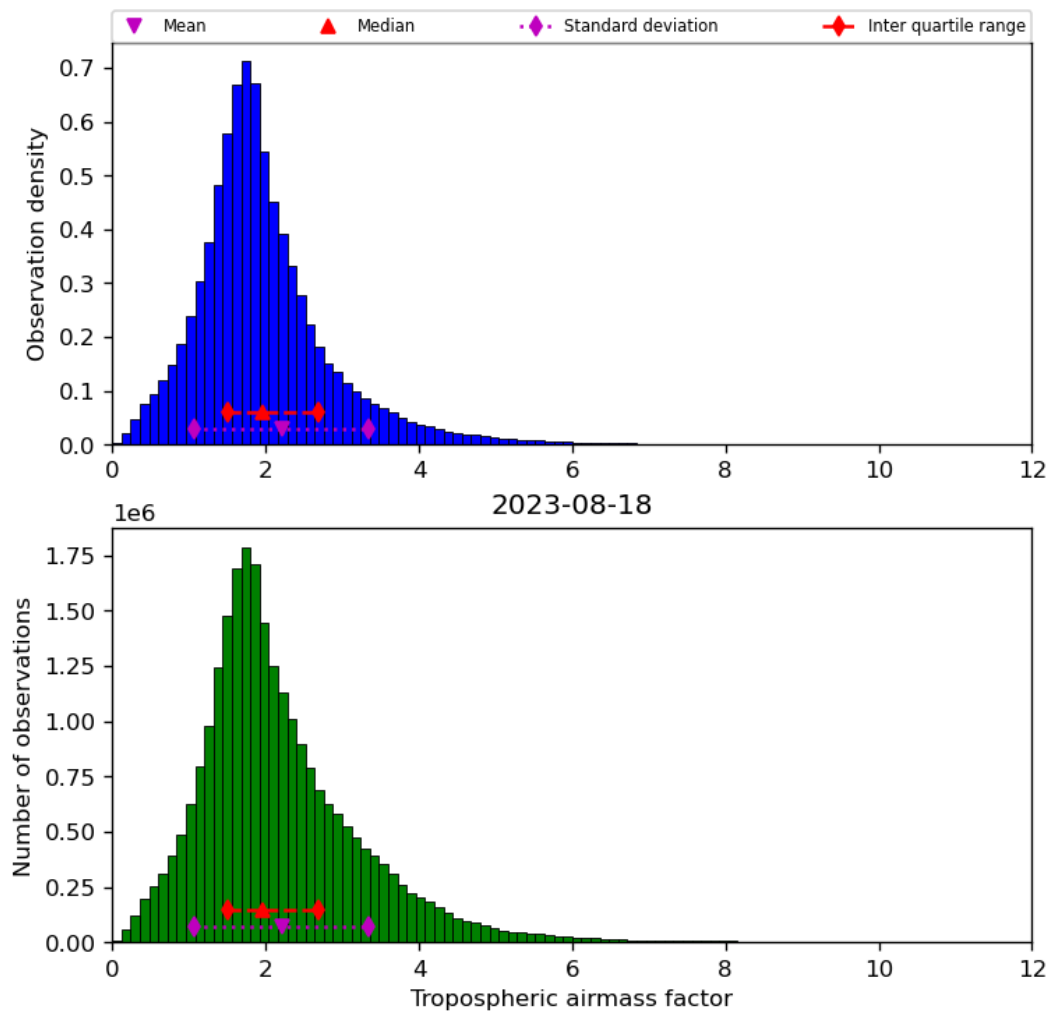
Figure 31: Histogram of “Tropospheric airmass factor” for 2023-08-17 to 2023-08-19
