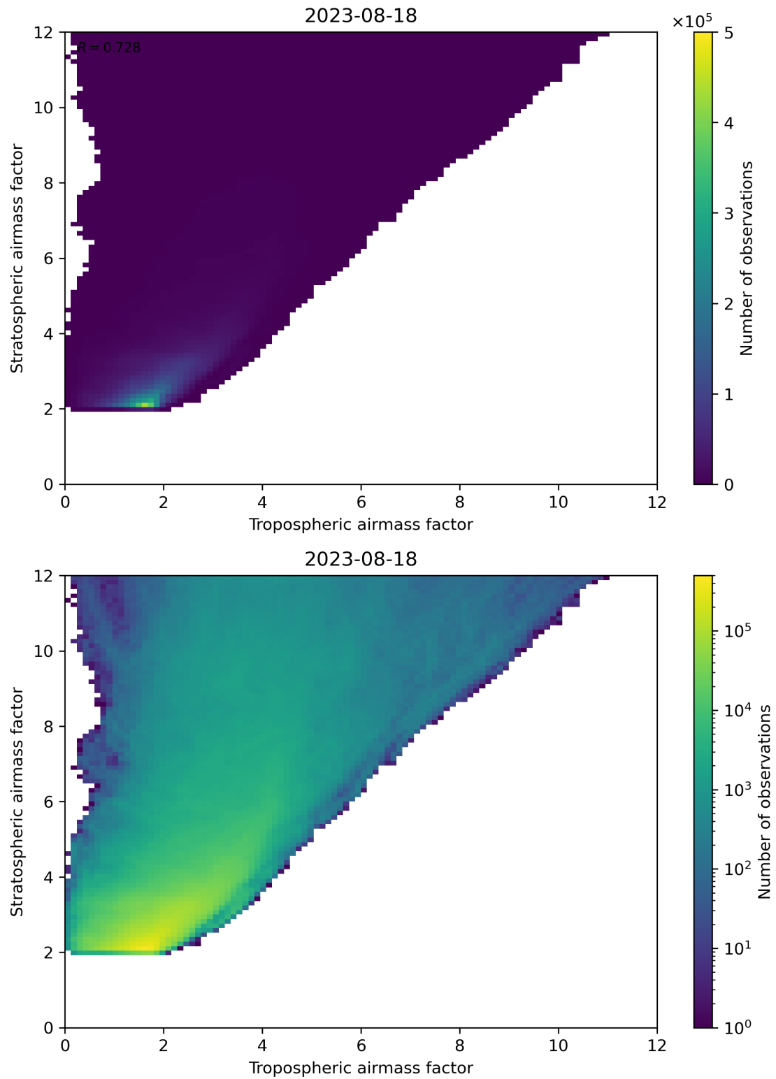
Figure 71: Scatter density plot of “Tropospheric airmass factor” against “Stratospheric airmass factor” for 2023-08-17 to 2023-08-19.
