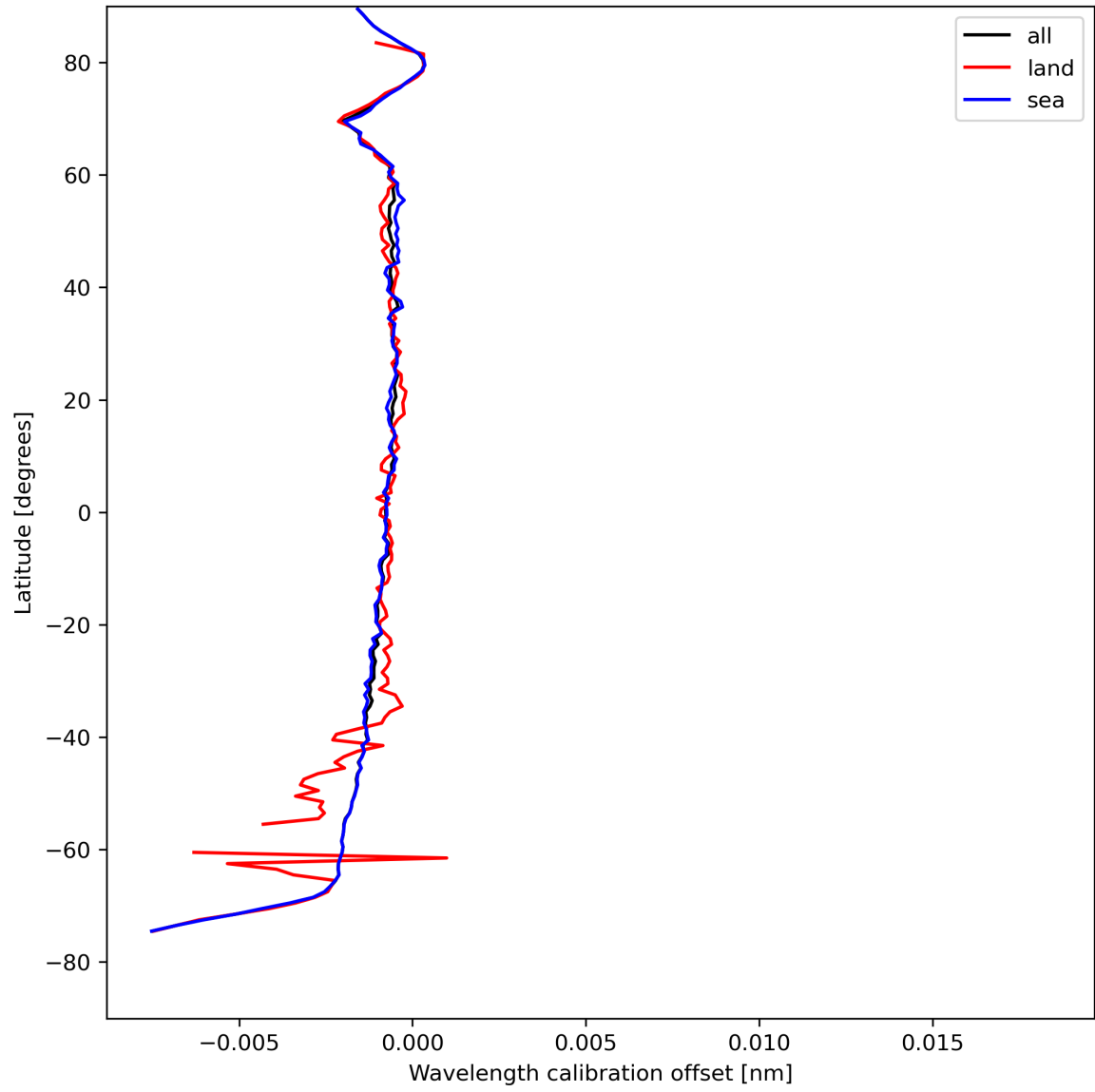
Figure 18: Zonal average of “Wavelength calibration offset” for 2023-08-17 to 2023-08-19.
