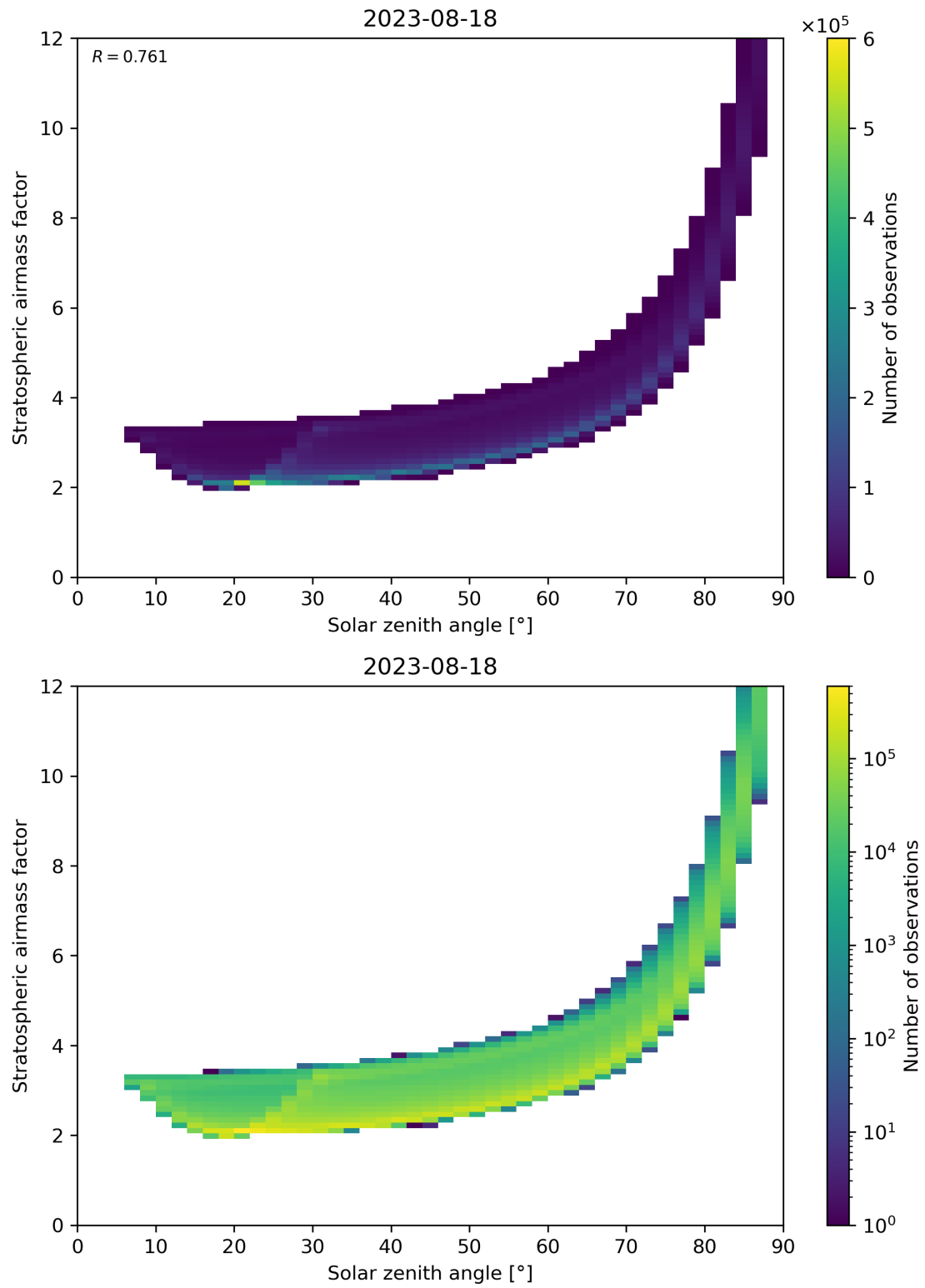
Figure 145: Scatter density plot of “Solar zenith angle” against “Stratospheric airmass factor” for 2023-08-17 to 2023-08-19.
