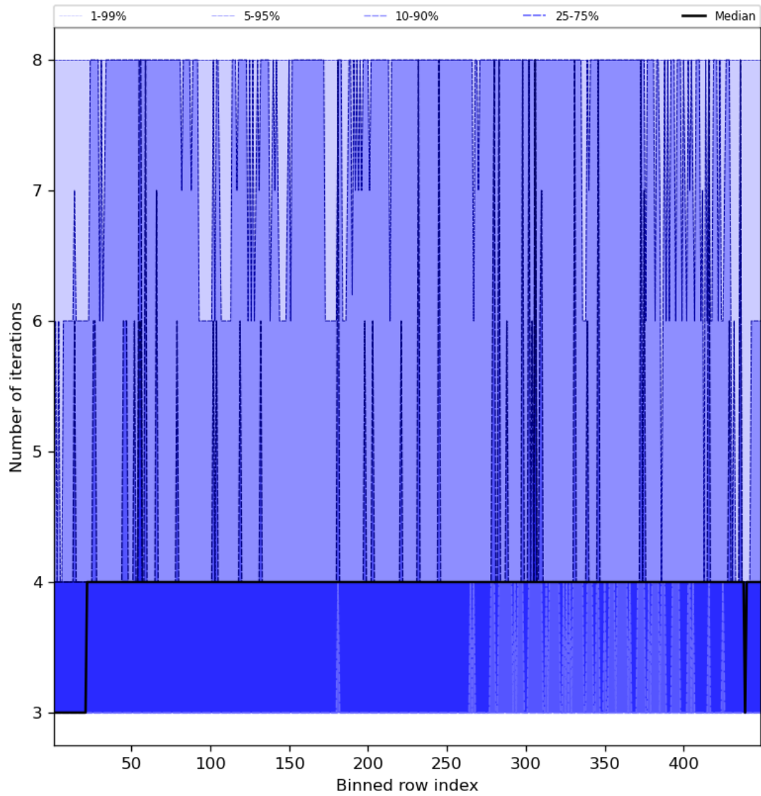
Figure 51: Along track statistics of “Number of iterations” for 2023-08-17 to 2023-08-19
