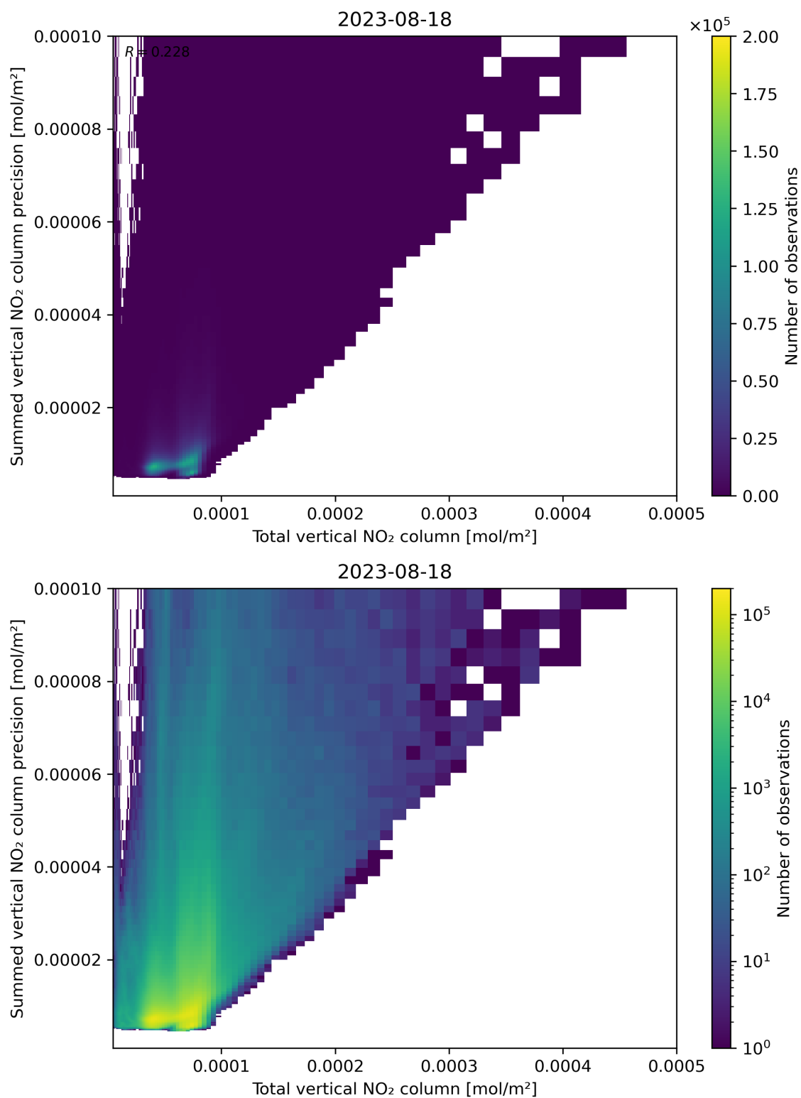
Figure 113: Scatter density plot of “Total vertical NO 2 column” against “Summed vertical NO 2 column precision” for 2023-08-17 to 2023-08-19.
