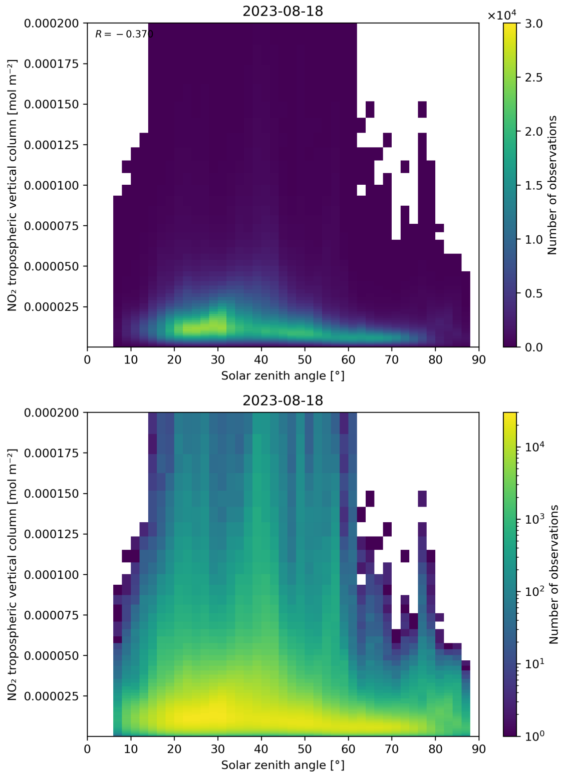
Figure 155: Scatter density plot of “Solar zenith angle” against “NO 2 tropospheric vertical column” for 2023-08-17 to 2023-08-19.
