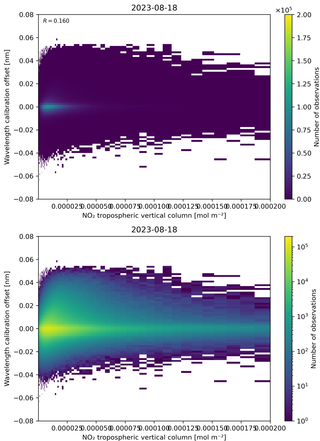
Figure 143: Scatter density plot of “NO 2 tropospheric vertical column” against “Wavelength calibration offset” for 2023-08-17 to 2023-08-19.
