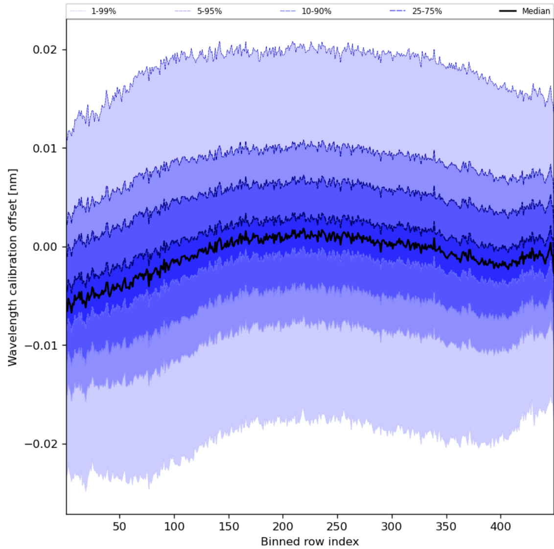
Figure 52: Along track statistics of "Wavelength calibration offset" for 2023-08-17 to 2023-08-19
