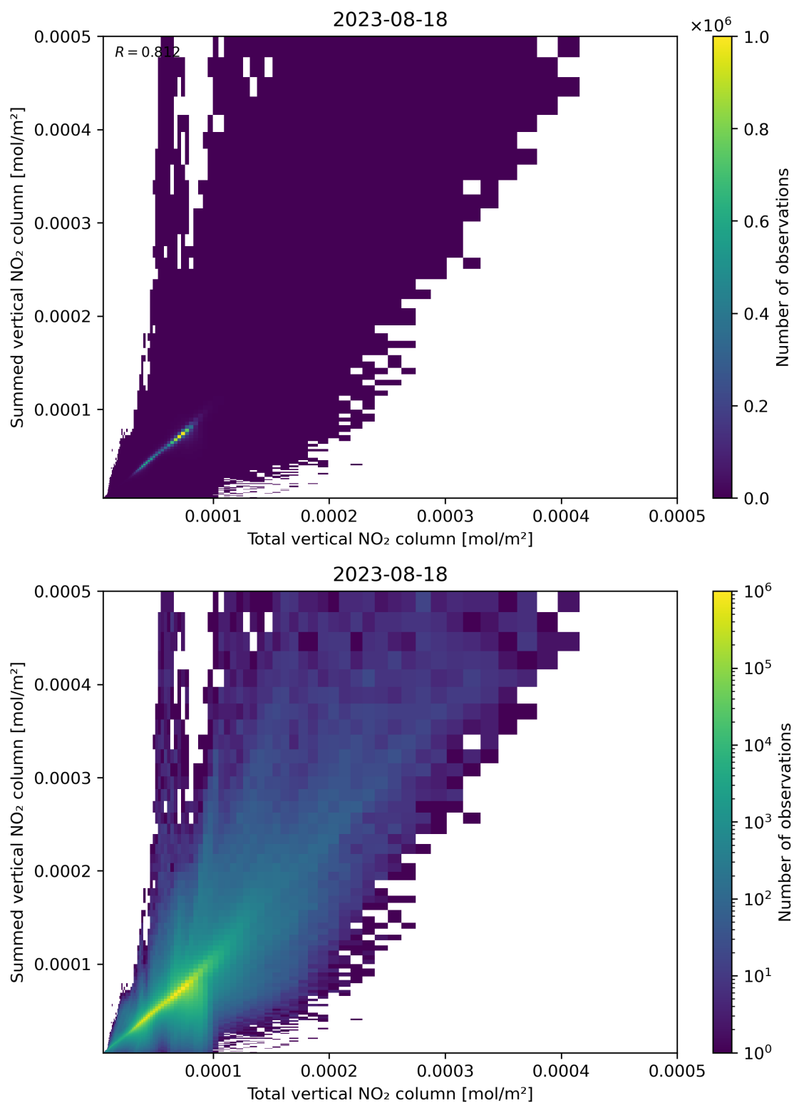
Figure 112: Scatter density plot of “Total vertical NO 2 column” against “Summed vertical NO 2 column” for 2023-08-17 to 2023-08-19.
