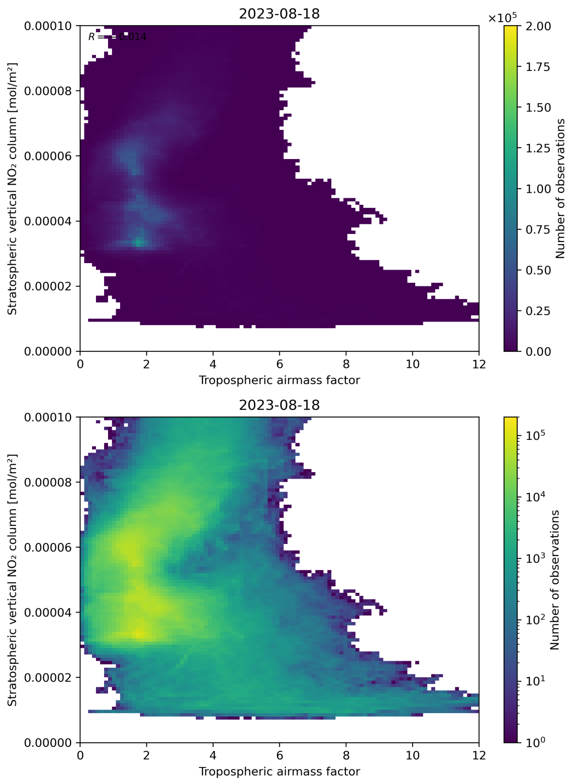
Figure 74: Scatter density plot of “Tropospheric air mass factor” against “Stratospheric vertical NO 2 column” for 2023-08-17 to 2023-08-19.
