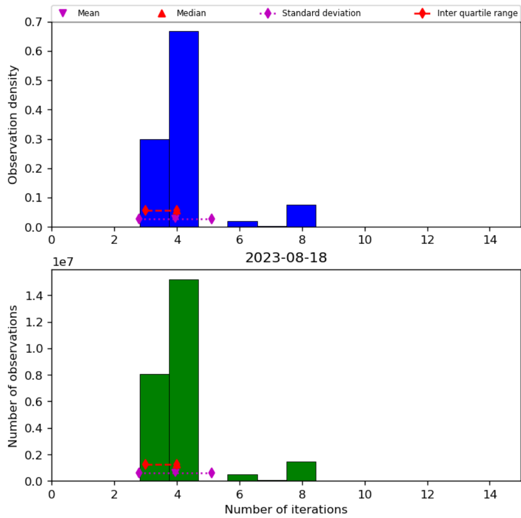
Figure 34: Histogram of “Number of iterations” for 2023-08-17 to 2023-08-19
