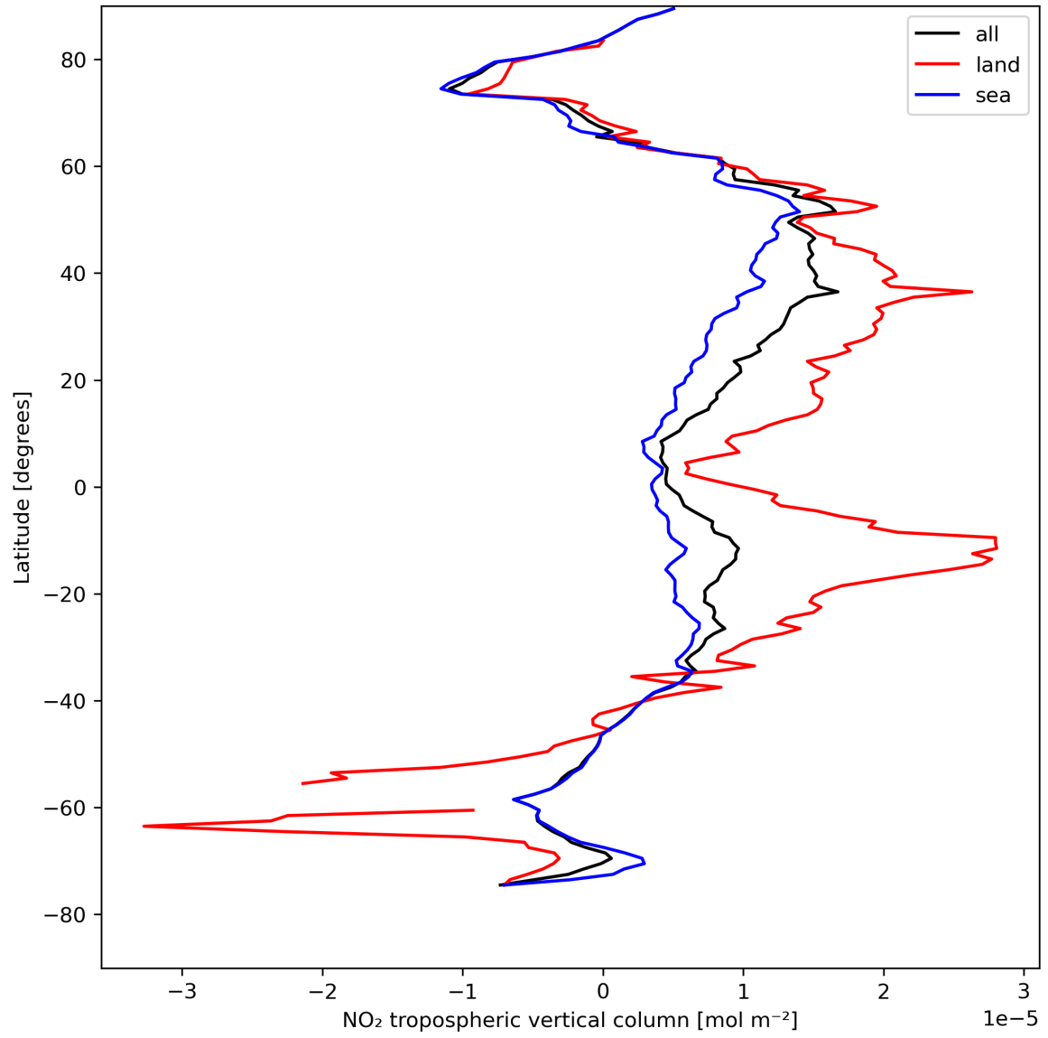
Figure 12: Zonal average of “NO 2 tropospheric vertical column” for 2023-08-17 to 2023-08-19.
