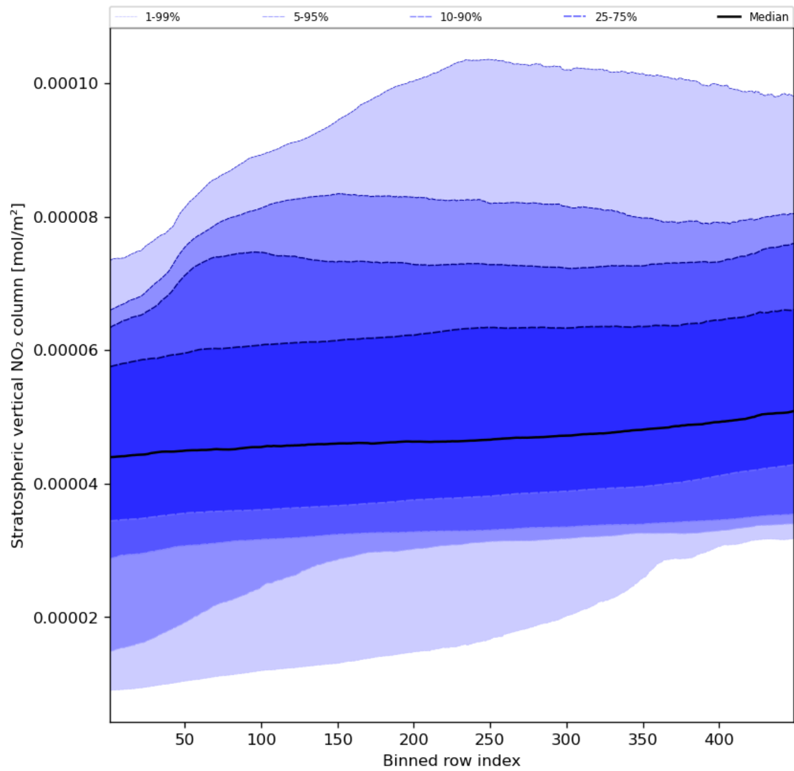
Figure 53: Along track statistics of “Stratospheric vertical NO 2 column” for 2023-08-17 to 2023-08-19
