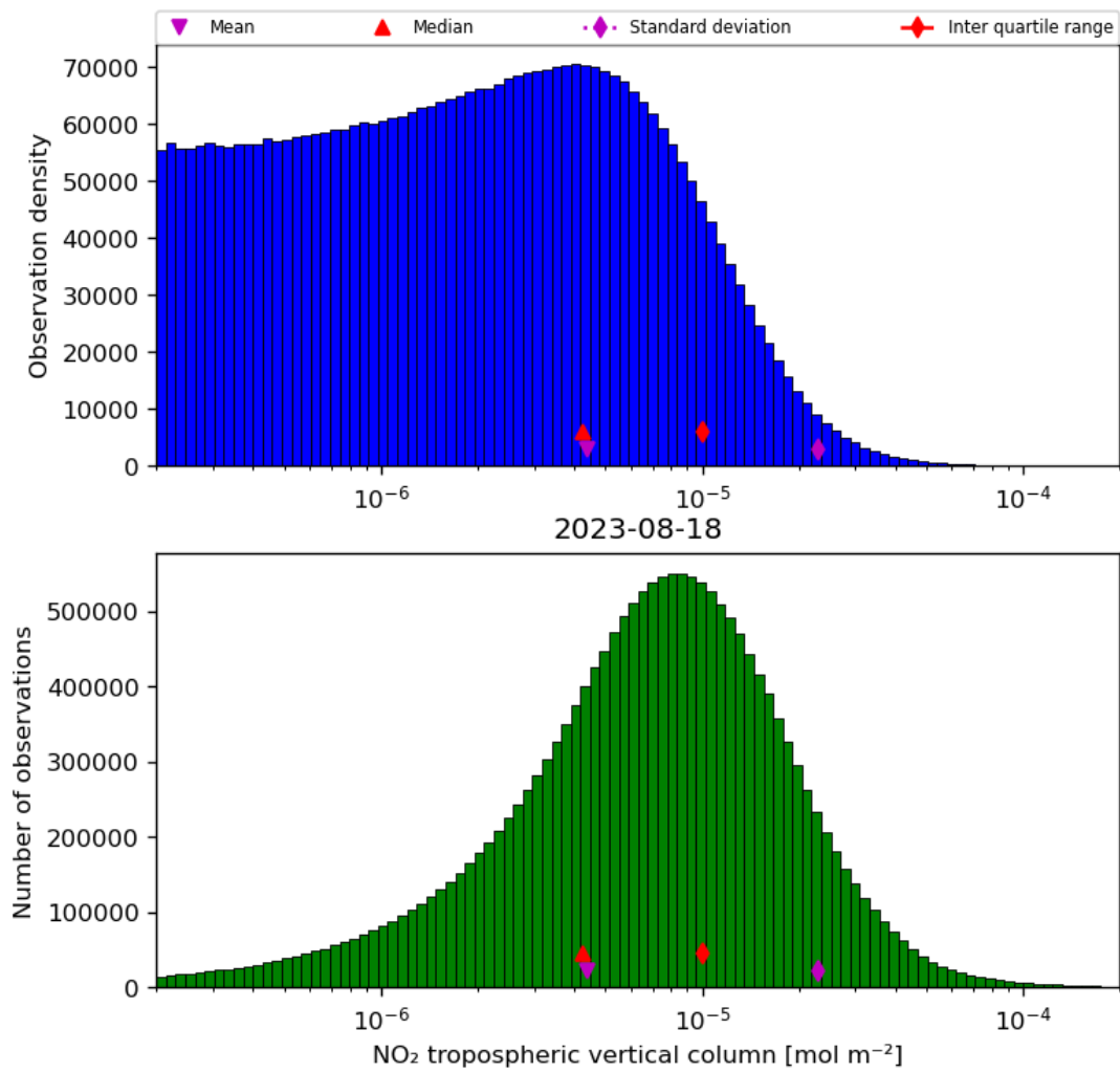
Figure 29: Histogram of “NO 2 tropospheric vertical column” for 2023-08-17 to 2023-08-19
