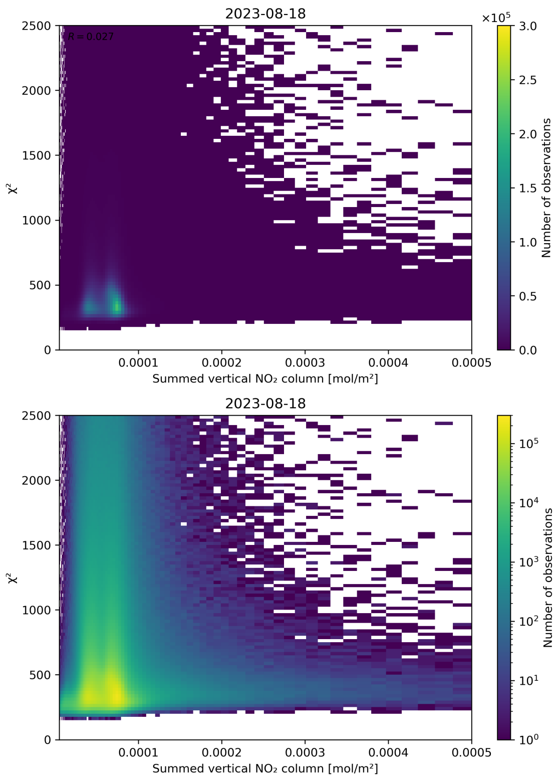
Figure 104: Scatter density plot of “Summed vertical NO 2 column” against “ \chi^2 ” for 2023-08-17 to 2023-08-19.
