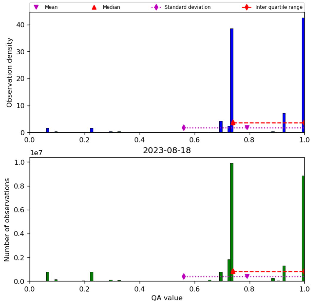
Figure 28: Histogram of “QA value” for 2023-08-17 to 2023-08-19
