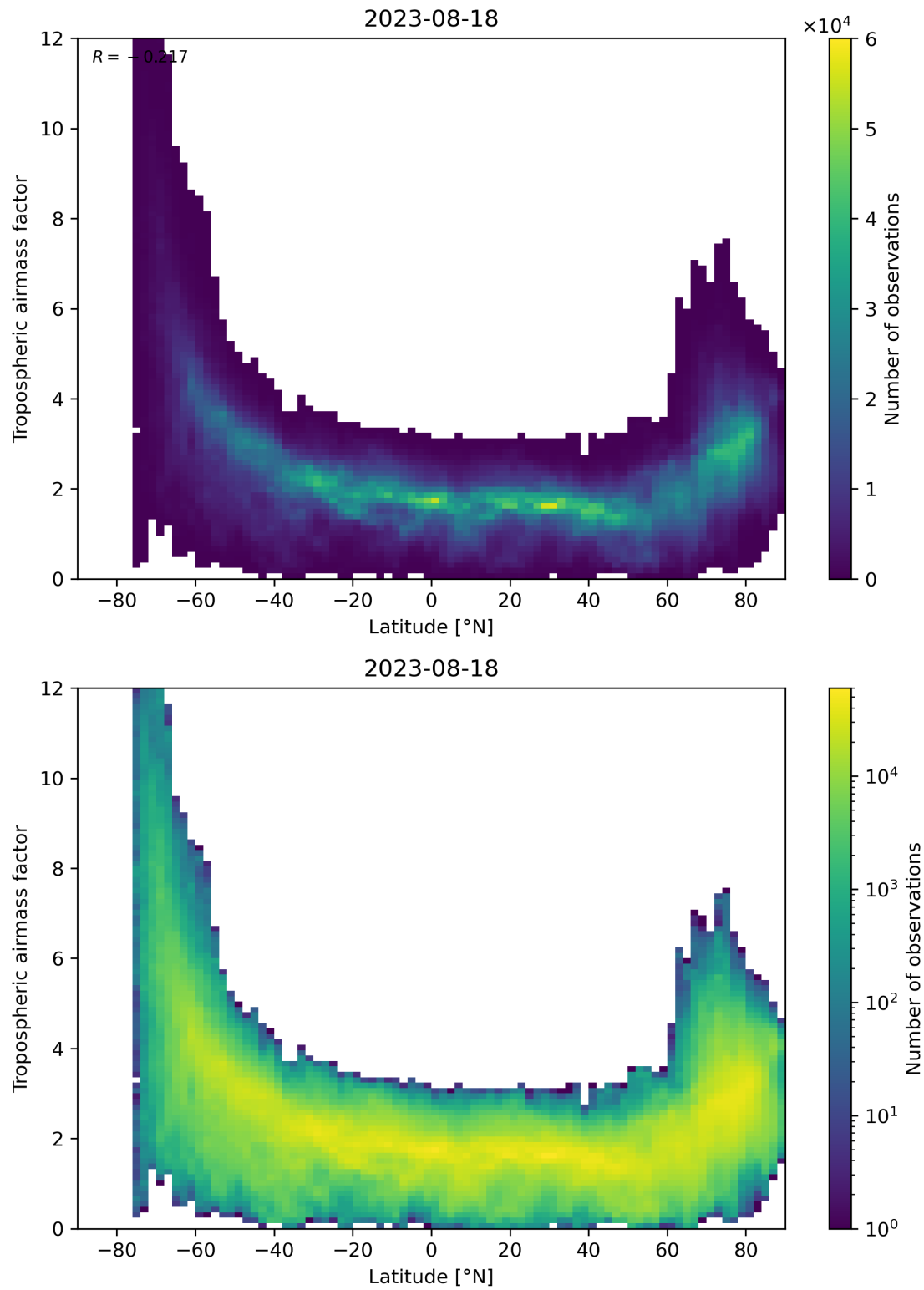
Figure 85: Scatter density plot of “Latitude” against “Tropospheric air mass factor” for 2023-08-17 to 2023-08-19.
