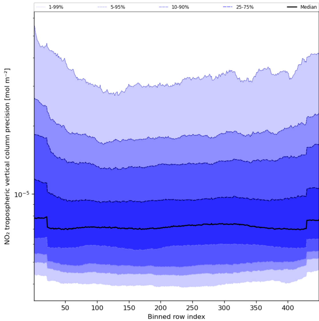
Figure 47: Along track statistics of “NO 2 tropospheric vertical column precision” for 2023-08-17 to 2023-08-19
