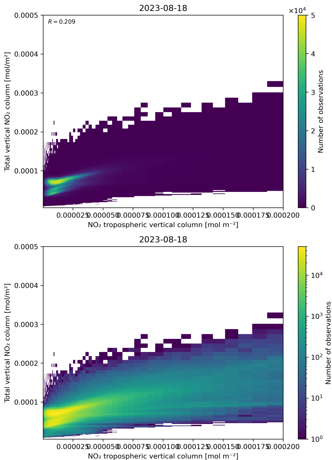
Figure 128: Scatter density plot of “NO 2 tropospheric vertical column” against “Total vertical NO 2 column” for 2023-08-17 to 2023-08-19.
