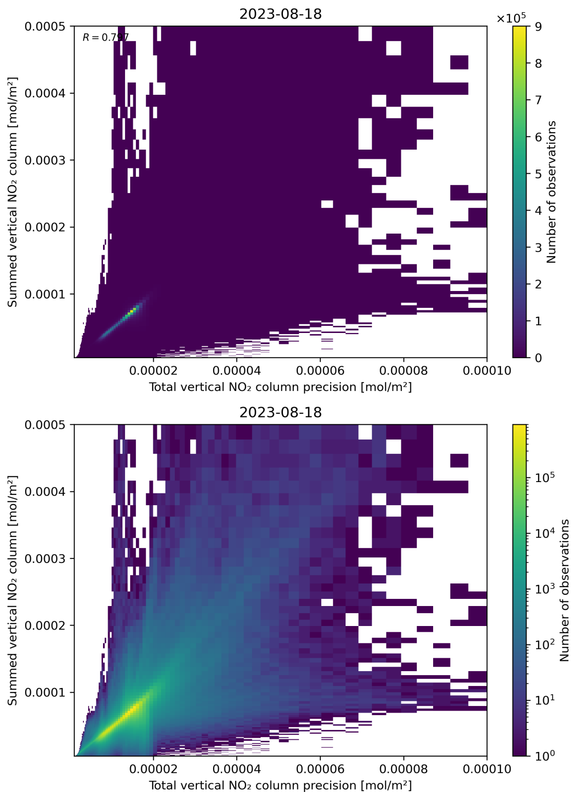
Figure 117: Scatter density plot of “Total vertical NO 2 column precision” against “Summed vertical NO 2 column” for 2023-08-17 to 2023-08-19.
