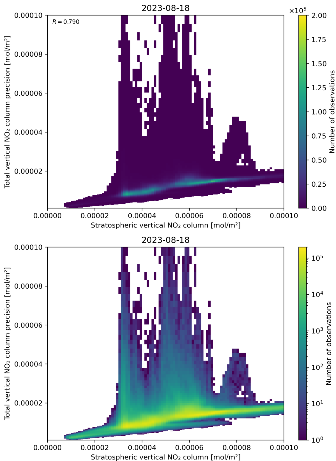
Figure 101: Scatter density plot of “Stratospheric vertical NO 2 column” against “Total vertical NO 2 column precision” for 2023-08-17 to 2023-08-19.
