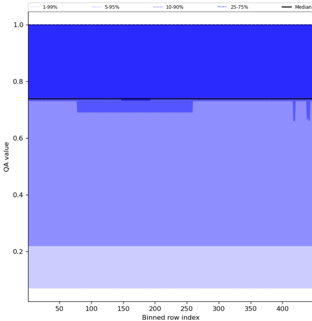
Figure 45: Along track statistics of “QA value” for 2023-08-17 to 2023-08-19
