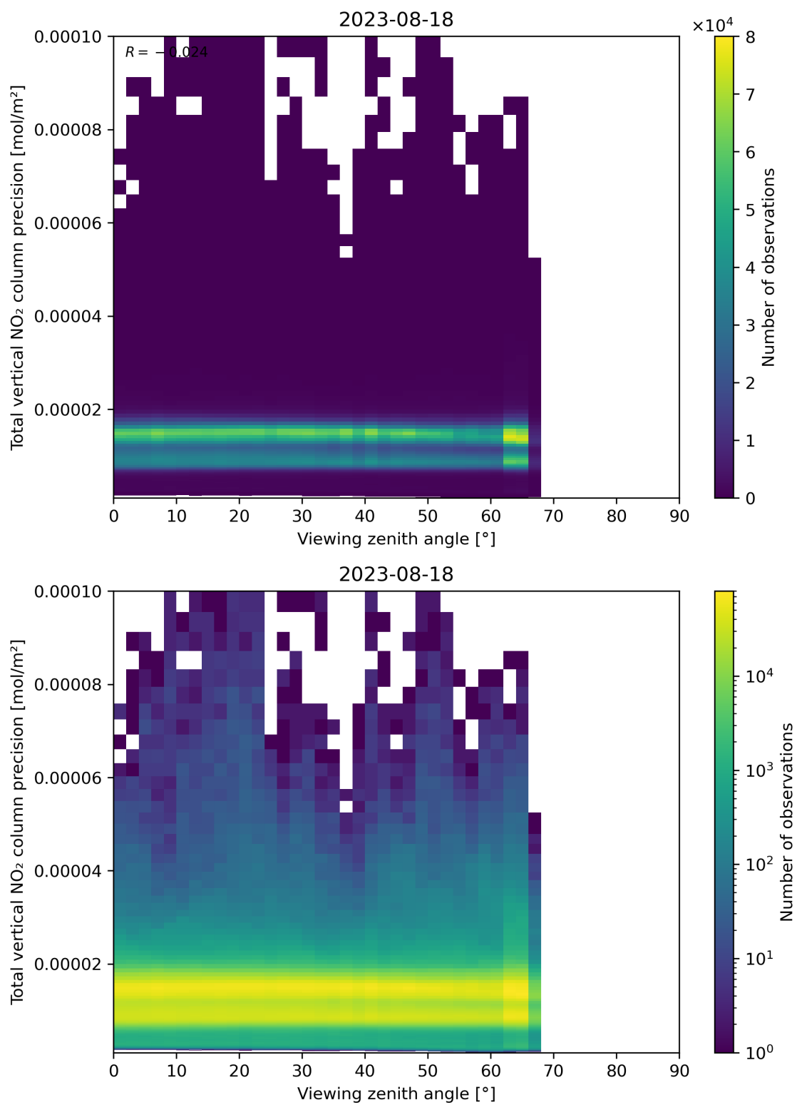
Figure 168: Scatter density plot of “Viewing zenith angle” against “Total vertical NO 2 column precision” for 2023-08-17 to 2023-08-19.
