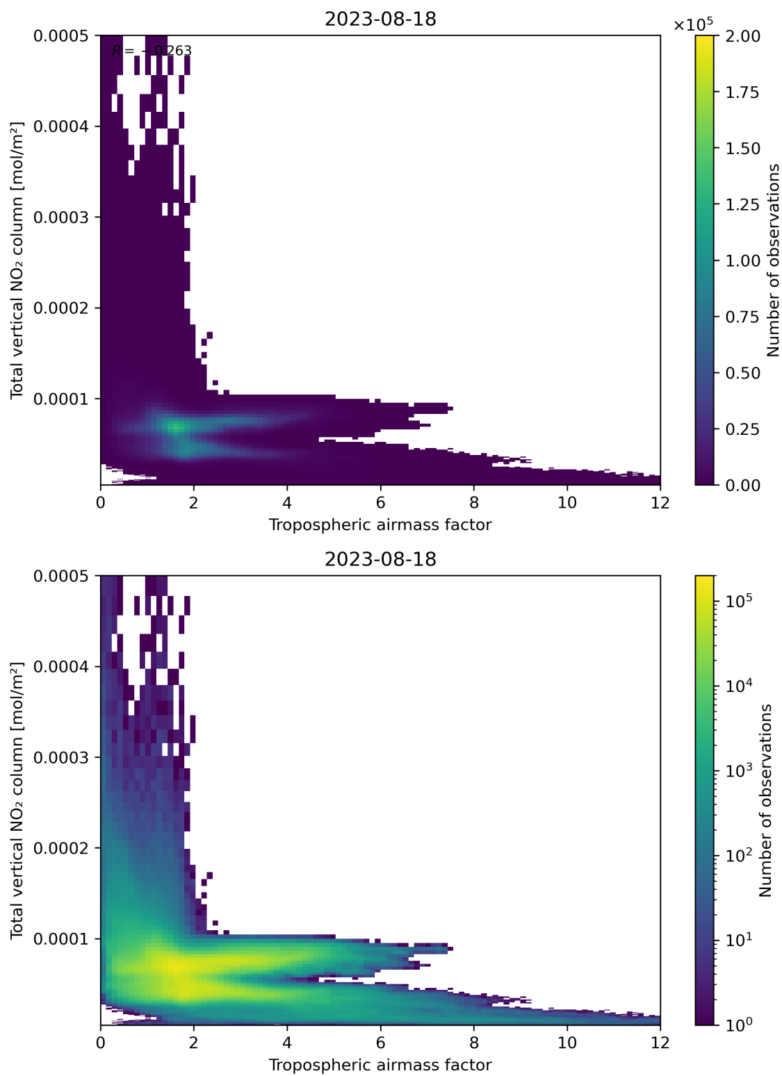
Figure 77: Scatter density plot of “Tropospheric airmass factor” against “Total vertical NO 2 column” for 2023-08-17 to 2023-08-19.
