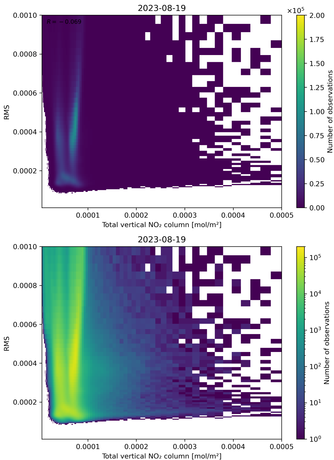
Figure 120: Scatter density plot of “Total vertical NO 2 column” against “RMS” for 2023-08-18 to 2023-08-20.
