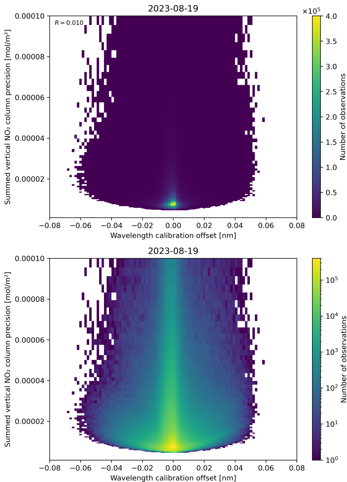
Figure 178: Scatter density plot of “Wavelength calibration offset” against “Summed vertical NO 2 column precision” for 2023-08-18 to 2023-08-20.
