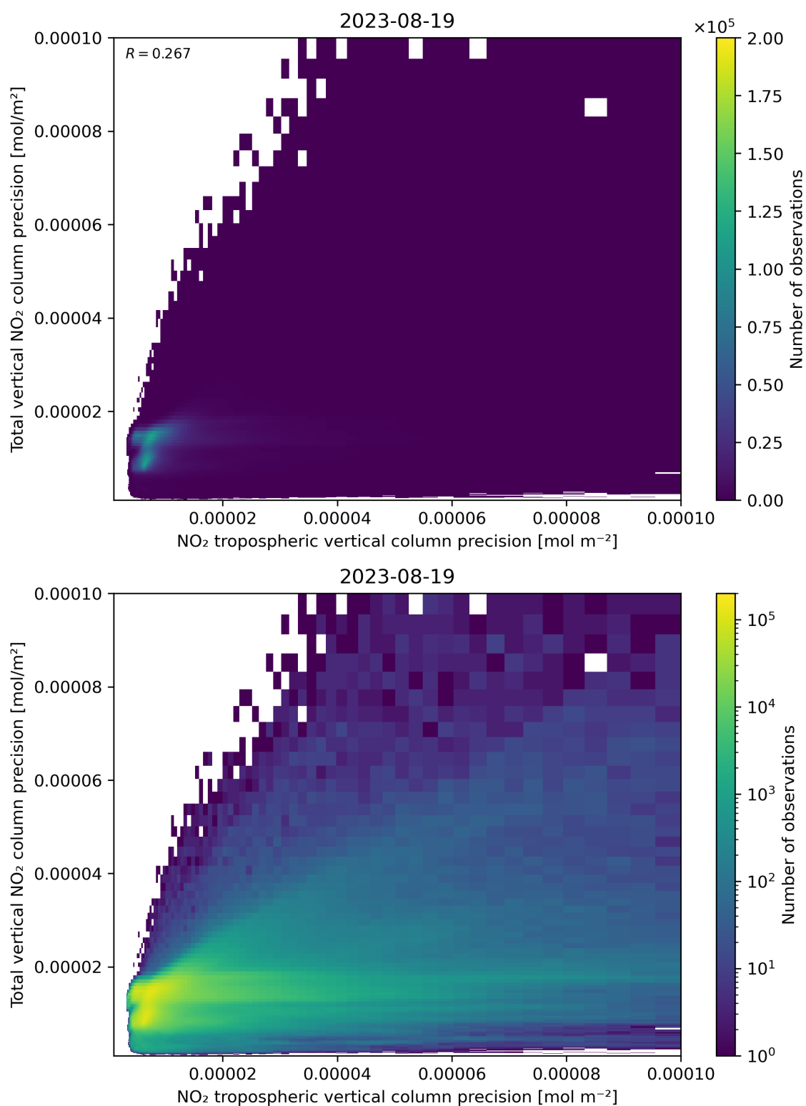
Figure 139: Scatter density plot of “NO 2 tropospheric vertical column precision” against “Total vertical NO 2 column precision” for 2023-08-18 to 2023-08-20.
