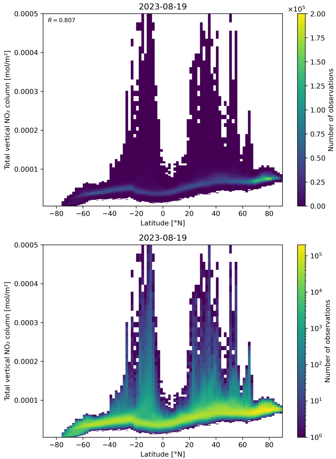
Figure 90: Scatter density plot of “Latitude” against “Total vertical NO 2 column” for 2023-08-18 to 2023-08-20.
