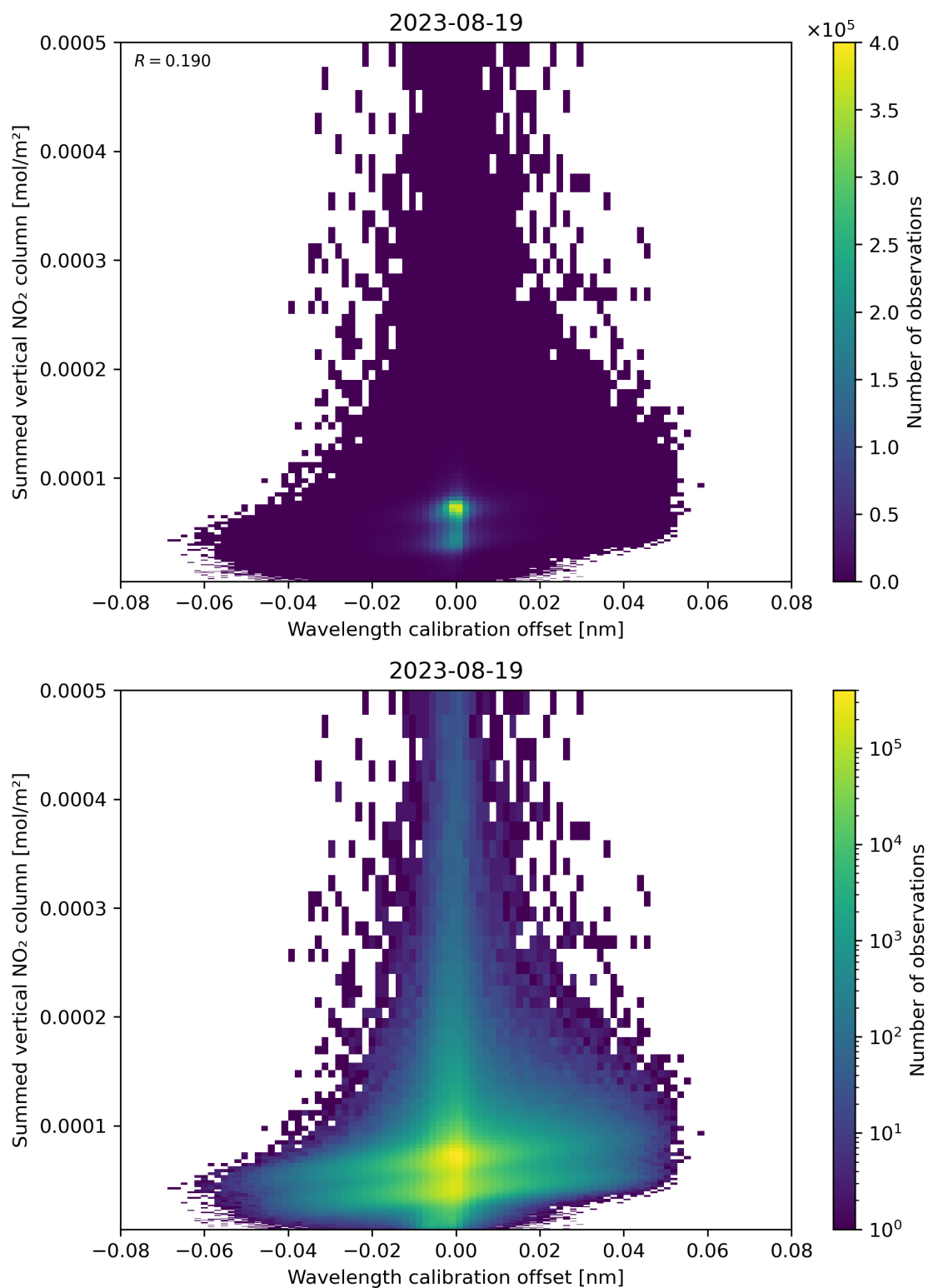
Figure 177: Scatter density plot of “Wavelength calibration offset” against “Summed vertical NO 2 column” for 2023-08-18 to 2023-08-20.
