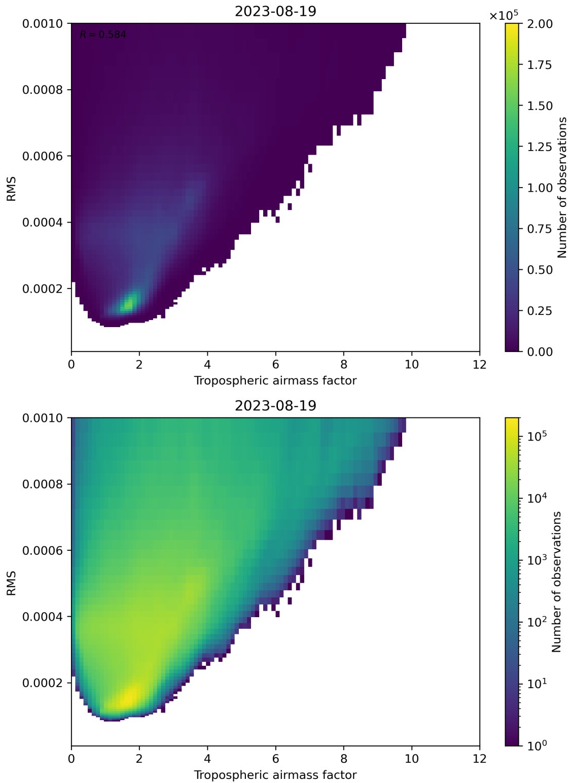
Figure 79: Scatter density plot of “Tropospheric airmass factor” against “RMS” for 2023-08-18 to 2023-08-20.
