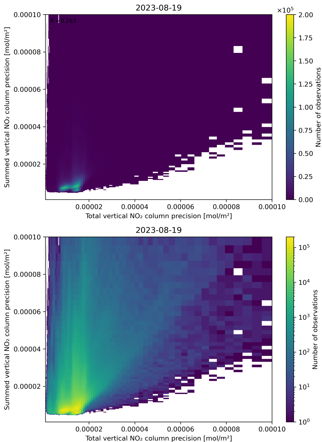
Figure 118: Scatter density plot of “Total vertical NO 2 column precision” against “Summed vertical NO 2 column precision” for 2023-08-18 to 2023-08-20.
