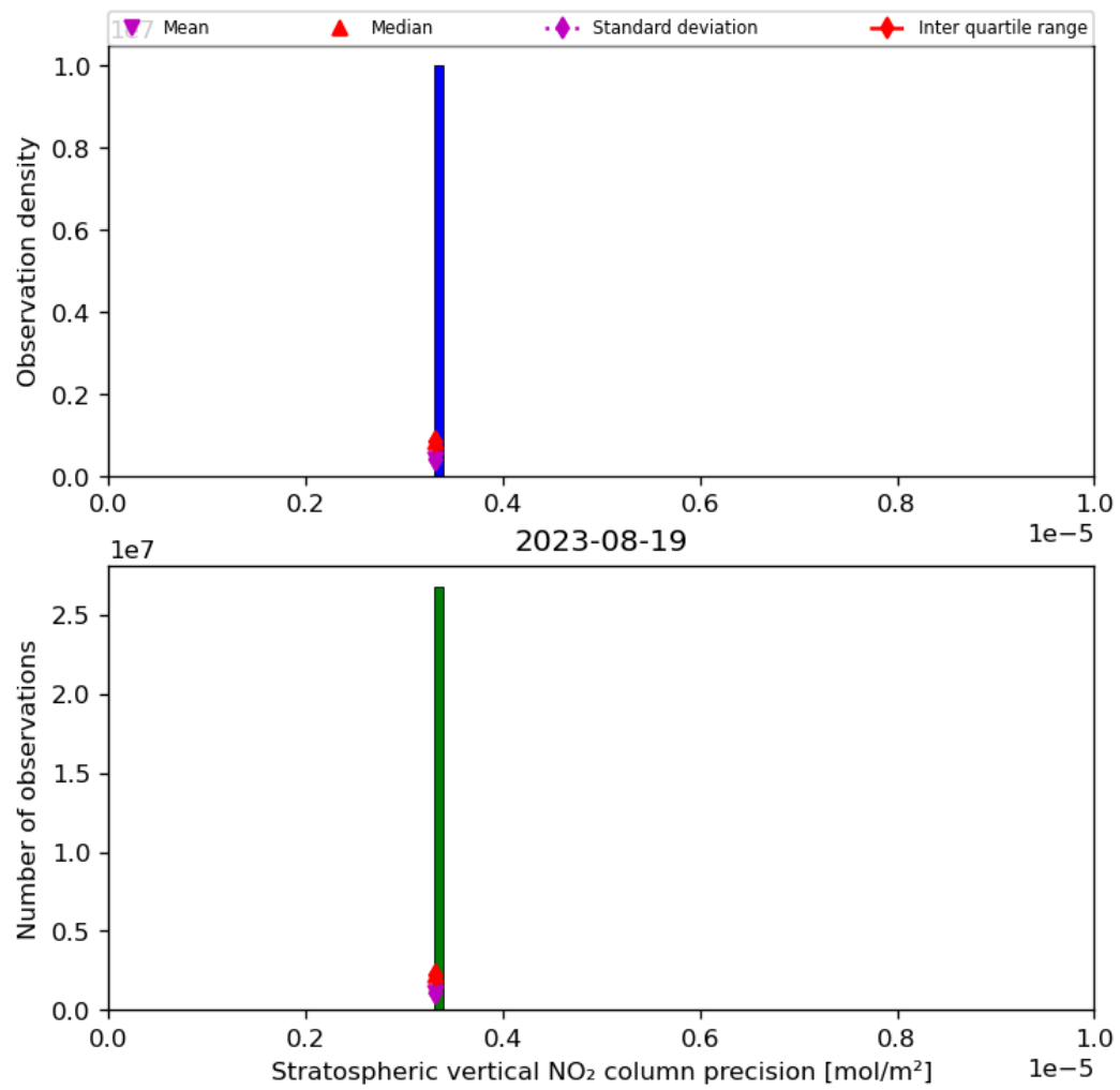
Figure 37: Histogram of “Stratospheric vertical NO 2 column precision” for 2023-08-18 to 2023-08-20
