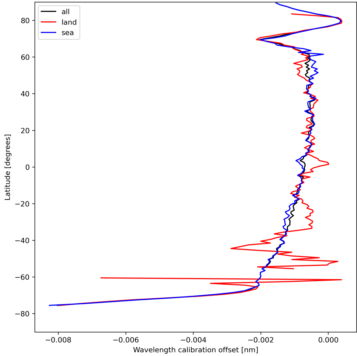
Figure 18: Zonal average of “Wavelength calibration offset” for 2023-08-18 to 2023-08-20.
