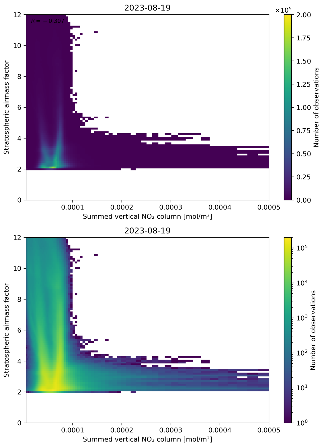
Figure 103: Scatter density plot of “Summed vertical NO 2 column” against “Stratospheric airmass factor” for 2023-08-18 to 2023-08-20.
