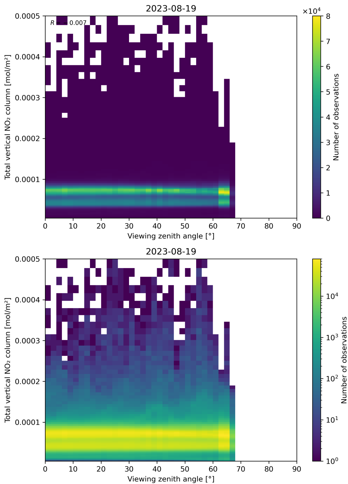
Figure 167: Scatter density plot of “Viewing zenith angle” against “Total vertical NO 2 column” for 2023-08-18 to 2023-08-20.
