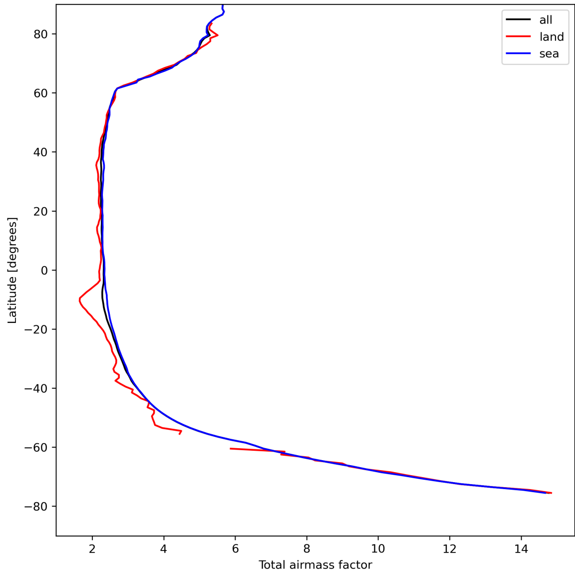
Figure 15: Zonal average of “Total airmass factor” for 2023-08-18 to 2023-08-20.
