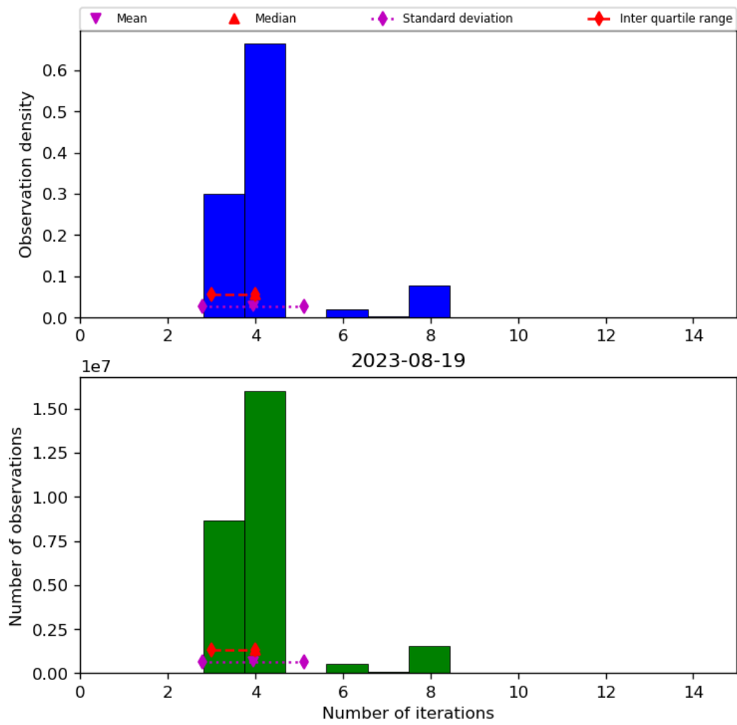
Figure 34: Histogram of “Number of iterations” for 2023-08-18 to 2023-08-20
