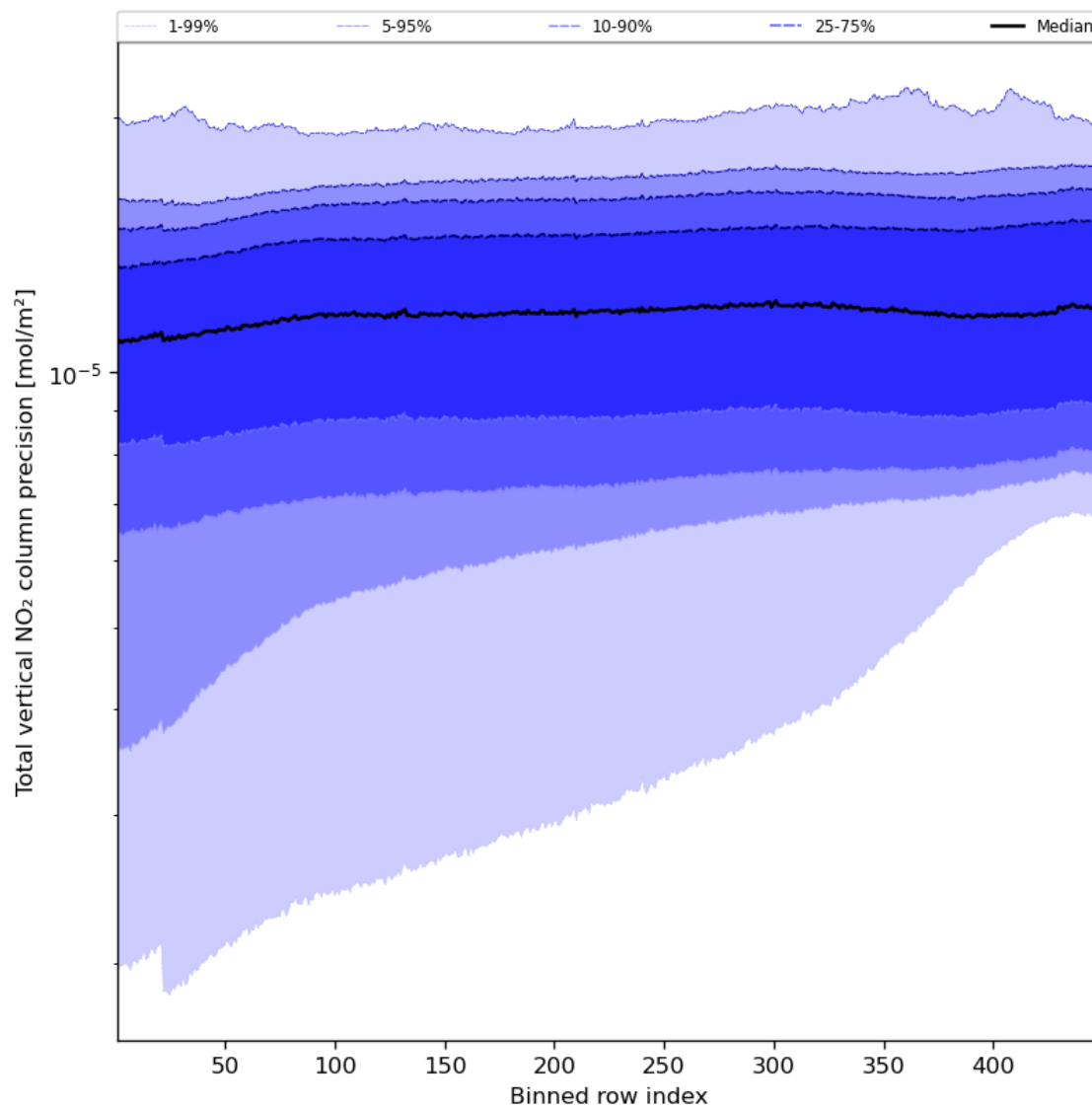
Figure 56: Along track statistics of “Total vertical NO 2 column precision” for 2023-08-18 to 2023-08-20
