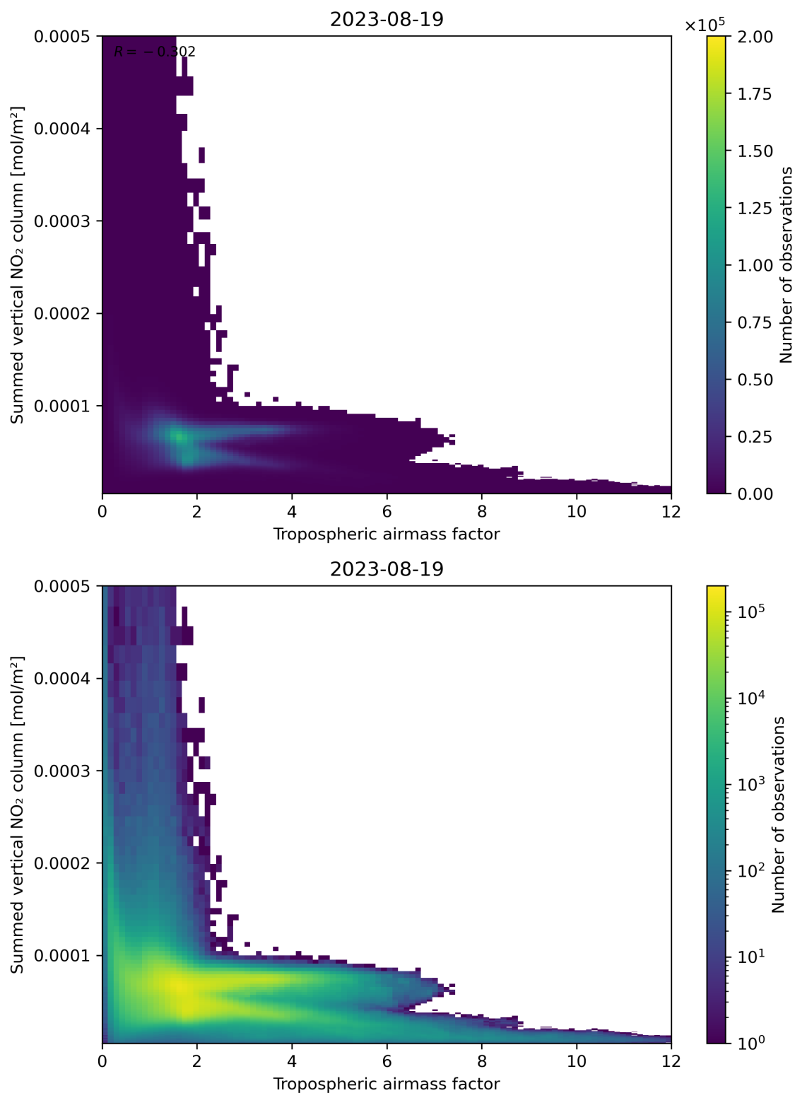
Figure 75: Scatter density plot of “Tropospheric air mass factor” against “Summed vertical NO 2 column” for 2023-08-18 to 2023-08-20.
