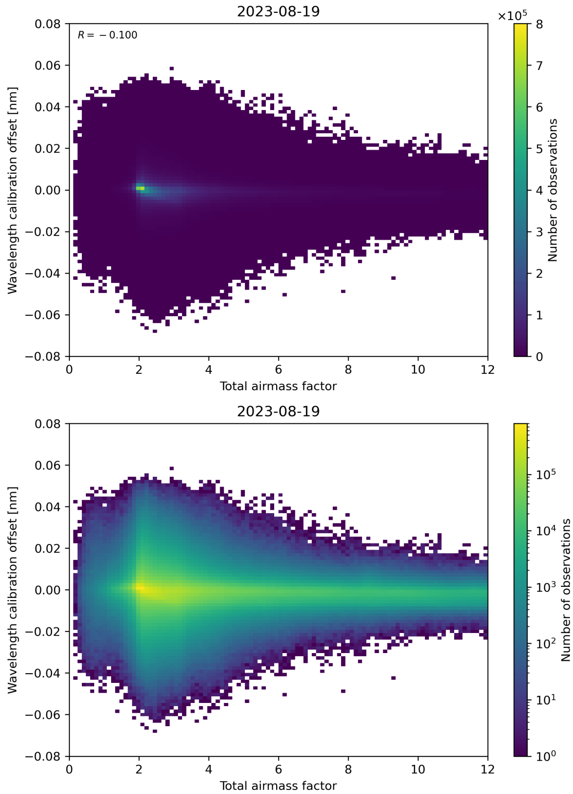
Figure 70: Scatter density plot of “Total airmass factor” against “Wavelength calibration offset” for 2023-08-18 to 2023-08-20.
