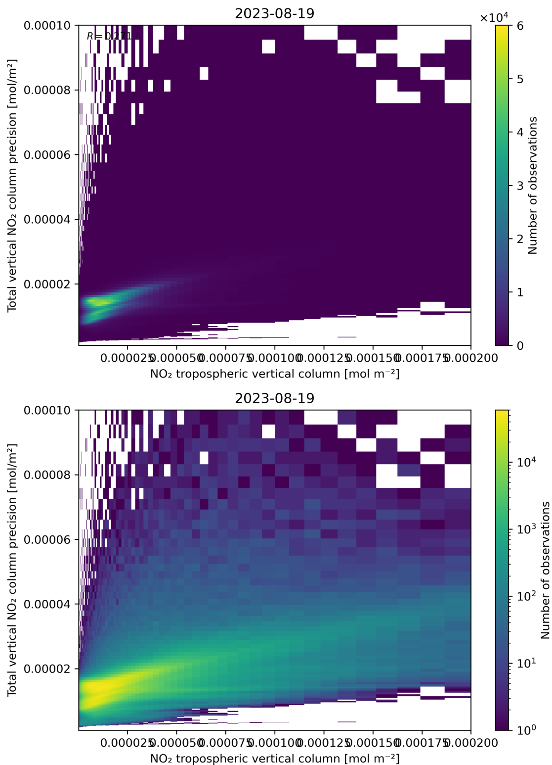
Figure 129: Scatter density plot of “NO 2 tropospheric vertical column” against “Total vertical NO 2 column precision” for 2023-08-18 to 2023-08-20.
