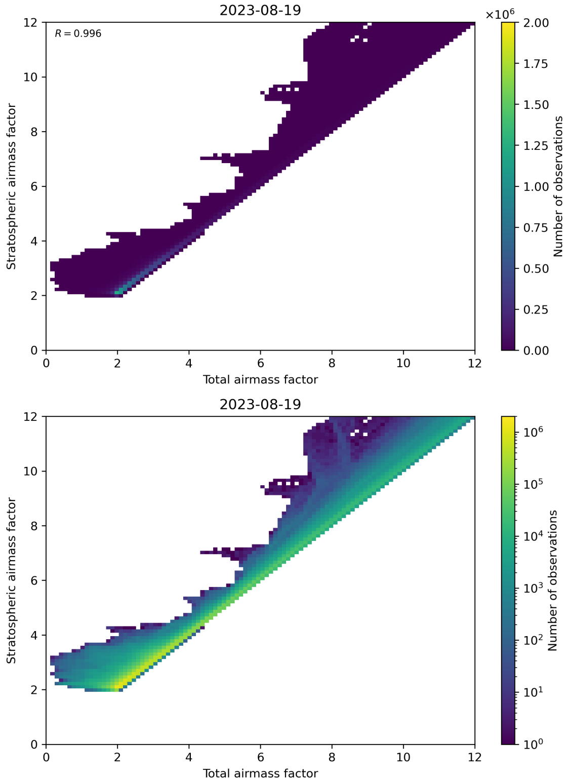
Figure 62: Scatter density plot of “Total airmass factor” against “Stratospheric airmass factor” for 2023-08-18 to 2023-08-20.
