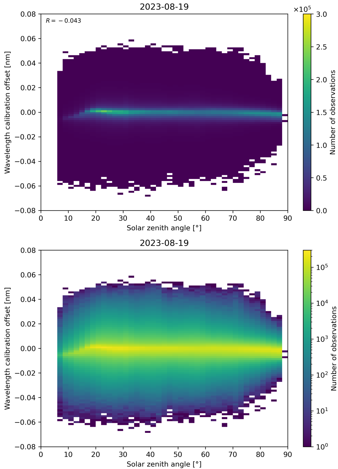
Figure 158: Scatter density plot of “Solar zenith angle” against “Wavelength calibration offset” for 2023-08-18 to 2023-08-20.
