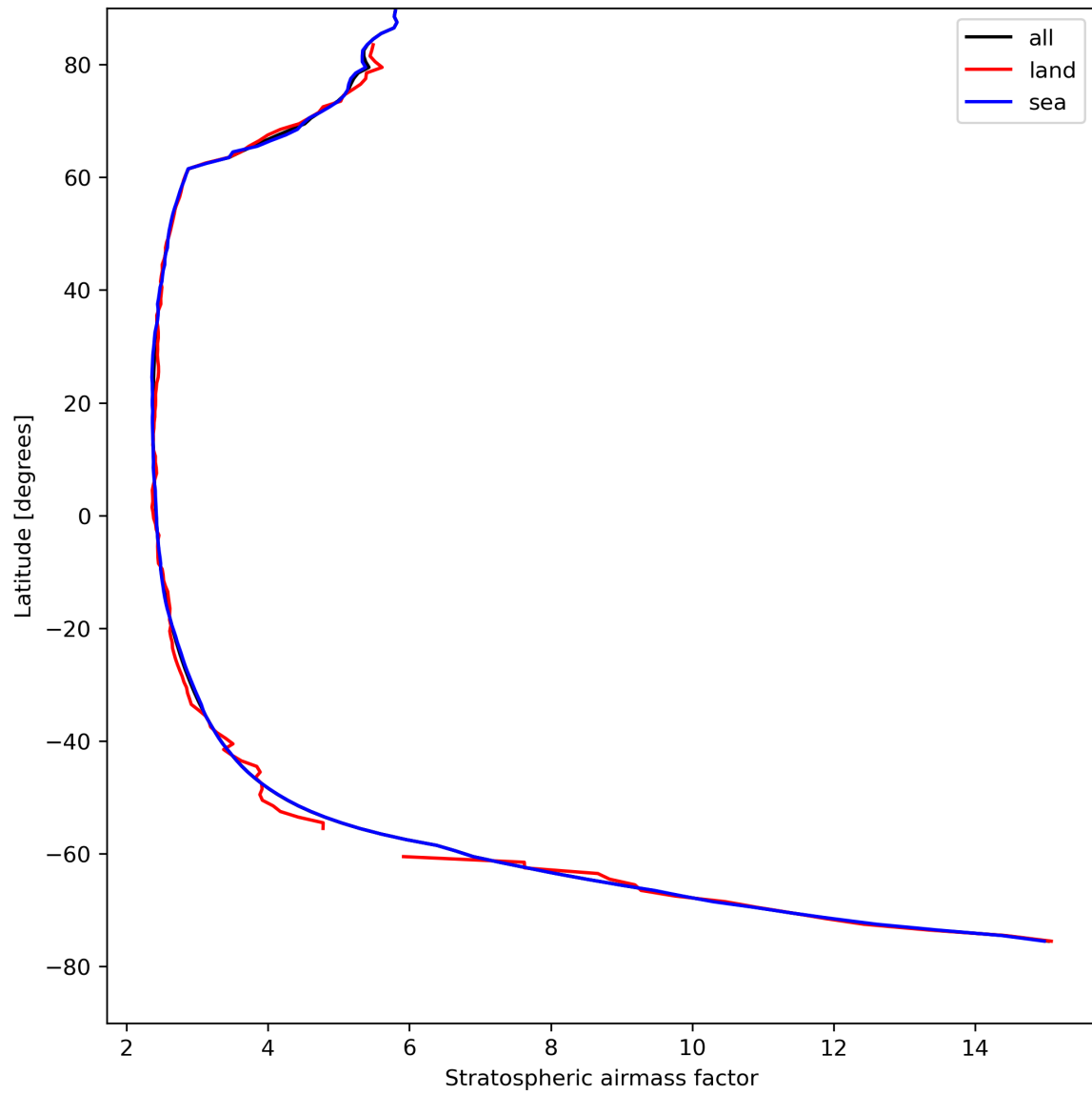
Figure 27: Zonal average of “Stratospheric air mass factor” for 2023-08-18 to 2023-08-20.
