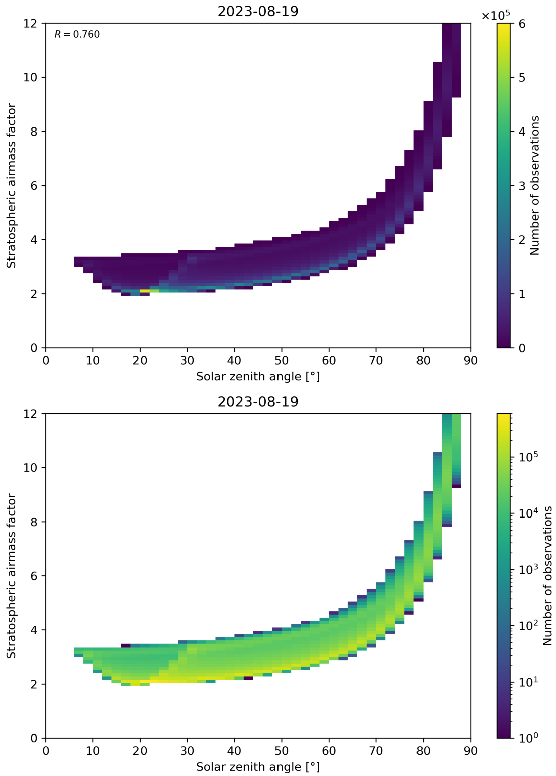
Figure 145: Scatter density plot of “Solar zenith angle” against “Stratospheric airmass factor” for 2023-08-18 to 2023-08-20.
