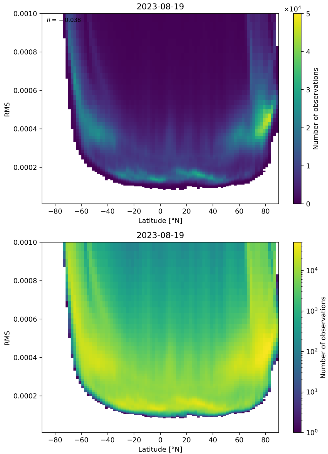
Figure 94: Scatter density plot of “Latitude” against “RMS” for 2023-08-18 to 2023-08-20.
