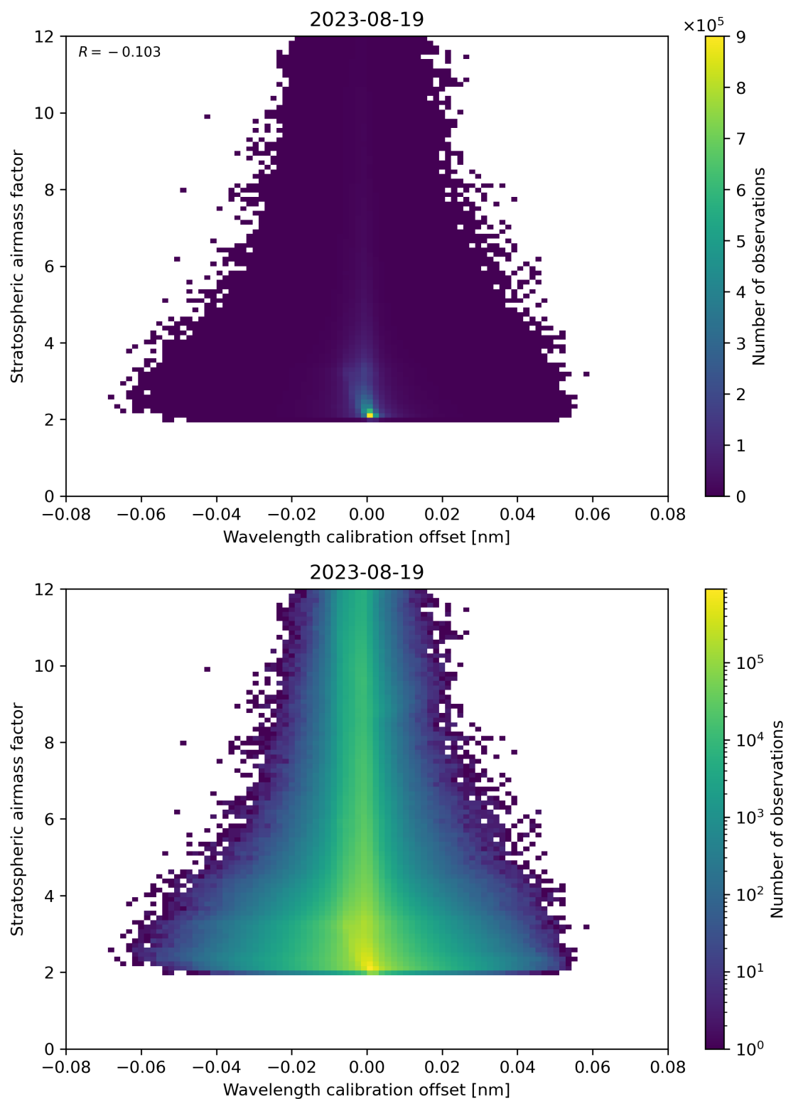
Figure 174: Scatter density plot of “Wavelength calibration offset” against “Stratospheric airmass factor” for 2023-08-18 to 2023-08-20.
