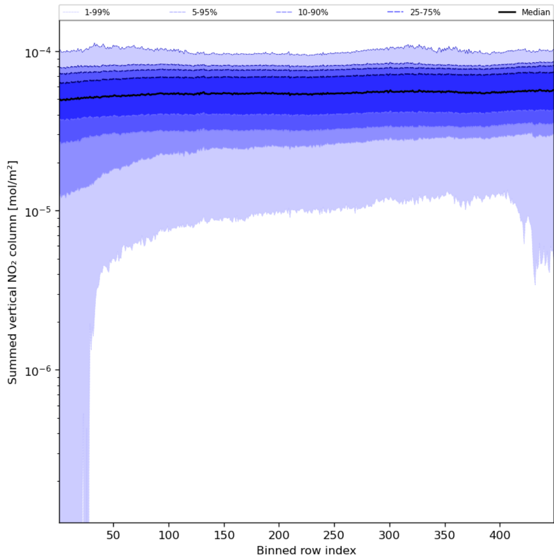
Figure 57: Along track statistics of “Summed vertical NO 2 column” for 2023-08-18 to 2023-08-20
