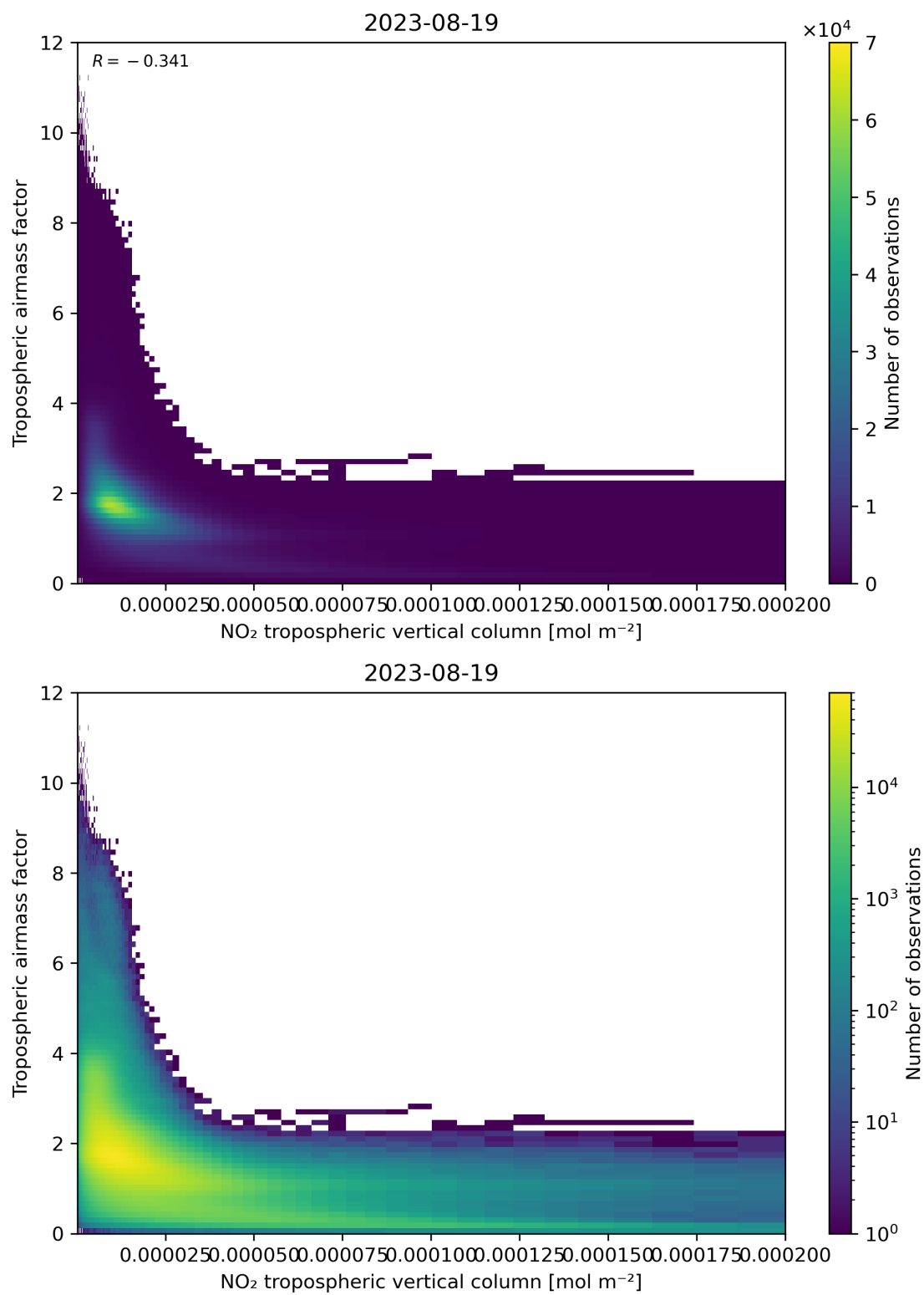
Figure 123: Scatter density plot of “NO 2 tropospheric vertical column” against “Tropospheric air mass factor” for 2023-08-18 to 2023-08-20.
