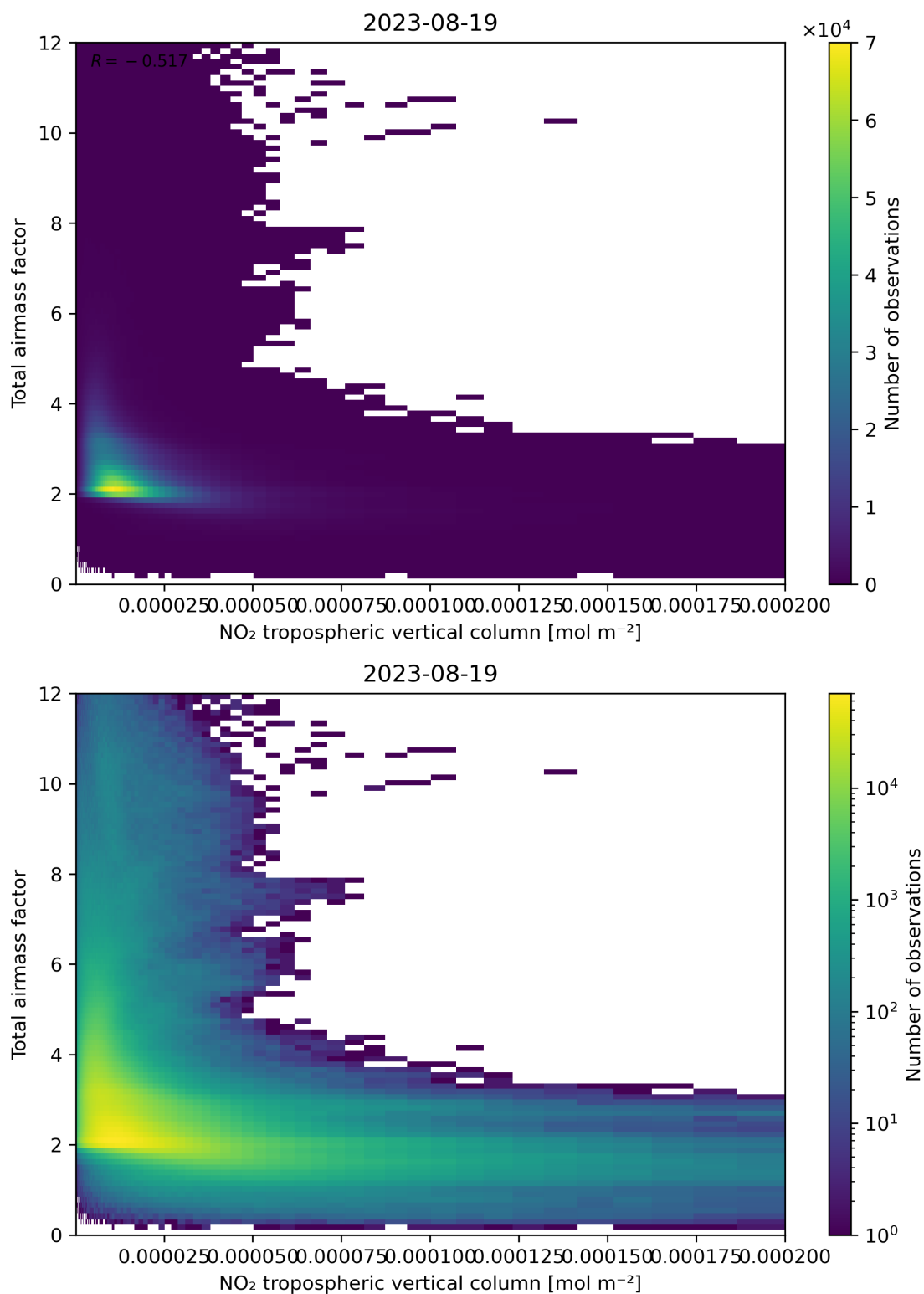
Figure 122: Scatter density plot of “NO 2 tropospheric vertical column” against “Total airmass factor” for 2023-08-18 to 2023-08-20.
