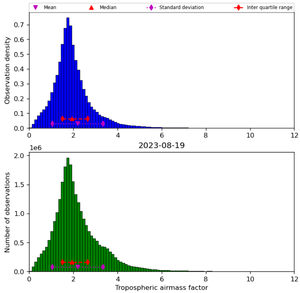
Figure 31: Histogram of “Tropospheric airmass factor” for 2023-08-18 to 2023-08-20
