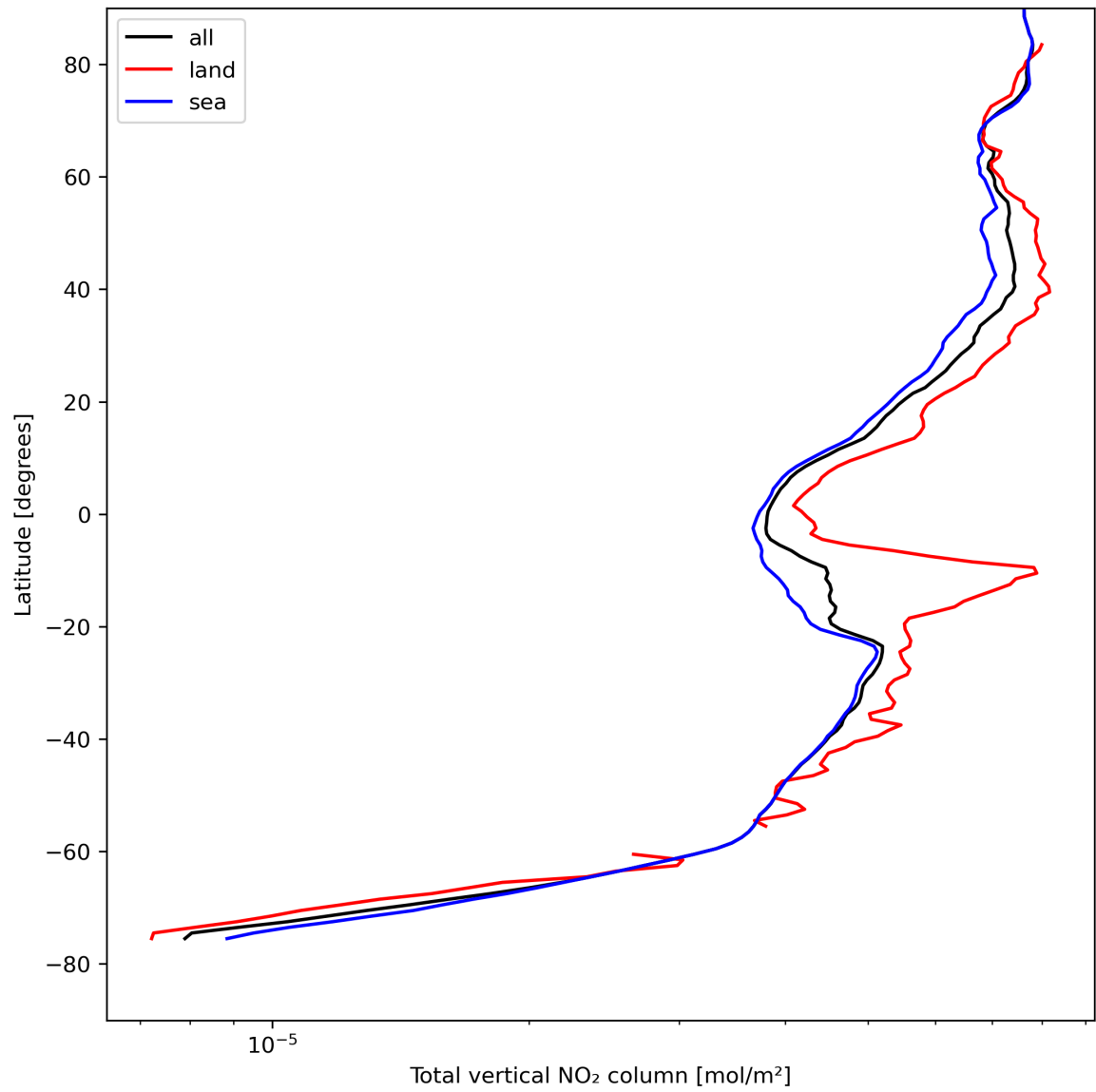
Figure 21: Zonal average of “Total vertical NO 2 column” for 2023-08-18 to 2023-08-20.
