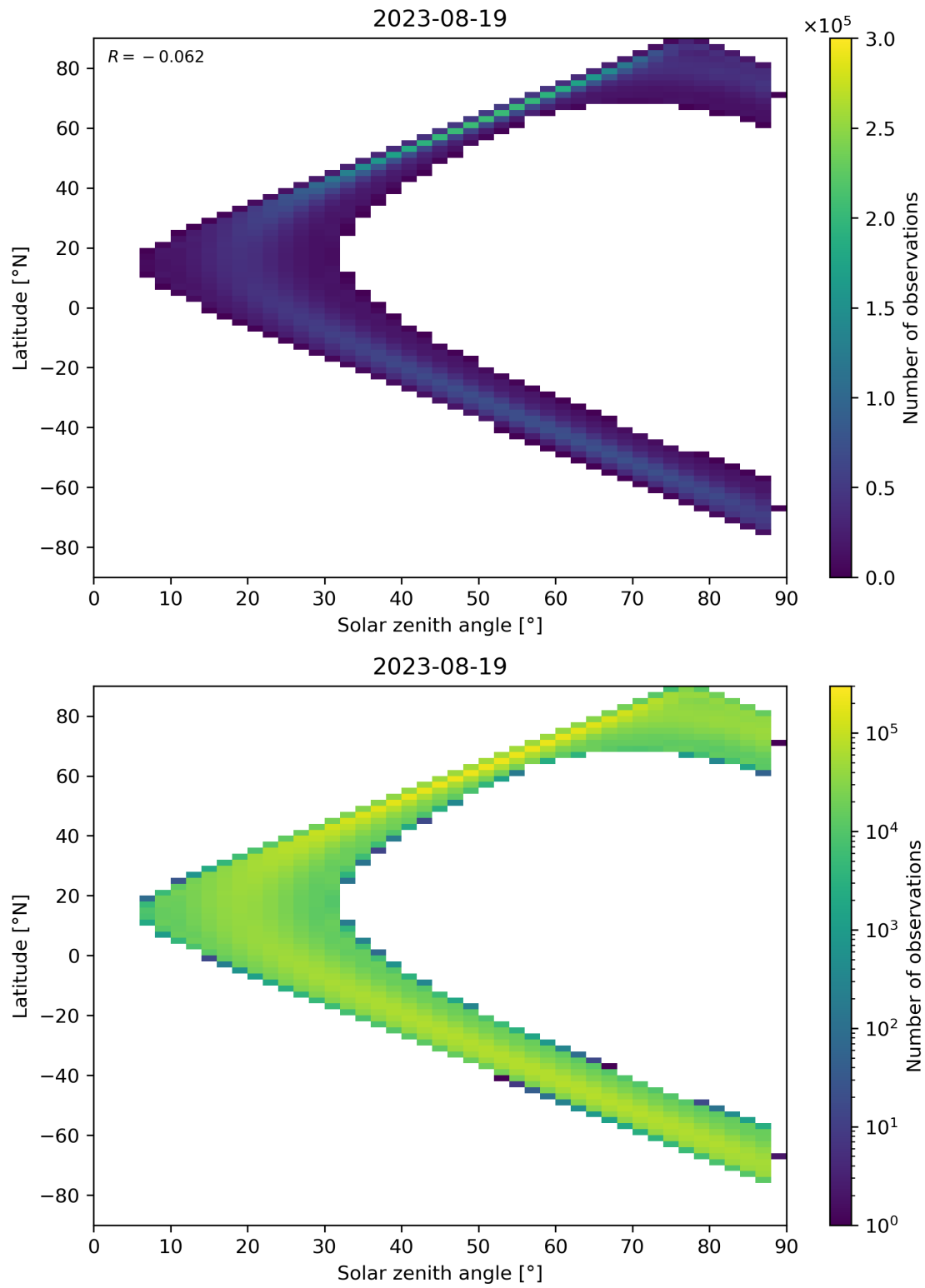
Figure 149: Scatter density plot of “Solar zenith angle” against “Latitude” for 2023-08-18 to 2023-08-20.
