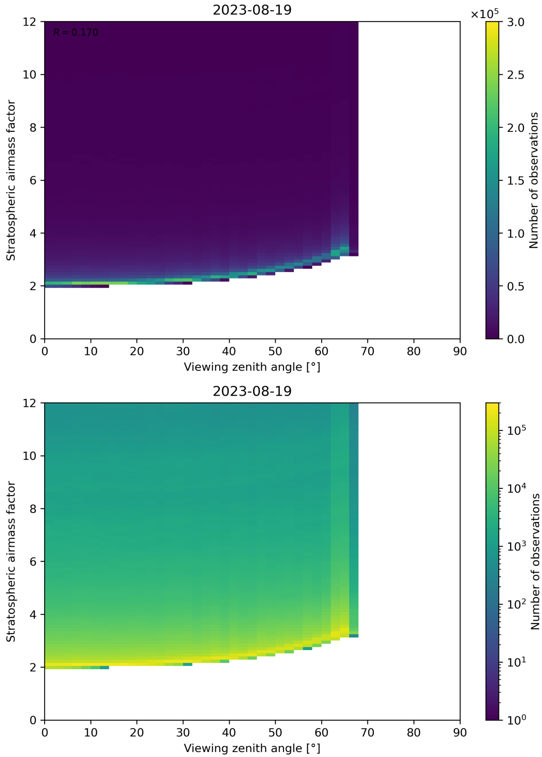
Figure 159: Scatter density plot of “Viewing zenith angle” against “Stratospheric airmass factor” for 2023-08-18 to 2023-08-20.
