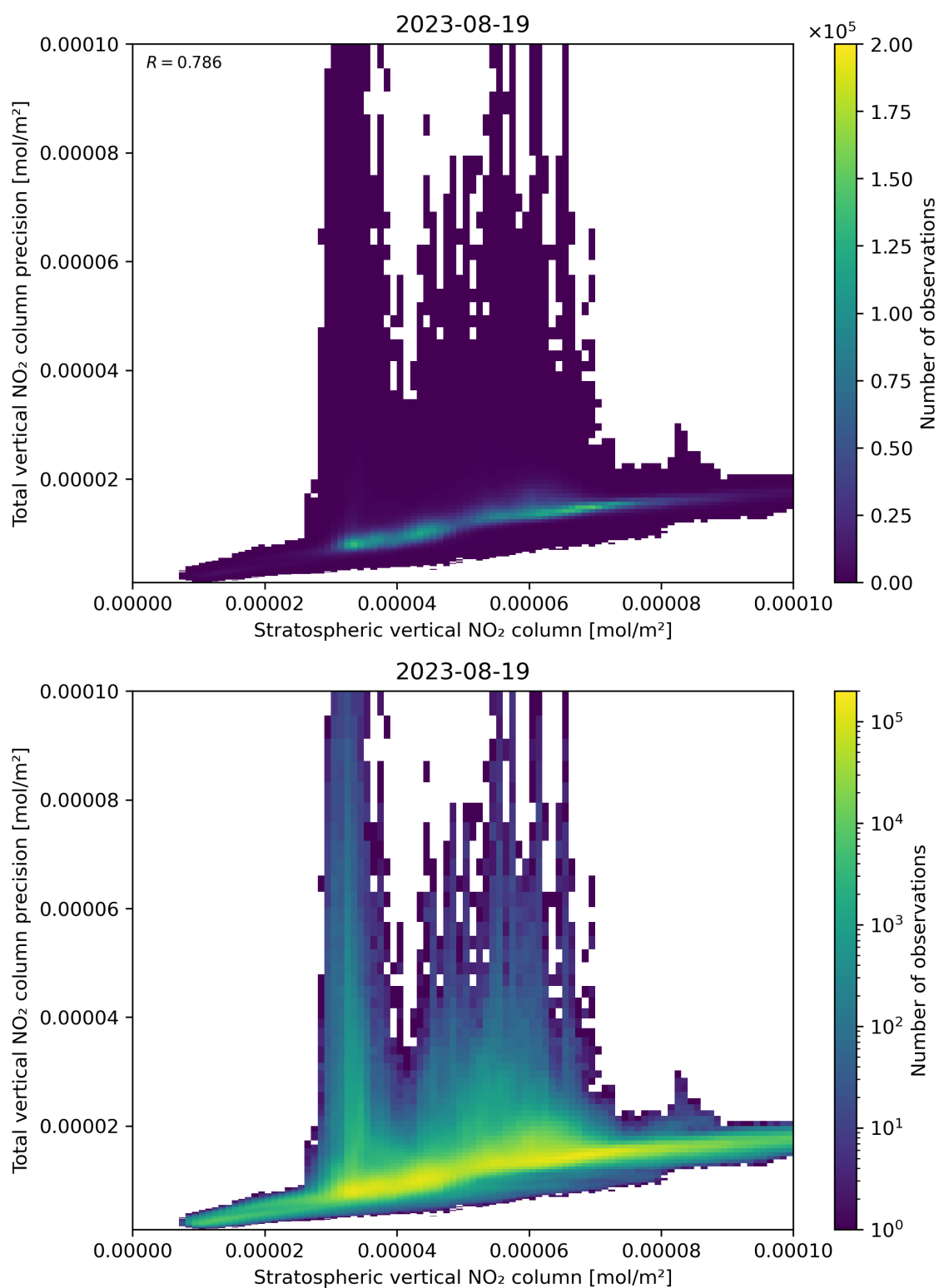
Figure 101: Scatter density plot of “Stratospheric vertical NO 2 column” against “Total vertical NO 2 column precision” for 2023-08-18 to 2023-08-20.
