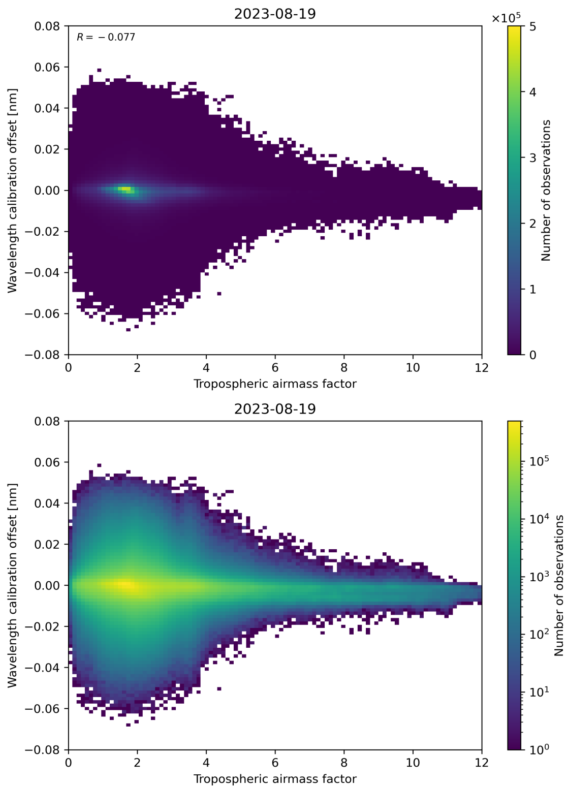
Figure 80: Scatter density plot of “Tropospheric airmass factor” against “Wavelength calibration offset” for 2023-08-18 to 2023-08-20.
