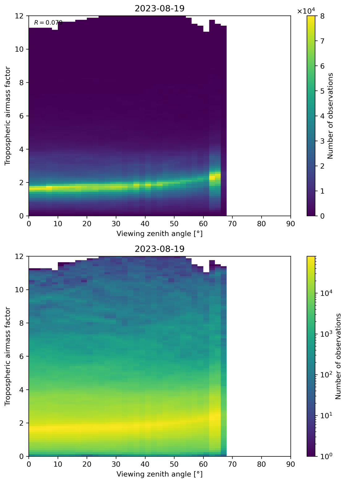
Figure 161: Scatter density plot of “Viewing zenith angle” against “Tropospheric airmass factor” for 2023-08-18 to 2023-08-20.
