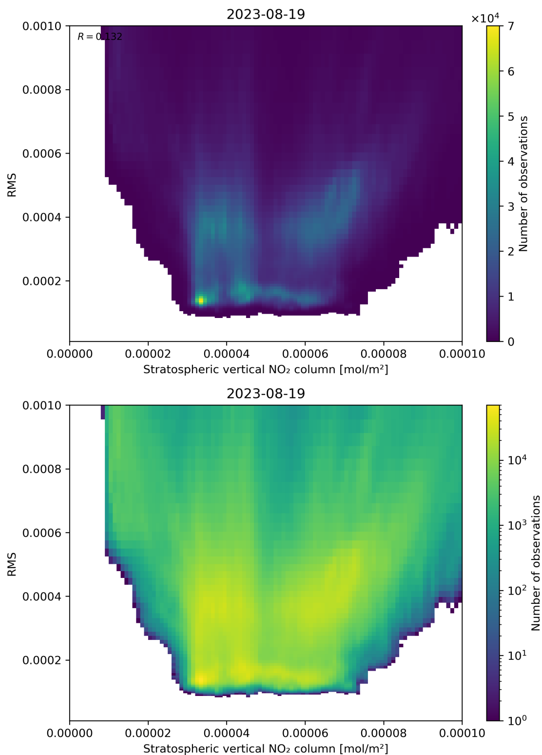
Figure 102: Scatter density plot of “Stratospheric vertical NO 2 column” against “RMS” for 2023-08-18 to 2023-08-20.
