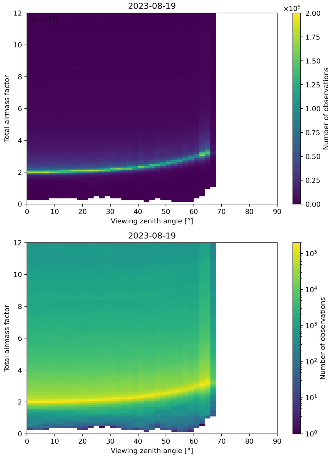
Figure 160: Scatter density plot of “Viewing zenith angle” against “Total airmass factor” for 2023-08-18 to 2023-08-20.
