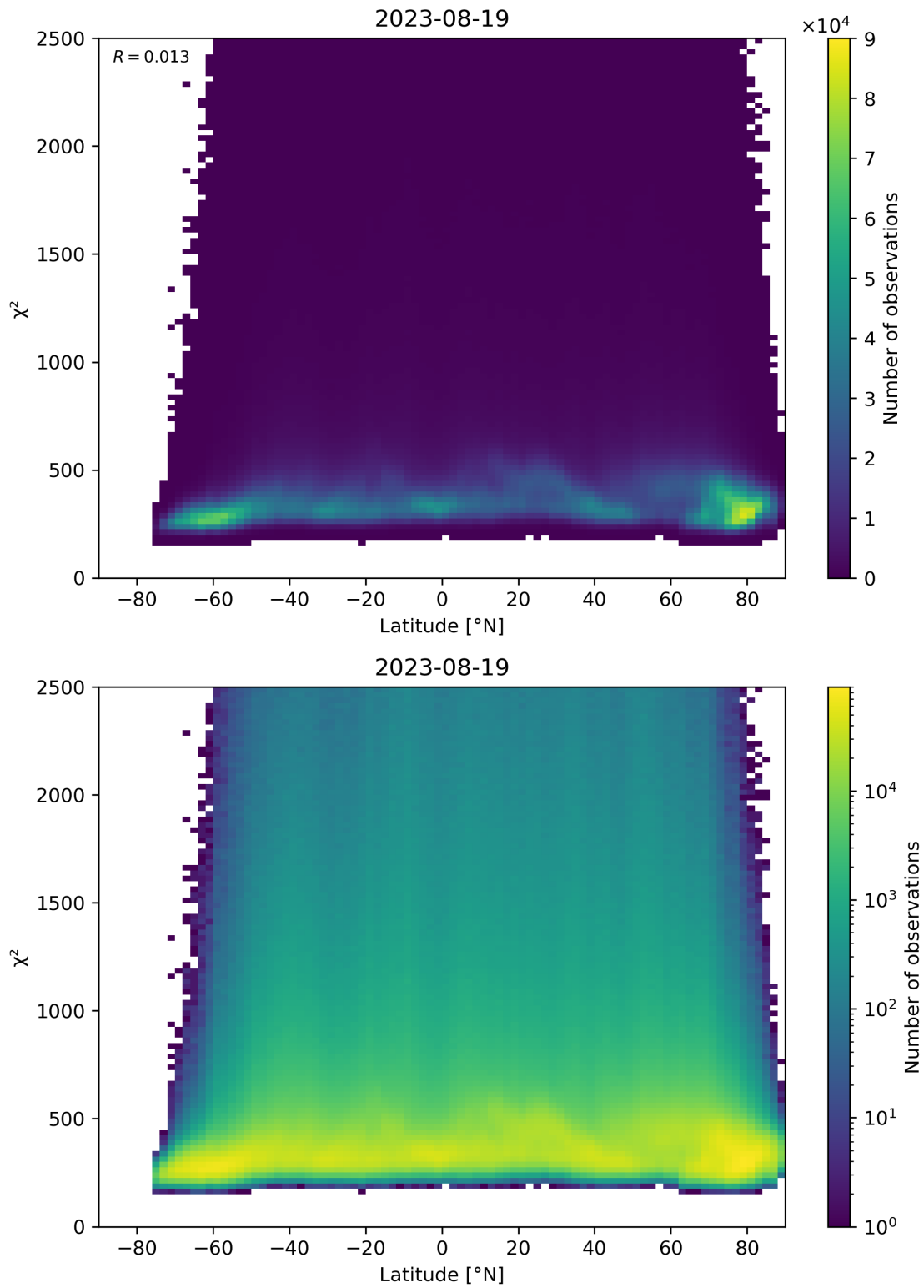
Figure 86: Scatter density plot of “Latitude” against “ \chi^2 ” for 2023-08-18 to 2023-08-20.
