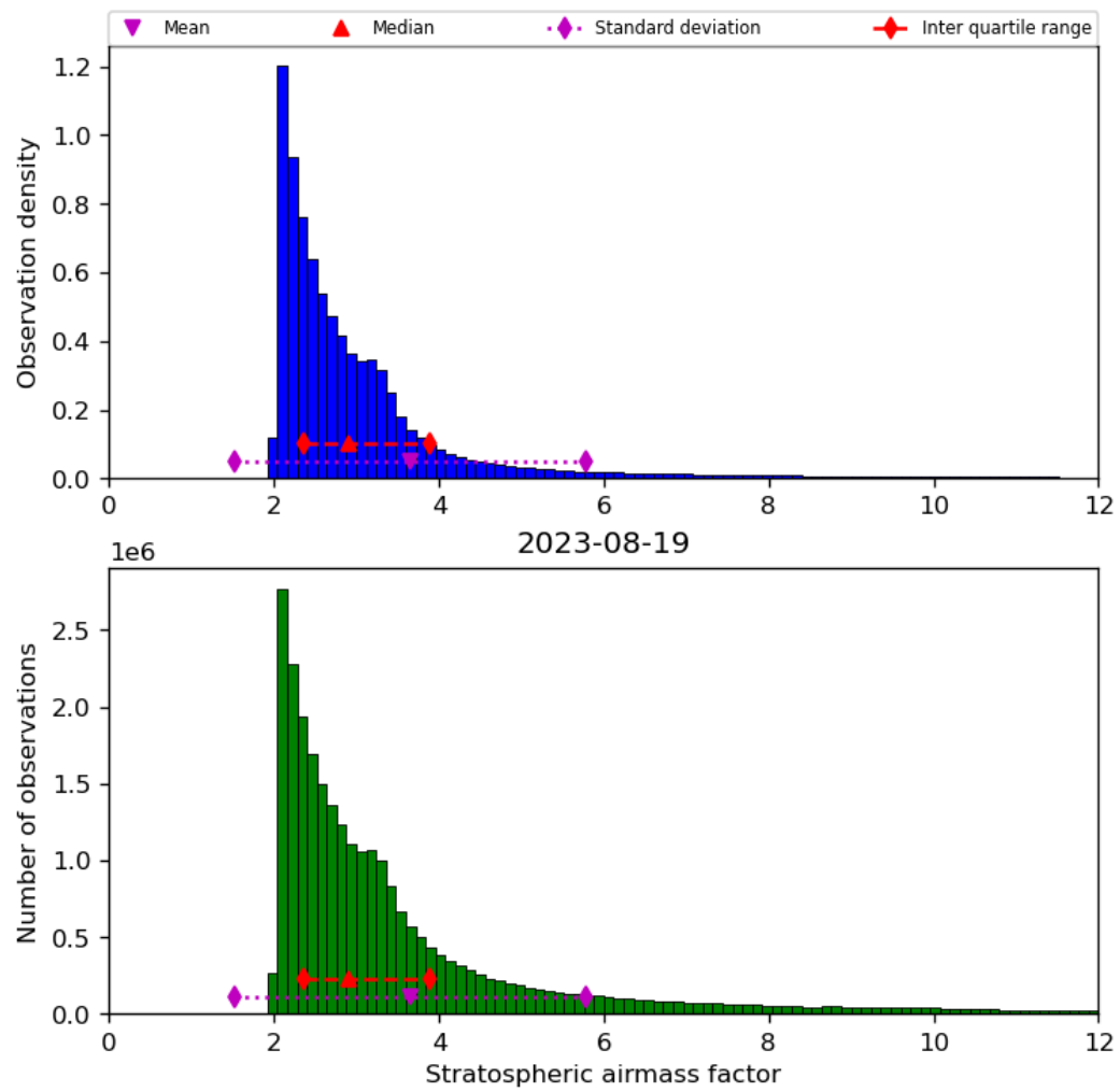
Figure 44: Histogram of “Stratospheric airmass factor” for 2023-08-18 to 2023-08-20
