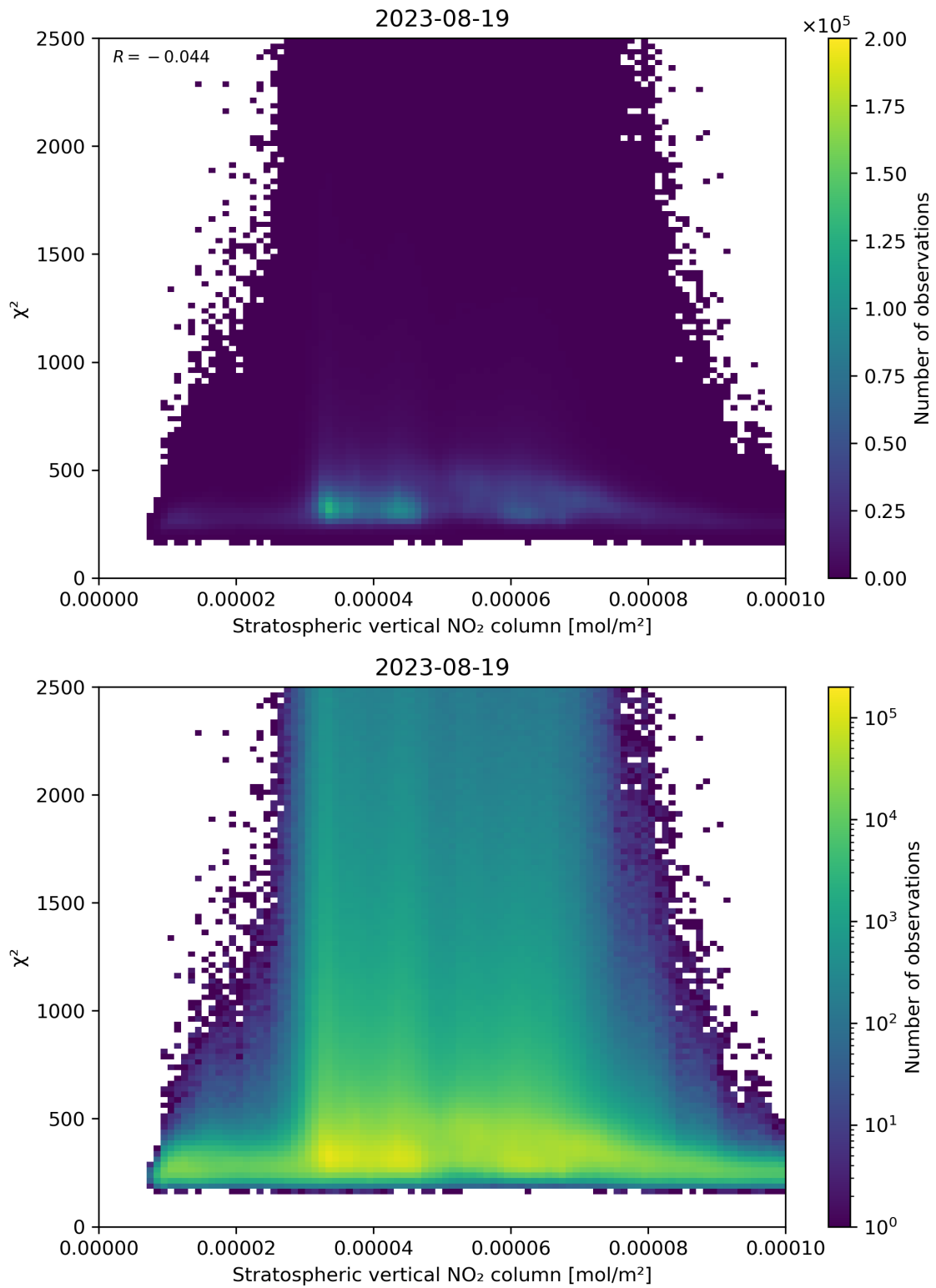
Figure 97: Scatter density plot of “Stratospheric vertical NO 2 column” against “ \chi^2 ” for 2023-08-18 to 2023-08-20.
