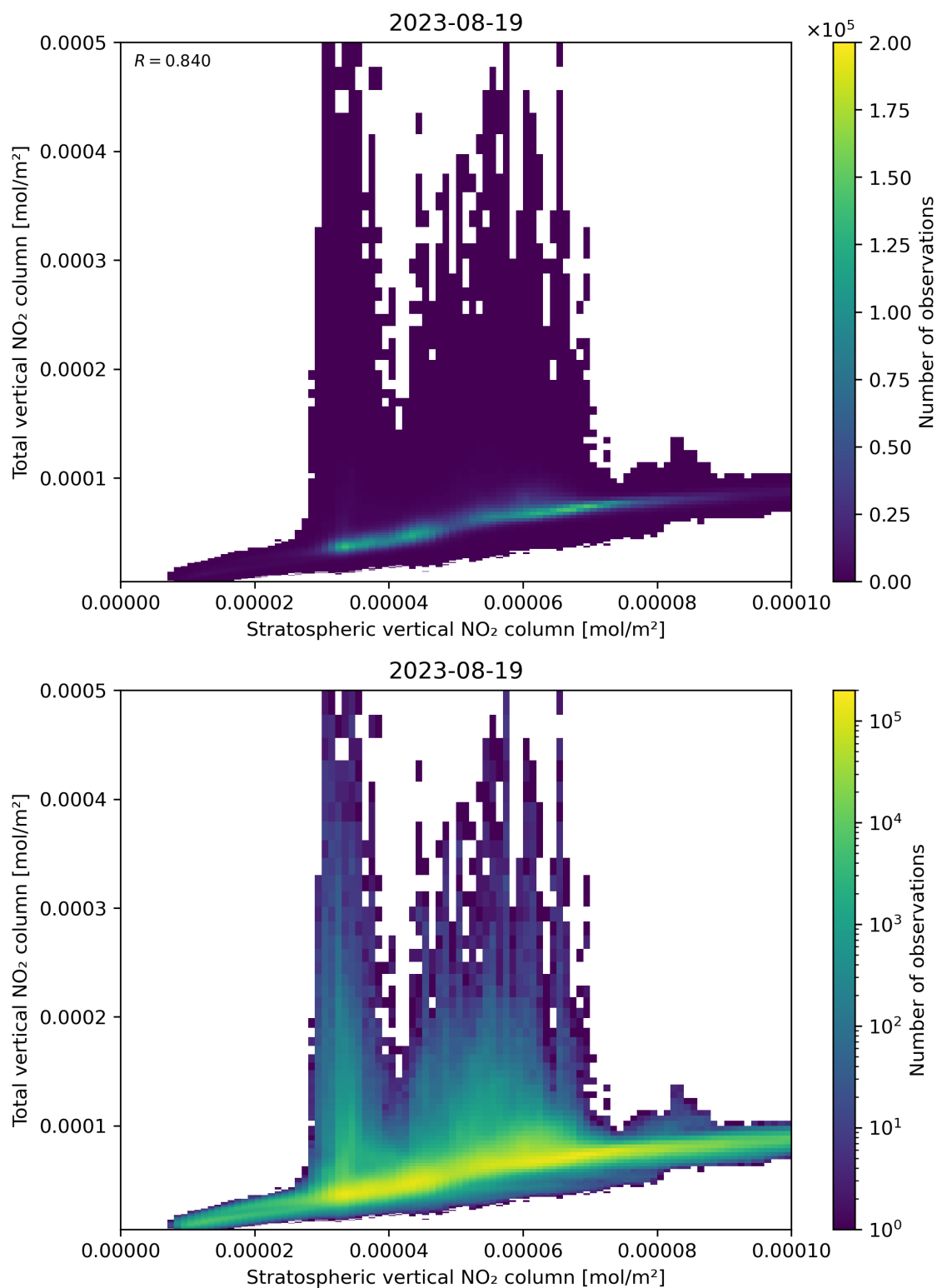
Figure 100: Scatter density plot of “Stratospheric vertical NO 2 column” against “Total vertical NO 2 column” for 2023-08-18 to 2023-08-20.
