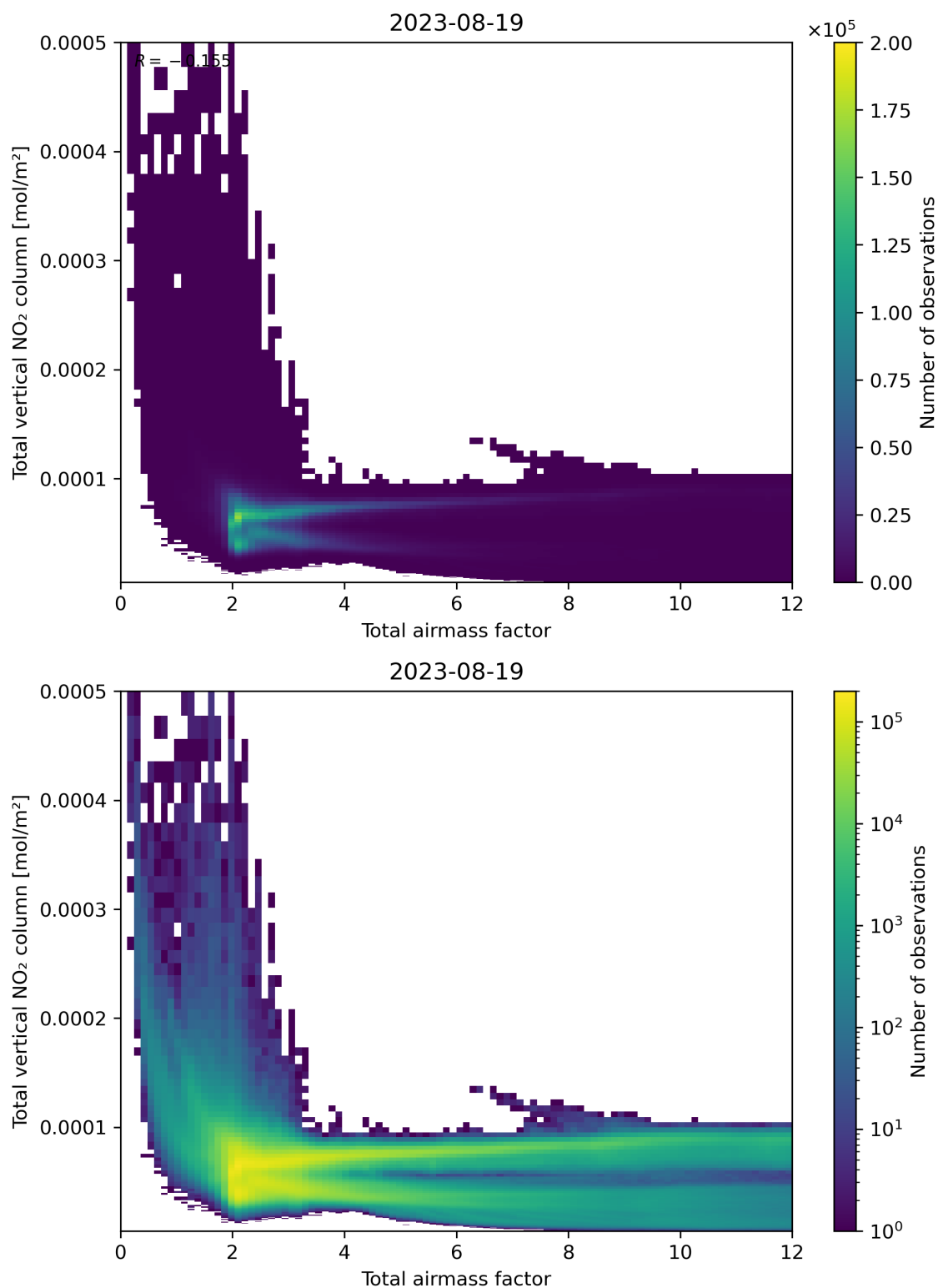
Figure 67: Scatter density plot of “Total airmass factor” against “Total vertical NO 2 column” for 2023-08-18 to 2023-08-20.
