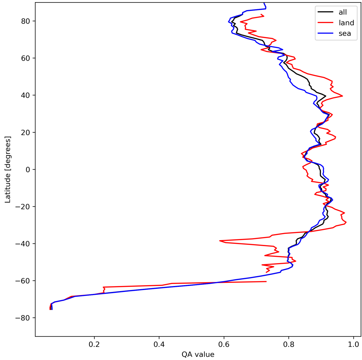
Figure 11: Zonal average of “QA value” for 2023-08-18 to 2023-08-20.
