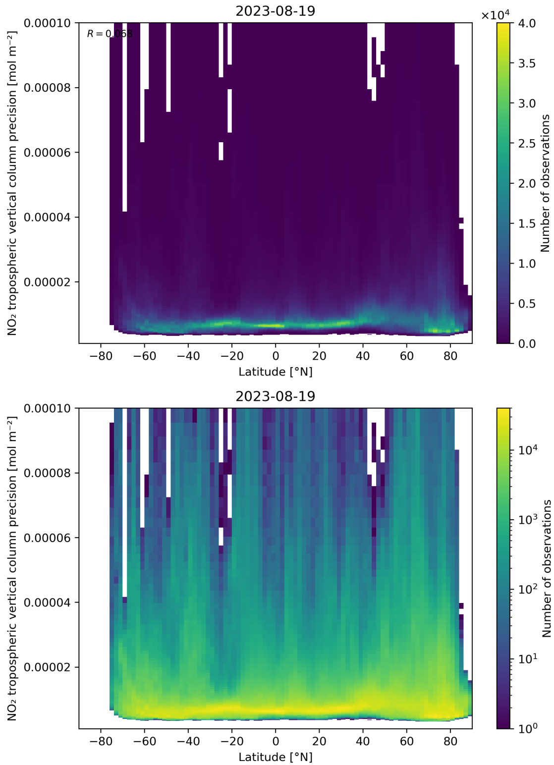
Figure 93: Scatter density plot of “Latitude” against “NO 2 tropospheric vertical column precision” for 2023-08-18 to 2023-08-20.
