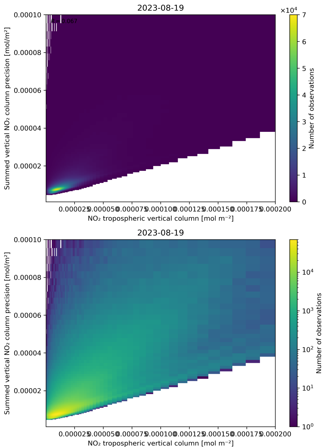
Figure 127: Scatter density plot of “NO 2 tropospheric vertical column” against “Summed vertical NO 2 column precision” for 2023-08-18 to 2023-08-20.
