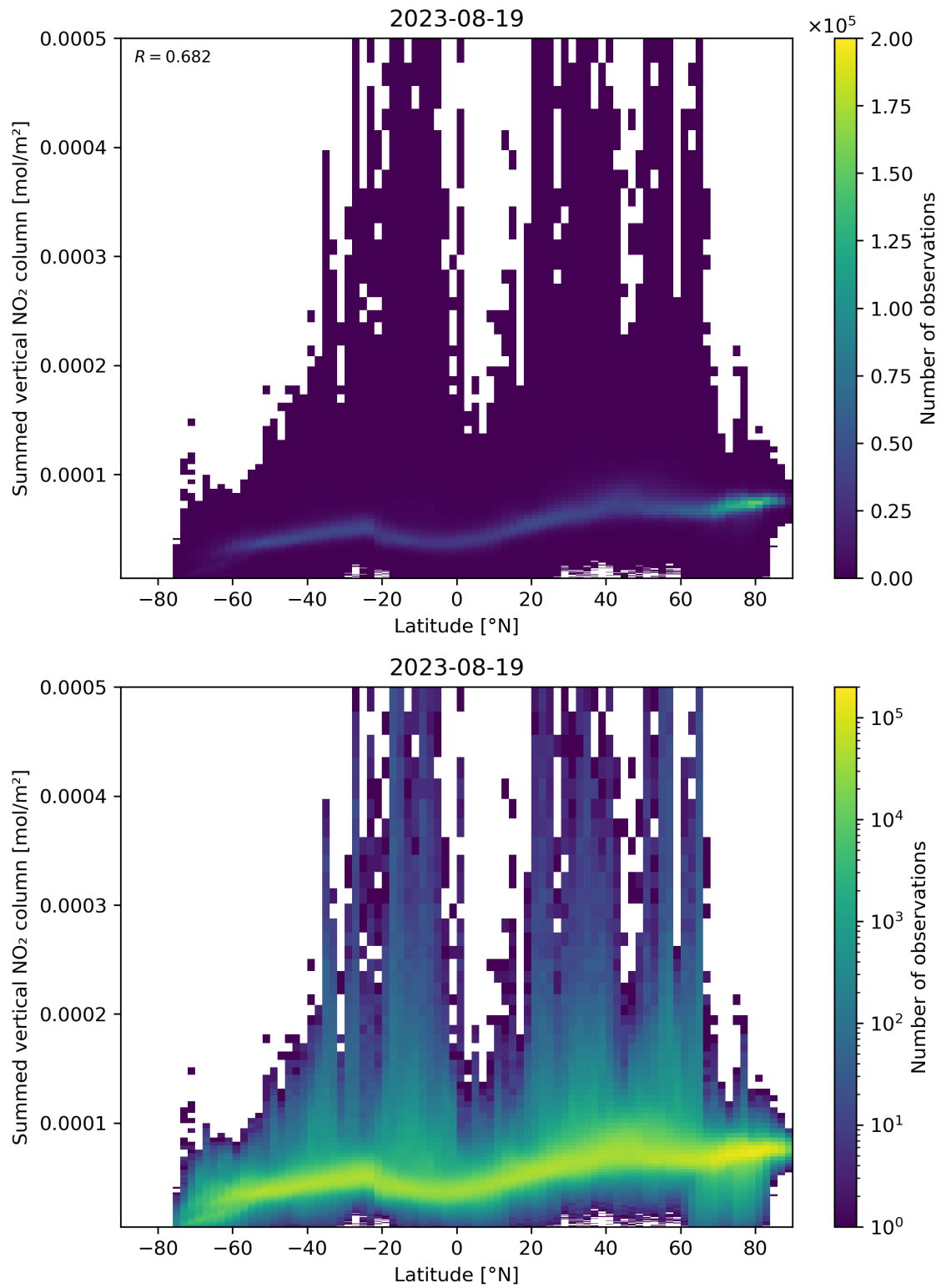
Figure 88: Scatter density plot of “Latitude” against “Summed vertical NO 2 column” for 2023-08-18 to 2023-08-20.
