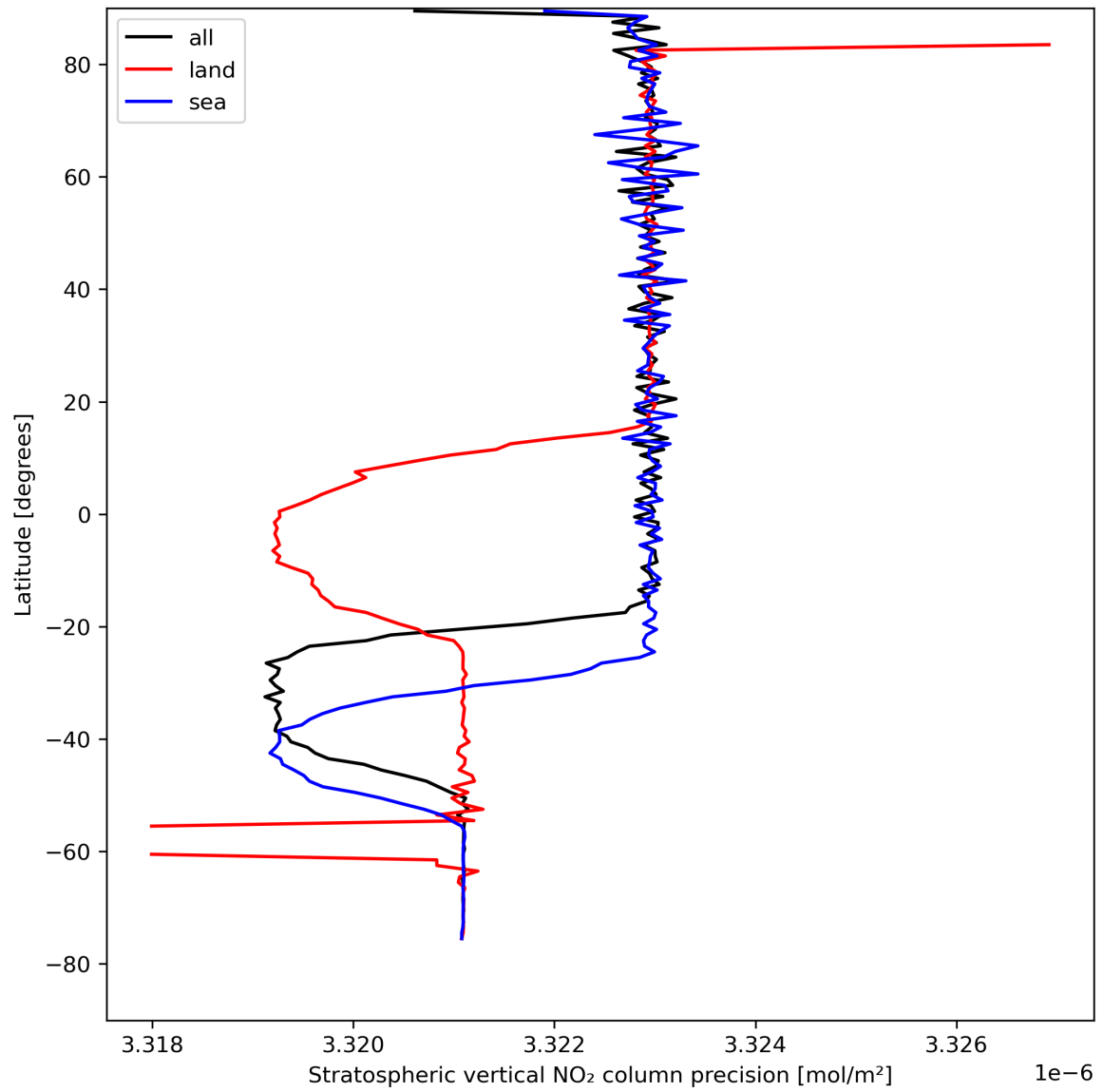
Figure 20: Zonal average of “Stratospheric vertical NO 2 column precision” for 2023-08-18 to 2023-08-20.
