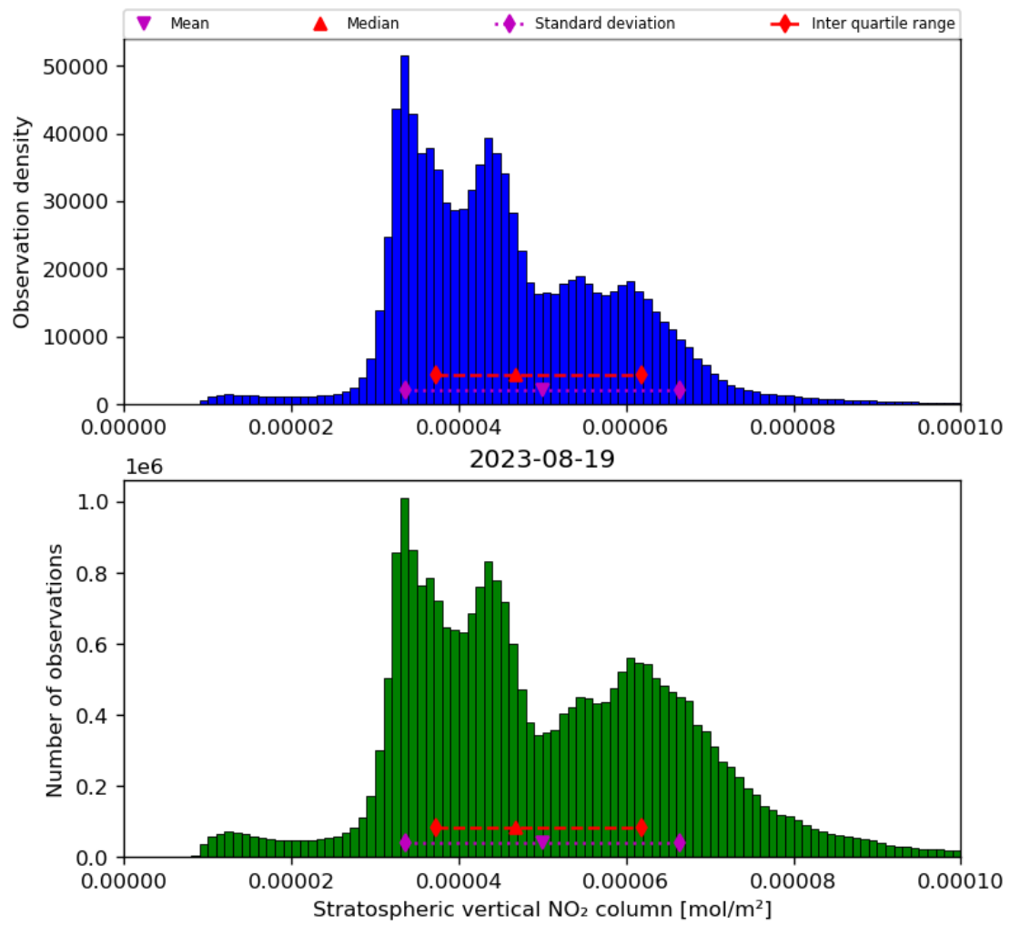
Figure 36: Histogram of “Stratospheric vertical NO 2 column” for 2023-08-18 to 2023-08-20
