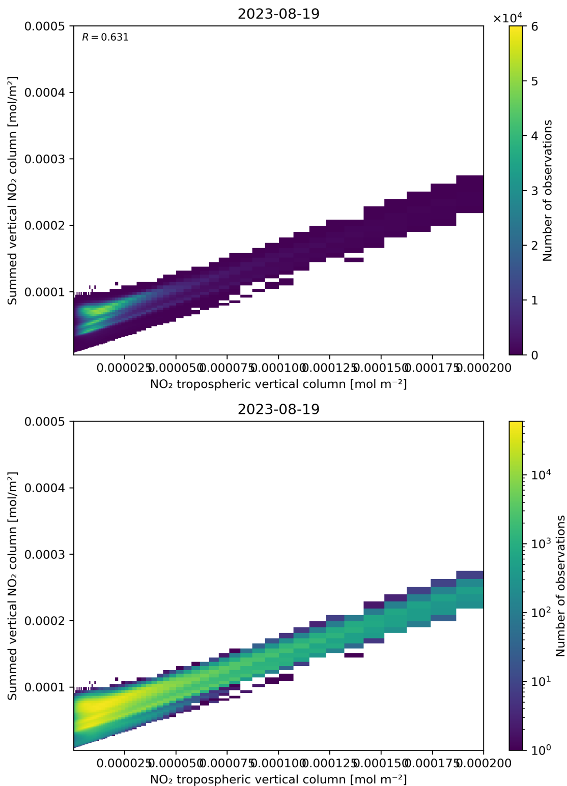
Figure 126: Scatter density plot of “NO 2 tropospheric vertical column” against “Summed vertical NO 2 column” for 2023-08-18 to 2023-08-20.
