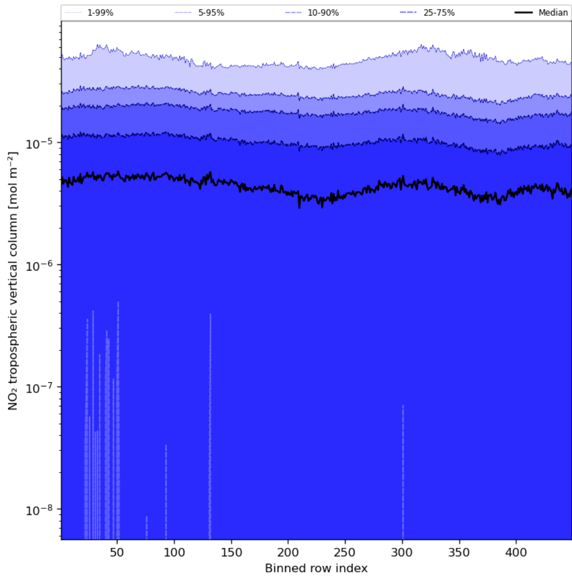
Figure 46: Along track statistics of “NO 2 tropospheric vertical column” for 2023-08-18 to 2023-08-20
