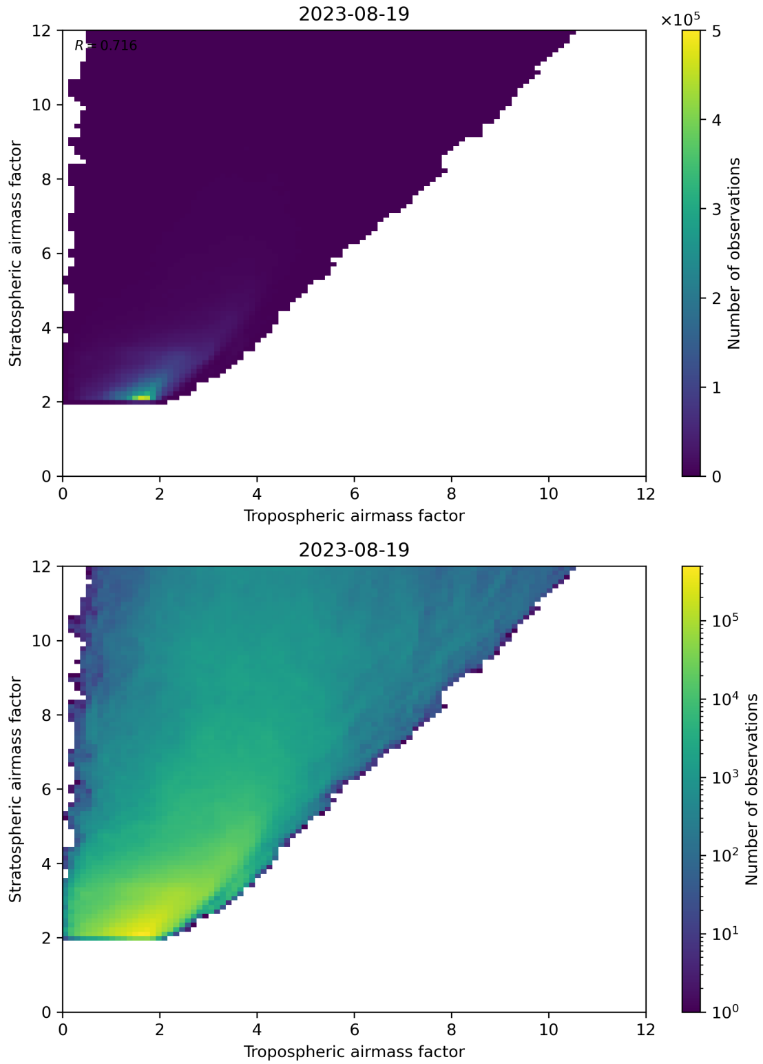
Figure 71: Scatter density plot of “Tropospheric airmass factor” against “Stratospheric airmass factor” for 2023-08-18 to 2023-08-20.
