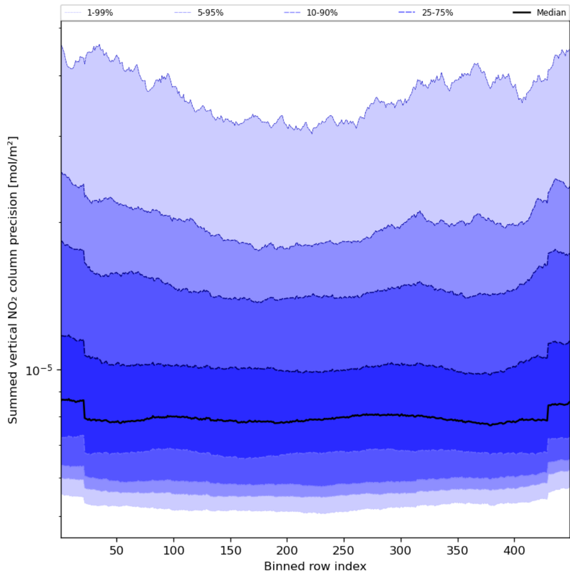
Figure 58: Along track statistics of “Summed vertical NO 2 column precision” for 2023-08-18 to 2023-08-20
