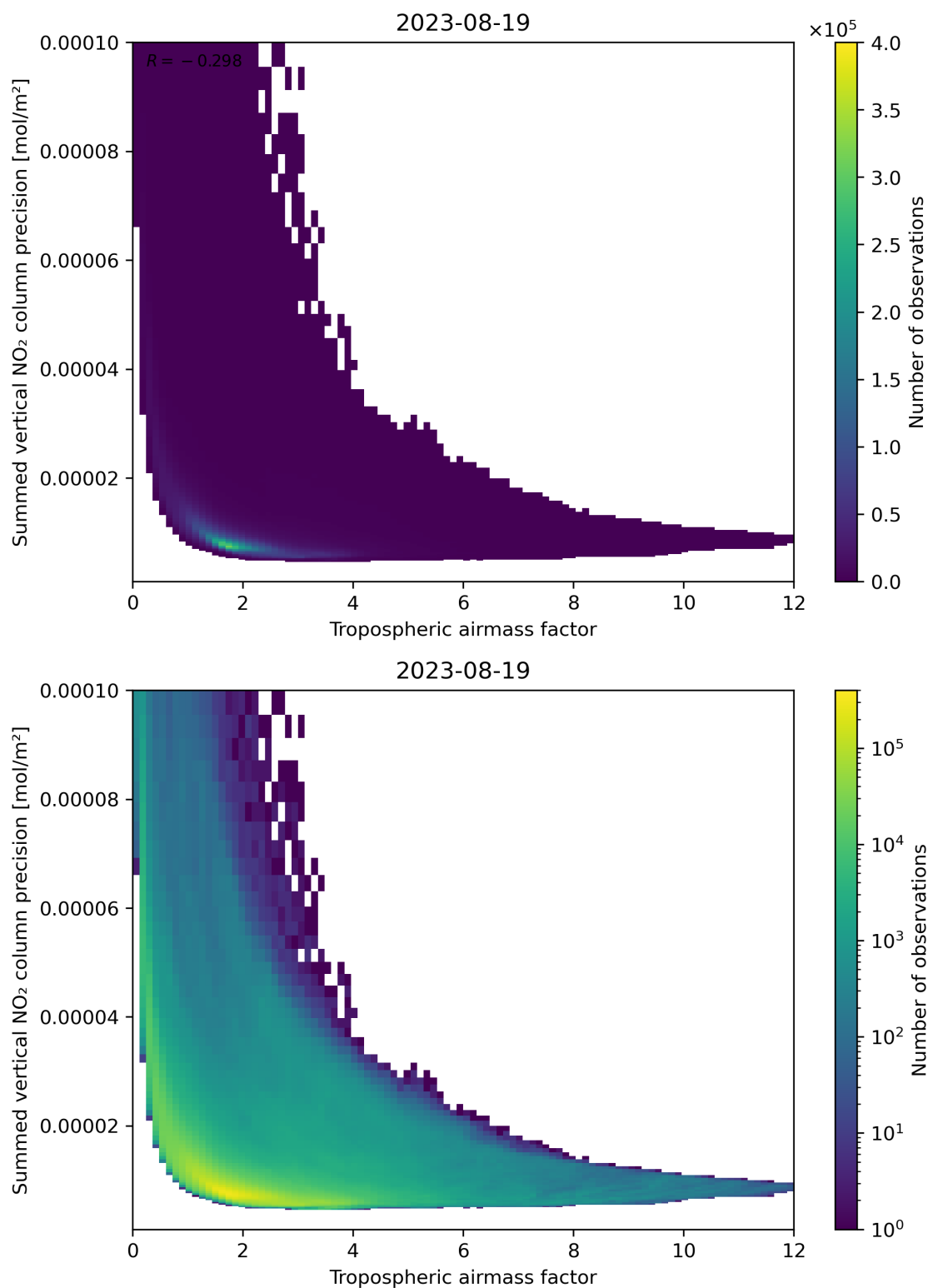
Figure 76: Scatter density plot of “Tropospheric air mass factor” against “Summed vertical NO 2 column precision” for 2023-08-18 to 2023-08-20.
