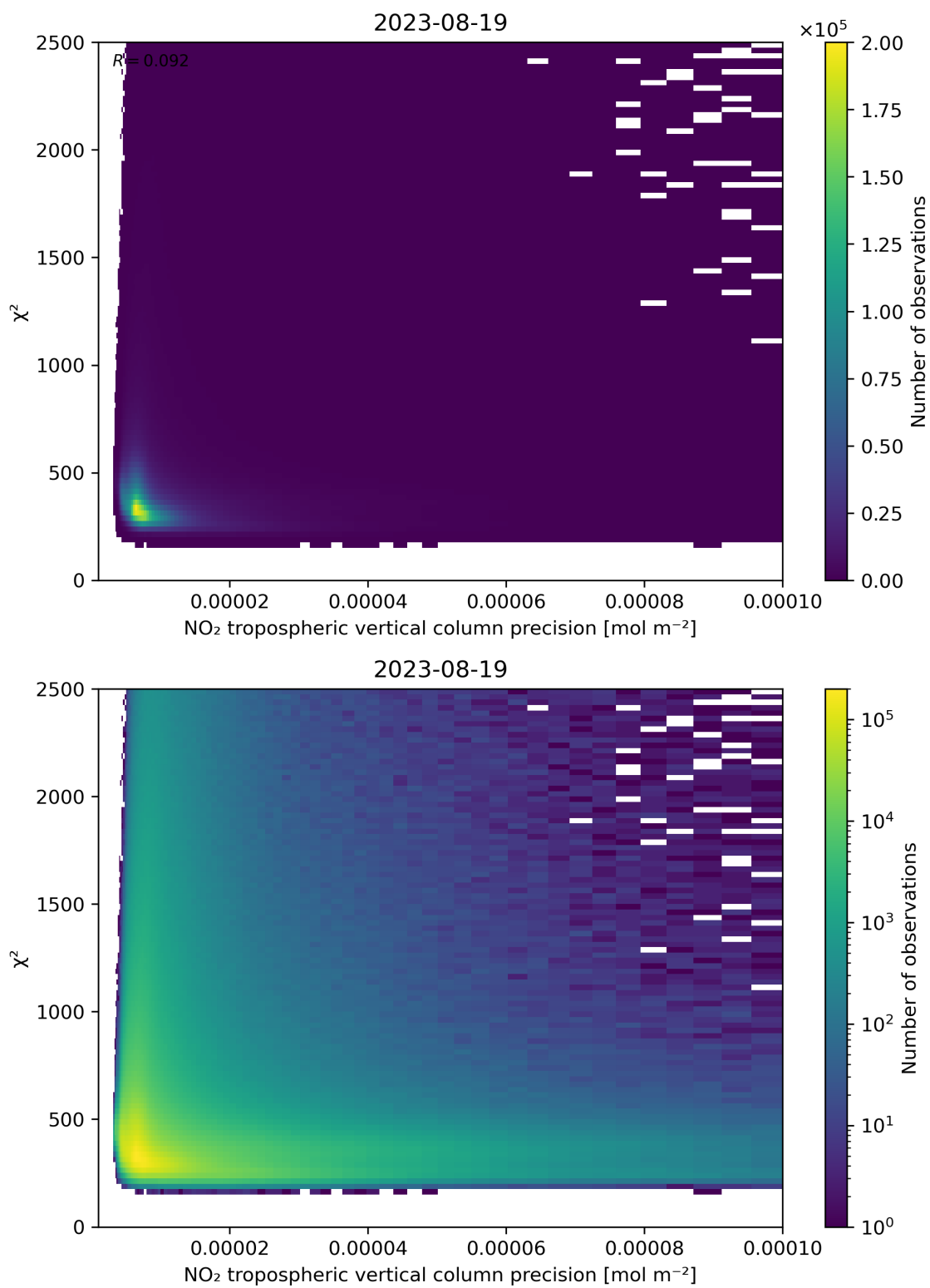
Figure 134: Scatter density plot of “NO 2 tropospheric vertical column precision” against “ \chi^2 ” for 2023-08-18 to 2023-08-20.
