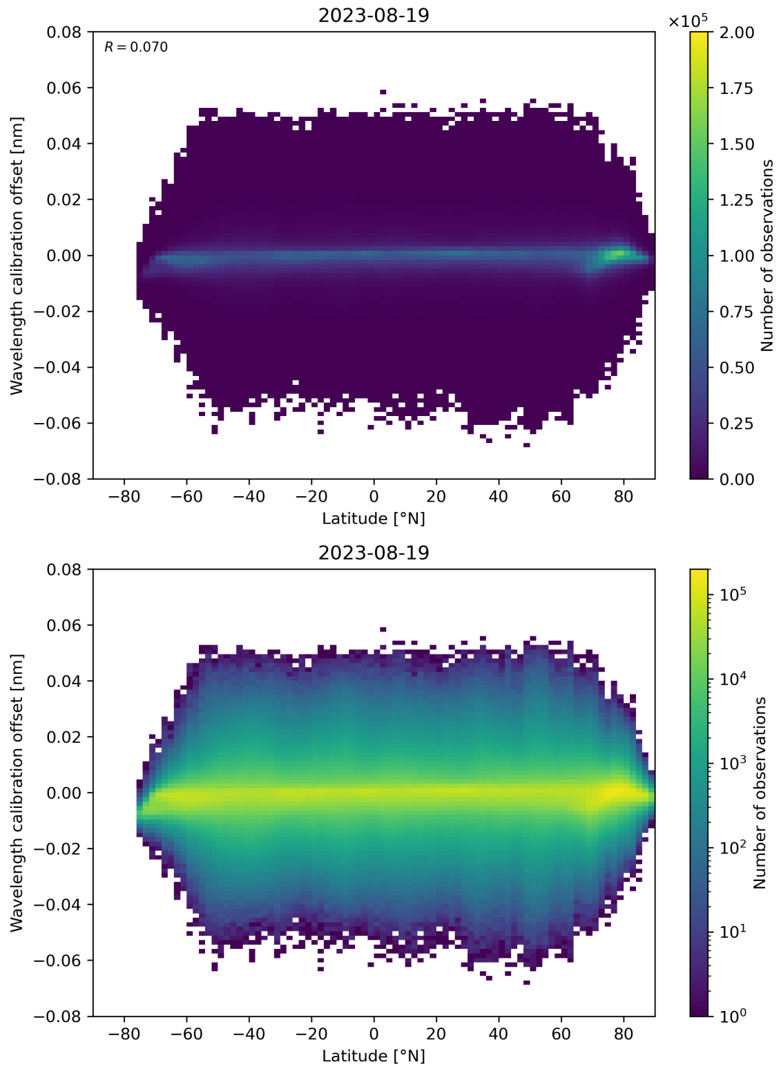
Figure 95: Scatter density plot of “Latitude” against “Wavelength calibration offset” for 2023-08-18 to 2023-08-20.
