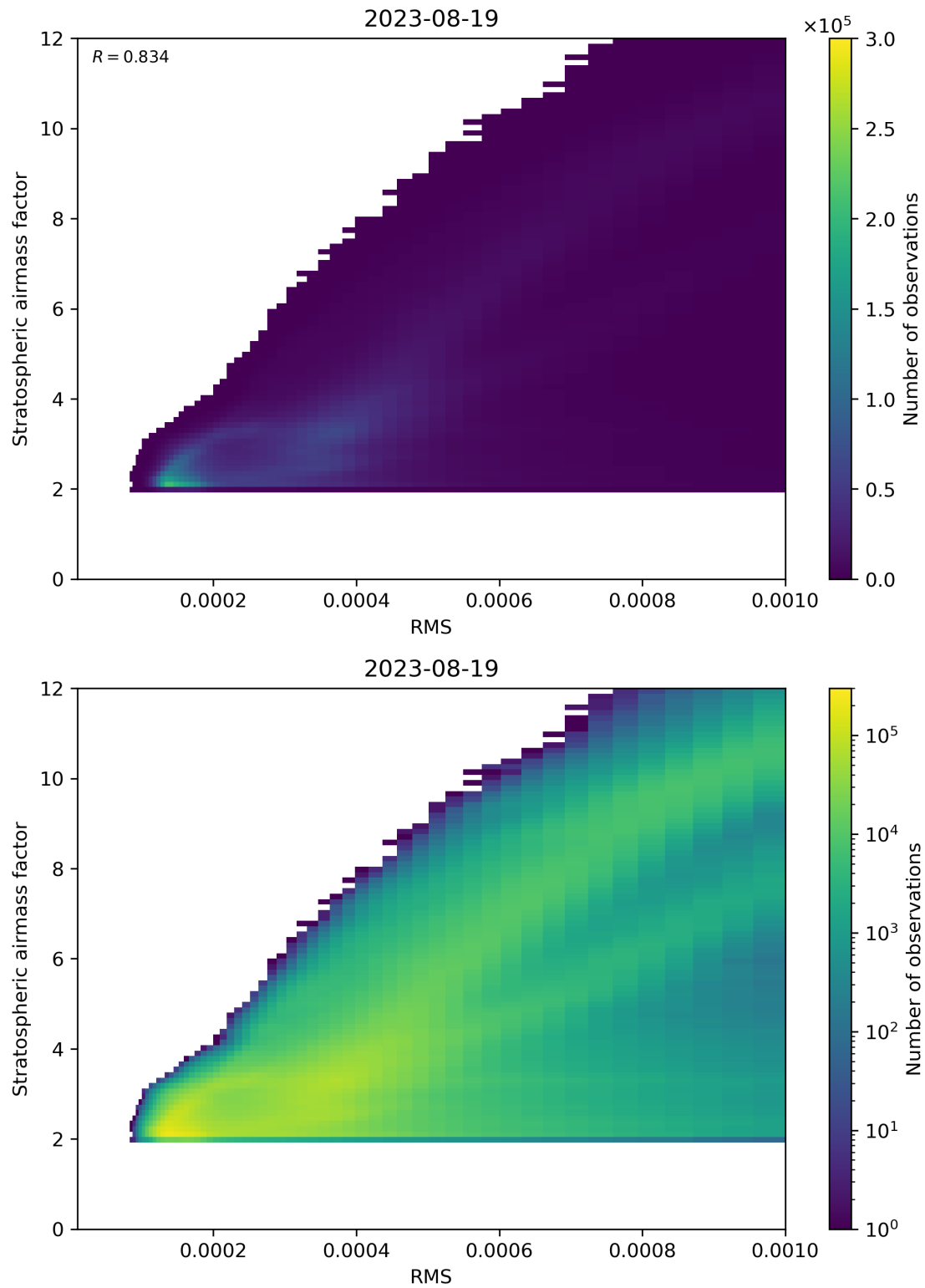
Figure 144: Scatter density plot of “RMS” against “Stratospheric airmass factor” for 2023-08-18 to 2023-08-20.
