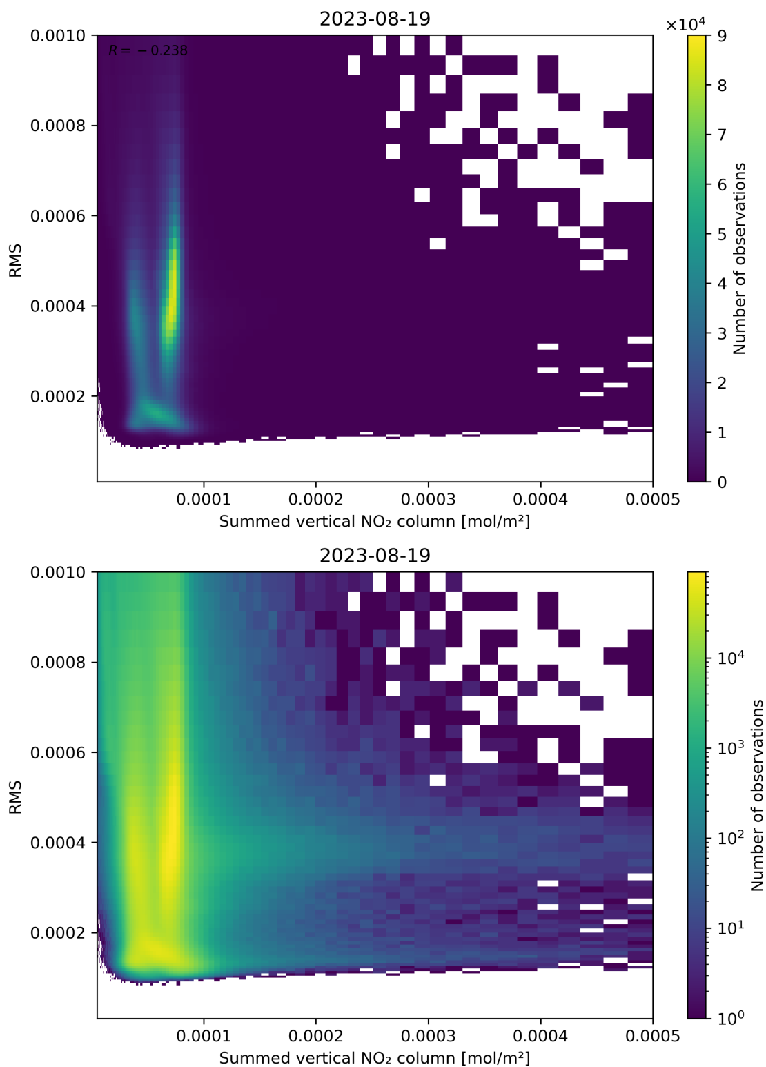
Figure 109: Scatter density plot of “Summed vertical NO 2 column” against “RMS” for 2023-08-18 to 2023-08-20.
