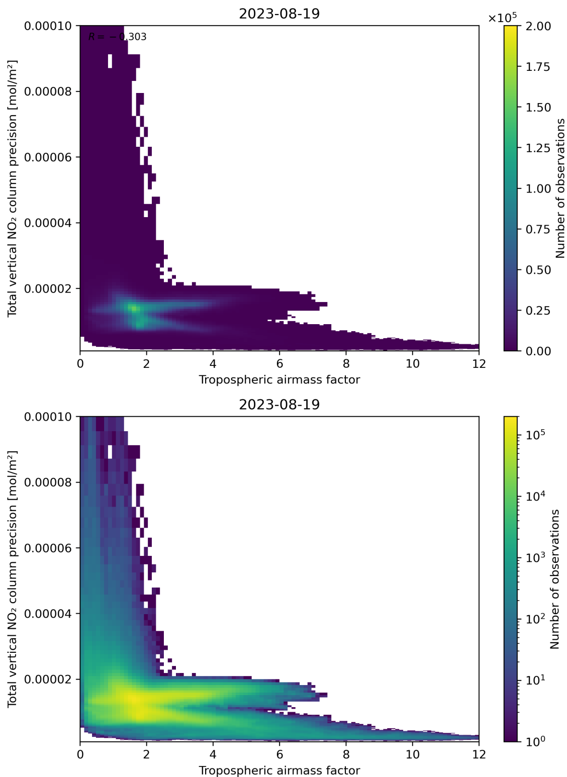
Figure 78: Scatter density plot of “Tropospheric airmass factor” against “Total vertical NO 2 column precision” for 2023-08-18 to 2023-08-20.
