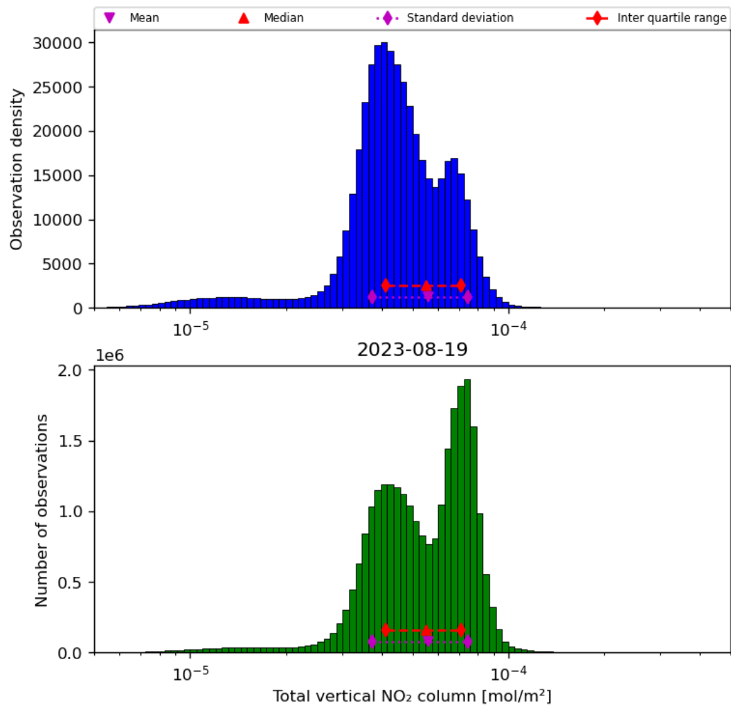
Figure 38: Histogram of "Total vertical NO 2 column" for 2023-08-18 to 2023-08-20
