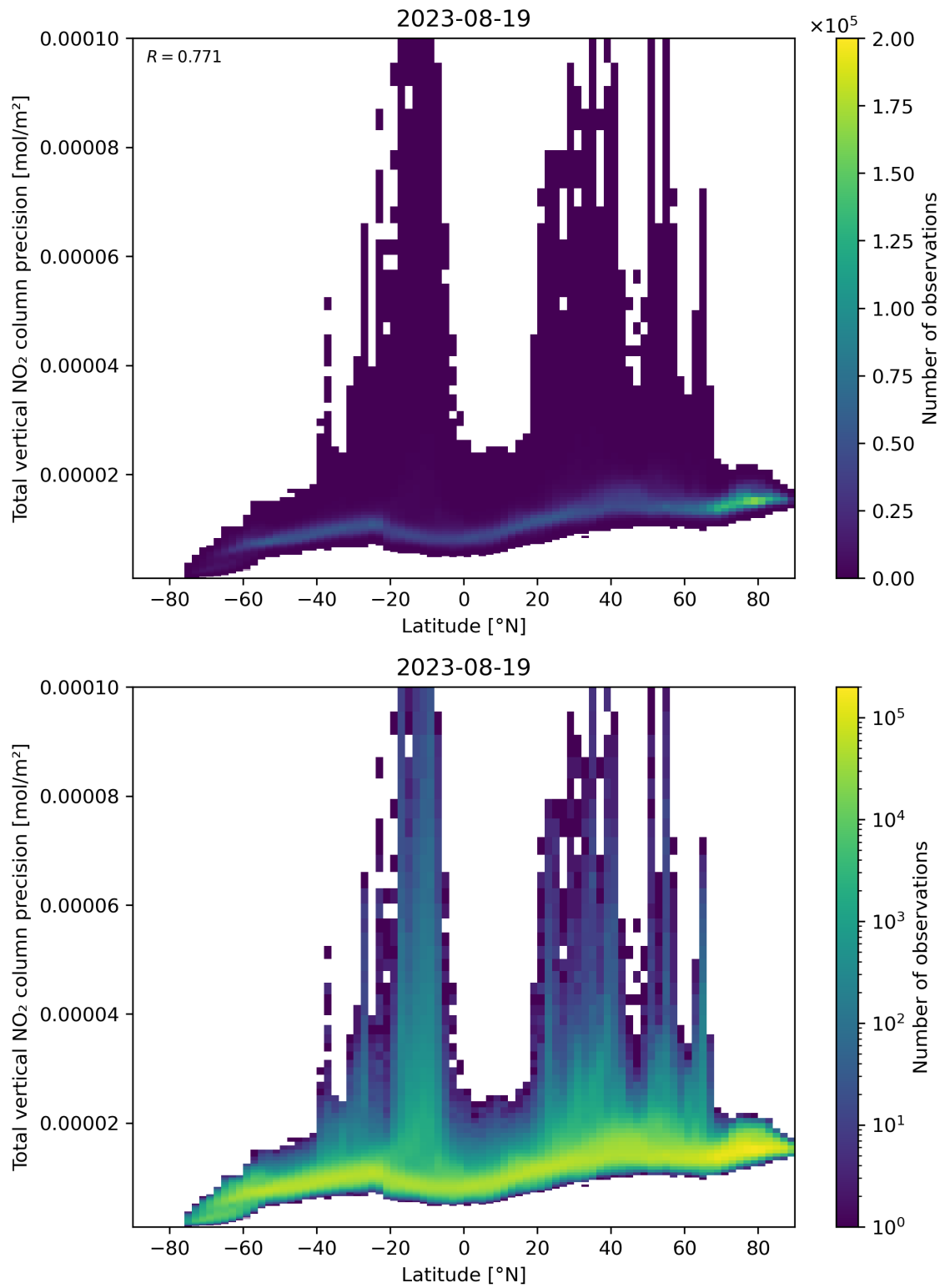
Figure 91: Scatter density plot of “Latitude” against “Total vertical NO 2 column precision” for 2023-08-18 to 2023-08-20.
