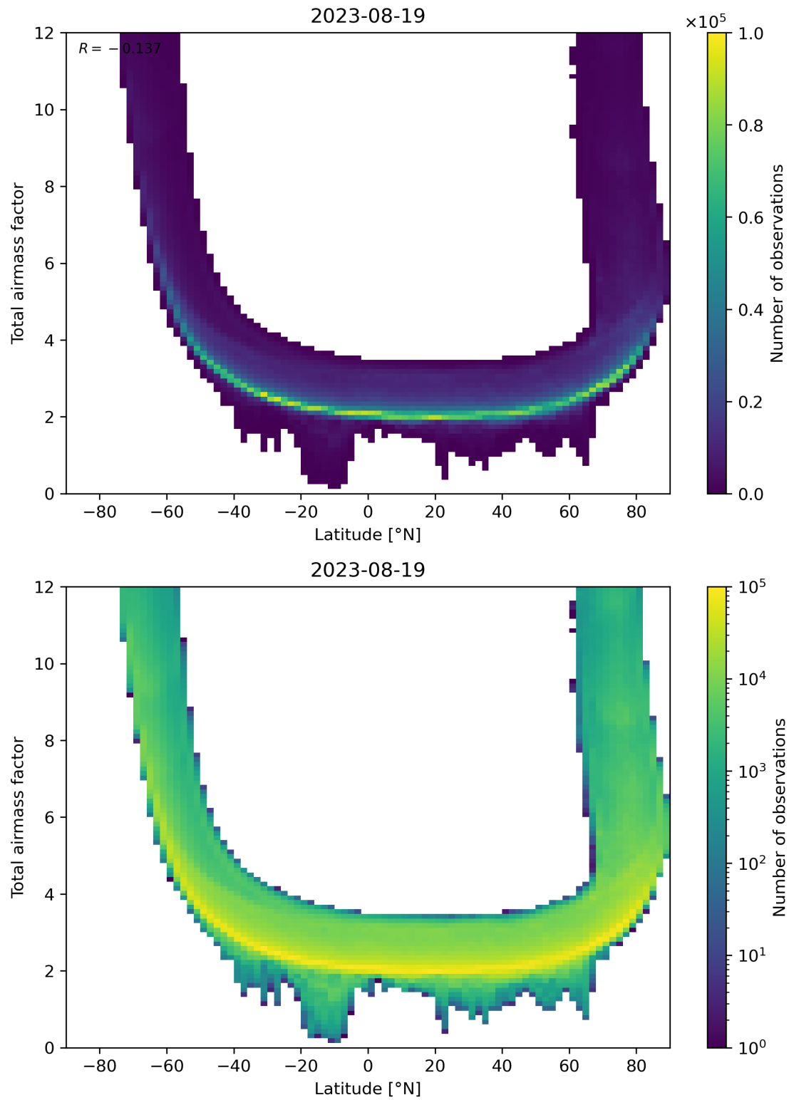
Figure 84: Scatter density plot of “Latitude” against “Total airmass factor” for 2023-08-18 to 2023-08-20.
