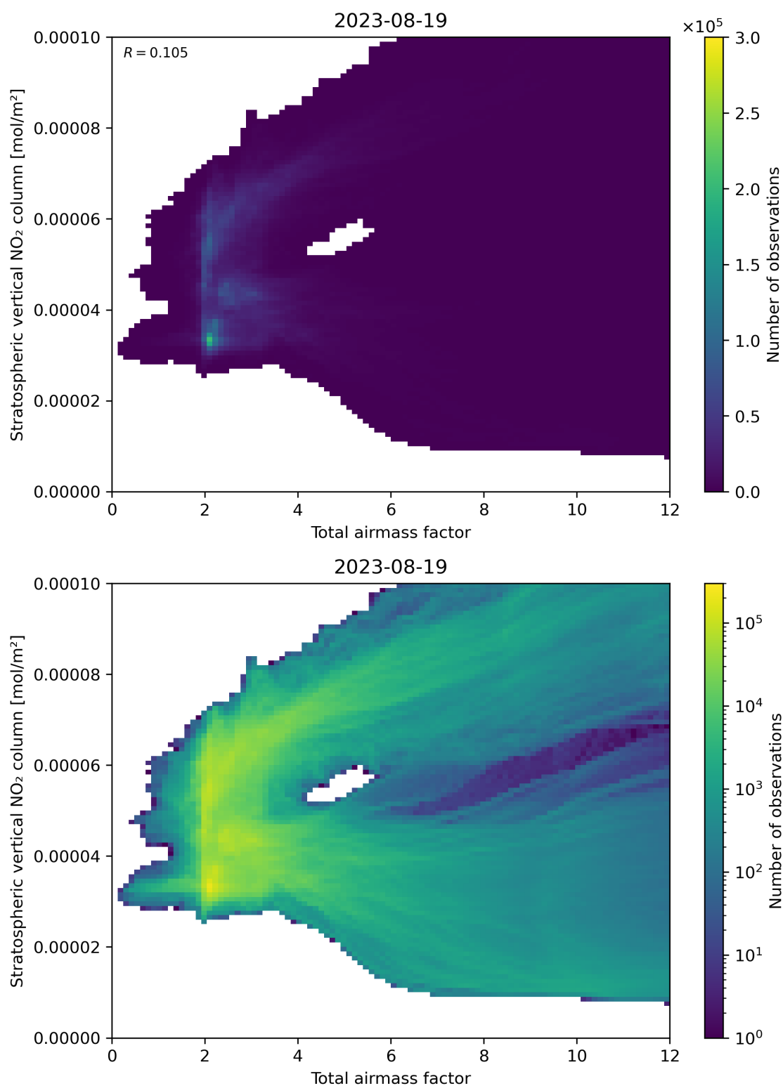
Figure 64: Scatter density plot of “Total airmass factor” against “Stratospheric vertical \text{NO}_2 column” for 2023-08-18 to 2023-08-20.
