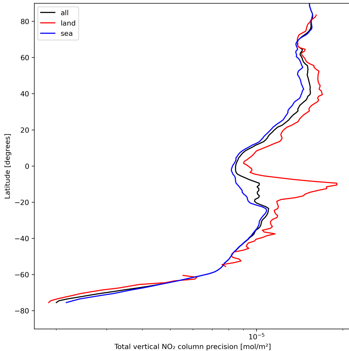
Figure 22: Zonal average of “Total vertical NO 2 column precision” for 2023-08-18 to 2023-08-20.
