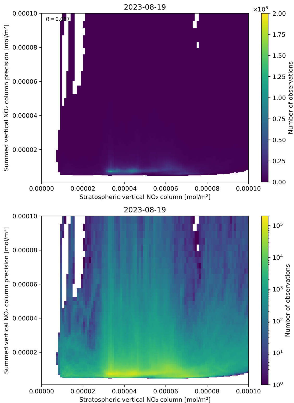
Figure 99: Scatter density plot of “Stratospheric vertical NO 2 column” against “Summed vertical NO 2 column precision” for 2023-08-18 to 2023-08-20.
