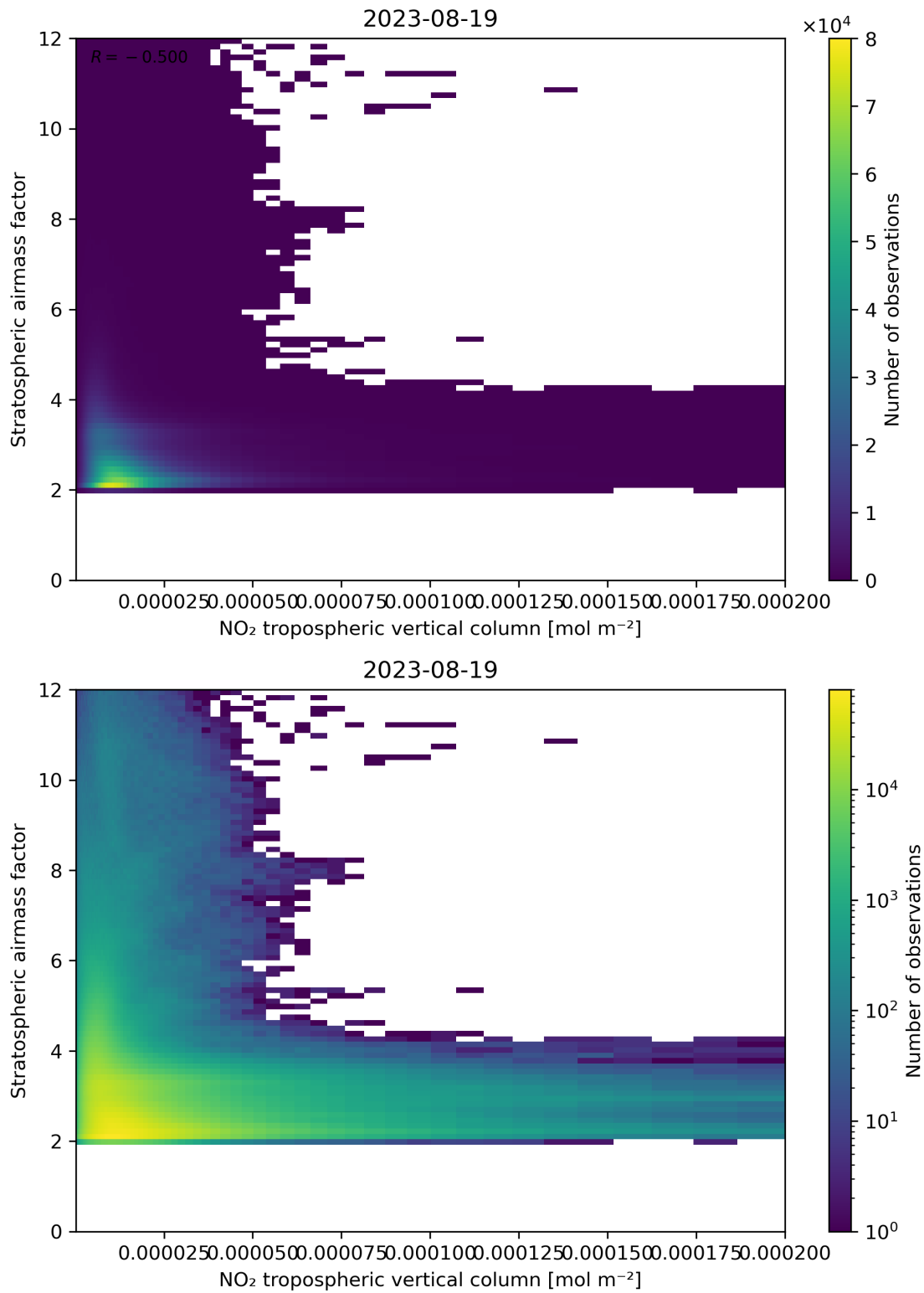
Figure 121: Scatter density plot of “NO 2 tropospheric vertical column” against “Stratospheric air mass factor” for 2023-08-18 to 2023-08-20.
