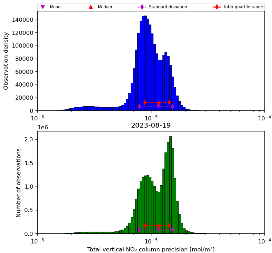
Figure 39: Histogram of “Total vertical NO 2 column precision” for 2023-08-18 to 2023-08-20
