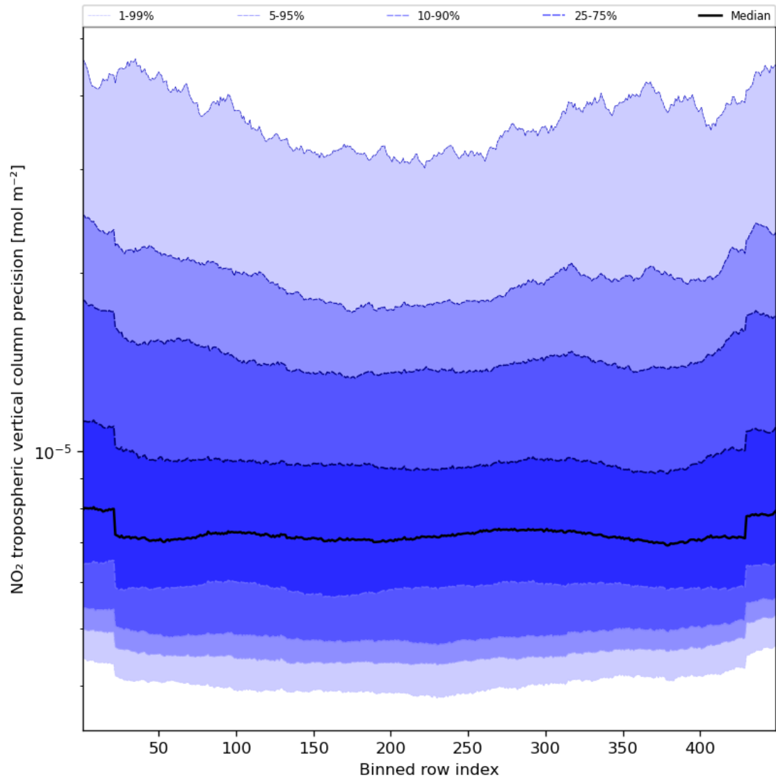
Figure 47: Along track statistics of “NO 2 tropospheric vertical column precision” for 2023-08-18 to 2023-08-20
