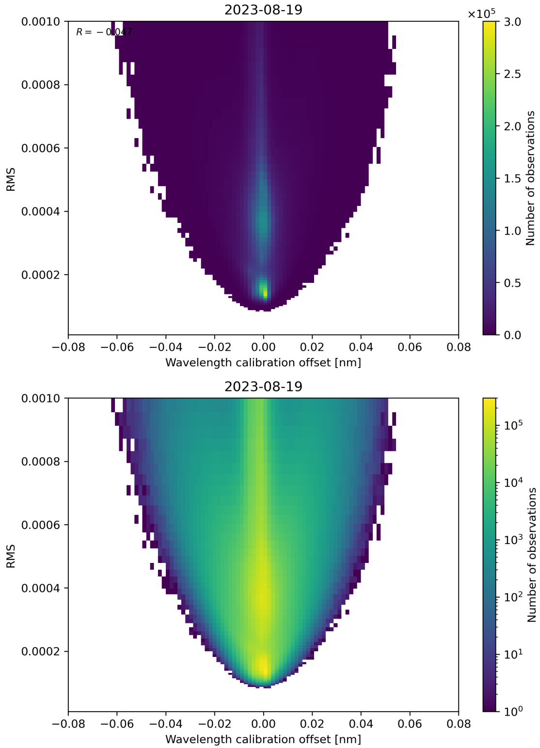
Figure 181: Scatter density plot of “Wavelength calibration offset” against “RMS” for 2023-08-18 to 2023-08-20.
