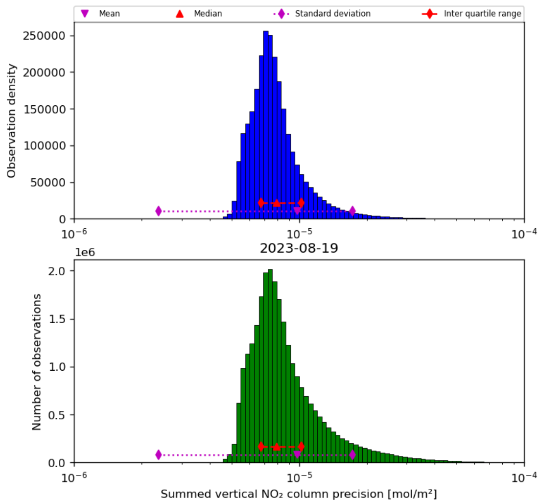
Figure 41: Histogram of “Summed vertical NO 2 column precision” for 2023-08-18 to 2023-08-20
