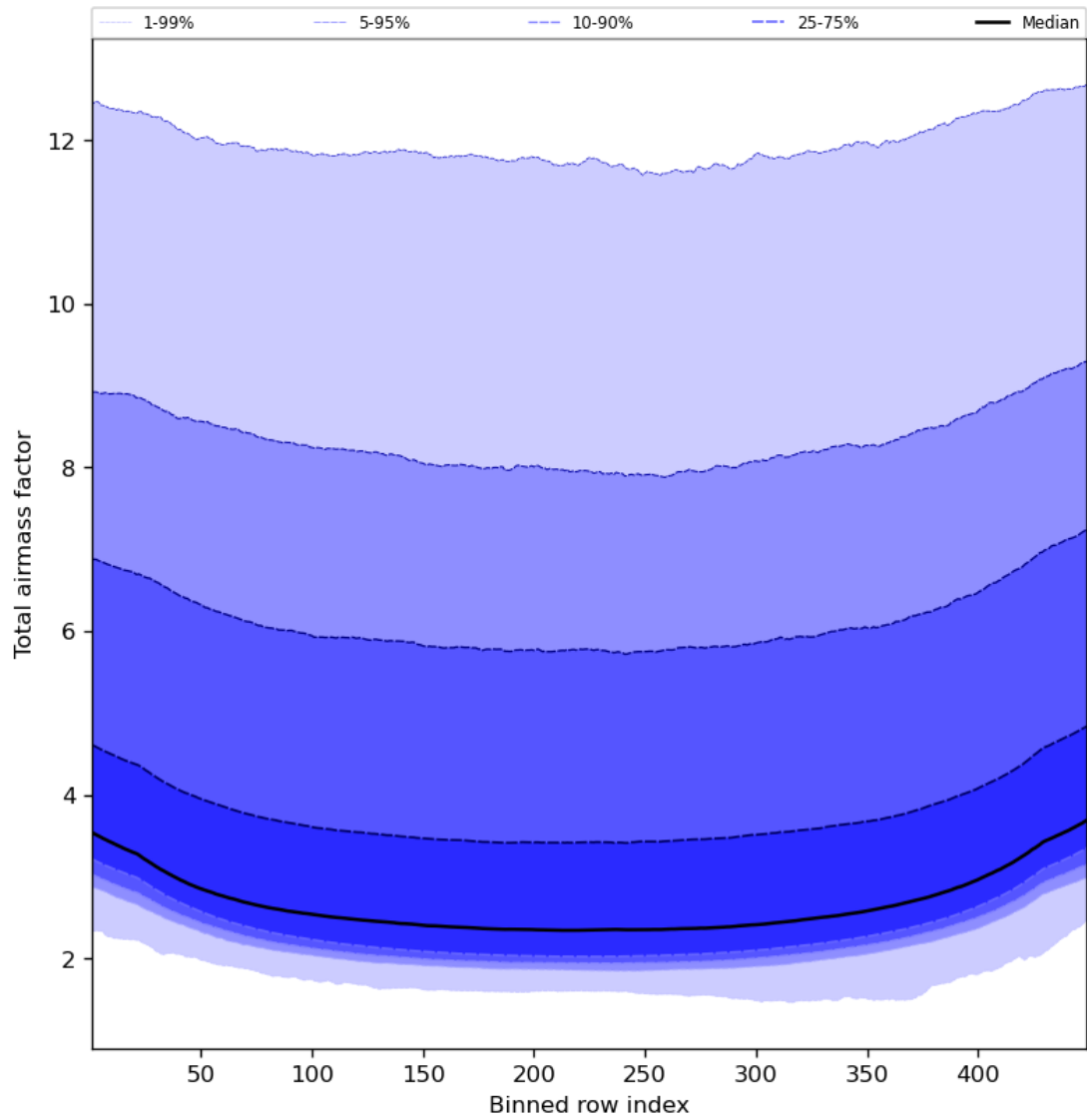
Figure 49: Along track statistics of “Total airmass factor” for 2023-08-18 to 2023-08-20
