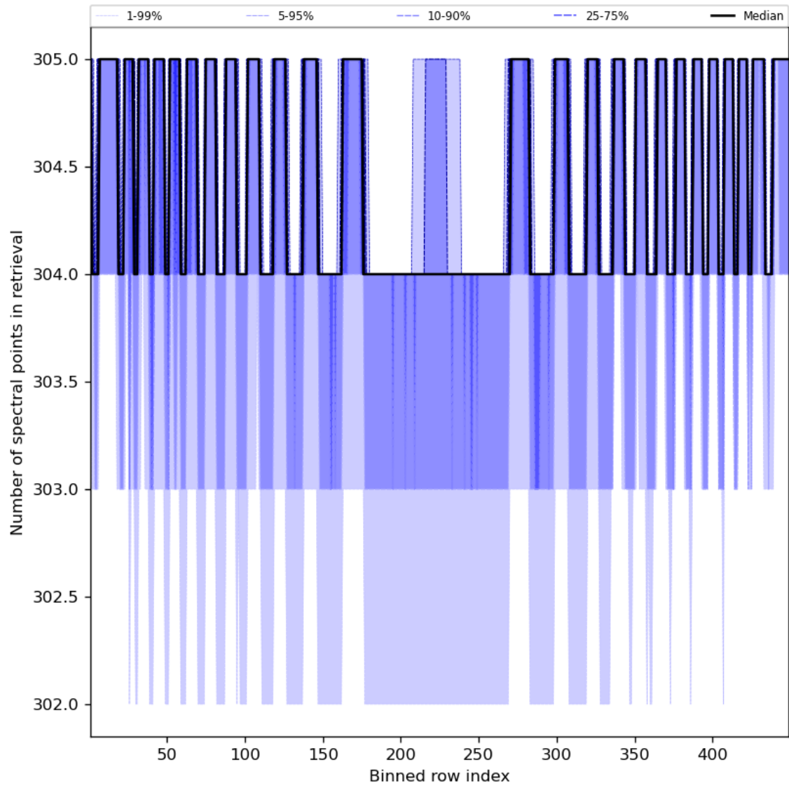
Figure 50: Along track statistics of “Number of spectral points in retrieval” for 2023-08-18 to 2023-08-20
