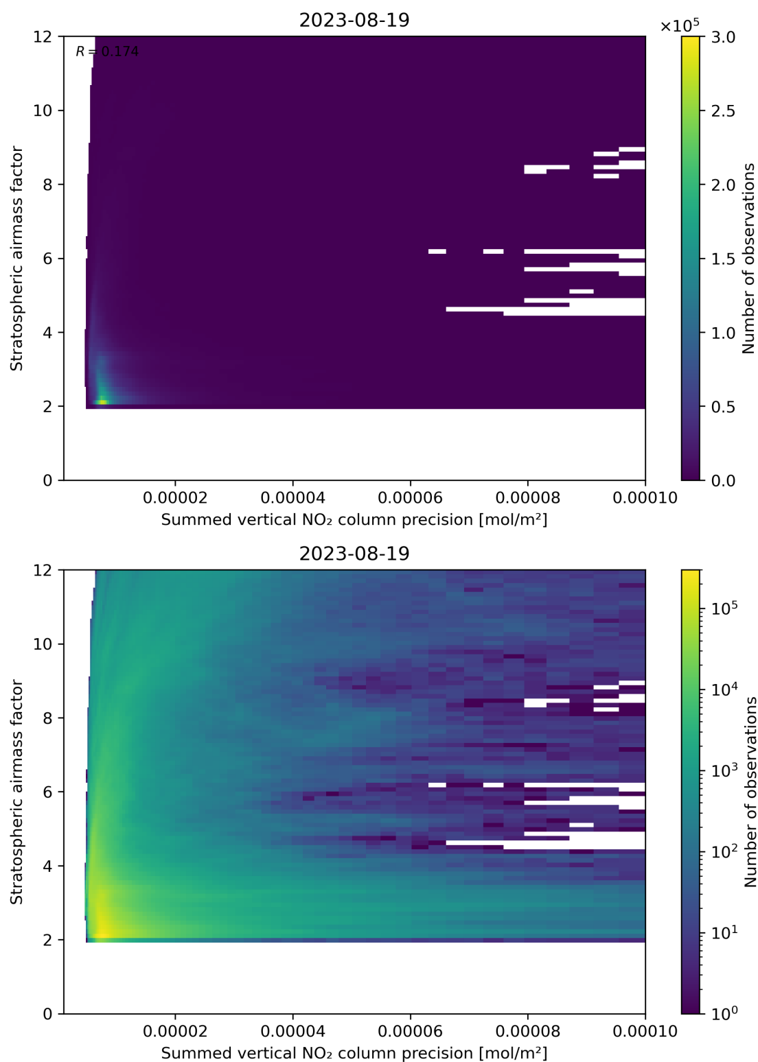
Figure 106: Scatter density plot of “Summed vertical NO 2 column precision” against “Stratospheric airmass factor” for 2023-08-18 to 2023-08-20.
