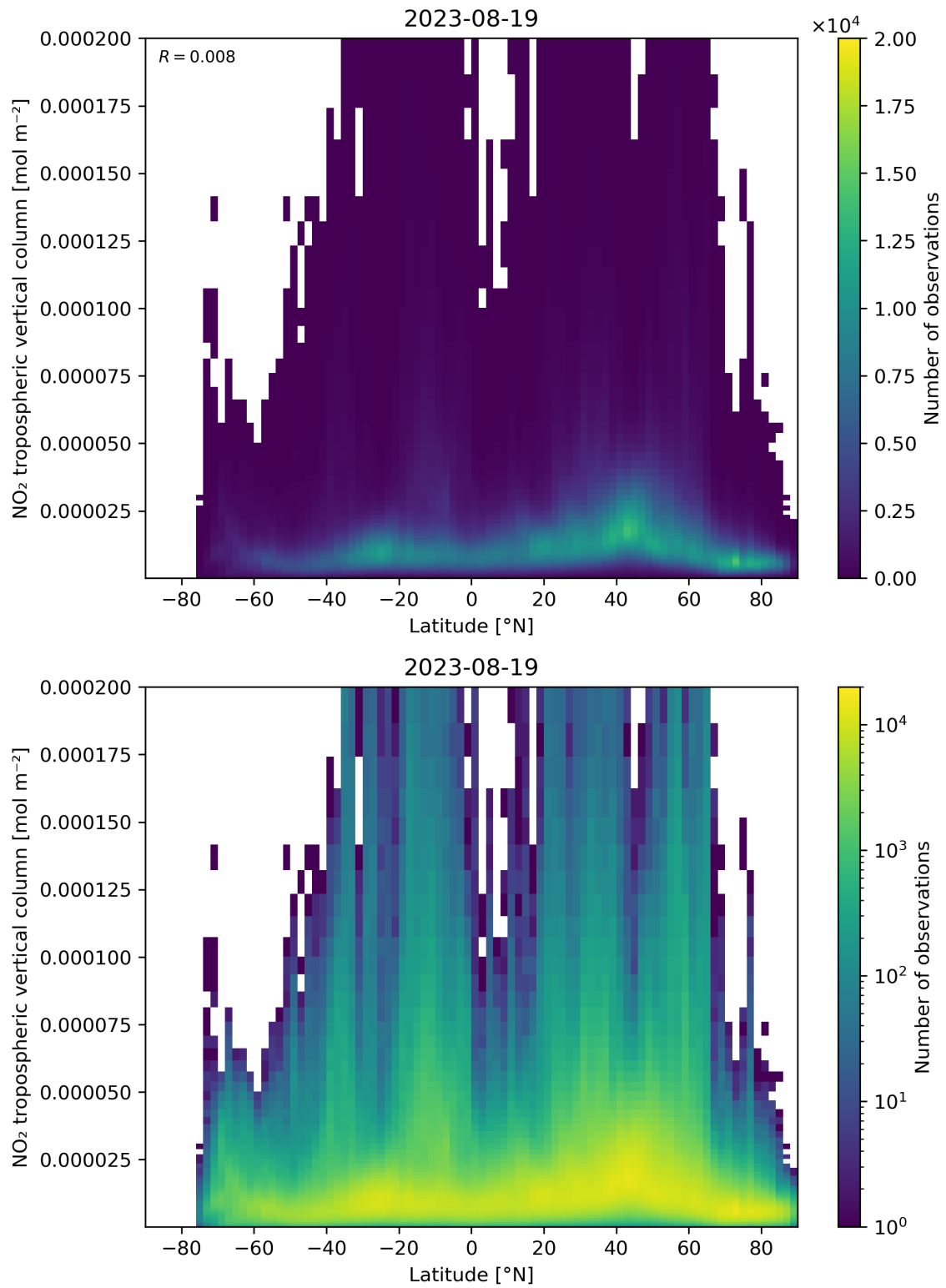
Figure 92: Scatter density plot of “Latitude” against “NO 2 tropospheric vertical column” for 2023-08-18 to 2023-08-20.
