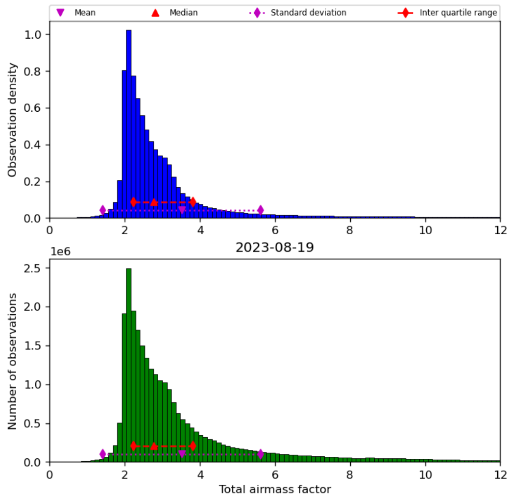
Figure 32: Histogram of “Total airmass factor” for 2023-08-18 to 2023-08-20
