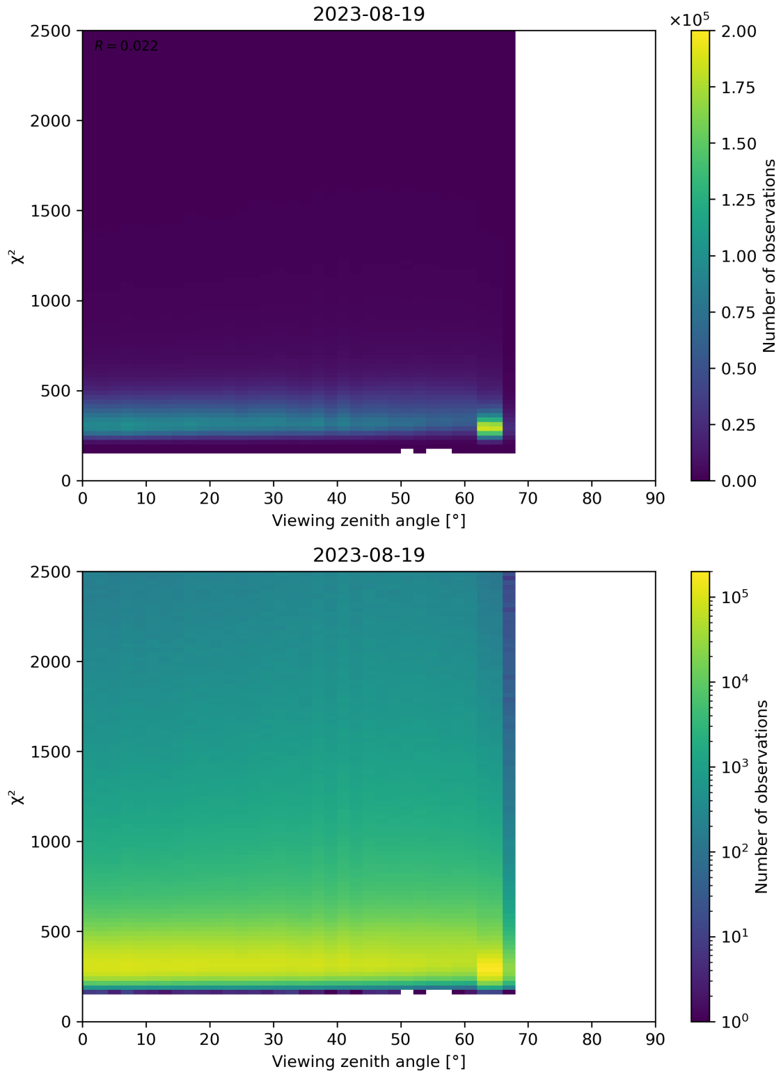
Figure 162: Scatter density plot of “Viewing zenith angle” against “ \chi^2 ” for 2023-08-18 to 2023-08-20.
