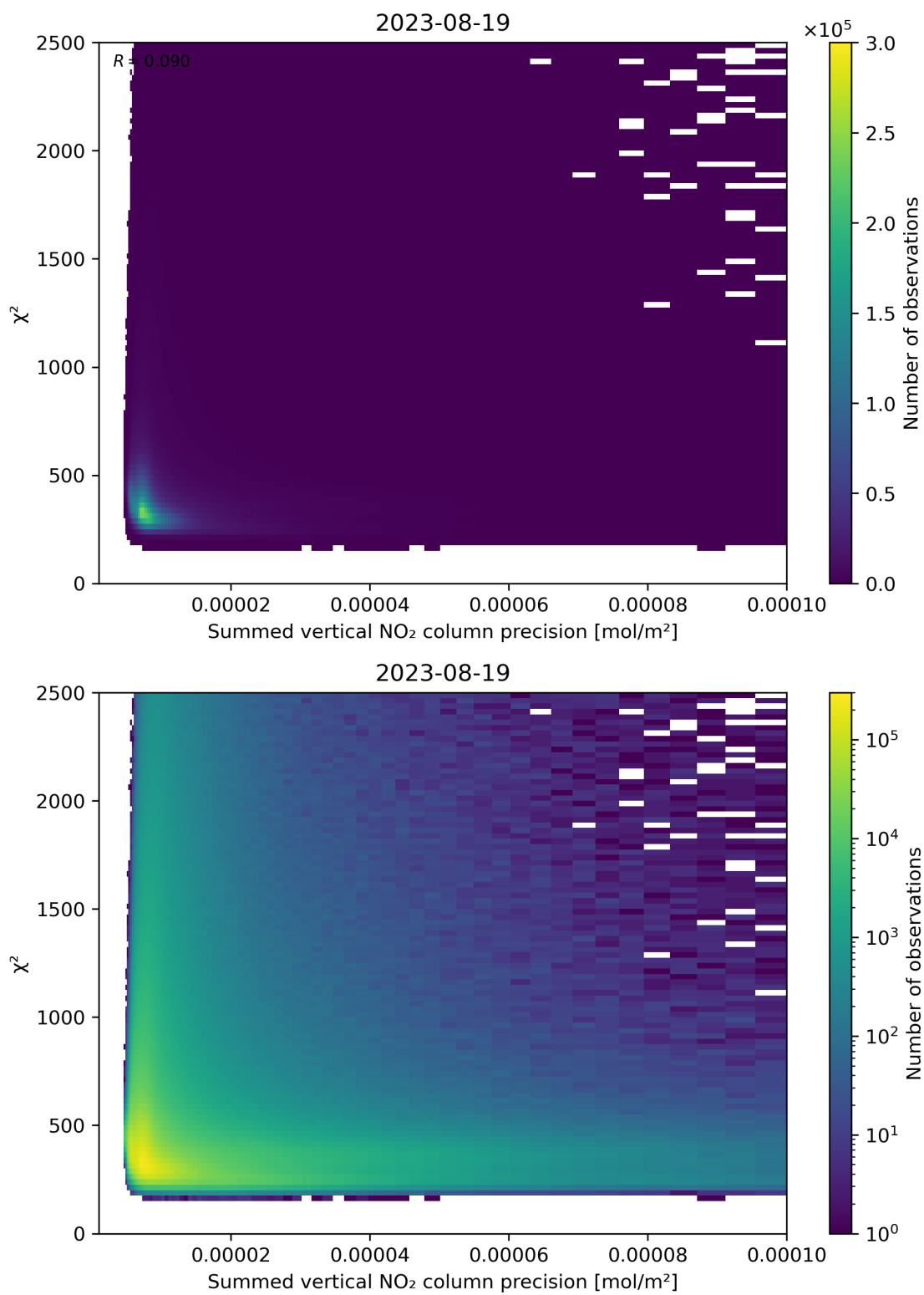
Figure 107: Scatter density plot of “Summed vertical NO 2 column precision” against “ \chi^2 ” for 2023-08-18 to 2023-08-20.
