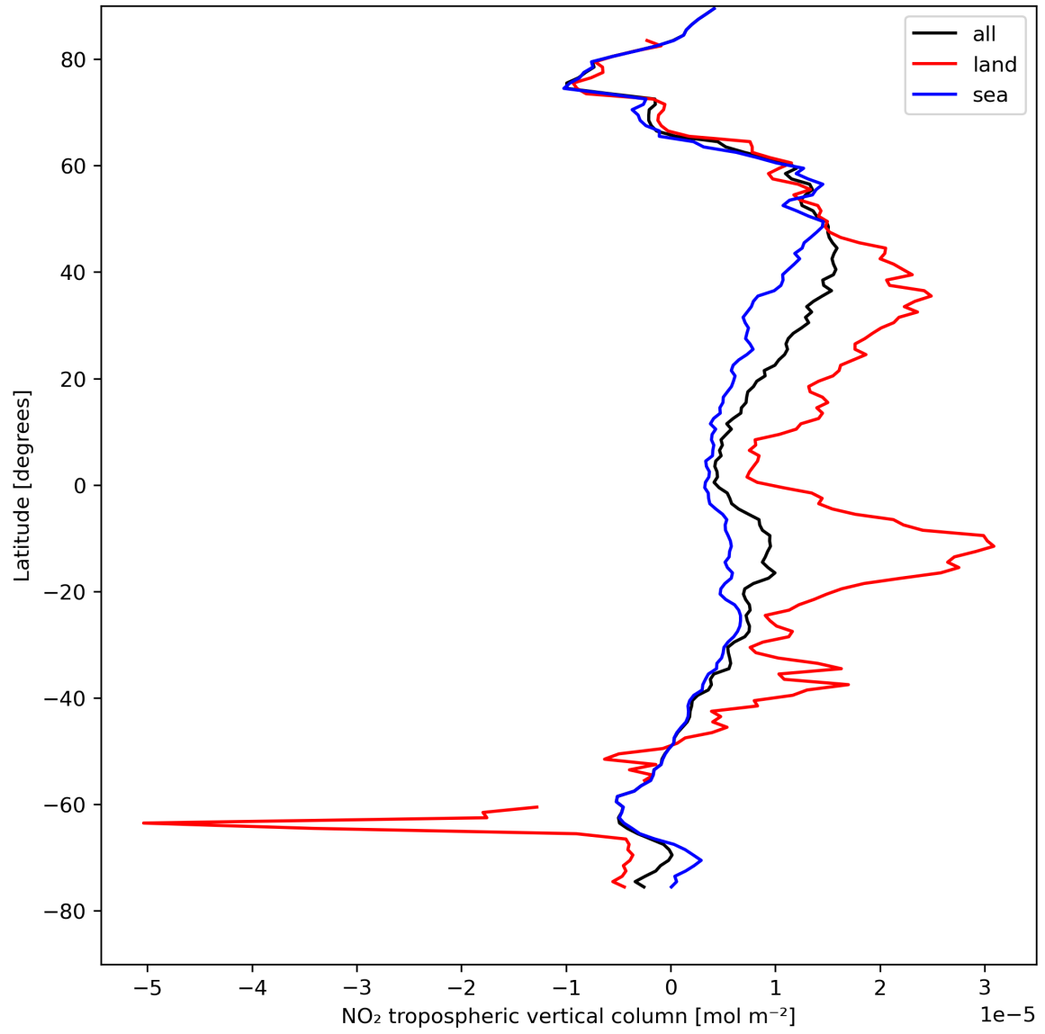
Figure 12: Zonal average of “NO 2 tropospheric vertical column” for 2023-08-18 to 2023-08-20.
