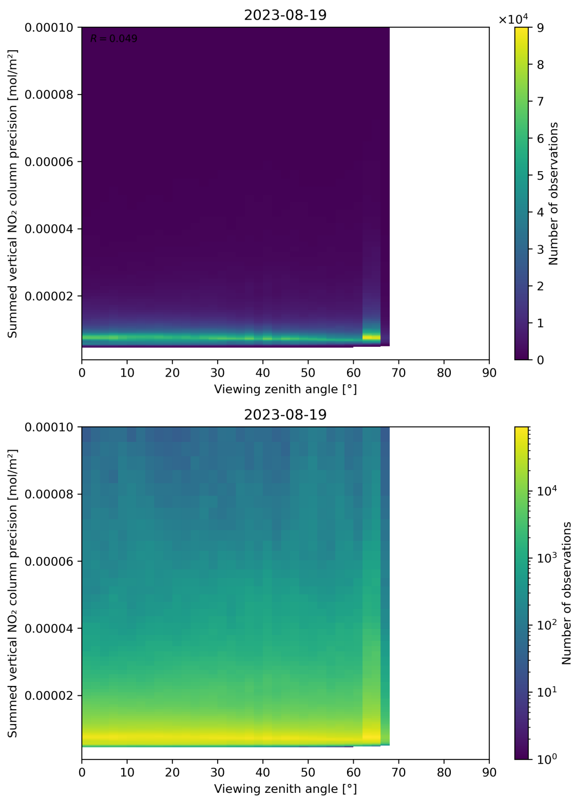
Figure 166: Scatter density plot of “Viewing zenith angle” against “Summed vertical NO 2 column precision” for 2023-08-18 to 2023-08-20.
