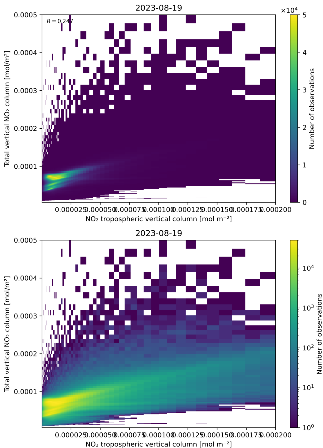
Figure 128: Scatter density plot of “NO 2 tropospheric vertical column” against “Total vertical NO 2 column” for 2023-08-18 to 2023-08-20.
