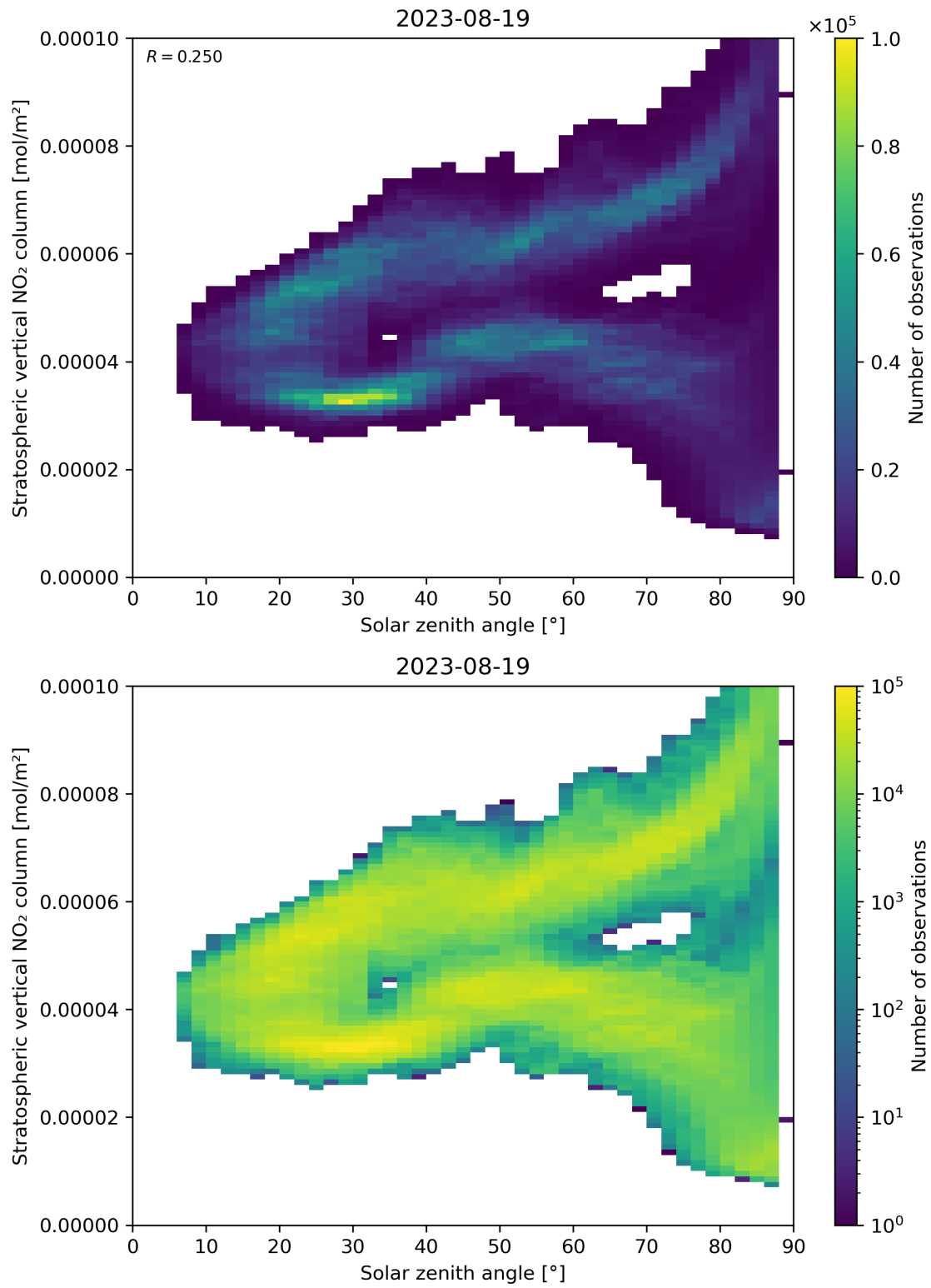
Figure 150: Scatter density plot of “Solar zenith angle” against “Stratospheric vertical \text{NO}_2 column” for 2023-08-18 to 2023-08-20.
