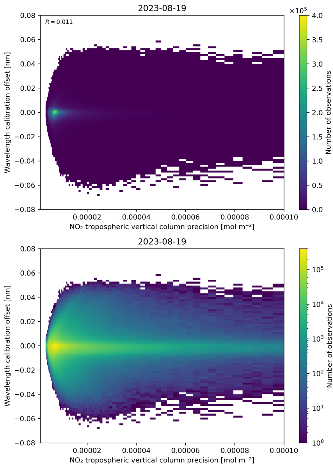
Figure 141: Scatter density plot of “NO 2 tropospheric vertical column precision” against “Wavelength calibration offset” for 2023-08-18 to 2023-08-20.
