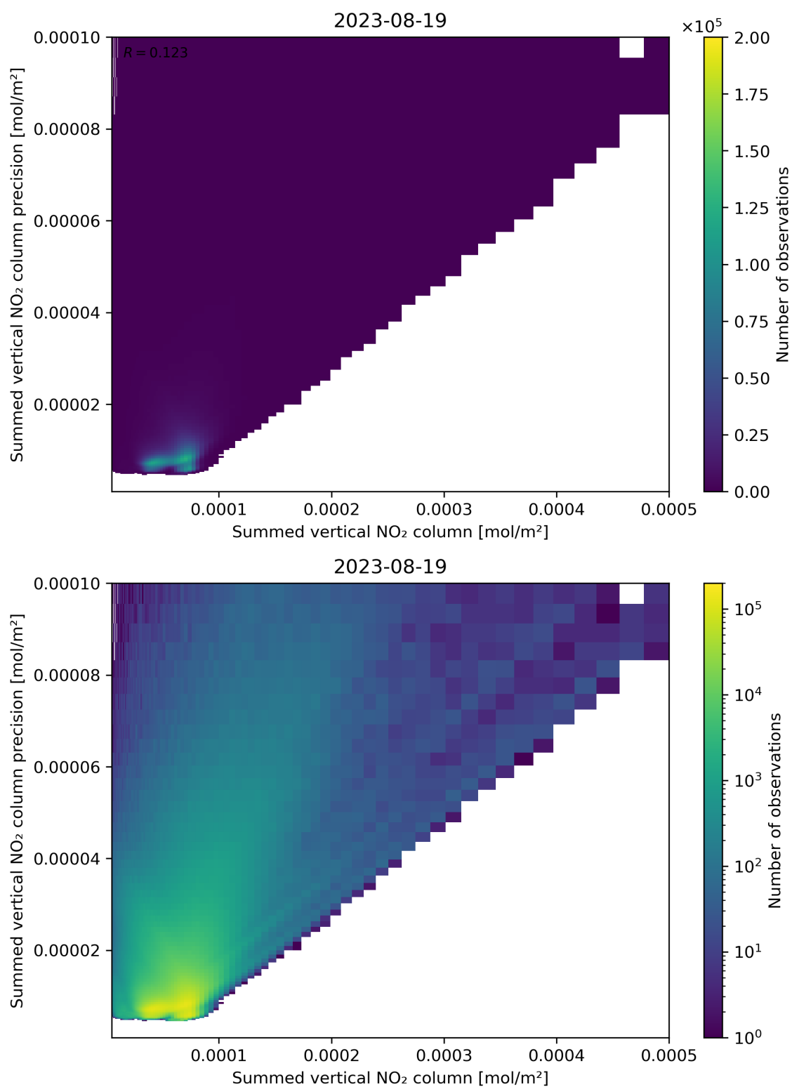
Figure 105: Scatter density plot of “Summed vertical NO 2 column” against “Summed vertical NO 2 column precision” for 2023-08-18 to 2023-08-20.
