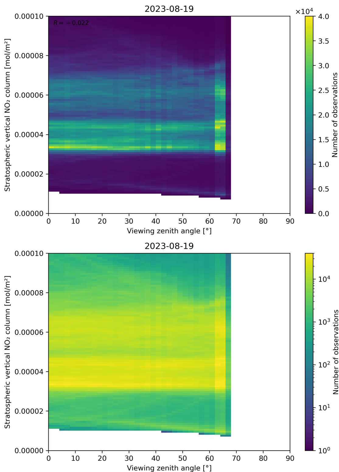
Figure 164: Scatter density plot of “Viewing zenith angle” against “Stratospheric vertical NO 2 column” for 2023-08-18 to 2023-08-20.
