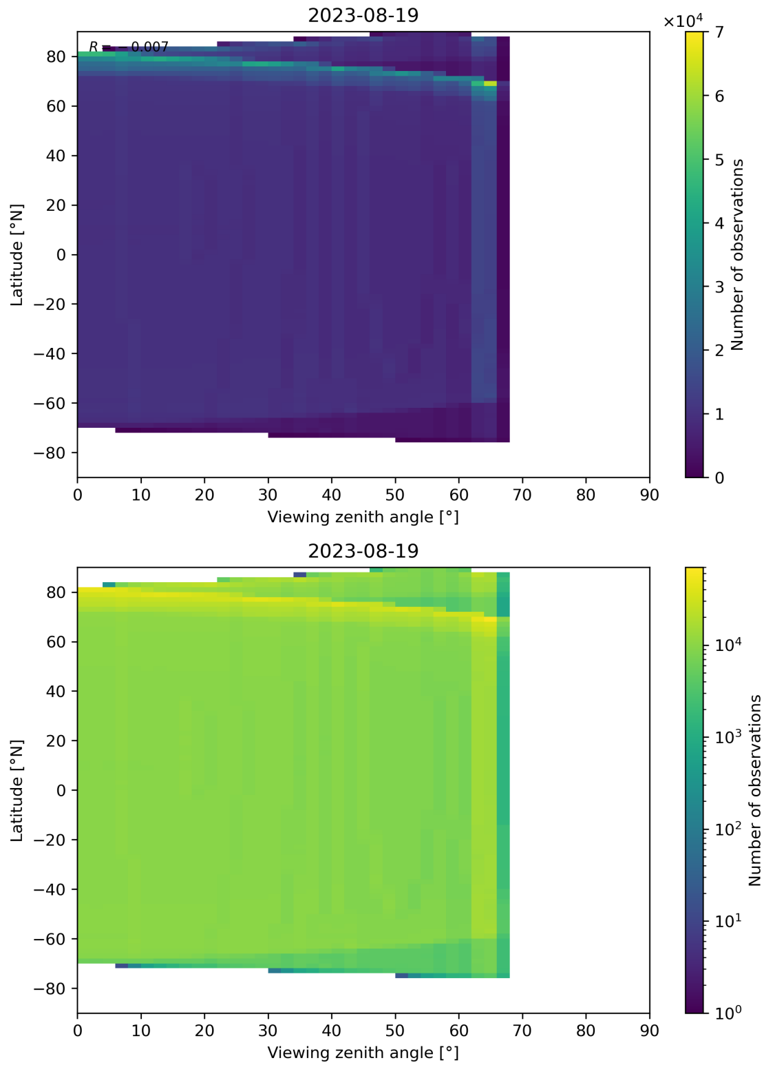
Figure 163: Scatter density plot of “Viewing zenith angle” against “Latitude” for 2023-08-18 to 2023-08-20.
