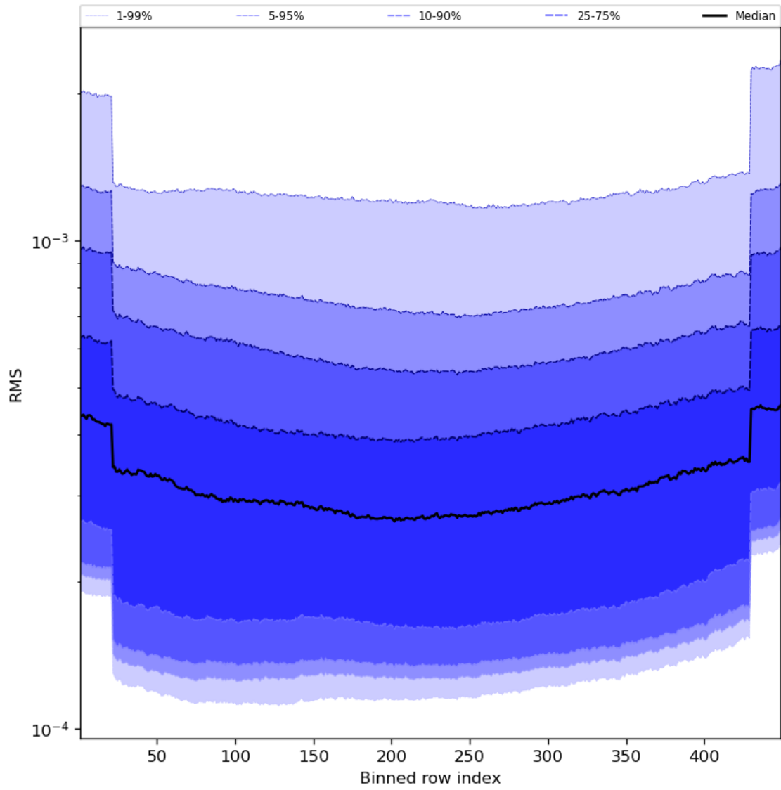
Figure 60: Along track statistics of “RMS” for 2023-08-18 to 2023-08-20
