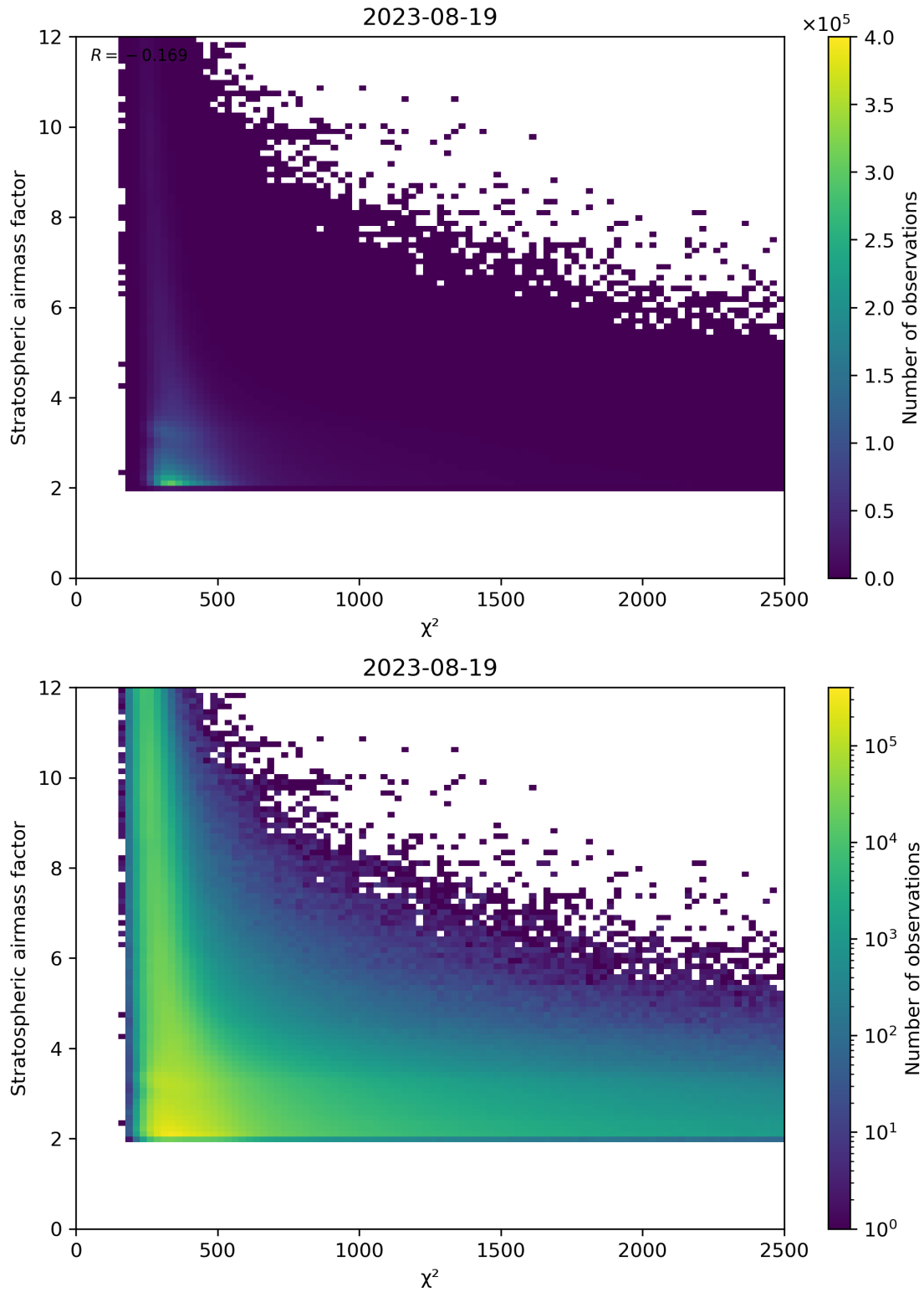
Figure 81: Scatter density plot of “ \chi^2 ” against “Stratospheric airmass factor” for 2023-08-18 to 2023-08-20.
