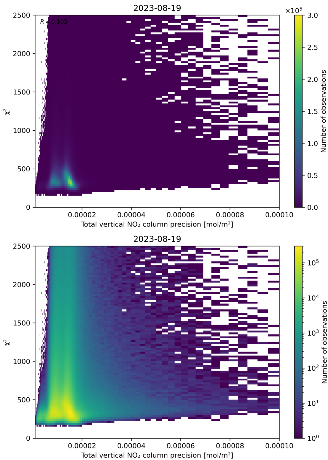
Figure 116: Scatter density plot of “Total vertical NO 2 column precision” against “ \chi^2 ” for 2023-08-18 to 2023-08-20.
