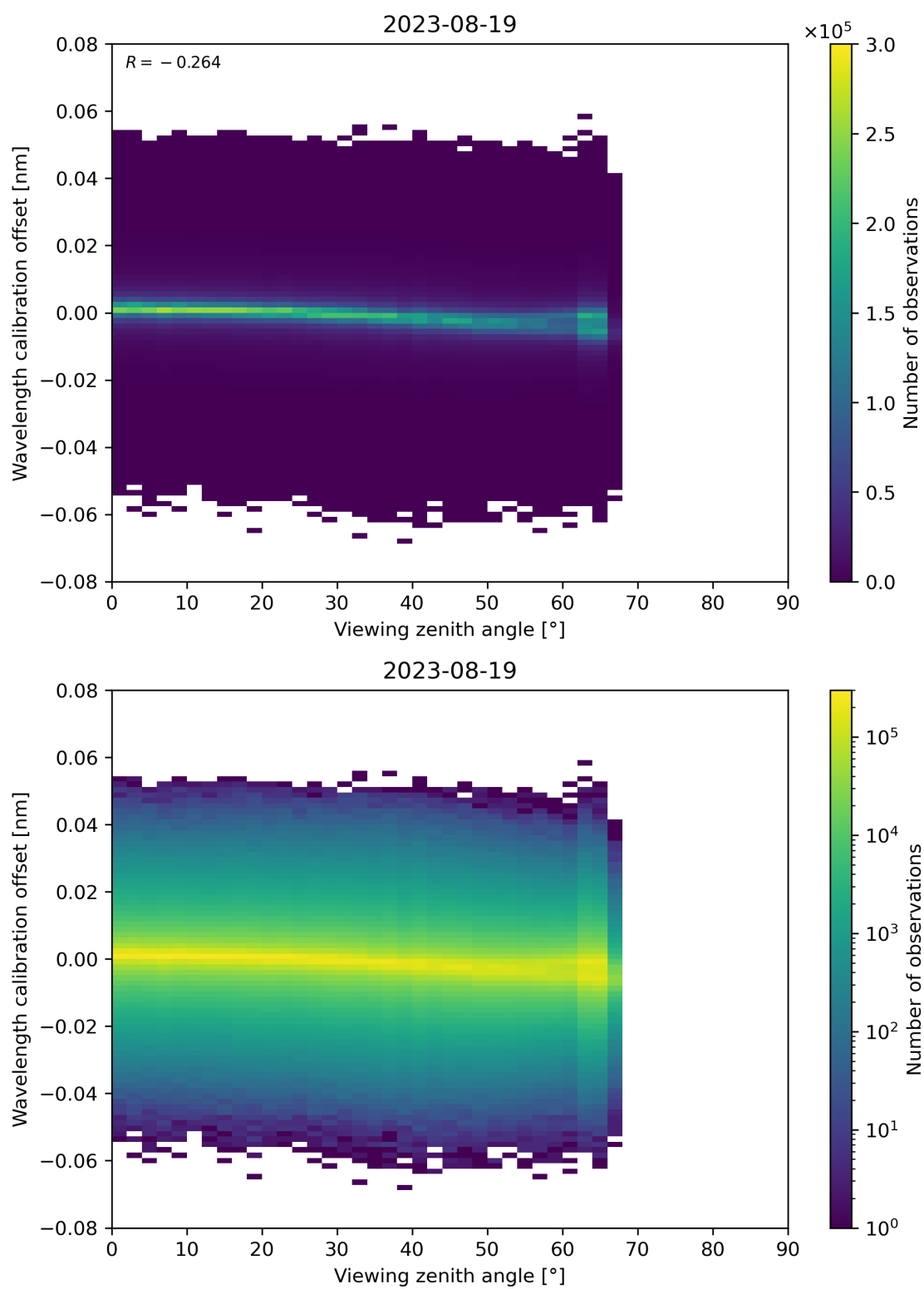
Figure 173: Scatter density plot of “Viewing zenith angle” against “Wavelength calibration offset” for 2023-08-18 to 2023-08-20.
