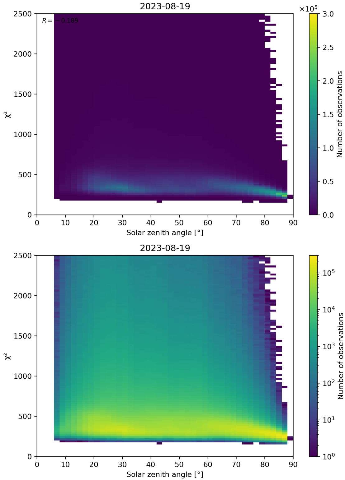
Figure 148: Scatter density plot of “Solar zenith angle” against “ \chi^2 ” for 2023-08-18 to 2023-08-20.
