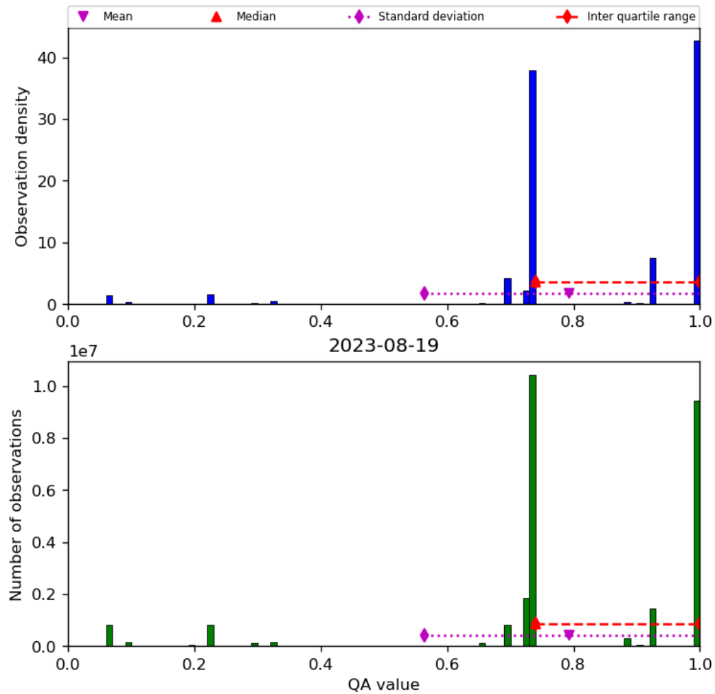
Figure 28: Histogram of “QA value” for 2023-08-18 to 2023-08-20
