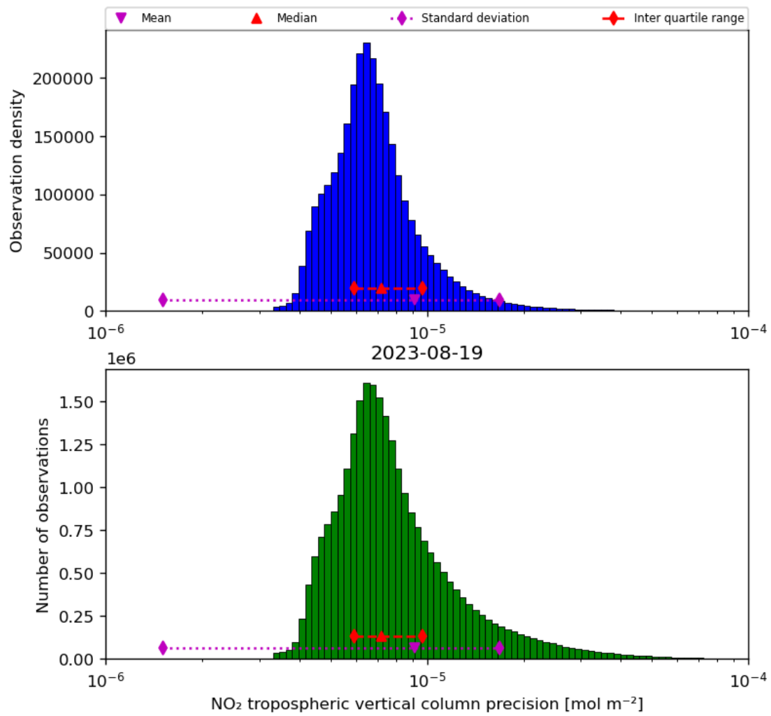
Figure 30: Histogram of “NO 2 tropospheric vertical column precision” for 2023-08-18 to 2023-08-20
