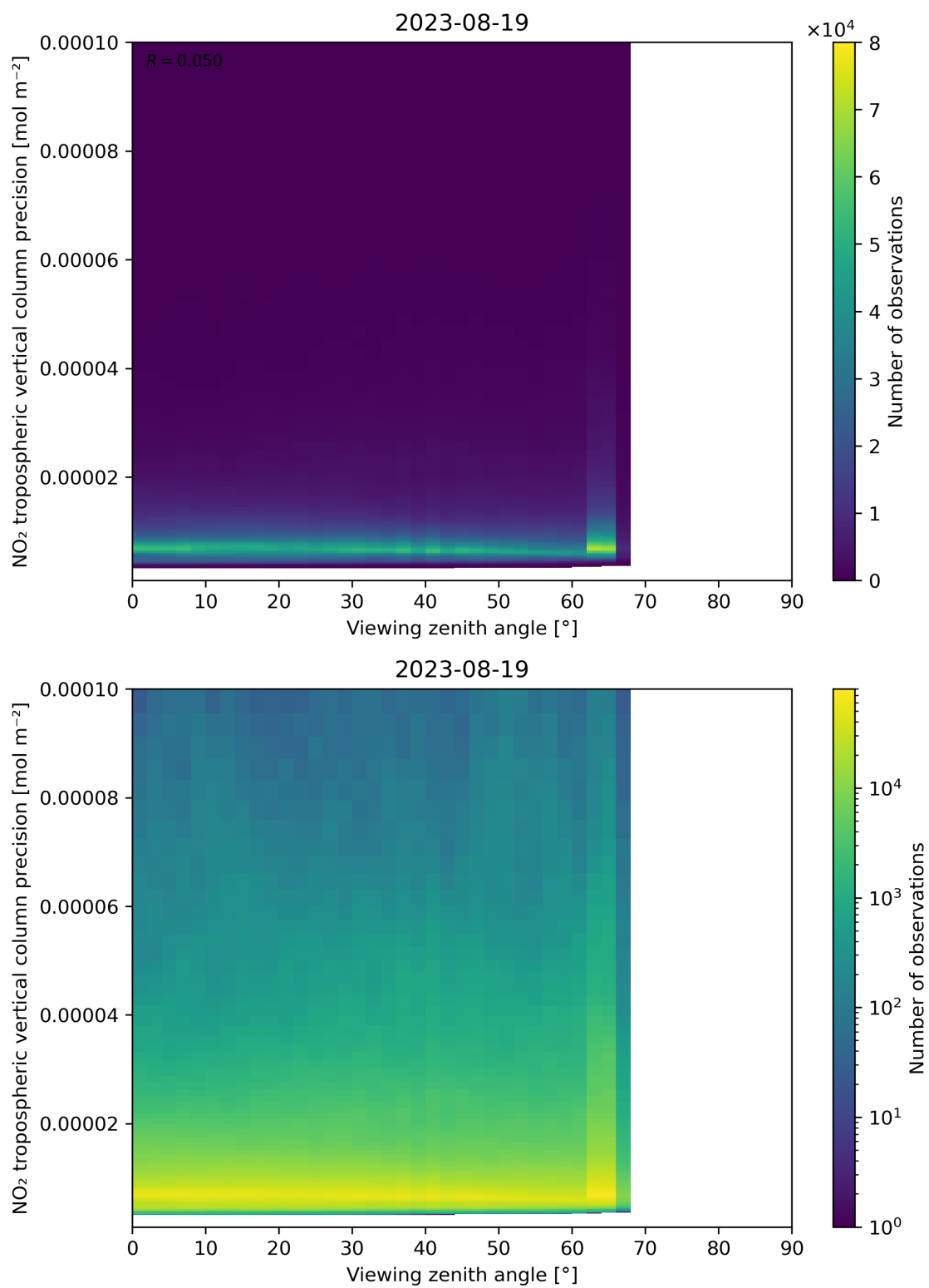
Figure 170: Scatter density plot of “Viewing zenith angle” against “NO 2 tropospheric vertical column precision” for 2023-08-18 to 2023-08-20.
