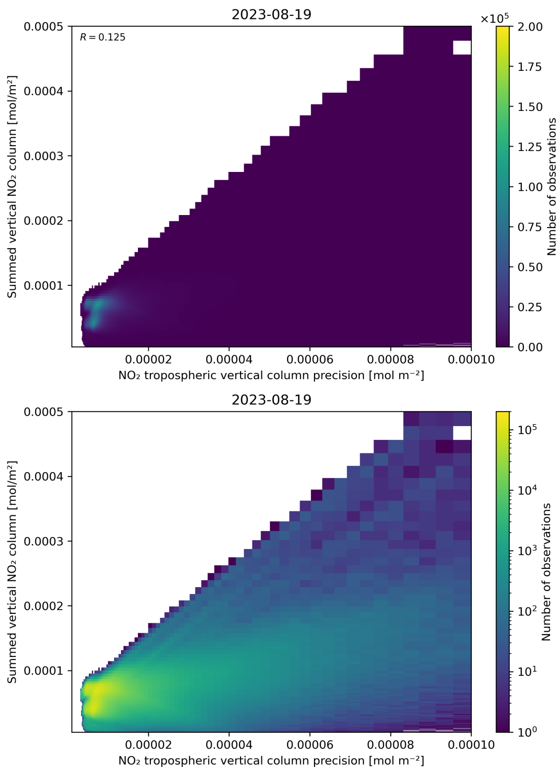
Figure 136: Scatter density plot of “NO 2 tropospheric vertical column precision” against “Summed vertical NO 2 column” for 2023-08-18 to 2023-08-20.
