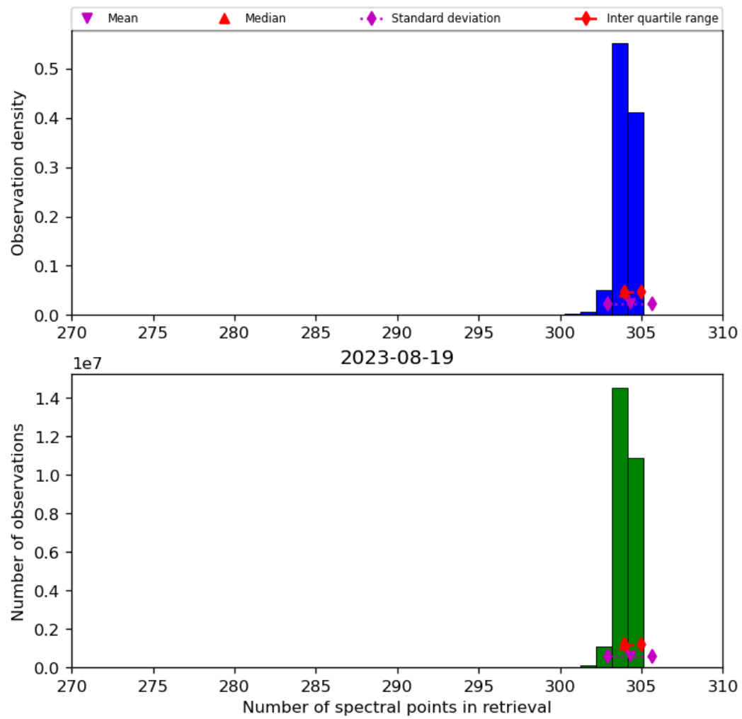
Figure 33: Histogram of “Number of spectral points in retrieval” for 2023-08-18 to 2023-08-20
