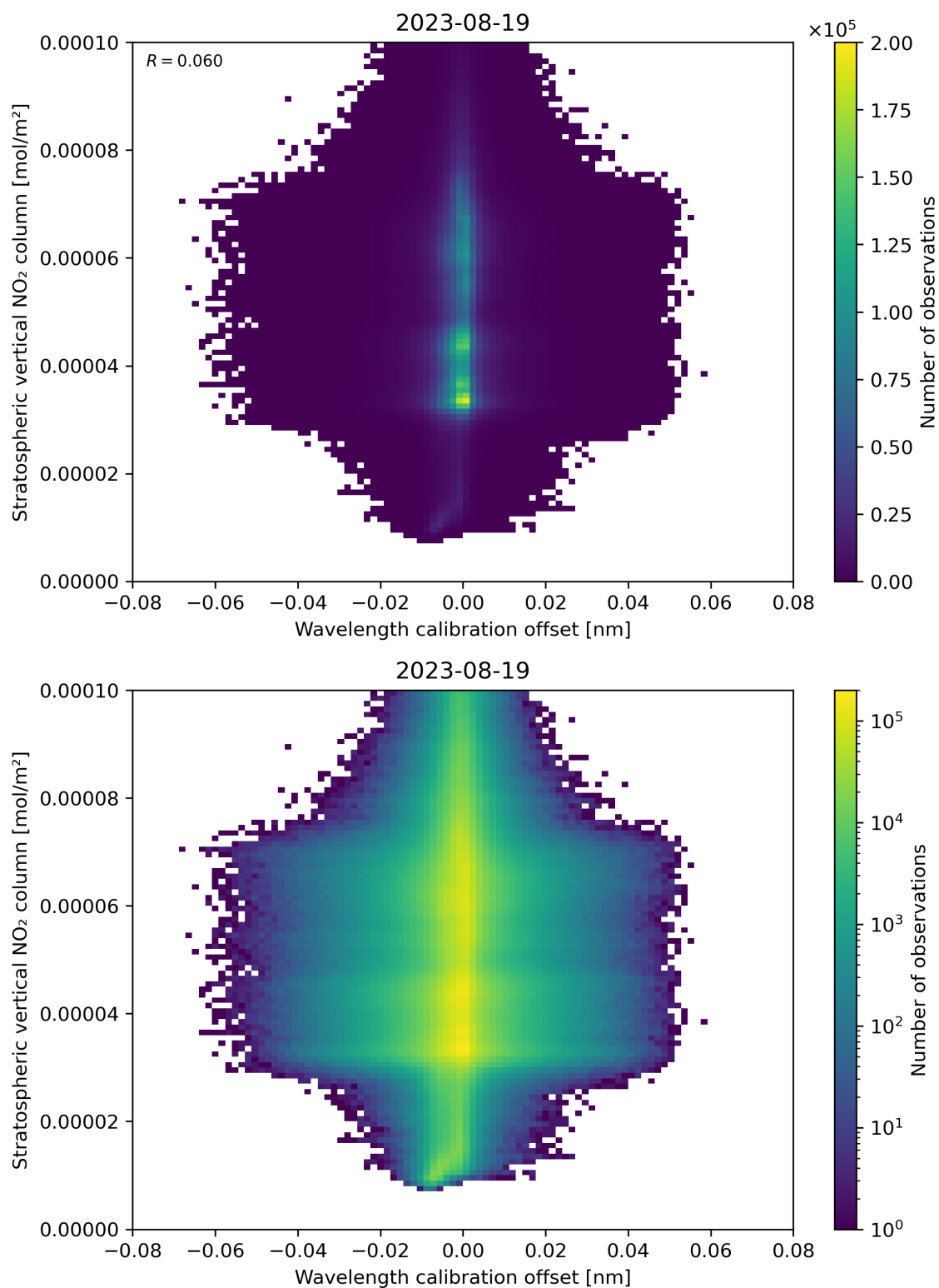
Figure 176: Scatter density plot of “Wavelength calibration offset” against “Stratospheric vertical NO 2 column” for 2023-08-18 to 2023-08-20.
