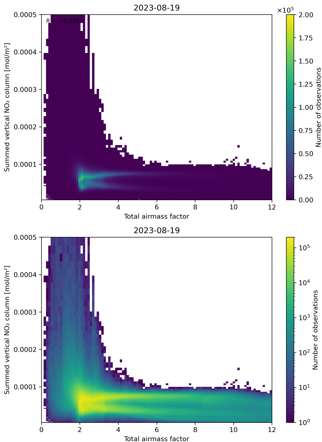
Figure 65: Scatter density plot of “Total airmass factor” against “Summed vertical NO 2 column” for 2023-08-18 to 2023-08-20.
