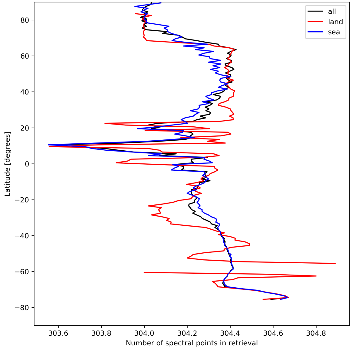
Figure 16: Zonal average of “Number of spectral points in retrieval” for 2023-08-18 to 2023-08-20.
