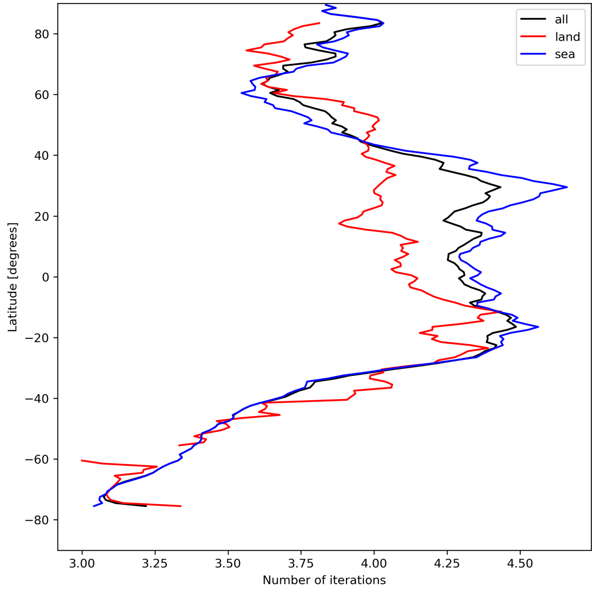
Figure 17: Zonal average of “Number of iterations” for 2023-08-18 to 2023-08-20.
