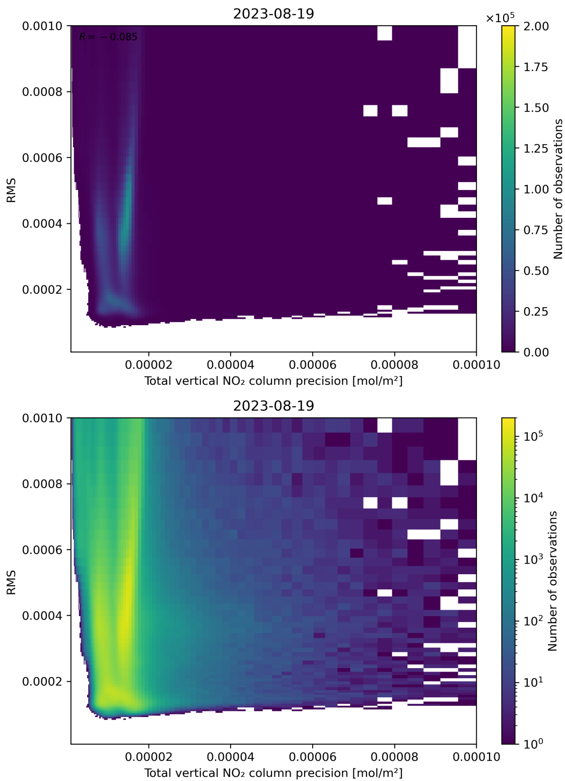
Figure 119: Scatter density plot of “Total vertical NO 2 column precision” against “RMS” for 2023-08-18 to 2023-08-20.
