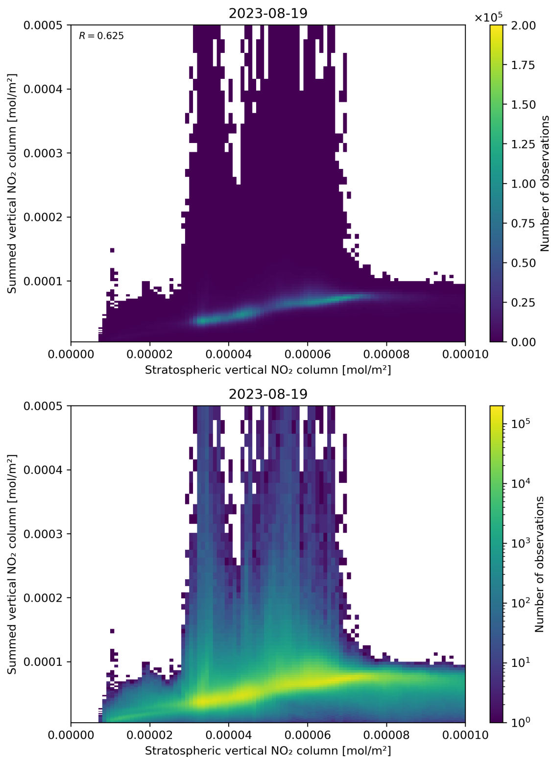
Figure 98: Scatter density plot of “Stratospheric vertical NO 2 column” against “Summed vertical NO 2 column” for 2023-08-18 to 2023-08-20.
