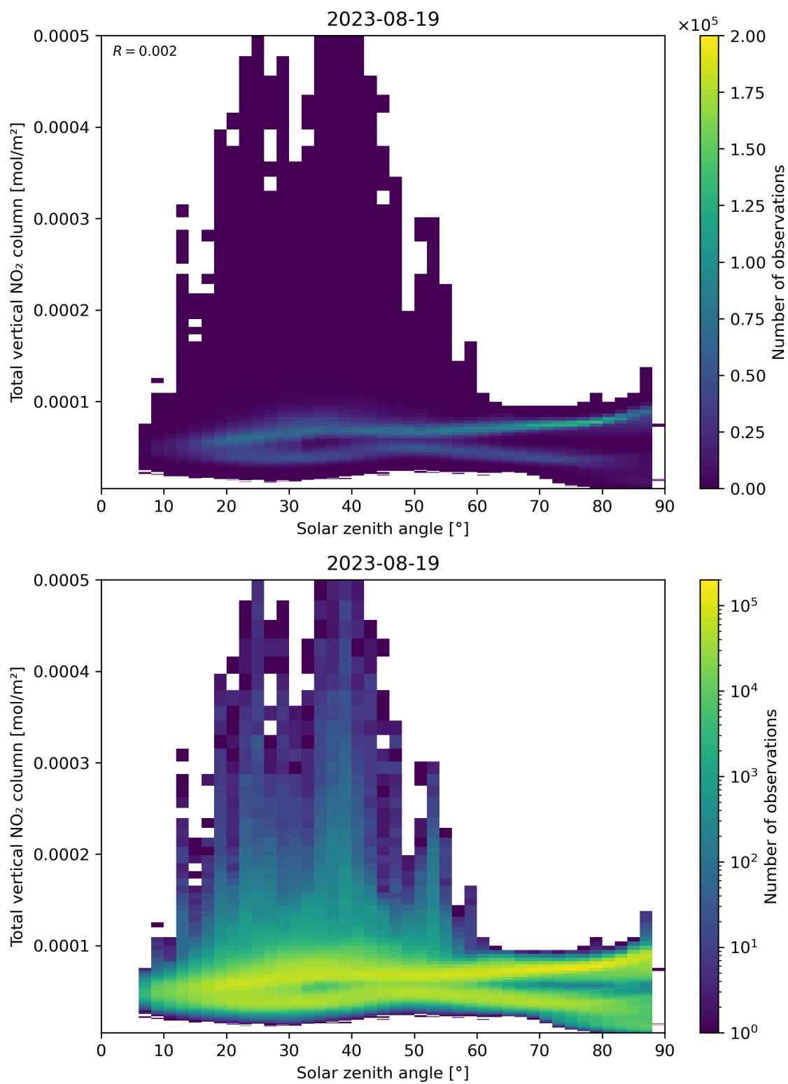
Figure 153: Scatter density plot of “Solar zenith angle” against “Total vertical NO 2 column” for 2023-08-18 to 2023-08-20.
