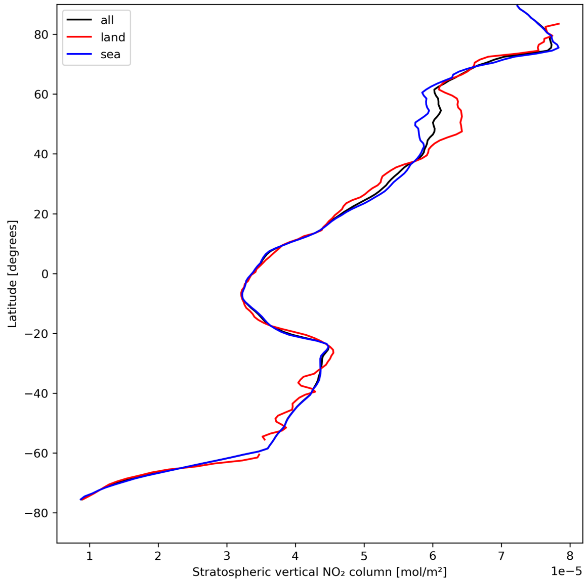
Figure 19: Zonal average of “Stratospheric vertical NO 2 column” for 2023-08-18 to 2023-08-20.
