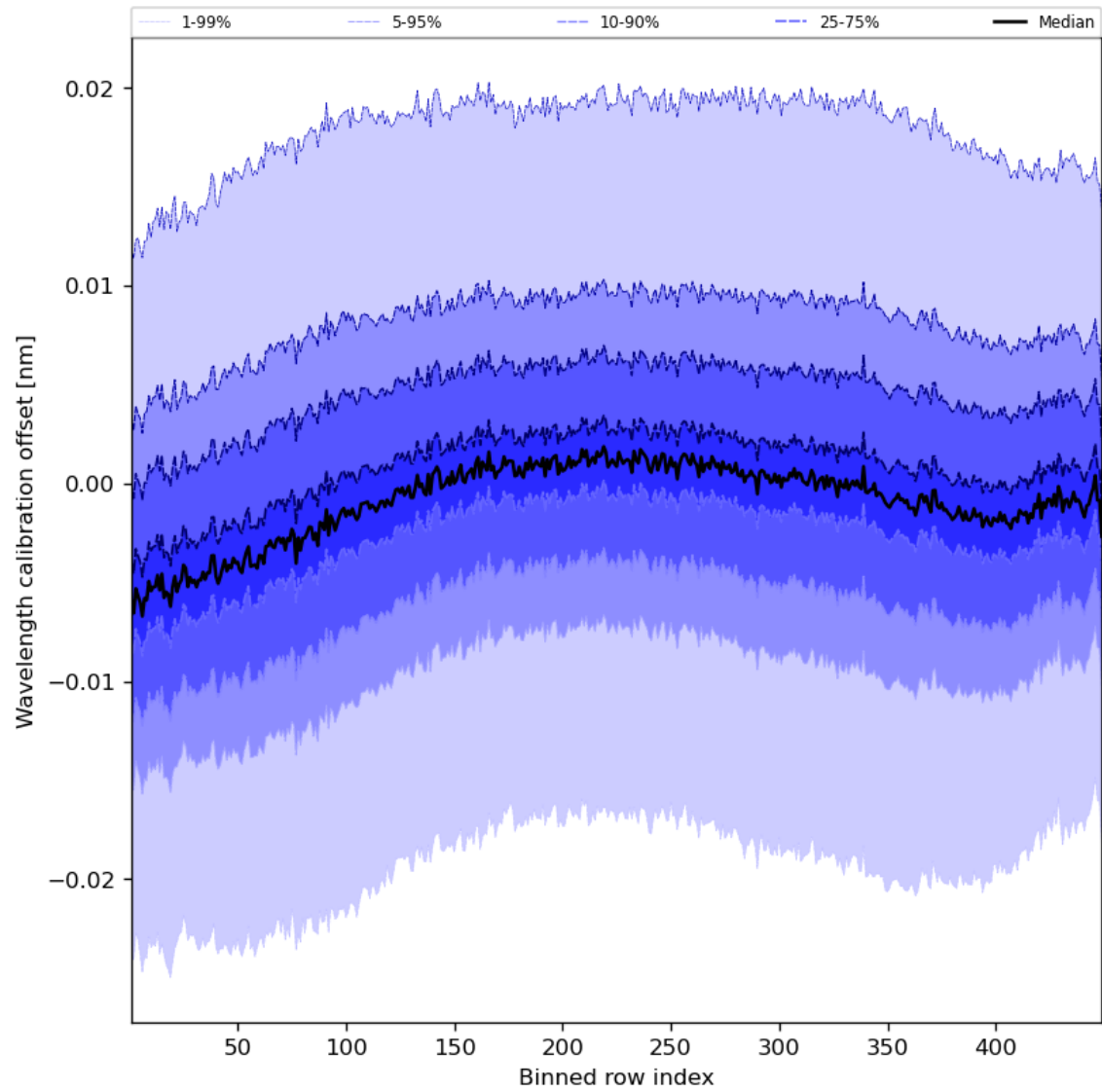
Figure 52: Along track statistics of “Wavelength calibration offset” for 2023-08-18 to 2023-08-20
