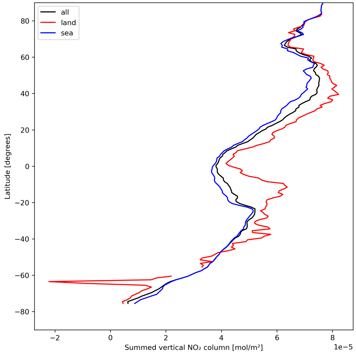
Figure 23: Zonal average of “Summed vertical NO 2 column” for 2023-08-18 to 2023-08-20.
