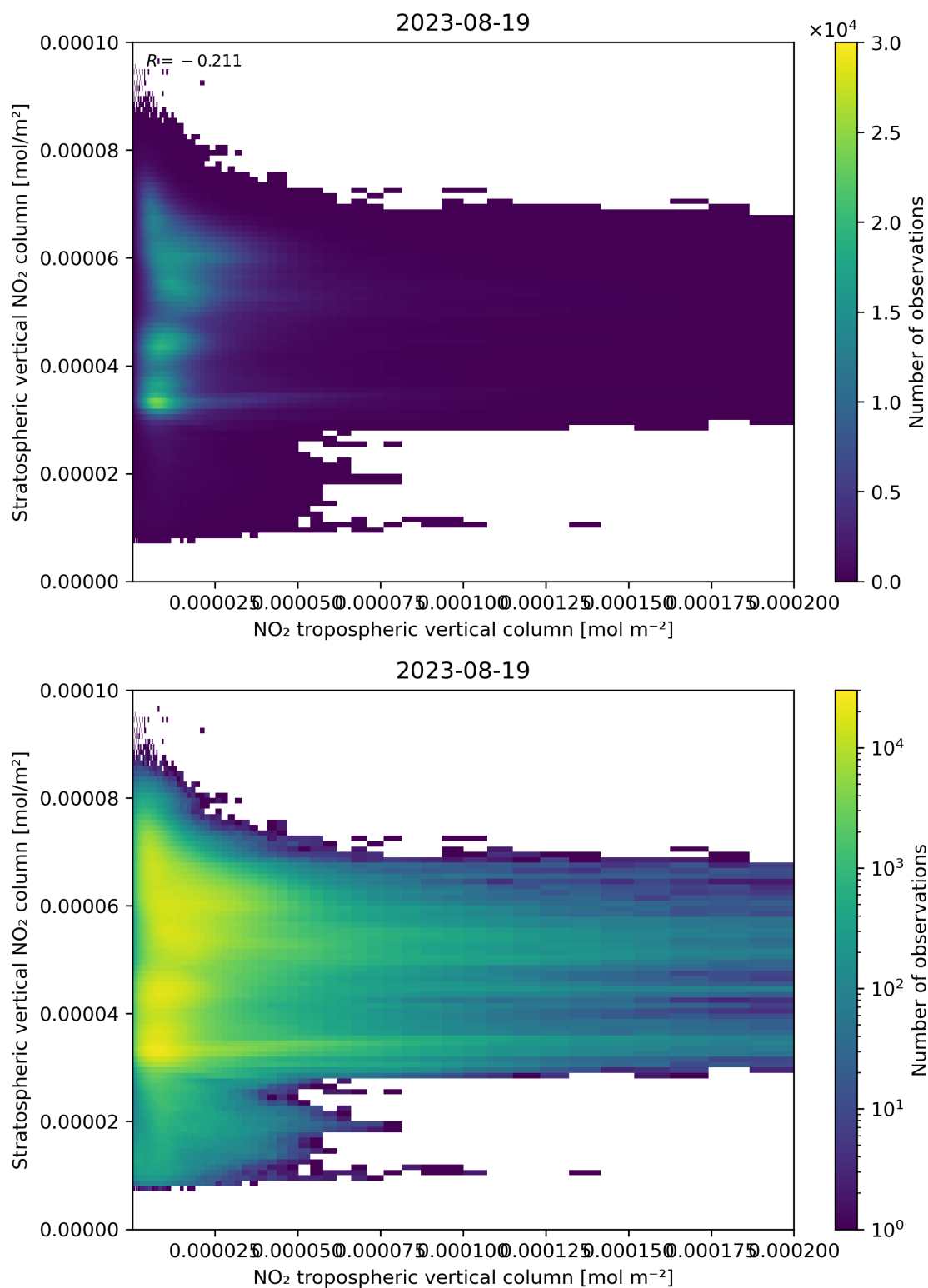
Figure 125: Scatter density plot of “NO 2 tropospheric vertical column” against “Stratospheric vertical NO 2 column” for 2023-08-18 to 2023-08-20.
