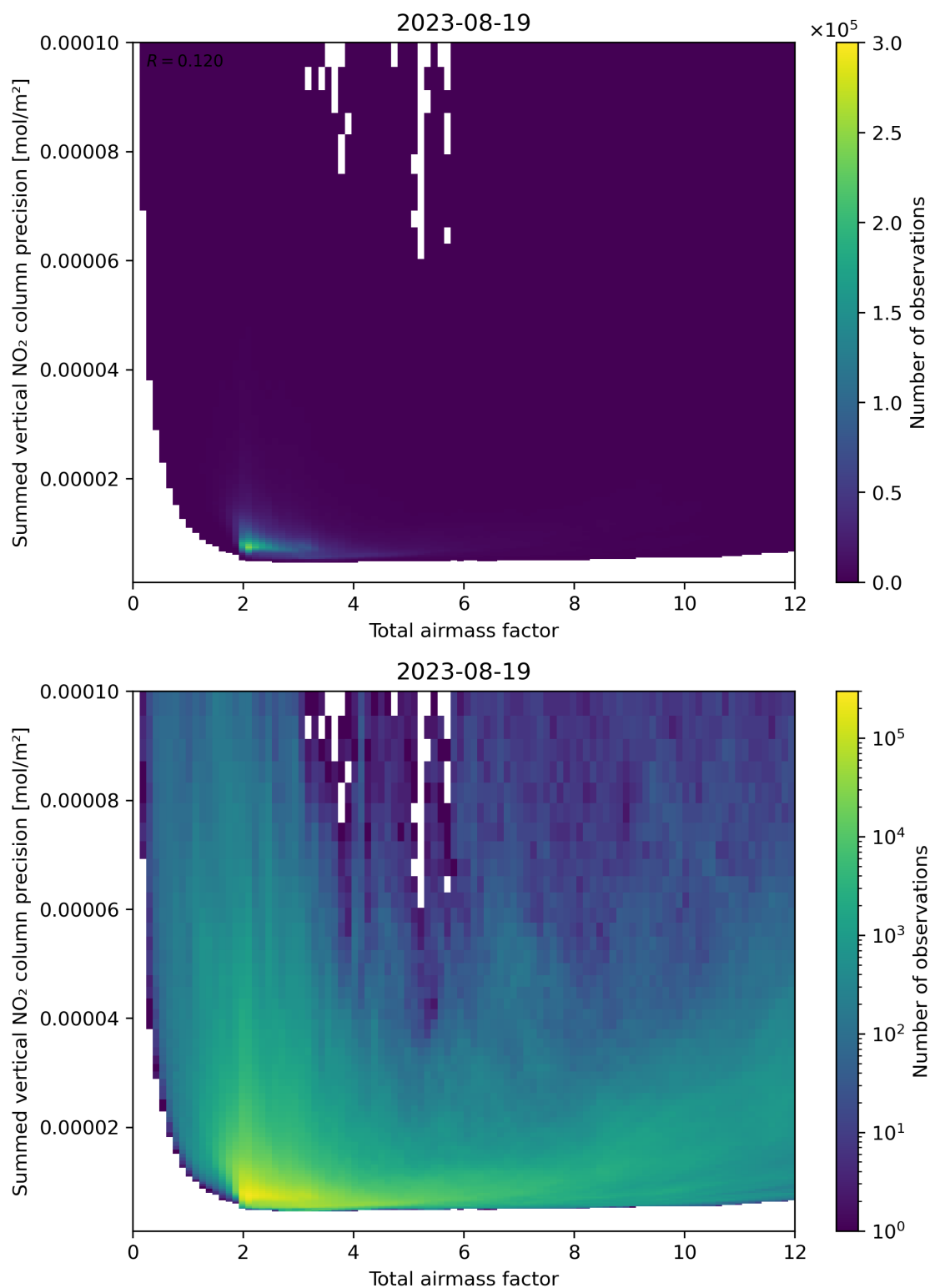
Figure 66: Scatter density plot of “Total airmass factor” against “Summed vertical NO 2 column precision” for 2023-08-18 to 2023-08-20.
