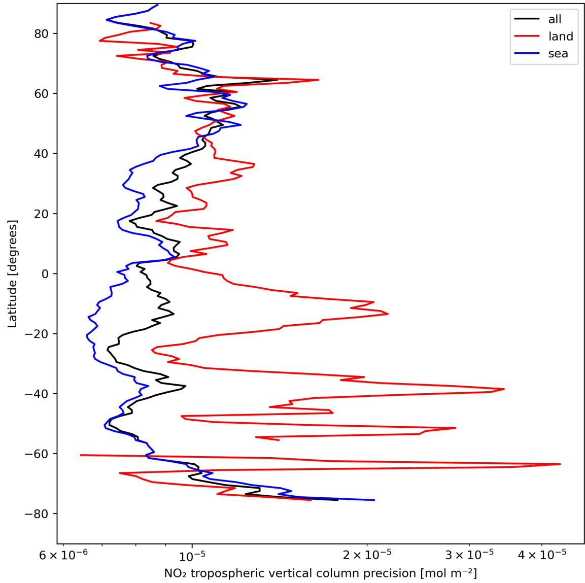
Figure 13: Zonal average of “NO 2 tropospheric vertical column precision” for 2023-08-18 to 2023-08-20.
