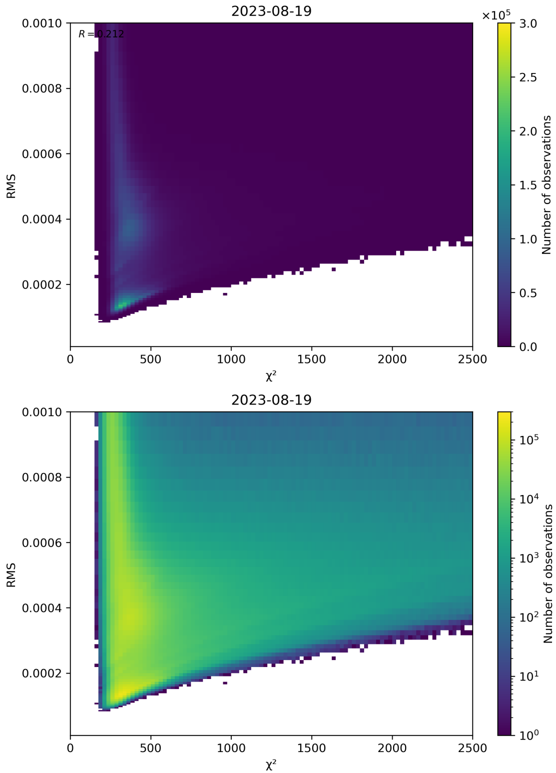
Figure 82: Scatter density plot of “ \chi^2 ” against “RMS” for 2023-08-18 to 2023-08-20.
