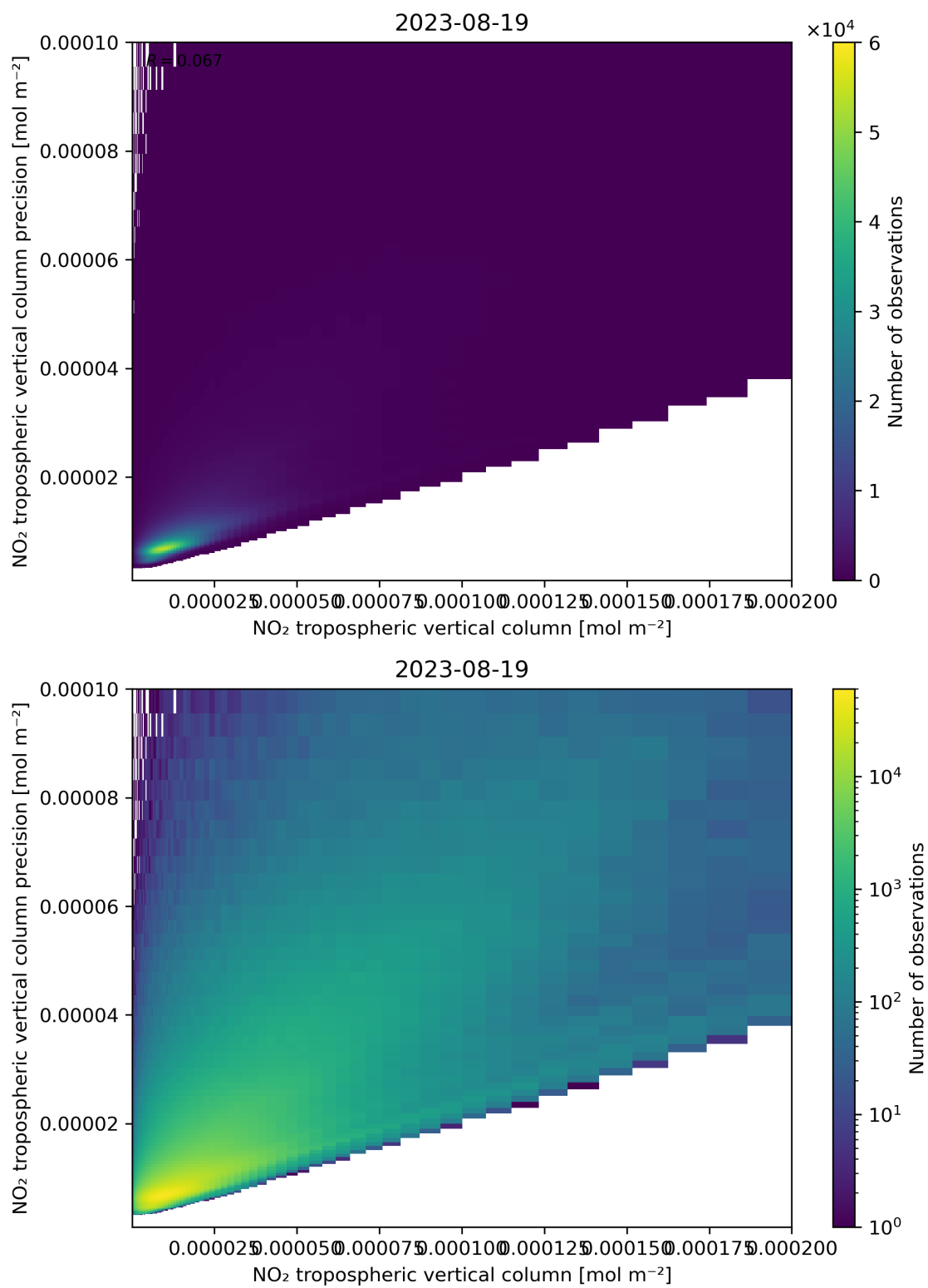
Figure 130: Scatter density plot of “NO 2 tropospheric vertical column” against “NO 2 tropospheric vertical column precision” for 2023-08-18 to 2023-08-20.
