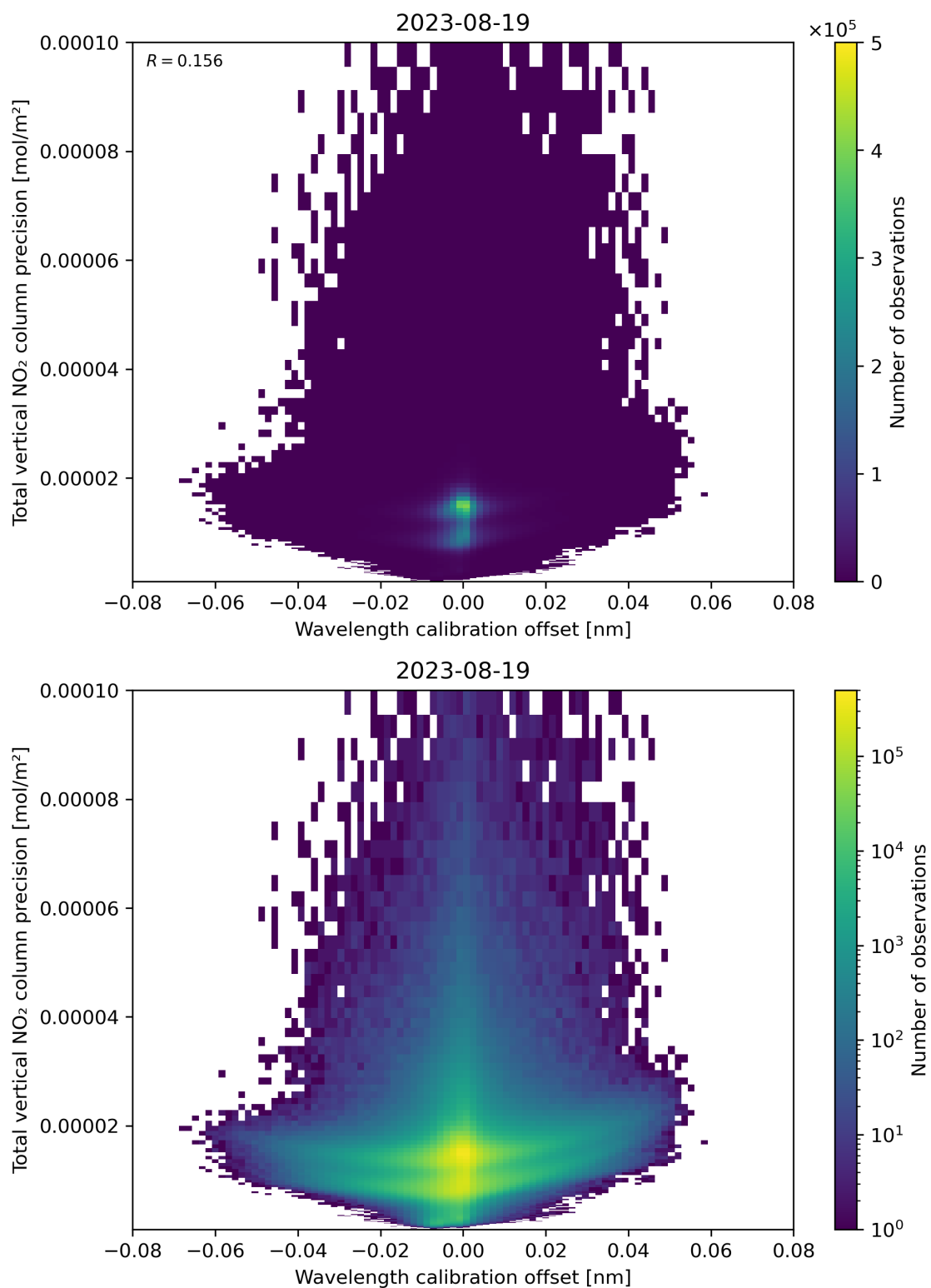
Figure 180: Scatter density plot of “Wavelength calibration offset” against “Total vertical NO 2 column precision” for 2023-08-18 to 2023-08-20.
