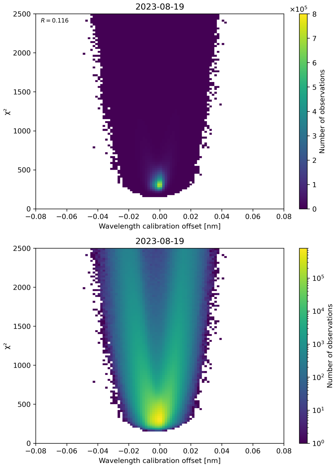
Figure 175: Scatter density plot of “Wavelength calibration offset” against “ \chi^2 ” for 2023-08-18 to 2023-08-20.
