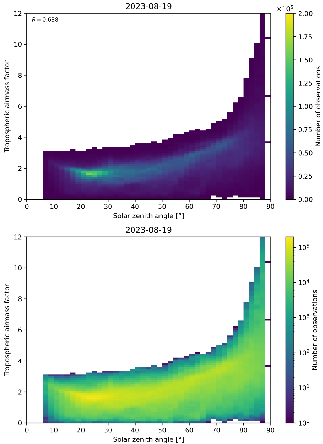
Figure 147: Scatter density plot of “Solar zenith angle” against “Tropospheric airmass factor” for 2023-08-18 to 2023-08-20.
