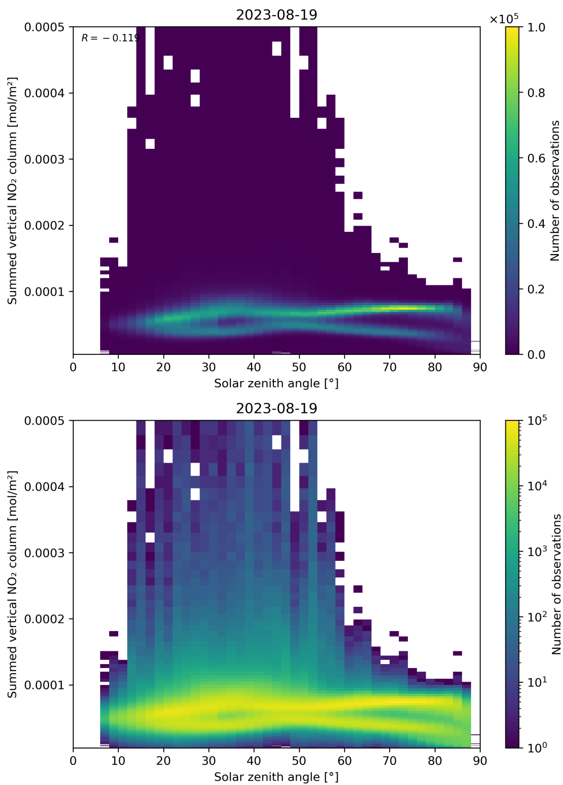
Figure 151: Scatter density plot of “Solar zenith angle” against “Summed vertical NO 2 column” for 2023-08-18 to 2023-08-20.
