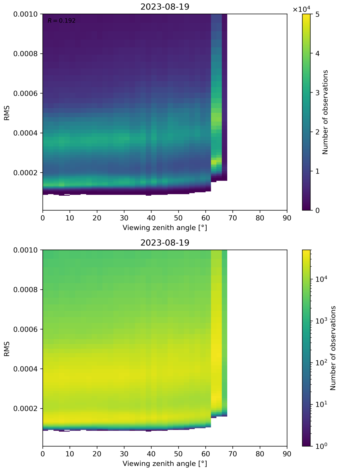
Figure 171: Scatter density plot of “Viewing zenith angle” against “RMS” for 2023-08-18 to 2023-08-20.
