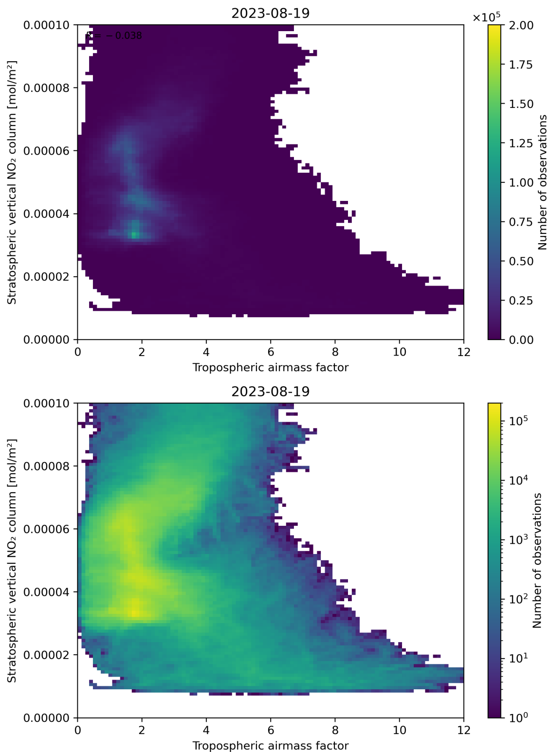
Figure 74: Scatter density plot of “Tropospheric airmass factor” against “Stratospheric vertical NO 2 column” for 2023-08-18 to 2023-08-20.
