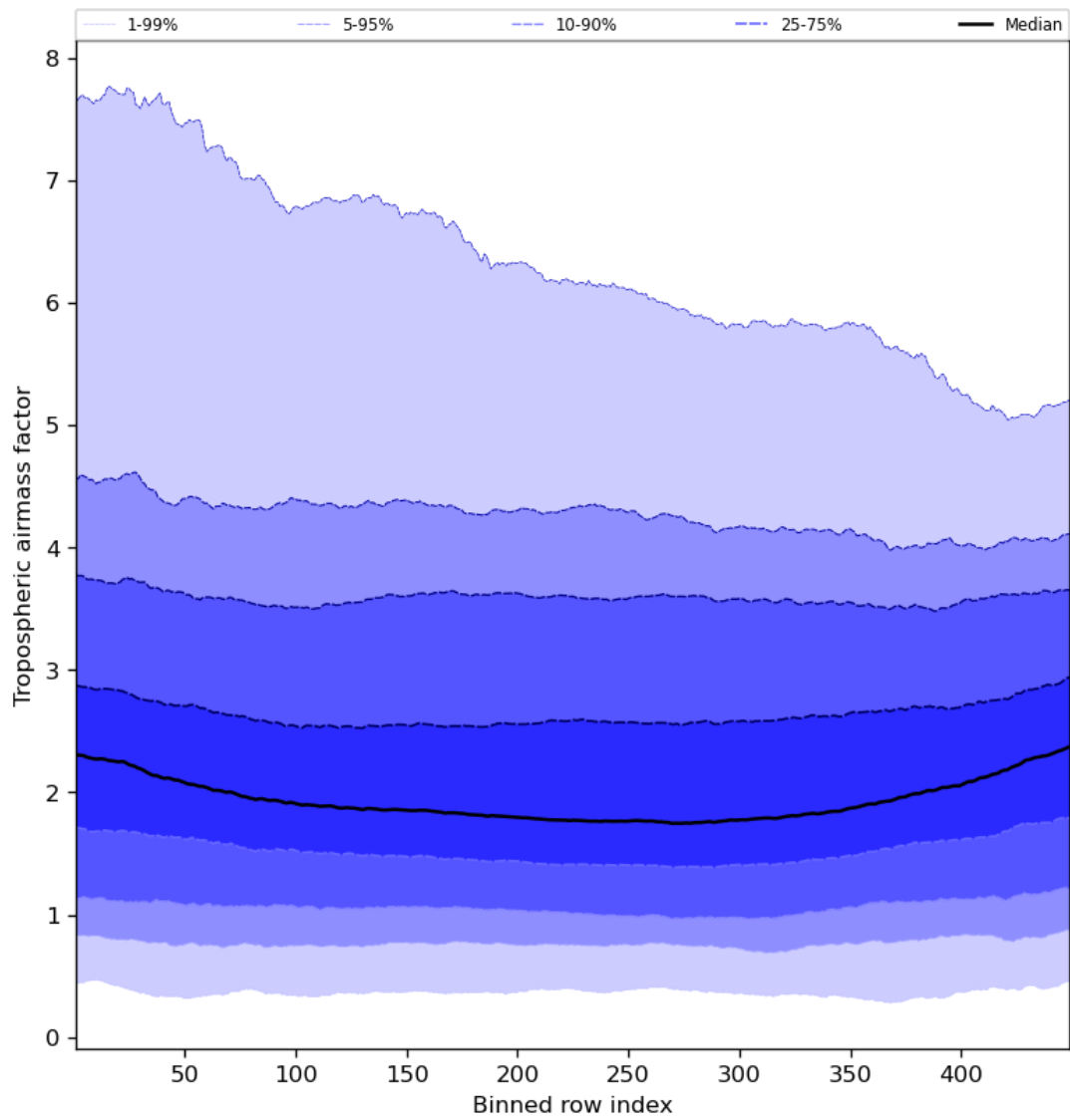
Figure 48: Along track statistics of “Tropospheric airmass factor” for 2023-08-18 to 2023-08-20
