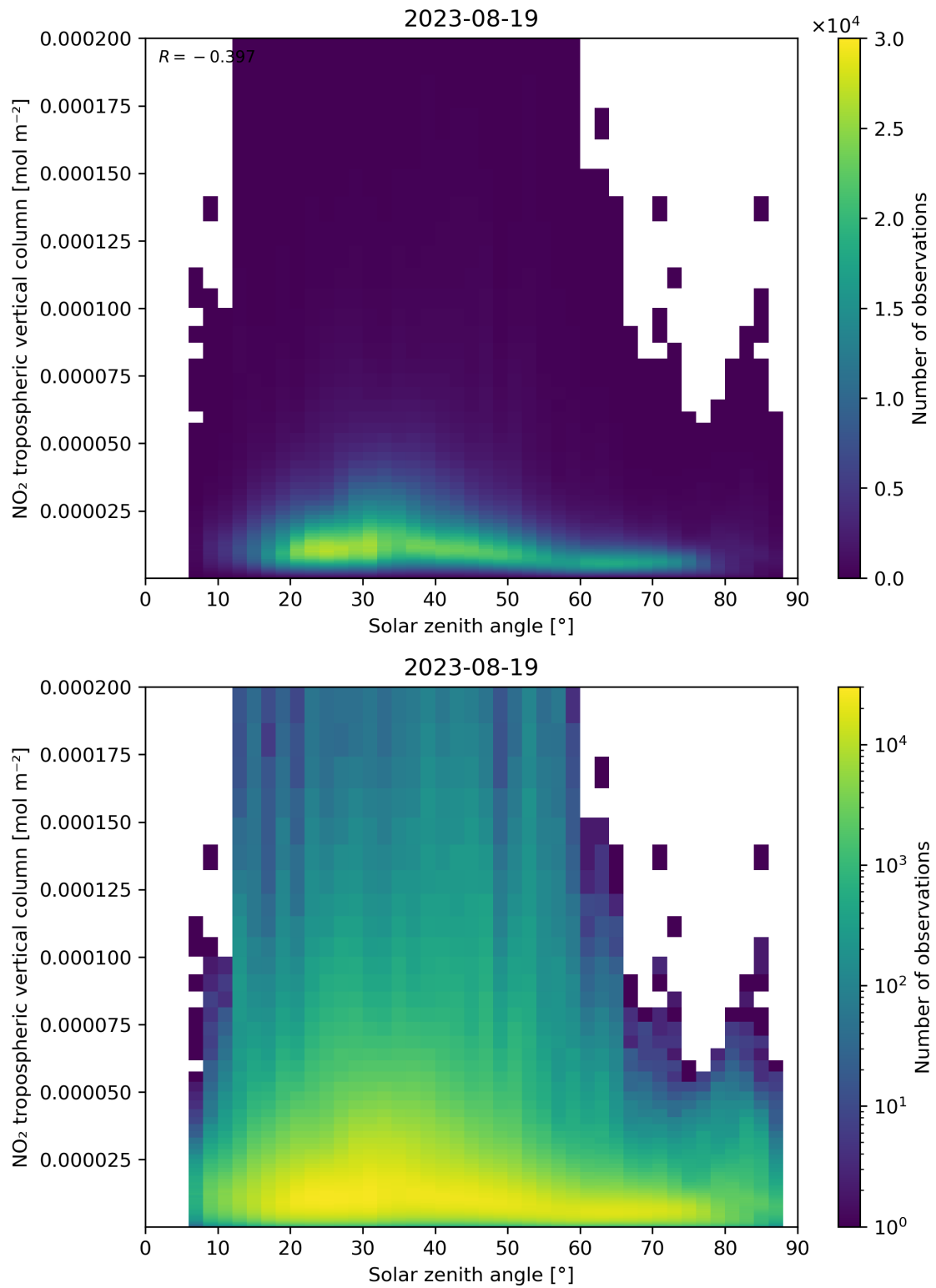
Figure 155: Scatter density plot of “Solar zenith angle” against “NO 2 tropospheric vertical column” for 2023-08-18 to 2023-08-20.
