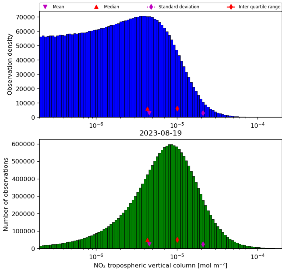
Figure 29: Histogram of “NO 2 tropospheric vertical column” for 2023-08-18 to 2023-08-20
