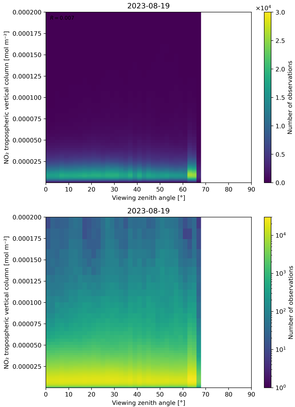
Figure 169: Scatter density plot of “Viewing zenith angle” against “NO 2 tropospheric vertical column” for 2023-08-18 to 2023-08-20.
