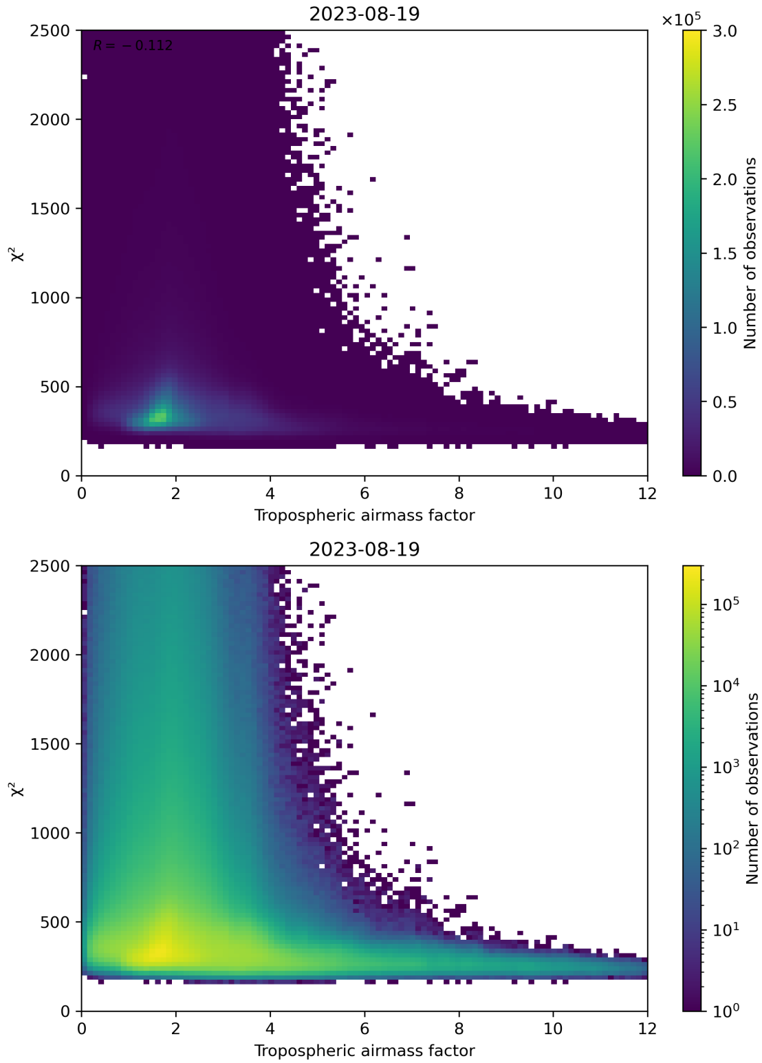
Figure 73: Scatter density plot of “Tropospheric airmass factor” against “ \chi^2 ” for 2023-08-18 to 2023-08-20.
