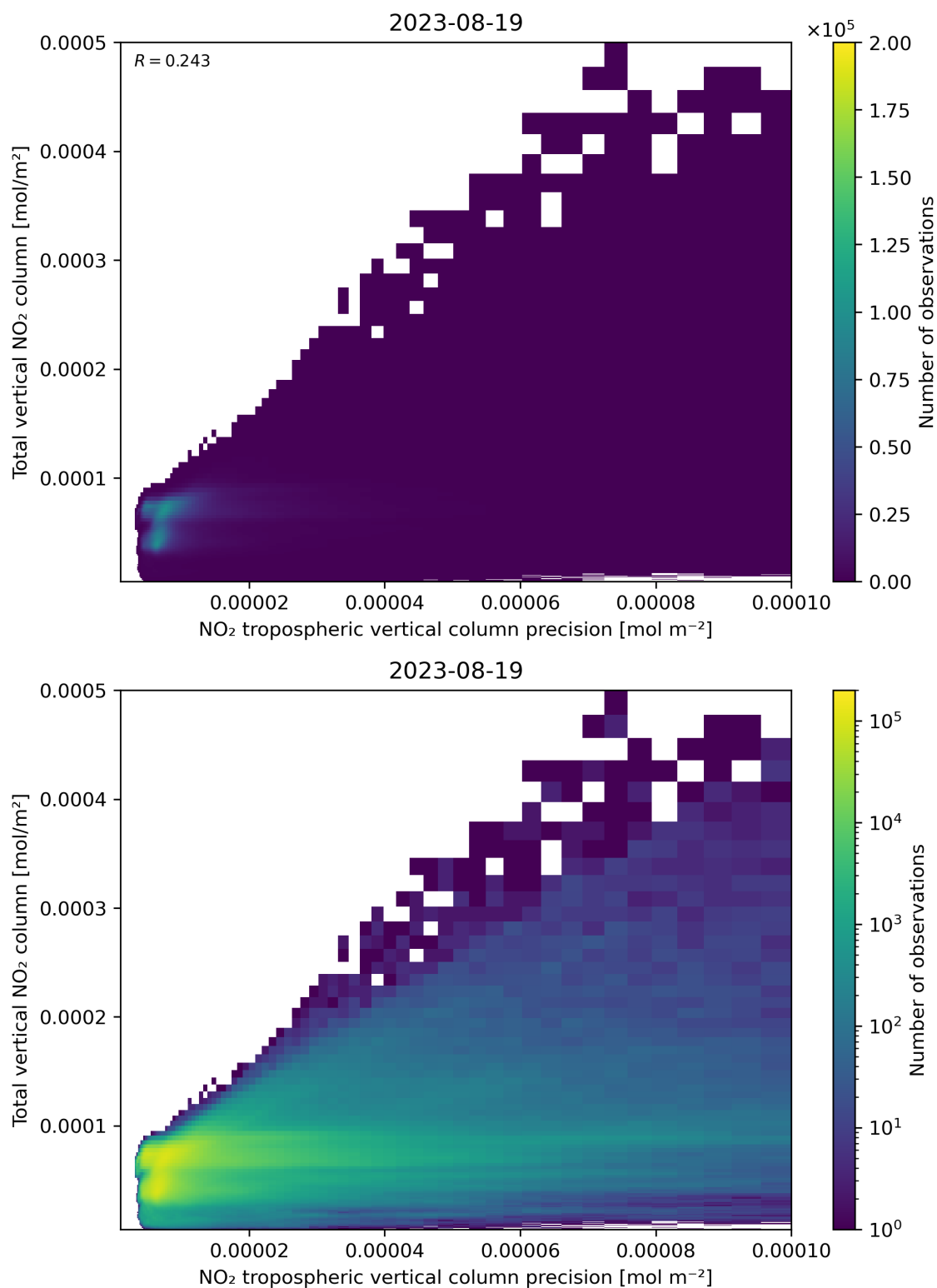
Figure 138: Scatter density plot of “NO 2 tropospheric vertical column precision” against “Total vertical NO 2 column” for 2023-08-18 to 2023-08-20.
