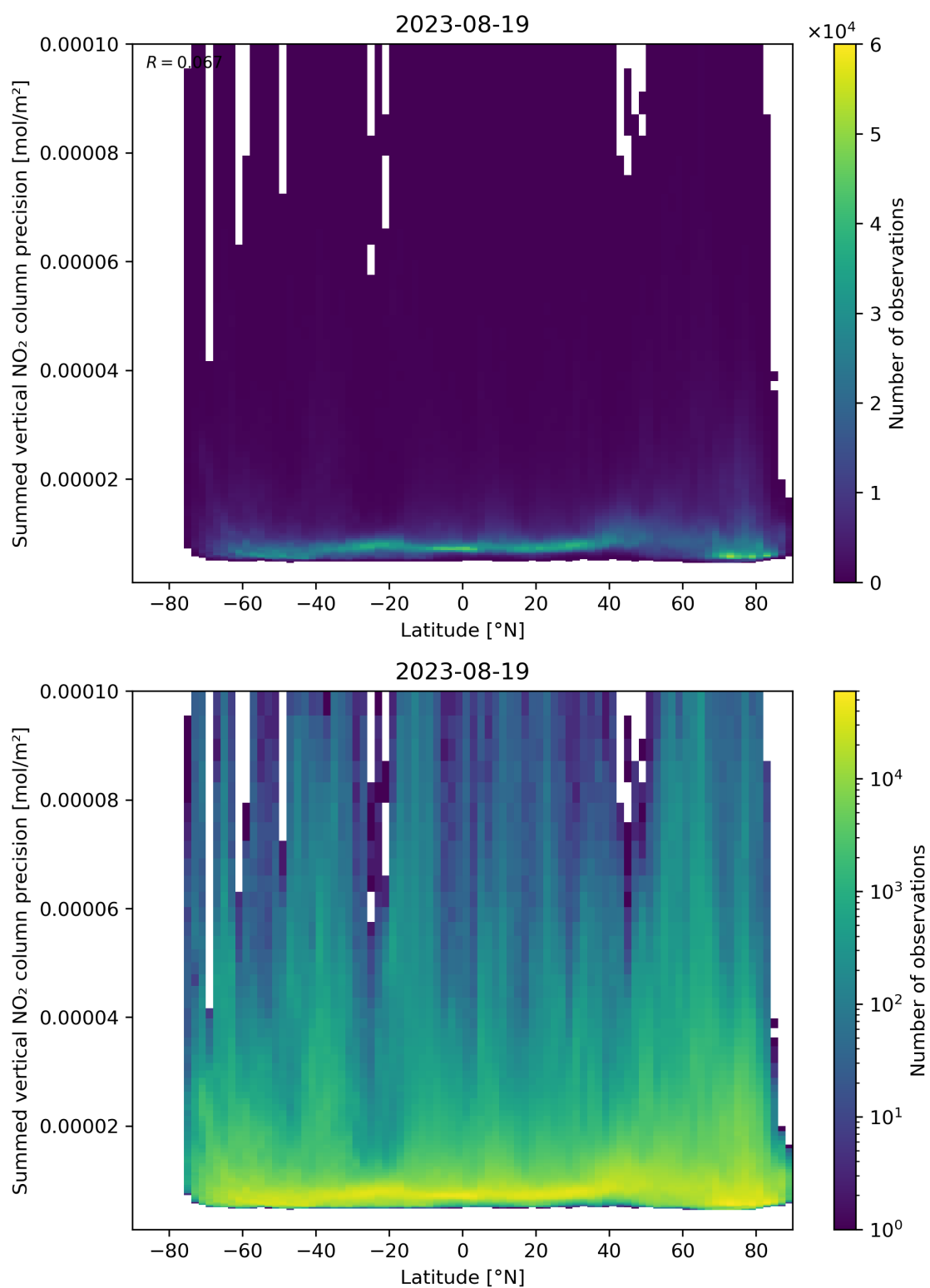
Figure 89: Scatter density plot of “Latitude” against “Summed vertical NO 2 column precision” for 2023-08-18 to 2023-08-20.
