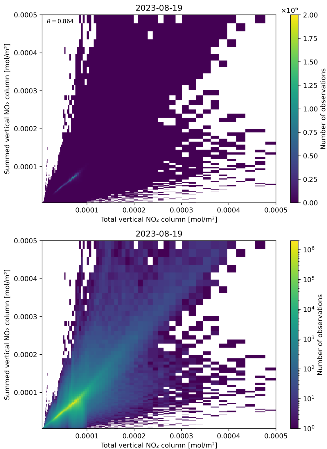
Figure 112: Scatter density plot of “Total vertical NO 2 column” against “Summed vertical NO 2 column” for 2023-08-18 to 2023-08-20.
