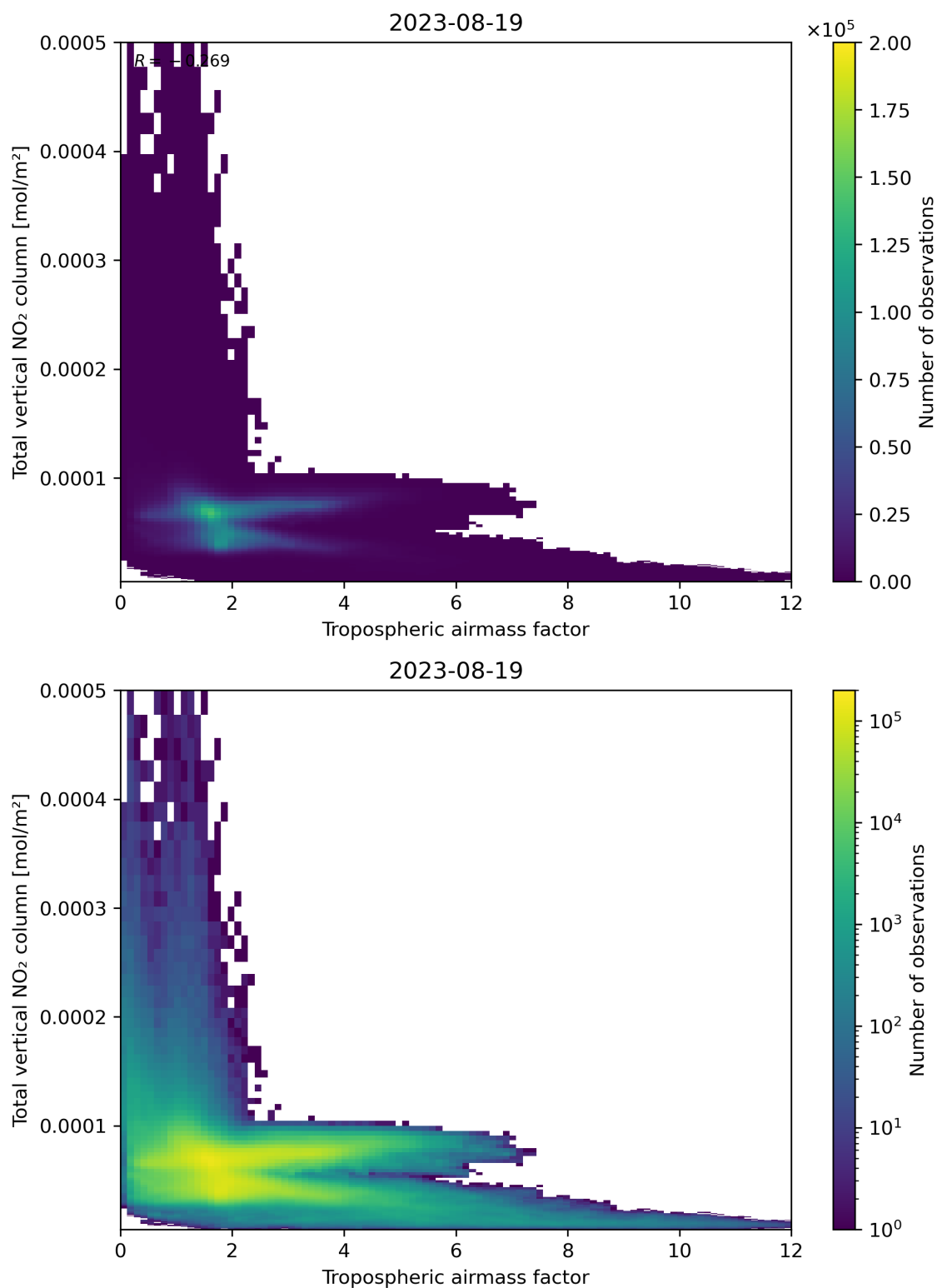
Figure 77: Scatter density plot of “Tropospheric airmass factor” against “Total vertical NO 2 column” for 2023-08-18 to 2023-08-20.
