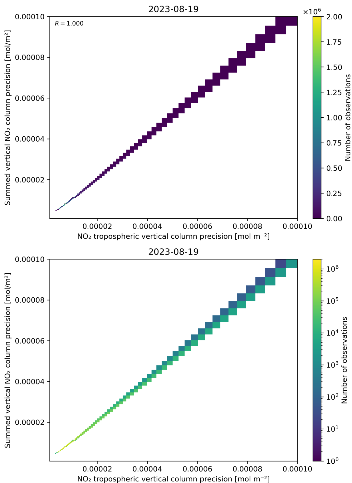
Figure 137: Scatter density plot of “NO 2 tropospheric vertical column precision” against “Summed vertical NO 2 column precision” for 2023-08-18 to 2023-08-20.
