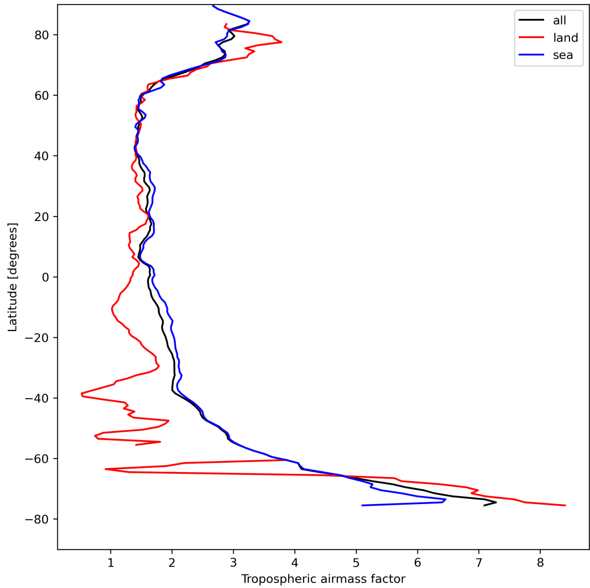
Figure 14: Zonal average of “Tropospheric airmass factor” for 2023-08-18 to 2023-08-20.
