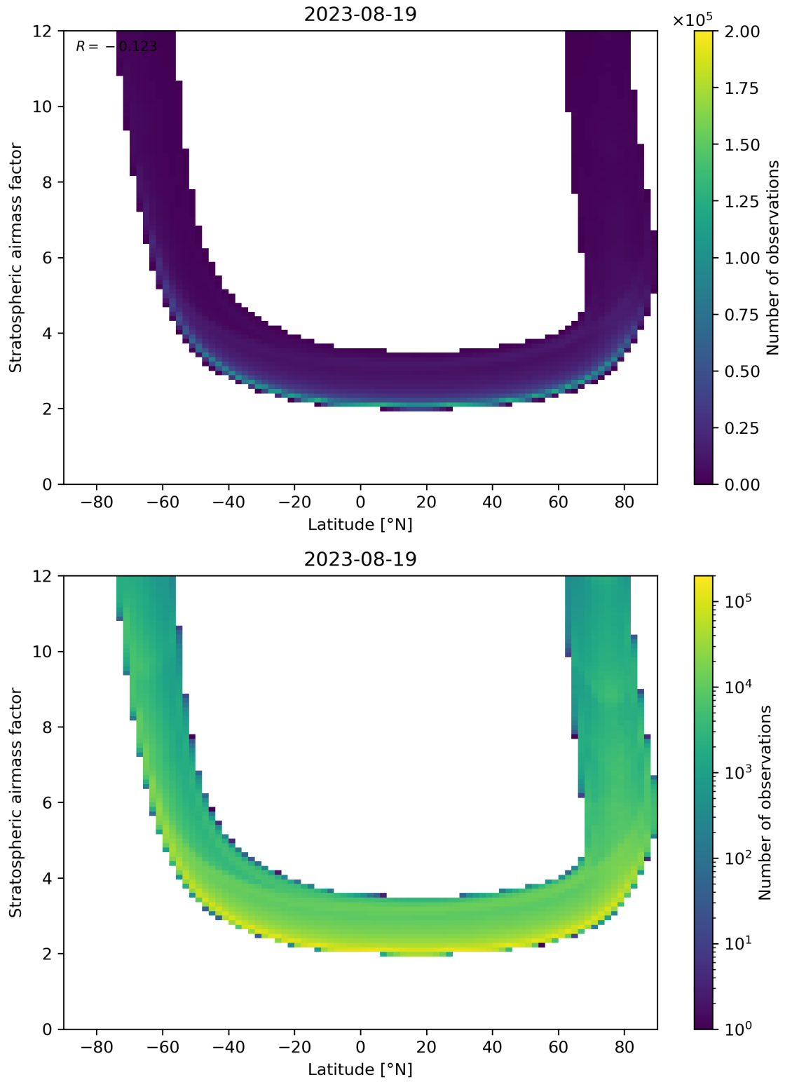
Figure 83: Scatter density plot of “Latitude” against “Stratospheric air mass factor” for 2023-08-18 to 2023-08-20.
