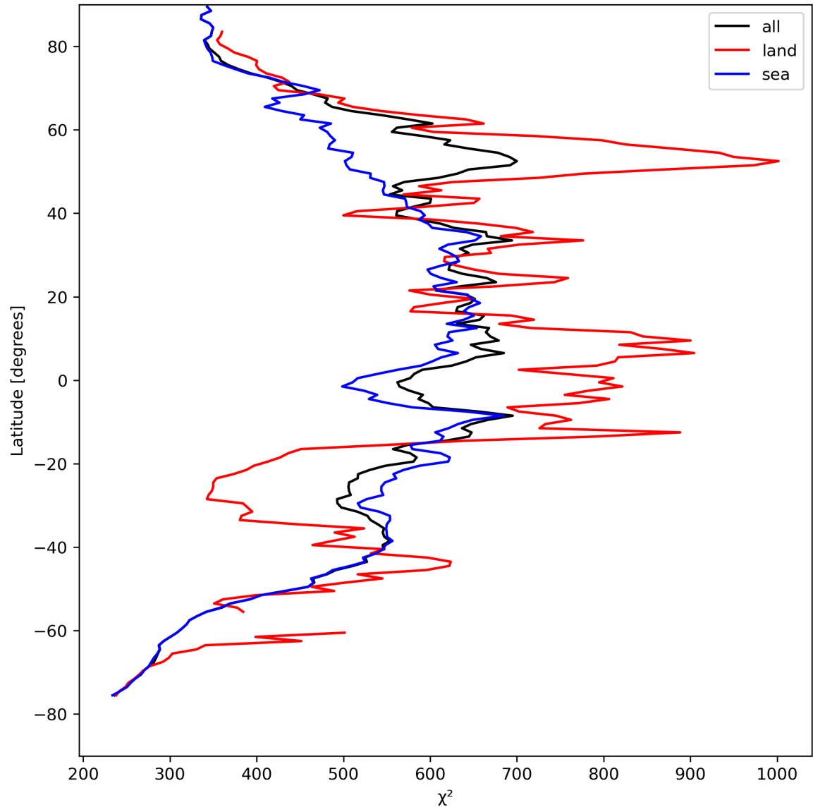
Figure 25: Zonal average of “ \chi^2 ” for 2023-08-18 to 2023-08-20.
