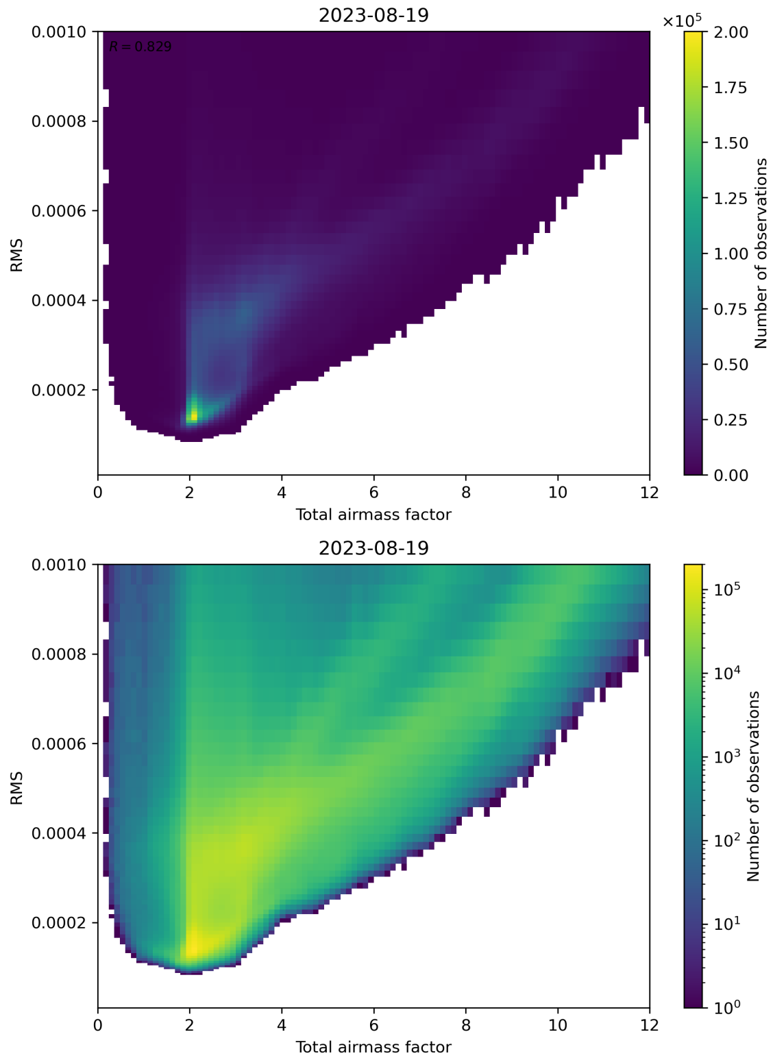
Figure 69: Scatter density plot of “Total airmass factor” against “RMS” for 2023-08-18 to 2023-08-20.
