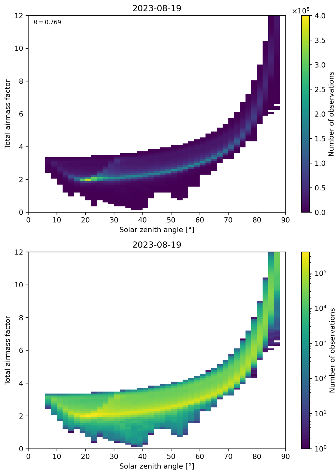
Figure 146: Scatter density plot of “Solar zenith angle” against “Total air mass factor” for 2023-08-18 to 2023-08-20.
