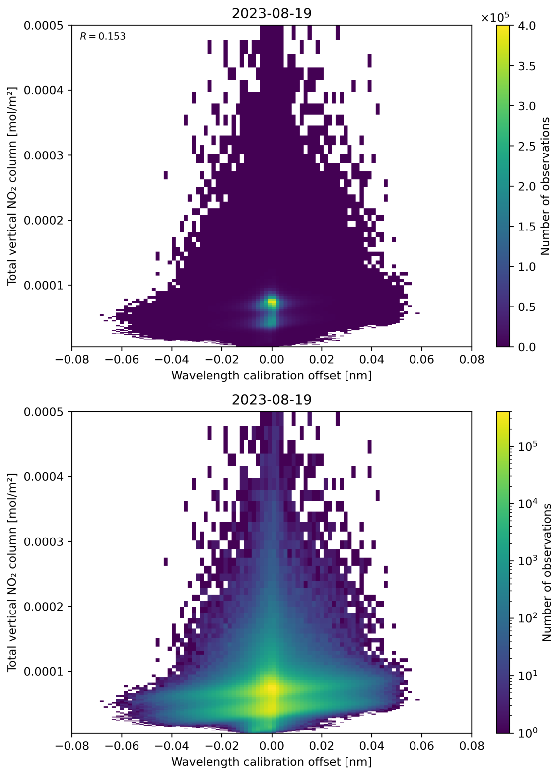
Figure 179: Scatter density plot of “Wavelength calibration offset” against “Total vertical NO 2 column” for 2023-08-18 to 2023-08-20.
