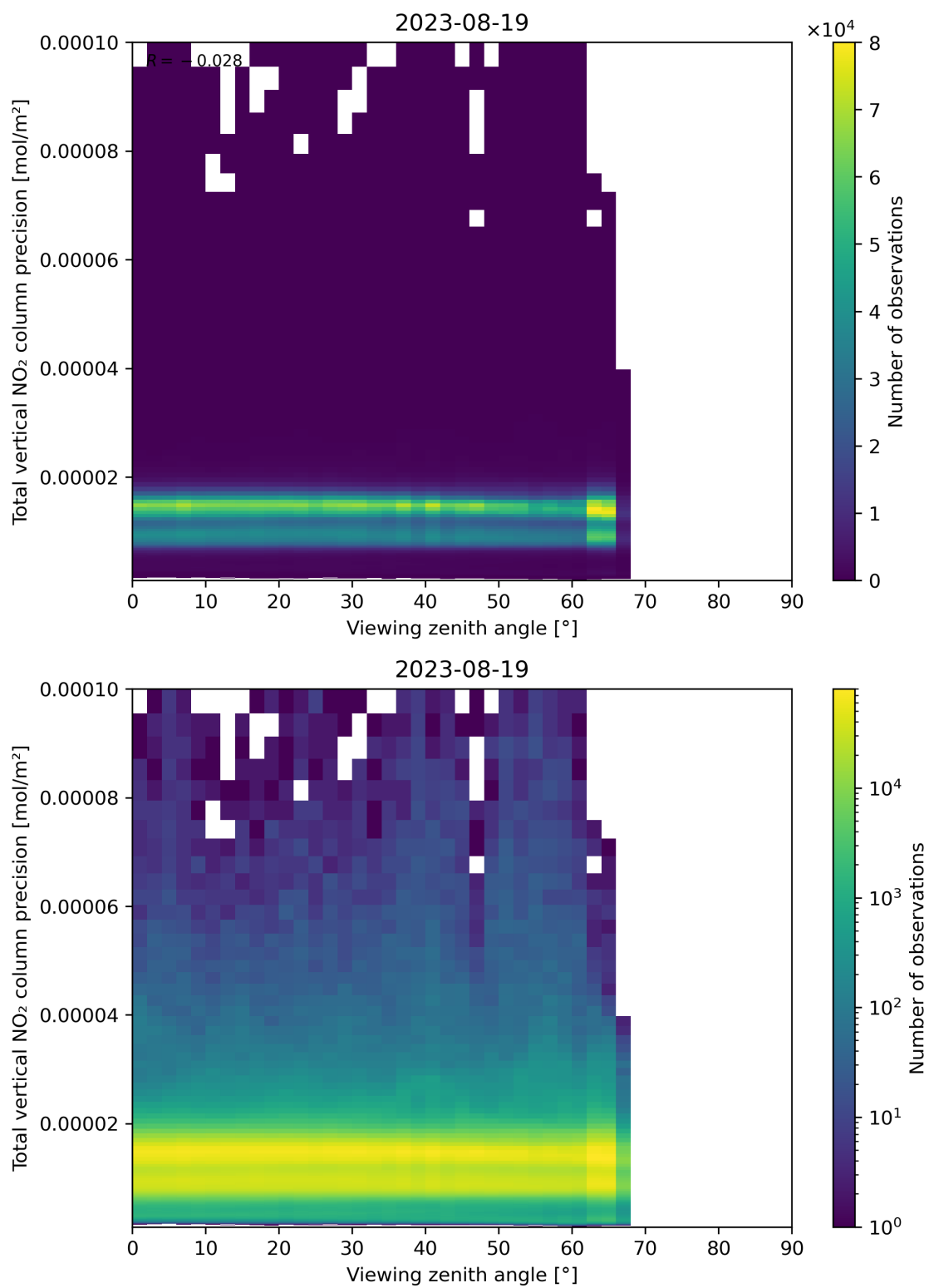
Figure 168: Scatter density plot of “Viewing zenith angle” against “Total vertical NO 2 column precision” for 2023-08-18 to 2023-08-20.
