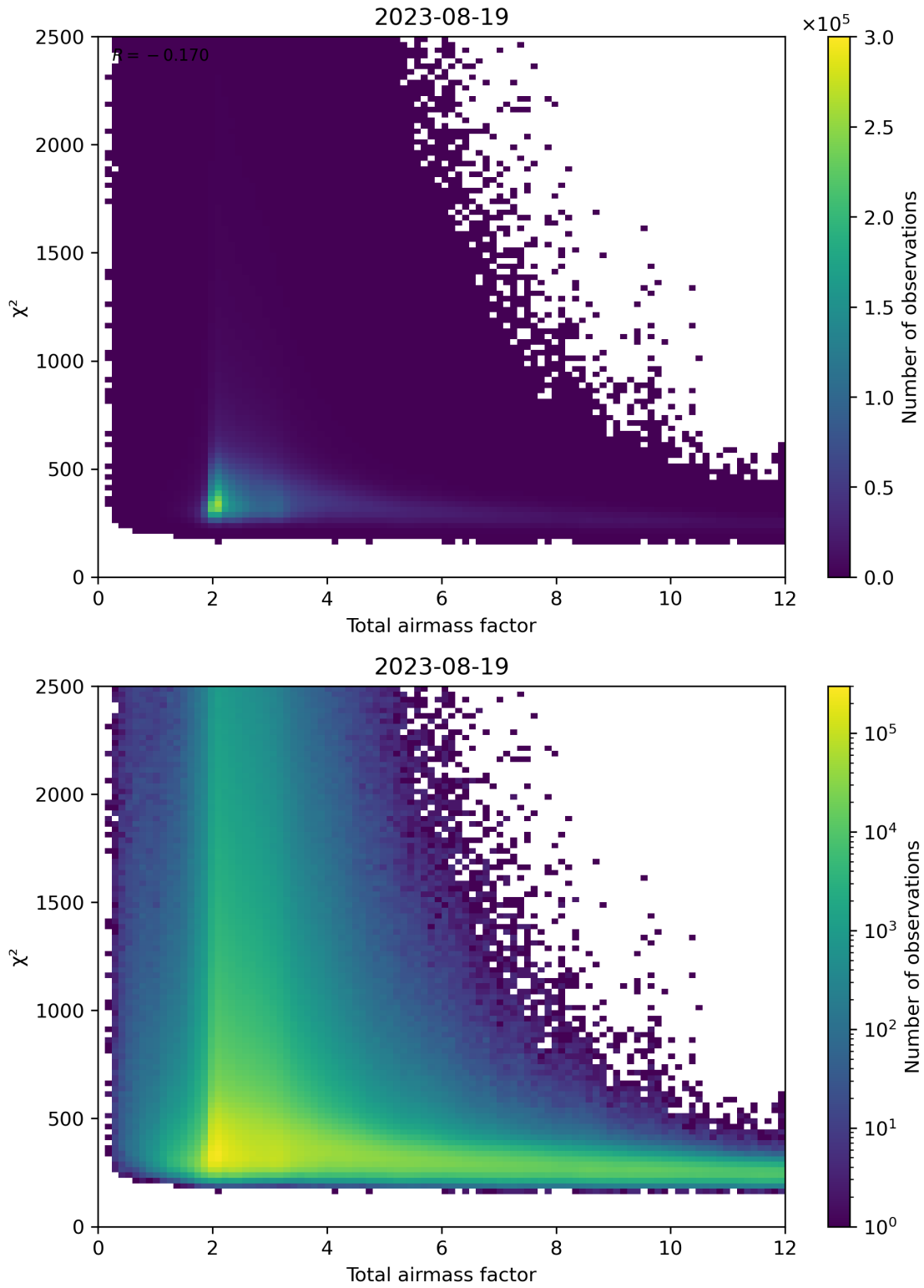
Figure 63: Scatter density plot of “Total airmass factor” against “ \chi^2 ” for 2023-08-18 to 2023-08-20.
