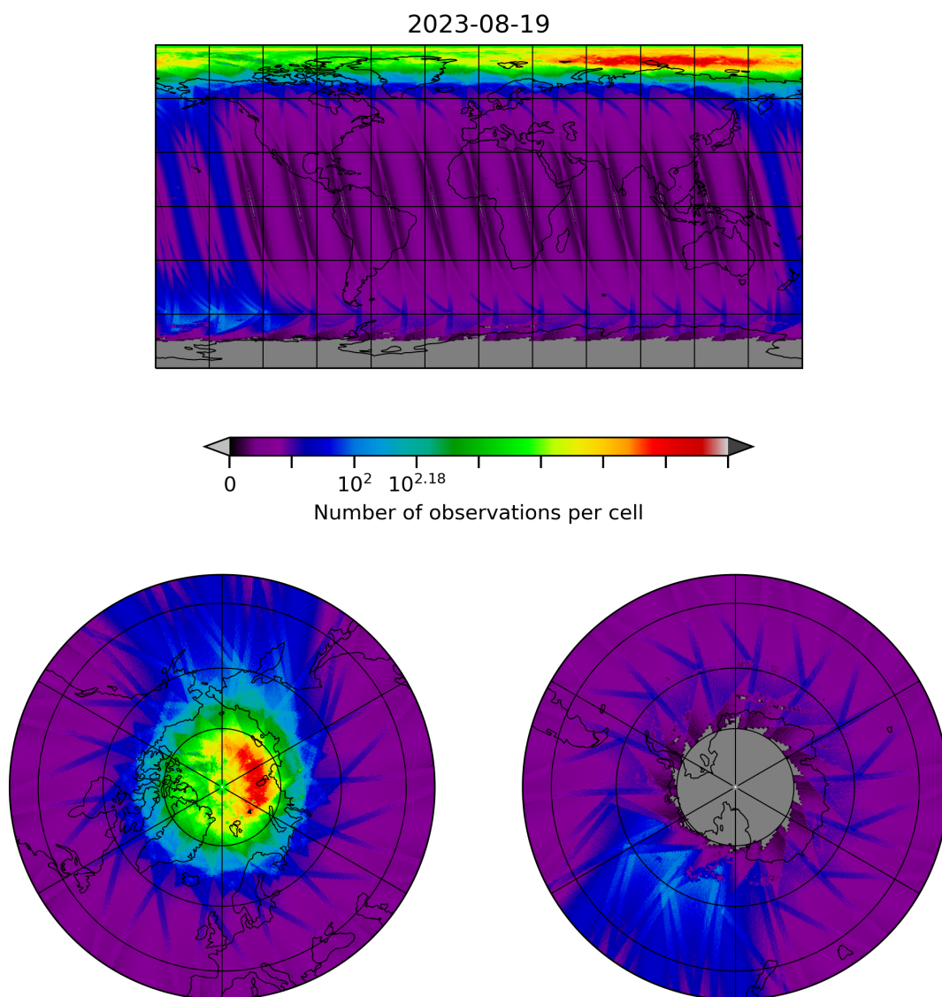
Figure 10: Map of the number of observations for 2023-08-18 to 2023-08-20
