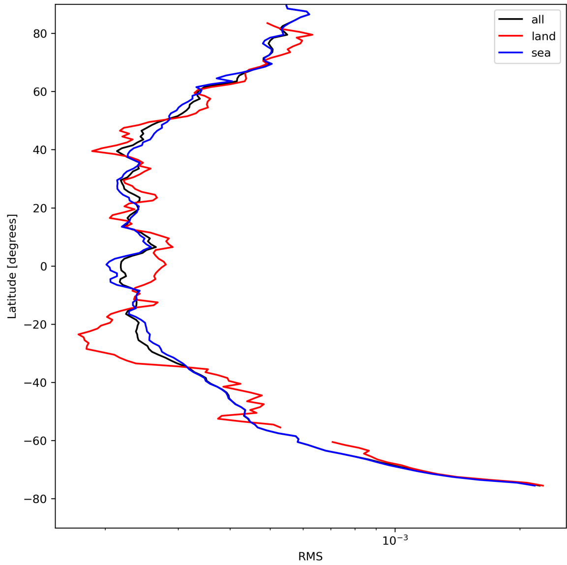
Figure 26: Zonal average of “RMS” for 2023-08-18 to 2023-08-20.
