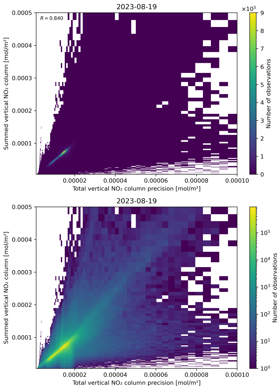
Figure 117: Scatter density plot of “Total vertical NO 2 column precision” against “Summed vertical NO 2 column” for 2023-08-18 to 2023-08-20.
