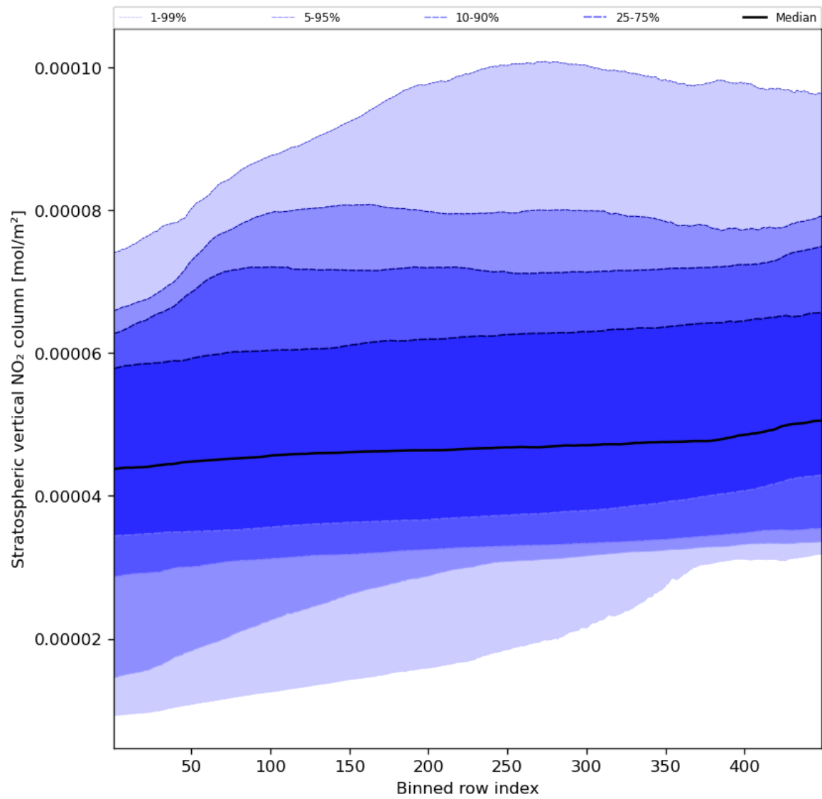
Figure 53: Along track statistics of “Stratospheric vertical NO 2 column” for 2023-08-18 to 2023-08-20
