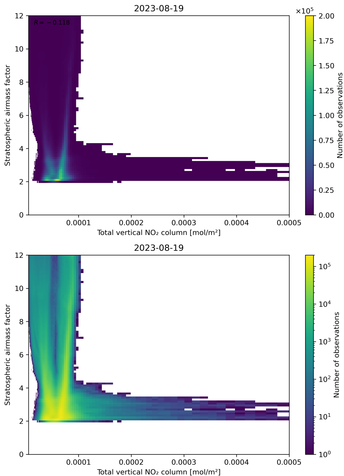
Figure 110: Scatter density plot of “Total vertical NO 2 column” against “Stratospheric airmass factor” for 2023-08-18 to 2023-08-20.
