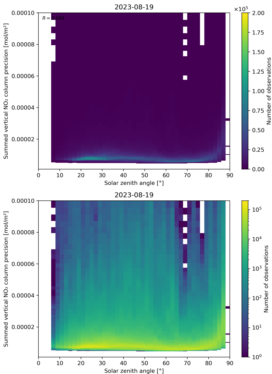
Figure 152: Scatter density plot of “Solar zenith angle” against “Summed vertical NO 2 column precision” for 2023-08-18 to 2023-08-20.
