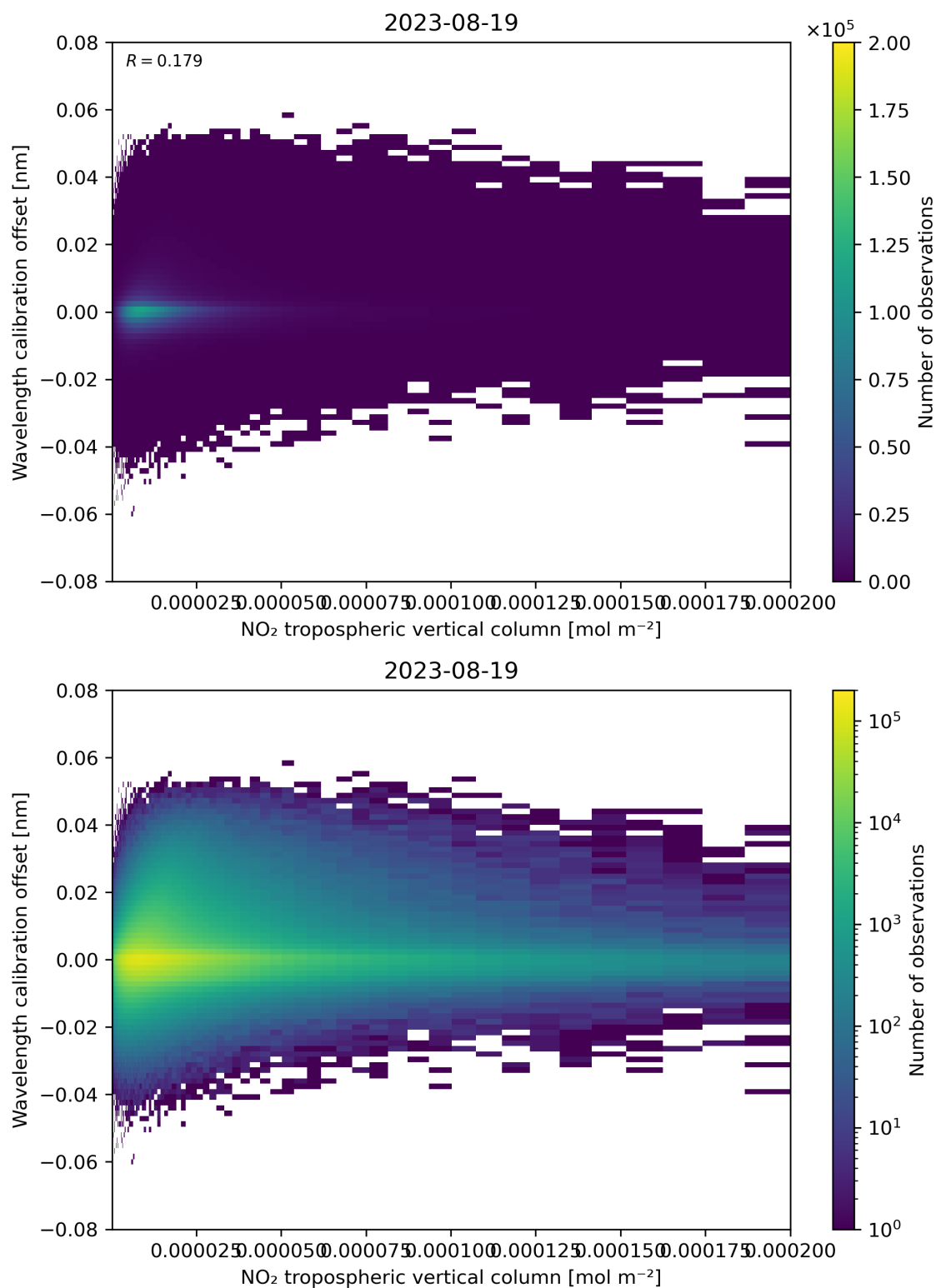
Figure 143: Scatter density plot of “NO 2 tropospheric vertical column” against “Wavelength calibration offset” for 2023-08-18 to 2023-08-20.
