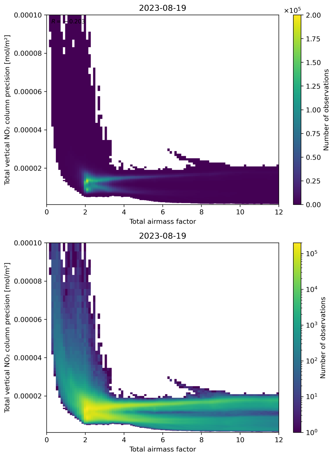
Figure 68: Scatter density plot of “Total airmass factor” against “Total vertical NO 2 column precision” for 2023-08-18 to 2023-08-20.
