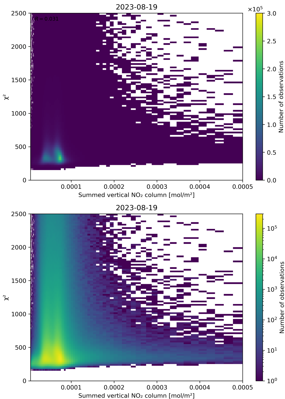
Figure 104: Scatter density plot of “Summed vertical NO 2 column” against “ \chi^2 ” for 2023-08-18 to 2023-08-20.
