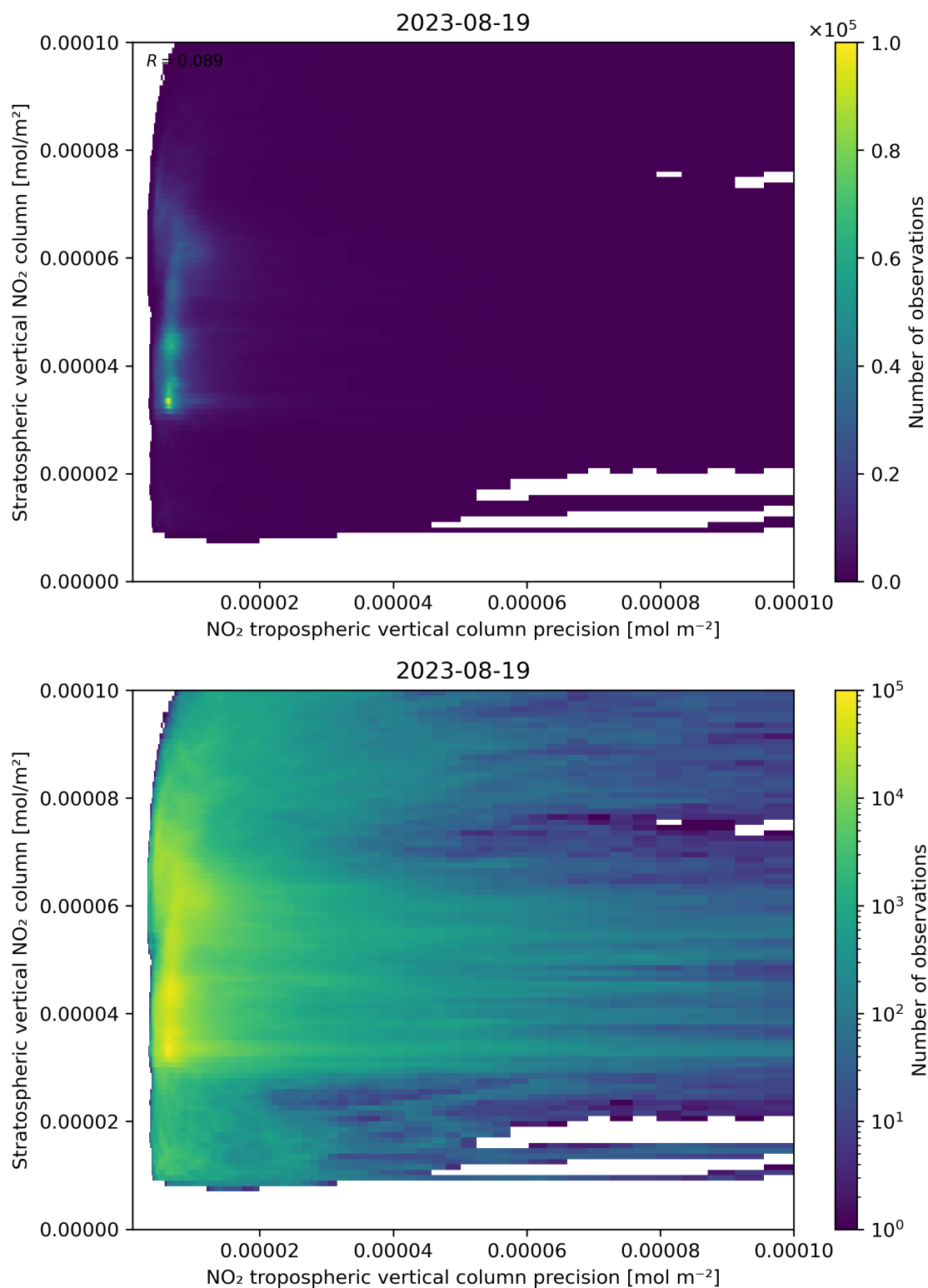
Figure 135: Scatter density plot of “NO 2 tropospheric vertical column precision” against “Stratospheric vertical NO 2 column” for 2023-08-18 to 2023-08-20.
