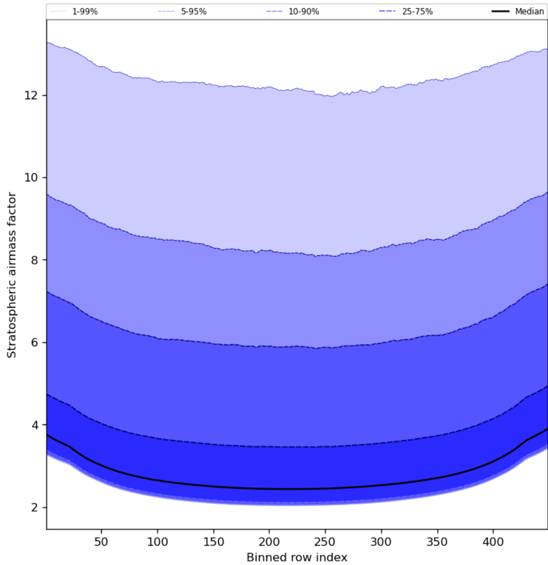
Figure 61: Along track statistics of “Stratospheric air mass factor” for 2023-08-18 to 2023-08-20
