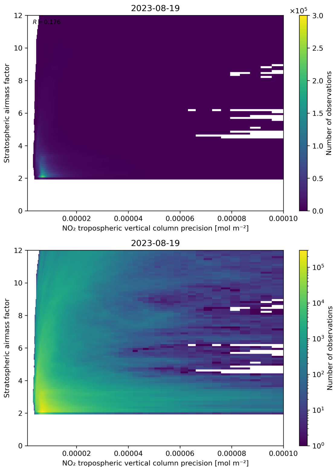
Figure 131: Scatter density plot of “NO 2 tropospheric vertical column precision” against “Stratospheric airmass factor” for 2023-08-18 to 2023-08-20.
