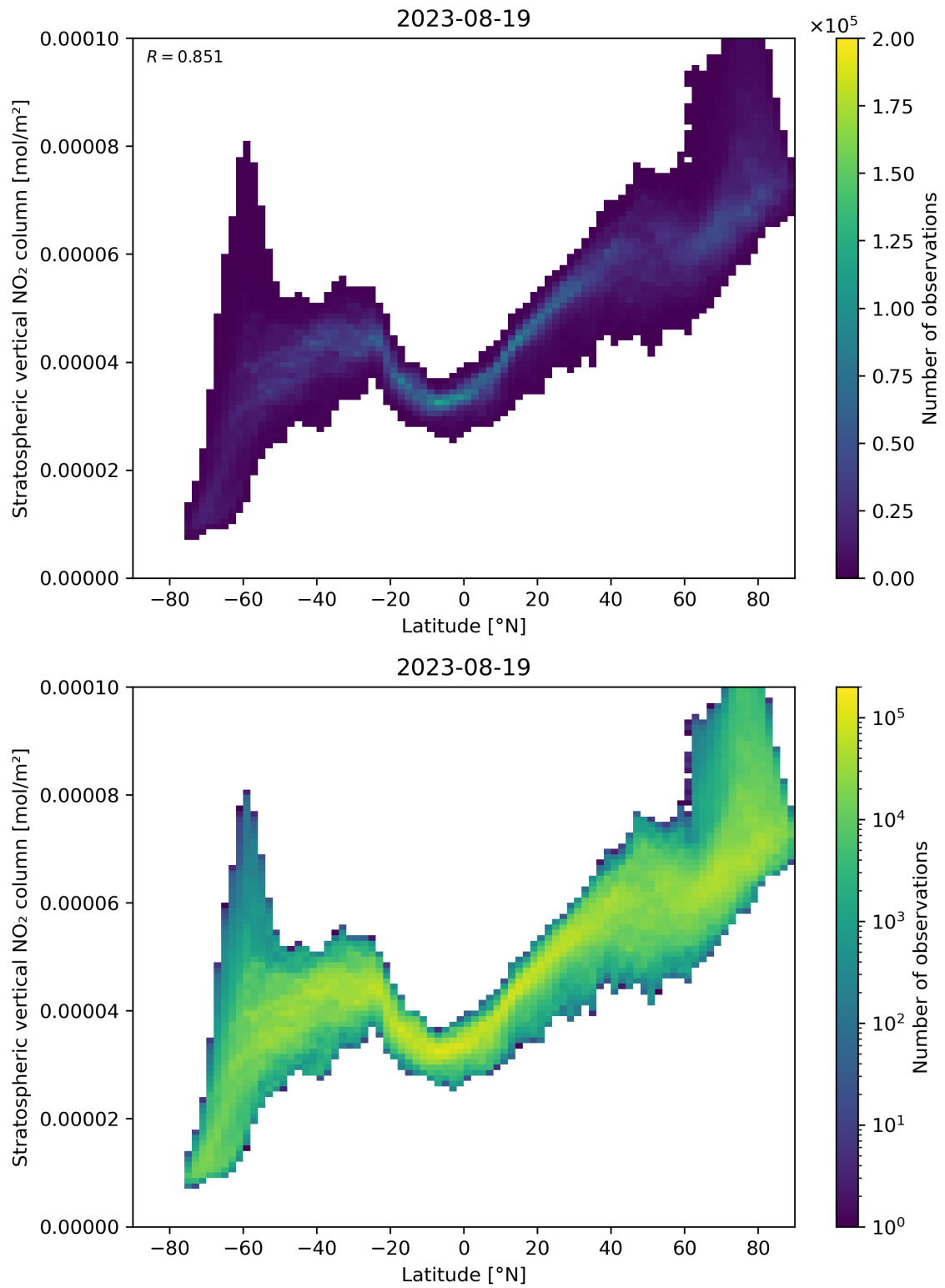
Figure 87: Scatter density plot of “Latitude” against “Stratospheric vertical NO 2 column” for 2023-08-18 to 2023-08-20.
