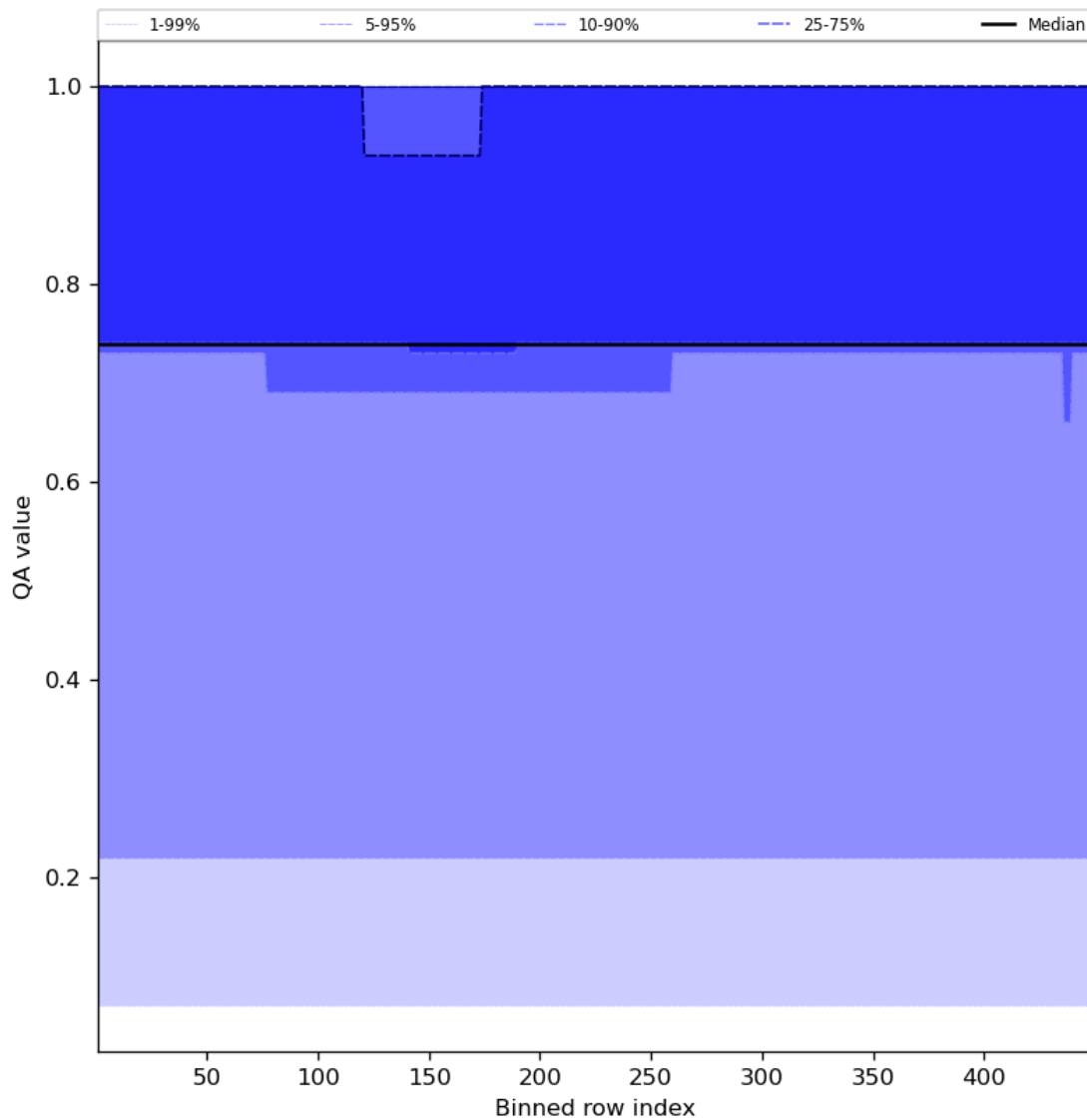
Figure 45: Along track statistics of “QA value” for 2023-08-18 to 2023-08-20
