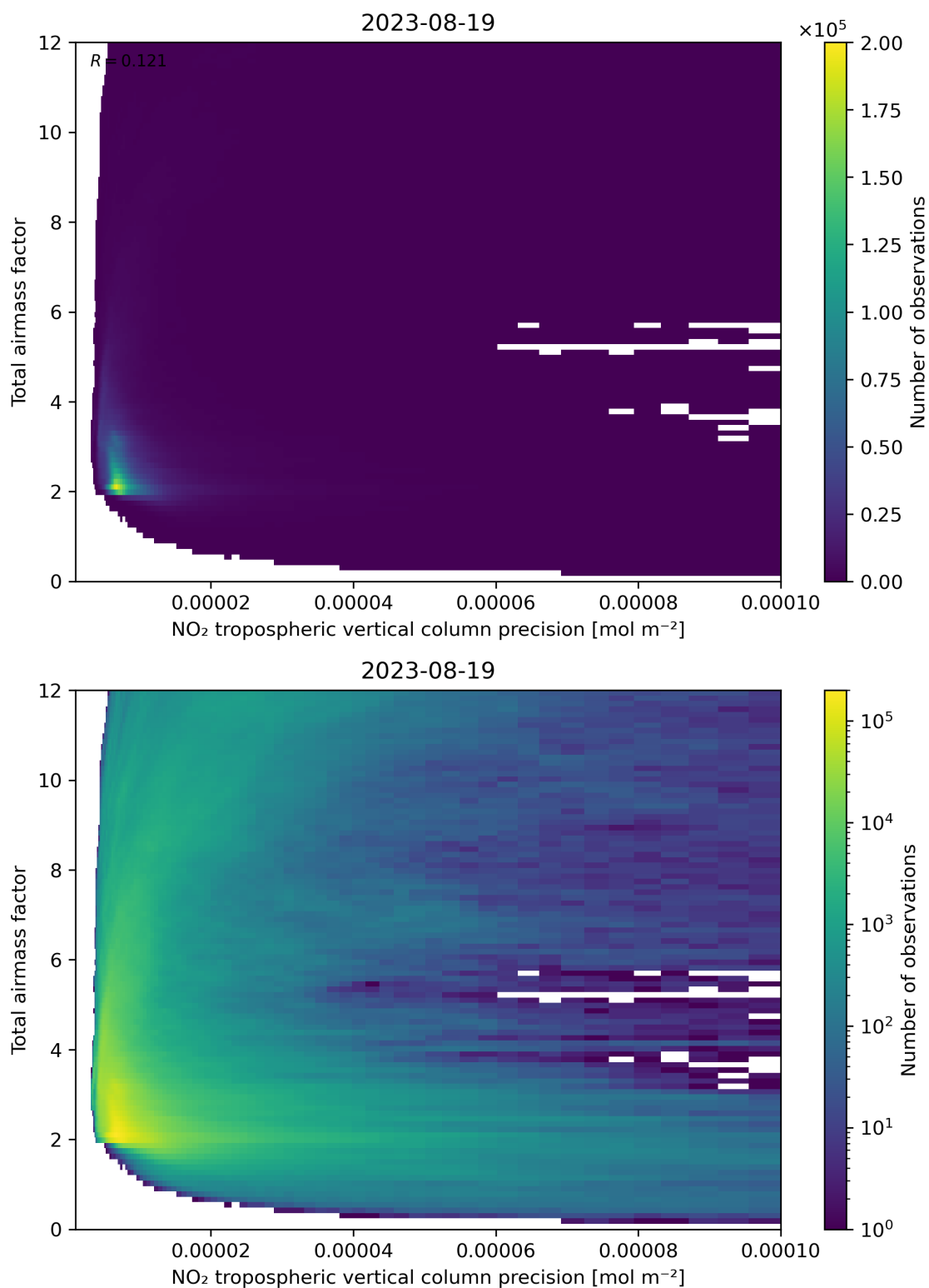
Figure 132: Scatter density plot of “NO 2 tropospheric vertical column precision” against “Total air mass factor” for 2023-08-18 to 2023-08-20.
