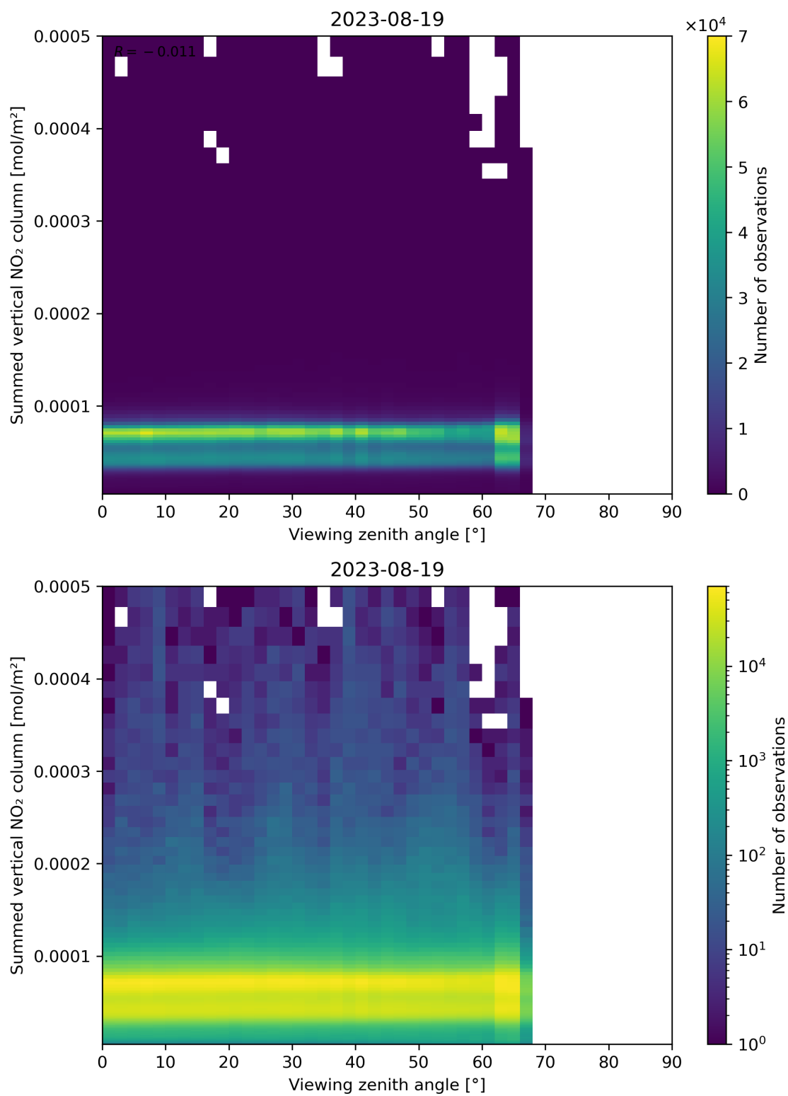
Figure 165: Scatter density plot of “Viewing zenith angle” against “Summed vertical NO 2 column” for 2023-08-18 to 2023-08-20.
