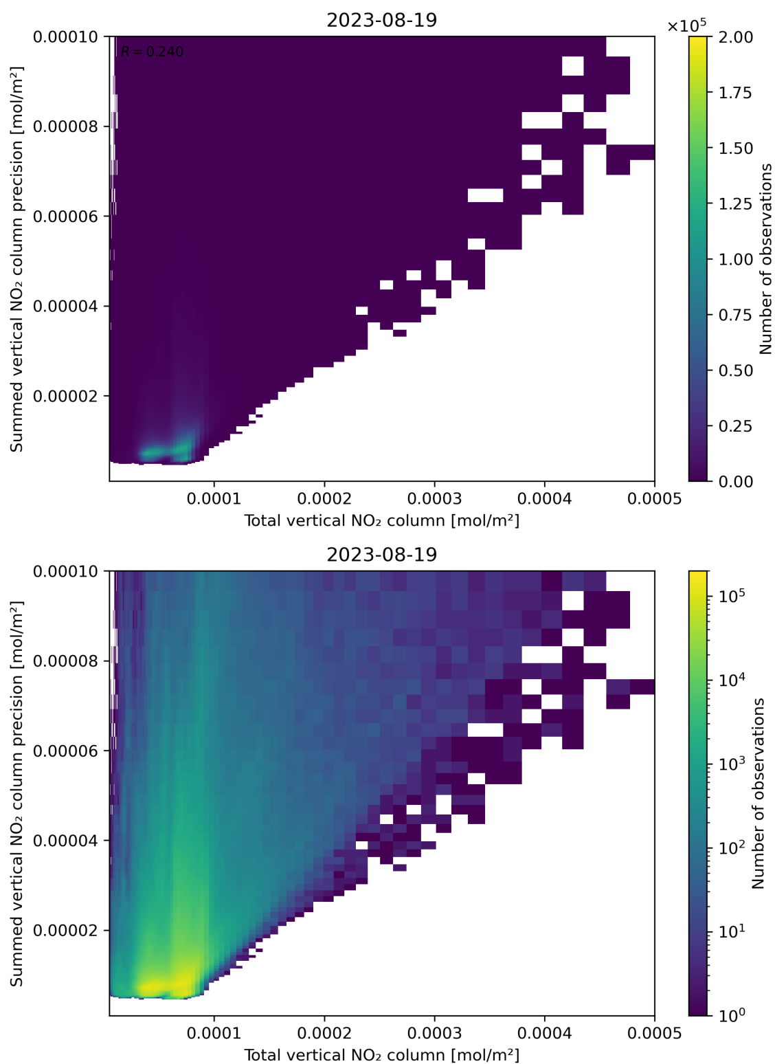
Figure 113: Scatter density plot of “Total vertical NO 2 column” against “Summed vertical NO 2 column precision” for 2023-08-18 to 2023-08-20.
