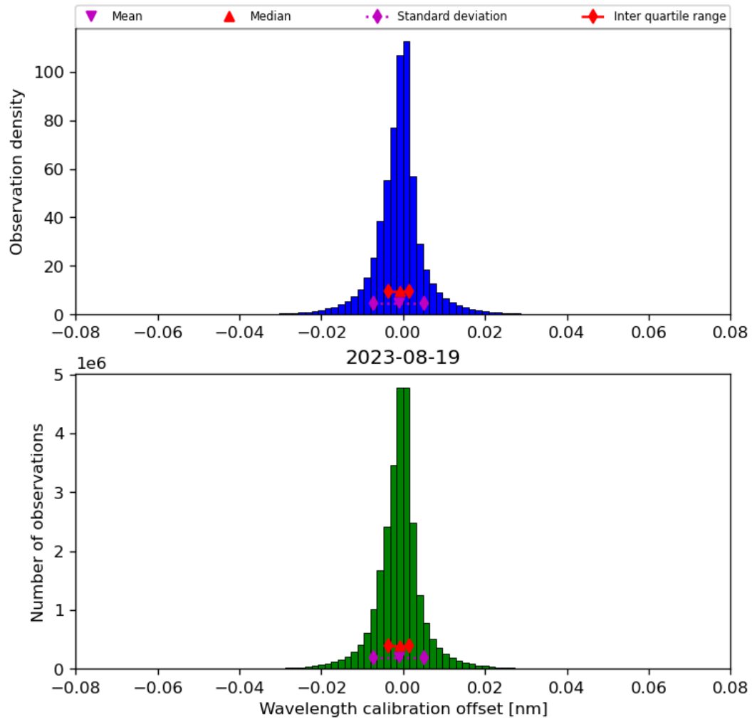
Figure 35: Histogram of “Wavelength calibration offset” for 2023-08-18 to 2023-08-20
