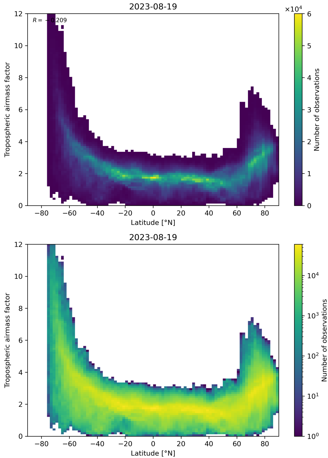
Figure 85: Scatter density plot of “Latitude” against “Tropospheric air mass factor” for 2023-08-18 to 2023-08-20.
