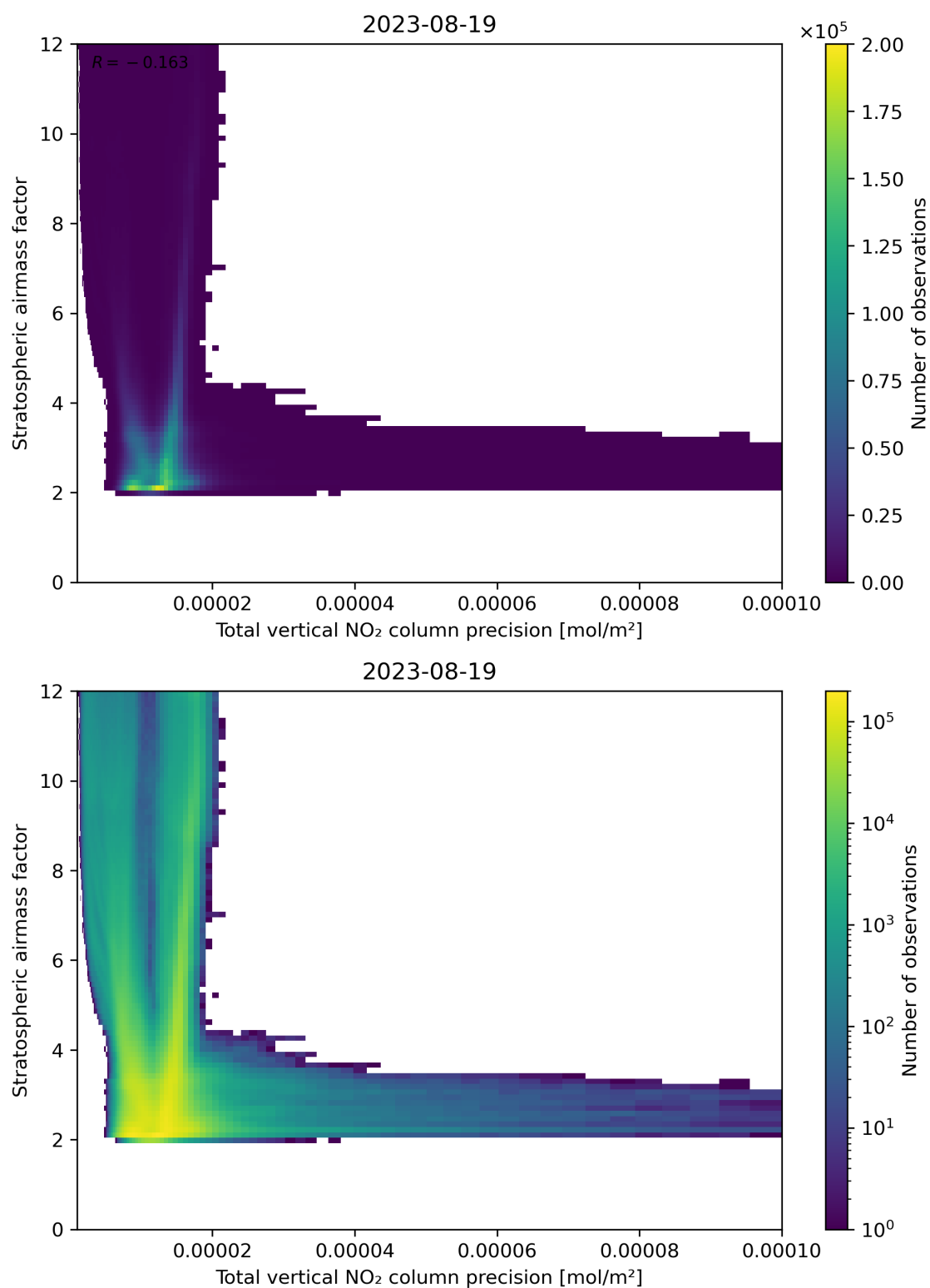
Figure 115: Scatter density plot of “Total vertical NO 2 column precision” against “Stratospheric airmass factor” for 2023-08-18 to 2023-08-20.
