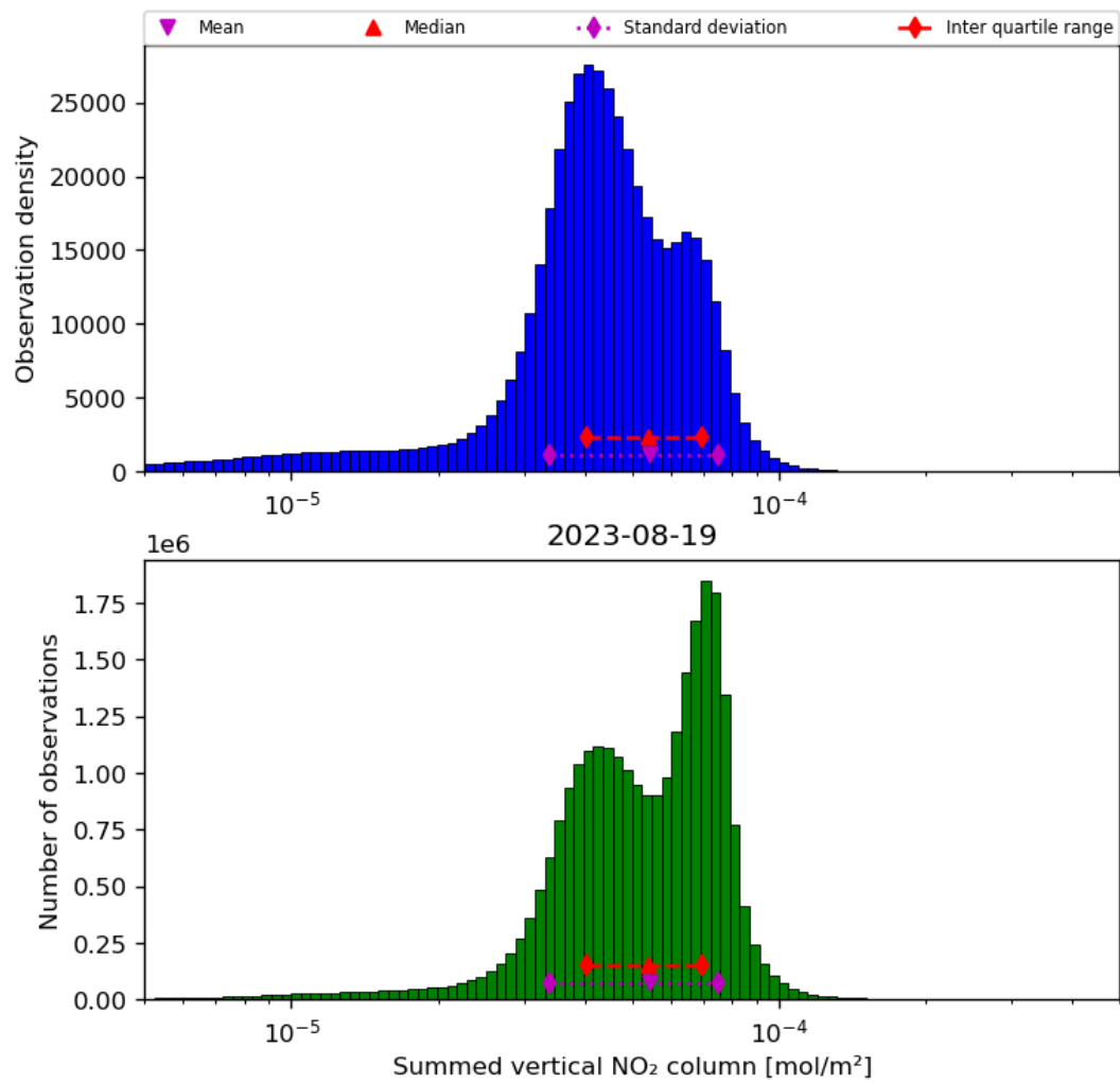
Figure 40: Histogram of “Summed vertical NO 2 column” for 2023-08-18 to 2023-08-20
