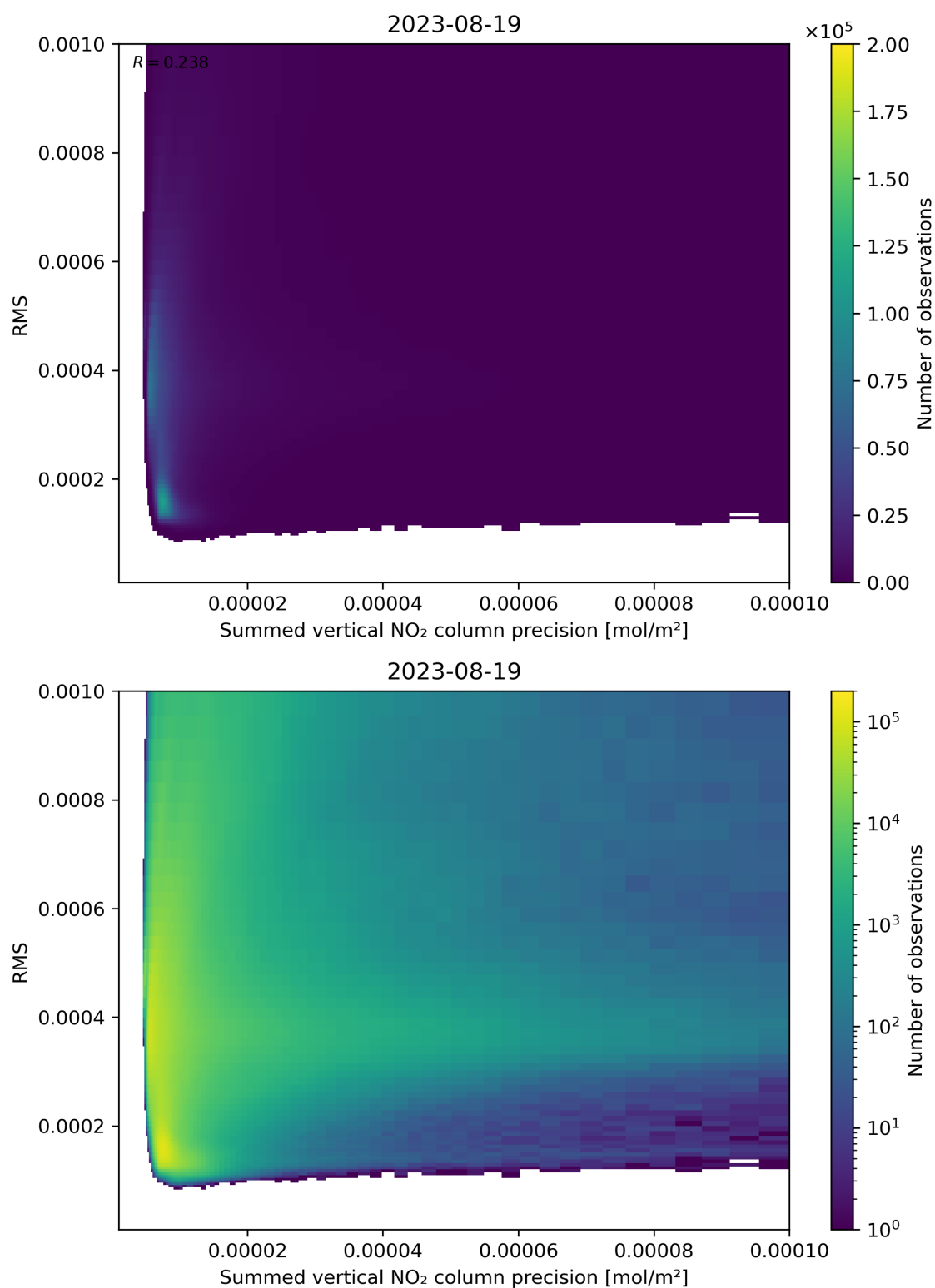
Figure 108: Scatter density plot of “Summed vertical NO 2 column precision” against “RMS” for 2023-08-18 to 2023-08-20.
