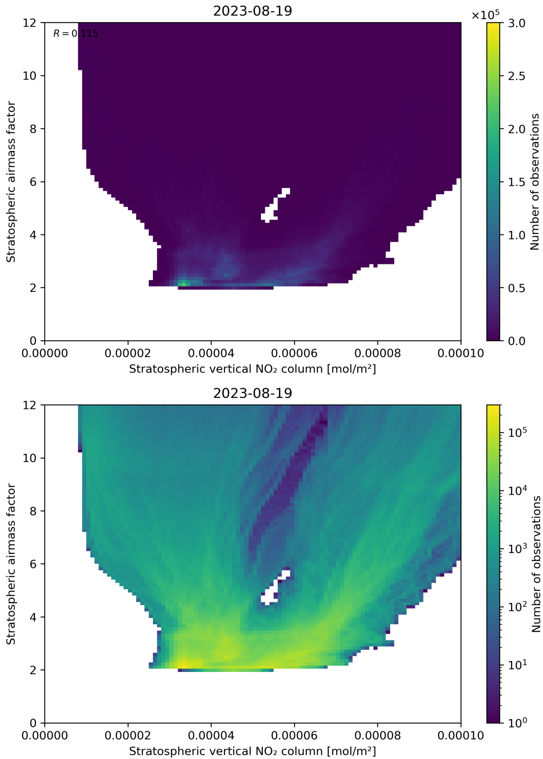
Figure 96: Scatter density plot of “Stratospheric vertical NO 2 column” against “Stratospheric airmass factor” for 2023-08-18 to 2023-08-20.
