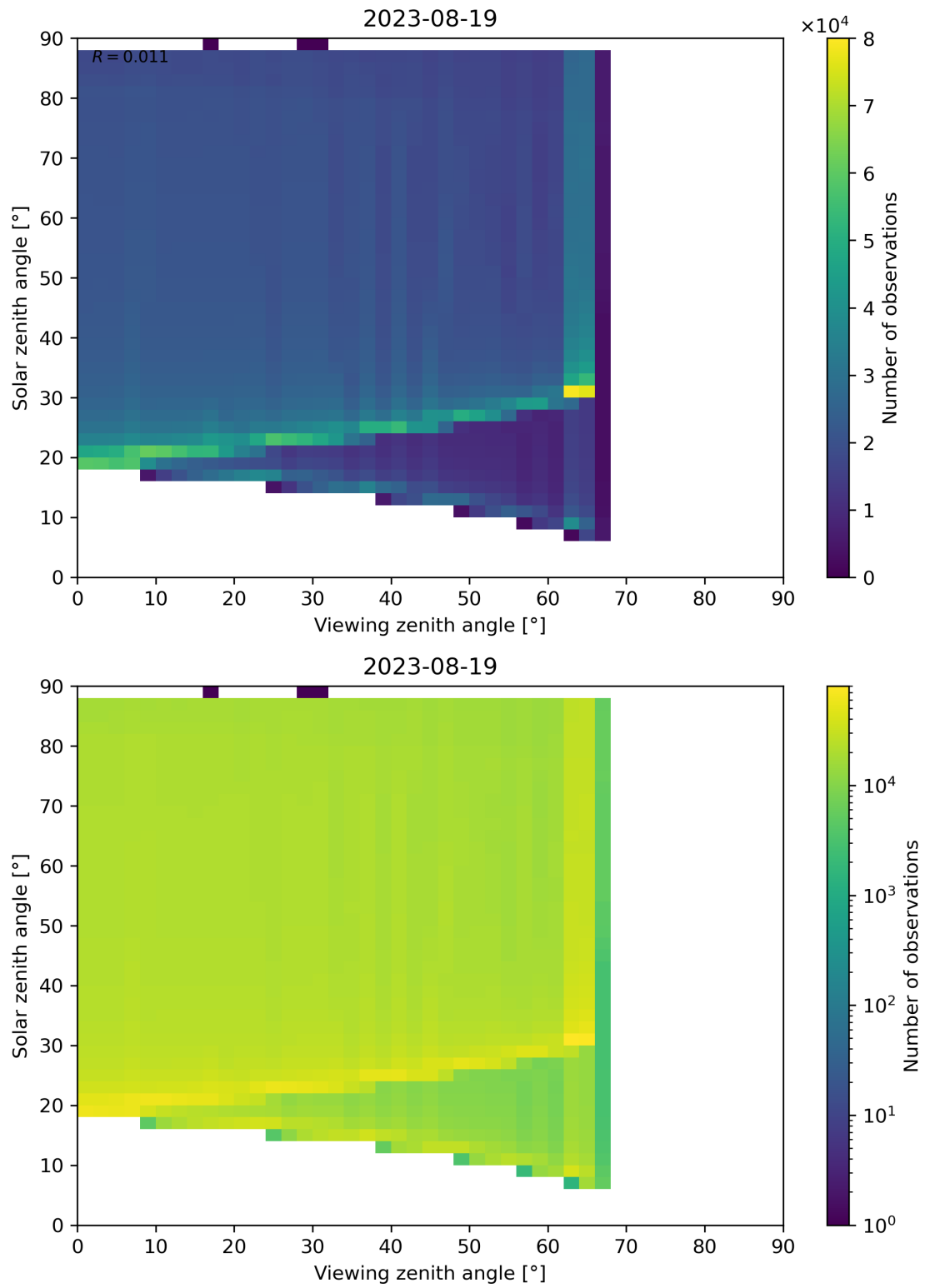
Figure 172: Scatter density plot of “Viewing zenith angle” against “Solar zenith angle” for 2023-08-18 to 2023-08-20.
