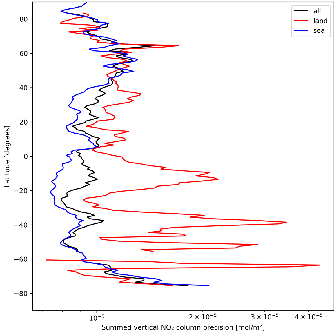
Figure 24: Zonal average of “Summed vertical NO 2 column precision” for 2023-08-18 to 2023-08-20.
