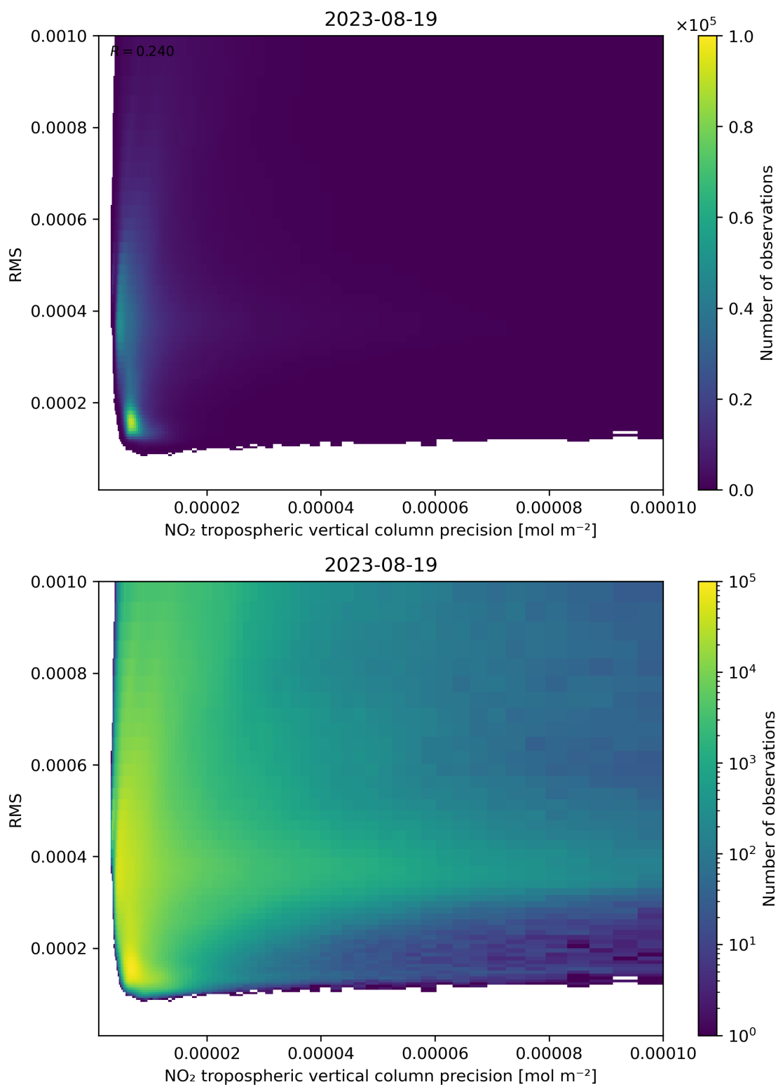
Figure 140: Scatter density plot of “NO 2 tropospheric vertical column precision” against “RMS” for 2023-08-18 to 2023-08-20.
