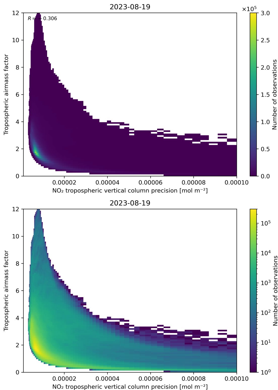
Figure 133: Scatter density plot of “NO 2 tropospheric vertical column precision” against “Tropospheric airmass factor” for 2023-08-18 to 2023-08-20.
