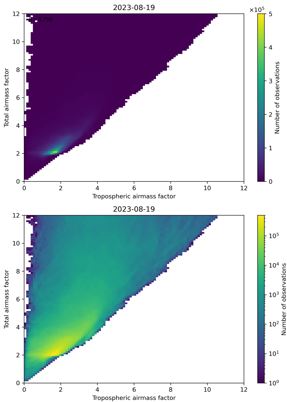
Figure 72: Scatter density plot of “Tropospheric airmass factor” against “Total airmass factor” for 2023-08-18 to 2023-08-20.
