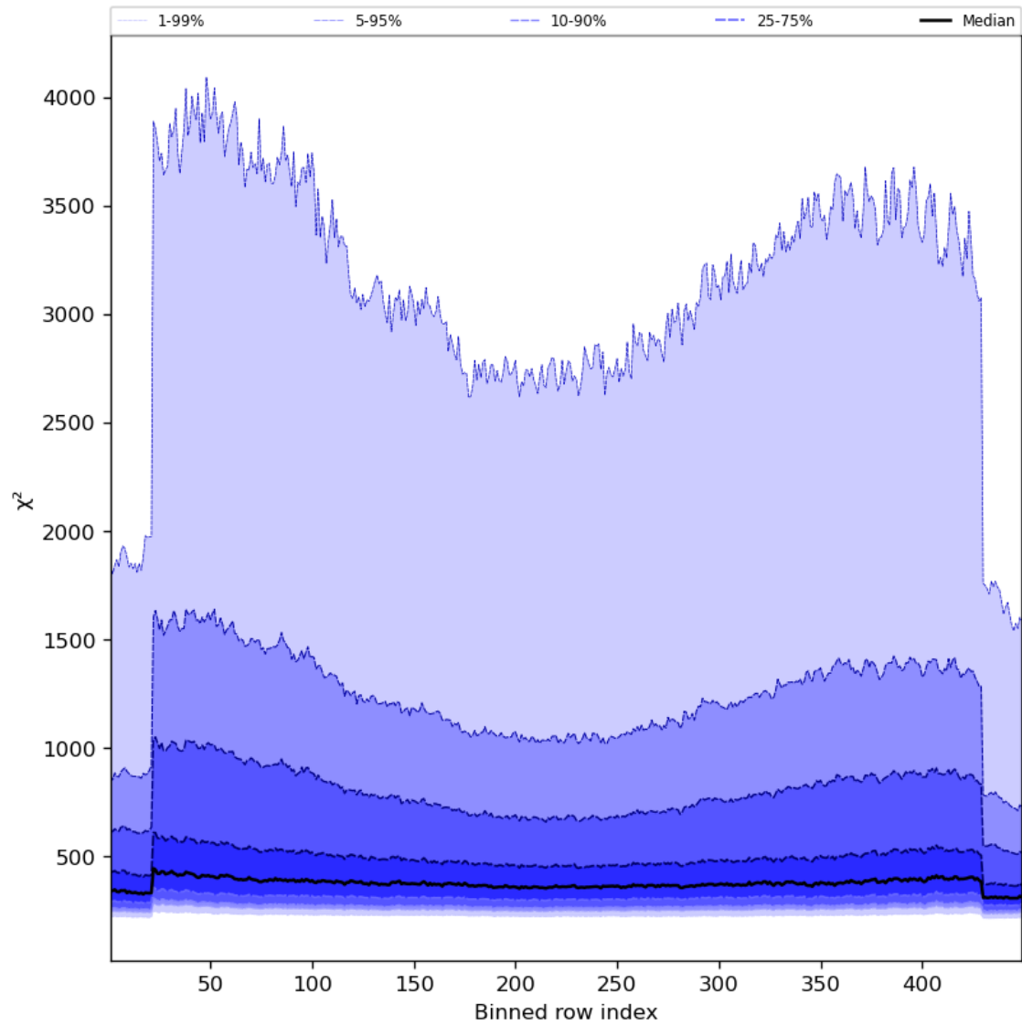
Figure 59: Along track statistics of “ \chi^2 ” for 2023-08-18 to 2023-08-20
