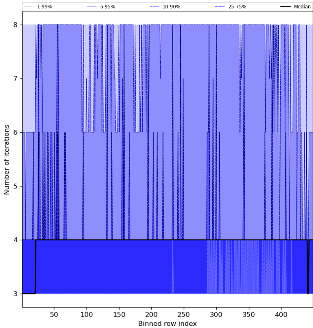
Figure 51: Along track statistics of “Number of iterations” for 2023-08-18 to 2023-08-20
