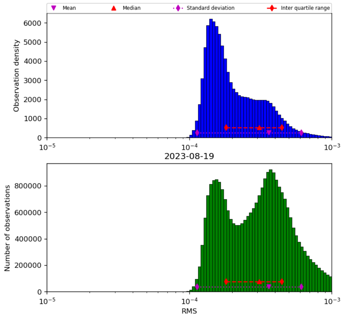
Figure 43: Histogram of “RMS” for 2023-08-18 to 2023-08-20
