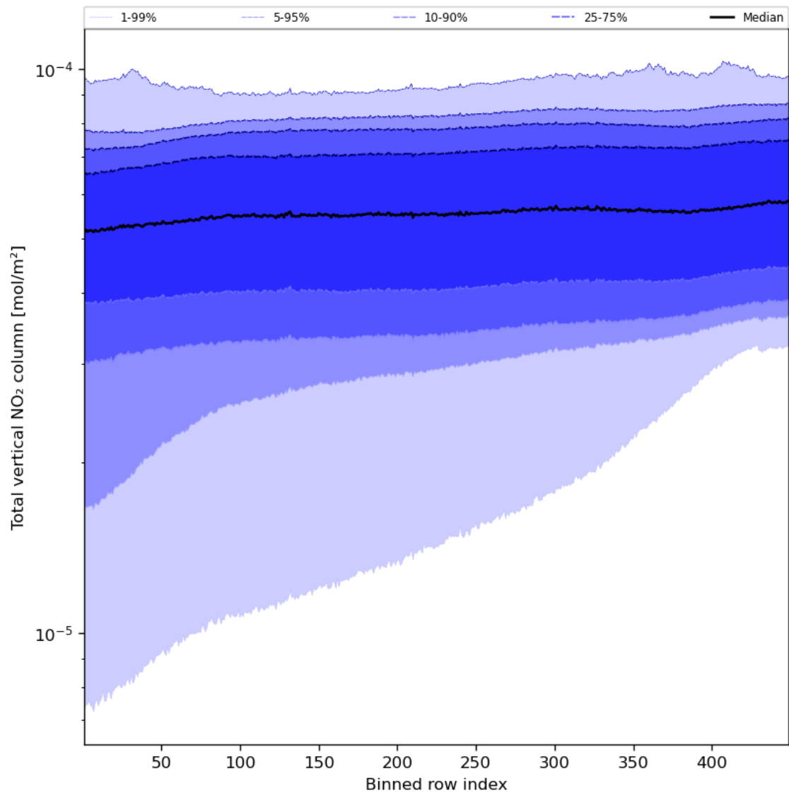
Figure 55: Along track statistics of “Total vertical NO 2 column” for 2023-08-18 to 2023-08-20
