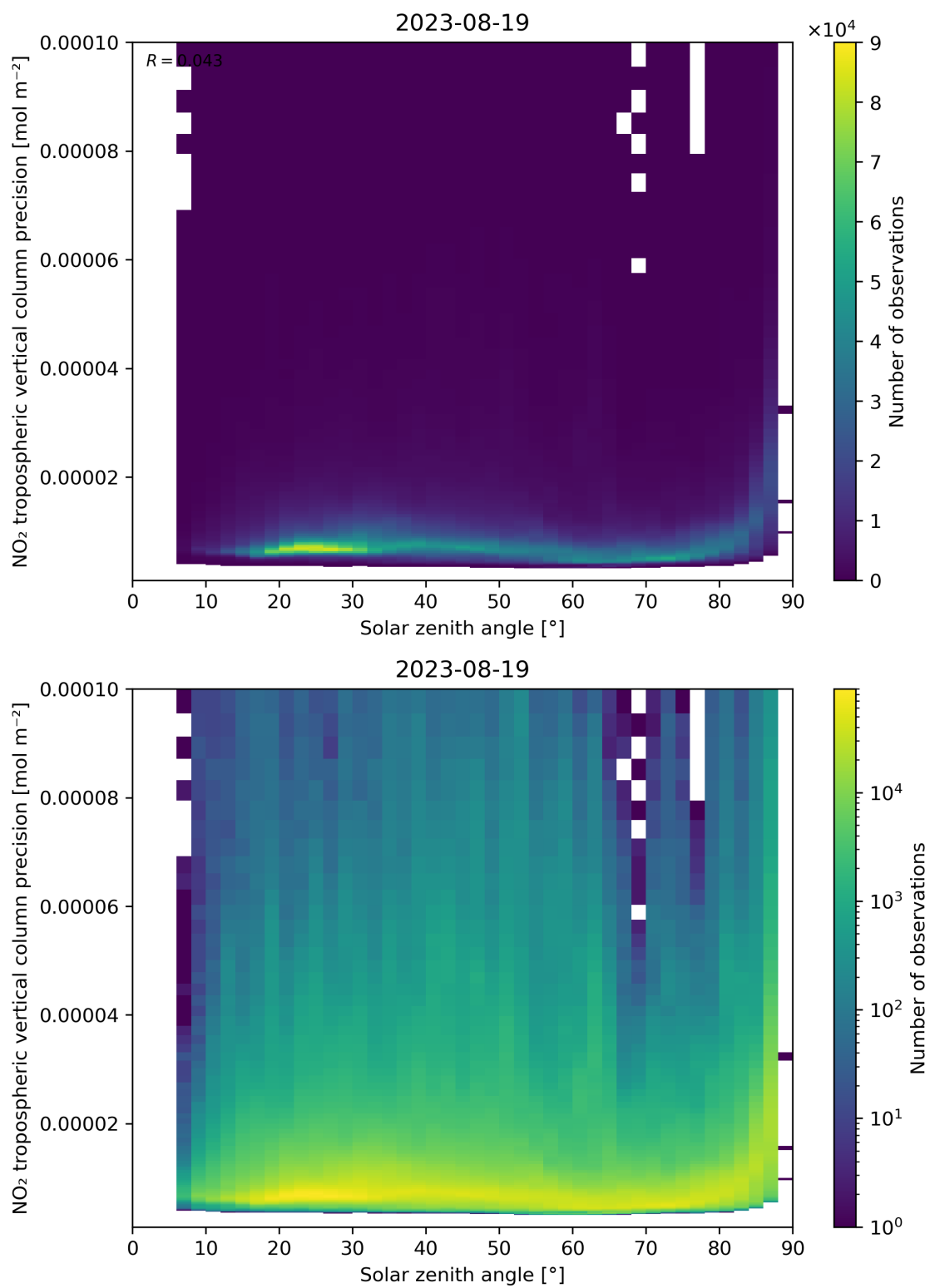
Figure 156: Scatter density plot of “Solar zenith angle” against “NO 2 tropospheric vertical column precision” for 2023-08-18 to 2023-08-20.
