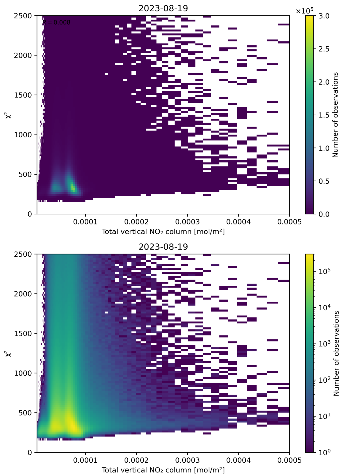
Figure 111: Scatter density plot of “Total vertical NO 2 column” against “ \chi^2 ” for 2023-08-18 to 2023-08-20.
