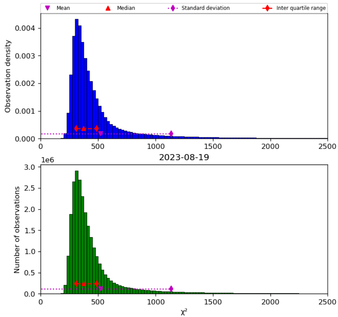
Figure 42: Histogram of “ \chi^2 ” for 2023-08-18 to 2023-08-20
