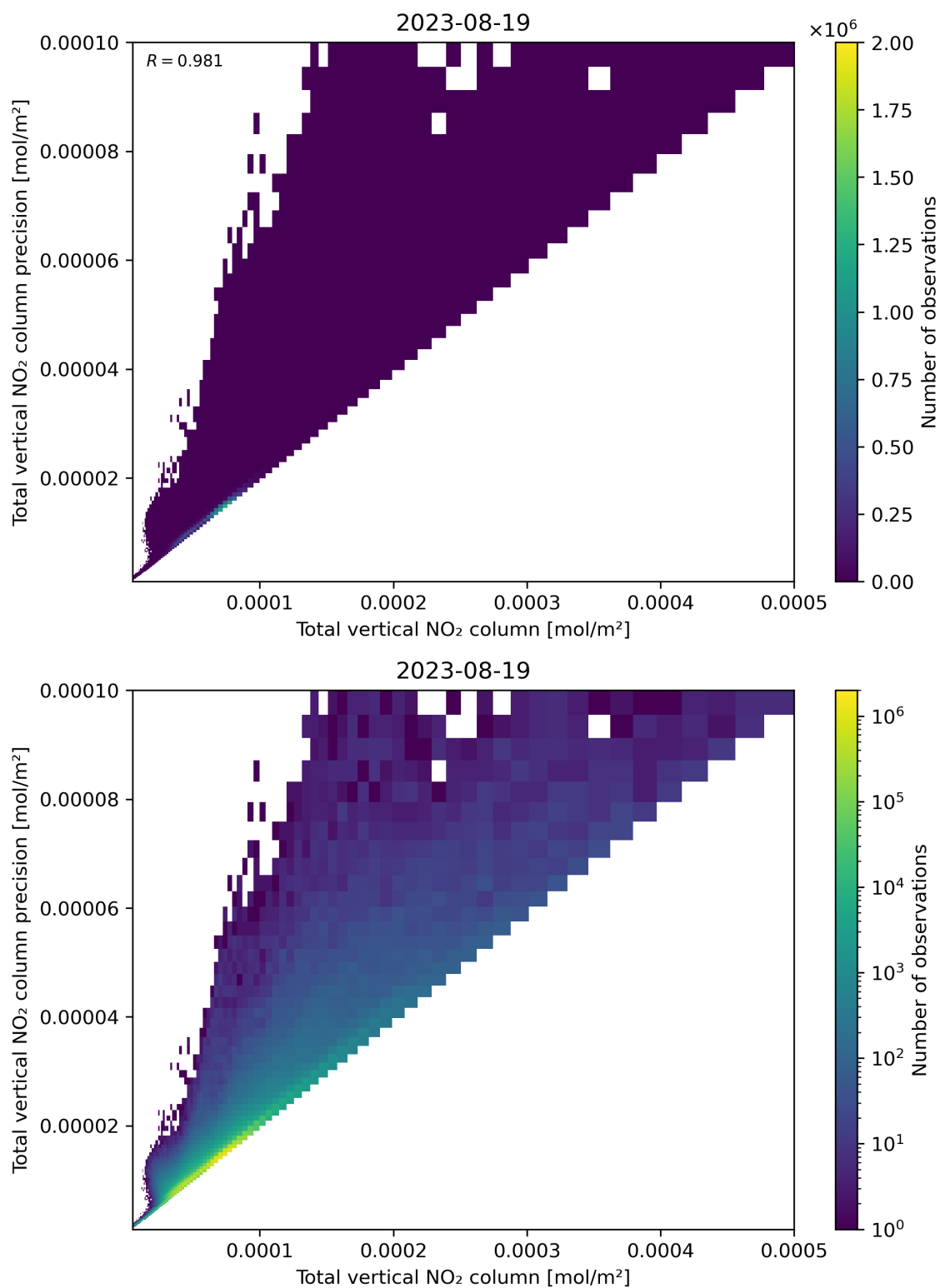
Figure 114: Scatter density plot of “Total vertical NO 2 column” against “Total vertical NO 2 column precision” for 2023-08-18 to 2023-08-20.
