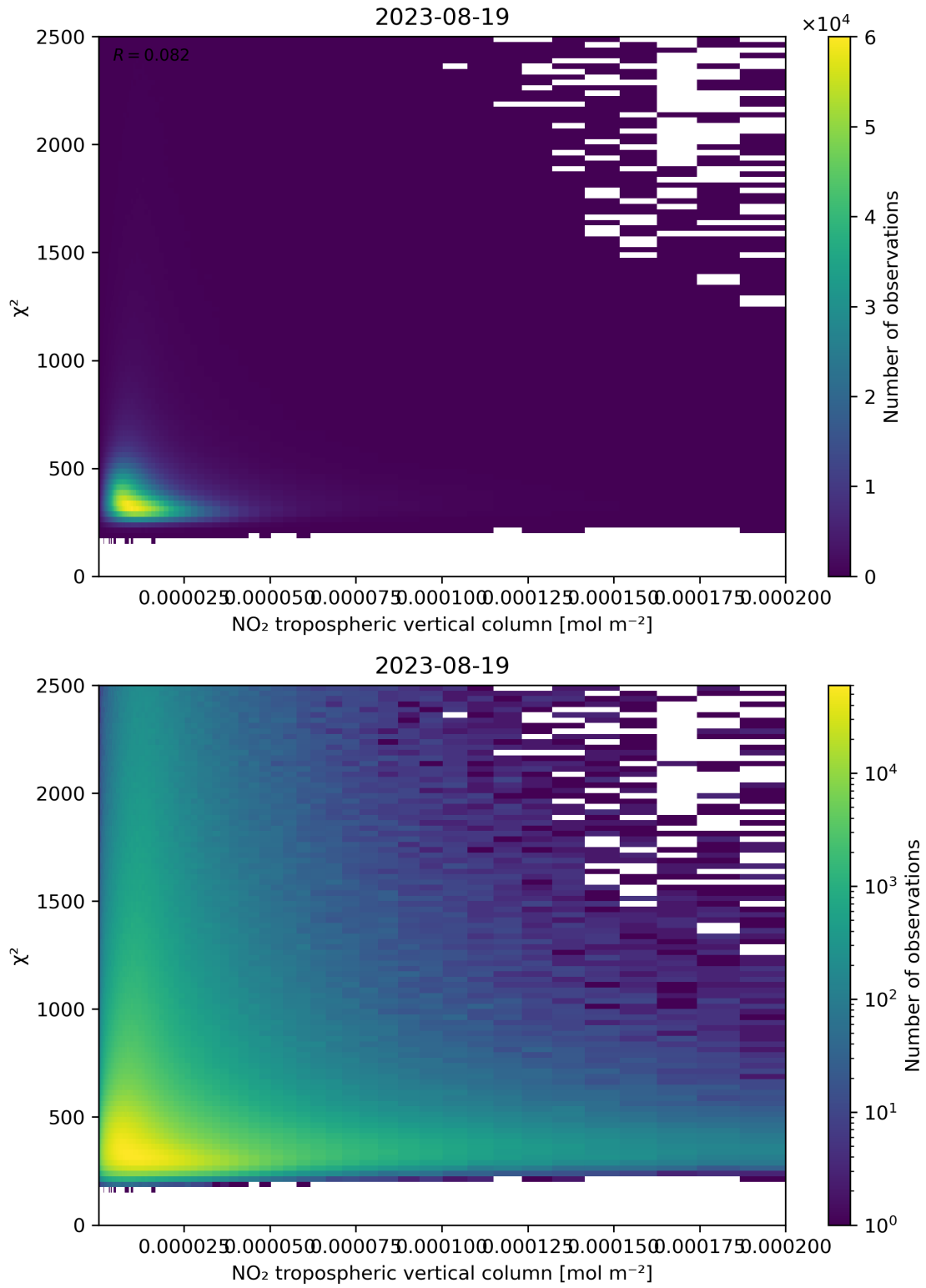
Figure 124: Scatter density plot of “NO 2 tropospheric vertical column” against “ \chi^2 ” for 2023-08-18 to 2023-08-20.
