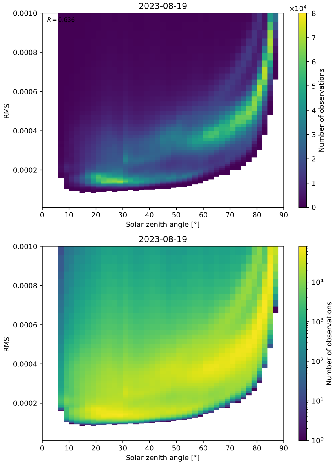
Figure 157: Scatter density plot of “Solar zenith angle” against “RMS” for 2023-08-18 to 2023-08-20.
