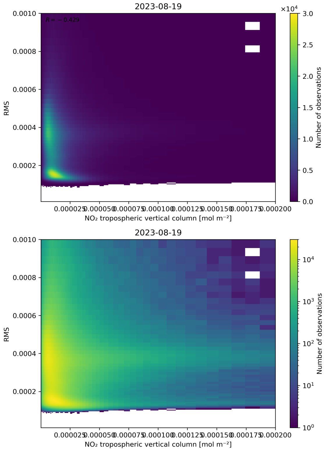
Figure 142: Scatter density plot of “NO 2 tropospheric vertical column” against “RMS” for 2023-08-18 to 2023-08-20.
