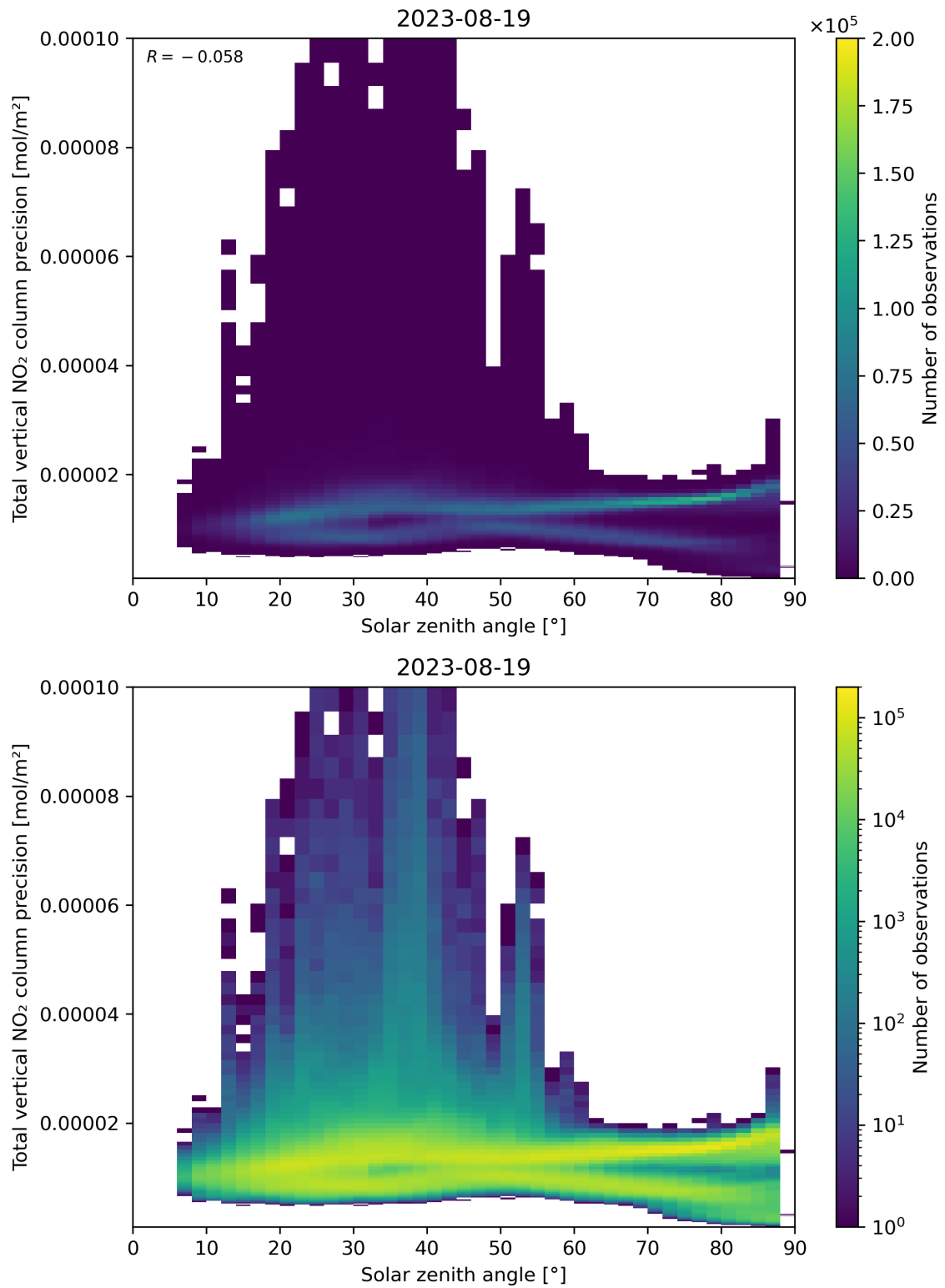
Figure 154: Scatter density plot of “Solar zenith angle” against “Total vertical NO 2 column precision” for 2023-08-18 to 2023-08-20.
