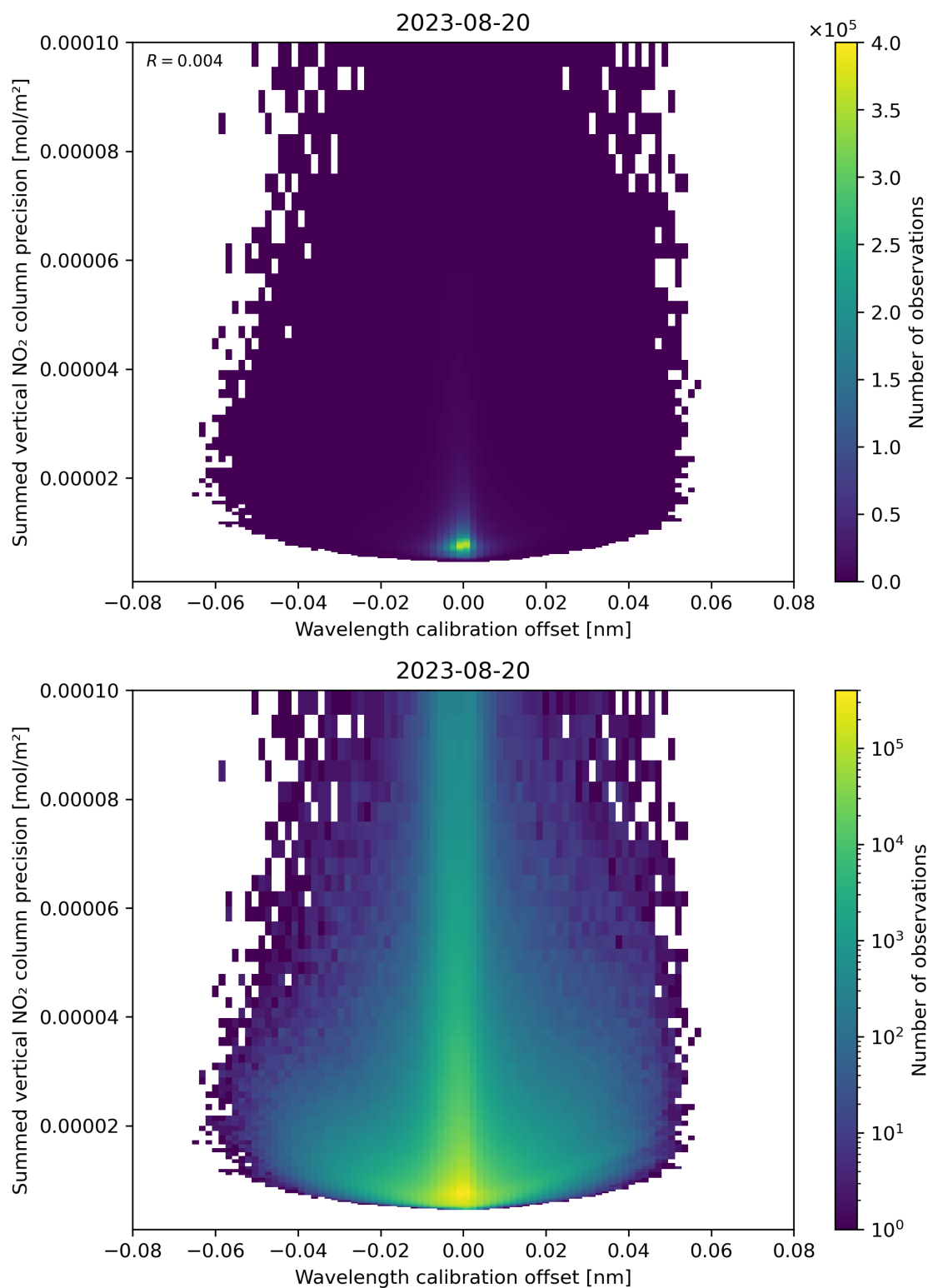
Figure 178: Scatter density plot of “Wavelength calibration offset” against “Summed vertical NO 2 column precision” for 2023-08-20 to 2023-08-21.
