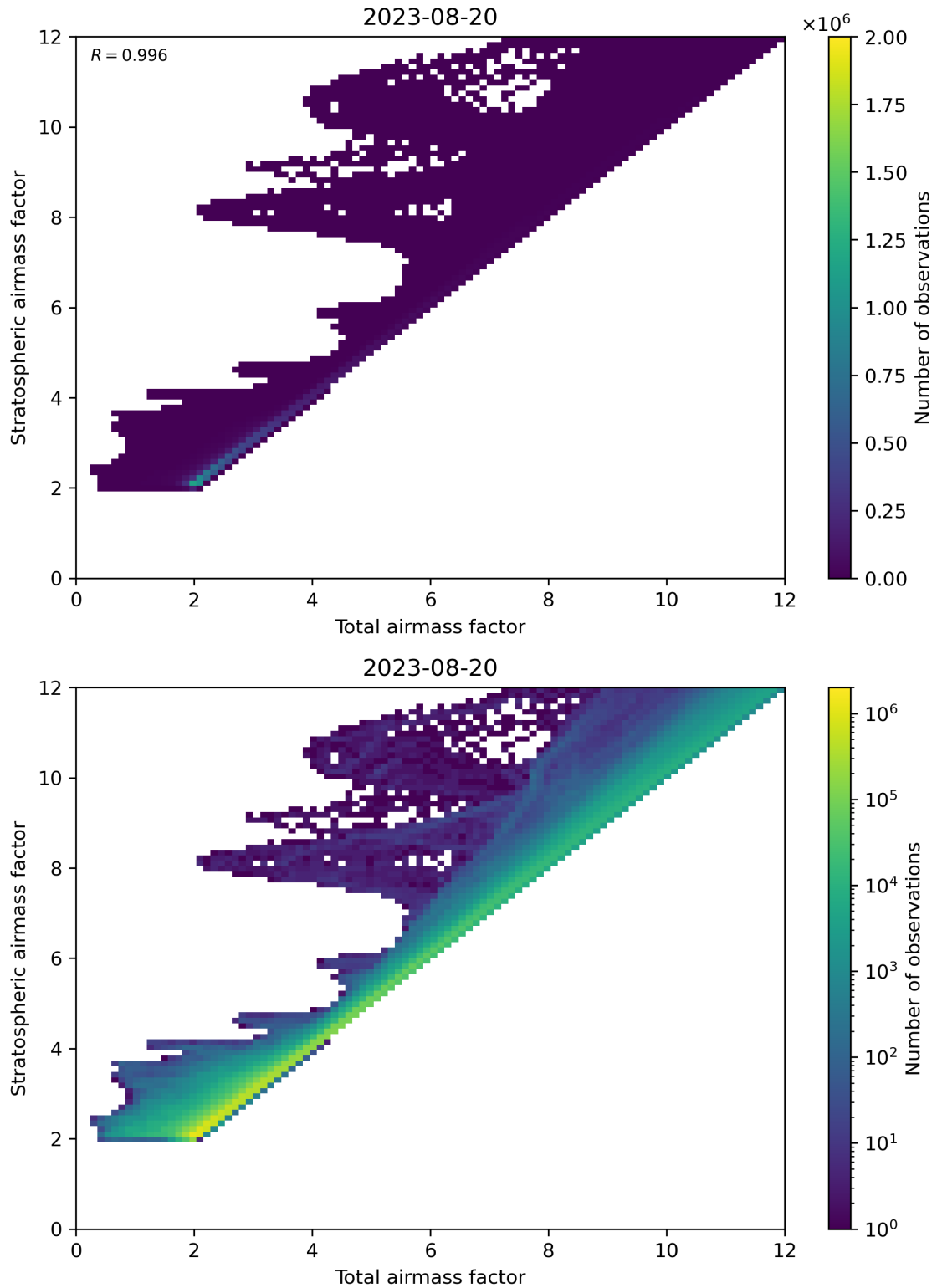
Figure 62: Scatter density plot of “Total airmass factor” against “Stratospheric airmass factor” for 2023-08-20 to 2023-08-21.
