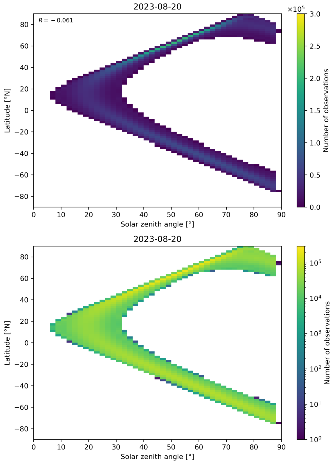
Figure 149: Scatter density plot of “Solar zenith angle” against “Latitude” for 2023-08-20 to 2023-08-21.
