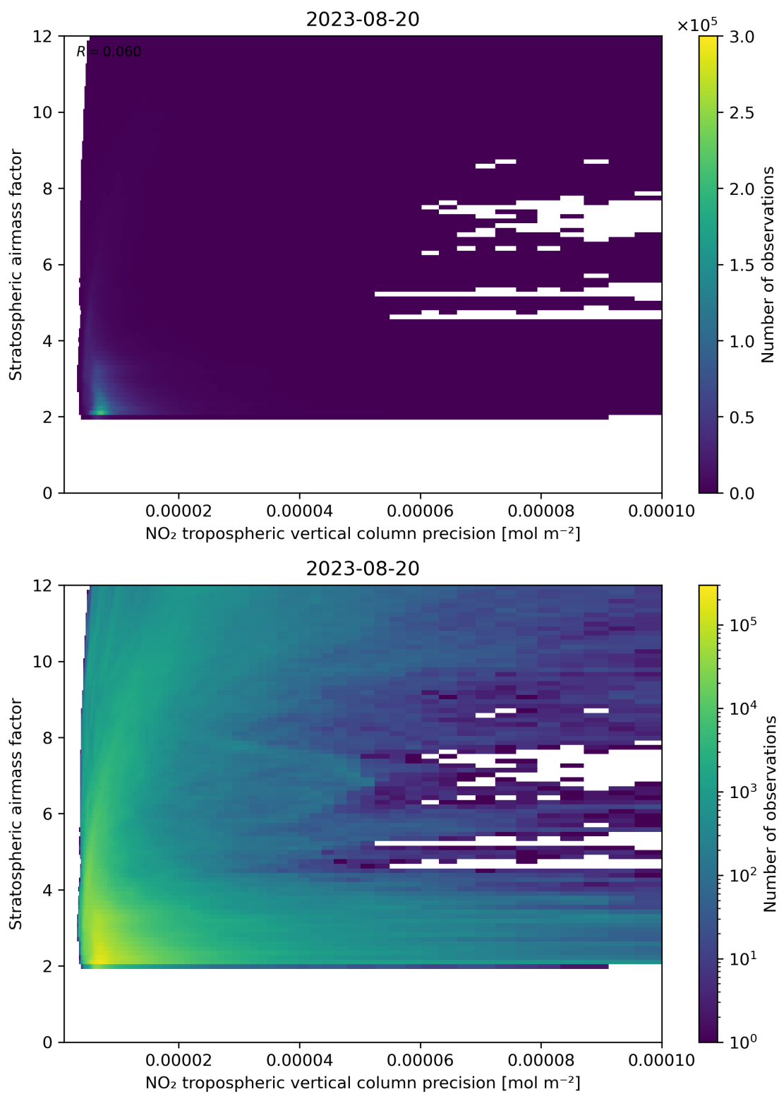
Figure 131: Scatter density plot of “NO 2 tropospheric vertical column precision” against “Stratospheric airmass factor” for 2023-08-20 to 2023-08-21.
