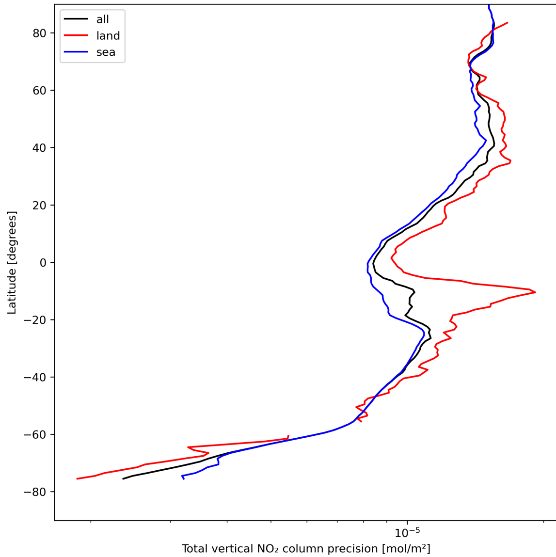
Figure 22: Zonal average of “Total vertical NO 2 column precision” for 2023-08-20 to 2023-08-21.
