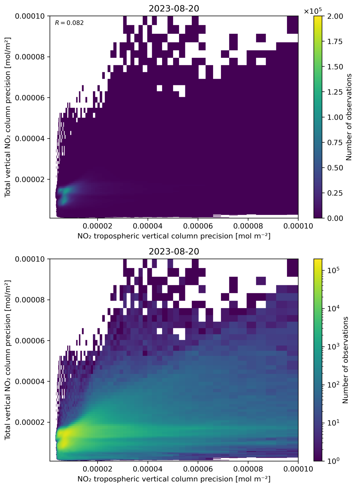
Figure 139: Scatter density plot of “NO 2 tropospheric vertical column precision” against “Total vertical NO 2 column precision” for 2023-08-20 to 2023-08-21.
