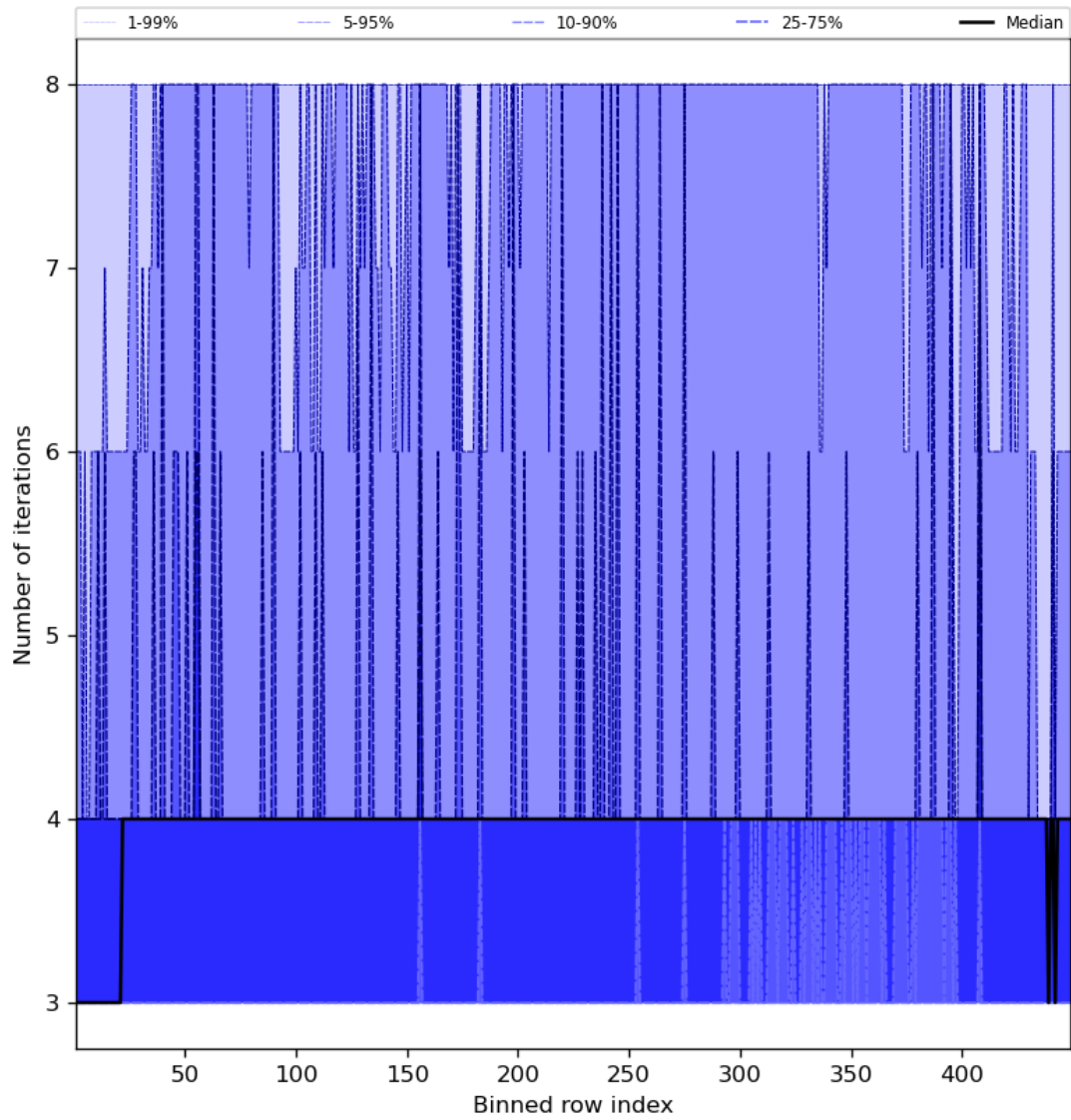
Figure 51: Along track statistics of “Number of iterations” for 2023-08-20 to 2023-08-21
