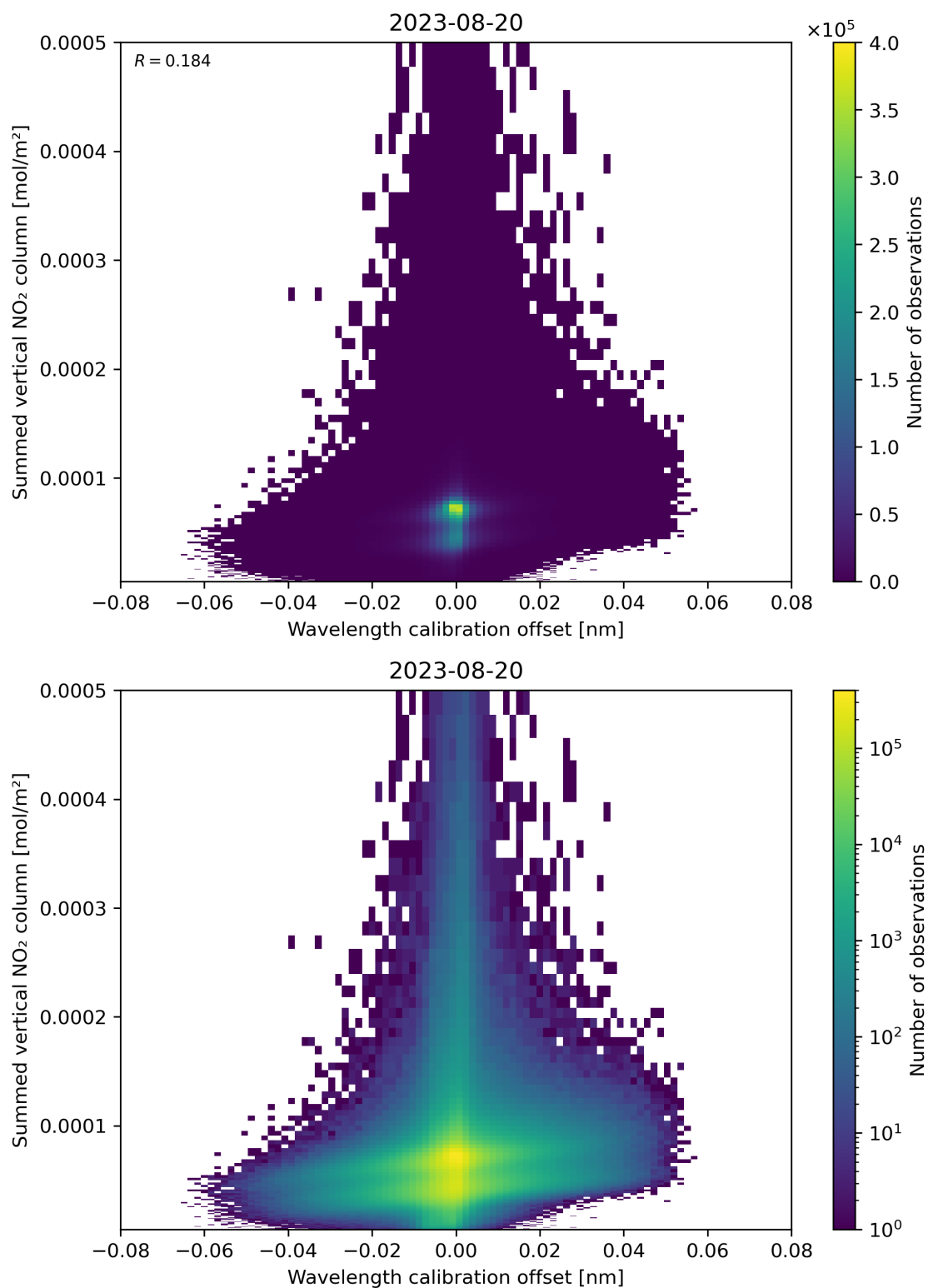
Figure 177: Scatter density plot of “Wavelength calibration offset” against “Summed vertical NO 2 column” for 2023-08-20 to 2023-08-21.
