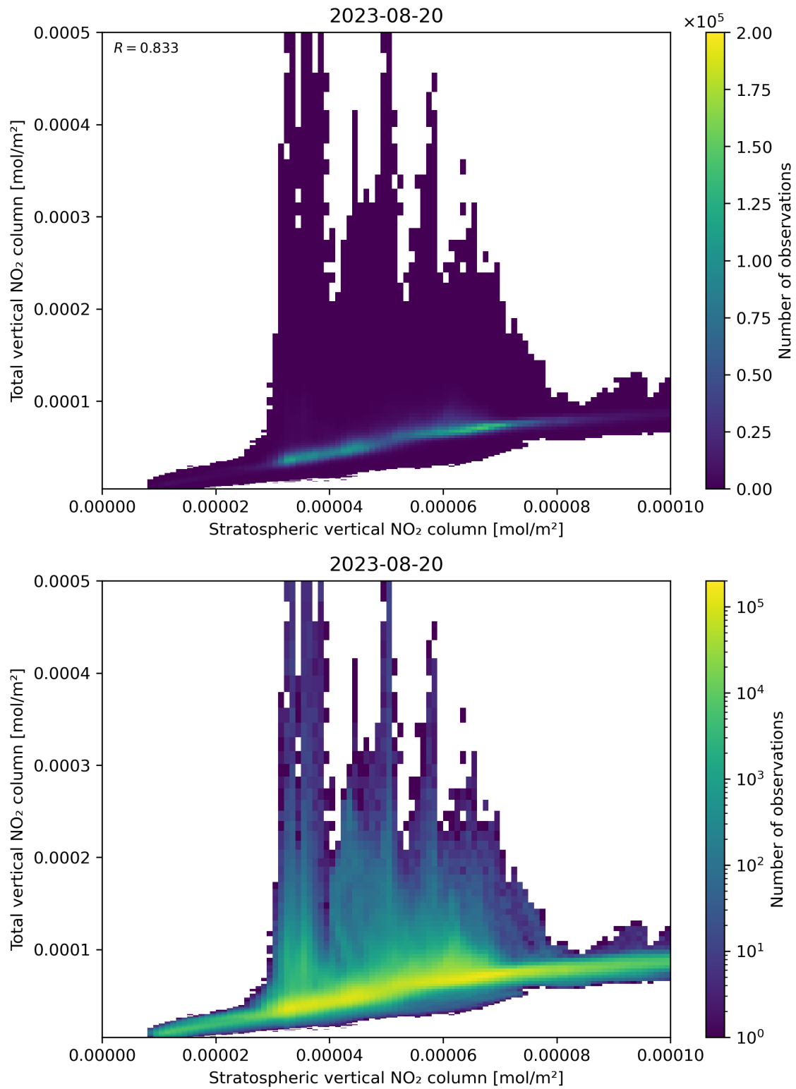
Figure 100: Scatter density plot of “Stratospheric vertical NO 2 column” against “Total vertical NO 2 column” for 2023-08-20 to 2023-08-21.
