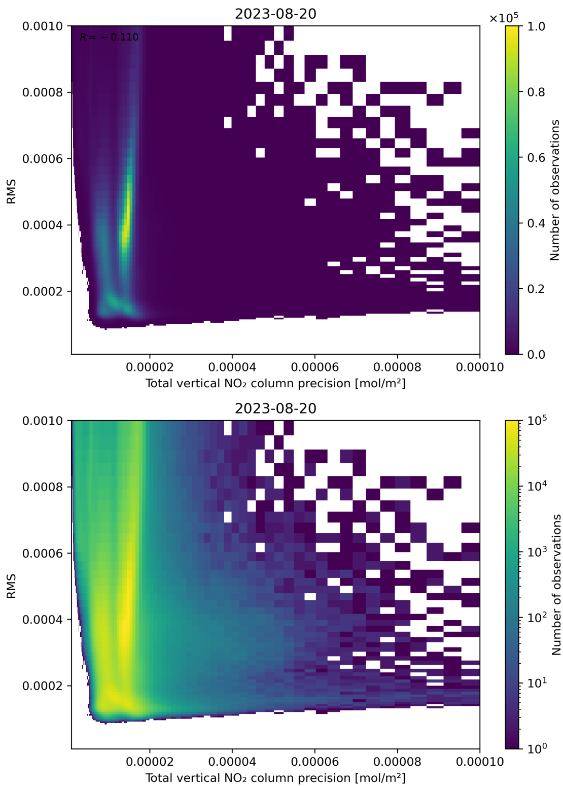
Figure 119: Scatter density plot of “Total vertical NO 2 column precision” against “RMS” for 2023-08-20 to 2023-08-21.
