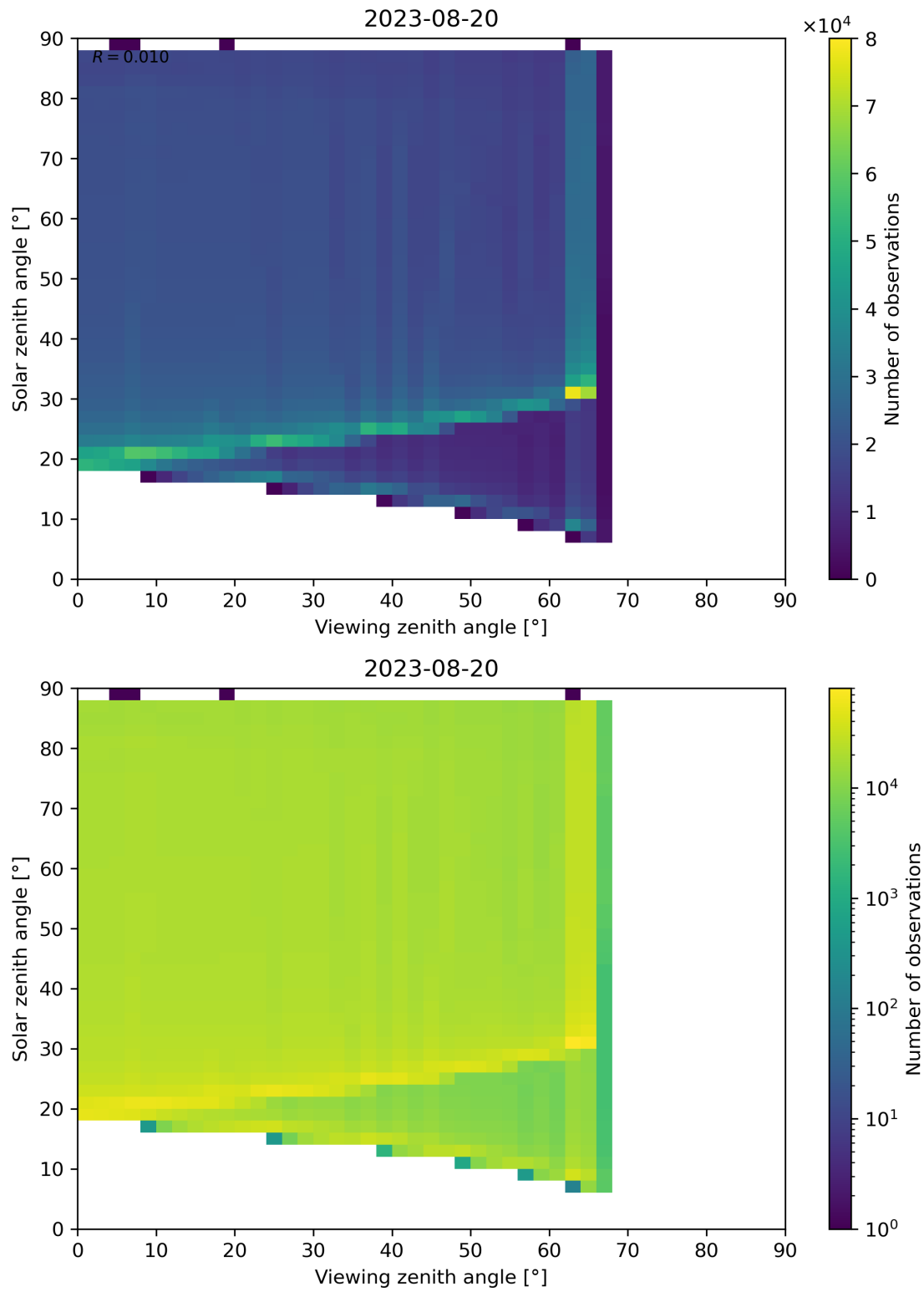
Figure 172: Scatter density plot of “Viewing zenith angle” against “Solar zenith angle” for 2023-08-20 to 2023-08-21.
