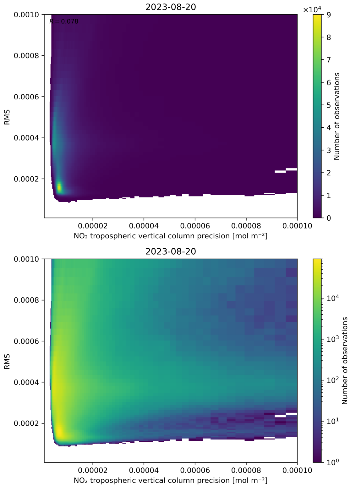
Figure 140: Scatter density plot of “NO 2 tropospheric vertical column precision” against “RMS” for 2023-08-20 to 2023-08-21.
