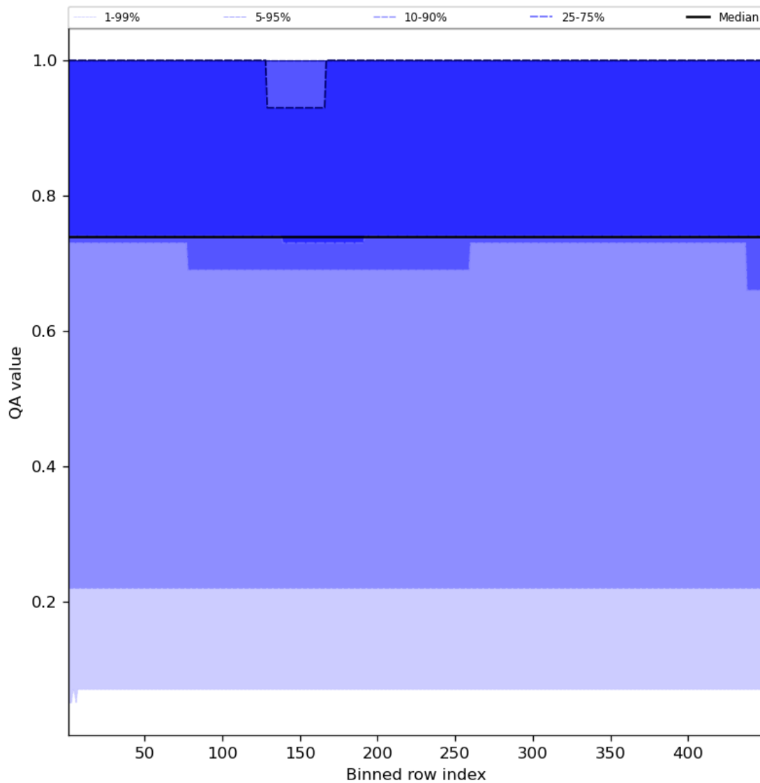
Figure 45: Along track statistics of “QA value” for 2023-08-20 to 2023-08-21
