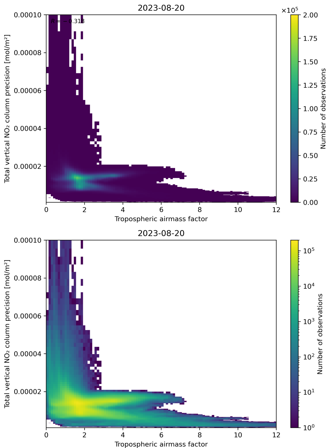
Figure 78: Scatter density plot of “Tropospheric air mass factor” against “Total vertical NO 2 column precision” for 2023-08-20 to 2023-08-21.
