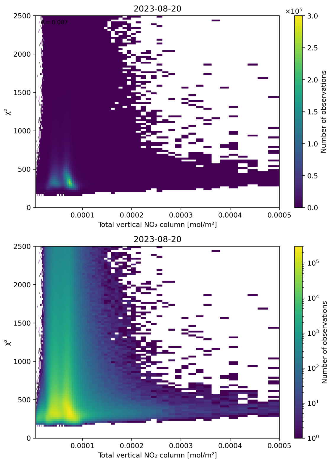
Figure 111: Scatter density plot of “Total vertical NO 2 column” against “ \chi^2 ” for 2023-08-20 to 2023-08-21.
