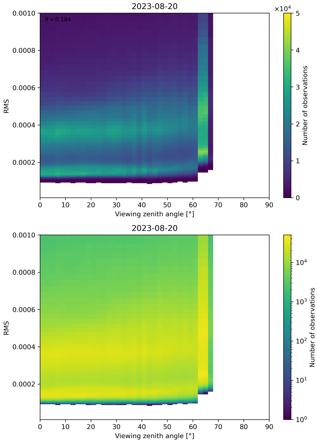
Figure 171: Scatter density plot of “Viewing zenith angle” against “RMS” for 2023-08-20 to 2023-08-21.
