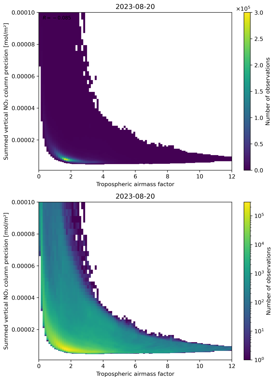
Figure 76: Scatter density plot of “Tropospheric air mass factor” against “Summed vertical NO 2 column precision” for 2023-08-20 to 2023-08-21.
