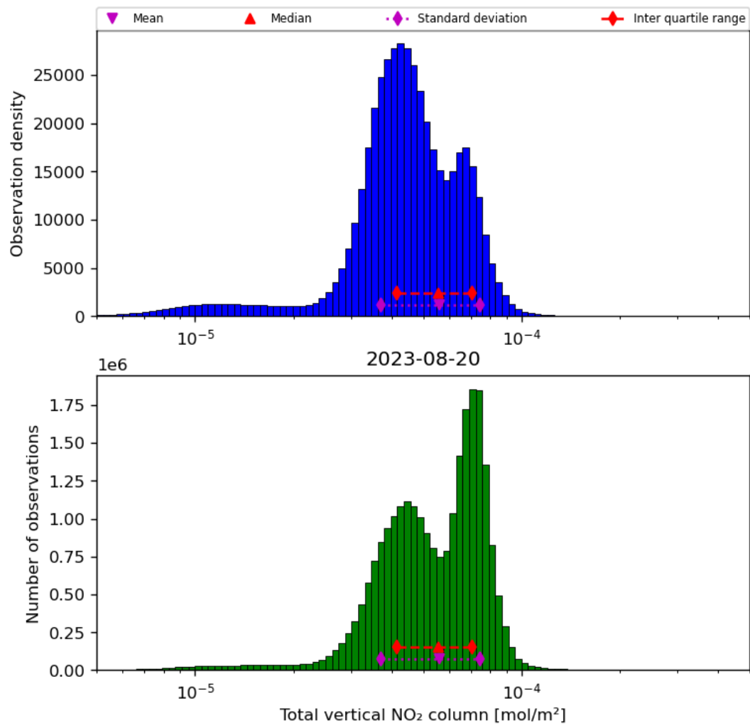
Figure 38: Histogram of “Total vertical NO 2 column” for 2023-08-20 to 2023-08-21
