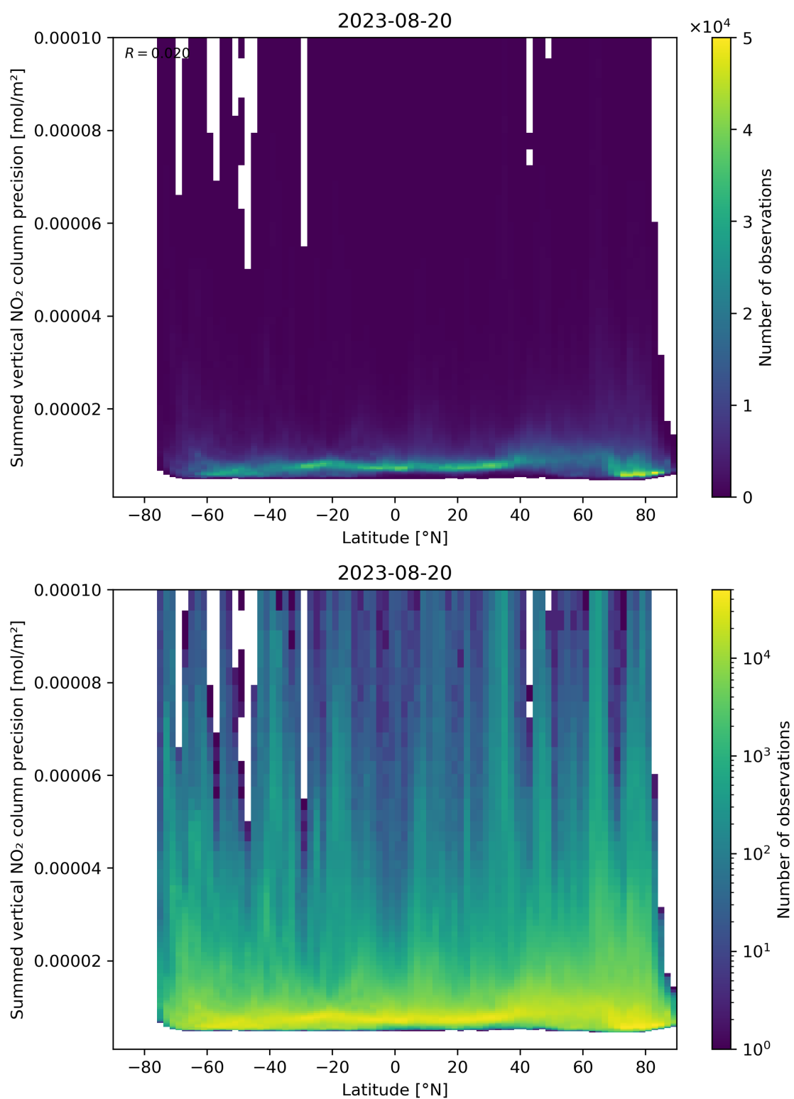
Figure 89: Scatter density plot of “Latitude” against “Summed vertical NO 2 column precision” for 2023-08-20 to 2023-08-21.
