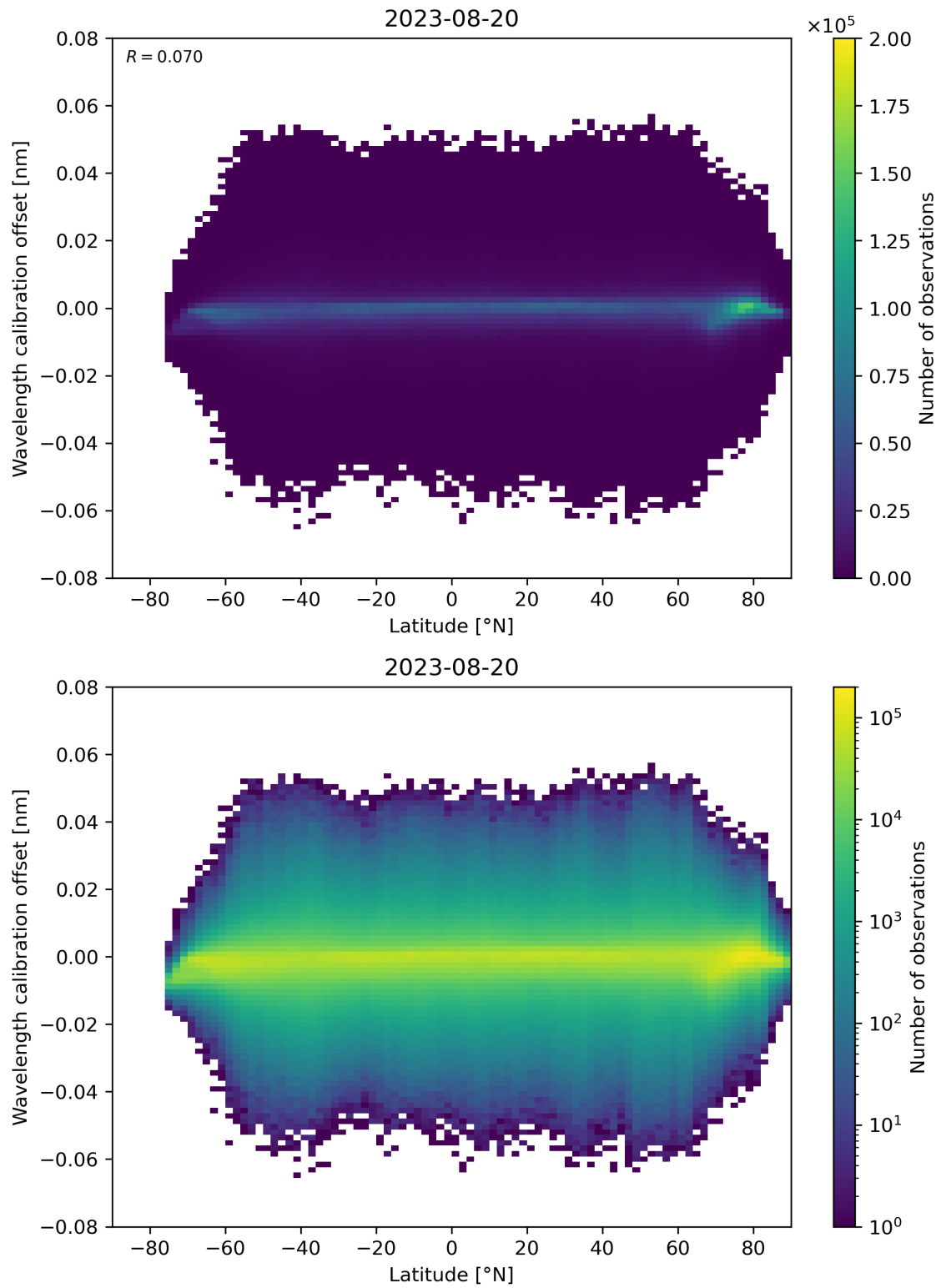
Figure 95: Scatter density plot of “Latitude” against “Wavelength calibration offset” for 2023-08-20 to 2023-08-21.
