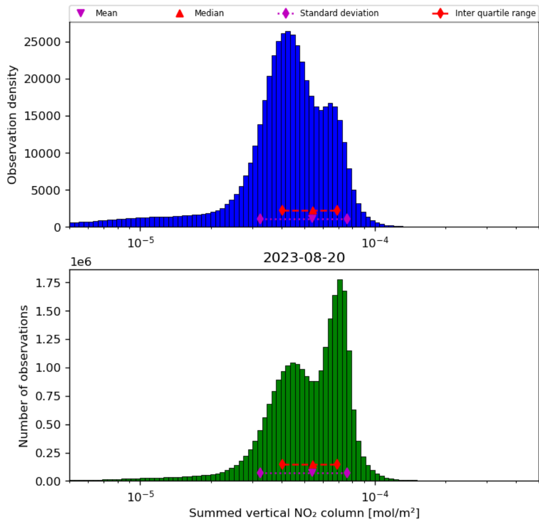
Figure 40: Histogram of “Summed vertical NO 2 column” for 2023-08-20 to 2023-08-21
