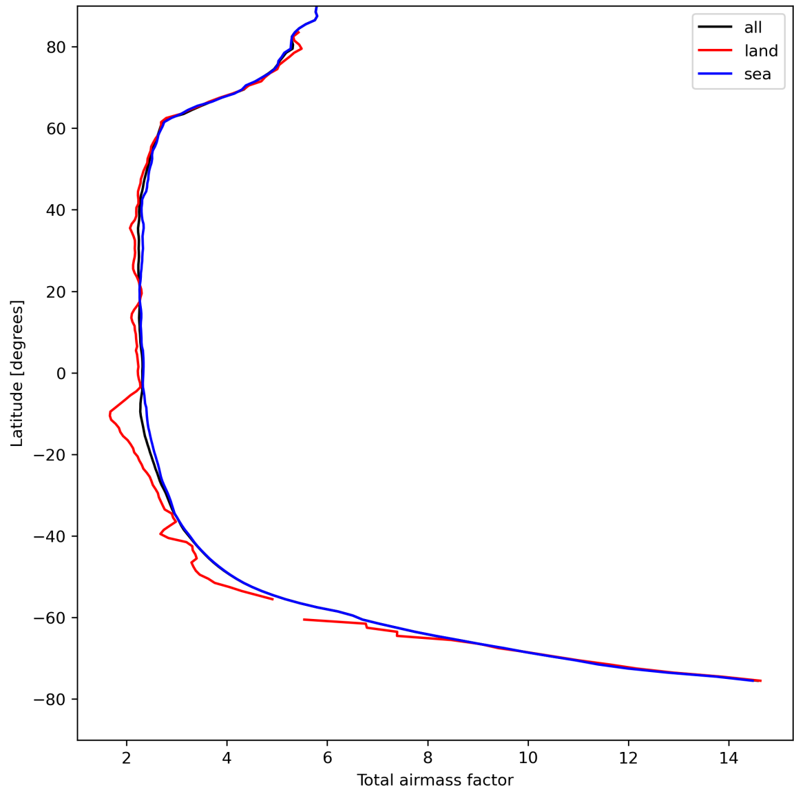
Figure 15: Zonal average of “Total airmass factor” for 2023-08-20 to 2023-08-21.
