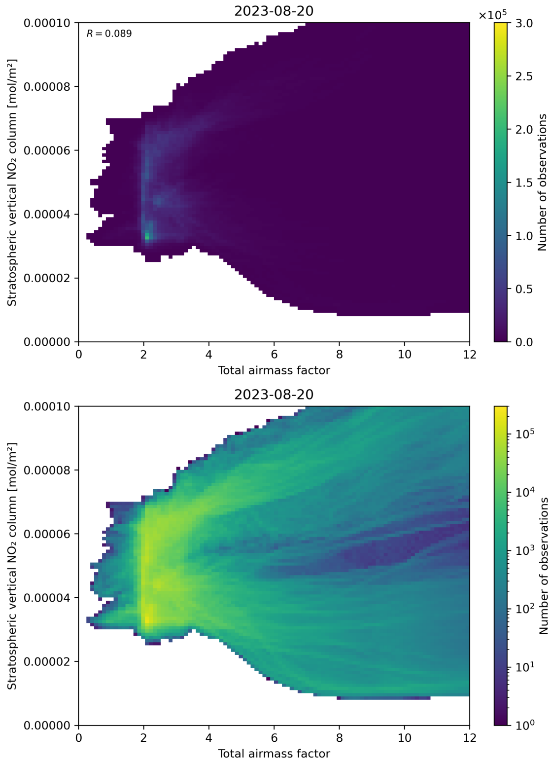
Figure 64: Scatter density plot of “Total airmass factor” against “Stratospheric vertical NO 2 column” for 2023-08-20 to 2023-08-21.
