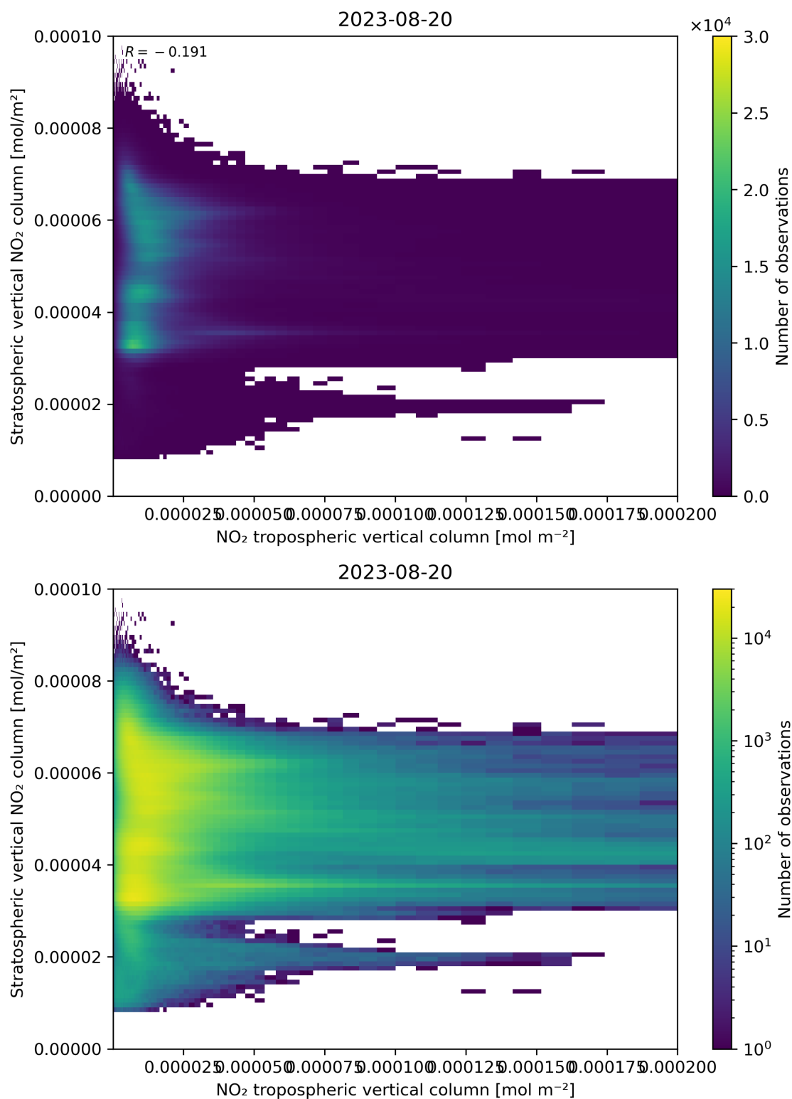
Figure 125: Scatter density plot of “NO 2 tropospheric vertical column” against “Stratospheric vertical NO 2 column” for 2023-08-20 to 2023-08-21.
