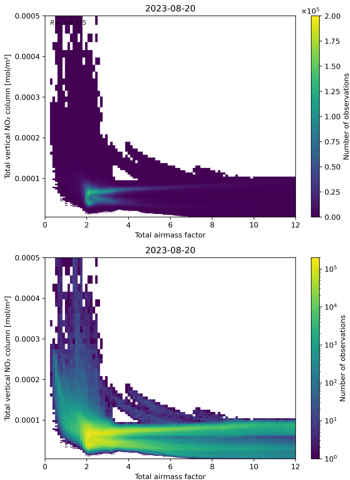
Figure 67: Scatter density plot of “Total airmass factor” against “Total vertical NO 2 column” for 2023-08-20 to 2023-08-21.
