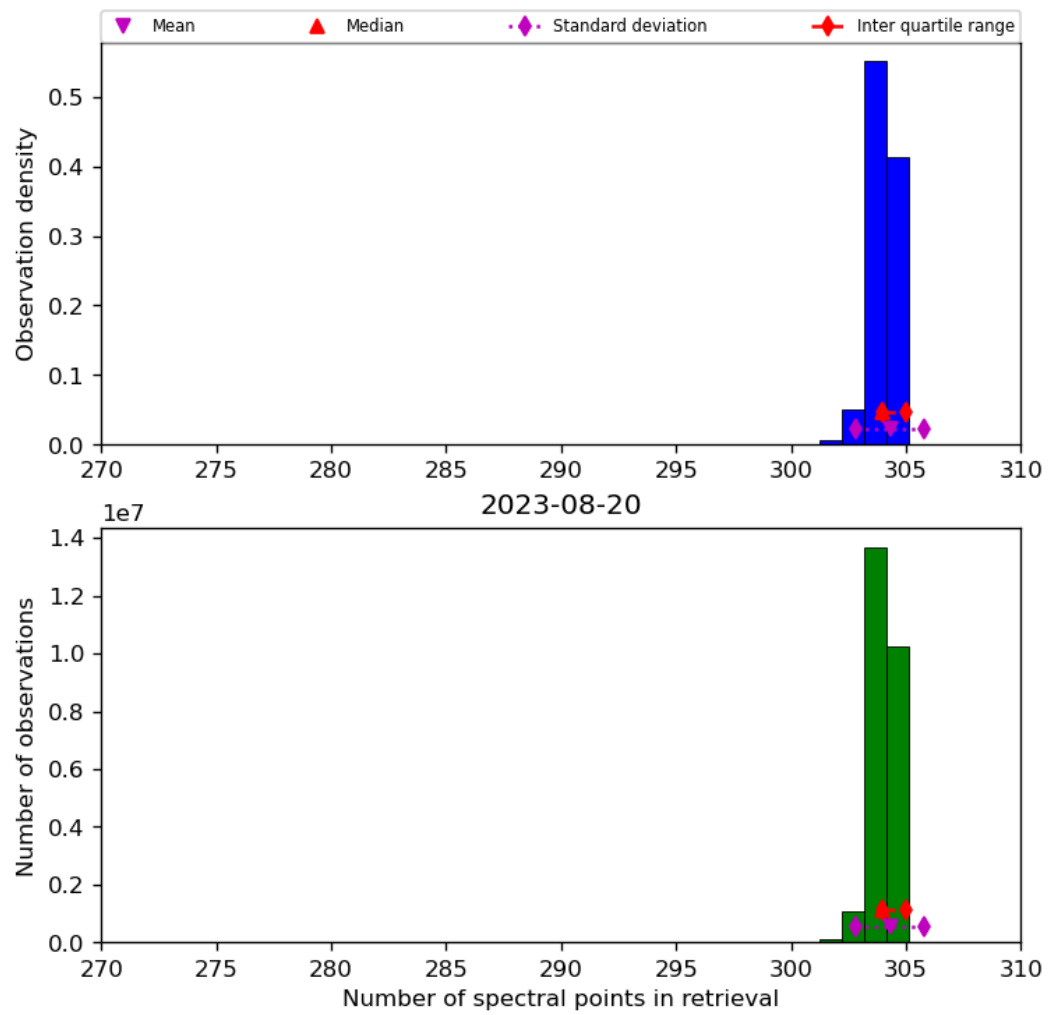
Figure 33: Histogram of “Number of spectral points in retrieval” for 2023-08-20 to 2023-08-21
