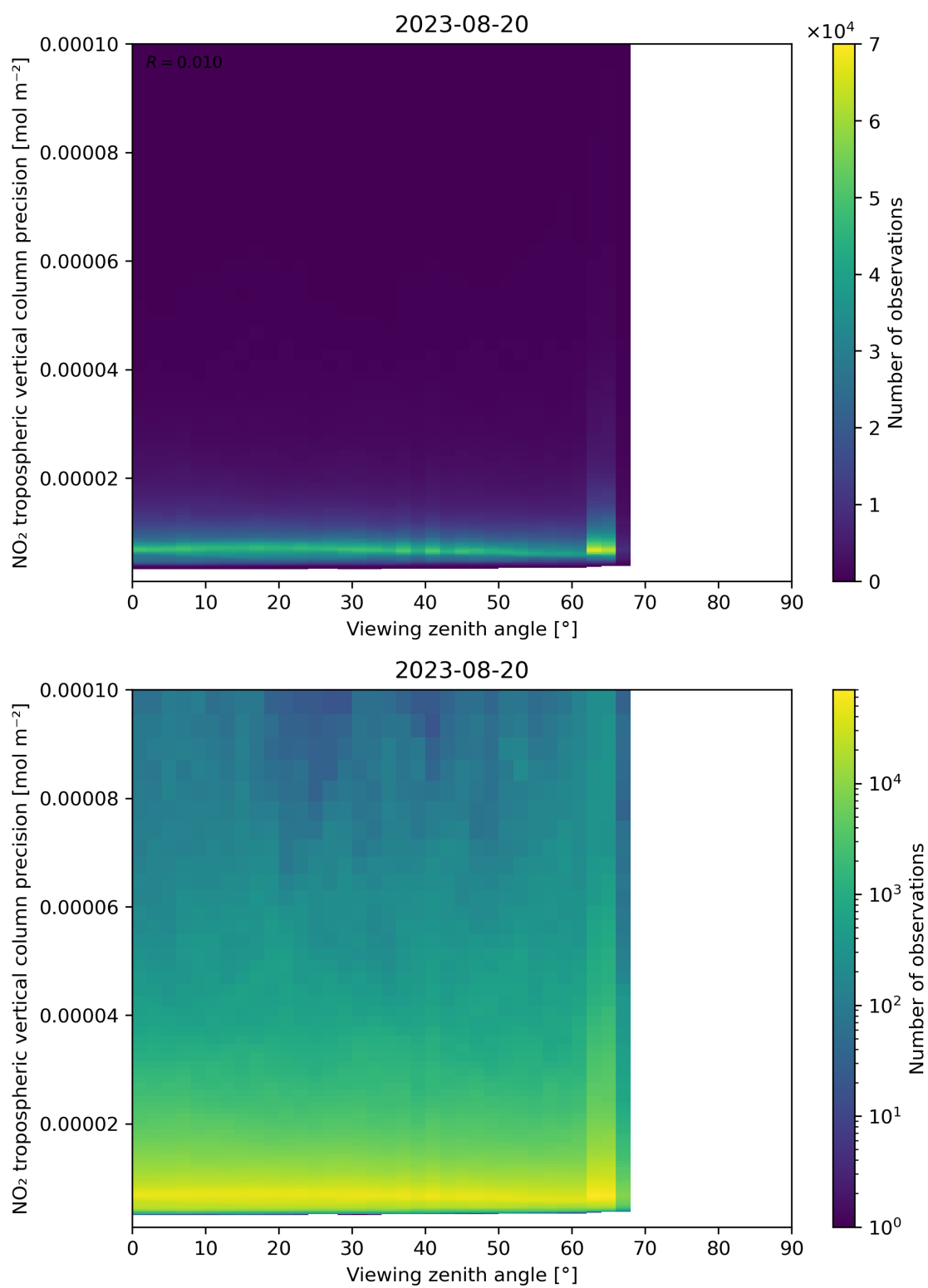
Figure 170: Scatter density plot of “Viewing zenith angle” against “NO 2 tropospheric vertical column precision” for 2023-08-20 to 2023-08-21.
