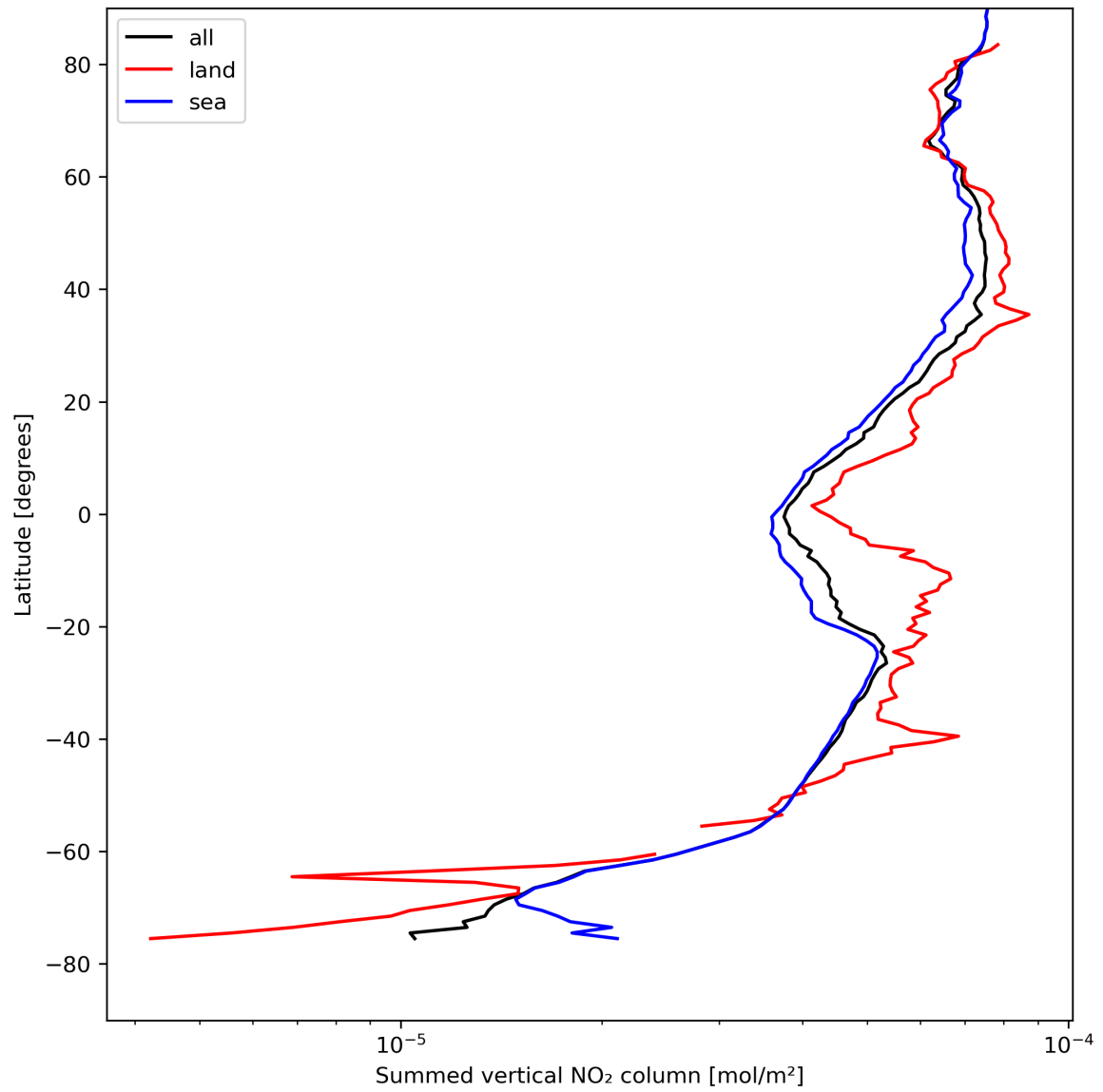
Figure 23: Zonal average of “Summed vertical NO 2 column” for 2023-08-20 to 2023-08-21.
