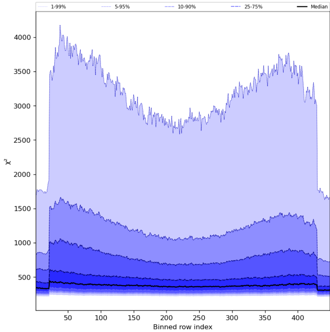
Figure 59: Along track statistics of “ \chi^2 ” for 2023-08-20 to 2023-08-21
