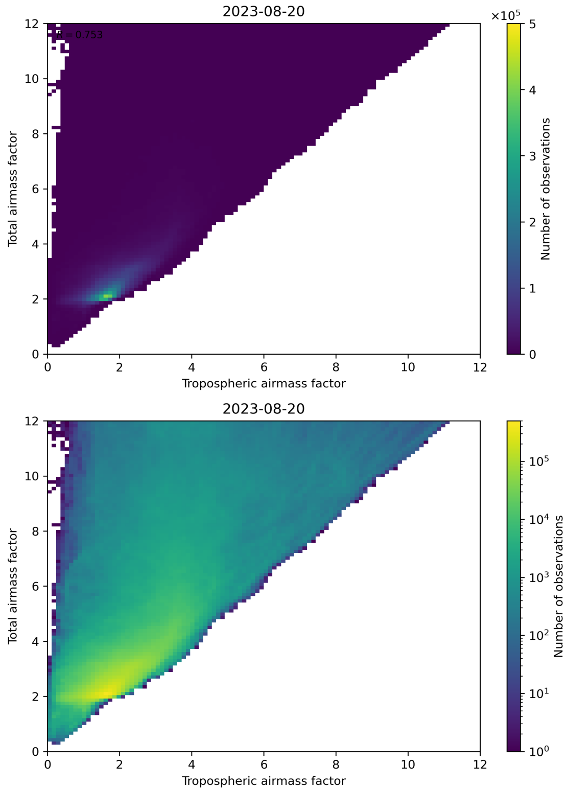
Figure 72: Scatter density plot of “Tropospheric airmass factor” against “Total airmass factor” for 2023-08-20 to 2023-08-21.
