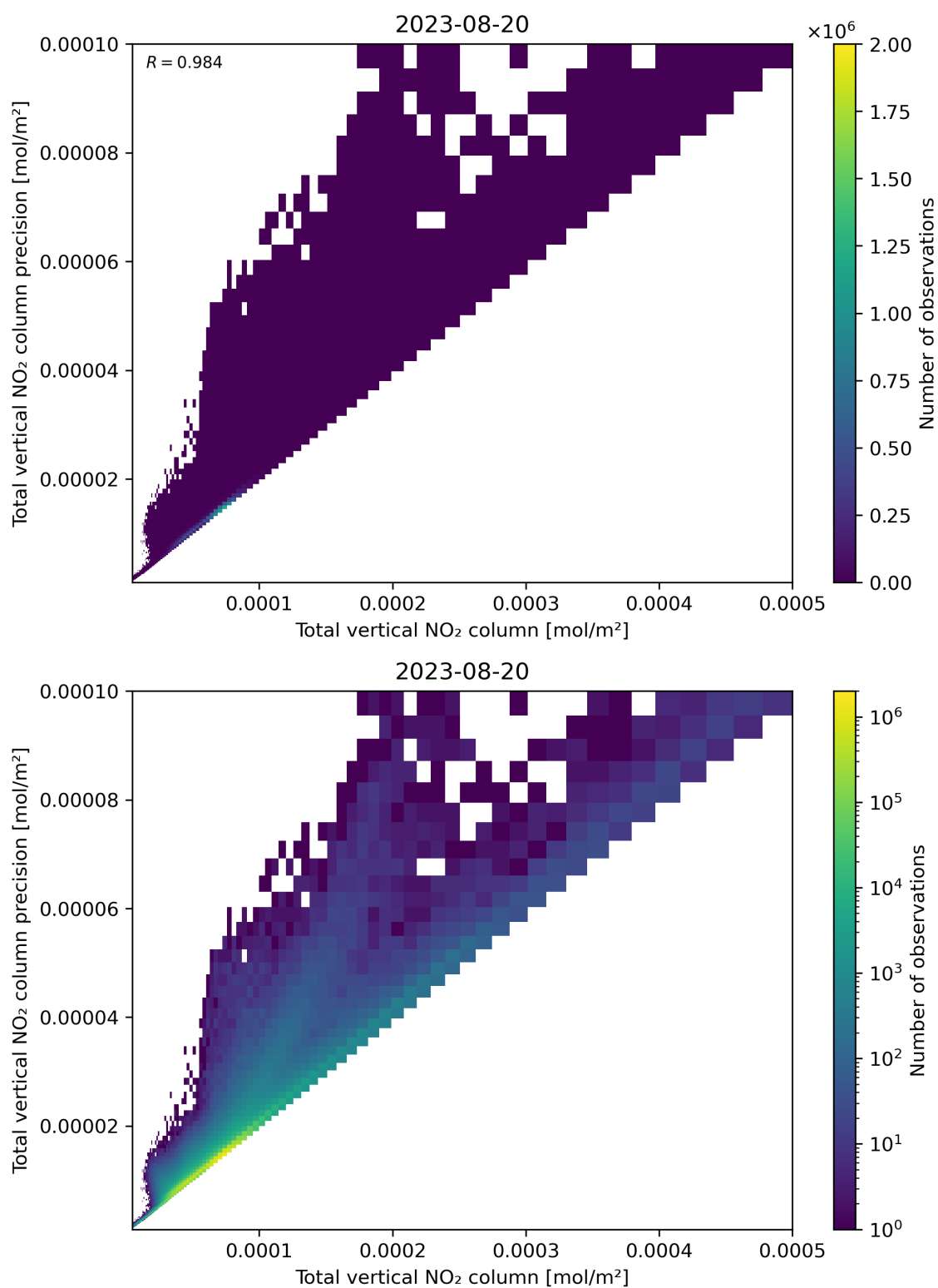
Figure 114: Scatter density plot of “Total vertical NO 2 column” against “Total vertical NO 2 column precision” for 2023-08-20 to 2023-08-21.
