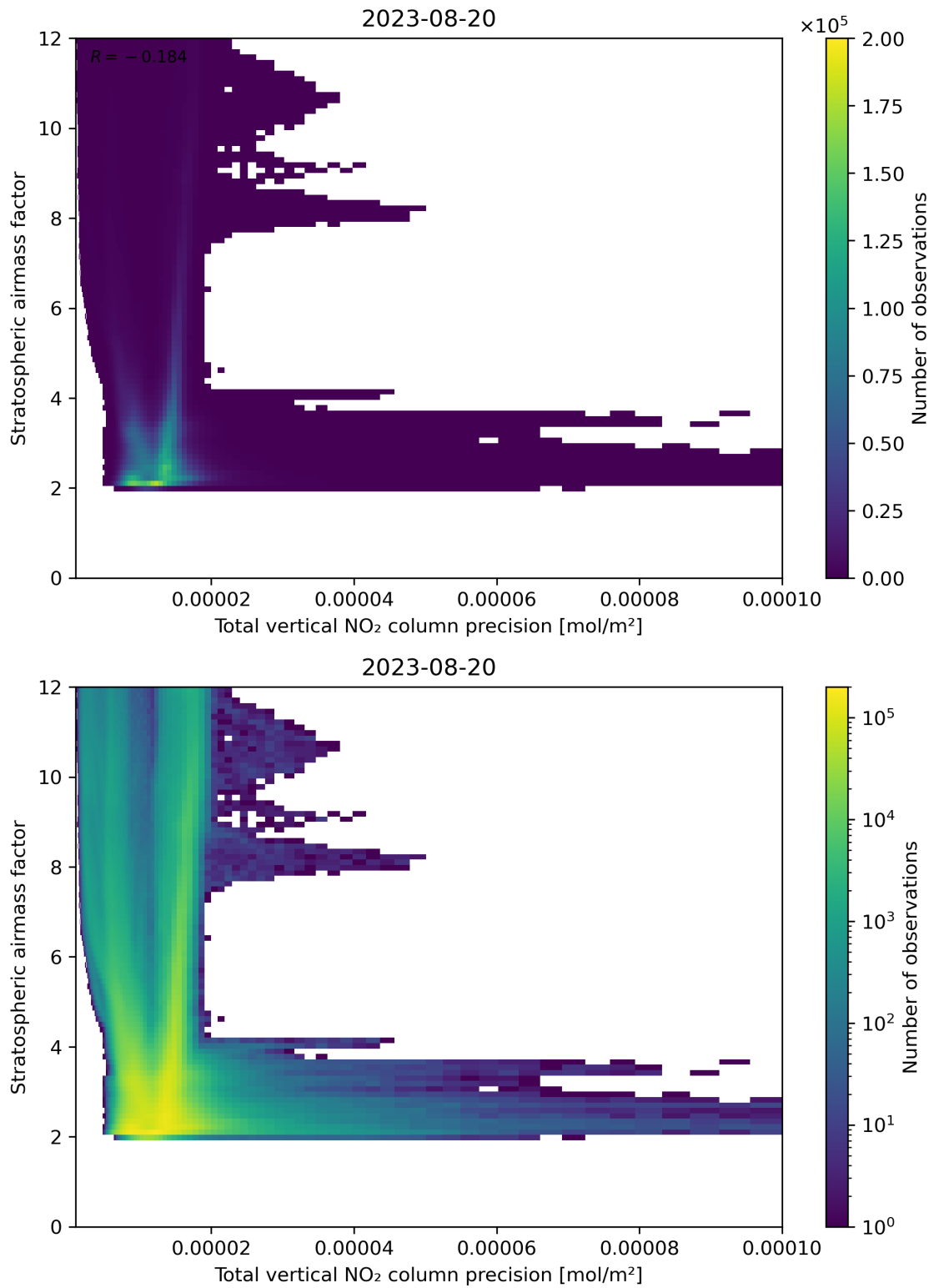
Figure 115: Scatter density plot of “Total vertical NO 2 column precision” against “Stratospheric air mass factor” for 2023-08-20 to 2023-08-21.
