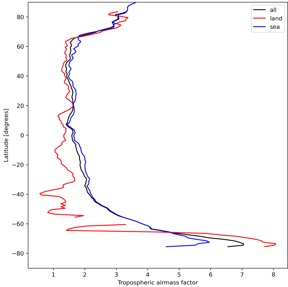
Figure 14: Zonal average of “Tropospheric air mass factor” for 2023-08-20 to 2023-08-21.
