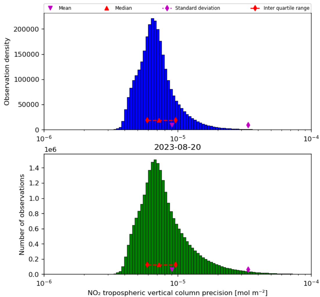
Figure 30: Histogram of “NO 2 tropospheric vertical column precision” for 2023-08-20 to 2023-08-21
