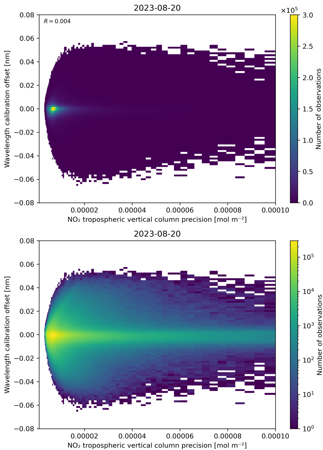
Figure 141: Scatter density plot of “NO 2 tropospheric vertical column precision” against “Wavelength calibration offset” for 2023-08-20 to 2023-08-21.
