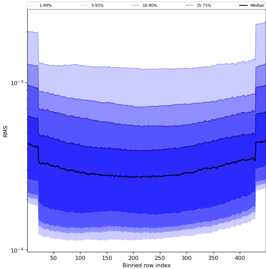
Figure 60: Along track statistics of “RMS” for 2023-08-20 to 2023-08-21
