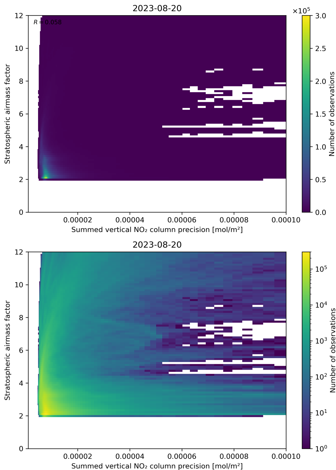
Figure 106: Scatter density plot of “Summed vertical NO 2 column precision” against “Stratospheric airmass factor” for 2023-08-20 to 2023-08-21.
