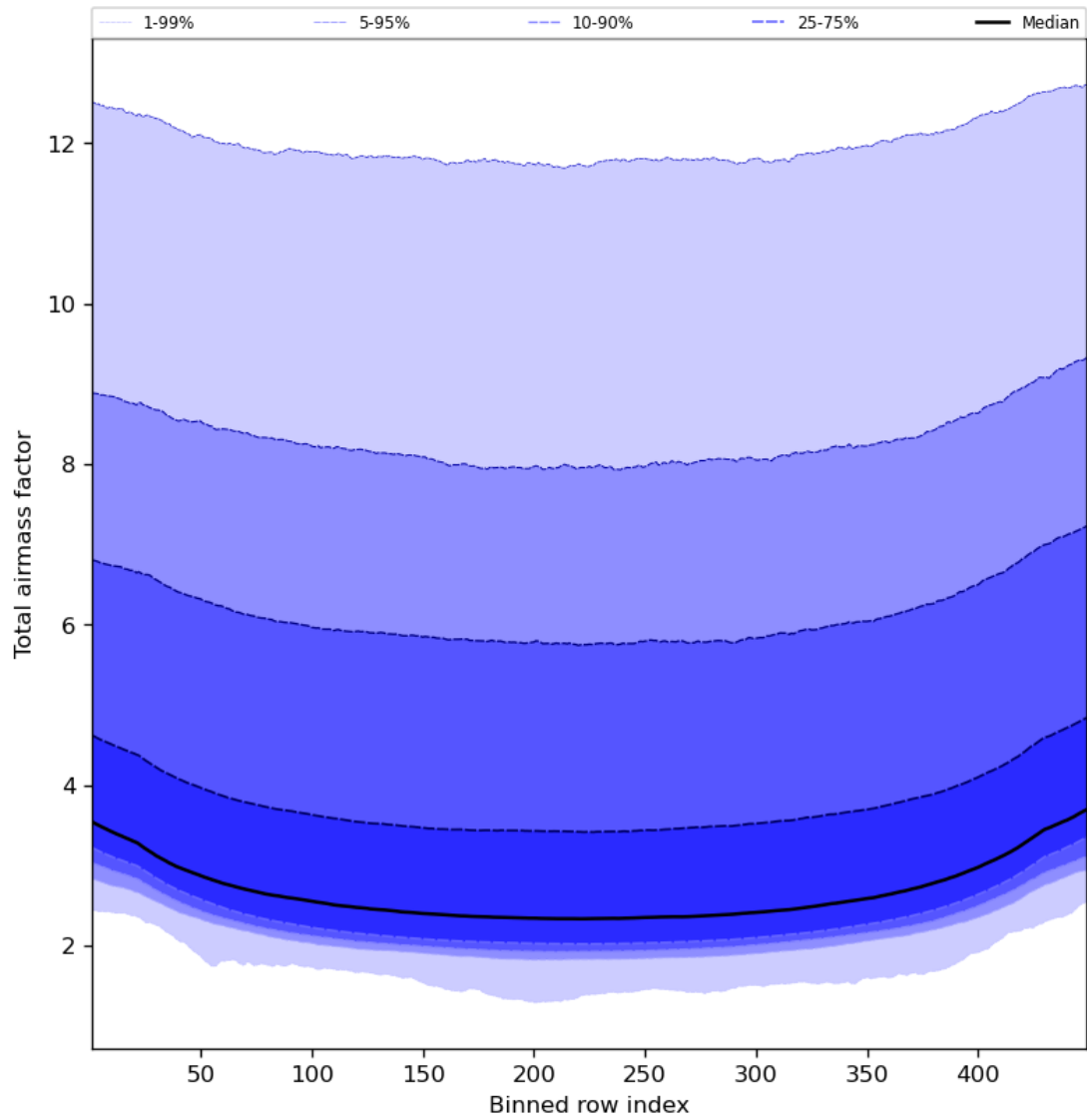
Figure 49: Along track statistics of “Total airmass factor” for 2023-08-20 to 2023-08-21
