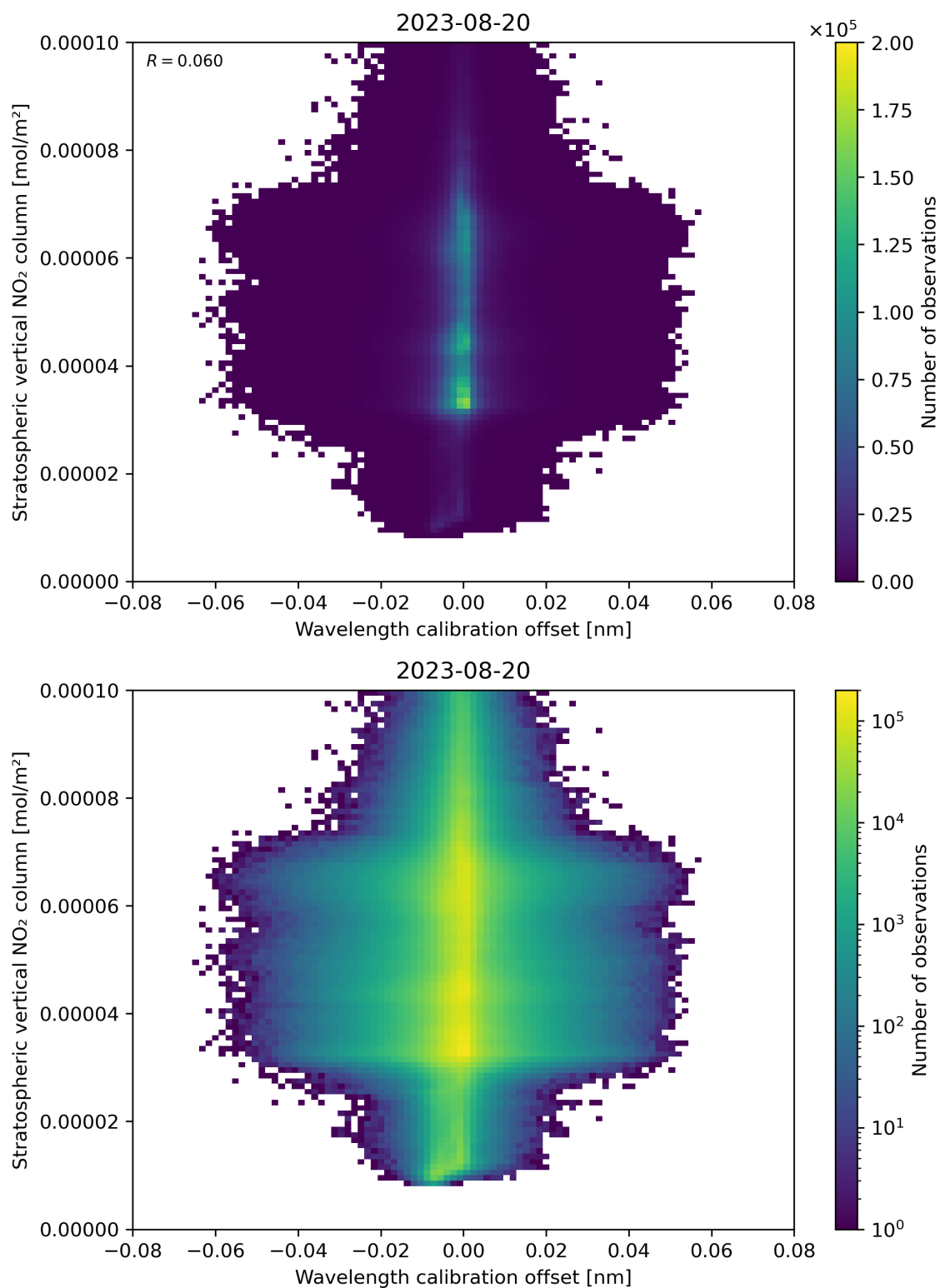
Figure 176: Scatter density plot of “Wavelength calibration offset” against “Stratospheric vertical NO 2 column” for 2023-08-20 to 2023-08-21.
