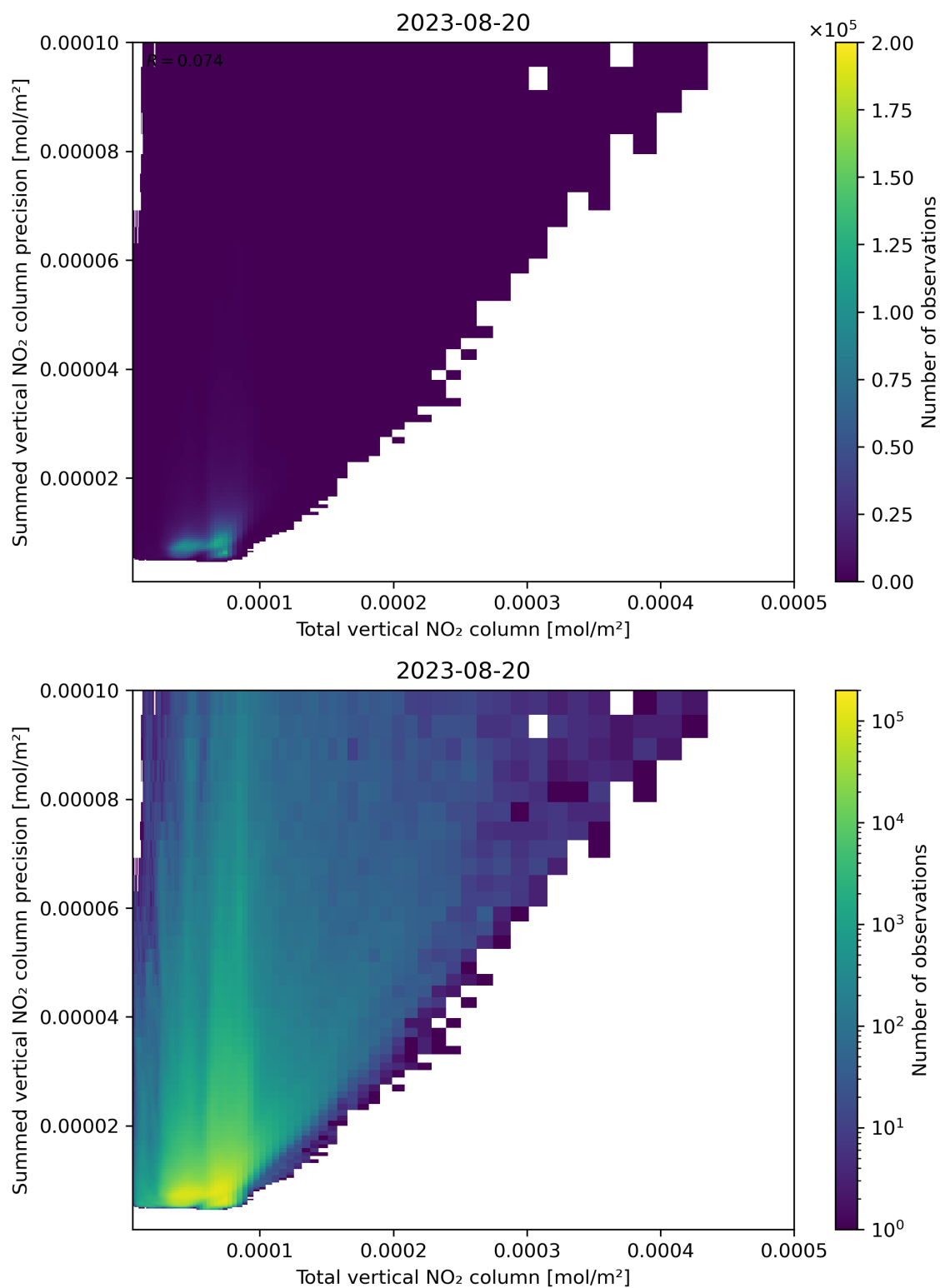
Figure 113: Scatter density plot of “Total vertical NO 2 column” against “Summed vertical NO 2 column precision” for 2023-08-20 to 2023-08-21.
