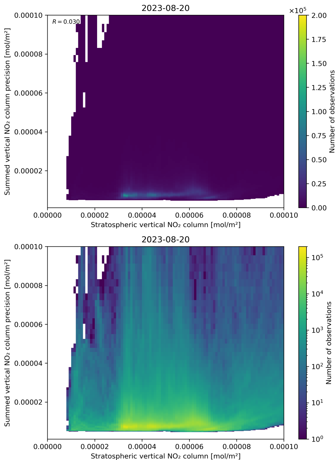
Figure 99: Scatter density plot of “Stratospheric vertical NO 2 column” against “Summed vertical NO 2 column precision” for 2023-08-20 to 2023-08-21.
