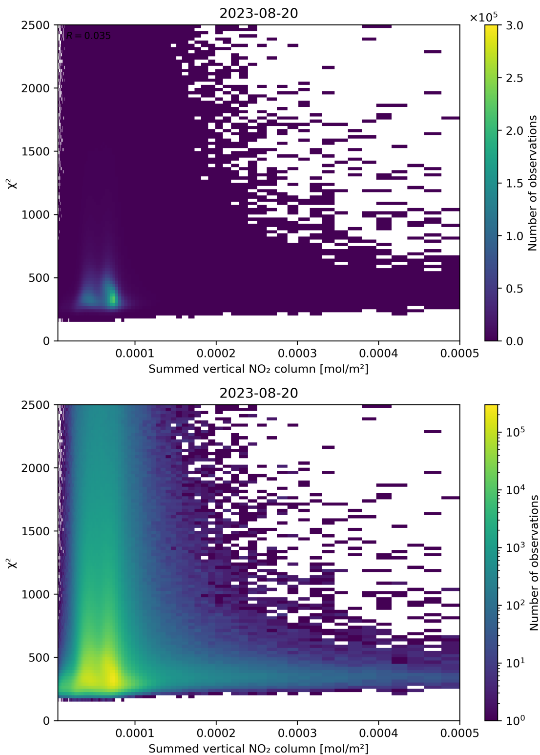
Figure 104: Scatter density plot of “Summed vertical NO 2 column” against “ \chi^2 ” for 2023-08-20 to 2023-08-21.
