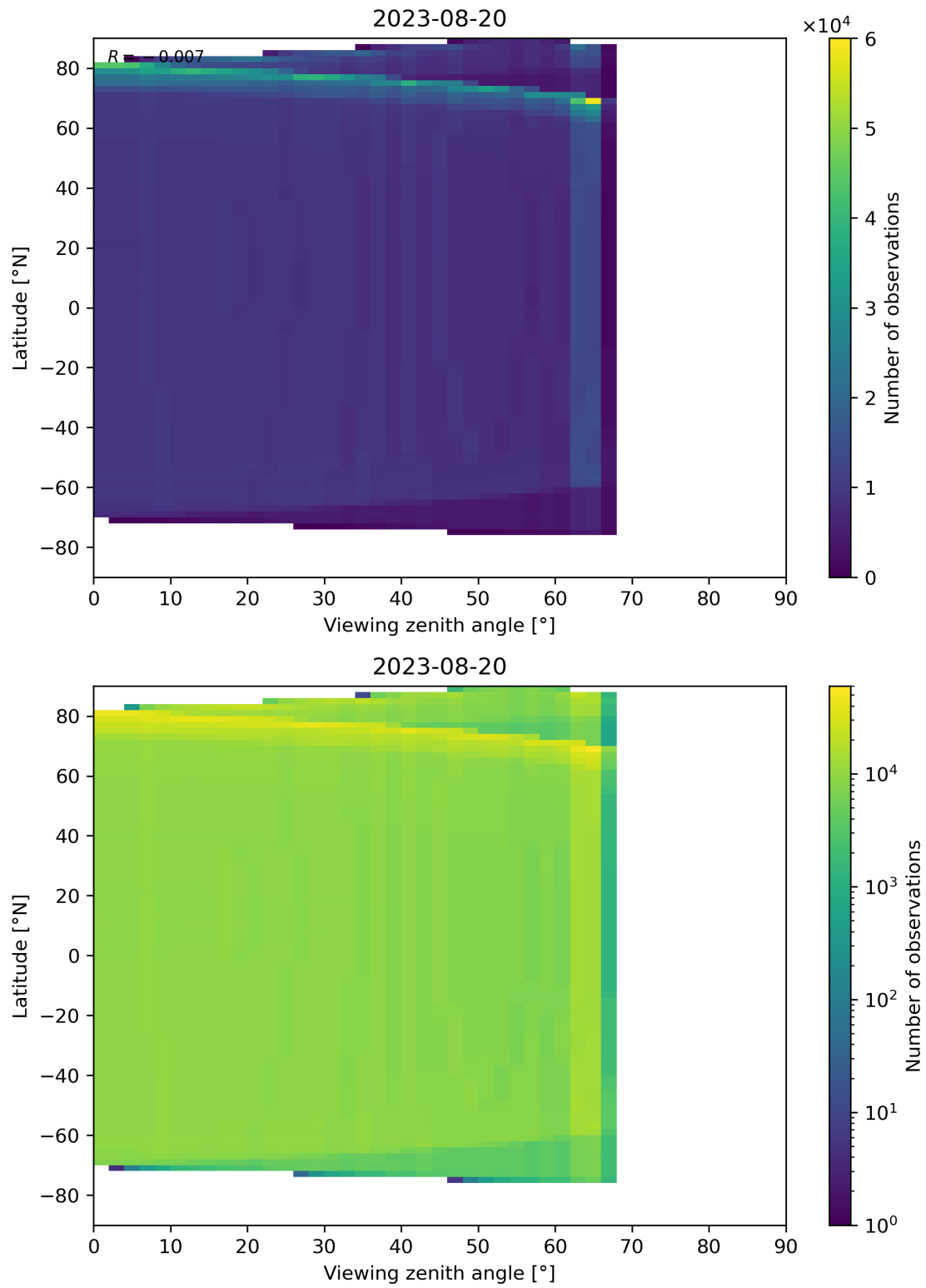
Figure 163: Scatter density plot of “Viewing zenith angle” against “Latitude” for 2023-08-20 to 2023-08-21.
