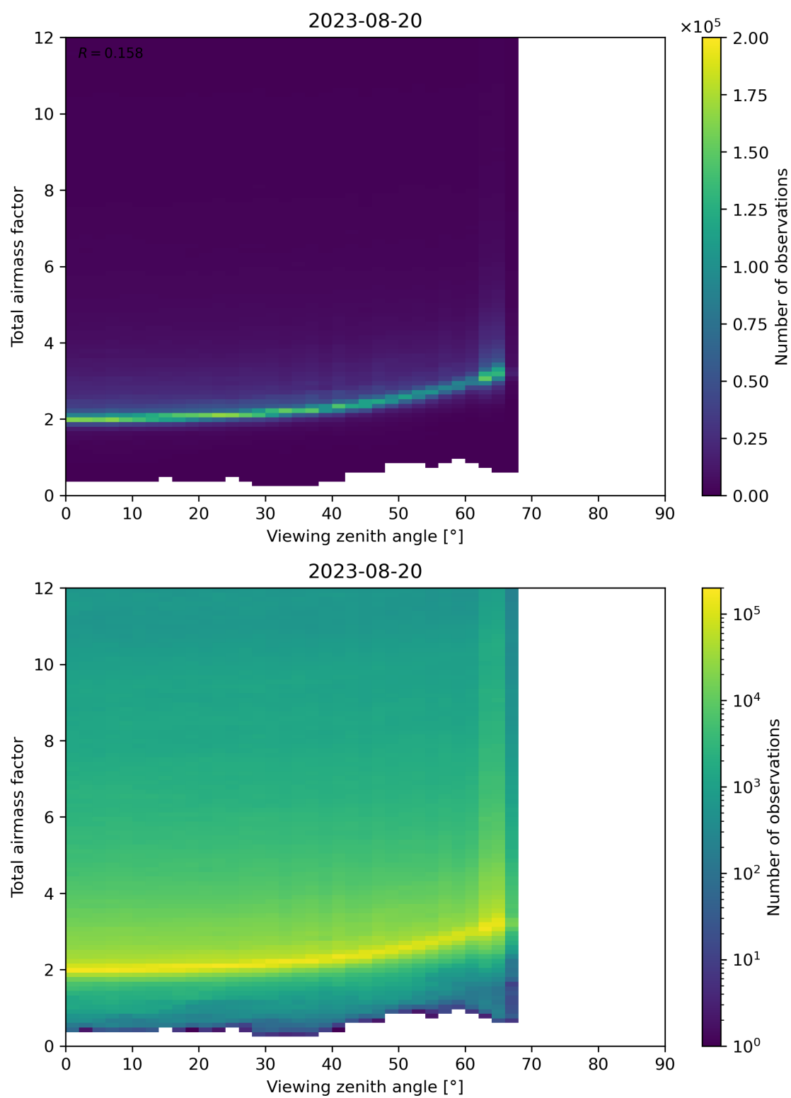
Figure 160: Scatter density plot of “Viewing zenith angle” against “Total airmass factor” for 2023-08-20 to 2023-08-21.
