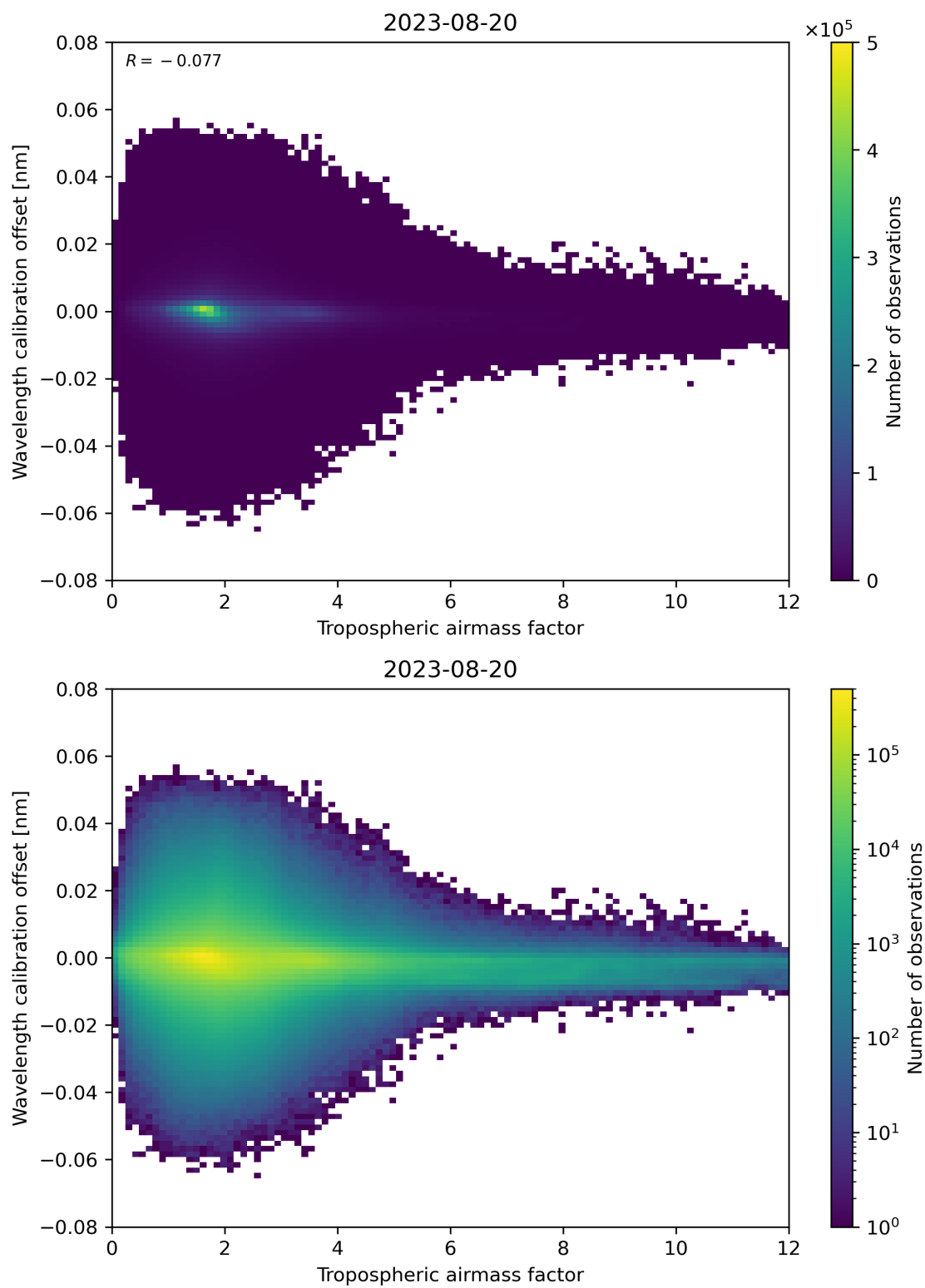
Figure 80: Scatter density plot of “Tropospheric airmass factor” against “Wavelength calibration offset” for 2023-08-20 to 2023-08-21.
