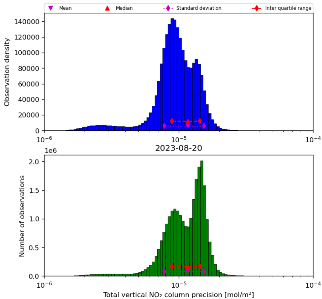
Figure 39: Histogram of “Total vertical NO 2 column precision” for 2023-08-20 to 2023-08-21
