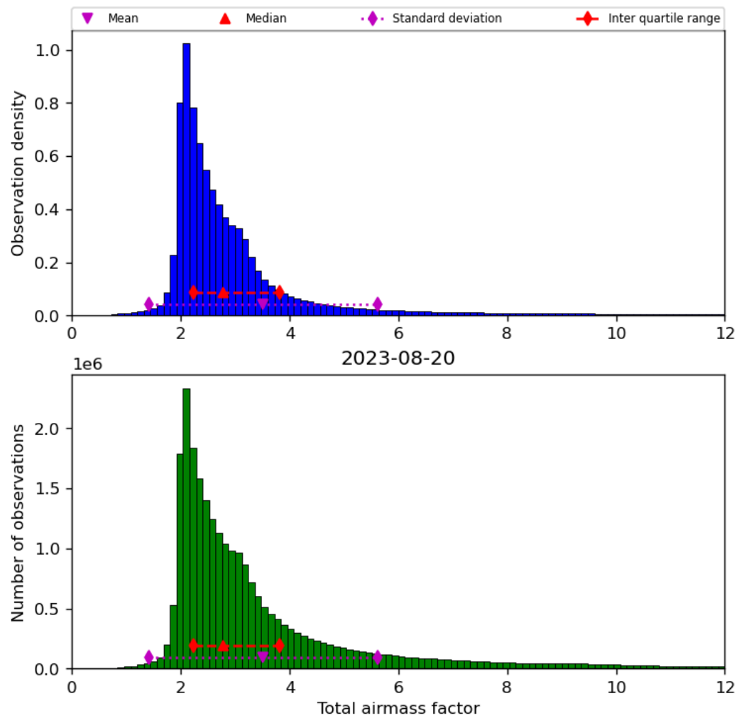
Figure 32: Histogram of “Total airmass factor” for 2023-08-20 to 2023-08-21
