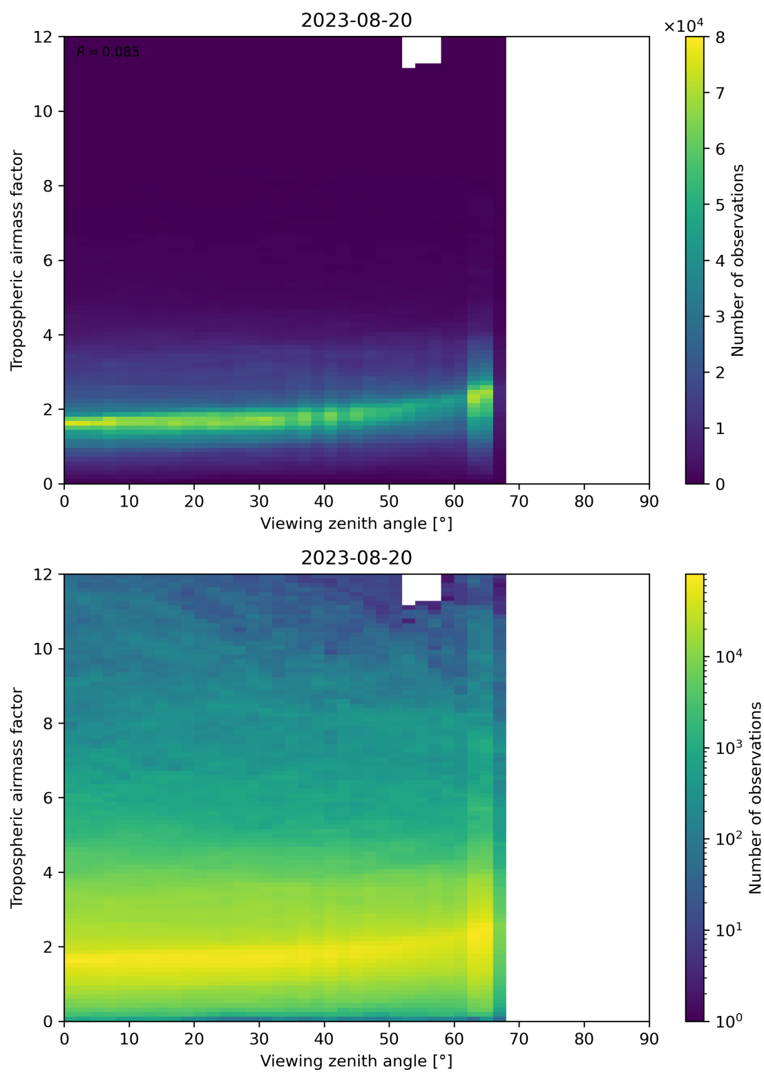
Figure 161: Scatter density plot of “Viewing zenith angle” against “Tropospheric airmass factor” for 2023-08-20 to 2023-08-21.
