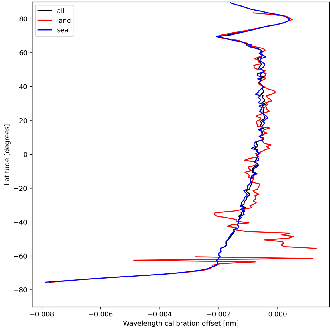
Figure 18: Zonal average of “Wavelength calibration offset” for 2023-08-20 to 2023-08-21.
