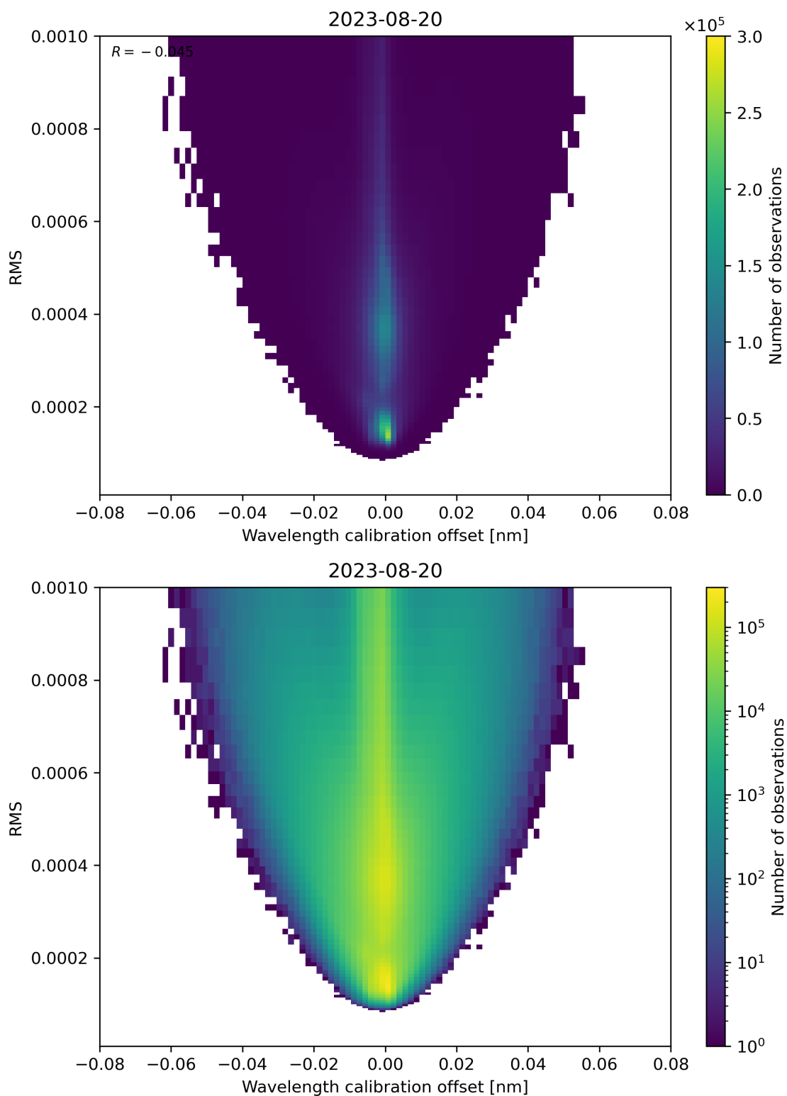
Figure 181: Scatter density plot of “Wavelength calibration offset” against “RMS” for 2023-08-20 to 2023-08-21.
