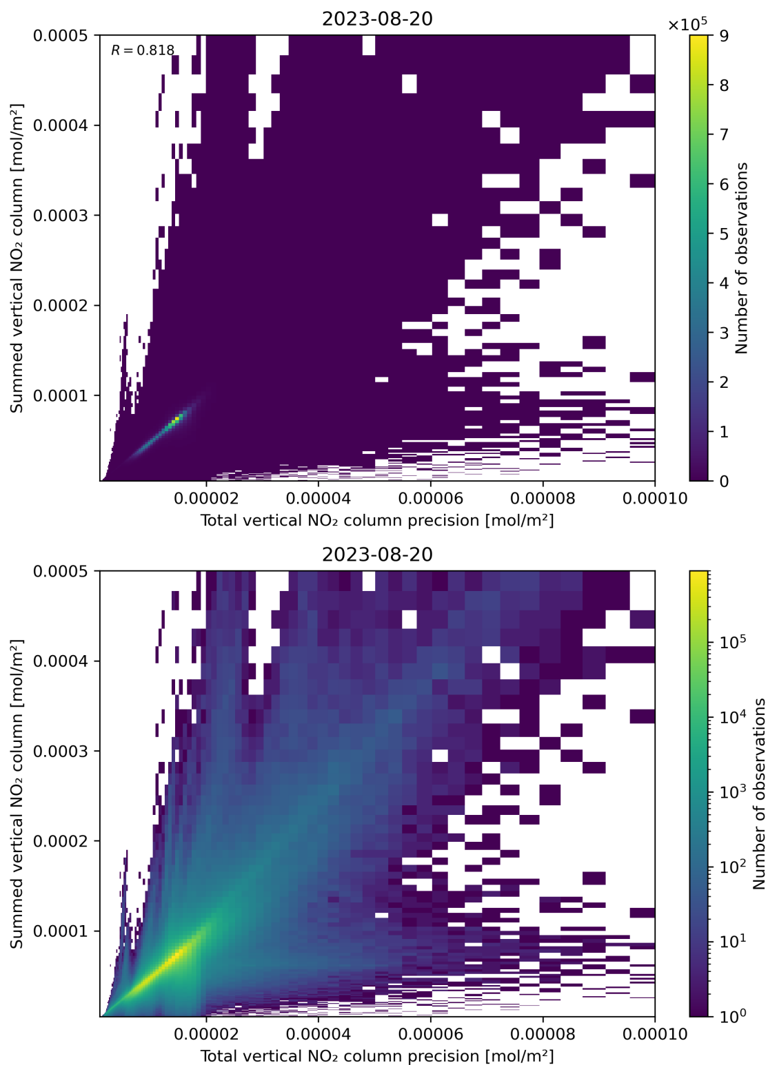
Figure 117: Scatter density plot of “Total vertical NO 2 column precision” against “Summed vertical NO 2 column” for 2023-08-20 to 2023-08-21.
