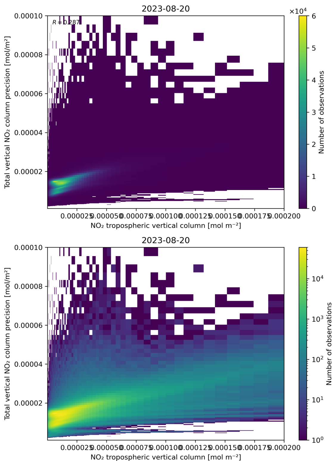
Figure 129: Scatter density plot of “NO 2 tropospheric vertical column” against “Total vertical NO 2 column precision” for 2023-08-20 to 2023-08-21.
