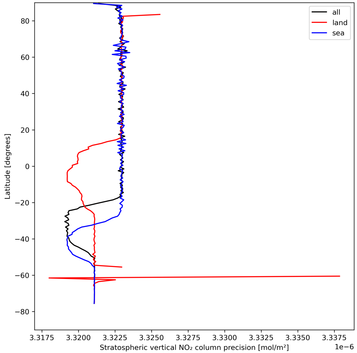
Figure 20: Zonal average of “Stratospheric vertical NO 2 column precision” for 2023-08-20 to 2023-08-21.
