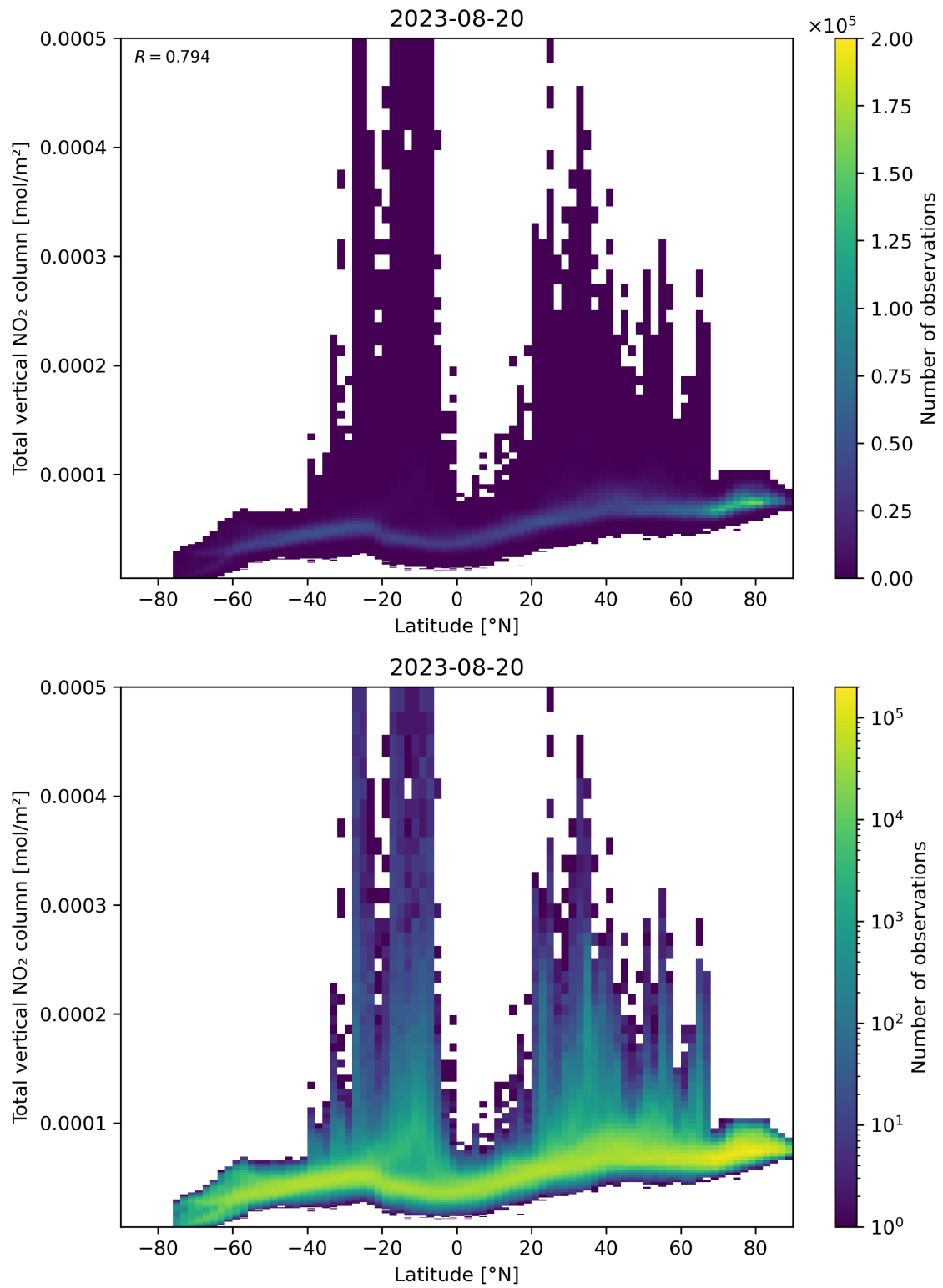
Figure 90: Scatter density plot of “Latitude” against “Total vertical NO 2 column” for 2023-08-20 to 2023-08-21.
