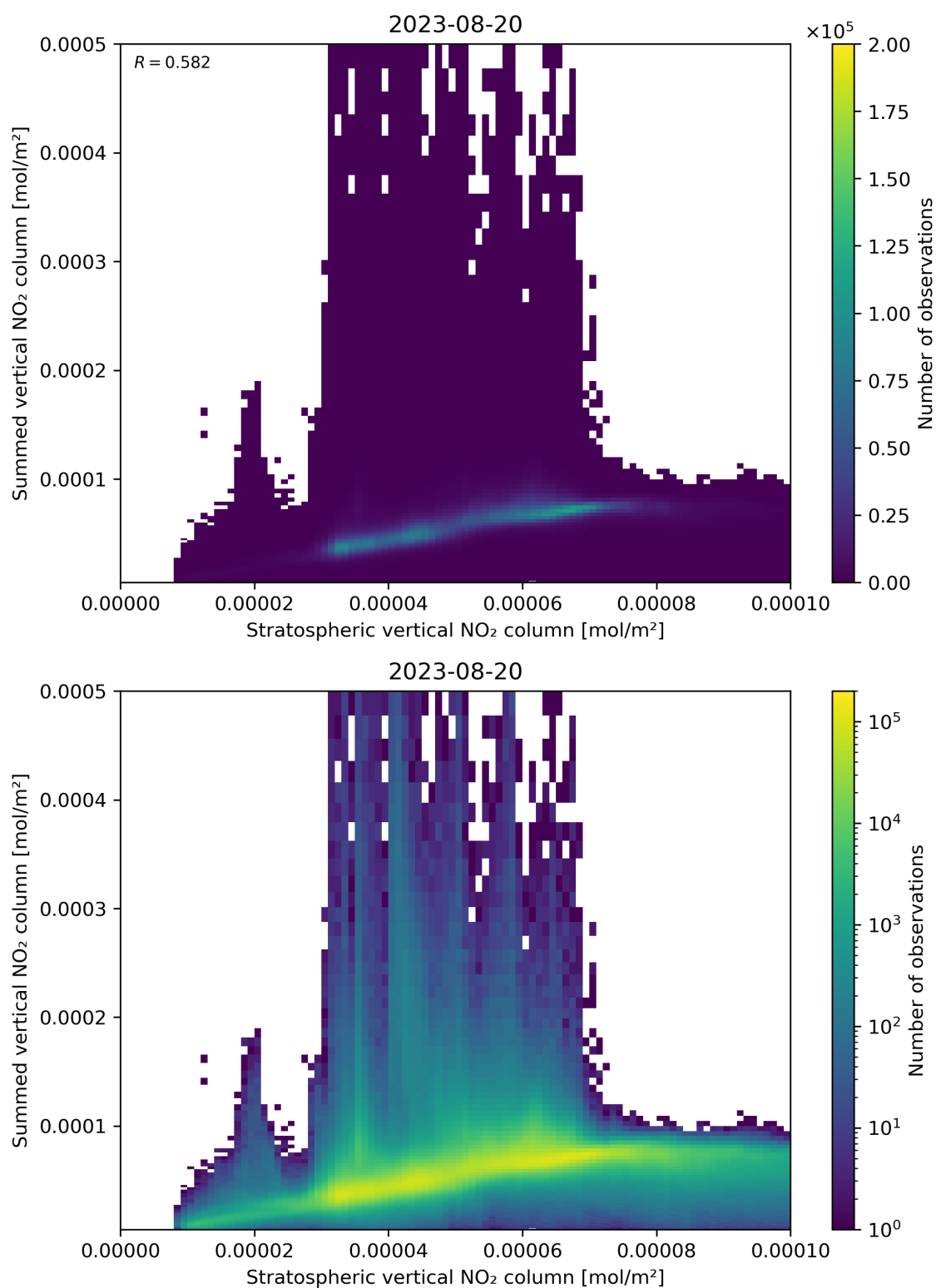
Figure 98: Scatter density plot of “Stratospheric vertical NO 2 column” against “Summed vertical NO 2 column” for 2023-08-20 to 2023-08-21.
