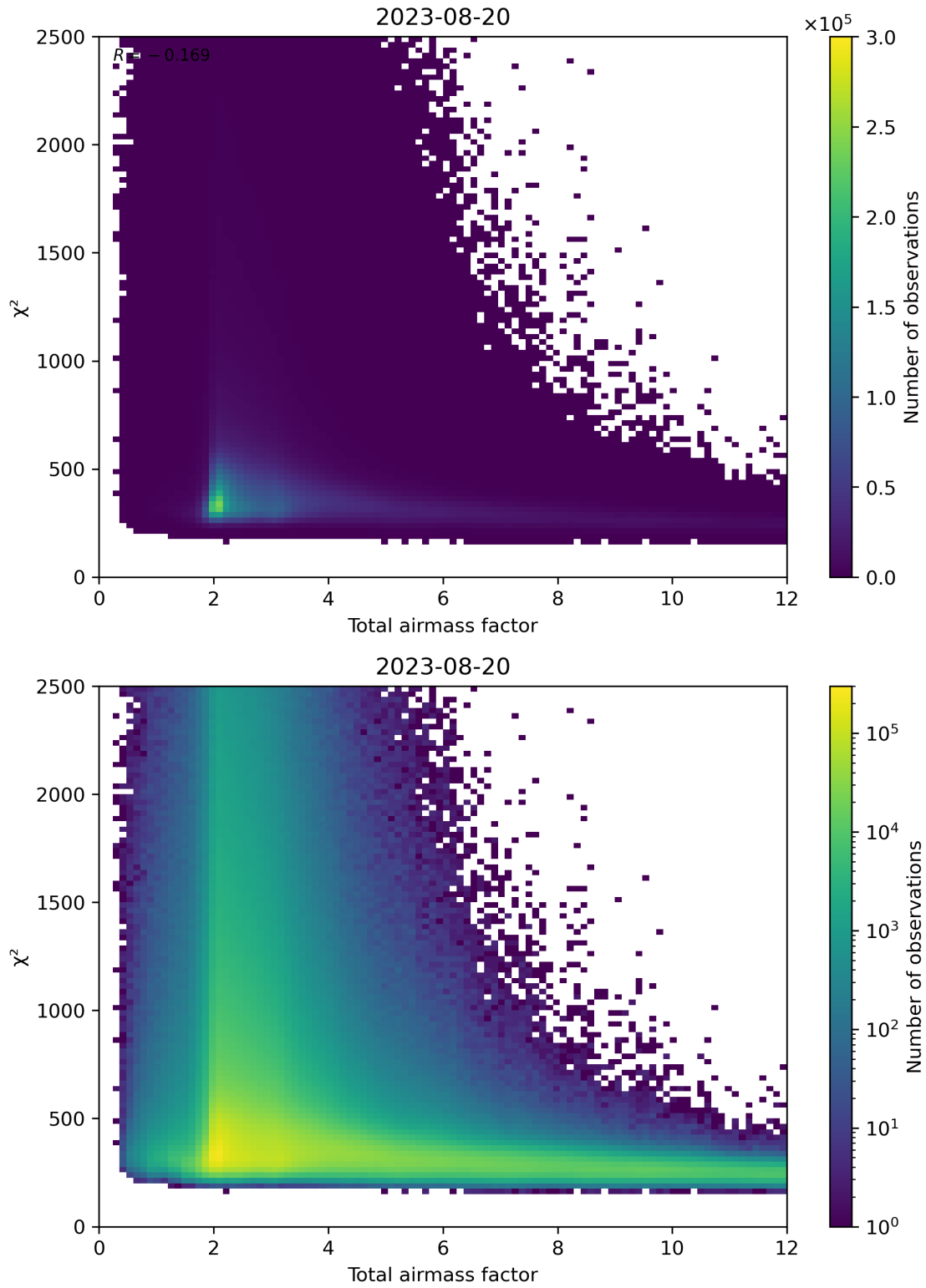
Figure 63: Scatter density plot of “Total airmass factor” against “ \chi^2 ” for 2023-08-20 to 2023-08-21.
