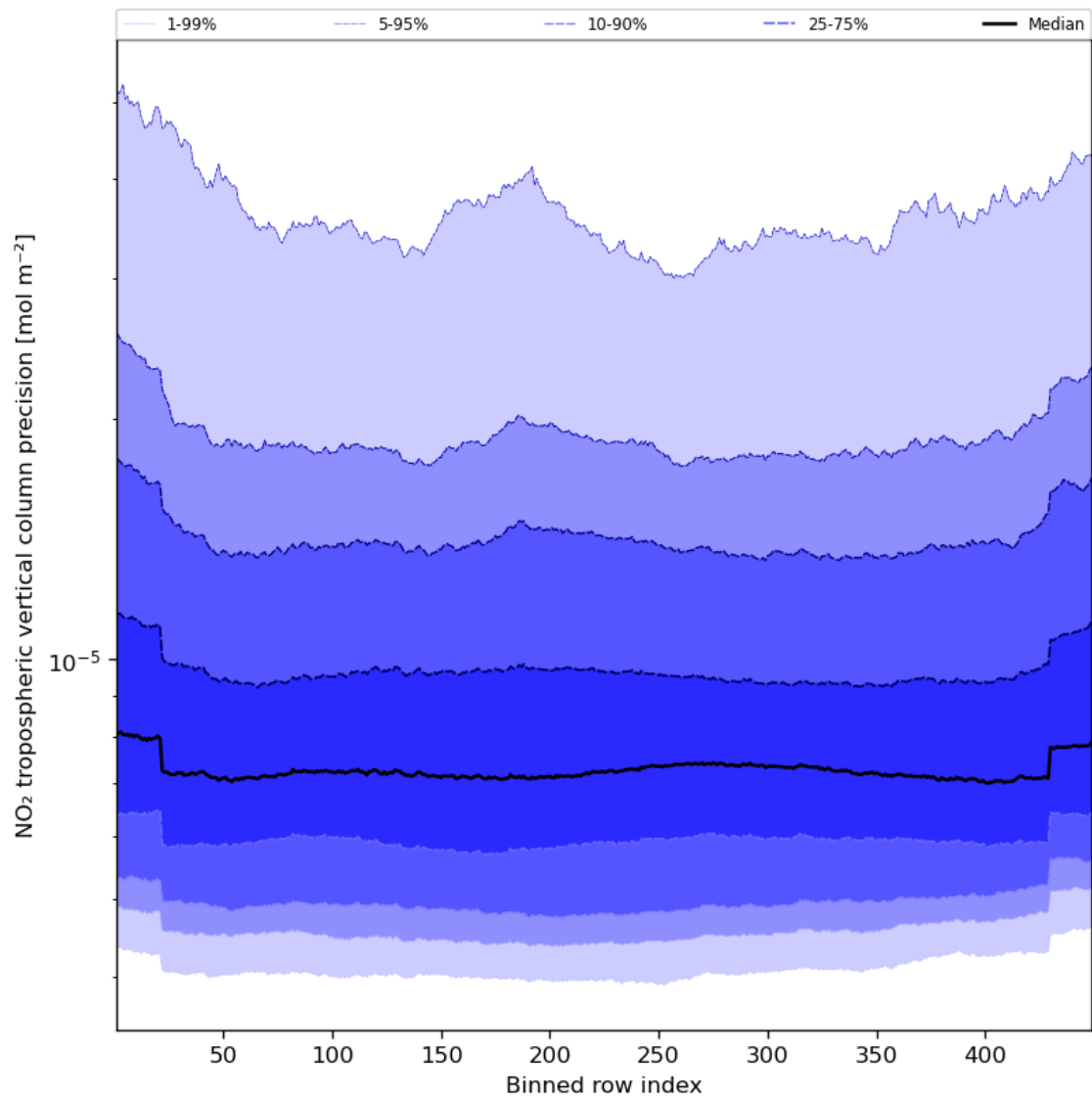
Figure 47: Along track statistics of “NO 2 tropospheric vertical column precision” for 2023-08-20 to 2023-08-21
