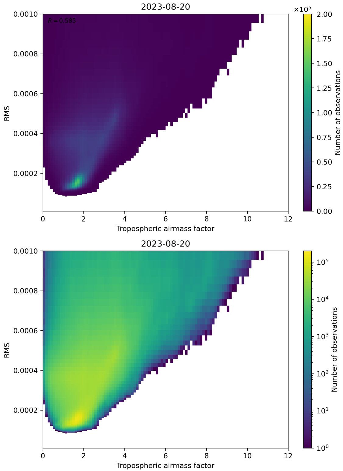
Figure 79: Scatter density plot of “Tropospheric airmass factor” against “RMS” for 2023-08-20 to 2023-08-21.
