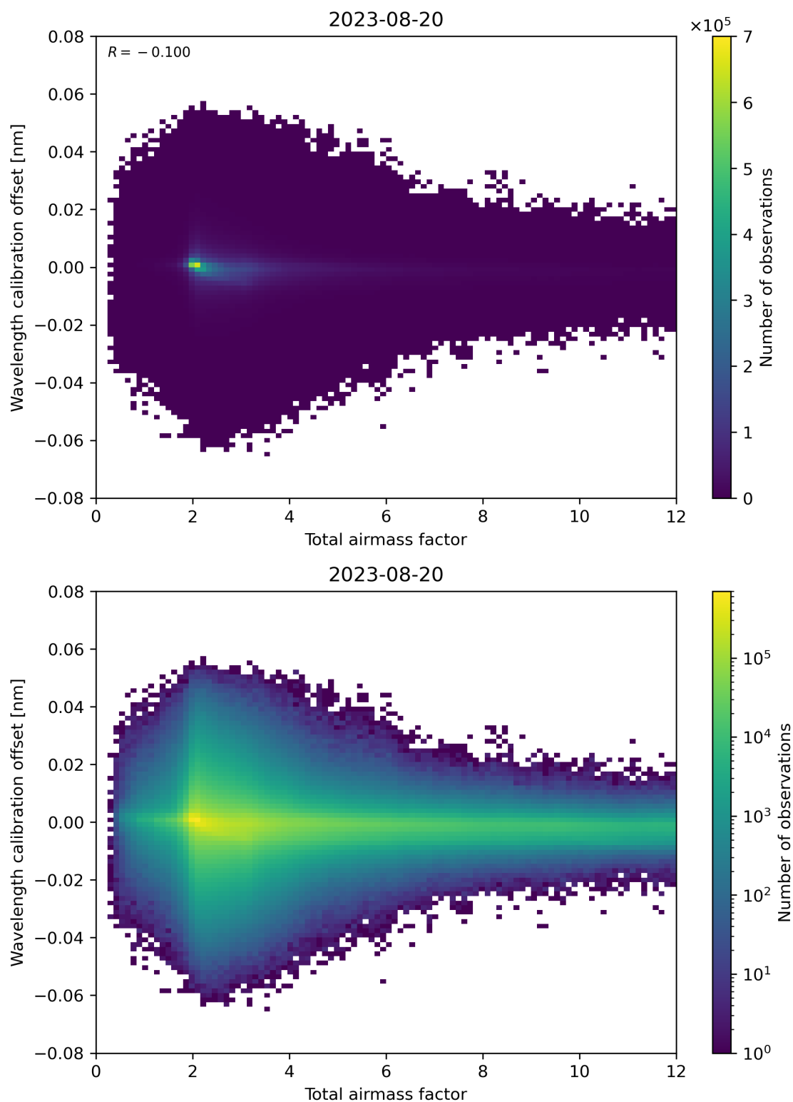
Figure 70: Scatter density plot of “Total airmass factor” against “Wavelength calibration offset” for 2023-08-20 to 2023-08-21.
