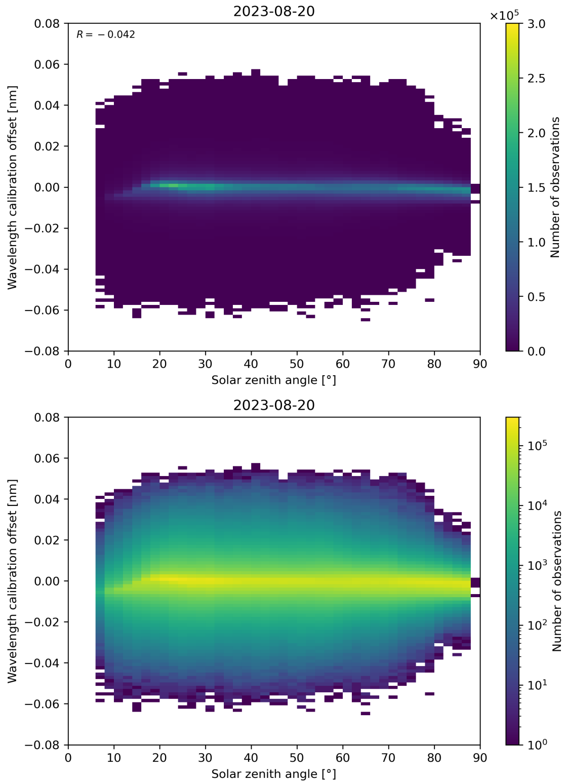
Figure 158: Scatter density plot of “Solar zenith angle” against “Wavelength calibration offset” for 2023-08-20 to 2023-08-21.
