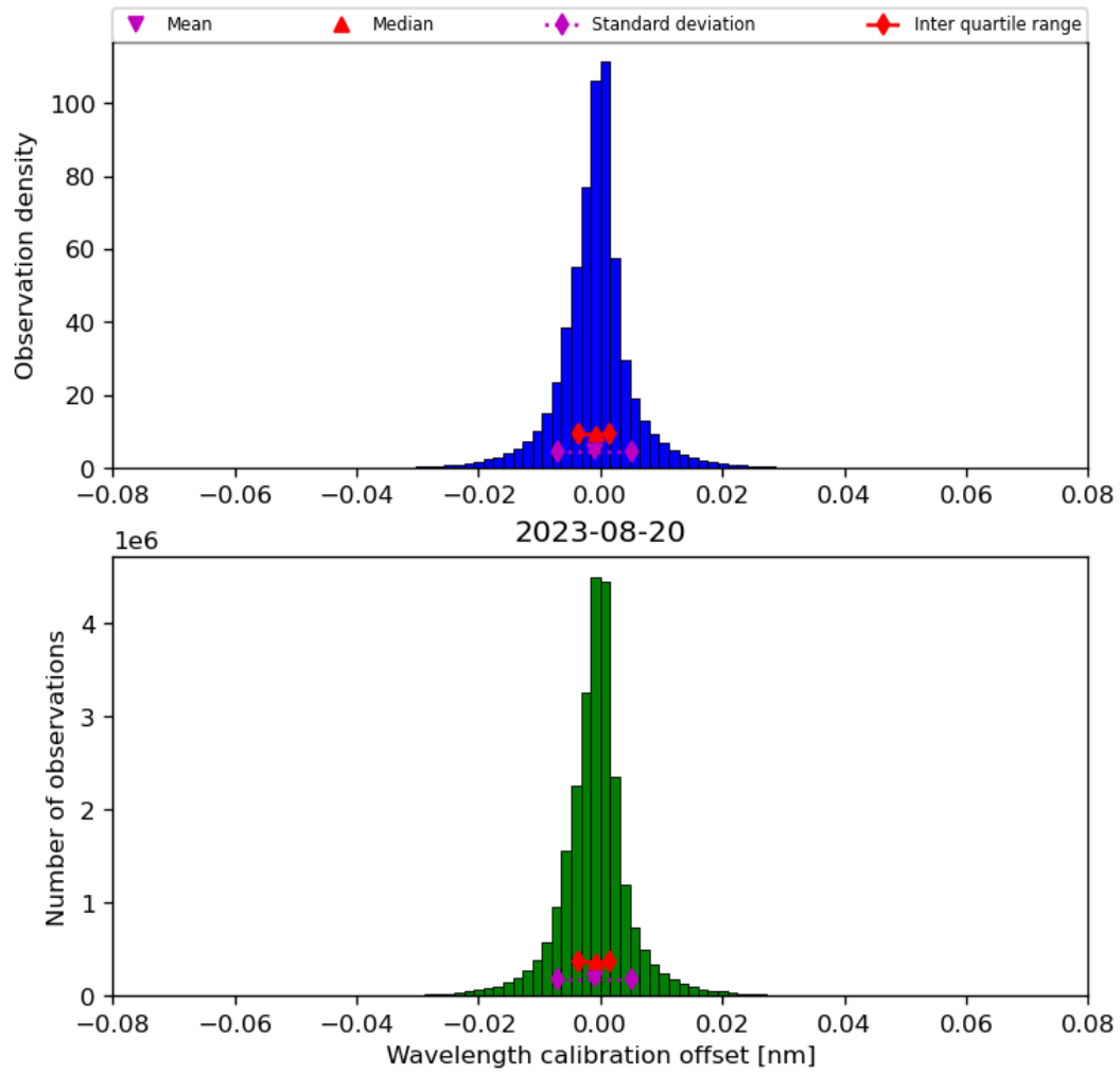
Figure 35: Histogram of “Wavelength calibration offset” for 2023-08-20 to 2023-08-21
