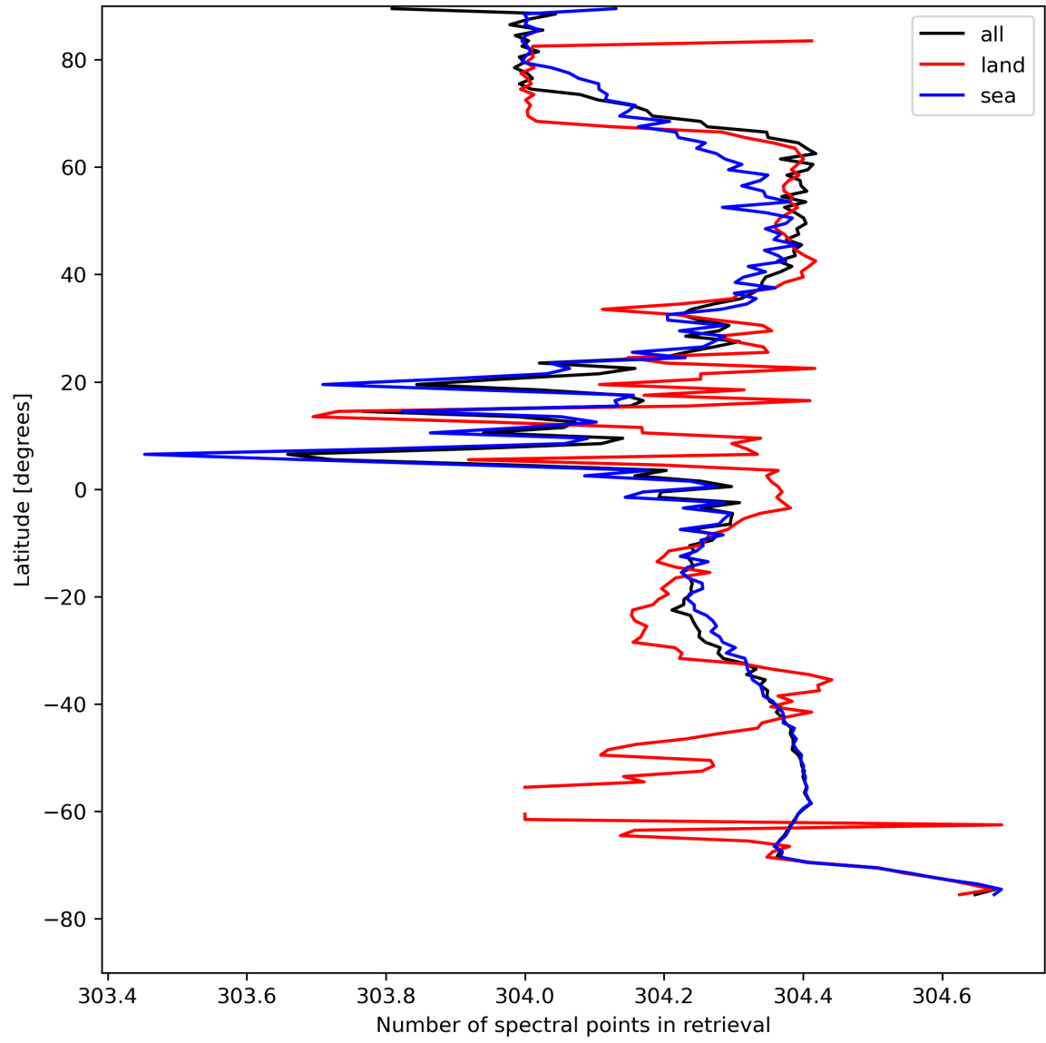
Figure 16: Zonal average of “Number of spectral points in retrieval” for 2023-08-20 to 2023-08-21.
