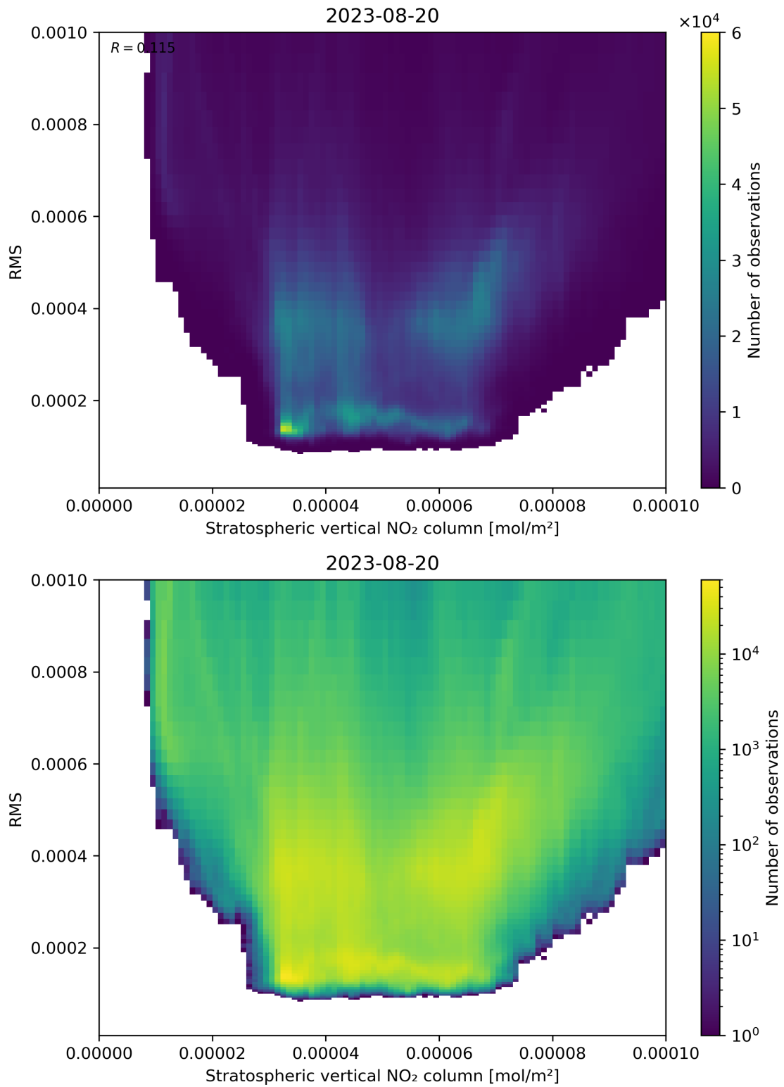
Figure 102: Scatter density plot of “Stratospheric vertical NO 2 column” against “RMS” for 2023-08-20 to 2023-08-21.
