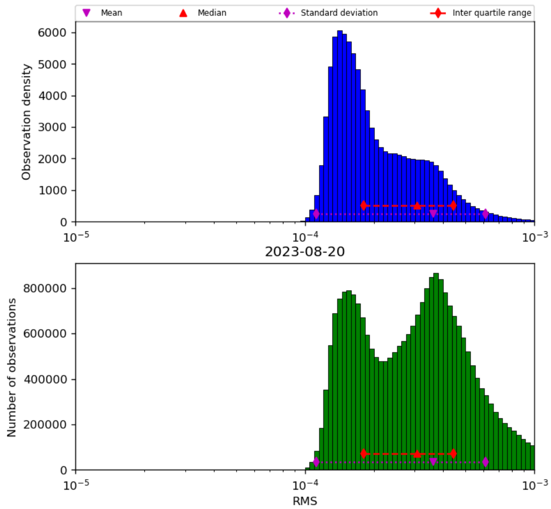
Figure 43: Histogram of “RMS” for 2023-08-20 to 2023-08-21
