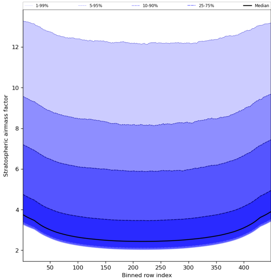
Figure 61: Along track statistics of “Stratospheric airmass factor” for 2023-08-20 to 2023-08-21
