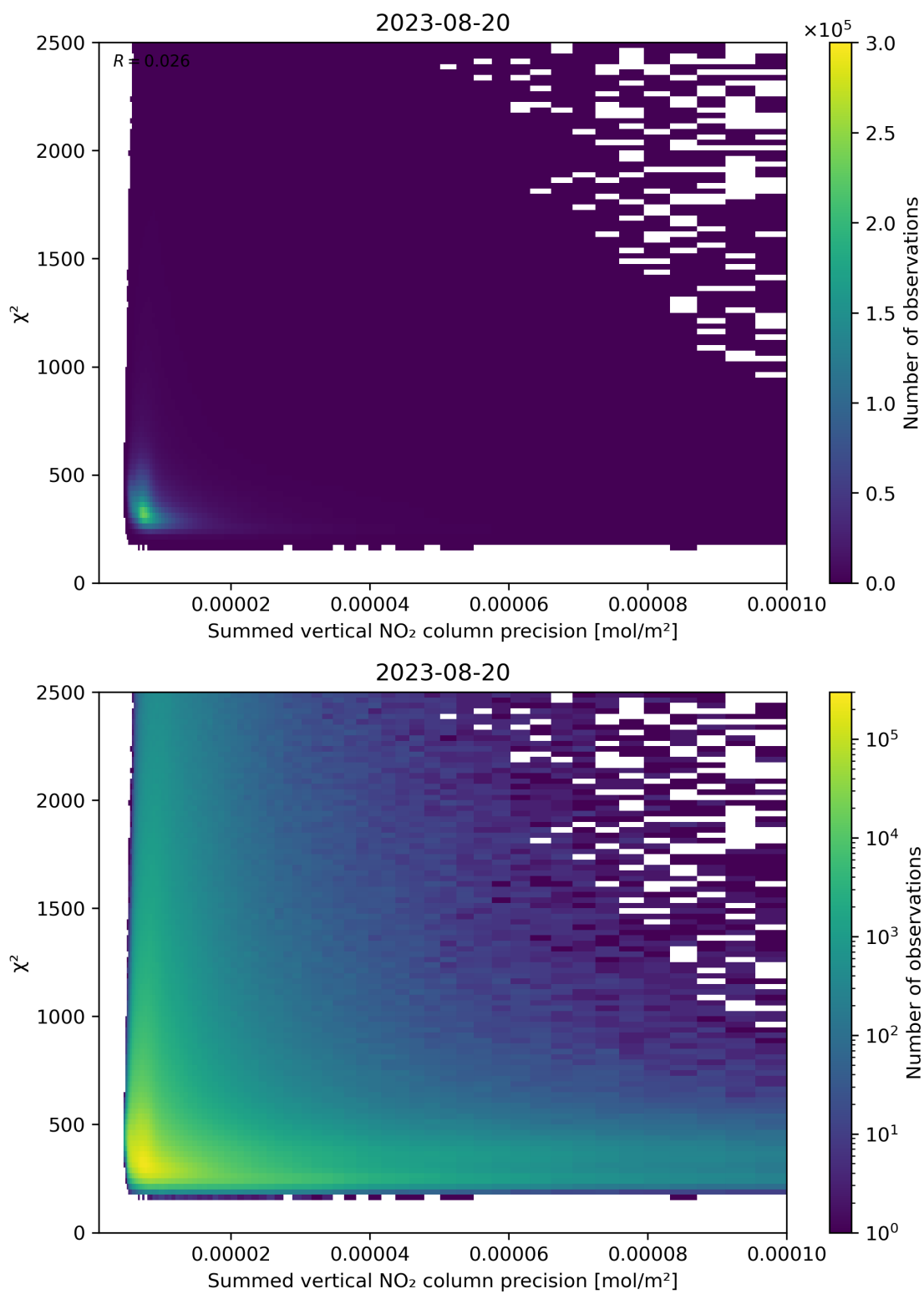
Figure 107: Scatter density plot of “Summed vertical NO 2 column precision” against “ \chi^2 ” for 2023-08-20 to 2023-08-21.
