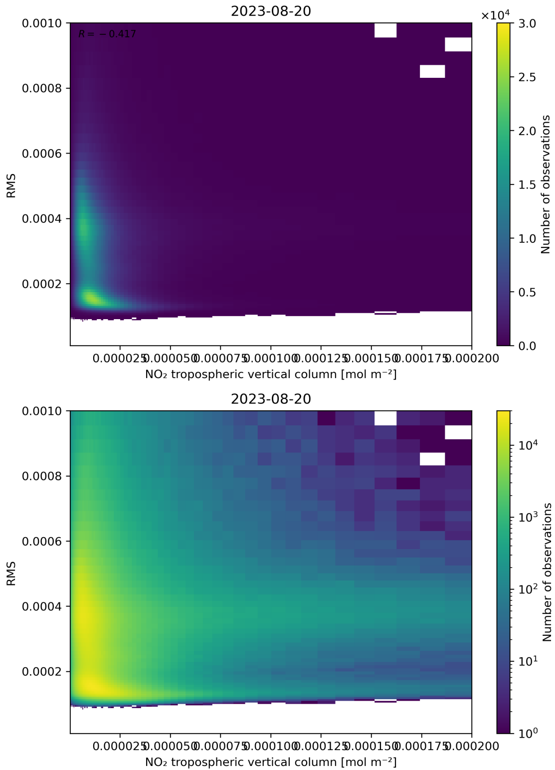
Figure 142: Scatter density plot of “NO 2 tropospheric vertical column” against “RMS” for 2023-08-20 to 2023-08-21.
