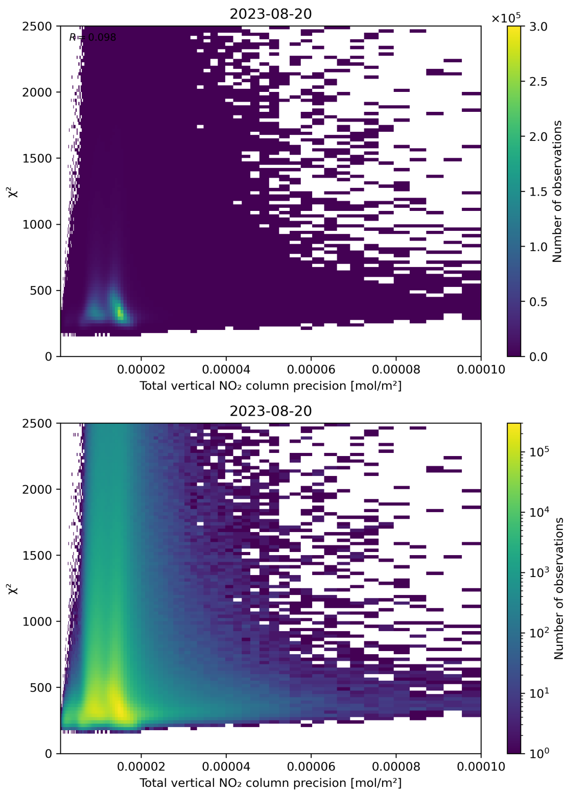
Figure 116: Scatter density plot of “Total vertical NO 2 column precision” against “ \chi^2 ” for 2023-08-20 to 2023-08-21.
