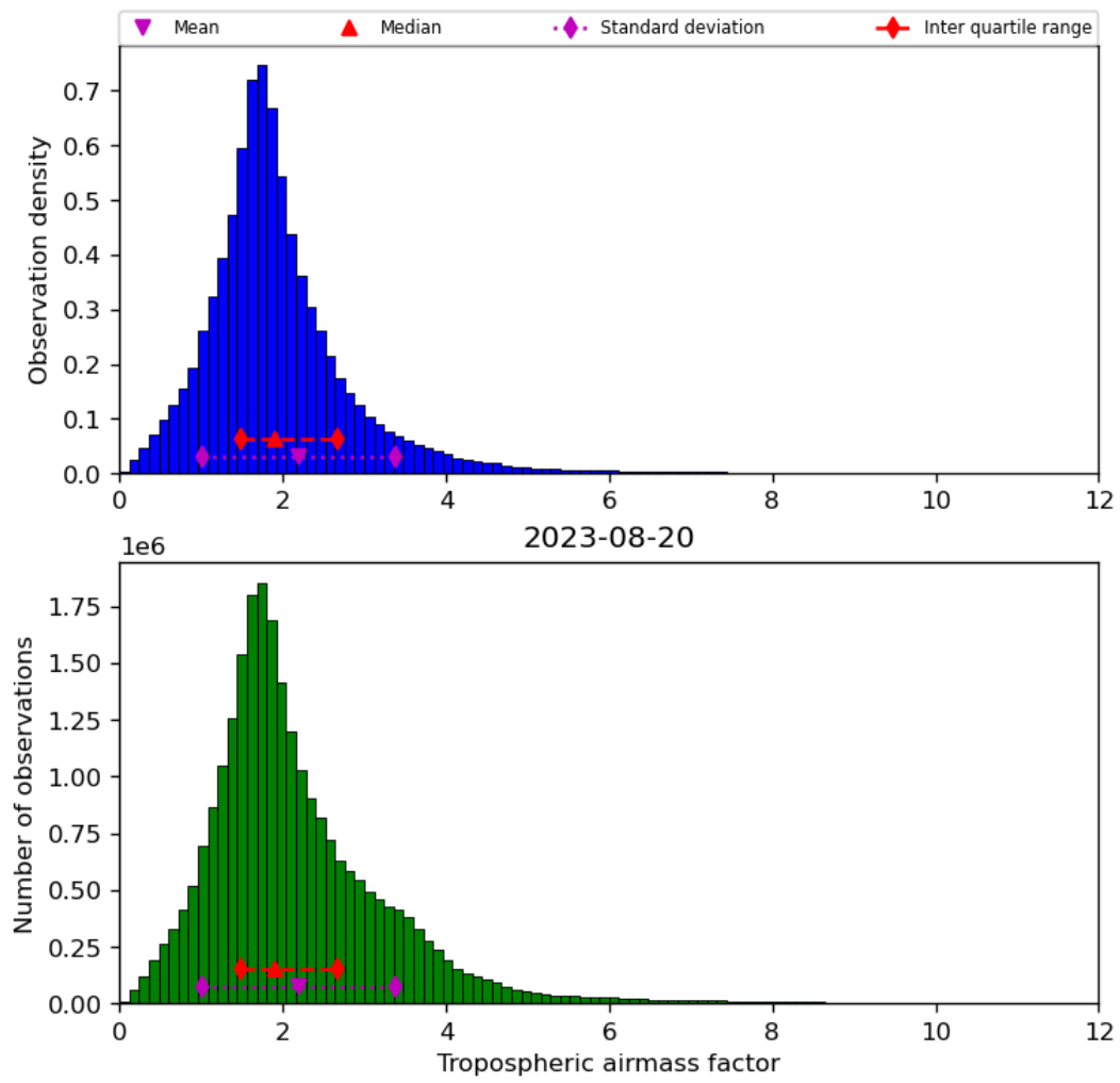
Figure 31: Histogram of “Tropospheric airmass factor” for 2023-08-20 to 2023-08-21
