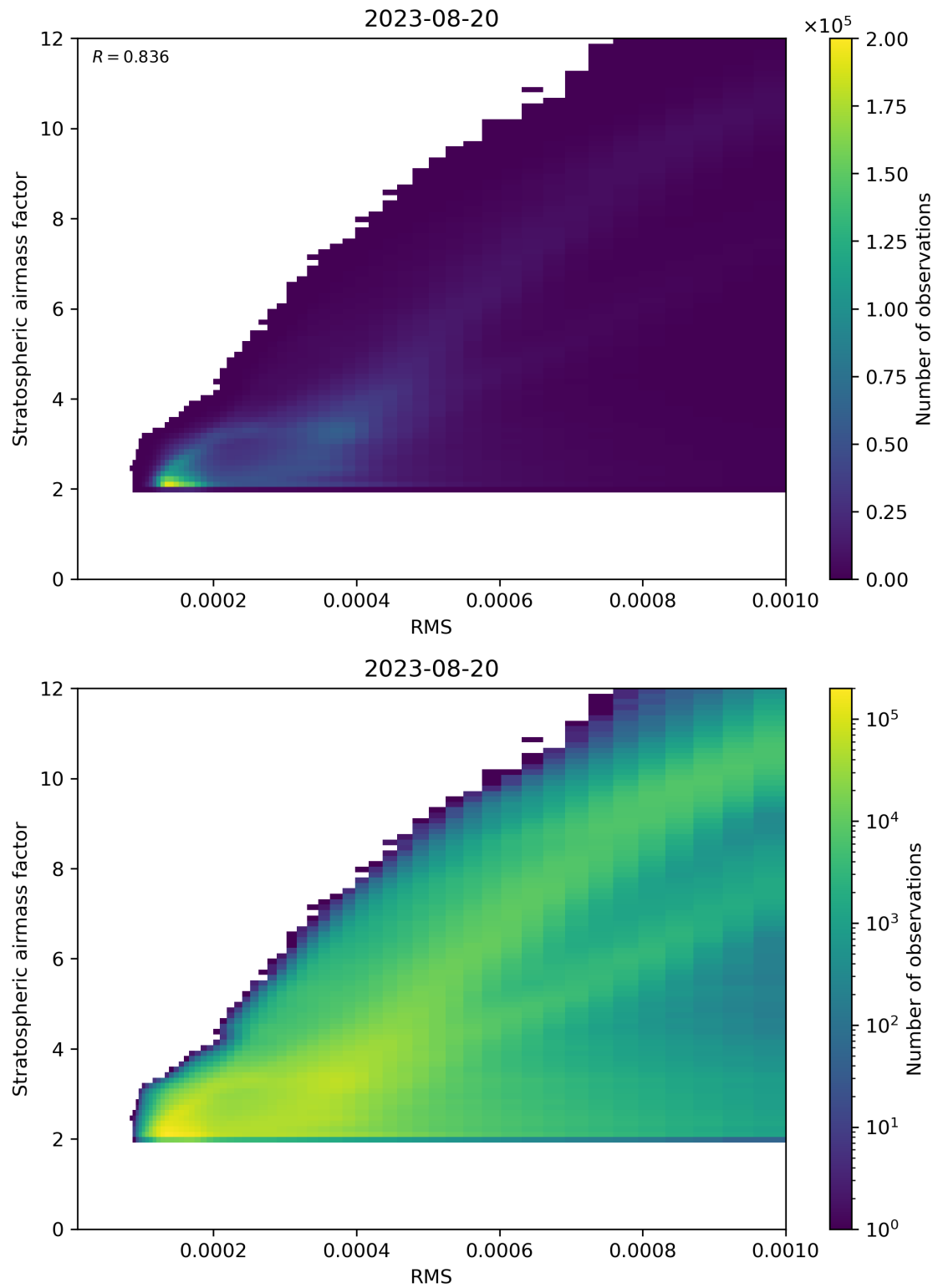
Figure 144: Scatter density plot of “RMS” against “Stratospheric airmass factor” for 2023-08-20 to 2023-08-21.
