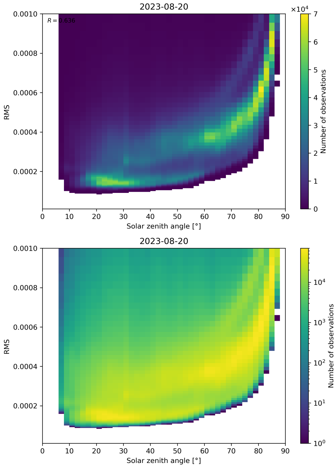
Figure 157: Scatter density plot of “Solar zenith angle” against “RMS” for 2023-08-20 to 2023-08-21.
