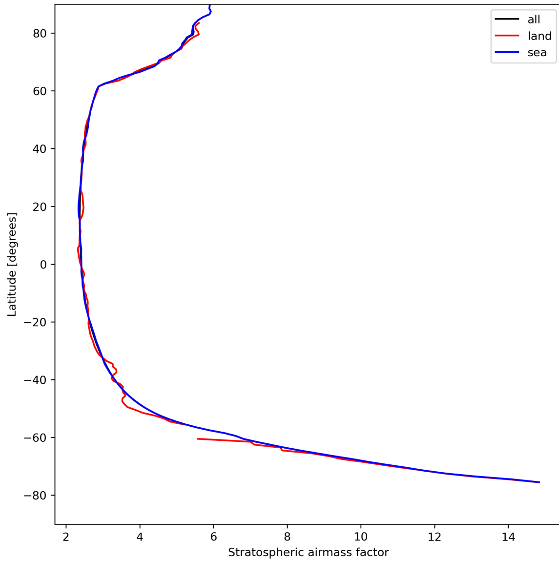
Figure 27: Zonal average of “Stratospheric air mass factor” for 2023-08-20 to 2023-08-21.
