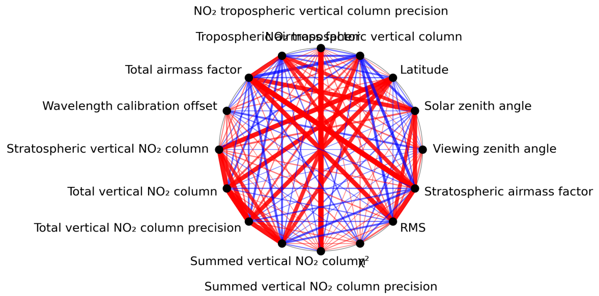
Figure 1: Map of correlation graph for 2023-08-20 to 2023-08-21.
