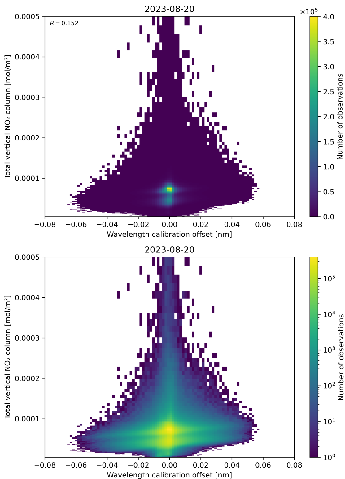
Figure 179: Scatter density plot of “Wavelength calibration offset” against “Total vertical NO 2 column” for 2023-08-20 to 2023-08-21.
