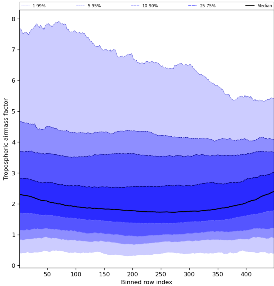
Figure 48: Along track statistics of “Tropospheric airmass factor” for 2023-08-20 to 2023-08-21
