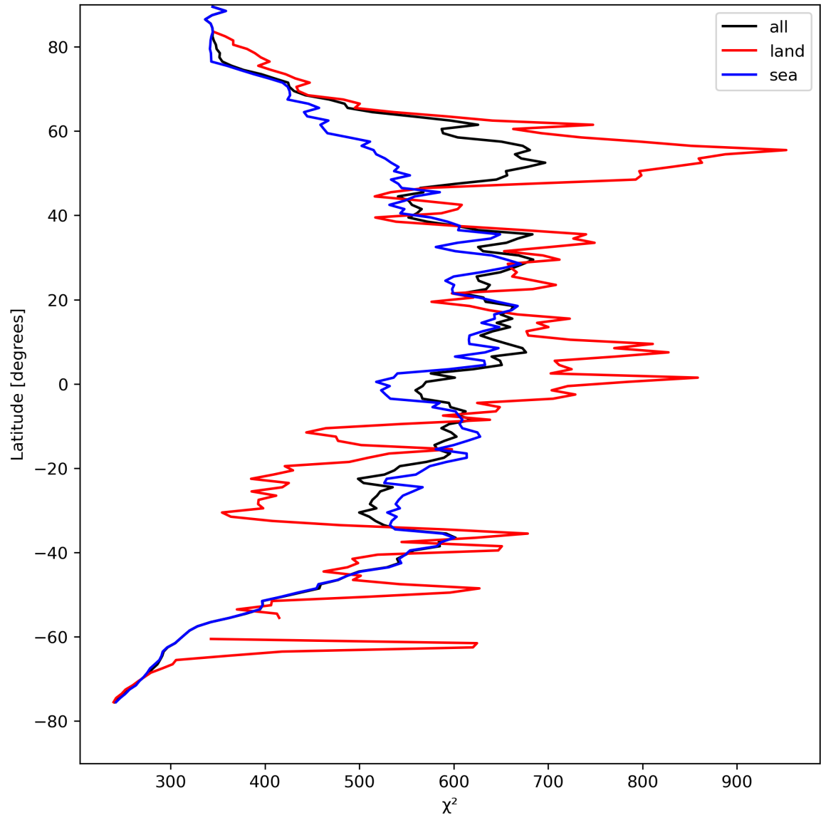
Figure 25: Zonal average of “ \chi^2 ” for 2023-08-20 to 2023-08-21.
