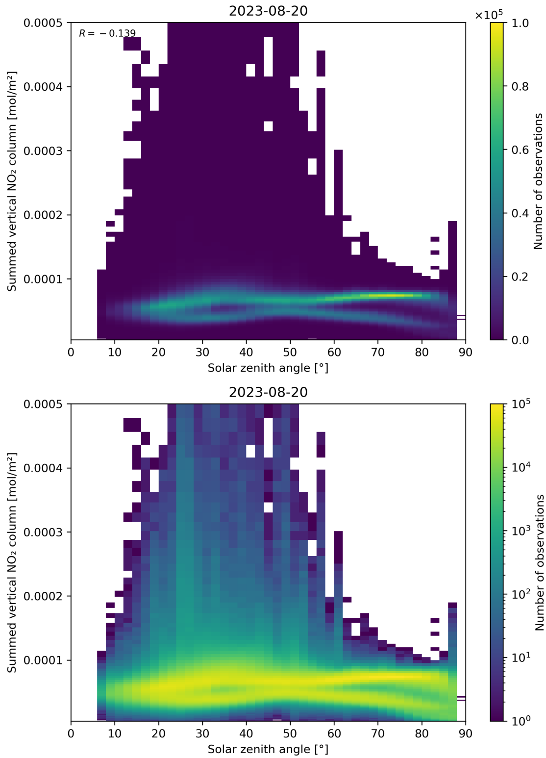
Figure 151: Scatter density plot of “Solar zenith angle” against “Summed vertical NO 2 column” for 2023-08-20 to 2023-08-21.
