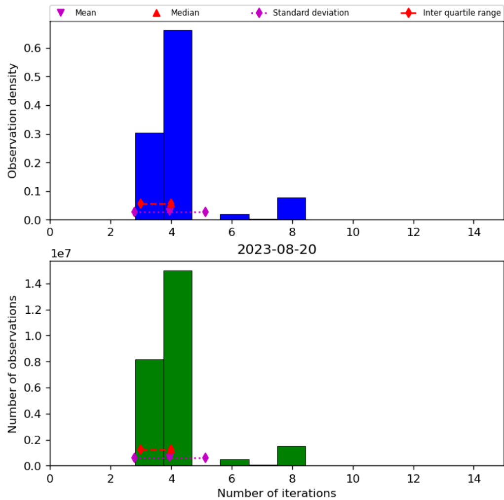
Figure 34: Histogram of “Number of iterations” for 2023-08-20 to 2023-08-21
