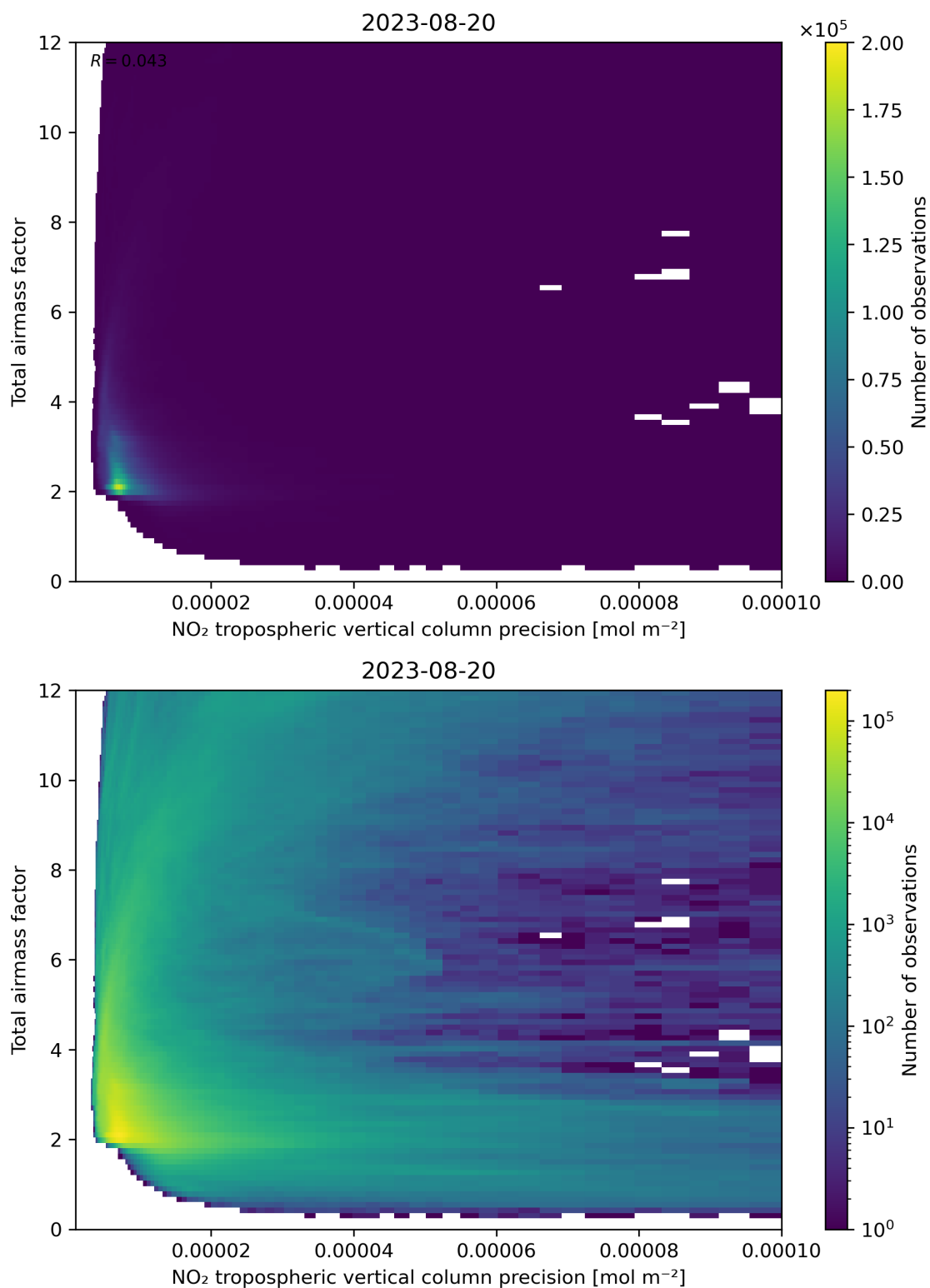
Figure 132: Scatter density plot of “NO 2 tropospheric vertical column precision” against “Total air mass factor” for 2023-08-20 to 2023-08-21.
