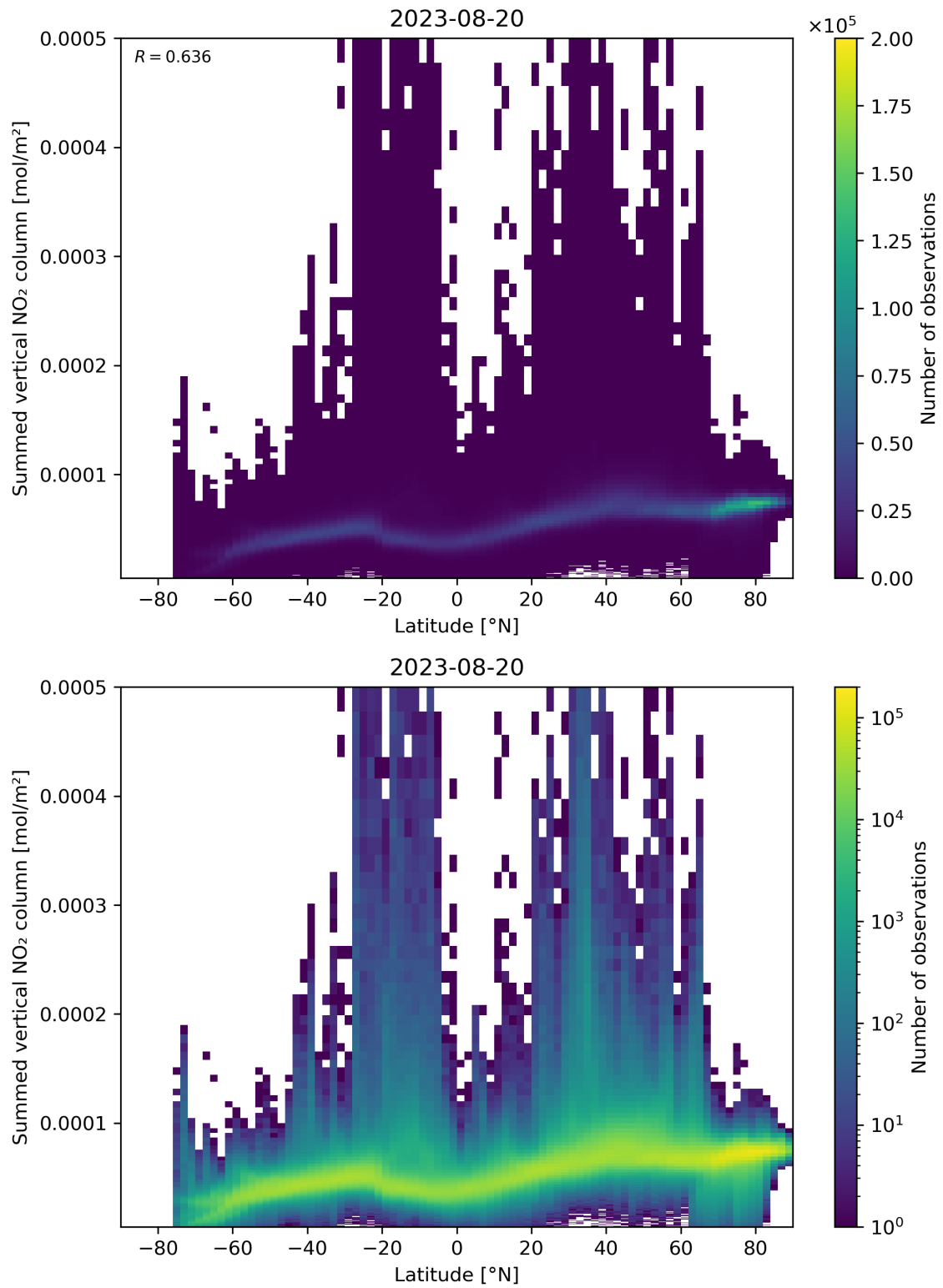
Figure 88: Scatter density plot of “Latitude” against “Summed vertical NO 2 column” for 2023-08-20 to 2023-08-21.
