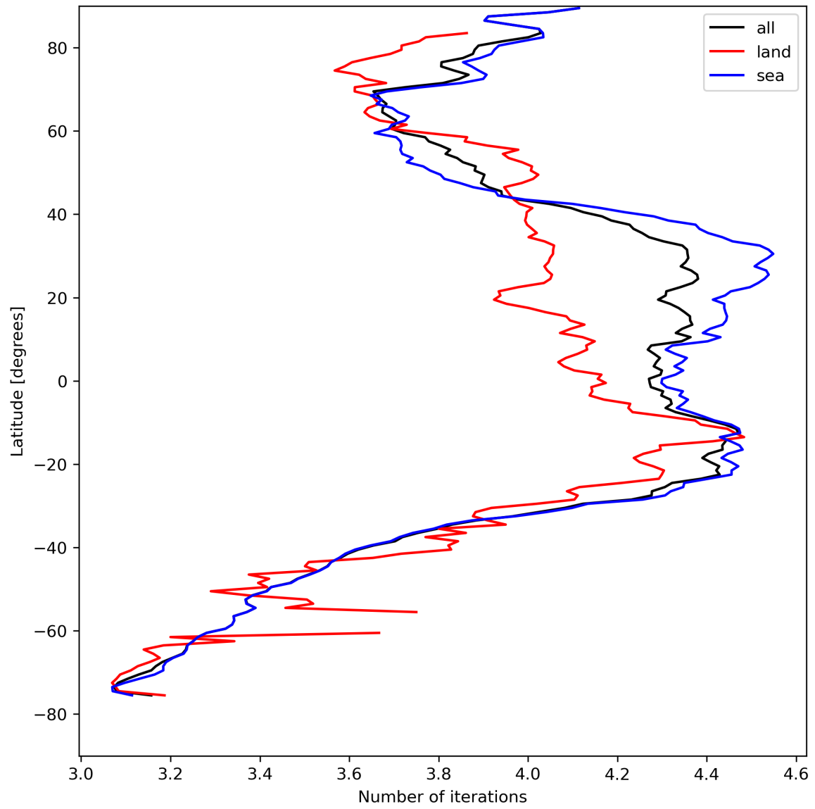
Figure 17: Zonal average of “Number of iterations” for 2023-08-20 to 2023-08-21.
