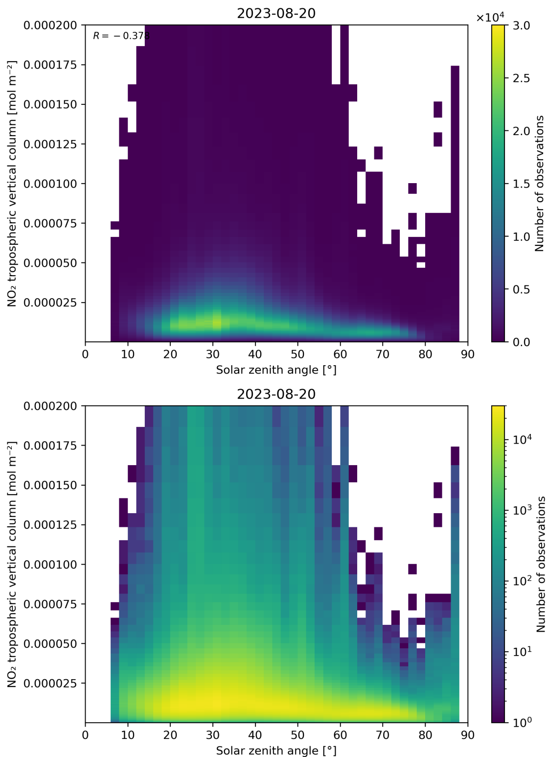
Figure 155: Scatter density plot of “Solar zenith angle” against “NO 2 tropospheric vertical column” for 2023-08-20 to 2023-08-21.
