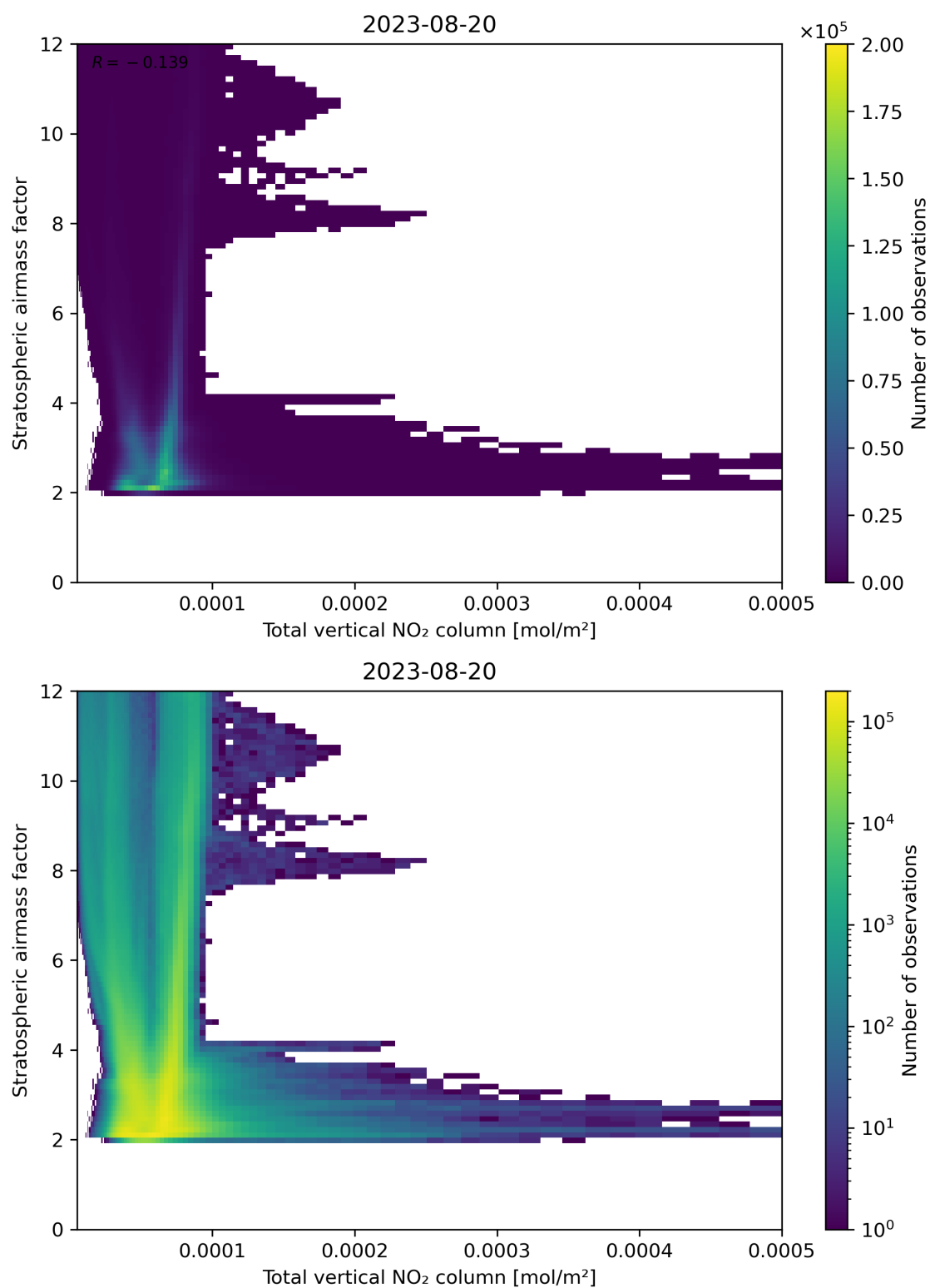
Figure 110: Scatter density plot of “Total vertical NO 2 column” against “Stratospheric airmass factor” for 2023-08-20 to 2023-08-21.
