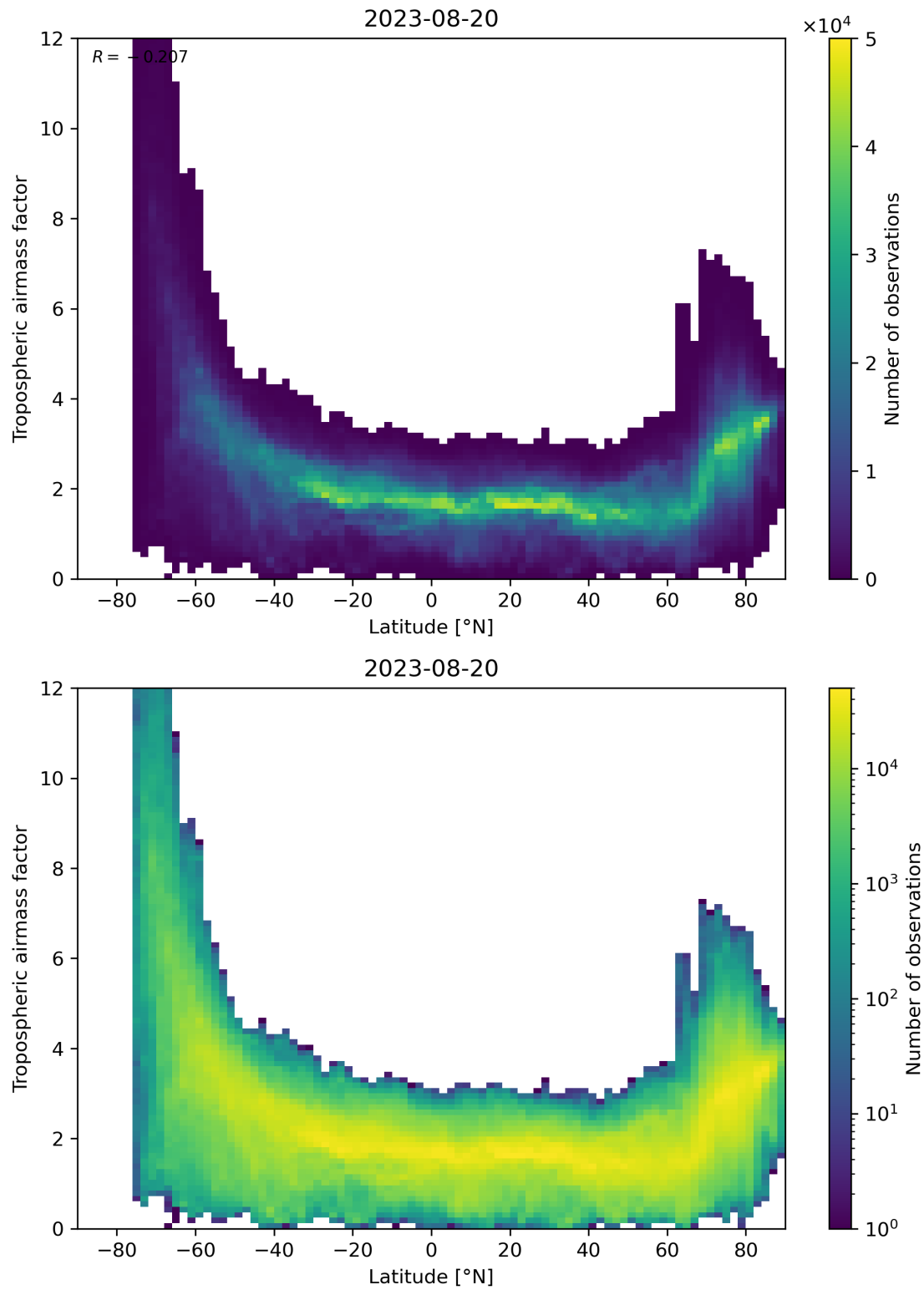
Figure 85: Scatter density plot of “Latitude” against “Tropospheric airmass factor” for 2023-08-20 to 2023-08-21.
