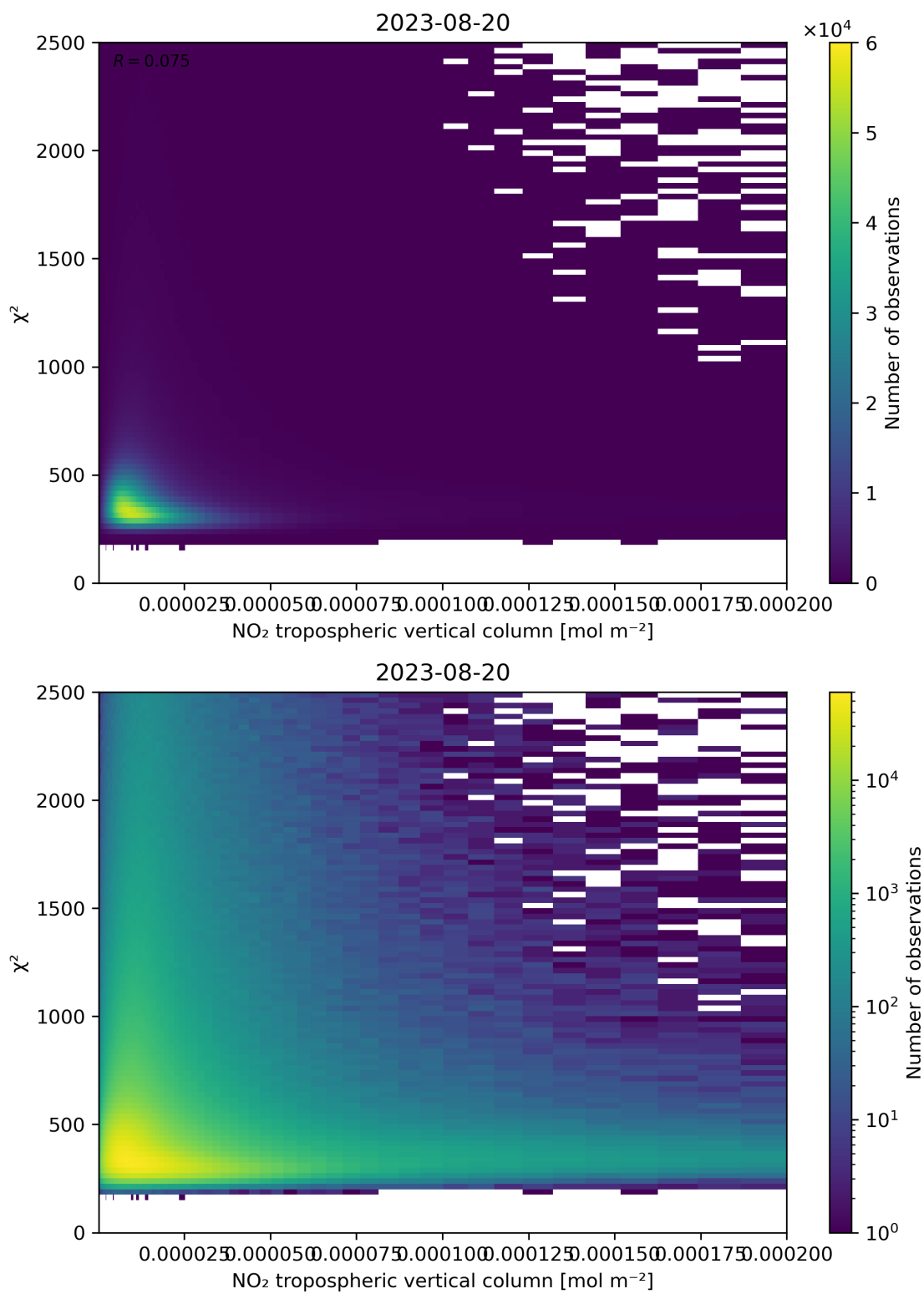
Figure 124: Scatter density plot of “NO 2 tropospheric vertical column” against “ \chi^2 ” for 2023-08-20 to 2023-08-21.
