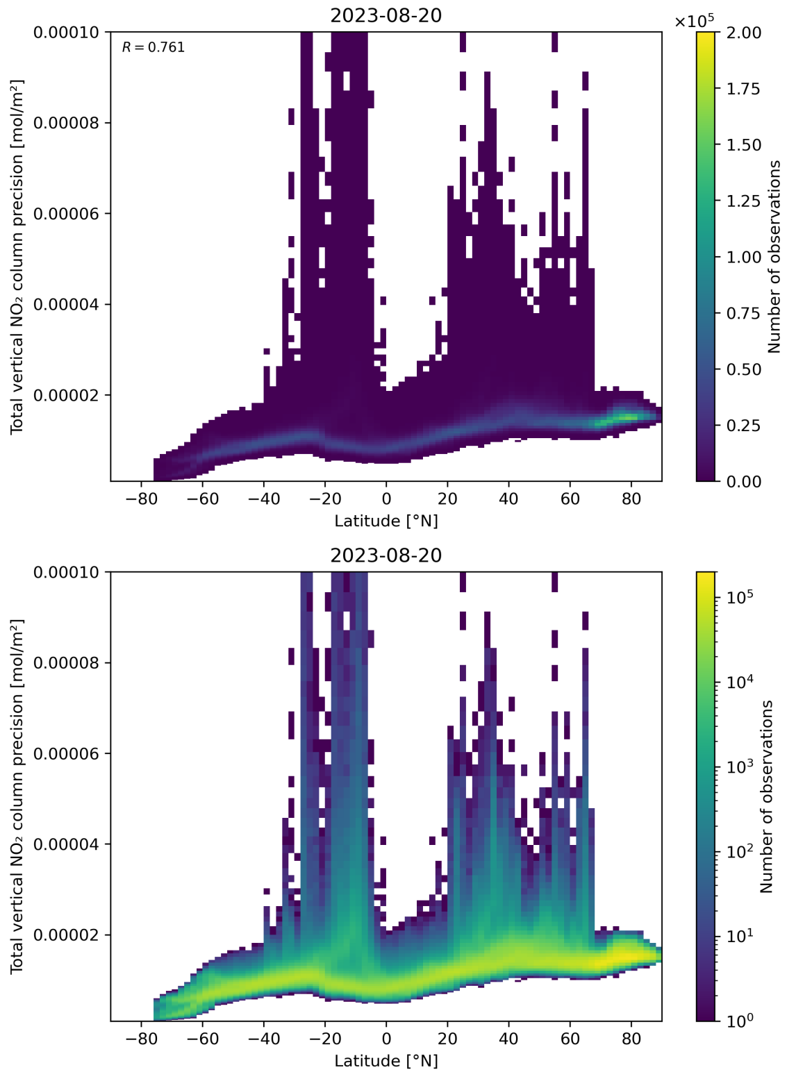
Figure 91: Scatter density plot of “Latitude” against “Total vertical NO 2 column precision” for 2023-08-20 to 2023-08-21.
