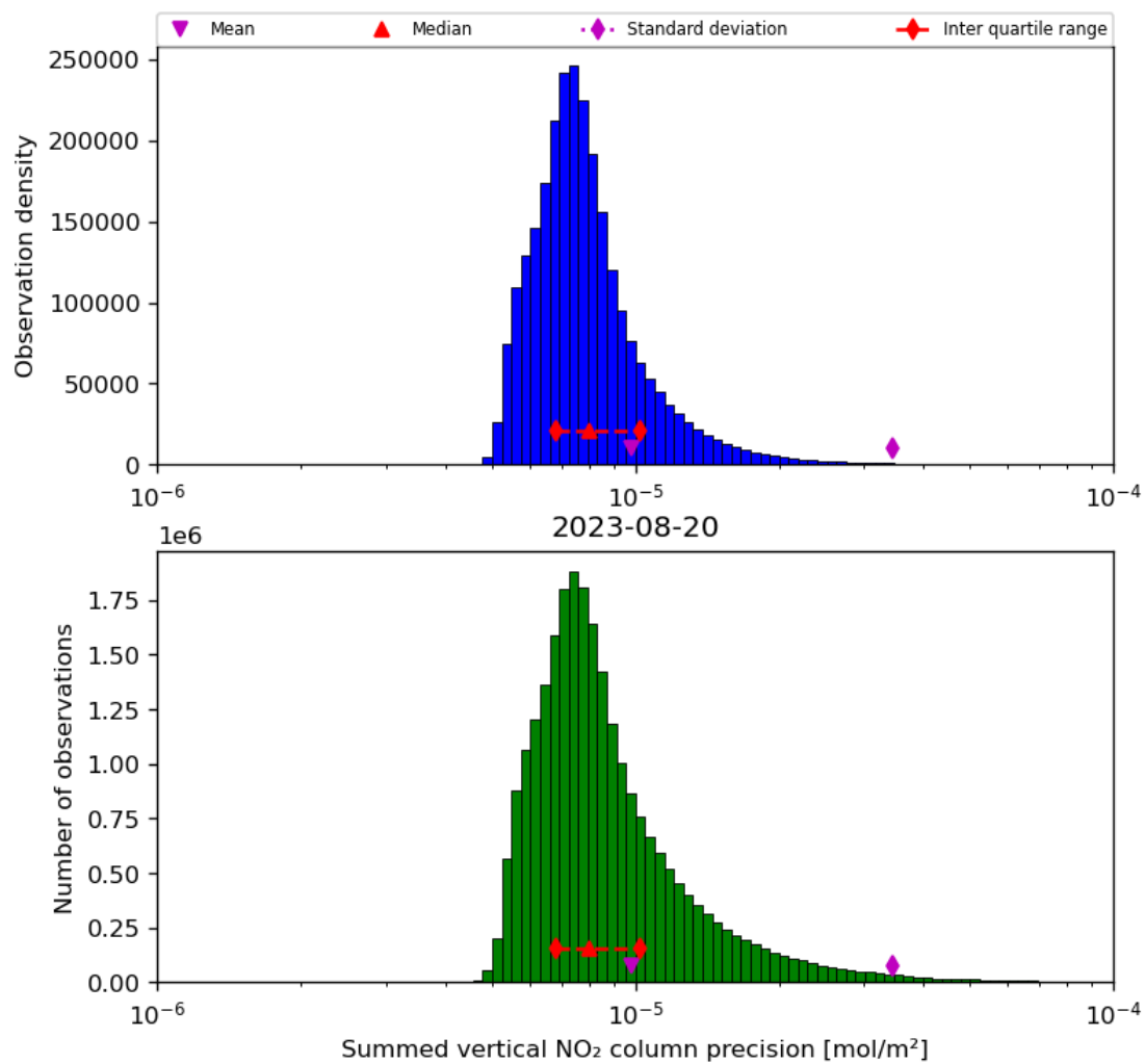
Figure 41: Histogram of “Summed vertical NO 2 column precision” for 2023-08-20 to 2023-08-21
