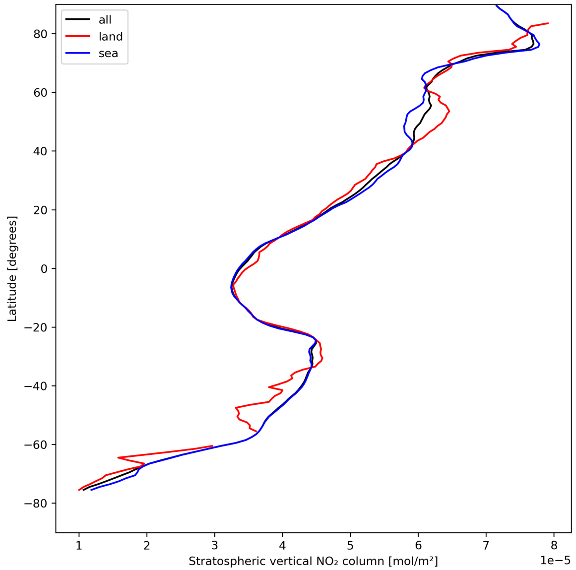
Figure 19: Zonal average of “Stratospheric vertical NO 2 column” for 2023-08-20 to 2023-08-21.
