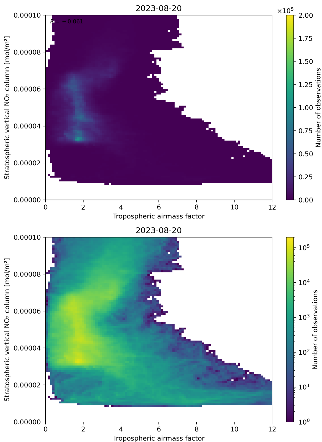
Figure 74: Scatter density plot of “Tropospheric air mass factor” against “Stratospheric vertical NO 2 column” for 2023-08-20 to 2023-08-21.
