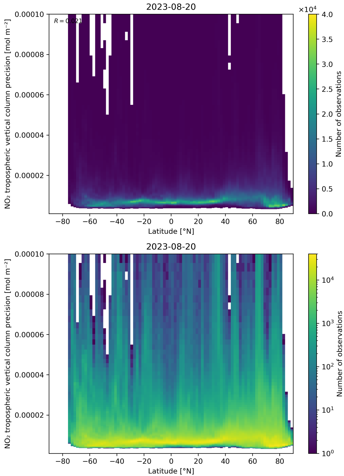
Figure 93: Scatter density plot of “Latitude” against “NO 2 tropospheric vertical column precision” for 2023-08-20 to 2023-08-21.
