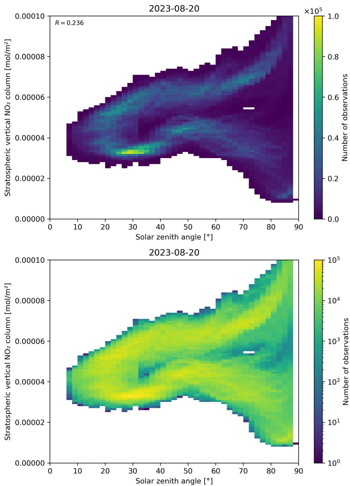
Figure 150: Scatter density plot of “Solar zenith angle” against “Stratospheric vertical NO 2 column” for 2023-08-20 to 2023-08-21.
