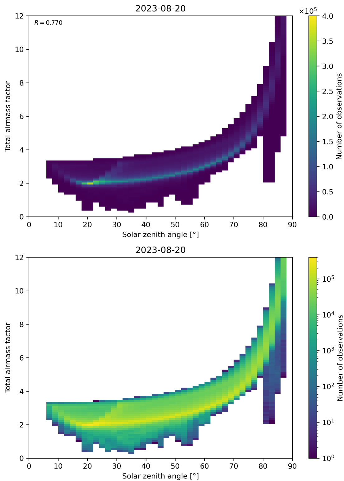
Figure 146: Scatter density plot of “Solar zenith angle” against “Total airmass factor” for 2023-08-20 to 2023-08-21.
