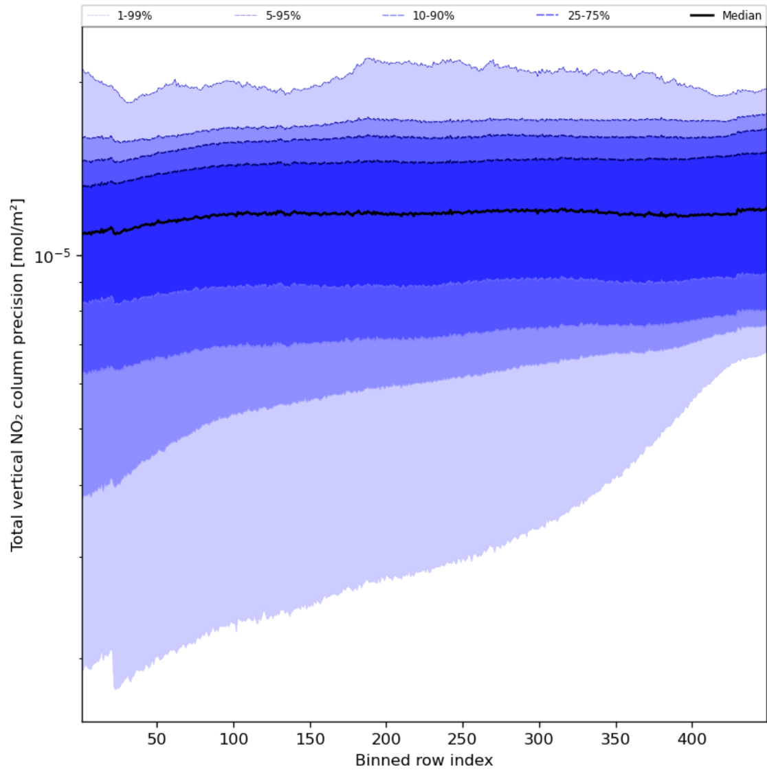
Figure 56: Along track statistics of “Total vertical NO 2 column precision” for 2023-08-20 to 2023-08-21
