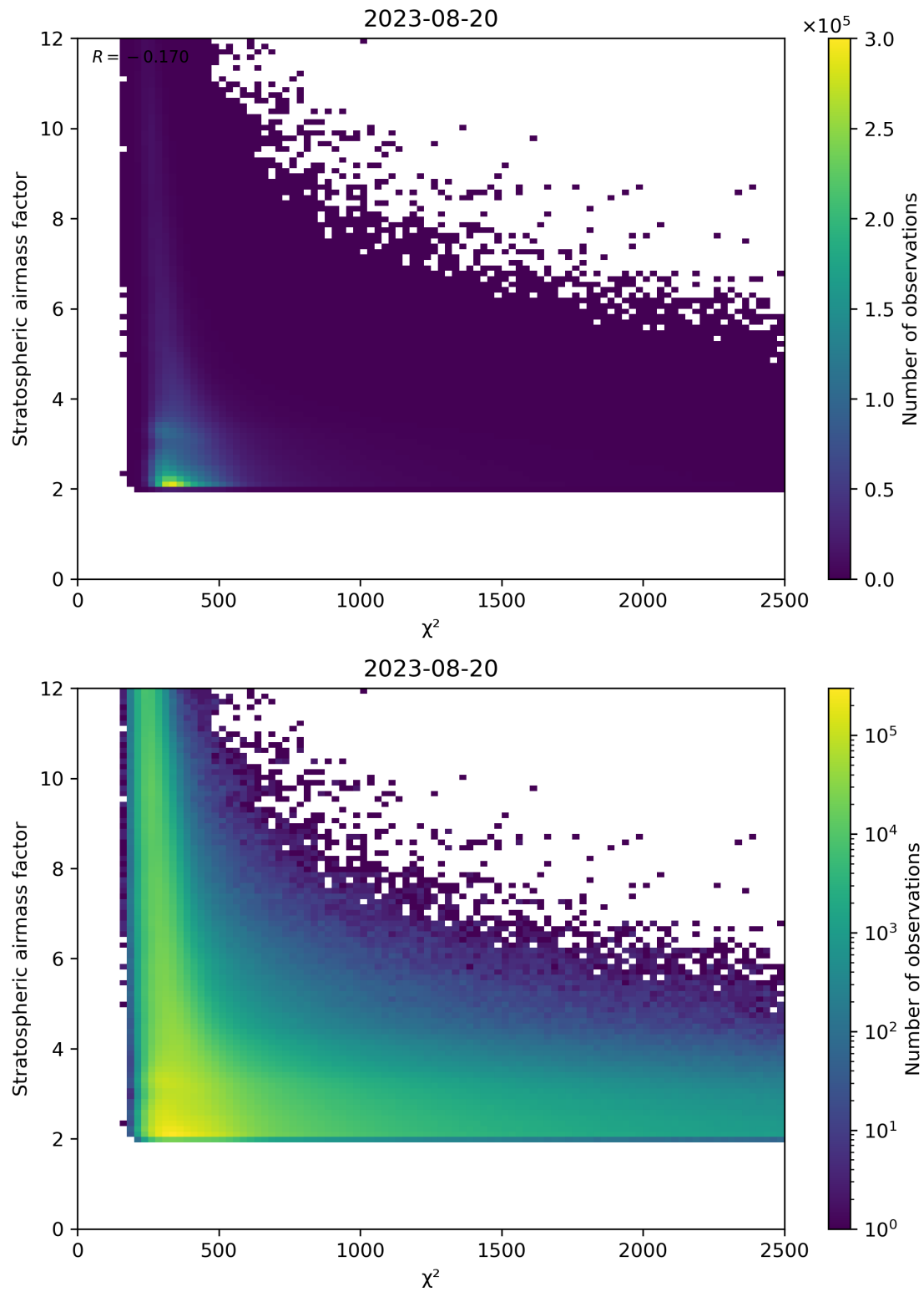
Figure 81: Scatter density plot of “ \chi^2 ” against “Stratospheric air mass factor” for 2023-08-20 to 2023-08-21.
