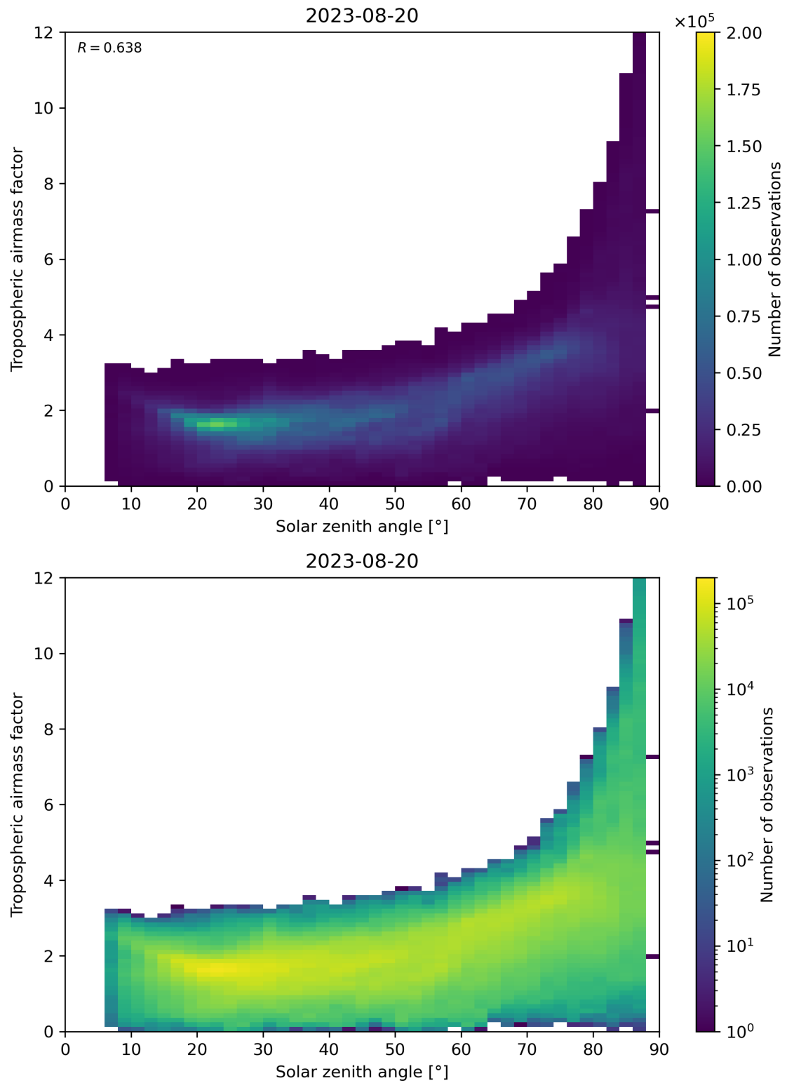
Figure 147: Scatter density plot of “Solar zenith angle” against “Tropospheric airmass factor” for 2023-08-20 to 2023-08-21.
