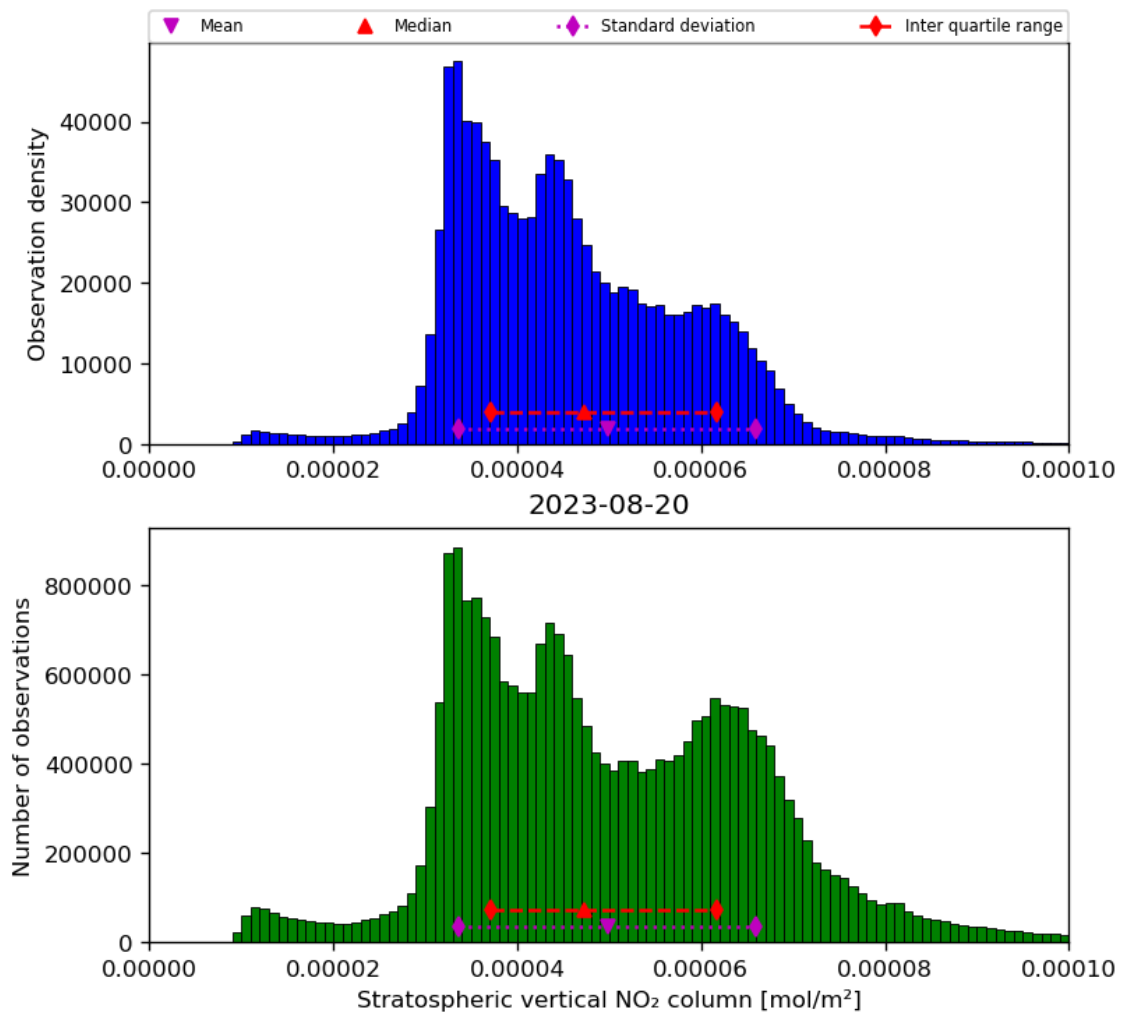
Figure 36: Histogram of “Stratospheric vertical NO 2 column” for 2023-08-20 to 2023-08-21
