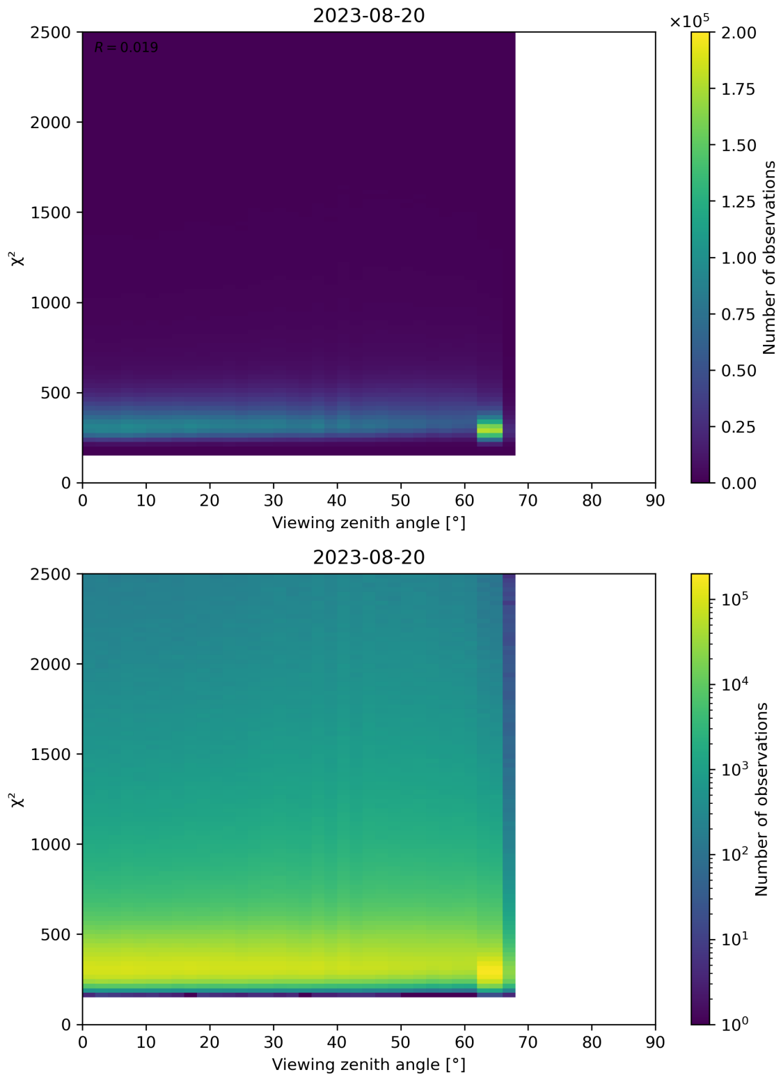
Figure 162: Scatter density plot of “Viewing zenith angle” against “ \chi^2 ” for 2023-08-20 to 2023-08-21.
