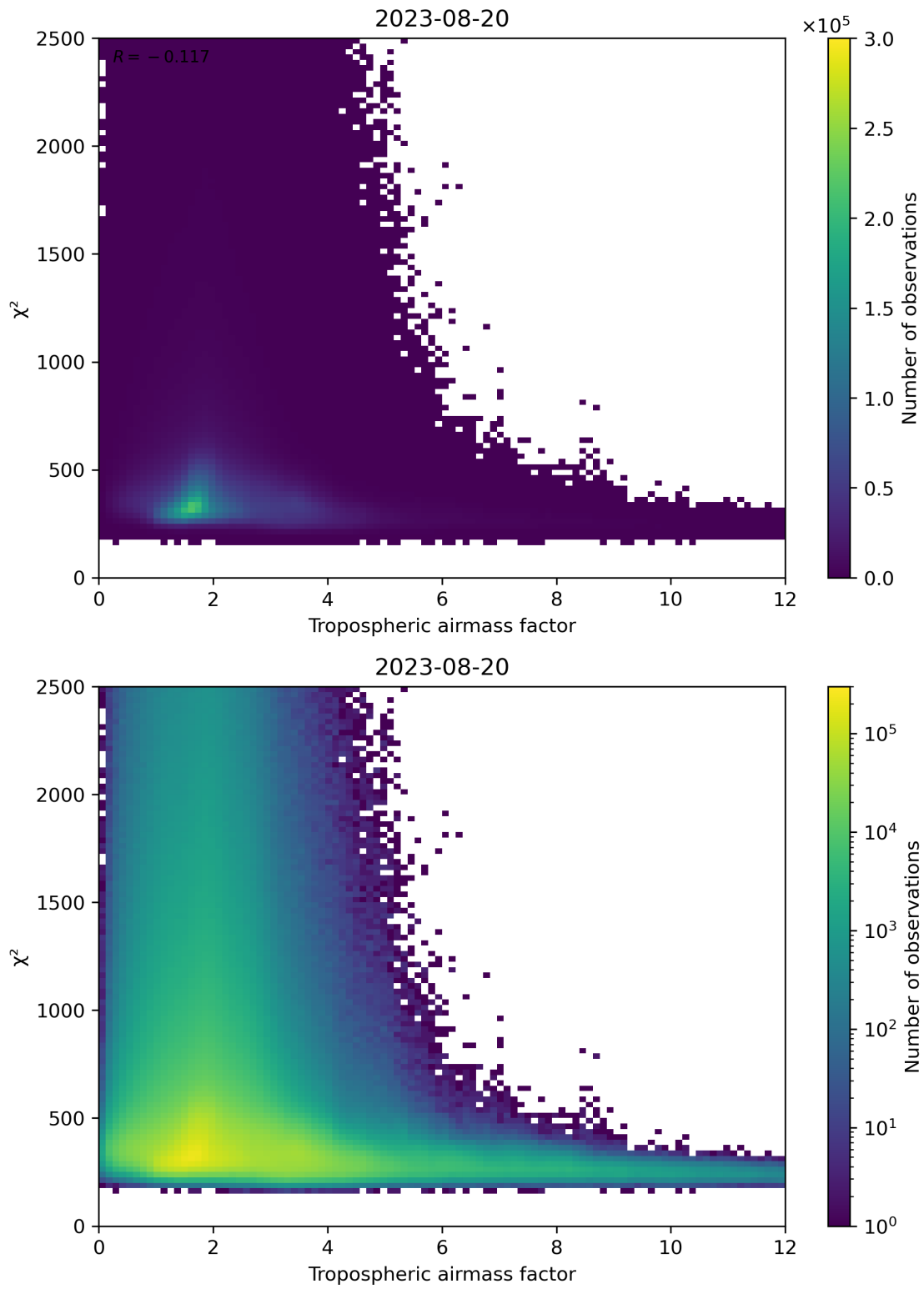
Figure 73: Scatter density plot of “Tropospheric airmass factor” against “ \chi^2 ” for 2023-08-20 to 2023-08-21.
