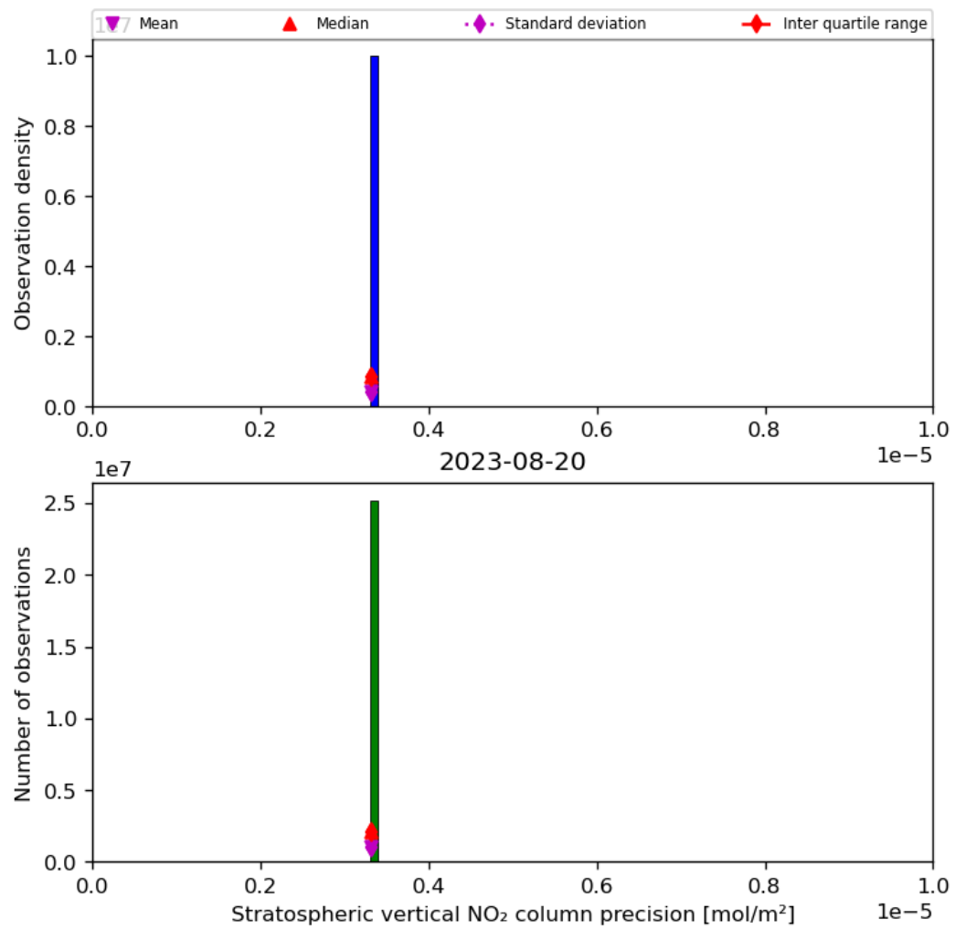
Figure 37: Histogram of “Stratospheric vertical NO 2 column precision” for 2023-08-20 to 2023-08-21
