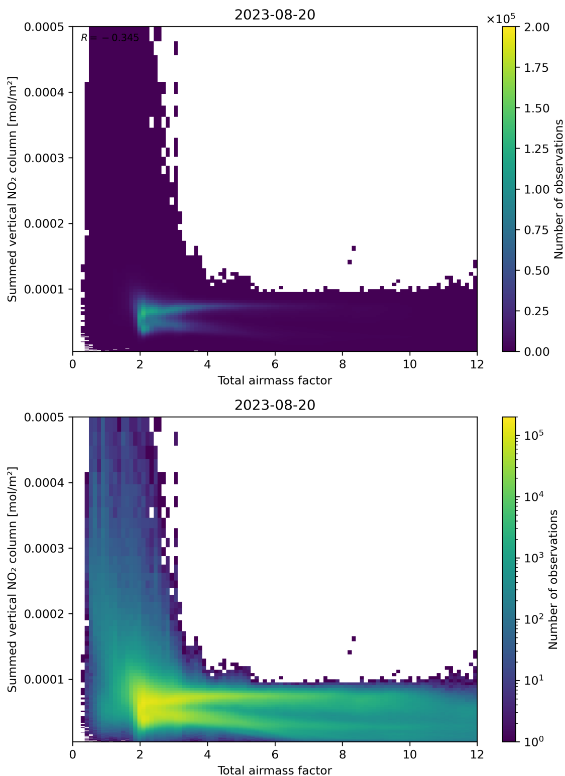
Figure 65: Scatter density plot of “Total airmass factor” against “Summed vertical NO 2 column” for 2023-08-20 to 2023-08-21.
