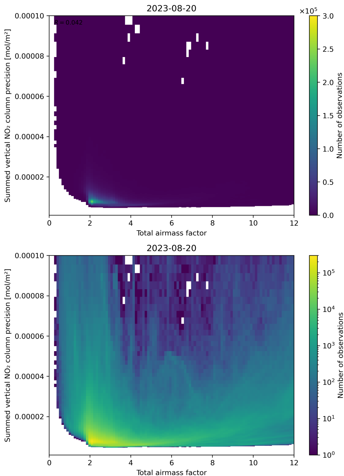
Figure 66: Scatter density plot of “Total airmass factor” against “Summed vertical NO 2 column precision” for 2023-08-20 to 2023-08-21.
