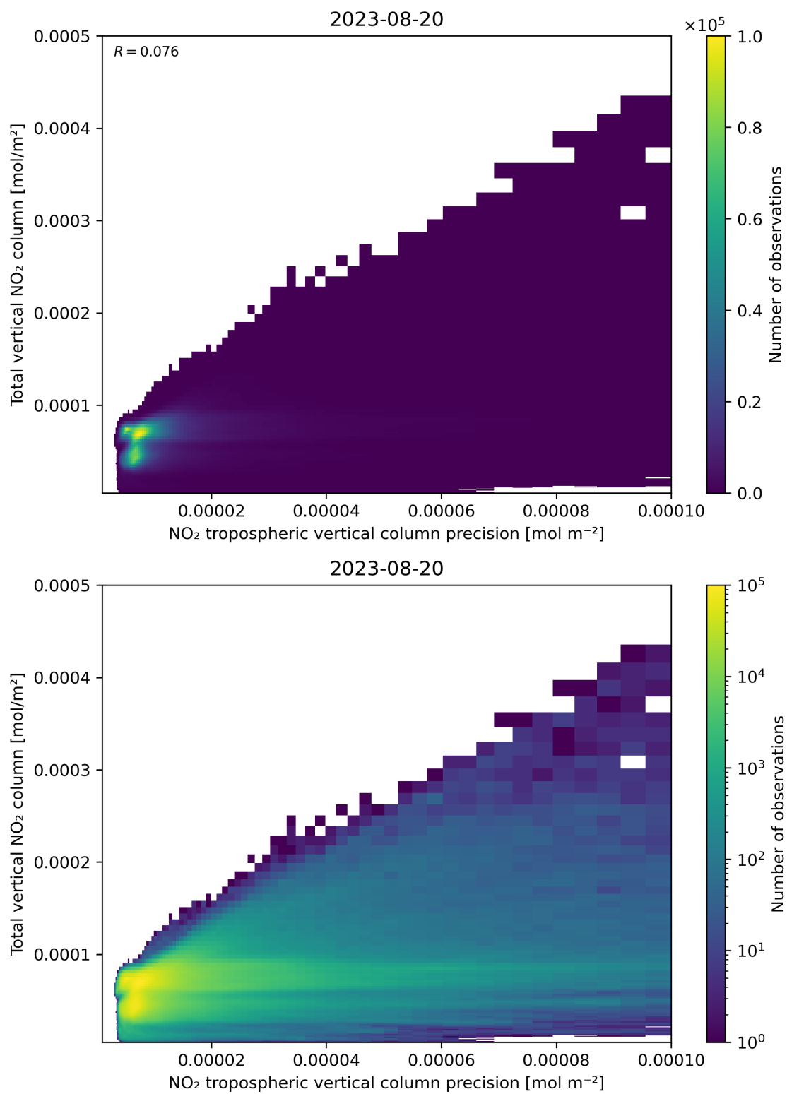
Figure 138: Scatter density plot of “NO 2 tropospheric vertical column precision” against “Total vertical NO 2 column” for 2023-08-20 to 2023-08-21.
