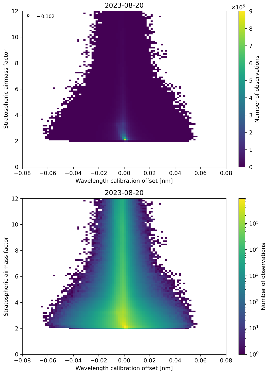
Figure 174: Scatter density plot of “Wavelength calibration offset” against “Stratospheric airmass factor” for 2023-08-20 to 2023-08-21.
