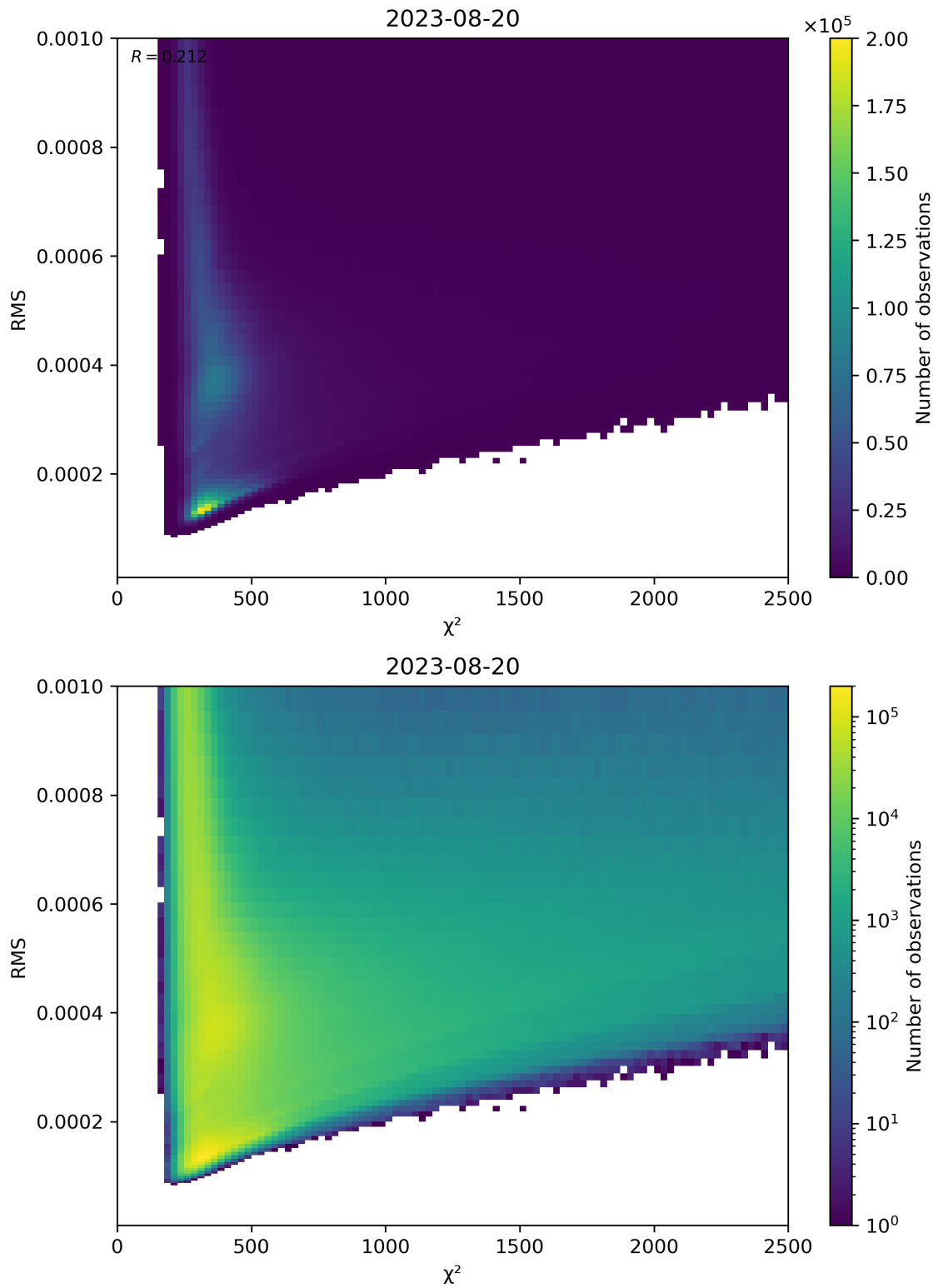
Figure 82: Scatter density plot of “ \chi^2 ” against “RMS” for 2023-08-20 to 2023-08-21.
