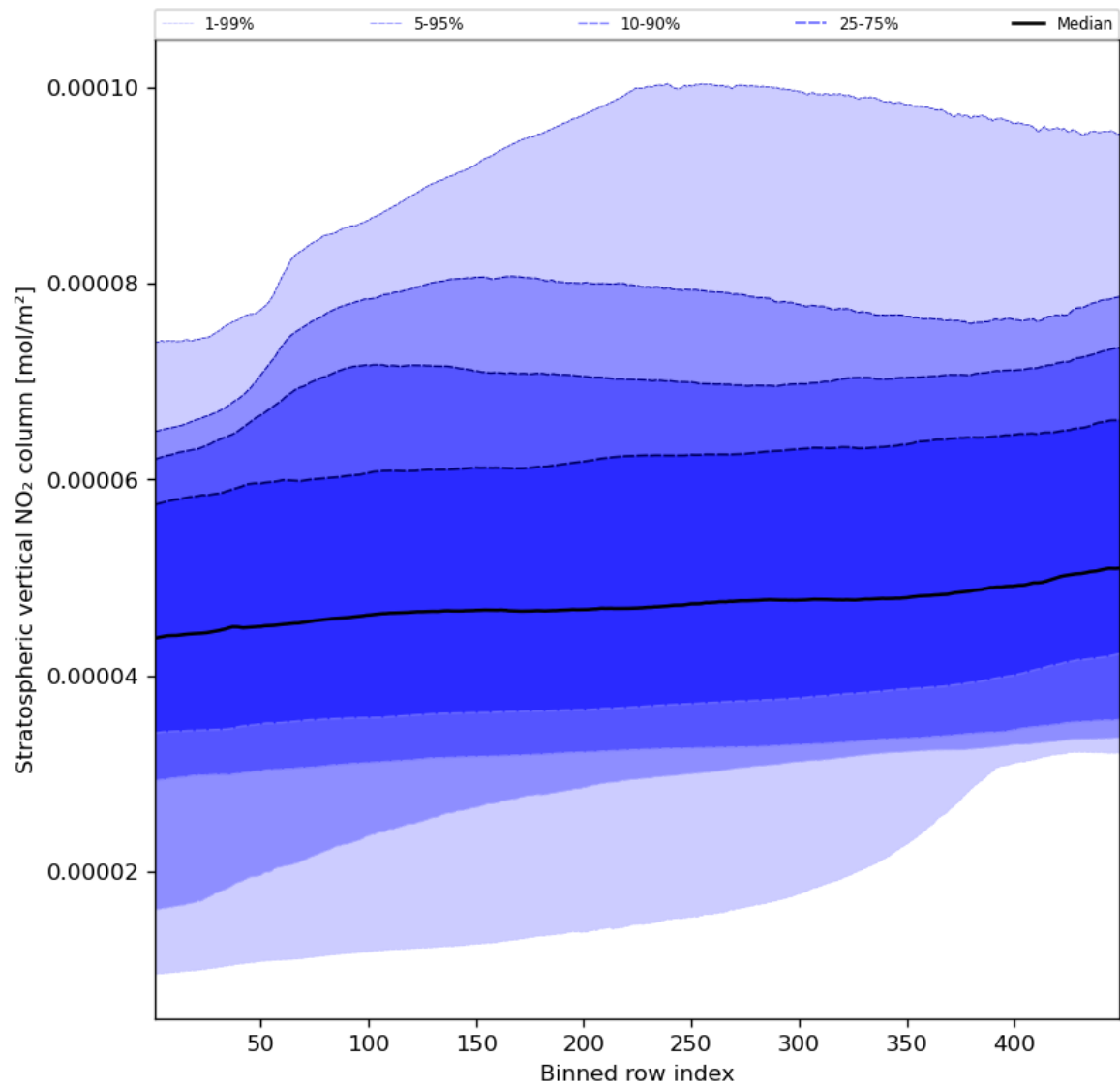
Figure 53: Along track statistics of “Stratospheric vertical NO 2 column” for 2023-08-20 to 2023-08-21
