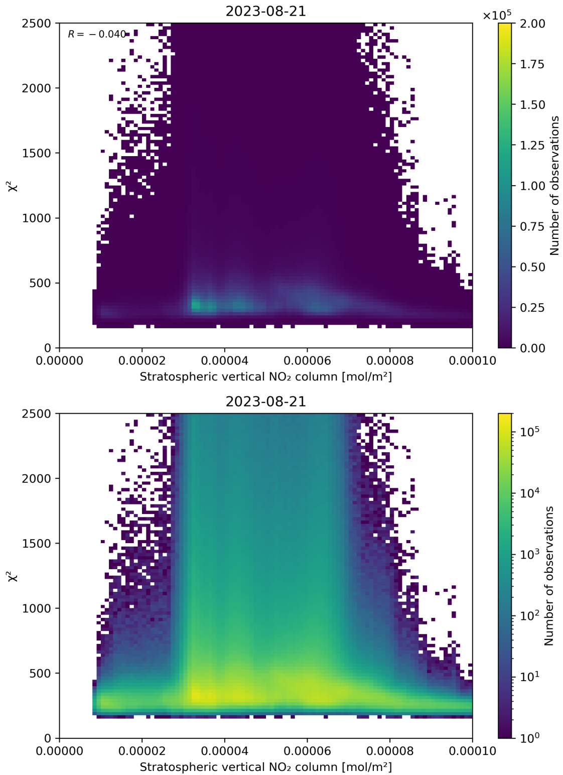
Figure 97: Scatter density plot of “Stratospheric vertical NO 2 column” against “ \chi^2 ” for 2023-08-20 to 2023-08-22.
