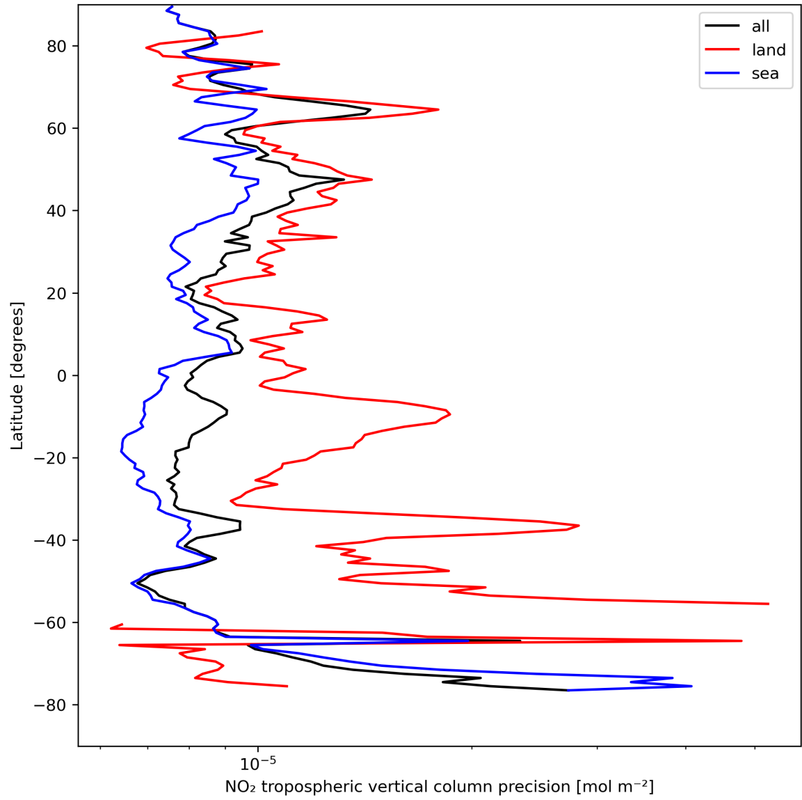
Figure 13: Zonal average of “NO 2 tropospheric vertical column precision” for 2023-08-20 to 2023-08-22.
