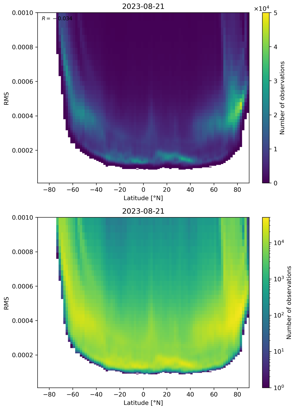
Figure 94: Scatter density plot of “Latitude” against “RMS” for 2023-08-20 to 2023-08-22.
