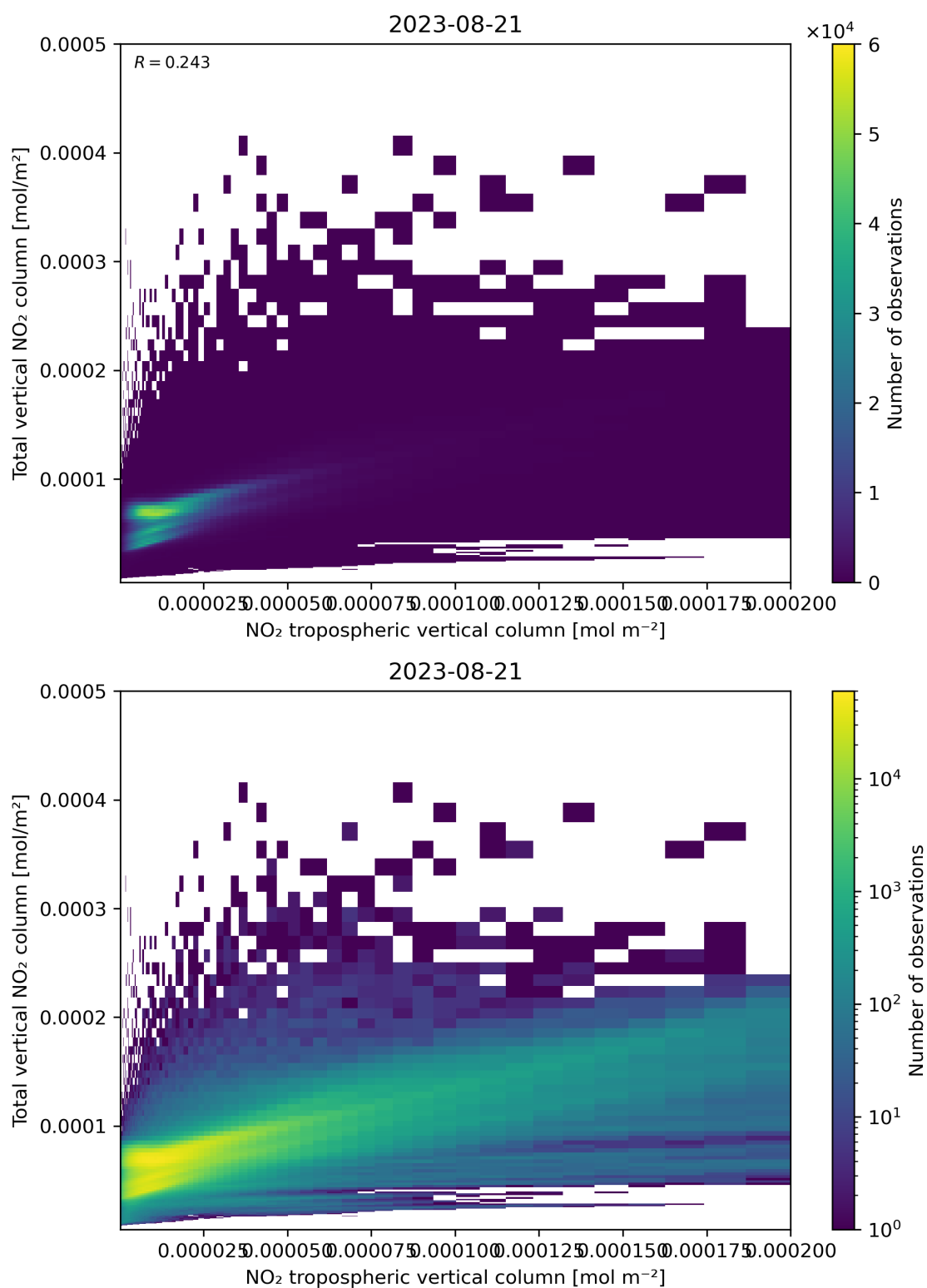
Figure 128: Scatter density plot of “NO 2 tropospheric vertical column” against “Total vertical NO 2 column” for 2023-08-20 to 2023-08-22.
