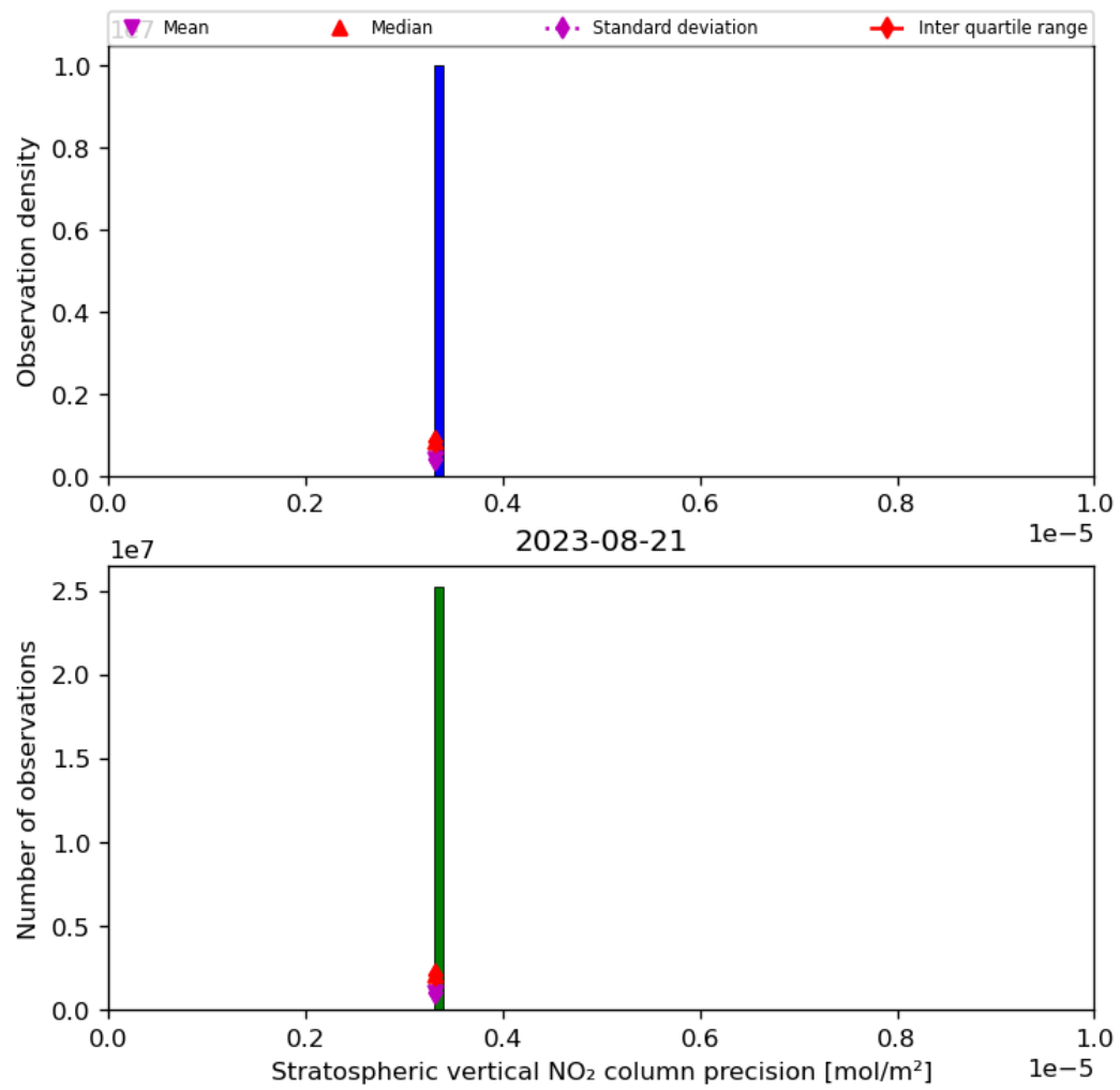
Figure 37: Histogram of “Stratospheric vertical NO 2 column precision” for 2023-08-20 to 2023-08-22
