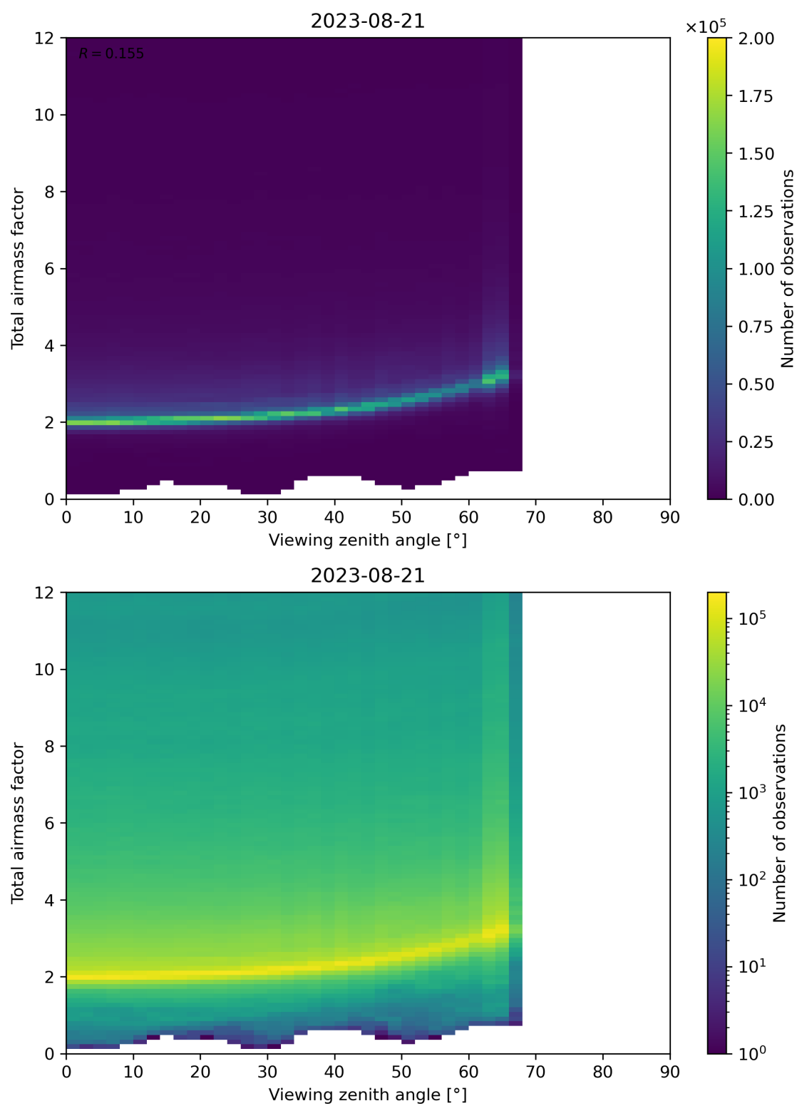
Figure 160: Scatter density plot of “Viewing zenith angle” against “Total airmass factor” for 2023-08-20 to 2023-08-22.
