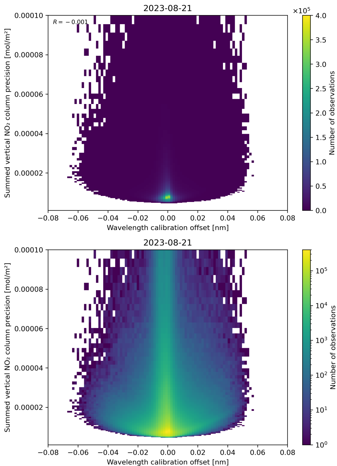
Figure 178: Scatter density plot of “Wavelength calibration offset” against “Summed vertical NO 2 column precision” for 2023-08-20 to 2023-08-22.
