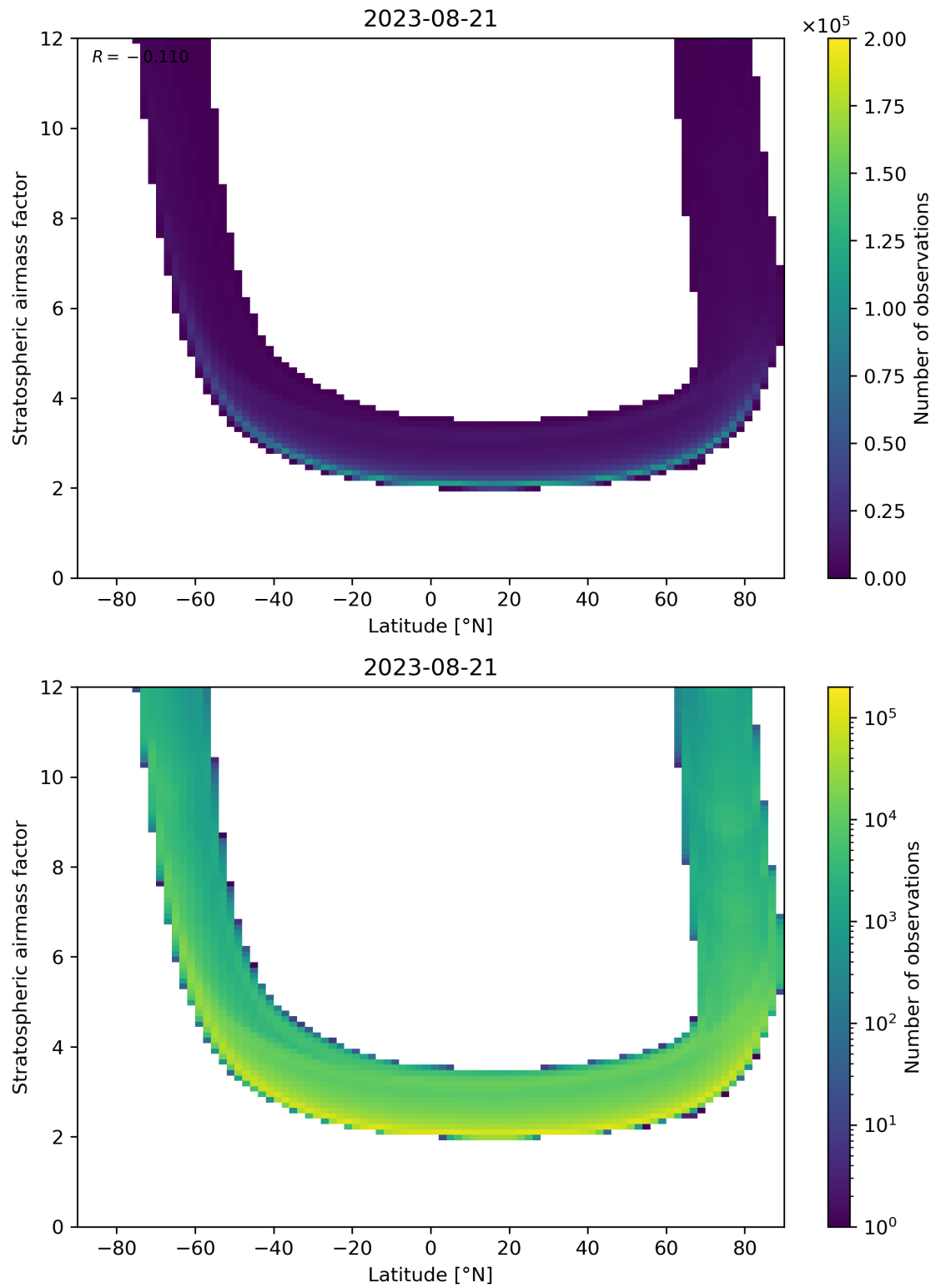
Figure 83: Scatter density plot of “Latitude” against “Stratospheric airmass factor” for 2023-08-20 to 2023-08-22.
