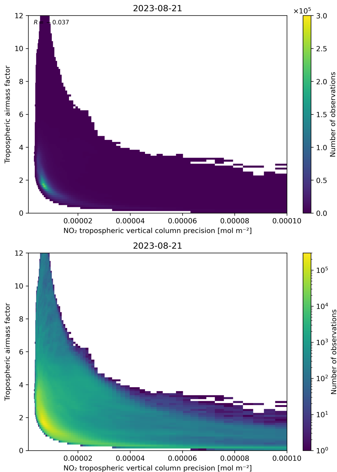
Figure 133: Scatter density plot of “NO 2 tropospheric vertical column precision” against “Tropospheric airmass factor” for 2023-08-20 to 2023-08-22.
