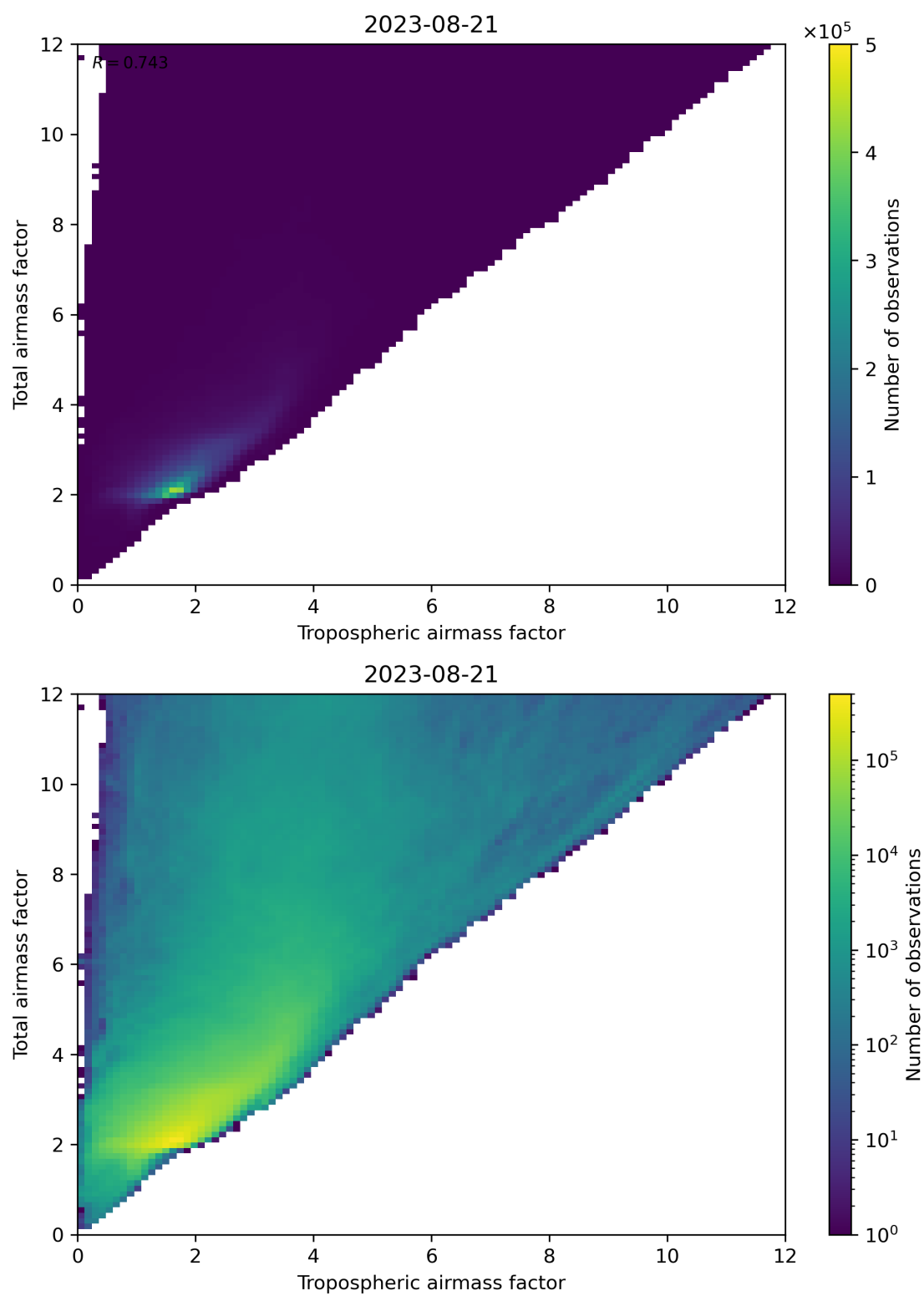
Figure 72: Scatter density plot of “Tropospheric airmass factor” against “Total airmass factor” for 2023-08-20 to 2023-08-22.
