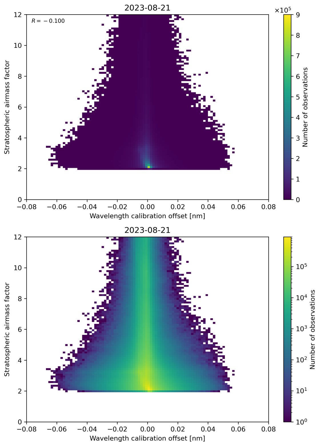
Figure 174: Scatter density plot of “Wavelength calibration offset” against “Stratospheric airmass factor” for 2023-08-20 to 2023-08-22.
