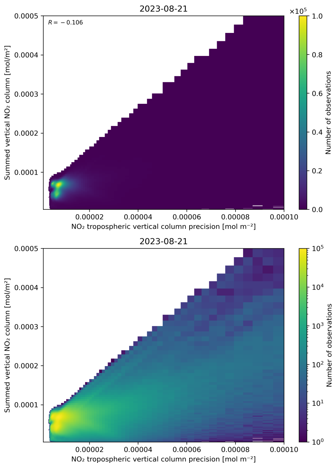
Figure 136: Scatter density plot of “NO 2 tropospheric vertical column precision” against “Summed vertical NO 2 column” for 2023-08-20 to 2023-08-22.
