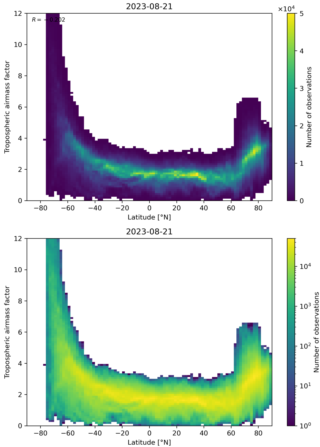
Figure 85: Scatter density plot of “Latitude” against “Tropospheric air mass factor” for 2023-08-20 to 2023-08-22.
