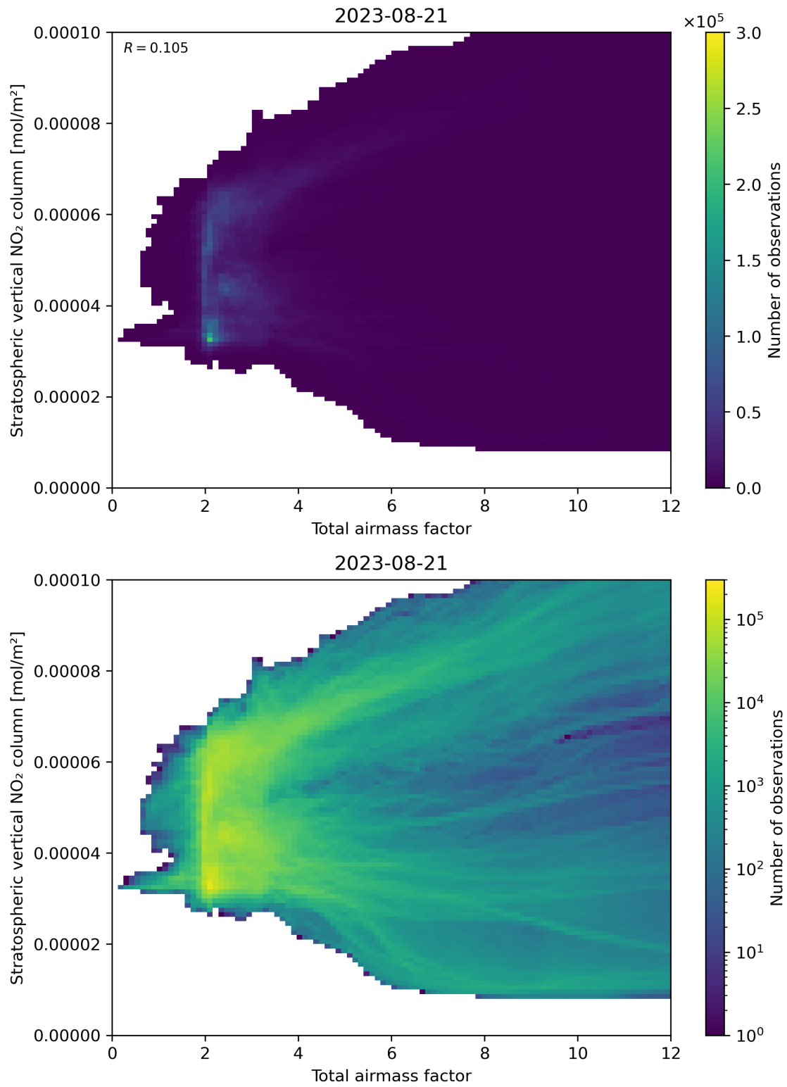
Figure 64: Scatter density plot of “Total airmass factor” against “Stratospheric vertical \text{NO}_2 column” for 2023-08-20 to 2023-08-22.
