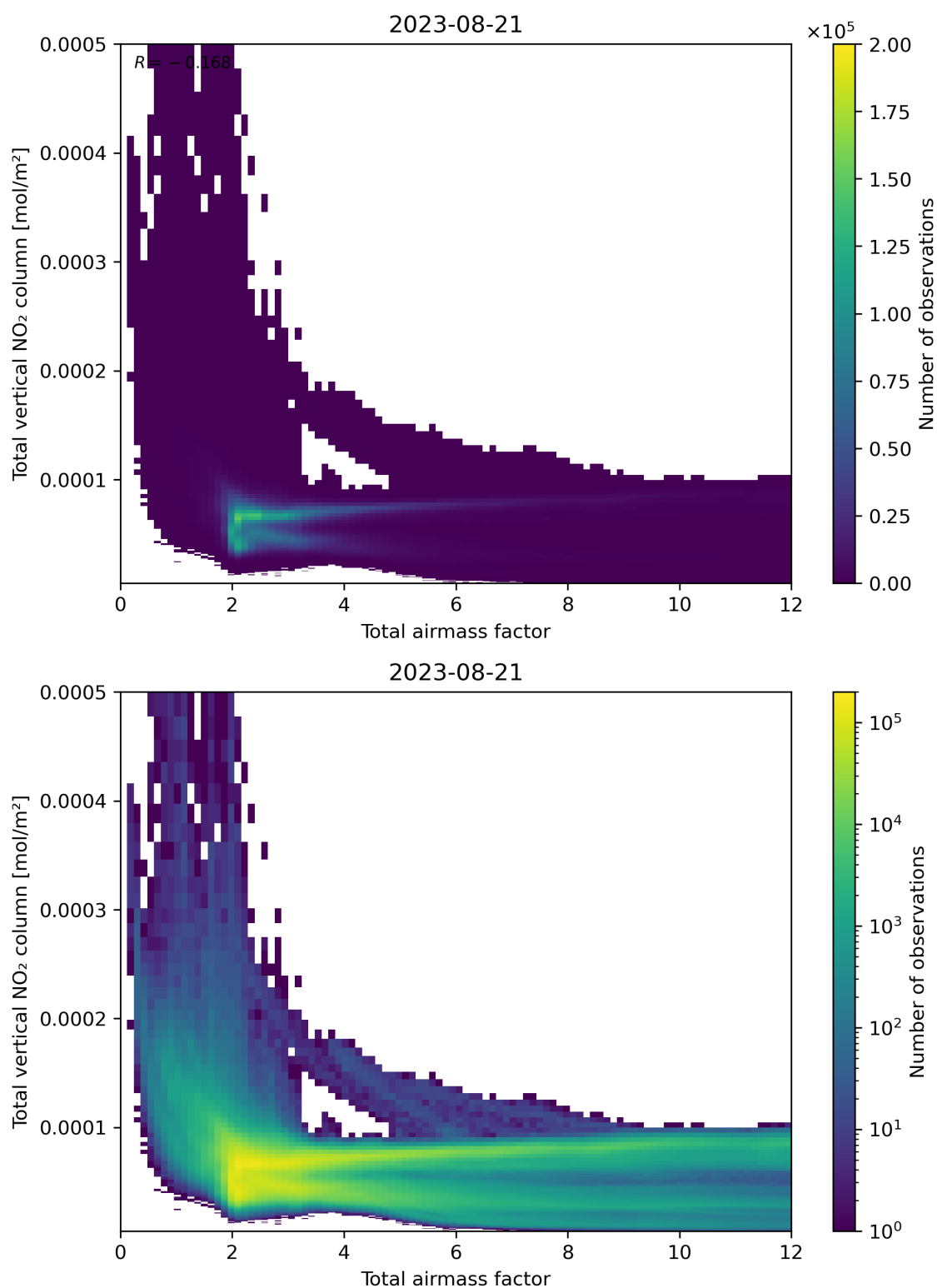
Figure 67: Scatter density plot of “Total airmass factor” against “Total vertical NO 2 column” for 2023-08-20 to 2023-08-22.
