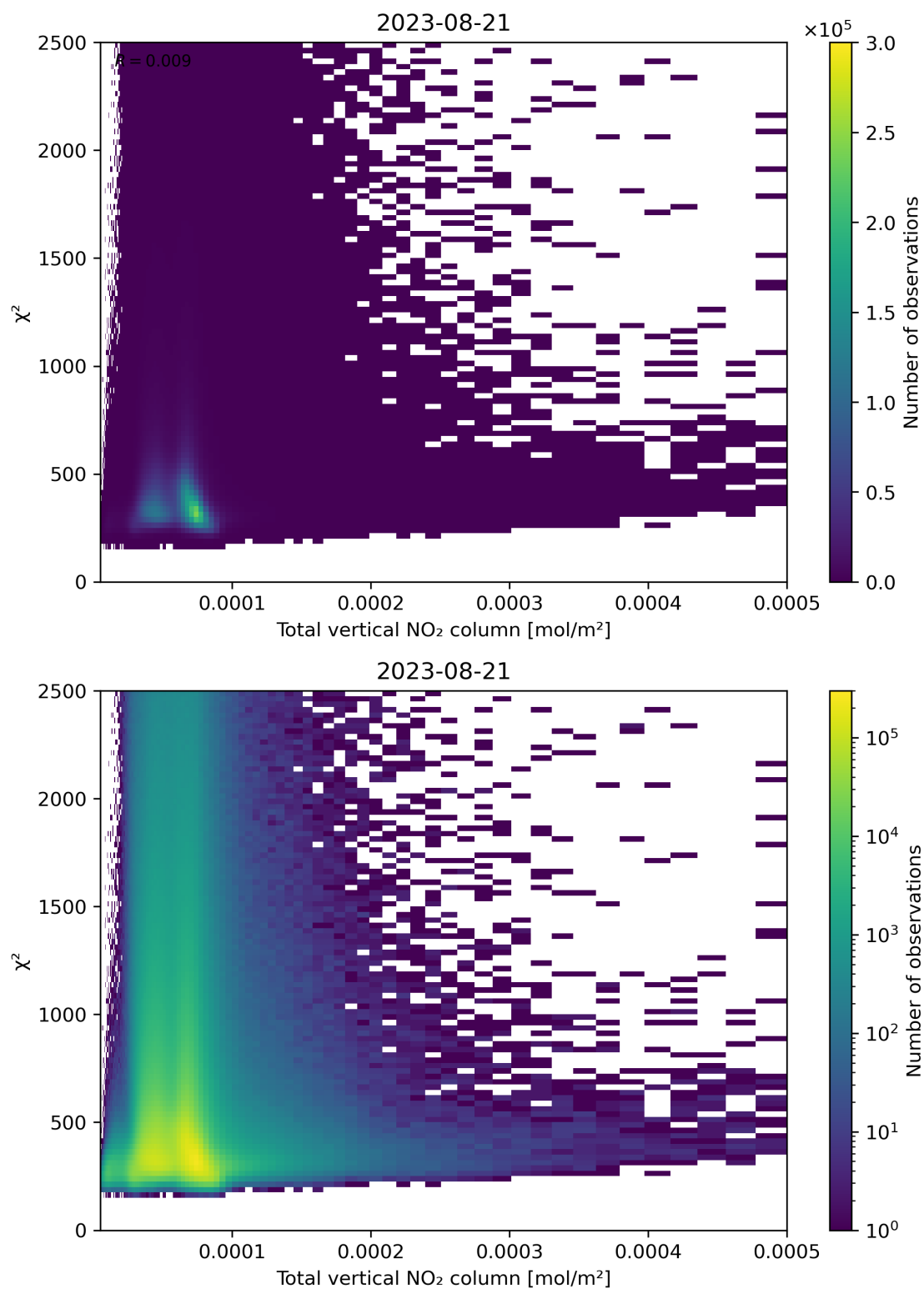
Figure 111: Scatter density plot of “Total vertical NO 2 column” against “ \chi^2 ” for 2023-08-20 to 2023-08-22.
