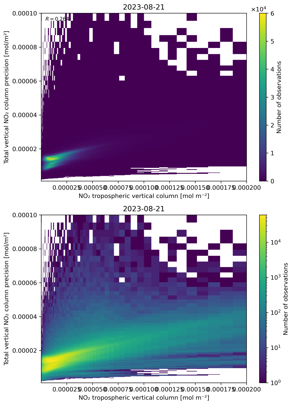
Figure 129: Scatter density plot of “NO 2 tropospheric vertical column” against “Total vertical NO 2 column precision” for 2023-08-20 to 2023-08-22.
