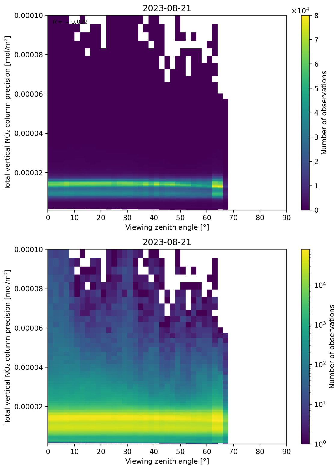
Figure 168: Scatter density plot of “Viewing zenith angle” against “Total vertical NO 2 column precision” for 2023-08-20 to 2023-08-22.
