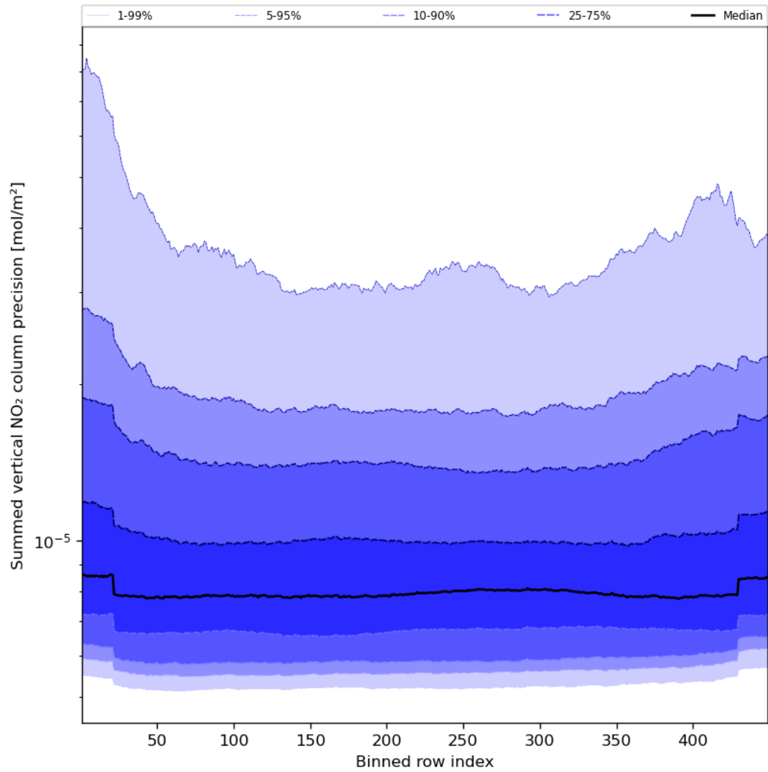
Figure 58: Along track statistics of “Summed vertical NO 2 column precision” for 2023-08-20 to 2023-08-22
