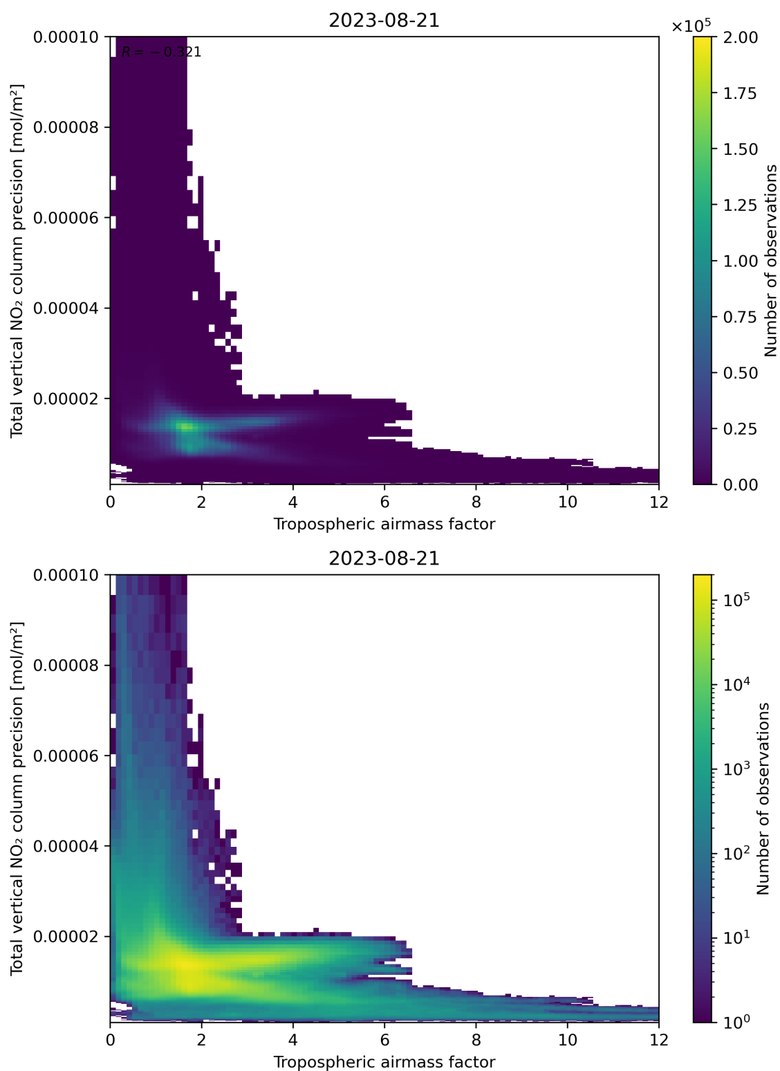
Figure 78: Scatter density plot of “Tropospheric air mass factor” against “Total vertical NO 2 column precision” for 2023-08-20 to 2023-08-22.
