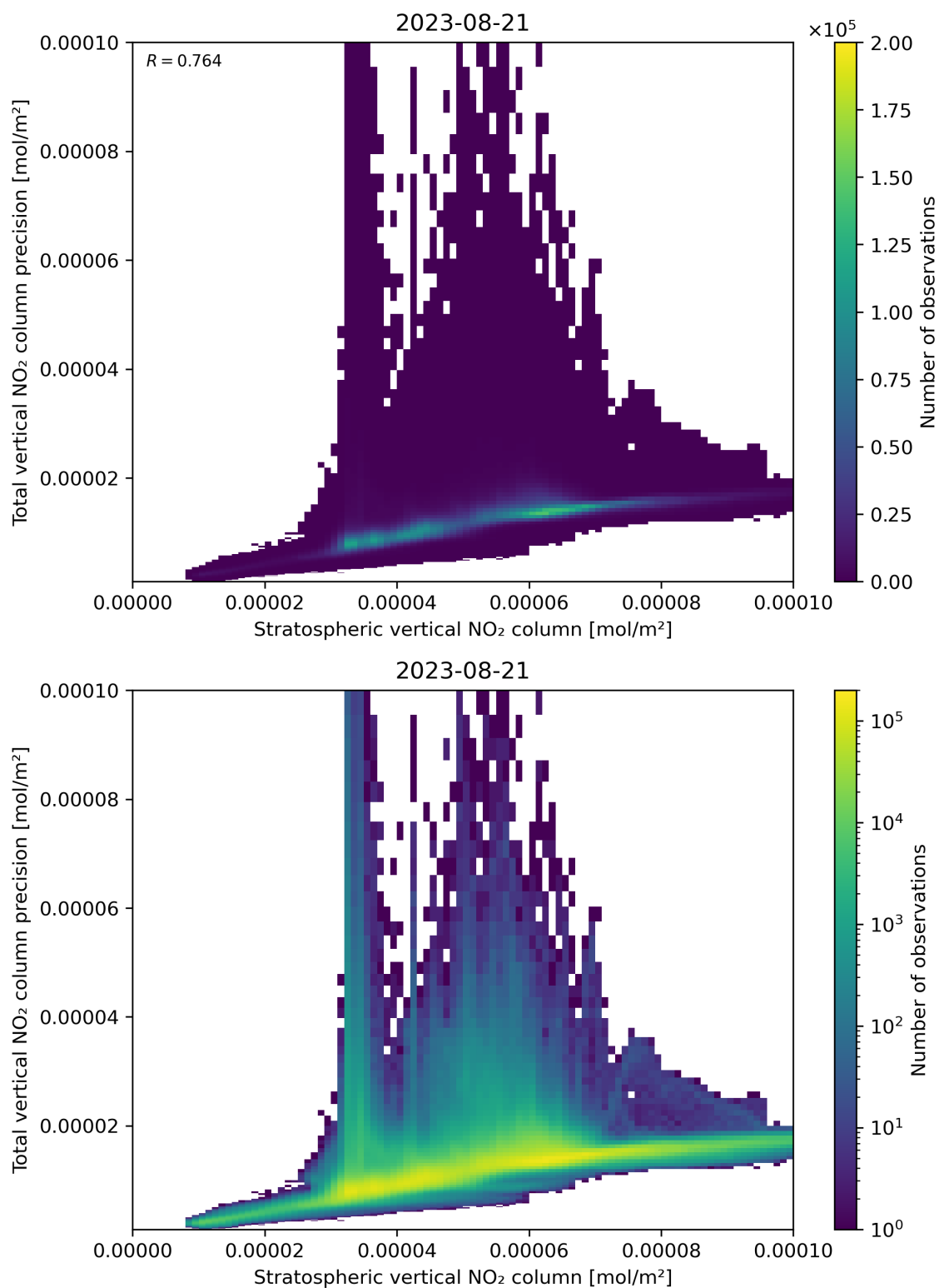
Figure 101: Scatter density plot of “Stratospheric vertical NO 2 column” against “Total vertical NO 2 column precision” for 2023-08-20 to 2023-08-22.
