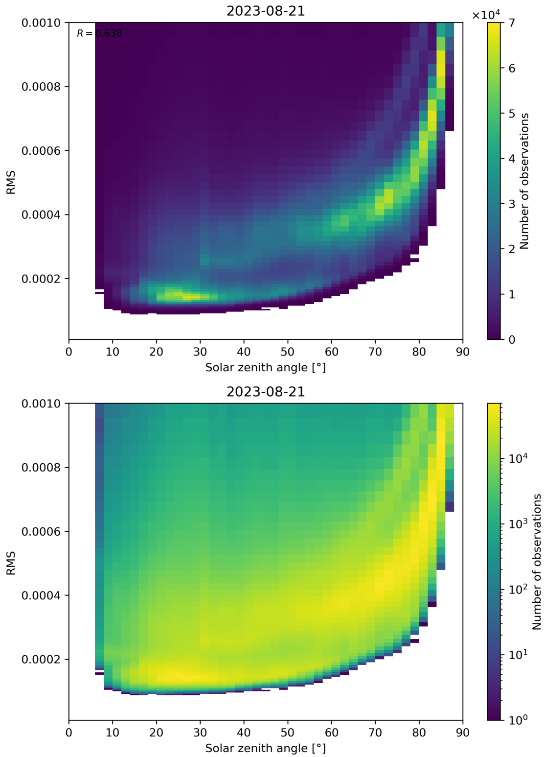
Figure 157: Scatter density plot of “Solar zenith angle” against “RMS” for 2023-08-20 to 2023-08-22.
