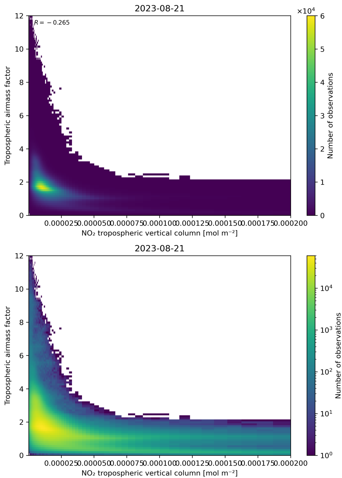
Figure 123: Scatter density plot of “NO 2 tropospheric vertical column” against “Tropospheric air mass factor” for 2023-08-20 to 2023-08-22.
