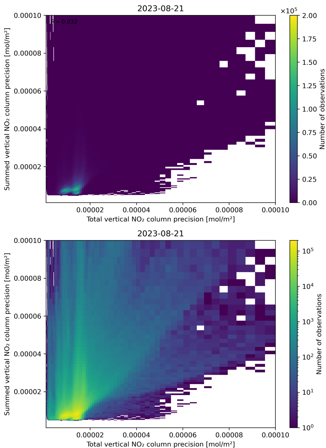
Figure 118: Scatter density plot of “Total vertical NO 2 column precision” against “Summed vertical NO 2 column precision” for 2023-08-20 to 2023-08-22.
