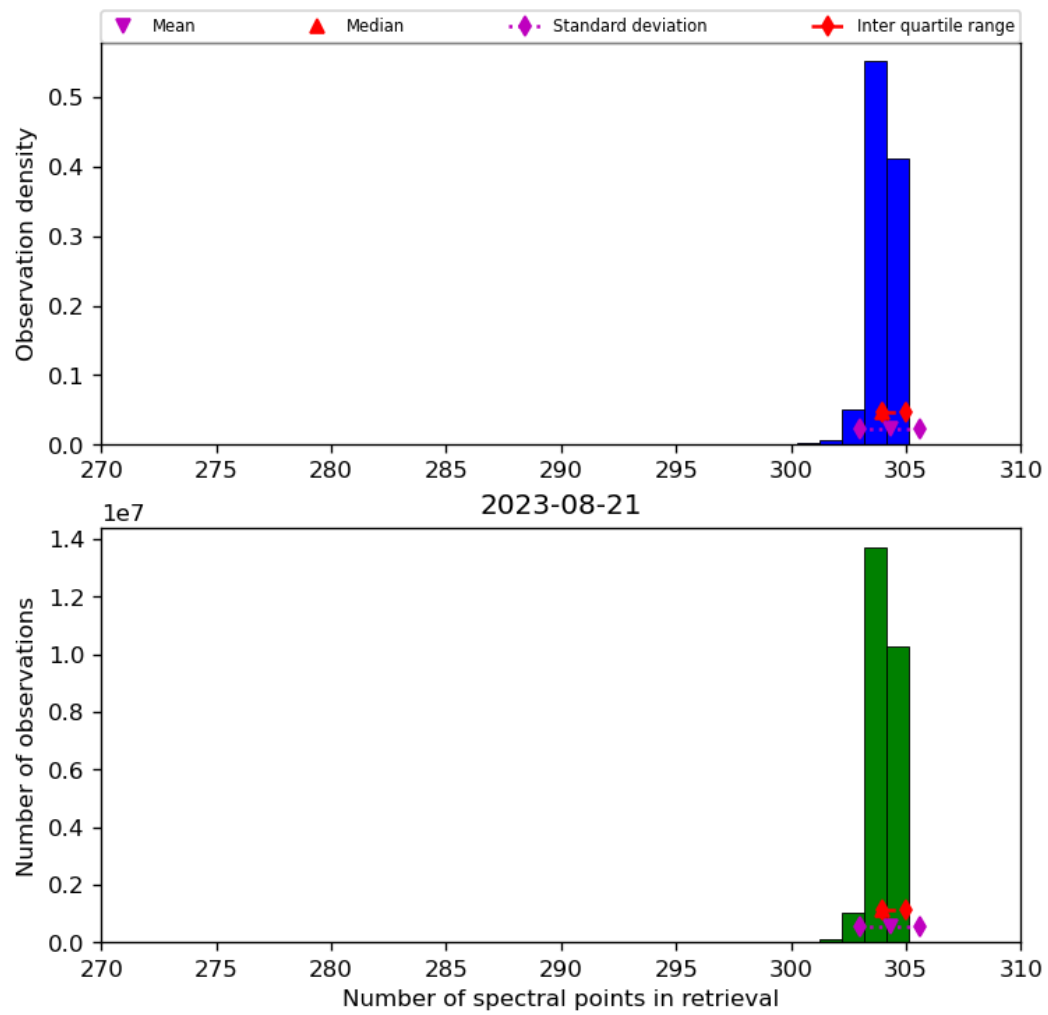
Figure 33: Histogram of “Number of spectral points in retrieval” for 2023-08-20 to 2023-08-22
