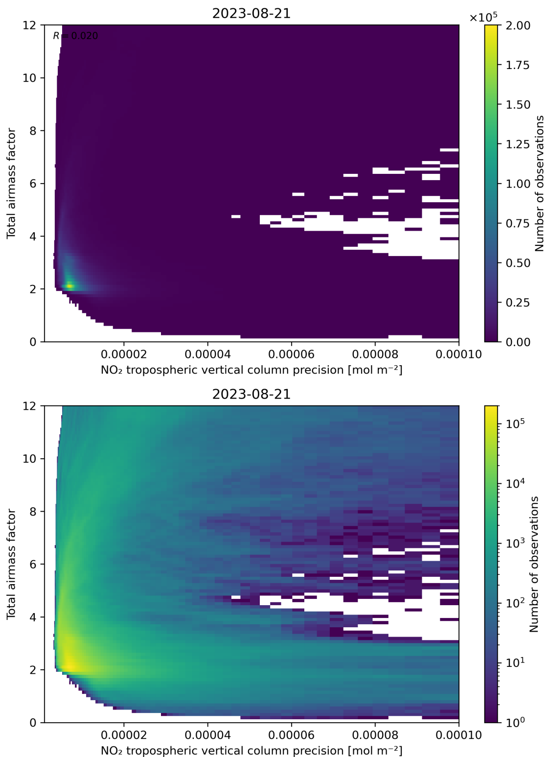
Figure 132: Scatter density plot of “NO 2 tropospheric vertical column precision” against “Total airmass factor” for 2023-08-20 to 2023-08-22.
