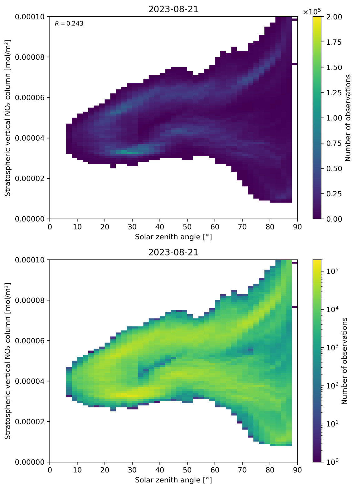
Figure 150: Scatter density plot of “Solar zenith angle” against “Stratospheric vertical NO 2 column” for 2023-08-20 to 2023-08-22.
