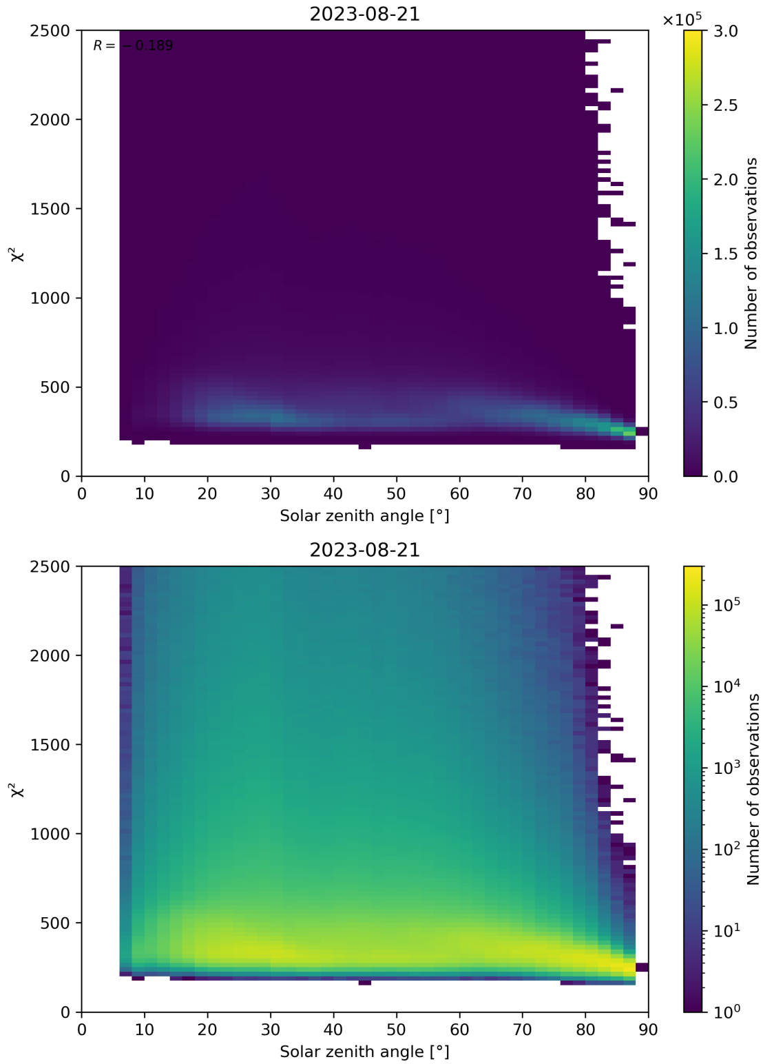
Figure 148: Scatter density plot of “Solar zenith angle” against “ \chi^2 ” for 2023-08-20 to 2023-08-22.
