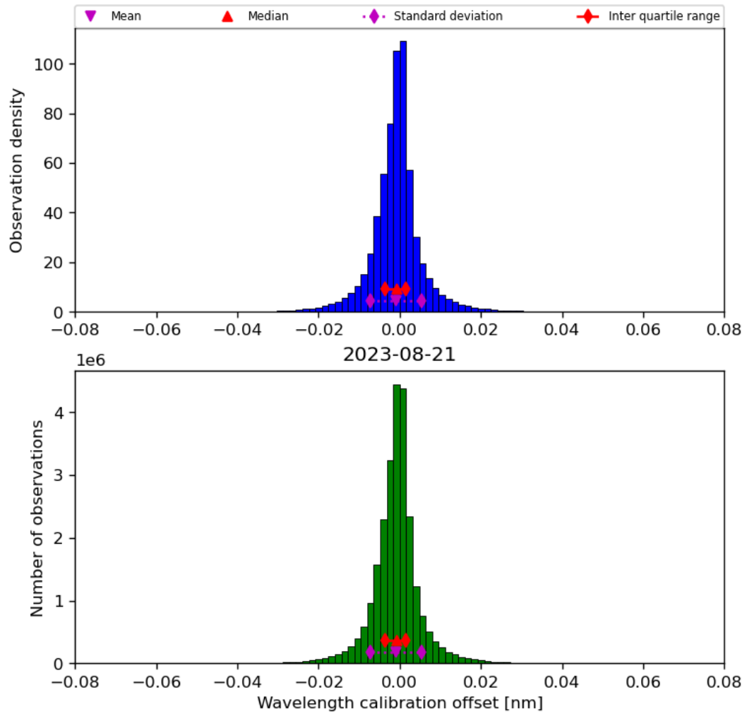
Figure 35: Histogram of “Wavelength calibration offset” for 2023-08-20 to 2023-08-22
