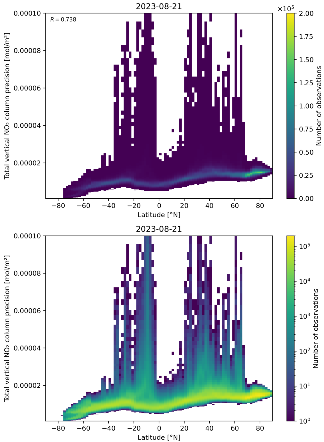
Figure 91: Scatter density plot of “Latitude” against “Total vertical NO 2 column precision” for 2023-08-20 to 2023-08-22.
