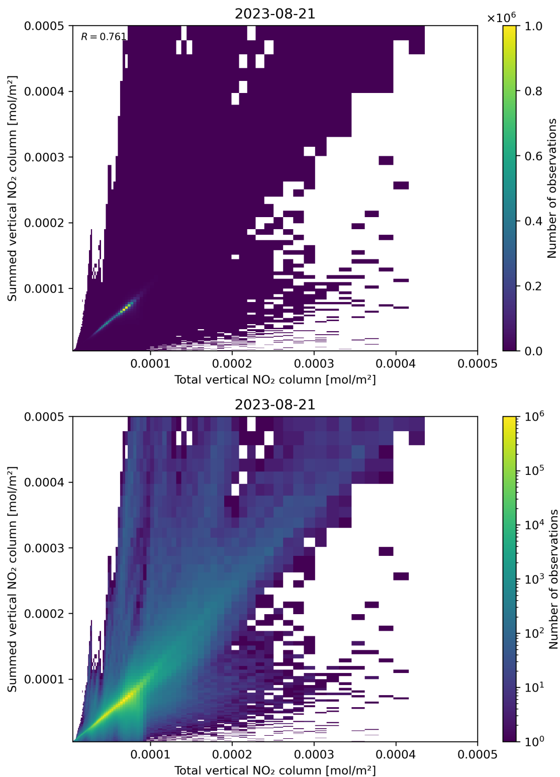
Figure 112: Scatter density plot of “Total vertical NO 2 column” against “Summed vertical NO 2 column” for 2023-08-20 to 2023-08-22.
