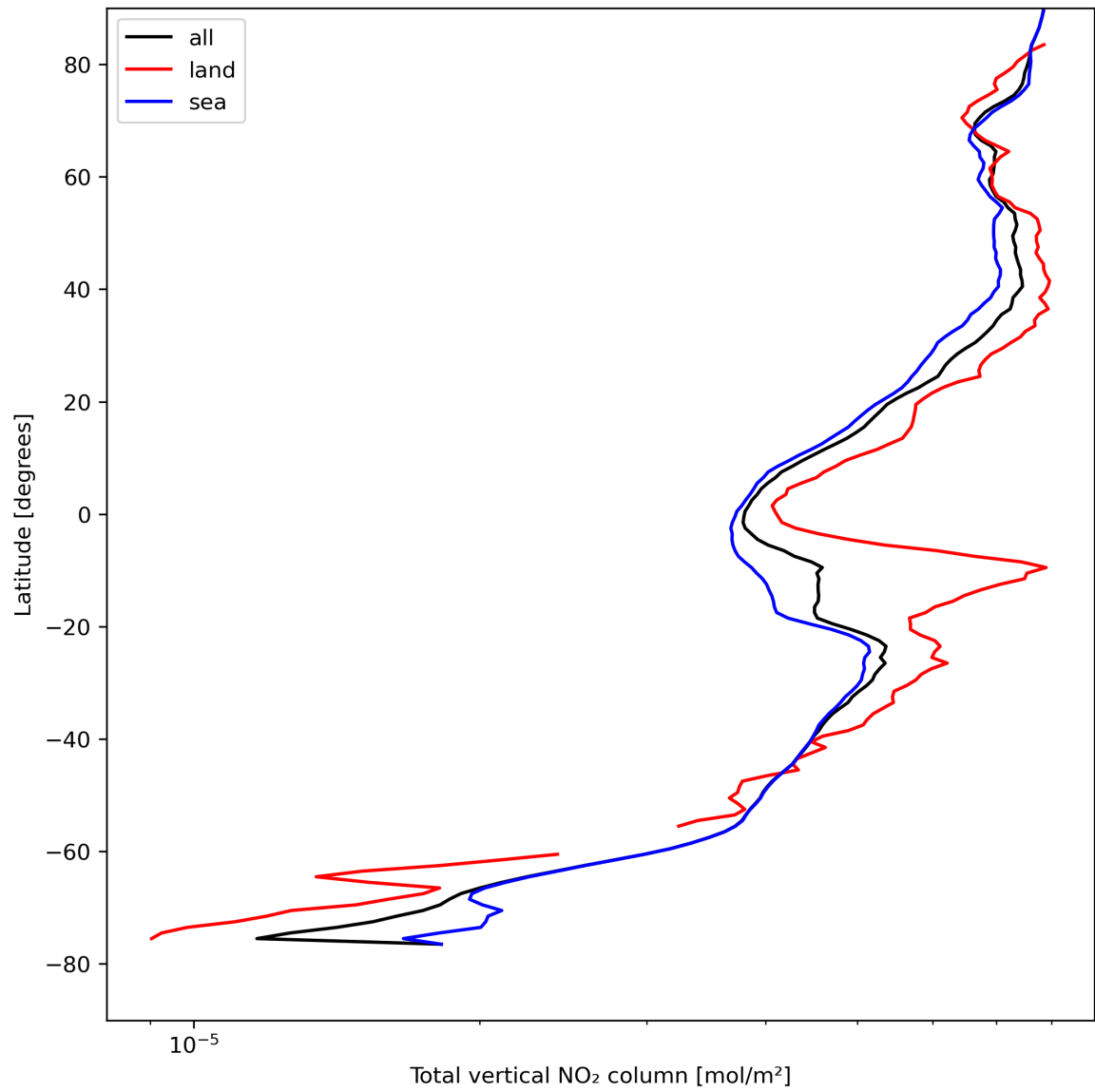
Figure 21: Zonal average of “Total vertical NO 2 column” for 2023-08-20 to 2023-08-22.
