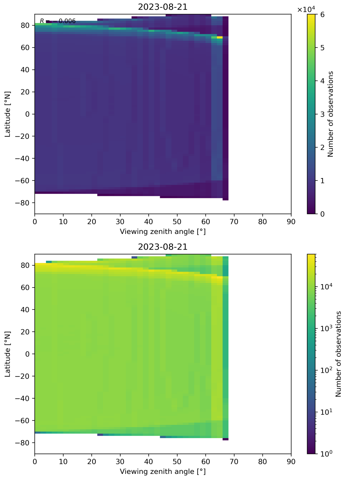
Figure 163: Scatter density plot of “Viewing zenith angle” against “Latitude” for 2023-08-20 to 2023-08-22.
