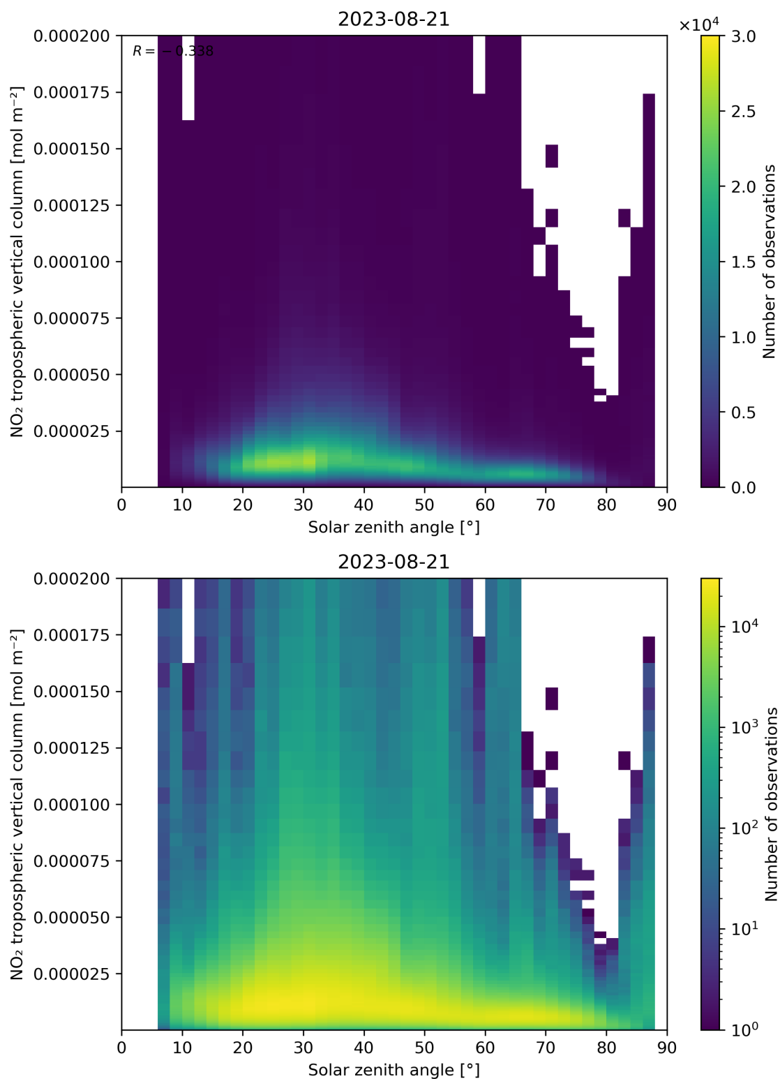
Figure 155: Scatter density plot of “Solar zenith angle” against “NO 2 tropospheric vertical column” for 2023-08-20 to 2023-08-22.
