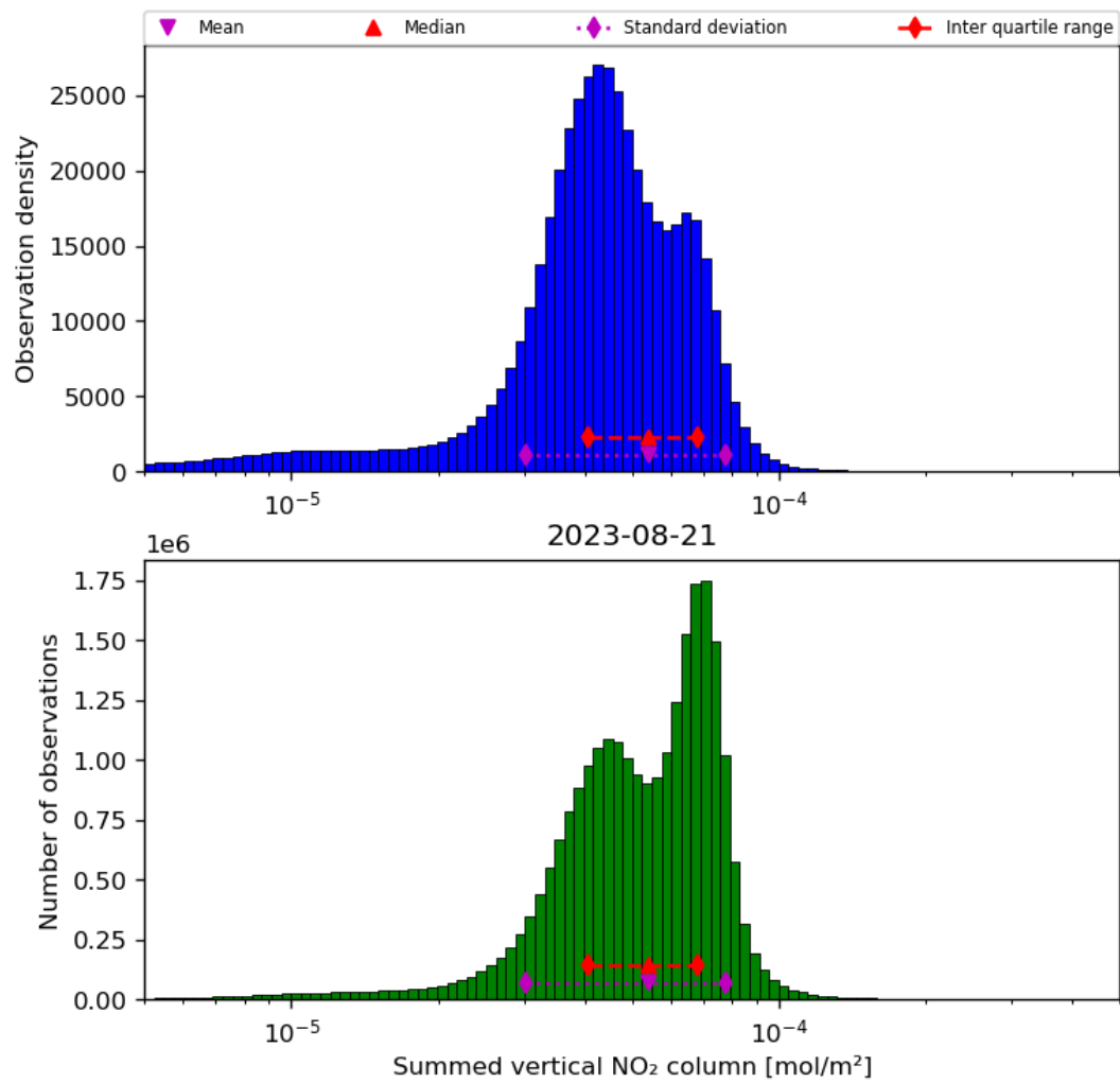
Figure 40: Histogram of “Summed vertical NO 2 column” for 2023-08-20 to 2023-08-22
