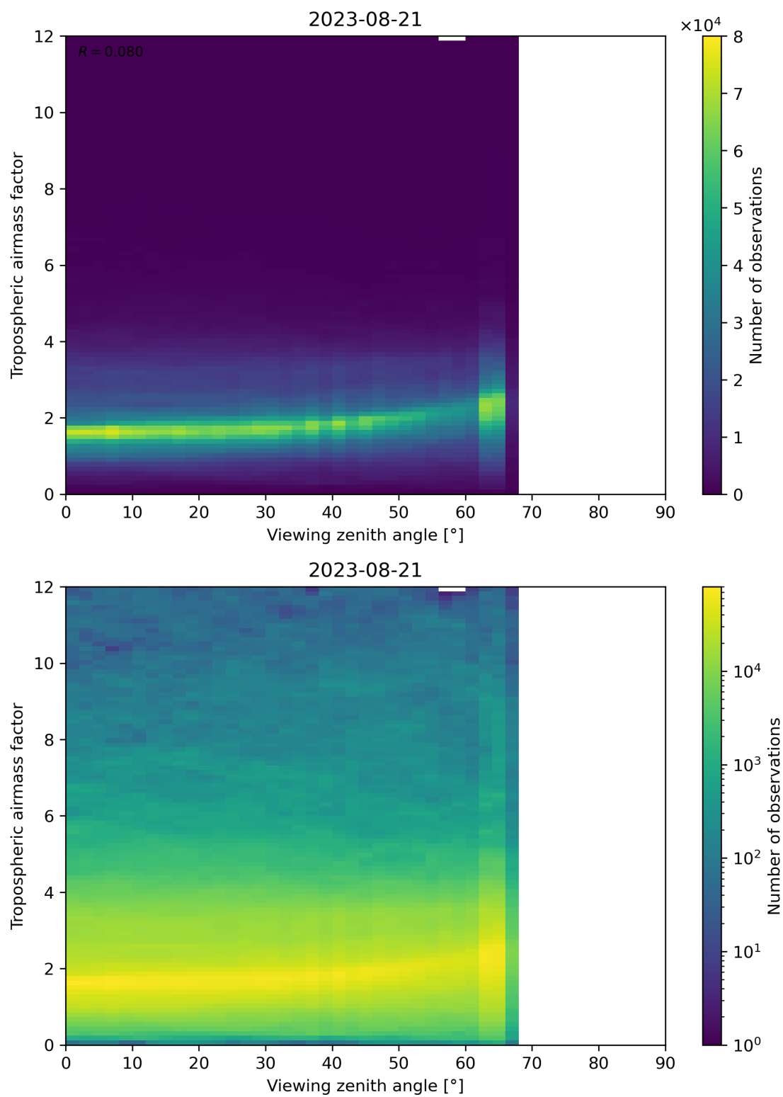
Figure 161: Scatter density plot of “Viewing zenith angle” against “Tropospheric airmass factor” for 2023-08-20 to 2023-08-22.
