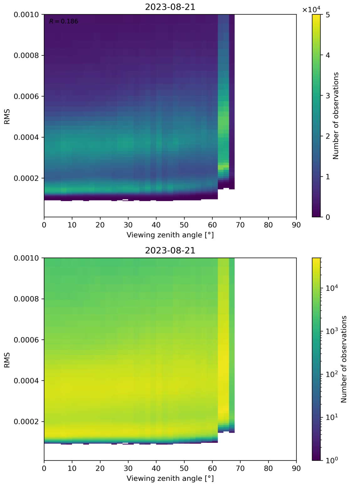
Figure 171: Scatter density plot of “Viewing zenith angle” against “RMS” for 2023-08-20 to 2023-08-22.
