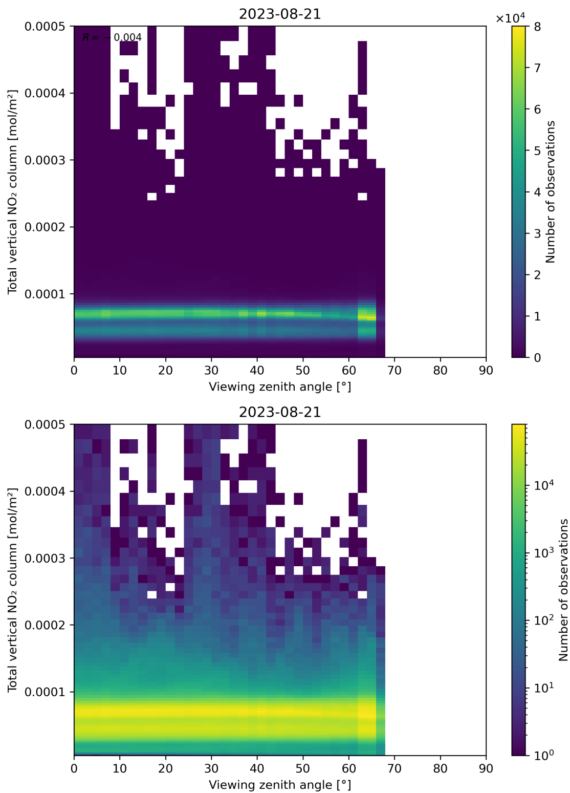
Figure 167: Scatter density plot of “Viewing zenith angle” against “Total vertical NO 2 column” for 2023-08-20 to 2023-08-22.
