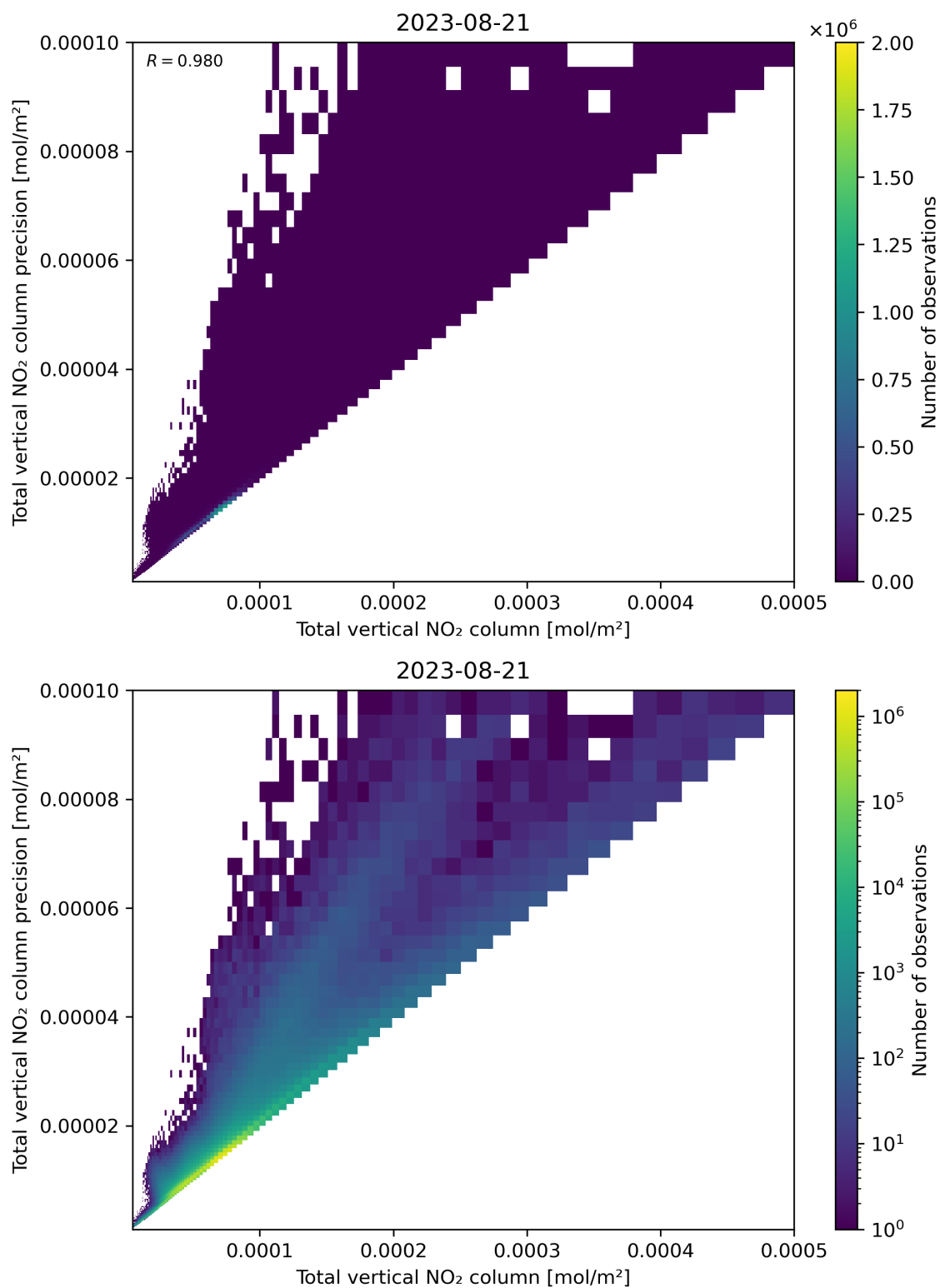
Figure 114: Scatter density plot of “Total vertical NO 2 column” against “Total vertical NO 2 column precision” for 2023-08-20 to 2023-08-22.
