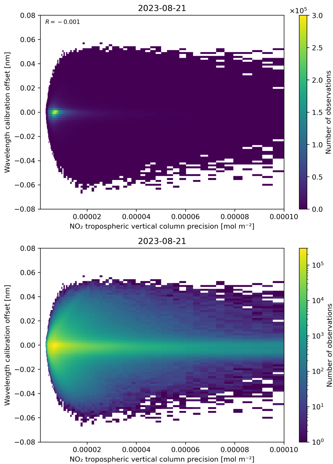
Figure 141: Scatter density plot of “NO 2 tropospheric vertical column precision” against “Wavelength calibration offset” for 2023-08-20 to 2023-08-22.
