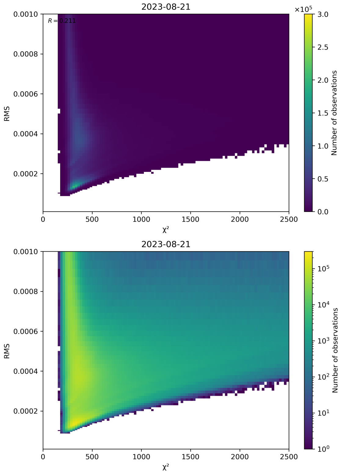
Figure 82: Scatter density plot of “ \chi^2 ” against “RMS” for 2023-08-20 to 2023-08-22.
