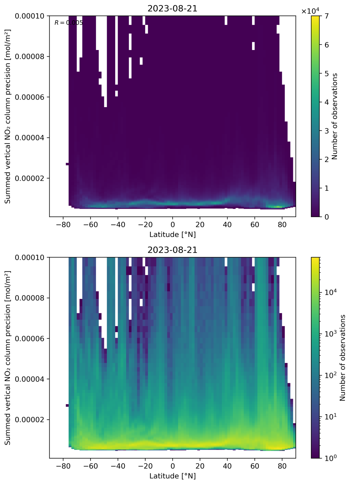
Figure 89: Scatter density plot of “Latitude” against “Summed vertical NO 2 column precision” for 2023-08-20 to 2023-08-22.
