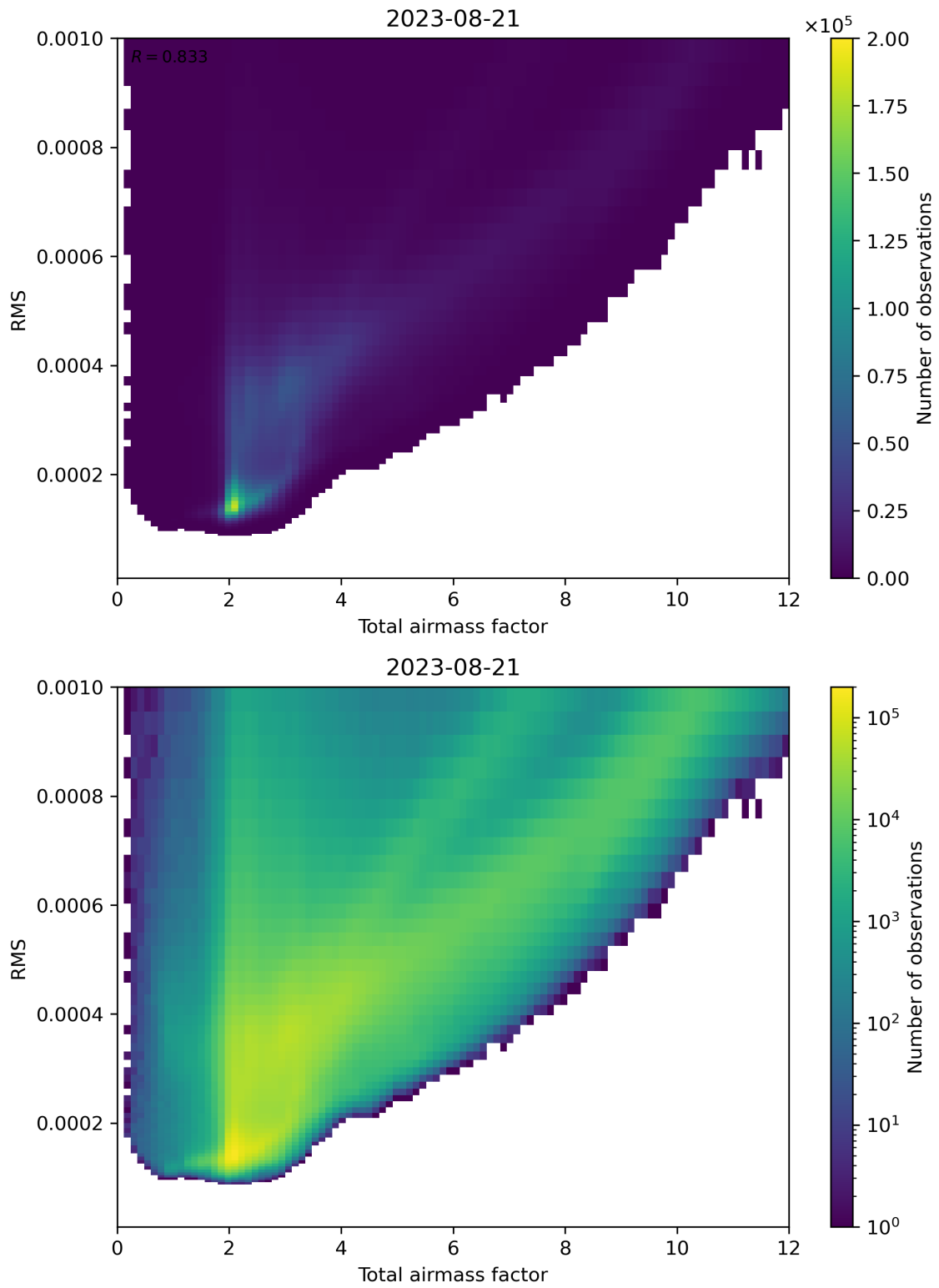
Figure 69: Scatter density plot of “Total airmass factor” against “RMS” for 2023-08-20 to 2023-08-22.
