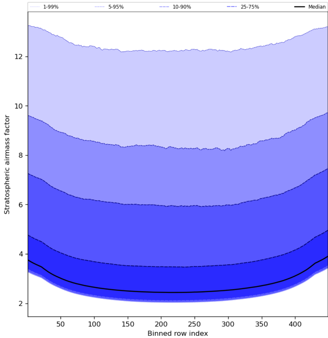
Figure 61: Along track statistics of “Stratospheric airmass factor” for 2023-08-20 to 2023-08-22
