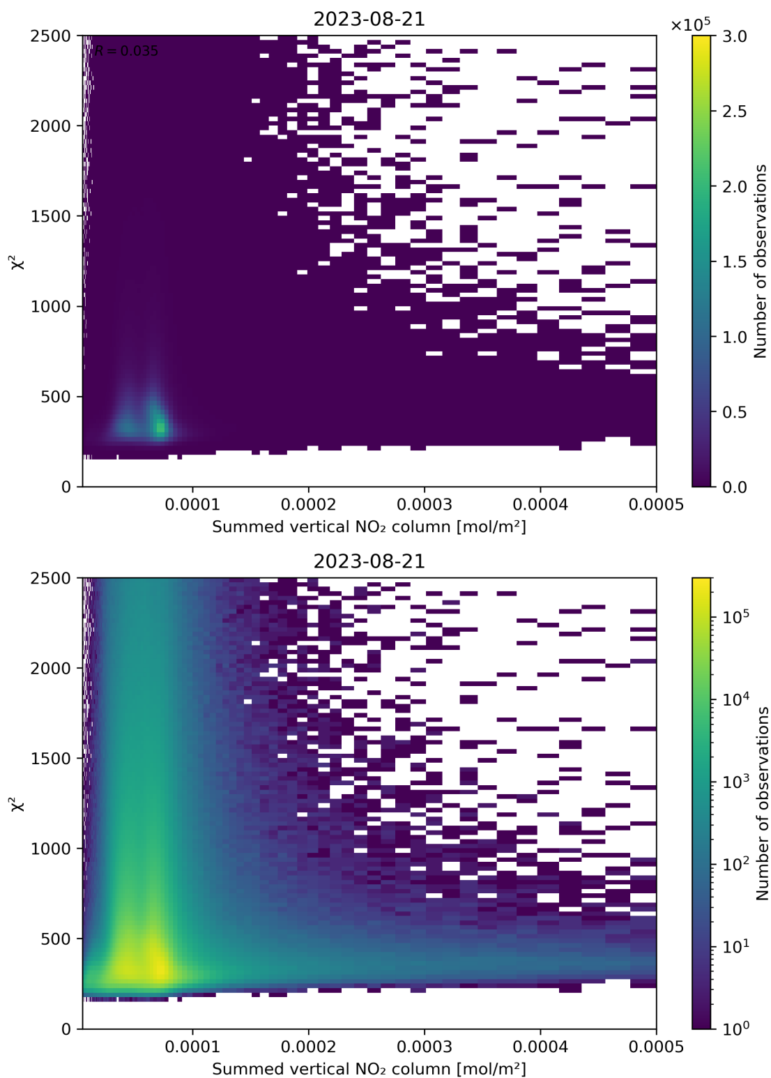
Figure 104: Scatter density plot of “Summed vertical NO 2 column” against “ \chi^2 ” for 2023-08-20 to 2023-08-22.
