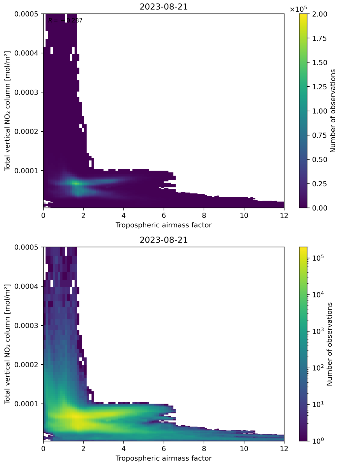
Figure 77: Scatter density plot of “Tropospheric airmass factor” against “Total vertical NO 2 column” for 2023-08-20 to 2023-08-22.
