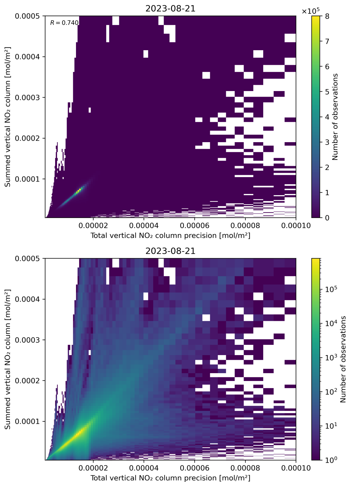
Figure 117: Scatter density plot of “Total vertical NO 2 column precision” against “Summed vertical NO 2 column” for 2023-08-20 to 2023-08-22.
