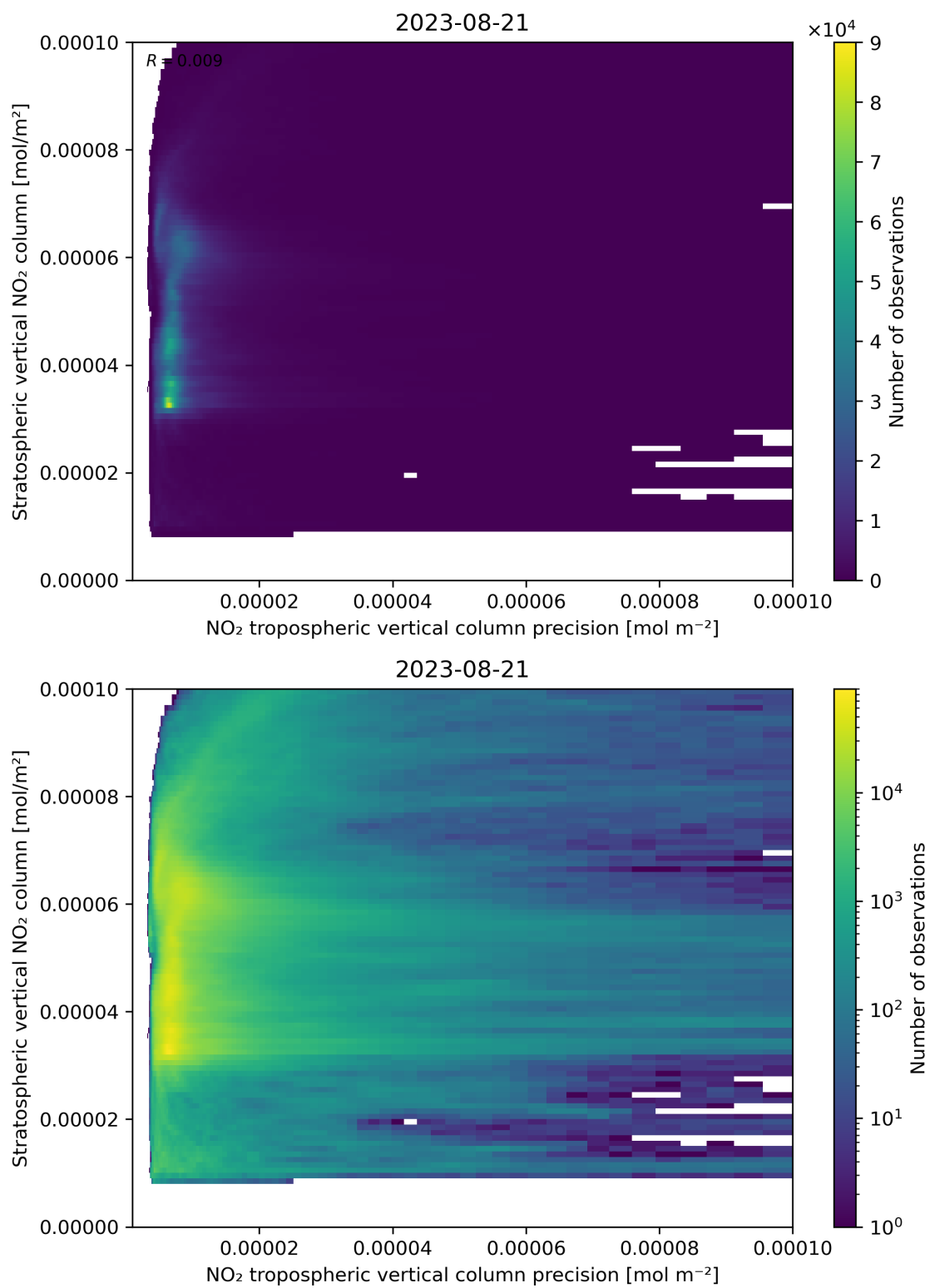
Figure 135: Scatter density plot of “NO 2 tropospheric vertical column precision” against “Stratospheric vertical NO 2 column” for 2023-08-20 to 2023-08-22.
