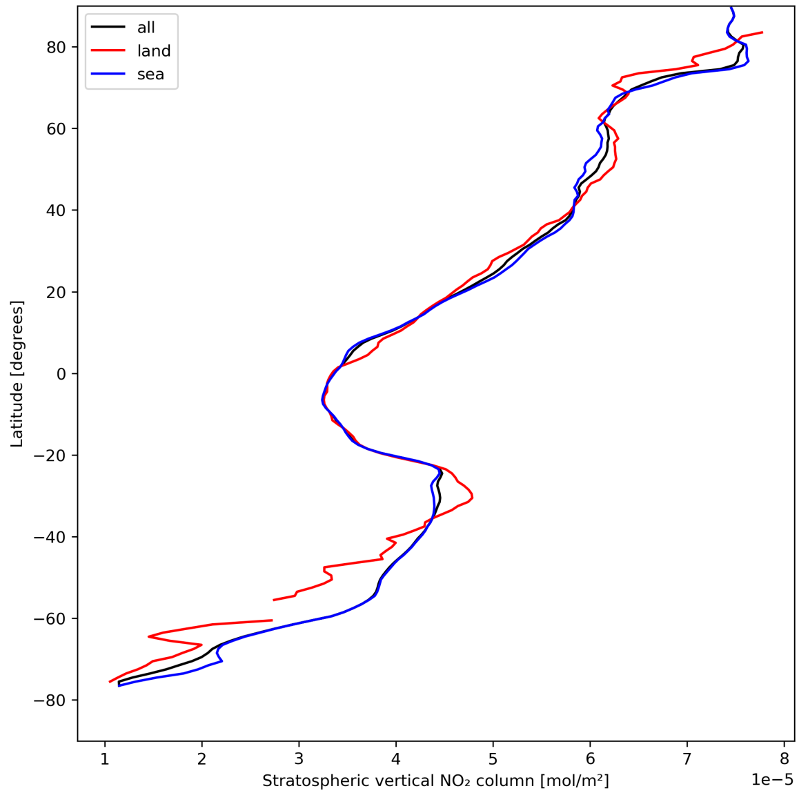
Figure 19: Zonal average of “Stratospheric vertical NO 2 column” for 2023-08-20 to 2023-08-22.
