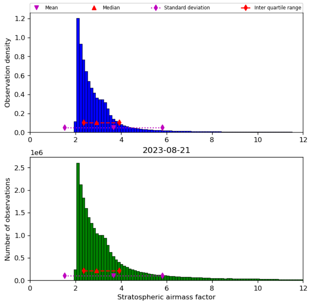
Figure 44: Histogram of “Stratospheric airmass factor” for 2023-08-20 to 2023-08-22
