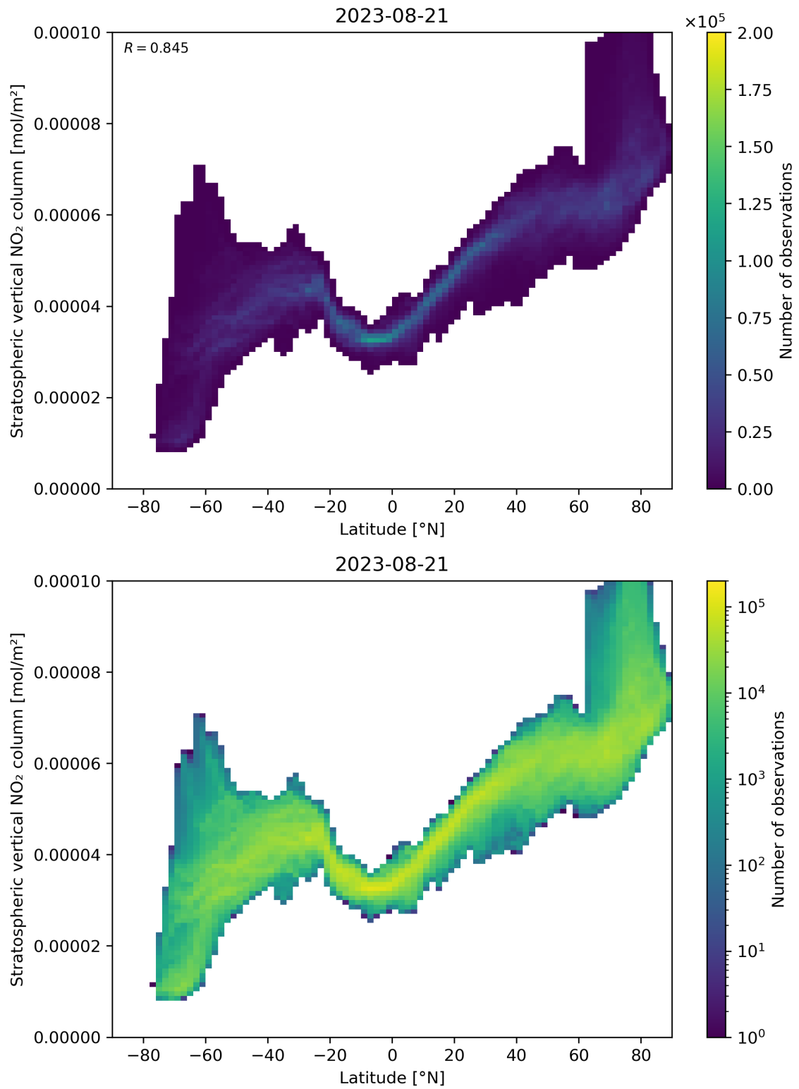
Figure 87: Scatter density plot of “Latitude” against “Stratospheric vertical NO 2 column” for 2023-08-20 to 2023-08-22.
