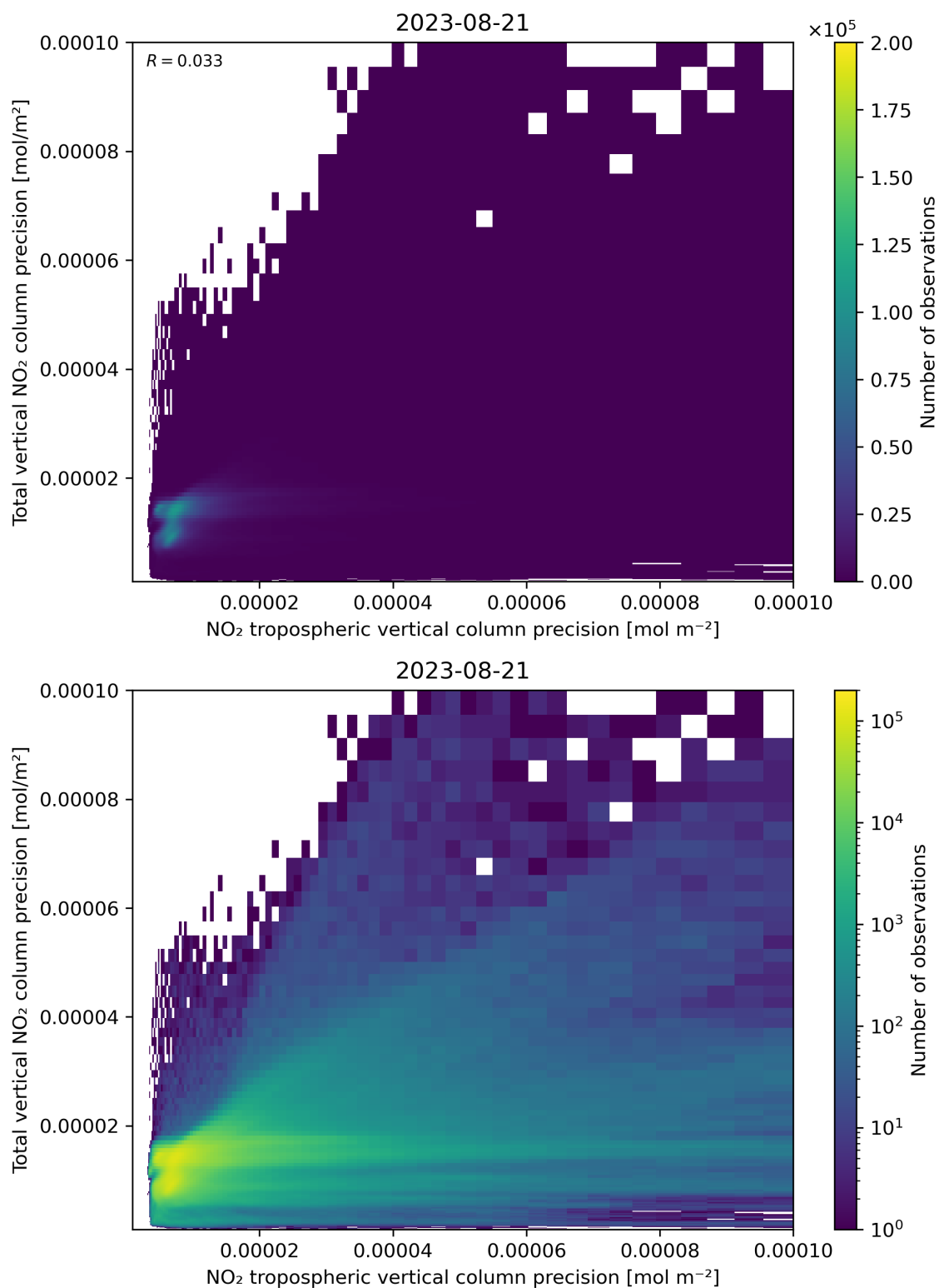
Figure 139: Scatter density plot of “NO 2 tropospheric vertical column precision” against “Total vertical NO 2 column precision” for 2023-08-20 to 2023-08-22.
