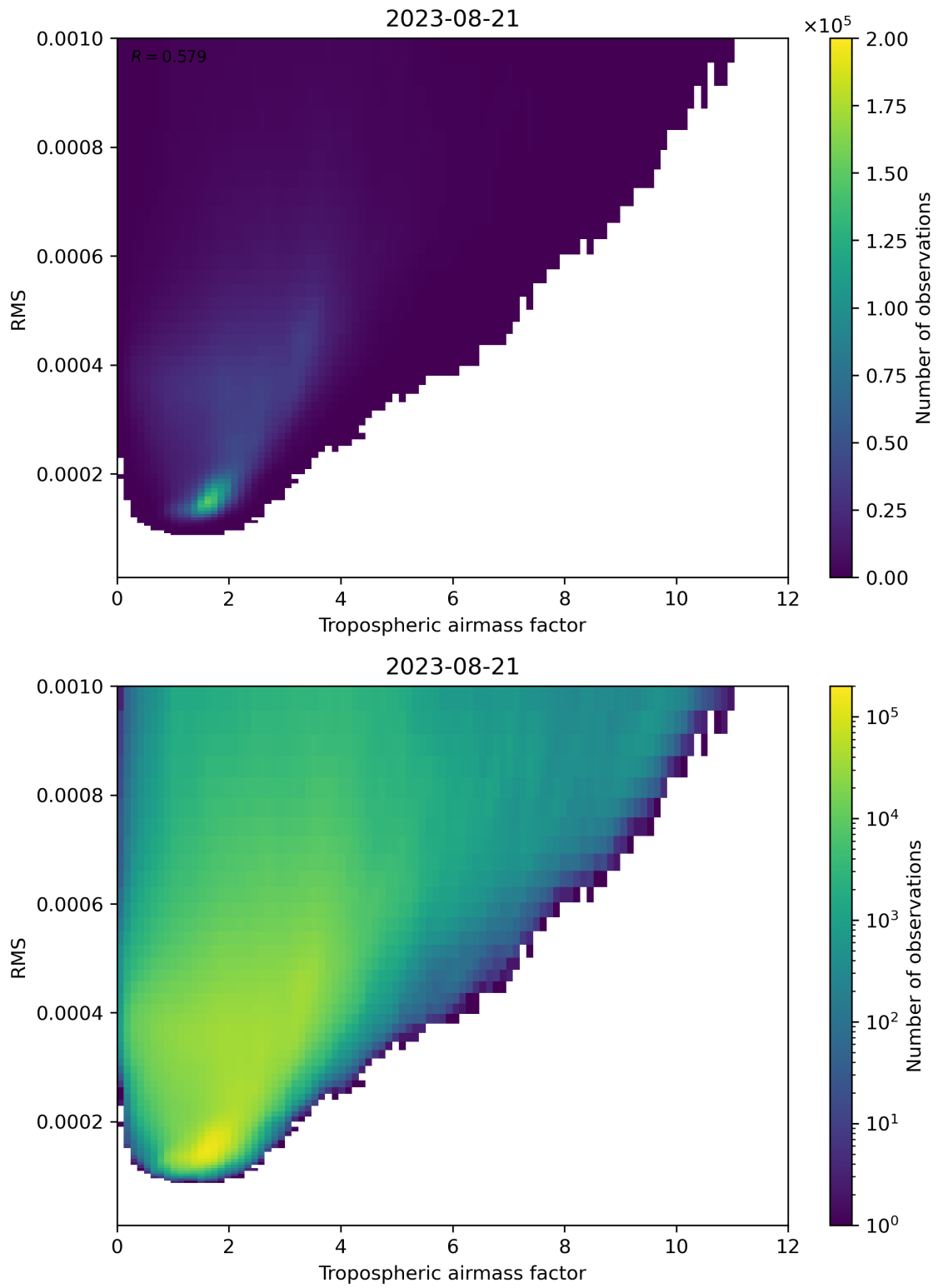
Figure 79: Scatter density plot of “Tropospheric airmass factor” against “RMS” for 2023-08-20 to 2023-08-22.
