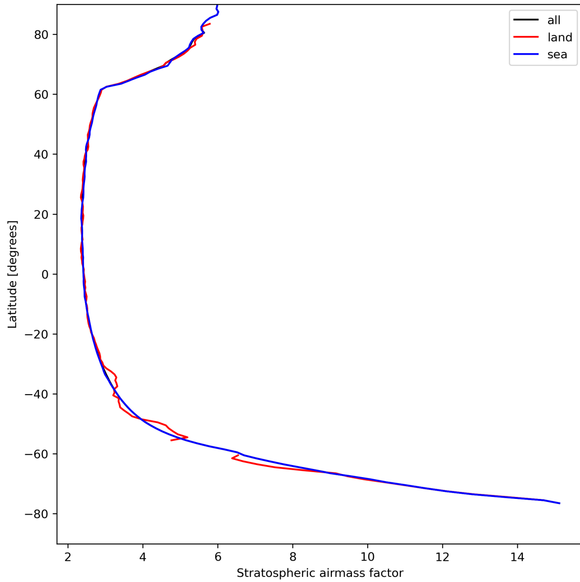
Figure 27: Zonal average of “Stratospheric airmass factor” for 2023-08-20 to 2023-08-22.
