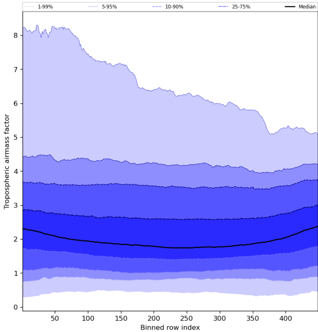
Figure 48: Along track statistics of “Tropospheric airmass factor” for 2023-08-20 to 2023-08-22
