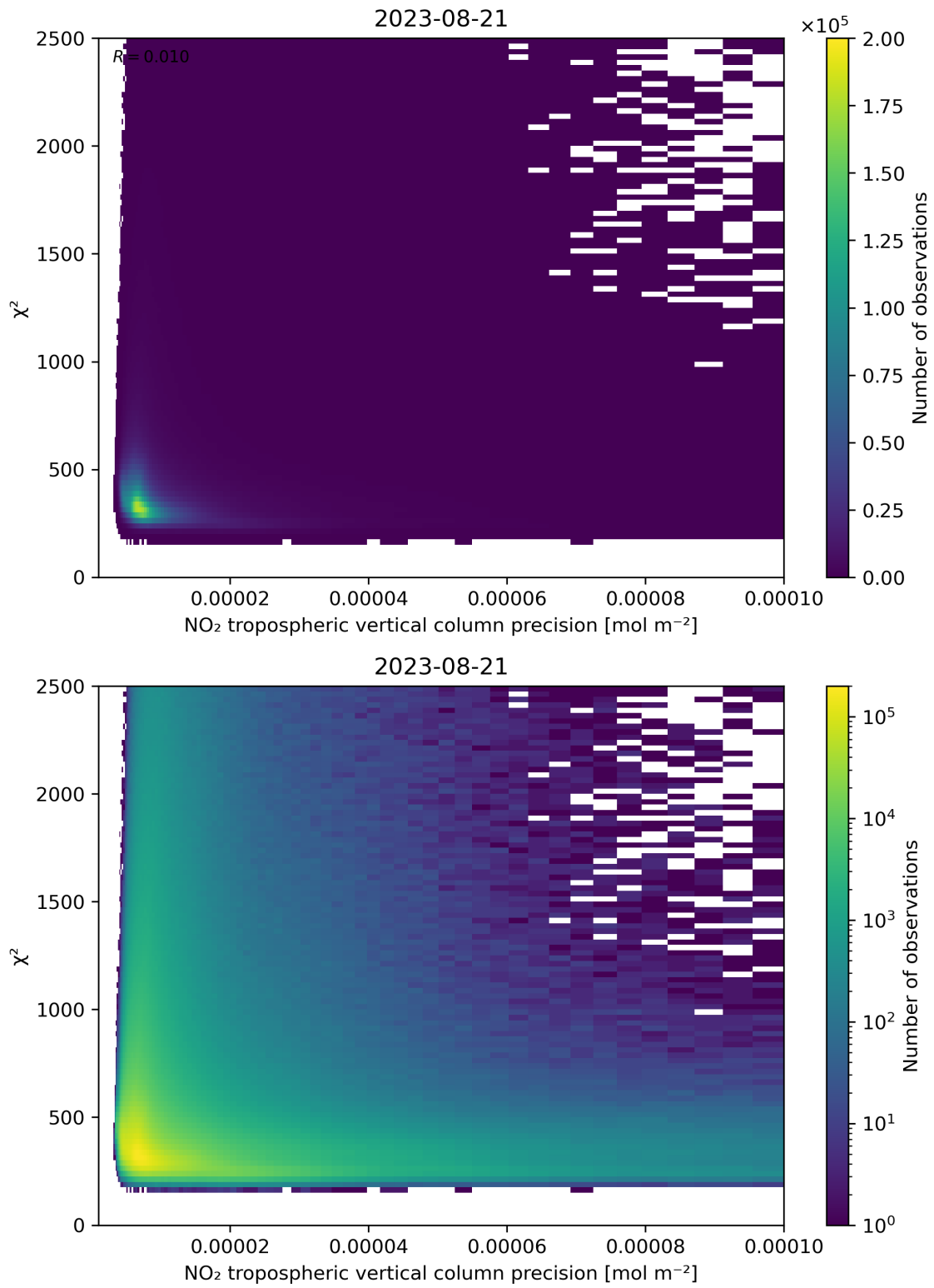
Figure 134: Scatter density plot of “NO 2 tropospheric vertical column precision” against “ \chi^2 ” for 2023-08-20 to 2023-08-22.
