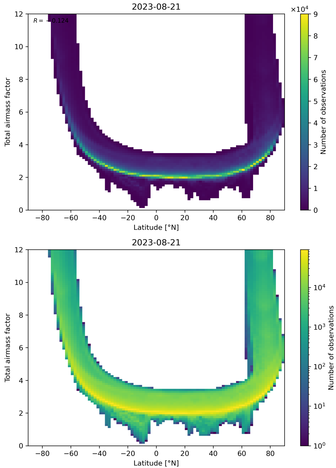
Figure 84: Scatter density plot of “Latitude” against “Total airmass factor” for 2023-08-20 to 2023-08-22.
