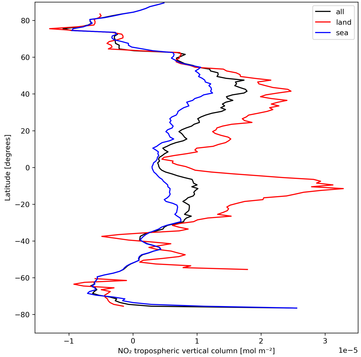
Figure 12: Zonal average of “NO 2 tropospheric vertical column” for 2023-08-20 to 2023-08-22.
