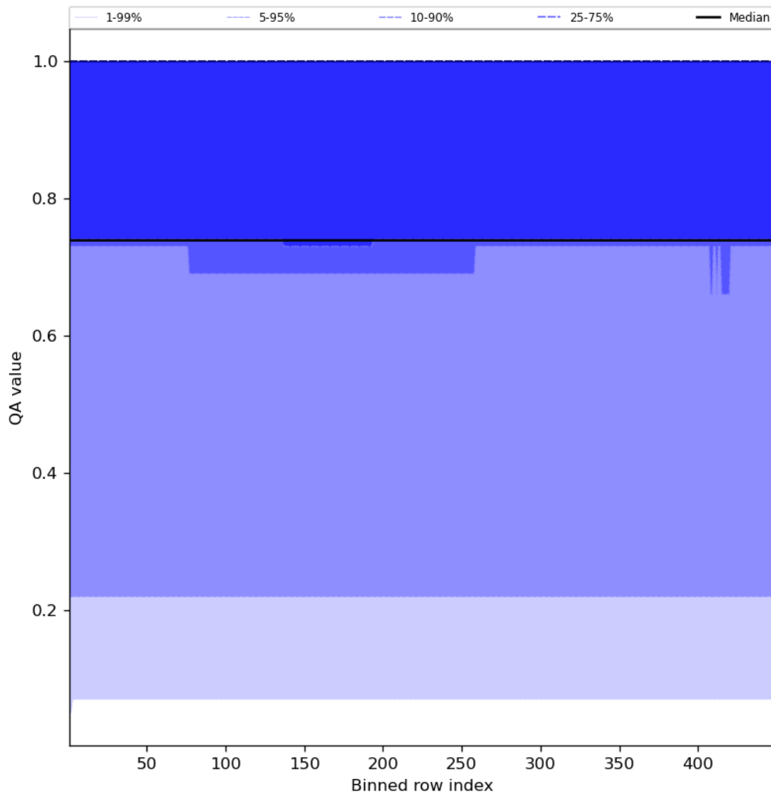
Figure 45: Along track statistics of “QA value” for 2023-08-20 to 2023-08-22
