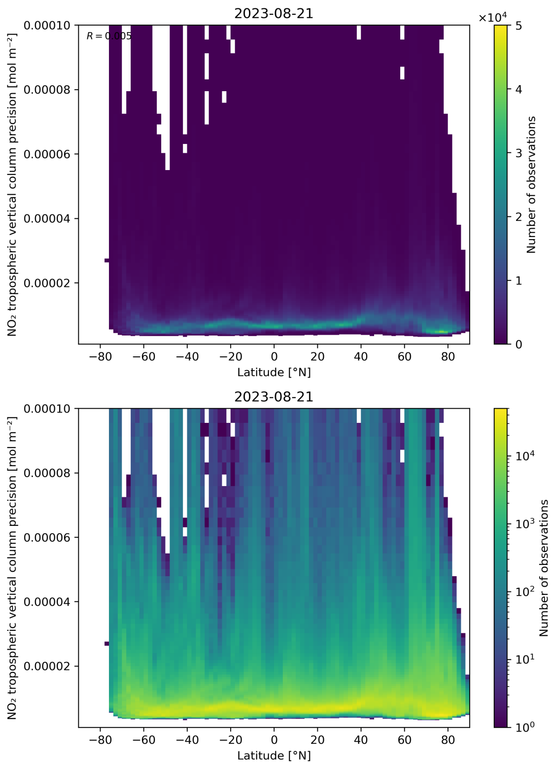
Figure 93: Scatter density plot of “Latitude” against “NO 2 tropospheric vertical column precision” for 2023-08-20 to 2023-08-22.
