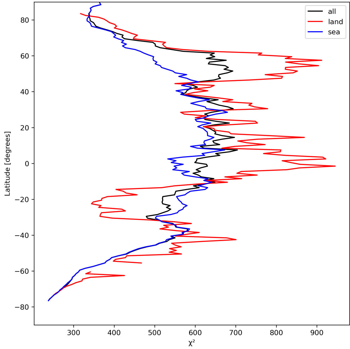
Figure 25: Zonal average of “ \chi^2 ” for 2023-08-20 to 2023-08-22.
