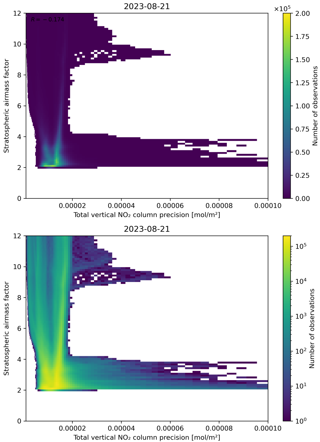
Figure 115: Scatter density plot of “Total vertical NO 2 column precision” against “Stratospheric air mass factor” for 2023-08-20 to 2023-08-22.
