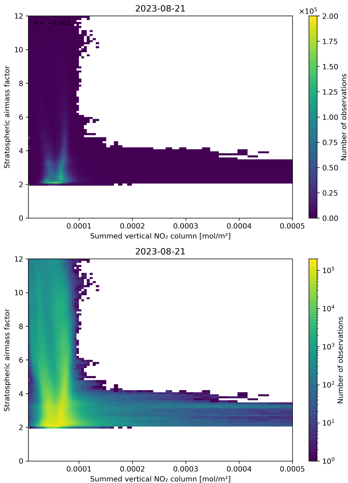
Figure 103: Scatter density plot of “Summed vertical NO 2 column” against “Stratospheric air mass factor” for 2023-08-20 to 2023-08-22.
