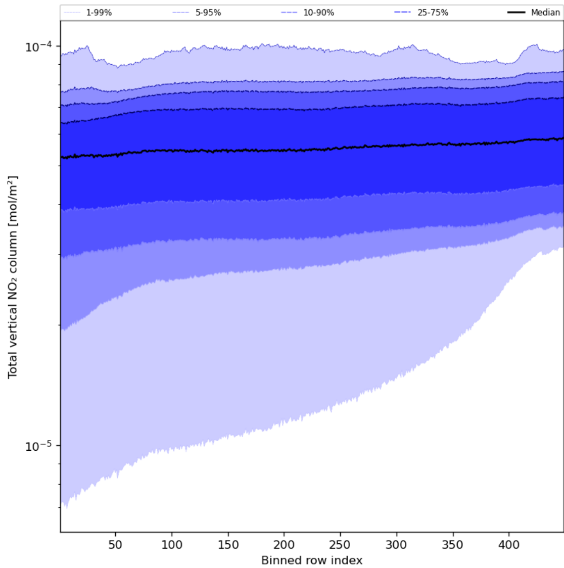
Figure 55: Along track statistics of “Total vertical NO 2 column” for 2023-08-20 to 2023-08-22
