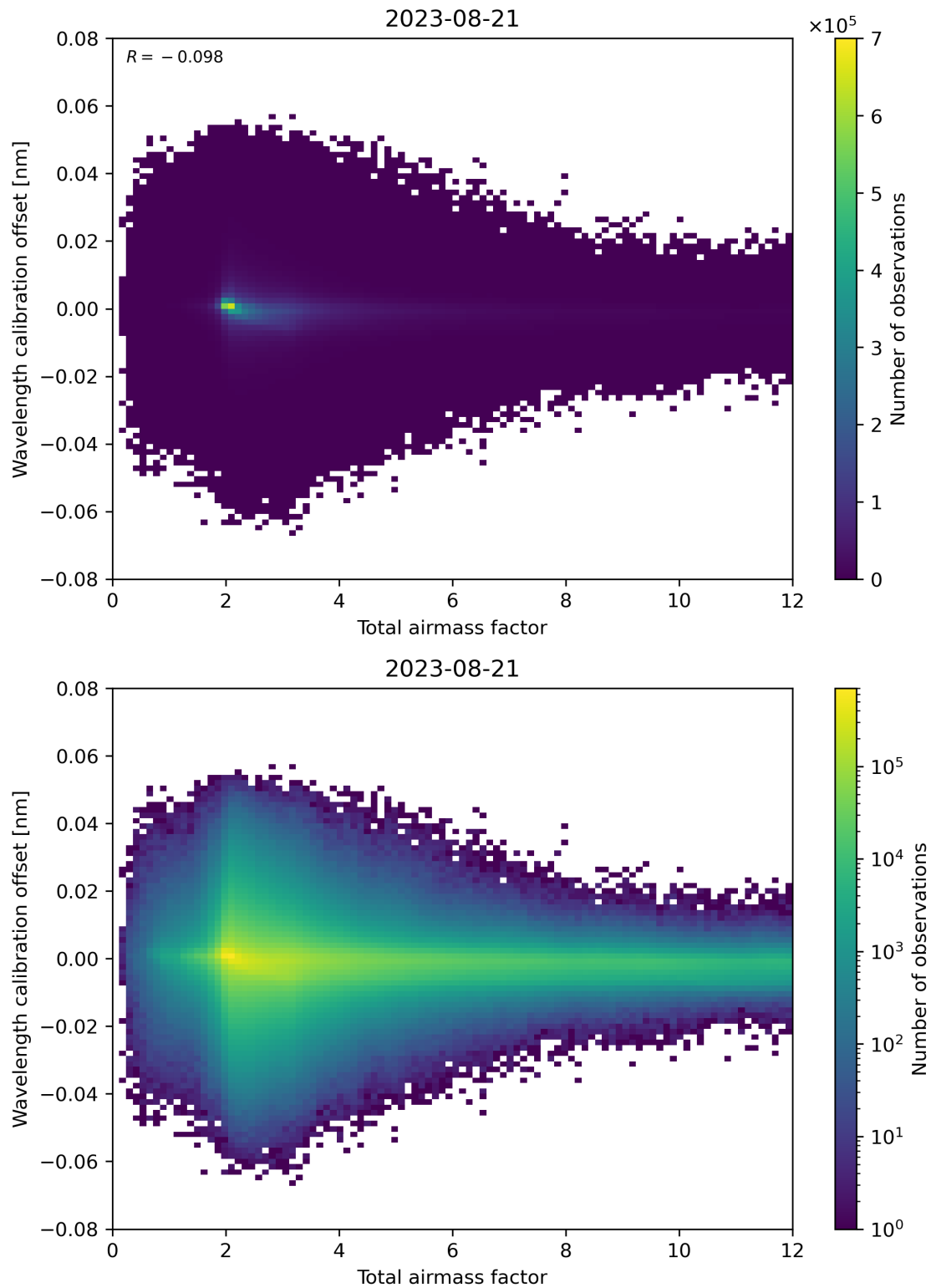
Figure 70: Scatter density plot of “Total airmass factor” against “Wavelength calibration offset” for 2023-08-20 to 2023-08-22.
