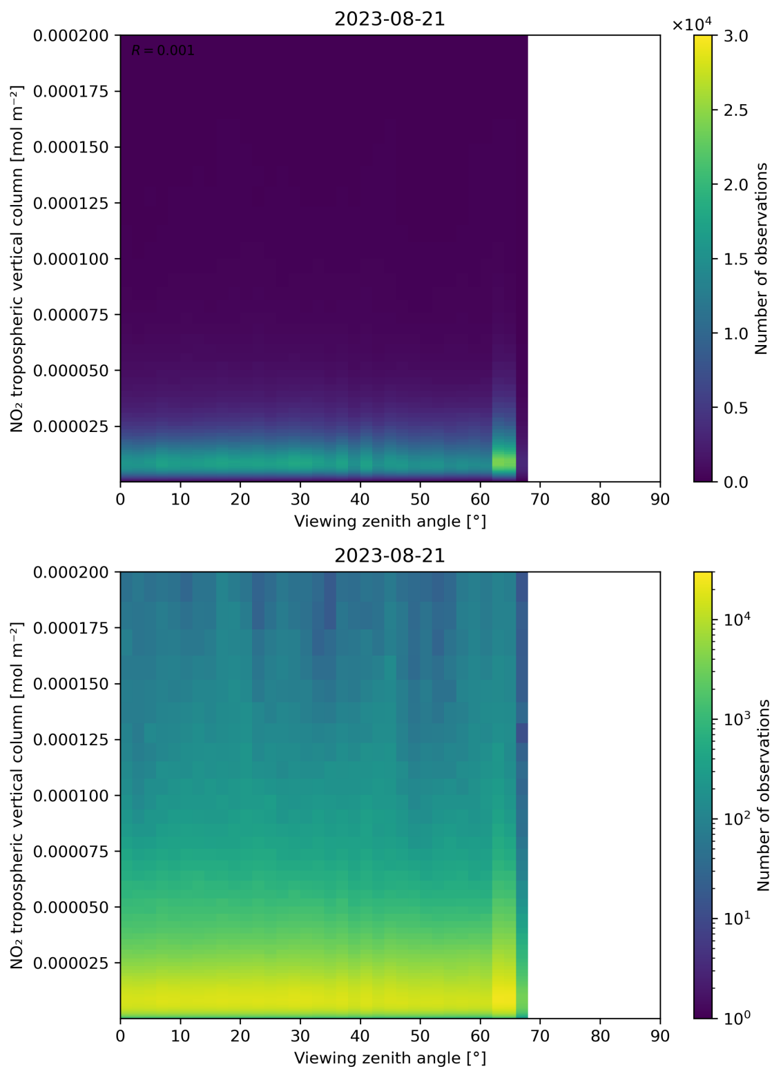
Figure 169: Scatter density plot of “Viewing zenith angle” against “NO 2 tropospheric vertical column” for 2023-08-20 to 2023-08-22.
