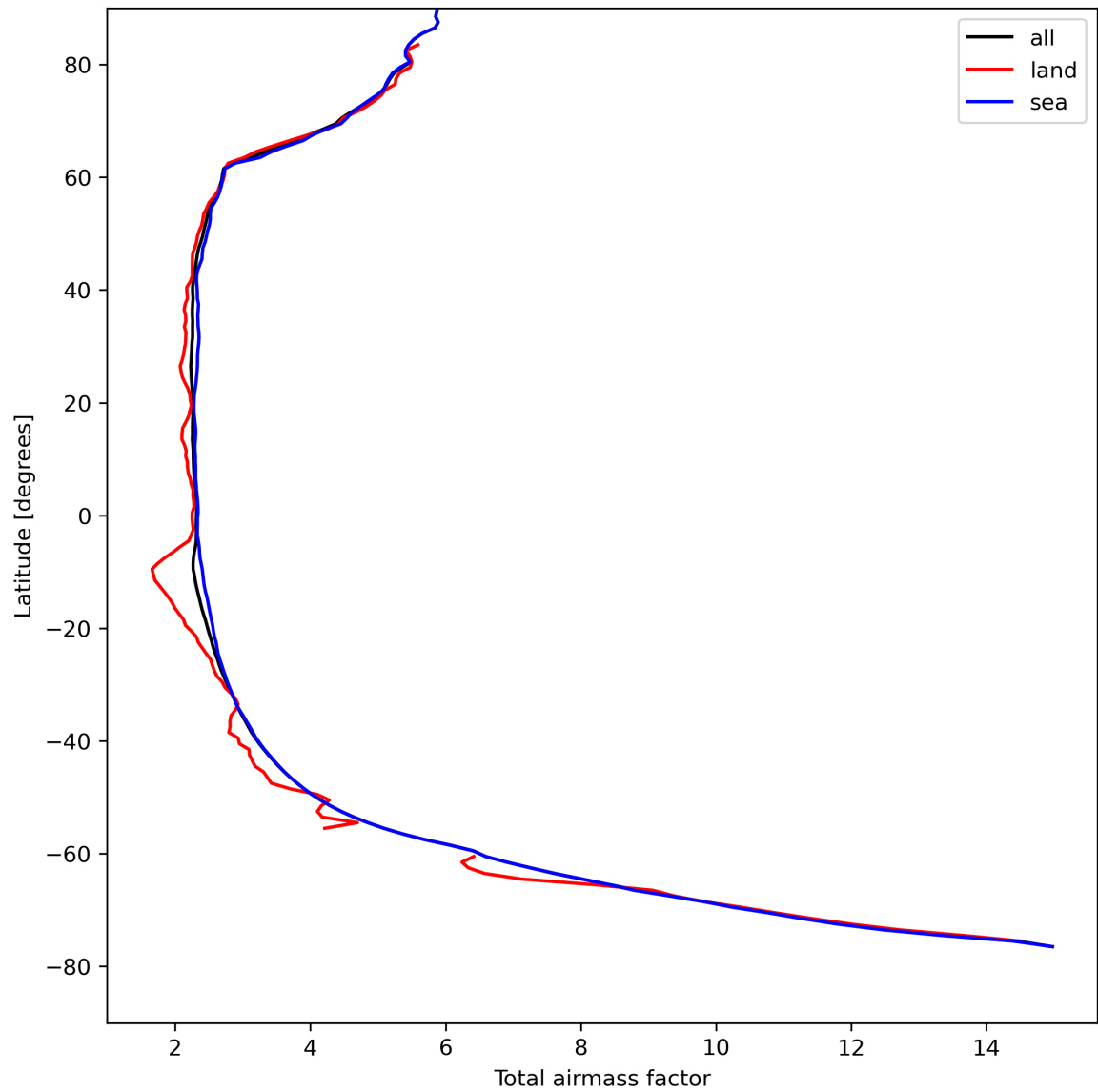
Figure 15: Zonal average of “Total airmass factor” for 2023-08-20 to 2023-08-22.
