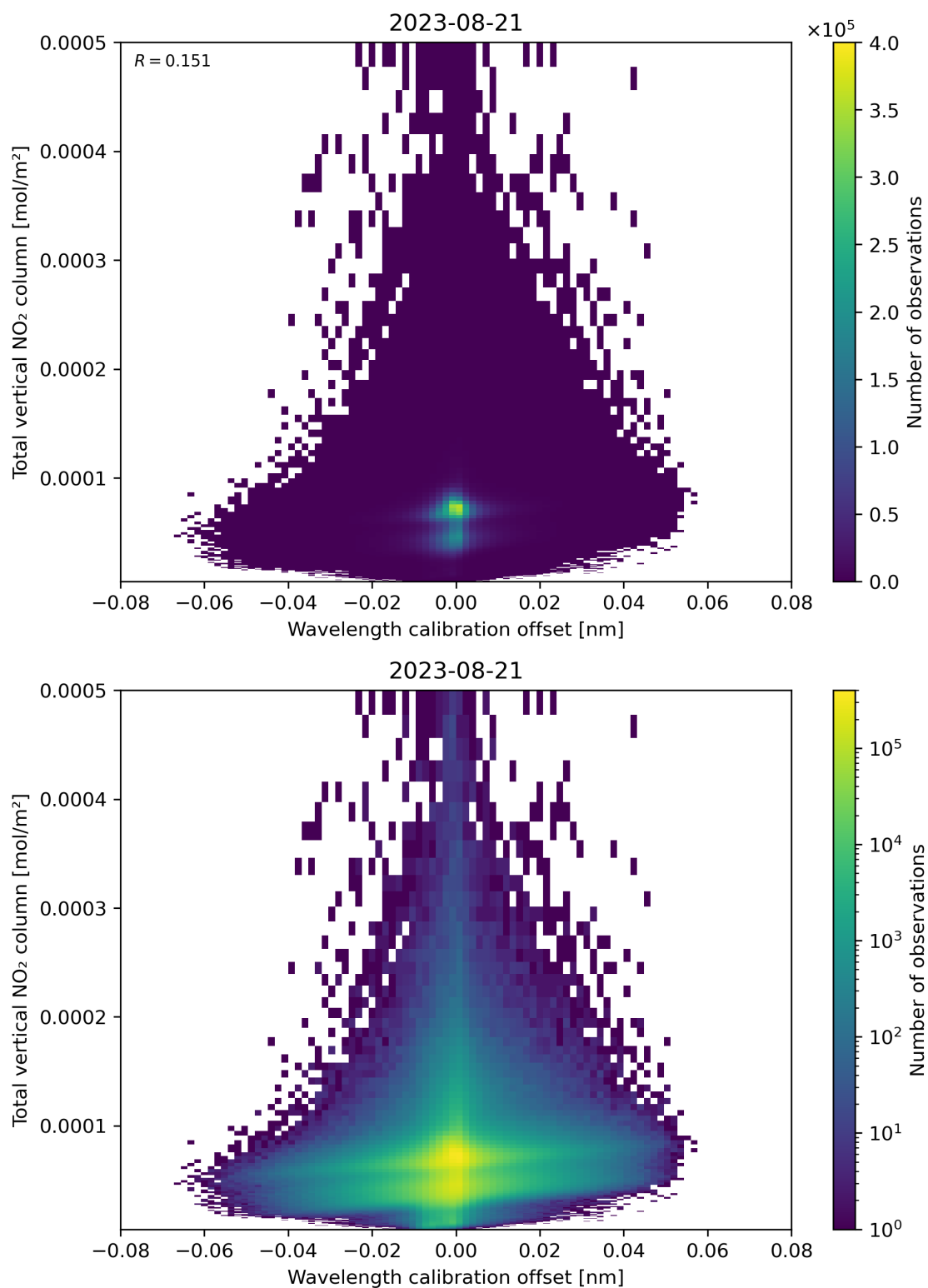
Figure 179: Scatter density plot of “Wavelength calibration offset” against “Total vertical NO 2 column” for 2023-08-20 to 2023-08-22.
