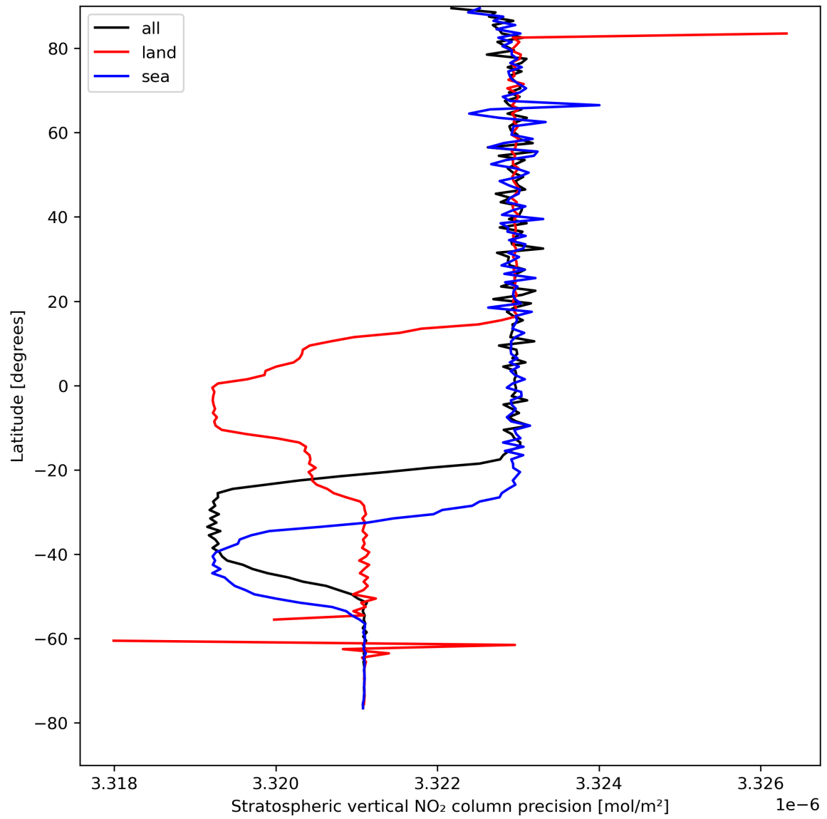
Figure 20: Zonal average of “Stratospheric vertical NO 2 column precision” for 2023-08-20 to 2023-08-22.
