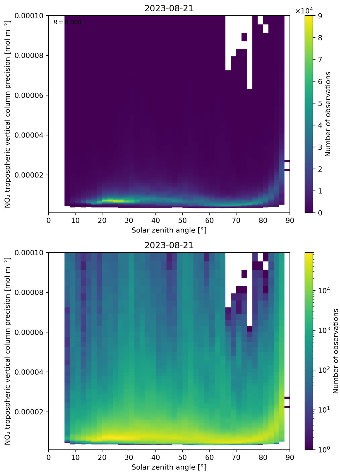
Figure 156: Scatter density plot of “Solar zenith angle” against “NO 2 tropospheric vertical column precision” for 2023-08-20 to 2023-08-22.
