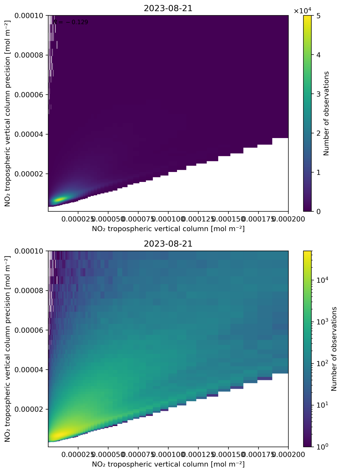
Figure 130: Scatter density plot of “NO 2 tropospheric vertical column” against “NO 2 tropospheric vertical column precision” for 2023-08-20 to 2023-08-22.
