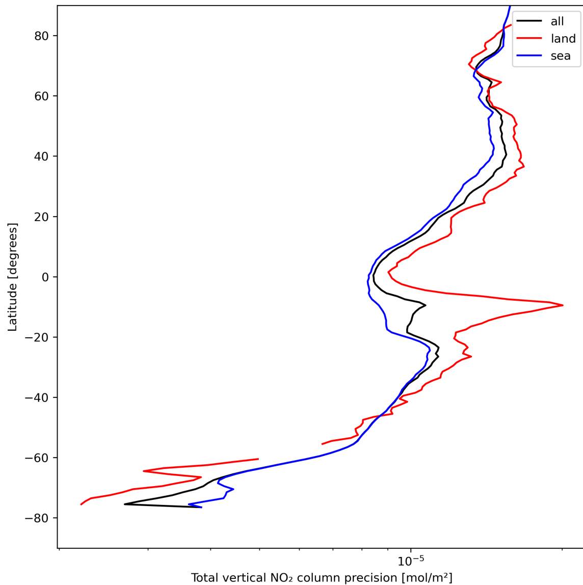
Figure 22: Zonal average of “Total vertical NO 2 column precision” for 2023-08-20 to 2023-08-22.
