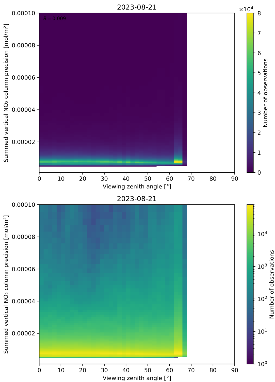
Figure 166: Scatter density plot of “Viewing zenith angle” against “Summed vertical NO 2 column precision” for 2023-08-20 to 2023-08-22.
