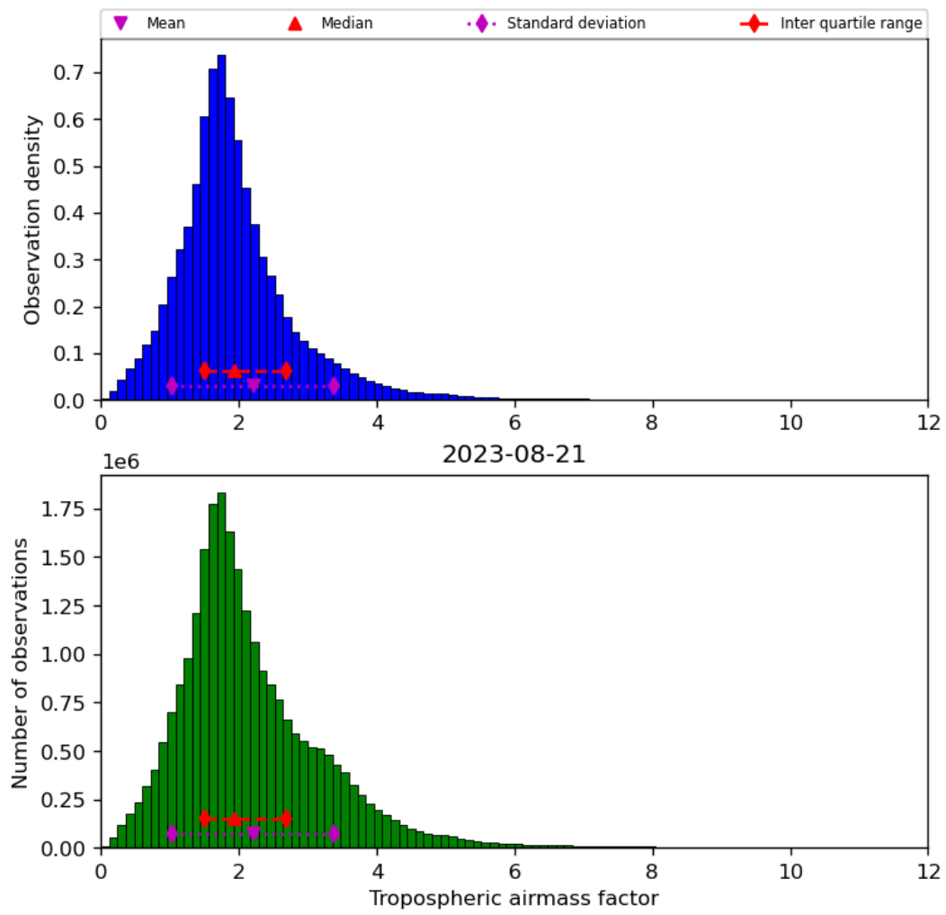
Figure 31: Histogram of “Tropospheric airmass factor” for 2023-08-20 to 2023-08-22
