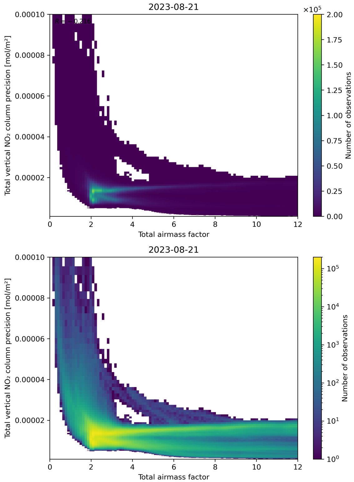
Figure 68: Scatter density plot of “Total airmass factor” against “Total vertical NO 2 column precision” for 2023-08-20 to 2023-08-22.
