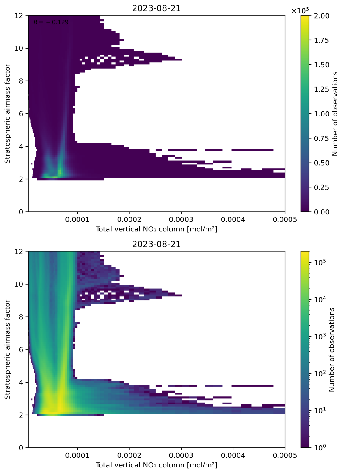
Figure 110: Scatter density plot of “Total vertical NO 2 column” against “Stratospheric airmass factor” for 2023-08-20 to 2023-08-22.
