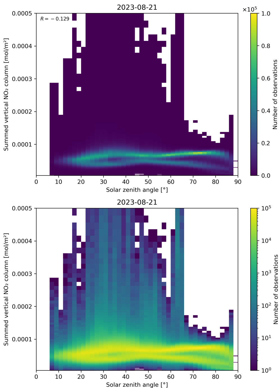
Figure 151: Scatter density plot of “Solar zenith angle” against “Summed vertical NO 2 column” for 2023-08-20 to 2023-08-22.
