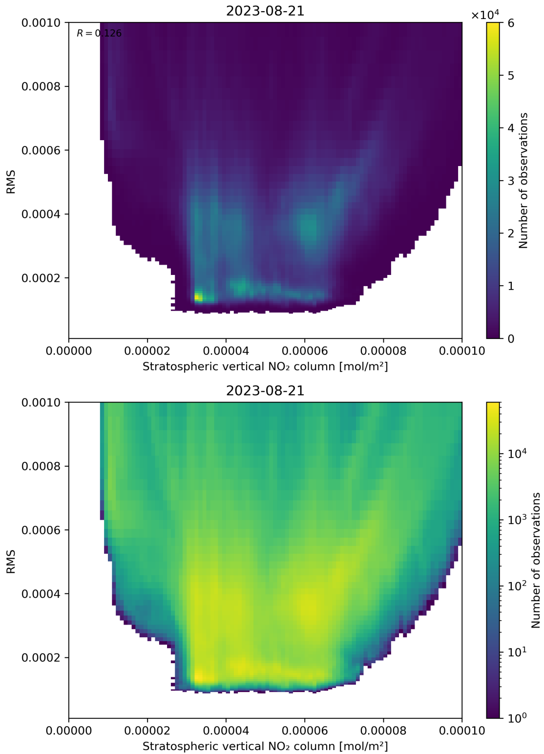
Figure 102: Scatter density plot of “Stratospheric vertical NO 2 column” against “RMS” for 2023-08-20 to 2023-08-22.
