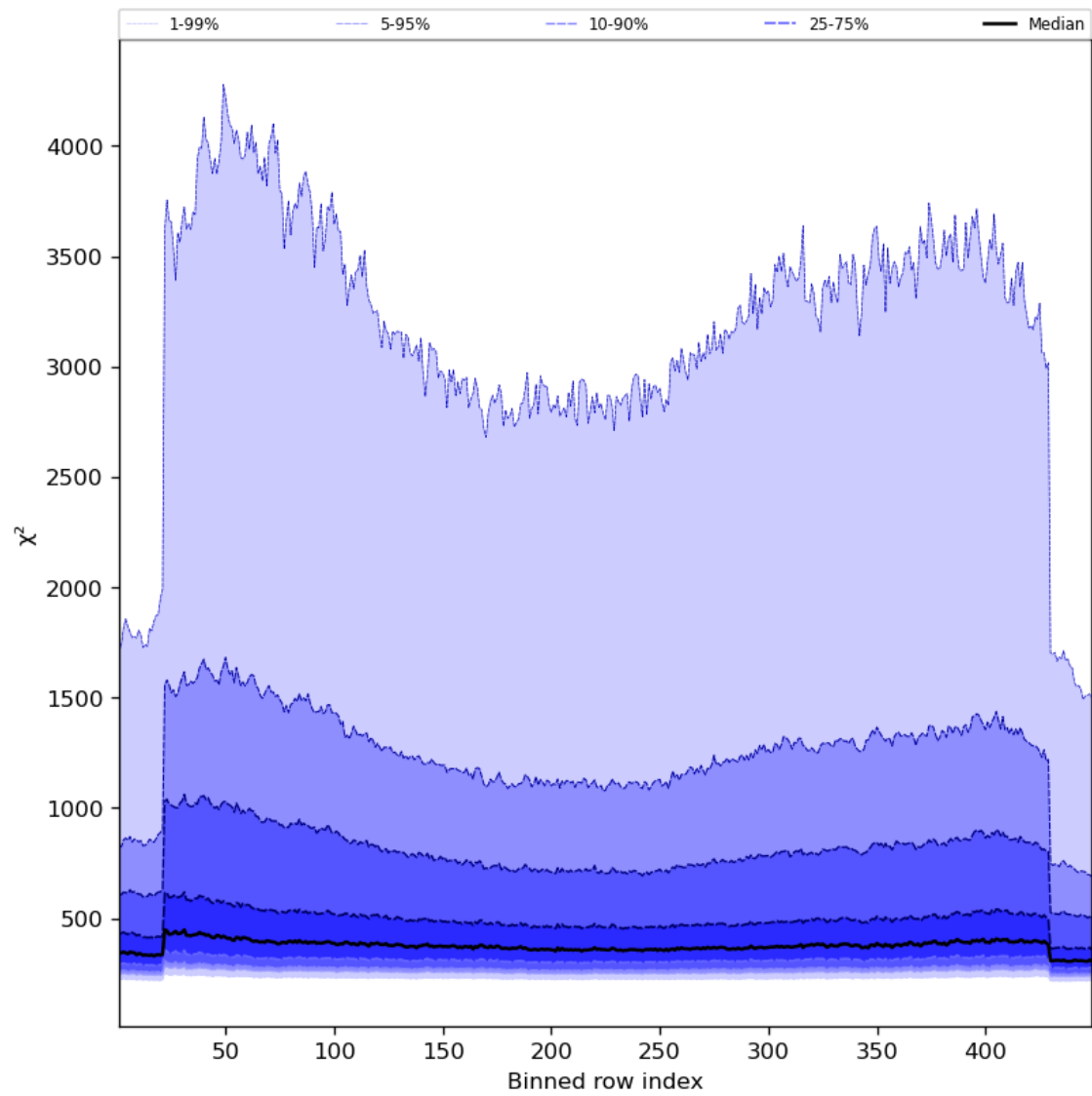
Figure 59: Along track statistics of “ \chi^2 ” for 2023-08-20 to 2023-08-22
