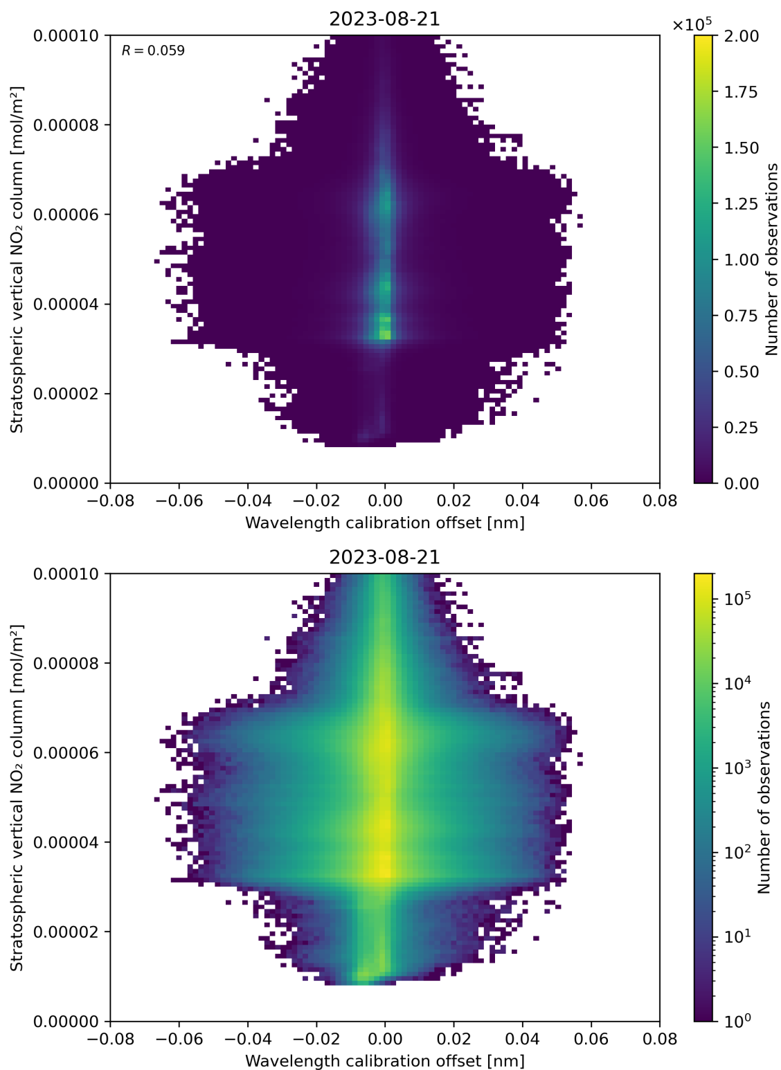
Figure 176: Scatter density plot of “Wavelength calibration offset” against “Stratospheric vertical NO 2 column” for 2023-08-20 to 2023-08-22.
