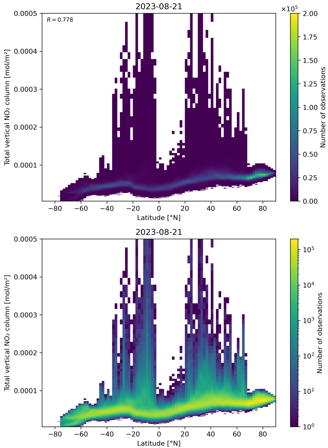
Figure 90: Scatter density plot of “Latitude” against “Total vertical NO 2 column” for 2023-08-20 to 2023-08-22.
