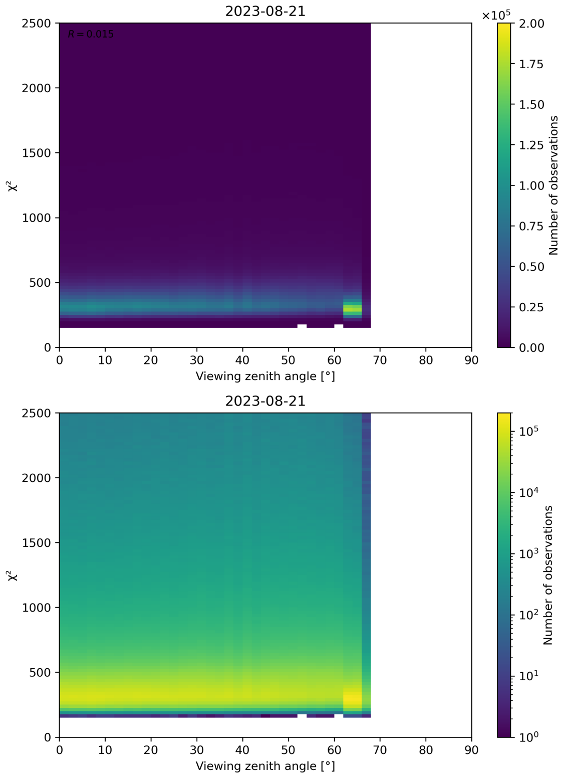
Figure 162: Scatter density plot of “Viewing zenith angle” against “ \chi^2 ” for 2023-08-20 to 2023-08-22.
