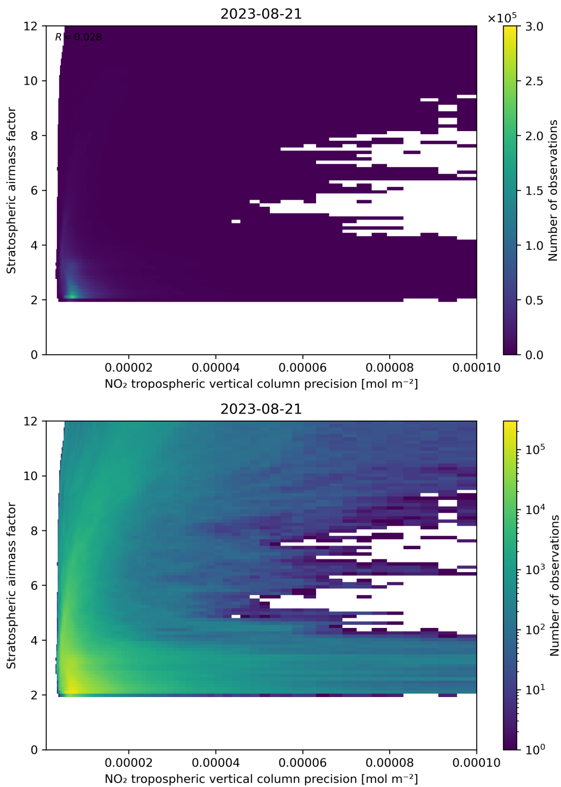
Figure 131: Scatter density plot of “NO 2 tropospheric vertical column precision” against “Stratospheric airmass factor” for 2023-08-20 to 2023-08-22.
