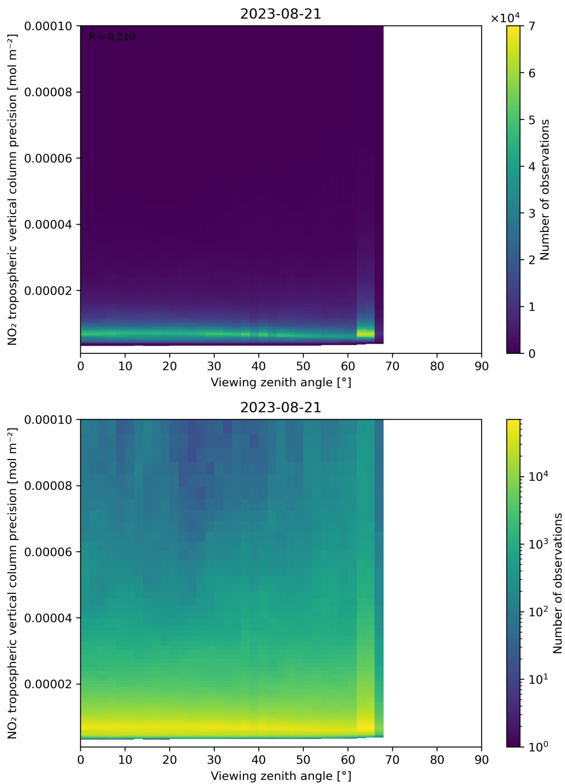
Figure 170: Scatter density plot of “Viewing zenith angle” against “NO 2 tropospheric vertical column precision” for 2023-08-20 to 2023-08-22.
