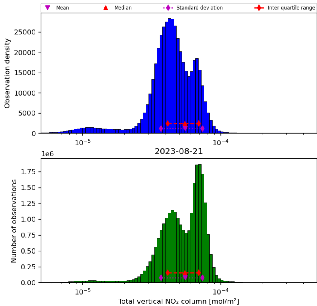
Figure 38: Histogram of “Total vertical NO 2 column” for 2023-08-20 to 2023-08-22
