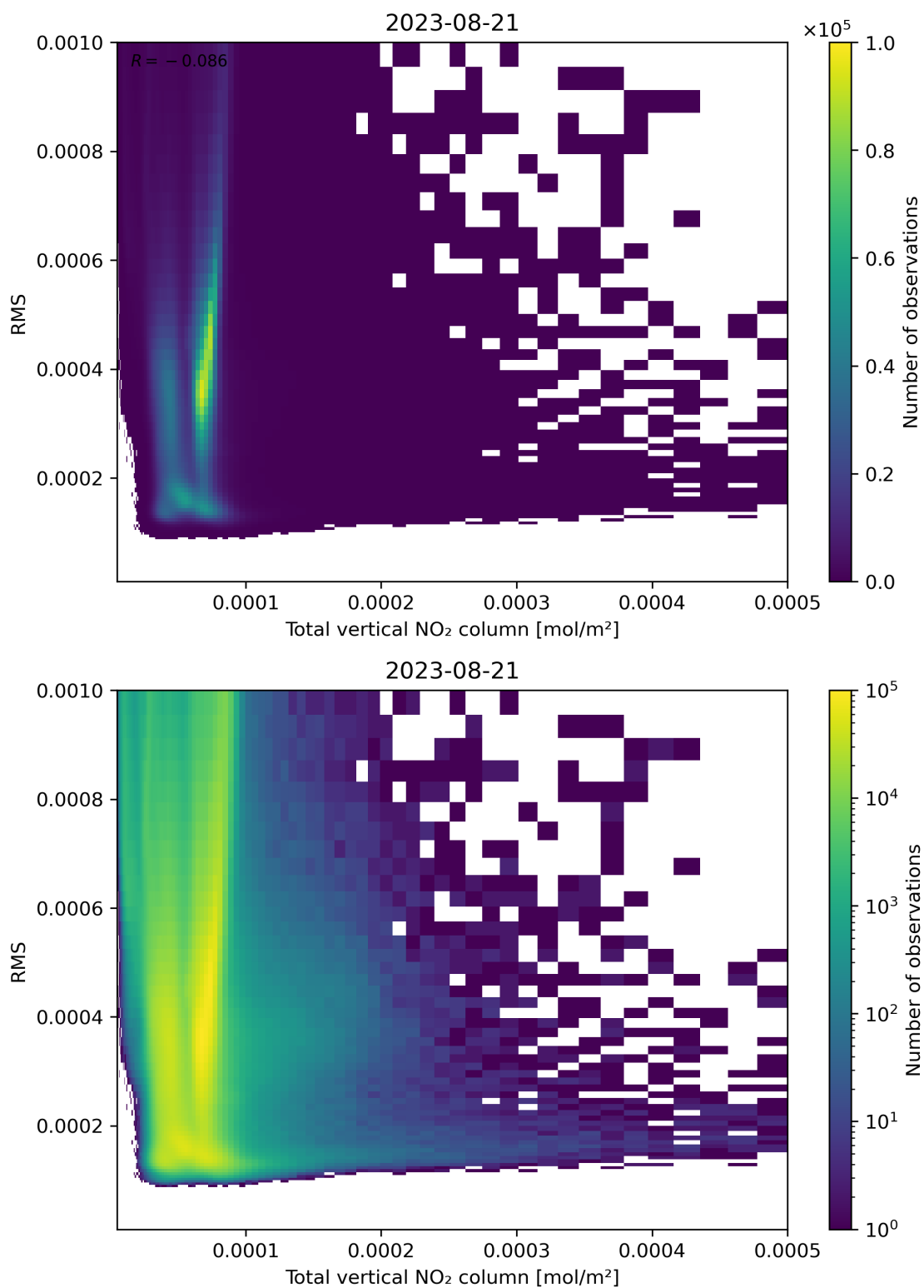
Figure 120: Scatter density plot of “Total vertical NO 2 column” against “RMS” for 2023-08-20 to 2023-08-22.
