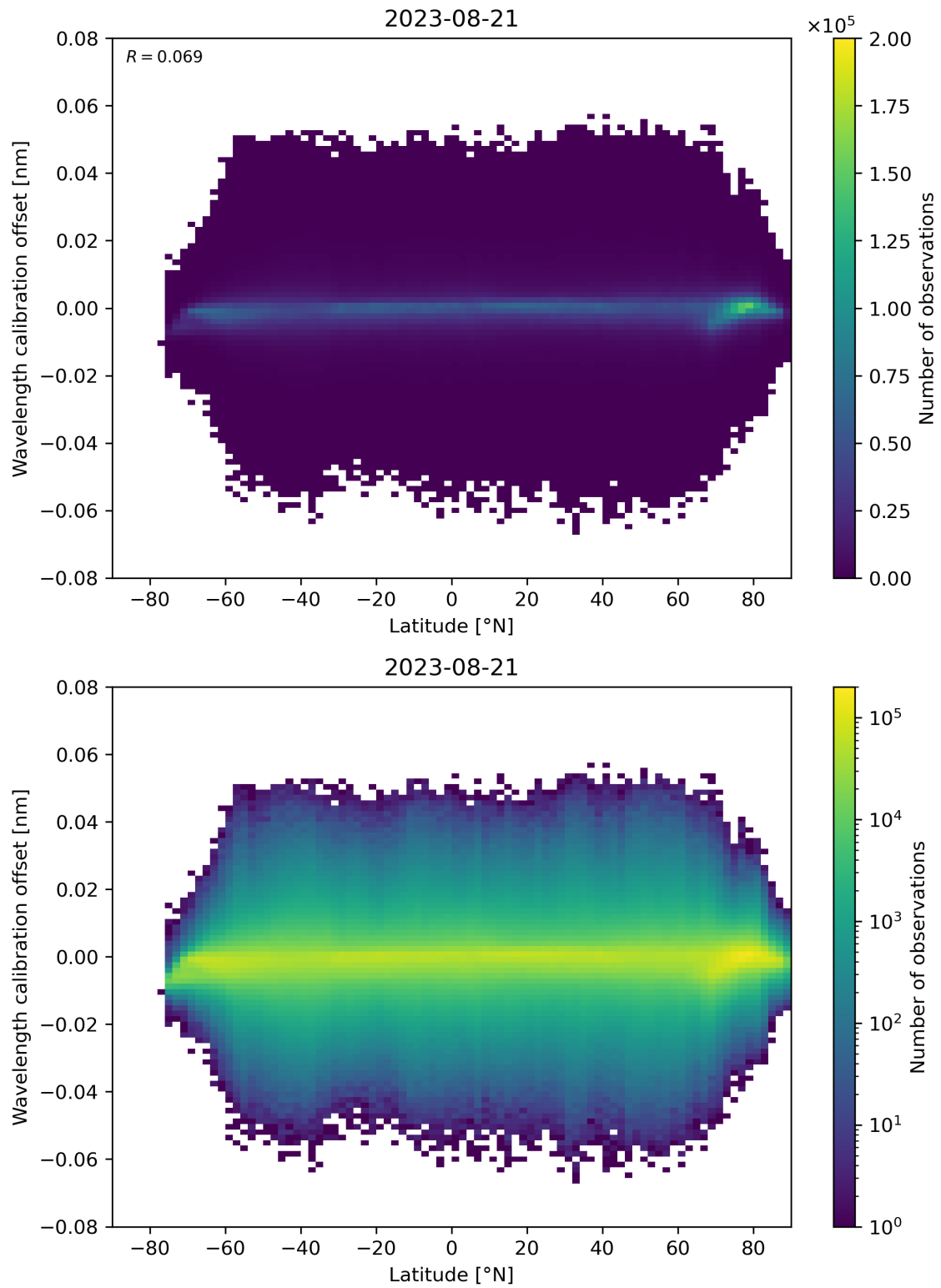
Figure 95: Scatter density plot of “Latitude” against “Wavelength calibration offset” for 2023-08-20 to 2023-08-22.
