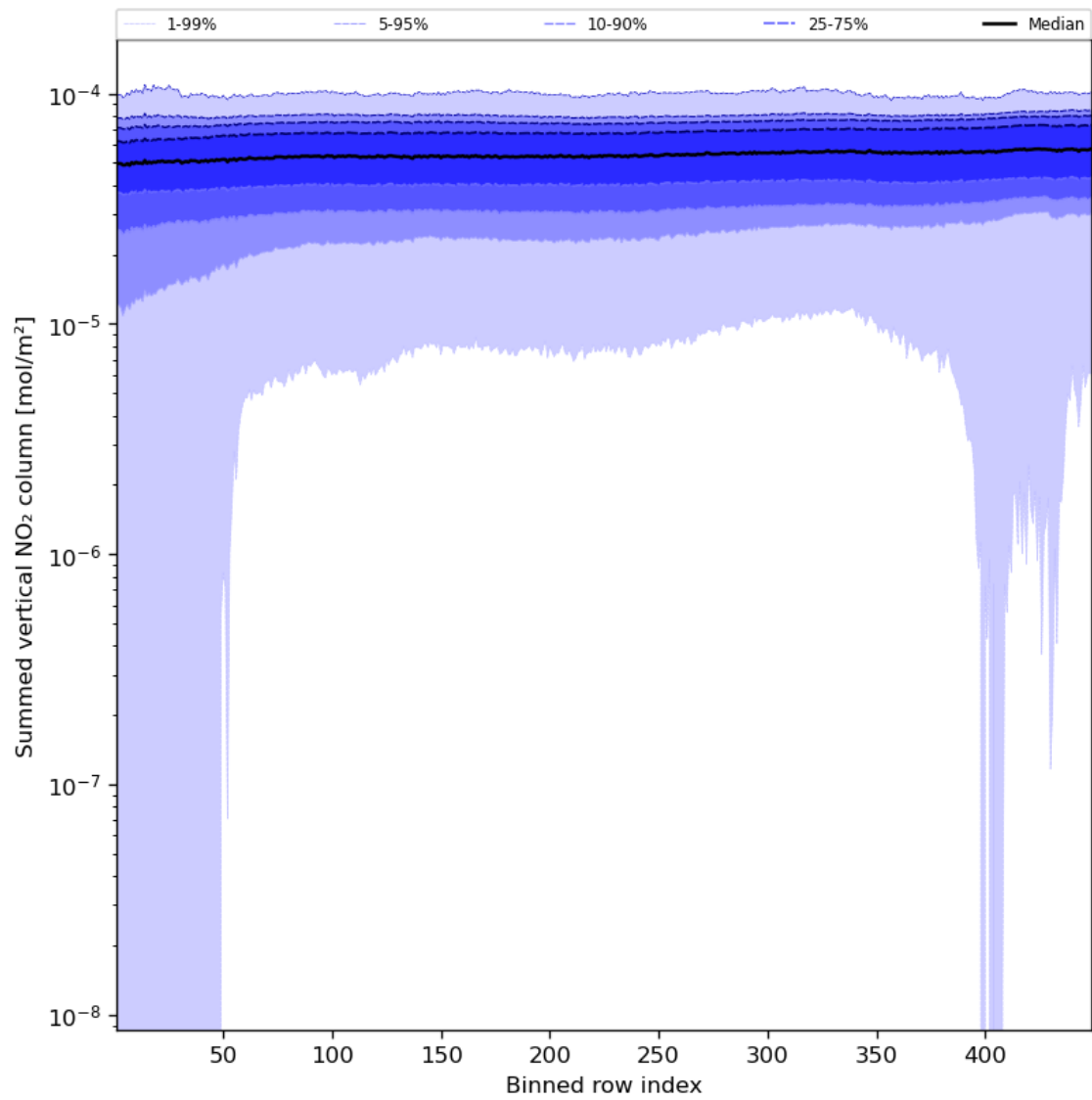
Figure 57: Along track statistics of “Summed vertical NO 2 column” for 2023-08-20 to 2023-08-22
