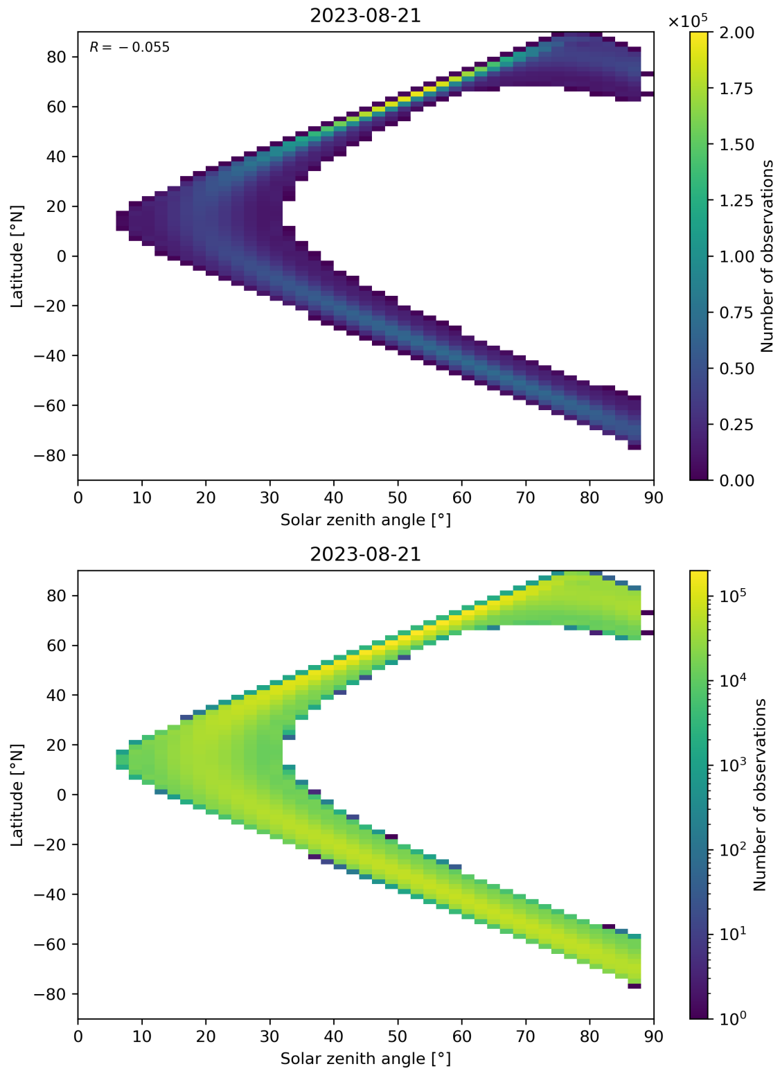
Figure 149: Scatter density plot of “Solar zenith angle” against “Latitude” for 2023-08-20 to 2023-08-22.
