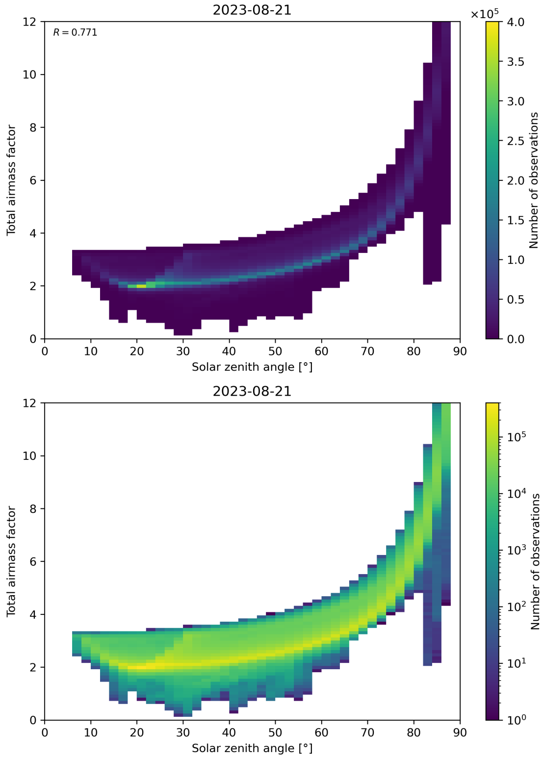
Figure 146: Scatter density plot of “Solar zenith angle” against “Total air mass factor” for 2023-08-20 to 2023-08-22.
