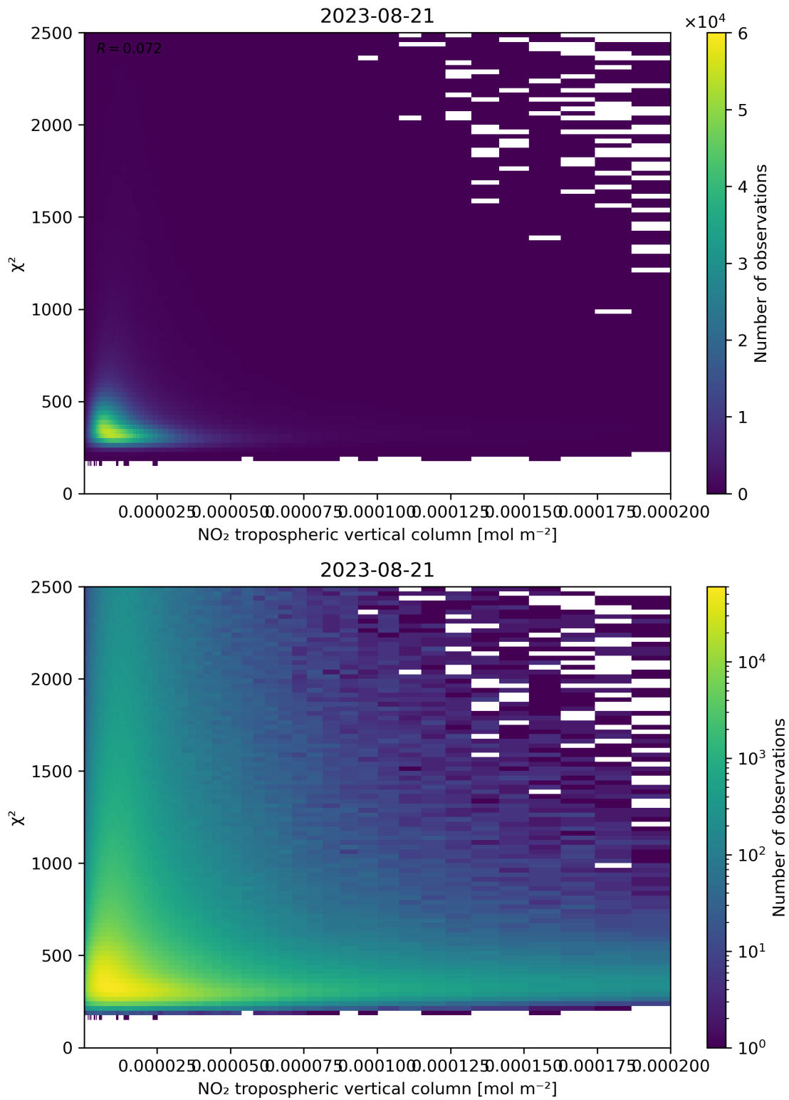
Figure 124: Scatter density plot of “NO 2 tropospheric vertical column” against “ \chi^2 ” for 2023-08-20 to 2023-08-22.
