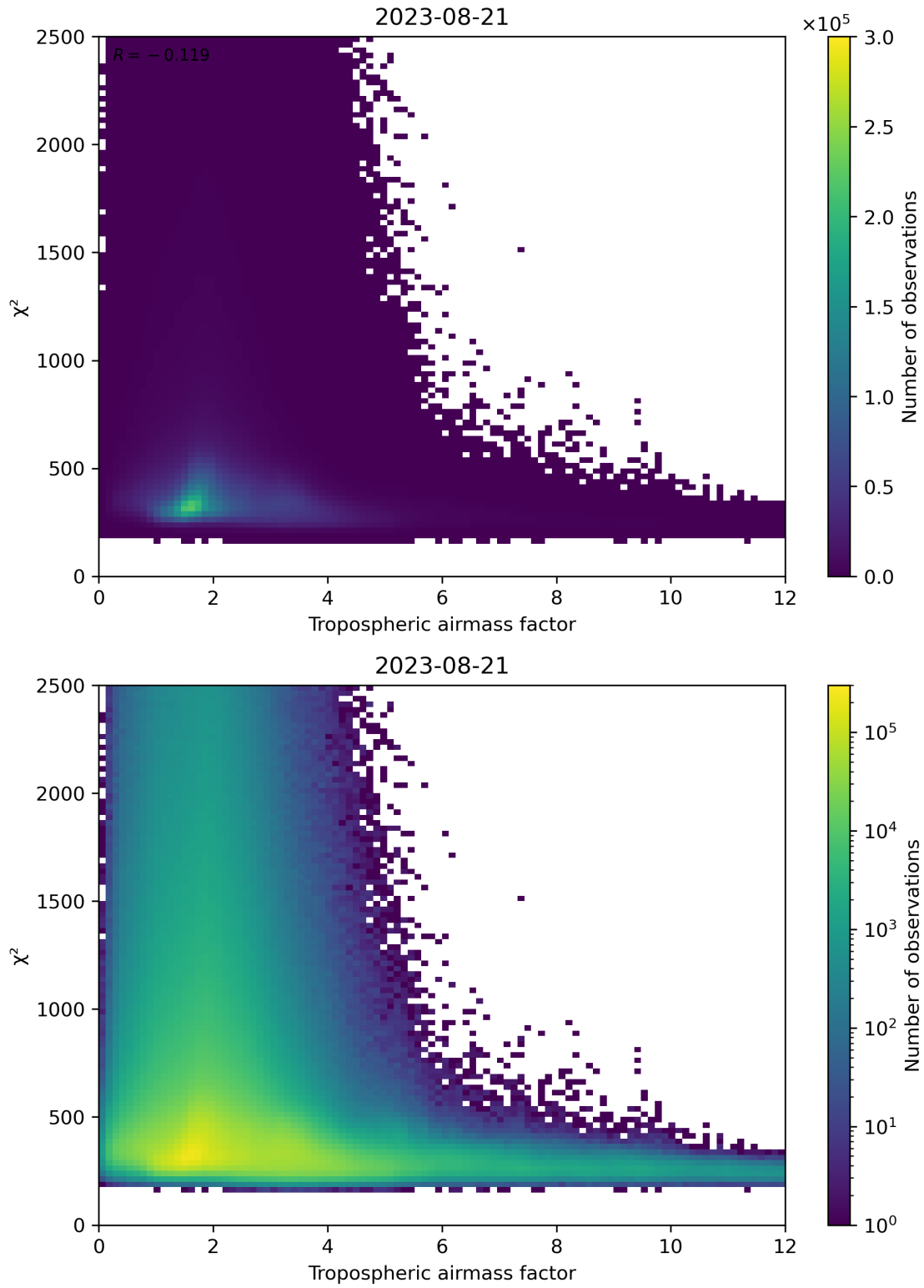
Figure 73: Scatter density plot of “Tropospheric airmass factor” against “ \chi^2 ” for 2023-08-20 to 2023-08-22.
