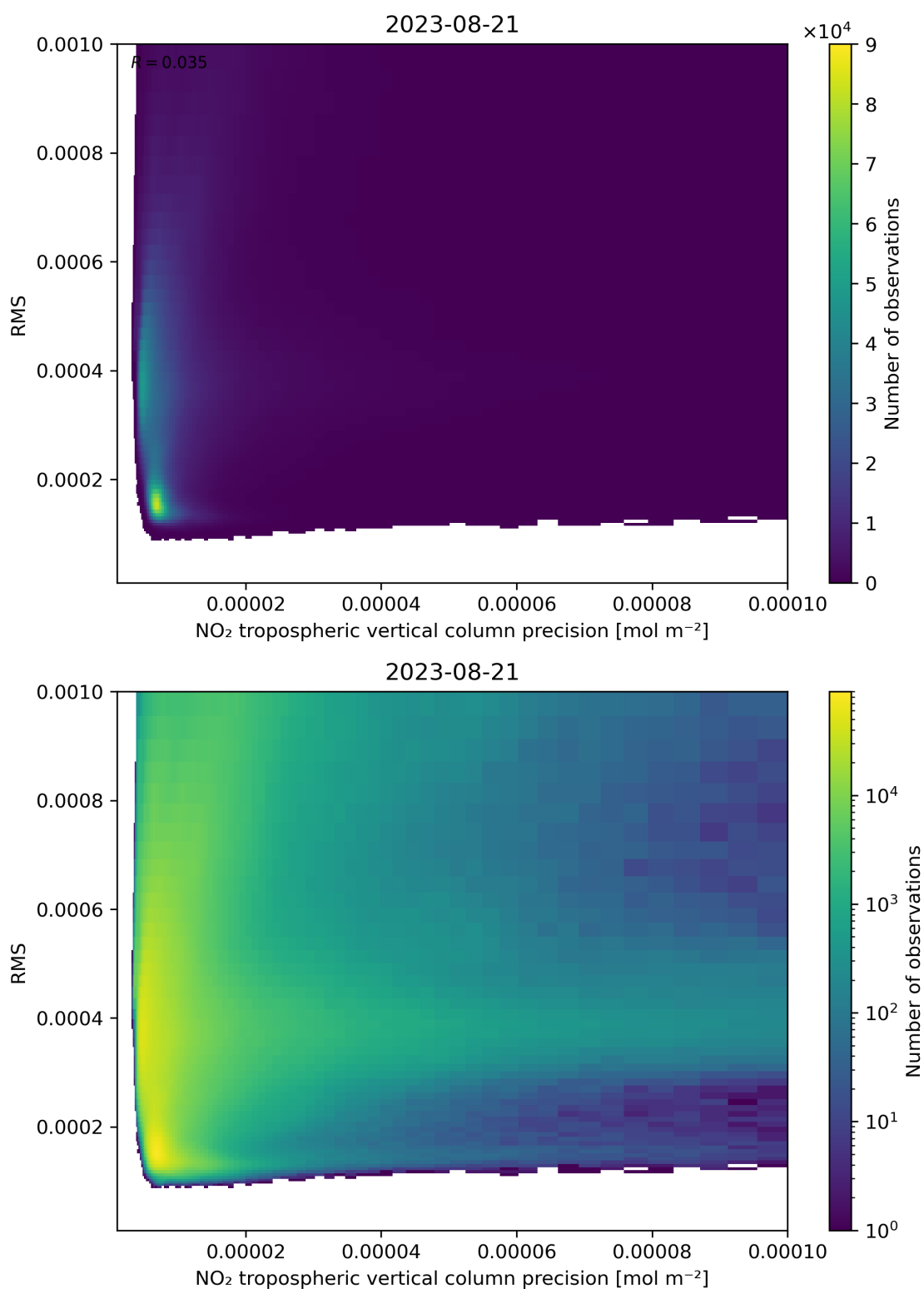
Figure 140: Scatter density plot of “NO 2 tropospheric vertical column precision” against “RMS” for 2023-08-20 to 2023-08-22.
