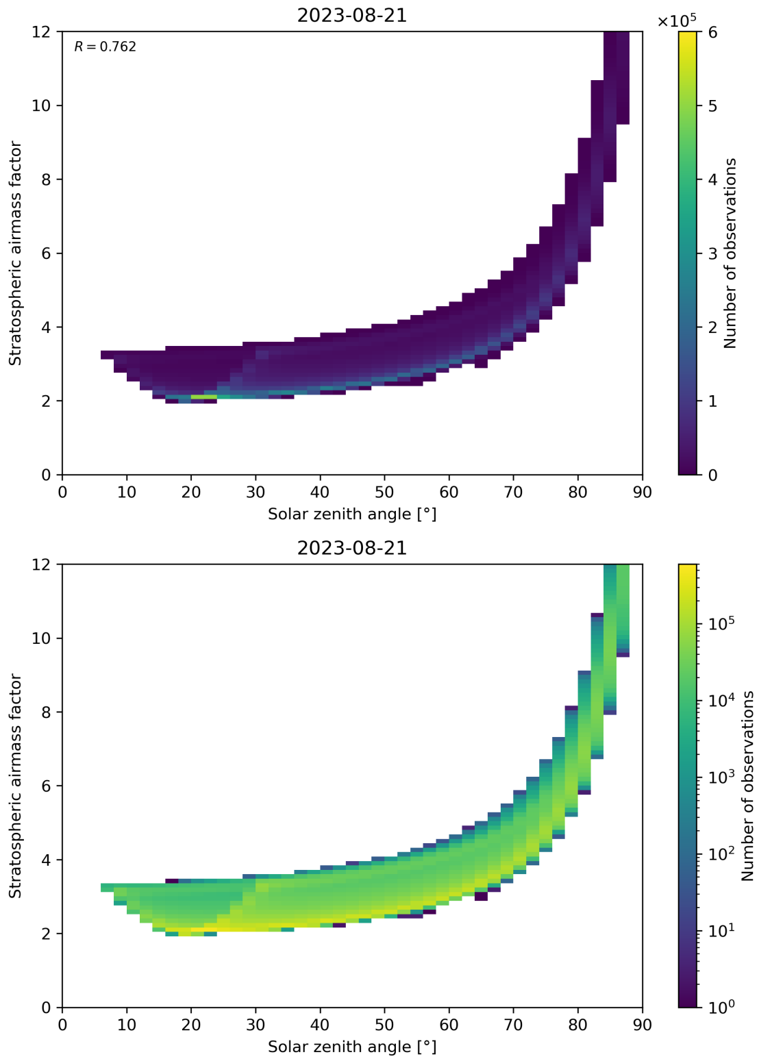
Figure 145: Scatter density plot of “Solar zenith angle” against “Stratospheric airmass factor” for 2023-08-20 to 2023-08-22.
