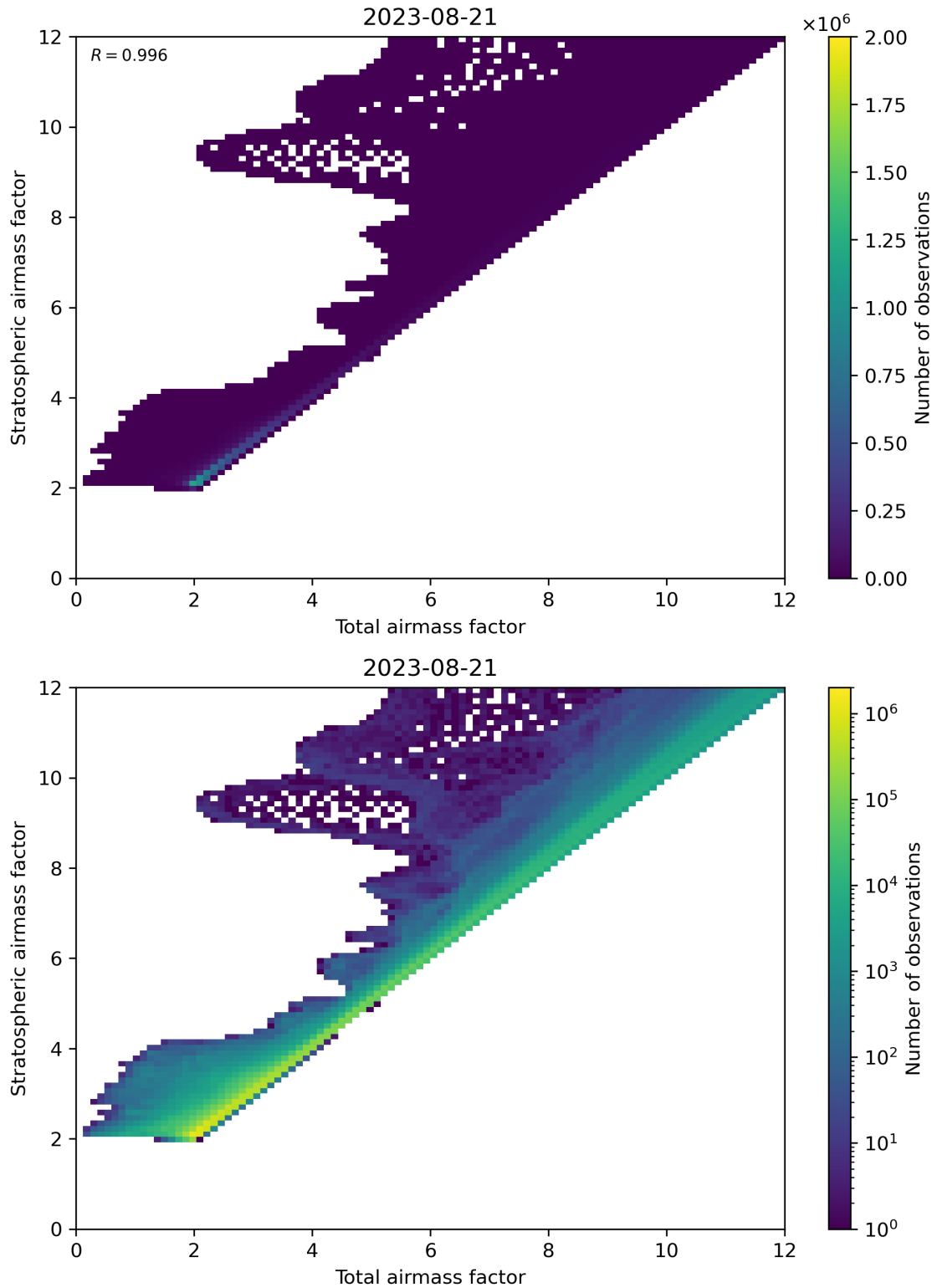
Figure 62: Scatter density plot of “Total airmass factor” against “Stratospheric airmass factor” for 2023-08-20 to 2023-08-22.
