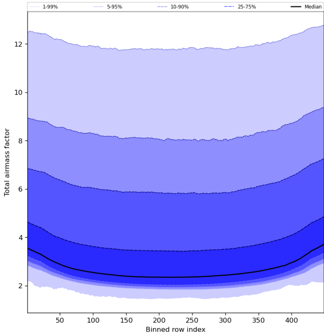
Figure 49: Along track statistics of “Total airmass factor” for 2023-08-20 to 2023-08-22
