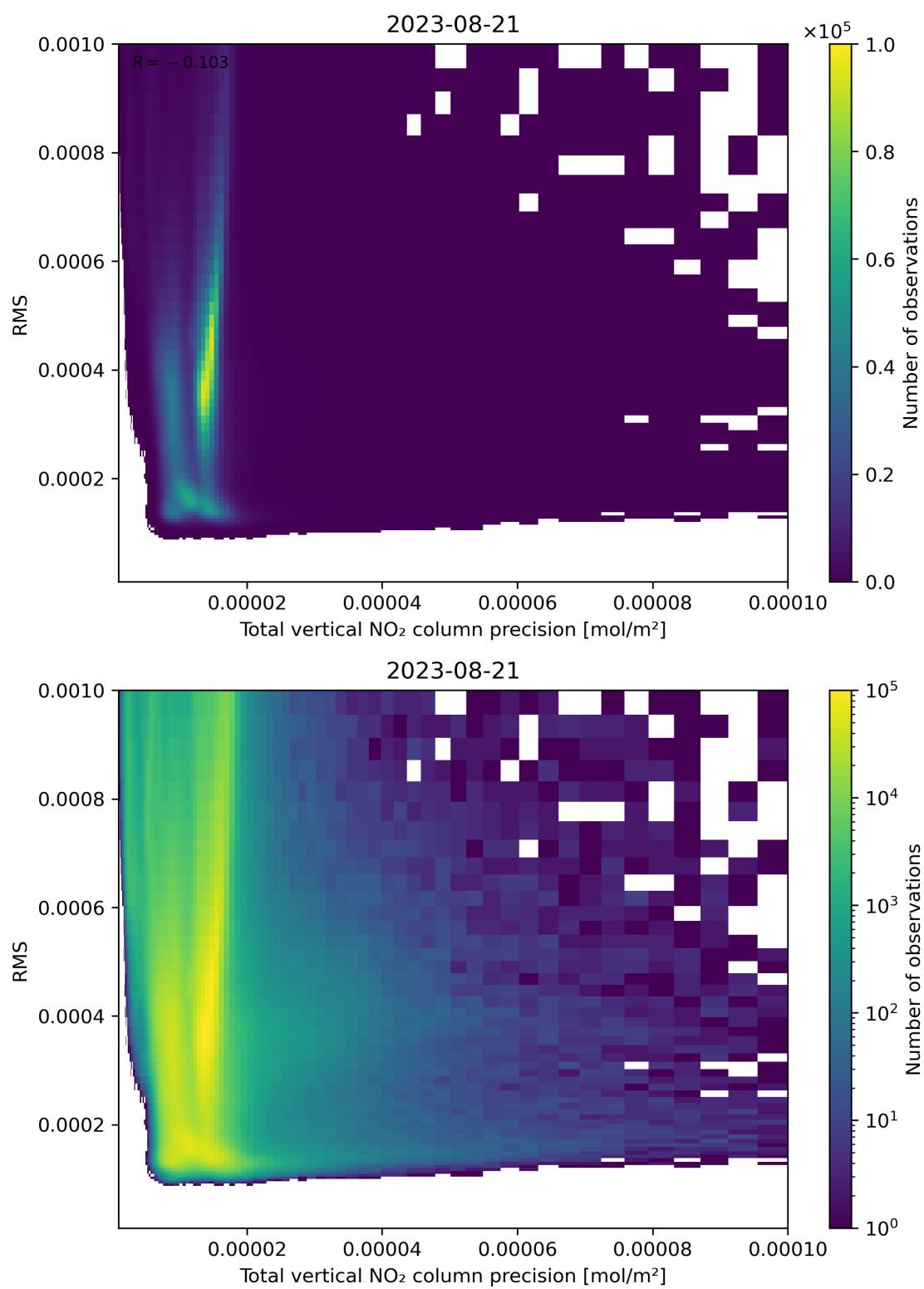
Figure 119: Scatter density plot of “Total vertical NO 2 column precision” against “RMS” for 2023-08-20 to 2023-08-22.
