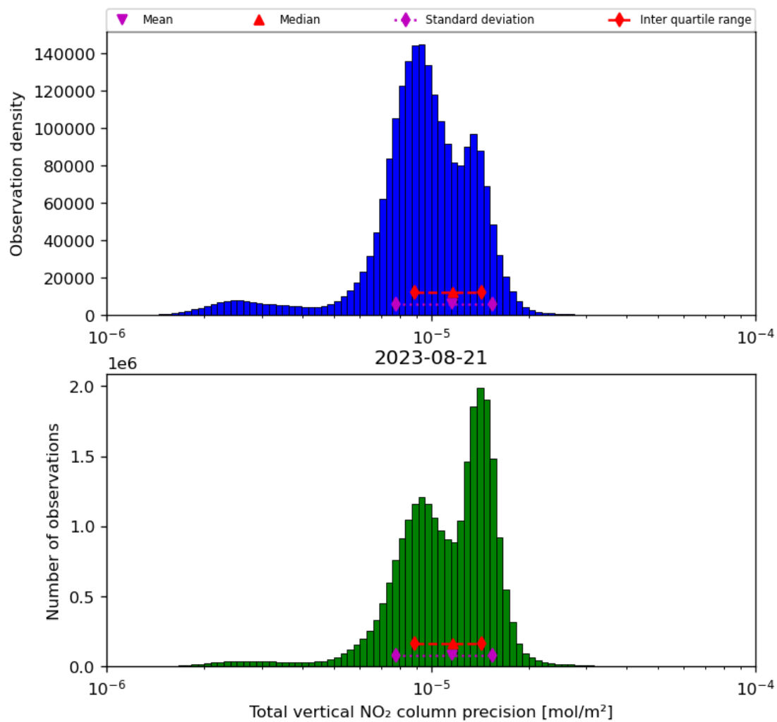
Figure 39: Histogram of “Total vertical NO 2 column precision” for 2023-08-20 to 2023-08-22
