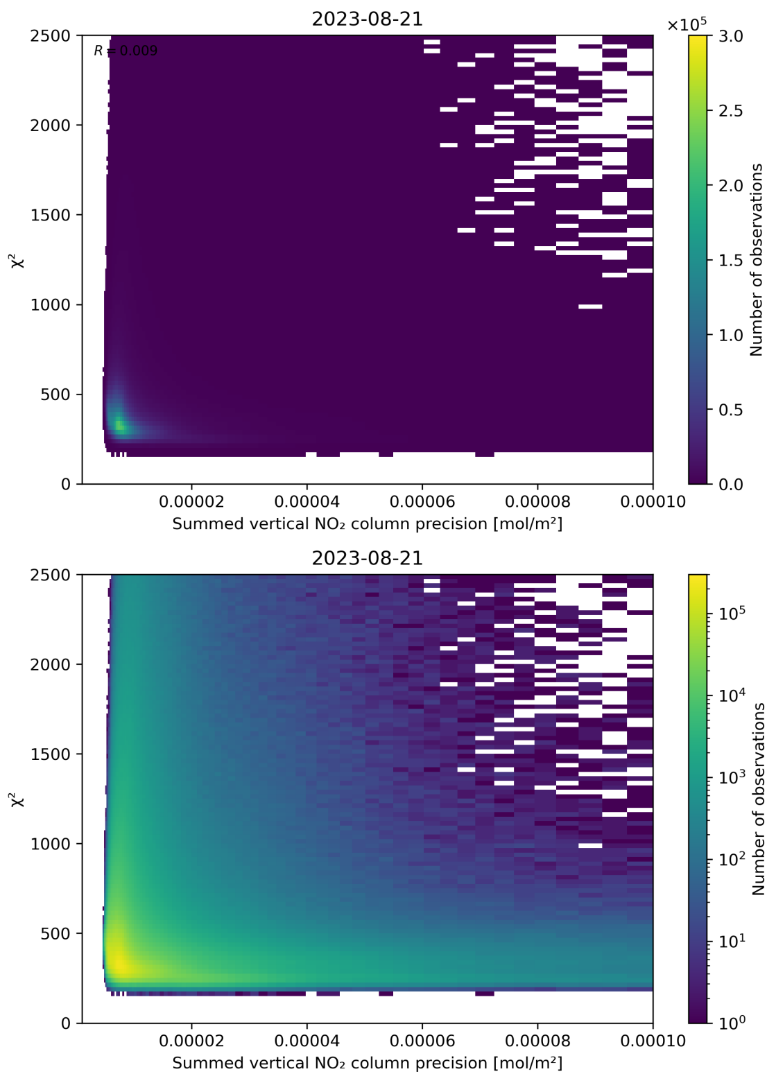
Figure 107: Scatter density plot of “Summed vertical NO 2 column precision” against “ \chi^2 ” for 2023-08-20 to 2023-08-22.
