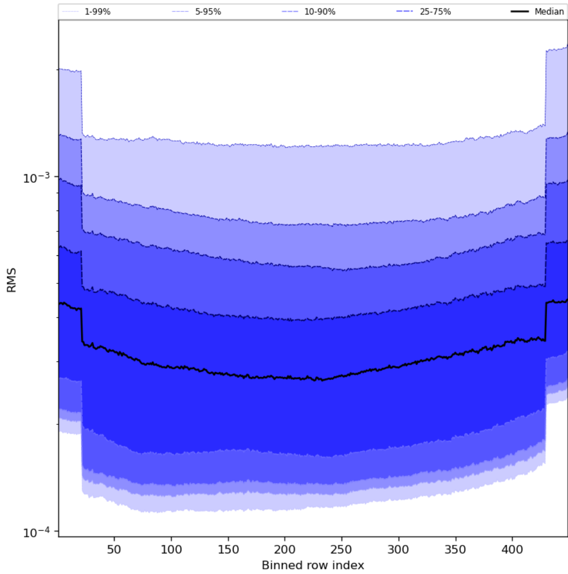
Figure 60: Along track statistics of “RMS” for 2023-08-20 to 2023-08-22
