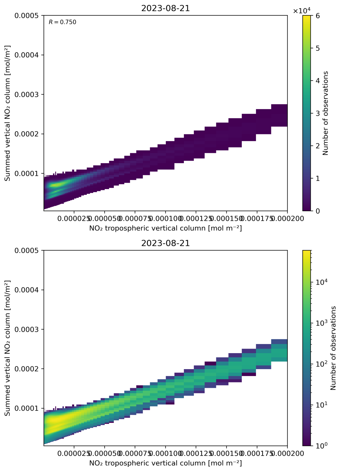
Figure 126: Scatter density plot of “NO 2 tropospheric vertical column” against “Summed vertical NO 2 column” for 2023-08-20 to 2023-08-22.
