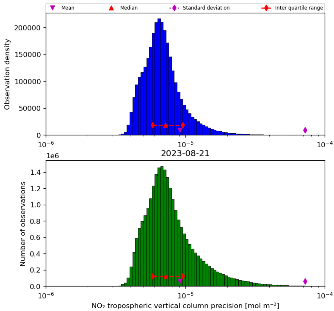
Figure 30: Histogram of “NO 2 tropospheric vertical column precision” for 2023-08-20 to 2023-08-22
