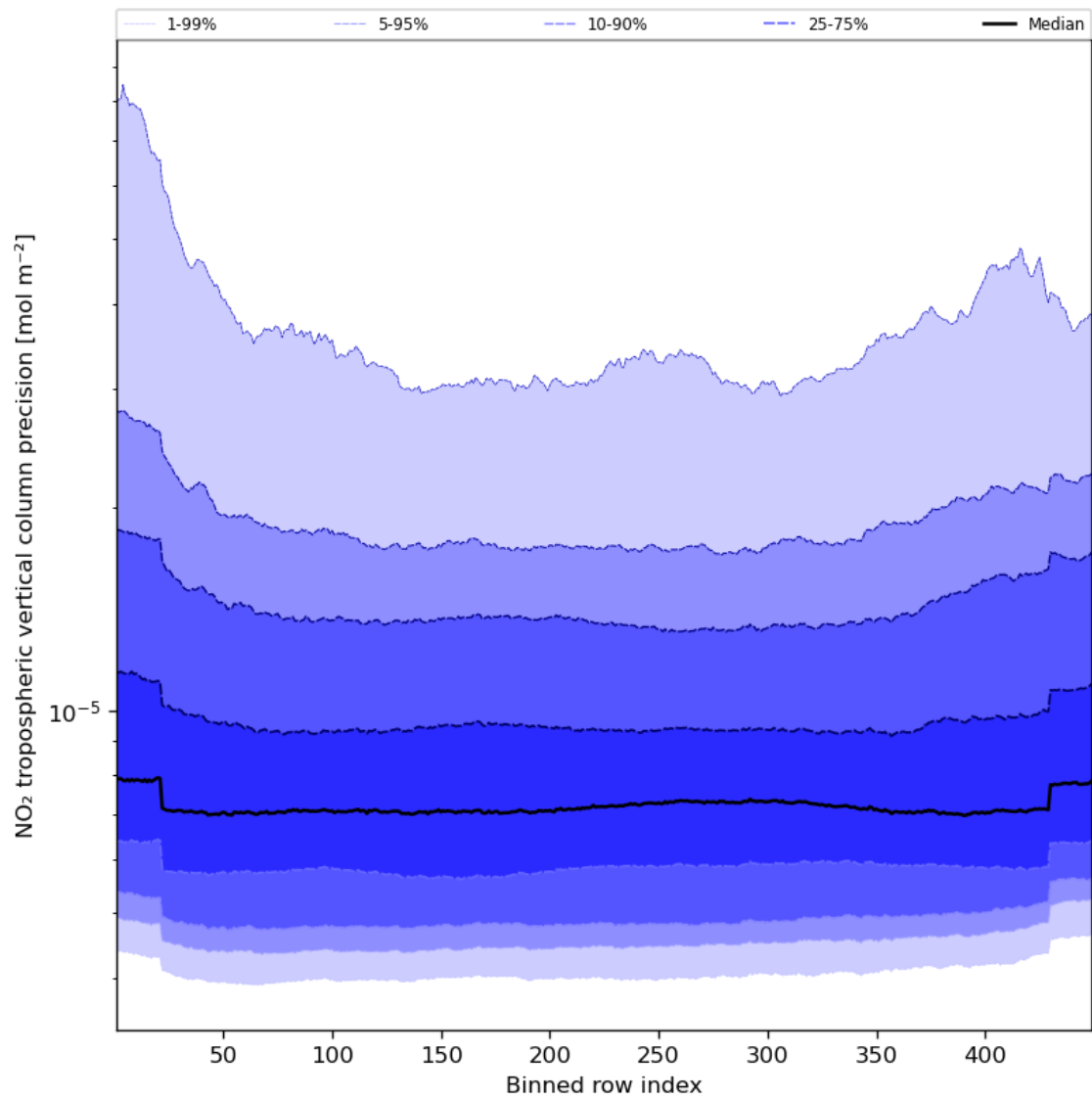
Figure 47: Along track statistics of “NO 2 tropospheric vertical column precision” for 2023-08-20 to 2023-08-22
