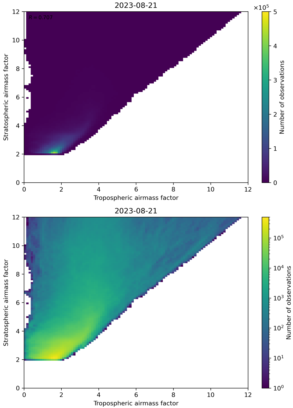
Figure 71: Scatter density plot of “Tropospheric airmass factor” against “Stratospheric airmass factor” for 2023-08-20 to 2023-08-22.
