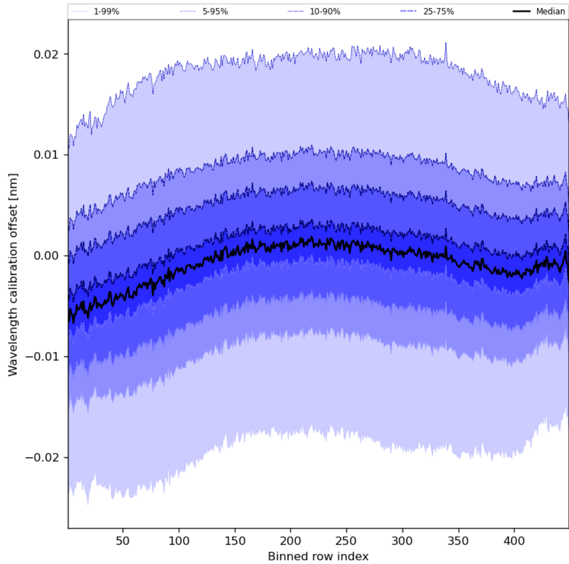
Figure 52: Along track statistics of “Wavelength calibration offset” for 2023-08-20 to 2023-08-22
