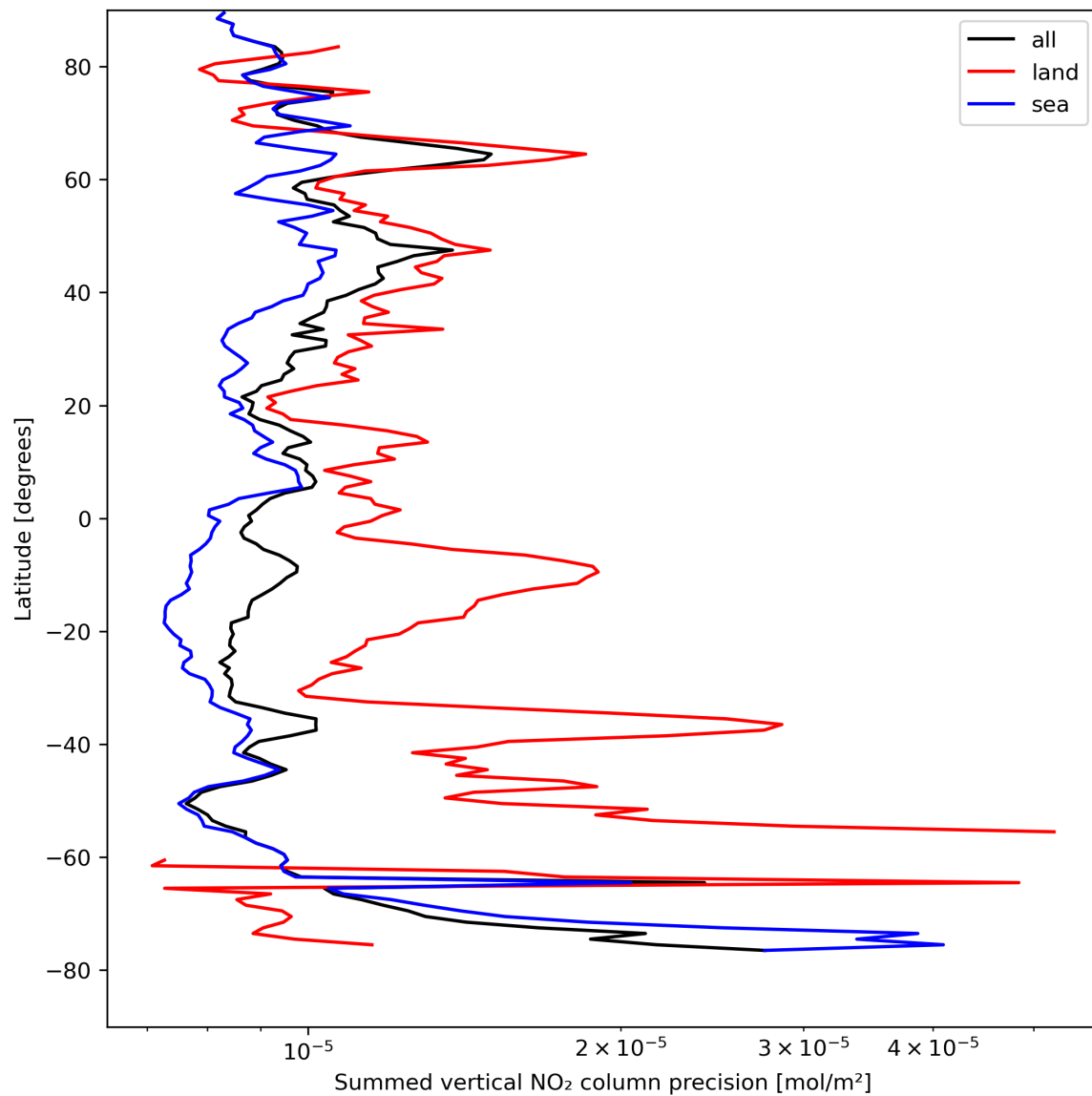
Figure 24: Zonal average of “Summed vertical NO 2 column precision” for 2023-08-20 to 2023-08-22.
