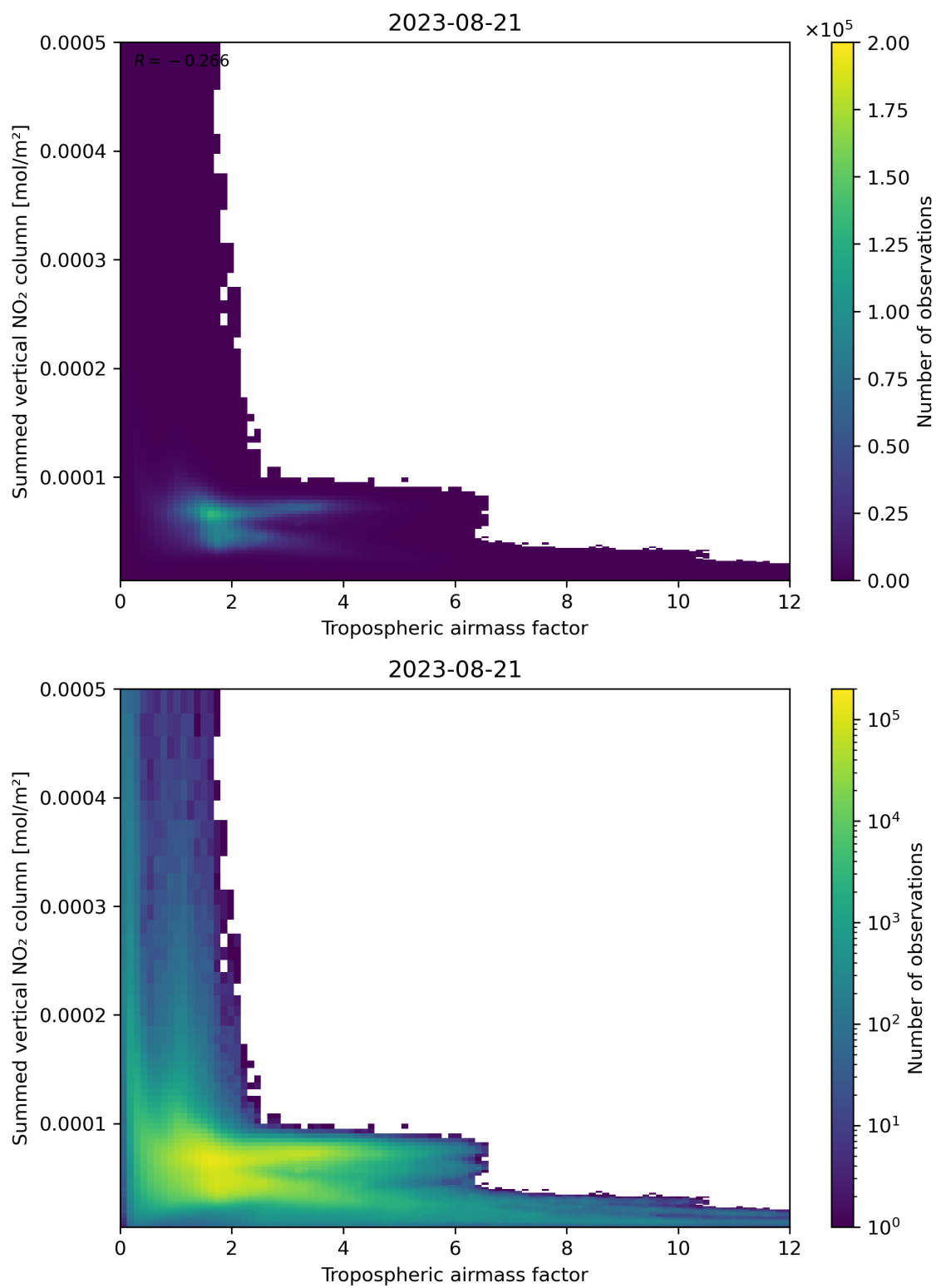
Figure 75: Scatter density plot of “Tropospheric airmass factor” against “Summed vertical NO 2 column” for 2023-08-20 to 2023-08-22.
