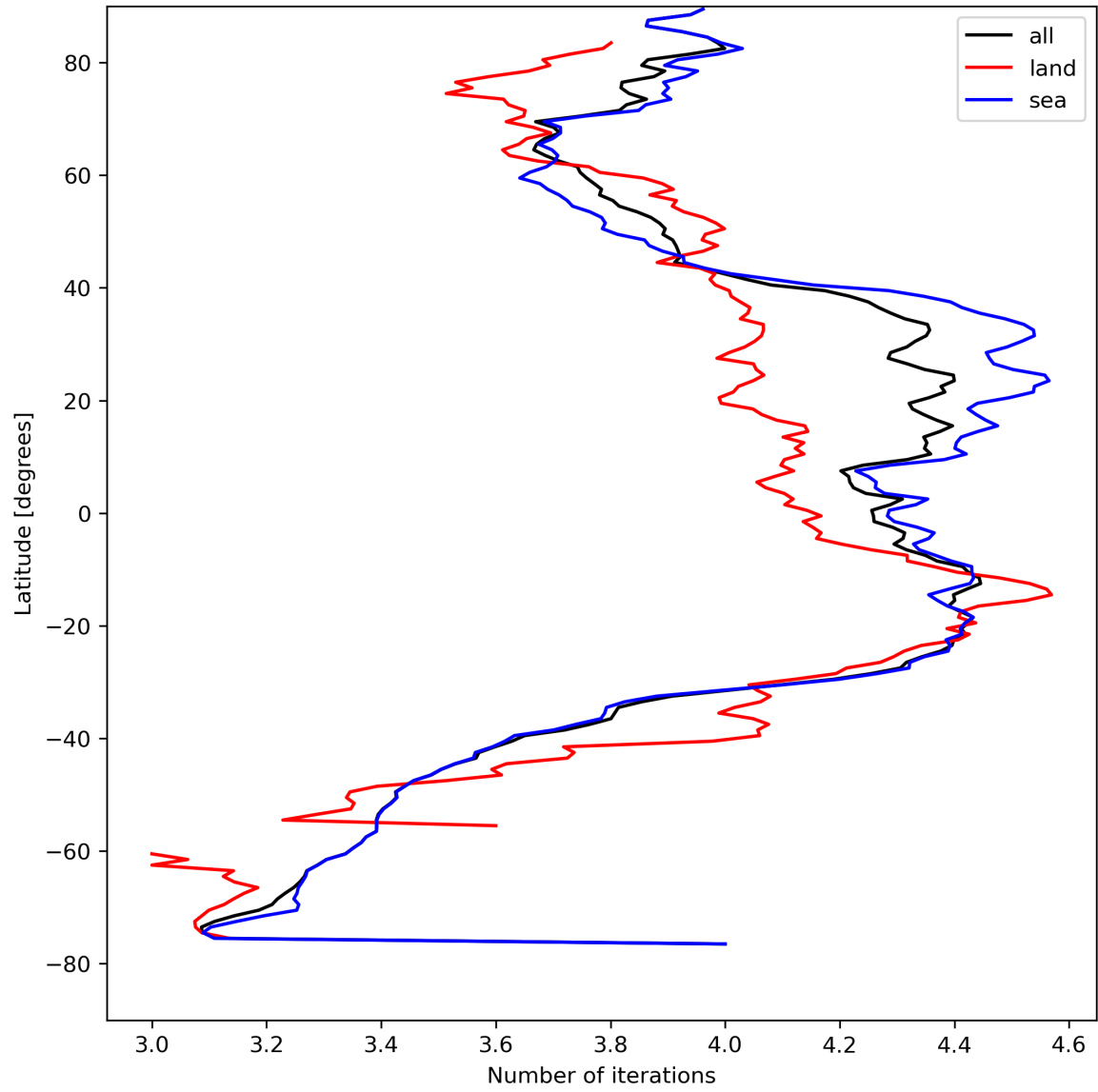
Figure 17: Zonal average of “Number of iterations” for 2023-08-20 to 2023-08-22.
