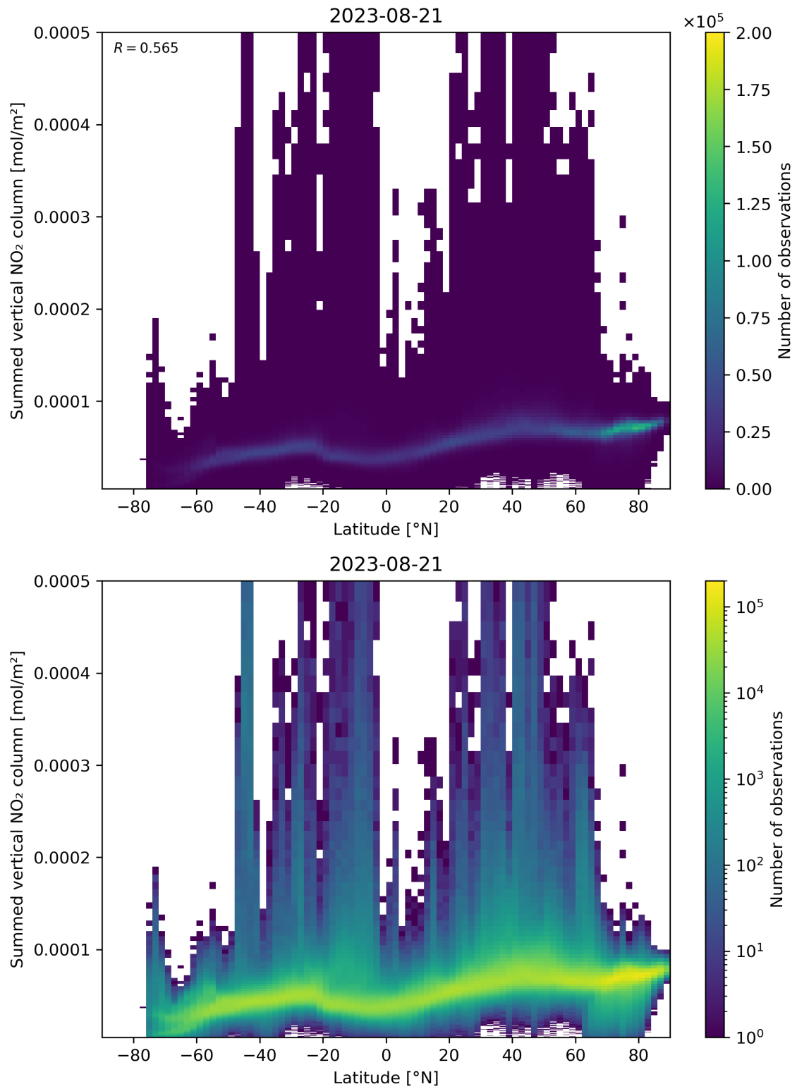
Figure 88: Scatter density plot of “Latitude” against “Summed vertical NO 2 column” for 2023-08-20 to 2023-08-22.
