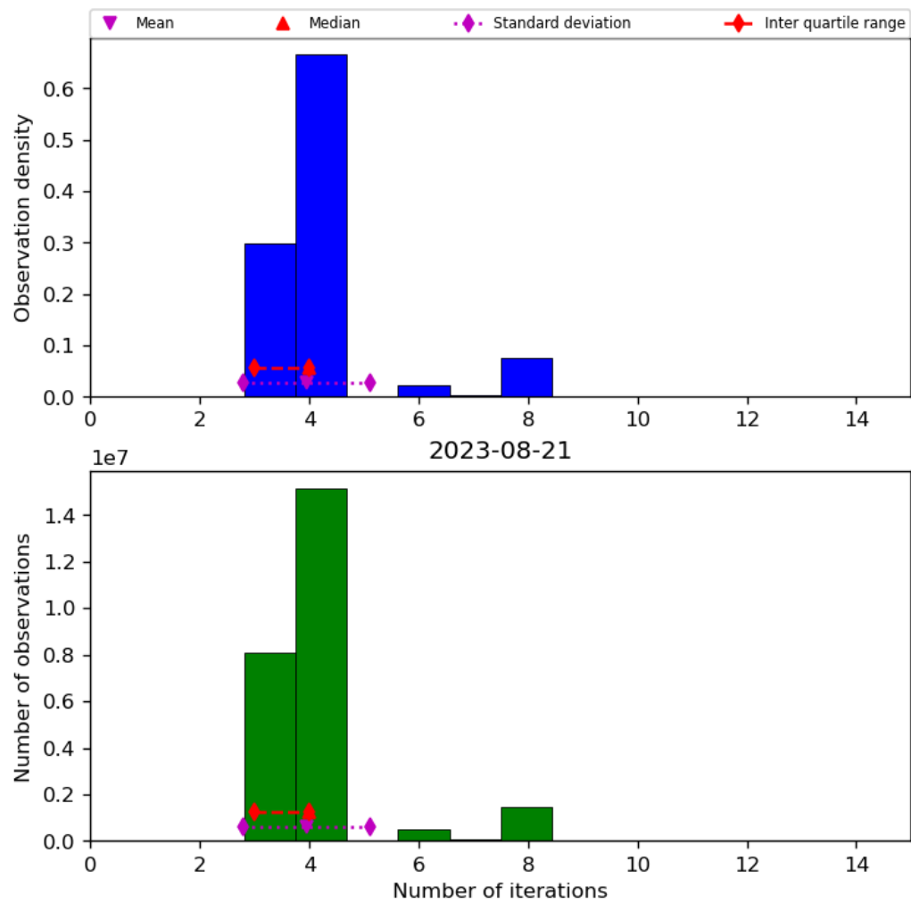
Figure 34: Histogram of “Number of iterations” for 2023-08-20 to 2023-08-22
