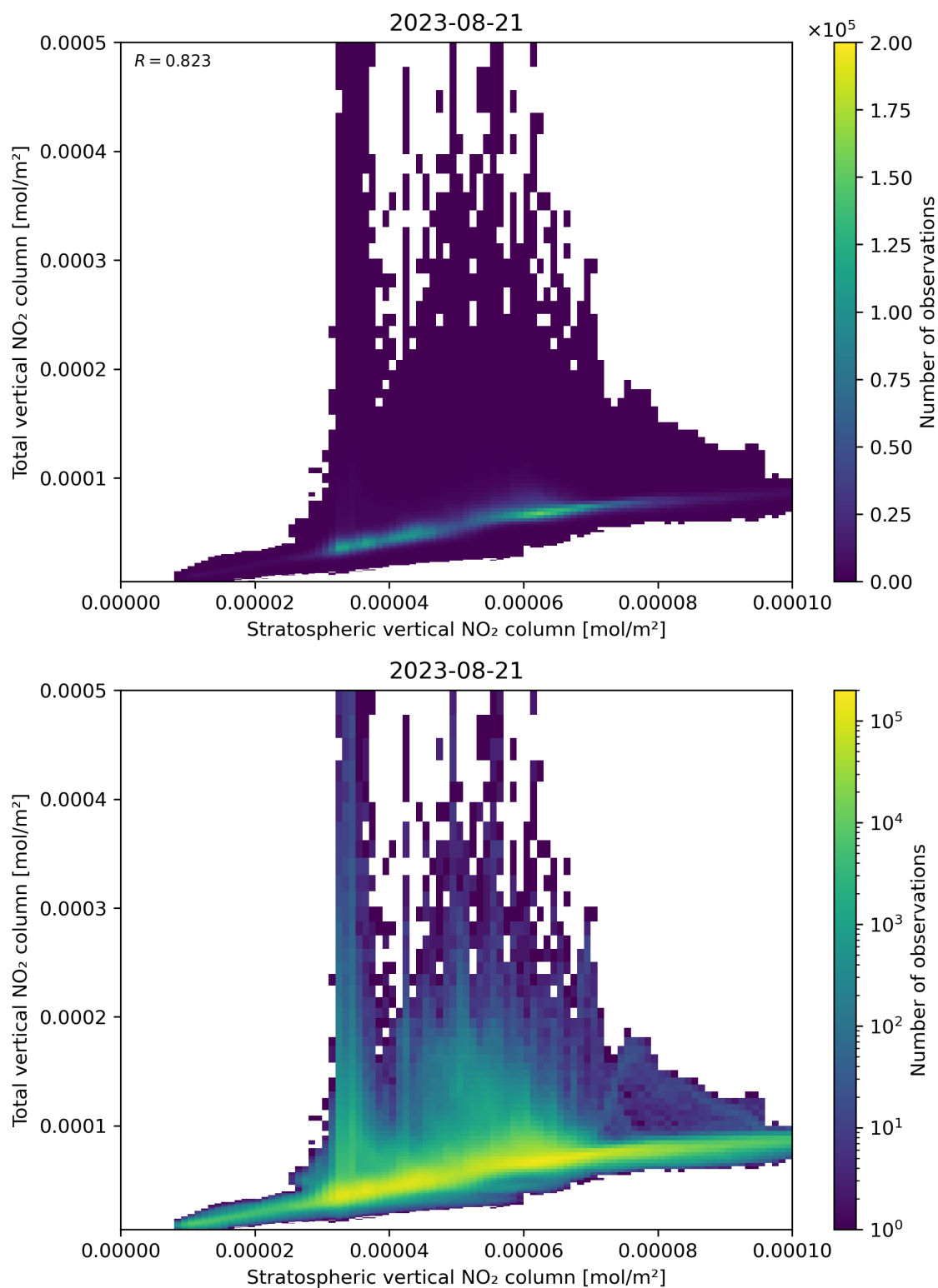
Figure 100: Scatter density plot of “Stratospheric vertical NO 2 column” against “Total vertical NO 2 column” for 2023-08-20 to 2023-08-22.
