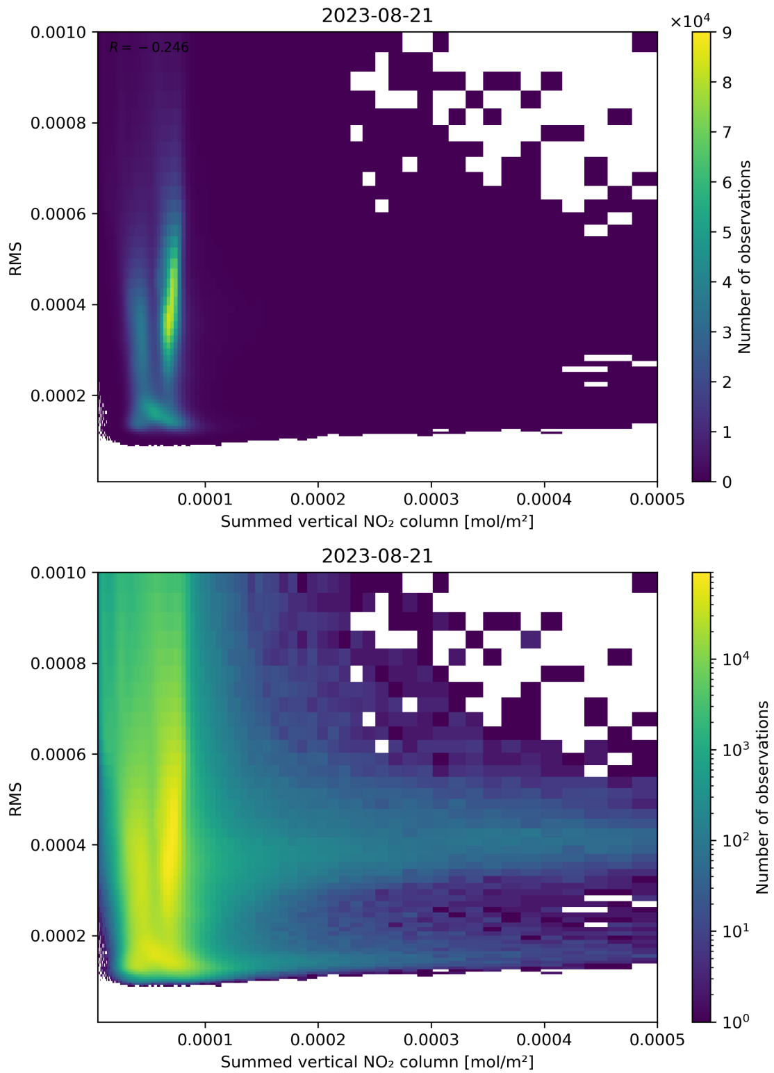
Figure 109: Scatter density plot of “Summed vertical NO 2 column” against “RMS” for 2023-08-20 to 2023-08-22.
