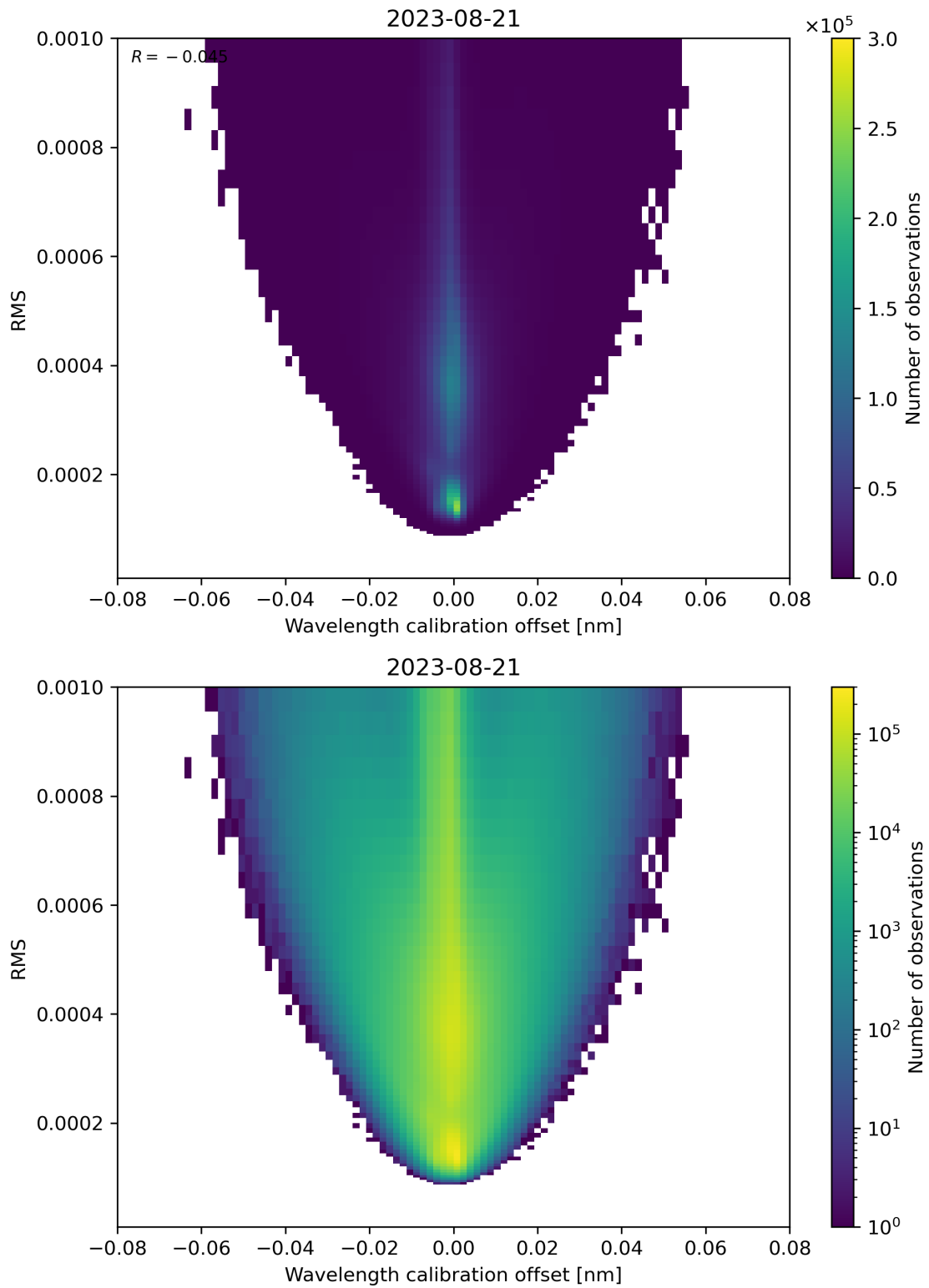
Figure 181: Scatter density plot of “Wavelength calibration offset” against “RMS” for 2023-08-20 to 2023-08-22.
