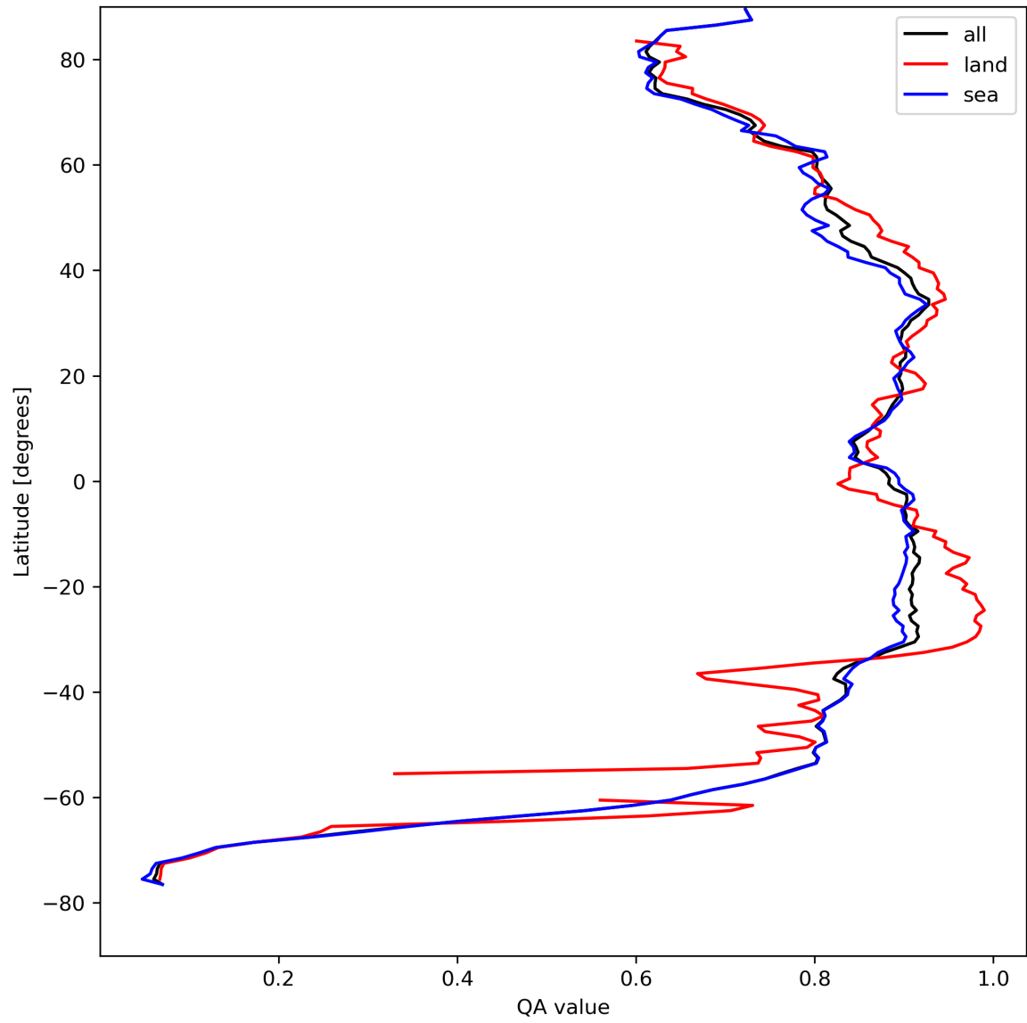
Figure 11: Zonal average of “QA value” for 2023-08-20 to 2023-08-22.
