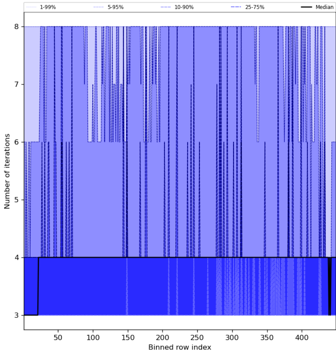
Figure 51: Along track statistics of “Number of iterations” for 2023-08-20 to 2023-08-22
