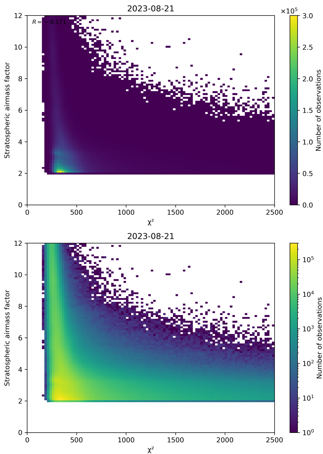
Figure 81: Scatter density plot of “ \chi^2 ” against “Stratospheric airmass factor” for 2023-08-20 to 2023-08-22.
