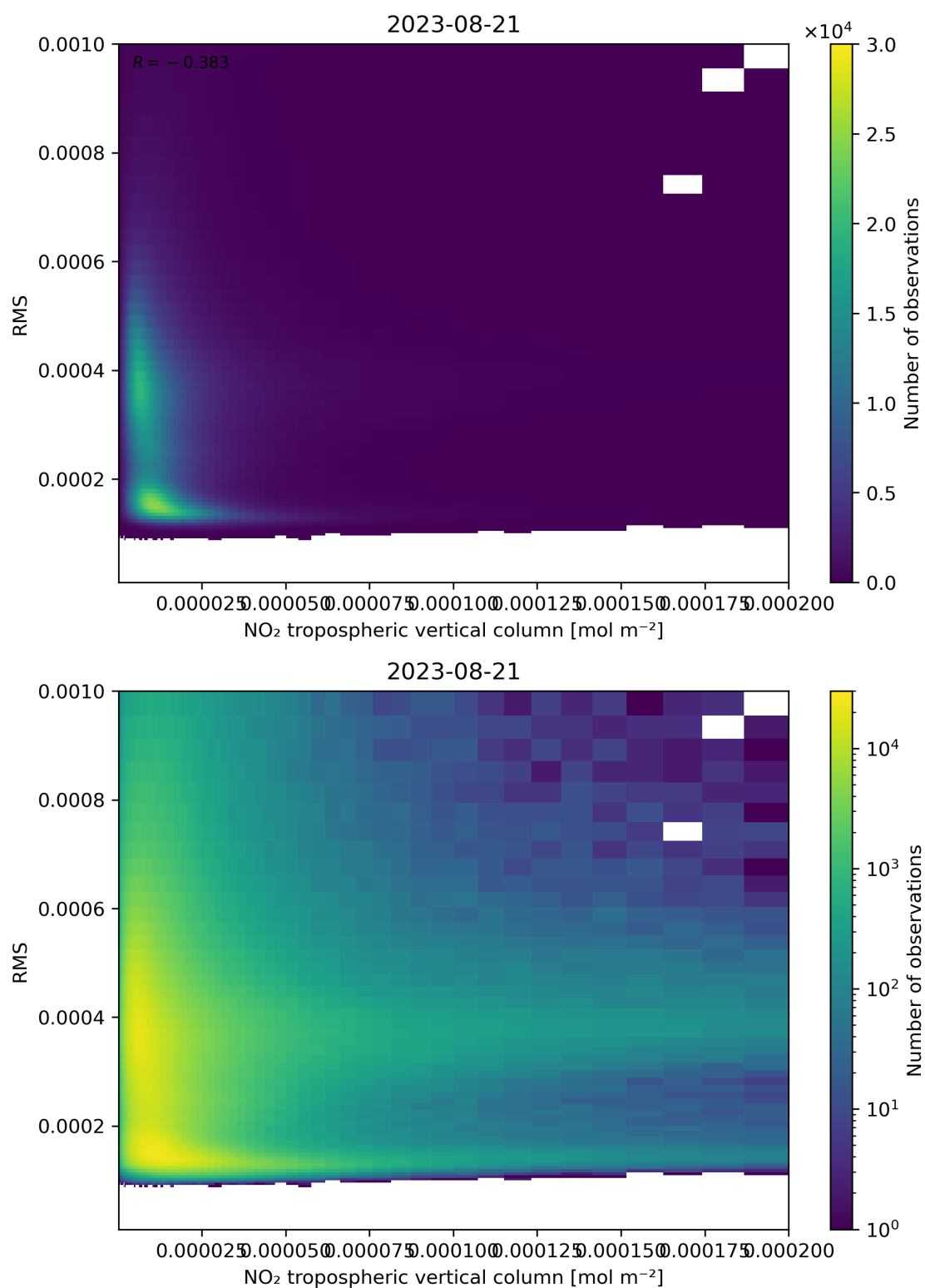
Figure 142: Scatter density plot of “NO 2 tropospheric vertical column” against “RMS” for 2023-08-20 to 2023-08-22.
