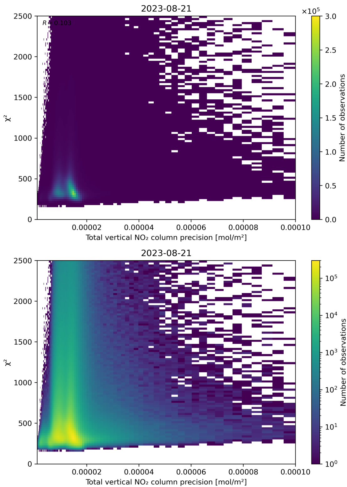
Figure 116: Scatter density plot of “Total vertical NO 2 column precision” against “ \chi^2 ” for 2023-08-20 to 2023-08-22.
