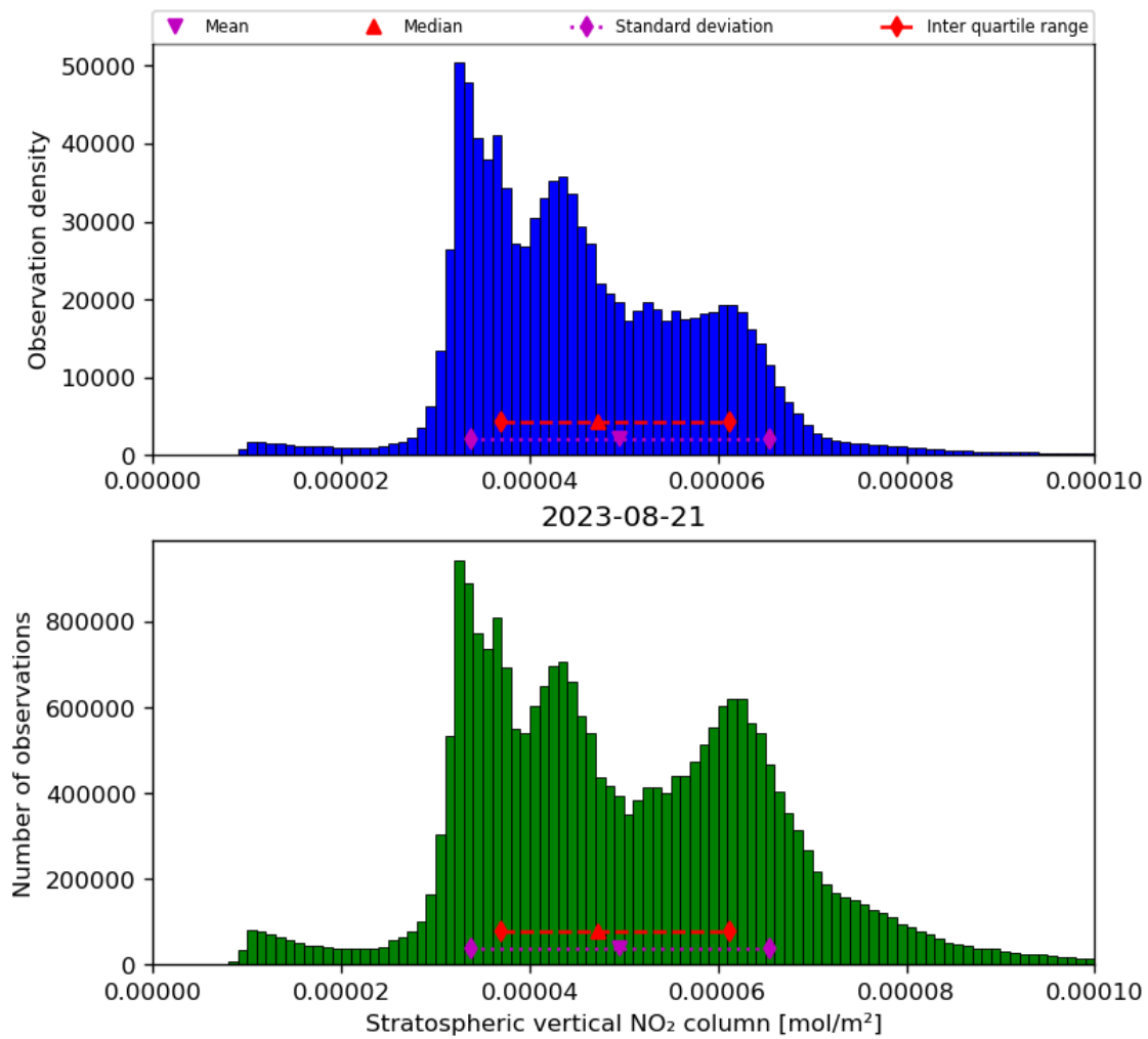
Figure 36: Histogram of “Stratospheric vertical NO 2 column” for 2023-08-20 to 2023-08-22
