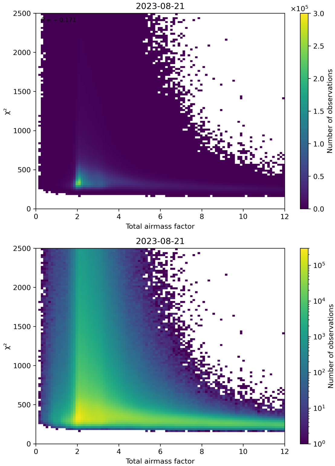
Figure 63: Scatter density plot of “Total airmass factor” against “ \chi^2 ” for 2023-08-20 to 2023-08-22.
