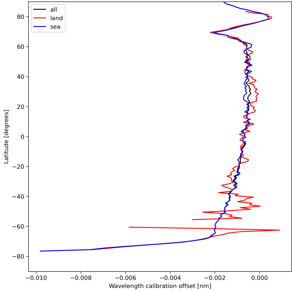
Figure 18: Zonal average of “Wavelength calibration offset” for 2023-08-20 to 2023-08-22.
