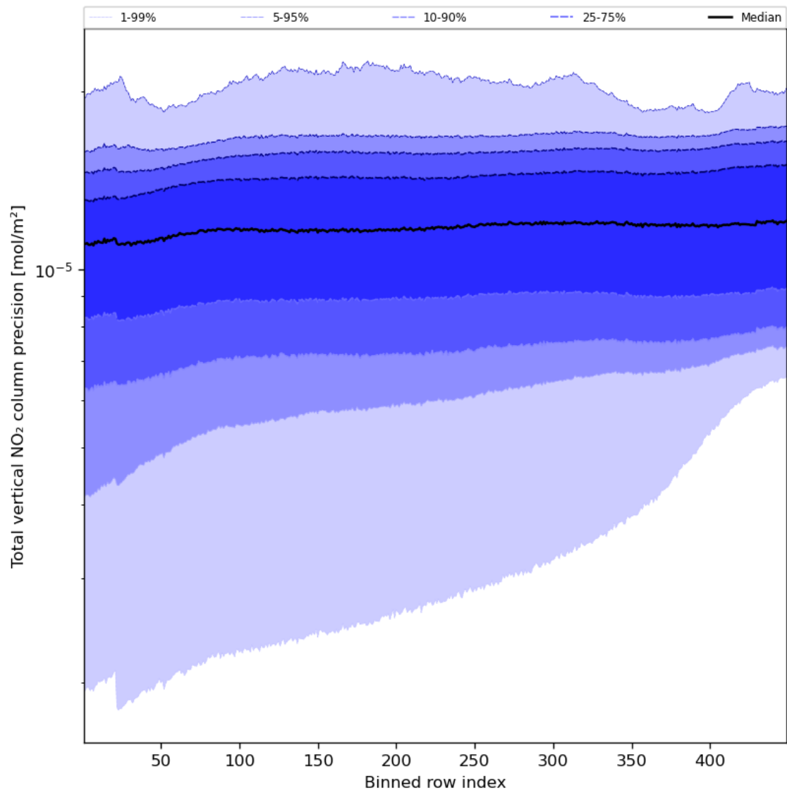
Figure 56: Along track statistics of “Total vertical NO 2 column precision” for 2023-08-20 to 2023-08-22
