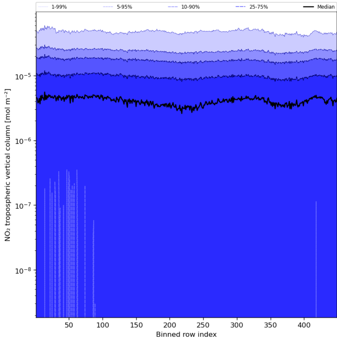
Figure 46: Along track statistics of “NO 2 tropospheric vertical column” for 2023-08-20 to 2023-08-22
