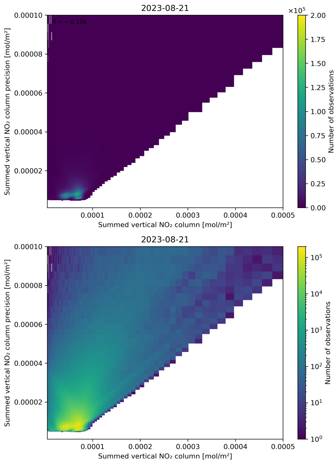
Figure 105: Scatter density plot of “Summed vertical NO 2 column” against “Summed vertical NO 2 column precision” for 2023-08-20 to 2023-08-22.
