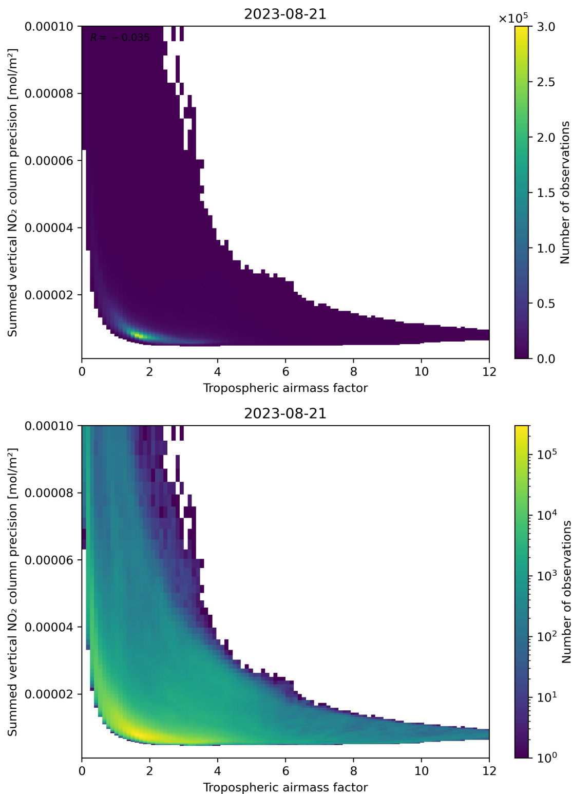
Figure 76: Scatter density plot of “Tropospheric air mass factor” against “Summed vertical NO 2 column precision” for 2023-08-20 to 2023-08-22.
