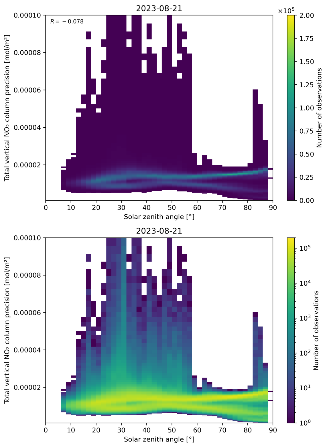
Figure 154: Scatter density plot of “Solar zenith angle” against “Total vertical NO 2 column precision” for 2023-08-20 to 2023-08-22.
