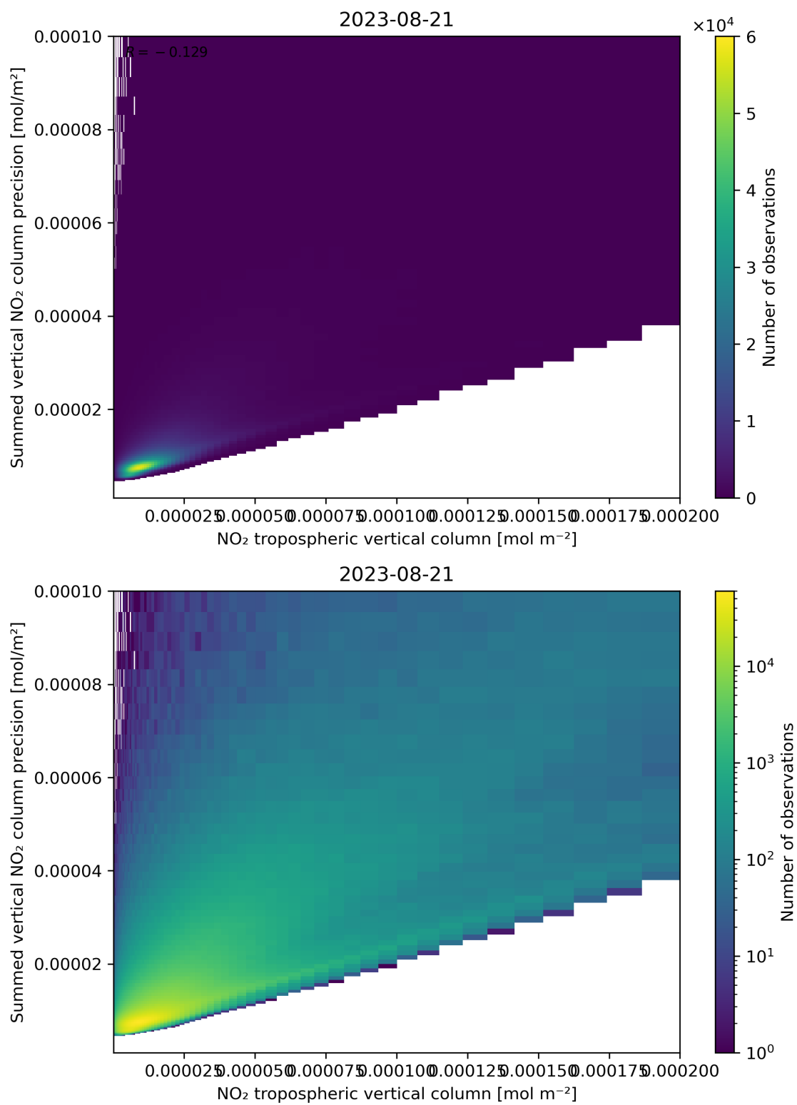
Figure 127: Scatter density plot of “NO 2 tropospheric vertical column” against “Summed vertical NO 2 column precision” for 2023-08-20 to 2023-08-22.
