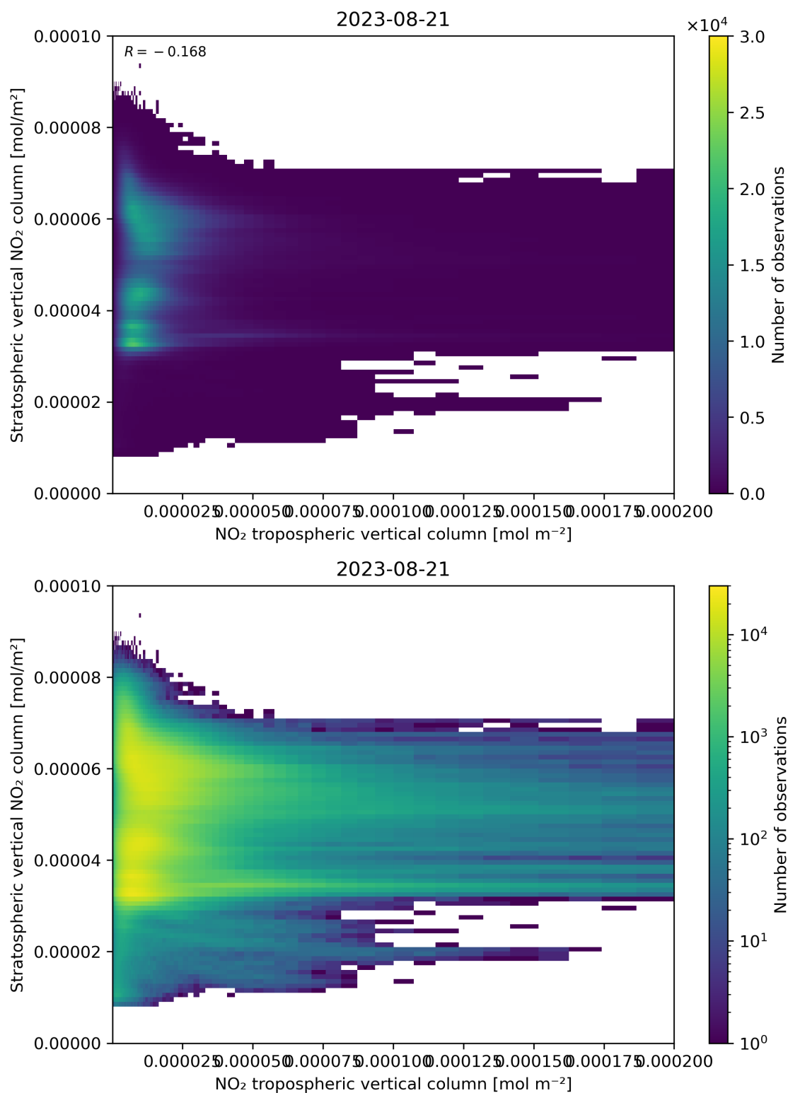
Figure 125: Scatter density plot of “NO 2 tropospheric vertical column” against “Stratospheric vertical NO 2 column” for 2023-08-20 to 2023-08-22.
