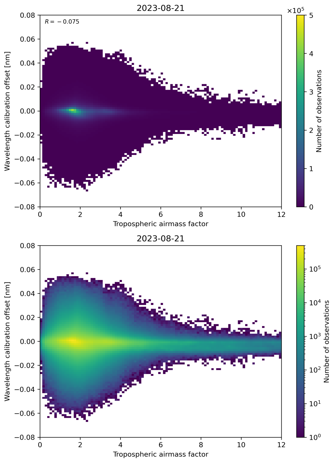
Figure 80: Scatter density plot of “Tropospheric airmass factor” against “Wavelength calibration offset” for 2023-08-20 to 2023-08-22.
