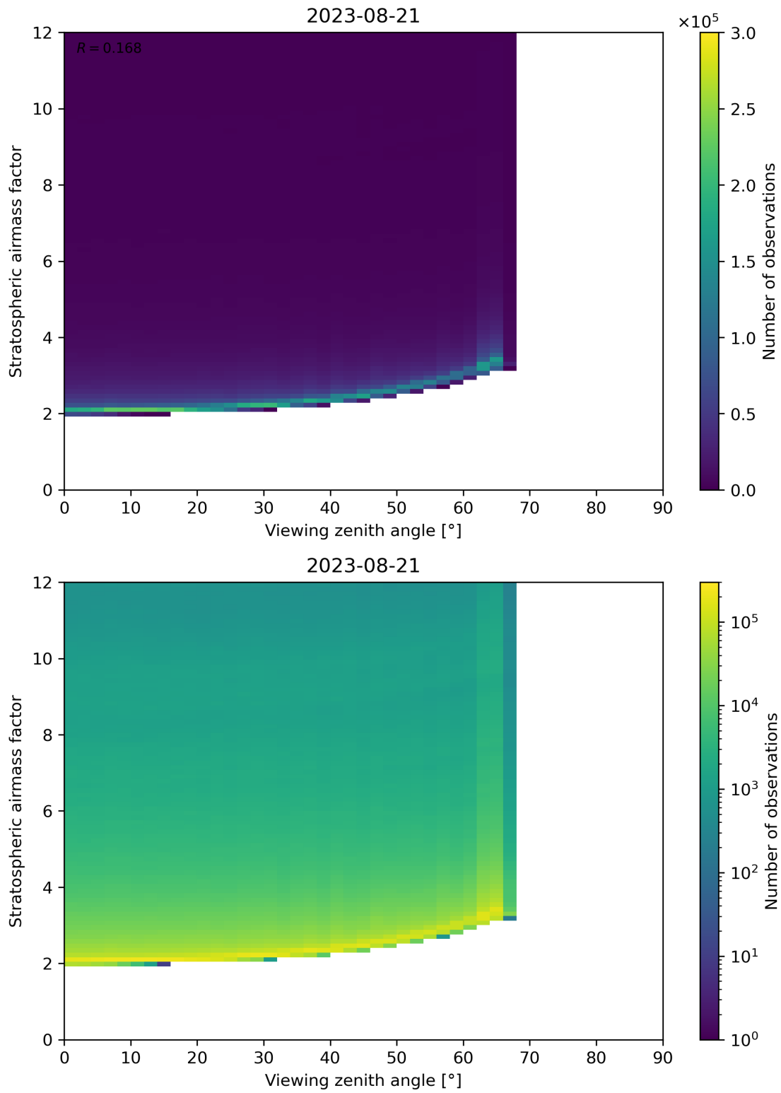
Figure 159: Scatter density plot of “Viewing zenith angle” against “Stratospheric airmass factor” for 2023-08-20 to 2023-08-22.
