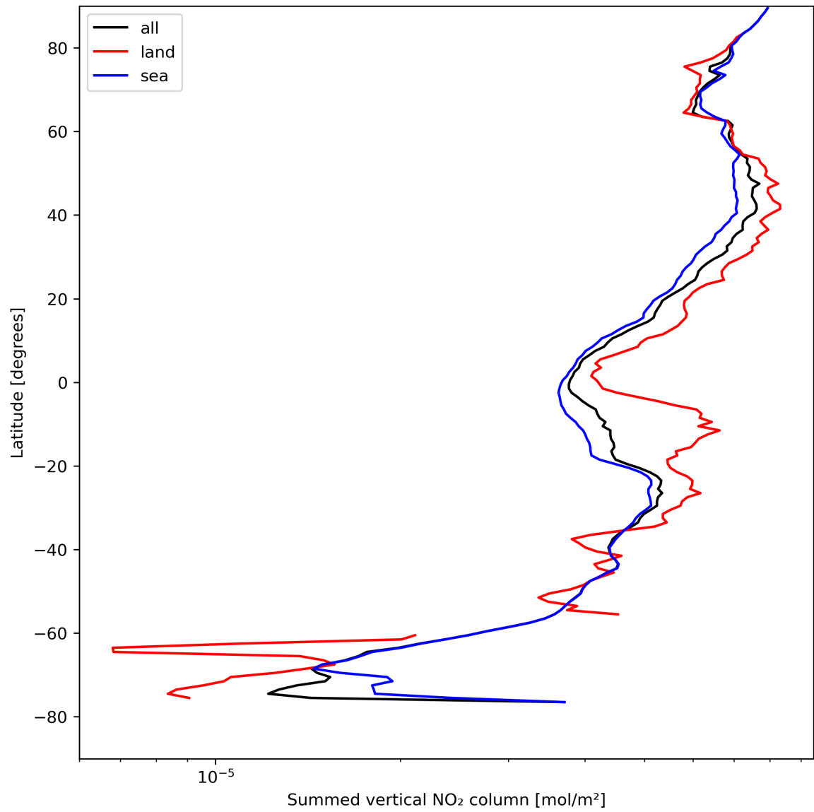
Figure 23: Zonal average of “Summed vertical NO 2 column” for 2023-08-20 to 2023-08-22.
