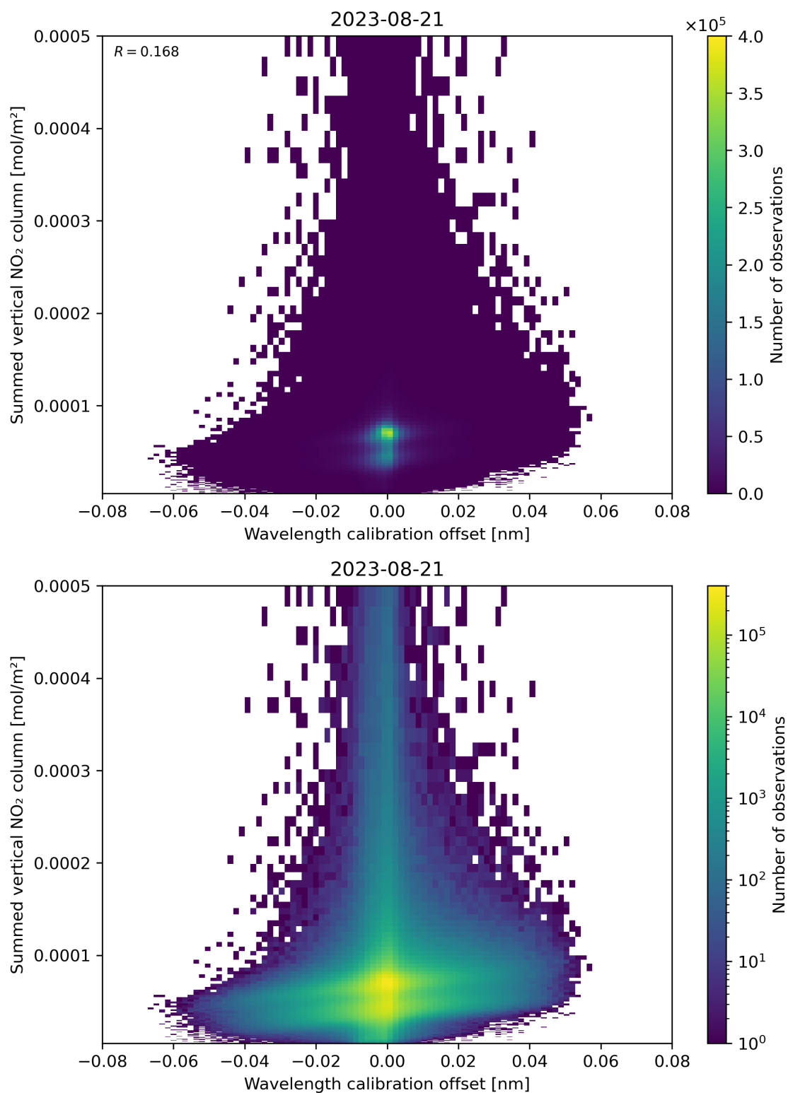
Figure 177: Scatter density plot of “Wavelength calibration offset” against “Summed vertical NO 2 column” for 2023-08-20 to 2023-08-22.
