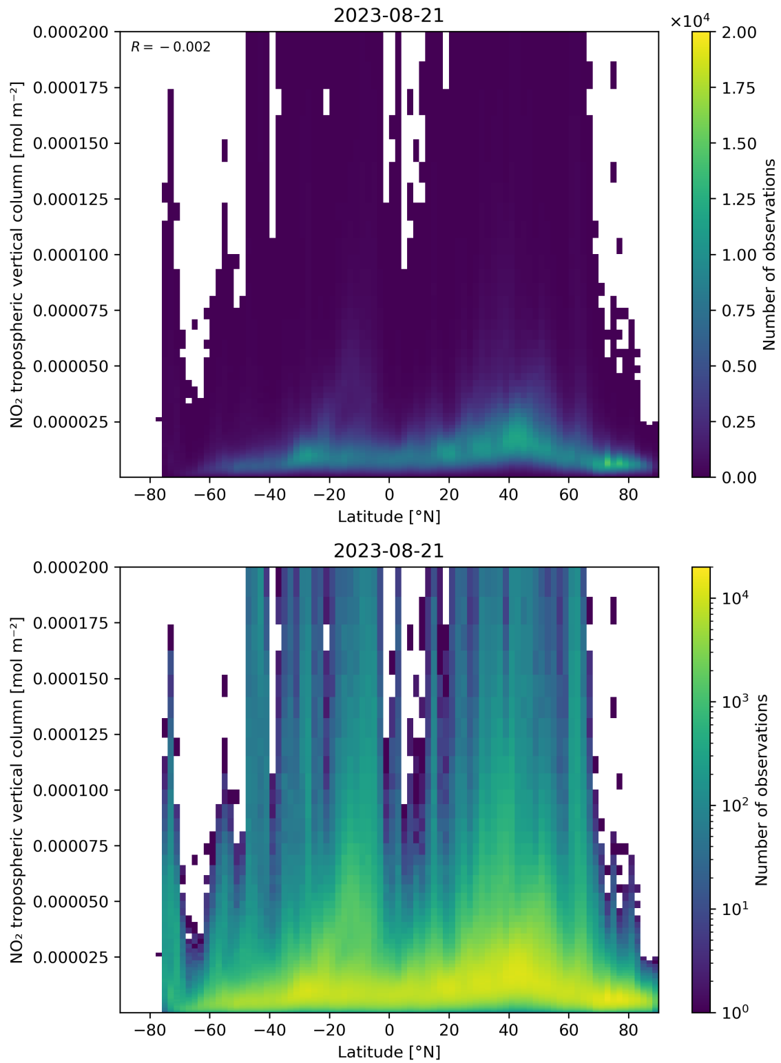
Figure 92: Scatter density plot of “Latitude” against “NO 2 tropospheric vertical column” for 2023-08-20 to 2023-08-22.
