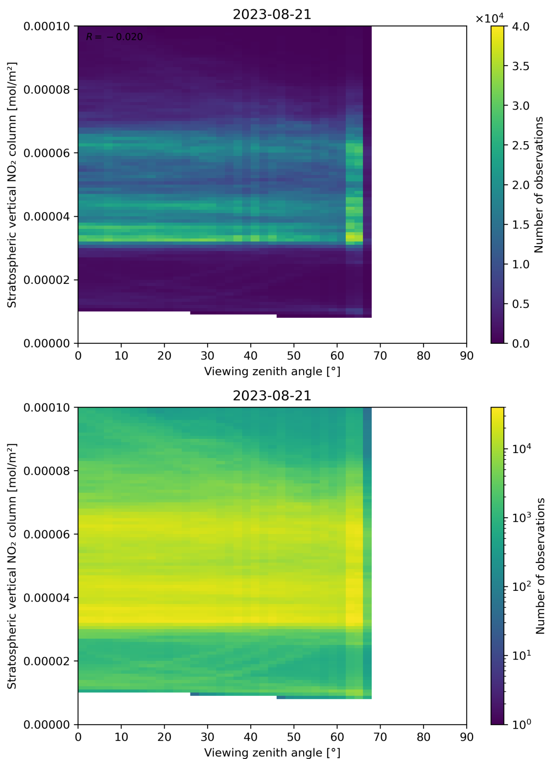
Figure 164: Scatter density plot of “Viewing zenith angle” against “Stratospheric vertical NO 2 column” for 2023-08-20 to 2023-08-22.
