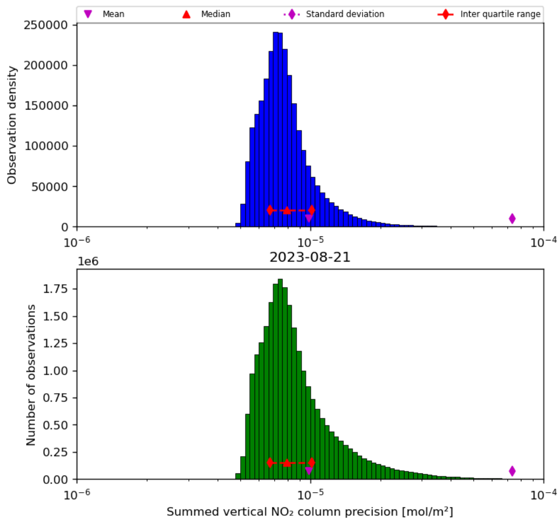
Figure 41: Histogram of “Summed vertical NO 2 column precision” for 2023-08-20 to 2023-08-22
