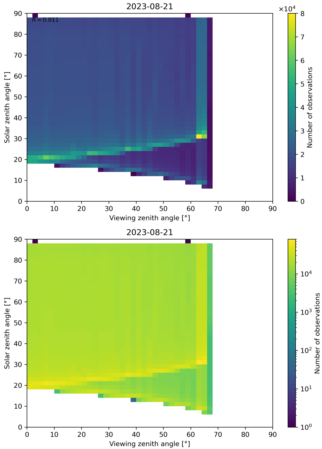
Figure 172: Scatter density plot of “Viewing zenith angle” against “Solar zenith angle” for 2023-08-20 to 2023-08-22.
