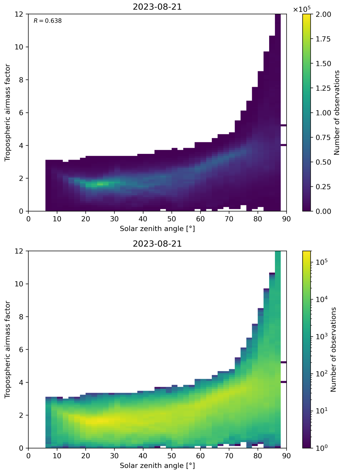
Figure 147: Scatter density plot of “Solar zenith angle” against “Tropospheric airmass factor” for 2023-08-20 to 2023-08-22.
