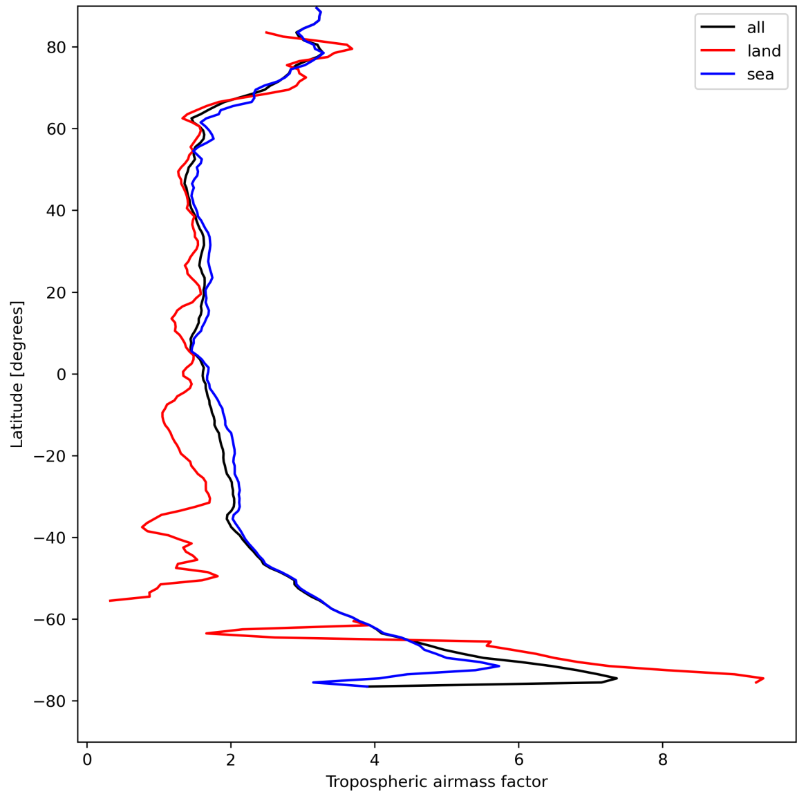
Figure 14: Zonal average of “Tropospheric airmass factor” for 2023-08-20 to 2023-08-22.
