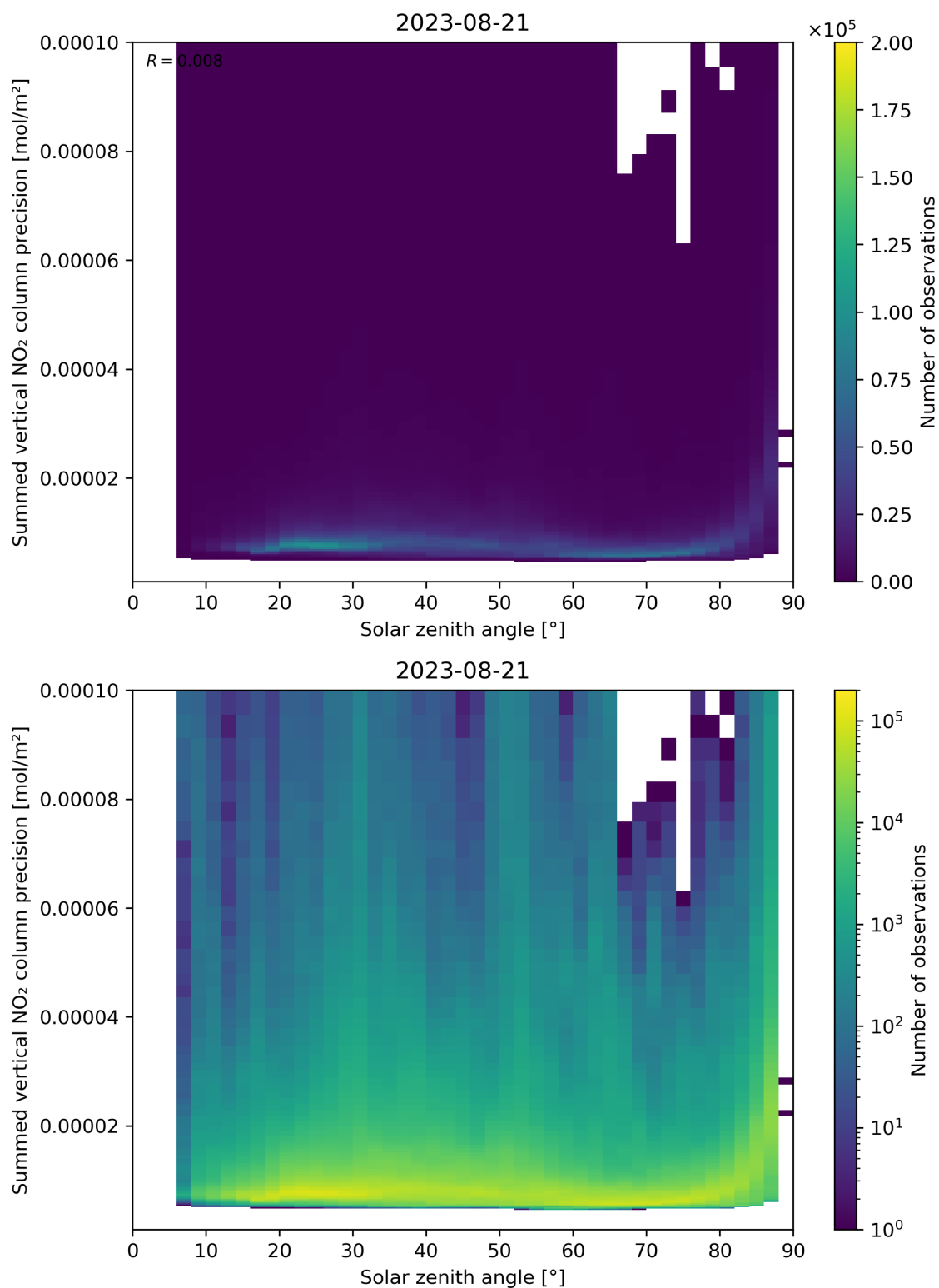
Figure 152: Scatter density plot of “Solar zenith angle” against “Summed vertical NO 2 column precision” for 2023-08-20 to 2023-08-22.
