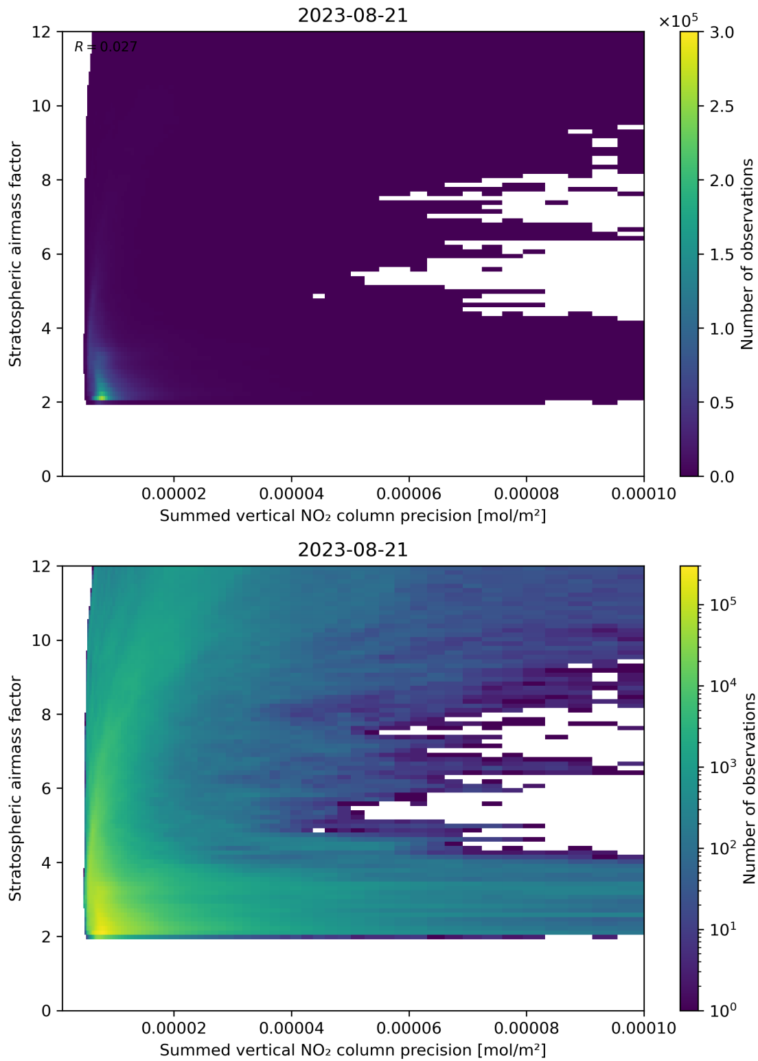
Figure 106: Scatter density plot of “Summed vertical NO 2 column precision” against “Stratospheric airmass factor” for 2023-08-20 to 2023-08-22.
