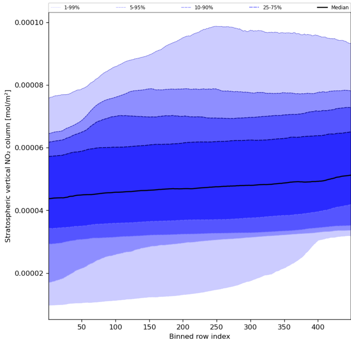
Figure 53: Along track statistics of “Stratospheric vertical NO 2 column” for 2023-08-20 to 2023-08-22
