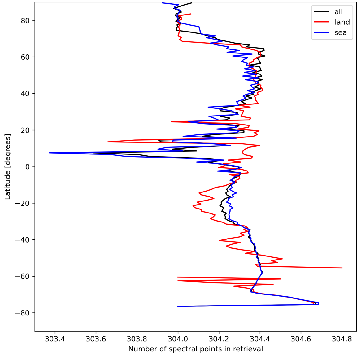
Figure 16: Zonal average of “Number of spectral points in retrieval” for 2023-08-20 to 2023-08-22.
