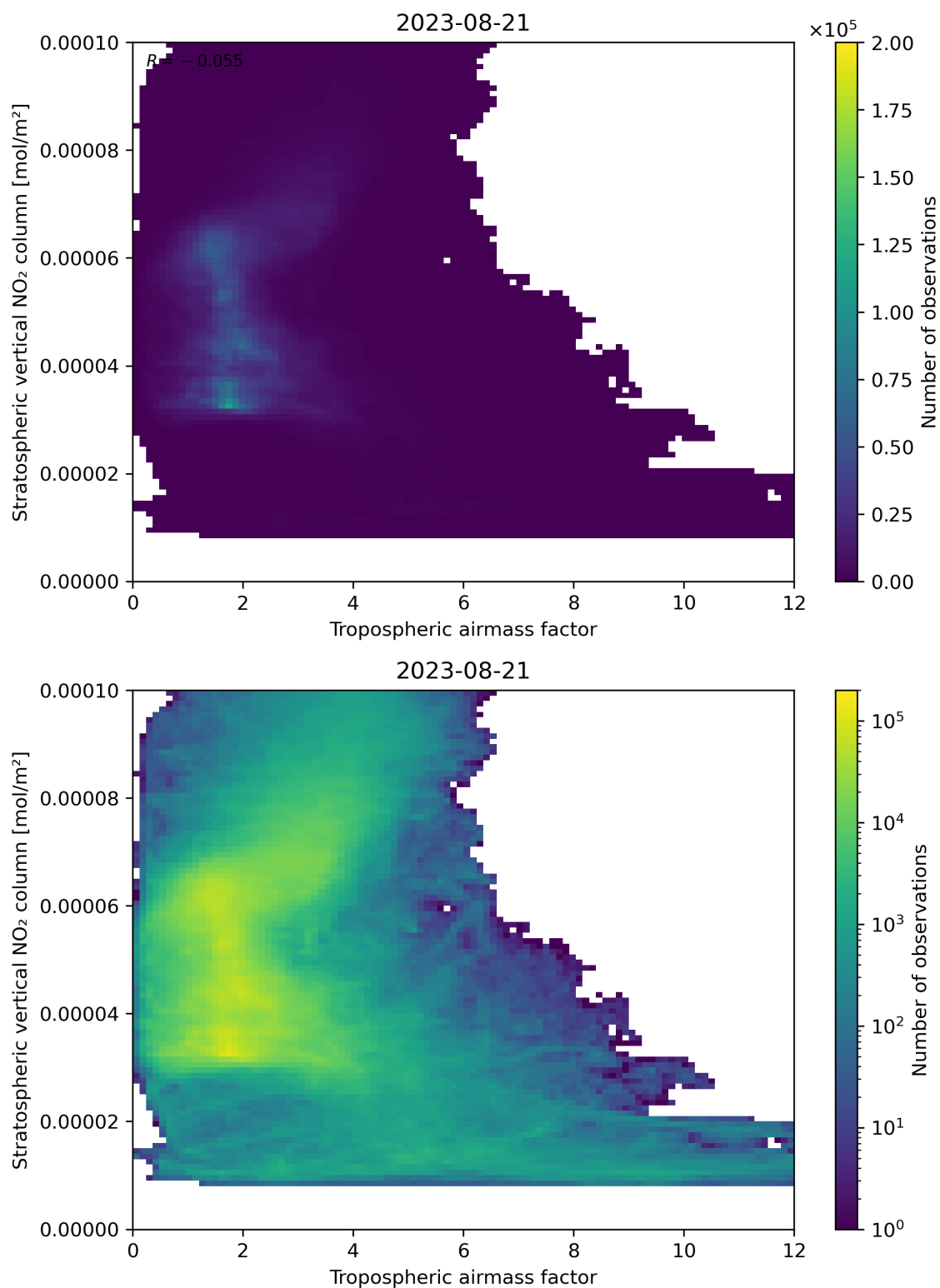
Figure 74: Scatter density plot of “Tropospheric air mass factor” against “Stratospheric vertical NO 2 column” for 2023-08-20 to 2023-08-22.
