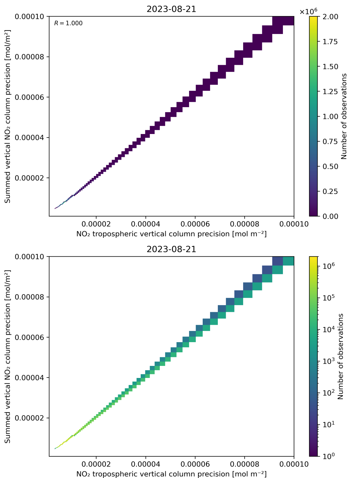
Figure 137: Scatter density plot of “NO 2 tropospheric vertical column precision” against “Summed vertical NO 2 column precision” for 2023-08-20 to 2023-08-22.
