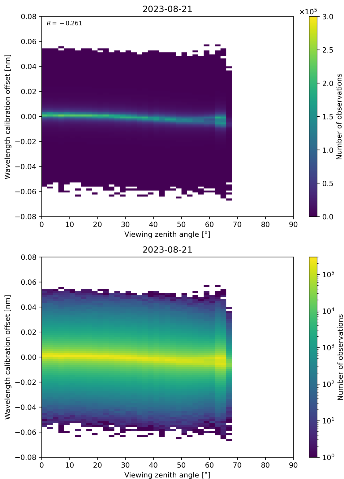
Figure 173: Scatter density plot of “Viewing zenith angle” against “Wavelength calibration offset” for 2023-08-20 to 2023-08-22.
