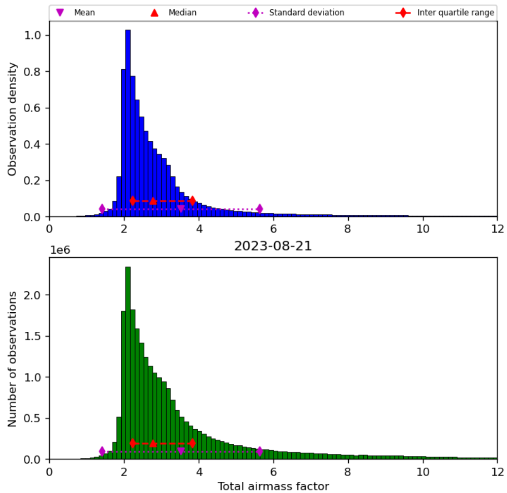
Figure 32: Histogram of “Total airmass factor” for 2023-08-20 to 2023-08-22
