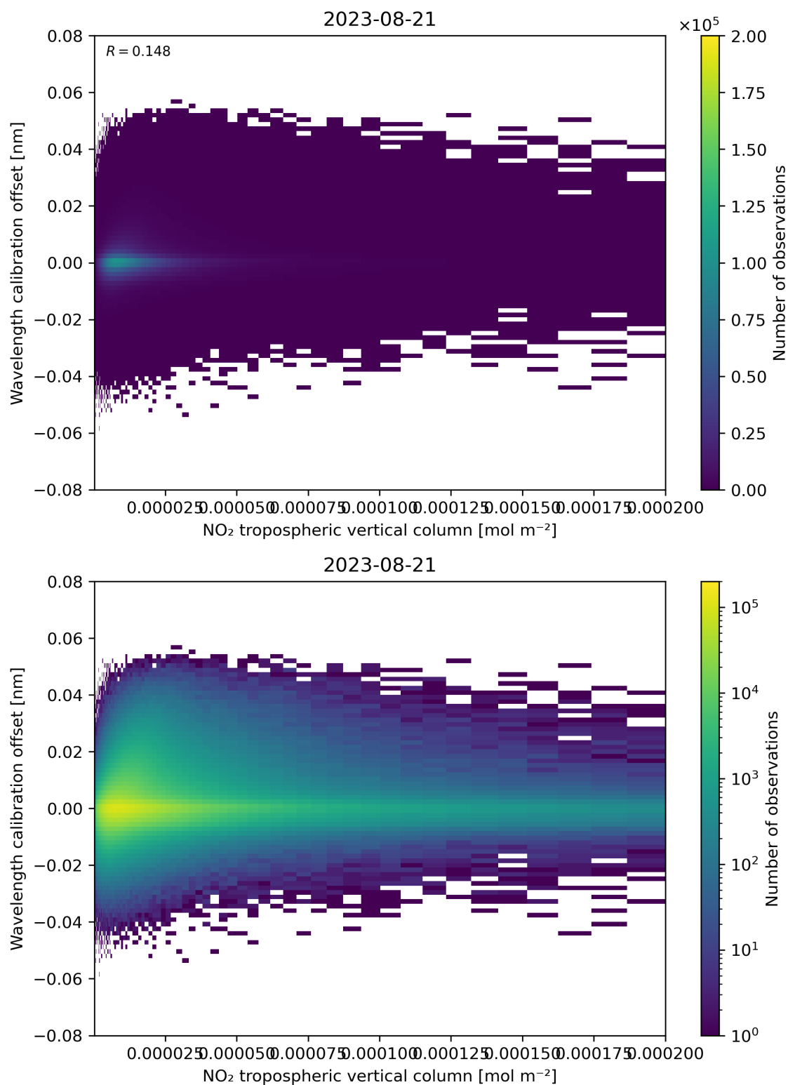
Figure 143: Scatter density plot of “NO 2 tropospheric vertical column” against “Wavelength calibration offset” for 2023-08-20 to 2023-08-22.
