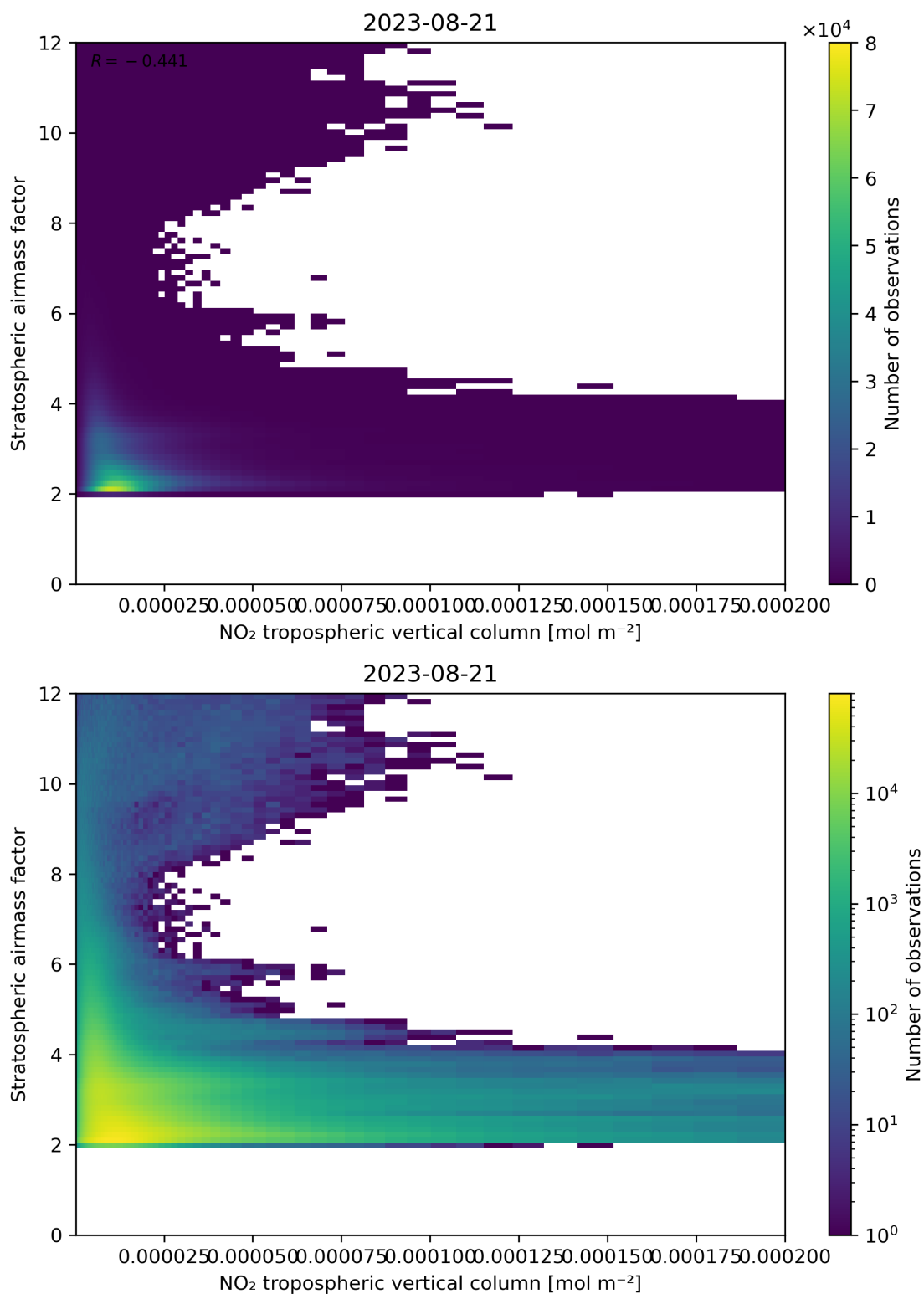
Figure 121: Scatter density plot of “NO 2 tropospheric vertical column” against “Stratospheric air mass factor” for 2023-08-20 to 2023-08-22.
