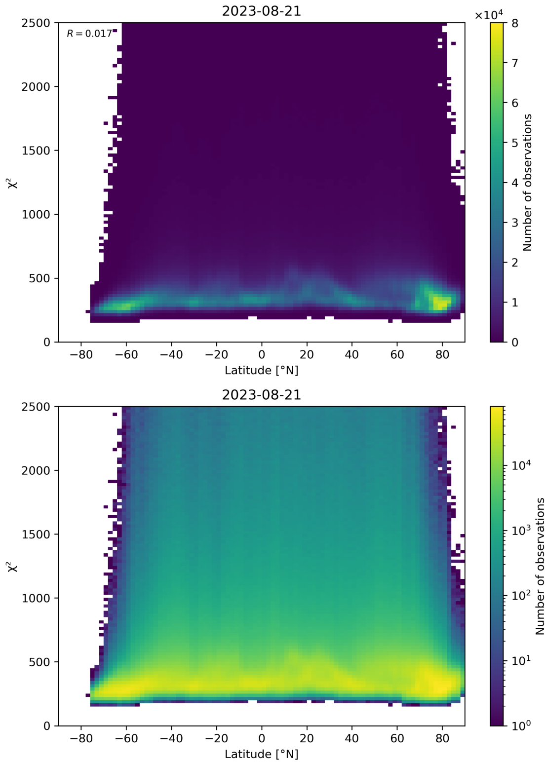
Figure 86: Scatter density plot of “Latitude” against “ \chi^2 ” for 2023-08-20 to 2023-08-22.
