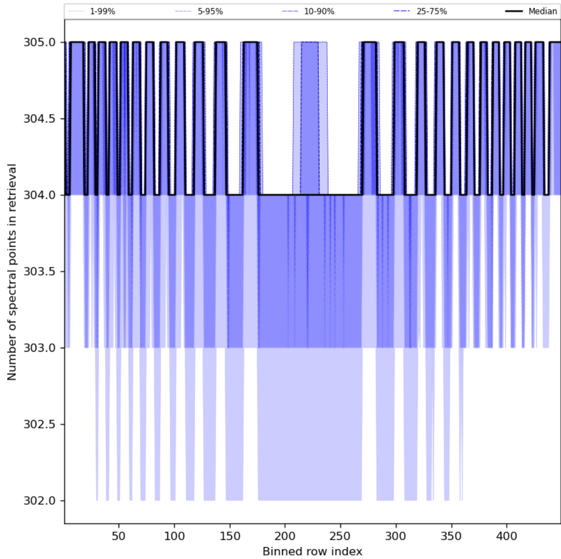
Figure 50: Along track statistics of “Number of spectral points in retrieval” for 2023-08-20 to 2023-08-22
