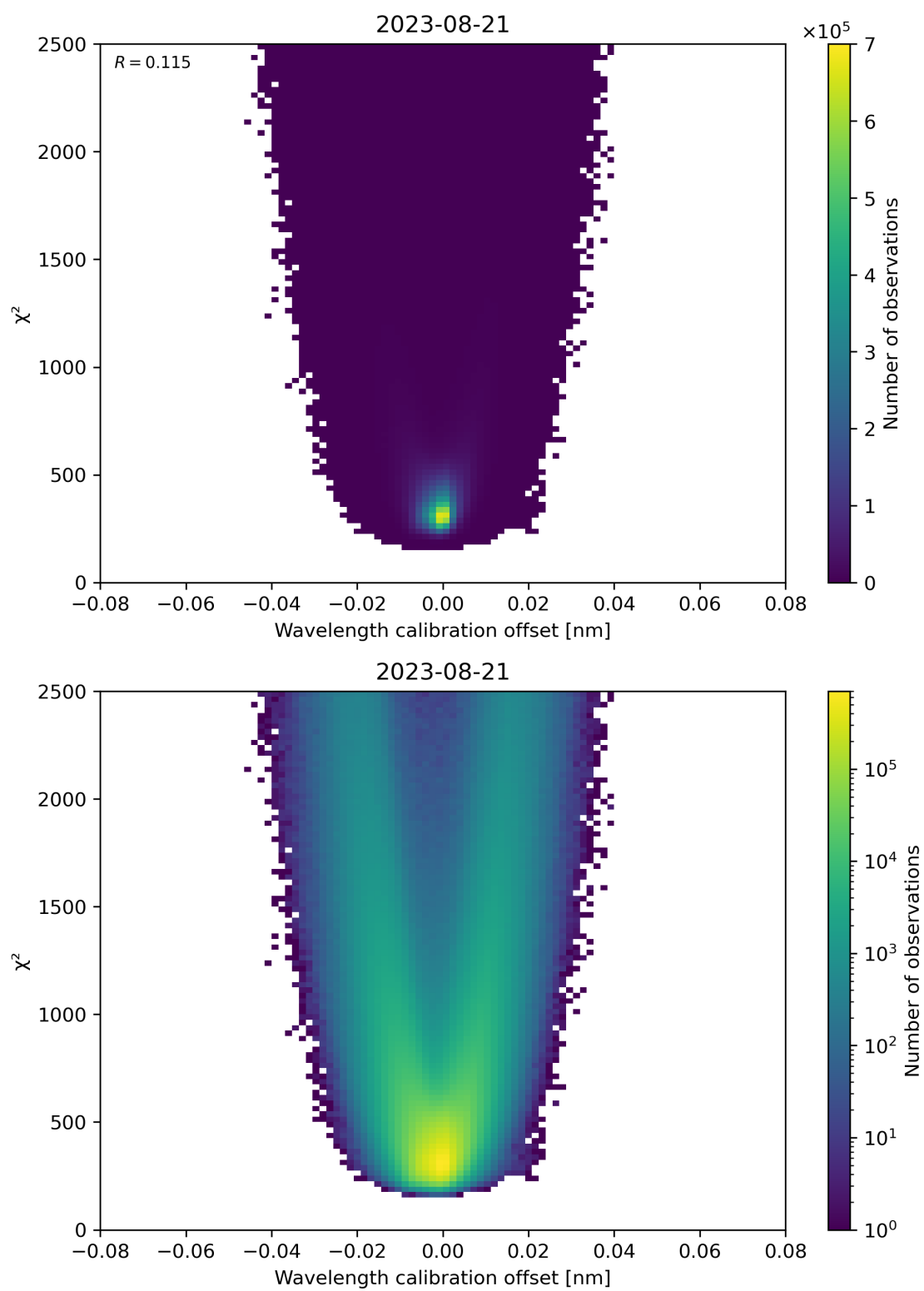
Figure 175: Scatter density plot of “Wavelength calibration offset” against “ \chi^2 ” for 2023-08-20 to 2023-08-22.
