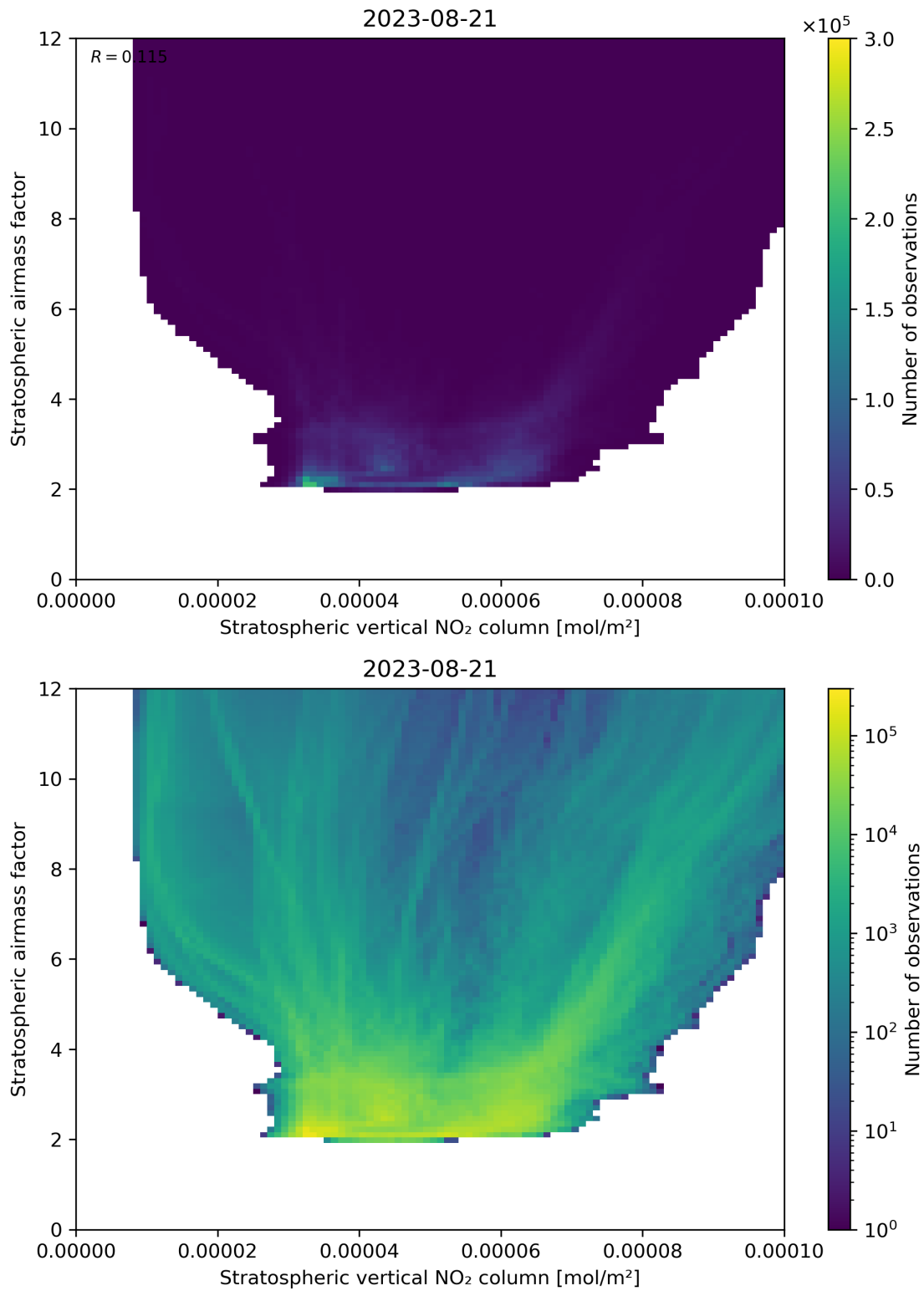
Figure 96: Scatter density plot of “Stratospheric vertical NO 2 column” against “Stratospheric airmass factor” for 2023-08-20 to 2023-08-22.
