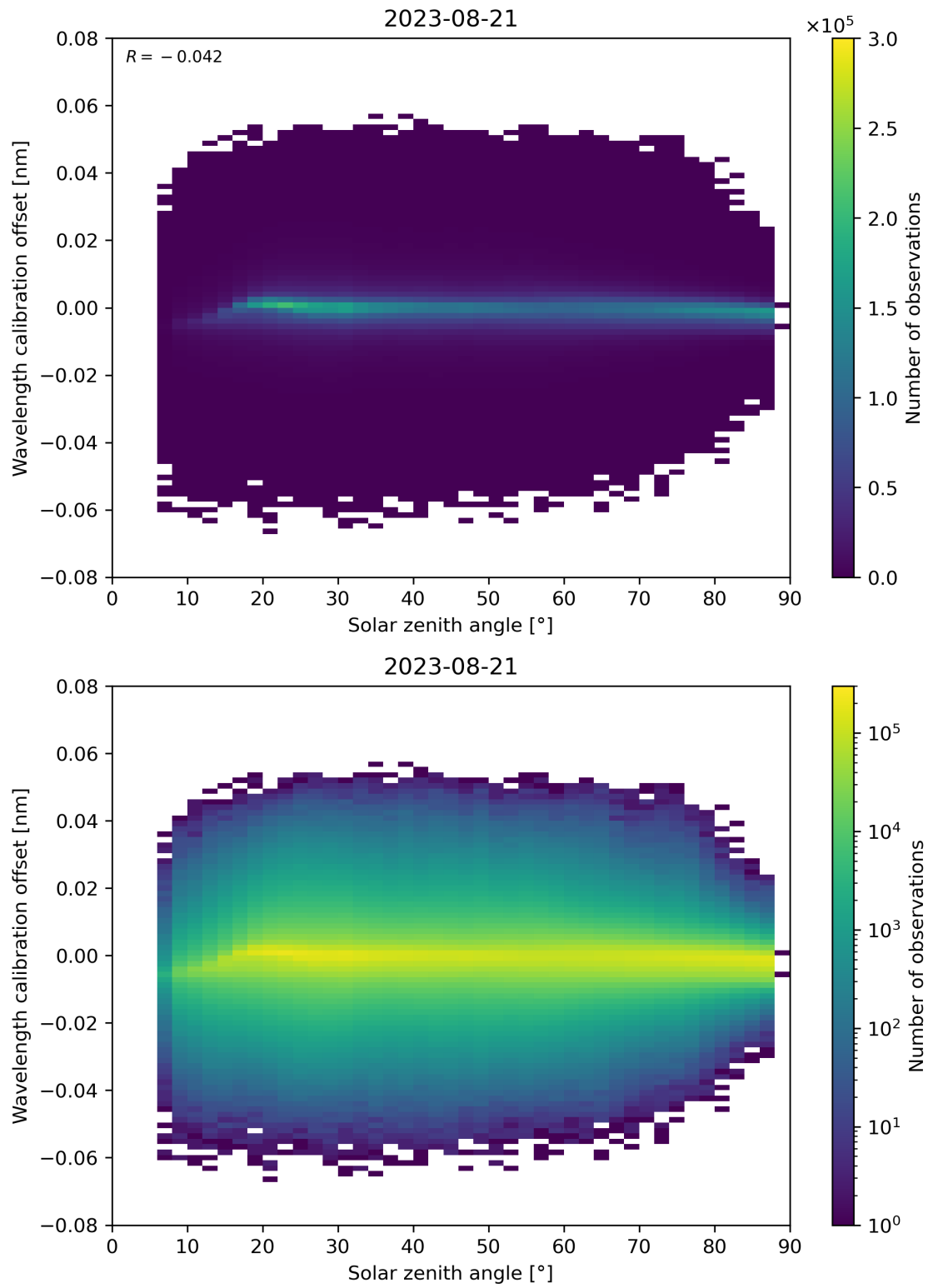
Figure 158: Scatter density plot of “Solar zenith angle” against “Wavelength calibration offset” for 2023-08-20 to 2023-08-22.
