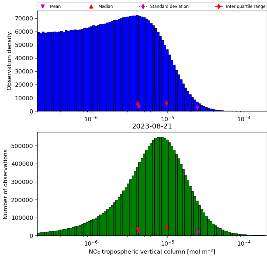
Figure 29: Histogram of “NO 2 tropospheric vertical column” for 2023-08-20 to 2023-08-22
