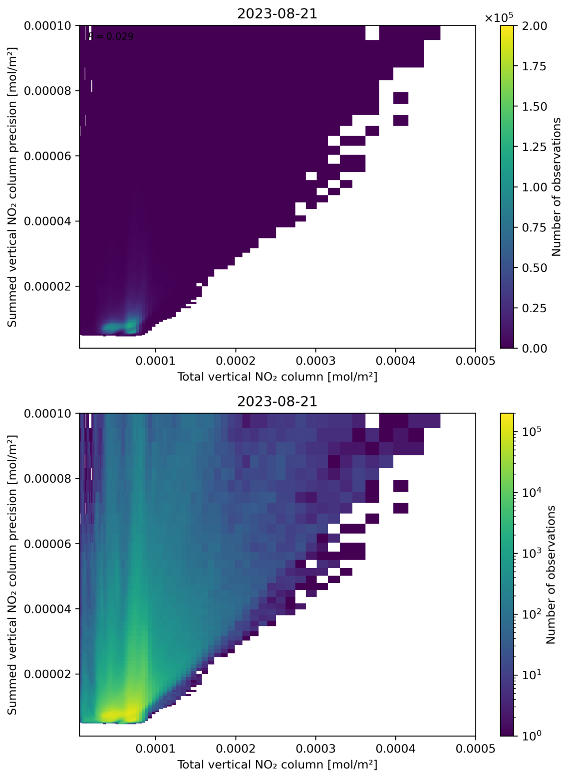
Figure 113: Scatter density plot of “Total vertical NO 2 column” against “Summed vertical NO 2 column precision” for 2023-08-20 to 2023-08-22.
