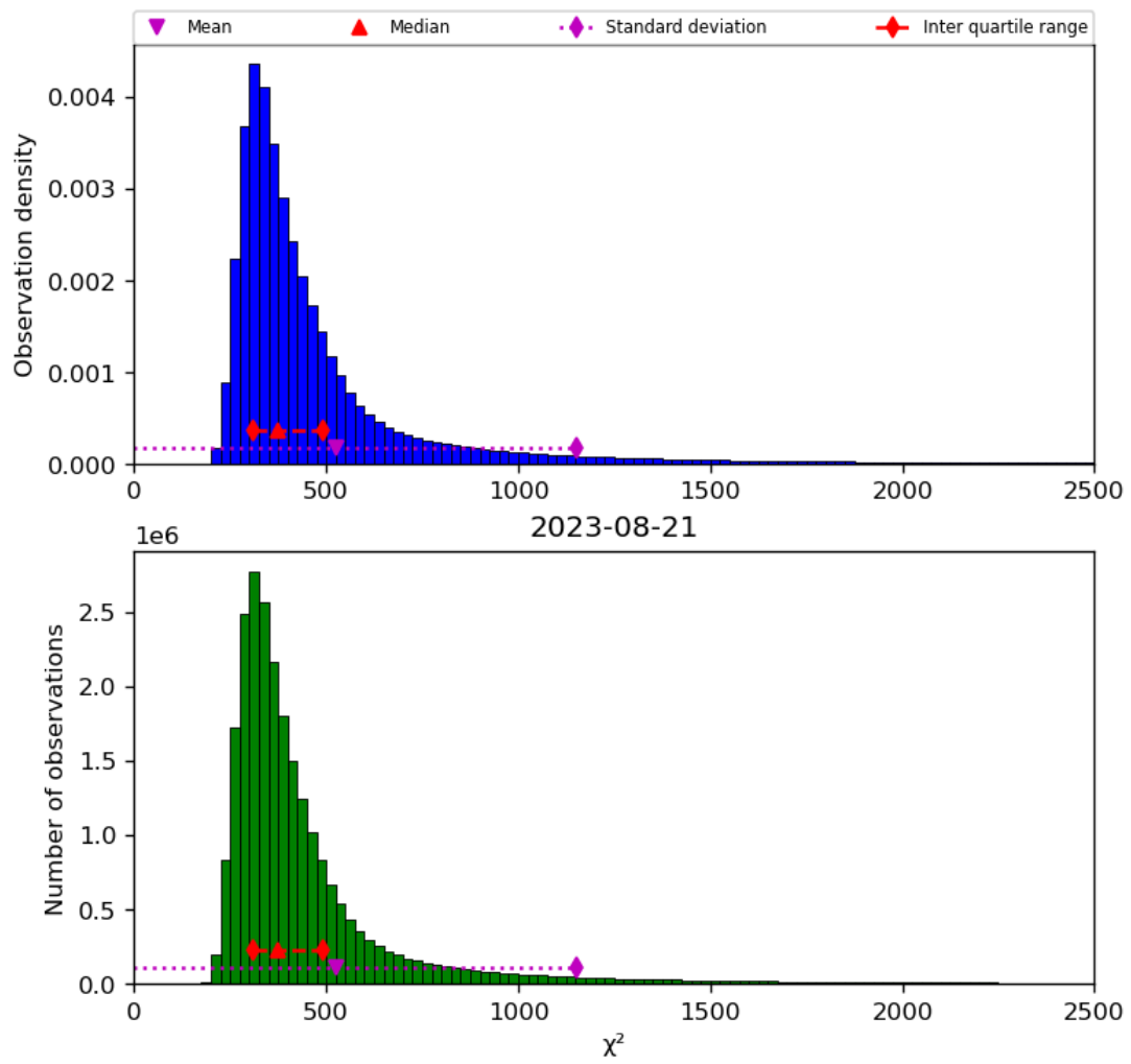
Figure 42: Histogram of “ \chi^2 ” for 2023-08-20 to 2023-08-22
