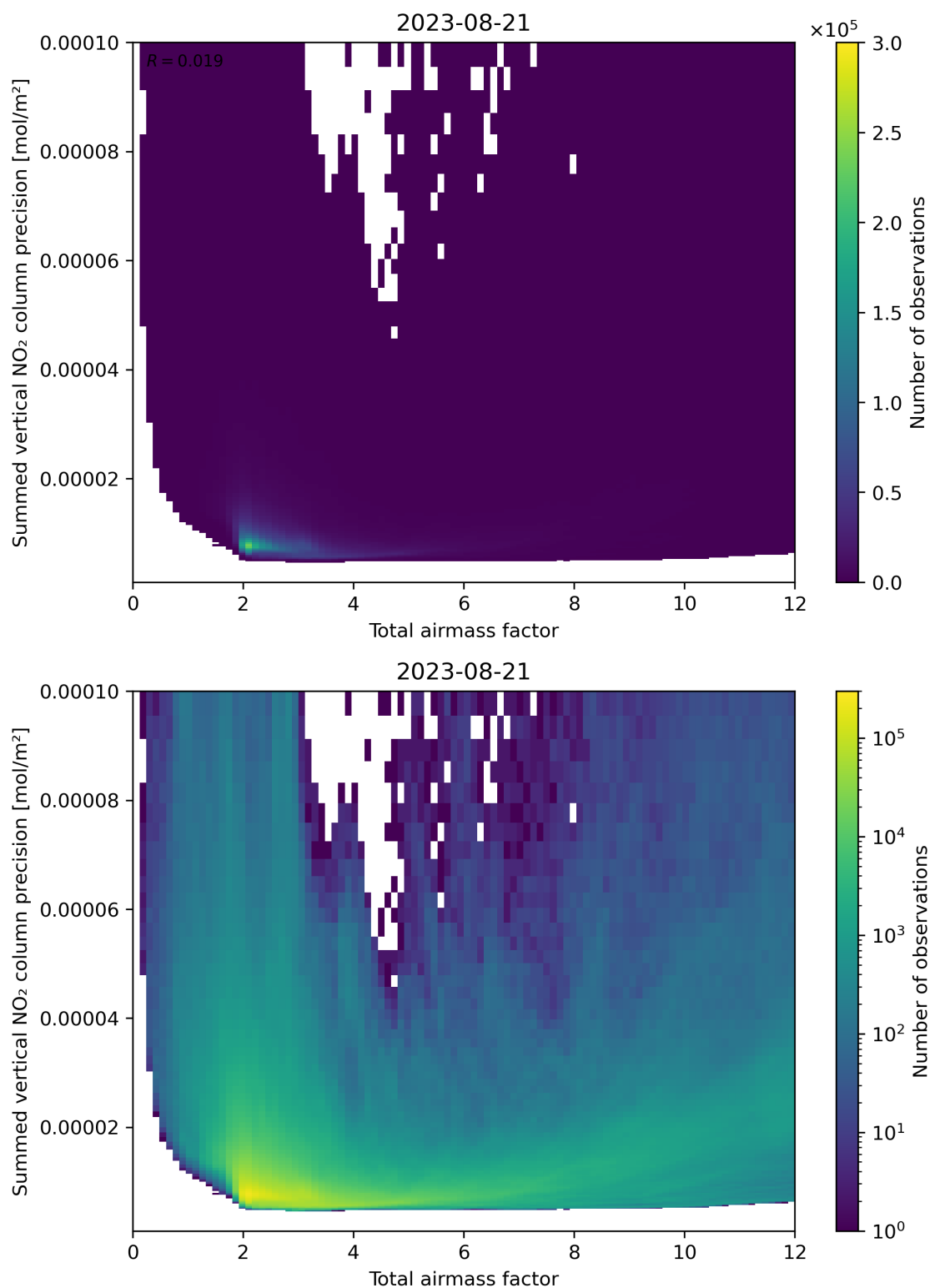
Figure 66: Scatter density plot of “Total airmass factor” against “Summed vertical NO 2 column precision” for 2023-08-20 to 2023-08-22.
