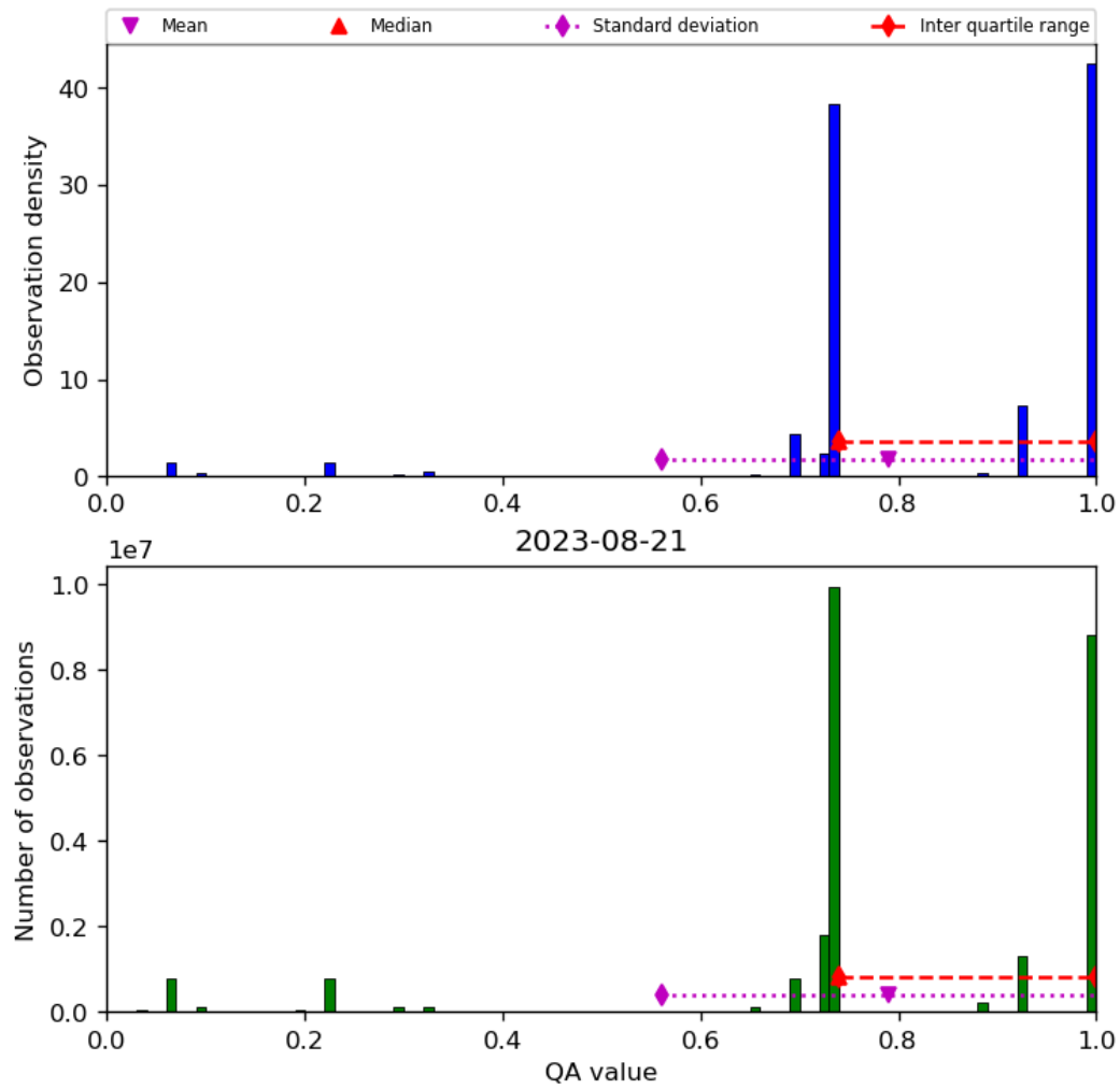
Figure 28: Histogram of “QA value” for 2023-08-20 to 2023-08-22
