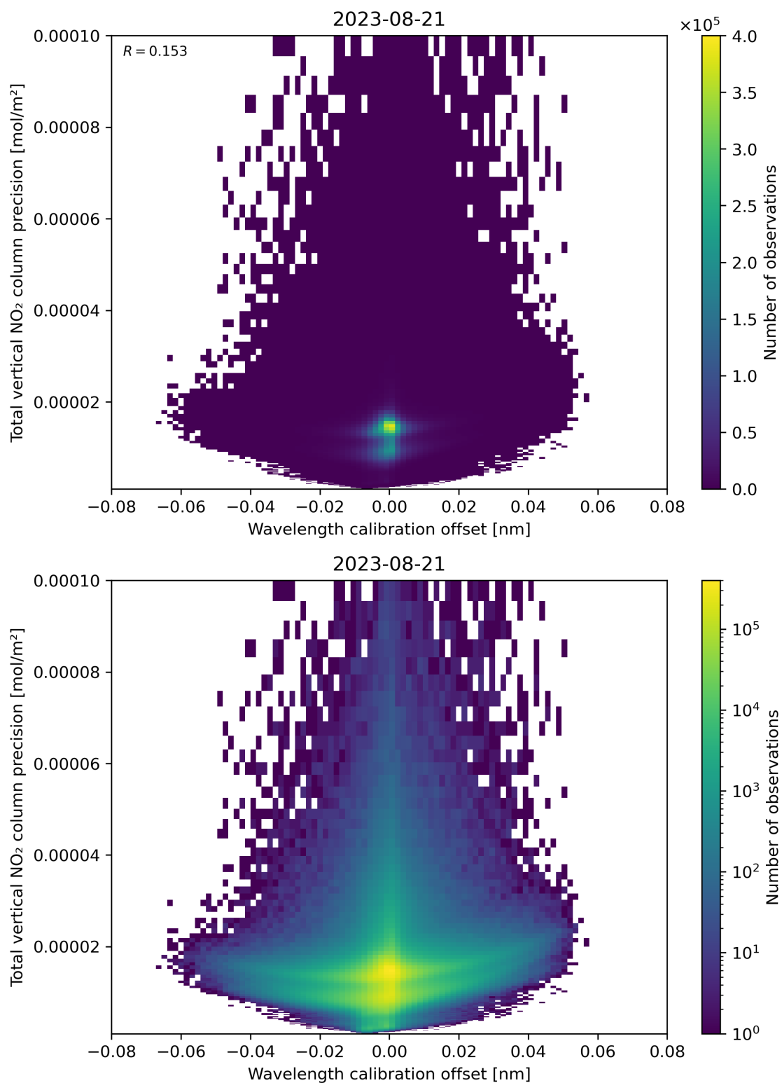
Figure 180: Scatter density plot of “Wavelength calibration offset” against “Total vertical NO 2 column precision” for 2023-08-20 to 2023-08-22.
