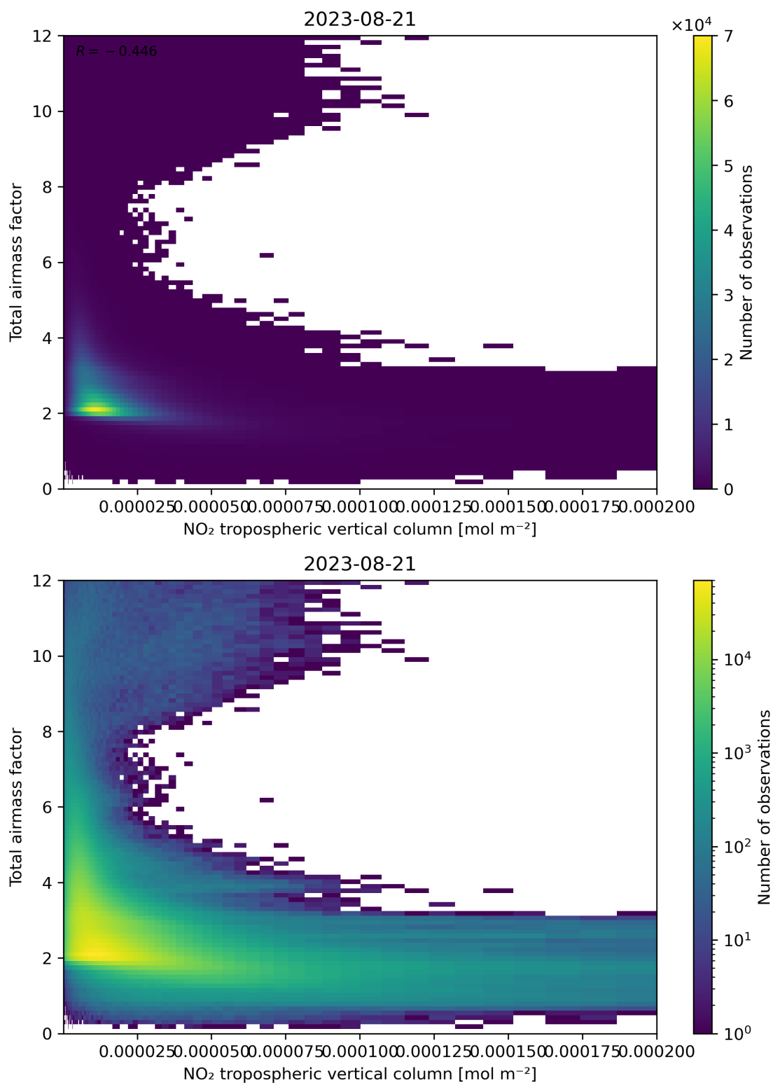
Figure 122: Scatter density plot of “NO 2 tropospheric vertical column” against “Total air mass factor” for 2023-08-20 to 2023-08-22.
