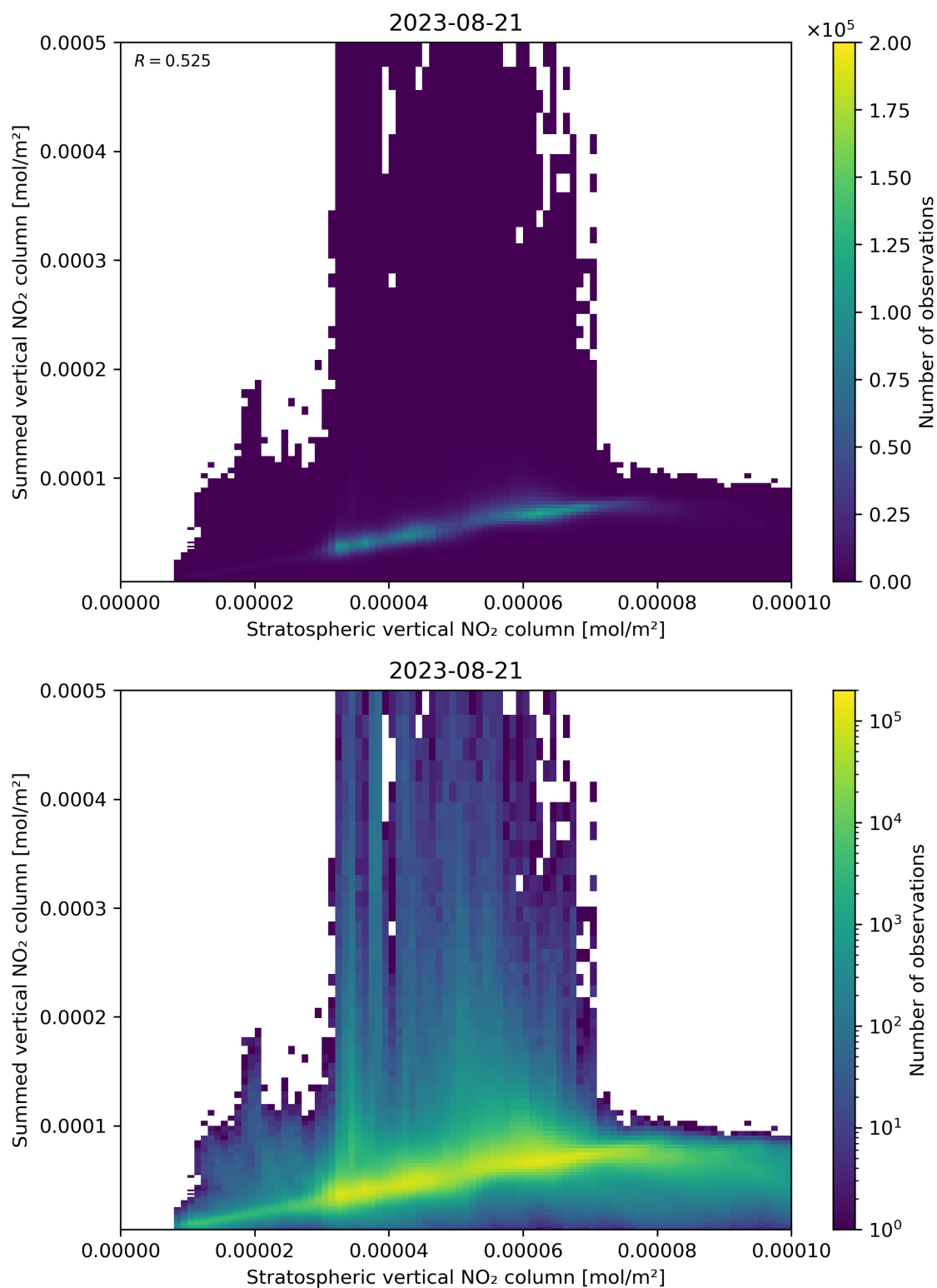
Figure 98: Scatter density plot of “Stratospheric vertical NO 2 column” against “Summed vertical NO 2 column” for 2023-08-20 to 2023-08-22.
