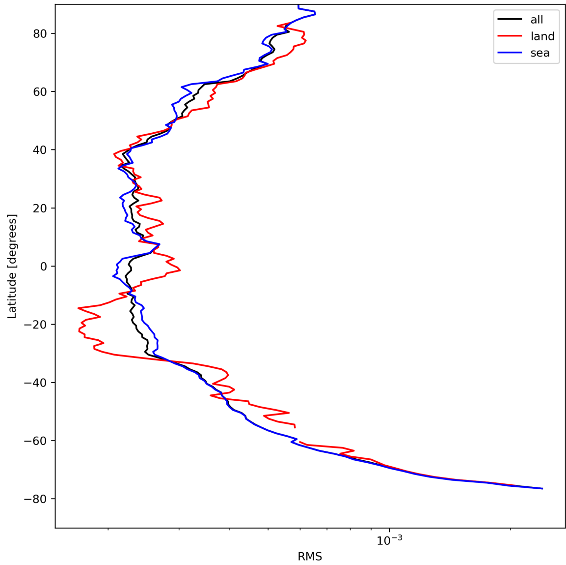
Figure 26: Zonal average of “RMS” for 2023-08-20 to 2023-08-22.
