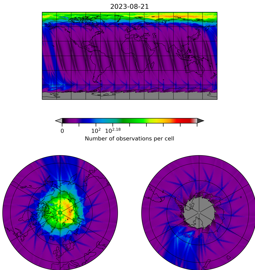
Figure 10: Map of the number of observations for 2023-08-20 to 2023-08-22
