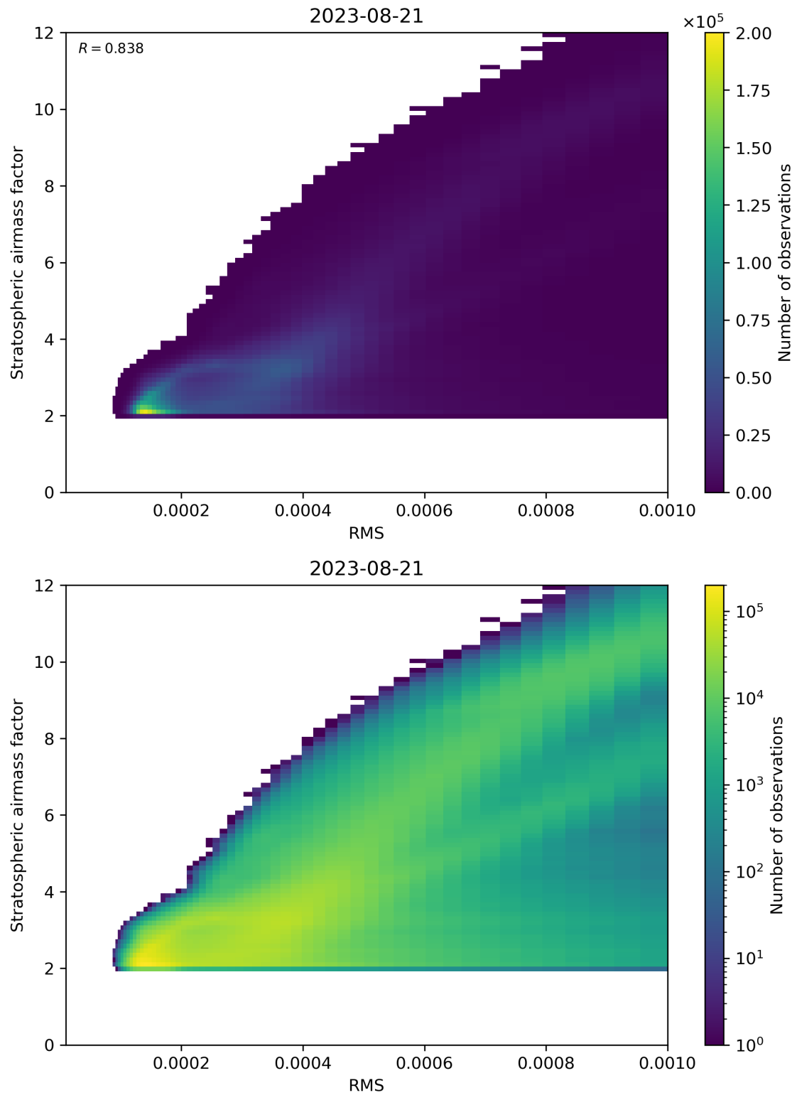
Figure 144: Scatter density plot of “RMS” against “Stratospheric airmass factor” for 2023-08-20 to 2023-08-22.
