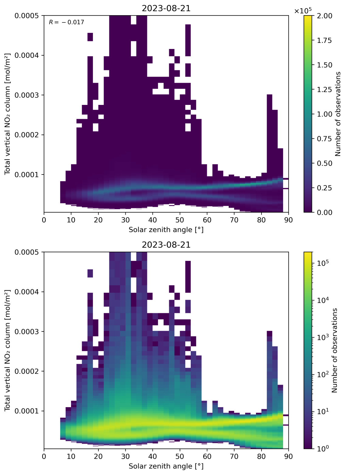
Figure 153: Scatter density plot of “Solar zenith angle” against “Total vertical NO 2 column” for 2023-08-20 to 2023-08-22.
