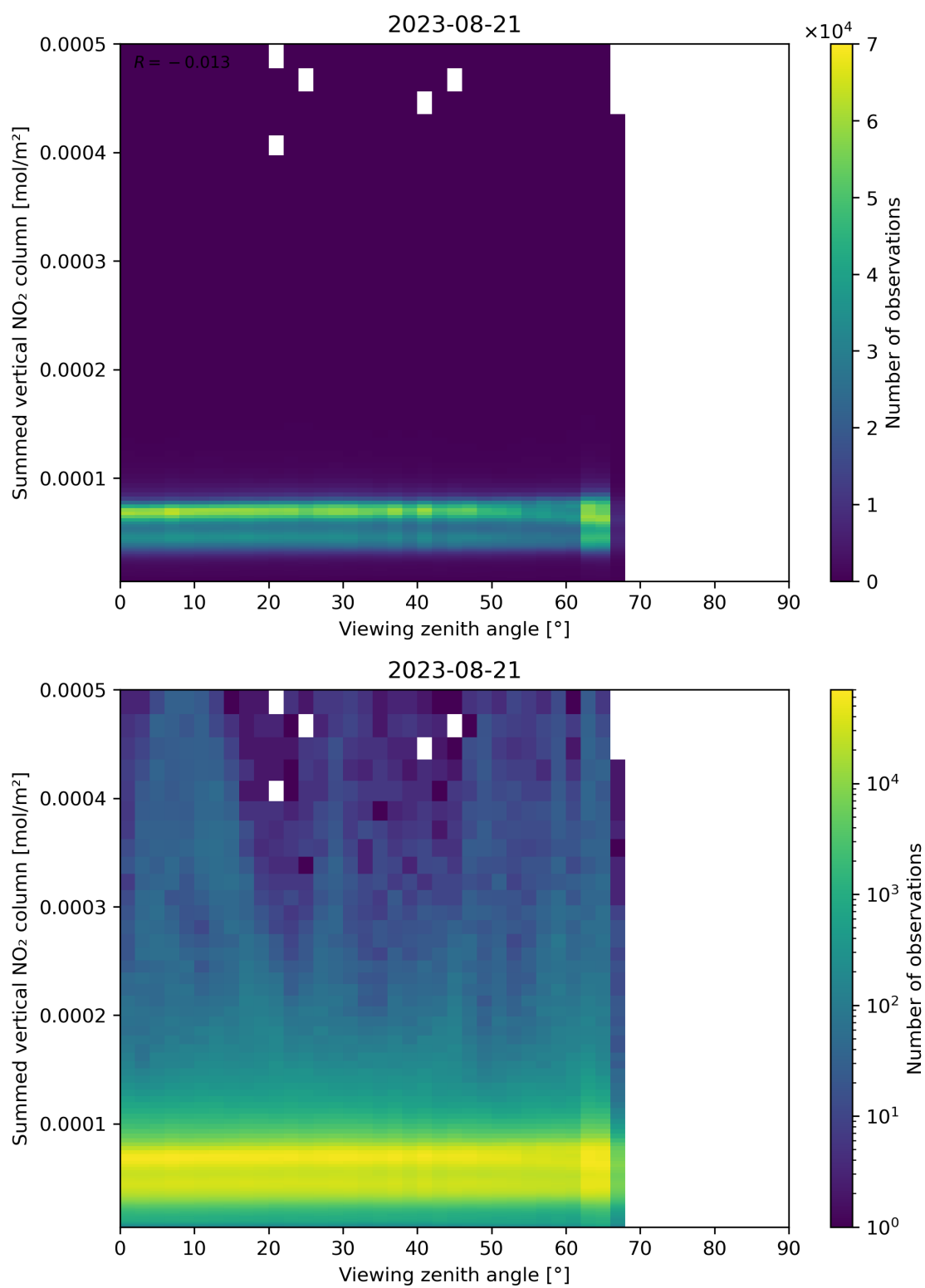
Figure 165: Scatter density plot of “Viewing zenith angle” against “Summed vertical NO 2 column” for 2023-08-20 to 2023-08-22.
