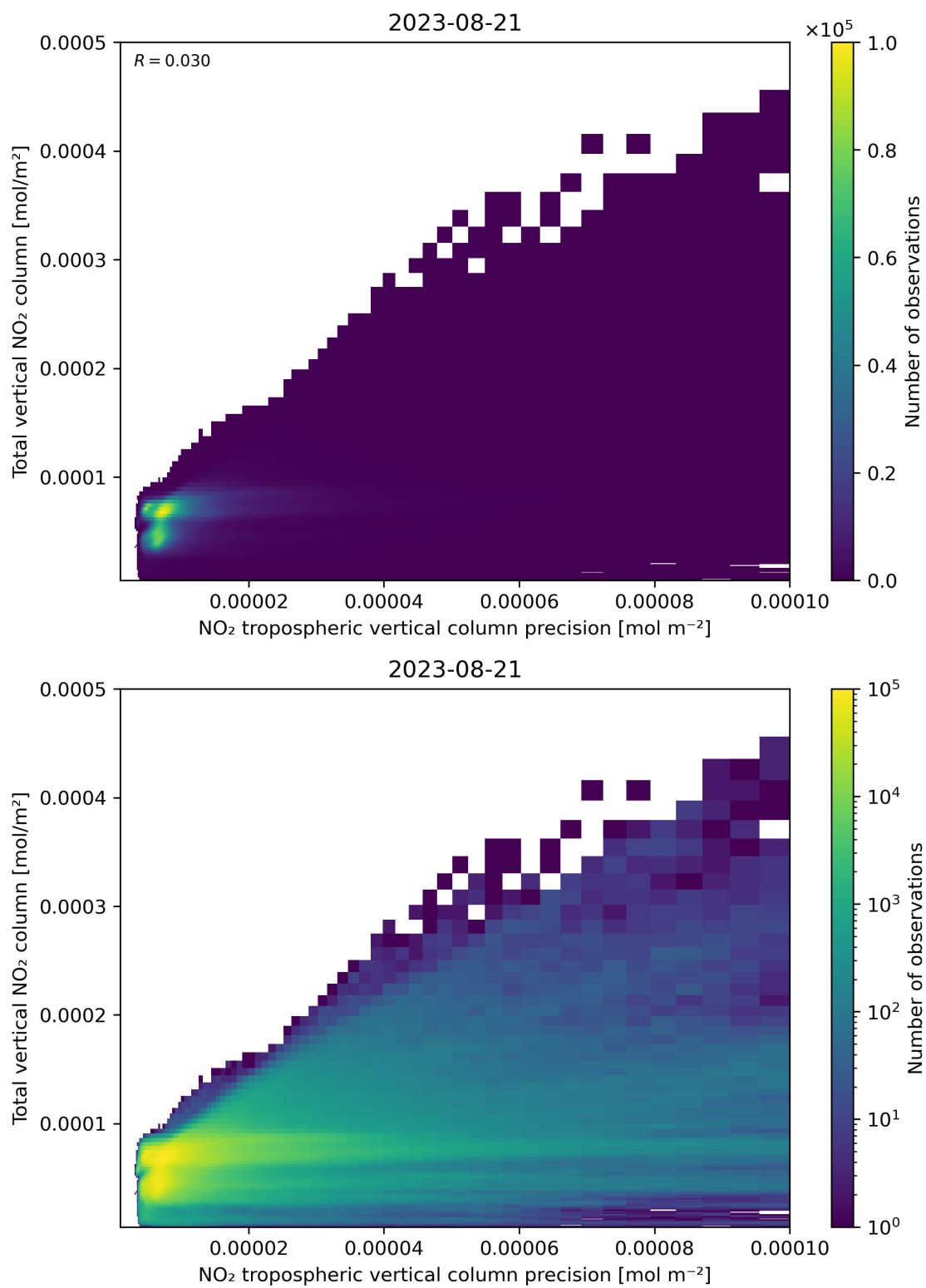
Figure 138: Scatter density plot of “NO 2 tropospheric vertical column precision” against “Total vertical NO 2 column” for 2023-08-20 to 2023-08-22.
