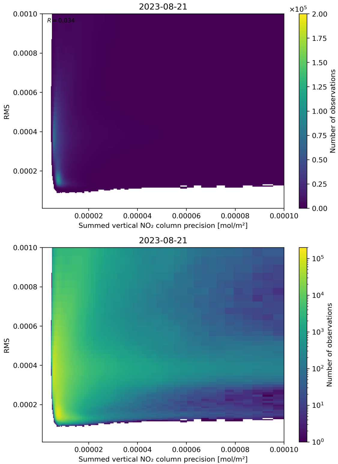
Figure 108: Scatter density plot of “Summed vertical NO 2 column precision” against “RMS” for 2023-08-20 to 2023-08-22.
