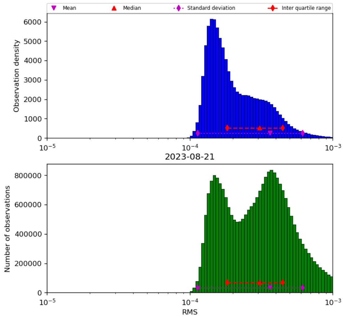
Figure 43: Histogram of “RMS” for 2023-08-20 to 2023-08-22
