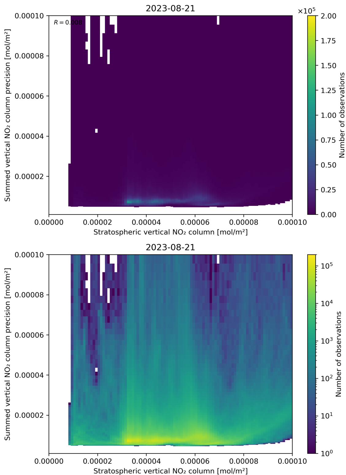
Figure 99: Scatter density plot of “Stratospheric vertical NO 2 column” against “Summed vertical NO 2 column precision” for 2023-08-20 to 2023-08-22.
