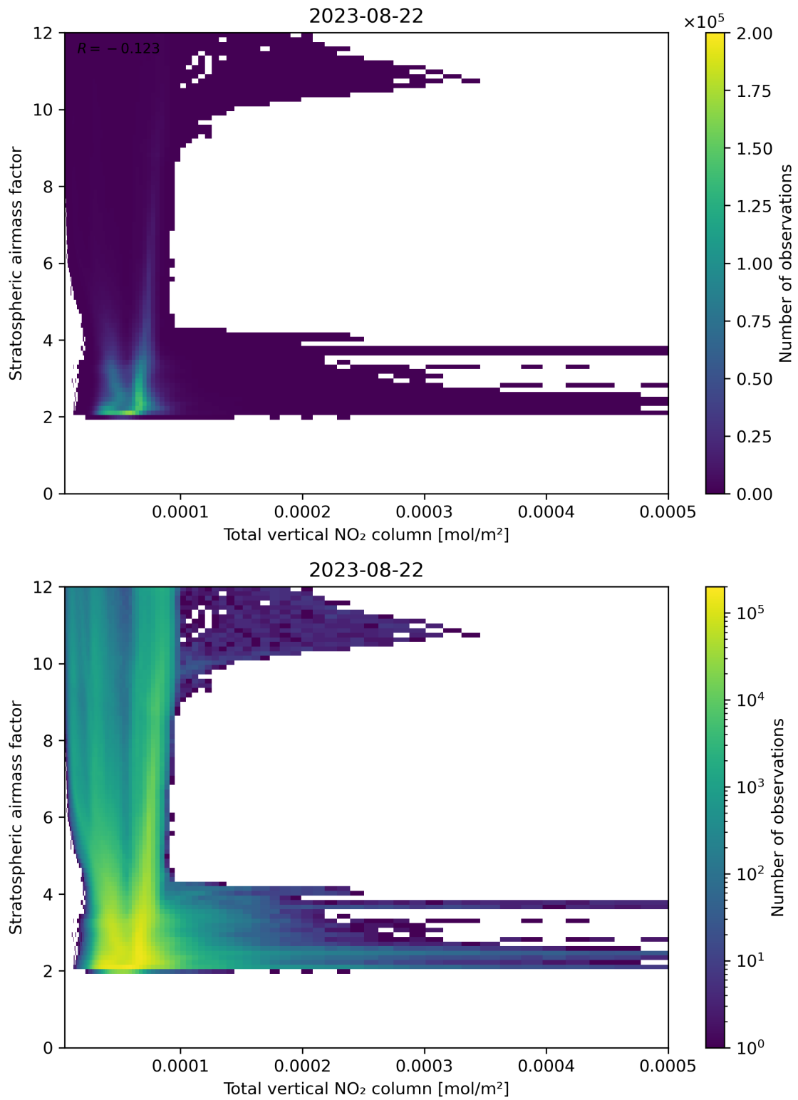
Figure 110: Scatter density plot of “Total vertical NO 2 column” against “Stratospheric airmass factor” for 2023-08-21 to 2023-08-23.
