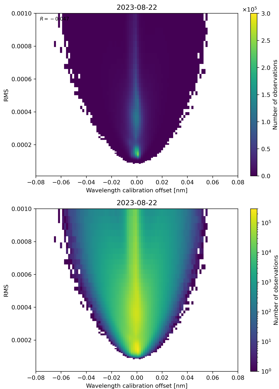
Figure 181: Scatter density plot of “Wavelength calibration offset” against “RMS” for 2023-08-21 to 2023-08-23.
