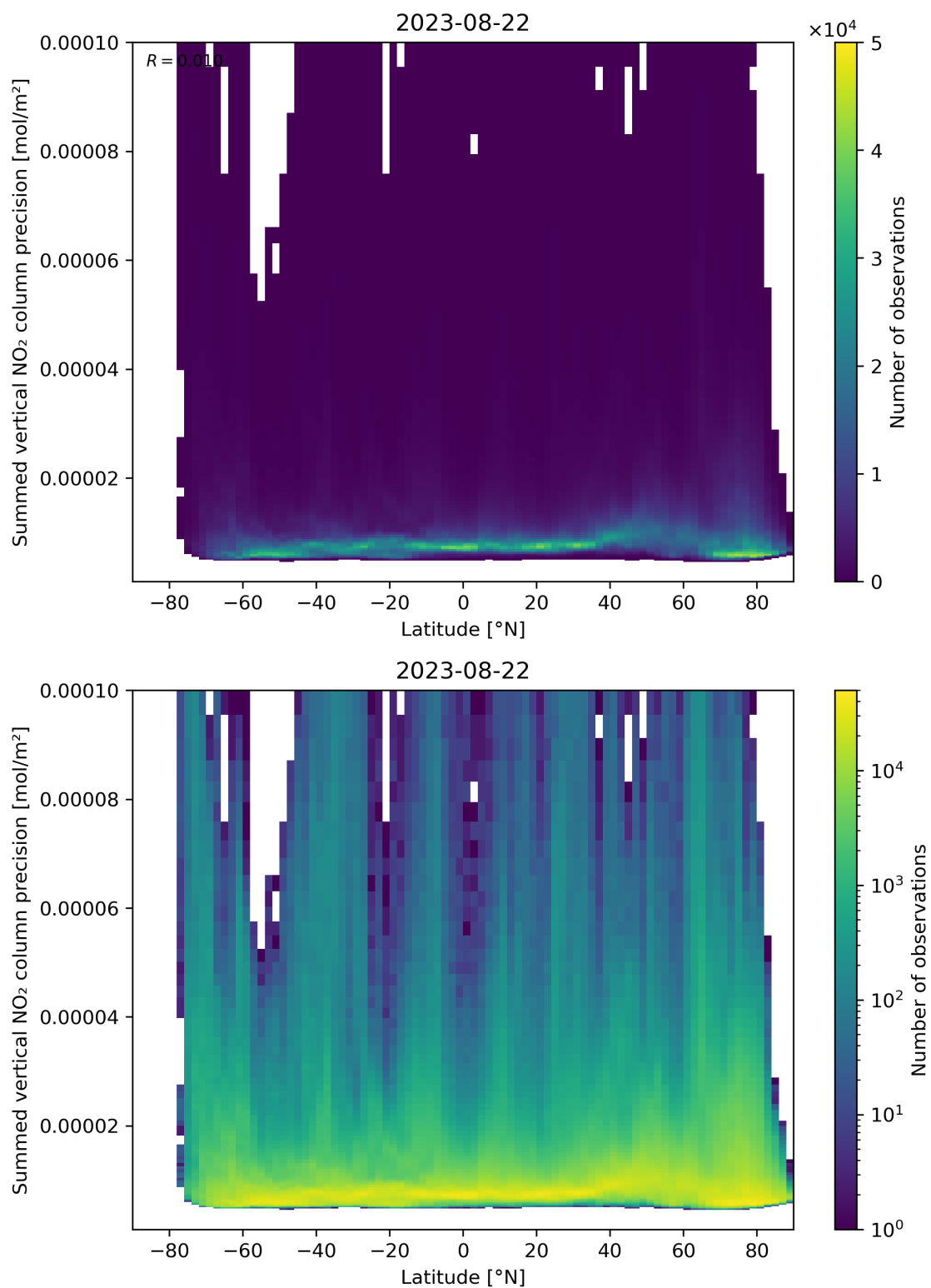
Figure 89: Scatter density plot of “Latitude” against “Summed vertical NO 2 column precision” for 2023-08-21 to 2023-08-23.
