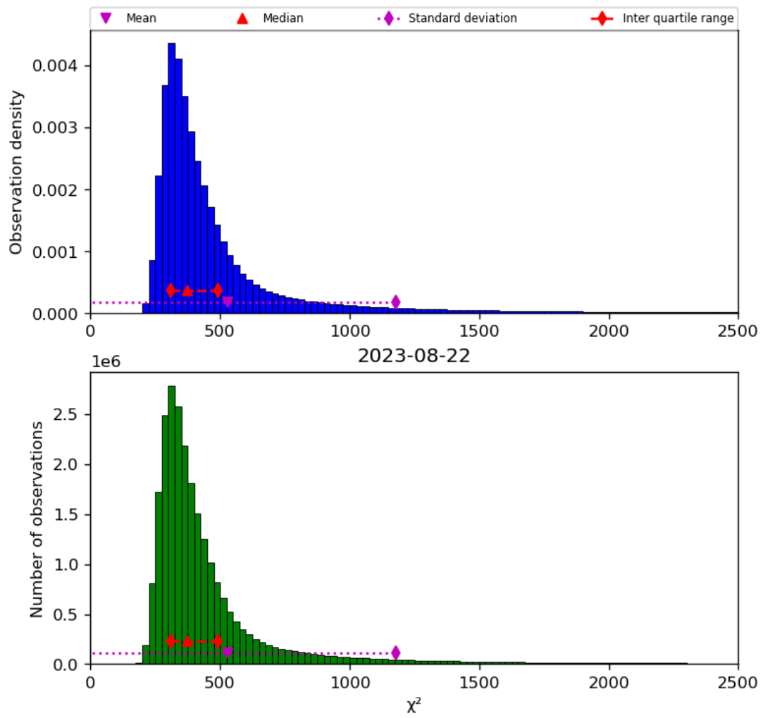
Figure 42: Histogram of “ \chi^2 ” for 2023-08-21 to 2023-08-23
