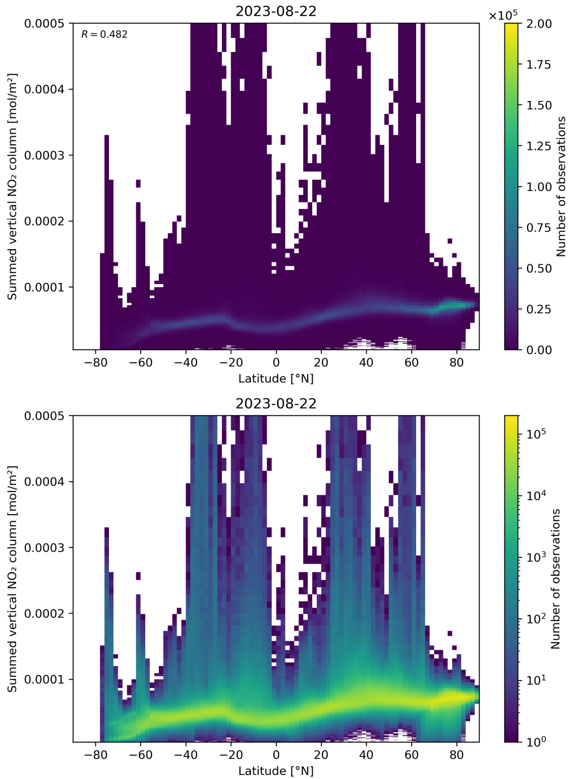
Figure 88: Scatter density plot of “Latitude” against “Summed vertical NO 2 column” for 2023-08-21 to 2023-08-23.
