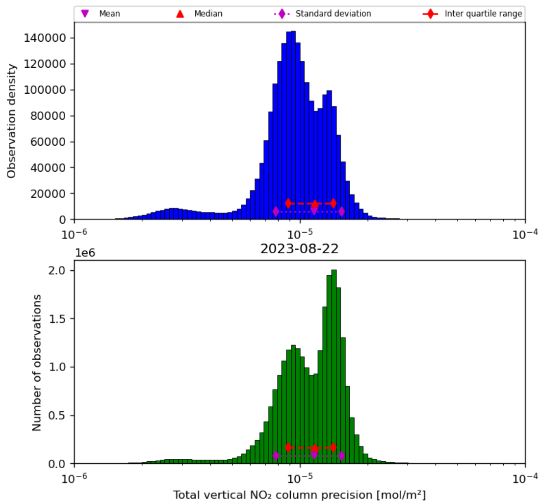
Figure 39: Histogram of “Total vertical NO 2 column precision” for 2023-08-21 to 2023-08-23
