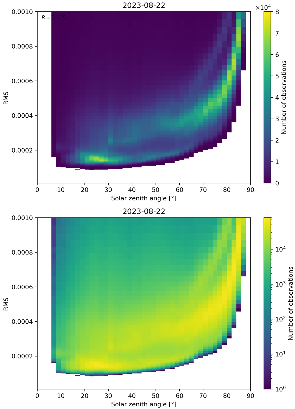
Figure 157: Scatter density plot of “Solar zenith angle” against “RMS” for 2023-08-21 to 2023-08-23.
