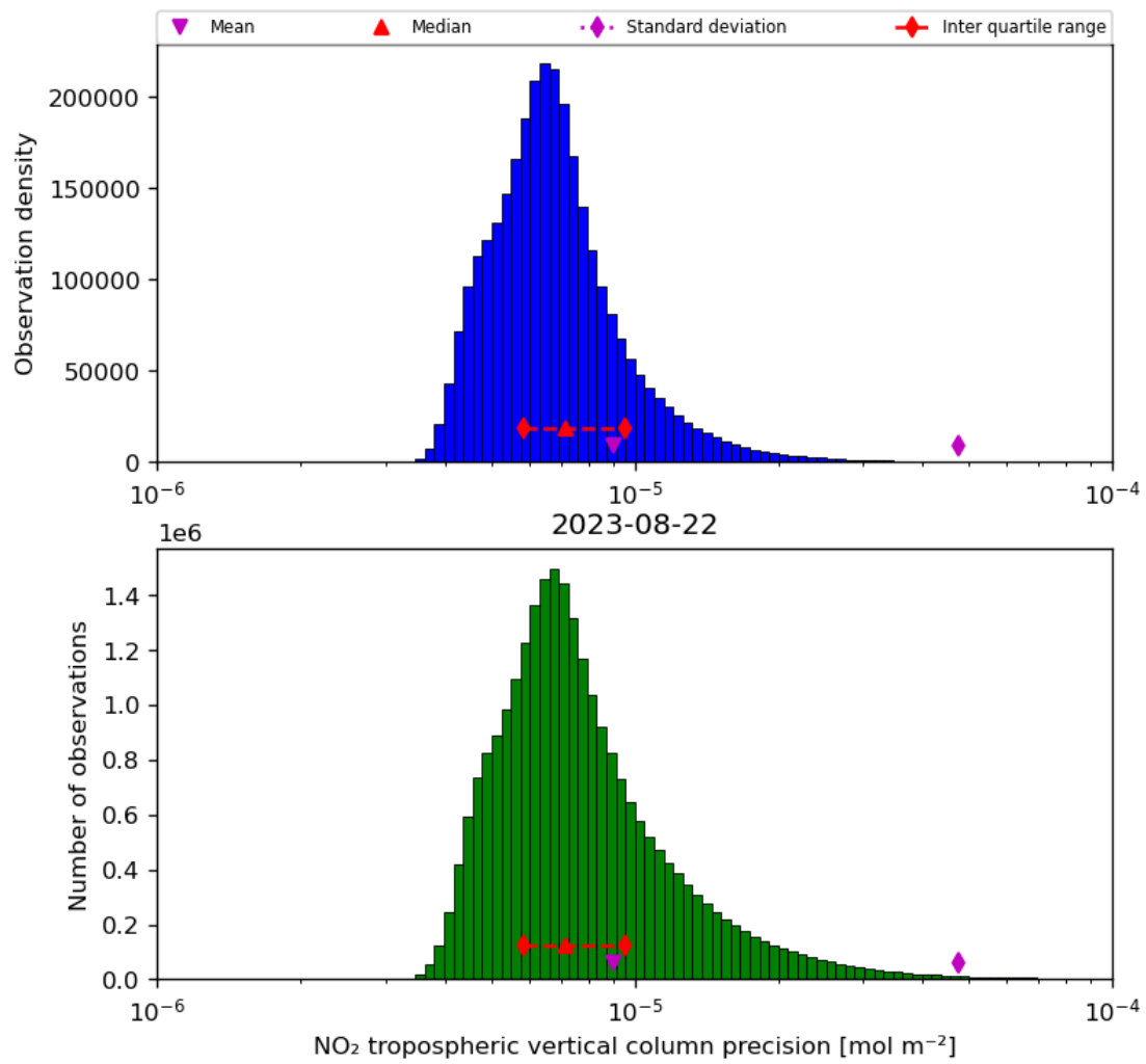
Figure 30: Histogram of “NO 2 tropospheric vertical column precision” for 2023-08-21 to 2023-08-23
