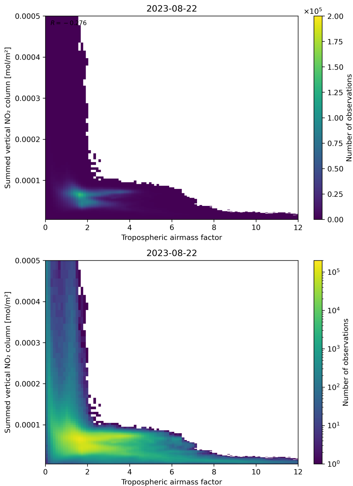
Figure 75: Scatter density plot of “Tropospheric airmass factor” against “Summed vertical NO 2 column” for 2023-08-21 to 2023-08-23.
