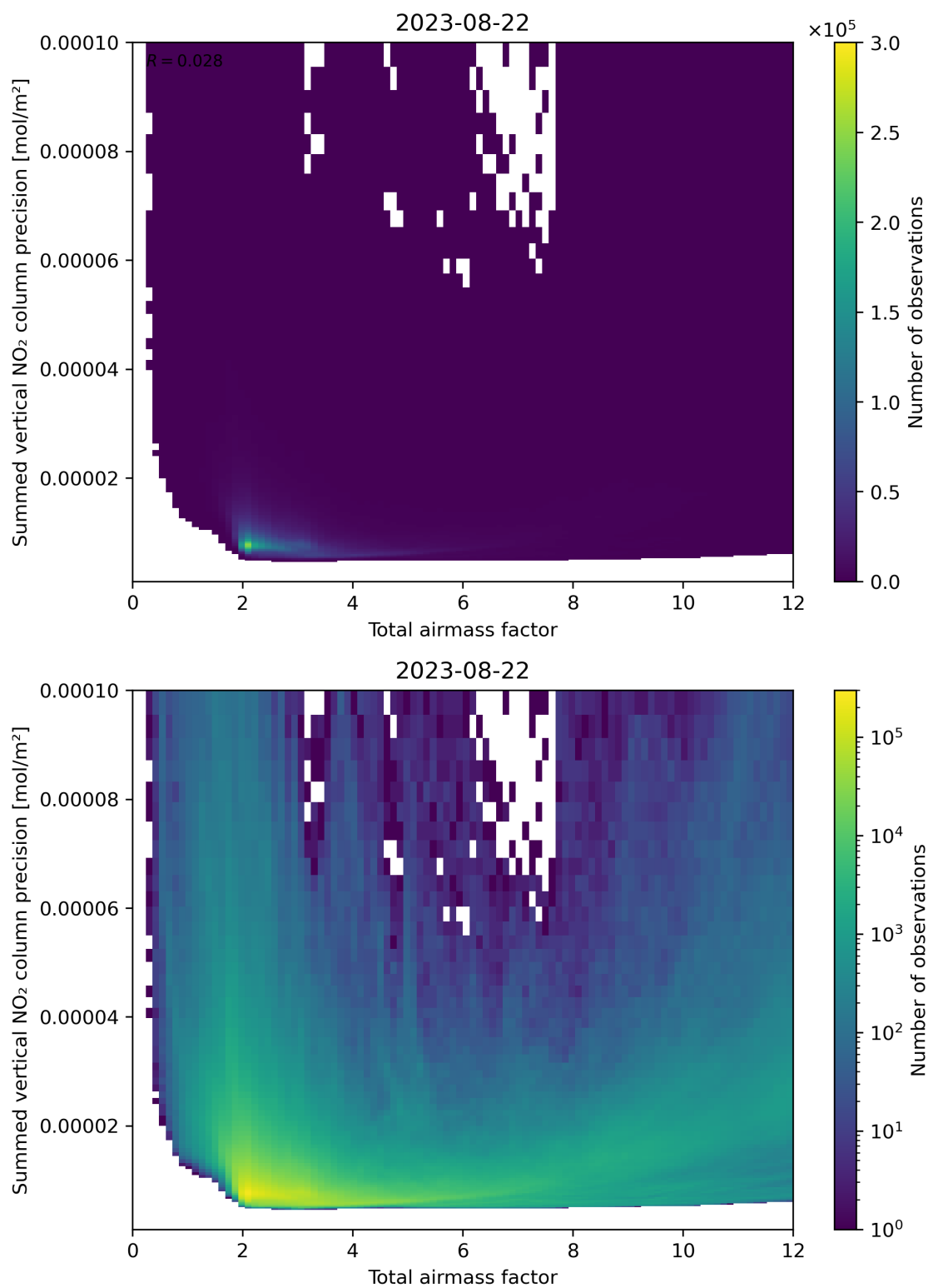
Figure 66: Scatter density plot of “Total airmass factor” against “Summed vertical NO 2 column precision” for 2023-08-21 to 2023-08-23.
