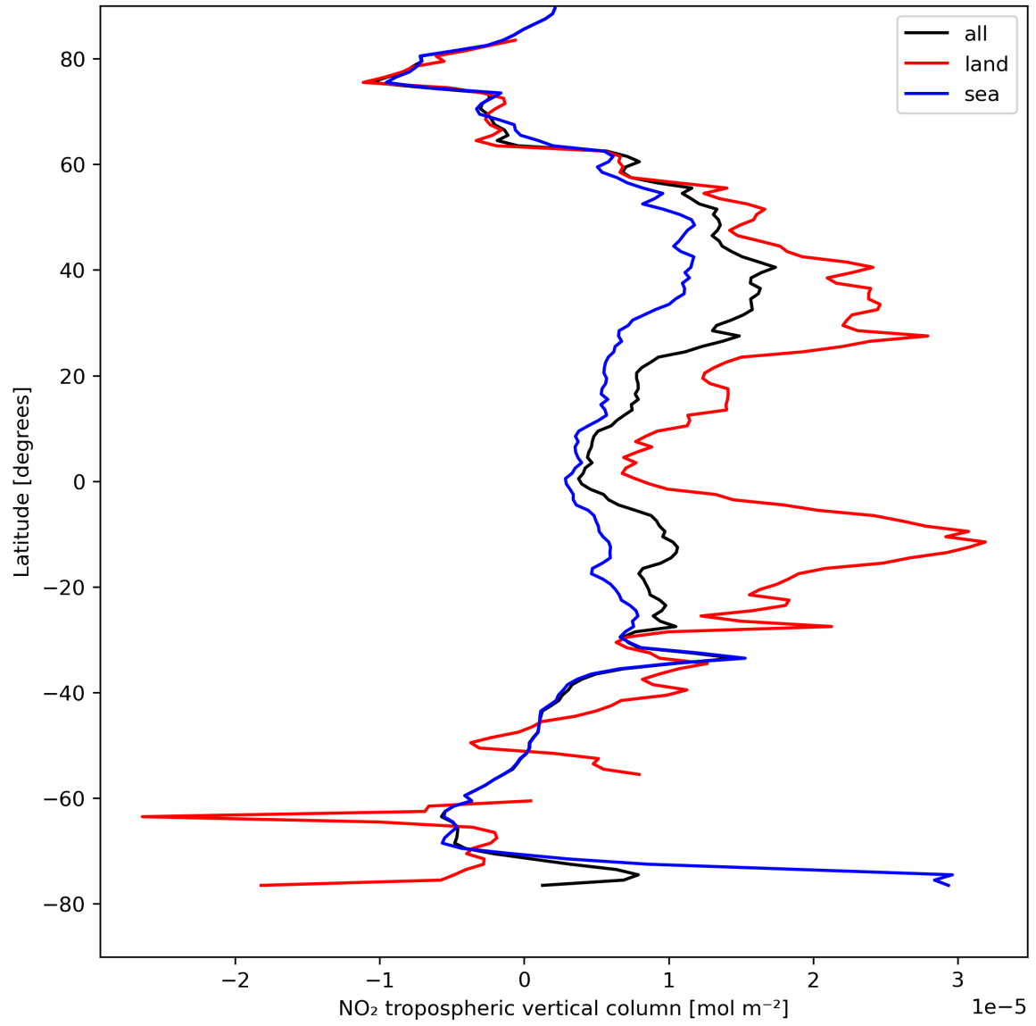
Figure 12: Zonal average of “NO 2 tropospheric vertical column” for 2023-08-21 to 2023-08-23.
