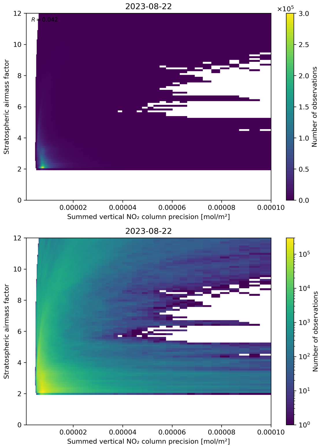
Figure 106: Scatter density plot of “Summed vertical NO 2 column precision” against “Stratospheric airmass factor” for 2023-08-21 to 2023-08-23.
