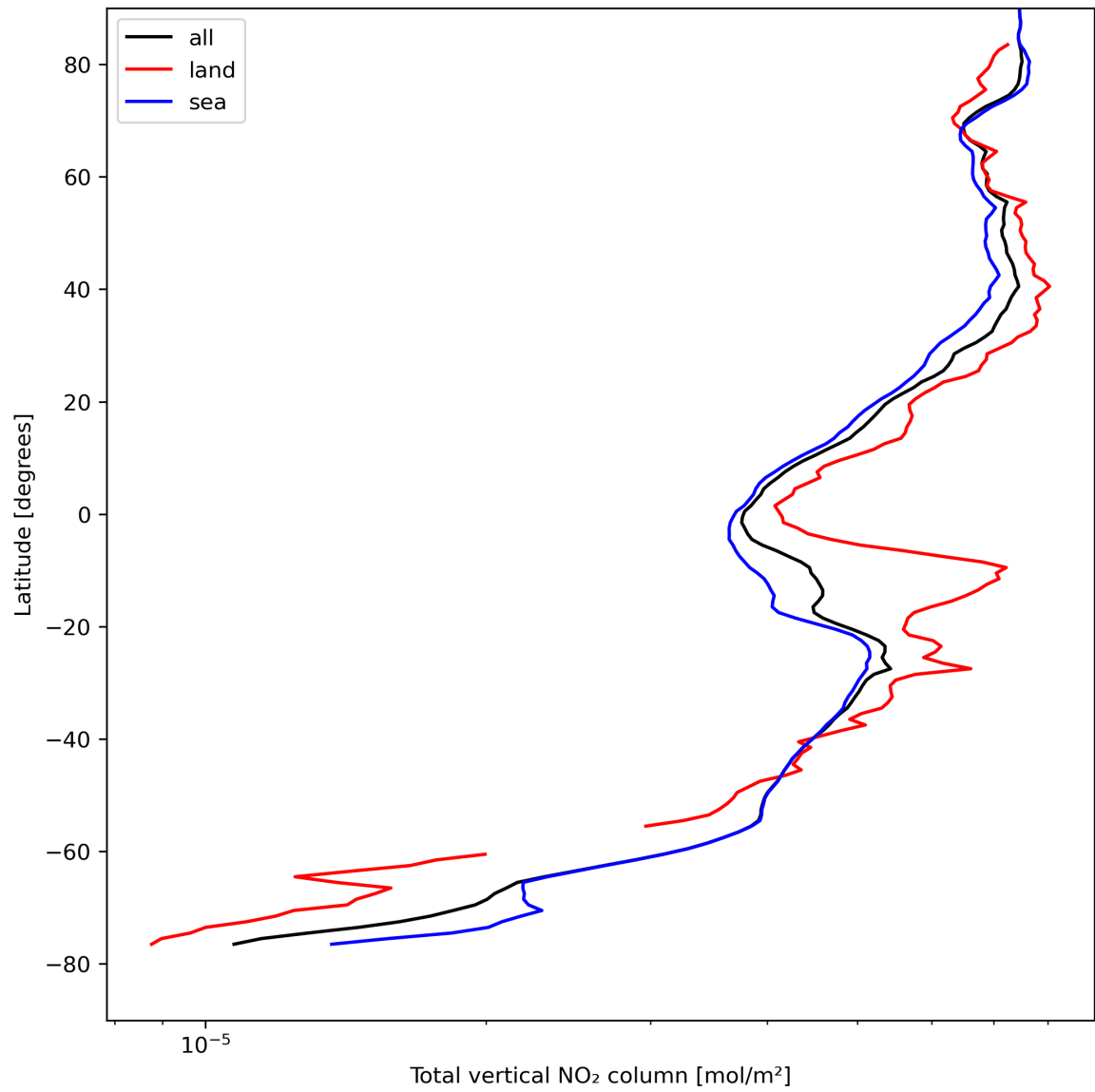
Figure 21: Zonal average of “Total vertical NO 2 column” for 2023-08-21 to 2023-08-23.
