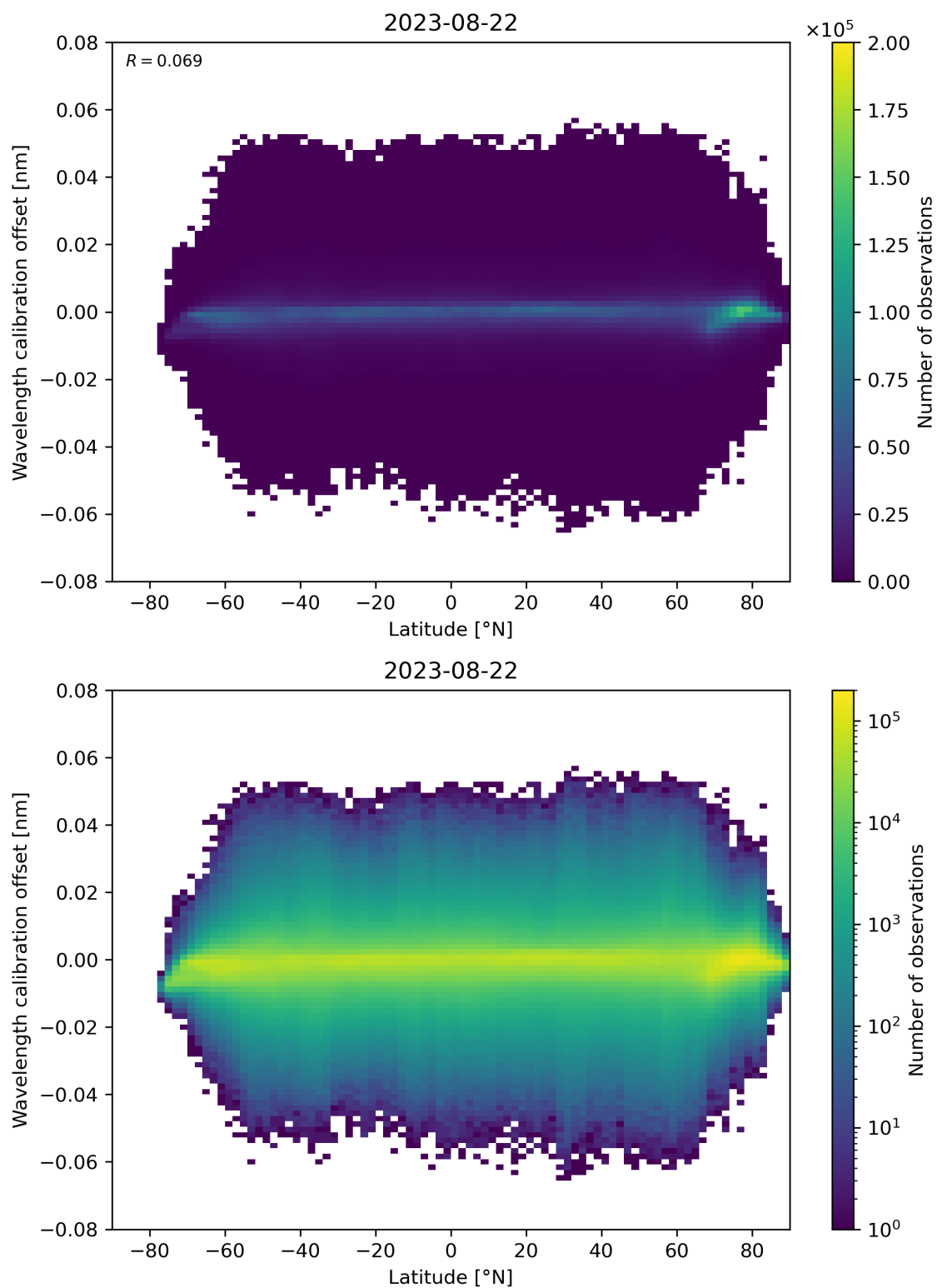
Figure 95: Scatter density plot of “Latitude” against “Wavelength calibration offset” for 2023-08-21 to 2023-08-23.
