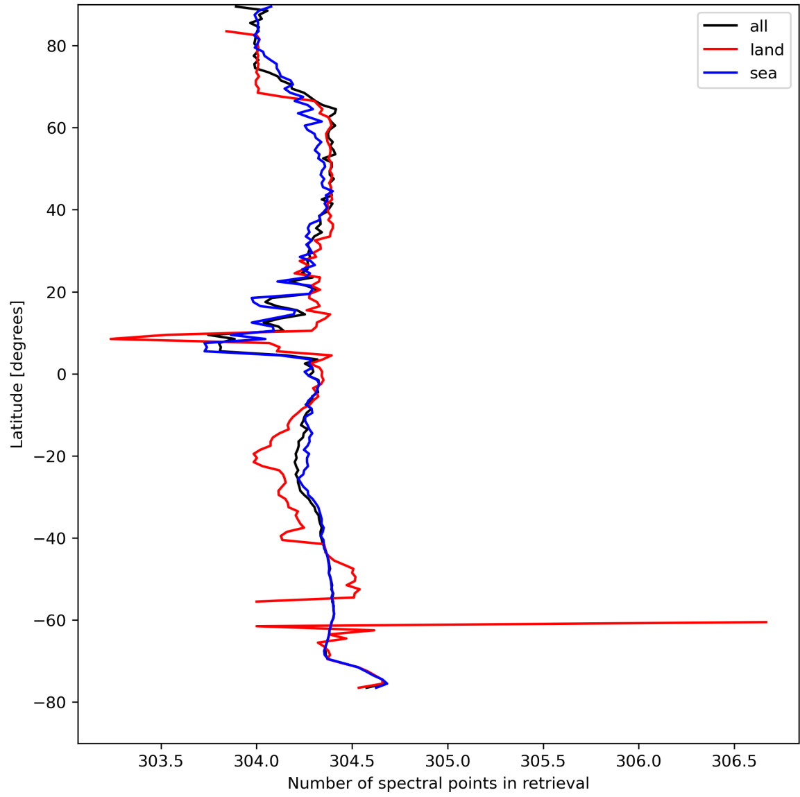
Figure 16: Zonal average of “Number of spectral points in retrieval” for 2023-08-21 to 2023-08-23.
