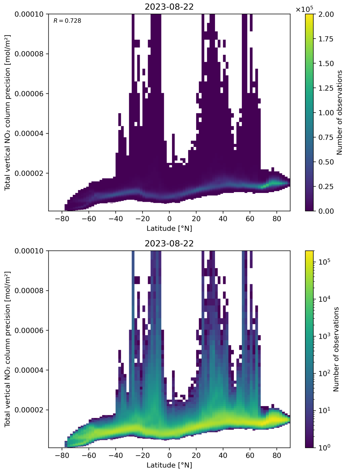
Figure 91: Scatter density plot of “Latitude” against “Total vertical NO 2 column precision” for 2023-08-21 to 2023-08-23.
