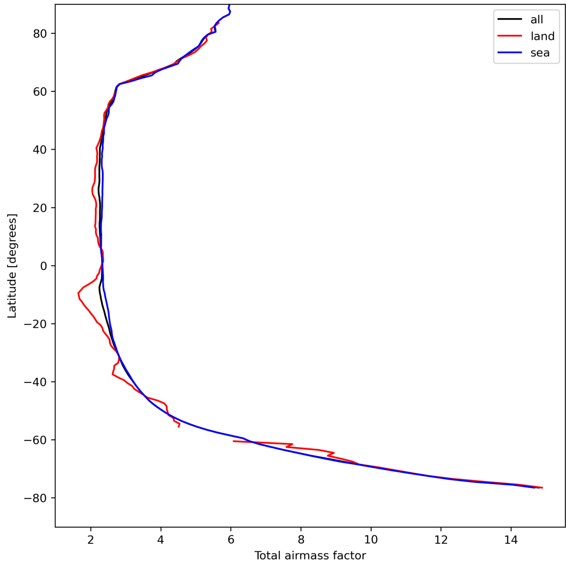
Figure 15: Zonal average of “Total airmass factor” for 2023-08-21 to 2023-08-23.
