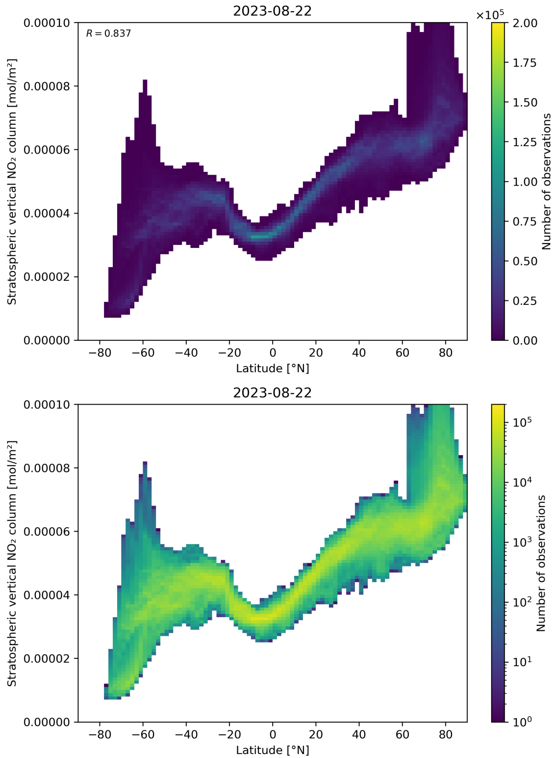
Figure 87: Scatter density plot of “Latitude” against “Stratospheric vertical \text{NO}_2 column” for 2023-08-21 to 2023-08-23.
