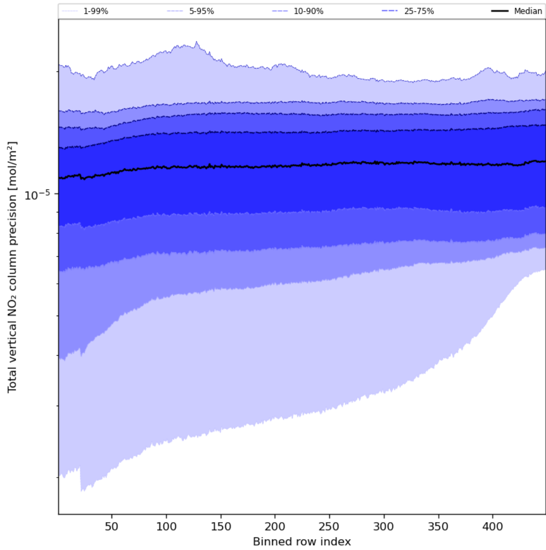
Figure 56: Along track statistics of “Total vertical NO 2 column precision” for 2023-08-21 to 2023-08-23
