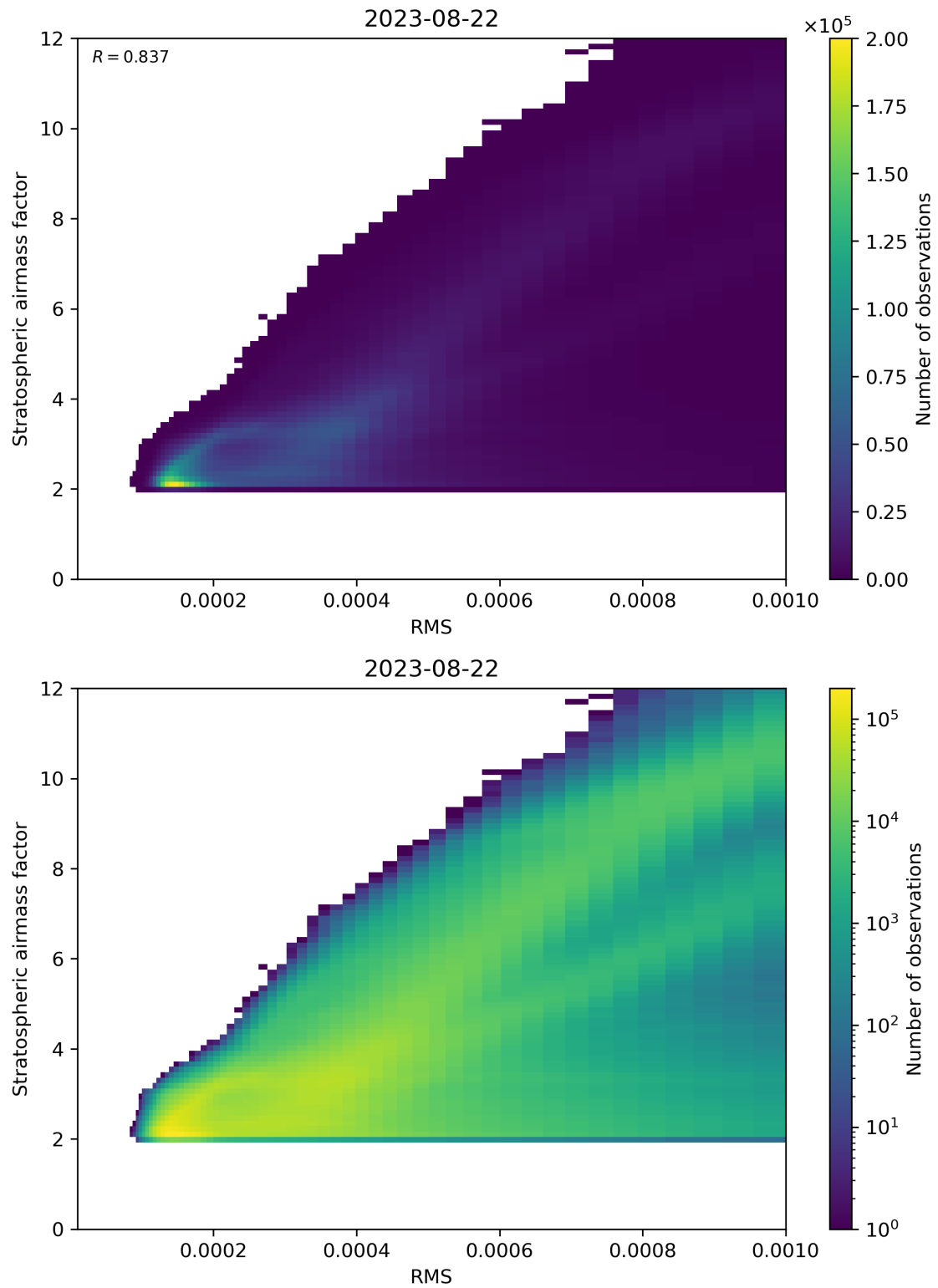
Figure 144: Scatter density plot of “RMS” against “Stratospheric airmass factor” for 2023-08-21 to 2023-08-23.
