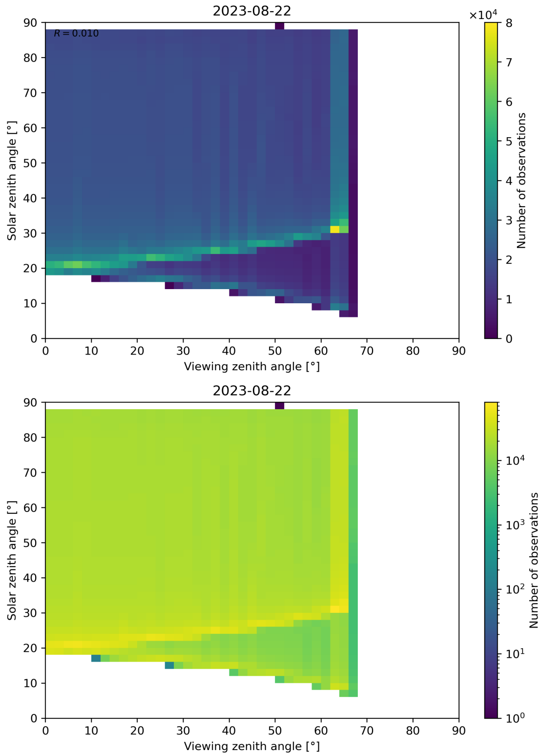
Figure 172: Scatter density plot of “Viewing zenith angle” against “Solar zenith angle” for 2023-08-21 to 2023-08-23.
