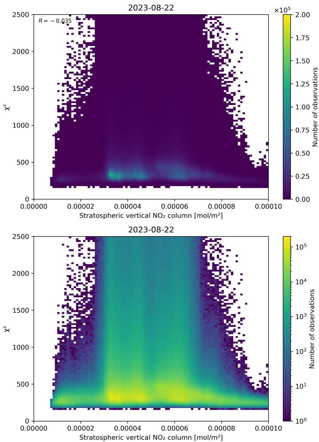
Figure 97: Scatter density plot of “Stratospheric vertical NO 2 column” against “ \chi^2 ” for 2023-08-21 to 2023-08-23.
