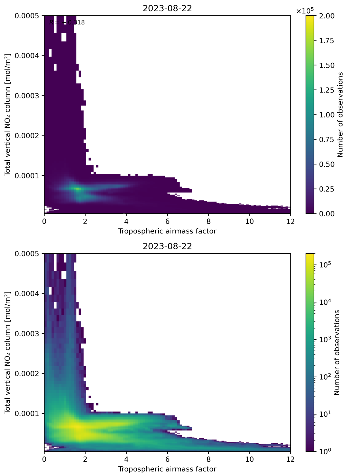
Figure 77: Scatter density plot of “Tropospheric airmass factor” against “Total vertical NO 2 column” for 2023-08-21 to 2023-08-23.
