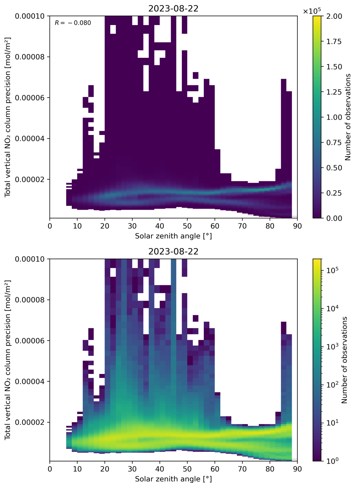
Figure 154: Scatter density plot of “Solar zenith angle” against “Total vertical NO 2 column precision” for 2023-08-21 to 2023-08-23.
