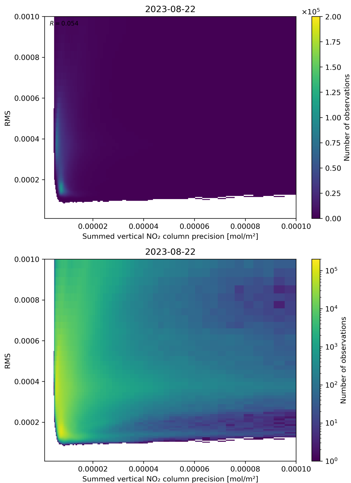
Figure 108: Scatter density plot of “Summed vertical NO 2 column precision” against “RMS” for 2023-08-21 to 2023-08-23.
