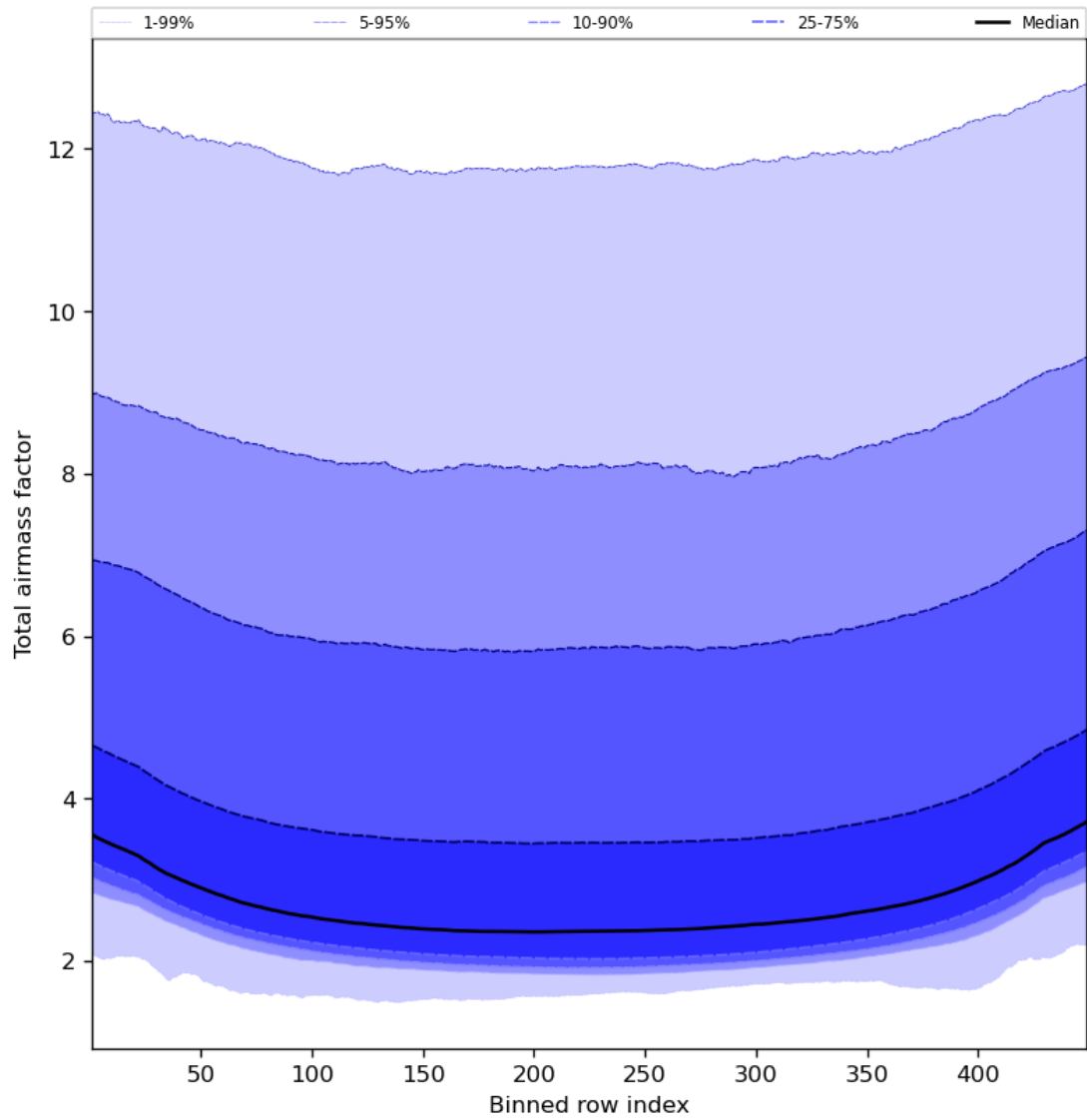
Figure 49: Along track statistics of “Total airmass factor” for 2023-08-21 to 2023-08-23
