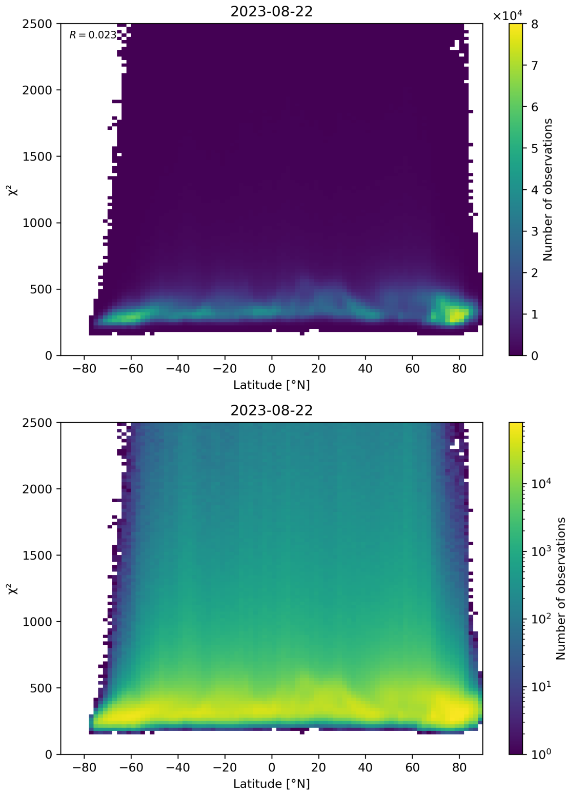
Figure 86: Scatter density plot of “Latitude” against “ \chi^2 ” for 2023-08-21 to 2023-08-23.
