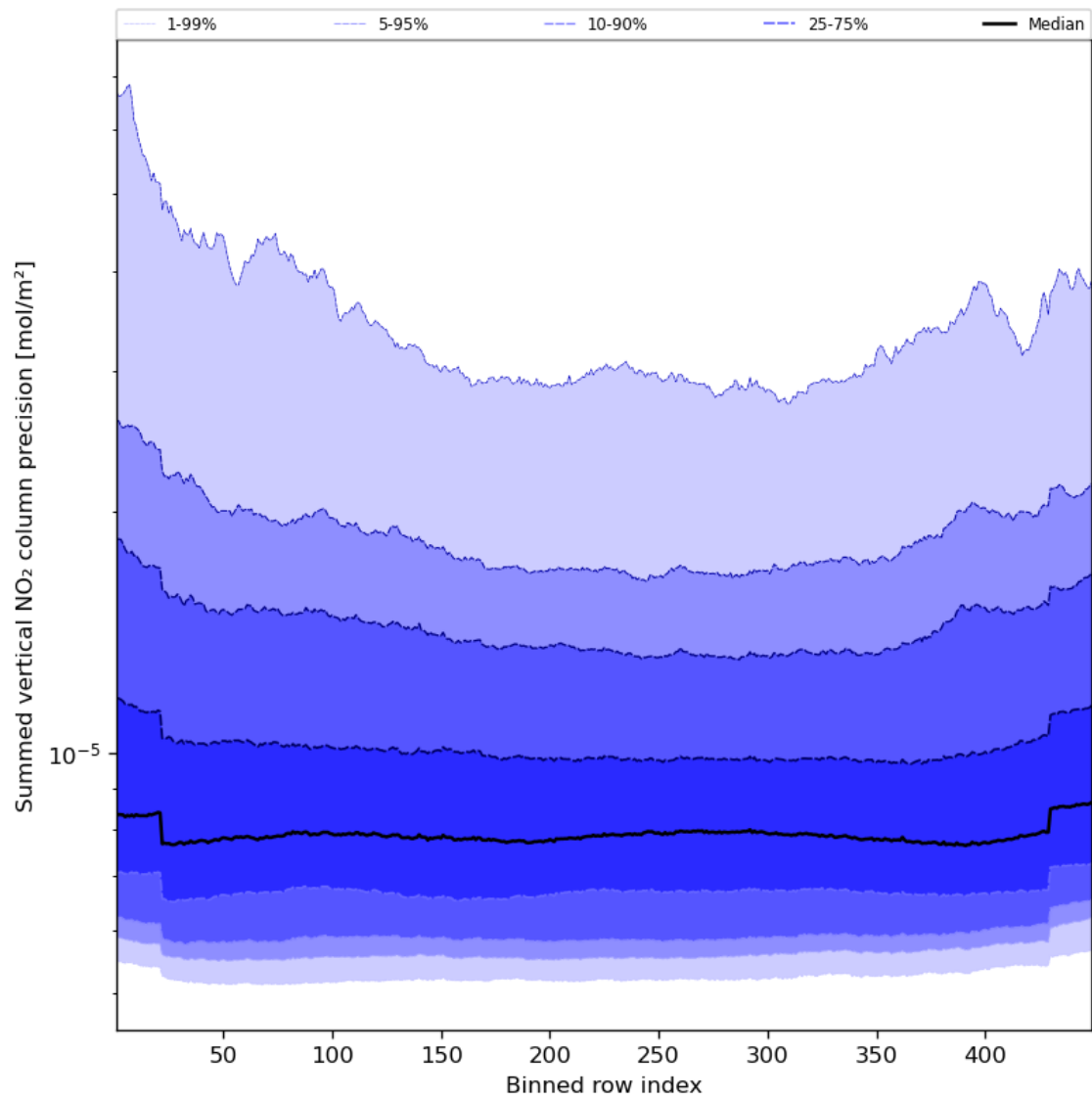
Figure 58: Along track statistics of “Summed vertical NO 2 column precision” for 2023-08-21 to 2023-08-23
