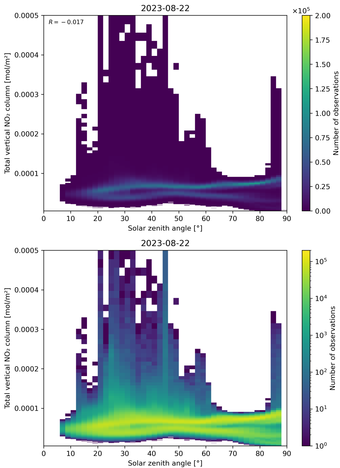
Figure 153: Scatter density plot of “Solar zenith angle” against “Total vertical NO 2 column” for 2023-08-21 to 2023-08-23.
