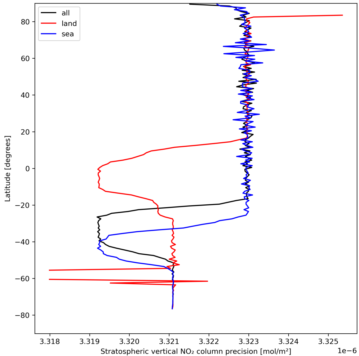
Figure 20: Zonal average of “Stratospheric vertical NO 2 column precision” for 2023-08-21 to 2023-08-23.
