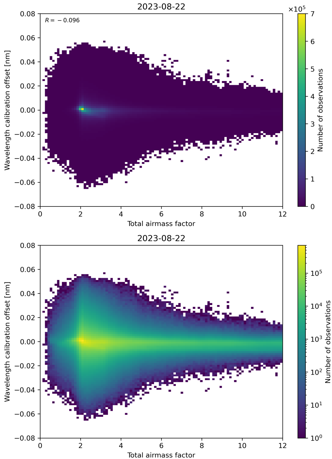
Figure 70: Scatter density plot of “Total airmass factor” against “Wavelength calibration offset” for 2023-08-21 to 2023-08-23.
