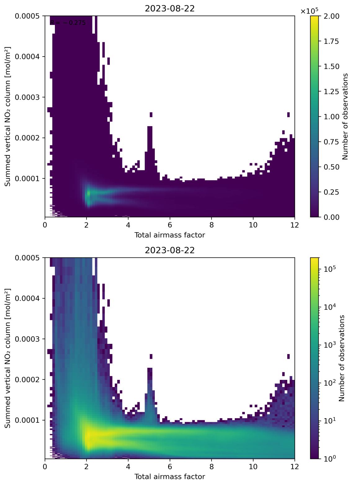
Figure 65: Scatter density plot of “Total airmass factor” against “Summed vertical NO 2 column” for 2023-08-21 to 2023-08-23.
