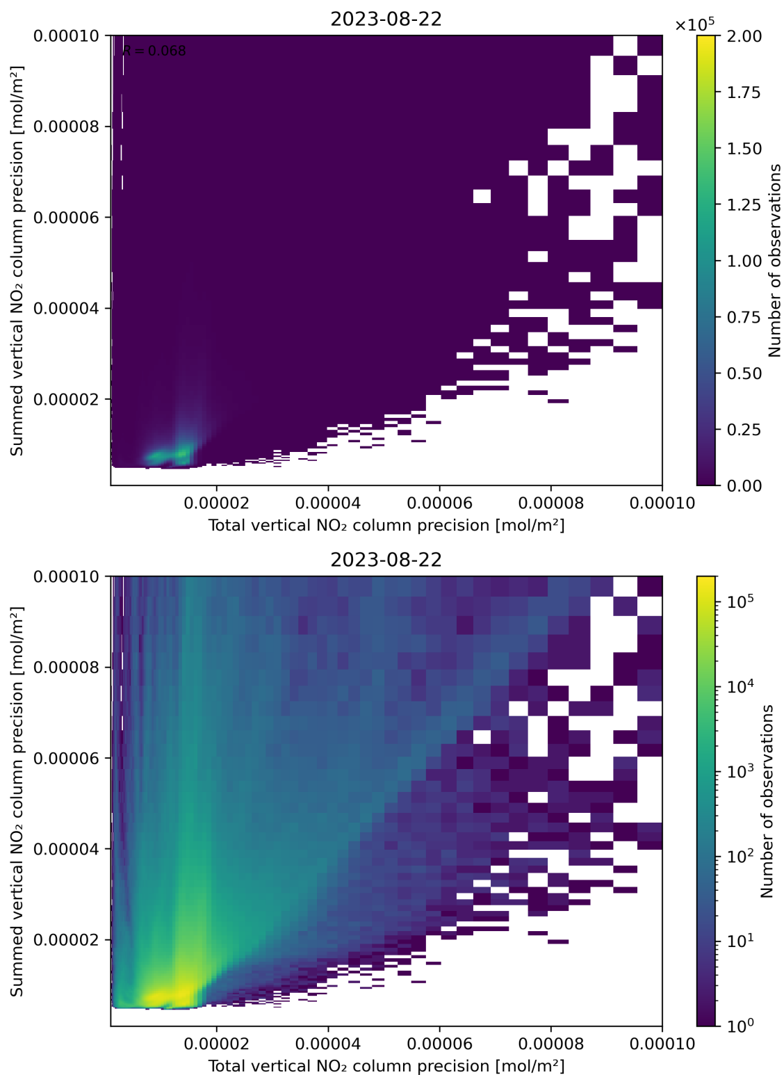
Figure 118: Scatter density plot of “Total vertical NO 2 column precision” against “Summed vertical NO 2 column precision” for 2023-08-21 to 2023-08-23.
