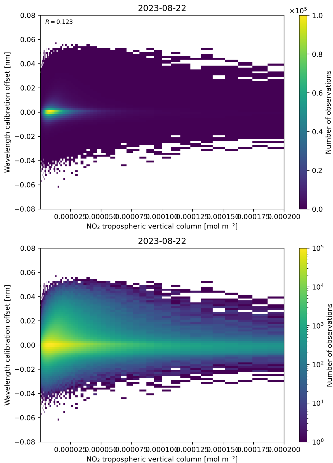
Figure 143: Scatter density plot of “NO 2 tropospheric vertical column” against “Wavelength calibration offset” for 2023-08-21 to 2023-08-23.
