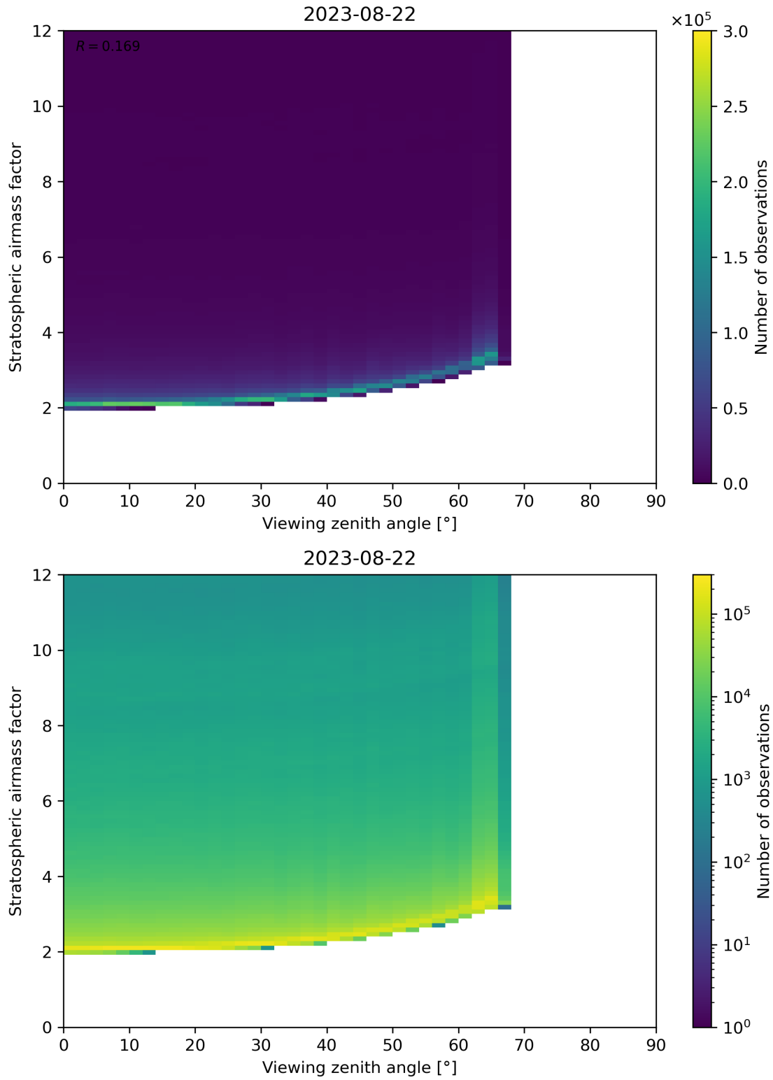
Figure 159: Scatter density plot of “Viewing zenith angle” against “Stratospheric airmass factor” for 2023-08-21 to 2023-08-23.
