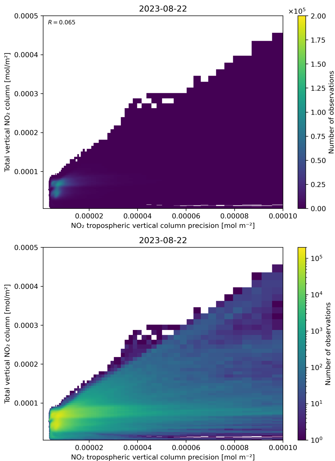
Figure 138: Scatter density plot of “NO 2 tropospheric vertical column precision” against “Total vertical NO 2 column” for 2023-08-21 to 2023-08-23.
