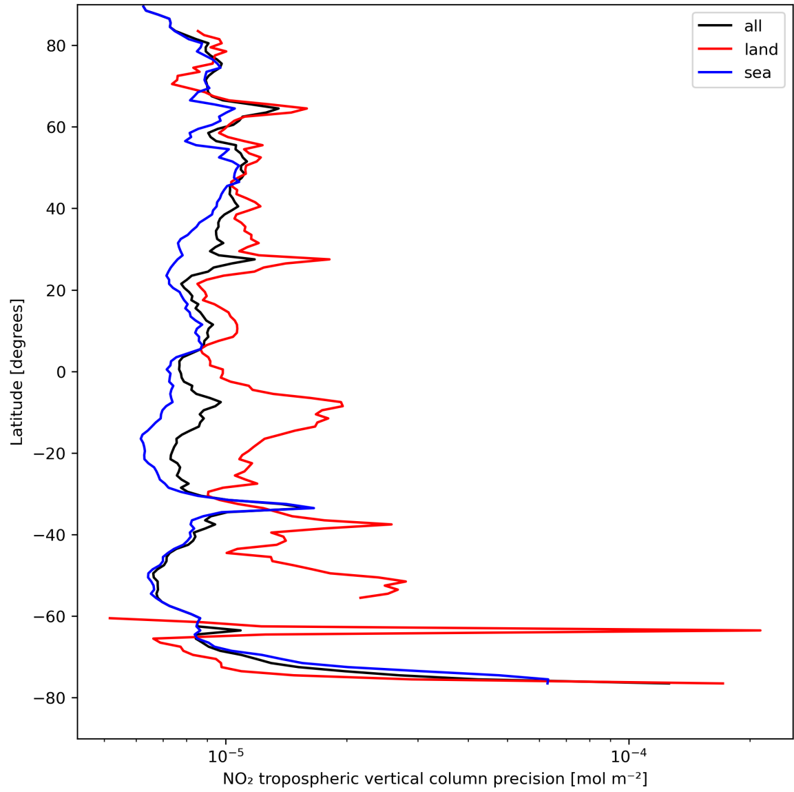
Figure 13: Zonal average of “NO 2 tropospheric vertical column precision” for 2023-08-21 to 2023-08-23.
