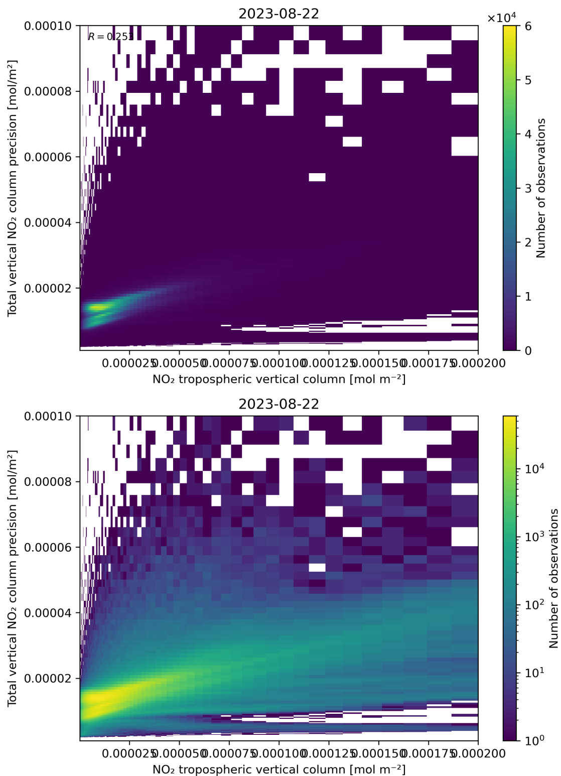
Figure 129: Scatter density plot of “NO 2 tropospheric vertical column” against “Total vertical NO 2 column precision” for 2023-08-21 to 2023-08-23.
