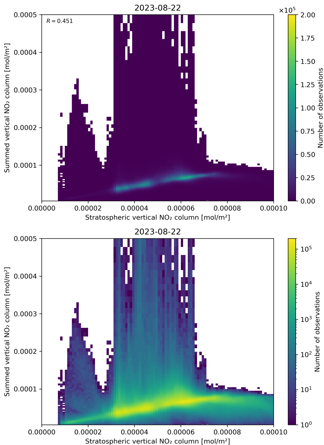
Figure 98: Scatter density plot of “Stratospheric vertical NO 2 column” against “Summed vertical NO 2 column” for 2023-08-21 to 2023-08-23.
