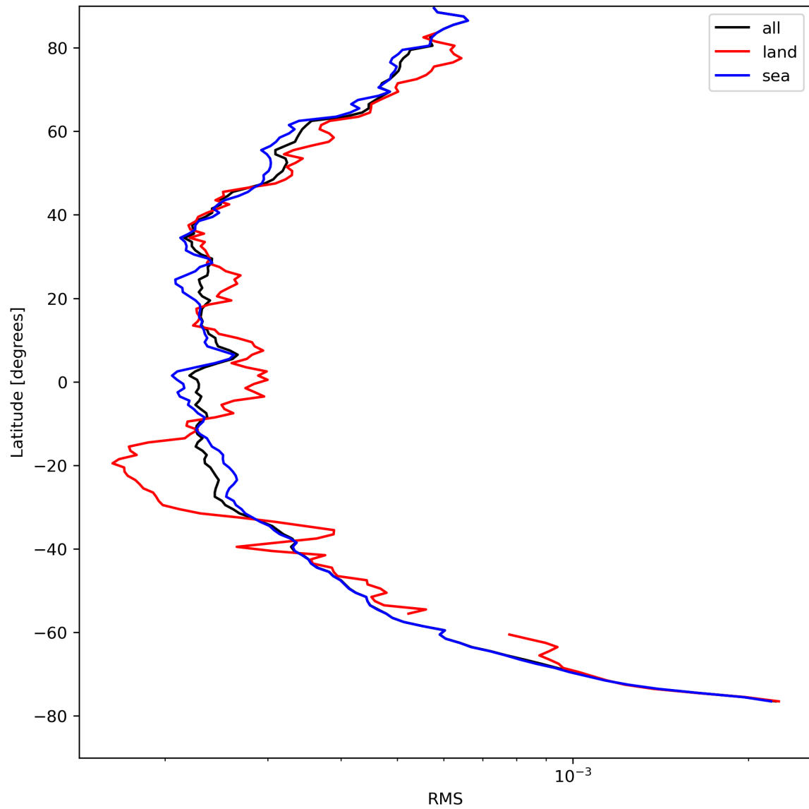
Figure 26: Zonal average of “RMS” for 2023-08-21 to 2023-08-23.
