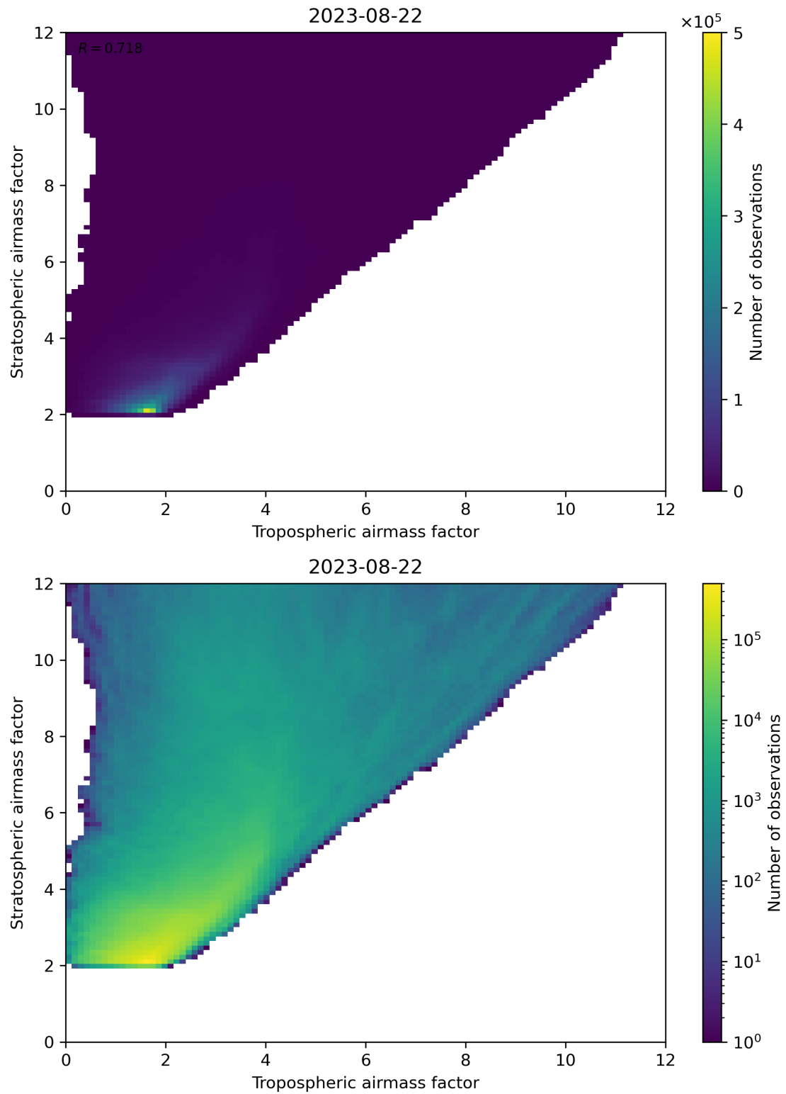
Figure 71: Scatter density plot of “Tropospheric airmass factor” against “Stratospheric airmass factor” for 2023-08-21 to 2023-08-23.
