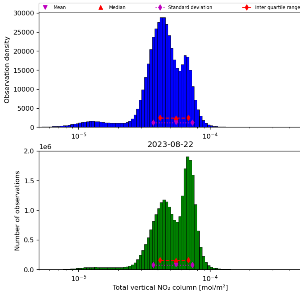
Figure 38: Histogram of "Total vertical NO 2 column" for 2023-08-21 to 2023-08-23
