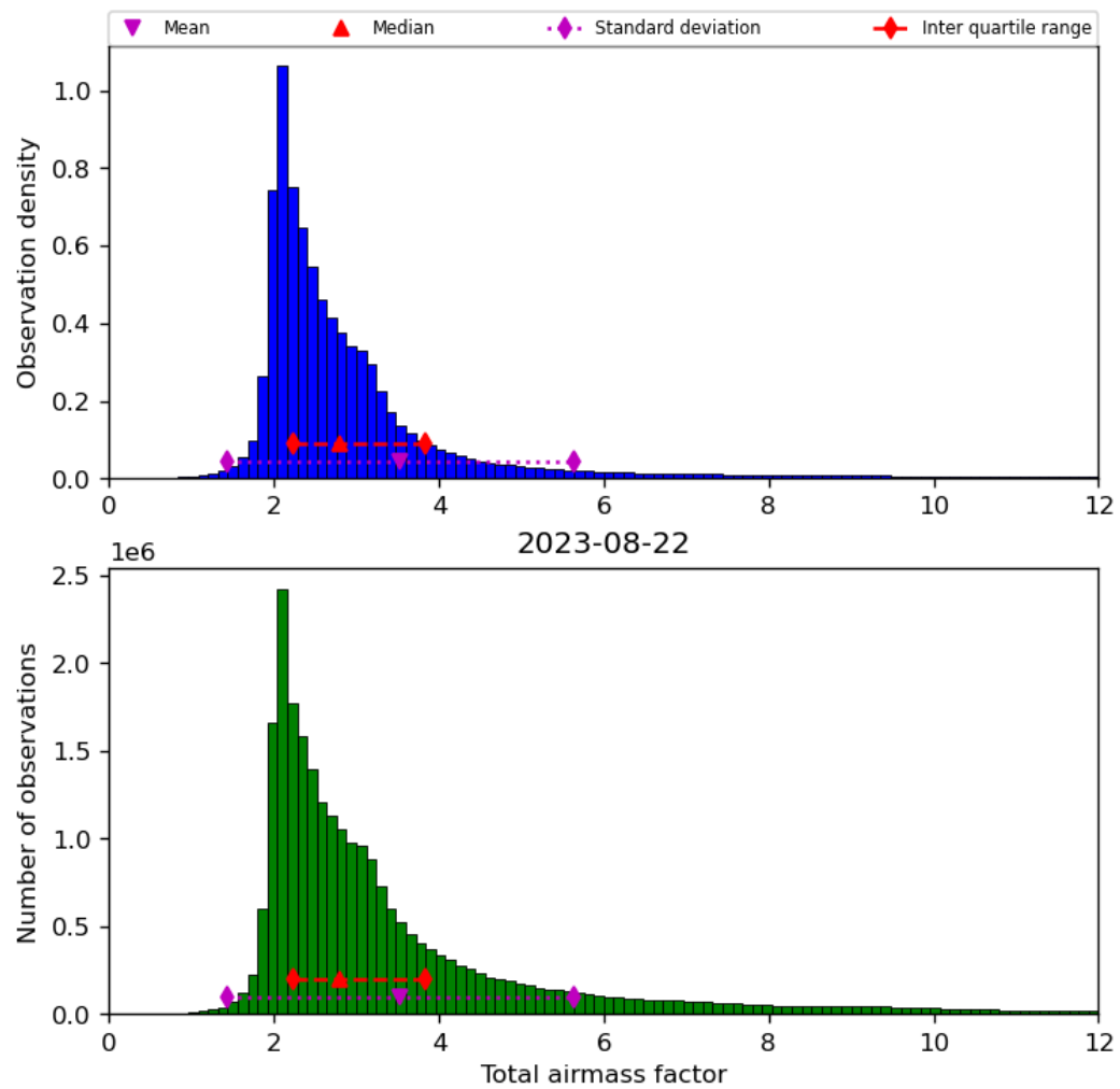
Figure 32: Histogram of “Total airmass factor” for 2023-08-21 to 2023-08-23
