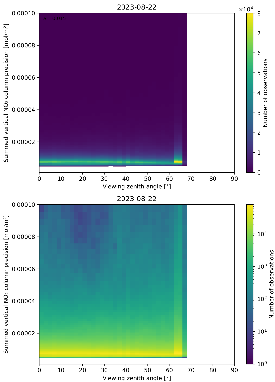
Figure 166: Scatter density plot of “Viewing zenith angle” against “Summed vertical NO 2 column precision” for 2023-08-21 to 2023-08-23.
