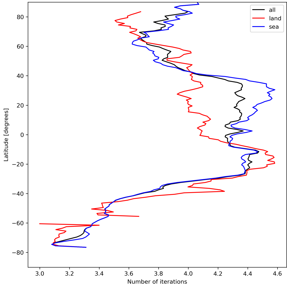
Figure 17: Zonal average of “Number of iterations” for 2023-08-21 to 2023-08-23.
