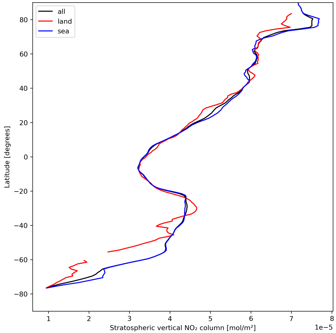
Figure 19: Zonal average of “Stratospheric vertical NO 2 column” for 2023-08-21 to 2023-08-23.
