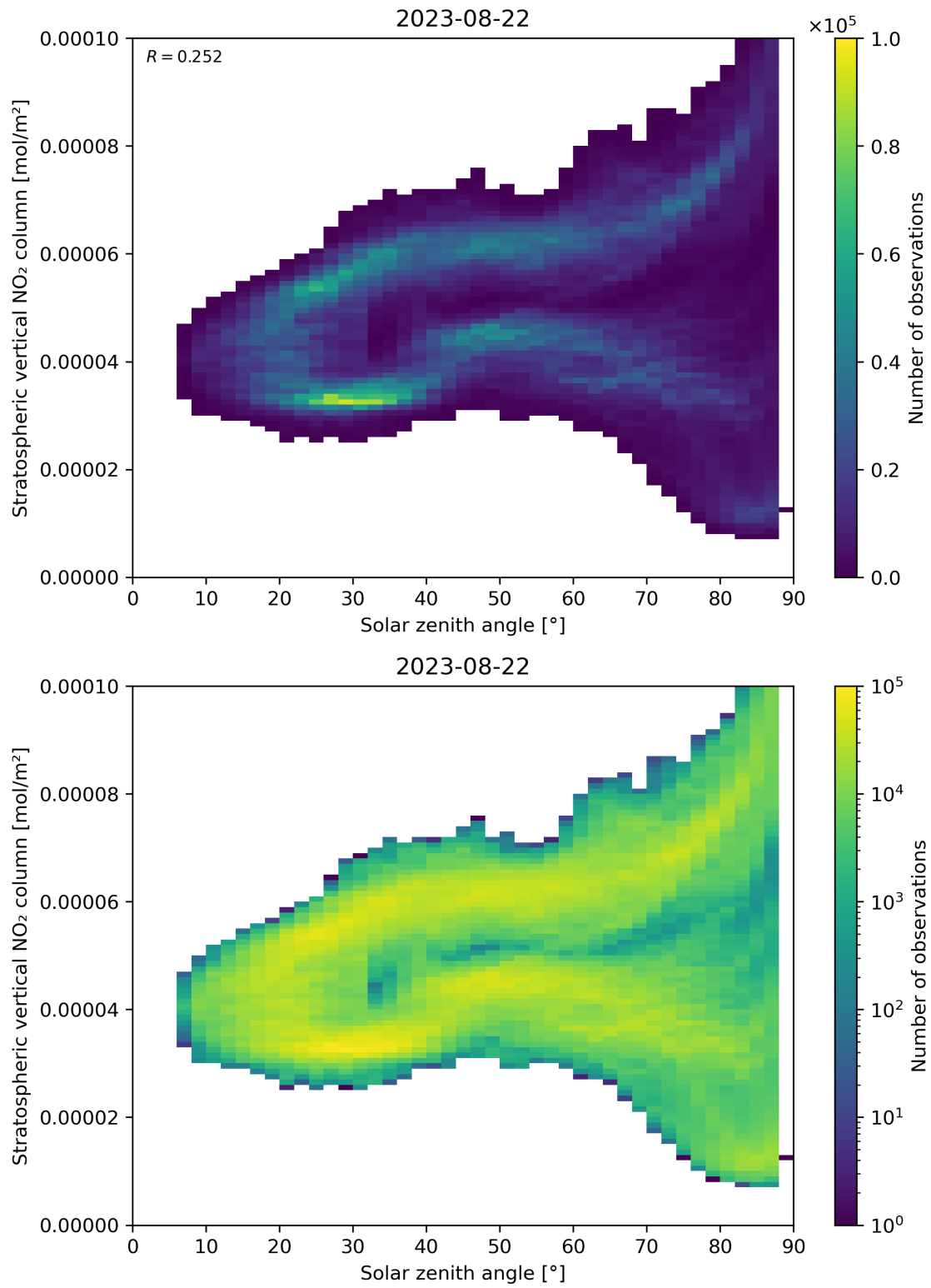
Figure 150: Scatter density plot of “Solar zenith angle” against “Stratospheric vertical NO 2 column” for 2023-08-21 to 2023-08-23.
