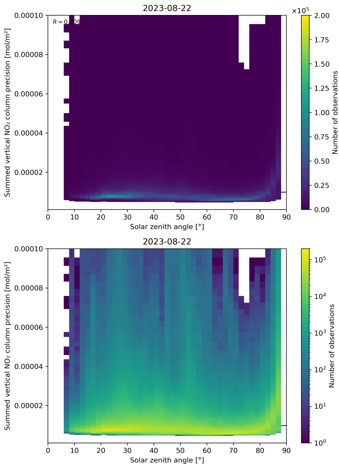
Figure 152: Scatter density plot of “Solar zenith angle” against “Summed vertical NO 2 column precision” for 2023-08-21 to 2023-08-23.
