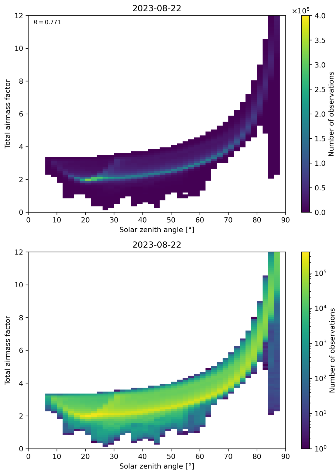
Figure 146: Scatter density plot of “Solar zenith angle” against “Total air mass factor” for 2023-08-21 to 2023-08-23.
