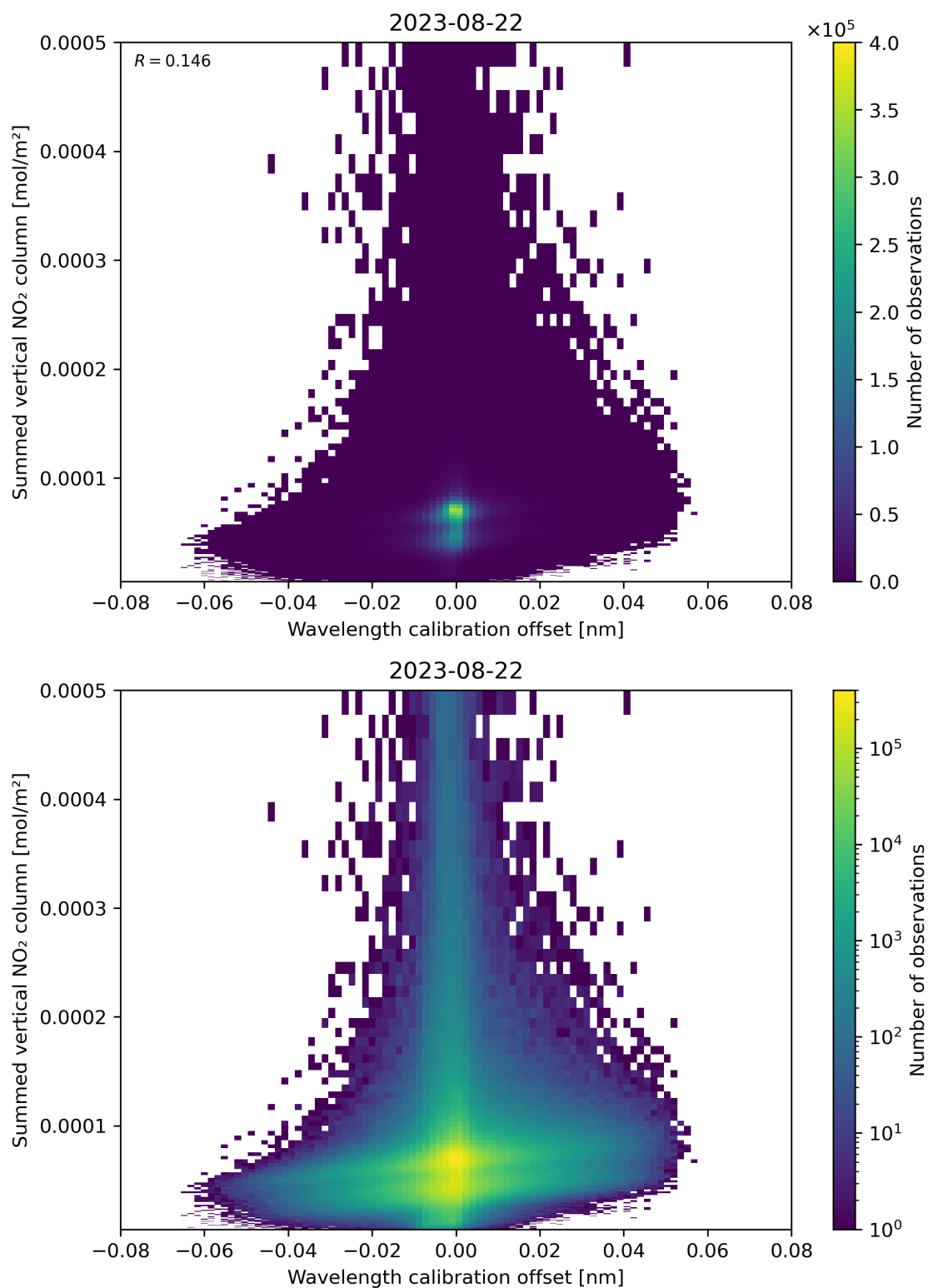
Figure 177: Scatter density plot of “Wavelength calibration offset” against “Summed vertical NO 2 column” for 2023-08-21 to 2023-08-23.
