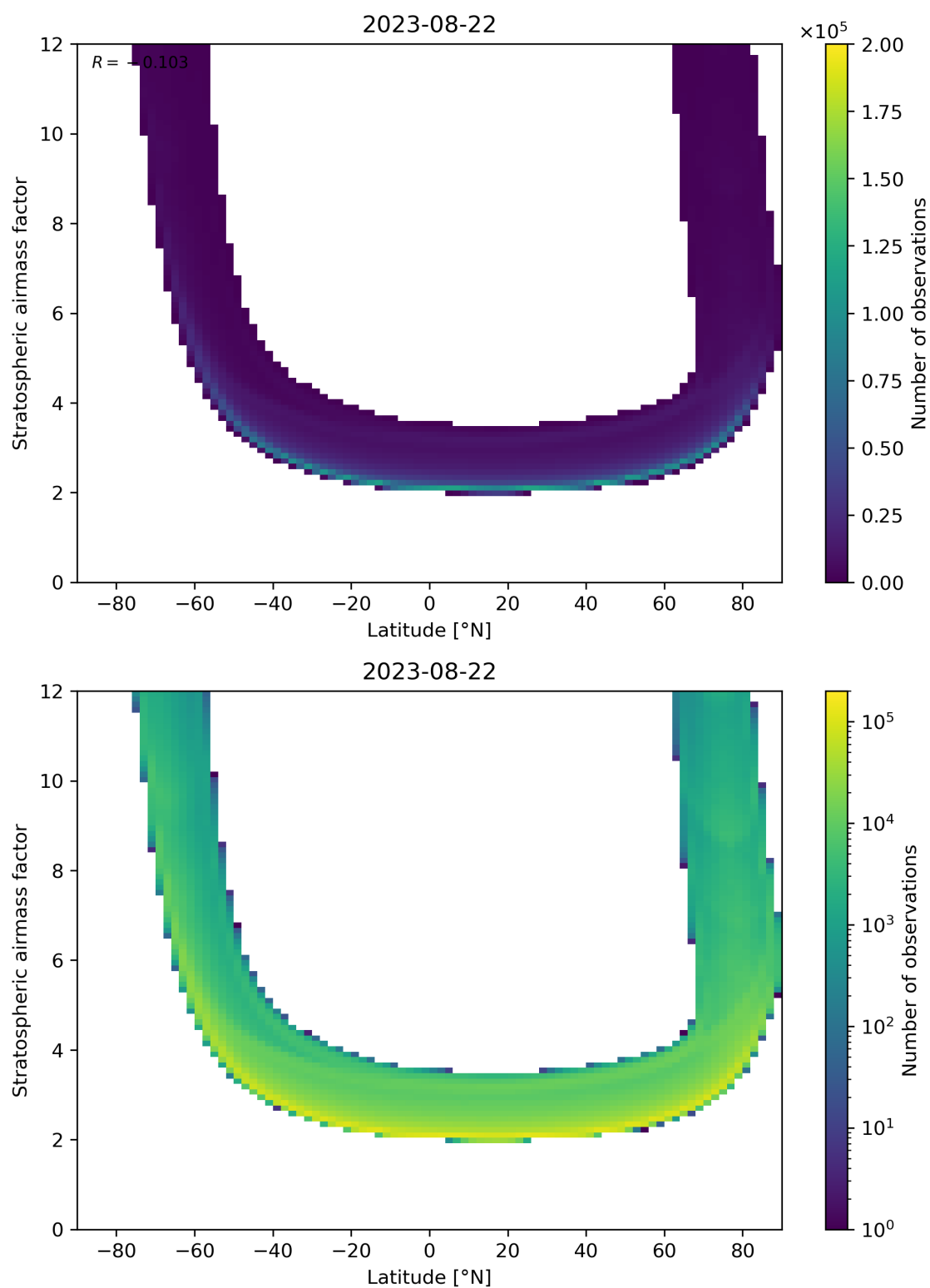
Figure 83: Scatter density plot of “Latitude” against “Stratospheric air mass factor” for 2023-08-21 to 2023-08-23.
