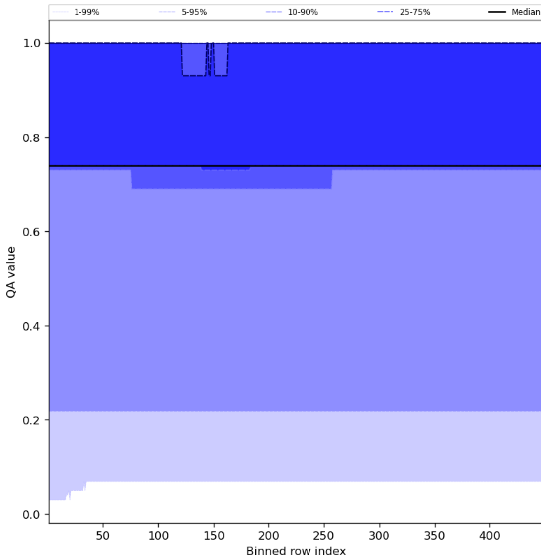
Figure 45: Along track statistics of “QA value” for 2023-08-21 to 2023-08-23
