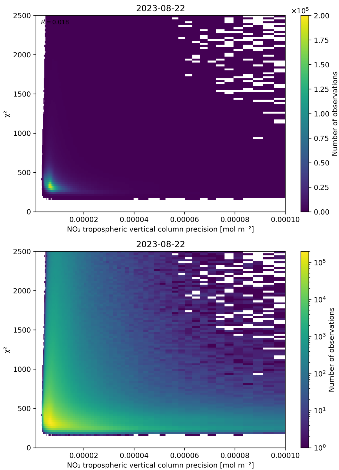
Figure 134: Scatter density plot of “NO 2 tropospheric vertical column precision” against “ \chi^2 ” for 2023-08-21 to 2023-08-23.
