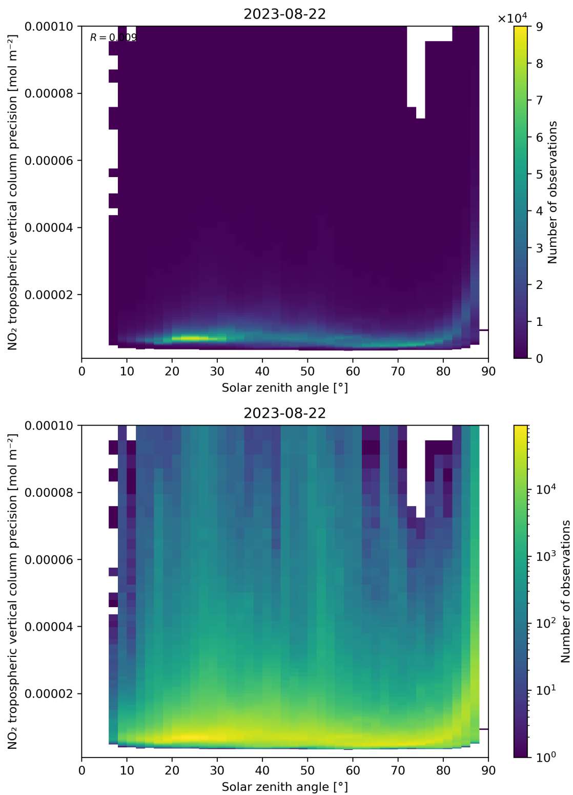
Figure 156: Scatter density plot of “Solar zenith angle” against “NO 2 tropospheric vertical column precision” for 2023-08-21 to 2023-08-23.
