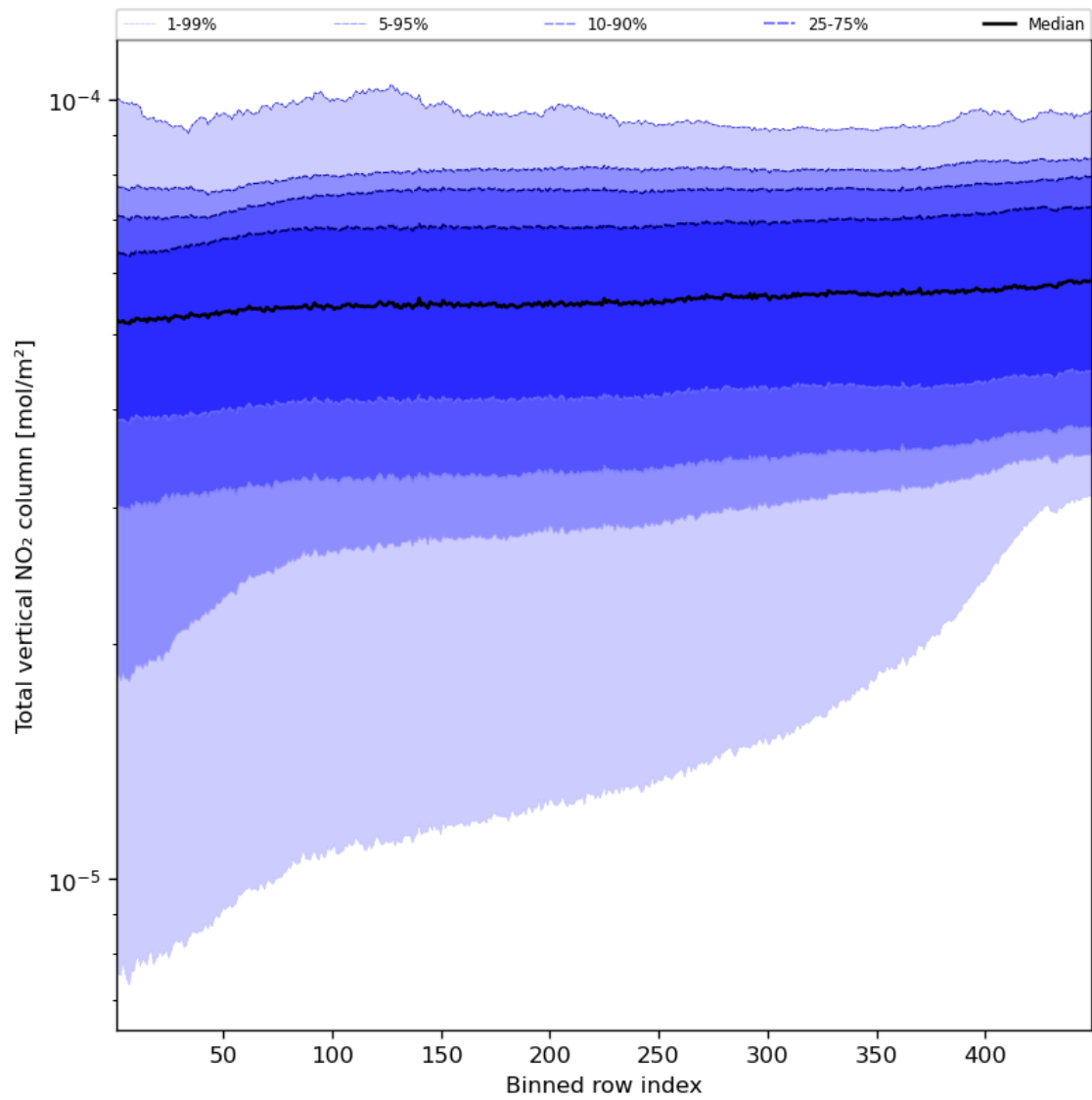
Figure 55: Along track statistics of “Total vertical NO 2 column” for 2023-08-21 to 2023-08-23
