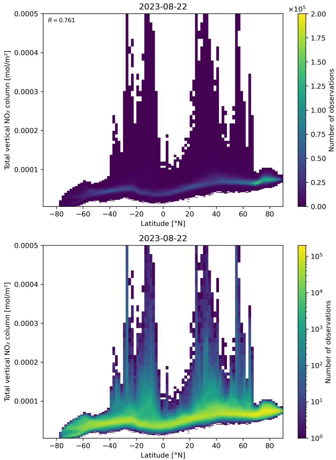
Figure 90: Scatter density plot of “Latitude” against “Total vertical NO 2 column” for 2023-08-21 to 2023-08-23.
