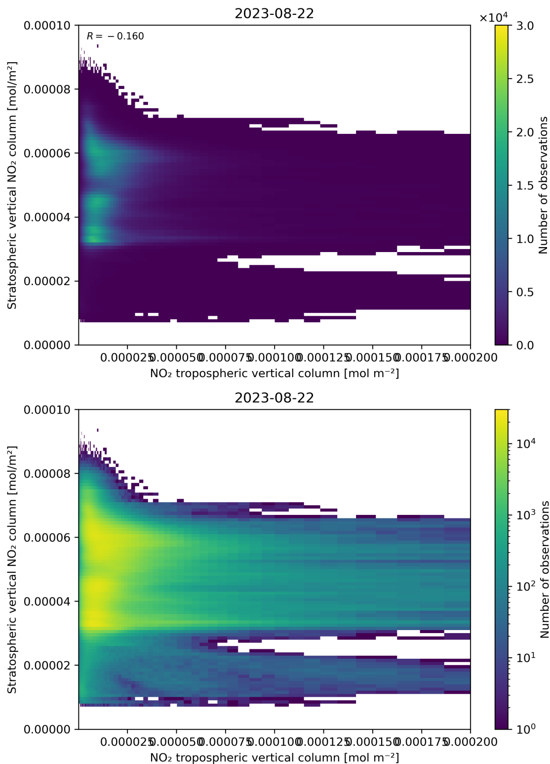
Figure 125: Scatter density plot of “NO 2 tropospheric vertical column” against “Stratospheric vertical NO 2 column” for 2023-08-21 to 2023-08-23.
