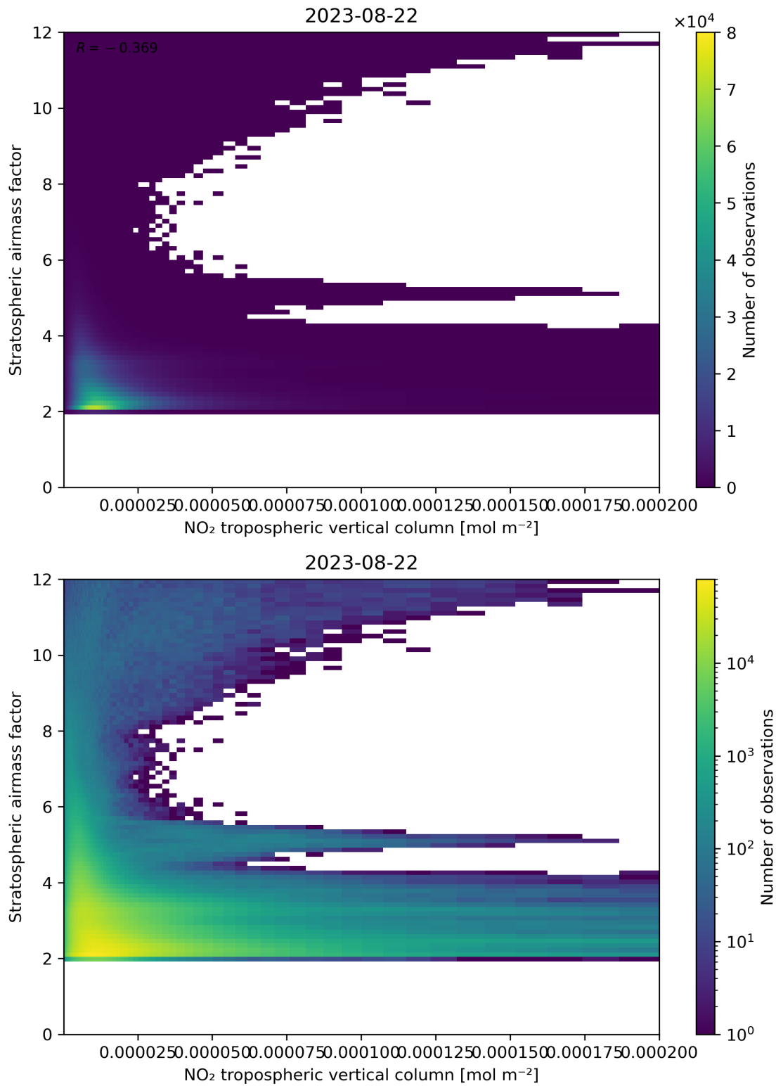
Figure 121: Scatter density plot of “NO 2 tropospheric vertical column” against “Stratospheric air mass factor” for 2023-08-21 to 2023-08-23.
