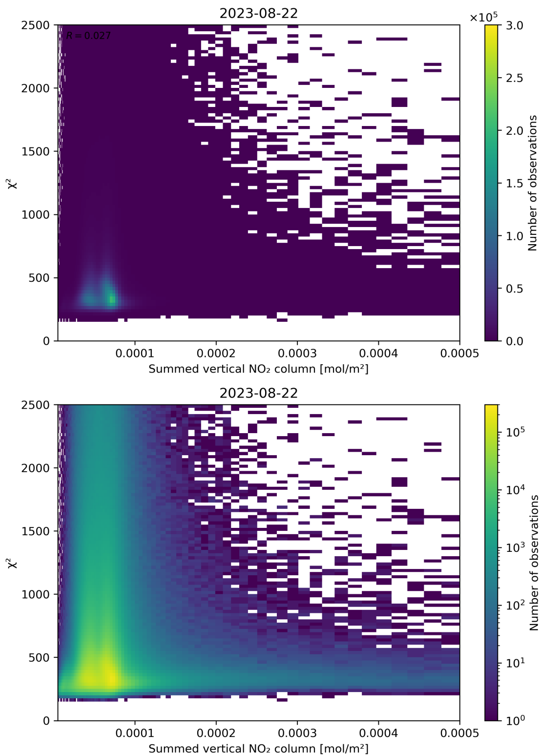
Figure 104: Scatter density plot of “Summed vertical NO 2 column” against “ \chi^2 ” for 2023-08-21 to 2023-08-23.
