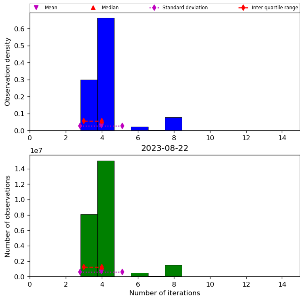
Figure 34: Histogram of “Number of iterations” for 2023-08-21 to 2023-08-23
