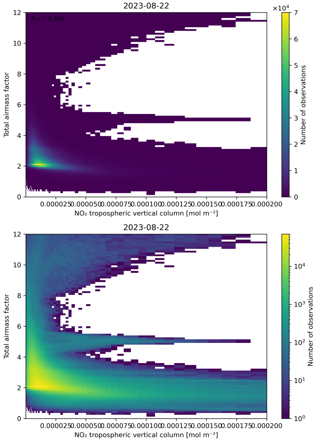
Figure 122: Scatter density plot of “NO 2 tropospheric vertical column” against “Total airmass factor” for 2023-08-21 to 2023-08-23.
