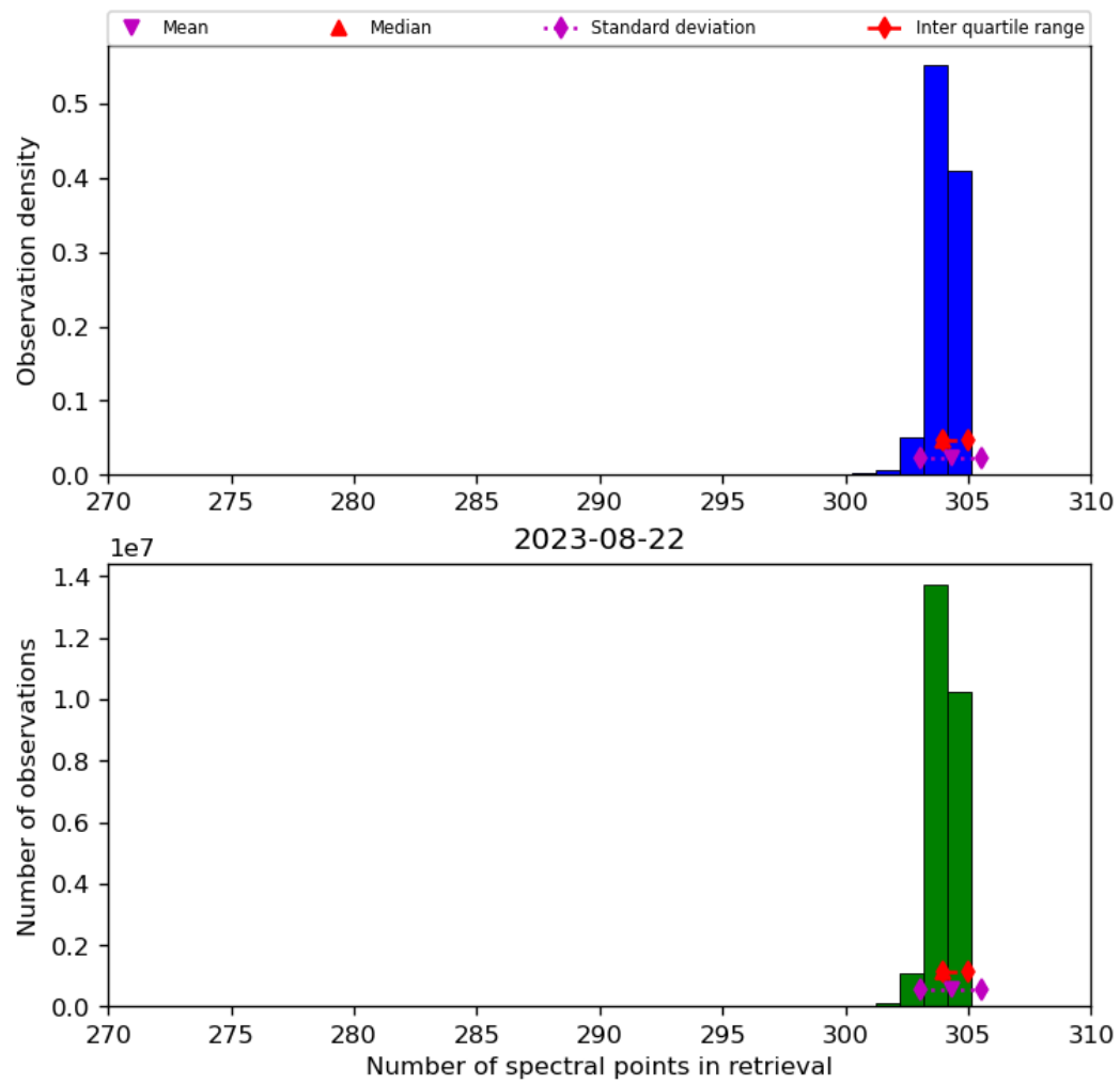
Figure 33: Histogram of “Number of spectral points in retrieval” for 2023-08-21 to 2023-08-23
