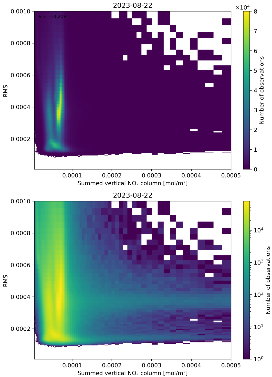
Figure 109: Scatter density plot of “Summed vertical NO 2 column” against “RMS” for 2023-08-21 to 2023-08-23.
