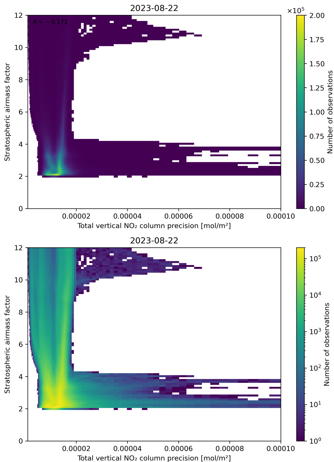
Figure 115: Scatter density plot of “Total vertical NO 2 column precision” against “Stratospheric air mass factor” for 2023-08-21 to 2023-08-23.
