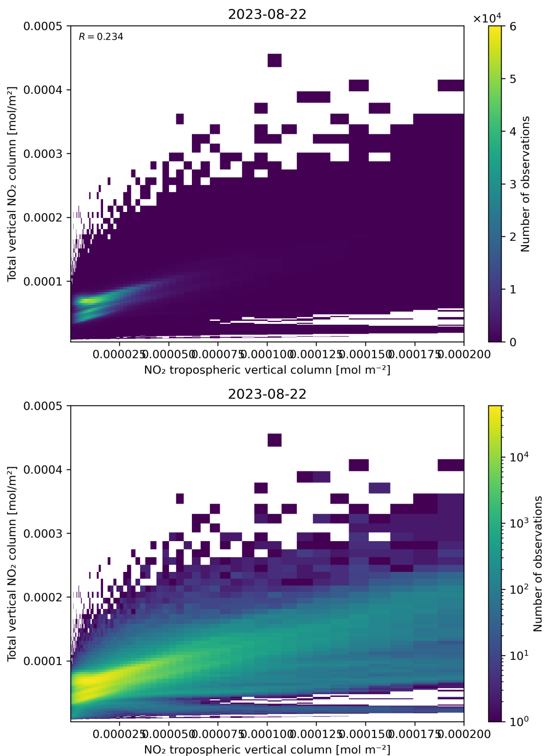
Figure 128: Scatter density plot of “NO 2 tropospheric vertical column” against “Total vertical NO 2 column” for 2023-08-21 to 2023-08-23.
