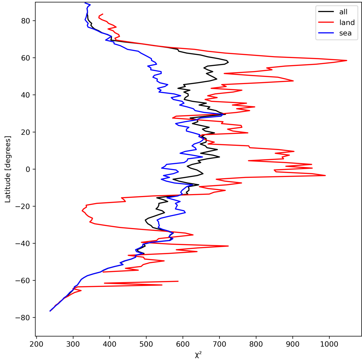
Figure 25: Zonal average of “ \chi^2 ” for 2023-08-21 to 2023-08-23.
