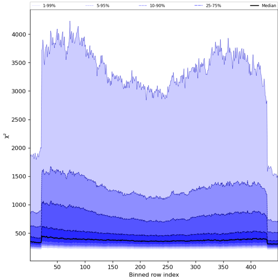
Figure 59: Along track statistics of “ \chi^2 ” for 2023-08-21 to 2023-08-23
