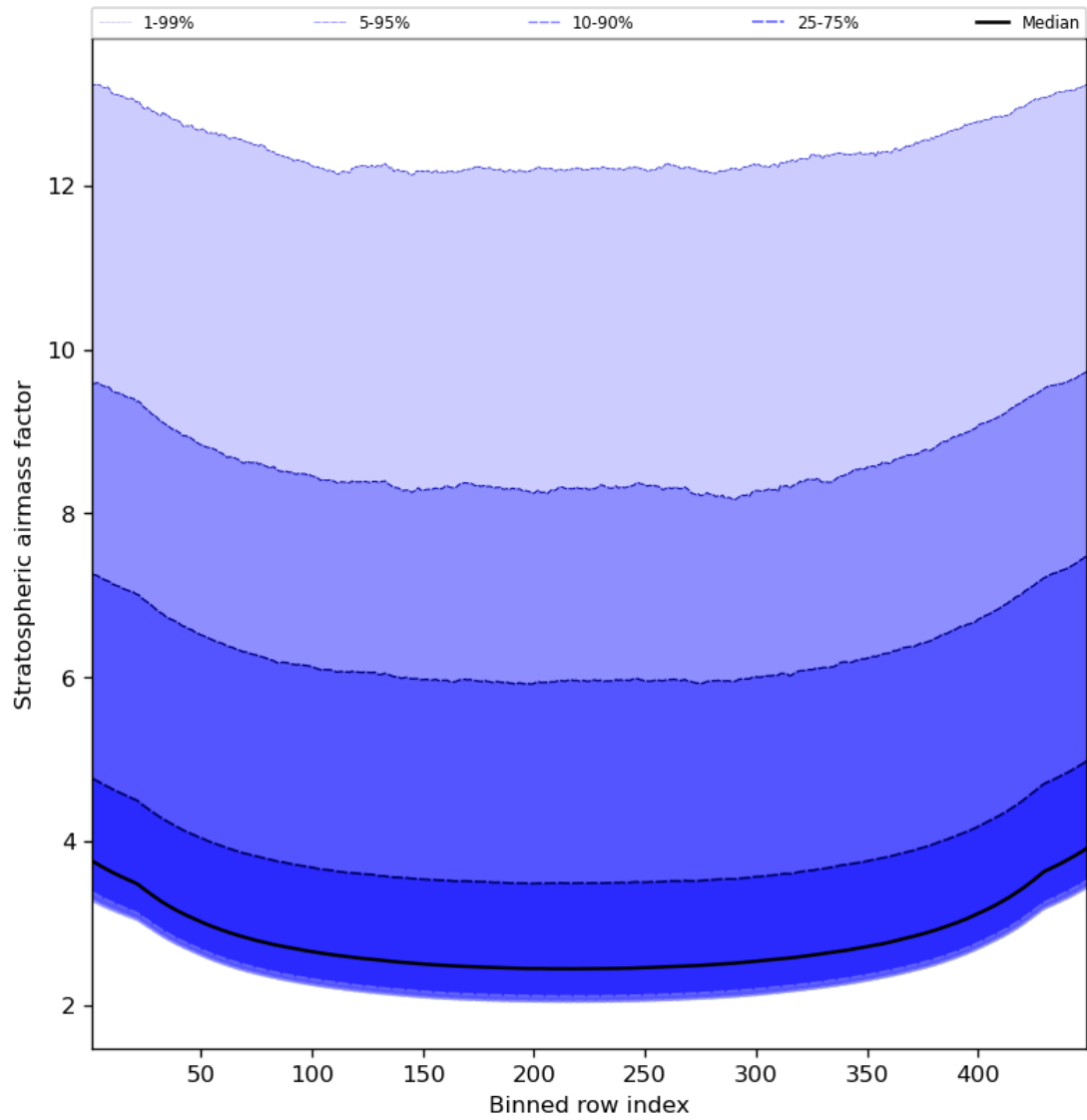
Figure 61: Along track statistics of “Stratospheric airmass factor” for 2023-08-21 to 2023-08-23
