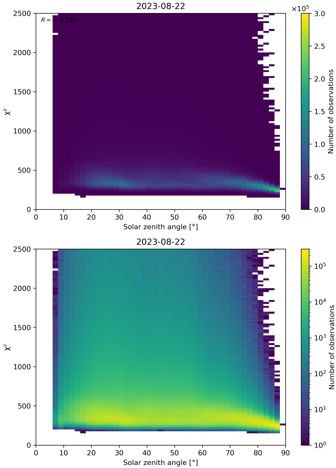
Figure 148: Scatter density plot of “Solar zenith angle” against “ \chi^2 ” for 2023-08-21 to 2023-08-23.
