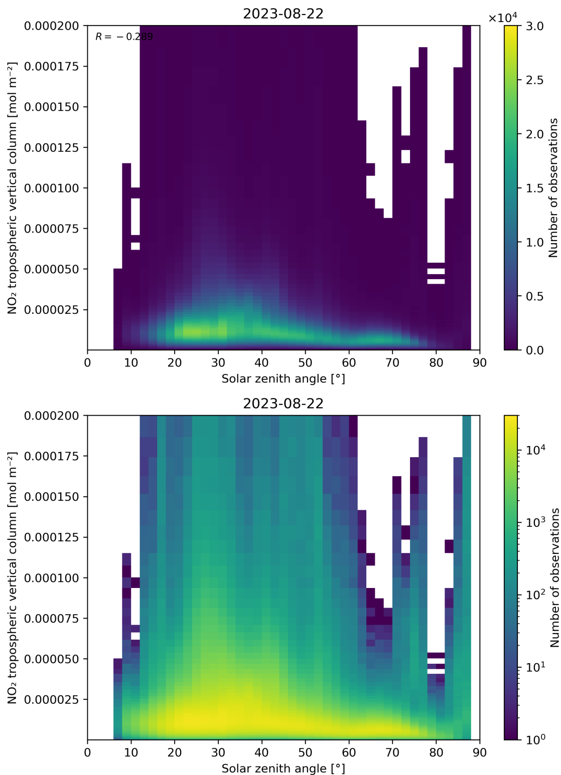
Figure 155: Scatter density plot of “Solar zenith angle” against “NO 2 tropospheric vertical column” for 2023-08-21 to 2023-08-23.
