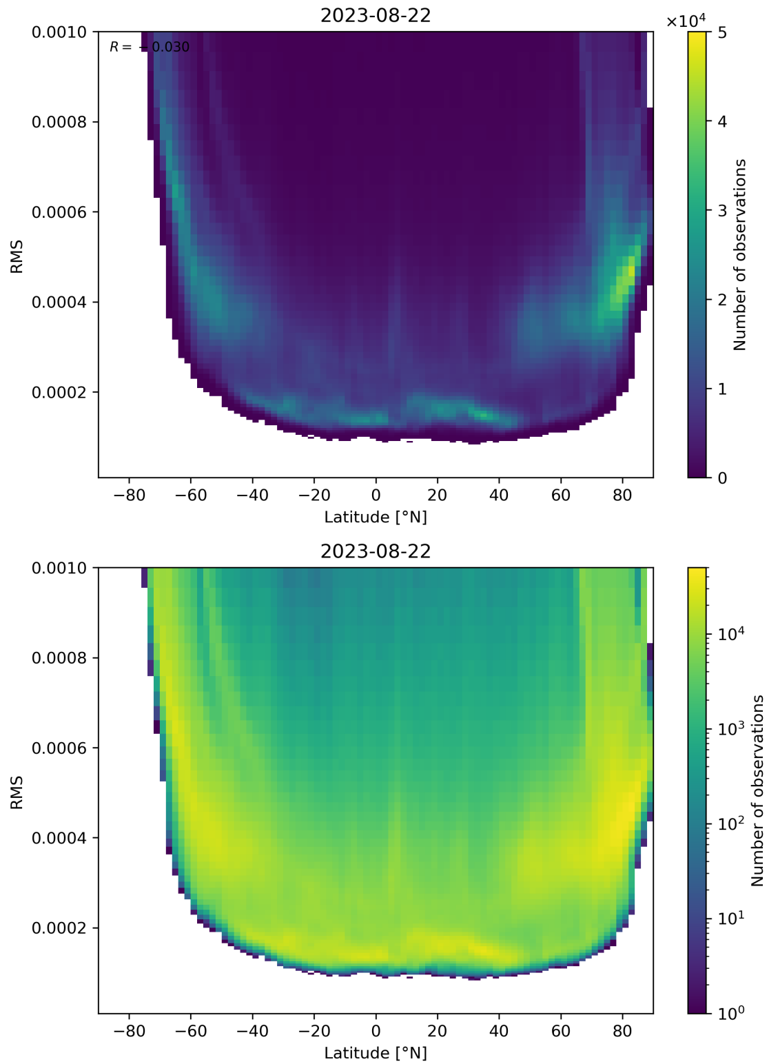
Figure 94: Scatter density plot of “Latitude” against “RMS” for 2023-08-21 to 2023-08-23.
