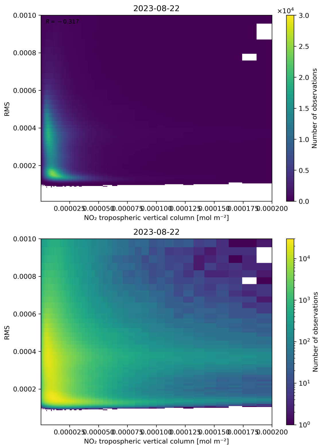
Figure 142: Scatter density plot of “NO 2 tropospheric vertical column” against “RMS” for 2023-08-21 to 2023-08-23.
