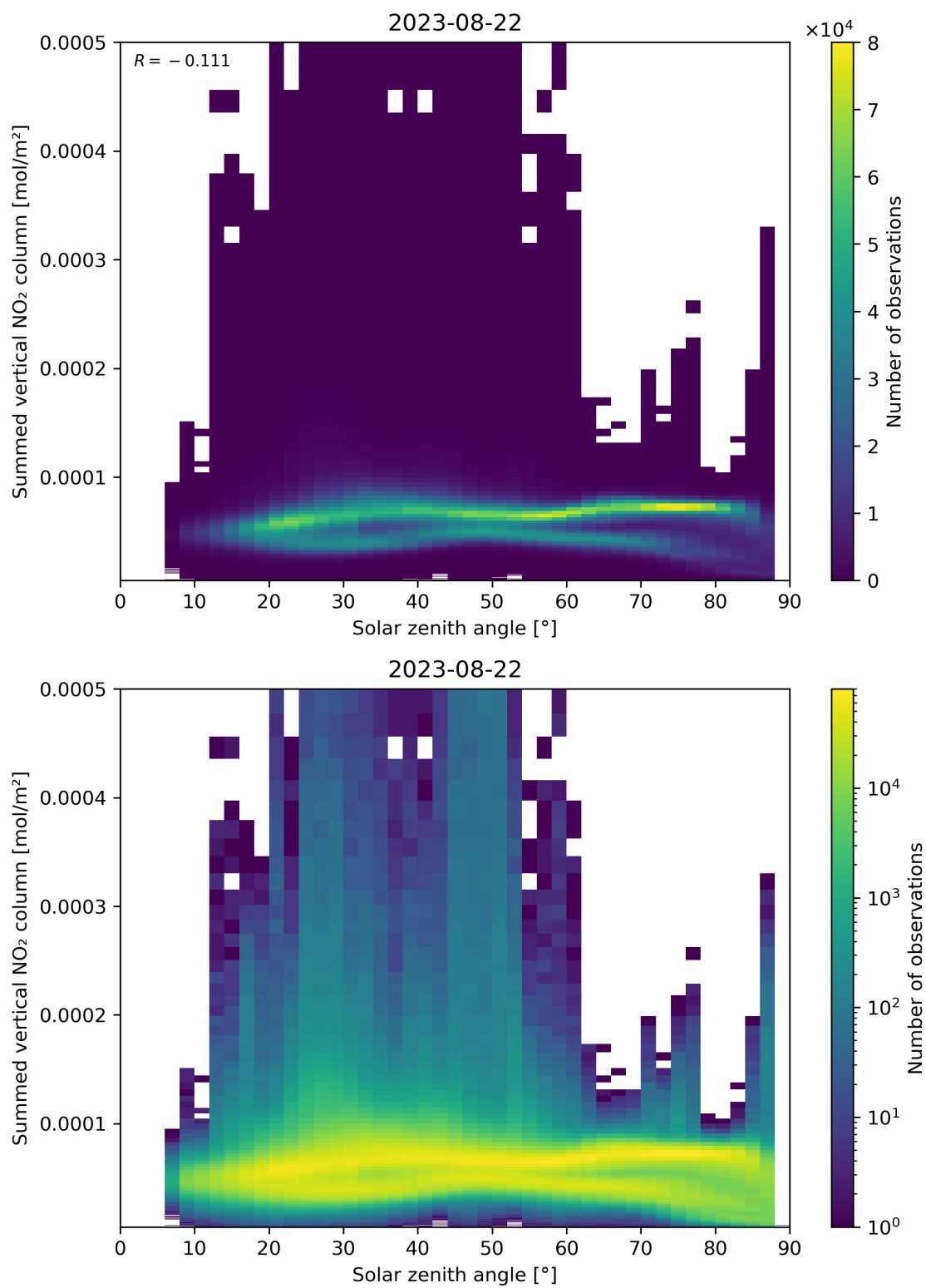
Figure 151: Scatter density plot of “Solar zenith angle” against “Summed vertical NO 2 column” for 2023-08-21 to 2023-08-23.
