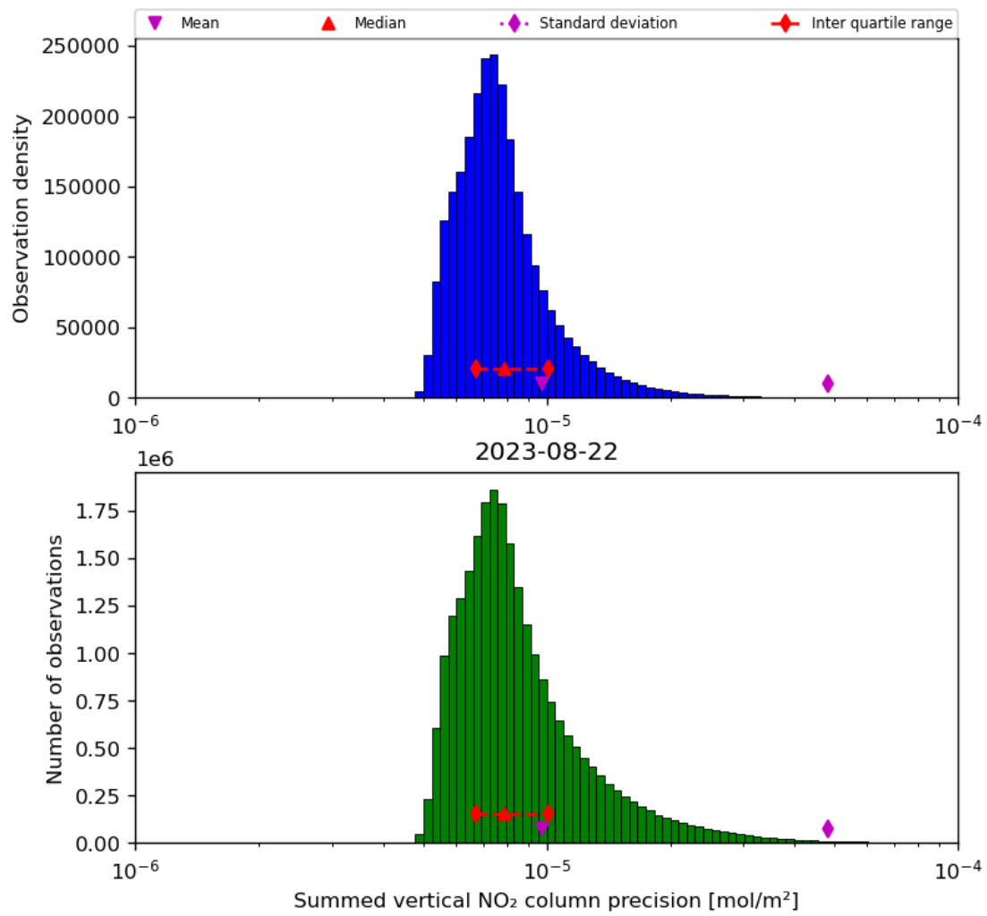
Figure 41: Histogram of “Summed vertical NO 2 column precision” for 2023-08-21 to 2023-08-23
