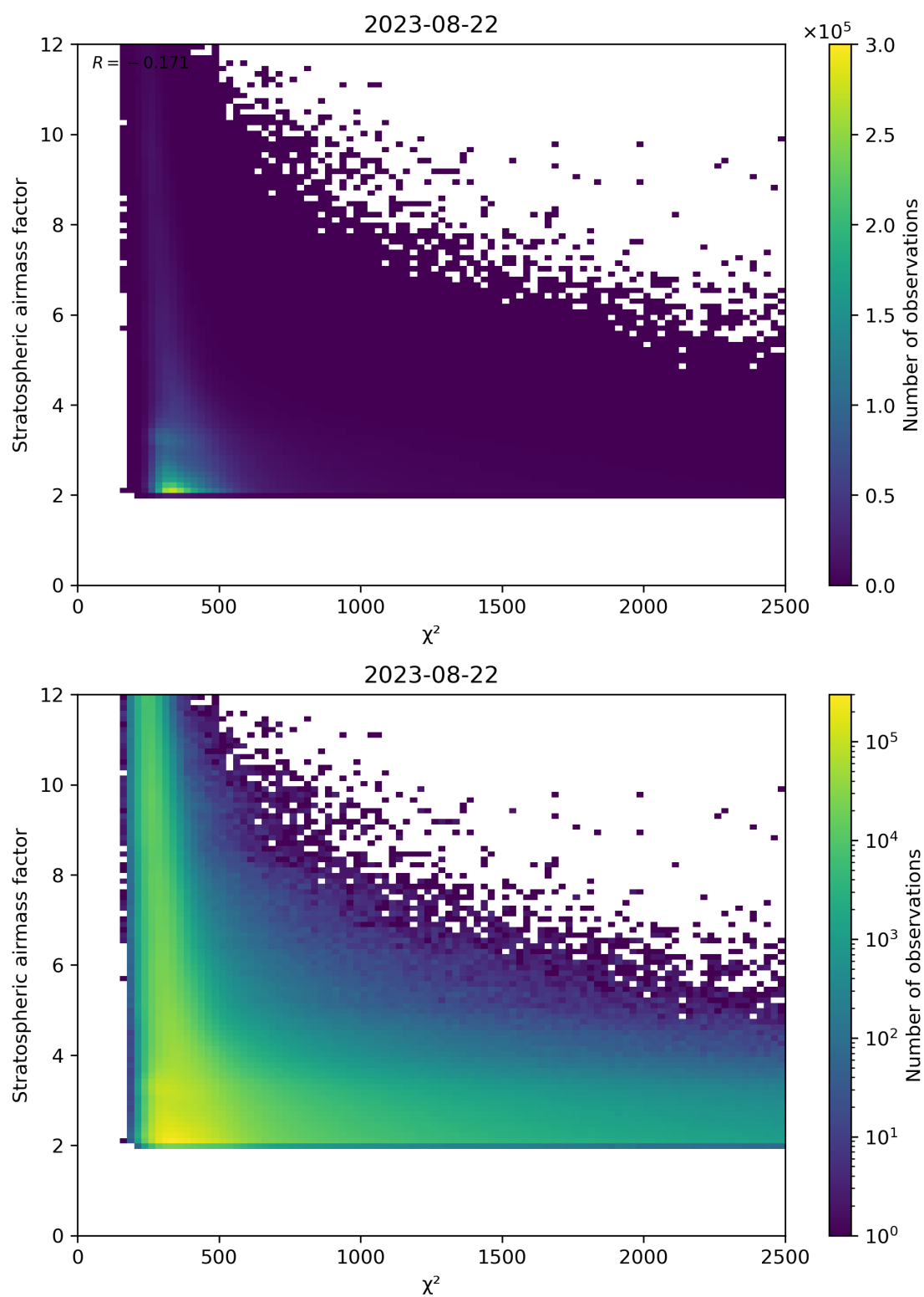
Figure 81: Scatter density plot of “ \chi^2 ” against “Stratospheric airmass factor” for 2023-08-21 to 2023-08-23.
