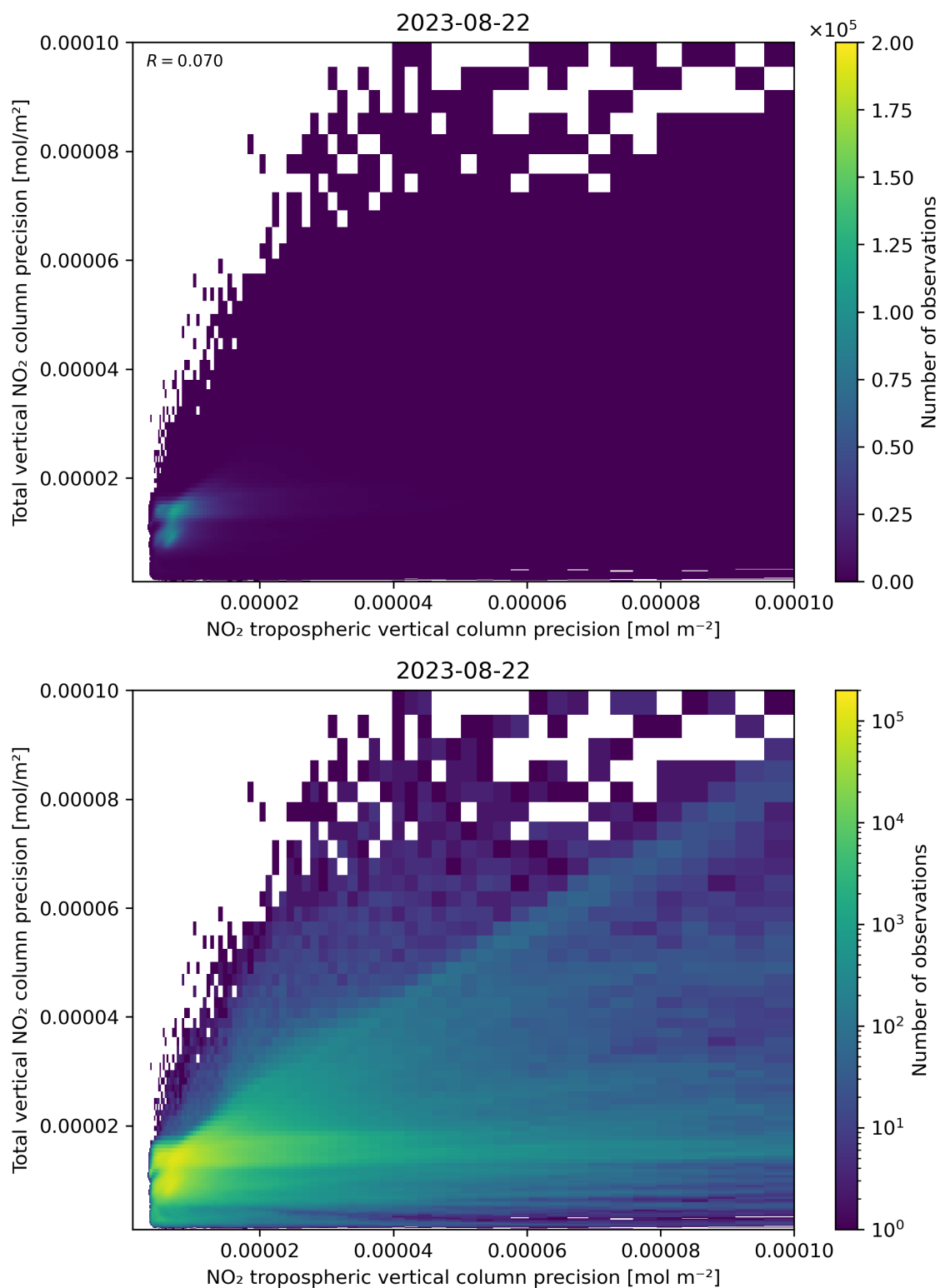
Figure 139: Scatter density plot of “NO 2 tropospheric vertical column precision” against “Total vertical NO 2 column precision” for 2023-08-21 to 2023-08-23.
