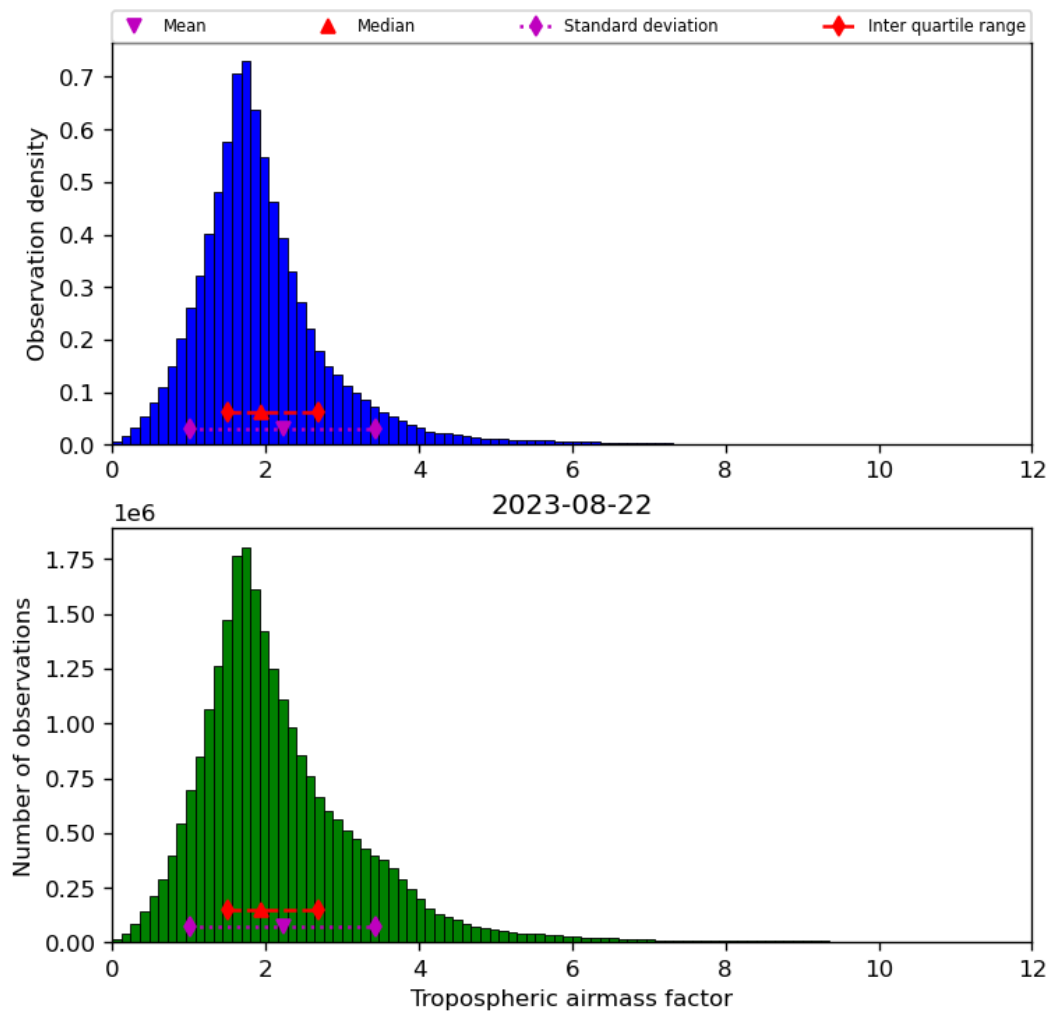
Figure 31: Histogram of “Tropospheric airmass factor” for 2023-08-21 to 2023-08-23
