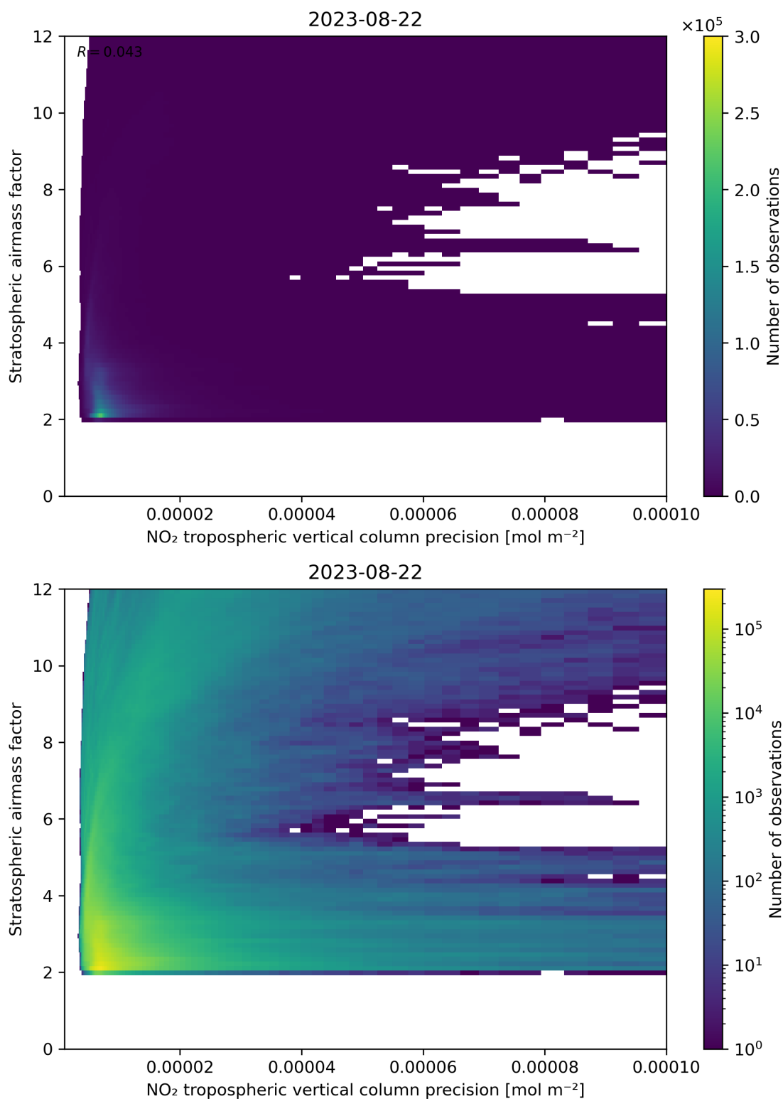
Figure 131: Scatter density plot of “NO 2 tropospheric vertical column precision” against “Stratospheric airmass factor” for 2023-08-21 to 2023-08-23.
