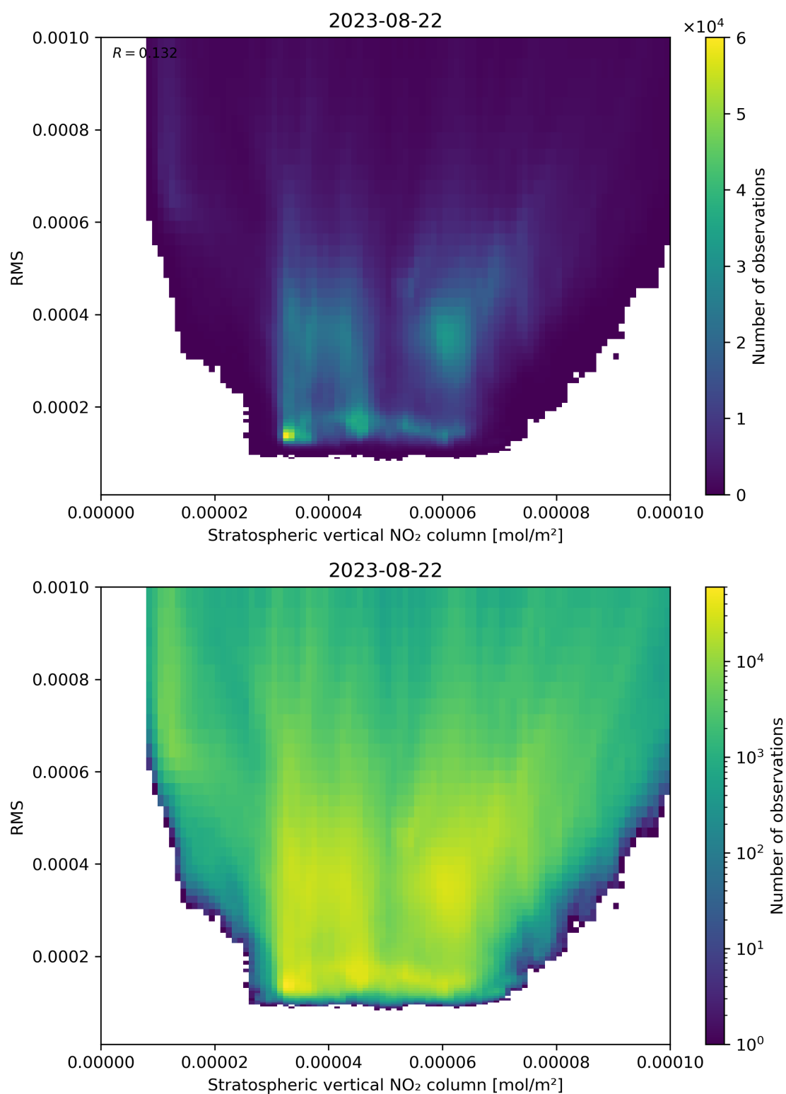
Figure 102: Scatter density plot of “Stratospheric vertical NO 2 column” against “RMS” for 2023-08-21 to 2023-08-23.
