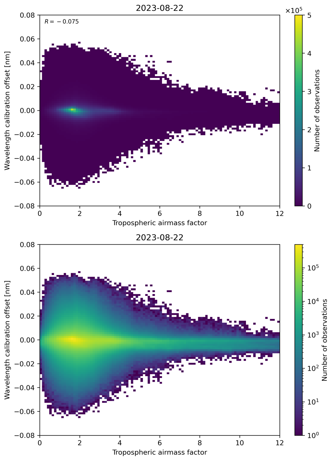
Figure 80: Scatter density plot of “Tropospheric airmass factor” against “Wavelength calibration offset” for 2023-08-21 to 2023-08-23.
