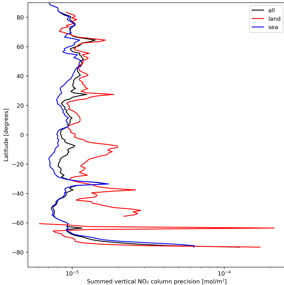
Figure 24: Zonal average of “Summed vertical NO 2 column precision” for 2023-08-21 to 2023-08-23.
