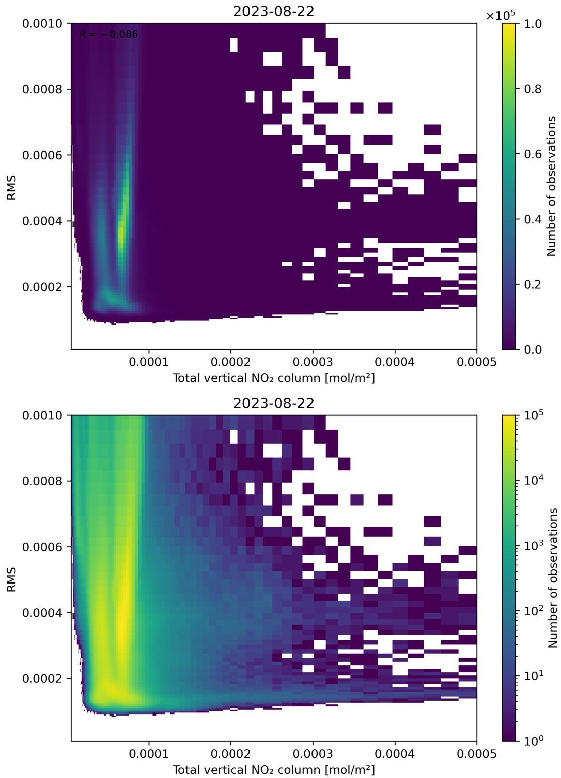
Figure 120: Scatter density plot of “Total vertical NO 2 column” against “RMS” for 2023-08-21 to 2023-08-23.
