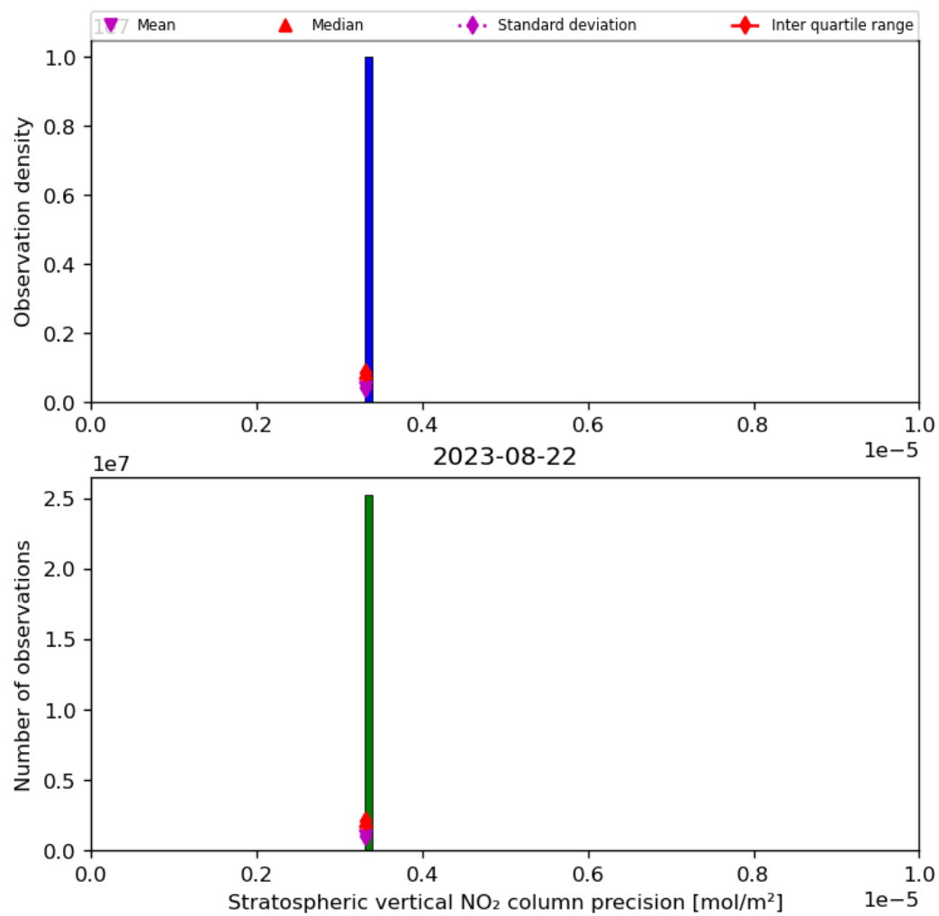
Figure 37: Histogram of “Stratospheric vertical NO 2 column precision” for 2023-08-21 to 2023-08-23
