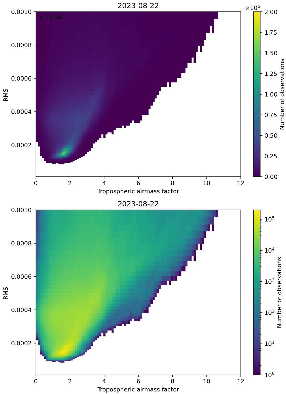
Figure 79: Scatter density plot of “Tropospheric airmass factor” against “RMS” for 2023-08-21 to 2023-08-23.
