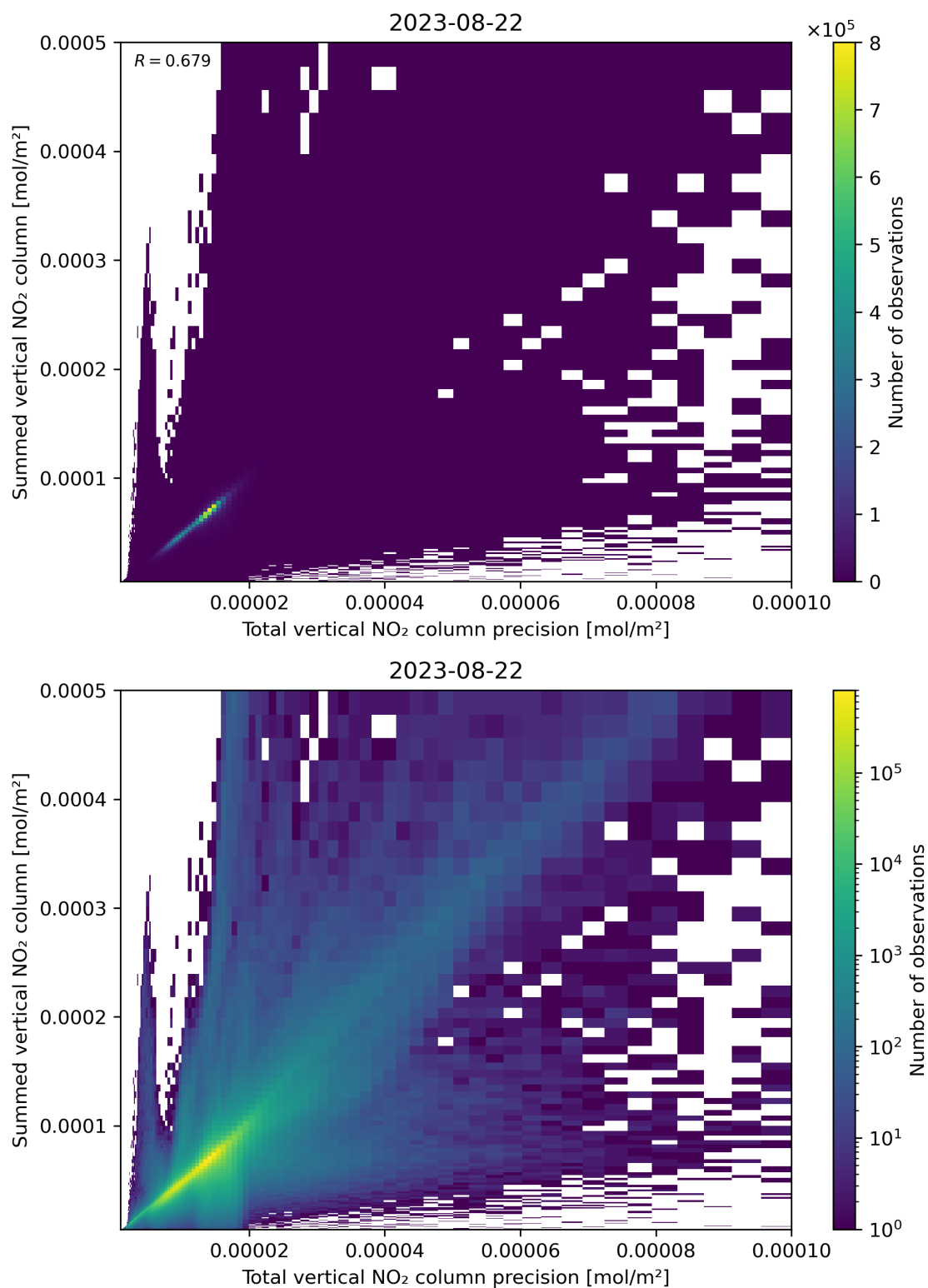
Figure 117: Scatter density plot of “Total vertical NO 2 column precision” against “Summed vertical NO 2 column” for 2023-08-21 to 2023-08-23.
