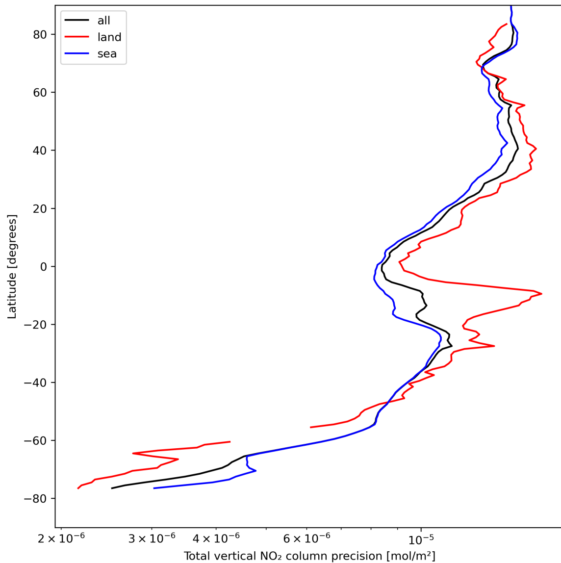
Figure 22: Zonal average of “Total vertical NO 2 column precision” for 2023-08-21 to 2023-08-23.
