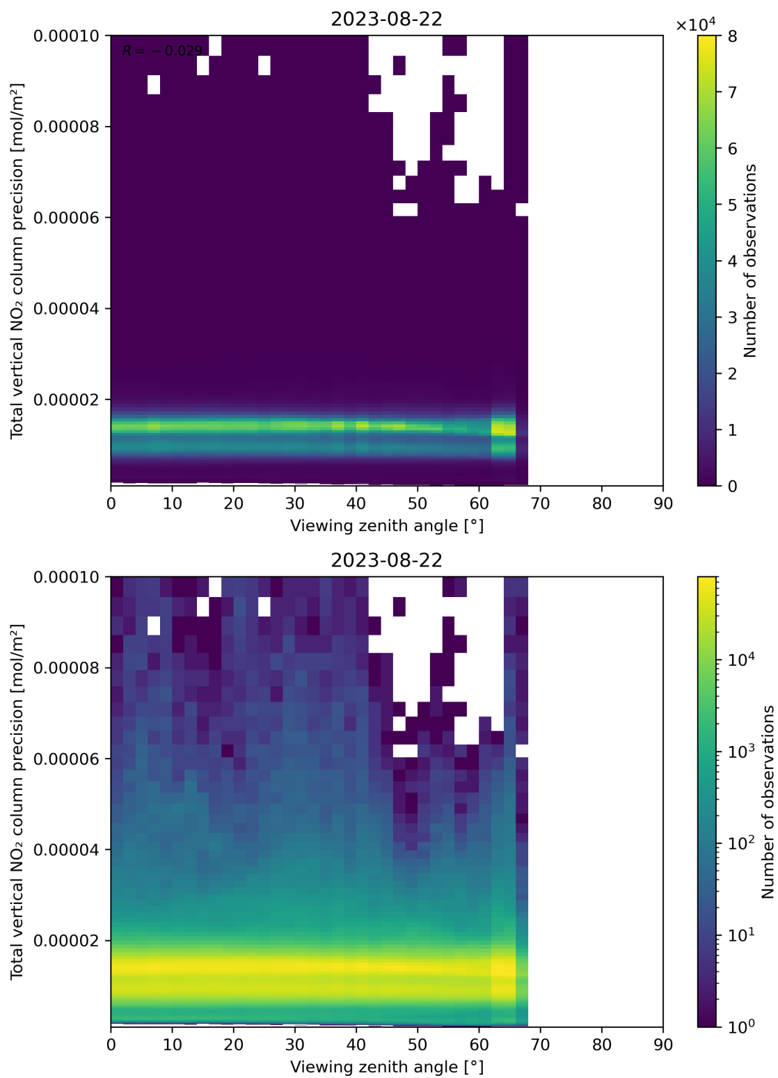
Figure 168: Scatter density plot of “Viewing zenith angle” against “Total vertical NO 2 column precision” for 2023-08-21 to 2023-08-23.
