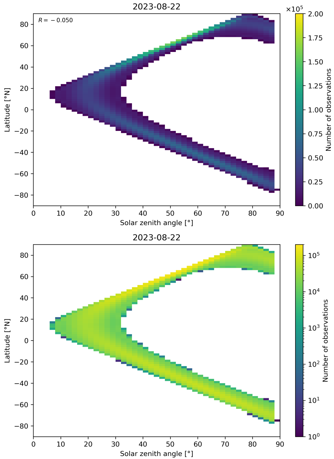
Figure 149: Scatter density plot of “Solar zenith angle” against “Latitude” for 2023-08-21 to 2023-08-23.
