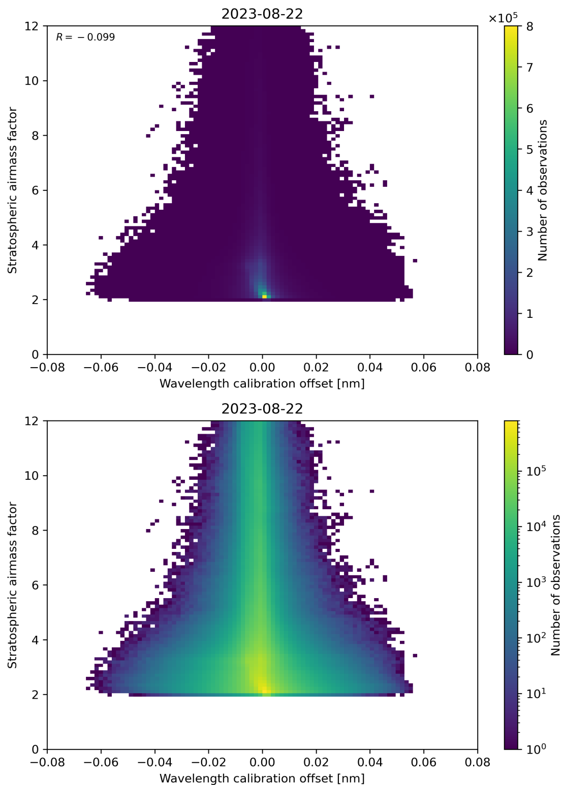
Figure 174: Scatter density plot of “Wavelength calibration offset” against “Stratospheric airmass factor” for 2023-08-21 to 2023-08-23.
