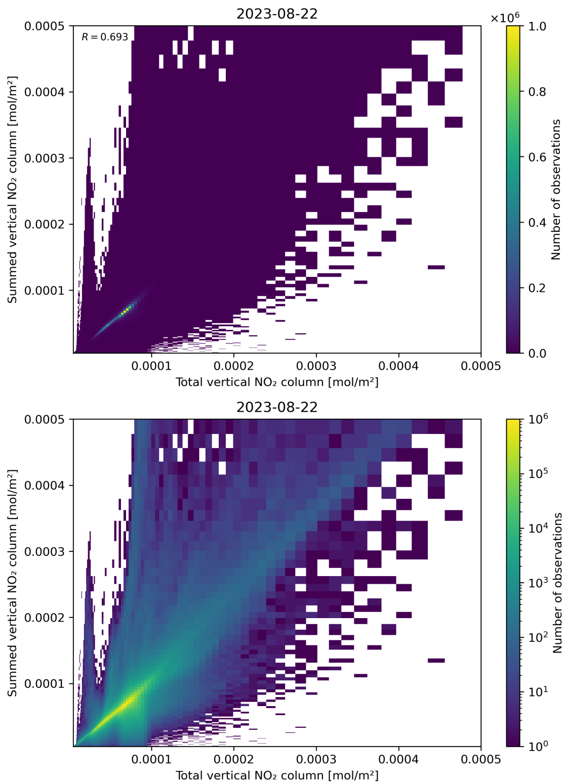
Figure 112: Scatter density plot of “Total vertical NO 2 column” against “Summed vertical NO 2 column” for 2023-08-21 to 2023-08-23.
