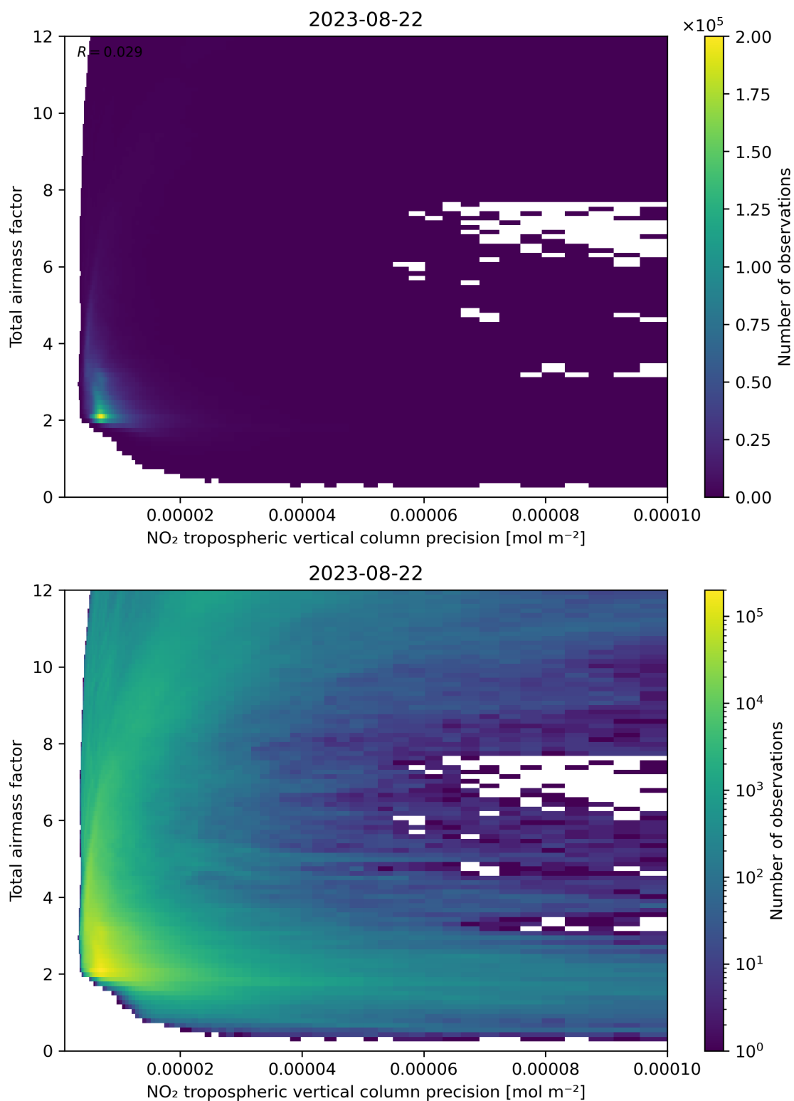
Figure 132: Scatter density plot of “NO 2 tropospheric vertical column precision” against “Total airmass factor” for 2023-08-21 to 2023-08-23.
