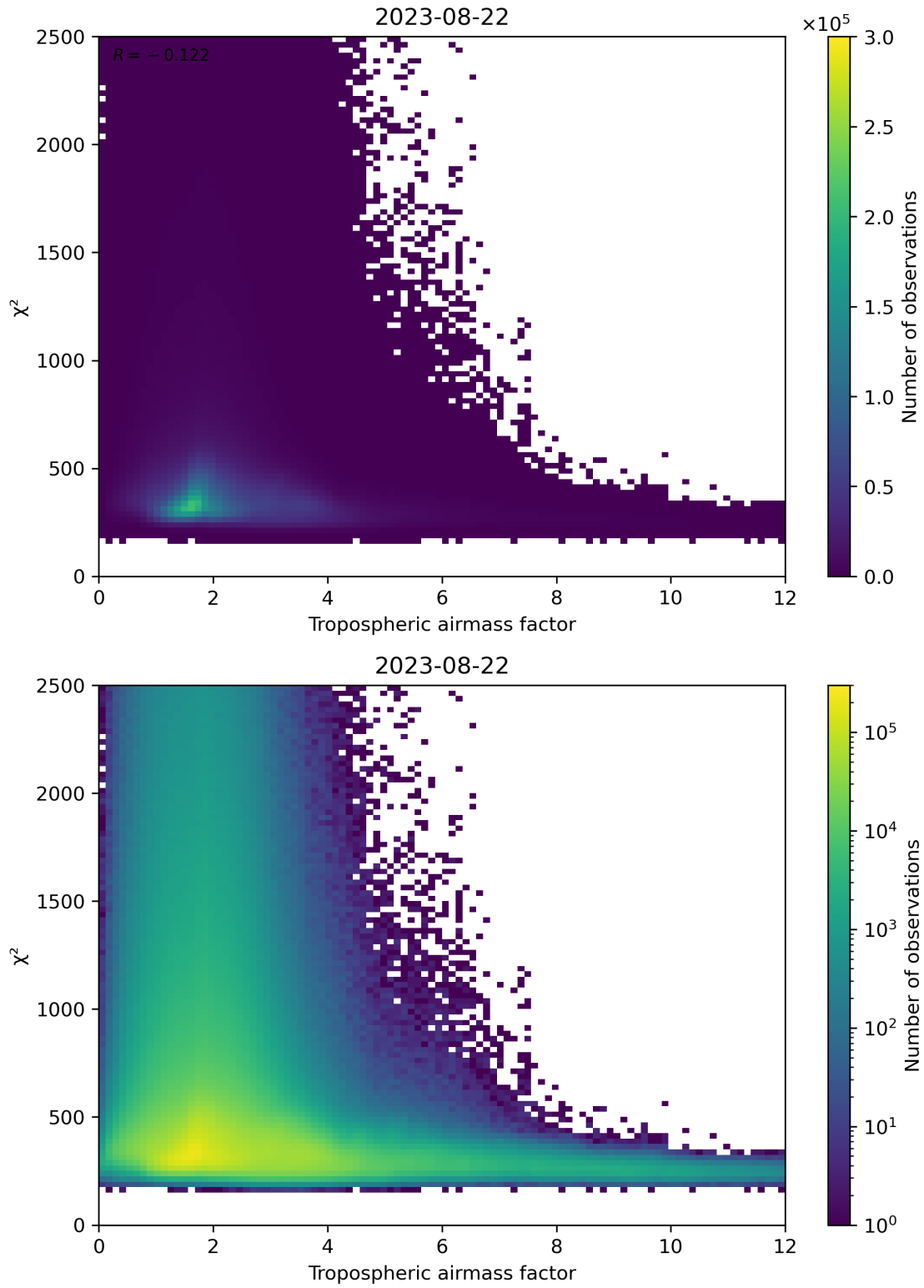
Figure 73: Scatter density plot of “Tropospheric airmass factor” against “ \chi^2 ” for 2023-08-21 to 2023-08-23.
