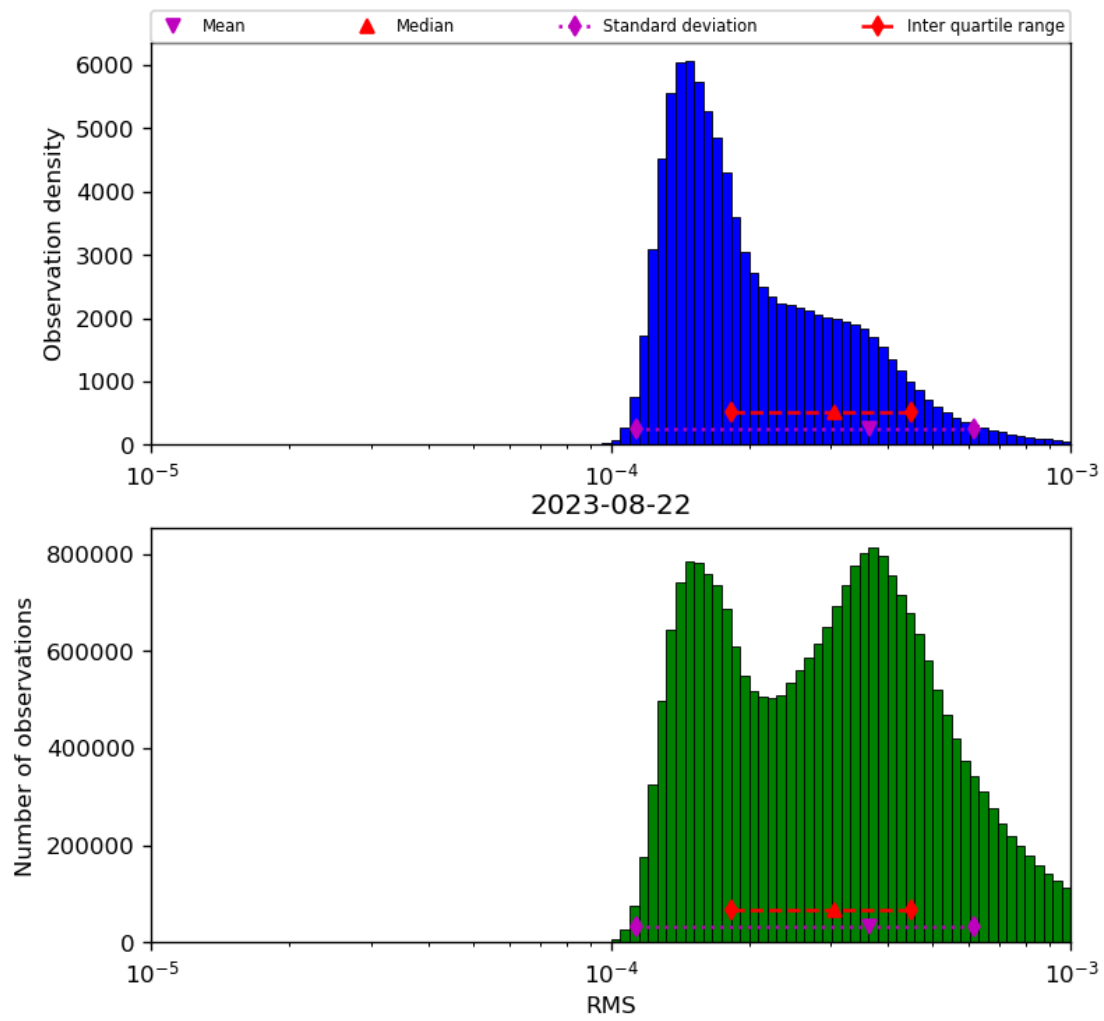
Figure 43: Histogram of “RMS” for 2023-08-21 to 2023-08-23
