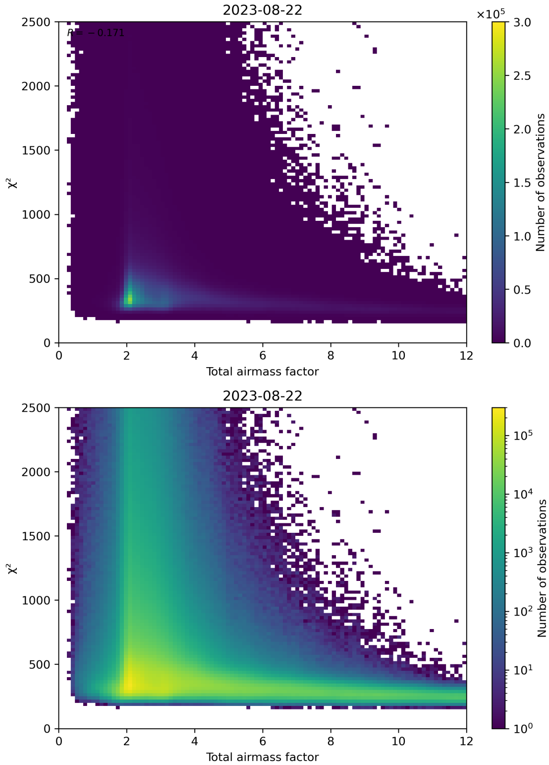
Figure 63: Scatter density plot of “Total airmass factor” against “ \chi^2 ” for 2023-08-21 to 2023-08-23.
