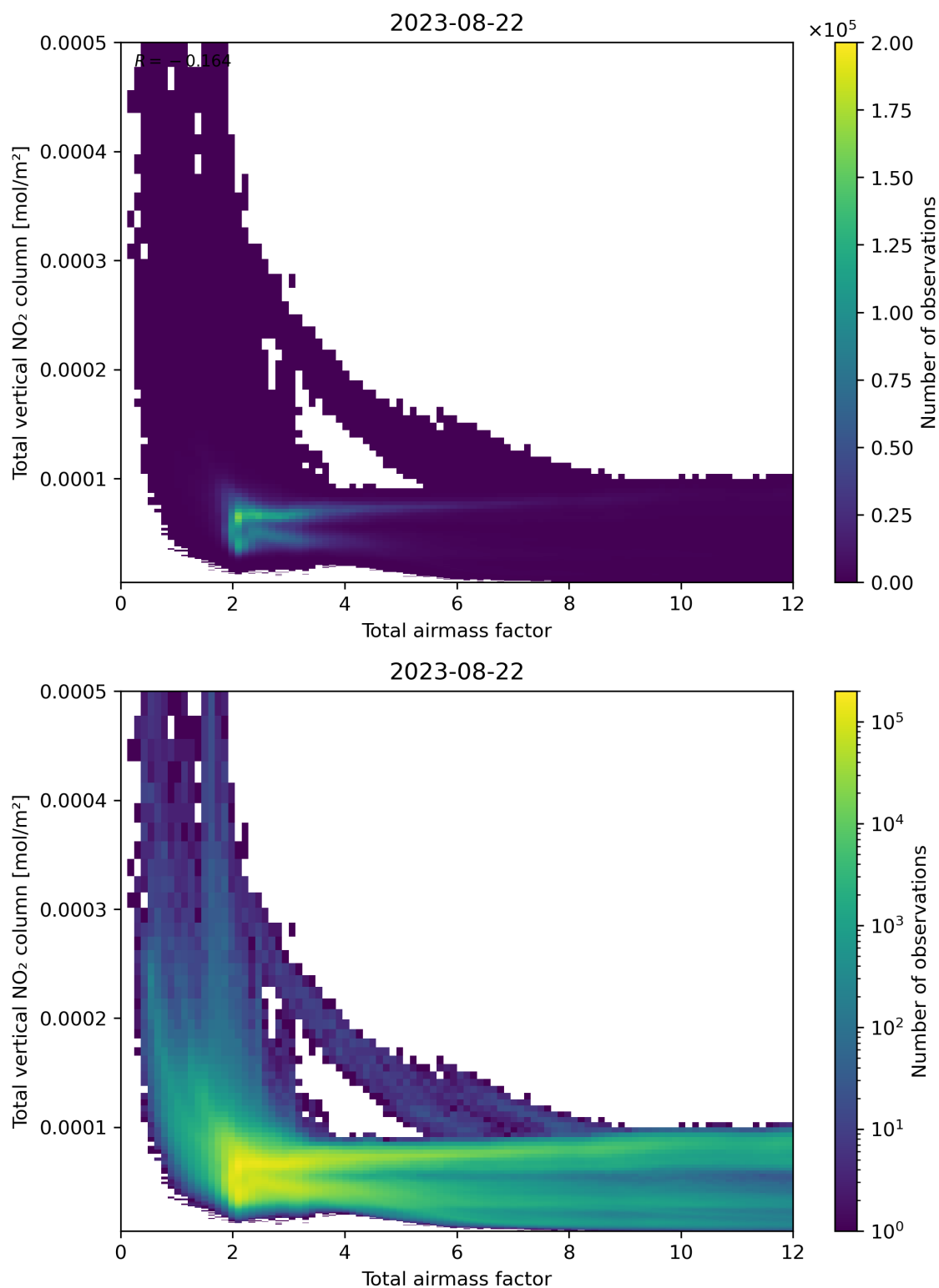
Figure 67: Scatter density plot of “Total airmass factor” against “Total vertical NO 2 column” for 2023-08-21 to 2023-08-23.
