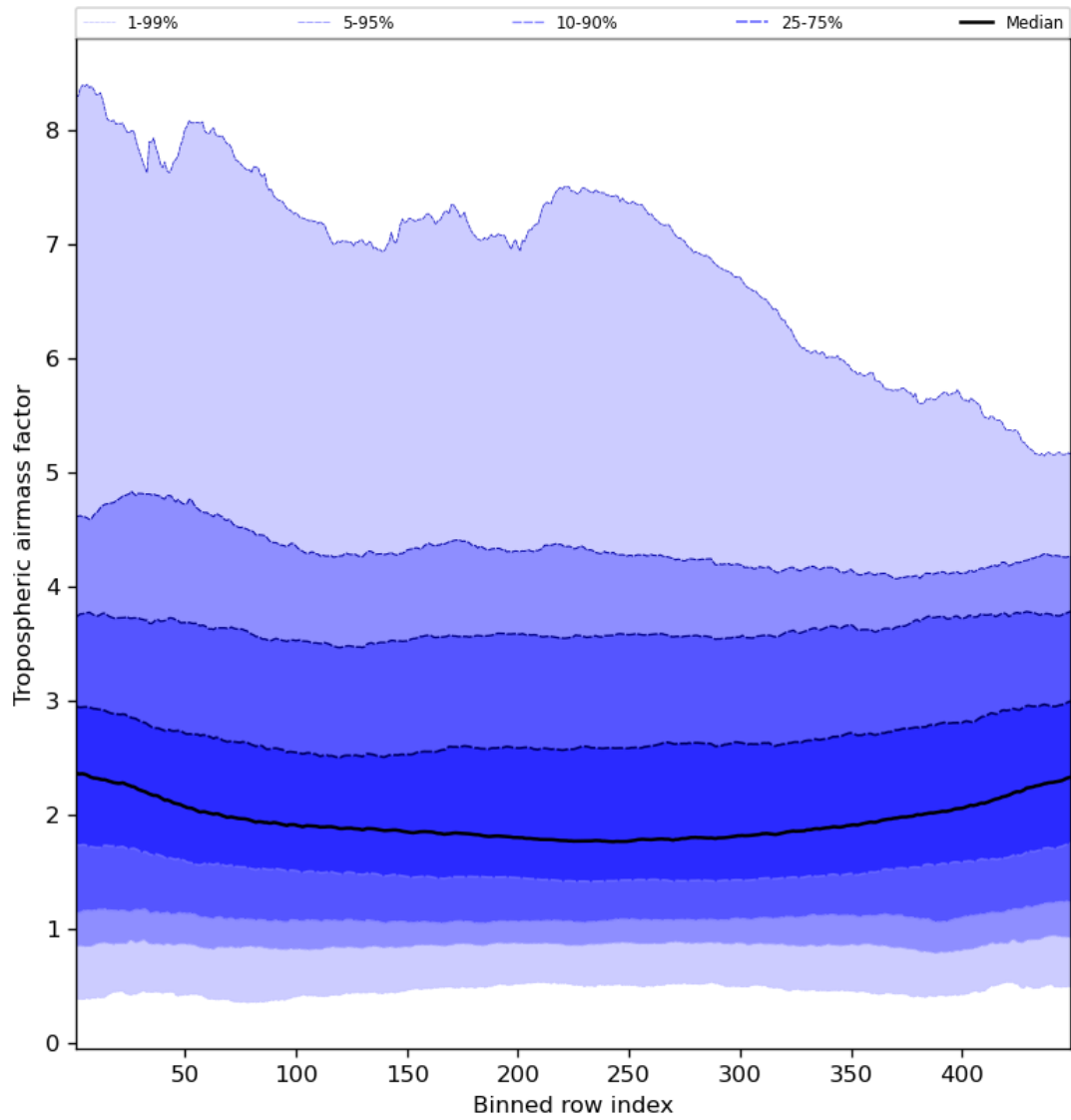
Figure 48: Along track statistics of “Tropospheric airmass factor” for 2023-08-21 to 2023-08-23
