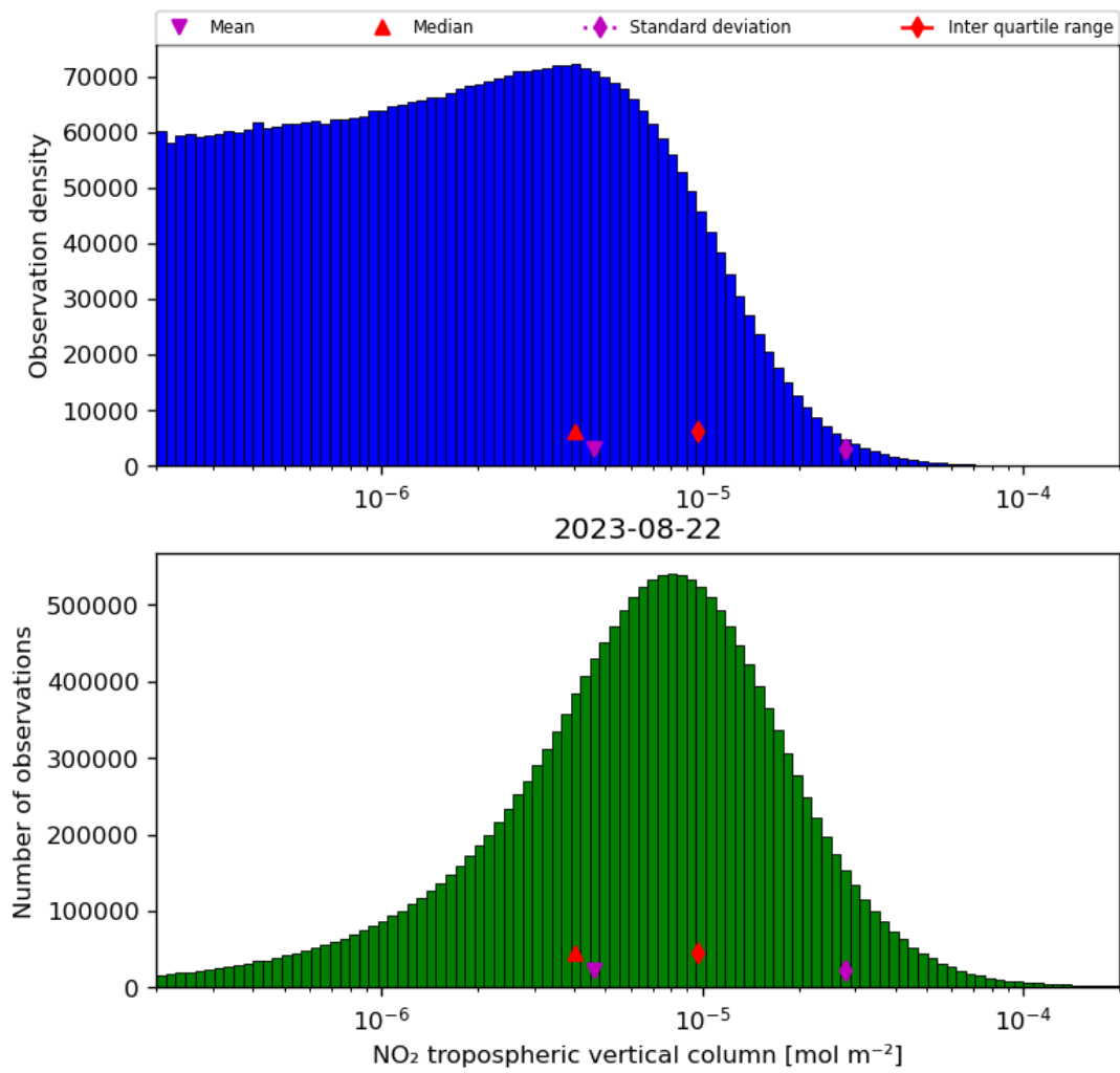
Figure 29: Histogram of “NO 2 tropospheric vertical column” for 2023-08-21 to 2023-08-23
