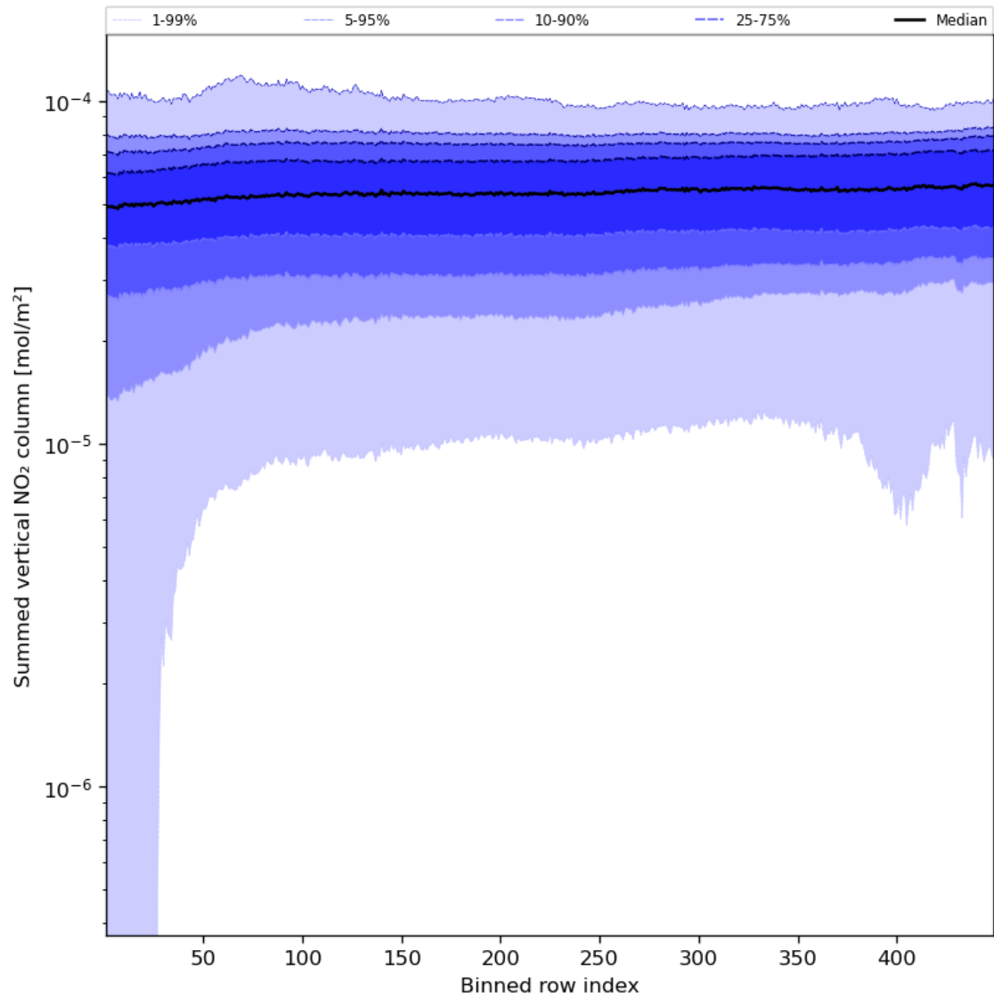
Figure 57: Along track statistics of “Summed vertical NO 2 column” for 2023-08-21 to 2023-08-23
