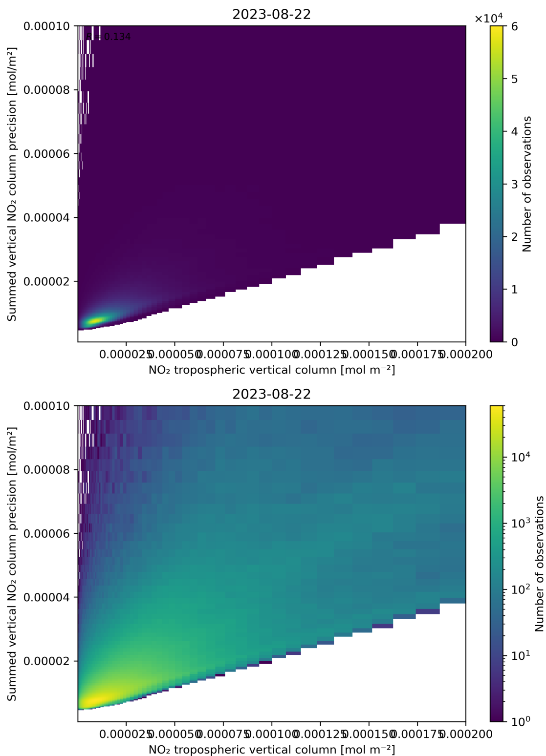
Figure 127: Scatter density plot of “NO 2 tropospheric vertical column” against “Summed vertical NO 2 column precision” for 2023-08-21 to 2023-08-23.
