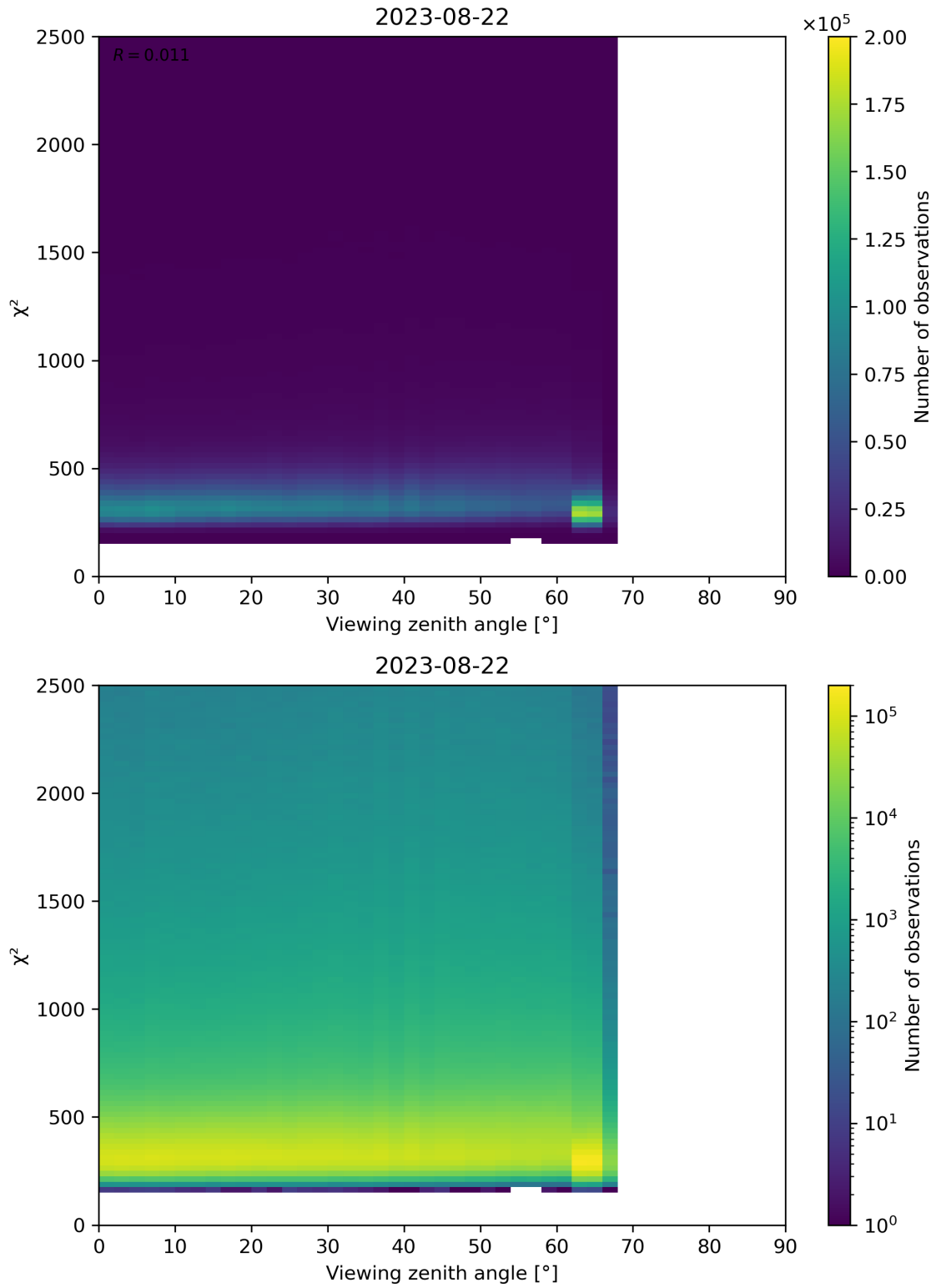
Figure 162: Scatter density plot of “Viewing zenith angle” against “ \chi^2 ” for 2023-08-21 to 2023-08-23.
