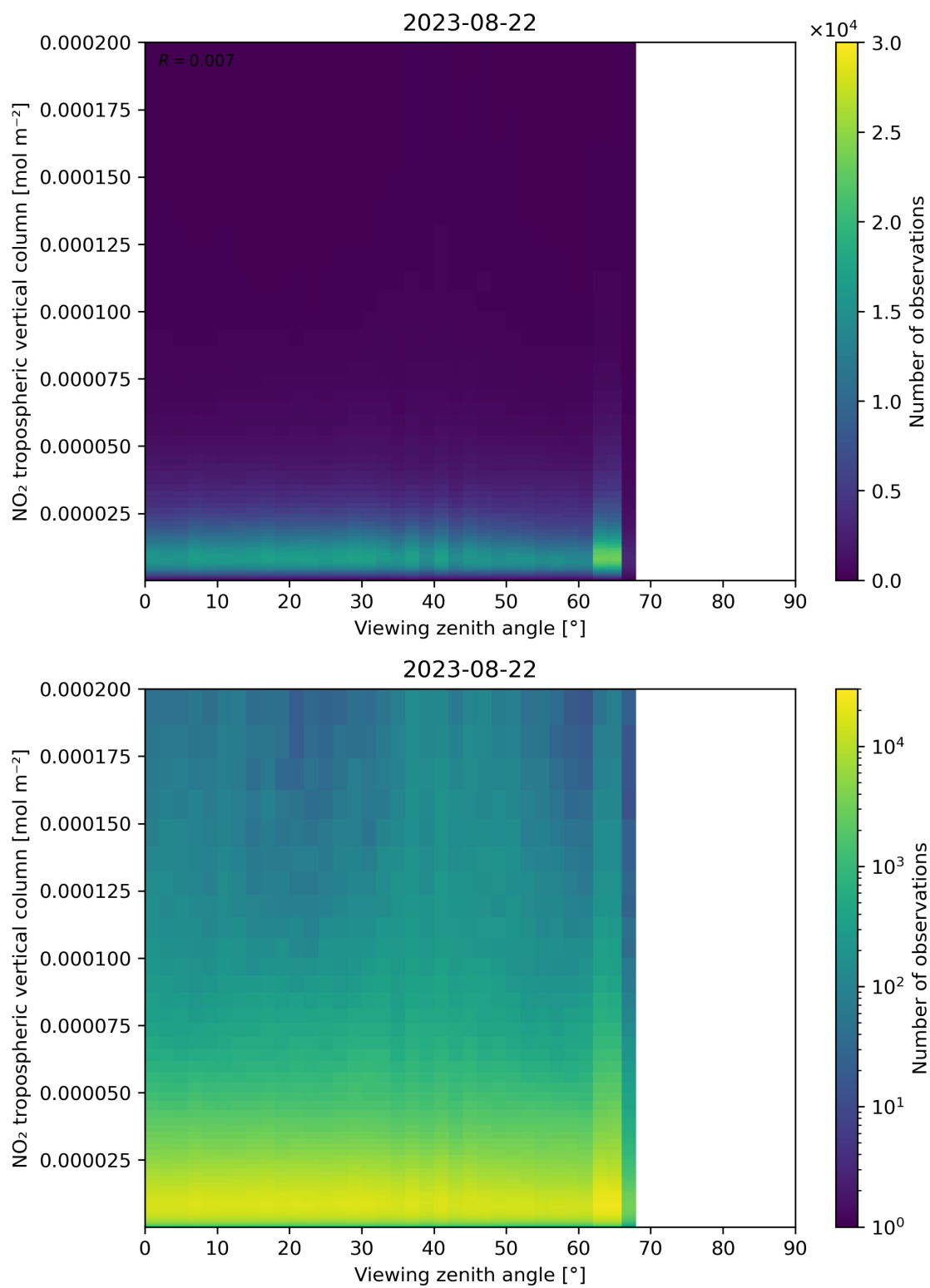
Figure 169: Scatter density plot of “Viewing zenith angle” against “NO 2 tropospheric vertical column” for 2023-08-21 to 2023-08-23.
