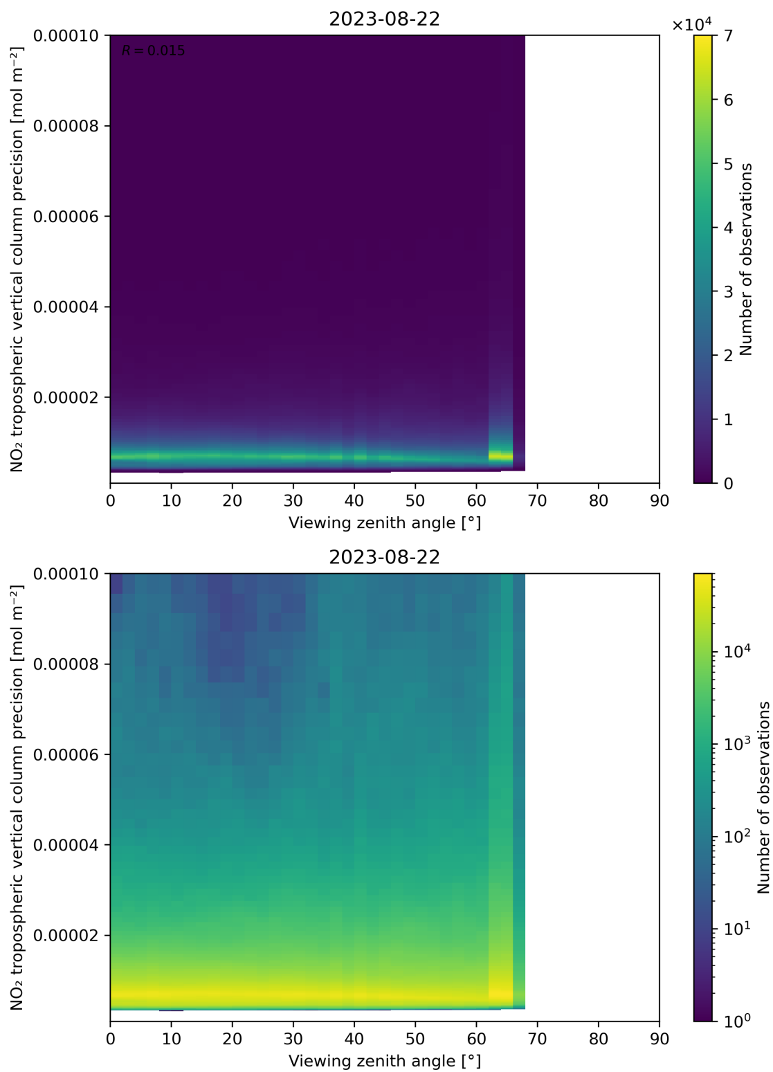
Figure 170: Scatter density plot of “Viewing zenith angle” against “NO 2 tropospheric vertical column precision” for 2023-08-21 to 2023-08-23.
