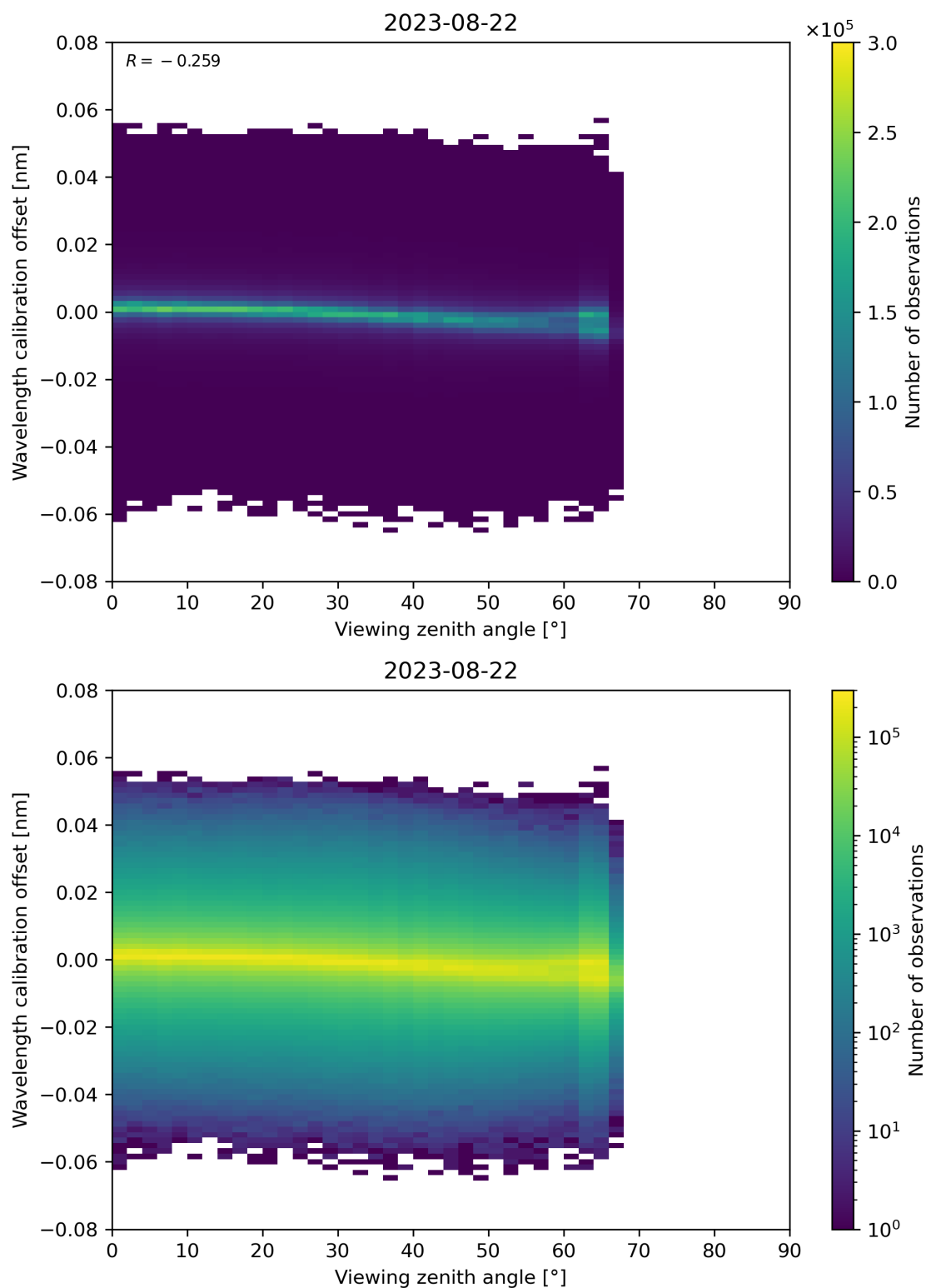
Figure 173: Scatter density plot of “Viewing zenith angle” against “Wavelength calibration offset” for 2023-08-21 to 2023-08-23.
