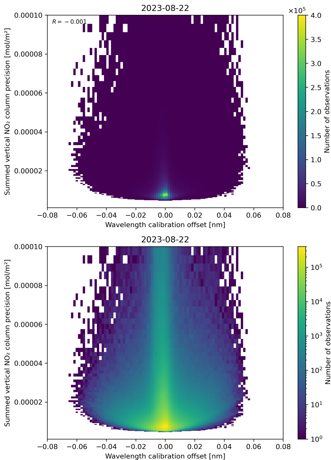
Figure 178: Scatter density plot of “Wavelength calibration offset” against “Summed vertical NO 2 column precision” for 2023-08-21 to 2023-08-23.
