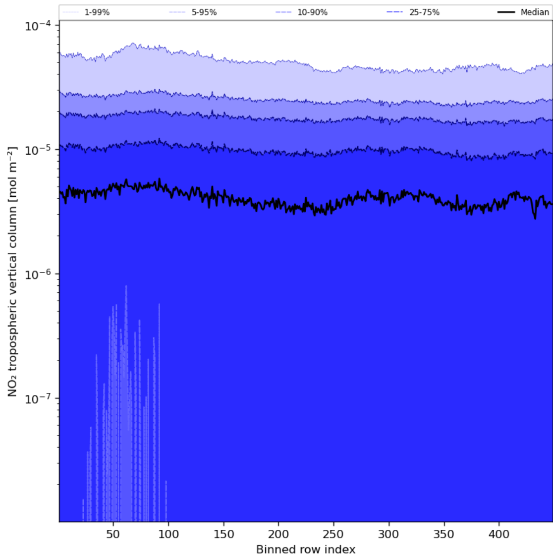
Figure 46: Along track statistics of “NO 2 tropospheric vertical column” for 2023-08-21 to 2023-08-23
