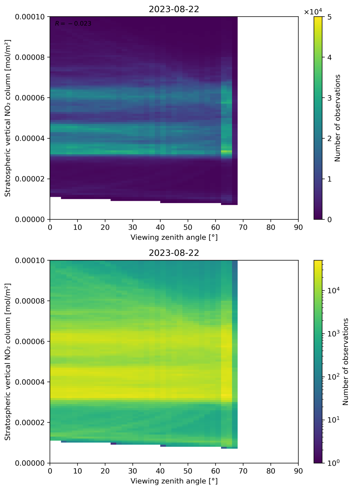
Figure 164: Scatter density plot of “Viewing zenith angle” against “Stratospheric vertical NO 2 column” for 2023-08-21 to 2023-08-23.
