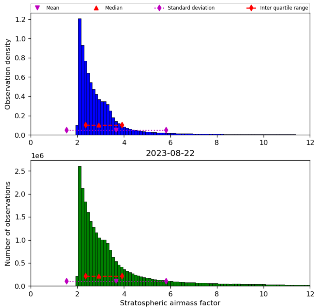
Figure 44: Histogram of “Stratospheric airmass factor” for 2023-08-21 to 2023-08-23
