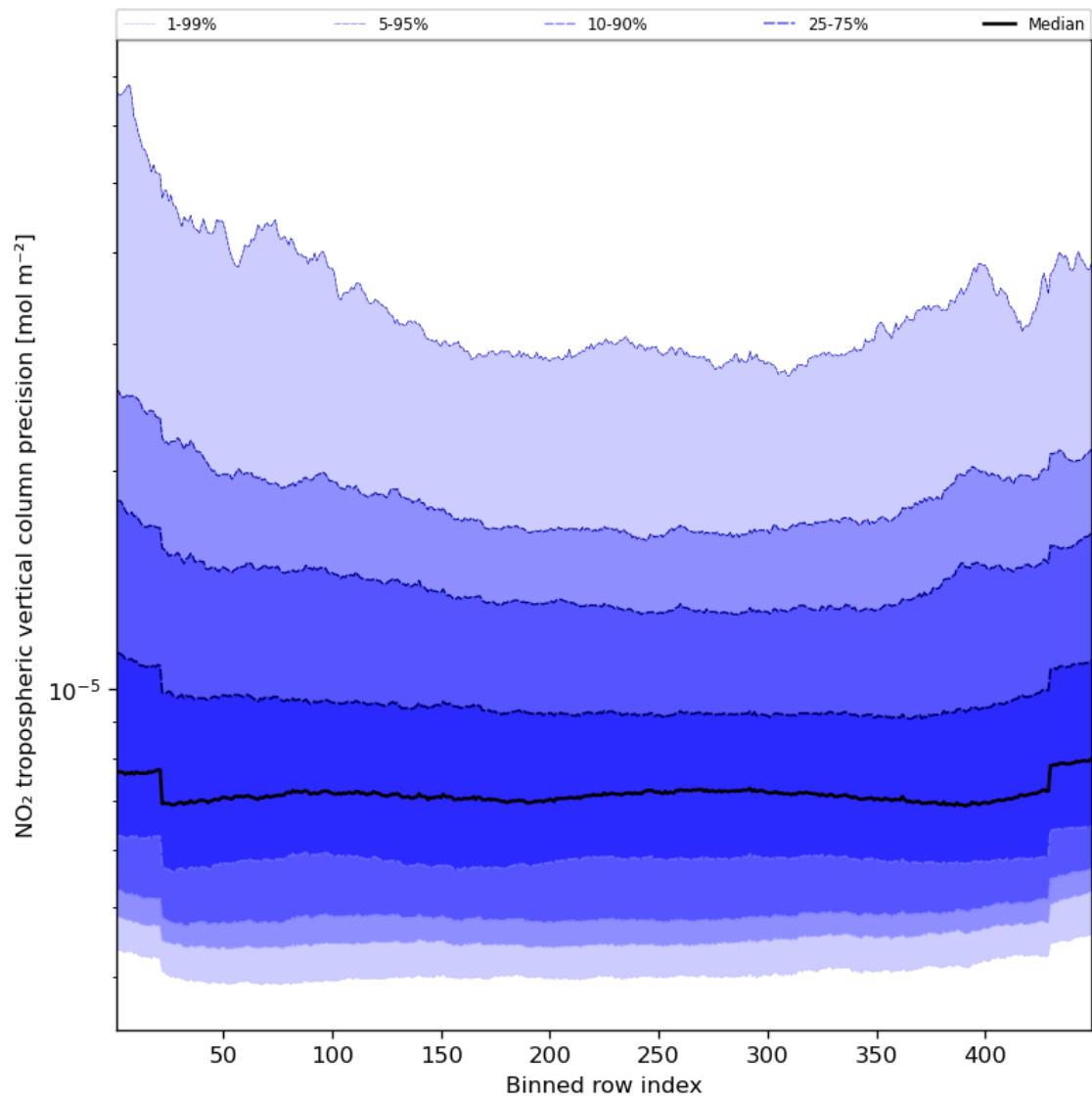
Figure 47: Along track statistics of “NO 2 tropospheric vertical column precision” for 2023-08-21 to 2023-08-23
