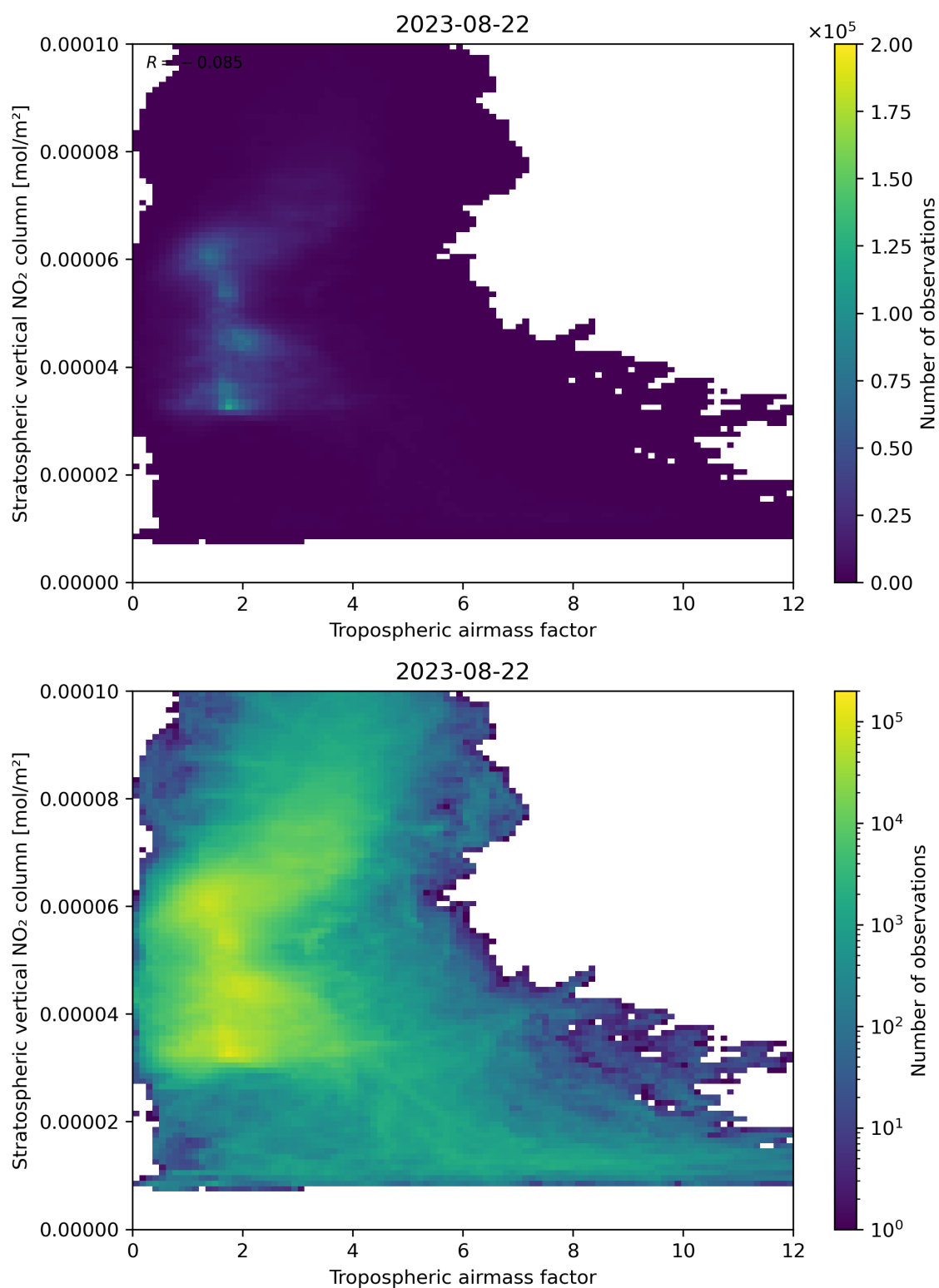
Figure 74: Scatter density plot of “Tropospheric air mass factor” against “Stratospheric vertical NO 2 column” for 2023-08-21 to 2023-08-23.
