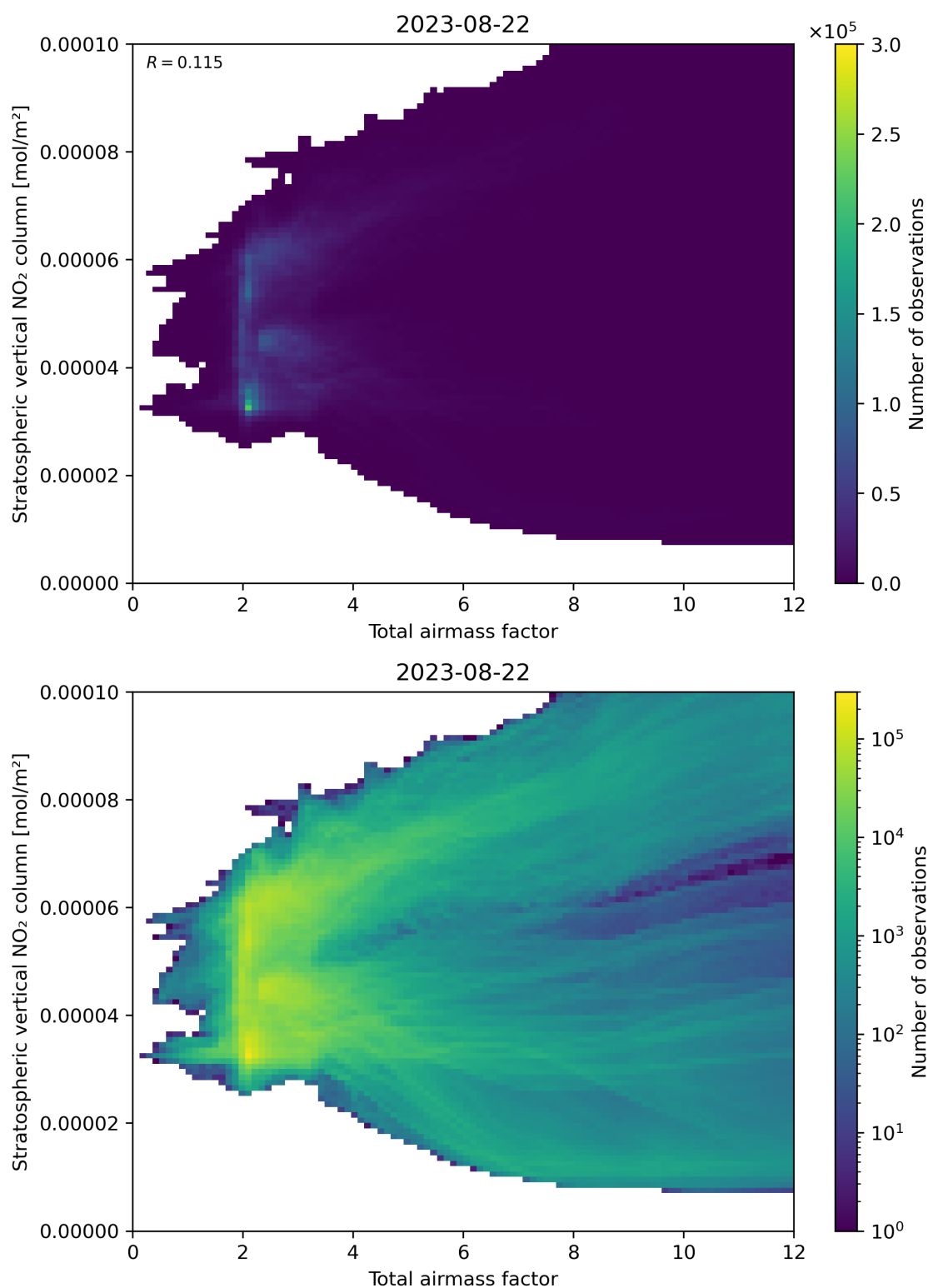
Figure 64: Scatter density plot of “Total airmass factor” against “Stratospheric vertical NO 2 column” for 2023-08-21 to 2023-08-23.
