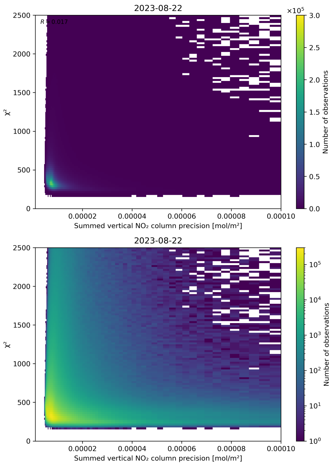
Figure 107: Scatter density plot of “Summed vertical NO 2 column precision” against “ \chi^2 ” for 2023-08-21 to 2023-08-23.
