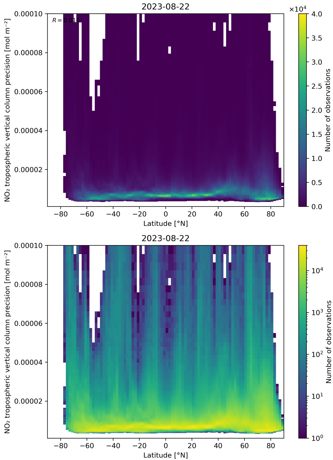
Figure 93: Scatter density plot of “Latitude” against “NO 2 tropospheric vertical column precision” for 2023-08-21 to 2023-08-23.
