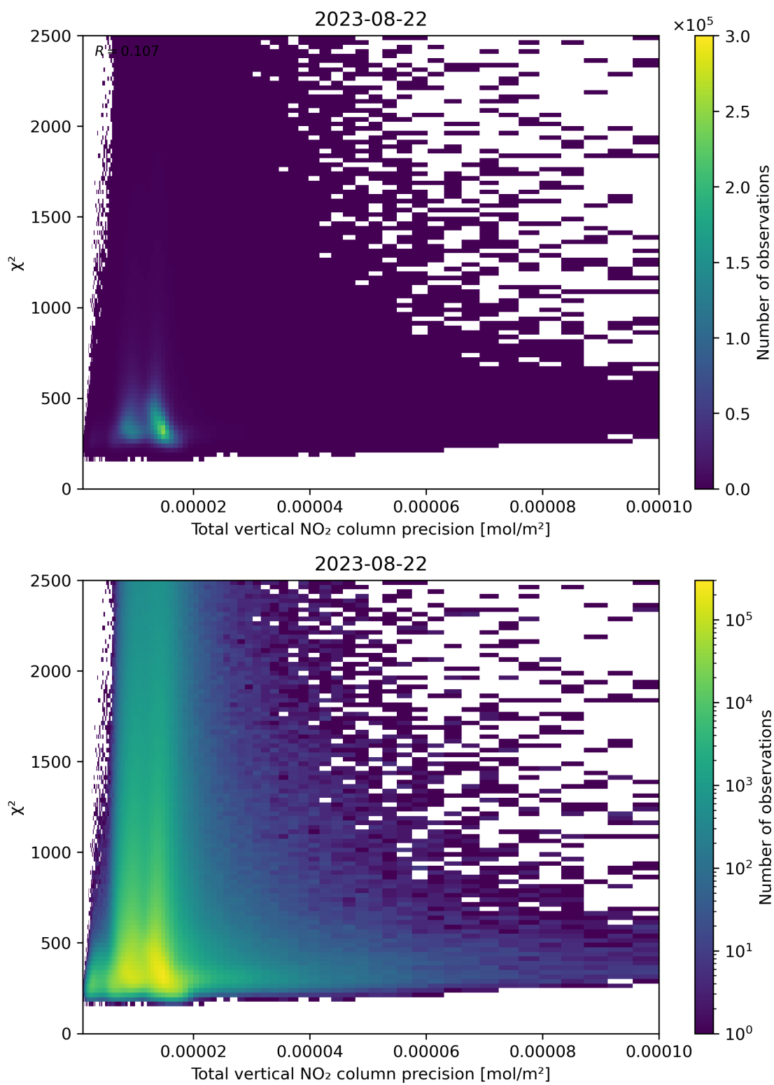
Figure 116: Scatter density plot of “Total vertical NO 2 column precision” against “ \chi^2 ” for 2023-08-21 to 2023-08-23.
