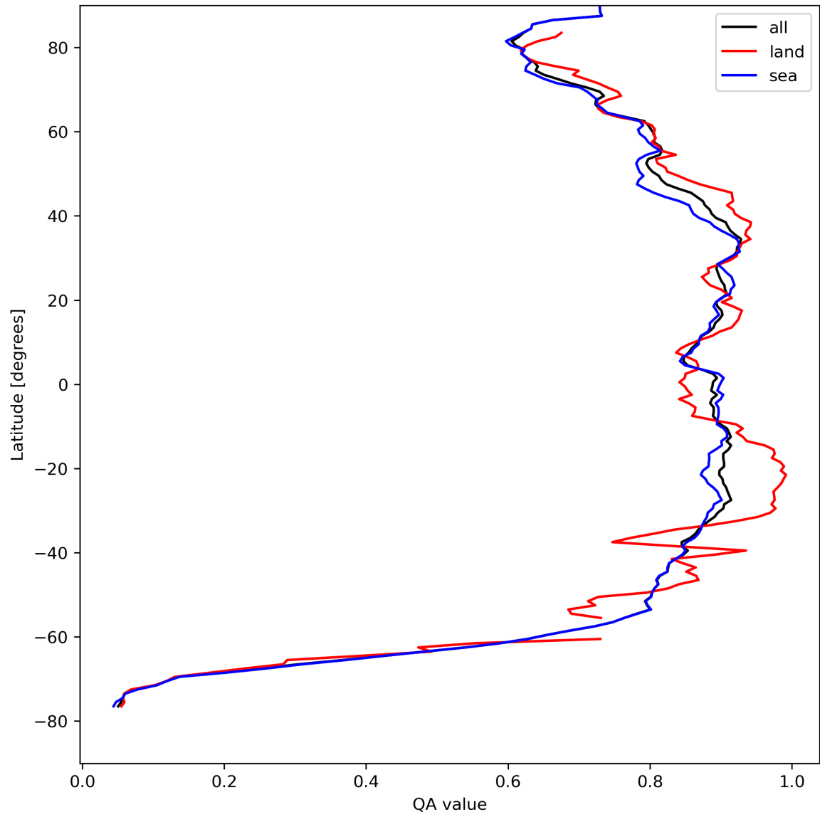
Figure 11: Zonal average of “QA value” for 2023-08-21 to 2023-08-23.
