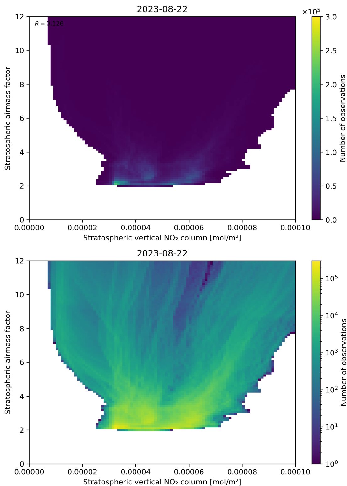
Figure 96: Scatter density plot of “Stratospheric vertical NO 2 column” against “Stratospheric airmass factor” for 2023-08-21 to 2023-08-23.
