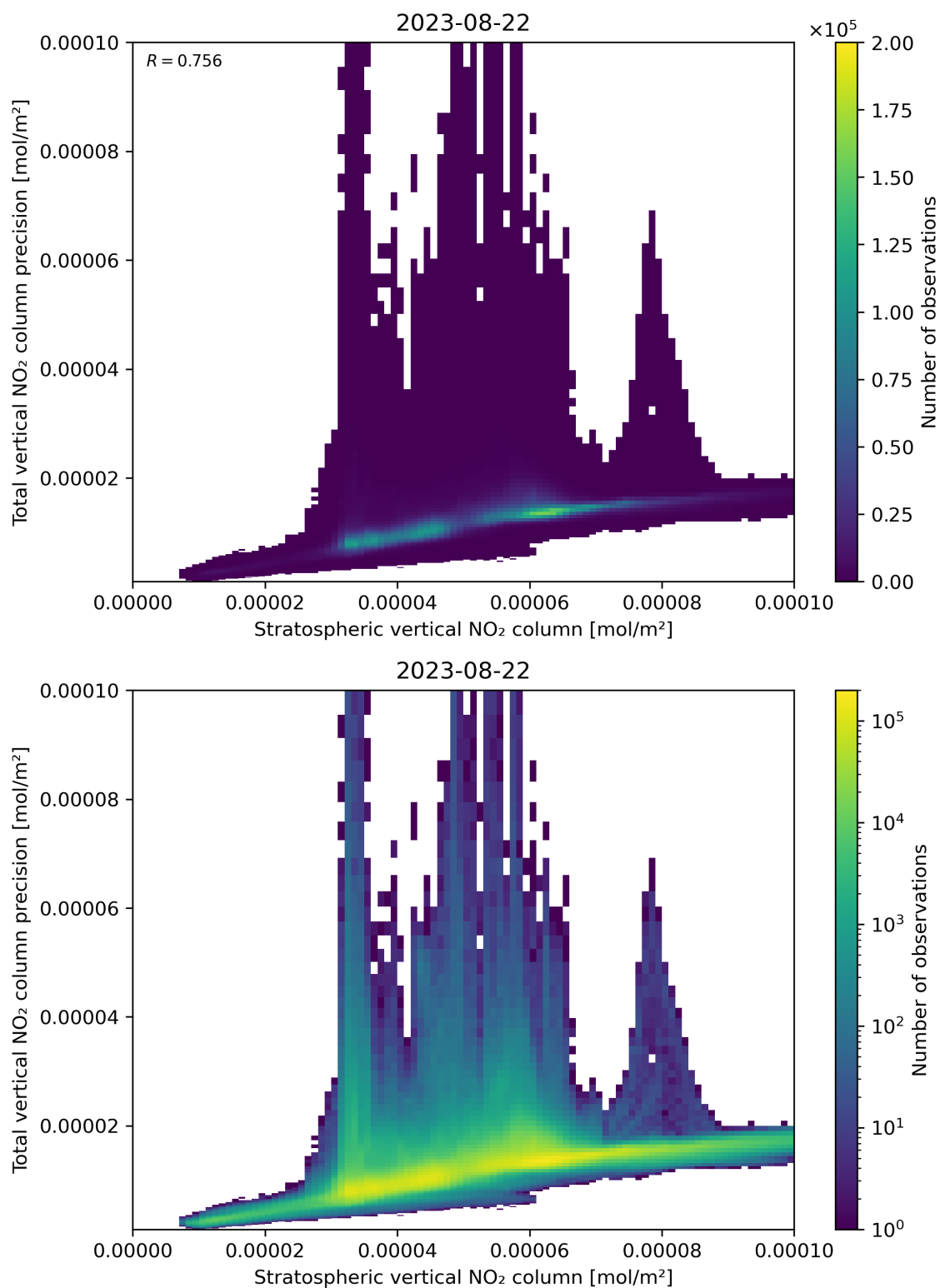
Figure 101: Scatter density plot of “Stratospheric vertical NO 2 column” against “Total vertical NO 2 column precision” for 2023-08-21 to 2023-08-23.
