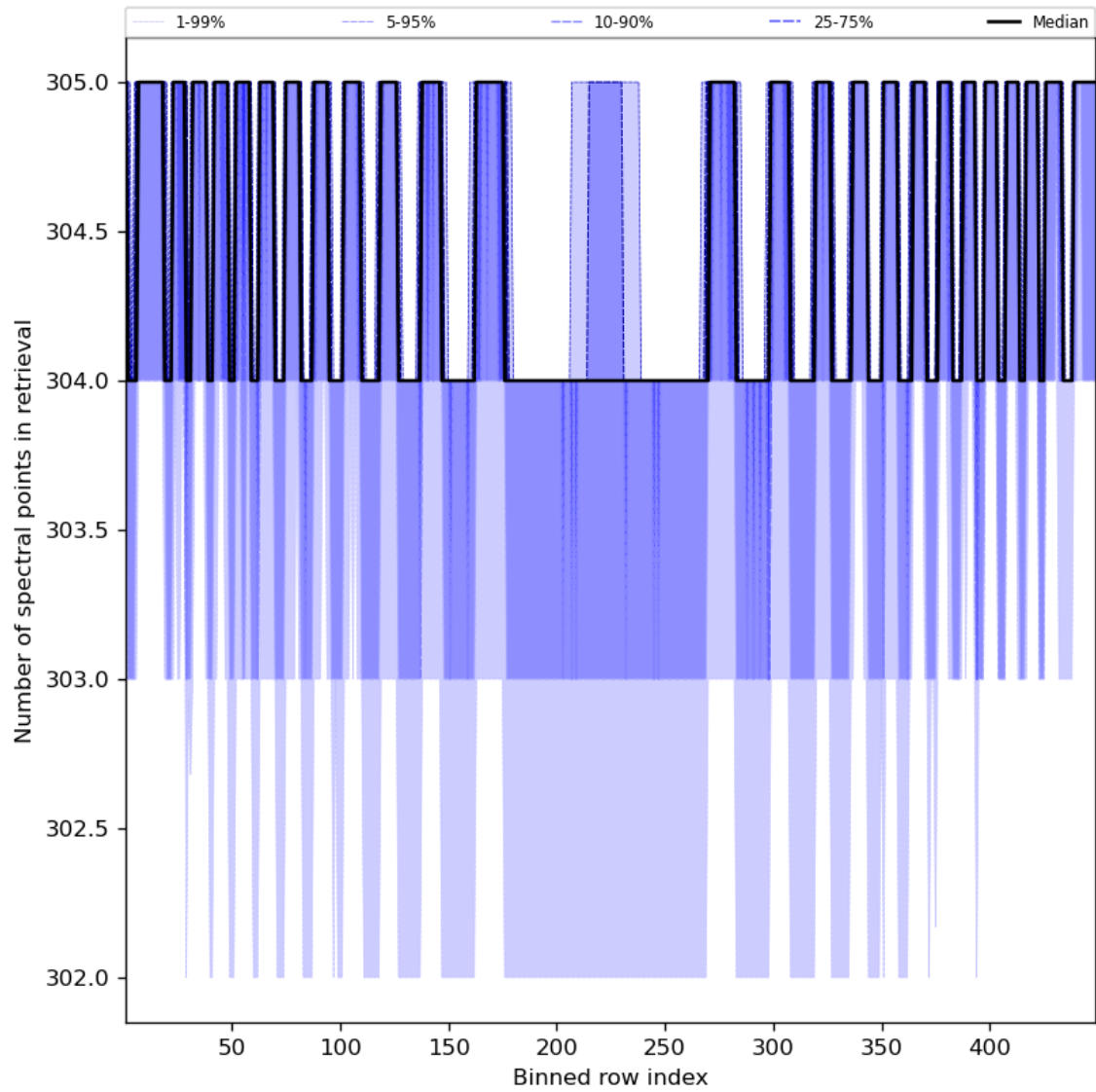
Figure 50: Along track statistics of “Number of spectral points in retrieval” for 2023-08-21 to 2023-08-23
