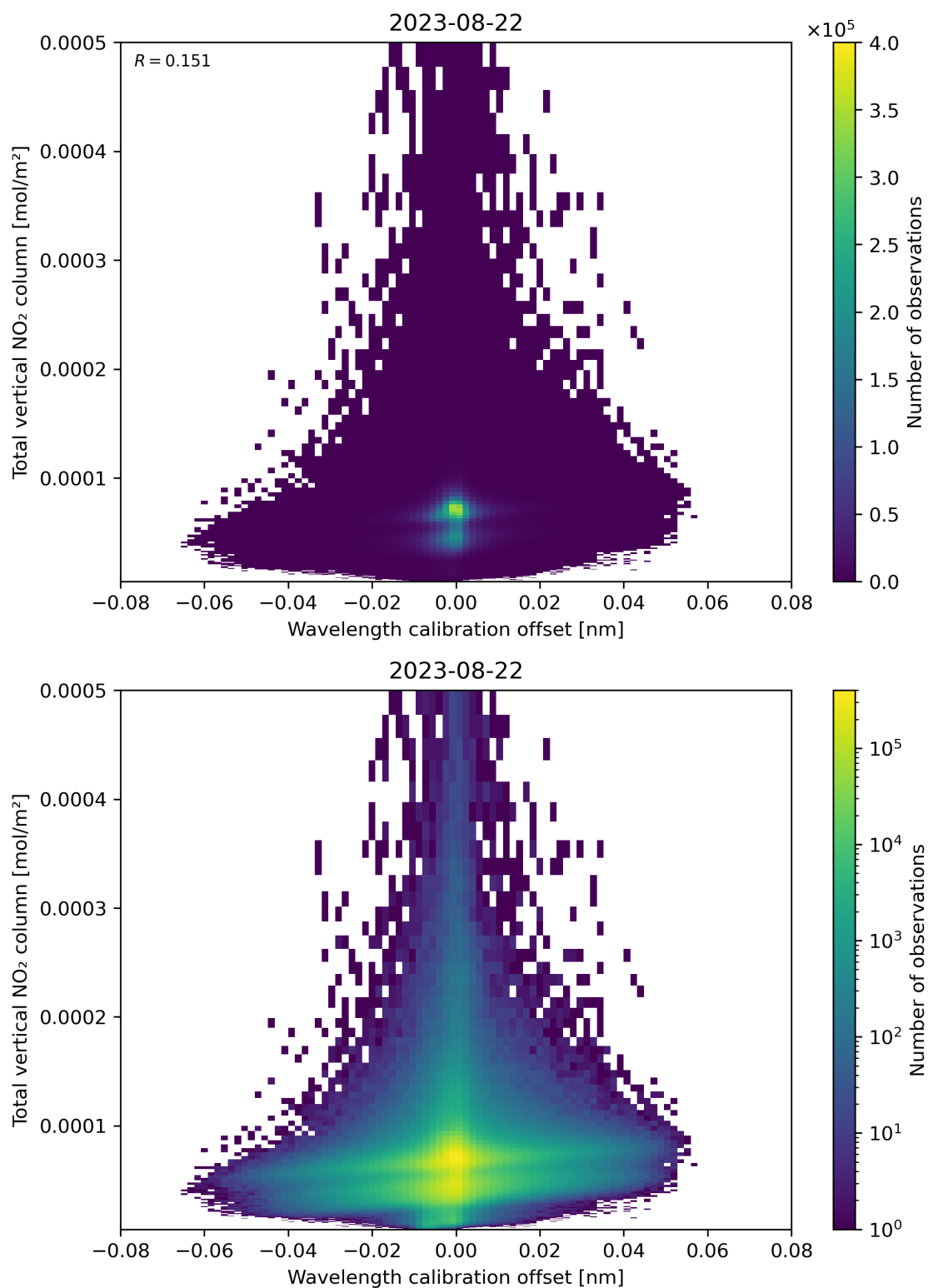
Figure 179: Scatter density plot of “Wavelength calibration offset” against “Total vertical NO 2 column” for 2023-08-21 to 2023-08-23.
