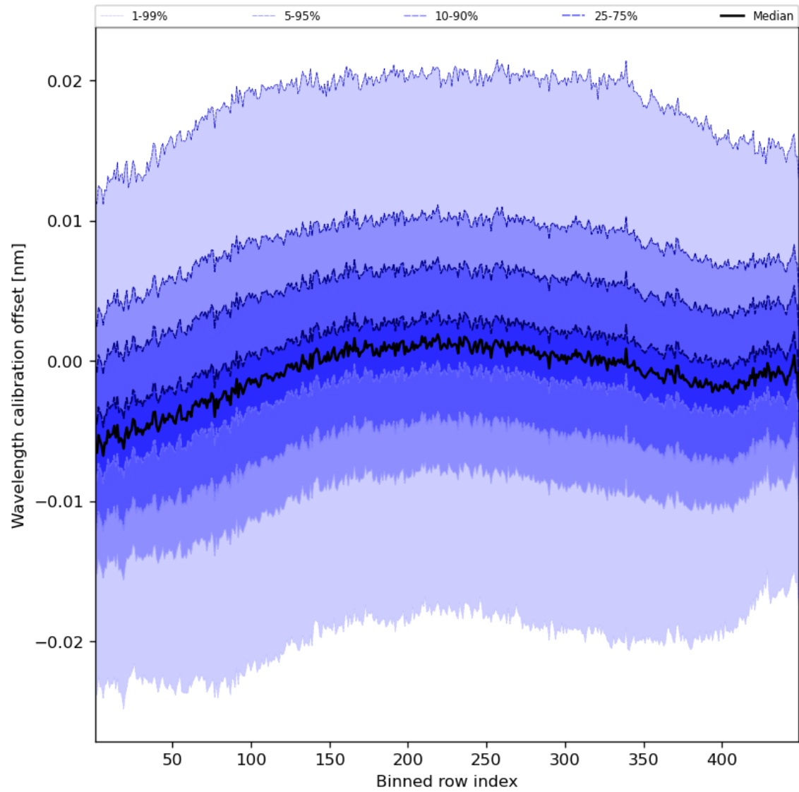
Figure 52: Along track statistics of “Wavelength calibration offset” for 2023-08-21 to 2023-08-23
