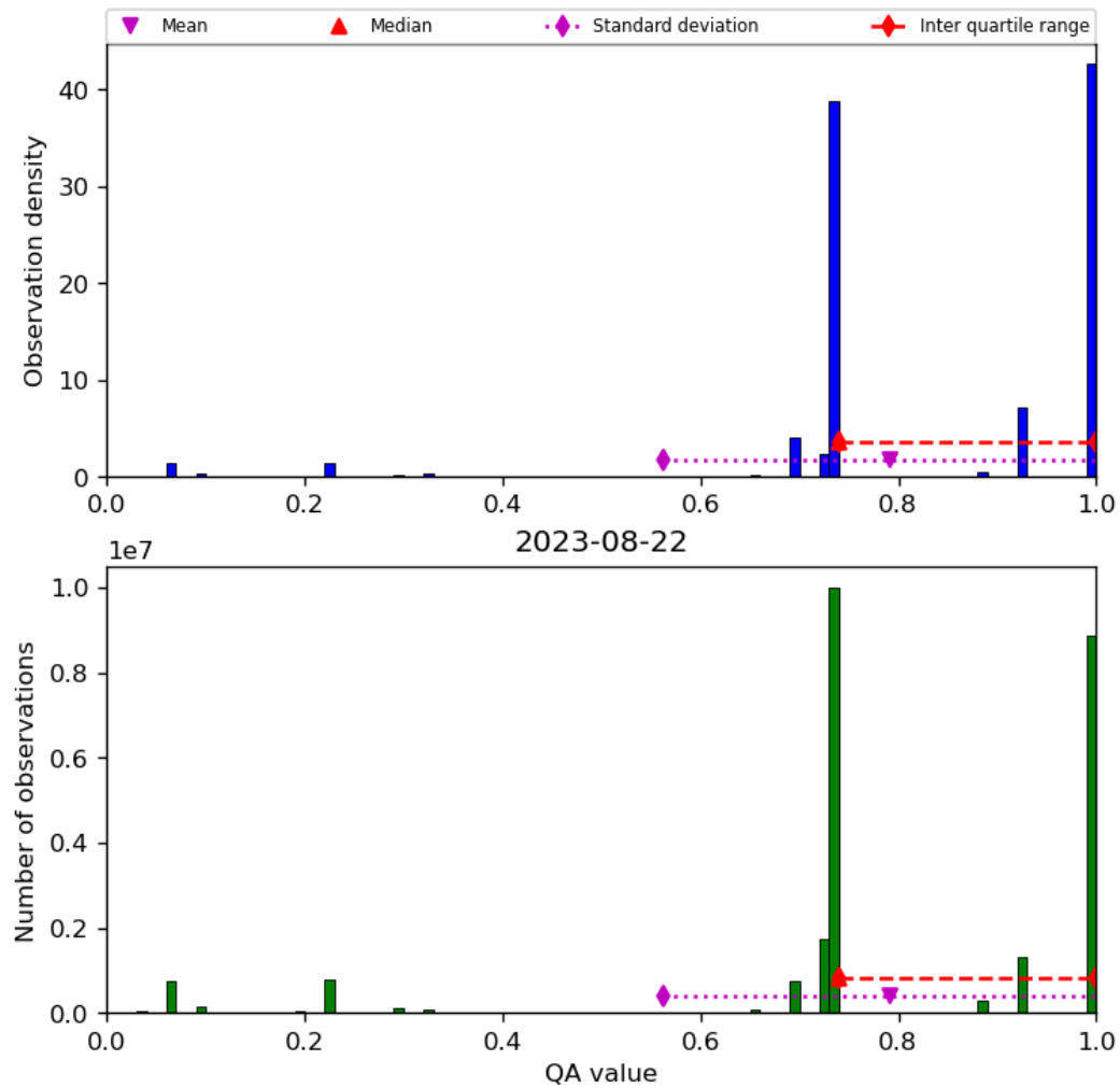
Figure 28: Histogram of “QA value” for 2023-08-21 to 2023-08-23
