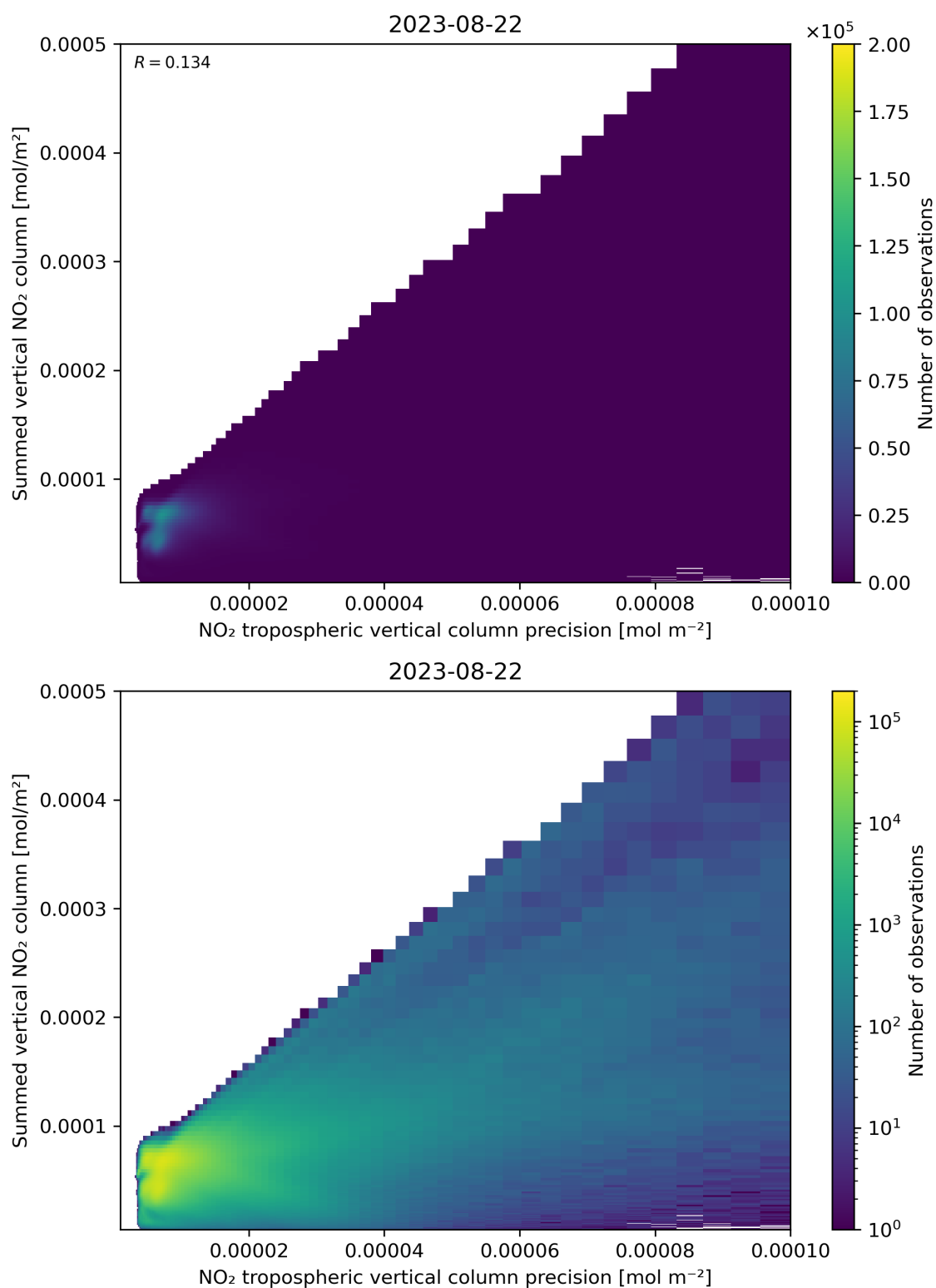
Figure 136: Scatter density plot of “NO 2 tropospheric vertical column precision” against “Summed vertical NO 2 column” for 2023-08-21 to 2023-08-23.
