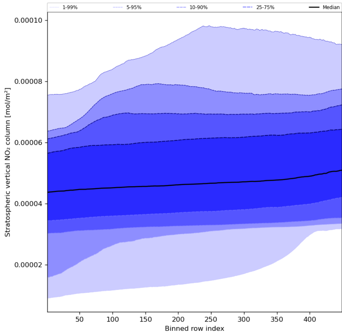
Figure 53: Along track statistics of “Stratospheric vertical NO 2 column” for 2023-08-21 to 2023-08-23
