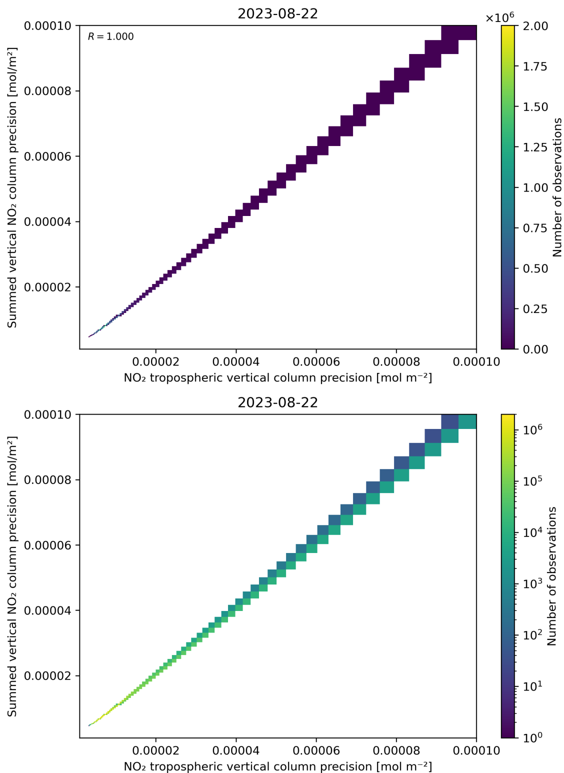
Figure 137: Scatter density plot of “NO 2 tropospheric vertical column precision” against “Summed vertical NO 2 column precision” for 2023-08-21 to 2023-08-23.
