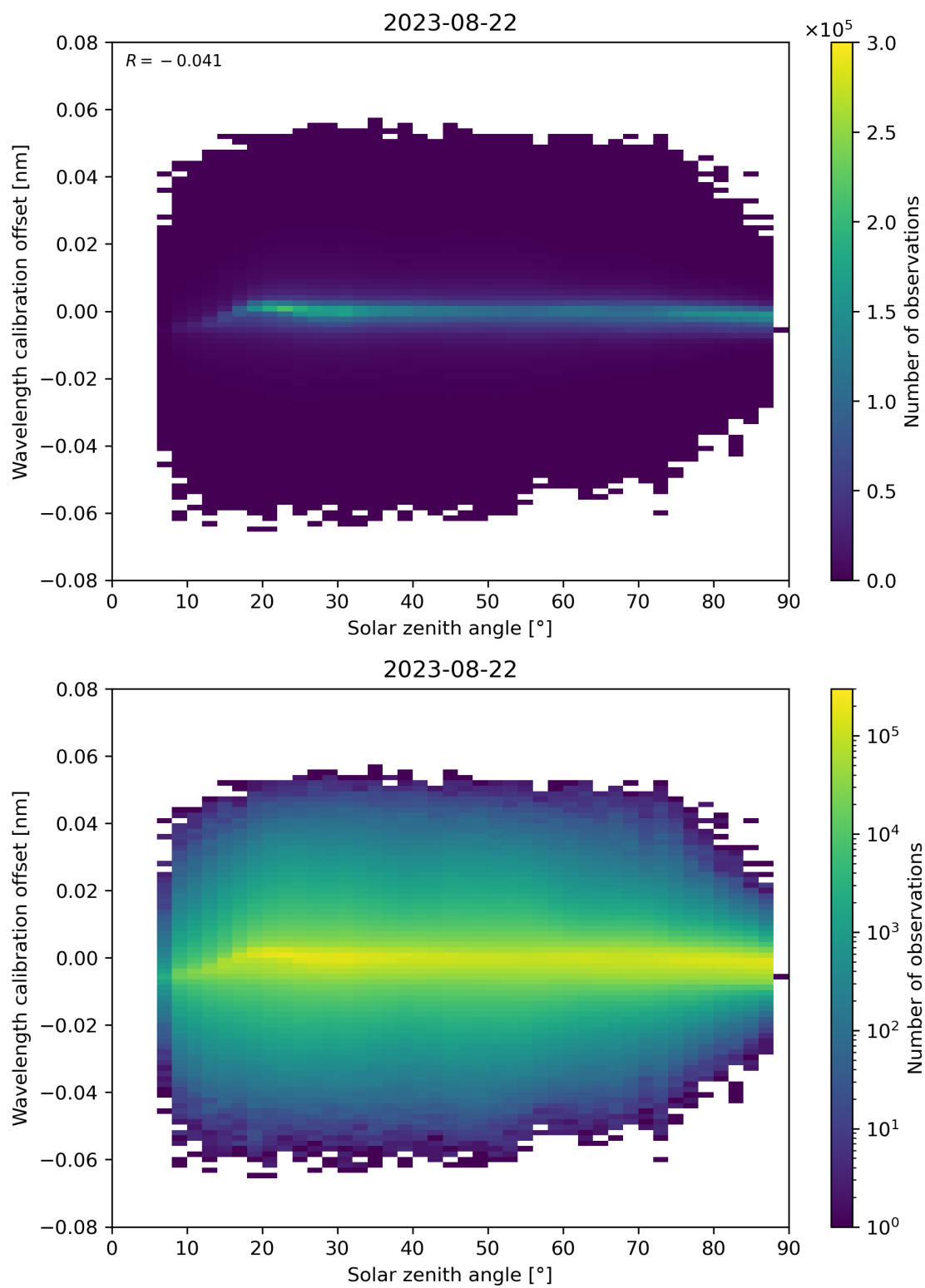
Figure 158: Scatter density plot of “Solar zenith angle” against “Wavelength calibration offset” for 2023-08-21 to 2023-08-23.
