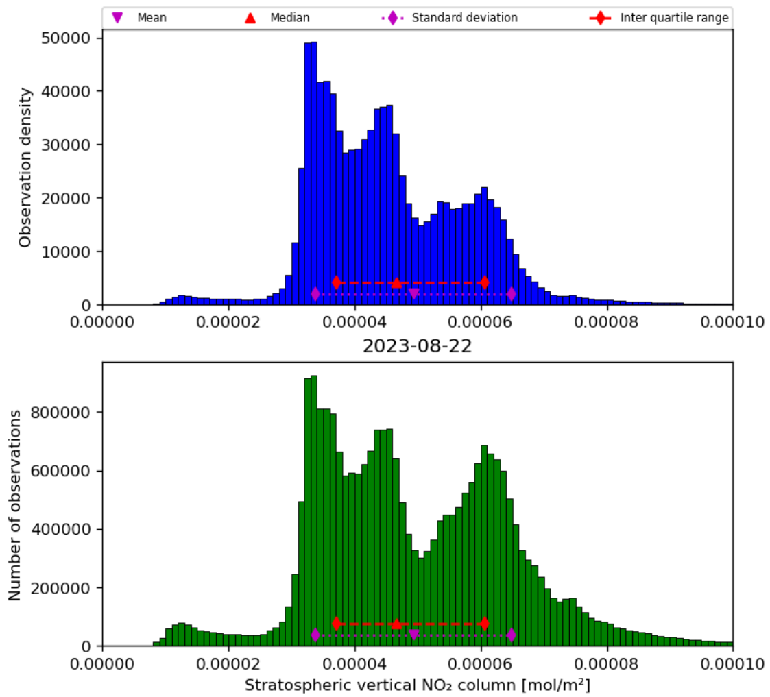
Figure 36: Histogram of “Stratospheric vertical NO 2 column” for 2023-08-21 to 2023-08-23
