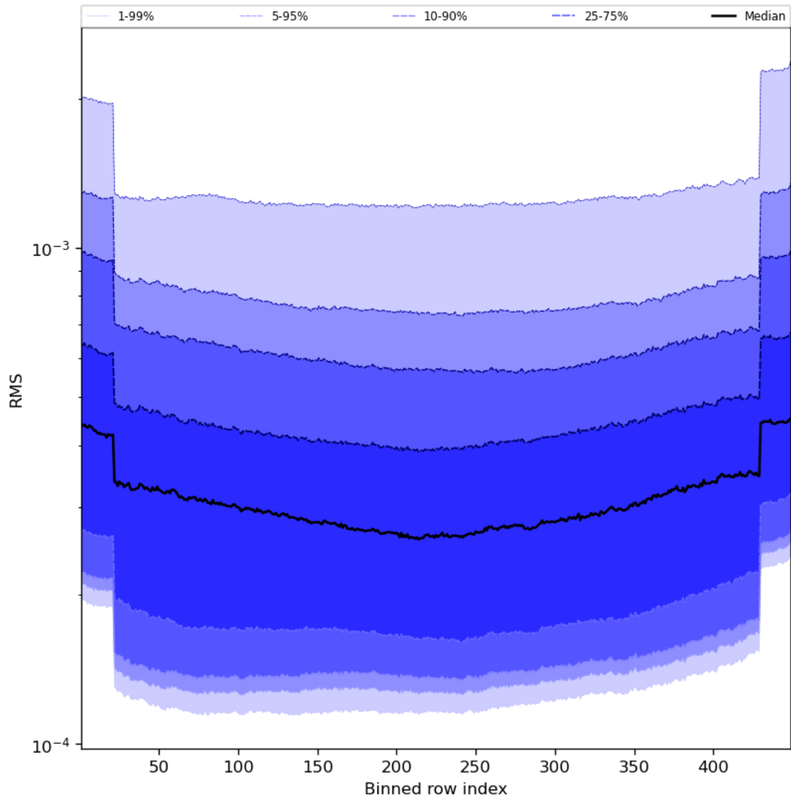
Figure 60: Along track statistics of “RMS” for 2023-08-21 to 2023-08-23
