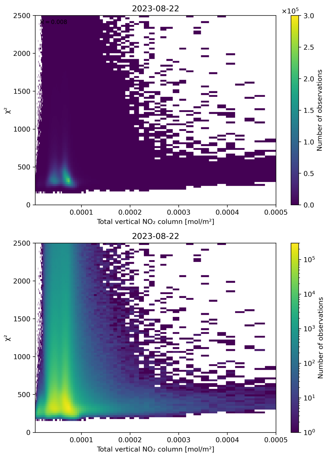
Figure 111: Scatter density plot of “Total vertical NO 2 column” against “ \chi^2 ” for 2023-08-21 to 2023-08-23.
