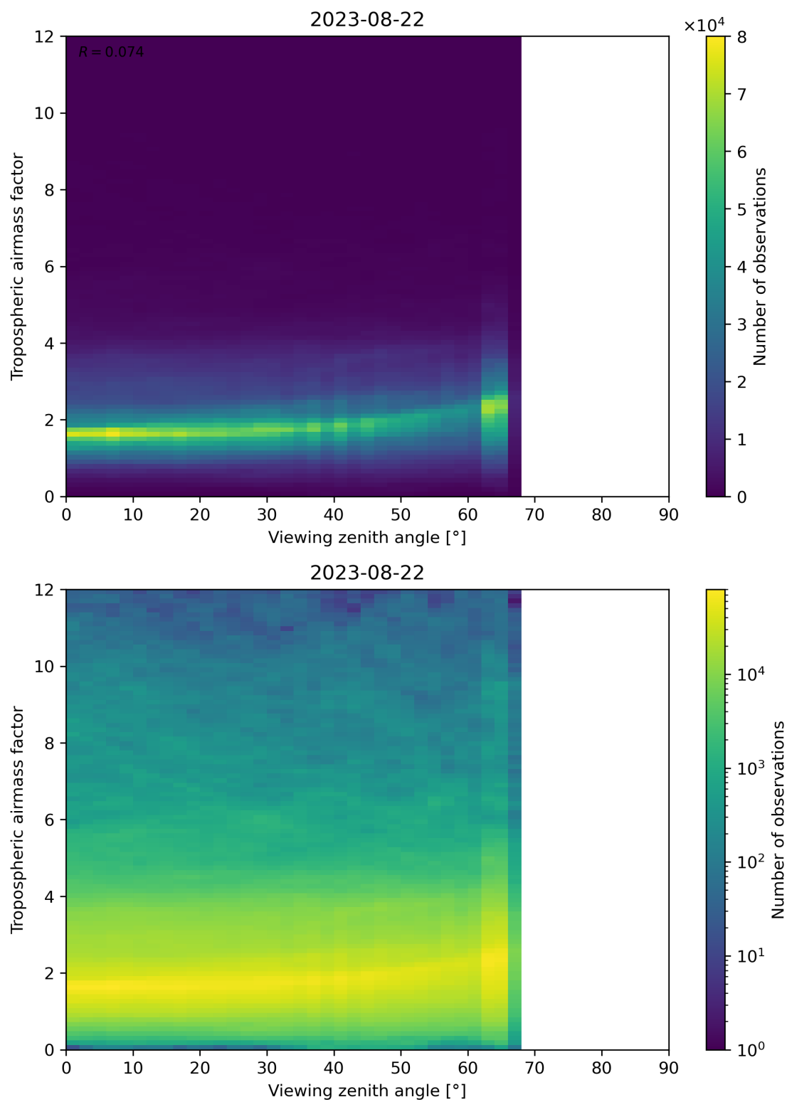
Figure 161: Scatter density plot of “Viewing zenith angle” against “Tropospheric airmass factor” for 2023-08-21 to 2023-08-23.
