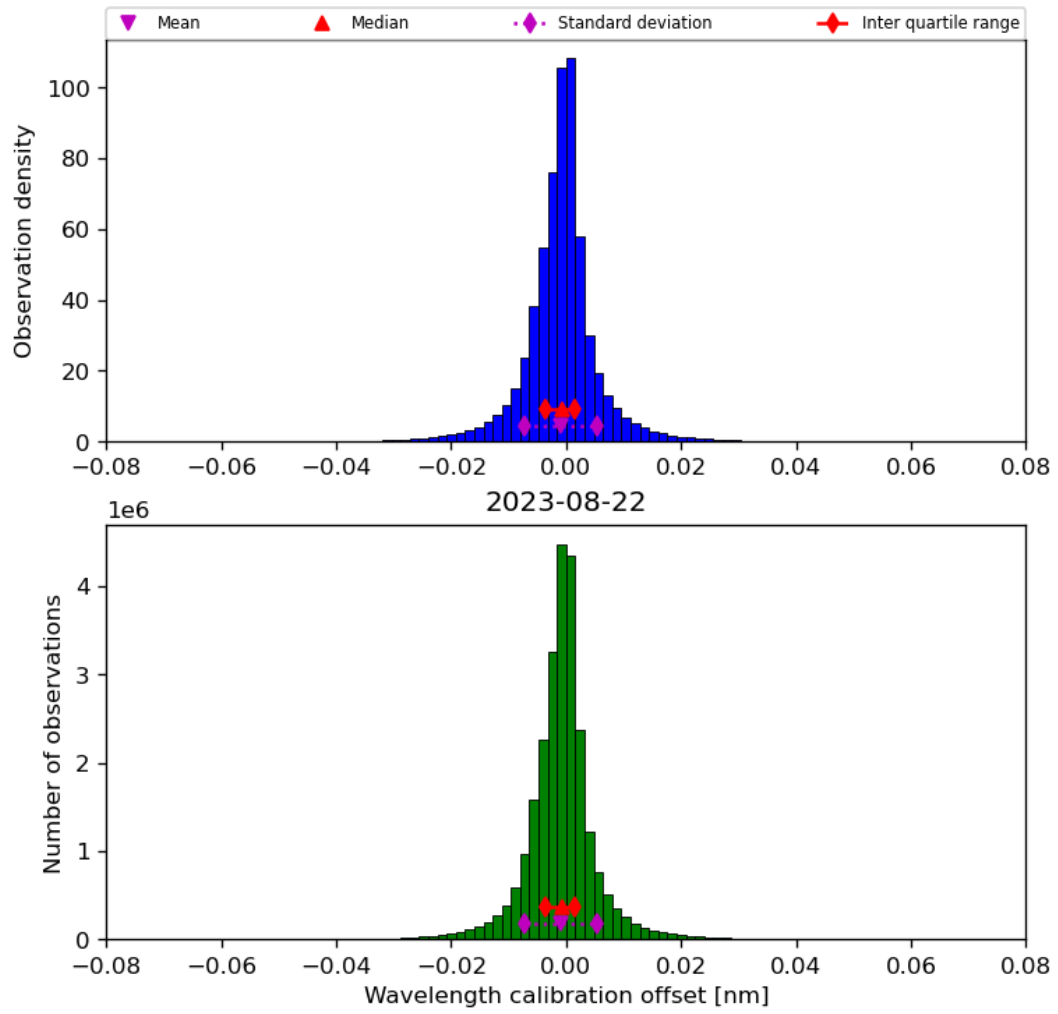
Figure 35: Histogram of “Wavelength calibration offset” for 2023-08-21 to 2023-08-23
