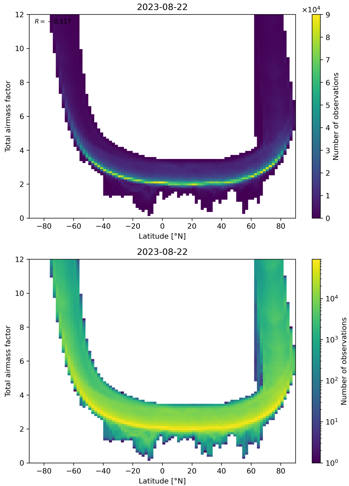
Figure 84: Scatter density plot of “Latitude” against “Total airmass factor” for 2023-08-21 to 2023-08-23.
