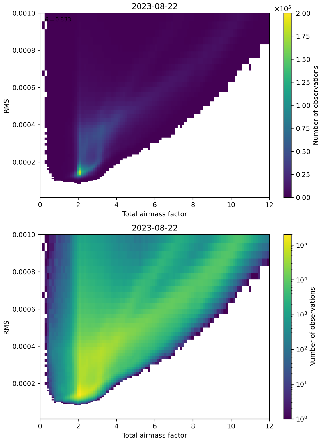
Figure 69: Scatter density plot of “Total airmass factor” against “RMS” for 2023-08-21 to 2023-08-23.
