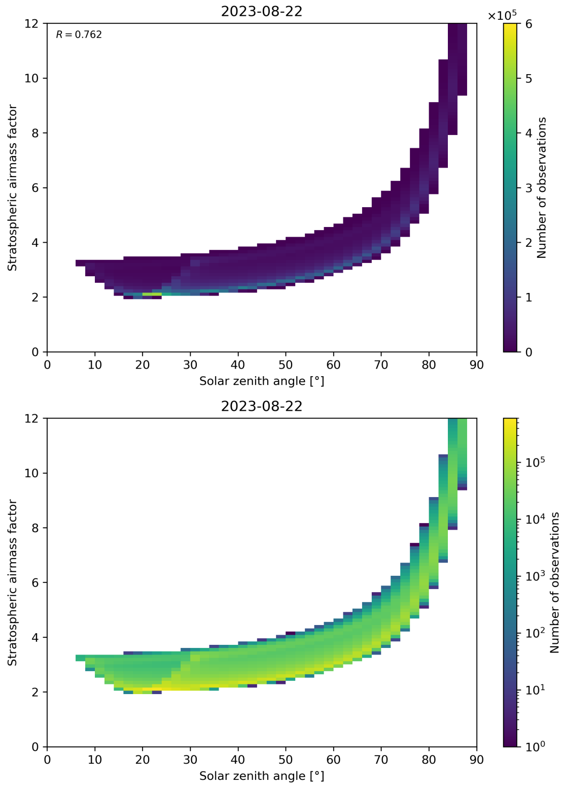
Figure 145: Scatter density plot of “Solar zenith angle” against “Stratospheric airmass factor” for 2023-08-21 to 2023-08-23.
