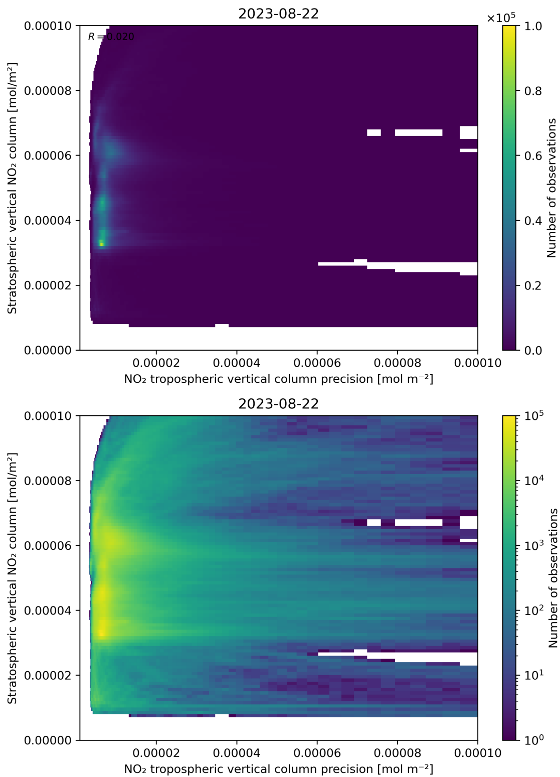
Figure 135: Scatter density plot of “NO 2 tropospheric vertical column precision” against “Stratospheric vertical NO 2 column” for 2023-08-21 to 2023-08-23.
