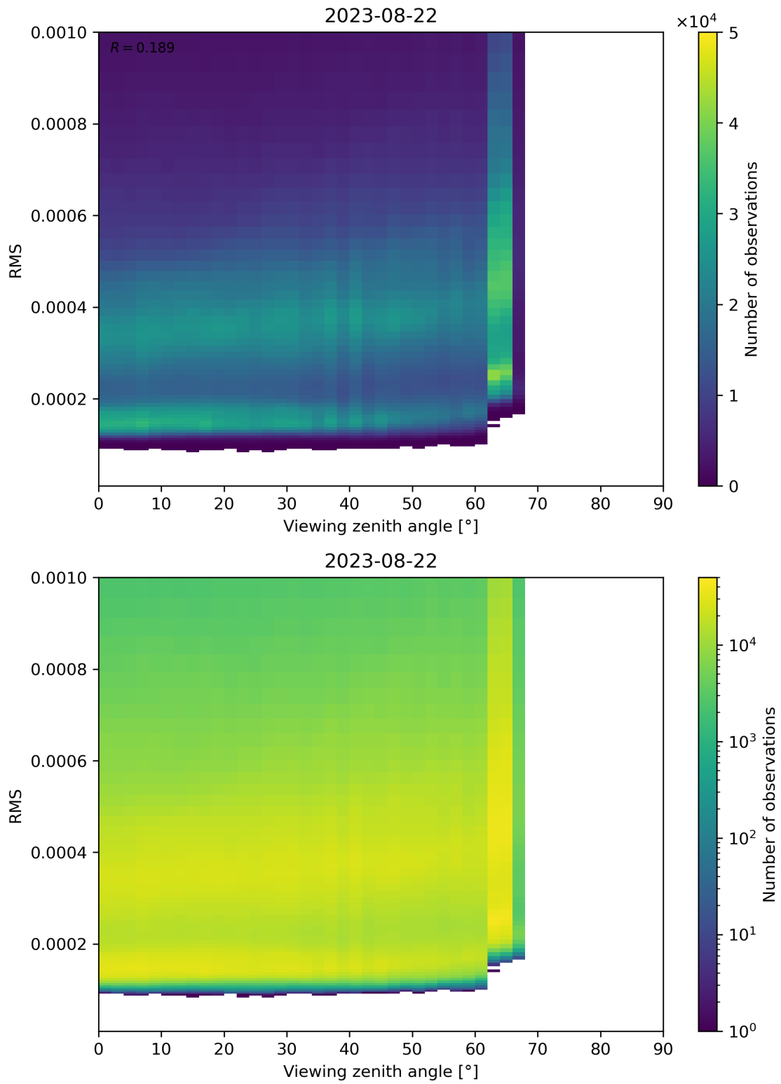
Figure 171: Scatter density plot of “Viewing zenith angle” against “RMS” for 2023-08-21 to 2023-08-23.
