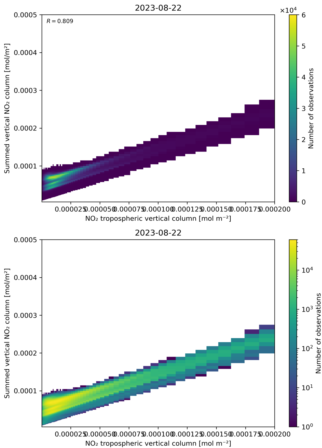
Figure 126: Scatter density plot of “NO 2 tropospheric vertical column” against “Summed vertical NO 2 column” for 2023-08-21 to 2023-08-23.
