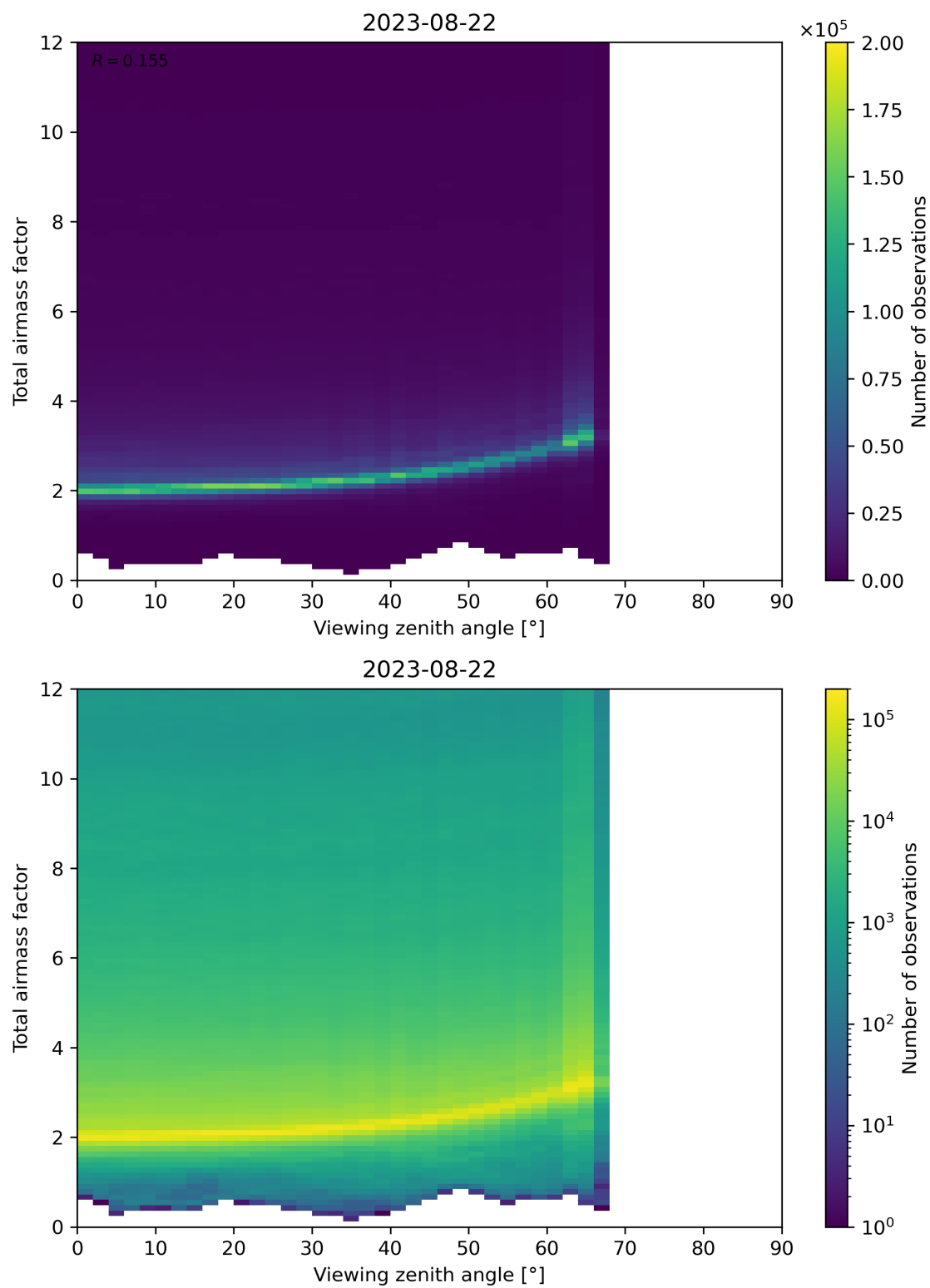
Figure 160: Scatter density plot of “Viewing zenith angle” against “Total airmass factor” for 2023-08-21 to 2023-08-23.
