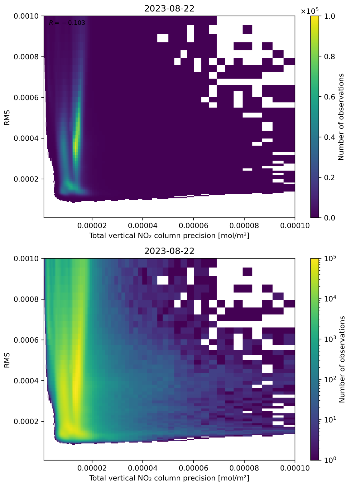
Figure 119: Scatter density plot of “Total vertical NO 2 column precision” against “RMS” for 2023-08-21 to 2023-08-23.
