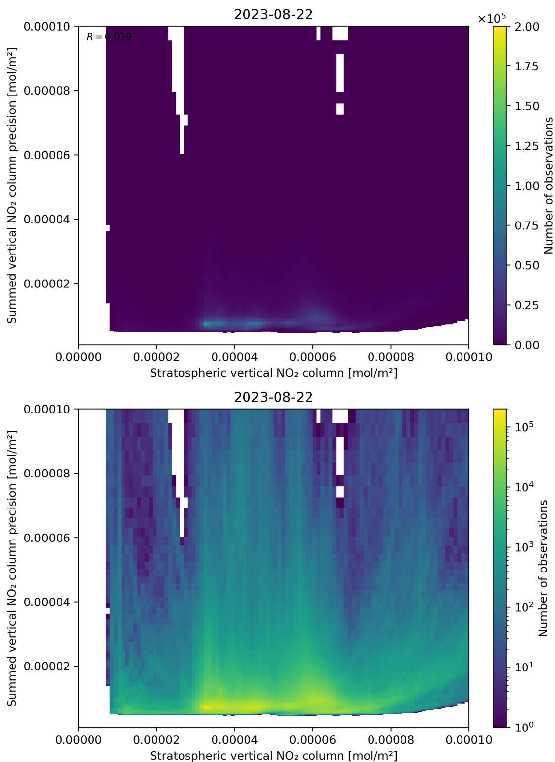
Figure 99: Scatter density plot of “Stratospheric vertical NO 2 column” against “Summed vertical NO 2 column precision” for 2023-08-21 to 2023-08-23.
