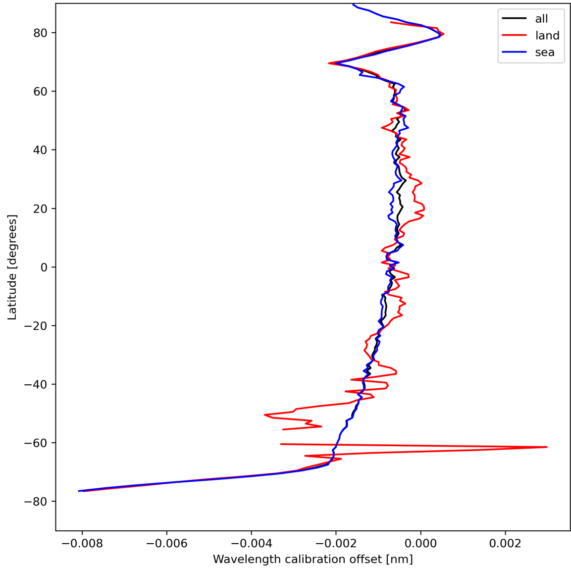
Figure 18: Zonal average of “Wavelength calibration offset” for 2023-08-21 to 2023-08-23.
