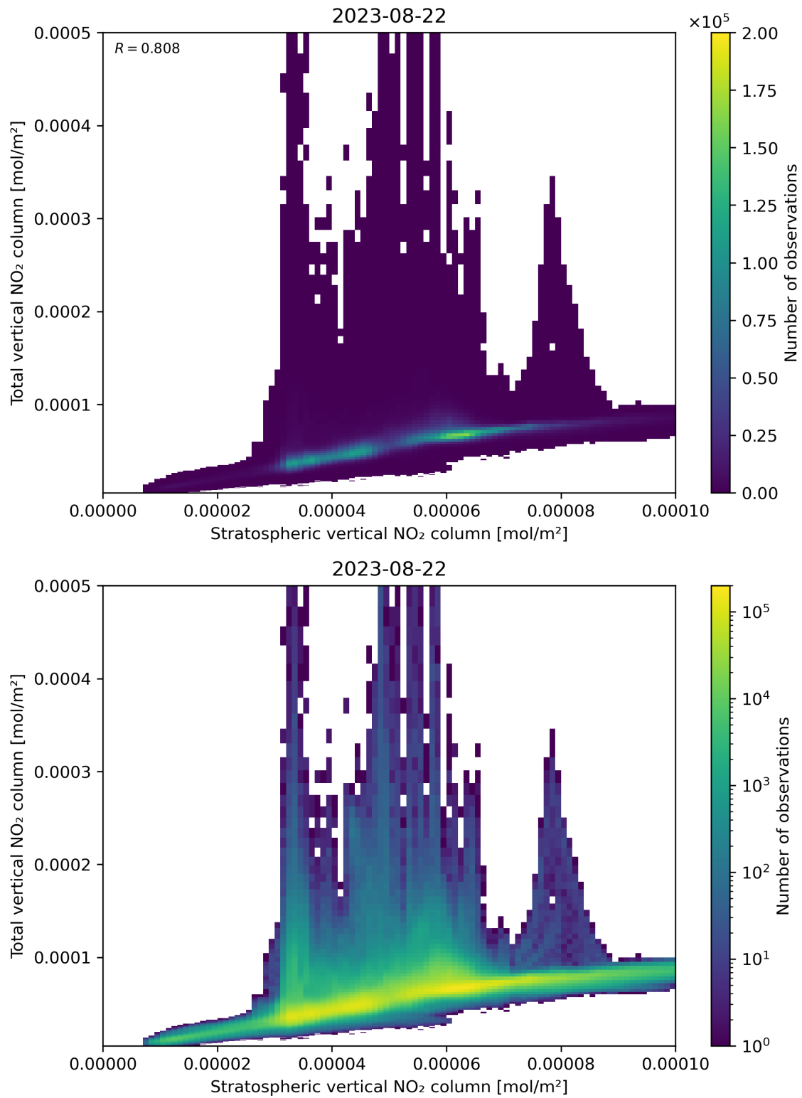
Figure 100: Scatter density plot of “Stratospheric vertical NO 2 column” against “Total vertical NO 2 column” for 2023-08-21 to 2023-08-23.
