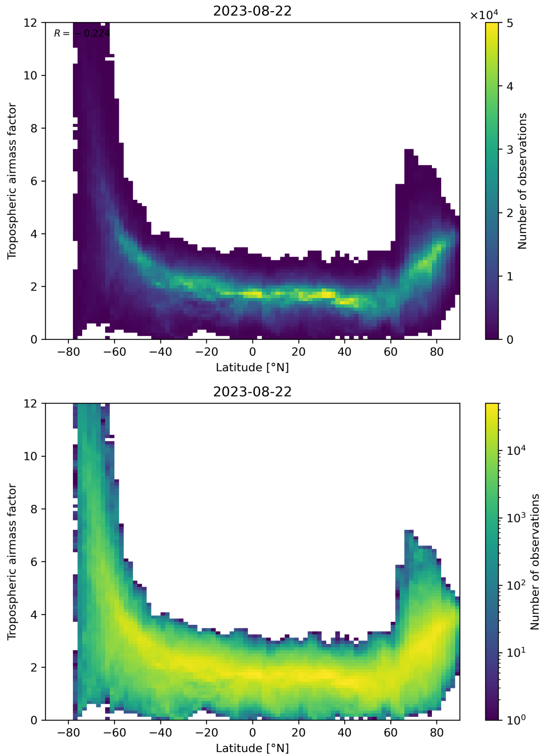
Figure 85: Scatter density plot of “Latitude” against “Tropospheric airmass factor” for 2023-08-21 to 2023-08-23.
