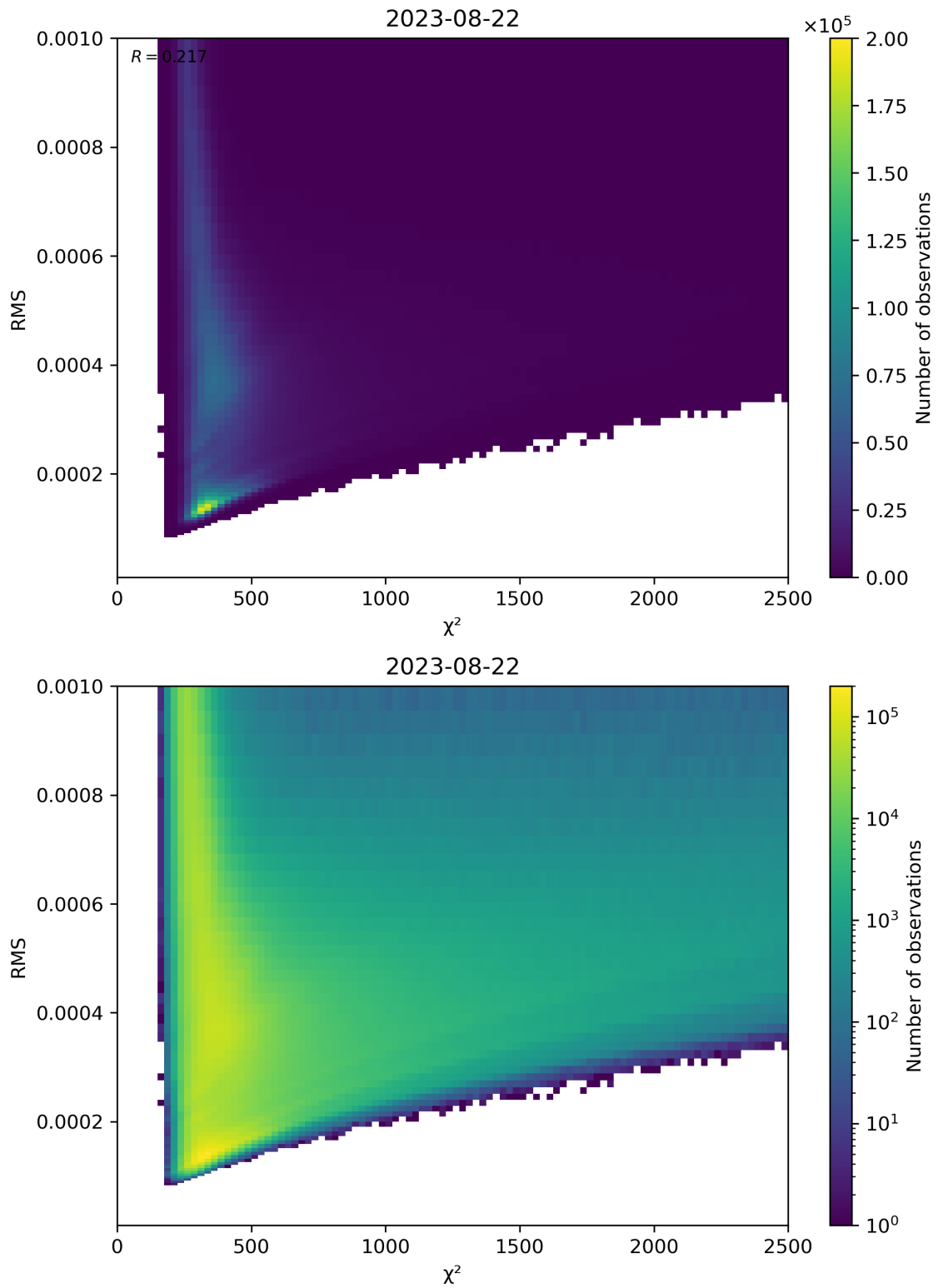
Figure 82: Scatter density plot of “ \chi^2 ” against “RMS” for 2023-08-21 to 2023-08-23.
