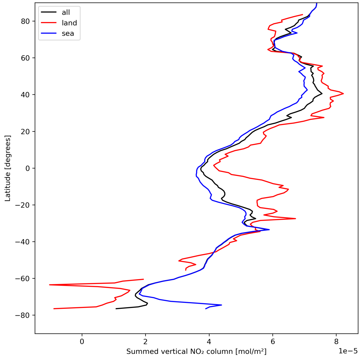
Figure 23: Zonal average of “Summed vertical NO 2 column” for 2023-08-21 to 2023-08-23.
