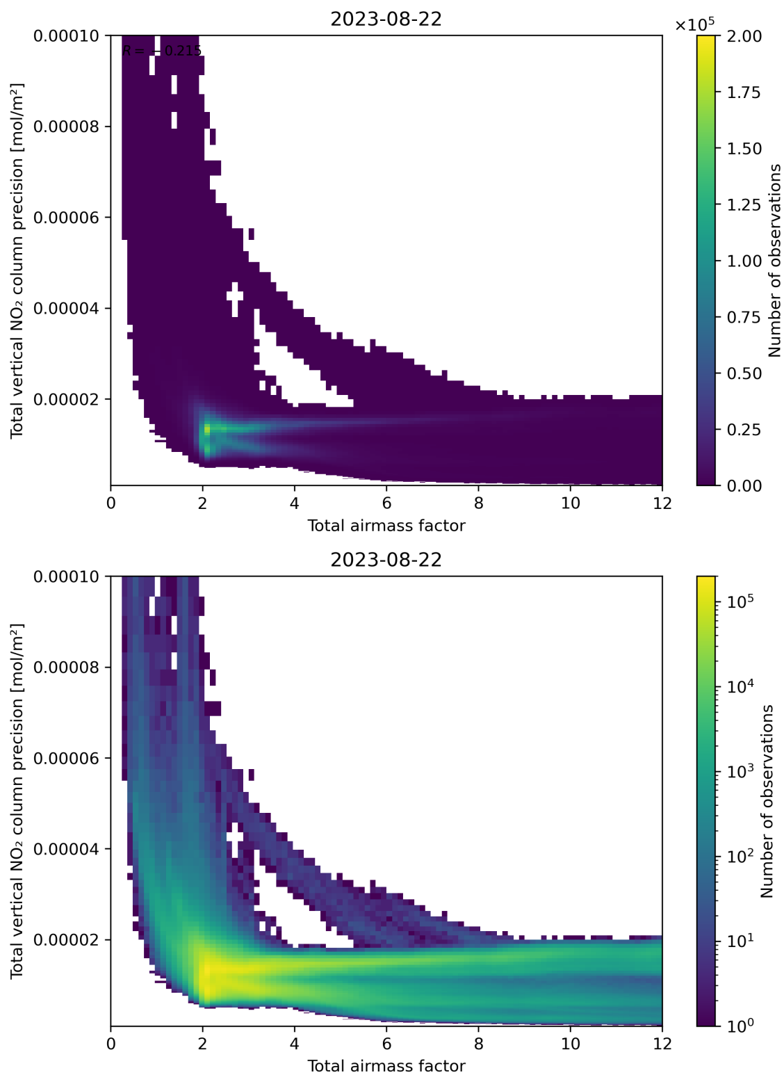
Figure 68: Scatter density plot of “Total airmass factor” against “Total vertical NO 2 column precision” for 2023-08-21 to 2023-08-23.
