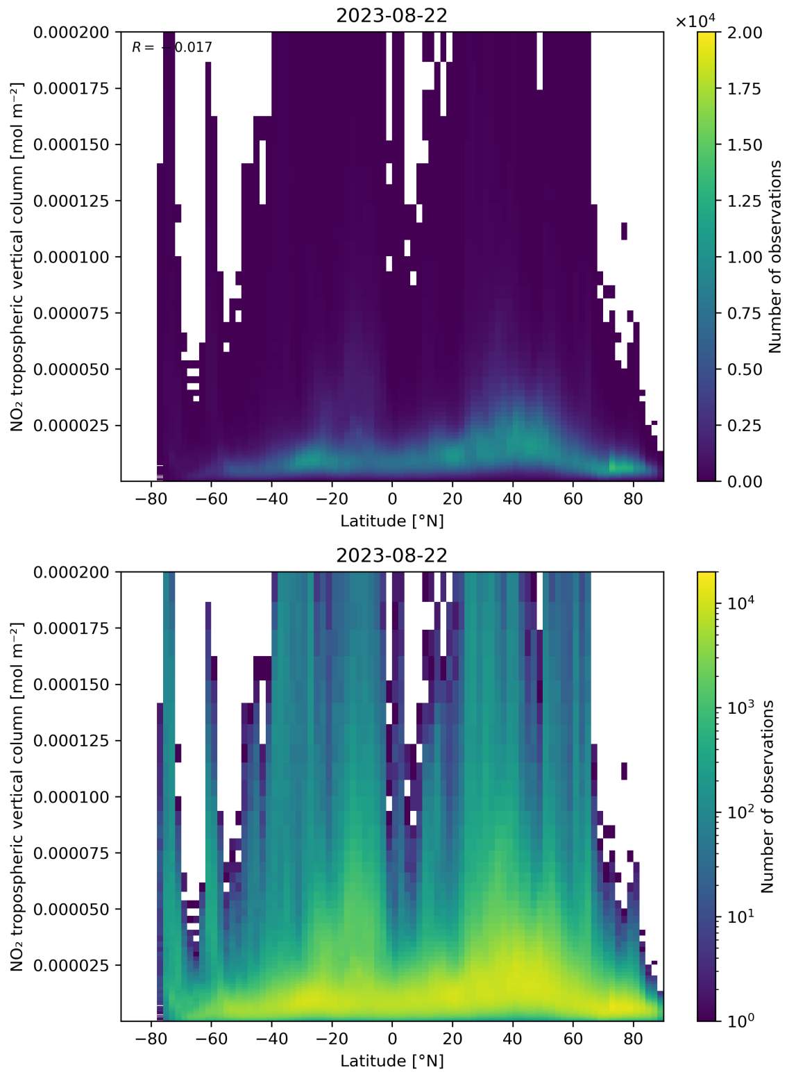
Figure 92: Scatter density plot of “Latitude” against “NO 2 tropospheric vertical column” for 2023-08-21 to 2023-08-23.
