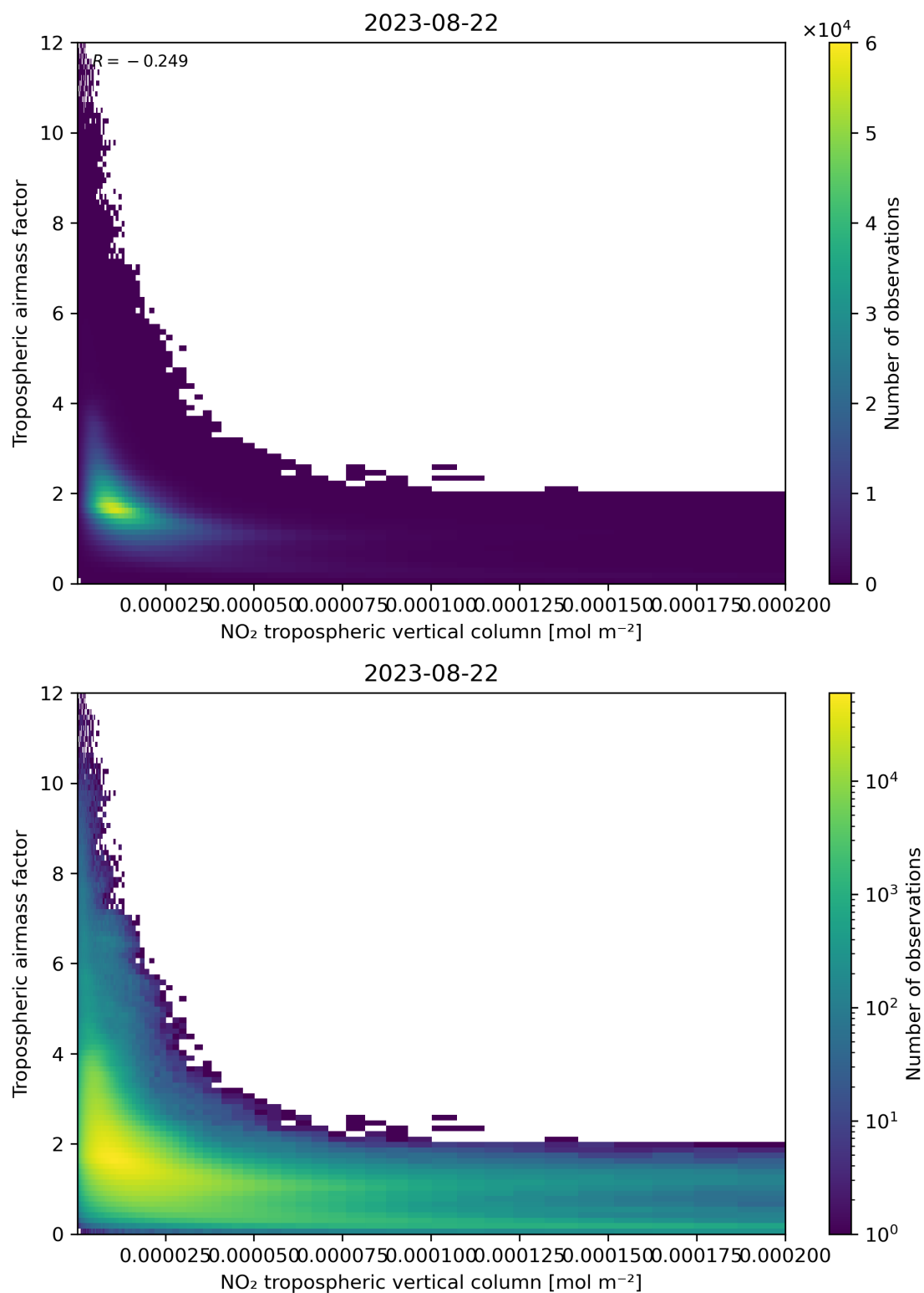
Figure 123: Scatter density plot of “NO 2 tropospheric vertical column” against “Tropospheric airmass factor” for 2023-08-21 to 2023-08-23.
