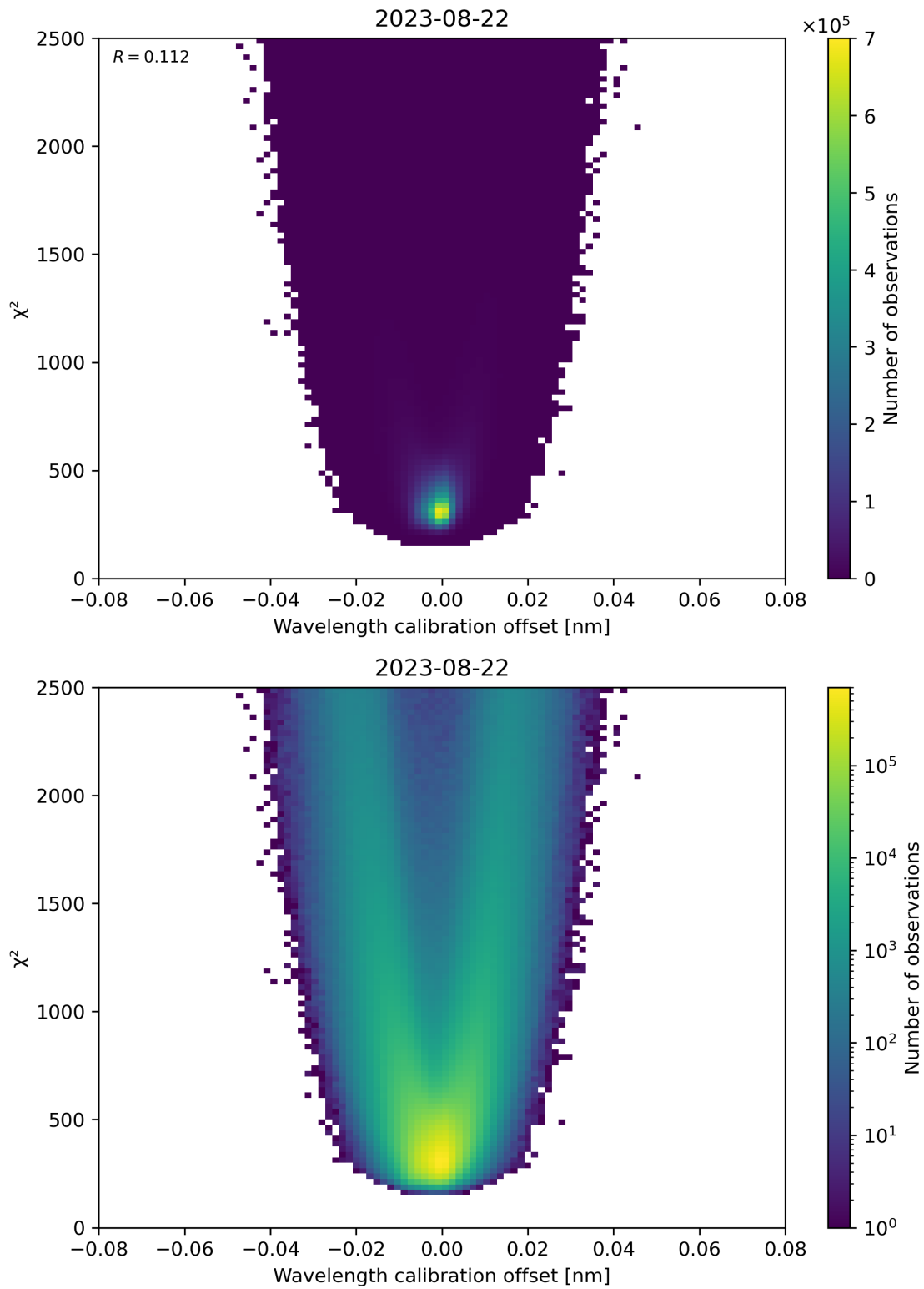
Figure 175: Scatter density plot of “Wavelength calibration offset” against “ \chi^2 ” for 2023-08-21 to 2023-08-23.
