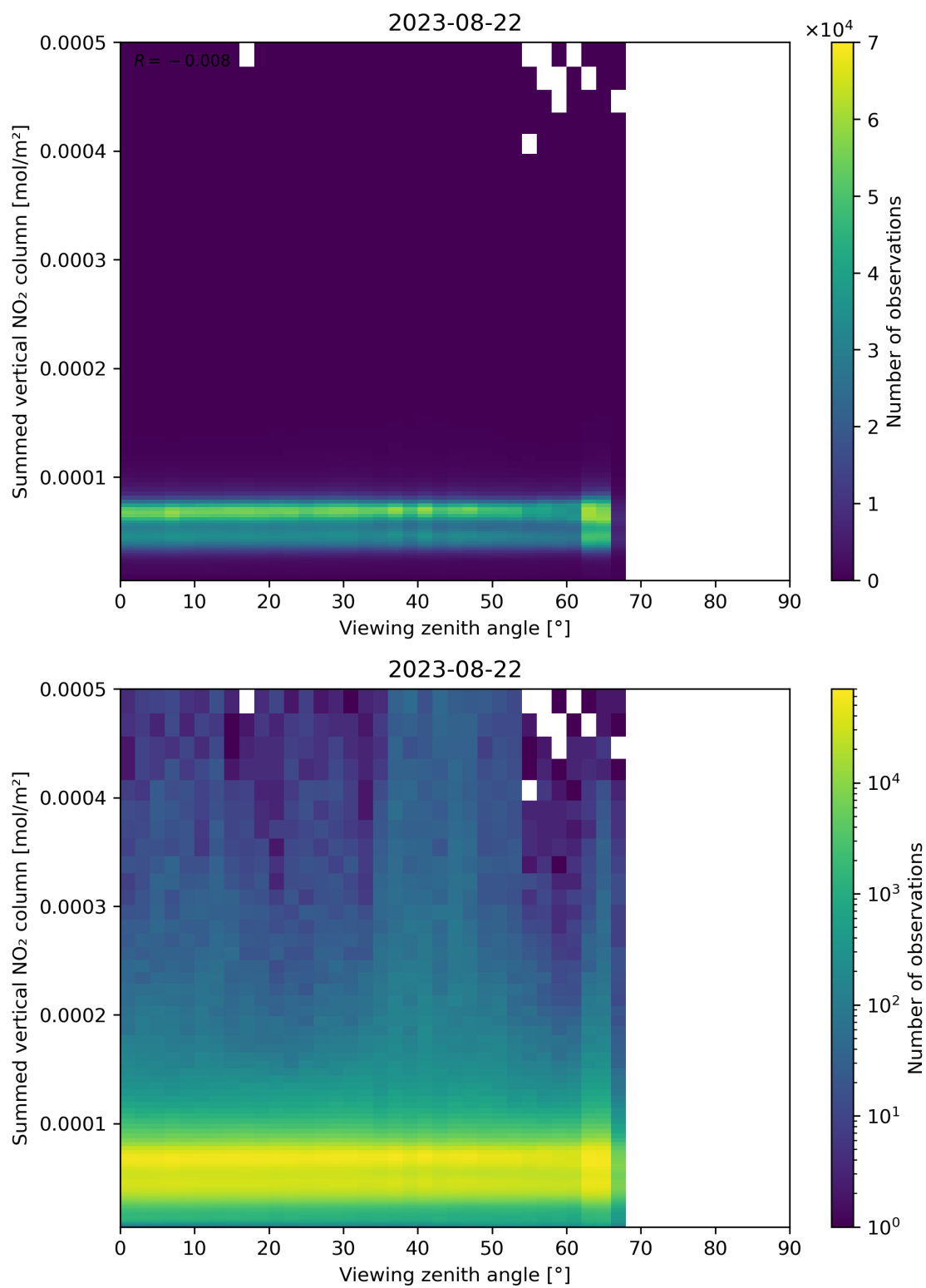
Figure 165: Scatter density plot of “Viewing zenith angle” against “Summed vertical NO 2 column” for 2023-08-21 to 2023-08-23.
