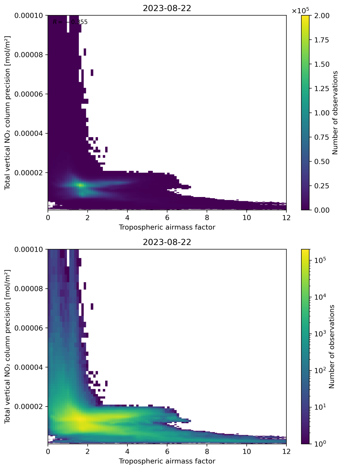
Figure 78: Scatter density plot of “Tropospheric air mass factor” against “Total vertical NO 2 column precision” for 2023-08-21 to 2023-08-23.
