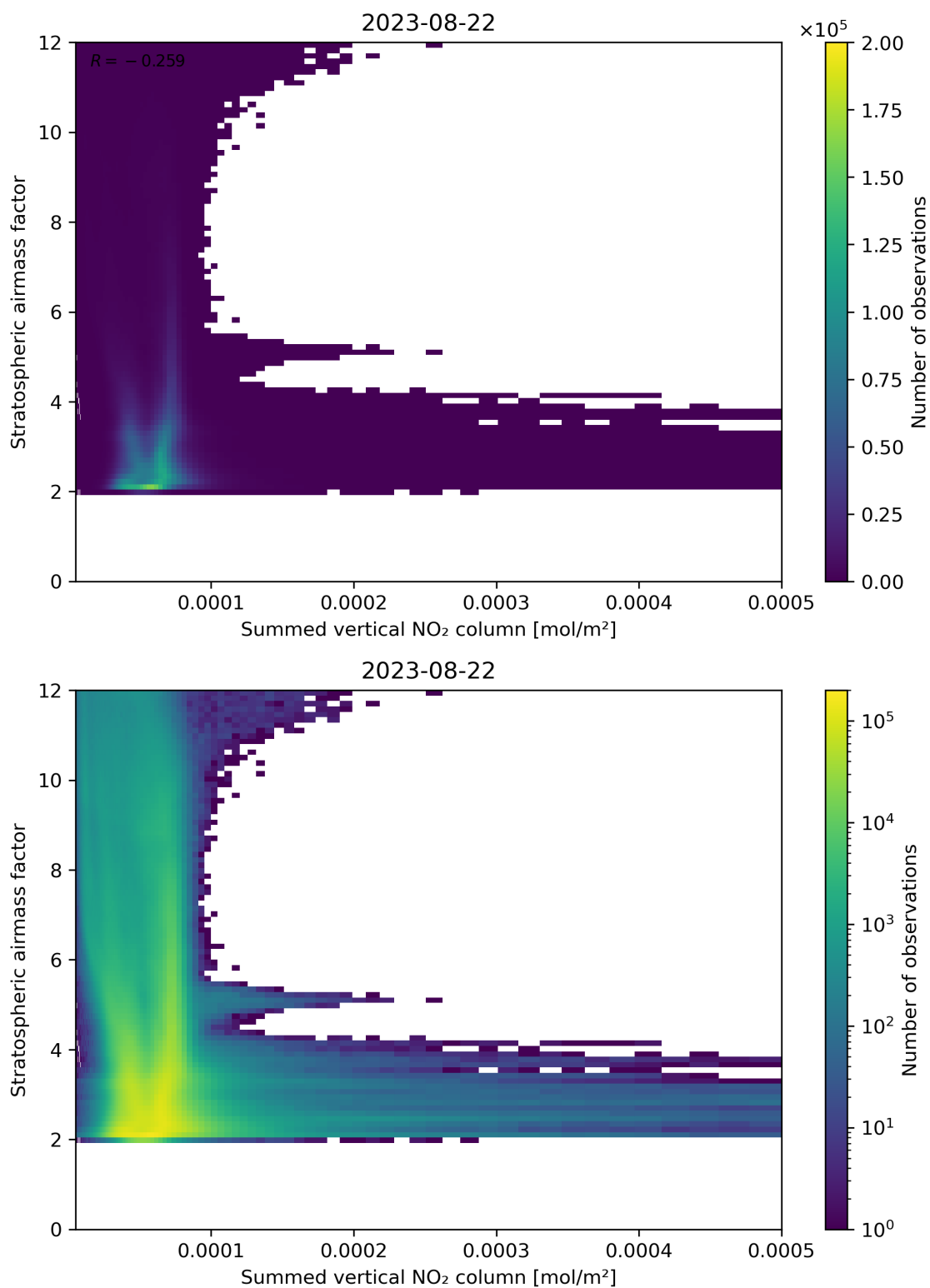
Figure 103: Scatter density plot of “Summed vertical NO 2 column” against “Stratospheric air mass factor” for 2023-08-21 to 2023-08-23.
