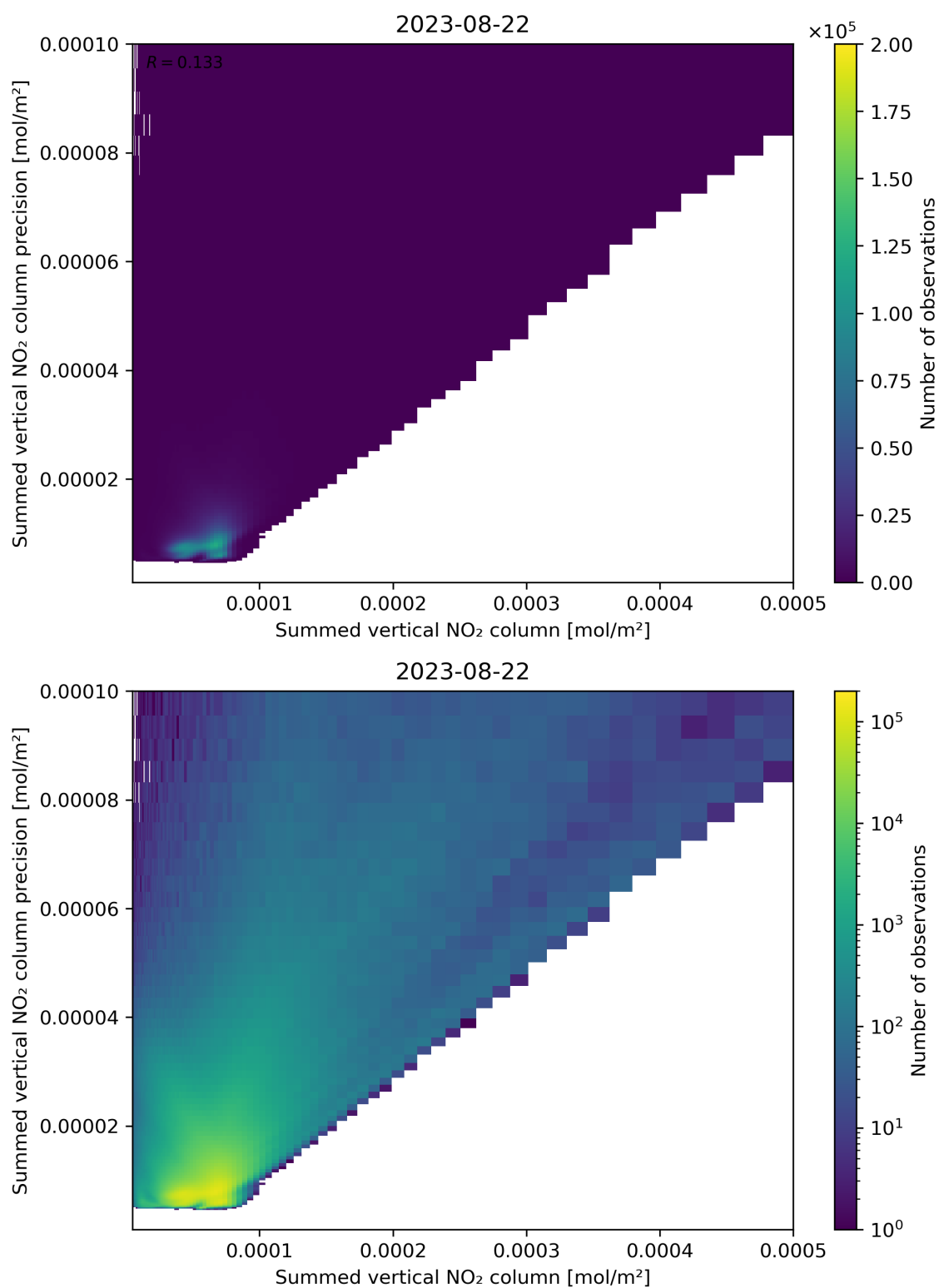
Figure 105: Scatter density plot of “Summed vertical NO 2 column” against “Summed vertical NO 2 column precision” for 2023-08-21 to 2023-08-23.
