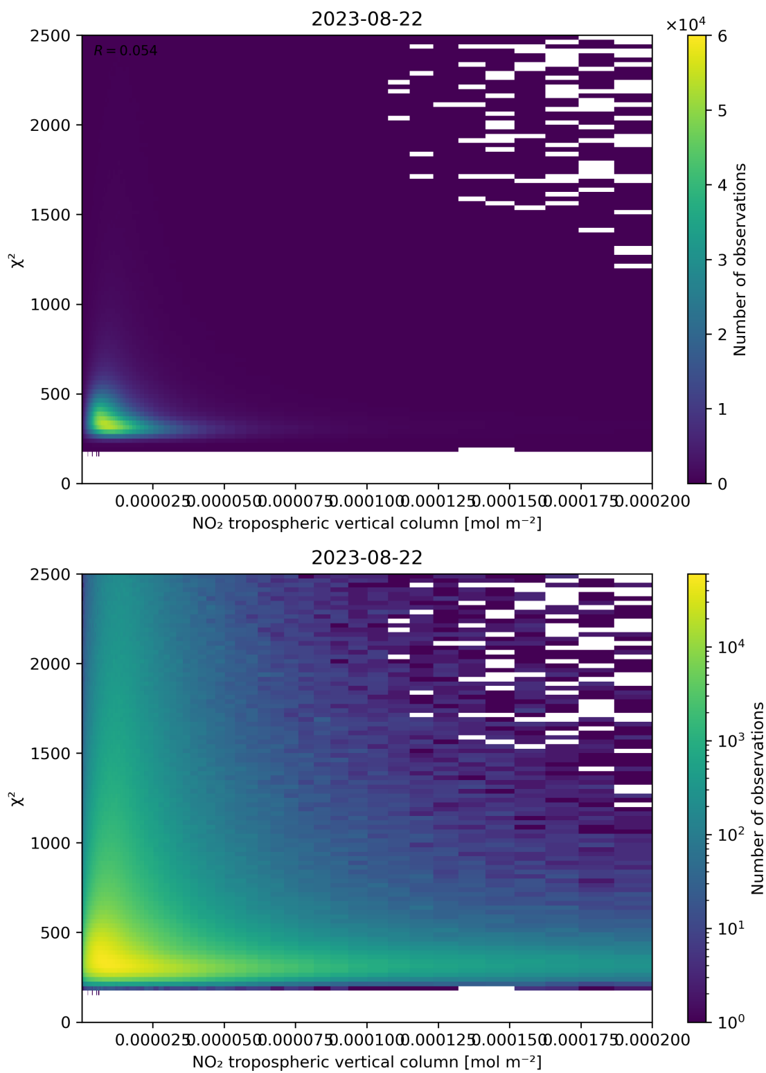
Figure 124: Scatter density plot of “NO 2 tropospheric vertical column” against “ \chi^2 ” for 2023-08-21 to 2023-08-23.
