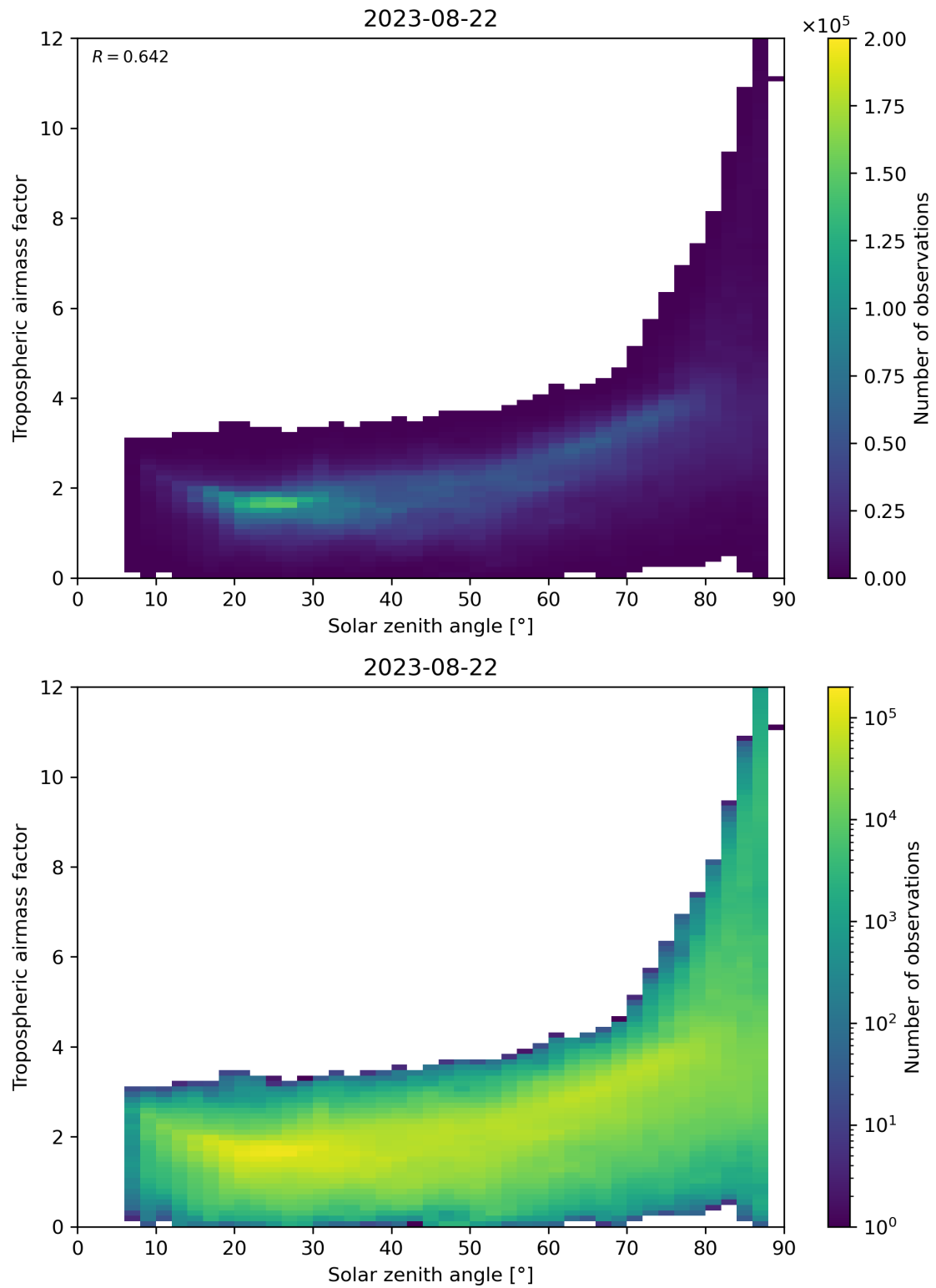
Figure 147: Scatter density plot of “Solar zenith angle” against “Tropospheric airmass factor” for 2023-08-21 to 2023-08-23.
