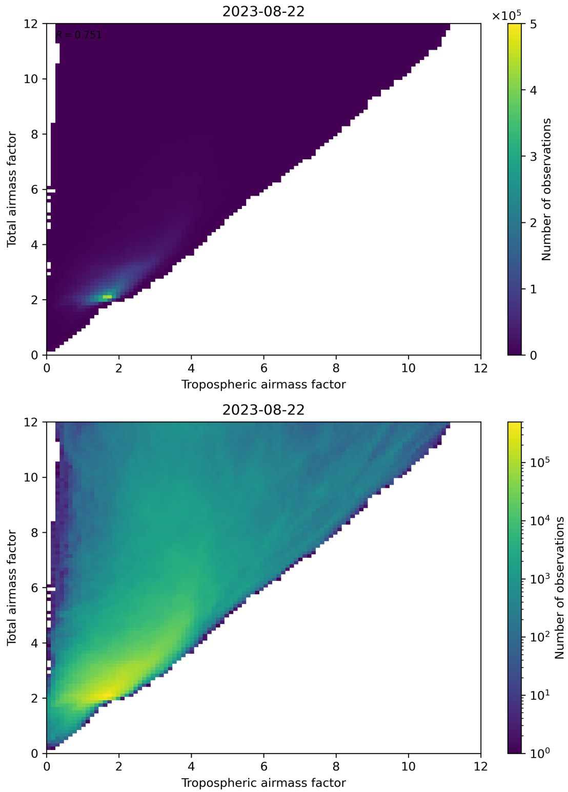
Figure 72: Scatter density plot of “Tropospheric airmass factor” against “Total airmass factor” for 2023-08-21 to 2023-08-23.
