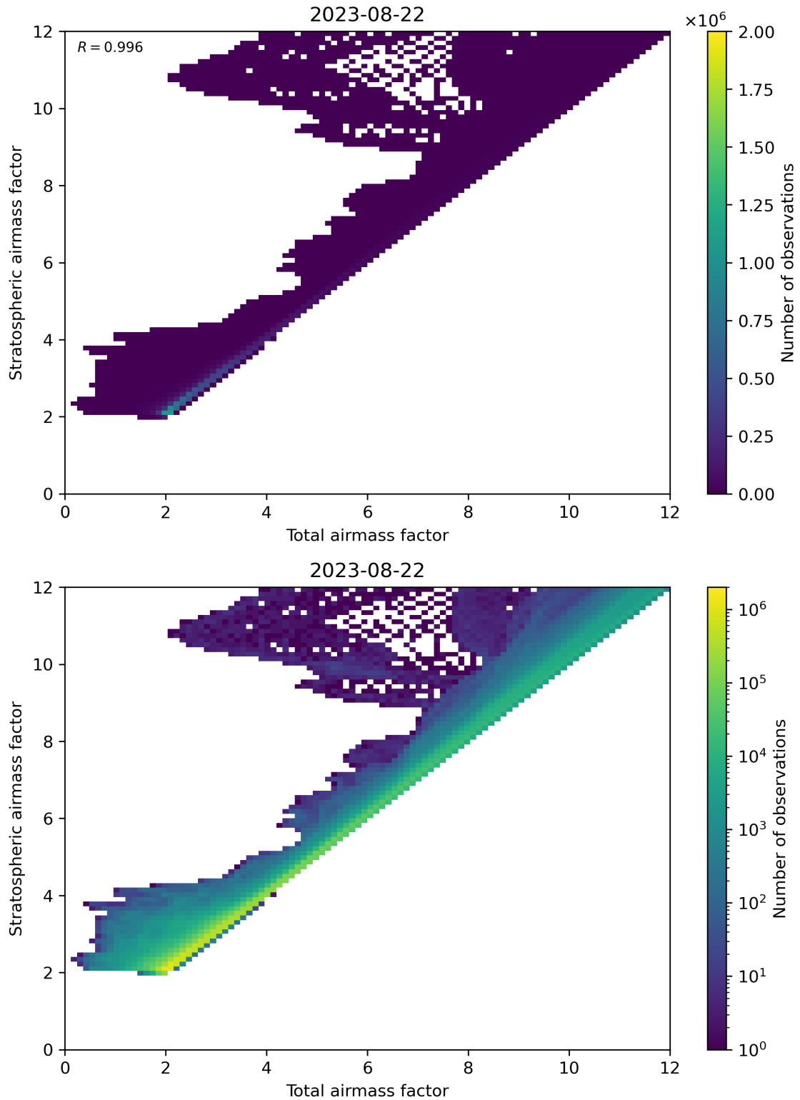
Figure 62: Scatter density plot of “Total airmass factor” against “Stratospheric airmass factor” for 2023-08-21 to 2023-08-23.
