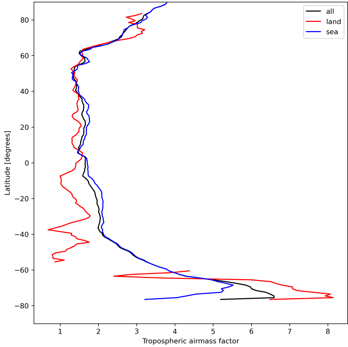
Figure 14: Zonal average of “Tropospheric airmass factor” for 2023-08-21 to 2023-08-23.
