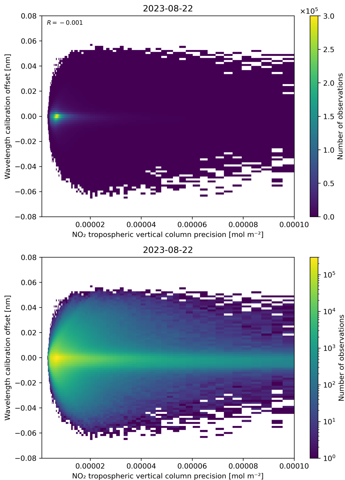
Figure 141: Scatter density plot of “NO 2 tropospheric vertical column precision” against “Wavelength calibration offset” for 2023-08-21 to 2023-08-23.
