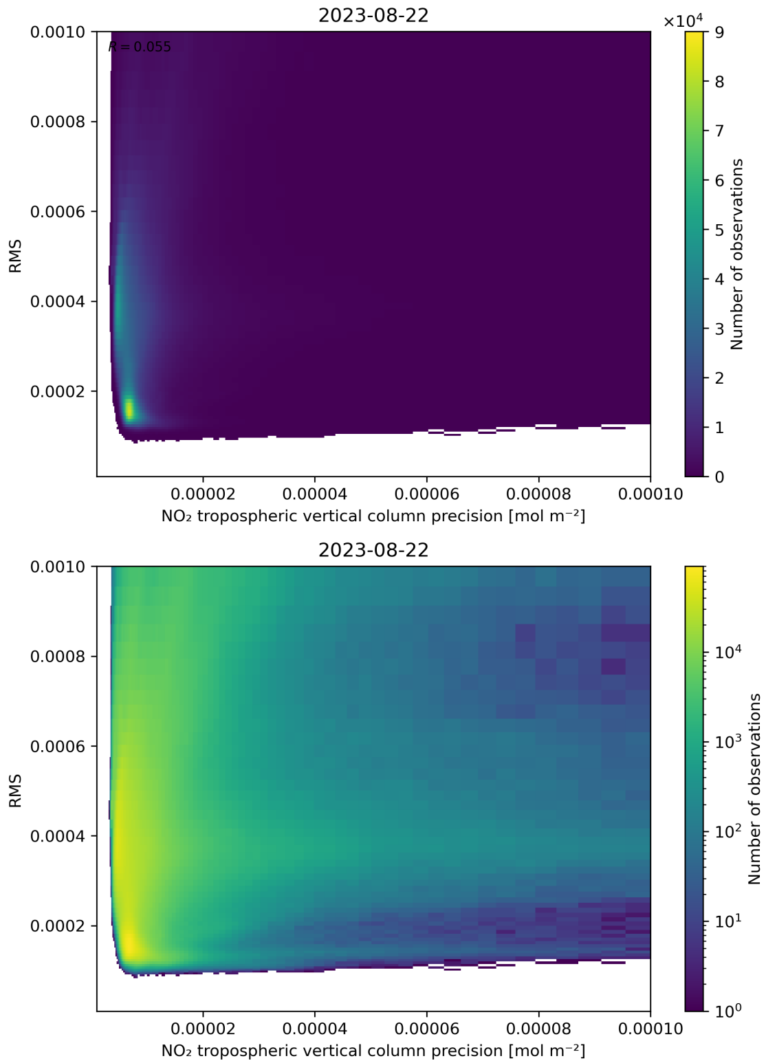
Figure 140: Scatter density plot of “NO 2 tropospheric vertical column precision” against “RMS” for 2023-08-21 to 2023-08-23.
