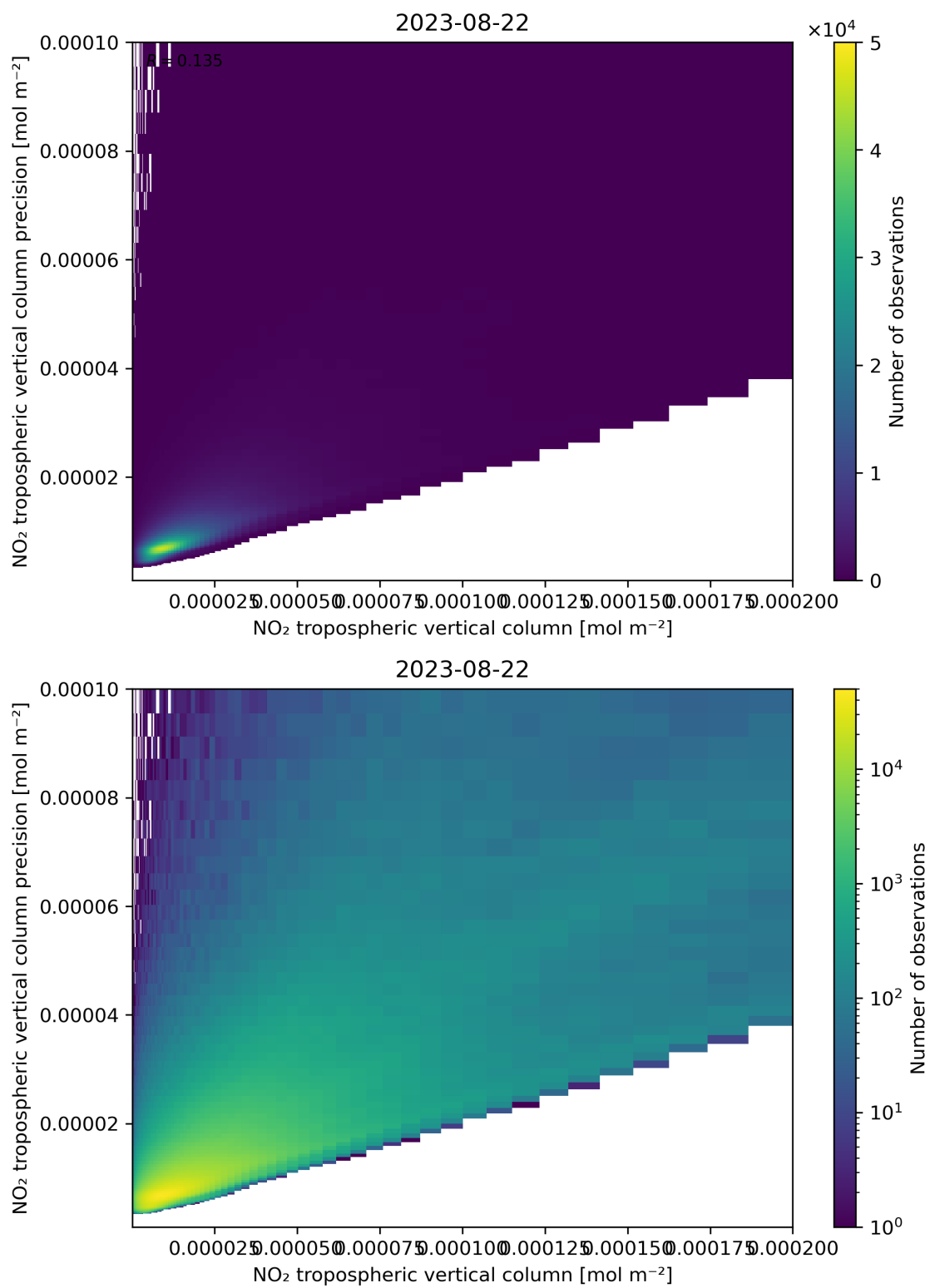
Figure 130: Scatter density plot of “NO 2 tropospheric vertical column” against “NO 2 tropospheric vertical column precision” for 2023-08-21 to 2023-08-23.
