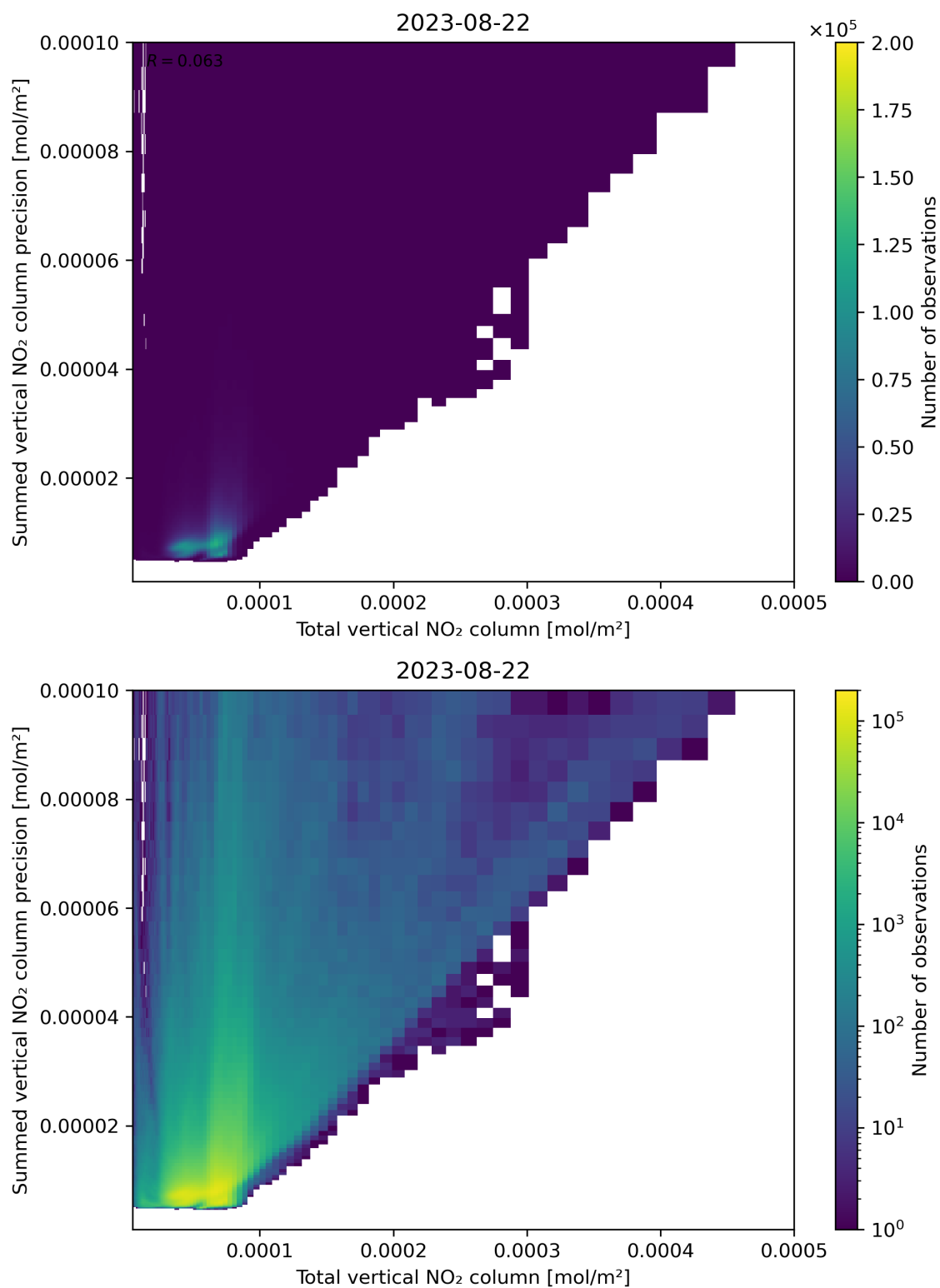
Figure 113: Scatter density plot of “Total vertical NO 2 column” against “Summed vertical NO 2 column precision” for 2023-08-21 to 2023-08-23.
