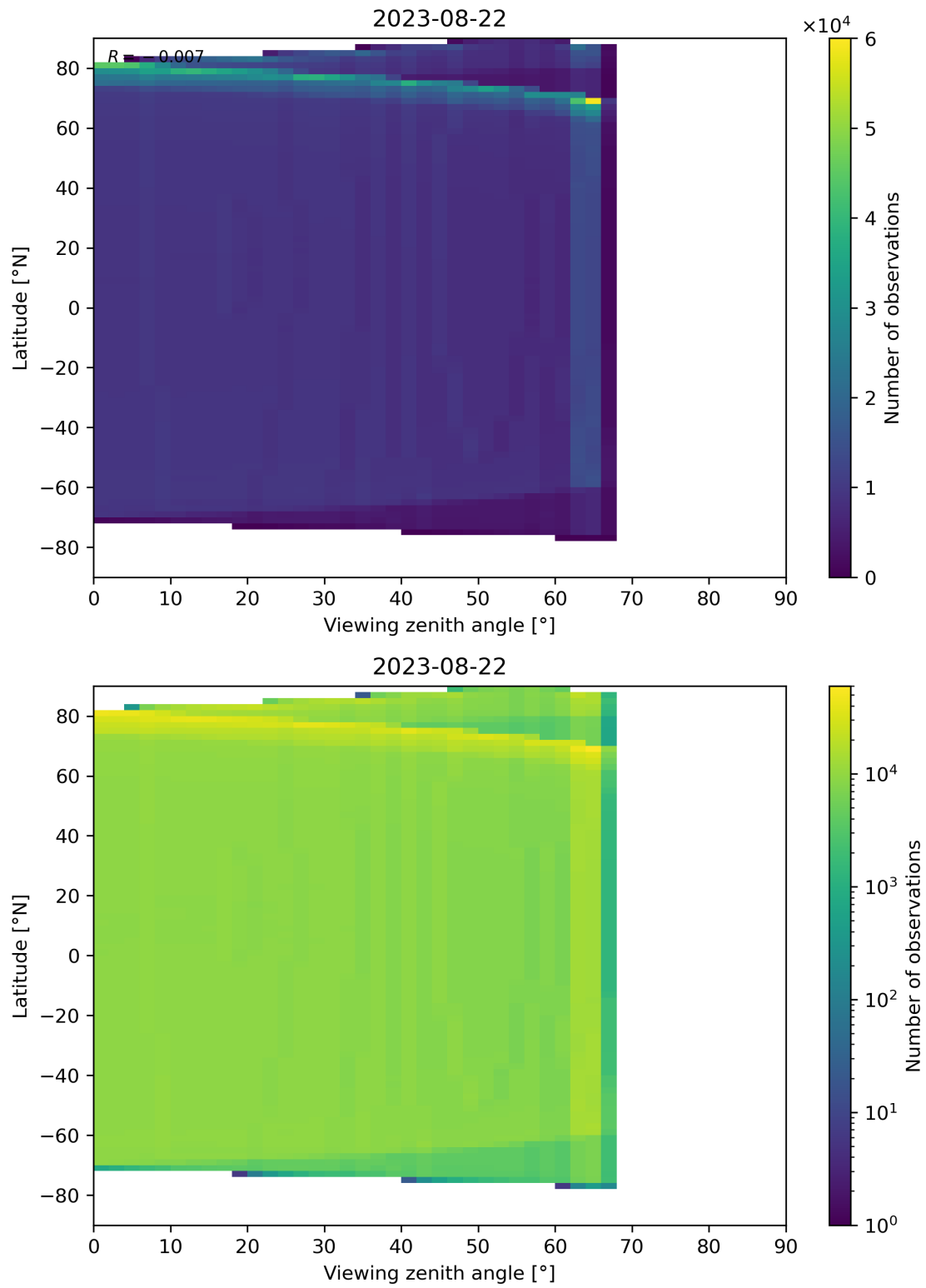
Figure 163: Scatter density plot of “Viewing zenith angle” against “Latitude” for 2023-08-21 to 2023-08-23.
