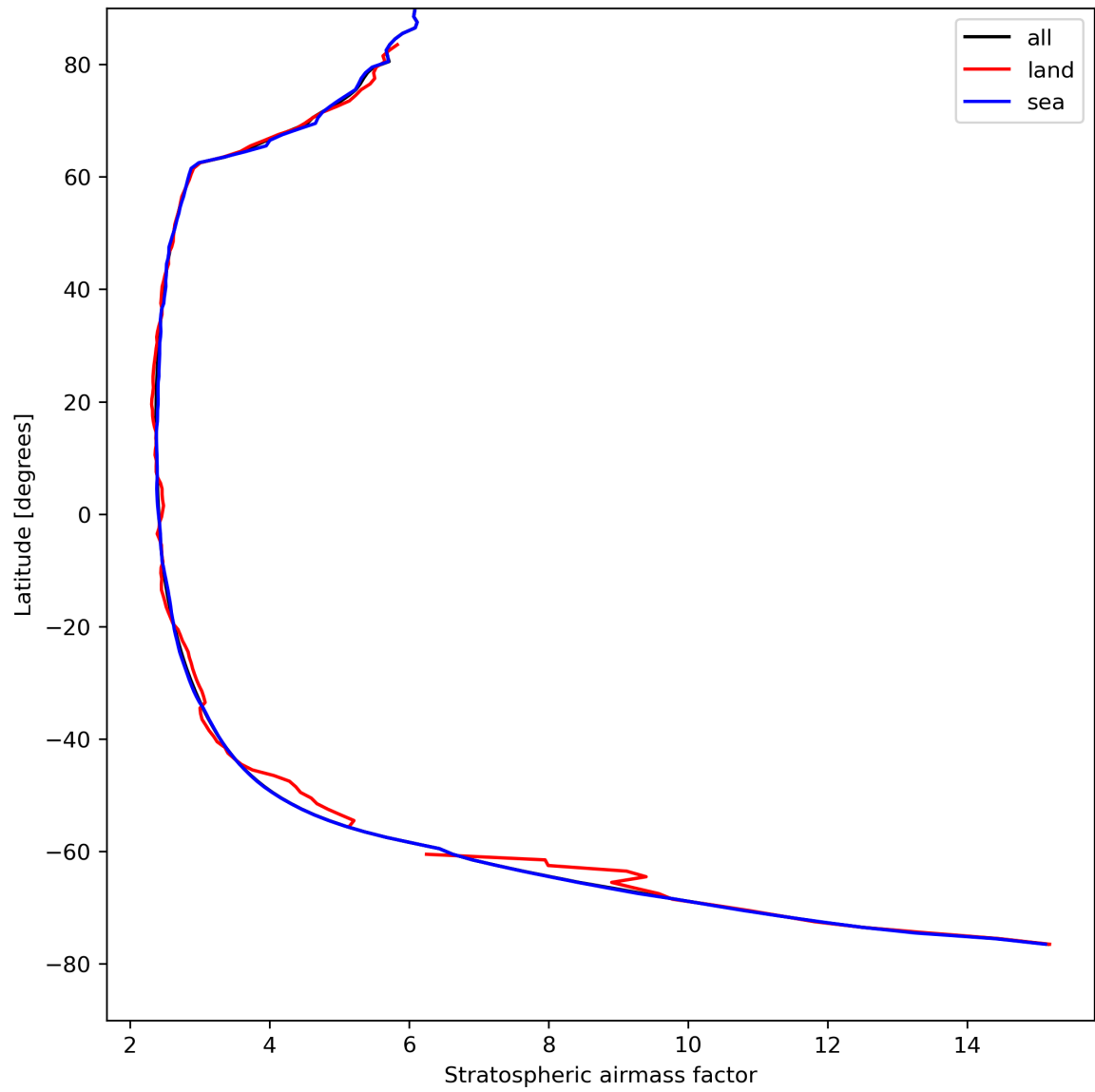
Figure 27: Zonal average of “Stratospheric airmass factor” for 2023-08-21 to 2023-08-23.
