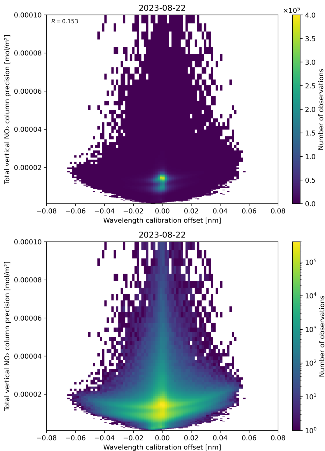
Figure 180: Scatter density plot of “Wavelength calibration offset” against “Total vertical NO 2 column precision” for 2023-08-21 to 2023-08-23.
