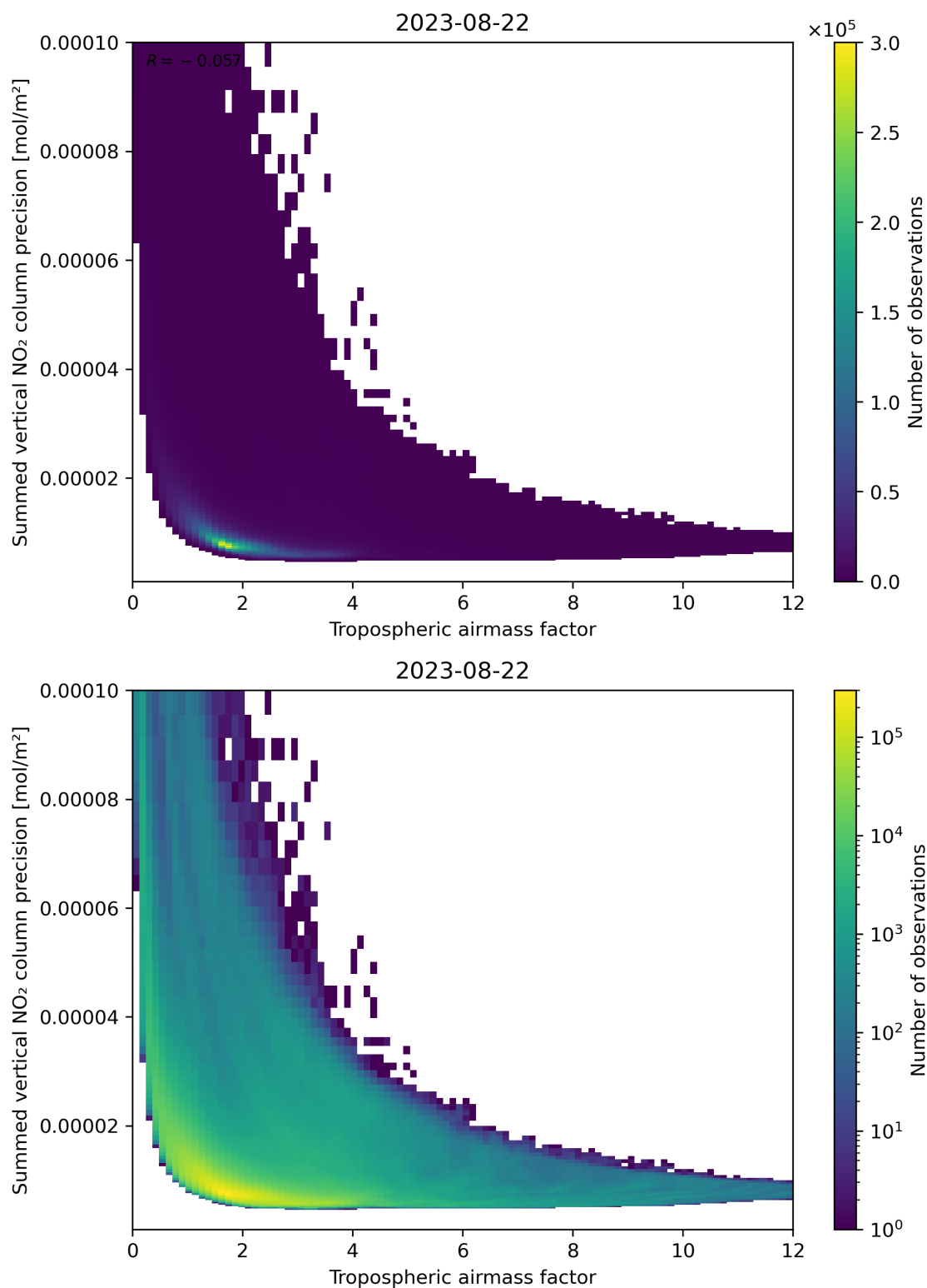
Figure 76: Scatter density plot of “Tropospheric air mass factor” against “Summed vertical NO 2 column precision” for 2023-08-21 to 2023-08-23.
