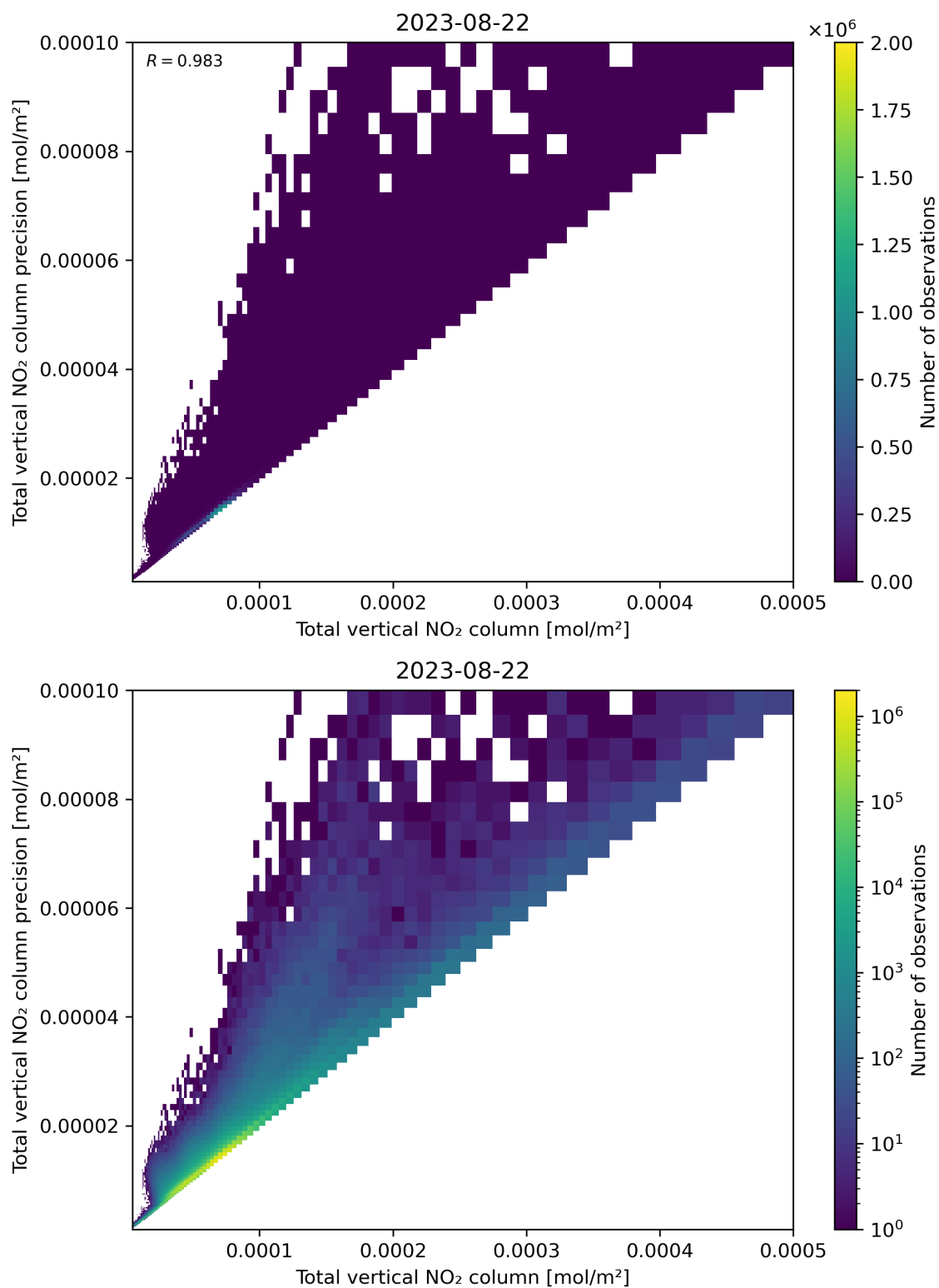
Figure 114: Scatter density plot of “Total vertical NO 2 column” against “Total vertical NO 2 column precision” for 2023-08-21 to 2023-08-23.
