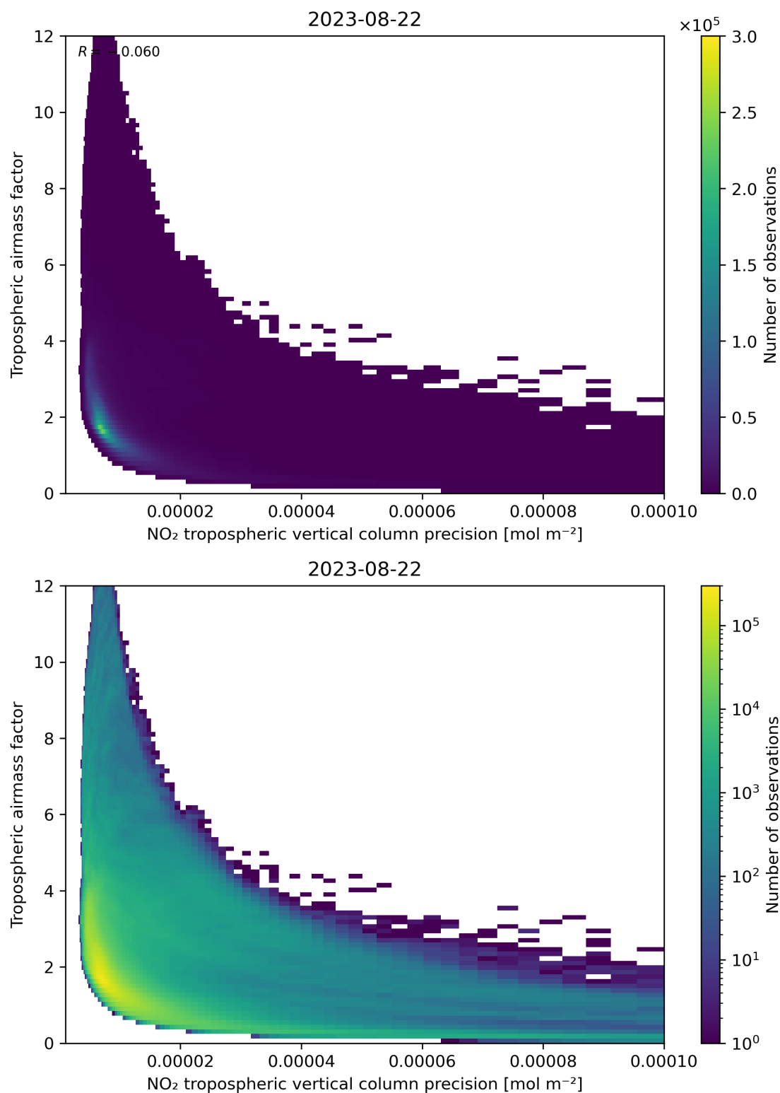
Figure 133: Scatter density plot of “NO 2 tropospheric vertical column precision” against “Tropospheric airmass factor” for 2023-08-21 to 2023-08-23.
