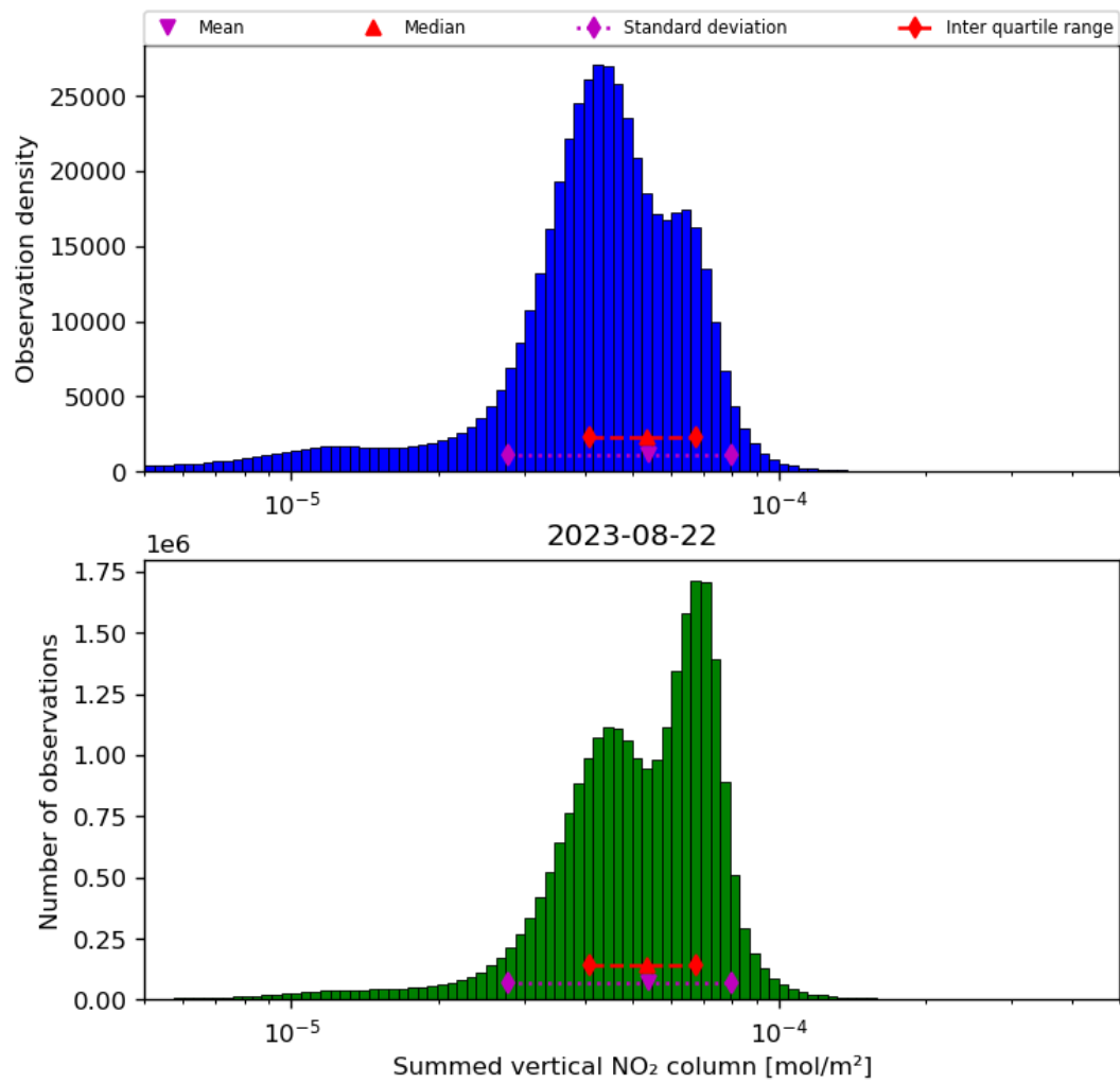
Figure 40: Histogram of “Summed vertical NO 2 column” for 2023-08-21 to 2023-08-23
