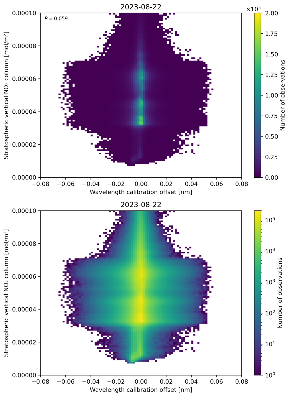
Figure 176: Scatter density plot of “Wavelength calibration offset” against “Stratospheric vertical NO 2 column” for 2023-08-21 to 2023-08-23.
