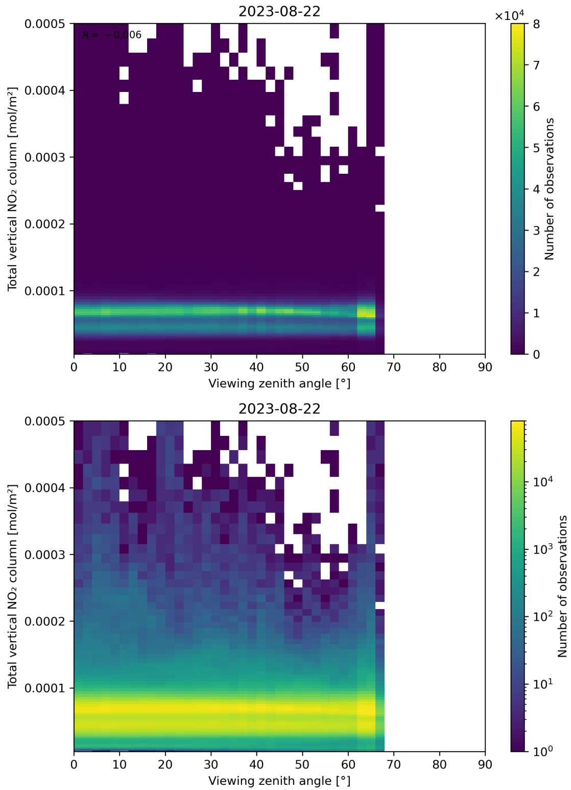
Figure 167: Scatter density plot of “Viewing zenith angle” against “Total vertical NO 2 column” for 2023-08-21 to 2023-08-23.
