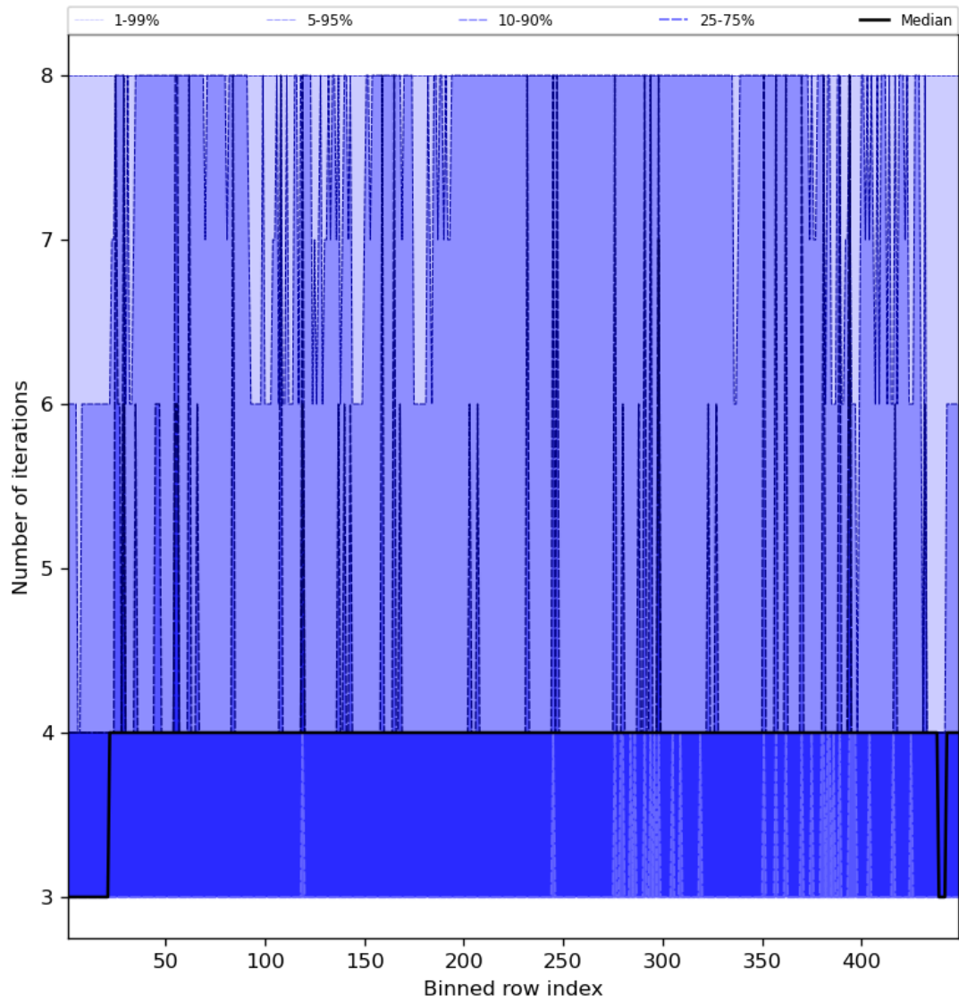
Figure 51: Along track statistics of “Number of iterations” for 2023-08-21 to 2023-08-23
