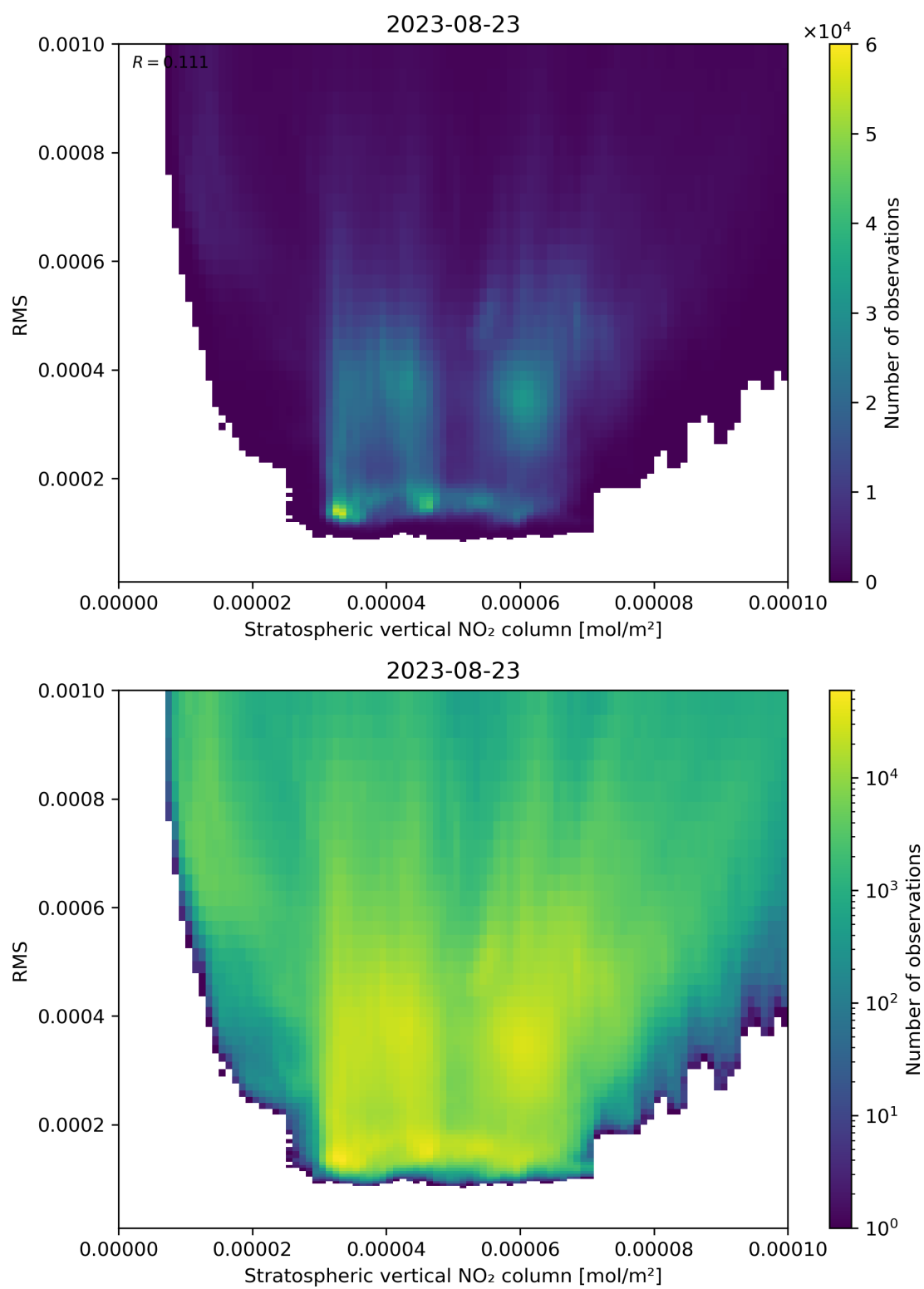
Figure 102: Scatter density plot of “Stratospheric vertical NO 2 column” against “RMS” for 2023-08-22 to 2023-08-24.
