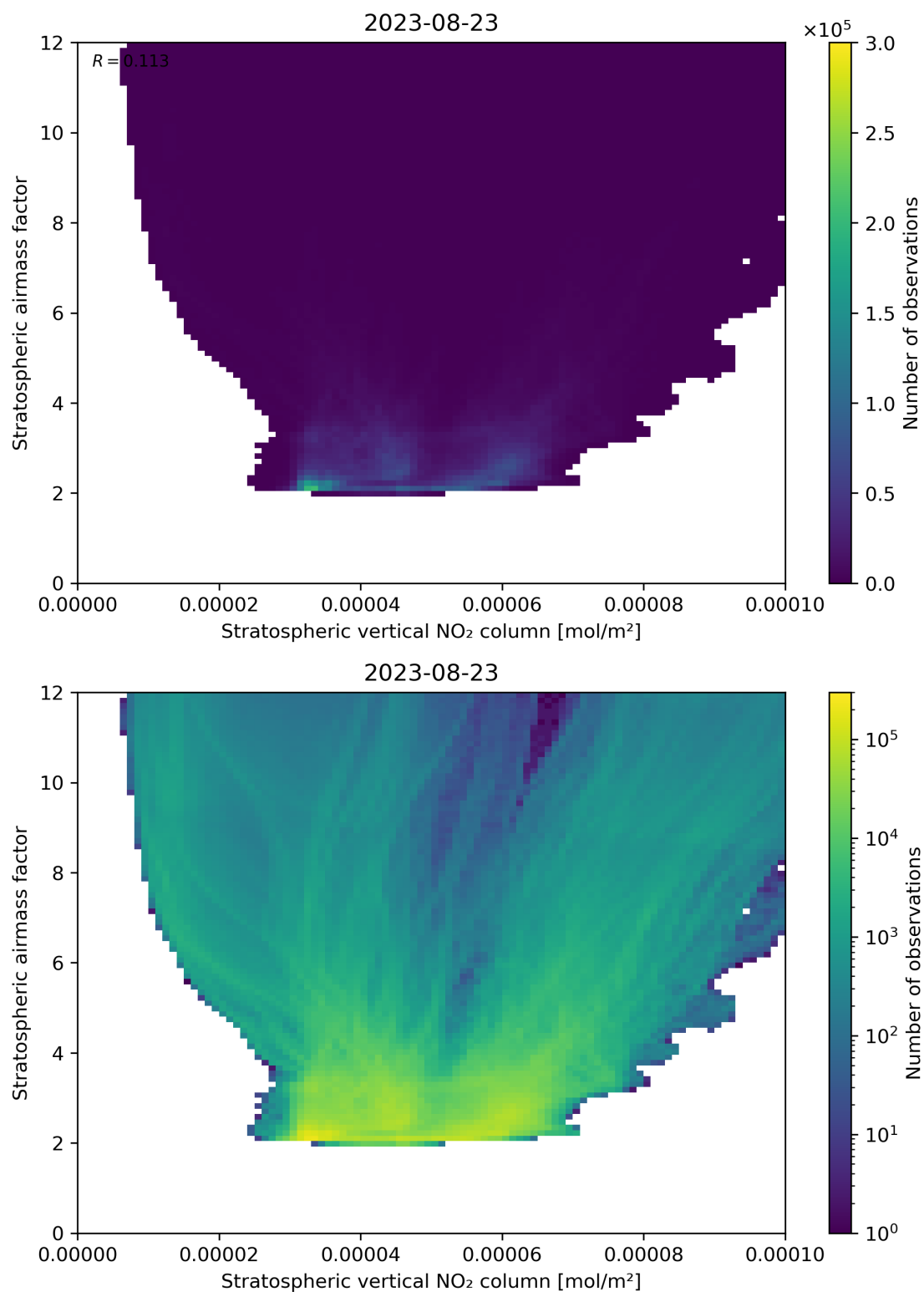
Figure 96: Scatter density plot of “Stratospheric vertical NO 2 column” against “Stratospheric airmass factor” for 2023-08-22 to 2023-08-24.
