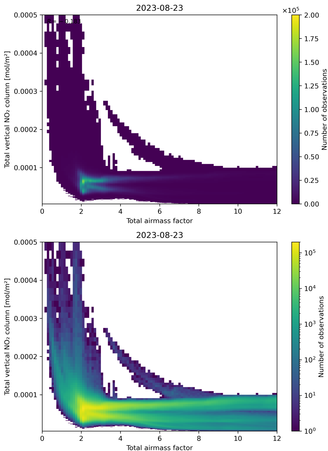
Figure 67: Scatter density plot of “Total airmass factor” against “Total vertical NO 2 column” for 2023-08-22 to 2023-08-24.
