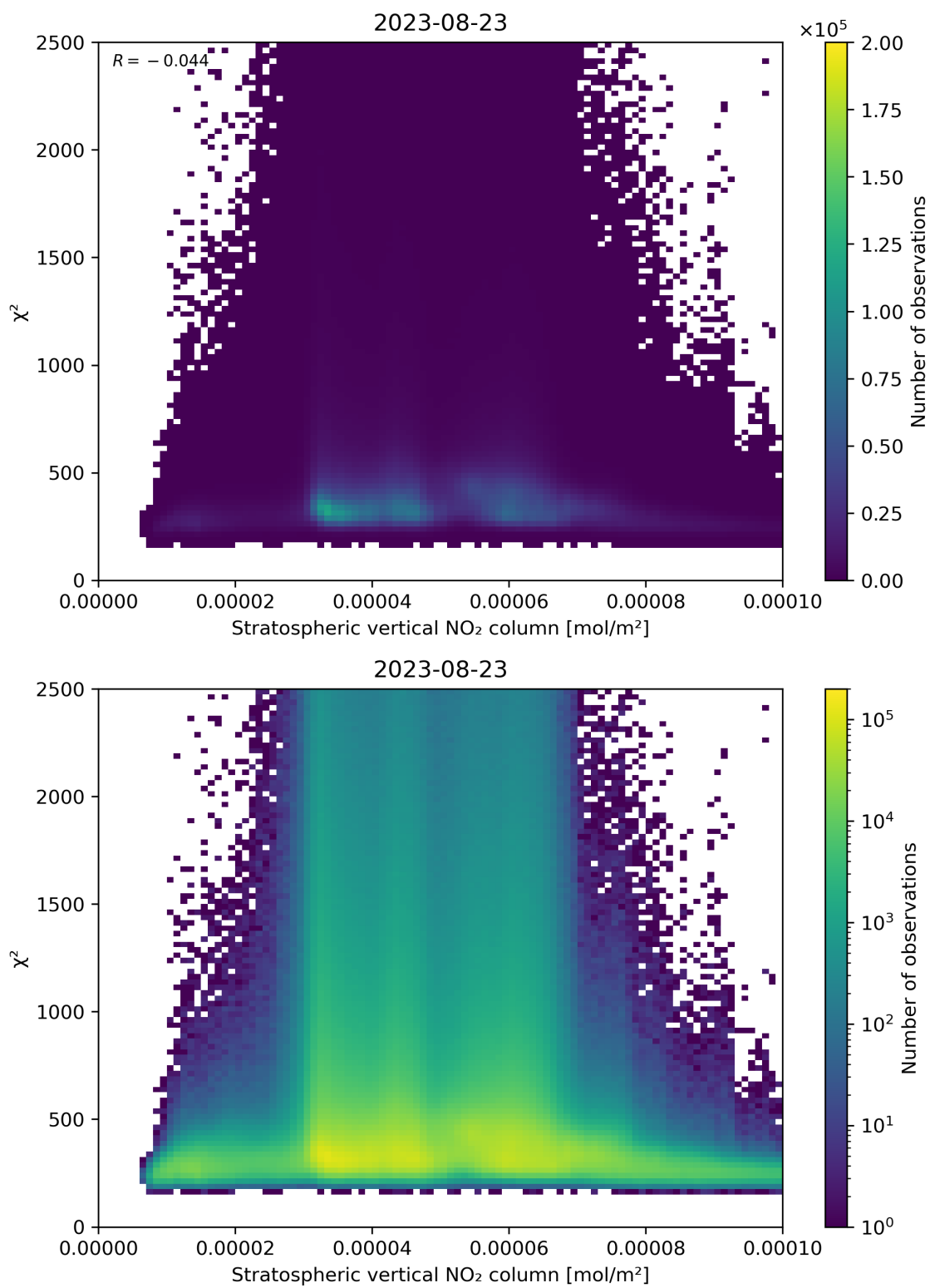
Figure 97: Scatter density plot of “Stratospheric vertical NO 2 column” against “ \chi^2 ” for 2023-08-22 to 2023-08-24.
