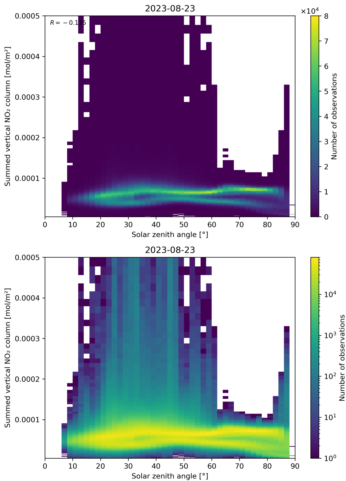
Figure 151: Scatter density plot of “Solar zenith angle” against “Summed vertical NO 2 column” for 2023-08-22 to 2023-08-24.
