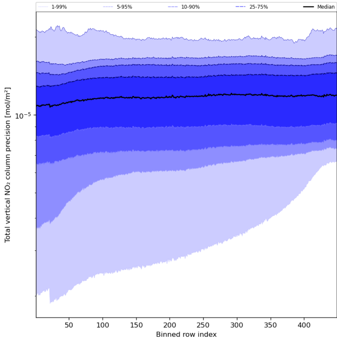
Figure 56: Along track statistics of “Total vertical NO 2 column precision” for 2023-08-22 to 2023-08-24
