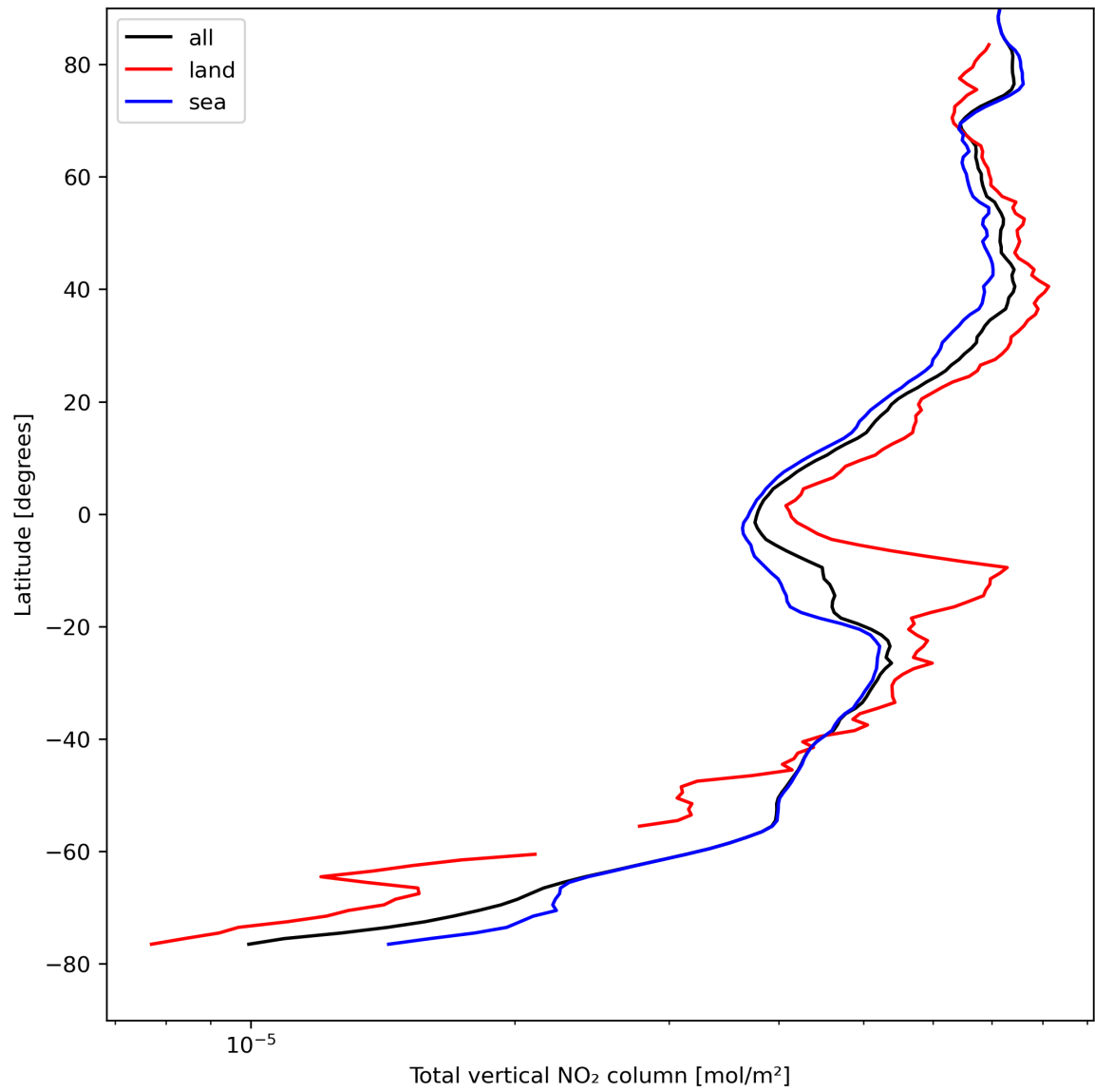
Figure 21: Zonal average of “Total vertical NO 2 column” for 2023-08-22 to 2023-08-24.
