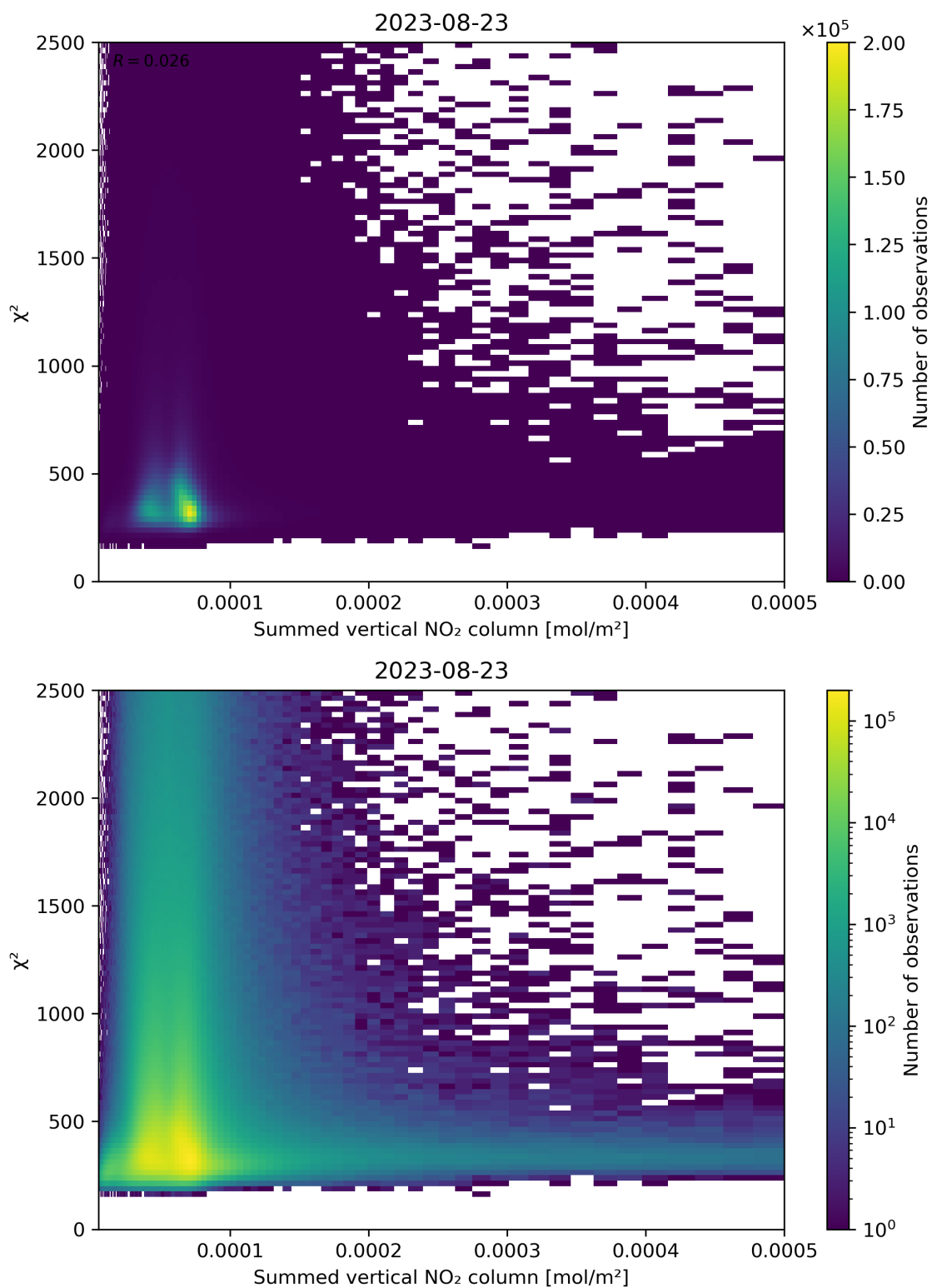
Figure 104: Scatter density plot of “Summed vertical NO 2 column” against “ \chi^2 ” for 2023-08-22 to 2023-08-24.
