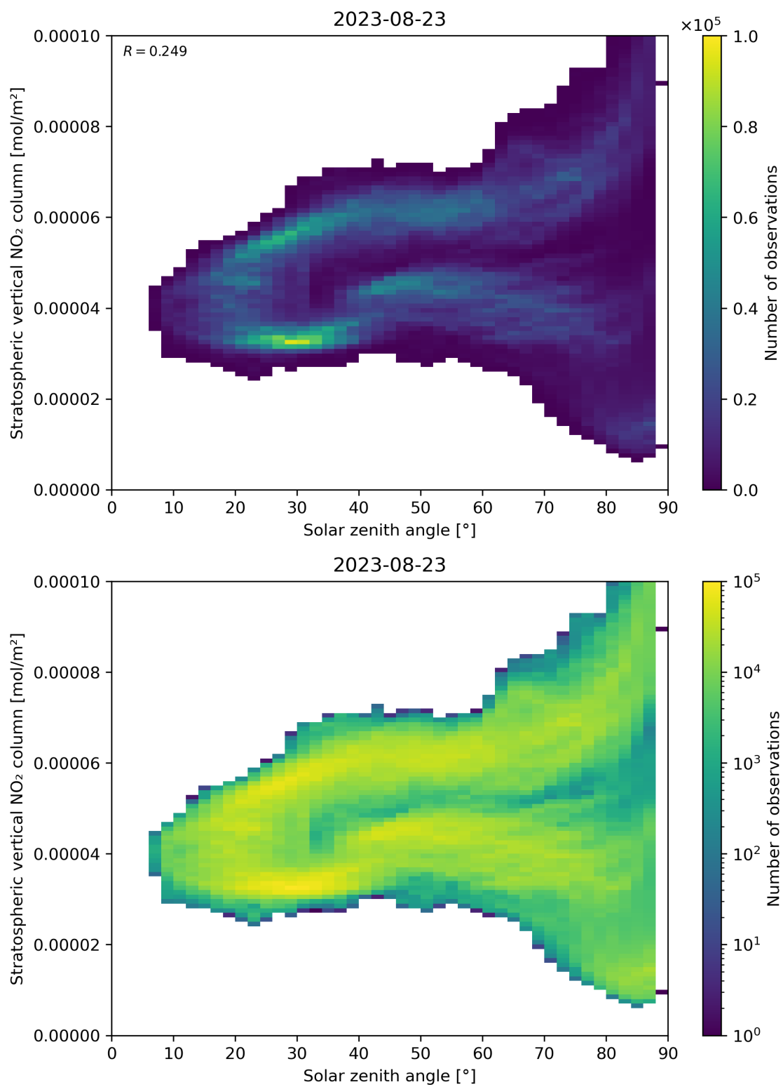
Figure 150: Scatter density plot of “Solar zenith angle” against “Stratospheric vertical NO 2 column” for 2023-08-22 to 2023-08-24.
