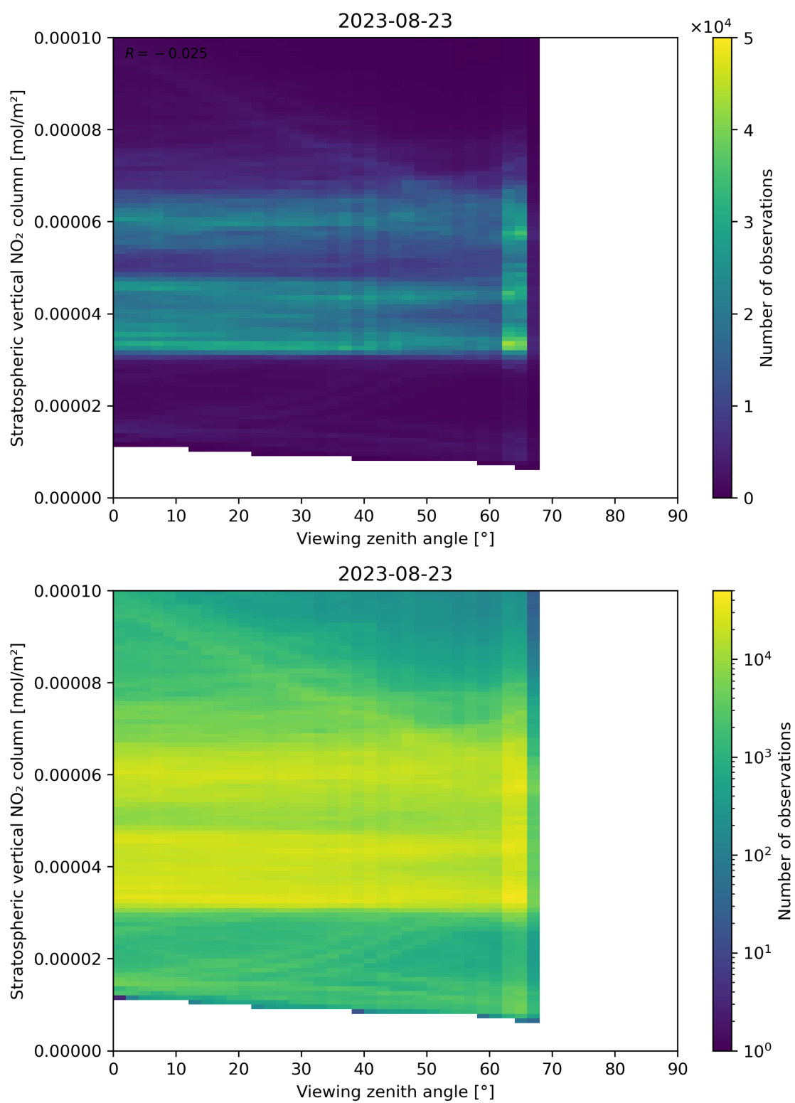
Figure 164: Scatter density plot of “Viewing zenith angle” against “Stratospheric vertical NO 2 column” for 2023-08-22 to 2023-08-24.
