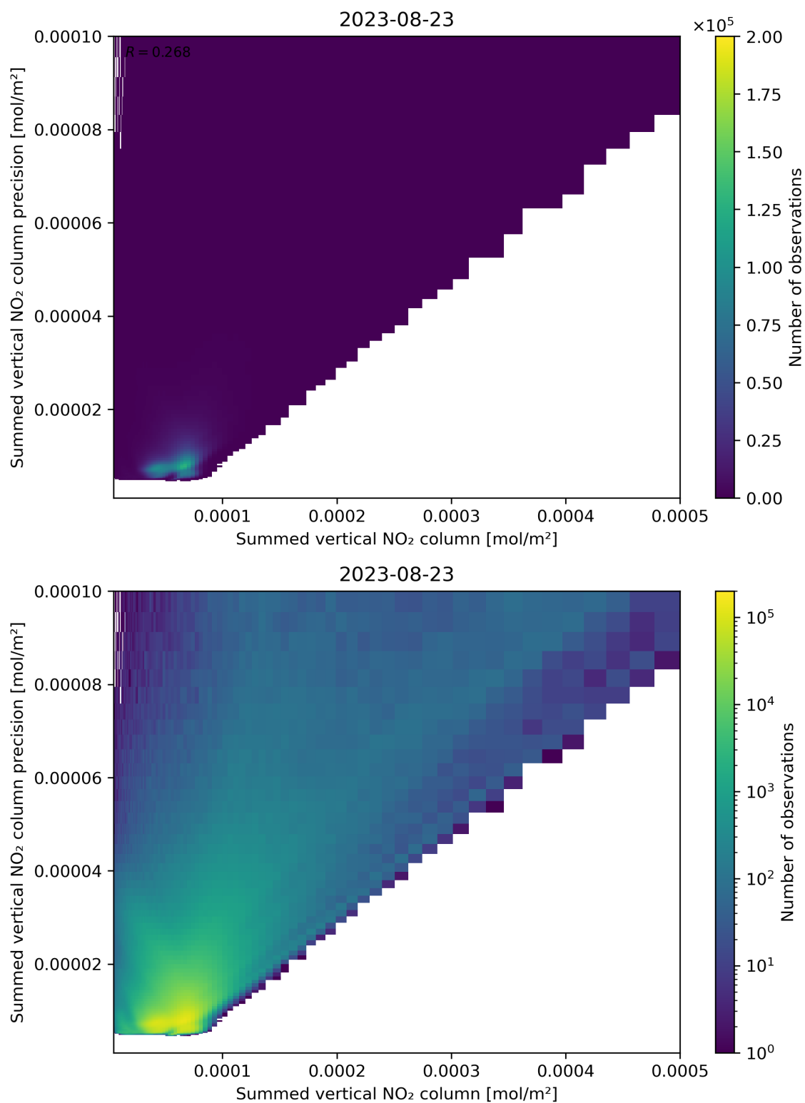
Figure 105: Scatter density plot of “Summed vertical NO 2 column” against “Summed vertical NO 2 column precision” for 2023-08-22 to 2023-08-24.
