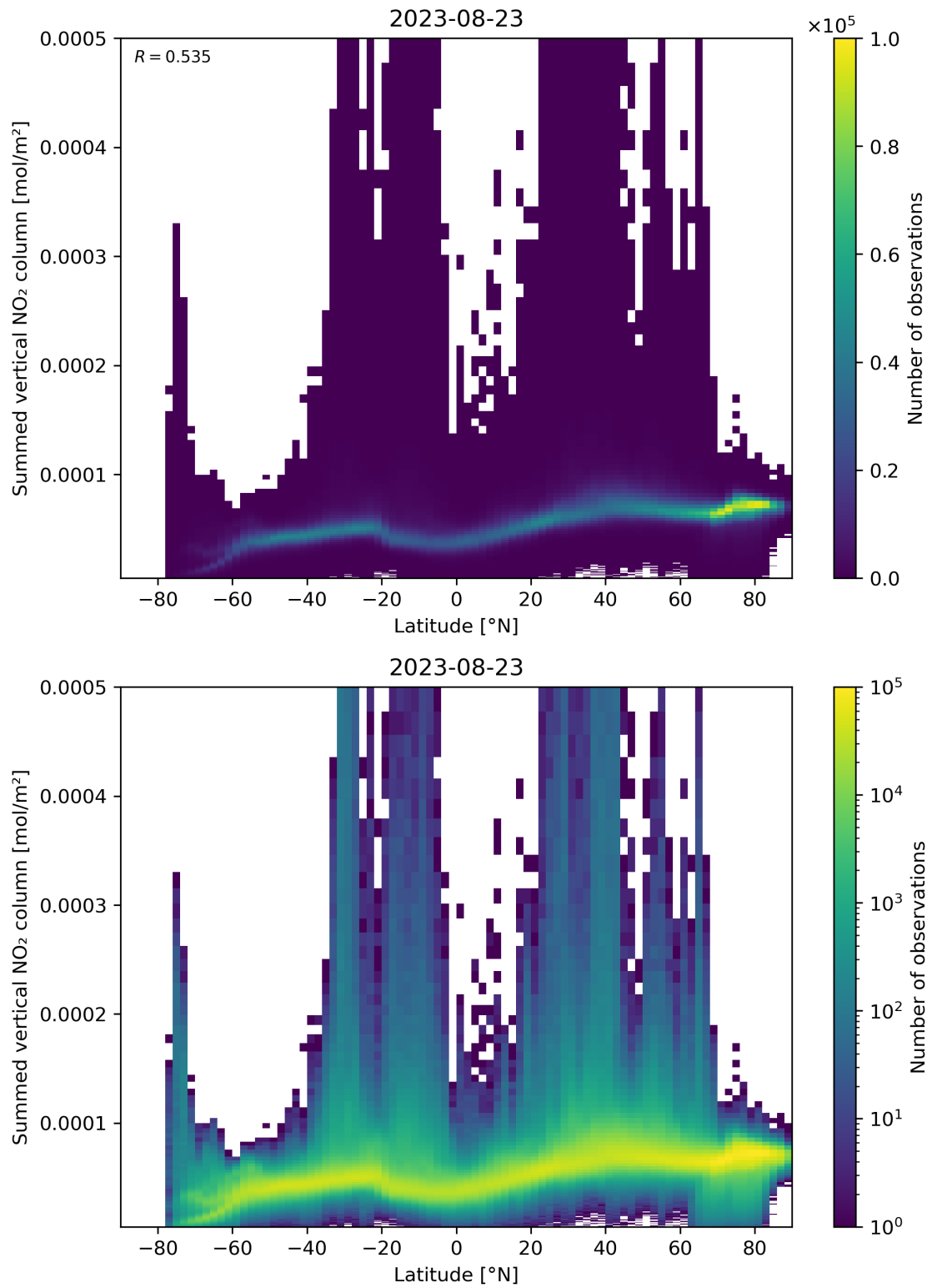
Figure 88: Scatter density plot of “Latitude” against “Summed vertical NO 2 column” for 2023-08-22 to 2023-08-24.
