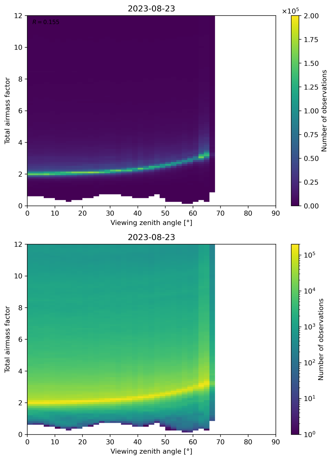
Figure 160: Scatter density plot of “Viewing zenith angle” against “Total airmass factor” for 2023-08-22 to 2023-08-24.
