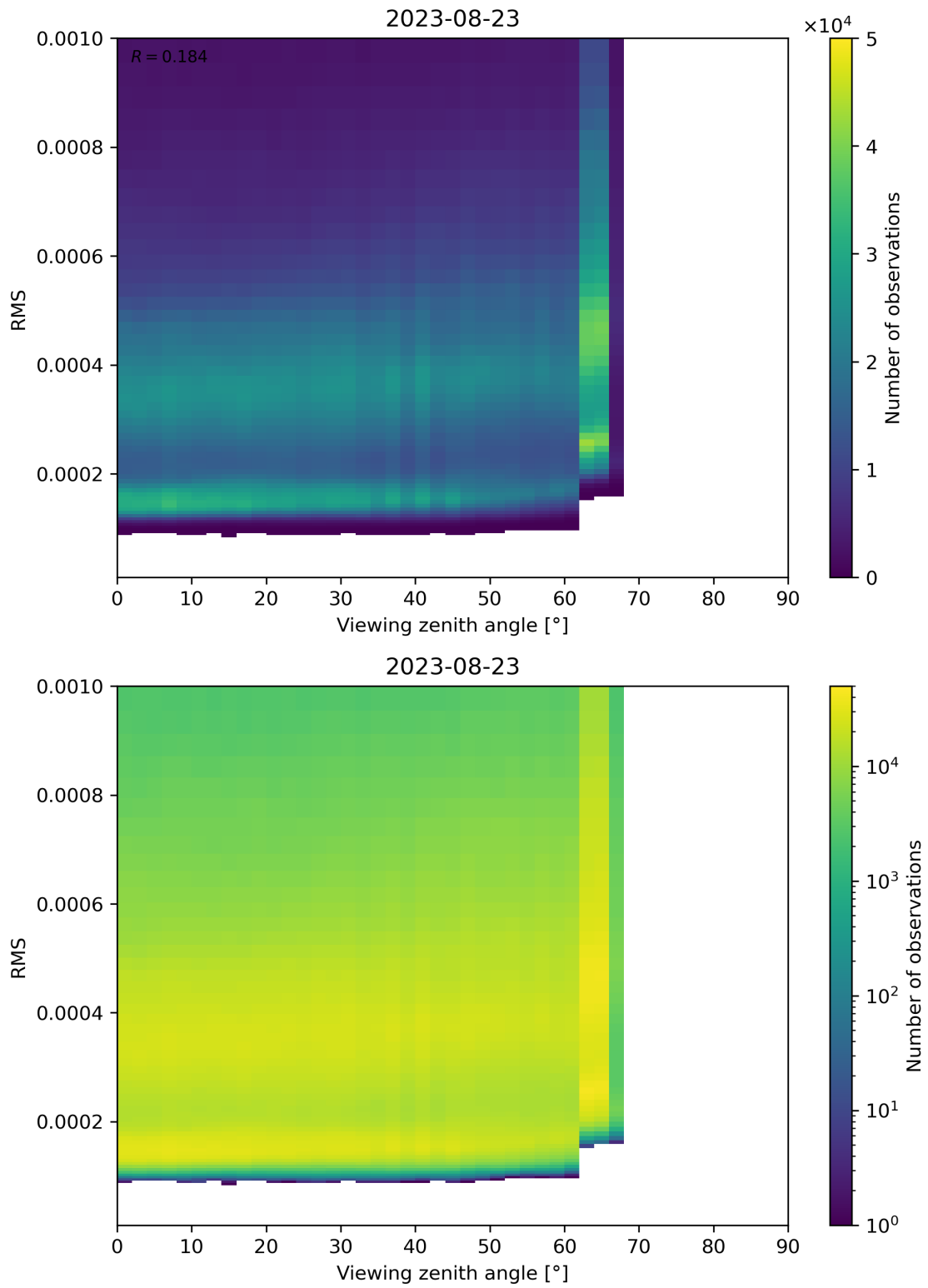
Figure 171: Scatter density plot of “Viewing zenith angle” against “RMS” for 2023-08-22 to 2023-08-24.
