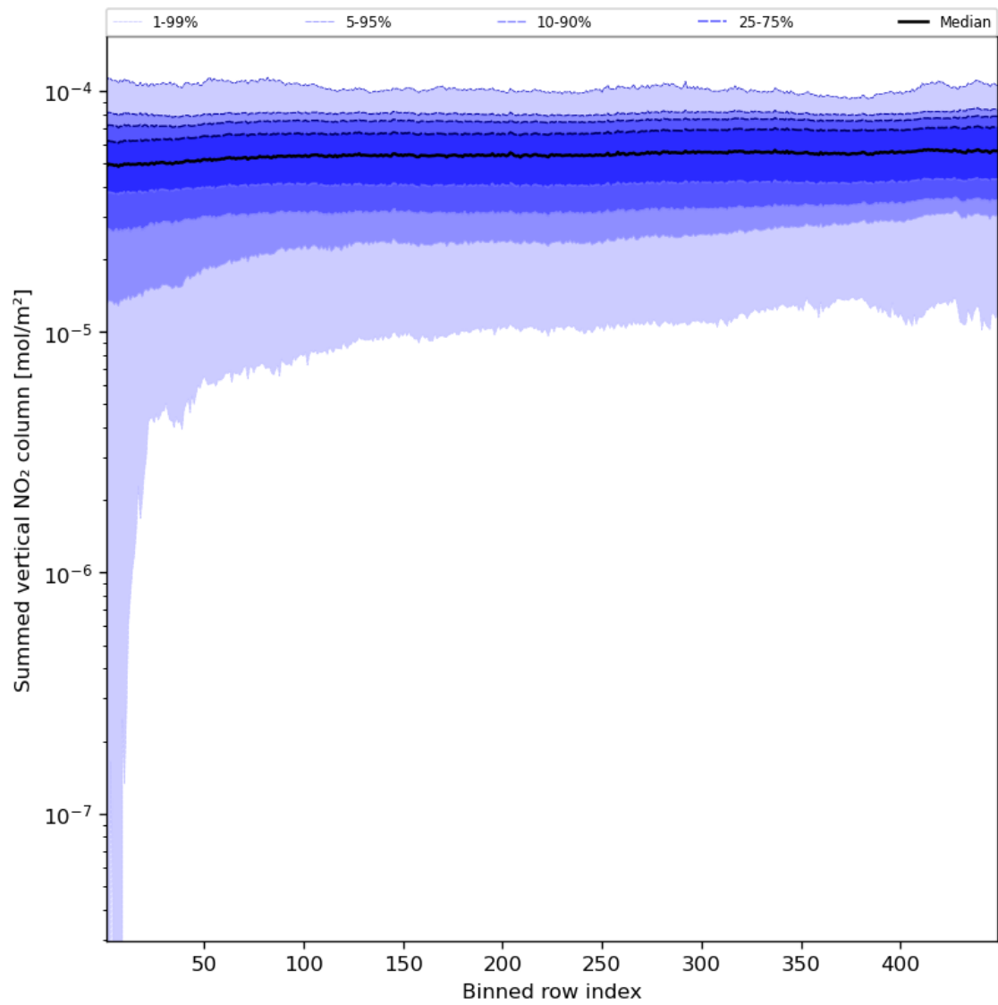
Figure 57: Along track statistics of “Summed vertical NO 2 column” for 2023-08-22 to 2023-08-24
