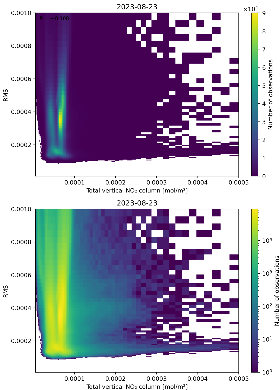
Figure 120: Scatter density plot of “Total vertical NO 2 column” against “RMS” for 2023-08-22 to 2023-08-24.
