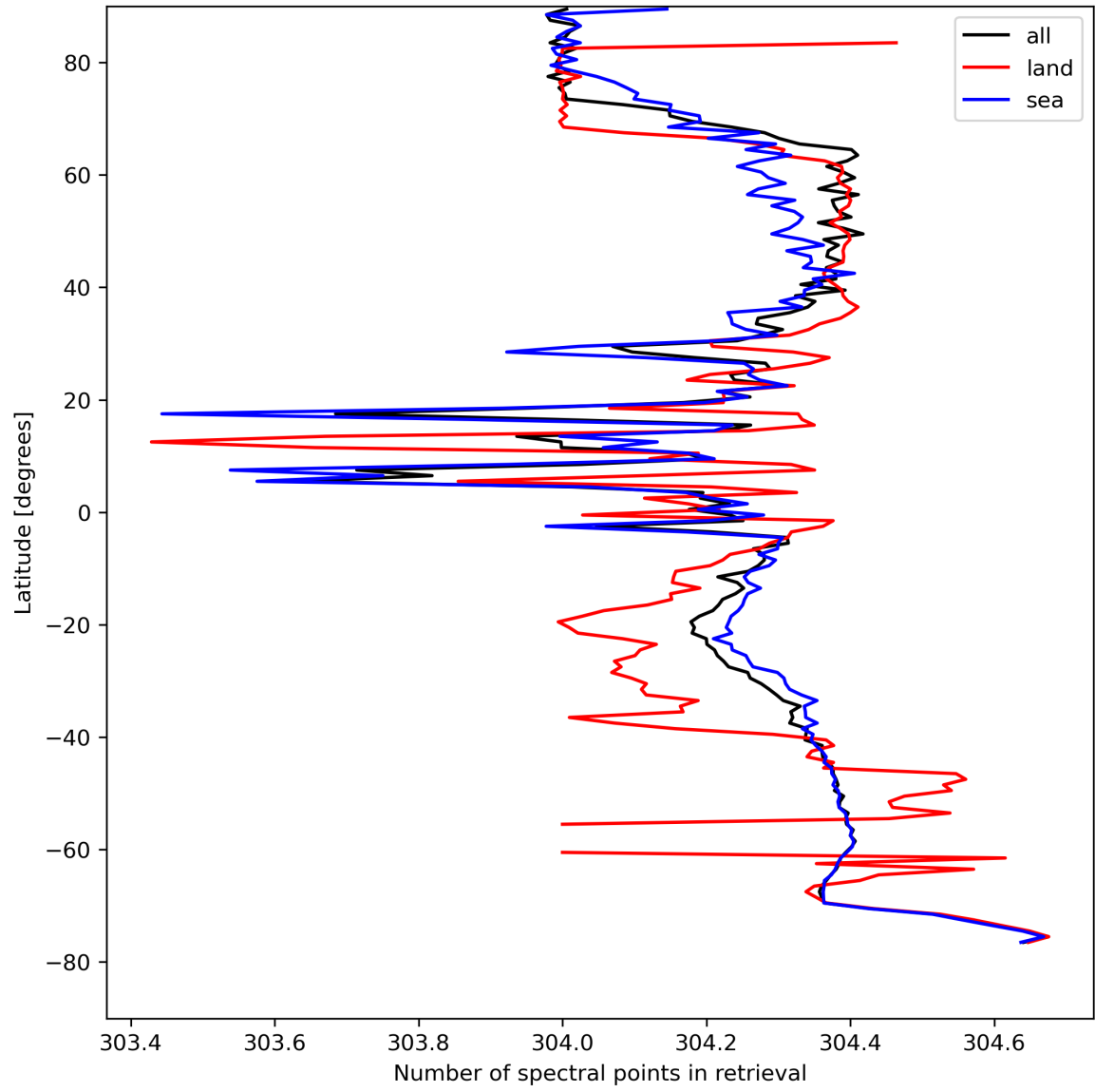
Figure 16: Zonal average of “Number of spectral points in retrieval” for 2023-08-22 to 2023-08-24.
