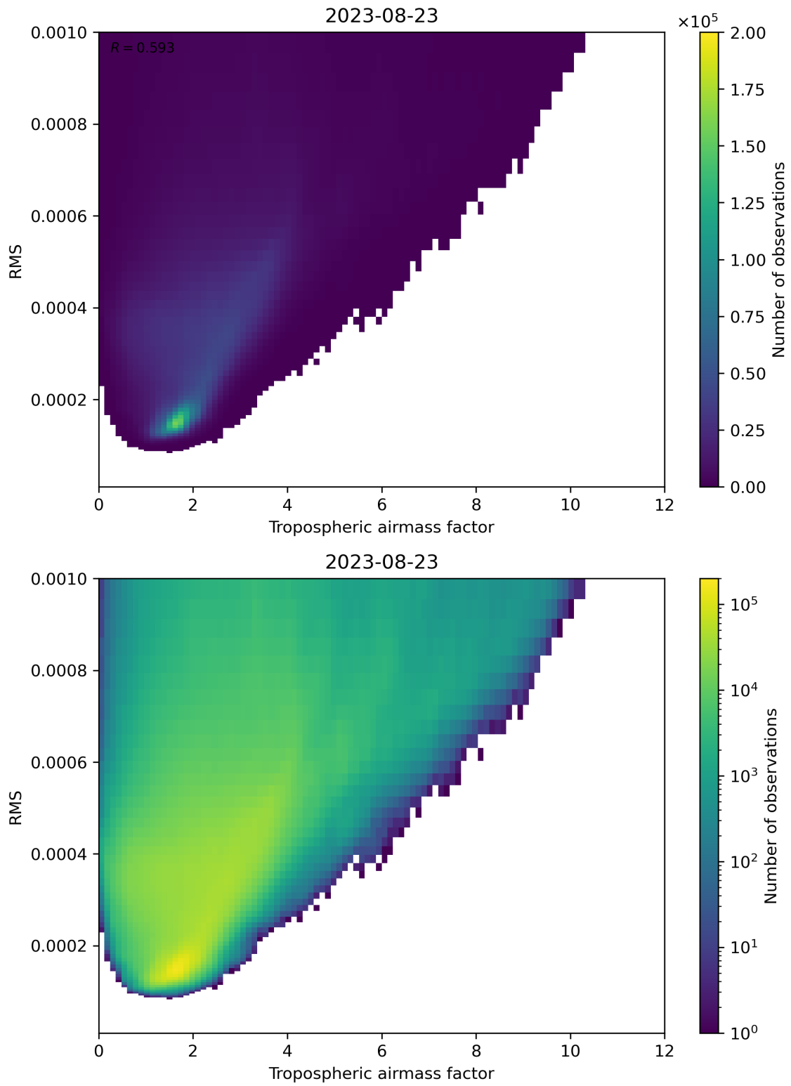
Figure 79: Scatter density plot of “Tropospheric airmass factor” against “RMS” for 2023-08-22 to 2023-08-24.
