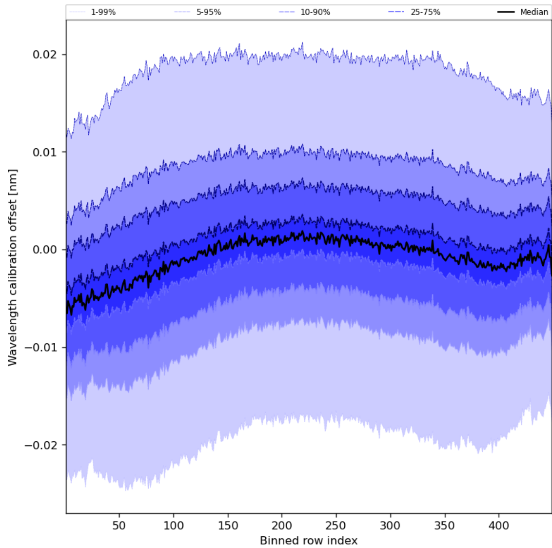
Figure 52: Along track statistics of “Wavelength calibration offset” for 2023-08-22 to 2023-08-24
