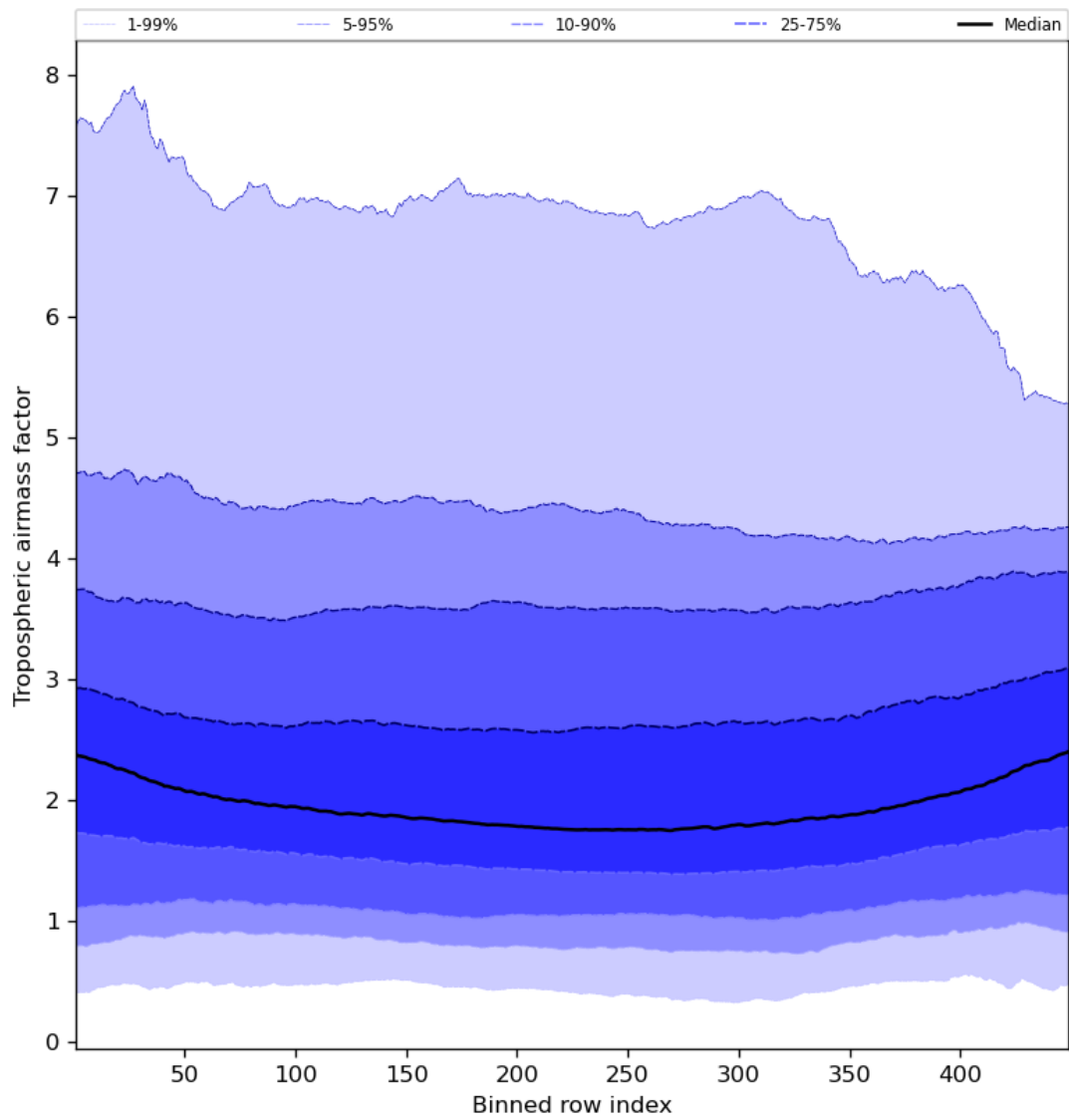
Figure 48: Along track statistics of “Tropospheric air mass factor” for 2023-08-22 to 2023-08-24
