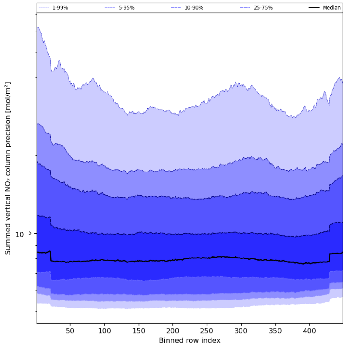
Figure 58: Along track statistics of “Summed vertical NO 2 column precision” for 2023-08-22 to 2023-08-24
