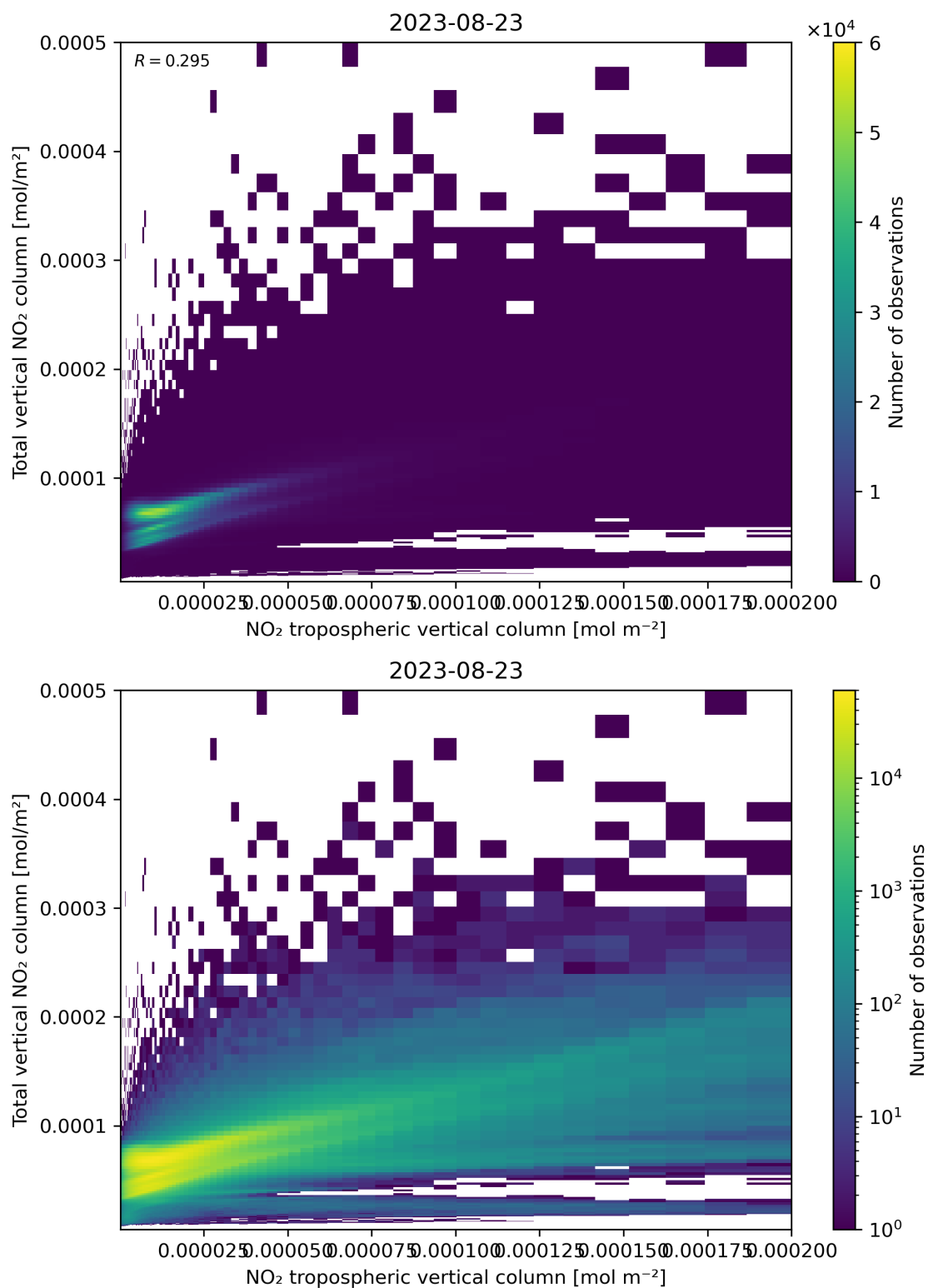
Figure 128: Scatter density plot of “NO 2 tropospheric vertical column” against “Total vertical NO 2 column” for 2023-08-22 to 2023-08-24.
