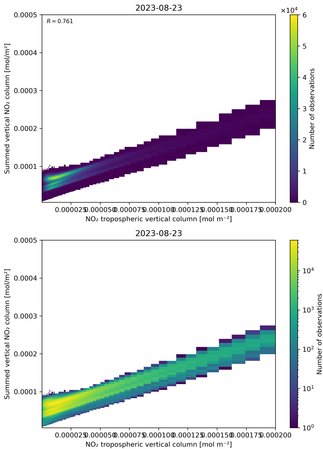
Figure 126: Scatter density plot of “NO 2 tropospheric vertical column” against “Summed vertical NO 2 column” for 2023-08-22 to 2023-08-24.
