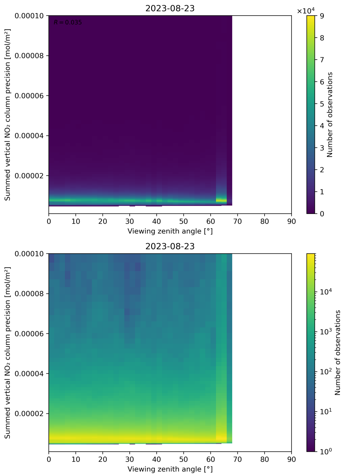
Figure 166: Scatter density plot of “Viewing zenith angle” against “Summed vertical NO 2 column precision” for 2023-08-22 to 2023-08-24.
