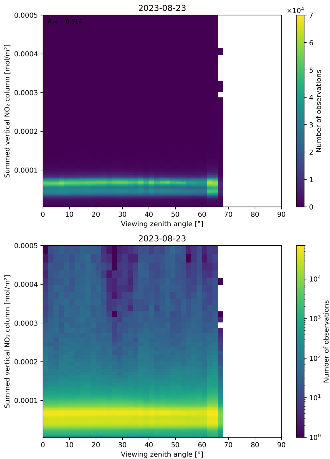
Figure 165: Scatter density plot of “Viewing zenith angle” against “Summed vertical NO 2 column” for 2023-08-22 to 2023-08-24.
