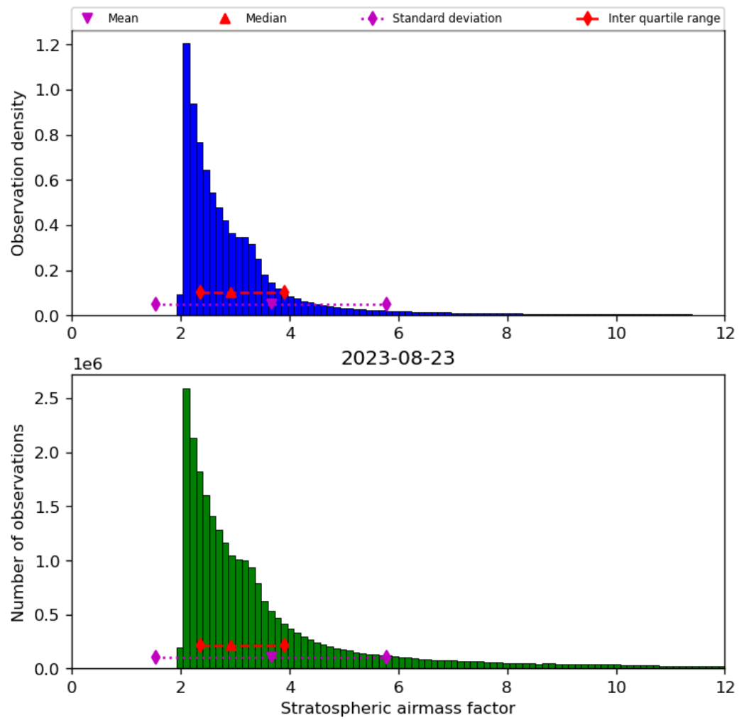
Figure 44: Histogram of “Stratospheric airmass factor” for 2023-08-22 to 2023-08-24
