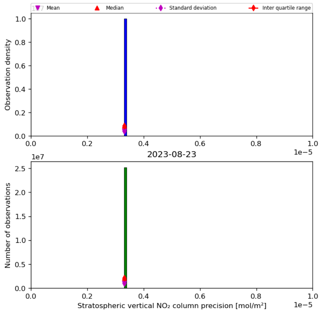
Figure 37: Histogram of “Stratospheric vertical NO 2 column precision” for 2023-08-22 to 2023-08-24
