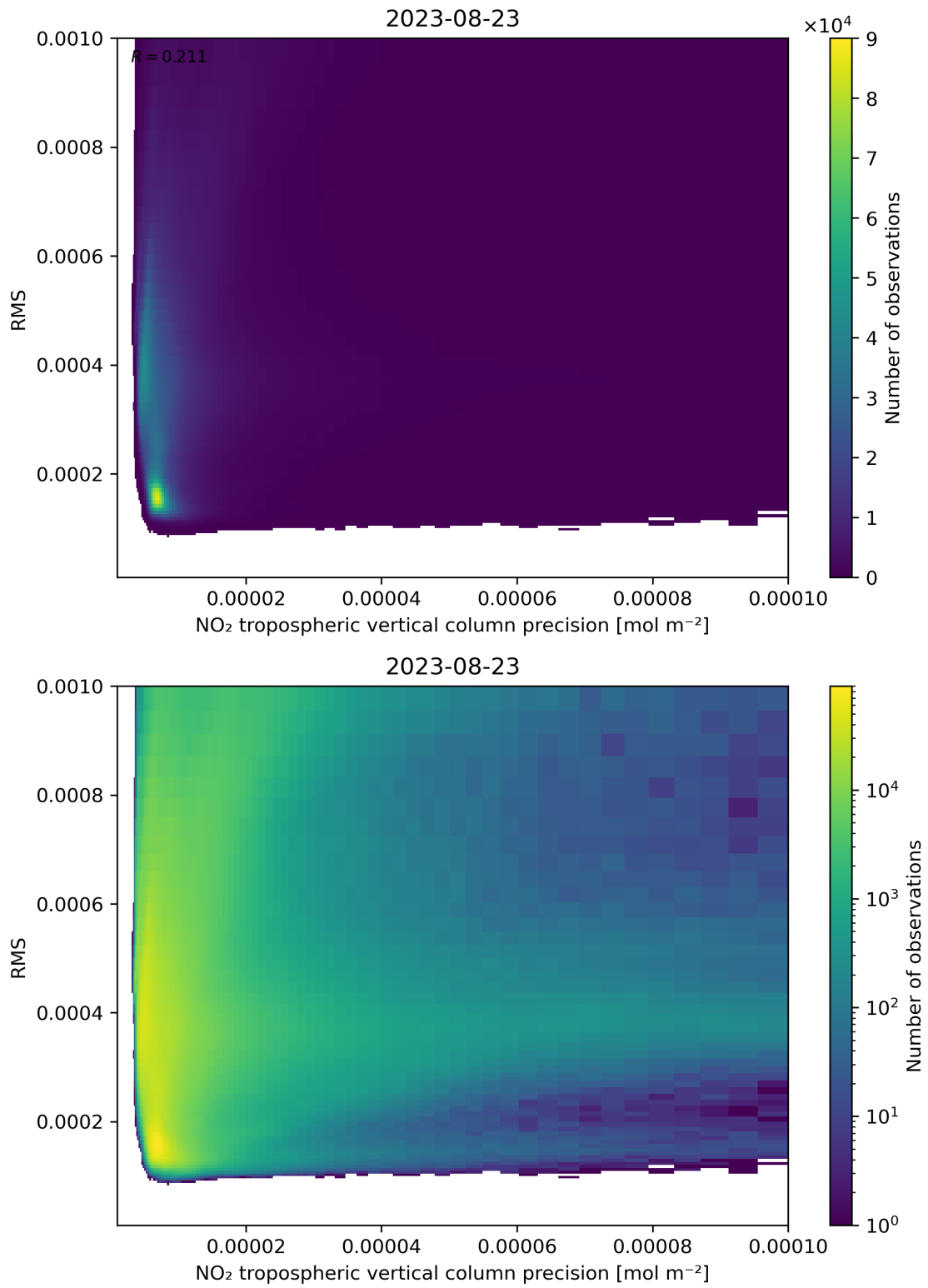
Figure 140: Scatter density plot of “NO 2 tropospheric vertical column precision” against “RMS” for 2023-08-22 to 2023-08-24.
