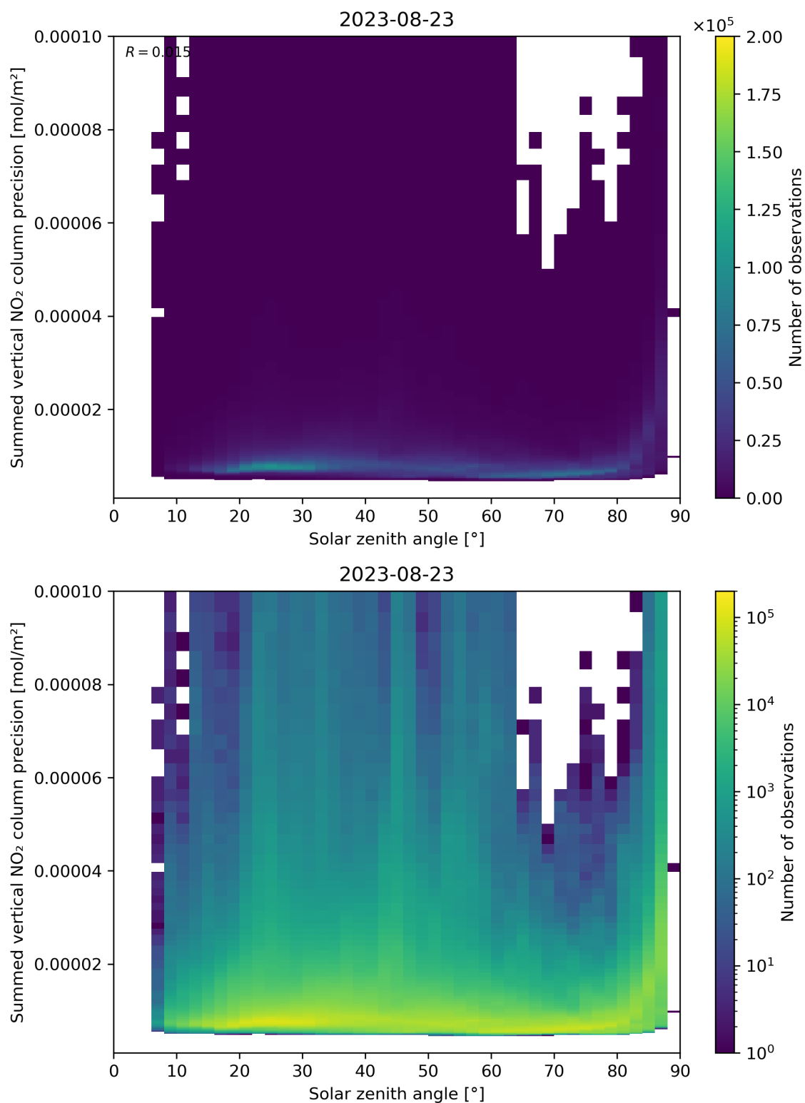
Figure 152: Scatter density plot of “Solar zenith angle” against “Summed vertical NO 2 column precision” for 2023-08-22 to 2023-08-24.
