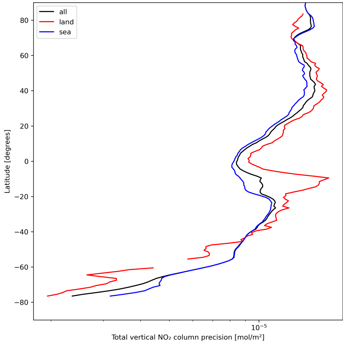
Figure 22: Zonal average of “Total vertical NO 2 column precision” for 2023-08-22 to 2023-08-24.
