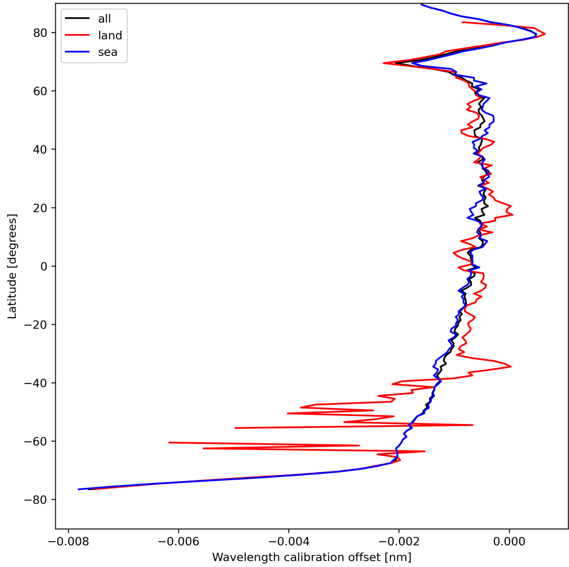
Figure 18: Zonal average of “Wavelength calibration offset” for 2023-08-22 to 2023-08-24.
