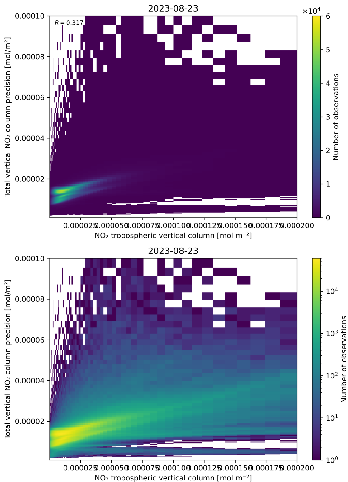
Figure 129: Scatter density plot of “NO 2 tropospheric vertical column” against “Total vertical NO 2 column precision” for 2023-08-22 to 2023-08-24.
