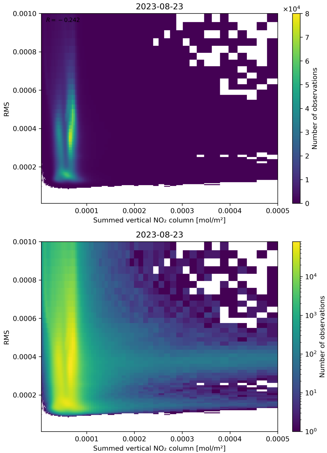
Figure 109: Scatter density plot of “Summed vertical NO 2 column” against “RMS” for 2023-08-22 to 2023-08-24.
