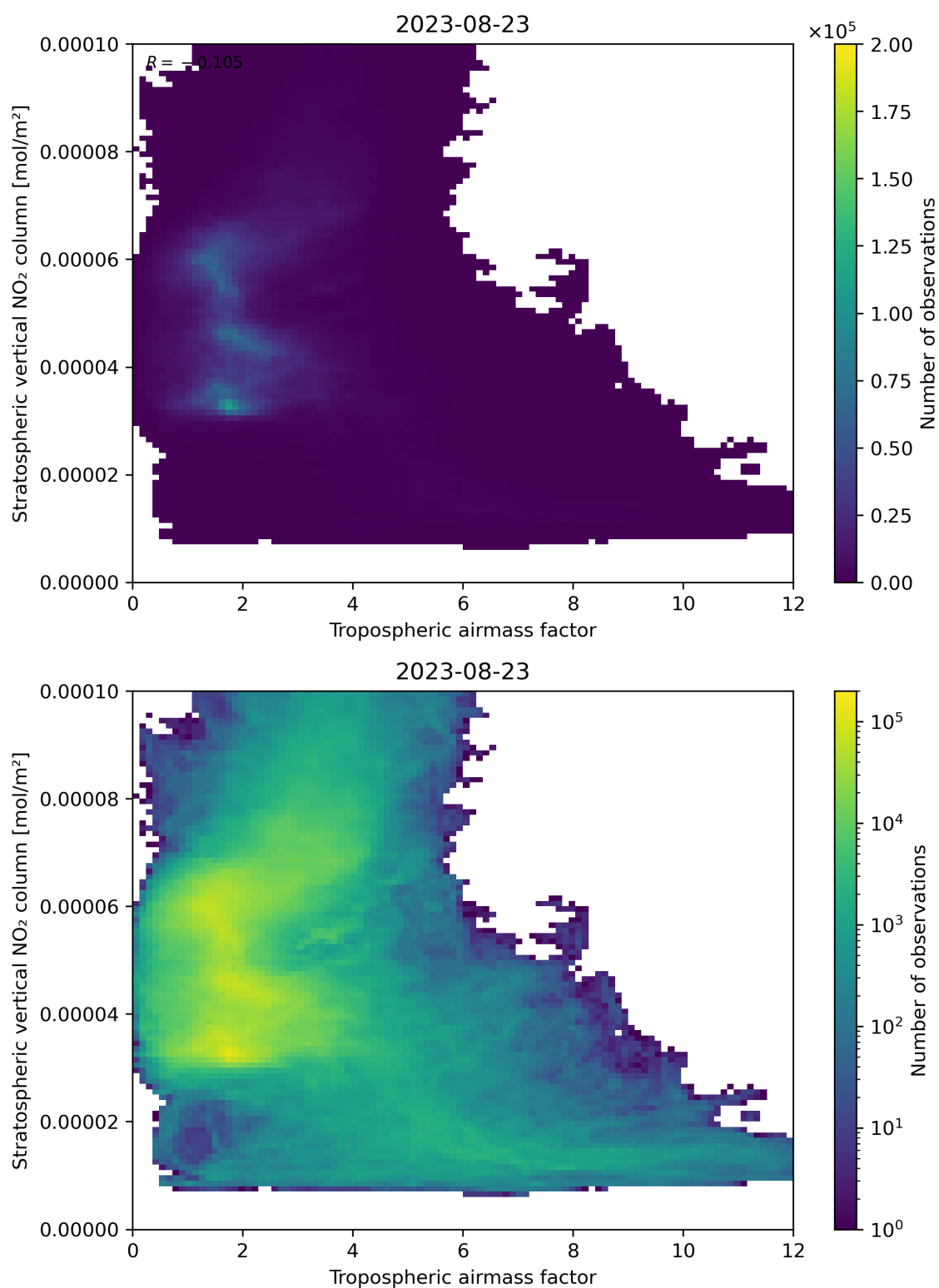
Figure 74: Scatter density plot of “Tropospheric air mass factor” against “Stratospheric vertical NO 2 column” for 2023-08-22 to 2023-08-24.
