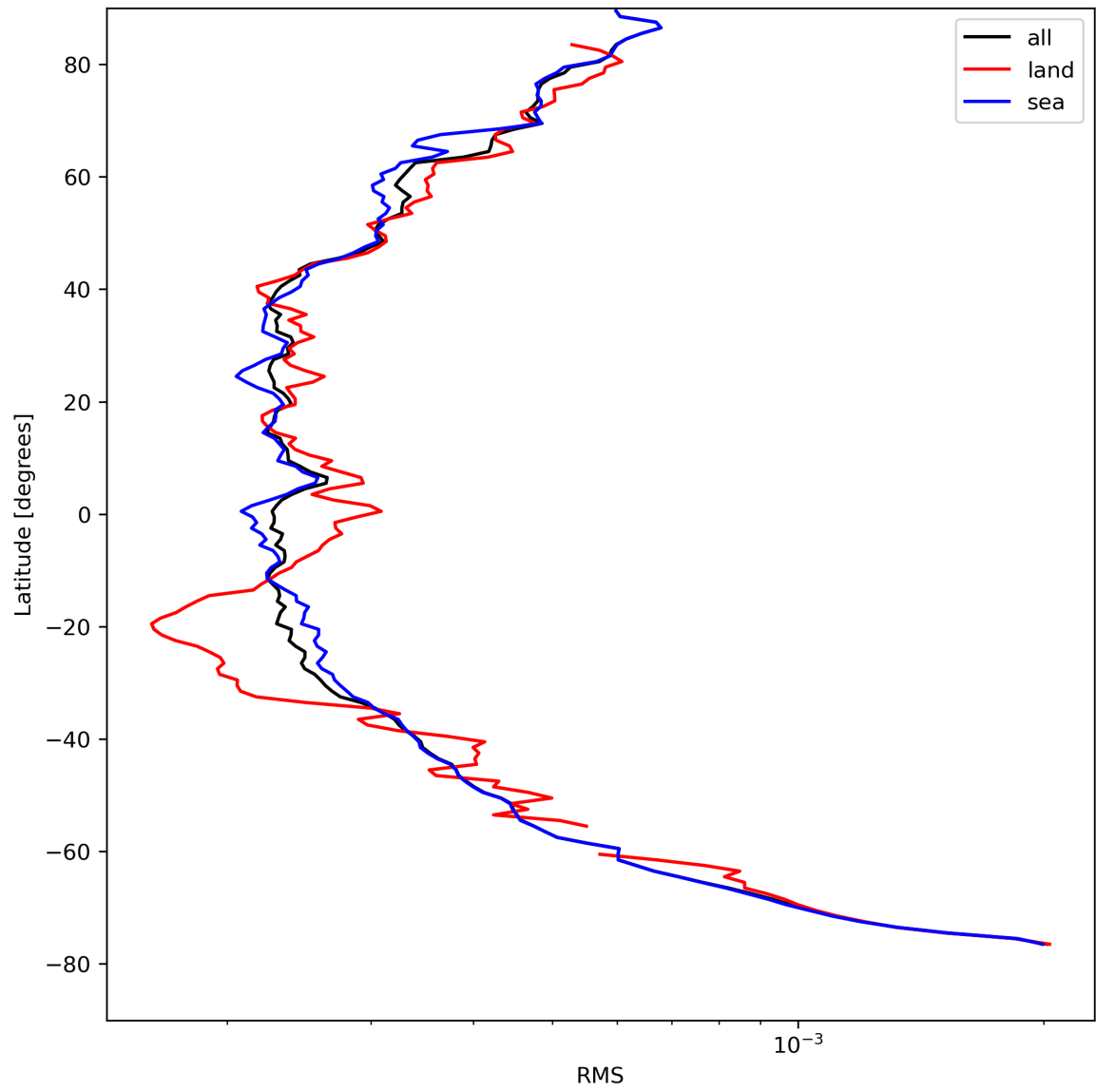
Figure 26: Zonal average of “RMS” for 2023-08-22 to 2023-08-24.
