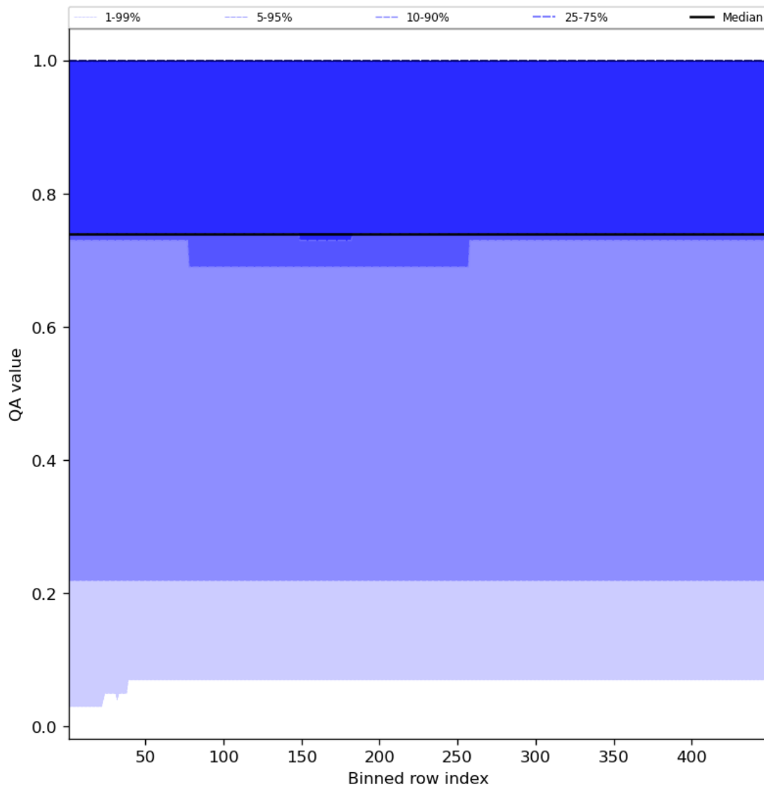
Figure 45: Along track statistics of “QA value” for 2023-08-22 to 2023-08-24
