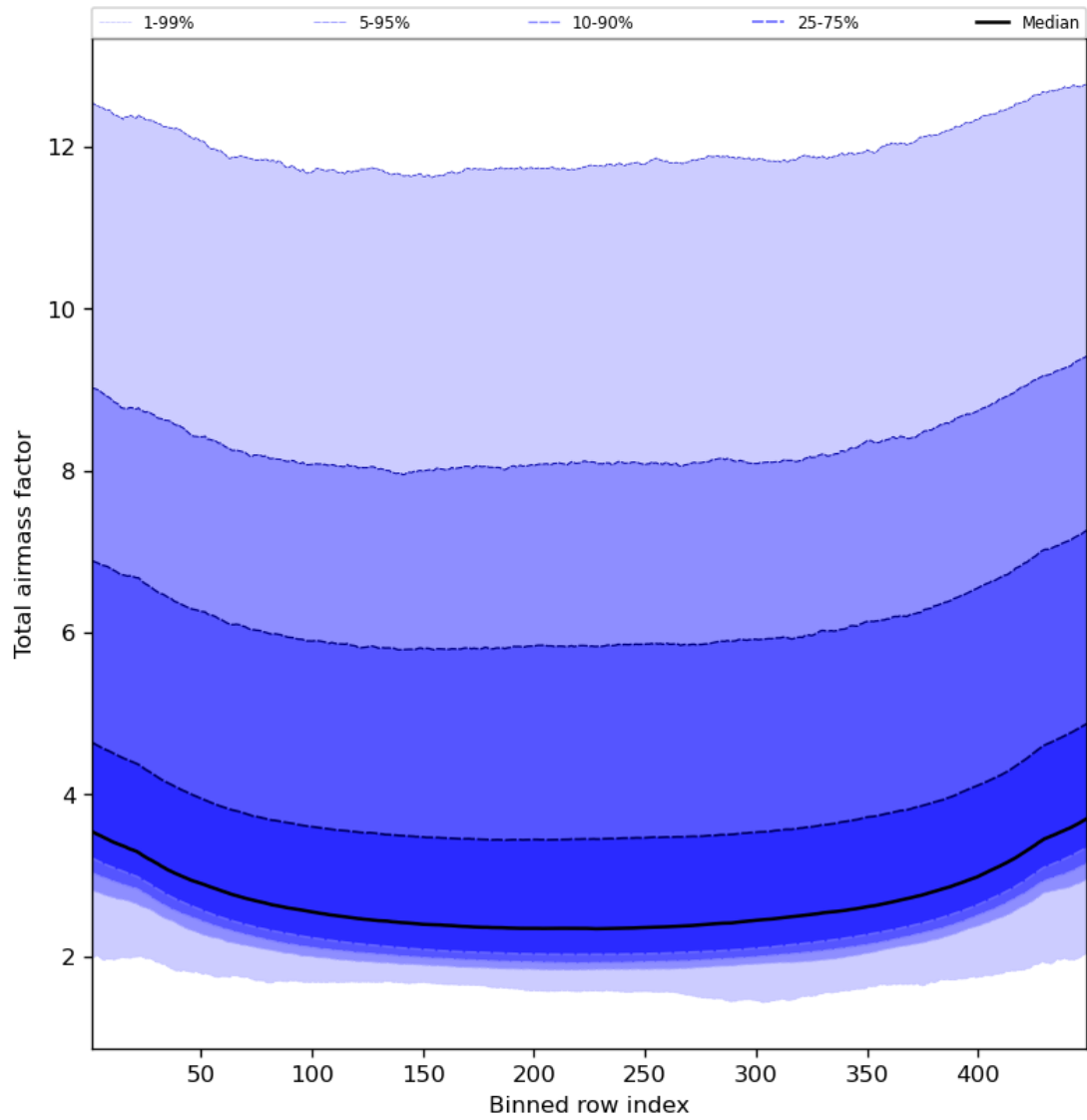
Figure 49: Along track statistics of “Total airmass factor” for 2023-08-22 to 2023-08-24
