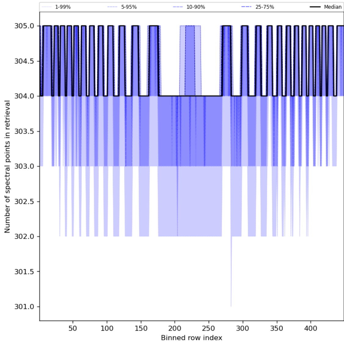
Figure 50: Along track statistics of “Number of spectral points in retrieval” for 2023-08-22 to 2023-08-24
