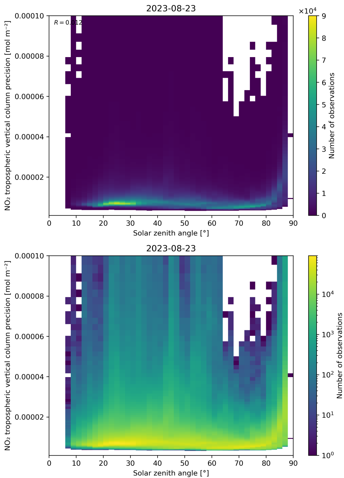
Figure 156: Scatter density plot of “Solar zenith angle” against “NO 2 tropospheric vertical column precision” for 2023-08-22 to 2023-08-24.
