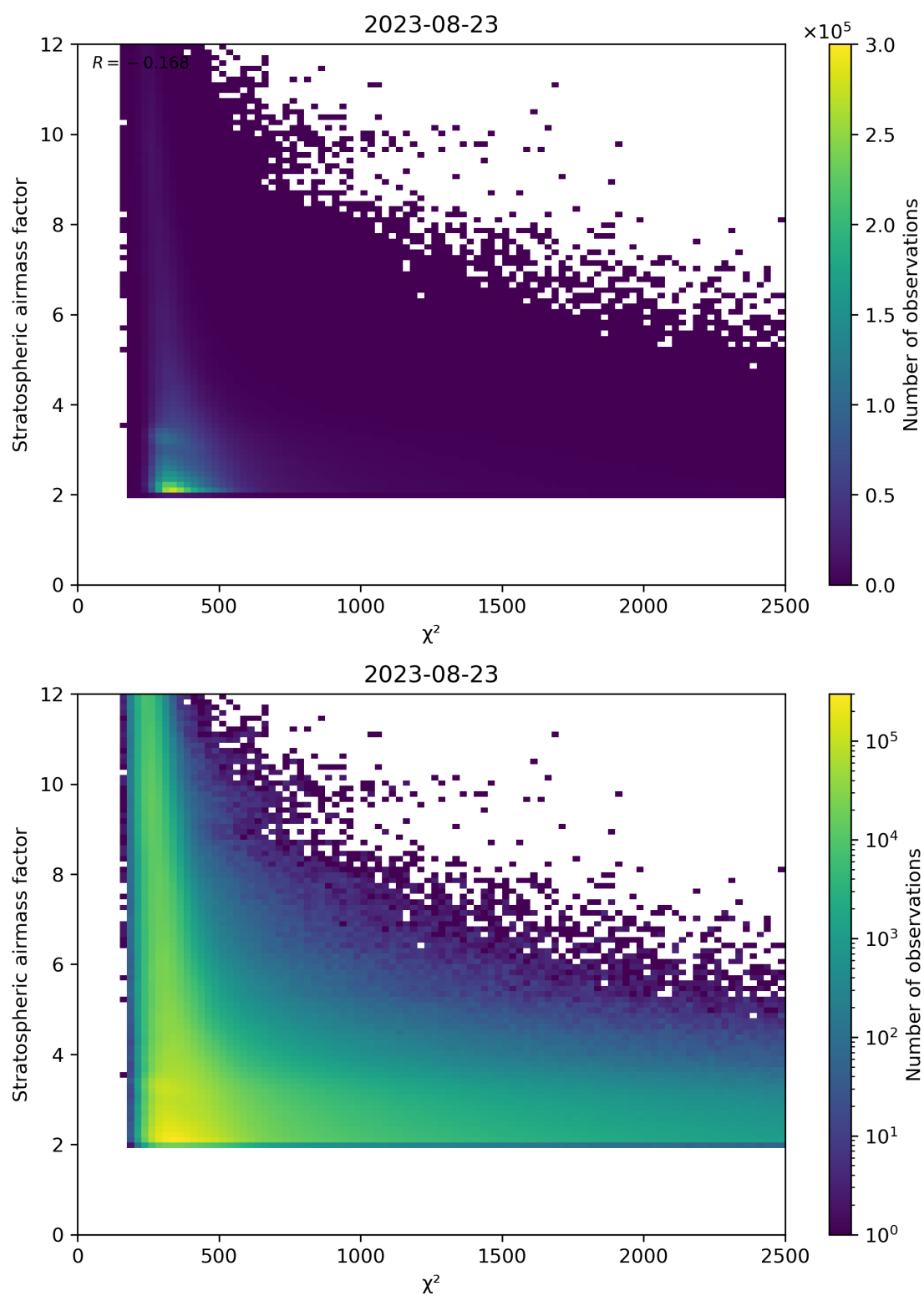
Figure 81: Scatter density plot of “ \chi^2 ” against “Stratospheric airmass factor” for 2023-08-22 to 2023-08-24.
