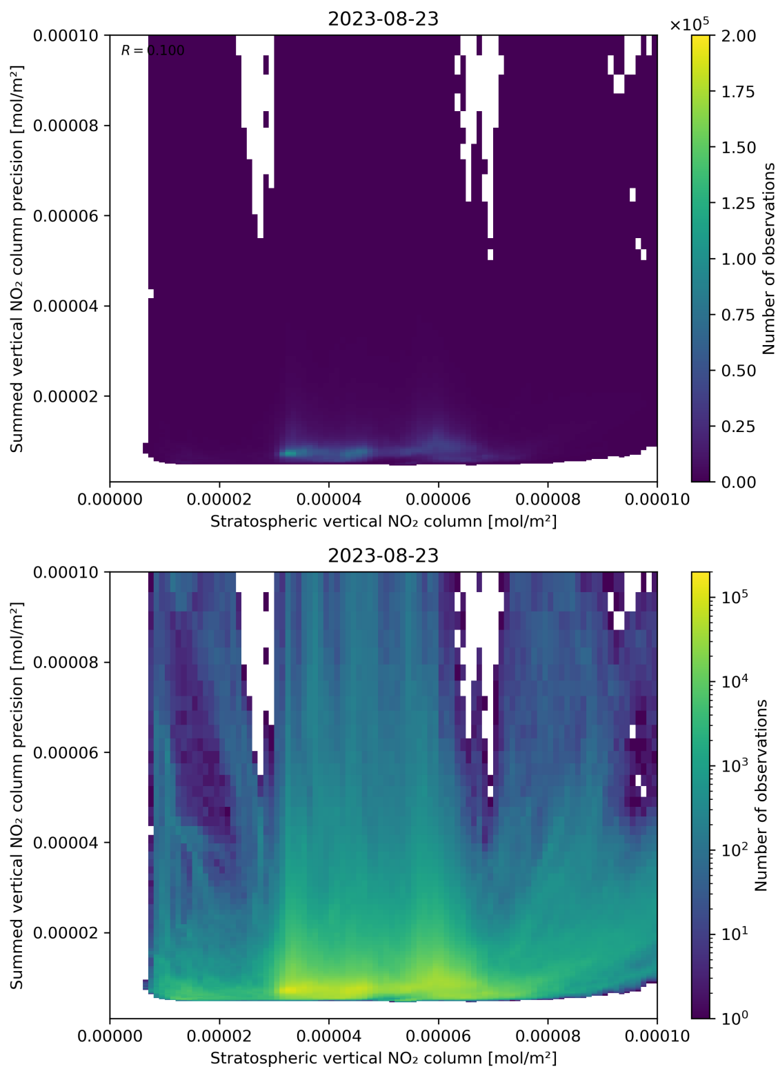
Figure 99: Scatter density plot of “Stratospheric vertical NO 2 column” against “Summed vertical NO 2 column precision” for 2023-08-22 to 2023-08-24.
