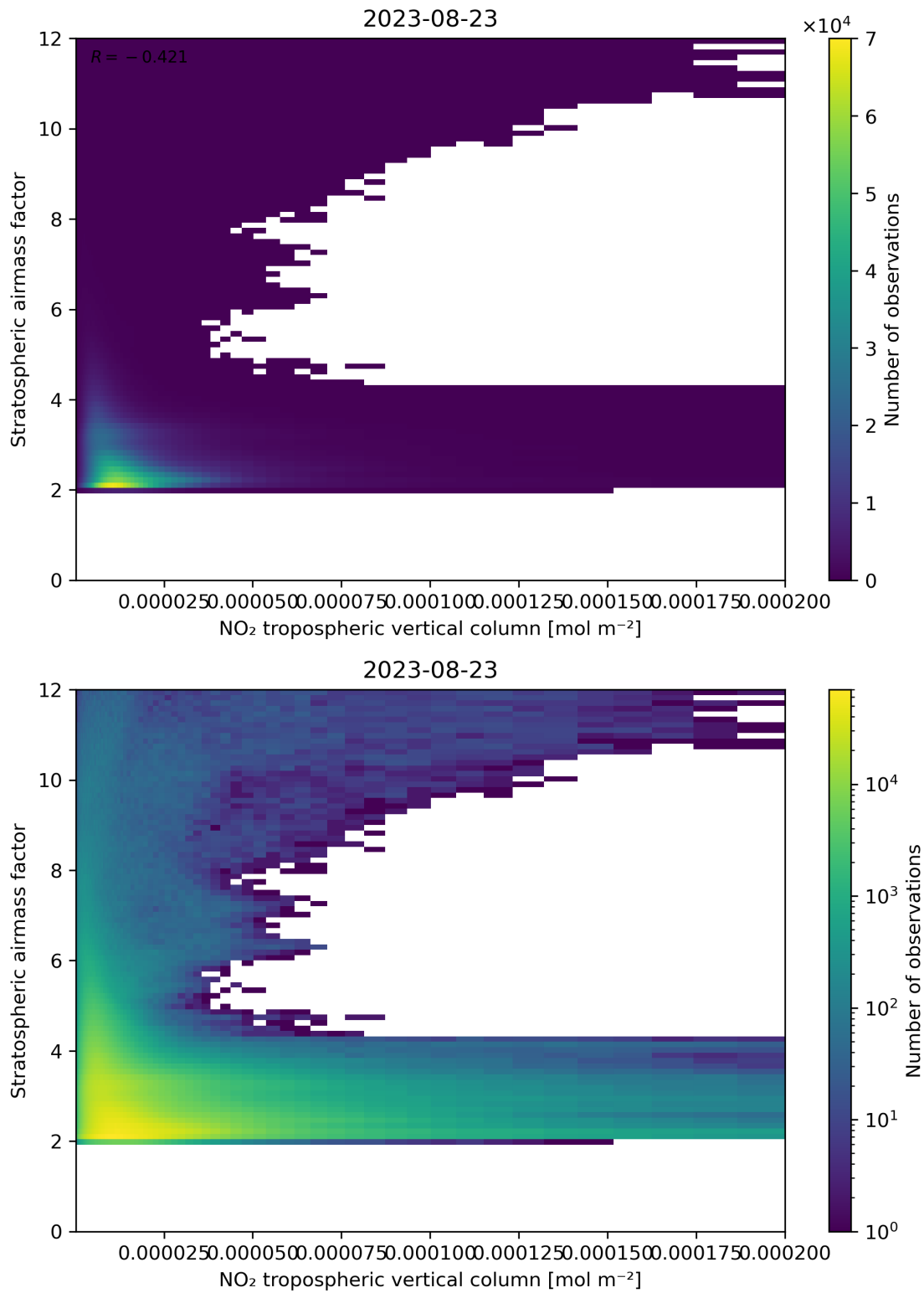
Figure 121: Scatter density plot of “NO 2 tropospheric vertical column” against “Stratospheric air mass factor” for 2023-08-22 to 2023-08-24.
