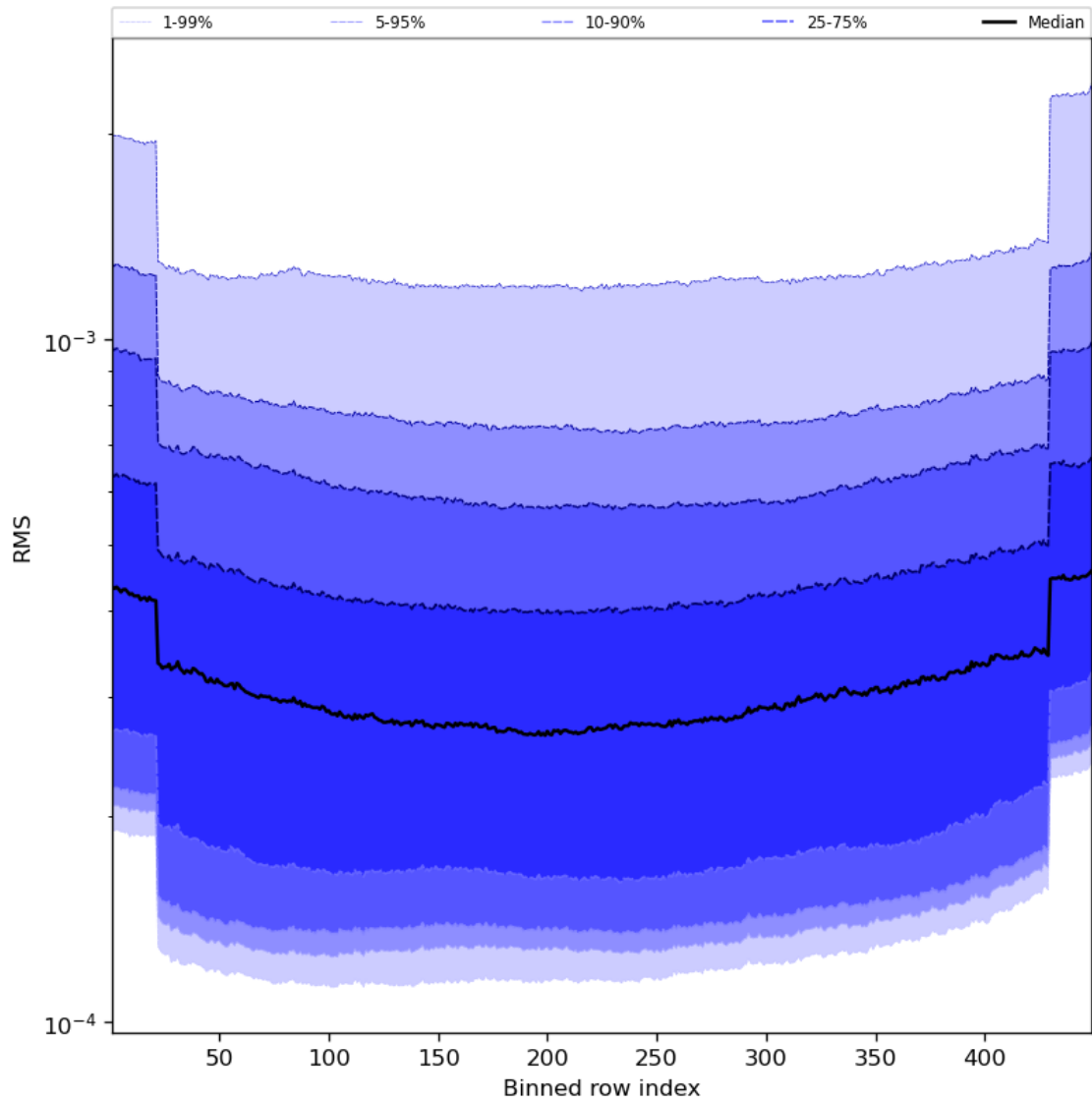
Figure 60: Along track statistics of “RMS” for 2023-08-22 to 2023-08-24
