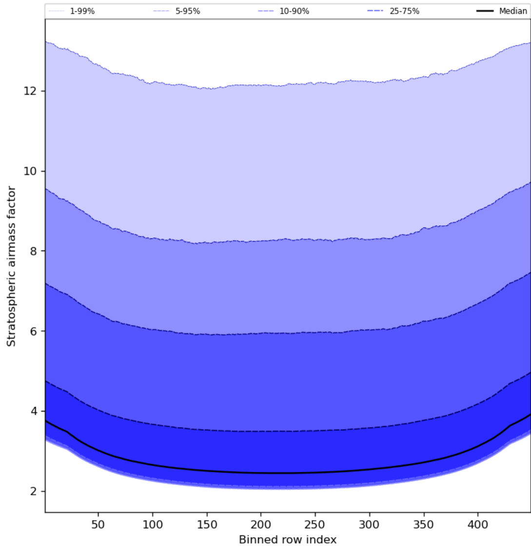
Figure 61: Along track statistics of “Stratospheric airmass factor” for 2023-08-22 to 2023-08-24
