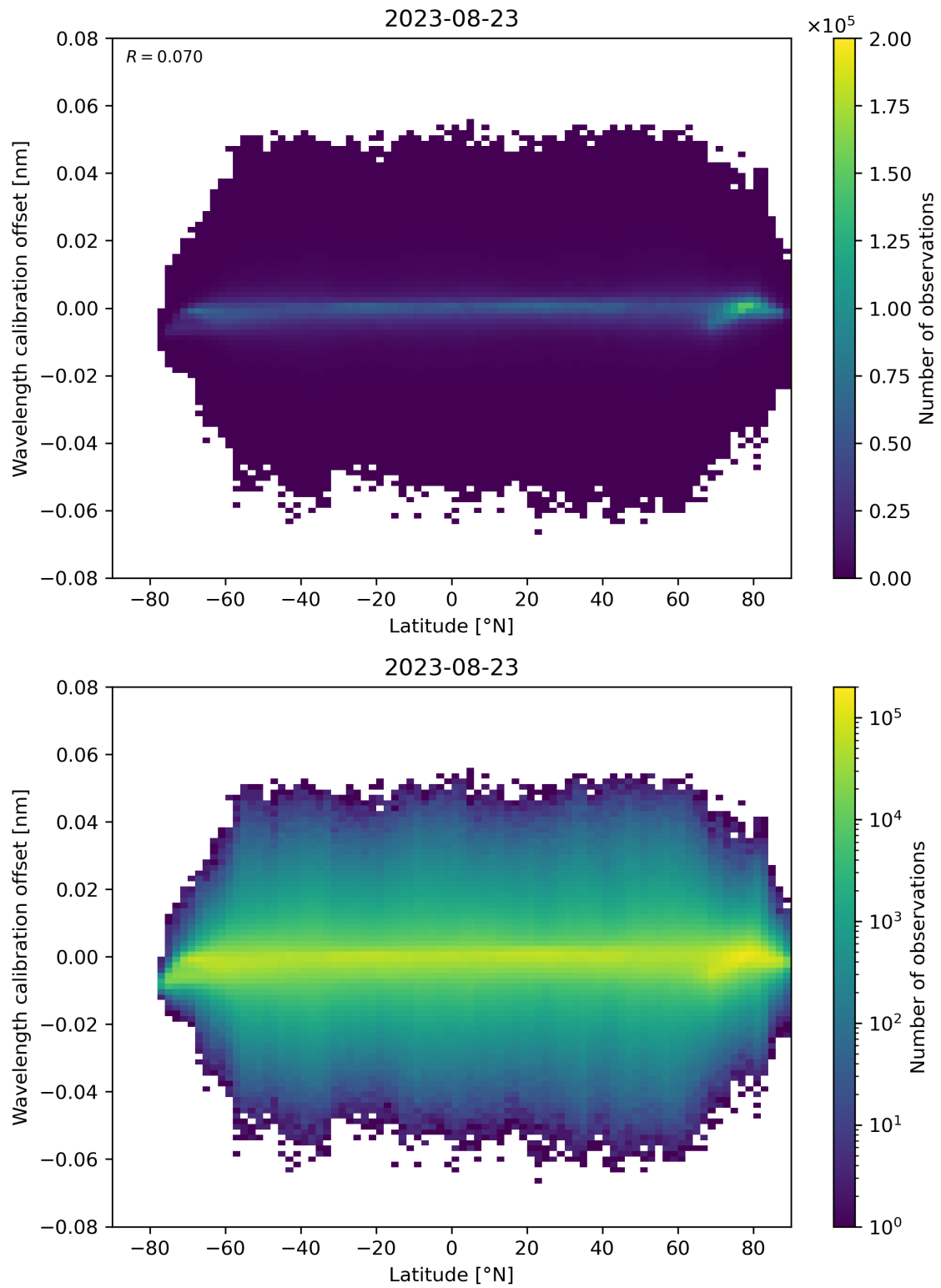
Figure 95: Scatter density plot of “Latitude” against “Wavelength calibration offset” for 2023-08-22 to 2023-08-24.
