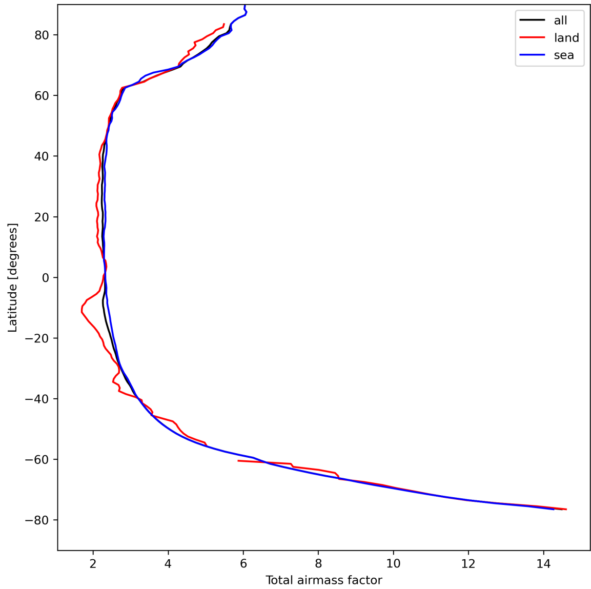
Figure 15: Zonal average of “Total airmass factor” for 2023-08-22 to 2023-08-24.
