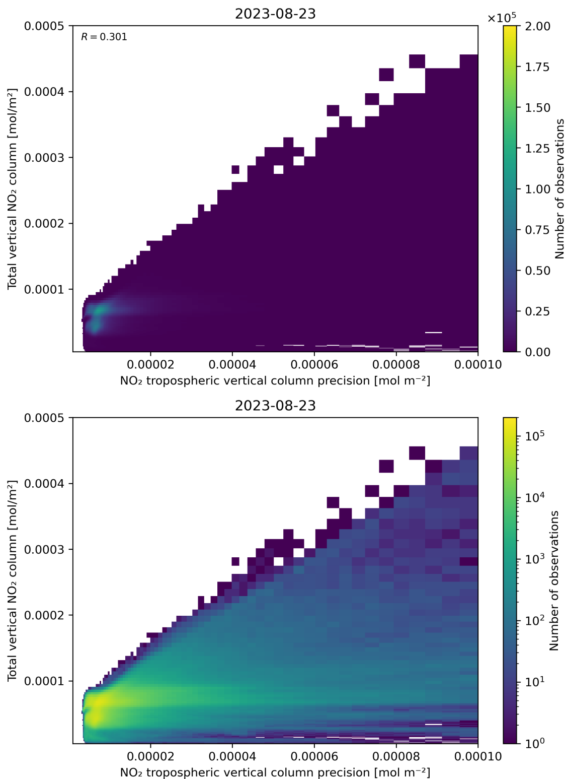
Figure 138: Scatter density plot of “NO 2 tropospheric vertical column precision” against “Total vertical NO 2 column” for 2023-08-22 to 2023-08-24.
