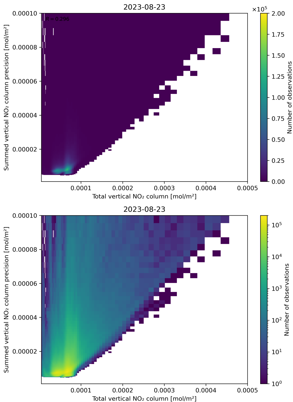
Figure 113: Scatter density plot of “Total vertical NO 2 column” against “Summed vertical NO 2 column precision” for 2023-08-22 to 2023-08-24.
