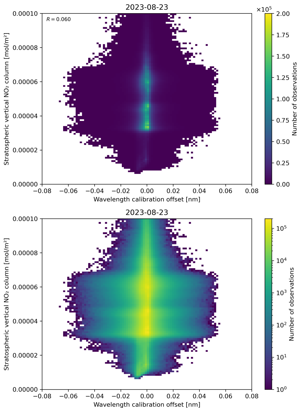
Figure 176: Scatter density plot of “Wavelength calibration offset” against “Stratospheric vertical NO 2 column” for 2023-08-22 to 2023-08-24.
