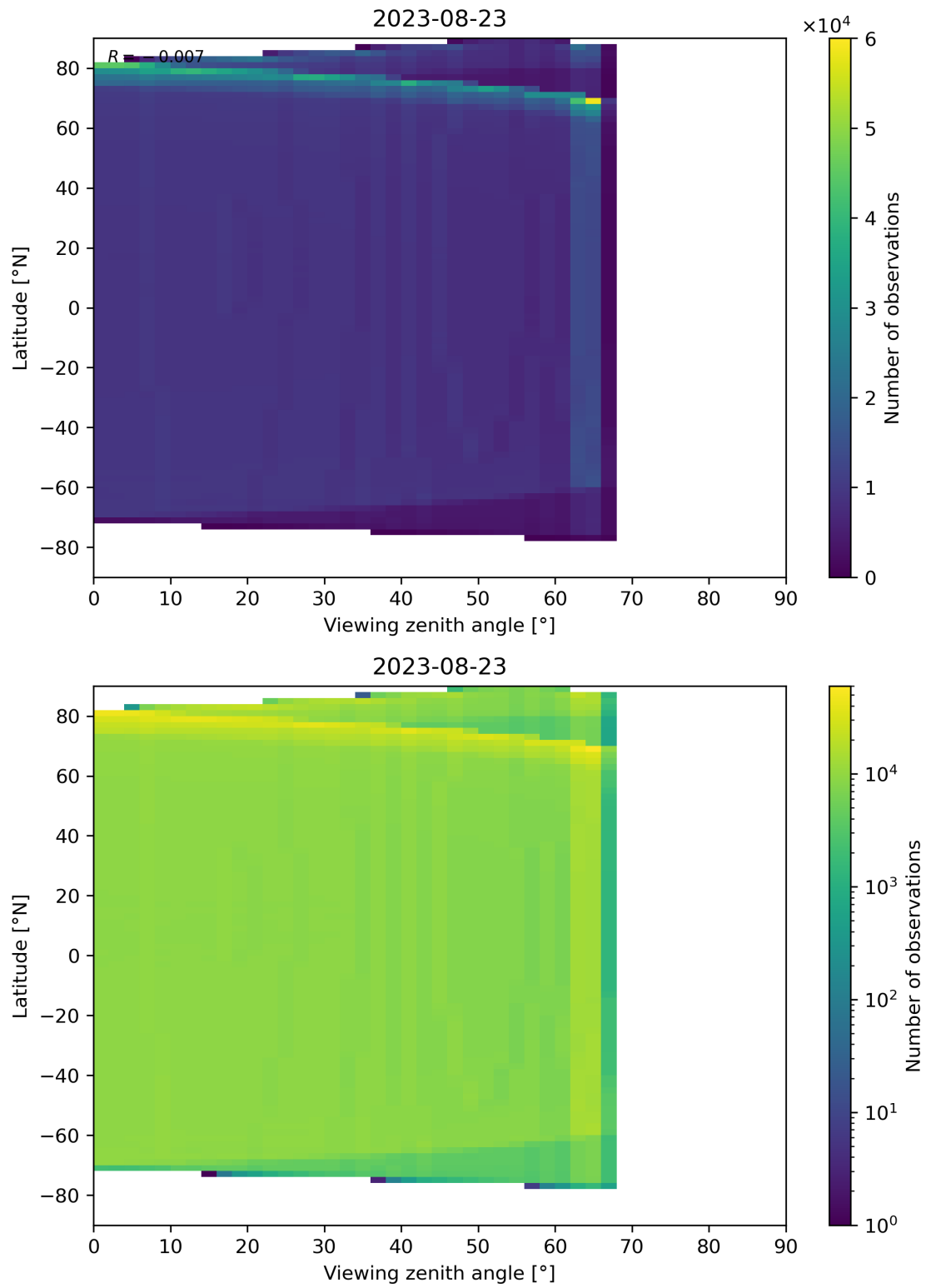
Figure 163: Scatter density plot of “Viewing zenith angle” against “Latitude” for 2023-08-22 to 2023-08-24.
