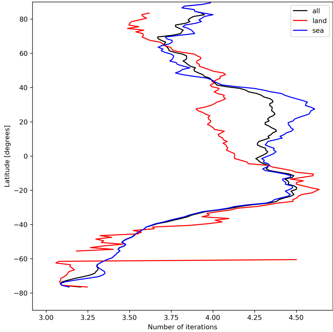
Figure 17: Zonal average of “Number of iterations” for 2023-08-22 to 2023-08-24.
