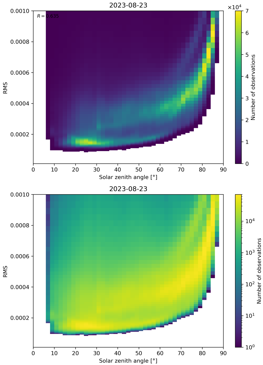
Figure 157: Scatter density plot of “Solar zenith angle” against “RMS” for 2023-08-22 to 2023-08-24.
