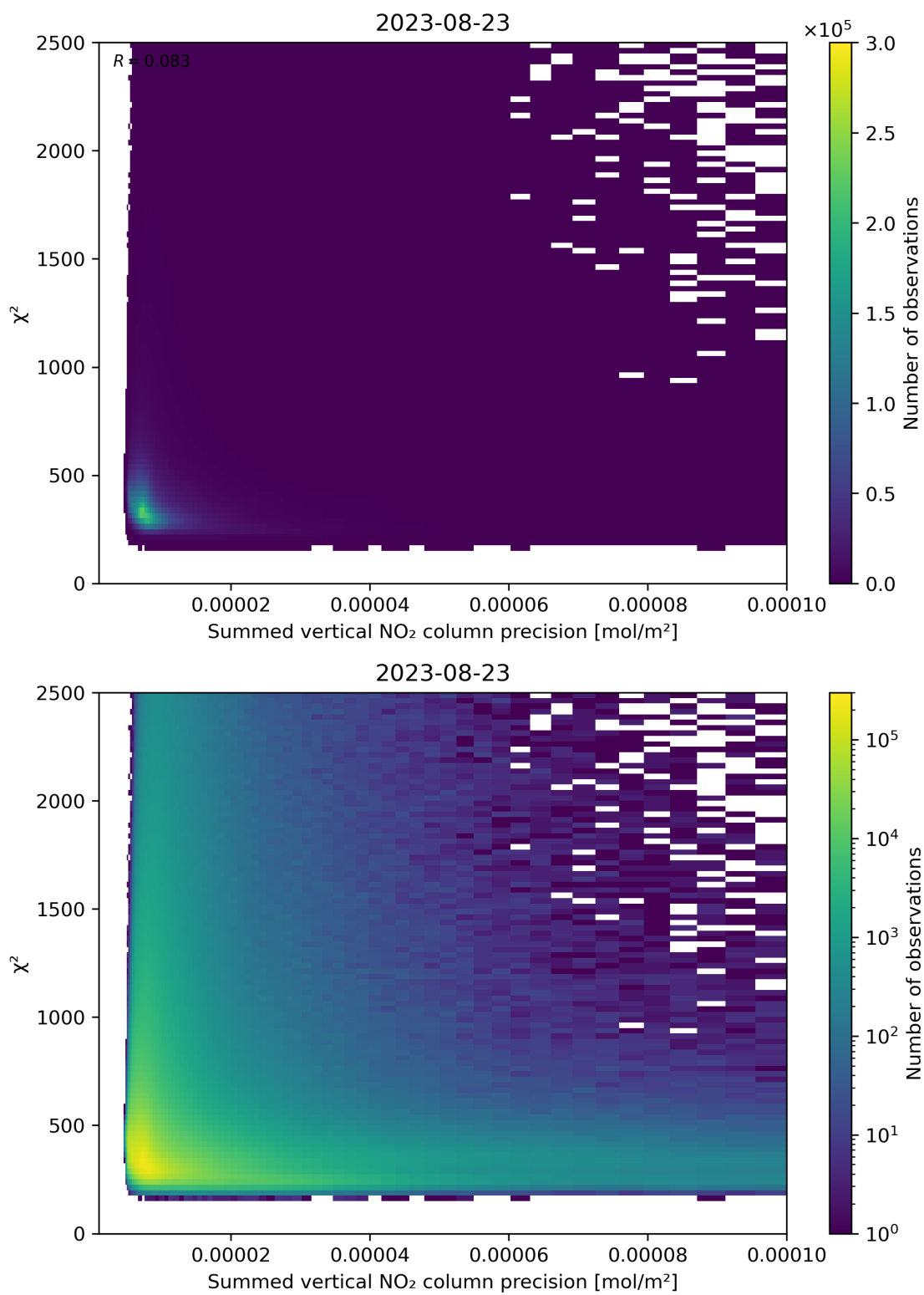
Figure 107: Scatter density plot of “Summed vertical NO 2 column precision” against “ \chi^2 ” for 2023-08-22 to 2023-08-24.
