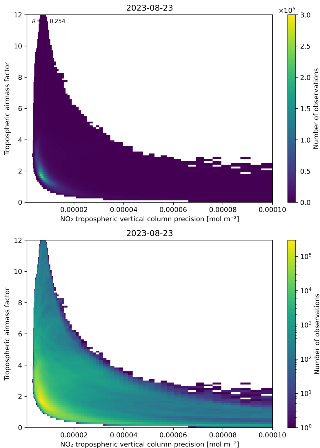
Figure 133: Scatter density plot of “NO 2 tropospheric vertical column precision” against “Tropospheric airmass factor” for 2023-08-22 to 2023-08-24.
