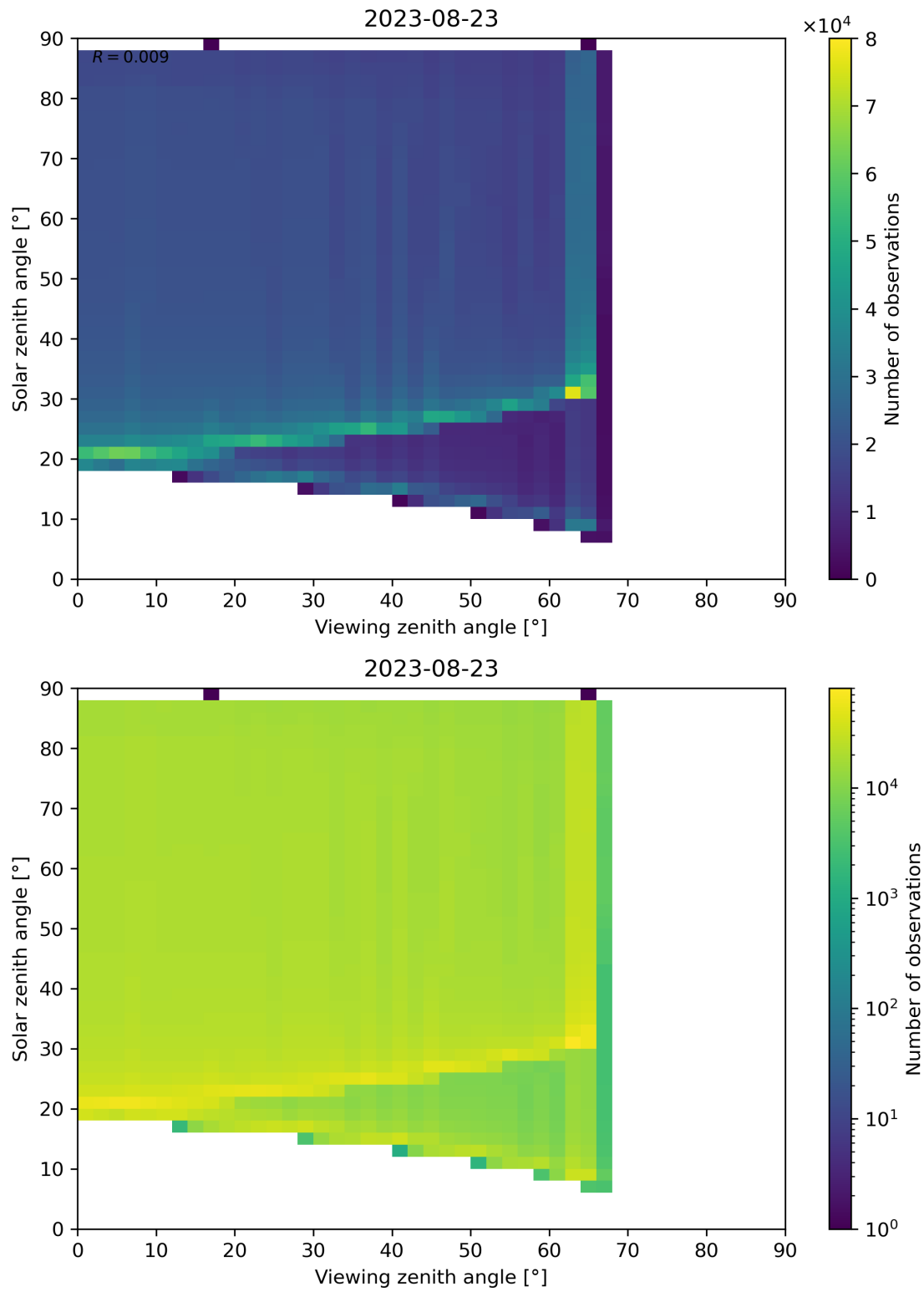
Figure 172: Scatter density plot of “Viewing zenith angle” against “Solar zenith angle” for 2023-08-22 to 2023-08-24.
