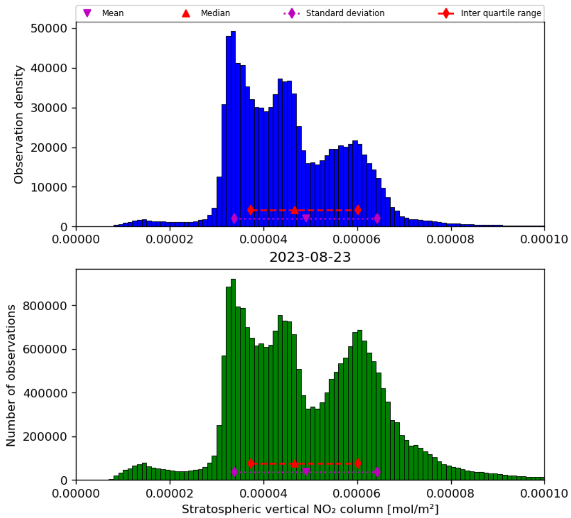
Figure 36: Histogram of “Stratospheric vertical NO 2 column” for 2023-08-22 to 2023-08-24
