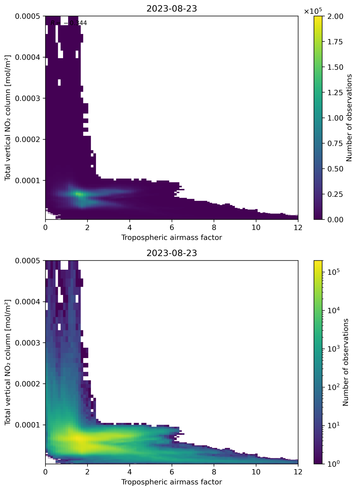
Figure 77: Scatter density plot of “Tropospheric airmass factor” against “Total vertical NO 2 column” for 2023-08-22 to 2023-08-24.
