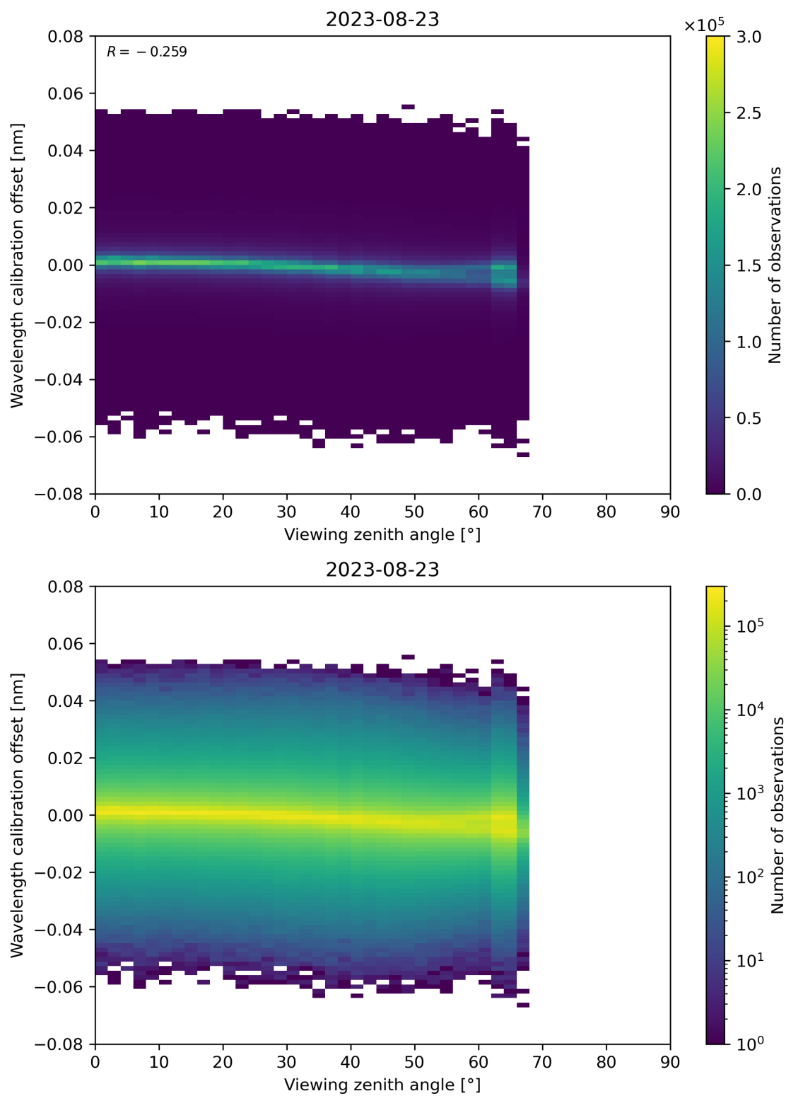
Figure 173: Scatter density plot of “Viewing zenith angle” against “Wavelength calibration offset” for 2023-08-22 to 2023-08-24.
