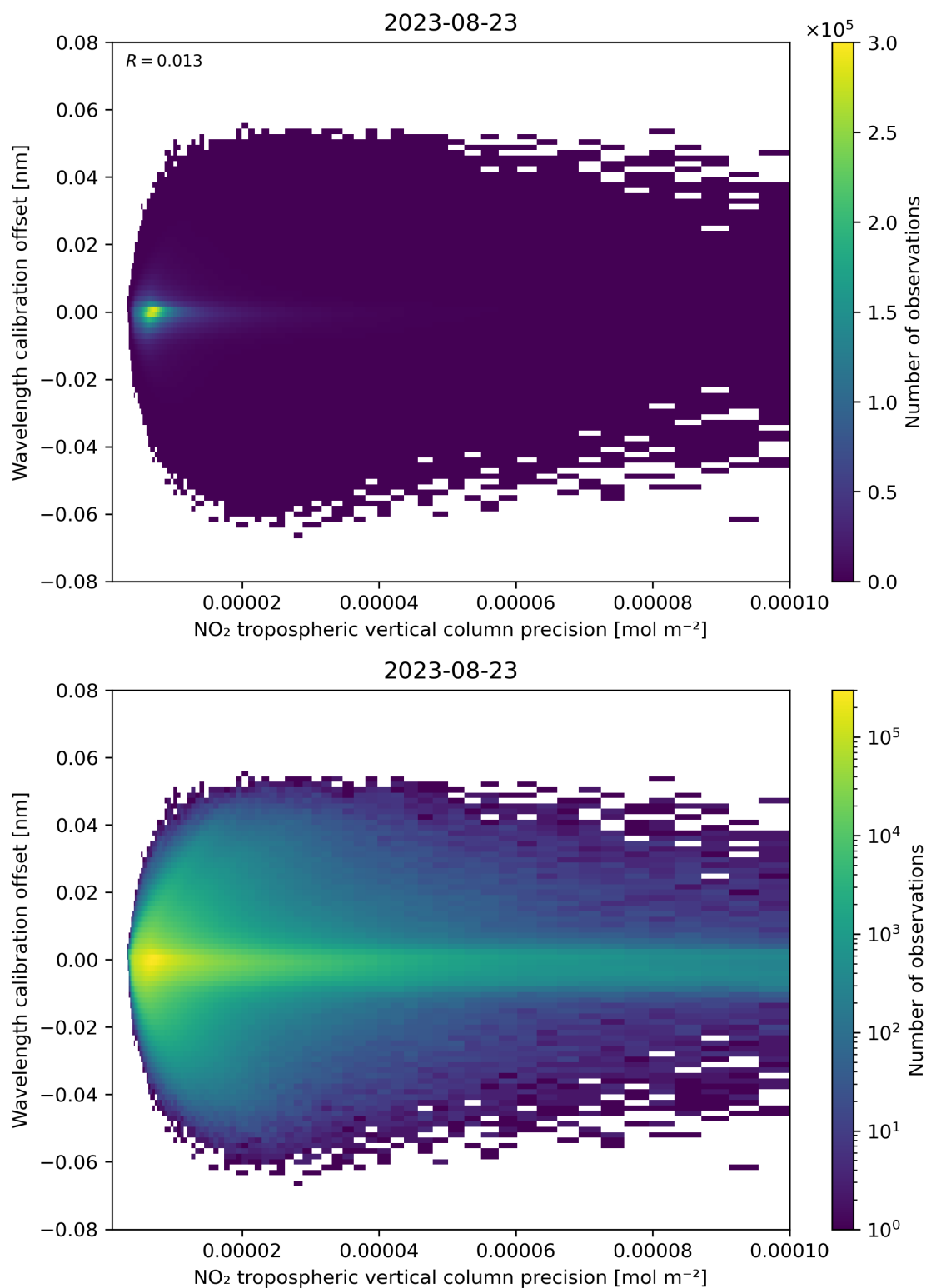
Figure 141: Scatter density plot of “NO 2 tropospheric vertical column precision” against “Wavelength calibration offset” for 2023-08-22 to 2023-08-24.
