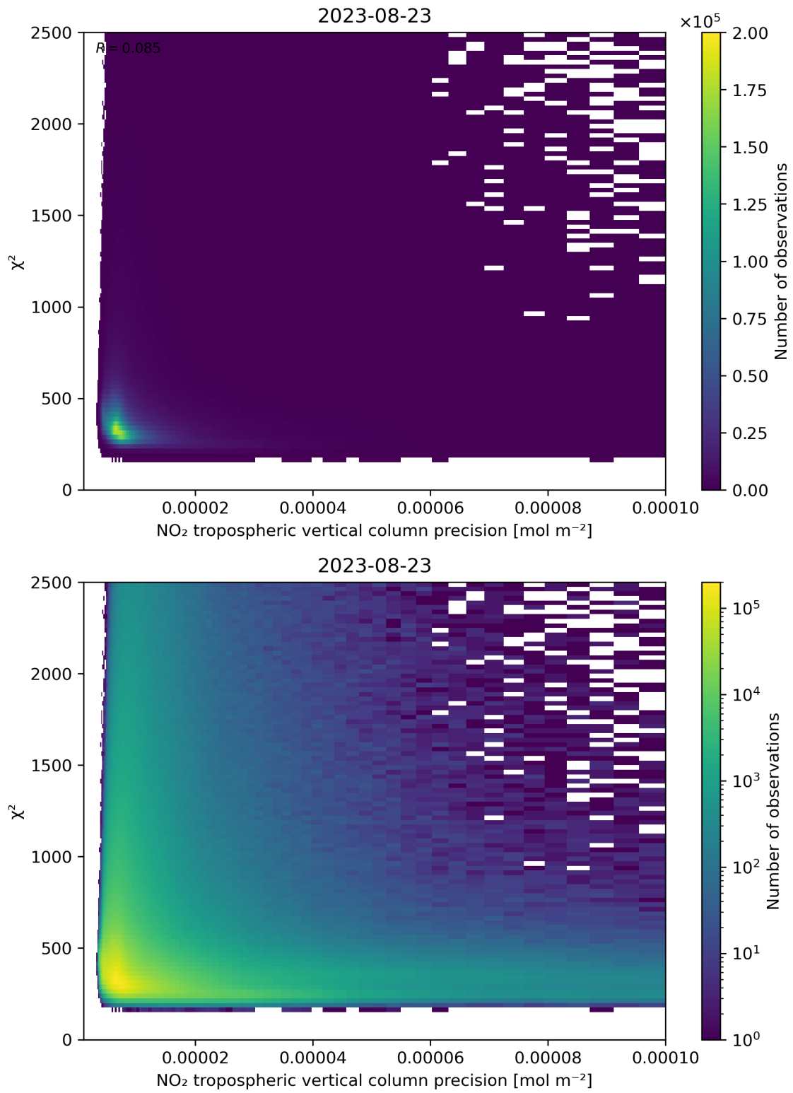
Figure 134: Scatter density plot of “NO 2 tropospheric vertical column precision” against “ \chi^2 ” for 2023-08-22 to 2023-08-24.
