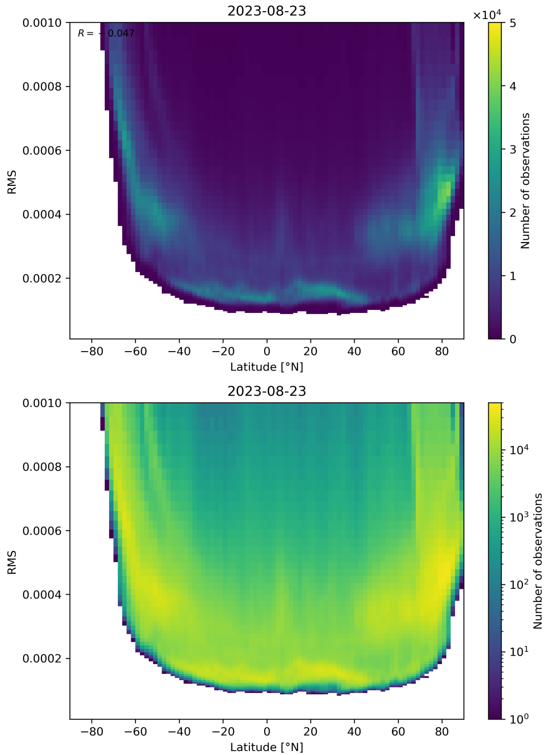
Figure 94: Scatter density plot of “Latitude” against “RMS” for 2023-08-22 to 2023-08-24.
