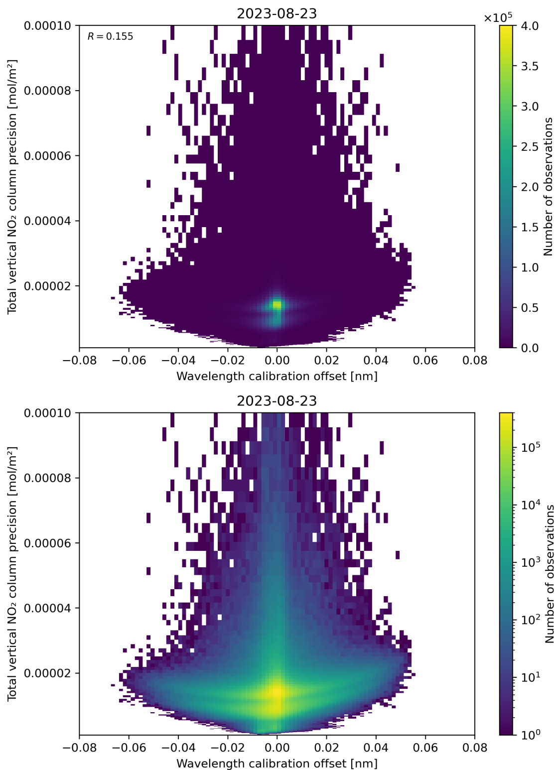
Figure 180: Scatter density plot of “Wavelength calibration offset” against “Total vertical NO 2 column precision” for 2023-08-22 to 2023-08-24.
