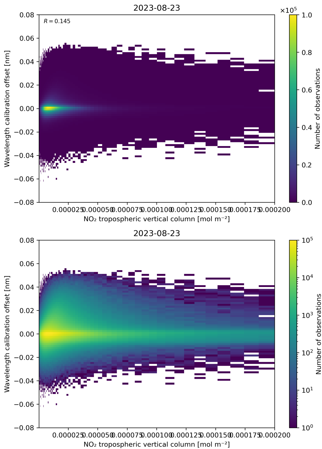
Figure 143: Scatter density plot of “NO 2 tropospheric vertical column” against “Wavelength calibration offset” for 2023-08-22 to 2023-08-24.
