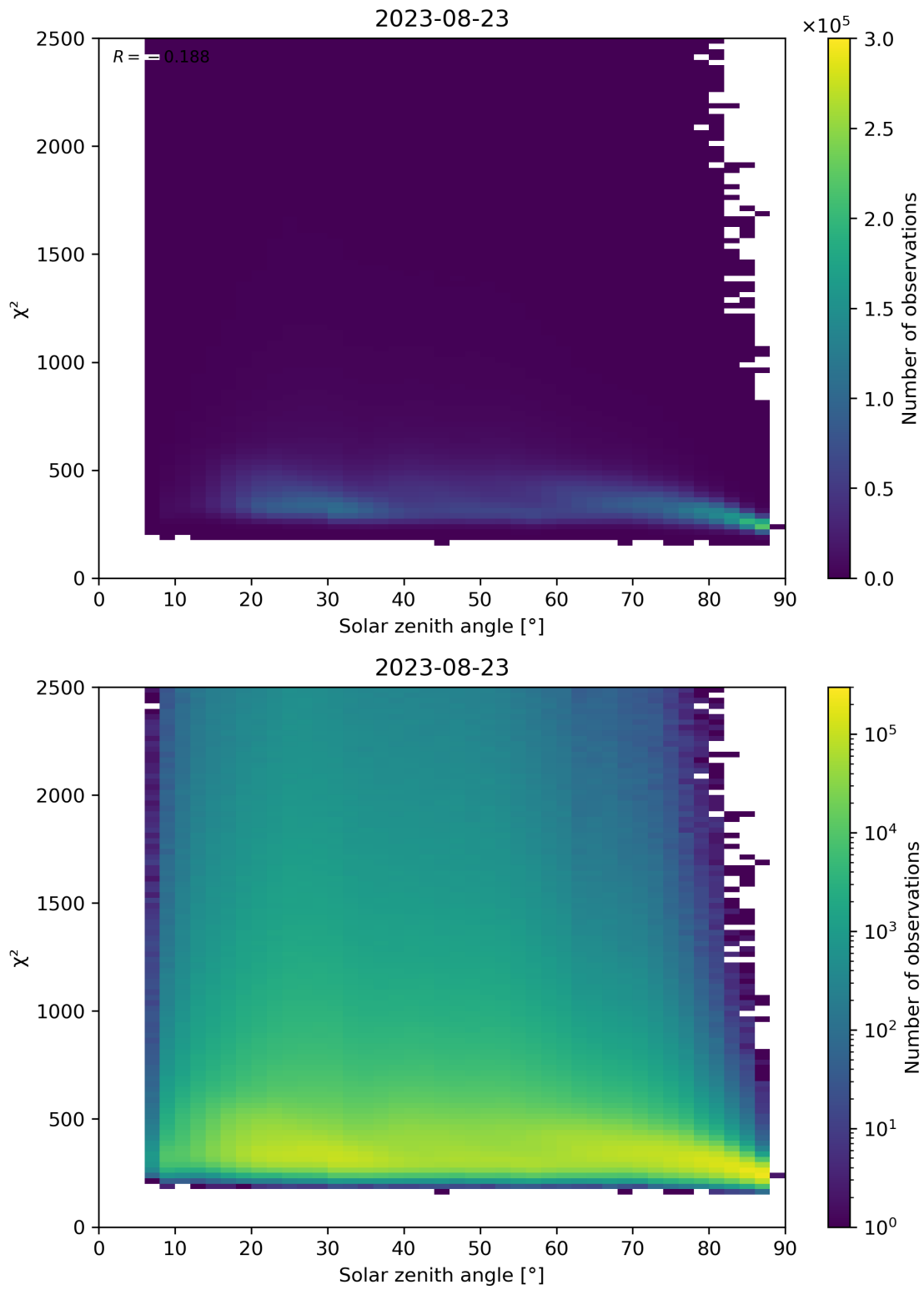
Figure 148: Scatter density plot of “Solar zenith angle” against “ \chi^2 ” for 2023-08-22 to 2023-08-24.
