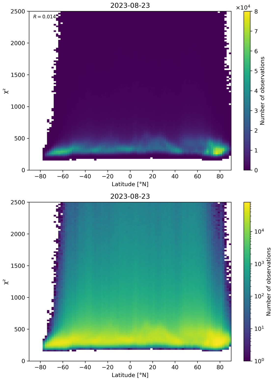
Figure 86: Scatter density plot of “Latitude” against “ \chi^2 ” for 2023-08-22 to 2023-08-24.
