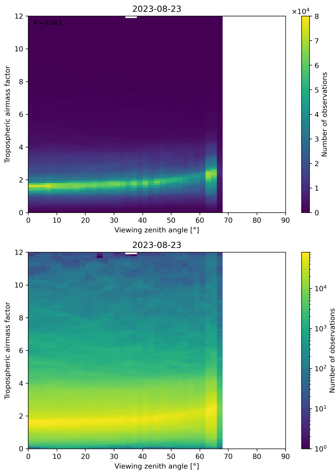
Figure 161: Scatter density plot of “Viewing zenith angle” against “Tropospheric airmass factor” for 2023-08-22 to 2023-08-24.
