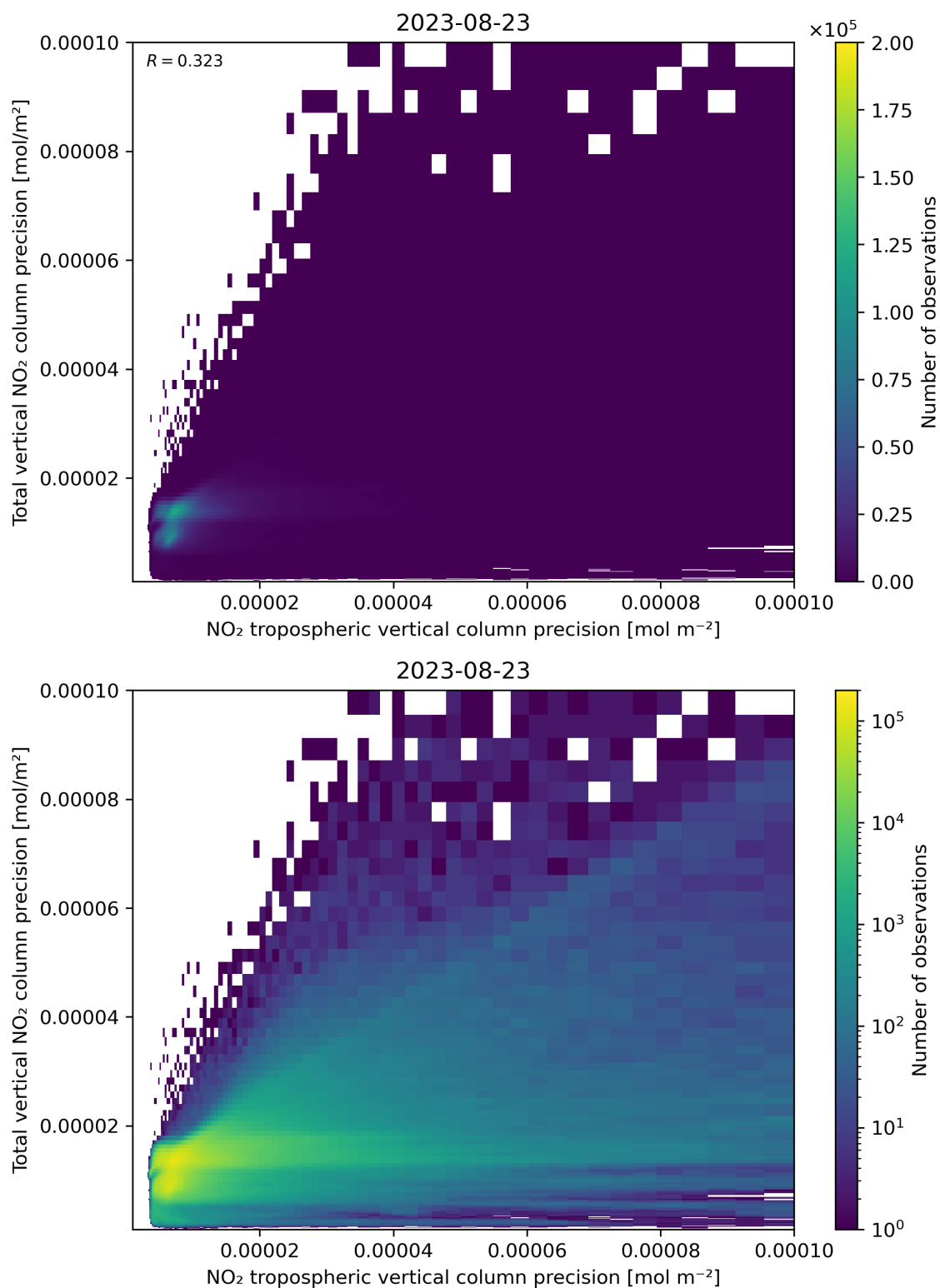
Figure 139: Scatter density plot of “NO 2 tropospheric vertical column precision” against “Total vertical NO 2 column precision” for 2023-08-22 to 2023-08-24.
