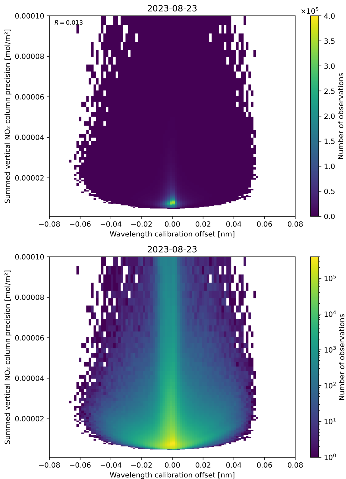
Figure 178: Scatter density plot of “Wavelength calibration offset” against “Summed vertical NO 2 column precision” for 2023-08-22 to 2023-08-24.
