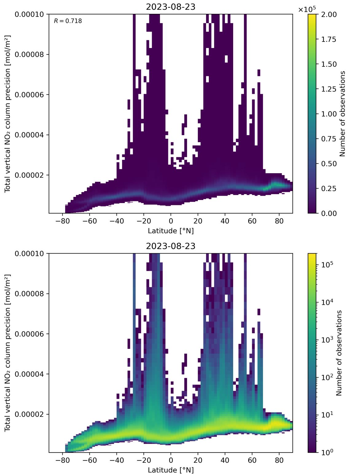
Figure 91: Scatter density plot of “Latitude” against “Total vertical NO 2 column precision” for 2023-08-22 to 2023-08-24.
