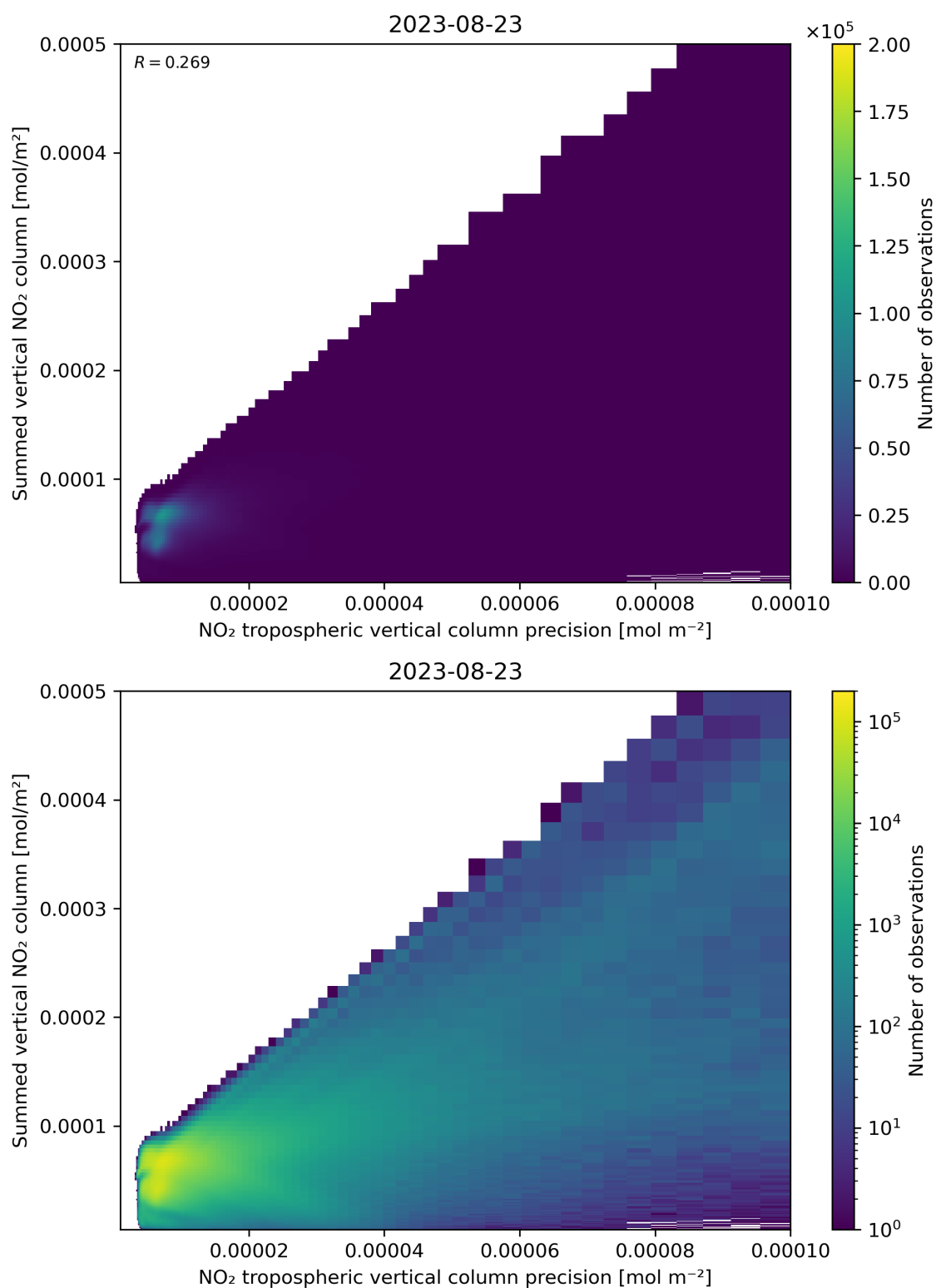
Figure 136: Scatter density plot of “NO 2 tropospheric vertical column precision” against “Summed vertical NO 2 column” for 2023-08-22 to 2023-08-24.
