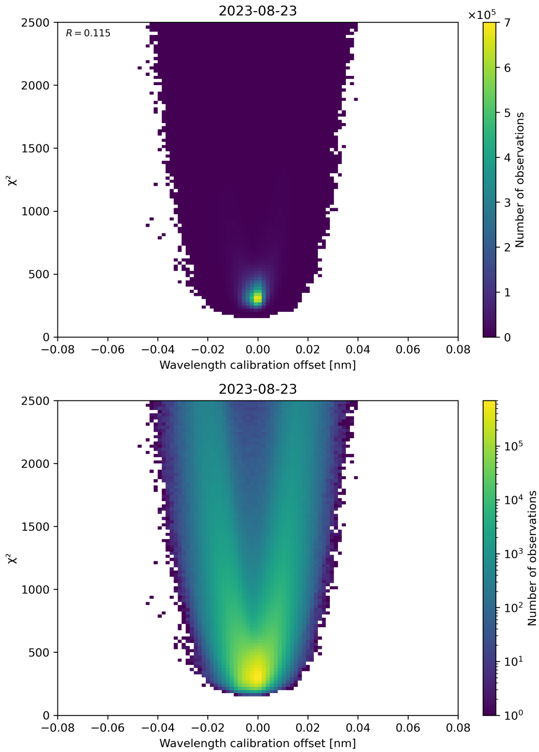
Figure 175: Scatter density plot of “Wavelength calibration offset” against “ \chi^2 ” for 2023-08-22 to 2023-08-24.
