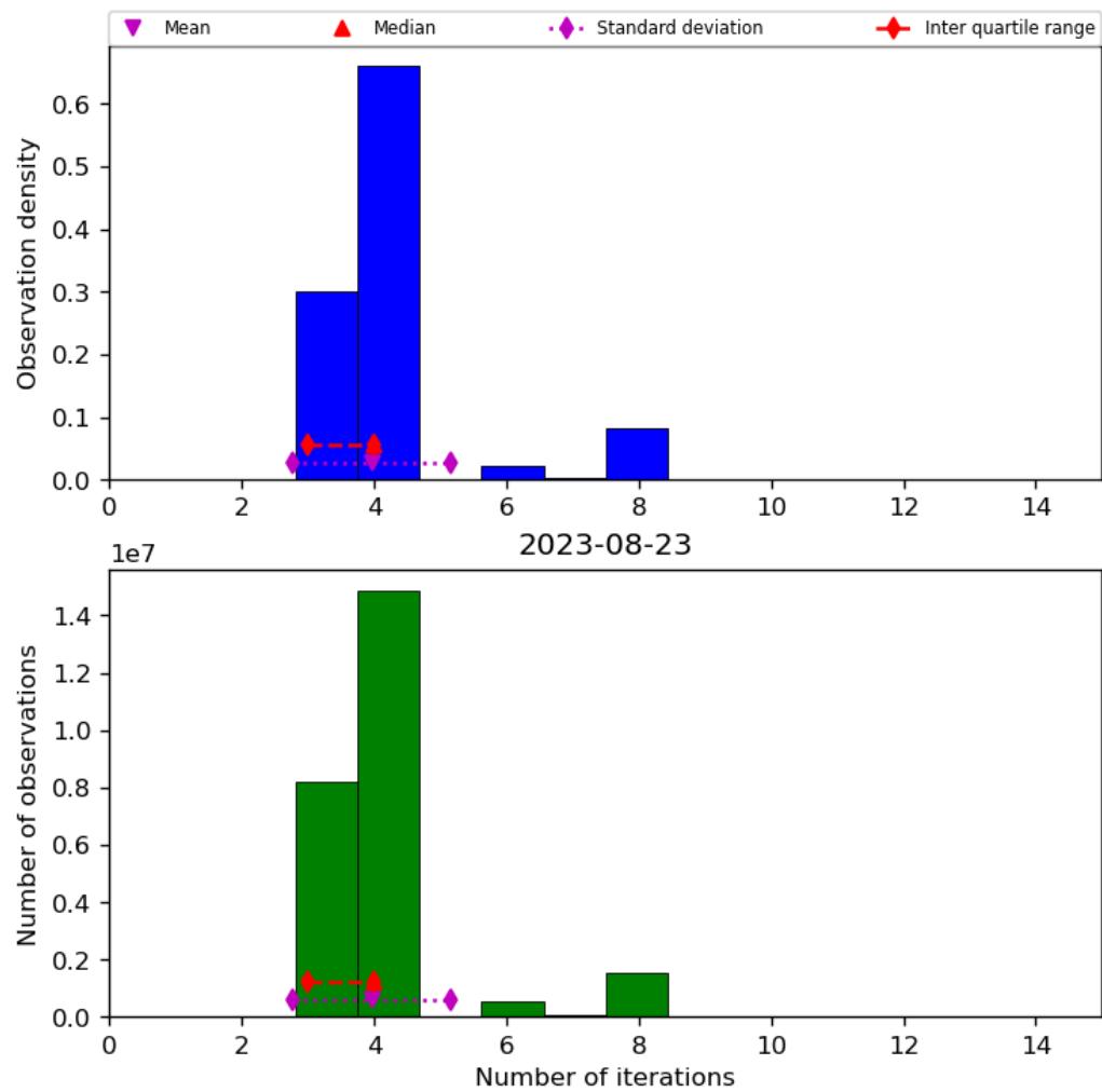
Figure 34: Histogram of “Number of iterations” for 2023-08-22 to 2023-08-24
