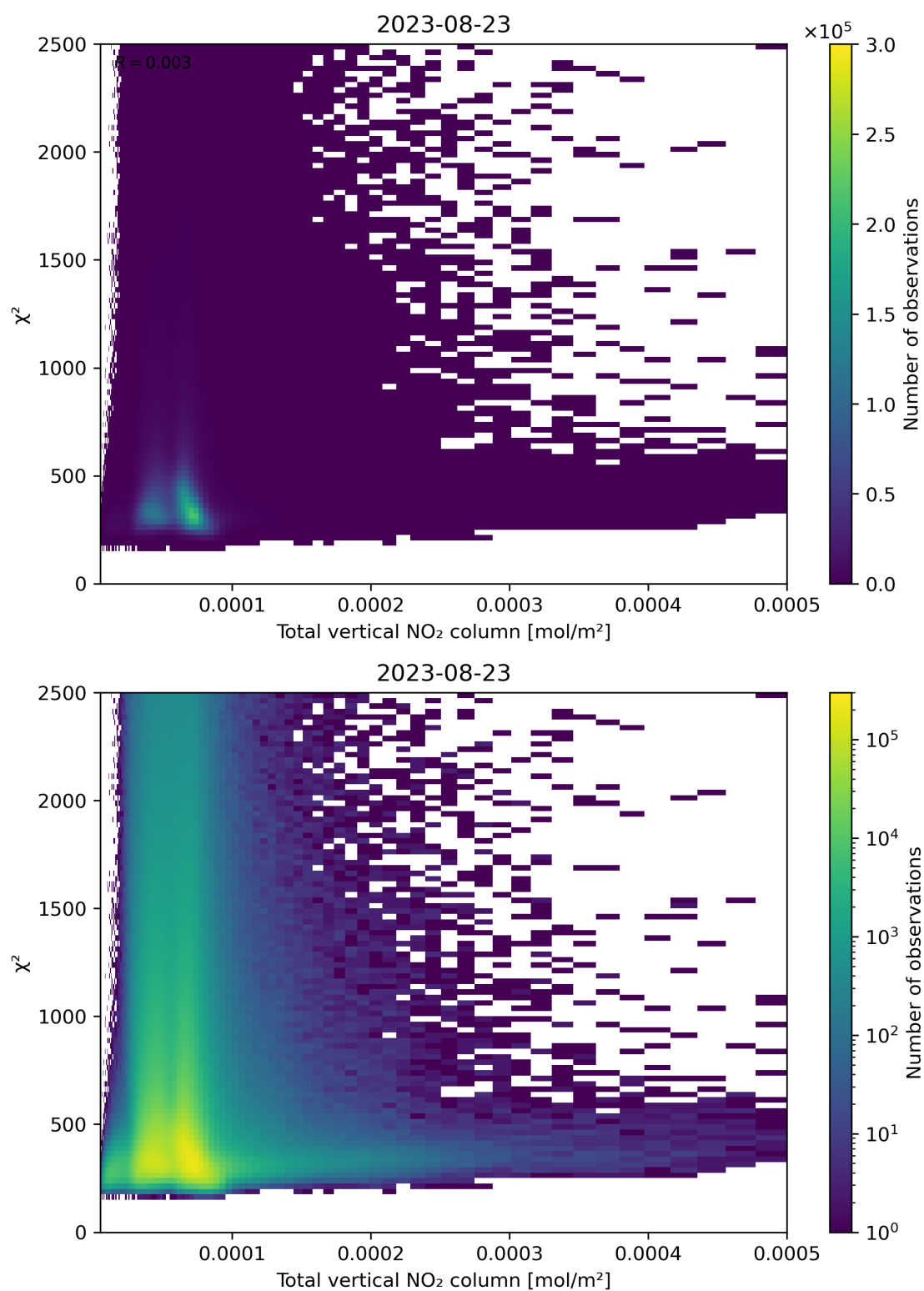
Figure 111: Scatter density plot of “Total vertical NO 2 column” against “ \chi^2 ” for 2023-08-22 to 2023-08-24.
