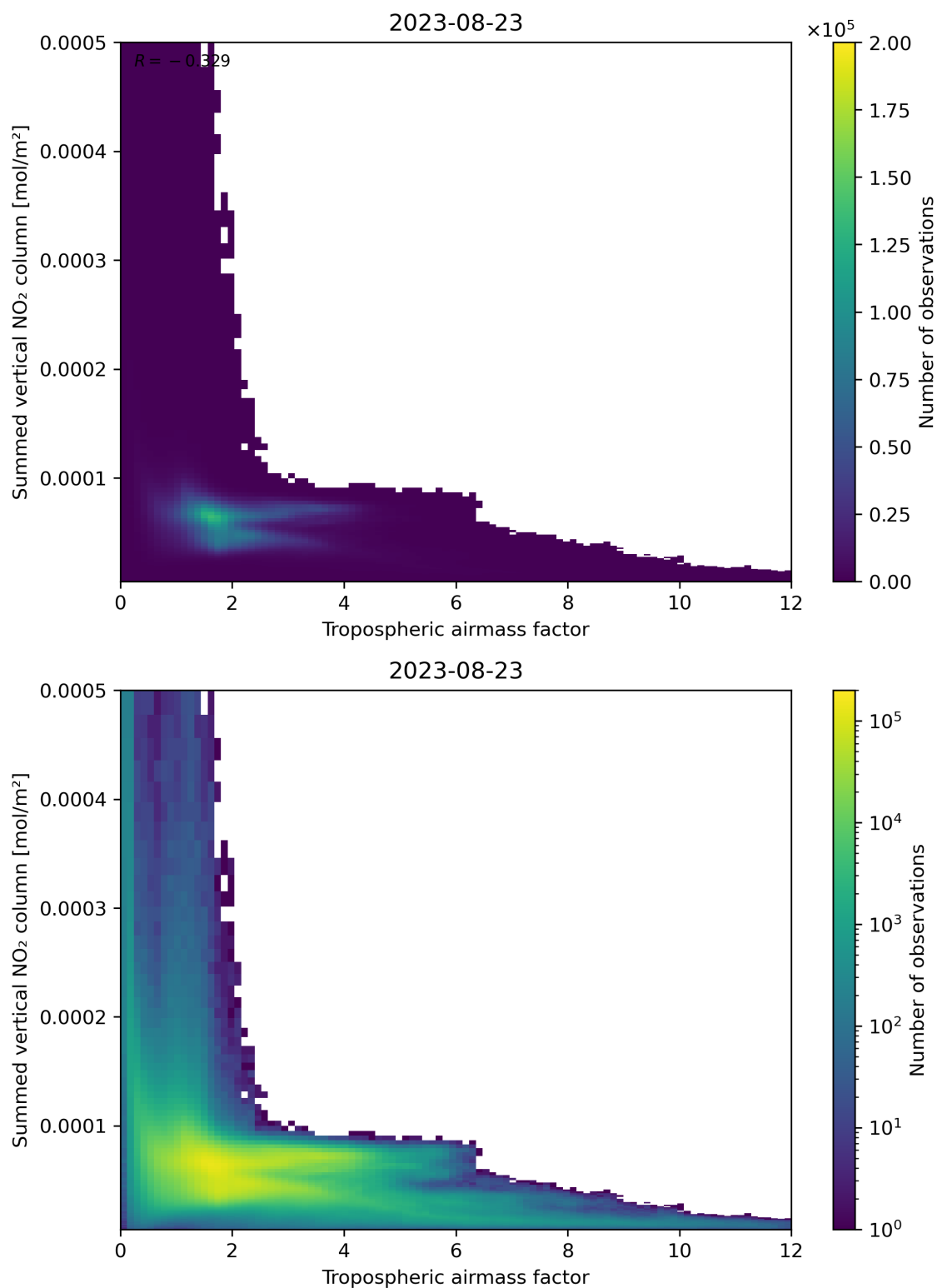
Figure 75: Scatter density plot of “Tropospheric air mass factor” against “Summed vertical NO 2 column” for 2023-08-22 to 2023-08-24.
