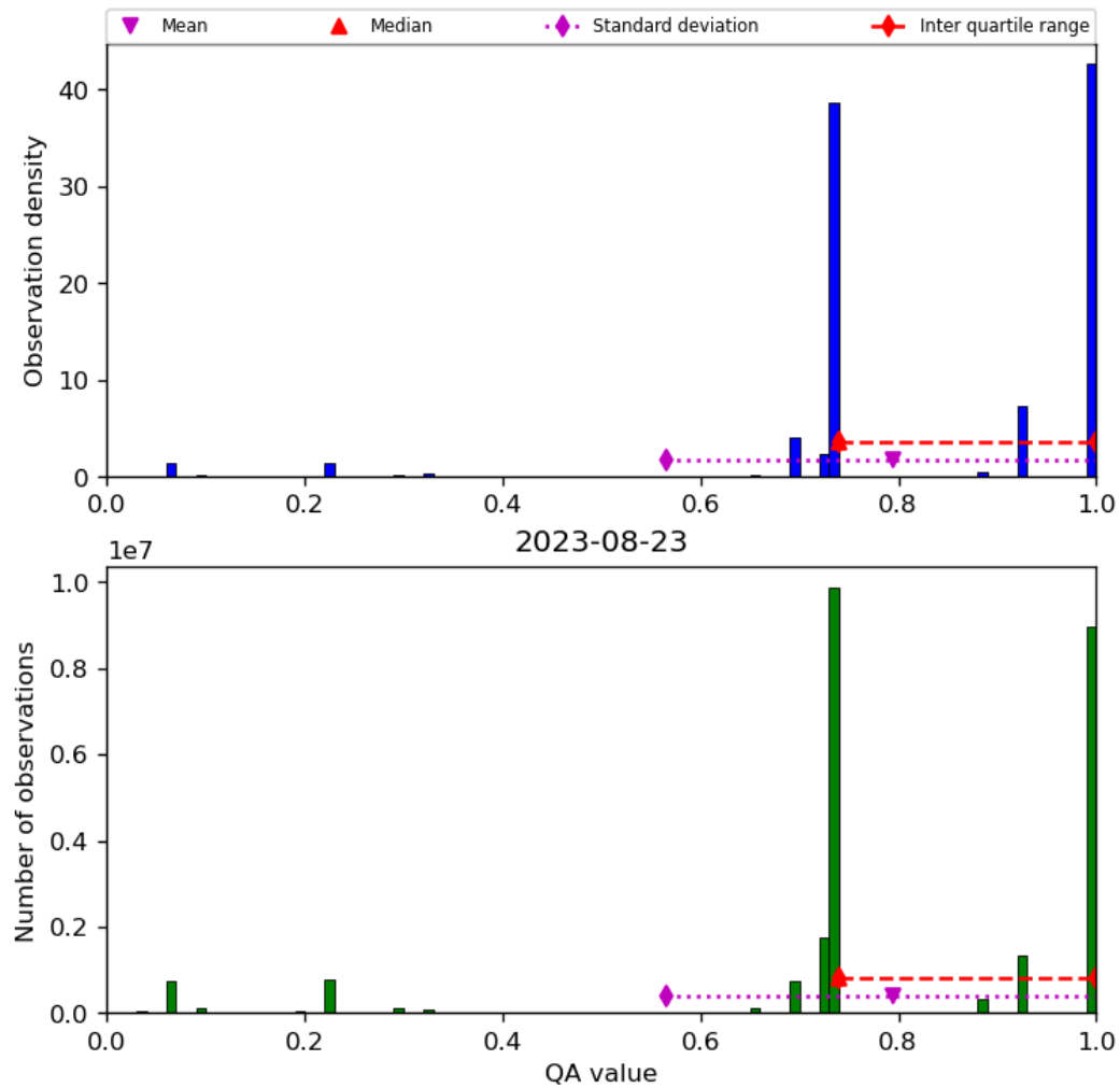
Figure 28: Histogram of “QA value” for 2023-08-22 to 2023-08-24
