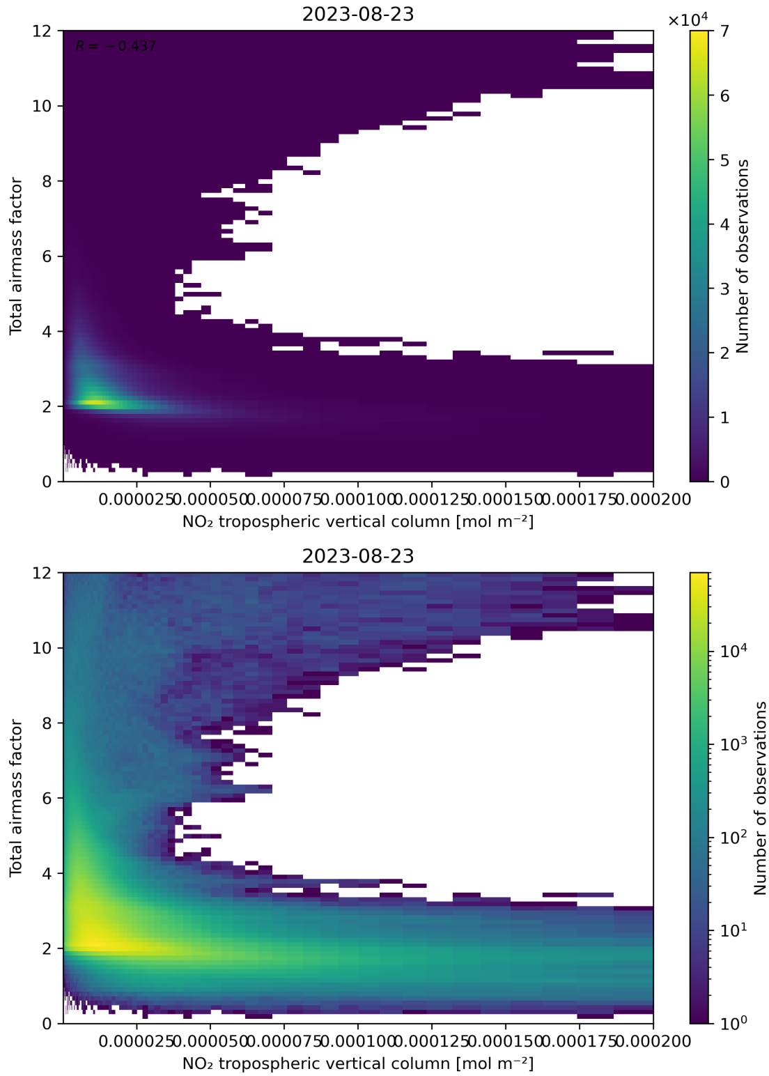
Figure 122: Scatter density plot of “NO 2 tropospheric vertical column” against “Total airmass factor” for 2023-08-22 to 2023-08-24.
