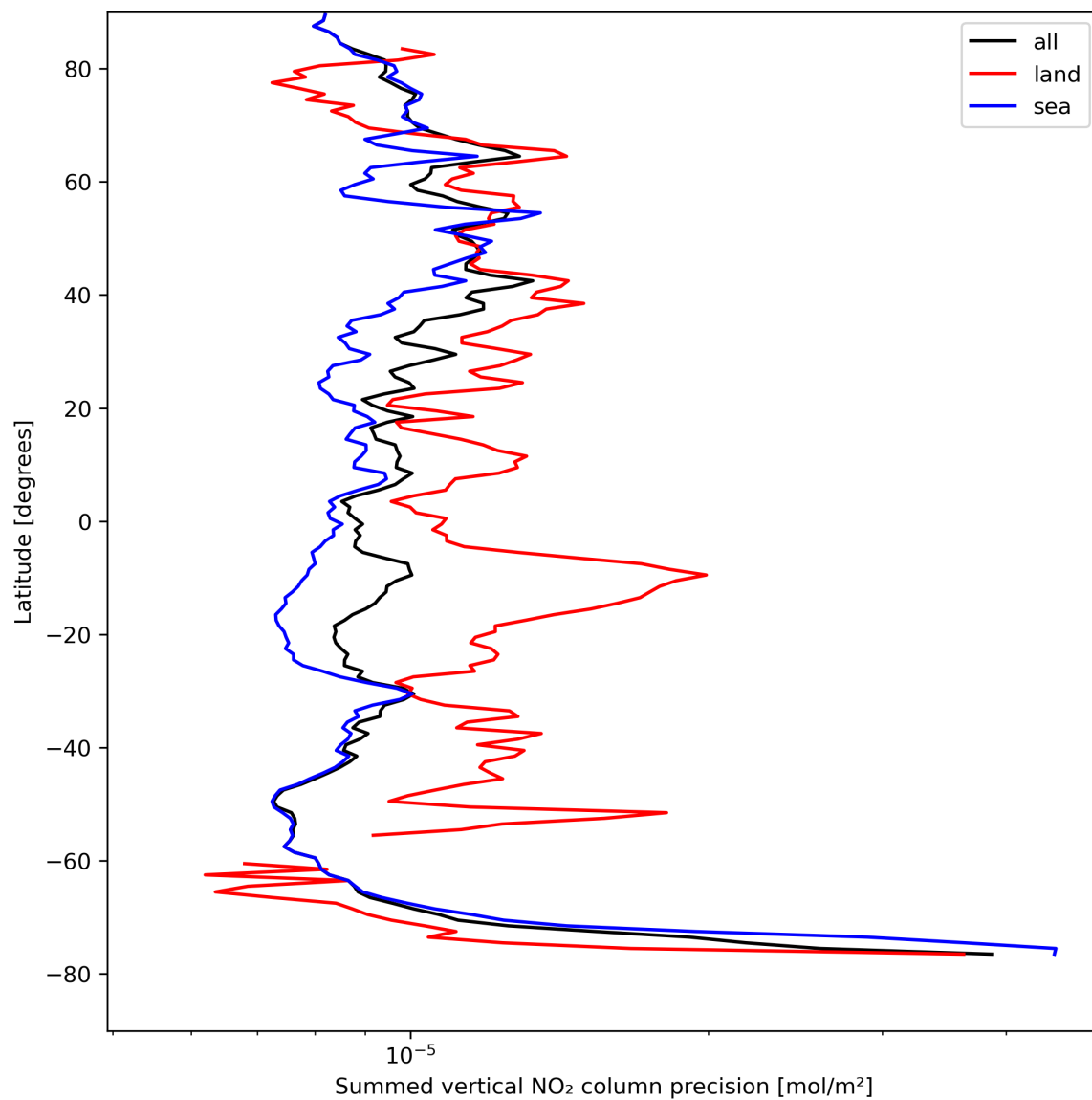
Figure 24: Zonal average of “Summed vertical NO 2 column precision” for 2023-08-22 to 2023-08-24.
