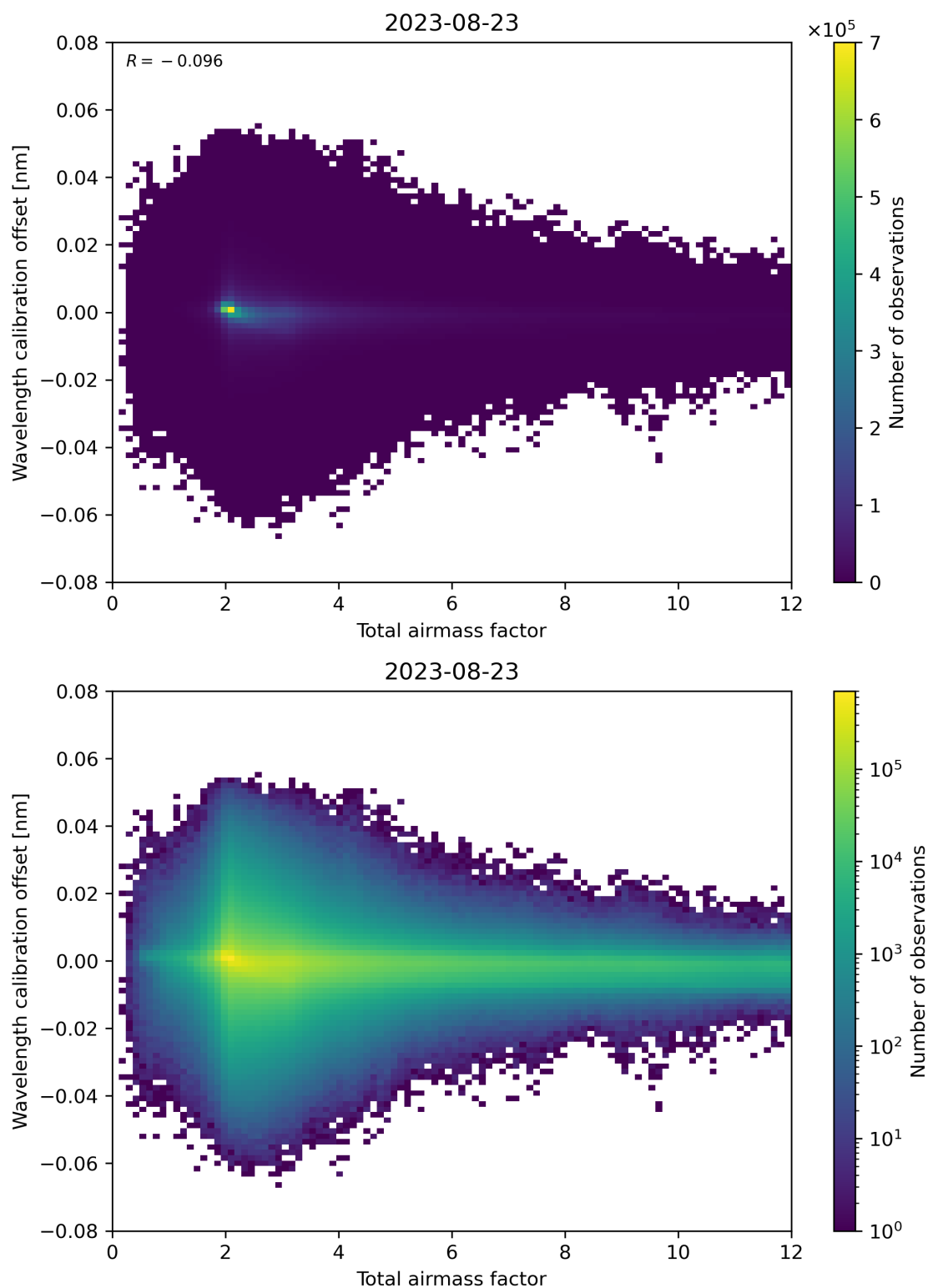
Figure 70: Scatter density plot of “Total airmass factor” against “Wavelength calibration offset” for 2023-08-22 to 2023-08-24.
