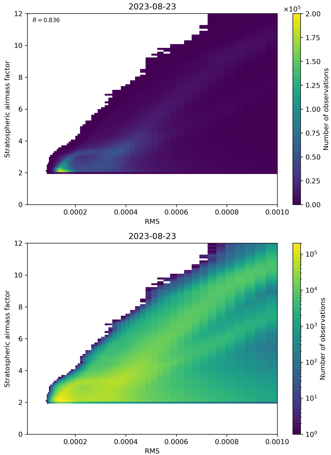
Figure 144: Scatter density plot of “RMS” against “Stratospheric airmass factor” for 2023-08-22 to 2023-08-24.
