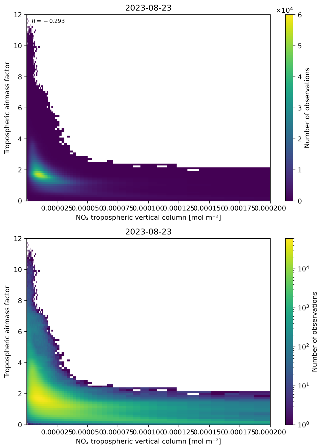
Figure 123: Scatter density plot of “NO 2 tropospheric vertical column” against “Tropospheric airmass factor” for 2023-08-22 to 2023-08-24.
