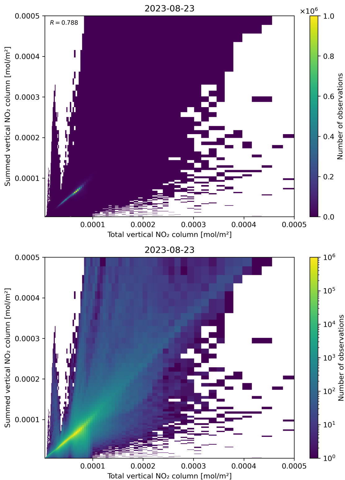
Figure 112: Scatter density plot of “Total vertical NO 2 column” against “Summed vertical NO 2 column” for 2023-08-22 to 2023-08-24.
