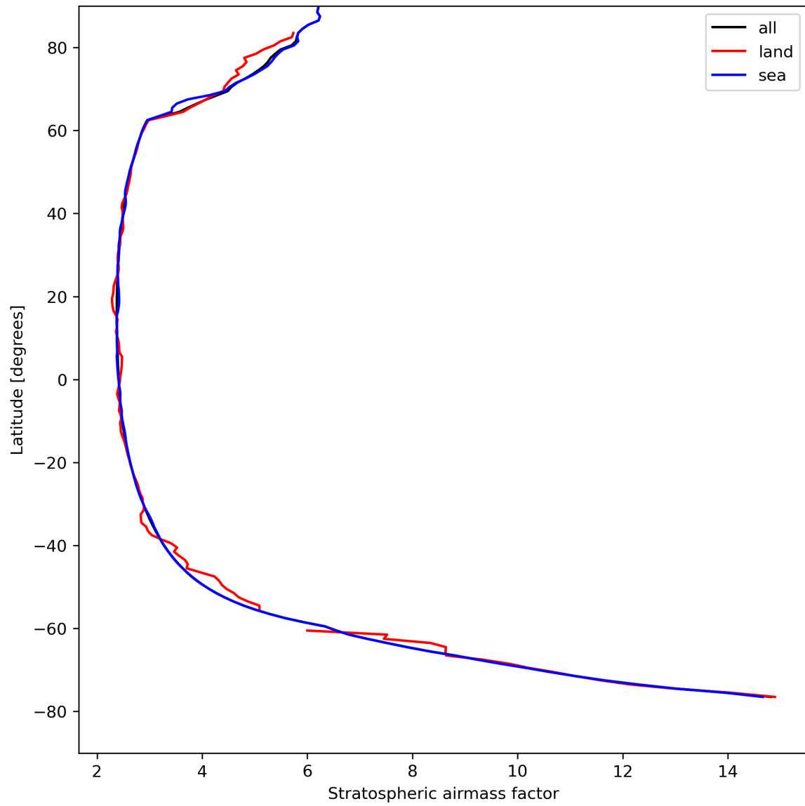
Figure 27: Zonal average of “Stratospheric air mass factor” for 2023-08-22 to 2023-08-24.
