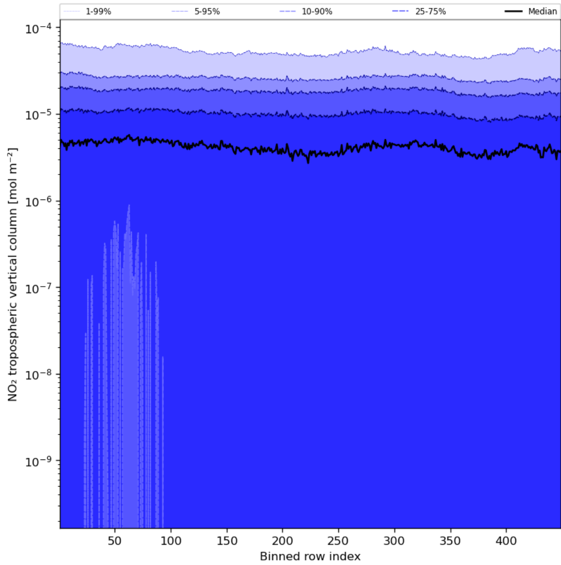
Figure 46: Along track statistics of “NO 2 tropospheric vertical column” for 2023-08-22 to 2023-08-24
