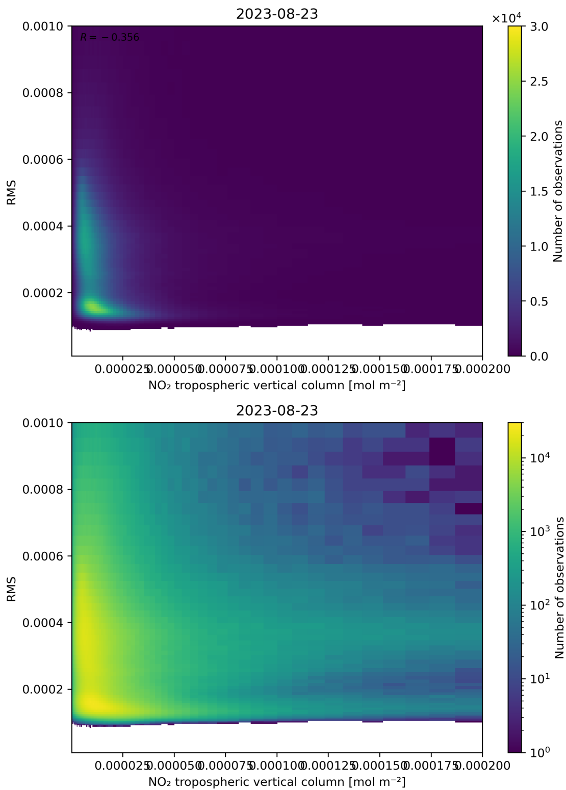
Figure 142: Scatter density plot of “NO 2 tropospheric vertical column” against “RMS” for 2023-08-22 to 2023-08-24.
