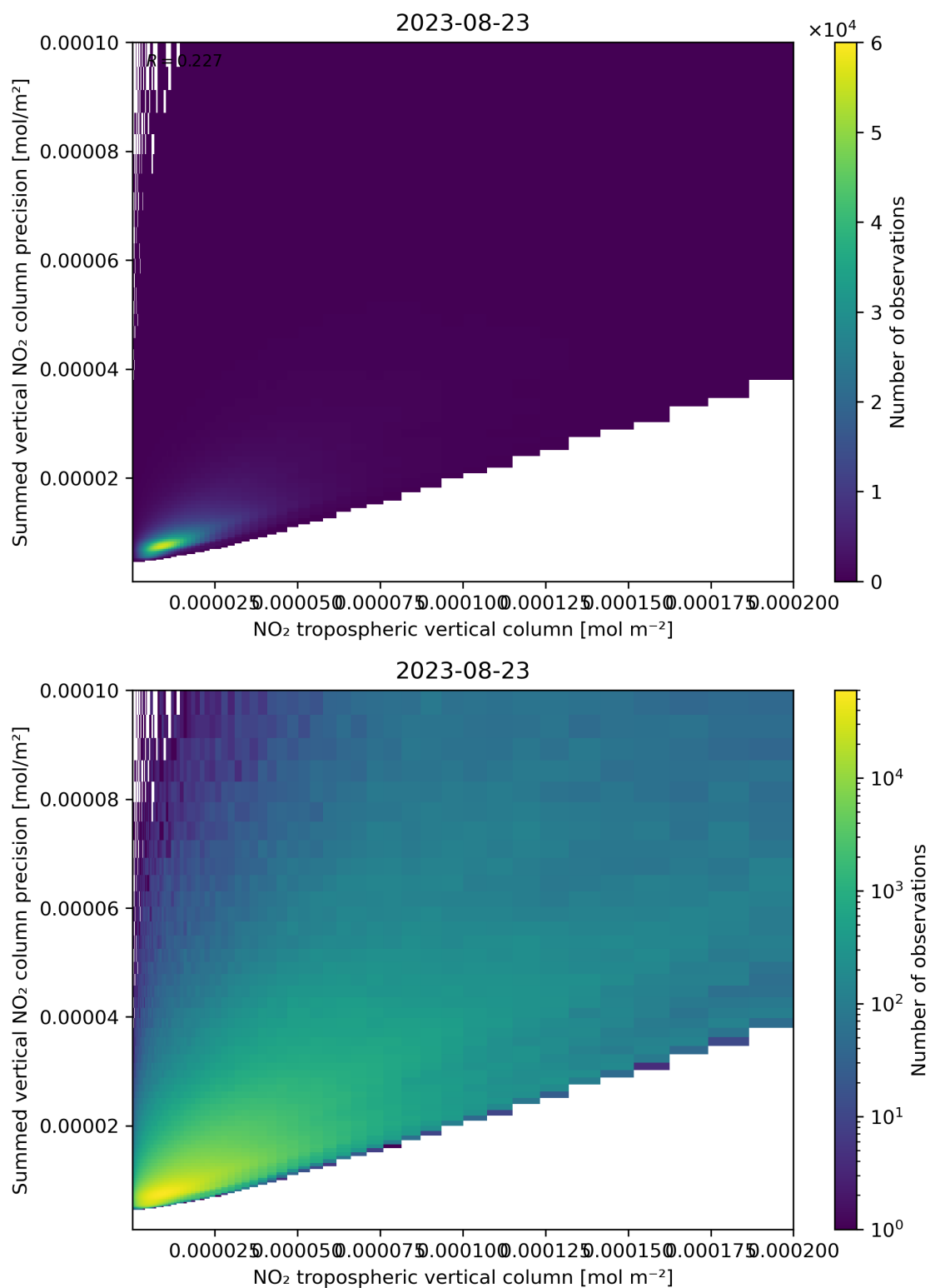
Figure 127: Scatter density plot of “NO 2 tropospheric vertical column” against “Summed vertical NO 2 column precision” for 2023-08-22 to 2023-08-24.
