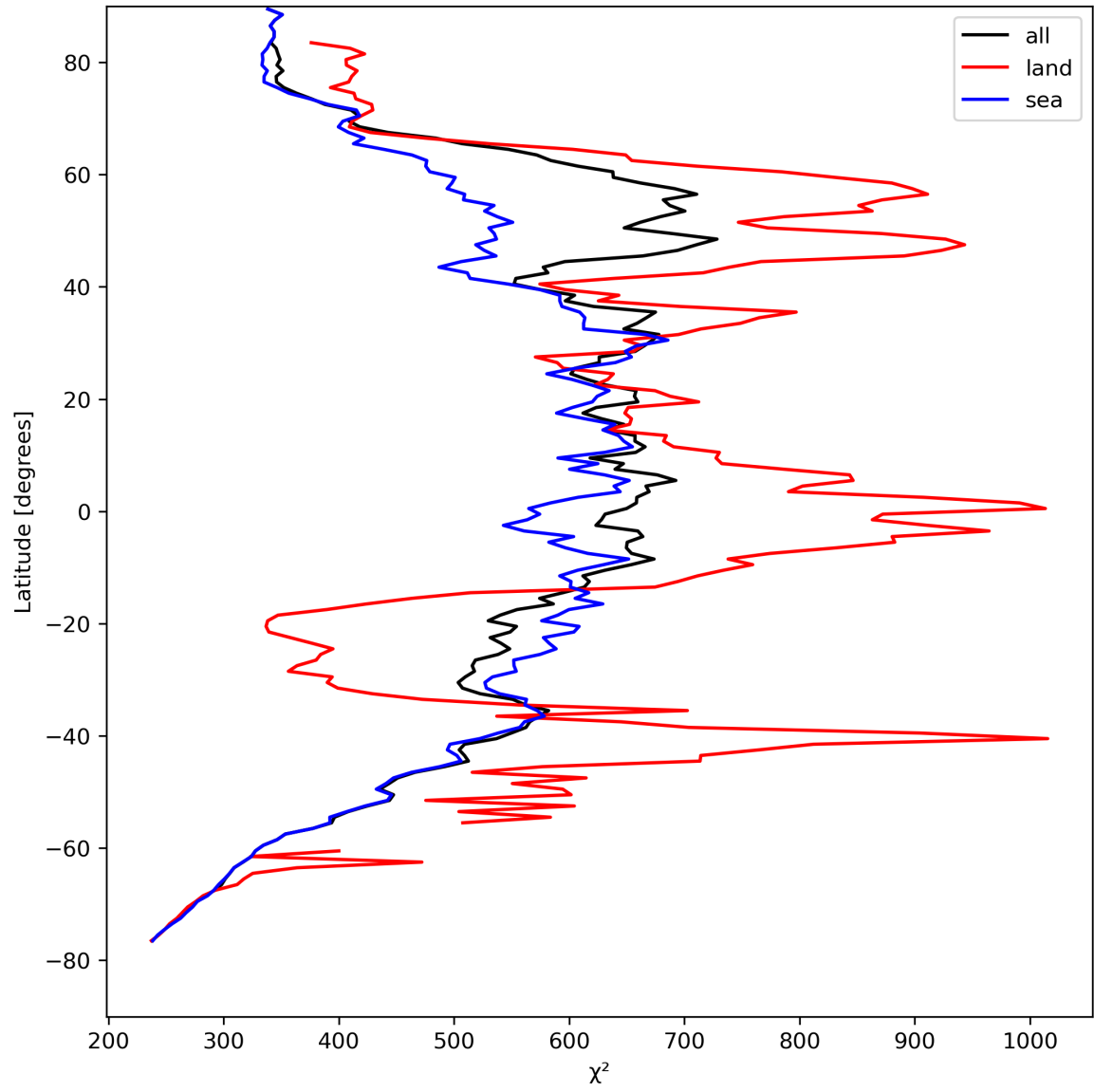
Figure 25: Zonal average of “ \chi^2 ” for 2023-08-22 to 2023-08-24.
