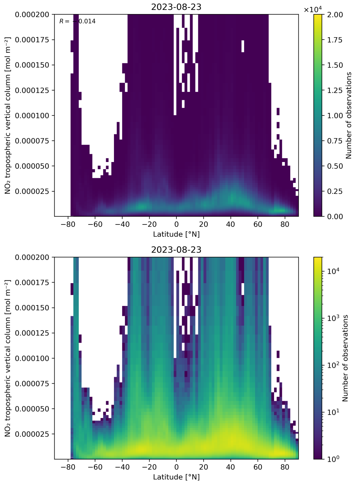
Figure 92: Scatter density plot of “Latitude” against “NO 2 tropospheric vertical column” for 2023-08-22 to 2023-08-24.
