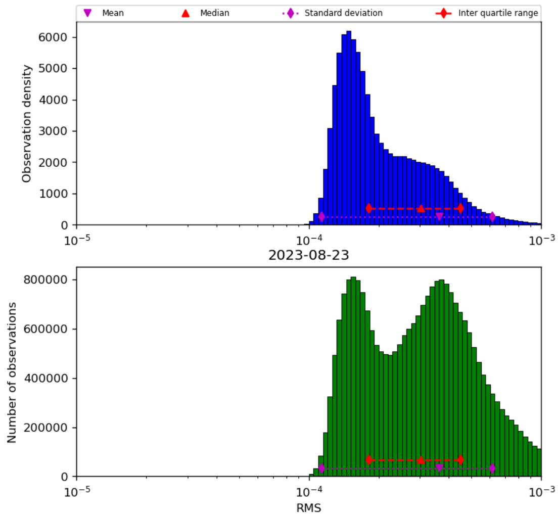
Figure 43: Histogram of “RMS” for 2023-08-22 to 2023-08-24
