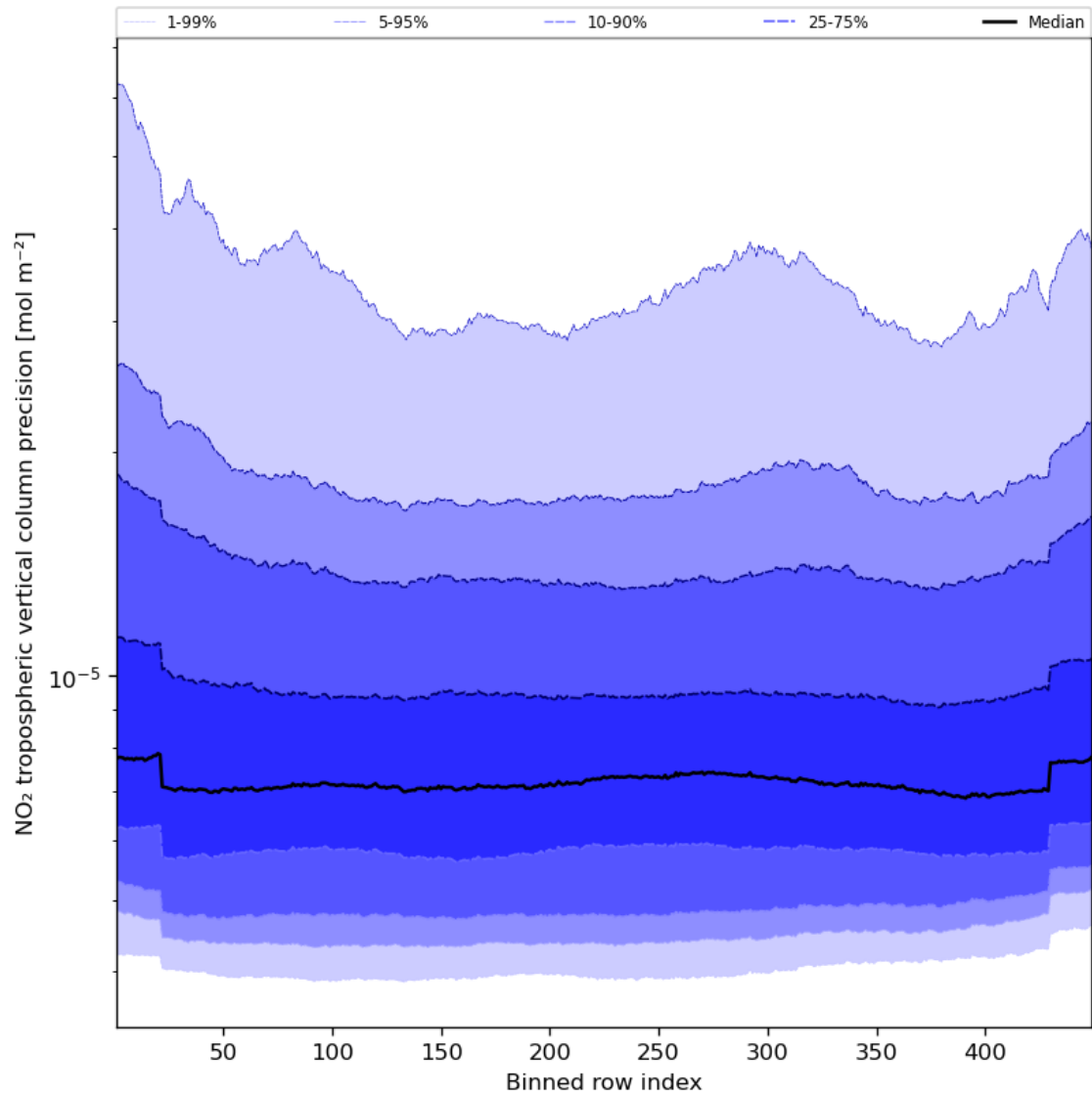
Figure 47: Along track statistics of “NO 2 tropospheric vertical column precision” for 2023-08-22 to 2023-08-24
