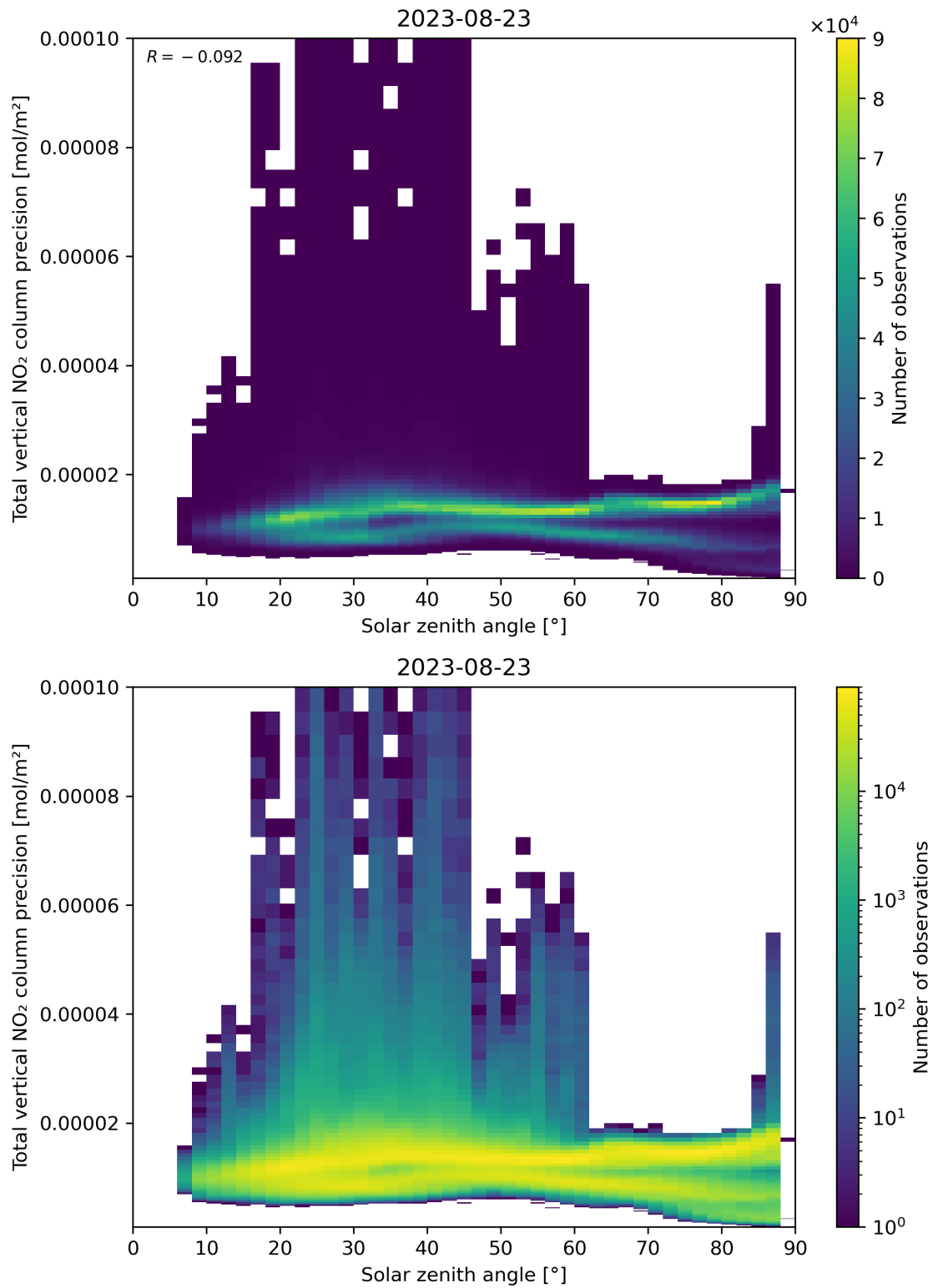
Figure 154: Scatter density plot of “Solar zenith angle” against “Total vertical NO 2 column precision” for 2023-08-22 to 2023-08-24.
