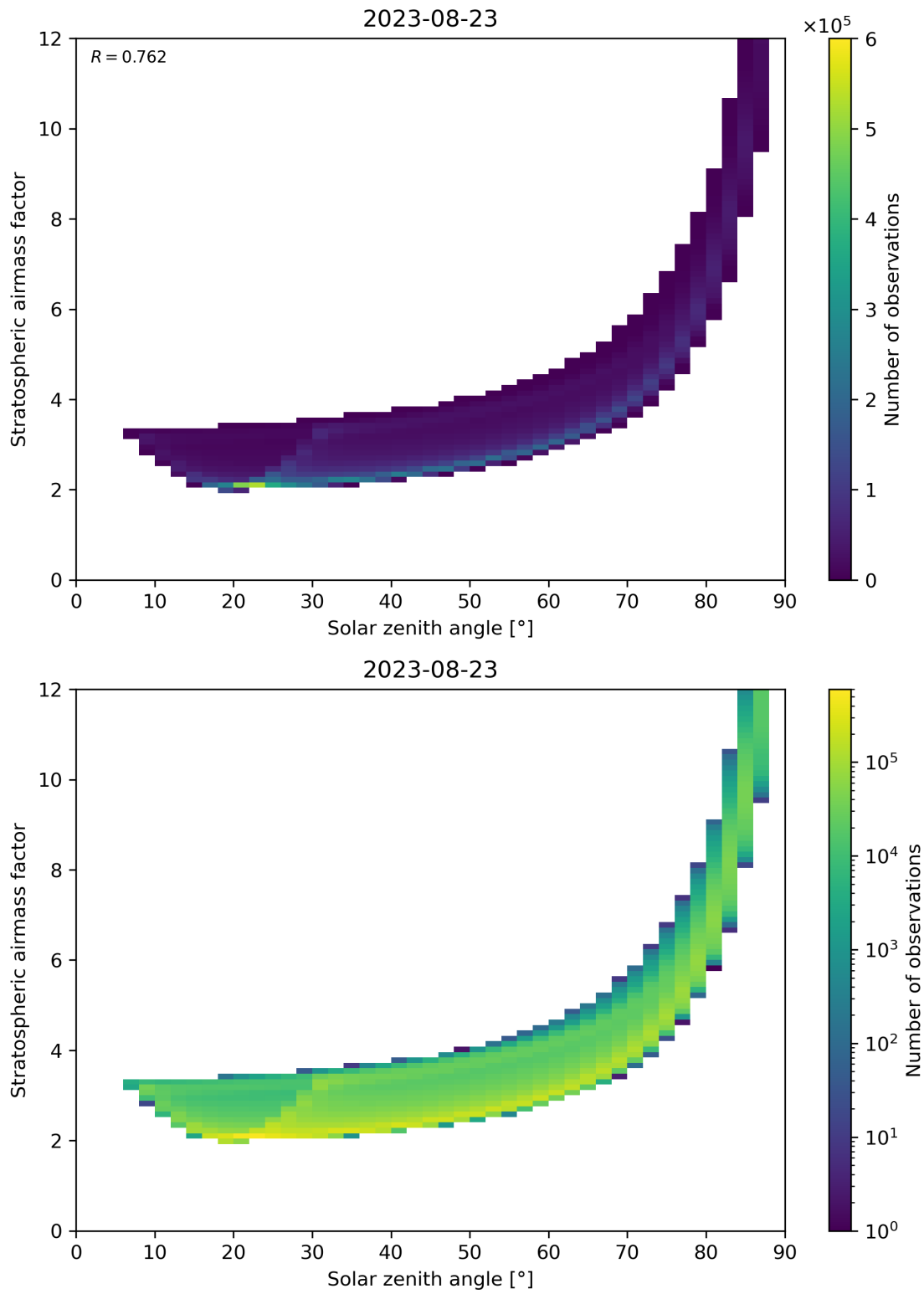
Figure 145: Scatter density plot of “Solar zenith angle” against “Stratospheric airmass factor” for 2023-08-22 to 2023-08-24.
