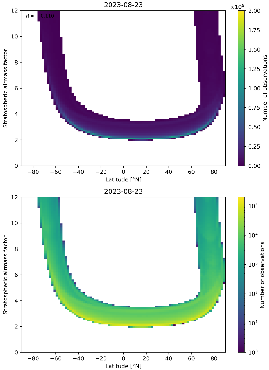
Figure 83: Scatter density plot of “Latitude” against “Stratospheric air mass factor” for 2023-08-22 to 2023-08-24.
