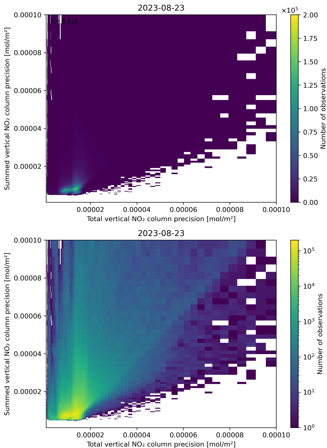
Figure 118: Scatter density plot of “Total vertical NO 2 column precision” against “Summed vertical NO 2 column precision” for 2023-08-22 to 2023-08-24.
