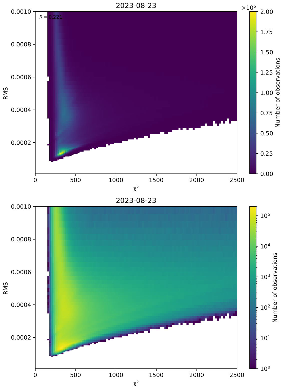
Figure 82: Scatter density plot of “ \chi^2 ” against “RMS” for 2023-08-22 to 2023-08-24.
