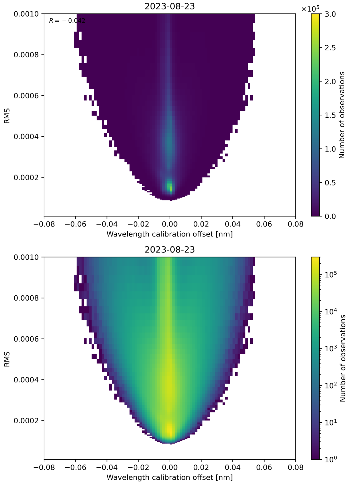
Figure 181: Scatter density plot of “Wavelength calibration offset” against “RMS” for 2023-08-22 to 2023-08-24.
