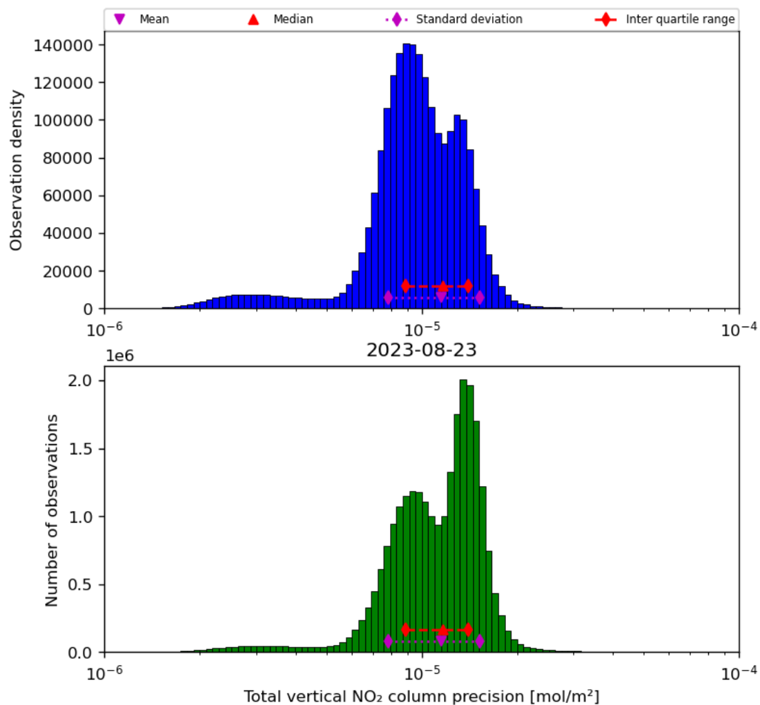
Figure 39: Histogram of “Total vertical NO 2 column precision” for 2023-08-22 to 2023-08-24
