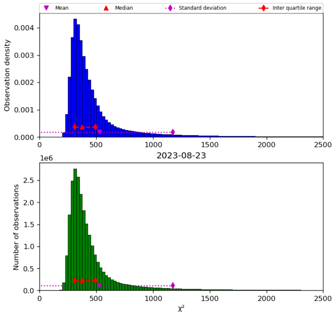
Figure 42: Histogram of “ \chi^2 ” for 2023-08-22 to 2023-08-24
