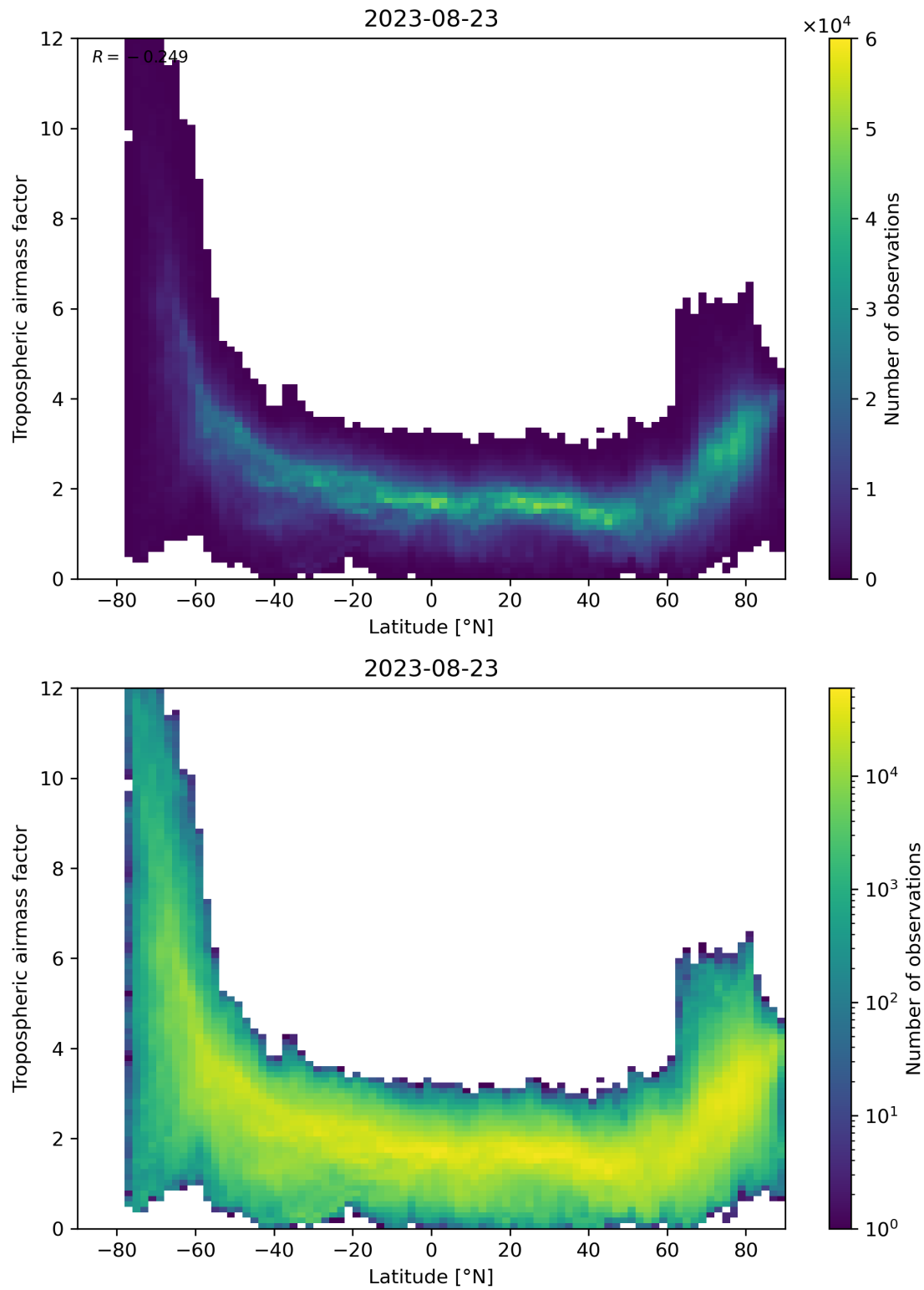
Figure 85: Scatter density plot of “Latitude” against “Tropospheric air mass factor” for 2023-08-22 to 2023-08-24.
