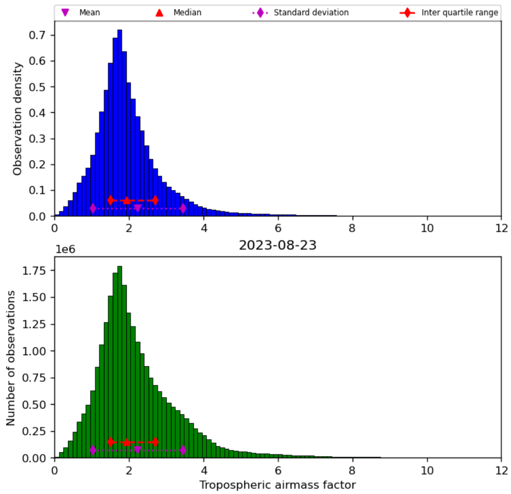
Figure 31: Histogram of “Tropospheric airmass factor” for 2023-08-22 to 2023-08-24
