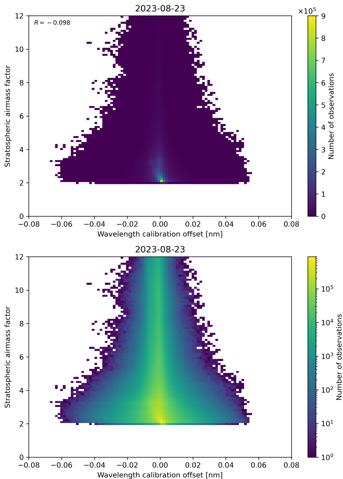
Figure 174: Scatter density plot of “Wavelength calibration offset” against “Stratospheric air mass factor” for 2023-08-22 to 2023-08-24.
