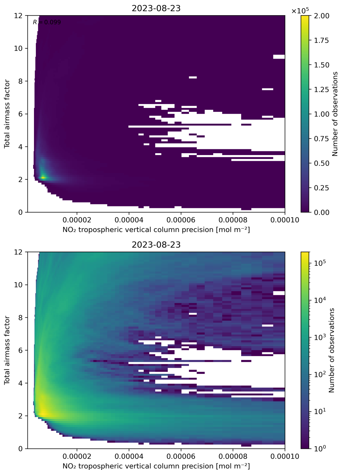
Figure 132: Scatter density plot of “NO 2 tropospheric vertical column precision” against “Total air mass factor” for 2023-08-22 to 2023-08-24.
