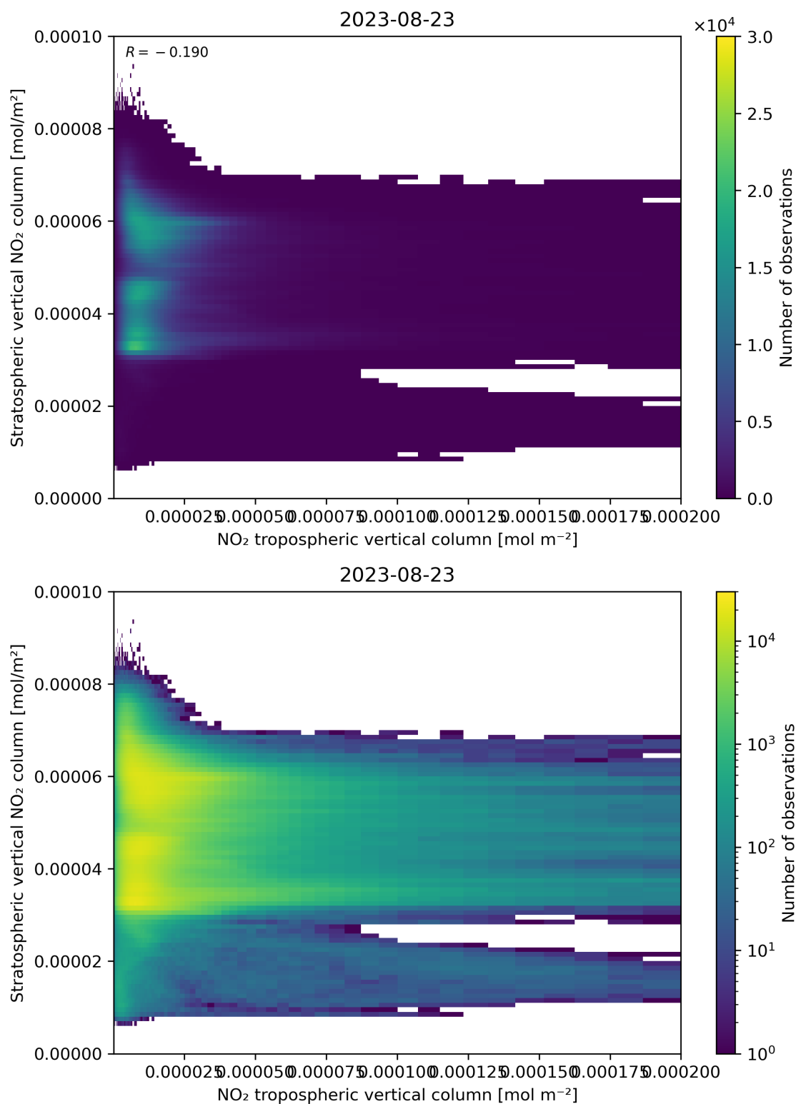
Figure 125: Scatter density plot of “NO 2 tropospheric vertical column” against “Stratospheric vertical NO 2 column” for 2023-08-22 to 2023-08-24.
