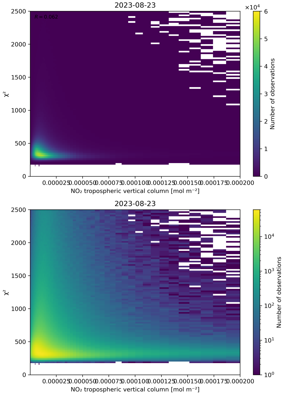
Figure 124: Scatter density plot of “NO 2 tropospheric vertical column” against “ \chi^2 ” for 2023-08-22 to 2023-08-24.
