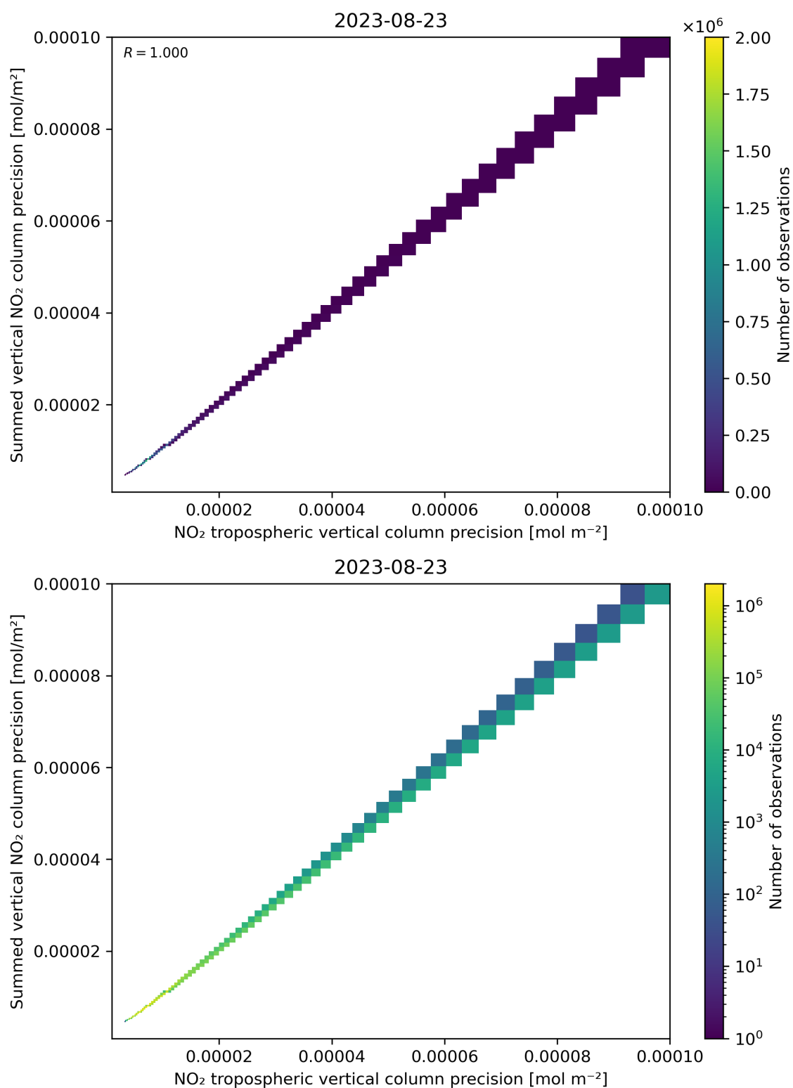
Figure 137: Scatter density plot of “NO 2 tropospheric vertical column precision” against “Summed vertical NO 2 column precision” for 2023-08-22 to 2023-08-24.
