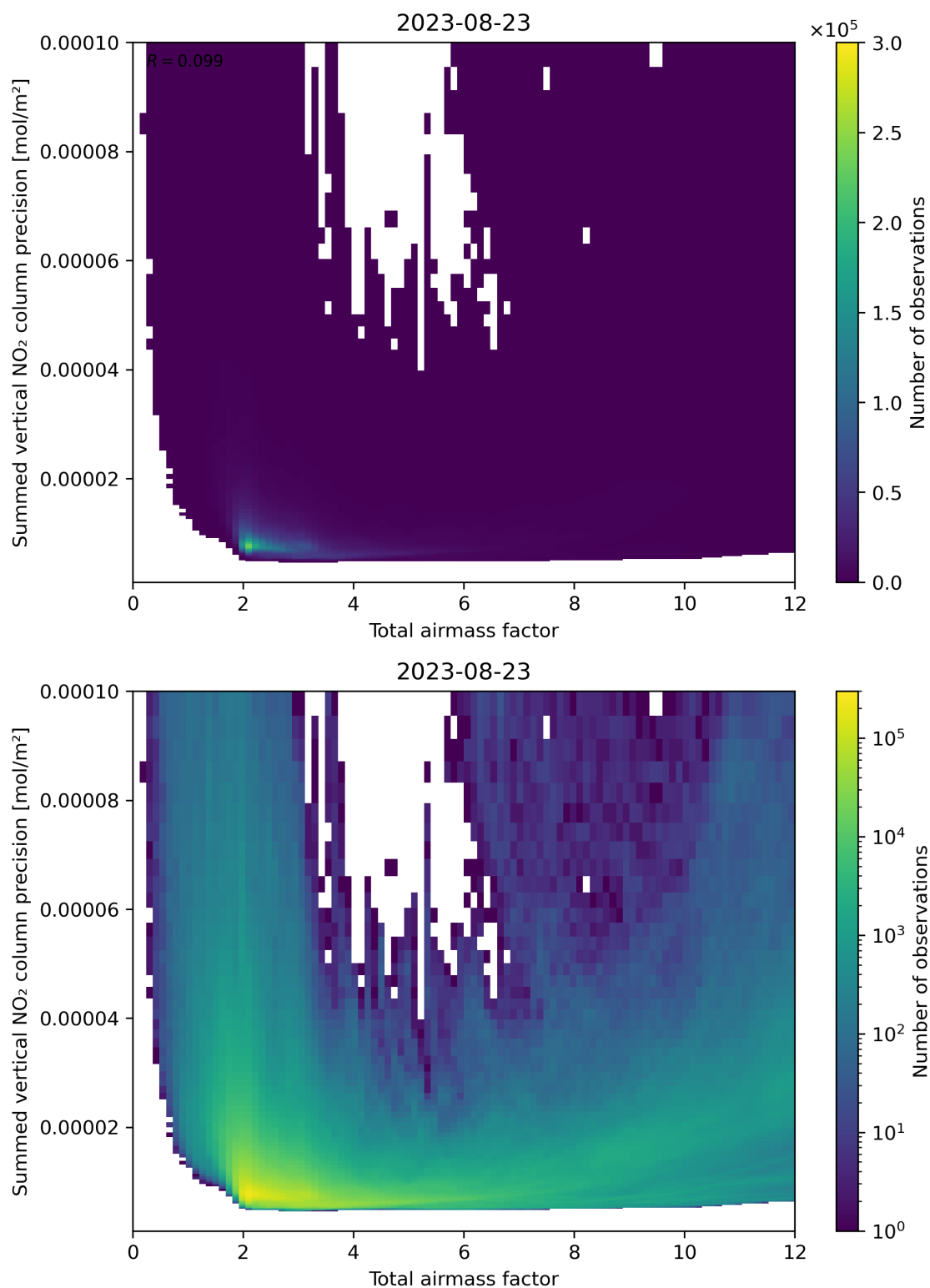
Figure 66: Scatter density plot of “Total airmass factor” against “Summed vertical NO 2 column precision” for 2023-08-22 to 2023-08-24.
