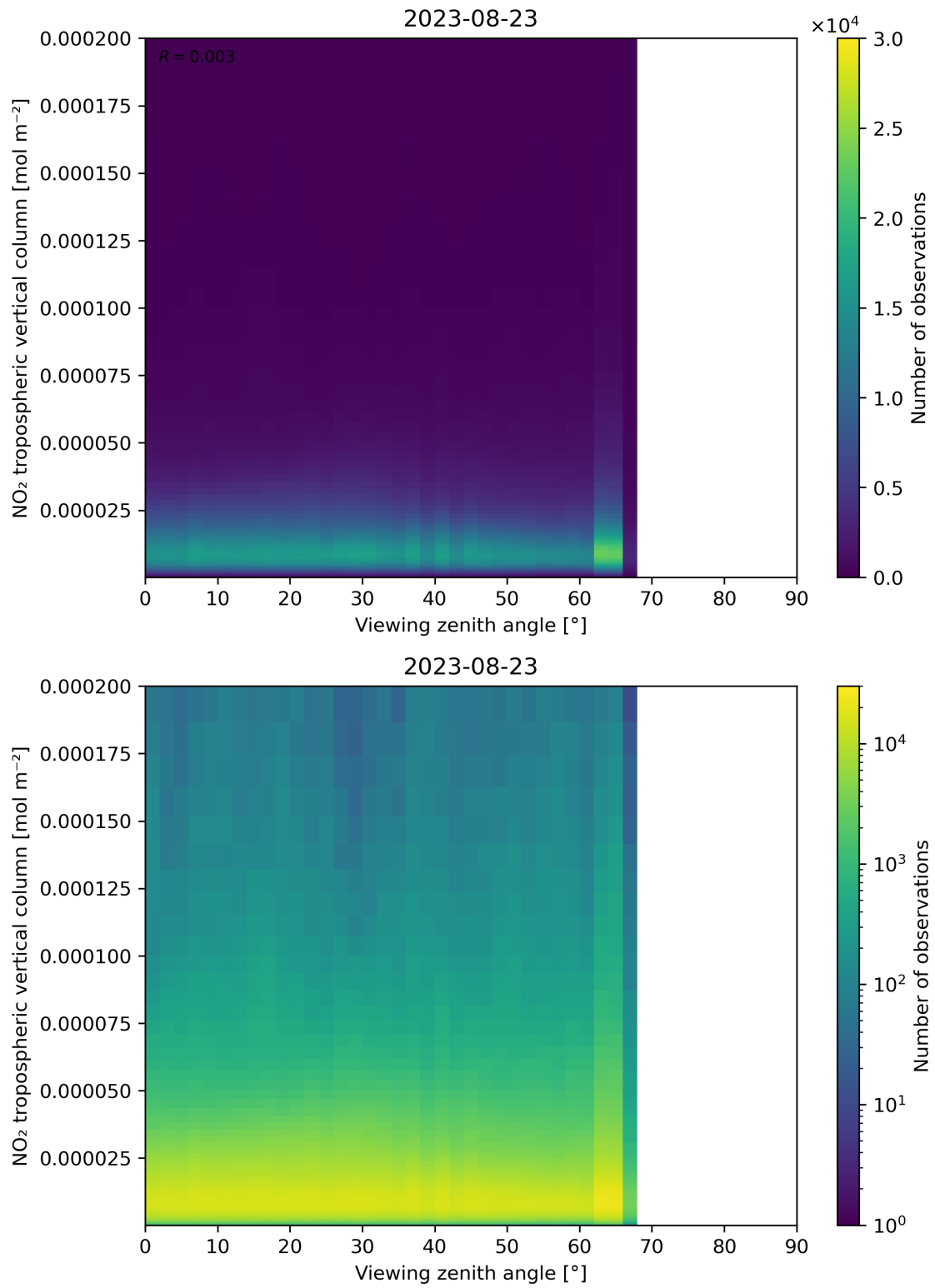
Figure 169: Scatter density plot of “Viewing zenith angle” against “NO 2 tropospheric vertical column” for 2023-08-22 to 2023-08-24.
