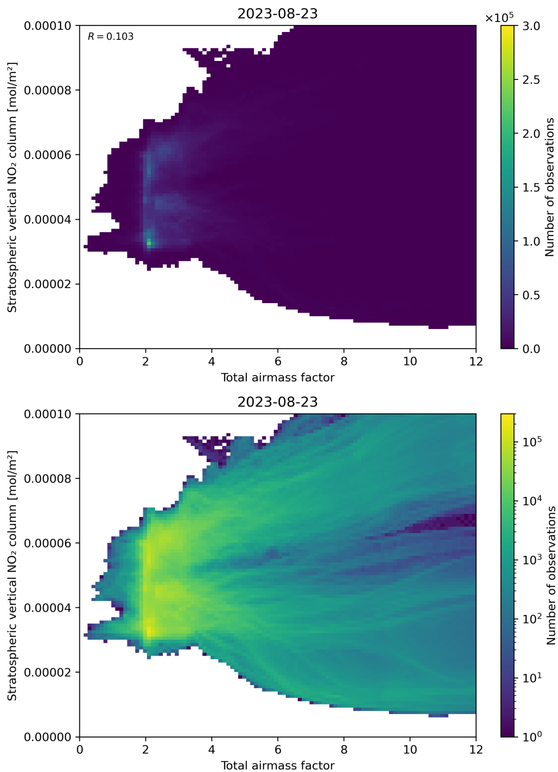
Figure 64: Scatter density plot of “Total airmass factor” against “Stratospheric vertical \text{NO}_2 column” for 2023-08-22 to 2023-08-24.
