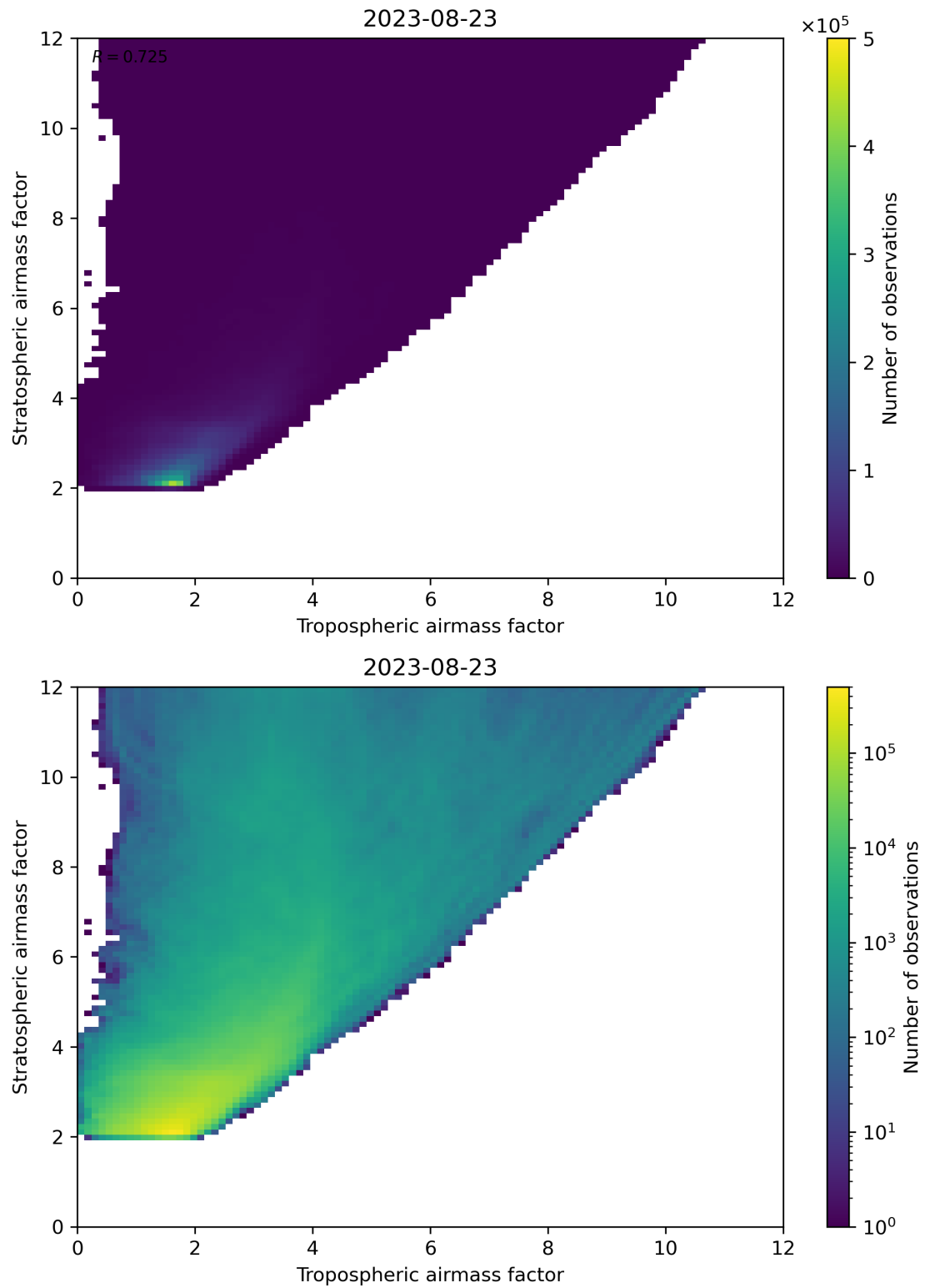
Figure 71: Scatter density plot of “Tropospheric airmass factor” against “Stratospheric airmass factor” for 2023-08-22 to 2023-08-24.
