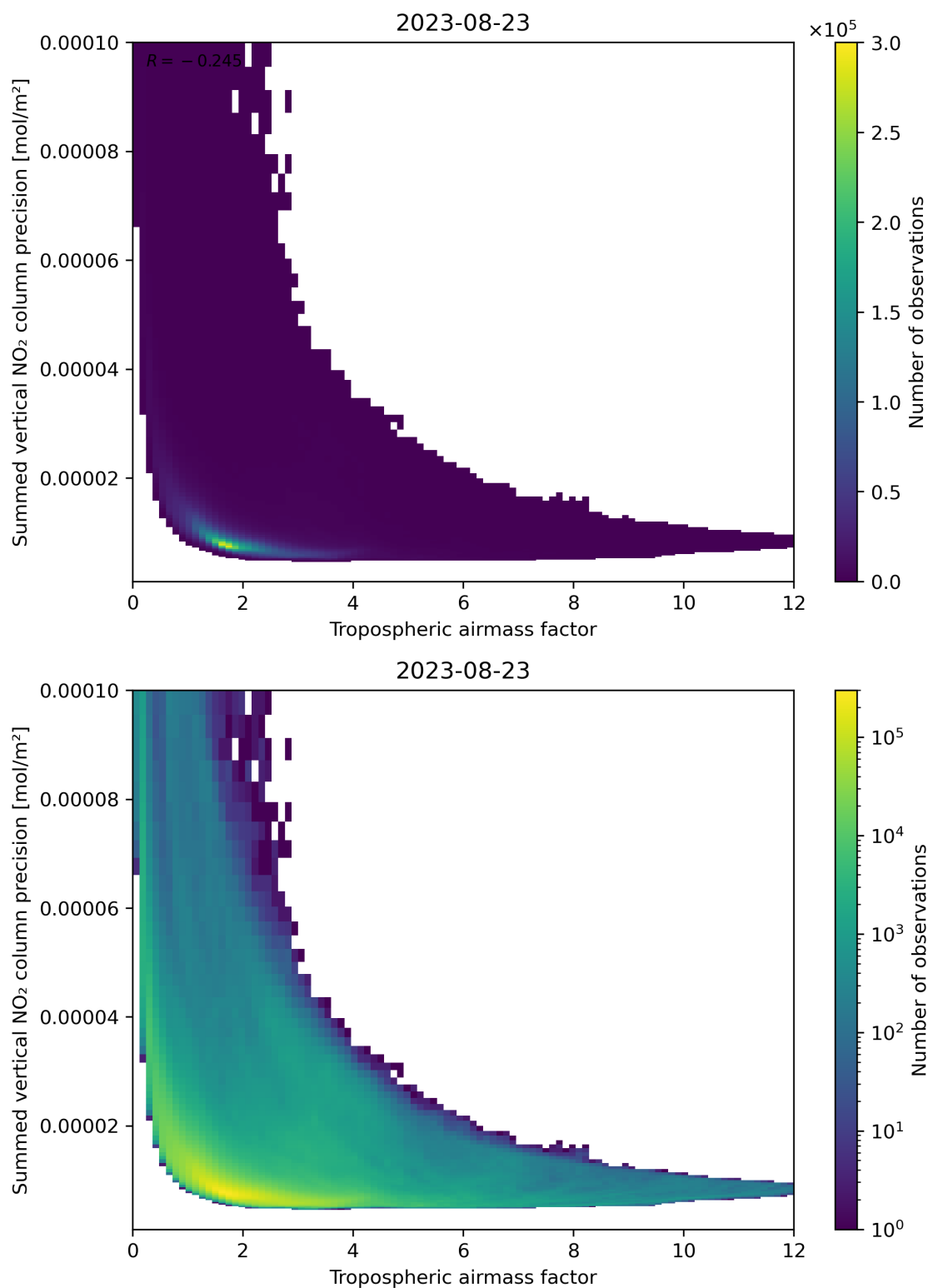
Figure 76: Scatter density plot of “Tropospheric air mass factor” against “Summed vertical NO 2 column precision” for 2023-08-22 to 2023-08-24.
