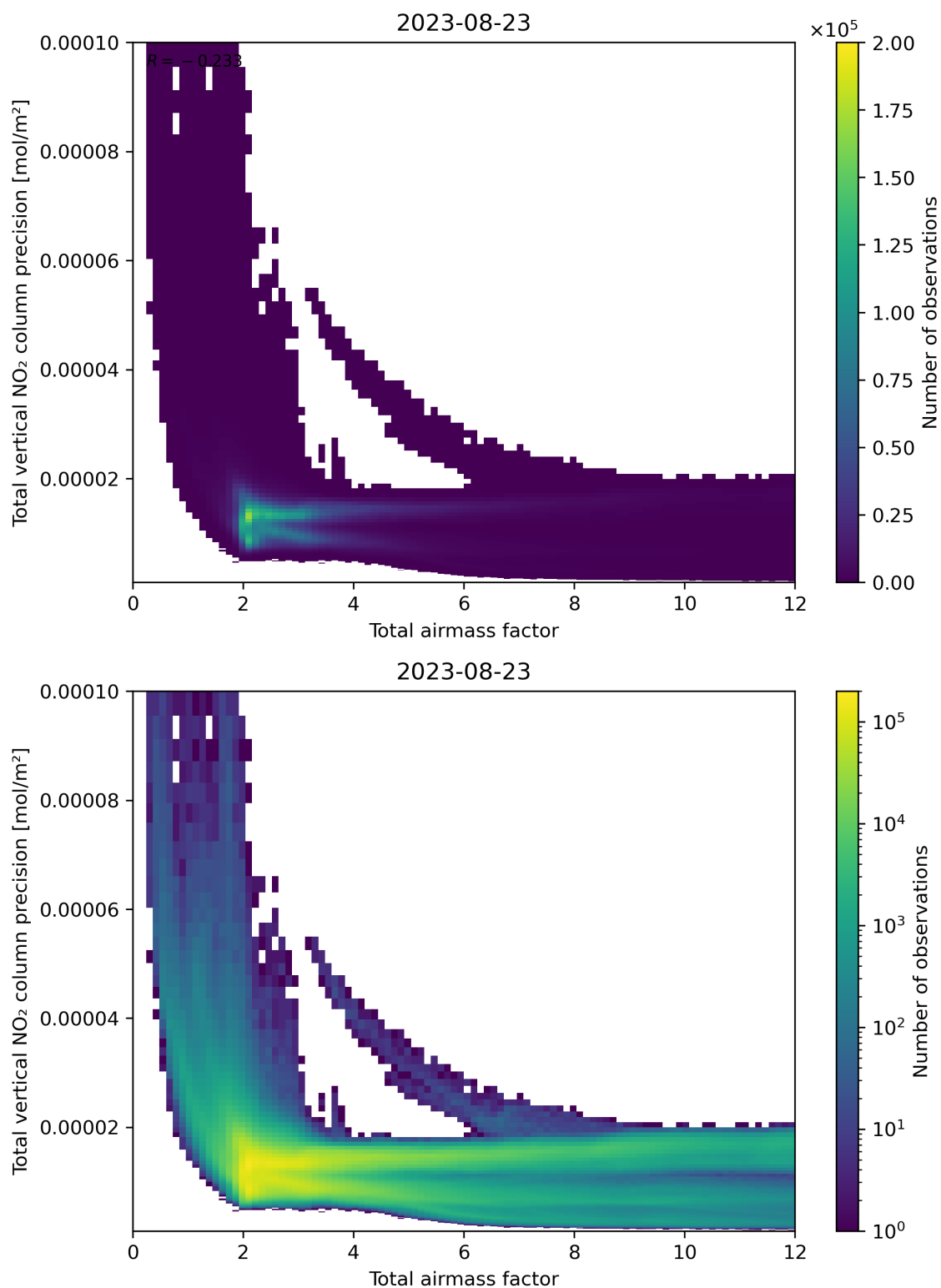
Figure 68: Scatter density plot of “Total airmass factor” against “Total vertical NO 2 column precision” for 2023-08-22 to 2023-08-24.
