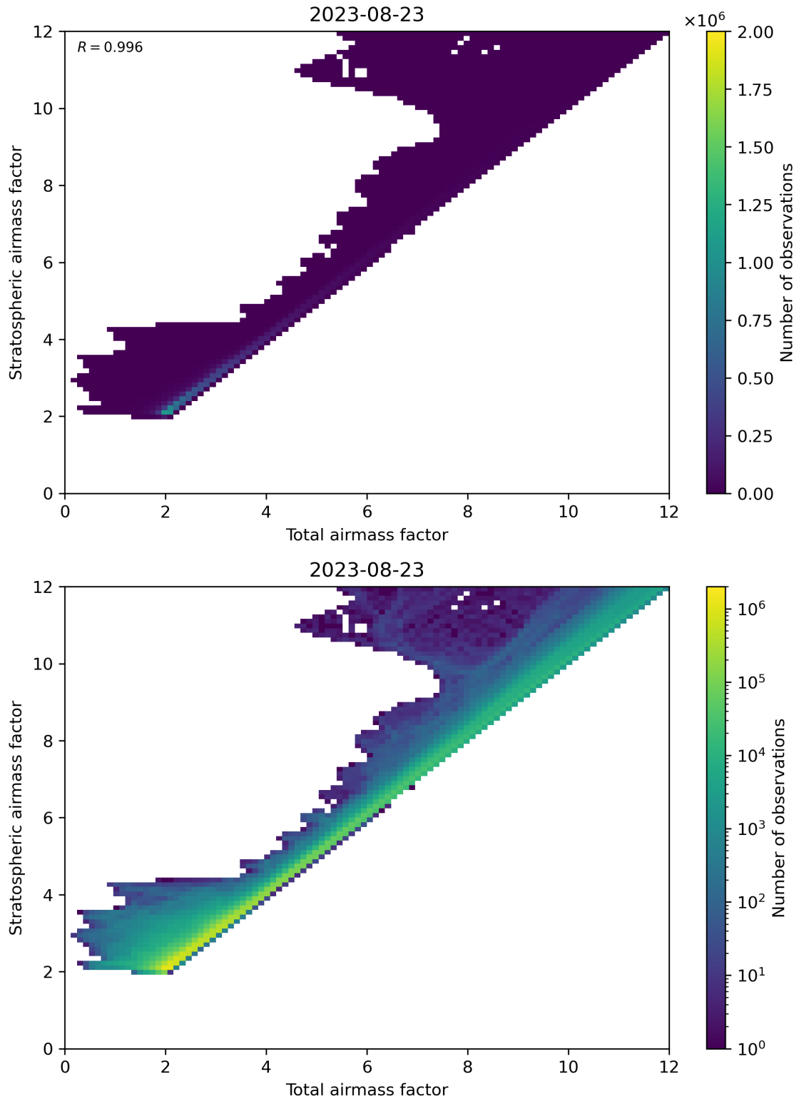
Figure 62: Scatter density plot of “Total airmass factor” against “Stratospheric airmass factor” for 2023-08-22 to 2023-08-24.
