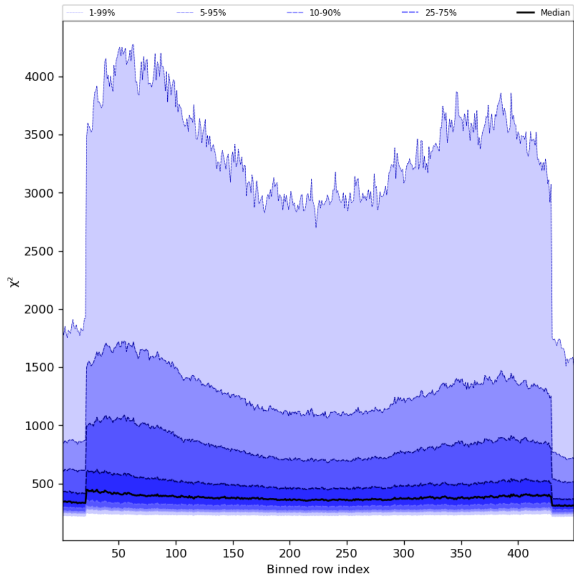
Figure 59: Along track statistics of “ \chi^2 ” for 2023-08-22 to 2023-08-24
