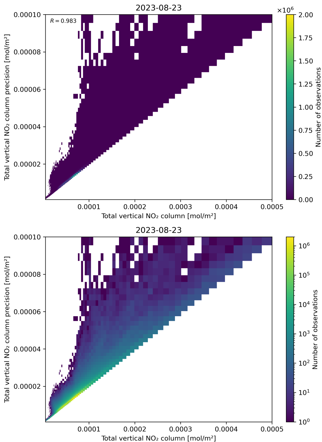
Figure 114: Scatter density plot of “Total vertical NO 2 column” against “Total vertical NO 2 column precision” for 2023-08-22 to 2023-08-24.
