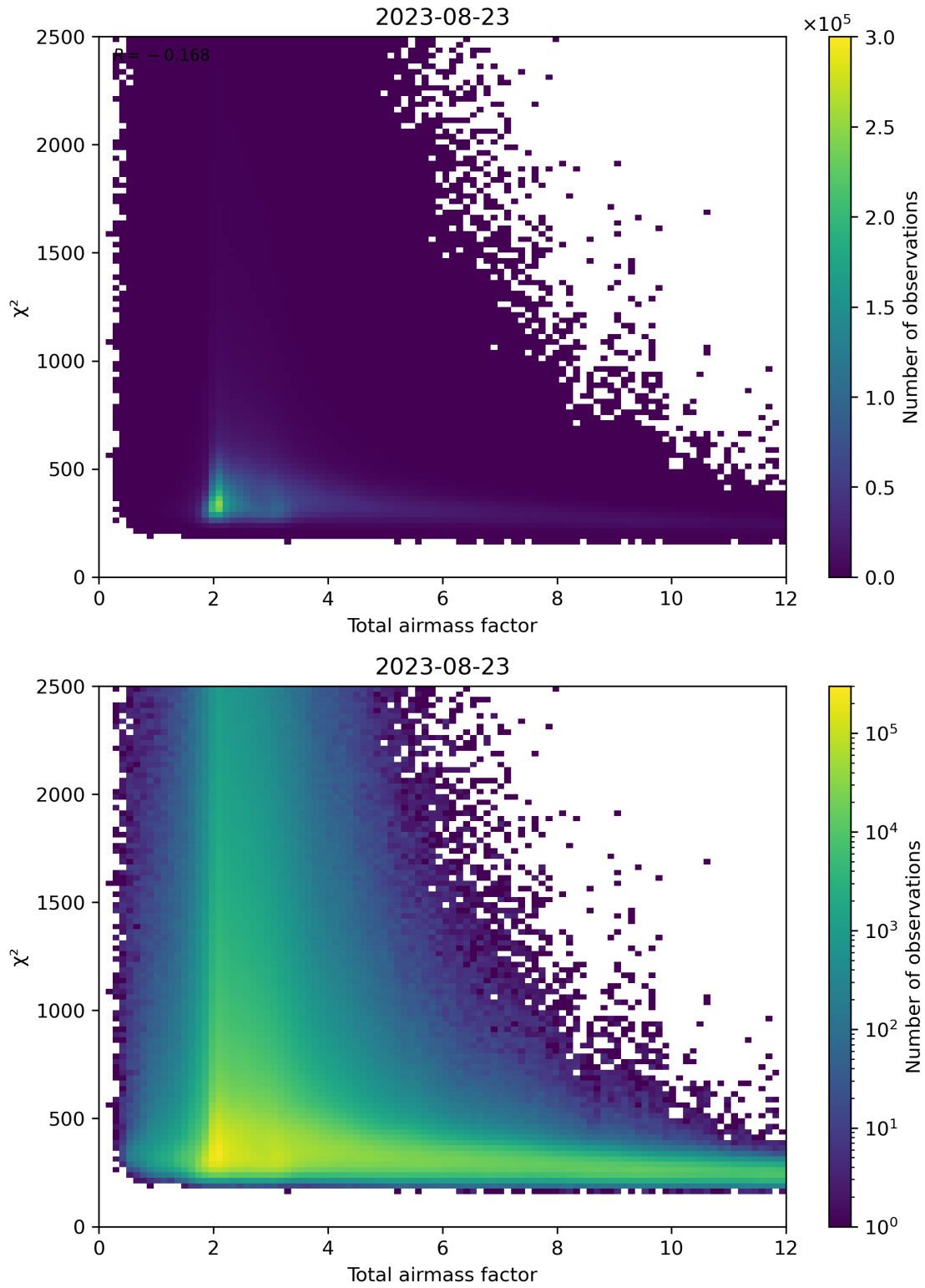
Figure 63: Scatter density plot of “Total airmass factor” against “ \chi^2 ” for 2023-08-22 to 2023-08-24.
