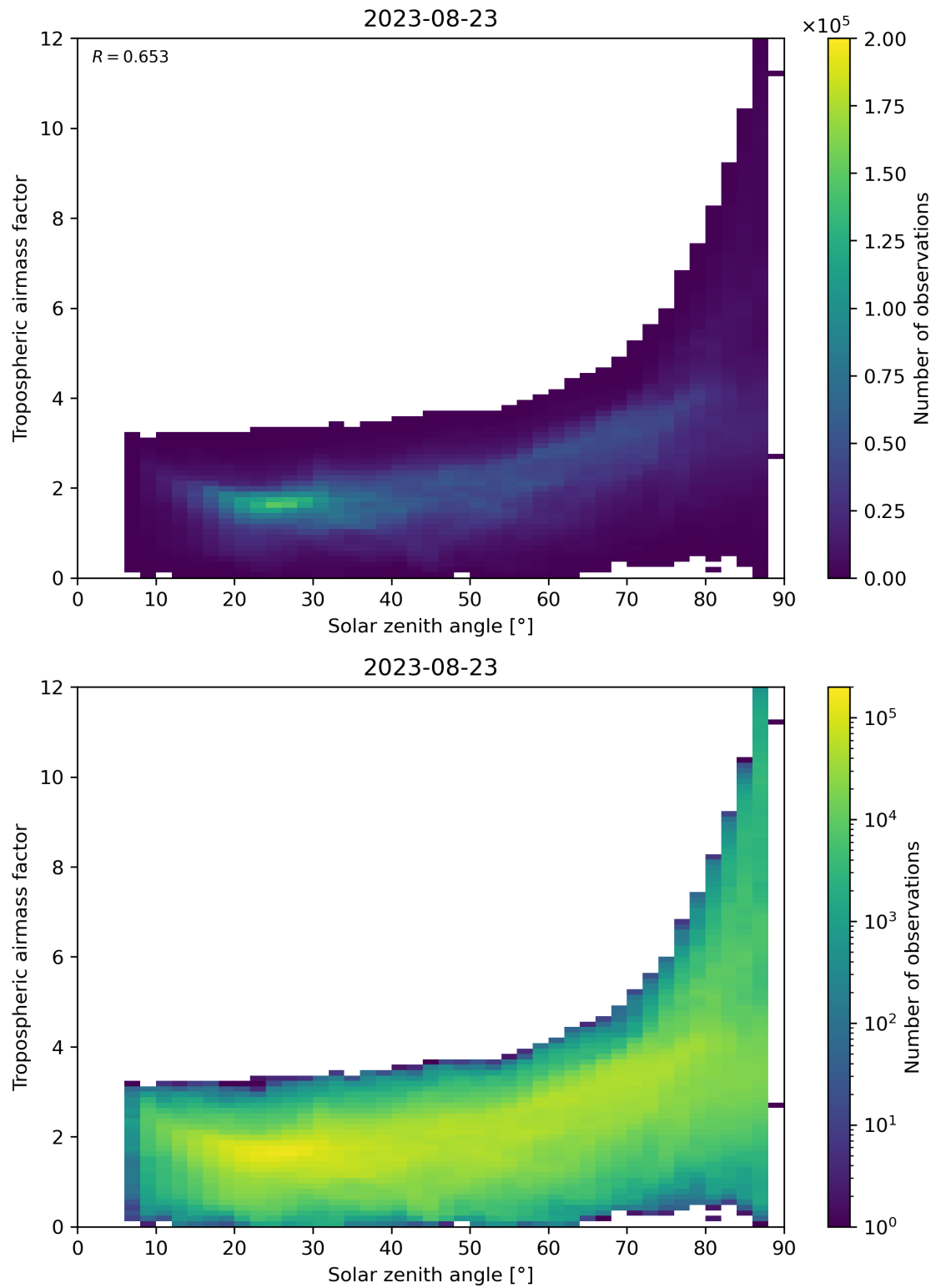
Figure 147: Scatter density plot of “Solar zenith angle” against “Tropospheric airmass factor” for 2023-08-22 to 2023-08-24.
