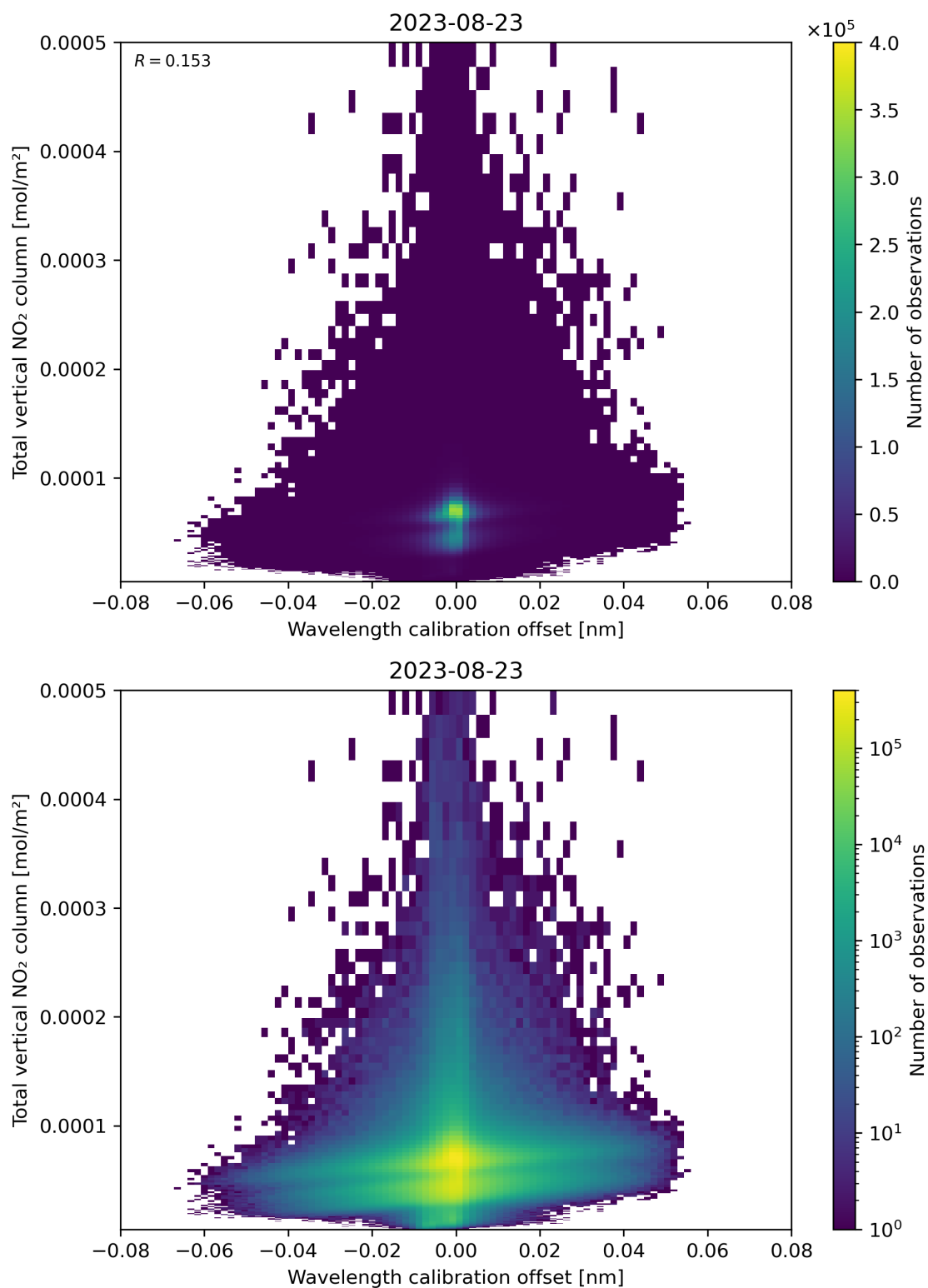
Figure 179: Scatter density plot of “Wavelength calibration offset” against “Total vertical NO 2 column” for 2023-08-22 to 2023-08-24.
