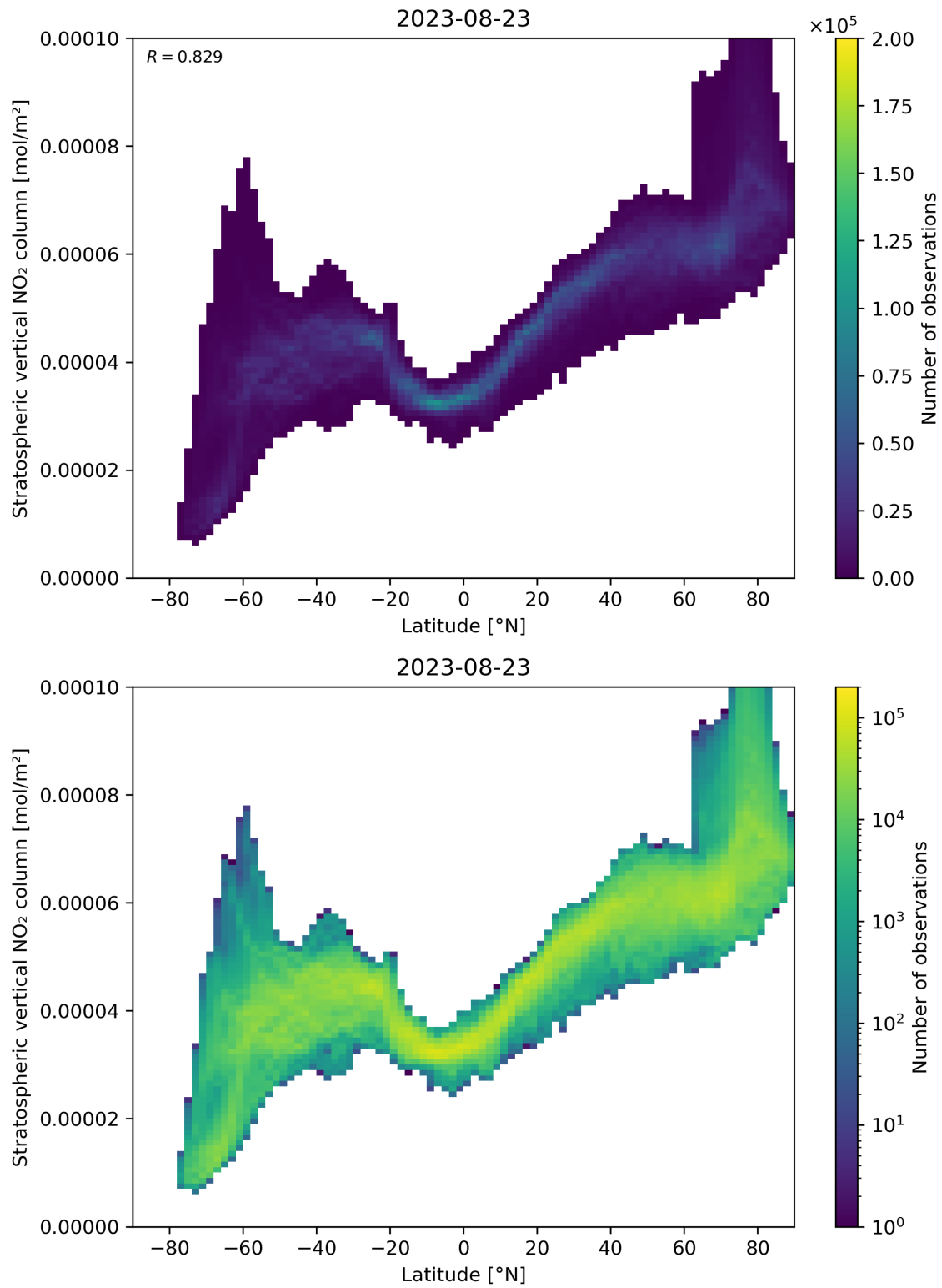
Figure 87: Scatter density plot of “Latitude” against “Stratospheric vertical NO 2 column” for 2023-08-22 to 2023-08-24.
