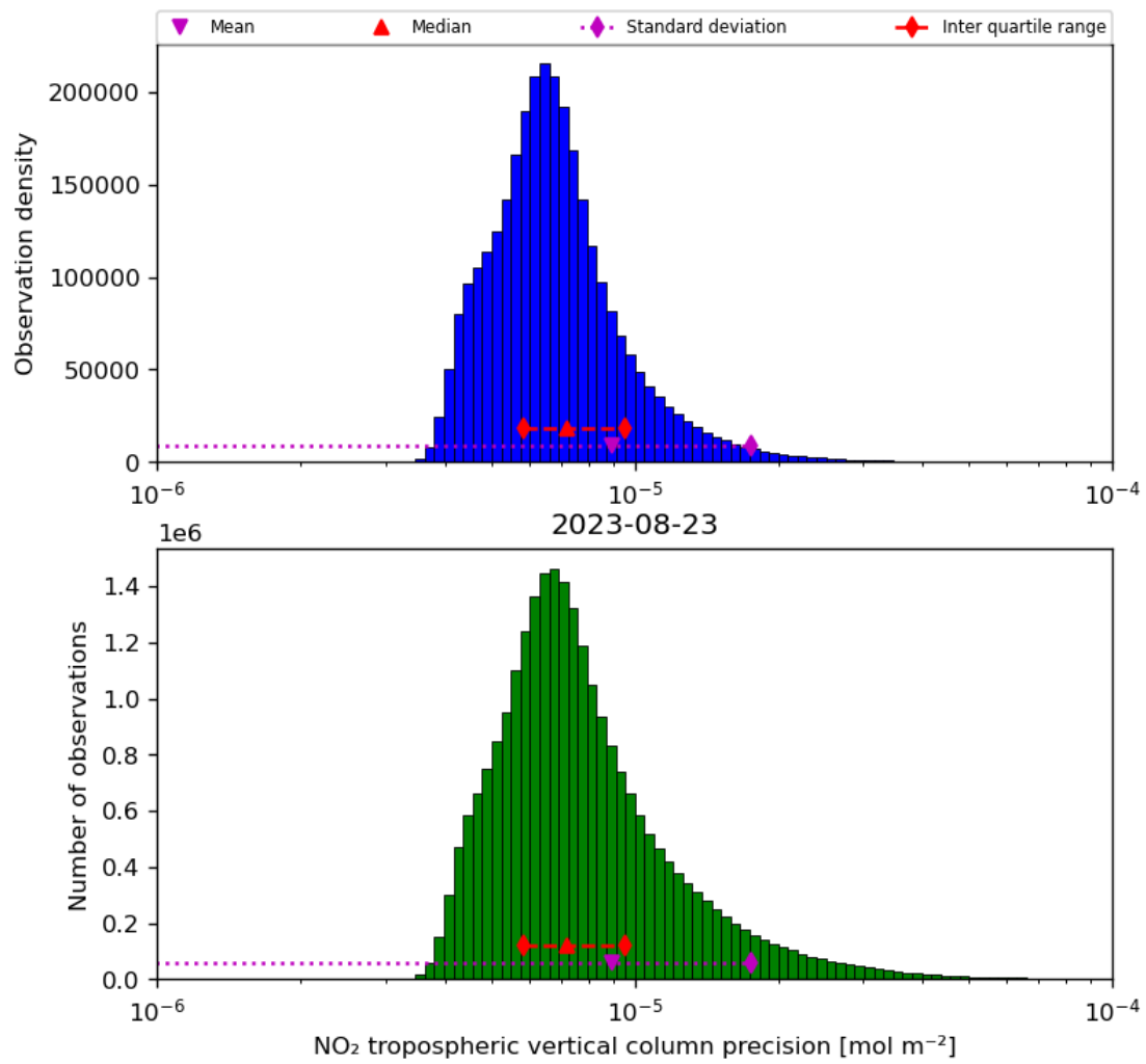
Figure 30: Histogram of “NO 2 tropospheric vertical column precision” for 2023-08-22 to 2023-08-24
