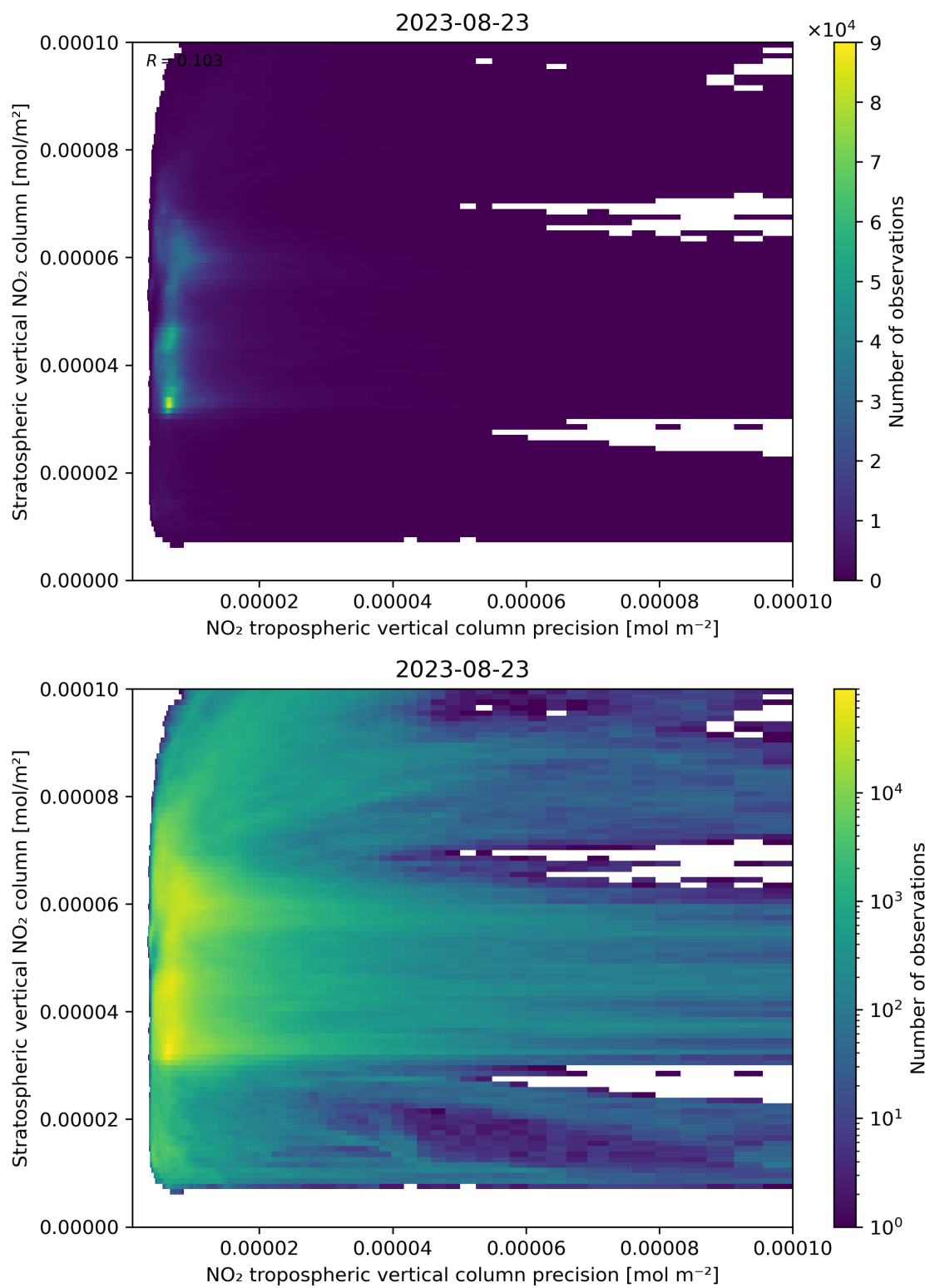
Figure 135: Scatter density plot of “NO 2 tropospheric vertical column precision” against “Stratospheric vertical NO 2 column” for 2023-08-22 to 2023-08-24.
