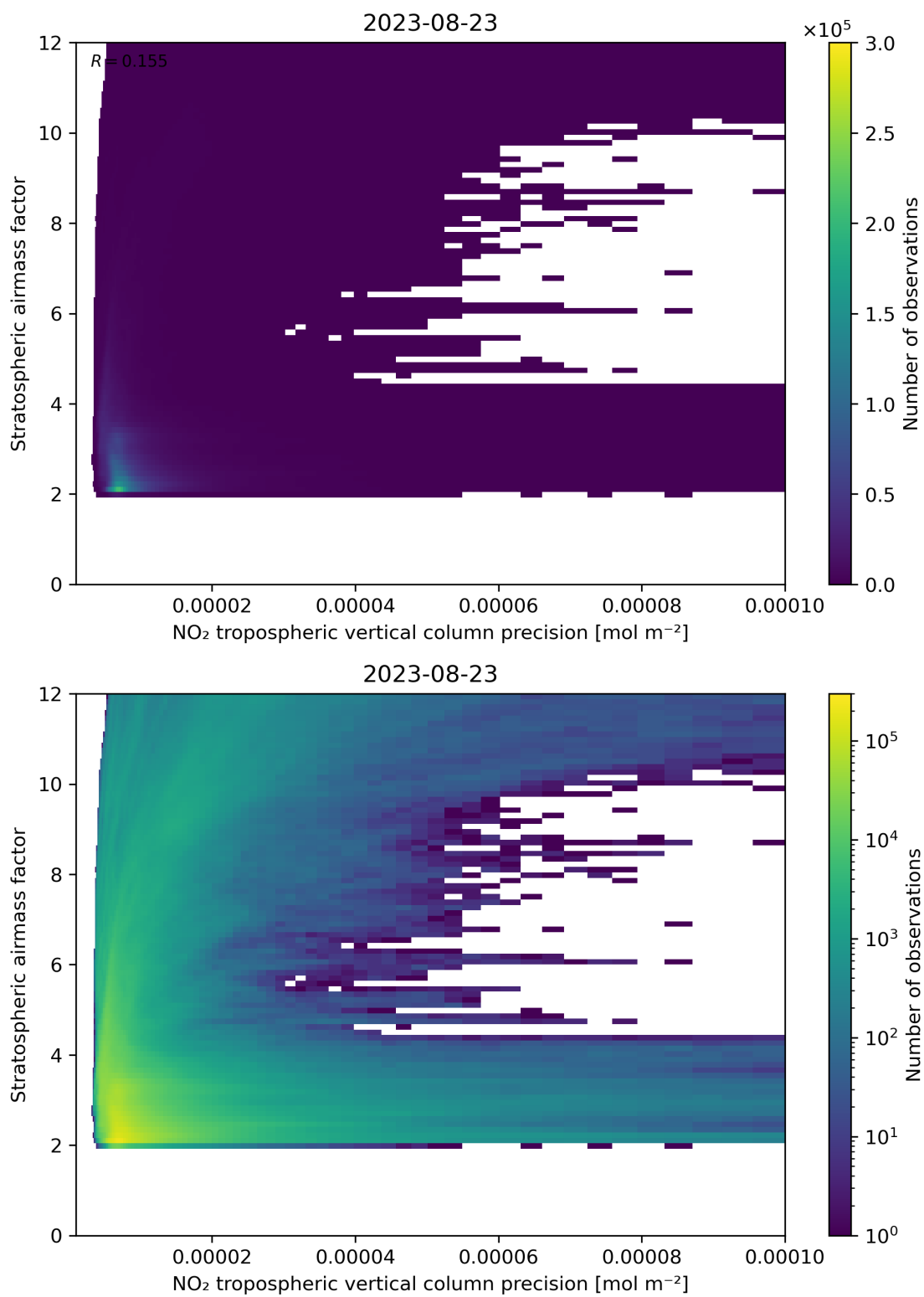
Figure 131: Scatter density plot of “NO 2 tropospheric vertical column precision” against “Stratospheric airmass factor” for 2023-08-22 to 2023-08-24.
