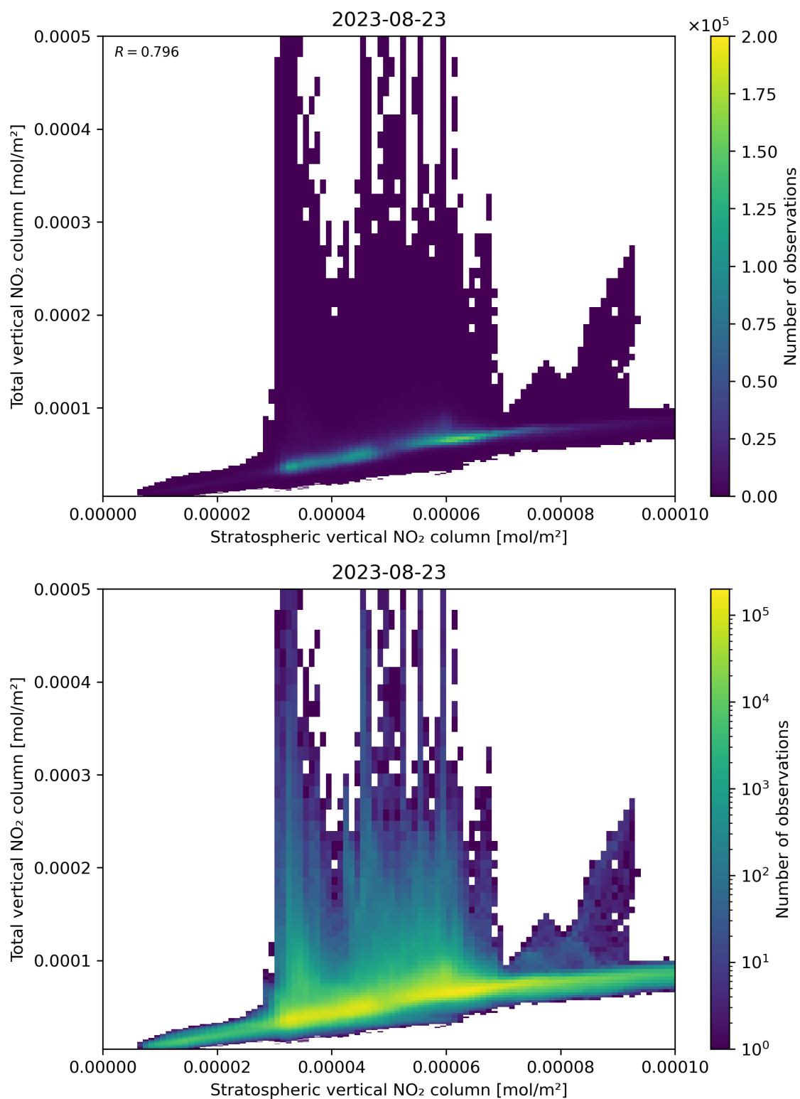
Figure 100: Scatter density plot of “Stratospheric vertical NO 2 column” against “Total vertical NO 2 column” for 2023-08-22 to 2023-08-24.
