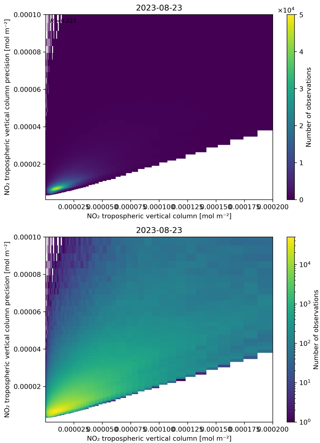
Figure 130: Scatter density plot of “NO 2 tropospheric vertical column” against “NO 2 tropospheric vertical column precision” for 2023-08-22 to 2023-08-24.
