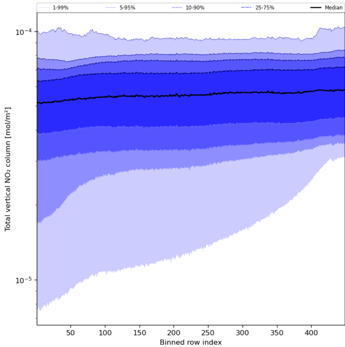
Figure 55: Along track statistics of “Total vertical NO 2 column” for 2023-08-22 to 2023-08-24
