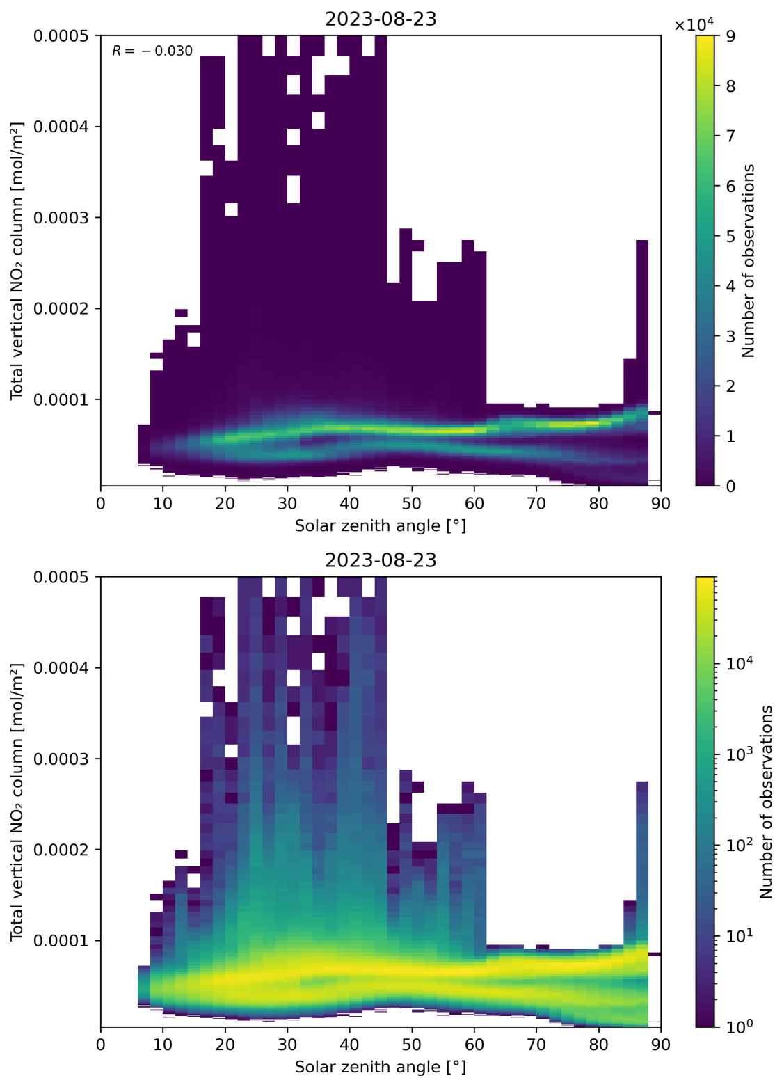
Figure 153: Scatter density plot of “Solar zenith angle” against “Total vertical NO 2 column” for 2023-08-22 to 2023-08-24.
