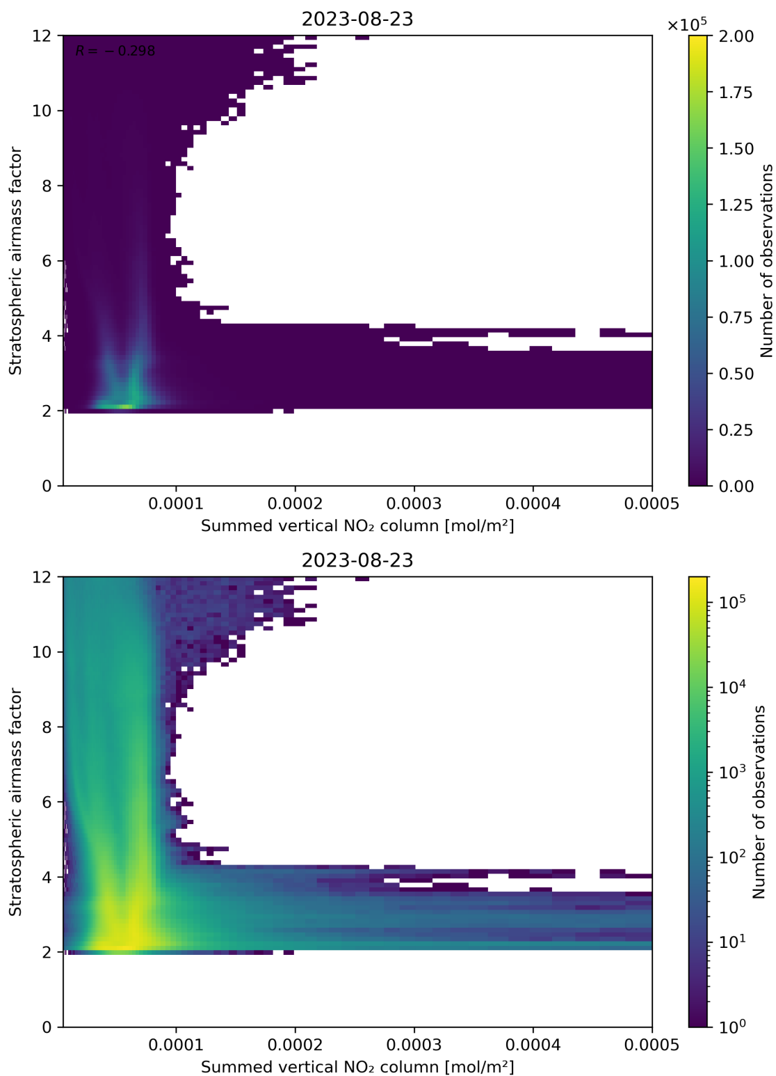
Figure 103: Scatter density plot of “Summed vertical NO 2 column” against “Stratospheric airmass factor” for 2023-08-22 to 2023-08-24.
