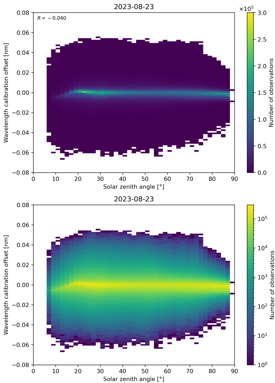
Figure 158: Scatter density plot of “Solar zenith angle” against “Wavelength calibration offset” for 2023-08-22 to 2023-08-24.
