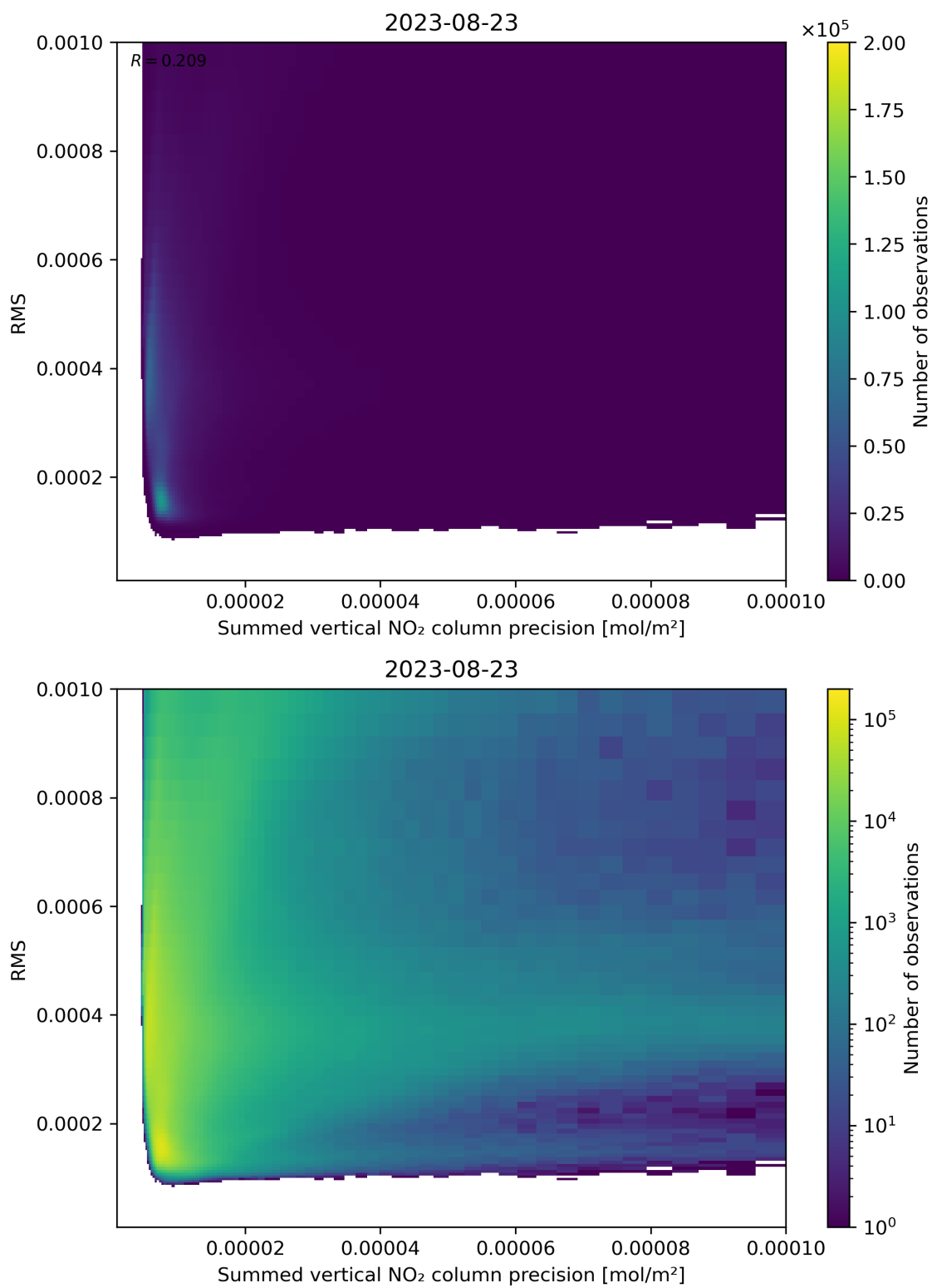
Figure 108: Scatter density plot of “Summed vertical NO 2 column precision” against “RMS” for 2023-08-22 to 2023-08-24.
