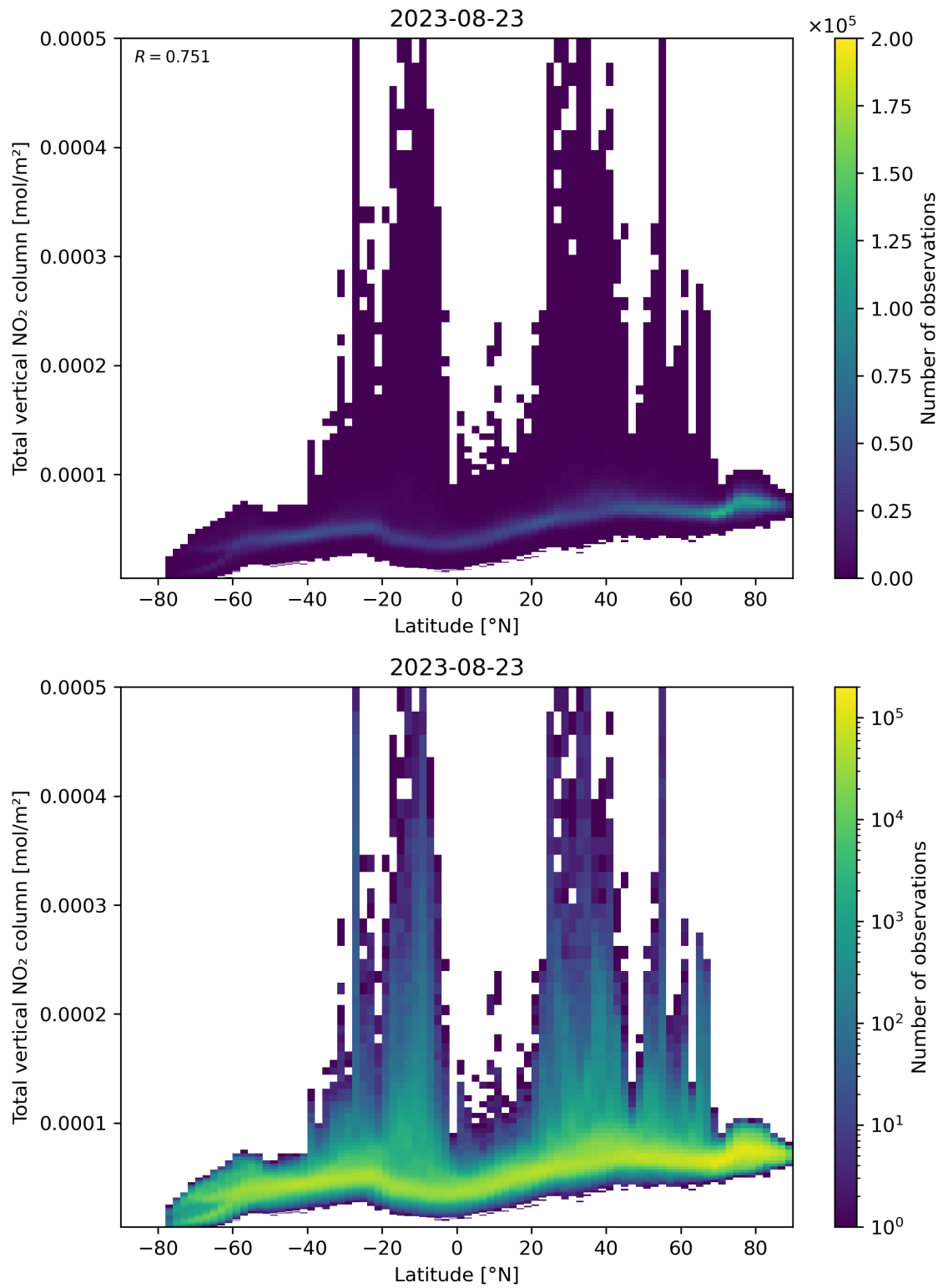
Figure 90: Scatter density plot of “Latitude” against “Total vertical NO 2 column” for 2023-08-22 to 2023-08-24.
