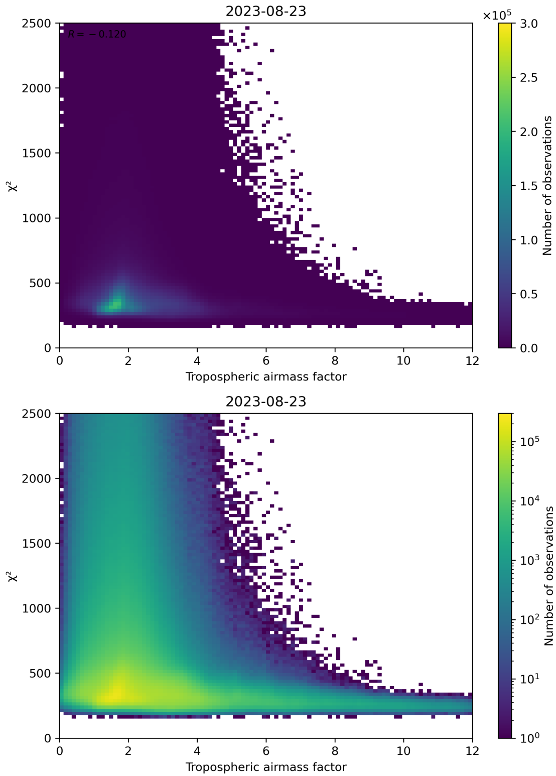
Figure 73: Scatter density plot of “Tropospheric airmass factor” against “ \chi^2 ” for 2023-08-22 to 2023-08-24.
