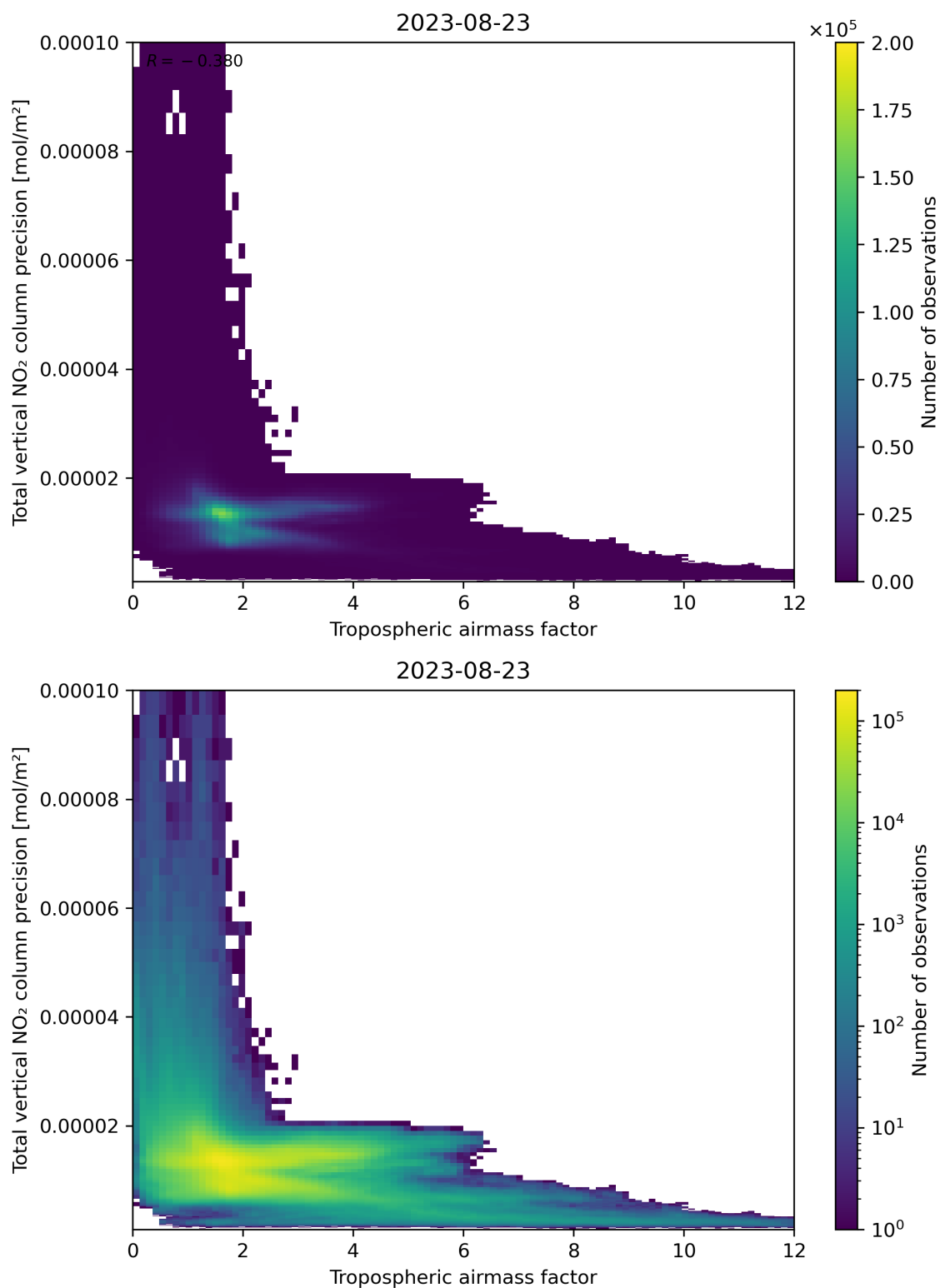
Figure 78: Scatter density plot of “Tropospheric airmass factor” against “Total vertical NO 2 column precision” for 2023-08-22 to 2023-08-24.
