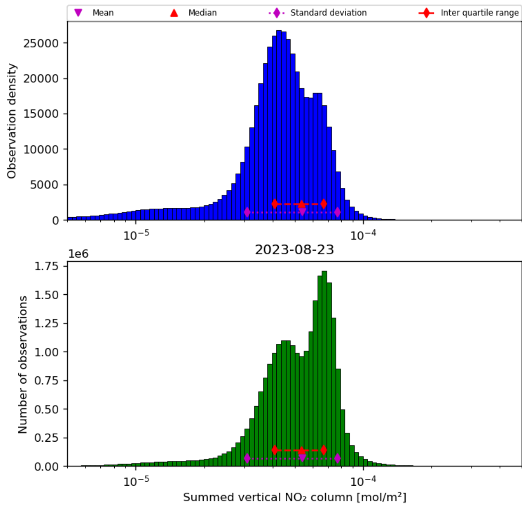
Figure 40: Histogram of “Summed vertical NO 2 column” for 2023-08-22 to 2023-08-24
