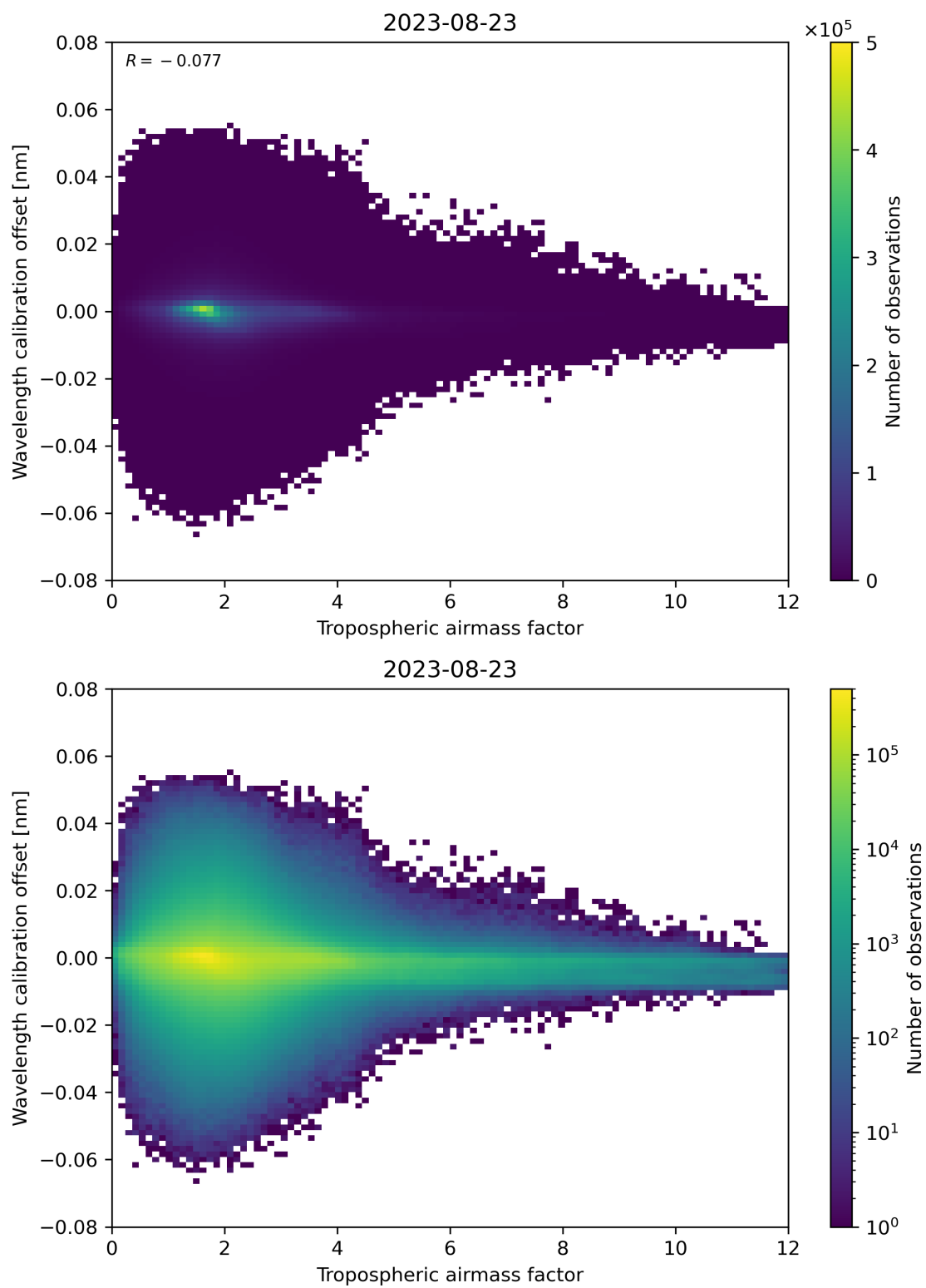
Figure 80: Scatter density plot of “Tropospheric airmass factor” against “Wavelength calibration offset” for 2023-08-22 to 2023-08-24.
