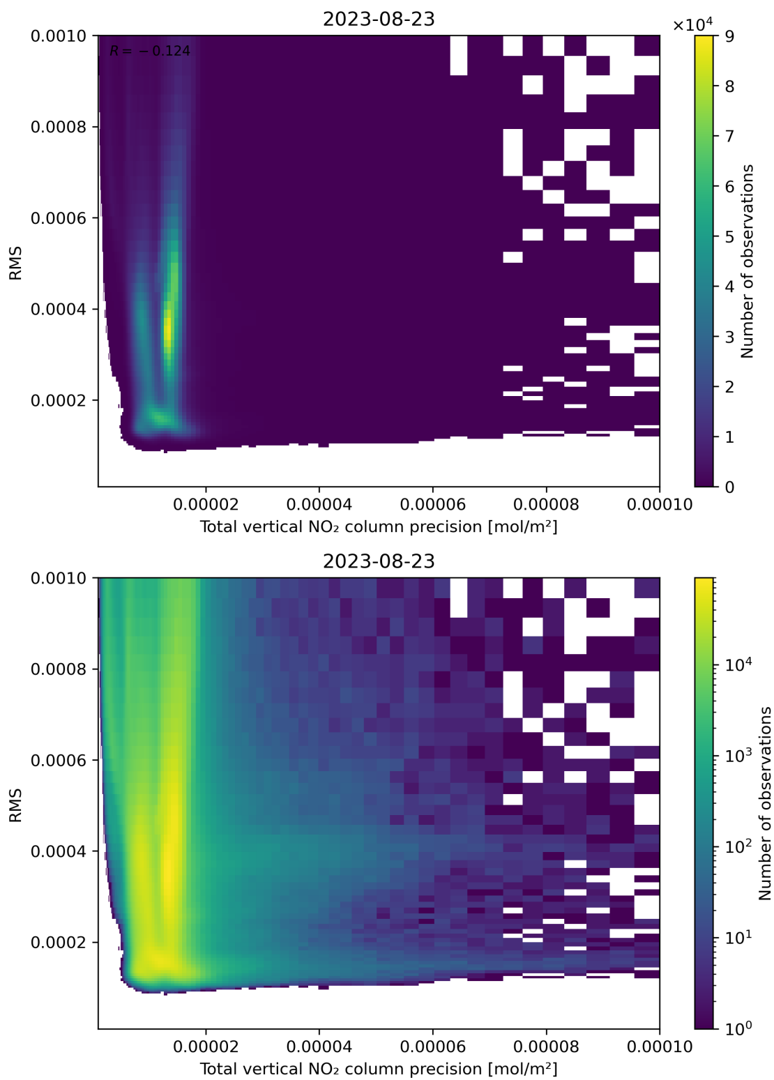
Figure 119: Scatter density plot of “Total vertical NO 2 column precision” against “RMS” for 2023-08-22 to 2023-08-24.
