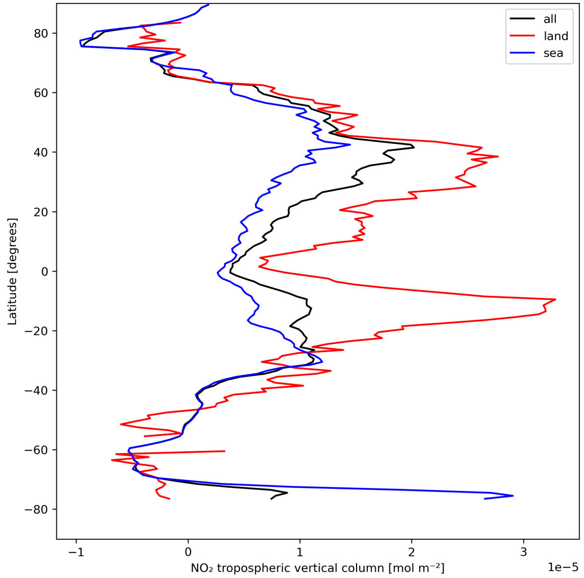
Figure 12: Zonal average of “NO 2 tropospheric vertical column” for 2023-08-22 to 2023-08-24.
