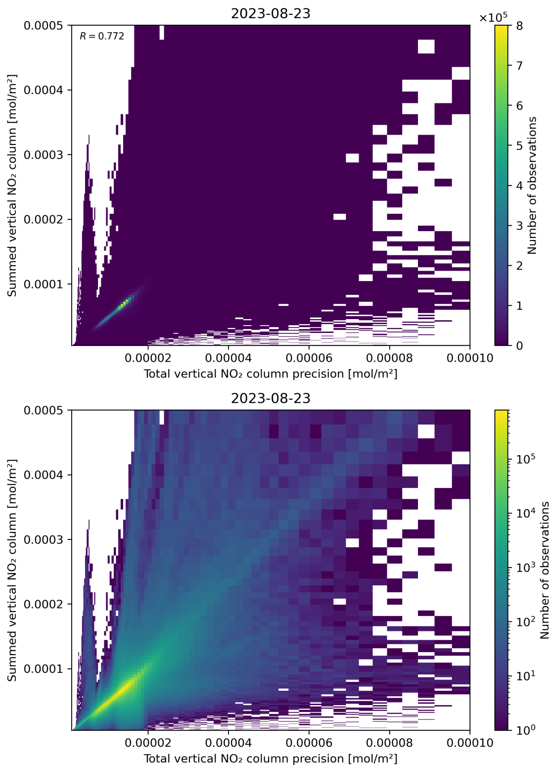
Figure 117: Scatter density plot of “Total vertical NO 2 column precision” against “Summed vertical NO 2 column” for 2023-08-22 to 2023-08-24.
