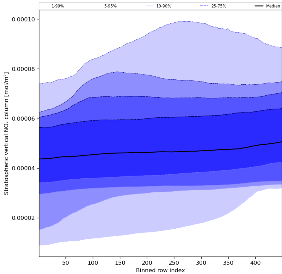
Figure 53: Along track statistics of “Stratospheric vertical NO 2 column” for 2023-08-22 to 2023-08-24
