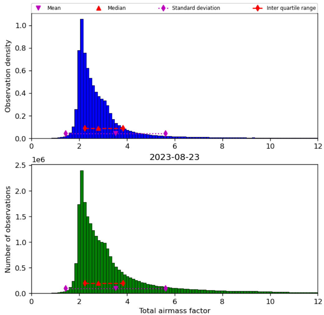
Figure 32: Histogram of “Total airmass factor” for 2023-08-22 to 2023-08-24
