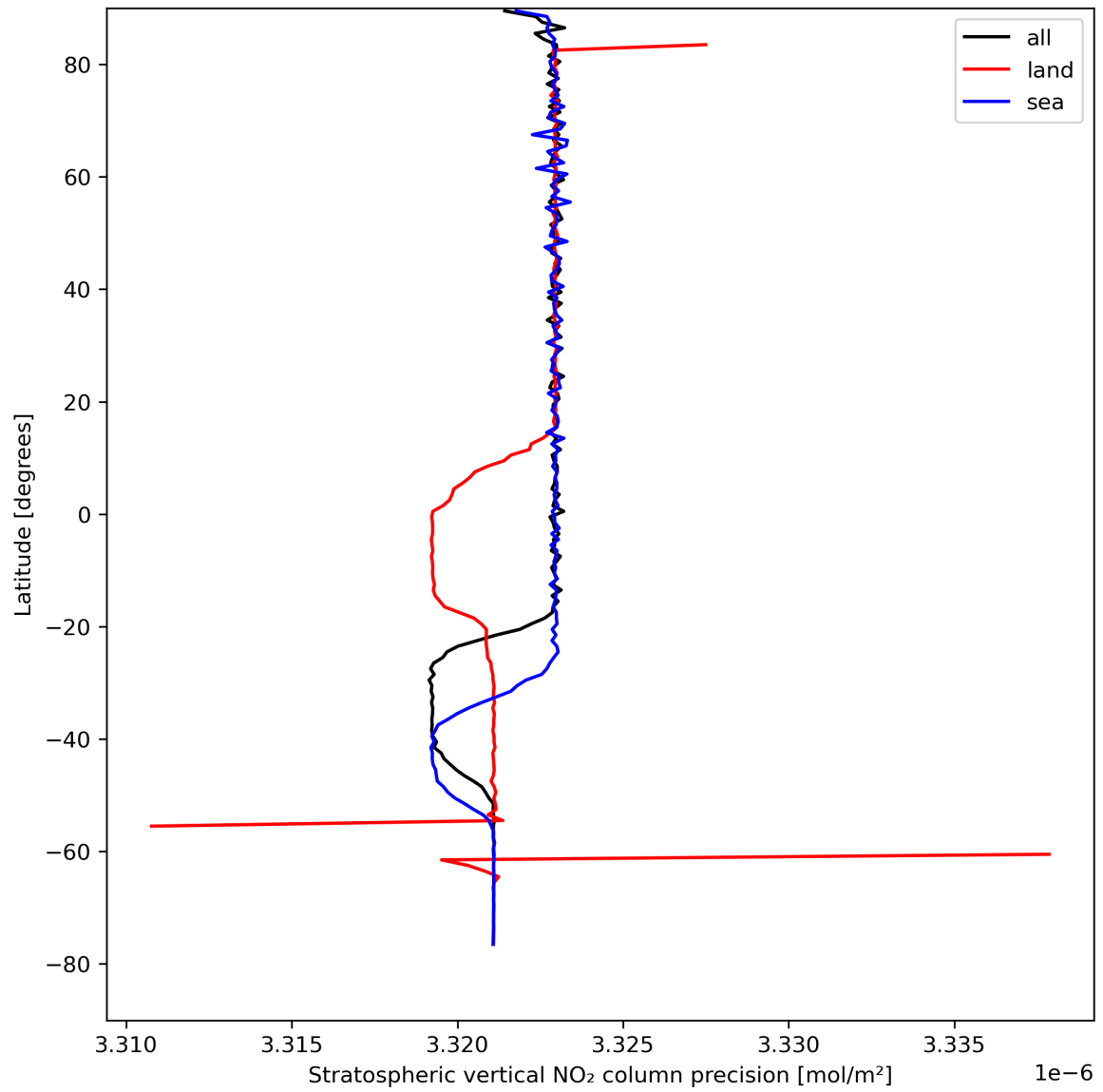
Figure 20: Zonal average of “Stratospheric vertical NO 2 column precision” for 2023-08-22 to 2023-08-24.
