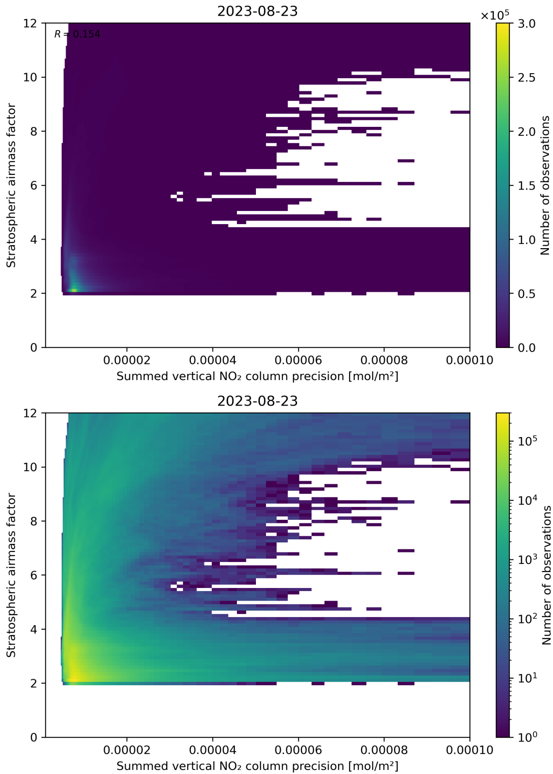
Figure 106: Scatter density plot of “Summed vertical NO 2 column precision” against “Stratospheric airmass factor” for 2023-08-22 to 2023-08-24.
