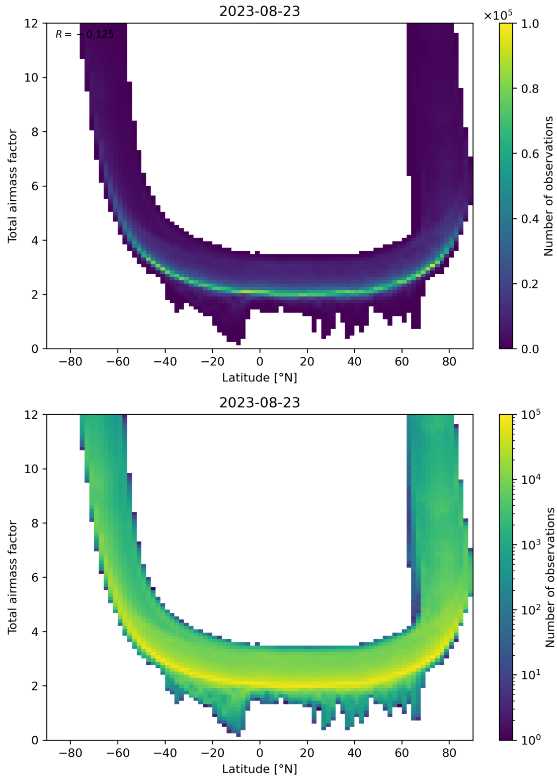
Figure 84: Scatter density plot of “Latitude” against “Total airmass factor” for 2023-08-22 to 2023-08-24.
