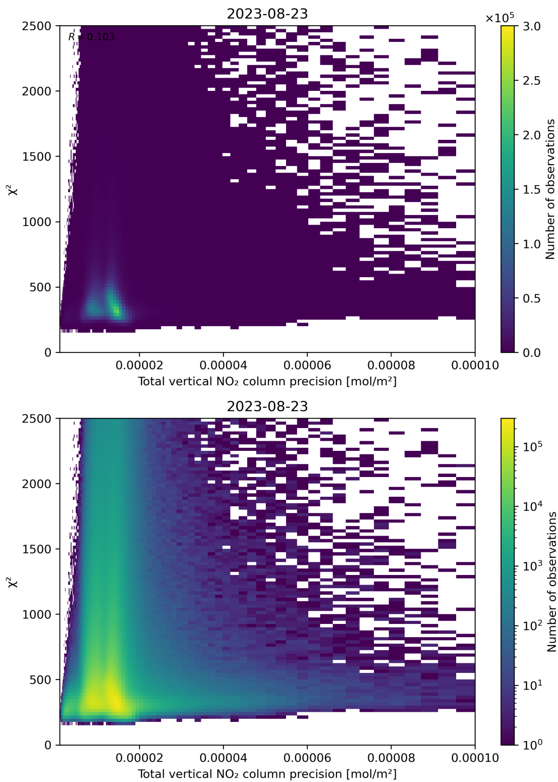
Figure 116: Scatter density plot of “Total vertical NO 2 column precision” against “ \chi^2 ” for 2023-08-22 to 2023-08-24.
