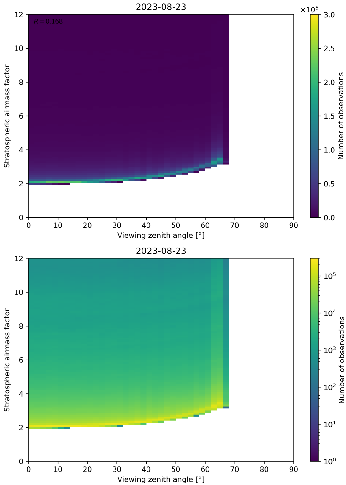
Figure 159: Scatter density plot of “Viewing zenith angle” against “Stratospheric airmass factor” for 2023-08-22 to 2023-08-24.
