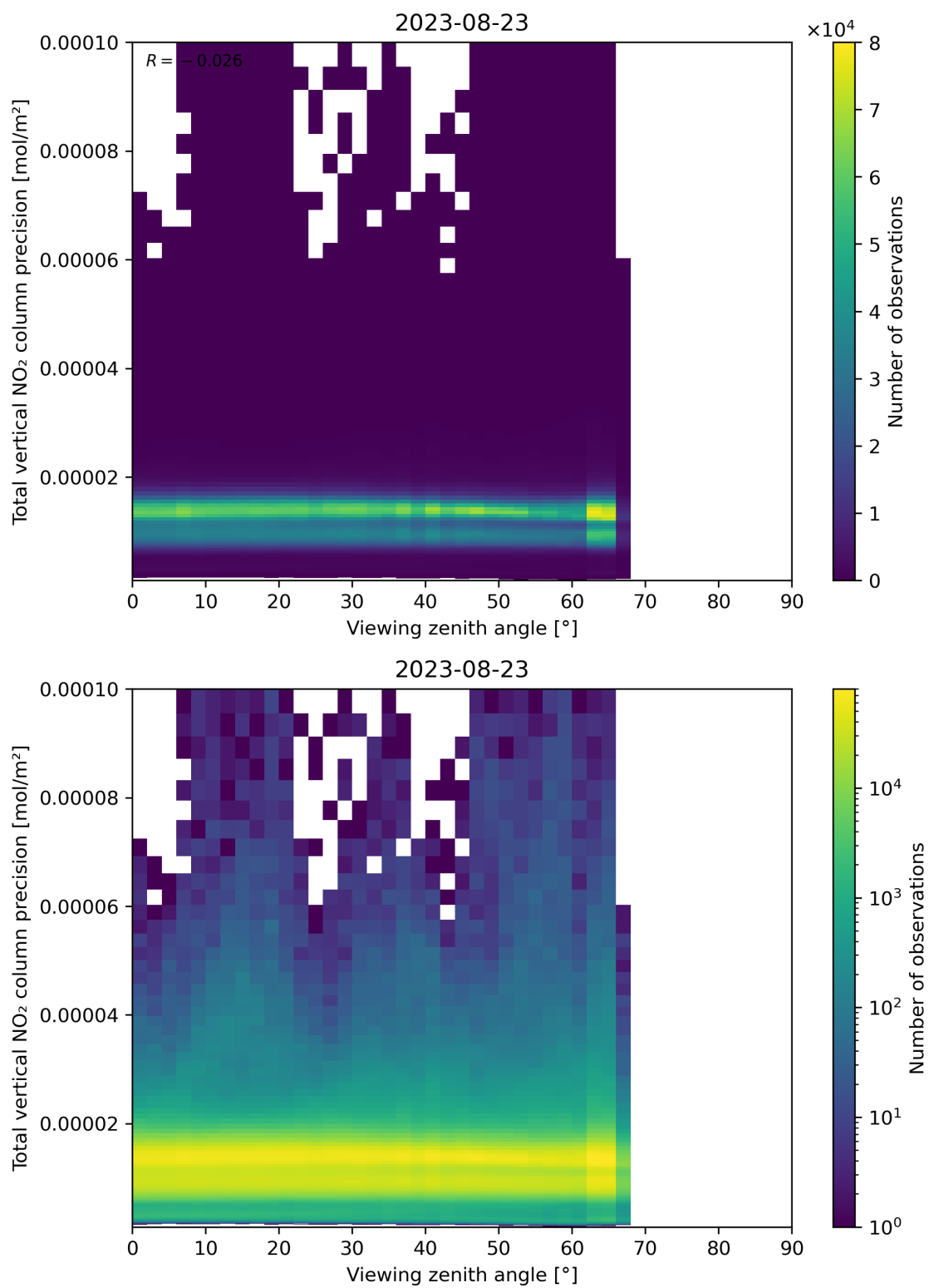
Figure 168: Scatter density plot of “Viewing zenith angle” against “Total vertical NO 2 column precision” for 2023-08-22 to 2023-08-24.
