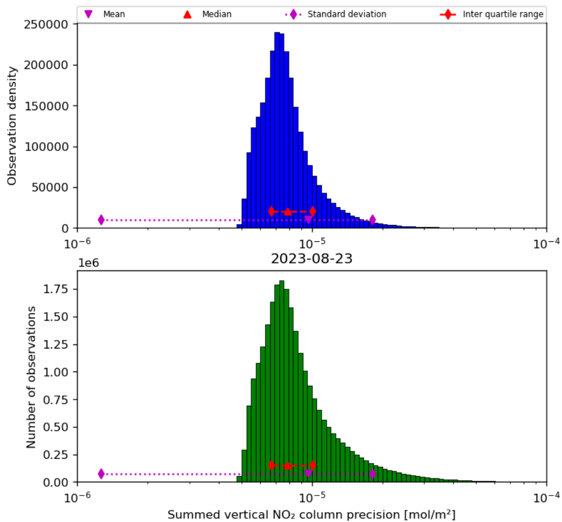
Figure 41: Histogram of "Summed vertical NO 2 column precision" for 2023-08-22 to 2023-08-24
