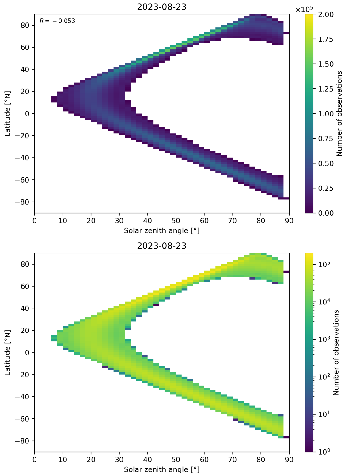
Figure 149: Scatter density plot of “Solar zenith angle” against “Latitude” for 2023-08-22 to 2023-08-24.
