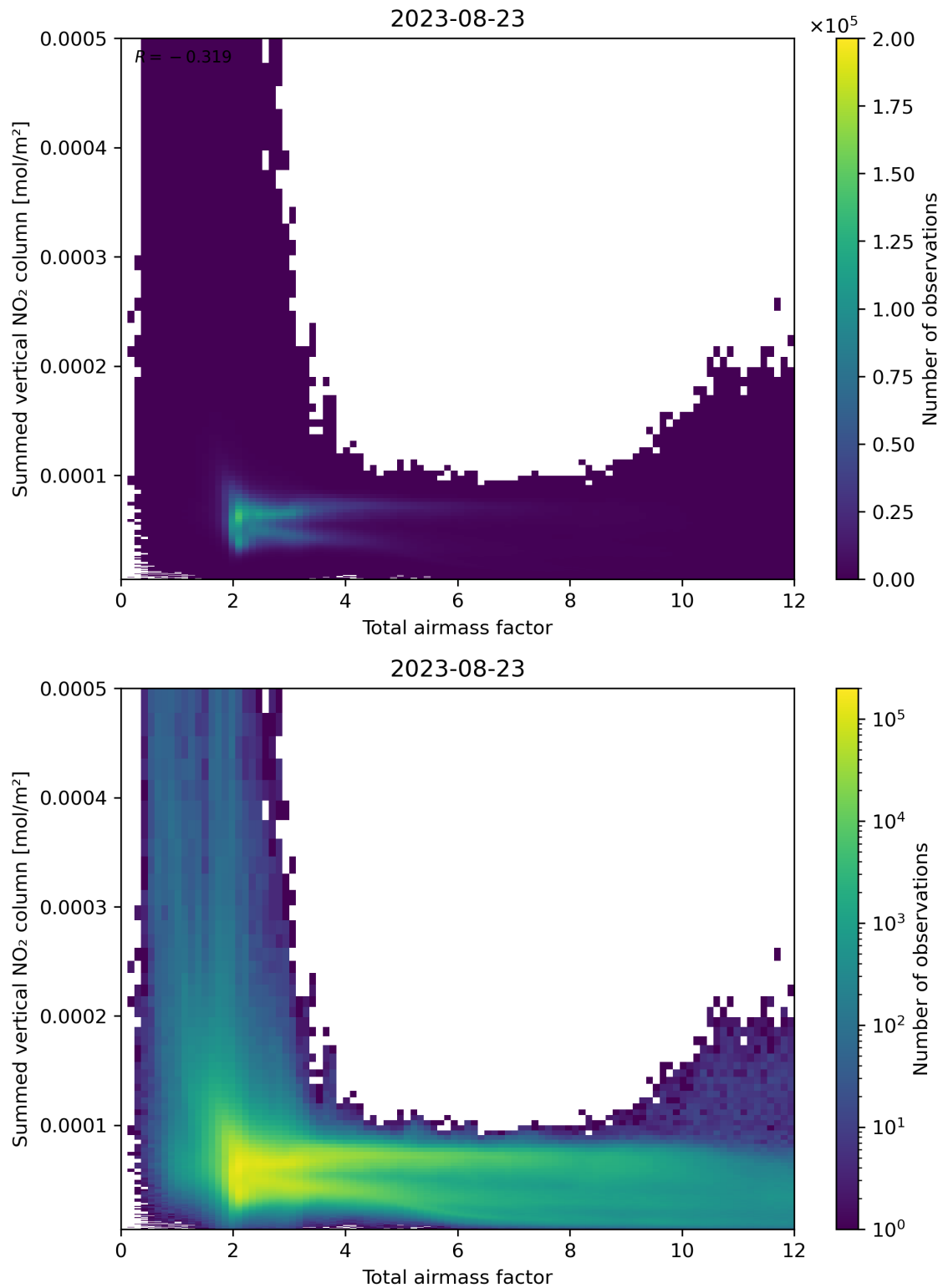
Figure 65: Scatter density plot of “Total airmass factor” against “Summed vertical NO 2 column” for 2023-08-22 to 2023-08-24.
