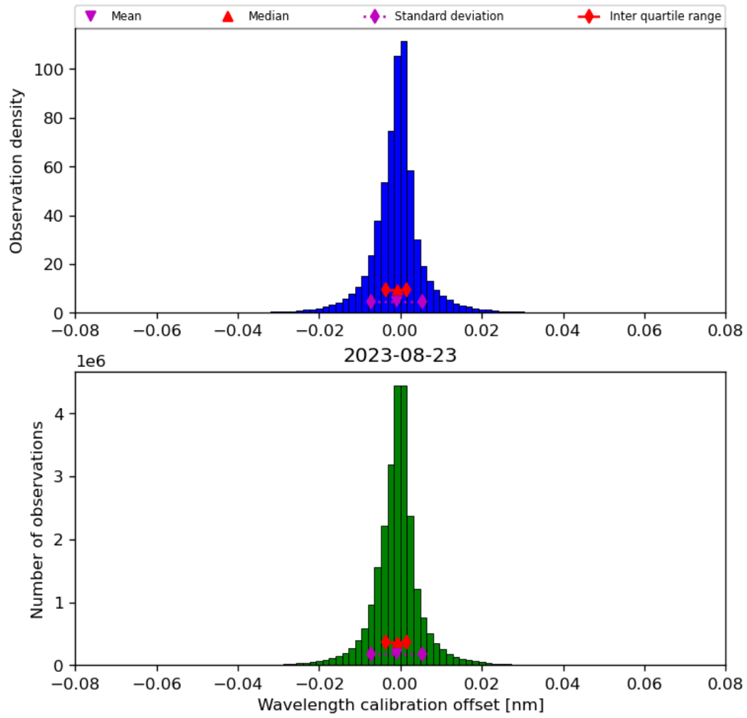
Figure 35: Histogram of “Wavelength calibration offset” for 2023-08-22 to 2023-08-24
