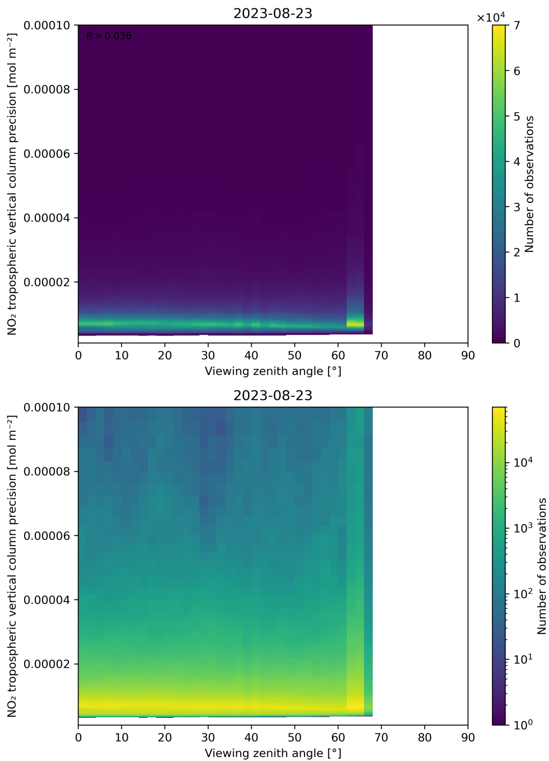
Figure 170: Scatter density plot of “Viewing zenith angle” against “NO 2 tropospheric vertical column precision” for 2023-08-22 to 2023-08-24.
