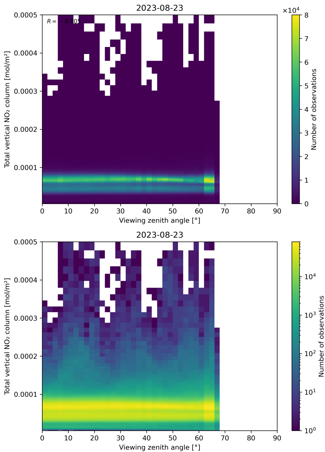
Figure 167: Scatter density plot of “Viewing zenith angle” against “Total vertical NO 2 column” for 2023-08-22 to 2023-08-24.
