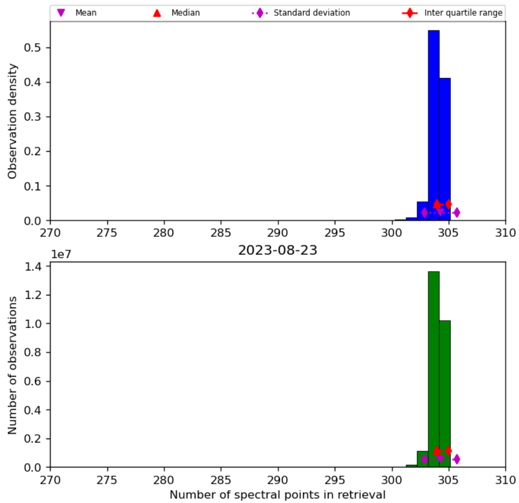
Figure 33: Histogram of “Number of spectral points in retrieval” for 2023-08-22 to 2023-08-24
