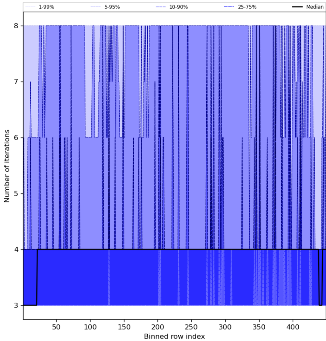
Figure 51: Along track statistics of “Number of iterations” for 2023-08-22 to 2023-08-24
