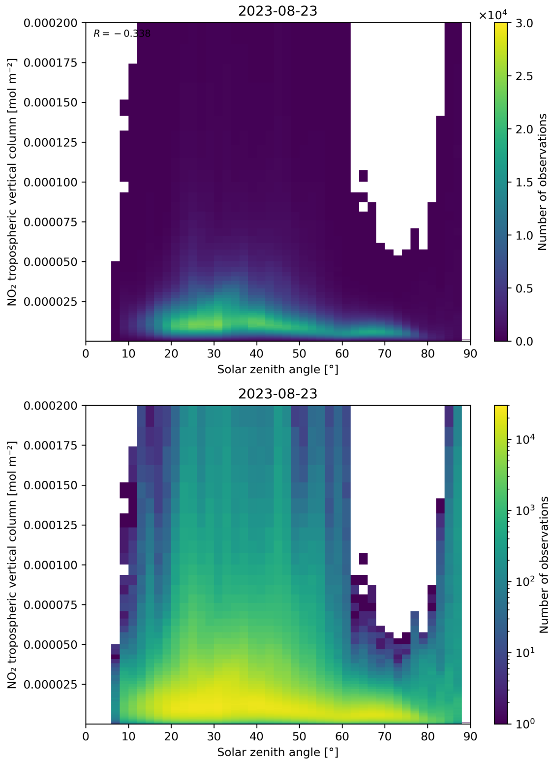
Figure 155: Scatter density plot of “Solar zenith angle” against “NO 2 tropospheric vertical column” for 2023-08-22 to 2023-08-24.
