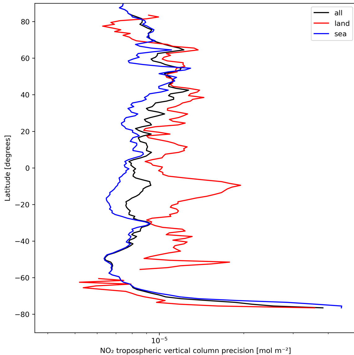
Figure 13: Zonal average of “NO 2 tropospheric vertical column precision” for 2023-08-22 to 2023-08-24.
