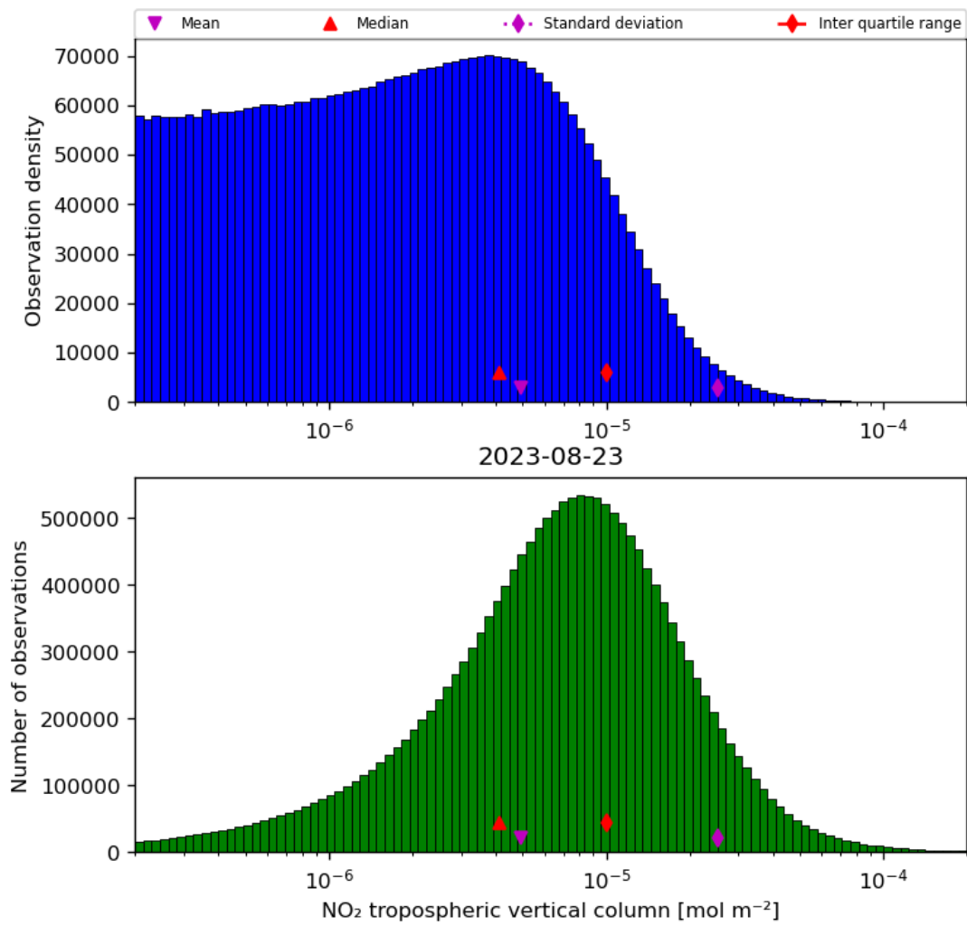
Figure 29: Histogram of “NO 2 tropospheric vertical column” for 2023-08-22 to 2023-08-24
