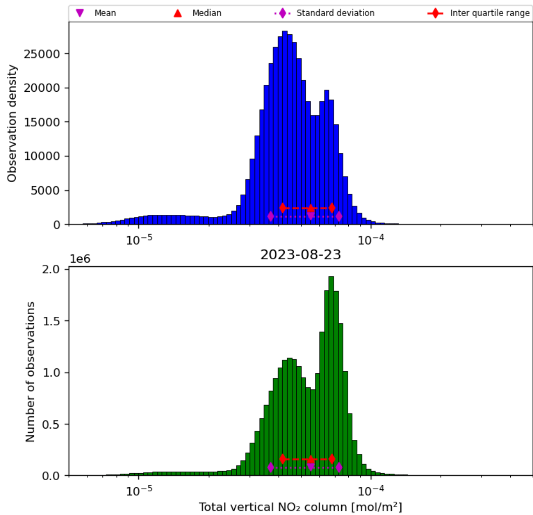
Figure 38: Histogram of “Total vertical NO 2 column” for 2023-08-22 to 2023-08-24
