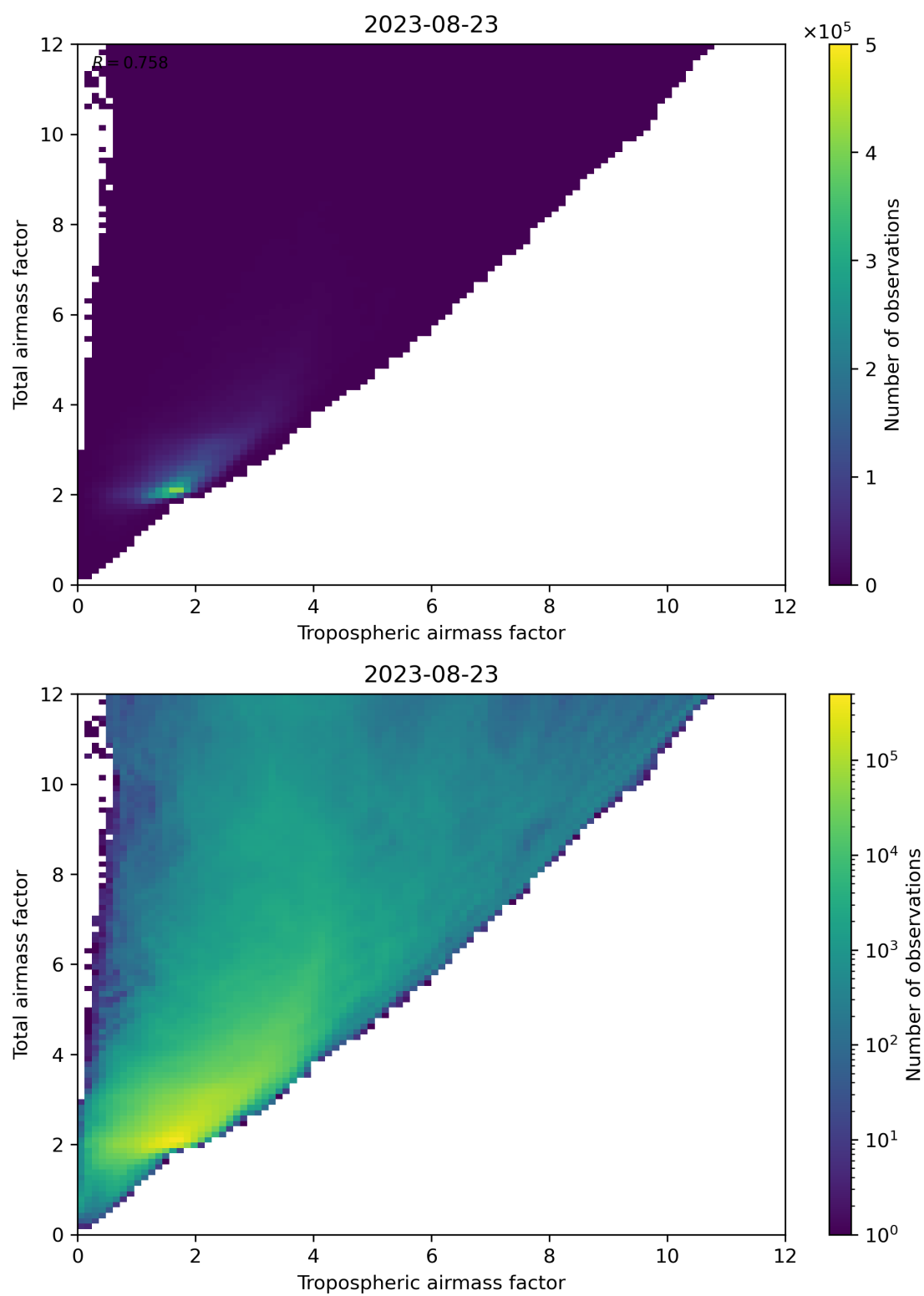
Figure 72: Scatter density plot of “Tropospheric airmass factor” against “Total airmass factor” for 2023-08-22 to 2023-08-24.
