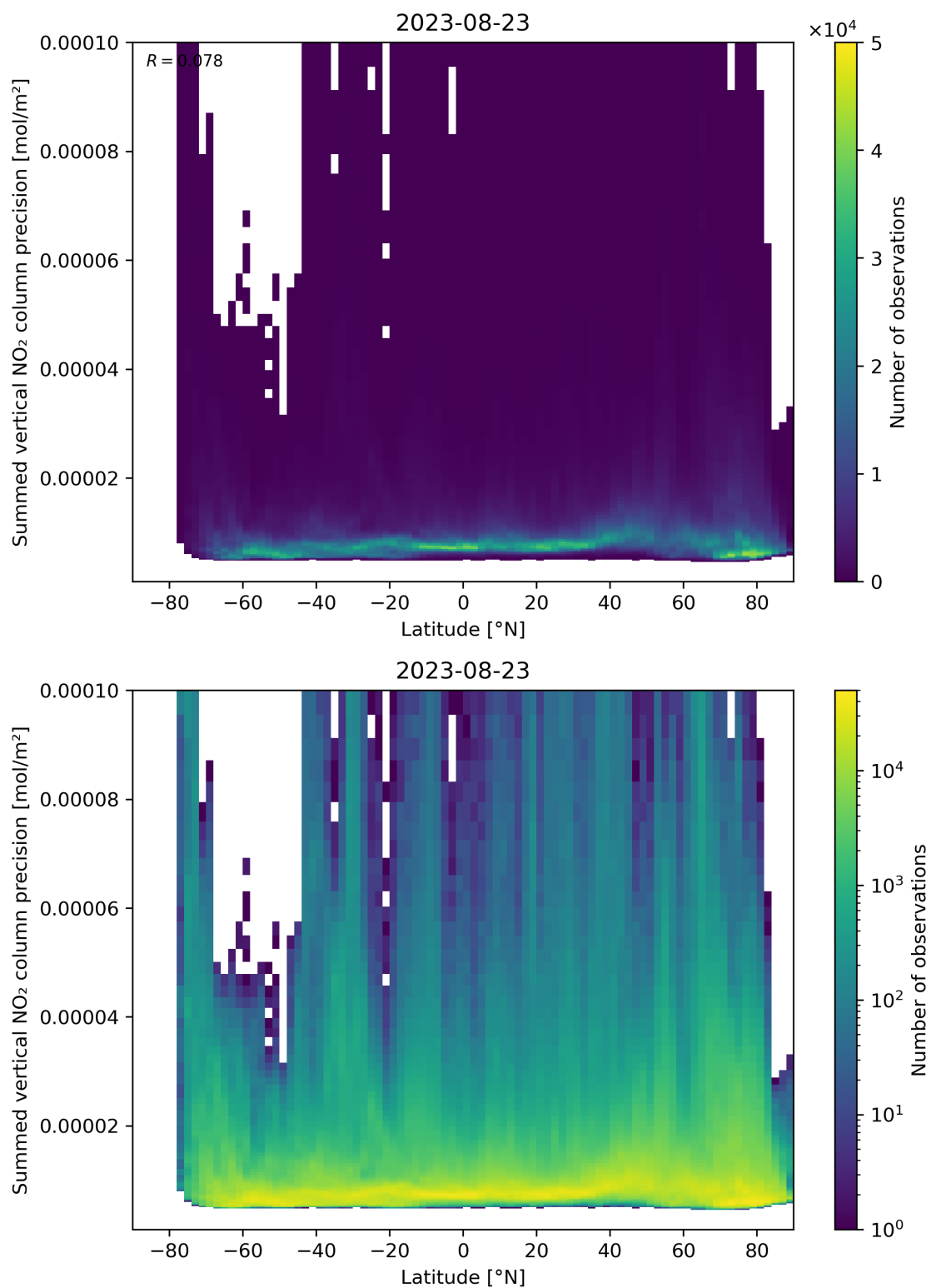
Figure 89: Scatter density plot of “Latitude” against “Summed vertical NO 2 column precision” for 2023-08-22 to 2023-08-24.
