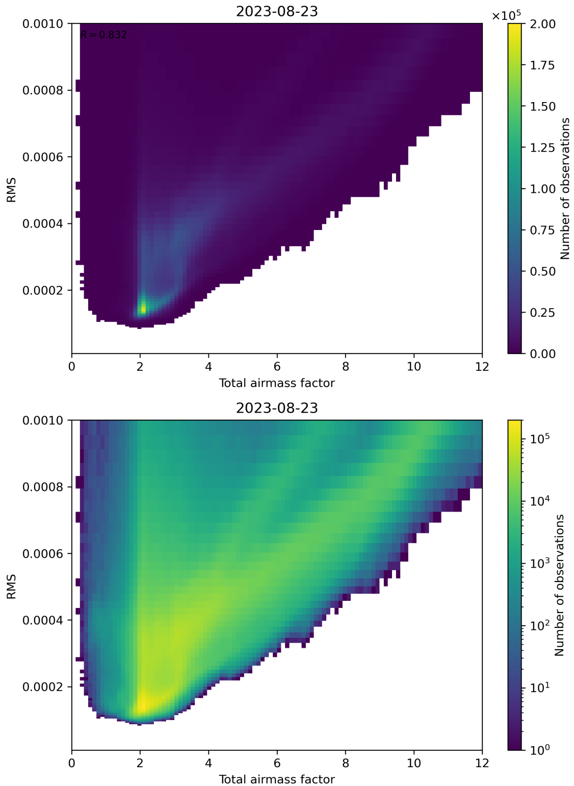
Figure 69: Scatter density plot of “Total airmass factor” against “RMS” for 2023-08-22 to 2023-08-24.
