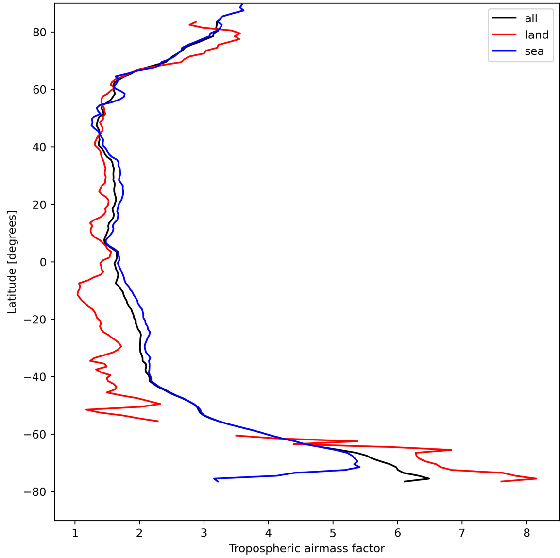
Figure 14: Zonal average of “Tropospheric airmass factor” for 2023-08-22 to 2023-08-24.
