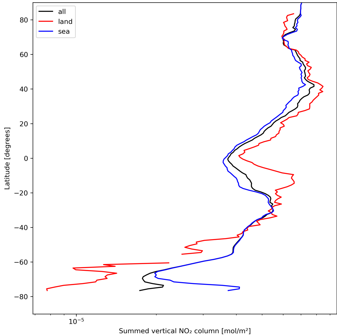
Figure 23: Zonal average of “Summed vertical NO 2 column” for 2023-08-22 to 2023-08-24.
