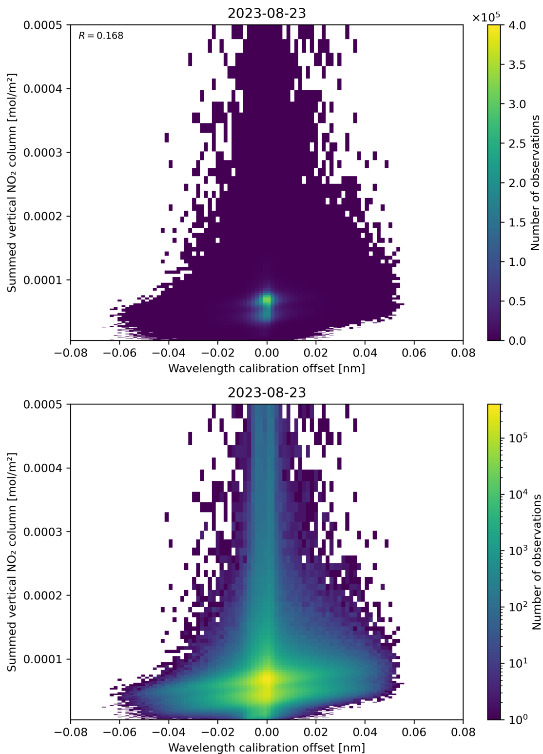
Figure 177: Scatter density plot of “Wavelength calibration offset” against “Summed vertical NO 2 column” for 2023-08-22 to 2023-08-24.
