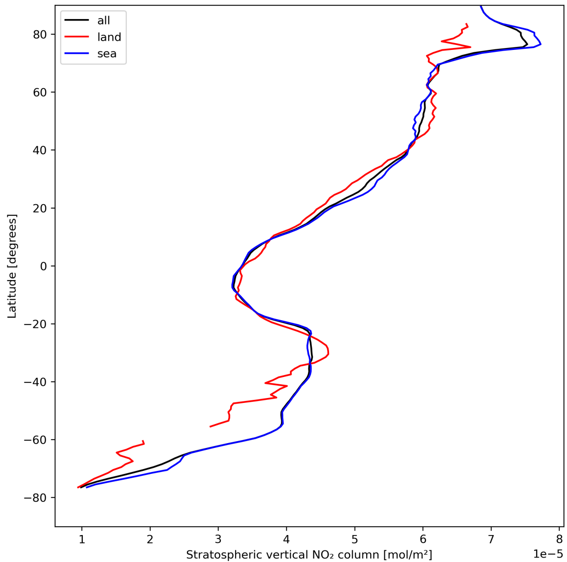
Figure 19: Zonal average of “Stratospheric vertical NO 2 column” for 2023-08-22 to 2023-08-24.
