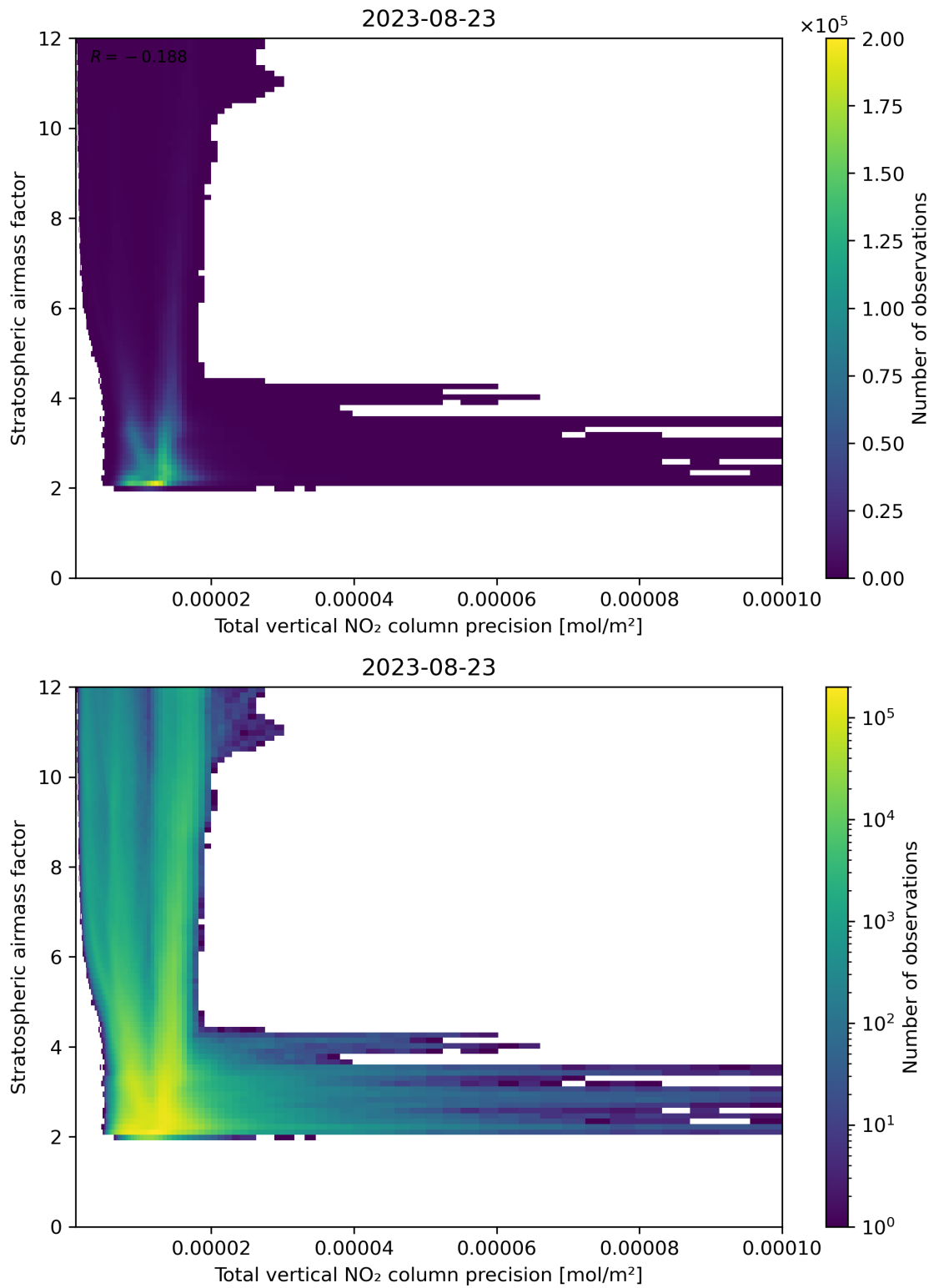
Figure 115: Scatter density plot of “Total vertical NO 2 column precision” against “Stratospheric air mass factor” for 2023-08-22 to 2023-08-24.
