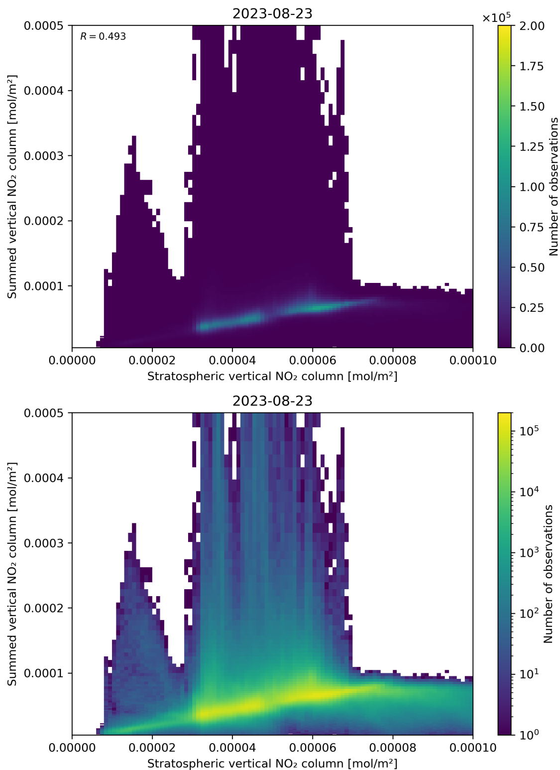
Figure 98: Scatter density plot of “Stratospheric vertical NO 2 column” against “Summed vertical NO 2 column” for 2023-08-22 to 2023-08-24.
