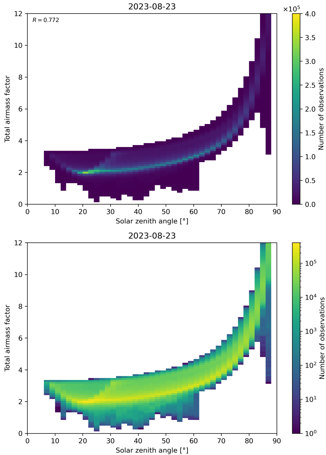
Figure 146: Scatter density plot of “Solar zenith angle” against “Total air mass factor” for 2023-08-22 to 2023-08-24.
