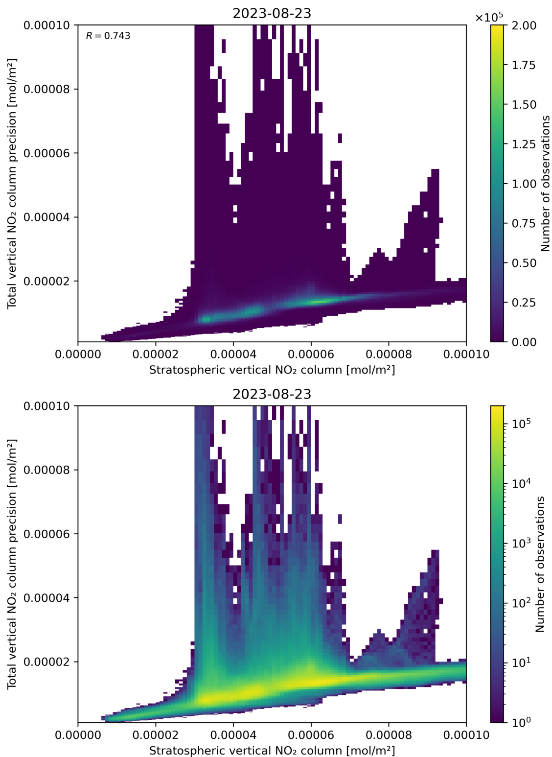
Figure 101: Scatter density plot of “Stratospheric vertical NO 2 column” against “Total vertical NO 2 column precision” for 2023-08-22 to 2023-08-24.
