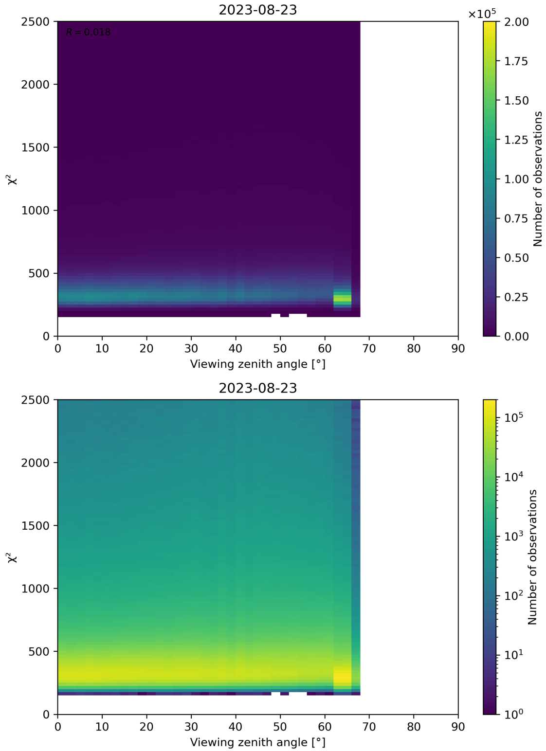
Figure 162: Scatter density plot of “Viewing zenith angle” against “ \chi^2 ” for 2023-08-22 to 2023-08-24.
