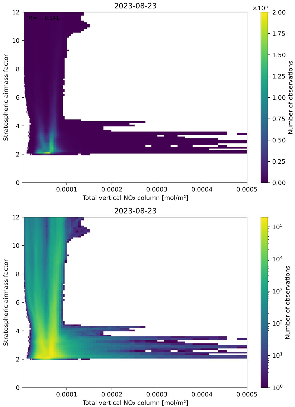
Figure 110: Scatter density plot of “Total vertical NO 2 column” against “Stratospheric air mass factor” for 2023-08-22 to 2023-08-24.
