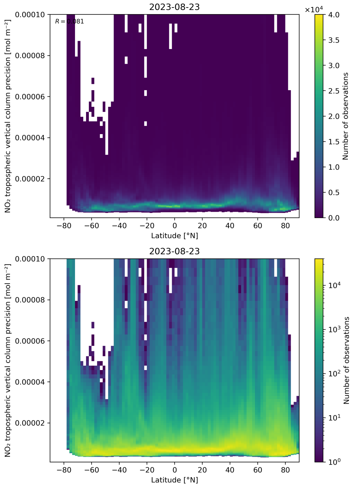
Figure 93: Scatter density plot of “Latitude” against “NO 2 tropospheric vertical column precision” for 2023-08-22 to 2023-08-24.
