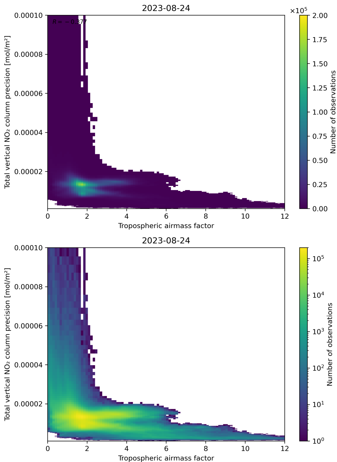
Figure 78: Scatter density plot of “Tropospheric air mass factor” against “Total vertical NO 2 column precision” for 2023-08-23 to 2023-08-25.
