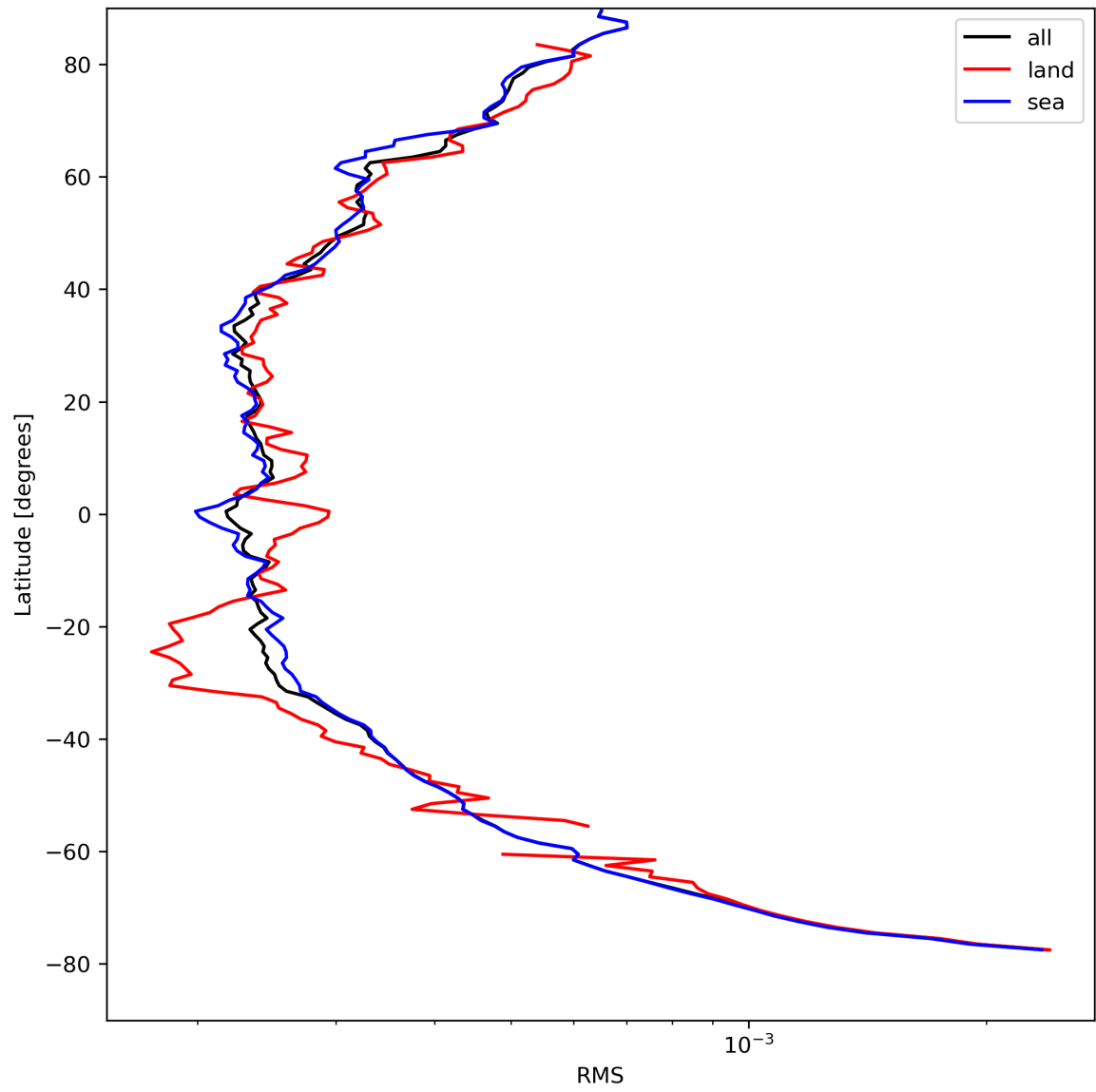
Figure 26: Zonal average of “RMS” for 2023-08-23 to 2023-08-25.
