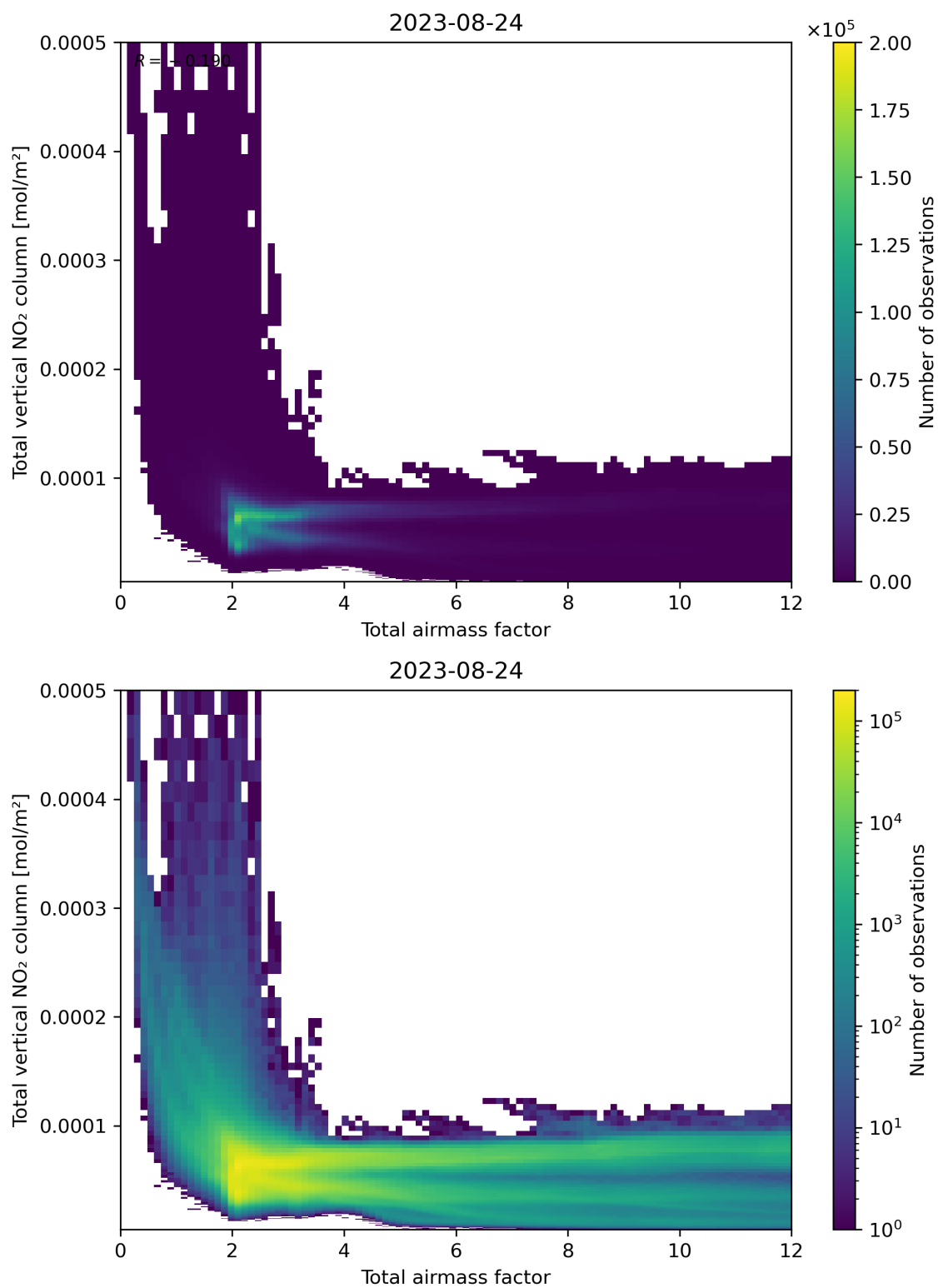
Figure 67: Scatter density plot of “Total airmass factor” against “Total vertical NO 2 column” for 2023-08-23 to 2023-08-25.
