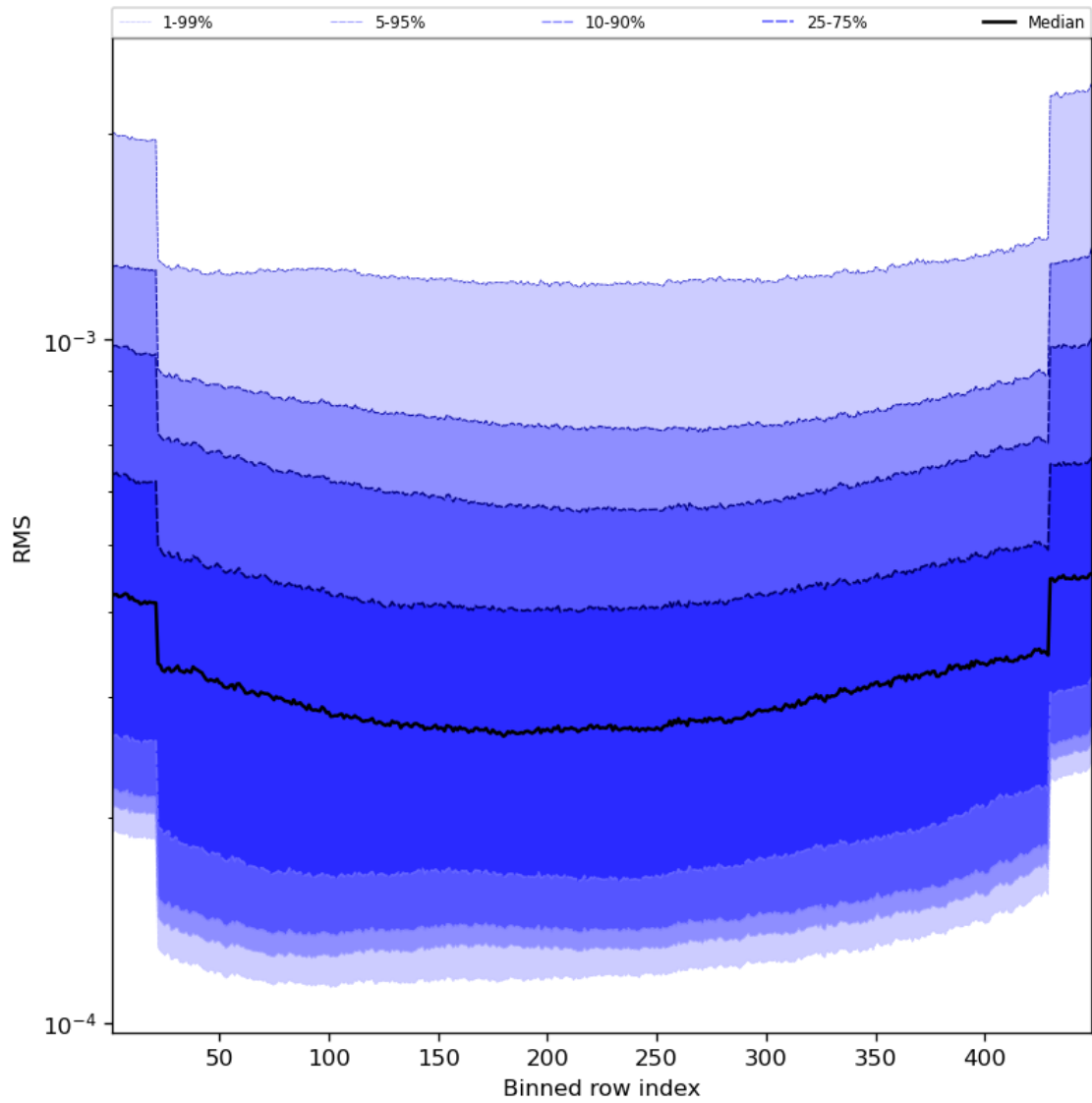
Figure 60: Along track statistics of “RMS” for 2023-08-23 to 2023-08-25
