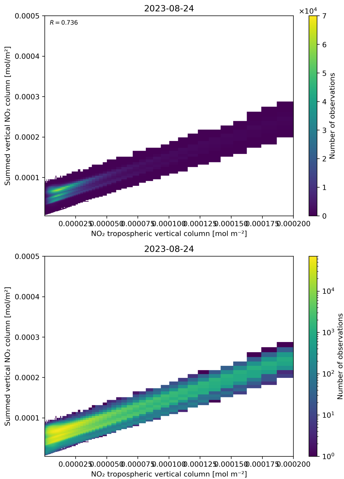
Figure 126: Scatter density plot of “NO 2 tropospheric vertical column” against “Summed vertical NO 2 column” for 2023-08-23 to 2023-08-25.
