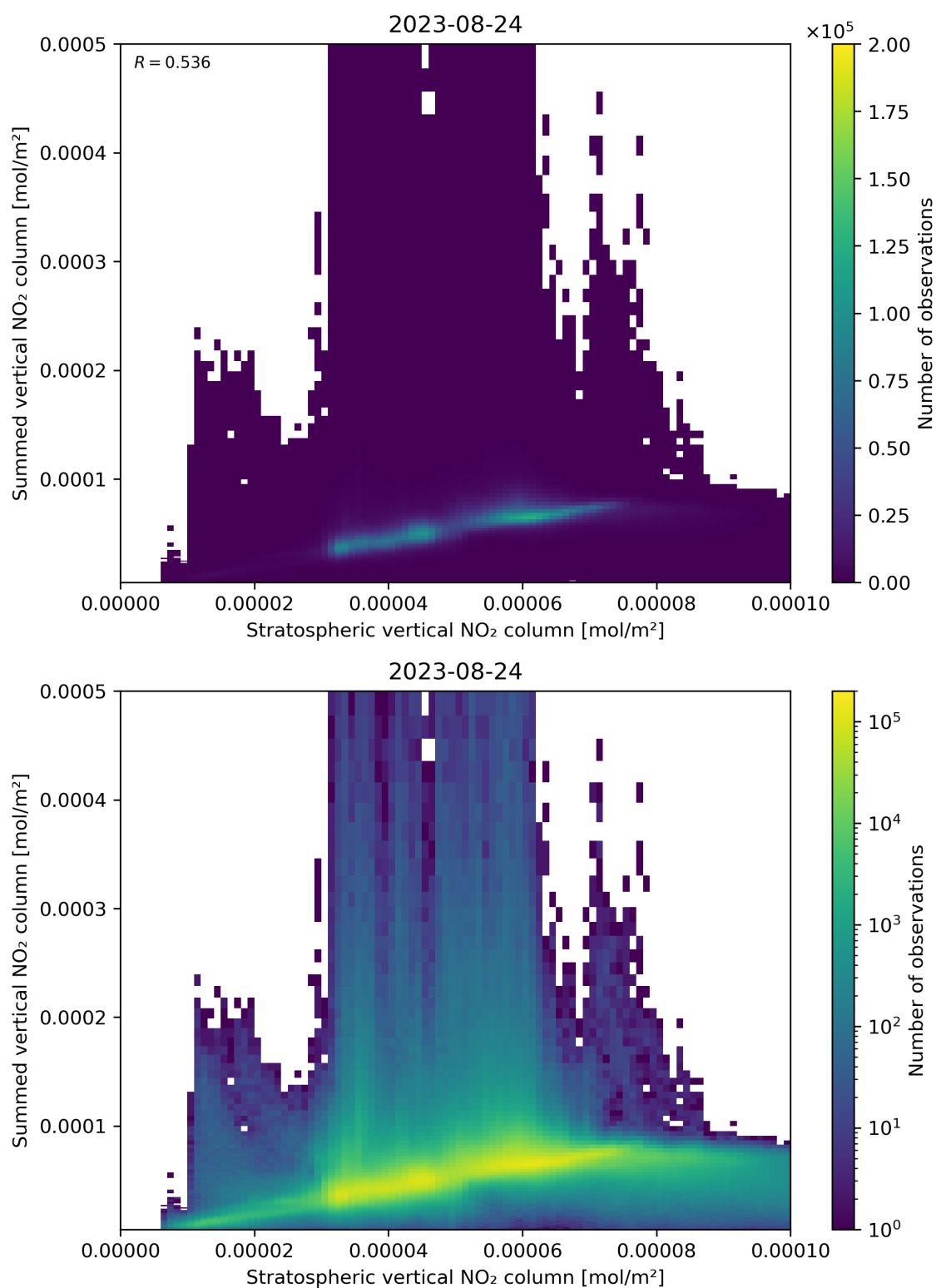
Figure 98: Scatter density plot of “Stratospheric vertical NO 2 column” against “Summed vertical NO 2 column” for 2023-08-23 to 2023-08-25.
