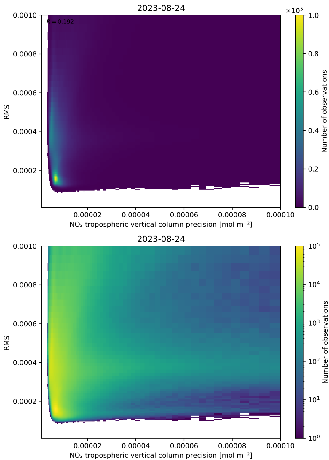
Figure 140: Scatter density plot of “NO 2 tropospheric vertical column precision” against “RMS” for 2023-08-23 to 2023-08-25.
