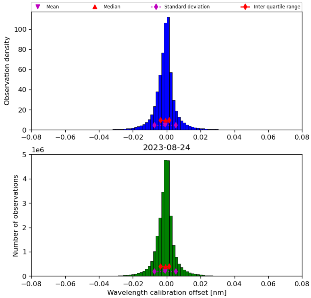
Figure 35: Histogram of “Wavelength calibration offset” for 2023-08-23 to 2023-08-25
