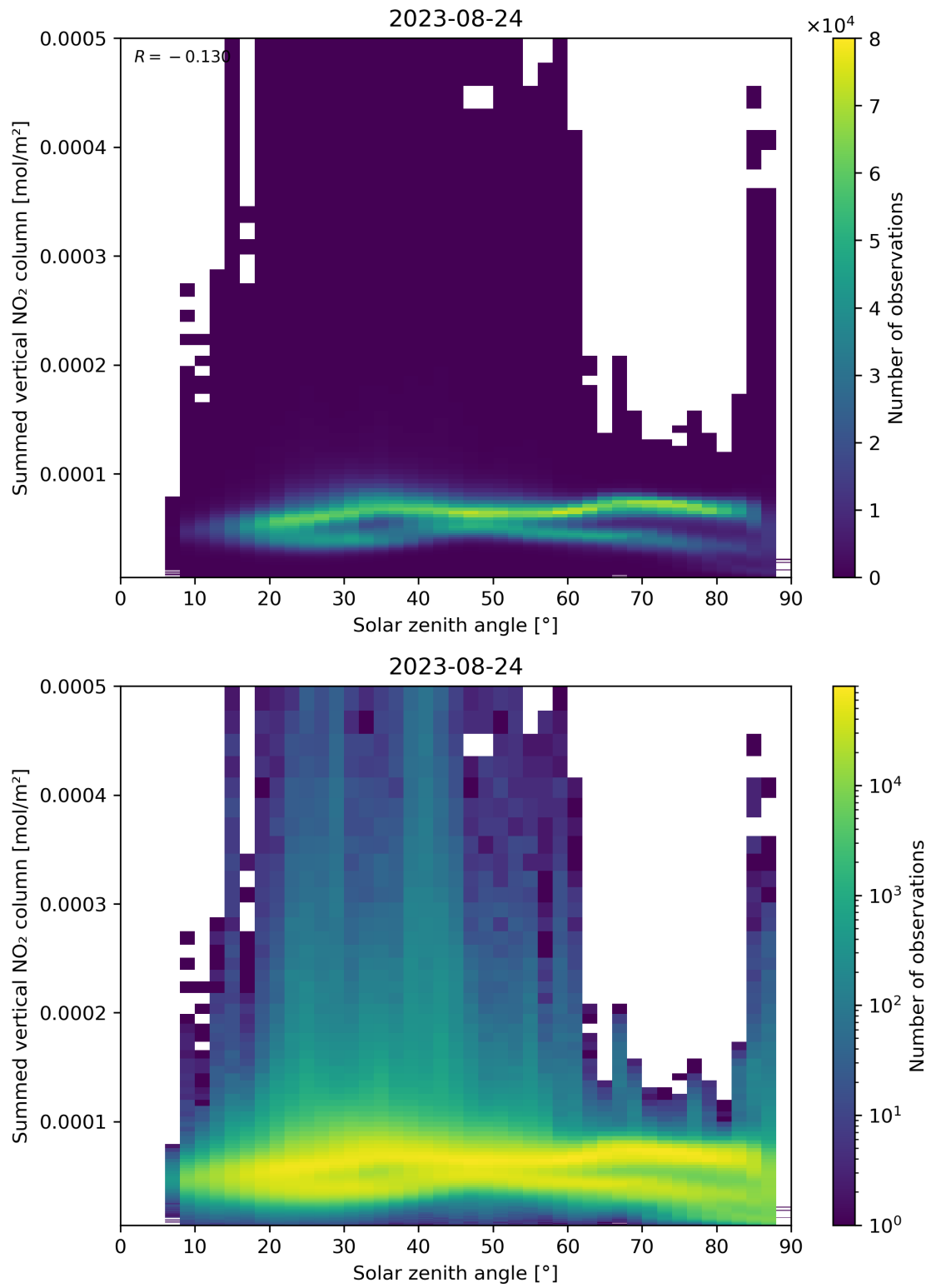
Figure 151: Scatter density plot of “Solar zenith angle” against “Summed vertical NO 2 column” for 2023-08-23 to 2023-08-25.
