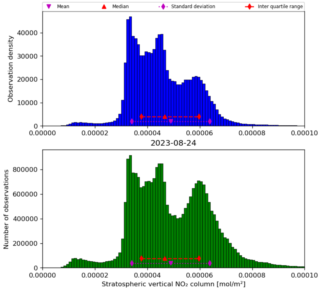
Figure 36: Histogram of “Stratospheric vertical NO 2 column” for 2023-08-23 to 2023-08-25
