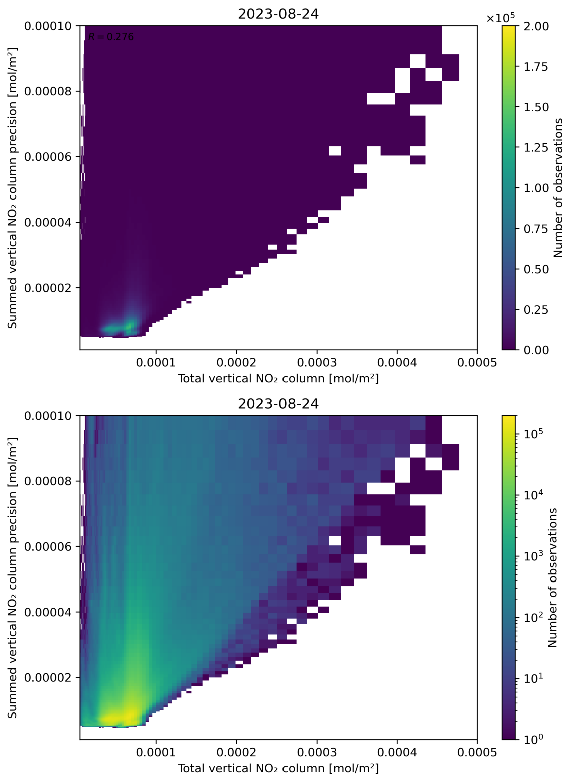
Figure 113: Scatter density plot of “Total vertical NO 2 column” against “Summed vertical NO 2 column precision” for 2023-08-23 to 2023-08-25.
