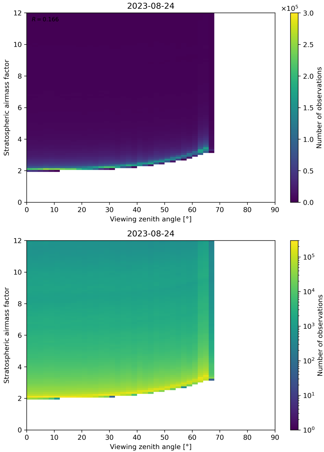
Figure 159: Scatter density plot of “Viewing zenith angle” against “Stratospheric airmass factor” for 2023-08-23 to 2023-08-25.
