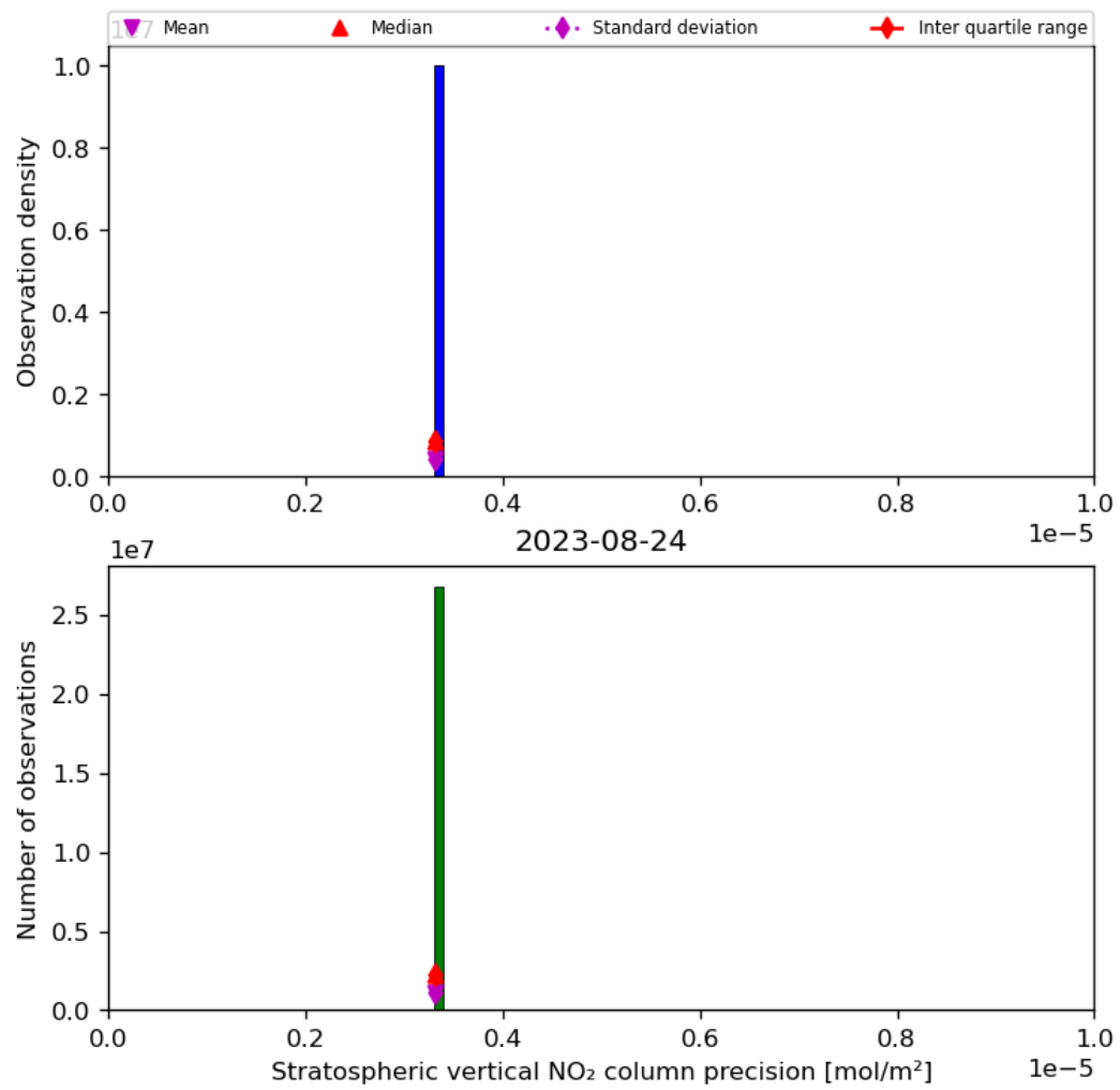
Figure 37: Histogram of “Stratospheric vertical NO 2 column precision” for 2023-08-23 to 2023-08-25
