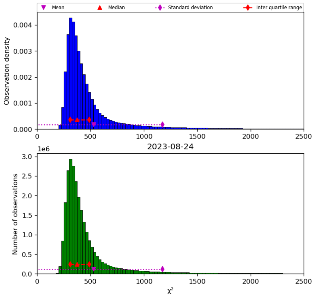
Figure 42: Histogram of " \chi^2 " for 2023-08-23 to 2023-08-25
