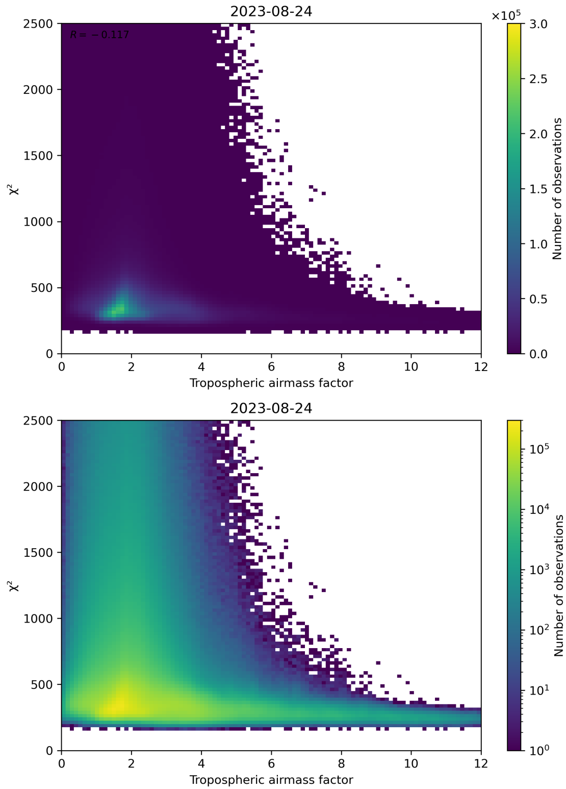
Figure 73: Scatter density plot of “Tropospheric airmass factor” against “ \chi^2 ” for 2023-08-23 to 2023-08-25.
