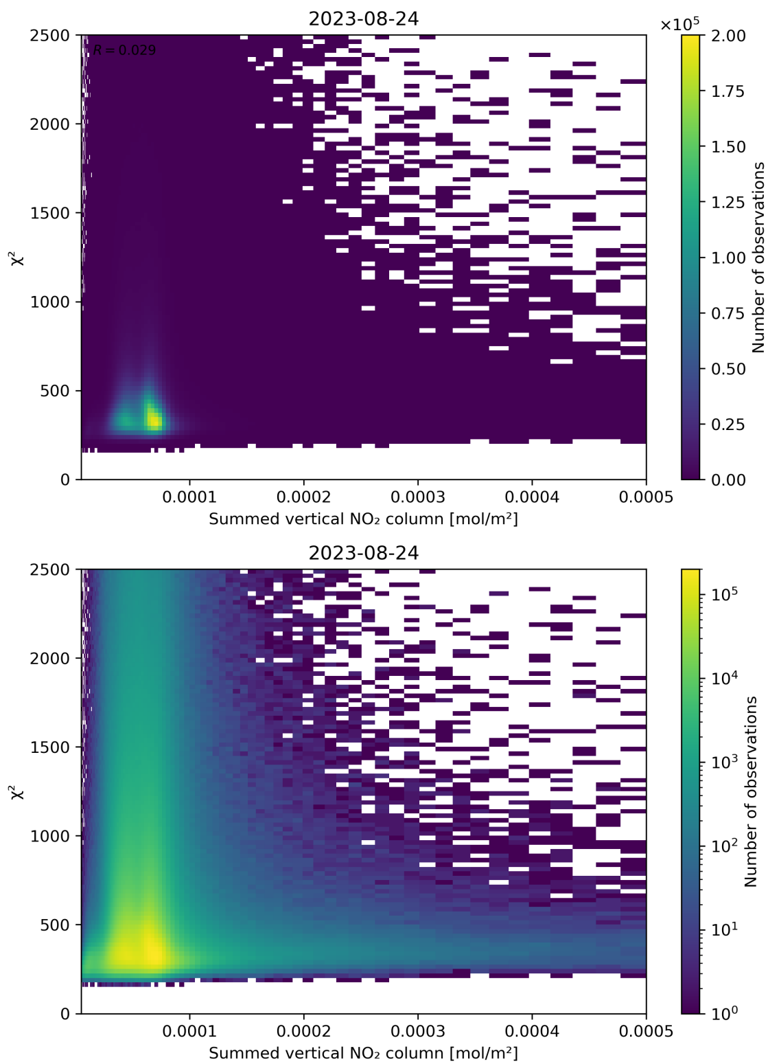
Figure 104: Scatter density plot of “Summed vertical NO 2 column” against “ \chi^2 ” for 2023-08-23 to 2023-08-25.
