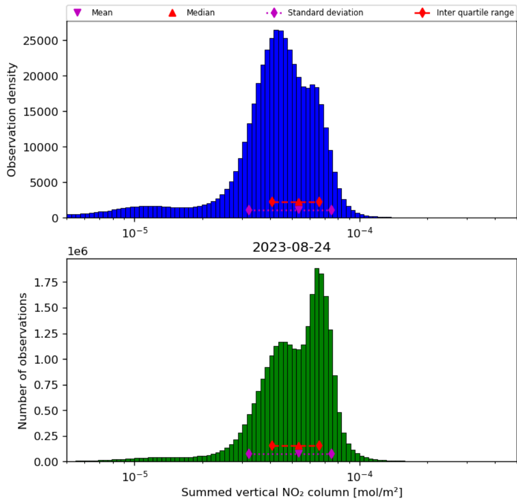
Figure 40: Histogram of "Summed vertical NO 2 column" for 2023-08-23 to 2023-08-25
