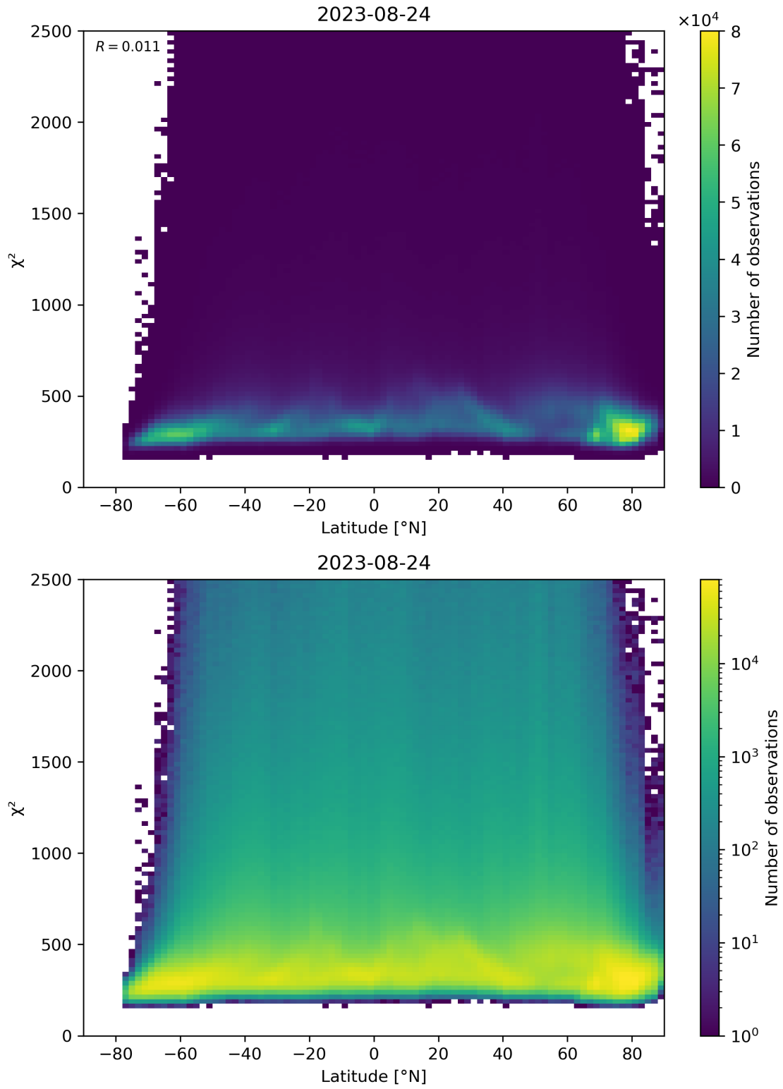
Figure 86: Scatter density plot of “Latitude” against “ \chi^2 ” for 2023-08-23 to 2023-08-25.
