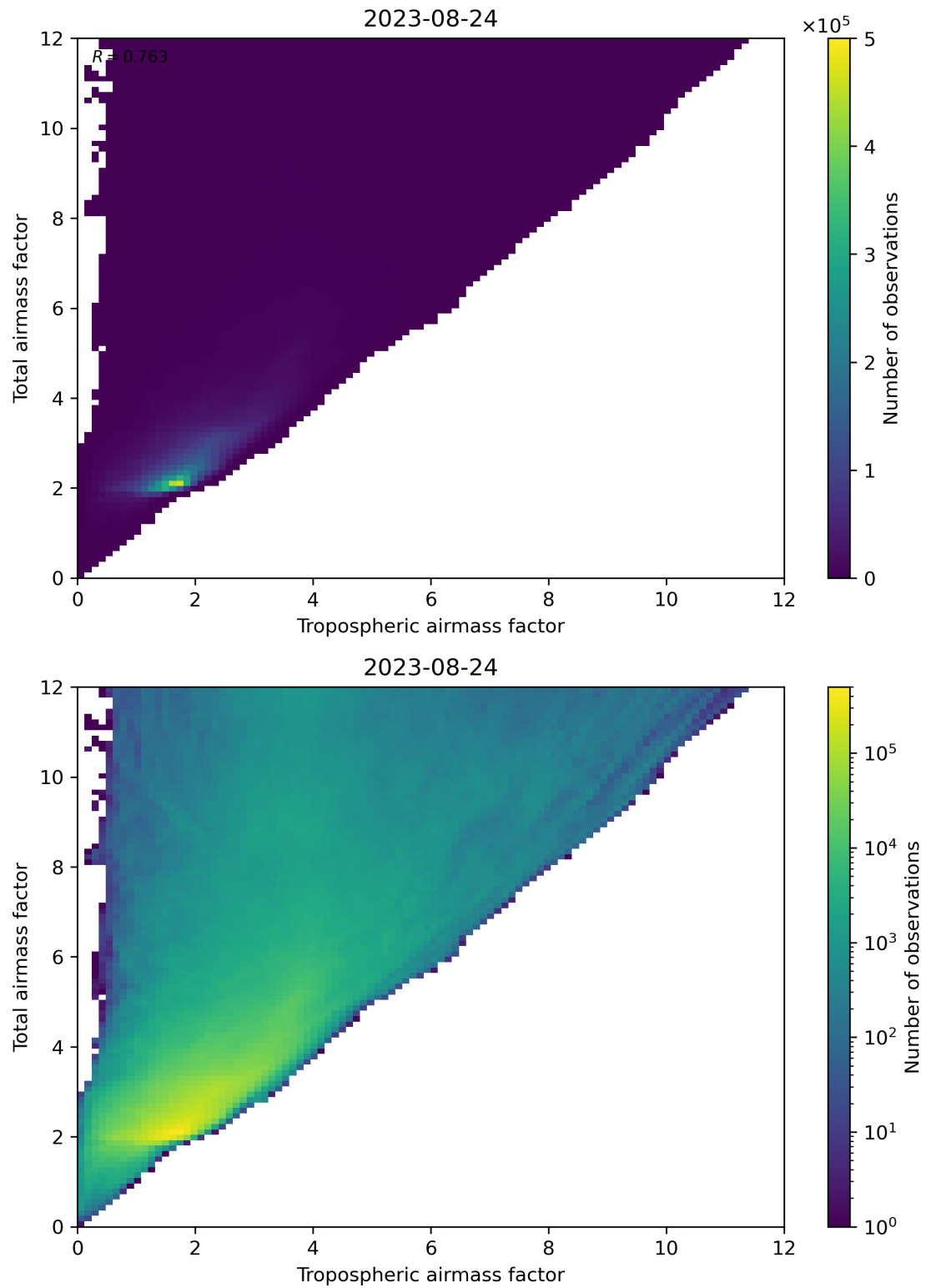
Figure 72: Scatter density plot of “Tropospheric airmass factor” against “Total airmass factor” for 2023-08-23 to 2023-08-25.
