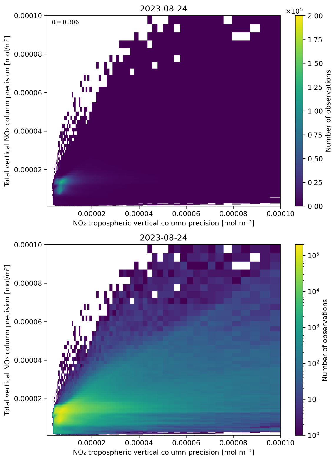
Figure 139: Scatter density plot of “NO 2 tropospheric vertical column precision” against “Total vertical NO 2 column precision” for 2023-08-23 to 2023-08-25.
