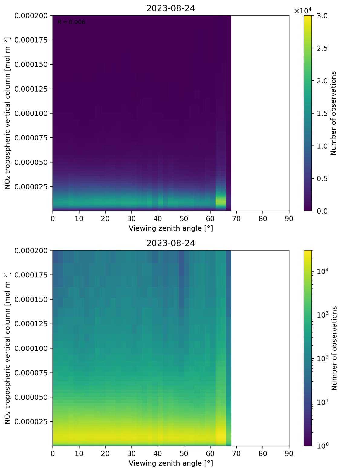
Figure 169: Scatter density plot of “Viewing zenith angle” against “NO 2 tropospheric vertical column” for 2023-08-23 to 2023-08-25.
