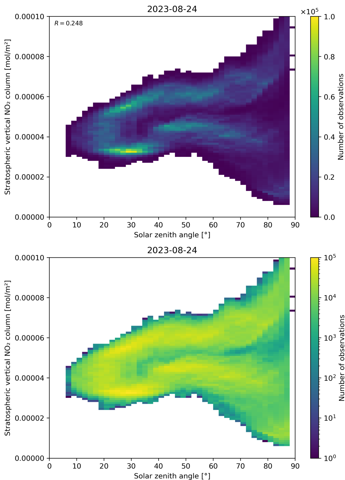
Figure 150: Scatter density plot of “Solar zenith angle” against “Stratospheric vertical NO 2 column” for 2023-08-23 to 2023-08-25.
