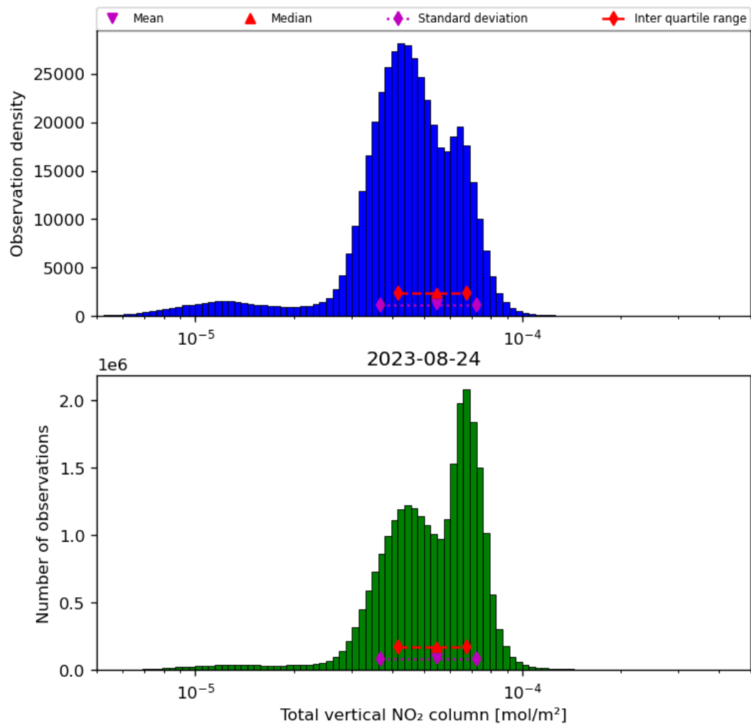
Figure 38: Histogram of “Total vertical NO 2 column” for 2023-08-23 to 2023-08-25
