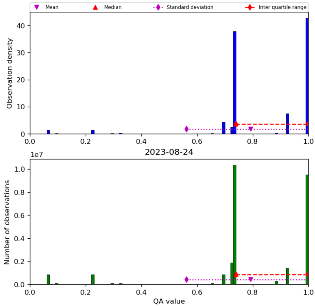
Figure 28: Histogram of “QA value” for 2023-08-23 to 2023-08-25
