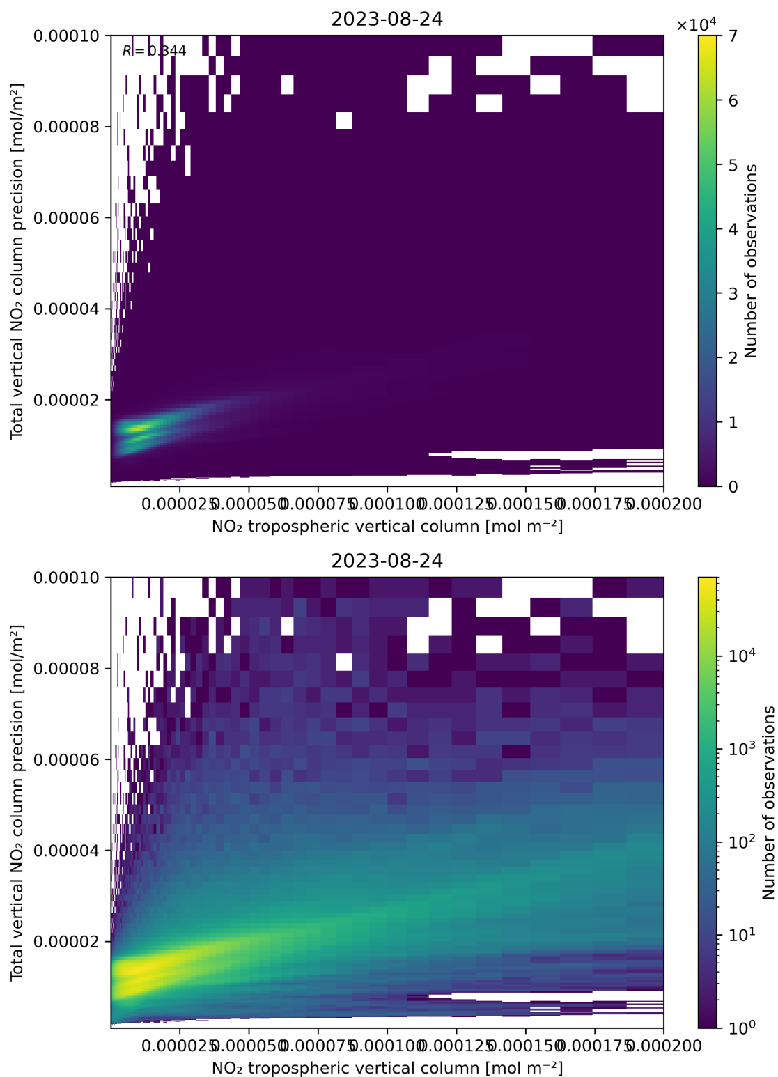
Figure 129: Scatter density plot of “NO 2 tropospheric vertical column” against “Total vertical NO 2 column precision” for 2023-08-23 to 2023-08-25.
