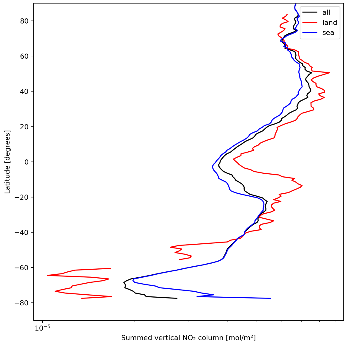
Figure 23: Zonal average of “Summed vertical NO 2 column” for 2023-08-23 to 2023-08-25.
