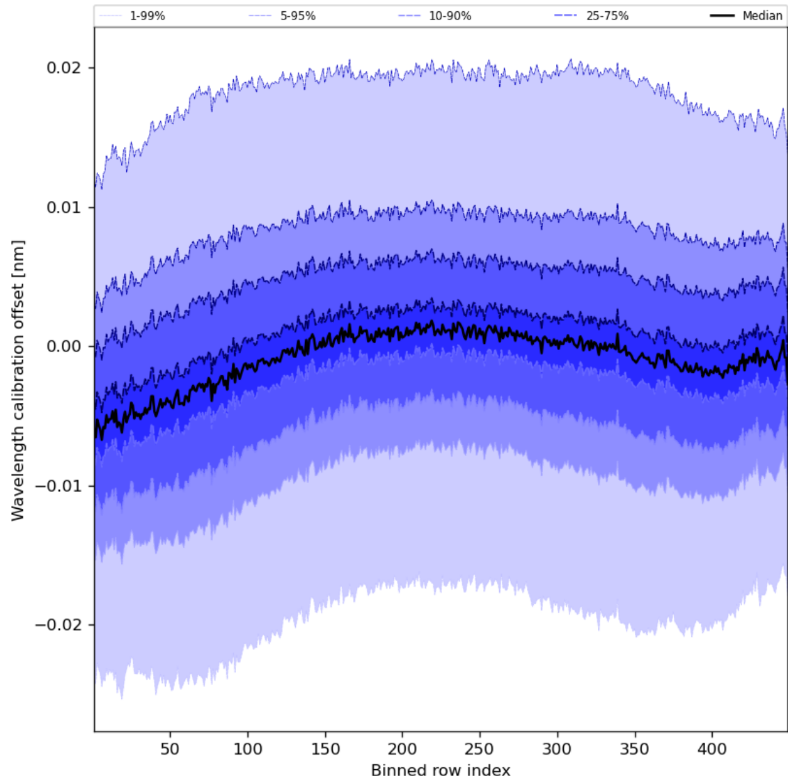
Figure 52: Along track statistics of “Wavelength calibration offset” for 2023-08-23 to 2023-08-25
