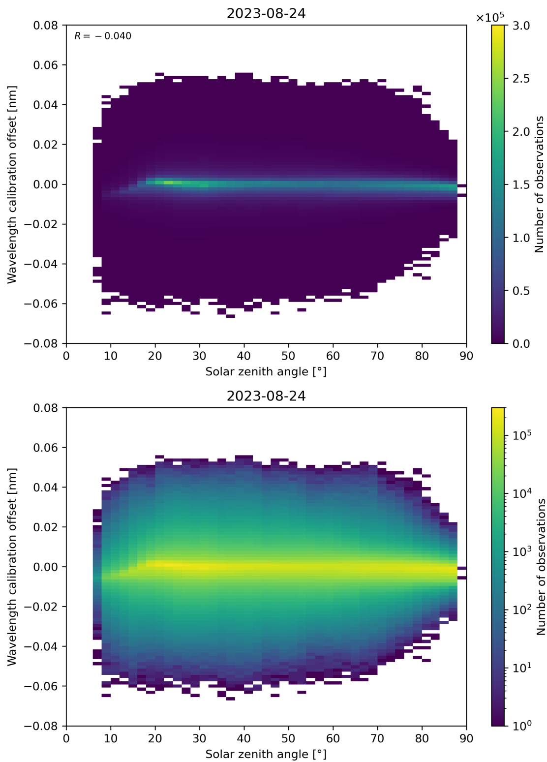
Figure 158: Scatter density plot of “Solar zenith angle” against “Wavelength calibration offset” for 2023-08-23 to 2023-08-25.
