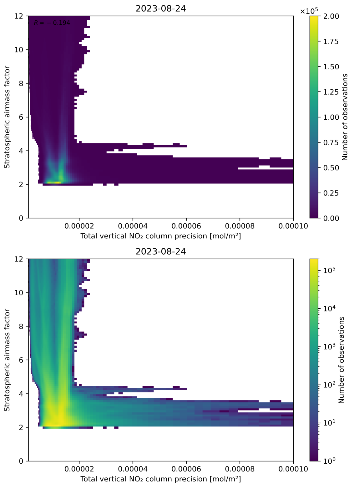
Figure 115: Scatter density plot of “Total vertical NO 2 column precision” against “Stratospheric air mass factor” for 2023-08-23 to 2023-08-25.
