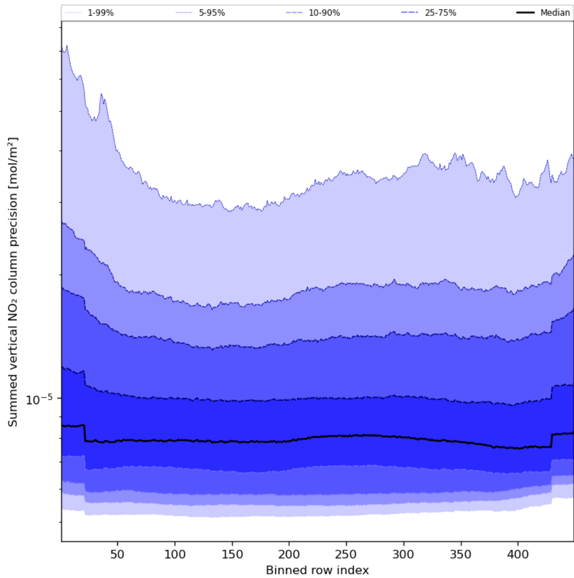
Figure 58: Along track statistics of “Summed vertical NO 2 column precision” for 2023-08-23 to 2023-08-25
