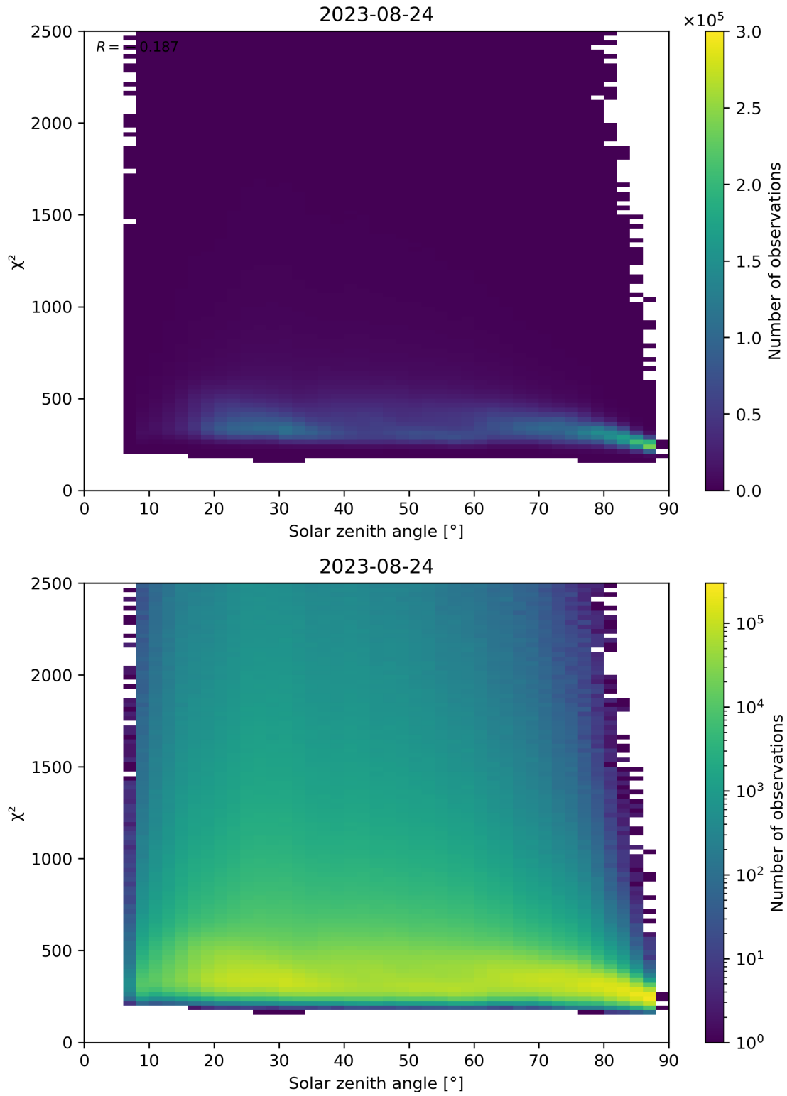
Figure 148: Scatter density plot of “Solar zenith angle” against “ \chi^2 ” for 2023-08-23 to 2023-08-25.
