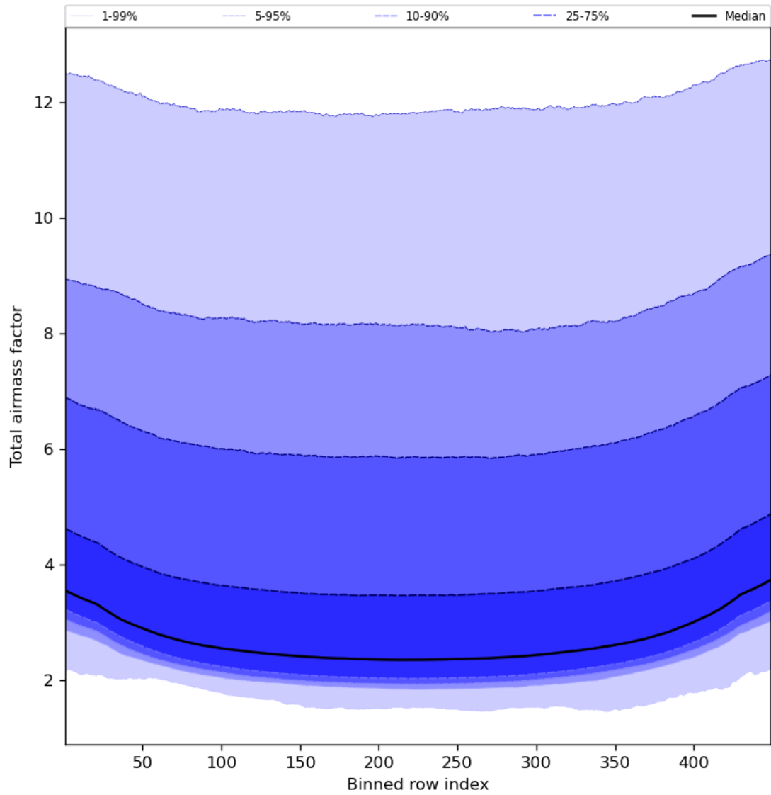
Figure 49: Along track statistics of “Total airmass factor” for 2023-08-23 to 2023-08-25
