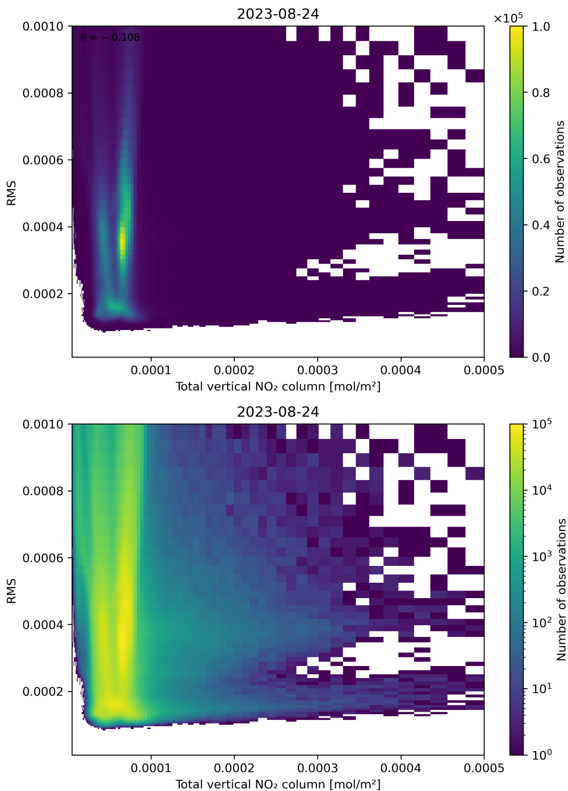
Figure 120: Scatter density plot of “Total vertical NO 2 column” against “RMS” for 2023-08-23 to 2023-08-25.
