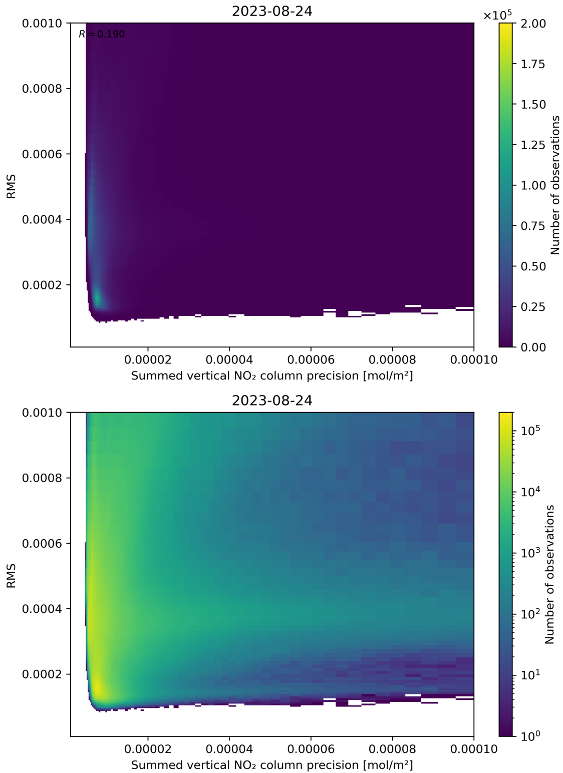
Figure 108: Scatter density plot of “Summed vertical NO 2 column precision” against “RMS” for 2023-08-23 to 2023-08-25.
