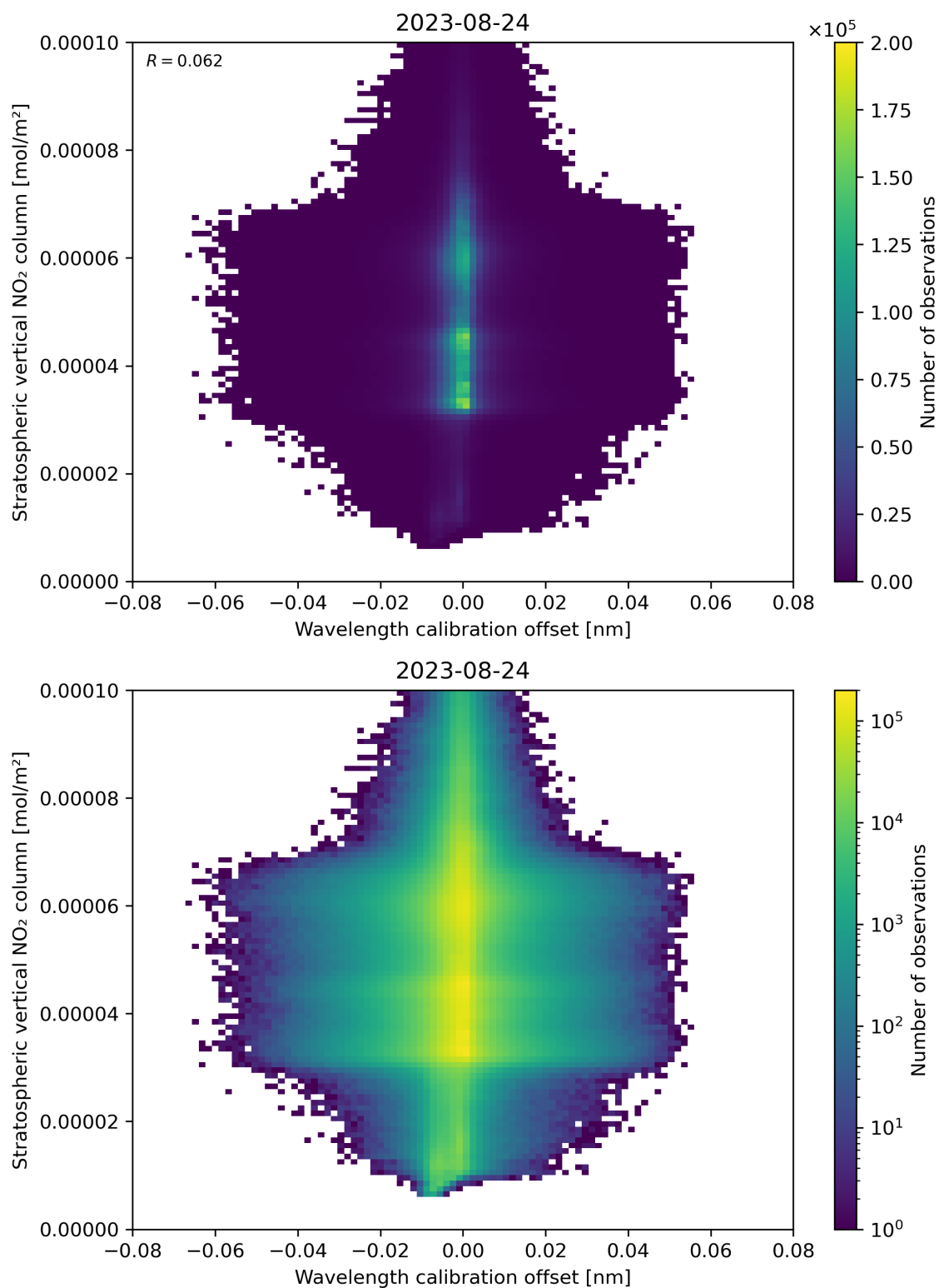
Figure 176: Scatter density plot of “Wavelength calibration offset” against “Stratospheric vertical NO 2 column” for 2023-08-23 to 2023-08-25.
