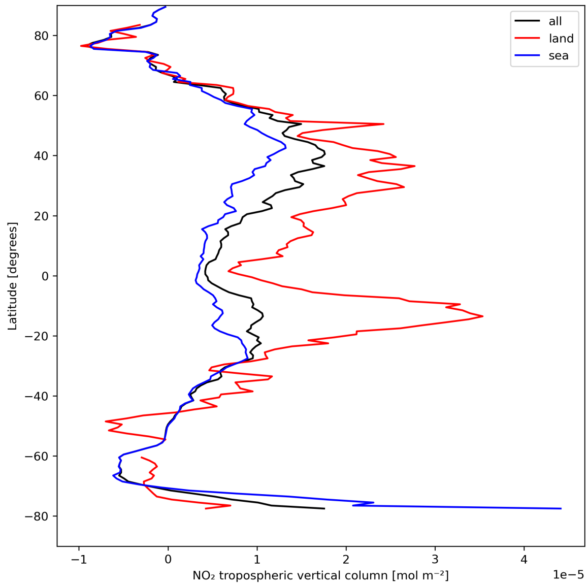
Figure 12: Zonal average of “NO 2 tropospheric vertical column” for 2023-08-23 to 2023-08-25.
