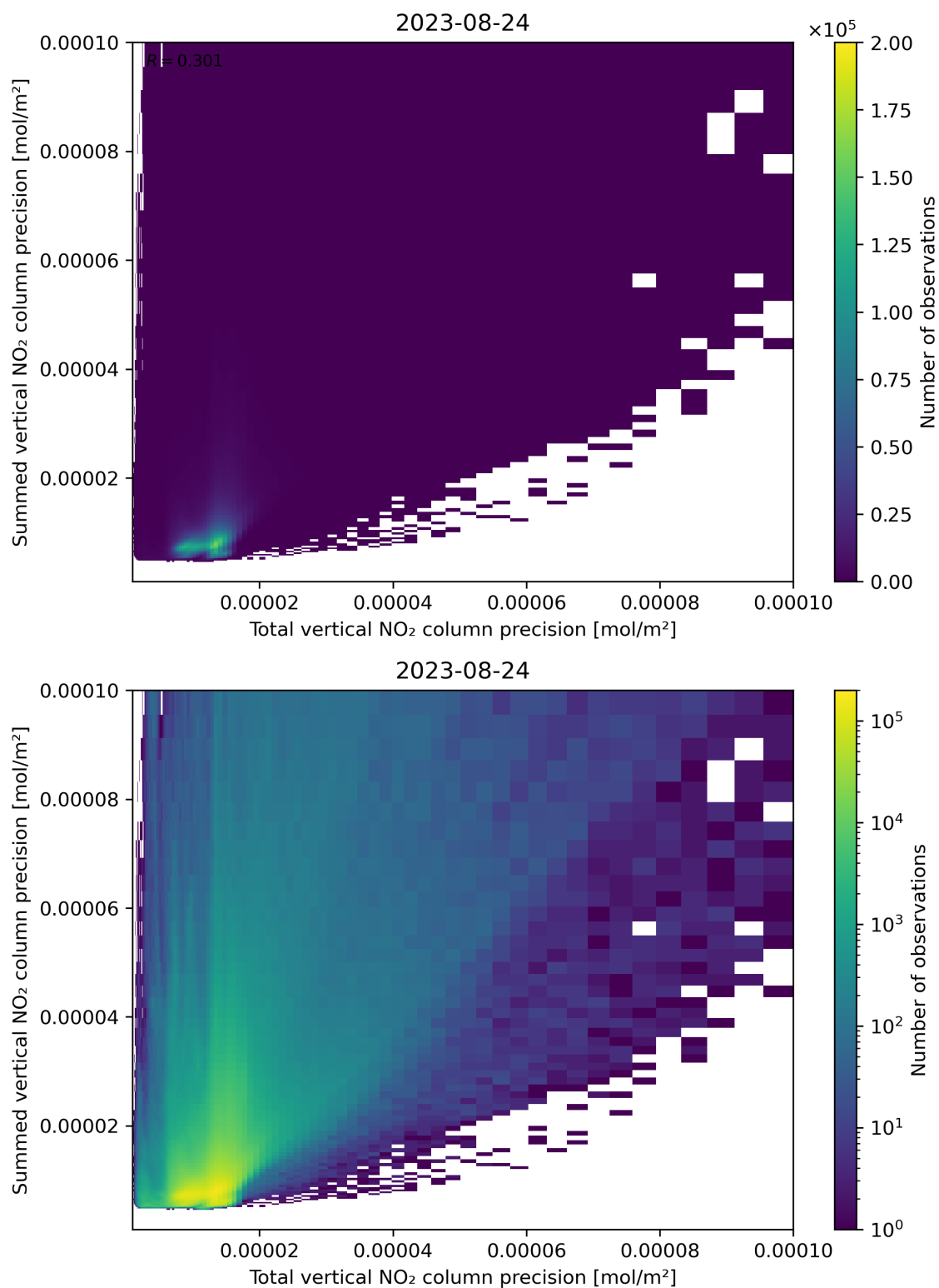
Figure 118: Scatter density plot of “Total vertical NO 2 column precision” against “Summed vertical NO 2 column precision” for 2023-08-23 to 2023-08-25.
