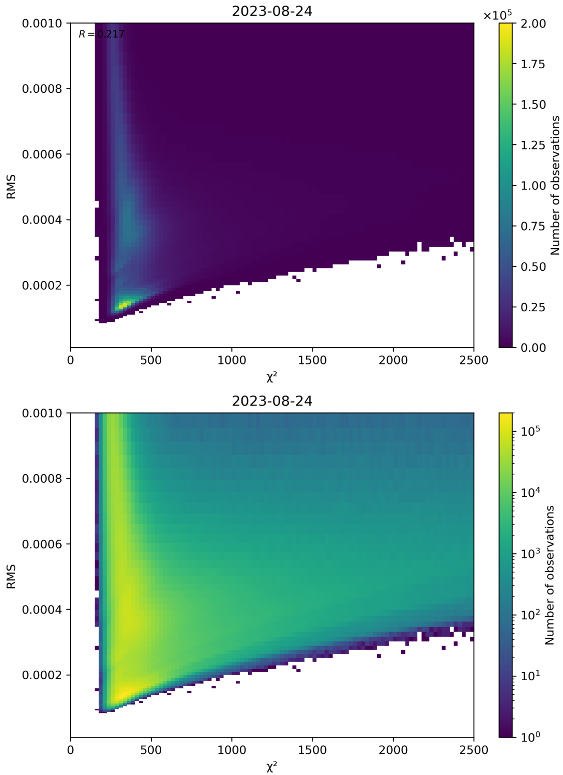
Figure 82: Scatter density plot of “ \chi^2 ” against “RMS” for 2023-08-23 to 2023-08-25.
