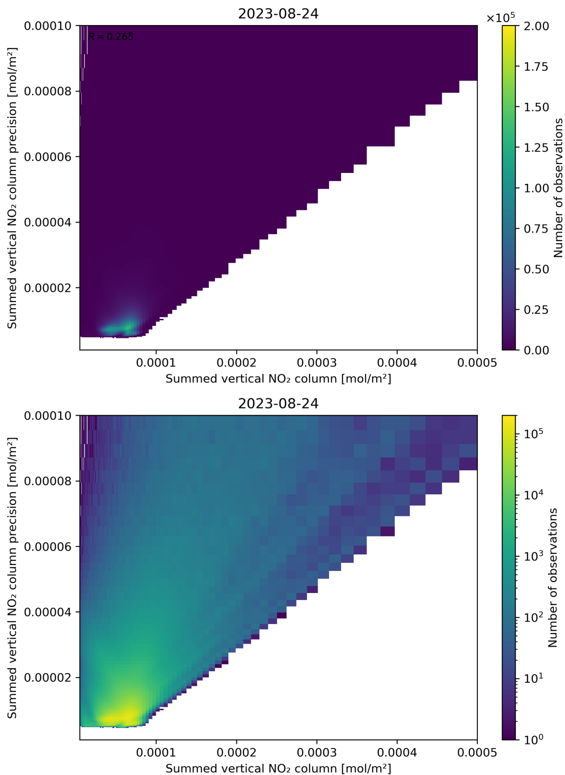
Figure 105: Scatter density plot of “Summed vertical NO 2 column” against “Summed vertical NO 2 column precision” for 2023-08-23 to 2023-08-25.
