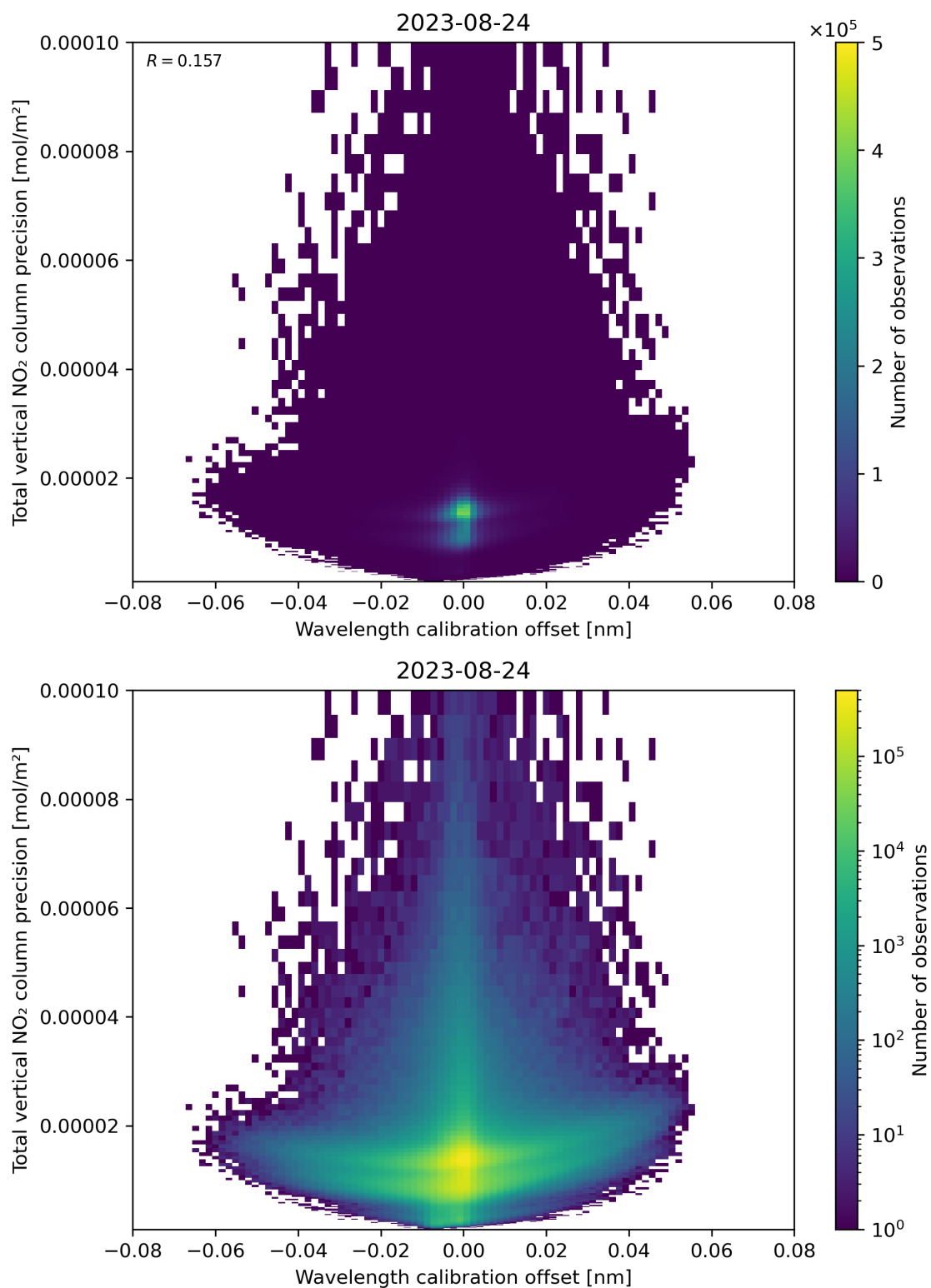
Figure 180: Scatter density plot of “Wavelength calibration offset” against “Total vertical NO 2 column precision” for 2023-08-23 to 2023-08-25.
