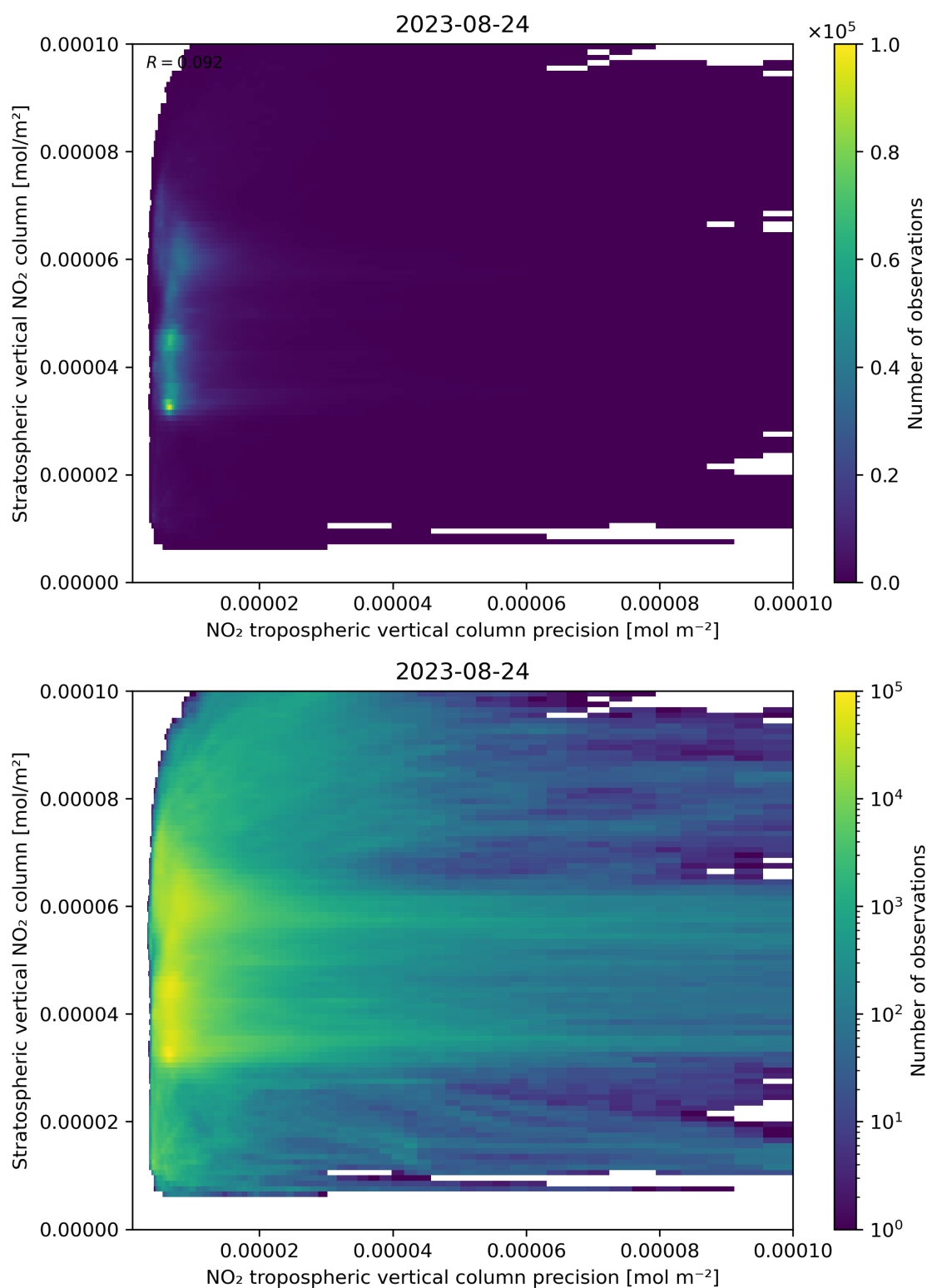
Figure 135: Scatter density plot of “NO 2 tropospheric vertical column precision” against “Stratospheric vertical NO 2 column” for 2023-08-23 to 2023-08-25.
