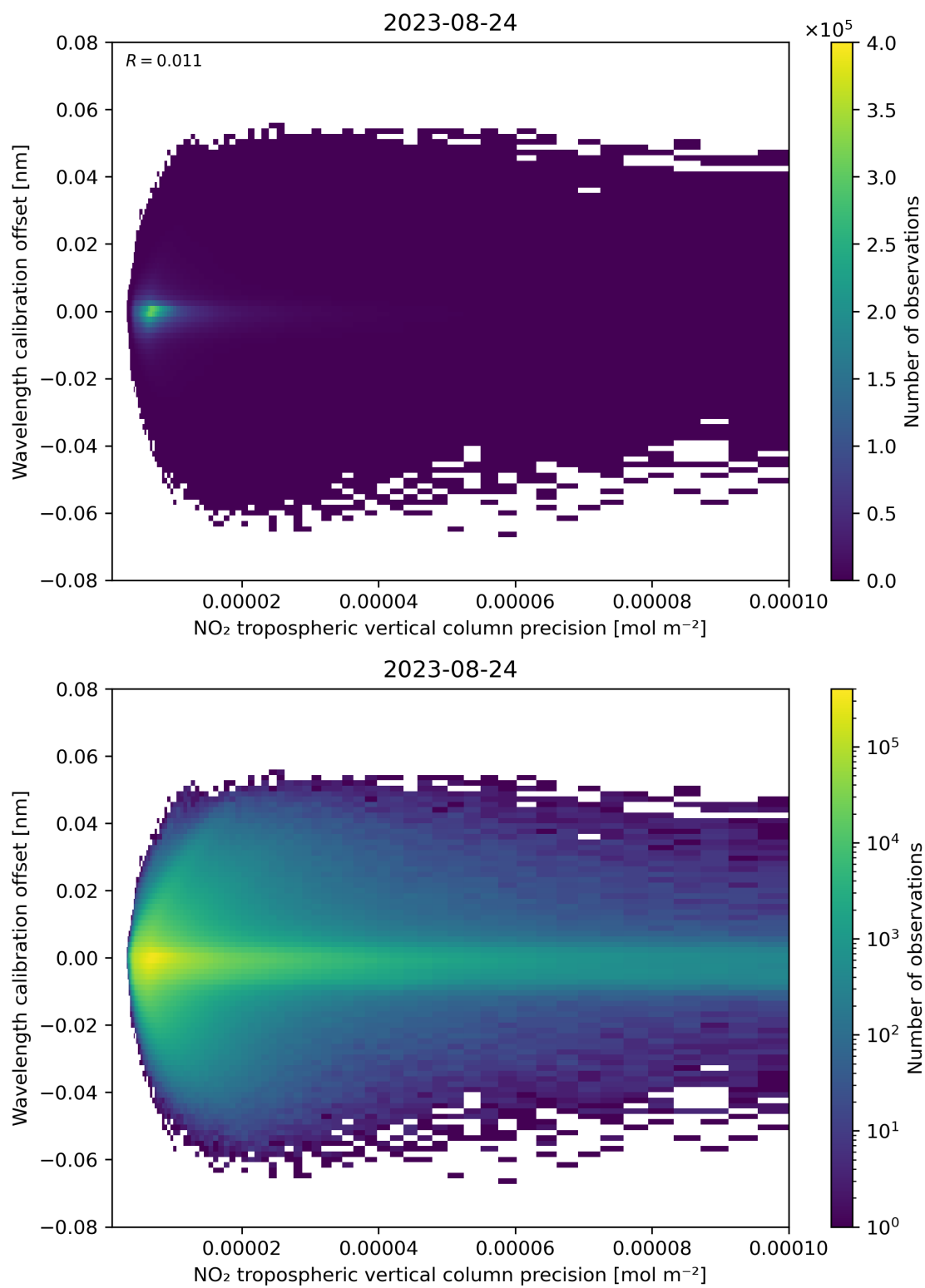
Figure 141: Scatter density plot of “NO 2 tropospheric vertical column precision” against “Wavelength calibration offset” for 2023-08-23 to 2023-08-25.
