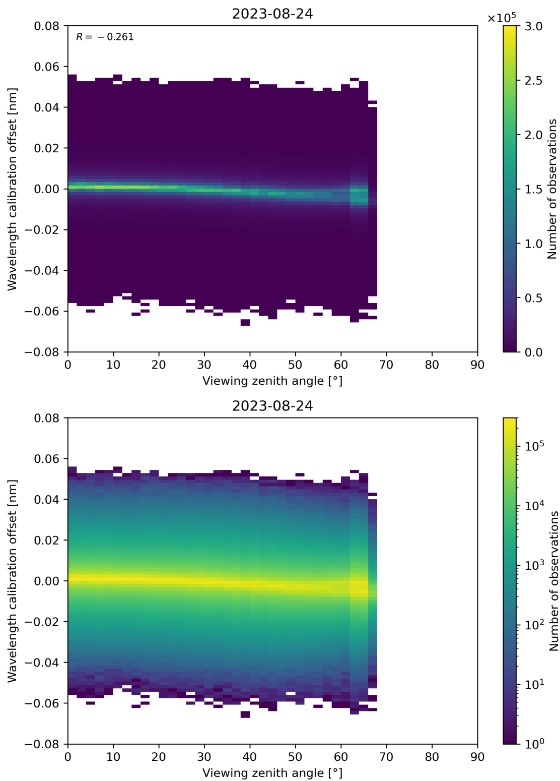
Figure 173: Scatter density plot of “Viewing zenith angle” against “Wavelength calibration offset” for 2023-08-23 to 2023-08-25.
