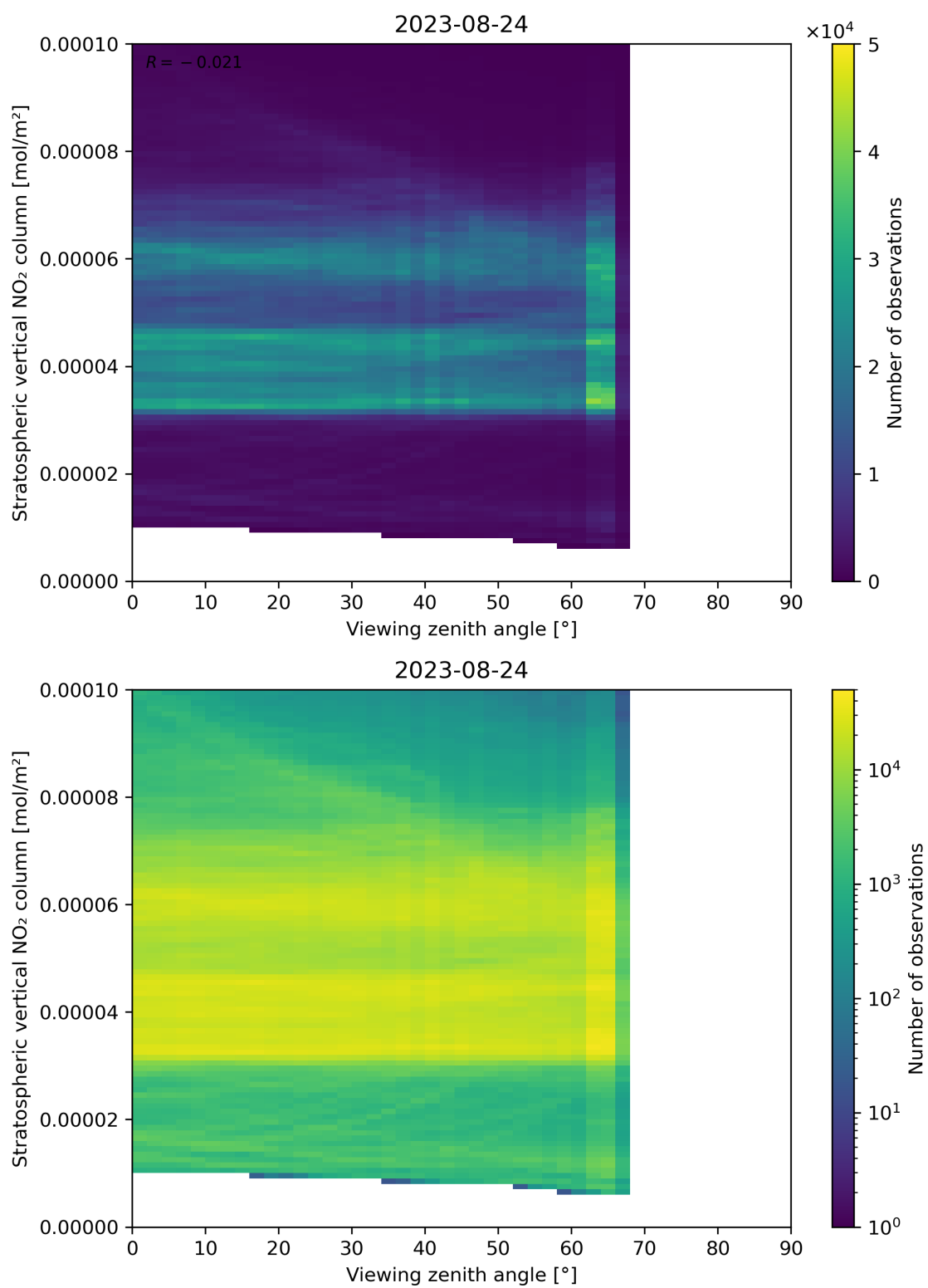
Figure 164: Scatter density plot of “Viewing zenith angle” against “Stratospheric vertical NO 2 column” for 2023-08-23 to 2023-08-25.
