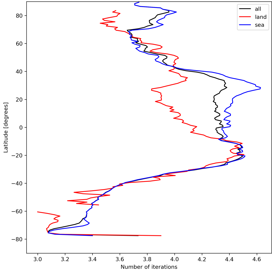
Figure 17: Zonal average of “Number of iterations” for 2023-08-23 to 2023-08-25.
