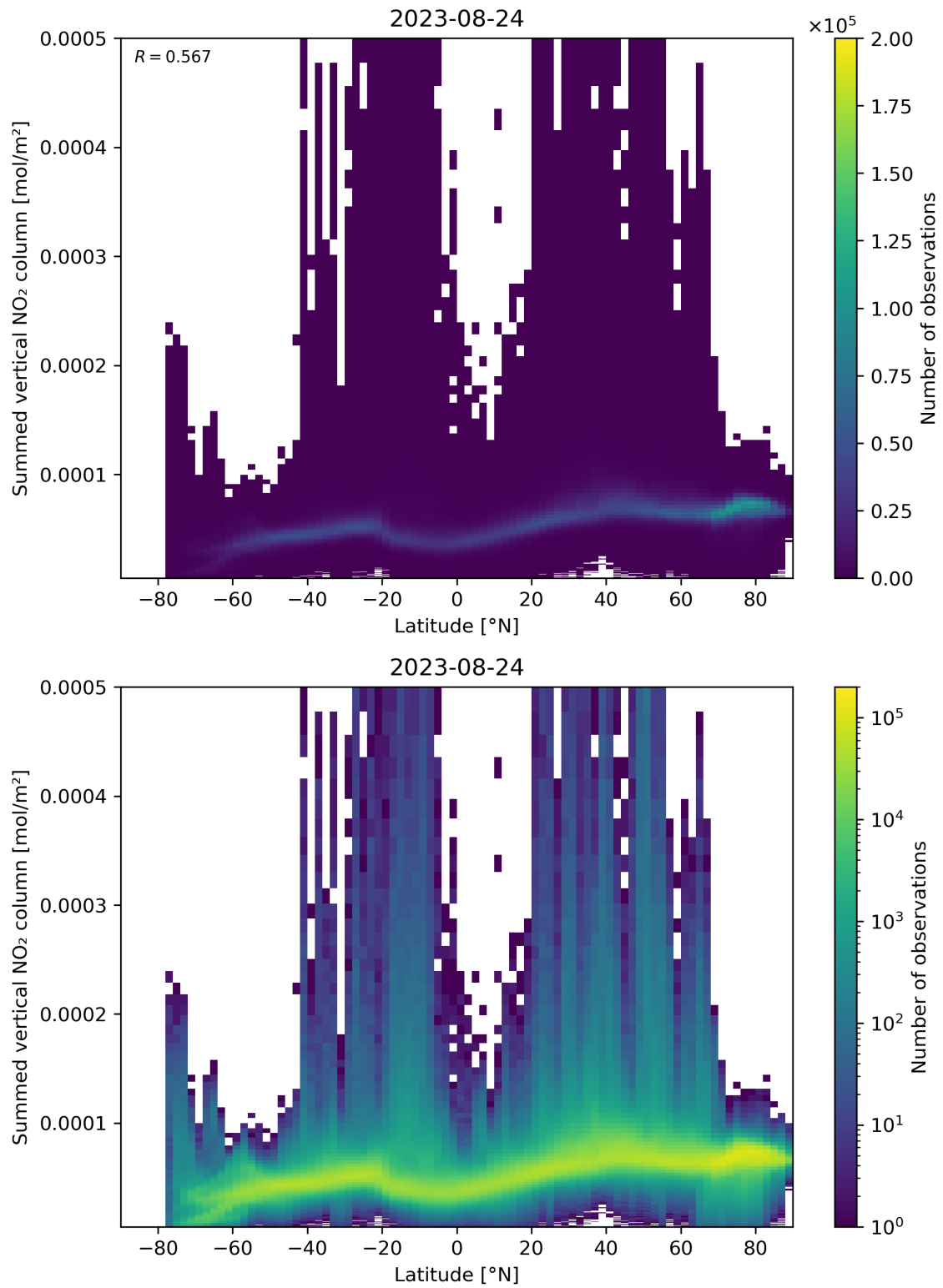
Figure 88: Scatter density plot of “Latitude” against “Summed vertical NO 2 column” for 2023-08-23 to 2023-08-25.
