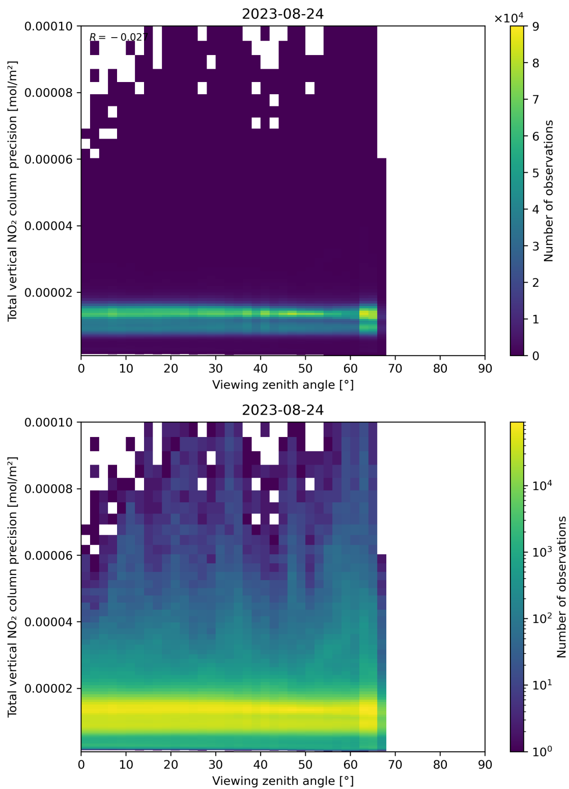
Figure 168: Scatter density plot of “Viewing zenith angle” against “Total vertical NO 2 column precision” for 2023-08-23 to 2023-08-25.
