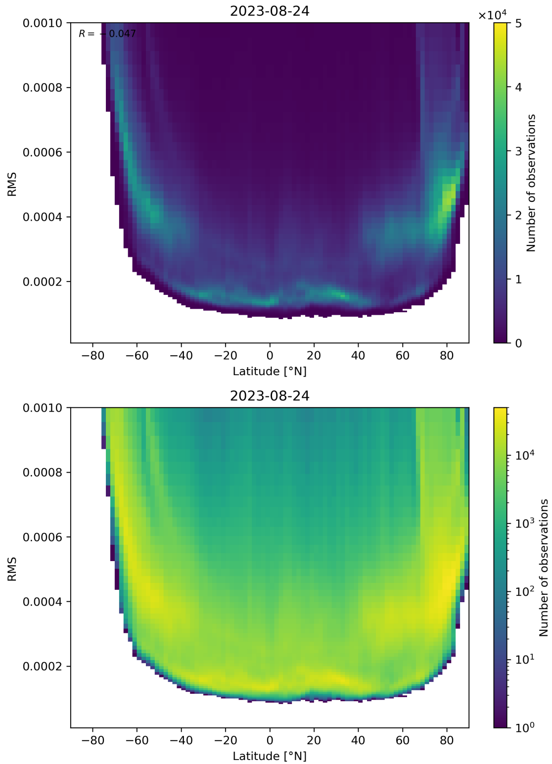
Figure 94: Scatter density plot of “Latitude” against “RMS” for 2023-08-23 to 2023-08-25.
