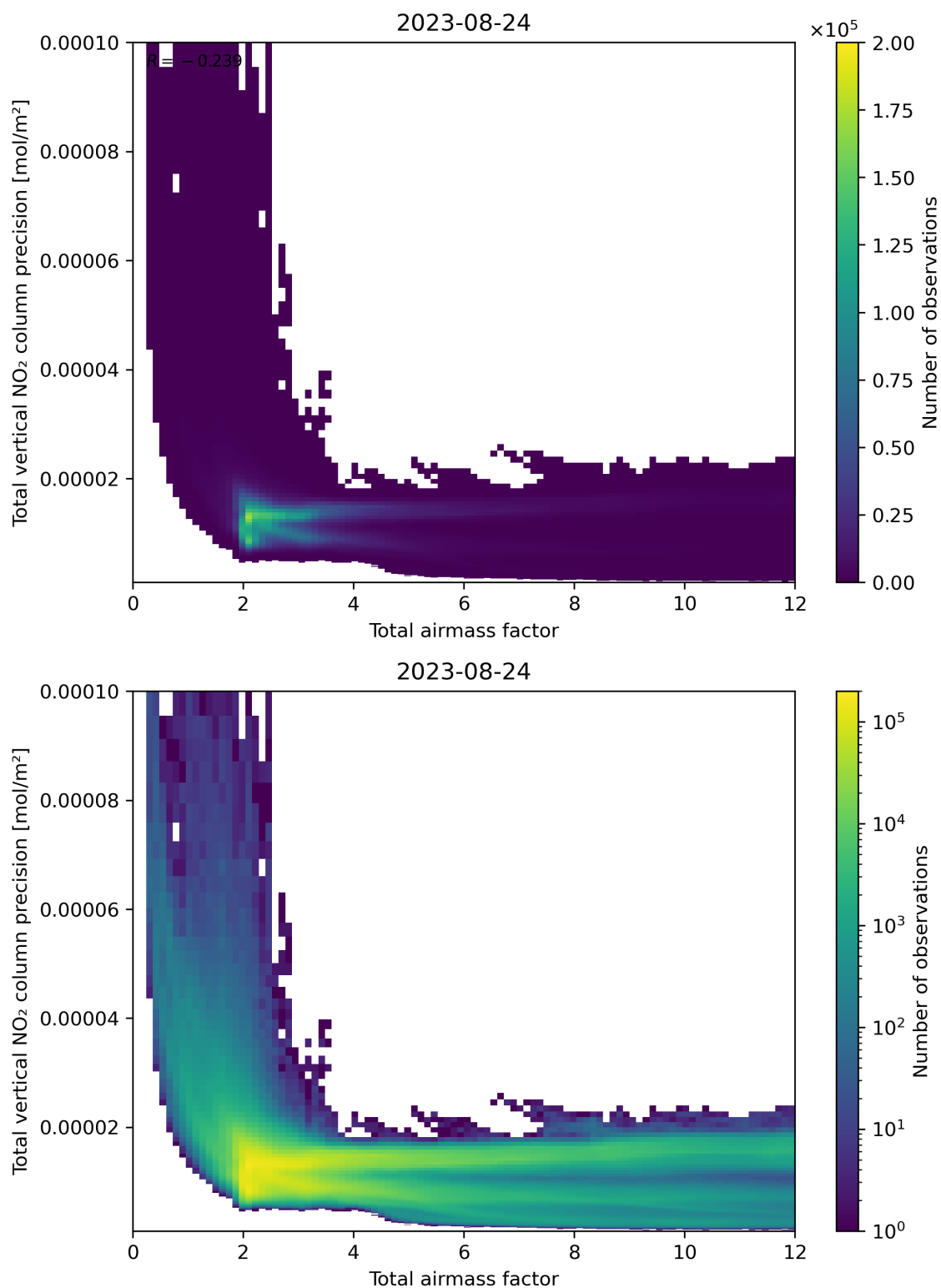
Figure 68: Scatter density plot of “Total airmass factor” against “Total vertical NO 2 column precision” for 2023-08-23 to 2023-08-25.
