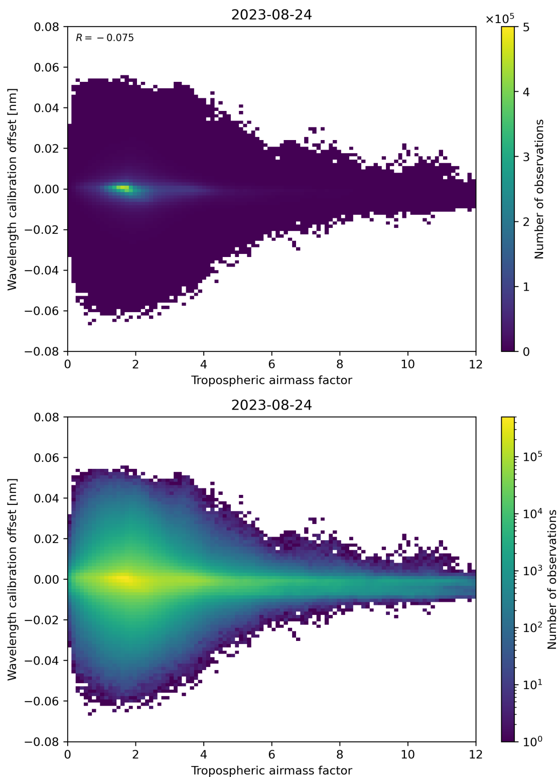
Figure 80: Scatter density plot of “Tropospheric airmass factor” against “Wavelength calibration offset” for 2023-08-23 to 2023-08-25.
