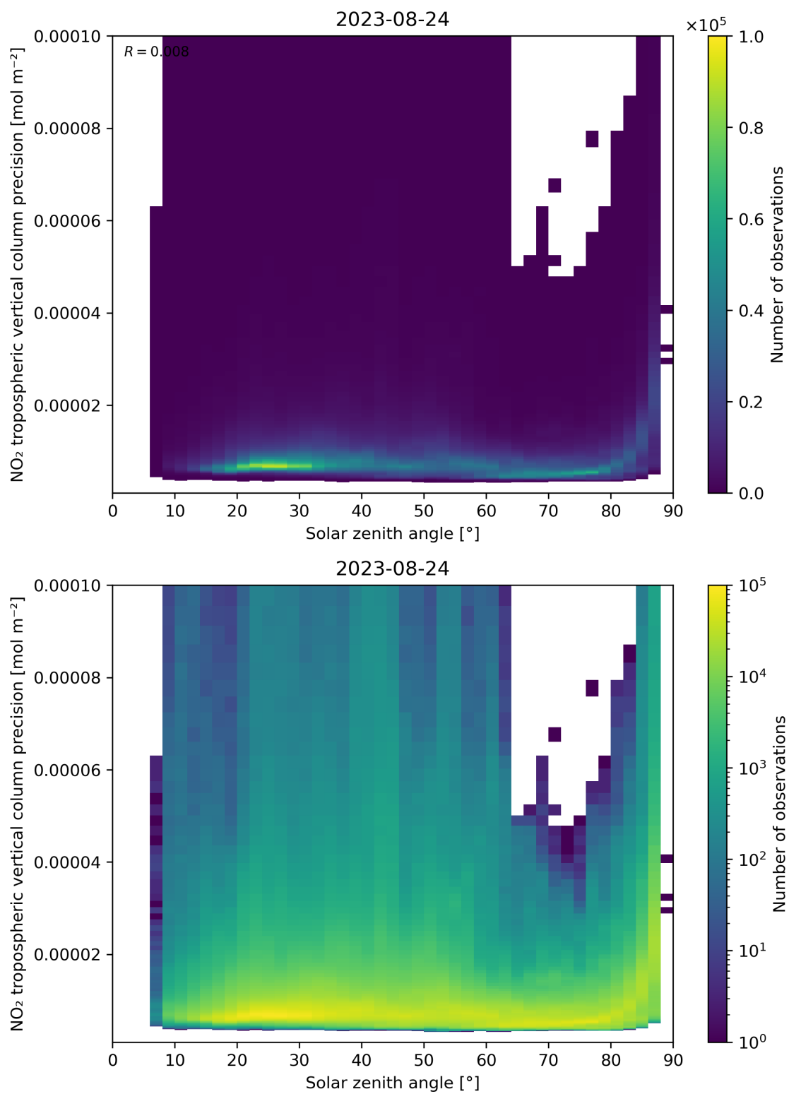
Figure 156: Scatter density plot of “Solar zenith angle” against “NO 2 tropospheric vertical column precision” for 2023-08-23 to 2023-08-25.
