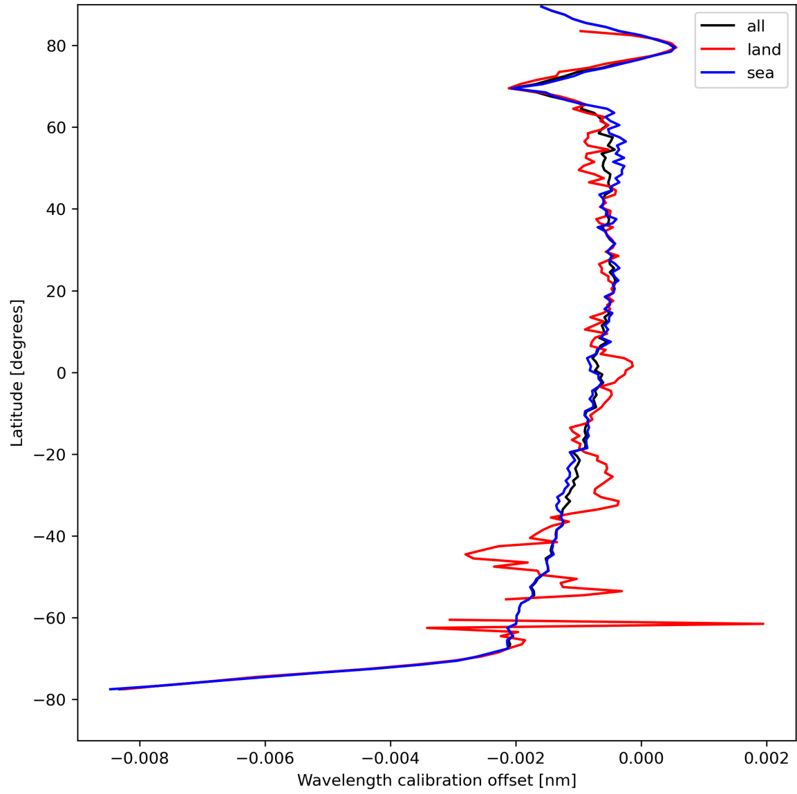
Figure 18: Zonal average of “Wavelength calibration offset” for 2023-08-23 to 2023-08-25.
