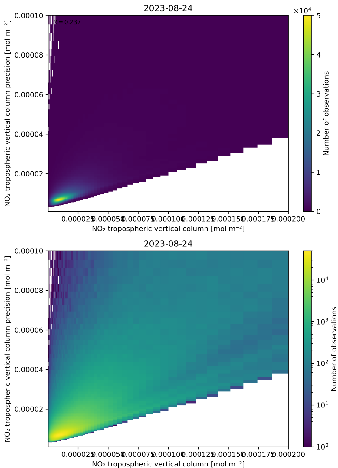
Figure 130: Scatter density plot of “NO 2 tropospheric vertical column” against “NO 2 tropospheric vertical column precision” for 2023-08-23 to 2023-08-25.
