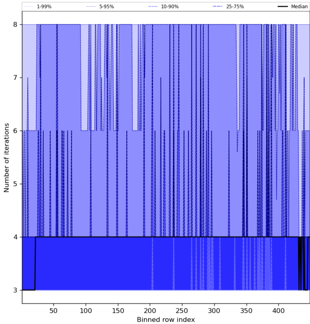
Figure 51: Along track statistics of “Number of iterations” for 2023-08-23 to 2023-08-25
