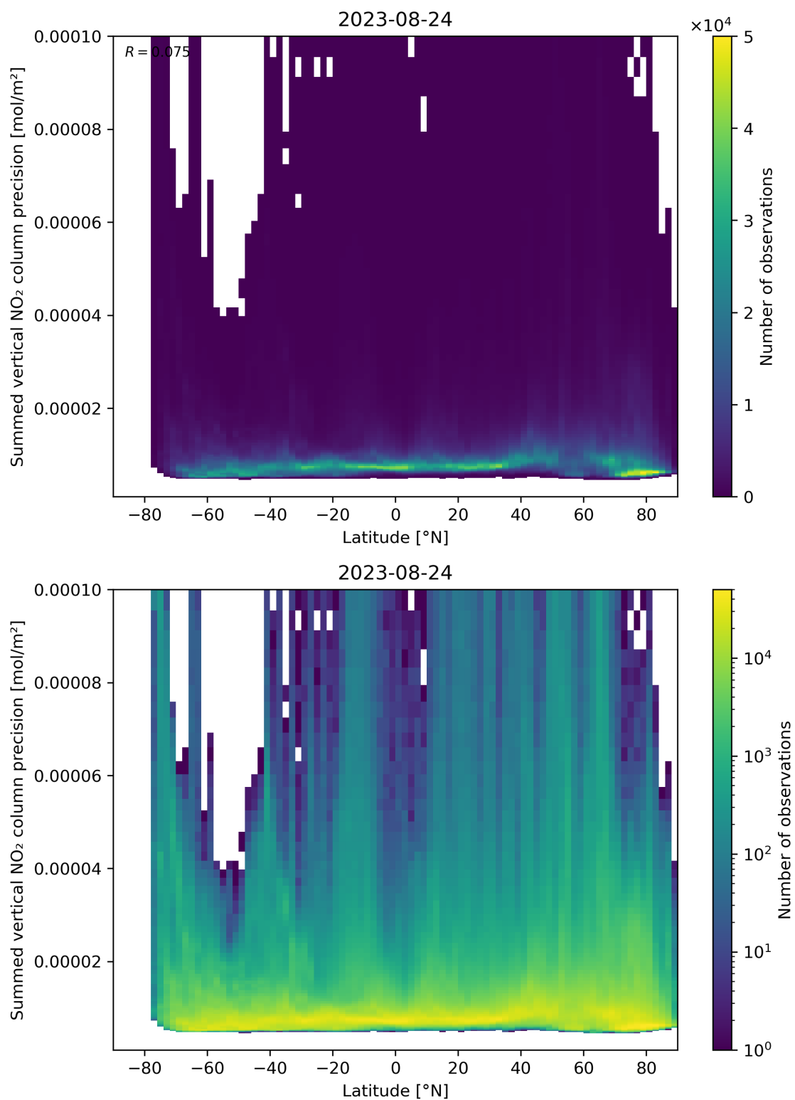
Figure 89: Scatter density plot of “Latitude” against “Summed vertical NO 2 column precision” for 2023-08-23 to 2023-08-25.
