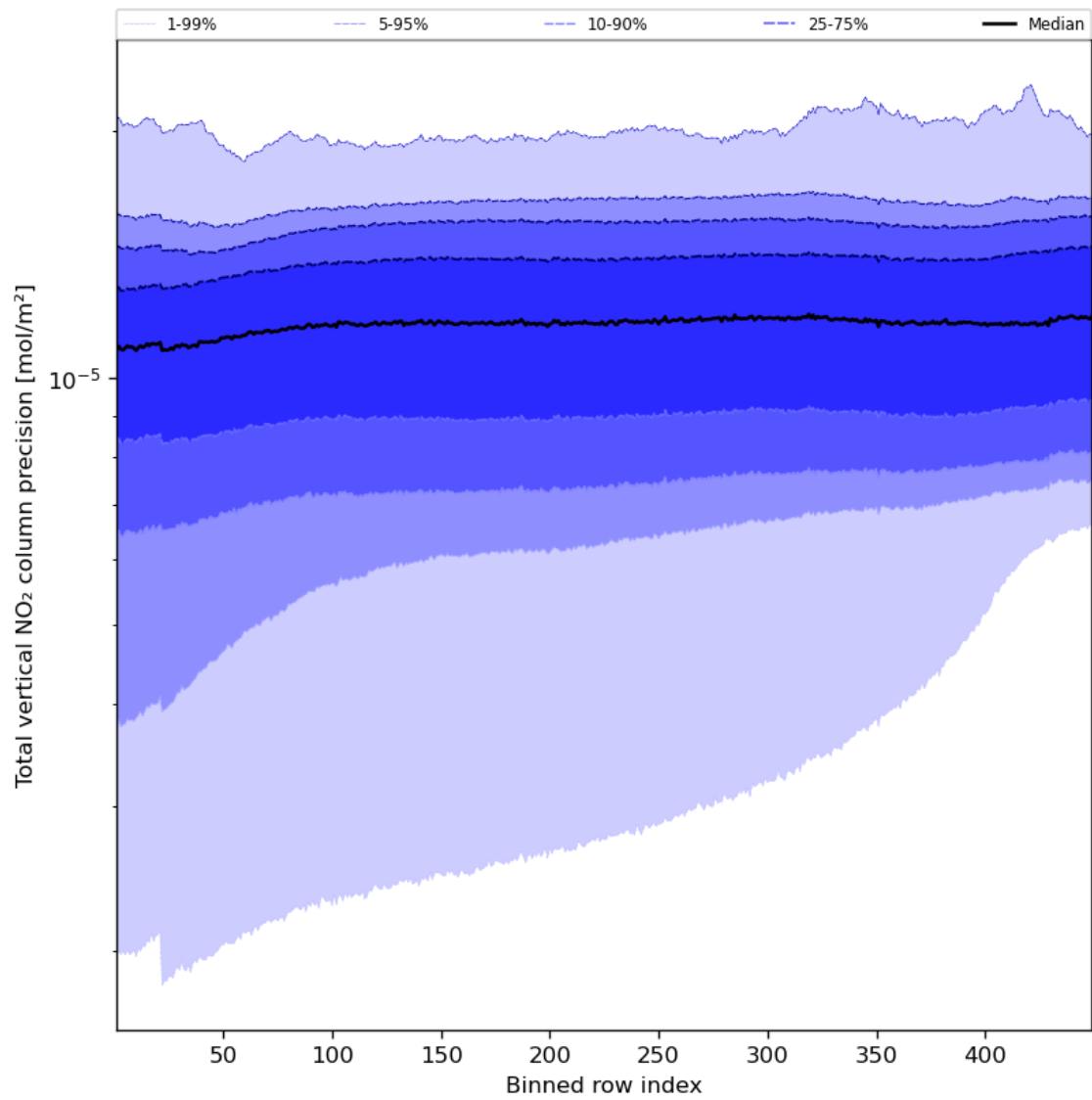
Figure 56: Along track statistics of “Total vertical NO 2 column precision” for 2023-08-23 to 2023-08-25
