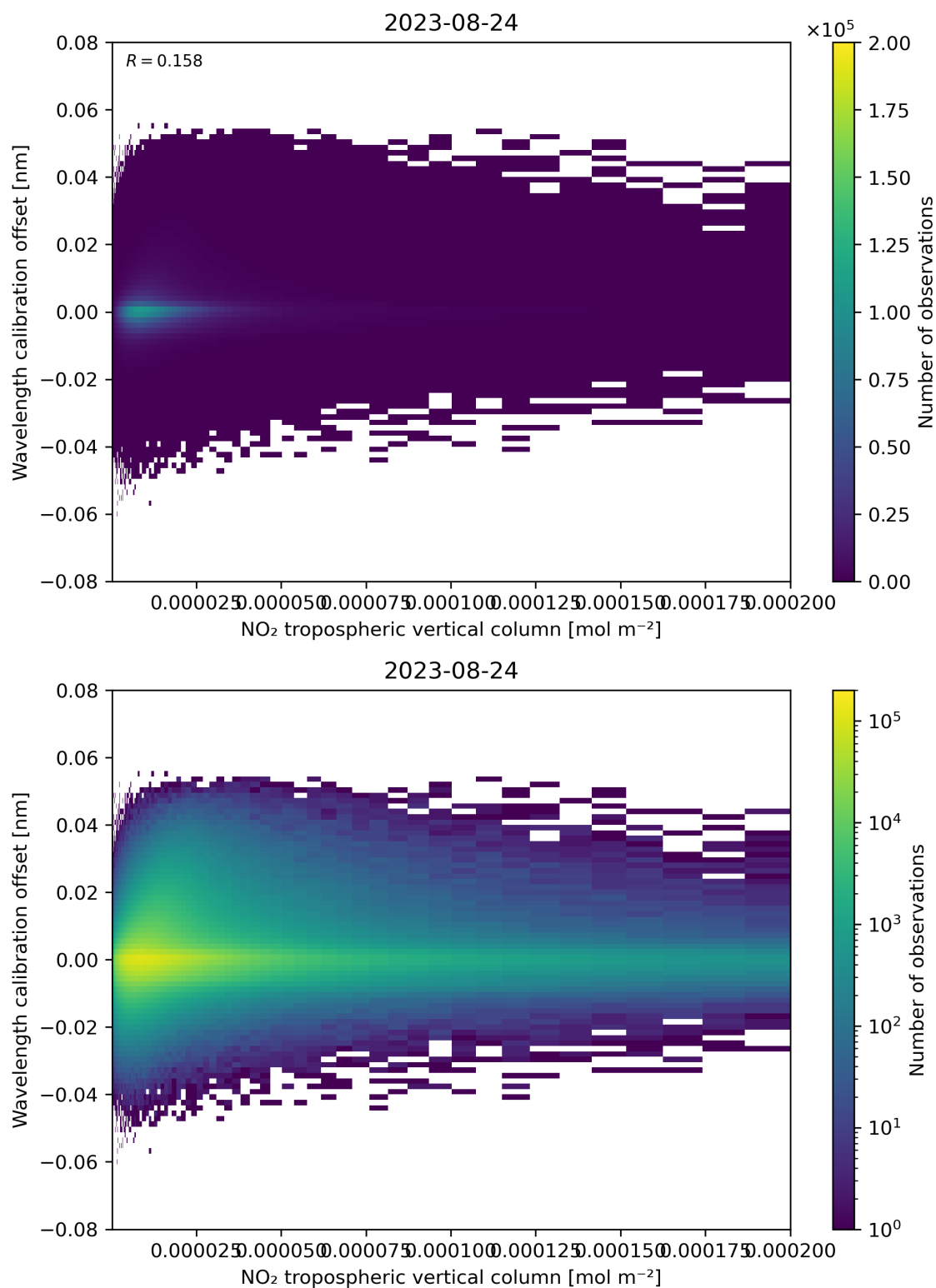
Figure 143: Scatter density plot of “NO 2 tropospheric vertical column” against “Wavelength calibration offset” for 2023-08-23 to 2023-08-25.
