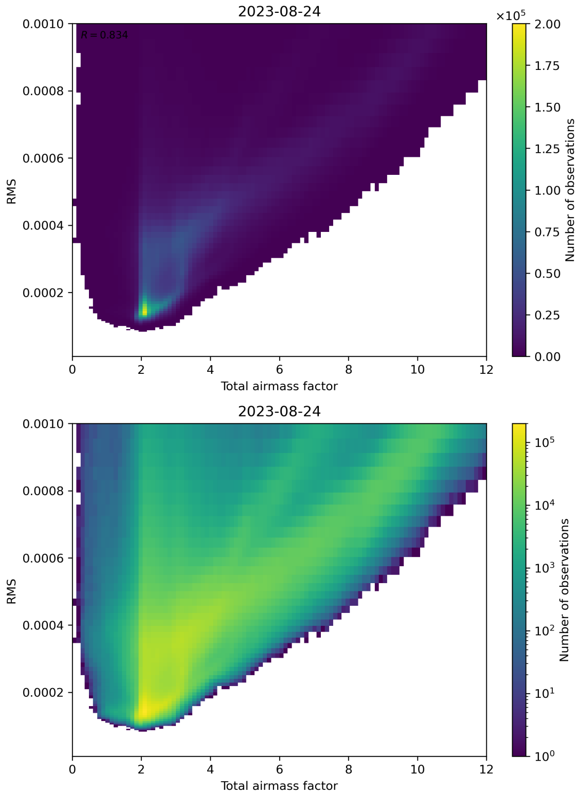
Figure 69: Scatter density plot of “Total airmass factor” against “RMS” for 2023-08-23 to 2023-08-25.
