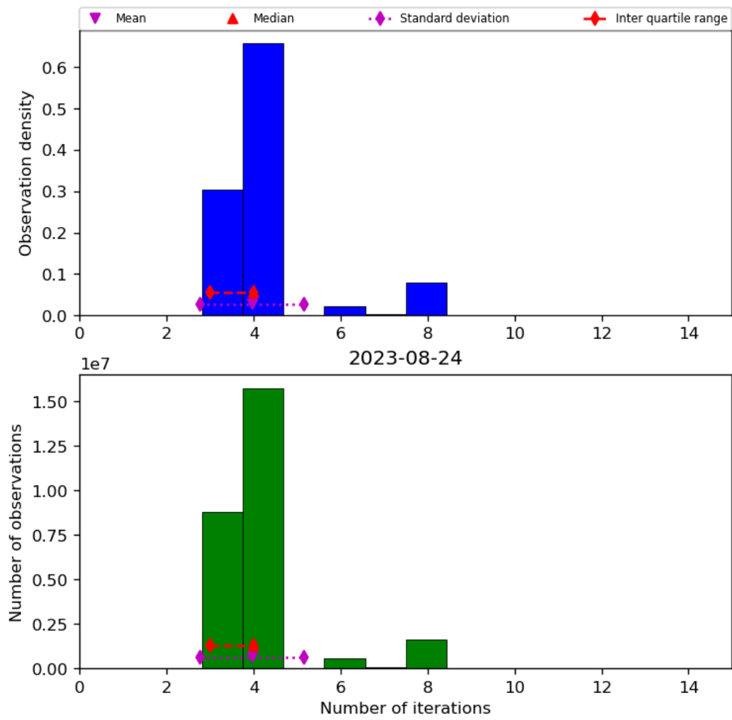
Figure 34: Histogram of “Number of iterations” for 2023-08-23 to 2023-08-25
