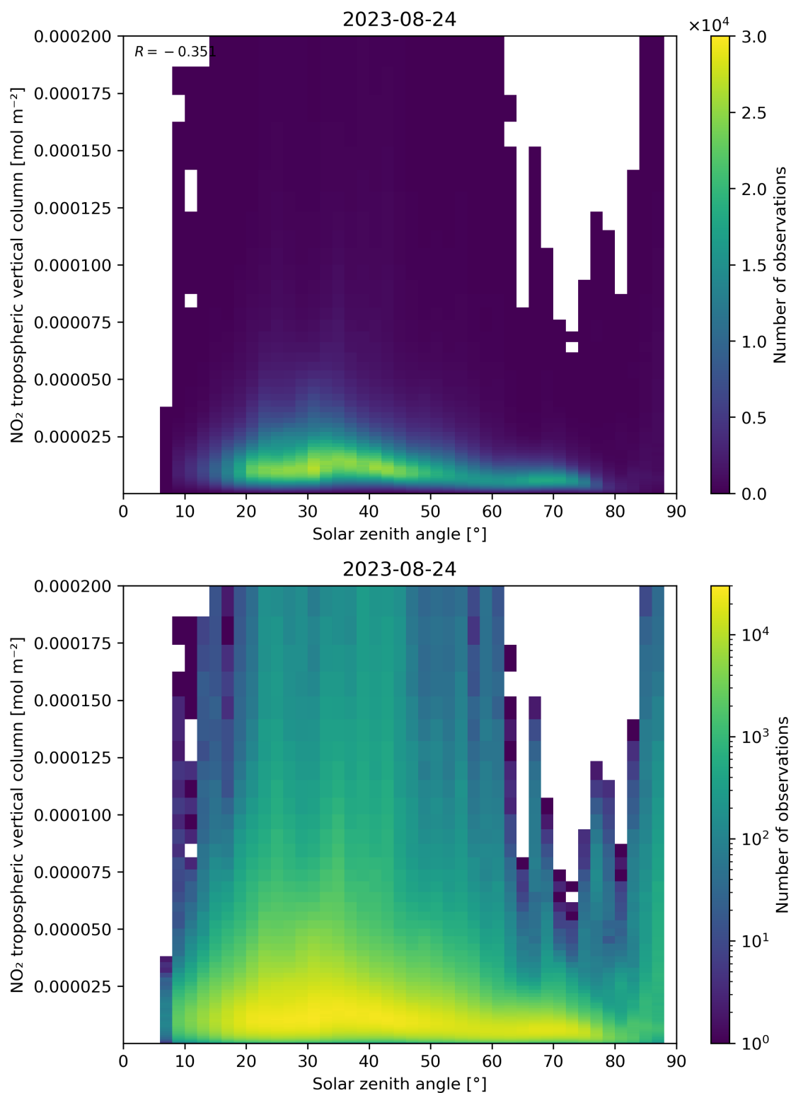
Figure 155: Scatter density plot of “Solar zenith angle” against “NO 2 tropospheric vertical column” for 2023-08-23 to 2023-08-25.
