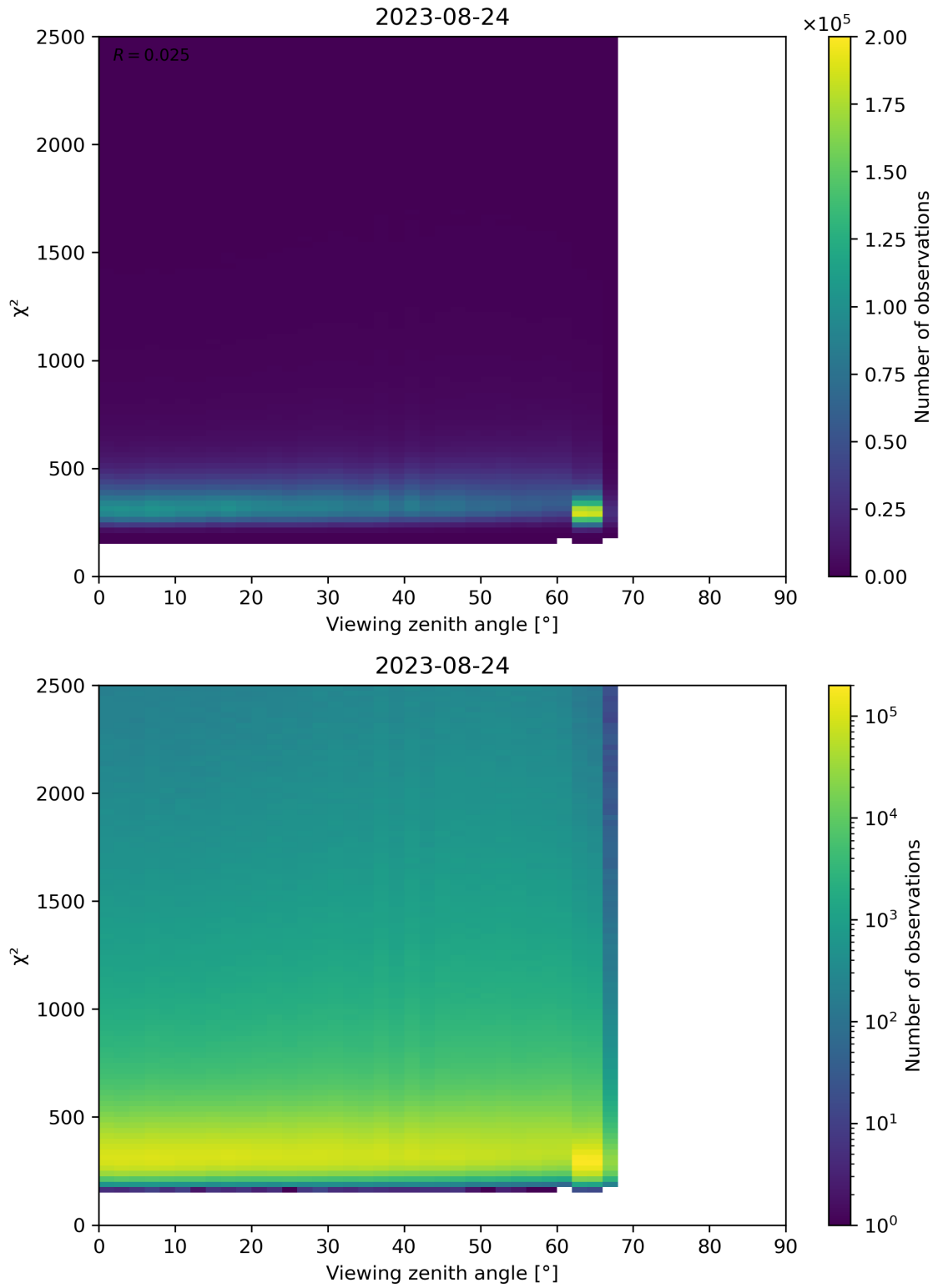
Figure 162: Scatter density plot of “Viewing zenith angle” against “ \chi^2 ” for 2023-08-23 to 2023-08-25.
