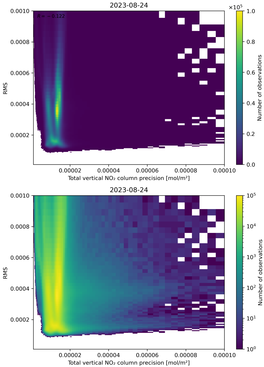
Figure 119: Scatter density plot of “Total vertical NO 2 column precision” against “RMS” for 2023-08-23 to 2023-08-25.
