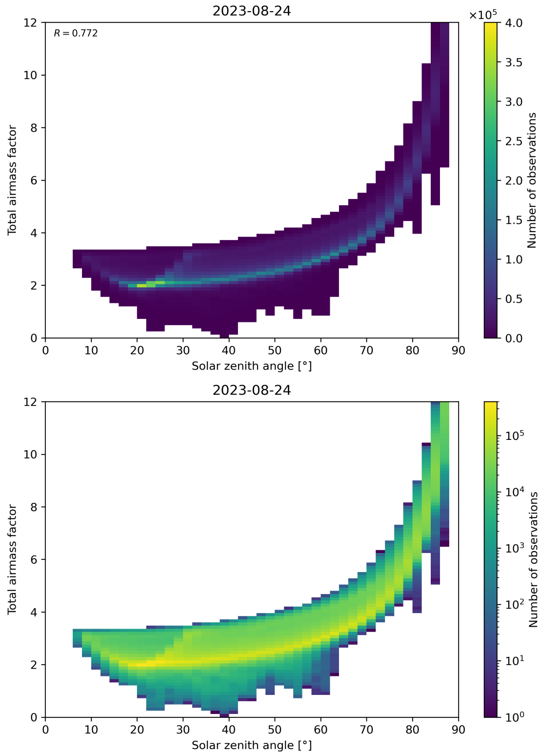
Figure 146: Scatter density plot of “Solar zenith angle” against “Total air mass factor” for 2023-08-23 to 2023-08-25.
