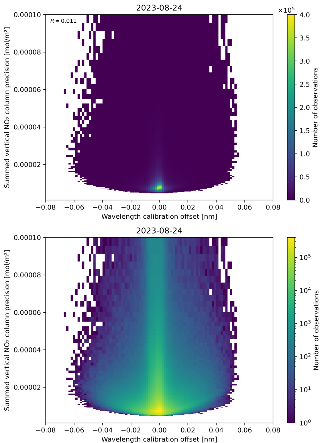
Figure 178: Scatter density plot of “Wavelength calibration offset” against “Summed vertical NO 2 column precision” for 2023-08-23 to 2023-08-25.
