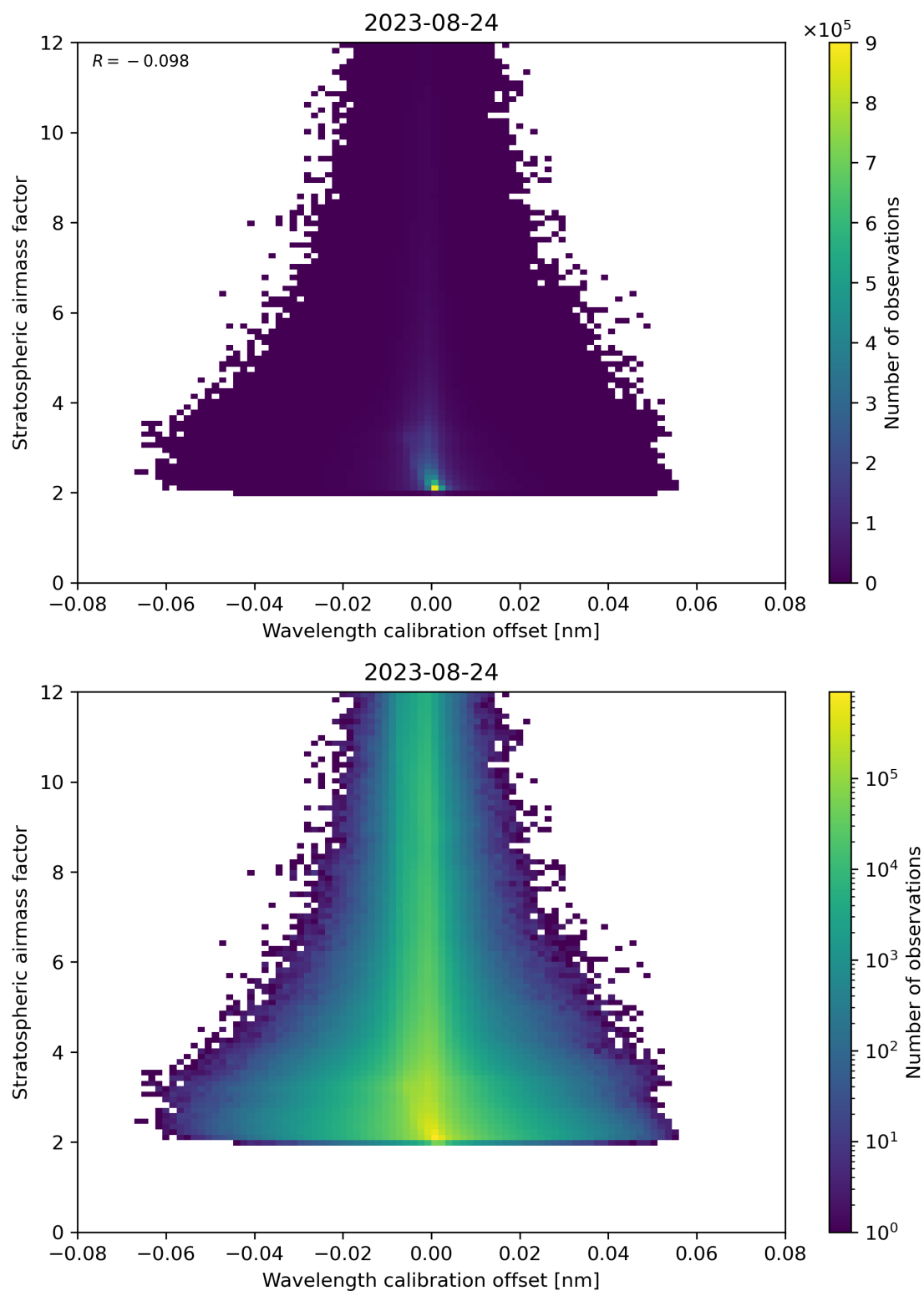
Figure 174: Scatter density plot of “Wavelength calibration offset” against “Stratospheric airmass factor” for 2023-08-23 to 2023-08-25.
