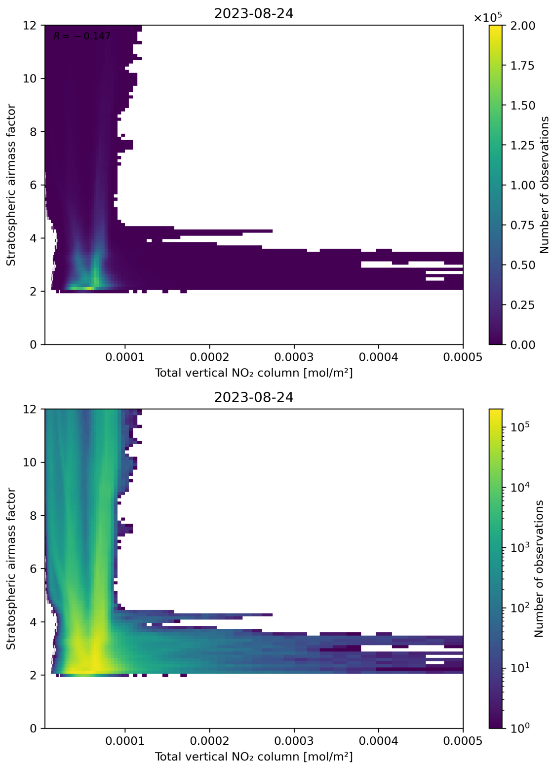
Figure 110: Scatter density plot of “Total vertical NO 2 column” against “Stratospheric airmass factor” for 2023-08-23 to 2023-08-25.
