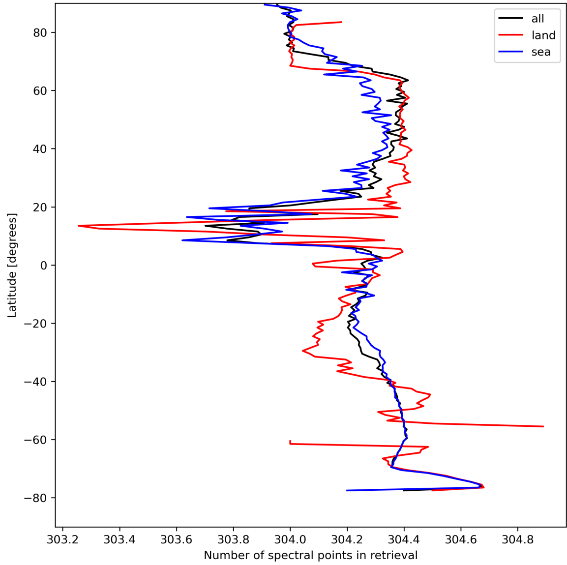
Figure 16: Zonal average of “Number of spectral points in retrieval” for 2023-08-23 to 2023-08-25.
