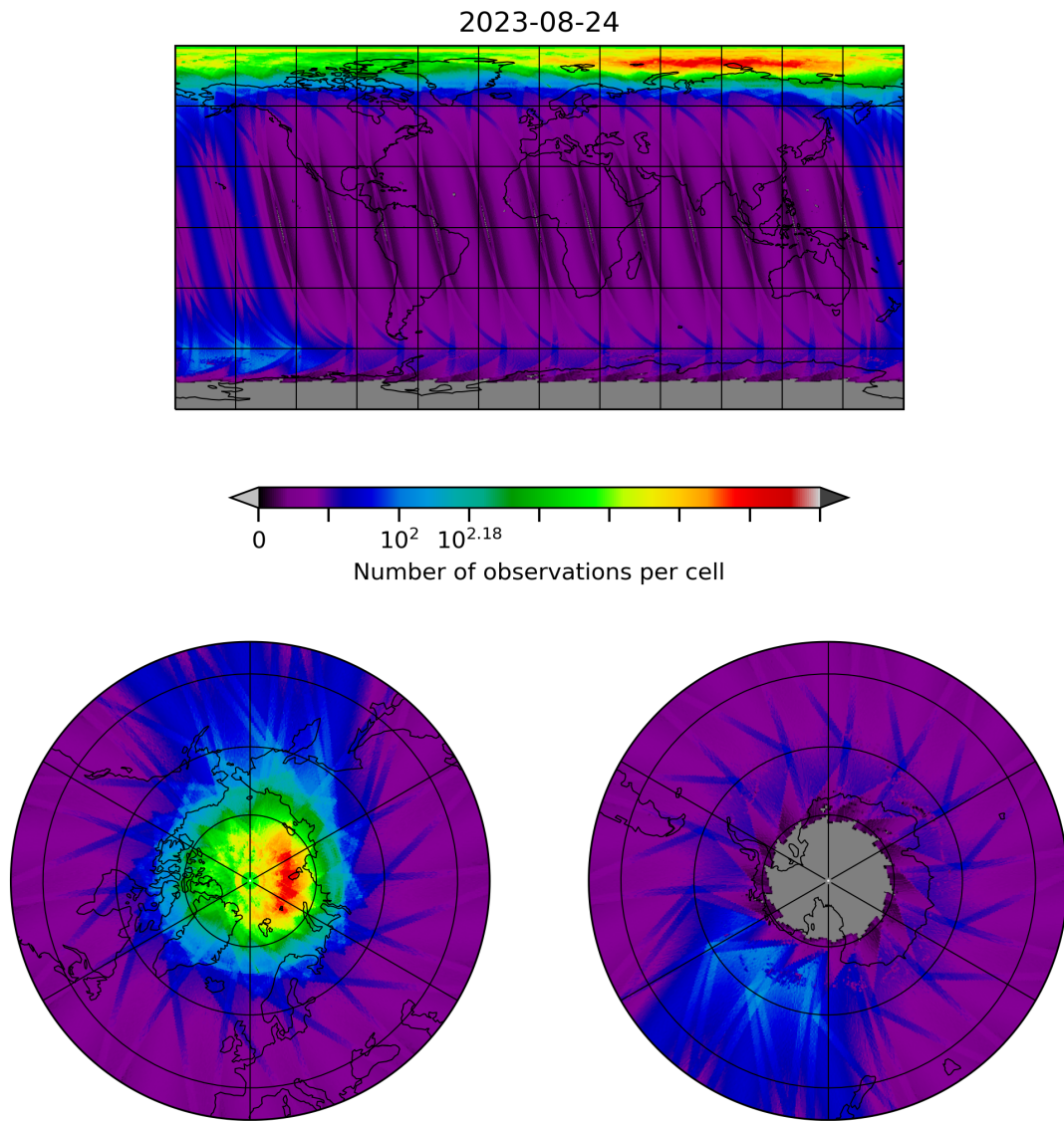
Figure 10: Map of the number of observations for 2023-08-23 to 2023-08-25
