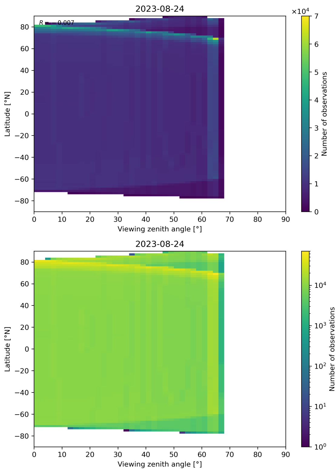
Figure 163: Scatter density plot of “Viewing zenith angle” against “Latitude” for 2023-08-23 to 2023-08-25.
