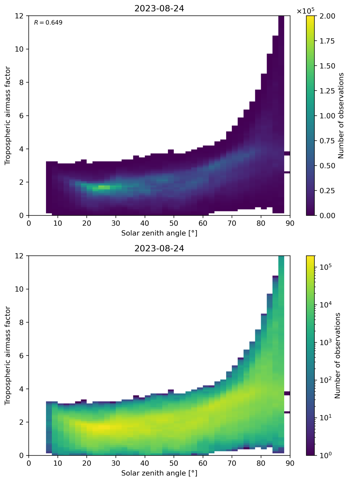
Figure 147: Scatter density plot of “Solar zenith angle” against “Tropospheric airmass factor” for 2023-08-23 to 2023-08-25.
