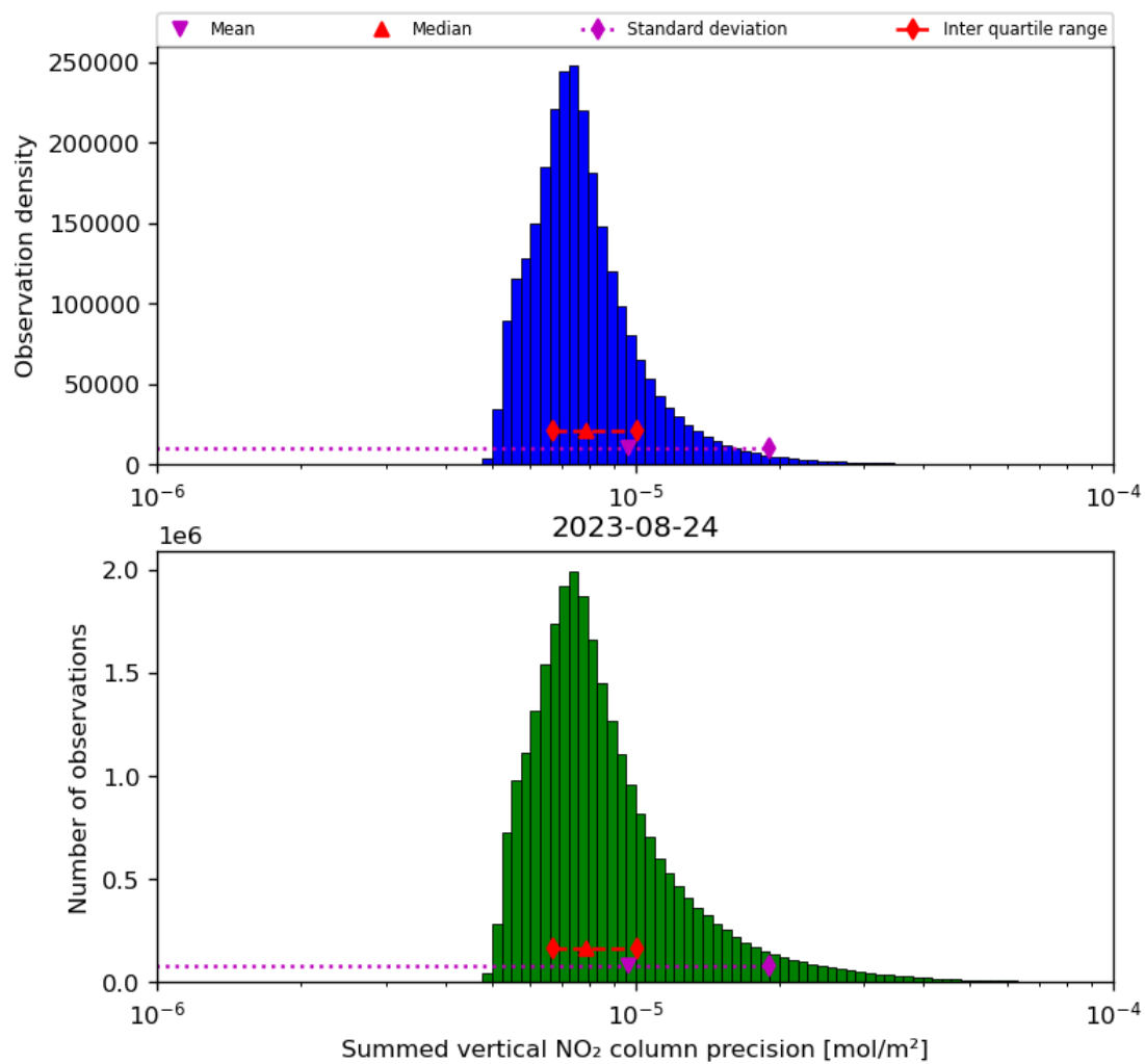
Figure 41: Histogram of "Summed vertical NO 2 column precision" for 2023-08-23 to 2023-08-25
