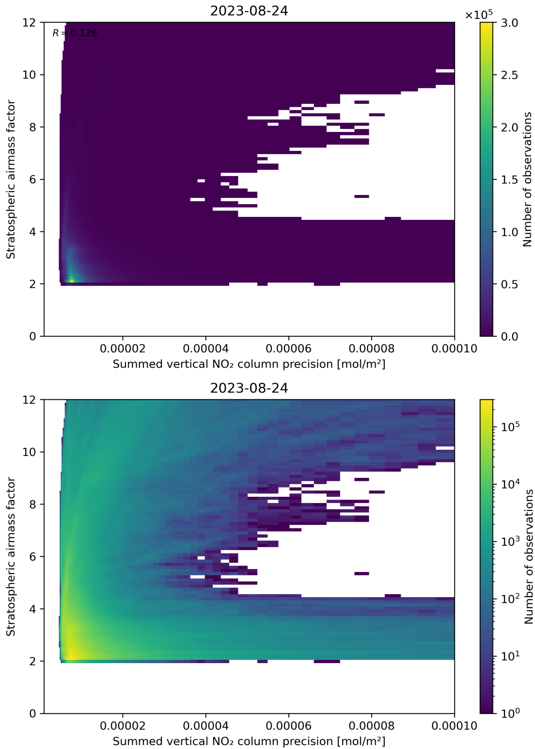
Figure 106: Scatter density plot of “Summed vertical NO 2 column precision” against “Stratospheric airmass factor” for 2023-08-23 to 2023-08-25.
