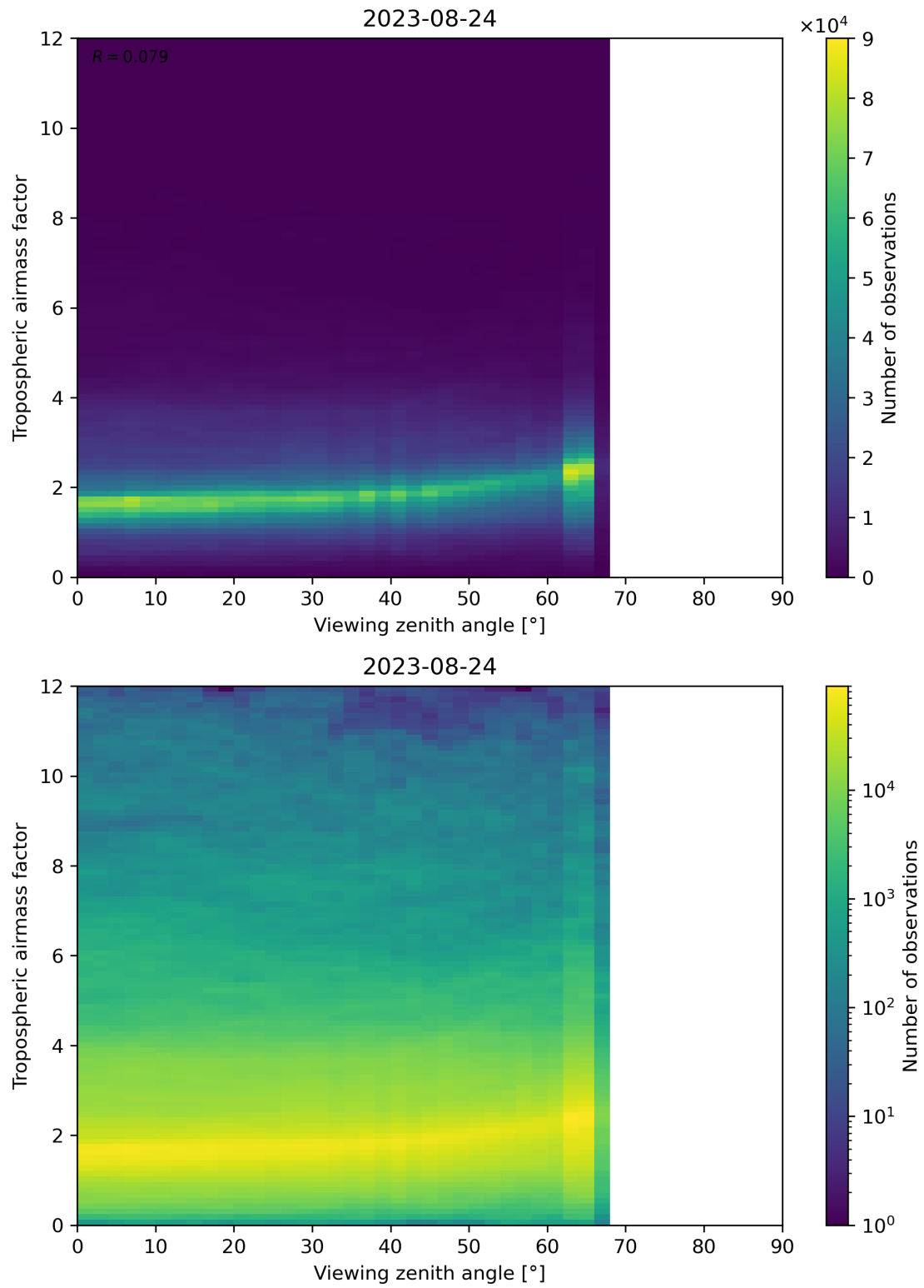
Figure 161: Scatter density plot of “Viewing zenith angle” against “Tropospheric airmass factor” for 2023-08-23 to 2023-08-25.
