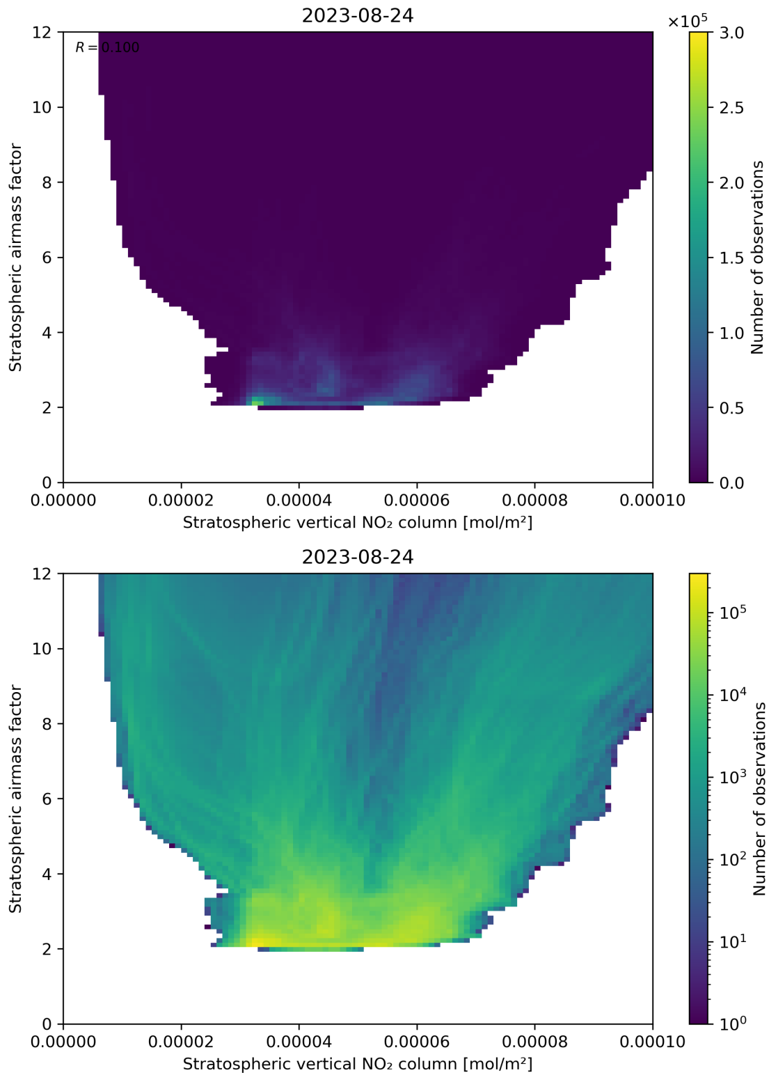
Figure 96: Scatter density plot of “Stratospheric vertical NO 2 column” against “Stratospheric airmass factor” for 2023-08-23 to 2023-08-25.
