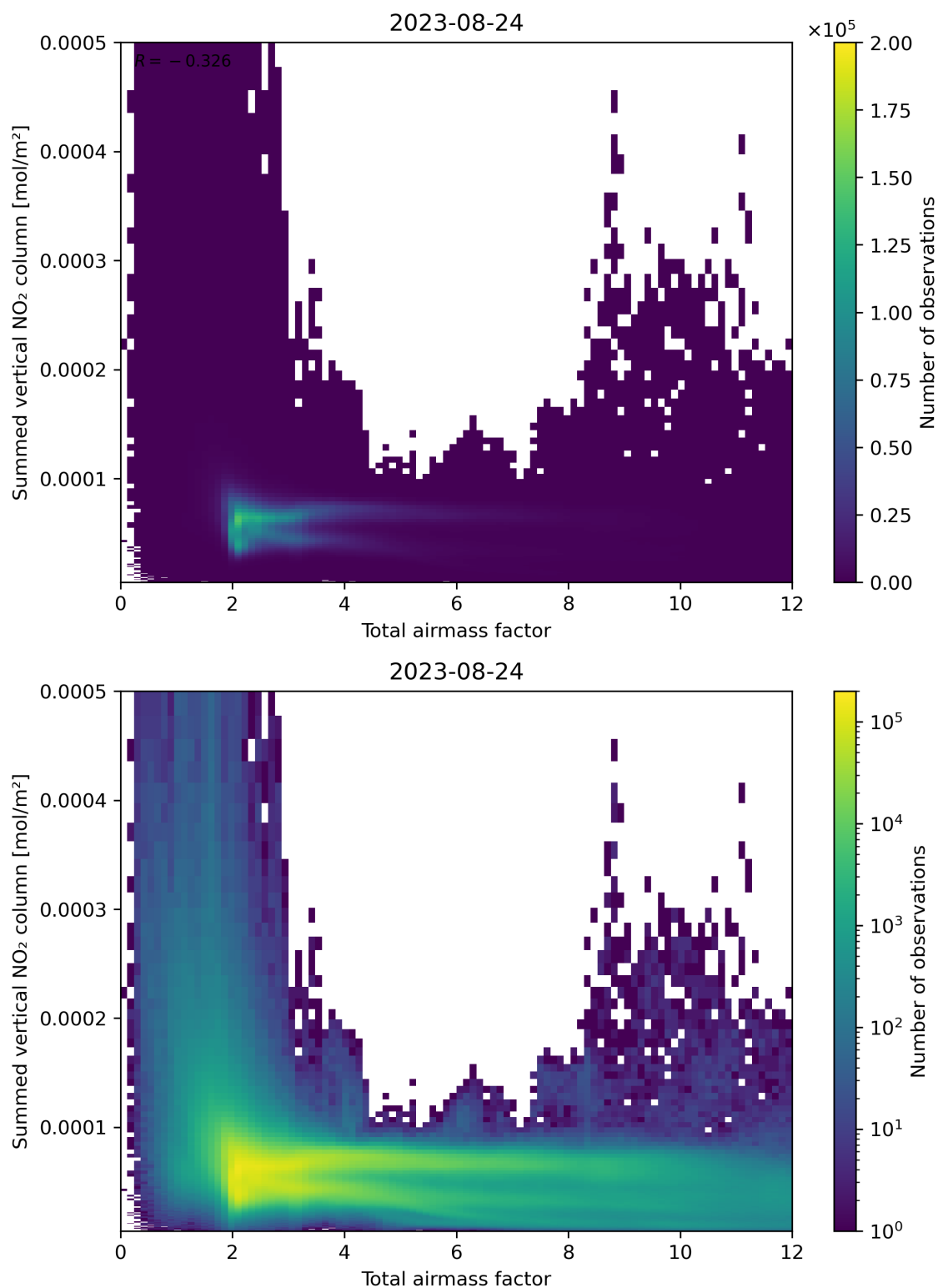
Figure 65: Scatter density plot of “Total airmass factor” against “Summed vertical NO 2 column” for 2023-08-23 to 2023-08-25.
