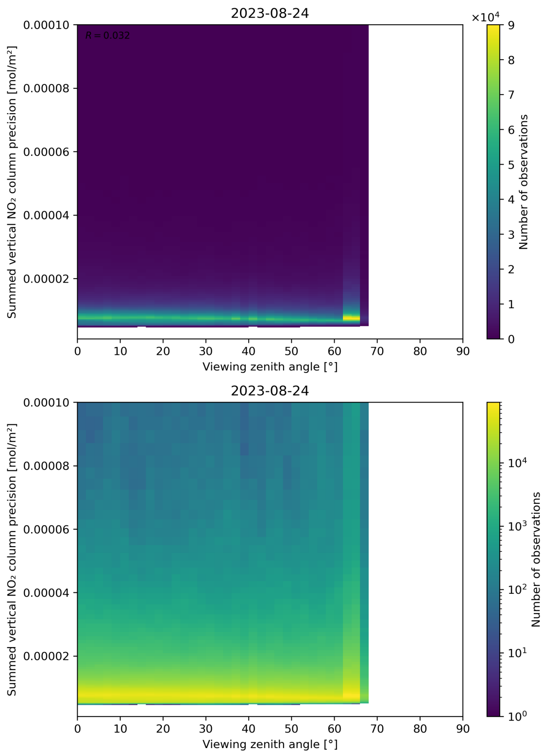
Figure 166: Scatter density plot of “Viewing zenith angle” against “Summed vertical NO 2 column precision” for 2023-08-23 to 2023-08-25.
