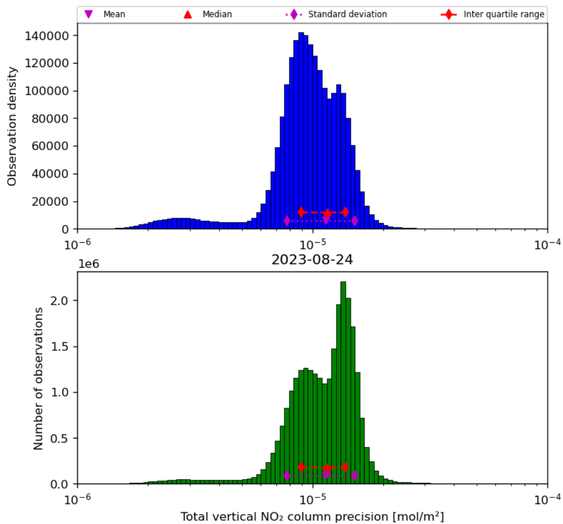
Figure 39: Histogram of “Total vertical NO 2 column precision” for 2023-08-23 to 2023-08-25
