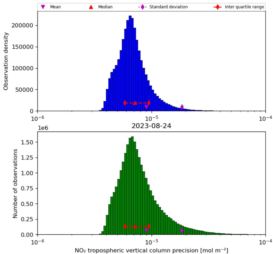
Figure 30: Histogram of “NO 2 tropospheric vertical column precision” for 2023-08-23 to 2023-08-25
