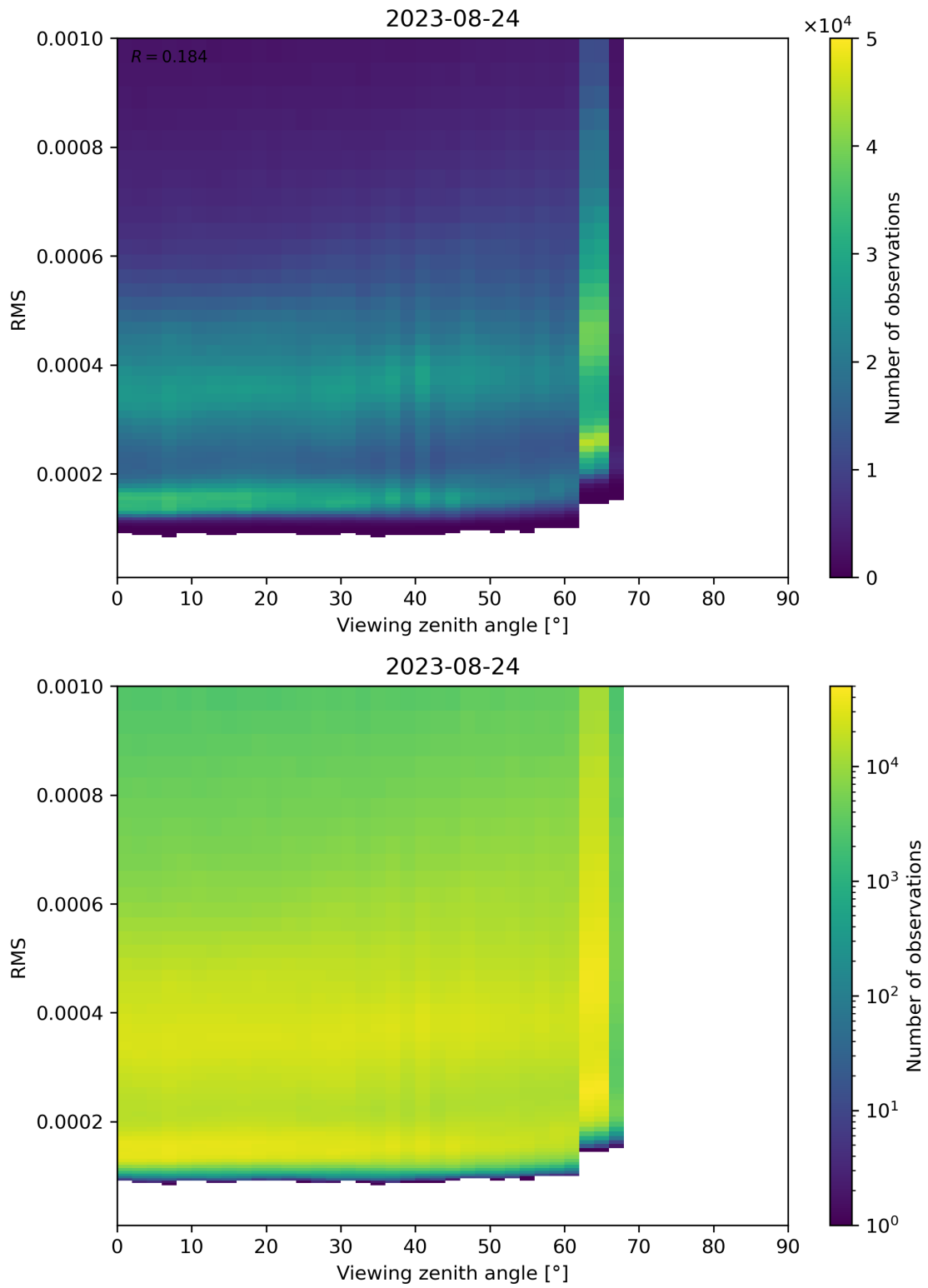
Figure 171: Scatter density plot of “Viewing zenith angle” against “RMS” for 2023-08-23 to 2023-08-25.
