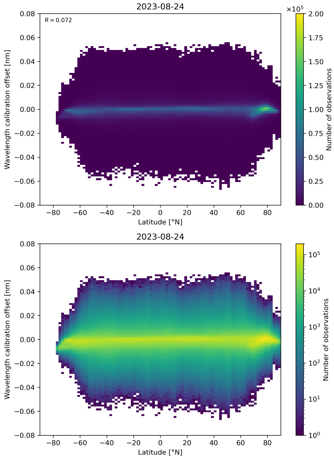
Figure 95: Scatter density plot of “Latitude” against “Wavelength calibration offset” for 2023-08-23 to 2023-08-25.
