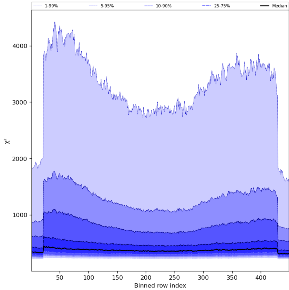
Figure 59: Along track statistics of “ \chi^2 ” for 2023-08-23 to 2023-08-25
