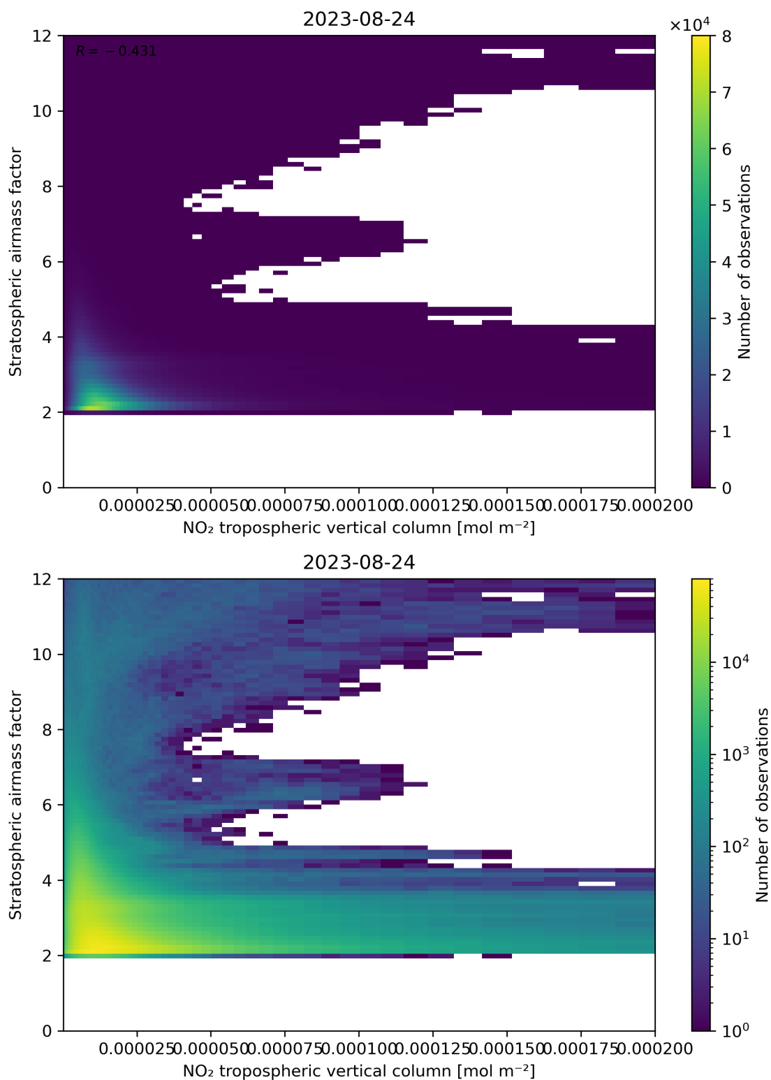
Figure 121: Scatter density plot of “NO 2 tropospheric vertical column” against “Stratospheric air mass factor” for 2023-08-23 to 2023-08-25.
