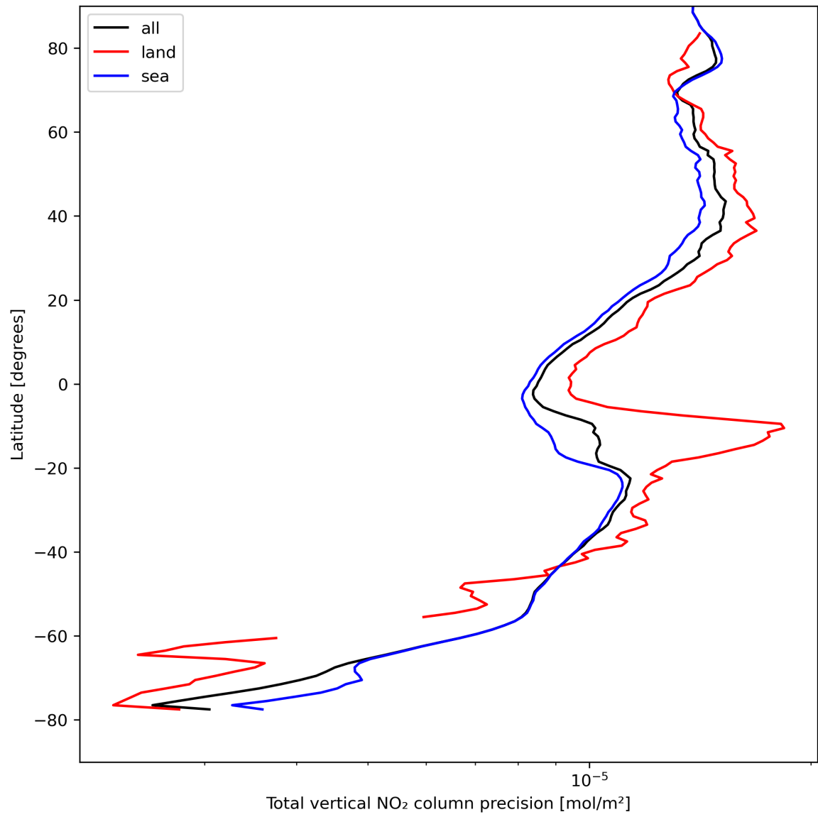
Figure 22: Zonal average of “Total vertical NO 2 column precision” for 2023-08-23 to 2023-08-25.
