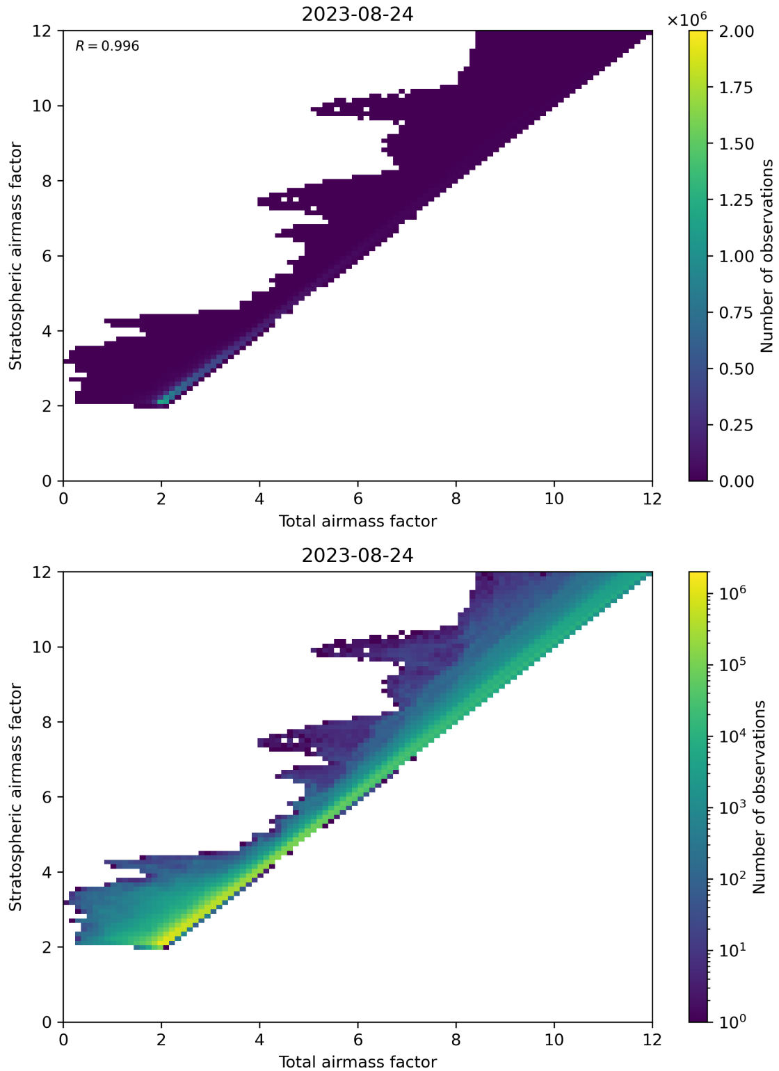
Figure 62: Scatter density plot of “Total airmass factor” against “Stratospheric airmass factor” for 2023-08-23 to 2023-08-25.
