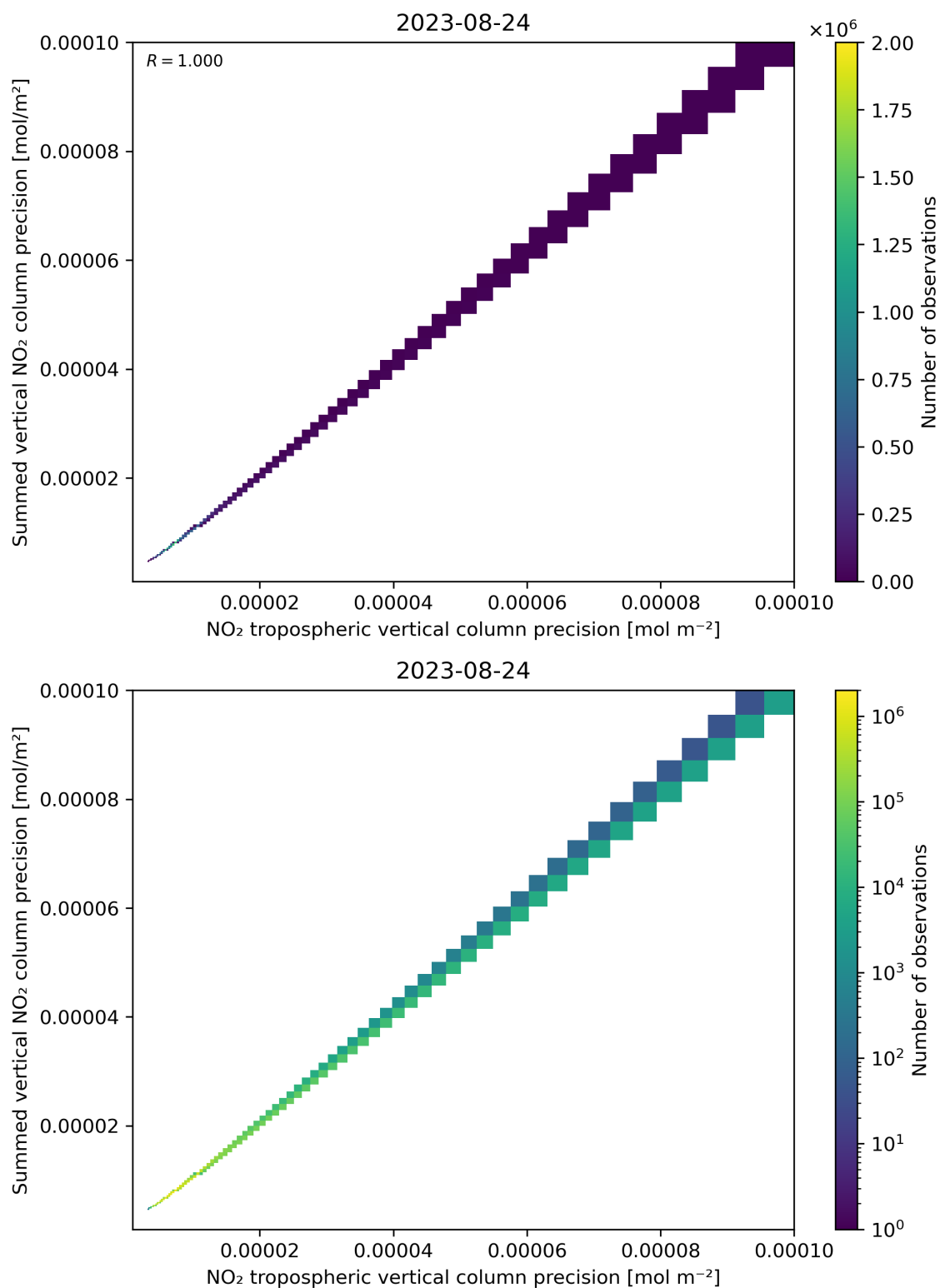
Figure 137: Scatter density plot of “NO 2 tropospheric vertical column precision” against “Summed vertical NO 2 column precision” for 2023-08-23 to 2023-08-25.
