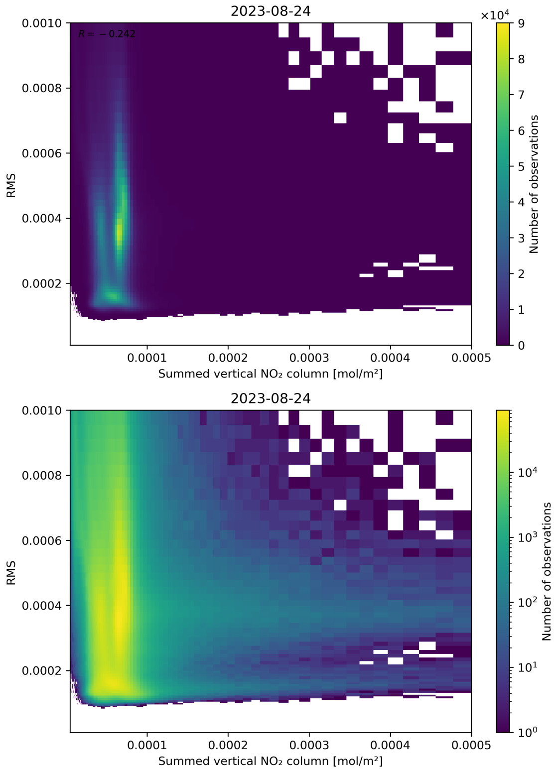
Figure 109: Scatter density plot of “Summed vertical NO 2 column” against “RMS” for 2023-08-23 to 2023-08-25.
