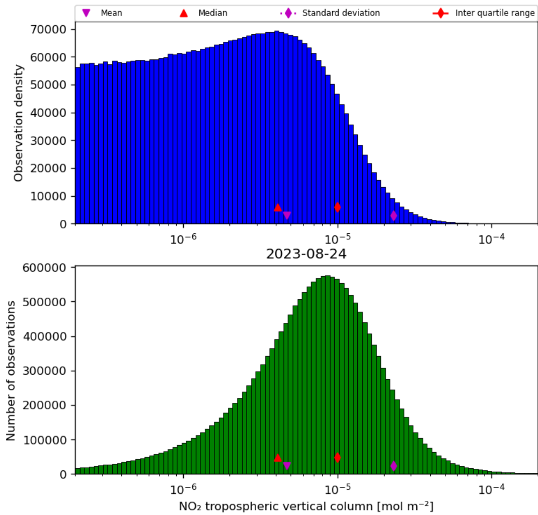
Figure 29: Histogram of “NO 2 tropospheric vertical column” for 2023-08-23 to 2023-08-25
