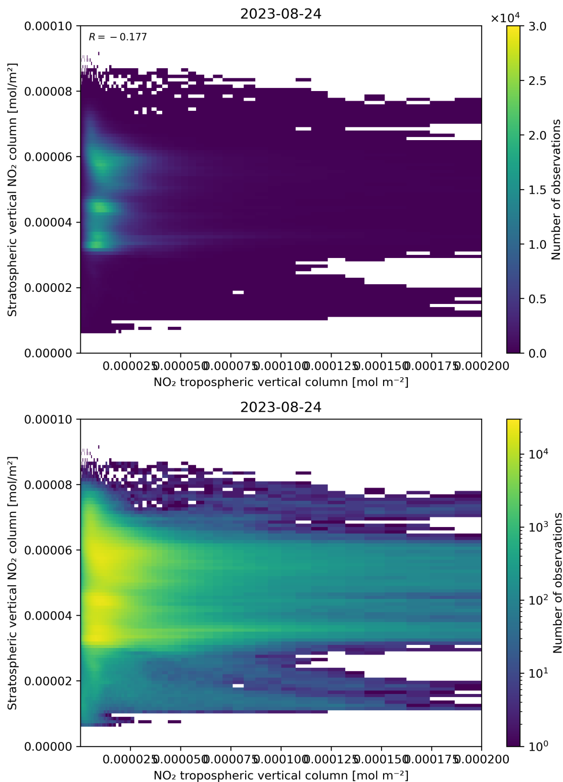
Figure 125: Scatter density plot of “NO 2 tropospheric vertical column” against “Stratospheric vertical NO 2 column” for 2023-08-23 to 2023-08-25.
