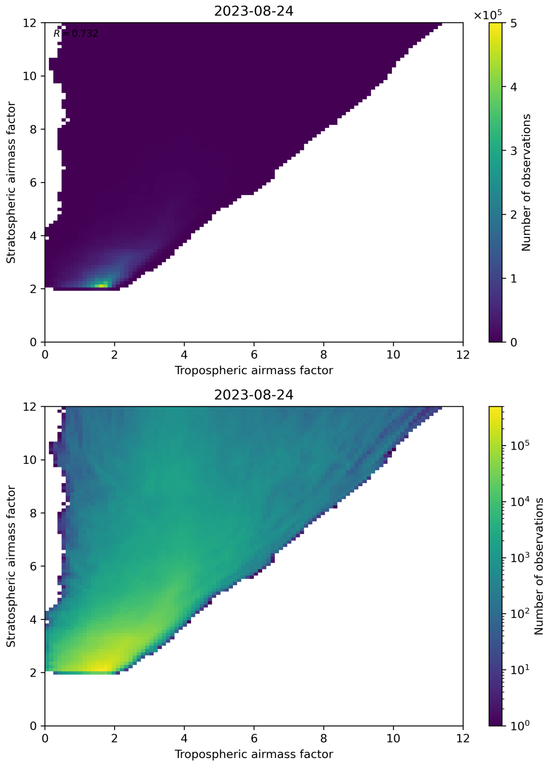
Figure 71: Scatter density plot of “Tropospheric airmass factor” against “Stratospheric airmass factor” for 2023-08-23 to 2023-08-25.
