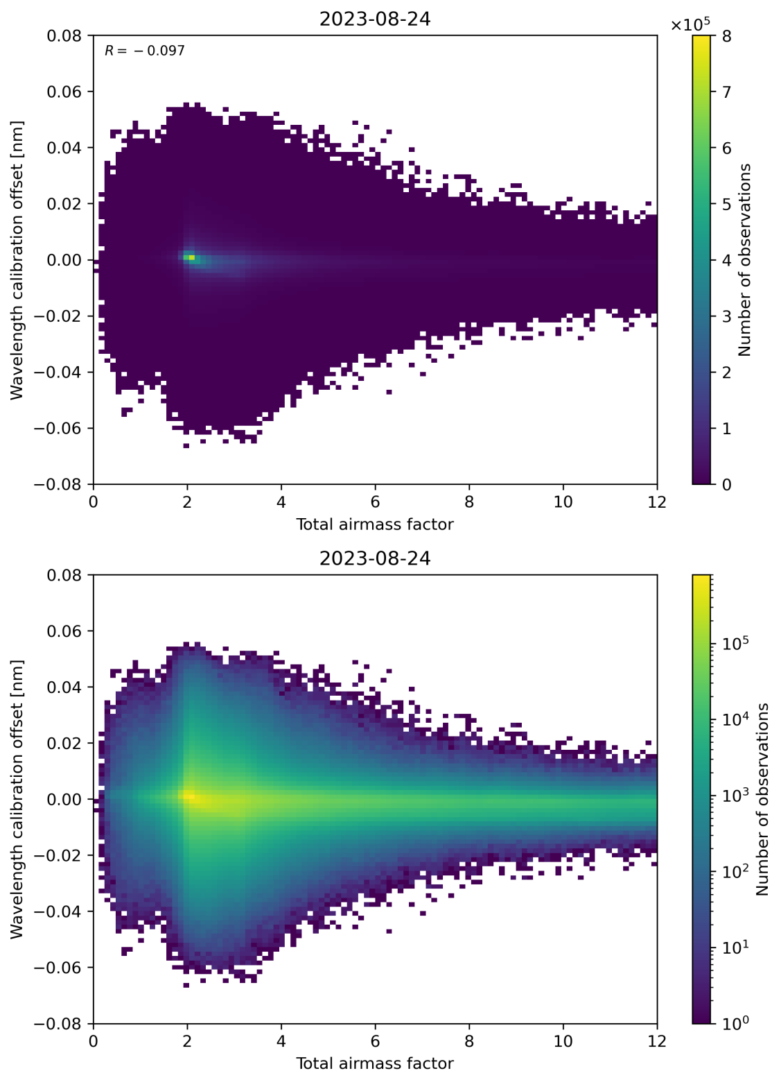
Figure 70: Scatter density plot of “Total airmass factor” against “Wavelength calibration offset” for 2023-08-23 to 2023-08-25.
