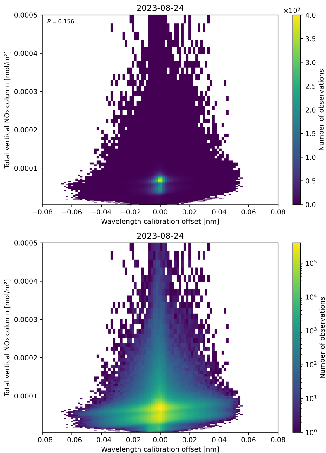
Figure 179: Scatter density plot of “Wavelength calibration offset” against “Total vertical NO 2 column” for 2023-08-23 to 2023-08-25.
