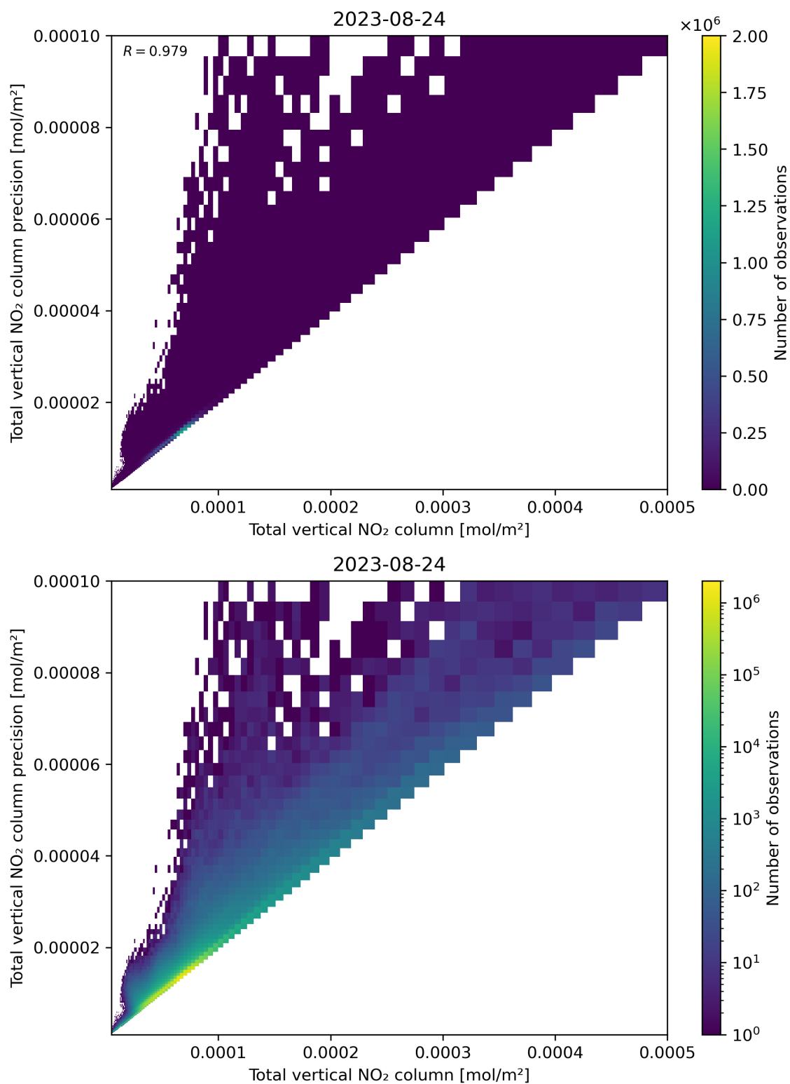
Figure 114: Scatter density plot of “Total vertical NO 2 column” against “Total vertical NO 2 column precision” for 2023-08-23 to 2023-08-25.
