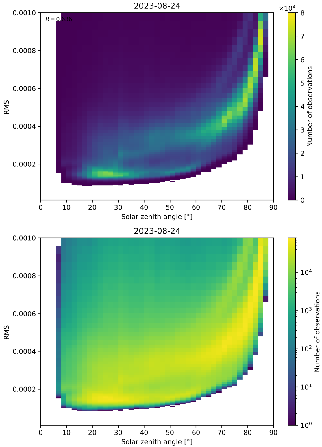
Figure 157: Scatter density plot of “Solar zenith angle” against “RMS” for 2023-08-23 to 2023-08-25.
