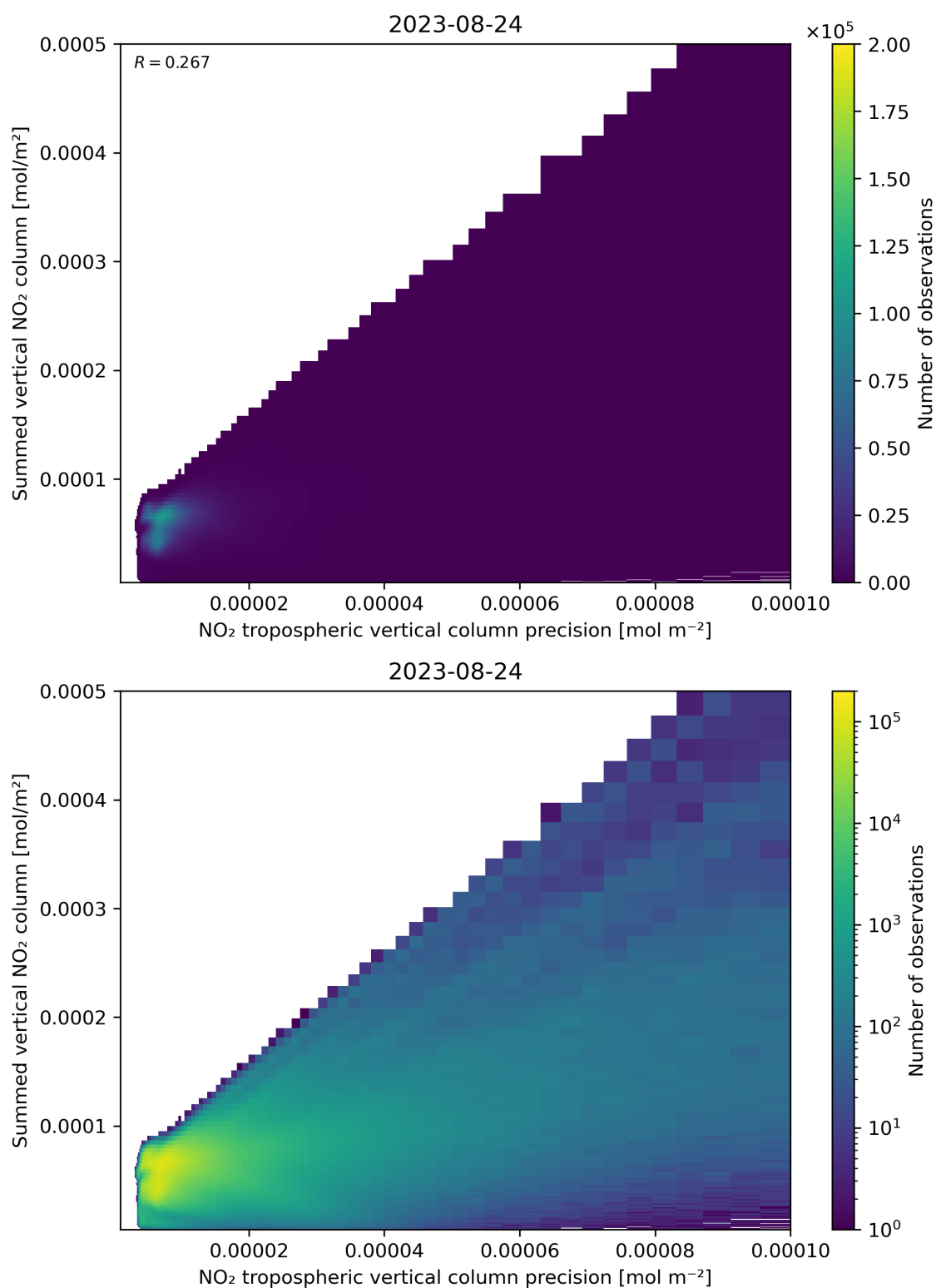
Figure 136: Scatter density plot of “NO 2 tropospheric vertical column precision” against “Summed vertical NO 2 column” for 2023-08-23 to 2023-08-25.
