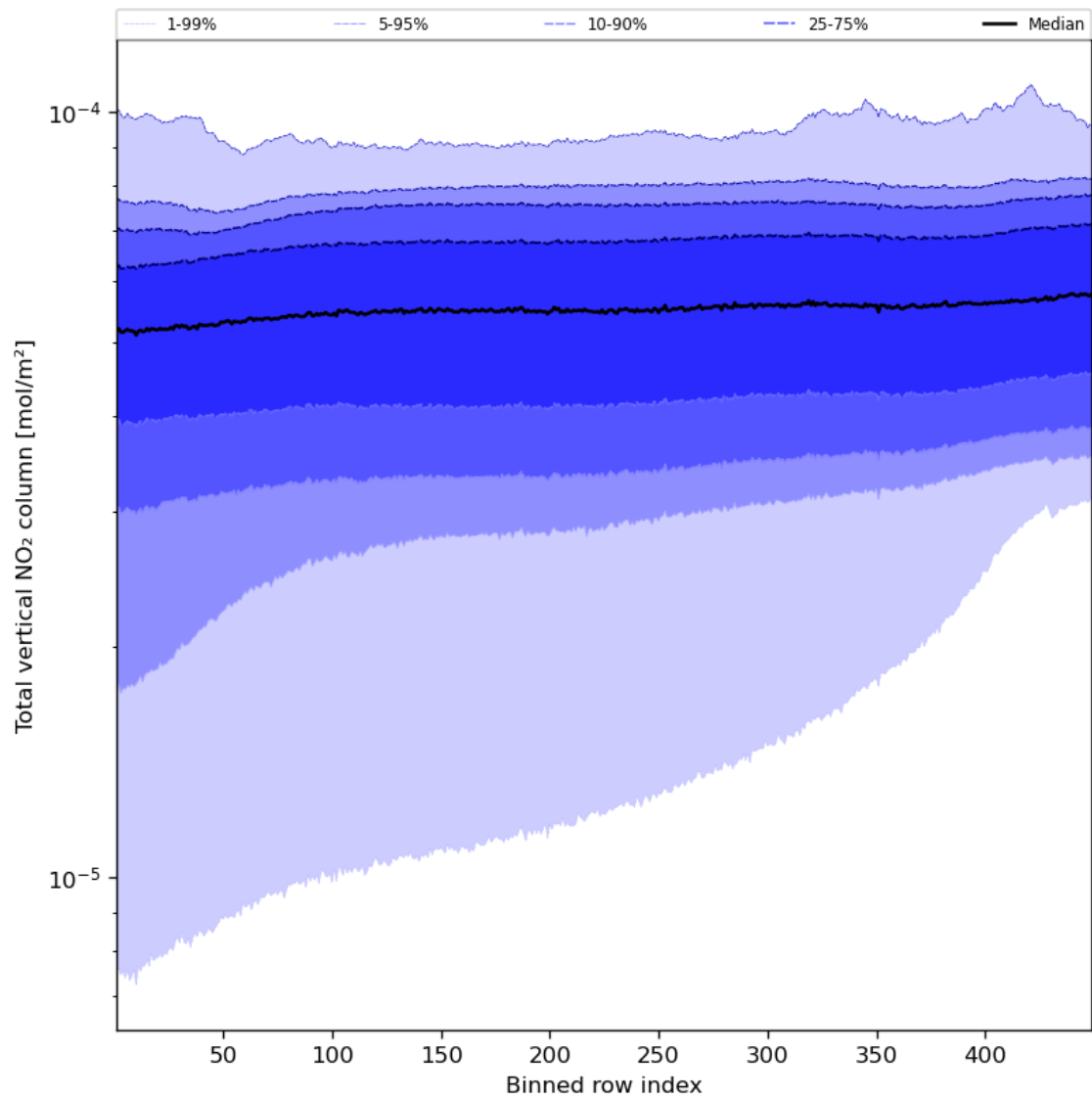
Figure 55: Along track statistics of “Total vertical NO 2 column” for 2023-08-23 to 2023-08-25
