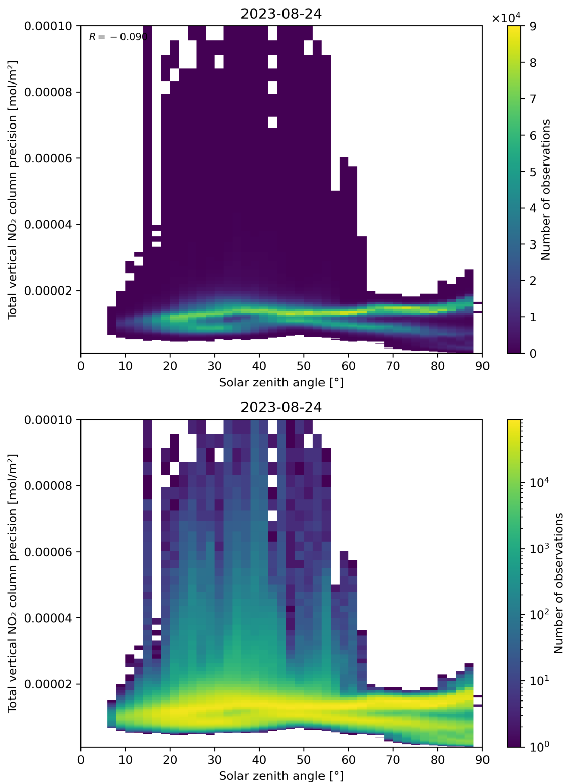
Figure 154: Scatter density plot of “Solar zenith angle” against “Total vertical NO 2 column precision” for 2023-08-23 to 2023-08-25.
