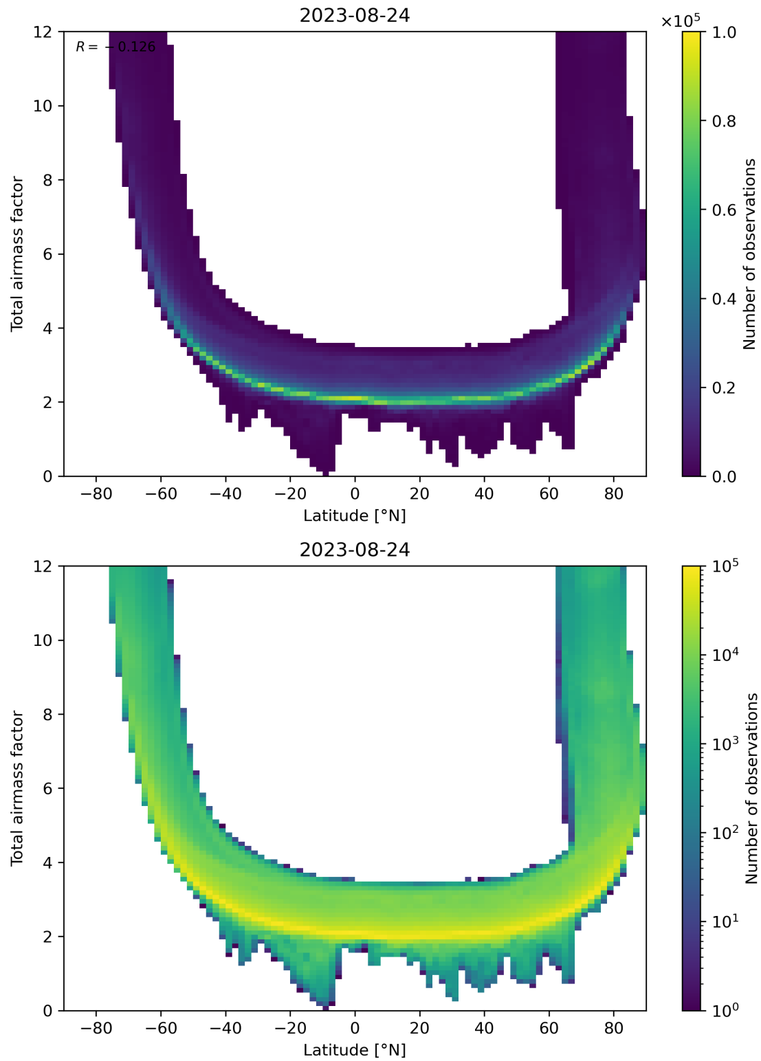
Figure 84: Scatter density plot of “Latitude” against “Total airmass factor” for 2023-08-23 to 2023-08-25.
