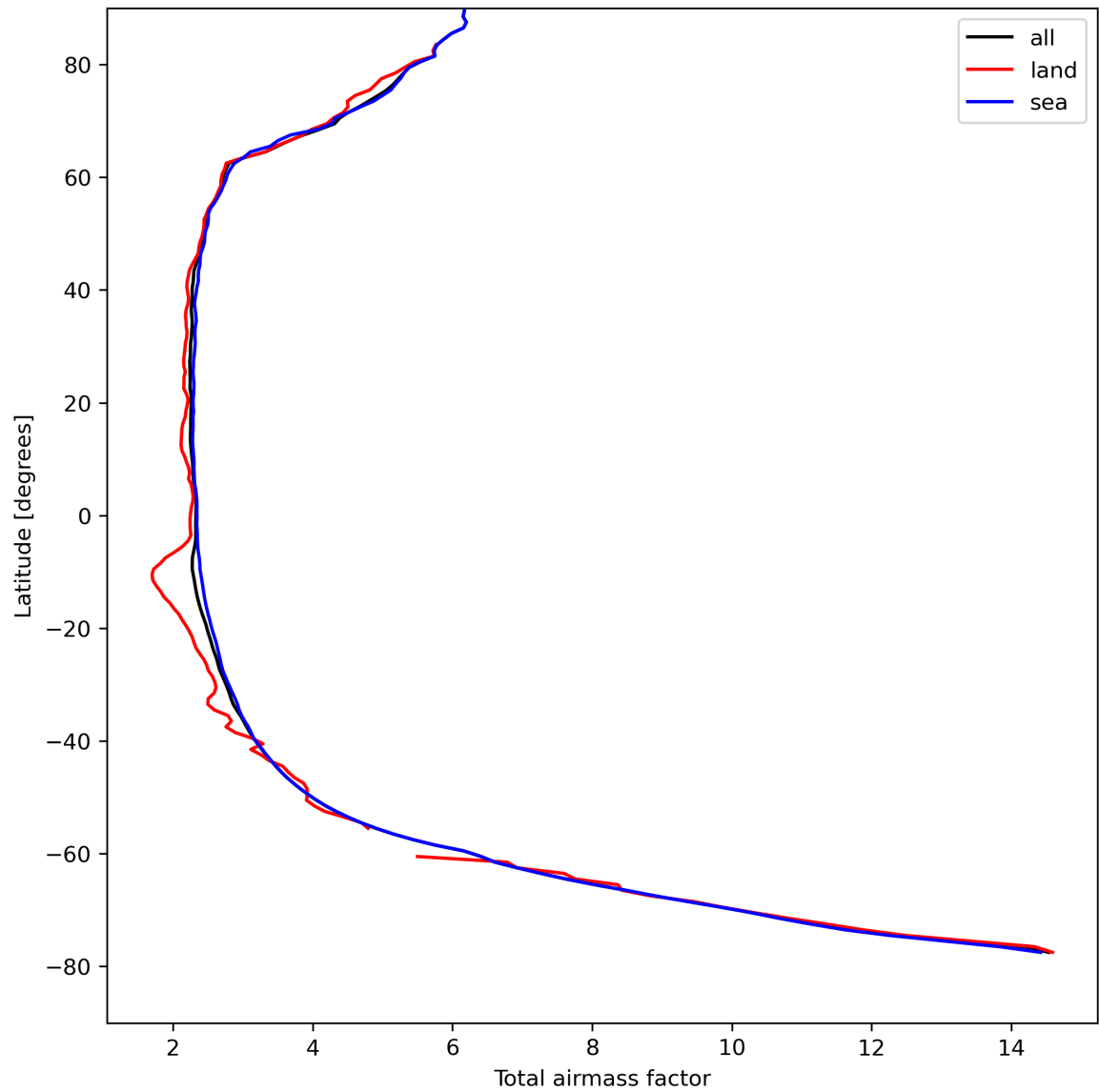
Figure 15: Zonal average of “Total airmass factor” for 2023-08-23 to 2023-08-25.
