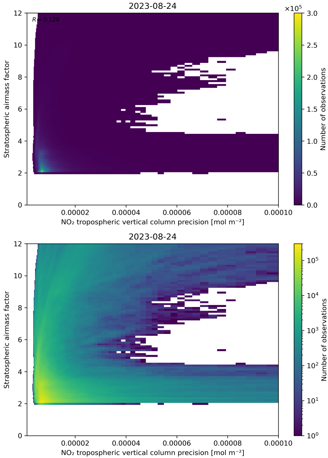
Figure 131: Scatter density plot of “NO 2 tropospheric vertical column precision” against “Stratospheric airmass factor” for 2023-08-23 to 2023-08-25.
