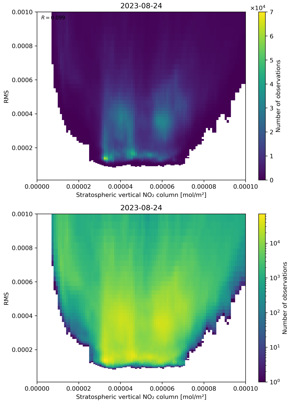
Figure 102: Scatter density plot of “Stratospheric vertical NO 2 column” against “RMS” for 2023-08-23 to 2023-08-25.
