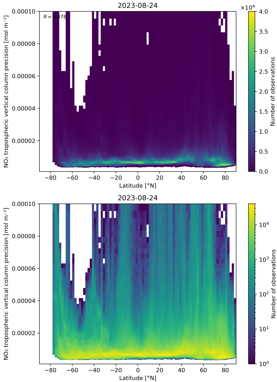
Figure 93: Scatter density plot of “Latitude” against “NO 2 tropospheric vertical column precision” for 2023-08-23 to 2023-08-25.
