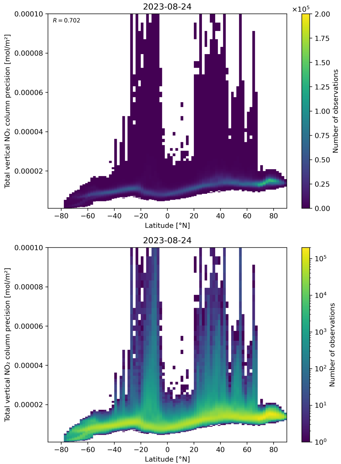
Figure 91: Scatter density plot of “Latitude” against “Total vertical NO 2 column precision” for 2023-08-23 to 2023-08-25.
