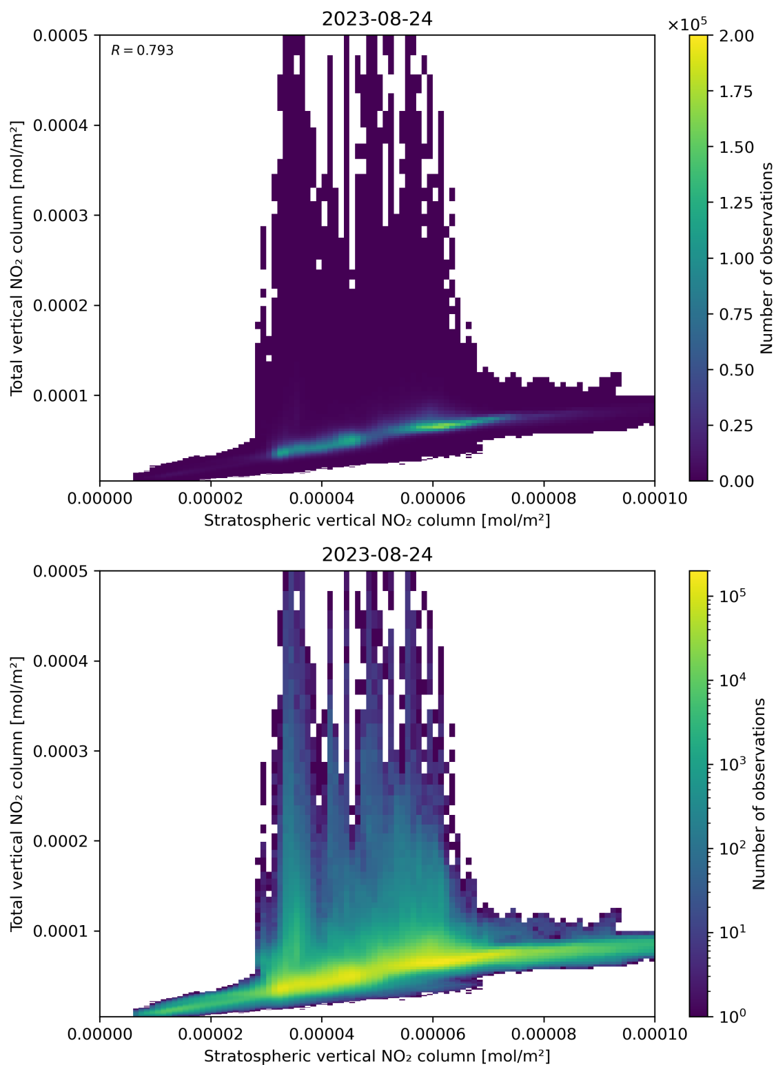
Figure 100: Scatter density plot of “Stratospheric vertical NO 2 column” against “Total vertical NO 2 column” for 2023-08-23 to 2023-08-25.
