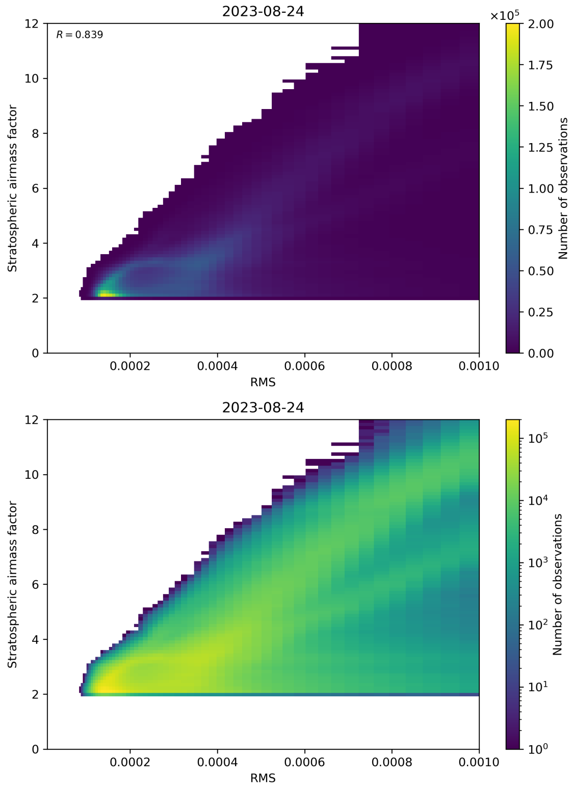
Figure 144: Scatter density plot of “RMS” against “Stratospheric airmass factor” for 2023-08-23 to 2023-08-25.
