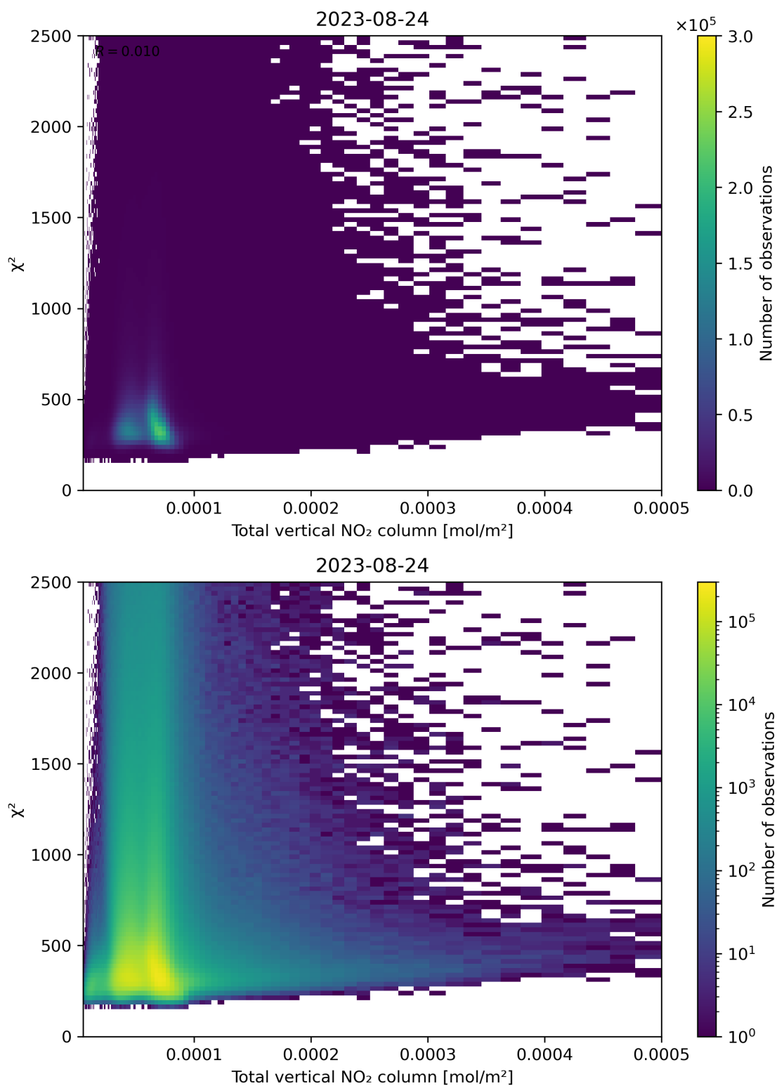
Figure 111: Scatter density plot of “Total vertical NO 2 column” against “ \chi^2 ” for 2023-08-23 to 2023-08-25.
