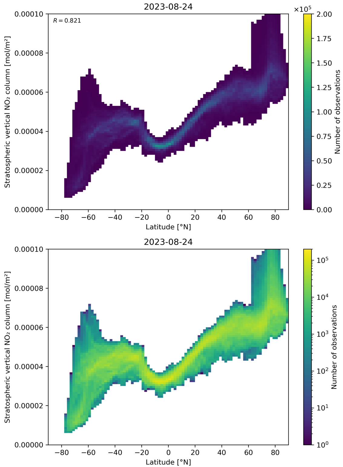
Figure 87: Scatter density plot of “Latitude” against “Stratospheric vertical NO 2 column” for 2023-08-23 to 2023-08-25.
