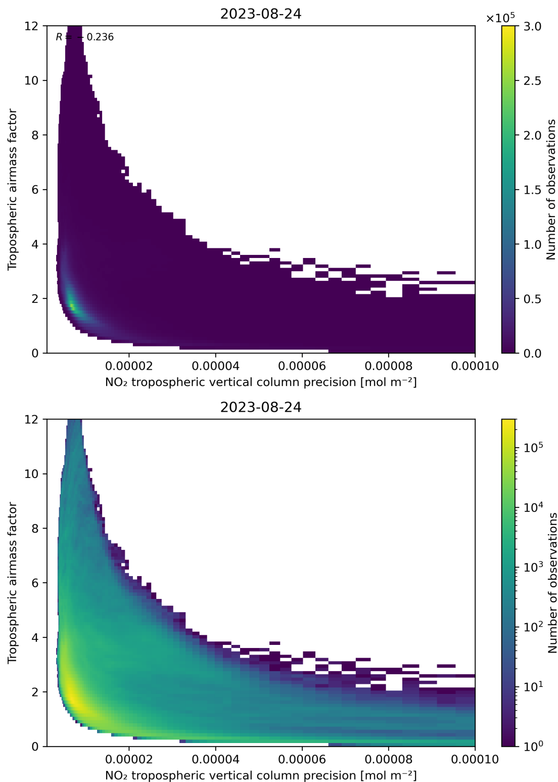
Figure 133: Scatter density plot of “NO 2 tropospheric vertical column precision” against “Tropospheric air mass factor” for 2023-08-23 to 2023-08-25.
