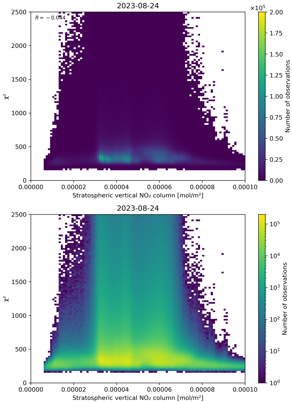
Figure 97: Scatter density plot of “Stratospheric vertical NO 2 column” against “ \chi^2 ” for 2023-08-23 to 2023-08-25.
