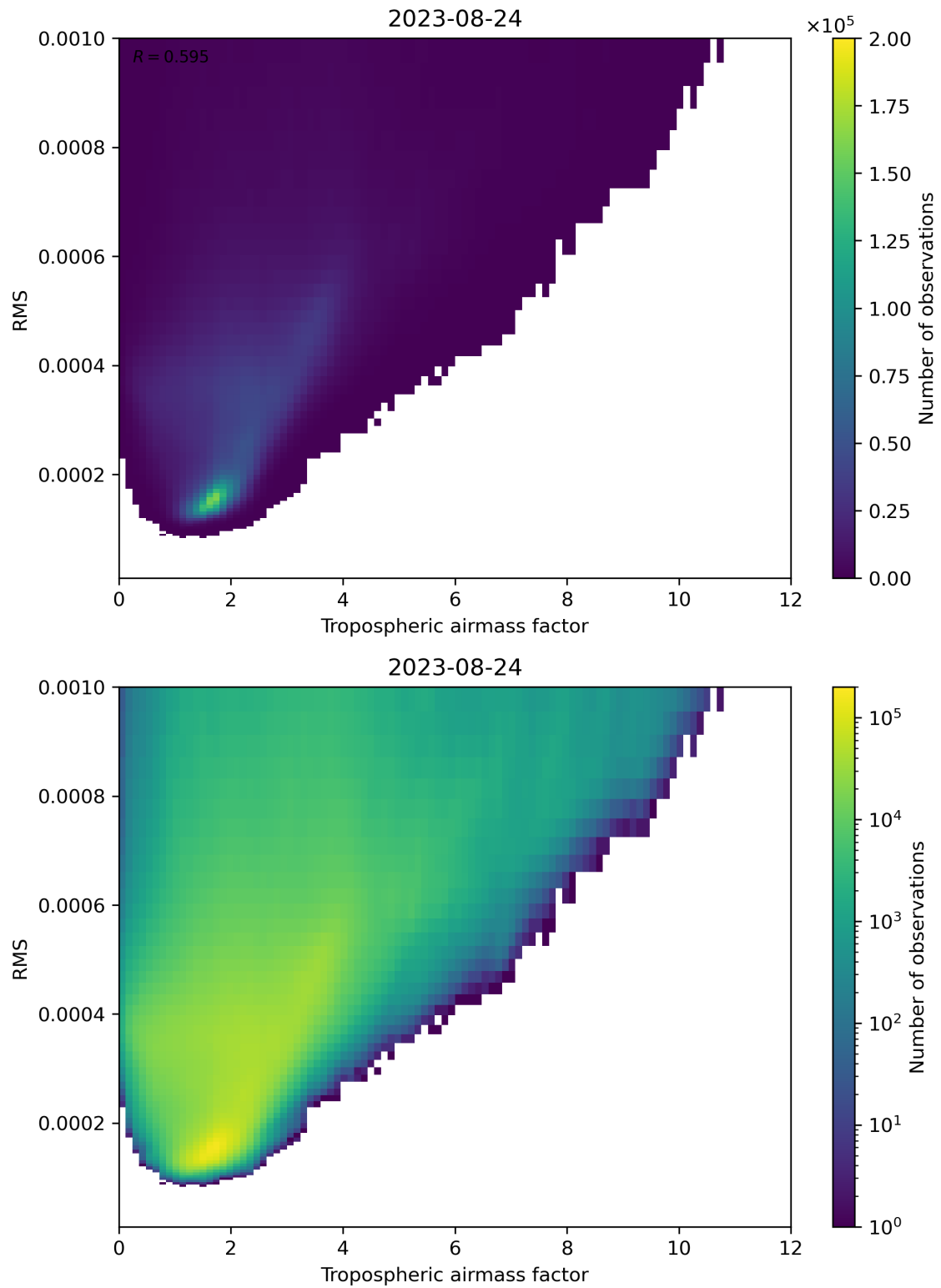
Figure 79: Scatter density plot of “Tropospheric airmass factor” against “RMS” for 2023-08-23 to 2023-08-25.
