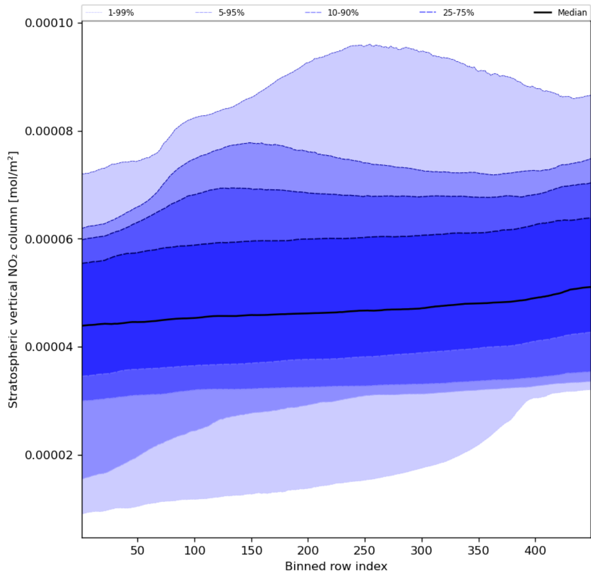
Figure 53: Along track statistics of “Stratospheric vertical NO 2 column” for 2023-08-23 to 2023-08-25
