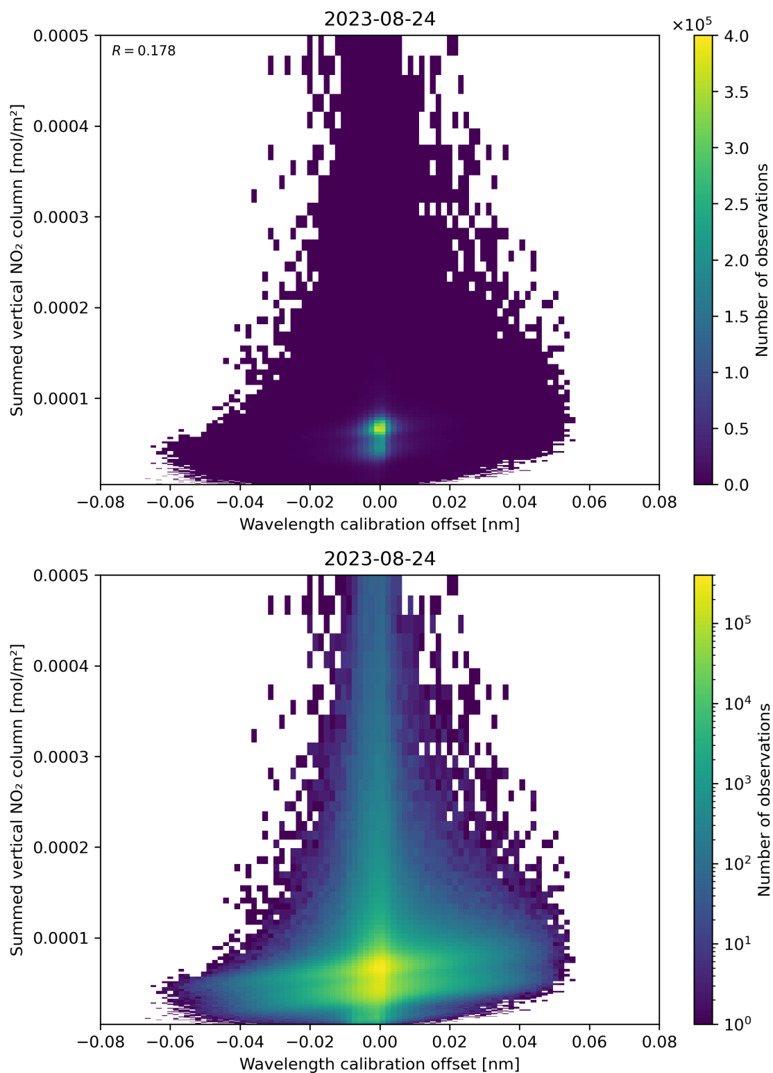
Figure 177: Scatter density plot of “Wavelength calibration offset” against “Summed vertical NO 2 column” for 2023-08-23 to 2023-08-25.
