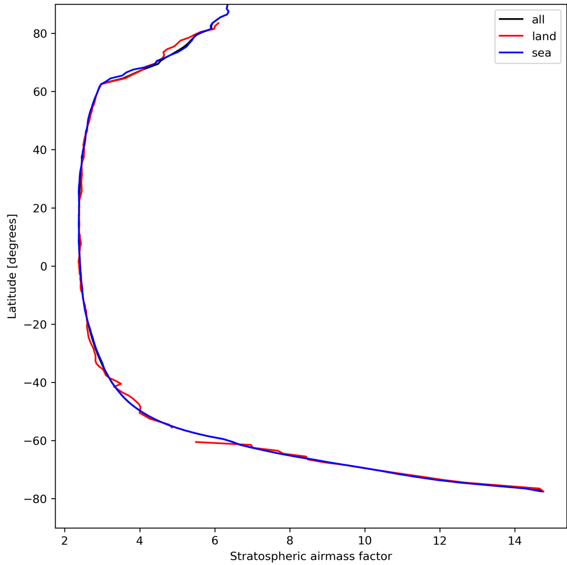
Figure 27: Zonal average of “Stratospheric air mass factor” for 2023-08-23 to 2023-08-25.
