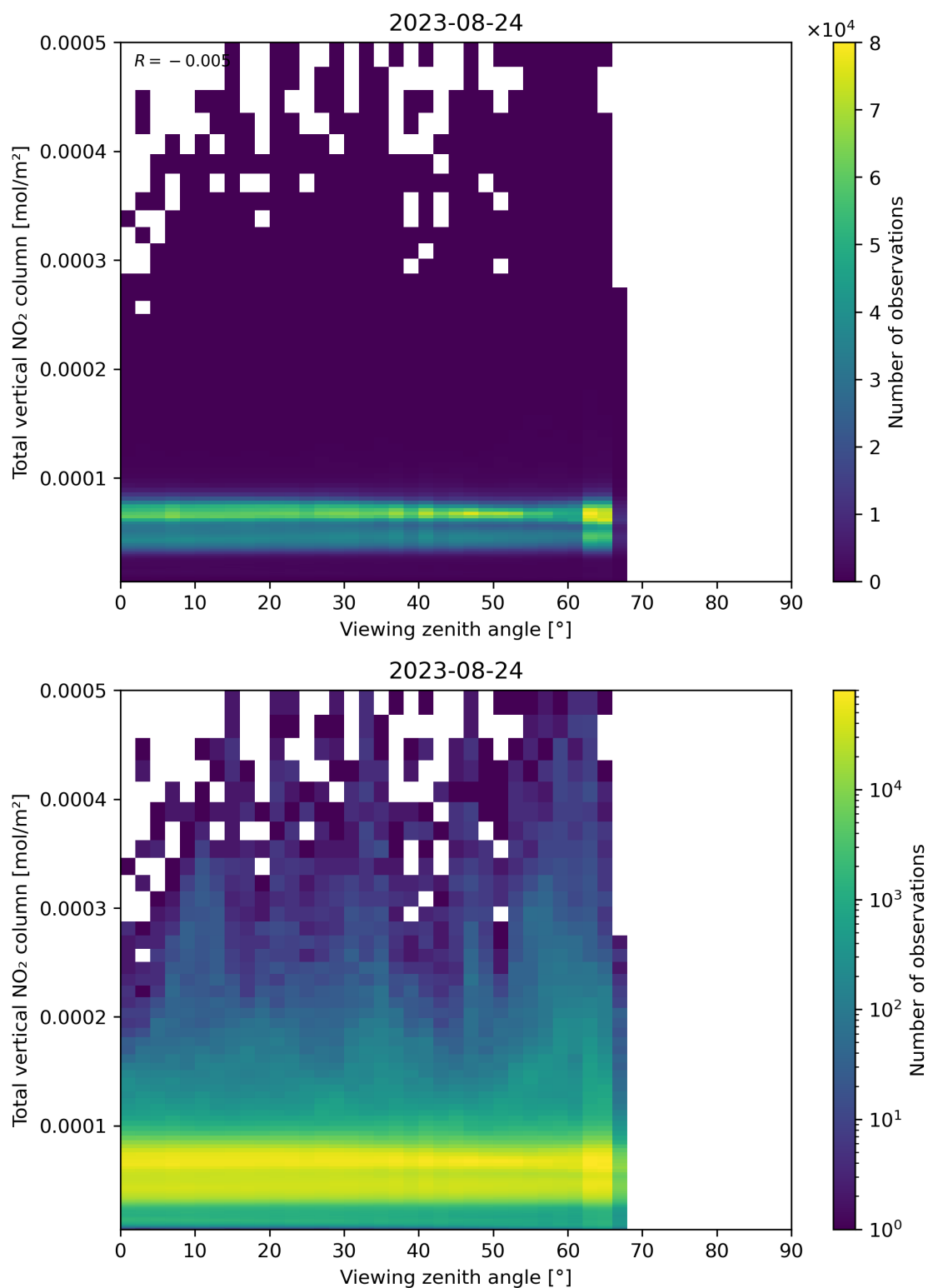
Figure 167: Scatter density plot of “Viewing zenith angle” against “Total vertical NO 2 column” for 2023-08-23 to 2023-08-25.
