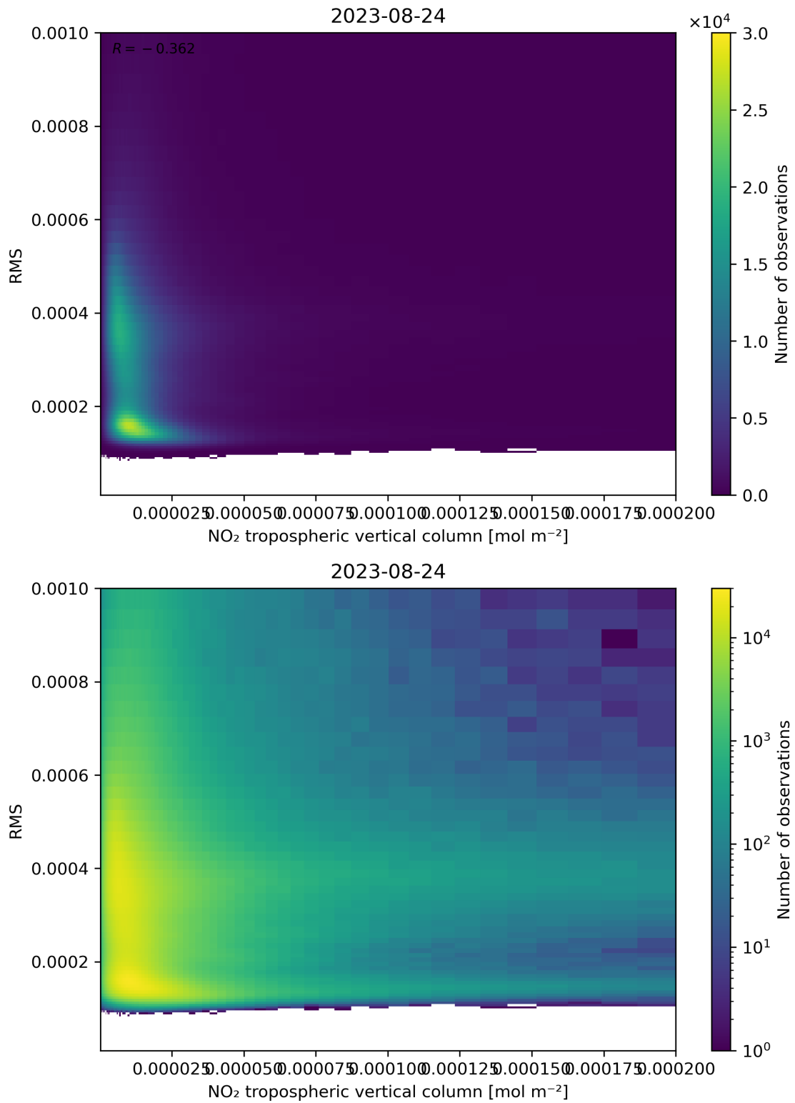
Figure 142: Scatter density plot of “NO 2 tropospheric vertical column” against “RMS” for 2023-08-23 to 2023-08-25.
