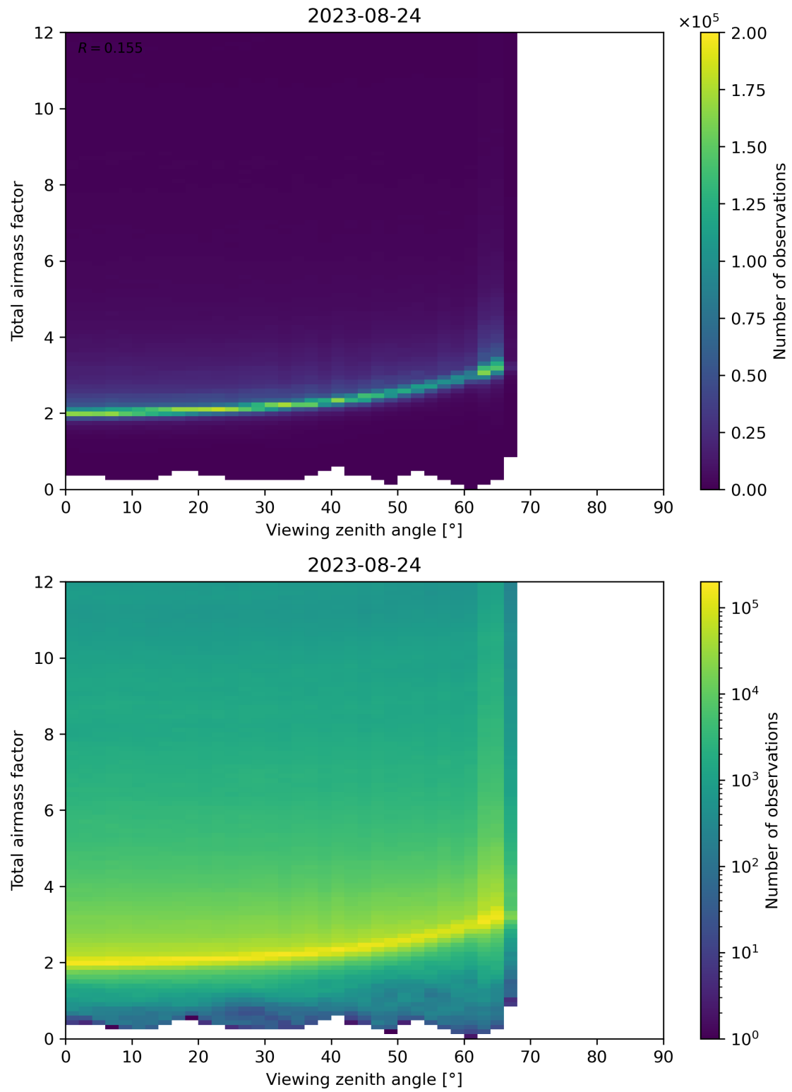
Figure 160: Scatter density plot of “Viewing zenith angle” against “Total airmass factor” for 2023-08-23 to 2023-08-25.
