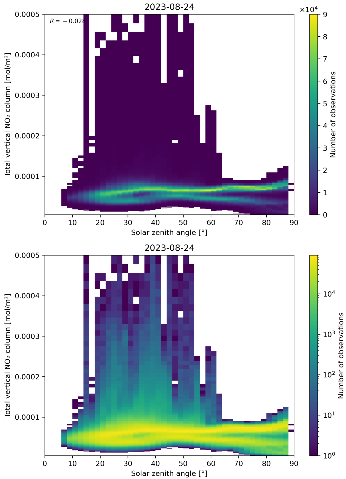
Figure 153: Scatter density plot of “Solar zenith angle” against “Total vertical NO 2 column” for 2023-08-23 to 2023-08-25.
