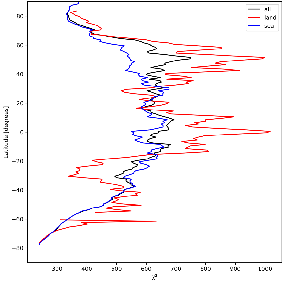
Figure 25: Zonal average of “ \chi^2 ” for 2023-08-23 to 2023-08-25.
