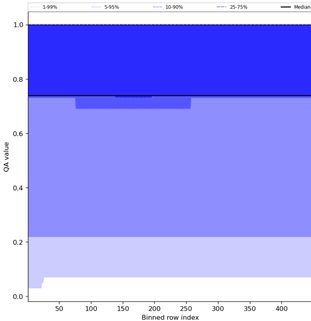
Figure 45: Along track statistics of “QA value” for 2023-08-23 to 2023-08-25
