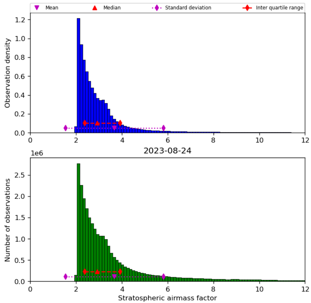
Figure 44: Histogram of “Stratospheric airmass factor” for 2023-08-23 to 2023-08-25
