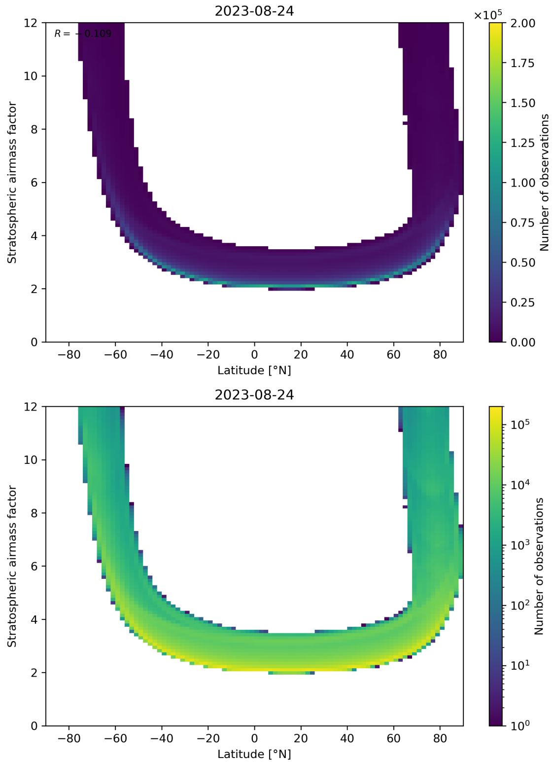
Figure 83: Scatter density plot of “Latitude” against “Stratospheric airmass factor” for 2023-08-23 to 2023-08-25.
