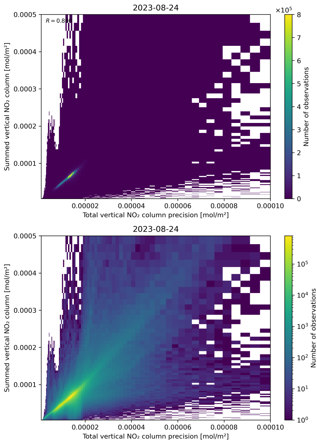
Figure 117: Scatter density plot of “Total vertical NO 2 column precision” against “Summed vertical NO 2 column” for 2023-08-23 to 2023-08-25.
