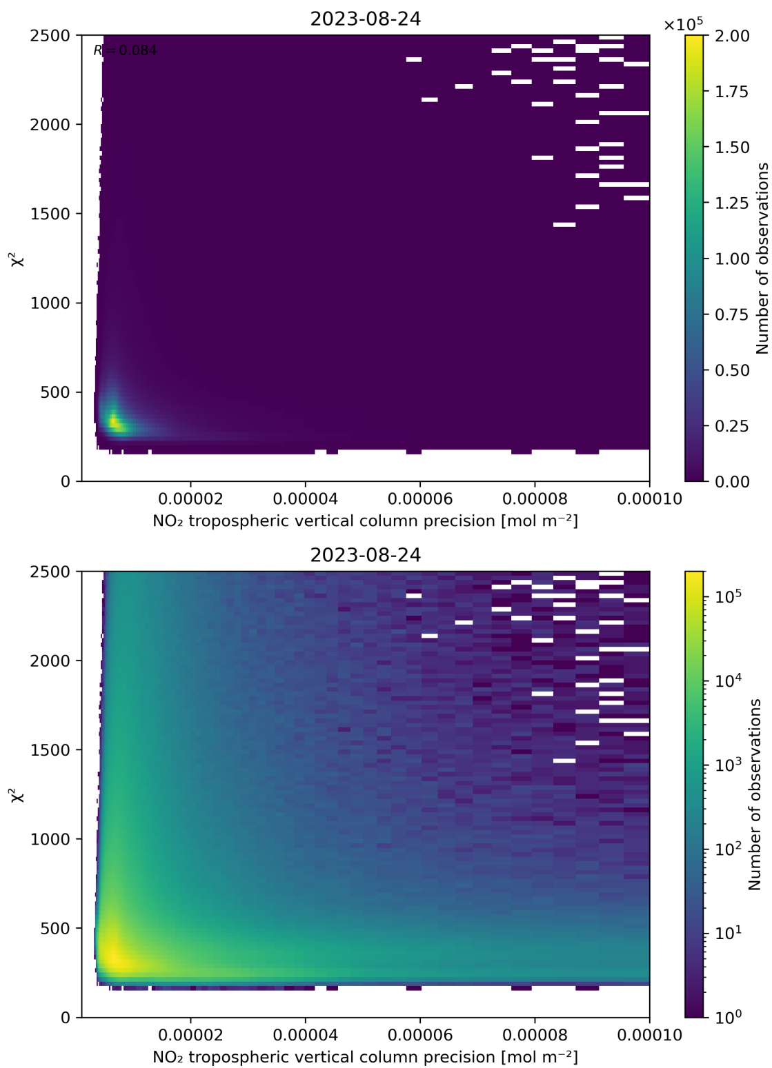
Figure 134: Scatter density plot of “NO 2 tropospheric vertical column precision” against “ \chi^2 ” for 2023-08-23 to 2023-08-25.
