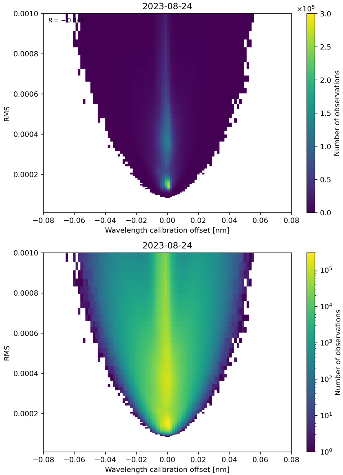
Figure 181: Scatter density plot of “Wavelength calibration offset” against “RMS” for 2023-08-23 to 2023-08-25.
