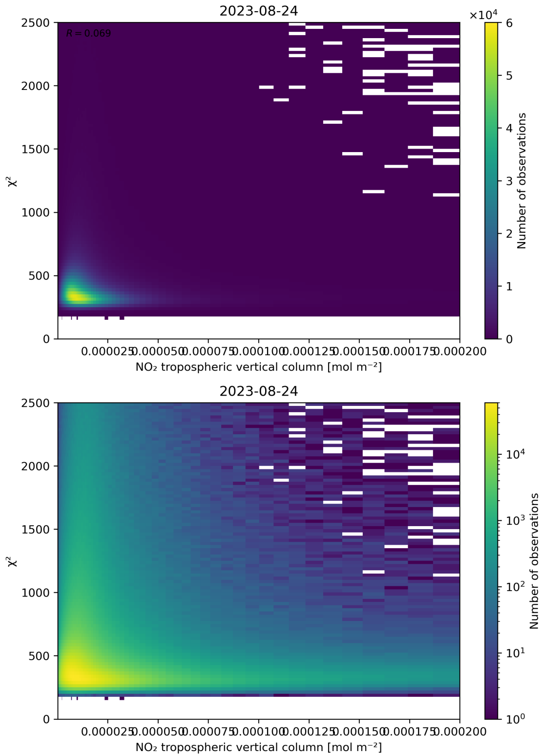
Figure 124: Scatter density plot of “NO 2 tropospheric vertical column” against “ \chi^2 ” for 2023-08-23 to 2023-08-25.
