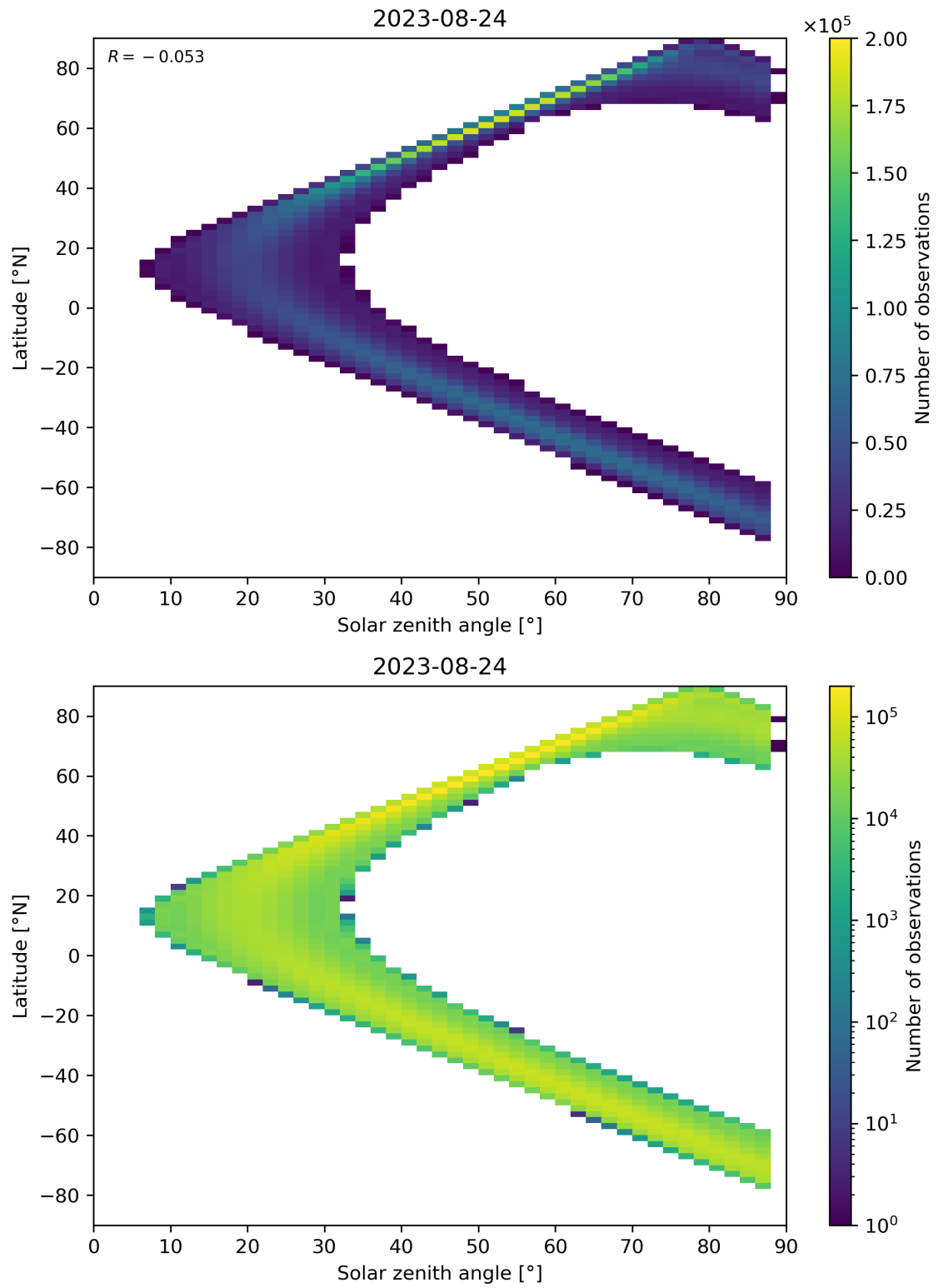
Figure 149: Scatter density plot of “Solar zenith angle” against “Latitude” for 2023-08-23 to 2023-08-25.
