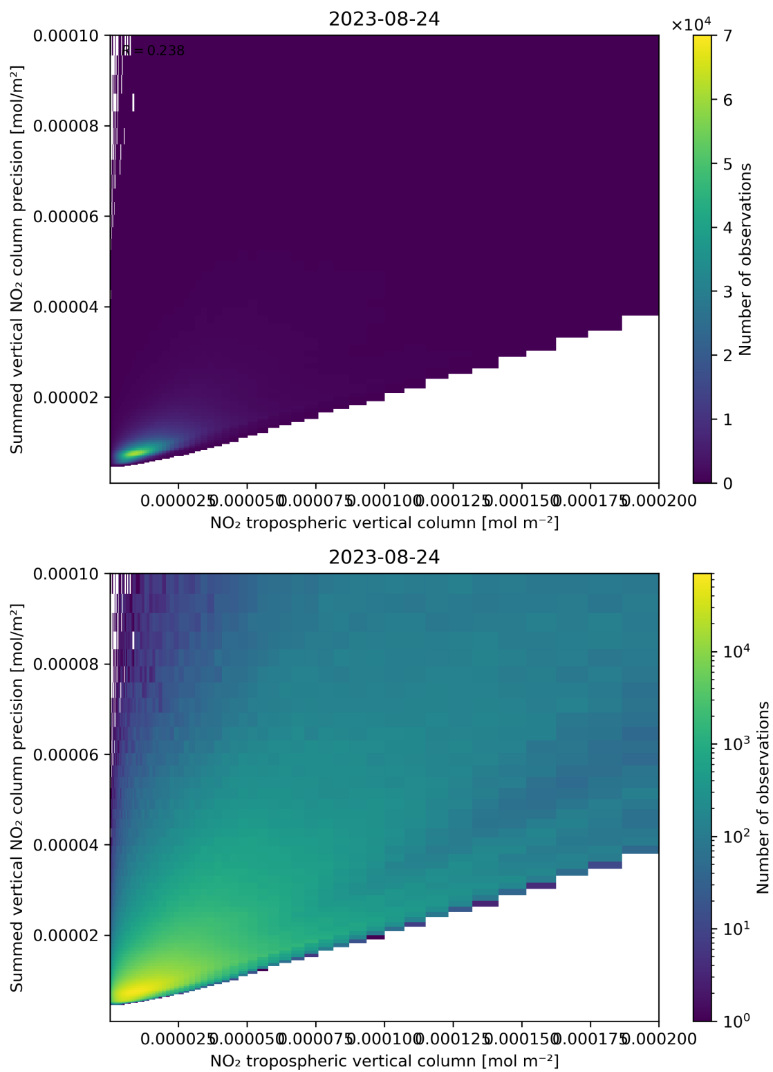
Figure 127: Scatter density plot of “NO 2 tropospheric vertical column” against “Summed vertical NO 2 column precision” for 2023-08-23 to 2023-08-25.
