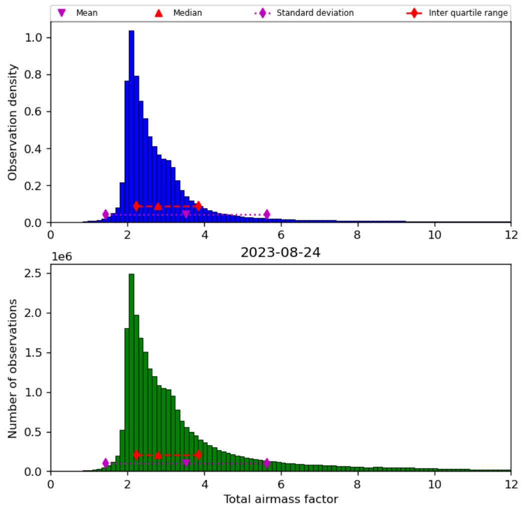
Figure 32: Histogram of “Total airmass factor” for 2023-08-23 to 2023-08-25
