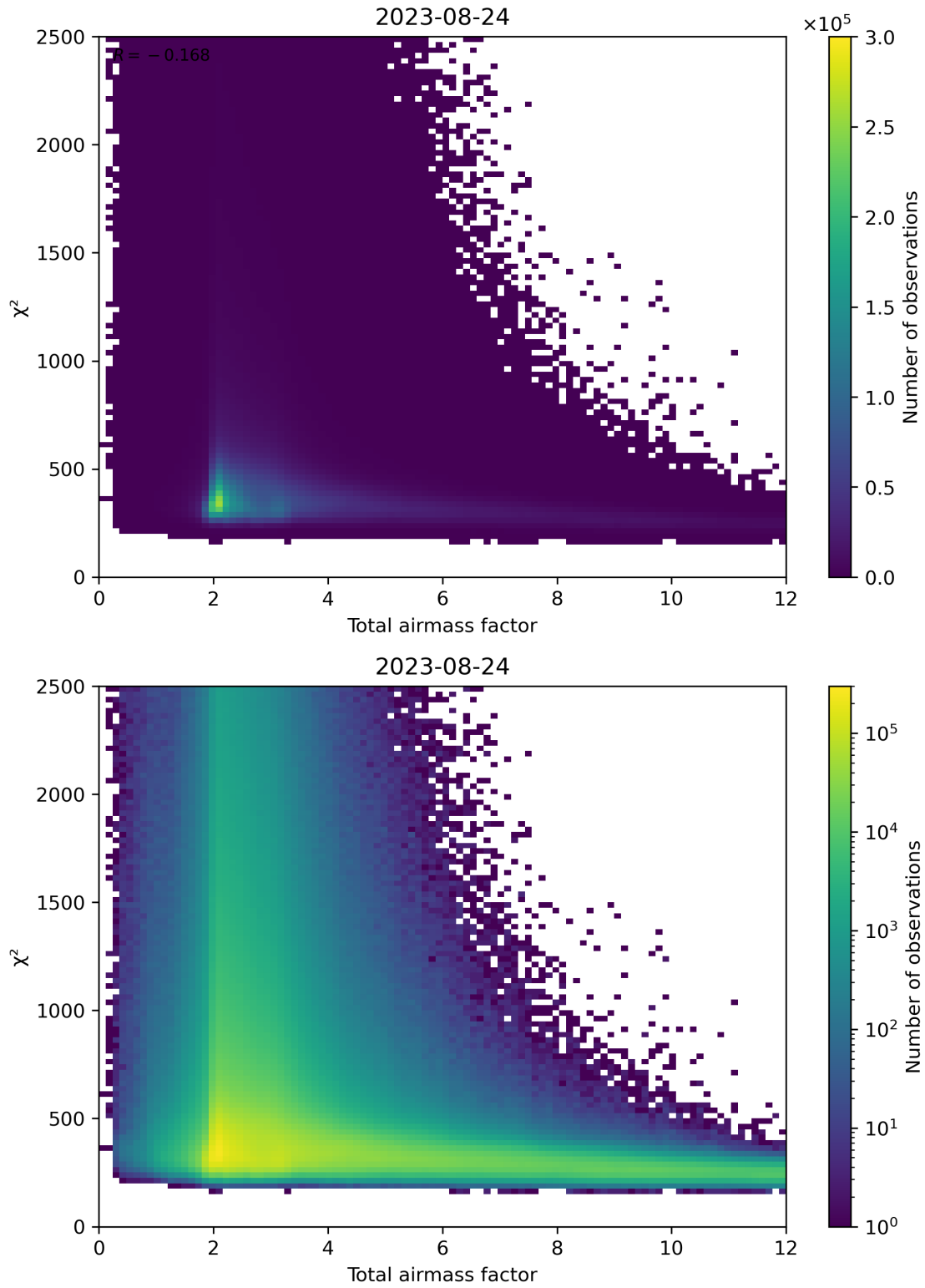
Figure 63: Scatter density plot of “Total airmass factor” against “ \chi^2 ” for 2023-08-23 to 2023-08-25.
