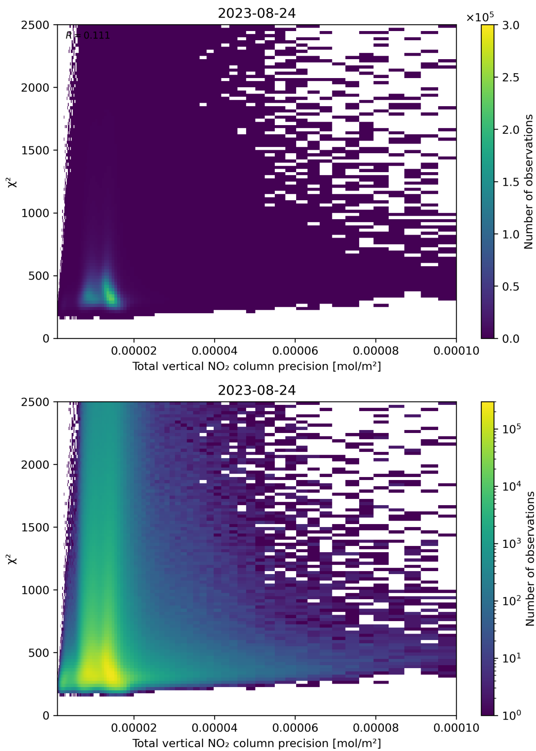
Figure 116: Scatter density plot of “Total vertical NO 2 column precision” against “ \chi^2 ” for 2023-08-23 to 2023-08-25.
