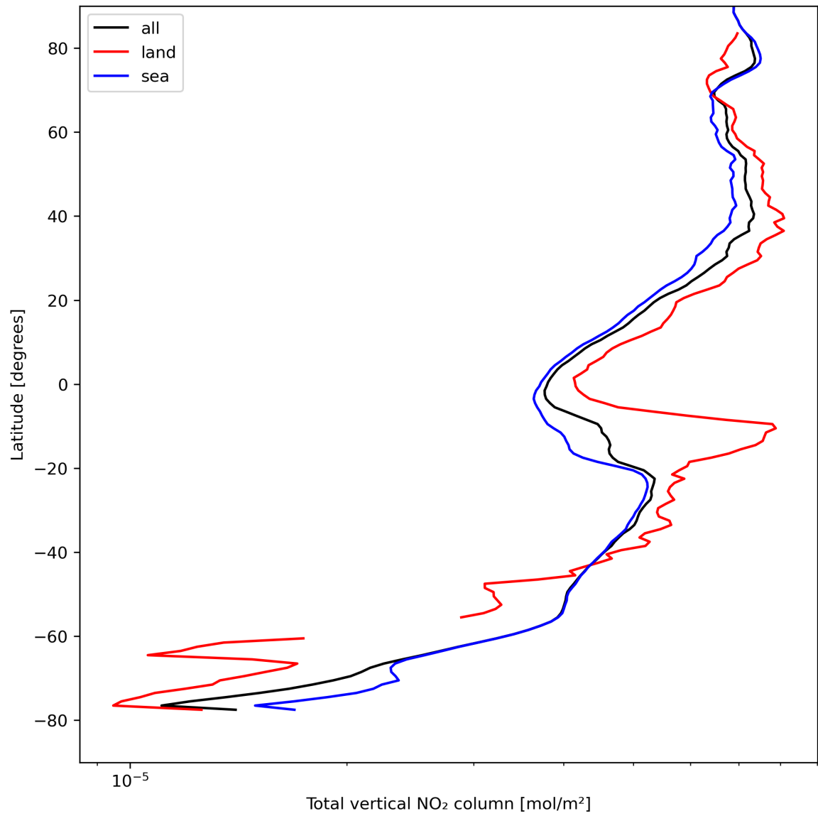
Figure 21: Zonal average of “Total vertical NO 2 column” for 2023-08-23 to 2023-08-25.
