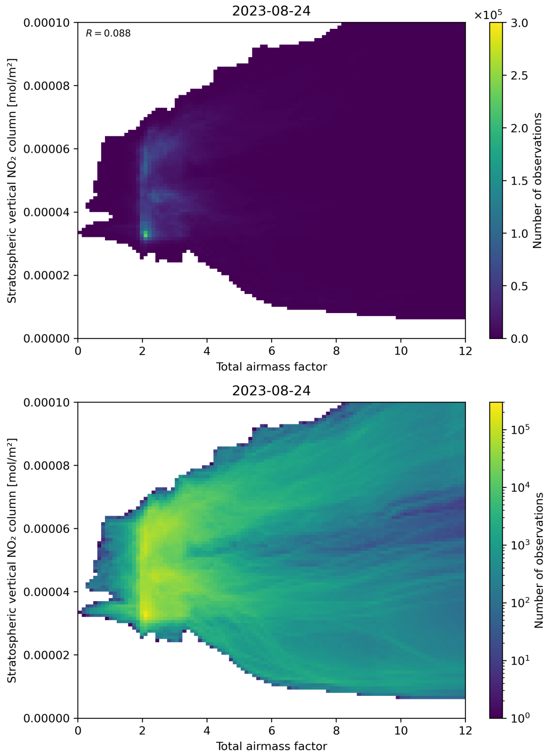
Figure 64: Scatter density plot of “Total airmass factor” against “Stratospheric vertical \text{NO}_2 column” for 2023-08-23 to 2023-08-25.
