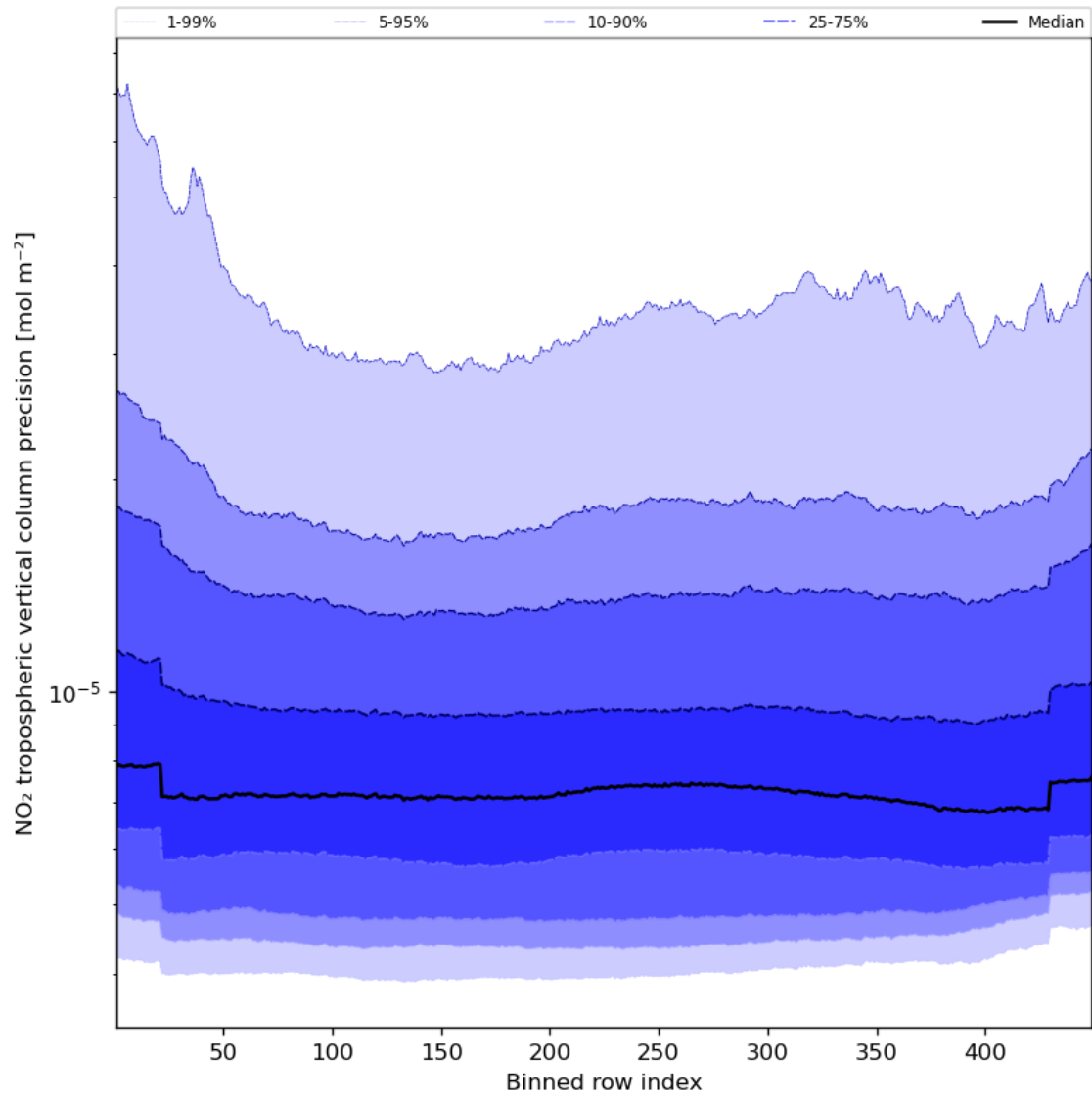
Figure 47: Along track statistics of “NO 2 tropospheric vertical column precision” for 2023-08-23 to 2023-08-25
