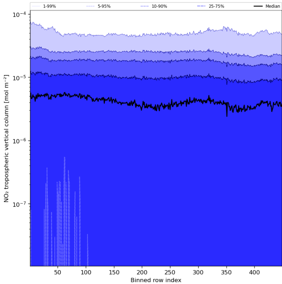
Figure 46: Along track statistics of “NO 2 tropospheric vertical column” for 2023-08-23 to 2023-08-25
