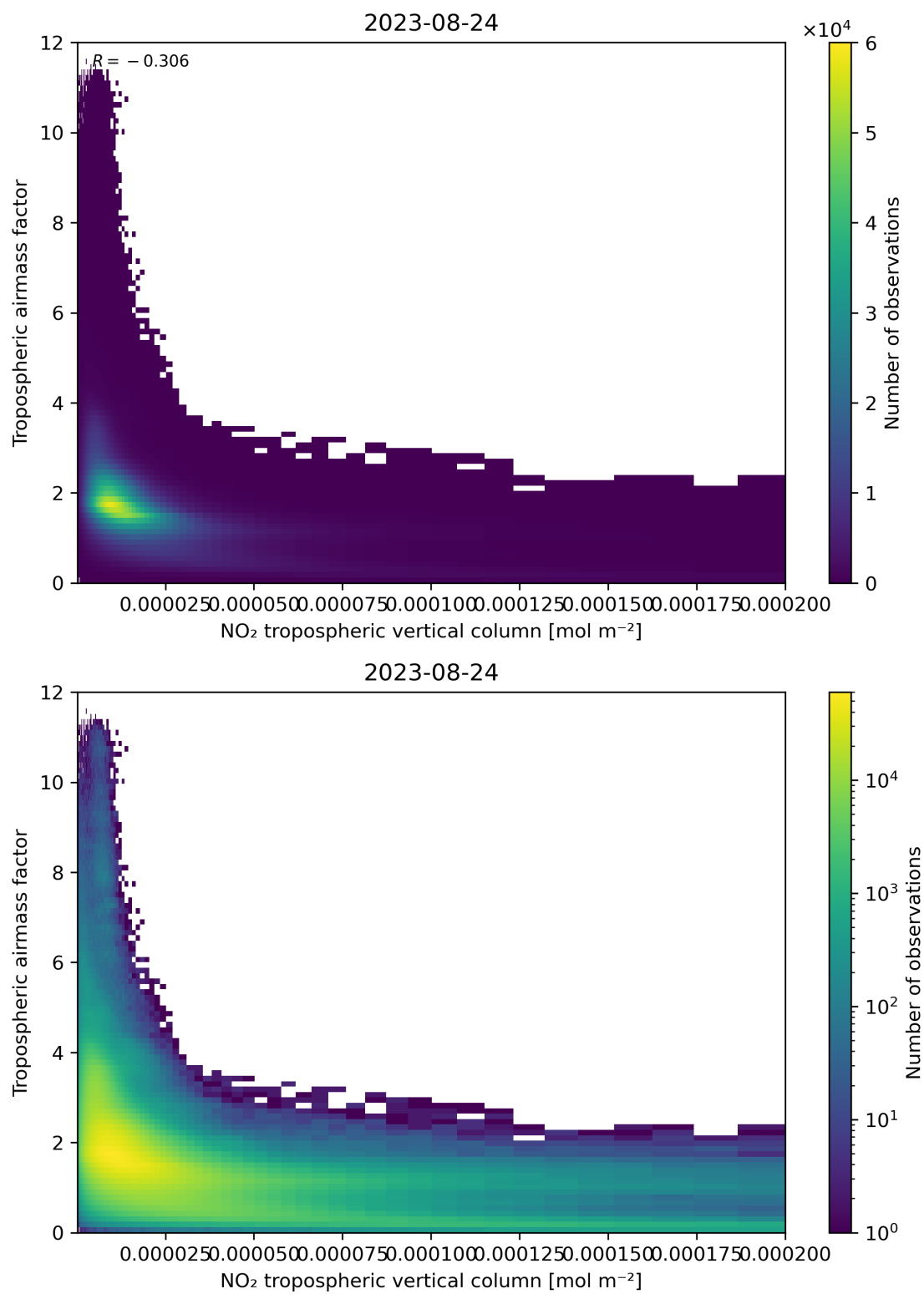
Figure 123: Scatter density plot of “NO 2 tropospheric vertical column” against “Tropospheric air mass factor” for 2023-08-23 to 2023-08-25.
