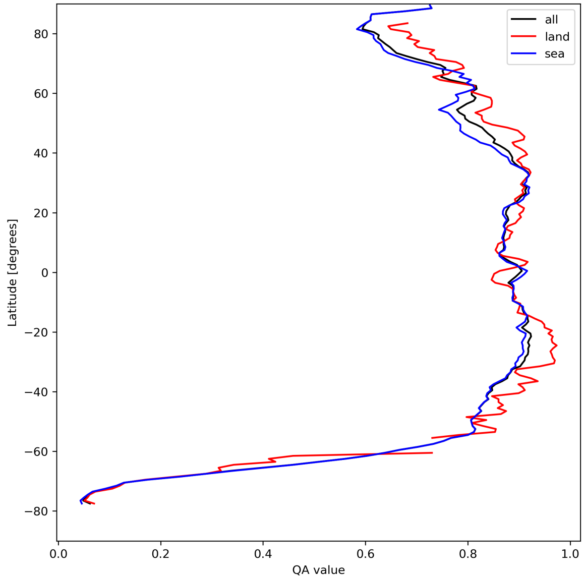
Figure 11: Zonal average of “QA value” for 2023-08-23 to 2023-08-25.
