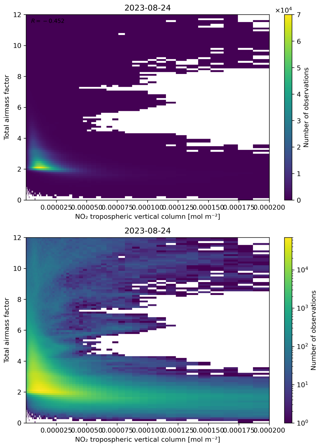
Figure 122: Scatter density plot of “NO 2 tropospheric vertical column” against “Total air mass factor” for 2023-08-23 to 2023-08-25.
