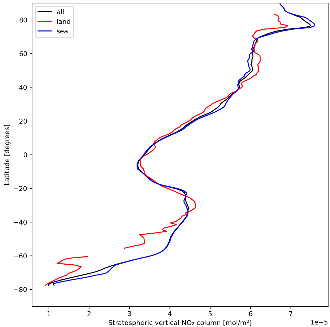
Figure 19: Zonal average of “Stratospheric vertical NO 2 column” for 2023-08-23 to 2023-08-25.
