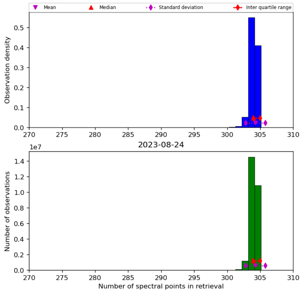
Figure 33: Histogram of “Number of spectral points in retrieval” for 2023-08-23 to 2023-08-25
