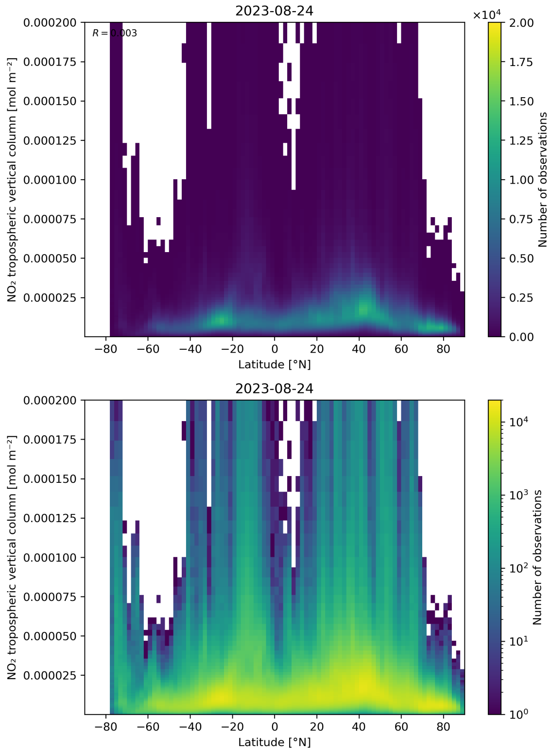
Figure 92: Scatter density plot of “Latitude” against “NO 2 tropospheric vertical column” for 2023-08-23 to 2023-08-25.
