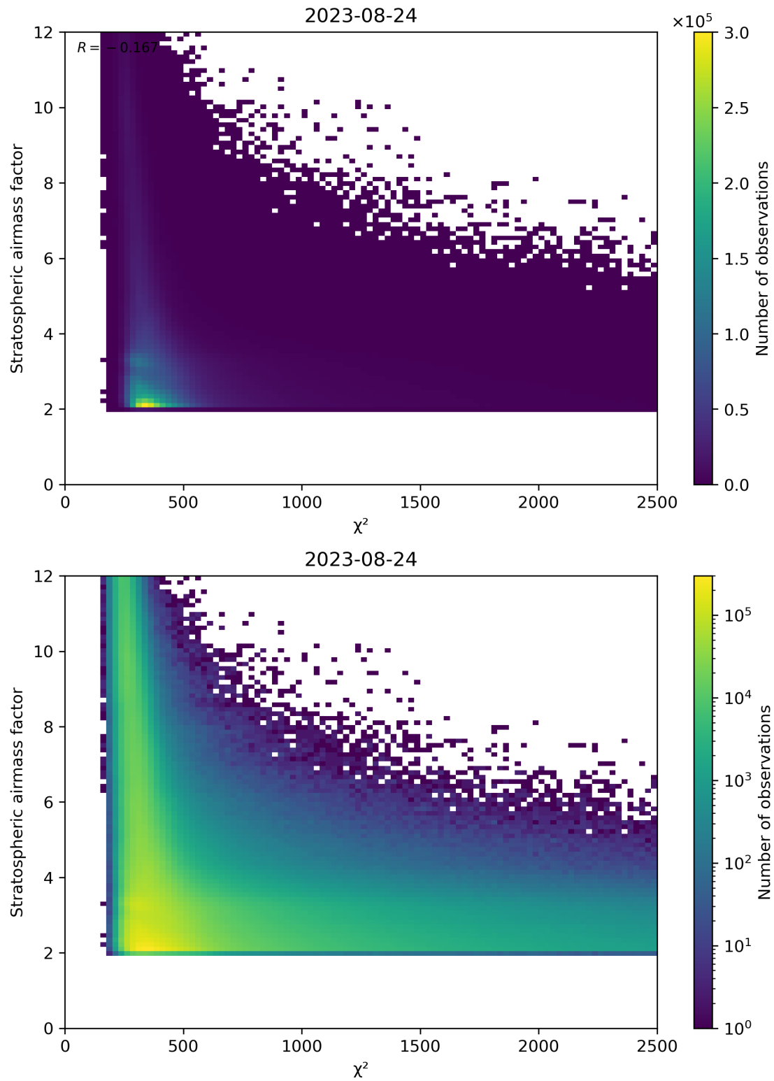
Figure 81: Scatter density plot of “ \chi^2 ” against “Stratospheric airmass factor” for 2023-08-23 to 2023-08-25.
