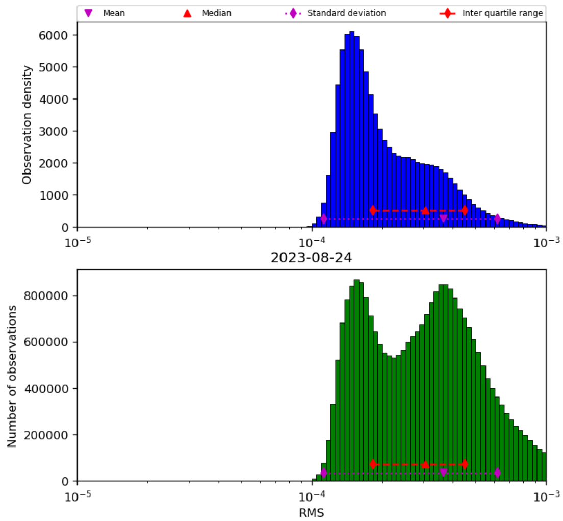
Figure 43: Histogram of “RMS” for 2023-08-23 to 2023-08-25
