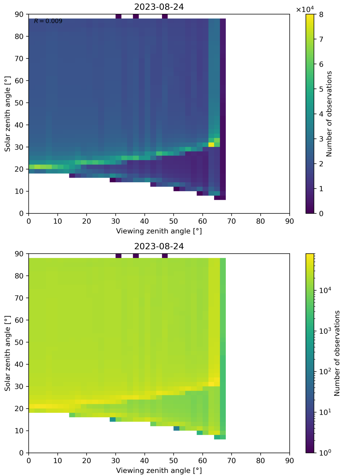
Figure 172: Scatter density plot of “Viewing zenith angle” against “Solar zenith angle” for 2023-08-23 to 2023-08-25.
