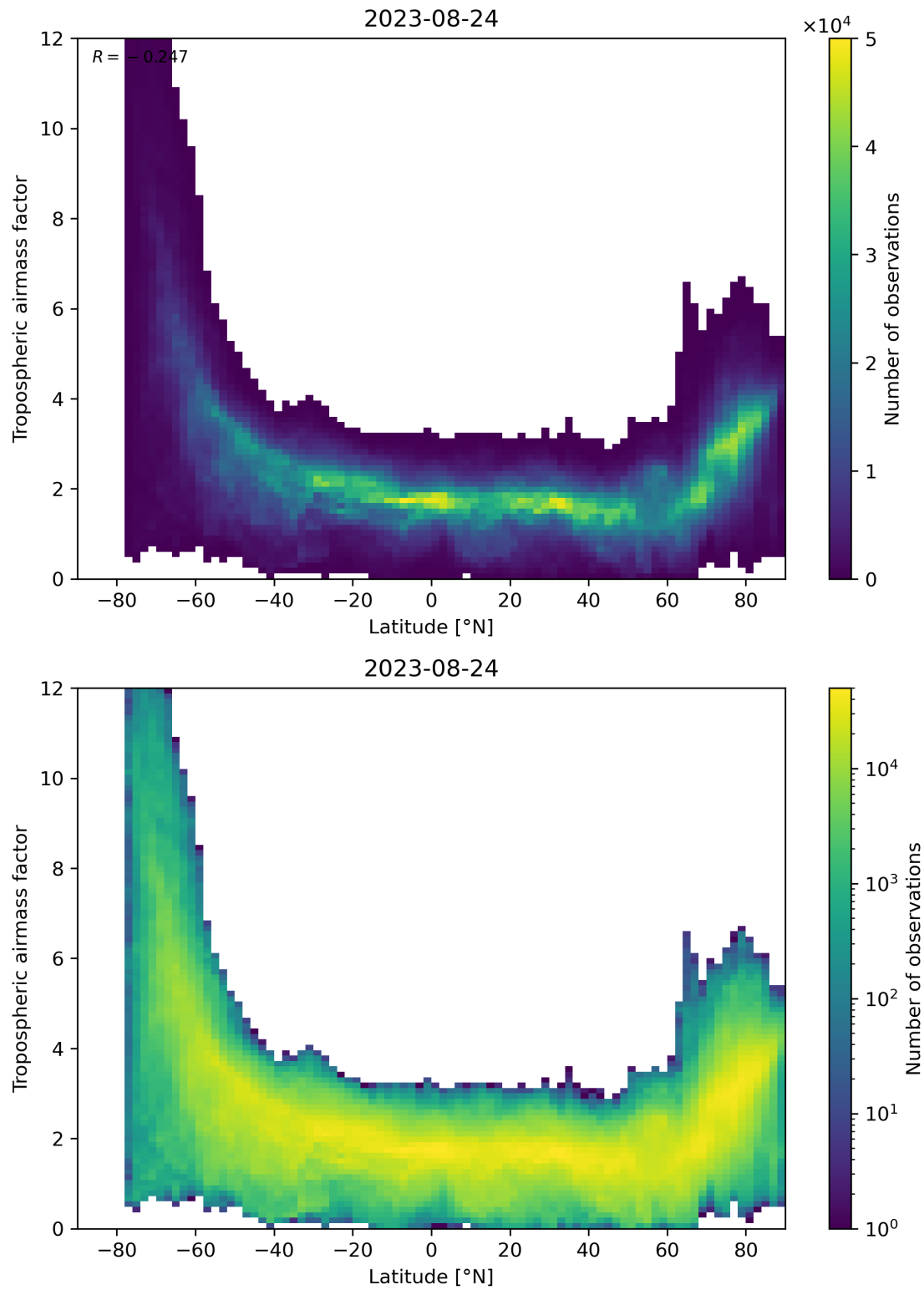
Figure 85: Scatter density plot of “Latitude” against “Tropospheric air mass factor” for 2023-08-23 to 2023-08-25.
