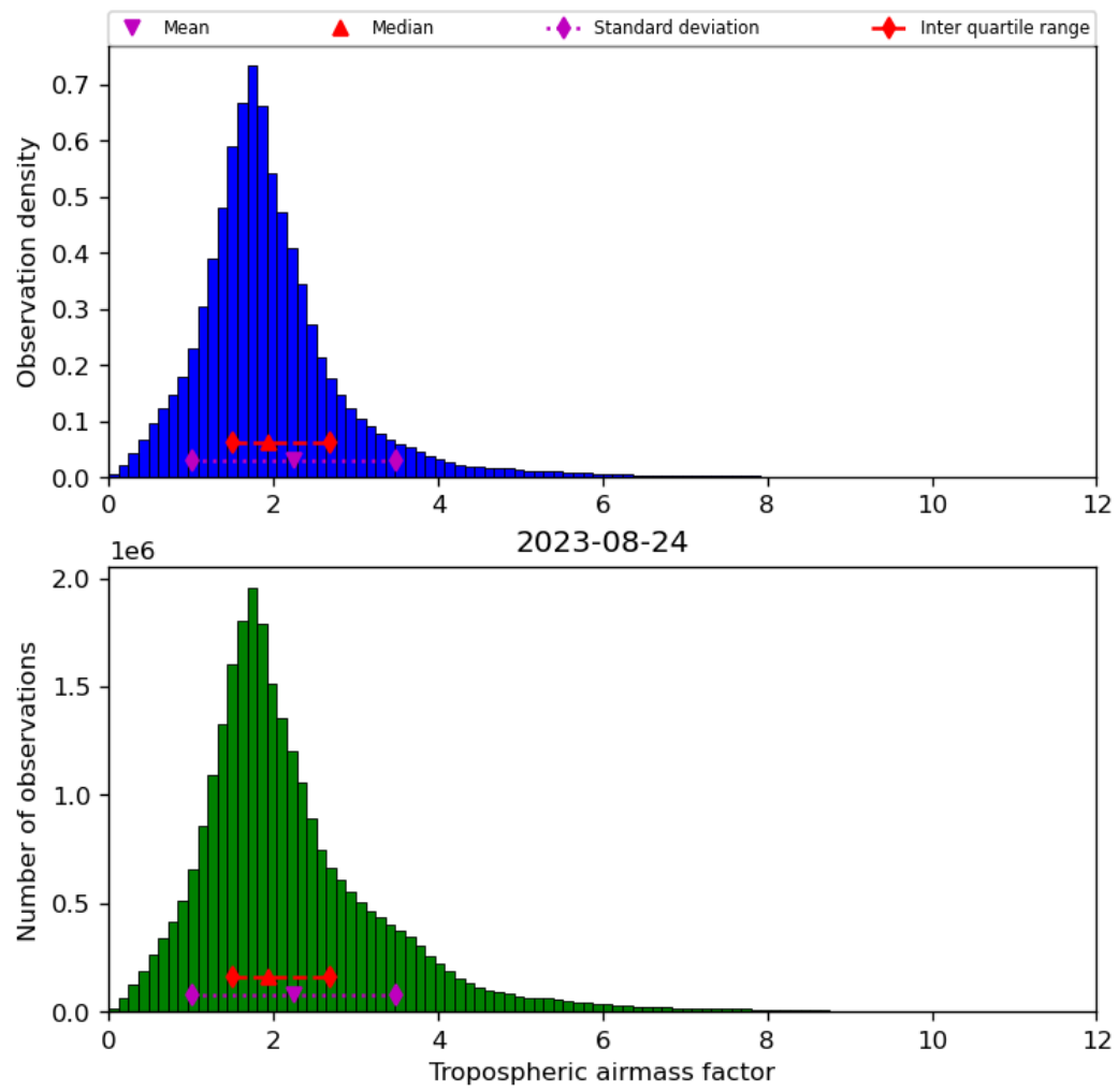
Figure 31: Histogram of “Tropospheric airmass factor” for 2023-08-23 to 2023-08-25
