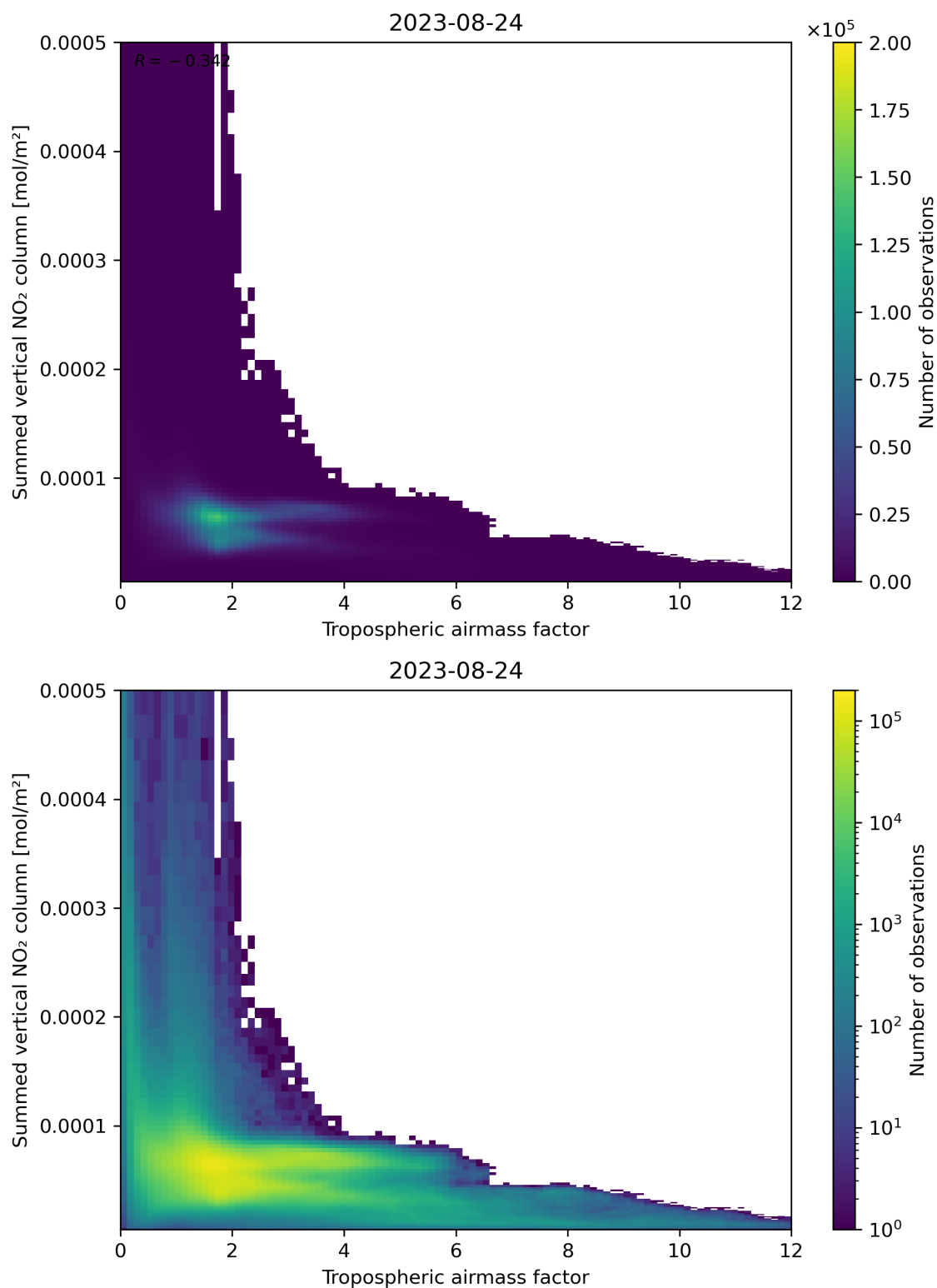
Figure 75: Scatter density plot of “Tropospheric air mass factor” against “Summed vertical NO 2 column” for 2023-08-23 to 2023-08-25.
