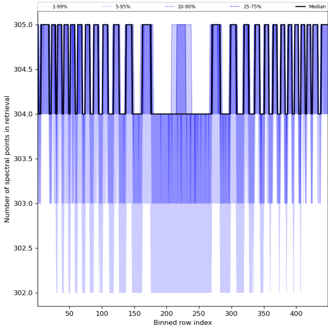
Figure 50: Along track statistics of “Number of spectral points in retrieval” for 2023-08-23 to 2023-08-25
