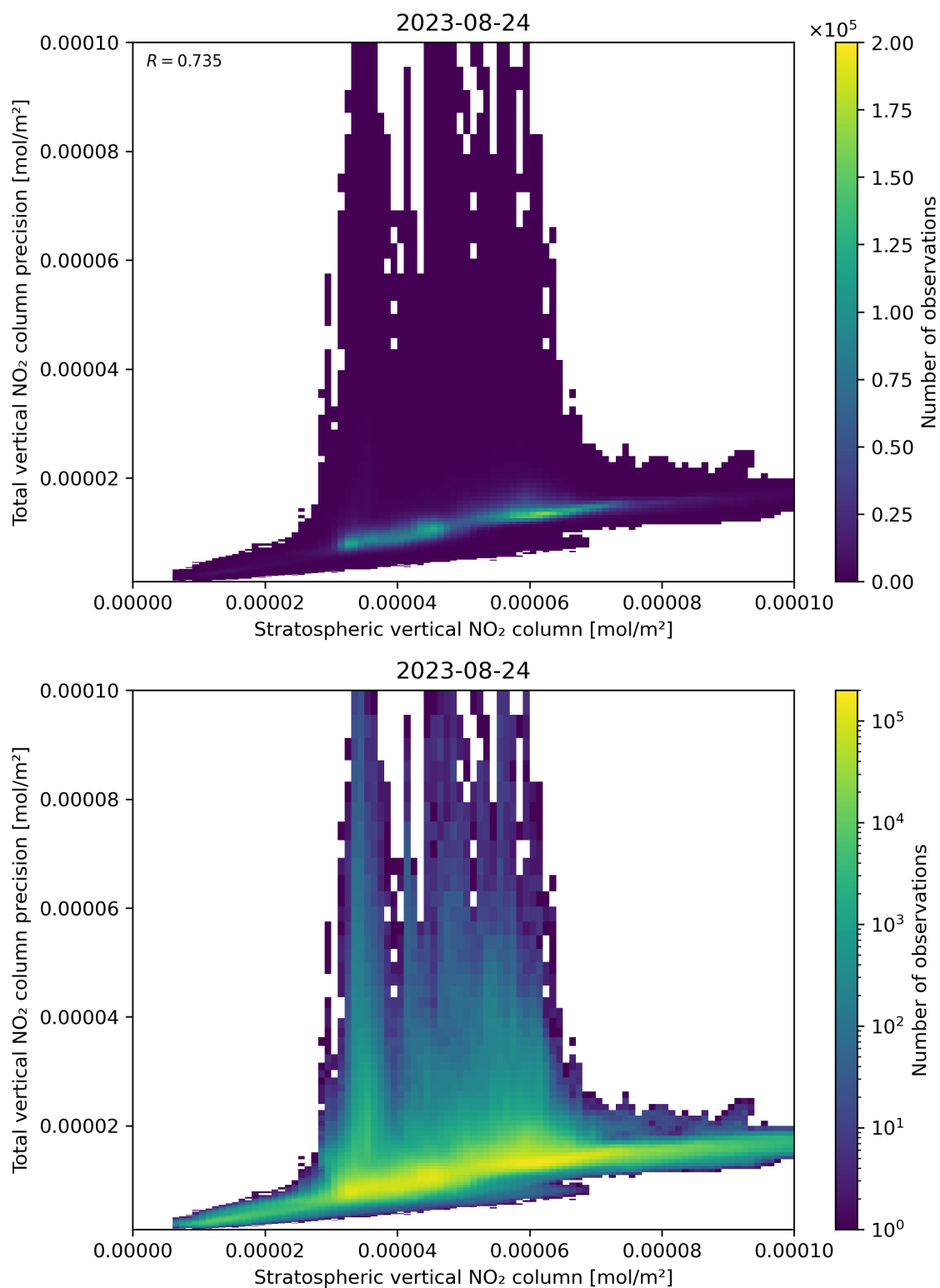
Figure 101: Scatter density plot of “Stratospheric vertical NO 2 column” against “Total vertical NO 2 column precision” for 2023-08-23 to 2023-08-25.
