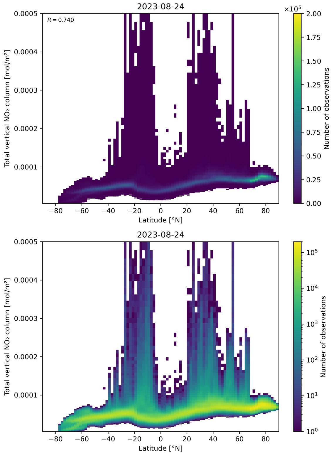
Figure 90: Scatter density plot of “Latitude” against “Total vertical NO 2 column” for 2023-08-23 to 2023-08-25.
