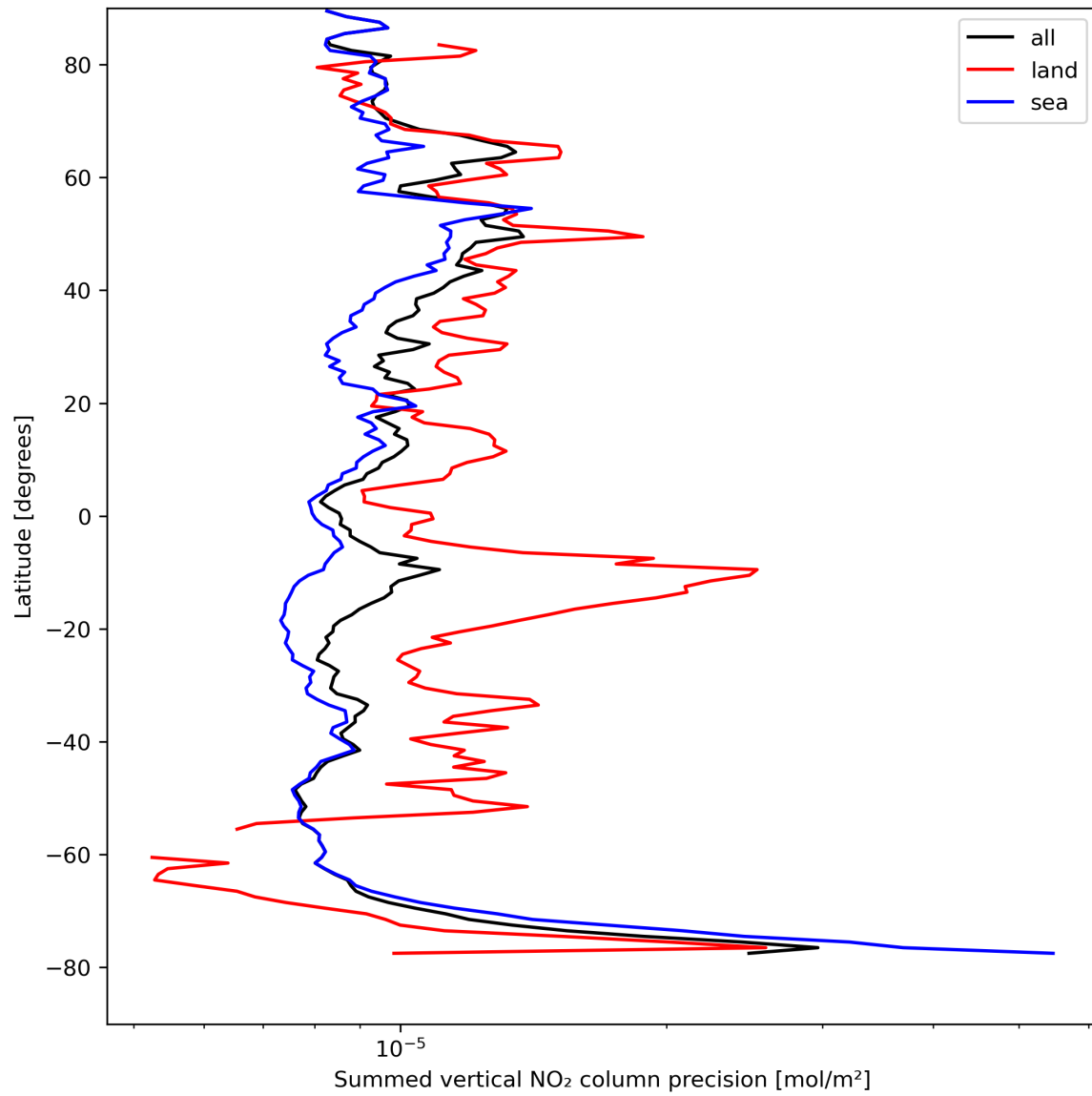
Figure 24: Zonal average of “Summed vertical NO 2 column precision” for 2023-08-23 to 2023-08-25.
