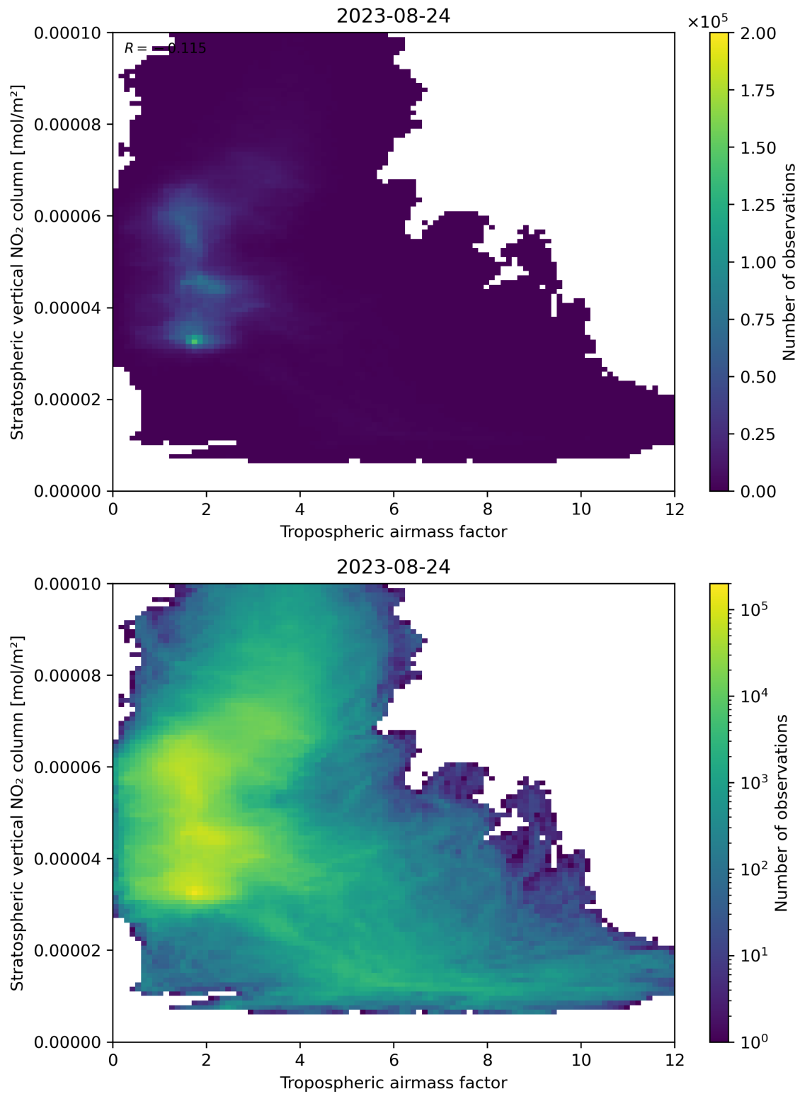
Figure 74: Scatter density plot of “Tropospheric air mass factor” against “Stratospheric vertical NO 2 column” for 2023-08-23 to 2023-08-25.
