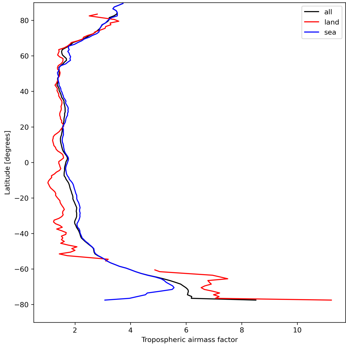
Figure 14: Zonal average of “Tropospheric airmass factor” for 2023-08-23 to 2023-08-25.
