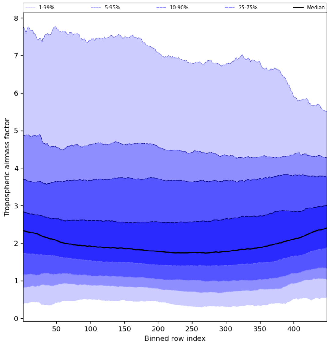
Figure 48: Along track statistics of “Tropospheric air mass factor” for 2023-08-23 to 2023-08-25
