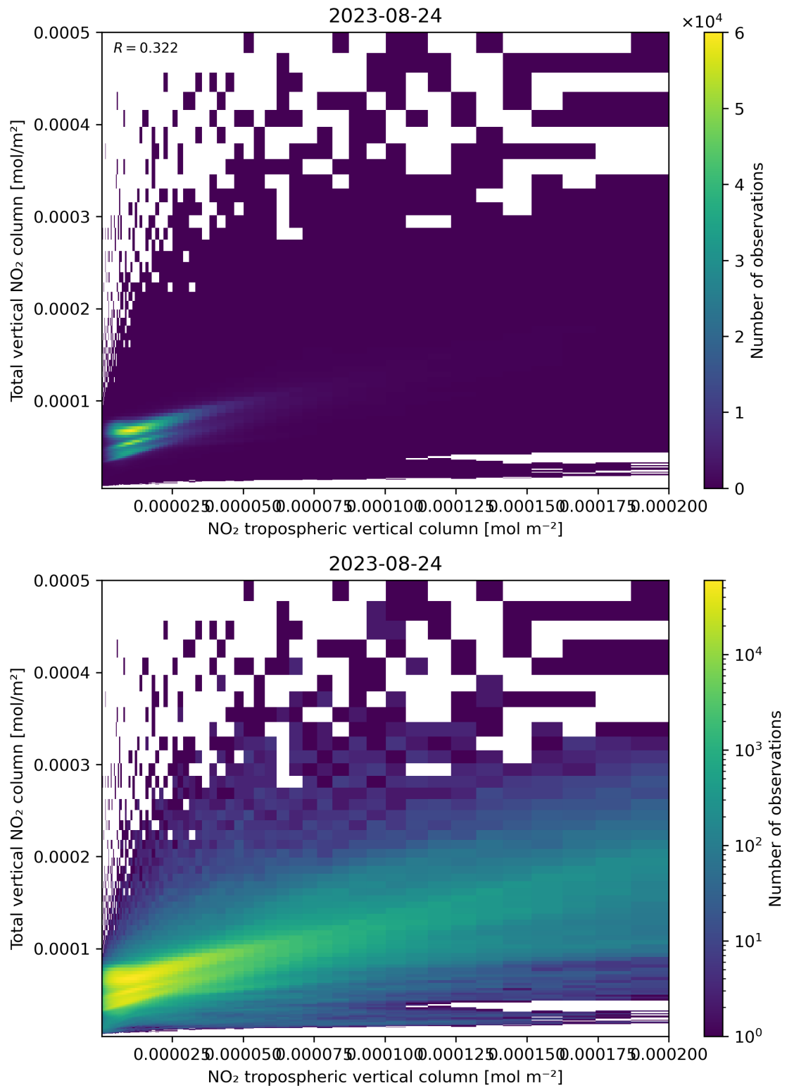
Figure 128: Scatter density plot of “NO 2 tropospheric vertical column” against “Total vertical NO 2 column” for 2023-08-23 to 2023-08-25.
