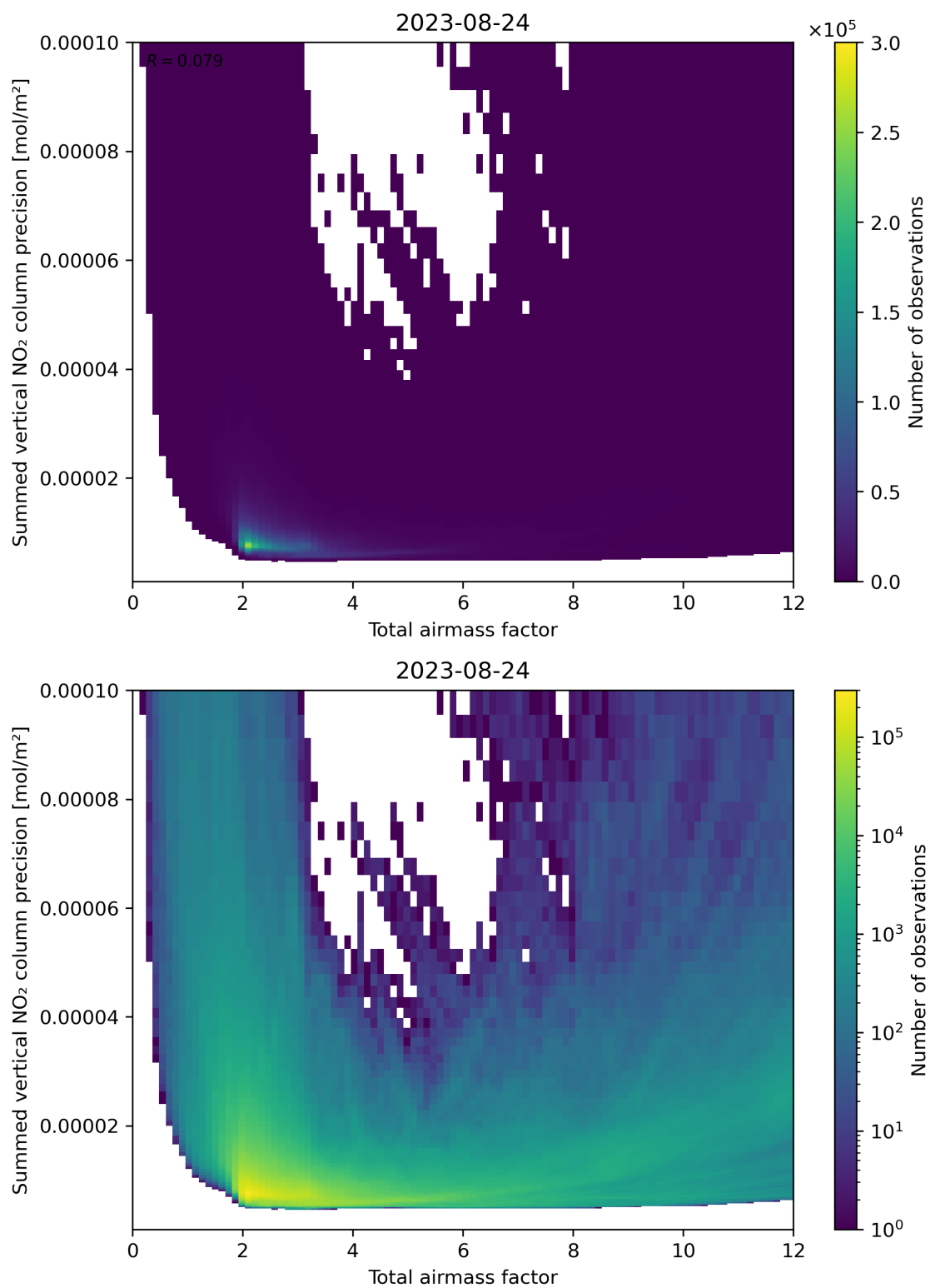
Figure 66: Scatter density plot of “Total airmass factor” against “Summed vertical NO 2 column precision” for 2023-08-23 to 2023-08-25.
