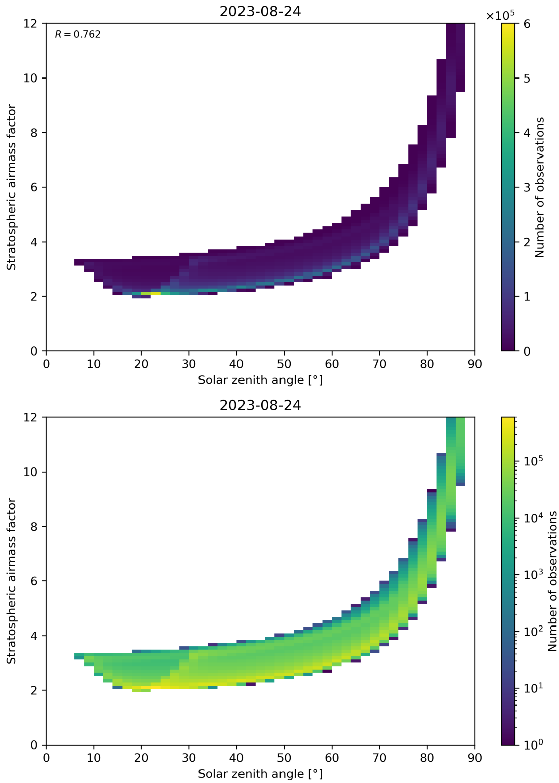
Figure 145: Scatter density plot of “Solar zenith angle” against “Stratospheric airmass factor” for 2023-08-23 to 2023-08-25.
