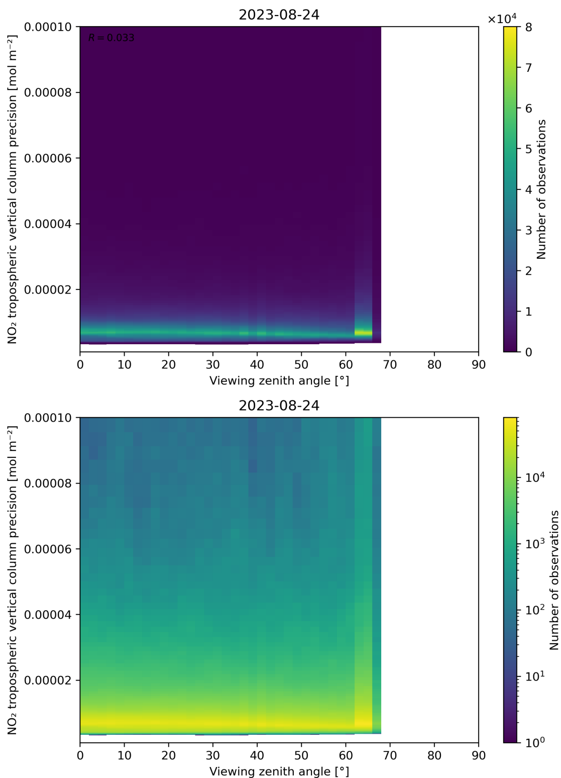
Figure 170: Scatter density plot of “Viewing zenith angle” against “NO 2 tropospheric vertical column precision” for 2023-08-23 to 2023-08-25.
