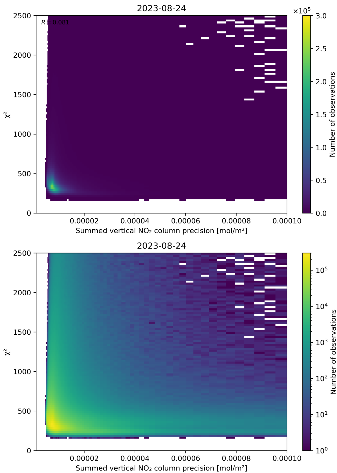
Figure 107: Scatter density plot of “Summed vertical NO 2 column precision” against “ \chi^2 ” for 2023-08-23 to 2023-08-25.
