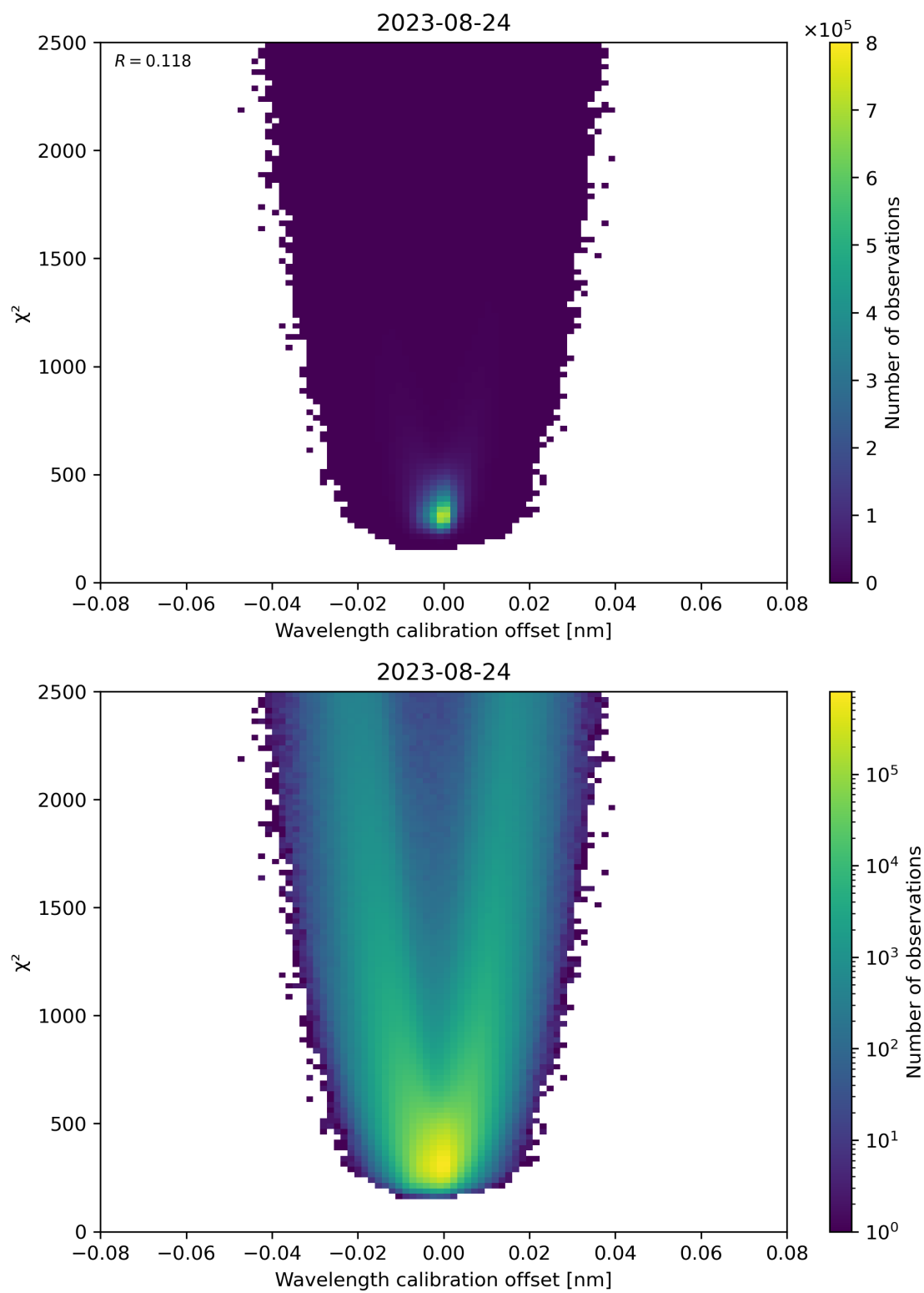
Figure 175: Scatter density plot of “Wavelength calibration offset” against “ \chi^2 ” for 2023-08-23 to 2023-08-25.
