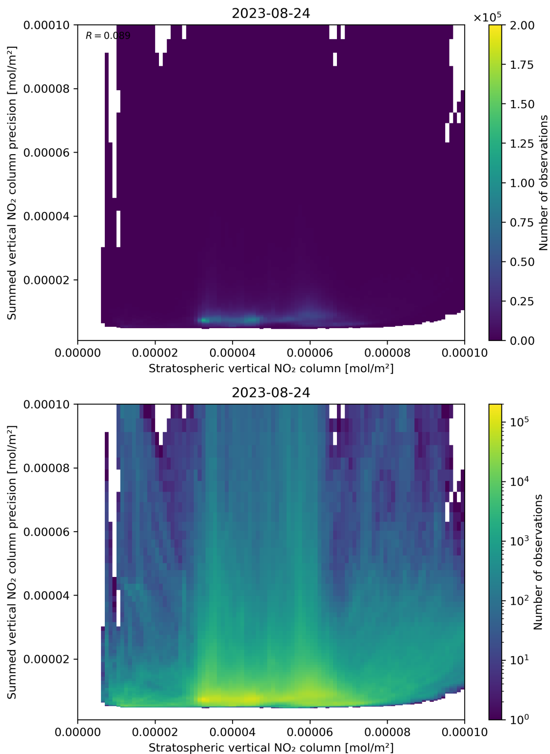
Figure 99: Scatter density plot of “Stratospheric vertical NO 2 column” against “Summed vertical NO 2 column precision” for 2023-08-23 to 2023-08-25.
