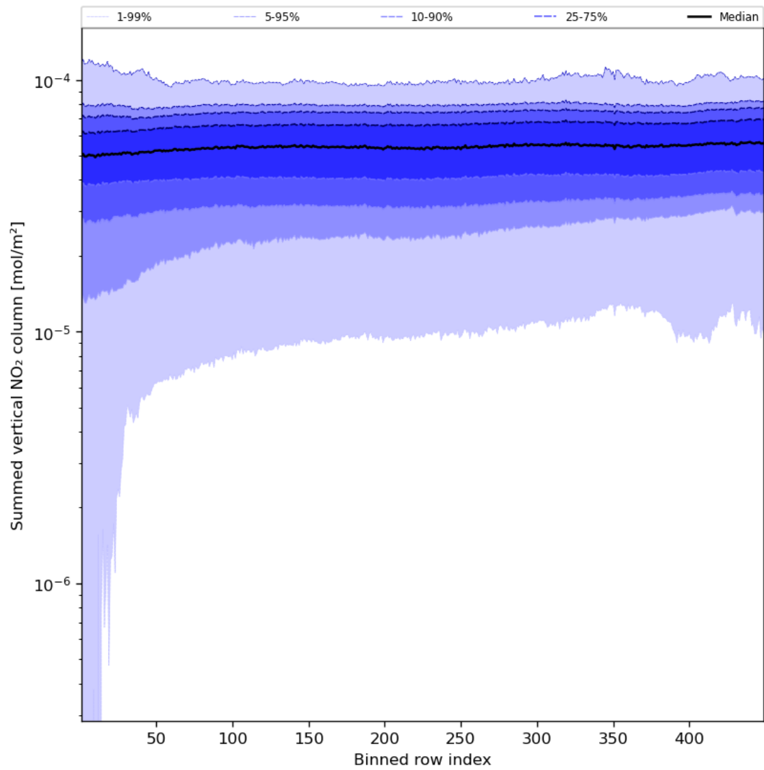
Figure 57: Along track statistics of “Summed vertical NO 2 column” for 2023-08-23 to 2023-08-25
