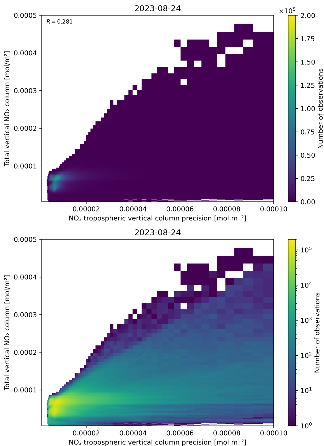
Figure 138: Scatter density plot of “NO 2 tropospheric vertical column precision” against “Total vertical NO 2 column” for 2023-08-23 to 2023-08-25.
