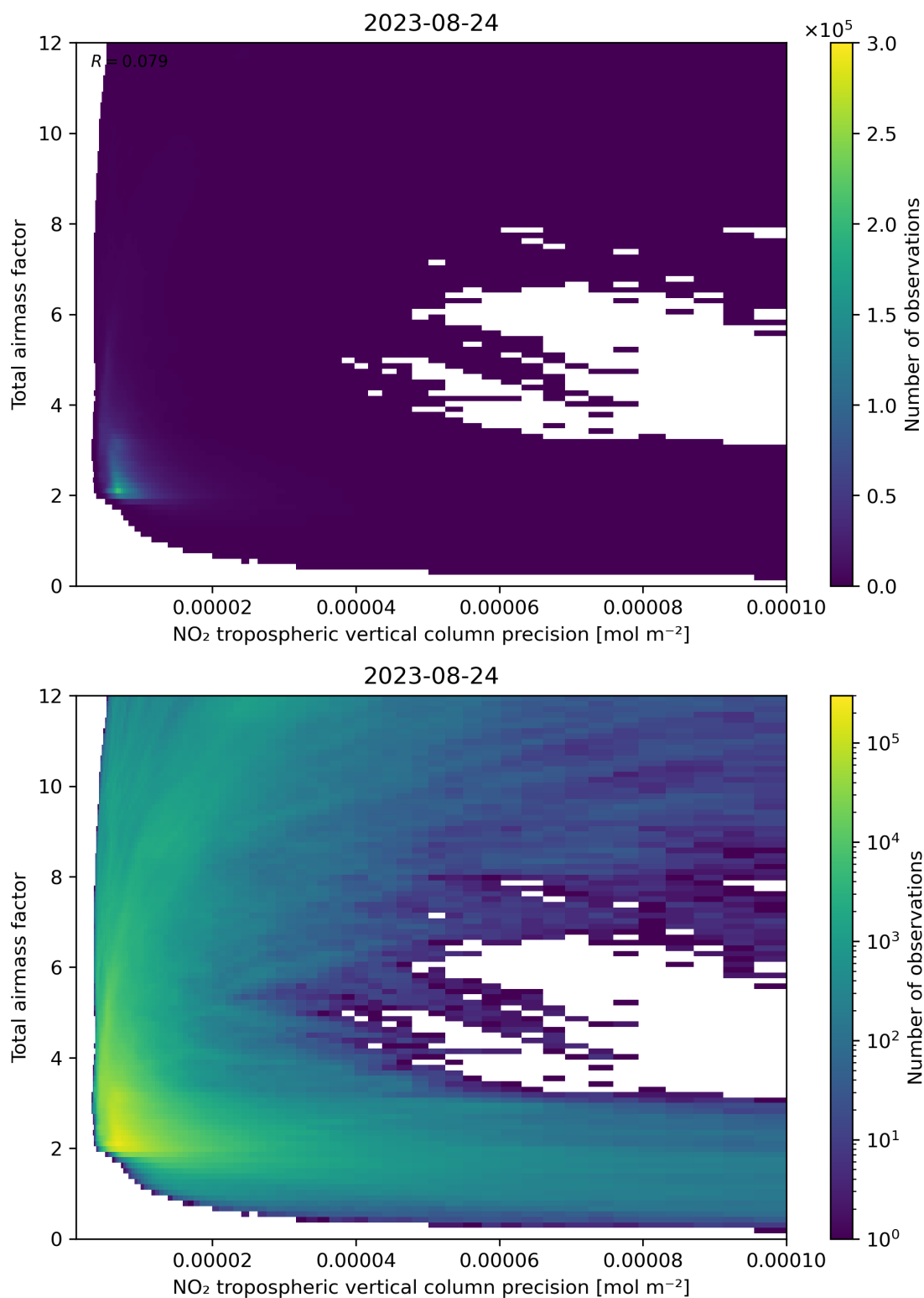
Figure 132: Scatter density plot of “NO 2 tropospheric vertical column precision” against “Total air mass factor” for 2023-08-23 to 2023-08-25.
