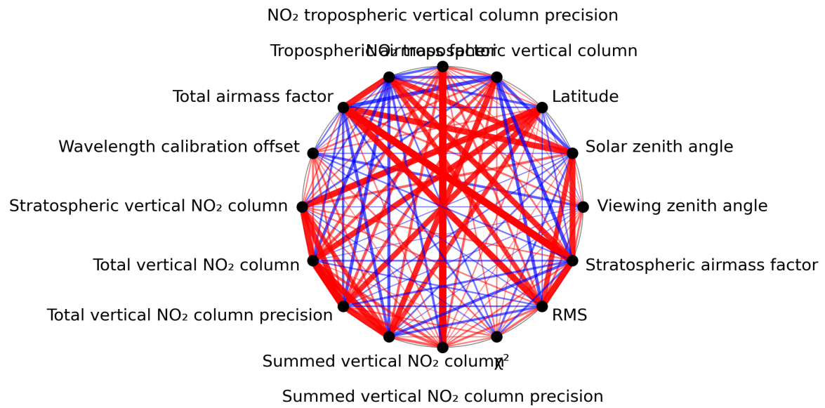
Figure 1: Map of correlation graph for 2023-08-23 to 2023-08-25.
