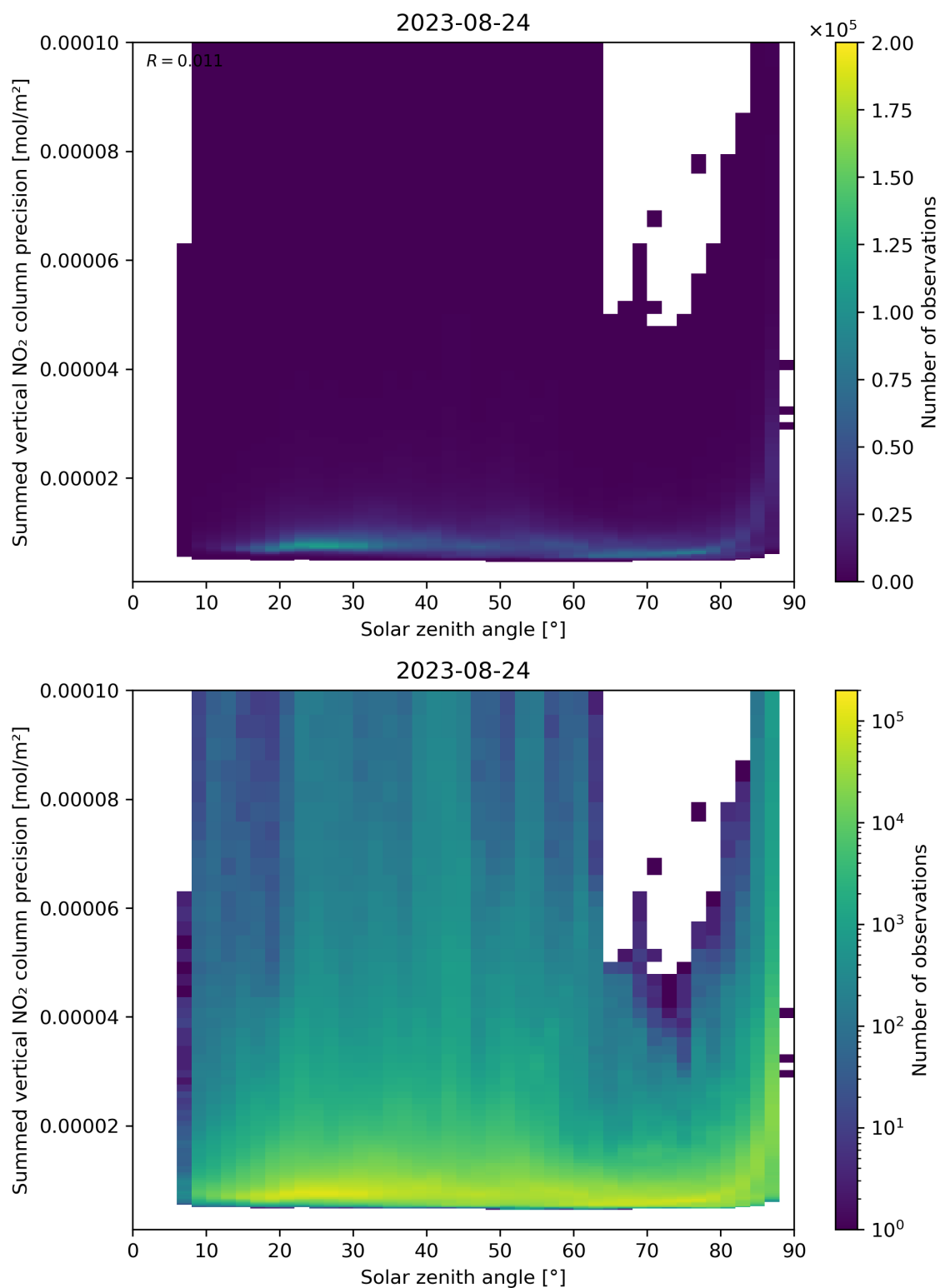
Figure 152: Scatter density plot of “Solar zenith angle” against “Summed vertical NO 2 column precision” for 2023-08-23 to 2023-08-25.
