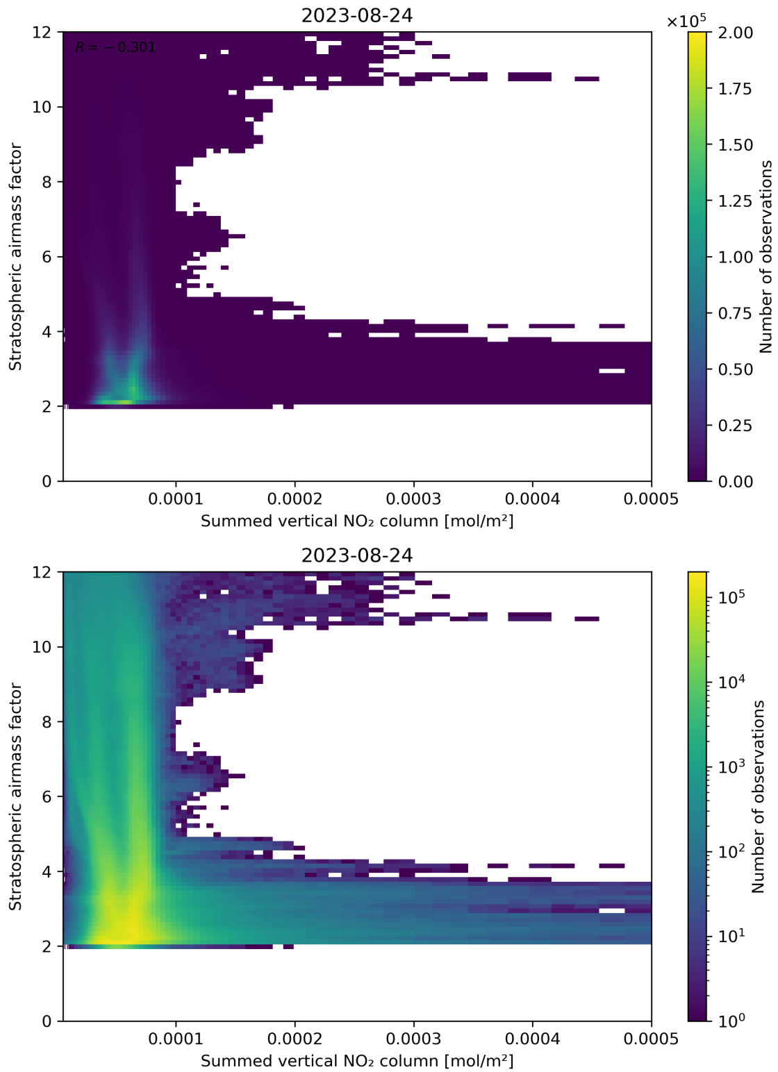
Figure 103: Scatter density plot of “Summed vertical NO 2 column” against “Stratospheric airmass factor” for 2023-08-23 to 2023-08-25.
