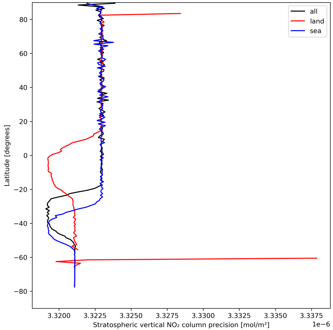
Figure 20: Zonal average of “Stratospheric vertical NO 2 column precision” for 2023-08-23 to 2023-08-25.
