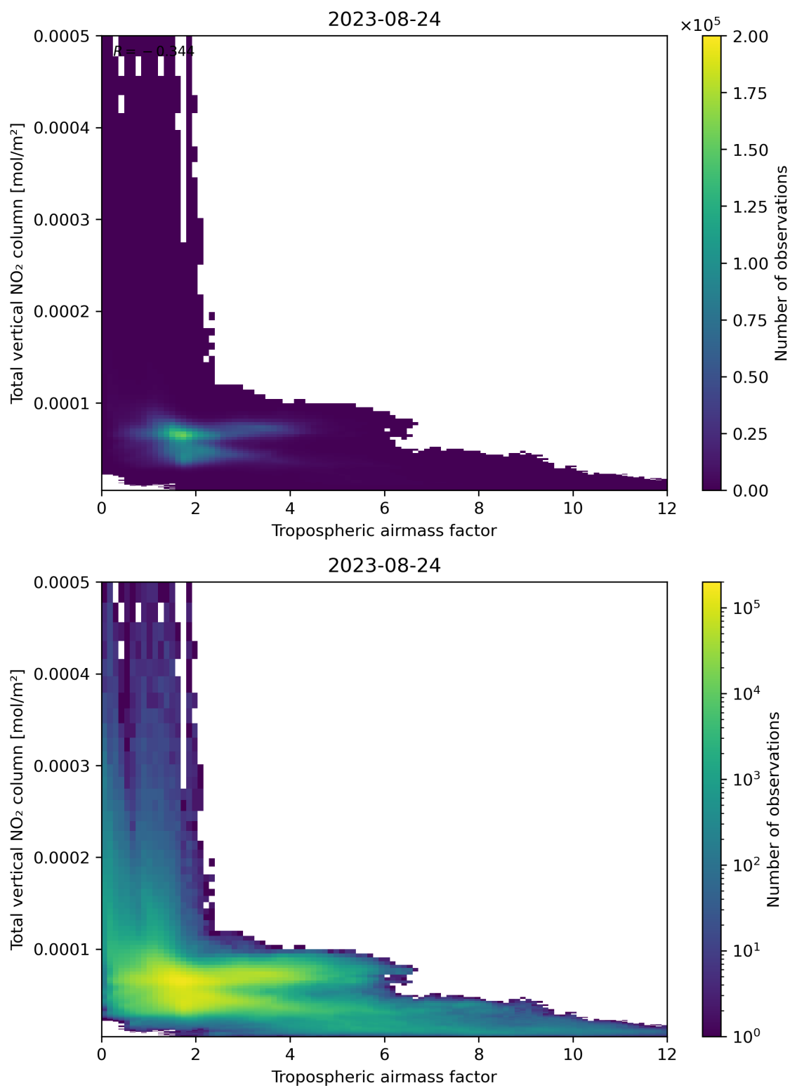
Figure 77: Scatter density plot of “Tropospheric airmass factor” against “Total vertical NO 2 column” for 2023-08-23 to 2023-08-25.
