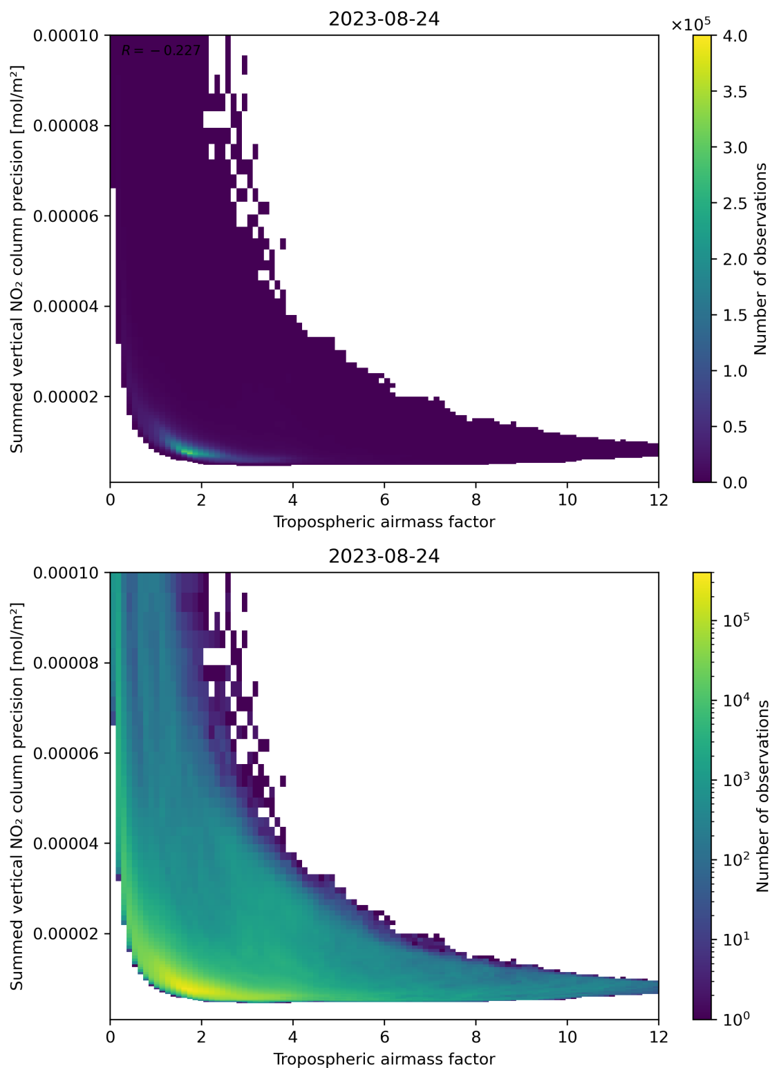
Figure 76: Scatter density plot of “Tropospheric air mass factor” against “Summed vertical NO 2 column precision” for 2023-08-23 to 2023-08-25.
