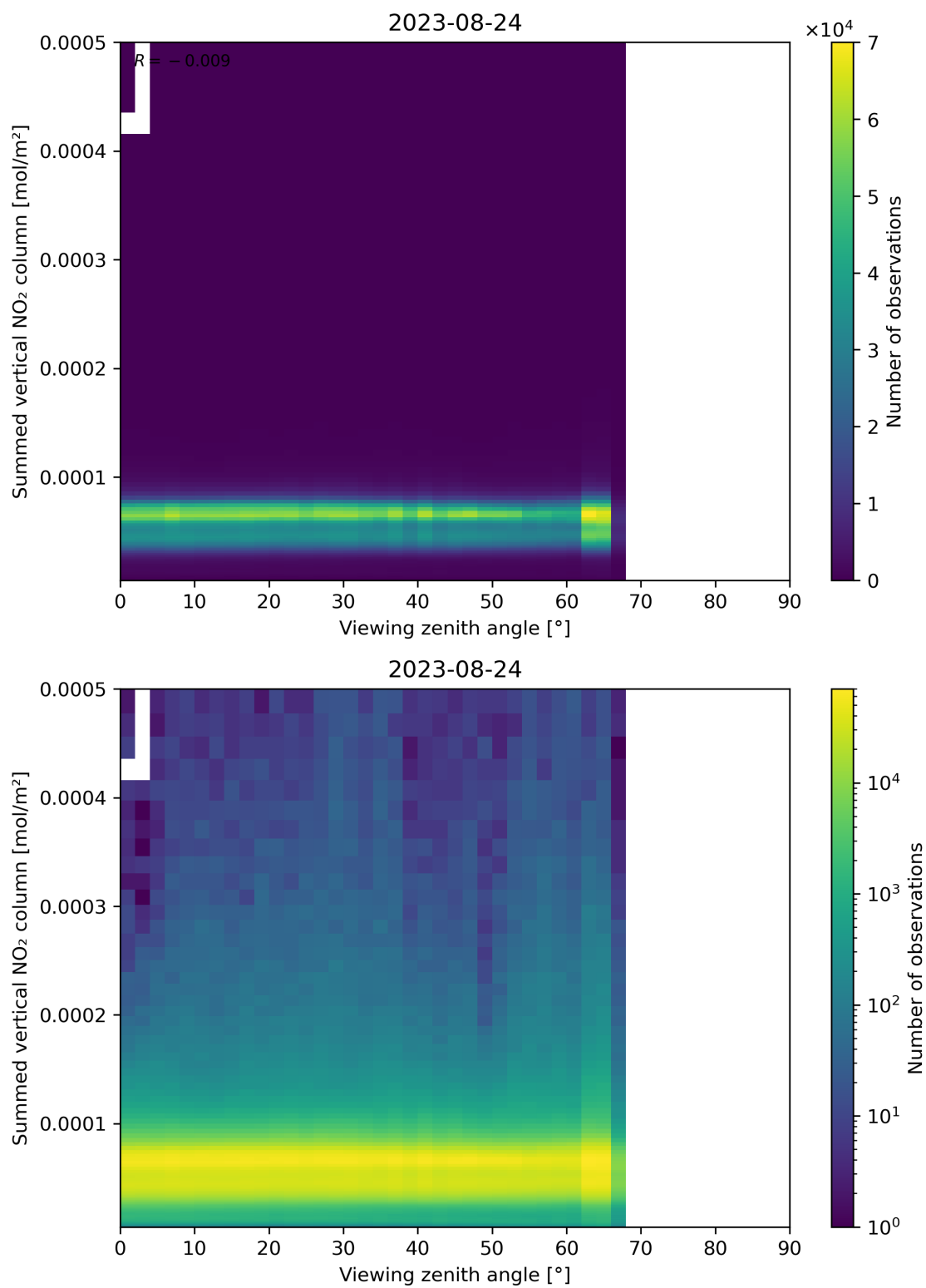
Figure 165: Scatter density plot of “Viewing zenith angle” against “Summed vertical NO 2 column” for 2023-08-23 to 2023-08-25.
