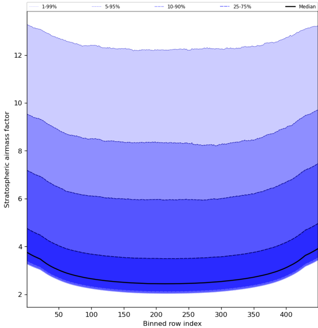
Figure 61: Along track statistics of “Stratospheric airmass factor” for 2023-08-23 to 2023-08-25
