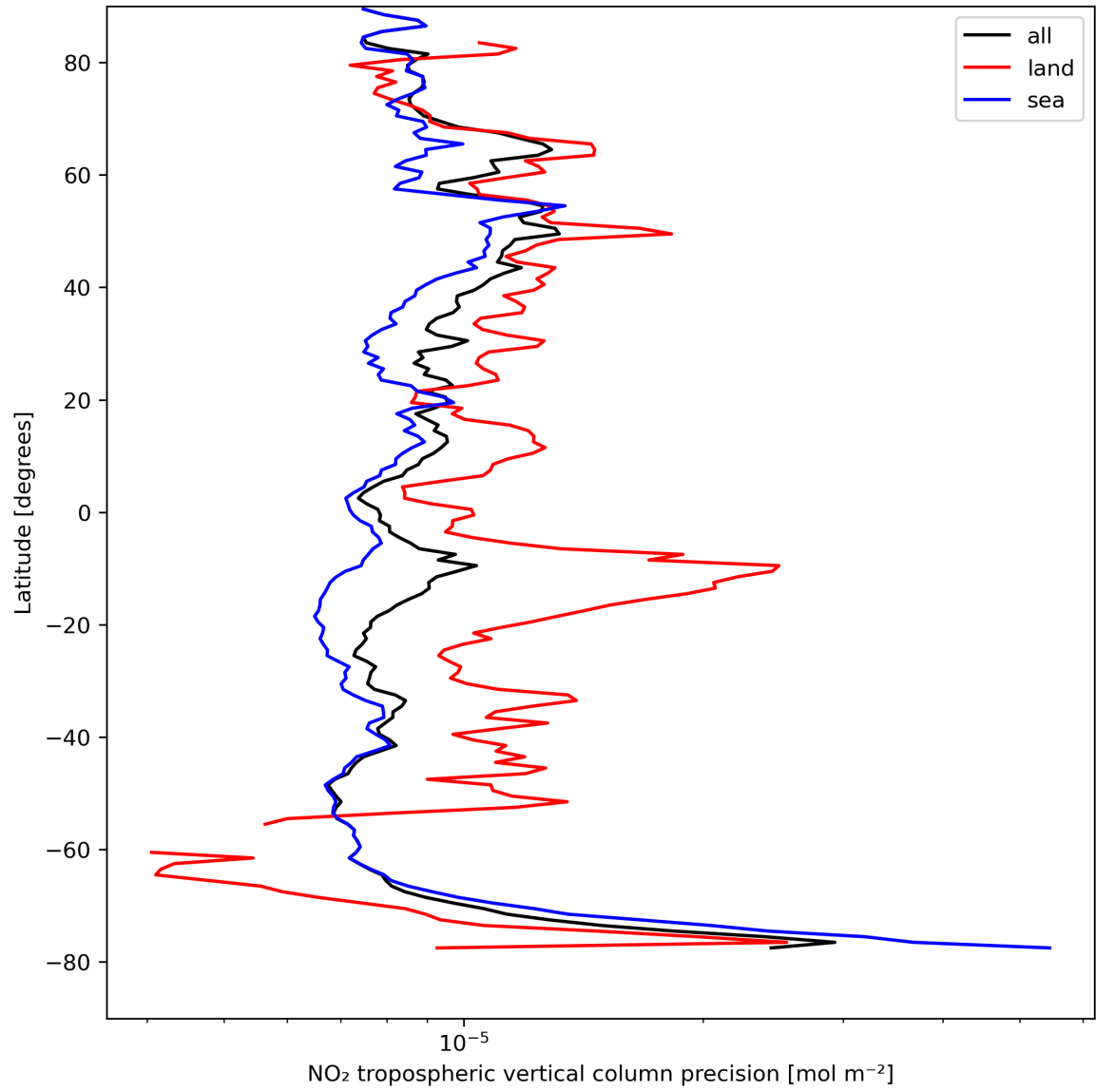
Figure 13: Zonal average of “NO 2 tropospheric vertical column precision” for 2023-08-23 to 2023-08-25.
