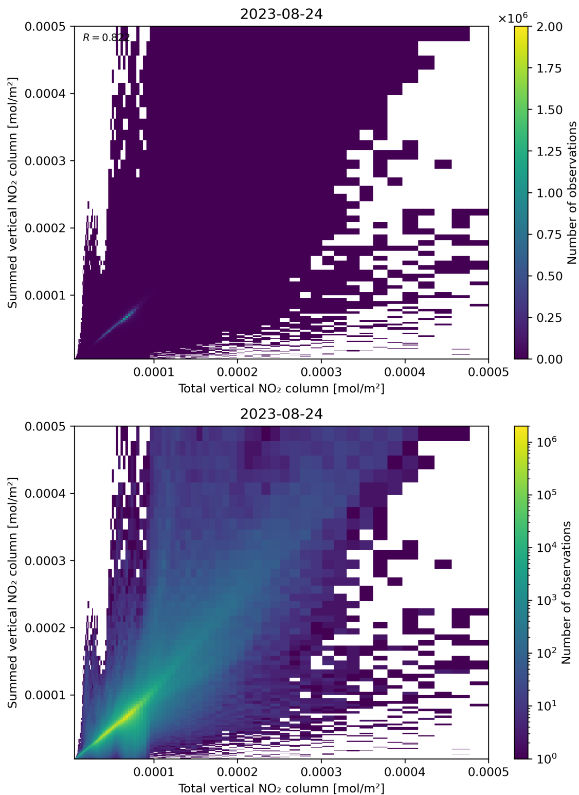
Figure 112: Scatter density plot of “Total vertical NO 2 column” against “Summed vertical NO 2 column” for 2023-08-23 to 2023-08-25.
