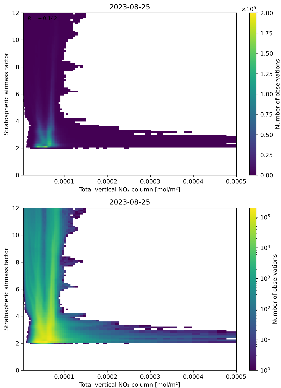
Figure 110: Scatter density plot of “Total vertical NO 2 column” against “Stratospheric airmass factor” for 2023-08-25 to 2023-08-26.
