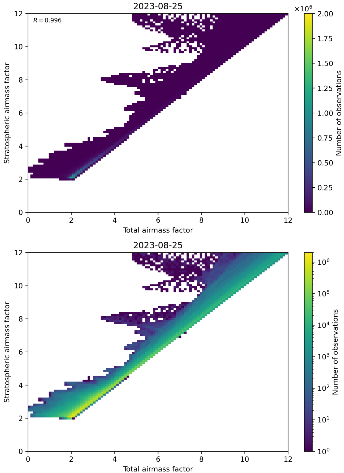
Figure 62: Scatter density plot of “Total airmass factor” against “Stratospheric airmass factor” for 2023-08-25 to 2023-08-26.
