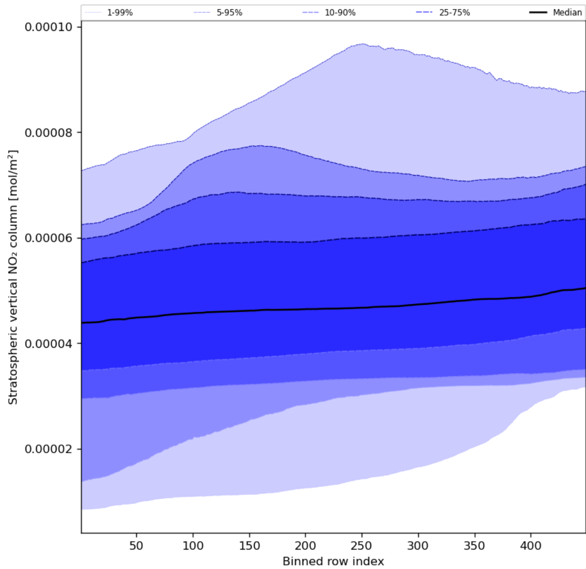
Figure 53: Along track statistics of “Stratospheric vertical NO 2 column” for 2023-08-25 to 2023-08-26
