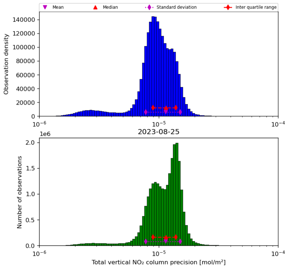
Figure 39: Histogram of "Total vertical NO 2 column precision" for 2023-08-25 to 2023-08-26
