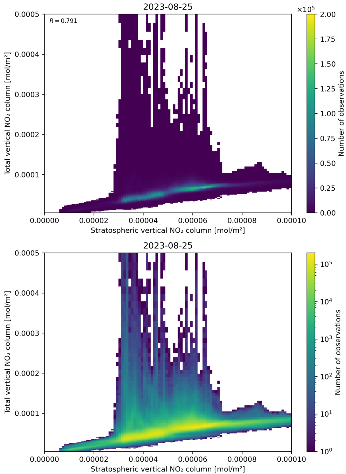
Figure 100: Scatter density plot of “Stratospheric vertical NO 2 column” against “Total vertical NO 2 column” for 2023-08-25 to 2023-08-26.
