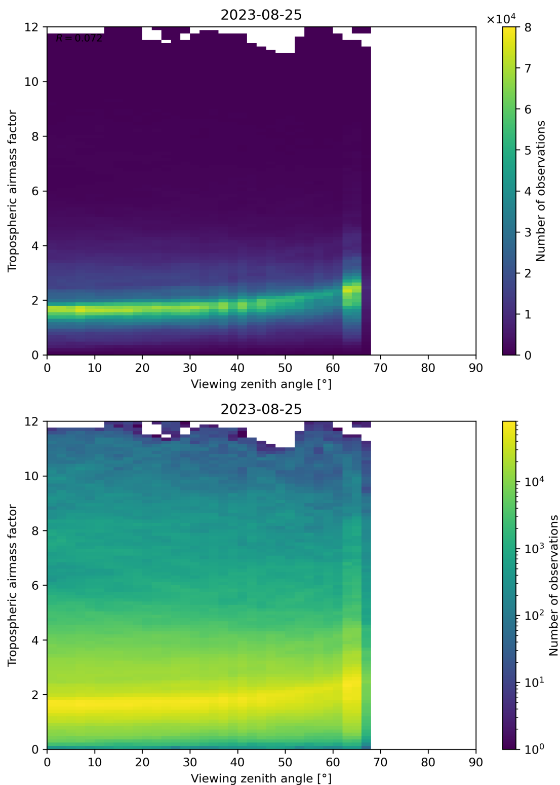
Figure 161: Scatter density plot of “Viewing zenith angle” against “Tropospheric airmass factor” for 2023-08-25 to 2023-08-26.
