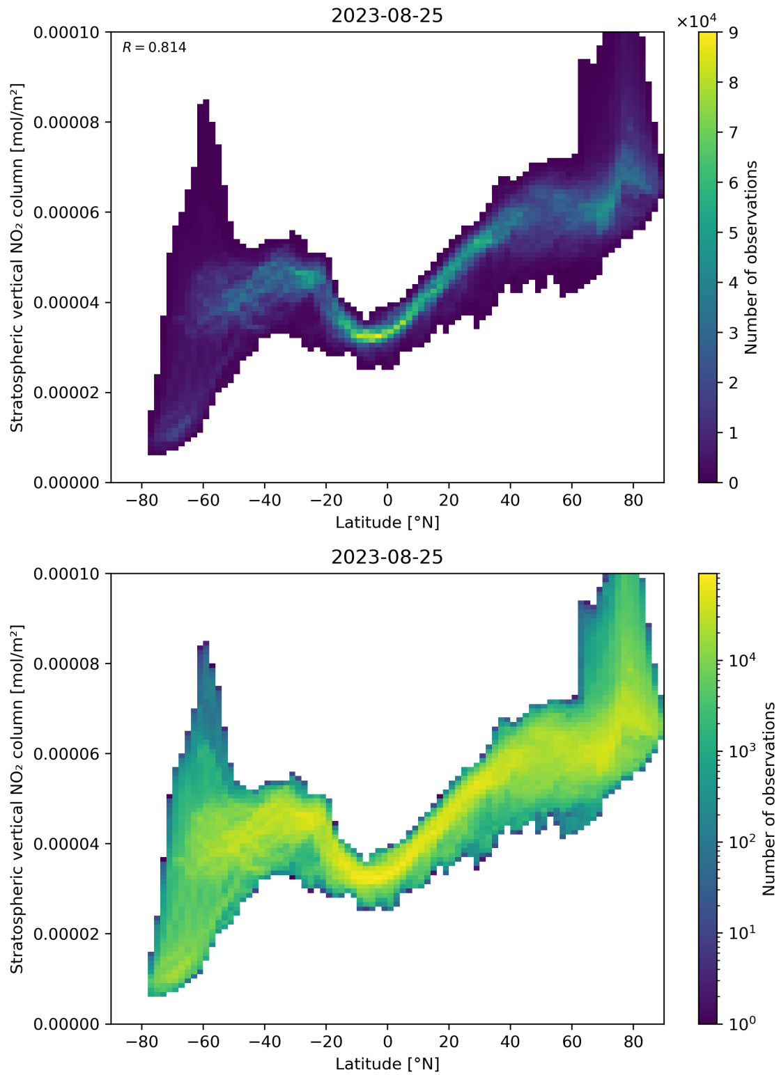
Figure 87: Scatter density plot of “Latitude” against “Stratospheric vertical NO 2 column” for 2023-08-25 to 2023-08-26.
