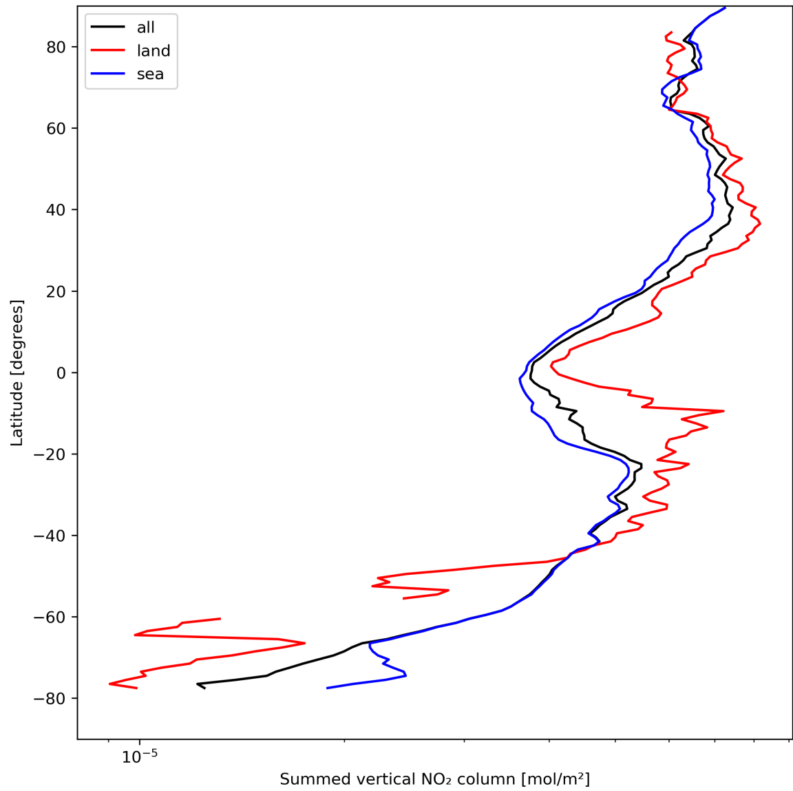
Figure 23: Zonal average of “Summed vertical NO 2 column” for 2023-08-25 to 2023-08-26.
