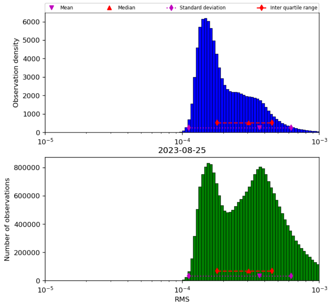
Figure 43: Histogram of “RMS” for 2023-08-25 to 2023-08-26
