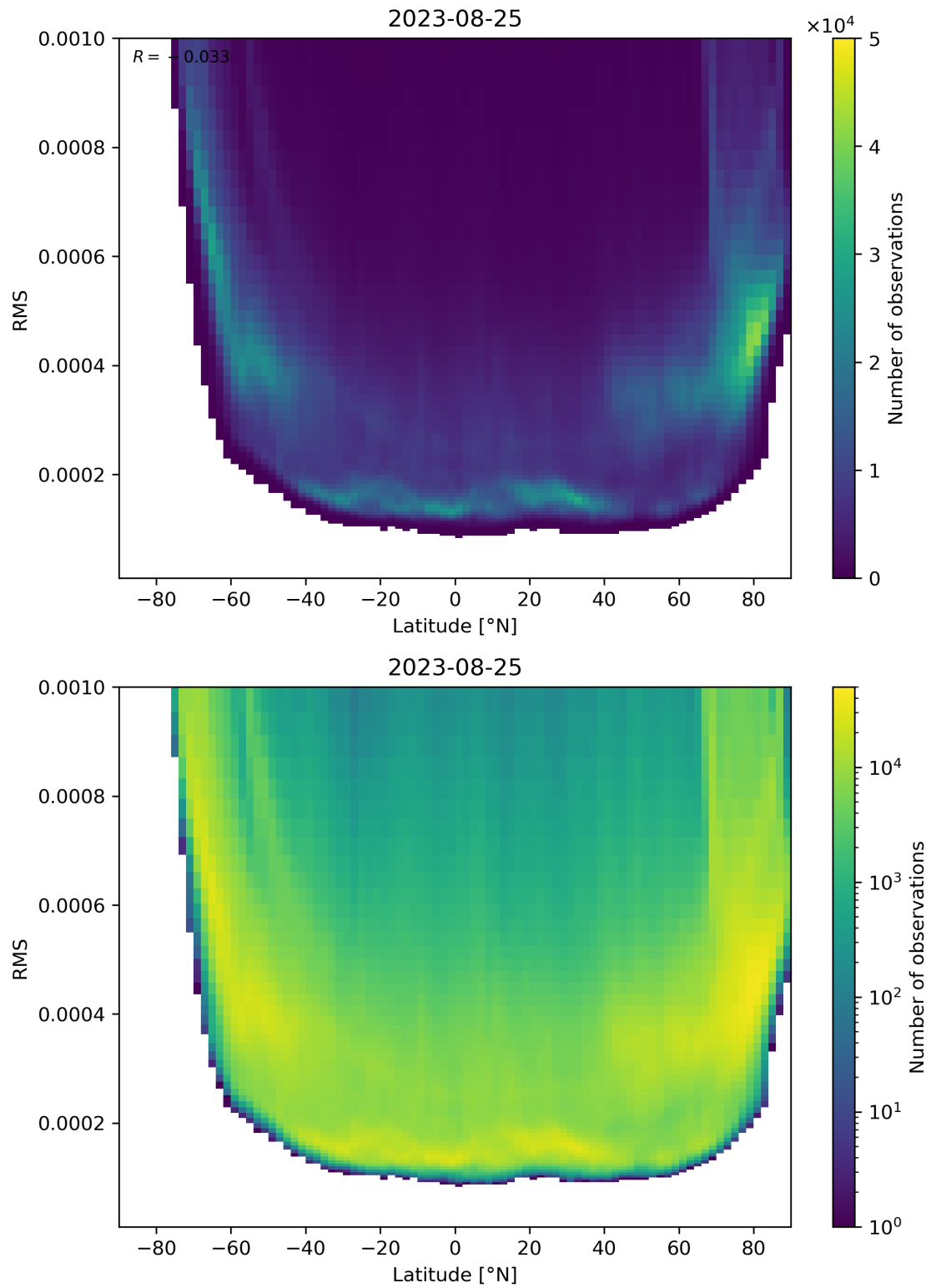
Figure 94: Scatter density plot of “Latitude” against “RMS” for 2023-08-25 to 2023-08-26.
