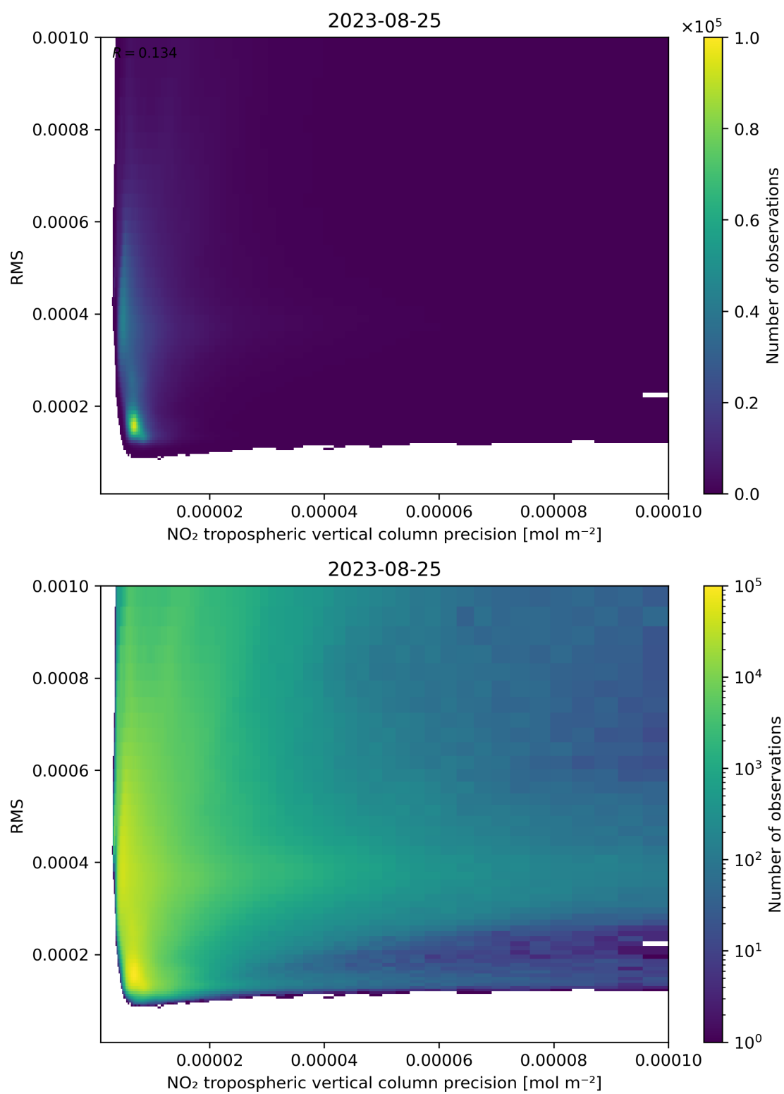
Figure 140: Scatter density plot of “NO 2 tropospheric vertical column precision” against “RMS” for 2023-08-25 to 2023-08-26.
