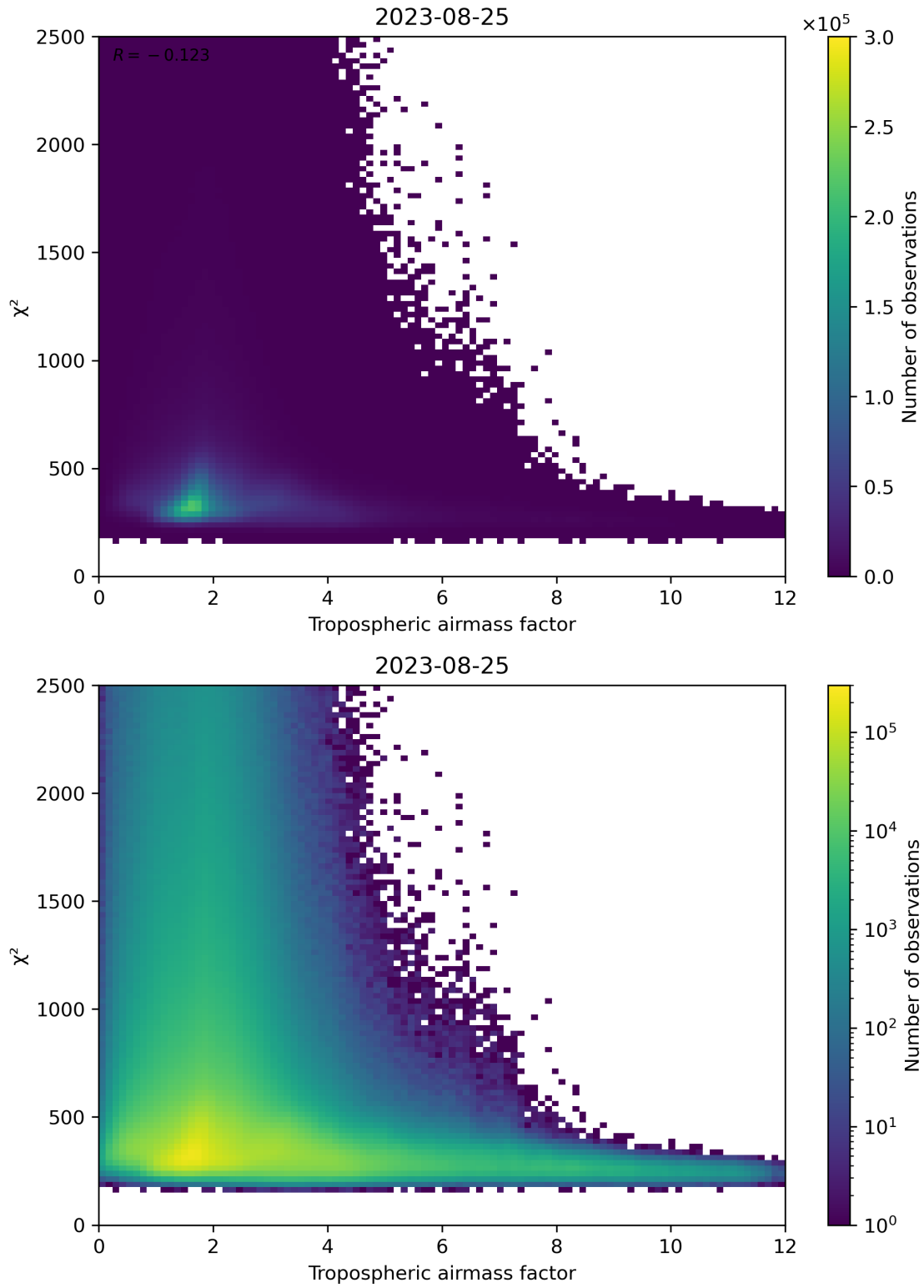
Figure 73: Scatter density plot of “Tropospheric airmass factor” against “ \chi^2 ” for 2023-08-25 to 2023-08-26.
