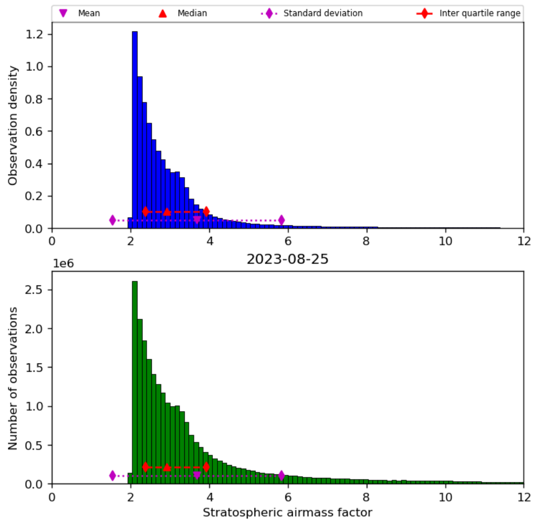
Figure 44: Histogram of “Stratospheric airmass factor” for 2023-08-25 to 2023-08-26
