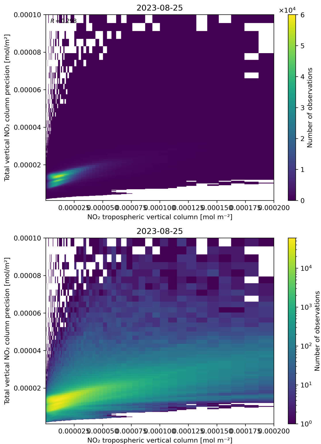
Figure 129: Scatter density plot of “NO 2 tropospheric vertical column” against “Total vertical NO 2 column precision” for 2023-08-25 to 2023-08-26.
