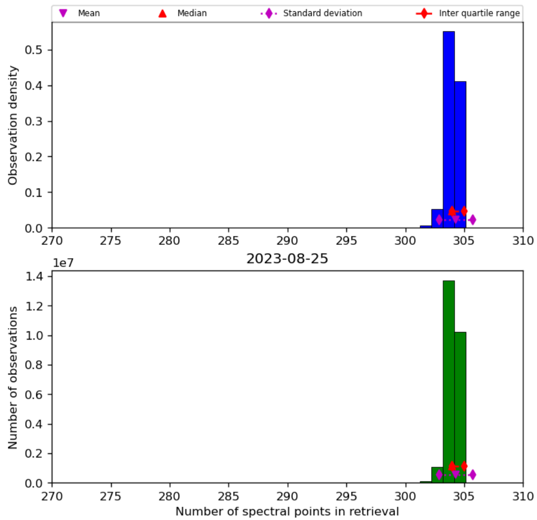
Figure 33: Histogram of “Number of spectral points in retrieval” for 2023-08-25 to 2023-08-26
