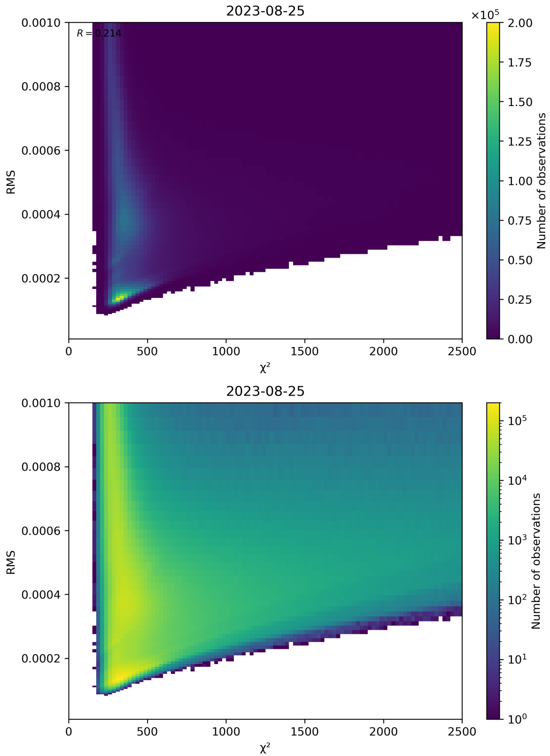
Figure 82: Scatter density plot of “ \chi^2 ” against “RMS” for 2023-08-25 to 2023-08-26.
