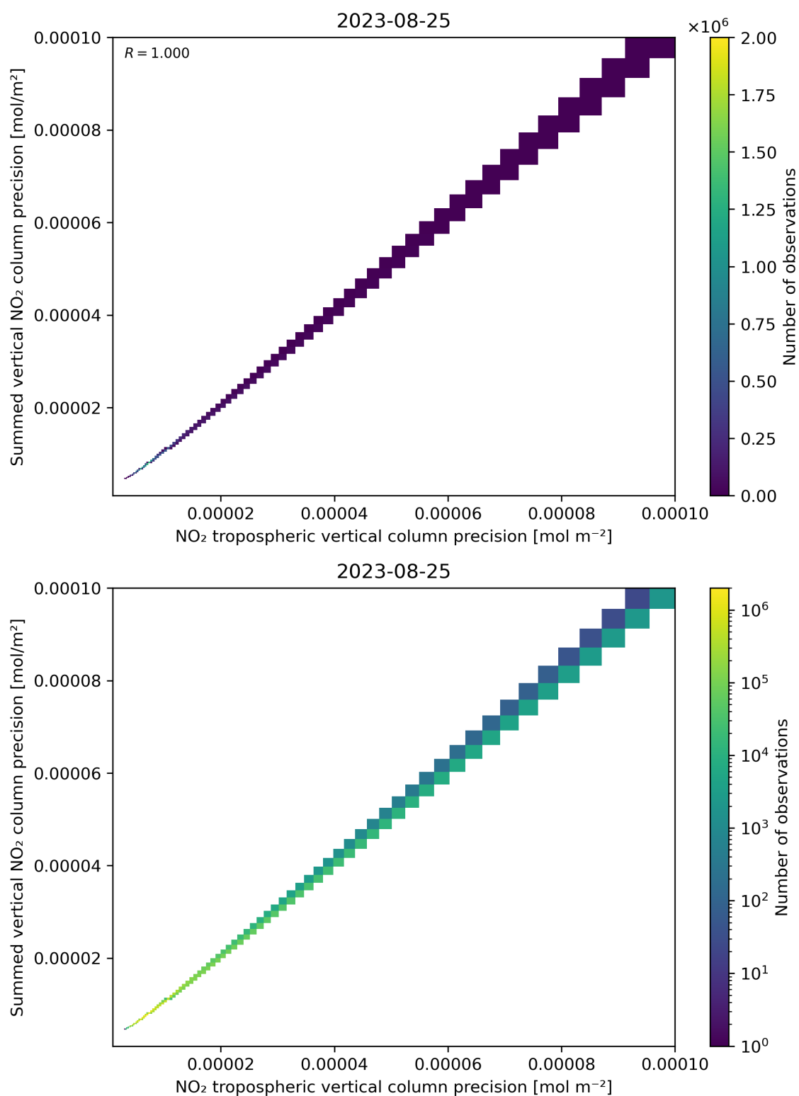
Figure 137: Scatter density plot of “NO 2 tropospheric vertical column precision” against “Summed vertical NO 2 column precision” for 2023-08-25 to 2023-08-26.
