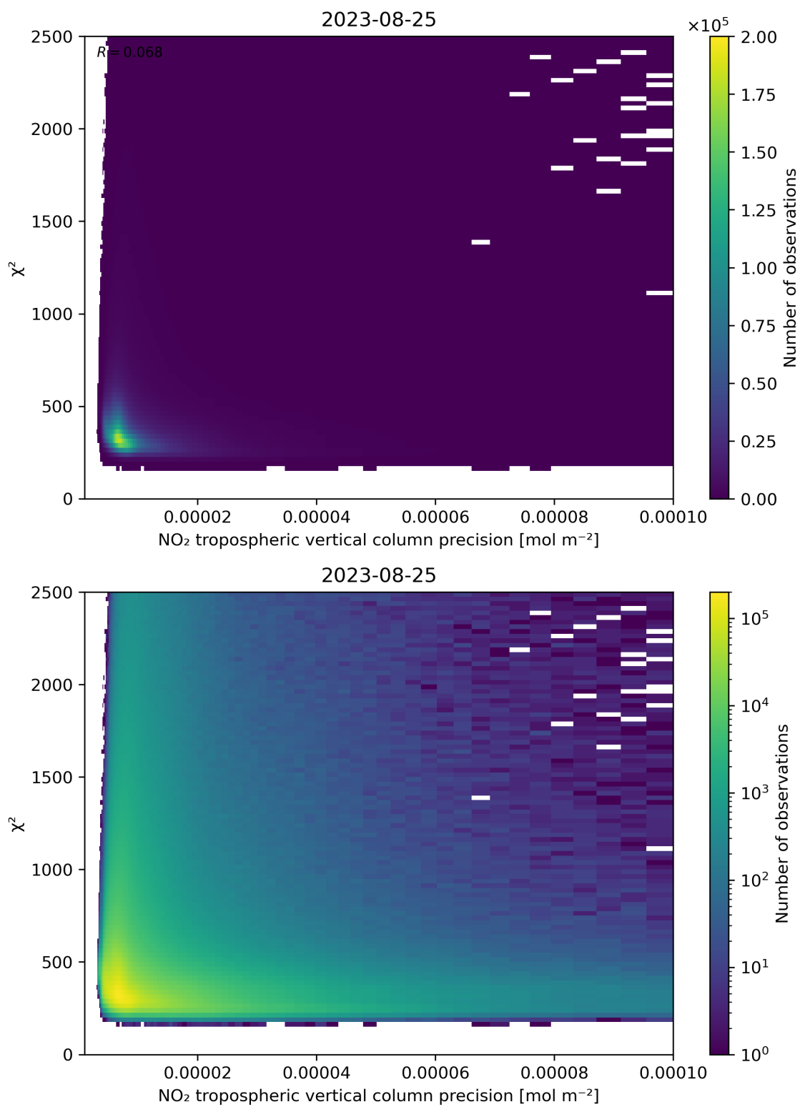
Figure 134: Scatter density plot of “NO 2 tropospheric vertical column precision” against “ \chi^2 ” for 2023-08-25 to 2023-08-26.
