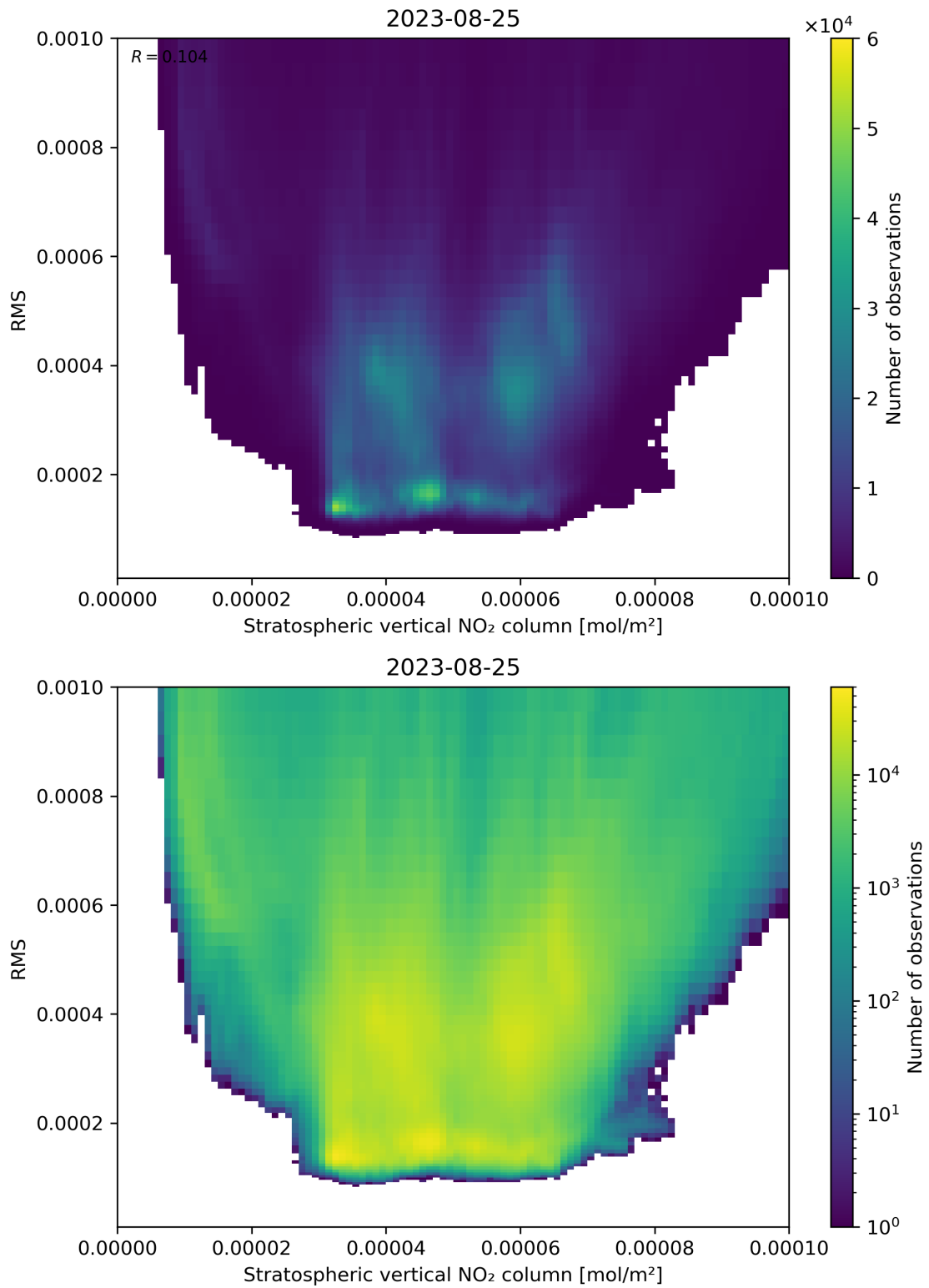
Figure 102: Scatter density plot of “Stratospheric vertical NO 2 column” against “RMS” for 2023-08-25 to 2023-08-26.
