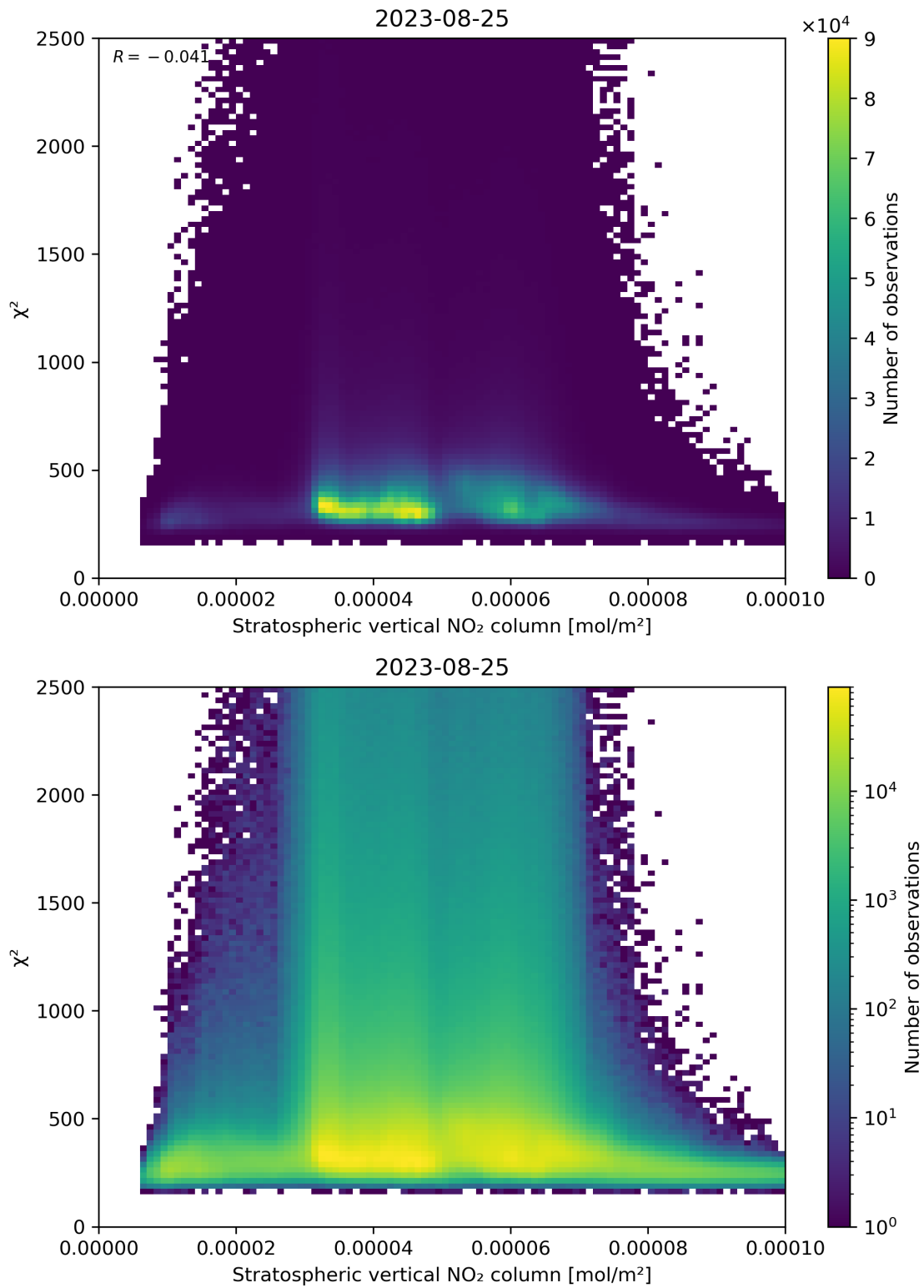
Figure 97: Scatter density plot of “Stratospheric vertical NO 2 column” against “ \chi^2 ” for 2023-08-25 to 2023-08-26.
