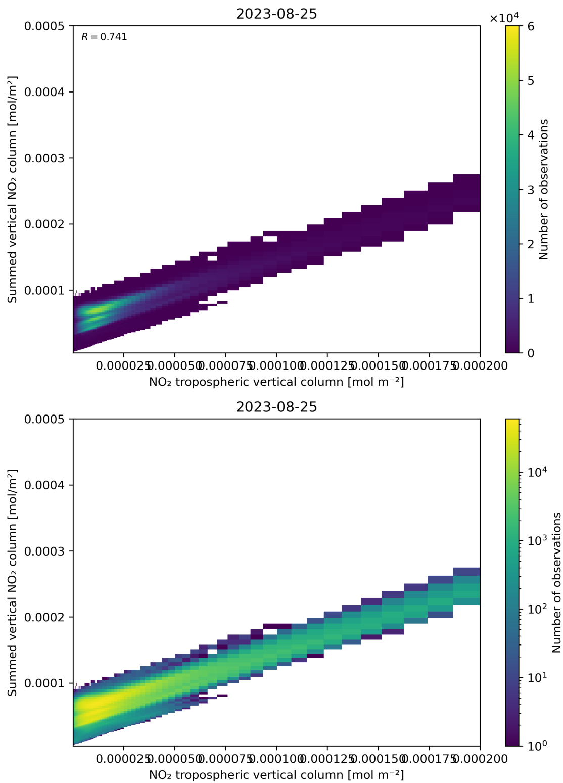
Figure 126: Scatter density plot of “NO 2 tropospheric vertical column” against “Summed vertical NO 2 column” for 2023-08-25 to 2023-08-26.
