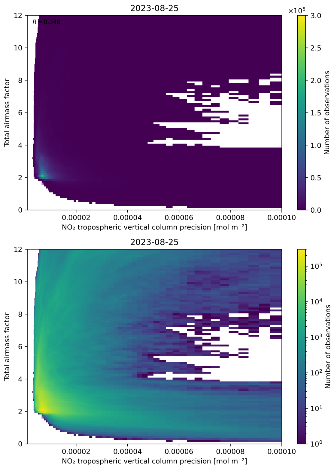
Figure 132: Scatter density plot of “NO 2 tropospheric vertical column precision” against “Total air mass factor” for 2023-08-25 to 2023-08-26.
