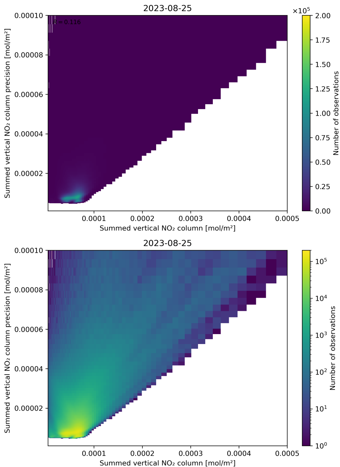
Figure 105: Scatter density plot of “Summed vertical NO 2 column” against “Summed vertical NO 2 column precision” for 2023-08-25 to 2023-08-26.
