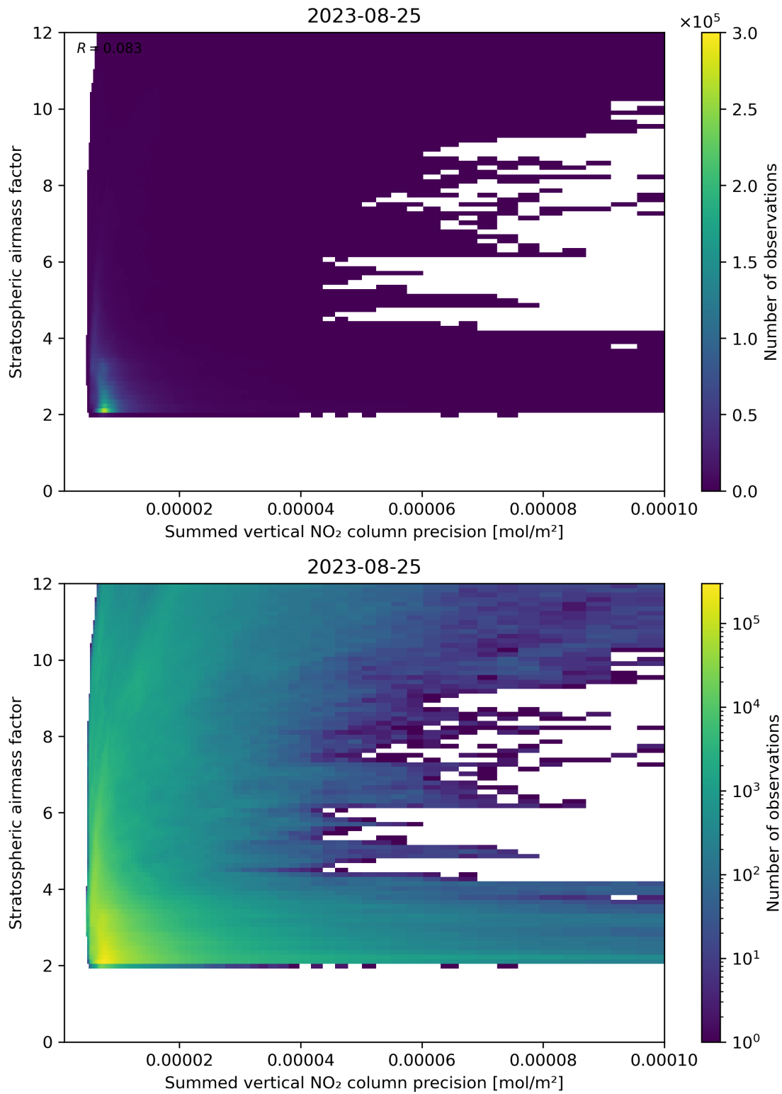
Figure 106: Scatter density plot of “Summed vertical NO 2 column precision” against “Stratospheric airmass factor” for 2023-08-25 to 2023-08-26.
