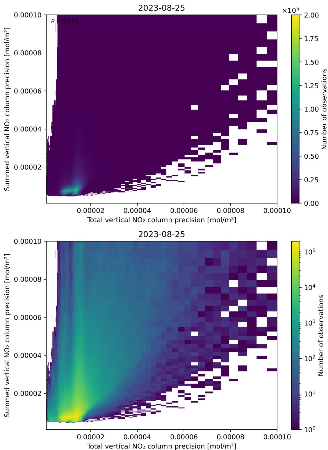
Figure 118: Scatter density plot of “Total vertical NO 2 column precision” against “Summed vertical NO 2 column precision” for 2023-08-25 to 2023-08-26.
