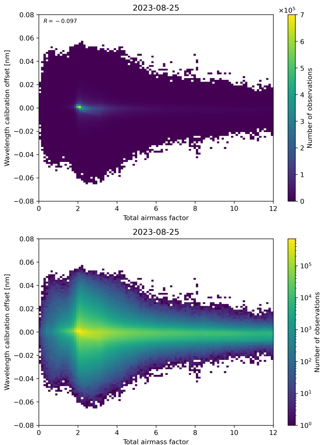
Figure 70: Scatter density plot of “Total airmass factor” against “Wavelength calibration offset” for 2023-08-25 to 2023-08-26.
