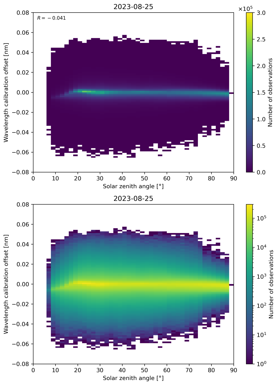
Figure 158: Scatter density plot of “Solar zenith angle” against “Wavelength calibration offset” for 2023-08-25 to 2023-08-26.
