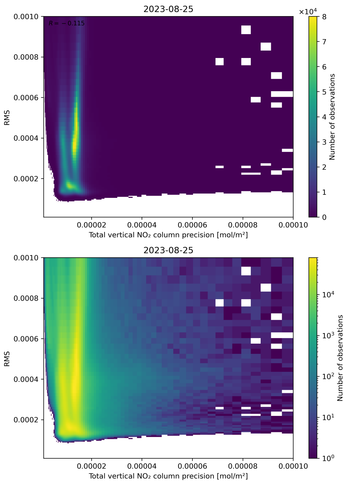
Figure 119: Scatter density plot of “Total vertical NO 2 column precision” against “RMS” for 2023-08-25 to 2023-08-26.
