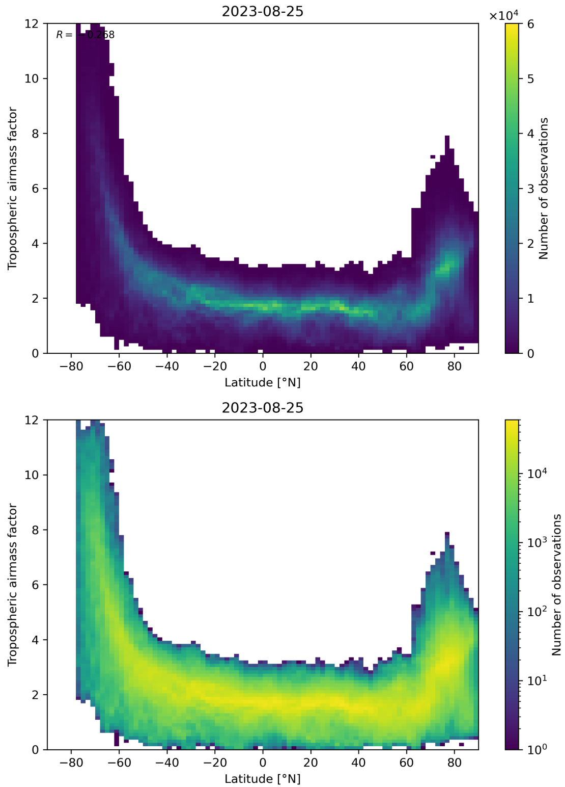
Figure 85: Scatter density plot of “Latitude” against “Tropospheric air mass factor” for 2023-08-25 to 2023-08-26.
