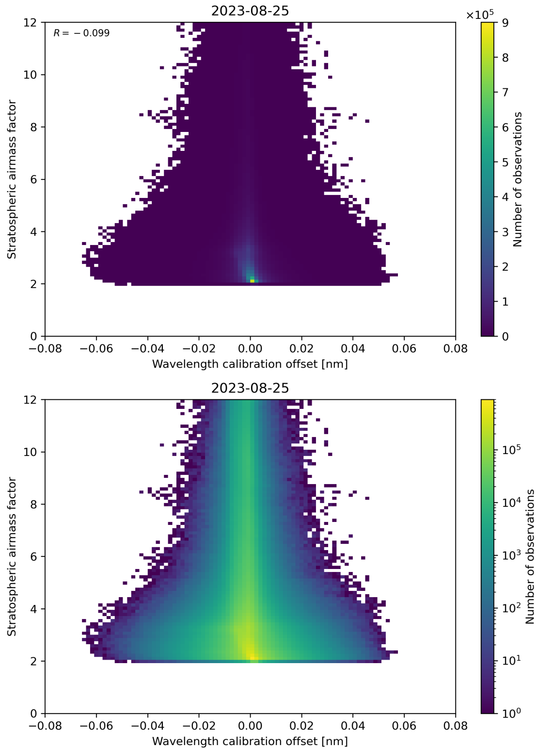
Figure 174: Scatter density plot of “Wavelength calibration offset” against “Stratospheric airmass factor” for 2023-08-25 to 2023-08-26.
