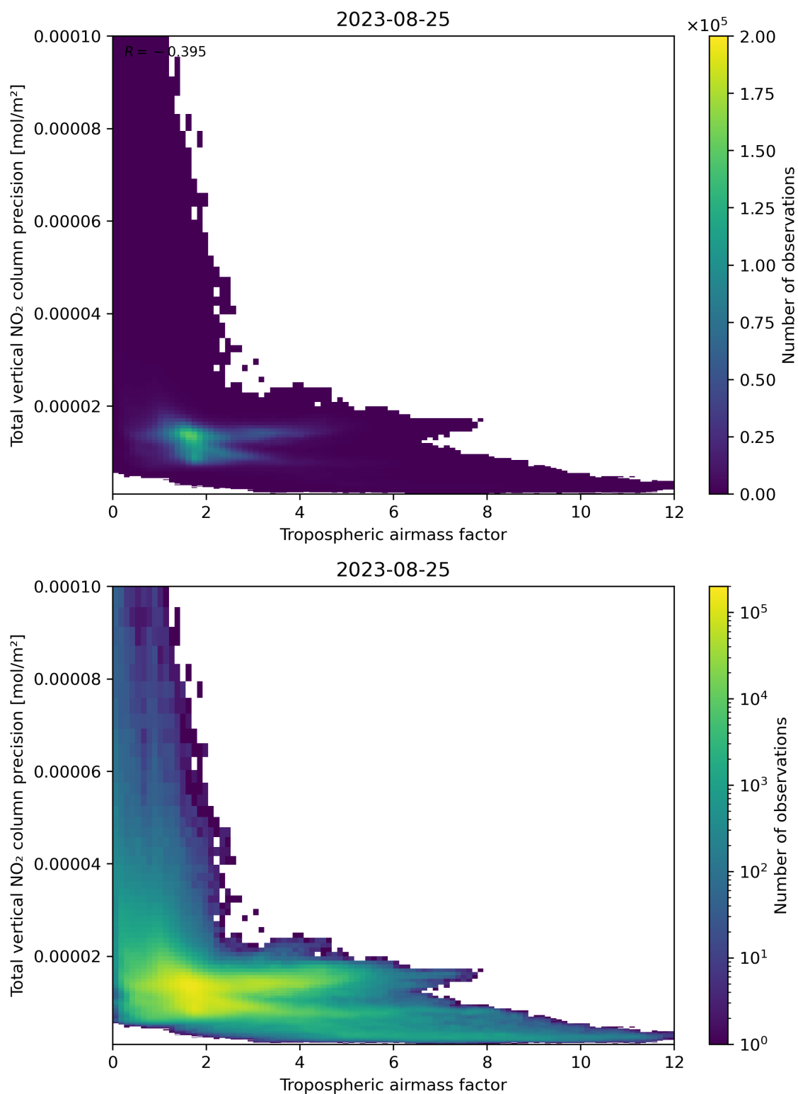
Figure 78: Scatter density plot of “Tropospheric air mass factor” against “Total vertical NO 2 column precision” for 2023-08-25 to 2023-08-26.
