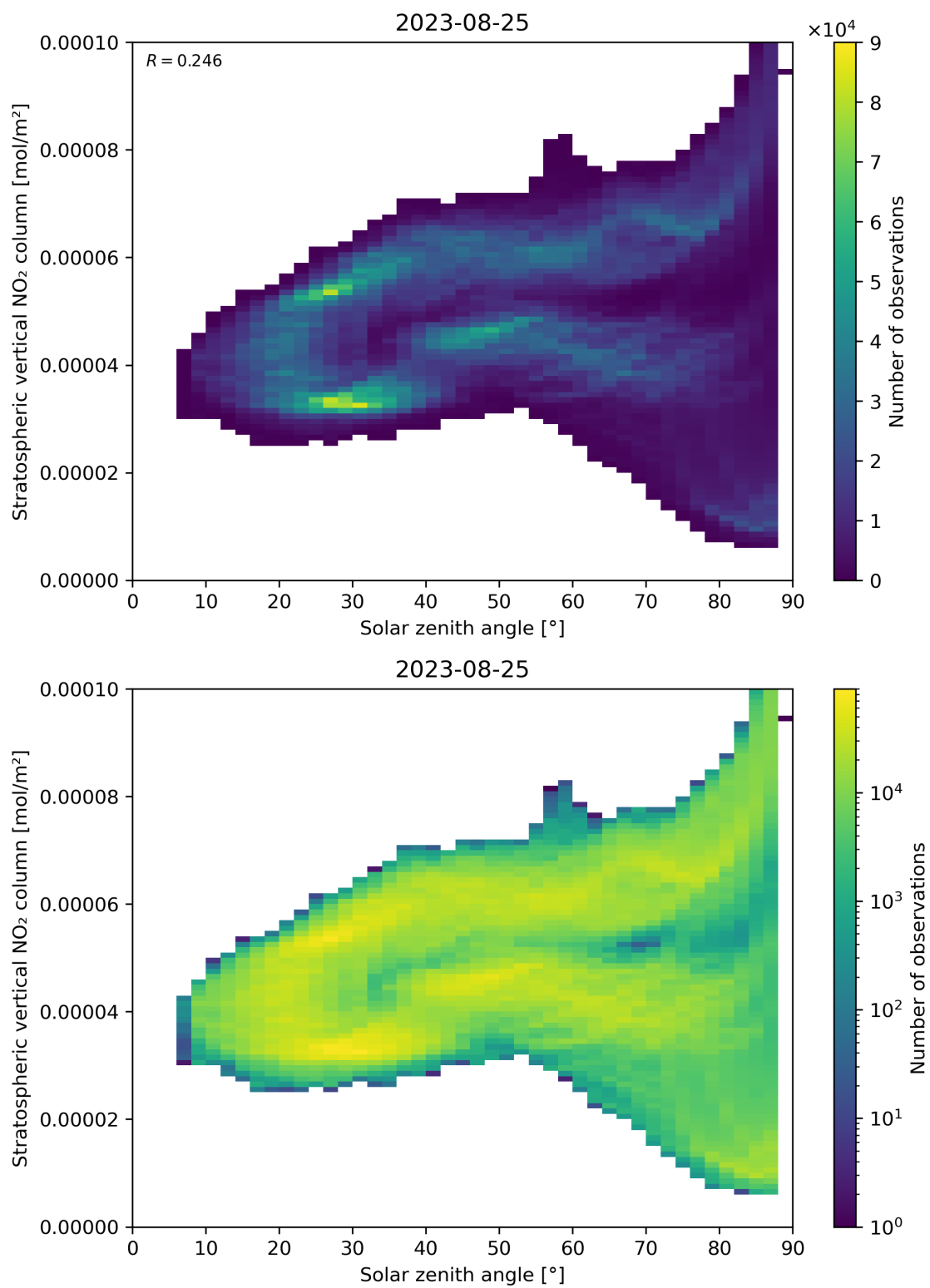
Figure 150: Scatter density plot of “Solar zenith angle” against “Stratospheric vertical NO 2 column” for 2023-08-25 to 2023-08-26.
