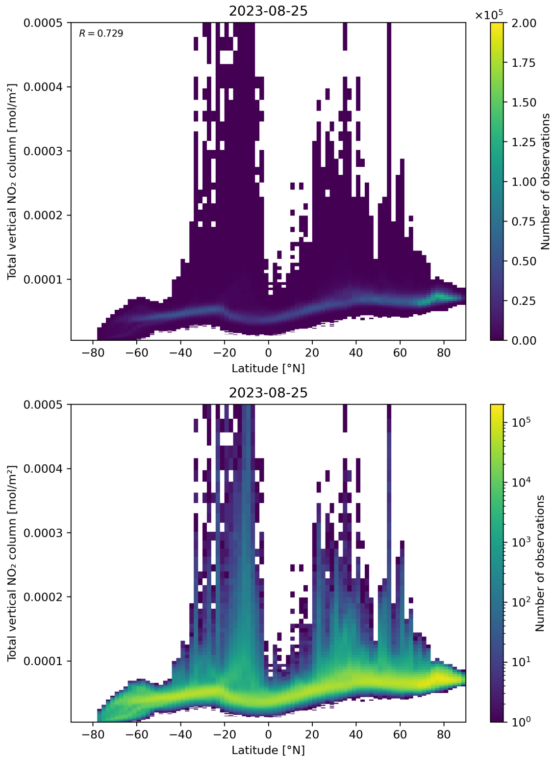
Figure 90: Scatter density plot of “Latitude” against “Total vertical NO 2 column” for 2023-08-25 to 2023-08-26.
