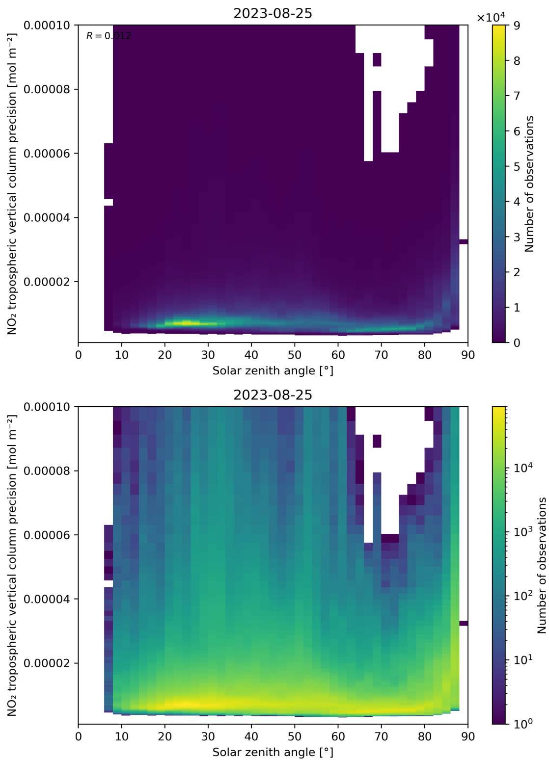
Figure 156: Scatter density plot of “Solar zenith angle” against “NO 2 tropospheric vertical column precision” for 2023-08-25 to 2023-08-26.
