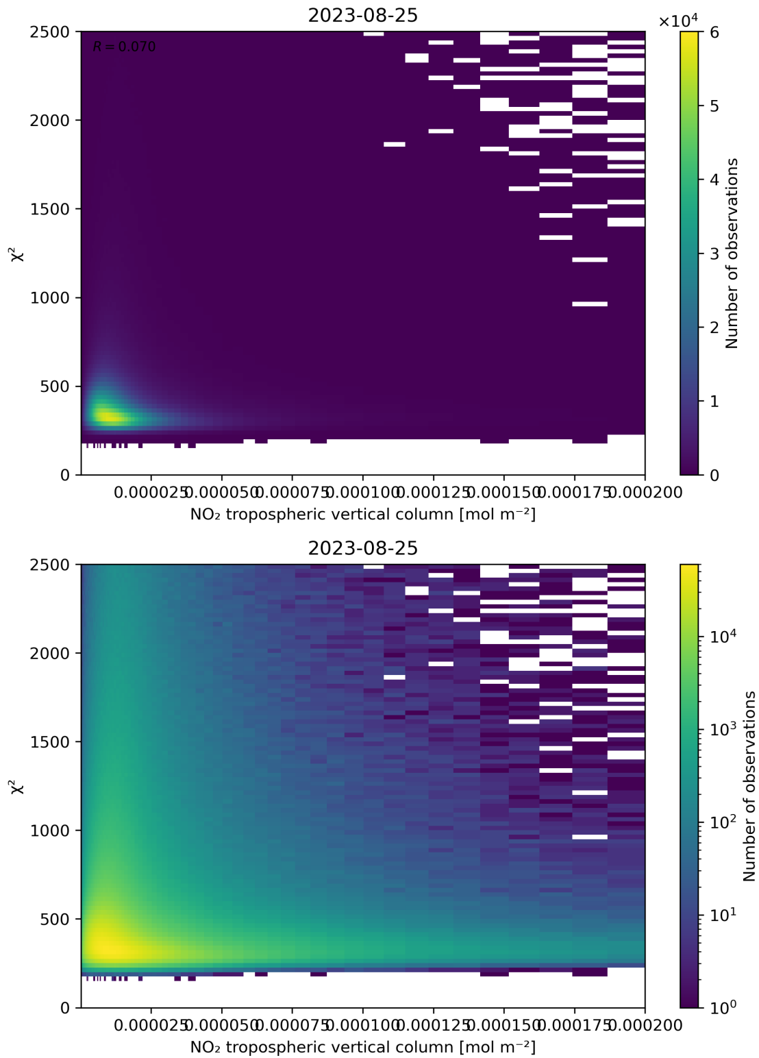
Figure 124: Scatter density plot of “NO 2 tropospheric vertical column” against “ \chi^2 ” for 2023-08-25 to 2023-08-26.
