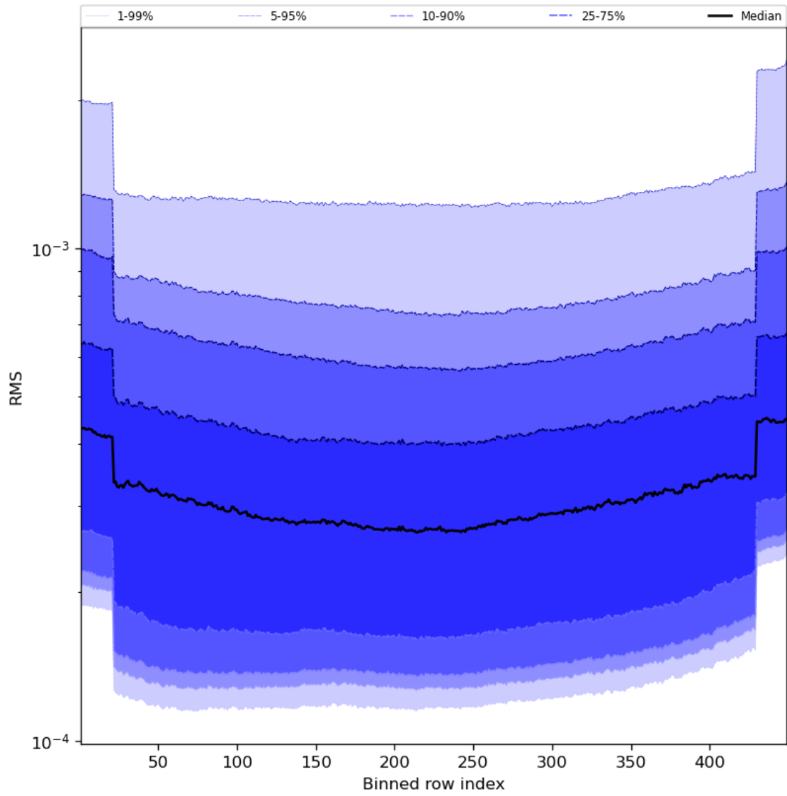
Figure 60: Along track statistics of “RMS” for 2023-08-25 to 2023-08-26
