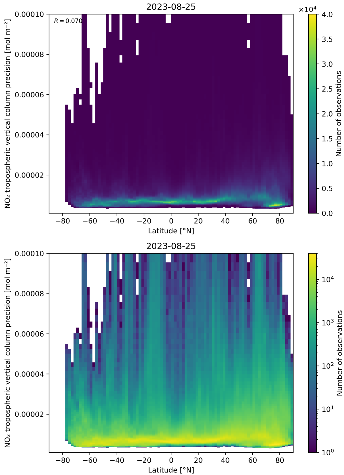
Figure 93: Scatter density plot of “Latitude” against “NO 2 tropospheric vertical column precision” for 2023-08-25 to 2023-08-26.
