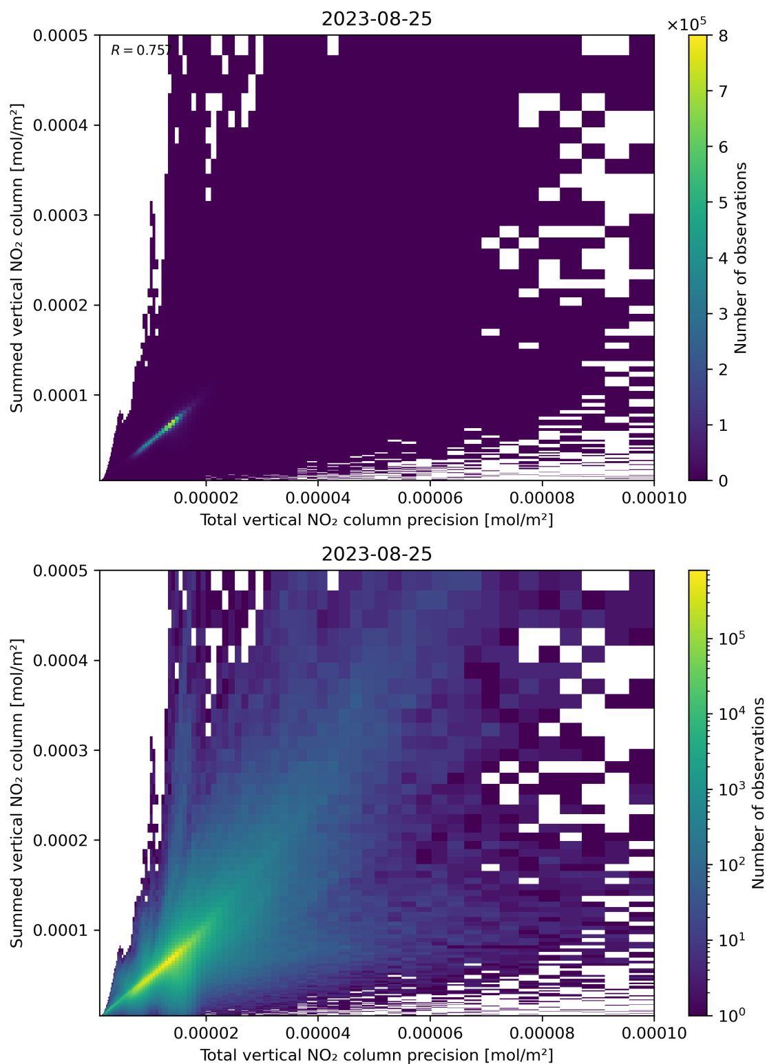
Figure 117: Scatter density plot of “Total vertical NO 2 column precision” against “Summed vertical NO 2 column” for 2023-08-25 to 2023-08-26.
