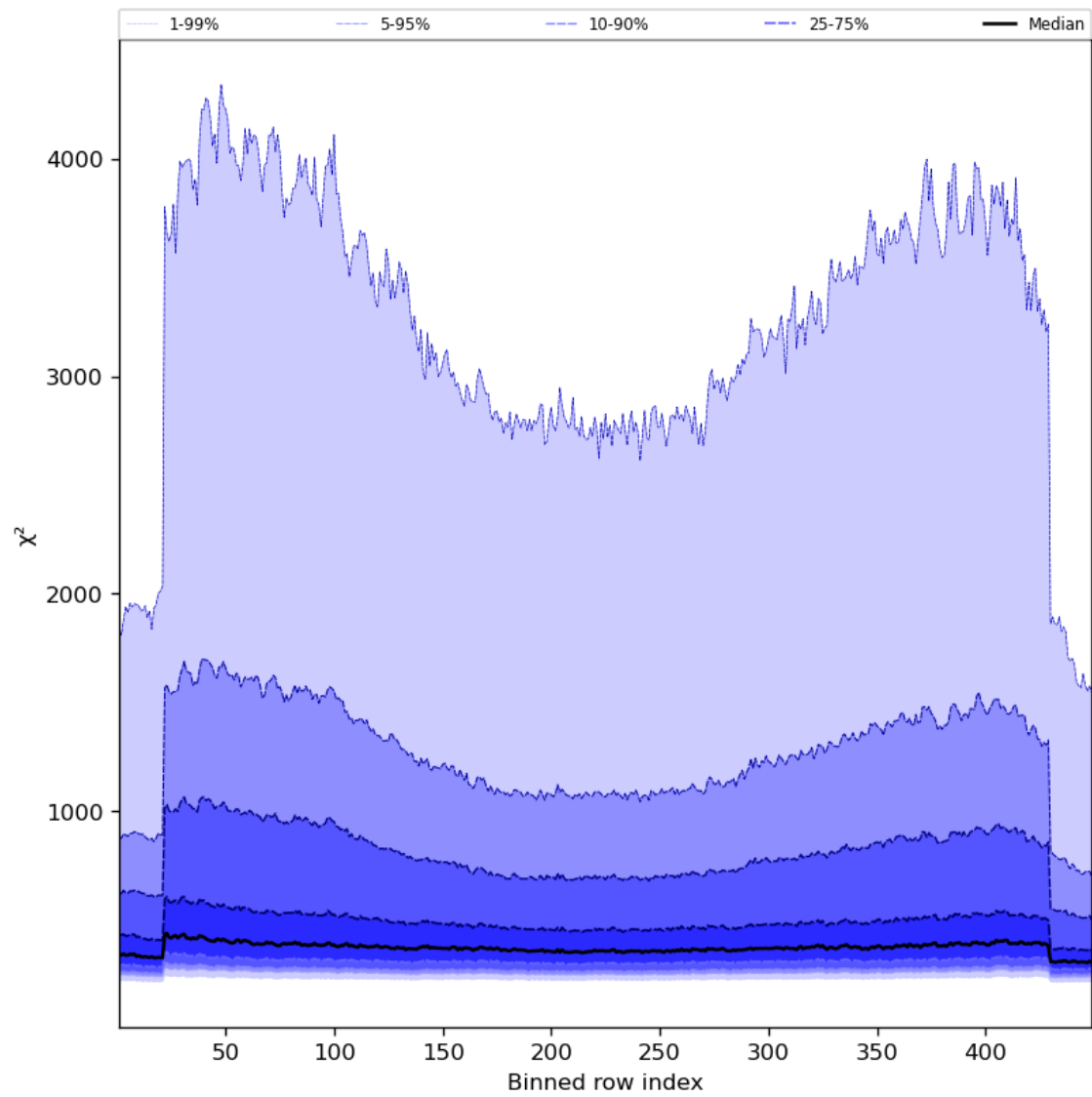
Figure 59: Along track statistics of “ \chi^2 ” for 2023-08-25 to 2023-08-26
