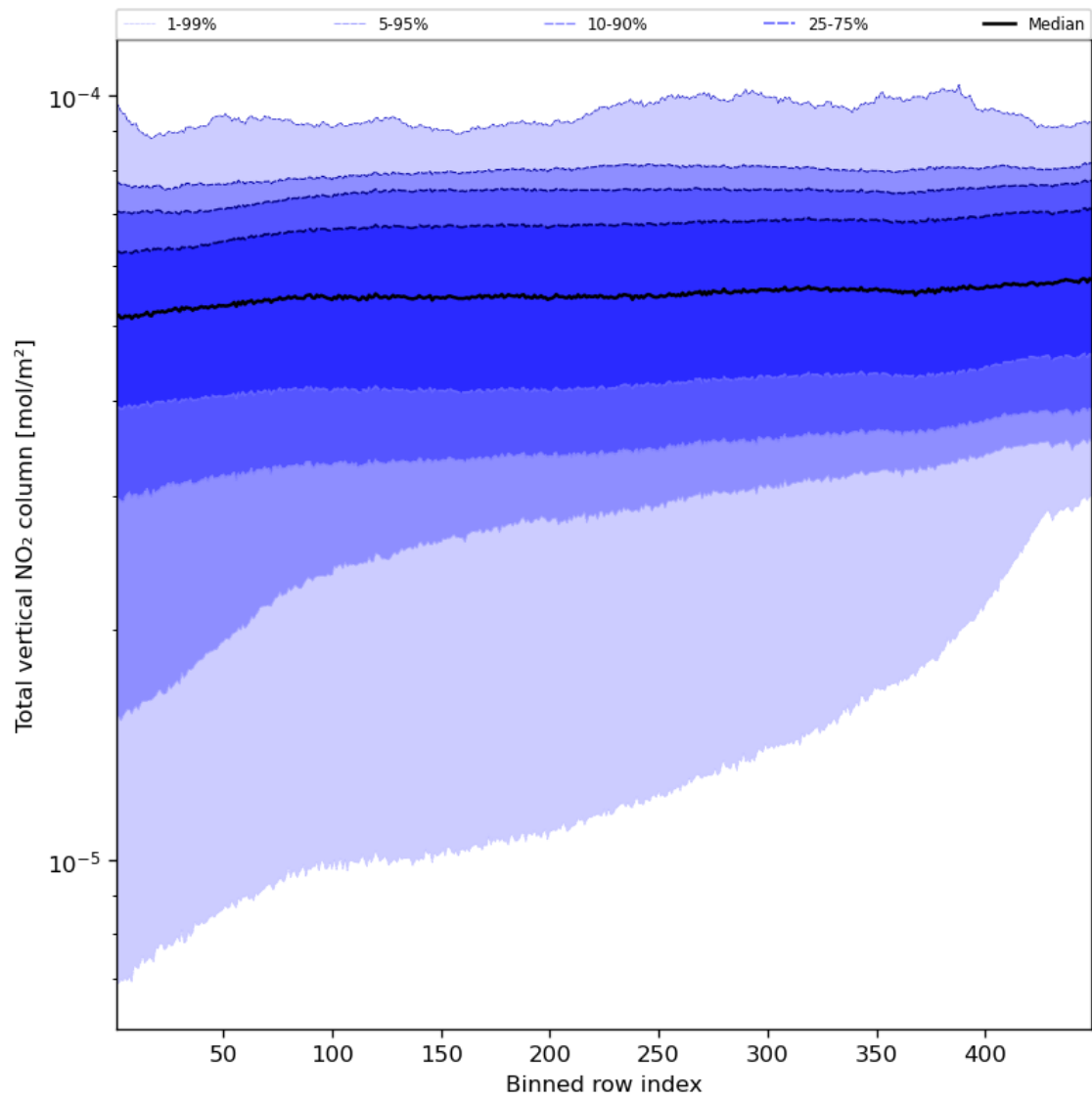
Figure 55: Along track statistics of “Total vertical NO 2 column” for 2023-08-25 to 2023-08-26
