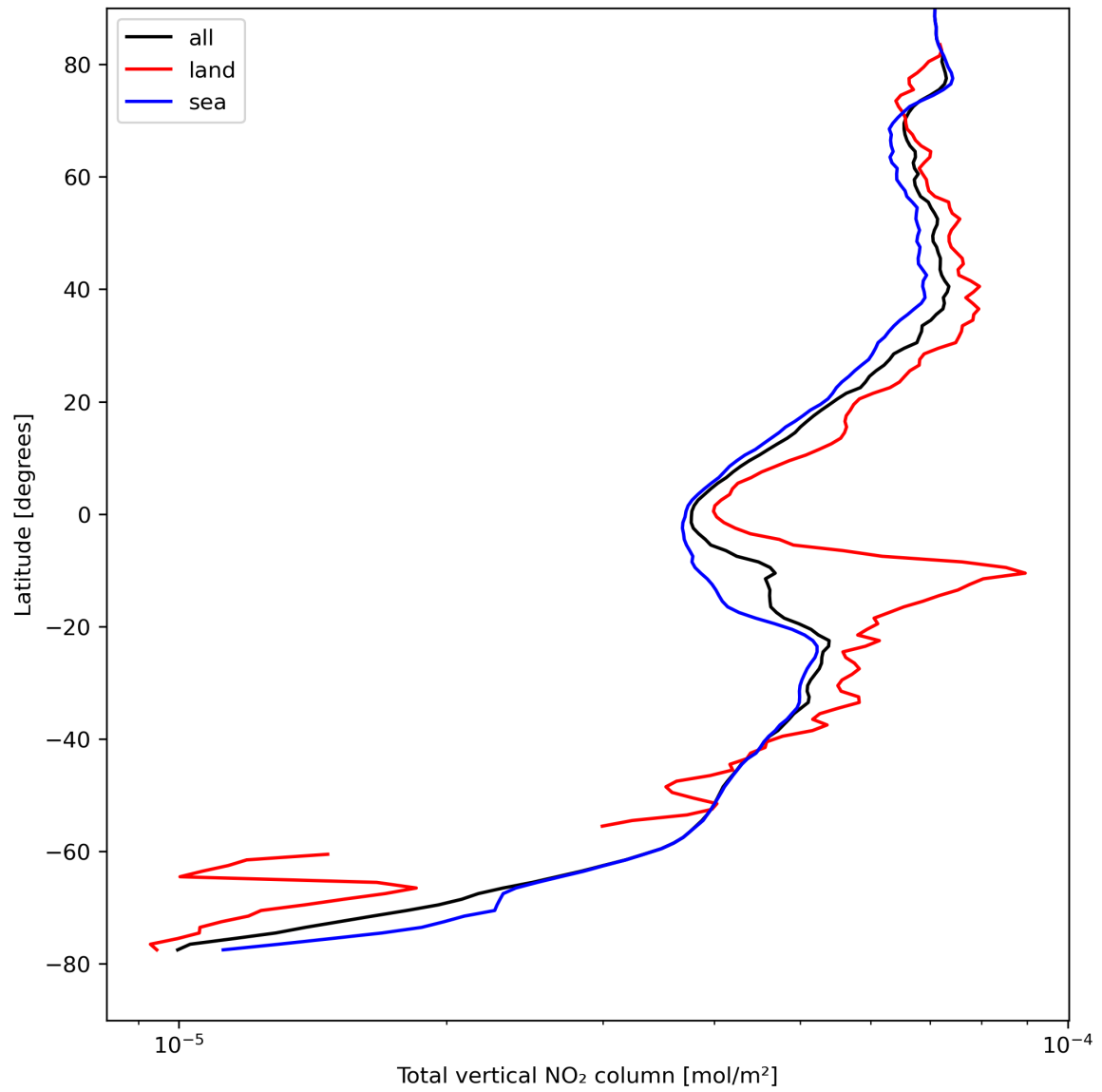
Figure 21: Zonal average of “Total vertical NO 2 column” for 2023-08-25 to 2023-08-26.
