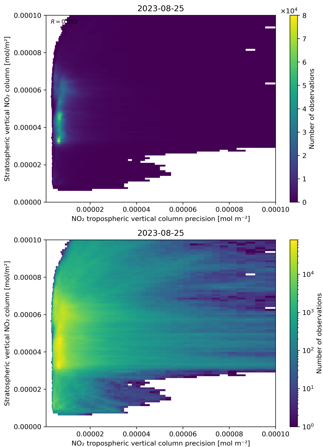
Figure 135: Scatter density plot of “NO 2 tropospheric vertical column precision” against “Stratospheric vertical NO 2 column” for 2023-08-25 to 2023-08-26.
