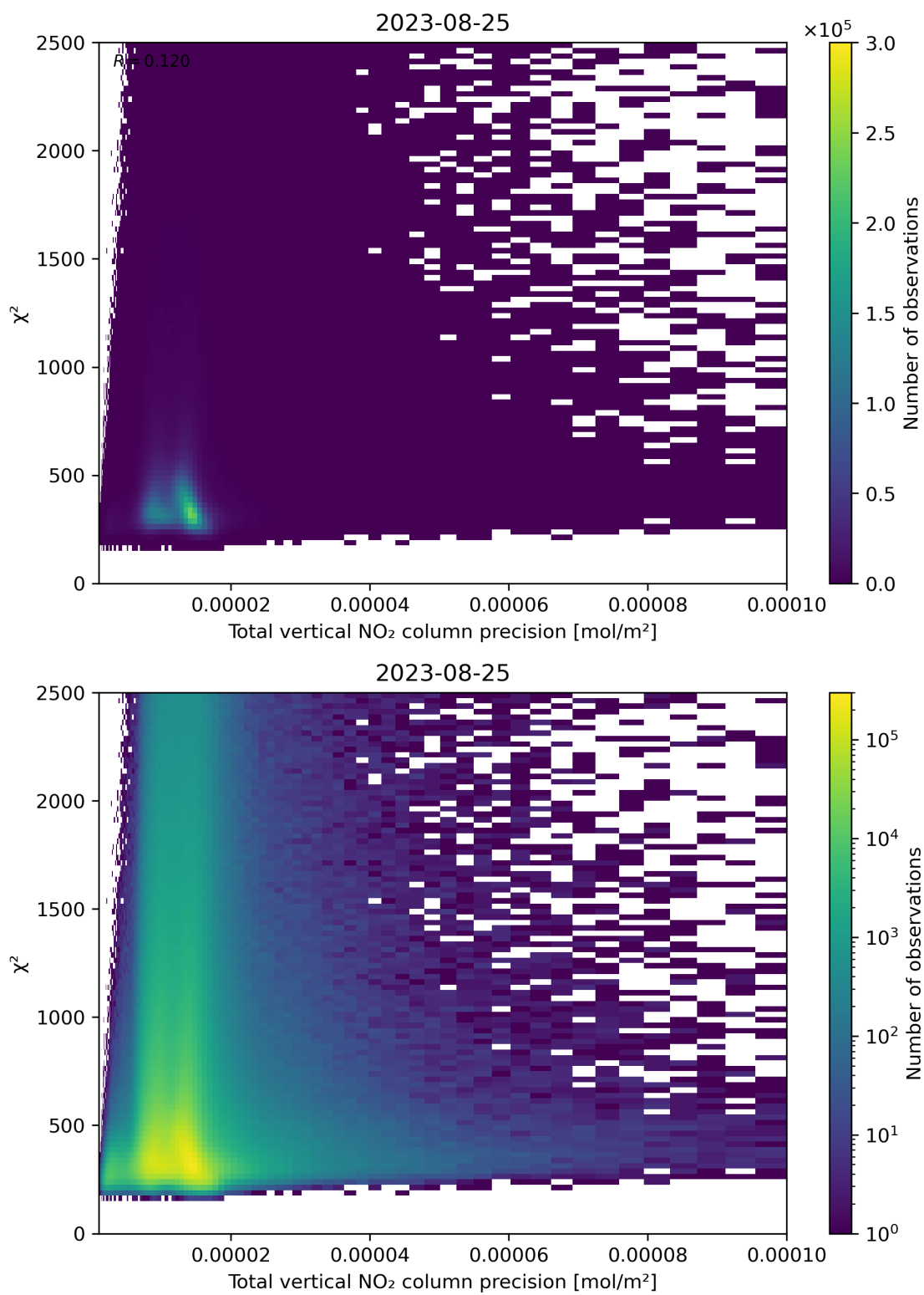
Figure 116: Scatter density plot of “Total vertical NO 2 column precision” against “ \chi^2 ” for 2023-08-25 to 2023-08-26.
