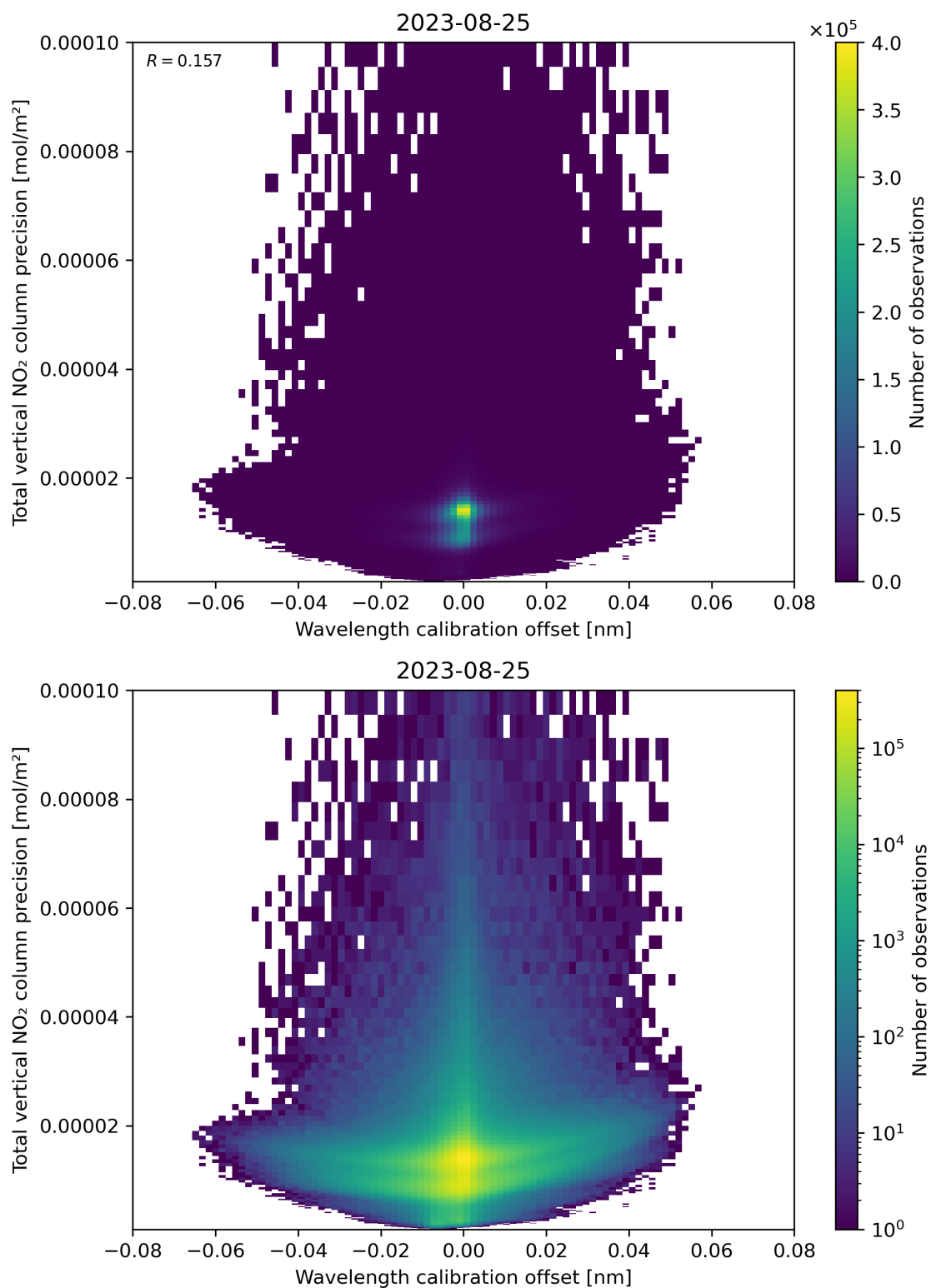
Figure 180: Scatter density plot of “Wavelength calibration offset” against “Total vertical NO 2 column precision” for 2023-08-25 to 2023-08-26.
