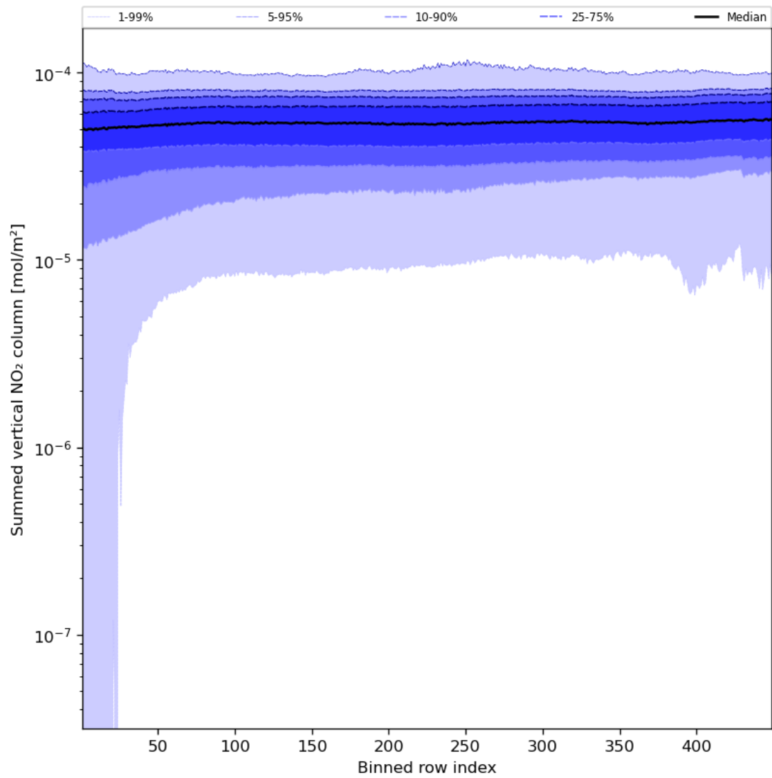
Figure 57: Along track statistics of “Summed vertical NO 2 column” for 2023-08-25 to 2023-08-26
