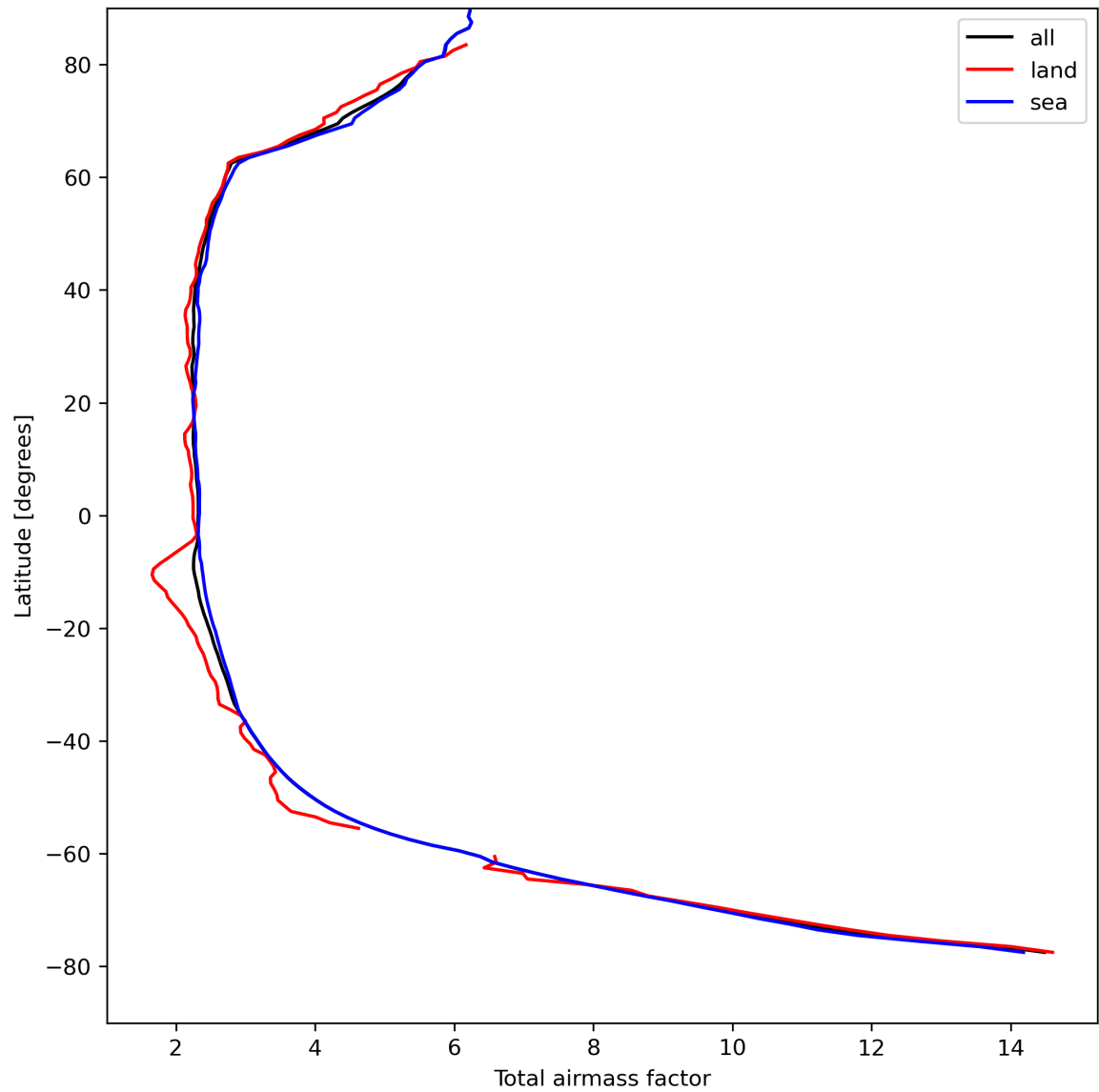
Figure 15: Zonal average of “Total airmass factor” for 2023-08-25 to 2023-08-26.
