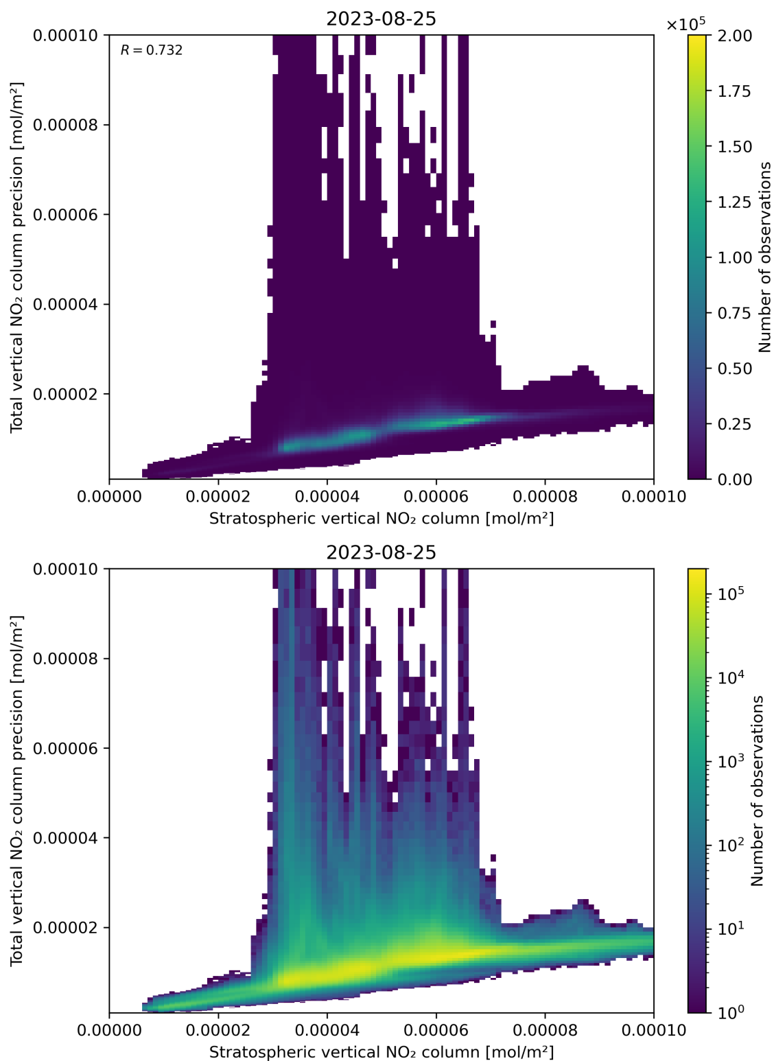
Figure 101: Scatter density plot of “Stratospheric vertical NO 2 column” against “Total vertical NO 2 column precision” for 2023-08-25 to 2023-08-26.
