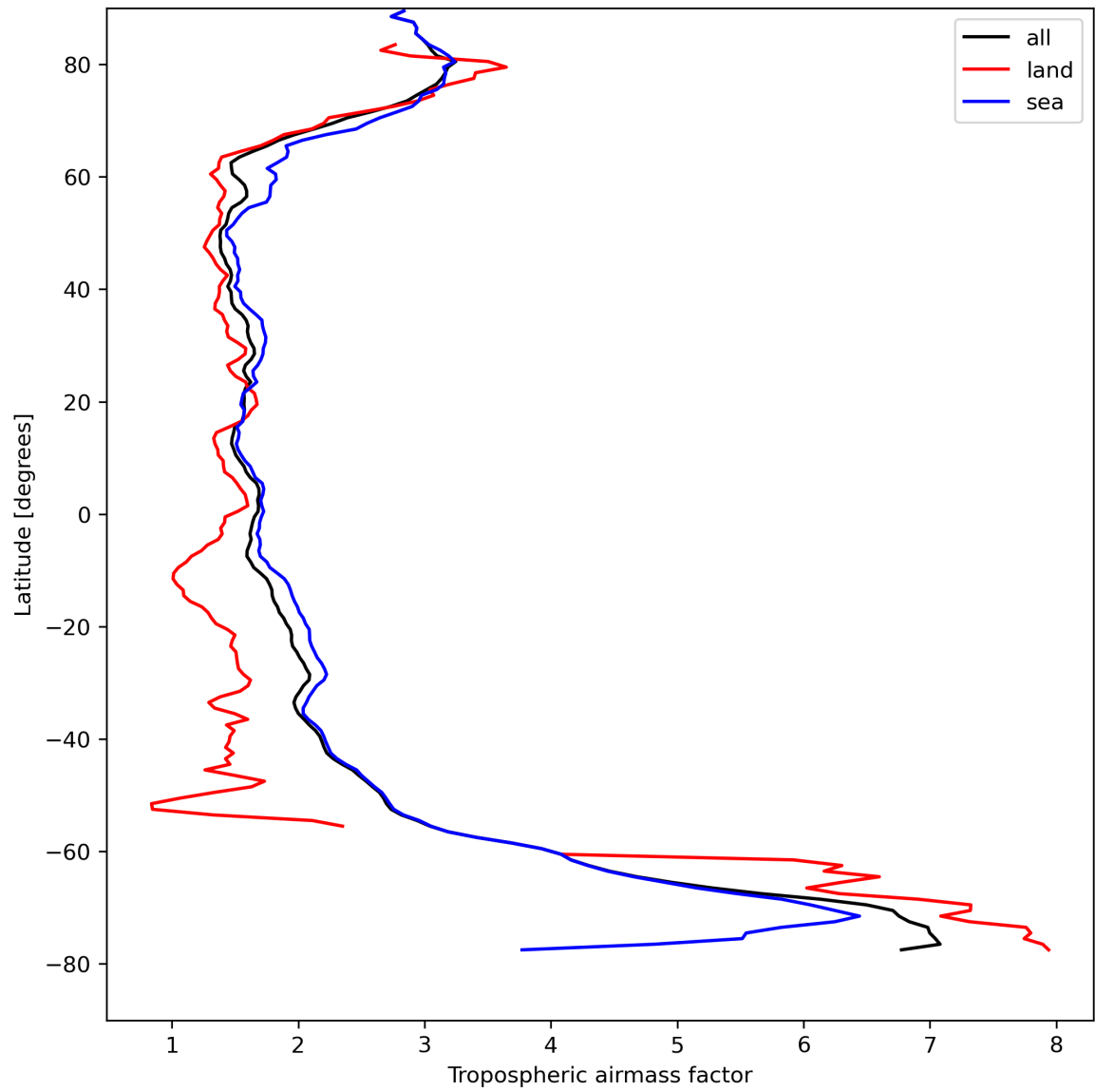
Figure 14: Zonal average of “Tropospheric airmass factor” for 2023-08-25 to 2023-08-26.
