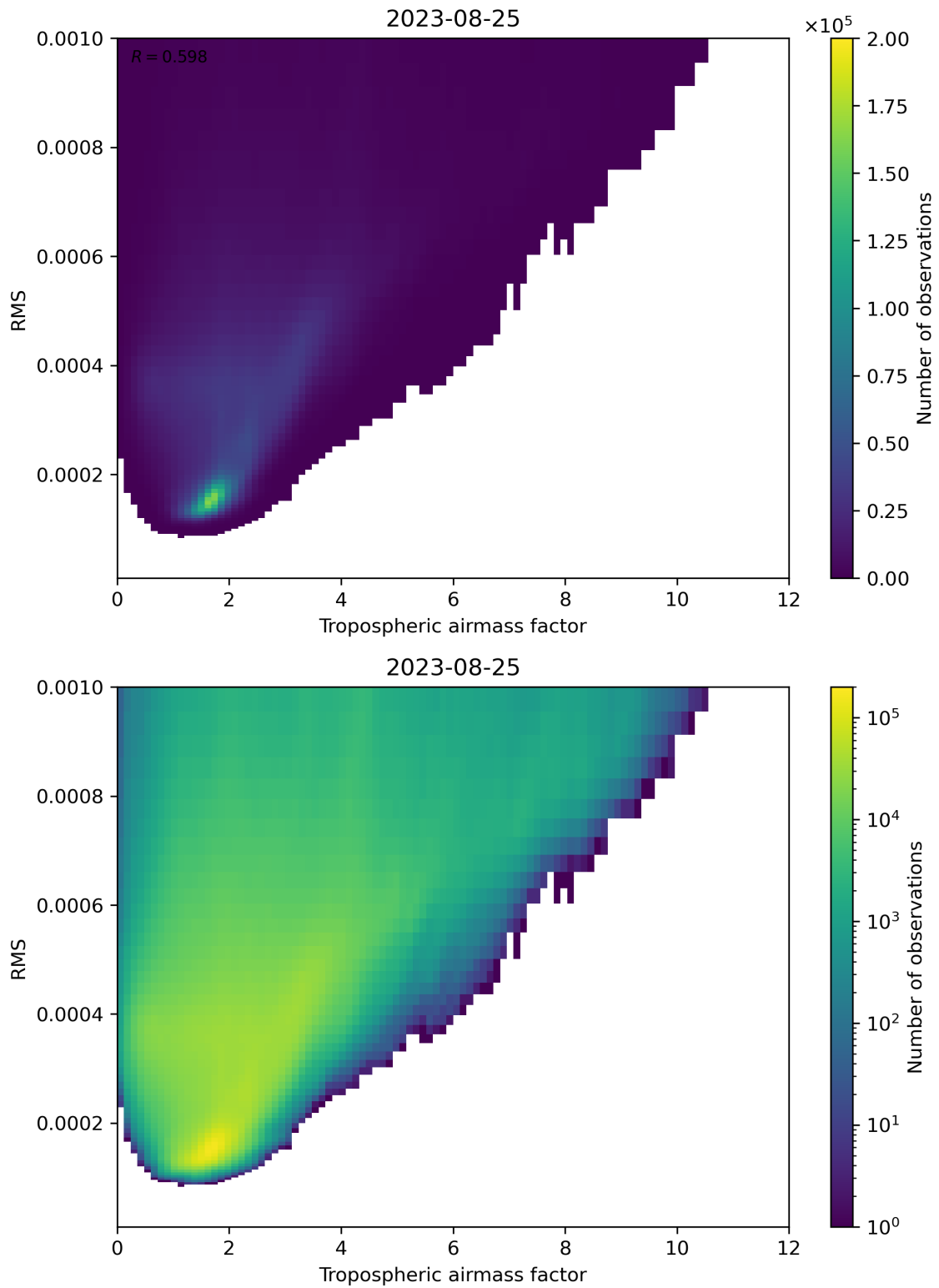
Figure 79: Scatter density plot of “Tropospheric airmass factor” against “RMS” for 2023-08-25 to 2023-08-26.
