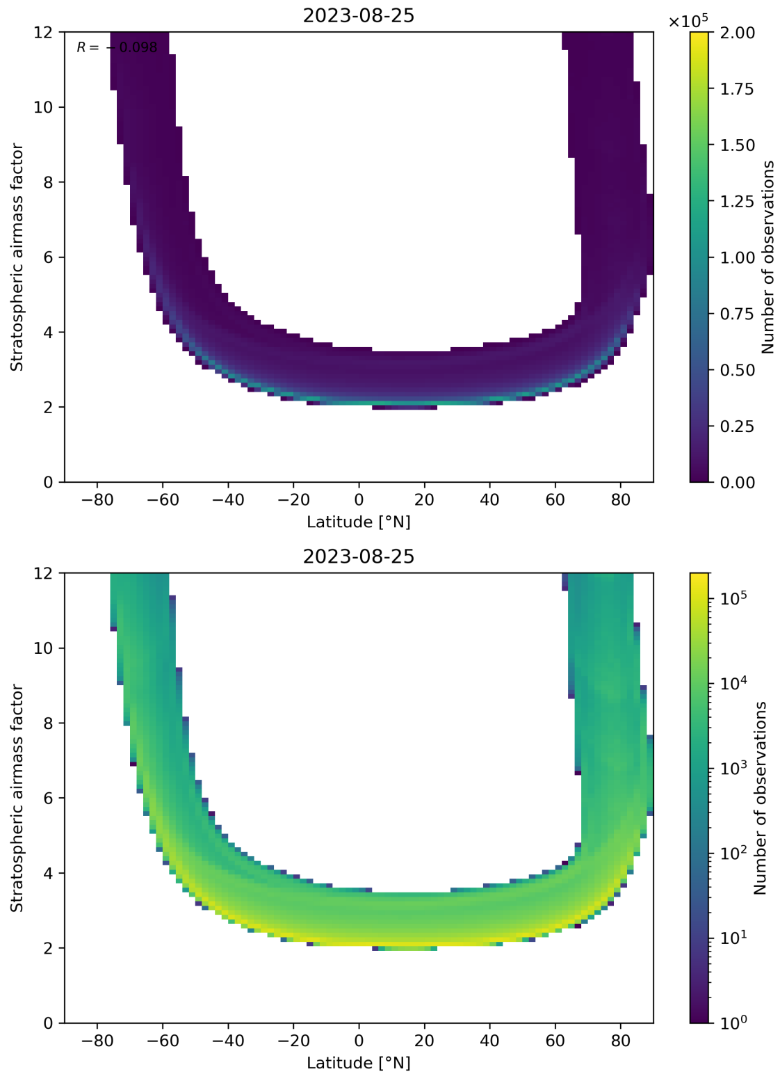
Figure 83: Scatter density plot of “Latitude” against “Stratospheric air mass factor” for 2023-08-25 to 2023-08-26.
