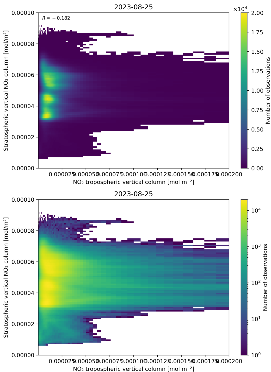
Figure 125: Scatter density plot of “NO 2 tropospheric vertical column” against “Stratospheric vertical NO 2 column” for 2023-08-25 to 2023-08-26.
