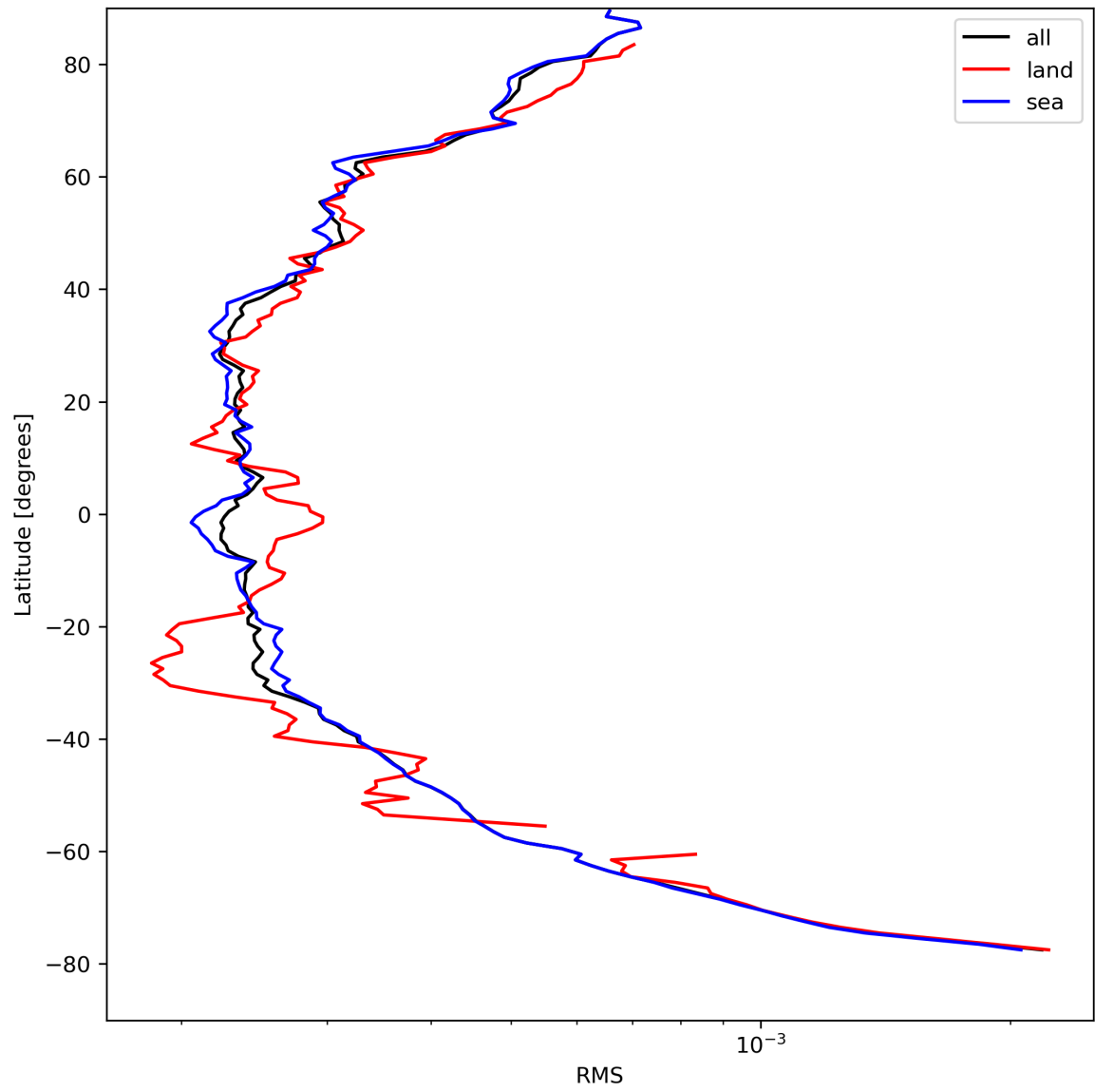
Figure 26: Zonal average of “RMS” for 2023-08-25 to 2023-08-26.
