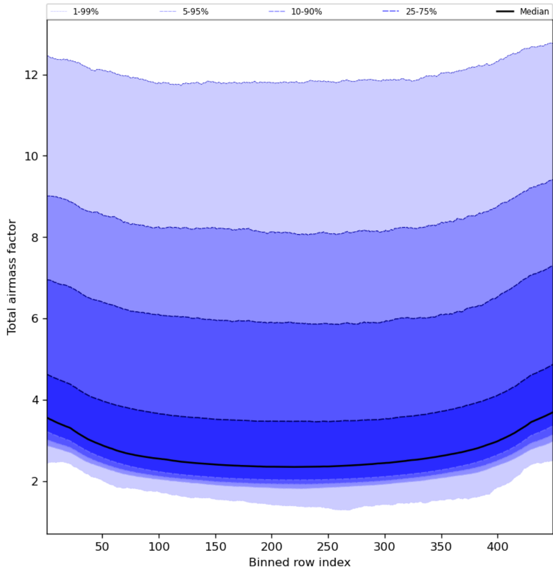
Figure 49: Along track statistics of “Total airmass factor” for 2023-08-25 to 2023-08-26
