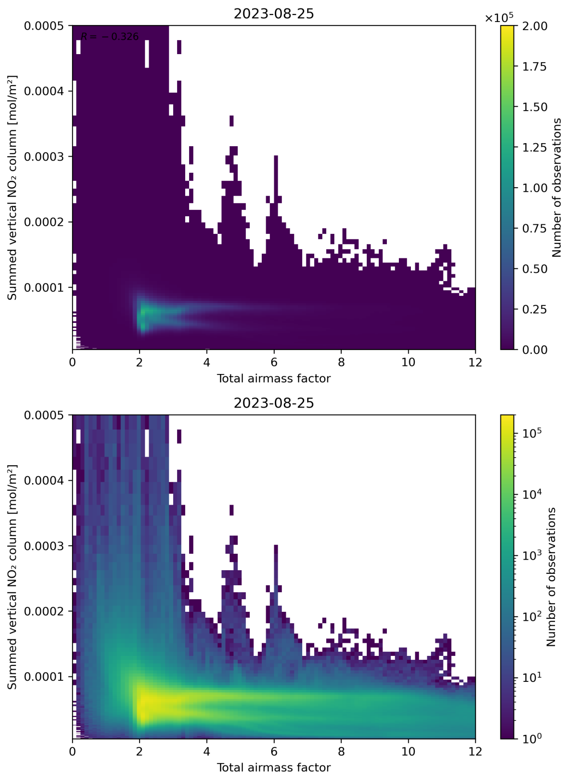
Figure 65: Scatter density plot of “Total airmass factor” against “Summed vertical NO 2 column” for 2023-08-25 to 2023-08-26.
