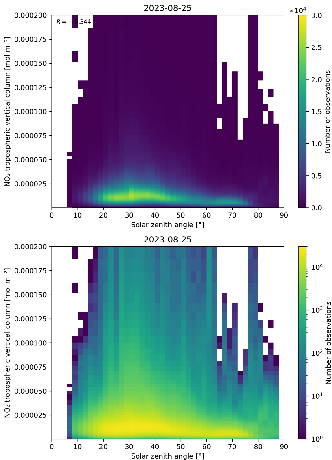
Figure 155: Scatter density plot of “Solar zenith angle” against “NO 2 tropospheric vertical column” for 2023-08-25 to 2023-08-26.
