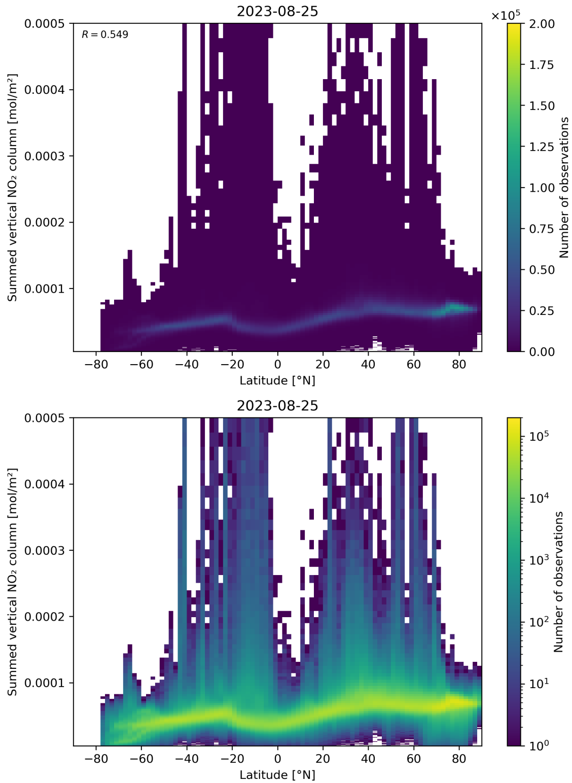
Figure 88: Scatter density plot of “Latitude” against “Summed vertical NO 2 column” for 2023-08-25 to 2023-08-26.
