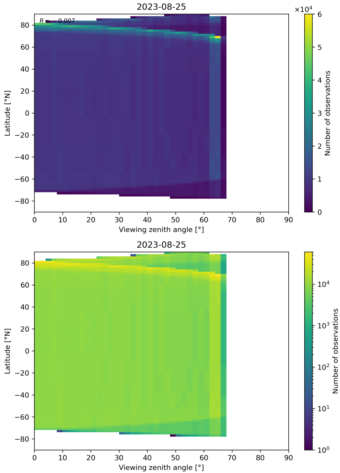
Figure 163: Scatter density plot of “Viewing zenith angle” against “Latitude” for 2023-08-25 to 2023-08-26.
