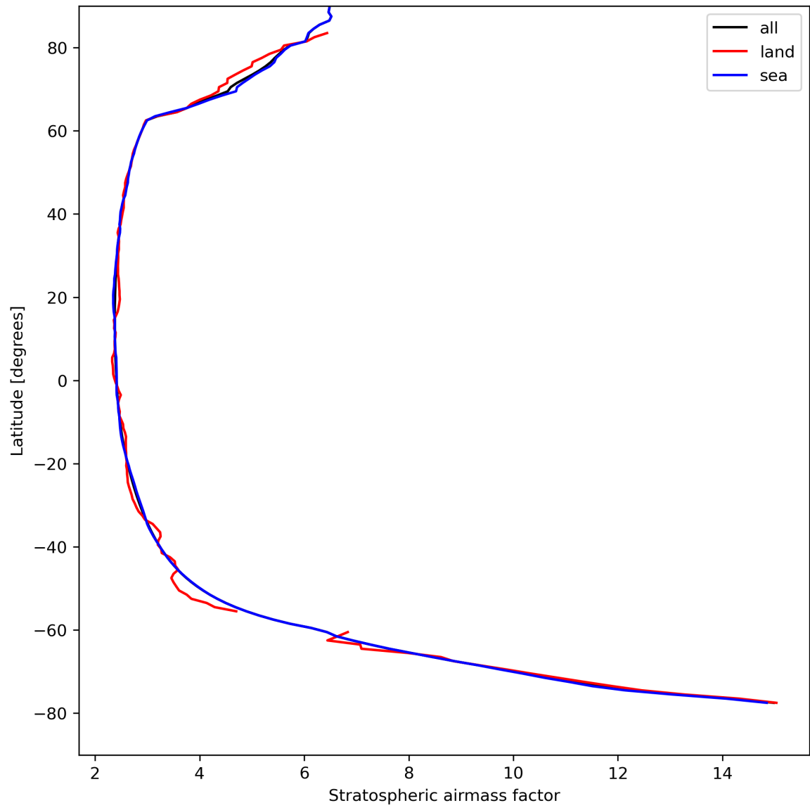
Figure 27: Zonal average of “Stratospheric airmass factor” for 2023-08-25 to 2023-08-26.
