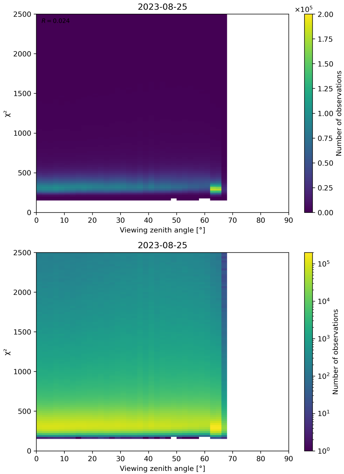
Figure 162: Scatter density plot of “Viewing zenith angle” against “ \chi^2 ” for 2023-08-25 to 2023-08-26.
