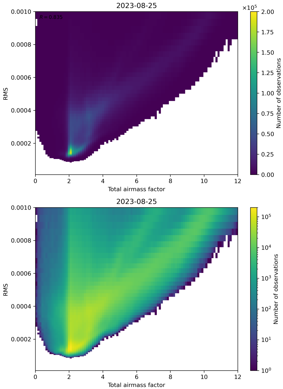
Figure 69: Scatter density plot of “Total airmass factor” against “RMS” for 2023-08-25 to 2023-08-26.
