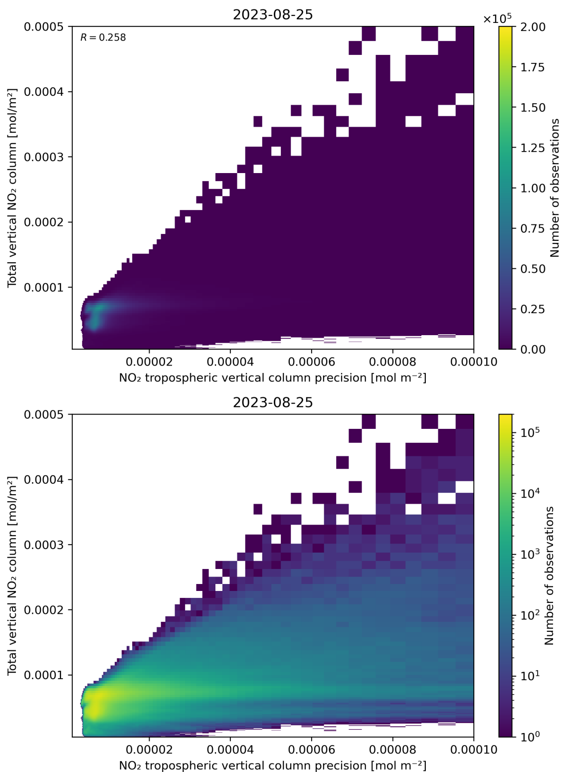
Figure 138: Scatter density plot of “NO 2 tropospheric vertical column precision” against “Total vertical NO 2 column” for 2023-08-25 to 2023-08-26.
