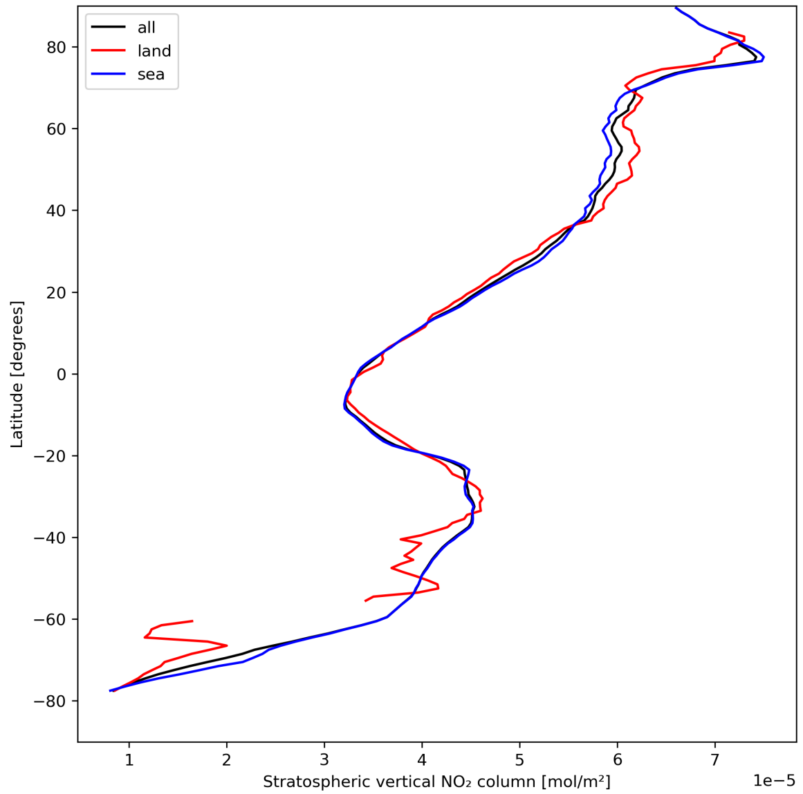
Figure 19: Zonal average of “Stratospheric vertical NO 2 column” for 2023-08-25 to 2023-08-26.
