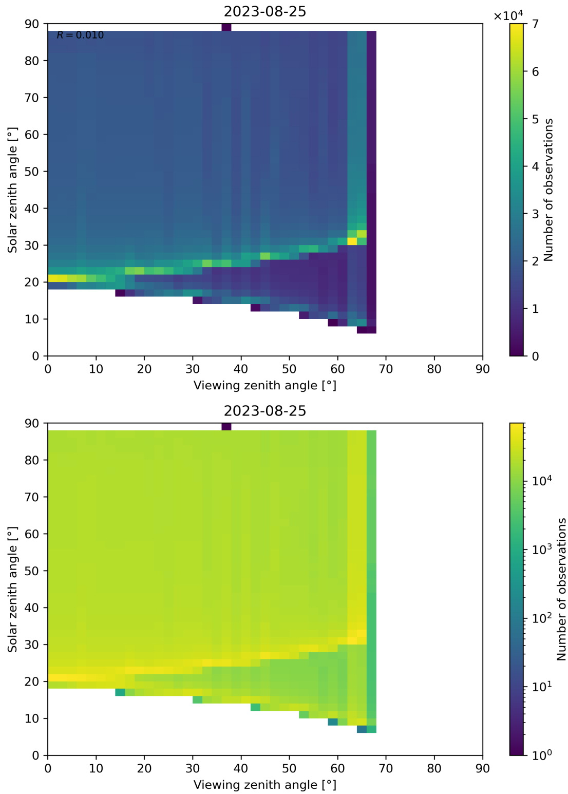
Figure 172: Scatter density plot of “Viewing zenith angle” against “Solar zenith angle” for 2023-08-25 to 2023-08-26.
