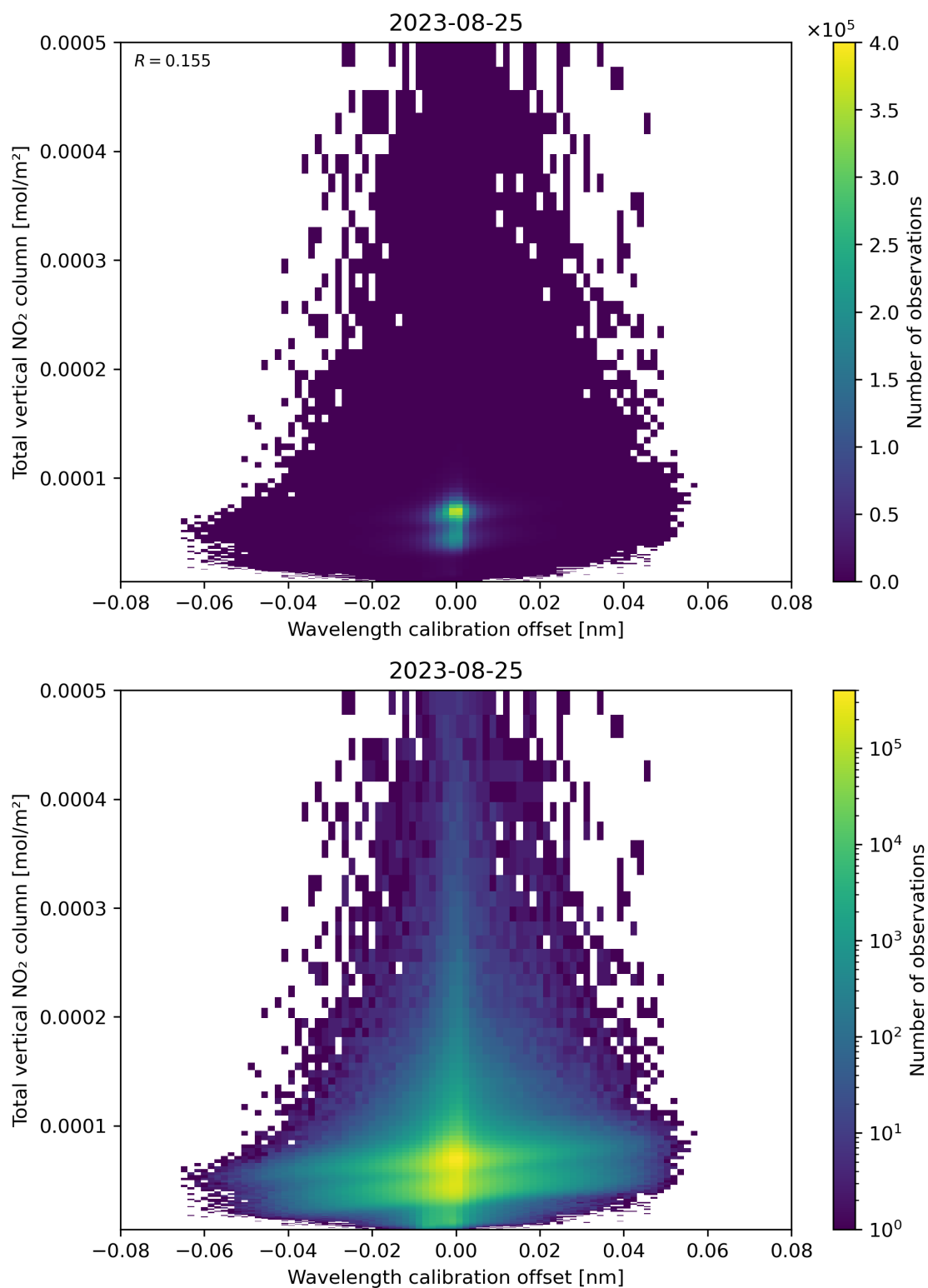
Figure 179: Scatter density plot of “Wavelength calibration offset” against “Total vertical NO 2 column” for 2023-08-25 to 2023-08-26.
