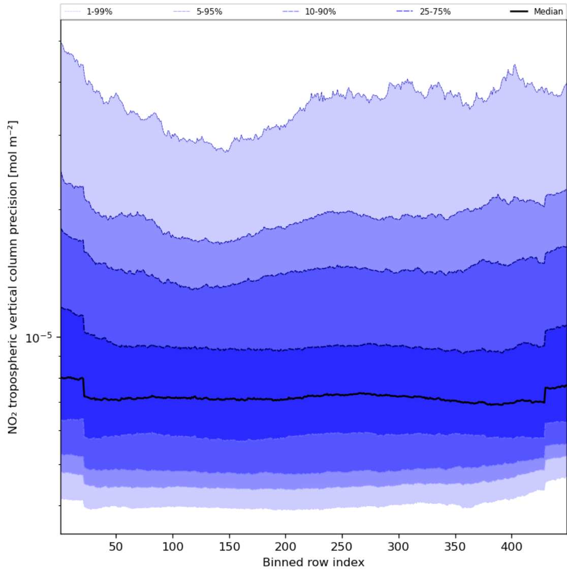
Figure 47: Along track statistics of “NO 2 tropospheric vertical column precision” for 2023-08-25 to 2023-08-26
