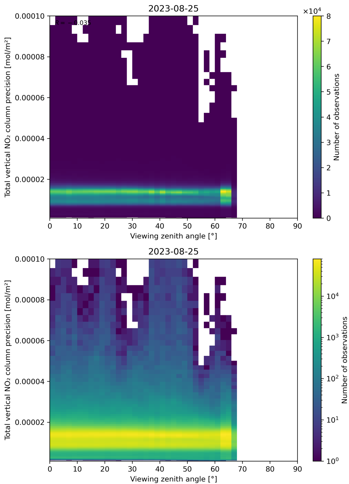
Figure 168: Scatter density plot of “Viewing zenith angle” against “Total vertical NO 2 column precision” for 2023-08-25 to 2023-08-26.
