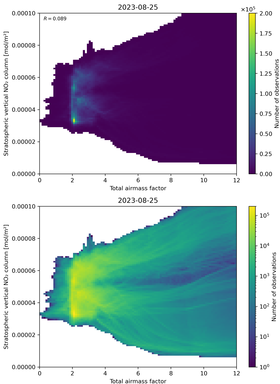
Figure 64: Scatter density plot of “Total airmass factor” against “Stratospheric vertical \text{NO}_2 column” for 2023-08-25 to 2023-08-26.
