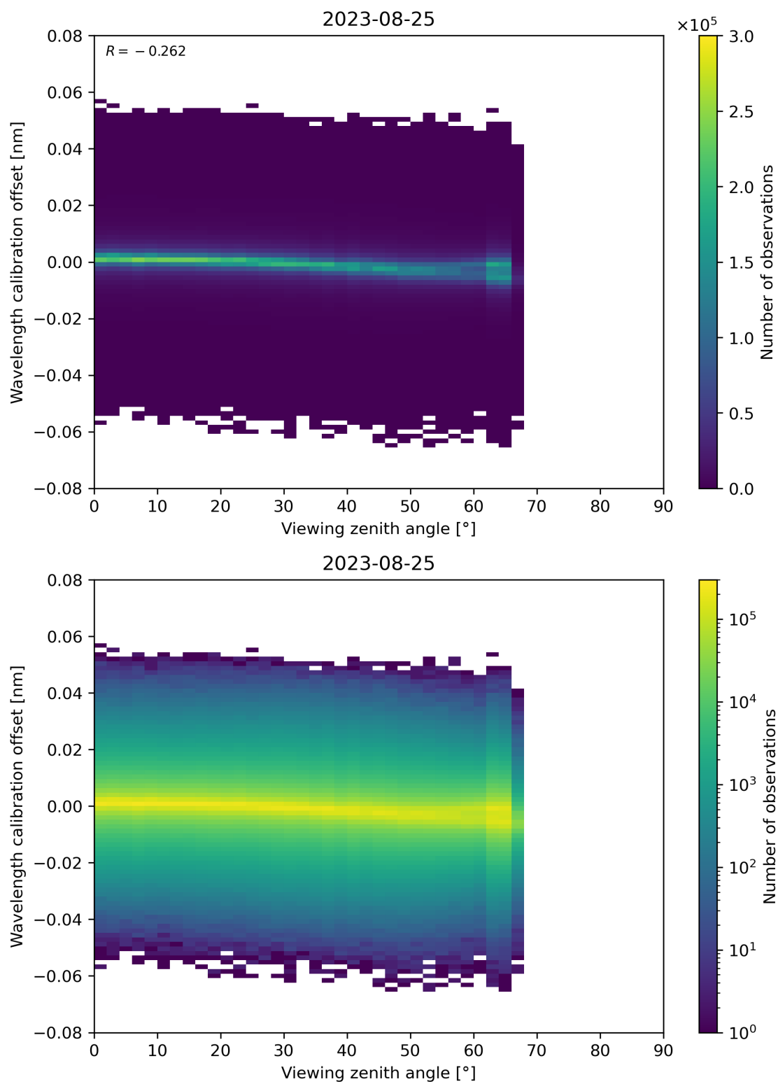
Figure 173: Scatter density plot of “Viewing zenith angle” against “Wavelength calibration offset” for 2023-08-25 to 2023-08-26.
