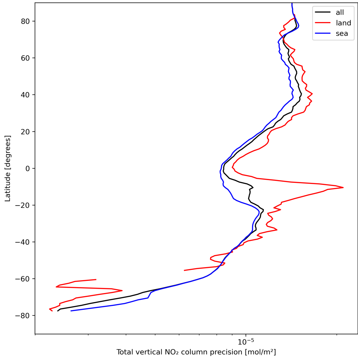
Figure 22: Zonal average of “Total vertical NO 2 column precision” for 2023-08-25 to 2023-08-26.
