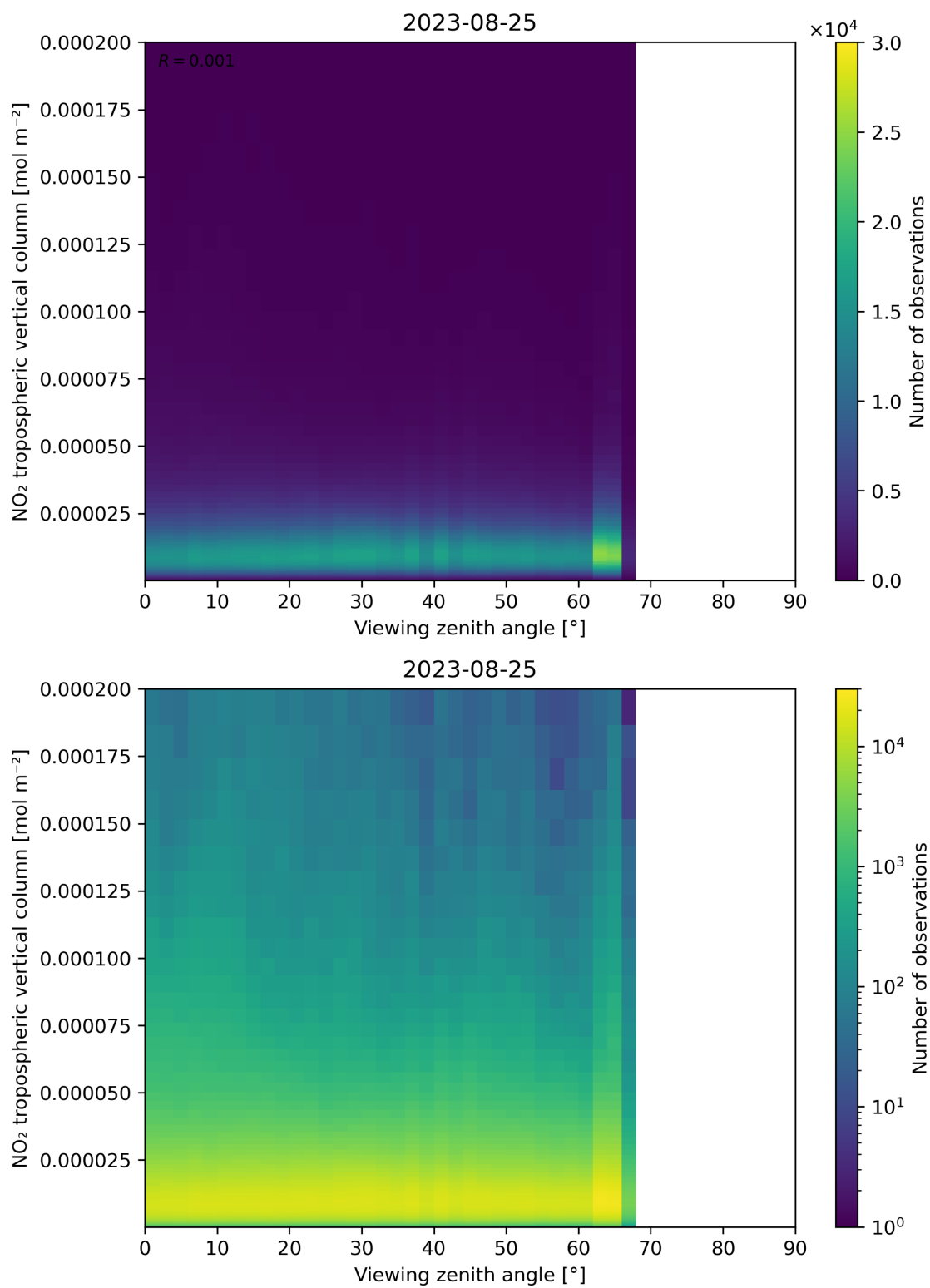
Figure 169: Scatter density plot of “Viewing zenith angle” against “NO 2 tropospheric vertical column” for 2023-08-25 to 2023-08-26.
