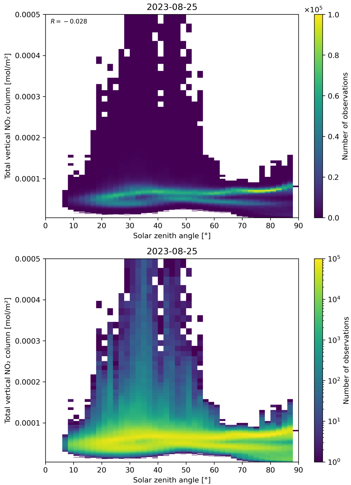
Figure 153: Scatter density plot of “Solar zenith angle” against “Total vertical NO 2 column” for 2023-08-25 to 2023-08-26.
