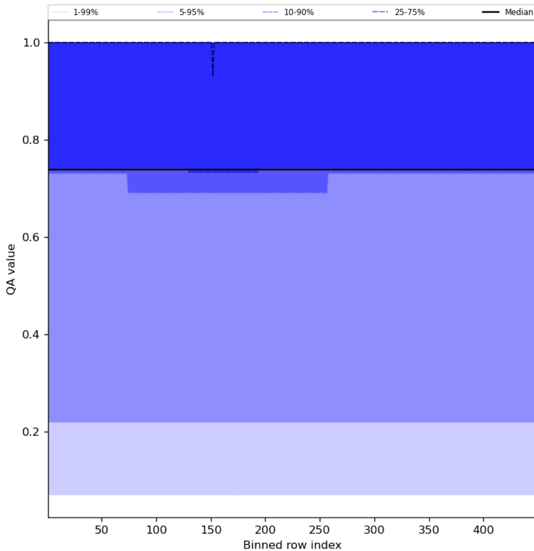
Figure 45: Along track statistics of “QA value” for 2023-08-25 to 2023-08-26
