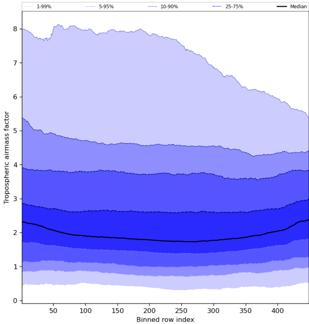
Figure 48: Along track statistics of “Tropospheric airmass factor” for 2023-08-25 to 2023-08-26
