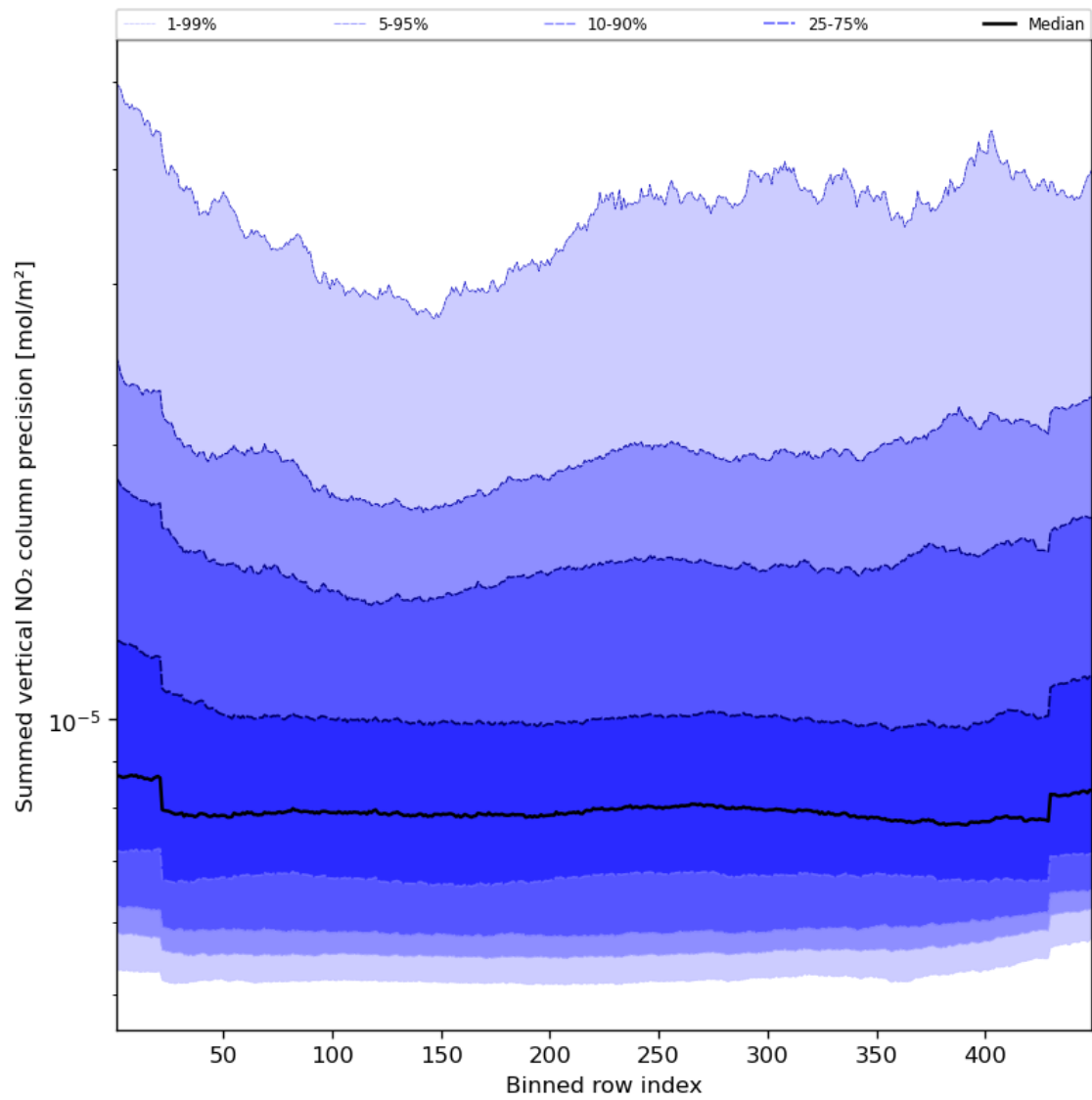
Figure 58: Along track statistics of “Summed vertical NO 2 column precision” for 2023-08-25 to 2023-08-26
