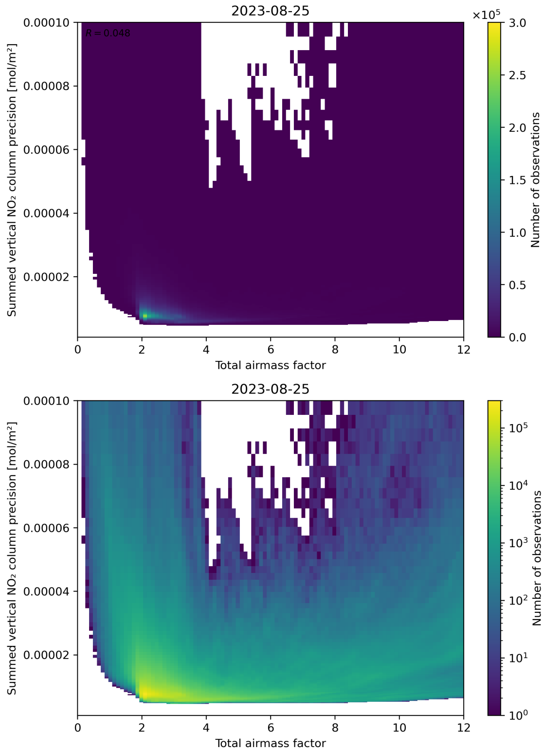
Figure 66: Scatter density plot of “Total airmass factor” against “Summed vertical NO 2 column precision” for 2023-08-25 to 2023-08-26.
