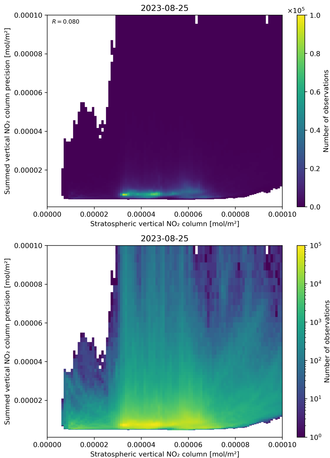
Figure 99: Scatter density plot of “Stratospheric vertical NO 2 column” against “Summed vertical NO 2 column precision” for 2023-08-25 to 2023-08-26.
