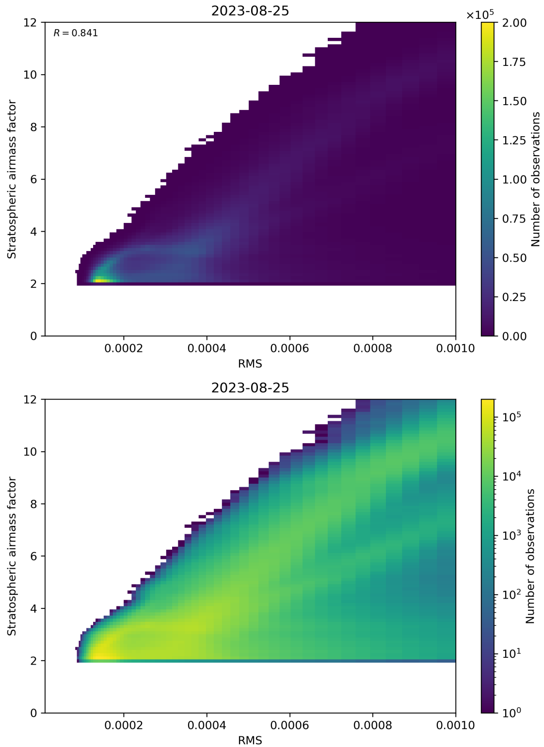
Figure 144: Scatter density plot of “RMS” against “Stratospheric airmass factor” for 2023-08-25 to 2023-08-26.
