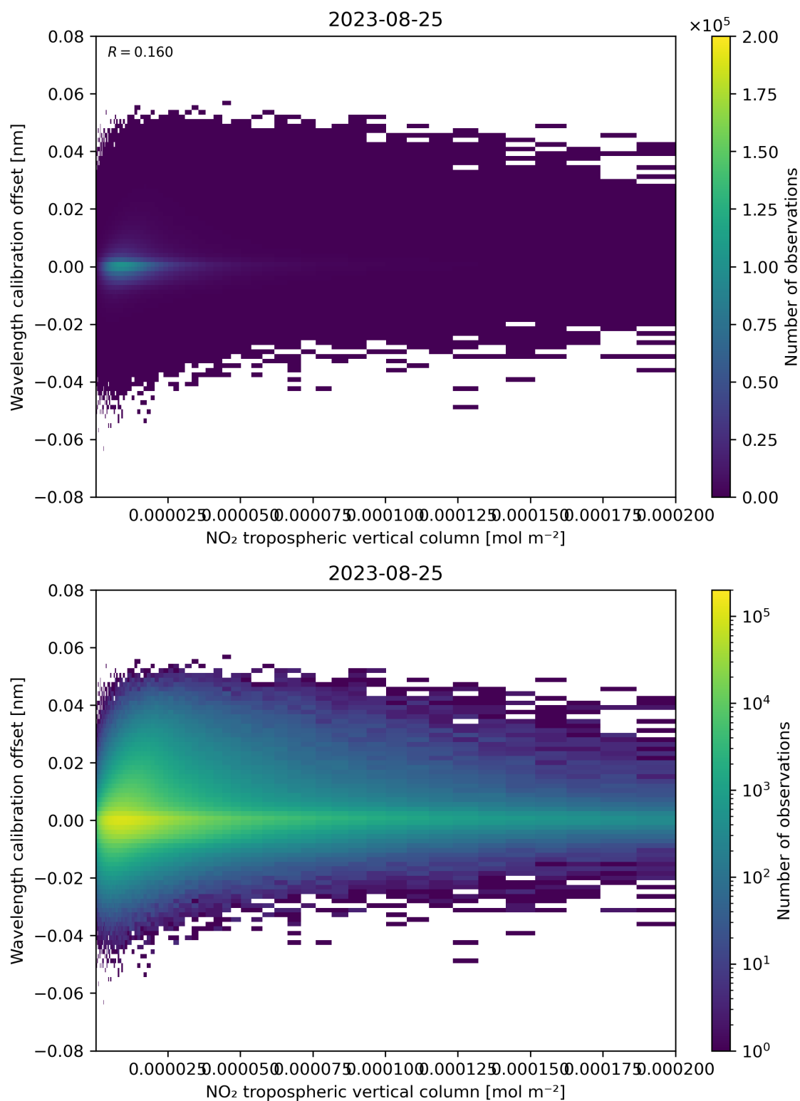
Figure 143: Scatter density plot of “NO 2 tropospheric vertical column” against “Wavelength calibration offset” for 2023-08-25 to 2023-08-26.
