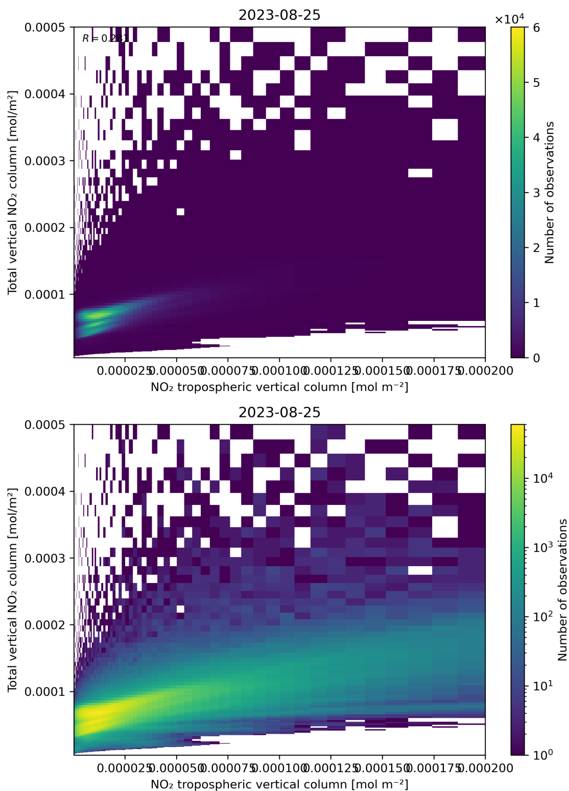
Figure 128: Scatter density plot of “NO 2 tropospheric vertical column” against “Total vertical NO 2 column” for 2023-08-25 to 2023-08-26.
