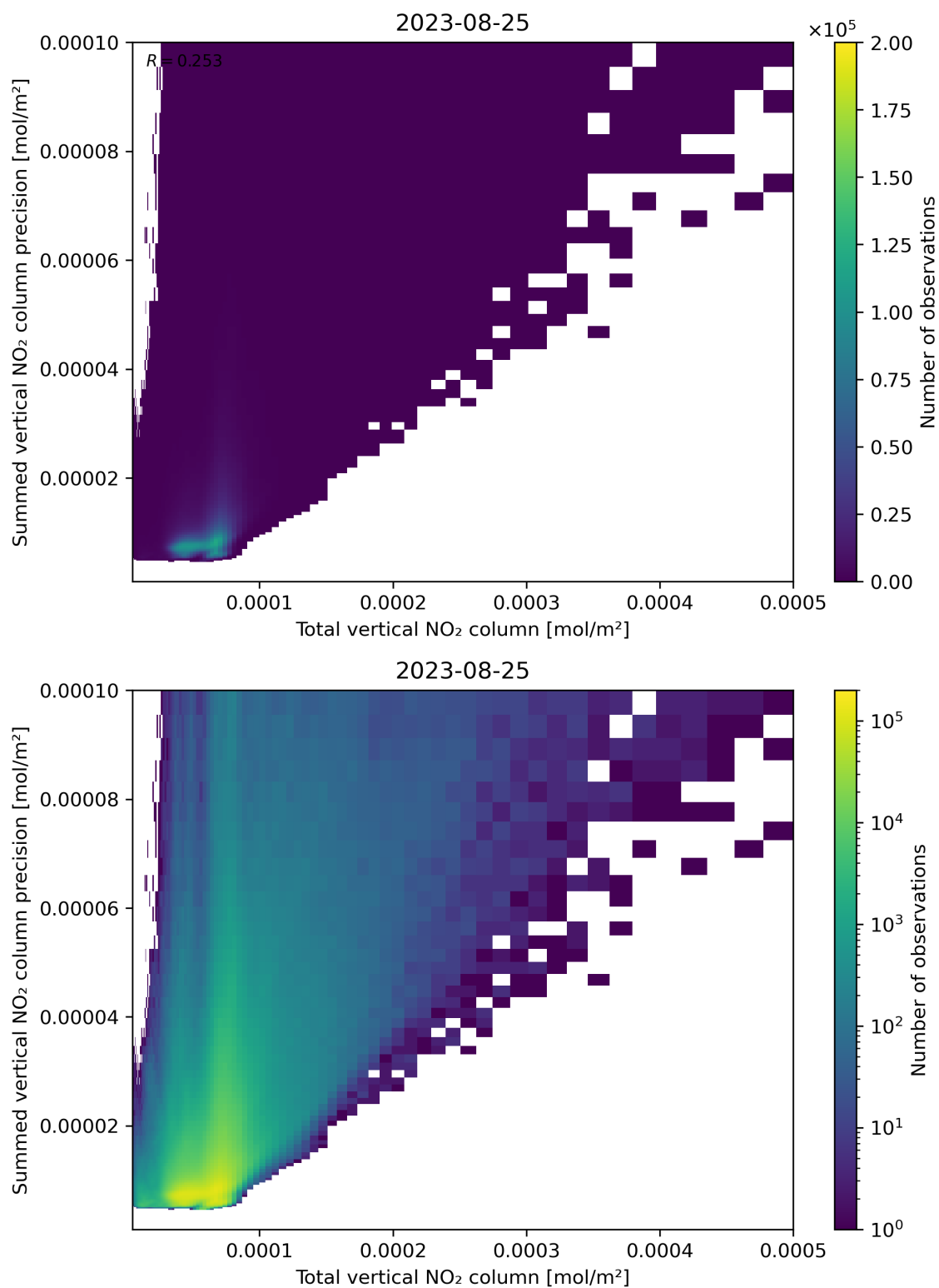
Figure 113: Scatter density plot of “Total vertical NO 2 column” against “Summed vertical NO 2 column precision” for 2023-08-25 to 2023-08-26.
