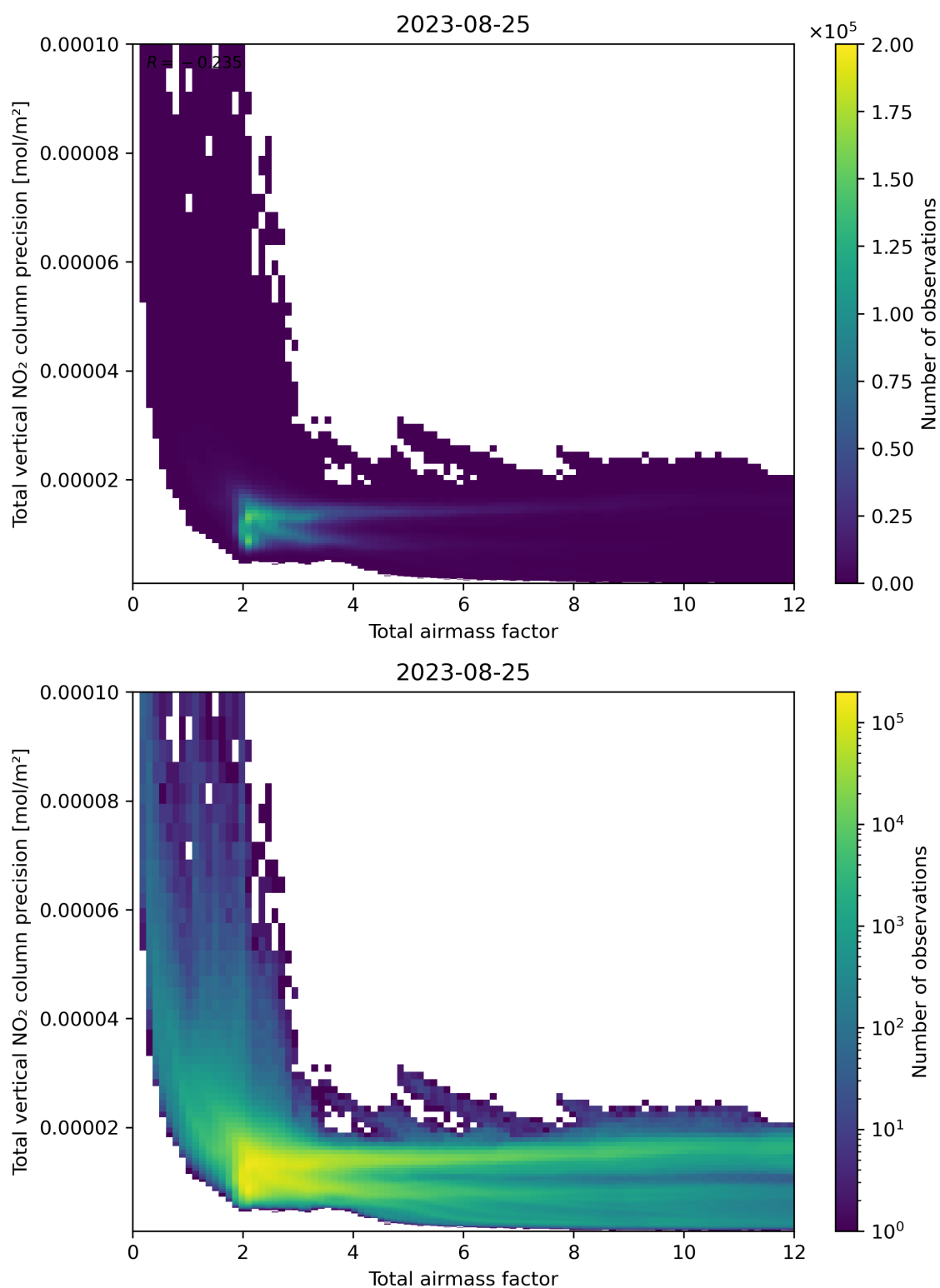
Figure 68: Scatter density plot of “Total airmass factor” against “Total vertical NO 2 column precision” for 2023-08-25 to 2023-08-26.
