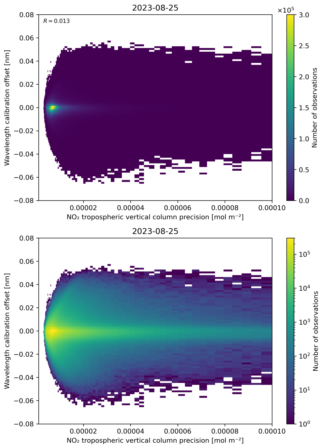
Figure 141: Scatter density plot of “NO 2 tropospheric vertical column precision” against “Wavelength calibration offset” for 2023-08-25 to 2023-08-26.
