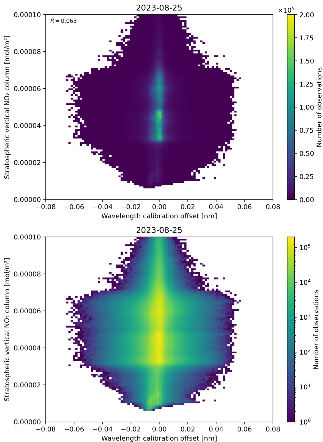
Figure 176: Scatter density plot of “Wavelength calibration offset” against “Stratospheric vertical NO 2 column” for 2023-08-25 to 2023-08-26.
