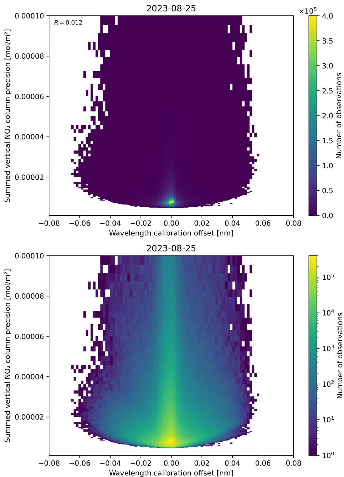
Figure 178: Scatter density plot of “Wavelength calibration offset” against “Summed vertical NO 2 column precision” for 2023-08-25 to 2023-08-26.
