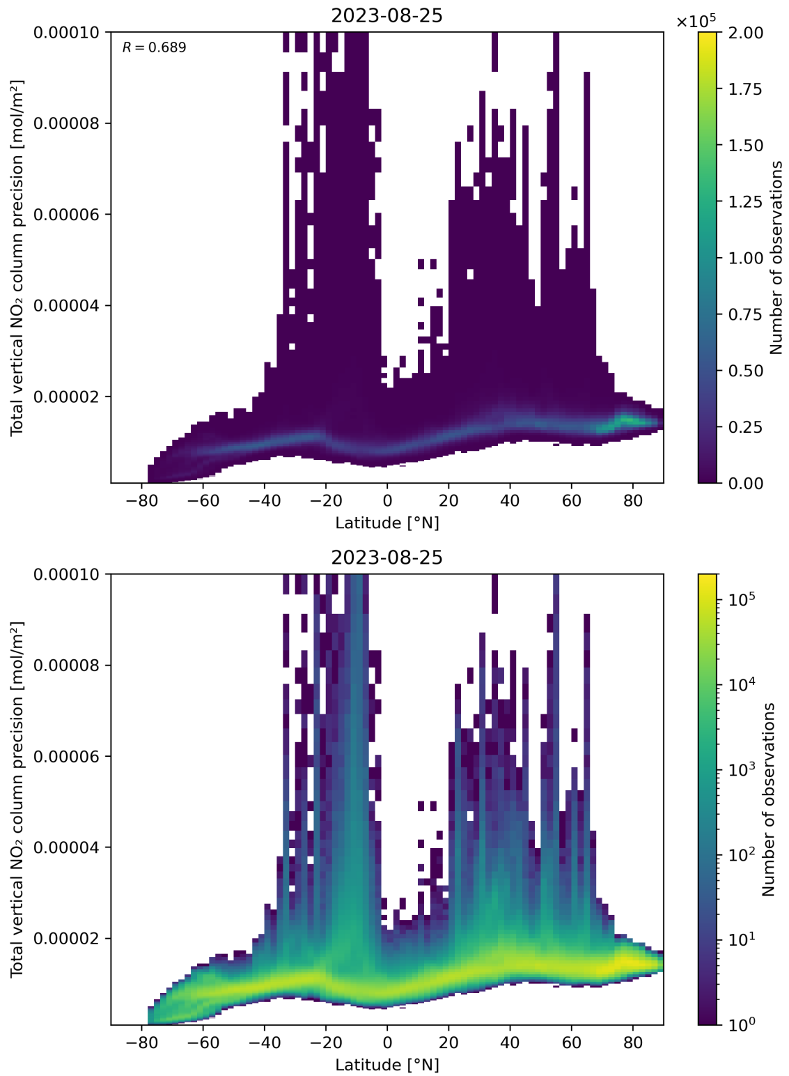
Figure 91: Scatter density plot of “Latitude” against “Total vertical NO 2 column precision” for 2023-08-25 to 2023-08-26.
