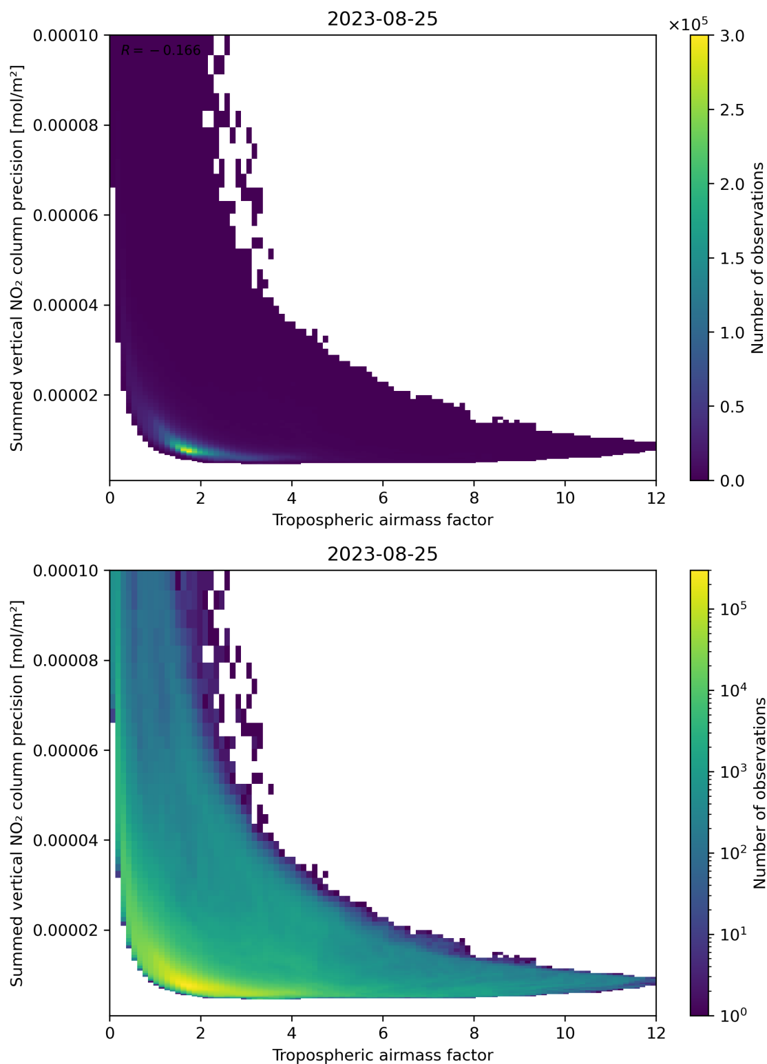
Figure 76: Scatter density plot of “Tropospheric air mass factor” against “Summed vertical NO 2 column precision” for 2023-08-25 to 2023-08-26.
