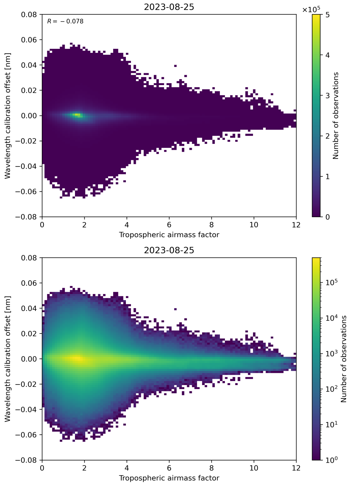
Figure 80: Scatter density plot of “Tropospheric airmass factor” against “Wavelength calibration offset” for 2023-08-25 to 2023-08-26.
