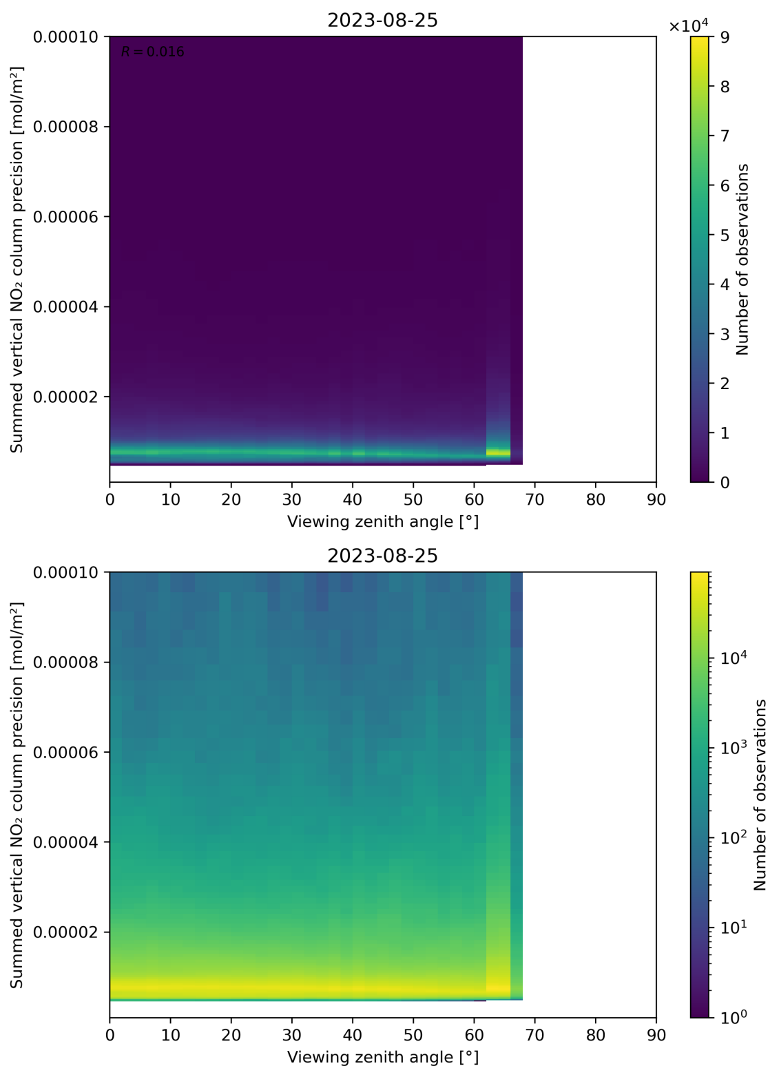
Figure 166: Scatter density plot of “Viewing zenith angle” against “Summed vertical NO 2 column precision” for 2023-08-25 to 2023-08-26.
