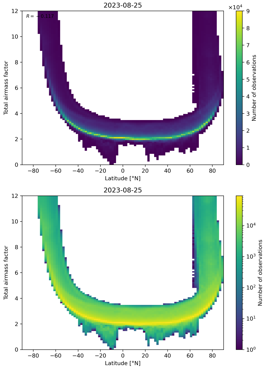
Figure 84: Scatter density plot of “Latitude” against “Total airmass factor” for 2023-08-25 to 2023-08-26.
