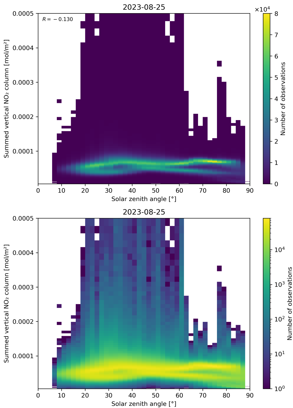
Figure 151: Scatter density plot of “Solar zenith angle” against “Summed vertical NO 2 column” for 2023-08-25 to 2023-08-26.
