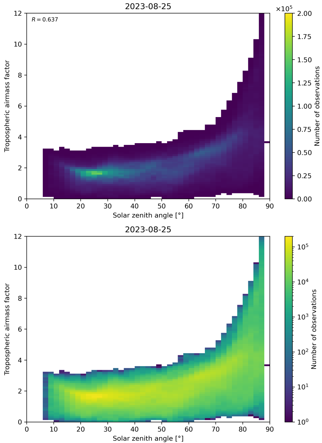
Figure 147: Scatter density plot of “Solar zenith angle” against “Tropospheric airmass factor” for 2023-08-25 to 2023-08-26.
