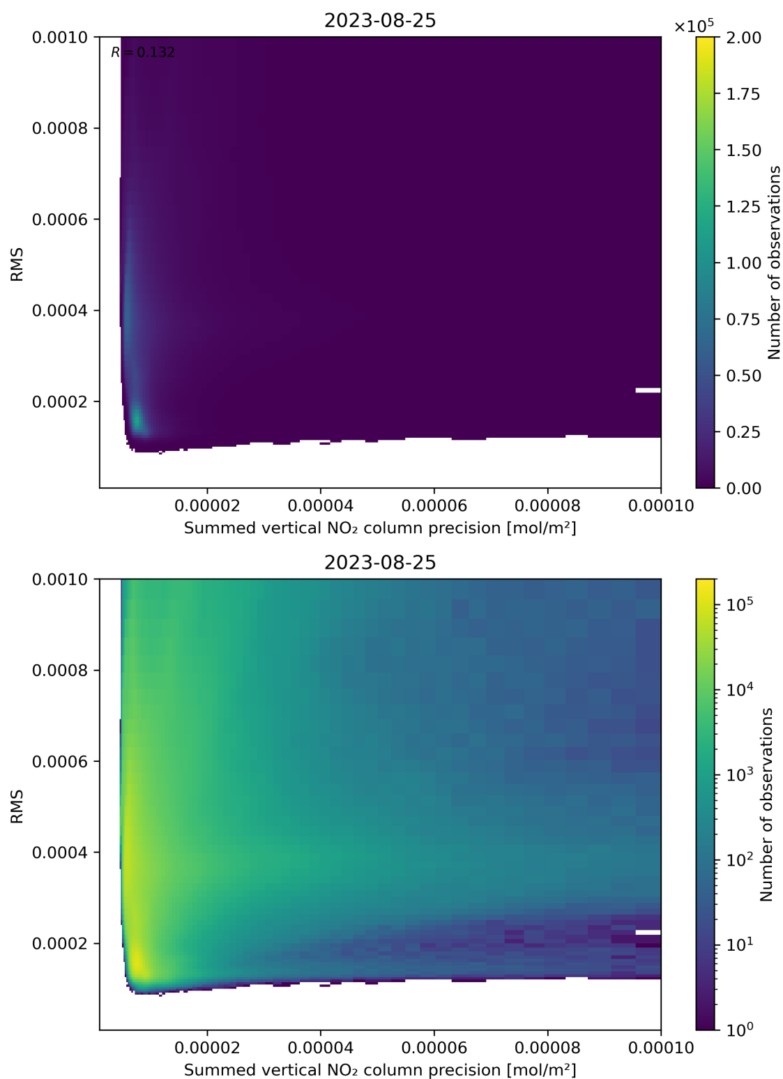
Figure 108: Scatter density plot of “Summed vertical NO 2 column precision” against “RMS” for 2023-08-25 to 2023-08-26.
