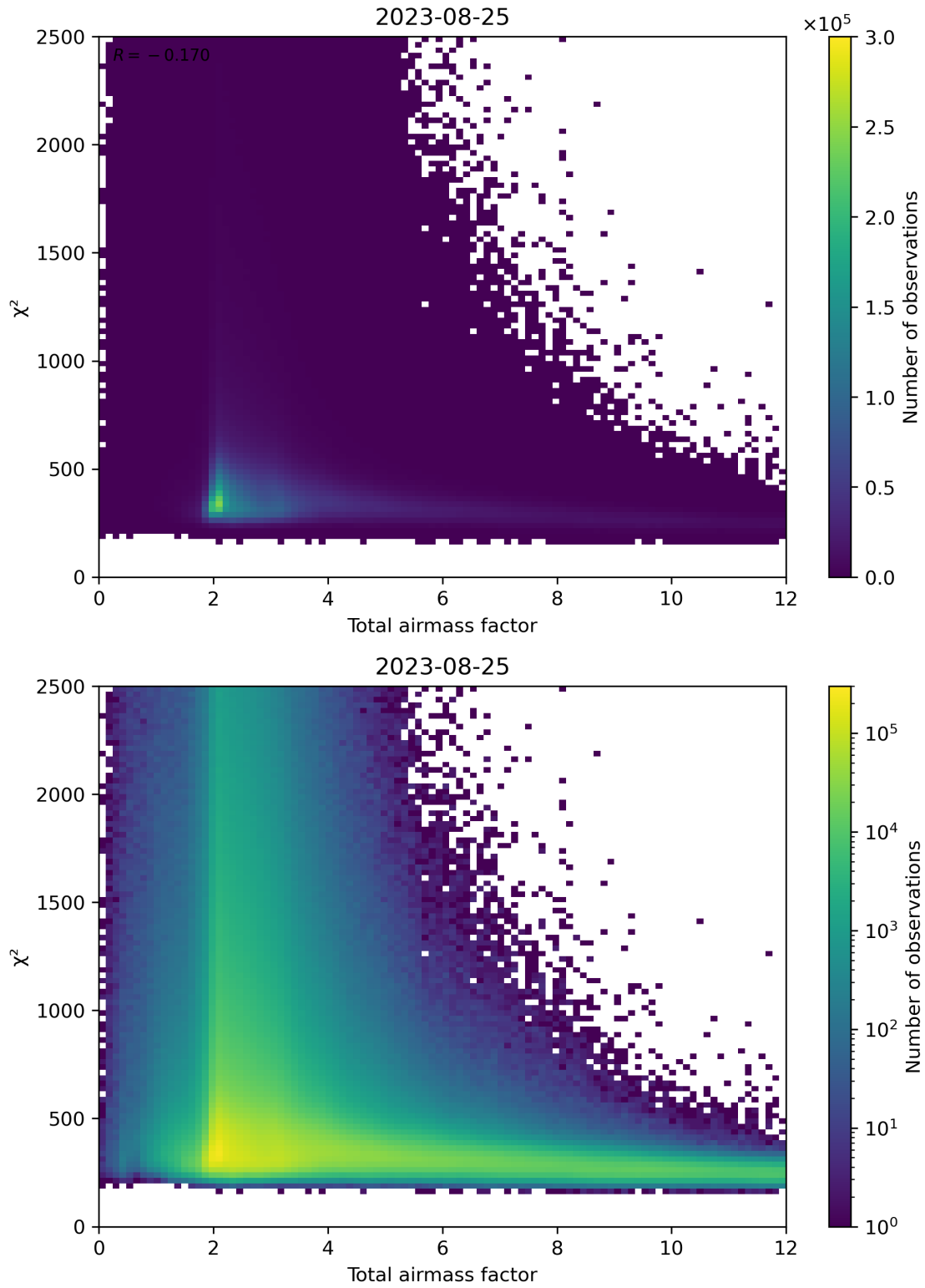
Figure 63: Scatter density plot of “Total airmass factor” against “ \chi^2 ” for 2023-08-25 to 2023-08-26.
