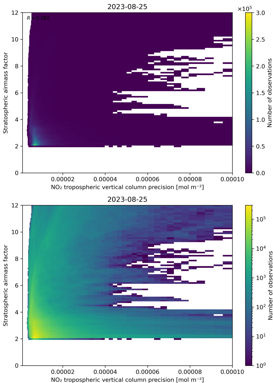
Figure 131: Scatter density plot of “NO 2 tropospheric vertical column precision” against “Stratospheric airmass factor” for 2023-08-25 to 2023-08-26.
