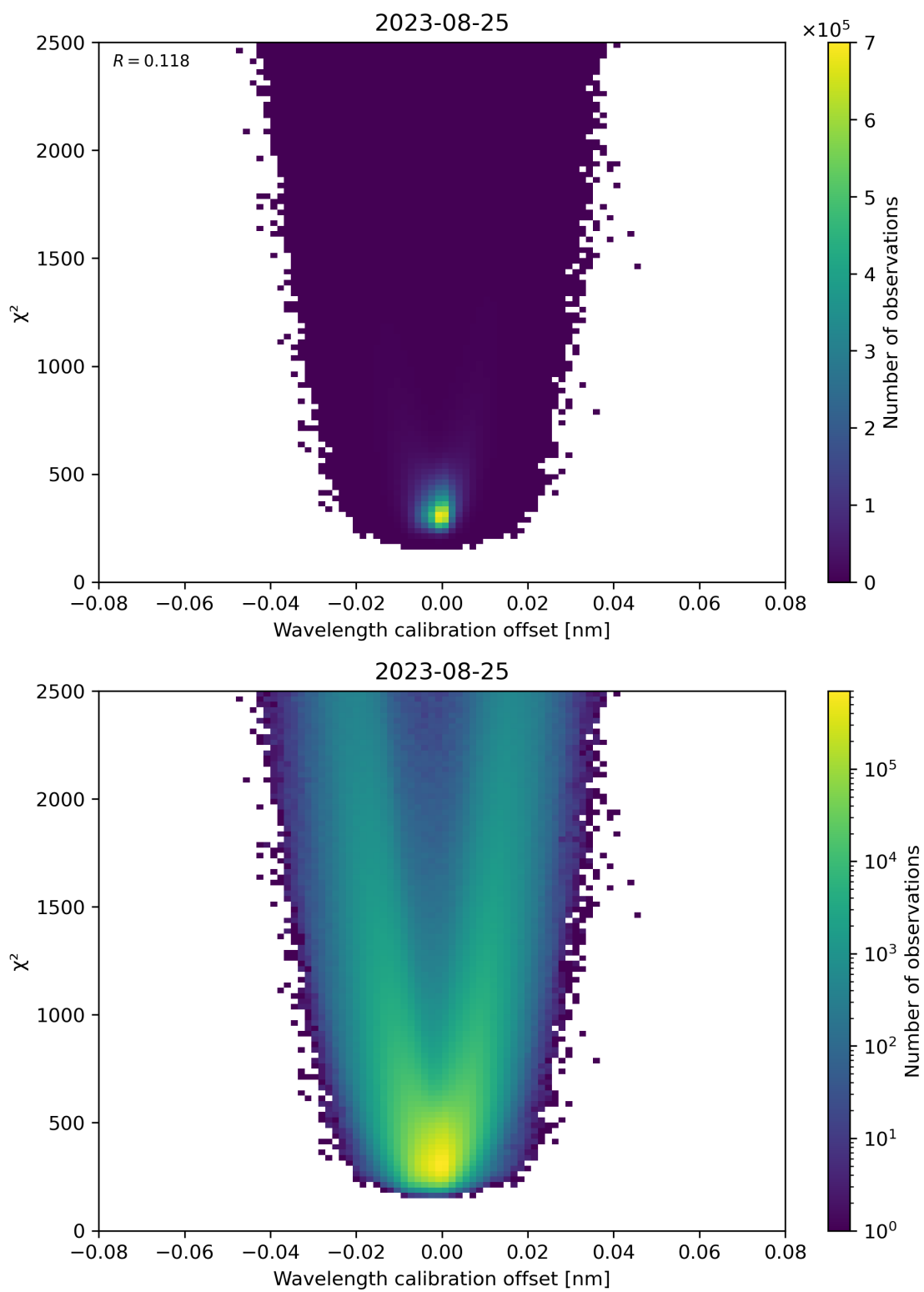
Figure 175: Scatter density plot of “Wavelength calibration offset” against “ \chi^2 ” for 2023-08-25 to 2023-08-26.
