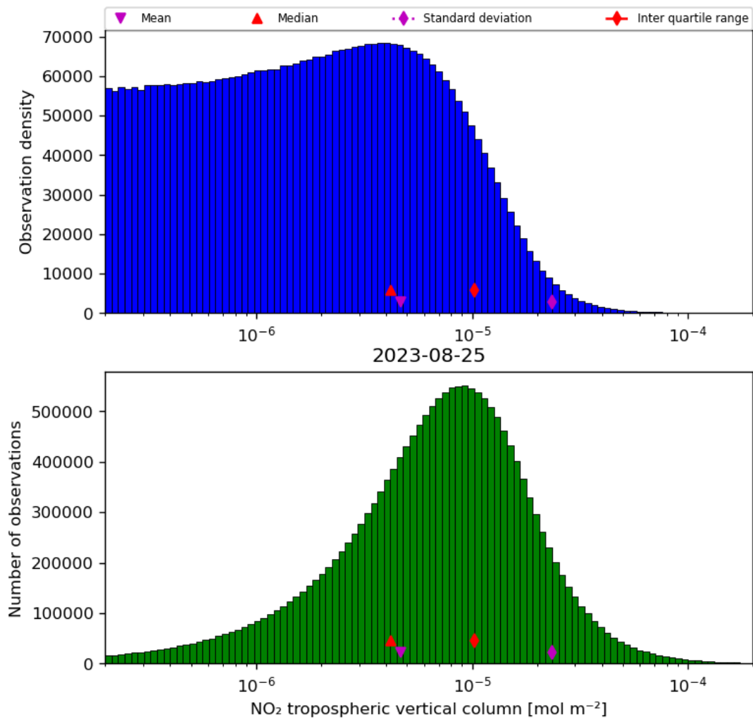
Figure 29: Histogram of “NO 2 tropospheric vertical column” for 2023-08-25 to 2023-08-26
