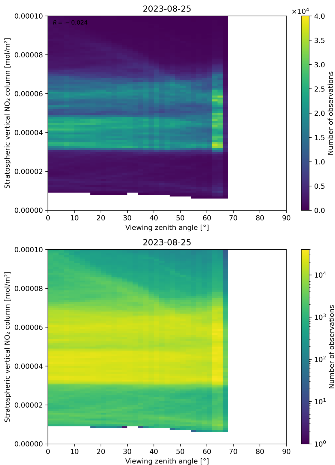
Figure 164: Scatter density plot of “Viewing zenith angle” against “Stratospheric vertical NO 2 column” for 2023-08-25 to 2023-08-26.
