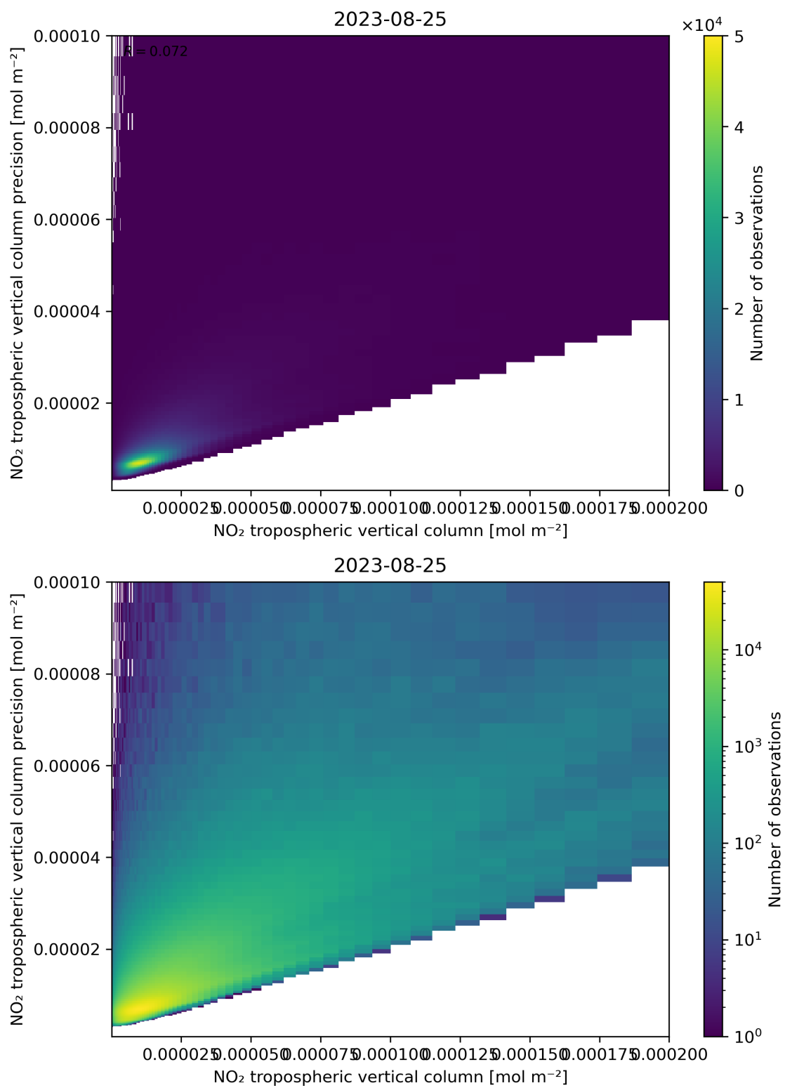
Figure 130: Scatter density plot of “NO 2 tropospheric vertical column” against “NO 2 tropospheric vertical column precision” for 2023-08-25 to 2023-08-26.
