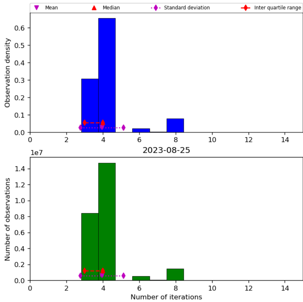
Figure 34: Histogram of “Number of iterations” for 2023-08-25 to 2023-08-26
