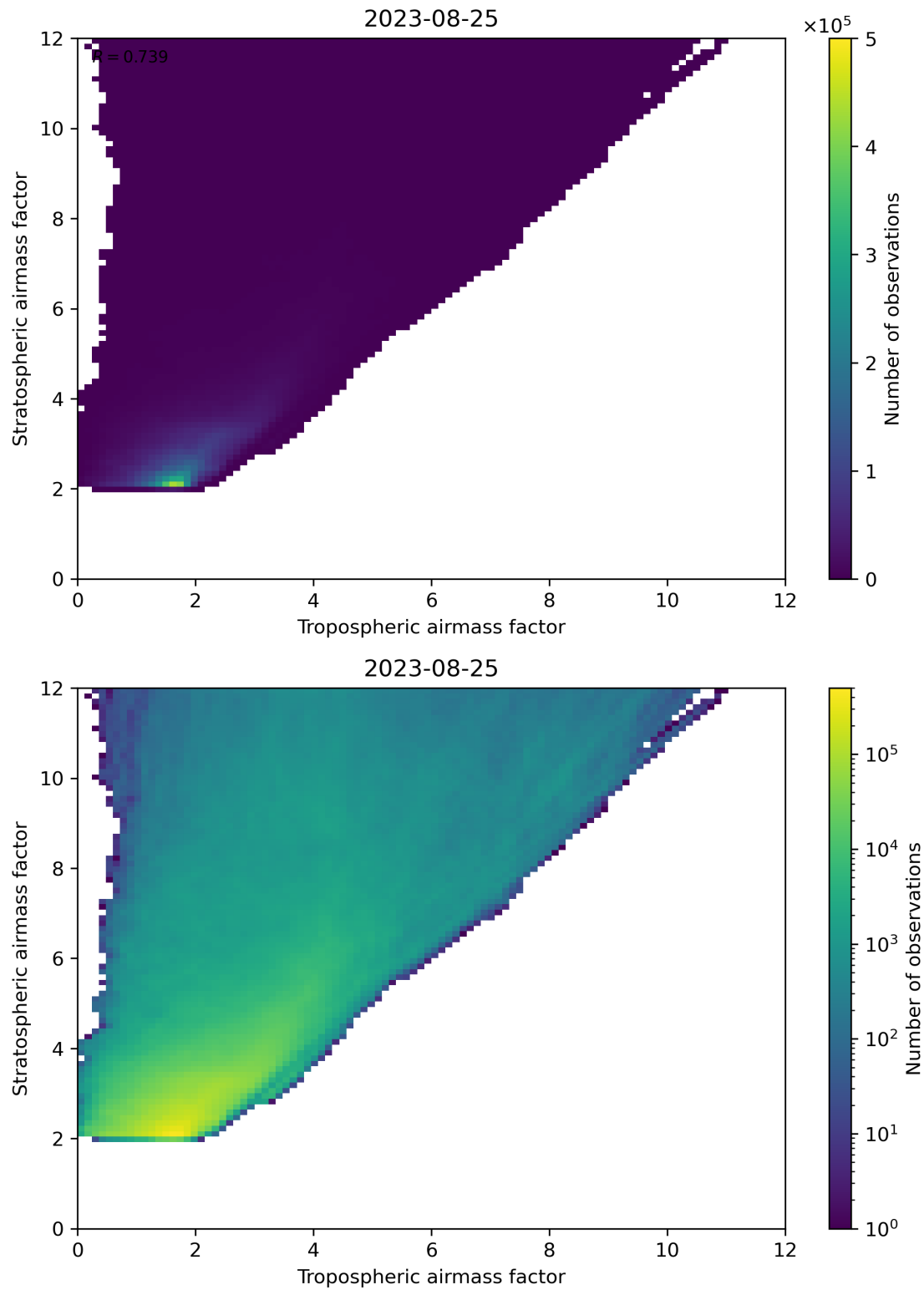
Figure 71: Scatter density plot of “Tropospheric airmass factor” against “Stratospheric airmass factor” for 2023-08-25 to 2023-08-26.
