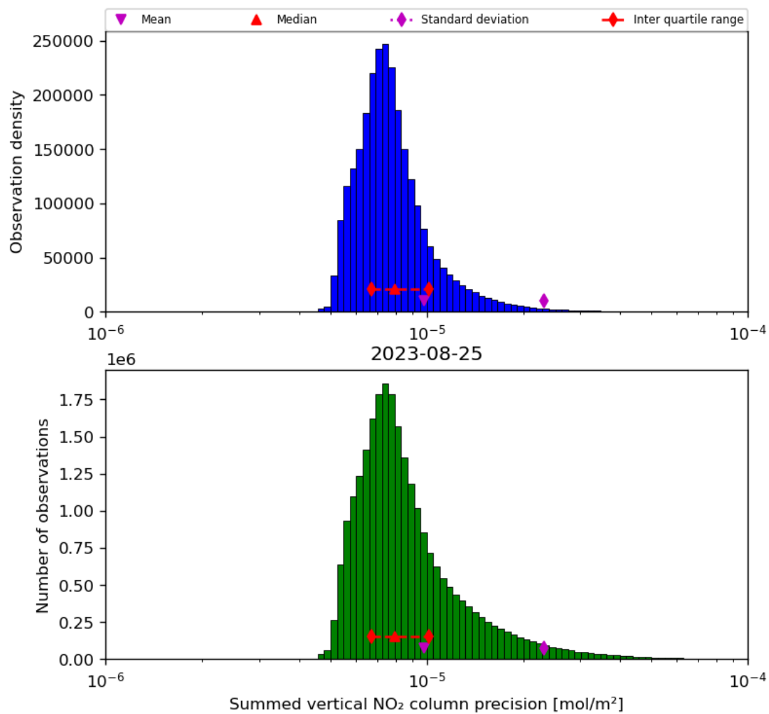
Figure 41: Histogram of "Summed vertical NO 2 column precision" for 2023-08-25 to 2023-08-26
