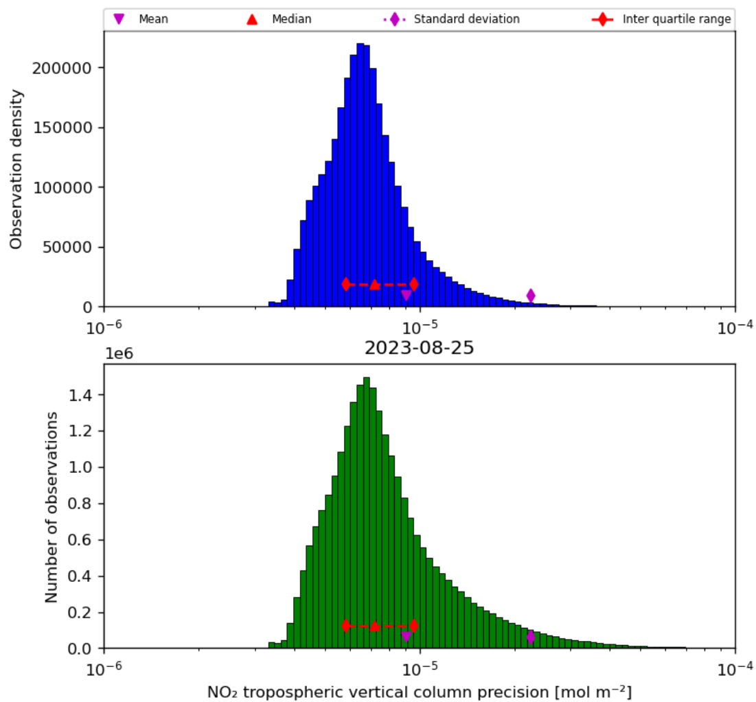
Figure 30: Histogram of “NO 2 tropospheric vertical column precision” for 2023-08-25 to 2023-08-26
