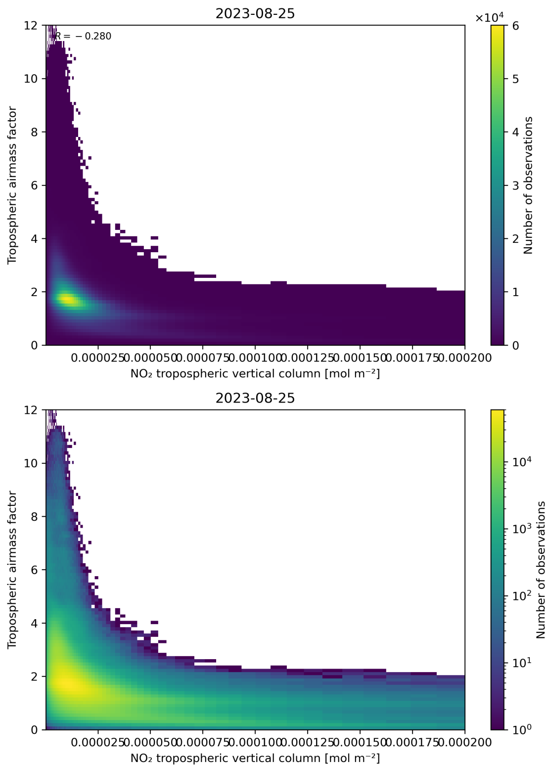
Figure 123: Scatter density plot of “NO 2 tropospheric vertical column” against “Tropospheric air mass factor” for 2023-08-25 to 2023-08-26.
