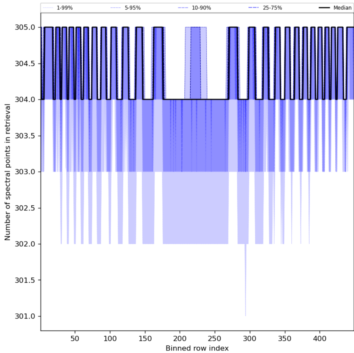
Figure 50: Along track statistics of “Number of spectral points in retrieval” for 2023-08-25 to 2023-08-26
