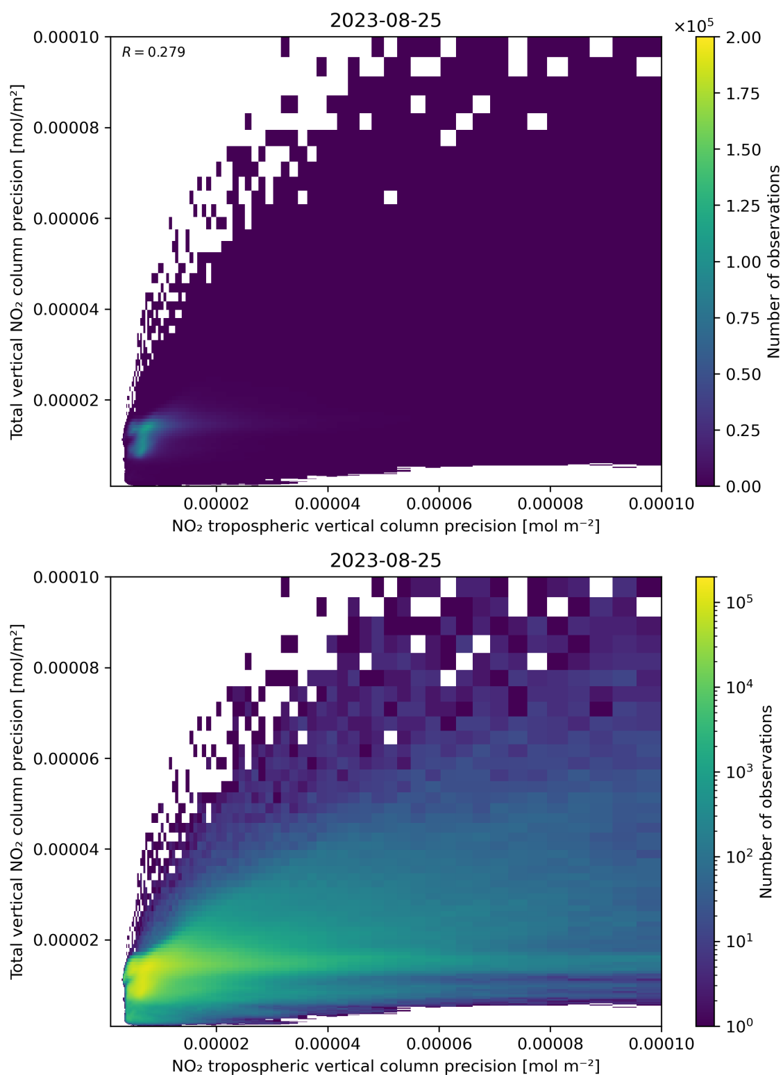
Figure 139: Scatter density plot of “NO 2 tropospheric vertical column precision” against “Total vertical NO 2 column precision” for 2023-08-25 to 2023-08-26.
