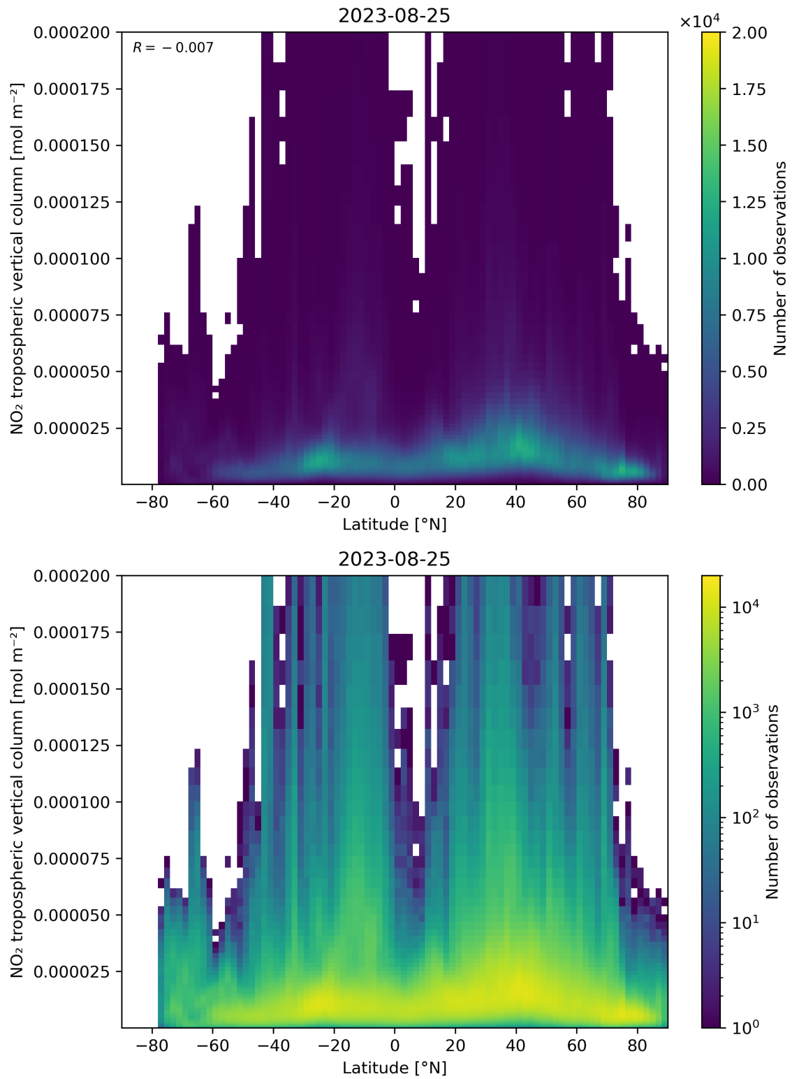
Figure 92: Scatter density plot of “Latitude” against “NO 2 tropospheric vertical column” for 2023-08-25 to 2023-08-26.
