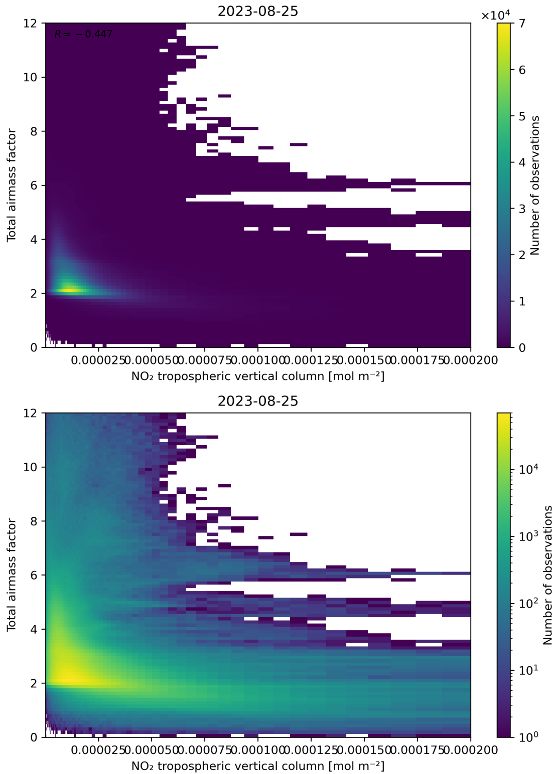
Figure 122: Scatter density plot of “NO 2 tropospheric vertical column” against “Total airmass factor” for 2023-08-25 to 2023-08-26.
