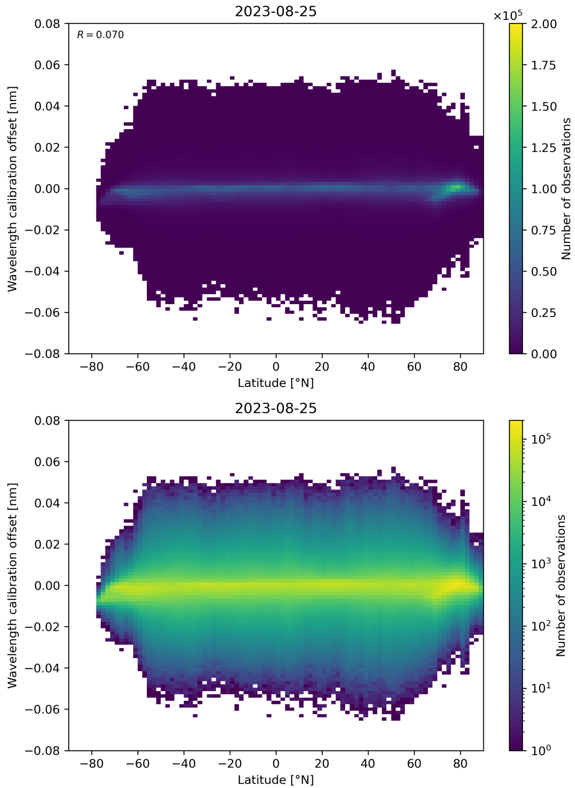
Figure 95: Scatter density plot of “Latitude” against “Wavelength calibration offset” for 2023-08-25 to 2023-08-26.
