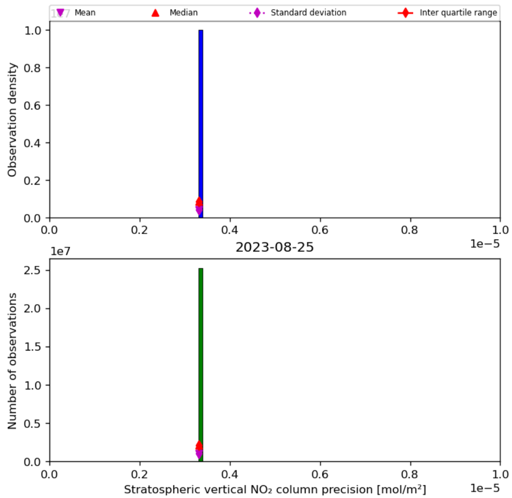
Figure 37: Histogram of “Stratospheric vertical NO 2 column precision” for 2023-08-25 to 2023-08-26
