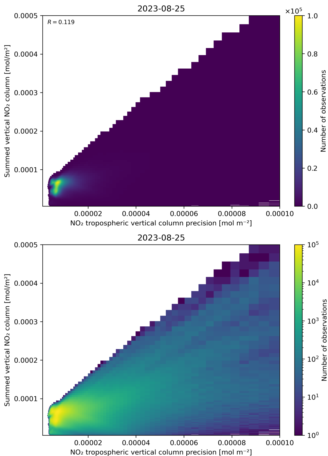
Figure 136: Scatter density plot of “NO 2 tropospheric vertical column precision” against “Summed vertical NO 2 column” for 2023-08-25 to 2023-08-26.
