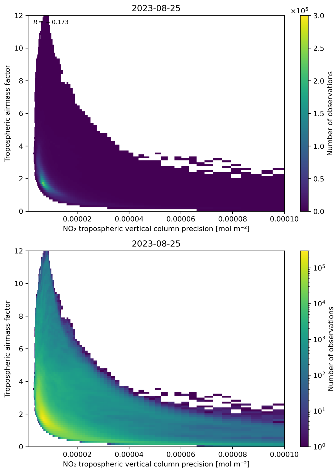
Figure 133: Scatter density plot of “NO 2 tropospheric vertical column precision” against “Tropospheric airmass factor” for 2023-08-25 to 2023-08-26.
