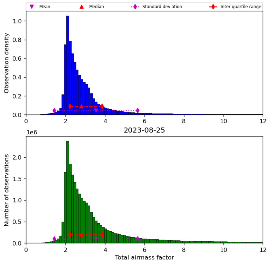
Figure 32: Histogram of “Total airmass factor” for 2023-08-25 to 2023-08-26
