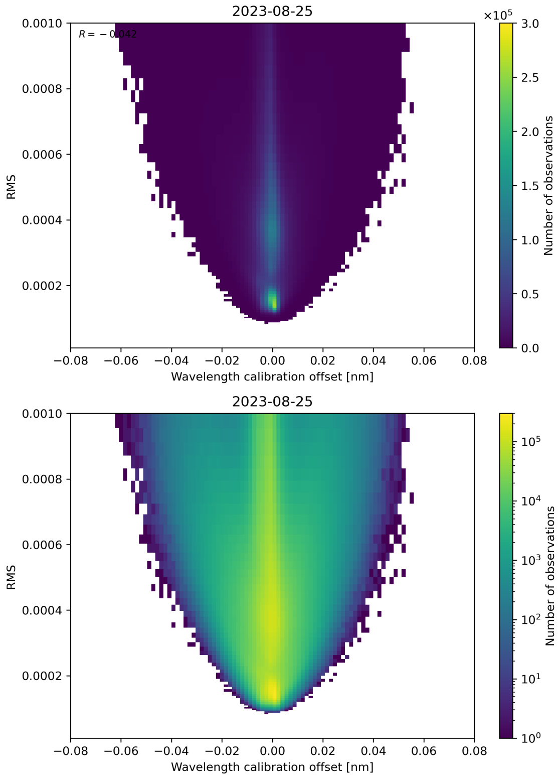
Figure 181: Scatter density plot of “Wavelength calibration offset” against “RMS” for 2023-08-25 to 2023-08-26.
