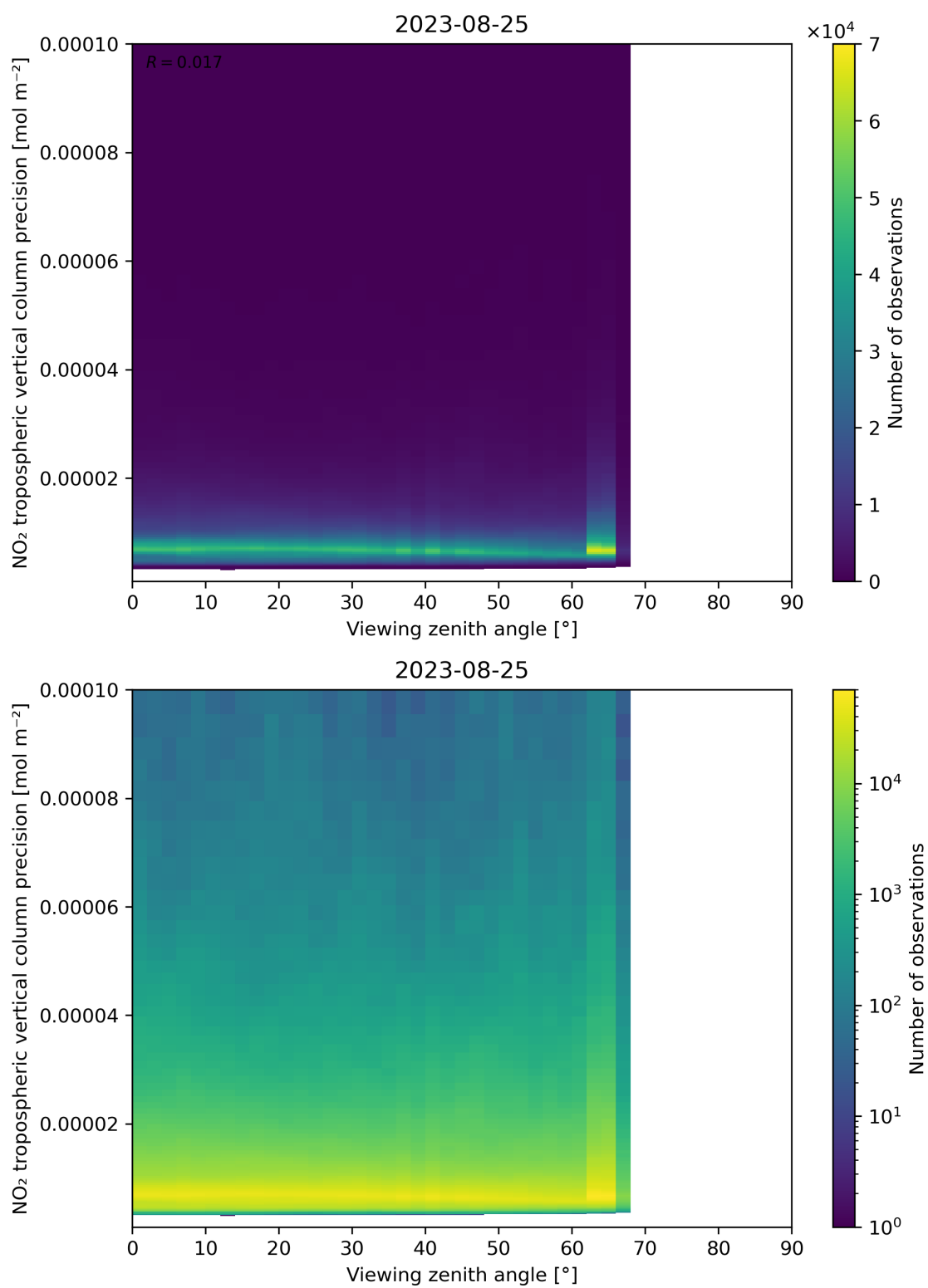
Figure 170: Scatter density plot of “Viewing zenith angle” against “NO 2 tropospheric vertical column precision” for 2023-08-25 to 2023-08-26.
