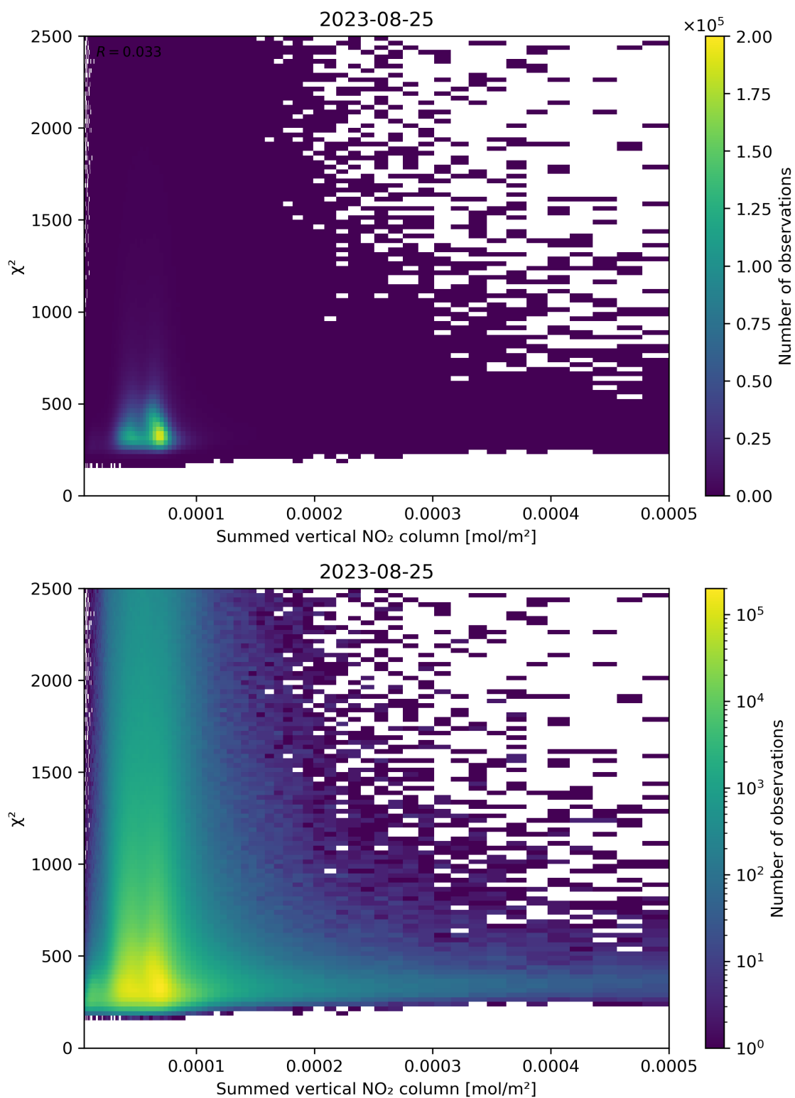
Figure 104: Scatter density plot of “Summed vertical NO 2 column” against “ \chi^2 ” for 2023-08-25 to 2023-08-26.
