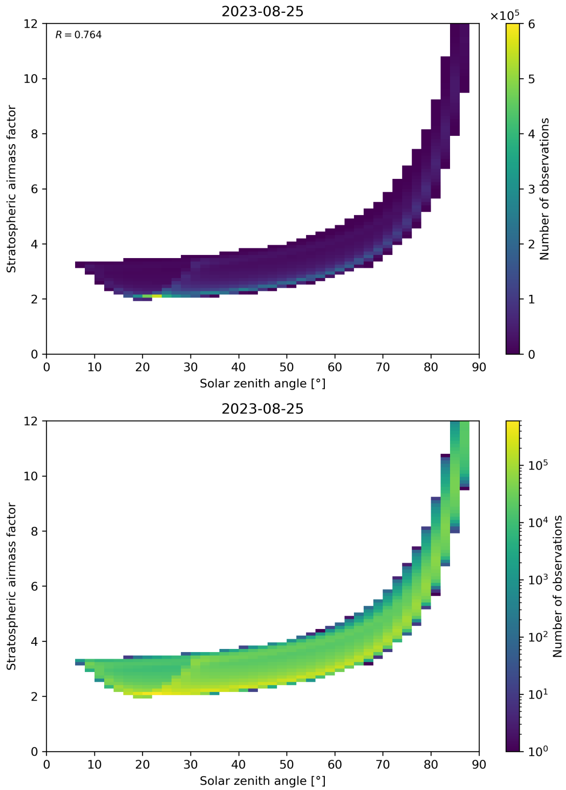
Figure 145: Scatter density plot of “Solar zenith angle” against “Stratospheric airmass factor” for 2023-08-25 to 2023-08-26.
