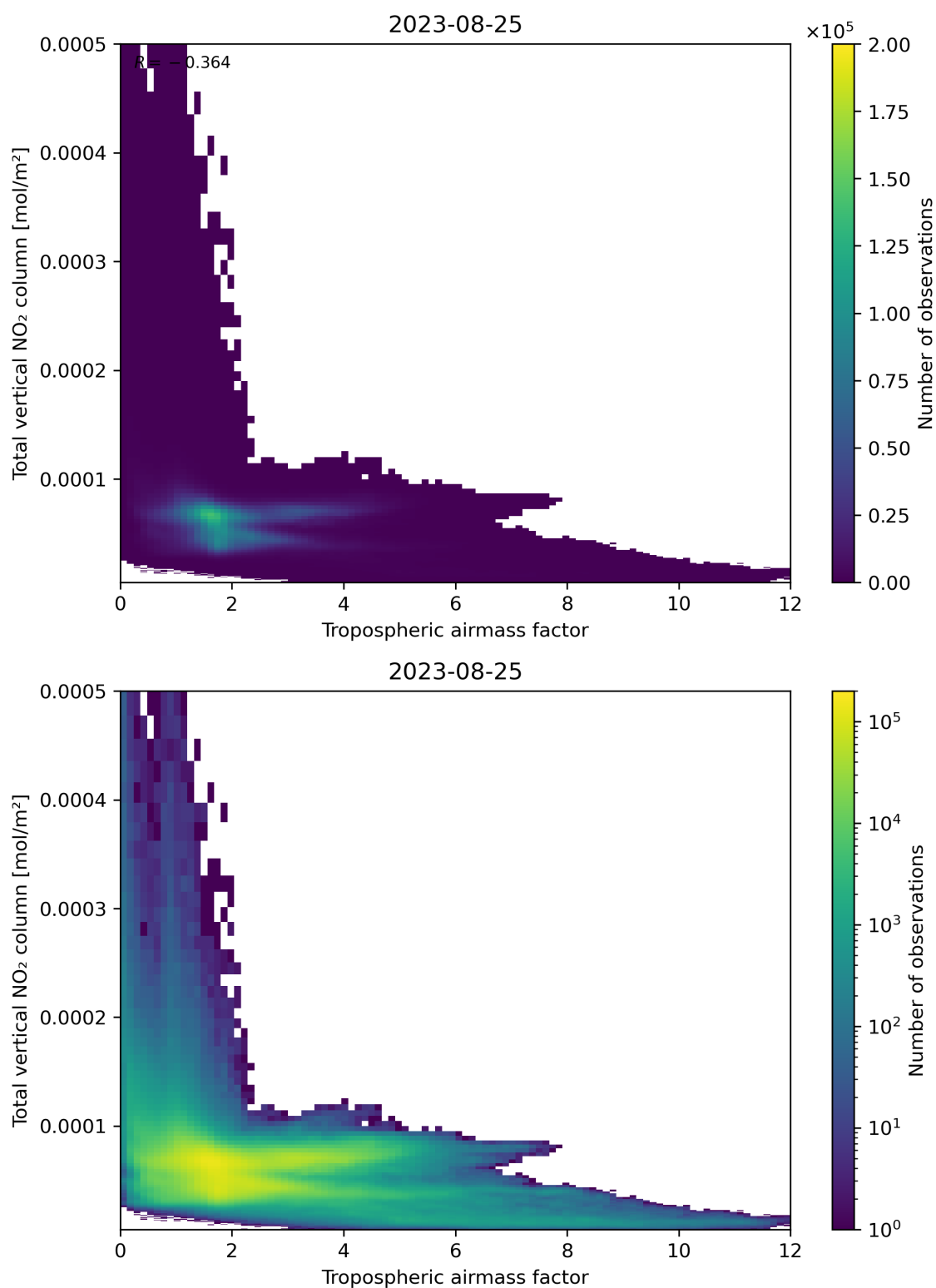
Figure 77: Scatter density plot of “Tropospheric airmass factor” against “Total vertical NO 2 column” for 2023-08-25 to 2023-08-26.
