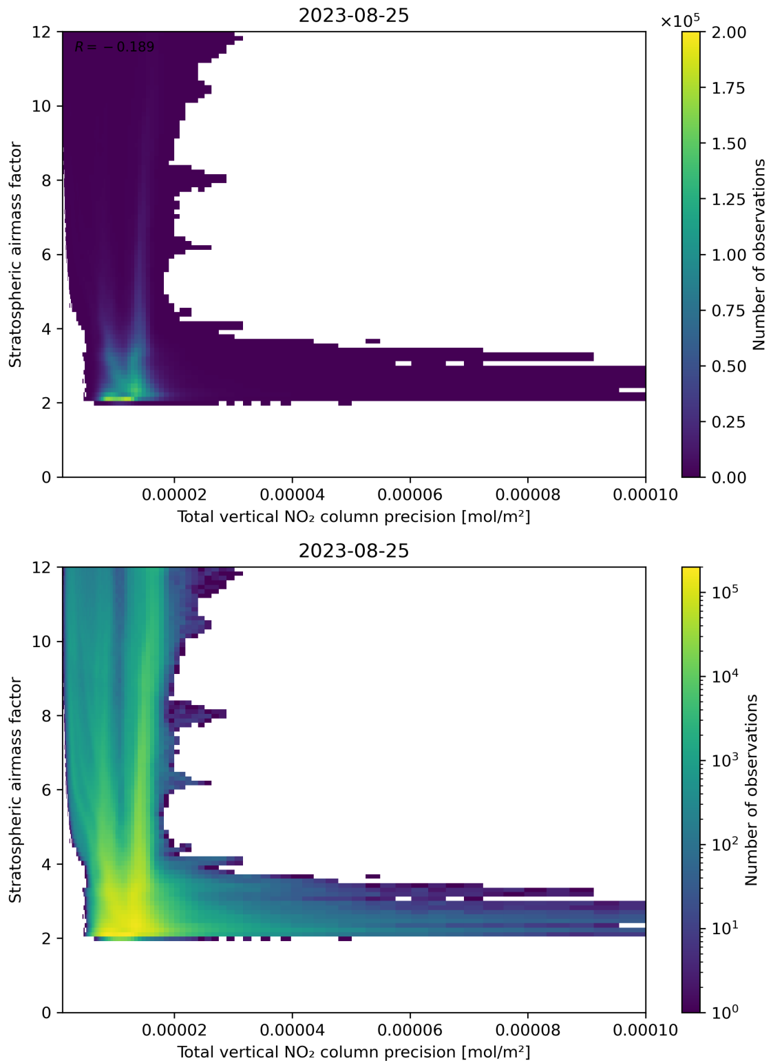
Figure 115: Scatter density plot of “Total vertical NO 2 column precision” against “Stratospheric air mass factor” for 2023-08-25 to 2023-08-26.
