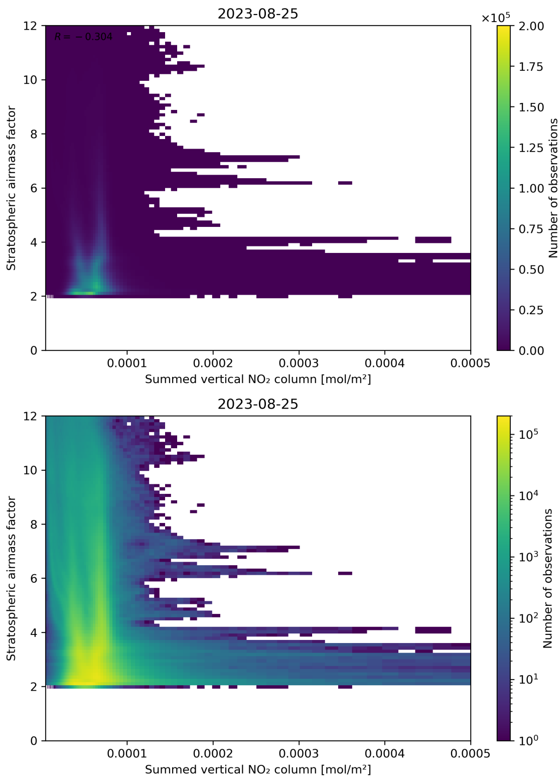
Figure 103: Scatter density plot of “Summed vertical NO 2 column” against “Stratospheric airmass factor” for 2023-08-25 to 2023-08-26.
