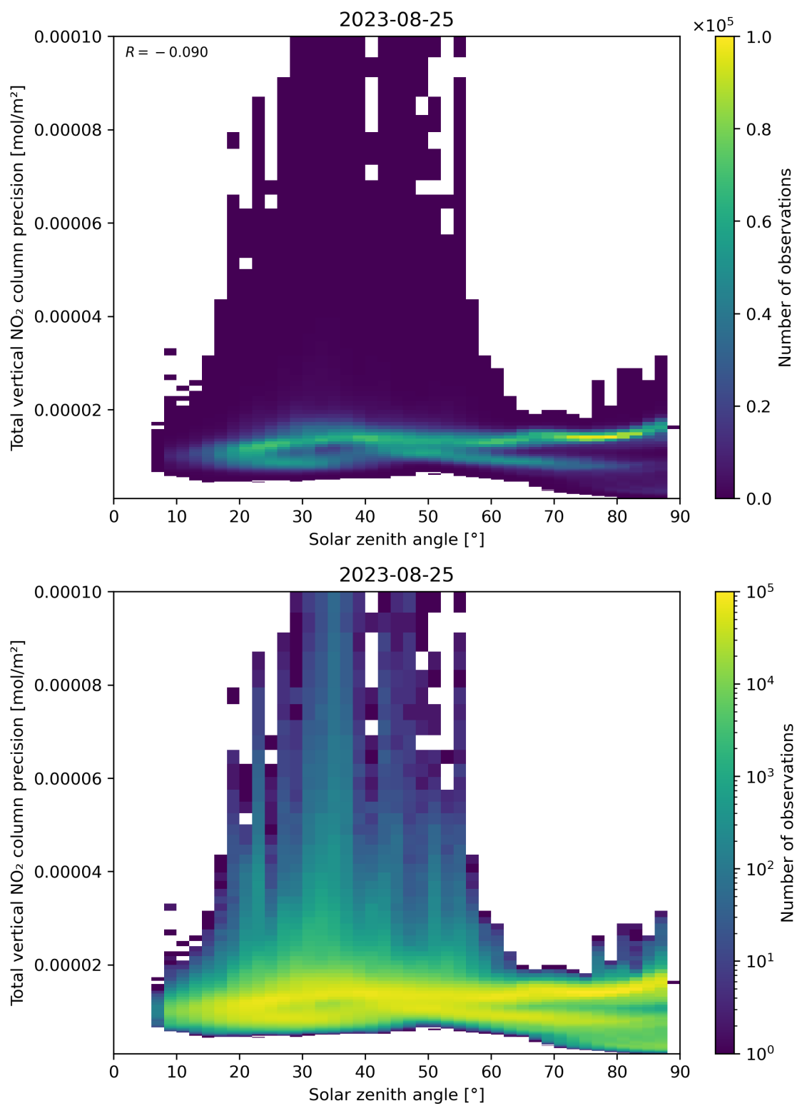
Figure 154: Scatter density plot of “Solar zenith angle” against “Total vertical NO 2 column precision” for 2023-08-25 to 2023-08-26.
