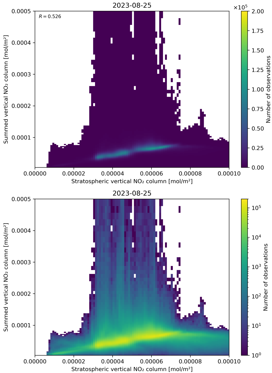
Figure 98: Scatter density plot of “Stratospheric vertical NO 2 column” against “Summed vertical NO 2 column” for 2023-08-25 to 2023-08-26.
