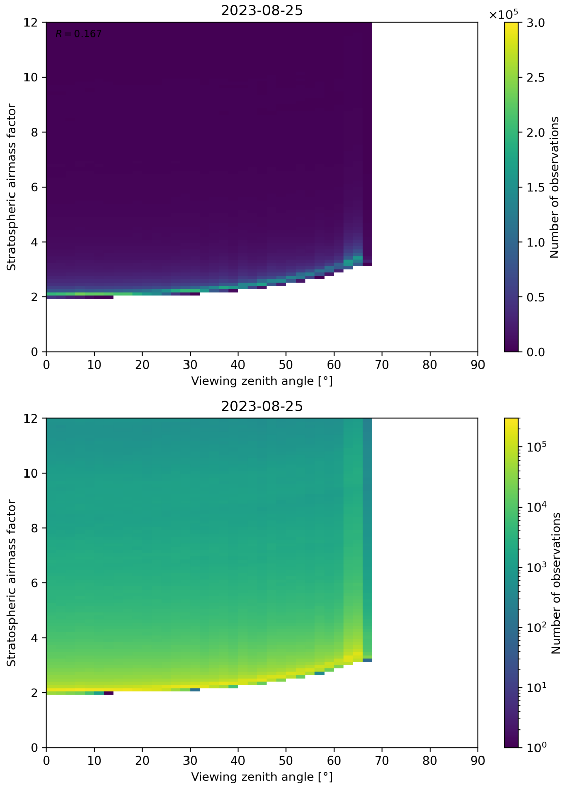
Figure 159: Scatter density plot of “Viewing zenith angle” against “Stratospheric airmass factor” for 2023-08-25 to 2023-08-26.
