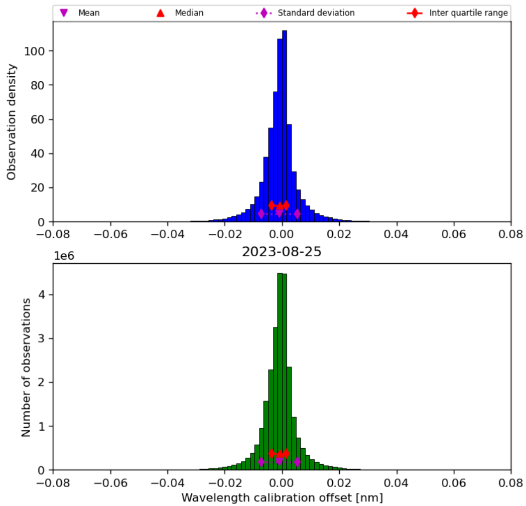
Figure 35: Histogram of “Wavelength calibration offset” for 2023-08-25 to 2023-08-26
