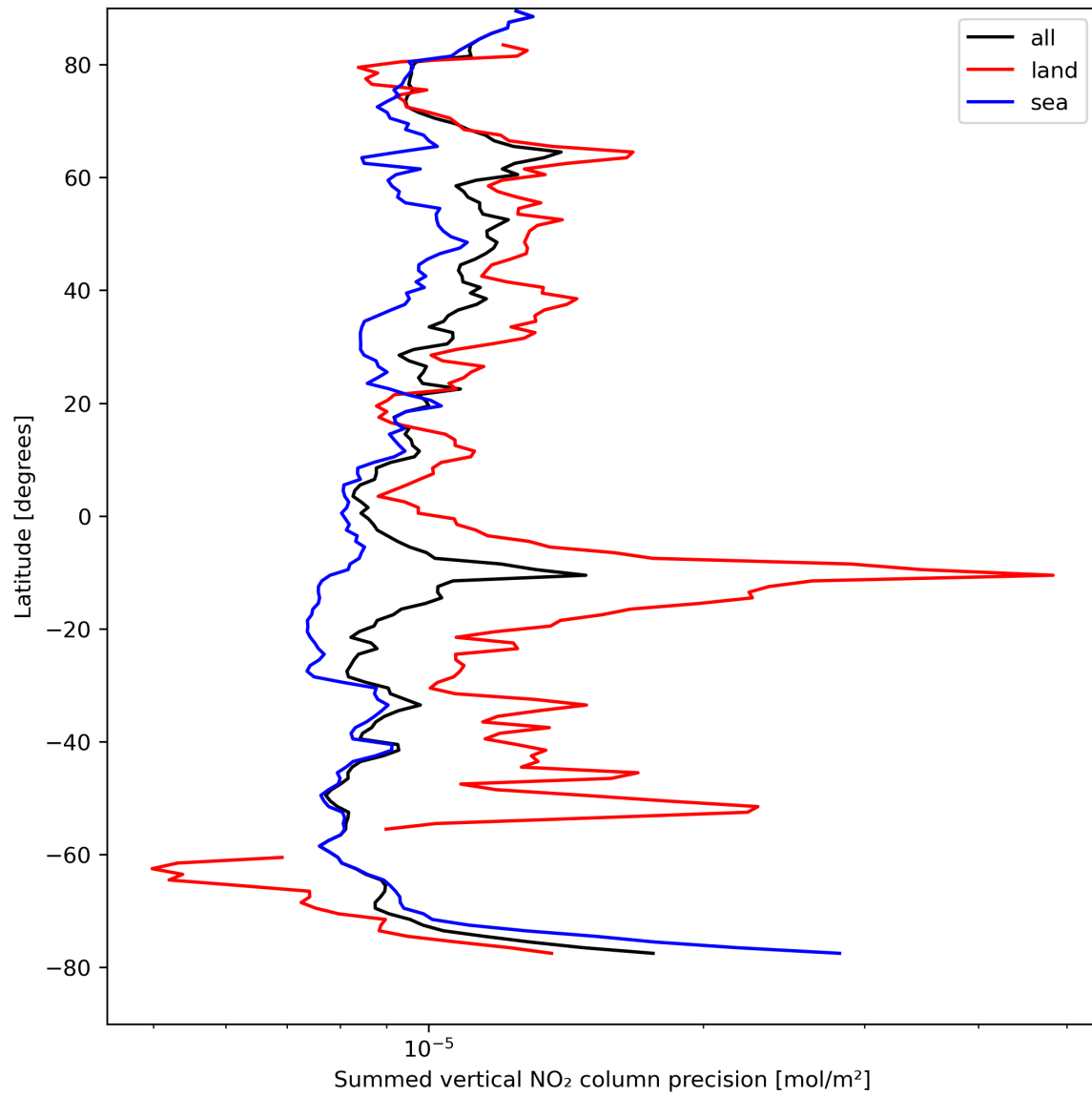
Figure 24: Zonal average of “Summed vertical NO 2 column precision” for 2023-08-25 to 2023-08-26.
