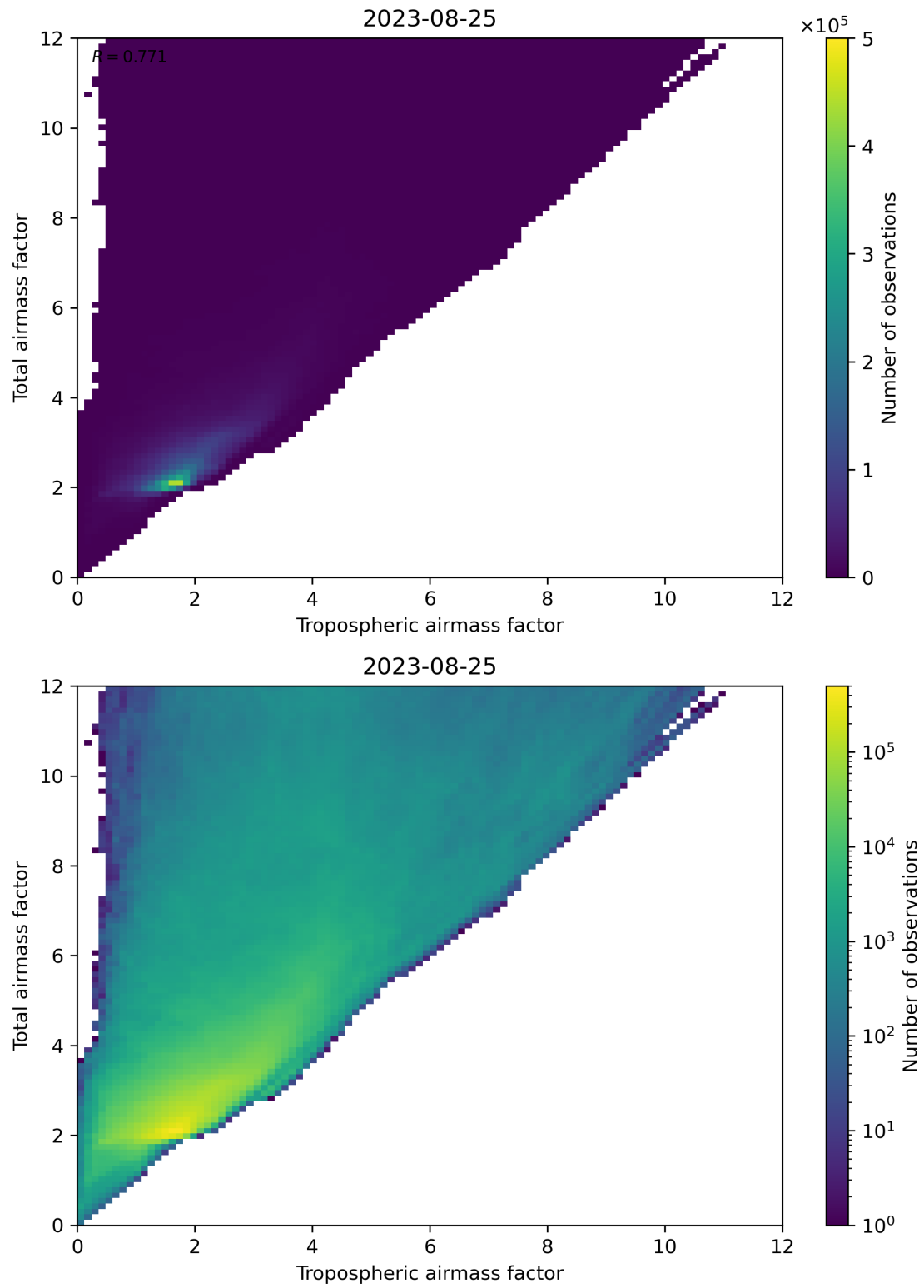
Figure 72: Scatter density plot of “Tropospheric airmass factor” against “Total airmass factor” for 2023-08-25 to 2023-08-26.
