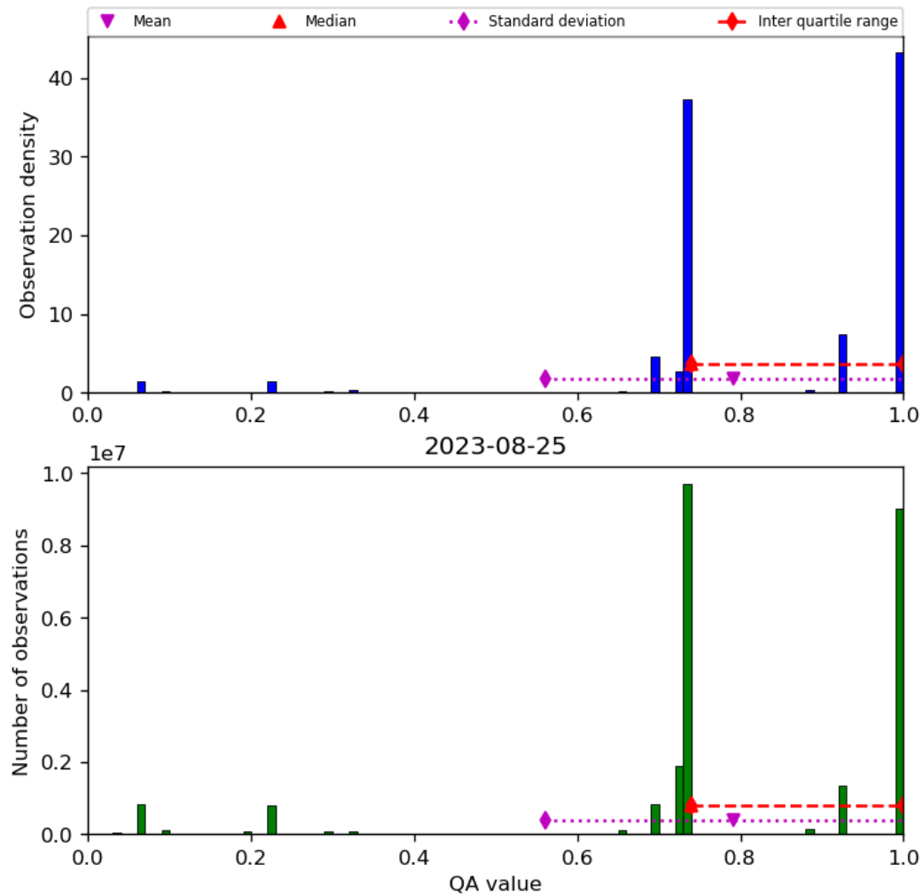
Figure 28: Histogram of “QA value” for 2023-08-25 to 2023-08-26
