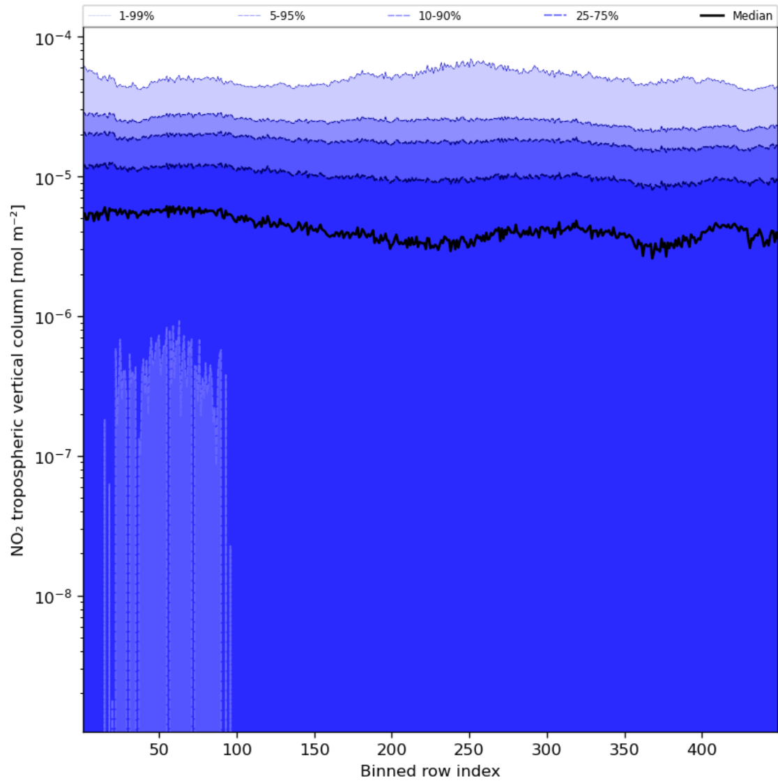
Figure 46: Along track statistics of “NO 2 tropospheric vertical column” for 2023-08-25 to 2023-08-26
