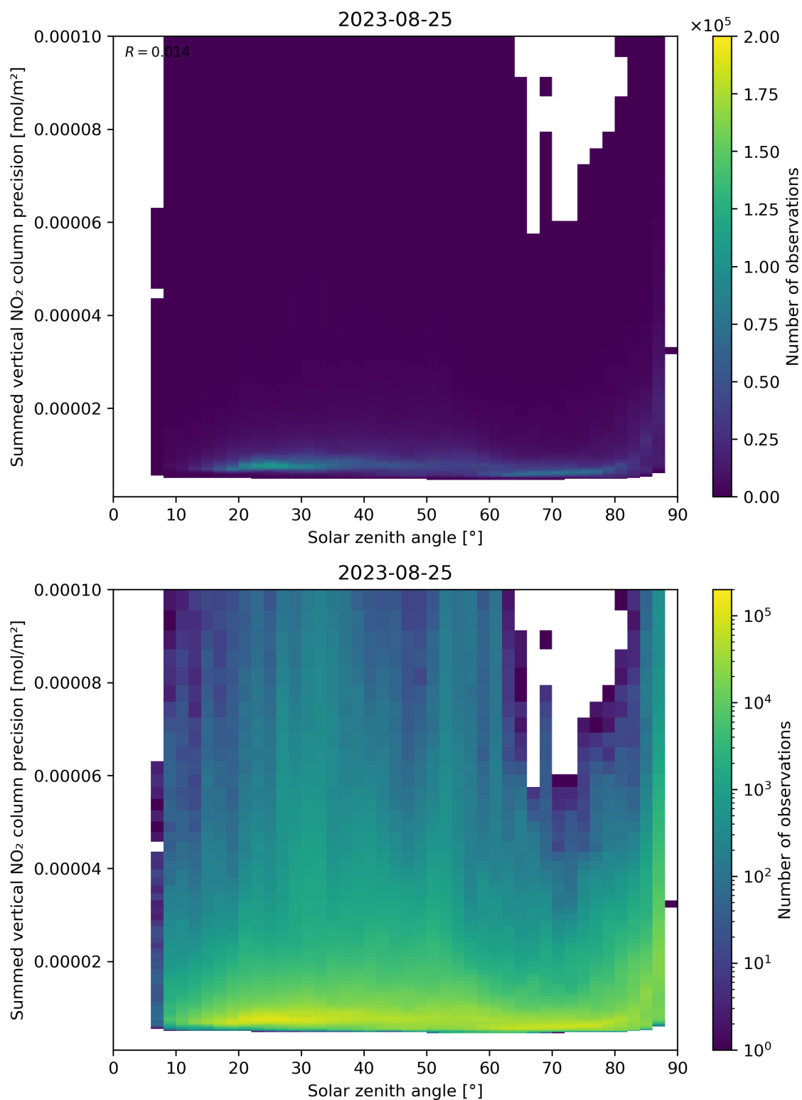
Figure 152: Scatter density plot of “Solar zenith angle” against “Summed vertical NO 2 column precision” for 2023-08-25 to 2023-08-26.
