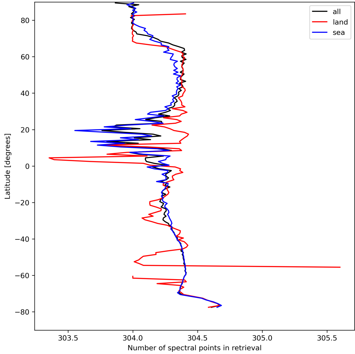
Figure 16: Zonal average of “Number of spectral points in retrieval” for 2023-08-25 to 2023-08-26.
