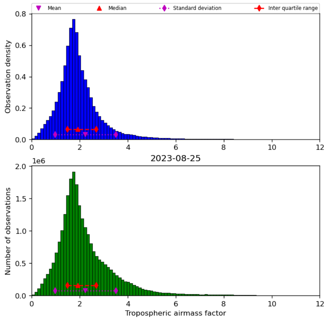
Figure 31: Histogram of “Tropospheric airmass factor” for 2023-08-25 to 2023-08-26
