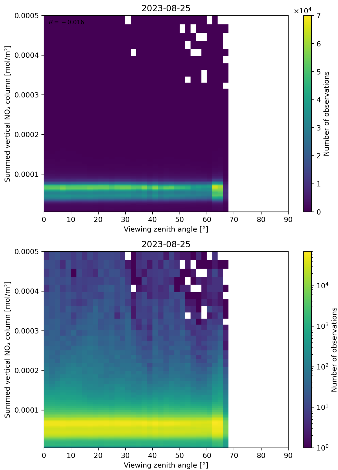
Figure 165: Scatter density plot of “Viewing zenith angle” against “Summed vertical NO 2 column” for 2023-08-25 to 2023-08-26.
