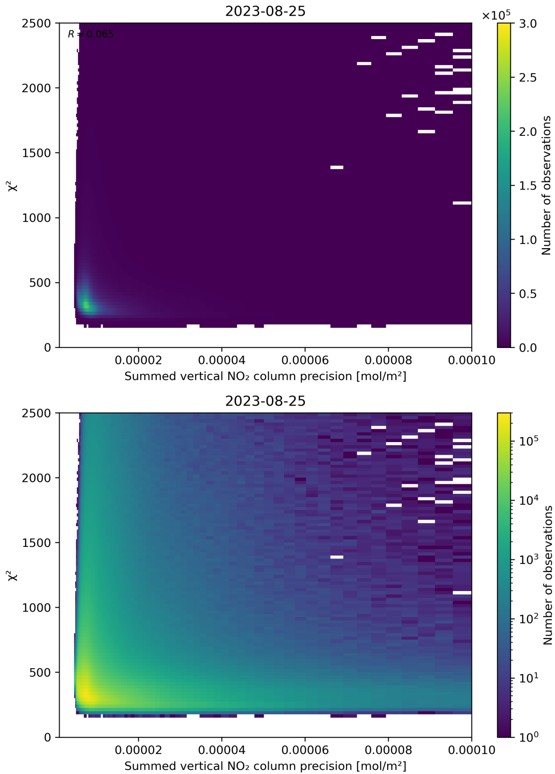
Figure 107: Scatter density plot of “Summed vertical NO 2 column precision” against “ \chi^2 ” for 2023-08-25 to 2023-08-26.
