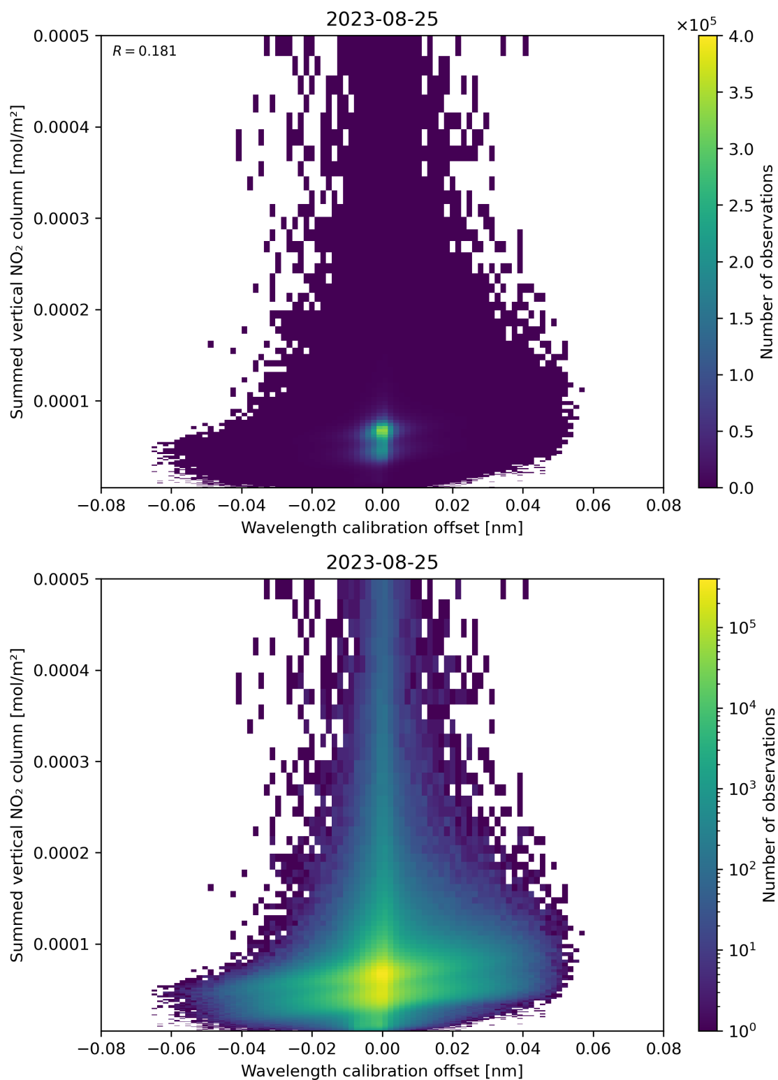
Figure 177: Scatter density plot of “Wavelength calibration offset” against “Summed vertical NO 2 column” for 2023-08-25 to 2023-08-26.
