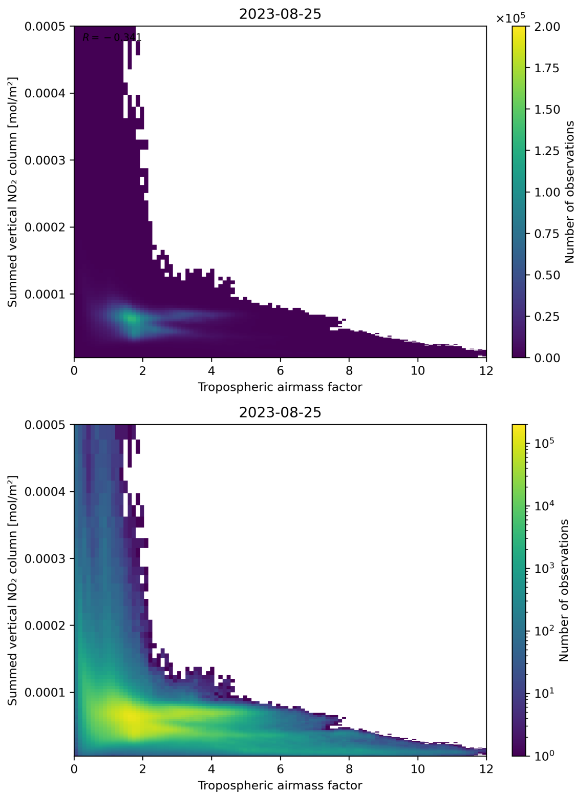
Figure 75: Scatter density plot of “Tropospheric airmass factor” against “Summed vertical NO 2 column” for 2023-08-25 to 2023-08-26.
