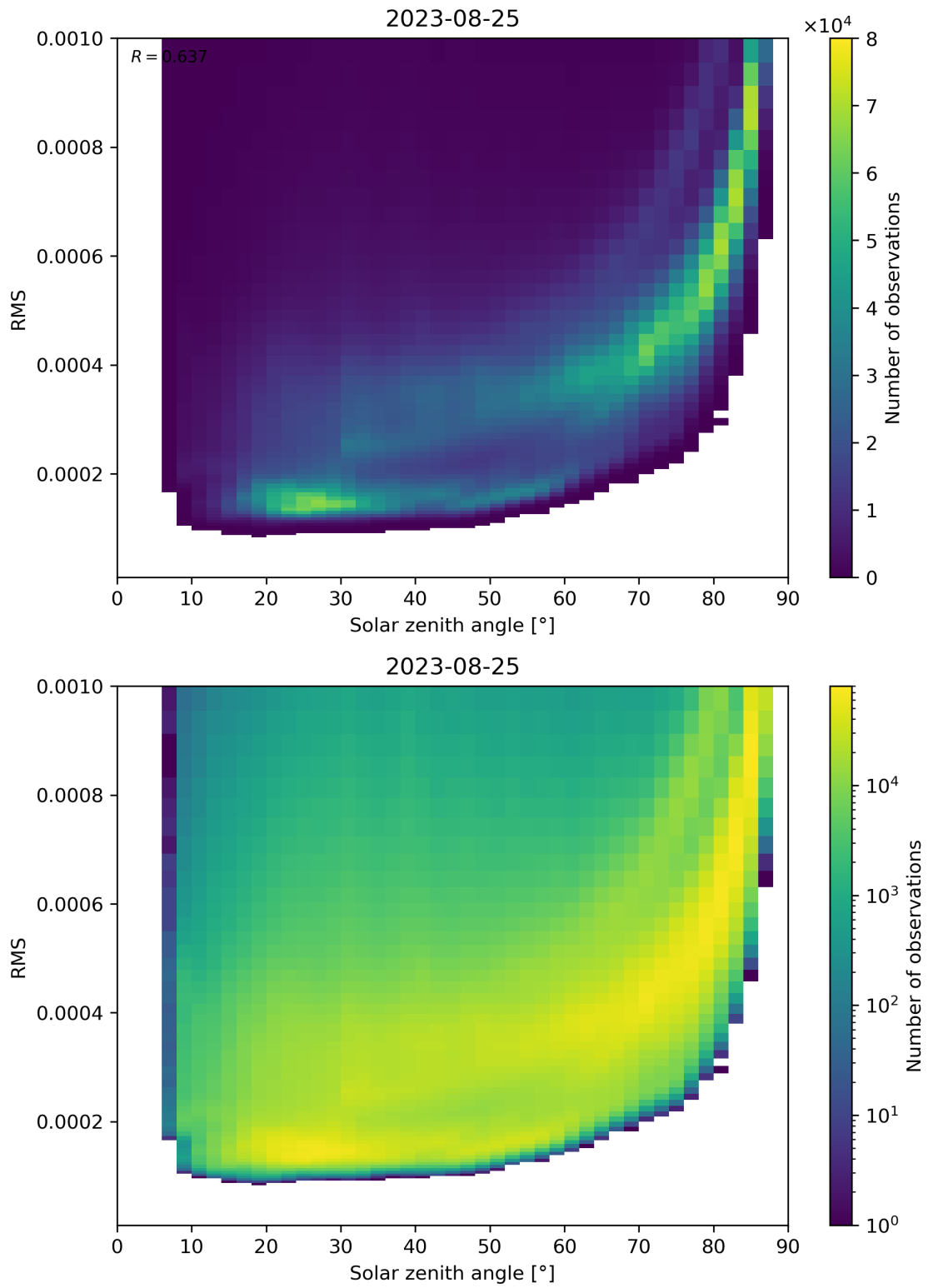
Figure 157: Scatter density plot of “Solar zenith angle” against “RMS” for 2023-08-25 to 2023-08-26.
