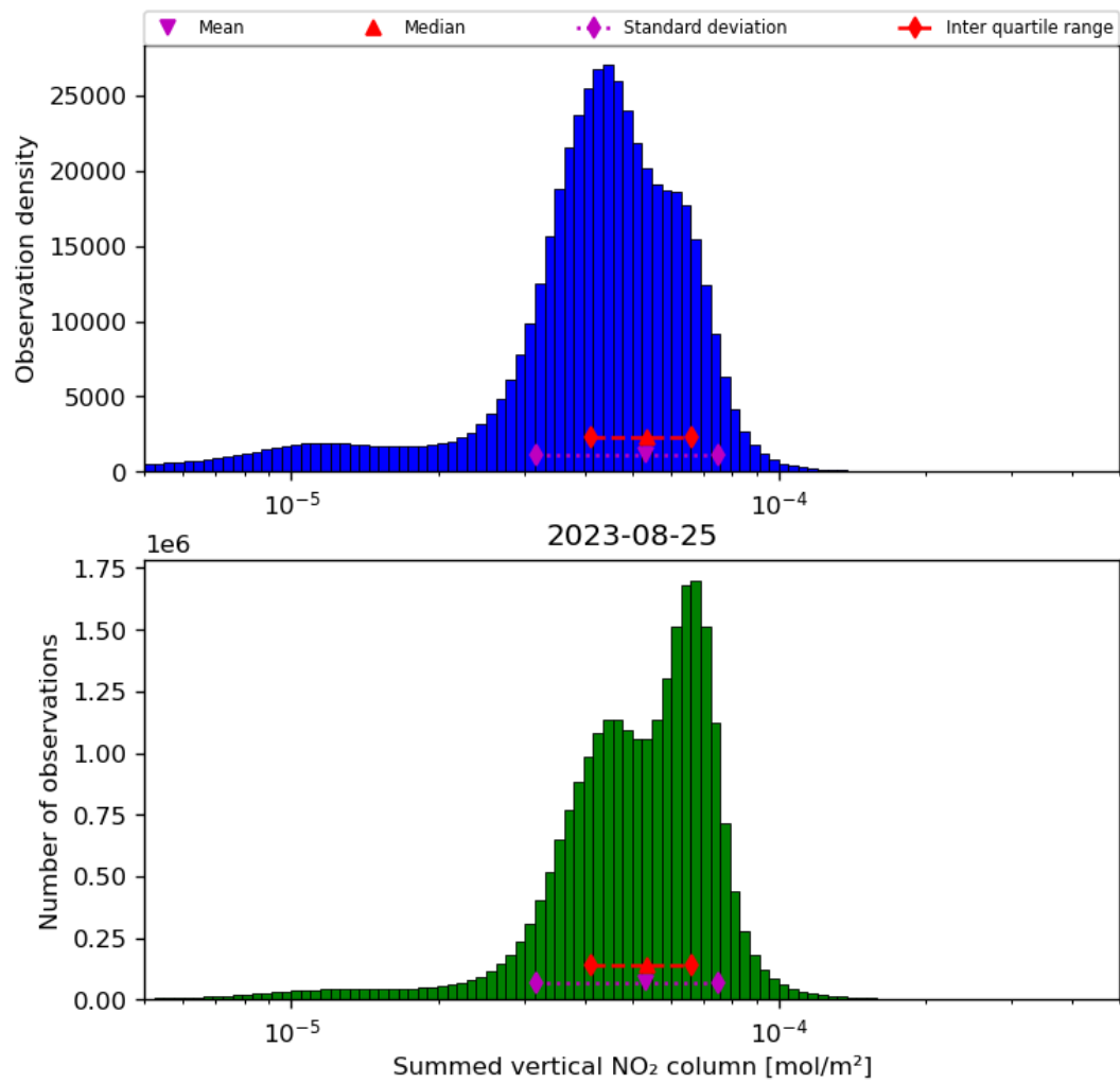
Figure 40: Histogram of “Summed vertical NO 2 column” for 2023-08-25 to 2023-08-26
