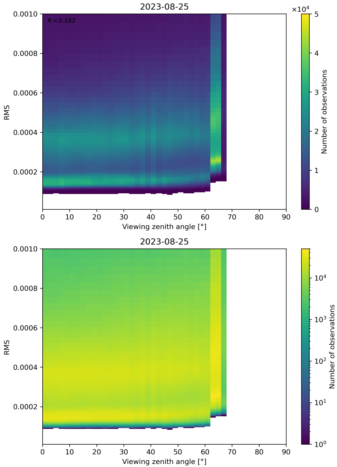
Figure 171: Scatter density plot of “Viewing zenith angle” against “RMS” for 2023-08-25 to 2023-08-26.
