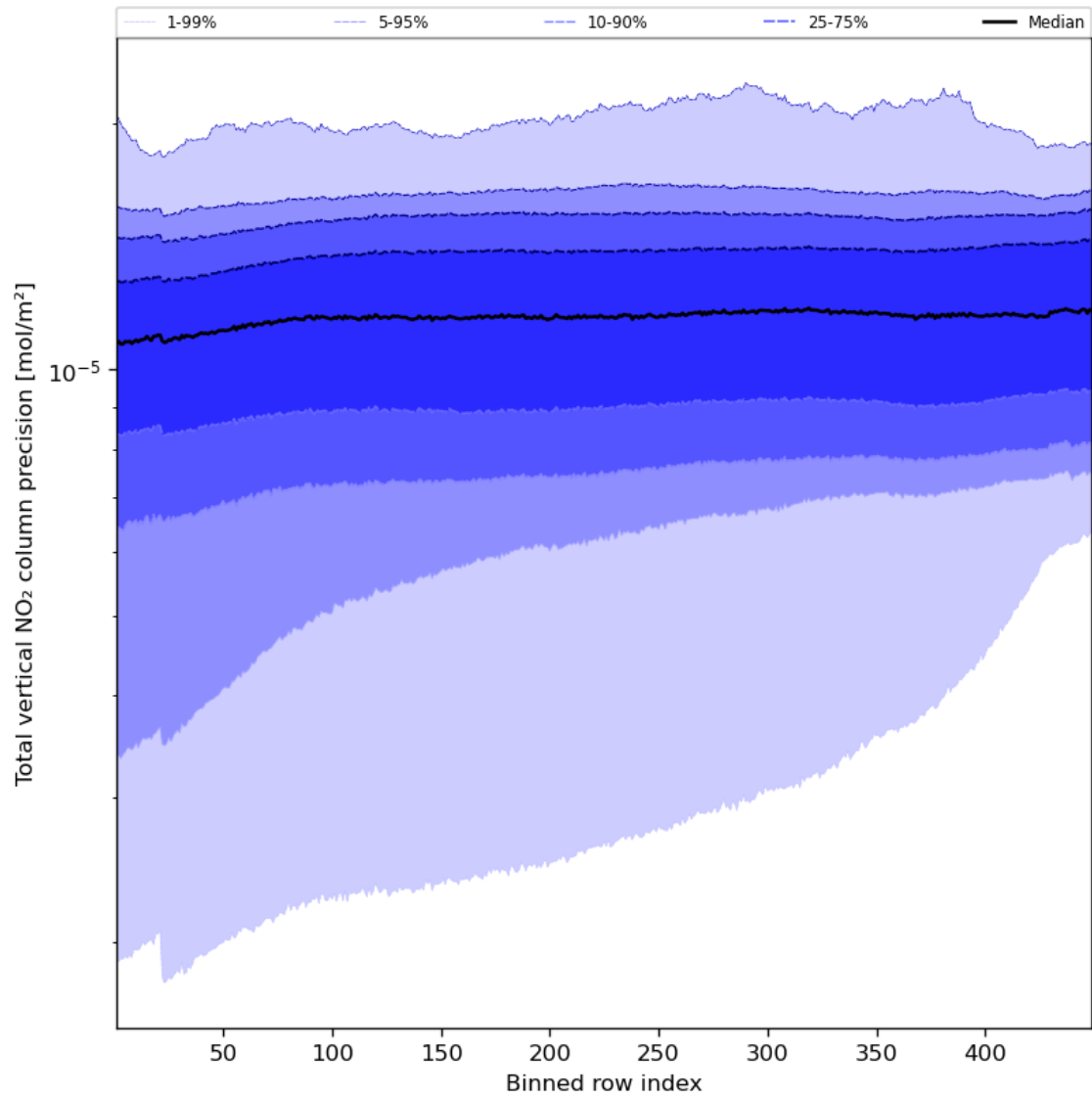
Figure 56: Along track statistics of “Total vertical NO 2 column precision” for 2023-08-25 to 2023-08-26
