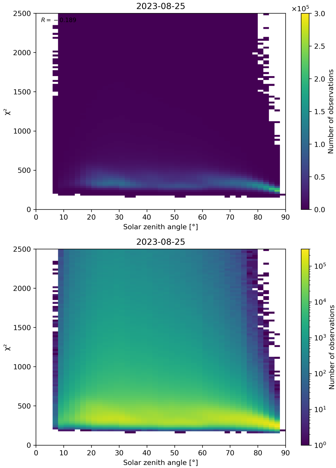
Figure 148: Scatter density plot of “Solar zenith angle” against “ \chi^2 ” for 2023-08-25 to 2023-08-26.
