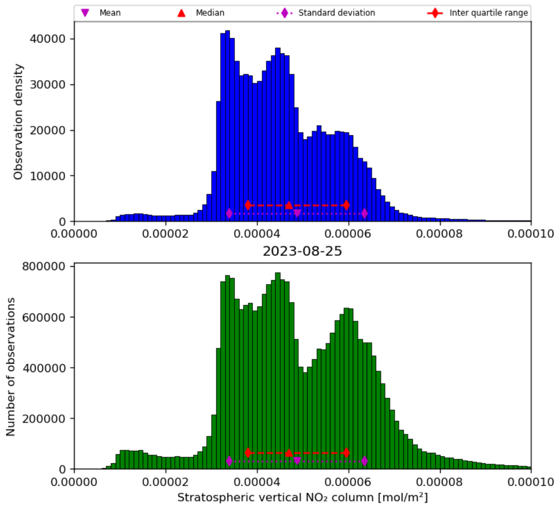
Figure 36: Histogram of “Stratospheric vertical NO 2 column” for 2023-08-25 to 2023-08-26
