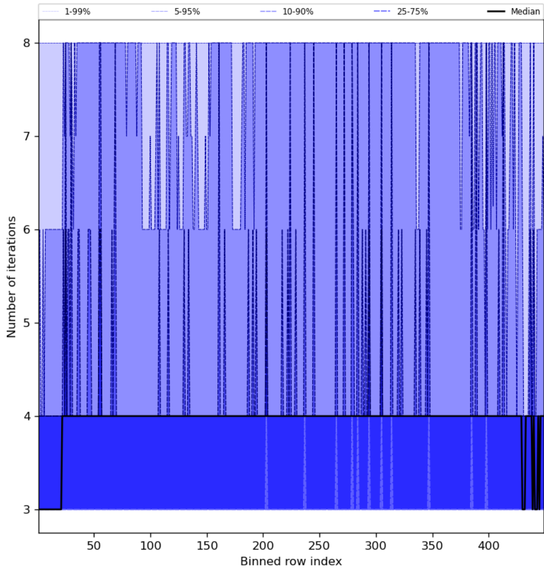
Figure 51: Along track statistics of “Number of iterations” for 2023-08-25 to 2023-08-26
