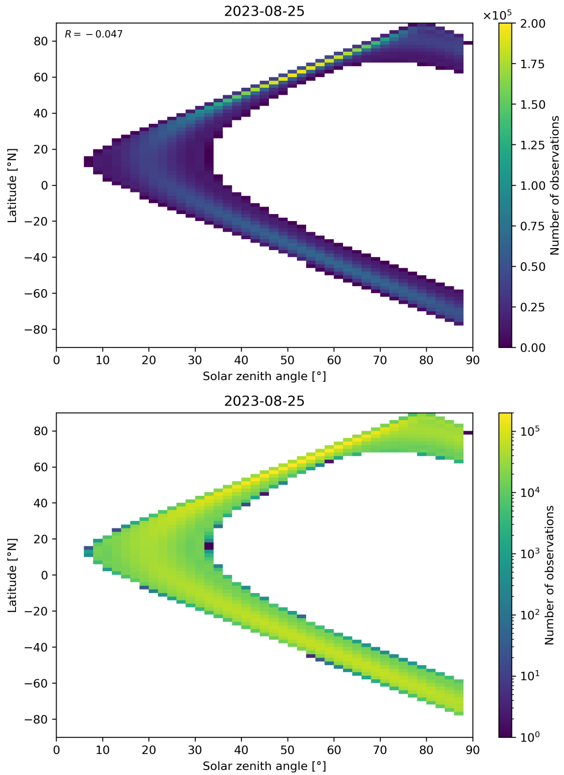
Figure 149: Scatter density plot of “Solar zenith angle” against “Latitude” for 2023-08-25 to 2023-08-26.
