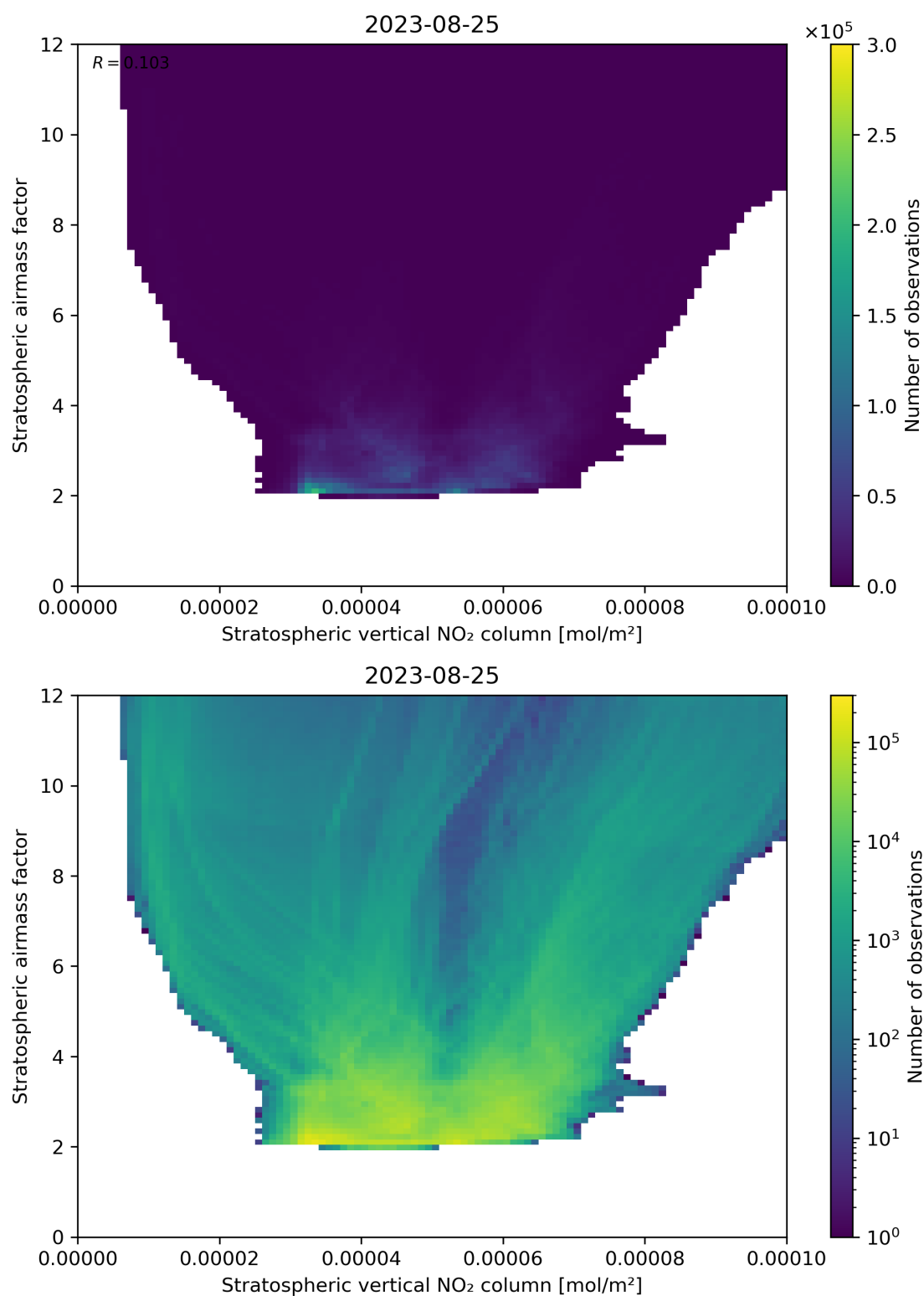
Figure 96: Scatter density plot of “Stratospheric vertical NO 2 column” against “Stratospheric airmass factor” for 2023-08-25 to 2023-08-26.
