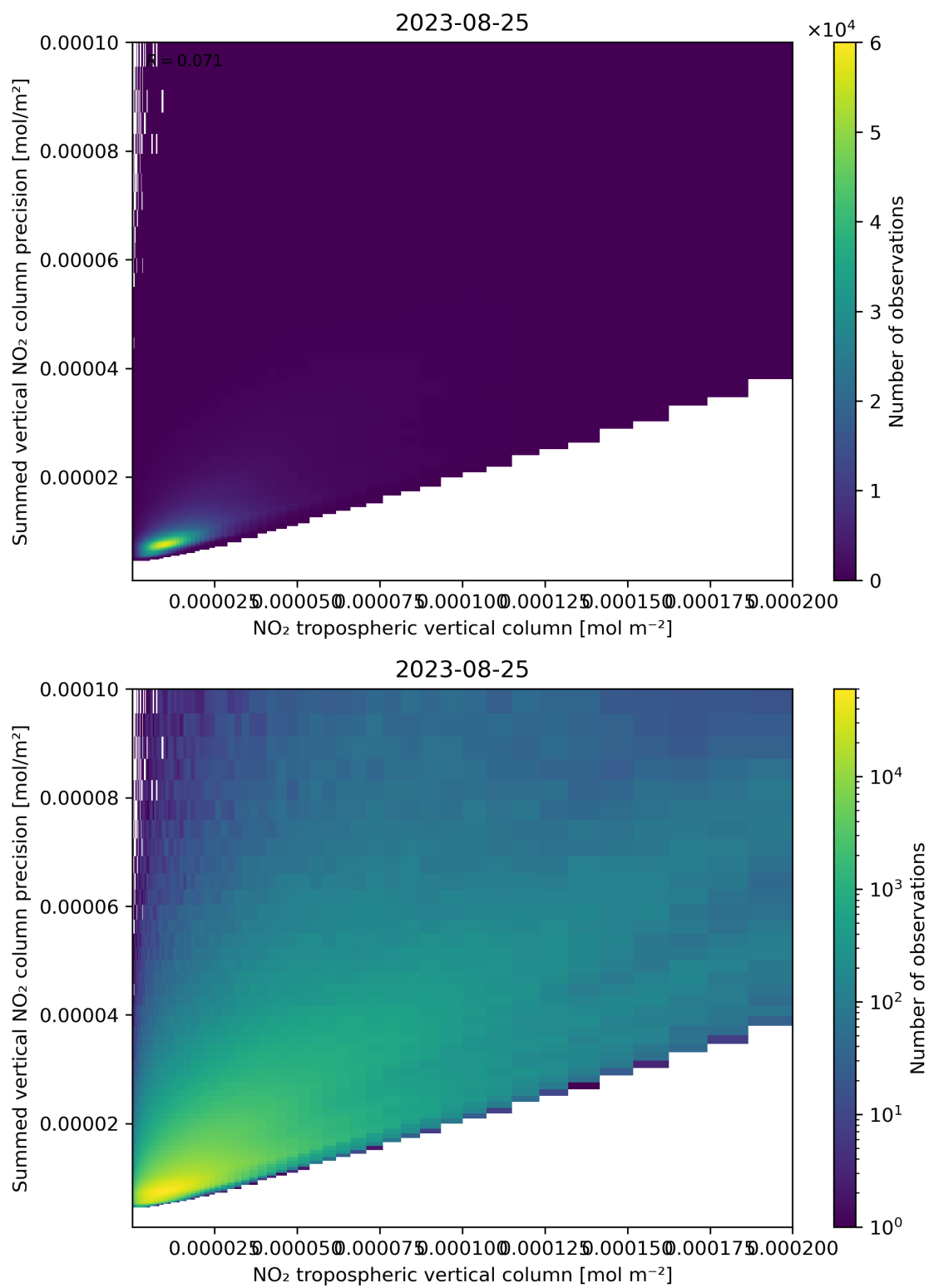
Figure 127: Scatter density plot of “NO 2 tropospheric vertical column” against “Summed vertical NO 2 column precision” for 2023-08-25 to 2023-08-26.
