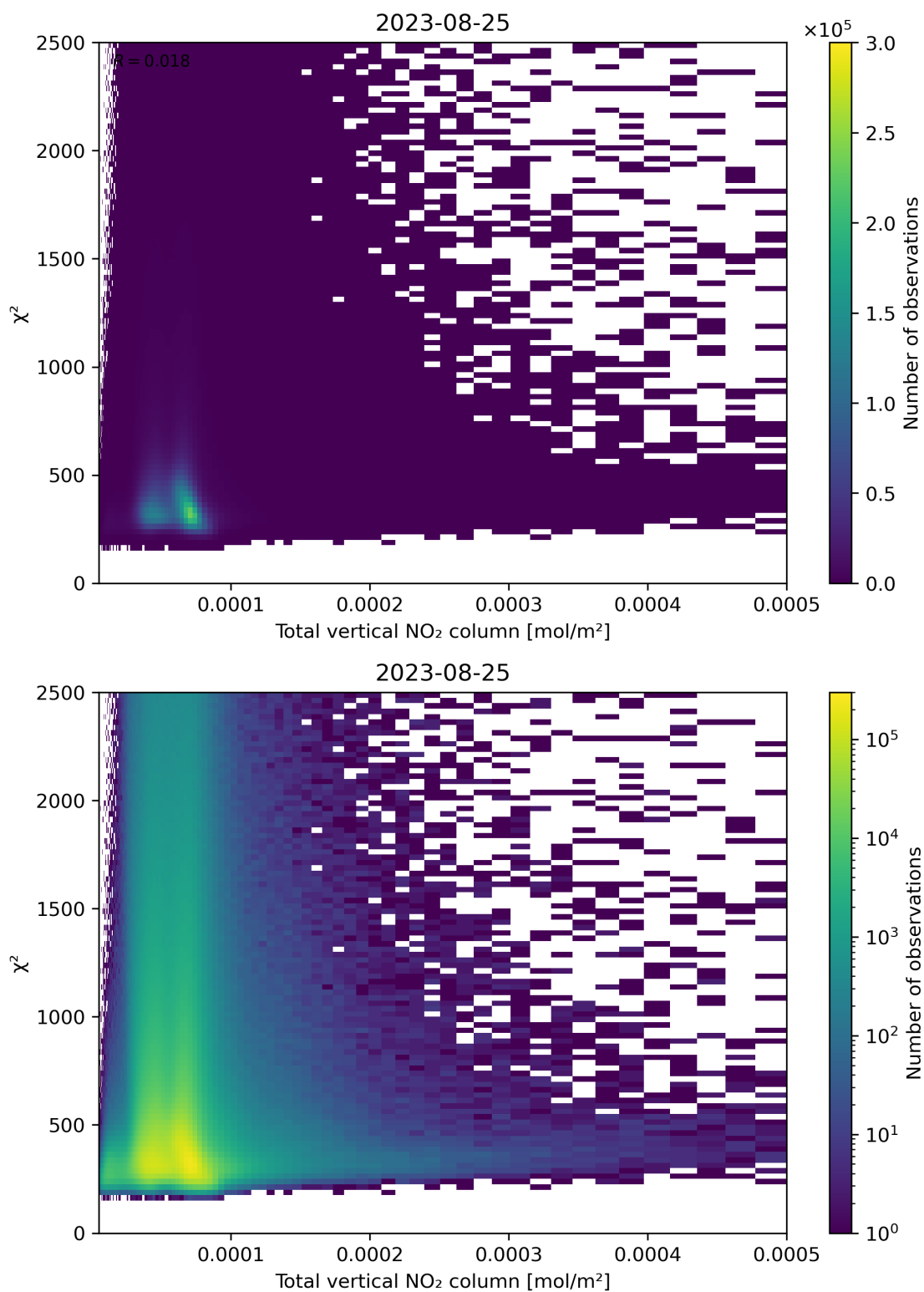
Figure 111: Scatter density plot of “Total vertical NO 2 column” against “ \chi^2 ” for 2023-08-25 to 2023-08-26.
