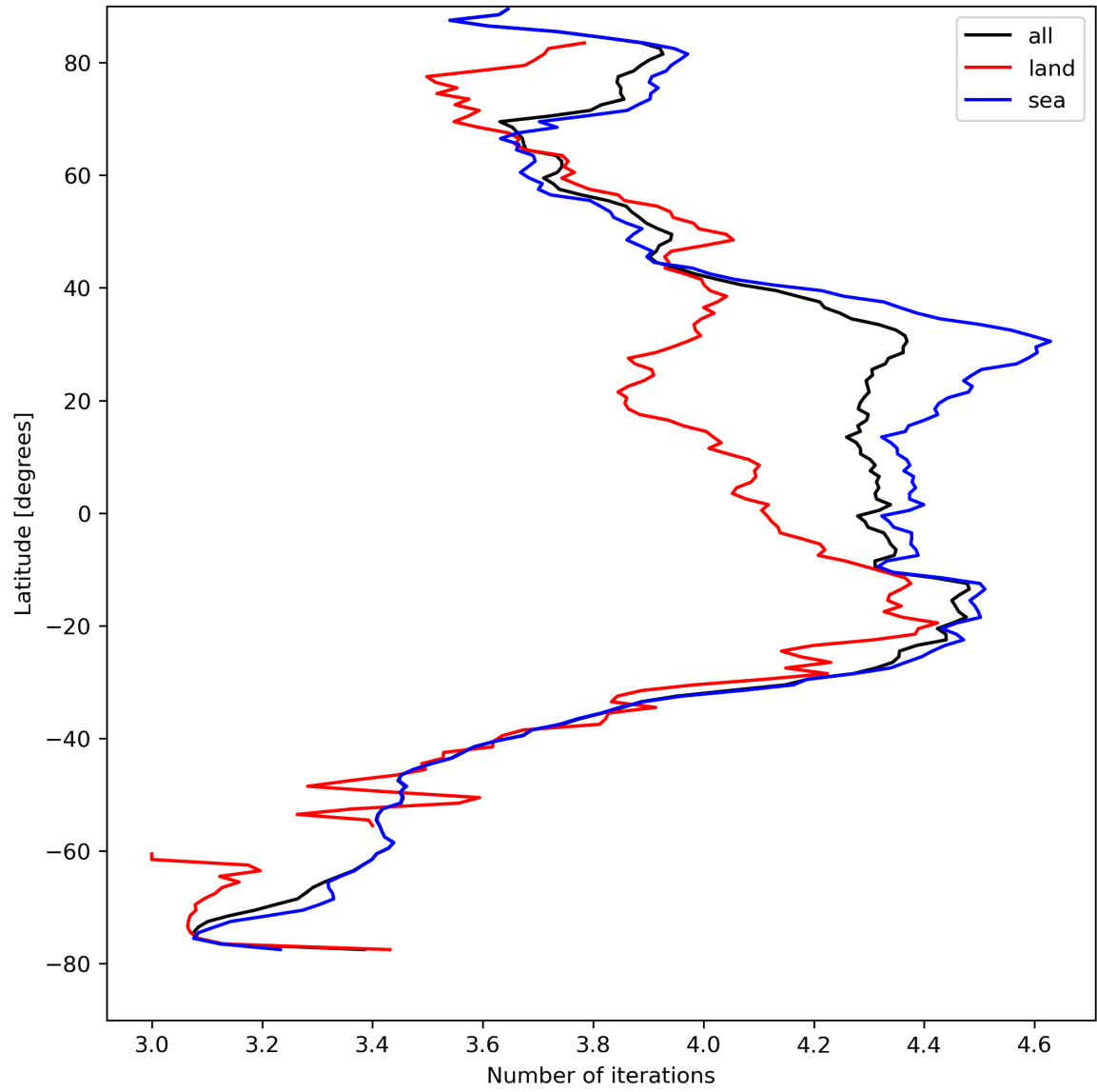
Figure 17: Zonal average of “Number of iterations” for 2023-08-25 to 2023-08-26.
