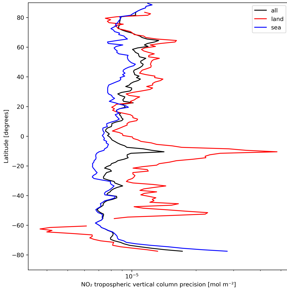
Figure 13: Zonal average of “NO 2 tropospheric vertical column precision” for 2023-08-25 to 2023-08-26.
