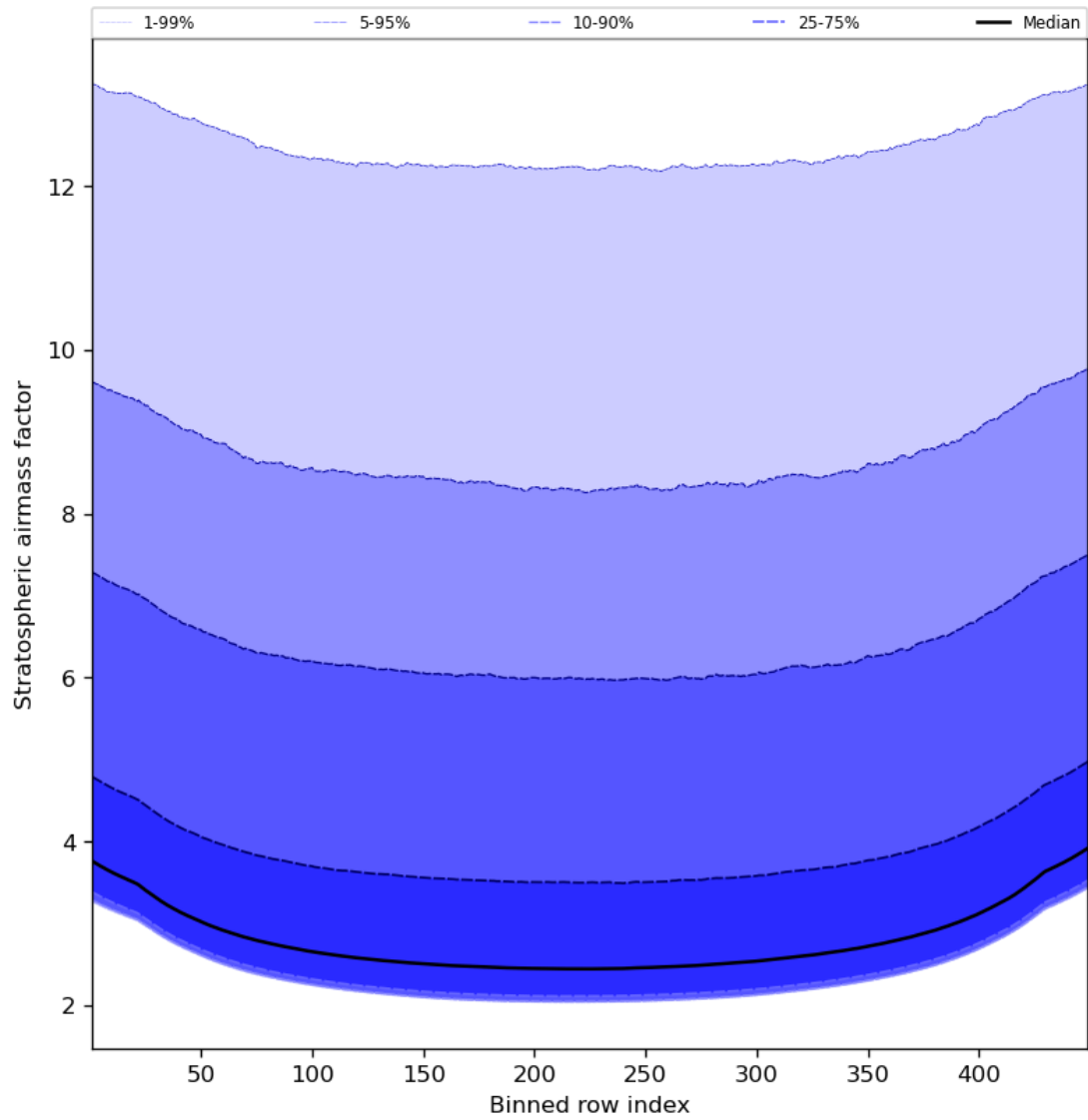
Figure 61: Along track statistics of “Stratospheric airmass factor” for 2023-08-25 to 2023-08-26
