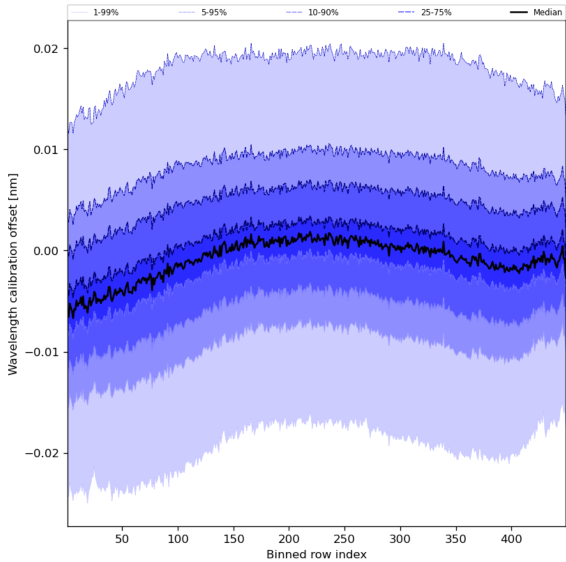
Figure 52: Along track statistics of “Wavelength calibration offset” for 2023-08-25 to 2023-08-26
