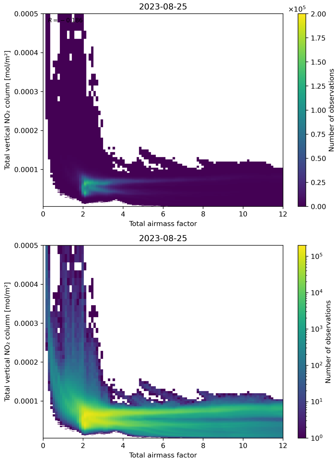
Figure 67: Scatter density plot of “Total airmass factor” against “Total vertical NO 2 column” for 2023-08-25 to 2023-08-26.
