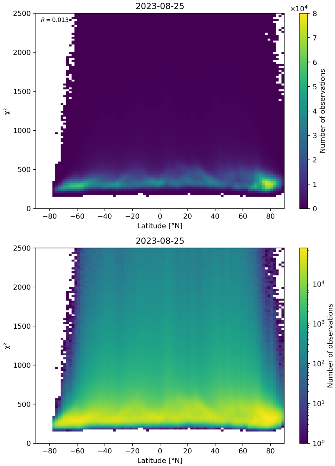
Figure 86: Scatter density plot of “Latitude” against “ \chi^2 ” for 2023-08-25 to 2023-08-26.
