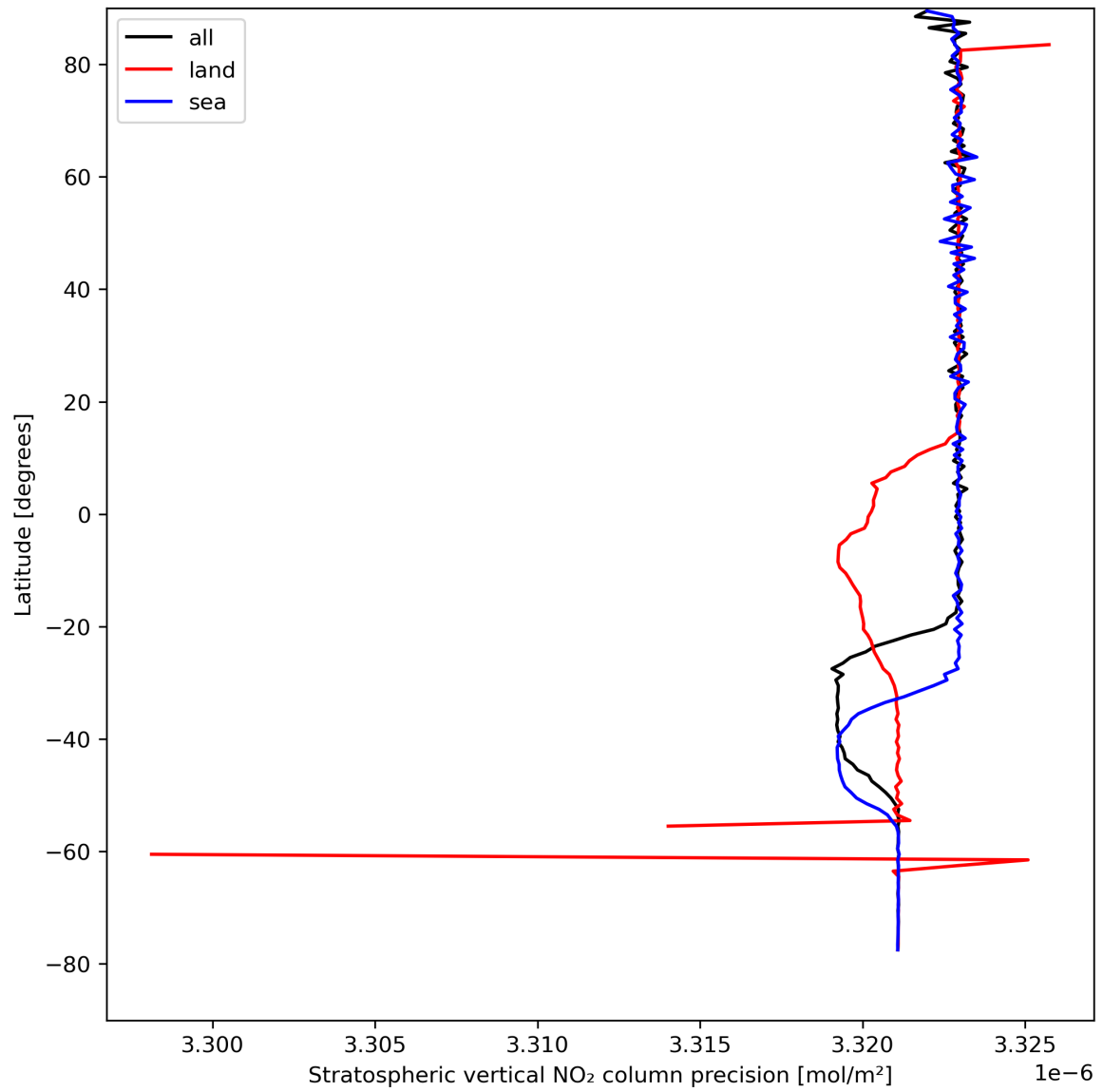
Figure 20: Zonal average of “Stratospheric vertical NO 2 column precision” for 2023-08-25 to 2023-08-26.
