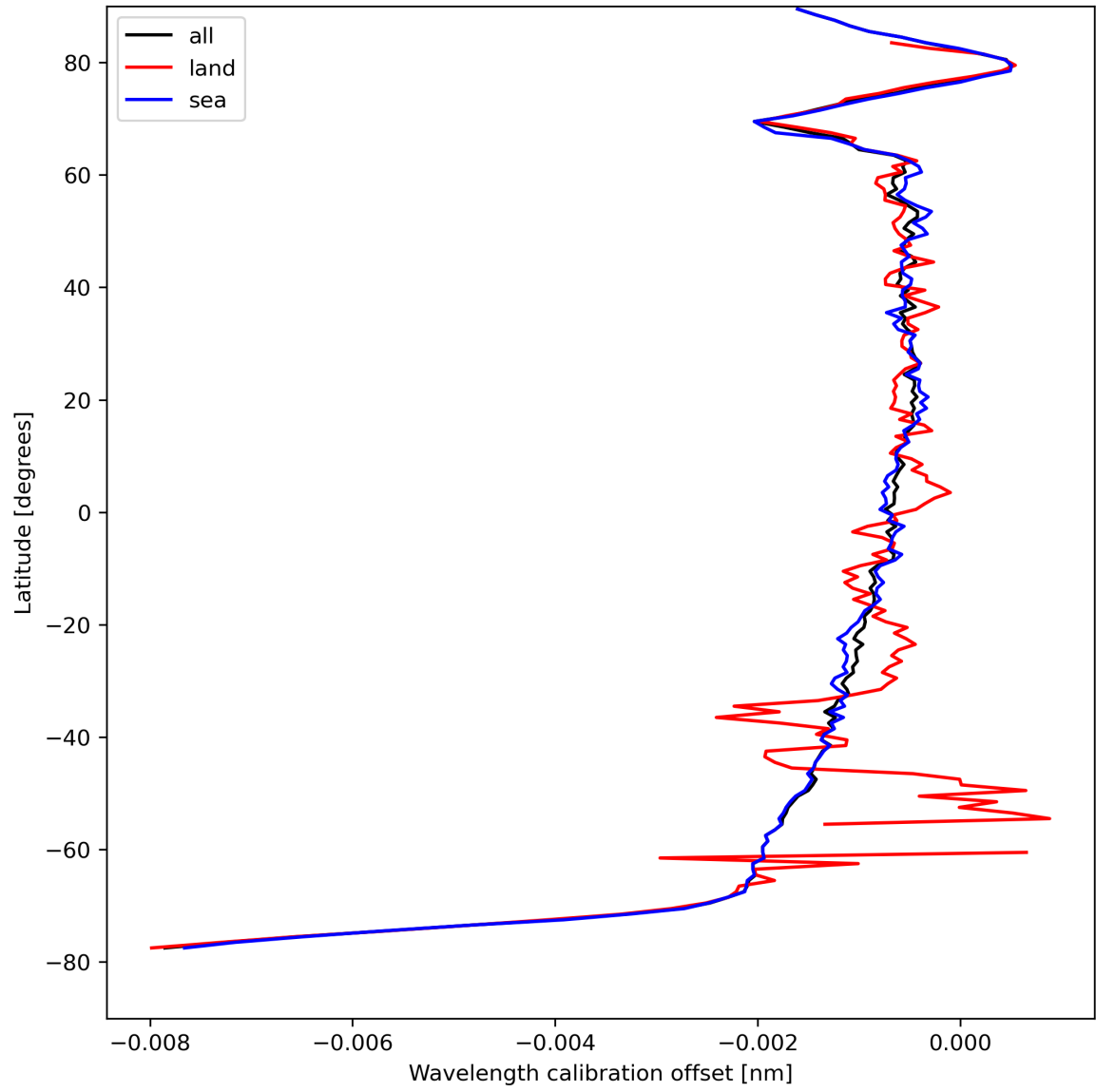
Figure 18: Zonal average of “Wavelength calibration offset” for 2023-08-25 to 2023-08-26.
