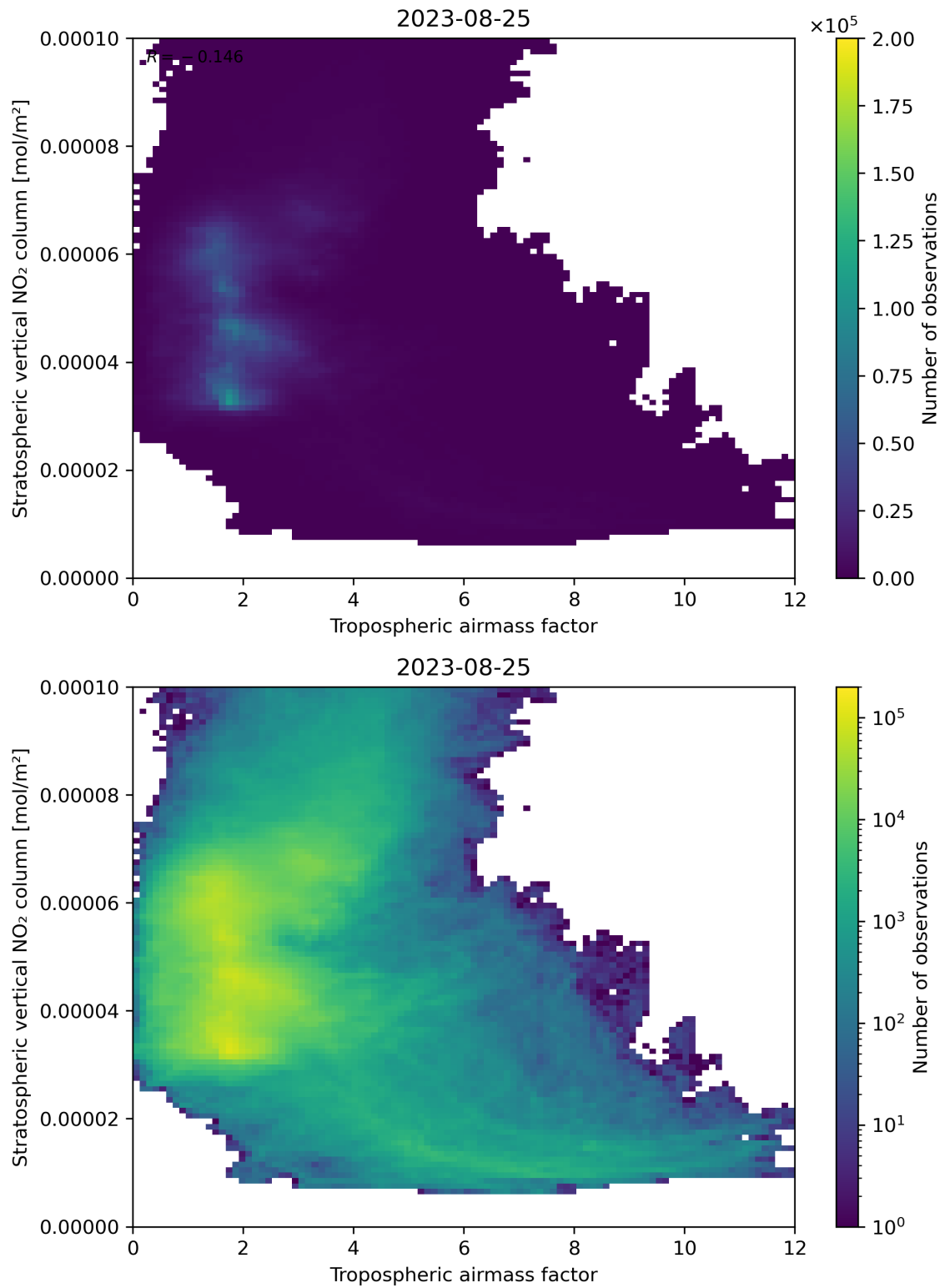
Figure 74: Scatter density plot of “Tropospheric air mass factor” against “Stratospheric vertical NO 2 column” for 2023-08-25 to 2023-08-26.
