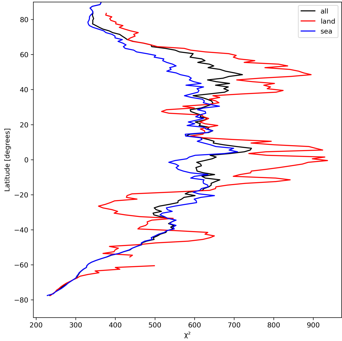
Figure 25: Zonal average of “ \chi^2 ” for 2023-08-25 to 2023-08-26.
