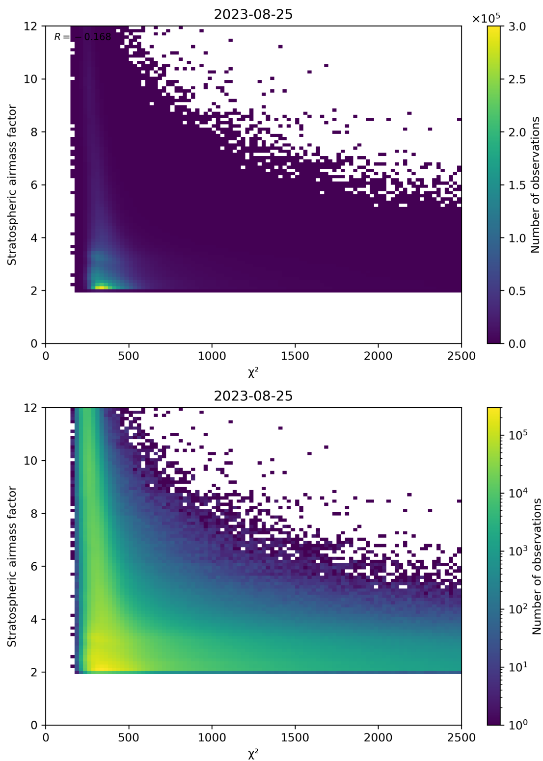
Figure 81: Scatter density plot of “ \chi^2 ” against “Stratospheric airmass factor” for 2023-08-25 to 2023-08-26.
