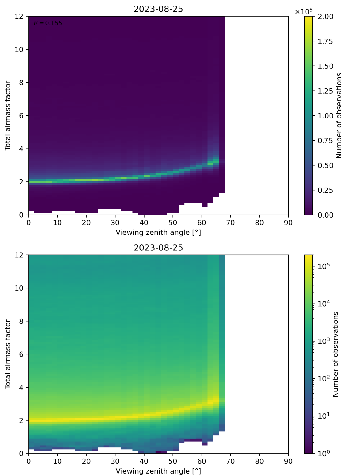
Figure 160: Scatter density plot of “Viewing zenith angle” against “Total airmass factor” for 2023-08-25 to 2023-08-26.
