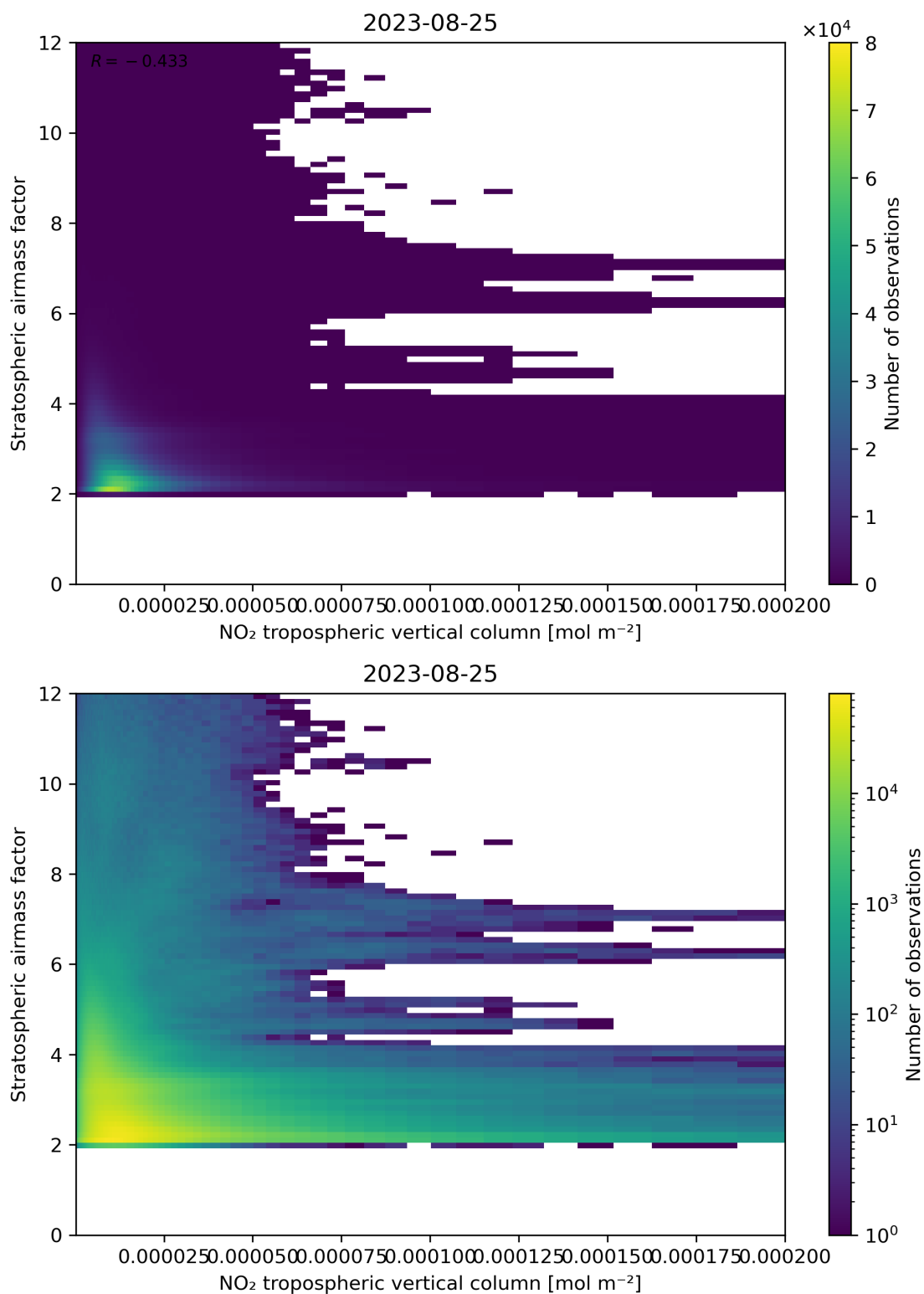
Figure 121: Scatter density plot of “NO 2 tropospheric vertical column” against “Stratospheric air mass factor” for 2023-08-25 to 2023-08-26.
