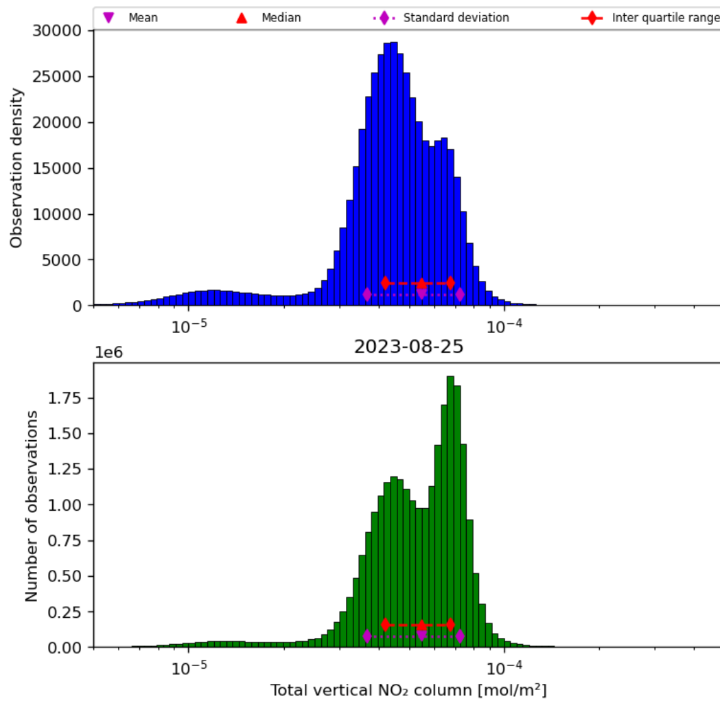
Figure 38: Histogram of “Total vertical NO 2 column” for 2023-08-25 to 2023-08-26
