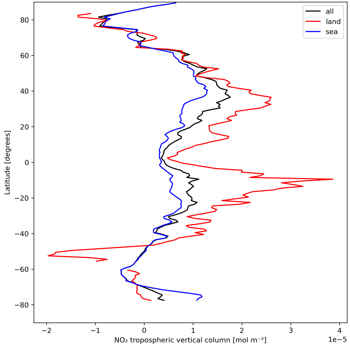
Figure 12: Zonal average of “NO 2 tropospheric vertical column” for 2023-08-25 to 2023-08-26.
