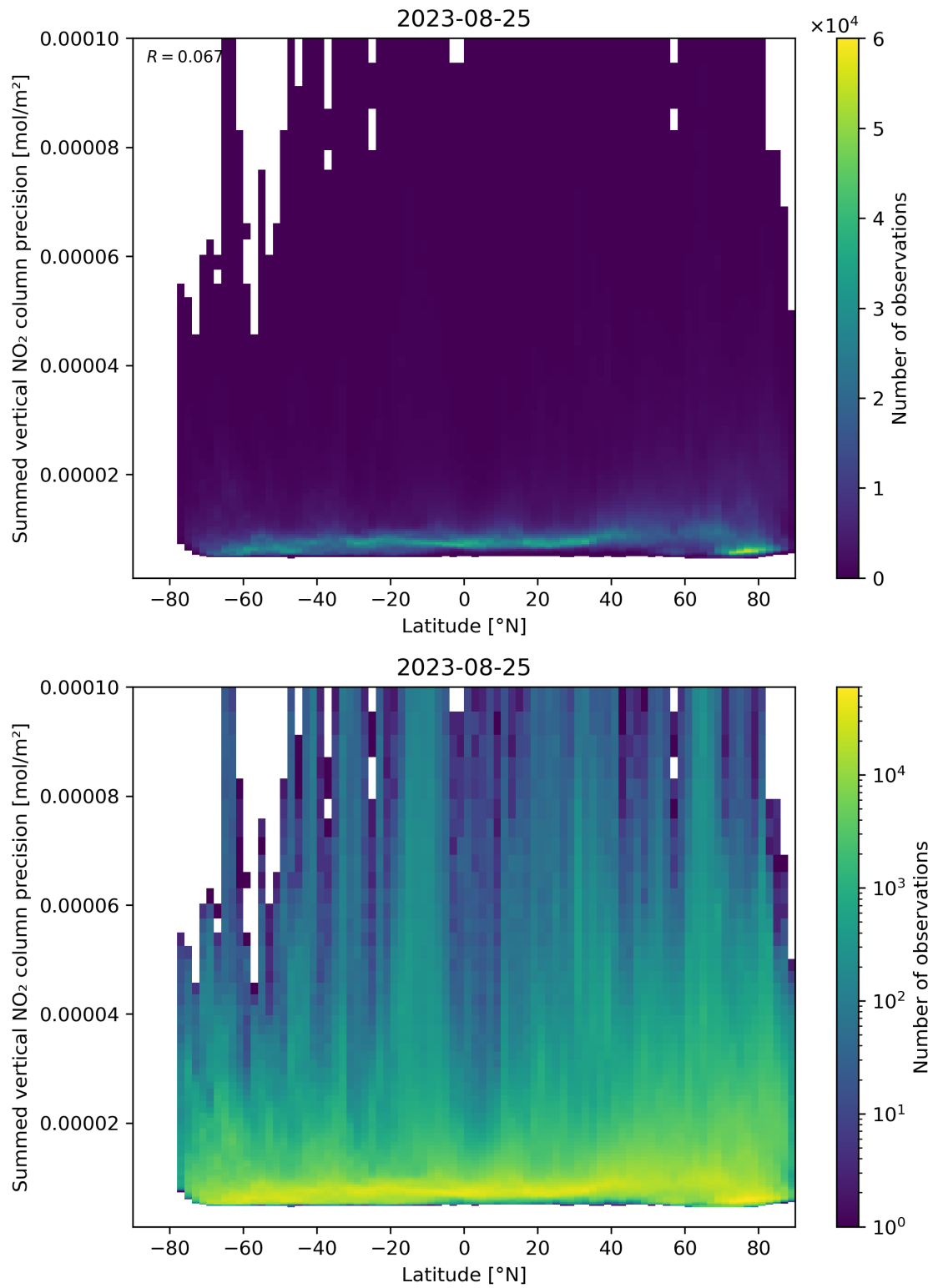
Figure 89: Scatter density plot of “Latitude” against “Summed vertical NO 2 column precision” for 2023-08-25 to 2023-08-26.
