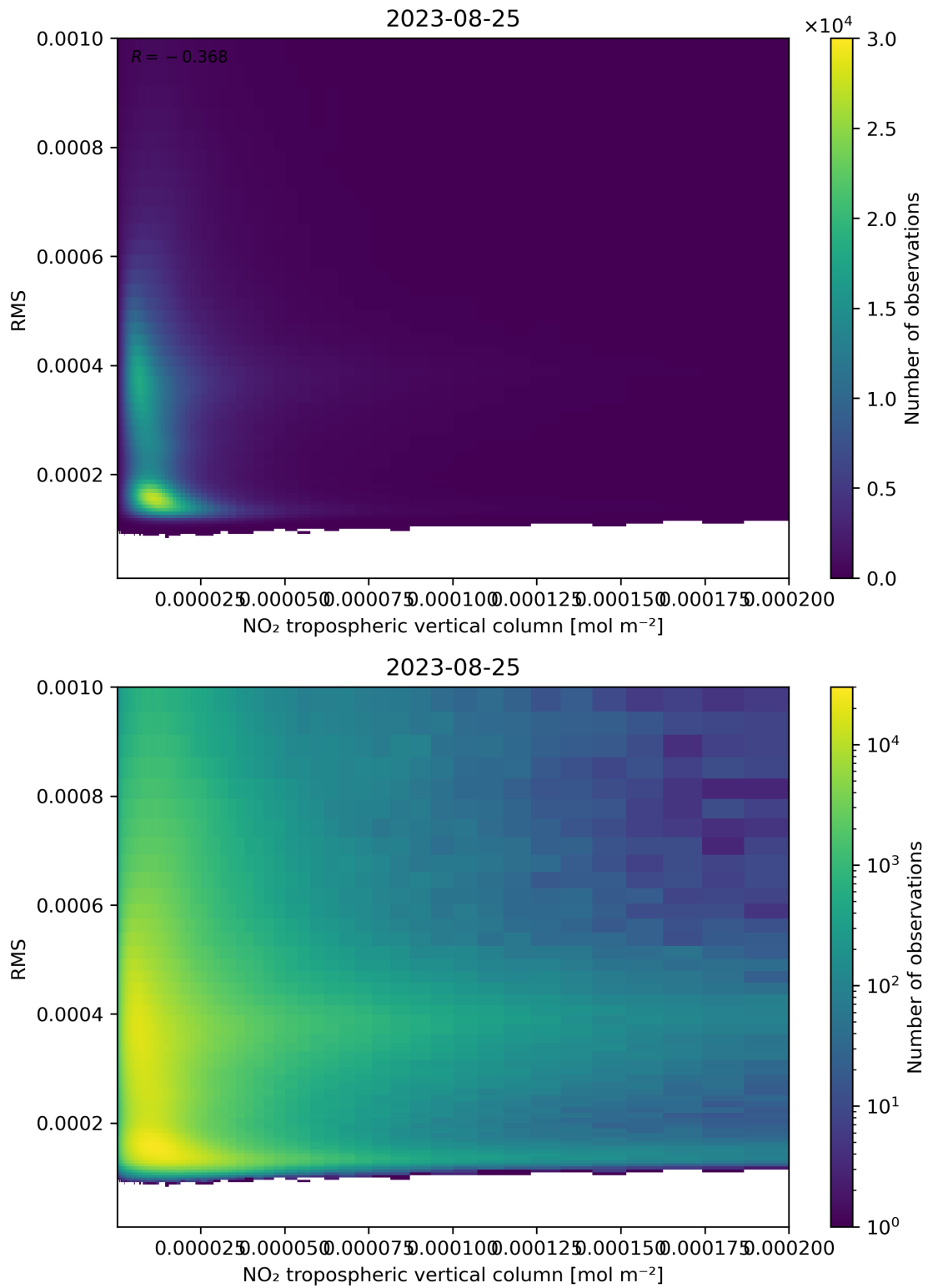
Figure 142: Scatter density plot of “NO 2 tropospheric vertical column” against “RMS” for 2023-08-25 to 2023-08-26.
