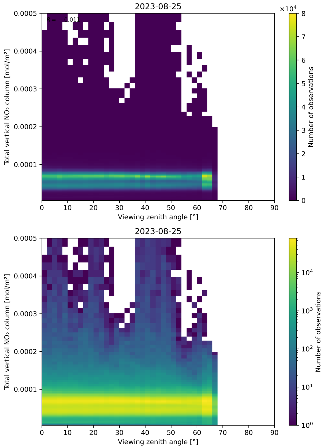
Figure 167: Scatter density plot of “Viewing zenith angle” against “Total vertical NO 2 column” for 2023-08-25 to 2023-08-26.
