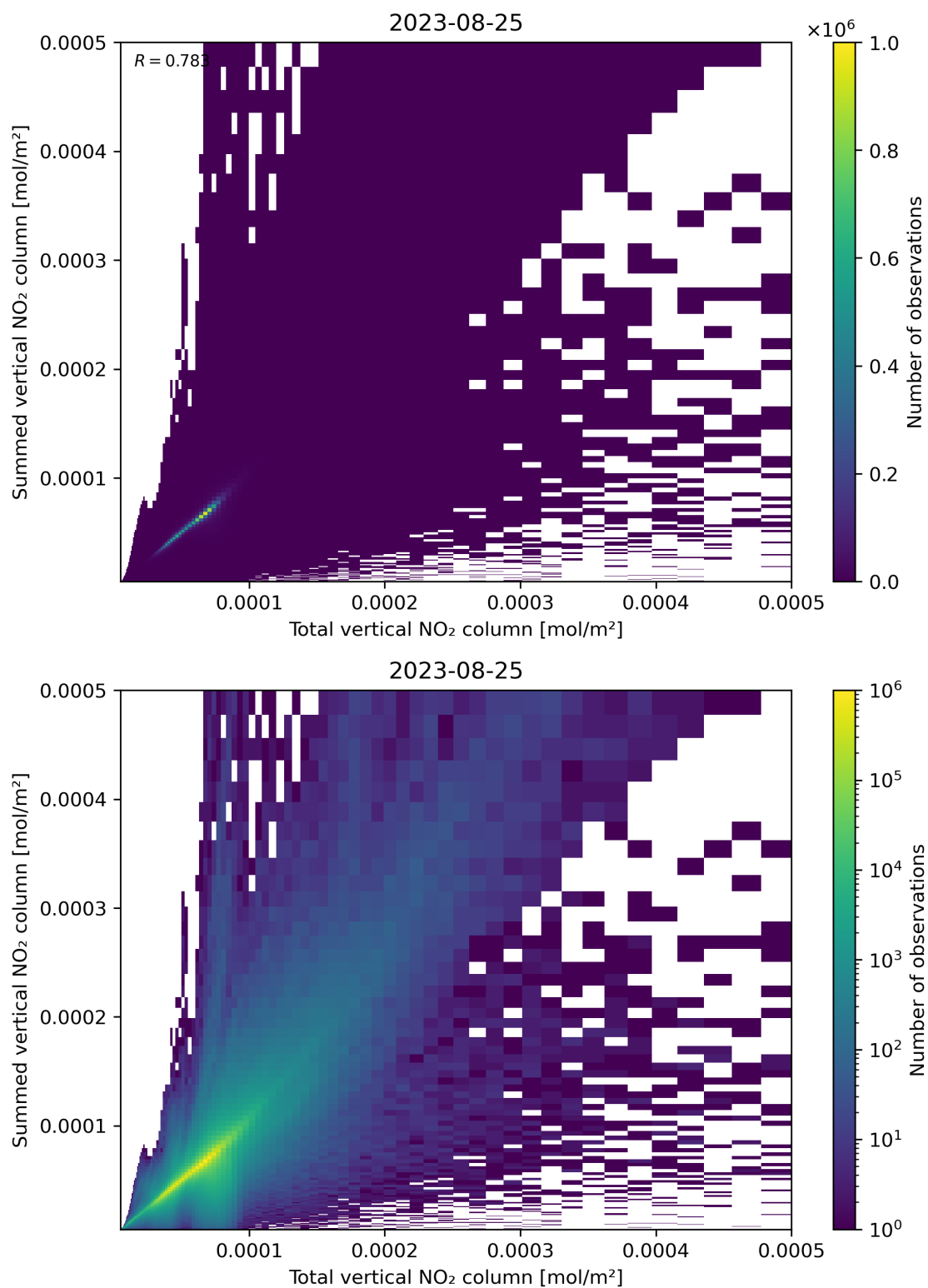
Figure 112: Scatter density plot of “Total vertical NO 2 column” against “Summed vertical NO 2 column” for 2023-08-25 to 2023-08-26.
