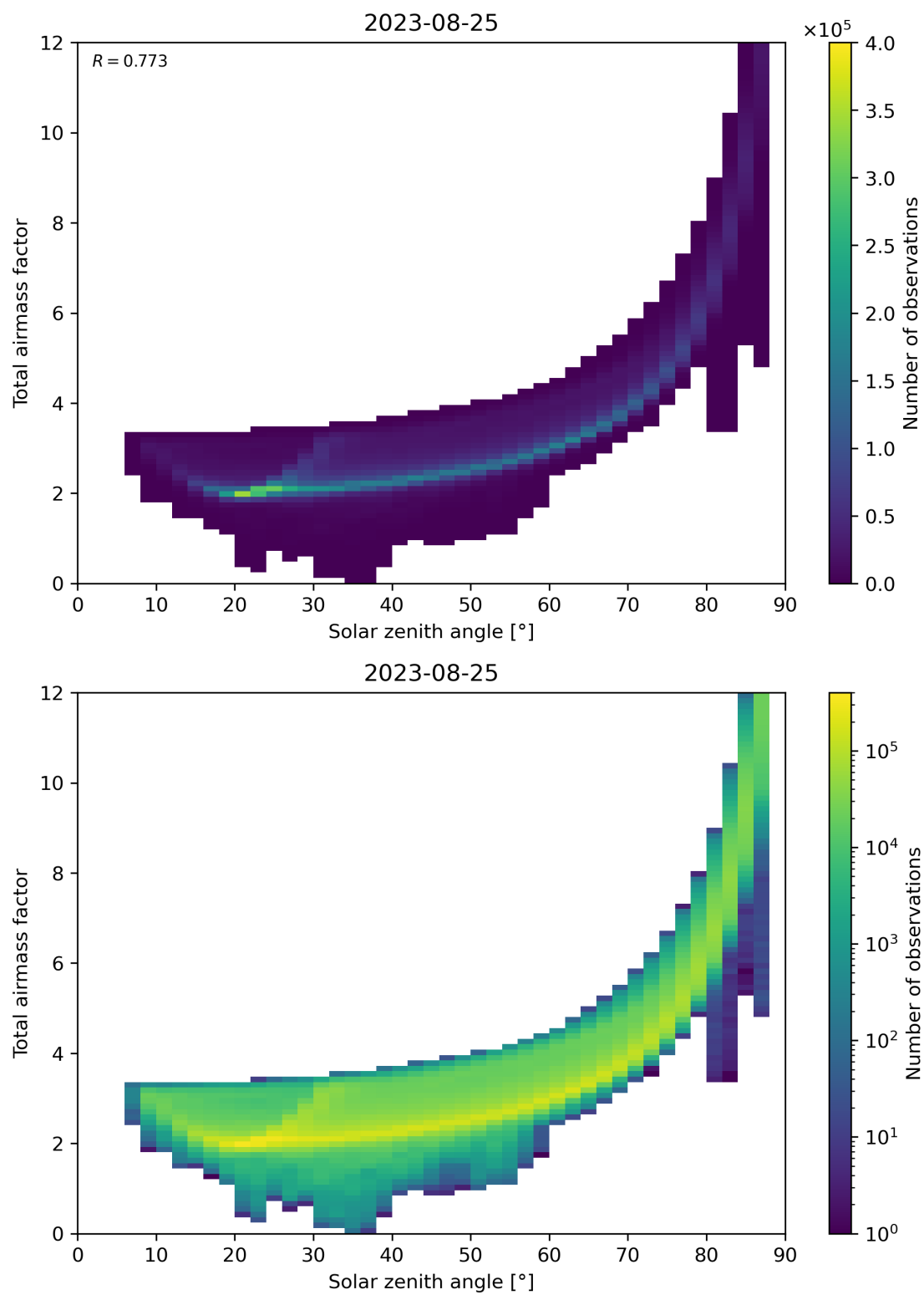
Figure 146: Scatter density plot of “Solar zenith angle” against “Total air mass factor” for 2023-08-25 to 2023-08-26.
