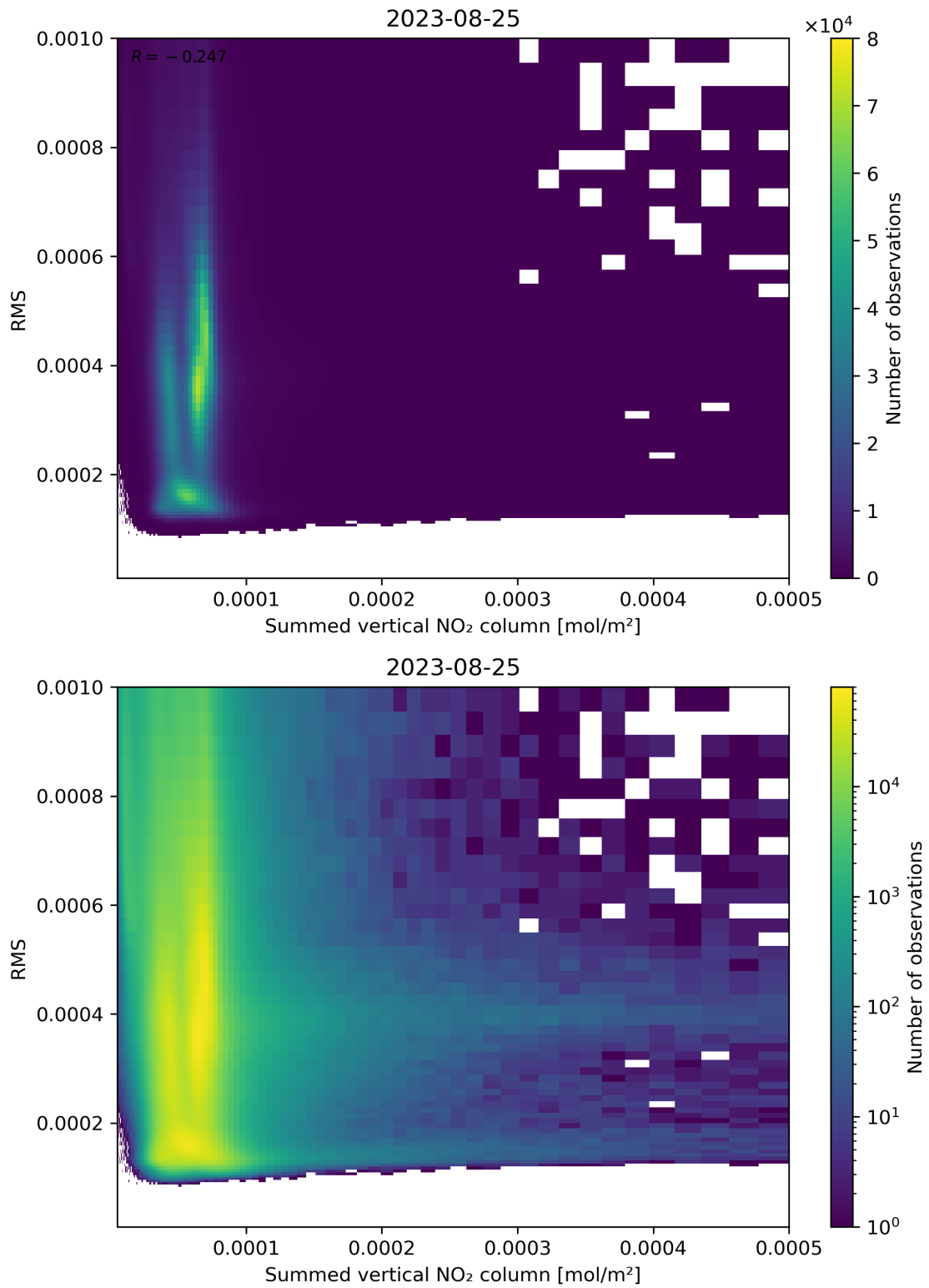
Figure 109: Scatter density plot of “Summed vertical NO 2 column” against “RMS” for 2023-08-25 to 2023-08-26.
