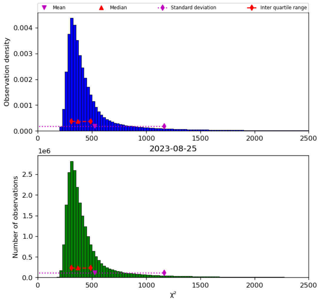
Figure 42: Histogram of " \chi^2 " for 2023-08-25 to 2023-08-26
