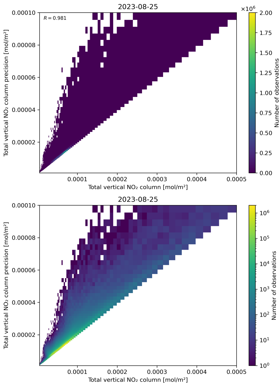
Figure 114: Scatter density plot of “Total vertical NO 2 column” against “Total vertical NO 2 column precision” for 2023-08-25 to 2023-08-26.
