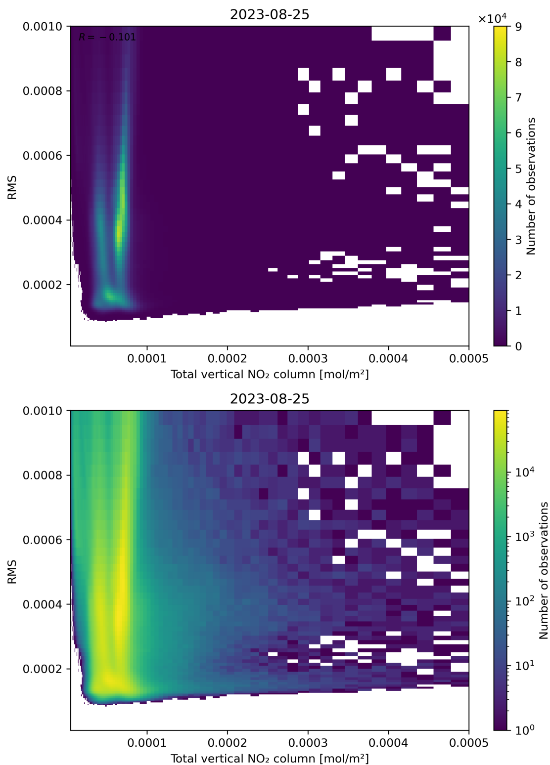
Figure 120: Scatter density plot of “Total vertical NO 2 column” against “RMS” for 2023-08-25 to 2023-08-26.
