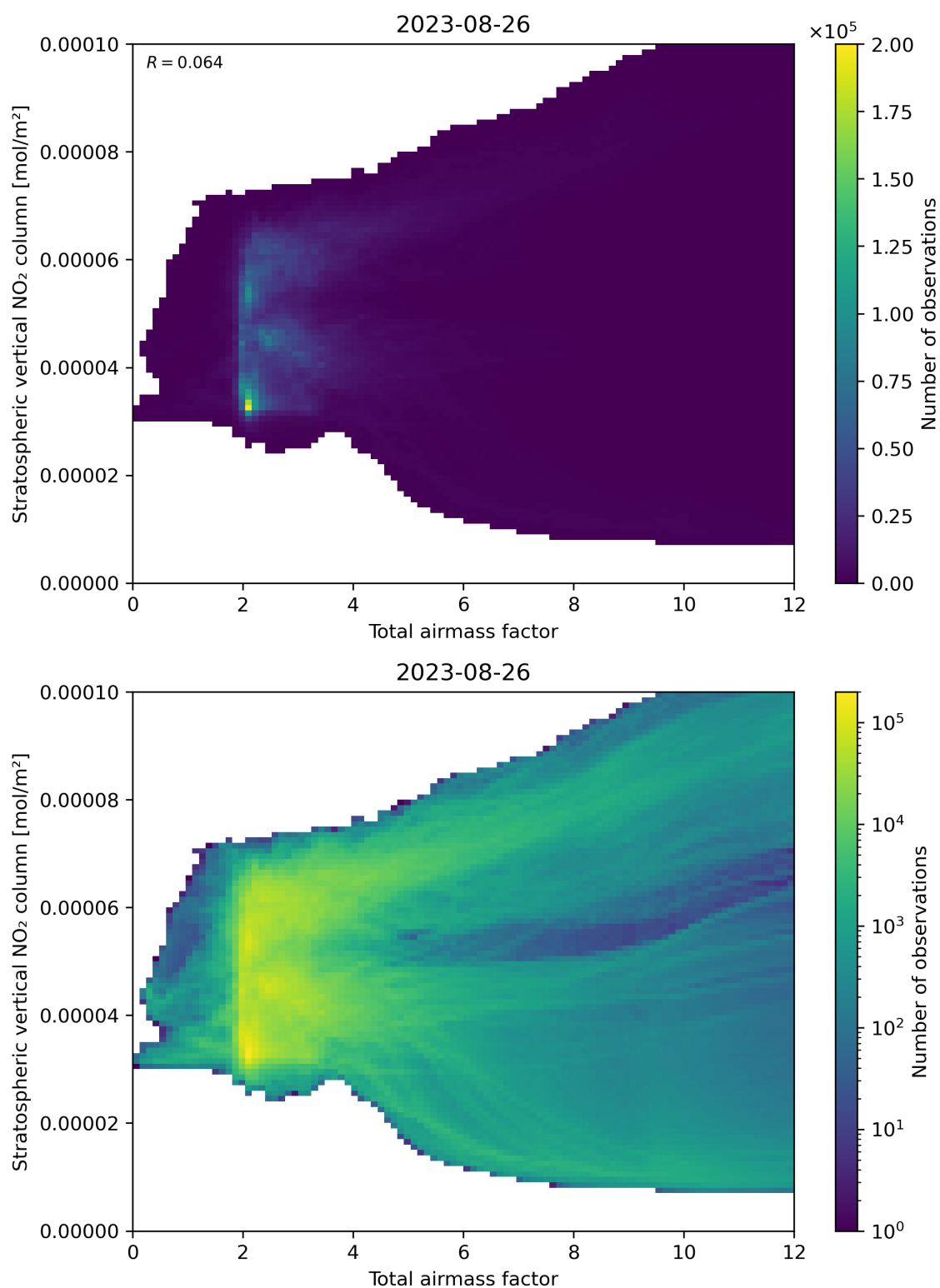
Figure 64: Scatter density plot of “Total airmass factor” against “Stratospheric vertical NO 2 column” for 2023-08-25 to 2023-08-27.
