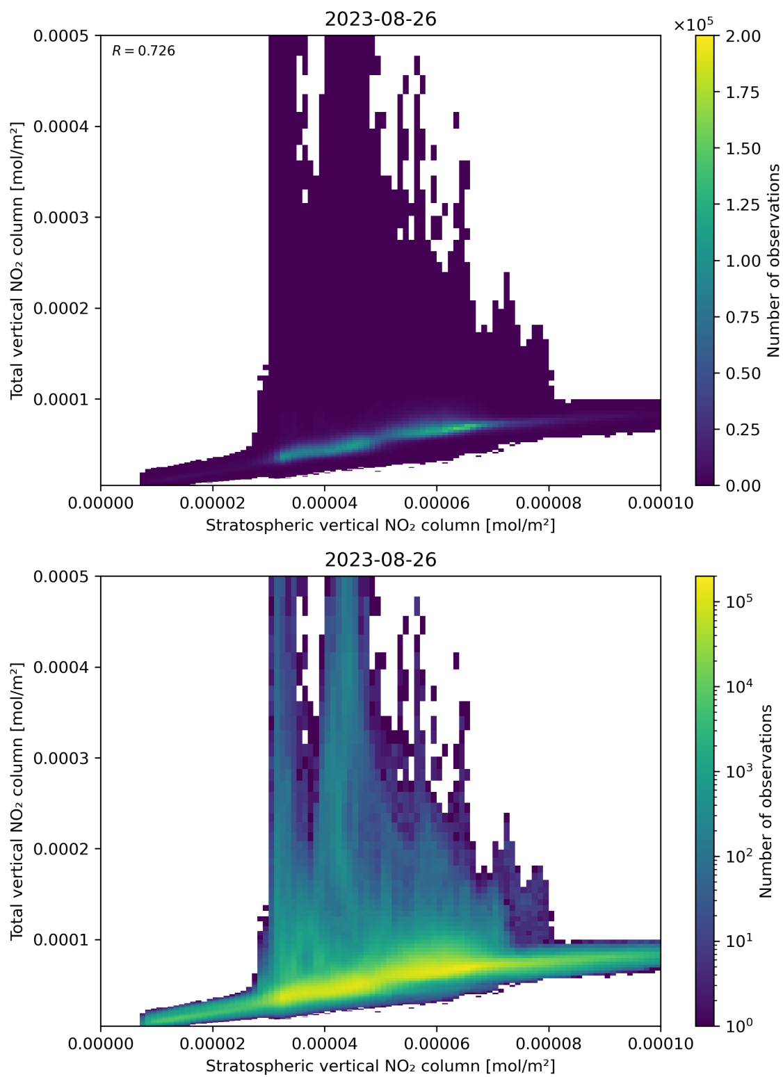
Figure 100: Scatter density plot of “Stratospheric vertical NO 2 column” against “Total vertical NO 2 column” for 2023-08-25 to 2023-08-27.
