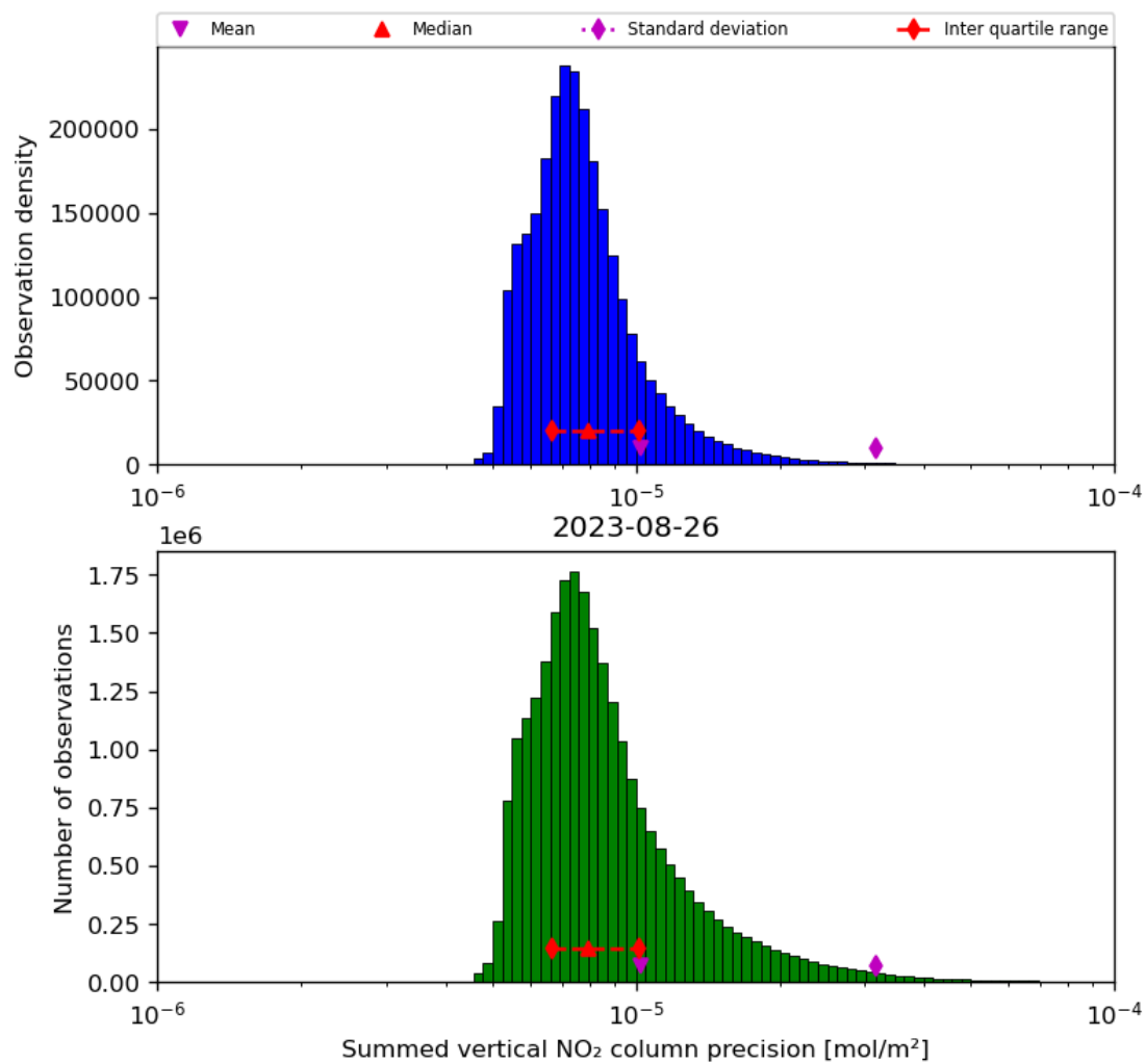
Figure 41: Histogram of "Summed vertical NO 2 column precision" for 2023-08-25 to 2023-08-27
