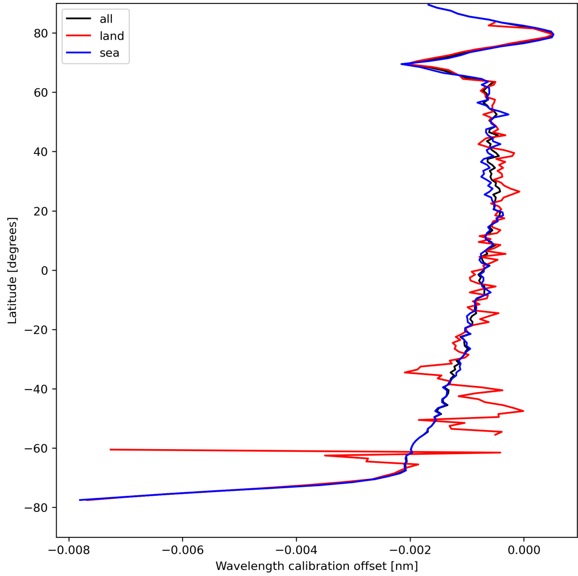
Figure 18: Zonal average of “Wavelength calibration offset” for 2023-08-25 to 2023-08-27.
