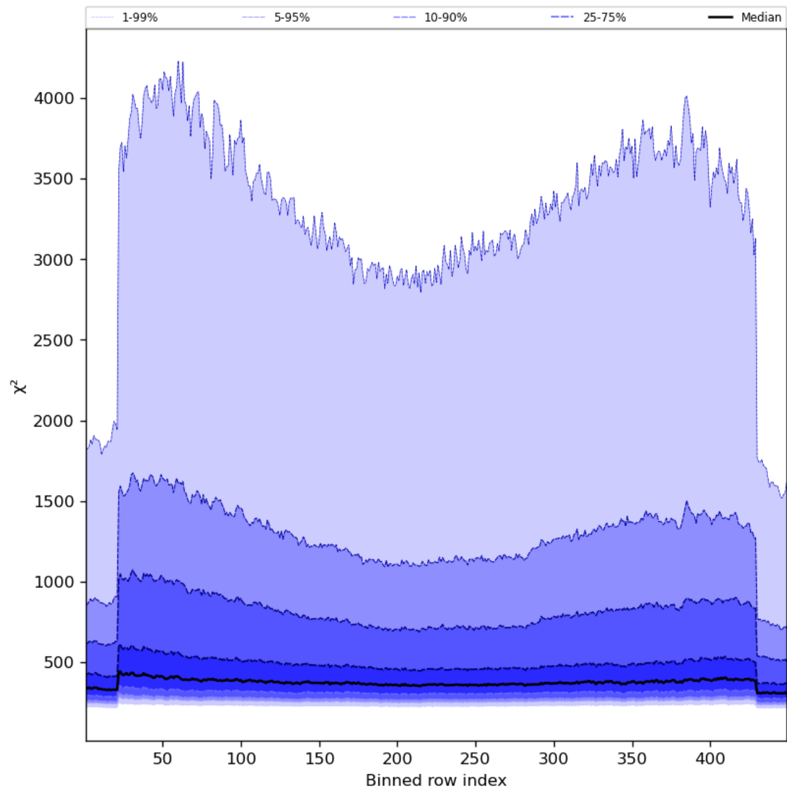
Figure 59: Along track statistics of “ \chi^2 ” for 2023-08-25 to 2023-08-27
