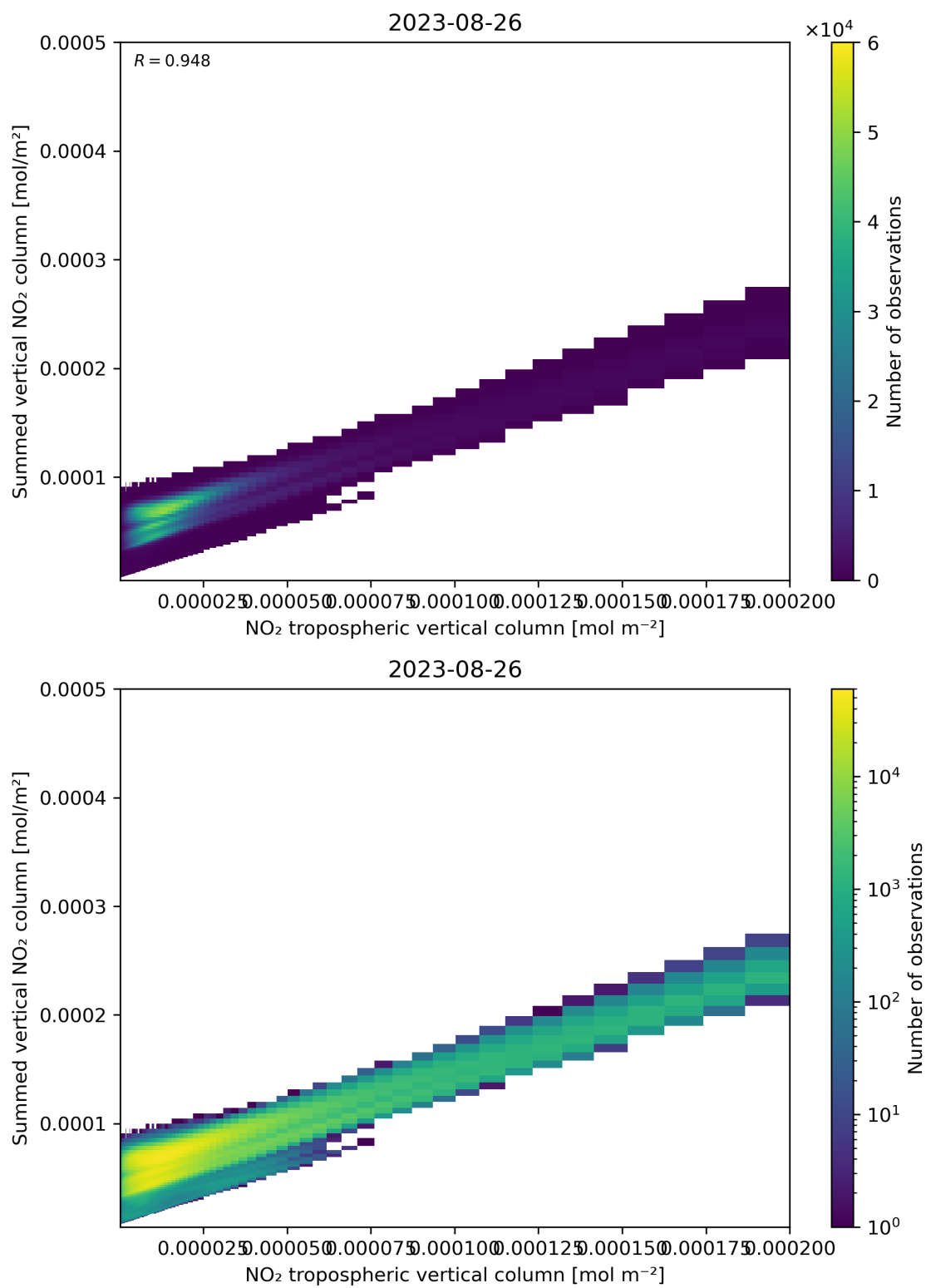
Figure 126: Scatter density plot of “NO 2 tropospheric vertical column” against “Summed vertical NO 2 column” for 2023-08-25 to 2023-08-27.
