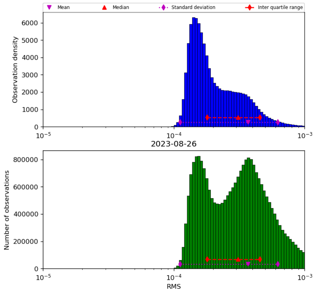
Figure 43: Histogram of “RMS” for 2023-08-25 to 2023-08-27
