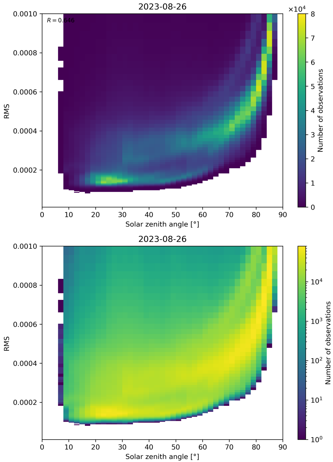
Figure 157: Scatter density plot of “Solar zenith angle” against “RMS” for 2023-08-25 to 2023-08-27.
