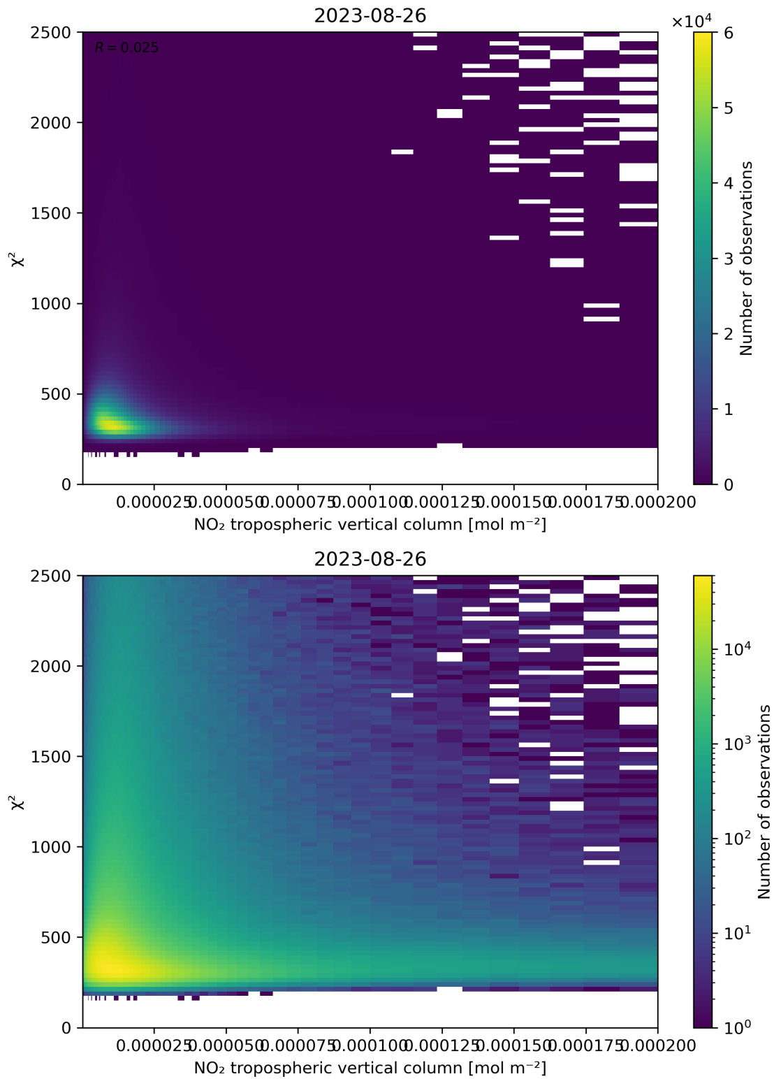
Figure 124: Scatter density plot of “NO 2 tropospheric vertical column” against “ \chi^2 ” for 2023-08-25 to 2023-08-27.
