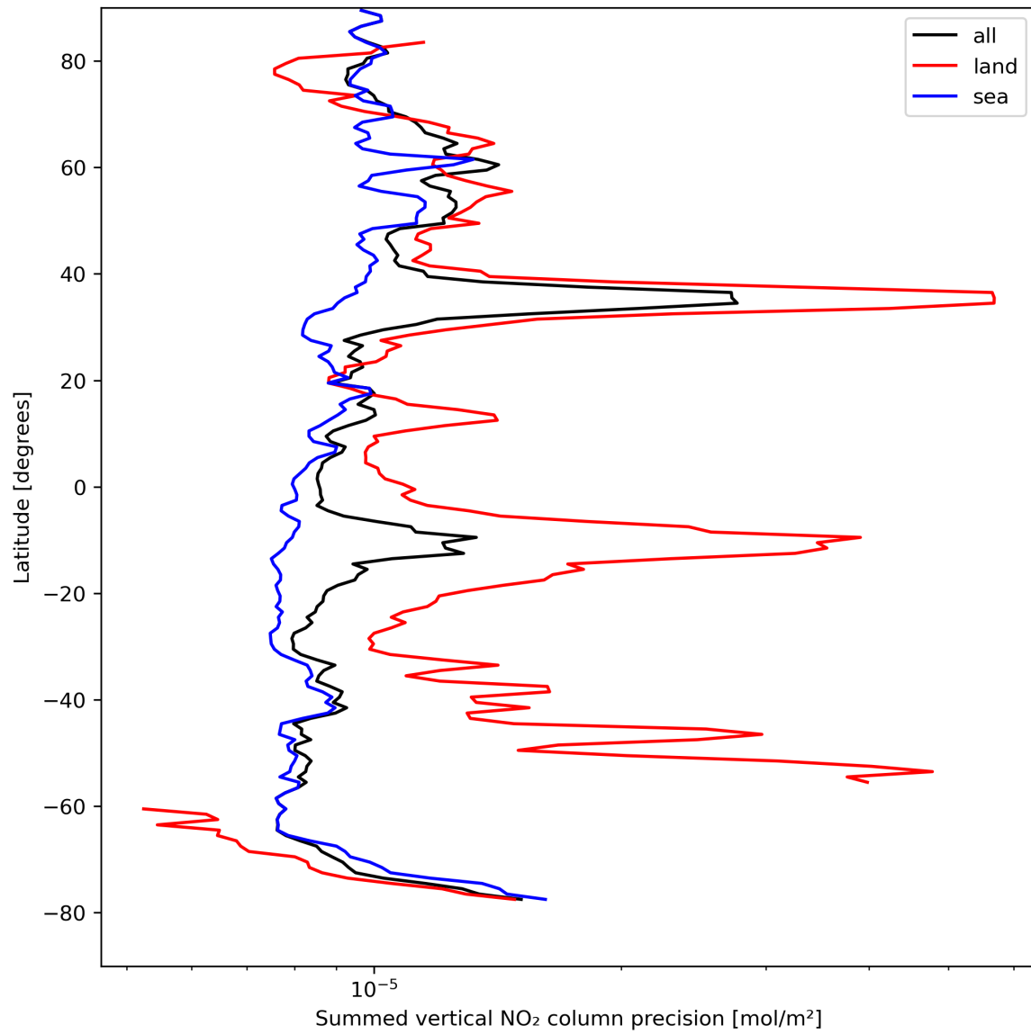
Figure 24: Zonal average of “Summed vertical NO 2 column precision” for 2023-08-25 to 2023-08-27.
