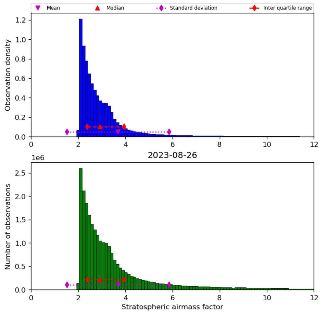
Figure 44: Histogram of “Stratospheric airmass factor” for 2023-08-25 to 2023-08-27
