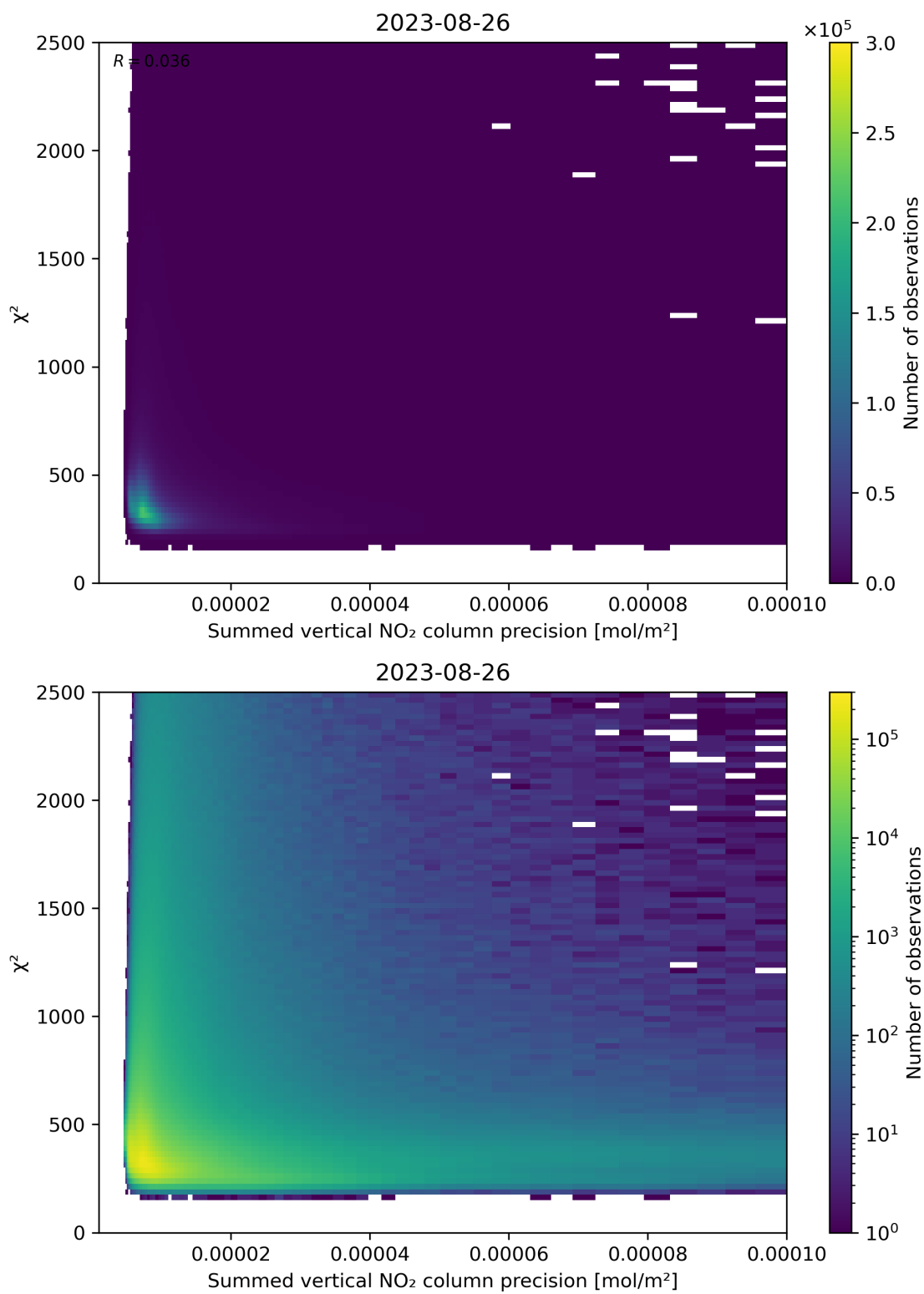
Figure 107: Scatter density plot of “Summed vertical NO 2 column precision” against “ \chi^2 ” for 2023-08-25 to 2023-08-27.
