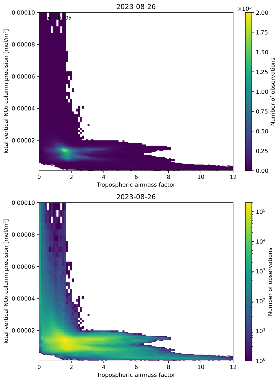
Figure 78: Scatter density plot of “Tropospheric airmass factor” against “Total vertical NO 2 column precision” for 2023-08-25 to 2023-08-27.
