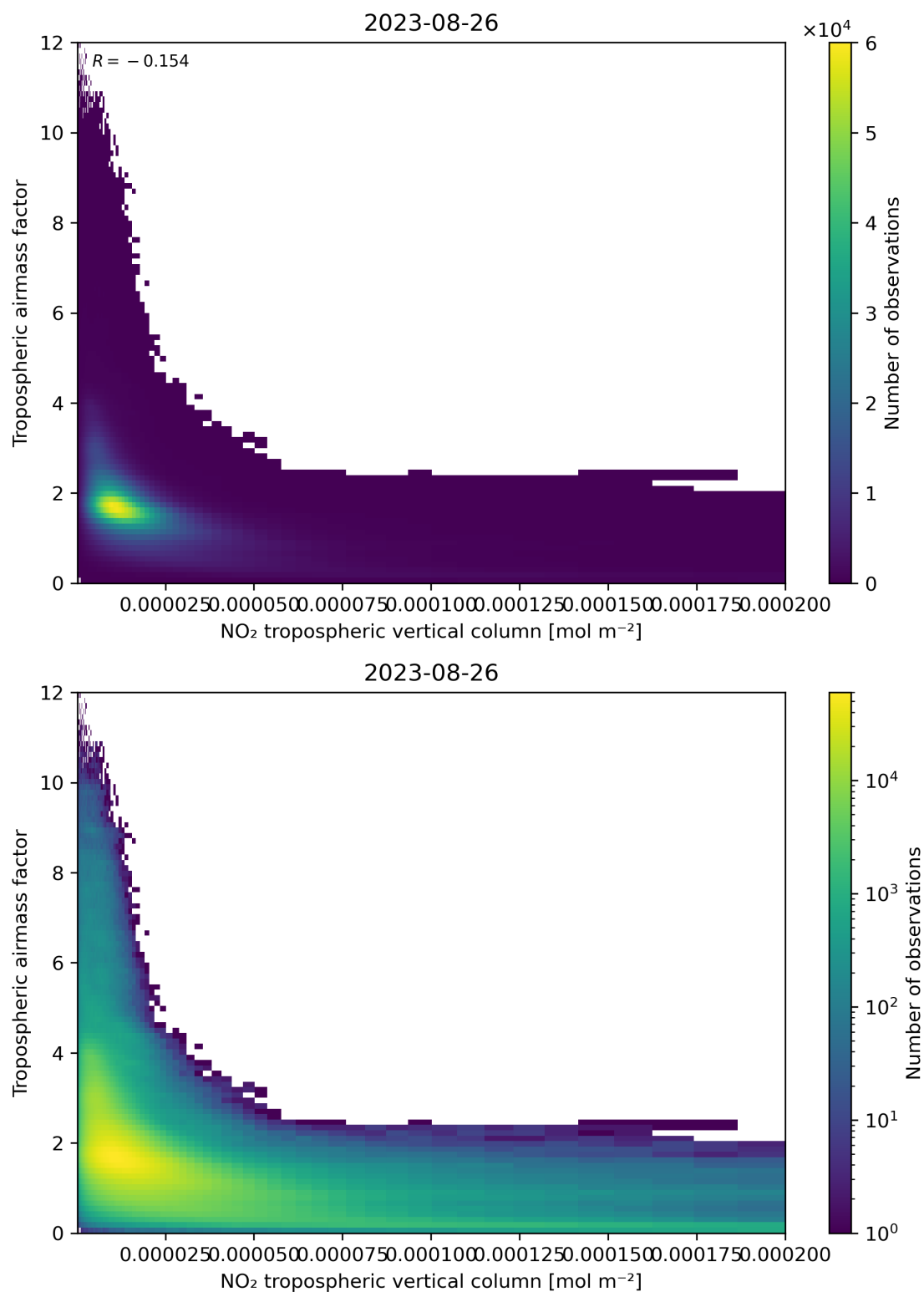
Figure 123: Scatter density plot of “NO 2 tropospheric vertical column” against “Tropospheric air mass factor” for 2023-08-25 to 2023-08-27.
