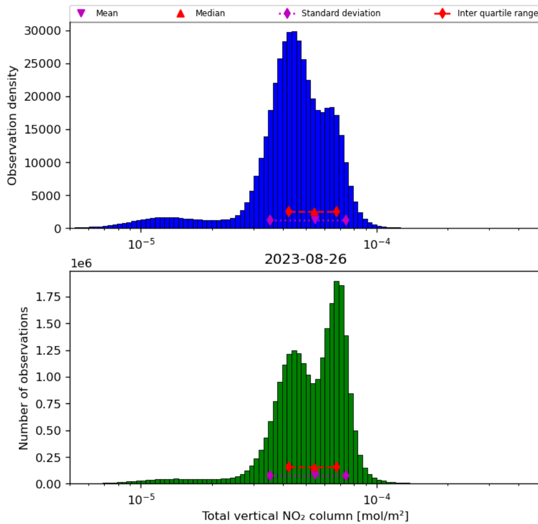
Figure 38: Histogram of “Total vertical NO 2 column” for 2023-08-25 to 2023-08-27
