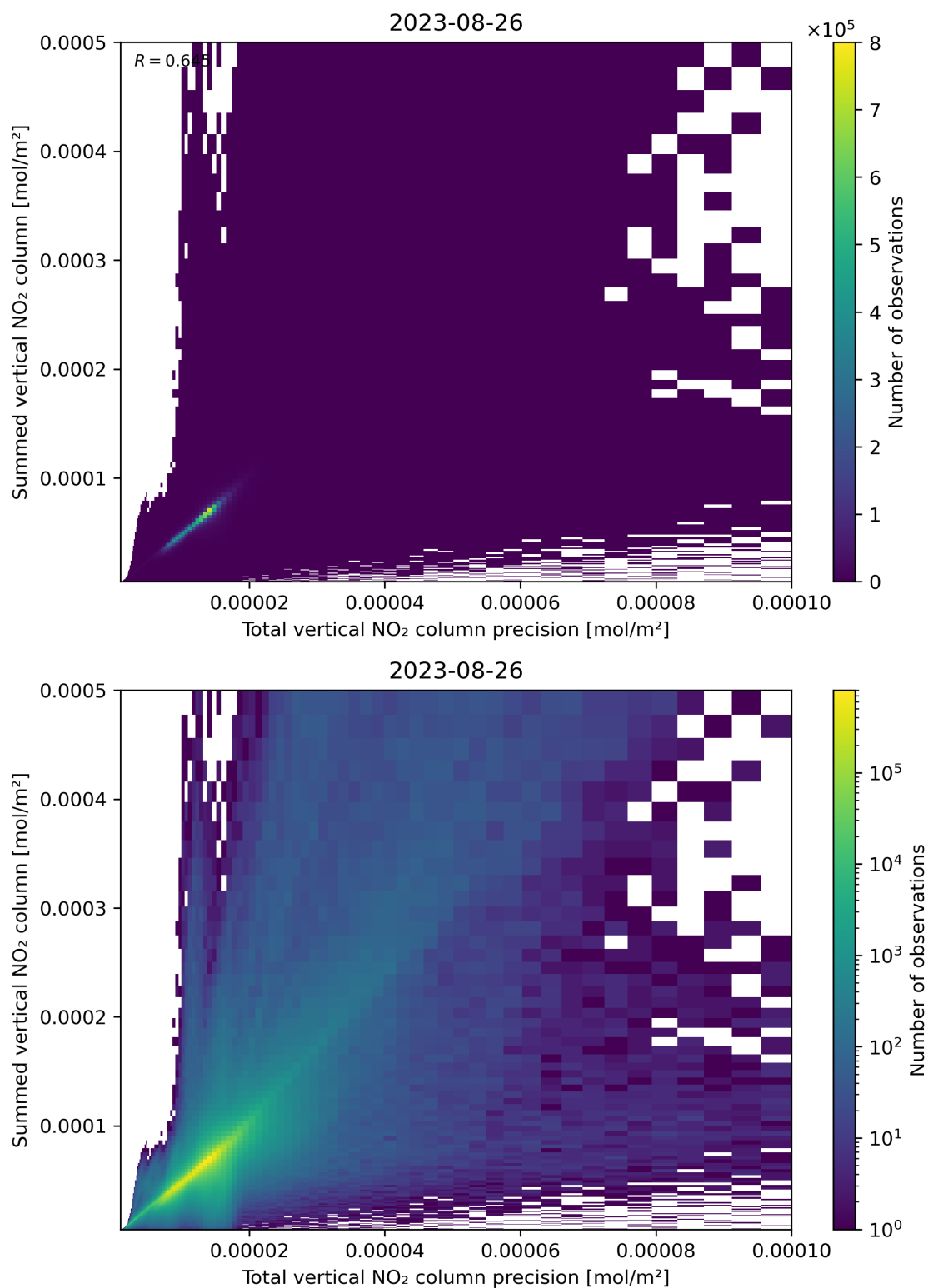
Figure 117: Scatter density plot of “Total vertical NO 2 column precision” against “Summed vertical NO 2 column” for 2023-08-25 to 2023-08-27.
