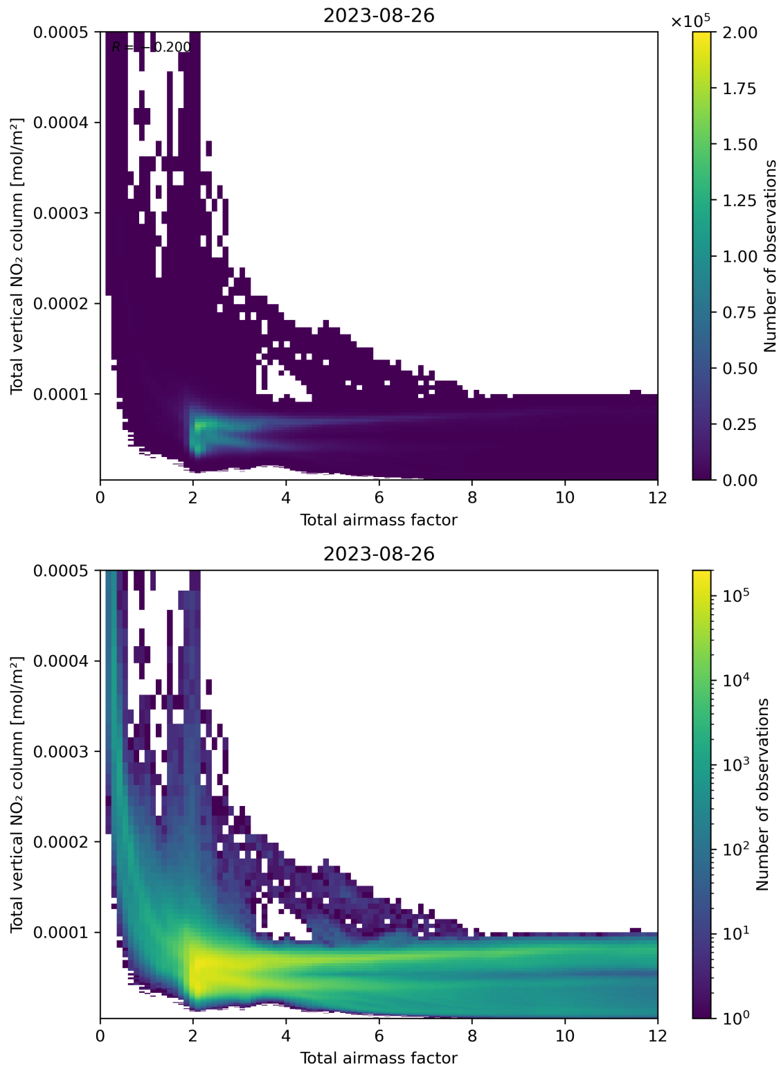
Figure 67: Scatter density plot of “Total airmass factor” against “Total vertical NO 2 column” for 2023-08-25 to 2023-08-27.
