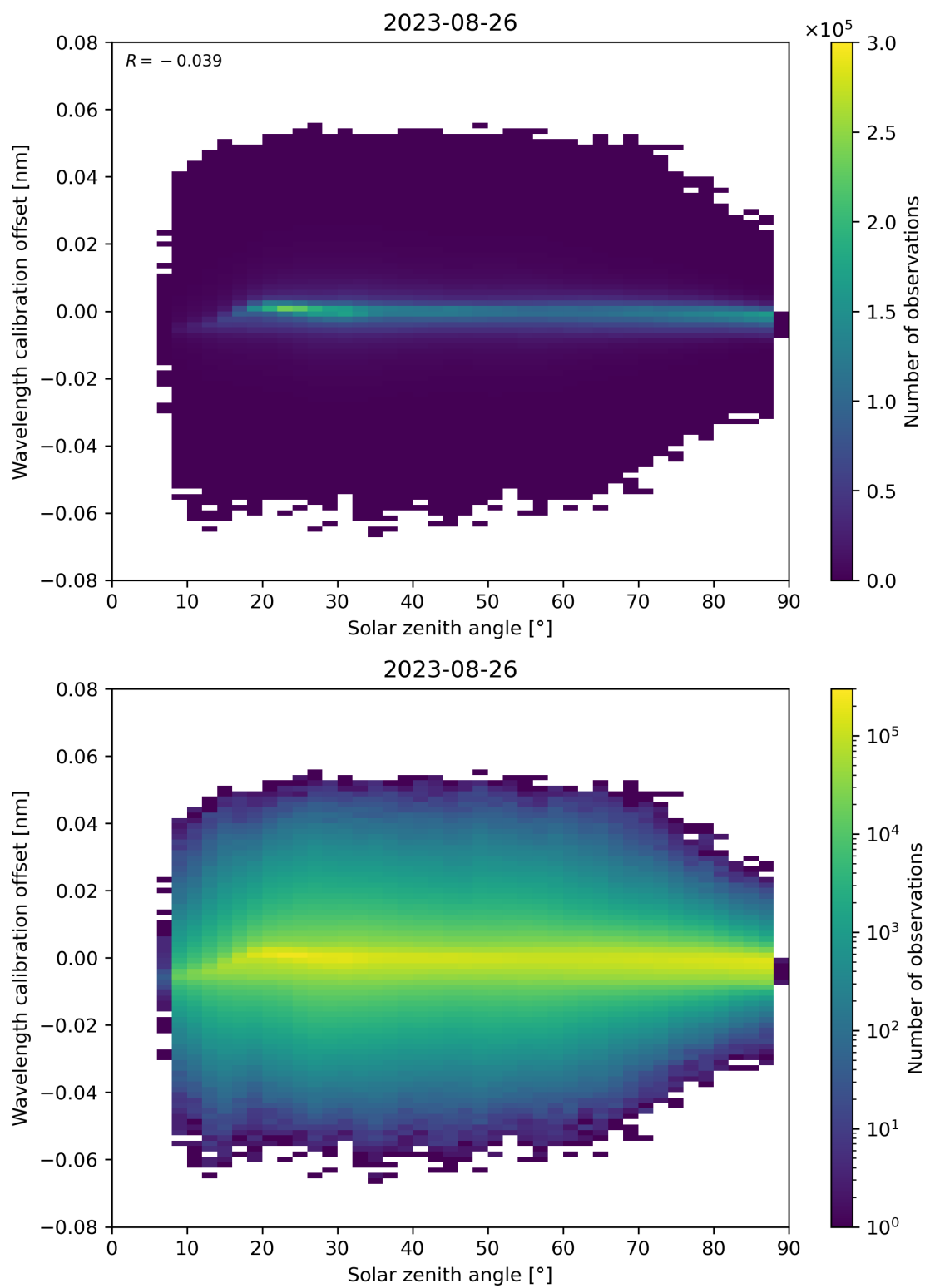
Figure 158: Scatter density plot of “Solar zenith angle” against “Wavelength calibration offset” for 2023-08-25 to 2023-08-27.
