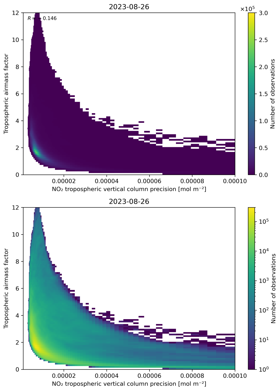
Figure 133: Scatter density plot of “NO 2 tropospheric vertical column precision” against “Tropospheric air mass factor” for 2023-08-25 to 2023-08-27.
