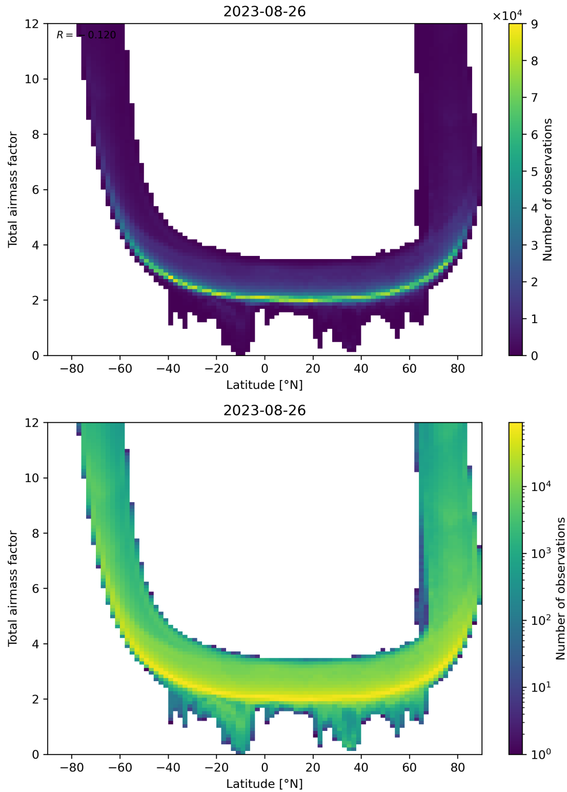
Figure 84: Scatter density plot of “Latitude” against “Total airmass factor” for 2023-08-25 to 2023-08-27.
