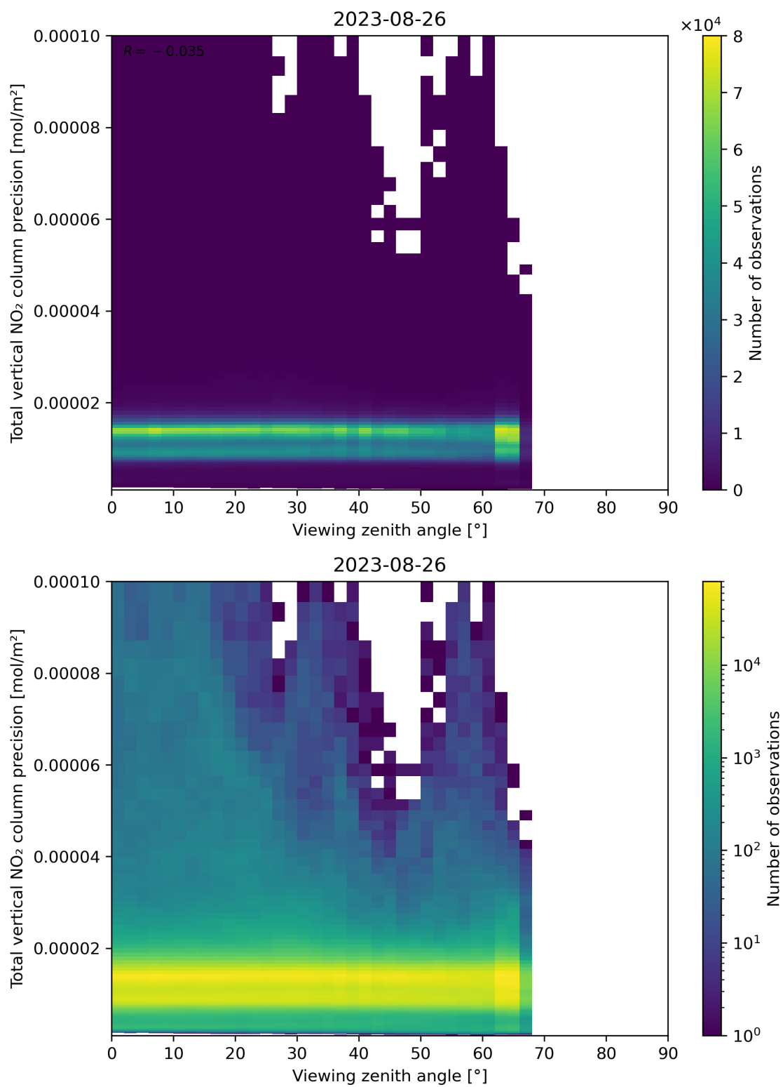
Figure 168: Scatter density plot of “Viewing zenith angle” against “Total vertical NO 2 column precision” for 2023-08-25 to 2023-08-27.
