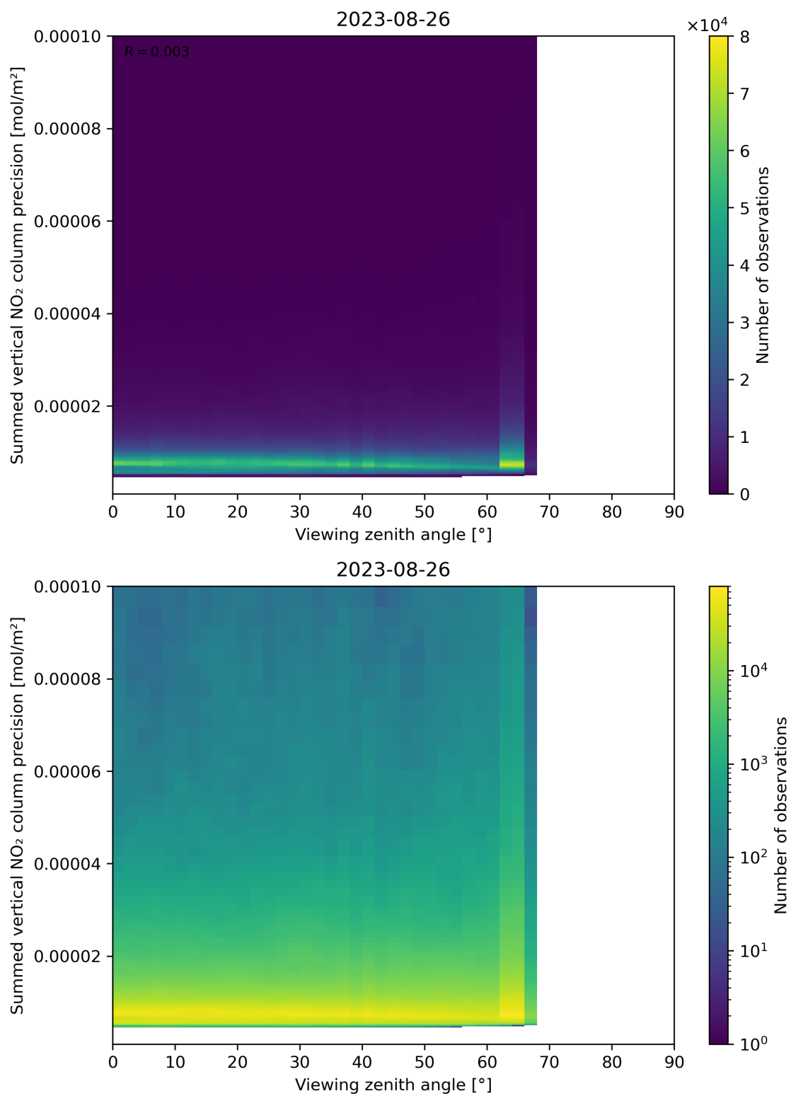
Figure 166: Scatter density plot of “Viewing zenith angle” against “Summed vertical NO 2 column precision” for 2023-08-25 to 2023-08-27.
