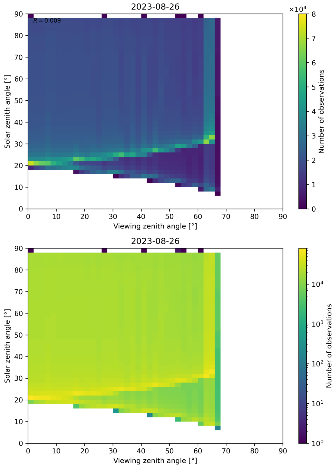
Figure 172: Scatter density plot of “Viewing zenith angle” against “Solar zenith angle” for 2023-08-25 to 2023-08-27.
