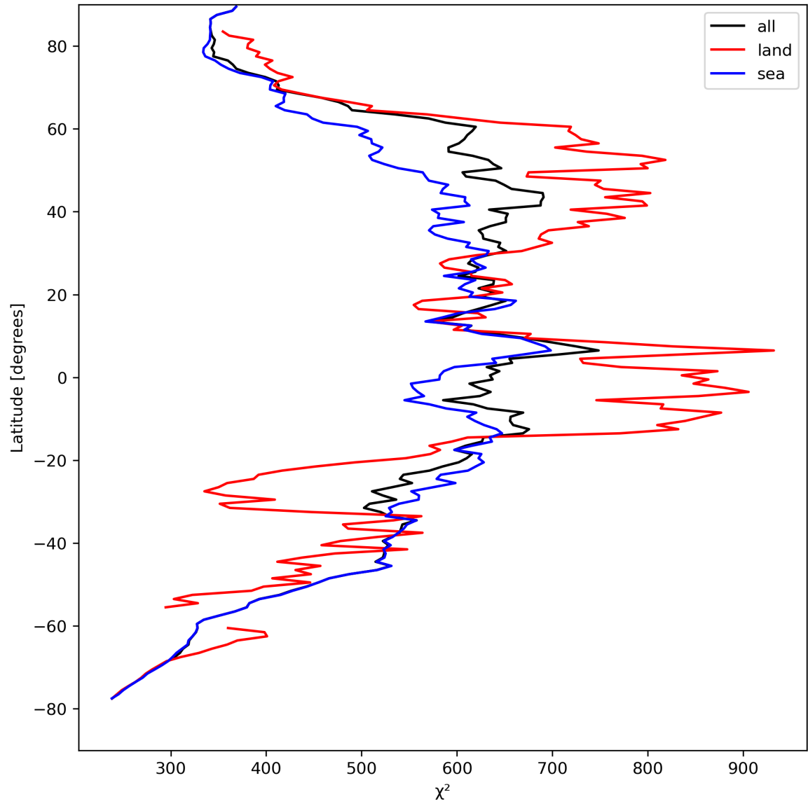
Figure 25: Zonal average of “ \chi^2 ” for 2023-08-25 to 2023-08-27.
