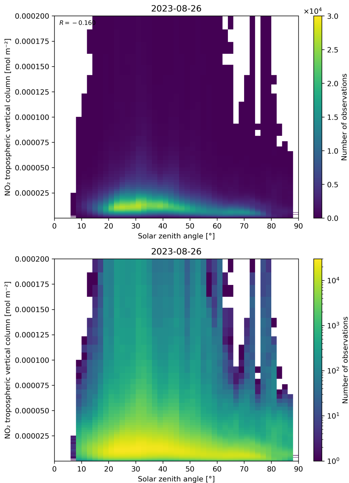
Figure 155: Scatter density plot of “Solar zenith angle” against “NO 2 tropospheric vertical column” for 2023-08-25 to 2023-08-27.
