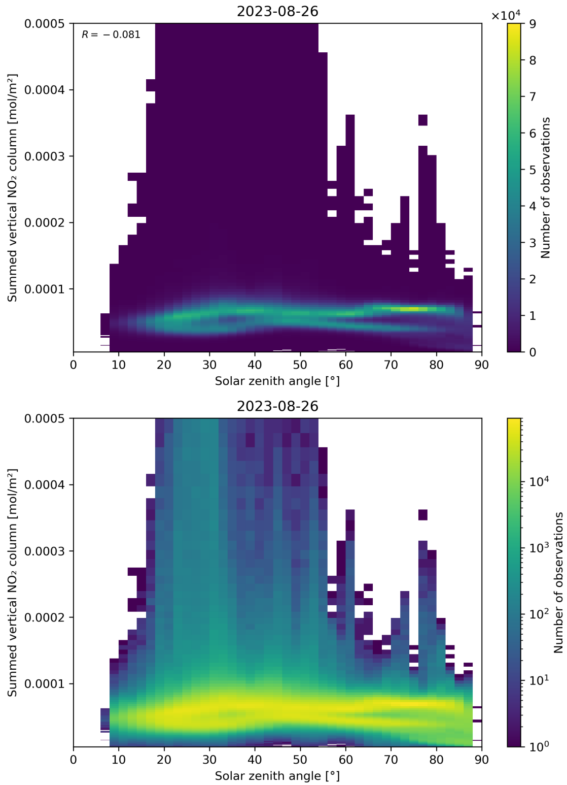
Figure 151: Scatter density plot of “Solar zenith angle” against “Summed vertical NO 2 column” for 2023-08-25 to 2023-08-27.
