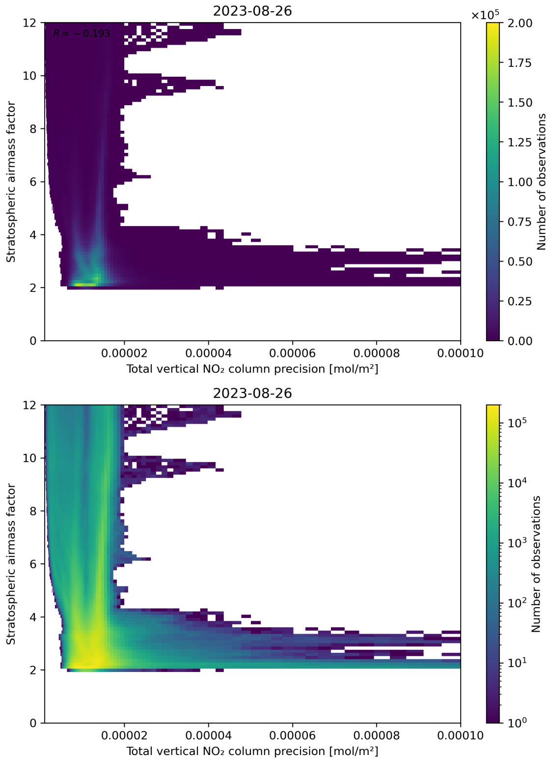
Figure 115: Scatter density plot of “Total vertical NO 2 column precision” against “Stratospheric air mass factor” for 2023-08-25 to 2023-08-27.
