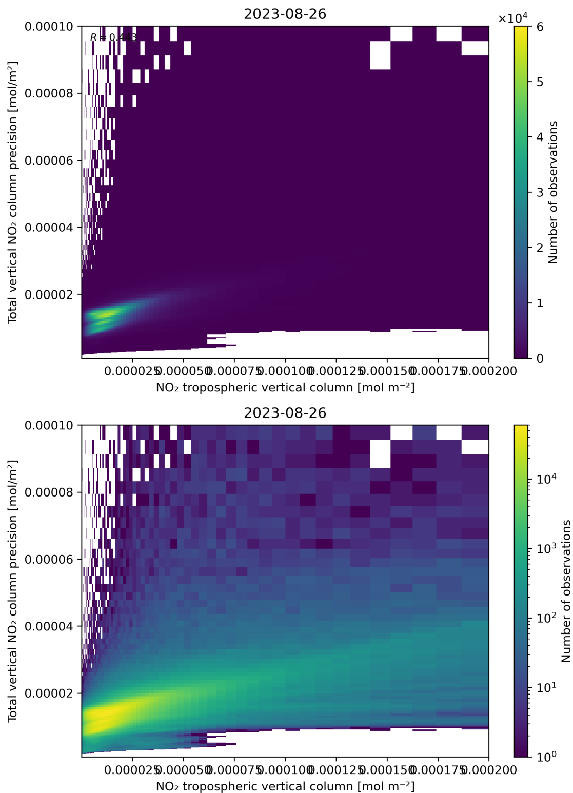
Figure 129: Scatter density plot of “NO 2 tropospheric vertical column” against “Total vertical NO 2 column precision” for 2023-08-25 to 2023-08-27.
