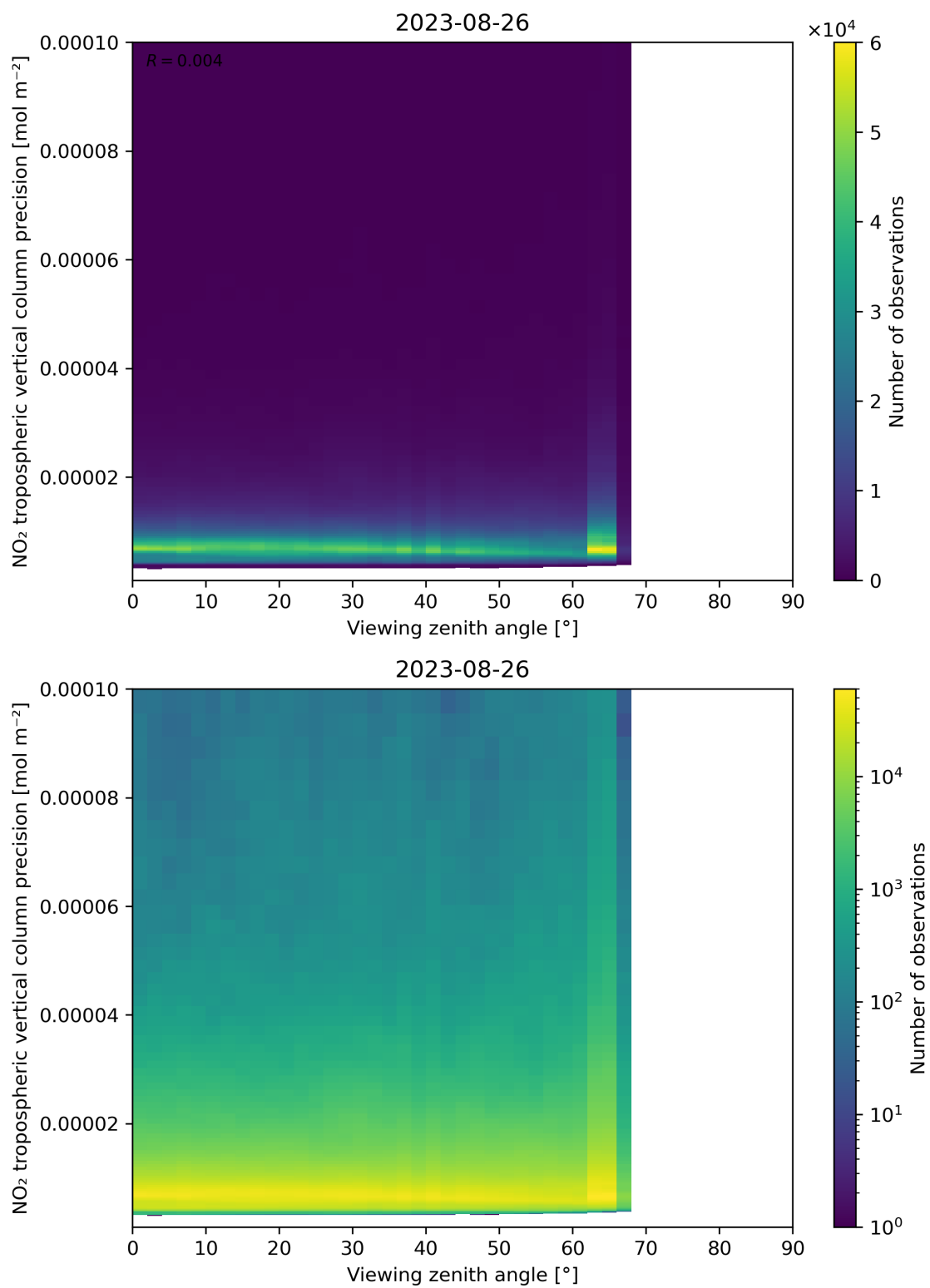
Figure 170: Scatter density plot of “Viewing zenith angle” against “NO 2 tropospheric vertical column precision” for 2023-08-25 to 2023-08-27.
