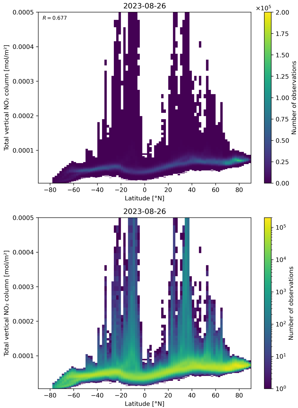
Figure 90: Scatter density plot of “Latitude” against “Total vertical NO 2 column” for 2023-08-25 to 2023-08-27.
