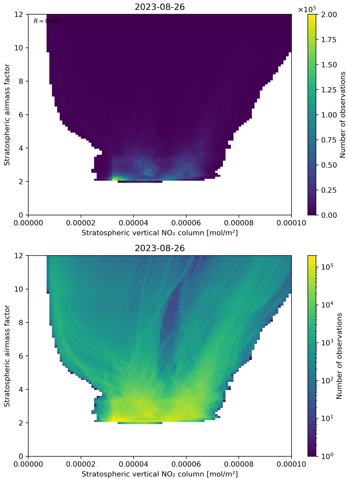
Figure 96: Scatter density plot of “Stratospheric vertical NO 2 column” against “Stratospheric airmass factor” for 2023-08-25 to 2023-08-27.
