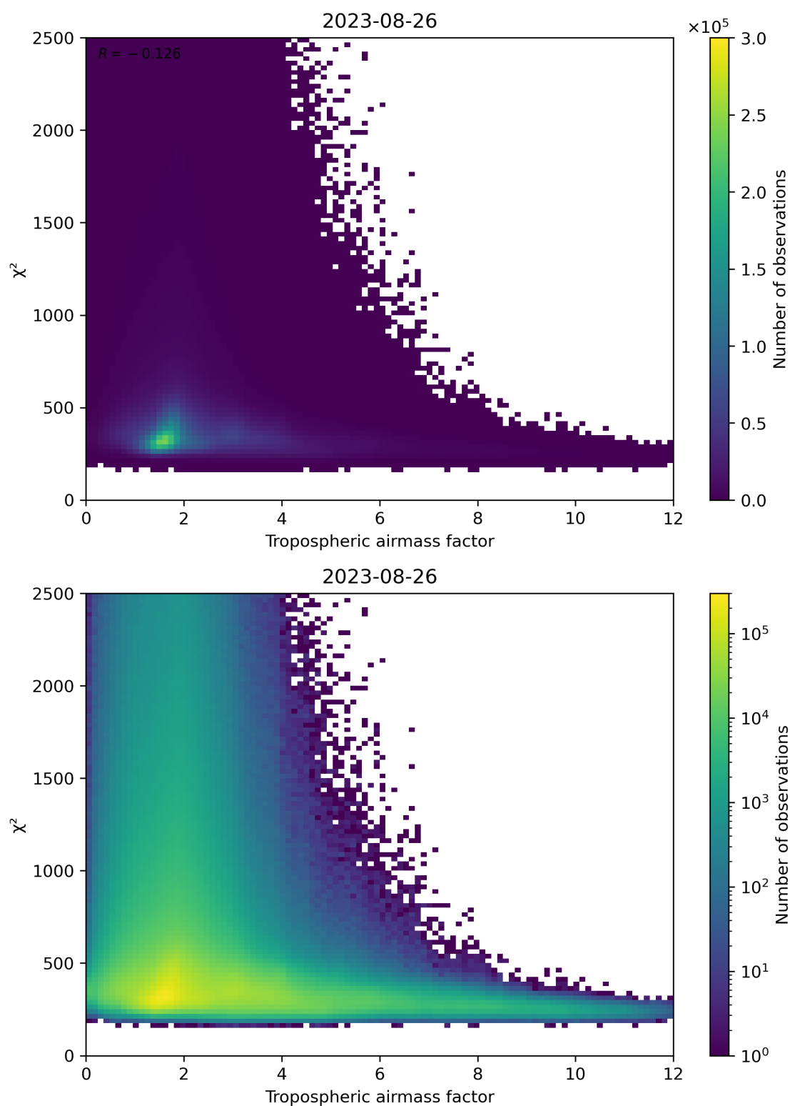
Figure 73: Scatter density plot of “Tropospheric airmass factor” against “ \chi^2 ” for 2023-08-25 to 2023-08-27.
