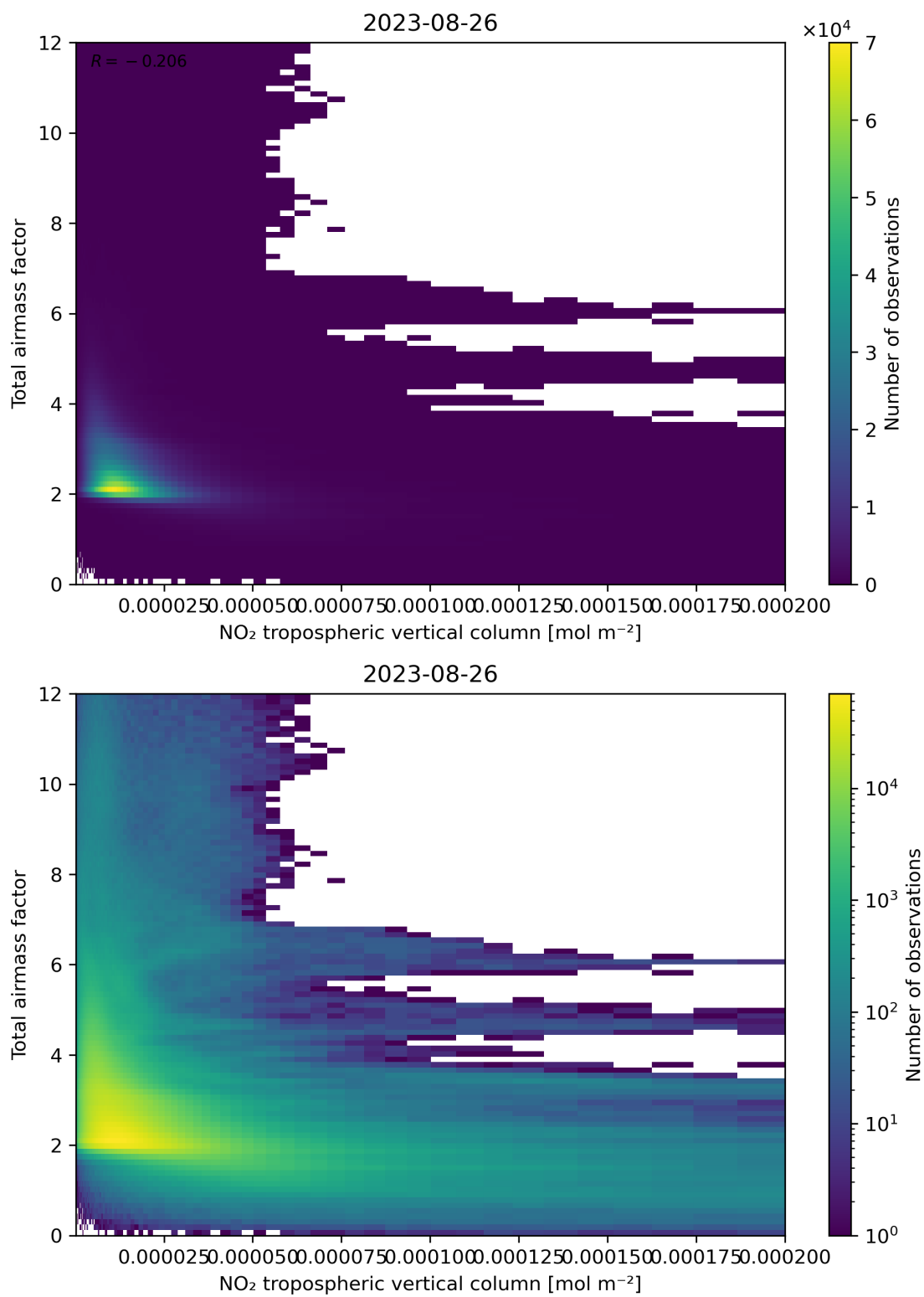
Figure 122: Scatter density plot of “NO 2 tropospheric vertical column” against “Total air mass factor” for 2023-08-25 to 2023-08-27.
