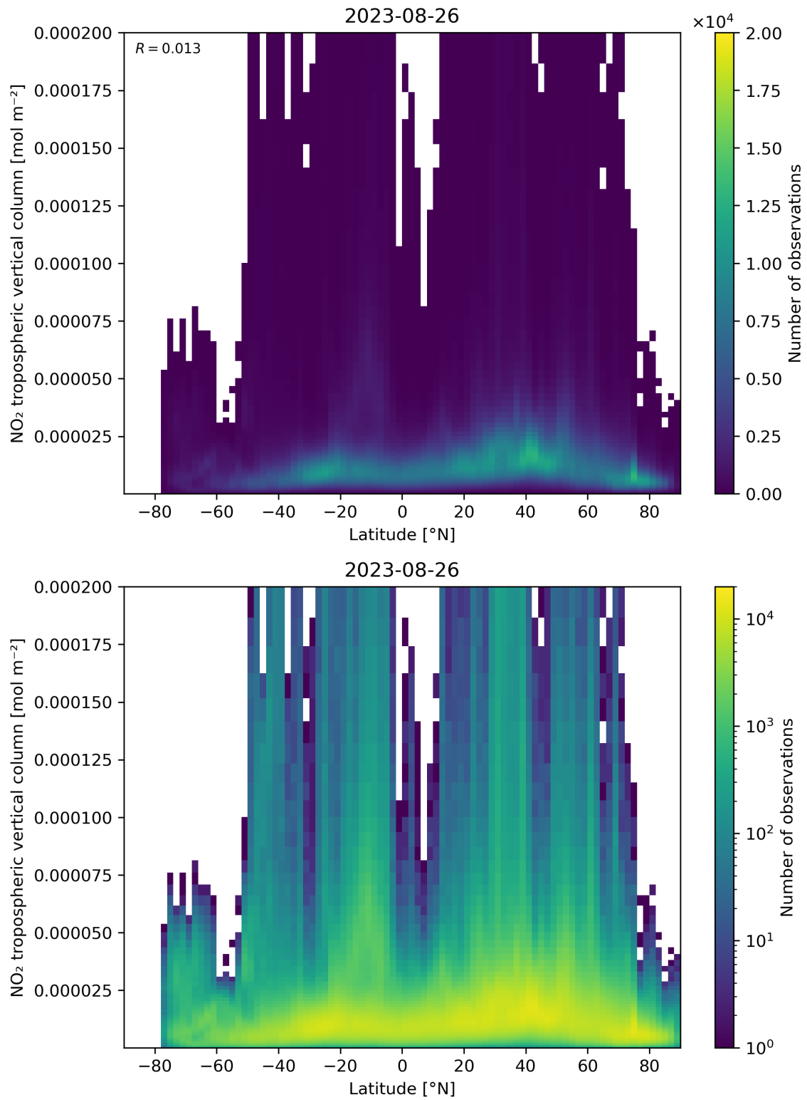
Figure 92: Scatter density plot of “Latitude” against “NO 2 tropospheric vertical column” for 2023-08-25 to 2023-08-27.
