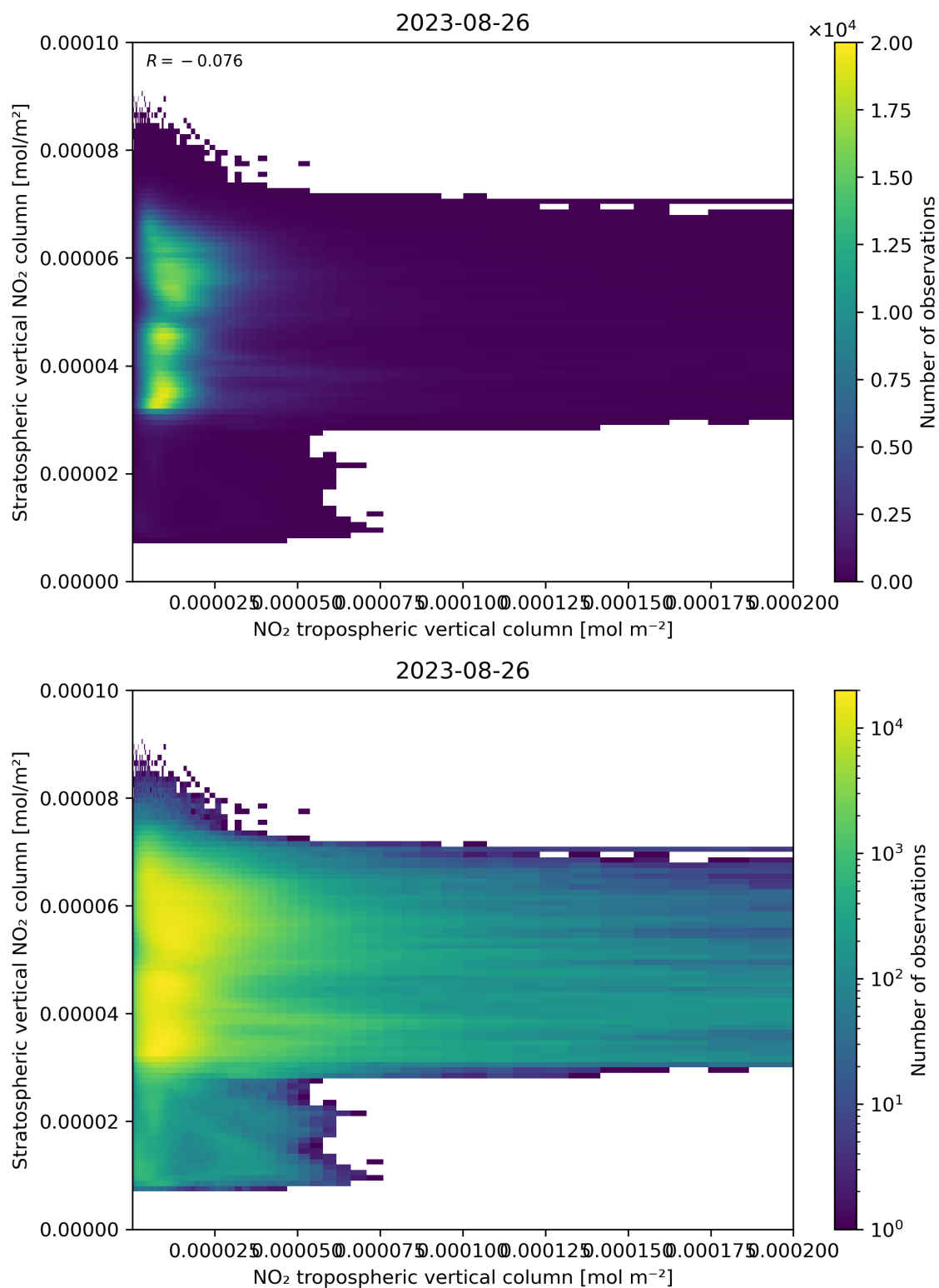
Figure 125: Scatter density plot of “NO 2 tropospheric vertical column” against “Stratospheric vertical NO 2 column” for 2023-08-25 to 2023-08-27.
