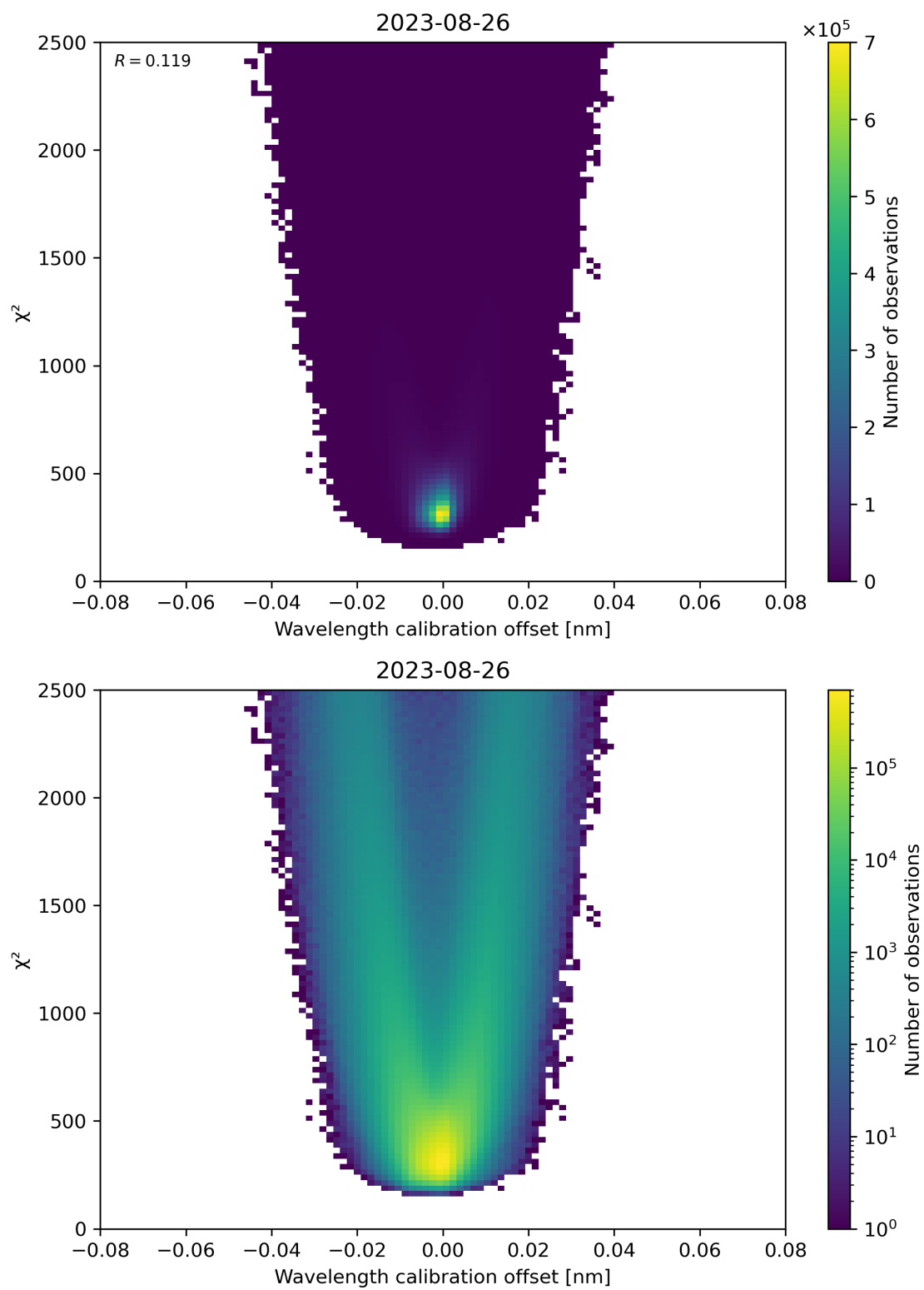
Figure 175: Scatter density plot of “Wavelength calibration offset” against “ \chi^2 ” for 2023-08-25 to 2023-08-27.
