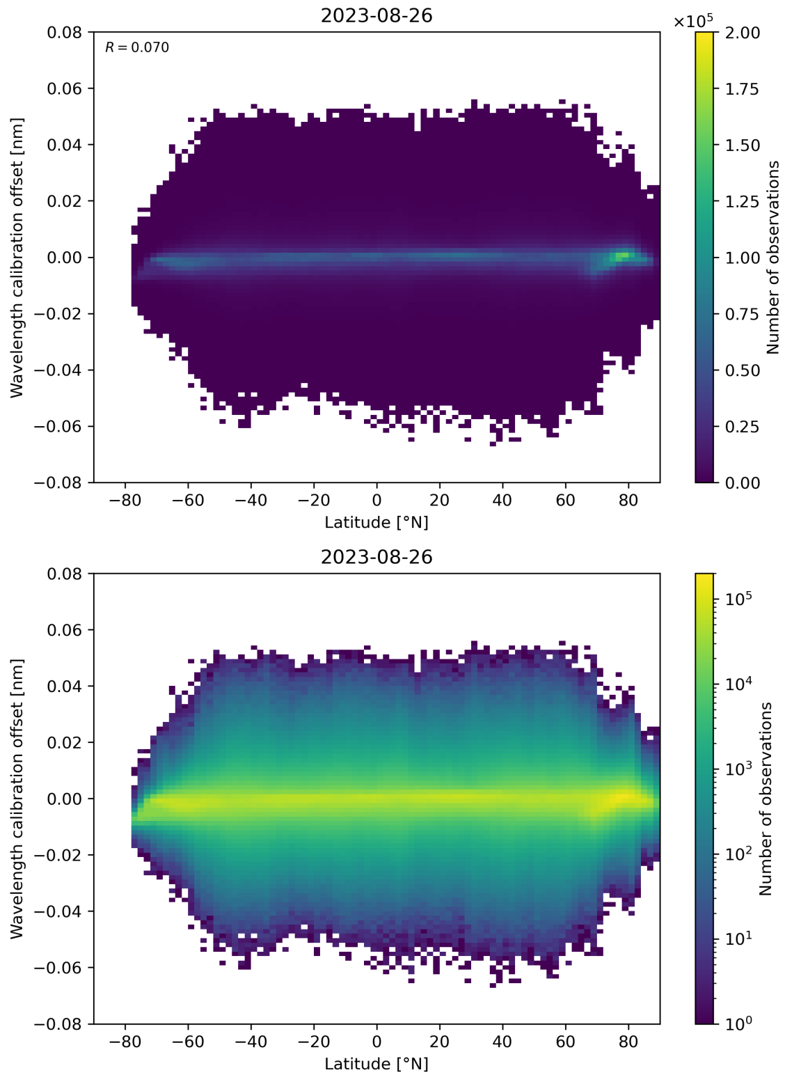
Figure 95: Scatter density plot of “Latitude” against “Wavelength calibration offset” for 2023-08-25 to 2023-08-27.
