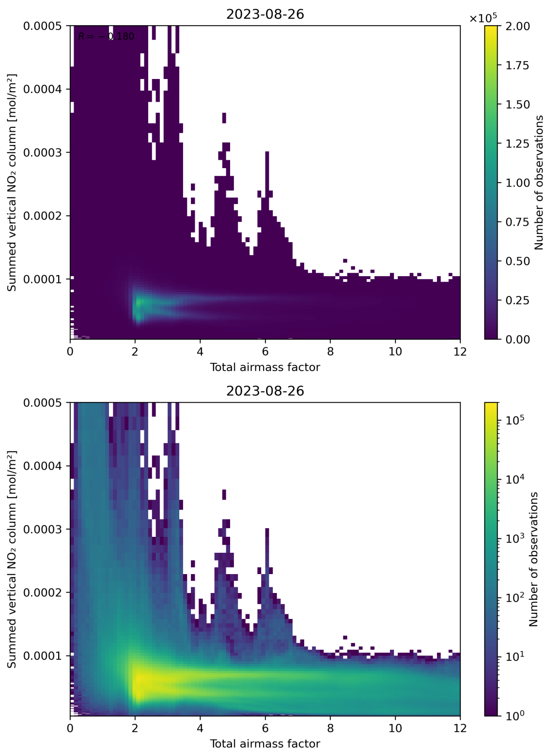
Figure 65: Scatter density plot of “Total airmass factor” against “Summed vertical NO 2 column” for 2023-08-25 to 2023-08-27.
