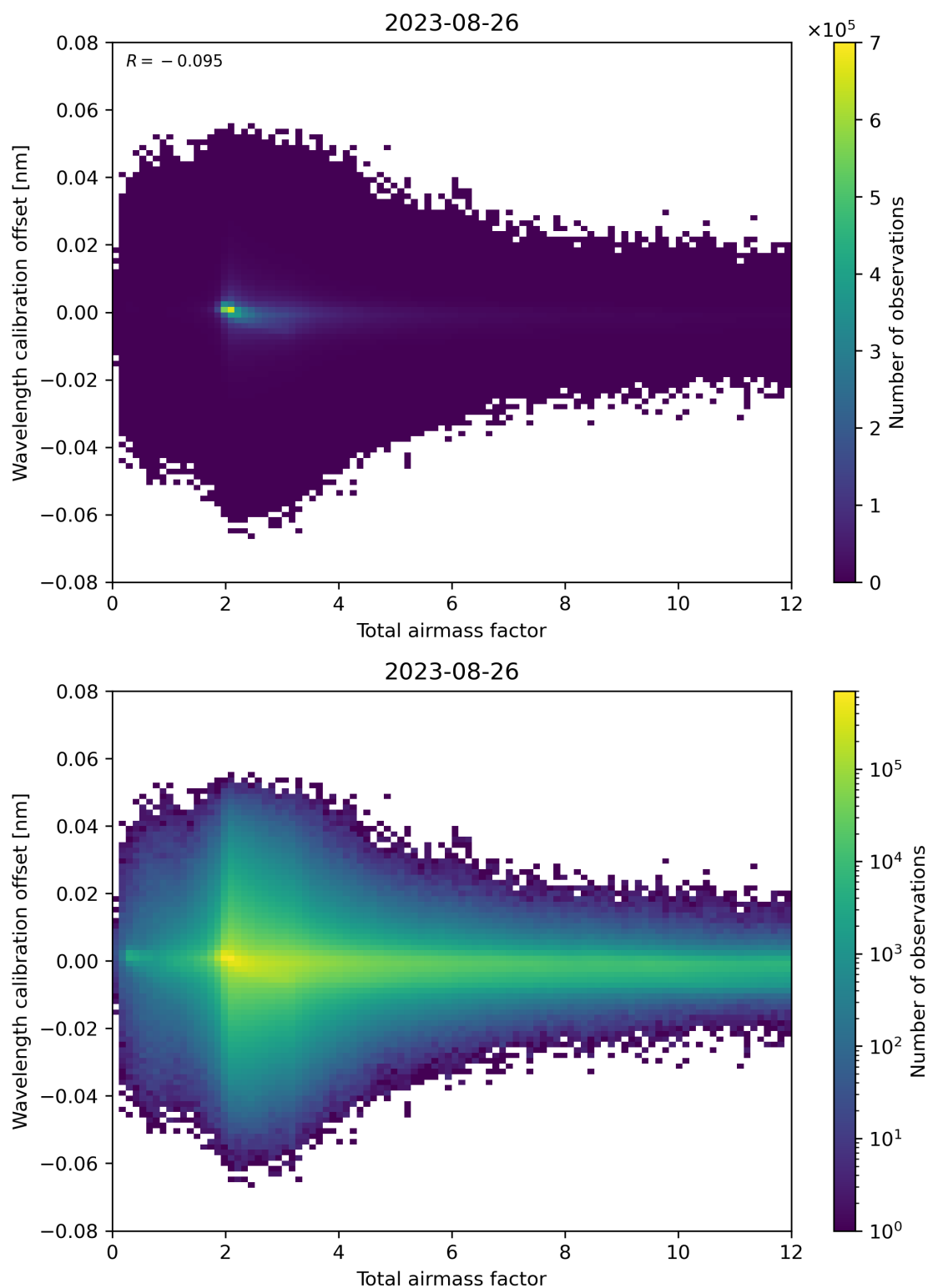
Figure 70: Scatter density plot of “Total airmass factor” against “Wavelength calibration offset” for 2023-08-25 to 2023-08-27.
