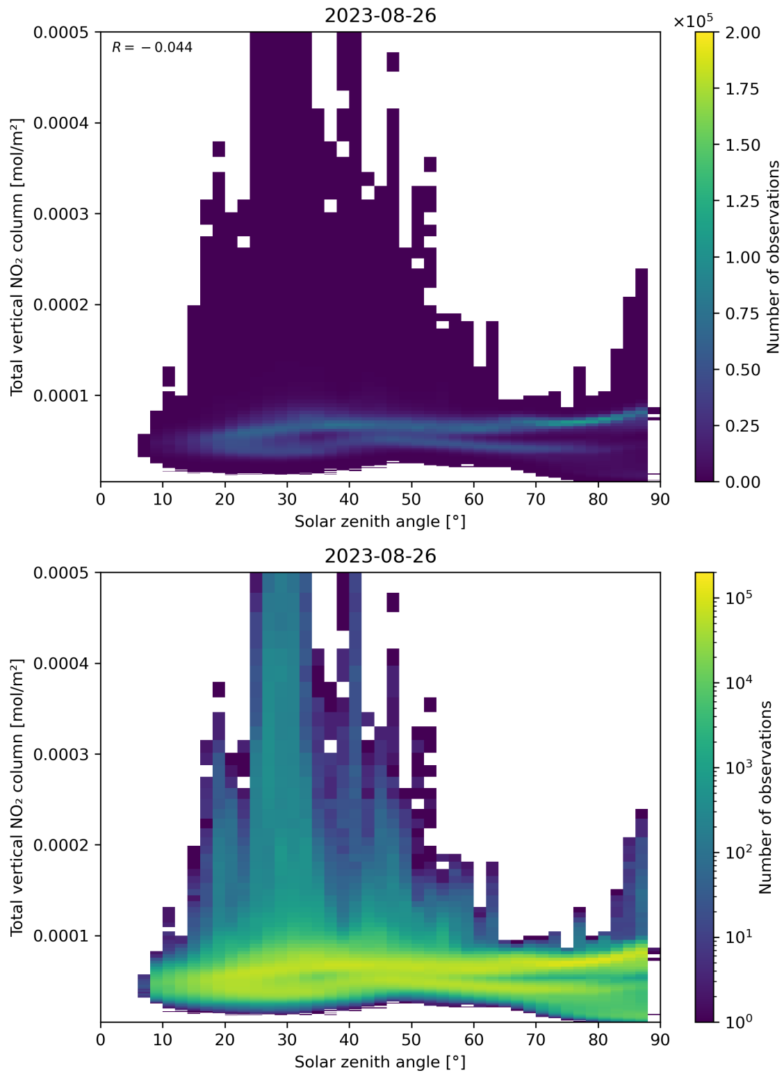
Figure 153: Scatter density plot of “Solar zenith angle” against “Total vertical NO 2 column” for 2023-08-25 to 2023-08-27.
