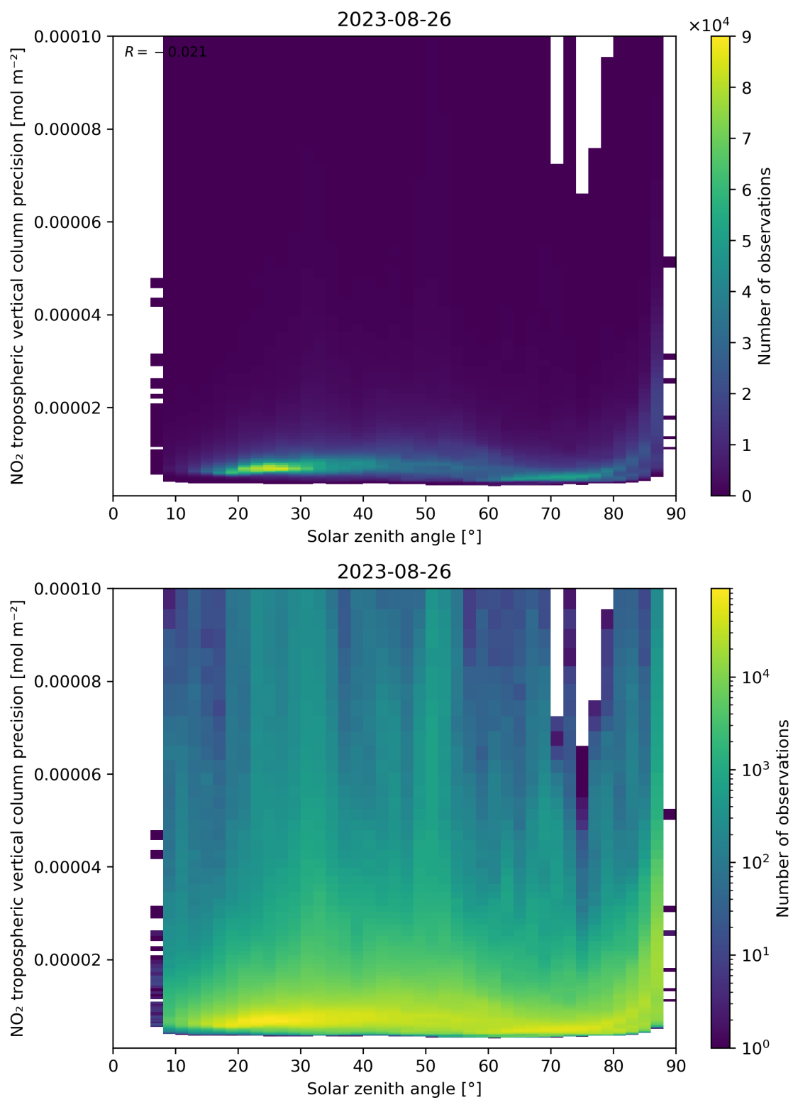
Figure 156: Scatter density plot of “Solar zenith angle” against “NO 2 tropospheric vertical column precision” for 2023-08-25 to 2023-08-27.
