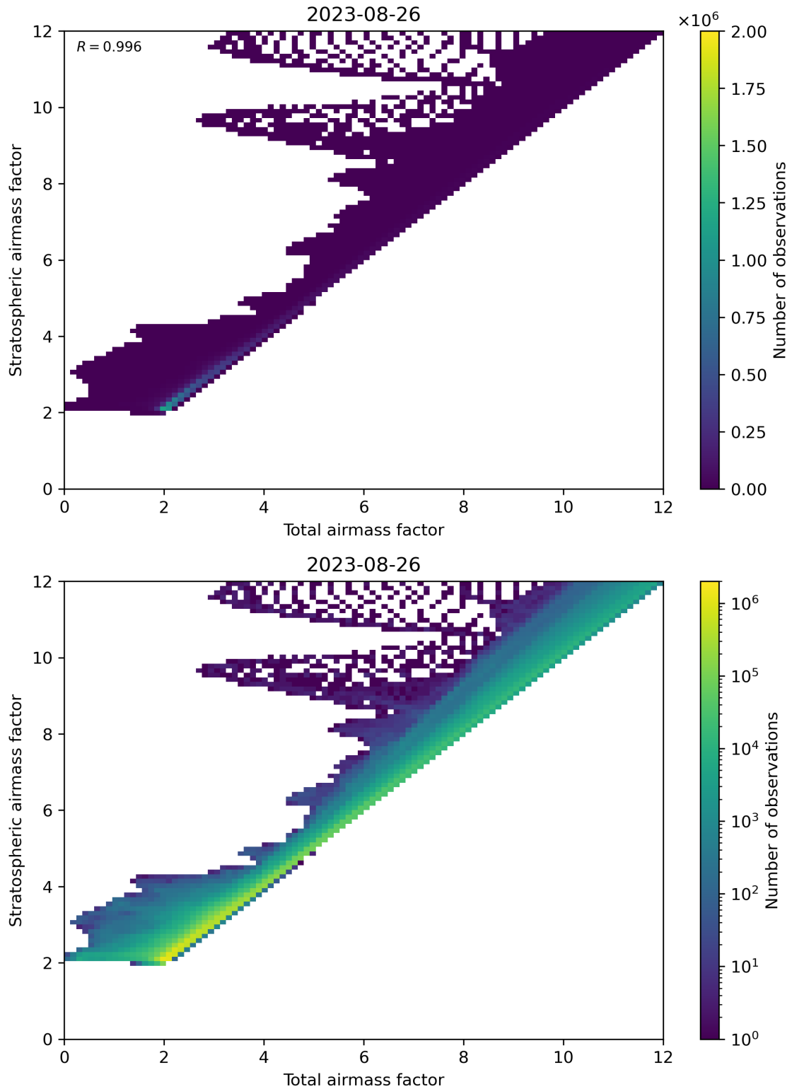
Figure 62: Scatter density plot of “Total airmass factor” against “Stratospheric airmass factor” for 2023-08-25 to 2023-08-27.
