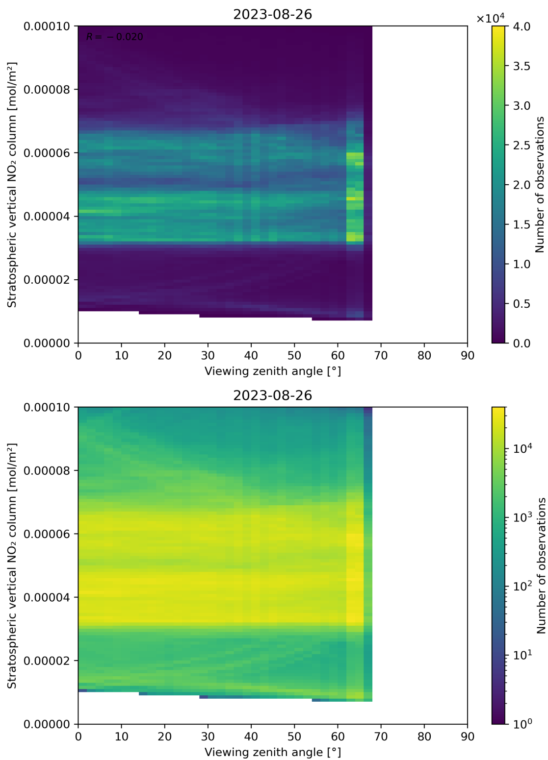
Figure 164: Scatter density plot of “Viewing zenith angle” against “Stratospheric vertical NO 2 column” for 2023-08-25 to 2023-08-27.
