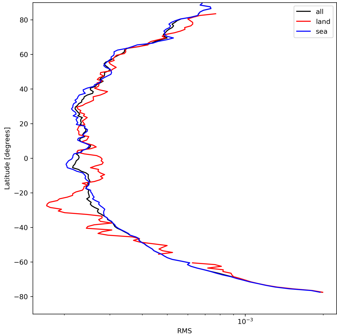
Figure 26: Zonal average of “RMS” for 2023-08-25 to 2023-08-27.
