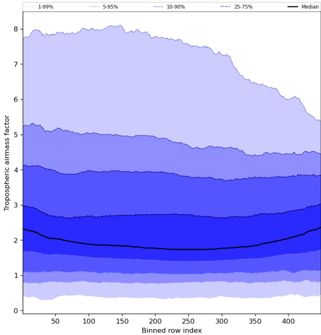
Figure 48: Along track statistics of “Tropospheric airmass factor” for 2023-08-25 to 2023-08-27
