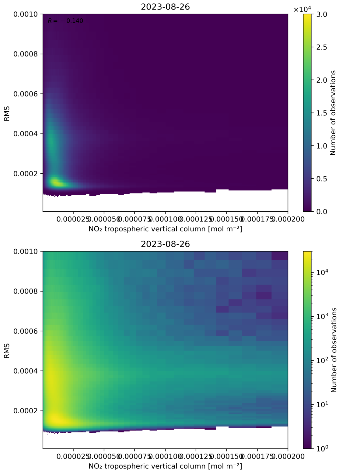
Figure 142: Scatter density plot of “NO 2 tropospheric vertical column” against “RMS” for 2023-08-25 to 2023-08-27.
