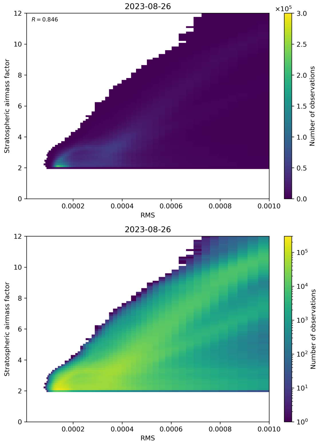
Figure 144: Scatter density plot of “RMS” against “Stratospheric airmass factor” for 2023-08-25 to 2023-08-27.
