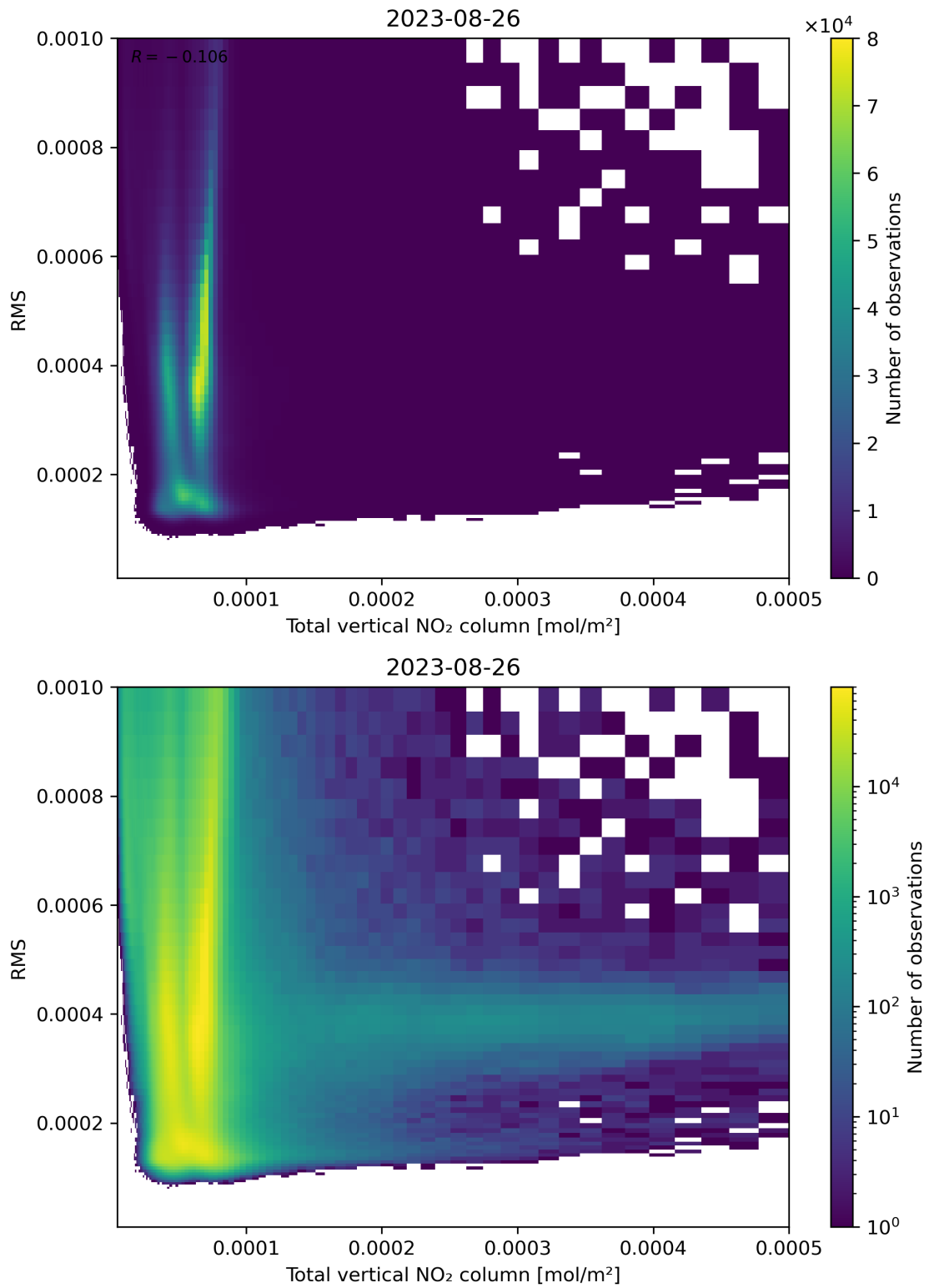
Figure 120: Scatter density plot of “Total vertical NO 2 column” against “RMS” for 2023-08-25 to 2023-08-27.
