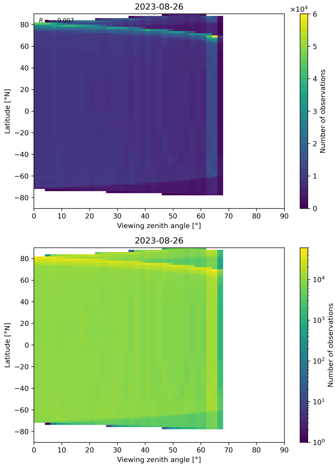
Figure 163: Scatter density plot of “Viewing zenith angle” against “Latitude” for 2023-08-25 to 2023-08-27.
