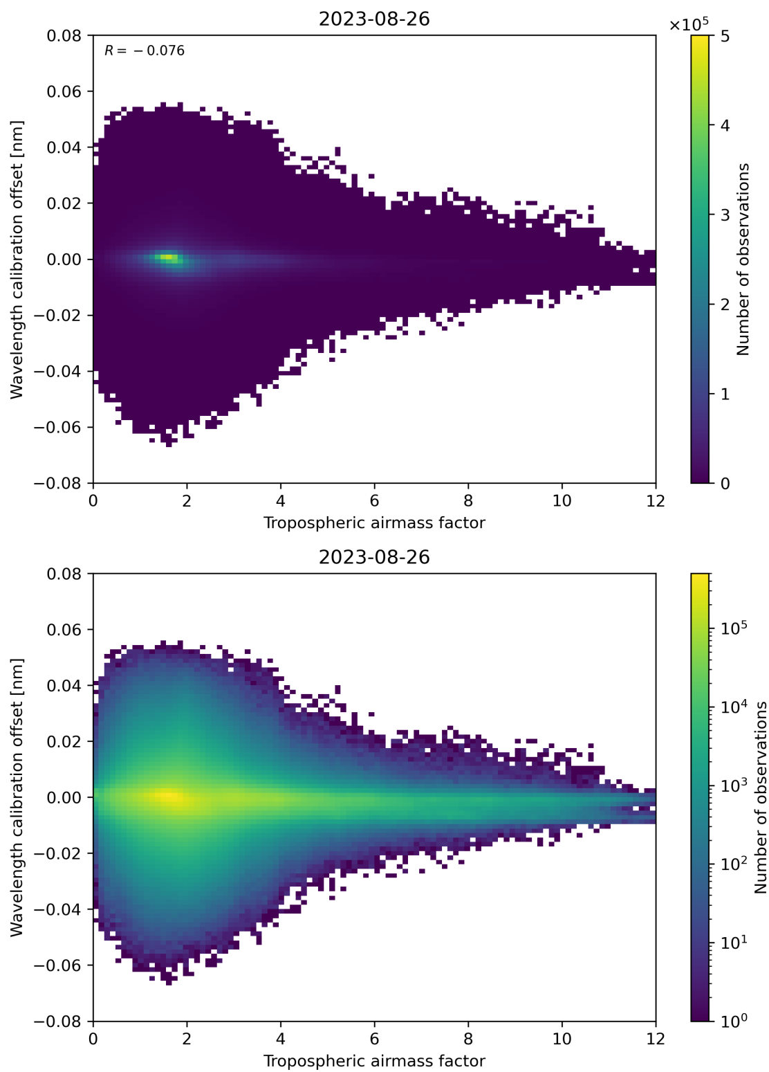
Figure 80: Scatter density plot of “Tropospheric airmass factor” against “Wavelength calibration offset” for 2023-08-25 to 2023-08-27.
