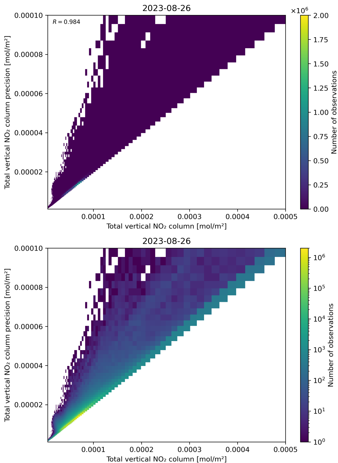
Figure 114: Scatter density plot of “Total vertical NO 2 column” against “Total vertical NO 2 column precision” for 2023-08-25 to 2023-08-27.
