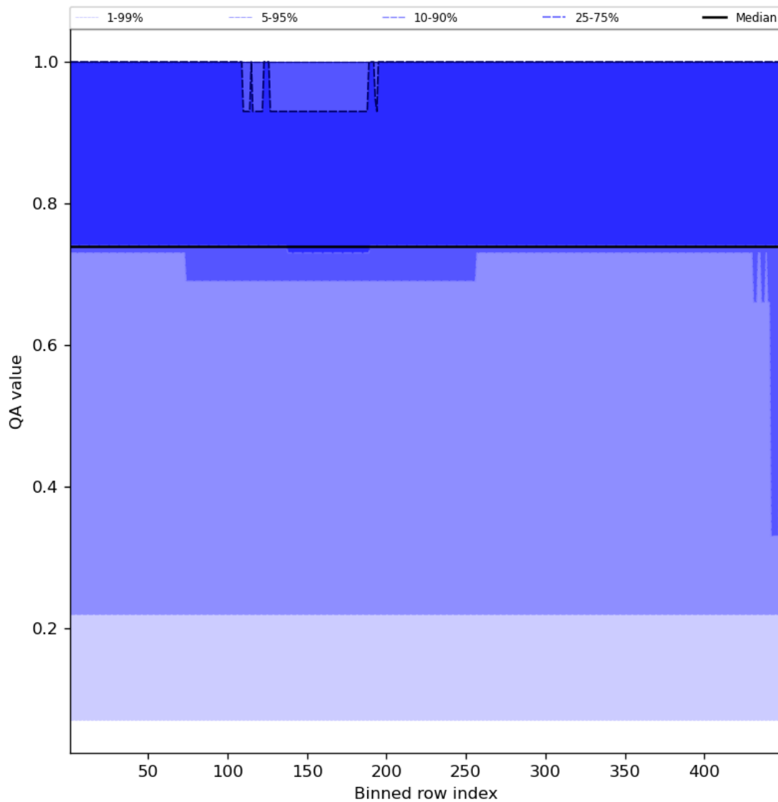
Figure 45: Along track statistics of “QA value” for 2023-08-25 to 2023-08-27
