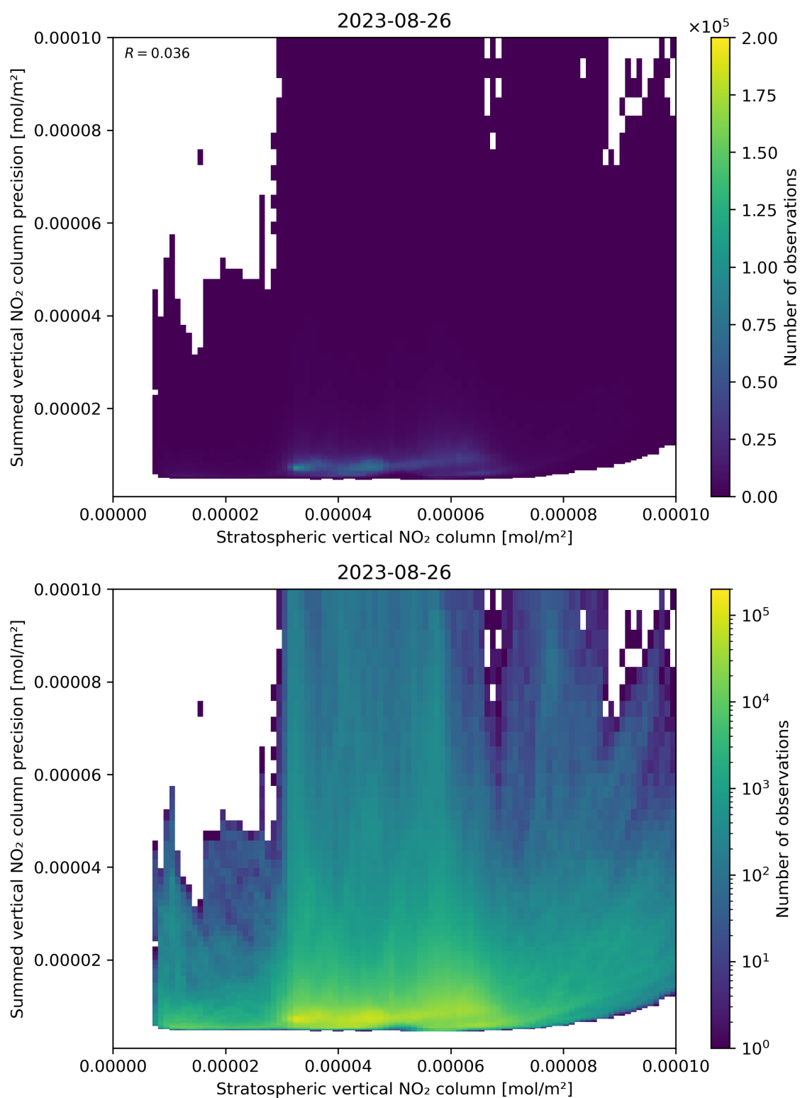
Figure 99: Scatter density plot of “Stratospheric vertical NO 2 column” against “Summed vertical NO 2 column precision” for 2023-08-25 to 2023-08-27.
