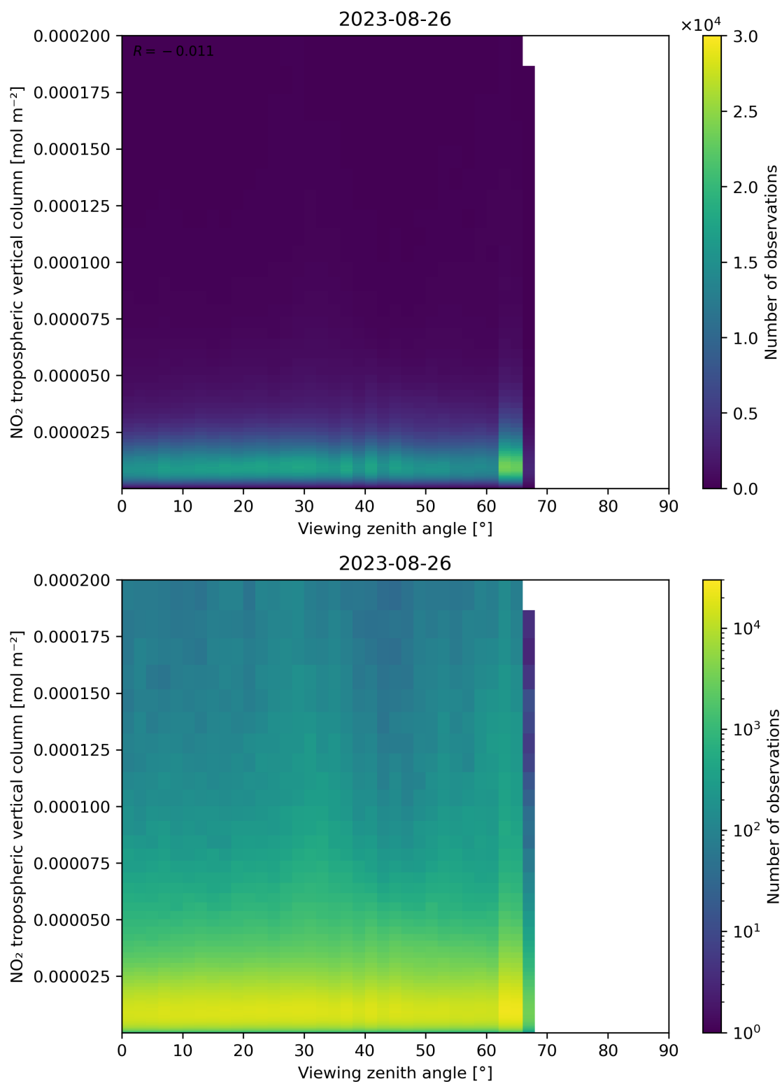
Figure 169: Scatter density plot of “Viewing zenith angle” against “NO 2 tropospheric vertical column” for 2023-08-25 to 2023-08-27.
