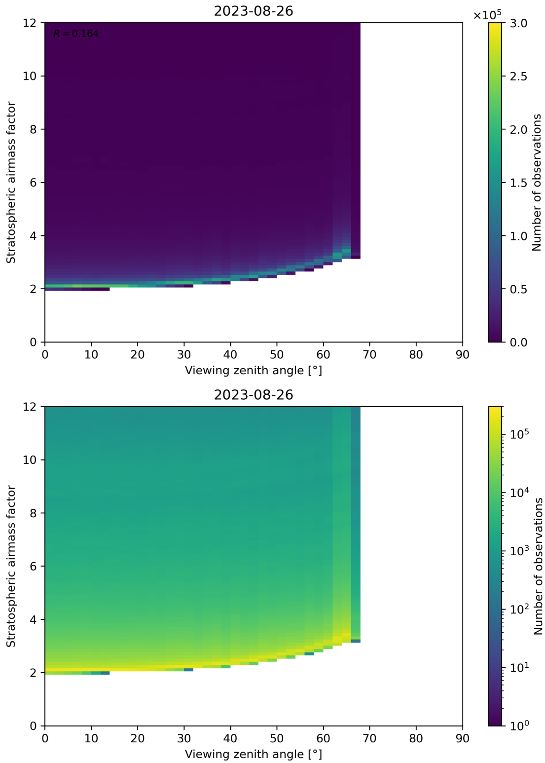
Figure 159: Scatter density plot of “Viewing zenith angle” against “Stratospheric airmass factor” for 2023-08-25 to 2023-08-27.
