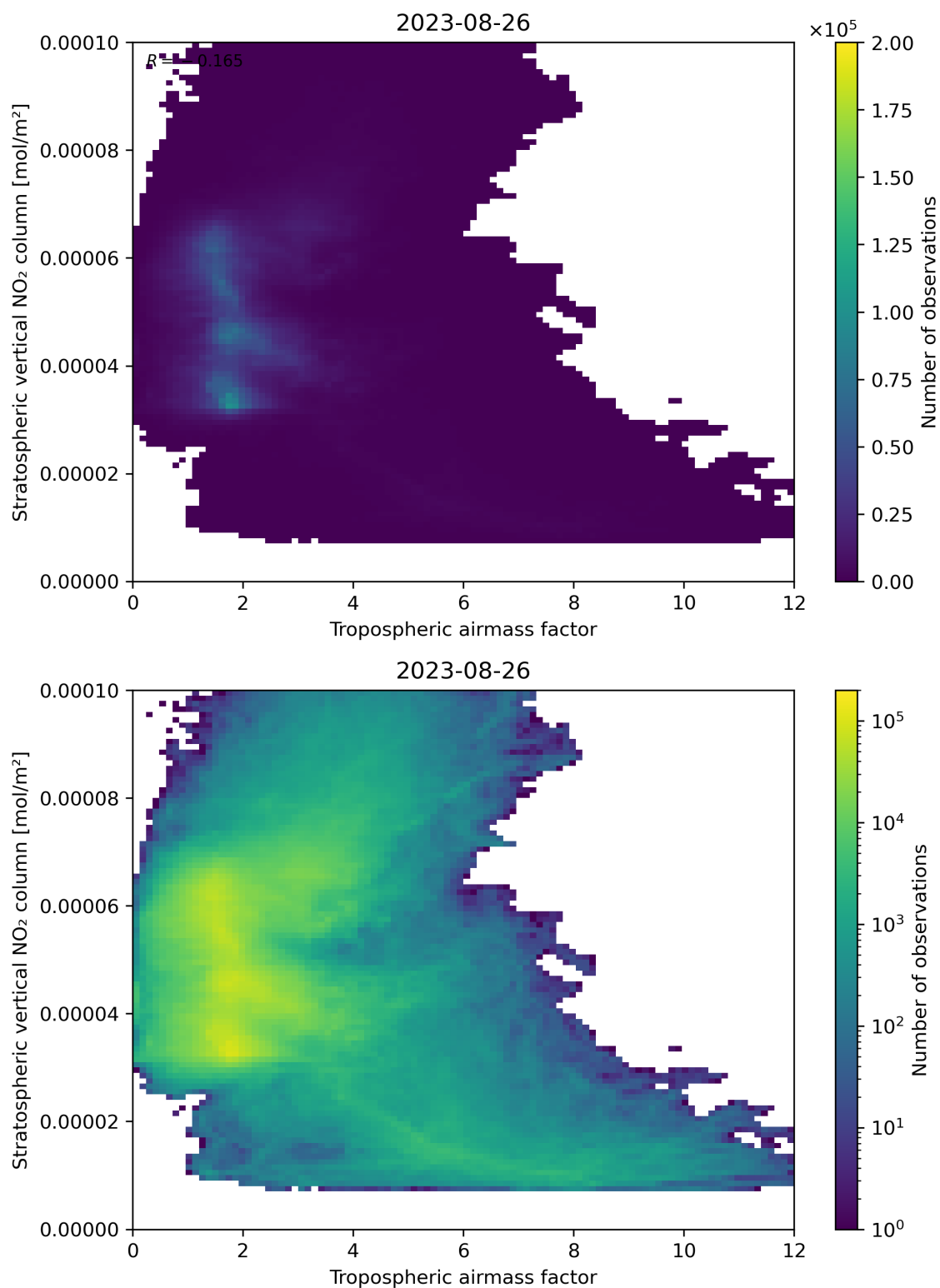
Figure 74: Scatter density plot of “Tropospheric air mass factor” against “Stratospheric vertical NO 2 column” for 2023-08-25 to 2023-08-27.
