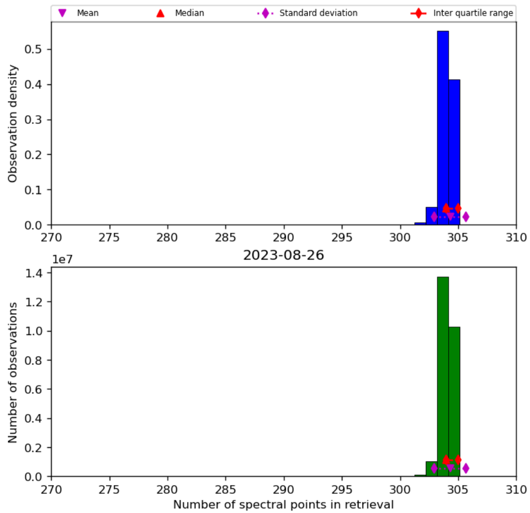
Figure 33: Histogram of “Number of spectral points in retrieval” for 2023-08-25 to 2023-08-27
