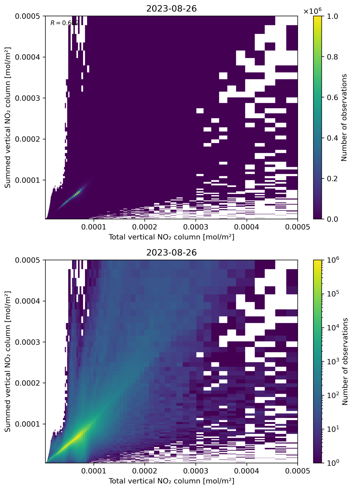
Figure 112: Scatter density plot of “Total vertical NO 2 column” against “Summed vertical NO 2 column” for 2023-08-25 to 2023-08-27.
