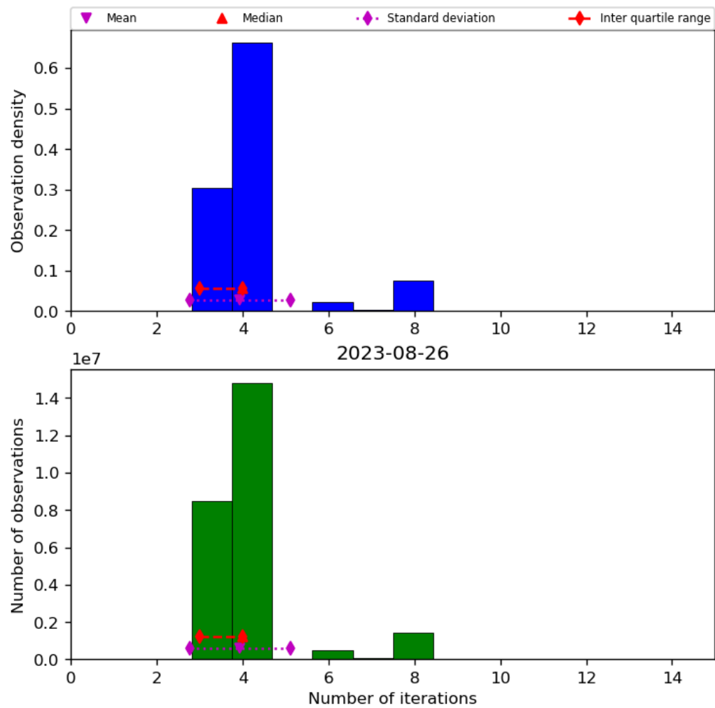
Figure 34: Histogram of “Number of iterations” for 2023-08-25 to 2023-08-27
