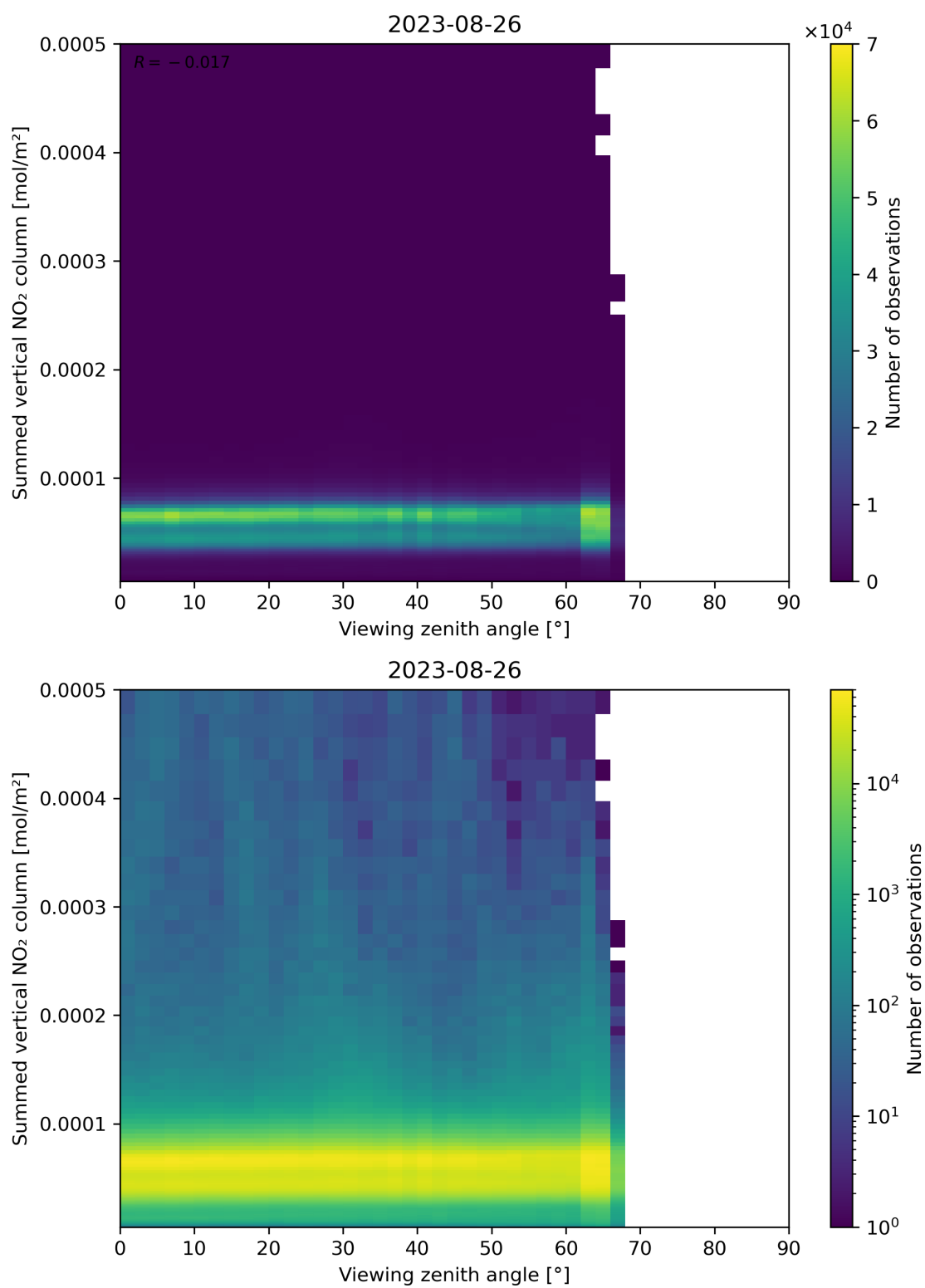
Figure 165: Scatter density plot of “Viewing zenith angle” against “Summed vertical NO 2 column” for 2023-08-25 to 2023-08-27.
