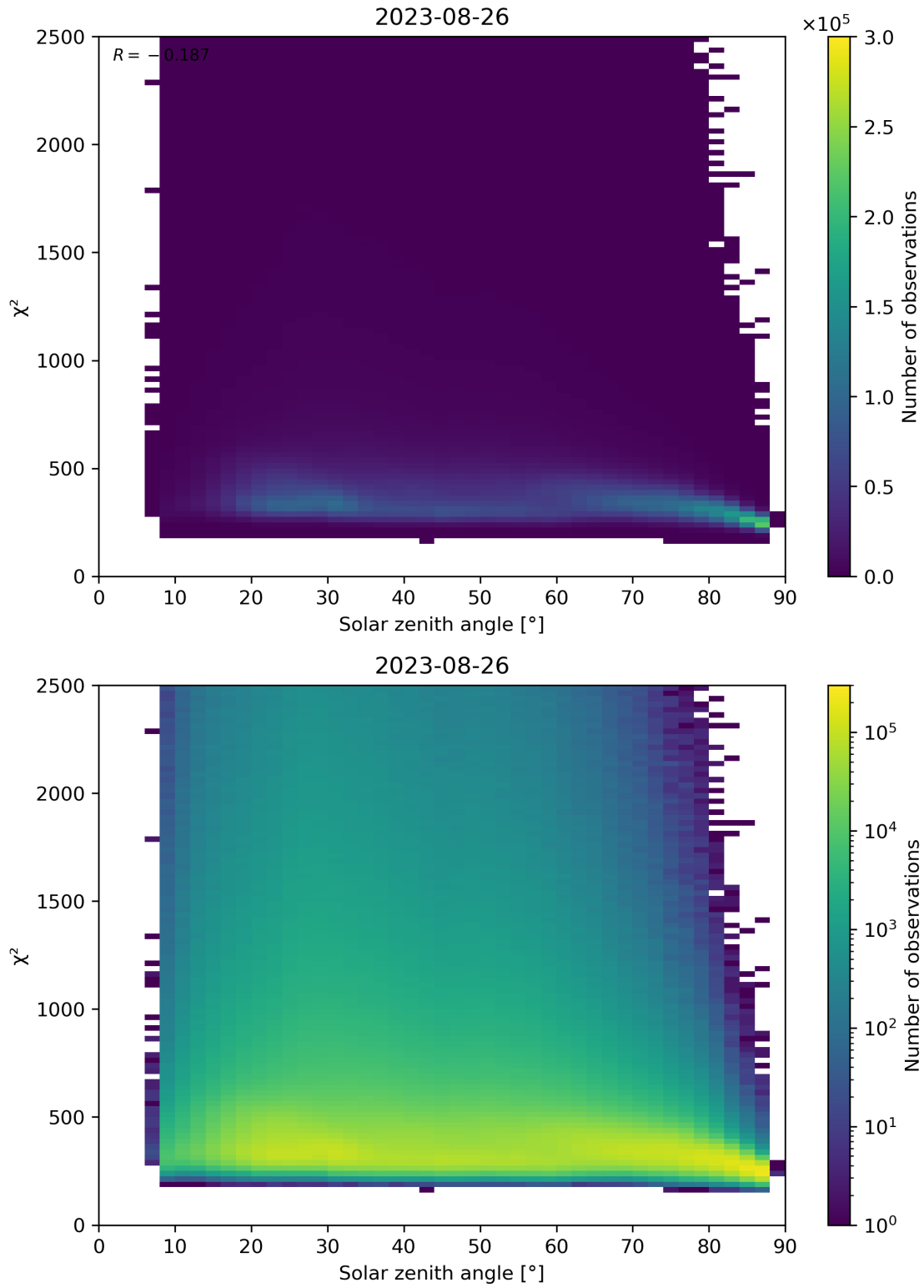
Figure 148: Scatter density plot of “Solar zenith angle” against “ \chi^2 ” for 2023-08-25 to 2023-08-27.
