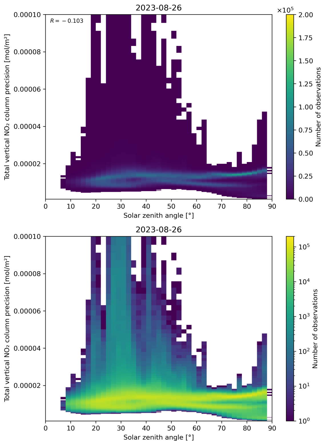
Figure 154: Scatter density plot of “Solar zenith angle” against “Total vertical NO 2 column precision” for 2023-08-25 to 2023-08-27.
