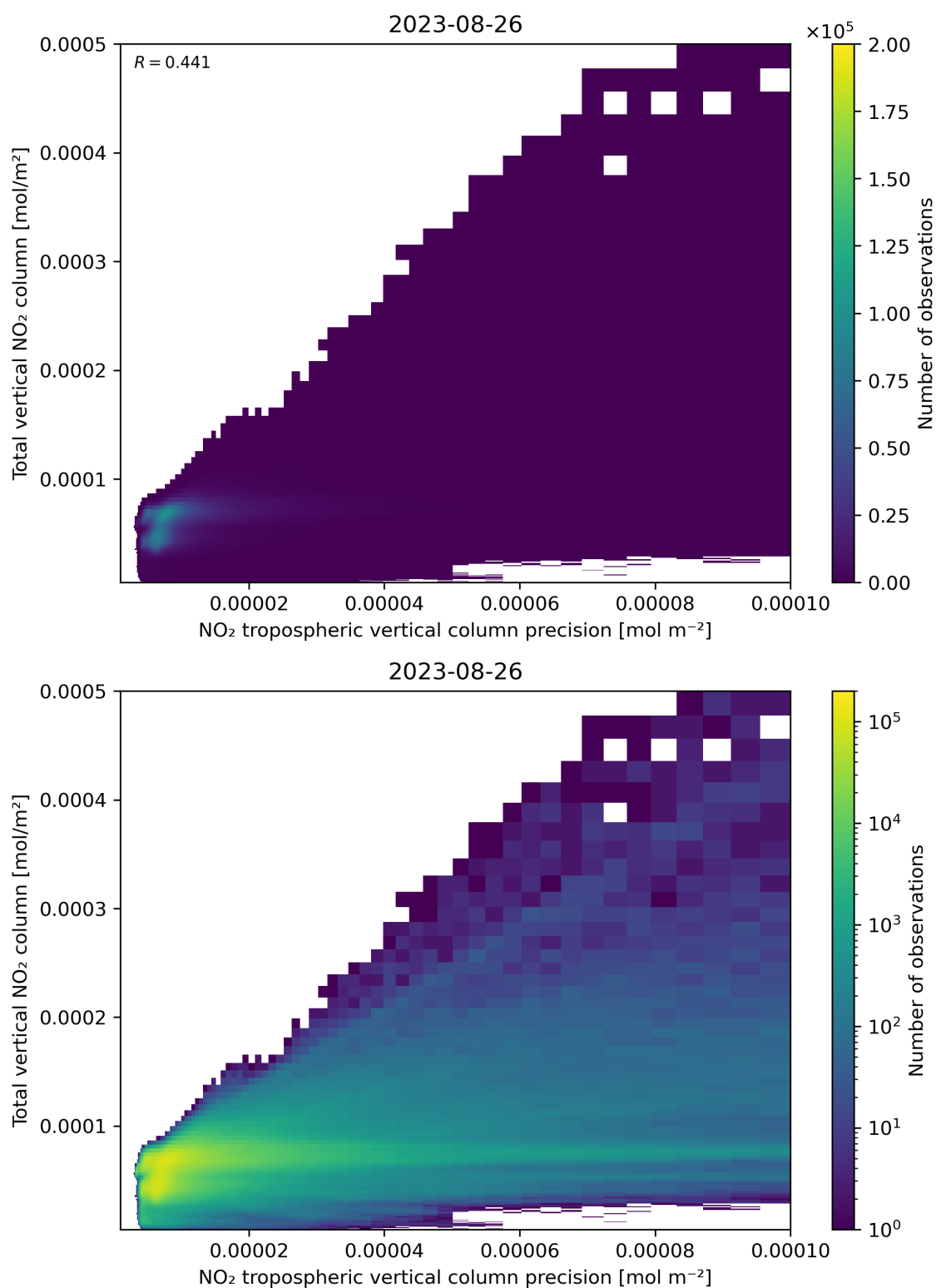
Figure 138: Scatter density plot of “NO 2 tropospheric vertical column precision” against “Total vertical NO 2 column” for 2023-08-25 to 2023-08-27.
