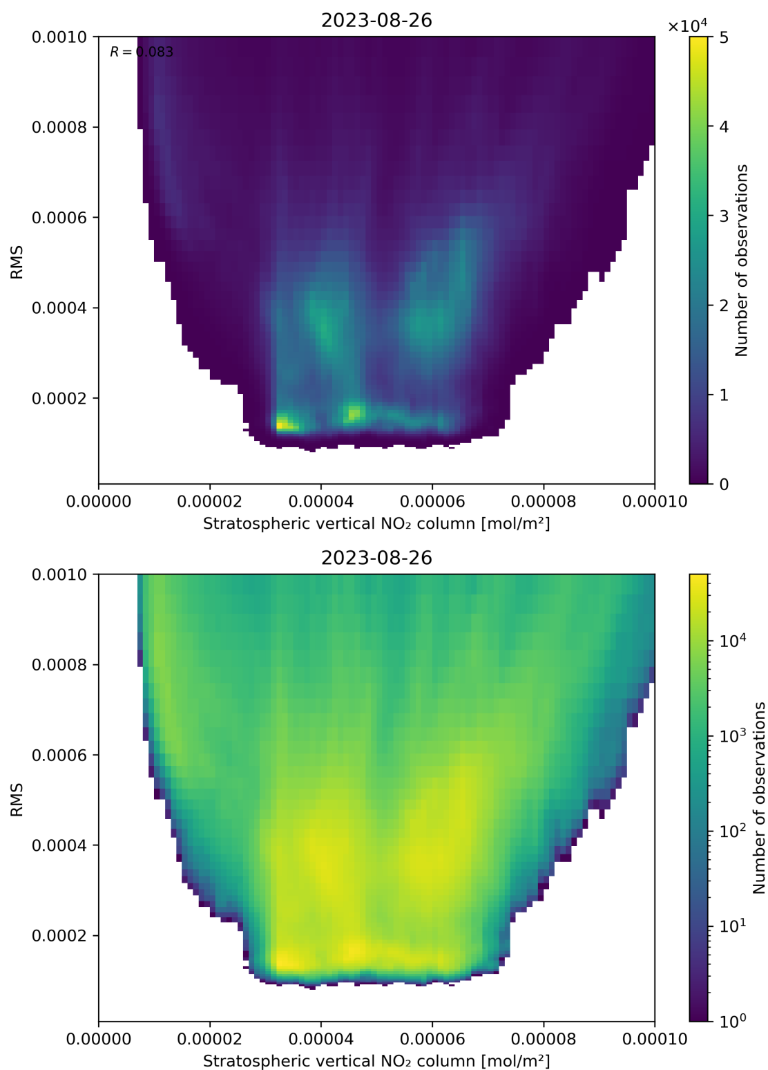
Figure 102: Scatter density plot of “Stratospheric vertical NO 2 column” against “RMS” for 2023-08-25 to 2023-08-27.
