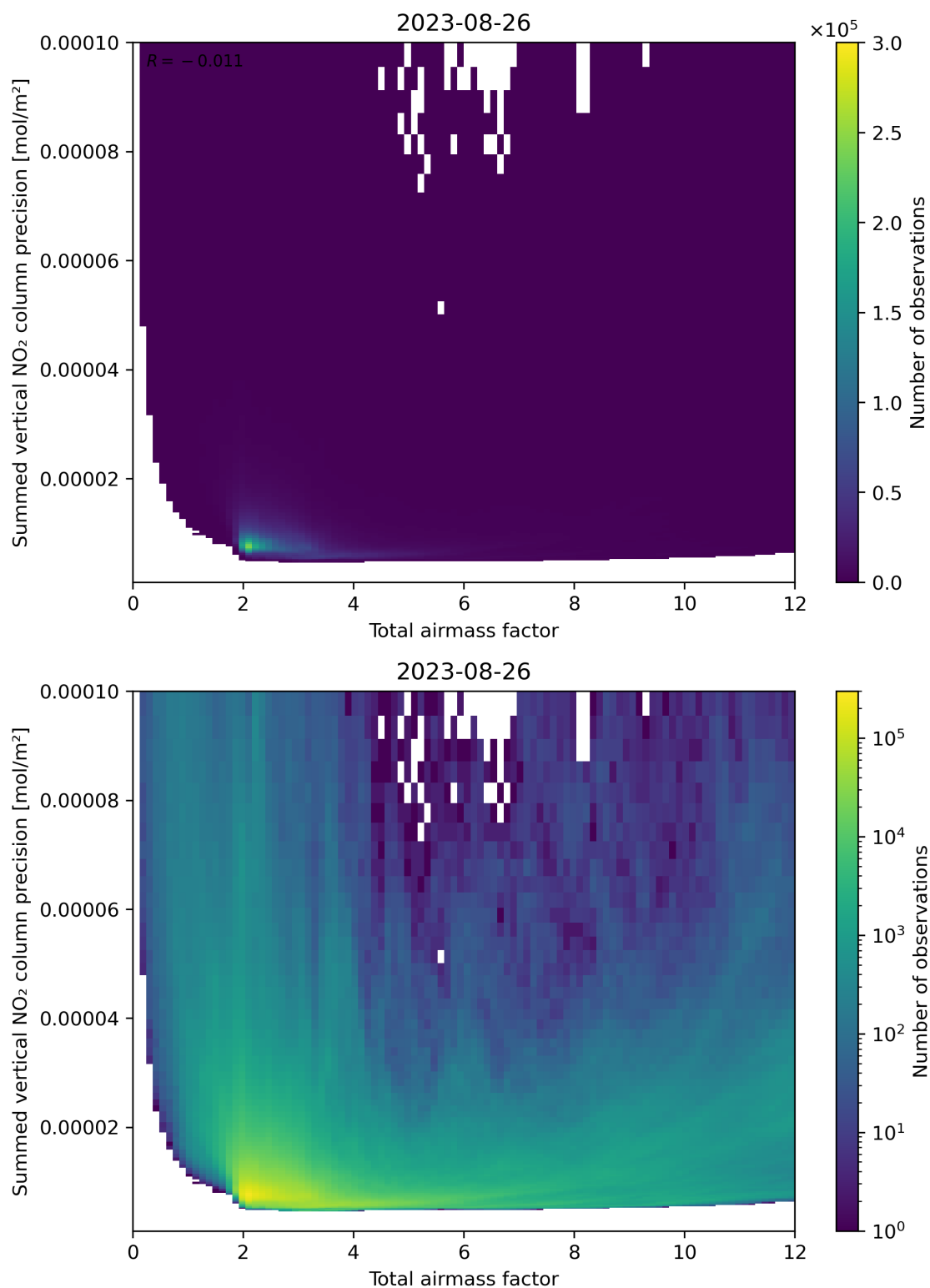
Figure 66: Scatter density plot of “Total airmass factor” against “Summed vertical NO 2 column precision” for 2023-08-25 to 2023-08-27.
