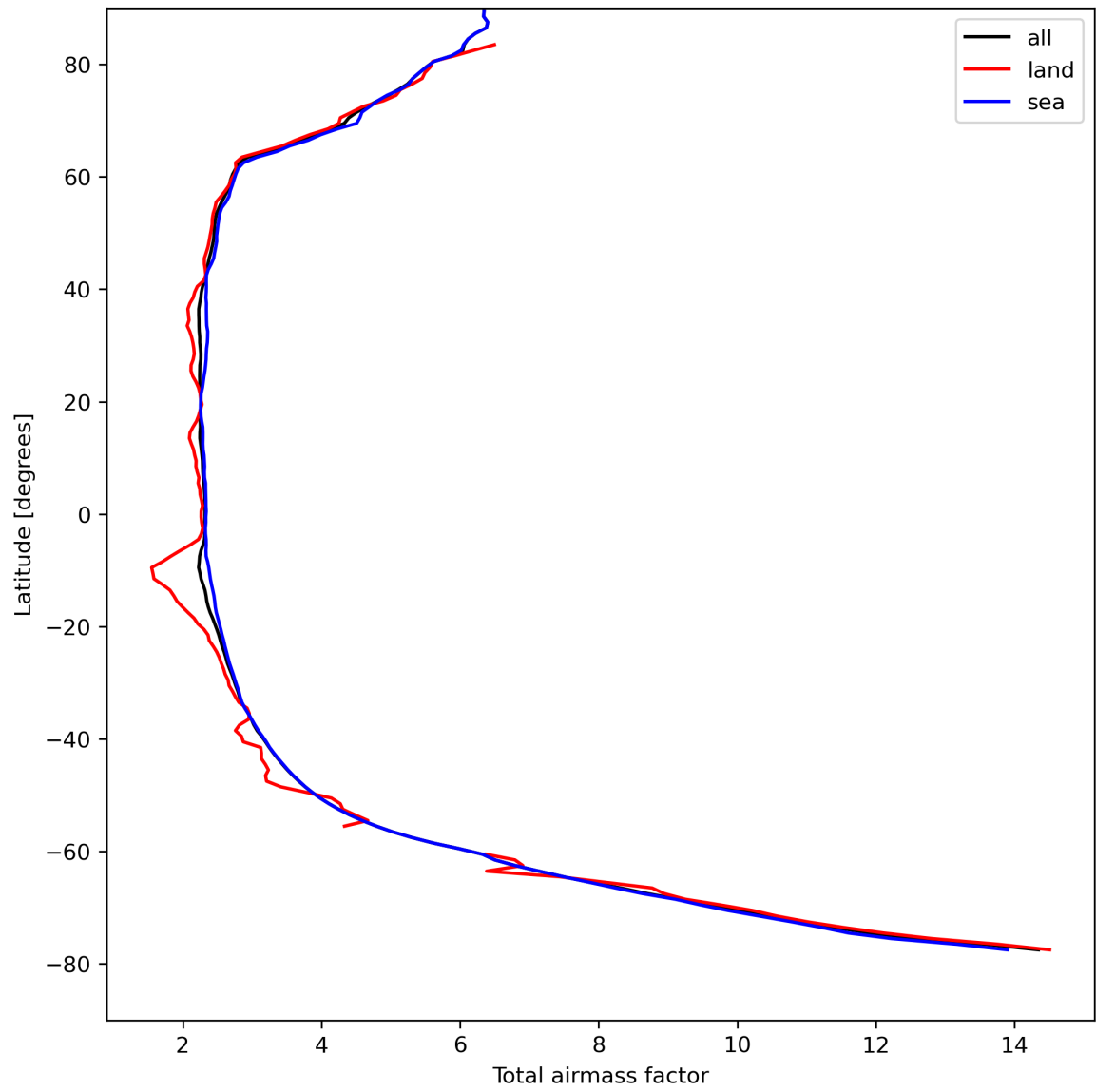
Figure 15: Zonal average of “Total airmass factor” for 2023-08-25 to 2023-08-27.
