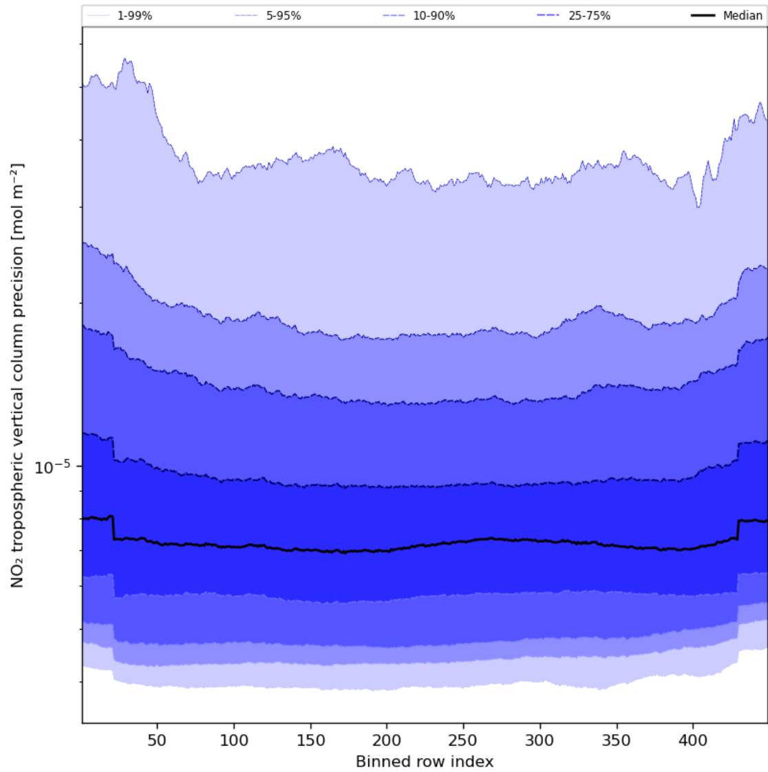
Figure 47: Along track statistics of “NO 2 tropospheric vertical column precision” for 2023-08-25 to 2023-08-27
