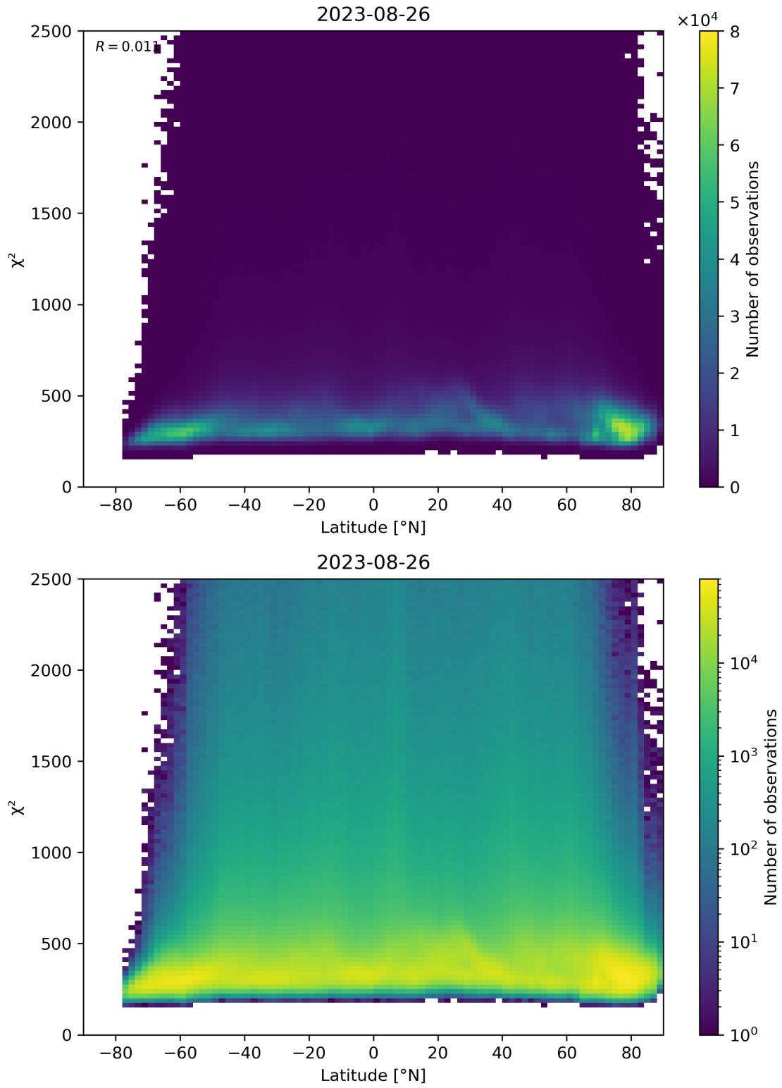
Figure 86: Scatter density plot of “Latitude” against “ \chi^2 ” for 2023-08-25 to 2023-08-27.
