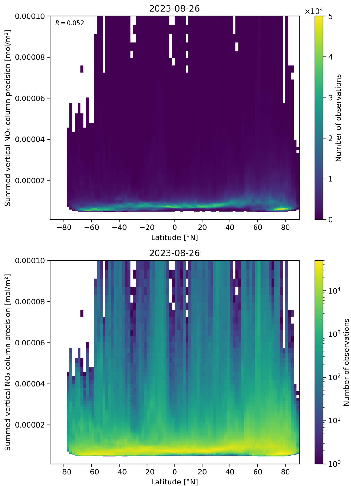
Figure 89: Scatter density plot of “Latitude” against “Summed vertical NO 2 column precision” for 2023-08-25 to 2023-08-27.
