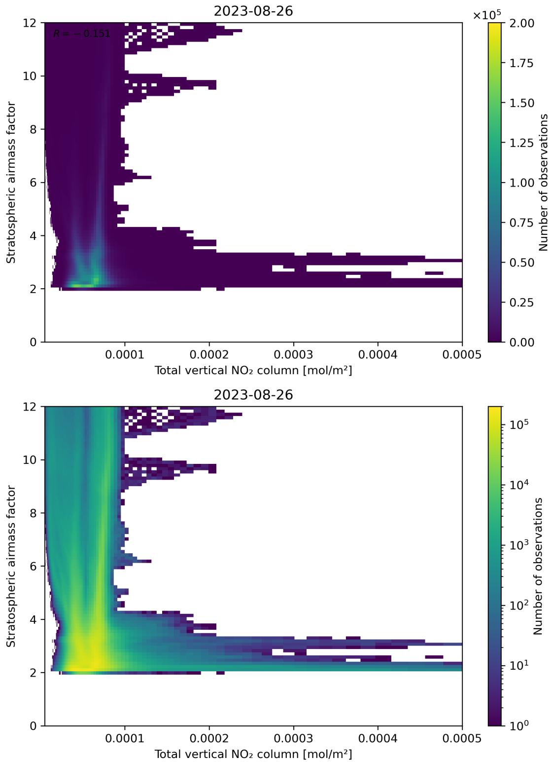
Figure 110: Scatter density plot of “Total vertical NO 2 column” against “Stratospheric airmass factor” for 2023-08-25 to 2023-08-27.
