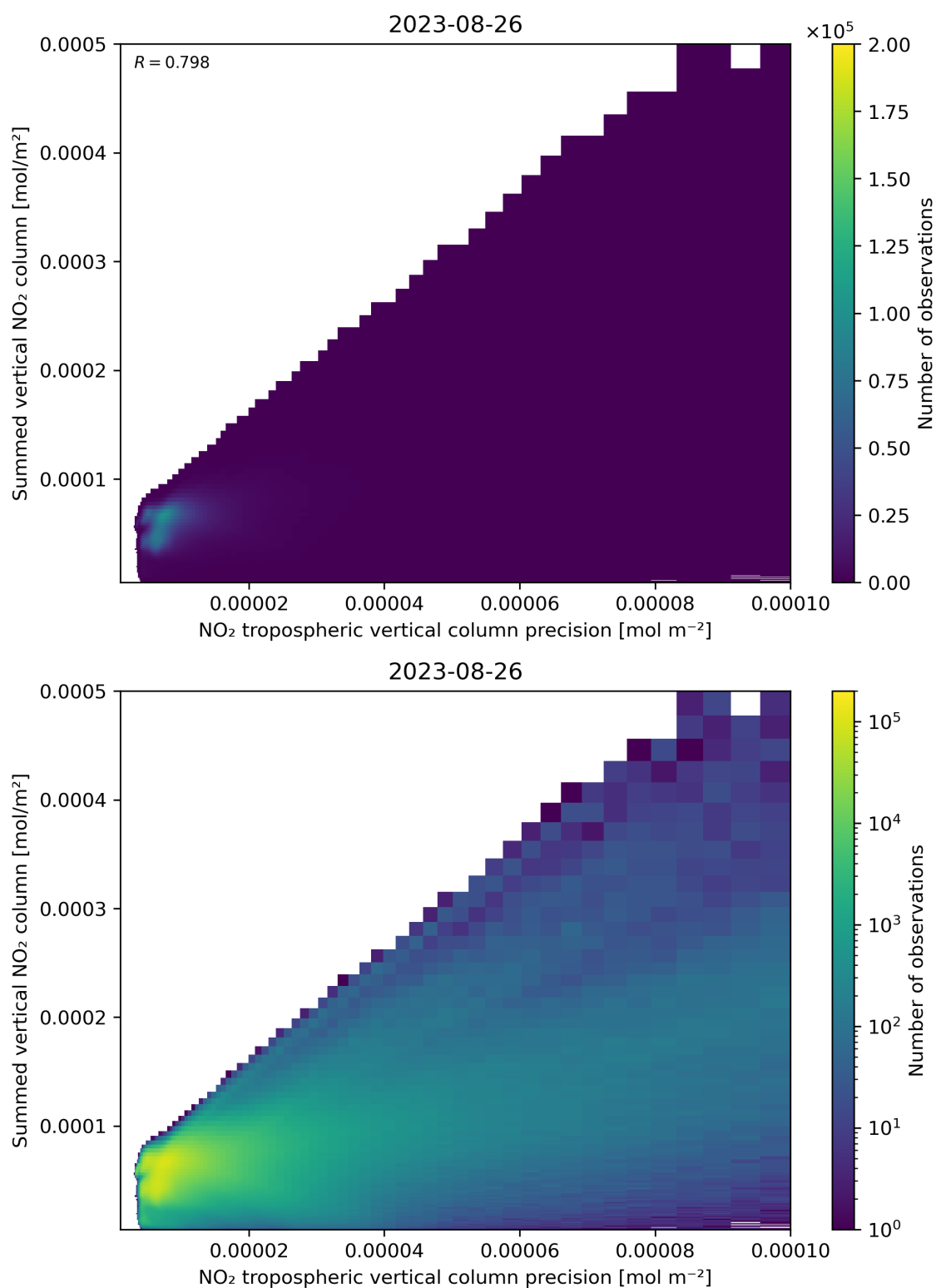
Figure 136: Scatter density plot of “NO 2 tropospheric vertical column precision” against “Summed vertical NO 2 column” for 2023-08-25 to 2023-08-27.
