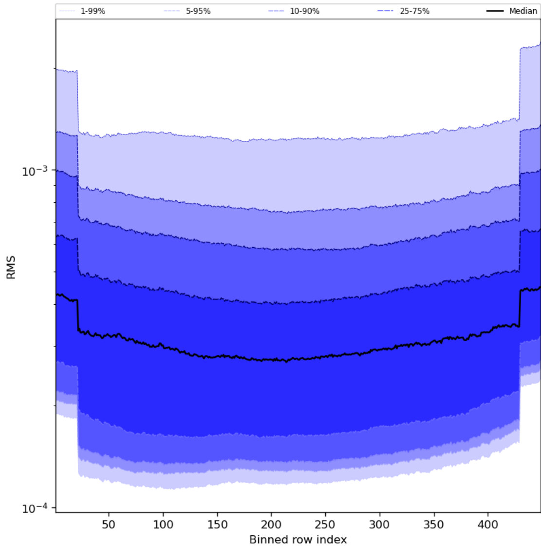
Figure 60: Along track statistics of “RMS” for 2023-08-25 to 2023-08-27
