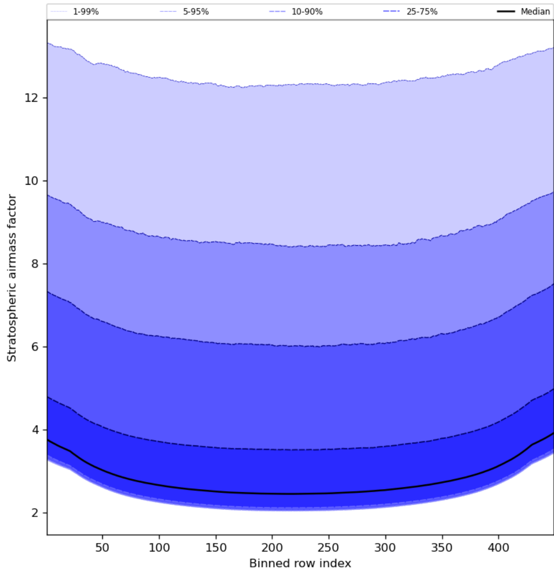
Figure 61: Along track statistics of “Stratospheric airmass factor” for 2023-08-25 to 2023-08-27
