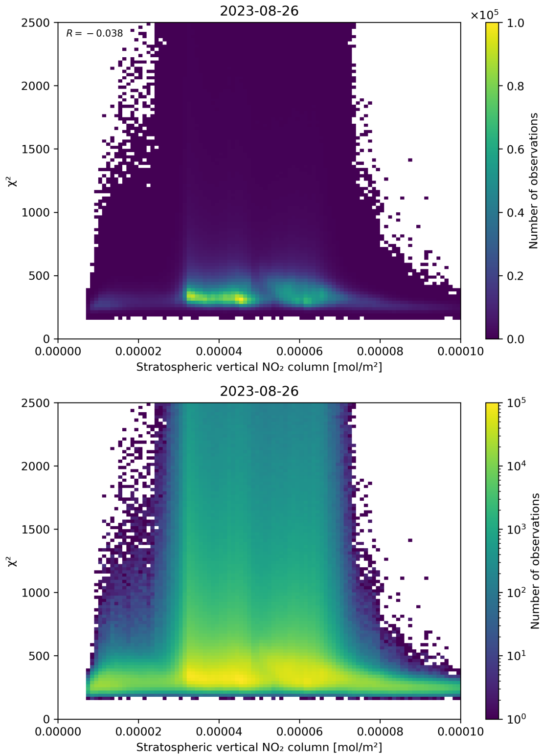
Figure 97: Scatter density plot of “Stratospheric vertical NO 2 column” against “ \chi^2 ” for 2023-08-25 to 2023-08-27.
