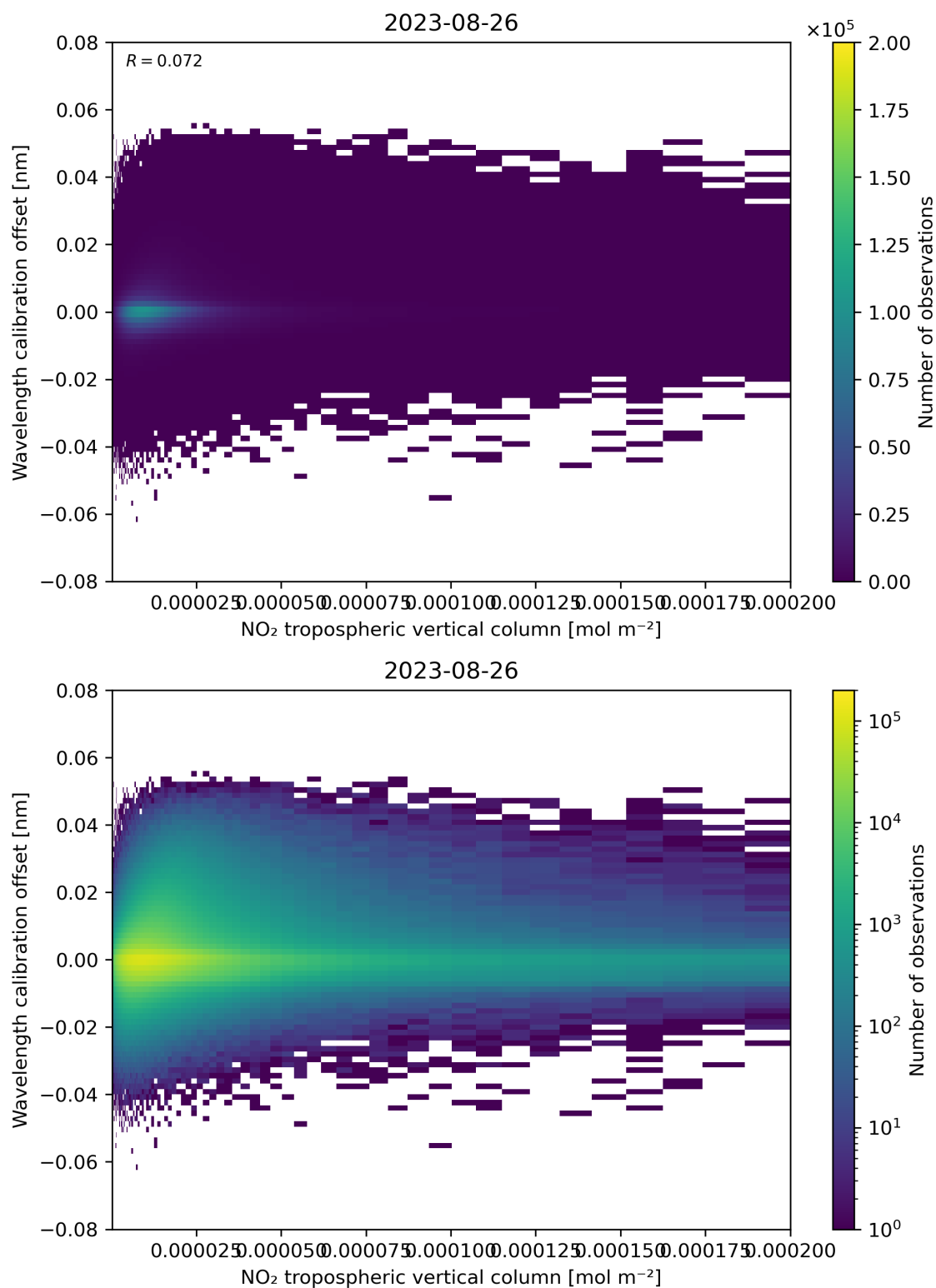
Figure 143: Scatter density plot of “NO 2 tropospheric vertical column” against “Wavelength calibration offset” for 2023-08-25 to 2023-08-27.
