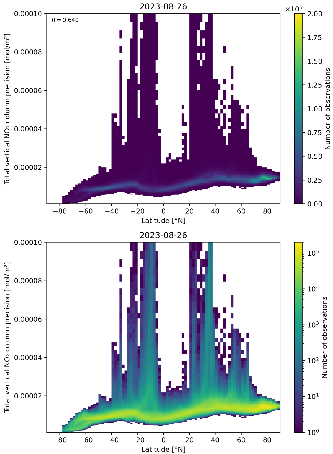
Figure 91: Scatter density plot of “Latitude” against “Total vertical NO 2 column precision” for 2023-08-25 to 2023-08-27.
