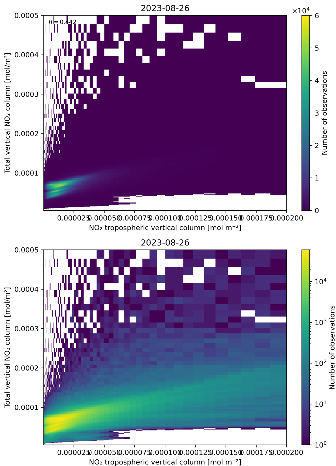
Figure 128: Scatter density plot of “NO 2 tropospheric vertical column” against “Total vertical NO 2 column” for 2023-08-25 to 2023-08-27.
