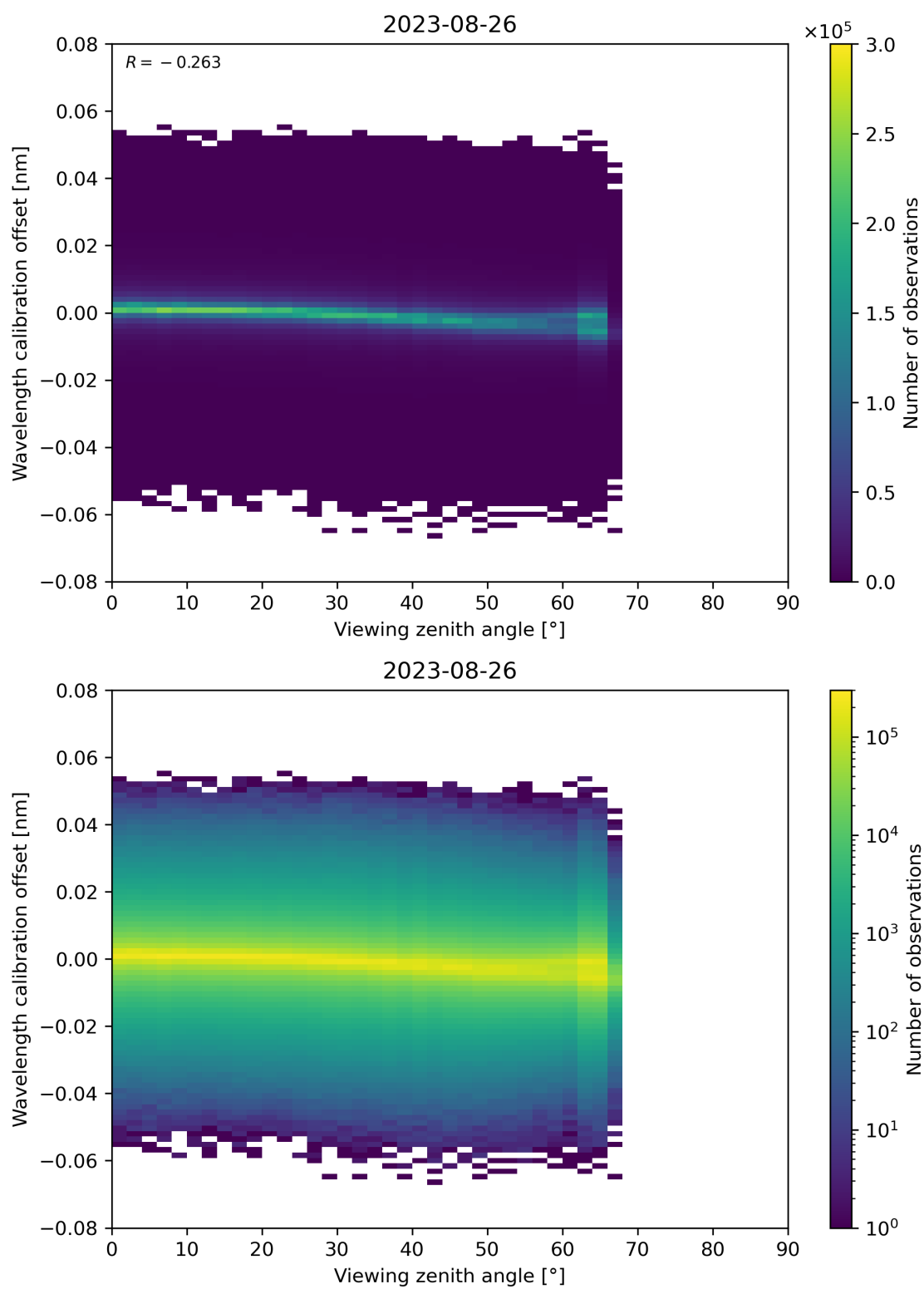
Figure 173: Scatter density plot of “Viewing zenith angle” against “Wavelength calibration offset” for 2023-08-25 to 2023-08-27.
