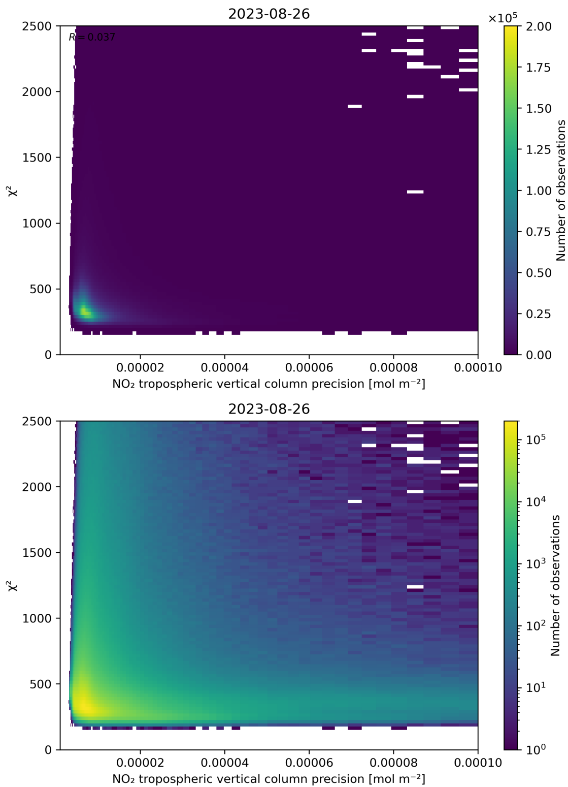
Figure 134: Scatter density plot of “NO 2 tropospheric vertical column precision” against “ \chi^2 ” for 2023-08-25 to 2023-08-27.
