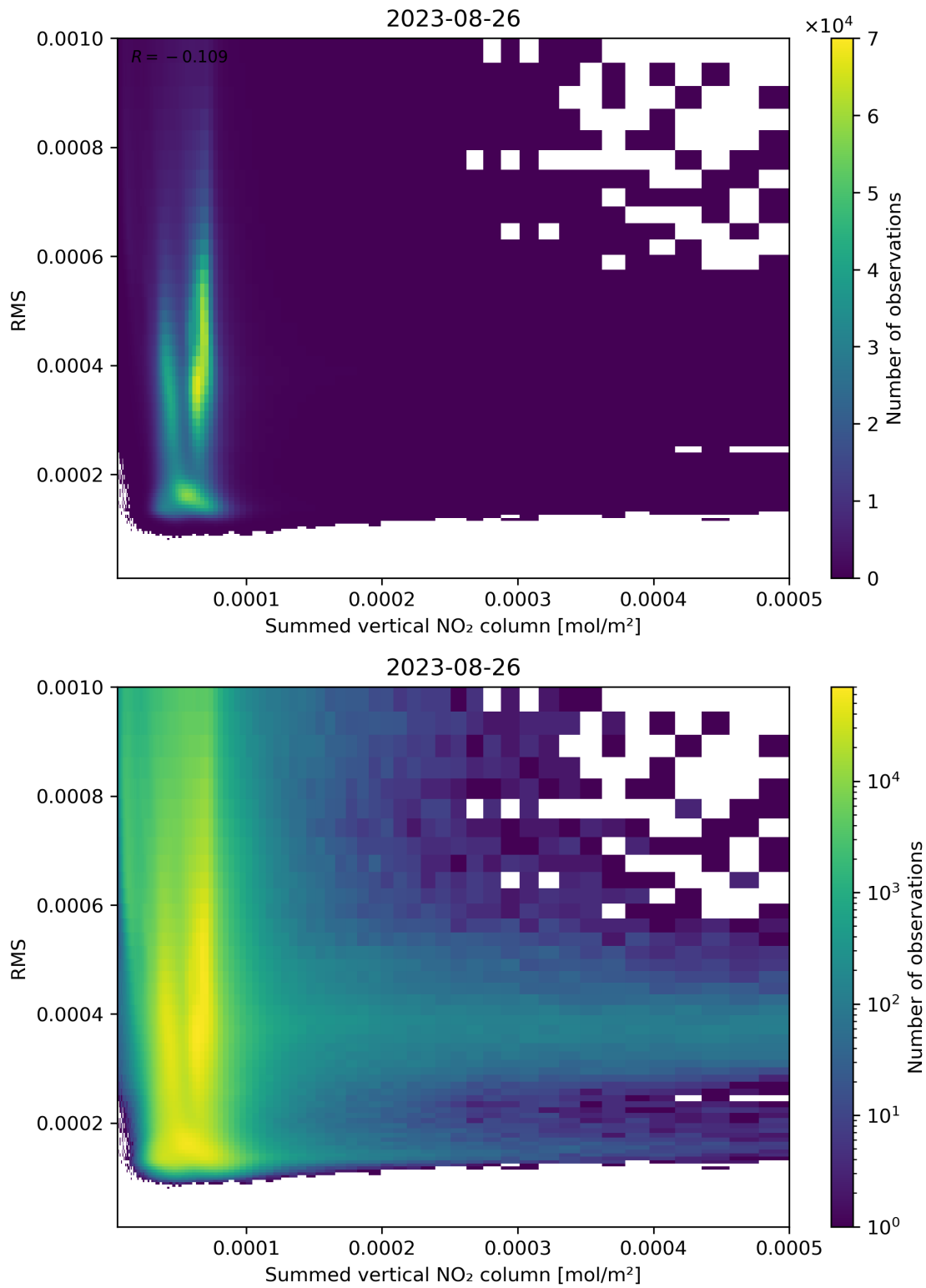
Figure 109: Scatter density plot of “Summed vertical NO 2 column” against “RMS” for 2023-08-25 to 2023-08-27.
