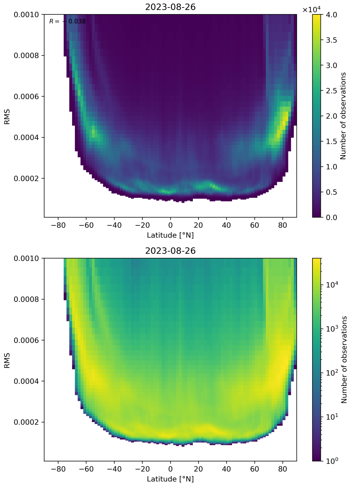
Figure 94: Scatter density plot of “Latitude” against “RMS” for 2023-08-25 to 2023-08-27.
