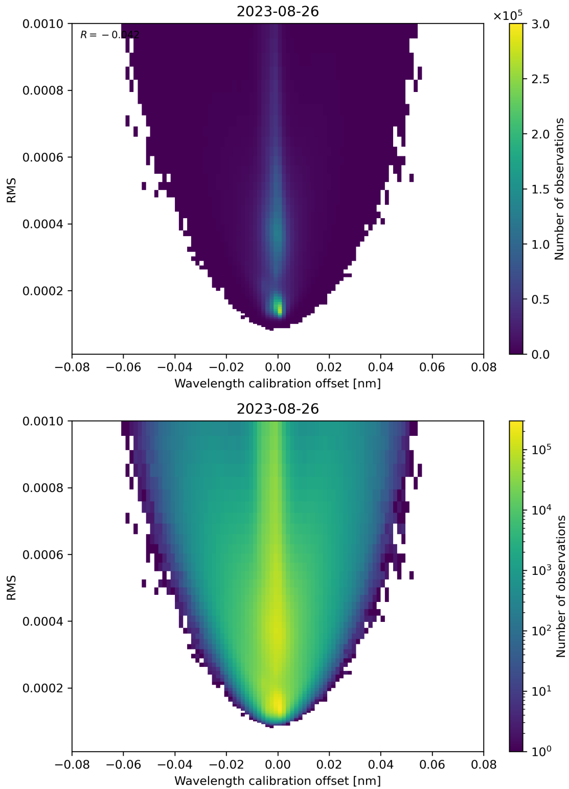
Figure 181: Scatter density plot of “Wavelength calibration offset” against “RMS” for 2023-08-25 to 2023-08-27.
