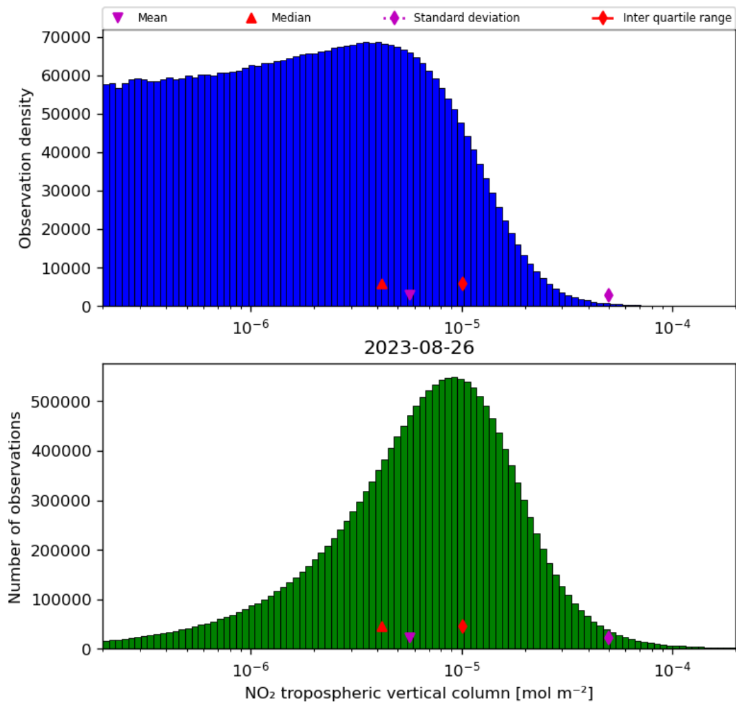
Figure 29: Histogram of “NO 2 tropospheric vertical column” for 2023-08-25 to 2023-08-27
