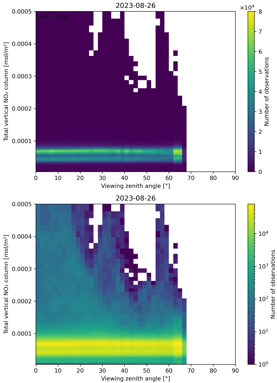
Figure 167: Scatter density plot of “Viewing zenith angle” against “Total vertical NO 2 column” for 2023-08-25 to 2023-08-27.
