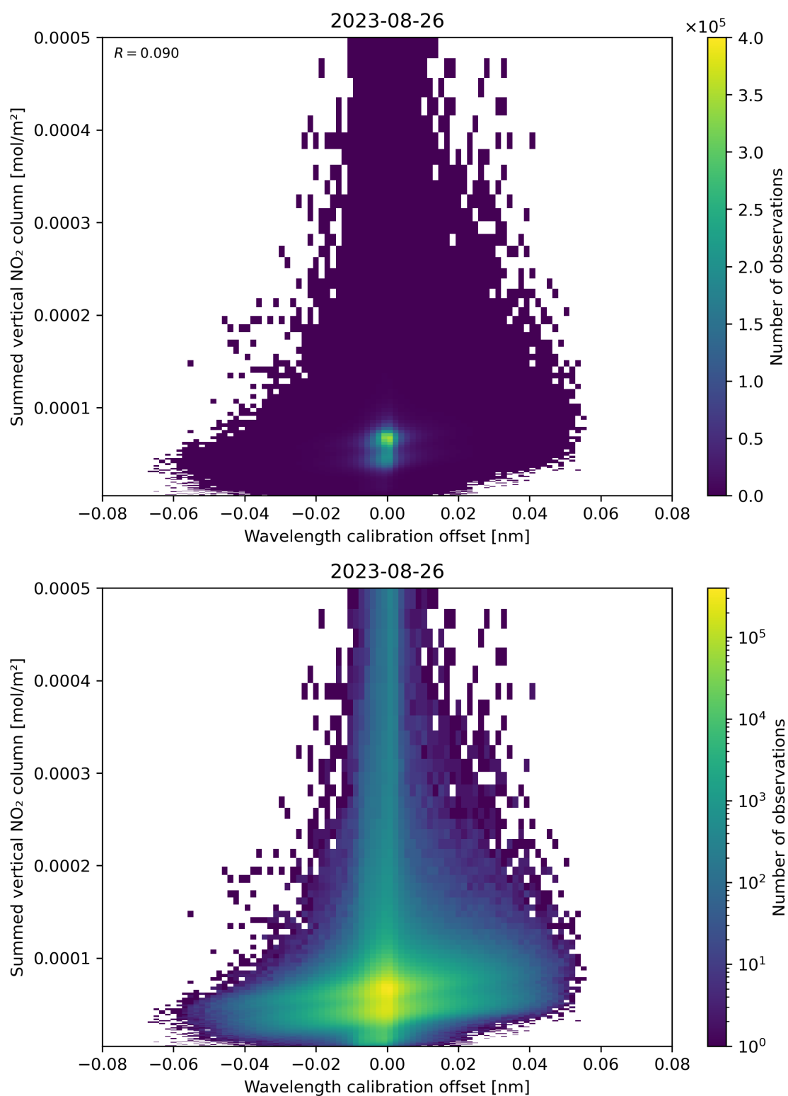
Figure 177: Scatter density plot of “Wavelength calibration offset” against “Summed vertical NO 2 column” for 2023-08-25 to 2023-08-27.
