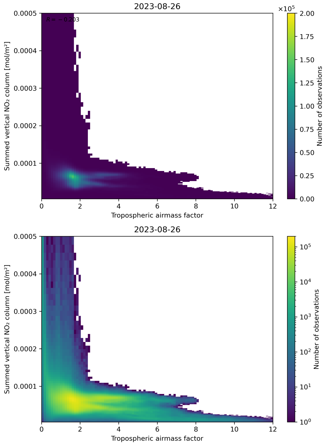
Figure 75: Scatter density plot of “Tropospheric air mass factor” against “Summed vertical NO 2 column” for 2023-08-25 to 2023-08-27.
