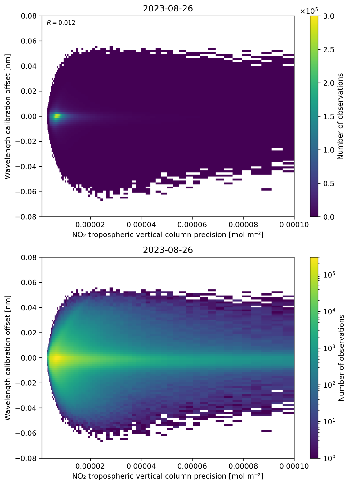
Figure 141: Scatter density plot of “NO 2 tropospheric vertical column precision” against “Wavelength calibration offset” for 2023-08-25 to 2023-08-27.
