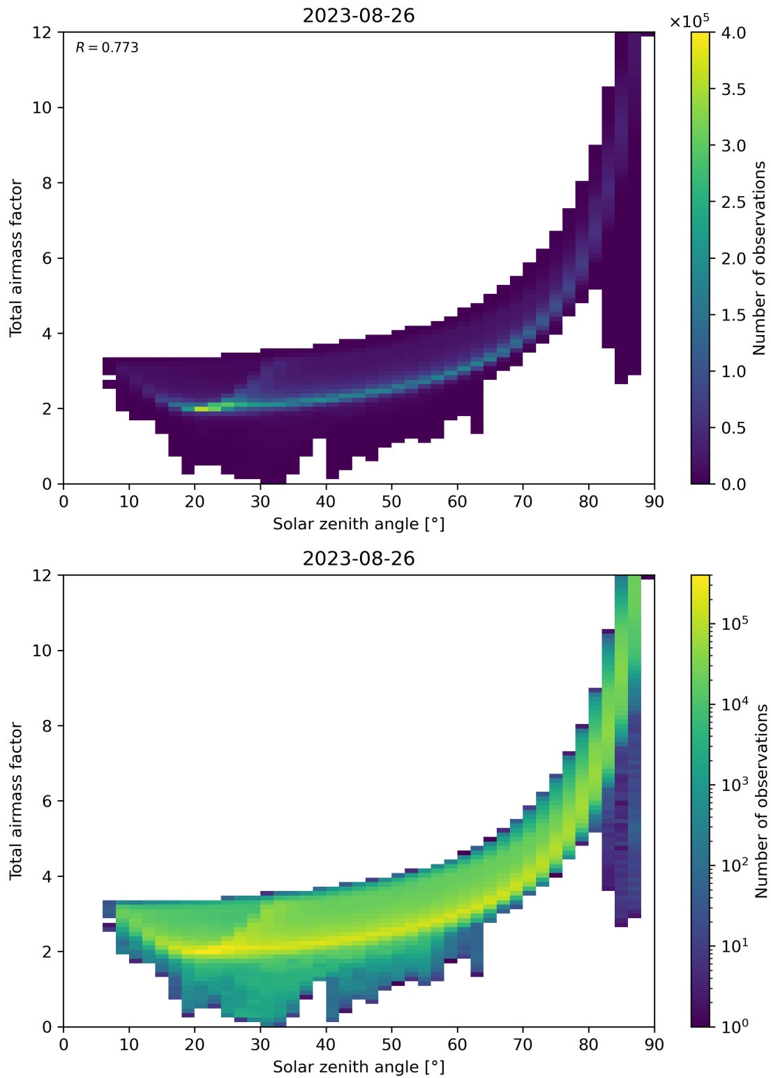
Figure 146: Scatter density plot of “Solar zenith angle” against “Total air mass factor” for 2023-08-25 to 2023-08-27.
