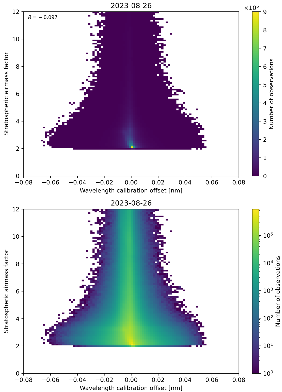
Figure 174: Scatter density plot of “Wavelength calibration offset” against “Stratospheric airmass factor” for 2023-08-25 to 2023-08-27.
