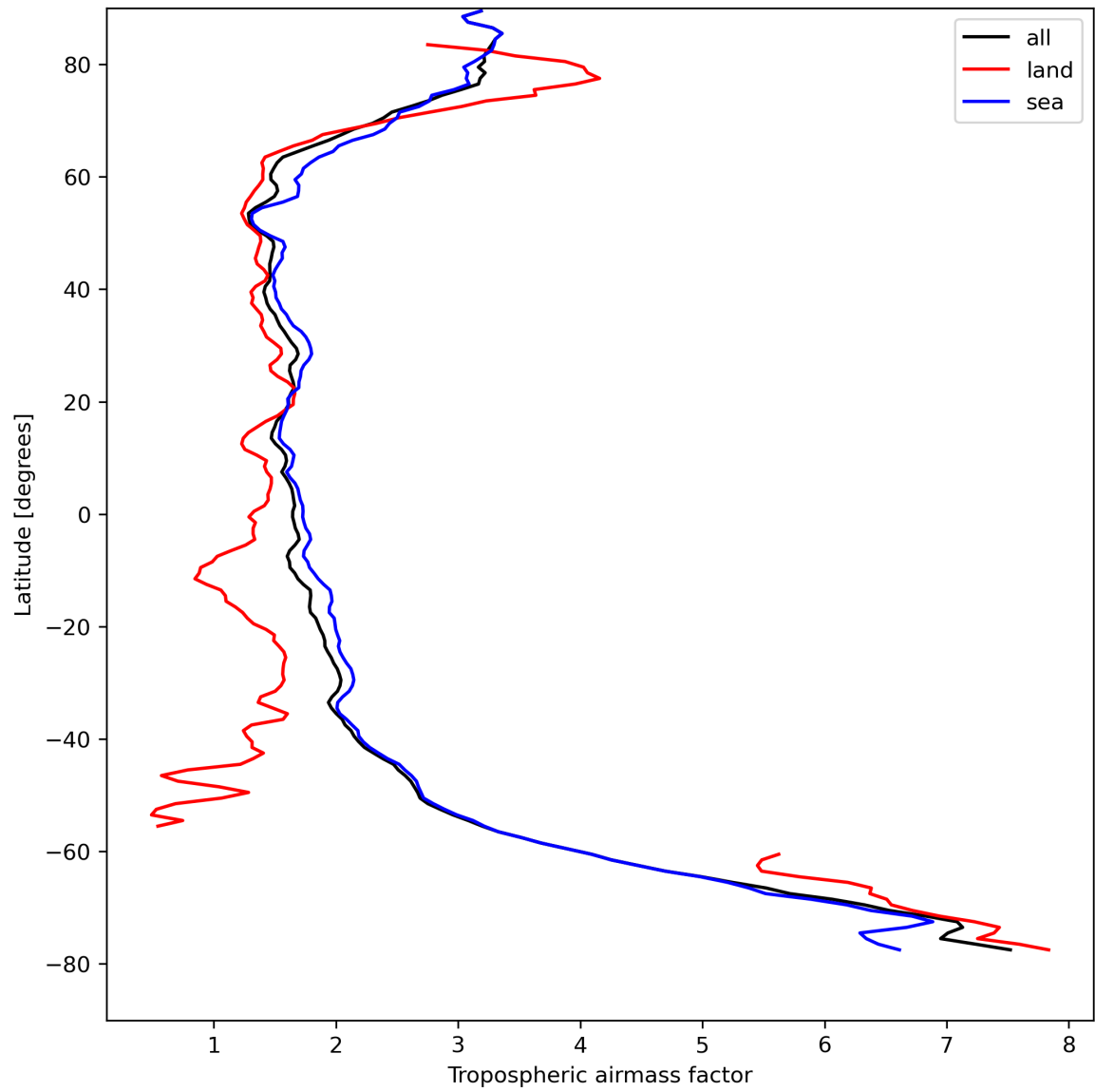
Figure 14: Zonal average of “Tropospheric airmass factor” for 2023-08-25 to 2023-08-27.
