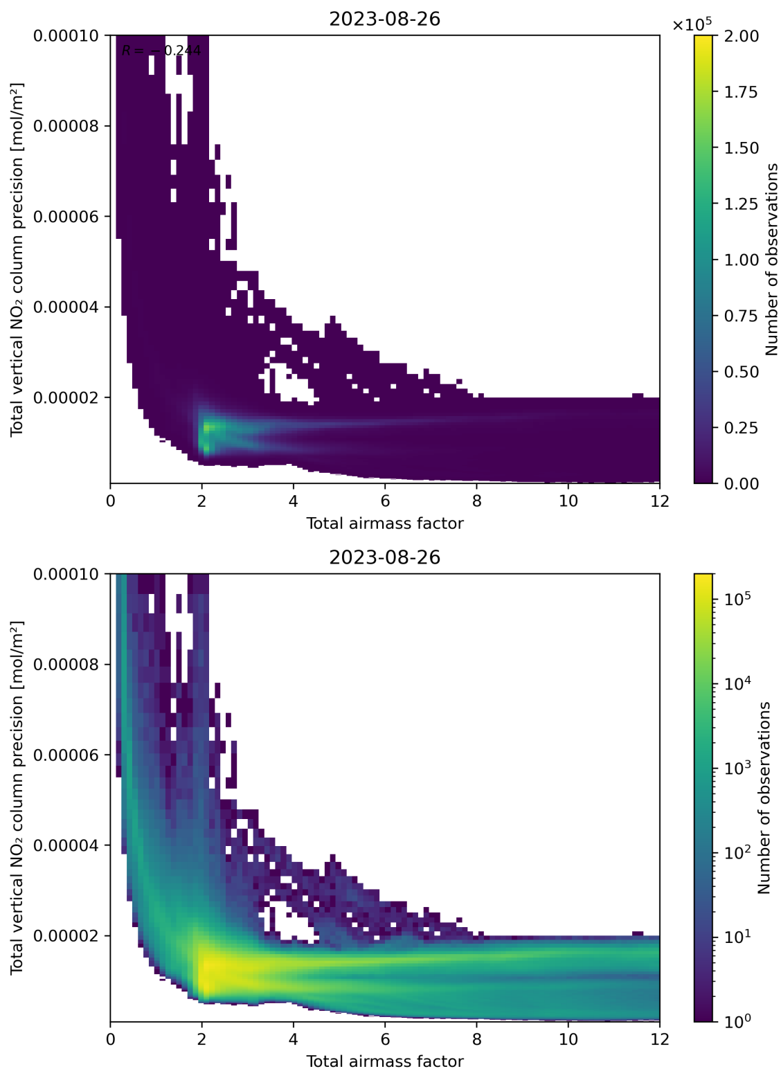
Figure 68: Scatter density plot of “Total airmass factor” against “Total vertical NO 2 column precision” for 2023-08-25 to 2023-08-27.
