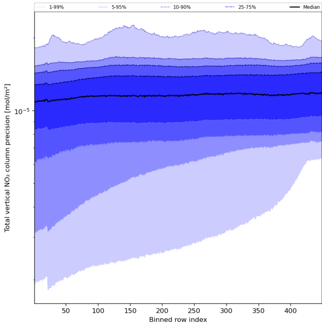
Figure 56: Along track statistics of “Total vertical NO 2 column precision” for 2023-08-25 to 2023-08-27
