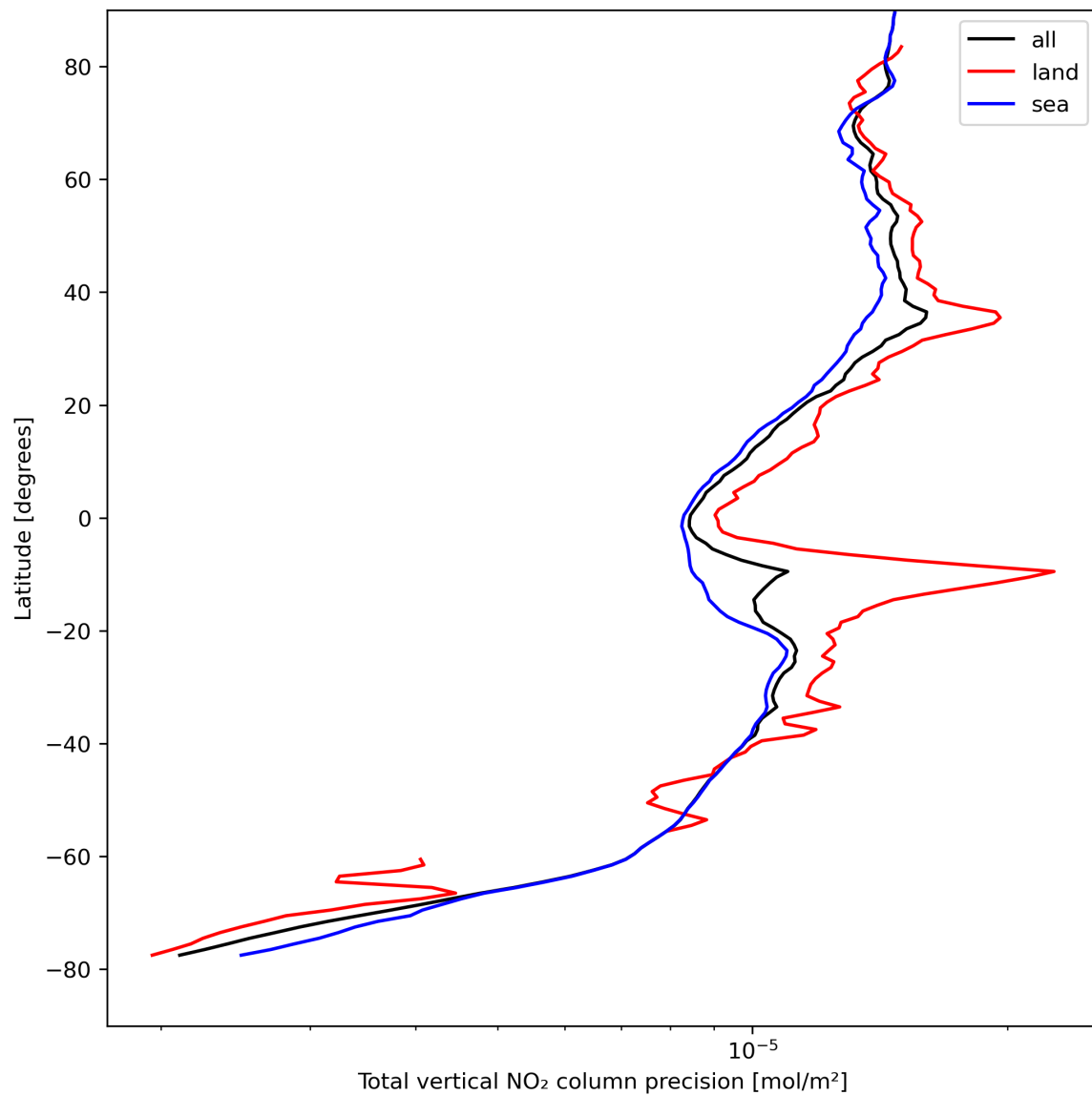
Figure 22: Zonal average of “Total vertical NO 2 column precision” for 2023-08-25 to 2023-08-27.
