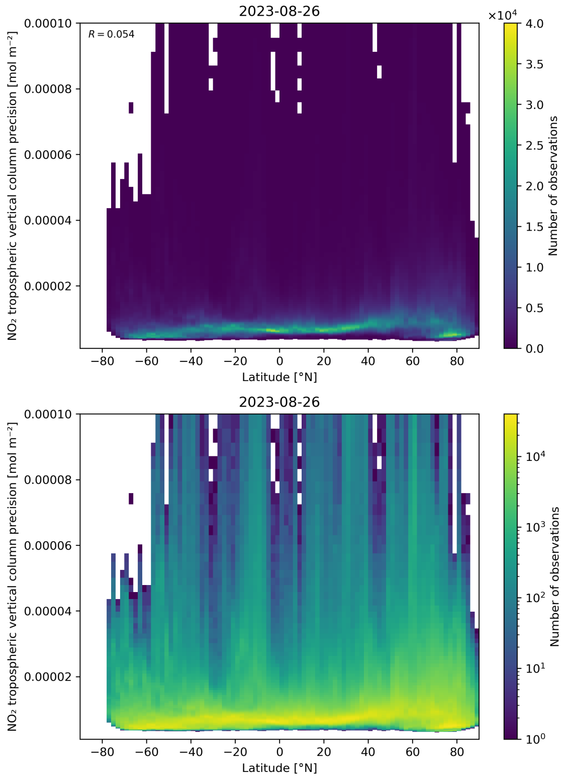
Figure 93: Scatter density plot of “Latitude” against “NO 2 tropospheric vertical column precision” for 2023-08-25 to 2023-08-27.
