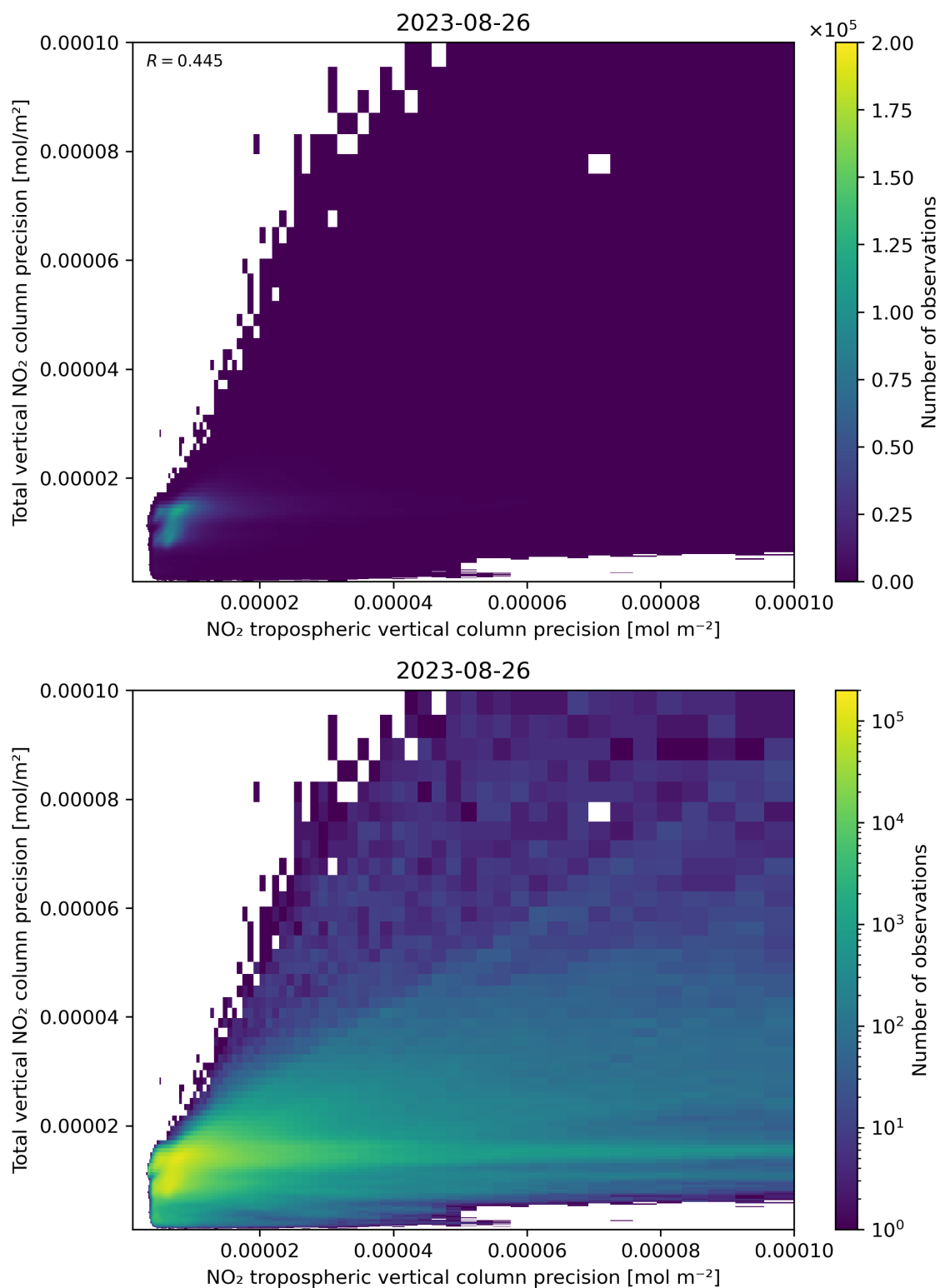
Figure 139: Scatter density plot of “NO 2 tropospheric vertical column precision” against “Total vertical NO 2 column precision” for 2023-08-25 to 2023-08-27.
