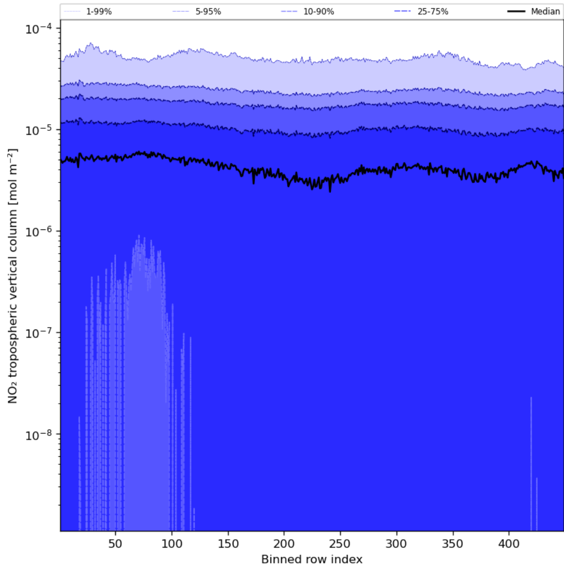
Figure 46: Along track statistics of “NO 2 tropospheric vertical column” for 2023-08-25 to 2023-08-27
