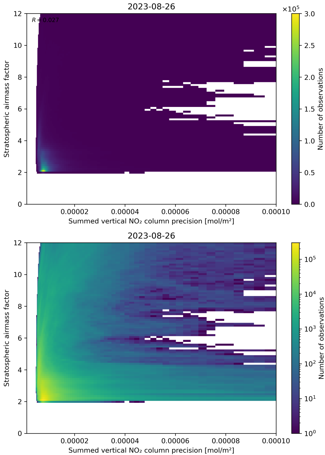
Figure 106: Scatter density plot of “Summed vertical NO 2 column precision” against “Stratospheric airmass factor” for 2023-08-25 to 2023-08-27.
