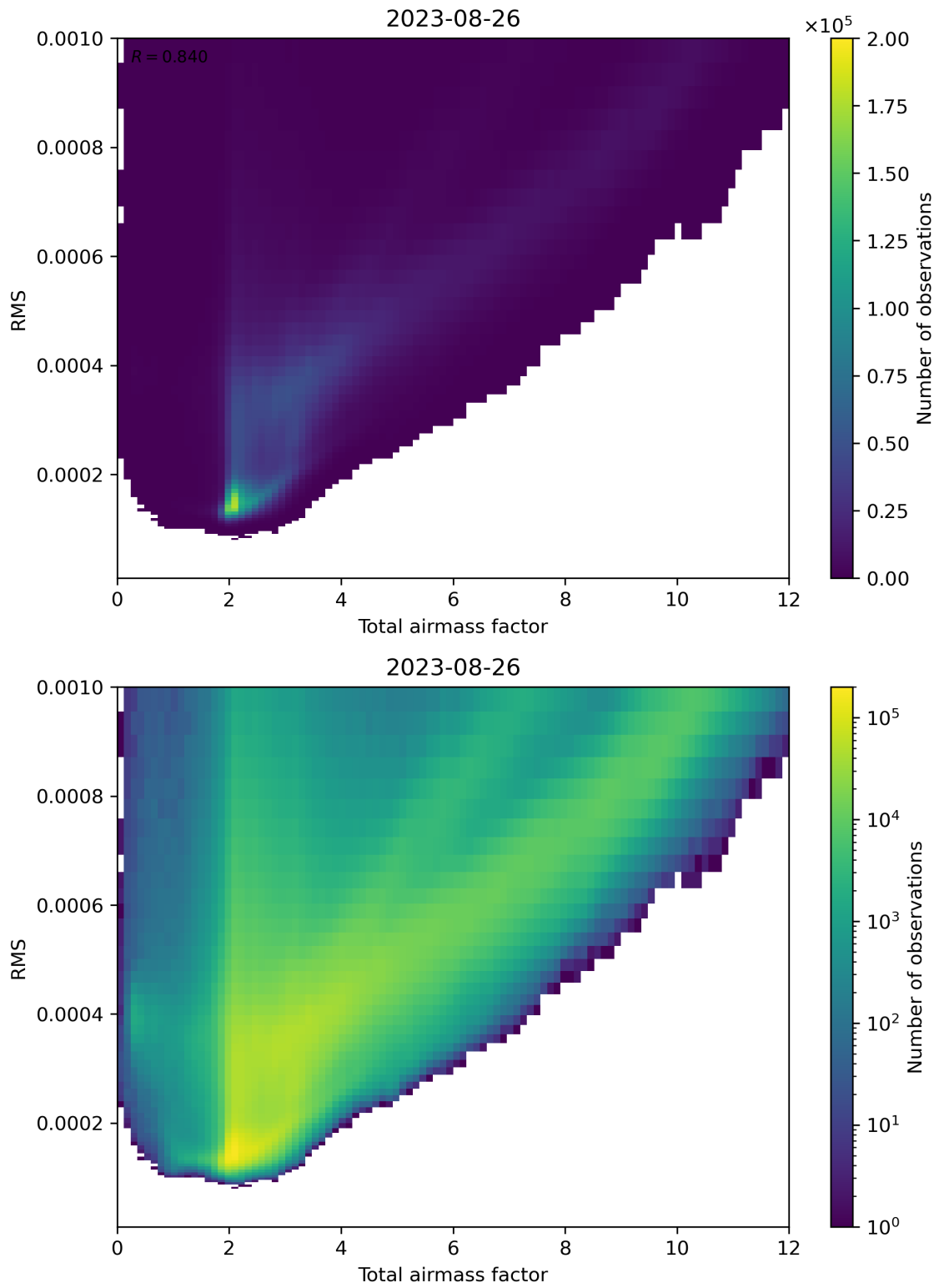
Figure 69: Scatter density plot of “Total airmass factor” against “RMS” for 2023-08-25 to 2023-08-27.
