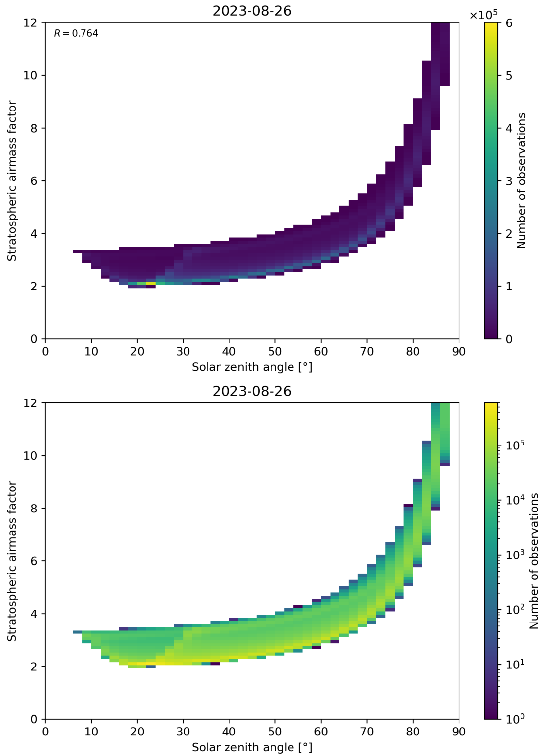
Figure 145: Scatter density plot of “Solar zenith angle” against “Stratospheric airmass factor” for 2023-08-25 to 2023-08-27.
