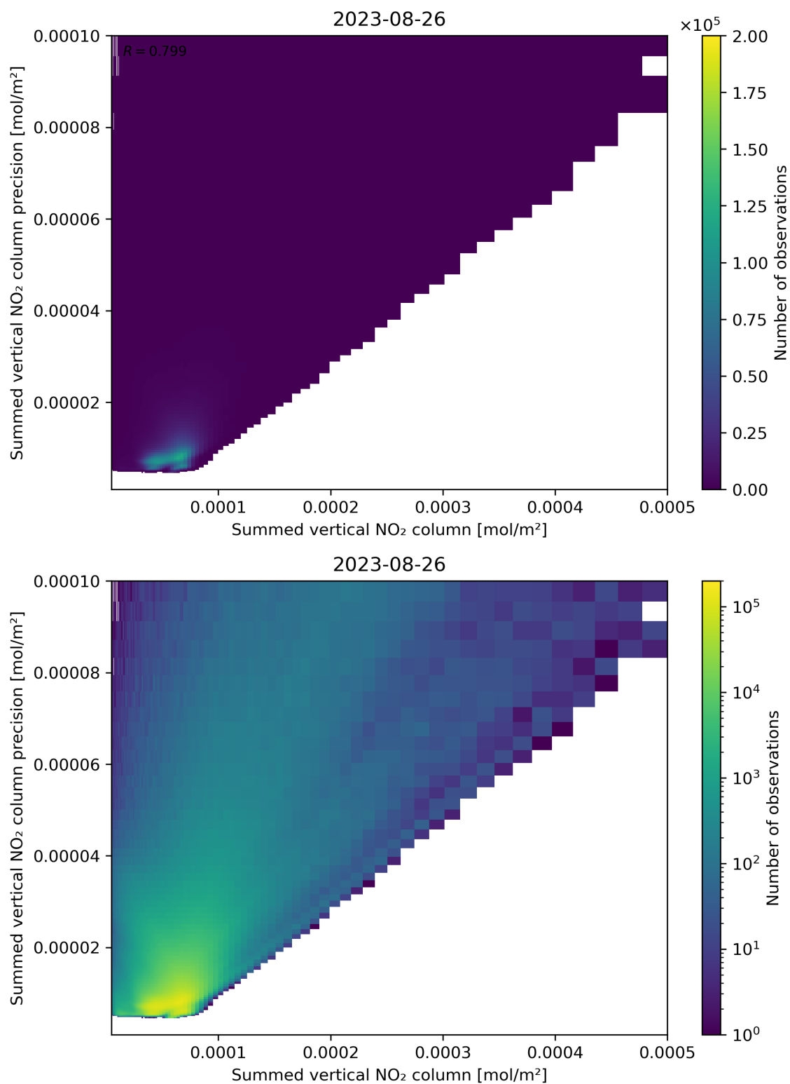
Figure 105: Scatter density plot of “Summed vertical NO 2 column” against “Summed vertical NO 2 column precision” for 2023-08-25 to 2023-08-27.
