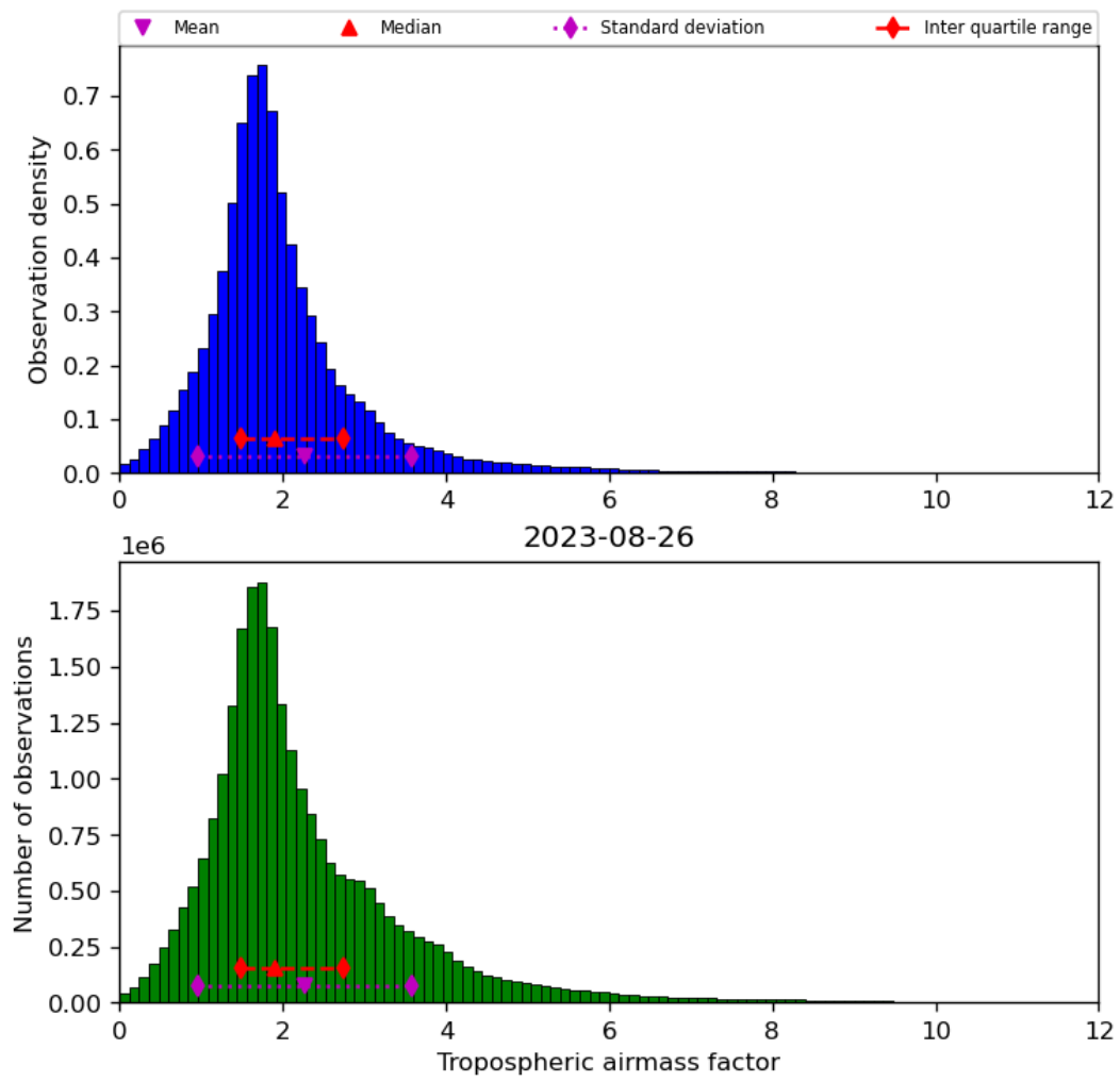
Figure 31: Histogram of “Tropospheric airmass factor” for 2023-08-25 to 2023-08-27
