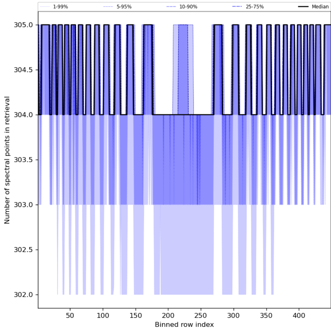
Figure 50: Along track statistics of “Number of spectral points in retrieval” for 2023-08-25 to 2023-08-27
