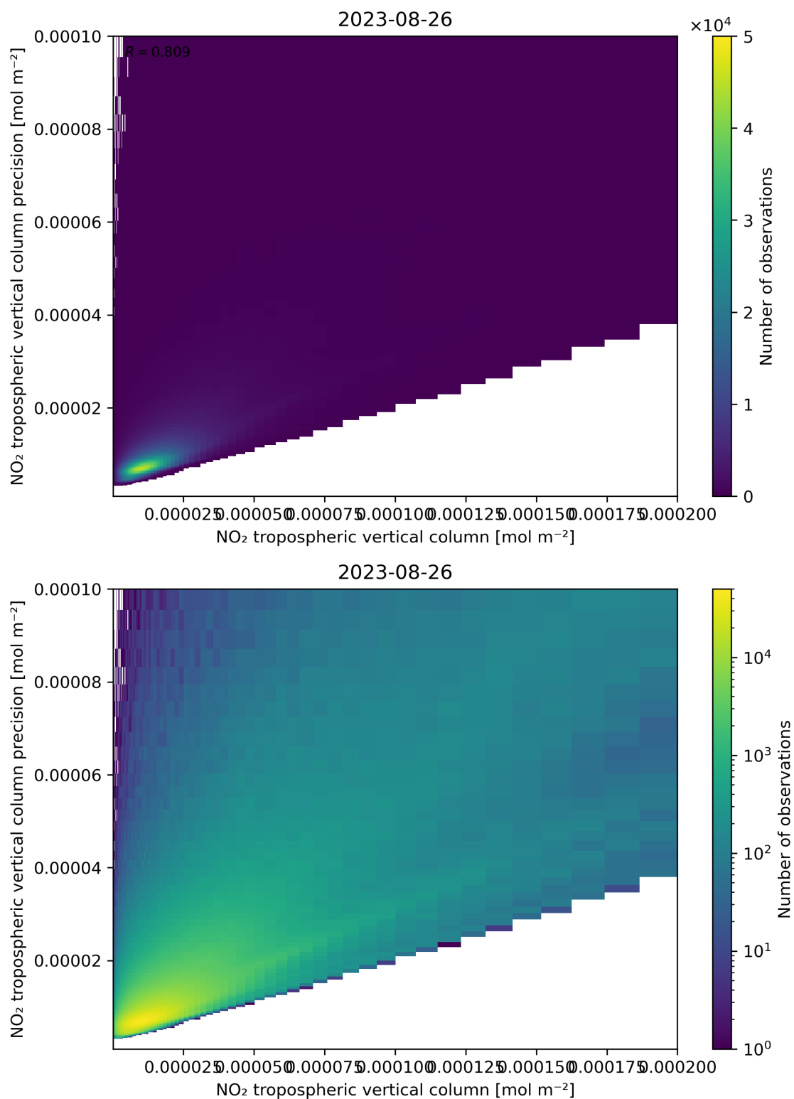
Figure 130: Scatter density plot of “NO 2 tropospheric vertical column” against “NO 2 tropospheric vertical column precision” for 2023-08-25 to 2023-08-27.
