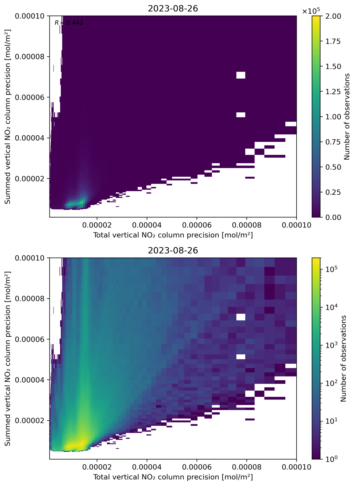
Figure 118: Scatter density plot of “Total vertical NO 2 column precision” against “Summed vertical NO 2 column precision” for 2023-08-25 to 2023-08-27.
