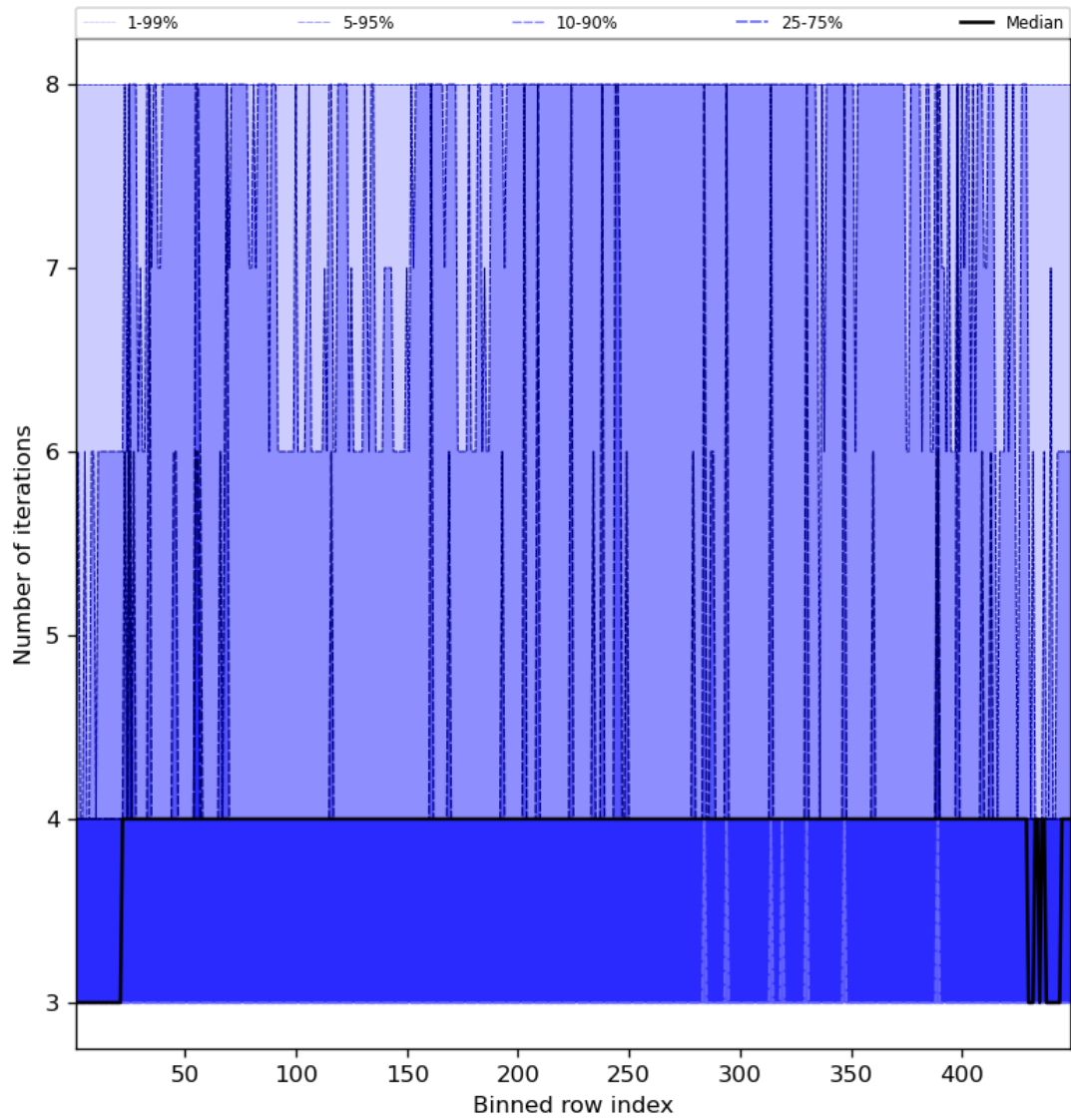
Figure 51: Along track statistics of “Number of iterations” for 2023-08-25 to 2023-08-27
