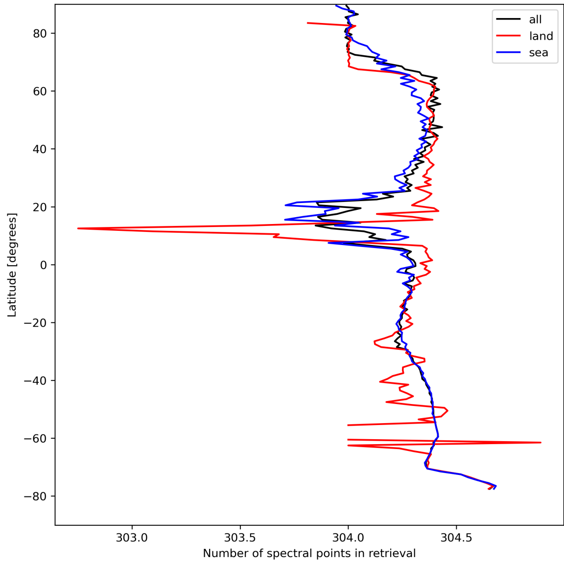
Figure 16: Zonal average of “Number of spectral points in retrieval” for 2023-08-25 to 2023-08-27.
