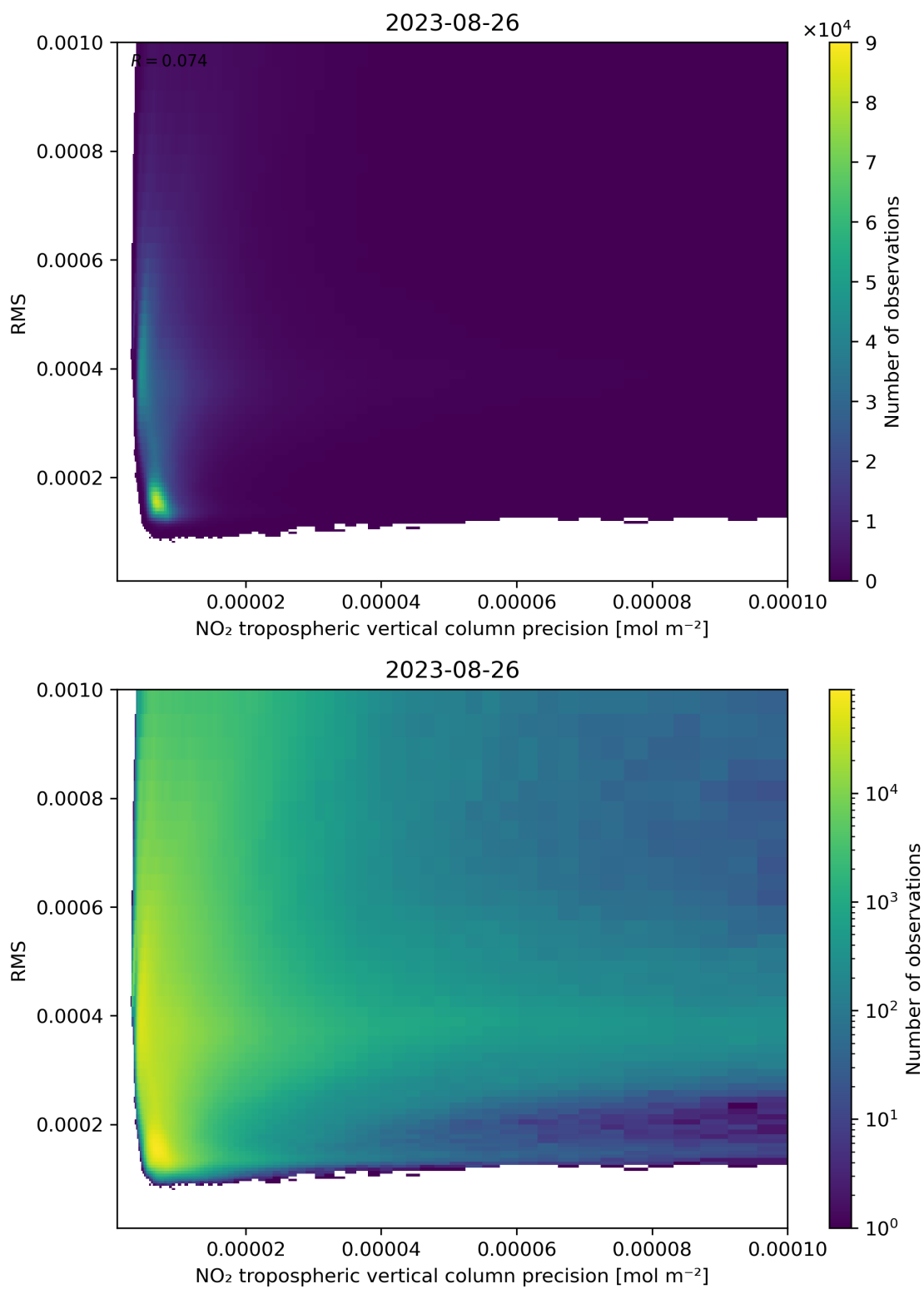
Figure 140: Scatter density plot of “NO 2 tropospheric vertical column precision” against “RMS” for 2023-08-25 to 2023-08-27.
