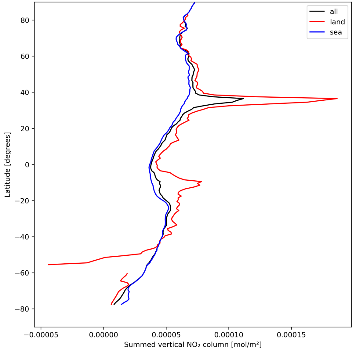
Figure 23: Zonal average of “Summed vertical NO 2 column” for 2023-08-25 to 2023-08-27.
