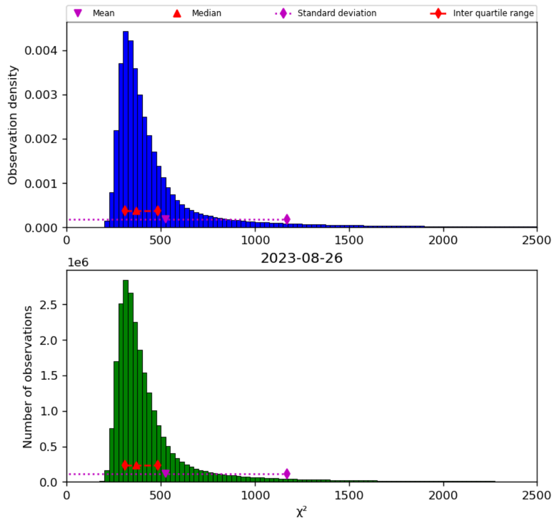
Figure 42: Histogram of “ \chi^2 ” for 2023-08-25 to 2023-08-27
