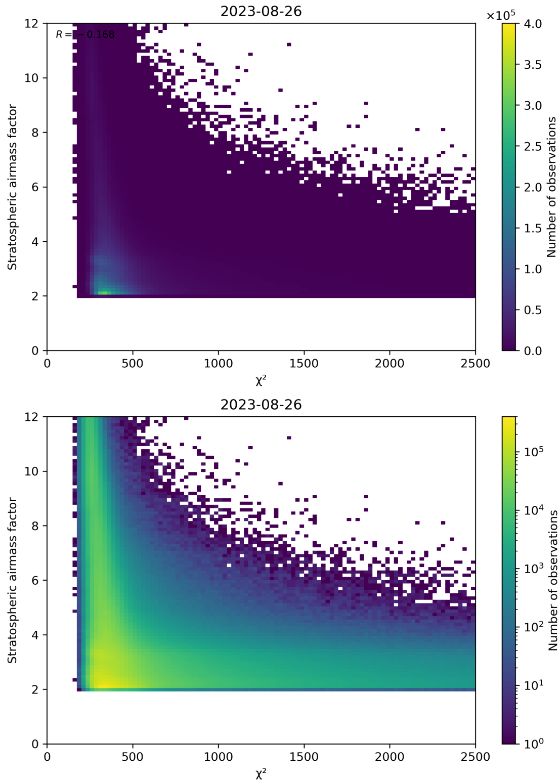
Figure 81: Scatter density plot of “ \chi^2 ” against “Stratospheric airmass factor” for 2023-08-25 to 2023-08-27.
