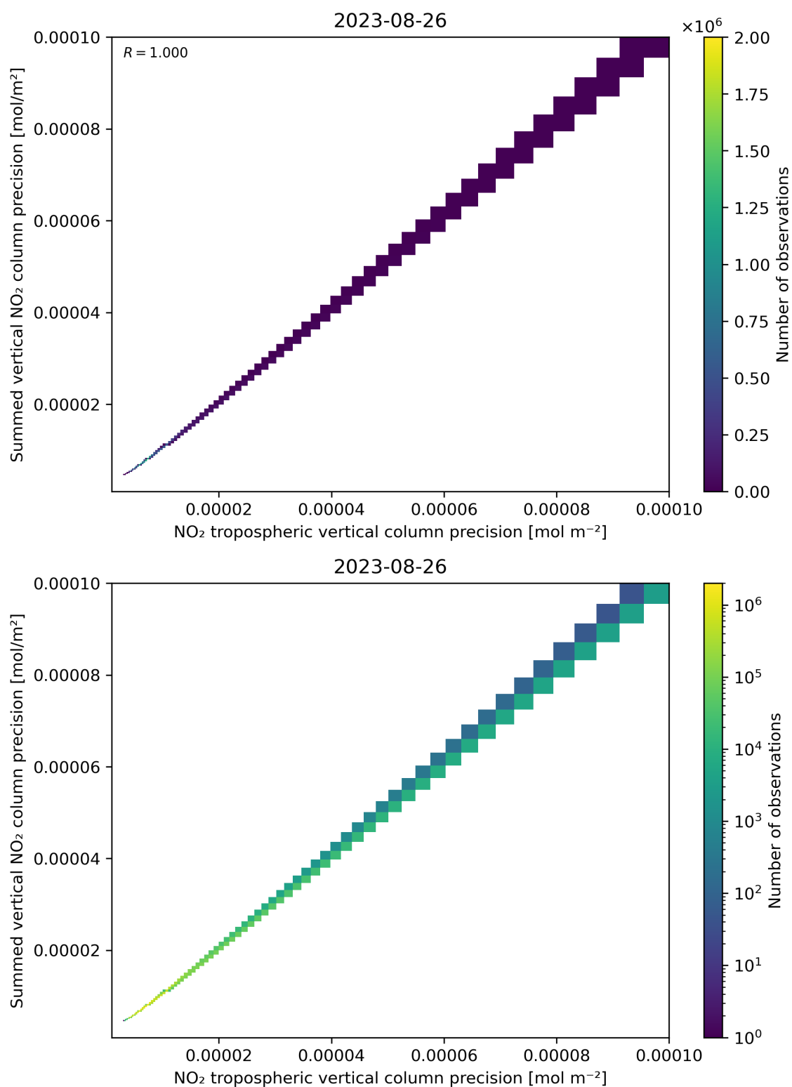
Figure 137: Scatter density plot of “NO 2 tropospheric vertical column precision” against “Summed vertical NO 2 column precision” for 2023-08-25 to 2023-08-27.
