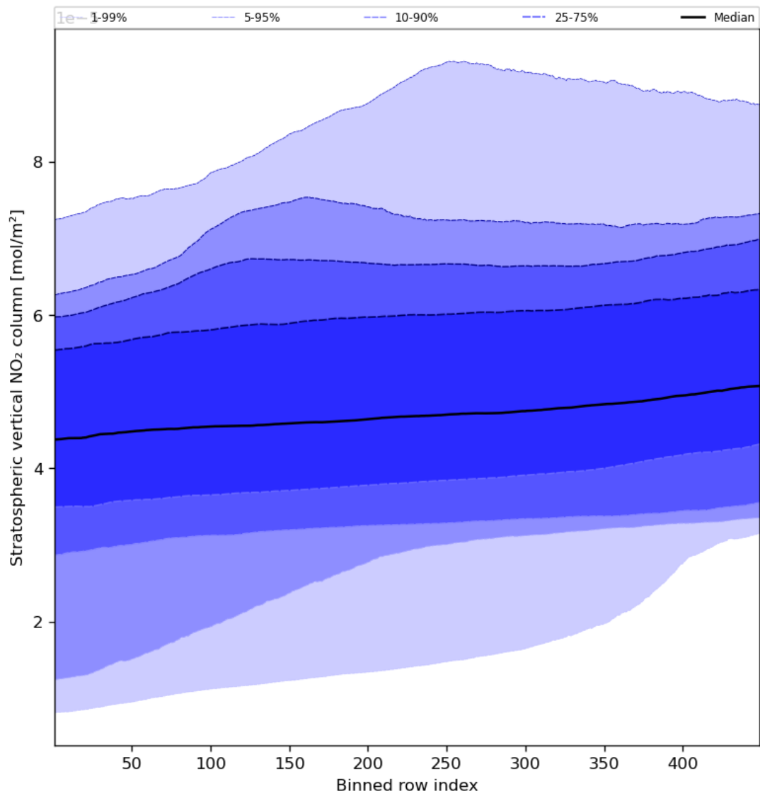
Figure 53: Along track statistics of “Stratospheric vertical NO 2 column” for 2023-08-25 to 2023-08-27
