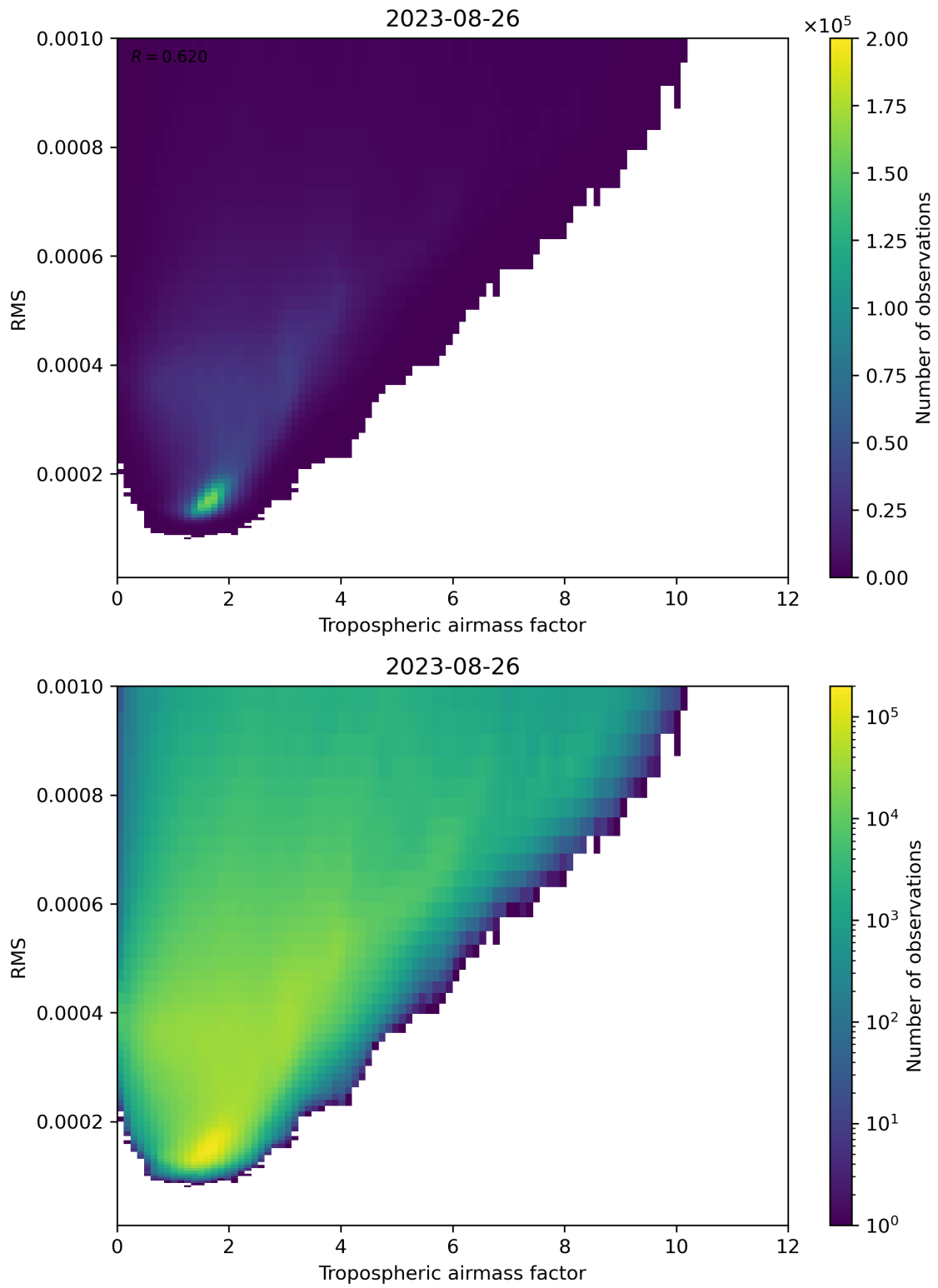
Figure 79: Scatter density plot of “Tropospheric airmass factor” against “RMS” for 2023-08-25 to 2023-08-27.
