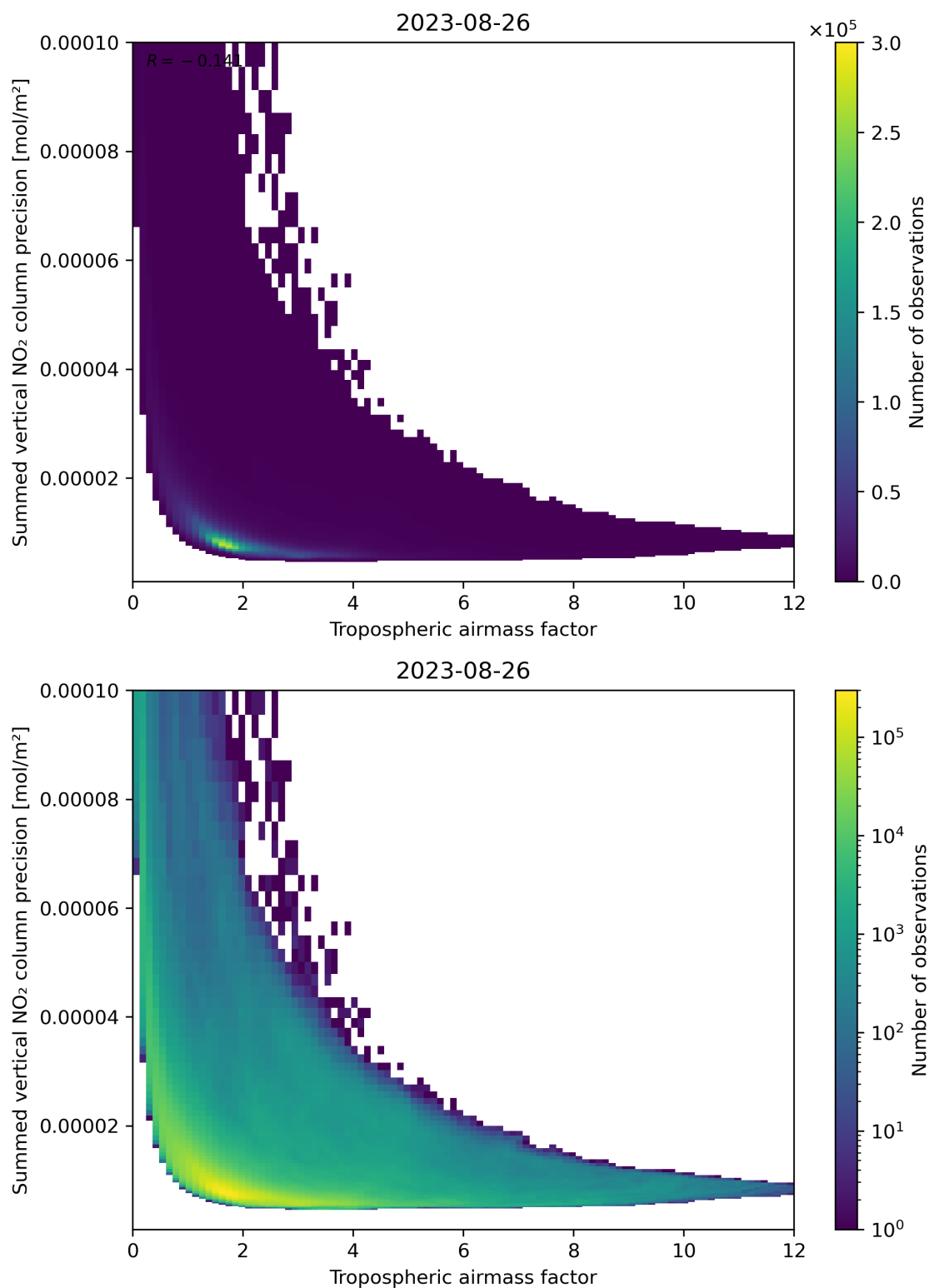
Figure 76: Scatter density plot of “Tropospheric air mass factor” against “Summed vertical NO 2 column precision” for 2023-08-25 to 2023-08-27.
