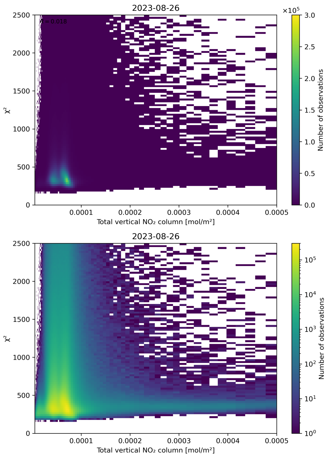
Figure 111: Scatter density plot of “Total vertical NO 2 column” against “ \chi^2 ” for 2023-08-25 to 2023-08-27.
