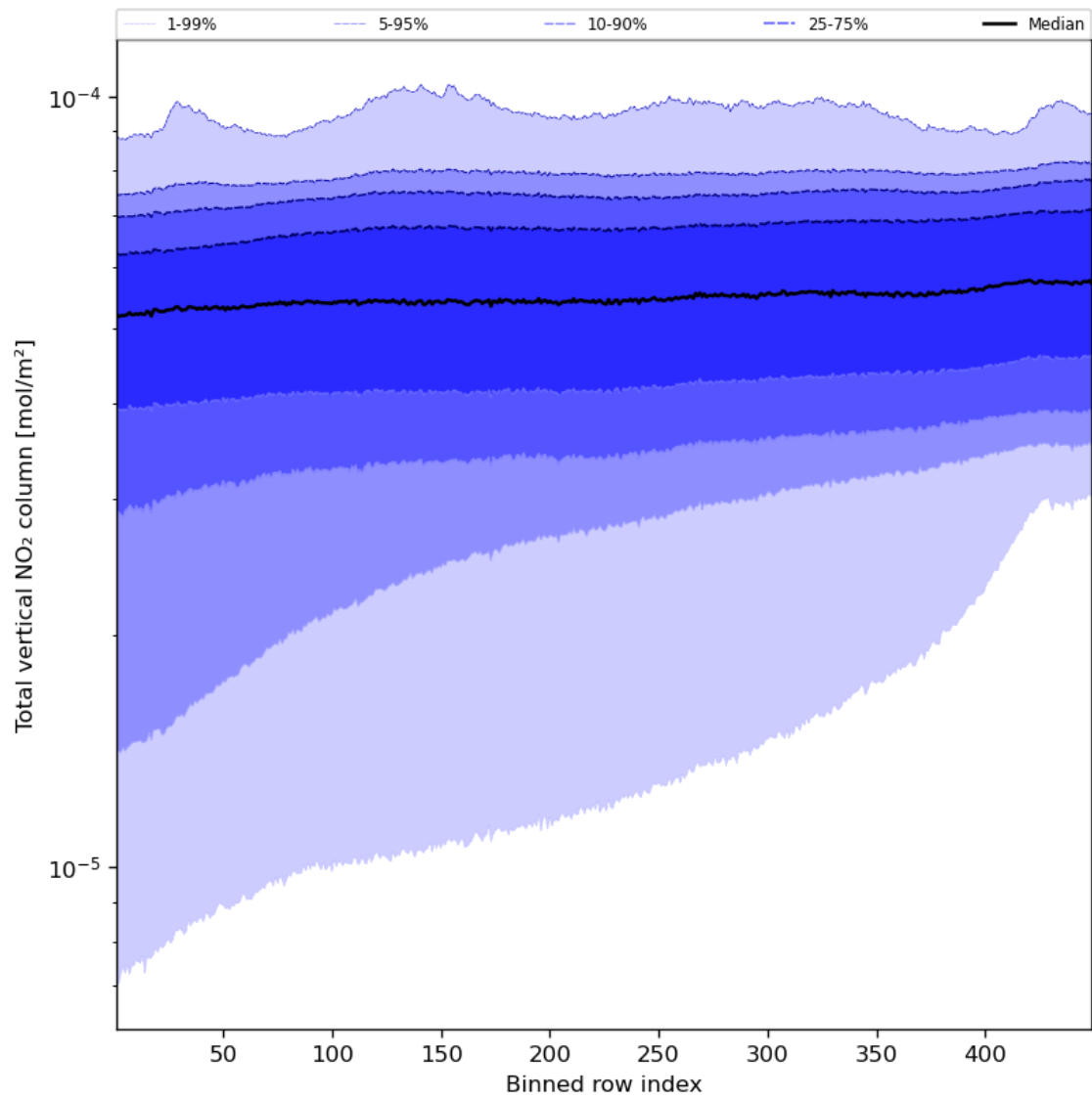
Figure 55: Along track statistics of “Total vertical NO 2 column” for 2023-08-25 to 2023-08-27
