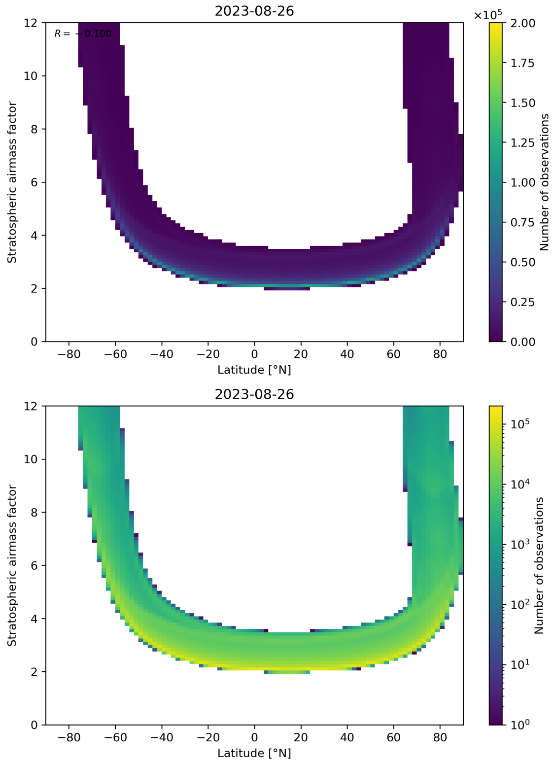
Figure 83: Scatter density plot of “Latitude” against “Stratospheric air mass factor” for 2023-08-25 to 2023-08-27.
