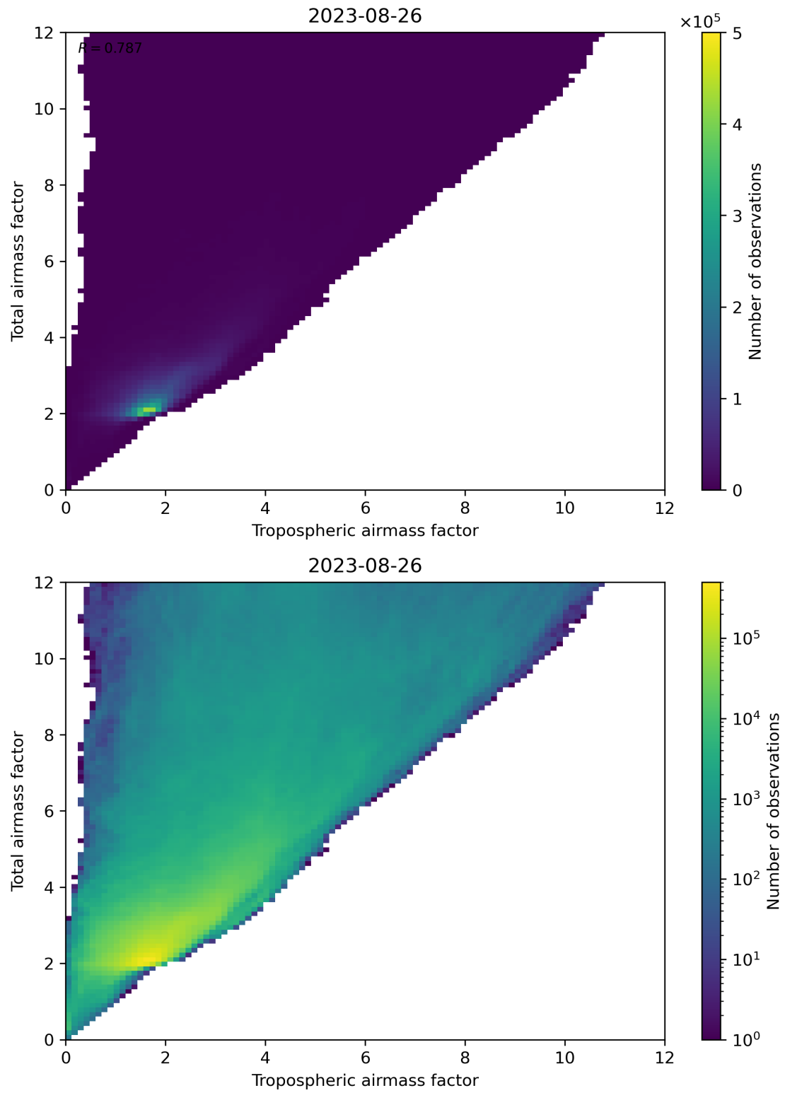
Figure 72: Scatter density plot of “Tropospheric airmass factor” against “Total airmass factor” for 2023-08-25 to 2023-08-27.
