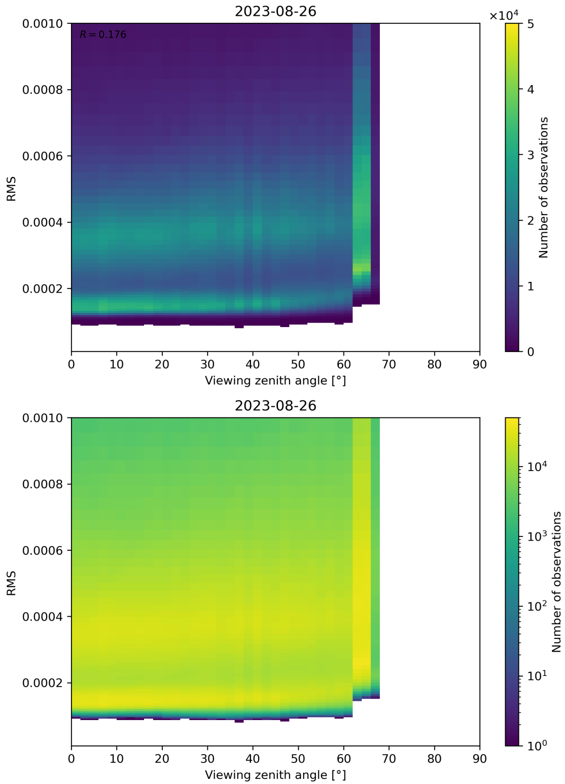
Figure 171: Scatter density plot of “Viewing zenith angle” against “RMS” for 2023-08-25 to 2023-08-27.
