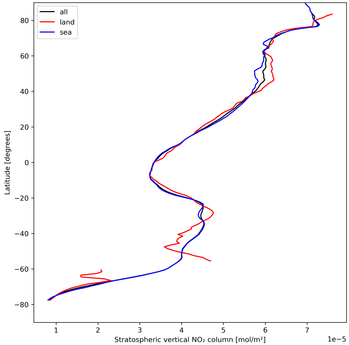
Figure 19: Zonal average of “Stratospheric vertical NO 2 column” for 2023-08-25 to 2023-08-27.
