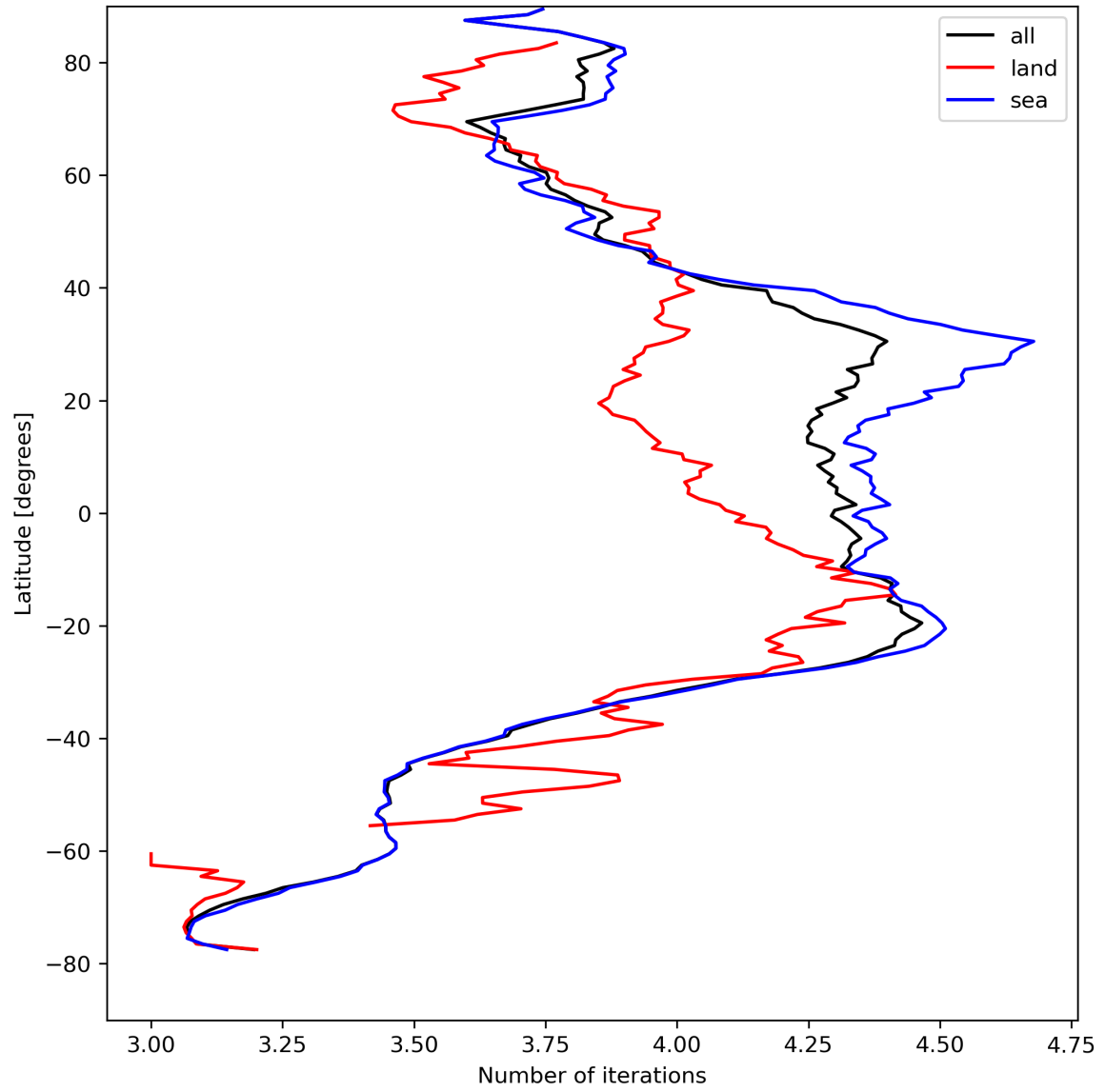
Figure 17: Zonal average of “Number of iterations” for 2023-08-25 to 2023-08-27.
