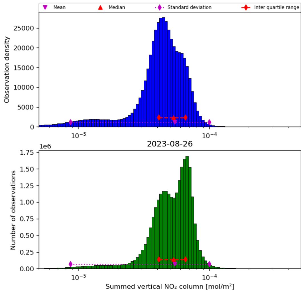
Figure 40: Histogram of “Summed vertical NO 2 column” for 2023-08-25 to 2023-08-27
