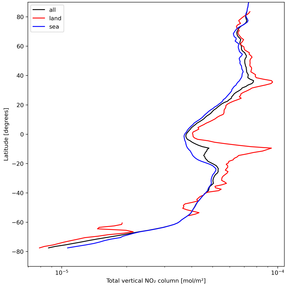
Figure 21: Zonal average of “Total vertical NO 2 column” for 2023-08-25 to 2023-08-27.
