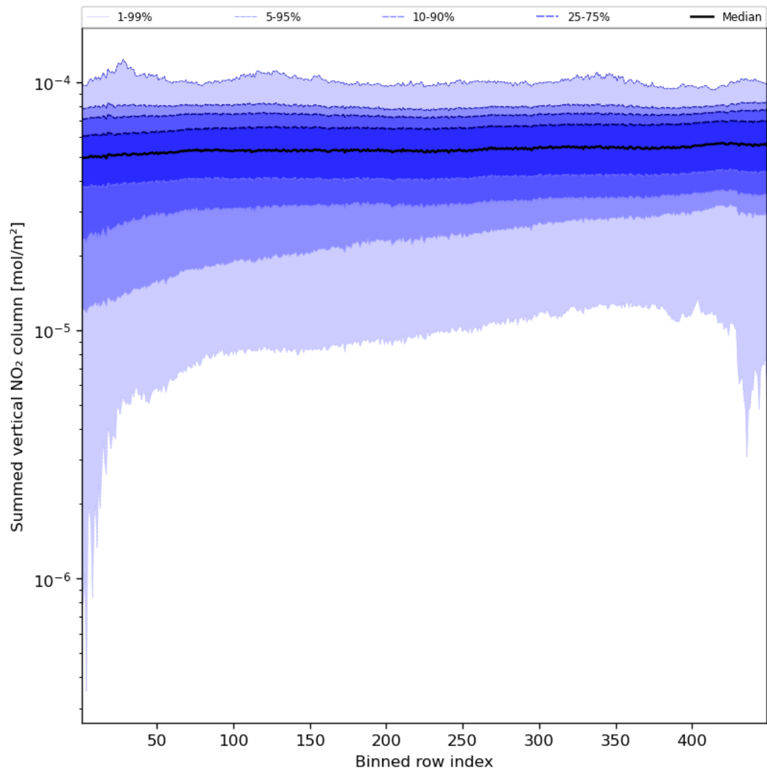
Figure 57: Along track statistics of “Summed vertical NO 2 column” for 2023-08-25 to 2023-08-27
