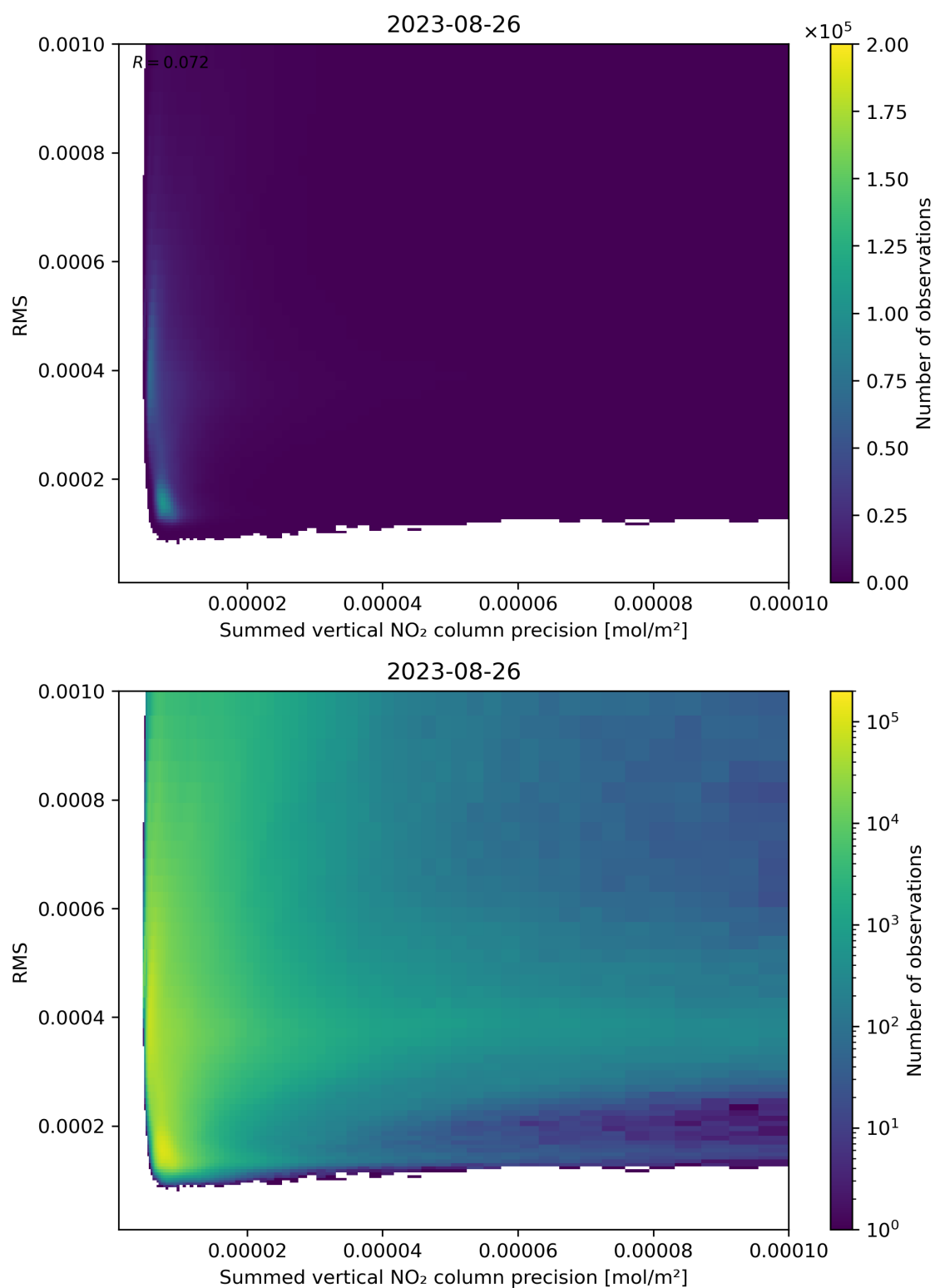
Figure 108: Scatter density plot of “Summed vertical NO 2 column precision” against “RMS” for 2023-08-25 to 2023-08-27.
