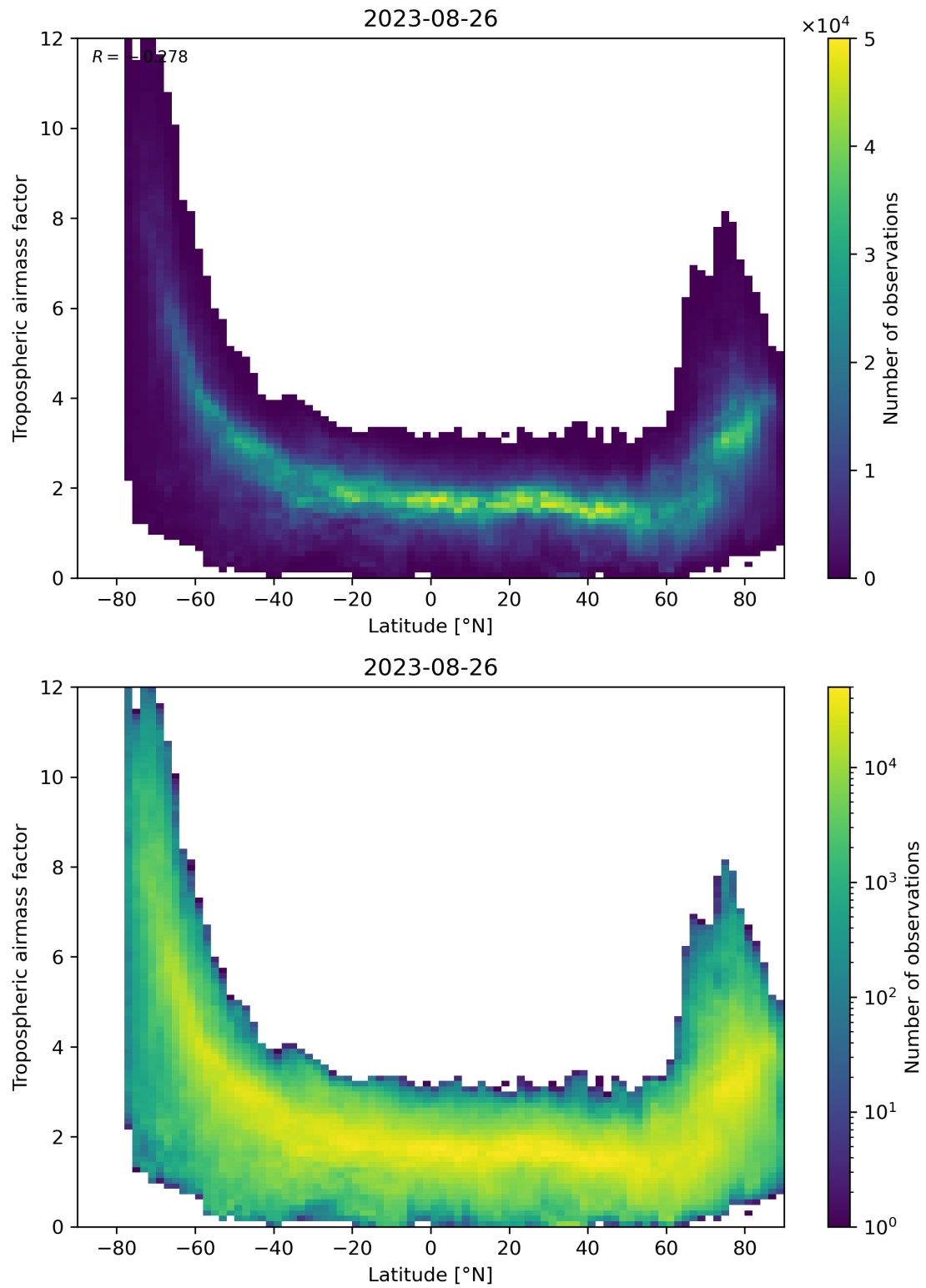
Figure 85: Scatter density plot of “Latitude” against “Tropospheric air mass factor” for 2023-08-25 to 2023-08-27.
