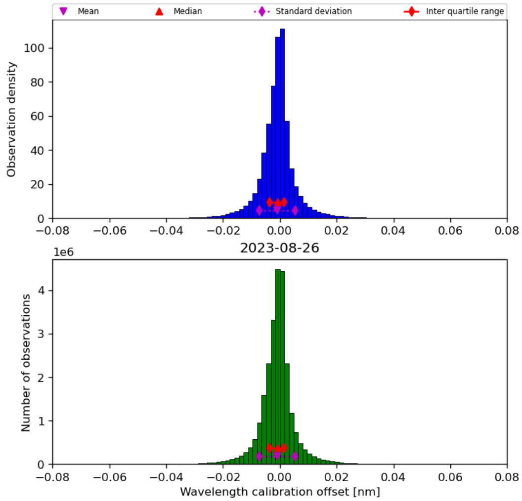
Figure 35: Histogram of “Wavelength calibration offset” for 2023-08-25 to 2023-08-27
