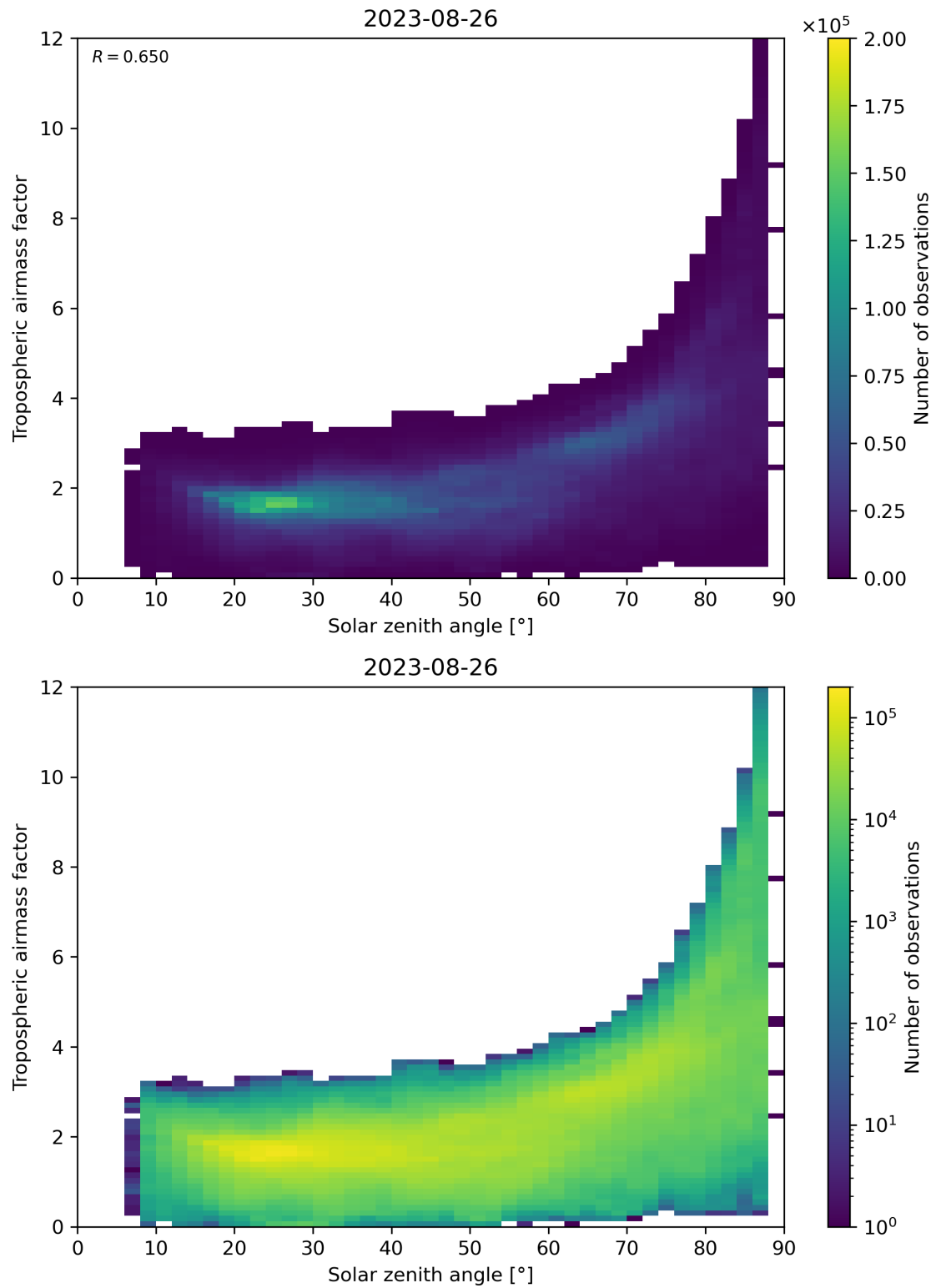
Figure 147: Scatter density plot of “Solar zenith angle” against “Tropospheric airmass factor” for 2023-08-25 to 2023-08-27.
