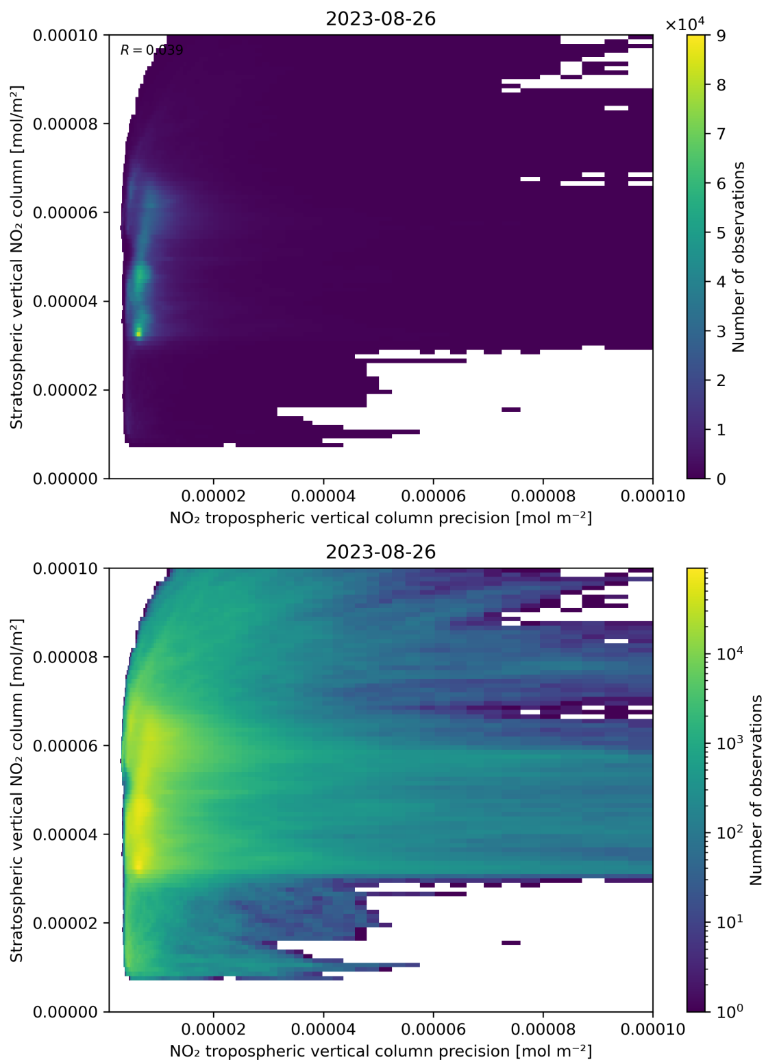
Figure 135: Scatter density plot of “NO 2 tropospheric vertical column precision” against “Stratospheric vertical NO 2 column” for 2023-08-25 to 2023-08-27.
