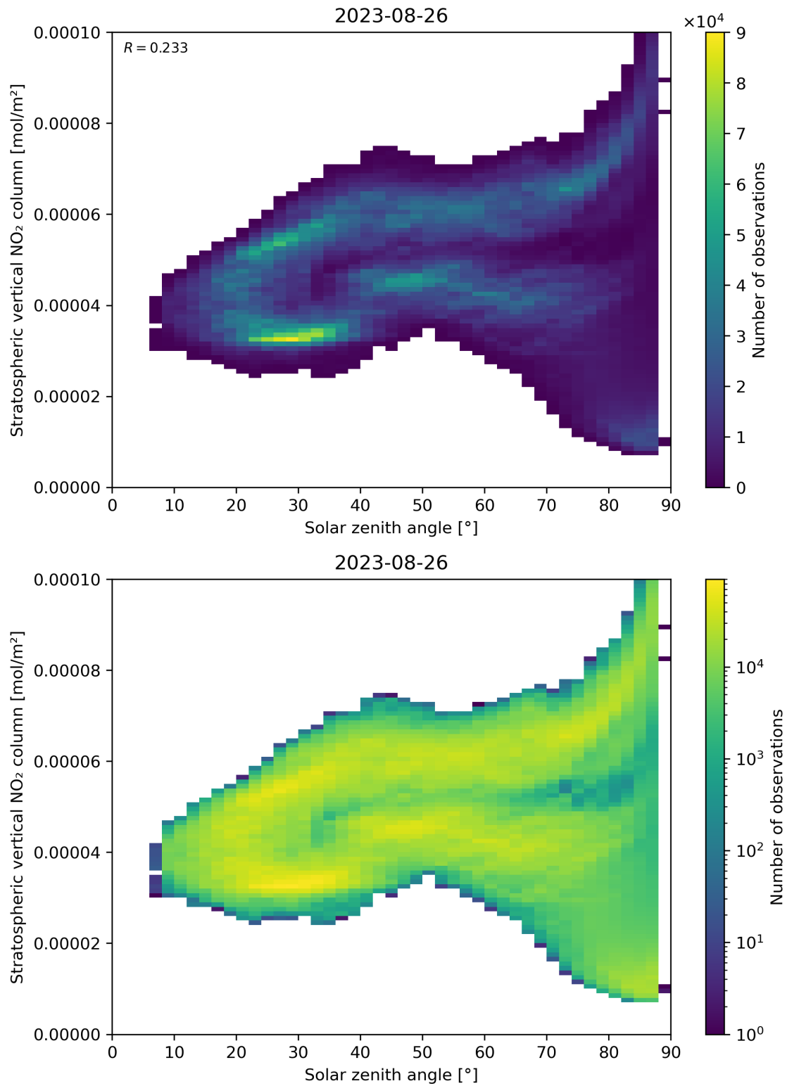
Figure 150: Scatter density plot of “Solar zenith angle” against “Stratospheric vertical \text{NO}_2 column” for 2023-08-25 to 2023-08-27.
