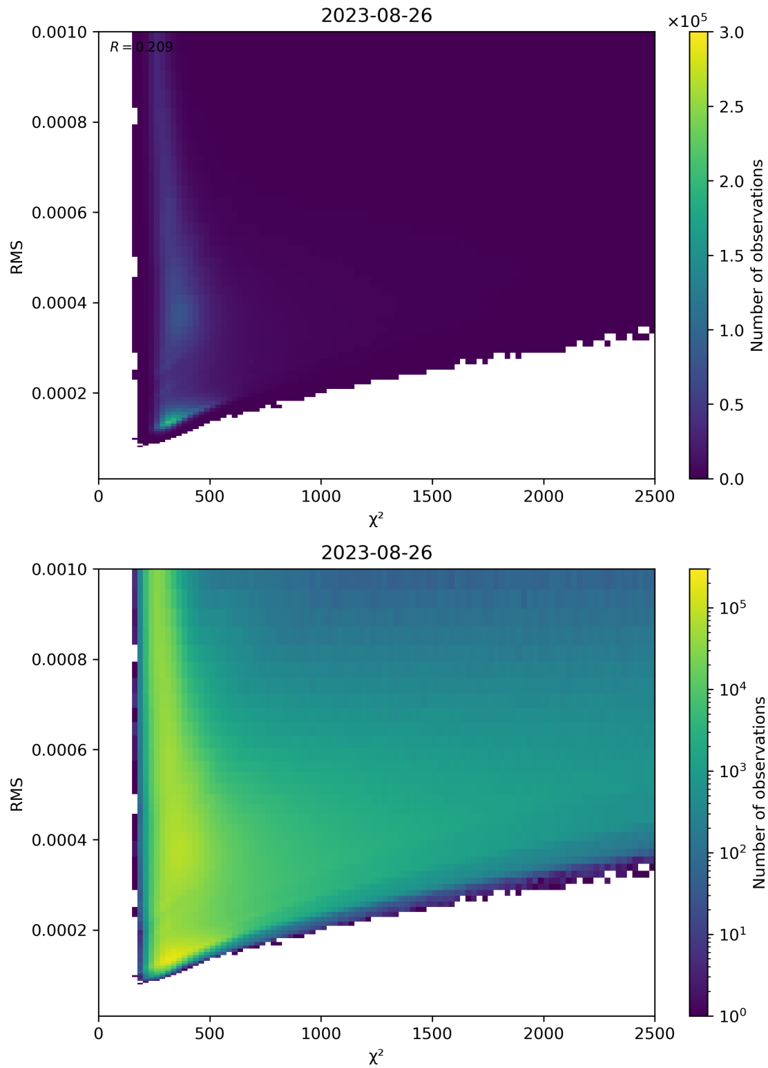
Figure 82: Scatter density plot of “ \chi^2 ” against “RMS” for 2023-08-25 to 2023-08-27.
