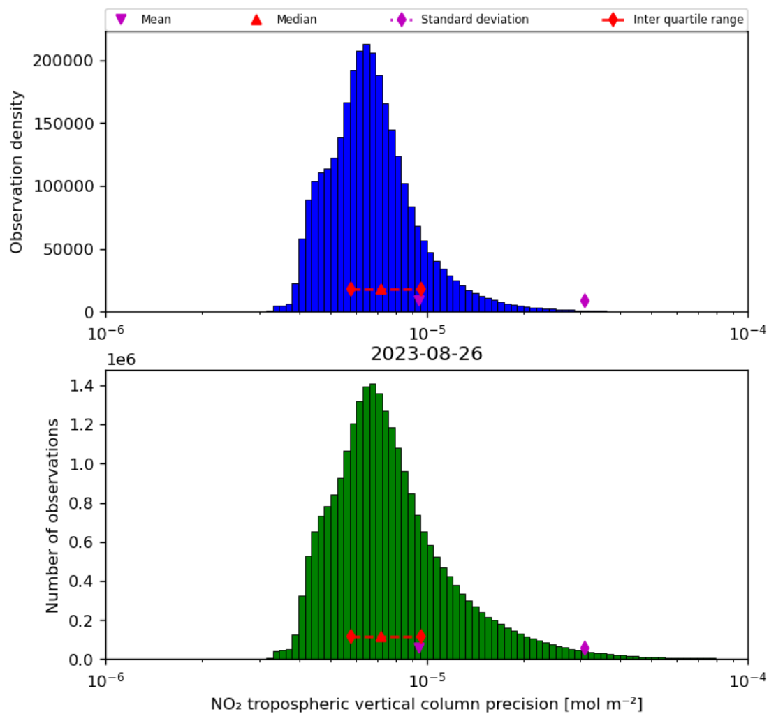
Figure 30: Histogram of “NO 2 tropospheric vertical column precision” for 2023-08-25 to 2023-08-27
