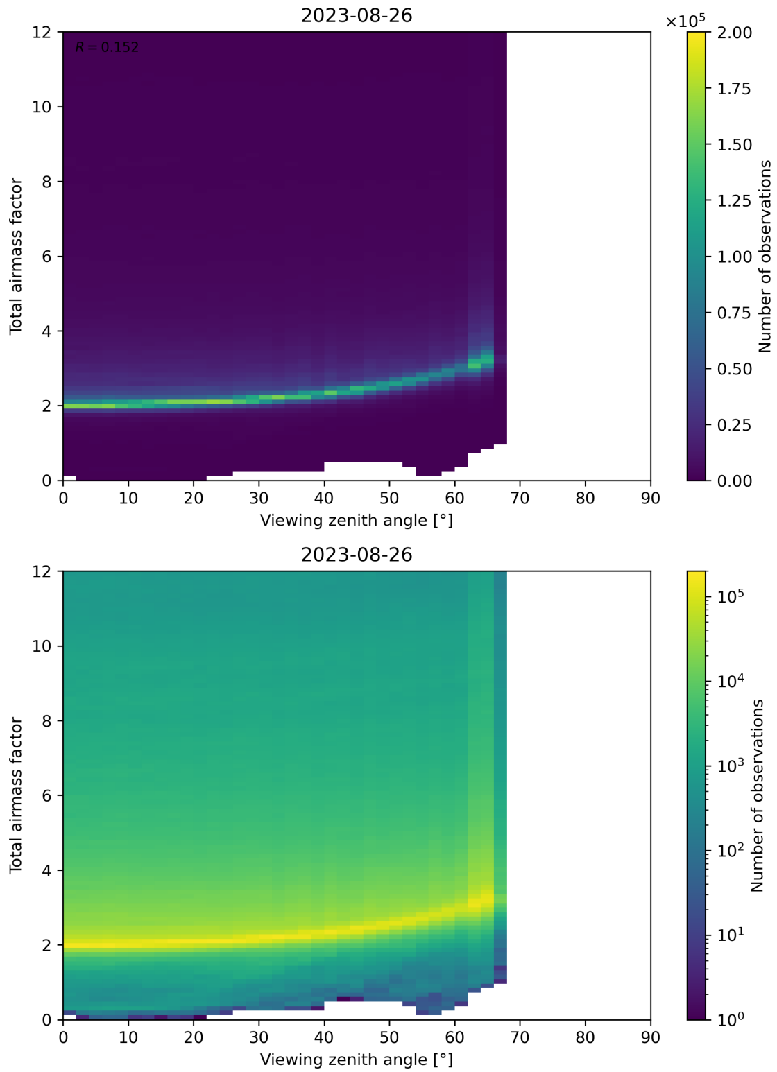
Figure 160: Scatter density plot of “Viewing zenith angle” against “Total airmass factor” for 2023-08-25 to 2023-08-27.
