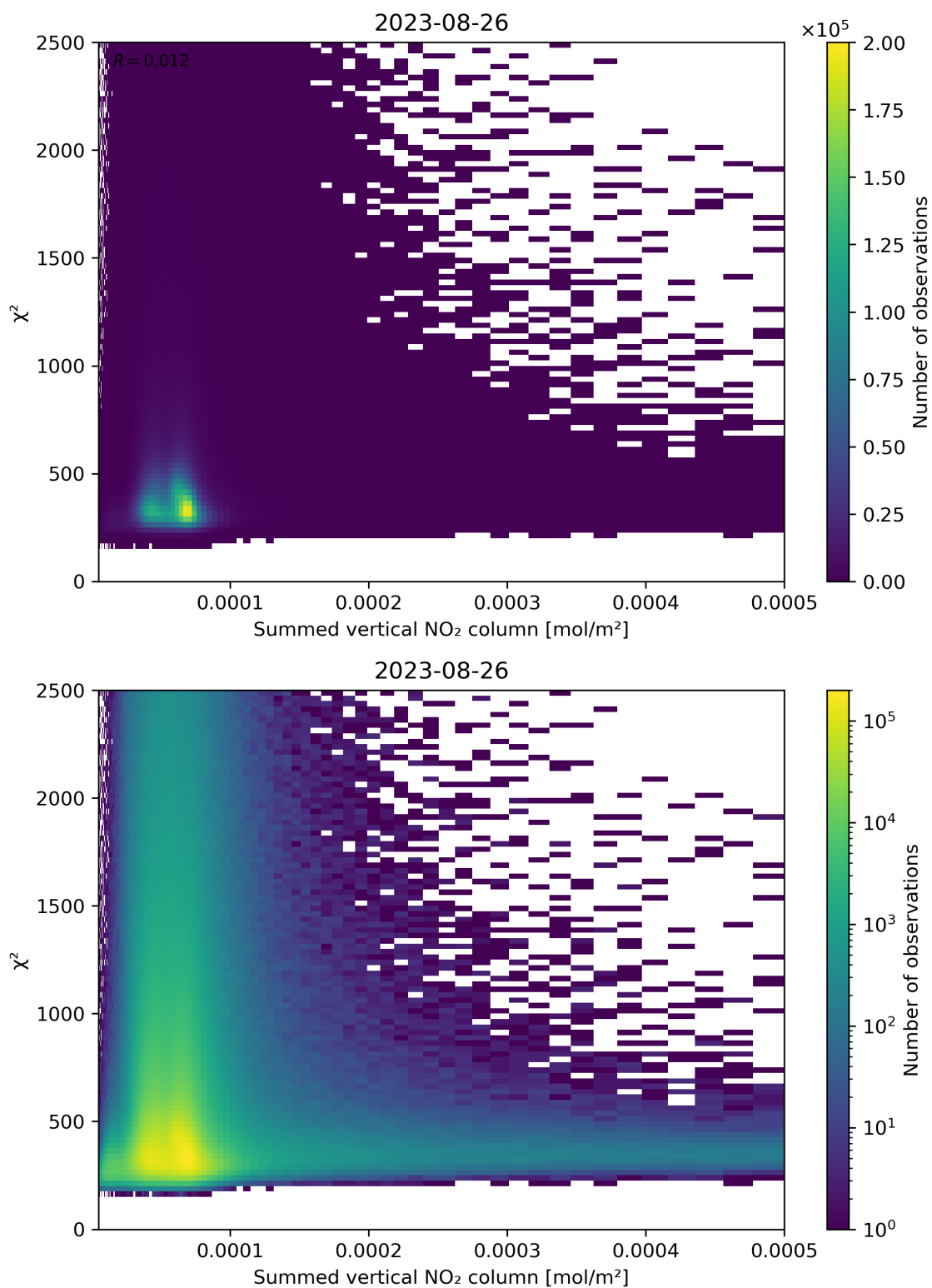
Figure 104: Scatter density plot of “Summed vertical NO 2 column” against “ \chi^2 ” for 2023-08-25 to 2023-08-27.
