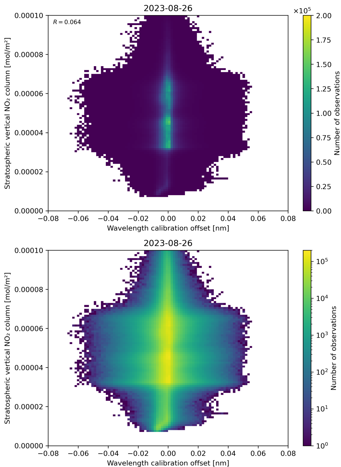
Figure 176: Scatter density plot of “Wavelength calibration offset” against “Stratospheric vertical NO 2 column” for 2023-08-25 to 2023-08-27.
