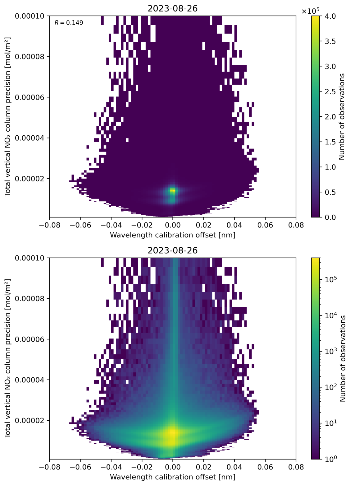
Figure 180: Scatter density plot of “Wavelength calibration offset” against “Total vertical NO 2 column precision” for 2023-08-25 to 2023-08-27.
