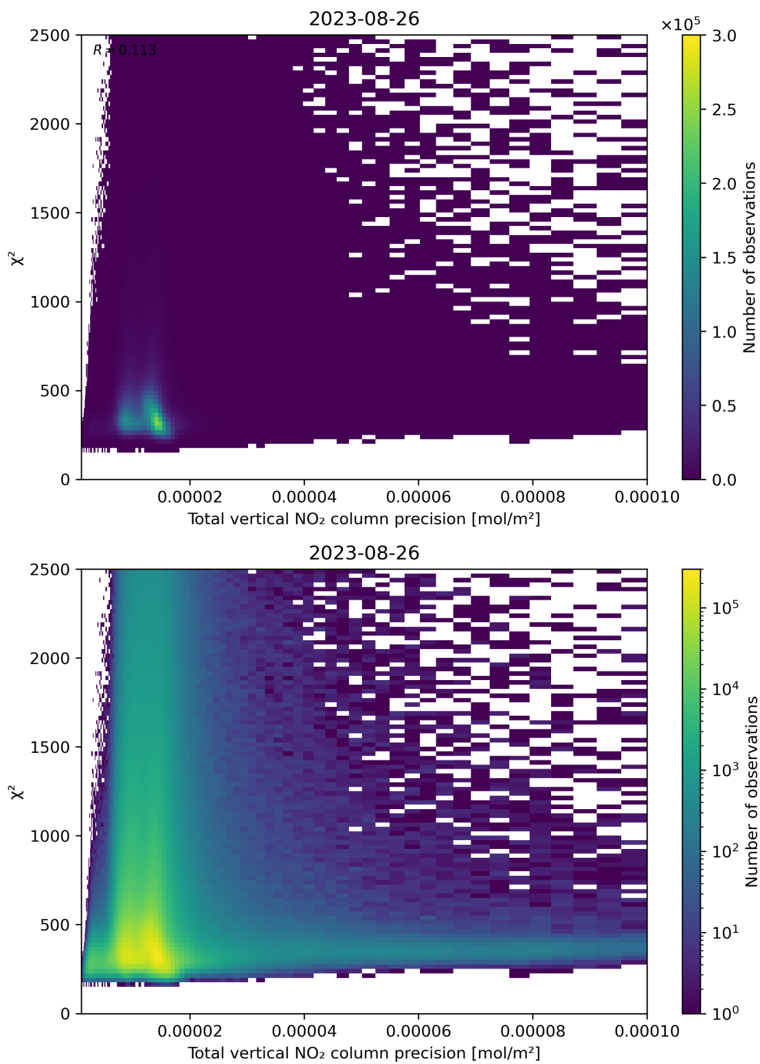
Figure 116: Scatter density plot of “Total vertical NO 2 column precision” against “ \chi^2 ” for 2023-08-25 to 2023-08-27.
