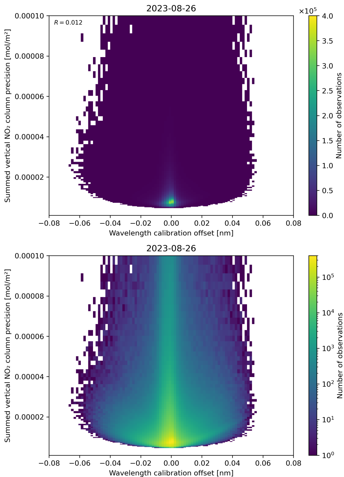
Figure 178: Scatter density plot of “Wavelength calibration offset” against “Summed vertical NO 2 column precision” for 2023-08-25 to 2023-08-27.
