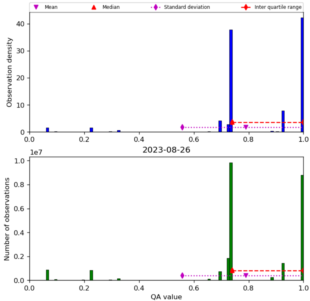
Figure 28: Histogram of “QA value” for 2023-08-25 to 2023-08-27
