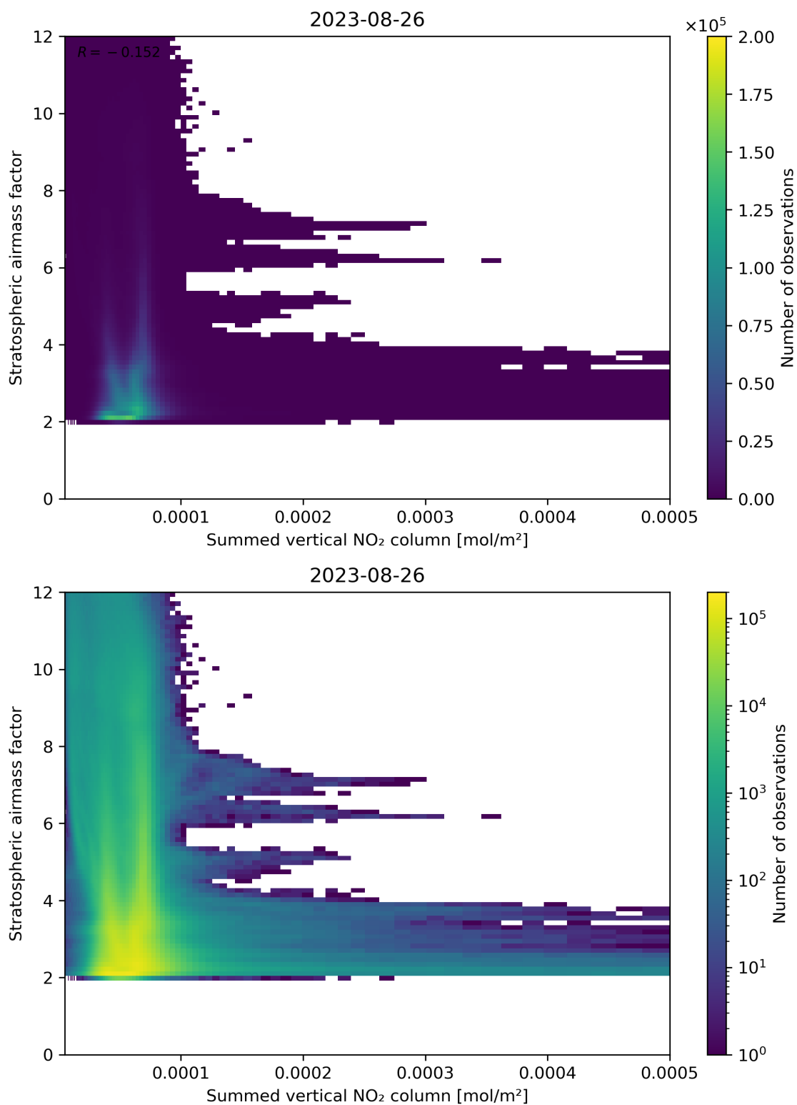
Figure 103: Scatter density plot of “Summed vertical NO 2 column” against “Stratospheric air mass factor” for 2023-08-25 to 2023-08-27.
