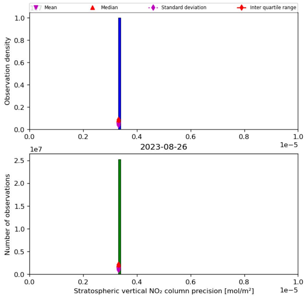
Figure 37: Histogram of “Stratospheric vertical NO 2 column precision” for 2023-08-25 to 2023-08-27
