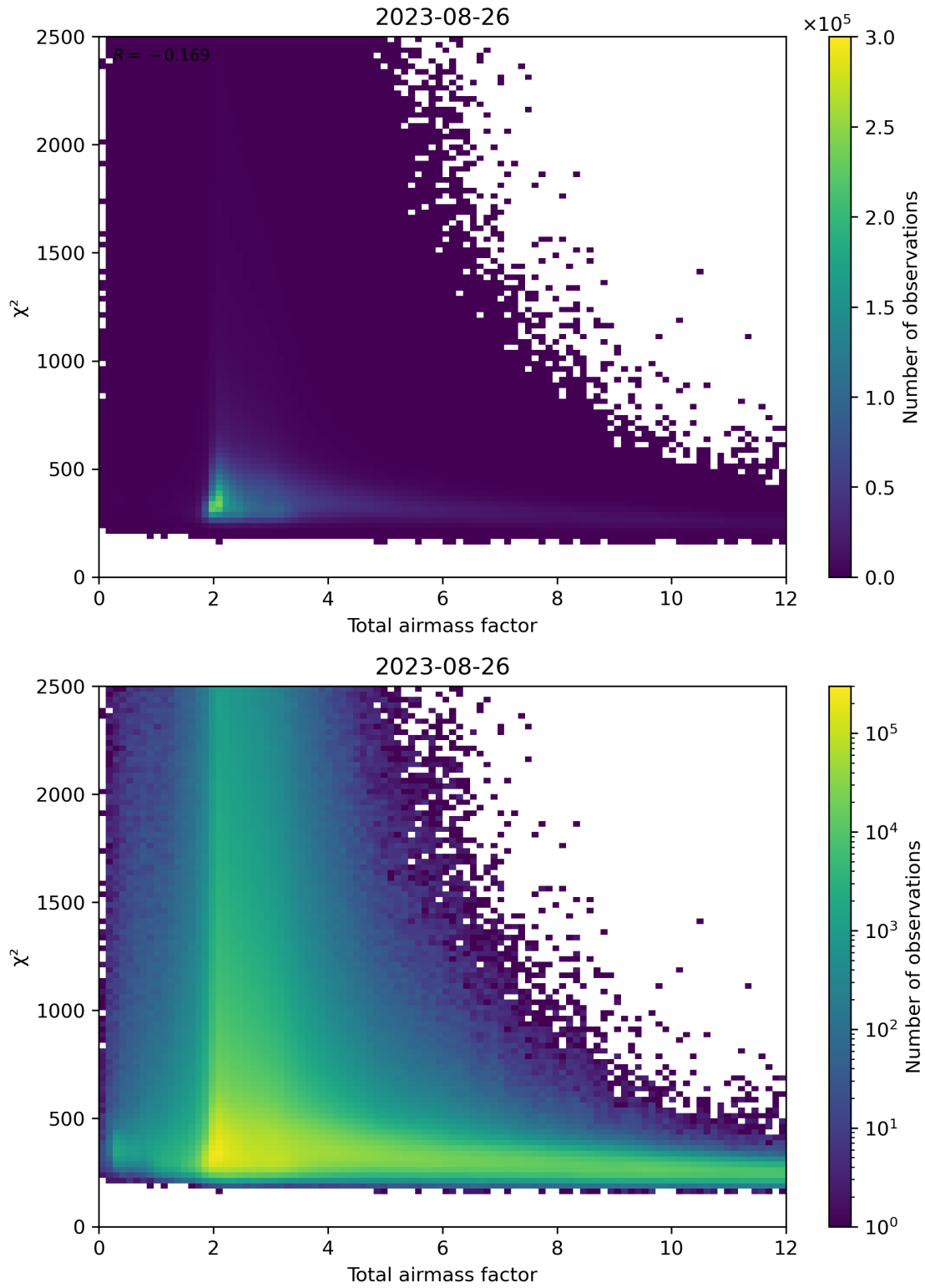
Figure 63: Scatter density plot of “Total airmass factor” against “ \chi^2 ” for 2023-08-25 to 2023-08-27.
