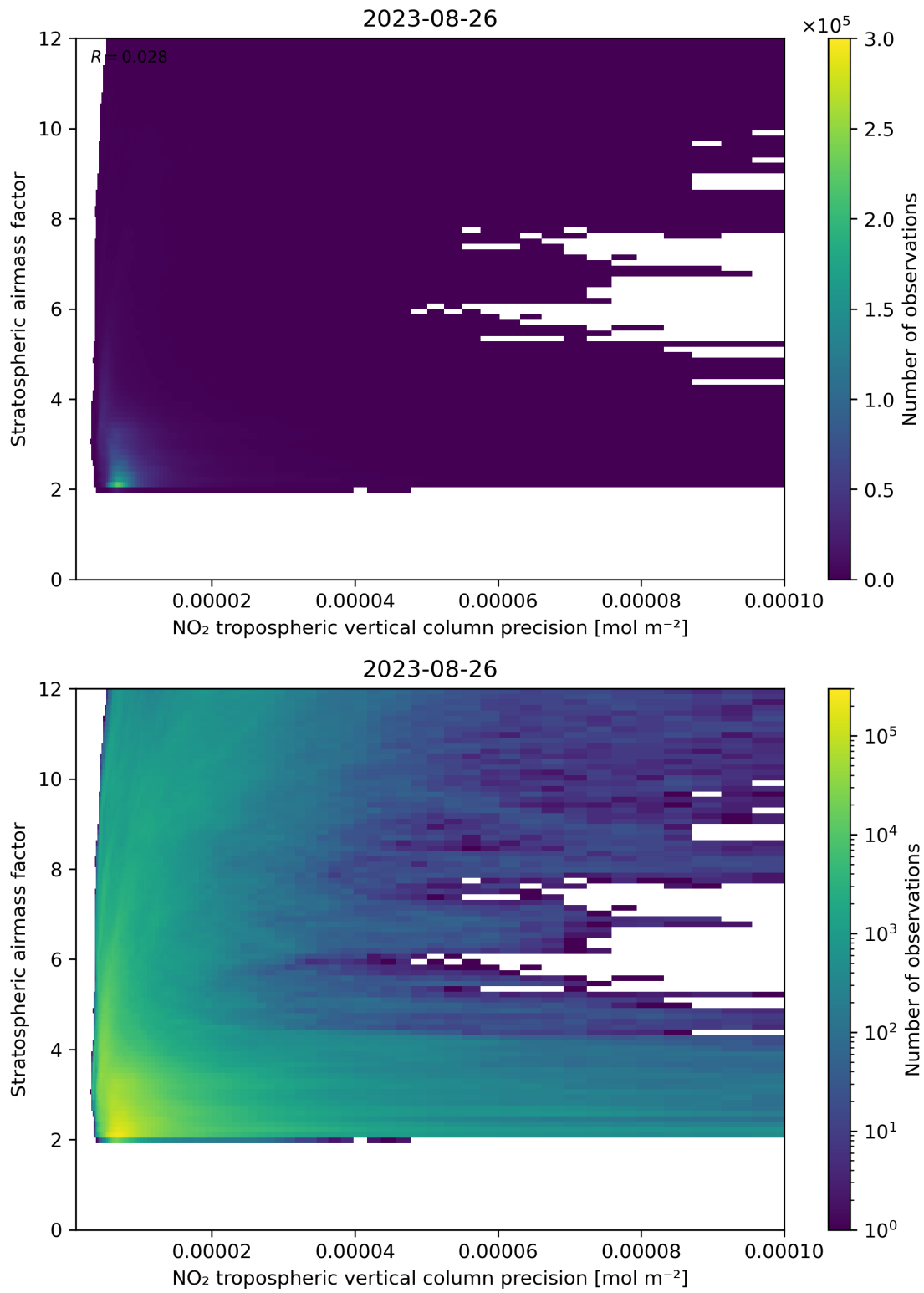
Figure 131: Scatter density plot of “NO 2 tropospheric vertical column precision” against “Stratospheric airmass factor” for 2023-08-25 to 2023-08-27.
