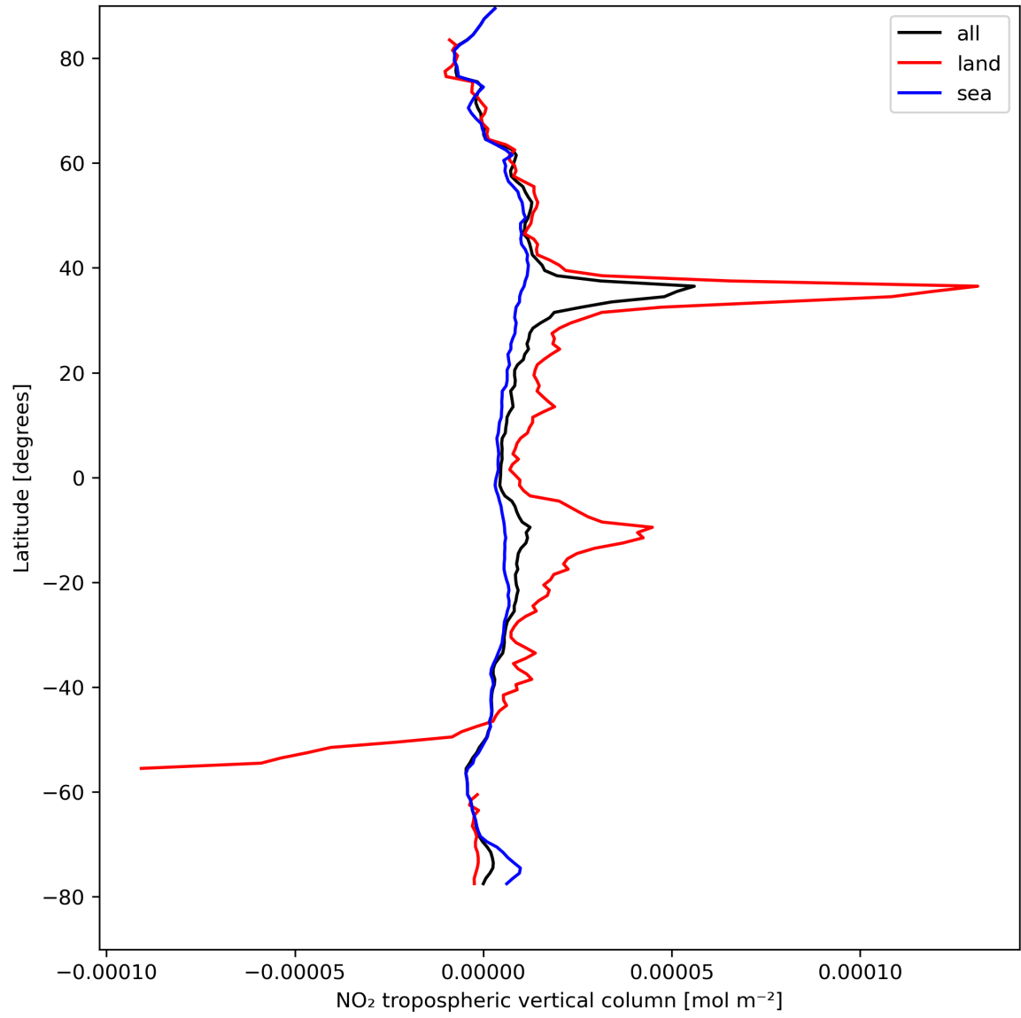
Figure 12: Zonal average of “NO 2 tropospheric vertical column” for 2023-08-25 to 2023-08-27.
