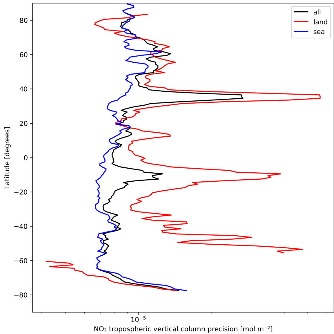
Figure 13: Zonal average of “NO 2 tropospheric vertical column precision” for 2023-08-25 to 2023-08-27.
