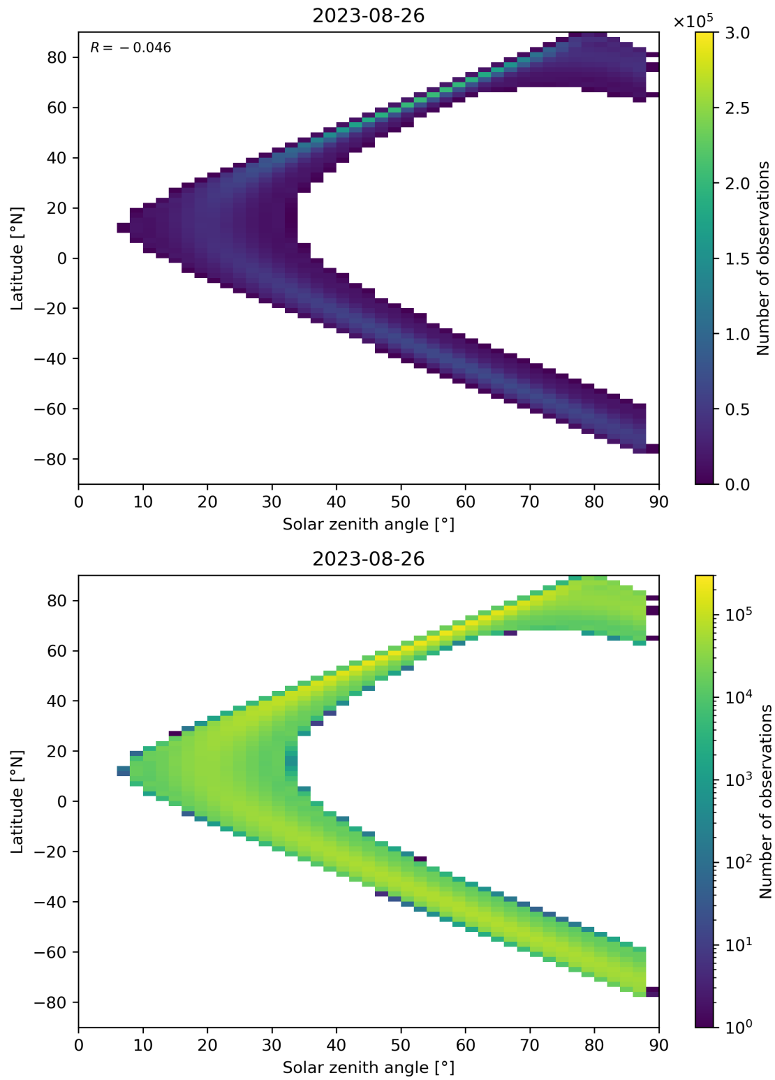
Figure 149: Scatter density plot of “Solar zenith angle” against “Latitude” for 2023-08-25 to 2023-08-27.
