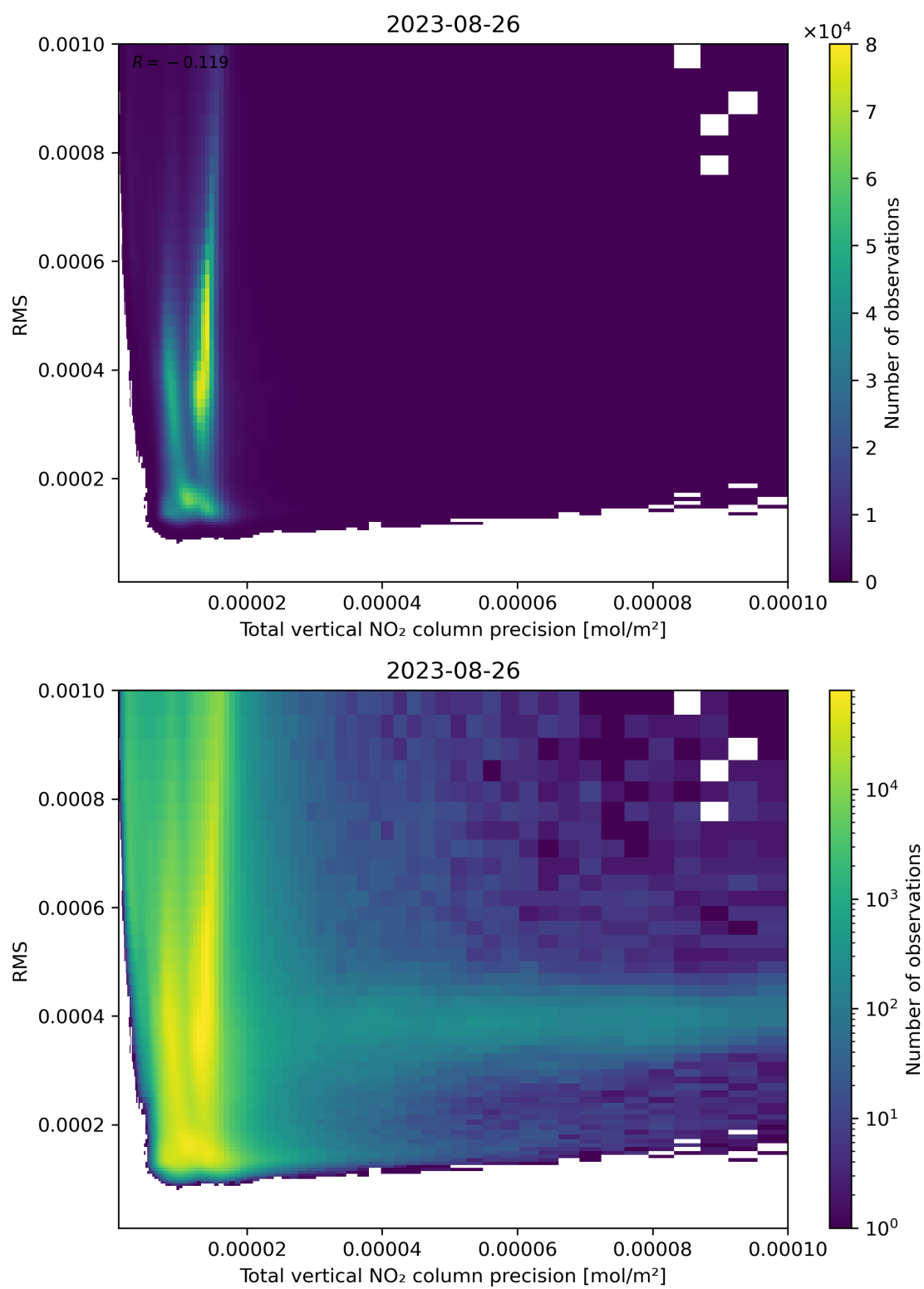
Figure 119: Scatter density plot of “Total vertical NO 2 column precision” against “RMS” for 2023-08-25 to 2023-08-27.
