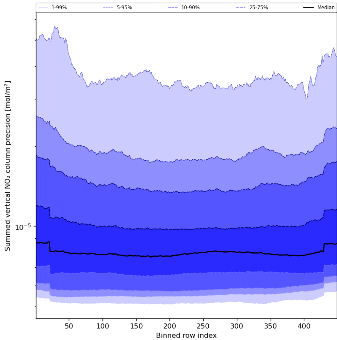
Figure 58: Along track statistics of “Summed vertical NO 2 column precision” for 2023-08-25 to 2023-08-27
