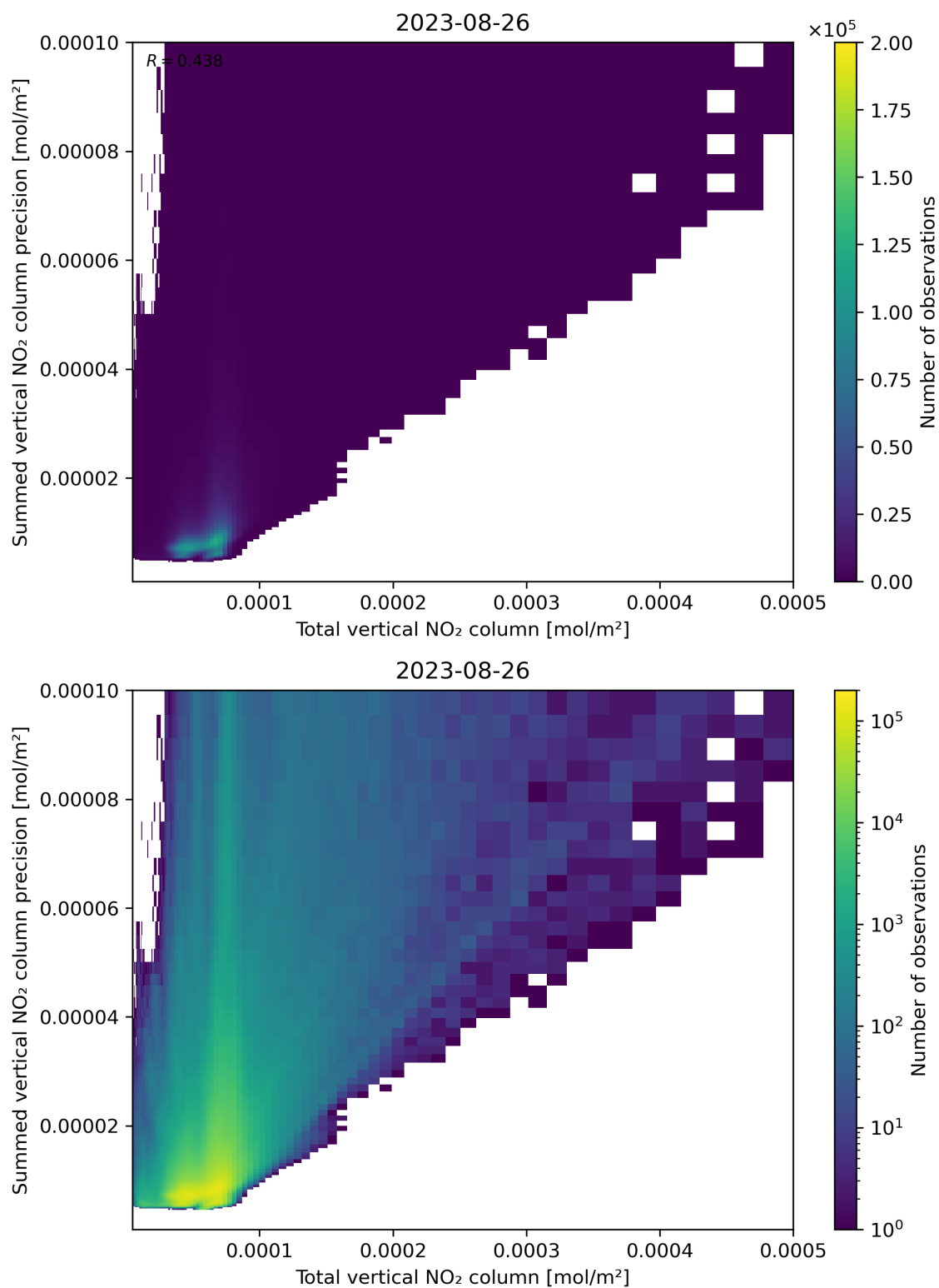
Figure 113: Scatter density plot of “Total vertical NO 2 column” against “Summed vertical NO 2 column precision” for 2023-08-25 to 2023-08-27.
