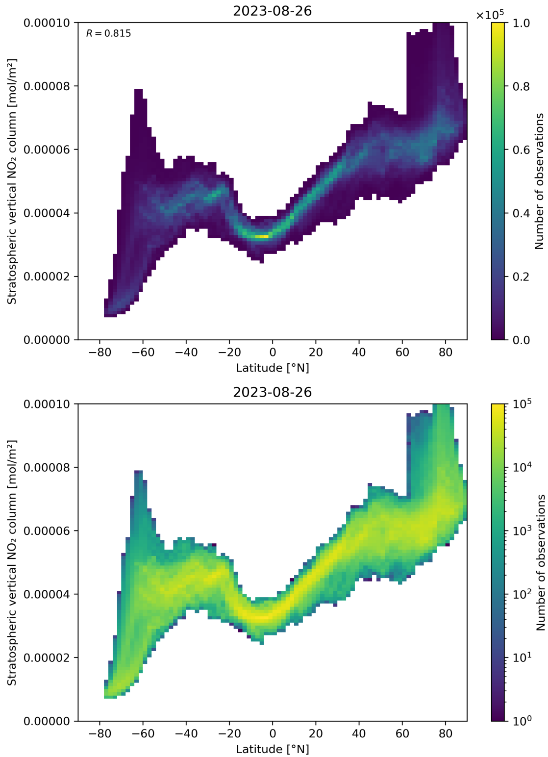
Figure 87: Scatter density plot of “Latitude” against “Stratospheric vertical \text{NO}_2 column” for 2023-08-25 to 2023-08-27.
