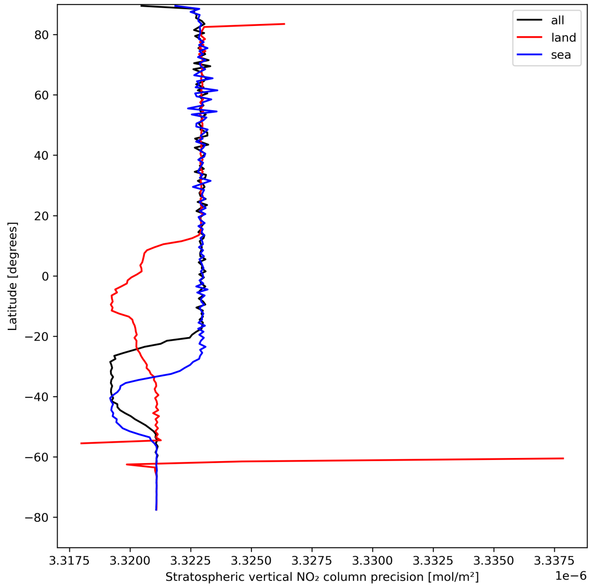
Figure 20: Zonal average of “Stratospheric vertical NO 2 column precision” for 2023-08-25 to 2023-08-27.
