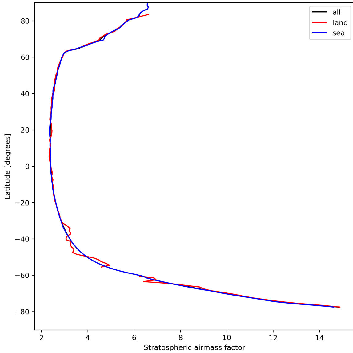
Figure 27: Zonal average of “Stratospheric air mass factor” for 2023-08-25 to 2023-08-27.
