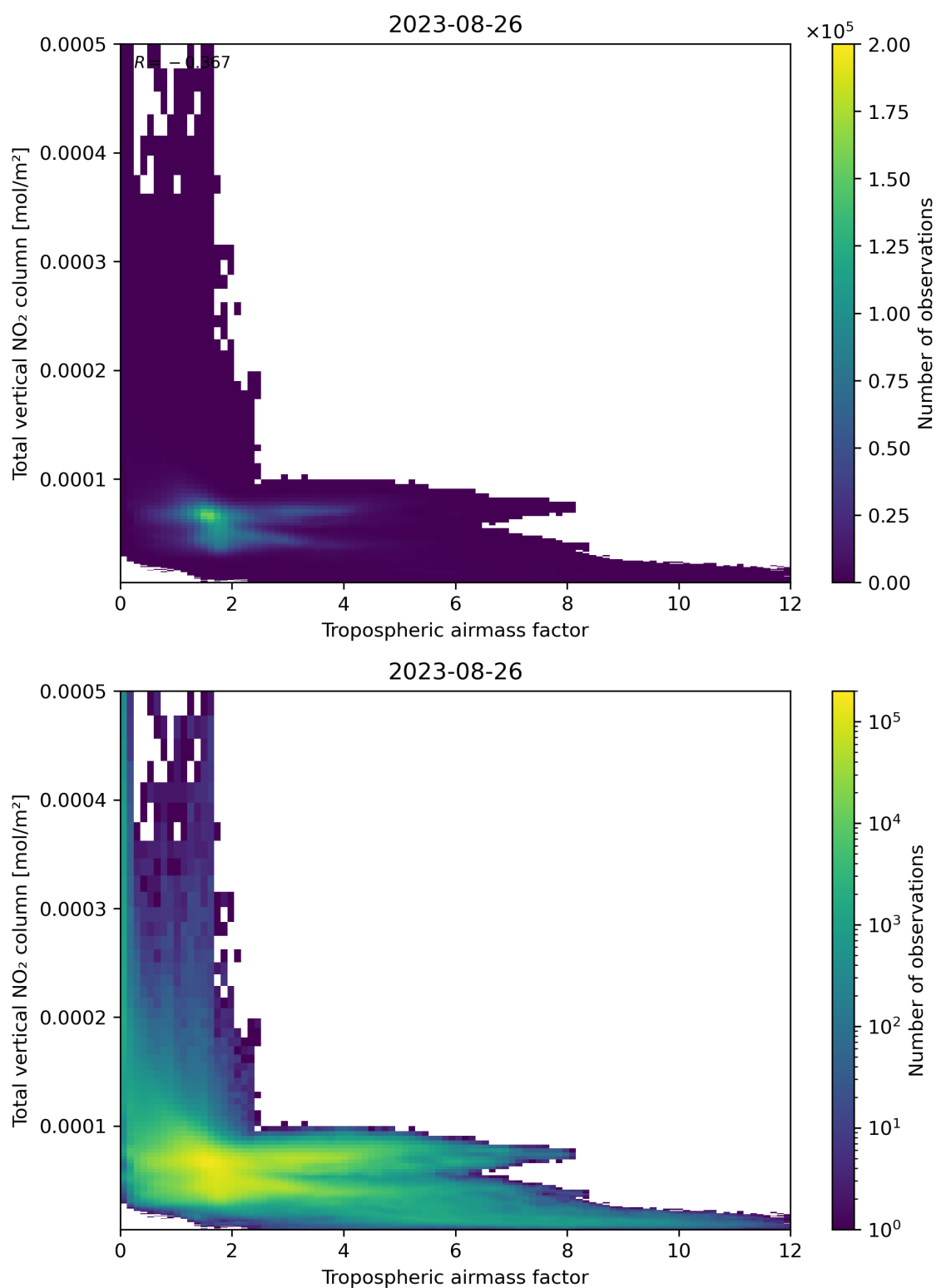
Figure 77: Scatter density plot of “Tropospheric airmass factor” against “Total vertical NO 2 column” for 2023-08-25 to 2023-08-27.
