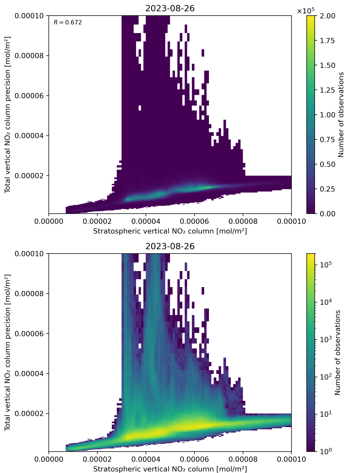
Figure 101: Scatter density plot of “Stratospheric vertical NO 2 column” against “Total vertical NO 2 column precision” for 2023-08-25 to 2023-08-27.
