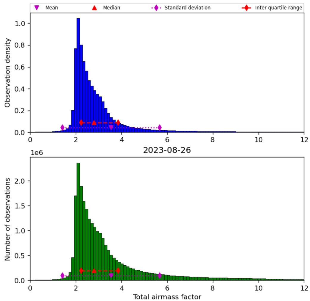
Figure 32: Histogram of “Total airmass factor” for 2023-08-25 to 2023-08-27
