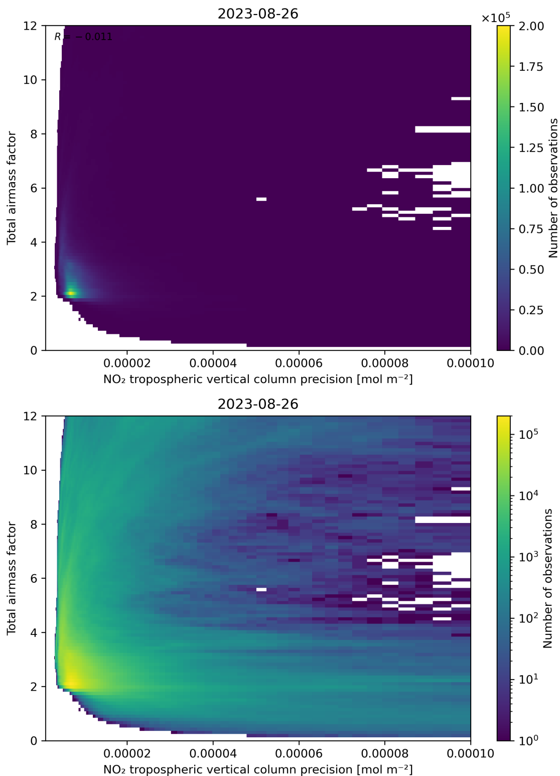
Figure 132: Scatter density plot of “NO 2 tropospheric vertical column precision” against “Total air mass factor” for 2023-08-25 to 2023-08-27.
