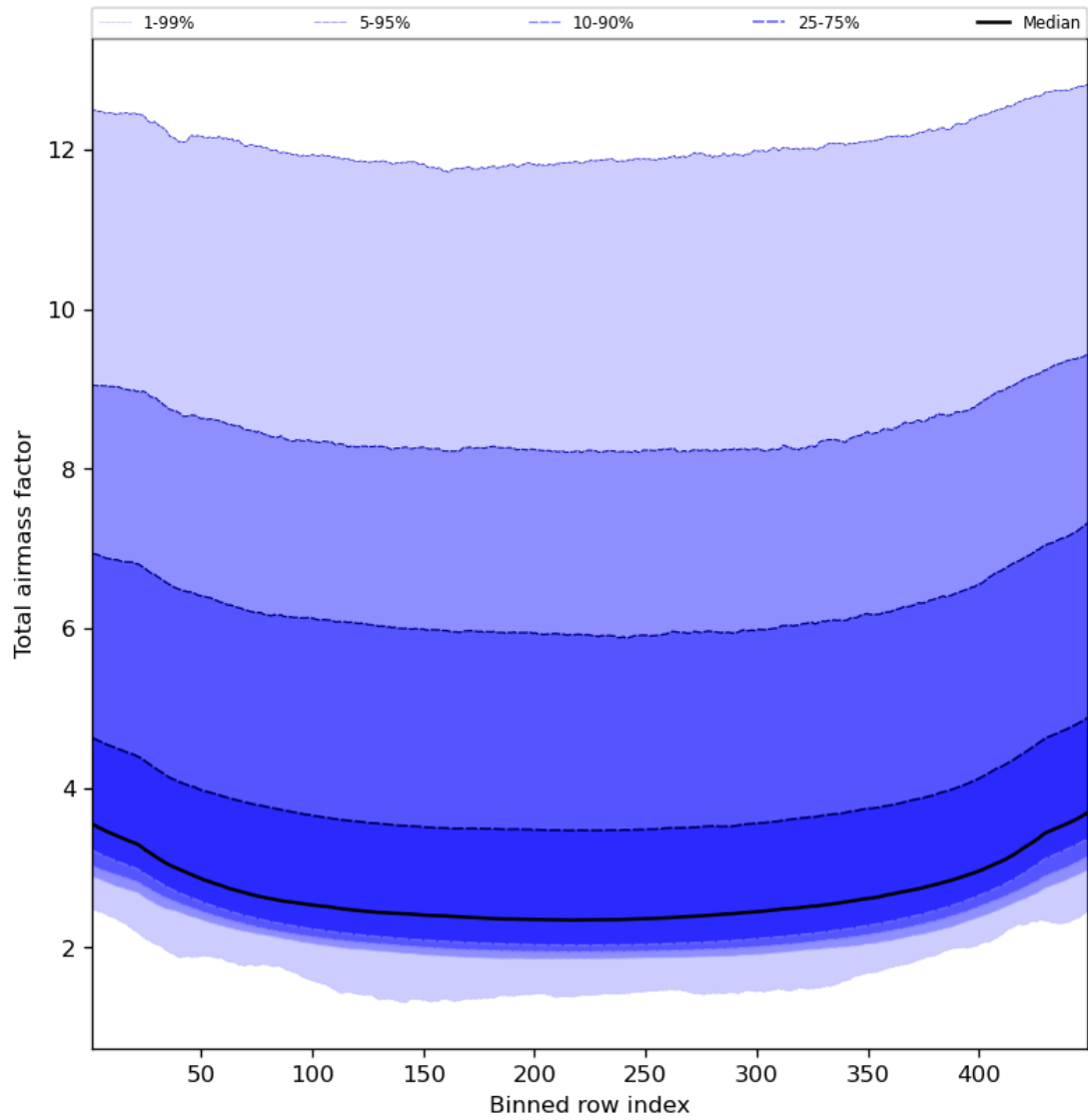
Figure 49: Along track statistics of “Total airmass factor” for 2023-08-25 to 2023-08-27
