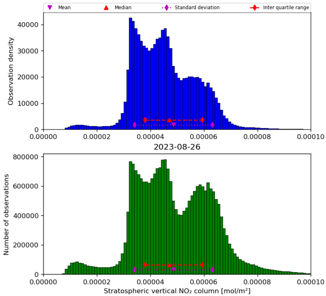
Figure 36: Histogram of “Stratospheric vertical NO 2 column” for 2023-08-25 to 2023-08-27
