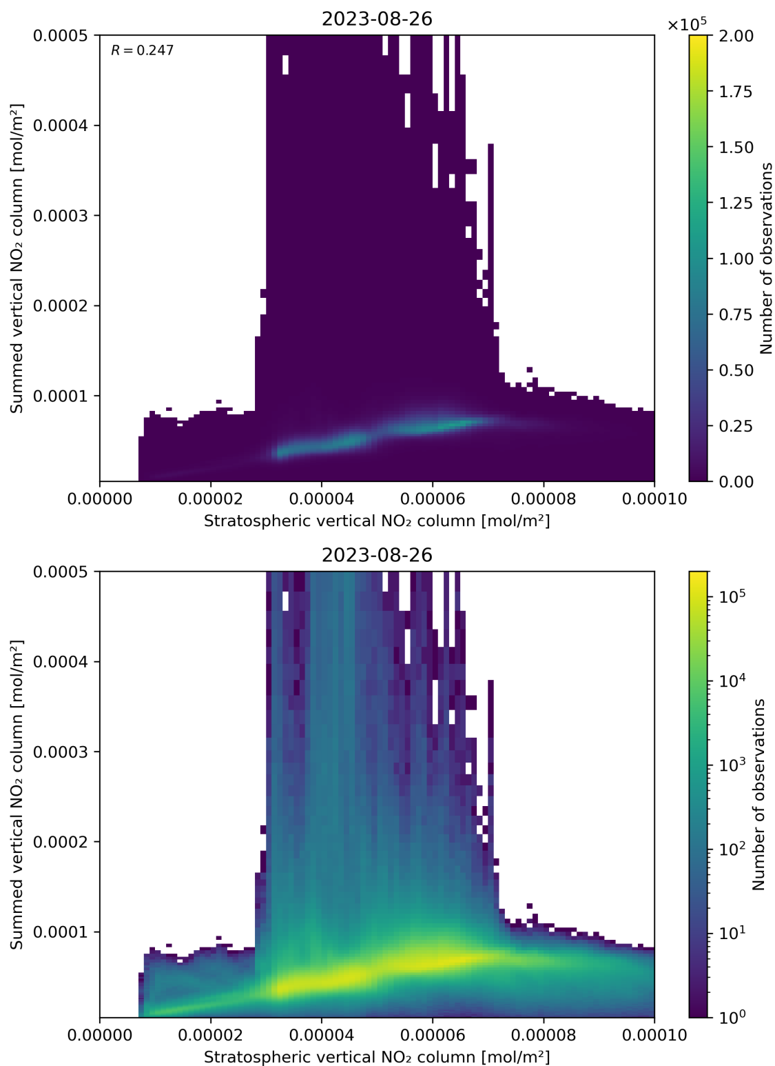
Figure 98: Scatter density plot of “Stratospheric vertical NO 2 column” against “Summed vertical NO 2 column” for 2023-08-25 to 2023-08-27.
