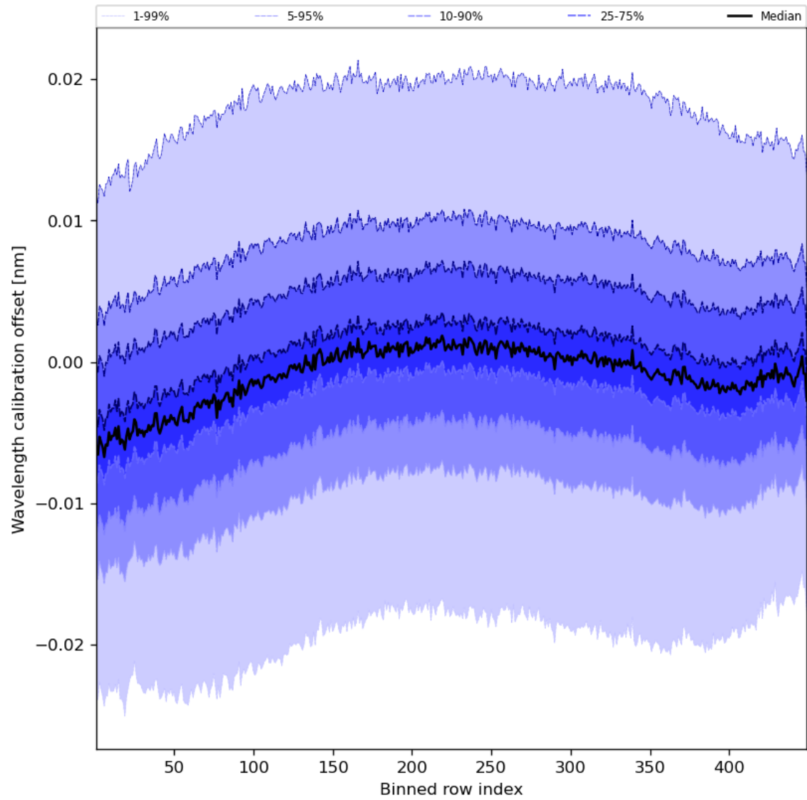
Figure 52: Along track statistics of “Wavelength calibration offset” for 2023-08-25 to 2023-08-27
