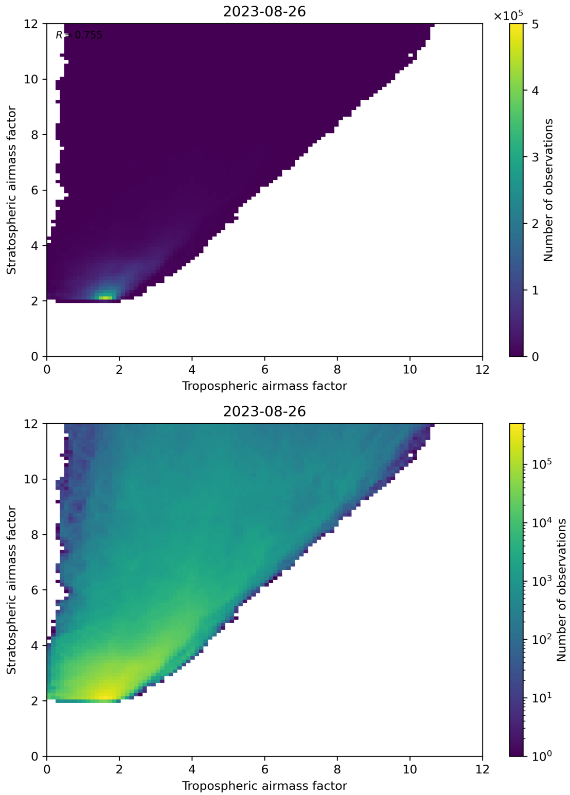
Figure 71: Scatter density plot of “Tropospheric airmass factor” against “Stratospheric airmass factor” for 2023-08-25 to 2023-08-27.
