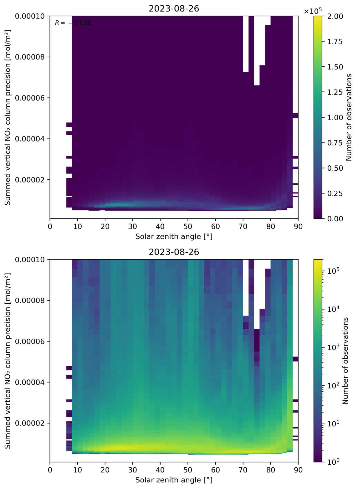
Figure 152: Scatter density plot of “Solar zenith angle” against “Summed vertical NO 2 column precision” for 2023-08-25 to 2023-08-27.
