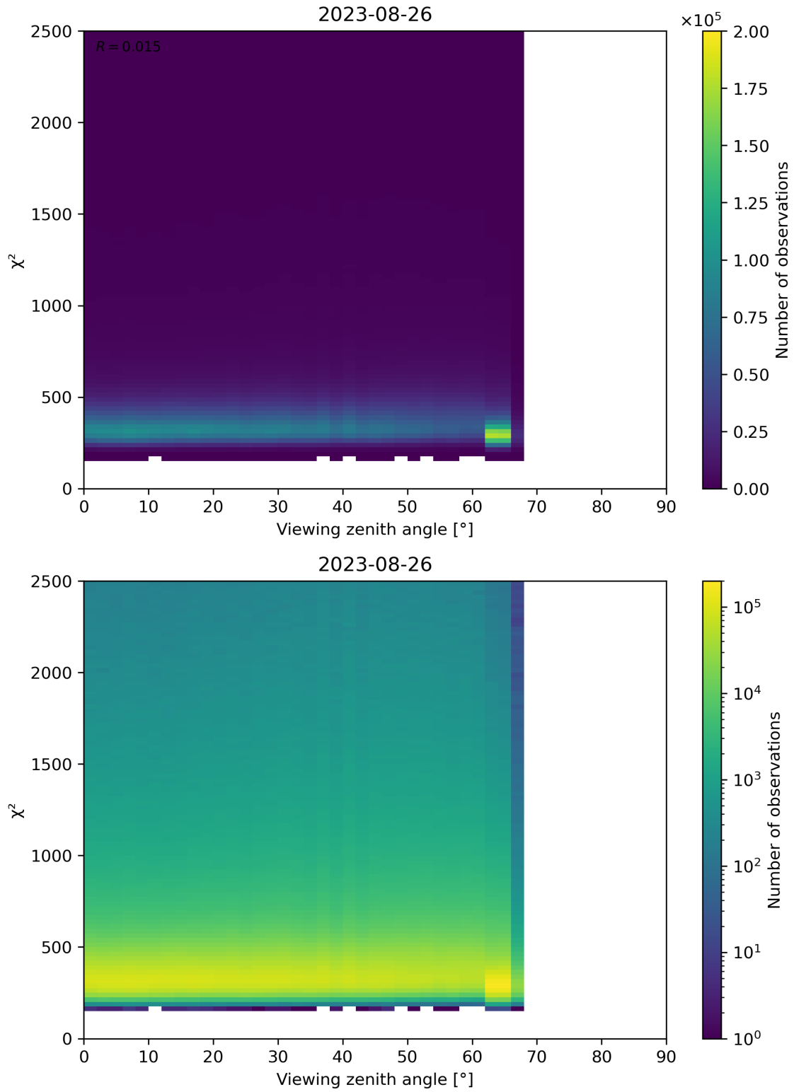
Figure 162: Scatter density plot of “Viewing zenith angle” against “ \chi^2 ” for 2023-08-25 to 2023-08-27.
