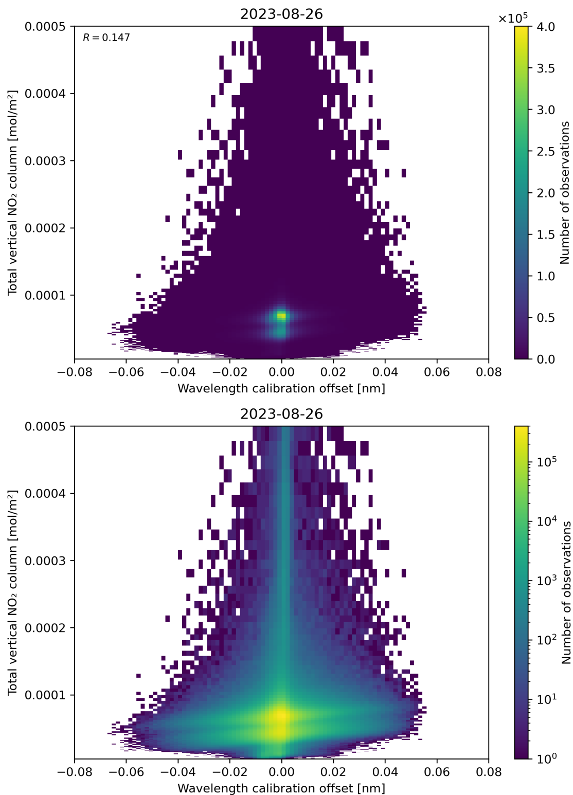
Figure 179: Scatter density plot of “Wavelength calibration offset” against “Total vertical NO 2 column” for 2023-08-25 to 2023-08-27.
