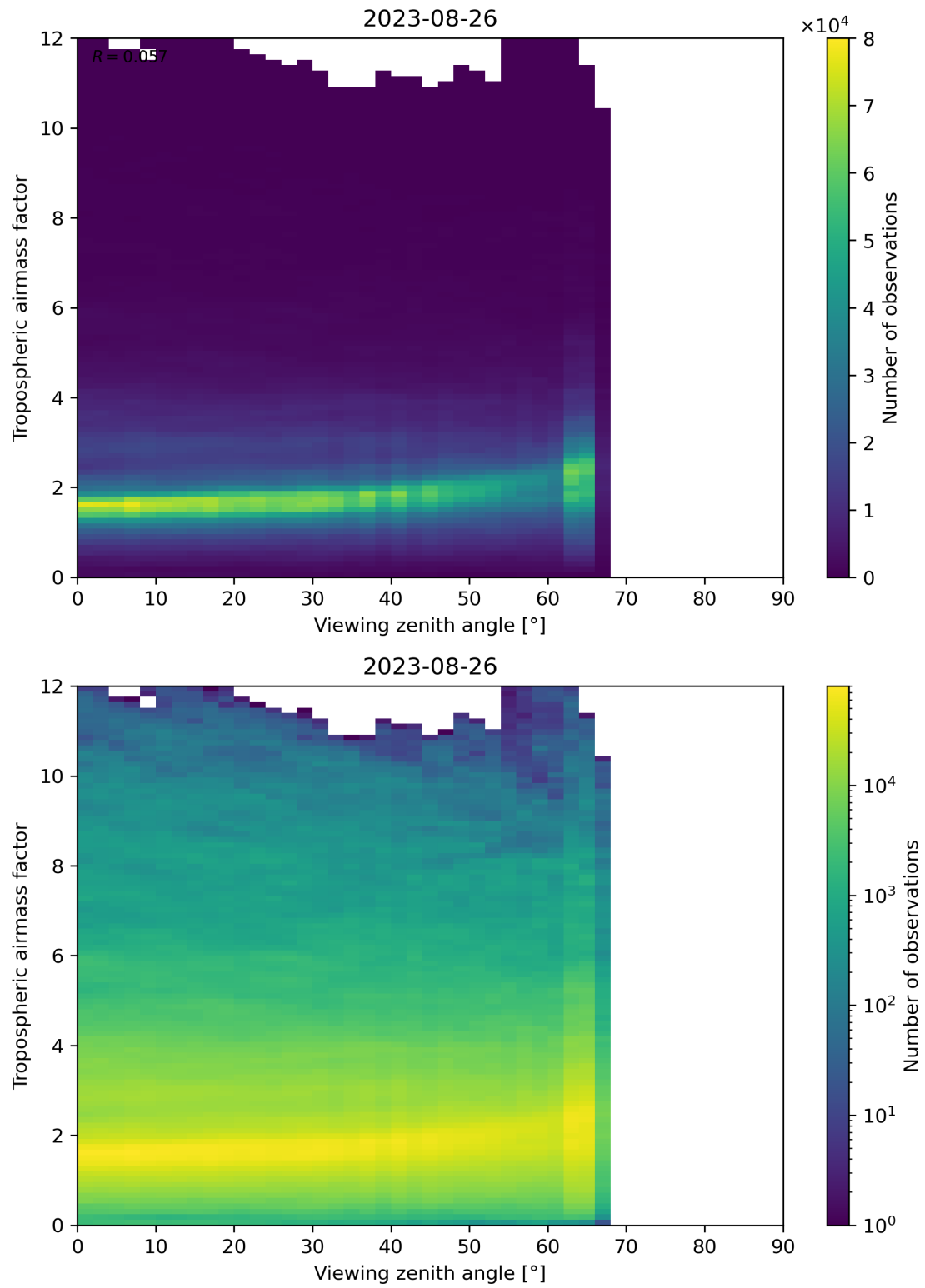
Figure 161: Scatter density plot of “Viewing zenith angle” against “Tropospheric airmass factor” for 2023-08-25 to 2023-08-27.
