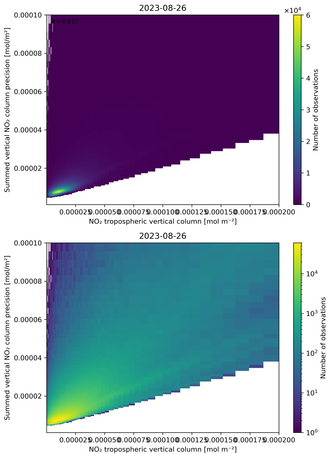
Figure 127: Scatter density plot of “NO 2 tropospheric vertical column” against “Summed vertical NO 2 column precision” for 2023-08-25 to 2023-08-27.
