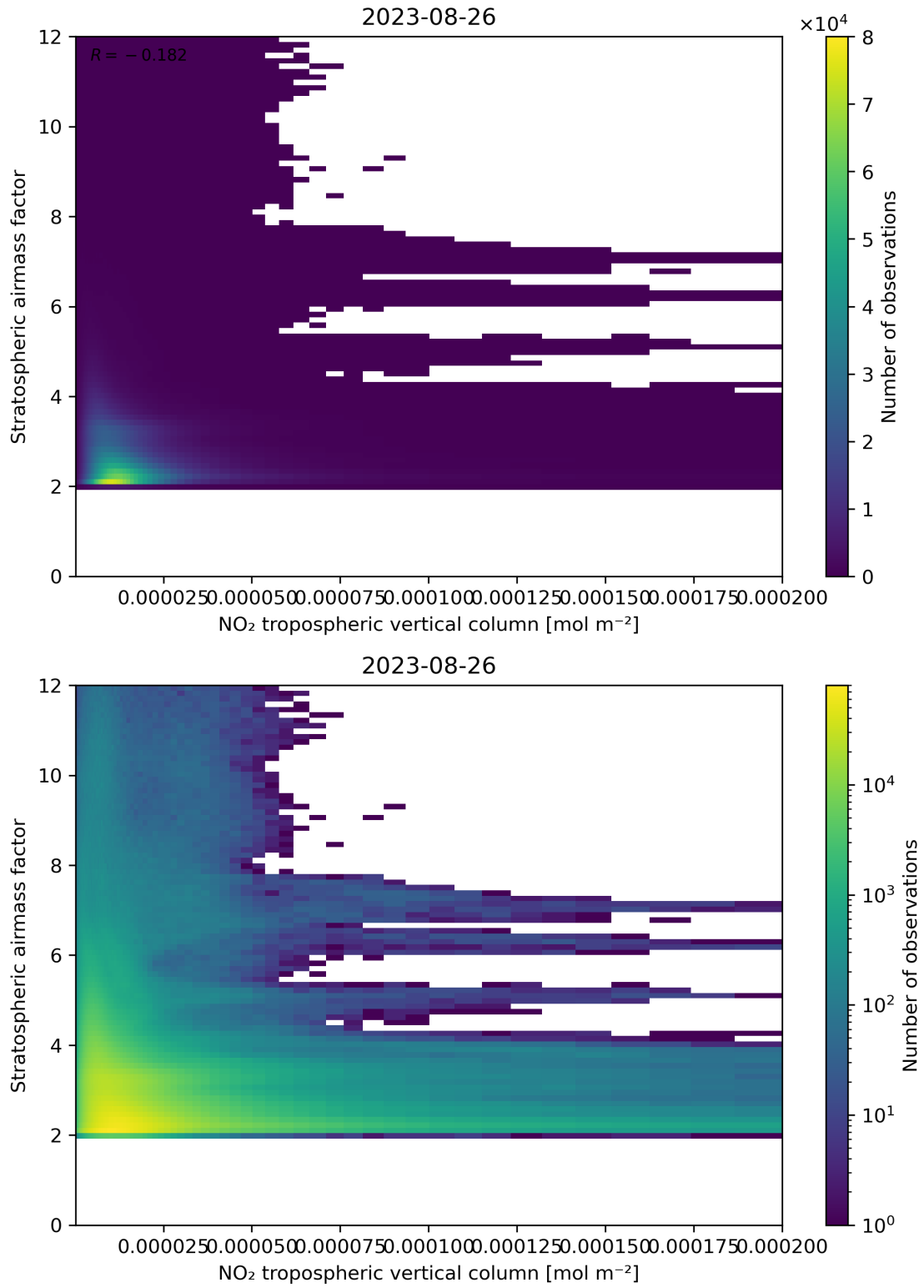
Figure 121: Scatter density plot of “NO 2 tropospheric vertical column” against “Stratospheric air mass factor” for 2023-08-25 to 2023-08-27.
