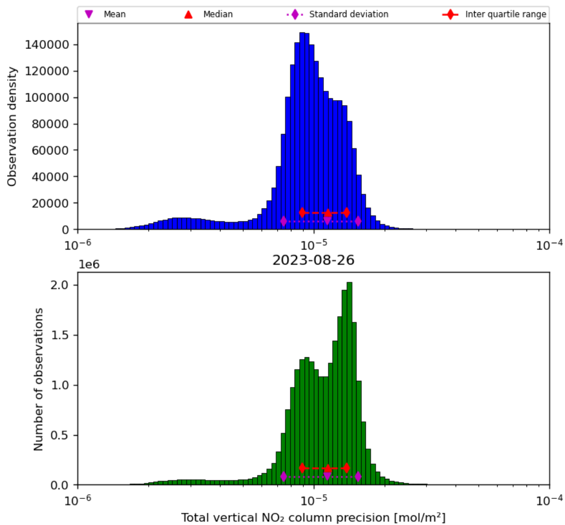
Figure 39: Histogram of “Total vertical NO 2 column precision” for 2023-08-25 to 2023-08-27
