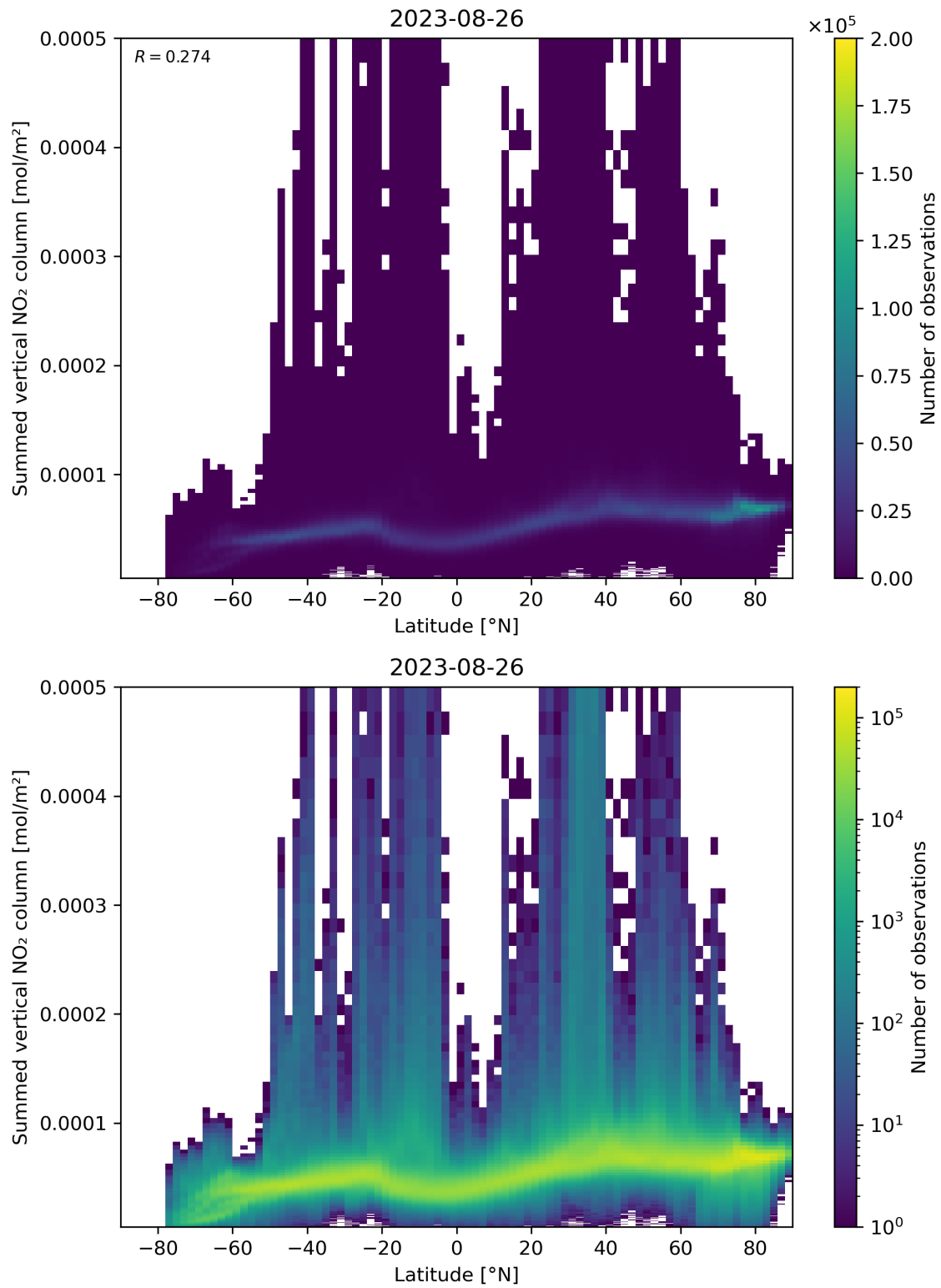
Figure 88: Scatter density plot of “Latitude” against “Summed vertical NO 2 column” for 2023-08-25 to 2023-08-27.
