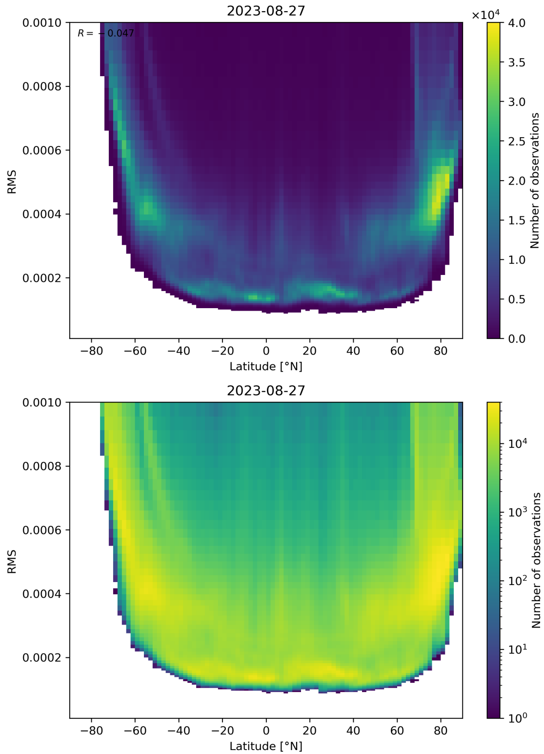
Figure 94: Scatter density plot of “Latitude” against “RMS” for 2023-08-26 to 2023-08-28.
