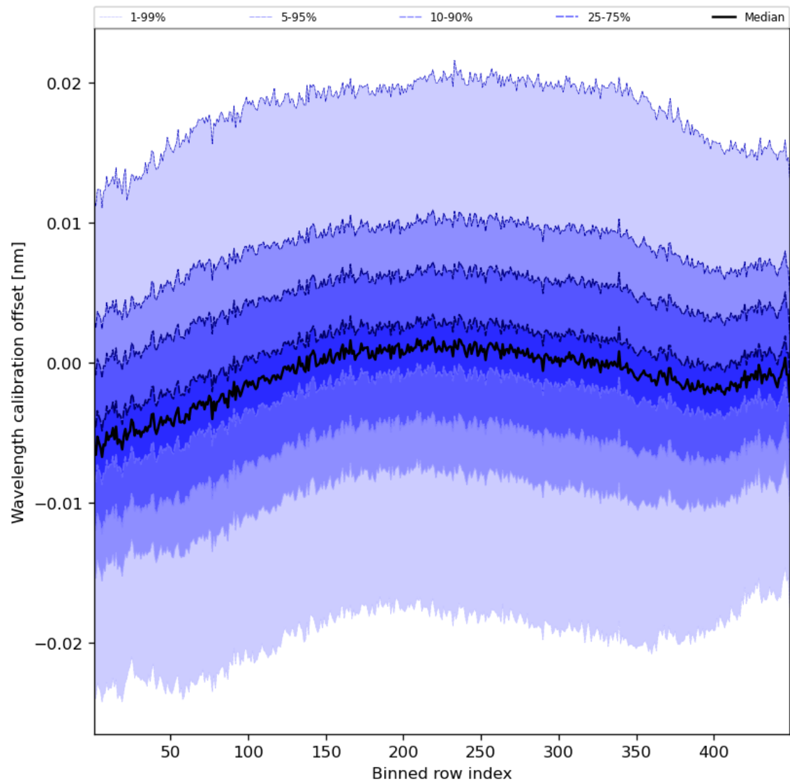
Figure 52: Along track statistics of “Wavelength calibration offset” for 2023-08-26 to 2023-08-28
