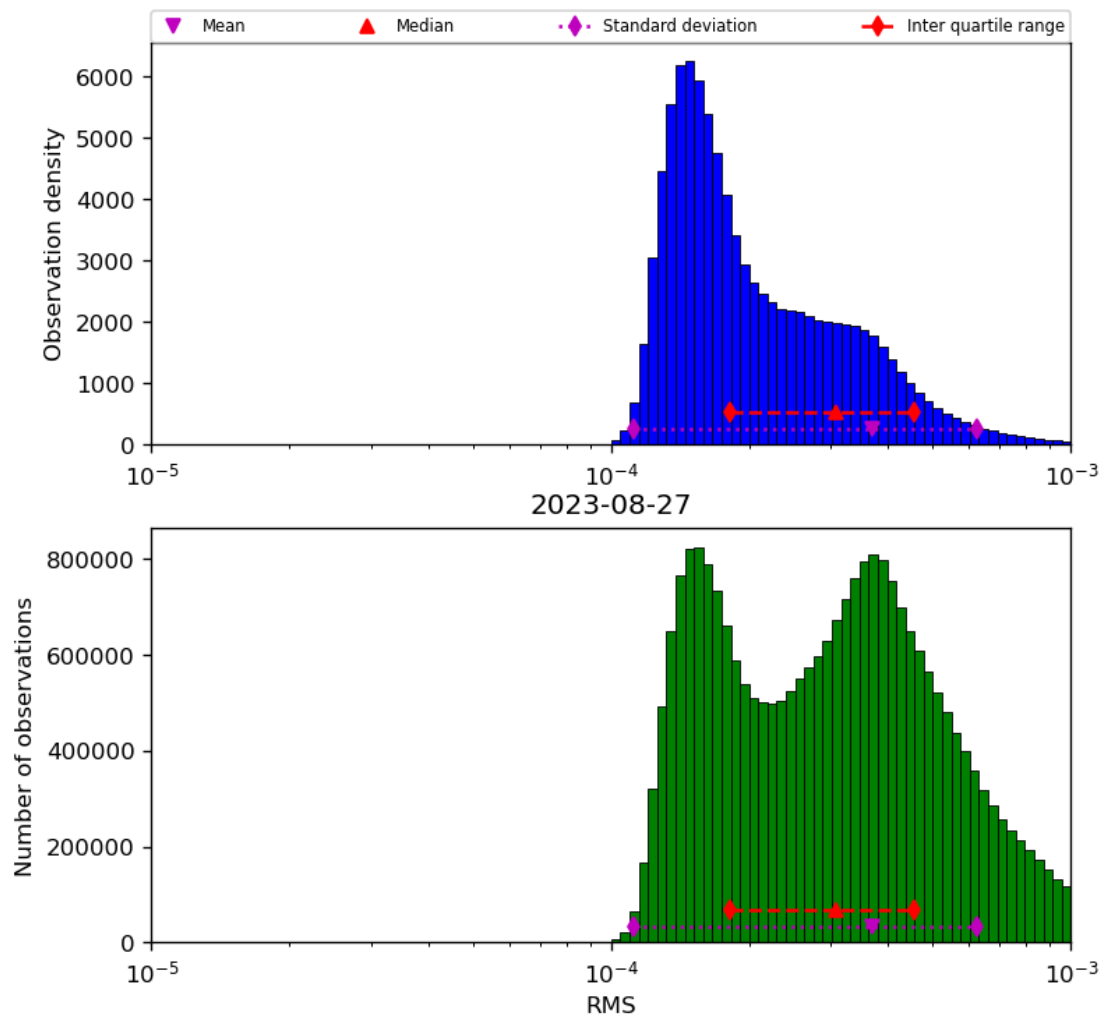
Figure 43: Histogram of “RMS” for 2023-08-26 to 2023-08-28
