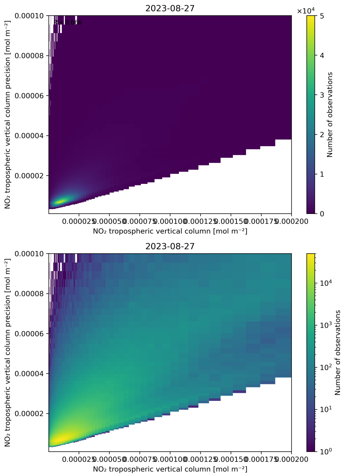
Figure 130: Scatter density plot of “NO 2 tropospheric vertical column” against “NO 2 tropospheric vertical column precision” for 2023-08-26 to 2023-08-28.
