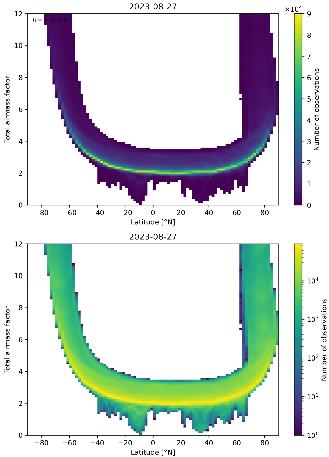
Figure 84: Scatter density plot of “Latitude” against “Total airmass factor” for 2023-08-26 to 2023-08-28.
