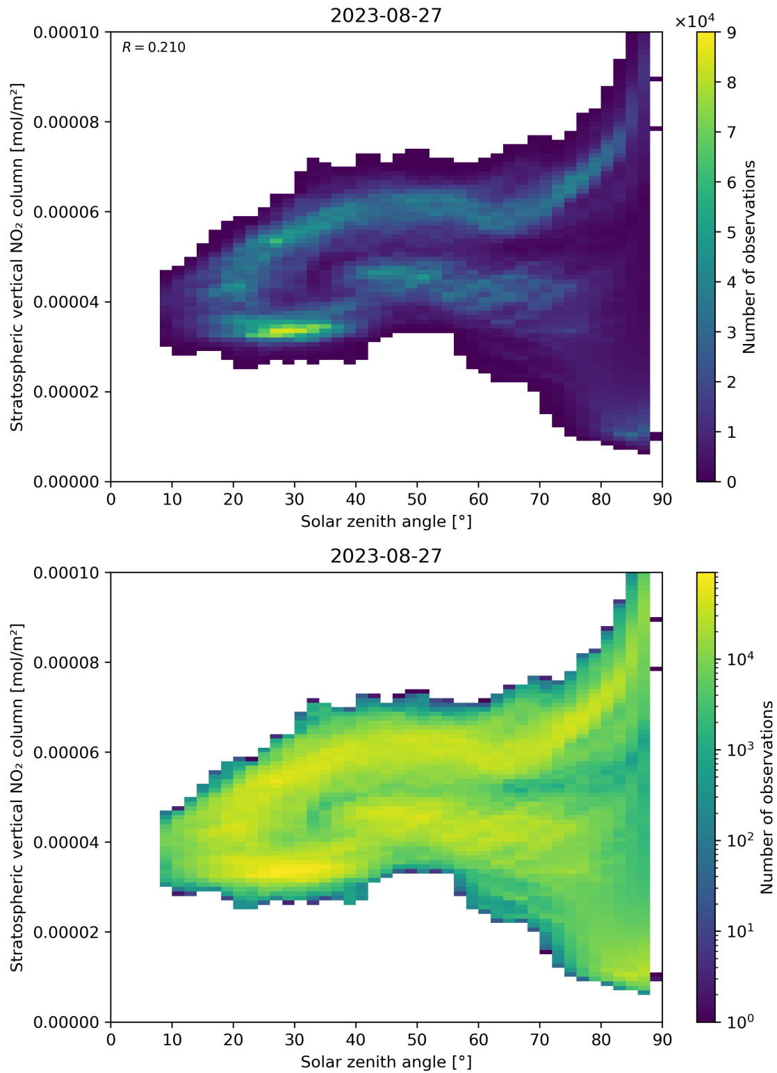
Figure 150: Scatter density plot of “Solar zenith angle” against “Stratospheric vertical NO 2 column” for 2023-08-26 to 2023-08-28.
