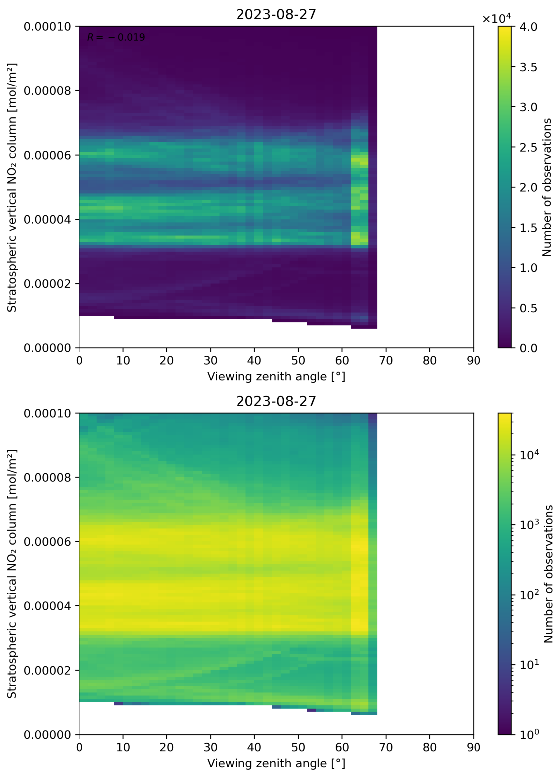
Figure 164: Scatter density plot of “Viewing zenith angle” against “Stratospheric vertical NO 2 column” for 2023-08-26 to 2023-08-28.
