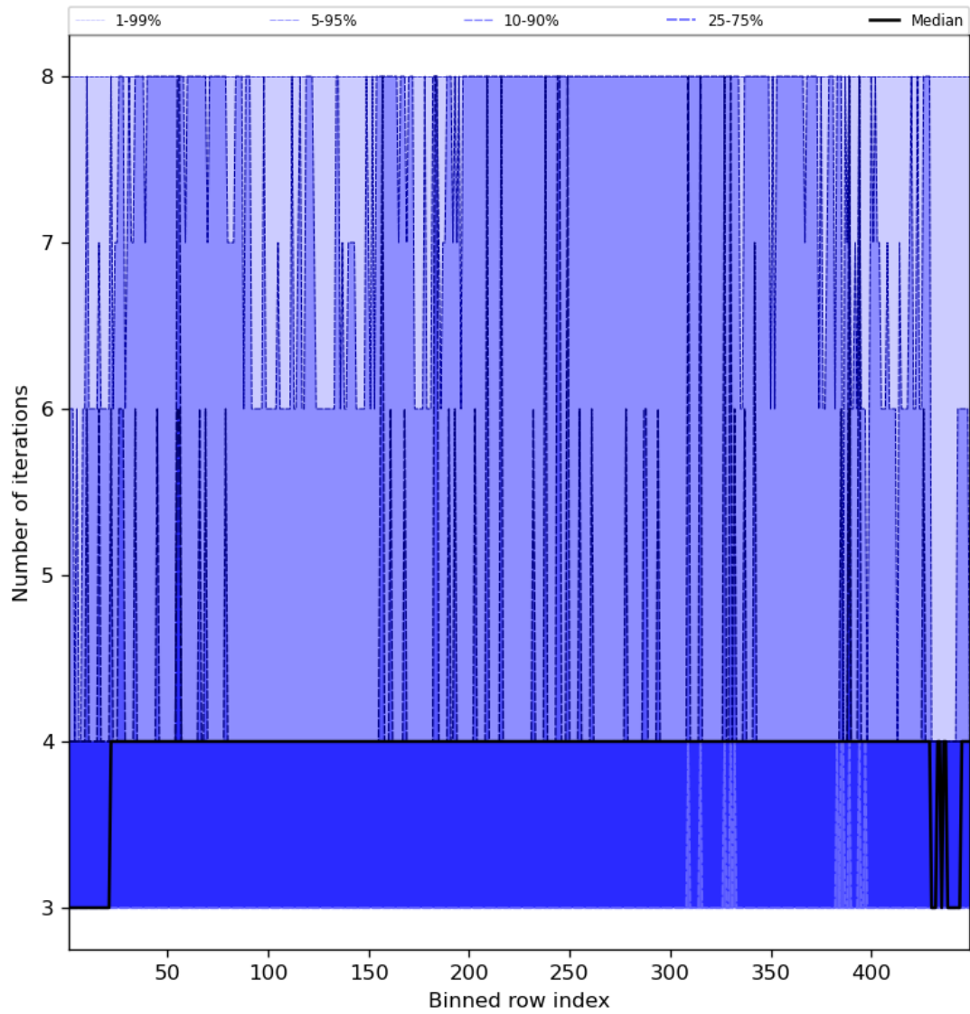
Figure 51: Along track statistics of “Number of iterations” for 2023-08-26 to 2023-08-28
