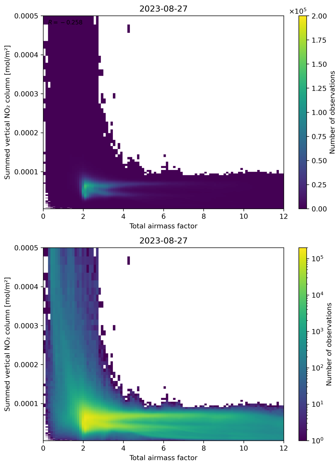
Figure 65: Scatter density plot of “Total airmass factor” against “Summed vertical NO 2 column” for 2023-08-26 to 2023-08-28.
