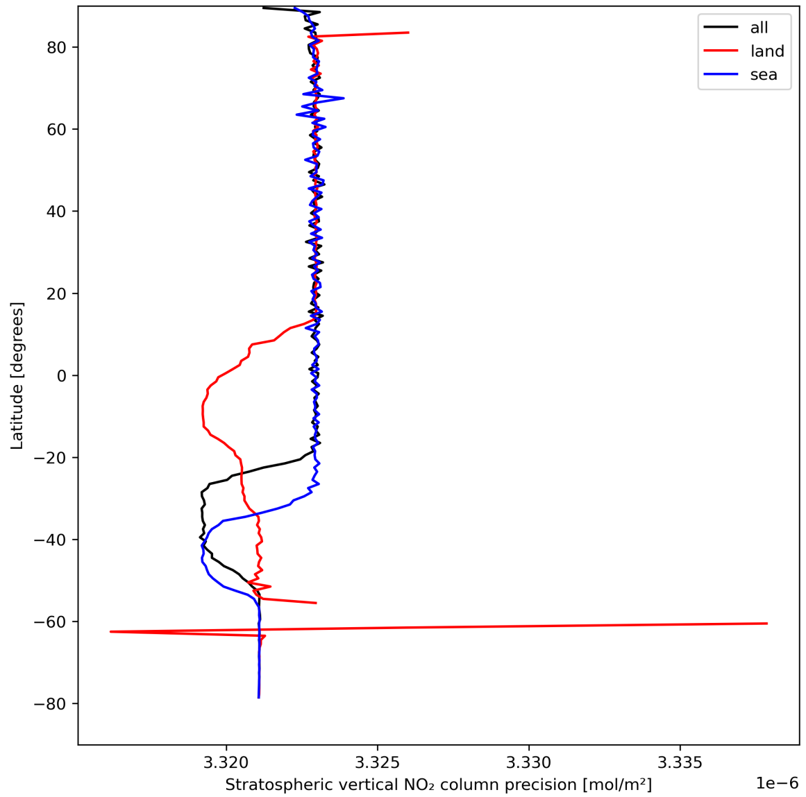
Figure 20: Zonal average of “Stratospheric vertical NO 2 column precision” for 2023-08-26 to 2023-08-28.
