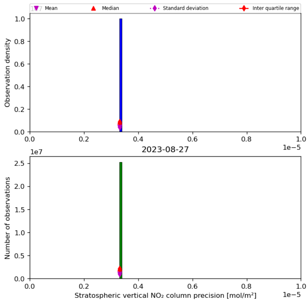
Figure 37: Histogram of “Stratospheric vertical NO 2 column precision” for 2023-08-26 to 2023-08-28
