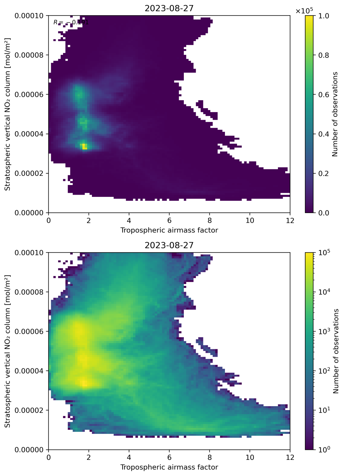
Figure 74: Scatter density plot of “Tropospheric air mass factor” against “Stratospheric vertical NO 2 column” for 2023-08-26 to 2023-08-28.
