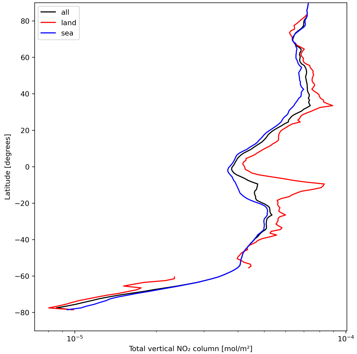
Figure 21: Zonal average of “Total vertical NO 2 column” for 2023-08-26 to 2023-08-28.
