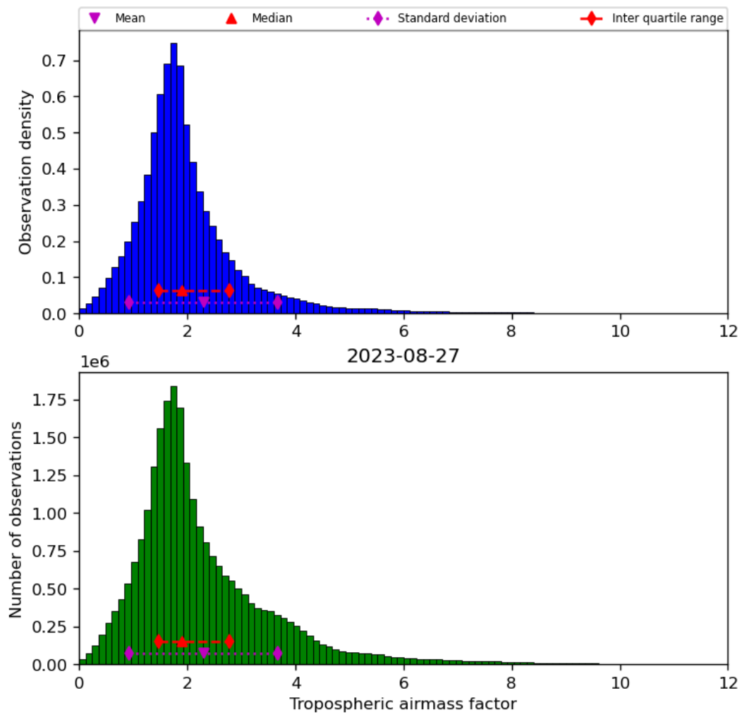
Figure 31: Histogram of “Tropospheric airmass factor” for 2023-08-26 to 2023-08-28
