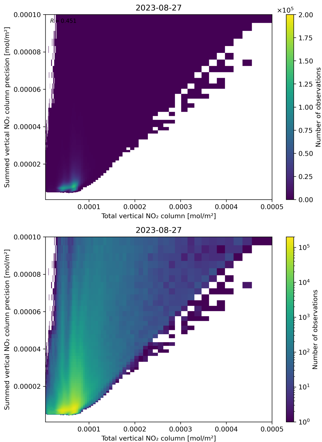
Figure 113: Scatter density plot of “Total vertical NO 2 column” against “Summed vertical NO 2 column precision” for 2023-08-26 to 2023-08-28.
