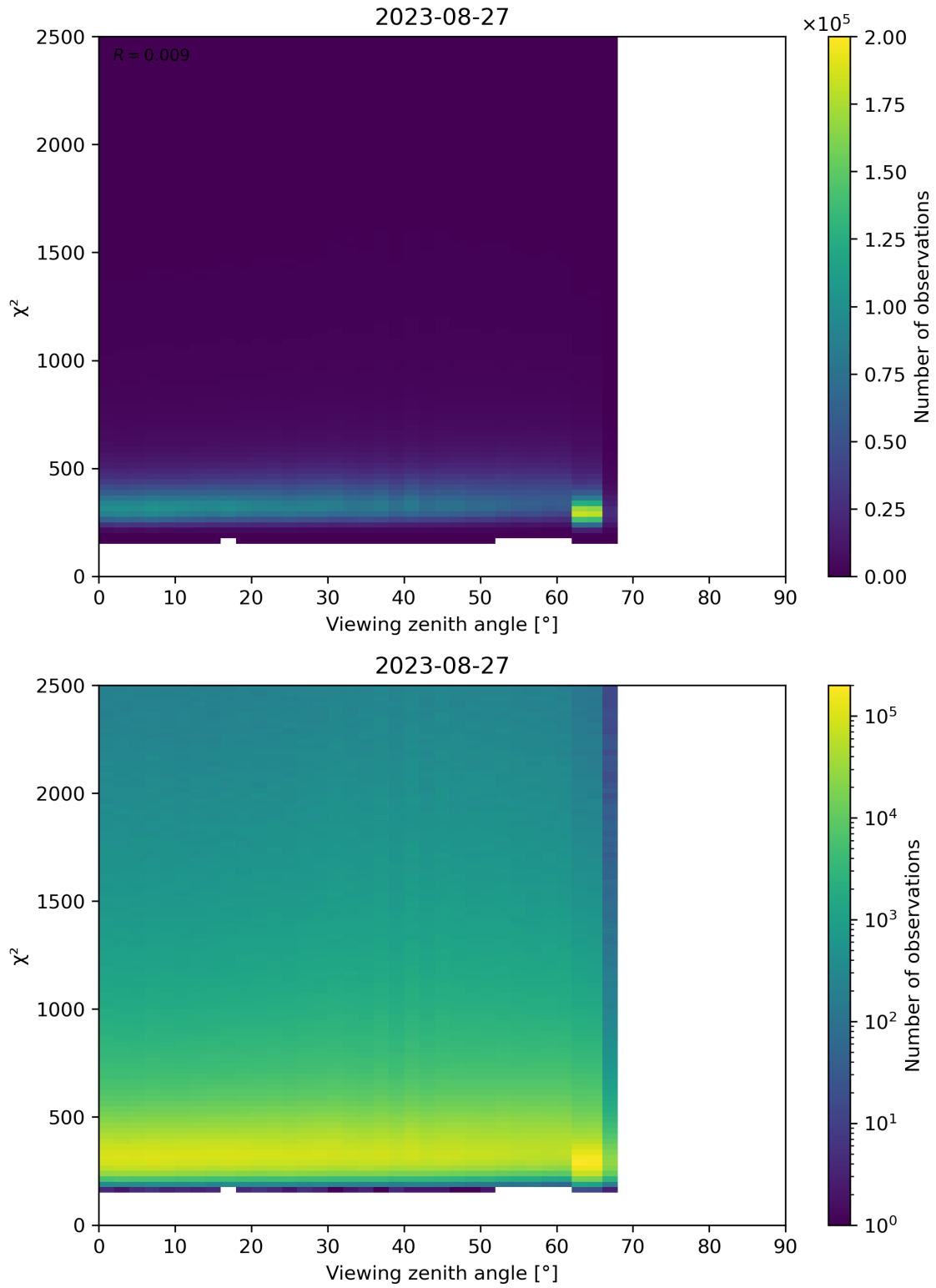
Figure 162: Scatter density plot of “Viewing zenith angle” against “ \chi^2 ” for 2023-08-26 to 2023-08-28.
