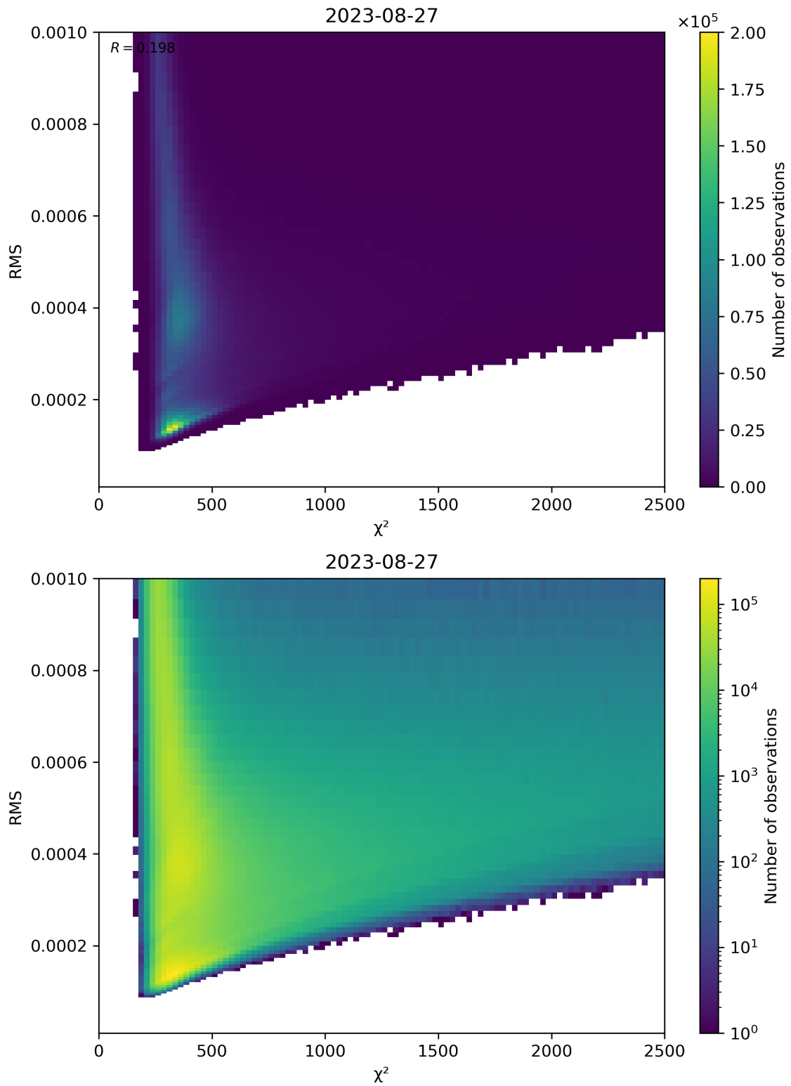
Figure 82: Scatter density plot of “ \chi^2 ” against “RMS” for 2023-08-26 to 2023-08-28.
