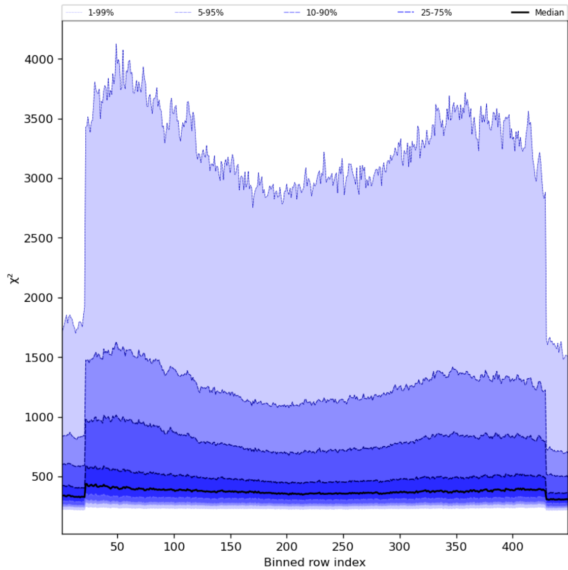
Figure 59: Along track statistics of “ \chi^2 ” for 2023-08-26 to 2023-08-28
