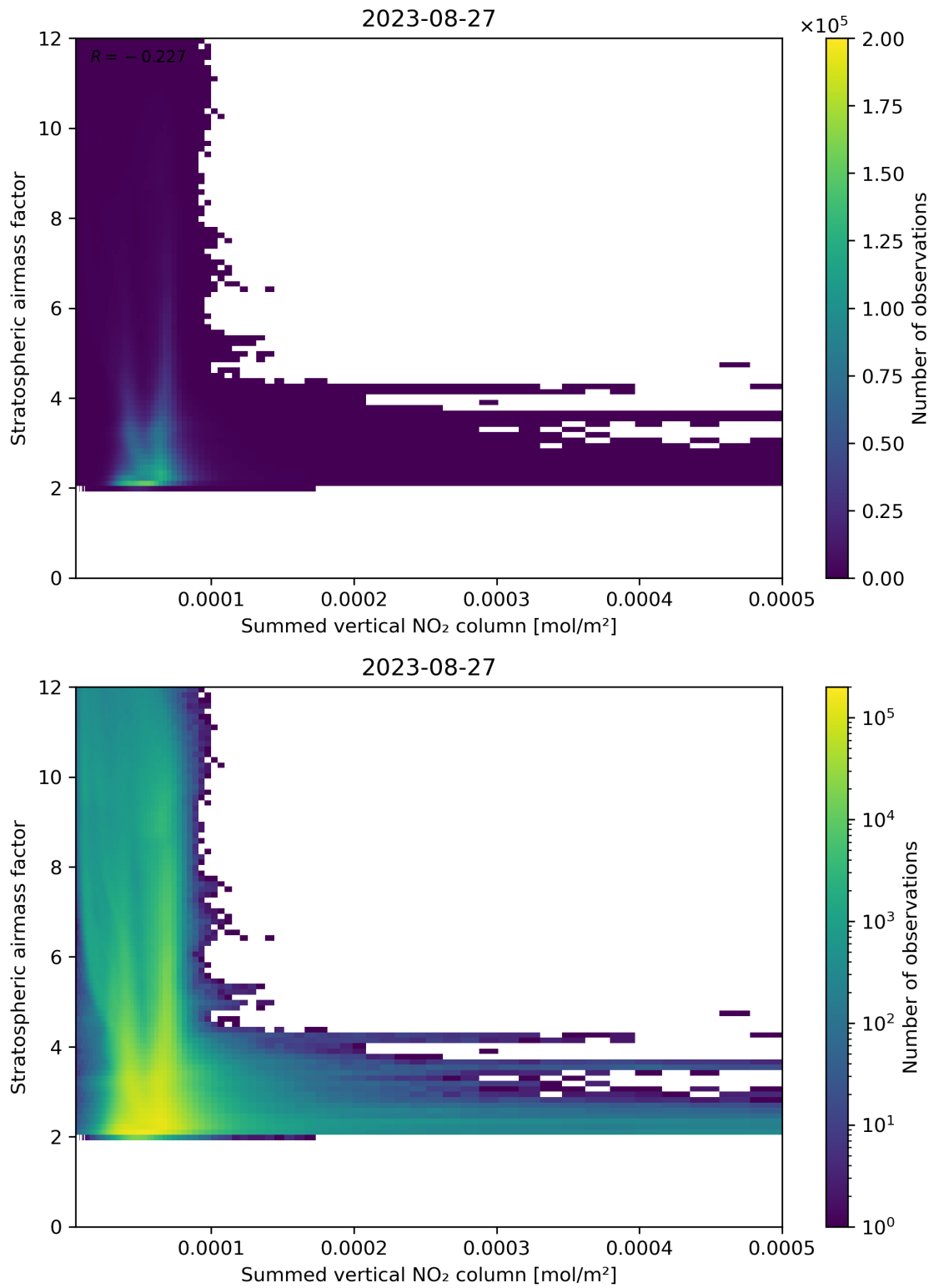
Figure 103: Scatter density plot of “Summed vertical NO 2 column” against “Stratospheric airmass factor” for 2023-08-26 to 2023-08-28.
