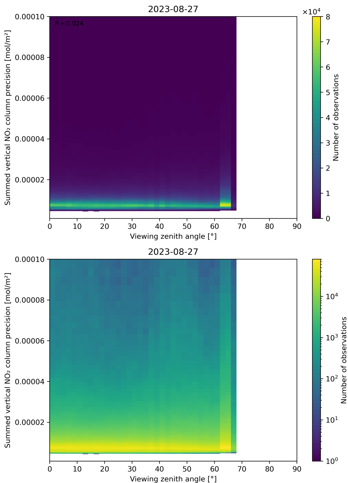
Figure 166: Scatter density plot of “Viewing zenith angle” against “Summed vertical NO 2 column precision” for 2023-08-26 to 2023-08-28.
