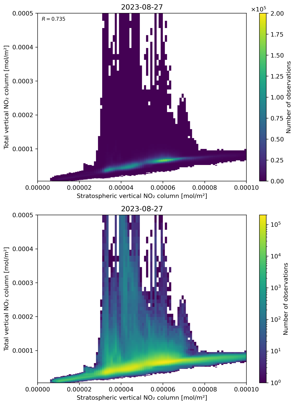
Figure 100: Scatter density plot of “Stratospheric vertical NO 2 column” against “Total vertical NO 2 column” for 2023-08-26 to 2023-08-28.
