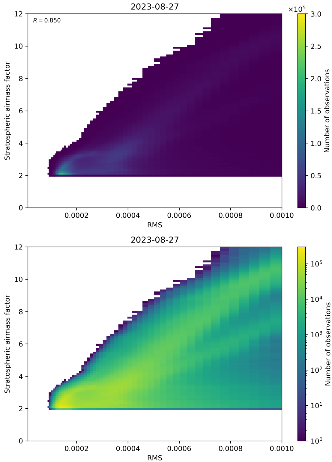
Figure 144: Scatter density plot of “RMS” against “Stratospheric airmass factor” for 2023-08-26 to 2023-08-28.
