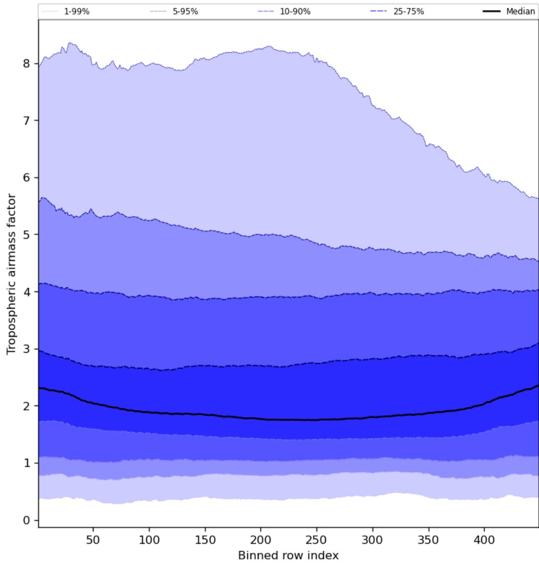
Figure 48: Along track statistics of “Tropospheric air mass factor” for 2023-08-26 to 2023-08-28
