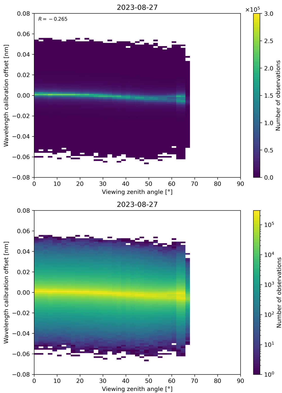
Figure 173: Scatter density plot of “Viewing zenith angle” against “Wavelength calibration offset” for 2023-08-26 to 2023-08-28.
