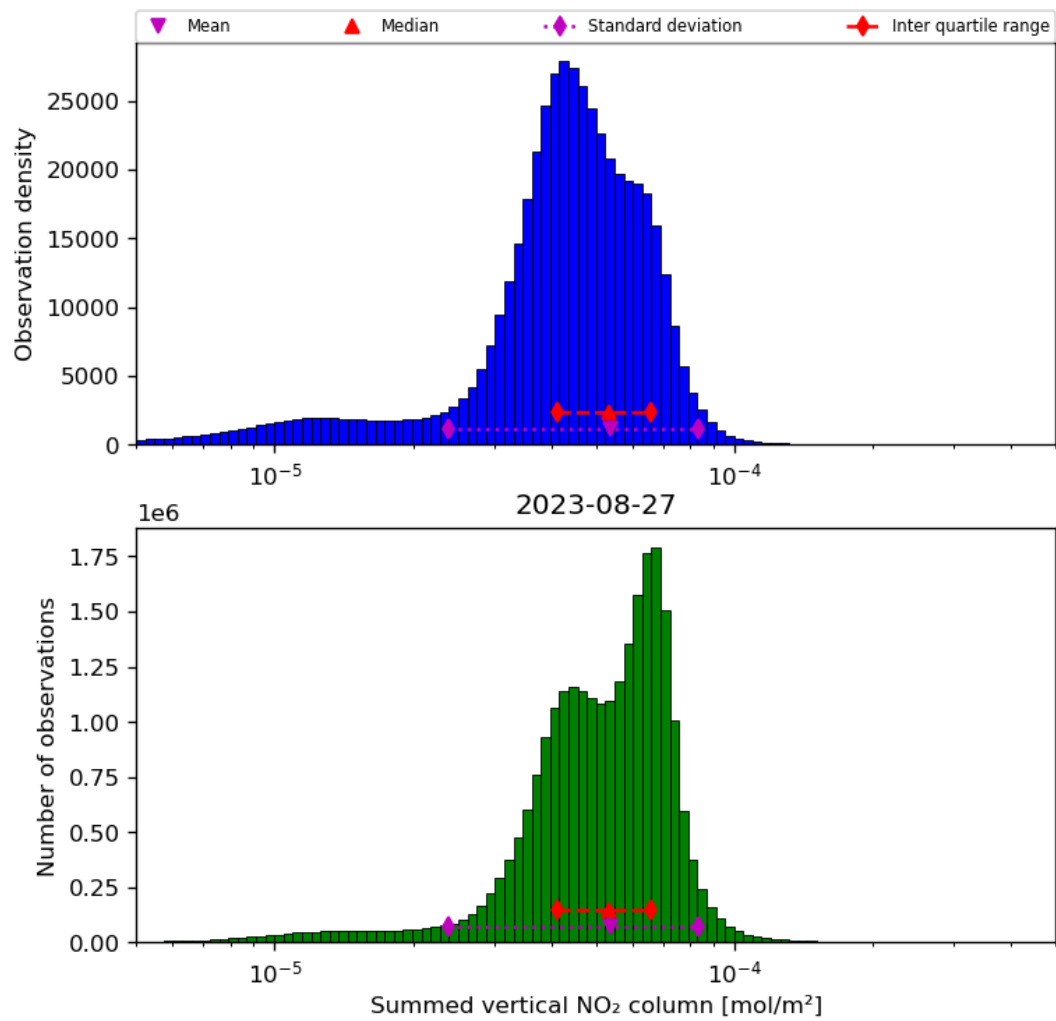
Figure 40: Histogram of “Summed vertical NO 2 column” for 2023-08-26 to 2023-08-28
