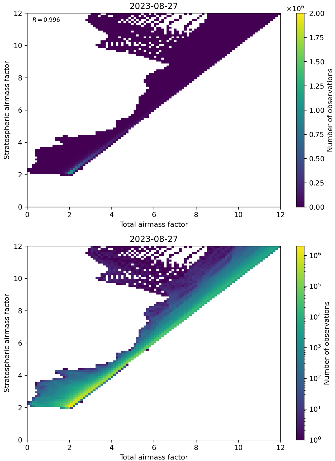
Figure 62: Scatter density plot of “Total airmass factor” against “Stratospheric airmass factor” for 2023-08-26 to 2023-08-28.
