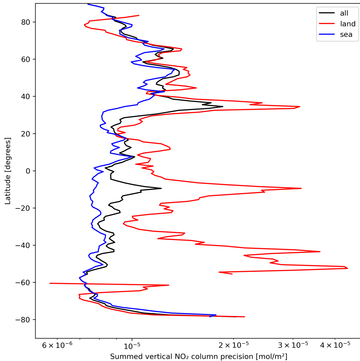
Figure 24: Zonal average of “Summed vertical NO 2 column precision” for 2023-08-26 to 2023-08-28.
