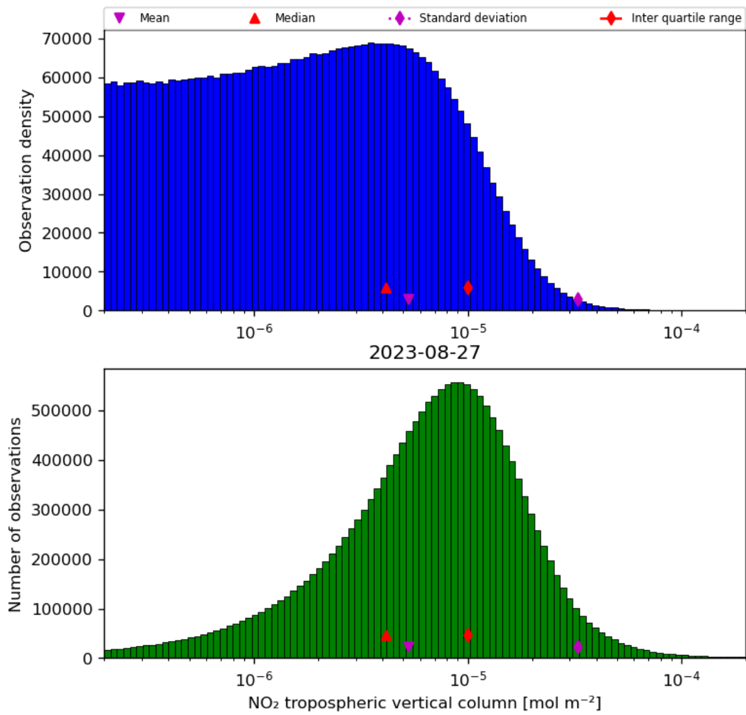
Figure 29: Histogram of “NO 2 tropospheric vertical column” for 2023-08-26 to 2023-08-28
