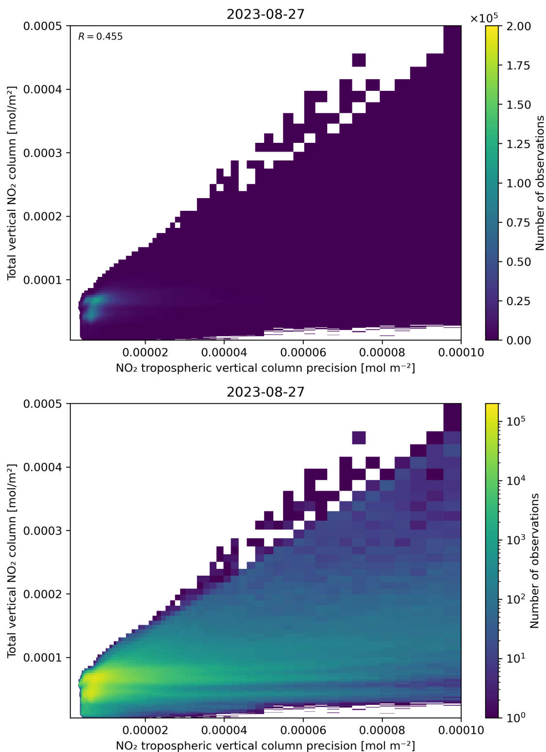
Figure 138: Scatter density plot of “NO 2 tropospheric vertical column precision” against “Total vertical NO 2 column” for 2023-08-26 to 2023-08-28.
