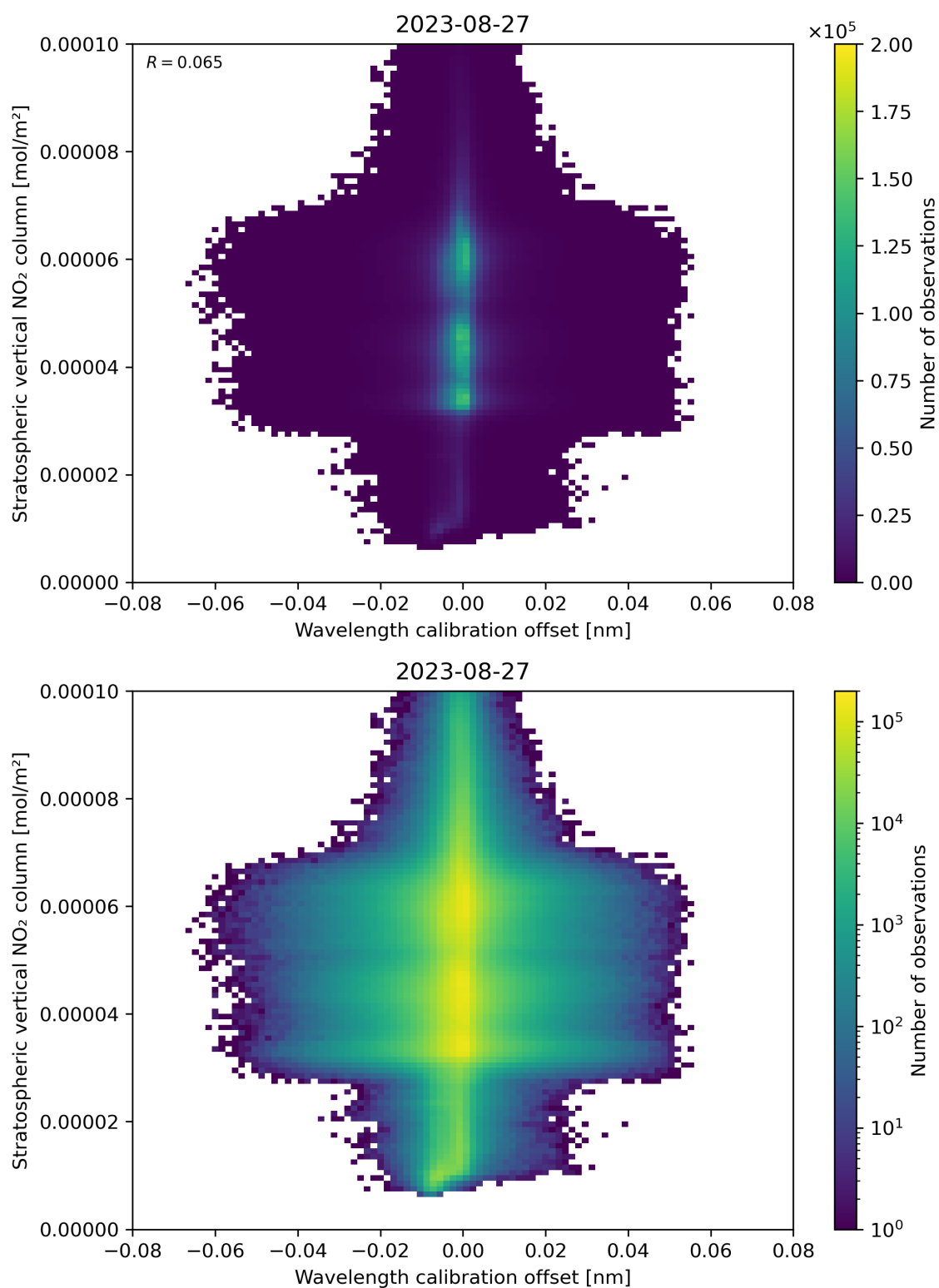
Figure 176: Scatter density plot of “Wavelength calibration offset” against “Stratospheric vertical NO 2 column” for 2023-08-26 to 2023-08-28.
