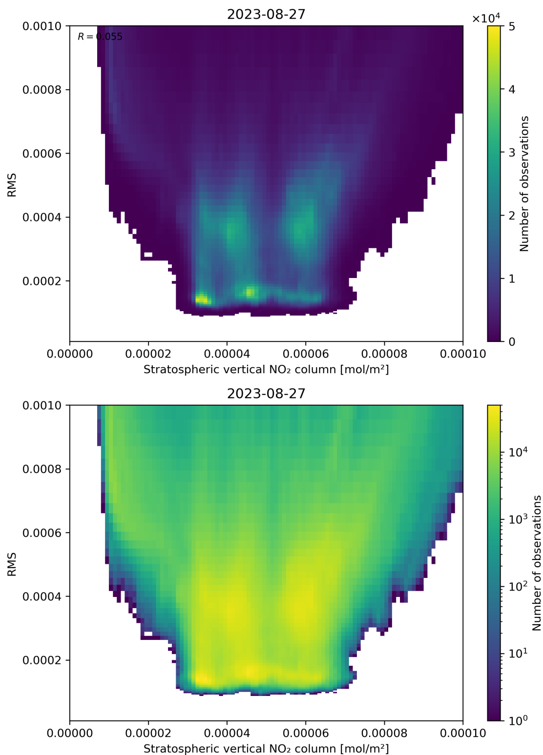
Figure 102: Scatter density plot of “Stratospheric vertical NO 2 column” against “RMS” for 2023-08-26 to 2023-08-28.
