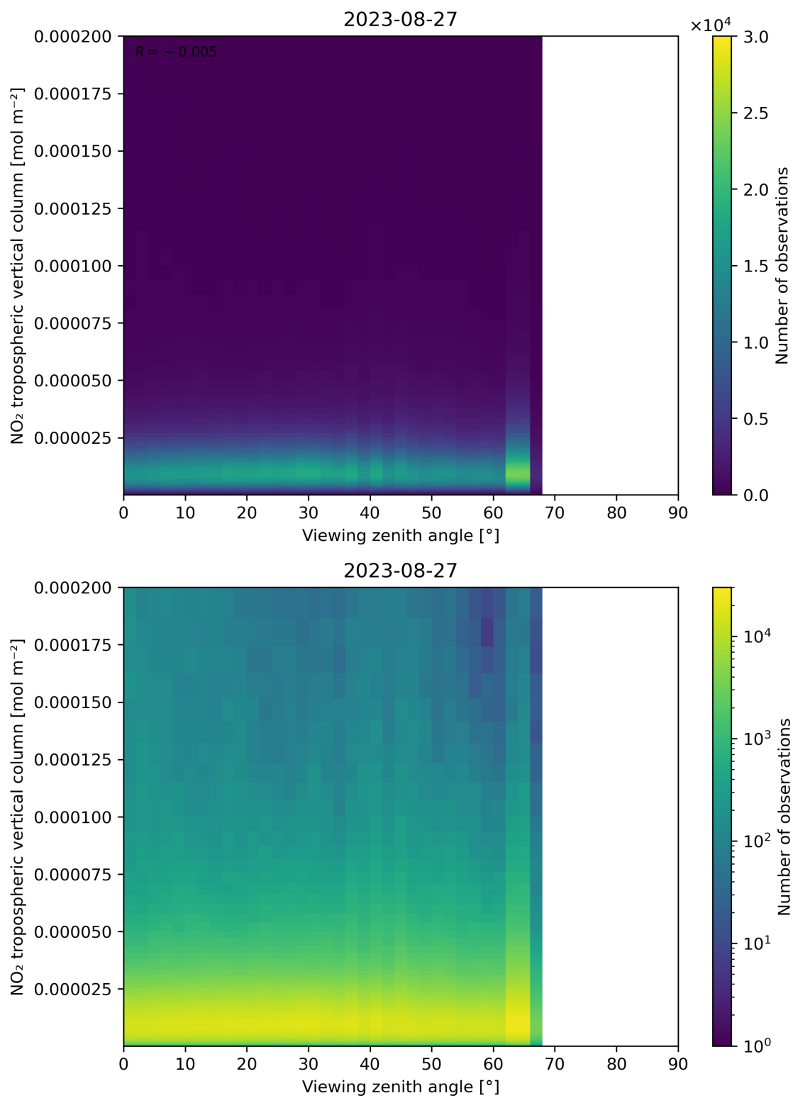
Figure 169: Scatter density plot of “Viewing zenith angle” against “NO 2 tropospheric vertical column” for 2023-08-26 to 2023-08-28.
