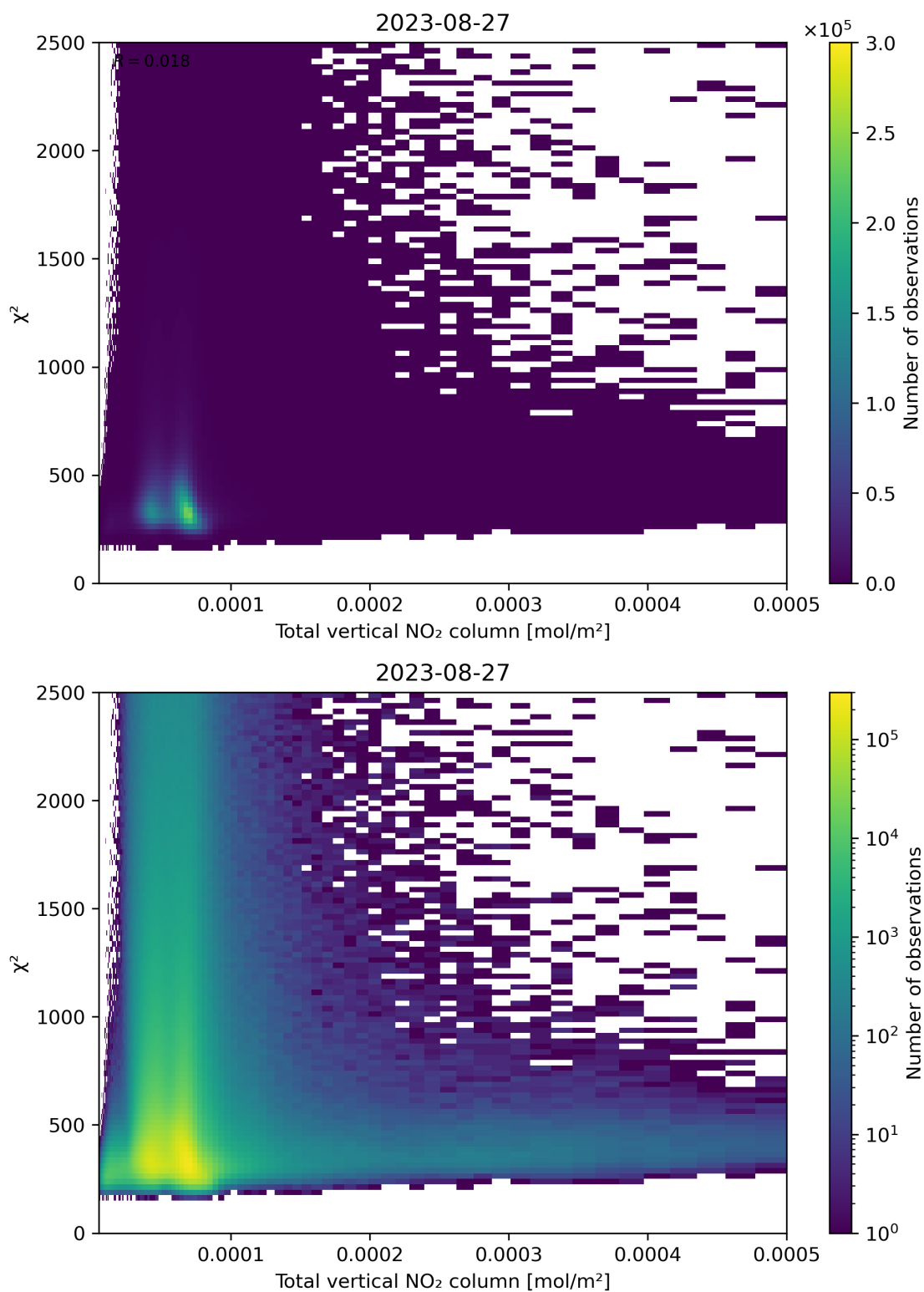
Figure 111: Scatter density plot of “Total vertical NO 2 column” against “ \chi^2 ” for 2023-08-26 to 2023-08-28.
