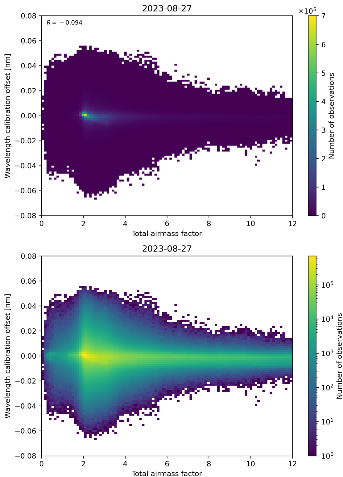
Figure 70: Scatter density plot of “Total airmass factor” against “Wavelength calibration offset” for 2023-08-26 to 2023-08-28.
