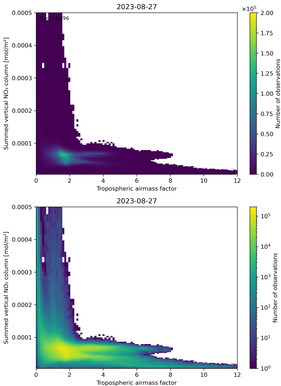
Figure 75: Scatter density plot of “Tropospheric air mass factor” against “Summed vertical NO 2 column” for 2023-08-26 to 2023-08-28.
