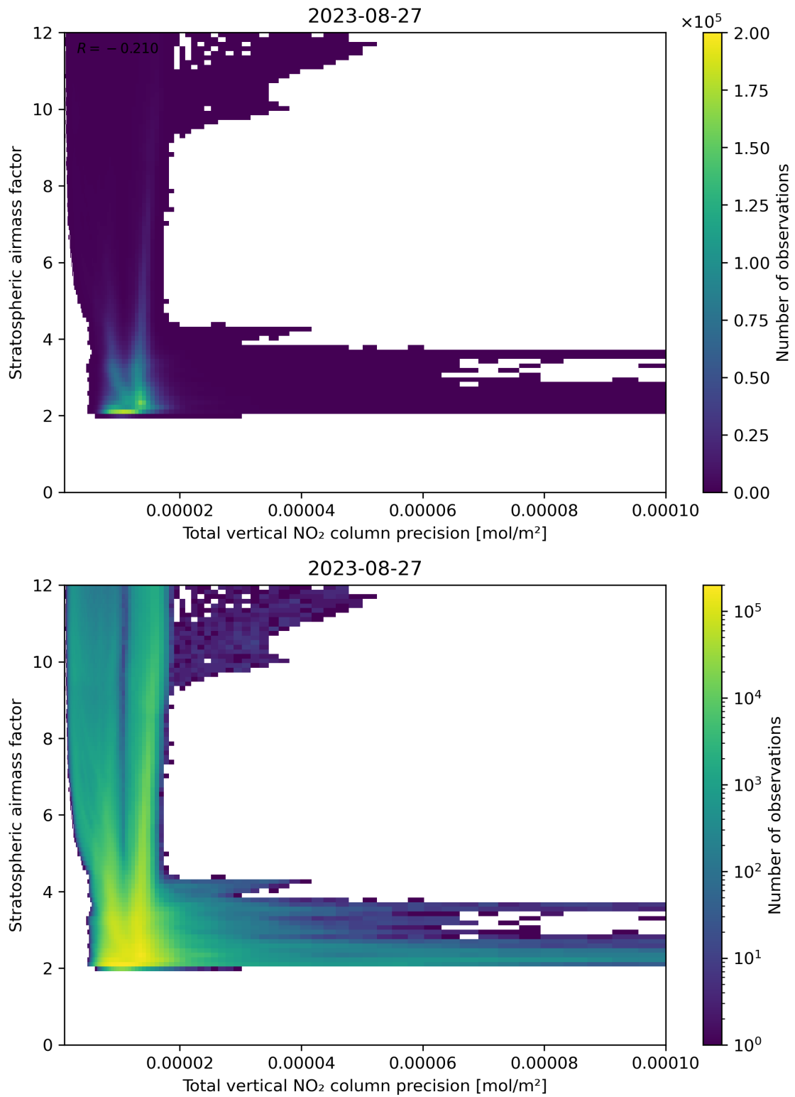
Figure 115: Scatter density plot of “Total vertical NO 2 column precision” against “Stratospheric air mass factor” for 2023-08-26 to 2023-08-28.
