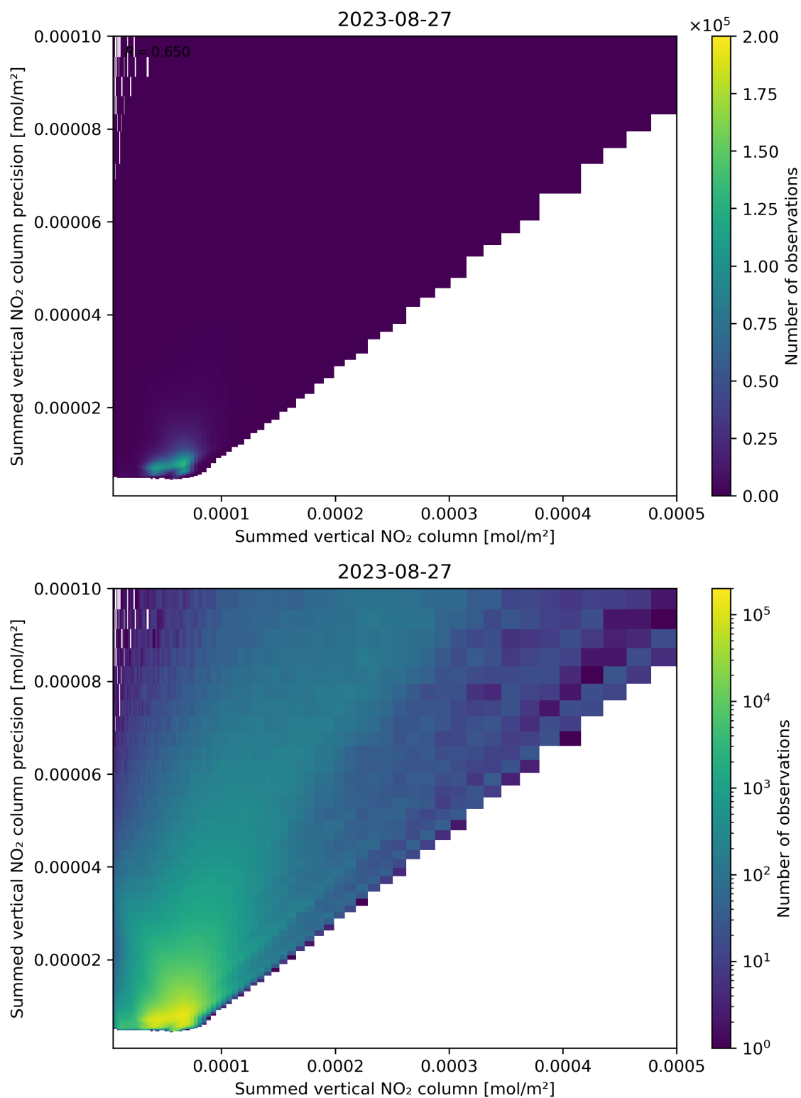
Figure 105: Scatter density plot of “Summed vertical NO 2 column” against “Summed vertical NO 2 column precision” for 2023-08-26 to 2023-08-28.
