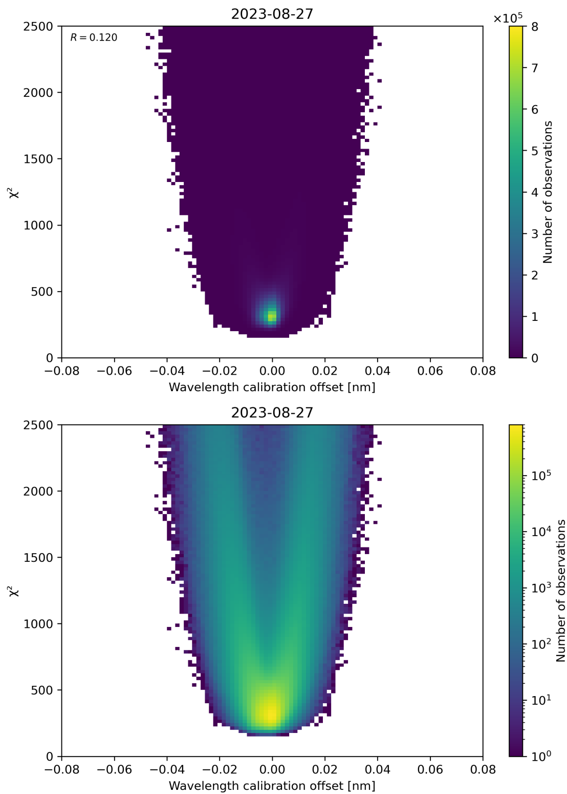
Figure 175: Scatter density plot of “Wavelength calibration offset” against “ \chi^2 ” for 2023-08-26 to 2023-08-28.
