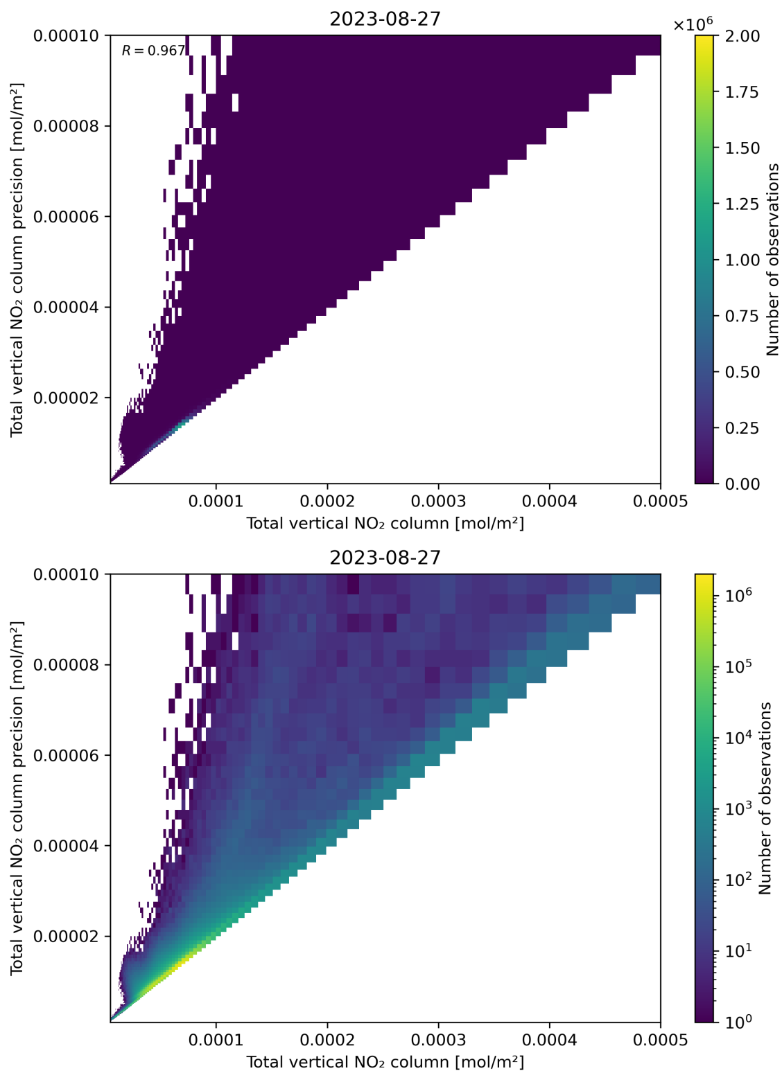
Figure 114: Scatter density plot of “Total vertical NO 2 column” against “Total vertical NO 2 column precision” for 2023-08-26 to 2023-08-28.
