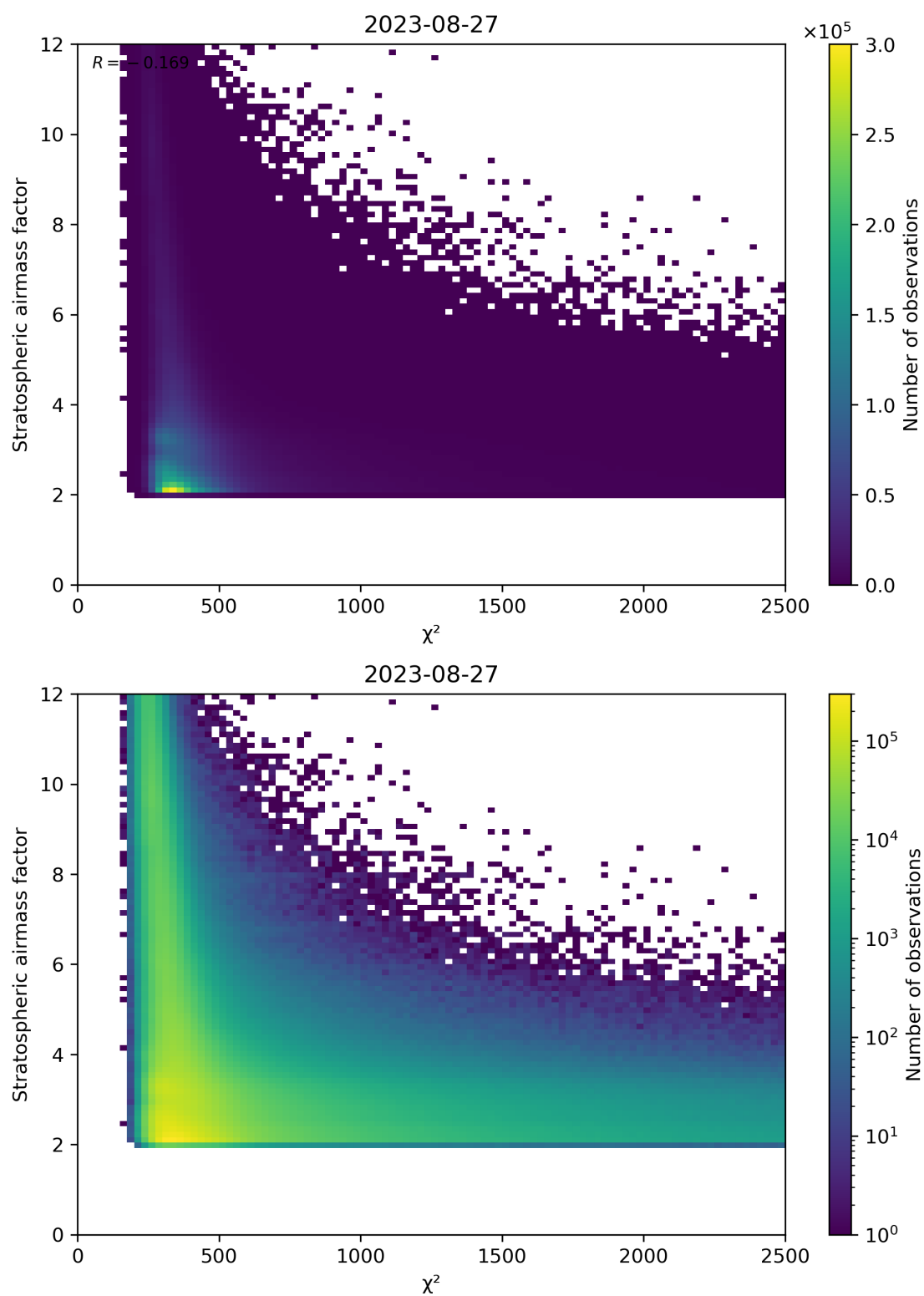
Figure 81: Scatter density plot of “ \chi^2 ” against “Stratospheric airmass factor” for 2023-08-26 to 2023-08-28.
