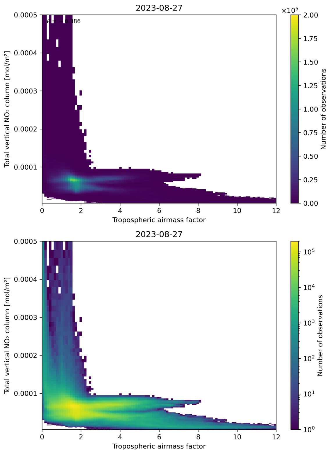
Figure 77: Scatter density plot of “Tropospheric airmass factor” against “Total vertical NO 2 column” for 2023-08-26 to 2023-08-28.
