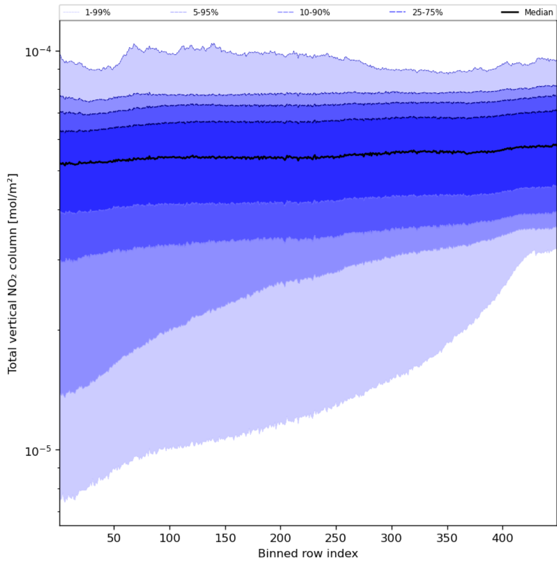
Figure 55: Along track statistics of “Total vertical NO 2 column” for 2023-08-26 to 2023-08-28
