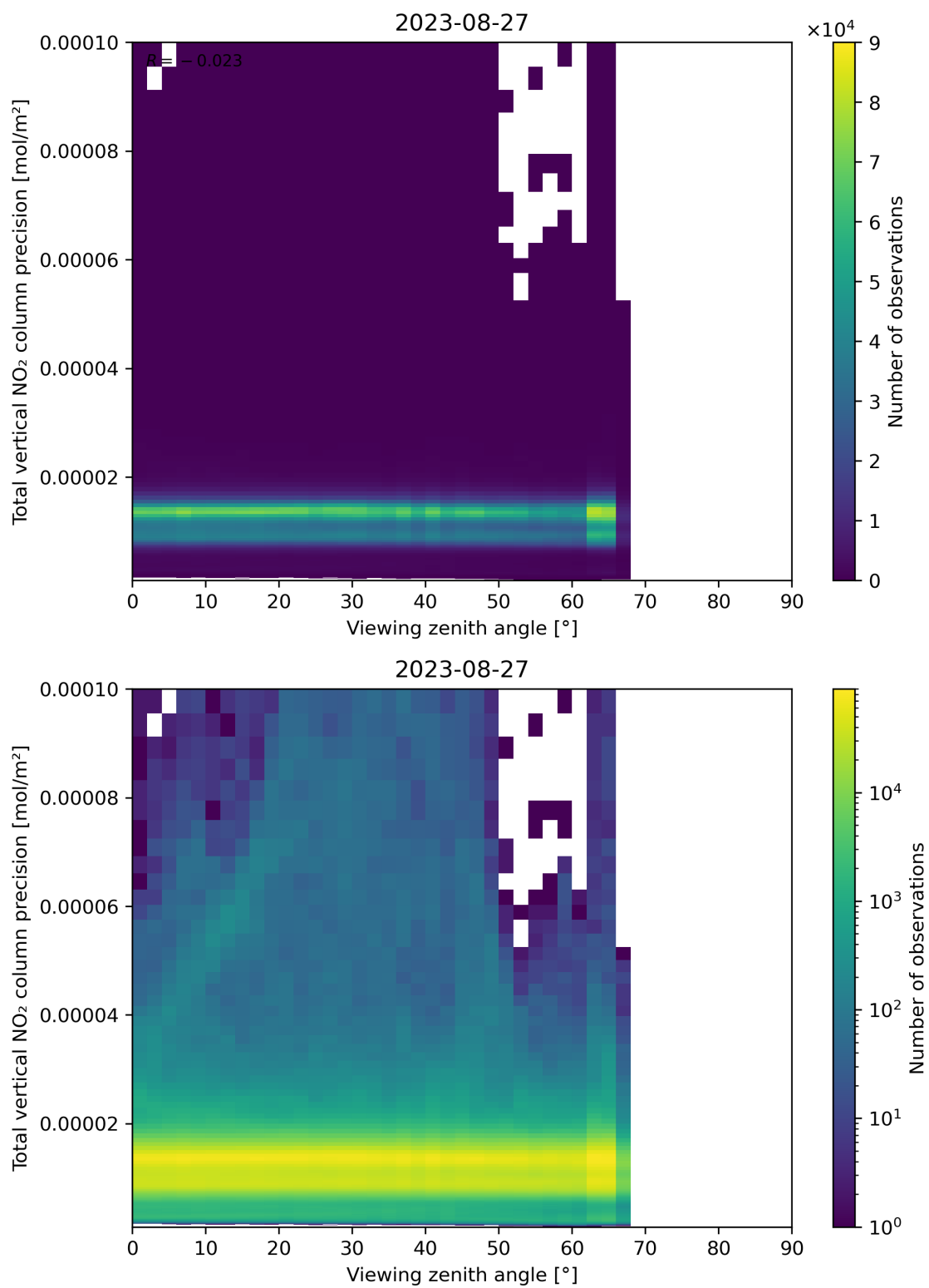
Figure 168: Scatter density plot of “Viewing zenith angle” against “Total vertical NO 2 column precision” for 2023-08-26 to 2023-08-28.
