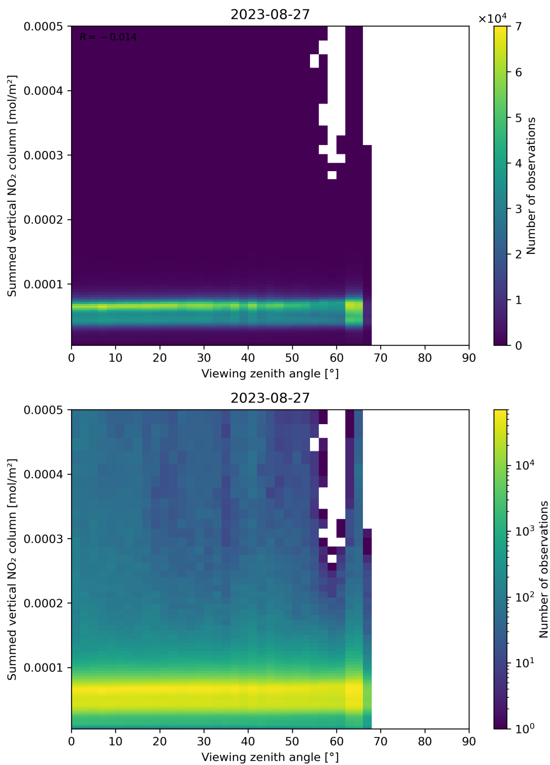
Figure 165: Scatter density plot of “Viewing zenith angle” against “Summed vertical NO 2 column” for 2023-08-26 to 2023-08-28.
