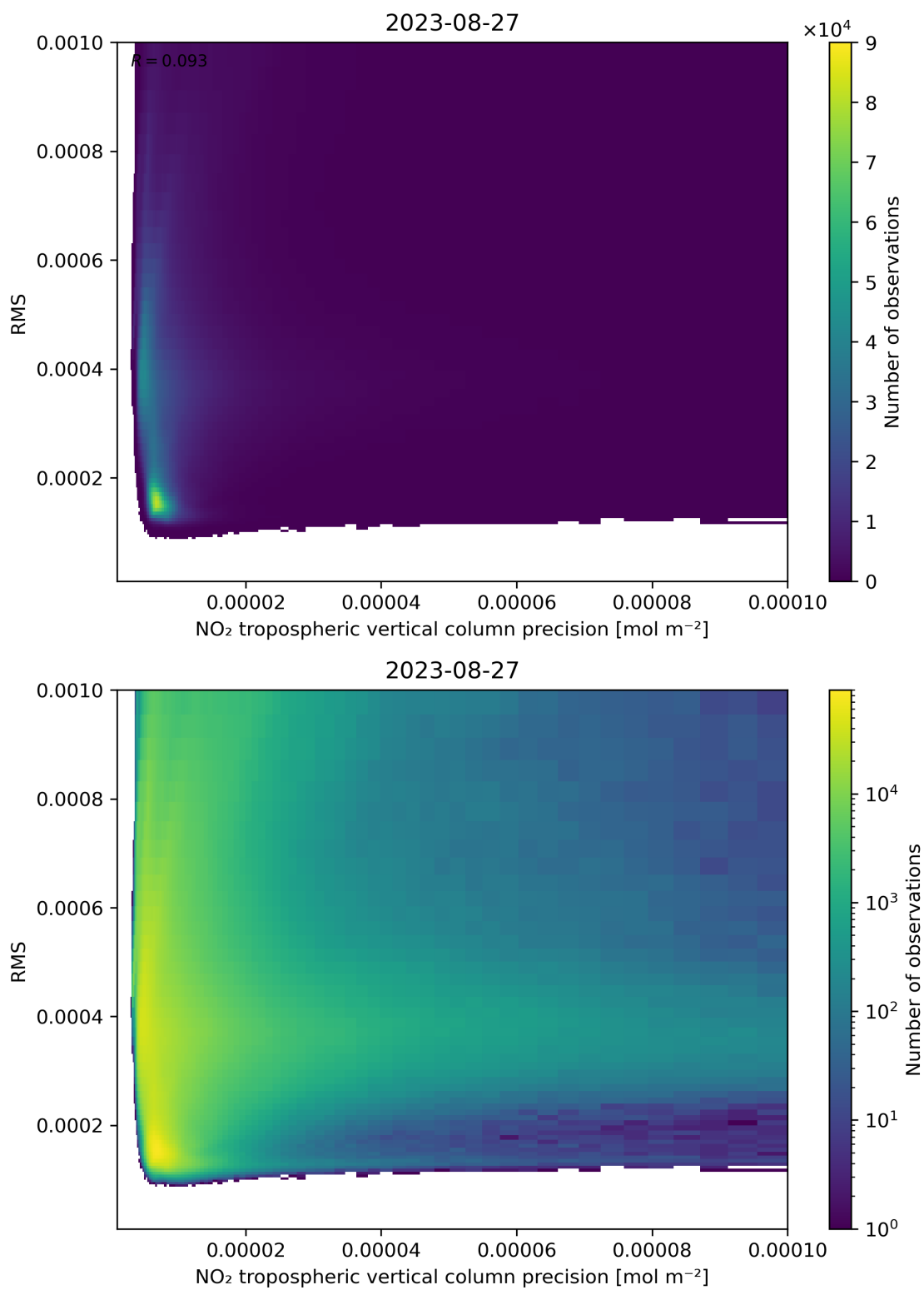
Figure 140: Scatter density plot of “NO 2 tropospheric vertical column precision” against “RMS” for 2023-08-26 to 2023-08-28.
