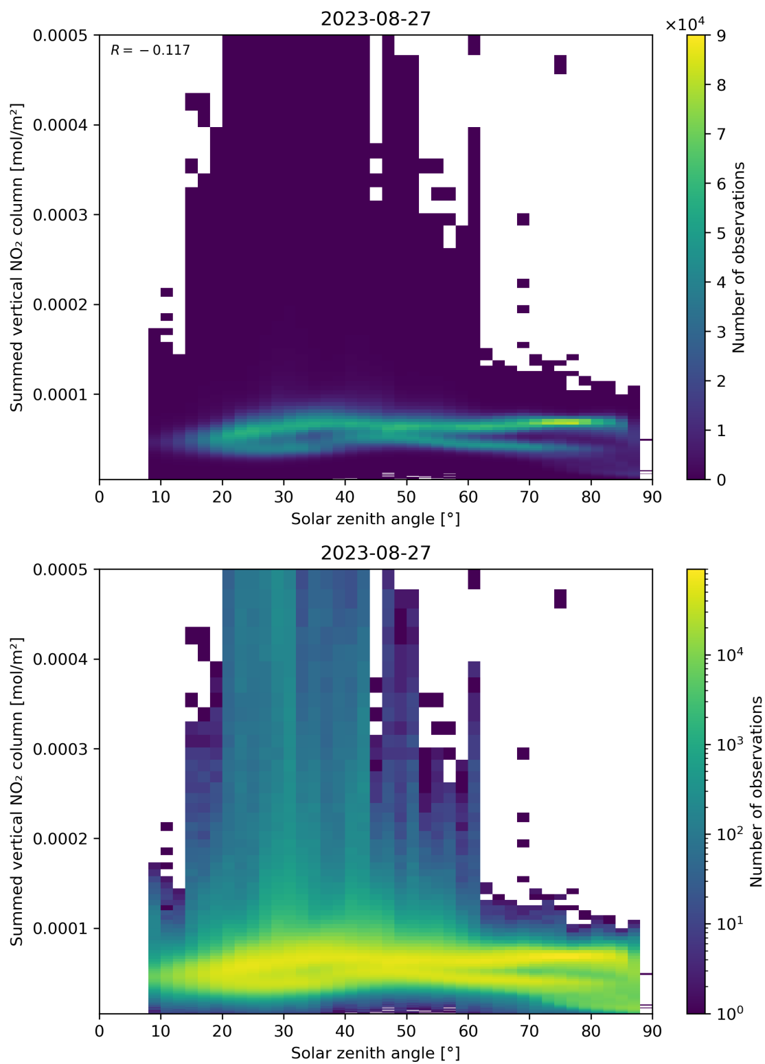
Figure 151: Scatter density plot of “Solar zenith angle” against “Summed vertical NO 2 column” for 2023-08-26 to 2023-08-28.
