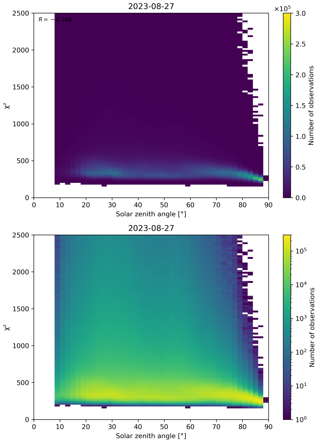
Figure 148: Scatter density plot of “Solar zenith angle” against “ \chi^2 ” for 2023-08-26 to 2023-08-28.
