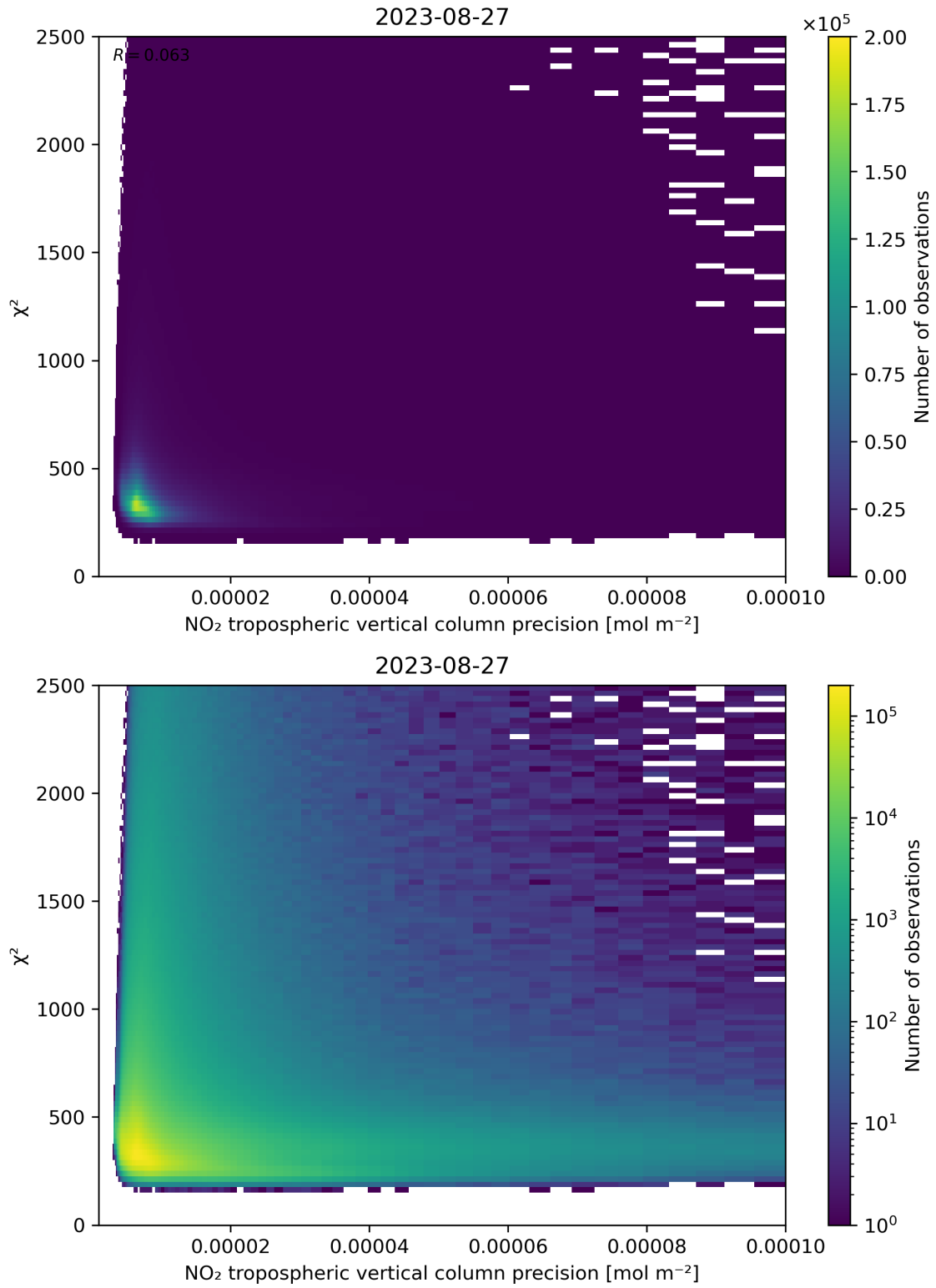
Figure 134: Scatter density plot of “NO 2 tropospheric vertical column precision” against “ \chi^2 ” for 2023-08-26 to 2023-08-28.
