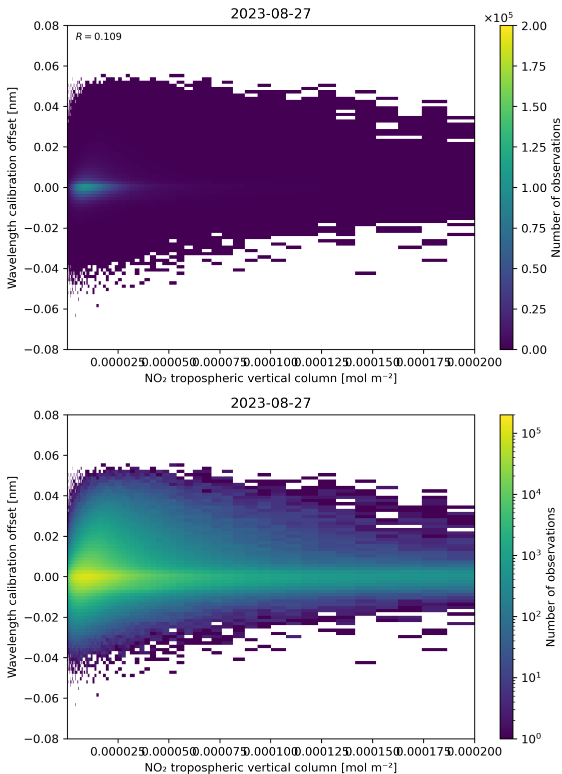
Figure 143: Scatter density plot of “NO 2 tropospheric vertical column” against “Wavelength calibration offset” for 2023-08-26 to 2023-08-28.
