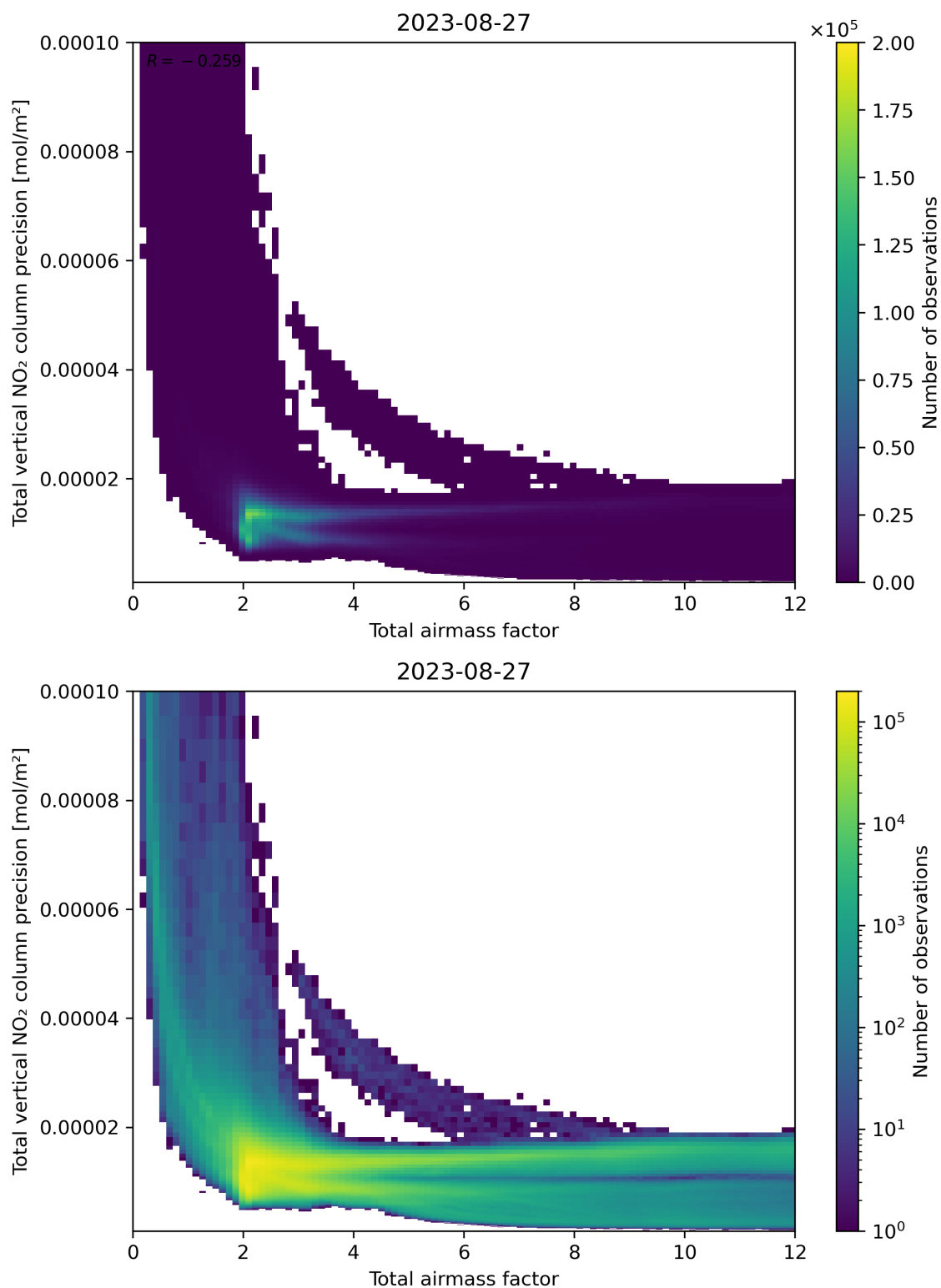
Figure 68: Scatter density plot of “Total airmass factor” against “Total vertical NO 2 column precision” for 2023-08-26 to 2023-08-28.
