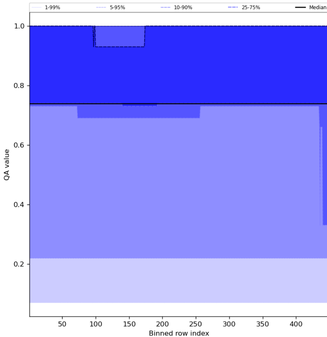
Figure 45: Along track statistics of “QA value” for 2023-08-26 to 2023-08-28
