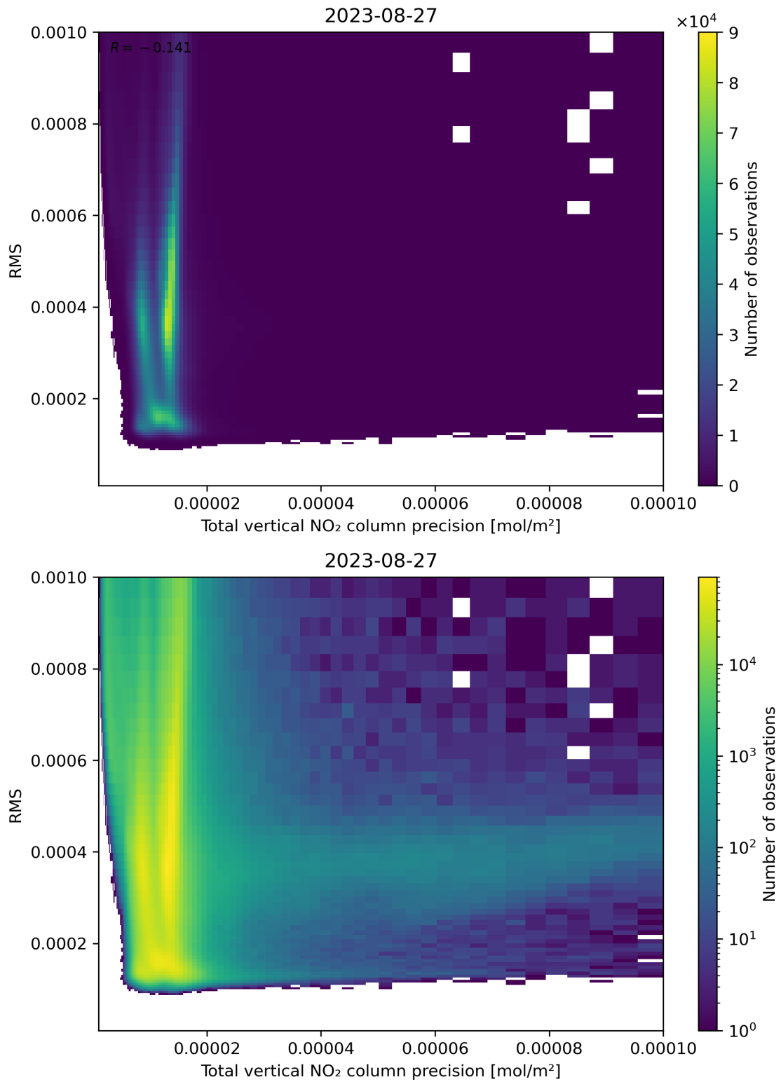
Figure 119: Scatter density plot of “Total vertical NO 2 column precision” against “RMS” for 2023-08-26 to 2023-08-28.
