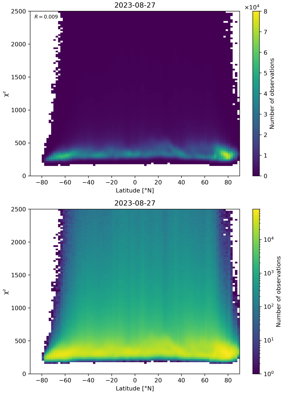
Figure 86: Scatter density plot of “Latitude” against “ \chi^2 ” for 2023-08-26 to 2023-08-28.
