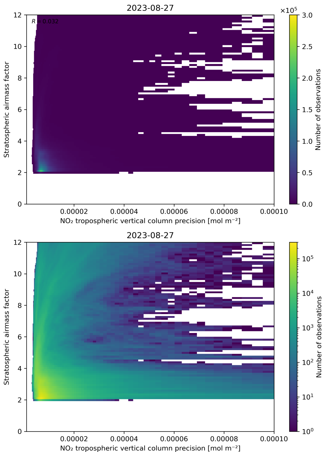
Figure 131: Scatter density plot of “NO 2 tropospheric vertical column precision” against “Stratospheric airmass factor” for 2023-08-26 to 2023-08-28.
