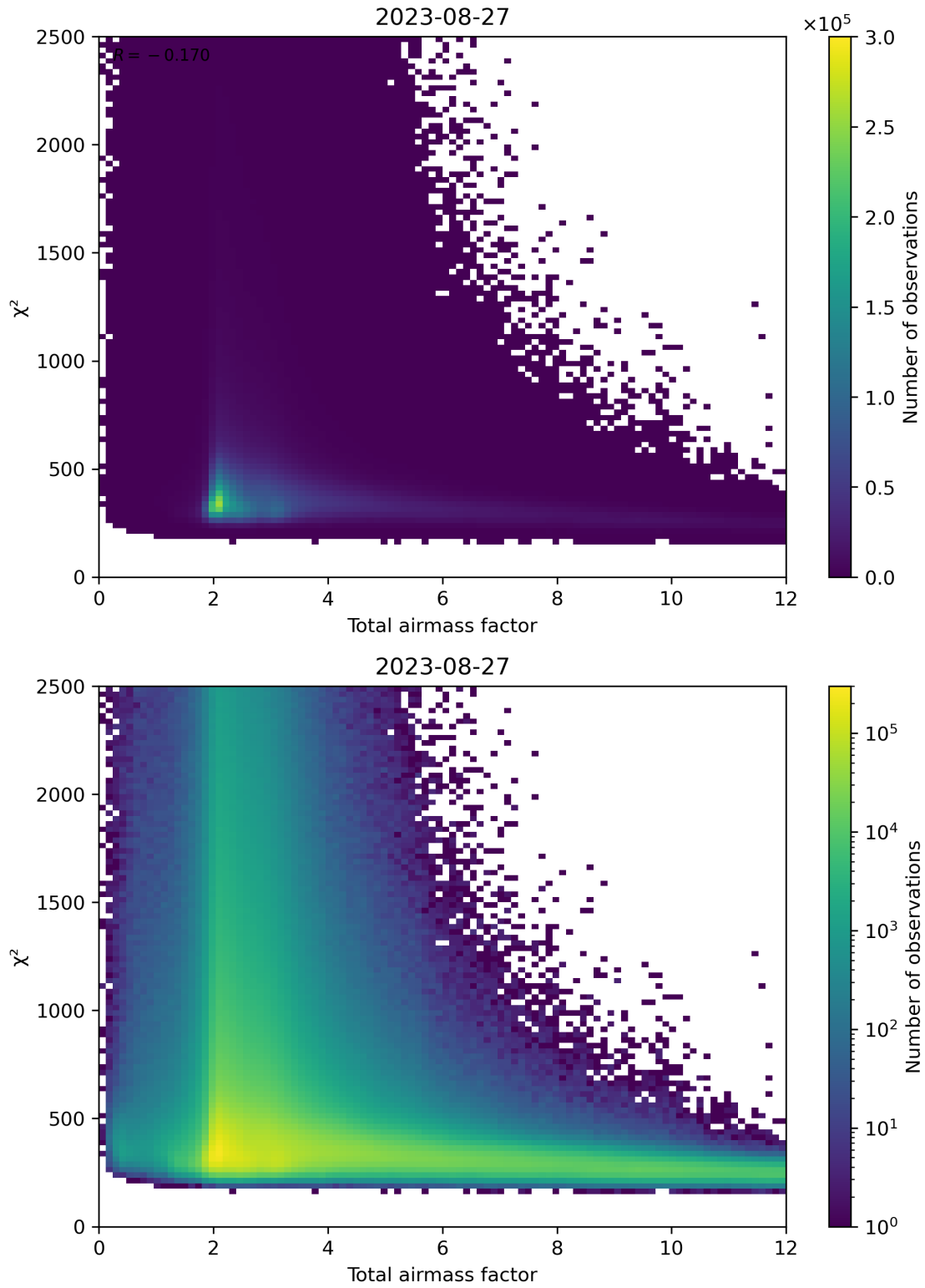
Figure 63: Scatter density plot of “Total airmass factor” against “ \chi^2 ” for 2023-08-26 to 2023-08-28.
