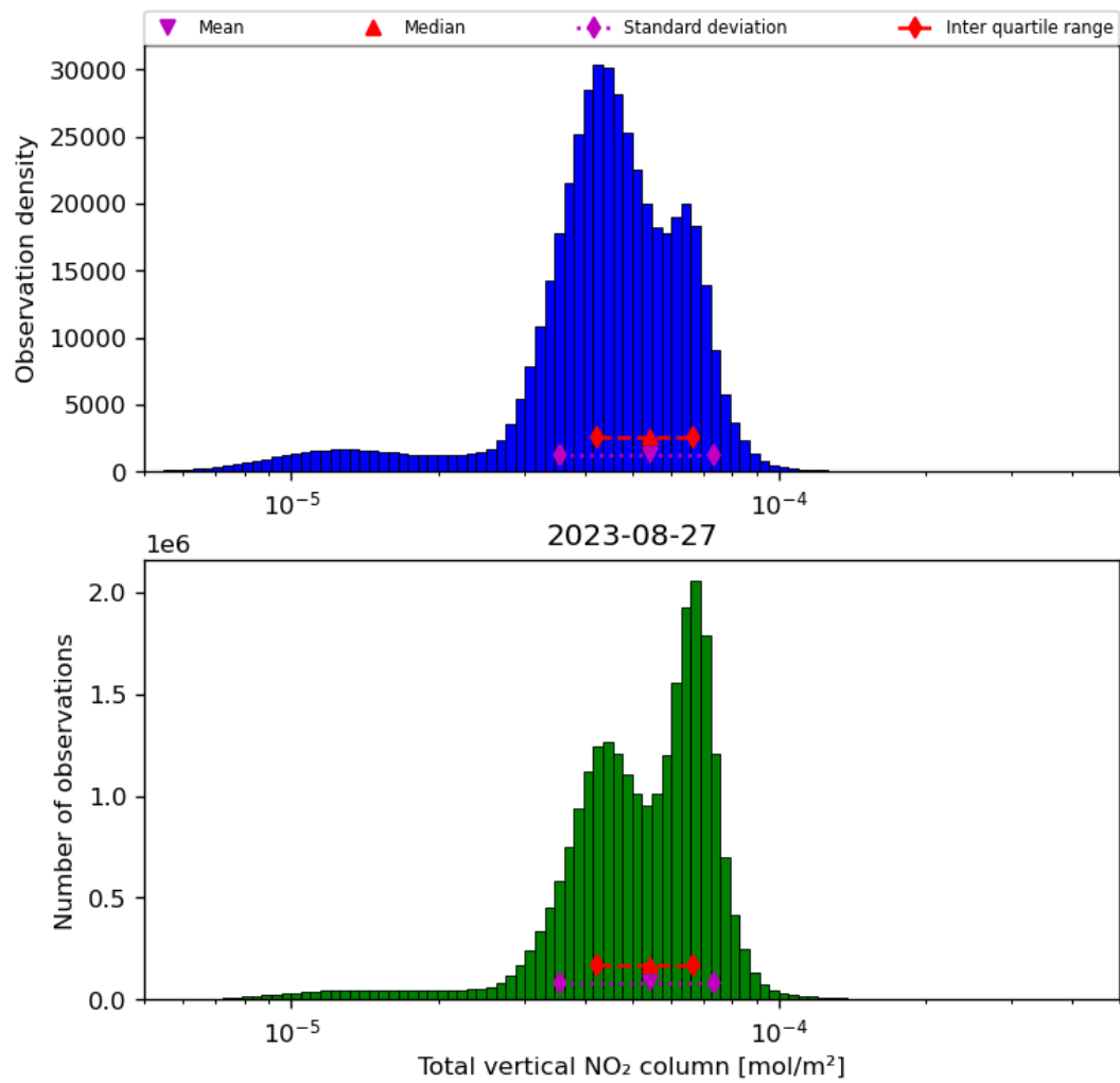
Figure 38: Histogram of “Total vertical NO 2 column” for 2023-08-26 to 2023-08-28
