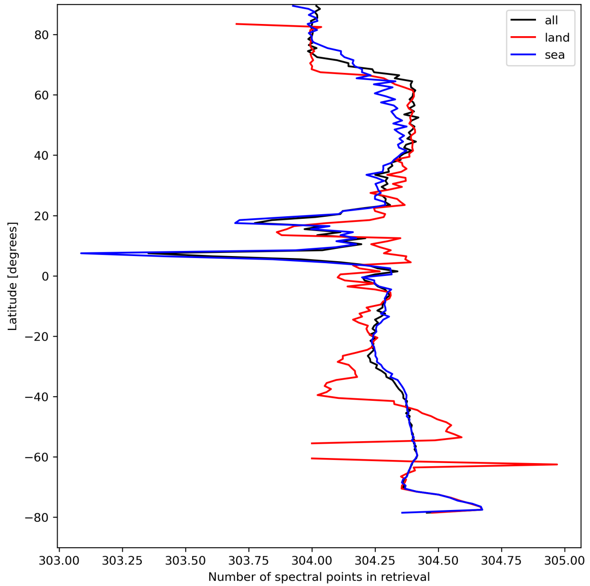
Figure 16: Zonal average of “Number of spectral points in retrieval” for 2023-08-26 to 2023-08-28.
