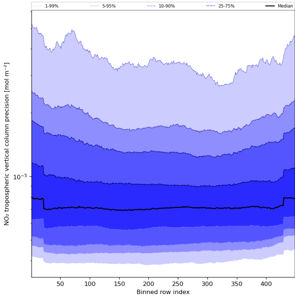
Figure 47: Along track statistics of “NO 2 tropospheric vertical column precision” for 2023-08-26 to 2023-08-28
