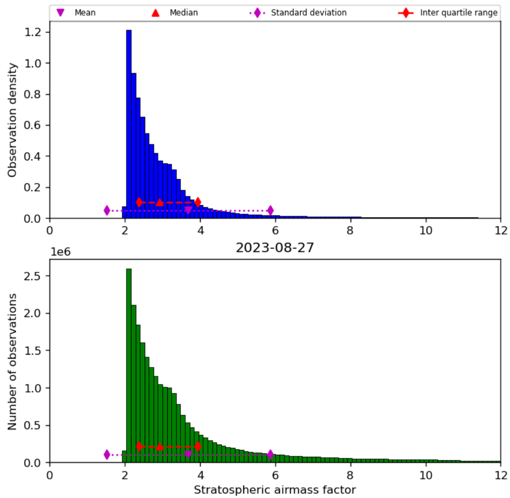
Figure 44: Histogram of “Stratospheric airmass factor” for 2023-08-26 to 2023-08-28
