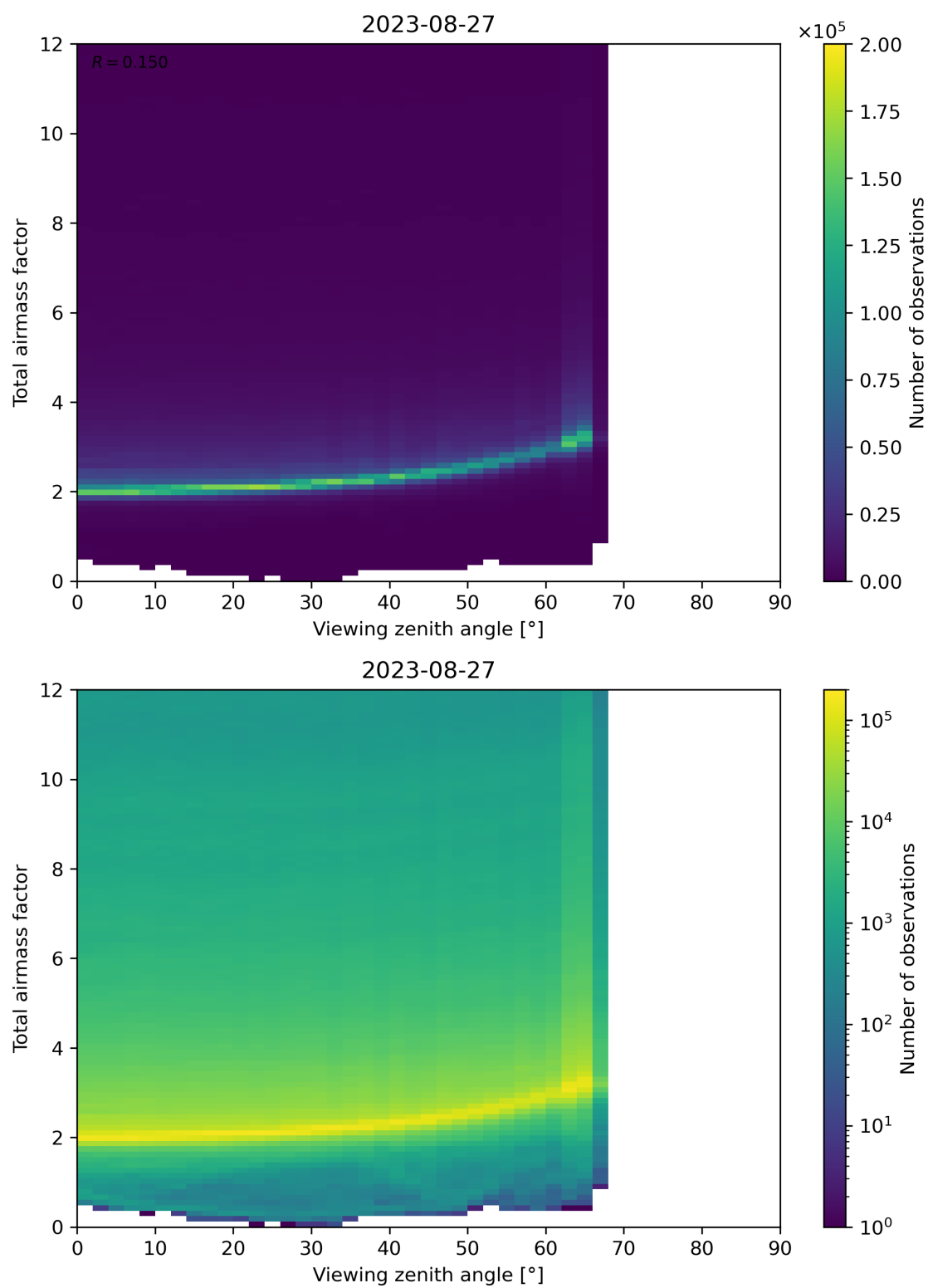
Figure 160: Scatter density plot of “Viewing zenith angle” against “Total airmass factor” for 2023-08-26 to 2023-08-28.
