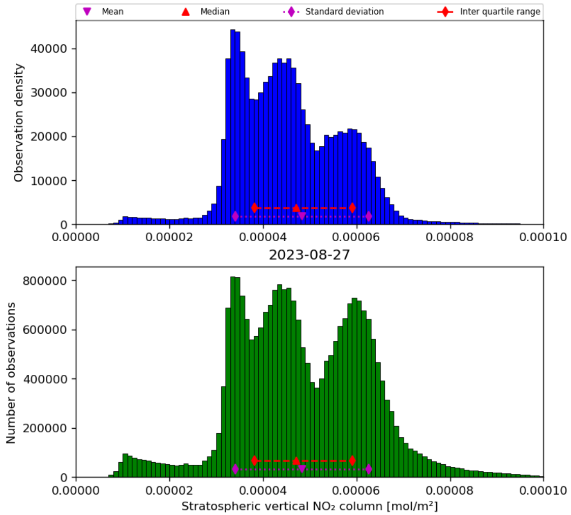
Figure 36: Histogram of “Stratospheric vertical NO 2 column” for 2023-08-26 to 2023-08-28
