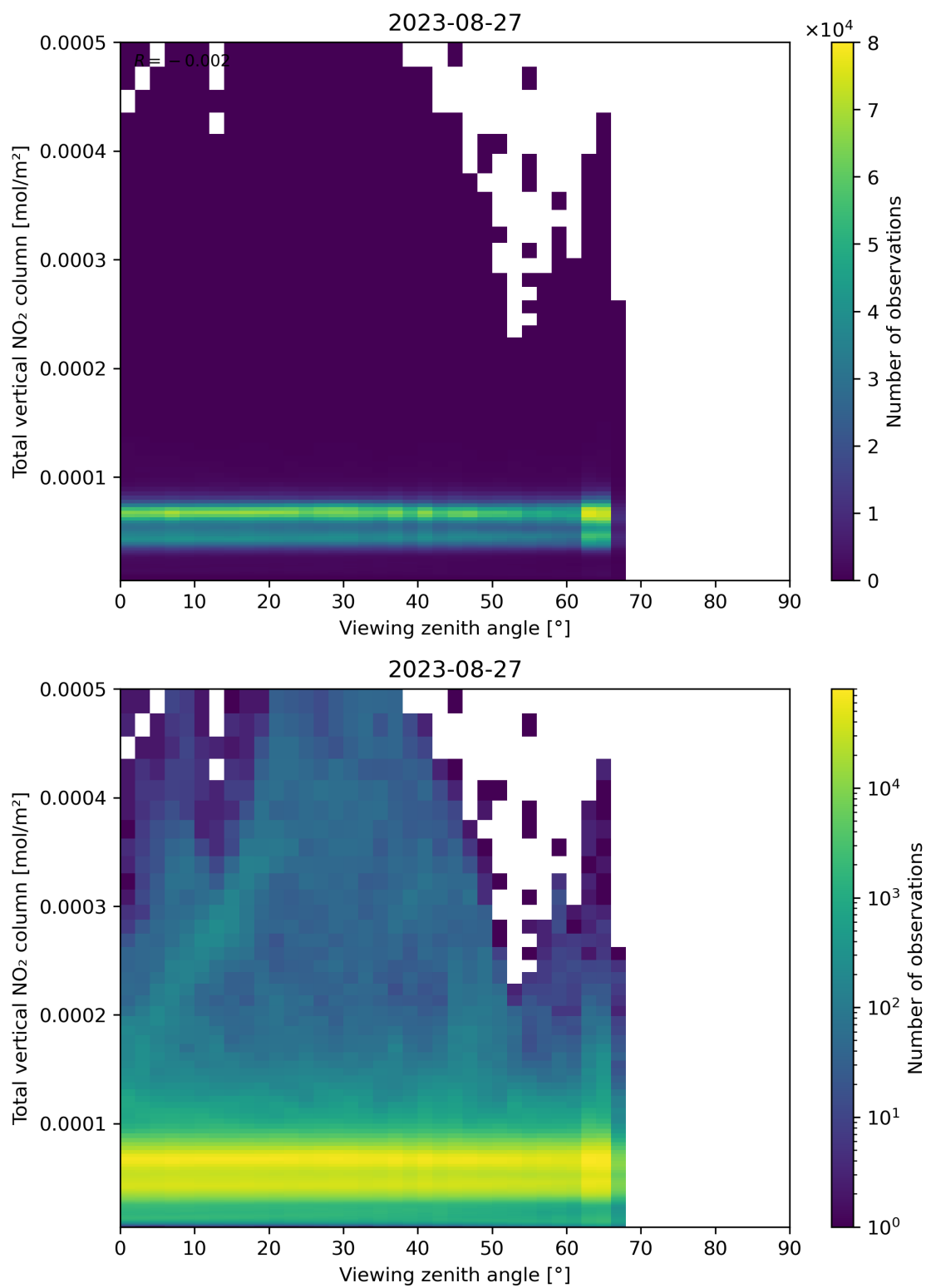
Figure 167: Scatter density plot of “Viewing zenith angle” against “Total vertical NO 2 column” for 2023-08-26 to 2023-08-28.
