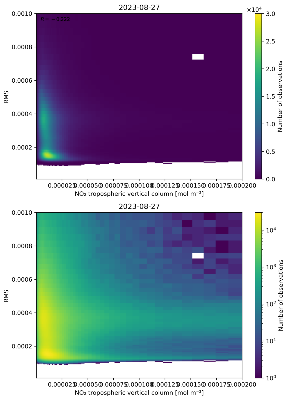
Figure 142: Scatter density plot of “NO 2 tropospheric vertical column” against “RMS” for 2023-08-26 to 2023-08-28.
