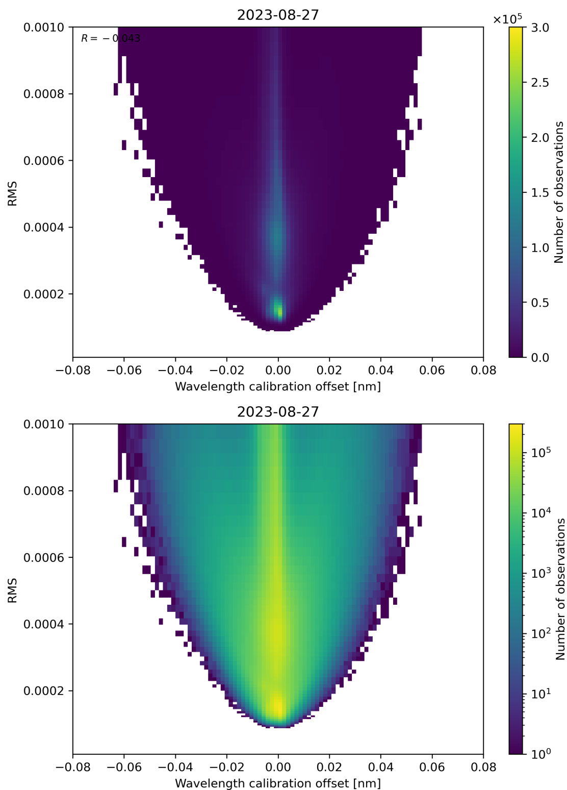
Figure 181: Scatter density plot of “Wavelength calibration offset” against “RMS” for 2023-08-26 to 2023-08-28.
