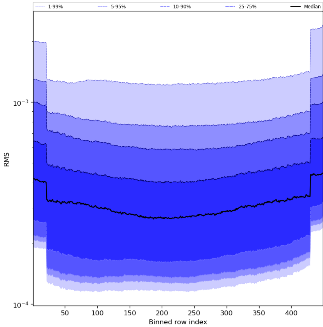
Figure 60: Along track statistics of “RMS” for 2023-08-26 to 2023-08-28
