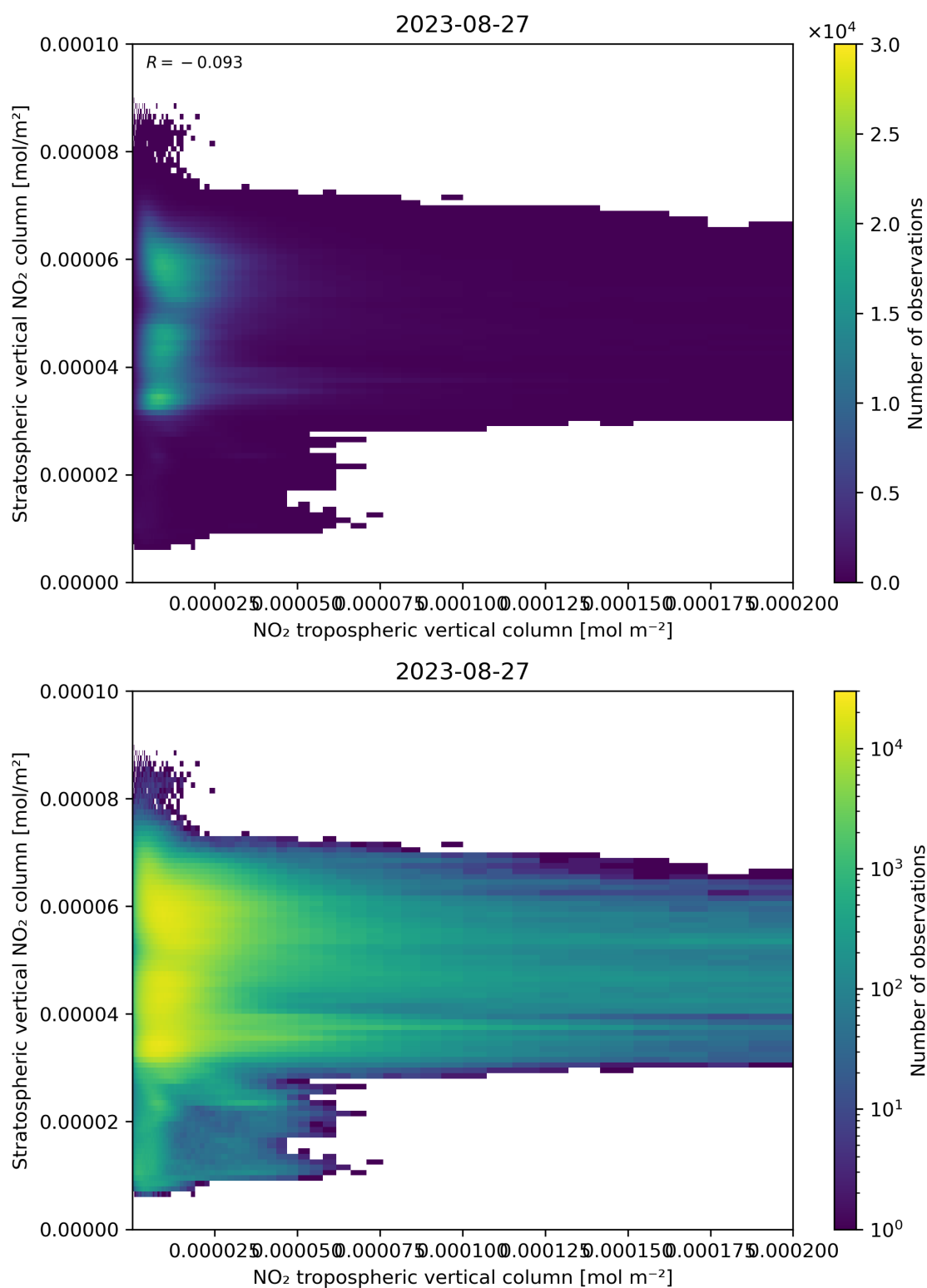
Figure 125: Scatter density plot of “NO 2 tropospheric vertical column” against “Stratospheric vertical NO 2 column” for 2023-08-26 to 2023-08-28.
