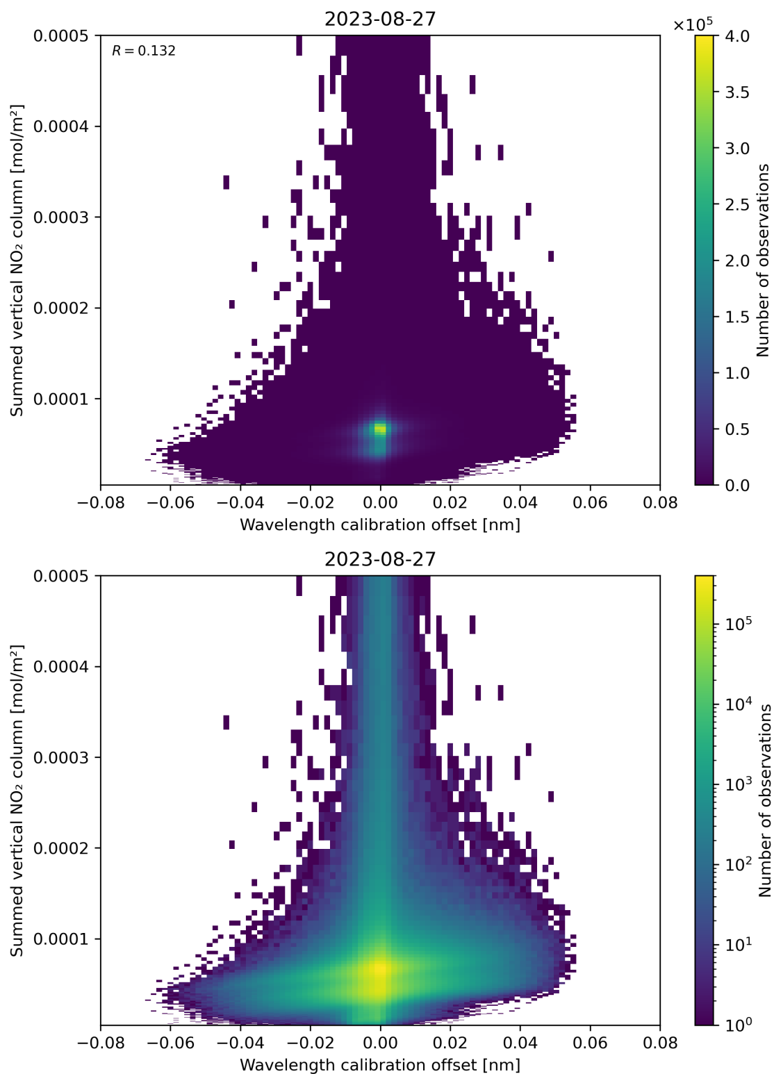
Figure 177: Scatter density plot of “Wavelength calibration offset” against “Summed vertical NO 2 column” for 2023-08-26 to 2023-08-28.
