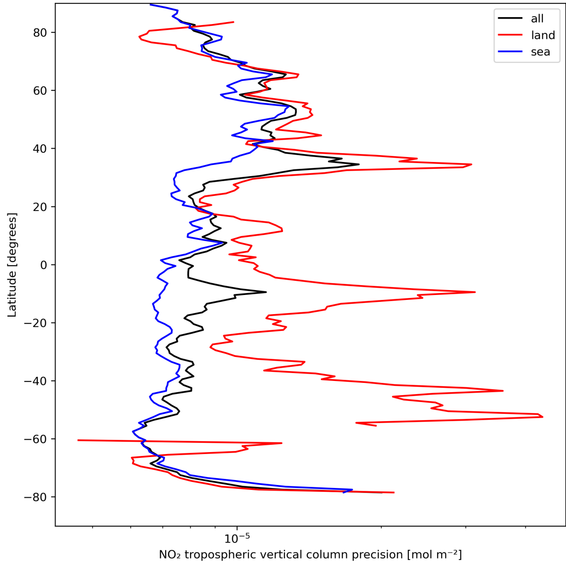
Figure 13: Zonal average of “NO 2 tropospheric vertical column precision” for 2023-08-26 to 2023-08-28.
