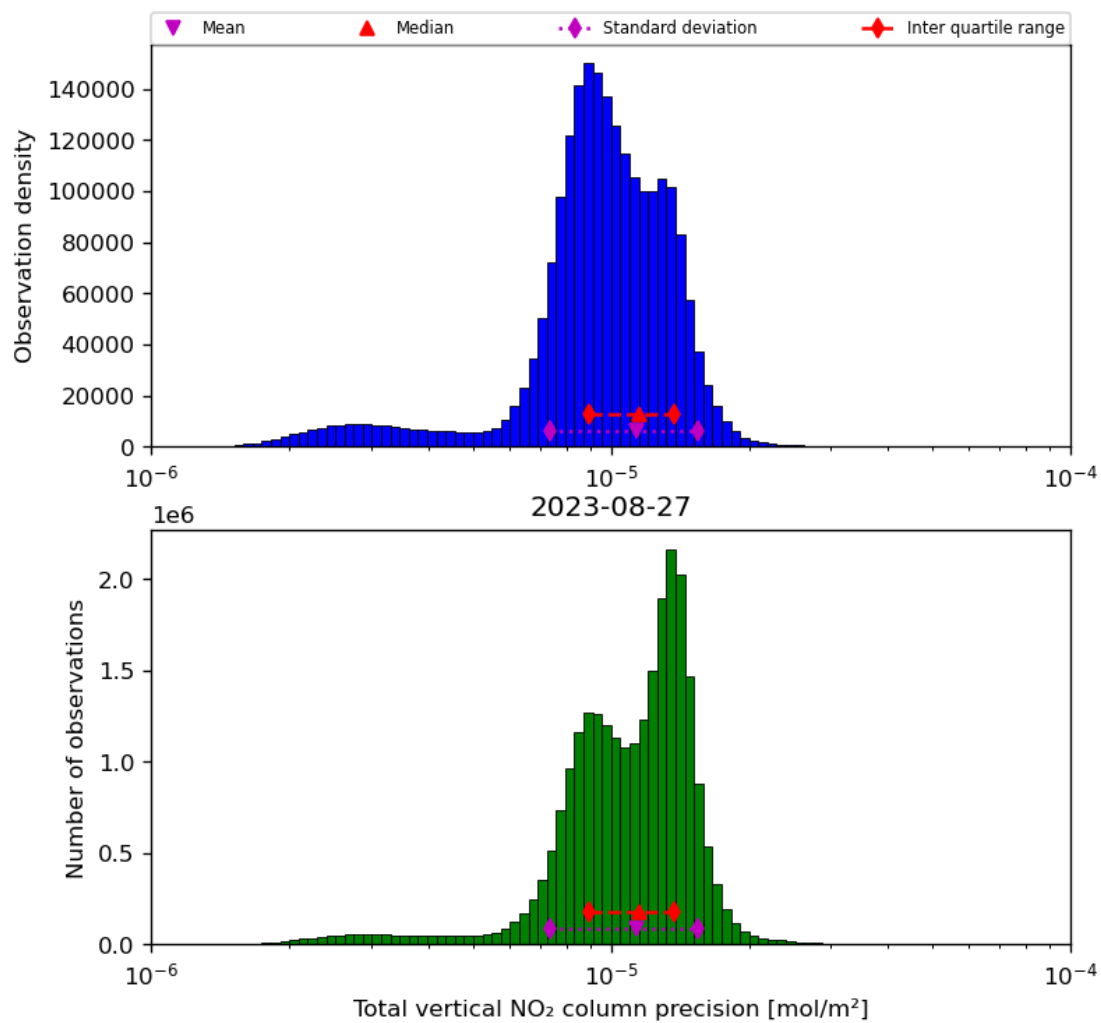
Figure 39: Histogram of "Total vertical NO 2 column precision" for 2023-08-26 to 2023-08-28
