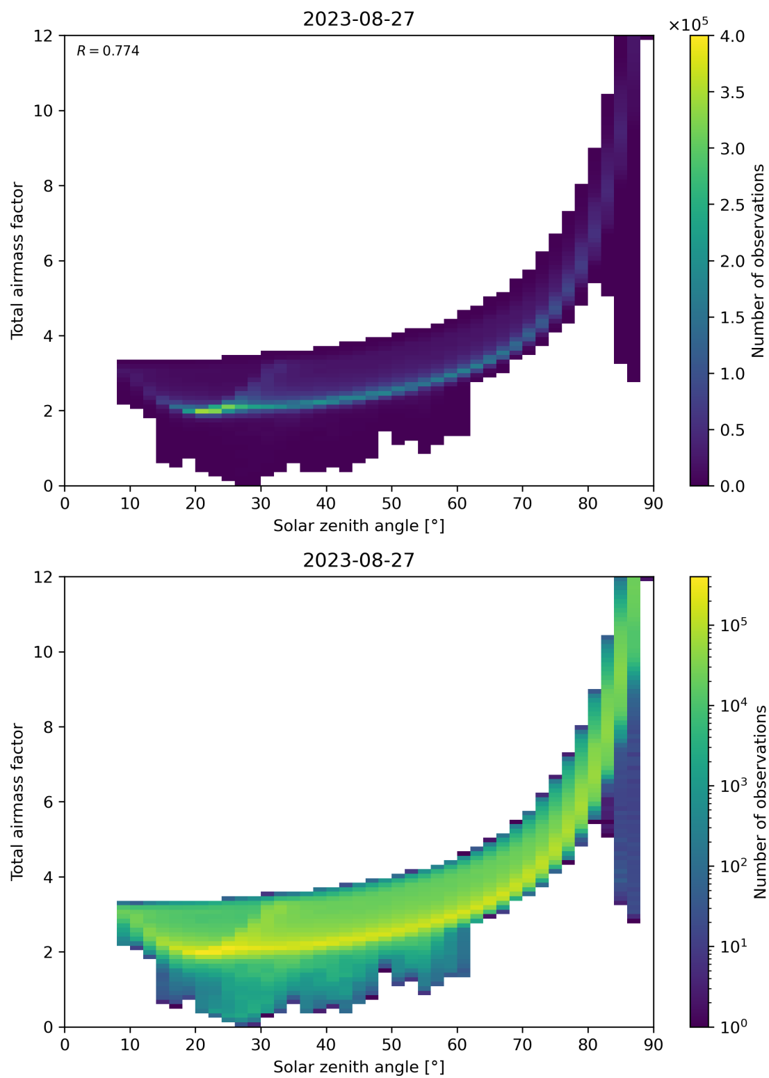
Figure 146: Scatter density plot of “Solar zenith angle” against “Total air mass factor” for 2023-08-26 to 2023-08-28.
