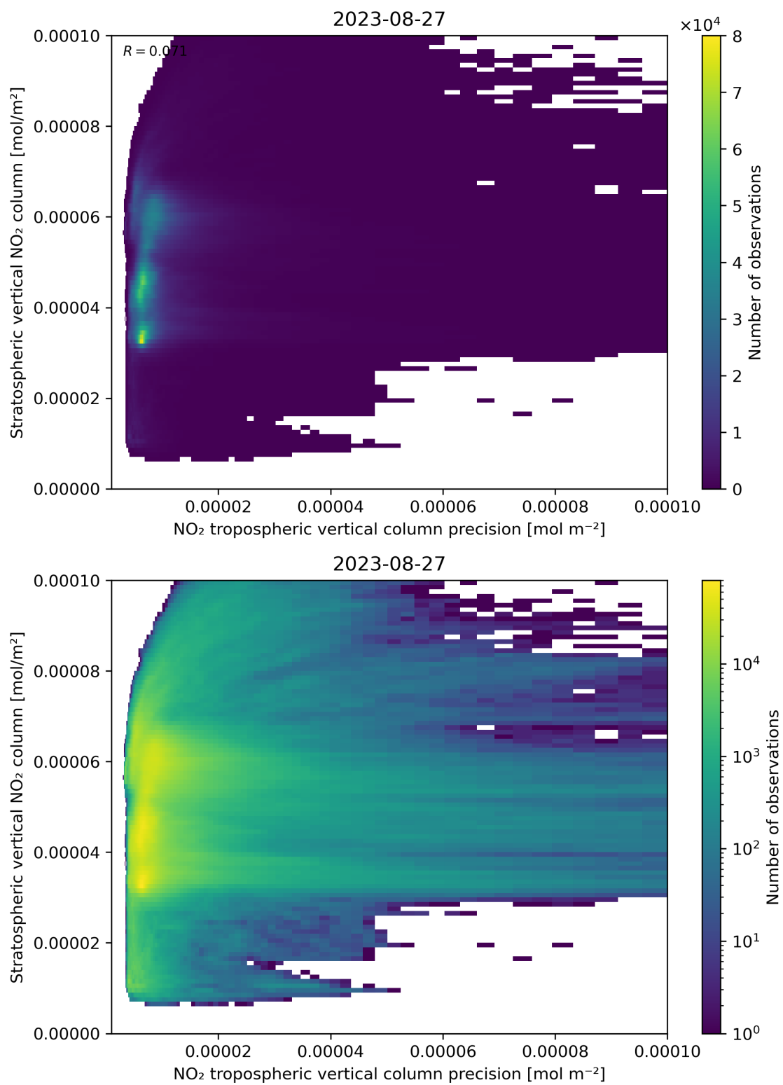
Figure 135: Scatter density plot of “NO 2 tropospheric vertical column precision” against “Stratospheric vertical NO 2 column” for 2023-08-26 to 2023-08-28.
