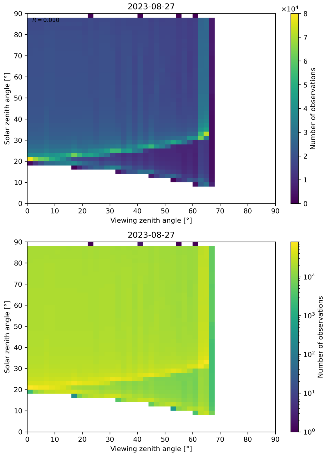
Figure 172: Scatter density plot of “Viewing zenith angle” against “Solar zenith angle” for 2023-08-26 to 2023-08-28.
