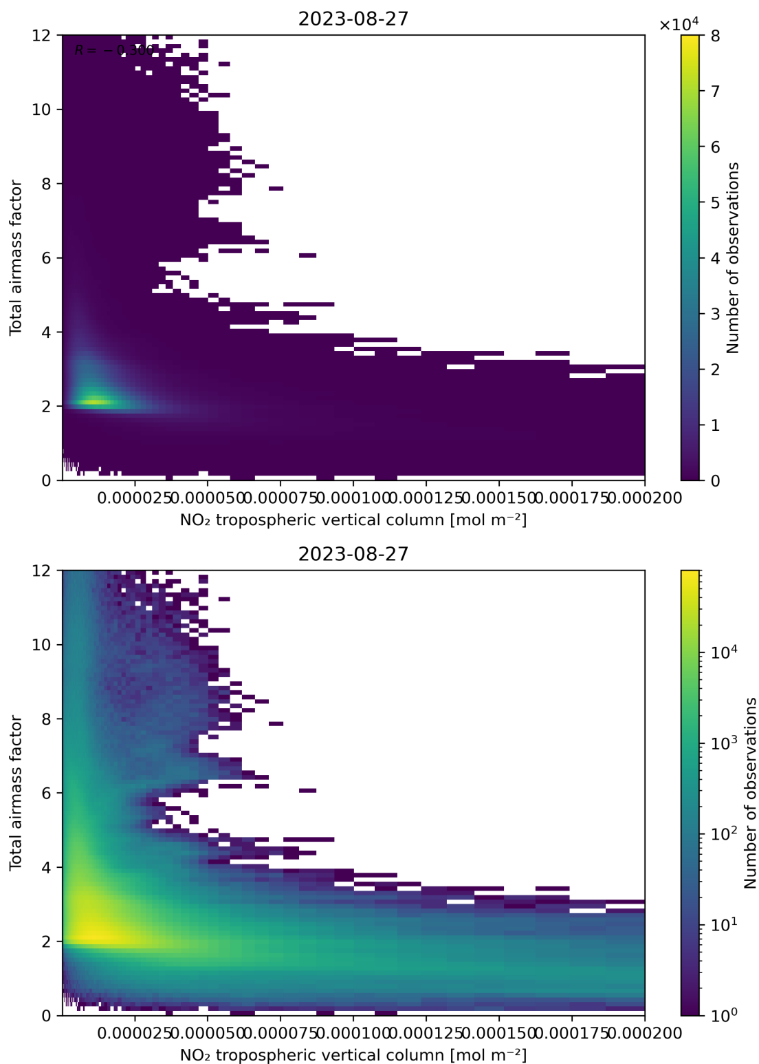
Figure 122: Scatter density plot of “NO 2 tropospheric vertical column” against “Total air mass factor” for 2023-08-26 to 2023-08-28.
