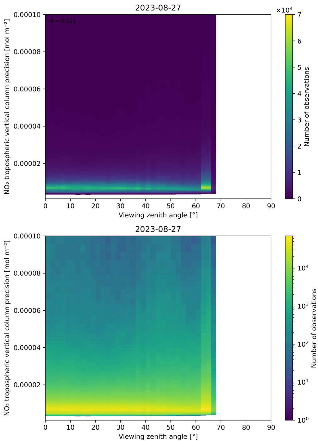
Figure 170: Scatter density plot of “Viewing zenith angle” against “NO 2 tropospheric vertical column precision” for 2023-08-26 to 2023-08-28.
