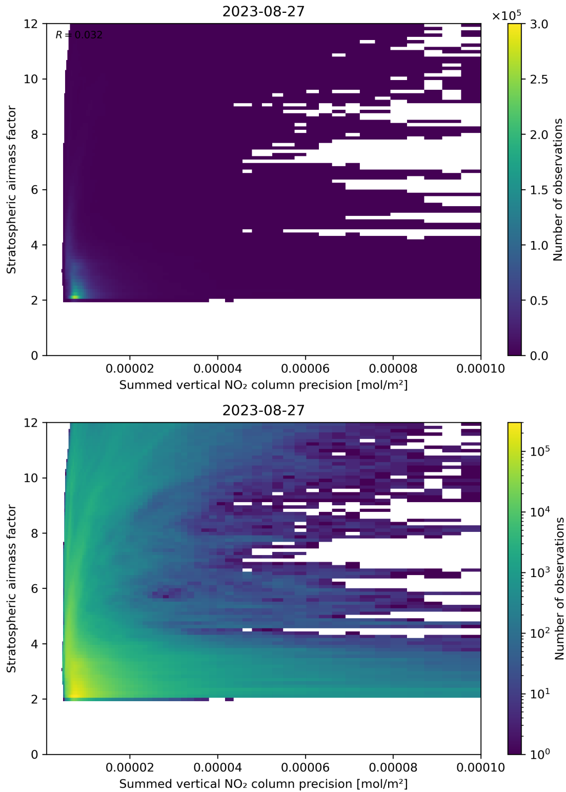
Figure 106: Scatter density plot of “Summed vertical NO 2 column precision” against “Stratospheric airmass factor” for 2023-08-26 to 2023-08-28.
