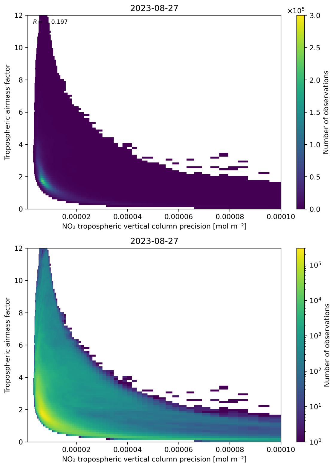
Figure 133: Scatter density plot of “NO 2 tropospheric vertical column precision” against “Tropospheric airmass factor” for 2023-08-26 to 2023-08-28.
