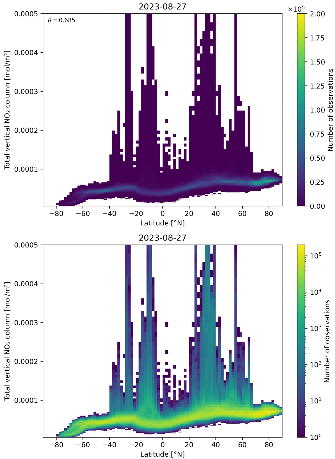
Figure 90: Scatter density plot of “Latitude” against “Total vertical NO 2 column” for 2023-08-26 to 2023-08-28.
