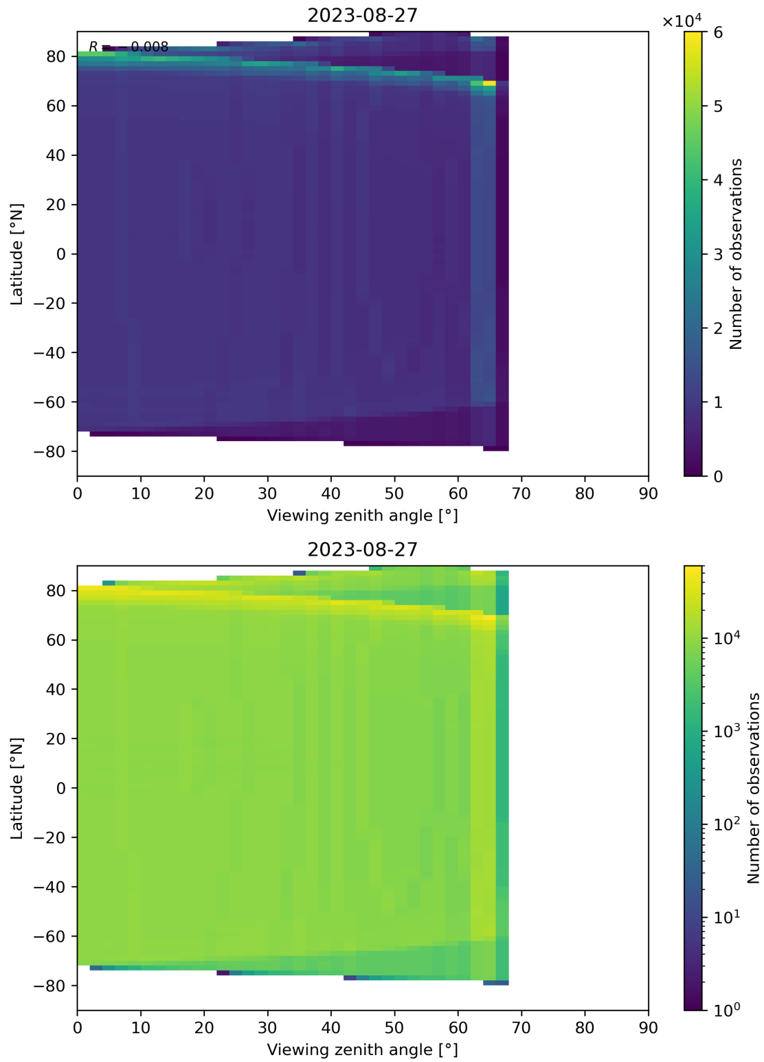
Figure 163: Scatter density plot of “Viewing zenith angle” against “Latitude” for 2023-08-26 to 2023-08-28.
