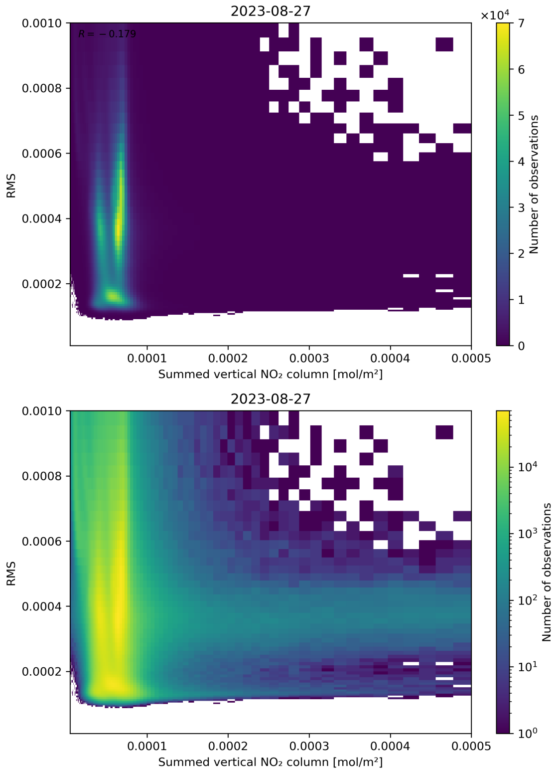
Figure 109: Scatter density plot of “Summed vertical NO 2 column” against “RMS” for 2023-08-26 to 2023-08-28.
