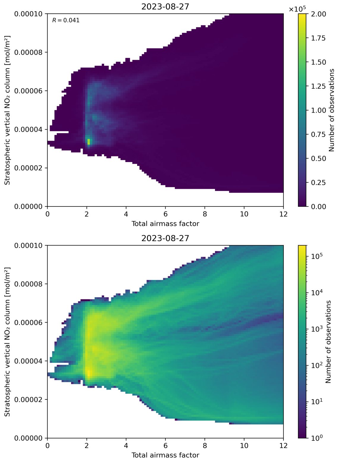
Figure 64: Scatter density plot of “Total airmass factor” against “Stratospheric vertical \text{NO}_2 column” for 2023-08-26 to 2023-08-28.
