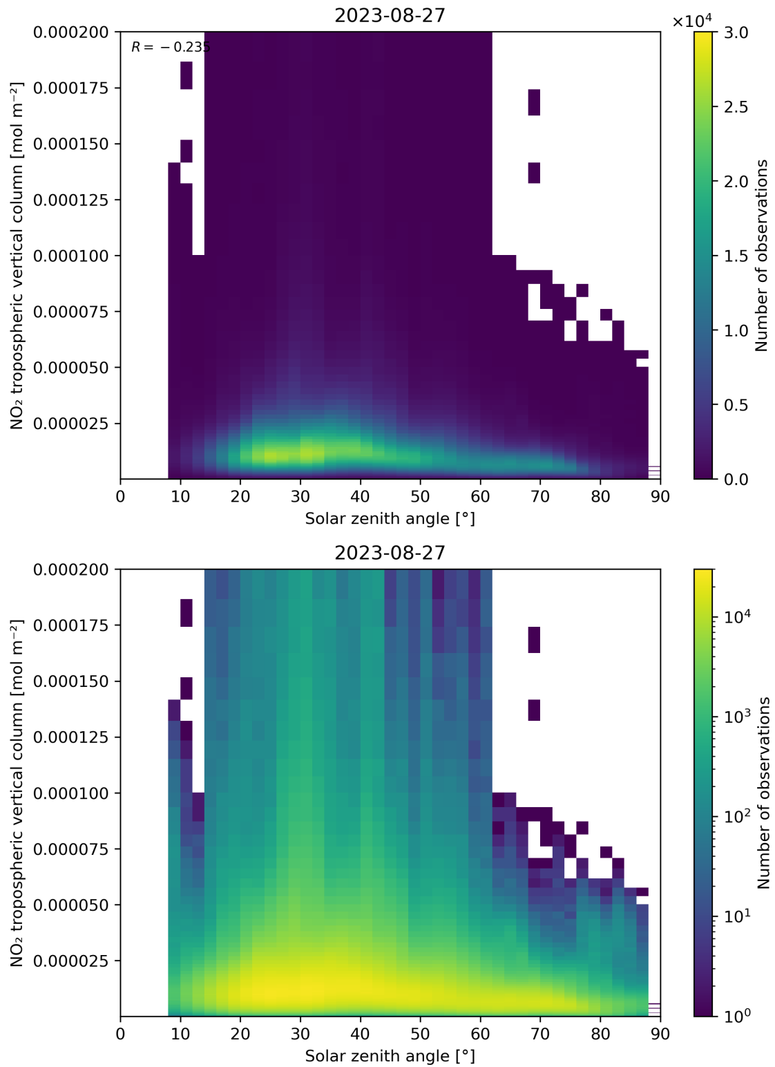
Figure 155: Scatter density plot of “Solar zenith angle” against “NO 2 tropospheric vertical column” for 2023-08-26 to 2023-08-28.
