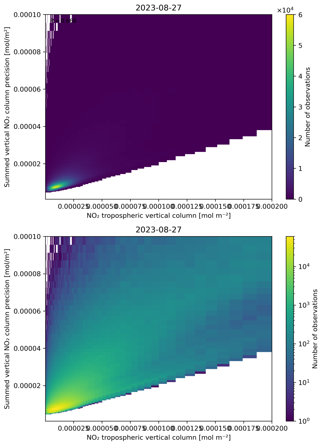
Figure 127: Scatter density plot of “NO 2 tropospheric vertical column” against “Summed vertical NO 2 column precision” for 2023-08-26 to 2023-08-28.
