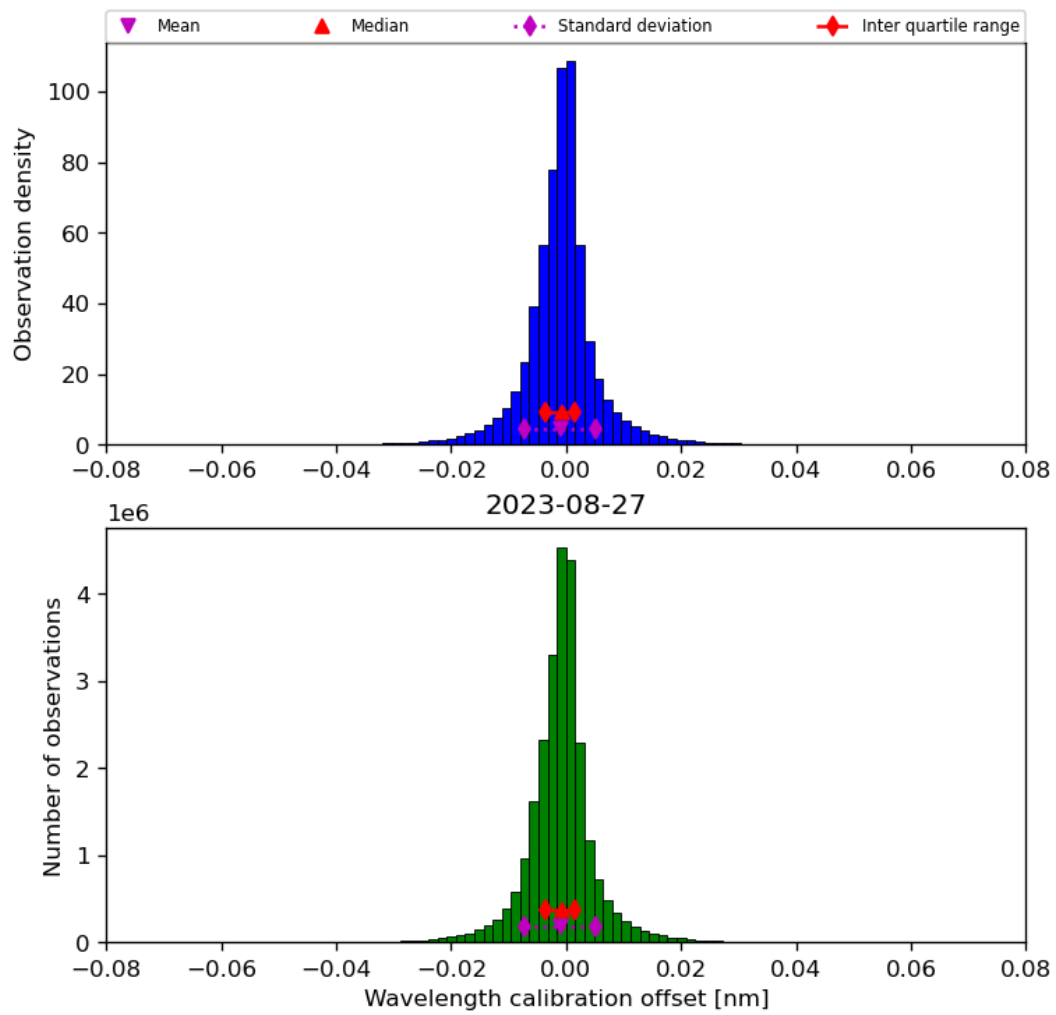
Figure 35: Histogram of “Wavelength calibration offset” for 2023-08-26 to 2023-08-28
