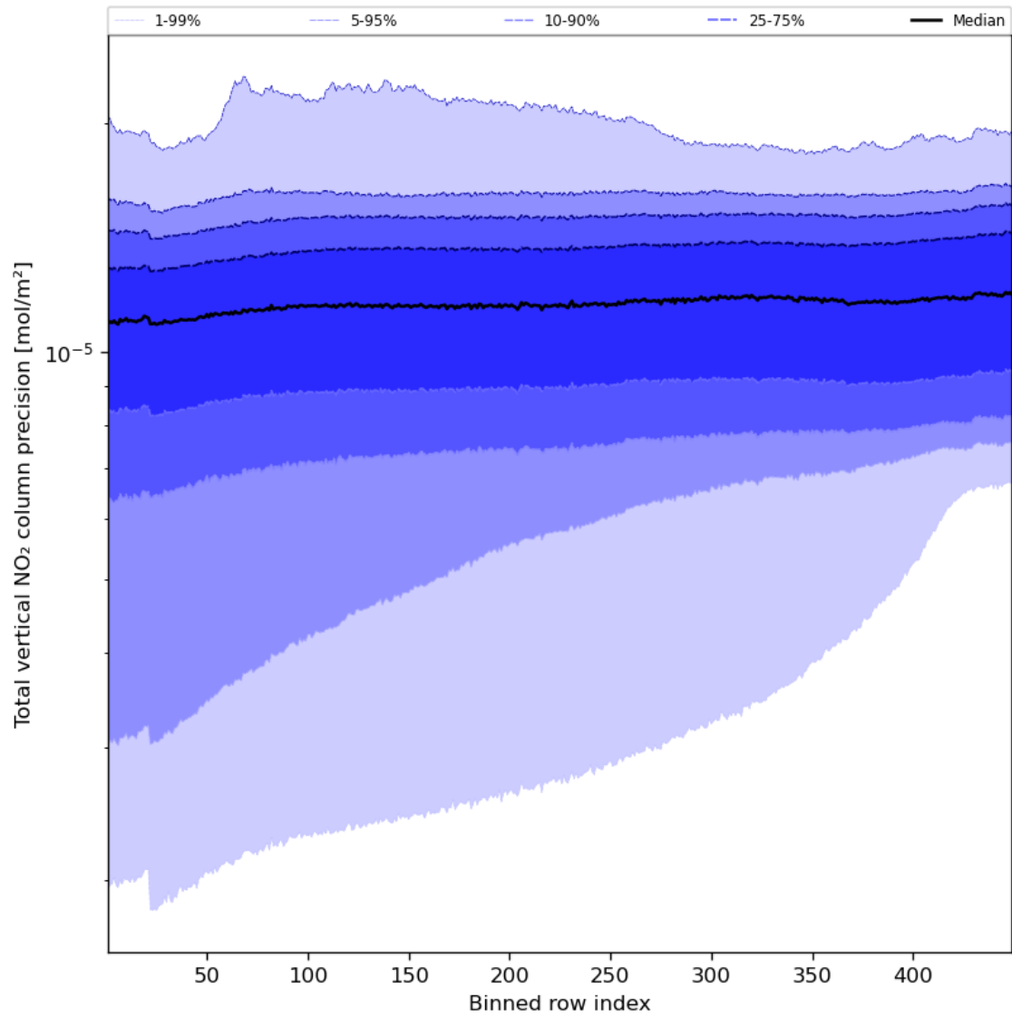
Figure 56: Along track statistics of “Total vertical NO 2 column precision” for 2023-08-26 to 2023-08-28
