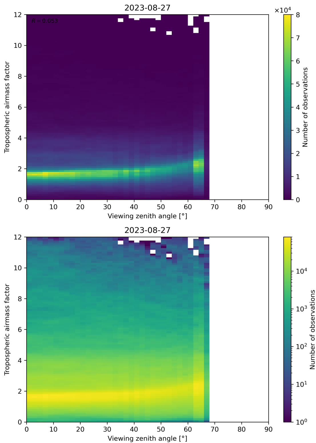
Figure 161: Scatter density plot of “Viewing zenith angle” against “Tropospheric airmass factor” for 2023-08-26 to 2023-08-28.
