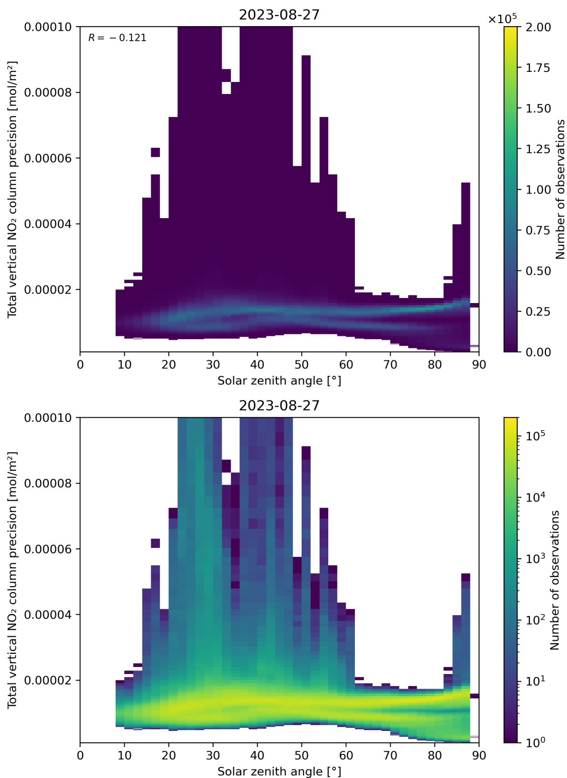
Figure 154: Scatter density plot of “Solar zenith angle” against “Total vertical NO 2 column precision” for 2023-08-26 to 2023-08-28.
