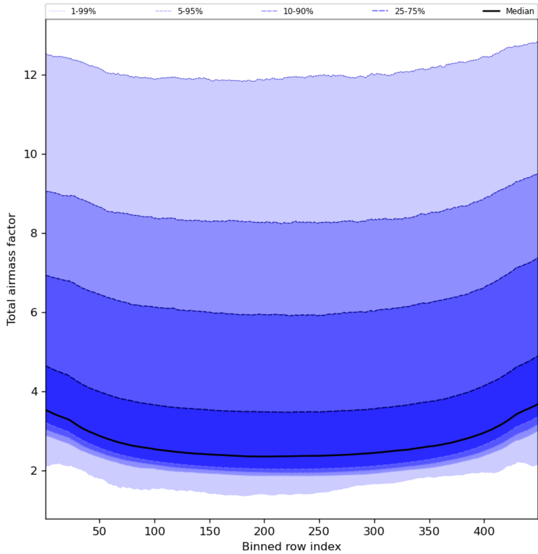
Figure 49: Along track statistics of “Total airmass factor” for 2023-08-26 to 2023-08-28
