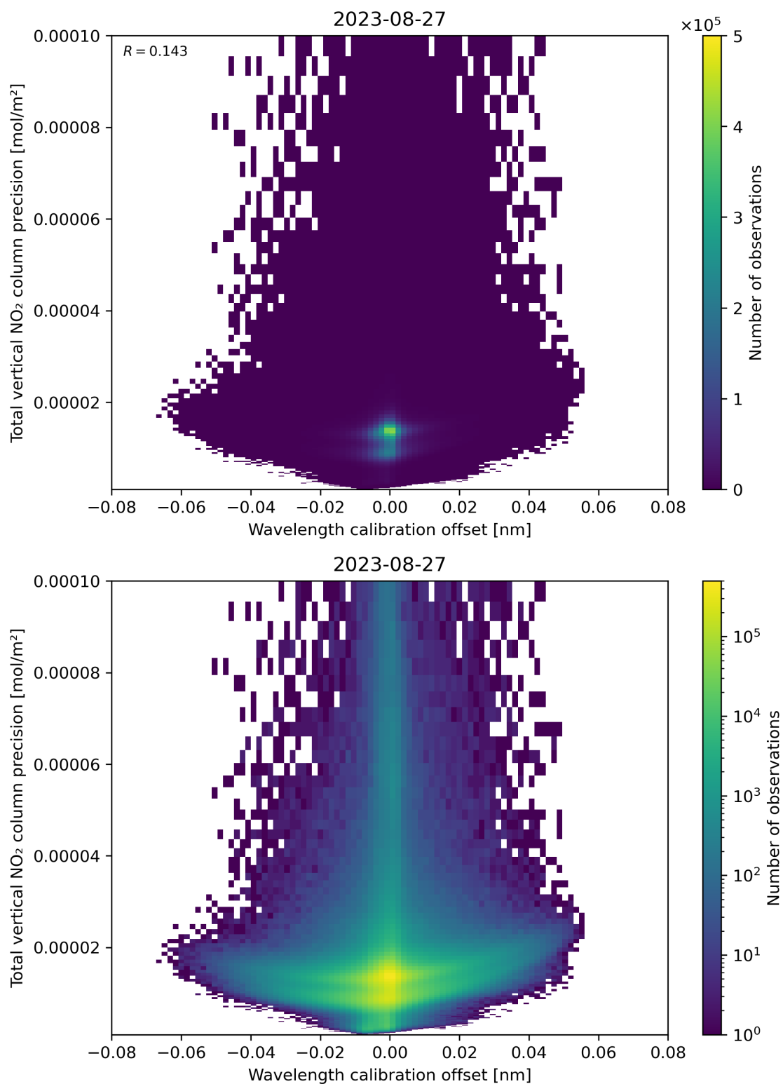
Figure 180: Scatter density plot of “Wavelength calibration offset” against “Total vertical NO 2 column precision” for 2023-08-26 to 2023-08-28.
