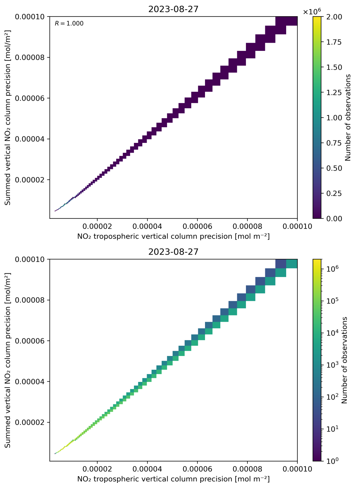
Figure 137: Scatter density plot of “NO 2 tropospheric vertical column precision” against “Summed vertical NO 2 column precision” for 2023-08-26 to 2023-08-28.
