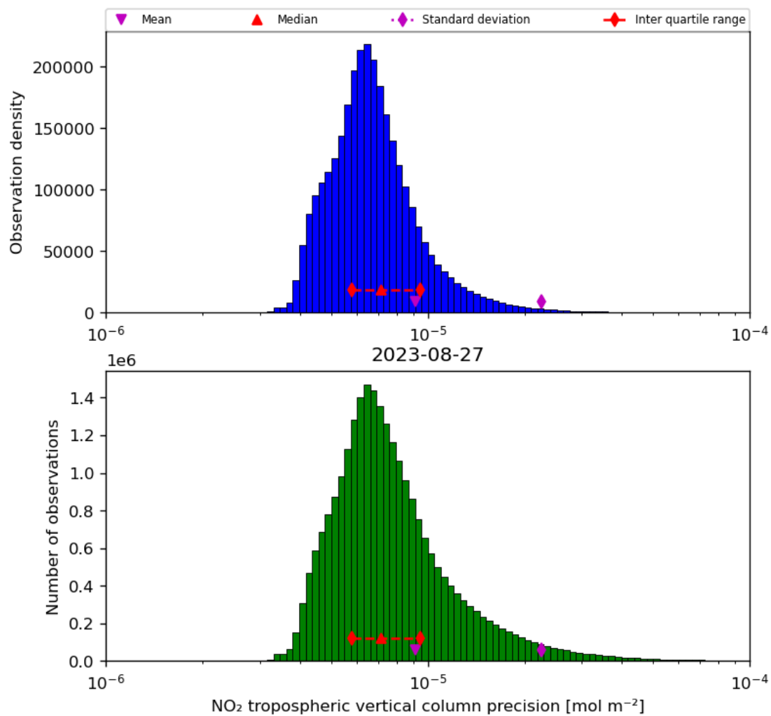
Figure 30: Histogram of “NO 2 tropospheric vertical column precision” for 2023-08-26 to 2023-08-28
