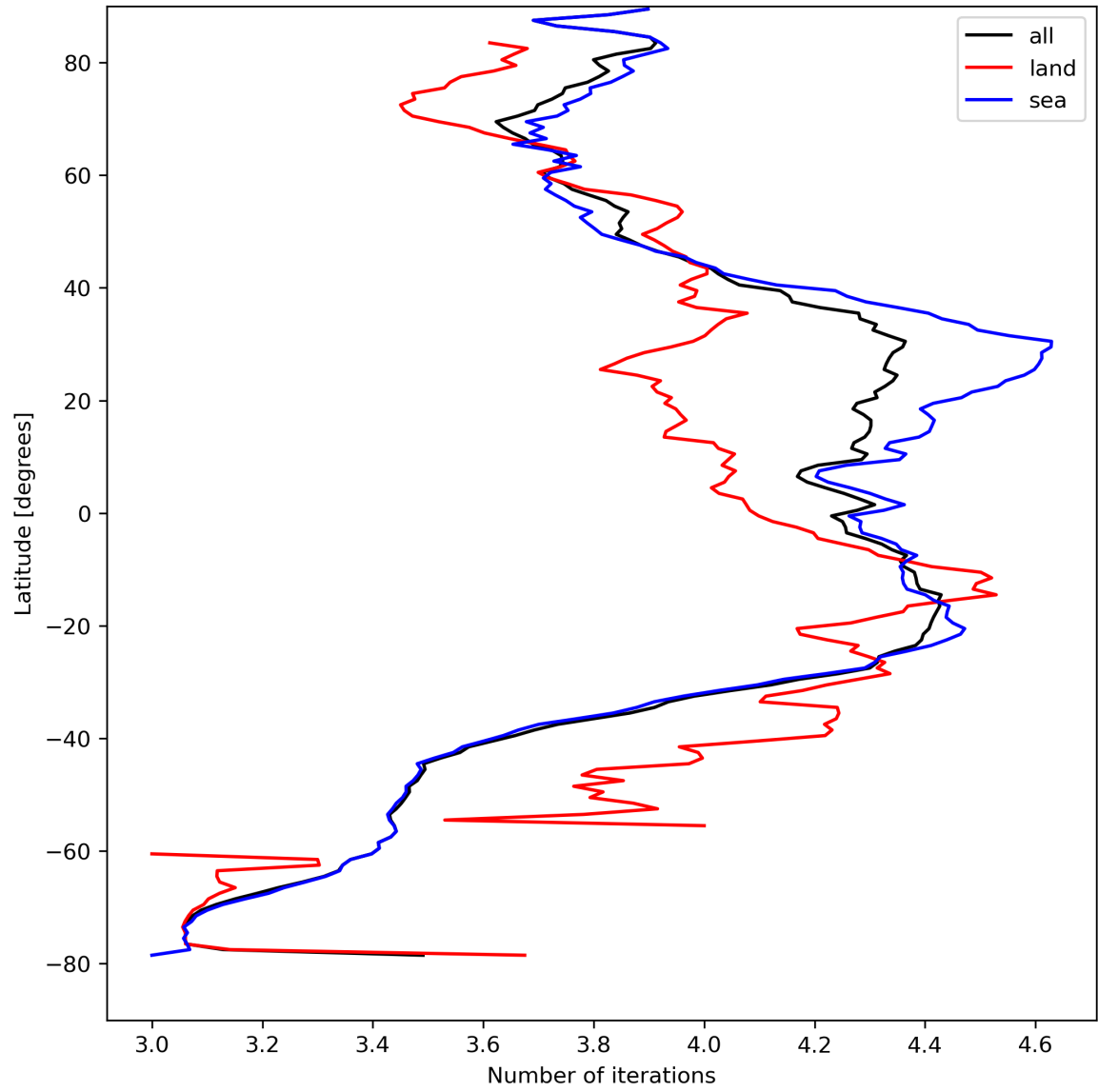
Figure 17: Zonal average of “Number of iterations” for 2023-08-26 to 2023-08-28.
