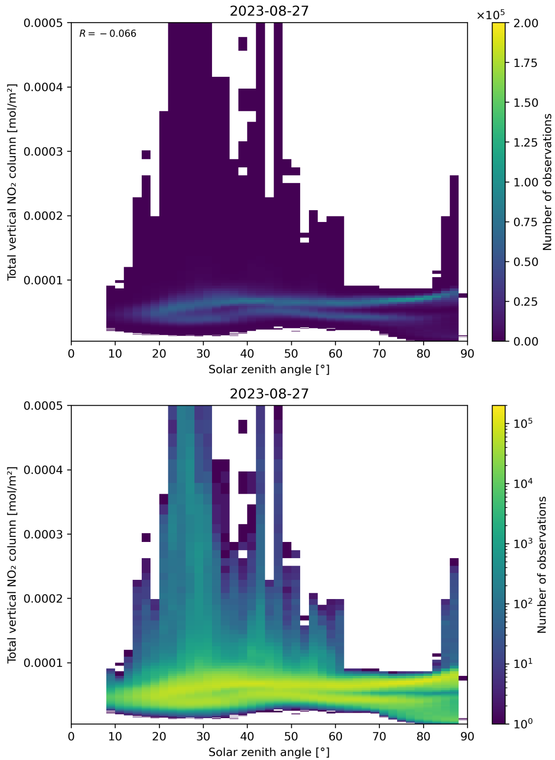
Figure 153: Scatter density plot of “Solar zenith angle” against “Total vertical NO 2 column” for 2023-08-26 to 2023-08-28.
