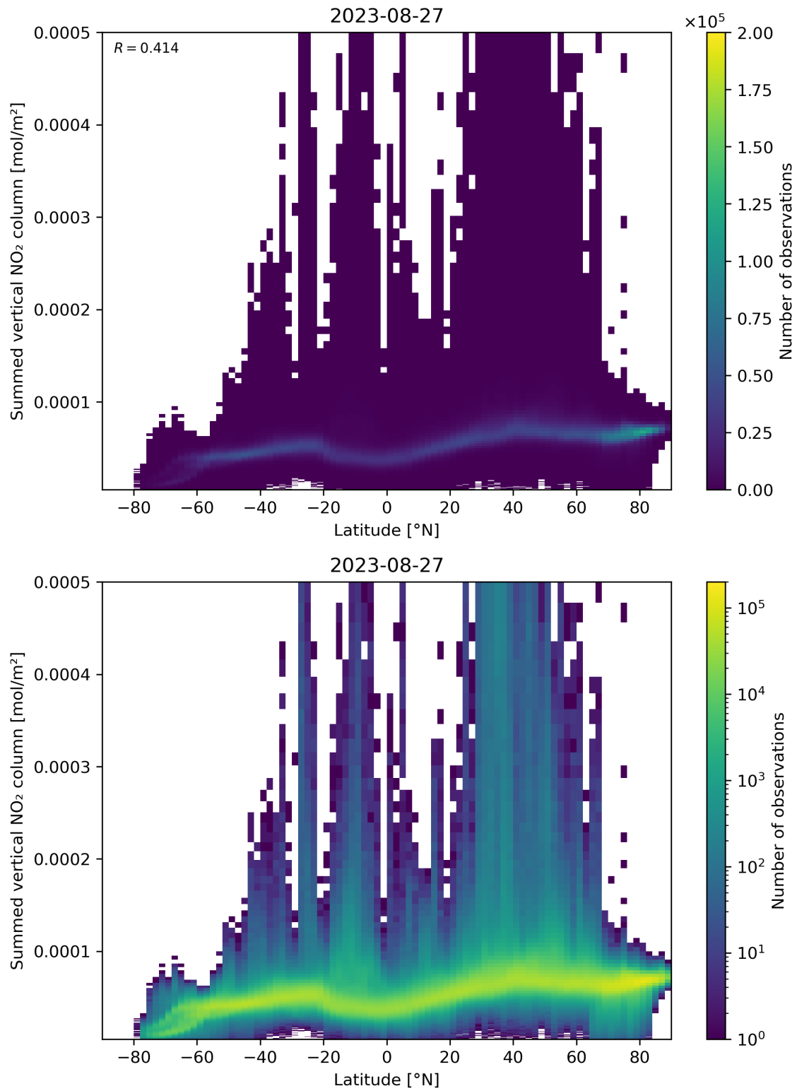
Figure 88: Scatter density plot of “Latitude” against “Summed vertical NO 2 column” for 2023-08-26 to 2023-08-28.
