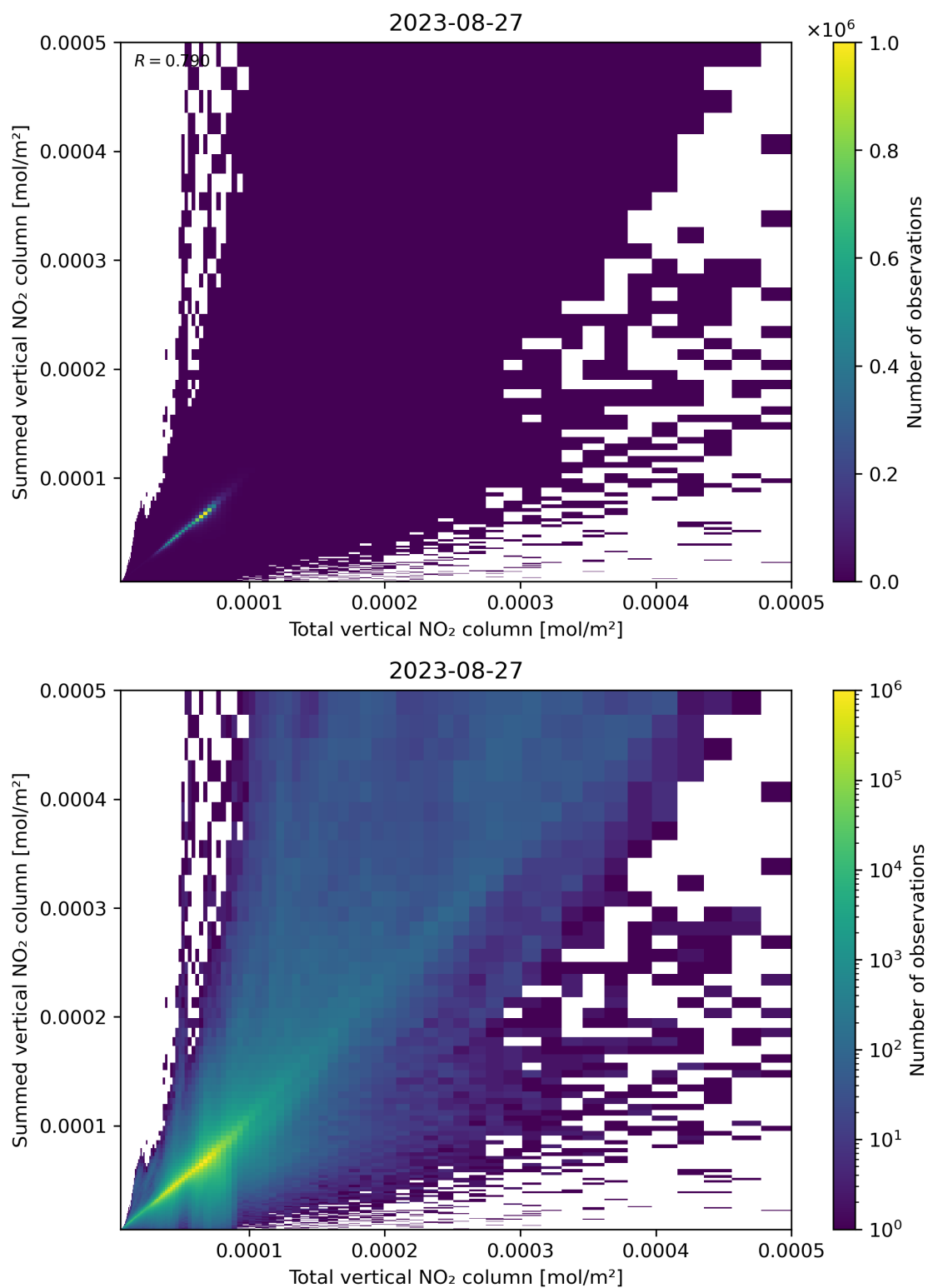
Figure 112: Scatter density plot of “Total vertical NO 2 column” against “Summed vertical NO 2 column” for 2023-08-26 to 2023-08-28.
