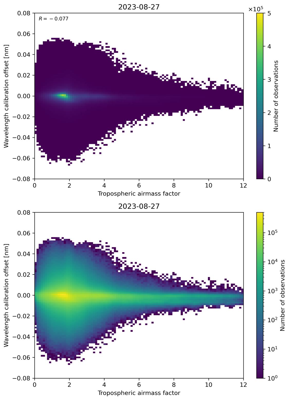
Figure 80: Scatter density plot of “Tropospheric air mass factor” against “Wavelength calibration offset” for 2023-08-26 to 2023-08-28.
