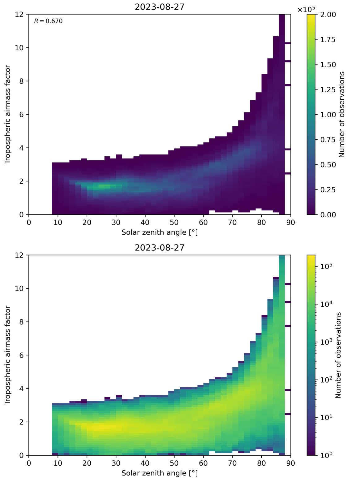
Figure 147: Scatter density plot of “Solar zenith angle” against “Tropospheric airmass factor” for 2023-08-26 to 2023-08-28.
