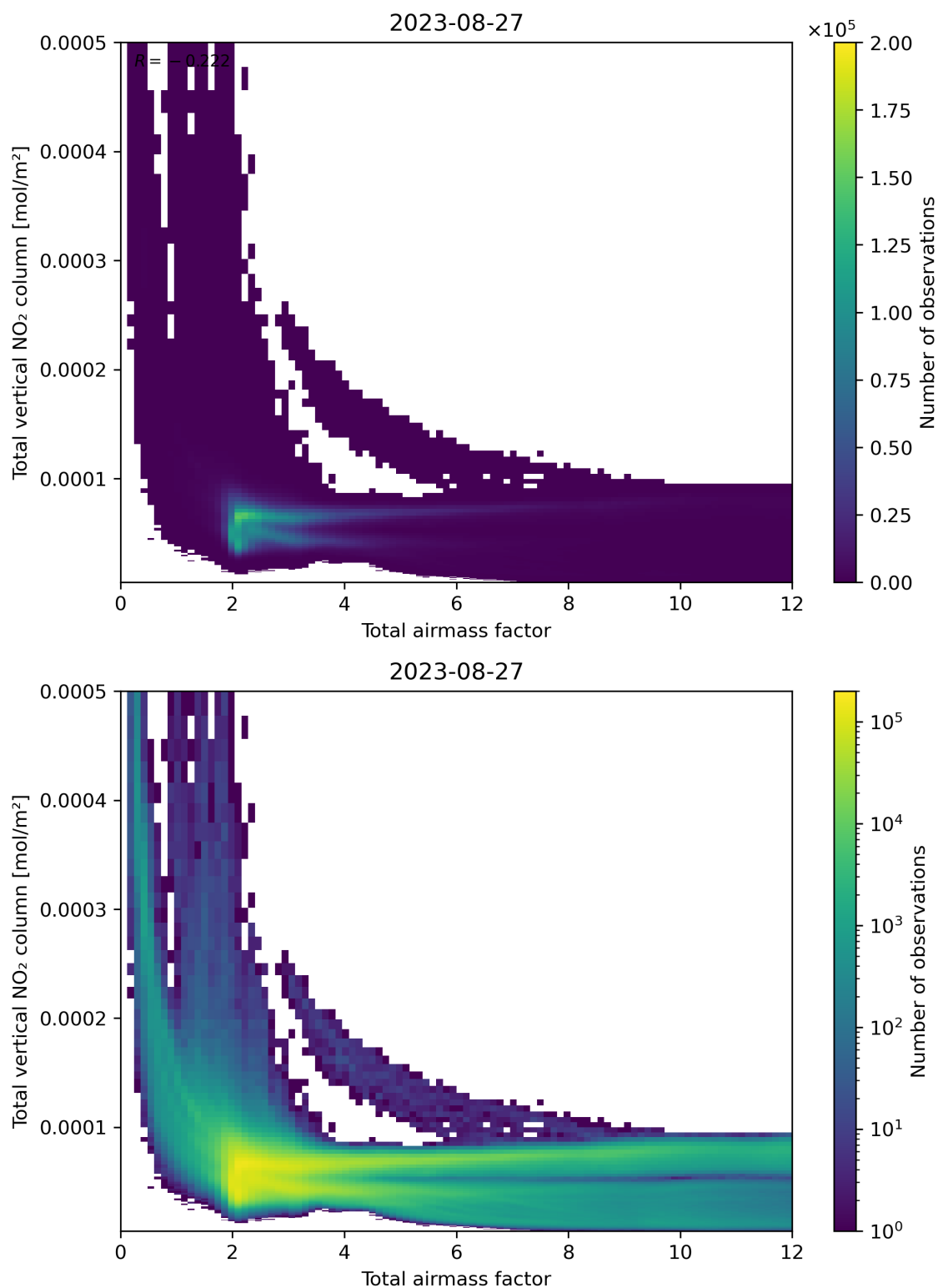
Figure 67: Scatter density plot of “Total airmass factor” against “Total vertical NO 2 column” for 2023-08-26 to 2023-08-28.
