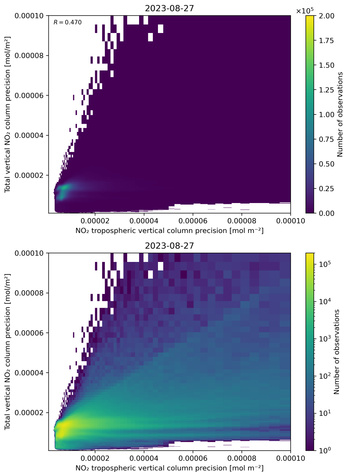
Figure 139: Scatter density plot of “NO 2 tropospheric vertical column precision” against “Total vertical NO 2 column precision” for 2023-08-26 to 2023-08-28.
