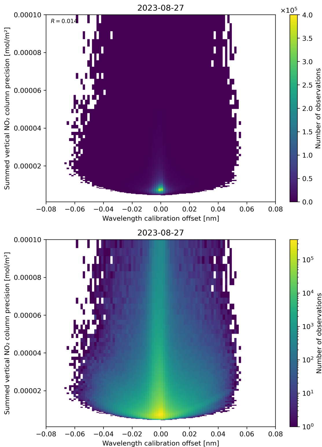
Figure 178: Scatter density plot of “Wavelength calibration offset” against “Summed vertical NO 2 column precision” for 2023-08-26 to 2023-08-28.
