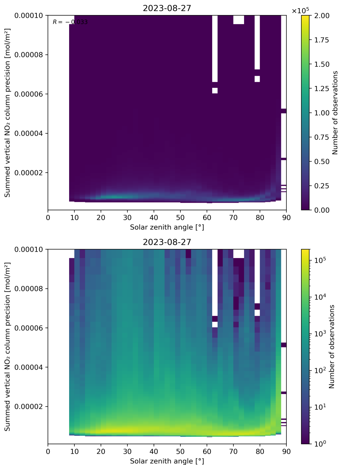
Figure 152: Scatter density plot of “Solar zenith angle” against “Summed vertical NO 2 column precision” for 2023-08-26 to 2023-08-28.
