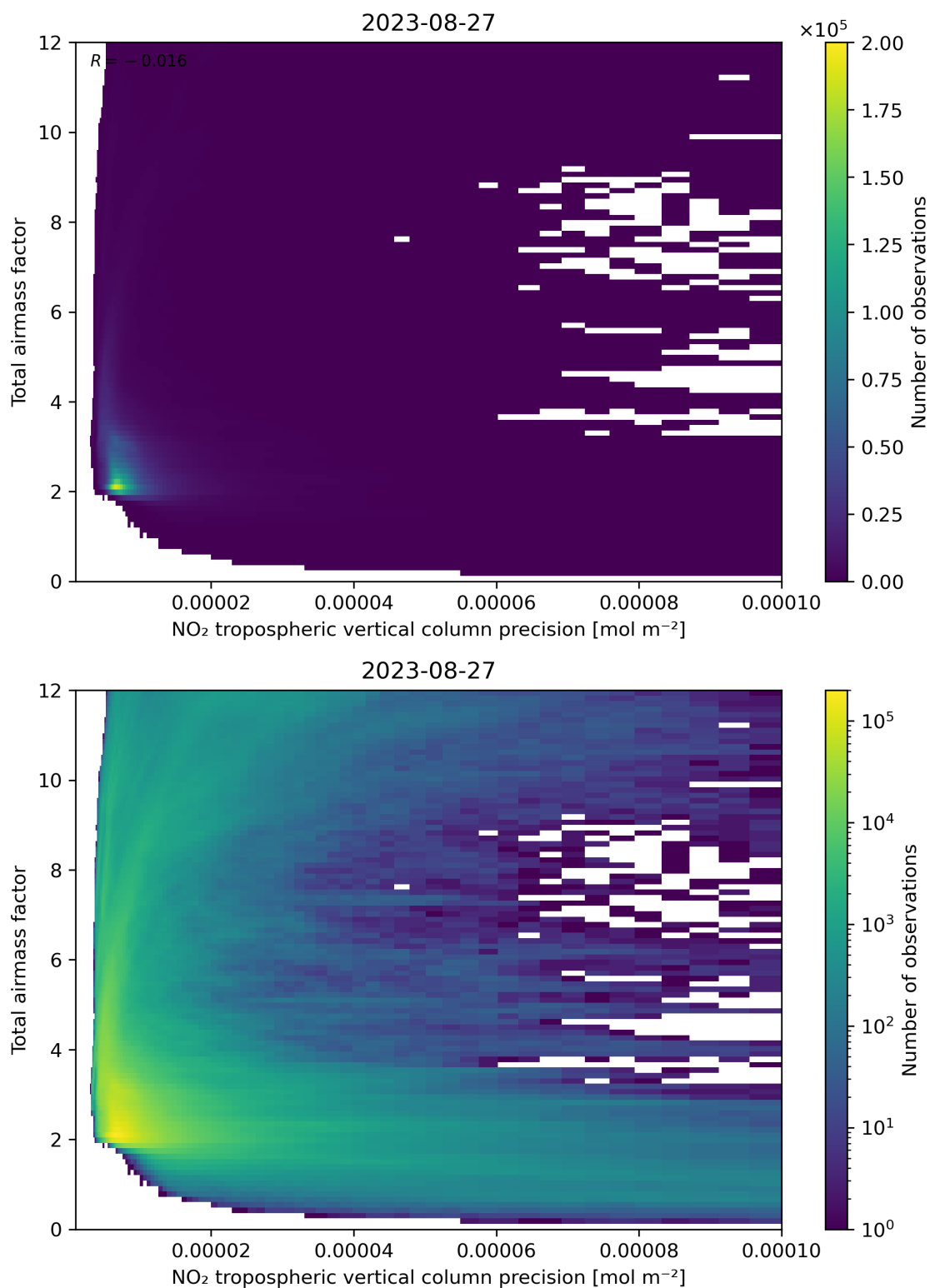
Figure 132: Scatter density plot of “NO 2 tropospheric vertical column precision” against “Total air mass factor” for 2023-08-26 to 2023-08-28.
