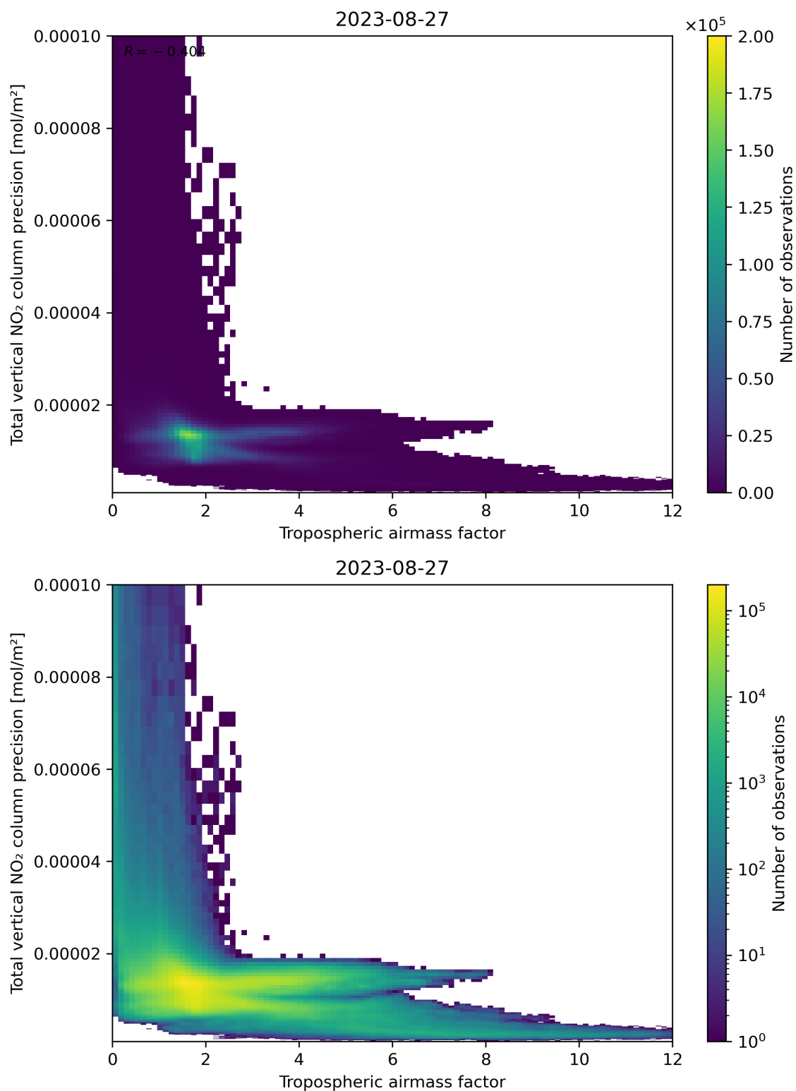
Figure 78: Scatter density plot of “Tropospheric air mass factor” against “Total vertical NO 2 column precision” for 2023-08-26 to 2023-08-28.
