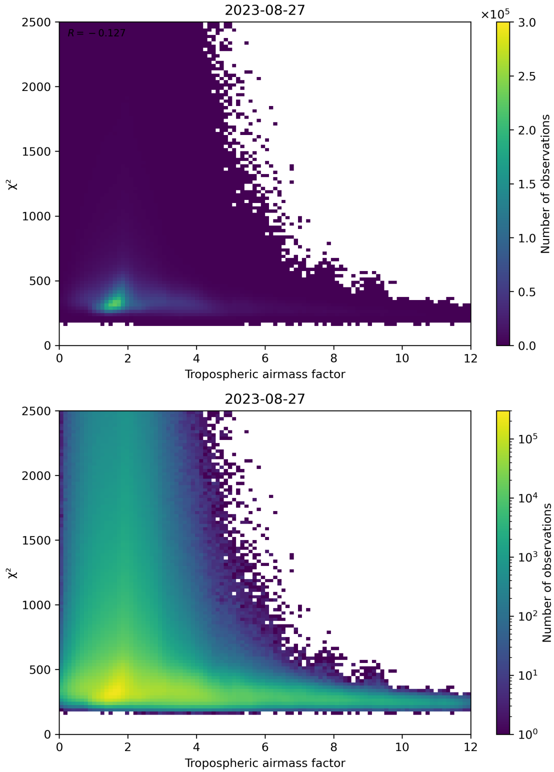
Figure 73: Scatter density plot of “Tropospheric airmass factor” against “ \chi^2 ” for 2023-08-26 to 2023-08-28.
