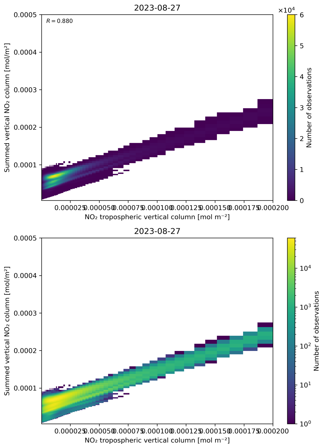
Figure 126: Scatter density plot of “NO 2 tropospheric vertical column” against “Summed vertical NO 2 column” for 2023-08-26 to 2023-08-28.
