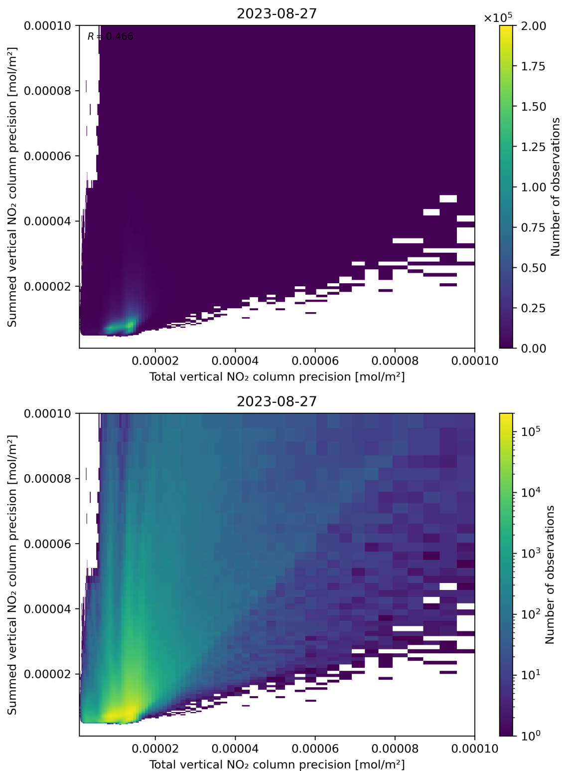
Figure 118: Scatter density plot of “Total vertical NO 2 column precision” against “Summed vertical NO 2 column precision” for 2023-08-26 to 2023-08-28.
