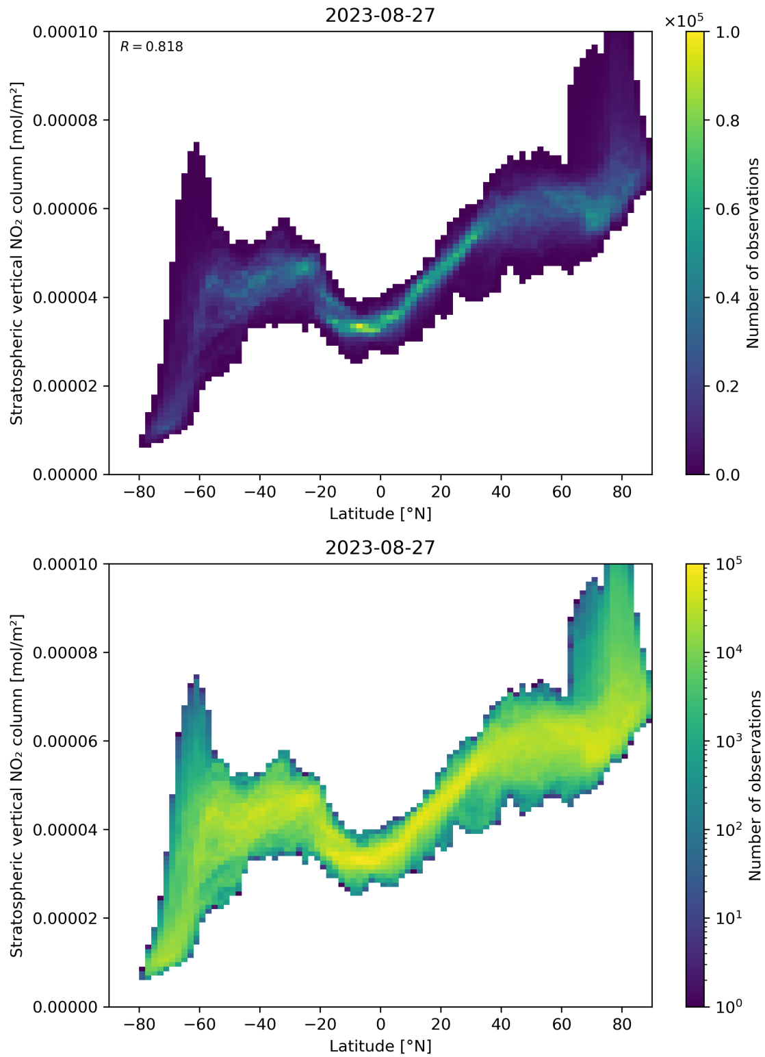
Figure 87: Scatter density plot of “Latitude” against “Stratospheric vertical \text{NO}_2 column” for 2023-08-26 to 2023-08-28.
