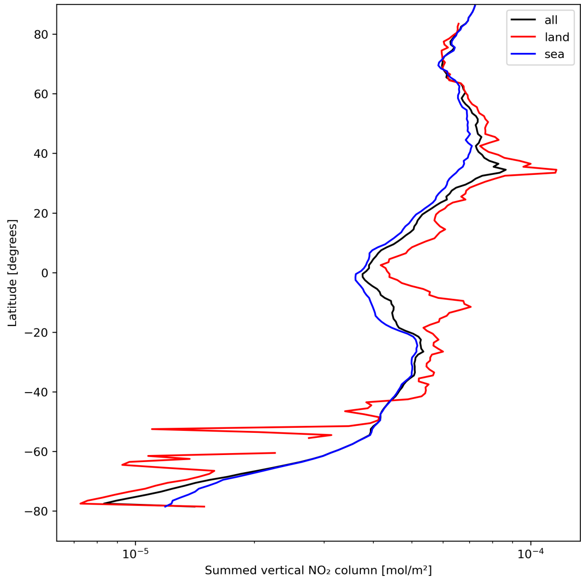
Figure 23: Zonal average of “Summed vertical NO 2 column” for 2023-08-26 to 2023-08-28.
