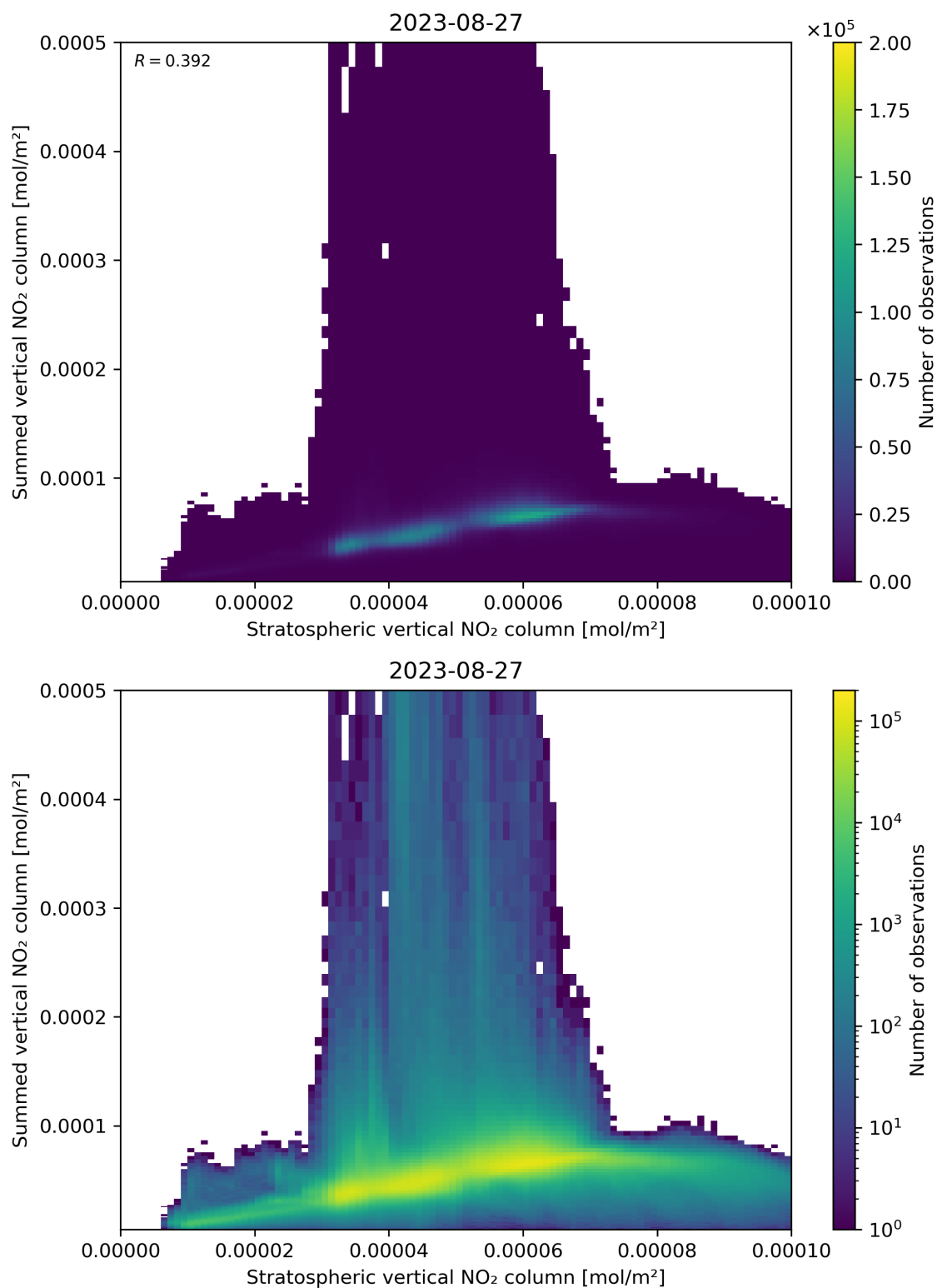
Figure 98: Scatter density plot of “Stratospheric vertical NO 2 column” against “Summed vertical NO 2 column” for 2023-08-26 to 2023-08-28.
