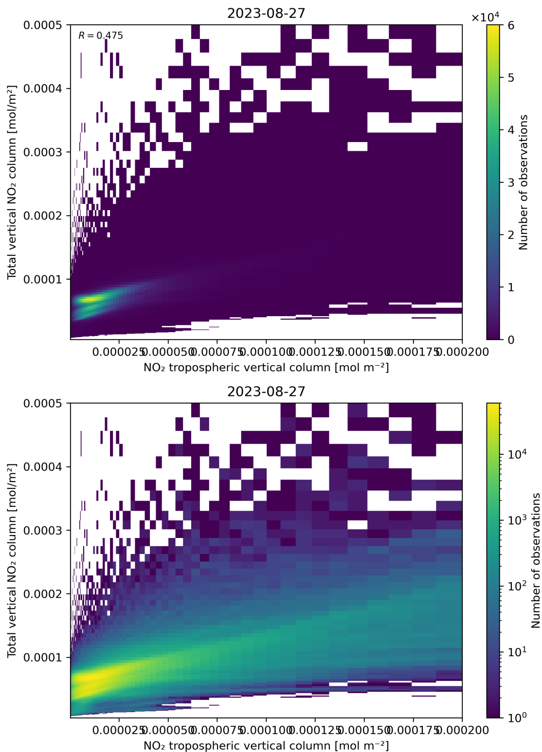
Figure 128: Scatter density plot of “NO 2 tropospheric vertical column” against “Total vertical NO 2 column” for 2023-08-26 to 2023-08-28.
