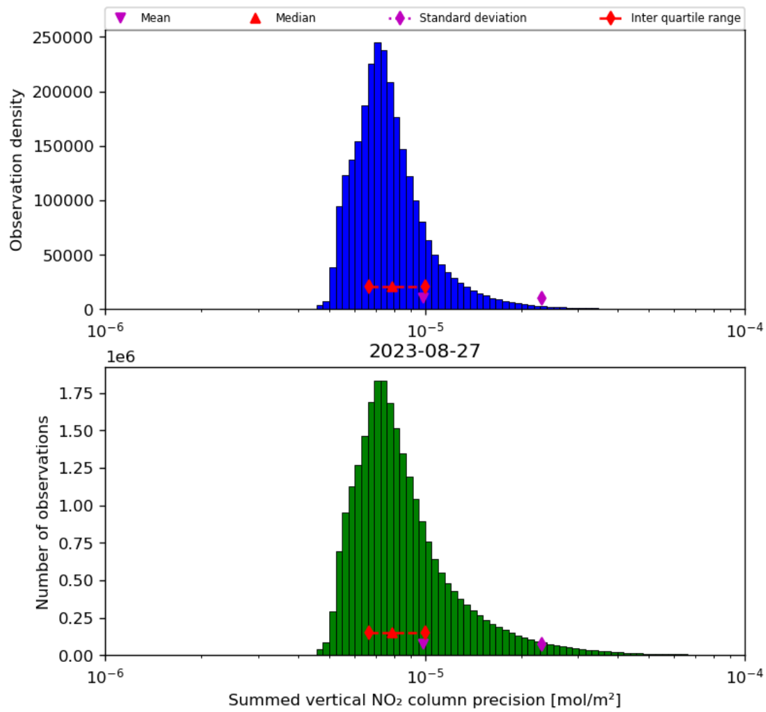
Figure 41: Histogram of “Summed vertical NO 2 column precision” for 2023-08-26 to 2023-08-28
