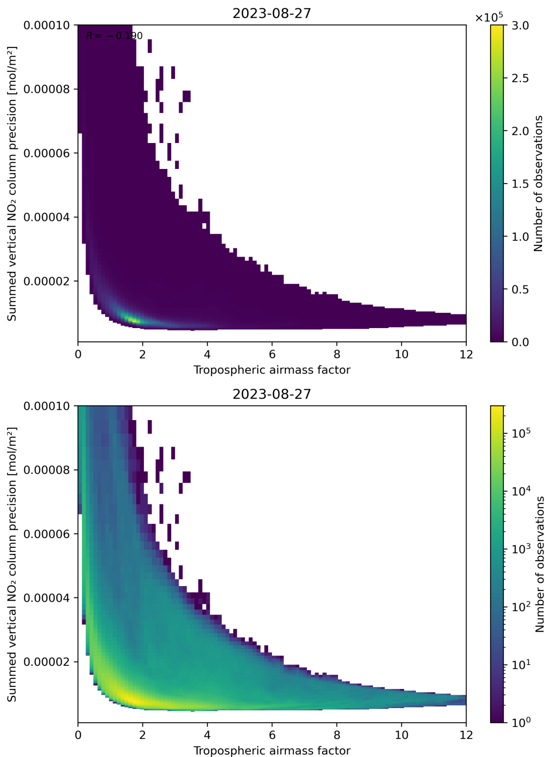
Figure 76: Scatter density plot of “Tropospheric air mass factor” against “Summed vertical NO 2 column precision” for 2023-08-26 to 2023-08-28.
