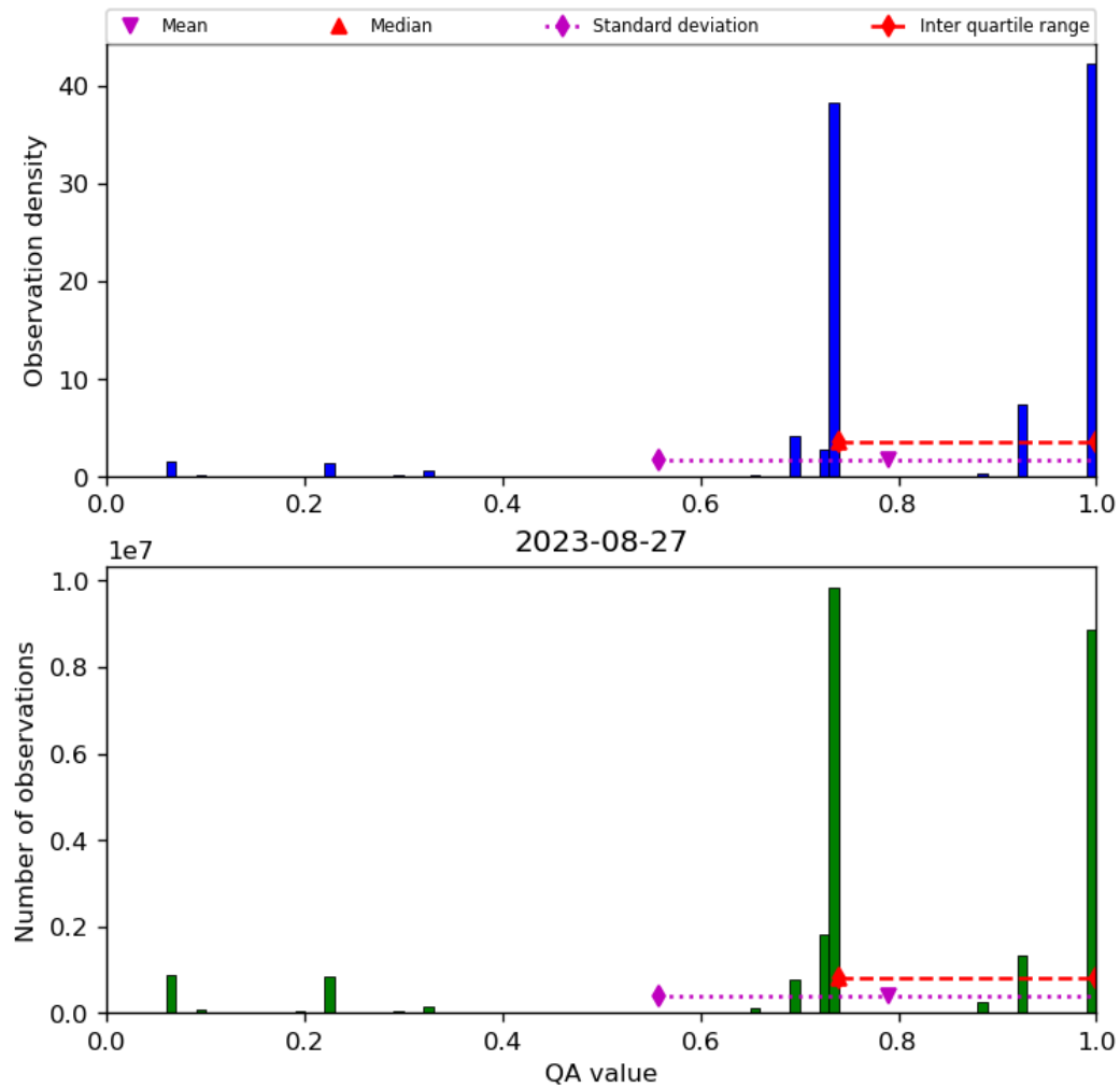
Figure 28: Histogram of “QA value” for 2023-08-26 to 2023-08-28
