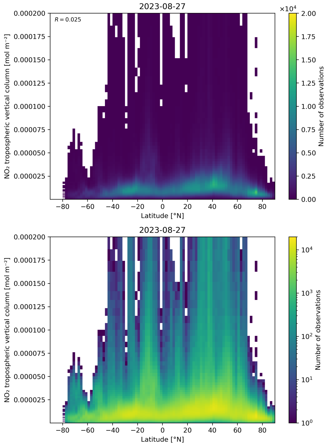
Figure 92: Scatter density plot of “Latitude” against “NO 2 tropospheric vertical column” for 2023-08-26 to 2023-08-28.
