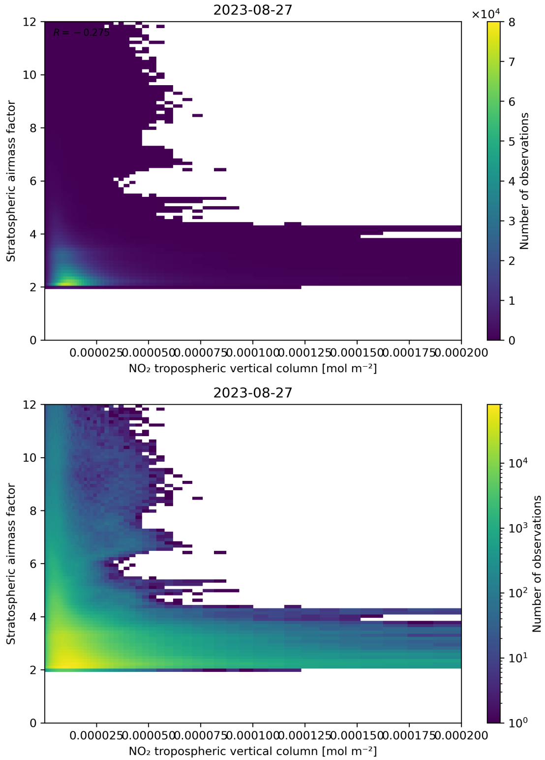
Figure 121: Scatter density plot of “NO 2 tropospheric vertical column” against “Stratospheric airmass factor” for 2023-08-26 to 2023-08-28.
