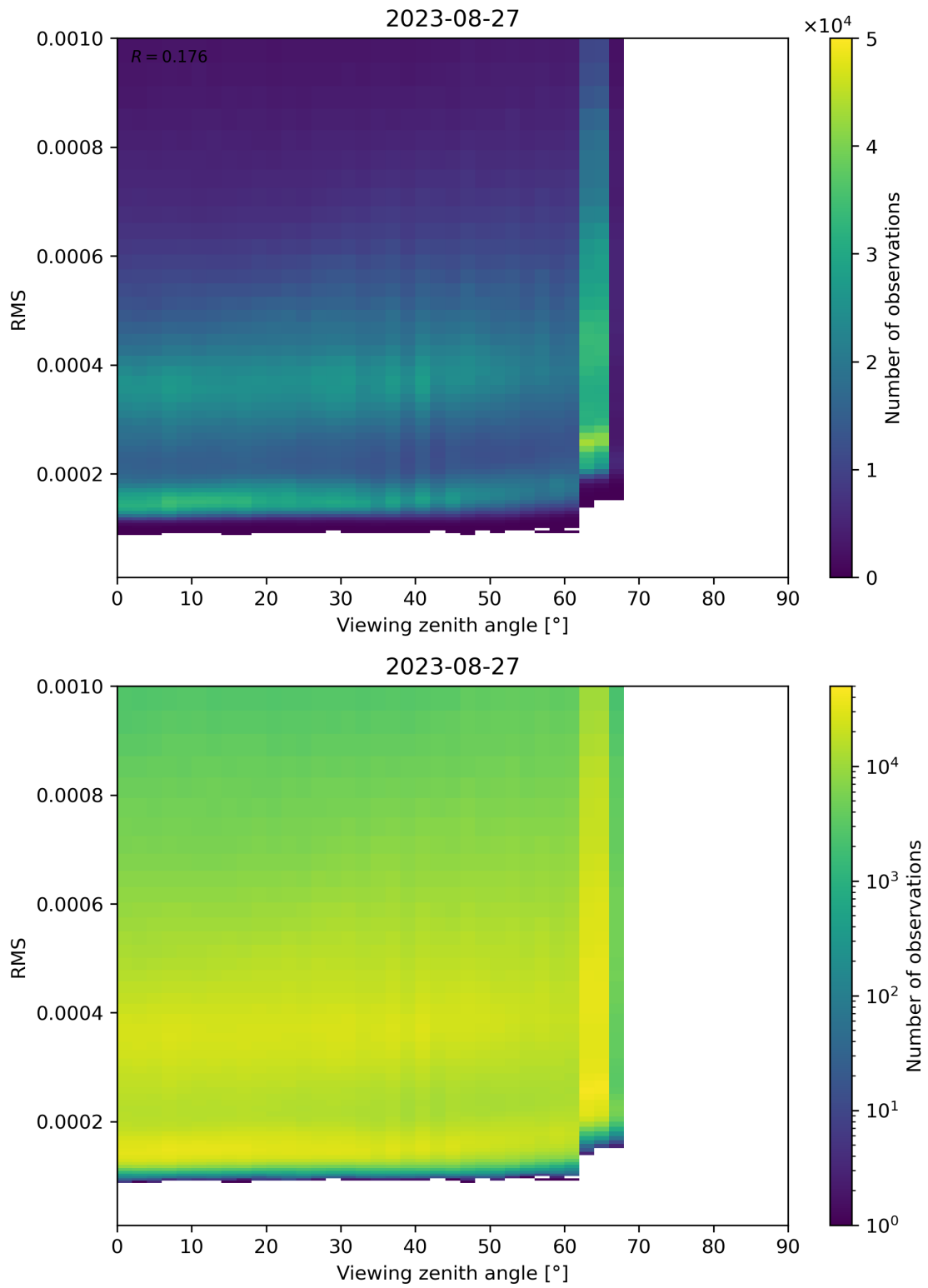
Figure 171: Scatter density plot of “Viewing zenith angle” against “RMS” for 2023-08-26 to 2023-08-28.
