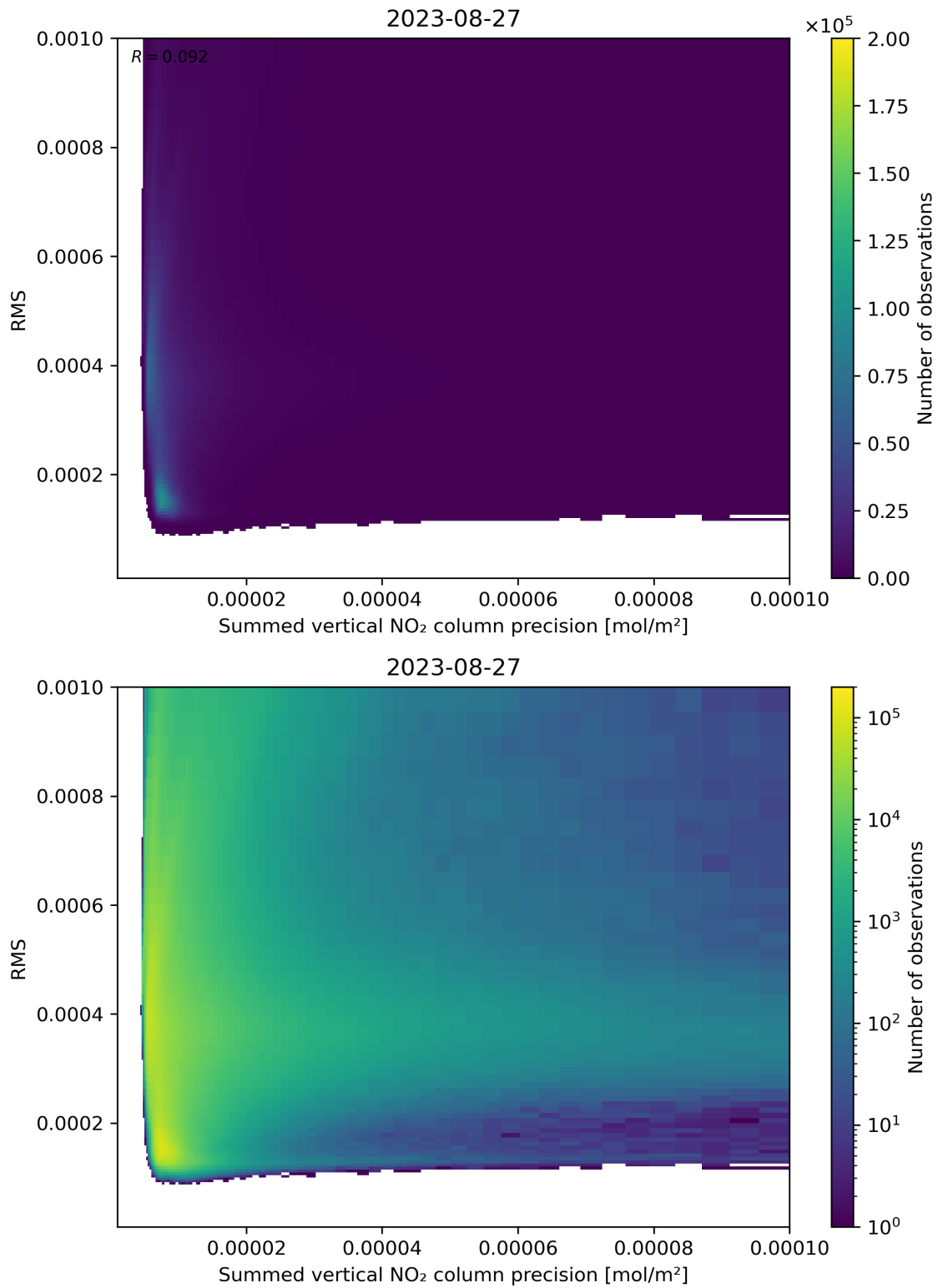
Figure 108: Scatter density plot of “Summed vertical NO 2 column precision” against “RMS” for 2023-08-26 to 2023-08-28.
