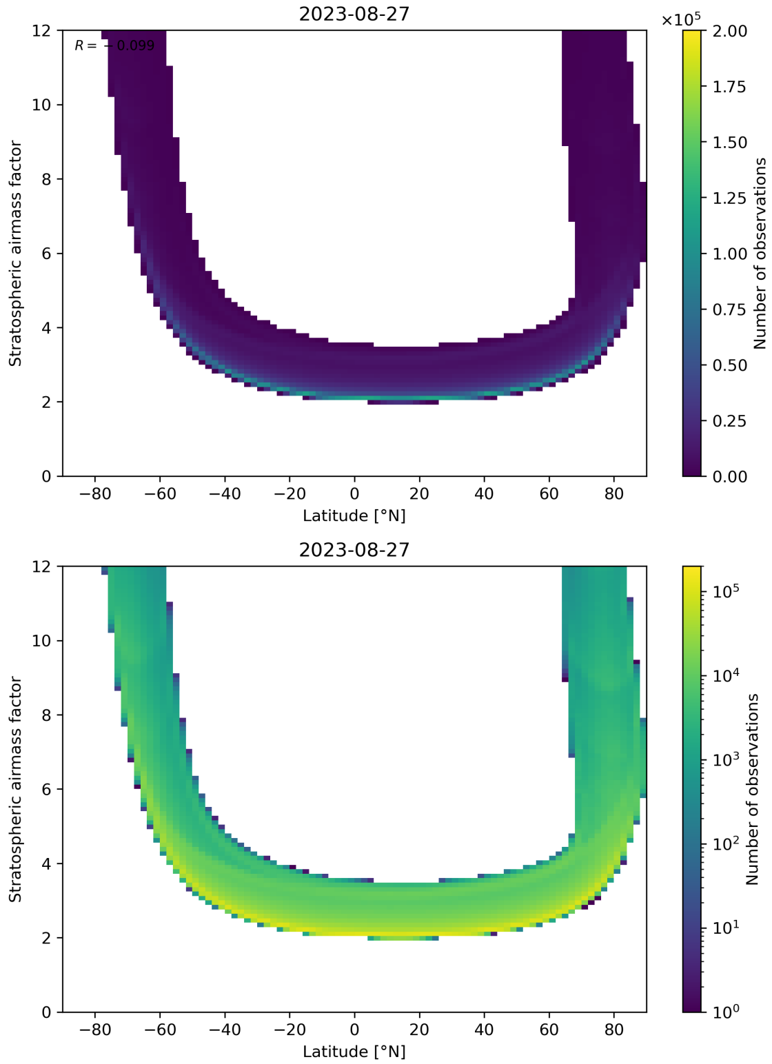
Figure 83: Scatter density plot of “Latitude” against “Stratospheric air mass factor” for 2023-08-26 to 2023-08-28.
