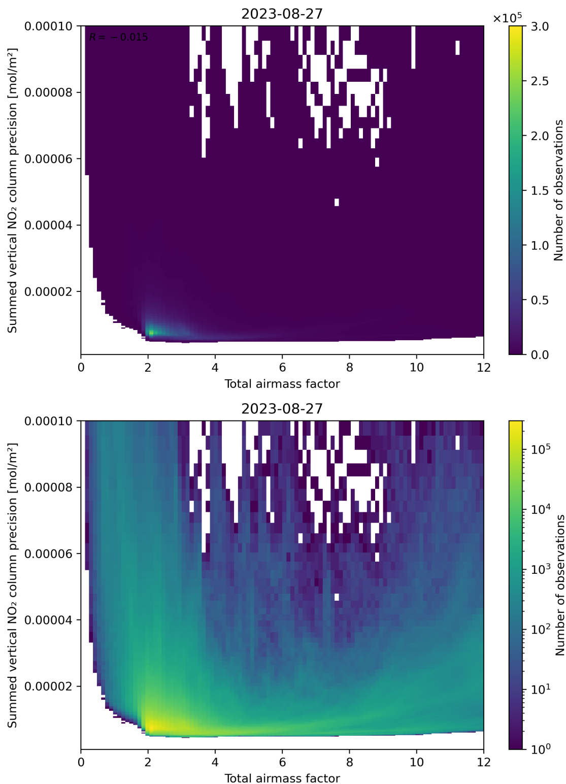
Figure 66: Scatter density plot of “Total airmass factor” against “Summed vertical NO 2 column precision” for 2023-08-26 to 2023-08-28.
