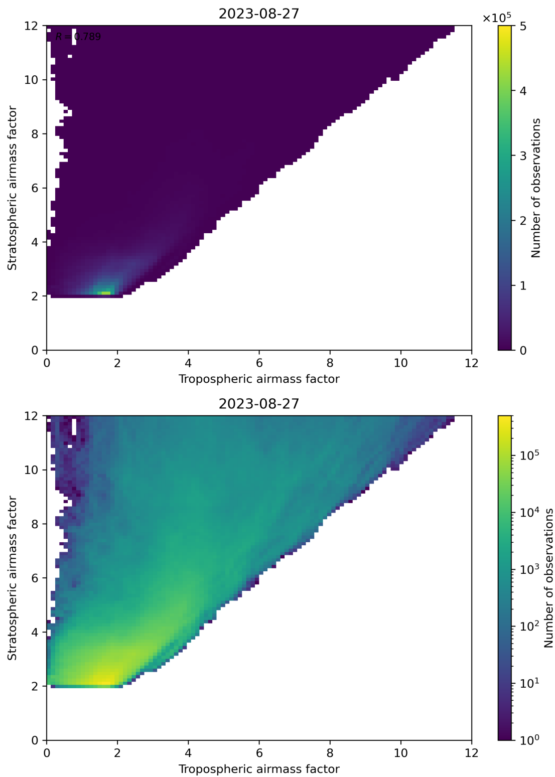
Figure 71: Scatter density plot of “Tropospheric airmass factor” against “Stratospheric airmass factor” for 2023-08-26 to 2023-08-28.
