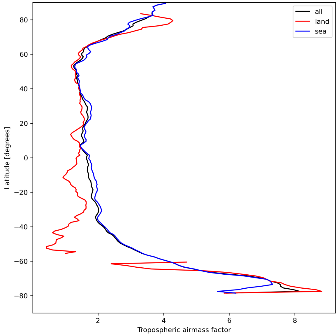
Figure 14: Zonal average of “Tropospheric airmass factor” for 2023-08-26 to 2023-08-28.
