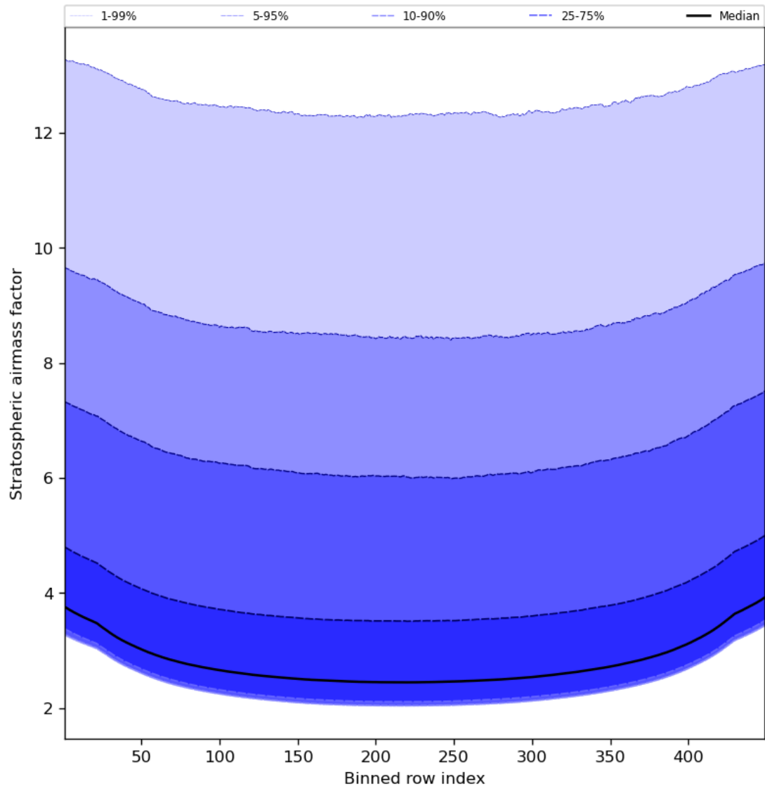
Figure 61: Along track statistics of “Stratospheric airmass factor” for 2023-08-26 to 2023-08-28
