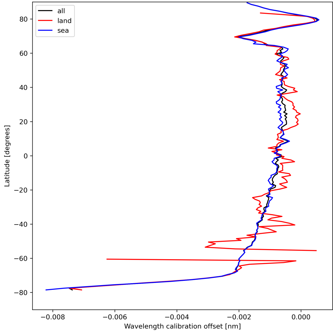
Figure 18: Zonal average of “Wavelength calibration offset” for 2023-08-26 to 2023-08-28.
