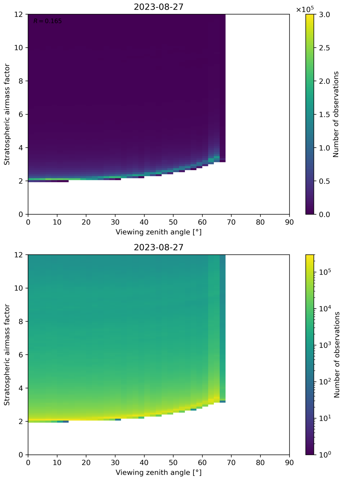
Figure 159: Scatter density plot of “Viewing zenith angle” against “Stratospheric airmass factor” for 2023-08-26 to 2023-08-28.
