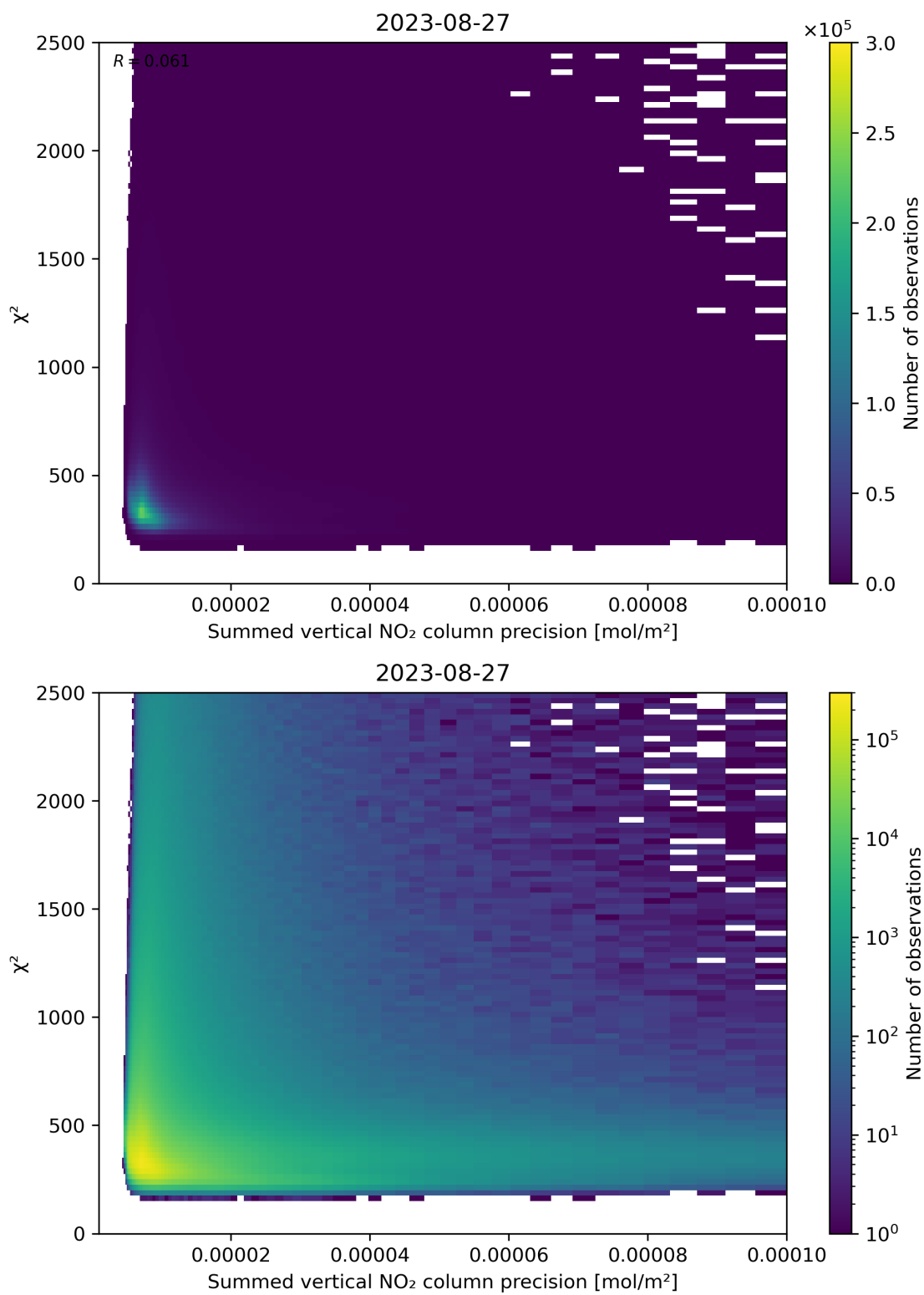
Figure 107: Scatter density plot of “Summed vertical NO 2 column precision” against “ \chi^2 ” for 2023-08-26 to 2023-08-28.
