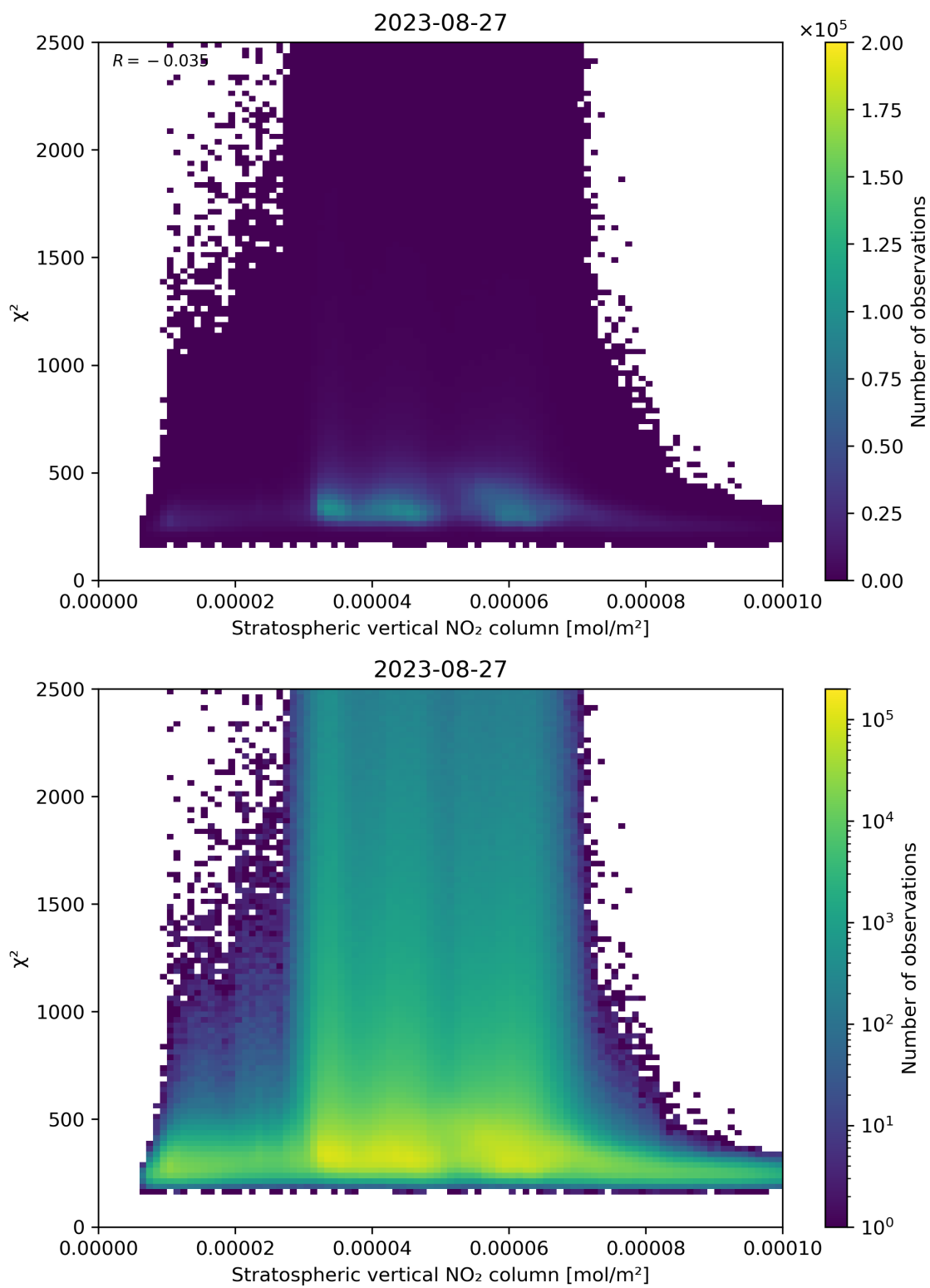
Figure 97: Scatter density plot of “Stratospheric vertical NO 2 column” against “ \chi^2 ” for 2023-08-26 to 2023-08-28.
