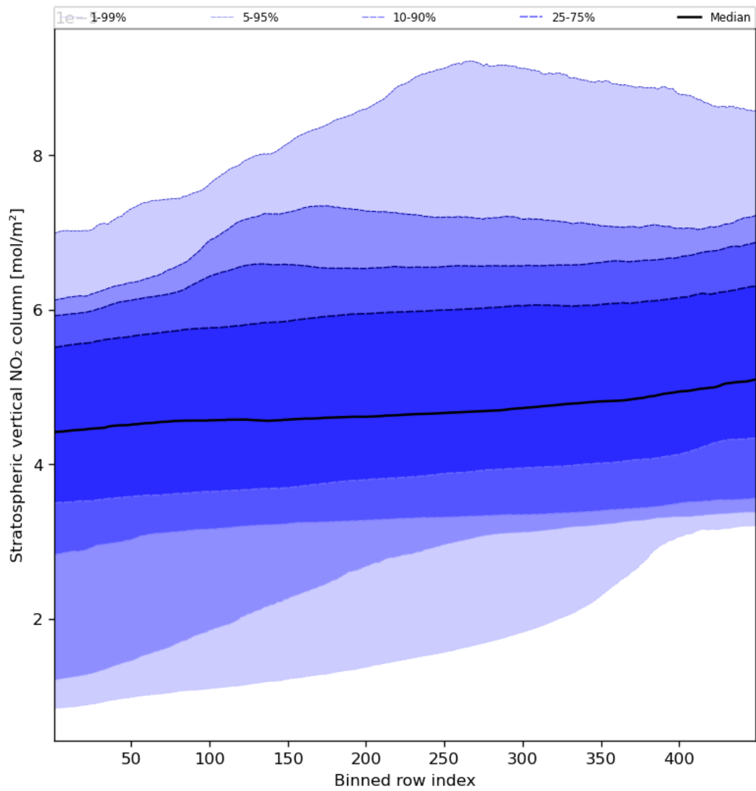
Figure 53: Along track statistics of “Stratospheric vertical NO 2 column” for 2023-08-26 to 2023-08-28
