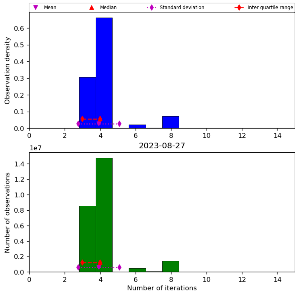
Figure 34: Histogram of “Number of iterations” for 2023-08-26 to 2023-08-28
