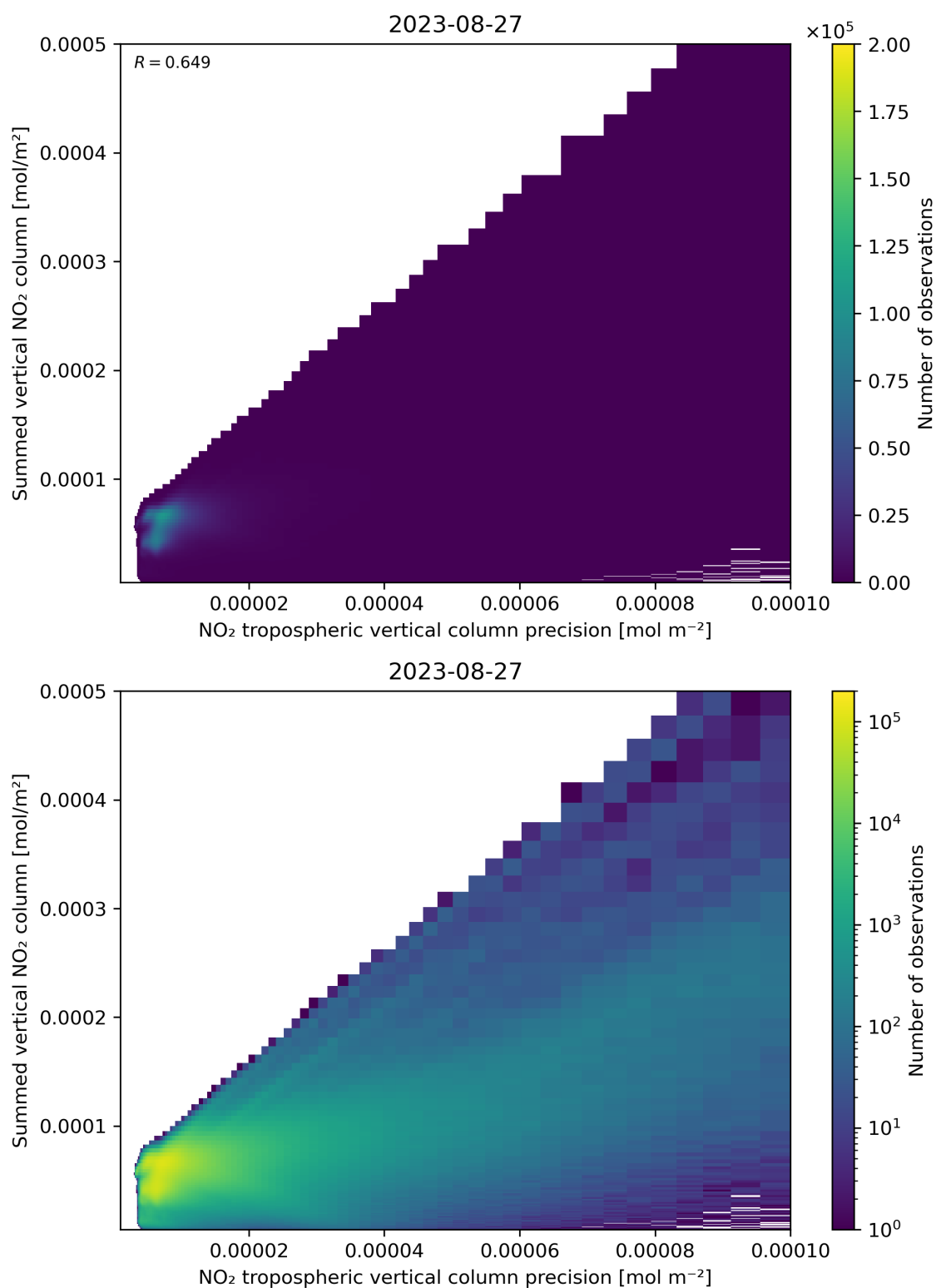
Figure 136: Scatter density plot of “NO 2 tropospheric vertical column precision” against “Summed vertical NO 2 column” for 2023-08-26 to 2023-08-28.
