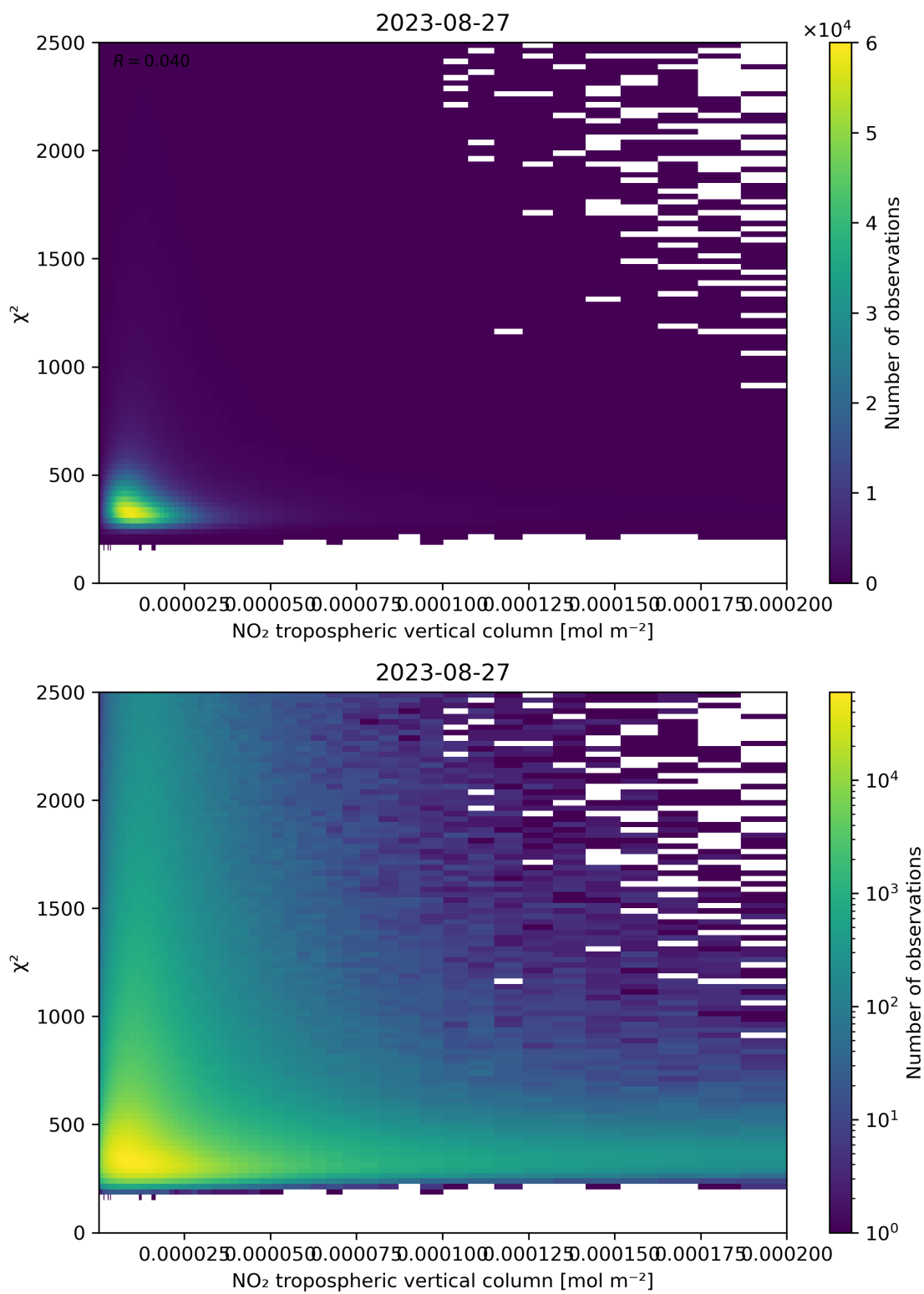
Figure 124: Scatter density plot of “NO 2 tropospheric vertical column” against “ \chi^2 ” for 2023-08-26 to 2023-08-28.
