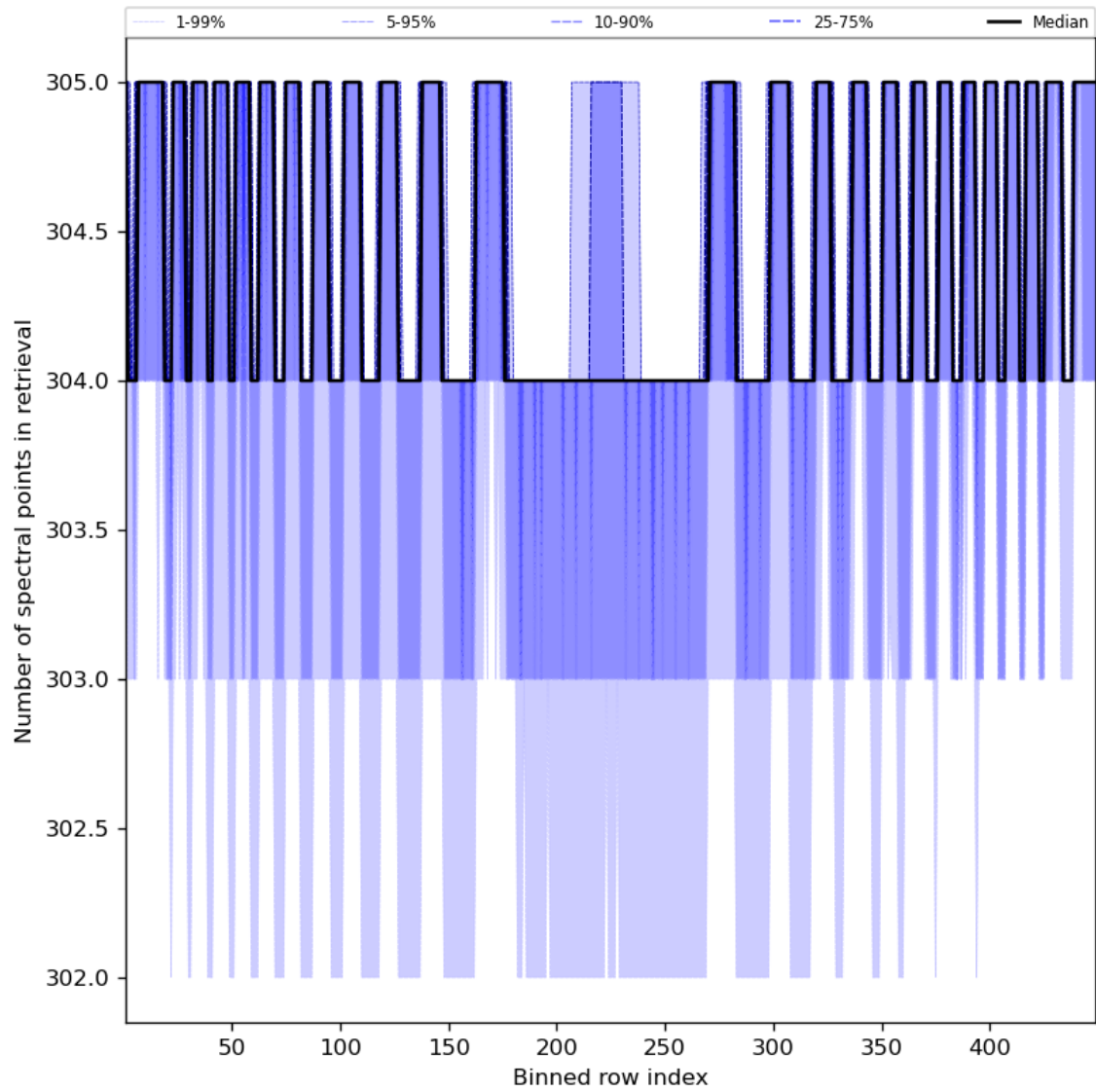
Figure 50: Along track statistics of “Number of spectral points in retrieval” for 2023-08-26 to 2023-08-28
