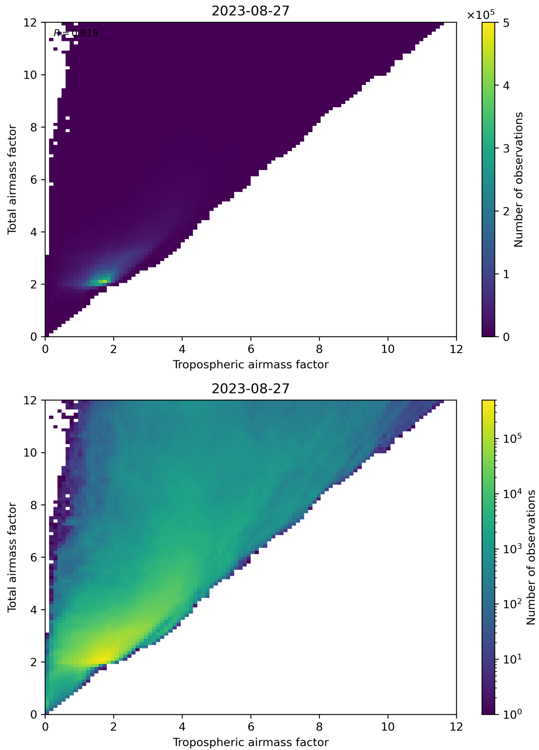
Figure 72: Scatter density plot of “Tropospheric airmass factor” against “Total airmass factor” for 2023-08-26 to 2023-08-28.
