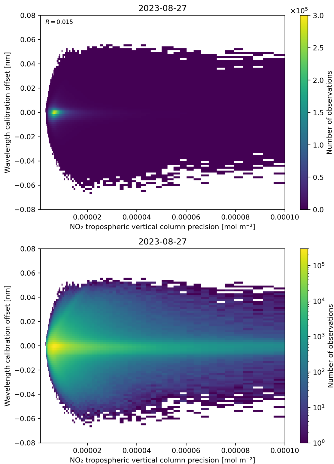
Figure 141: Scatter density plot of “NO 2 tropospheric vertical column precision” against “Wavelength calibration offset” for 2023-08-26 to 2023-08-28.
