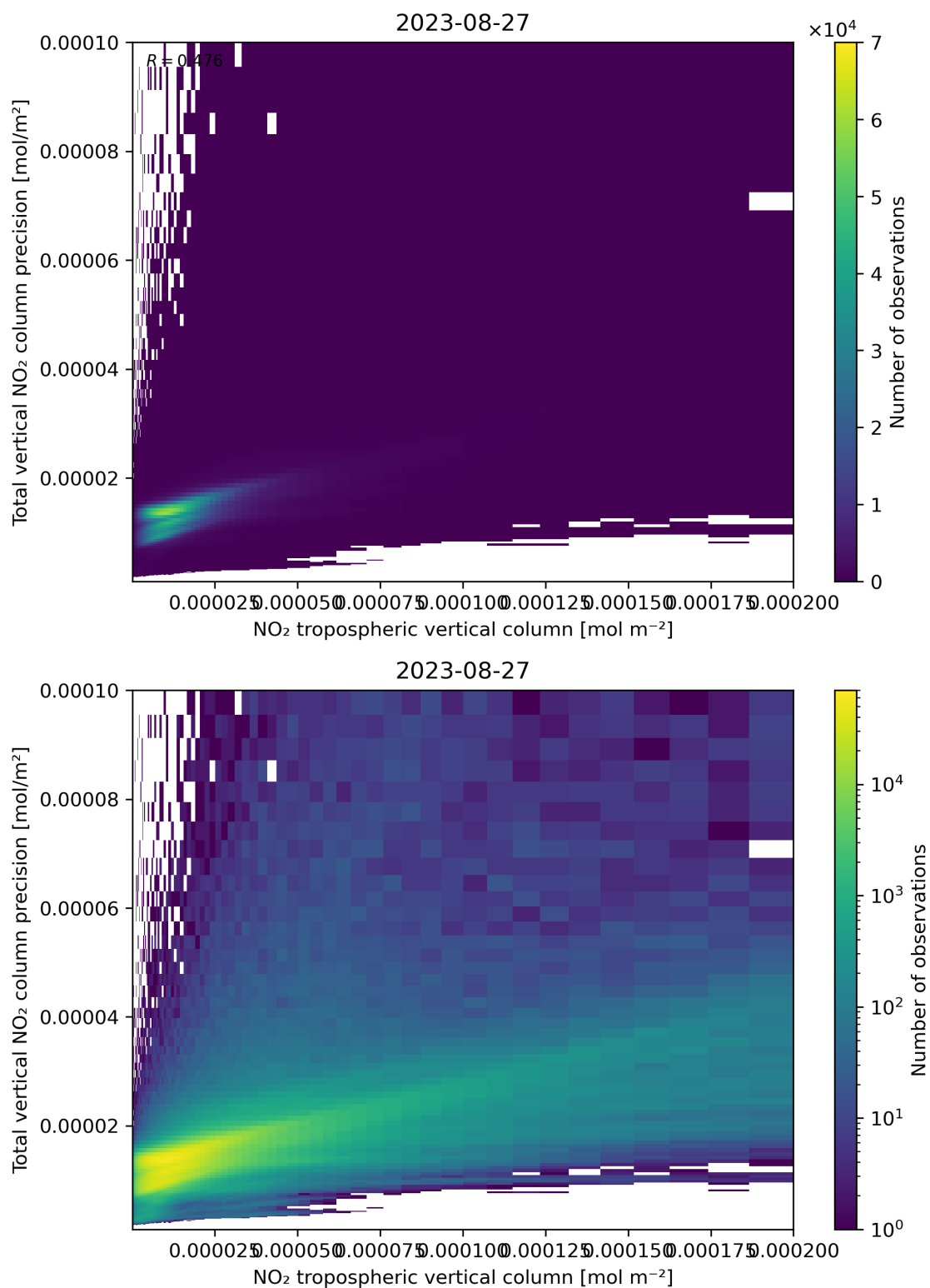
Figure 129: Scatter density plot of “NO 2 tropospheric vertical column” against “Total vertical NO 2 column precision” for 2023-08-26 to 2023-08-28.
