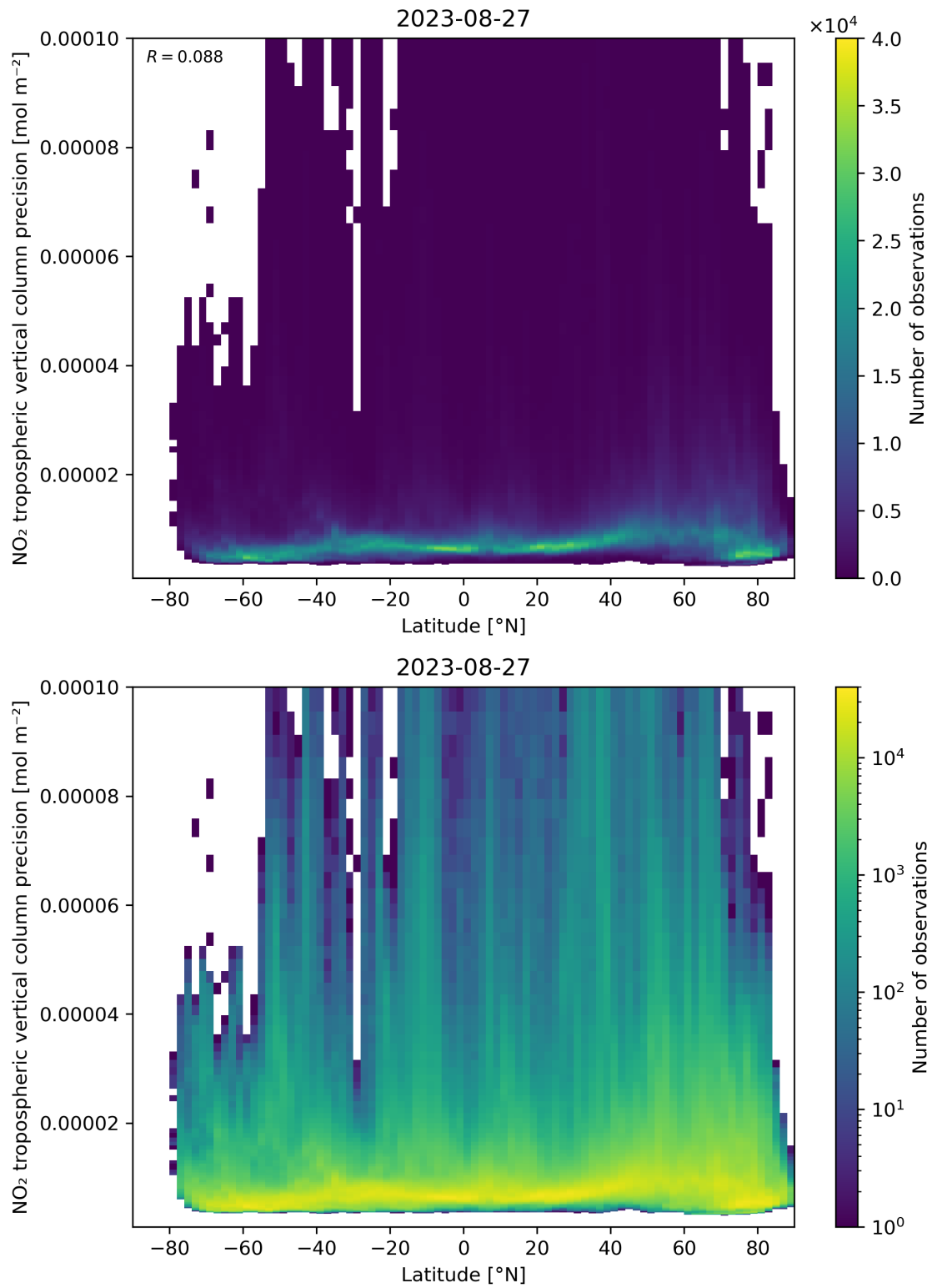
Figure 93: Scatter density plot of “Latitude” against “NO 2 tropospheric vertical column precision” for 2023-08-26 to 2023-08-28.
