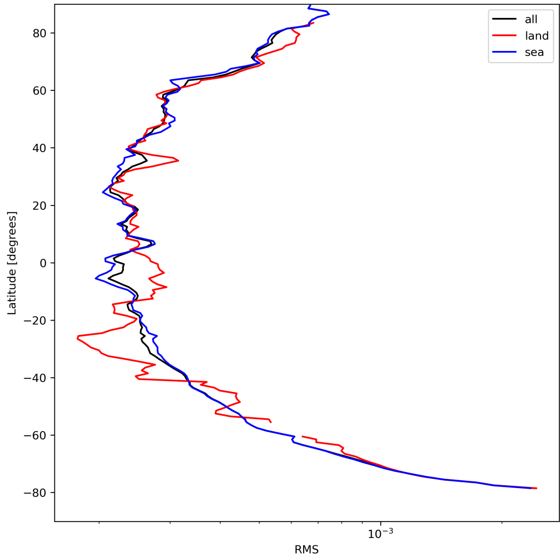
Figure 26: Zonal average of “RMS” for 2023-08-26 to 2023-08-28.
