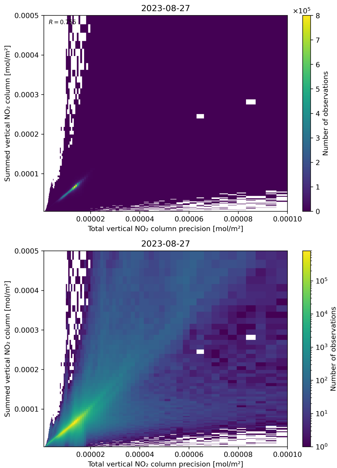
Figure 117: Scatter density plot of “Total vertical NO 2 column precision” against “Summed vertical NO 2 column” for 2023-08-26 to 2023-08-28.
