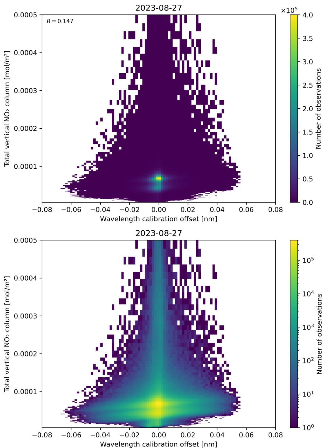
Figure 179: Scatter density plot of “Wavelength calibration offset” against “Total vertical NO 2 column” for 2023-08-26 to 2023-08-28.
