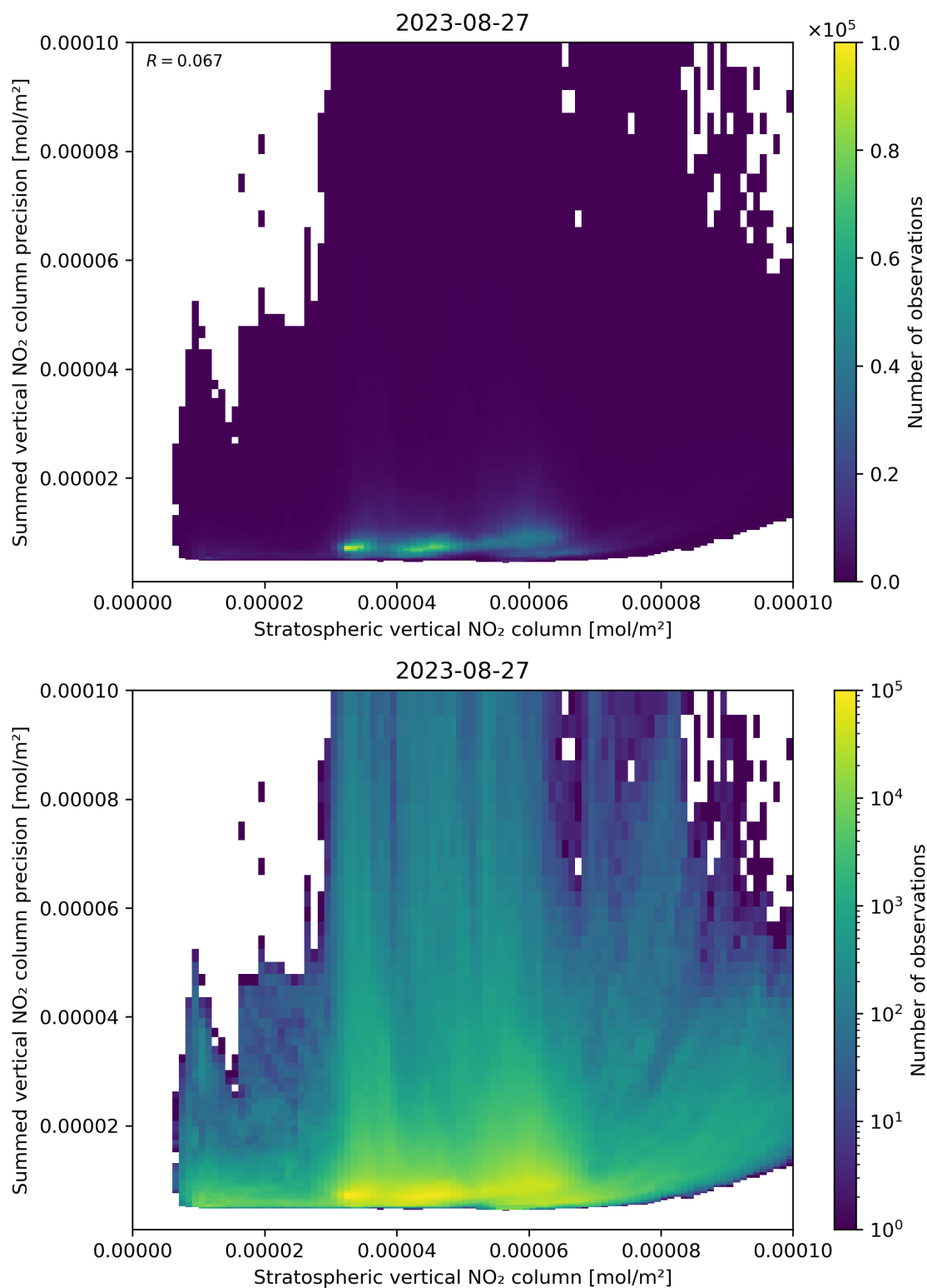
Figure 99: Scatter density plot of “Stratospheric vertical NO 2 column” against “Summed vertical NO 2 column precision” for 2023-08-26 to 2023-08-28.
