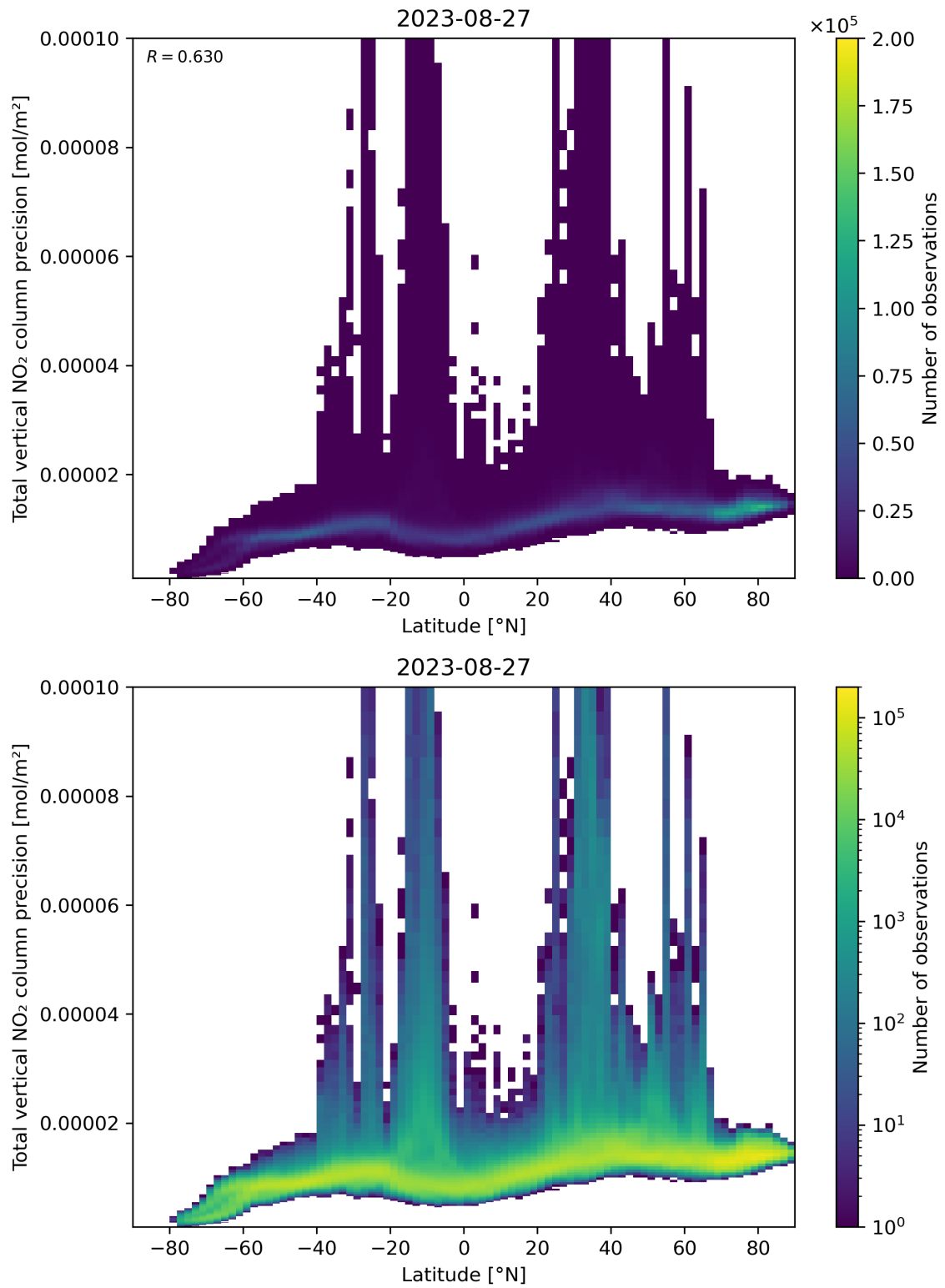
Figure 91: Scatter density plot of “Latitude” against “Total vertical NO 2 column precision” for 2023-08-26 to 2023-08-28.
