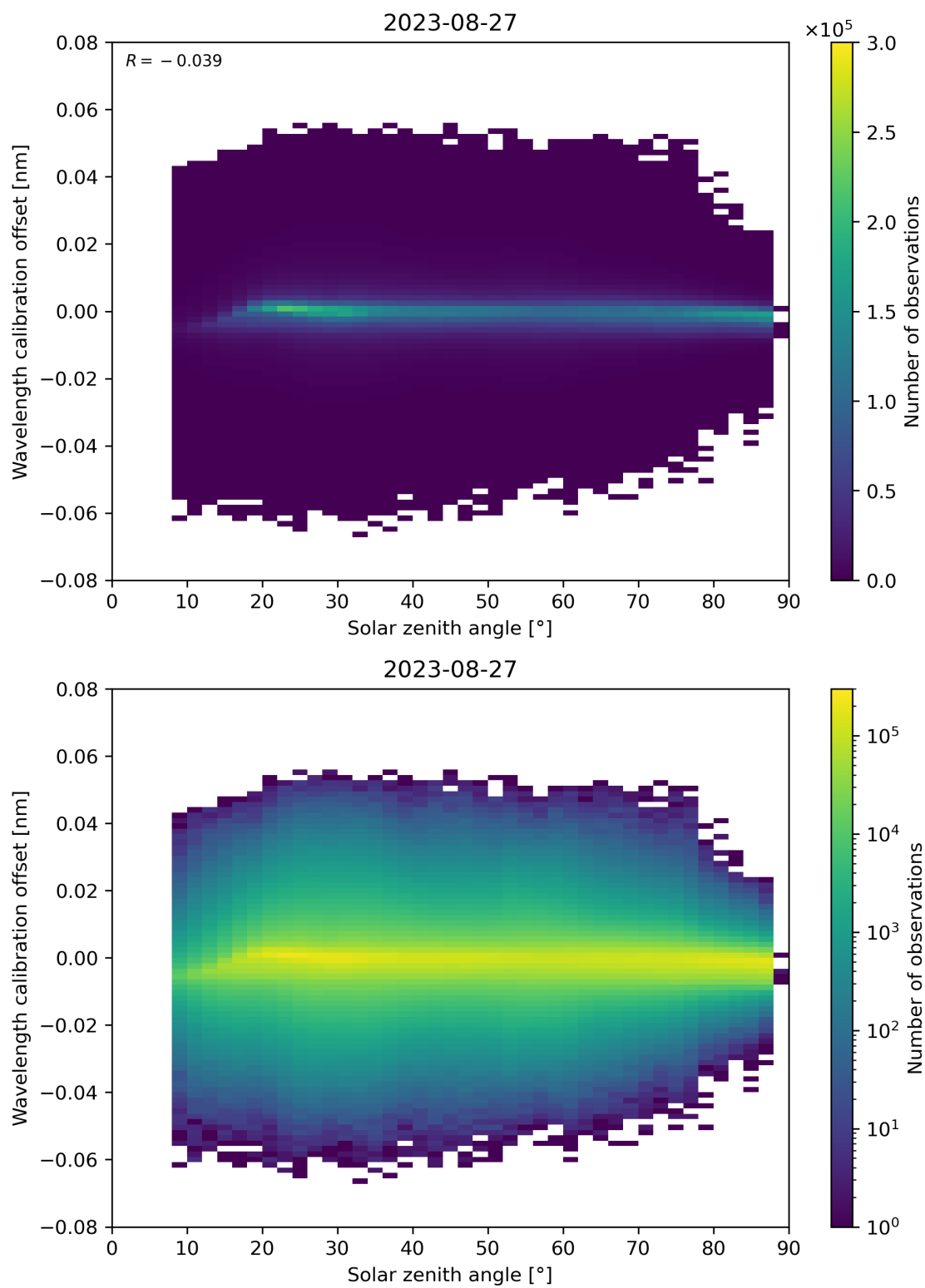
Figure 158: Scatter density plot of “Solar zenith angle” against “Wavelength calibration offset” for 2023-08-26 to 2023-08-28.
