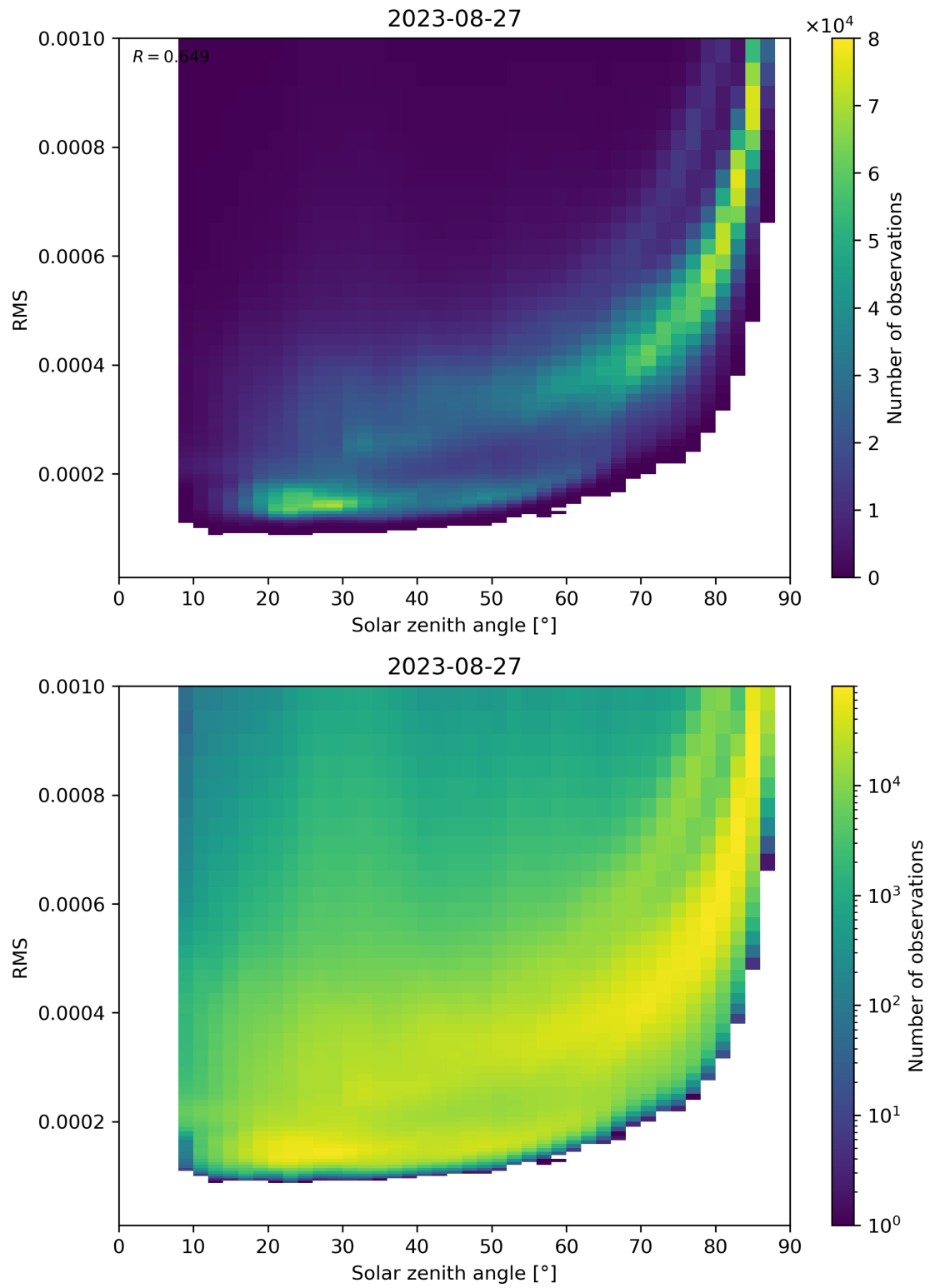
Figure 157: Scatter density plot of “Solar zenith angle” against “RMS” for 2023-08-26 to 2023-08-28.
