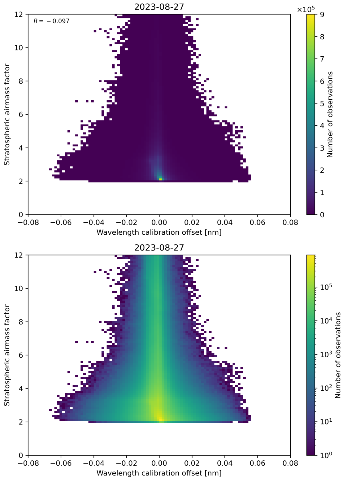
Figure 174: Scatter density plot of “Wavelength calibration offset” against “Stratospheric airmass factor” for 2023-08-26 to 2023-08-28.
