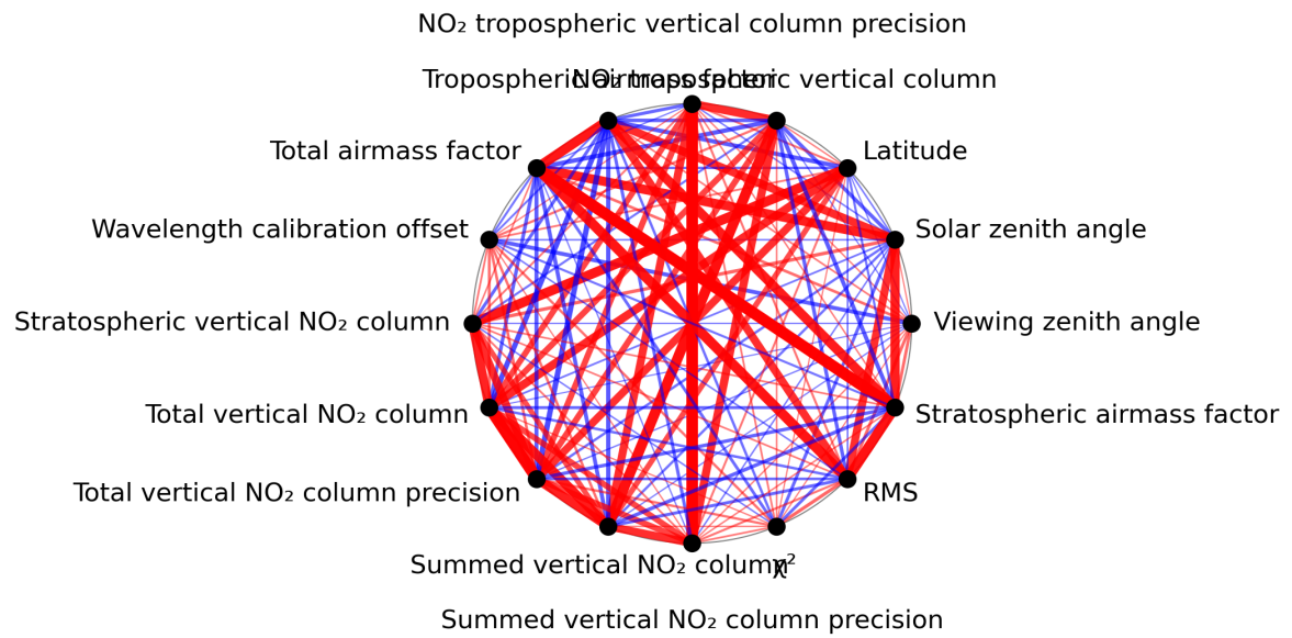
Figure 1: Map of correlation graph for 2023-08-26 to 2023-08-28.
