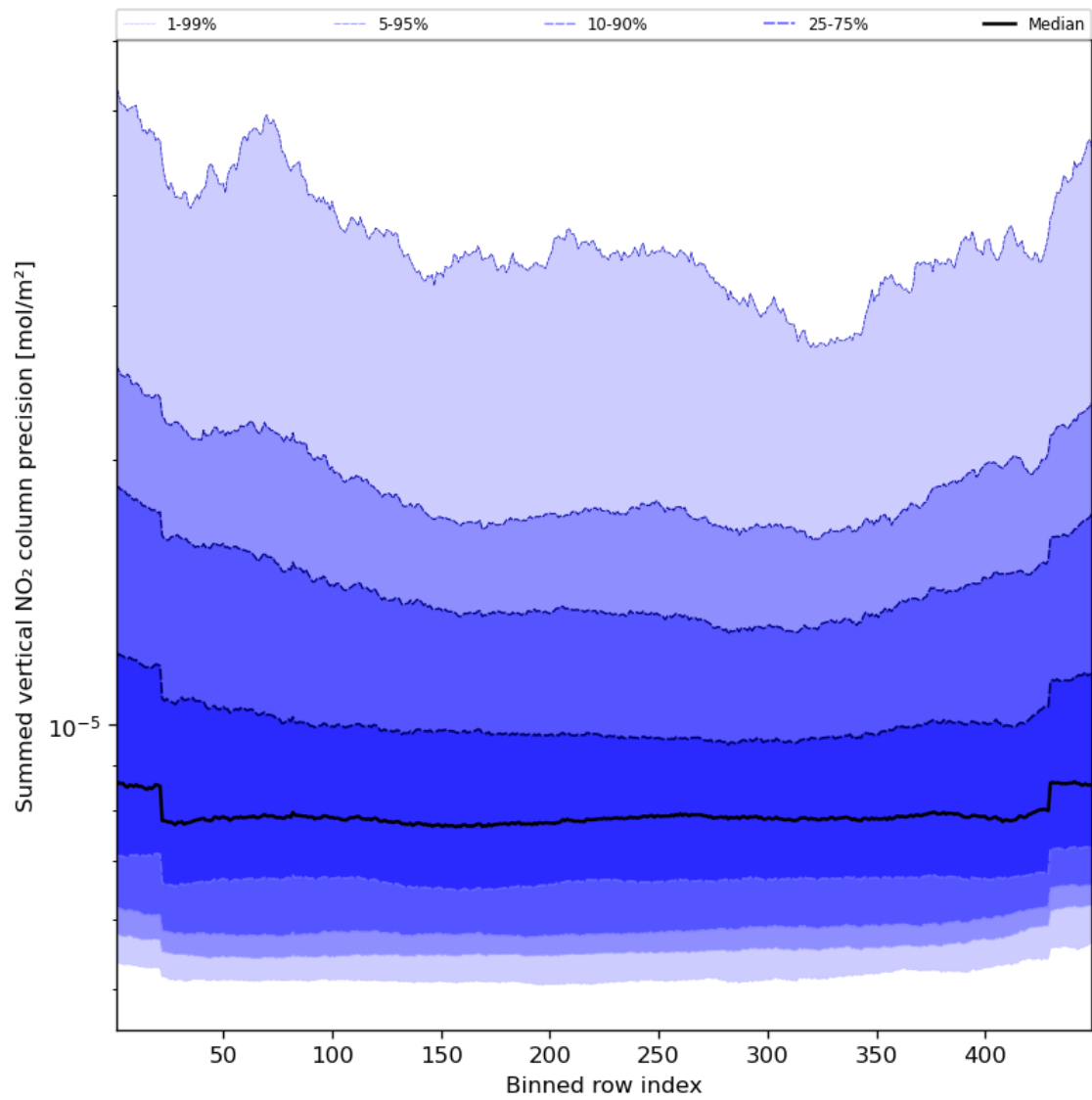
Figure 58: Along track statistics of “Summed vertical NO 2 column precision” for 2023-08-26 to 2023-08-28
