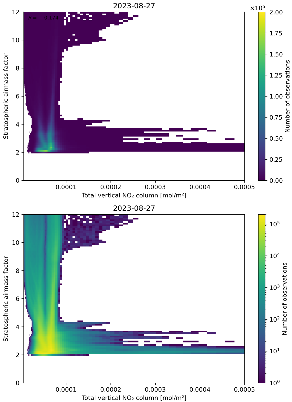
Figure 110: Scatter density plot of “Total vertical NO 2 column” against “Stratospheric airmass factor” for 2023-08-26 to 2023-08-28.
