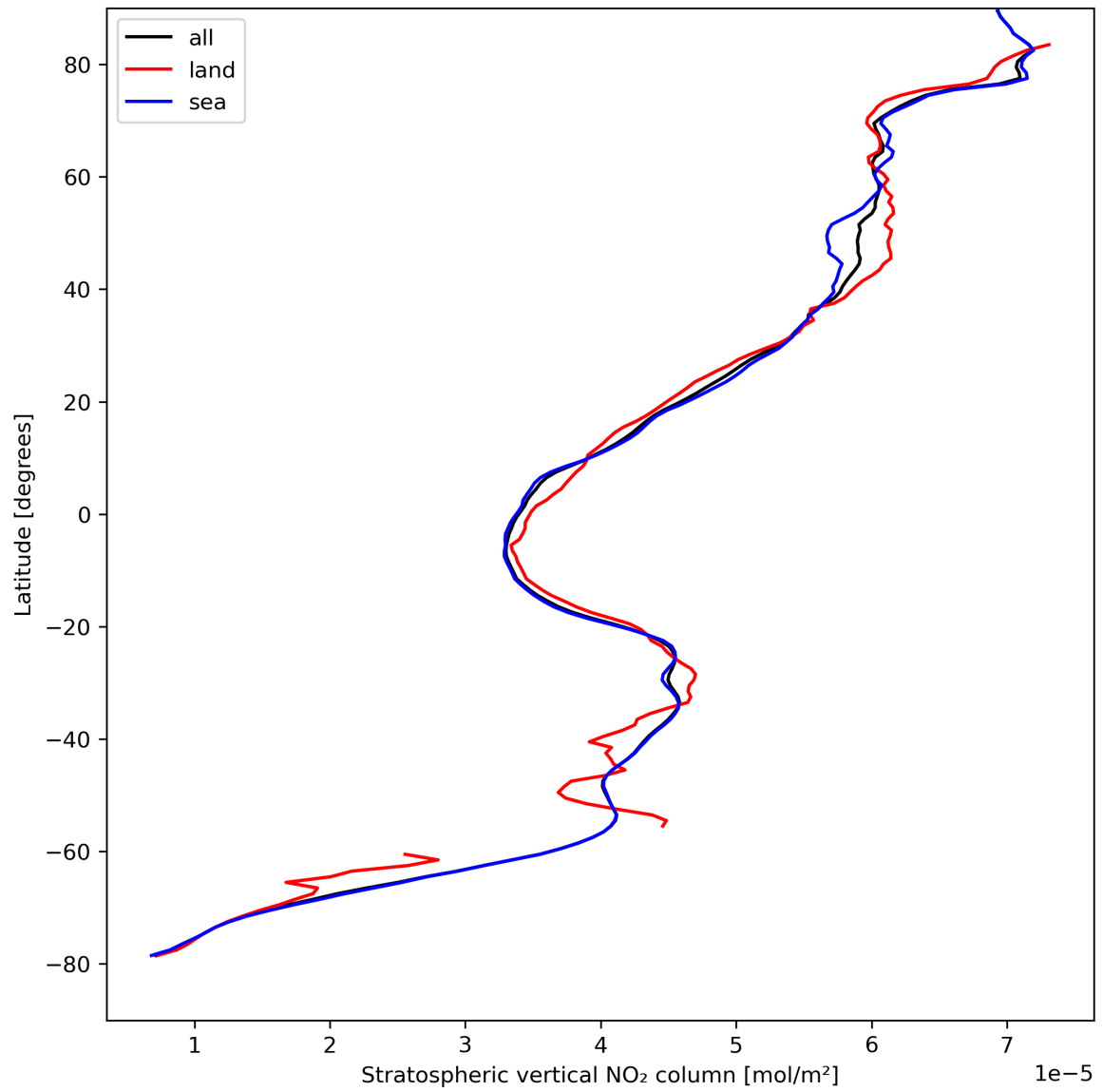
Figure 19: Zonal average of “Stratospheric vertical NO 2 column” for 2023-08-26 to 2023-08-28.
