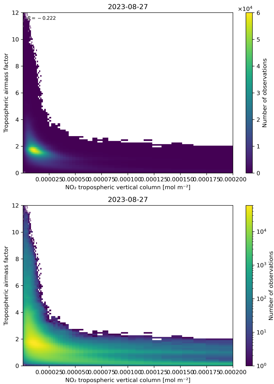
Figure 123: Scatter density plot of “NO 2 tropospheric vertical column” against “Tropospheric airmass factor” for 2023-08-26 to 2023-08-28.
