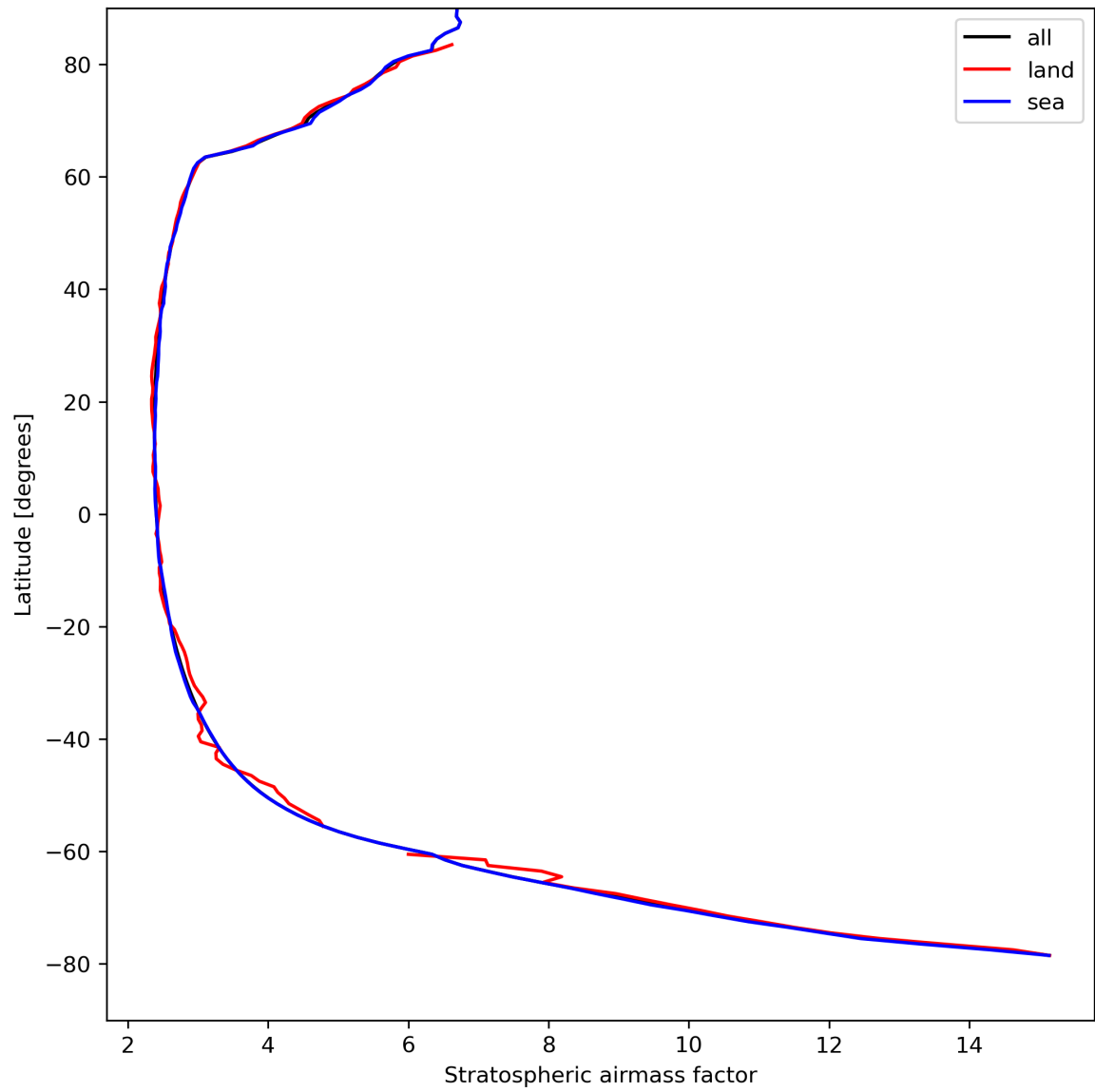
Figure 27: Zonal average of “Stratospheric airmass factor” for 2023-08-26 to 2023-08-28.
