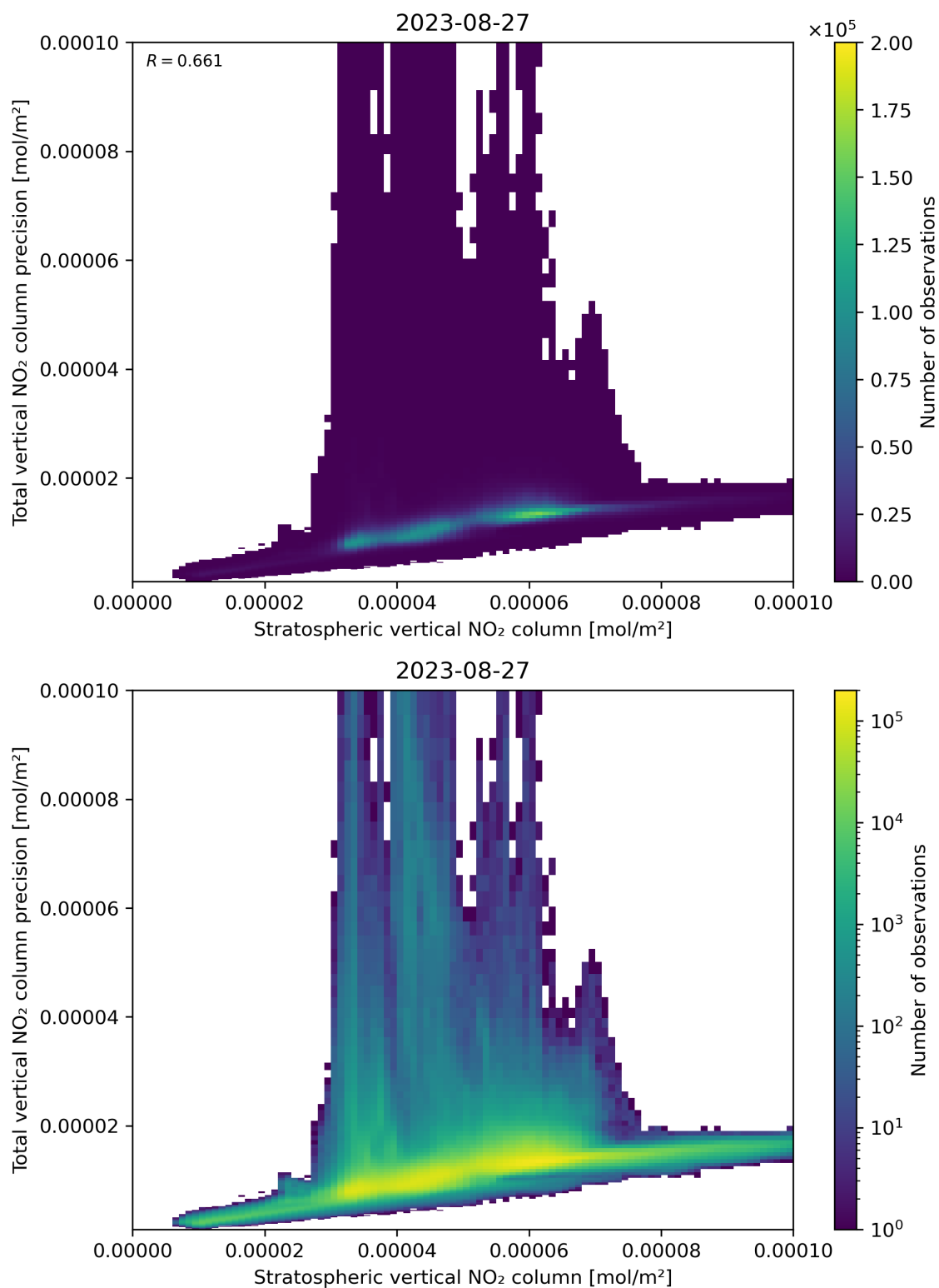
Figure 101: Scatter density plot of “Stratospheric vertical NO 2 column” against “Total vertical NO 2 column precision” for 2023-08-26 to 2023-08-28.
