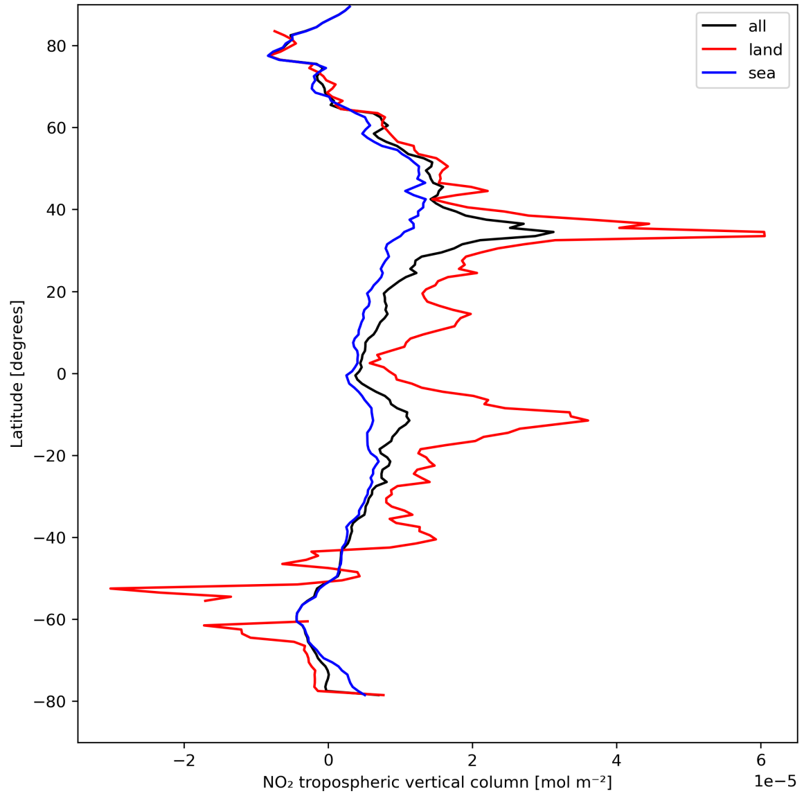
Figure 12: Zonal average of “NO 2 tropospheric vertical column” for 2023-08-26 to 2023-08-28.
