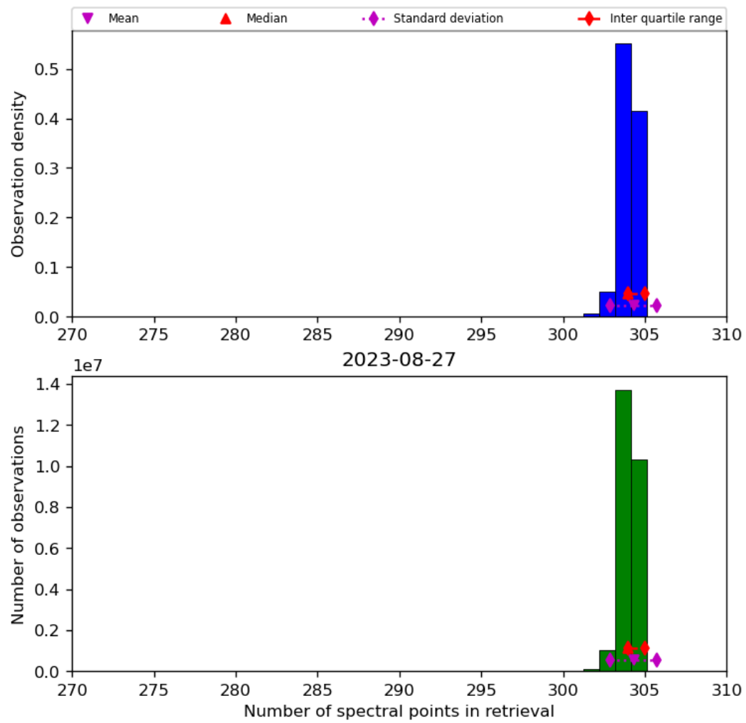
Figure 33: Histogram of “Number of spectral points in retrieval” for 2023-08-26 to 2023-08-28
