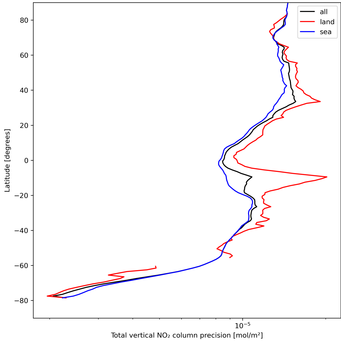
Figure 22: Zonal average of “Total vertical NO 2 column precision” for 2023-08-26 to 2023-08-28.
