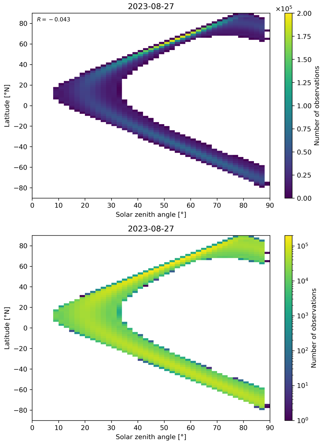
Figure 149: Scatter density plot of “Solar zenith angle” against “Latitude” for 2023-08-26 to 2023-08-28.
