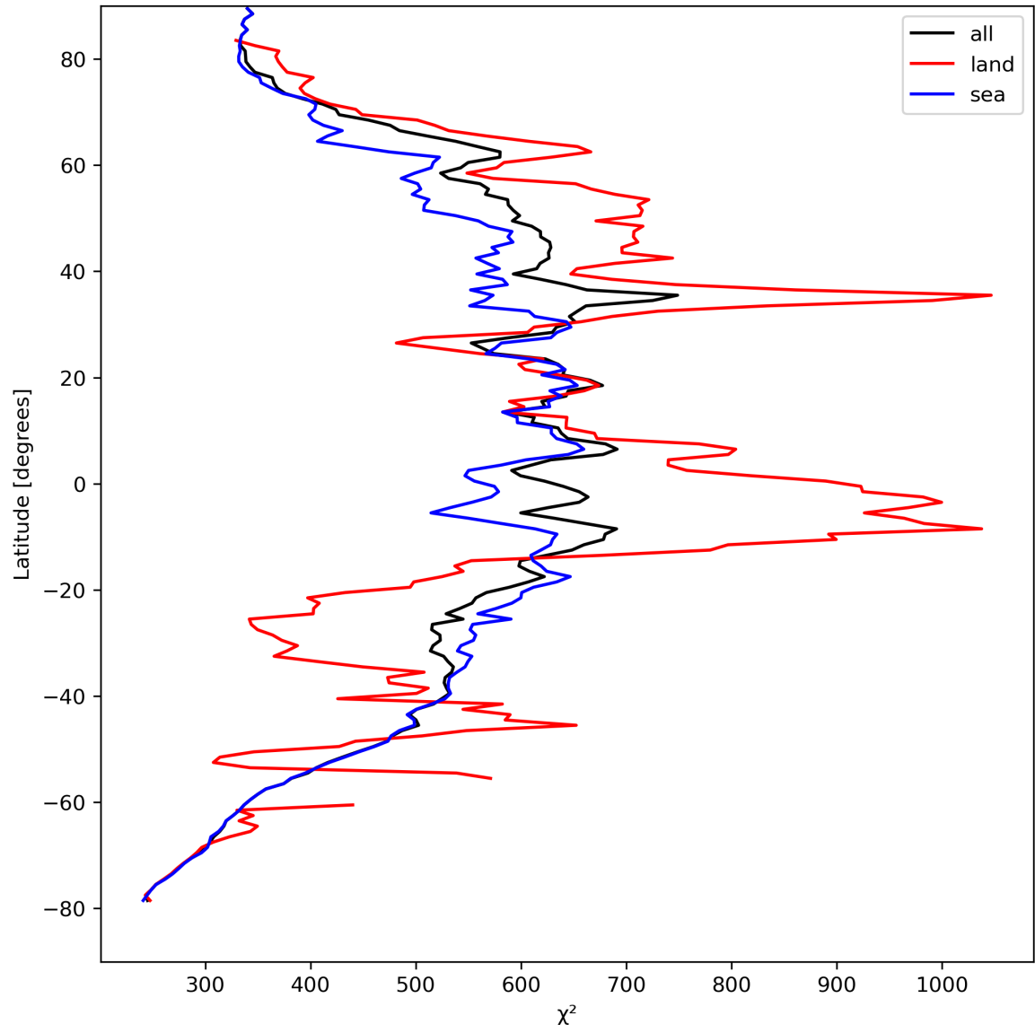
Figure 25: Zonal average of “ \chi^2 ” for 2023-08-26 to 2023-08-28.
