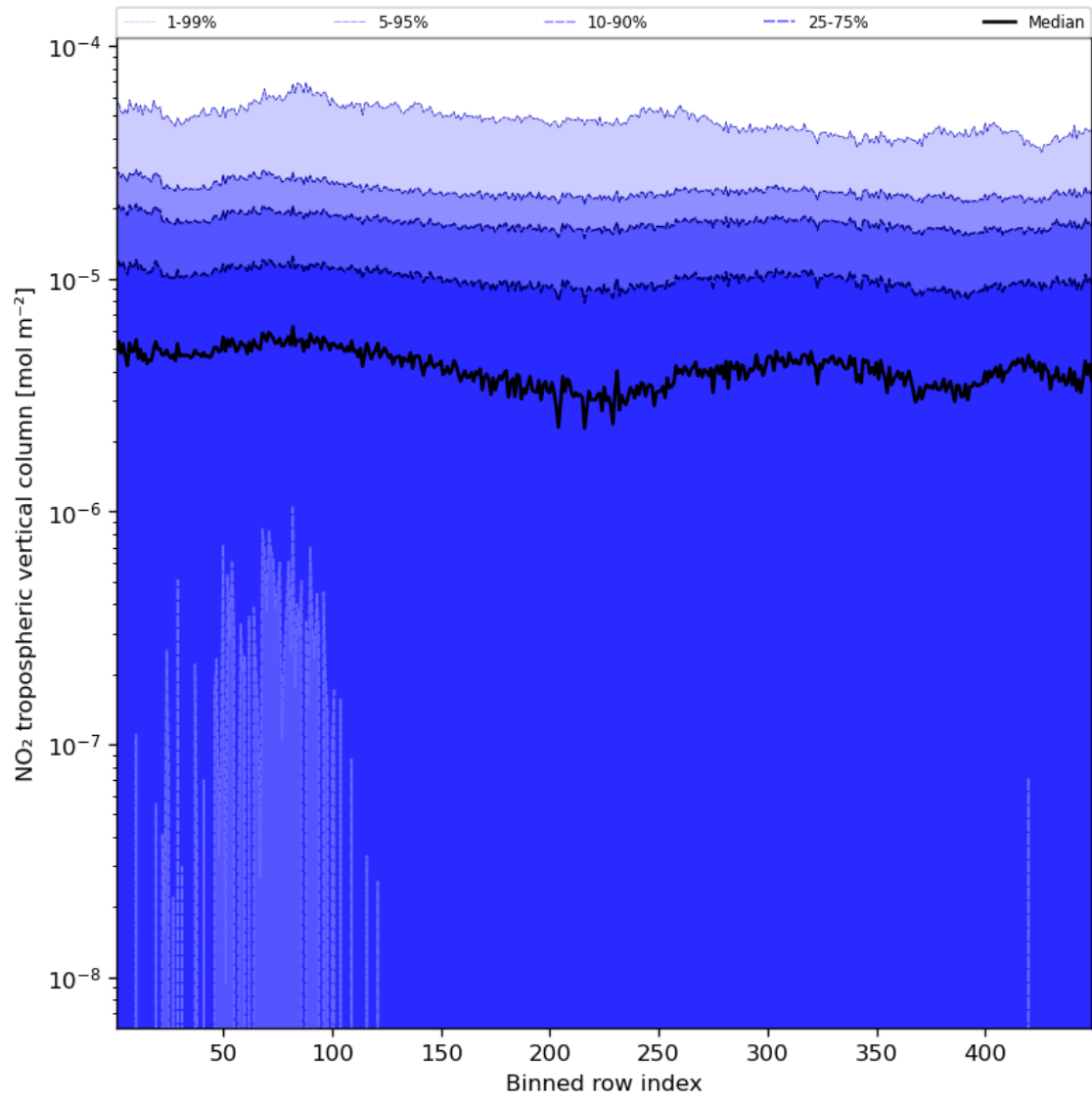
Figure 46: Along track statistics of “NO 2 tropospheric vertical column” for 2023-08-26 to 2023-08-28
