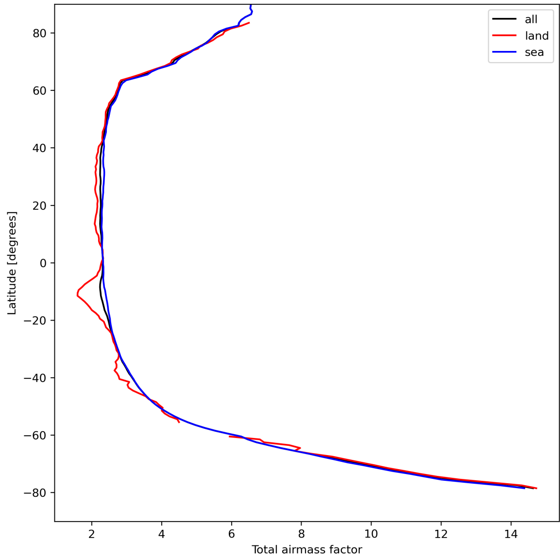
Figure 15: Zonal average of “Total airmass factor” for 2023-08-26 to 2023-08-28.
