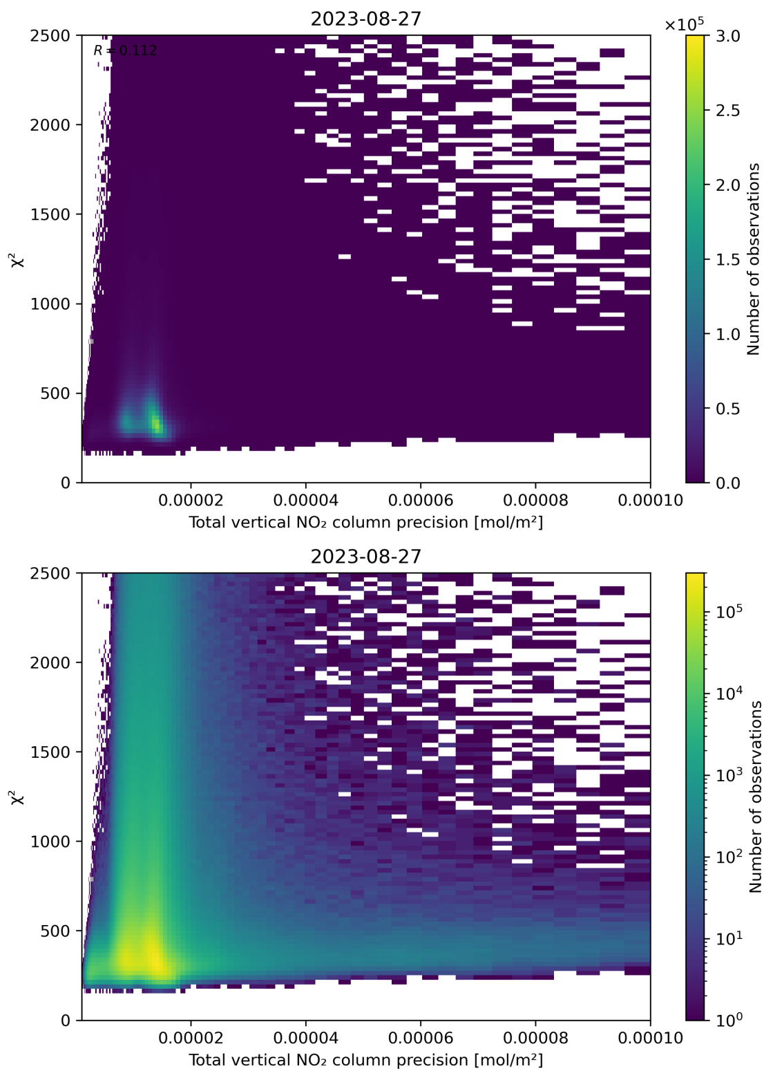
Figure 116: Scatter density plot of “Total vertical NO 2 column precision” against “ \chi^2 ” for 2023-08-26 to 2023-08-28.
