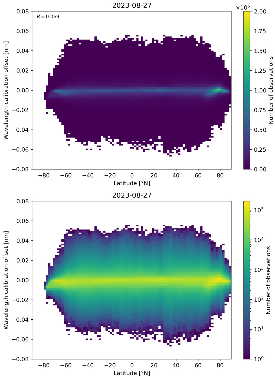
Figure 95: Scatter density plot of “Latitude” against “Wavelength calibration offset” for 2023-08-26 to 2023-08-28.
