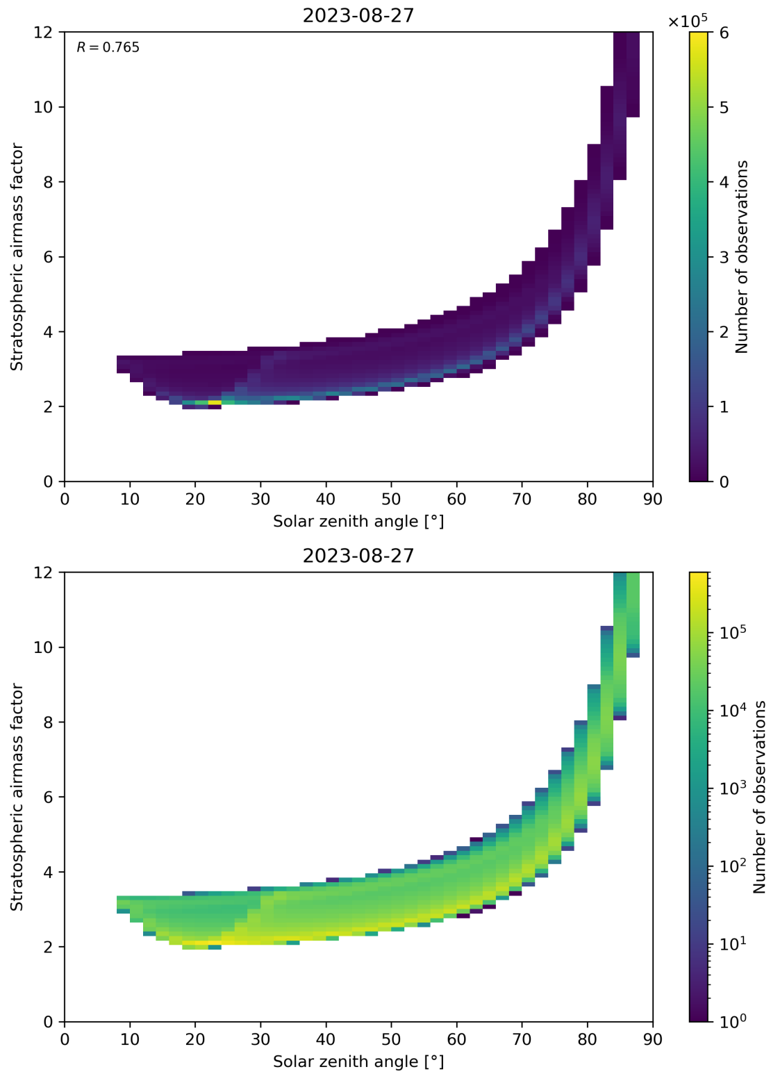
Figure 145: Scatter density plot of “Solar zenith angle” against “Stratospheric airmass factor” for 2023-08-26 to 2023-08-28.
