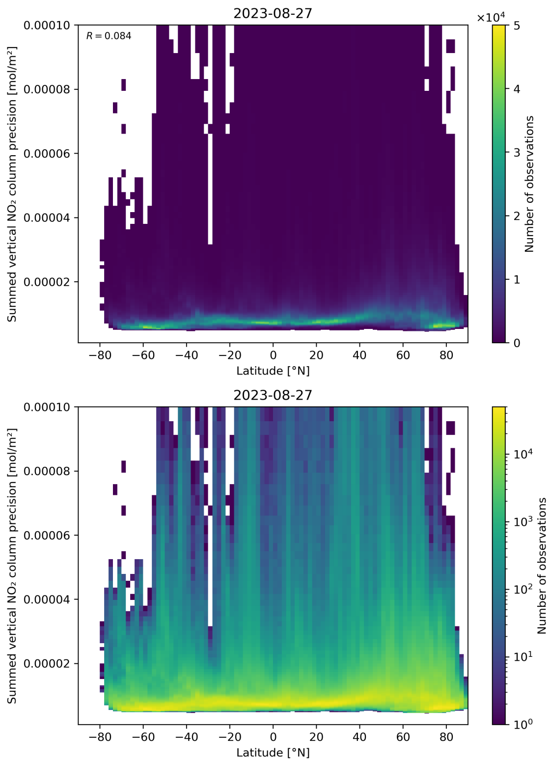
Figure 89: Scatter density plot of “Latitude” against “Summed vertical NO 2 column precision” for 2023-08-26 to 2023-08-28.
