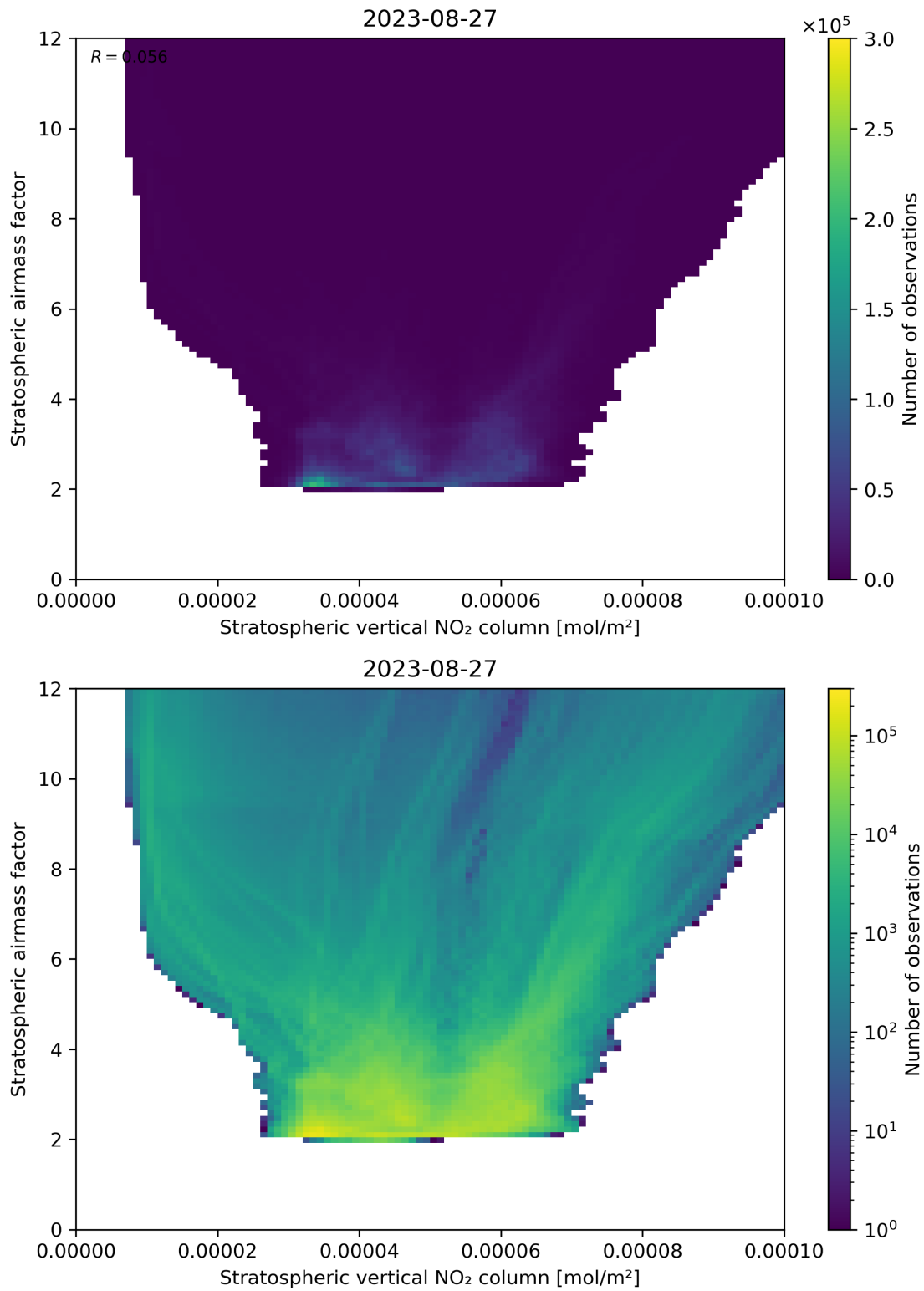
Figure 96: Scatter density plot of “Stratospheric vertical NO 2 column” against “Stratospheric airmass factor” for 2023-08-26 to 2023-08-28.
