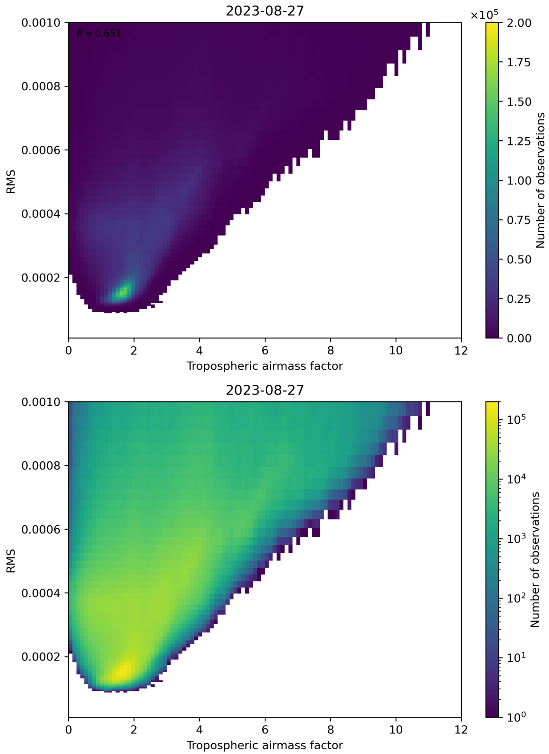
Figure 79: Scatter density plot of “Tropospheric airmass factor” against “RMS” for 2023-08-26 to 2023-08-28.
