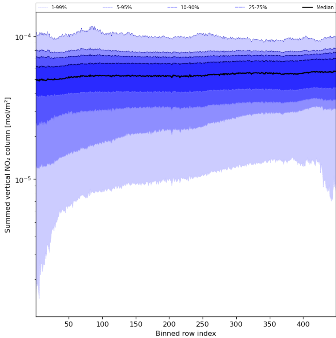
Figure 57: Along track statistics of “Summed vertical NO 2 column” for 2023-08-26 to 2023-08-28
