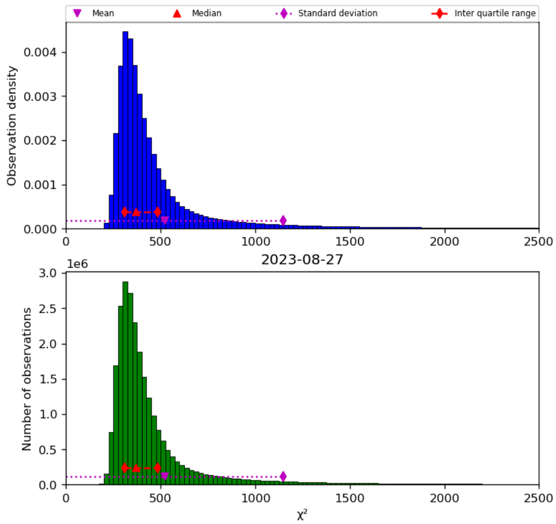
Figure 42: Histogram of “ \chi^2 ” for 2023-08-26 to 2023-08-28
