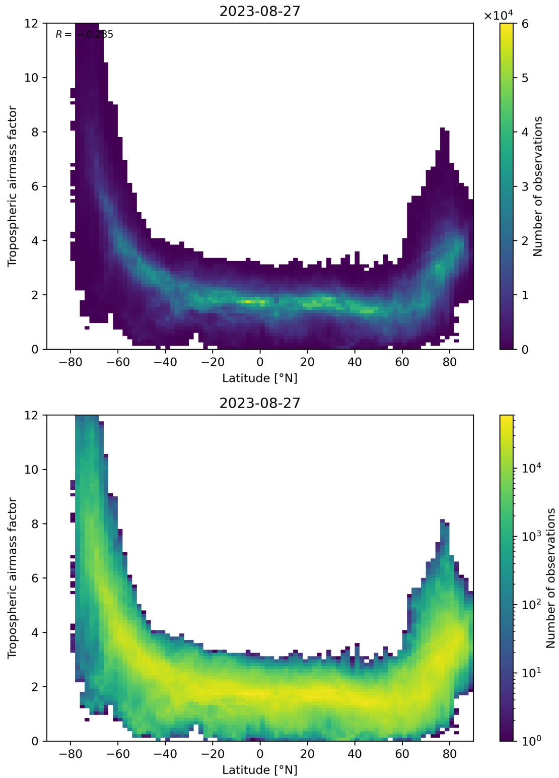
Figure 85: Scatter density plot of “Latitude” against “Tropospheric airmass factor” for 2023-08-26 to 2023-08-28.
