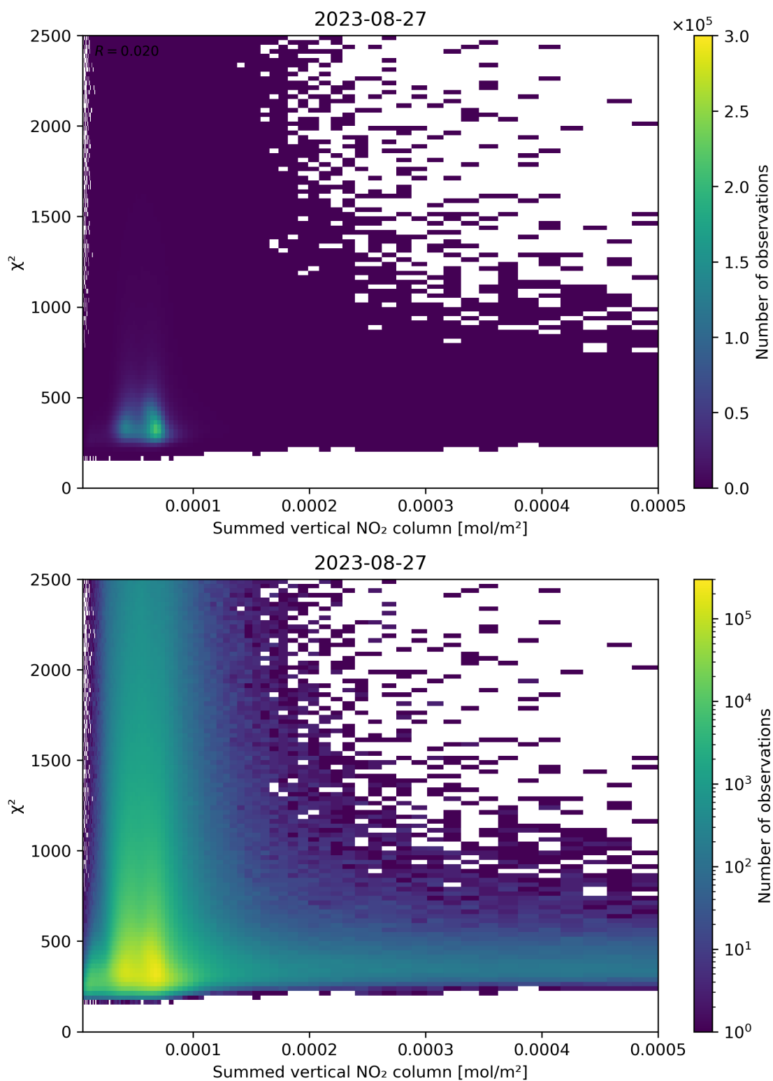
Figure 104: Scatter density plot of “Summed vertical NO 2 column” against “ \chi^2 ” for 2023-08-26 to 2023-08-28.
