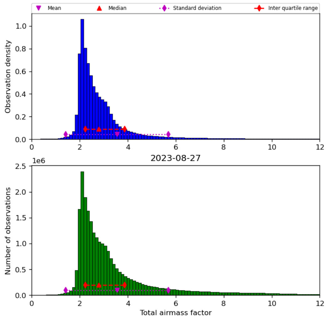
Figure 32: Histogram of “Total airmass factor” for 2023-08-26 to 2023-08-28
