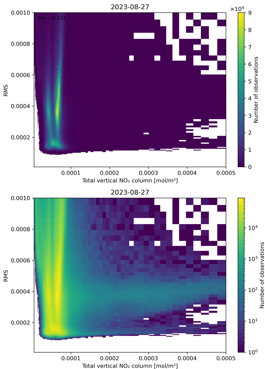
Figure 120: Scatter density plot of “Total vertical NO 2 column” against “RMS” for 2023-08-26 to 2023-08-28.
