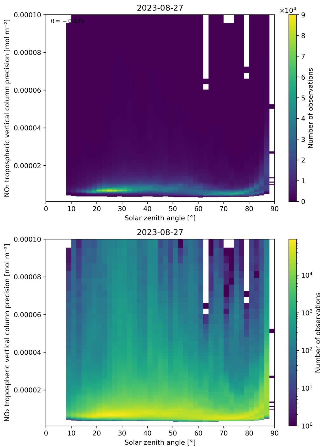
Figure 156: Scatter density plot of “Solar zenith angle” against “NO 2 tropospheric vertical column precision” for 2023-08-26 to 2023-08-28.
