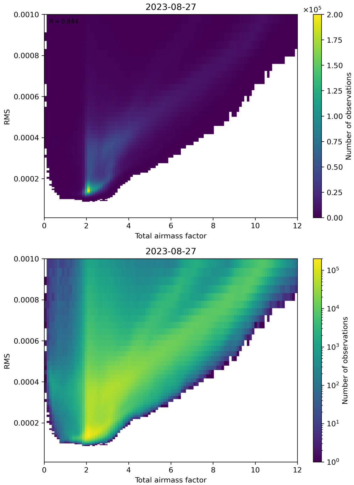
Figure 69: Scatter density plot of “Total airmass factor” against “RMS” for 2023-08-26 to 2023-08-28.
