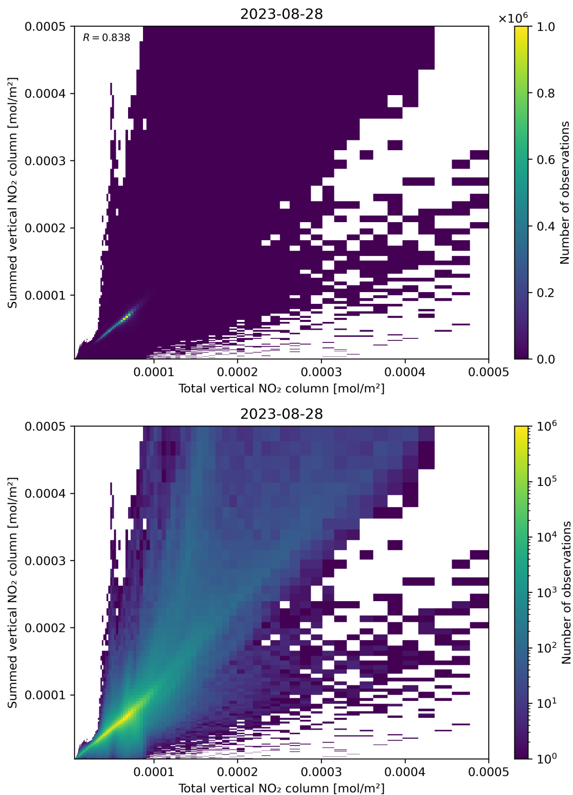
Figure 112: Scatter density plot of “Total vertical NO 2 column” against “Summed vertical NO 2 column” for 2023-08-27 to 2023-08-29.
