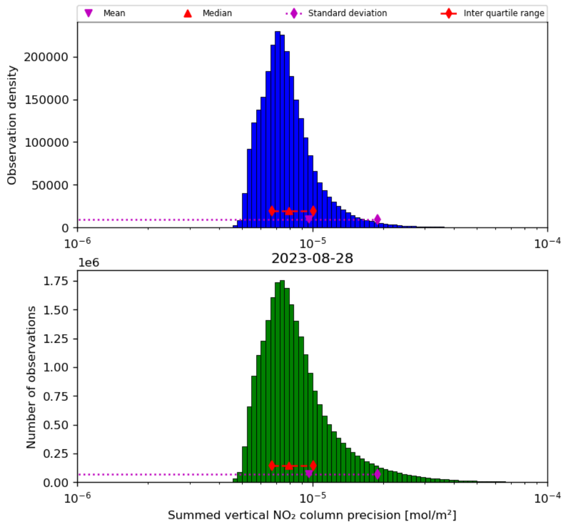
Figure 41: Histogram of “Summed vertical NO 2 column precision” for 2023-08-27 to 2023-08-29
