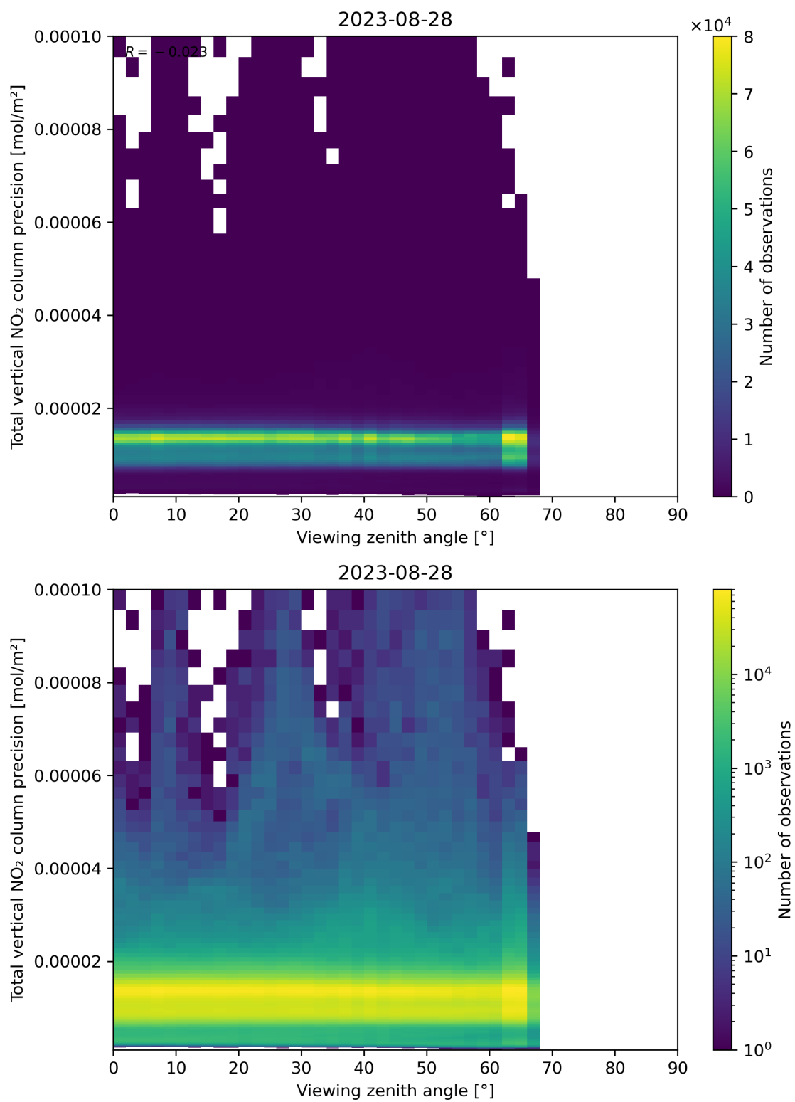
Figure 168: Scatter density plot of “Viewing zenith angle” against “Total vertical NO 2 column precision” for 2023-08-27 to 2023-08-29.
