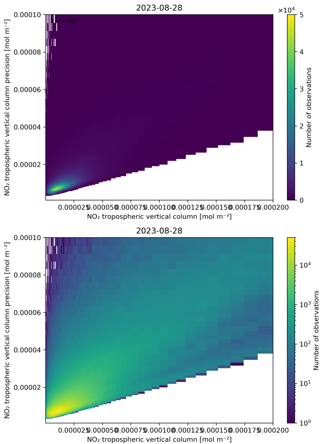
Figure 130: Scatter density plot of “NO 2 tropospheric vertical column” against “NO 2 tropospheric vertical column precision” for 2023-08-27 to 2023-08-29.
