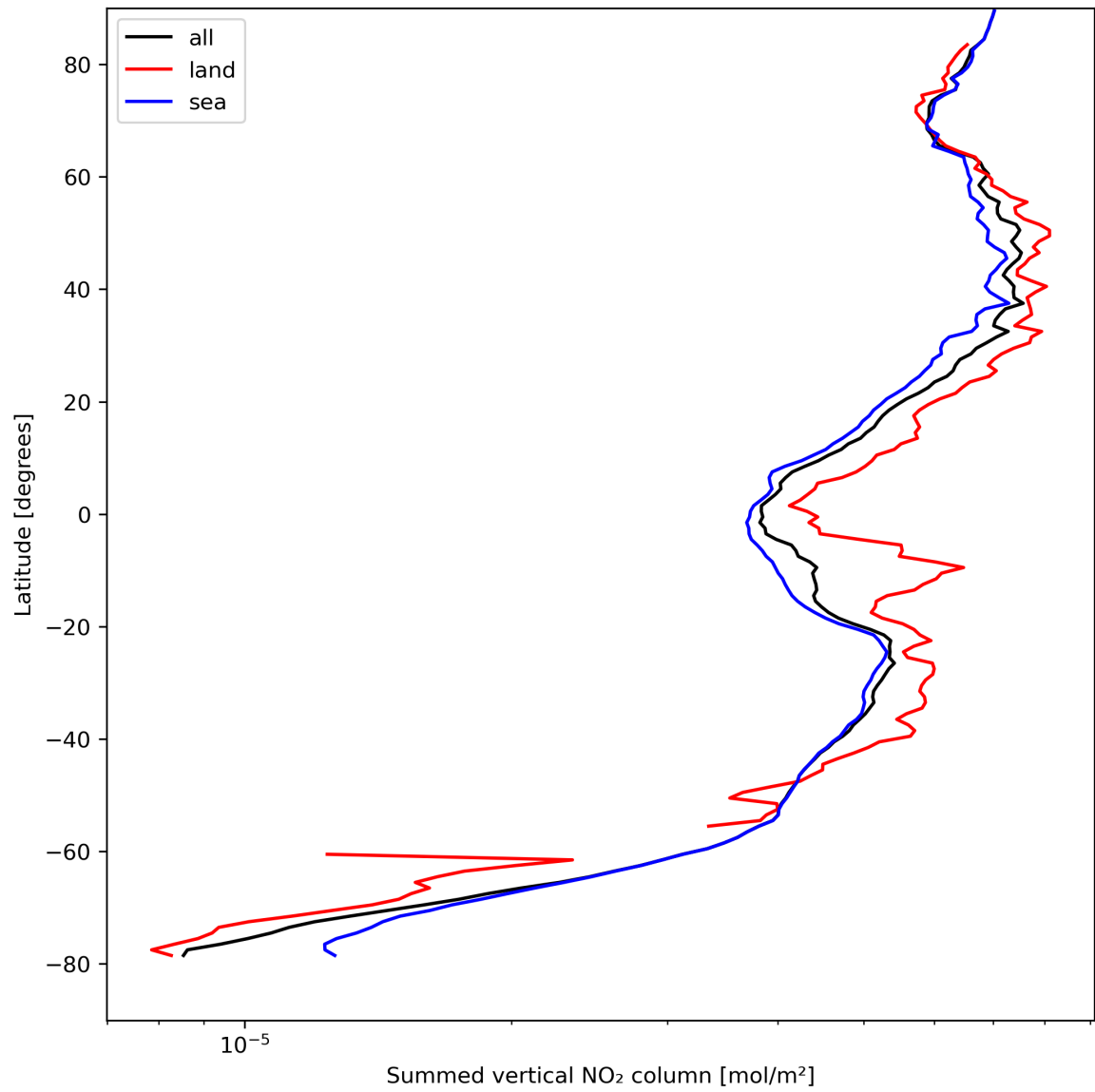
Figure 23: Zonal average of “Summed vertical NO 2 column” for 2023-08-27 to 2023-08-29.
