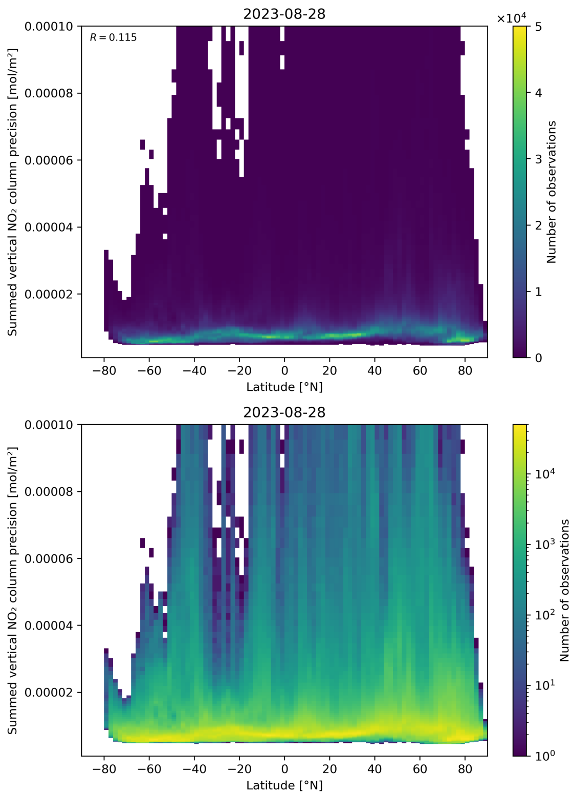
Figure 89: Scatter density plot of “Latitude” against “Summed vertical NO 2 column precision” for 2023-08-27 to 2023-08-29.
