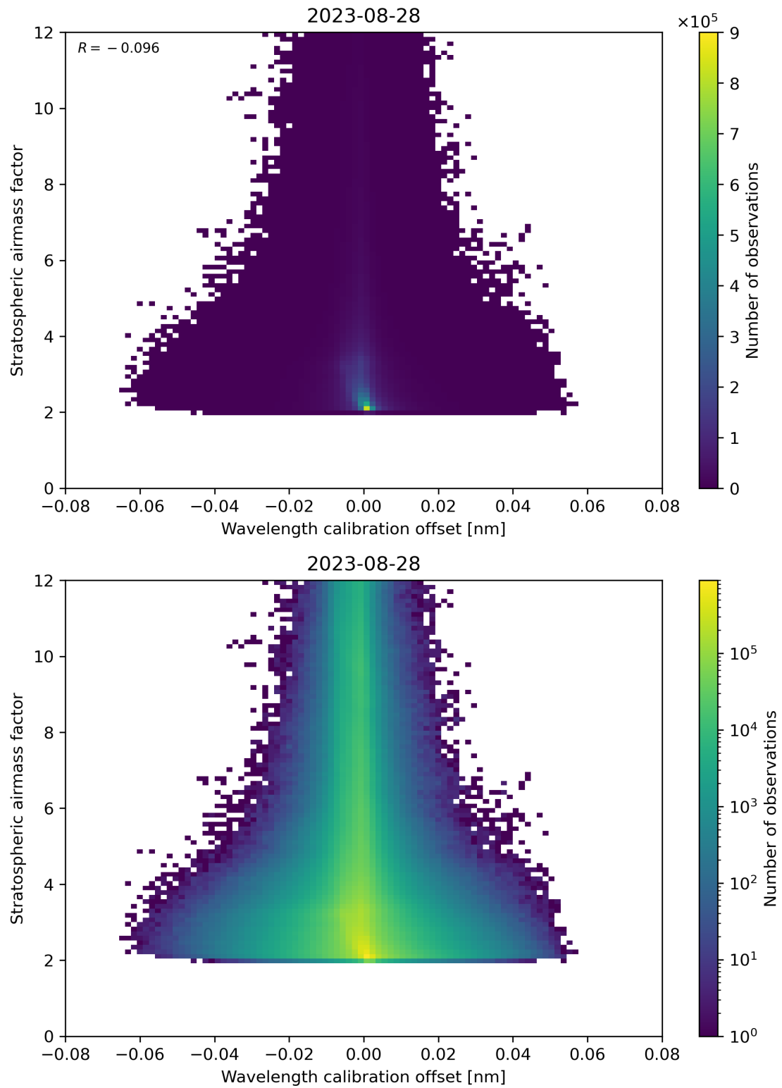
Figure 174: Scatter density plot of “Wavelength calibration offset” against “Stratospheric airmass factor” for 2023-08-27 to 2023-08-29.
