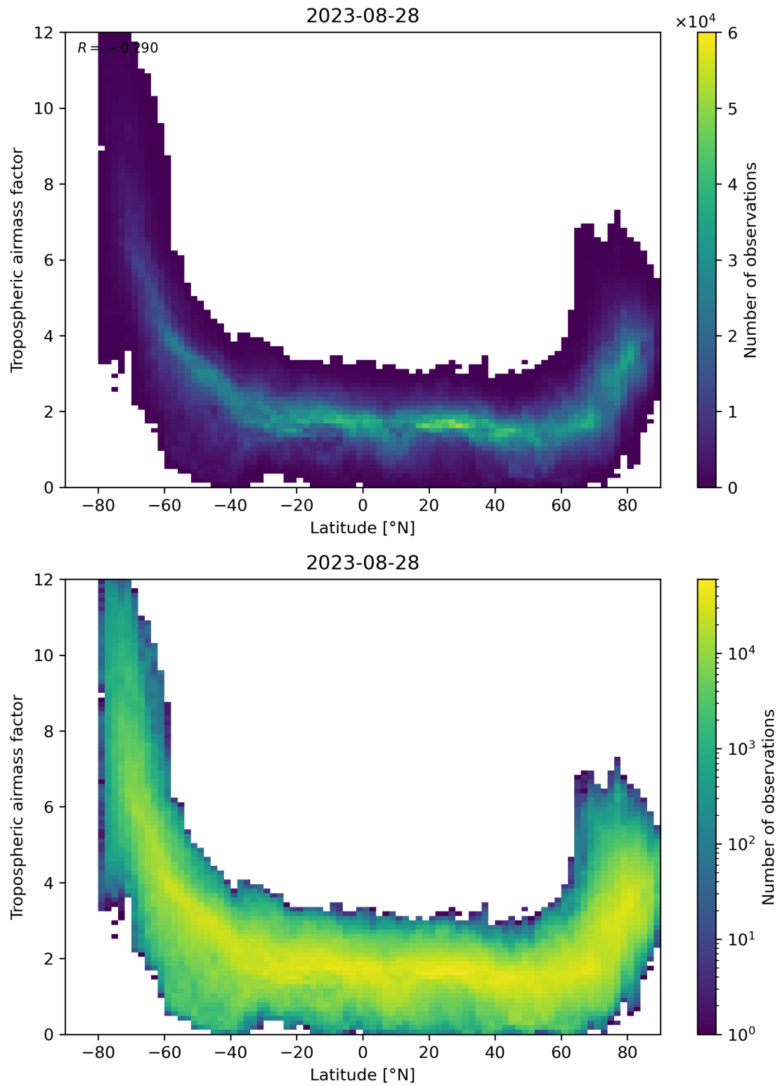
Figure 85: Scatter density plot of “Latitude” against “Tropospheric air mass factor” for 2023-08-27 to 2023-08-29.
