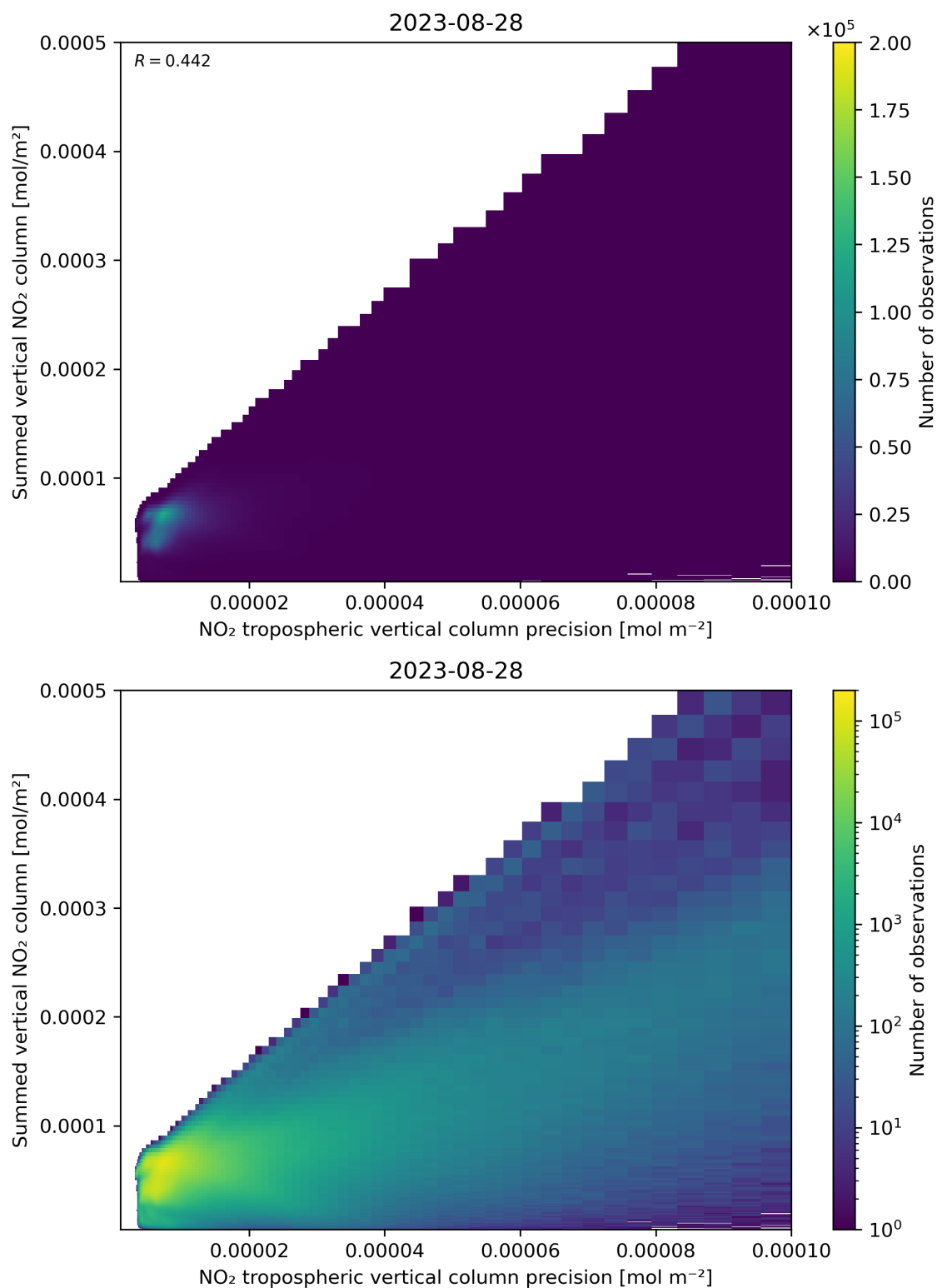
Figure 136: Scatter density plot of “NO 2 tropospheric vertical column precision” against “Summed vertical NO 2 column” for 2023-08-27 to 2023-08-29.
