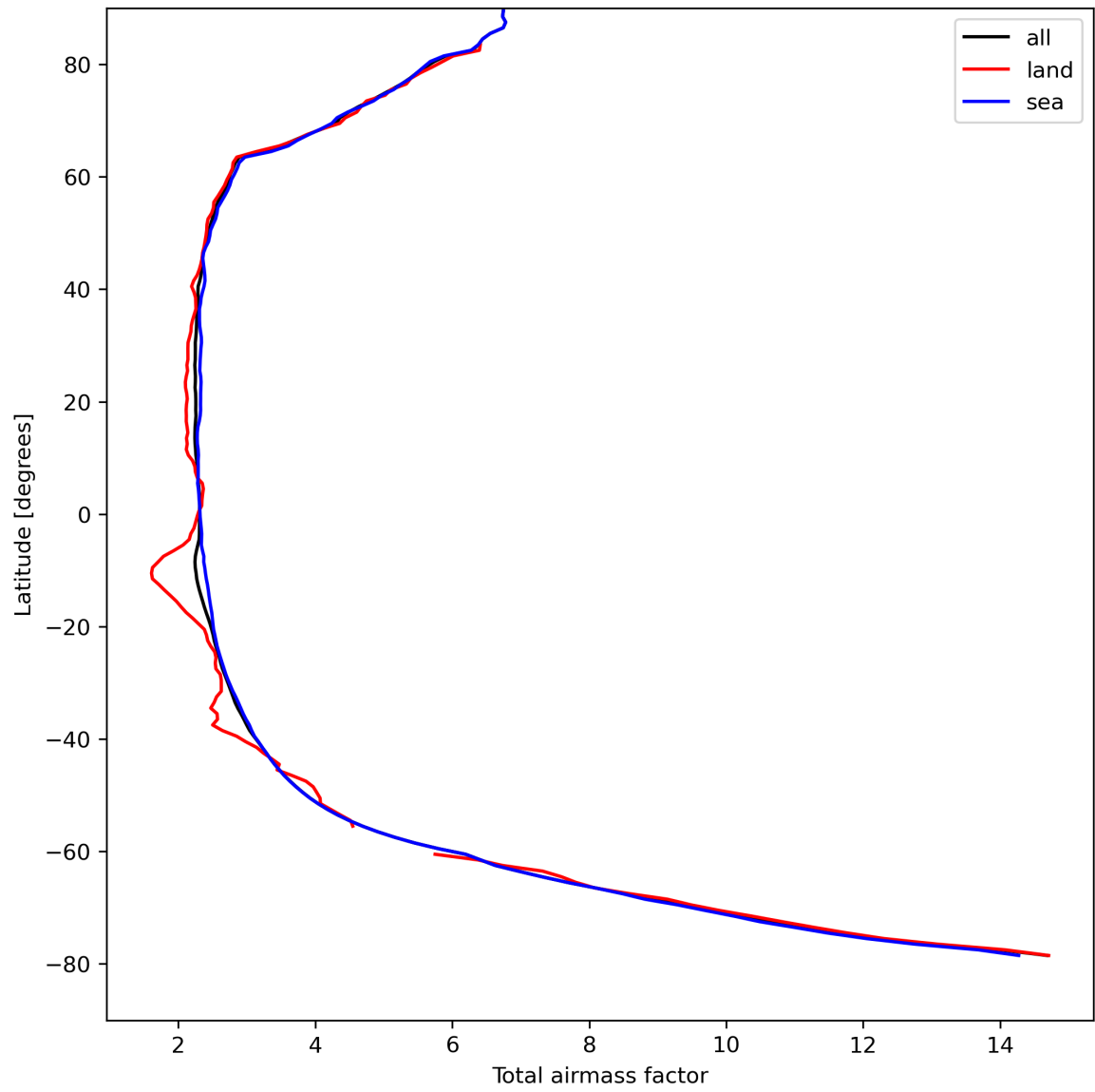
Figure 15: Zonal average of “Total airmass factor” for 2023-08-27 to 2023-08-29.
