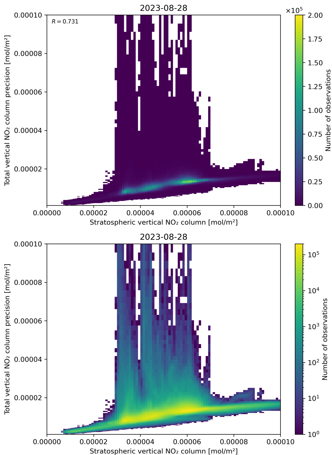
Figure 101: Scatter density plot of “Stratospheric vertical NO 2 column” against “Total vertical NO 2 column precision” for 2023-08-27 to 2023-08-29.
