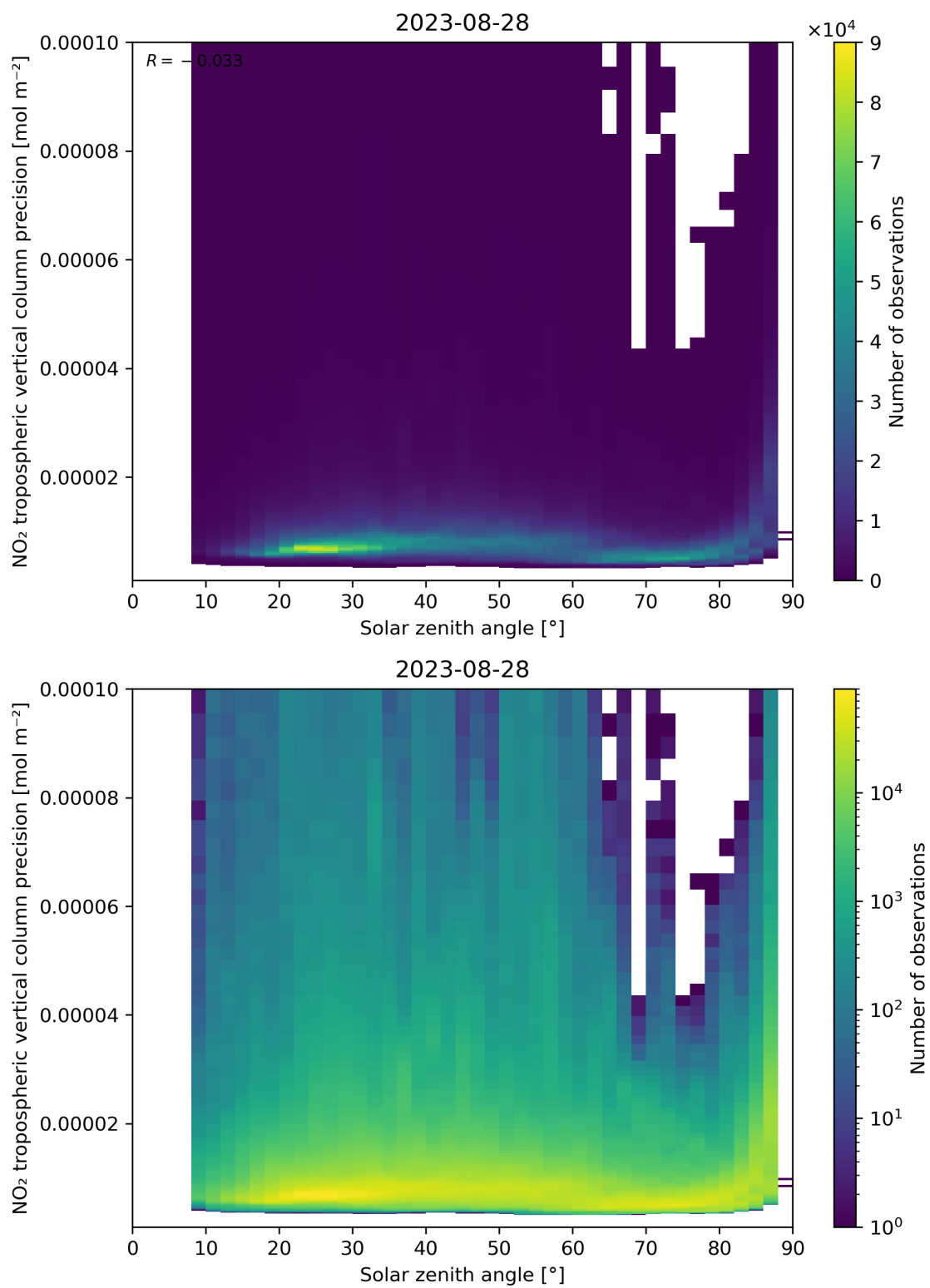
Figure 156: Scatter density plot of “Solar zenith angle” against “NO 2 tropospheric vertical column precision” for 2023-08-27 to 2023-08-29.
