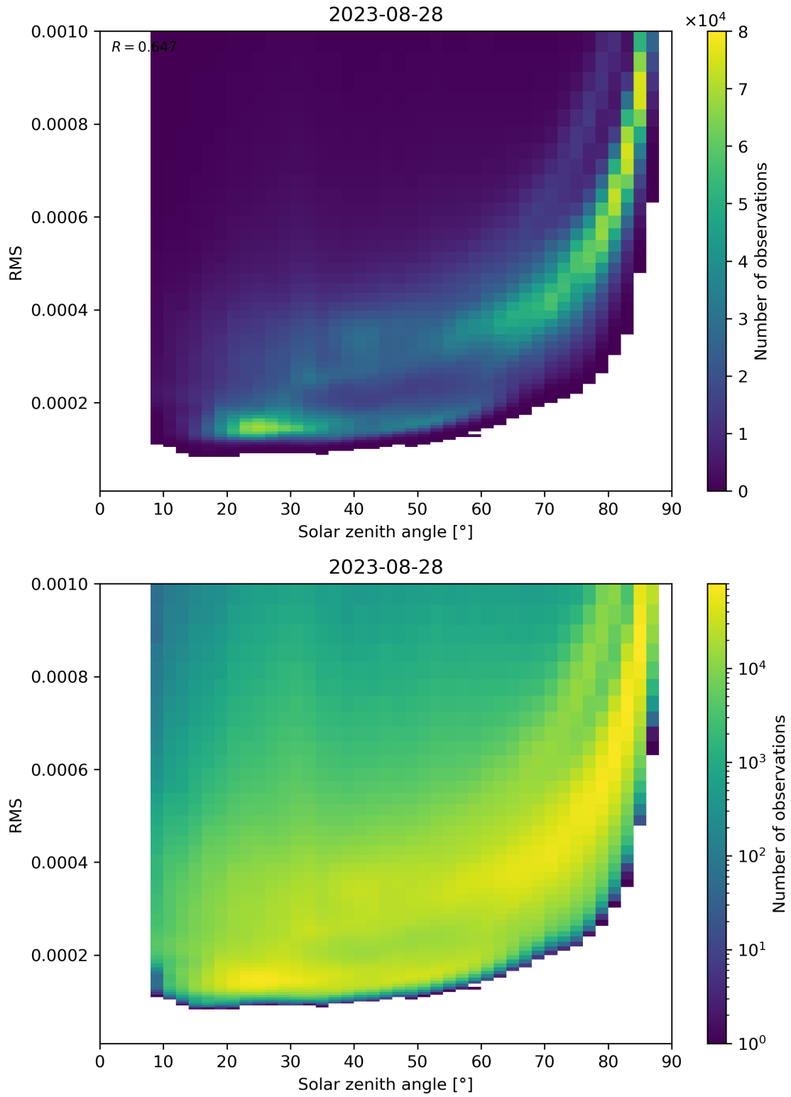
Figure 157: Scatter density plot of “Solar zenith angle” against “RMS” for 2023-08-27 to 2023-08-29.
