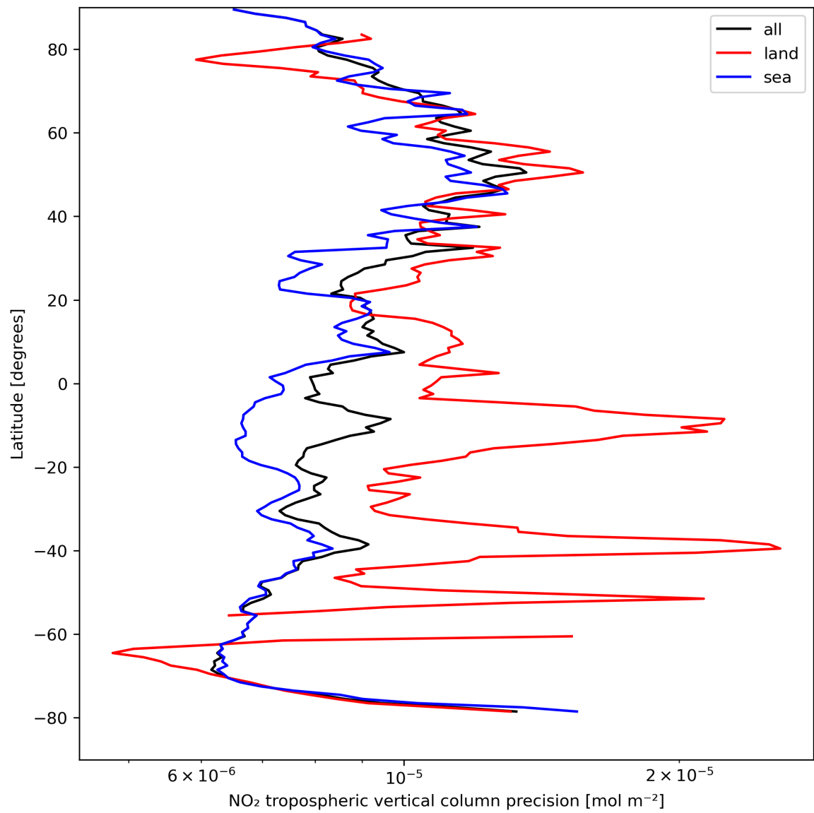
Figure 13: Zonal average of “NO 2 tropospheric vertical column precision” for 2023-08-27 to 2023-08-29.
