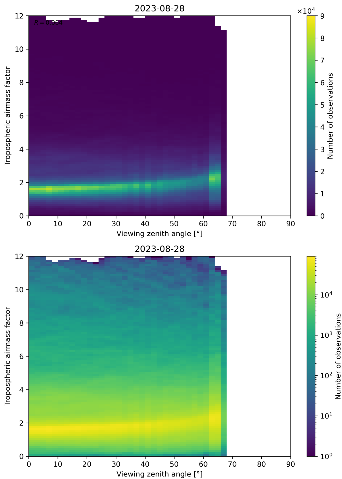
Figure 161: Scatter density plot of “Viewing zenith angle” against “Tropospheric airmass factor” for 2023-08-27 to 2023-08-29.
