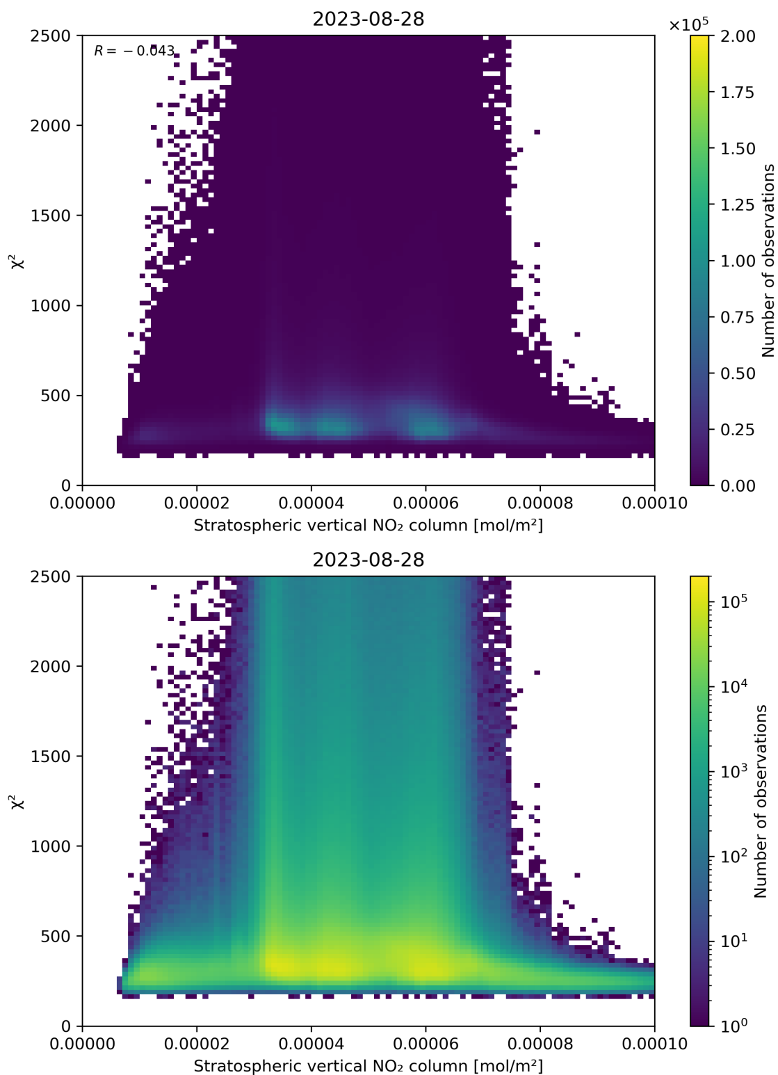
Figure 97: Scatter density plot of “Stratospheric vertical NO 2 column” against “ \chi^2 ” for 2023-08-27 to 2023-08-29.
