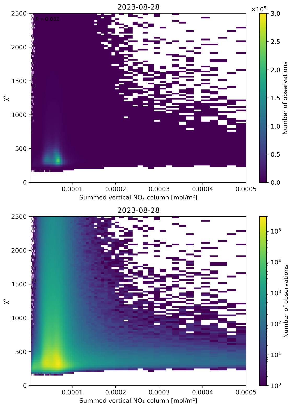
Figure 104: Scatter density plot of “Summed vertical NO 2 column” against “ \chi^2 ” for 2023-08-27 to 2023-08-29.
