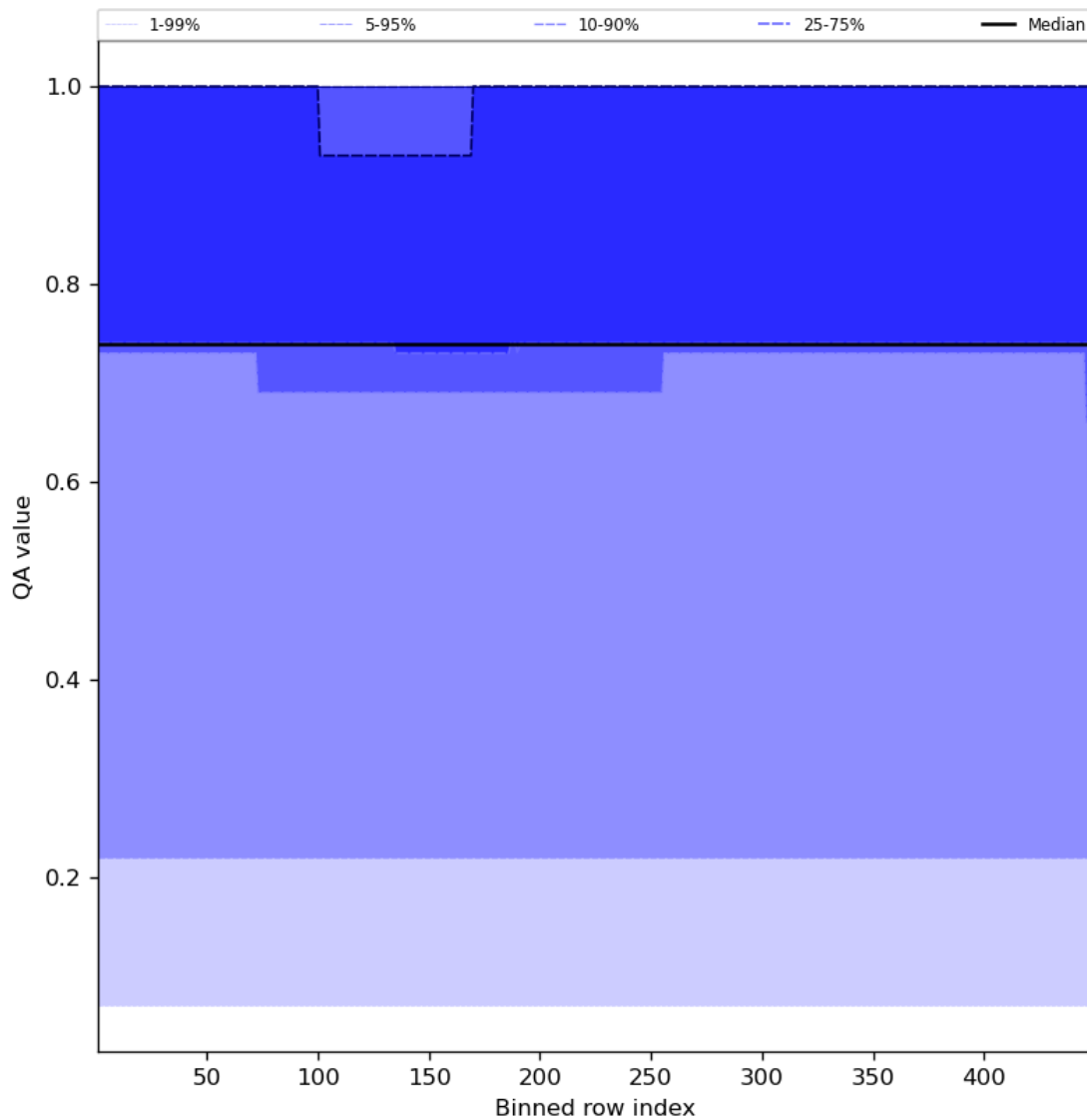
Figure 45: Along track statistics of “QA value” for 2023-08-27 to 2023-08-29
