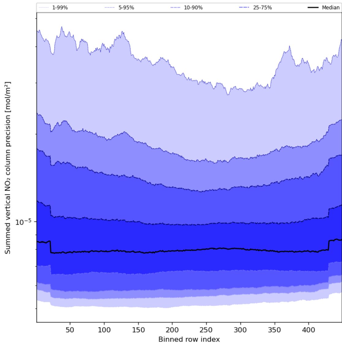
Figure 58: Along track statistics of “Summed vertical NO 2 column precision” for 2023-08-27 to 2023-08-29
