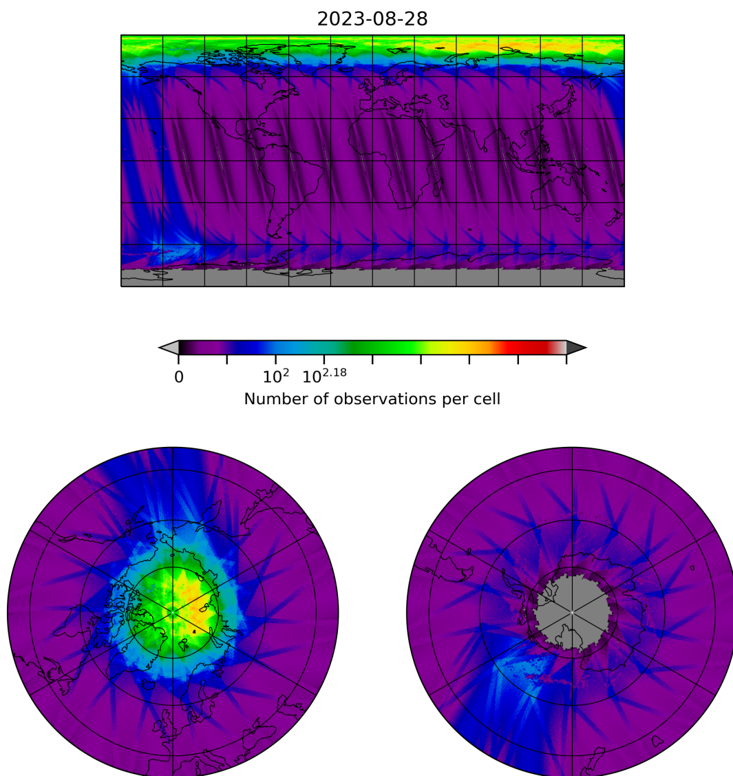
Figure 10: Map of the number of observations for 2023-08-27 to 2023-08-29
