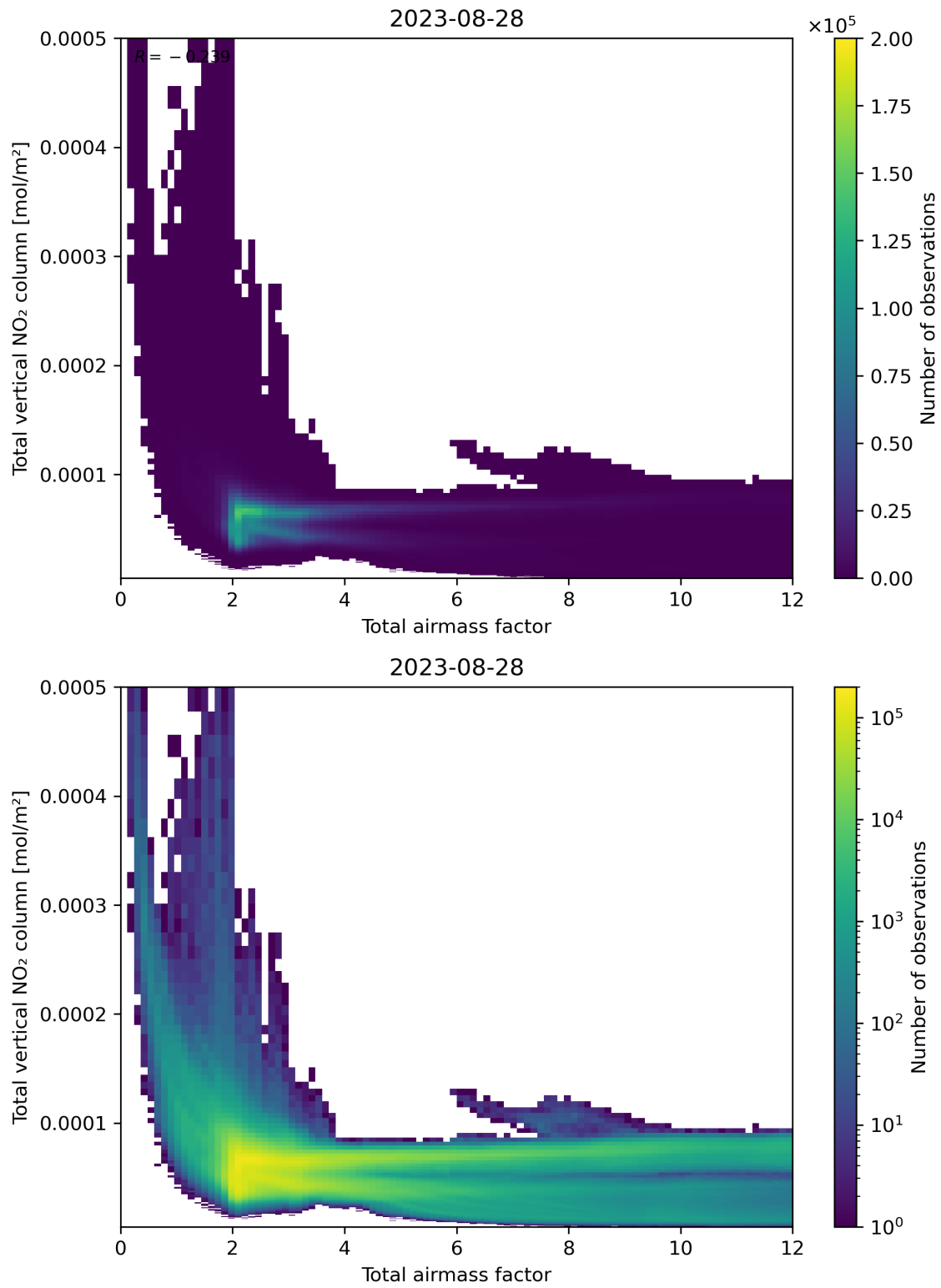
Figure 67: Scatter density plot of “Total airmass factor” against “Total vertical NO 2 column” for 2023-08-27 to 2023-08-29.
