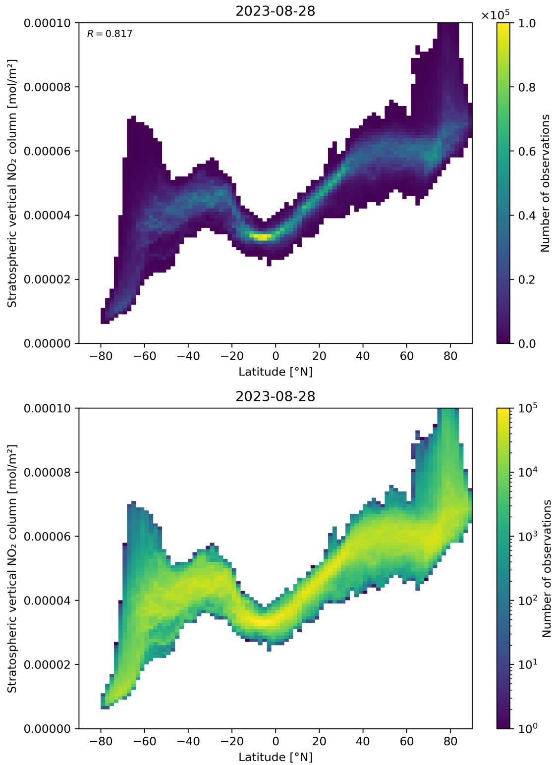
Figure 87: Scatter density plot of “Latitude” against “Stratospheric vertical NO 2 column” for 2023-08-27 to 2023-08-29.
