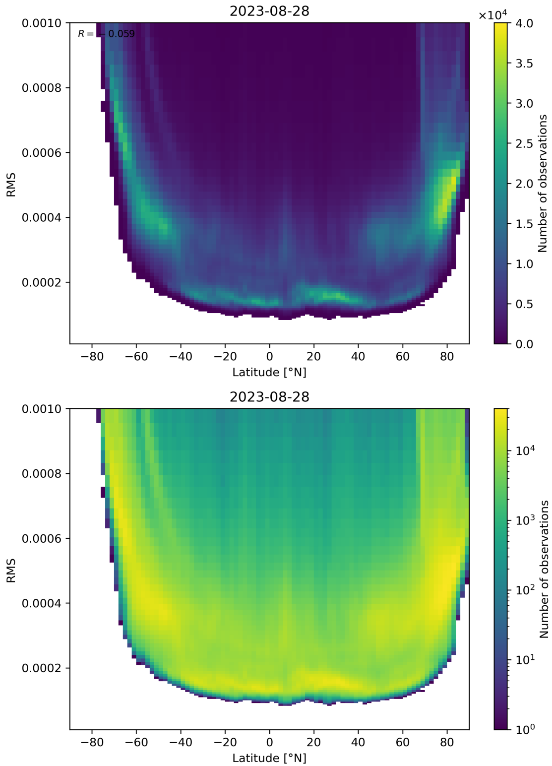
Figure 94: Scatter density plot of “Latitude” against “RMS” for 2023-08-27 to 2023-08-29.
