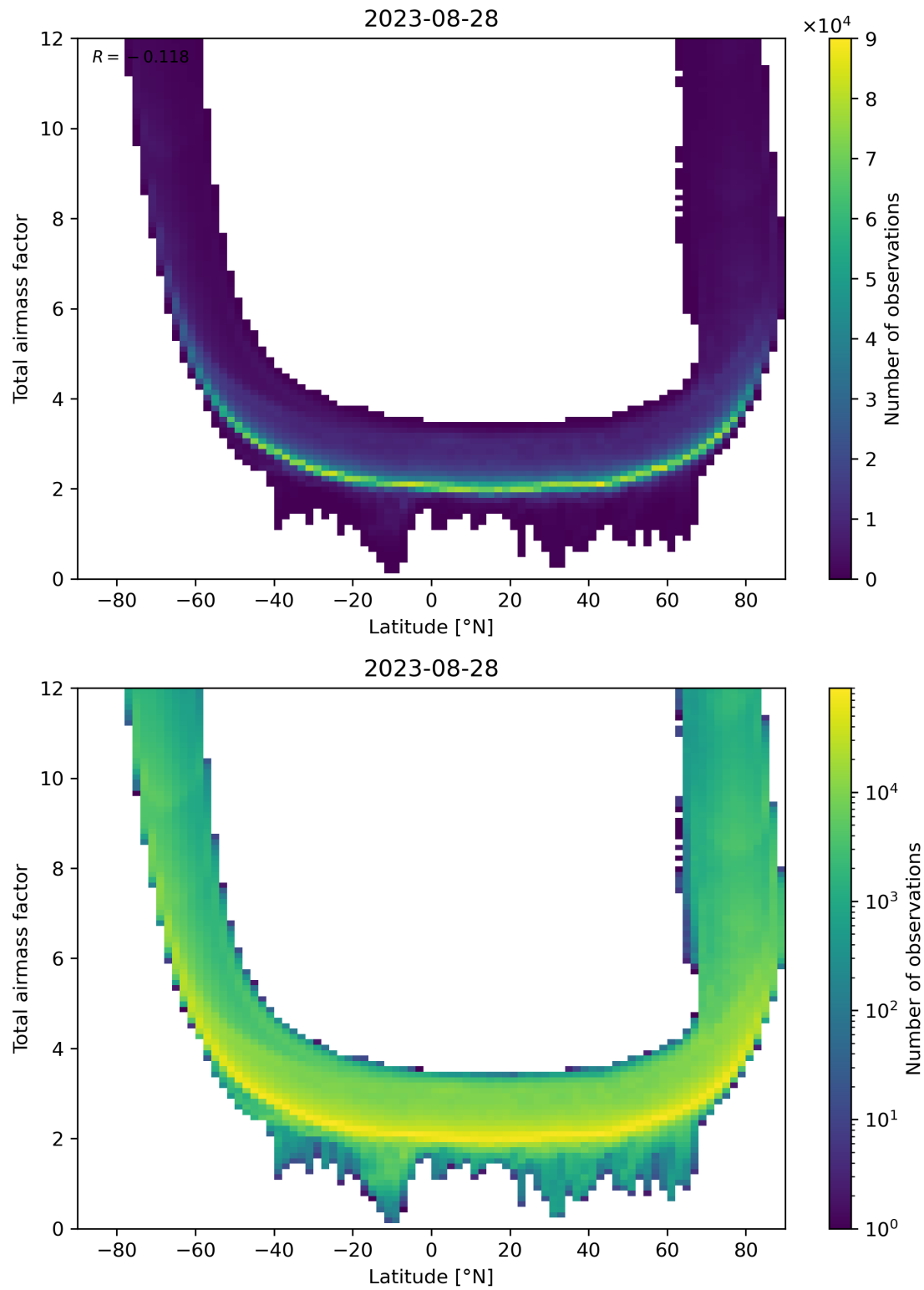
Figure 84: Scatter density plot of “Latitude” against “Total airmass factor” for 2023-08-27 to 2023-08-29.
