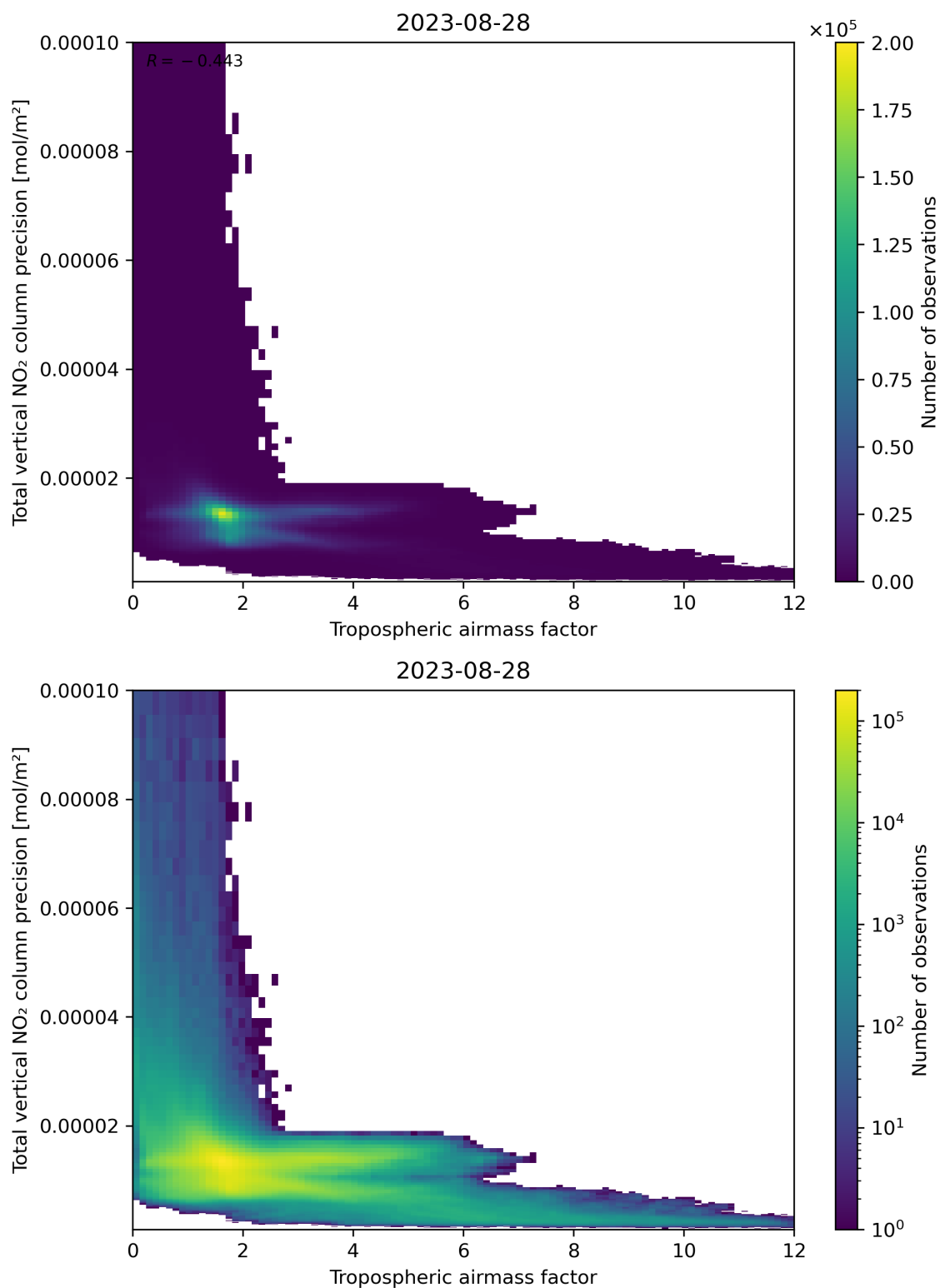
Figure 78: Scatter density plot of “Tropospheric air mass factor” against “Total vertical NO 2 column precision” for 2023-08-27 to 2023-08-29.
