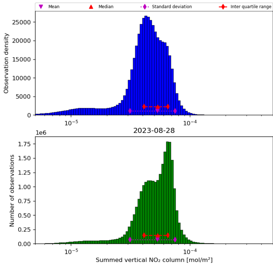
Figure 40: Histogram of “Summed vertical NO 2 column” for 2023-08-27 to 2023-08-29
