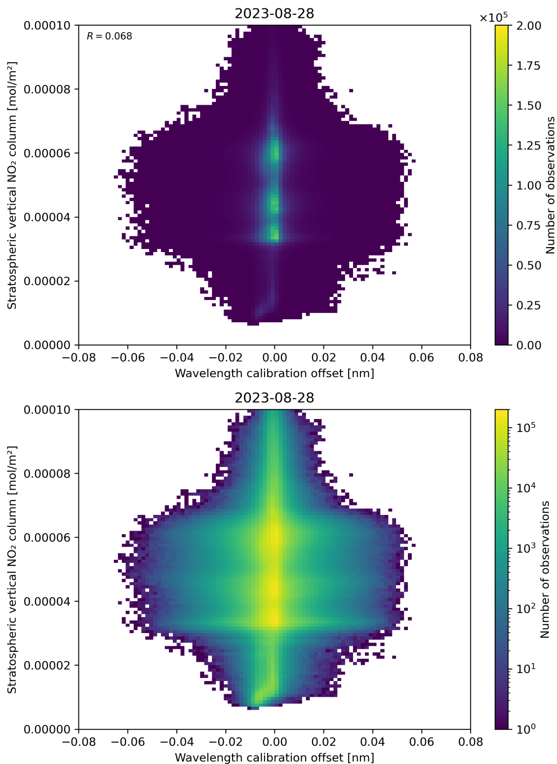
Figure 176: Scatter density plot of “Wavelength calibration offset” against “Stratospheric vertical NO 2 column” for 2023-08-27 to 2023-08-29.
