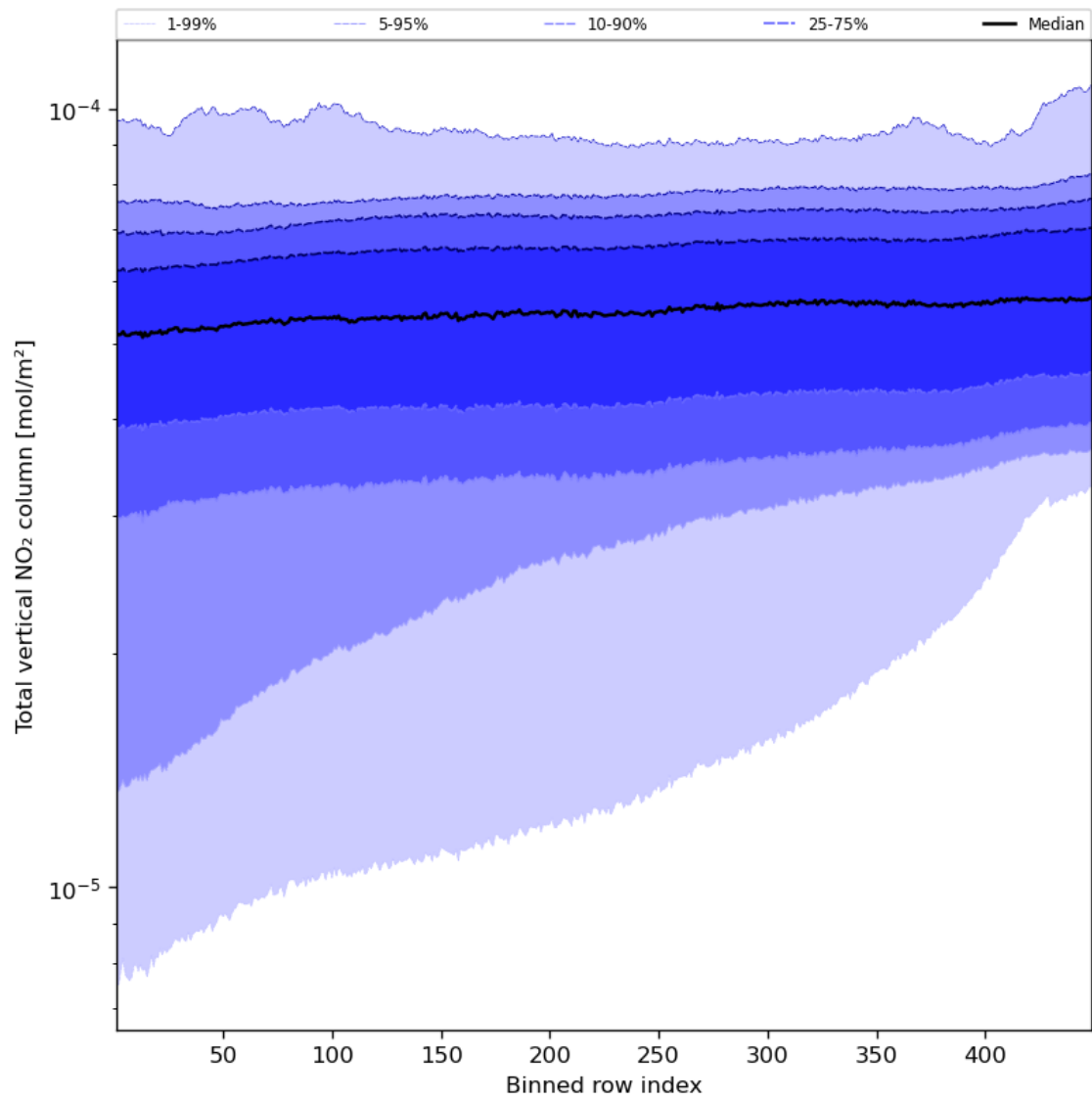
Figure 55: Along track statistics of “Total vertical NO 2 column” for 2023-08-27 to 2023-08-29
