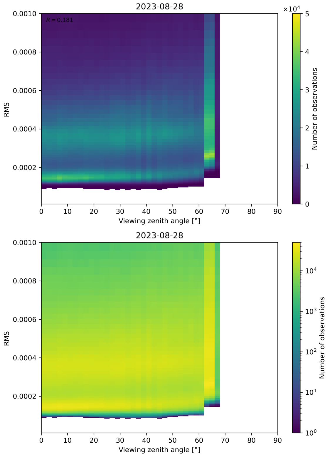
Figure 171: Scatter density plot of “Viewing zenith angle” against “RMS” for 2023-08-27 to 2023-08-29.
