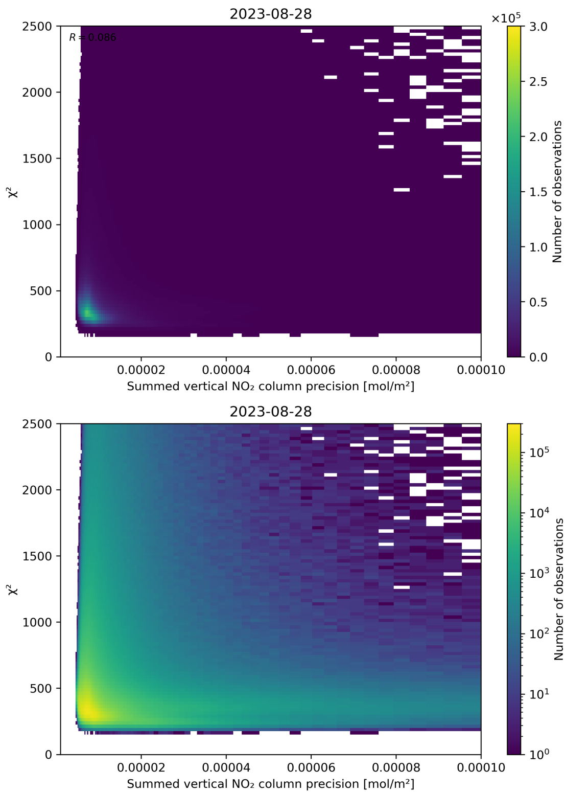
Figure 107: Scatter density plot of “Summed vertical NO 2 column precision” against “ \chi^2 ” for 2023-08-27 to 2023-08-29.
