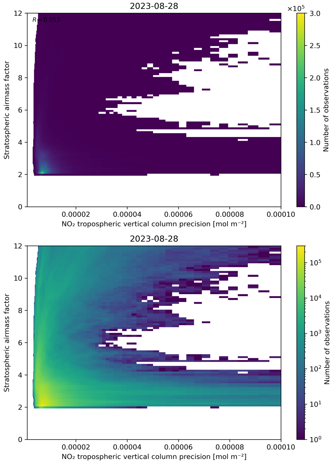
Figure 131: Scatter density plot of “NO 2 tropospheric vertical column precision” against “Stratospheric airmass factor” for 2023-08-27 to 2023-08-29.
