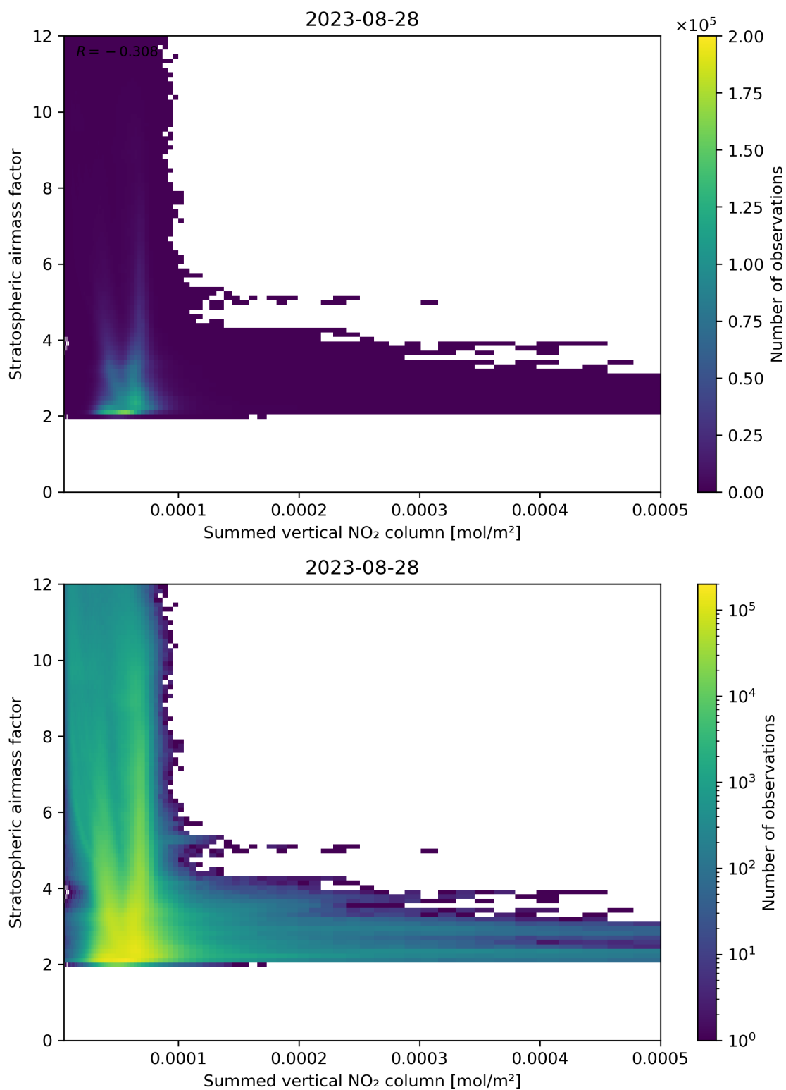
Figure 103: Scatter density plot of “Summed vertical NO 2 column” against “Stratospheric airmass factor” for 2023-08-27 to 2023-08-29.
