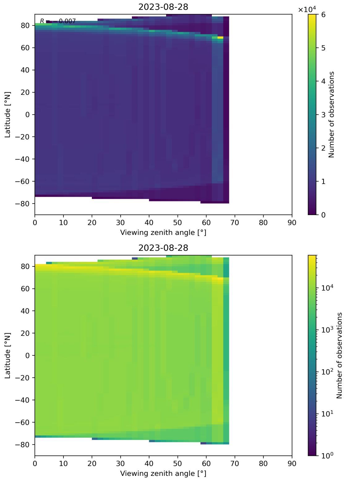
Figure 163: Scatter density plot of “Viewing zenith angle” against “Latitude” for 2023-08-27 to 2023-08-29.
