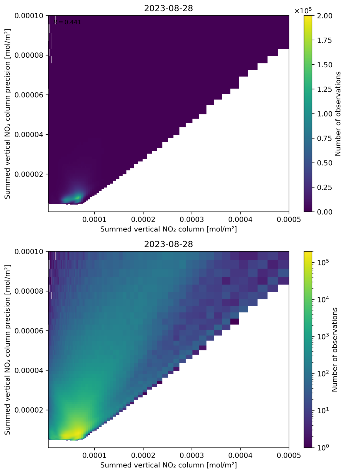
Figure 105: Scatter density plot of “Summed vertical NO 2 column” against “Summed vertical NO 2 column precision” for 2023-08-27 to 2023-08-29.
