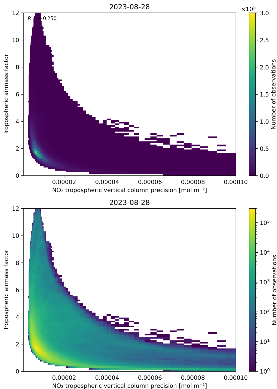
Figure 133: Scatter density plot of “NO 2 tropospheric vertical column precision” against “Tropospheric air mass factor” for 2023-08-27 to 2023-08-29.
