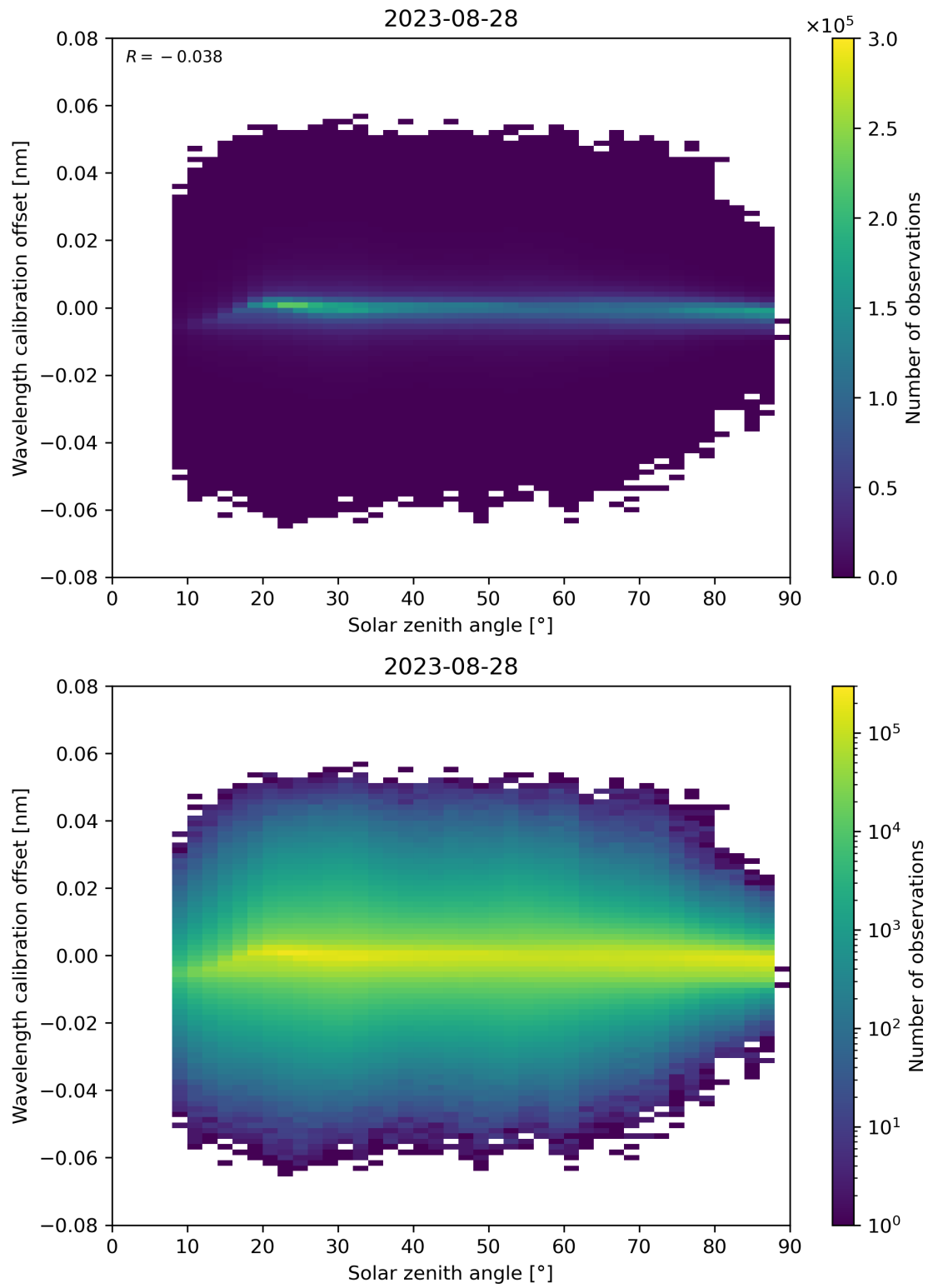
Figure 158: Scatter density plot of “Solar zenith angle” against “Wavelength calibration offset” for 2023-08-27 to 2023-08-29.
