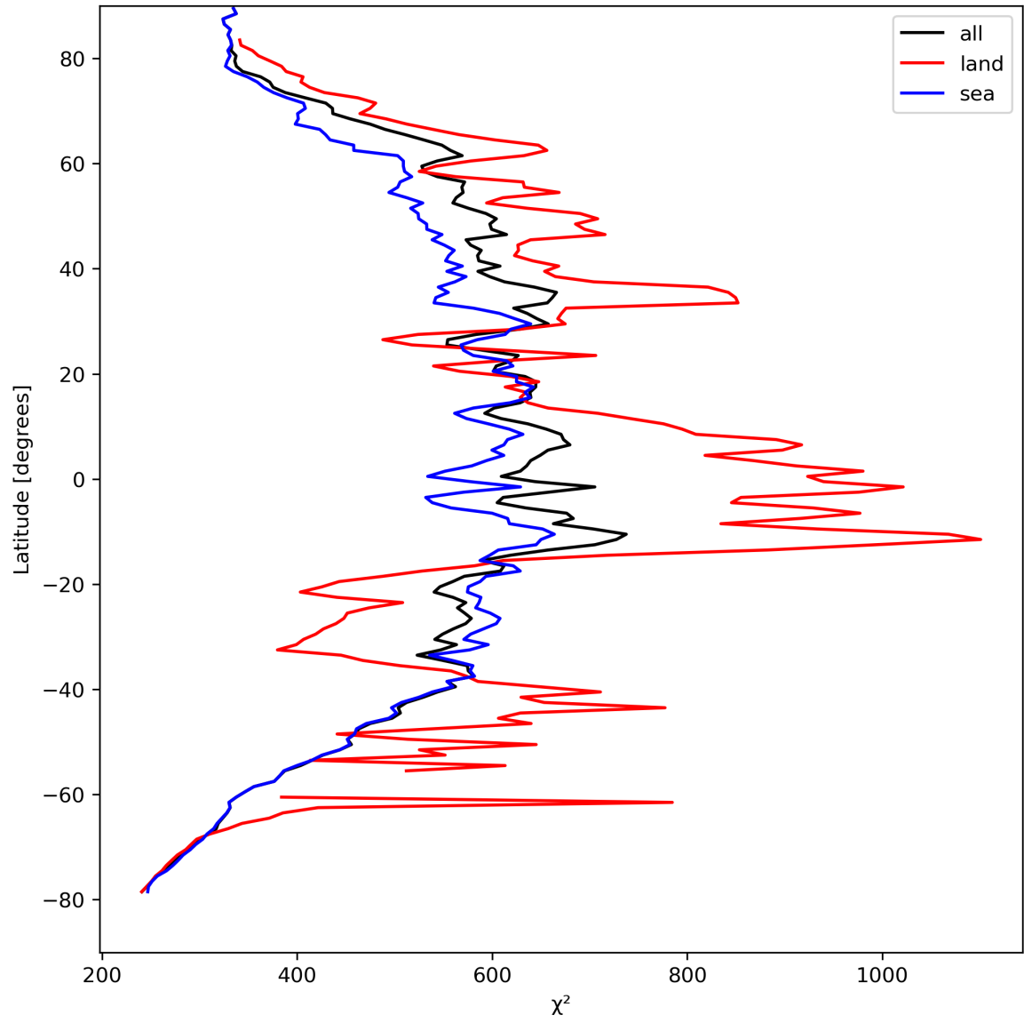
Figure 25: Zonal average of “ \chi^2 ” for 2023-08-27 to 2023-08-29.
