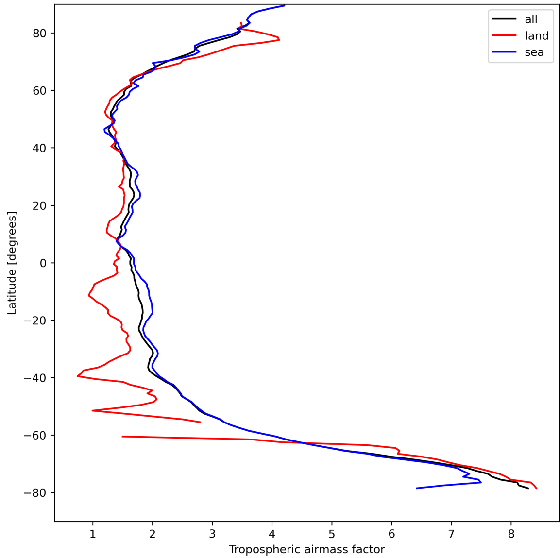
Figure 14: Zonal average of “Tropospheric airmass factor” for 2023-08-27 to 2023-08-29.
