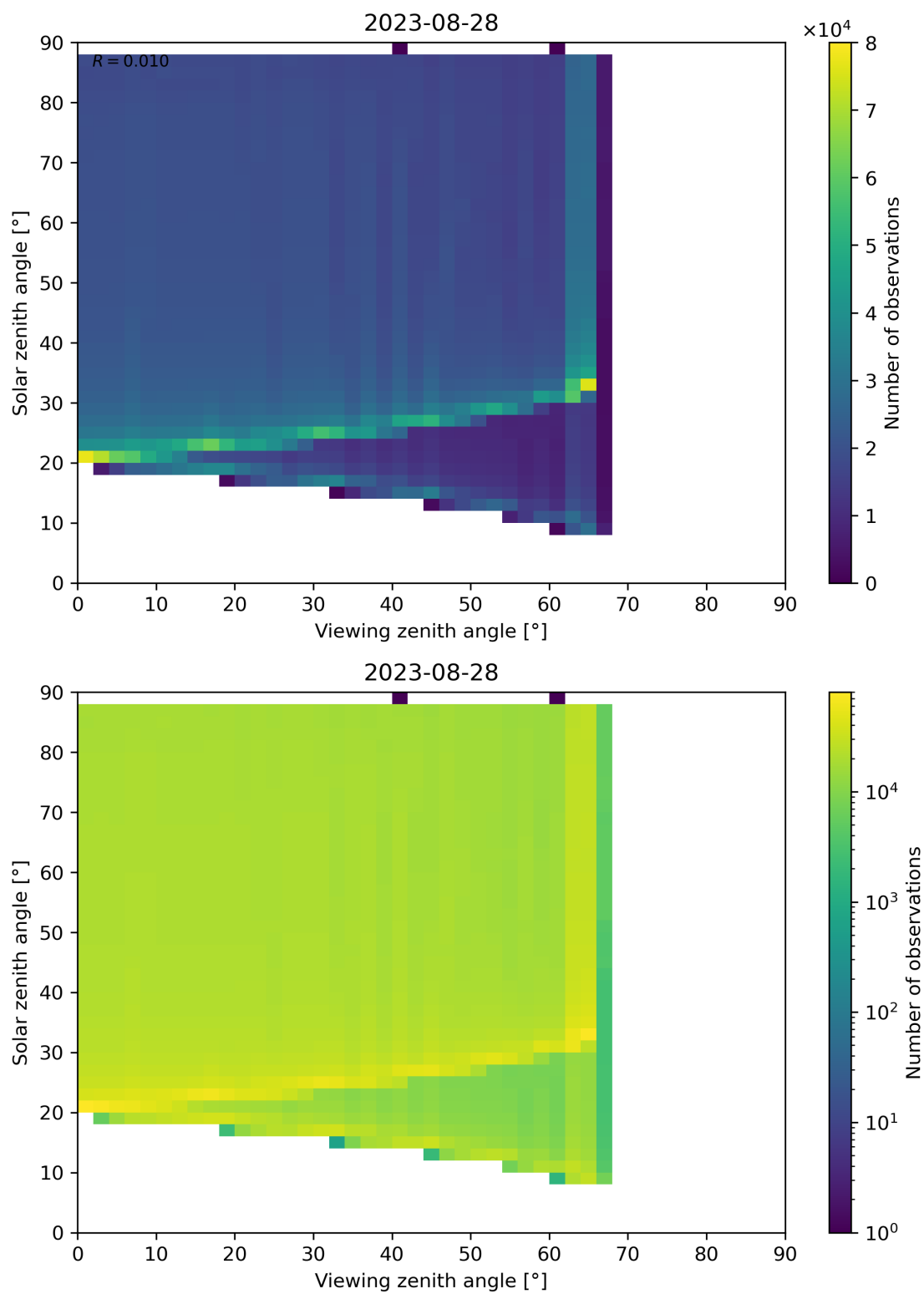
Figure 172: Scatter density plot of “Viewing zenith angle” against “Solar zenith angle” for 2023-08-27 to 2023-08-29.
