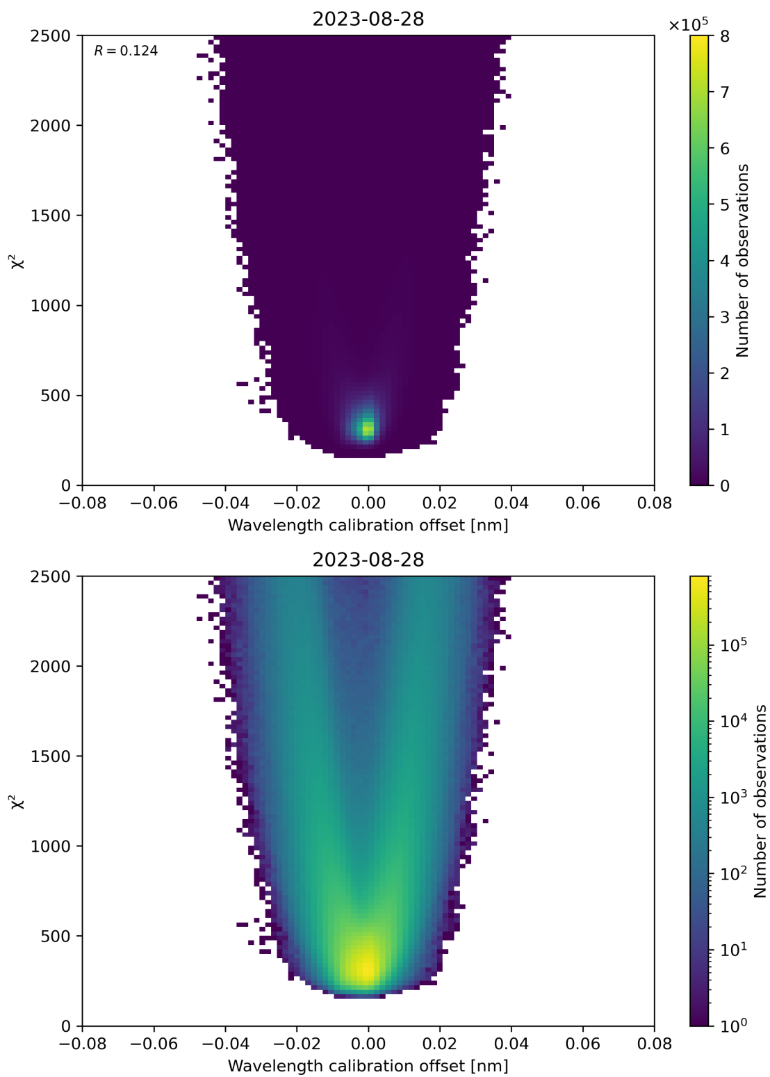
Figure 175: Scatter density plot of “Wavelength calibration offset” against “ \chi^2 ” for 2023-08-27 to 2023-08-29.
