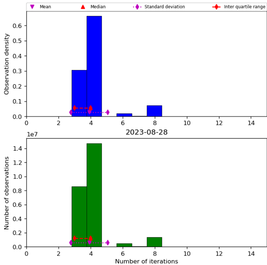
Figure 34: Histogram of “Number of iterations” for 2023-08-27 to 2023-08-29
