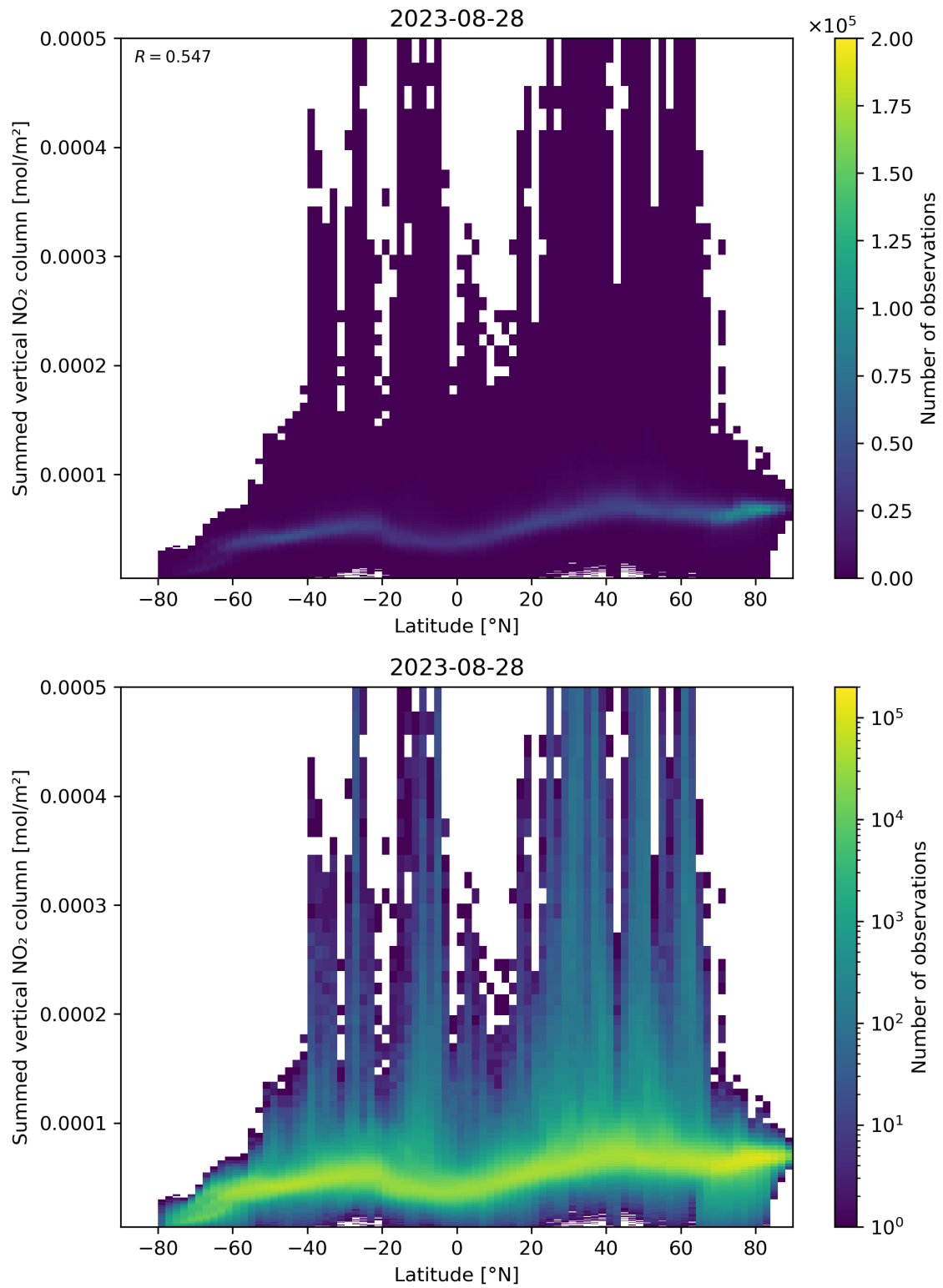
Figure 88: Scatter density plot of “Latitude” against “Summed vertical NO 2 column” for 2023-08-27 to 2023-08-29.
