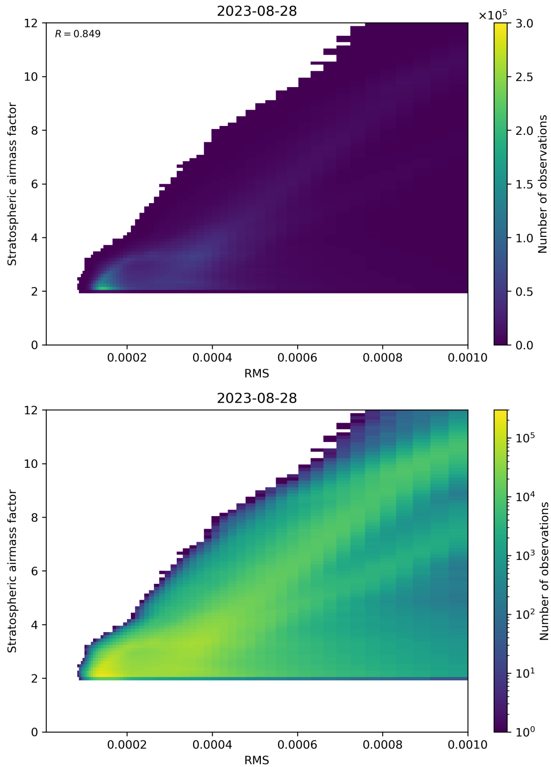
Figure 144: Scatter density plot of “RMS” against “Stratospheric airmass factor” for 2023-08-27 to 2023-08-29.
