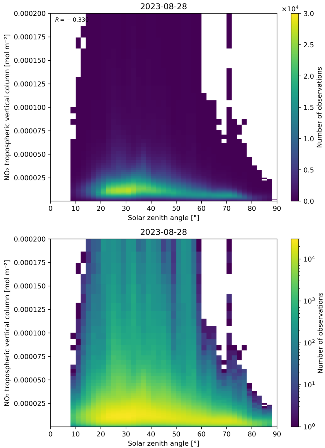
Figure 155: Scatter density plot of “Solar zenith angle” against “NO 2 tropospheric vertical column” for 2023-08-27 to 2023-08-29.
