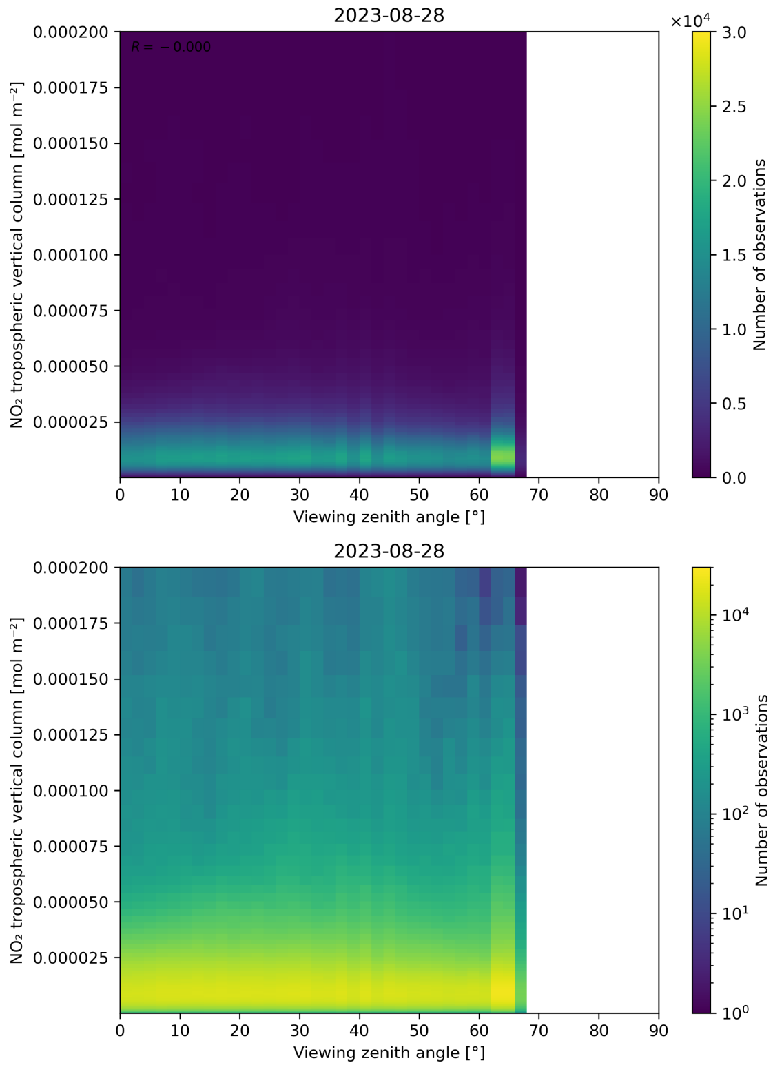
Figure 169: Scatter density plot of “Viewing zenith angle” against “NO 2 tropospheric vertical column” for 2023-08-27 to 2023-08-29.
