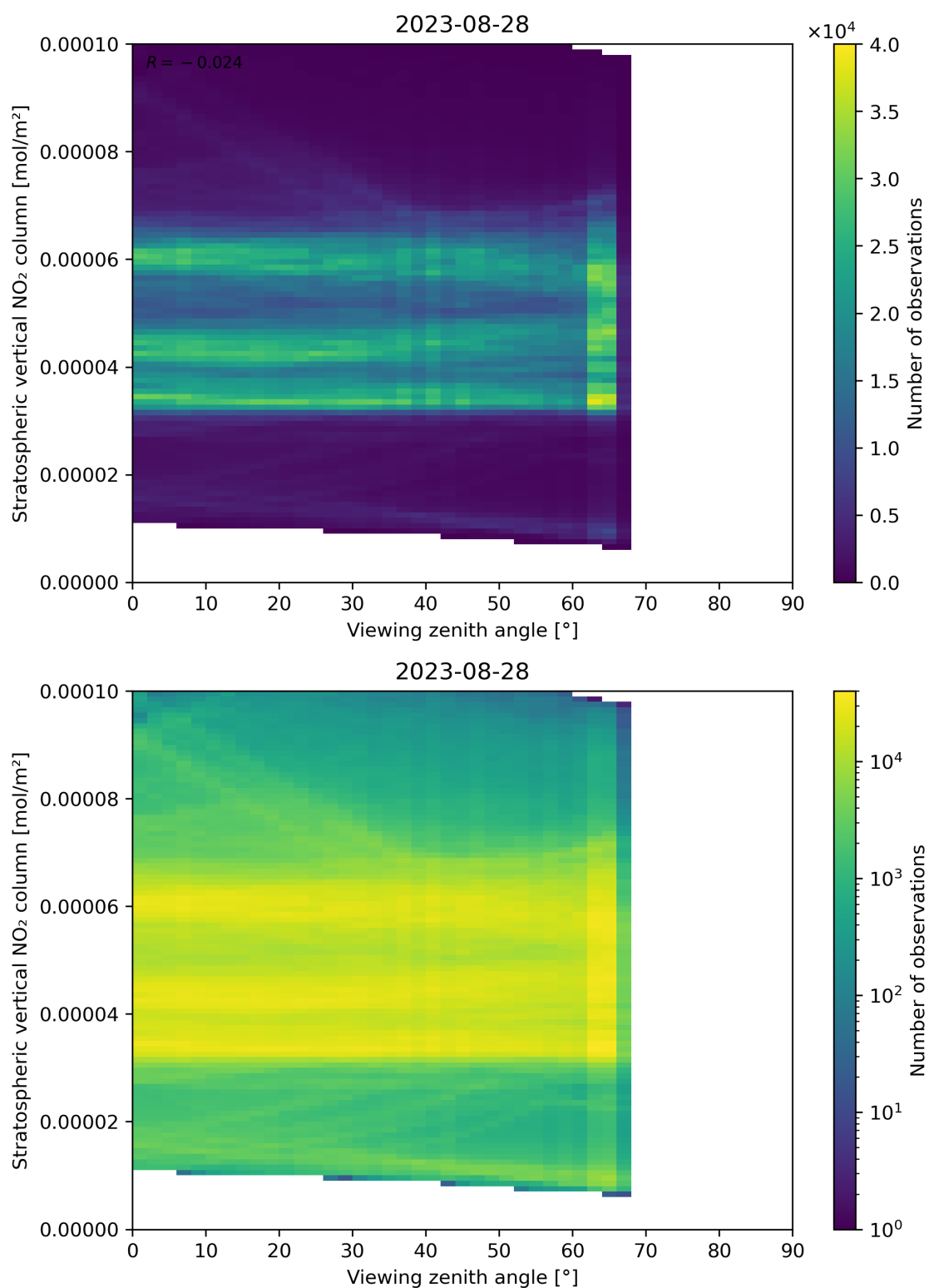
Figure 164: Scatter density plot of “Viewing zenith angle” against “Stratospheric vertical NO 2 column” for 2023-08-27 to 2023-08-29.
