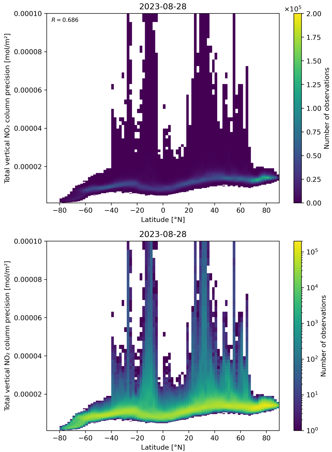
Figure 91: Scatter density plot of “Latitude” against “Total vertical NO 2 column precision” for 2023-08-27 to 2023-08-29.
