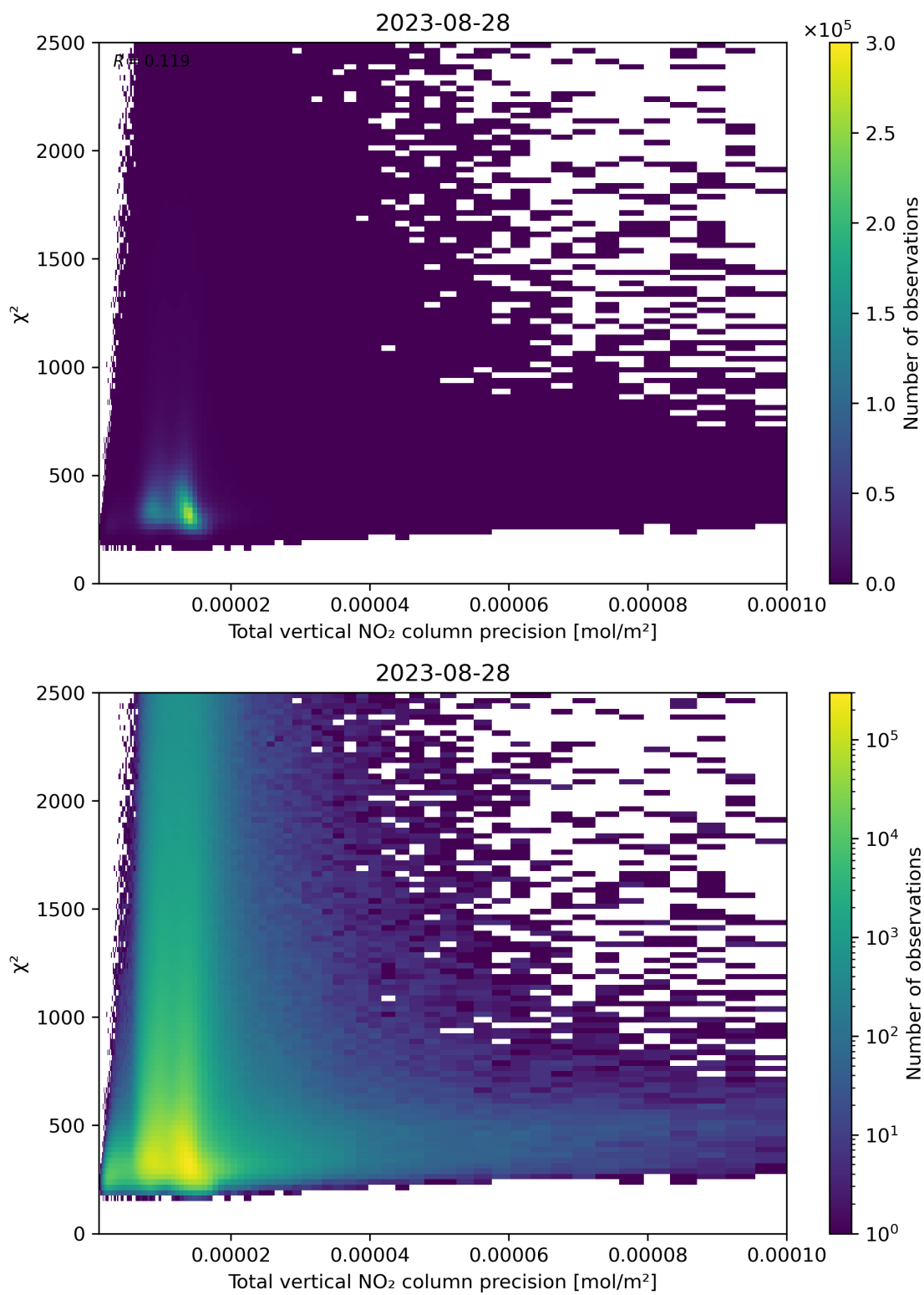
Figure 116: Scatter density plot of “Total vertical NO 2 column precision” against “ \chi^2 ” for 2023-08-27 to 2023-08-29.
