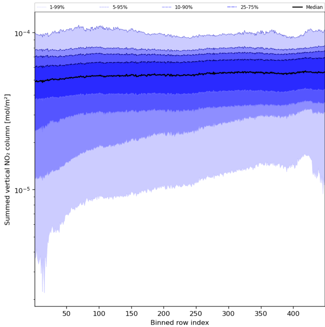
Figure 57: Along track statistics of “Summed vertical NO 2 column” for 2023-08-27 to 2023-08-29
