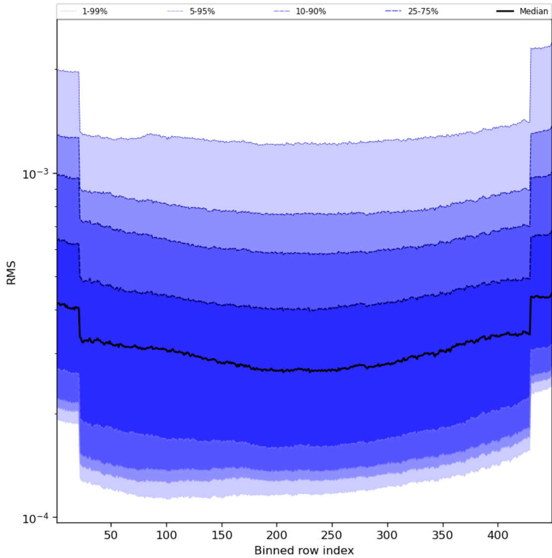
Figure 60: Along track statistics of “RMS” for 2023-08-27 to 2023-08-29
