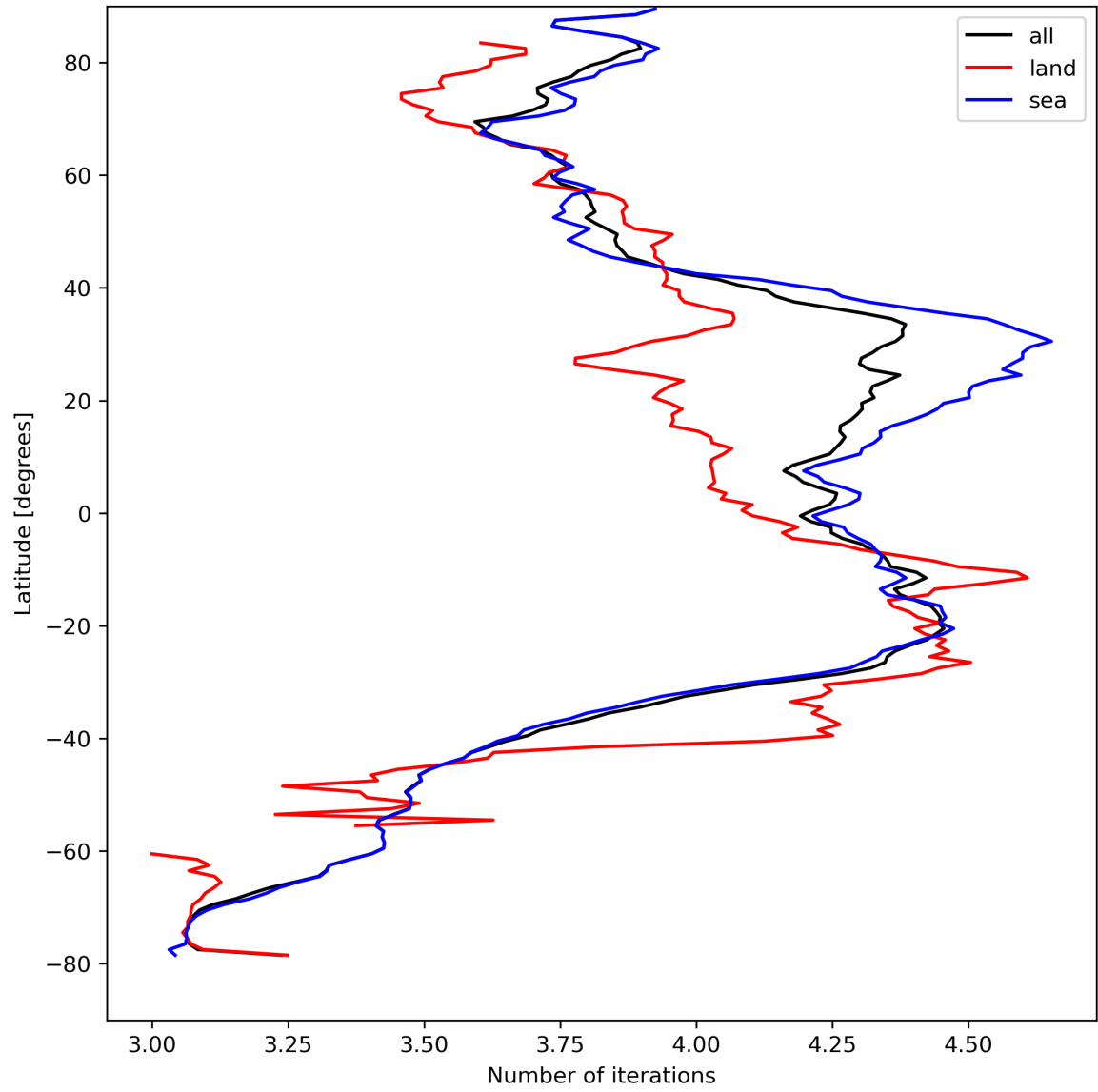
Figure 17: Zonal average of “Number of iterations” for 2023-08-27 to 2023-08-29.
