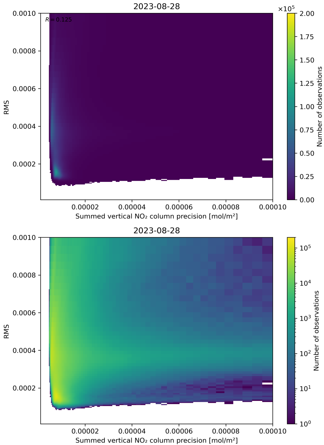
Figure 108: Scatter density plot of “Summed vertical NO 2 column precision” against “RMS” for 2023-08-27 to 2023-08-29.
