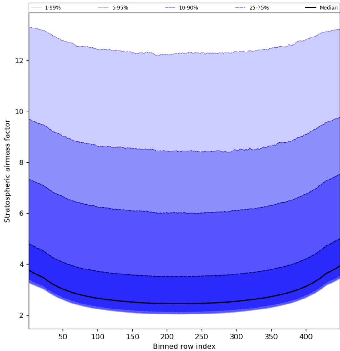
Figure 61: Along track statistics of “Stratospheric airmass factor” for 2023-08-27 to 2023-08-29
