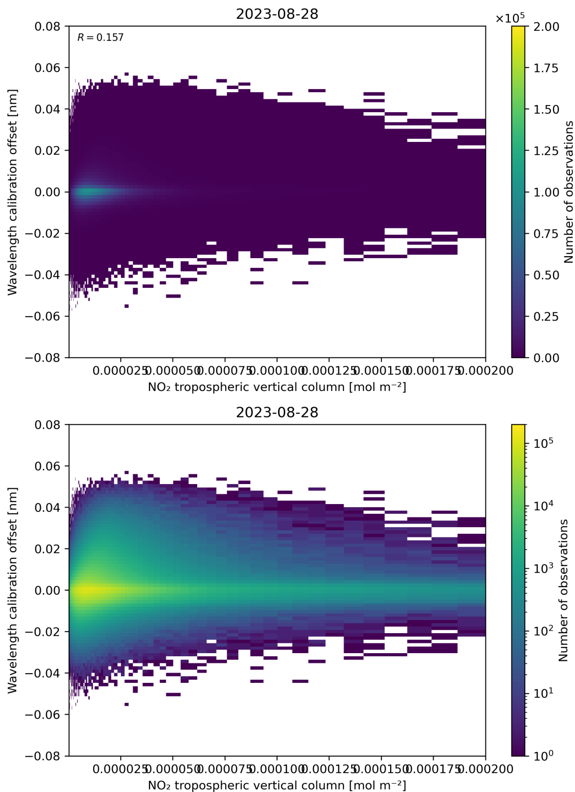
Figure 143: Scatter density plot of “NO 2 tropospheric vertical column” against “Wavelength calibration offset” for 2023-08-27 to 2023-08-29.
