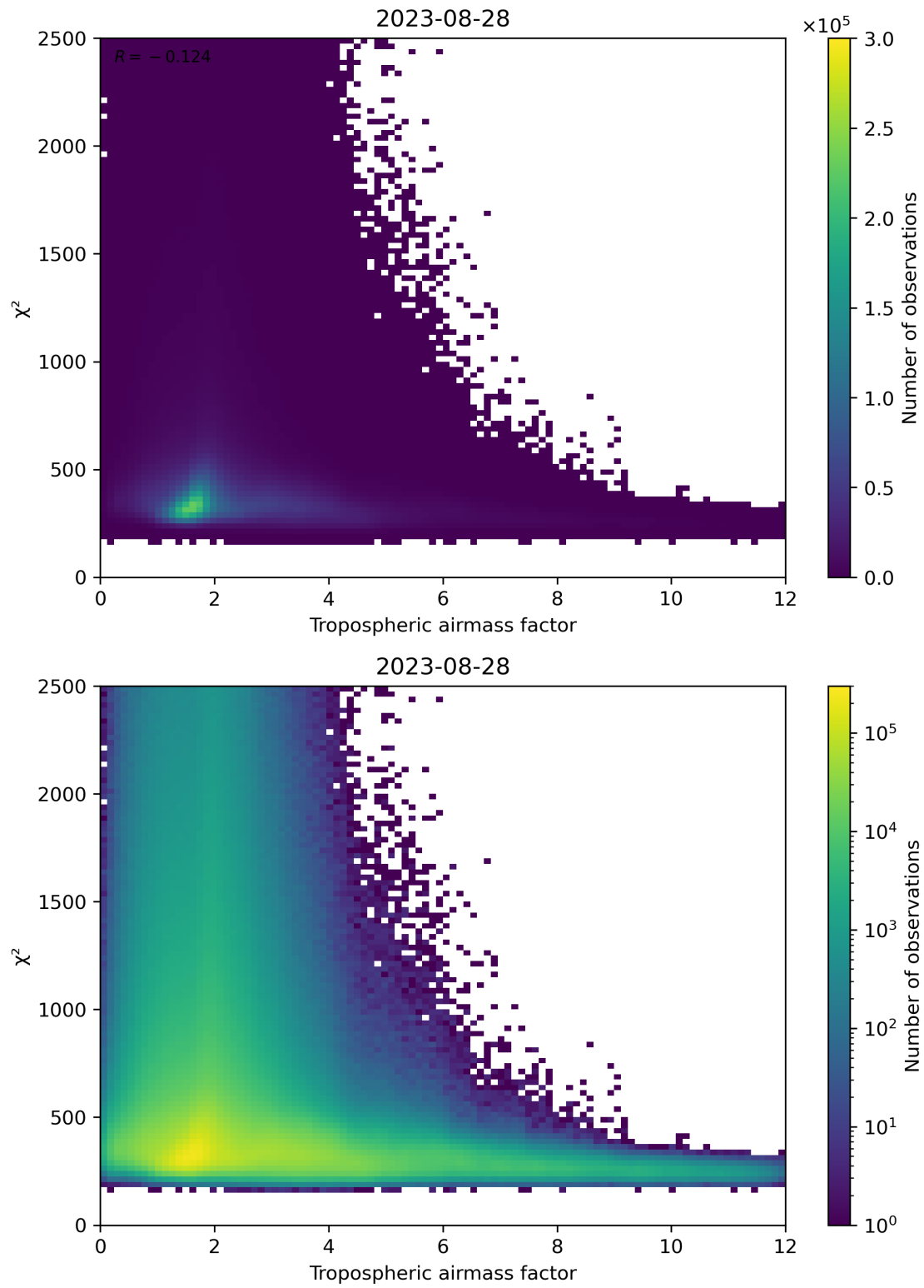
Figure 73: Scatter density plot of “Tropospheric airmass factor” against “ \chi^2 ” for 2023-08-27 to 2023-08-29.
