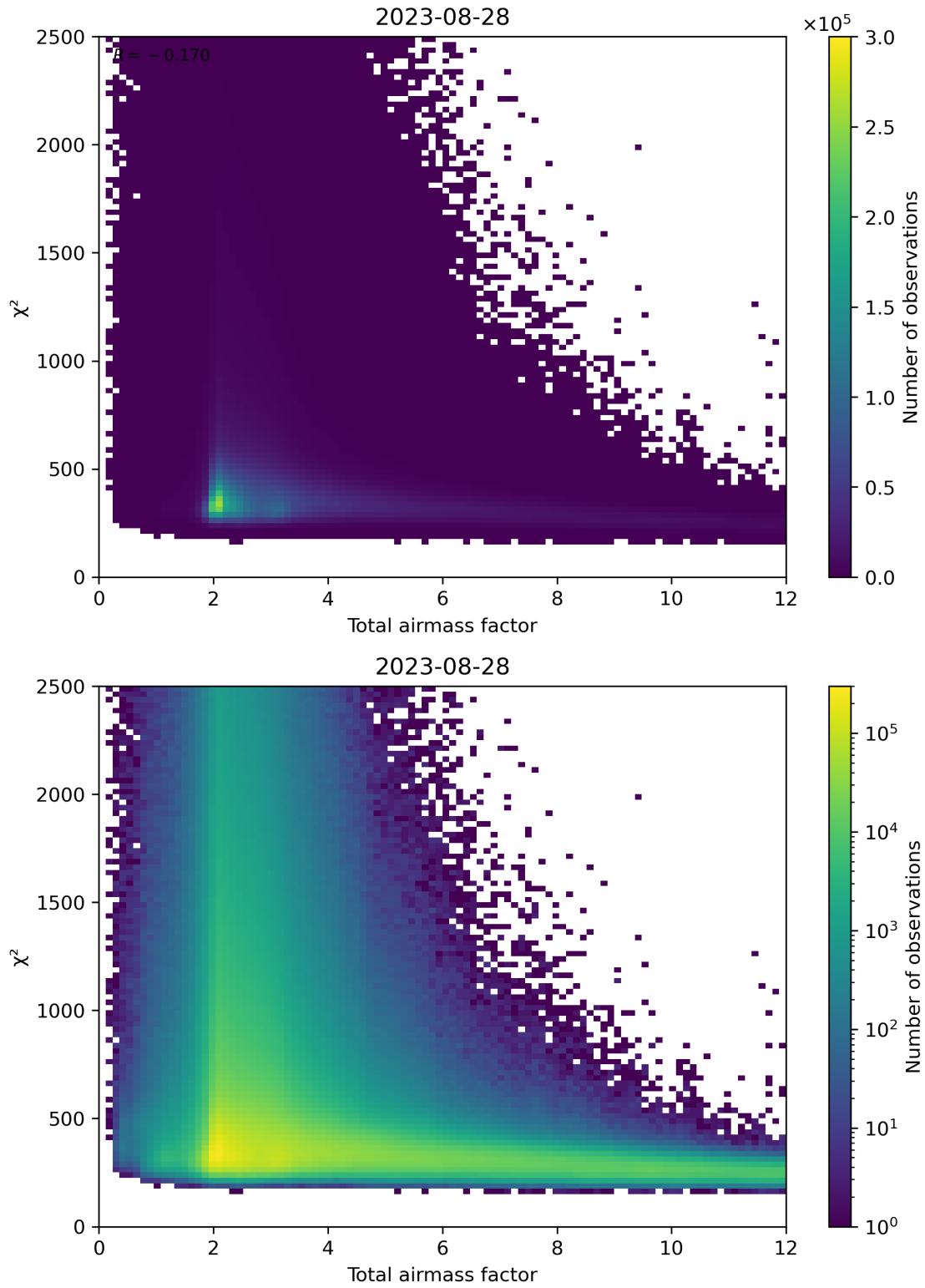
Figure 63: Scatter density plot of “Total airmass factor” against “ \chi^2 ” for 2023-08-27 to 2023-08-29.
