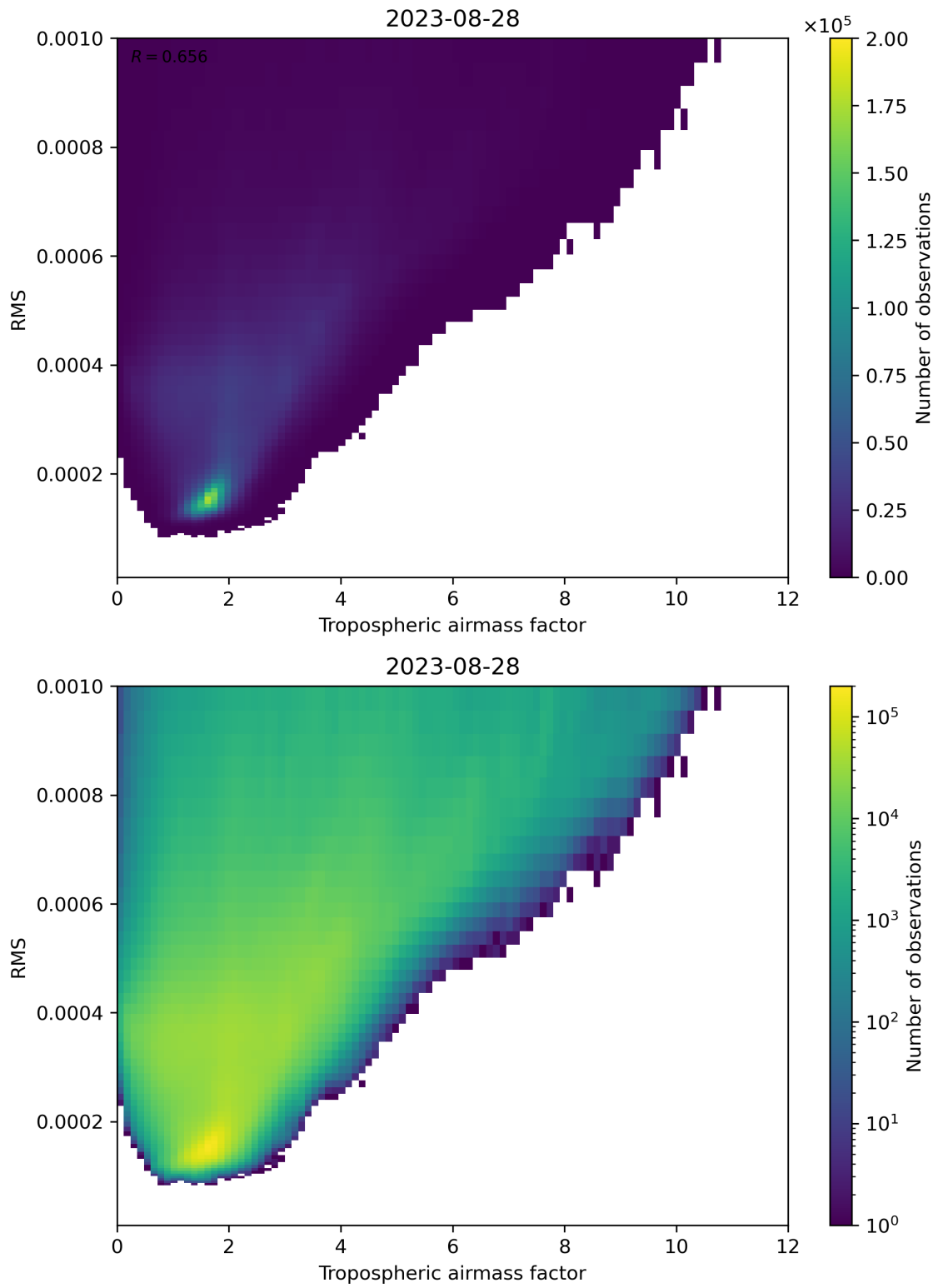
Figure 79: Scatter density plot of “Tropospheric airmass factor” against “RMS” for 2023-08-27 to 2023-08-29.
