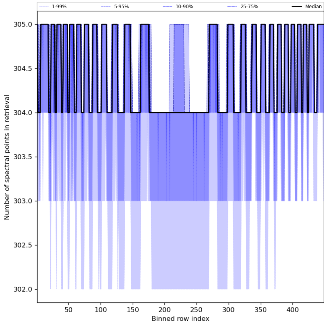
Figure 50: Along track statistics of “Number of spectral points in retrieval” for 2023-08-27 to 2023-08-29
