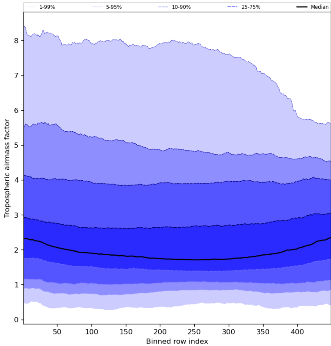
Figure 48: Along track statistics of “Tropospheric air mass factor” for 2023-08-27 to 2023-08-29
