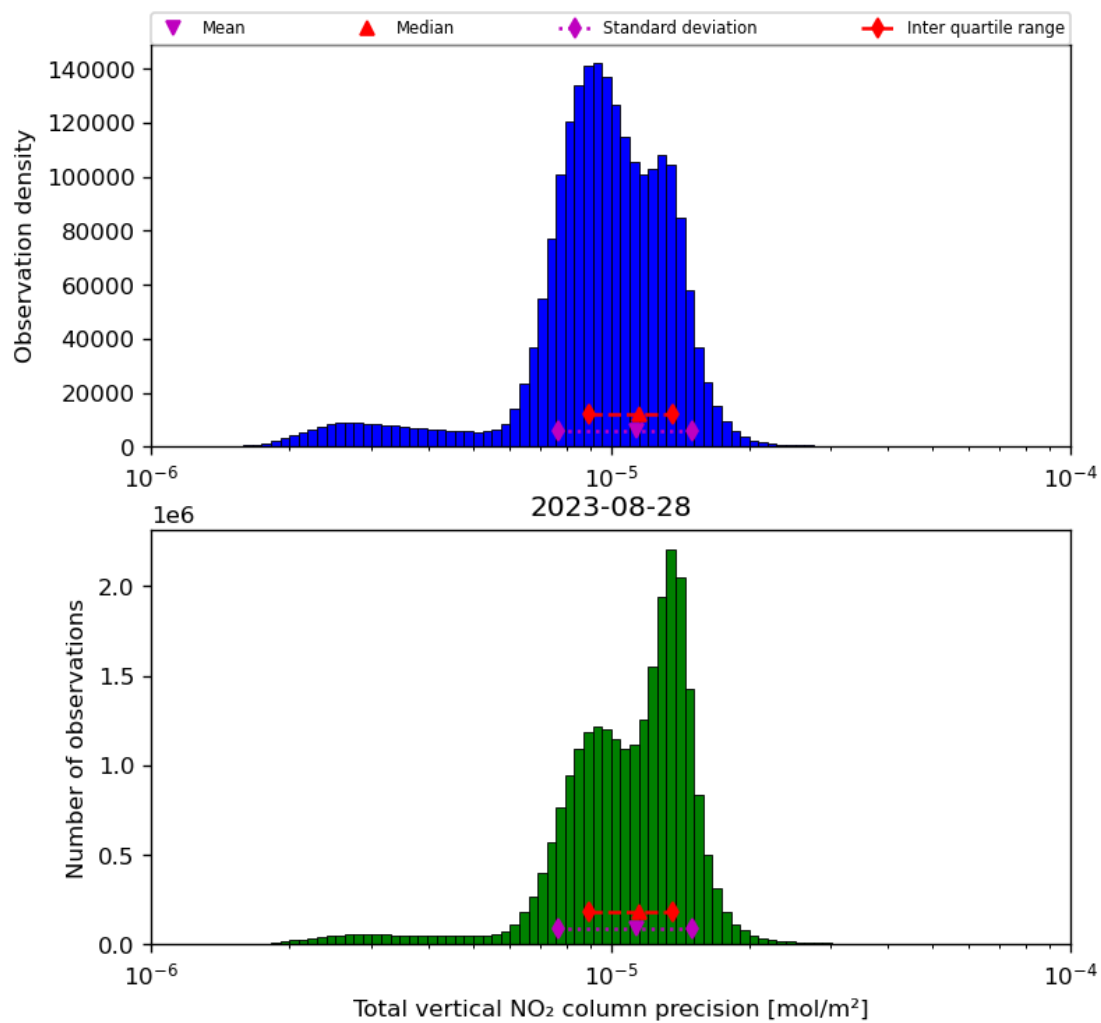
Figure 39: Histogram of “Total vertical NO 2 column precision” for 2023-08-27 to 2023-08-29
