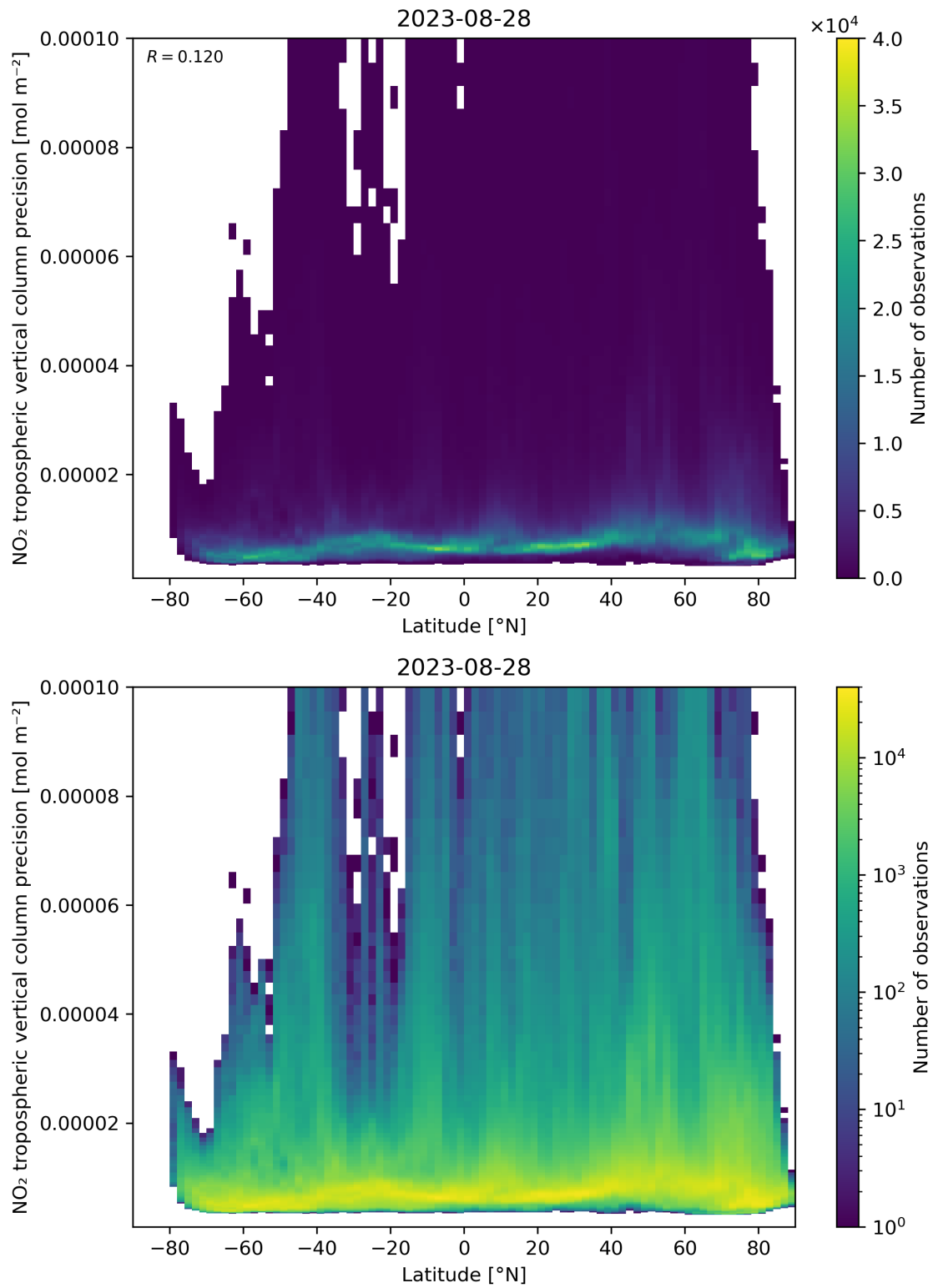
Figure 93: Scatter density plot of “Latitude” against “NO 2 tropospheric vertical column precision” for 2023-08-27 to 2023-08-29.
