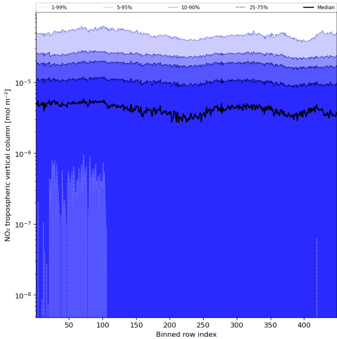
Figure 46: Along track statistics of “NO 2 tropospheric vertical column” for 2023-08-27 to 2023-08-29
