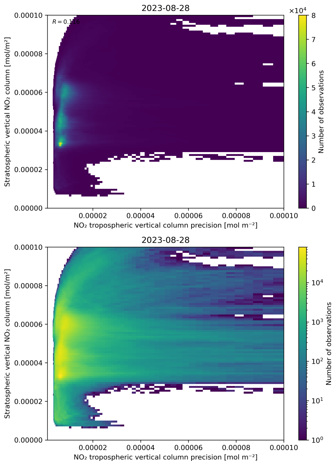
Figure 135: Scatter density plot of “NO 2 tropospheric vertical column precision” against “Stratospheric vertical NO 2 column” for 2023-08-27 to 2023-08-29.
