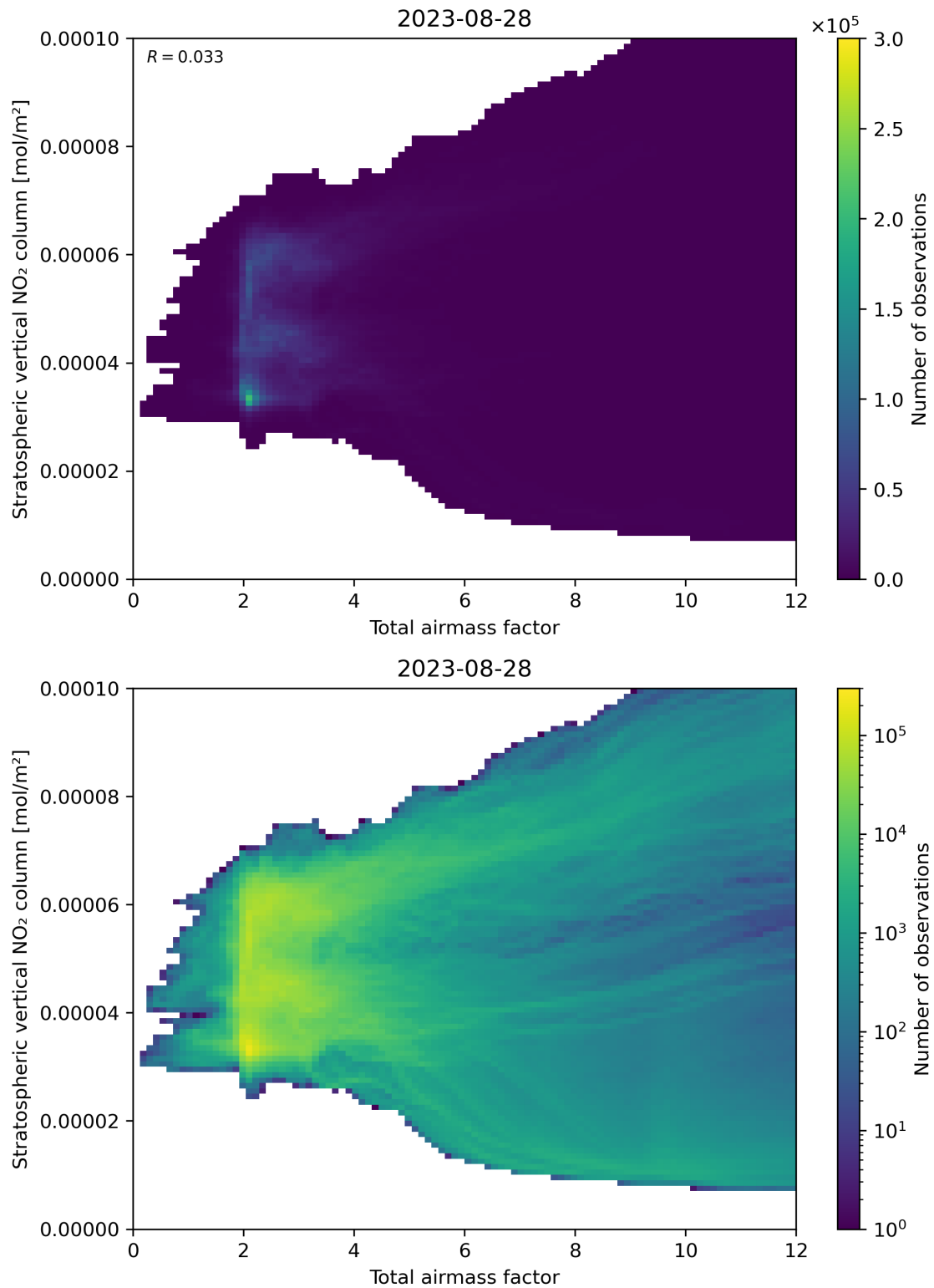
Figure 64: Scatter density plot of “Total airmass factor” against “Stratospheric vertical NO 2 column” for 2023-08-27 to 2023-08-29.
