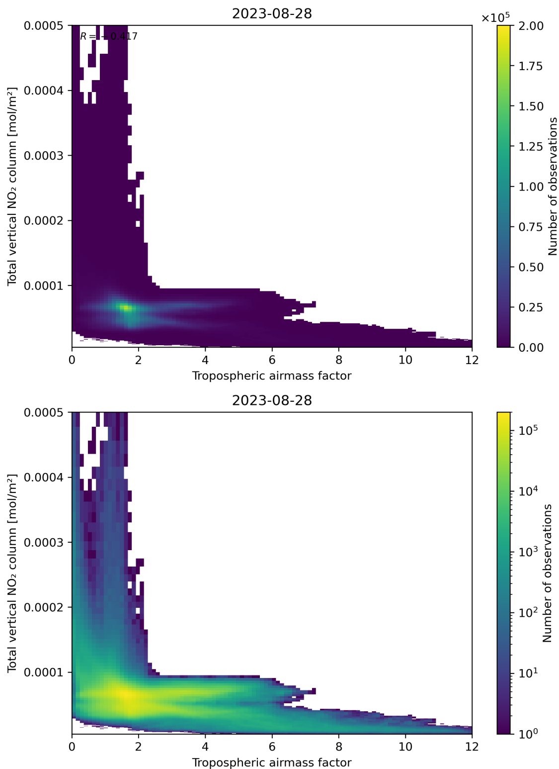
Figure 77: Scatter density plot of “Tropospheric airmass factor” against “Total vertical NO 2 column” for 2023-08-27 to 2023-08-29.
