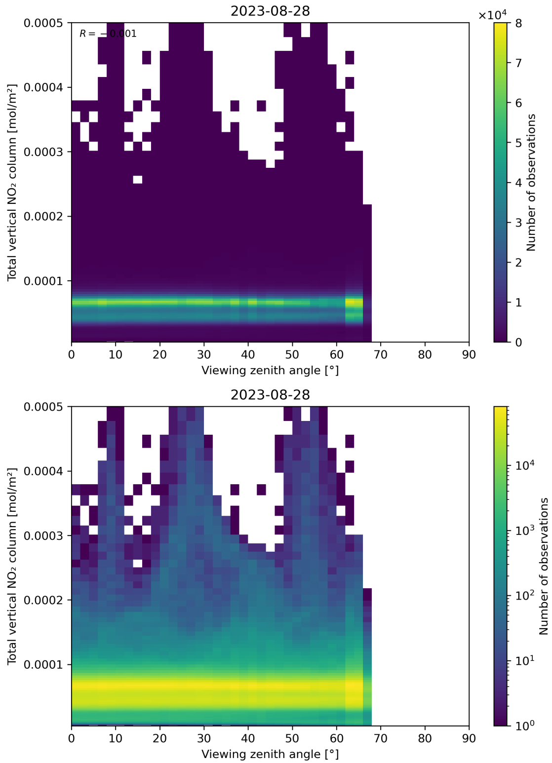
Figure 167: Scatter density plot of “Viewing zenith angle” against “Total vertical NO 2 column” for 2023-08-27 to 2023-08-29.
