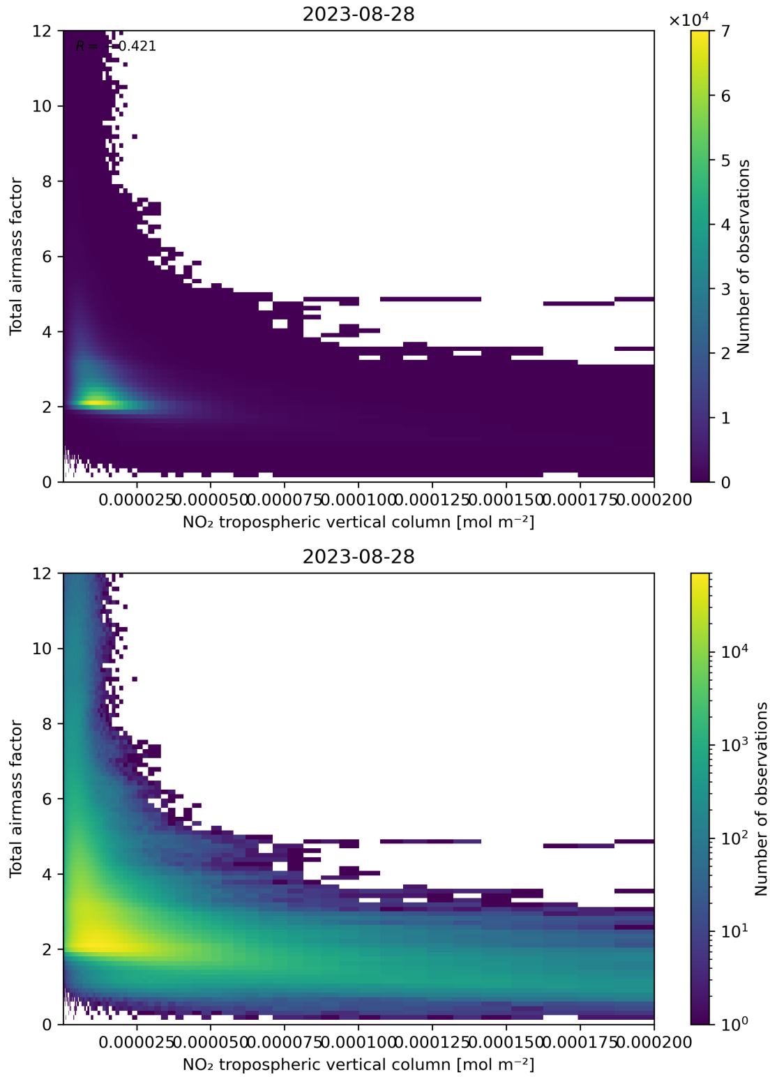
Figure 122: Scatter density plot of “NO 2 tropospheric vertical column” against “Total air mass factor” for 2023-08-27 to 2023-08-29.
