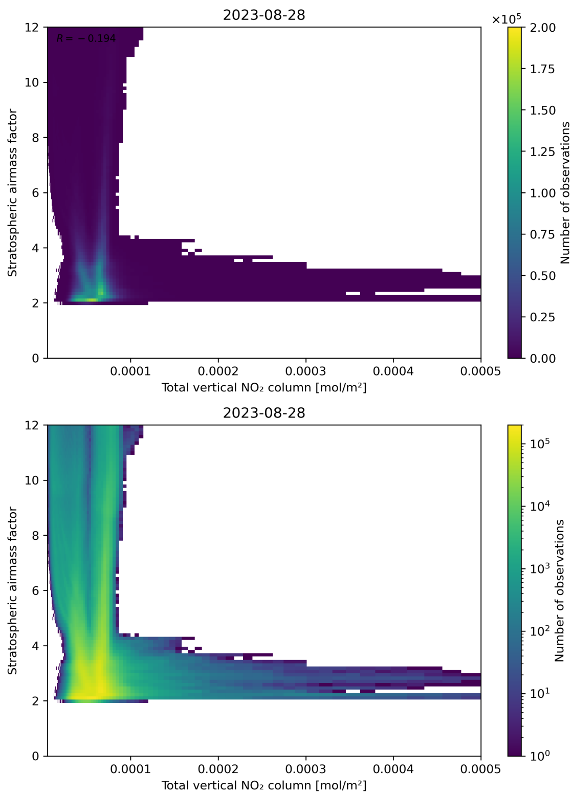
Figure 110: Scatter density plot of “Total vertical NO 2 column” against “Stratospheric airmass factor” for 2023-08-27 to 2023-08-29.
