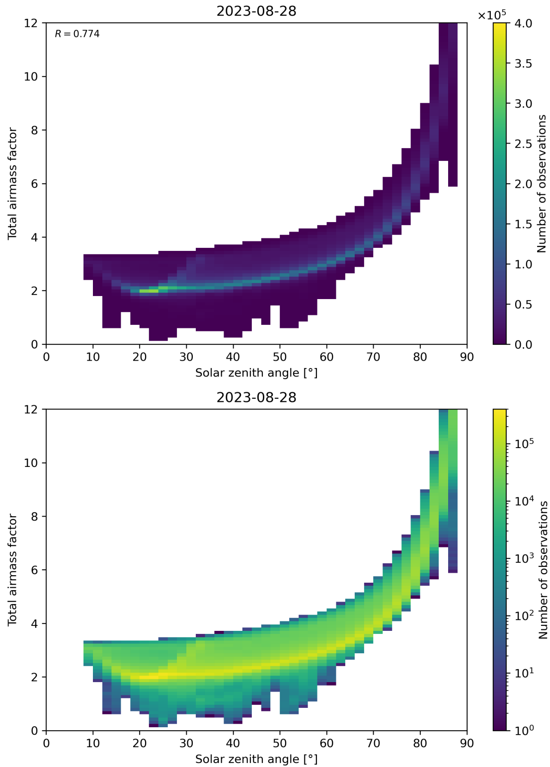
Figure 146: Scatter density plot of “Solar zenith angle” against “Total air mass factor” for 2023-08-27 to 2023-08-29.
