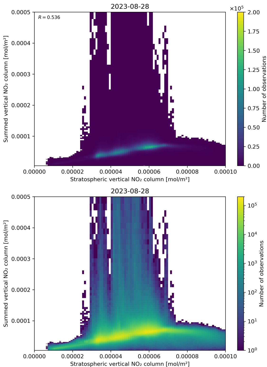
Figure 98: Scatter density plot of “Stratospheric vertical NO 2 column” against “Summed vertical NO 2 column” for 2023-08-27 to 2023-08-29.
