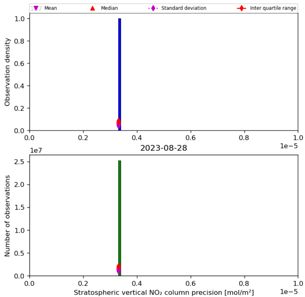
Figure 37: Histogram of “Stratospheric vertical NO 2 column precision” for 2023-08-27 to 2023-08-29
