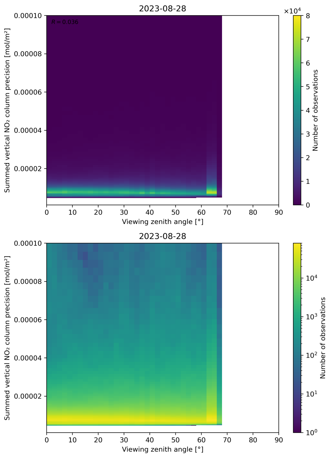
Figure 166: Scatter density plot of “Viewing zenith angle” against “Summed vertical NO 2 column precision” for 2023-08-27 to 2023-08-29.
