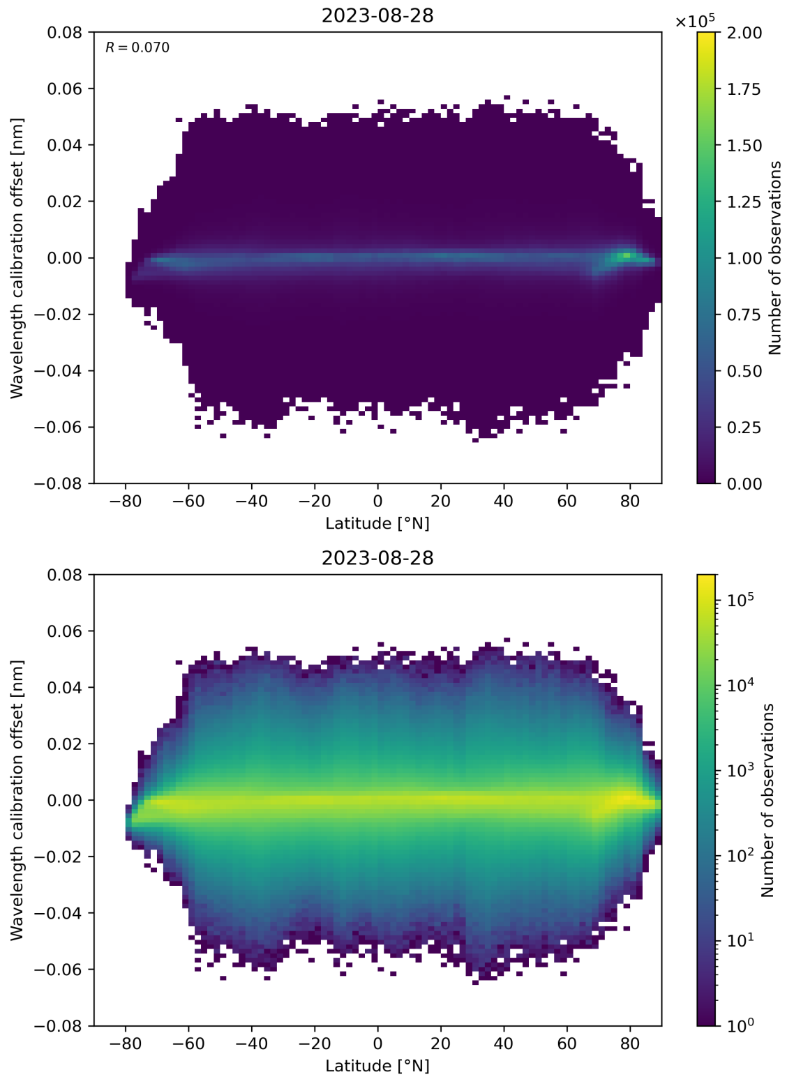
Figure 95: Scatter density plot of “Latitude” against “Wavelength calibration offset” for 2023-08-27 to 2023-08-29.
