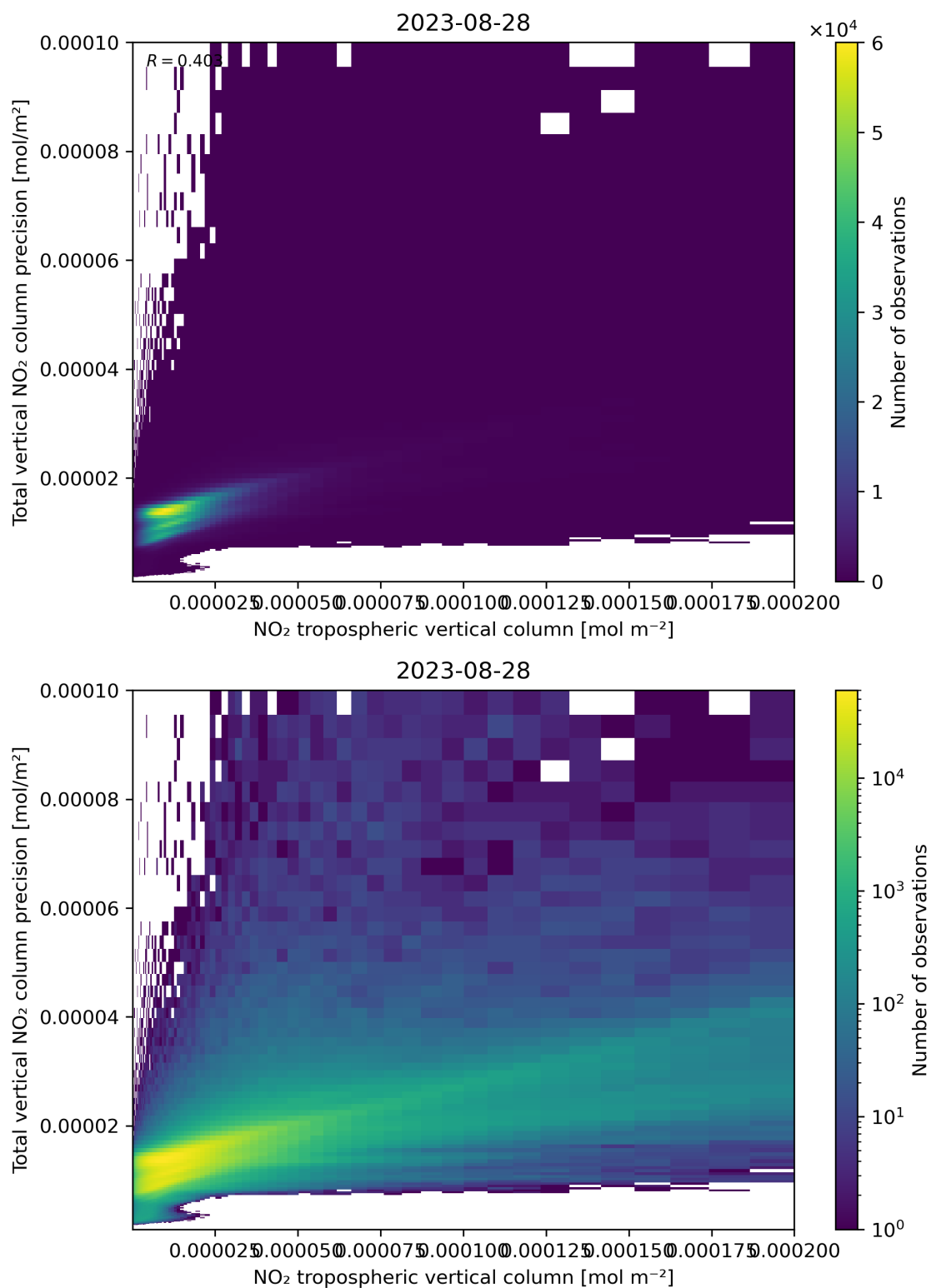
Figure 129: Scatter density plot of “NO 2 tropospheric vertical column” against “Total vertical NO 2 column precision” for 2023-08-27 to 2023-08-29.
