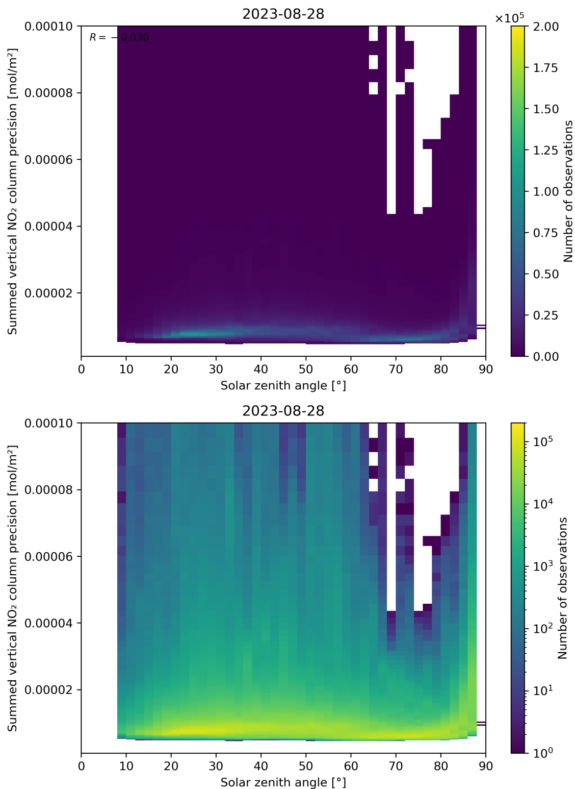
Figure 152: Scatter density plot of “Solar zenith angle” against “Summed vertical NO 2 column precision” for 2023-08-27 to 2023-08-29.
