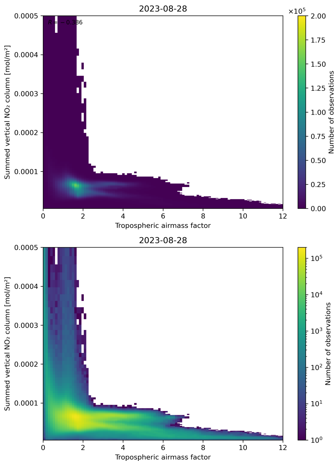
Figure 75: Scatter density plot of “Tropospheric airmass factor” against “Summed vertical NO 2 column” for 2023-08-27 to 2023-08-29.
