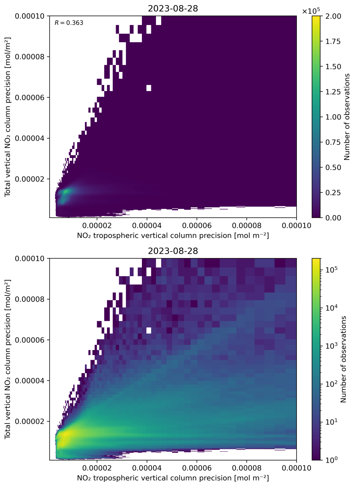
Figure 139: Scatter density plot of “NO 2 tropospheric vertical column precision” against “Total vertical NO 2 column precision” for 2023-08-27 to 2023-08-29.
