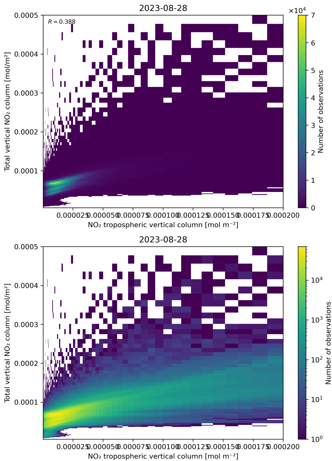
Figure 128: Scatter density plot of “NO 2 tropospheric vertical column” against “Total vertical NO 2 column” for 2023-08-27 to 2023-08-29.
