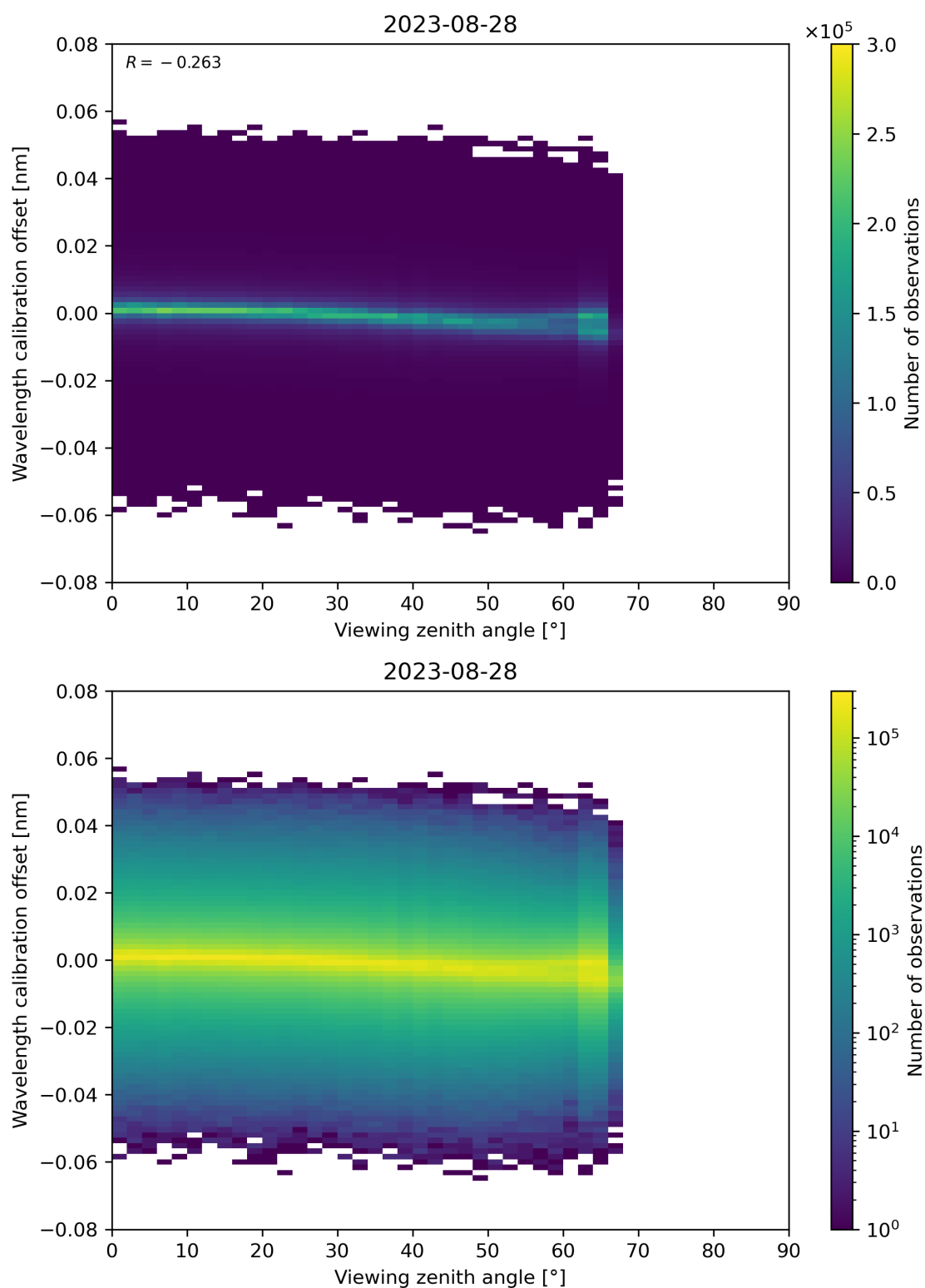
Figure 173: Scatter density plot of “Viewing zenith angle” against “Wavelength calibration offset” for 2023-08-27 to 2023-08-29.
