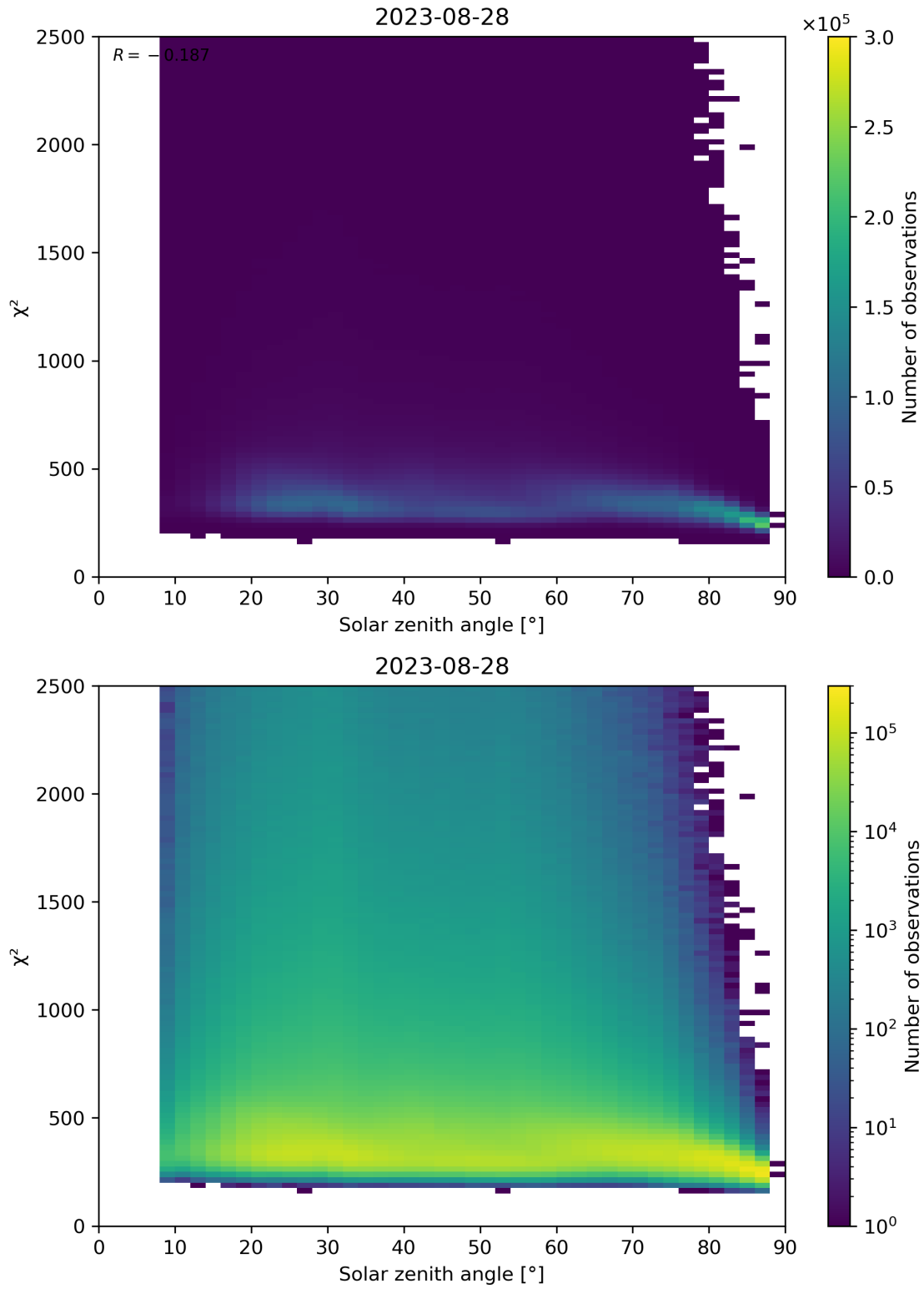
Figure 148: Scatter density plot of “Solar zenith angle” against “ \chi^2 ” for 2023-08-27 to 2023-08-29.
