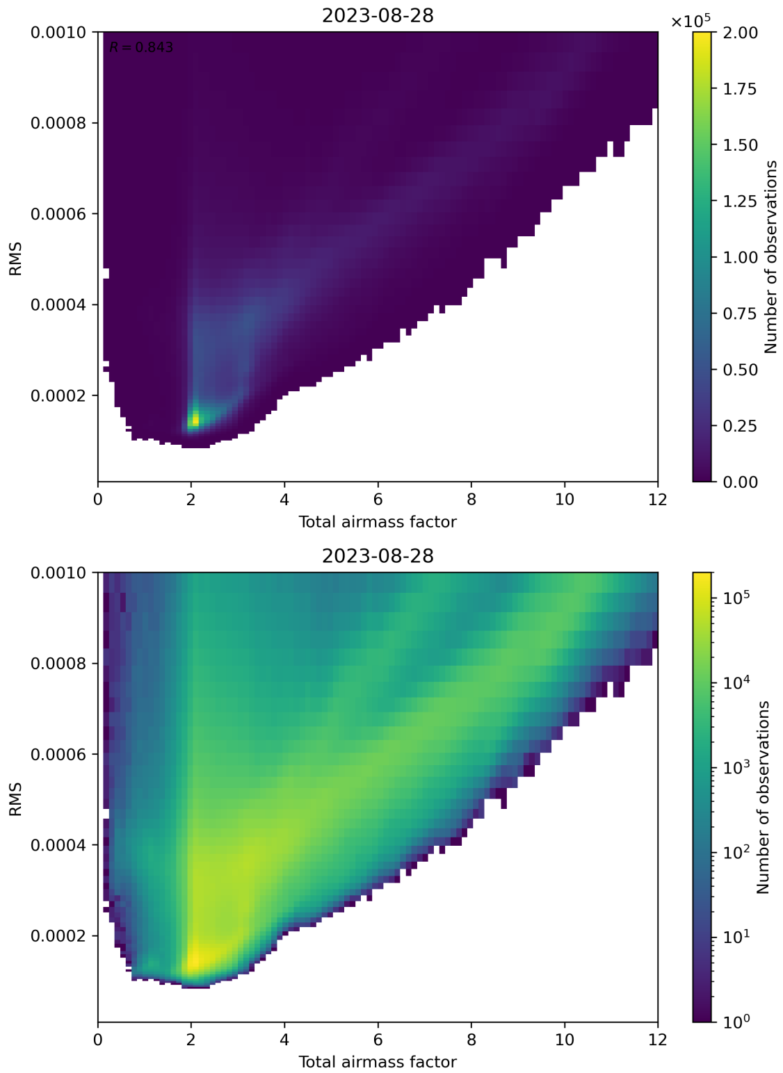
Figure 69: Scatter density plot of “Total airmass factor” against “RMS” for 2023-08-27 to 2023-08-29.
