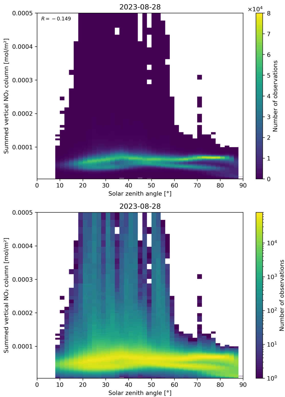
Figure 151: Scatter density plot of “Solar zenith angle” against “Summed vertical NO 2 column” for 2023-08-27 to 2023-08-29.
