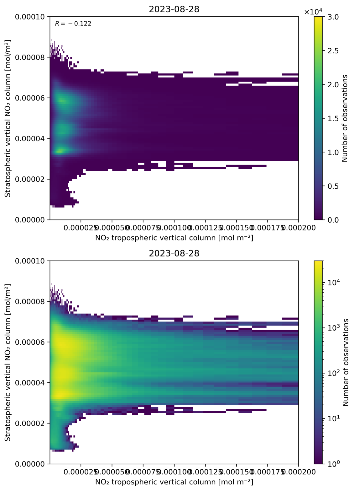
Figure 125: Scatter density plot of “NO 2 tropospheric vertical column” against “Stratospheric vertical NO 2 column” for 2023-08-27 to 2023-08-29.
