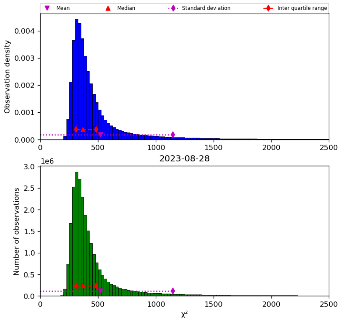
Figure 42: Histogram of “ \chi^2 ” for 2023-08-27 to 2023-08-29
