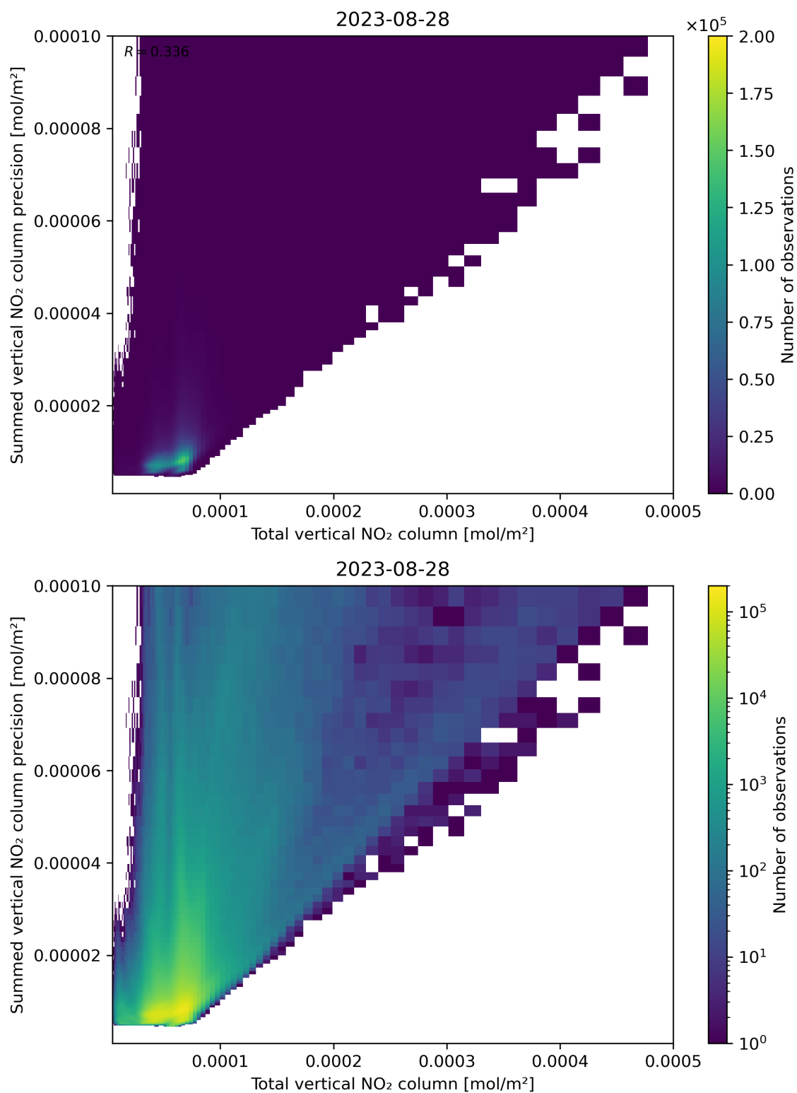
Figure 113: Scatter density plot of “Total vertical NO 2 column” against “Summed vertical NO 2 column precision” for 2023-08-27 to 2023-08-29.
