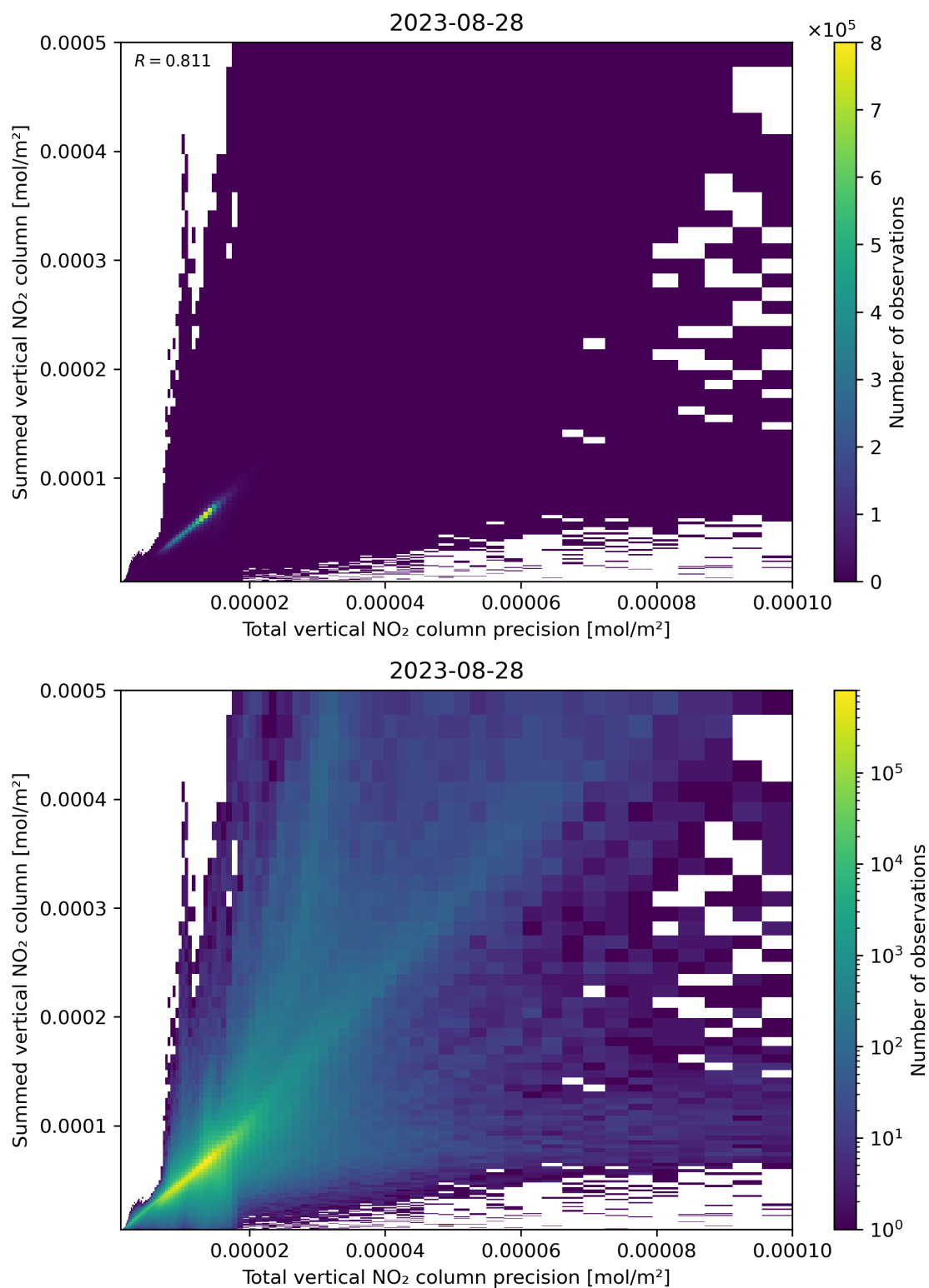
Figure 117: Scatter density plot of “Total vertical NO 2 column precision” against “Summed vertical NO 2 column” for 2023-08-27 to 2023-08-29.
