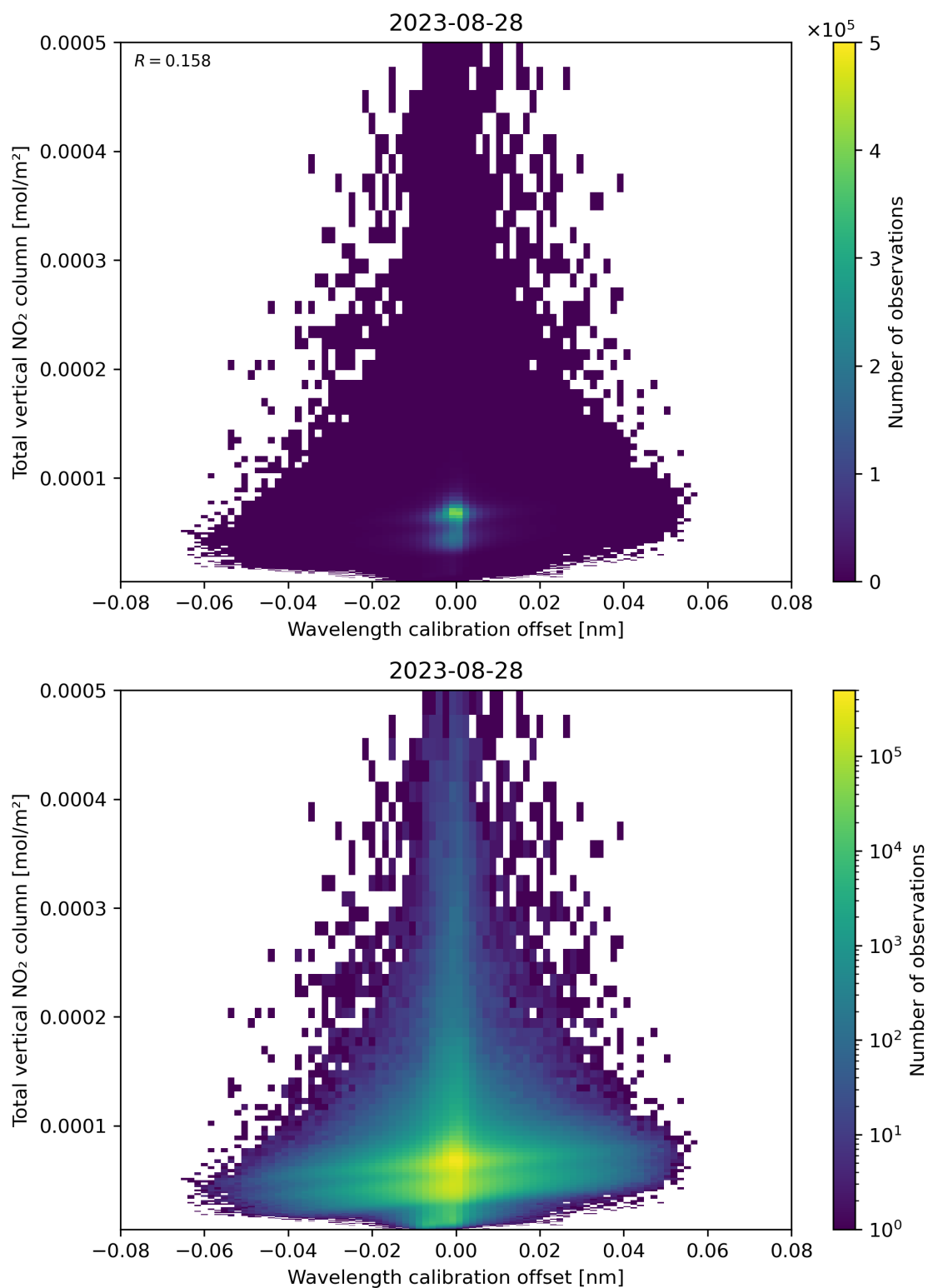
Figure 179: Scatter density plot of “Wavelength calibration offset” against “Total vertical NO 2 column” for 2023-08-27 to 2023-08-29.
