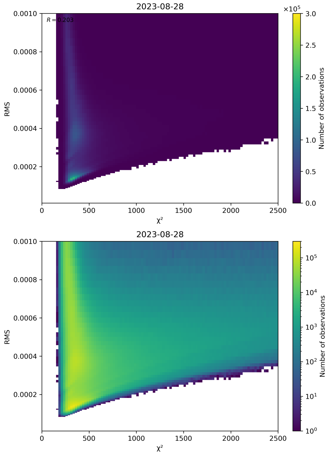
Figure 82: Scatter density plot of “ \chi^2 ” against “RMS” for 2023-08-27 to 2023-08-29.
