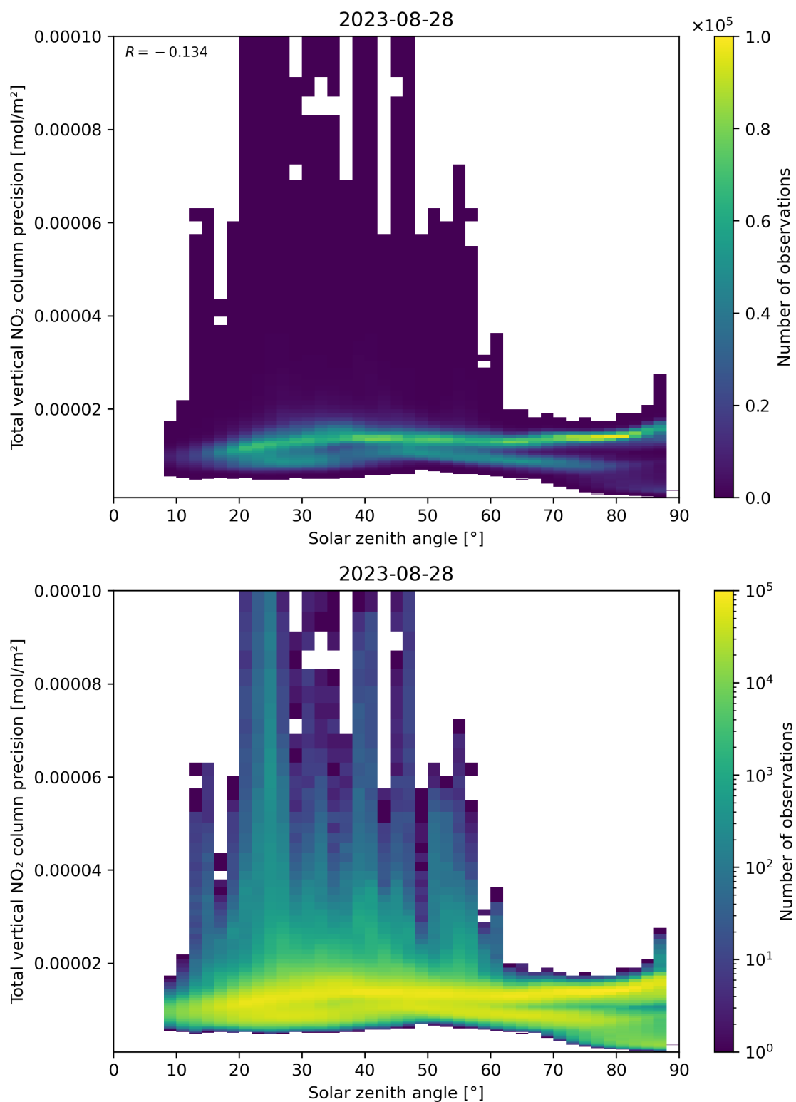
Figure 154: Scatter density plot of “Solar zenith angle” against “Total vertical NO 2 column precision” for 2023-08-27 to 2023-08-29.
