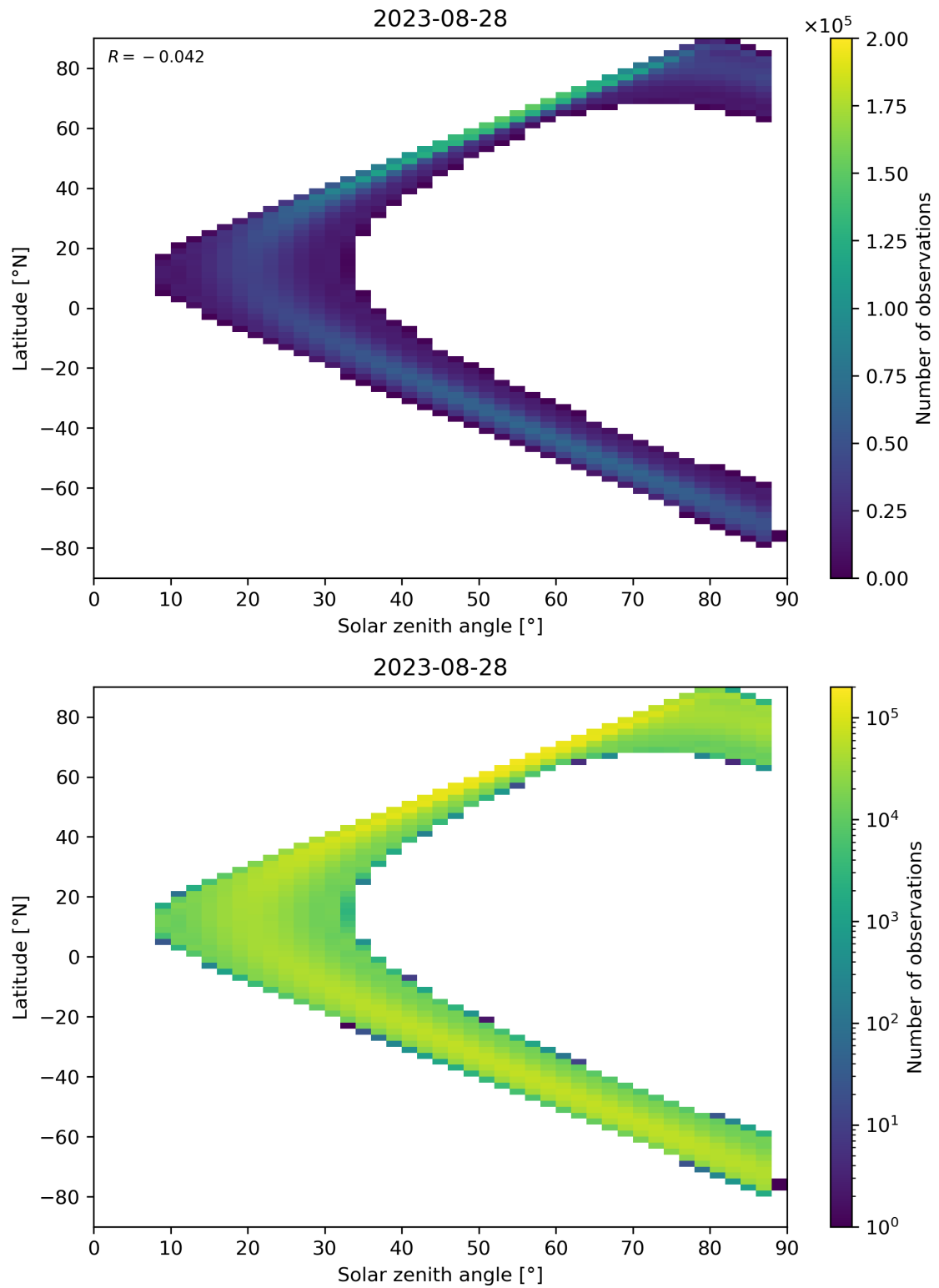
Figure 149: Scatter density plot of “Solar zenith angle” against “Latitude” for 2023-08-27 to 2023-08-29.
