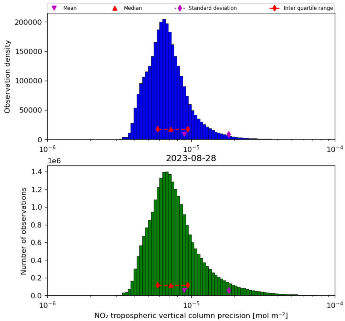
Figure 30: Histogram of “NO 2 tropospheric vertical column precision” for 2023-08-27 to 2023-08-29
