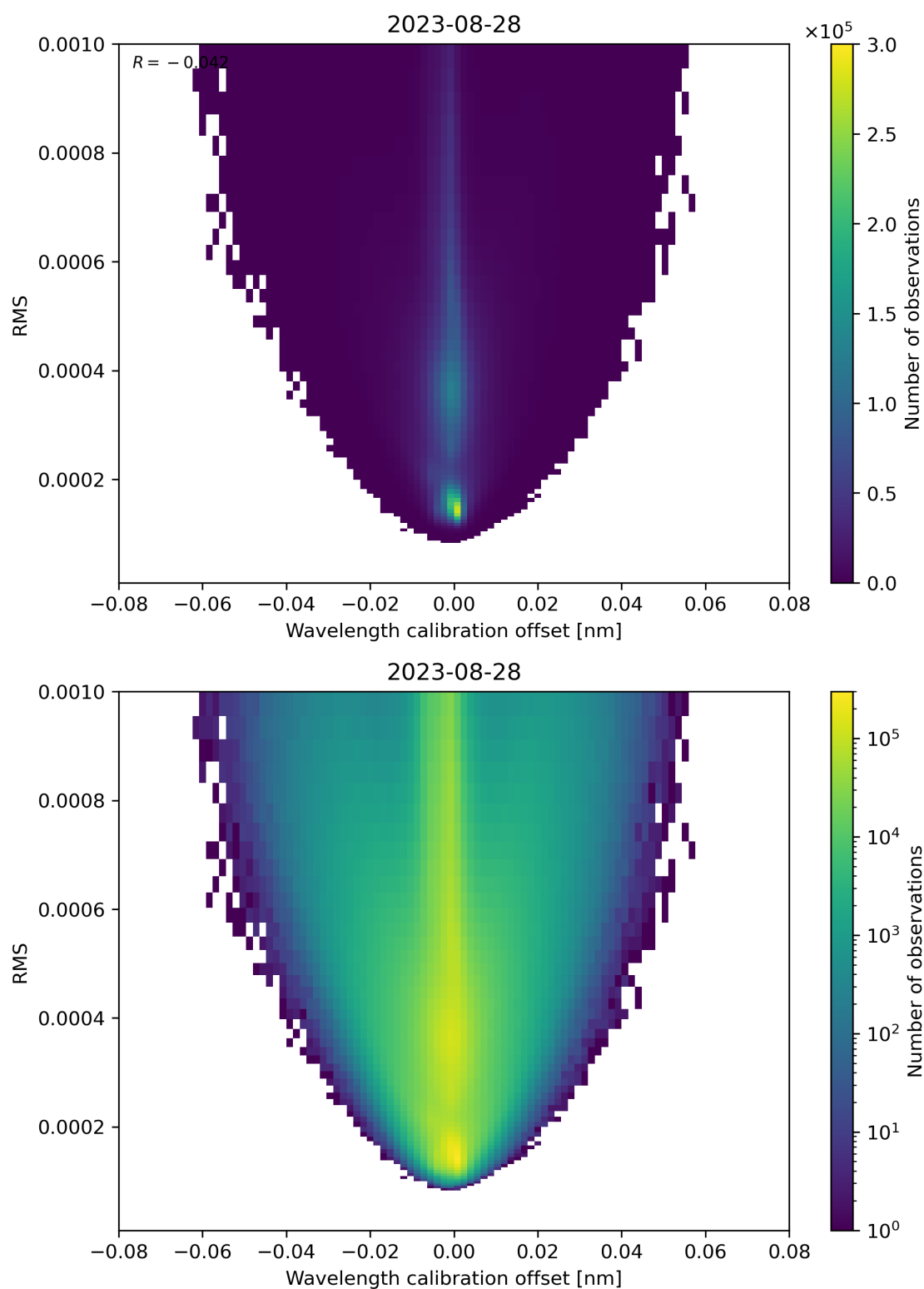
Figure 181: Scatter density plot of “Wavelength calibration offset” against “RMS” for 2023-08-27 to 2023-08-29.
