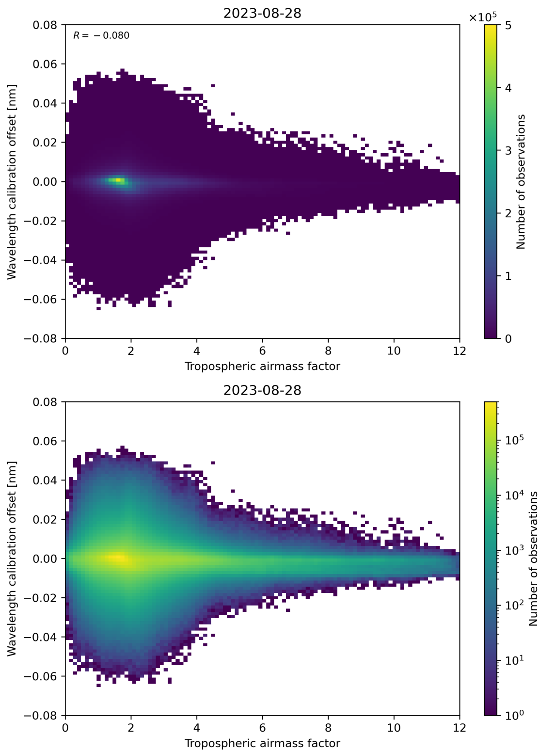
Figure 80: Scatter density plot of “Tropospheric airmass factor” against “Wavelength calibration offset” for 2023-08-27 to 2023-08-29.
