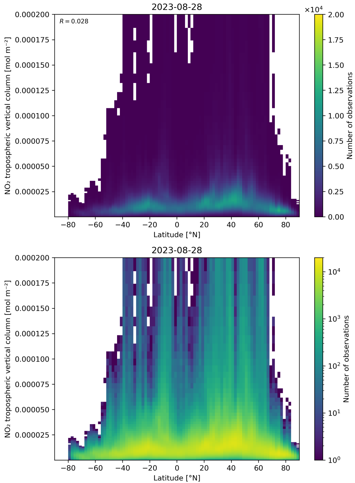
Figure 92: Scatter density plot of “Latitude” against “NO 2 tropospheric vertical column” for 2023-08-27 to 2023-08-29.
