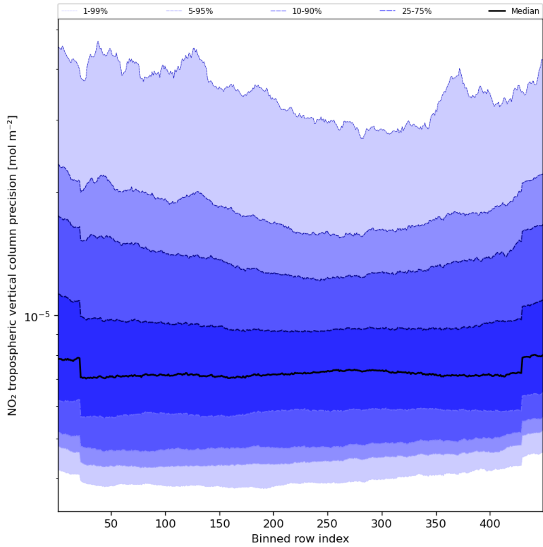
Figure 47: Along track statistics of “NO 2 tropospheric vertical column precision” for 2023-08-27 to 2023-08-29
