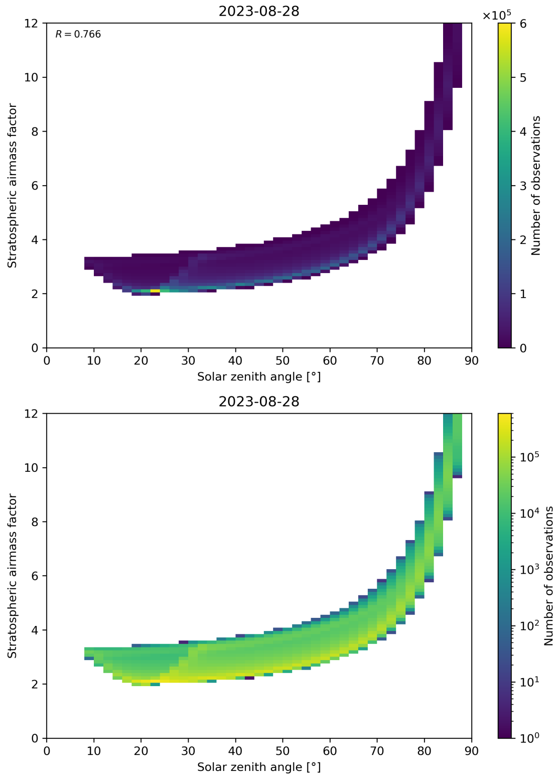
Figure 145: Scatter density plot of “Solar zenith angle” against “Stratospheric airmass factor” for 2023-08-27 to 2023-08-29.
