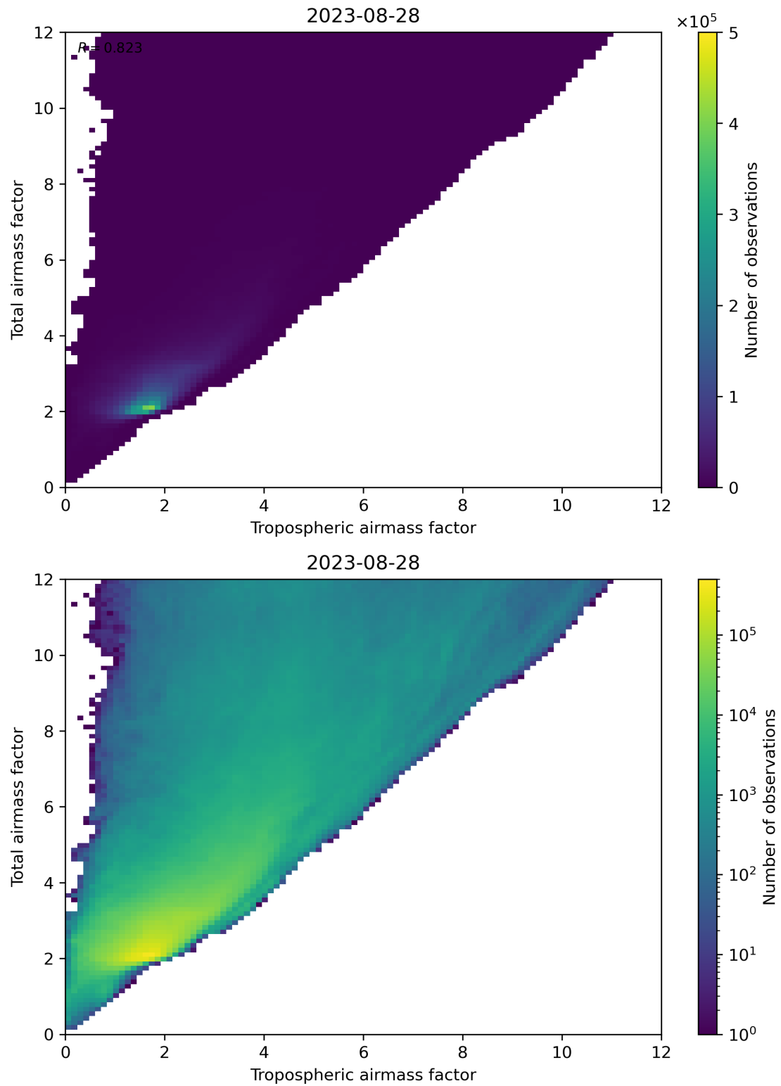
Figure 72: Scatter density plot of “Tropospheric airmass factor” against “Total airmass factor” for 2023-08-27 to 2023-08-29.
