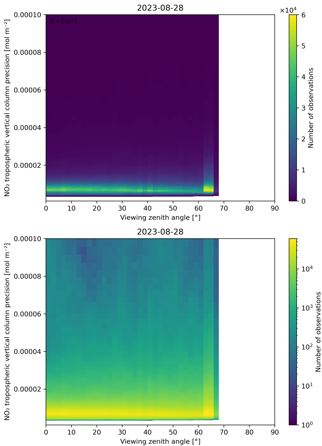
Figure 170: Scatter density plot of “Viewing zenith angle” against “NO 2 tropospheric vertical column precision” for 2023-08-27 to 2023-08-29.
