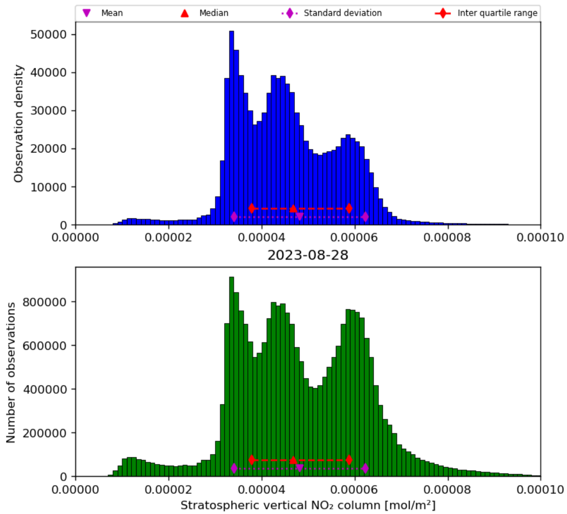
Figure 36: Histogram of “Stratospheric vertical NO 2 column” for 2023-08-27 to 2023-08-29
