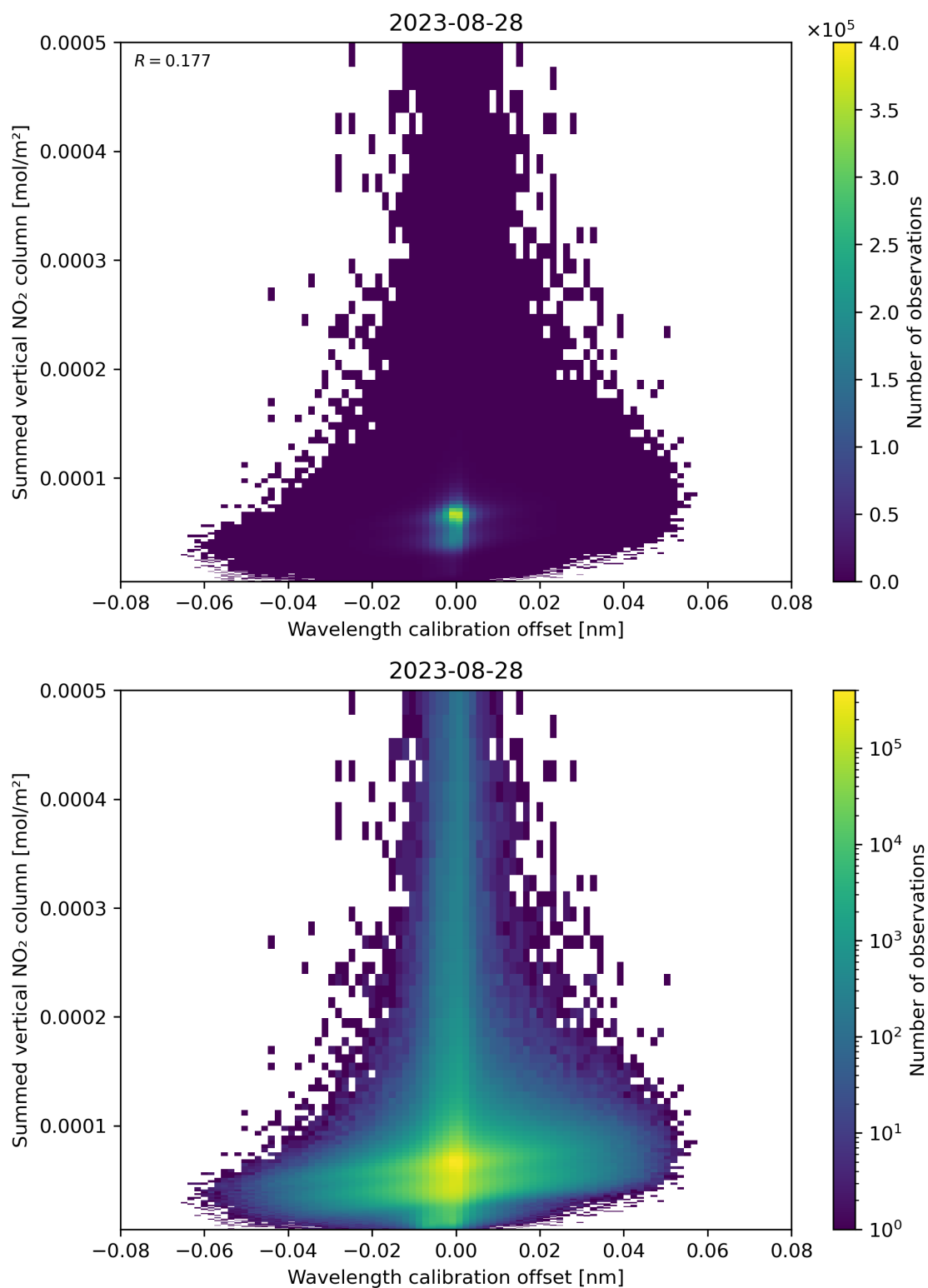
Figure 177: Scatter density plot of “Wavelength calibration offset” against “Summed vertical NO 2 column” for 2023-08-27 to 2023-08-29.
