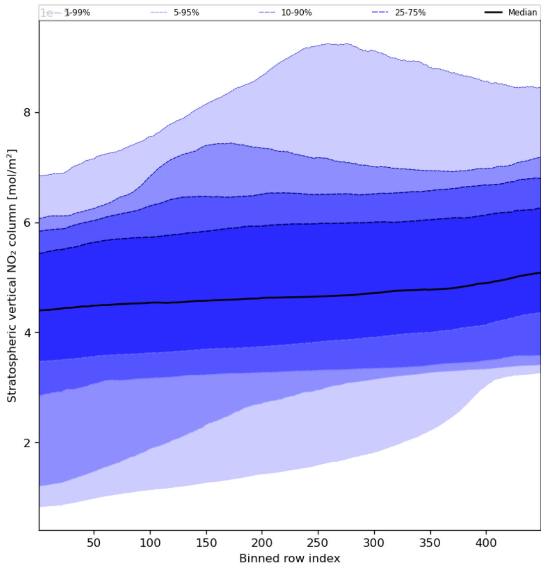
Figure 53: Along track statistics of “Stratospheric vertical NO 2 column” for 2023-08-27 to 2023-08-29
