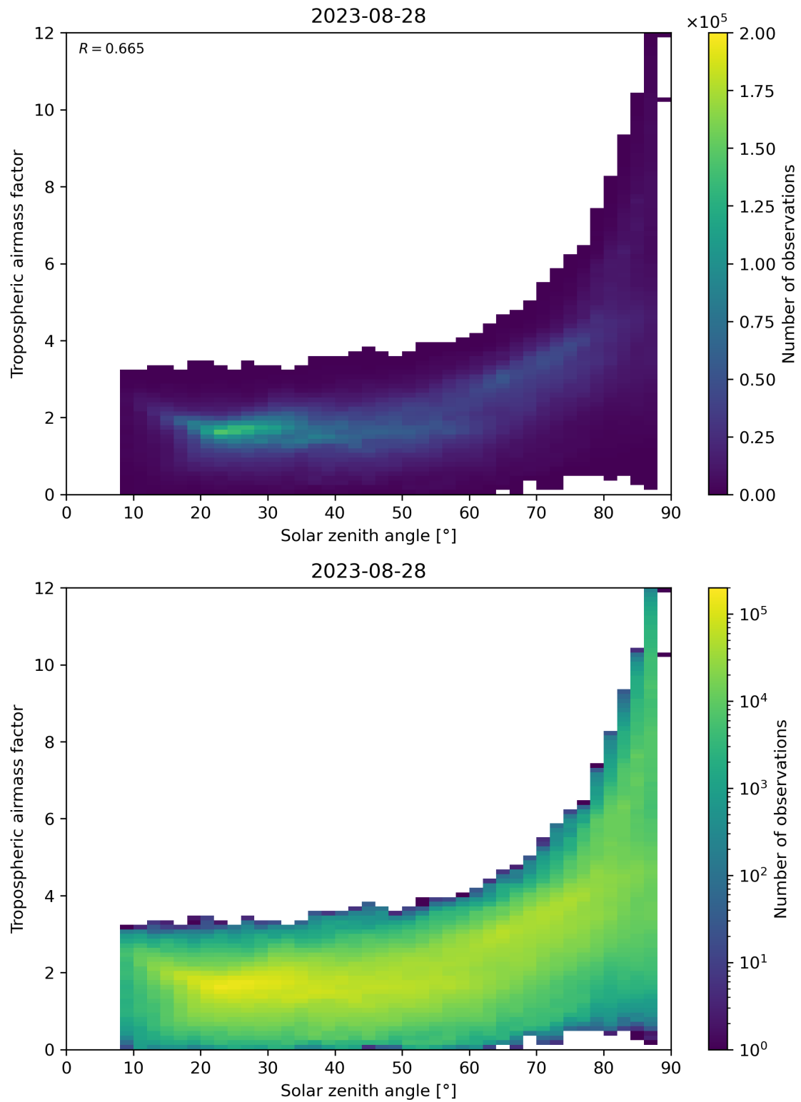
Figure 147: Scatter density plot of “Solar zenith angle” against “Tropospheric airmass factor” for 2023-08-27 to 2023-08-29.
