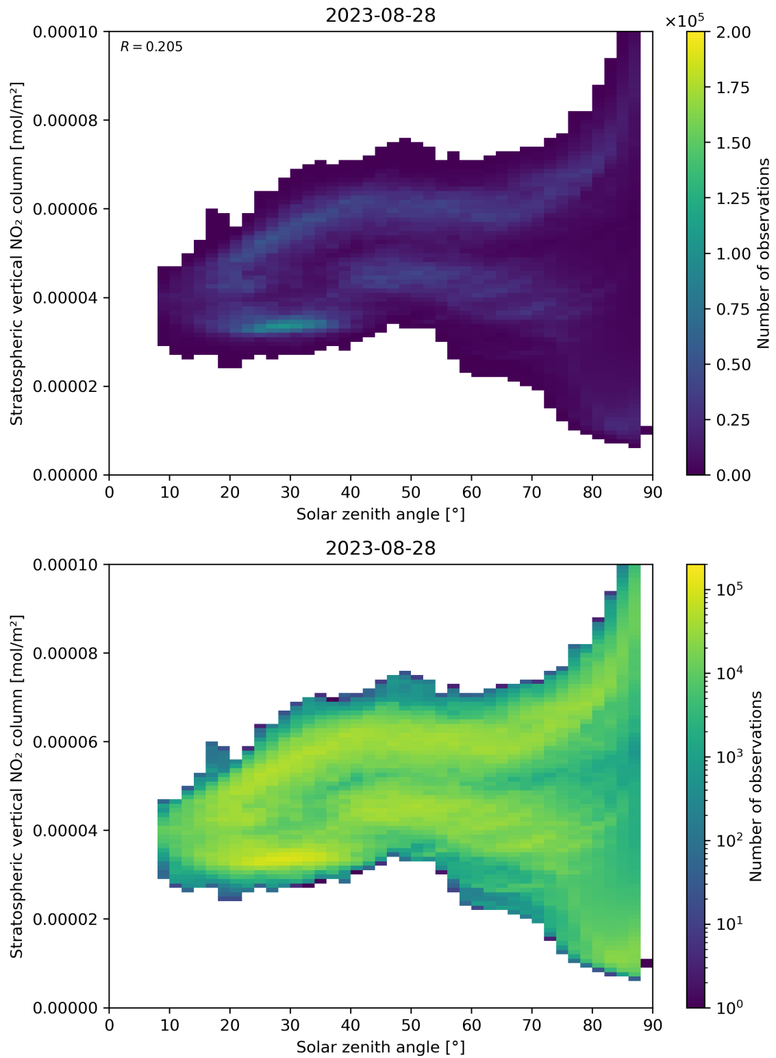
Figure 150: Scatter density plot of “Solar zenith angle” against “Stratospheric vertical NO 2 column” for 2023-08-27 to 2023-08-29.
