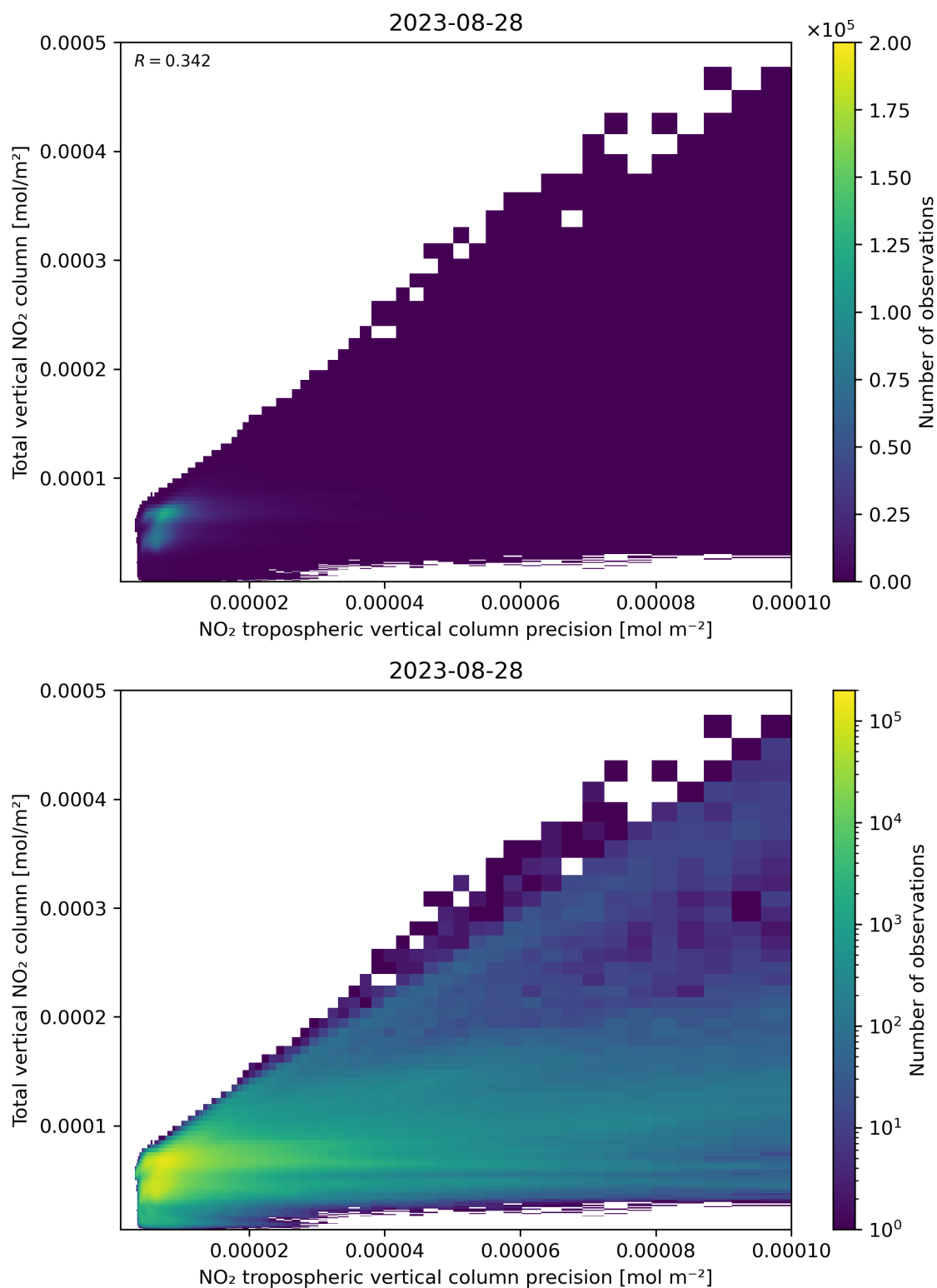
Figure 138: Scatter density plot of “NO 2 tropospheric vertical column precision” against “Total vertical NO 2 column” for 2023-08-27 to 2023-08-29.
