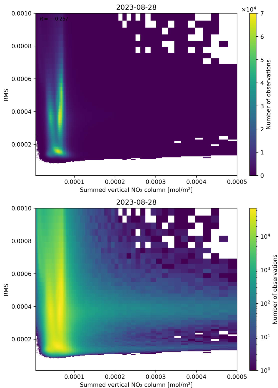
Figure 109: Scatter density plot of “Summed vertical NO 2 column” against “RMS” for 2023-08-27 to 2023-08-29.
