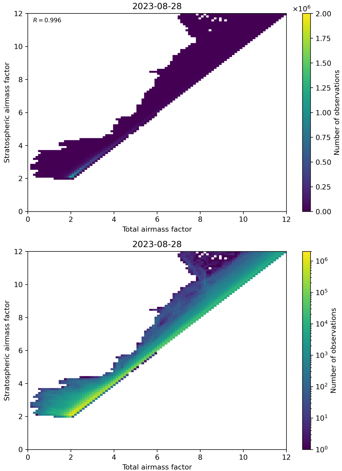
Figure 62: Scatter density plot of “Total airmass factor” against “Stratospheric airmass factor” for 2023-08-27 to 2023-08-29.
