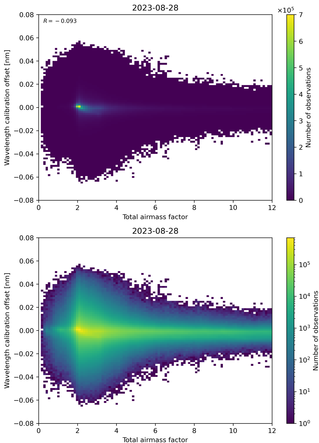
Figure 70: Scatter density plot of “Total airmass factor” against “Wavelength calibration offset” for 2023-08-27 to 2023-08-29.
