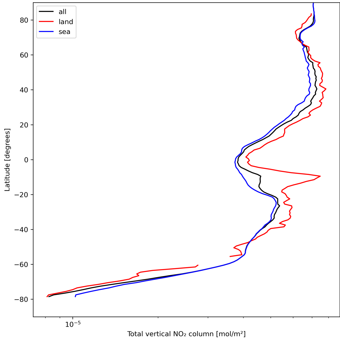
Figure 21: Zonal average of “Total vertical NO 2 column” for 2023-08-27 to 2023-08-29.
