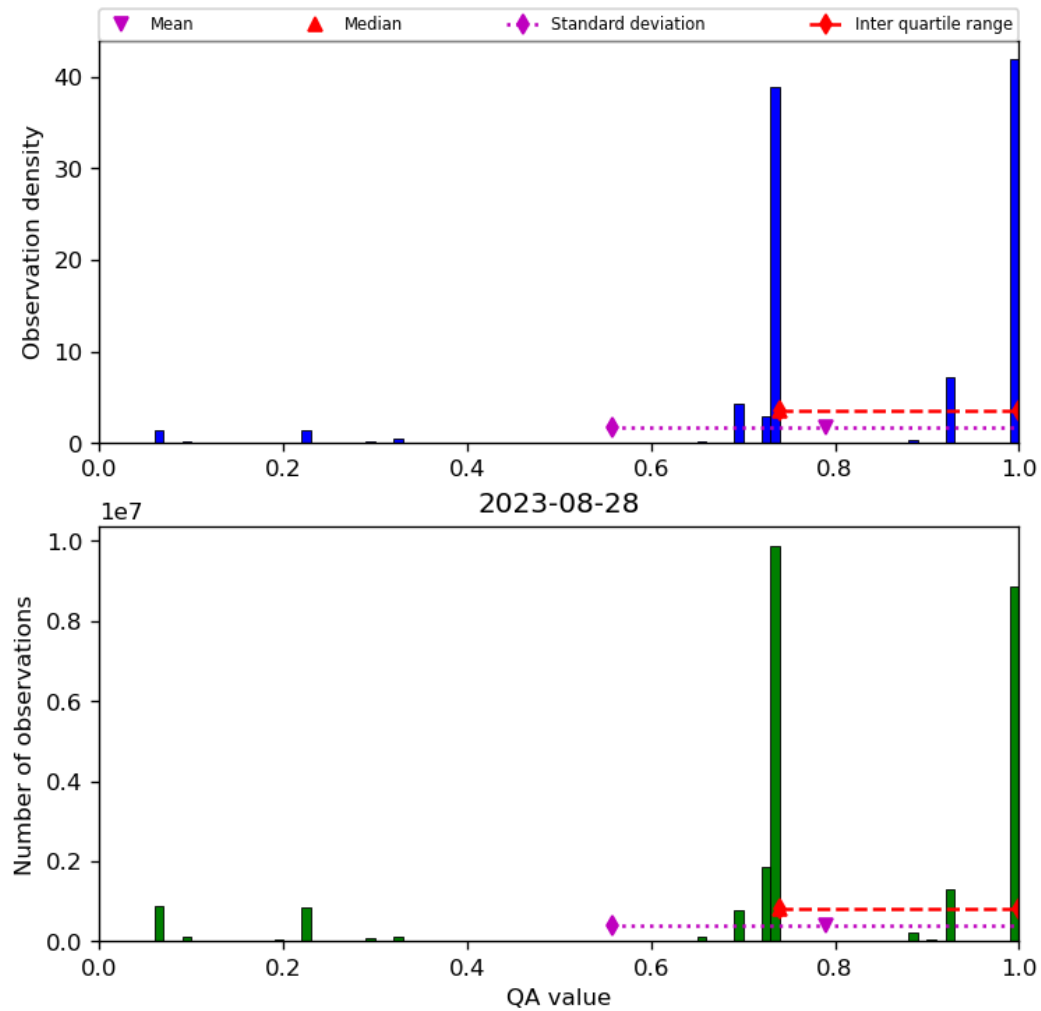
Figure 28: Histogram of “QA value” for 2023-08-27 to 2023-08-29
