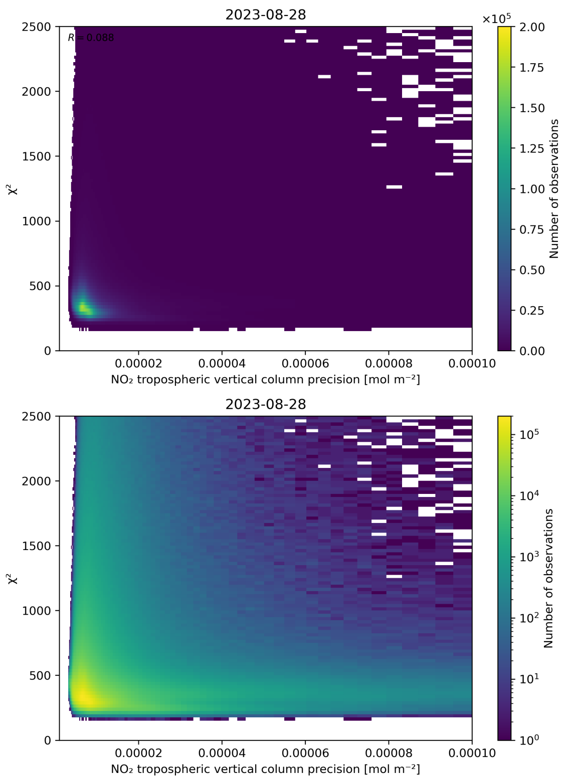
Figure 134: Scatter density plot of “NO 2 tropospheric vertical column precision” against “ \chi^2 ” for 2023-08-27 to 2023-08-29.
