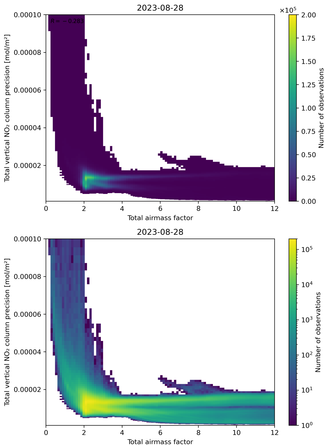
Figure 68: Scatter density plot of “Total airmass factor” against “Total vertical NO 2 column precision” for 2023-08-27 to 2023-08-29.
