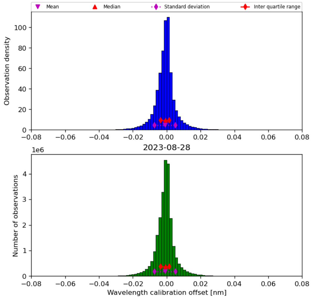
Figure 35: Histogram of “Wavelength calibration offset” for 2023-08-27 to 2023-08-29
