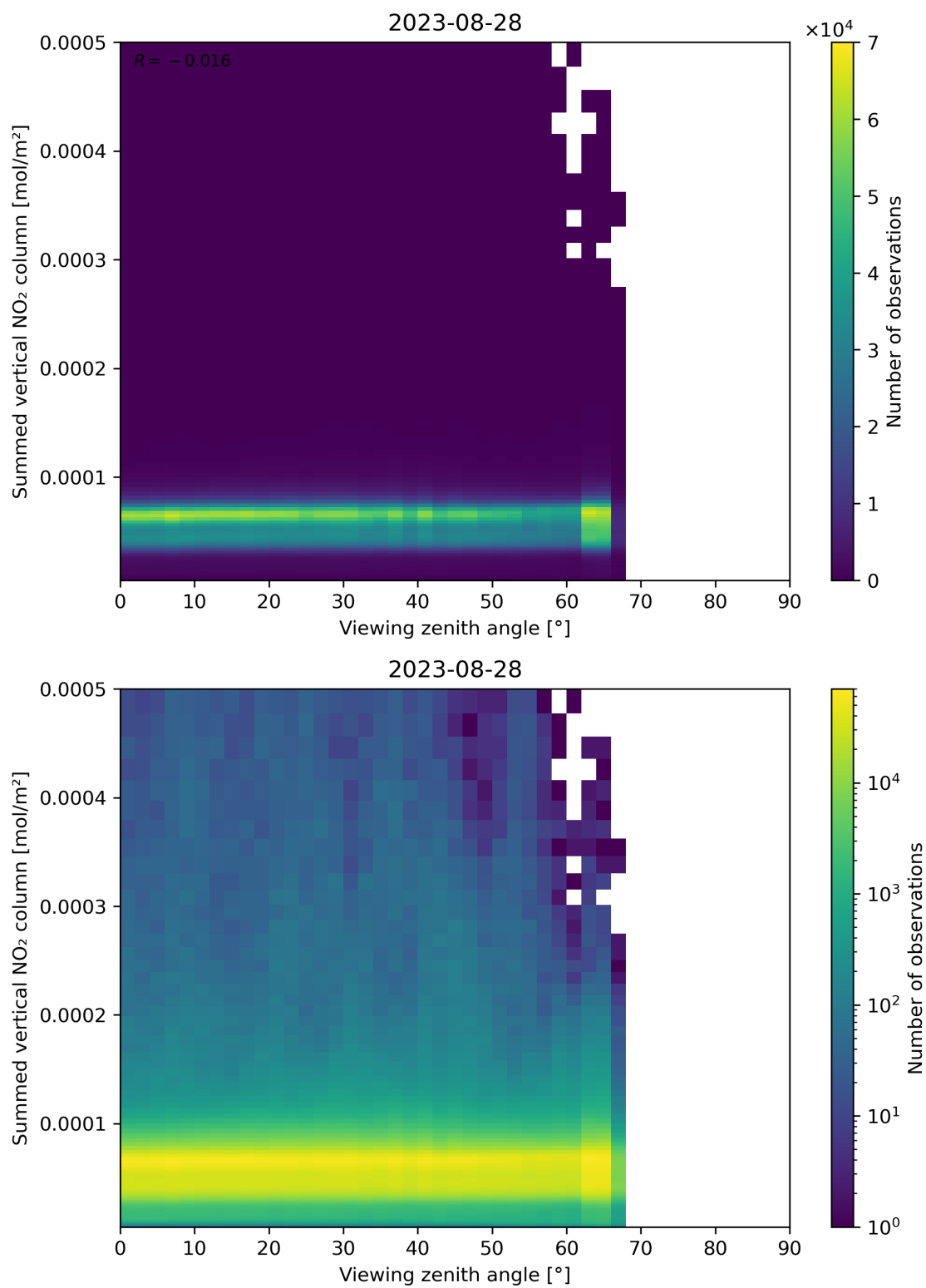
Figure 165: Scatter density plot of “Viewing zenith angle” against “Summed vertical NO 2 column” for 2023-08-27 to 2023-08-29.
