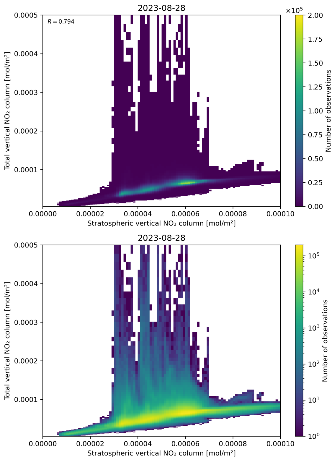
Figure 100: Scatter density plot of “Stratospheric vertical NO 2 column” against “Total vertical NO 2 column” for 2023-08-27 to 2023-08-29.
