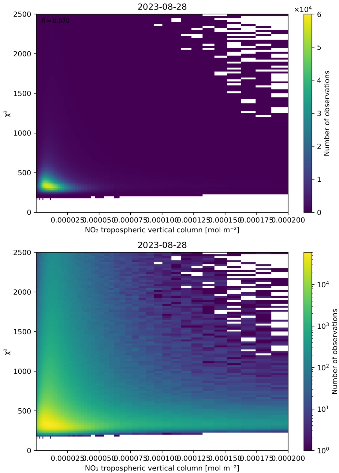
Figure 124: Scatter density plot of “NO 2 tropospheric vertical column” against “ \chi^2 ” for 2023-08-27 to 2023-08-29.
