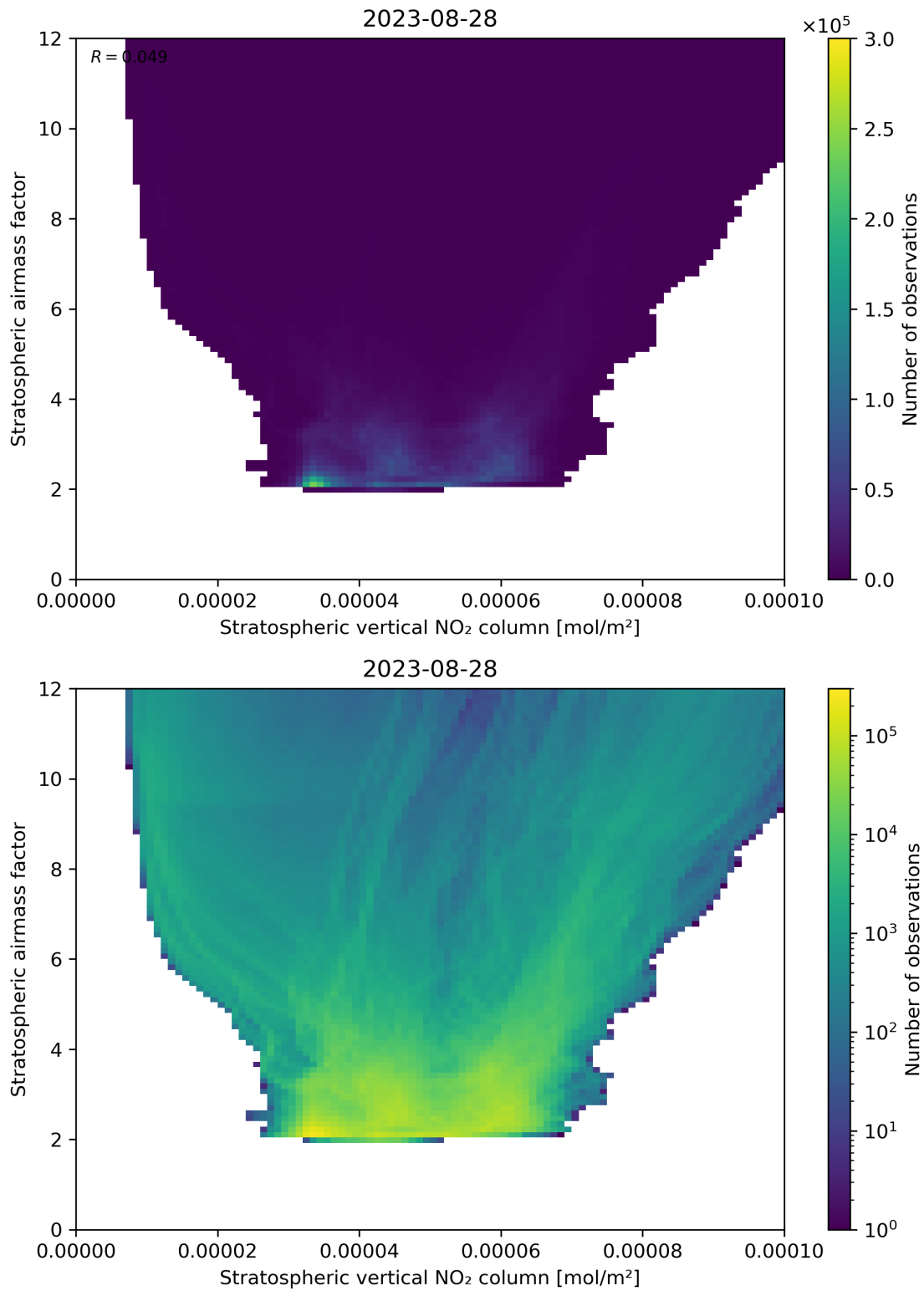
Figure 96: Scatter density plot of “Stratospheric vertical NO 2 column” against “Stratospheric airmass factor” for 2023-08-27 to 2023-08-29.
