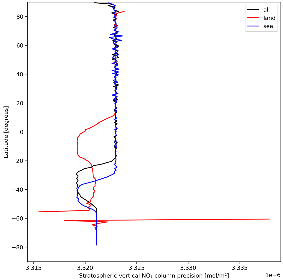
Figure 20: Zonal average of “Stratospheric vertical NO 2 column precision” for 2023-08-27 to 2023-08-29.
