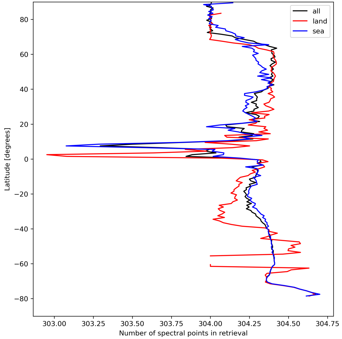
Figure 16: Zonal average of “Number of spectral points in retrieval” for 2023-08-27 to 2023-08-29.
