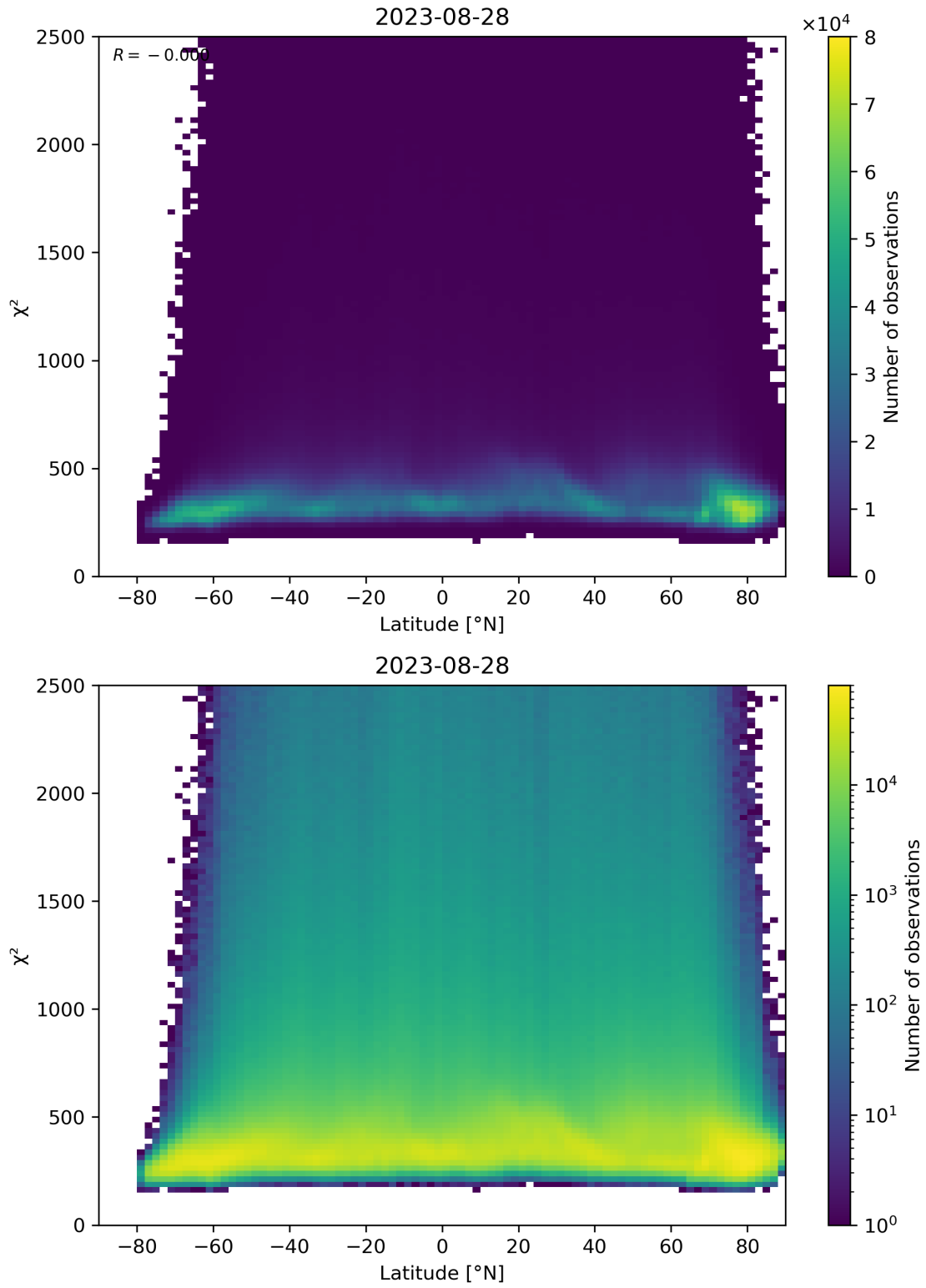
Figure 86: Scatter density plot of “Latitude” against “ \chi^2 ” for 2023-08-27 to 2023-08-29.
