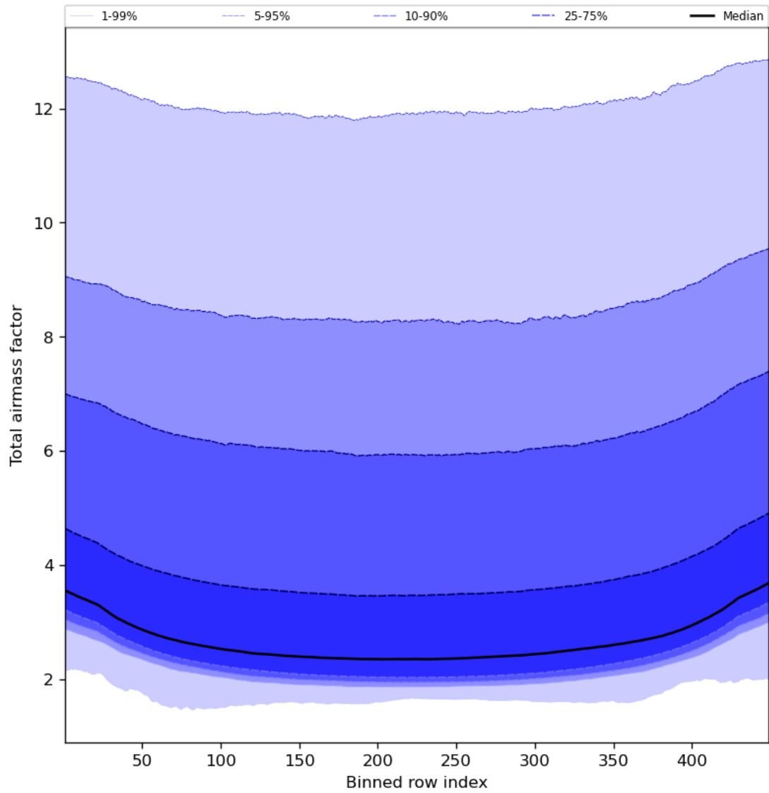
Figure 49: Along track statistics of “Total airmass factor” for 2023-08-27 to 2023-08-29
