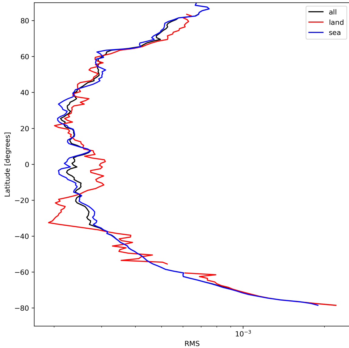
Figure 26: Zonal average of “RMS” for 2023-08-27 to 2023-08-29.
