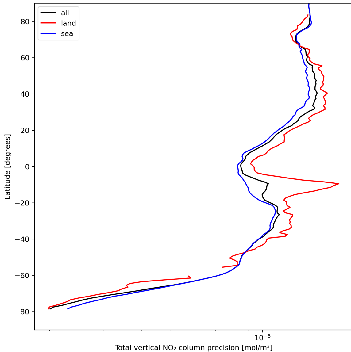
Figure 22: Zonal average of “Total vertical NO 2 column precision” for 2023-08-27 to 2023-08-29.
