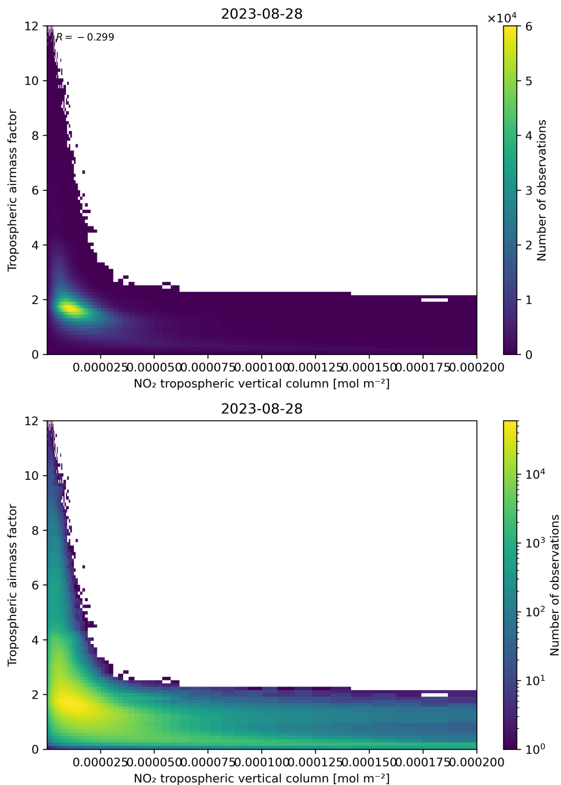
Figure 123: Scatter density plot of “NO 2 tropospheric vertical column” against “Tropospheric air mass factor” for 2023-08-27 to 2023-08-29.
