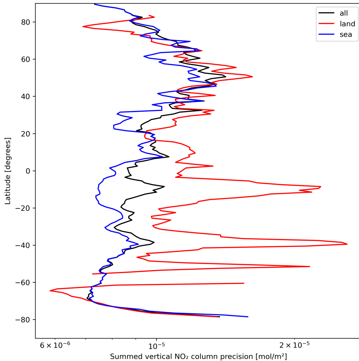
Figure 24: Zonal average of “Summed vertical NO 2 column precision” for 2023-08-27 to 2023-08-29.
