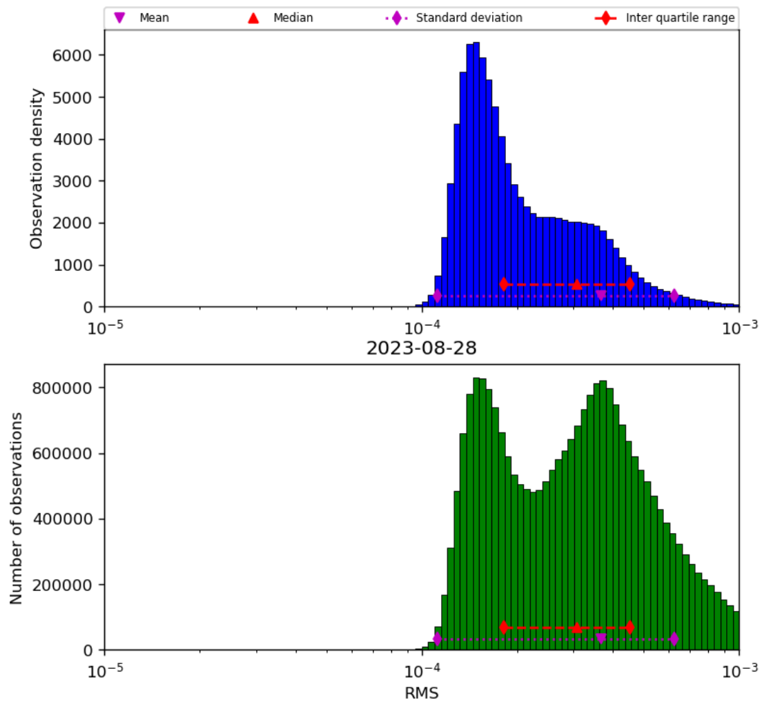
Figure 43: Histogram of “RMS” for 2023-08-27 to 2023-08-29
