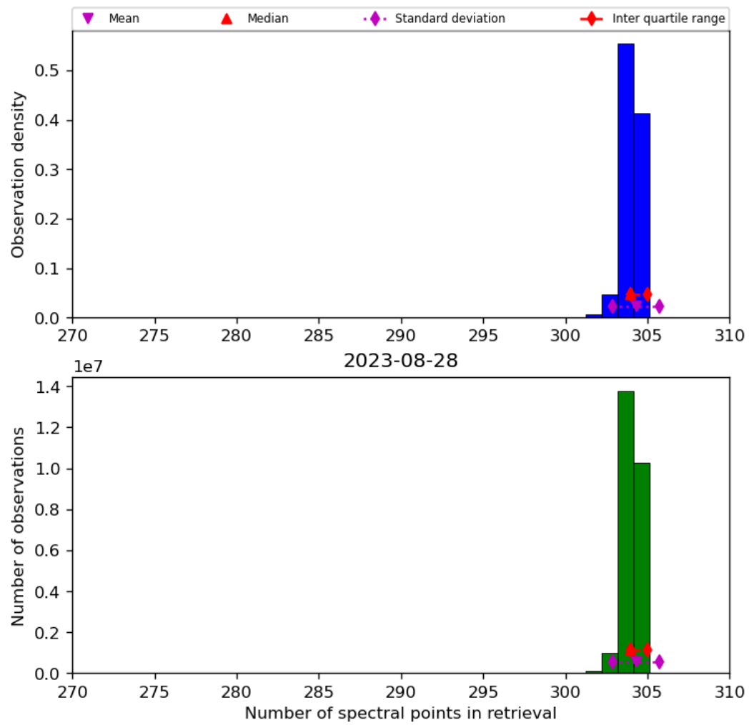
Figure 33: Histogram of “Number of spectral points in retrieval” for 2023-08-27 to 2023-08-29
