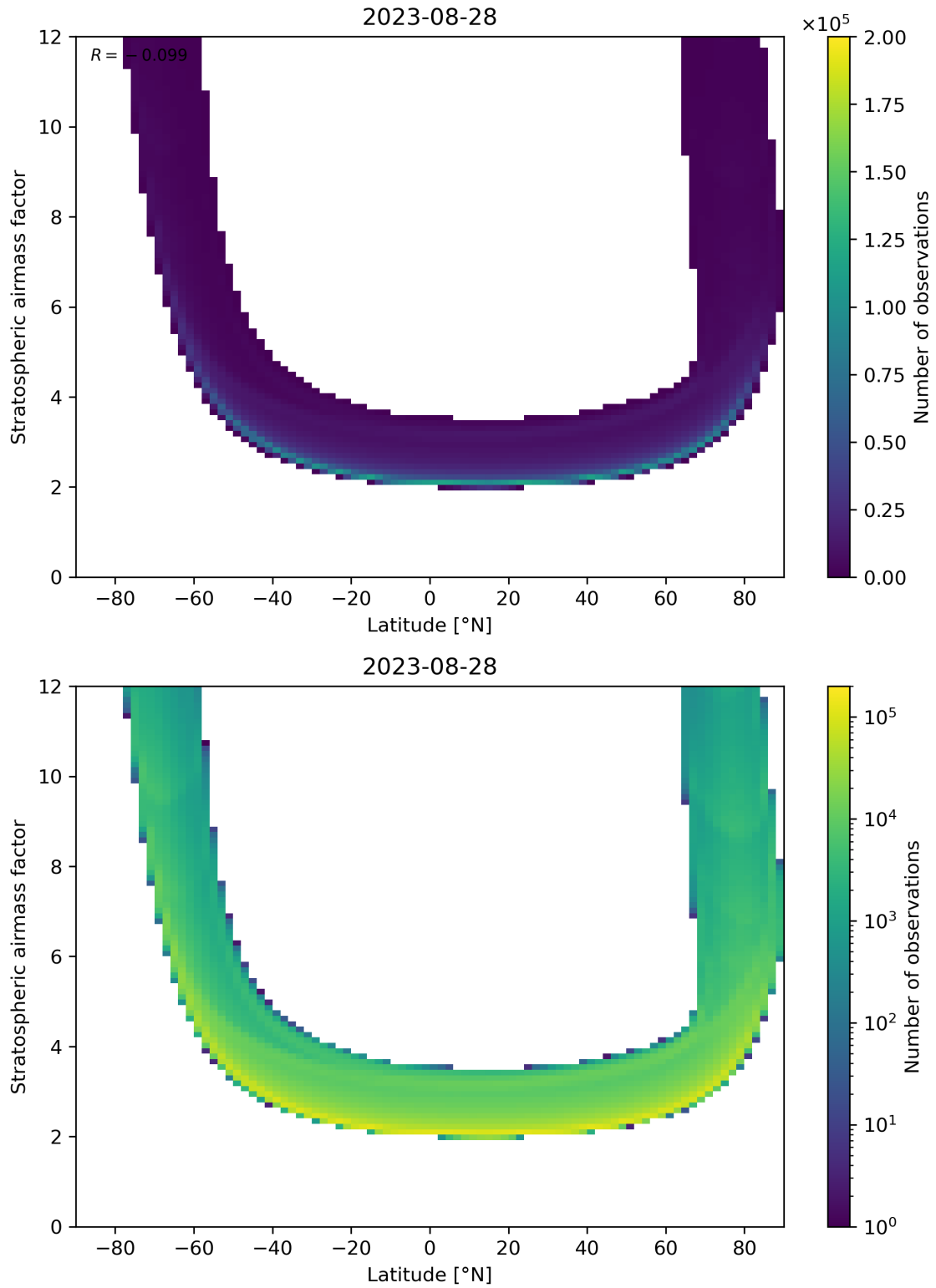
Figure 83: Scatter density plot of “Latitude” against “Stratospheric air mass factor” for 2023-08-27 to 2023-08-29.
