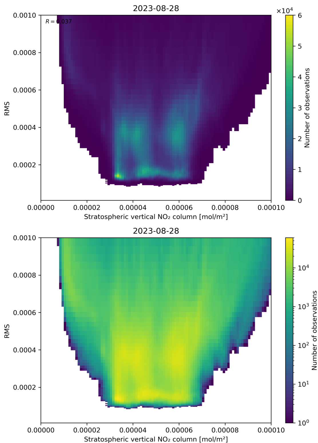
Figure 102: Scatter density plot of “Stratospheric vertical NO 2 column” against “RMS” for 2023-08-27 to 2023-08-29.
