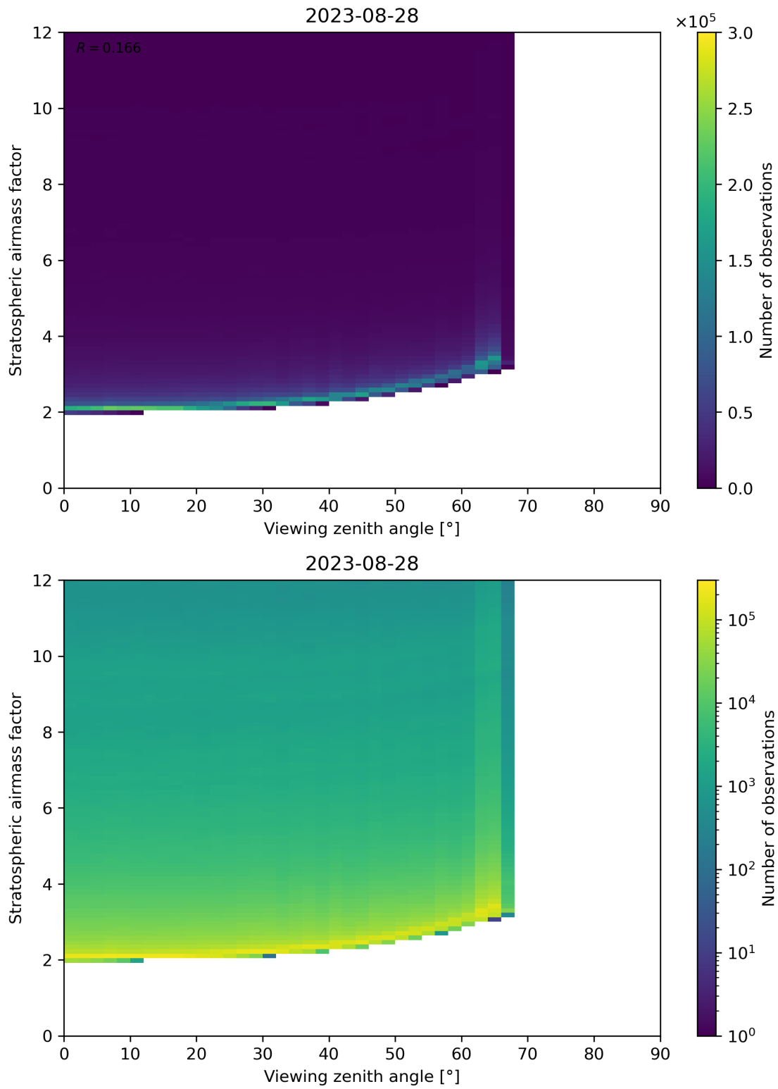
Figure 159: Scatter density plot of “Viewing zenith angle” against “Stratospheric airmass factor” for 2023-08-27 to 2023-08-29.
