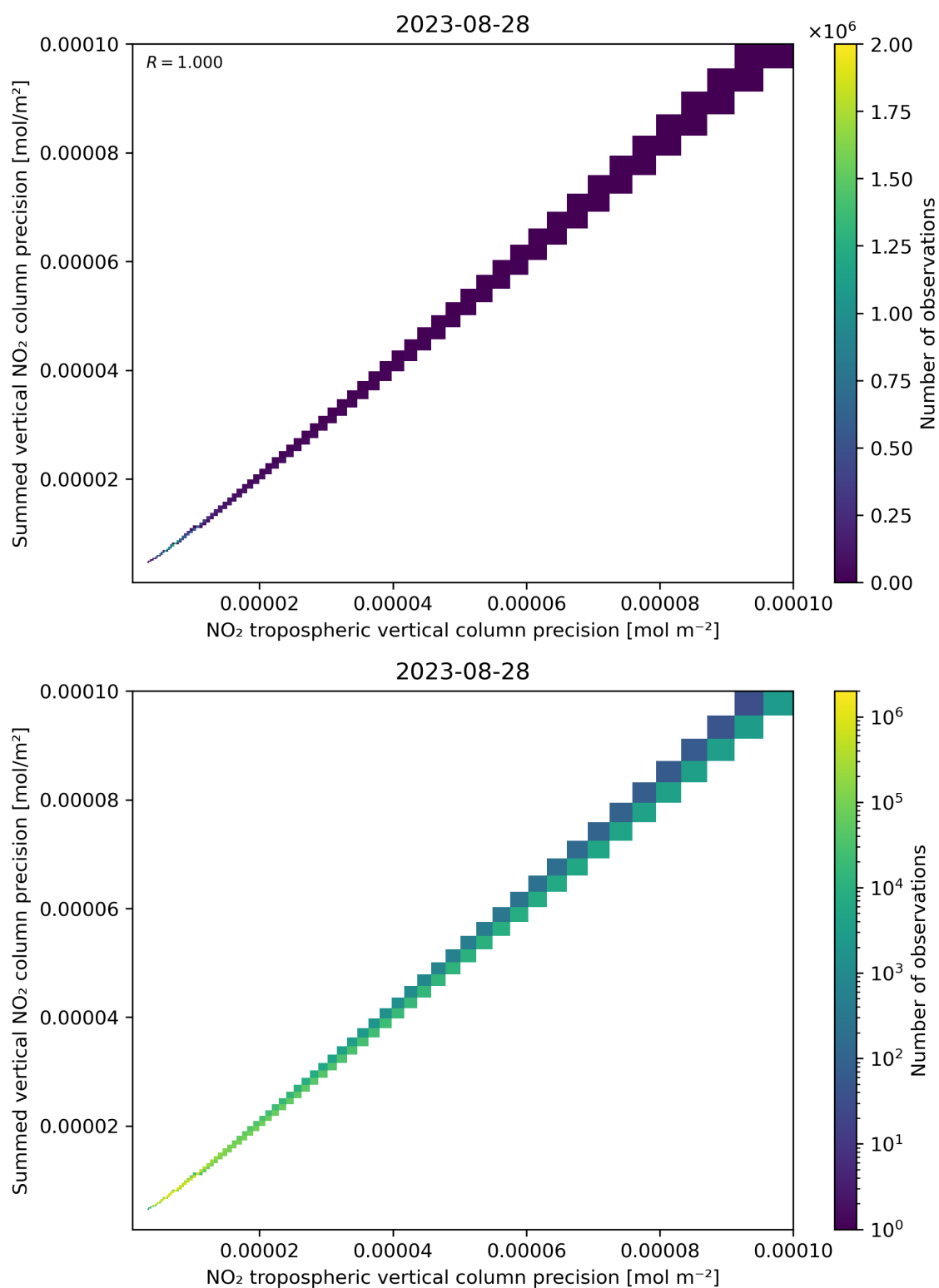
Figure 137: Scatter density plot of “NO 2 tropospheric vertical column precision” against “Summed vertical NO 2 column precision” for 2023-08-27 to 2023-08-29.
