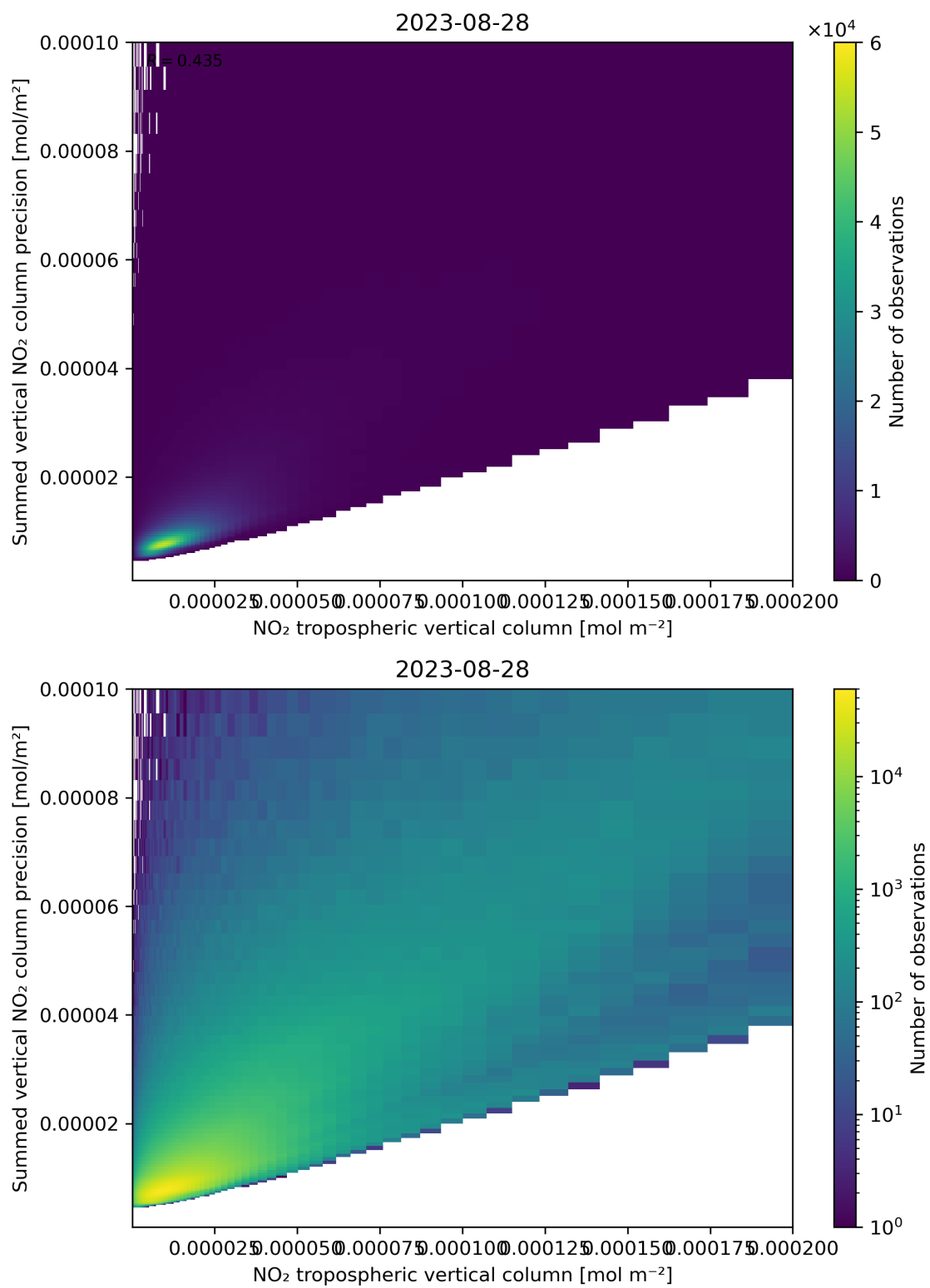
Figure 127: Scatter density plot of “NO 2 tropospheric vertical column” against “Summed vertical NO 2 column precision” for 2023-08-27 to 2023-08-29.
