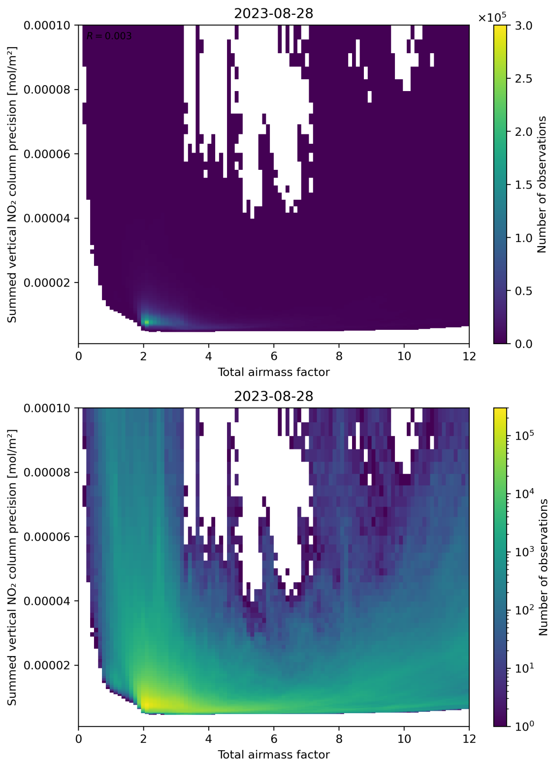
Figure 66: Scatter density plot of “Total airmass factor” against “Summed vertical NO 2 column precision” for 2023-08-27 to 2023-08-29.
