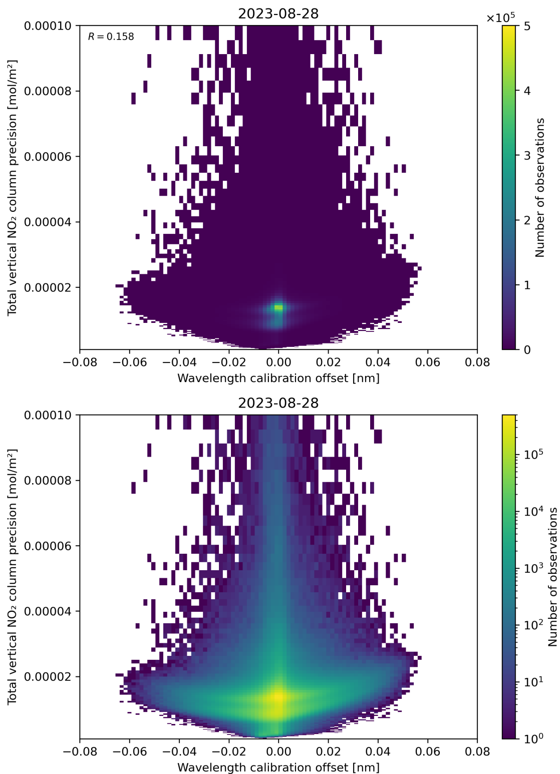
Figure 180: Scatter density plot of “Wavelength calibration offset” against “Total vertical NO 2 column precision” for 2023-08-27 to 2023-08-29.
