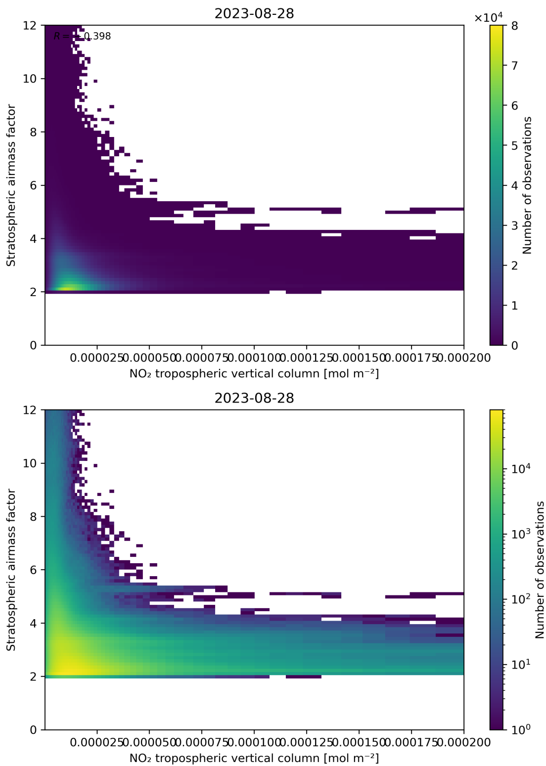
Figure 121: Scatter density plot of “NO 2 tropospheric vertical column” against “Stratospheric air mass factor” for 2023-08-27 to 2023-08-29.
