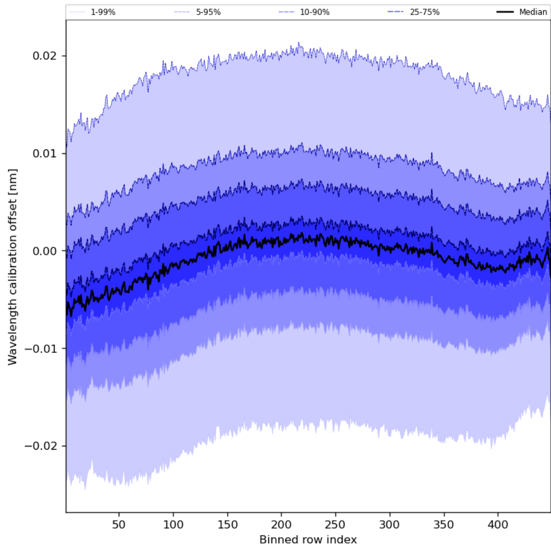
Figure 52: Along track statistics of “Wavelength calibration offset” for 2023-08-27 to 2023-08-29
