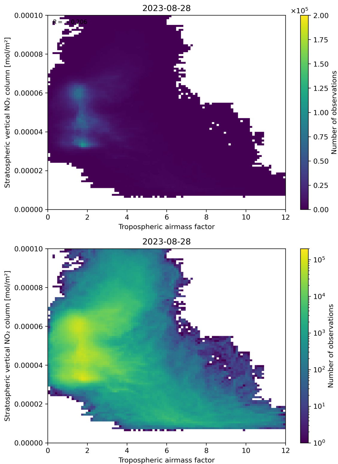
Figure 74: Scatter density plot of “Tropospheric air mass factor” against “Stratospheric vertical NO 2 column” for 2023-08-27 to 2023-08-29.
