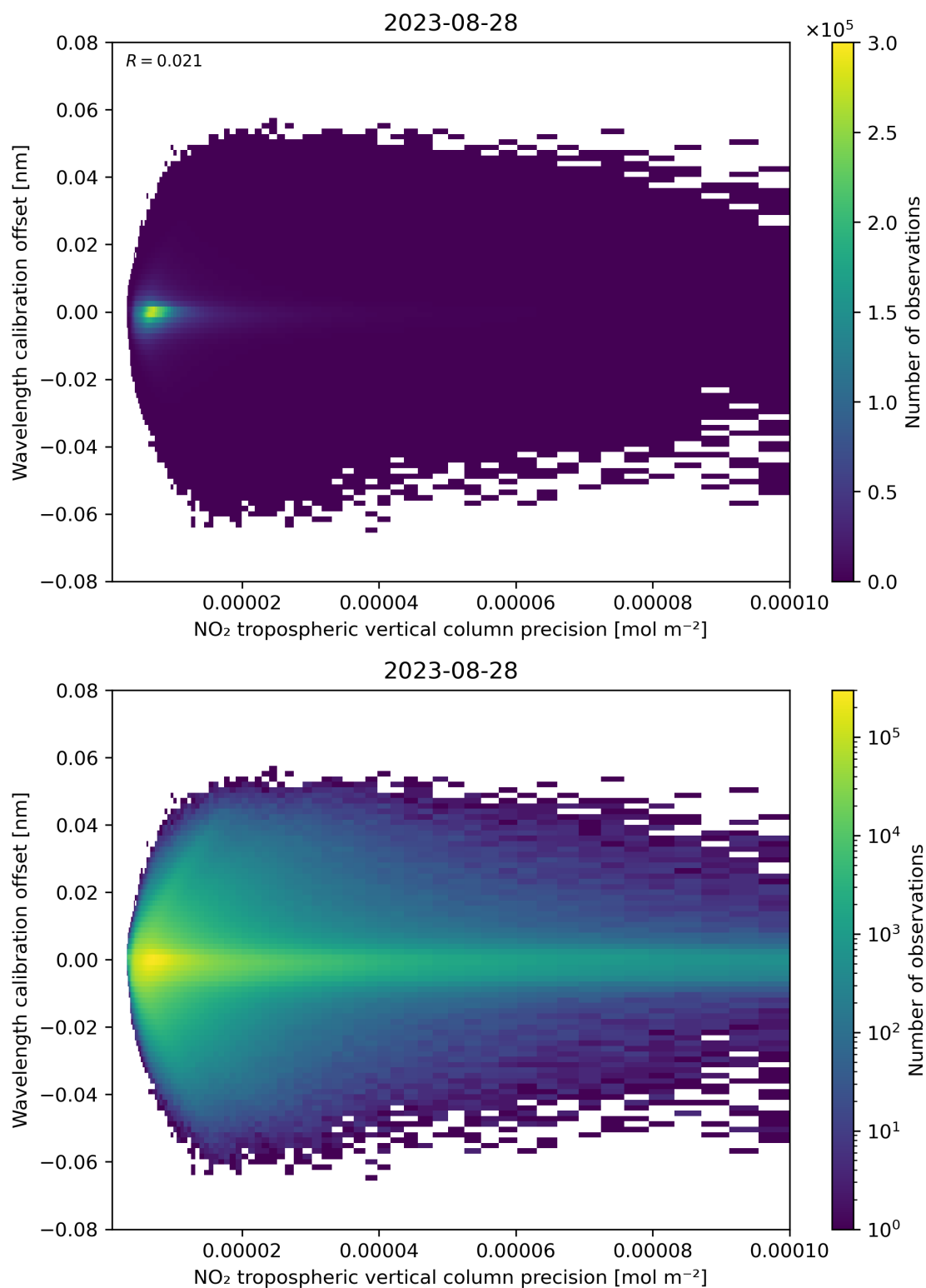
Figure 141: Scatter density plot of “NO 2 tropospheric vertical column precision” against “Wavelength calibration offset” for 2023-08-27 to 2023-08-29.
