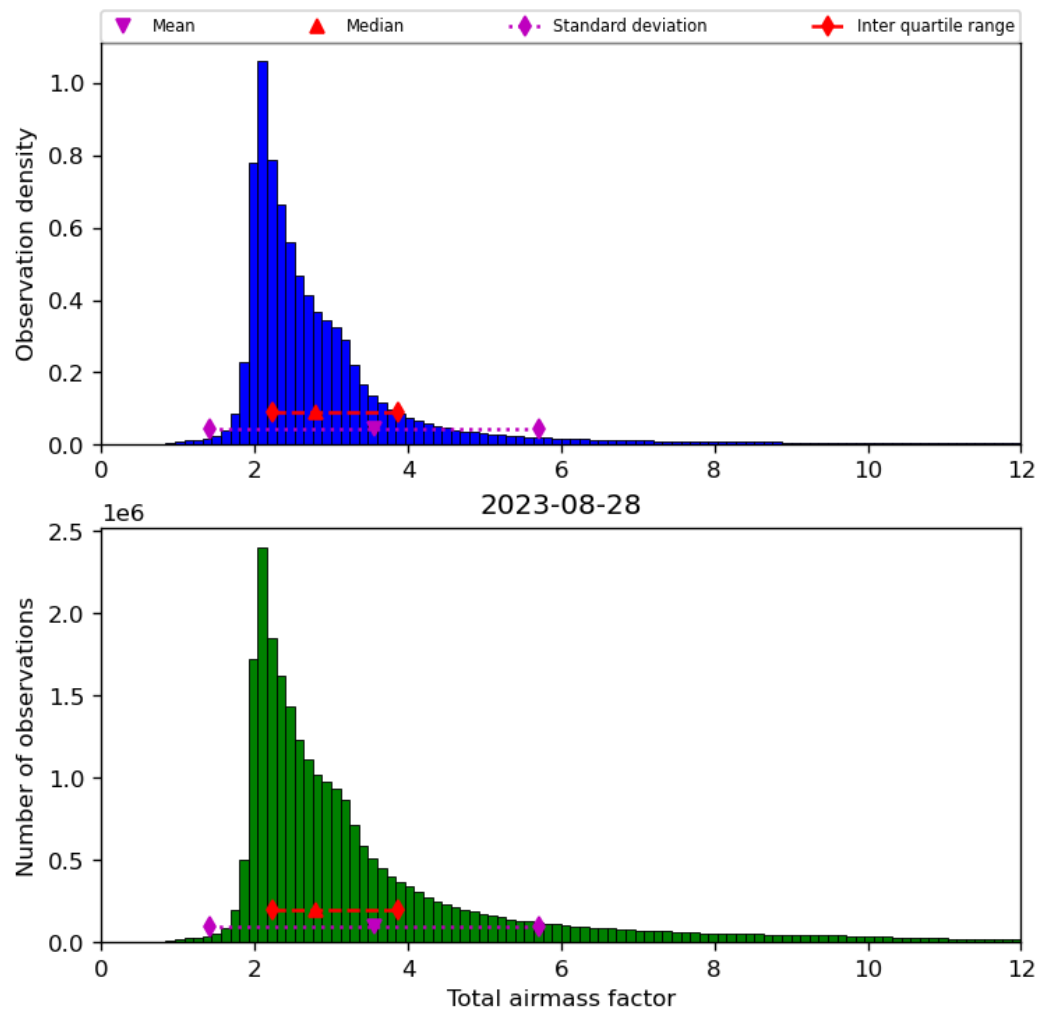
Figure 32: Histogram of “Total airmass factor” for 2023-08-27 to 2023-08-29
