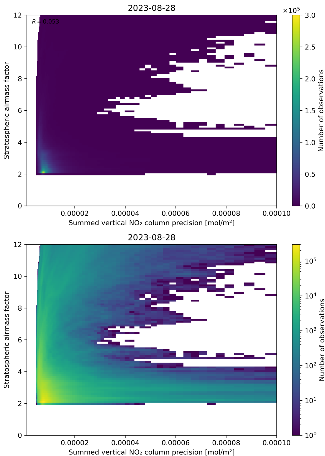
Figure 106: Scatter density plot of “Summed vertical NO 2 column precision” against “Stratospheric airmass factor” for 2023-08-27 to 2023-08-29.
