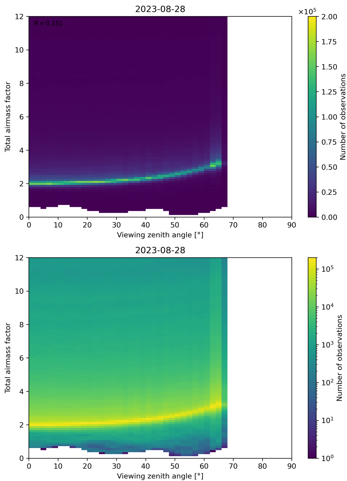
Figure 160: Scatter density plot of “Viewing zenith angle” against “Total airmass factor” for 2023-08-27 to 2023-08-29.
