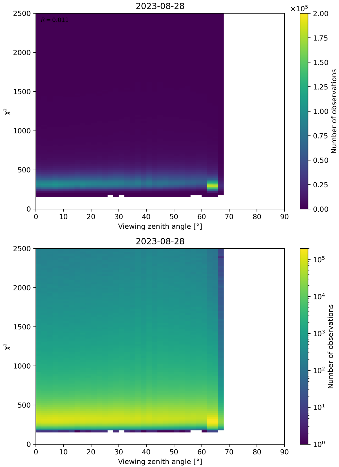
Figure 162: Scatter density plot of “Viewing zenith angle” against “ \chi^2 ” for 2023-08-27 to 2023-08-29.
