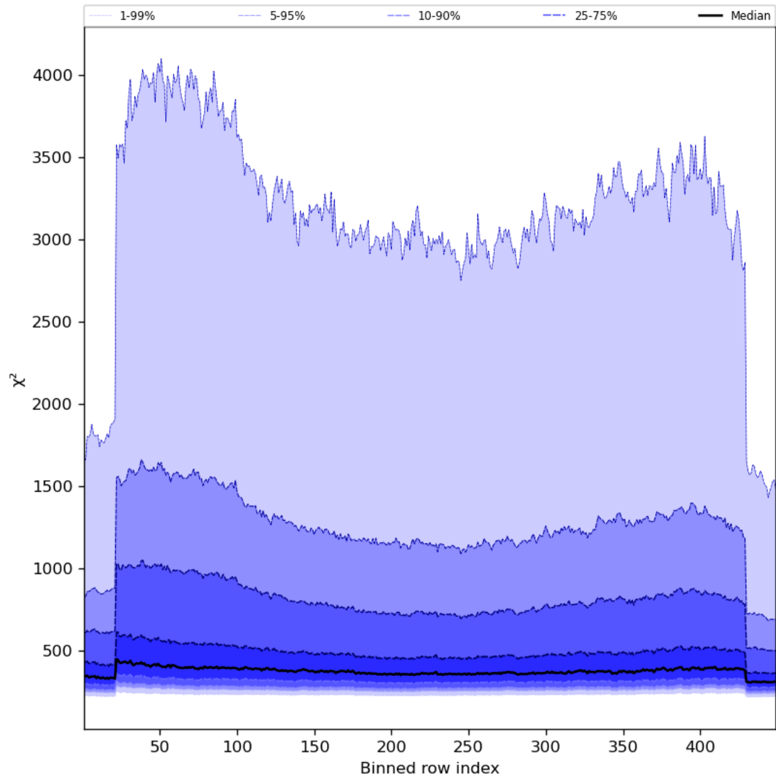
Figure 59: Along track statistics of “ \chi^2 ” for 2023-08-27 to 2023-08-29
