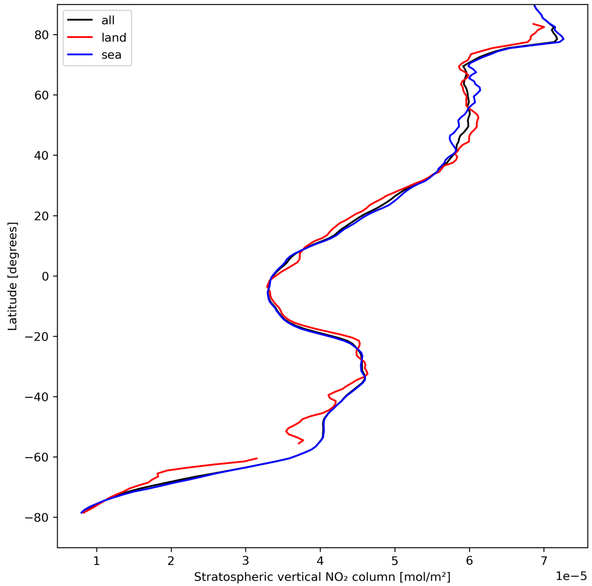
Figure 19: Zonal average of “Stratospheric vertical NO 2 column” for 2023-08-27 to 2023-08-29.
