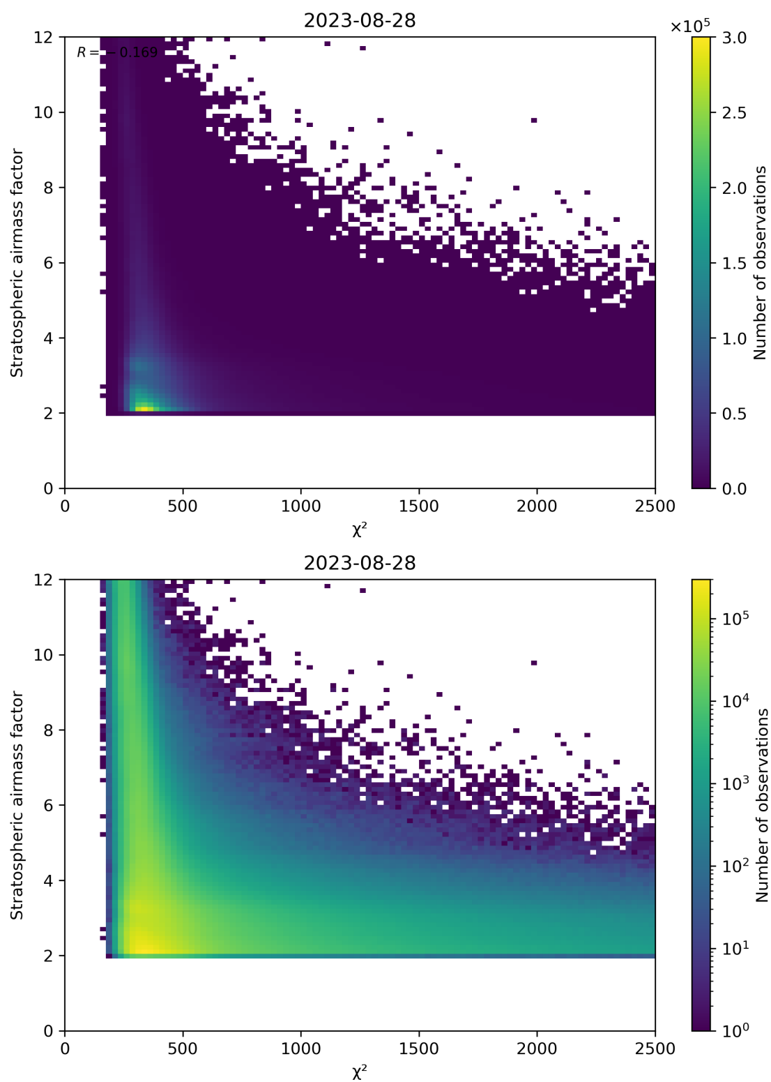
Figure 81: Scatter density plot of “ \chi^2 ” against “Stratospheric airmass factor” for 2023-08-27 to 2023-08-29.
