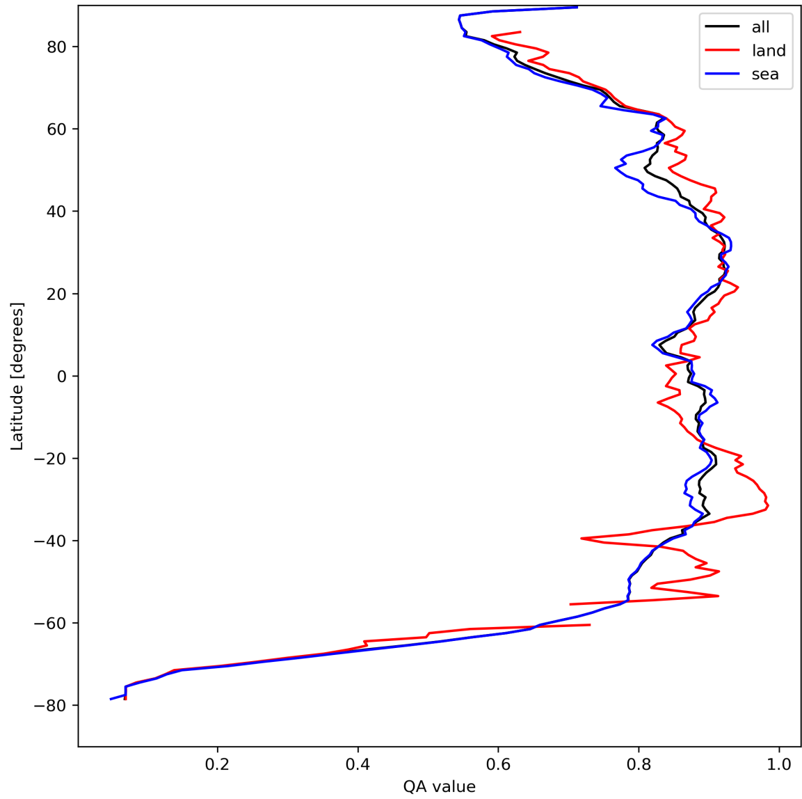
Figure 11: Zonal average of “QA value” for 2023-08-27 to 2023-08-29.
