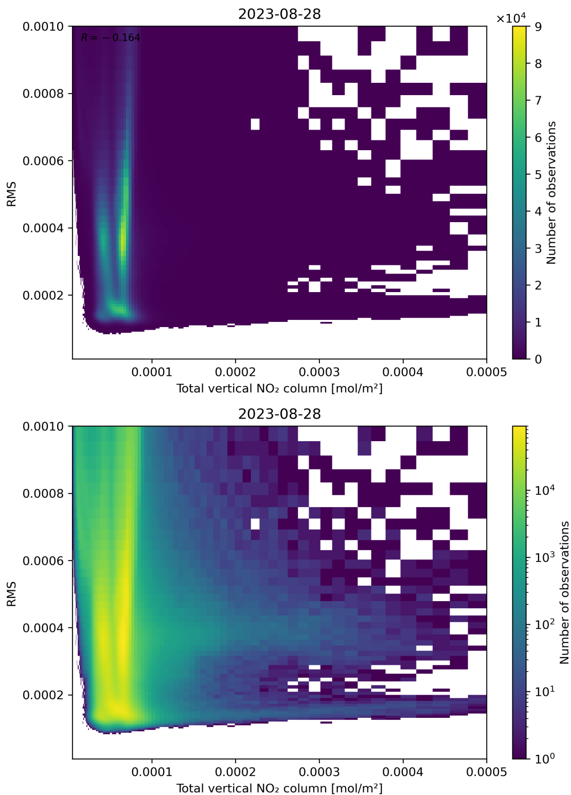
Figure 120: Scatter density plot of “Total vertical NO 2 column” against “RMS” for 2023-08-27 to 2023-08-29.
