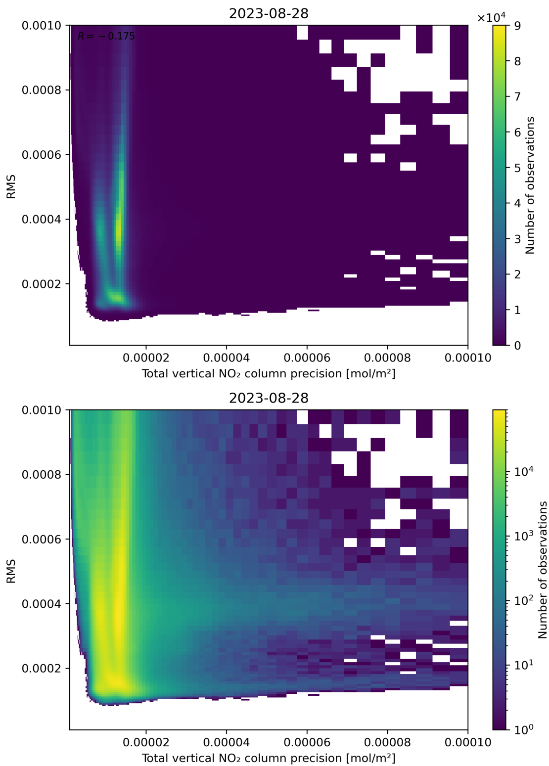
Figure 119: Scatter density plot of “Total vertical NO 2 column precision” against “RMS” for 2023-08-27 to 2023-08-29.
