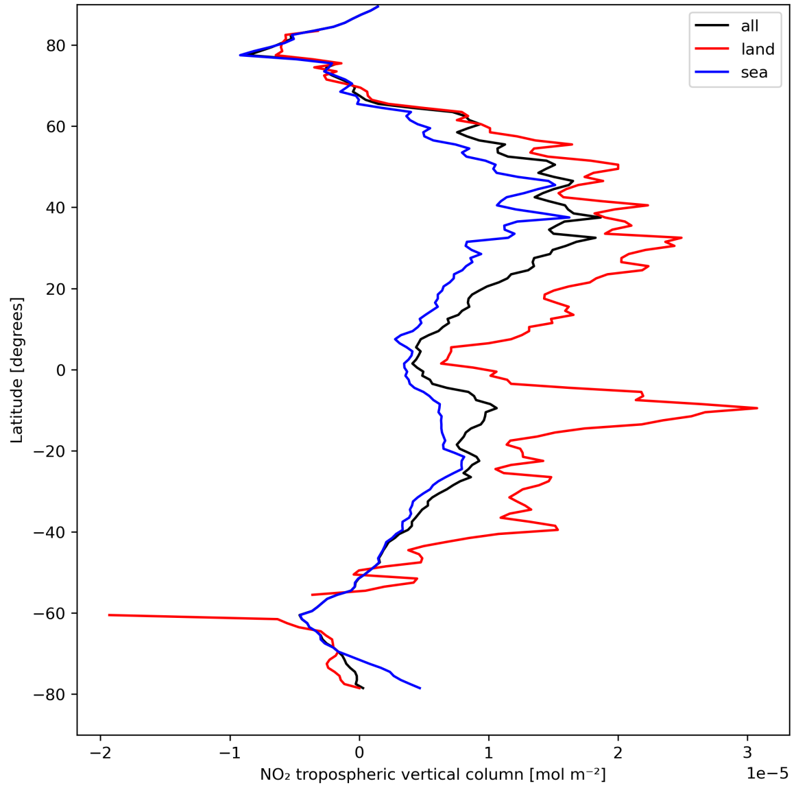
Figure 12: Zonal average of “NO 2 tropospheric vertical column” for 2023-08-27 to 2023-08-29.
