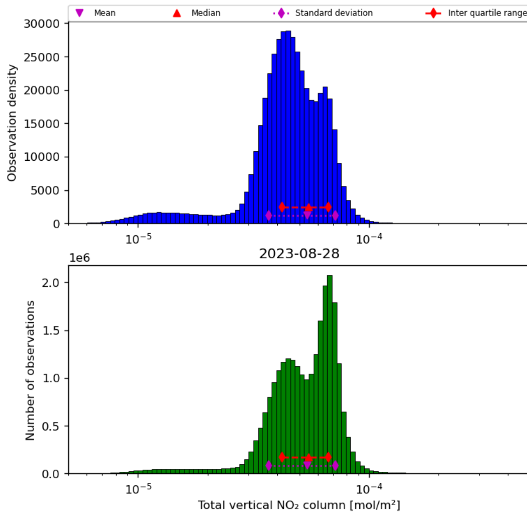
Figure 38: Histogram of “Total vertical NO 2 column” for 2023-08-27 to 2023-08-29
