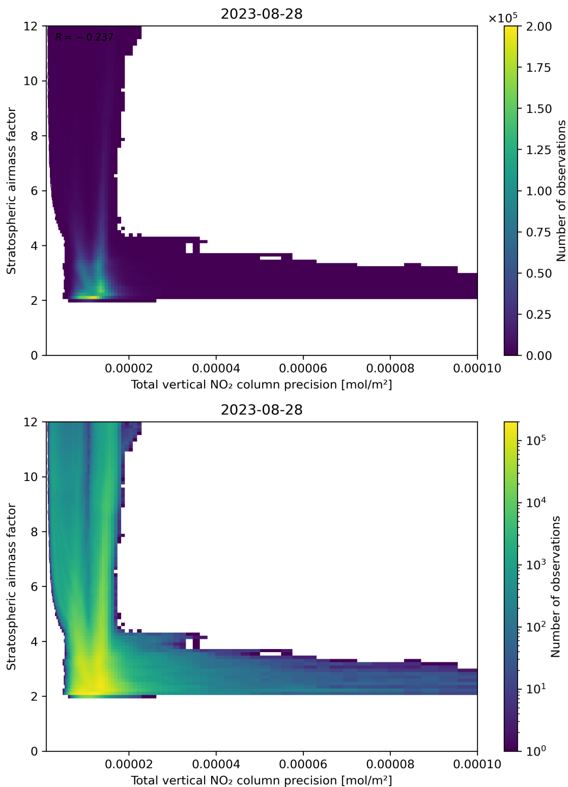
Figure 115: Scatter density plot of “Total vertical NO 2 column precision” against “Stratospheric air mass factor” for 2023-08-27 to 2023-08-29.
