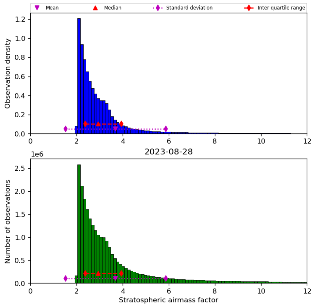
Figure 44: Histogram of “Stratospheric airmass factor” for 2023-08-27 to 2023-08-29
