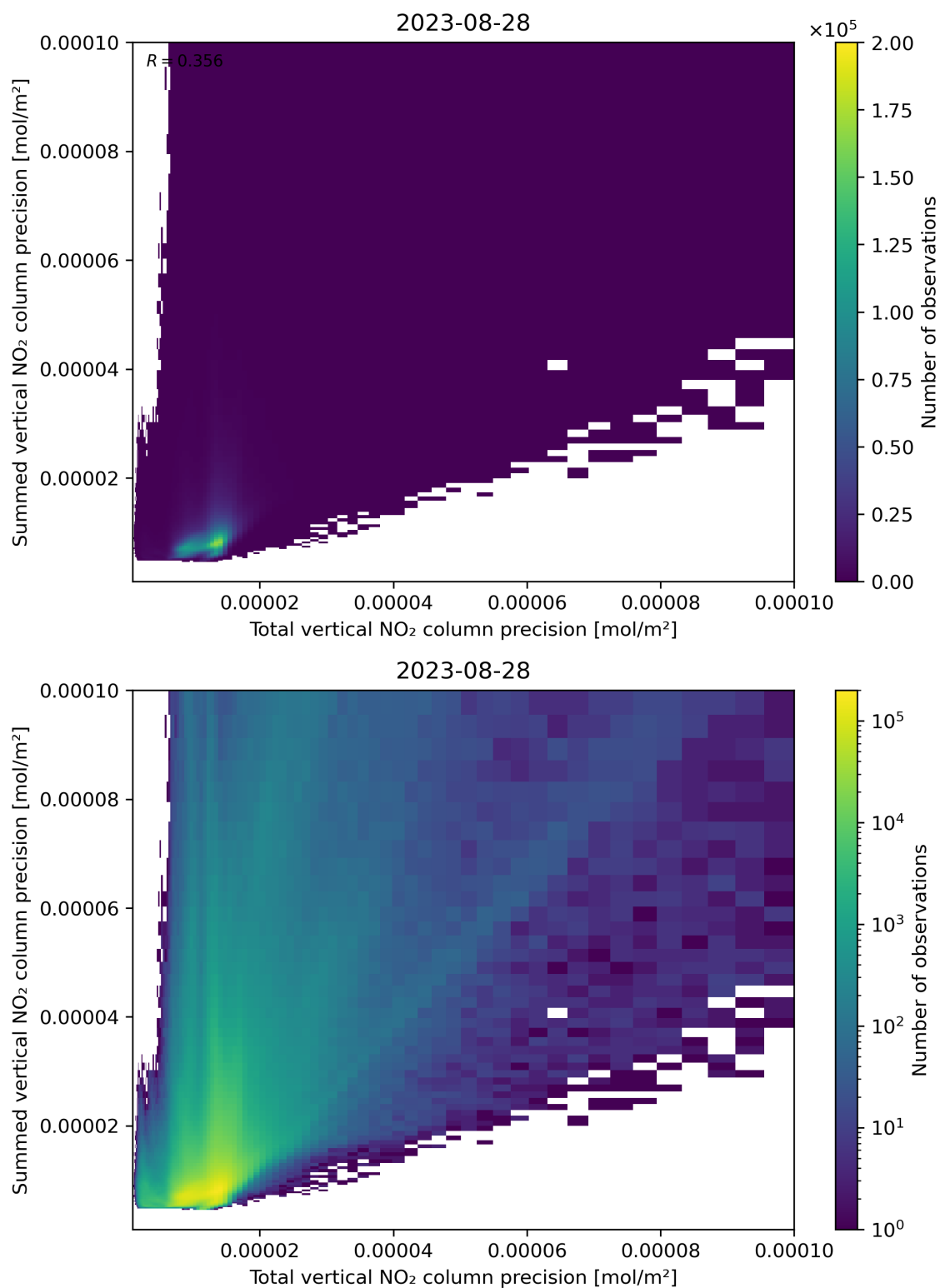
Figure 118: Scatter density plot of “Total vertical NO 2 column precision” against “Summed vertical NO 2 column precision” for 2023-08-27 to 2023-08-29.
