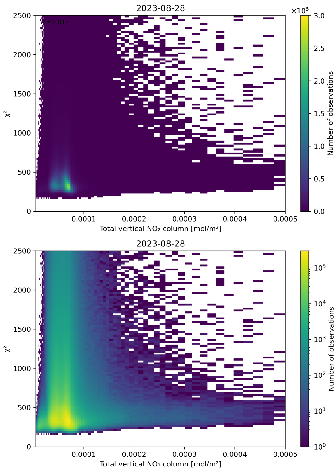
Figure 111: Scatter density plot of “Total vertical NO 2 column” against “ \chi^2 ” for 2023-08-27 to 2023-08-29.
