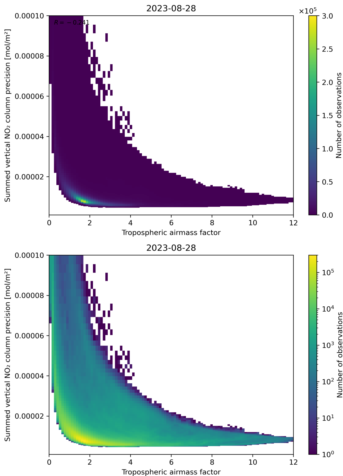
Figure 76: Scatter density plot of “Tropospheric air mass factor” against “Summed vertical NO 2 column precision” for 2023-08-27 to 2023-08-29.
