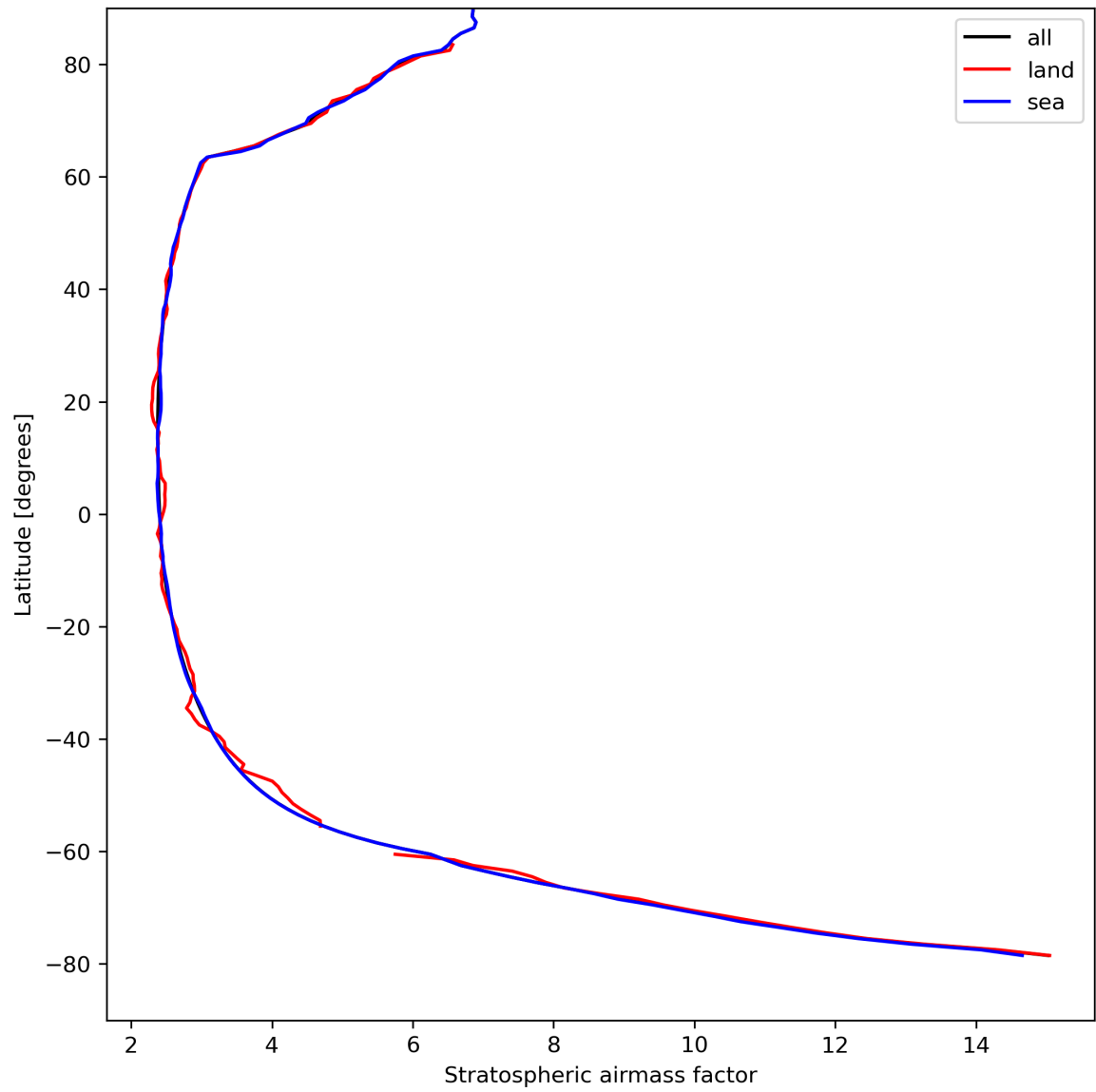
Figure 27: Zonal average of “Stratospheric airmass factor” for 2023-08-27 to 2023-08-29.
