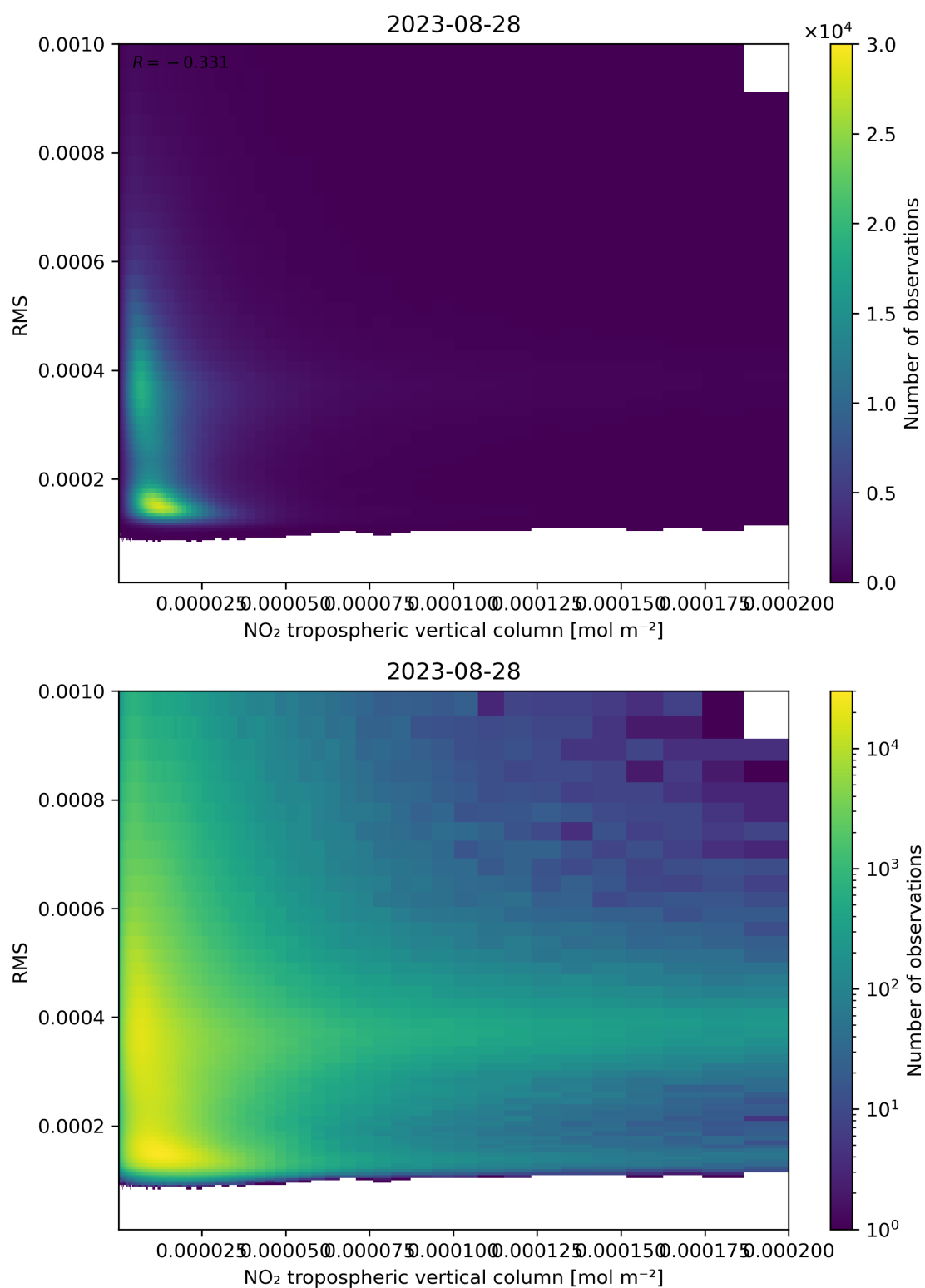
Figure 142: Scatter density plot of “NO 2 tropospheric vertical column” against “RMS” for 2023-08-27 to 2023-08-29.
