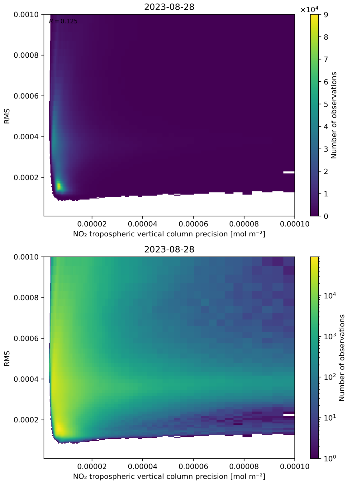
Figure 140: Scatter density plot of “NO 2 tropospheric vertical column precision” against “RMS” for 2023-08-27 to 2023-08-29.
