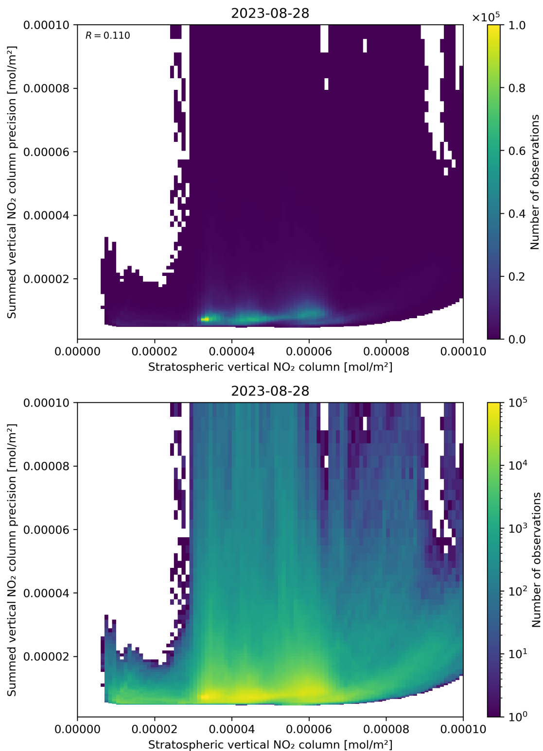
Figure 99: Scatter density plot of “Stratospheric vertical NO 2 column” against “Summed vertical NO 2 column precision” for 2023-08-27 to 2023-08-29.
