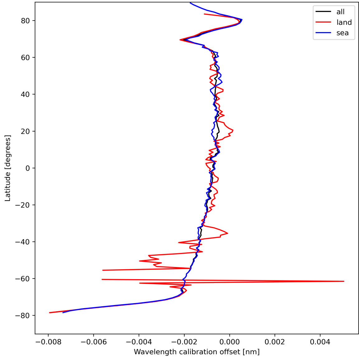
Figure 18: Zonal average of “Wavelength calibration offset” for 2023-08-27 to 2023-08-29.
