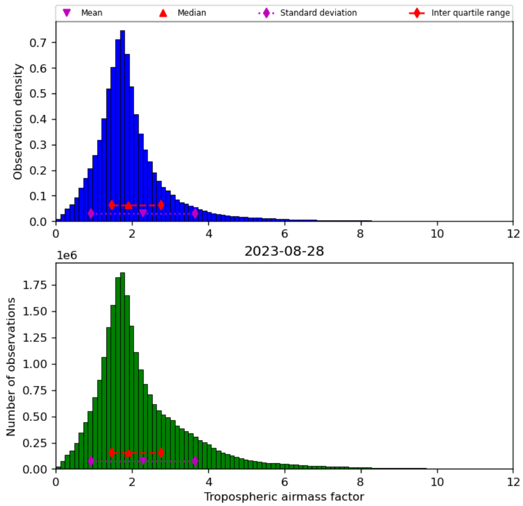
Figure 31: Histogram of “Tropospheric airmass factor” for 2023-08-27 to 2023-08-29
