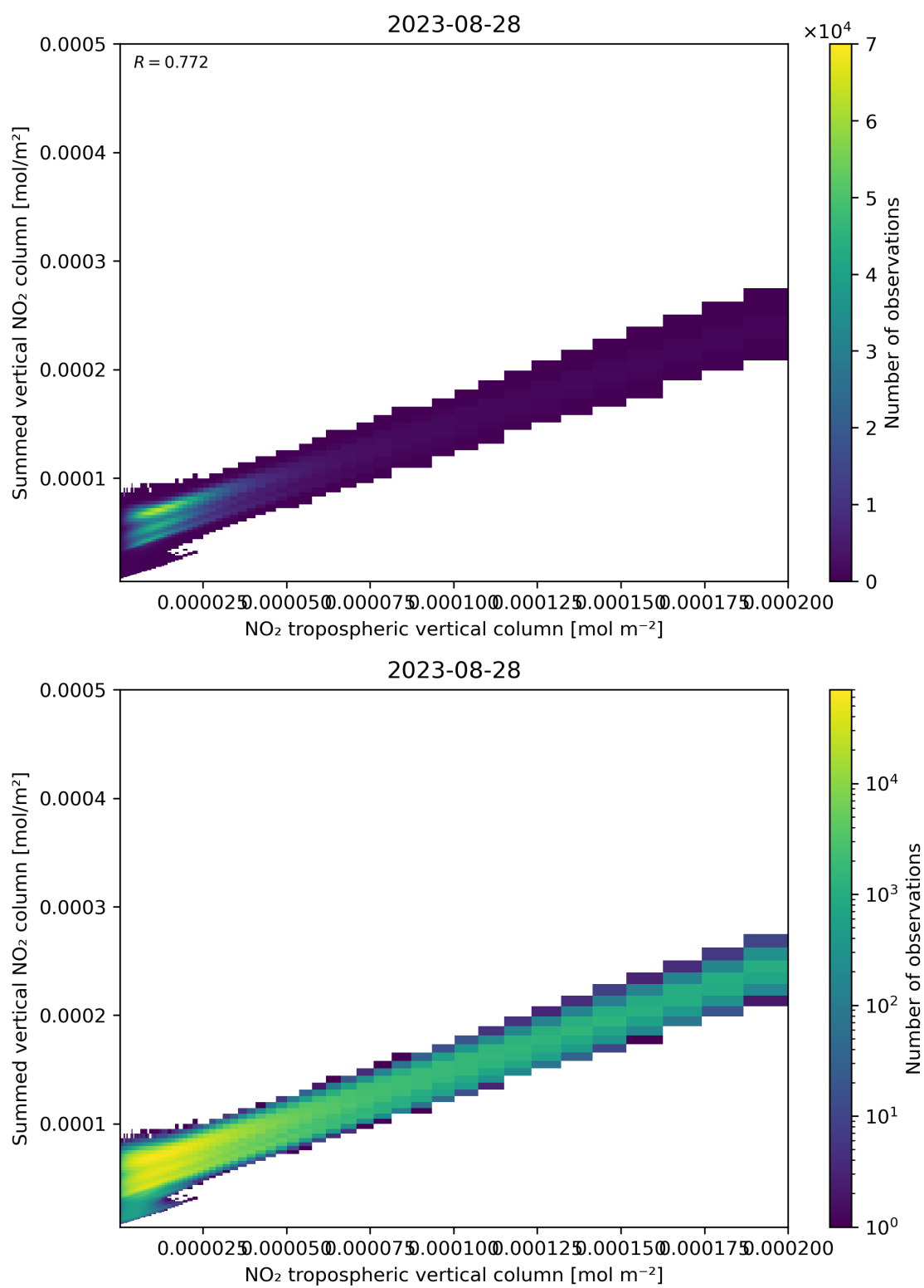
Figure 126: Scatter density plot of “NO 2 tropospheric vertical column” against “Summed vertical NO 2 column” for 2023-08-27 to 2023-08-29.
