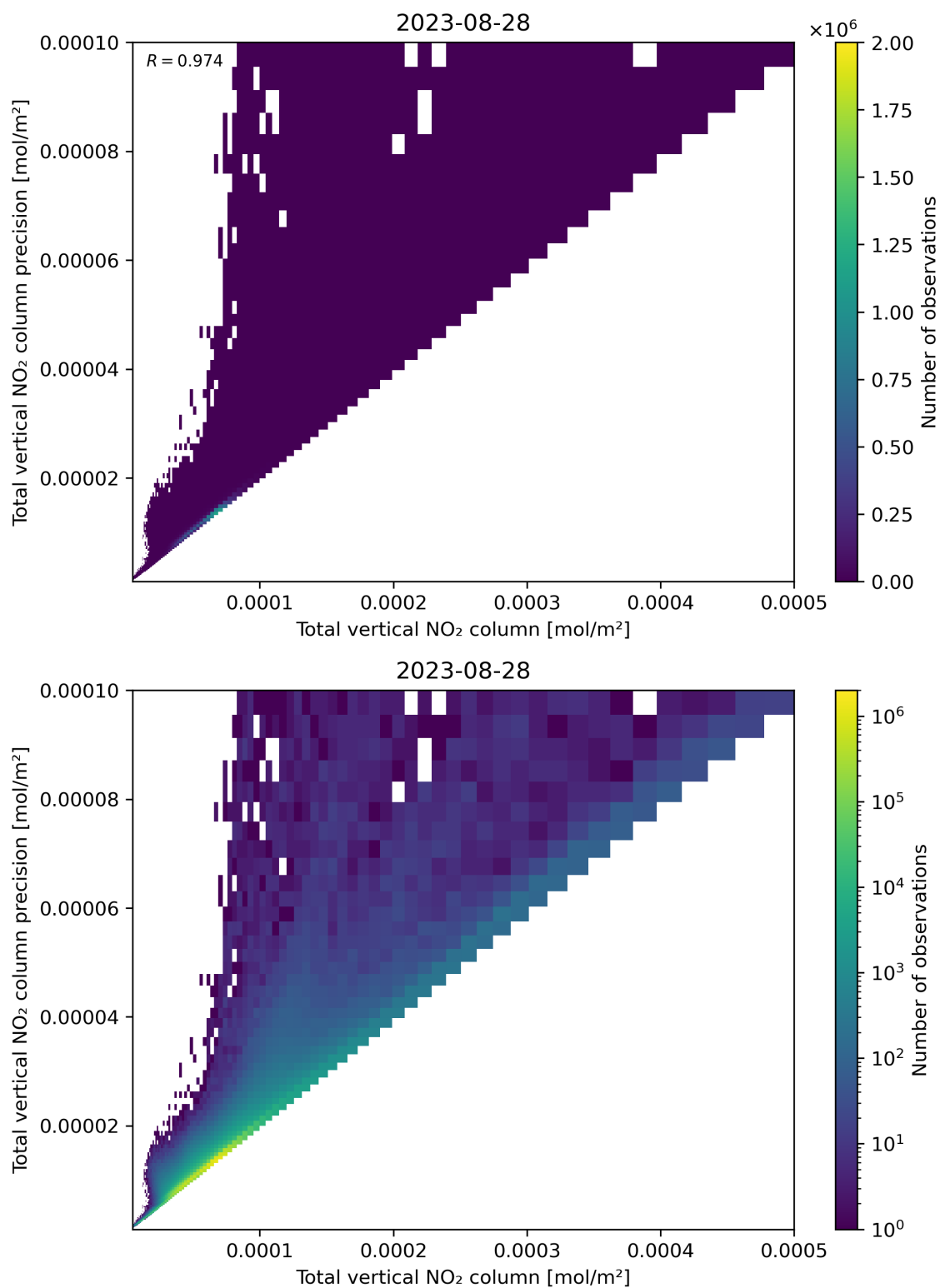
Figure 114: Scatter density plot of “Total vertical NO 2 column” against “Total vertical NO 2 column precision” for 2023-08-27 to 2023-08-29.
