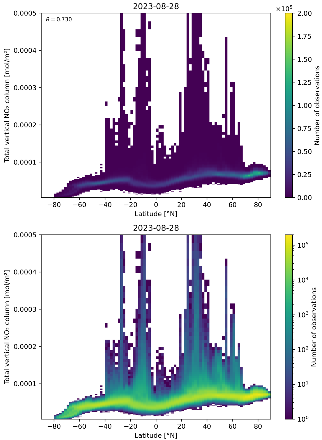
Figure 90: Scatter density plot of “Latitude” against “Total vertical NO 2 column” for 2023-08-27 to 2023-08-29.
