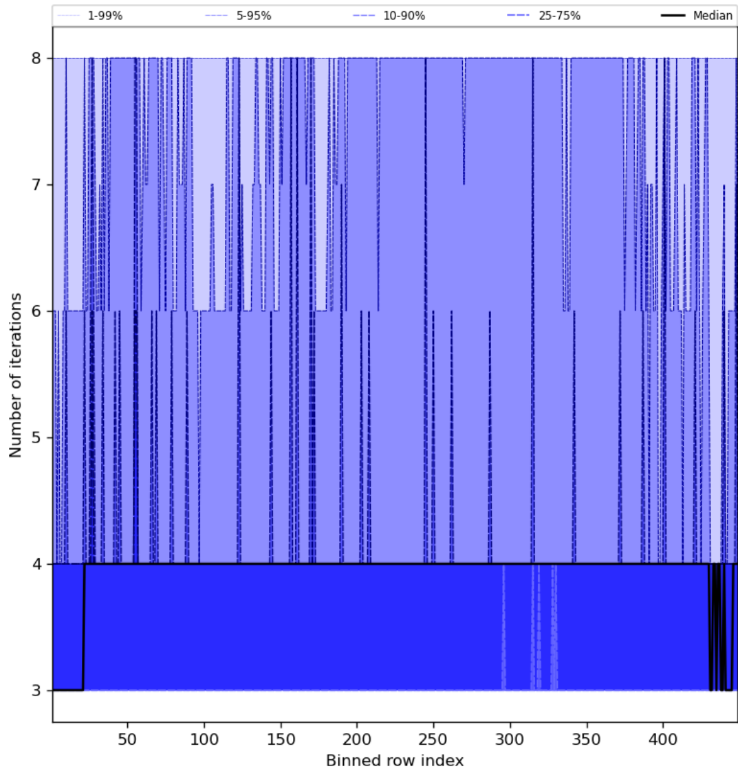
Figure 51: Along track statistics of “Number of iterations” for 2023-08-27 to 2023-08-29
