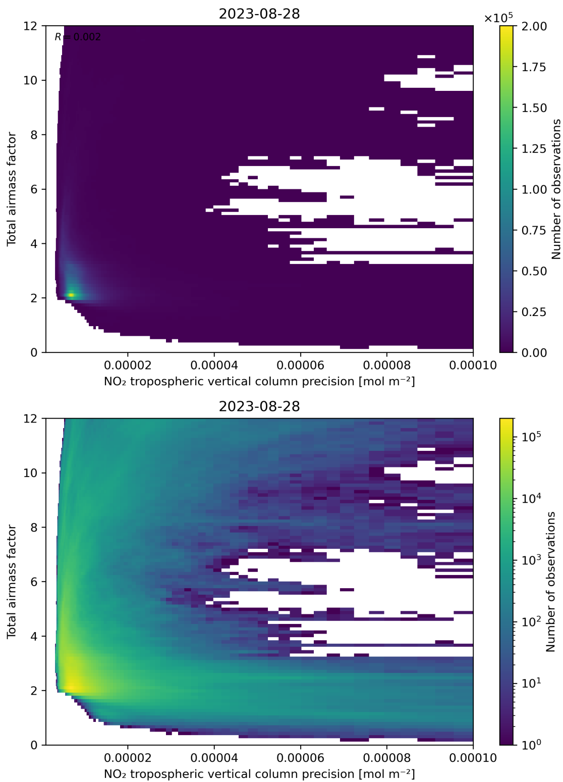
Figure 132: Scatter density plot of “NO 2 tropospheric vertical column precision” against “Total air mass factor” for 2023-08-27 to 2023-08-29.
