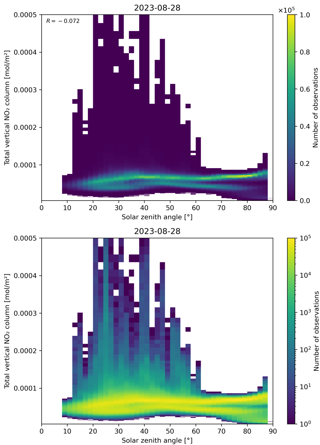
Figure 153: Scatter density plot of “Solar zenith angle” against “Total vertical NO 2 column” for 2023-08-27 to 2023-08-29.
