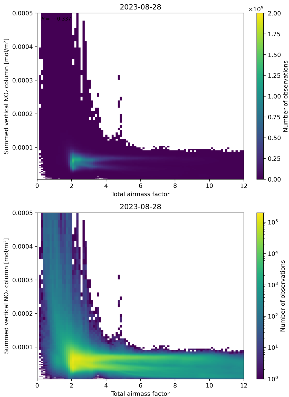
Figure 65: Scatter density plot of “Total airmass factor” against “Summed vertical NO 2 column” for 2023-08-27 to 2023-08-29.
