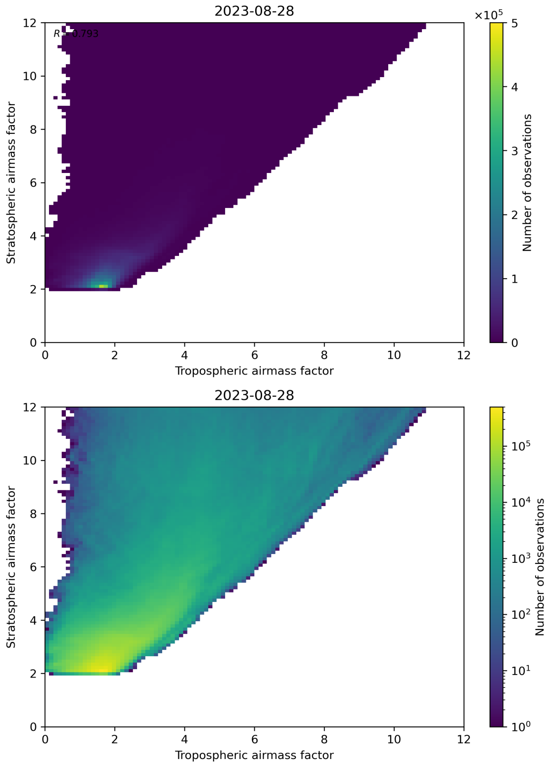
Figure 71: Scatter density plot of “Tropospheric airmass factor” against “Stratospheric airmass factor” for 2023-08-27 to 2023-08-29.
