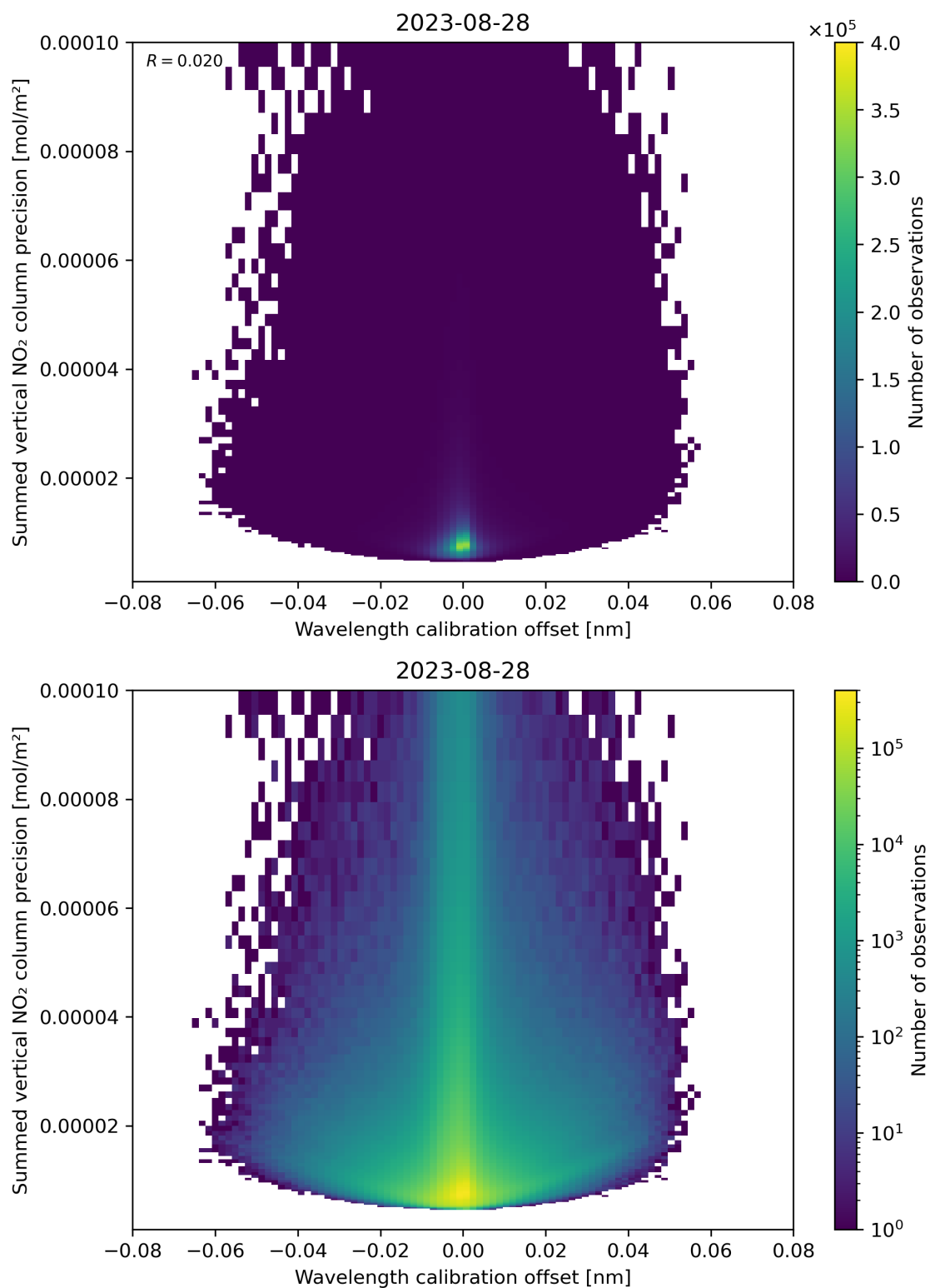
Figure 178: Scatter density plot of “Wavelength calibration offset” against “Summed vertical NO 2 column precision” for 2023-08-27 to 2023-08-29.
