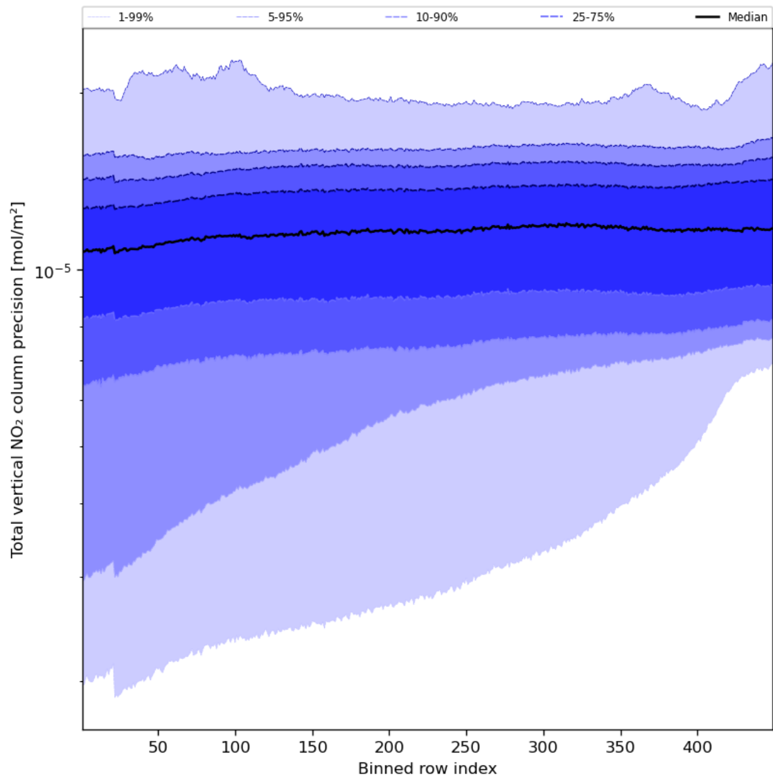
Figure 56: Along track statistics of “Total vertical NO 2 column precision” for 2023-08-27 to 2023-08-29
