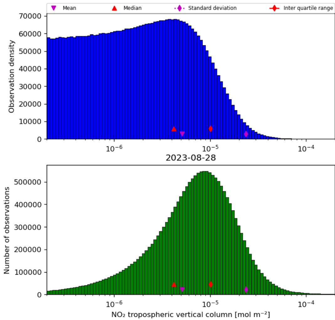
Figure 29: Histogram of “NO 2 tropospheric vertical column” for 2023-08-27 to 2023-08-29
