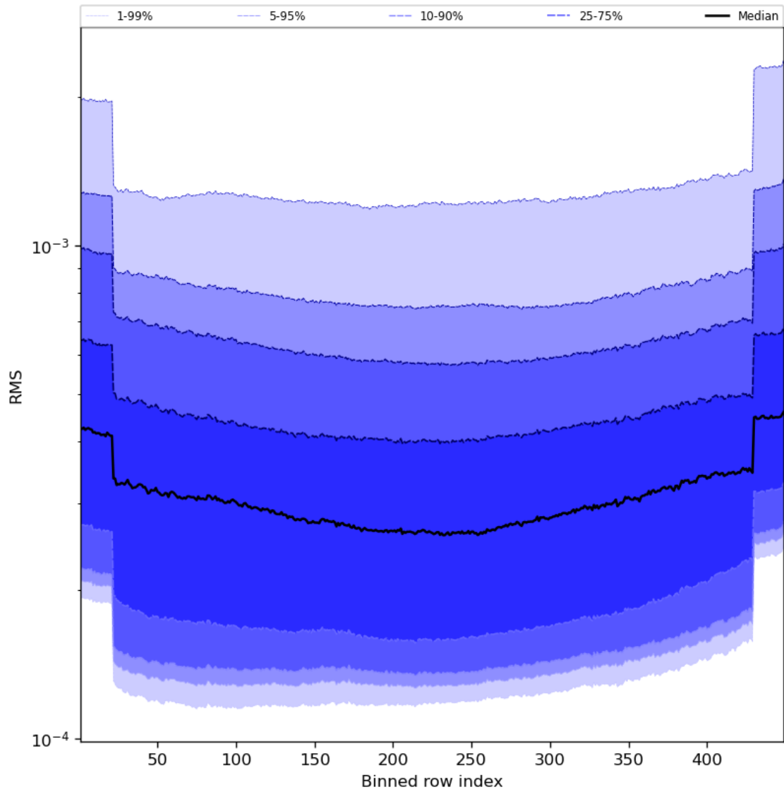
Figure 60: Along track statistics of “RMS” for 2023-08-28 to 2023-08-30
