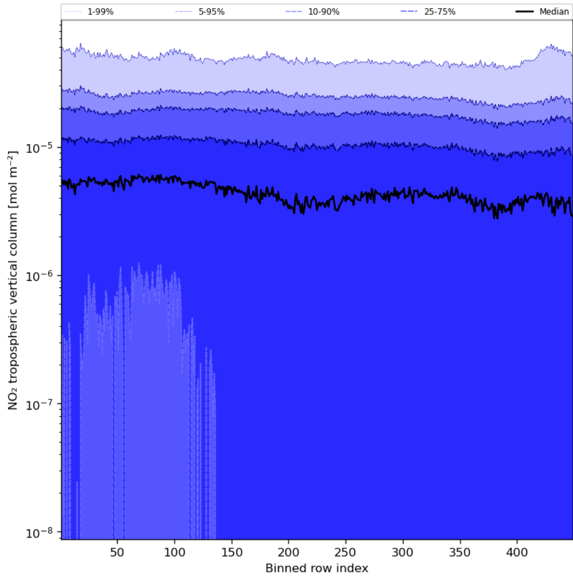
Figure 46: Along track statistics of “NO 2 tropospheric vertical column” for 2023-08-28 to 2023-08-30
