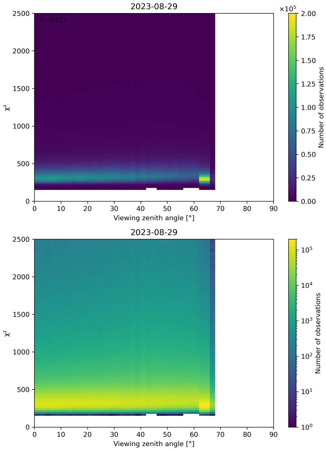
Figure 162: Scatter density plot of “Viewing zenith angle” against “ \chi^2 ” for 2023-08-28 to 2023-08-30.
