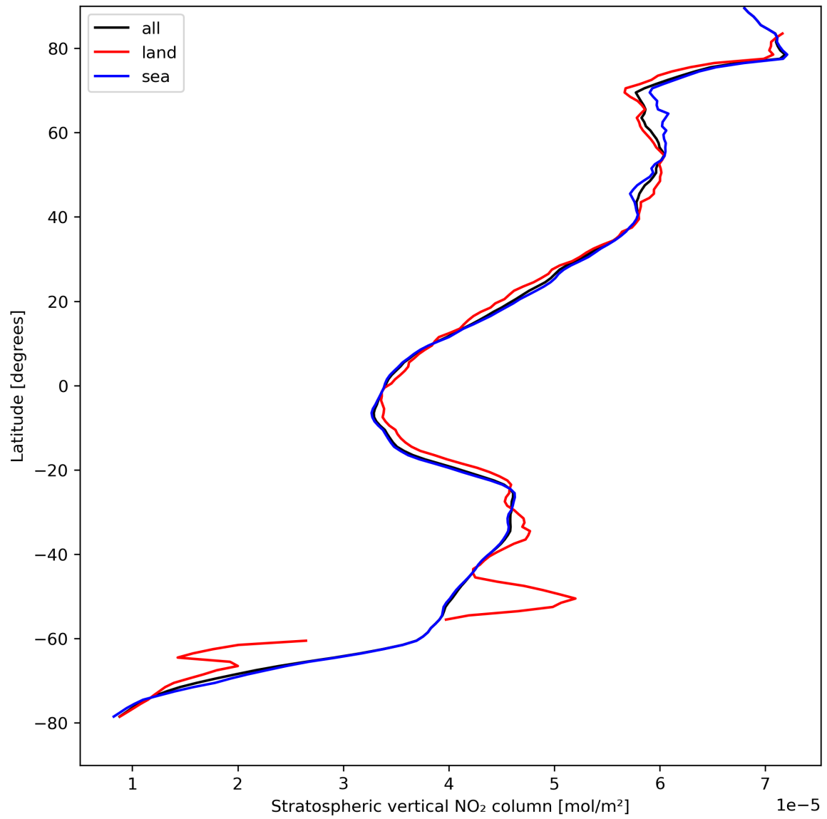
Figure 19: Zonal average of “Stratospheric vertical NO 2 column” for 2023-08-28 to 2023-08-30.
