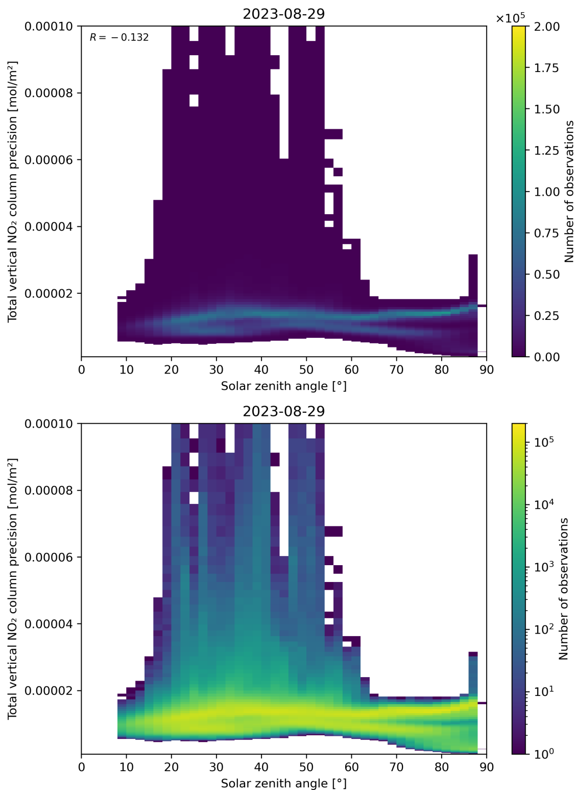
Figure 154: Scatter density plot of “Solar zenith angle” against “Total vertical NO 2 column precision” for 2023-08-28 to 2023-08-30.
