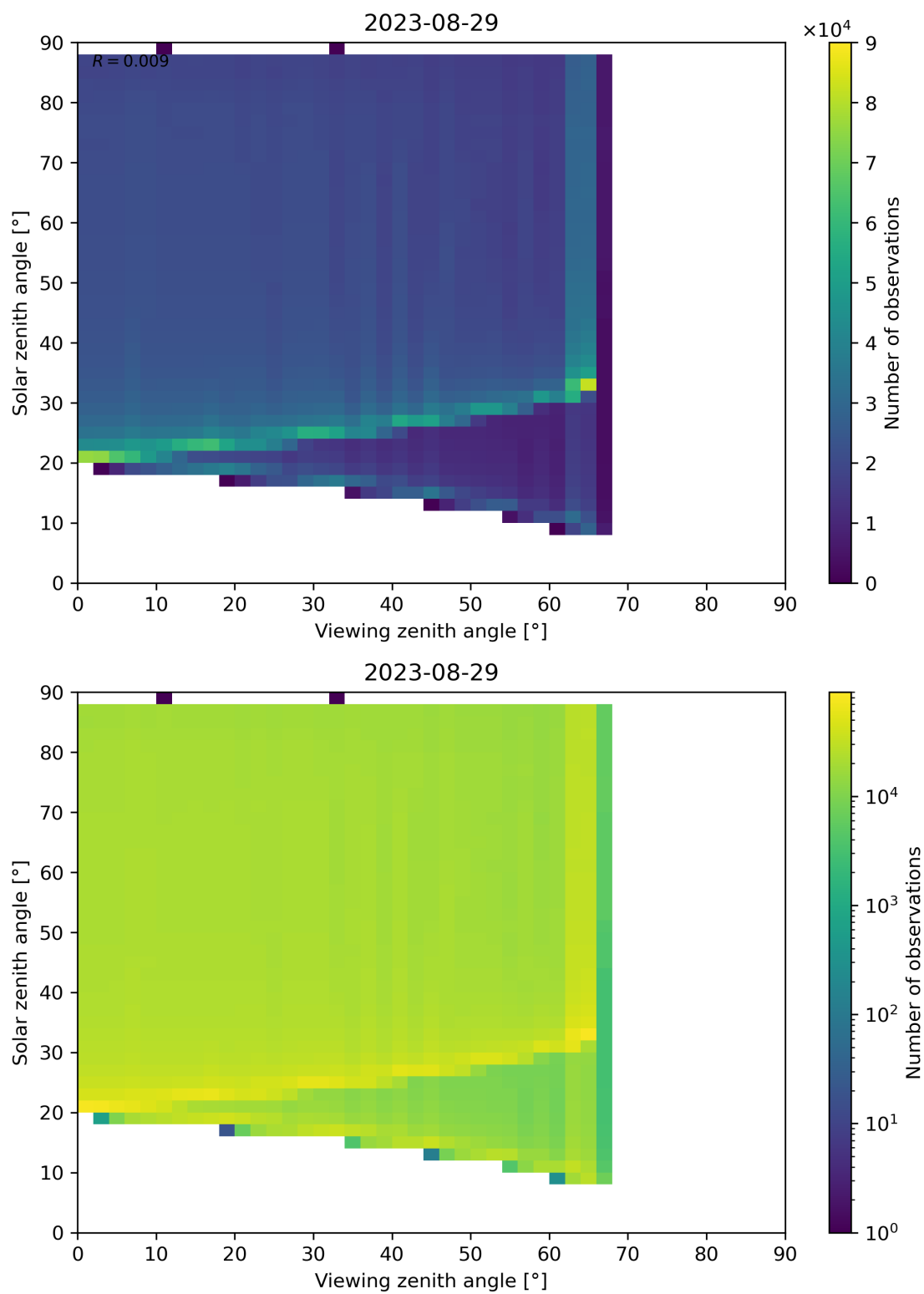
Figure 172: Scatter density plot of “Viewing zenith angle” against “Solar zenith angle” for 2023-08-28 to 2023-08-30.
