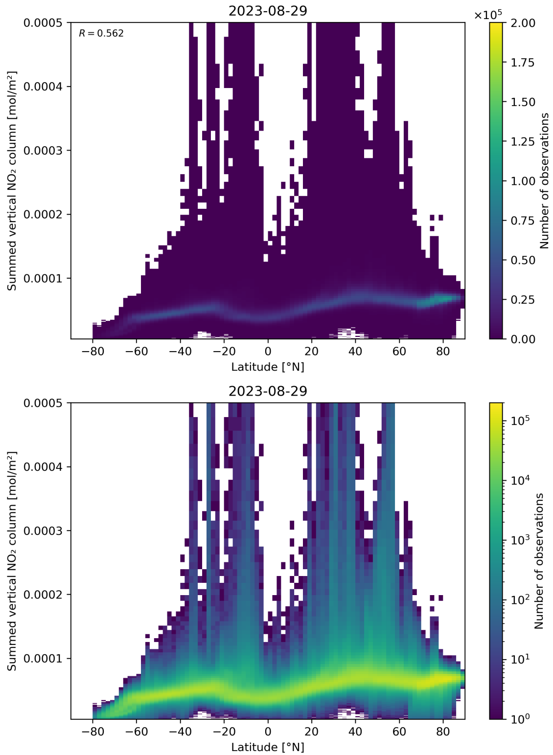
Figure 88: Scatter density plot of “Latitude” against “Summed vertical NO 2 column” for 2023-08-28 to 2023-08-30.
