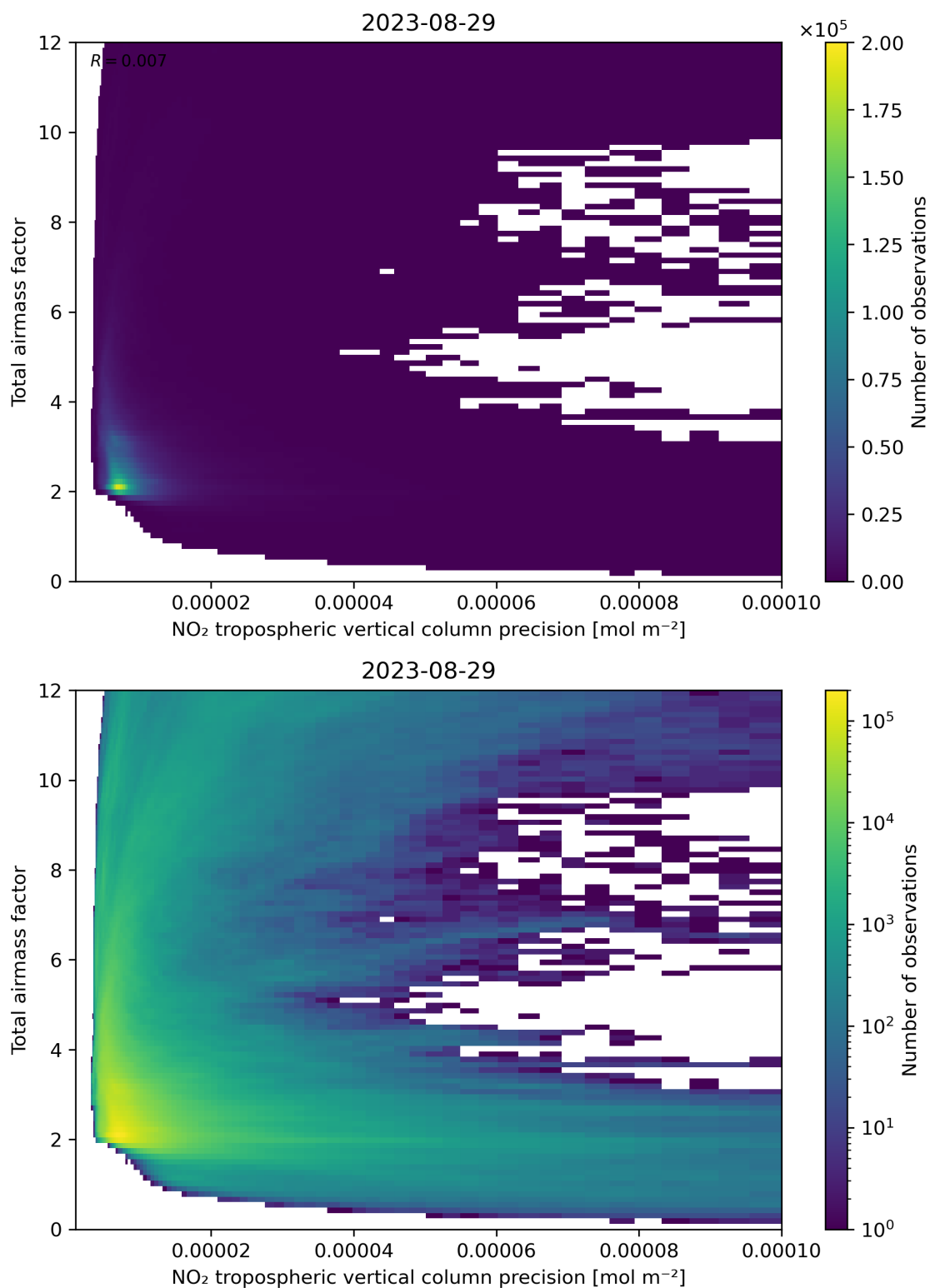
Figure 132: Scatter density plot of “NO 2 tropospheric vertical column precision” against “Total air mass factor” for 2023-08-28 to 2023-08-30.
