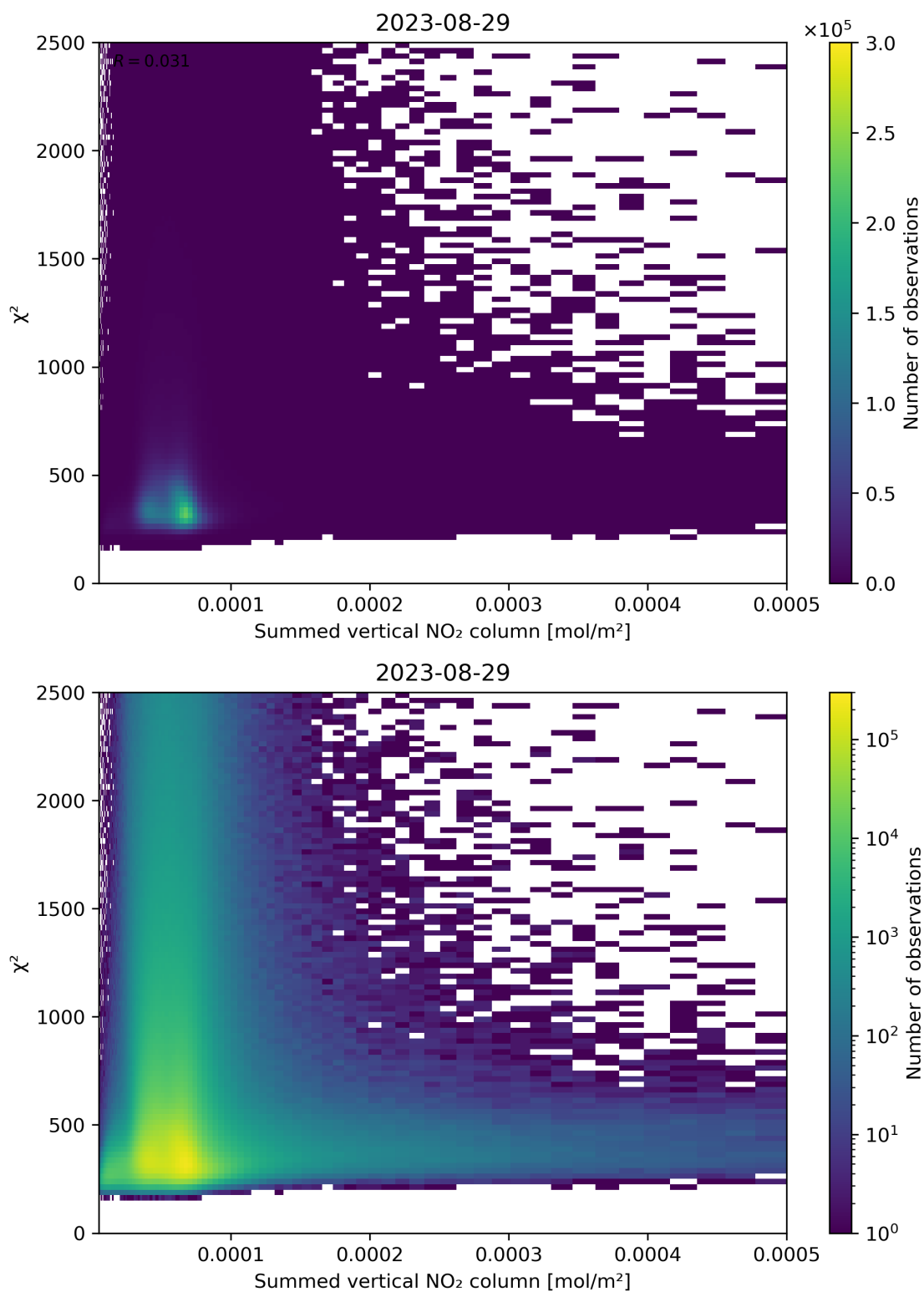
Figure 104: Scatter density plot of “Summed vertical NO 2 column” against “ \chi^2 ” for 2023-08-28 to 2023-08-30.
