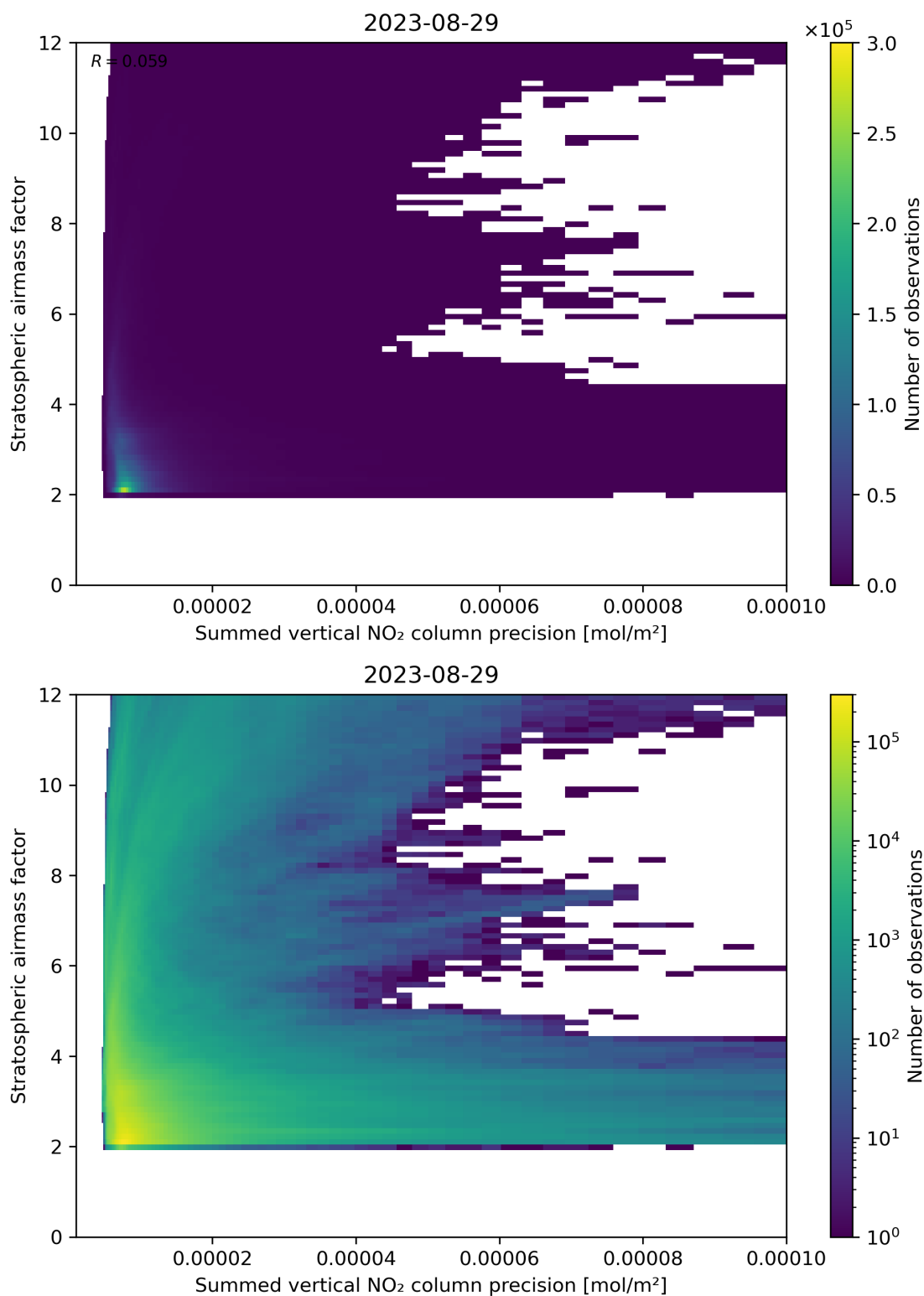
Figure 106: Scatter density plot of “Summed vertical NO 2 column precision” against “Stratospheric airmass factor” for 2023-08-28 to 2023-08-30.
