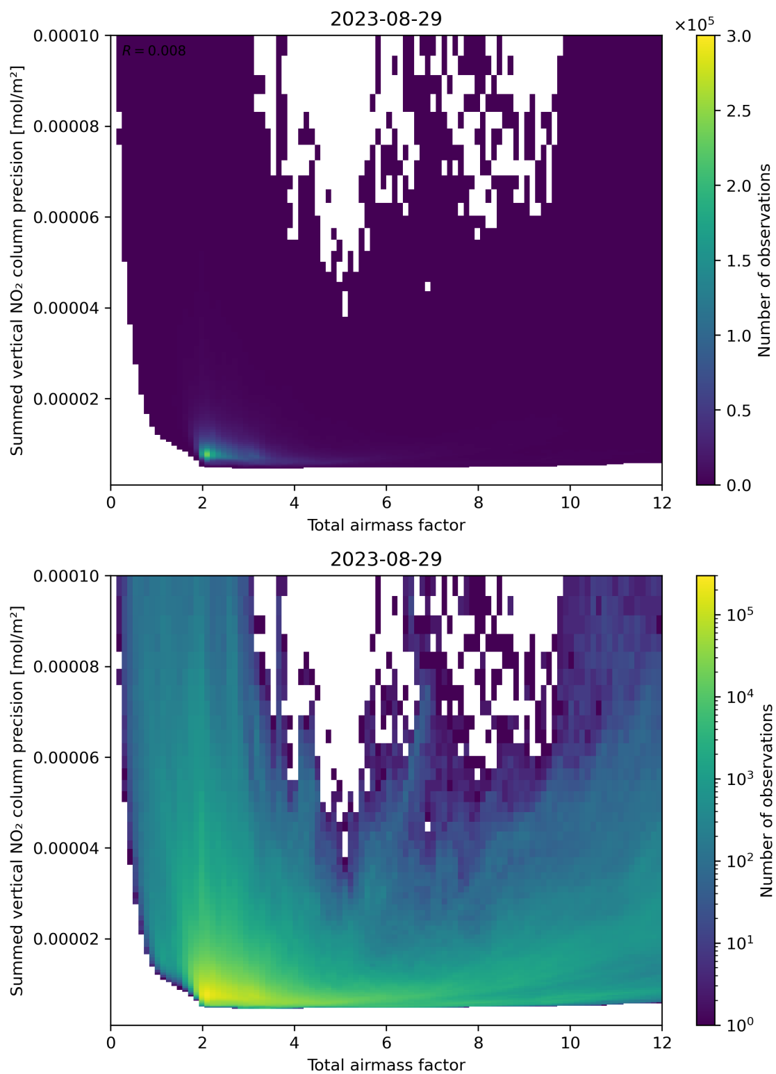
Figure 66: Scatter density plot of “Total airmass factor” against “Summed vertical NO 2 column precision” for 2023-08-28 to 2023-08-30.
