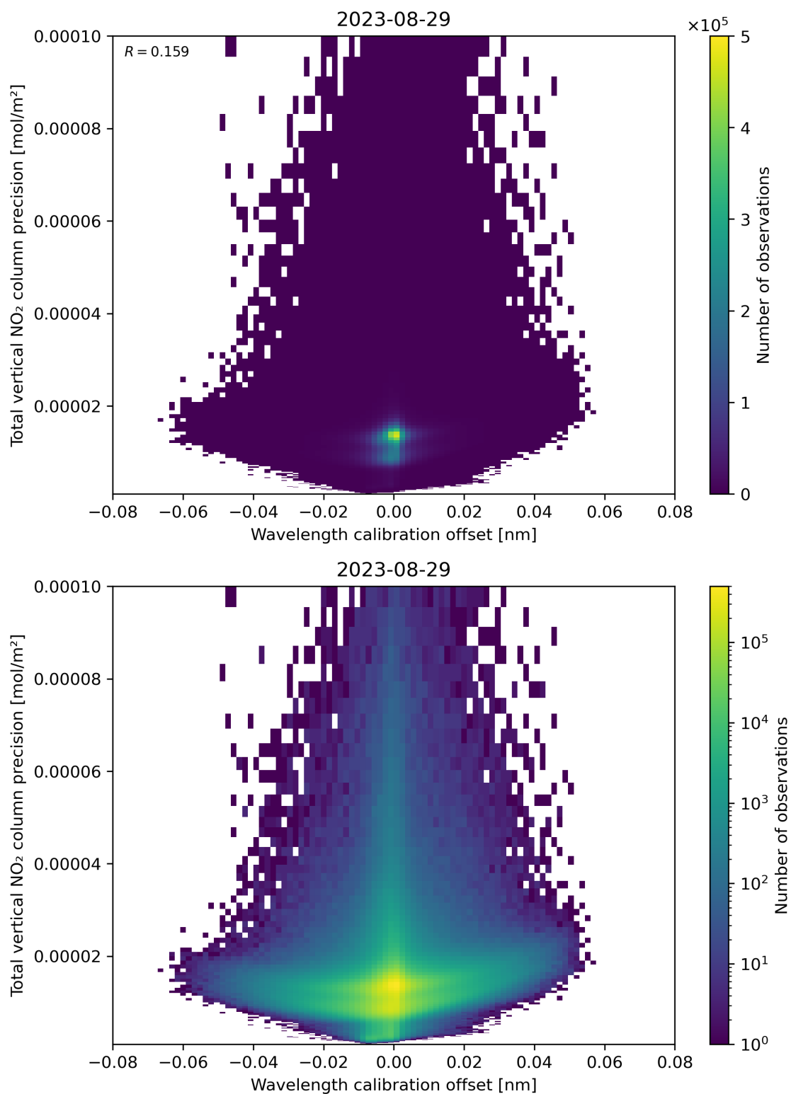
Figure 180: Scatter density plot of “Wavelength calibration offset” against “Total vertical NO 2 column precision” for 2023-08-28 to 2023-08-30.
