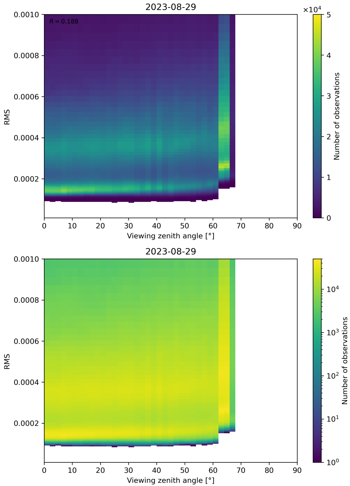
Figure 171: Scatter density plot of “Viewing zenith angle” against “RMS” for 2023-08-28 to 2023-08-30.
