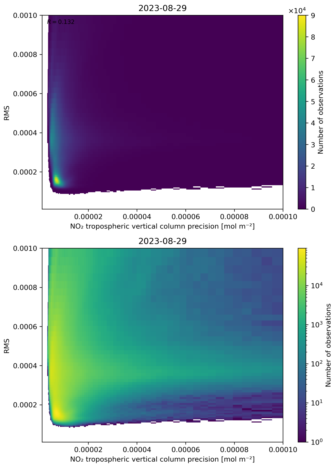
Figure 140: Scatter density plot of “NO 2 tropospheric vertical column precision” against “RMS” for 2023-08-28 to 2023-08-30.
