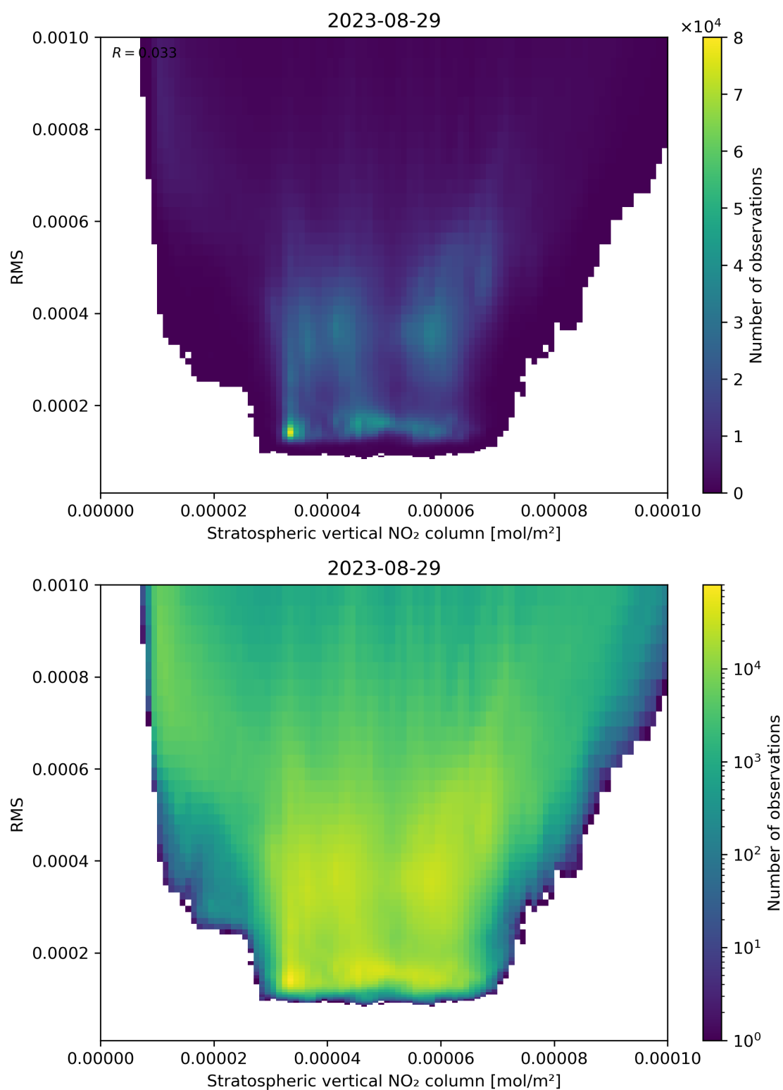
Figure 102: Scatter density plot of “Stratospheric vertical NO 2 column” against “RMS” for 2023-08-28 to 2023-08-30.
