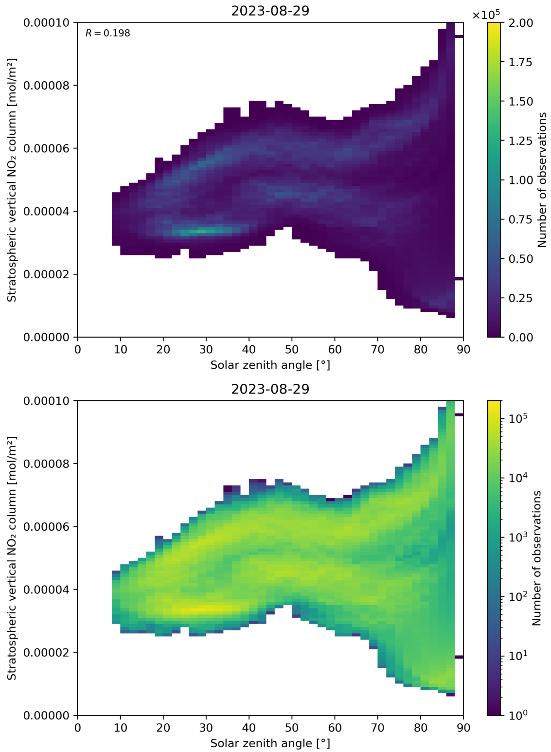
Figure 150: Scatter density plot of “Solar zenith angle” against “Stratospheric vertical NO 2 column” for 2023-08-28 to 2023-08-30.
