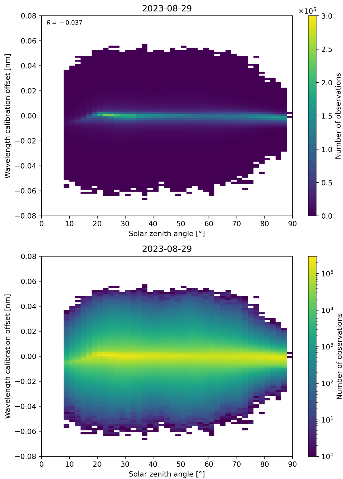
Figure 158: Scatter density plot of “Solar zenith angle” against “Wavelength calibration offset” for 2023-08-28 to 2023-08-30.
