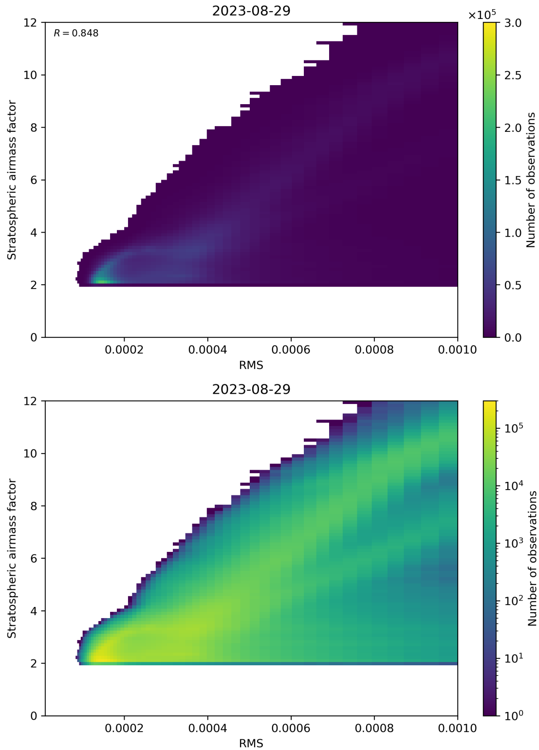
Figure 144: Scatter density plot of “RMS” against “Stratospheric airmass factor” for 2023-08-28 to 2023-08-30.
