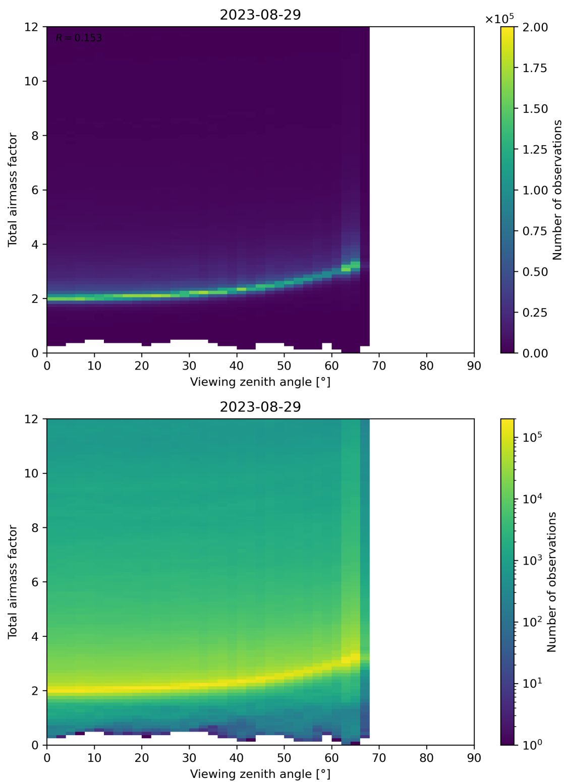
Figure 160: Scatter density plot of “Viewing zenith angle” against “Total airmass factor” for 2023-08-28 to 2023-08-30.
