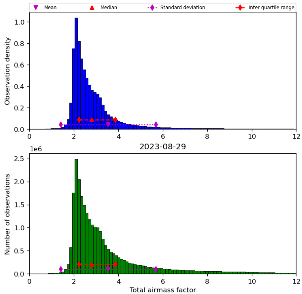
Figure 32: Histogram of “Total airmass factor” for 2023-08-28 to 2023-08-30
