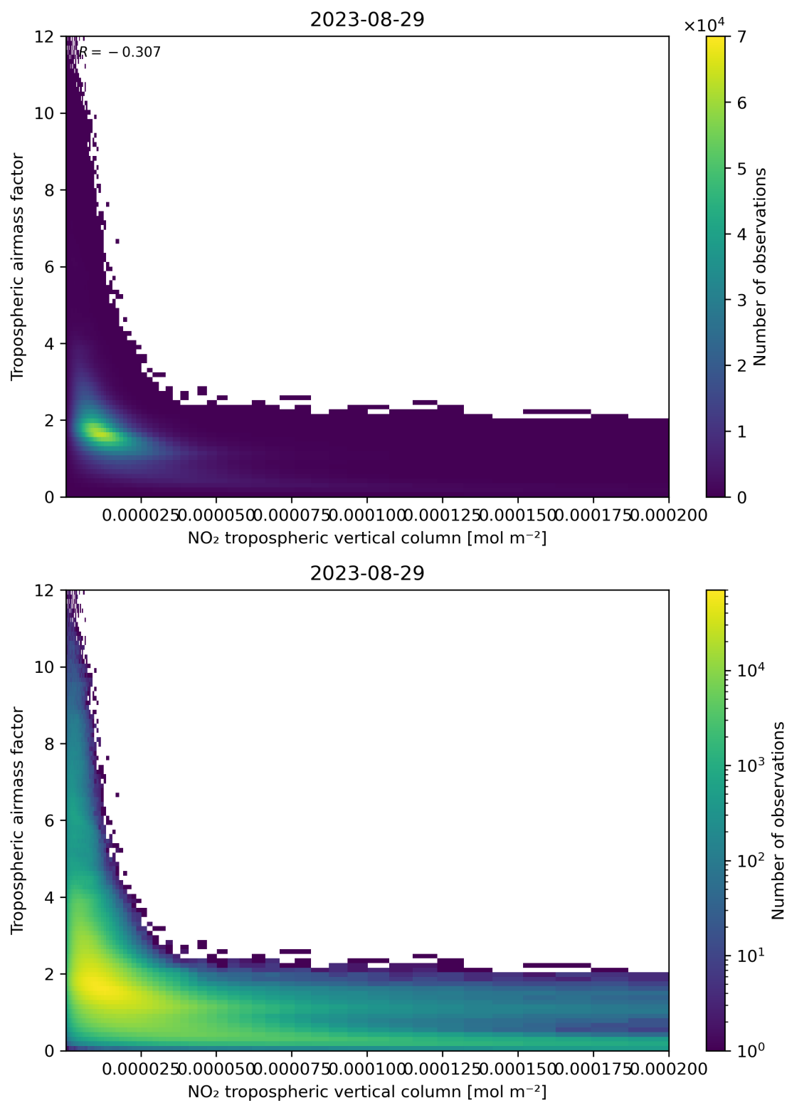
Figure 123: Scatter density plot of “NO 2 tropospheric vertical column” against “Tropospheric air mass factor” for 2023-08-28 to 2023-08-30.
