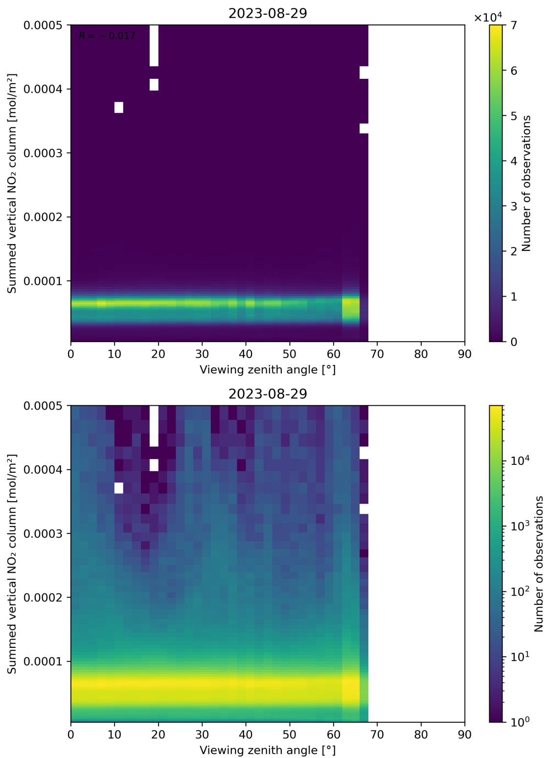
Figure 165: Scatter density plot of “Viewing zenith angle” against “Summed vertical NO 2 column” for 2023-08-28 to 2023-08-30.
