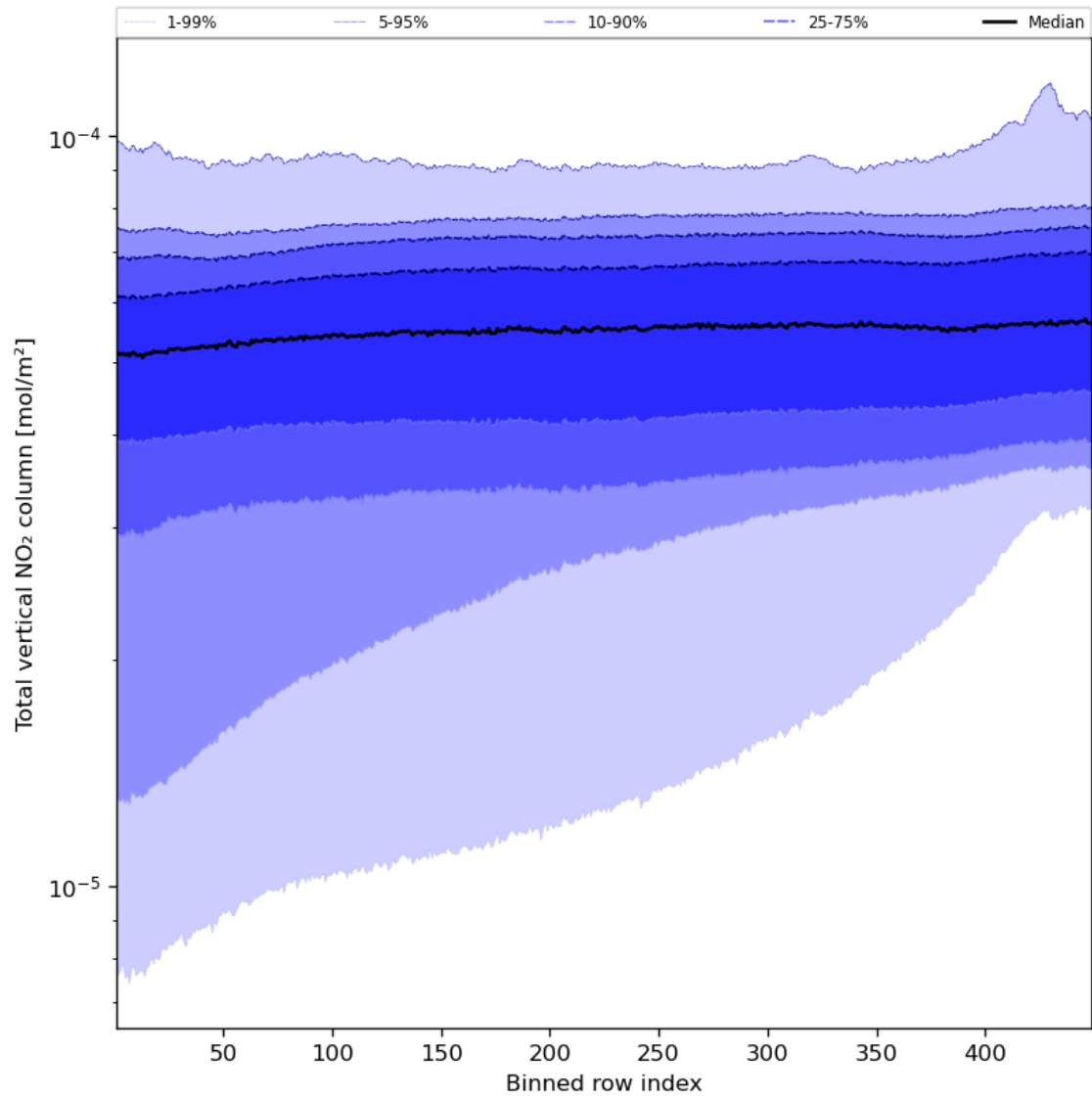
Figure 55: Along track statistics of “Total vertical NO 2 column” for 2023-08-28 to 2023-08-30
