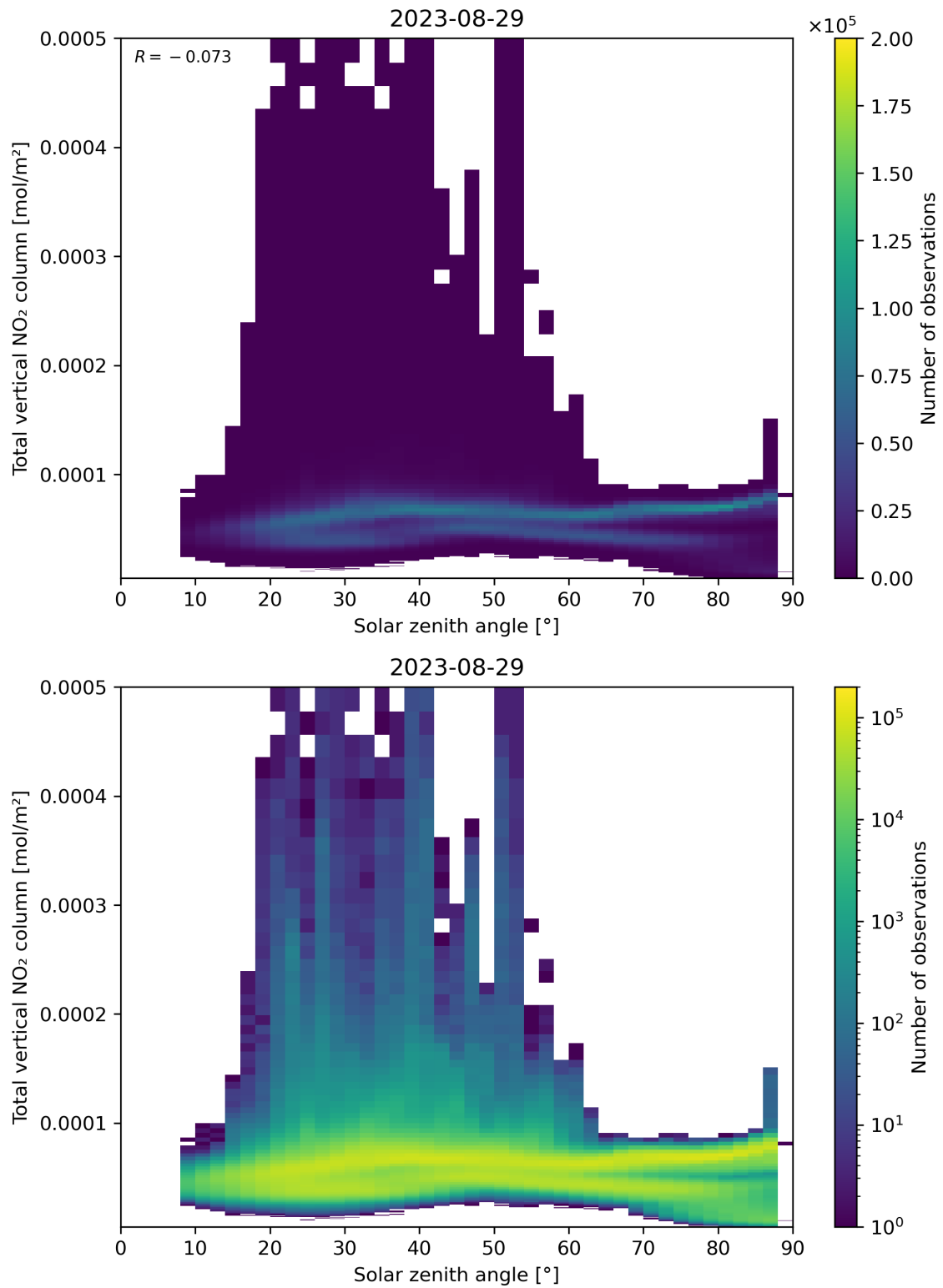
Figure 153: Scatter density plot of “Solar zenith angle” against “Total vertical NO 2 column” for 2023-08-28 to 2023-08-30.
