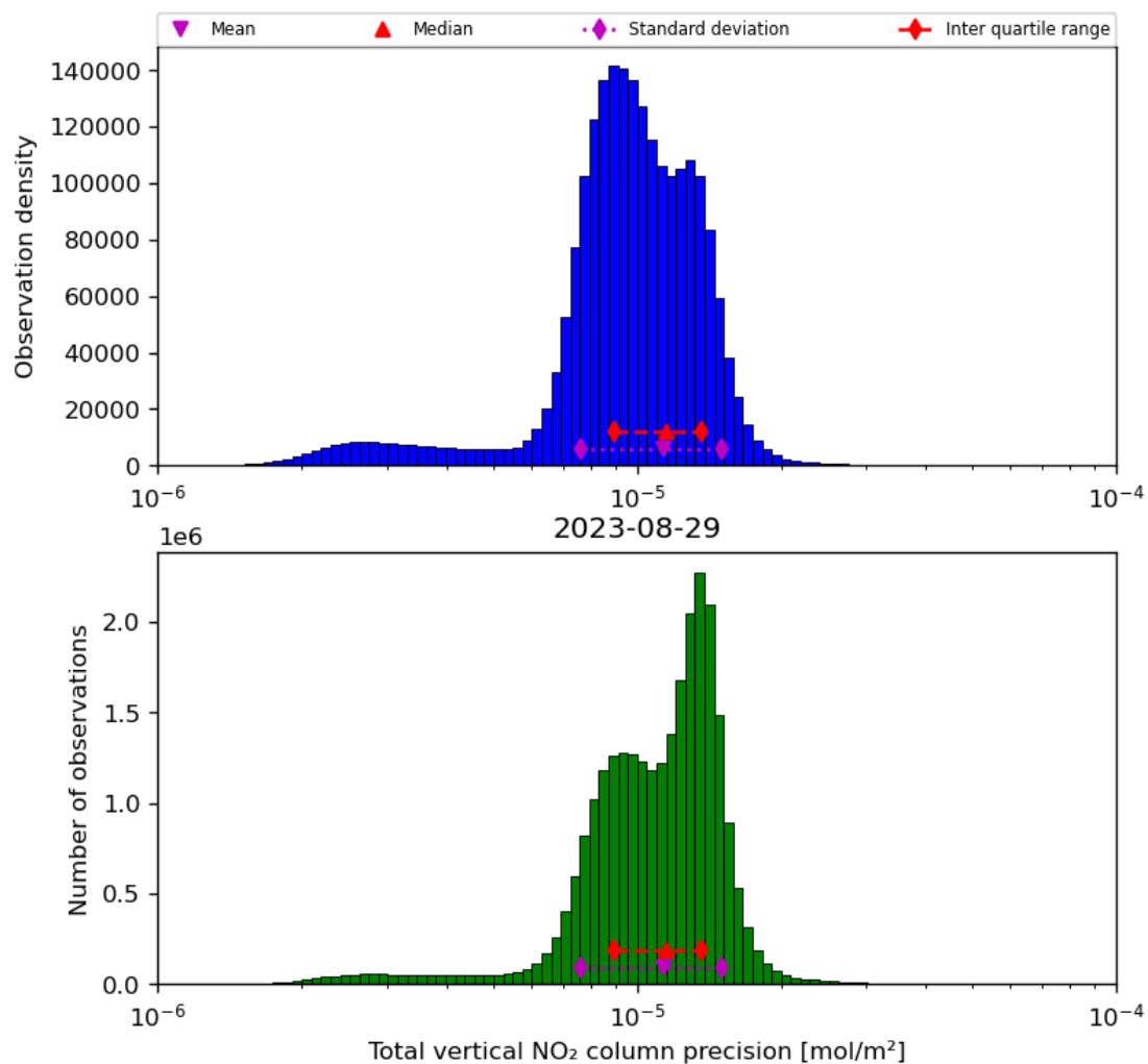
Figure 39: Histogram of “Total vertical NO 2 column precision” for 2023-08-28 to 2023-08-30
