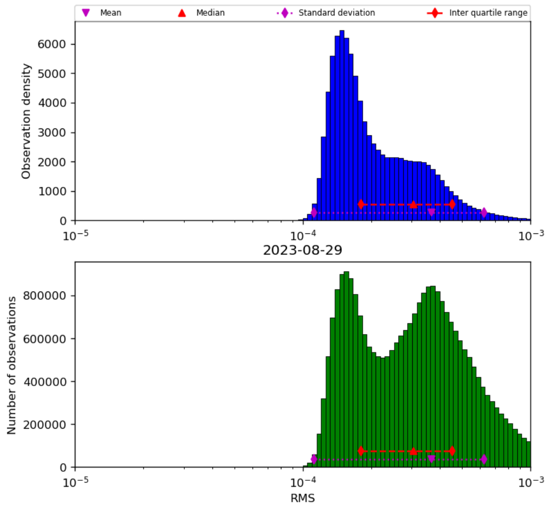
Figure 43: Histogram of “RMS” for 2023-08-28 to 2023-08-30
