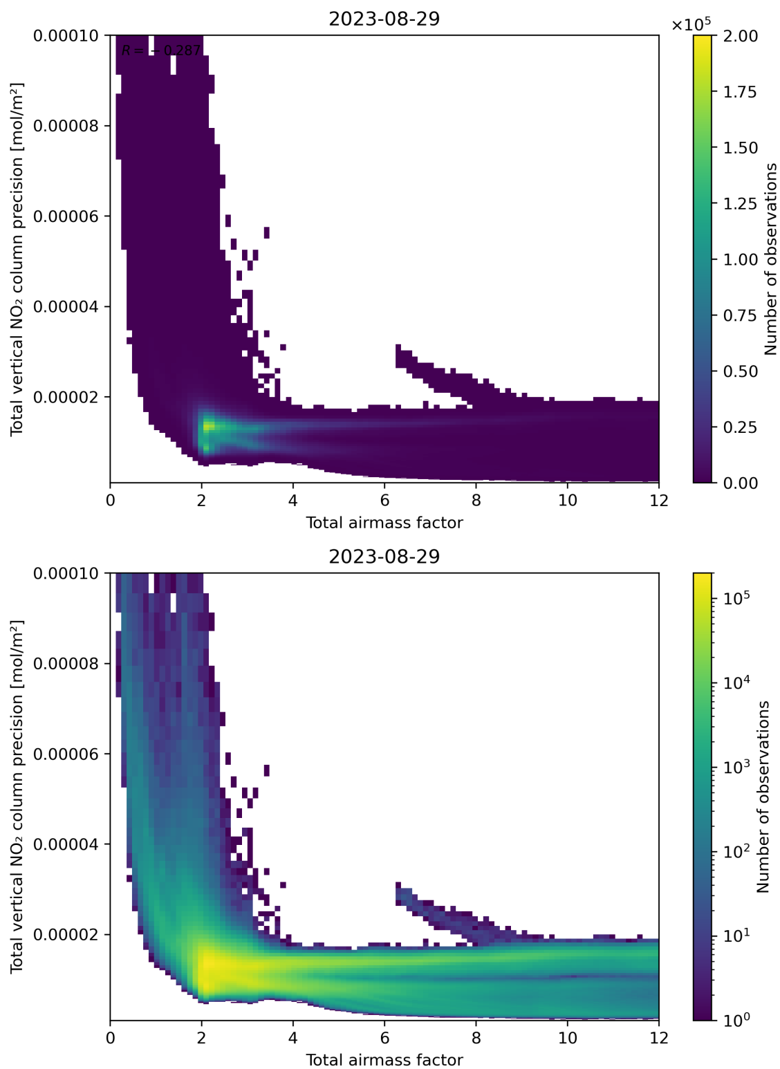
Figure 68: Scatter density plot of “Total airmass factor” against “Total vertical NO 2 column precision” for 2023-08-28 to 2023-08-30.
