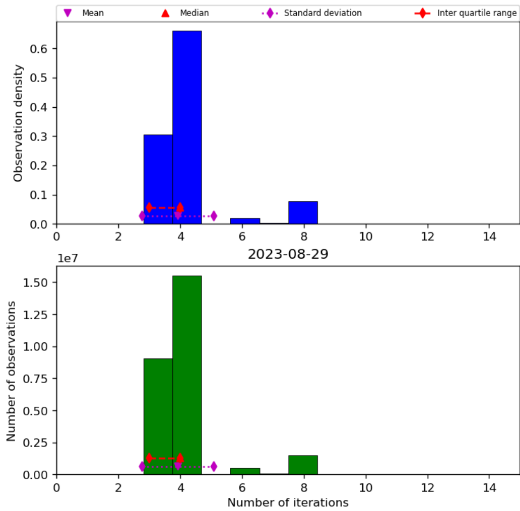
Figure 34: Histogram of “Number of iterations” for 2023-08-28 to 2023-08-30
