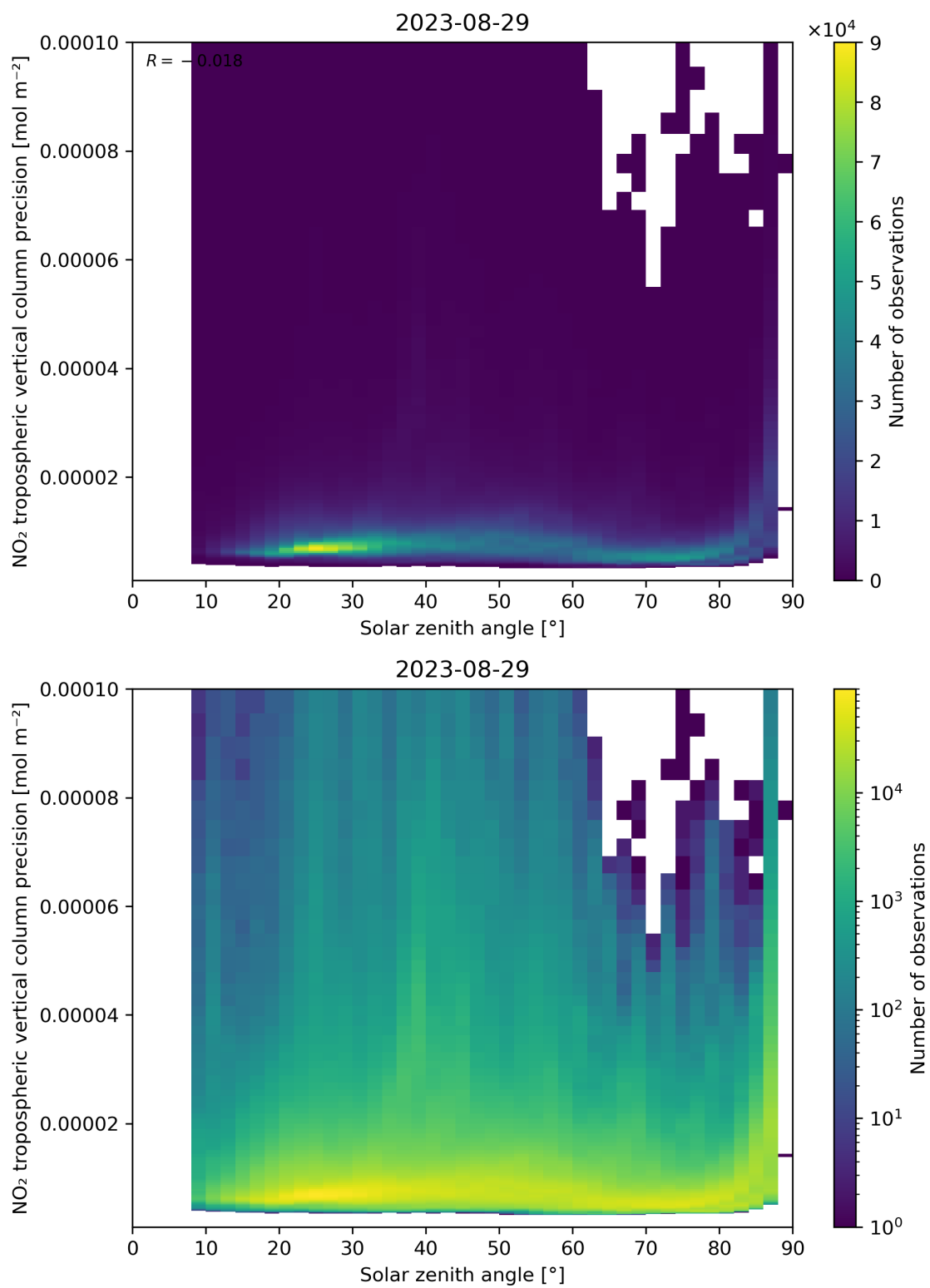
Figure 156: Scatter density plot of “Solar zenith angle” against “NO 2 tropospheric vertical column precision” for 2023-08-28 to 2023-08-30.
