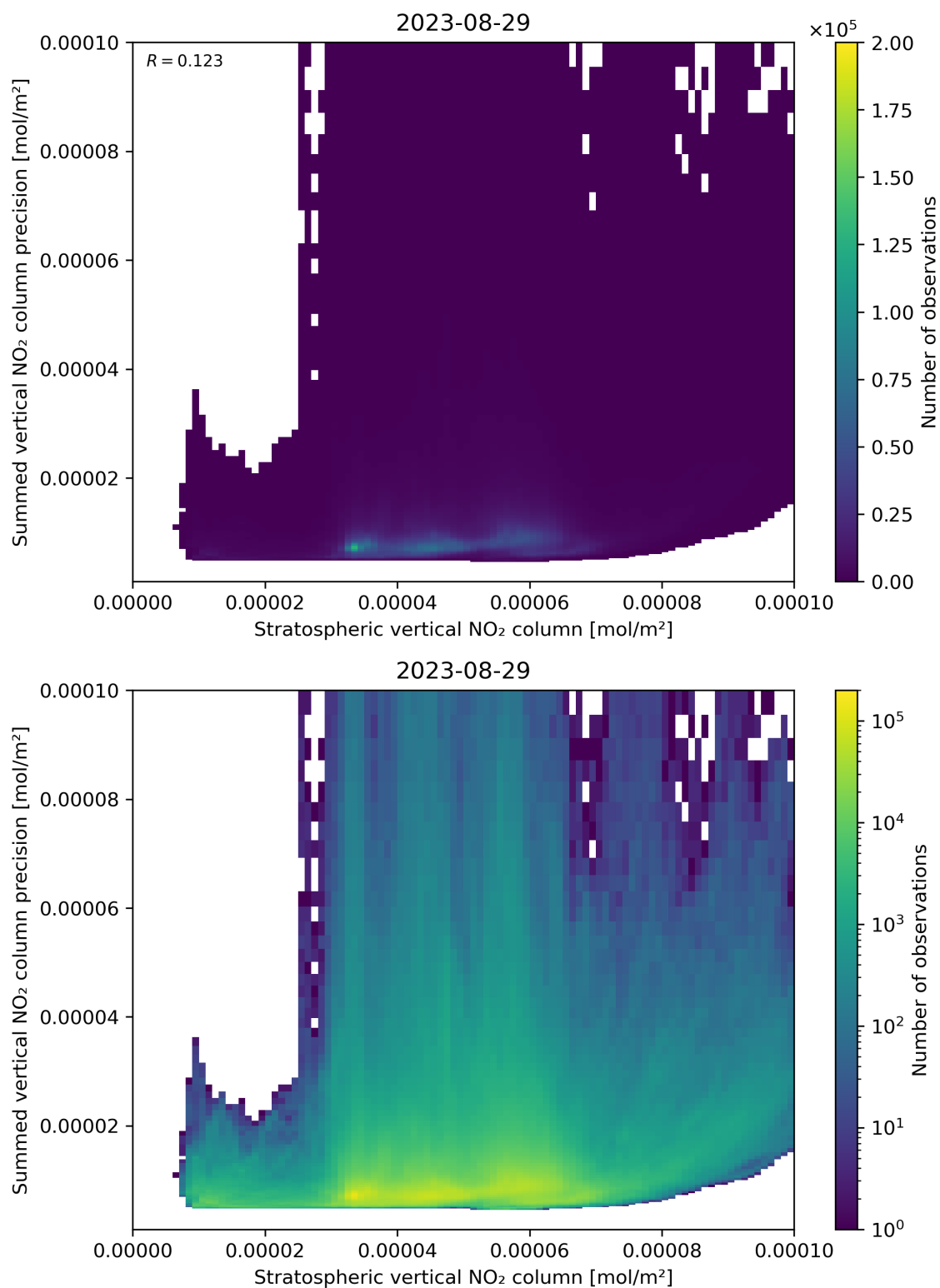
Figure 99: Scatter density plot of “Stratospheric vertical NO 2 column” against “Summed vertical NO 2 column precision” for 2023-08-28 to 2023-08-30.
