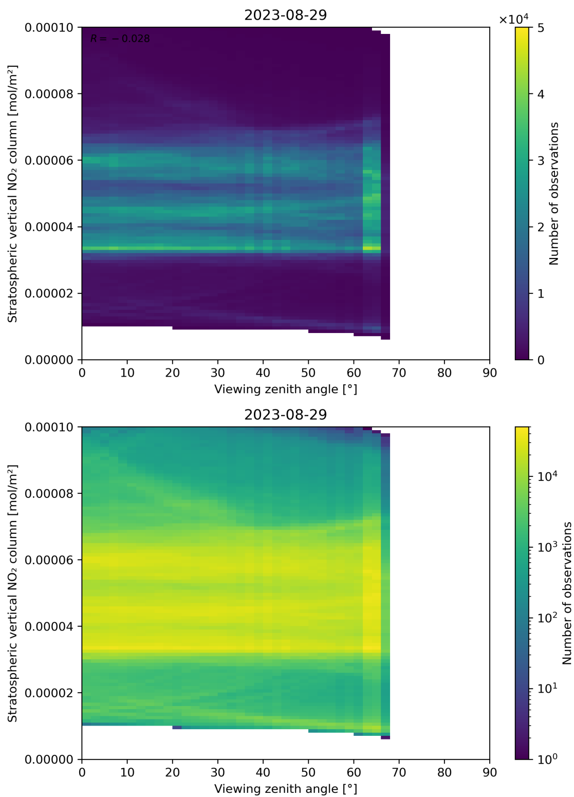
Figure 164: Scatter density plot of “Viewing zenith angle” against “Stratospheric vertical NO 2 column” for 2023-08-28 to 2023-08-30.
