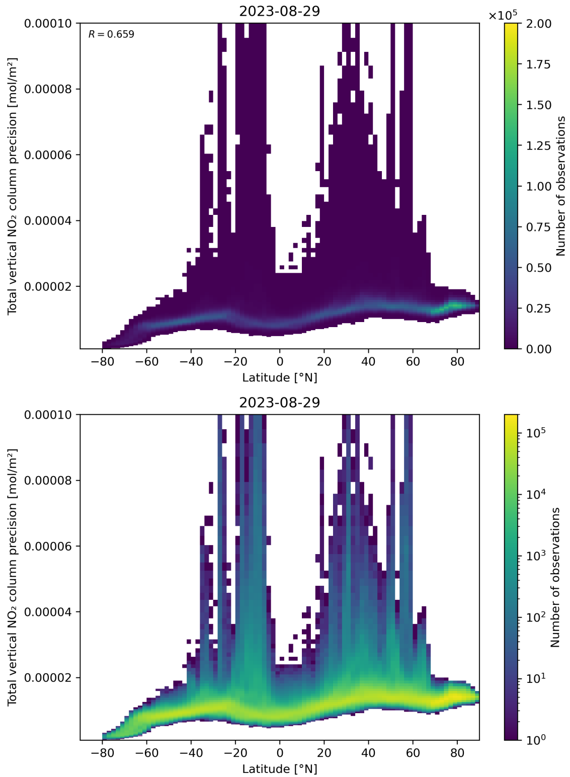
Figure 91: Scatter density plot of “Latitude” against “Total vertical NO 2 column precision” for 2023-08-28 to 2023-08-30.
