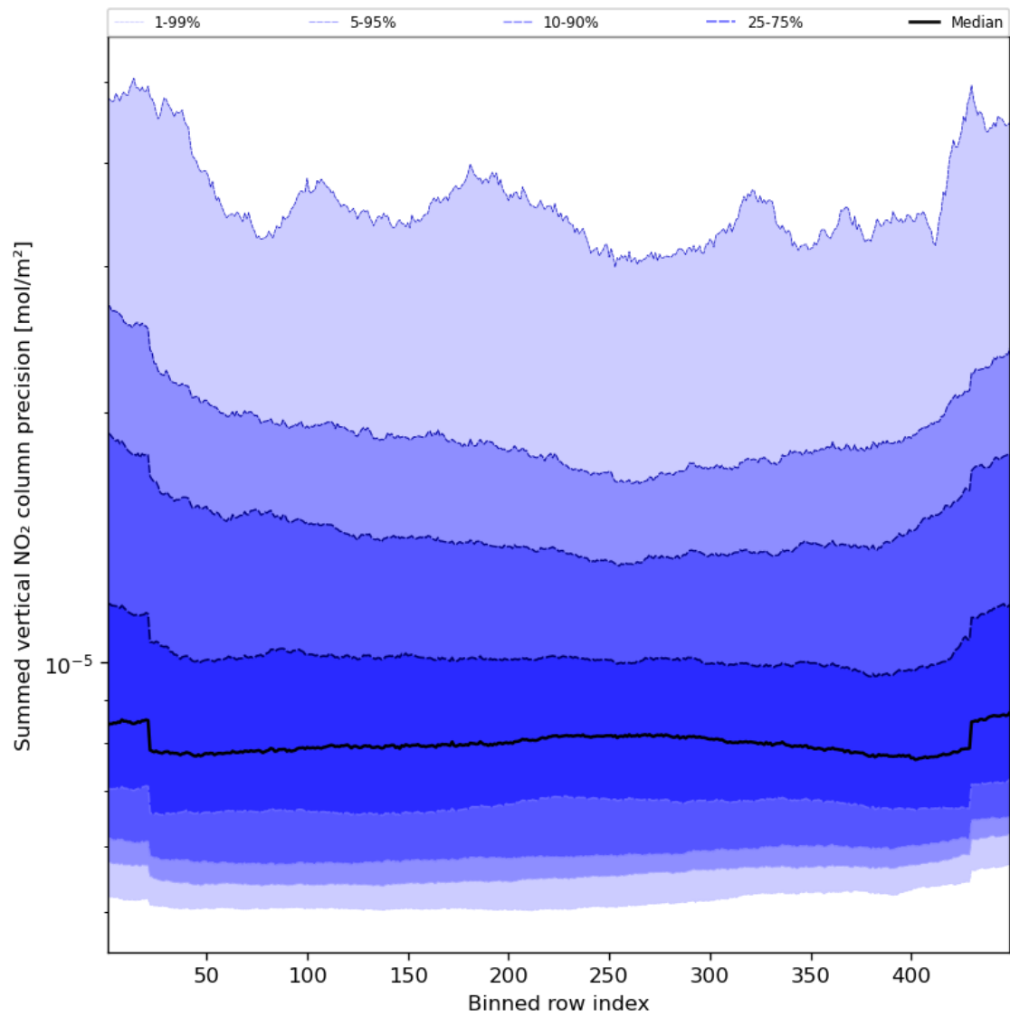
Figure 58: Along track statistics of “Summed vertical NO 2 column precision” for 2023-08-28 to 2023-08-30
