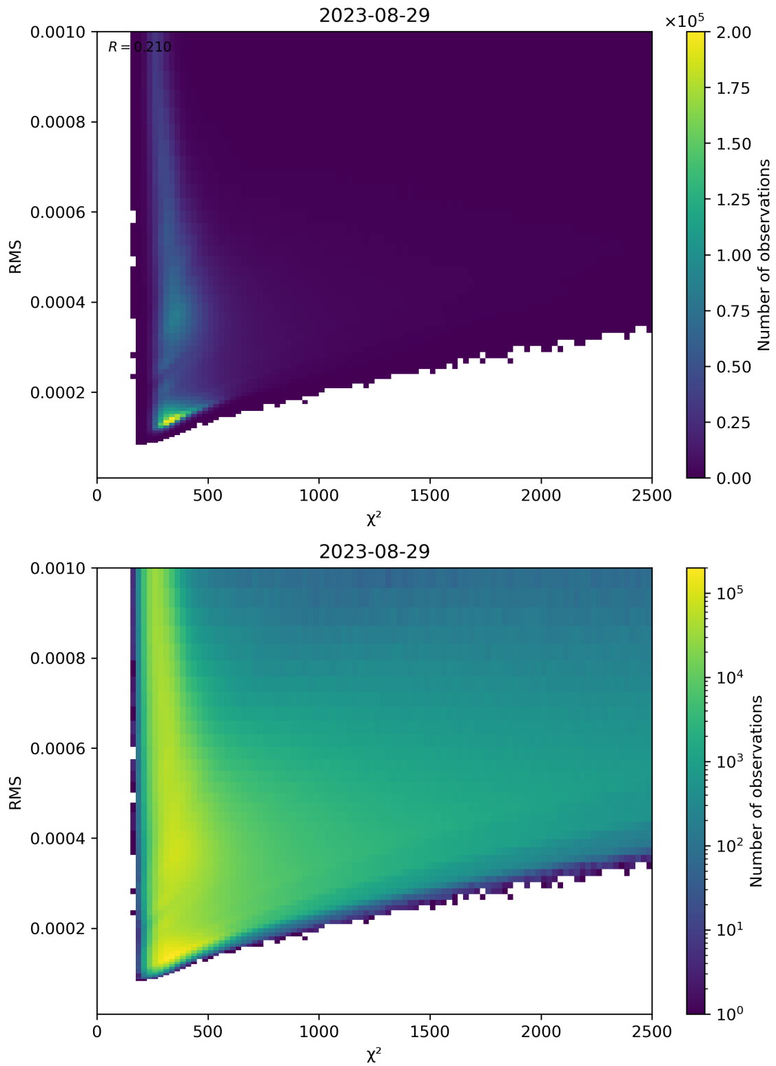
Figure 82: Scatter density plot of “ \chi^2 ” against “RMS” for 2023-08-28 to 2023-08-30.
