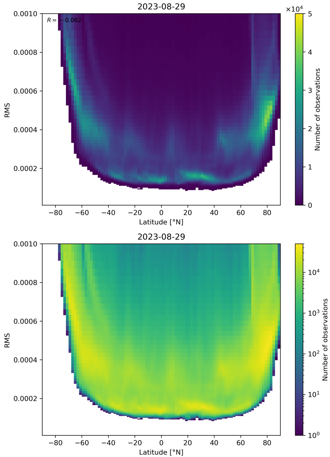
Figure 94: Scatter density plot of “Latitude” against “RMS” for 2023-08-28 to 2023-08-30.
