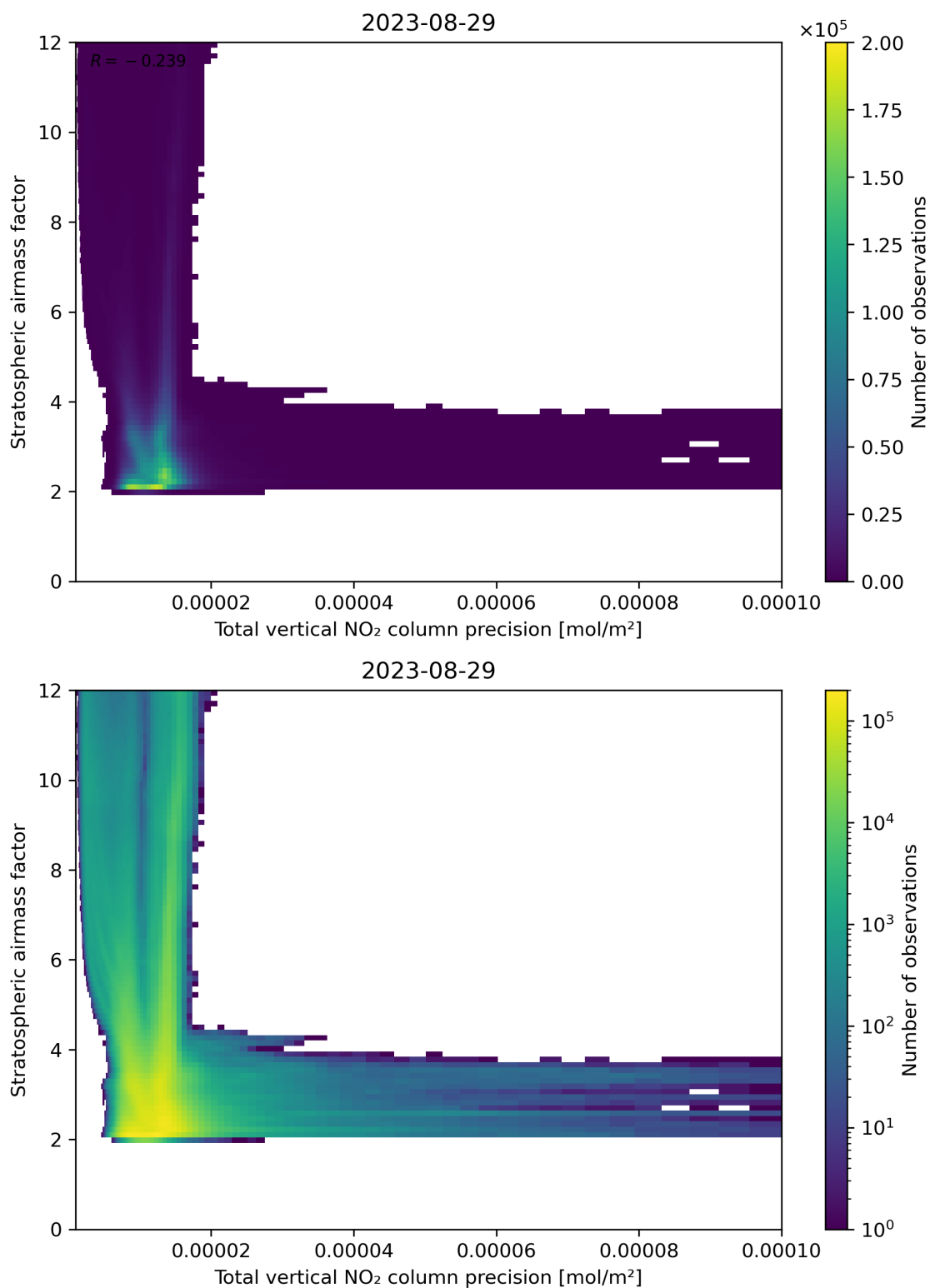
Figure 115: Scatter density plot of “Total vertical NO 2 column precision” against “Stratospheric airmass factor” for 2023-08-28 to 2023-08-30.
