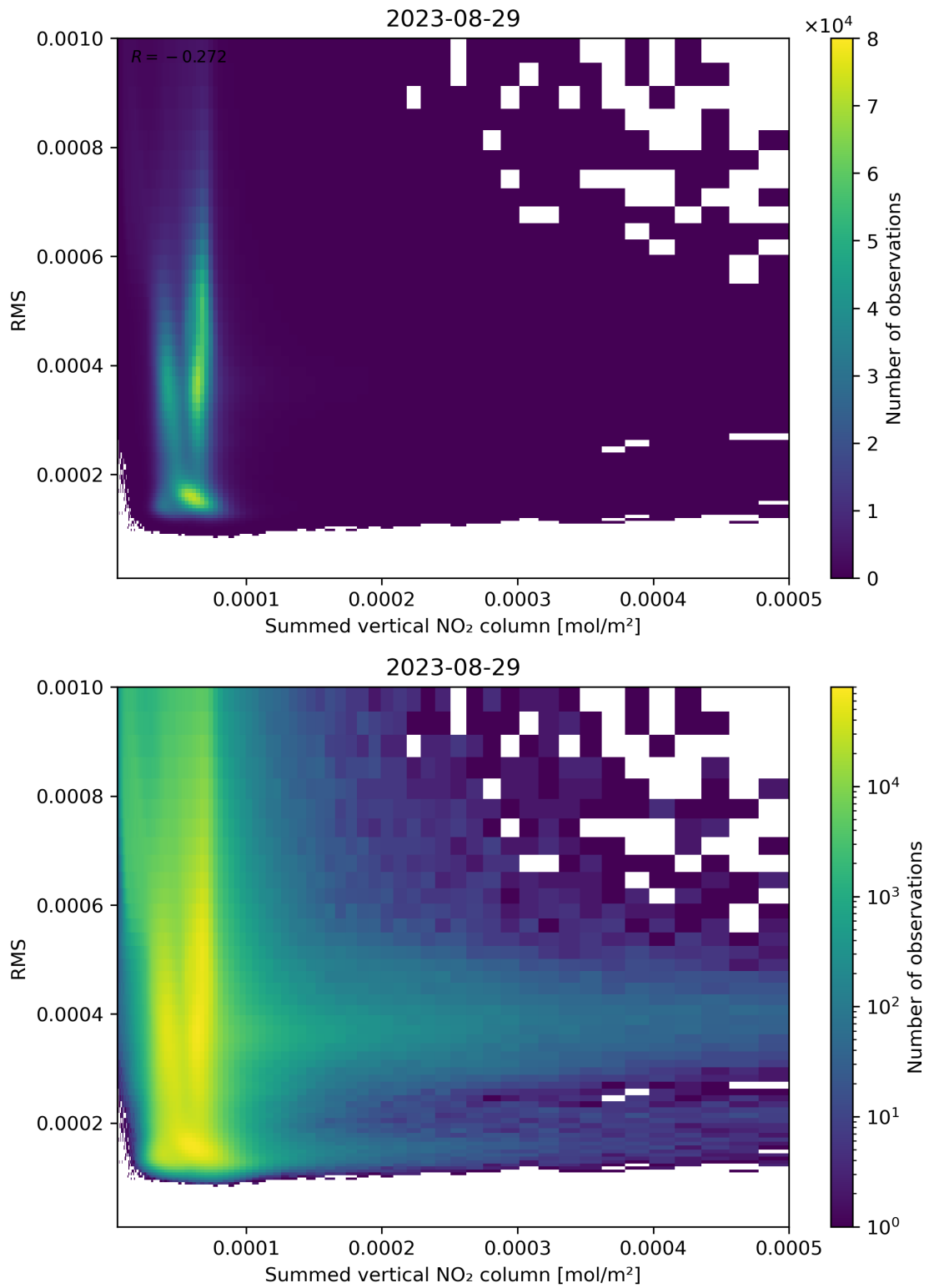
Figure 109: Scatter density plot of “Summed vertical NO 2 column” against “RMS” for 2023-08-28 to 2023-08-30.
