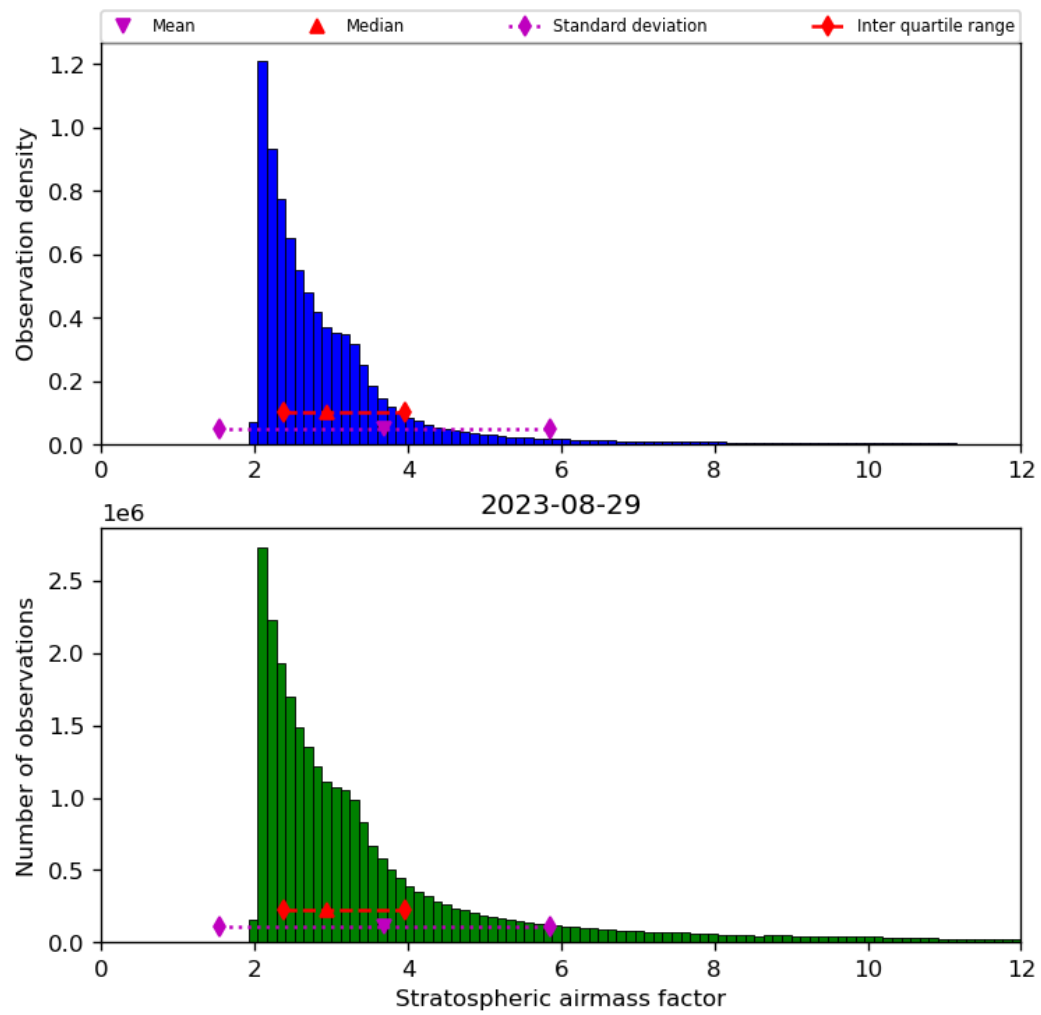
Figure 44: Histogram of “Stratospheric airmass factor” for 2023-08-28 to 2023-08-30
