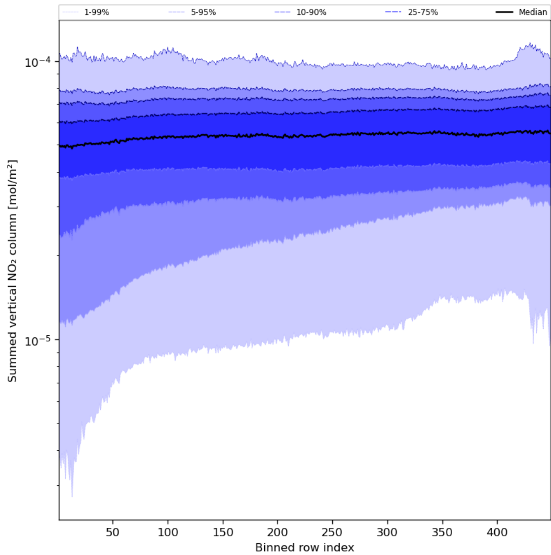
Figure 57: Along track statistics of “Summed vertical NO 2 column” for 2023-08-28 to 2023-08-30
