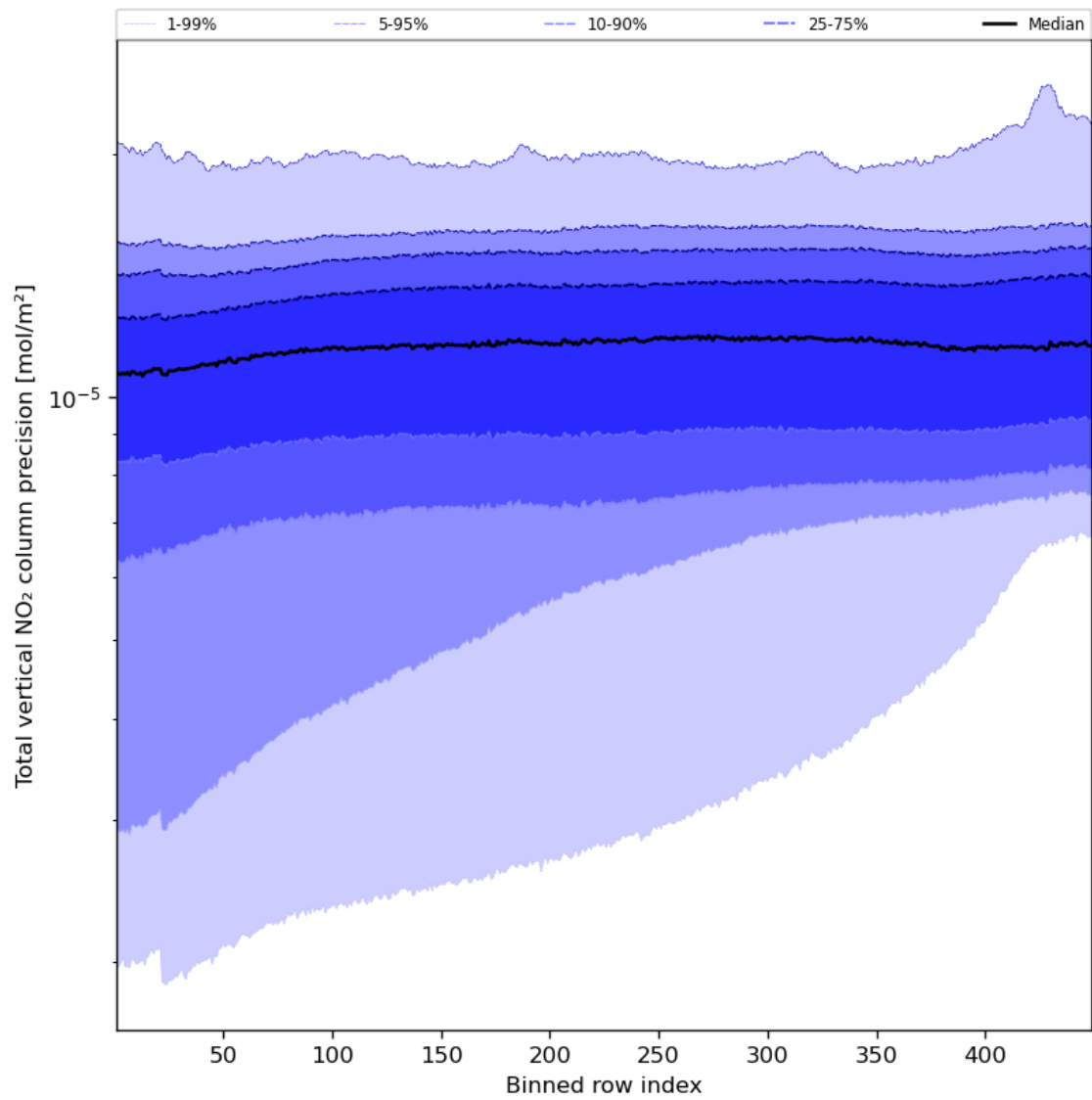
Figure 56: Along track statistics of “Total vertical NO 2 column precision” for 2023-08-28 to 2023-08-30
