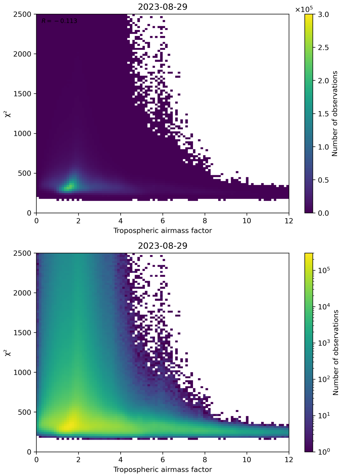
Figure 73: Scatter density plot of “Tropospheric airmass factor” against “ \chi^2 ” for 2023-08-28 to 2023-08-30.
