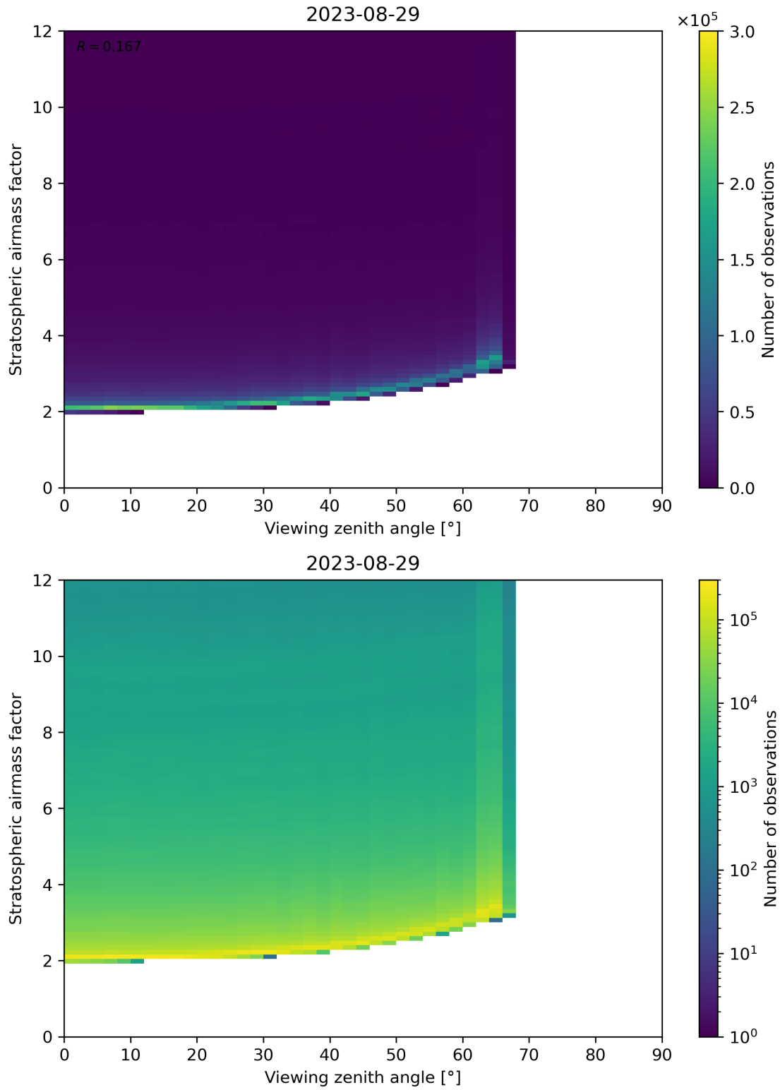
Figure 159: Scatter density plot of “Viewing zenith angle” against “Stratospheric airmass factor” for 2023-08-28 to 2023-08-30.
