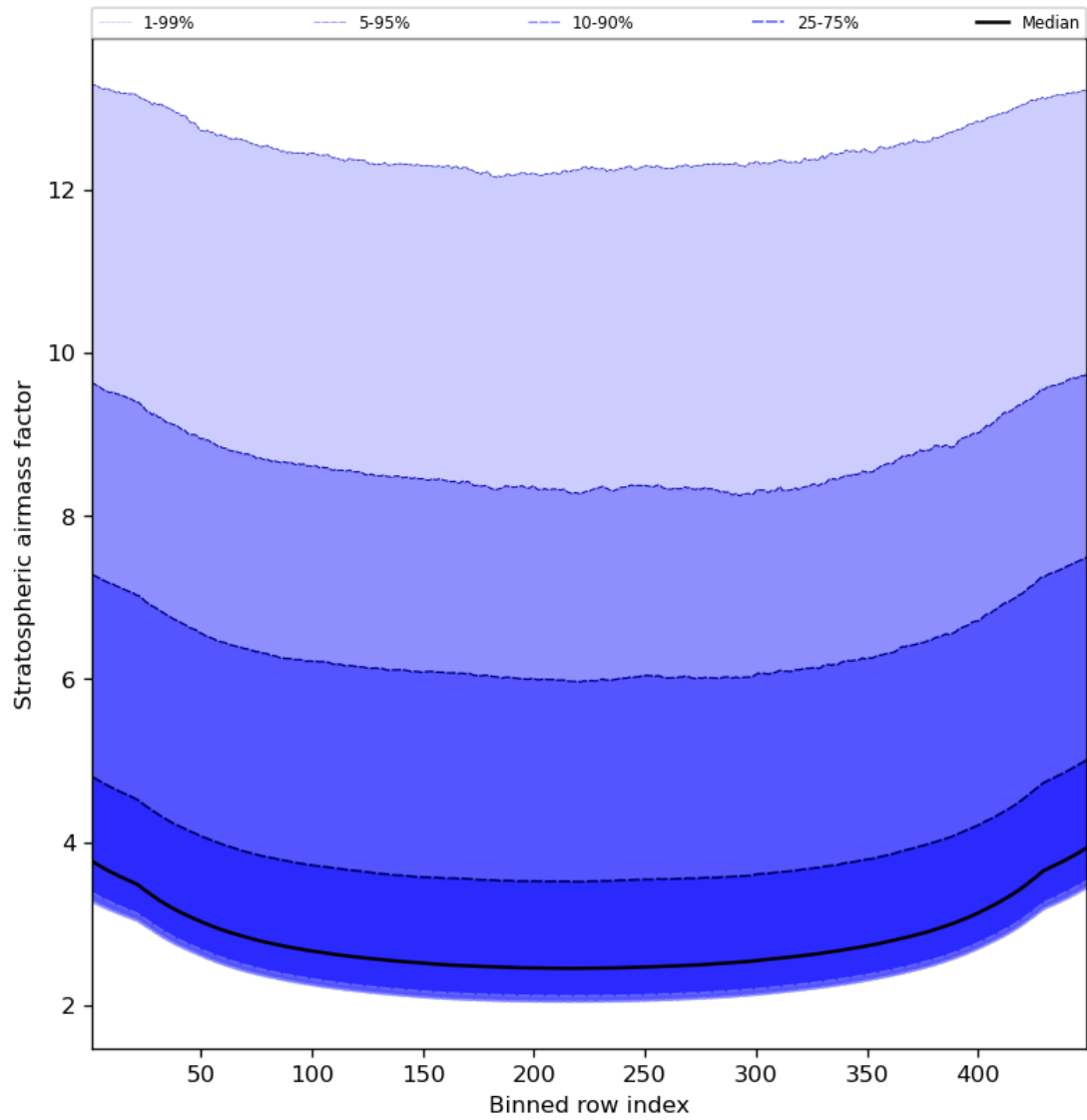
Figure 61: Along track statistics of “Stratospheric airmass factor” for 2023-08-28 to 2023-08-30
