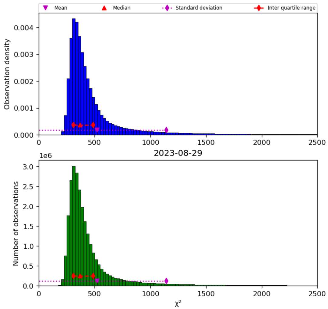
Figure 42: Histogram of “ \chi^2 ” for 2023-08-28 to 2023-08-30
