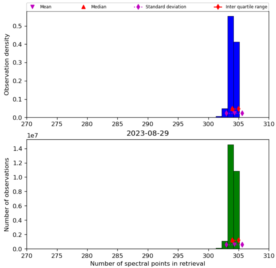
Figure 33: Histogram of “Number of spectral points in retrieval” for 2023-08-28 to 2023-08-30
