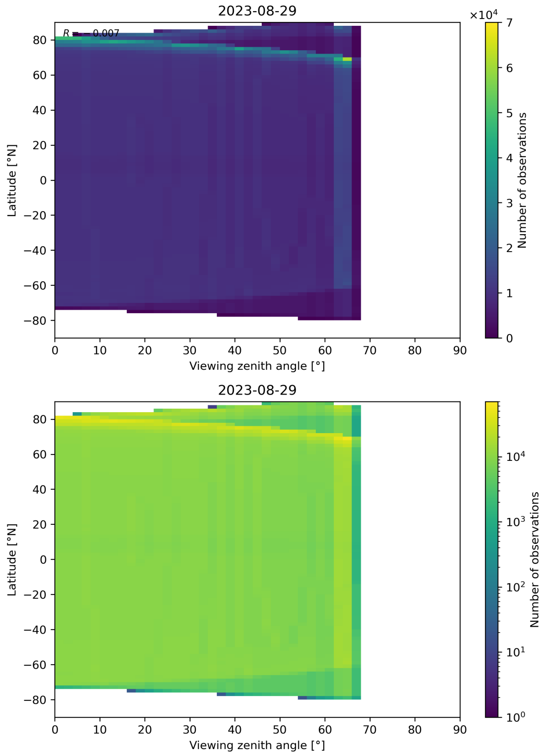
Figure 163: Scatter density plot of “Viewing zenith angle” against “Latitude” for 2023-08-28 to 2023-08-30.
