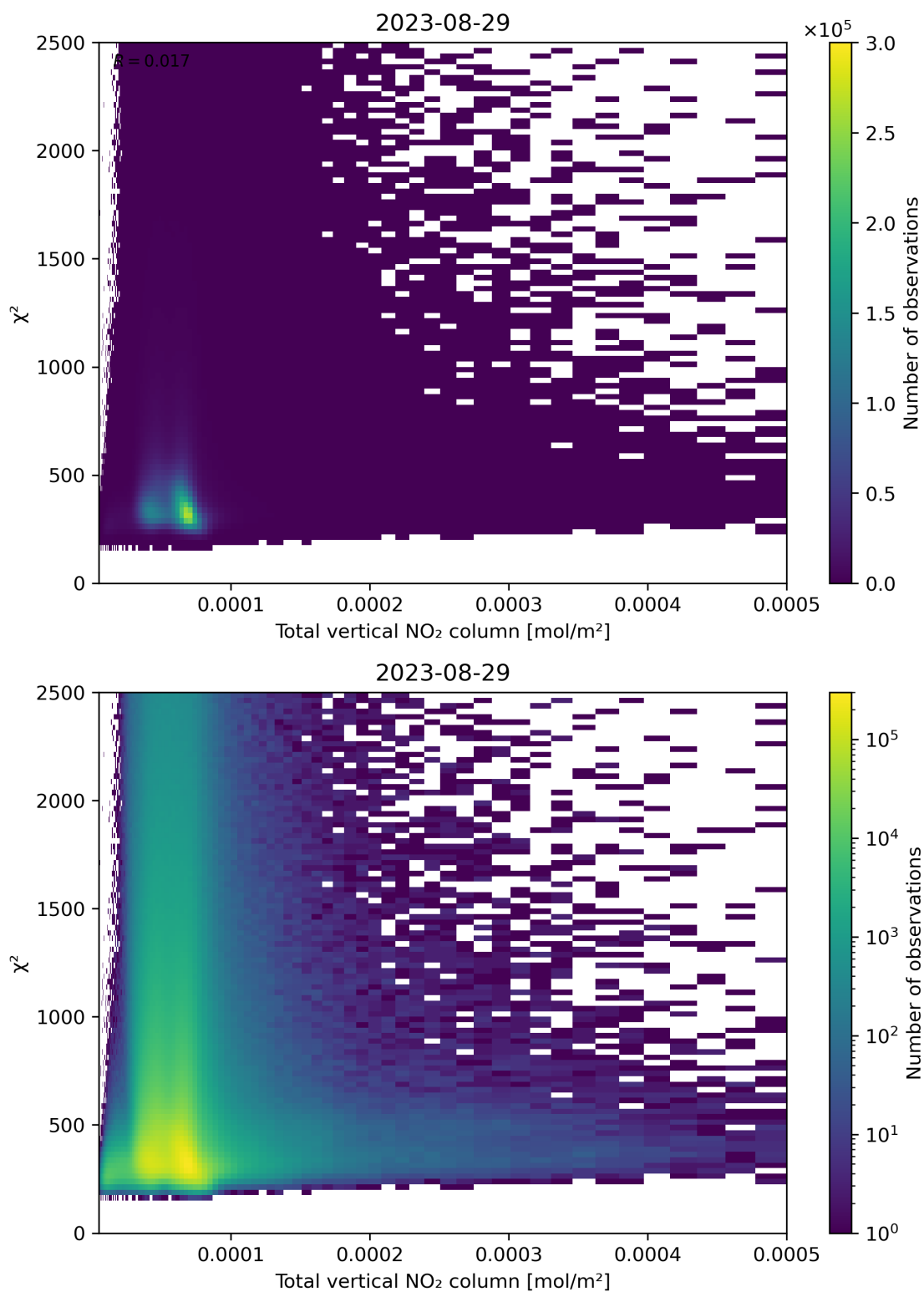
Figure 111: Scatter density plot of “Total vertical NO 2 column” against “ \chi^2 ” for 2023-08-28 to 2023-08-30.
