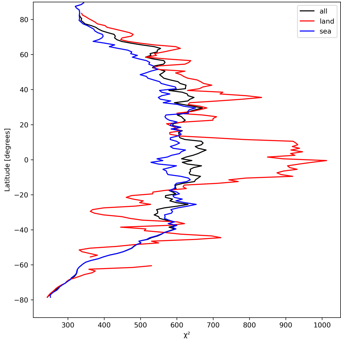
Figure 25: Zonal average of “ \chi^2 ” for 2023-08-28 to 2023-08-30.
