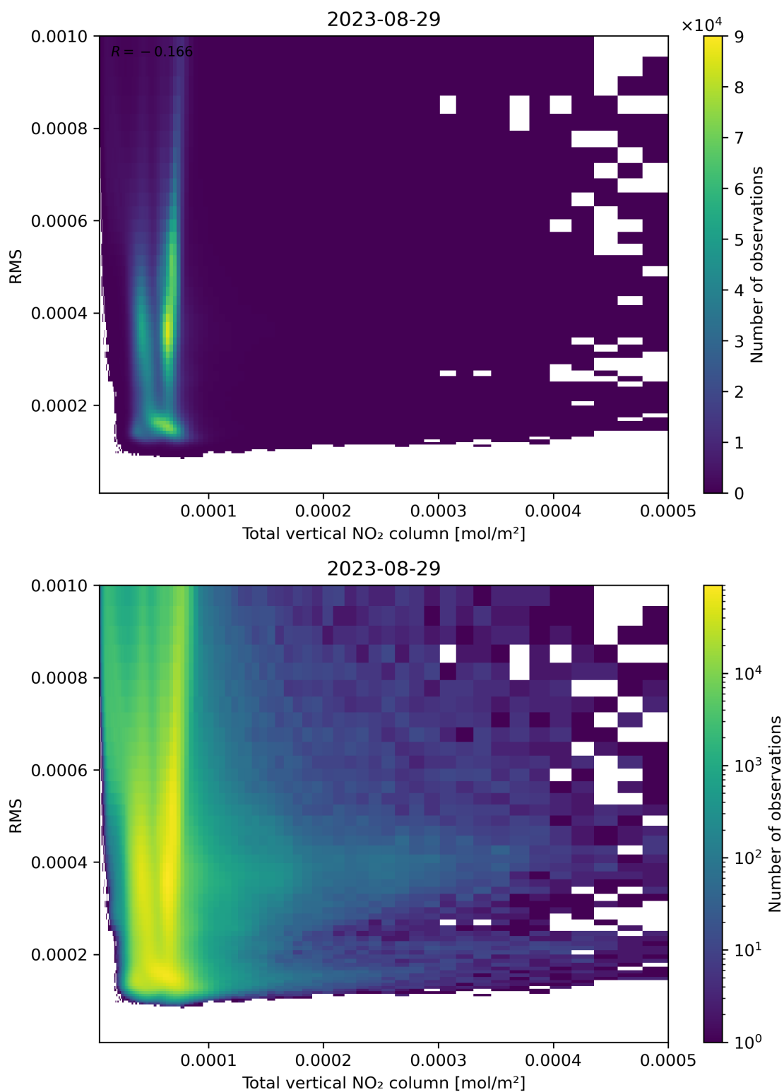
Figure 120: Scatter density plot of “Total vertical NO 2 column” against “RMS” for 2023-08-28 to 2023-08-30.
