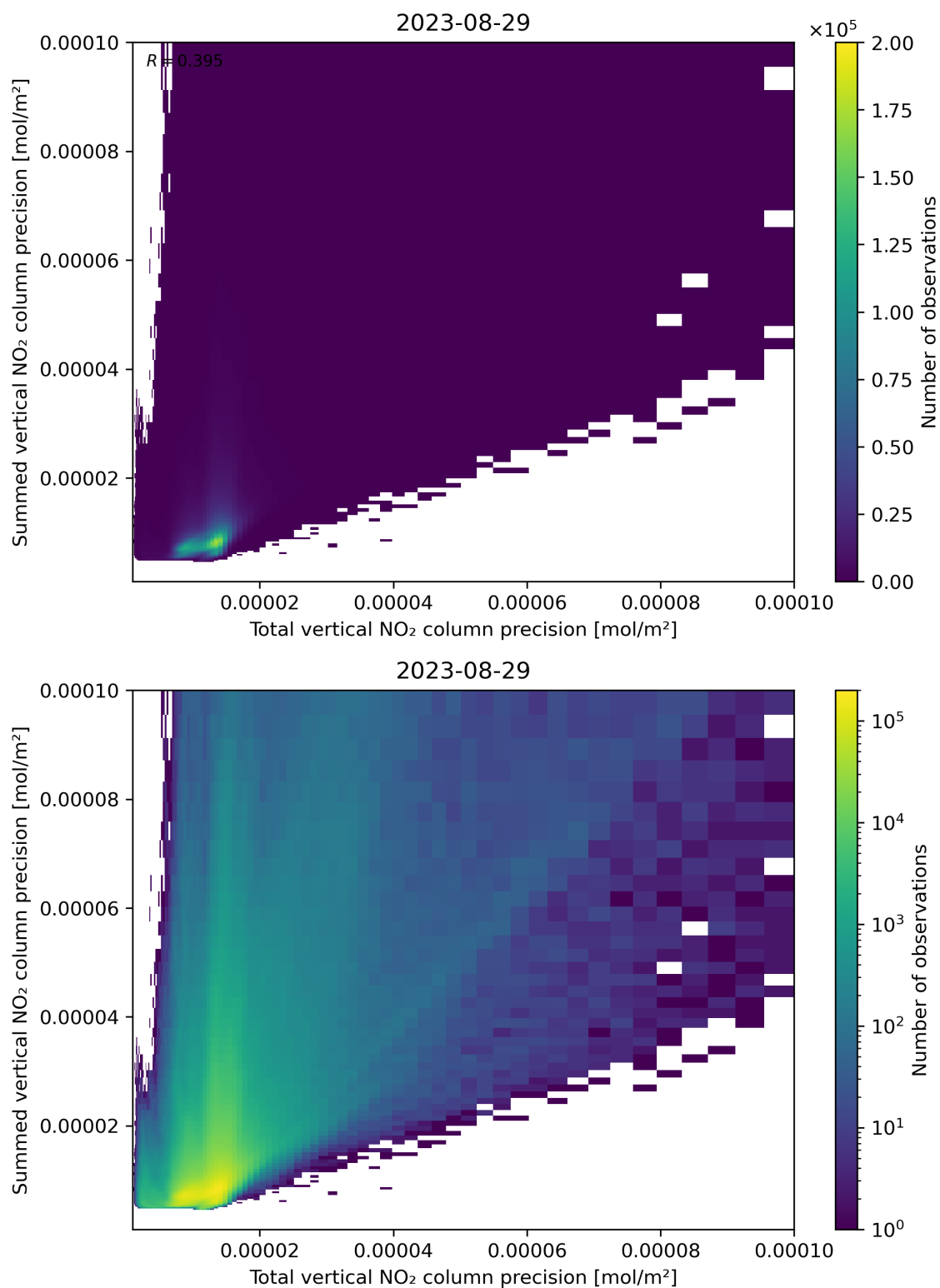
Figure 118: Scatter density plot of “Total vertical NO 2 column precision” against “Summed vertical NO 2 column precision” for 2023-08-28 to 2023-08-30.
