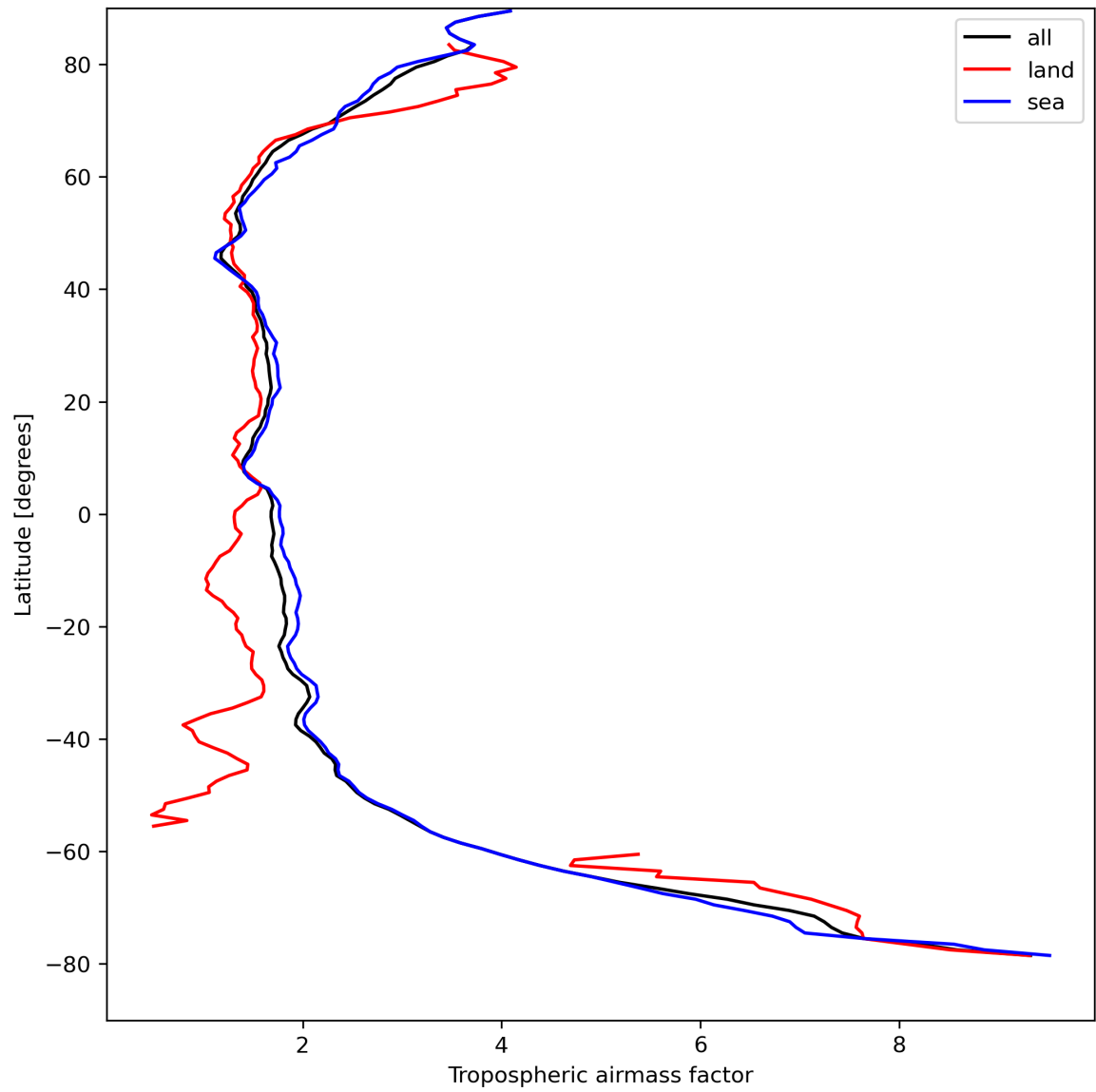
Figure 14: Zonal average of “Tropospheric airmass factor” for 2023-08-28 to 2023-08-30.
