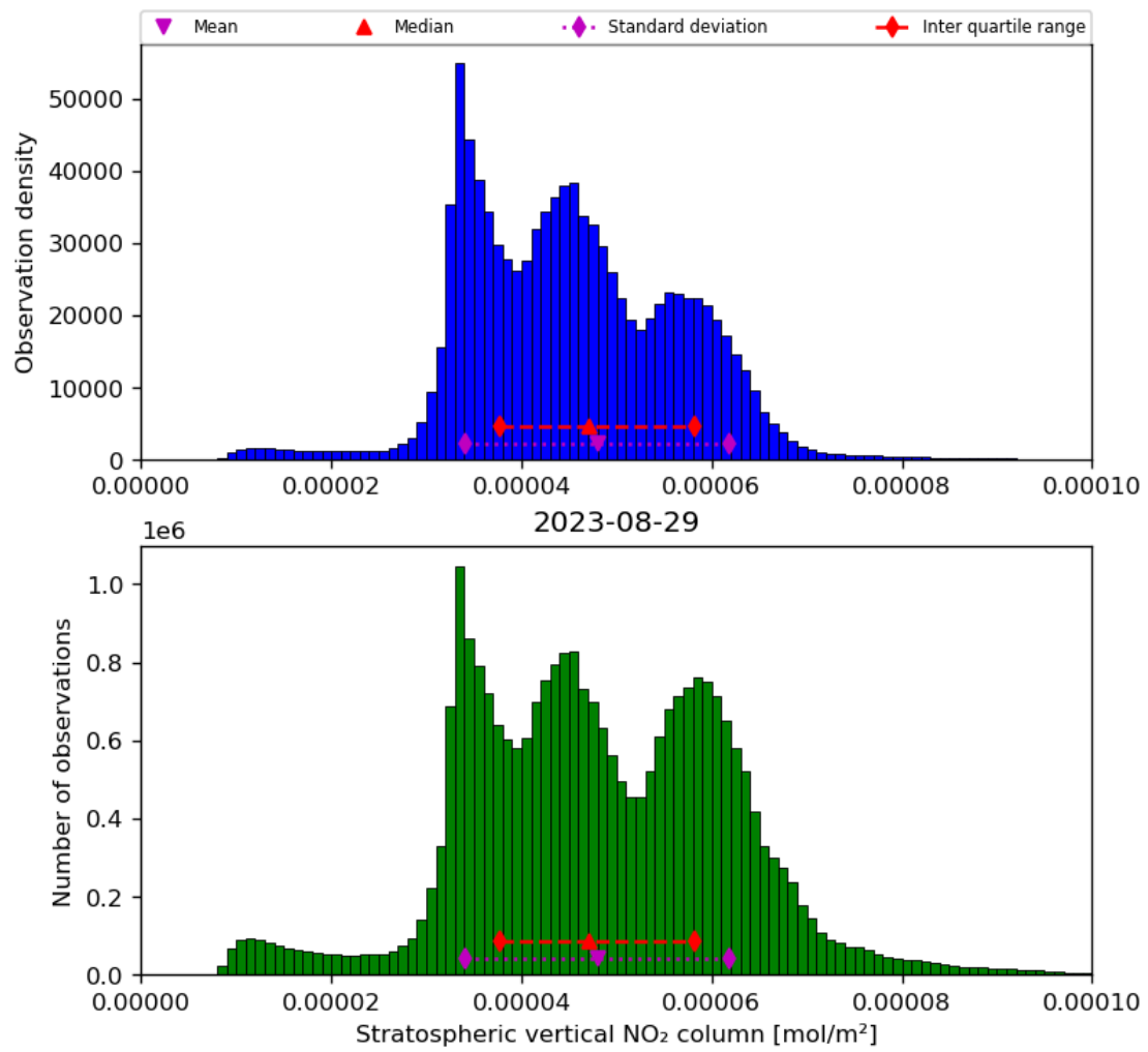
Figure 36: Histogram of “Stratospheric vertical NO 2 column” for 2023-08-28 to 2023-08-30
