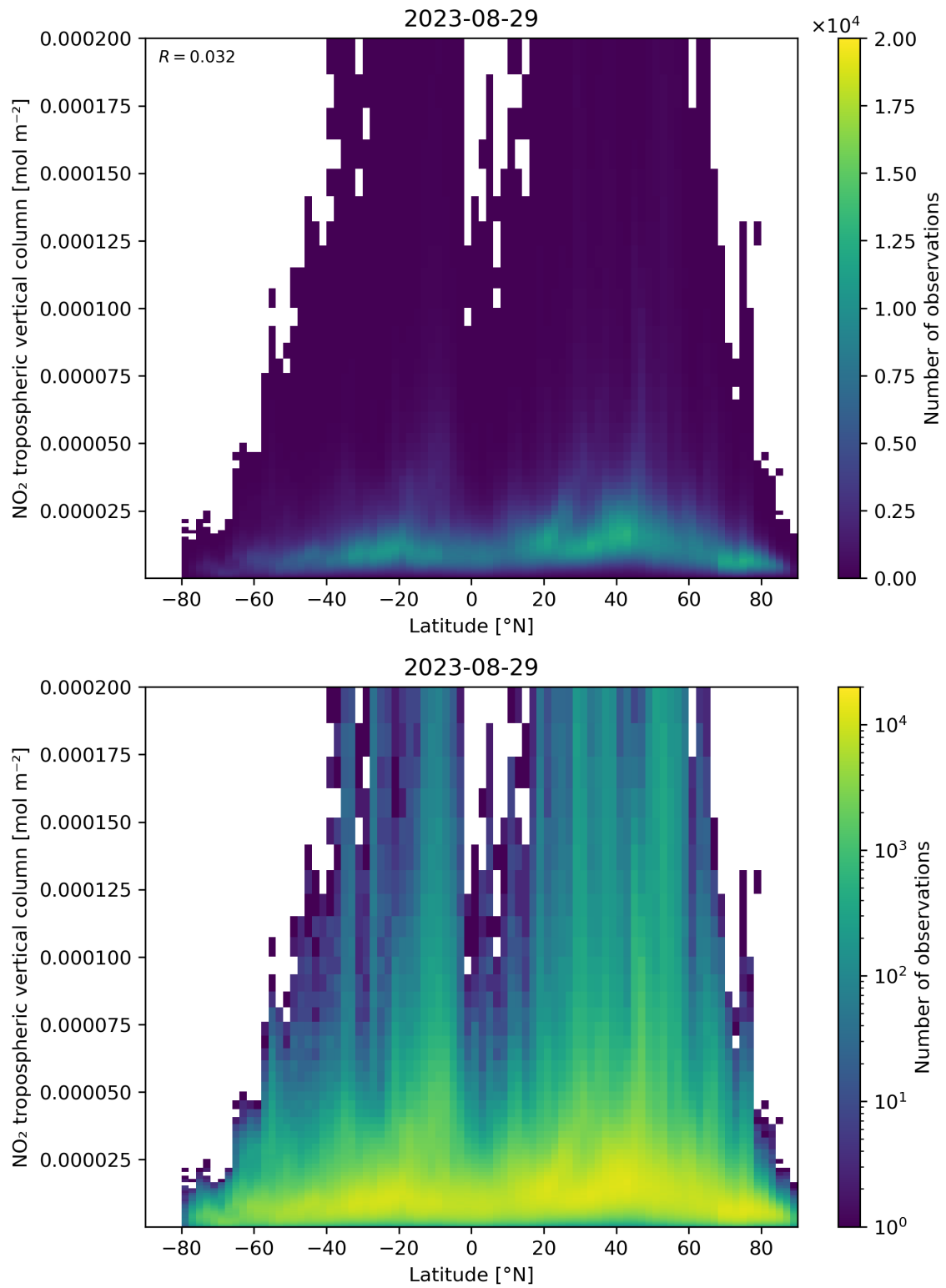
Figure 92: Scatter density plot of “Latitude” against “NO 2 tropospheric vertical column” for 2023-08-28 to 2023-08-30.
