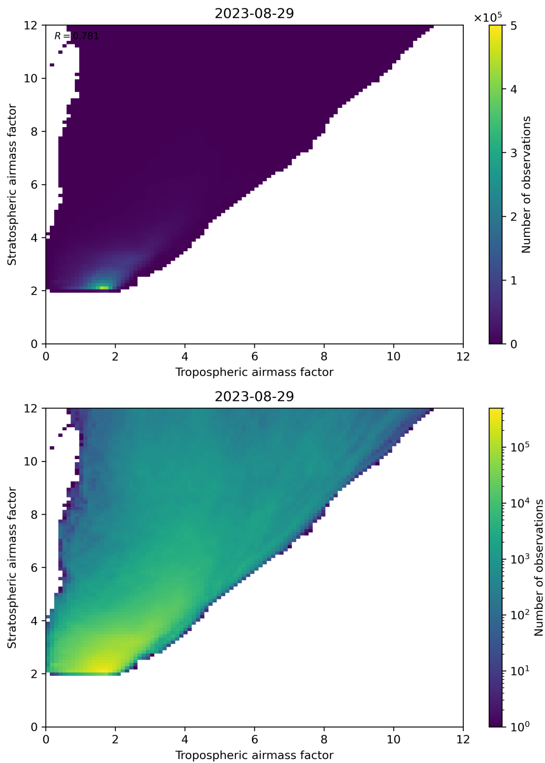
Figure 71: Scatter density plot of “Tropospheric airmass factor” against “Stratospheric airmass factor” for 2023-08-28 to 2023-08-30.
