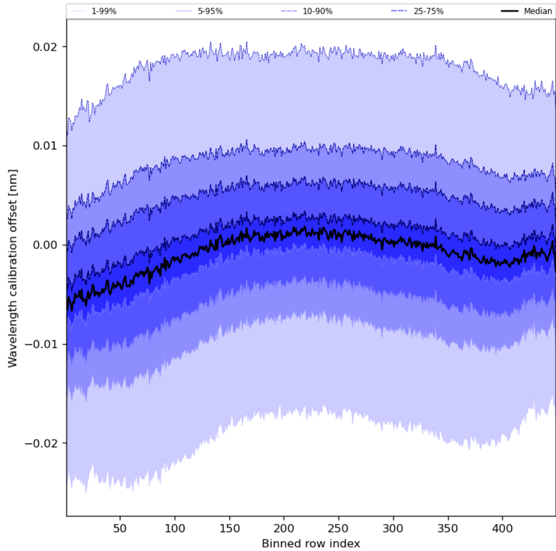
Figure 52: Along track statistics of “Wavelength calibration offset” for 2023-08-28 to 2023-08-30
