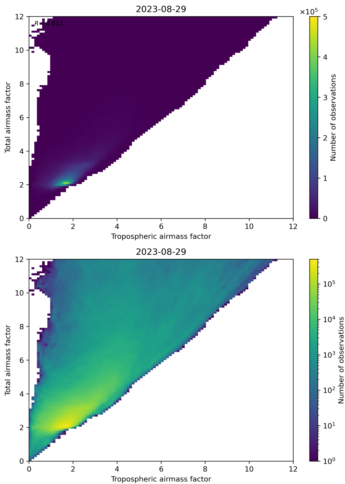
Figure 72: Scatter density plot of “Tropospheric airmass factor” against “Total airmass factor” for 2023-08-28 to 2023-08-30.
