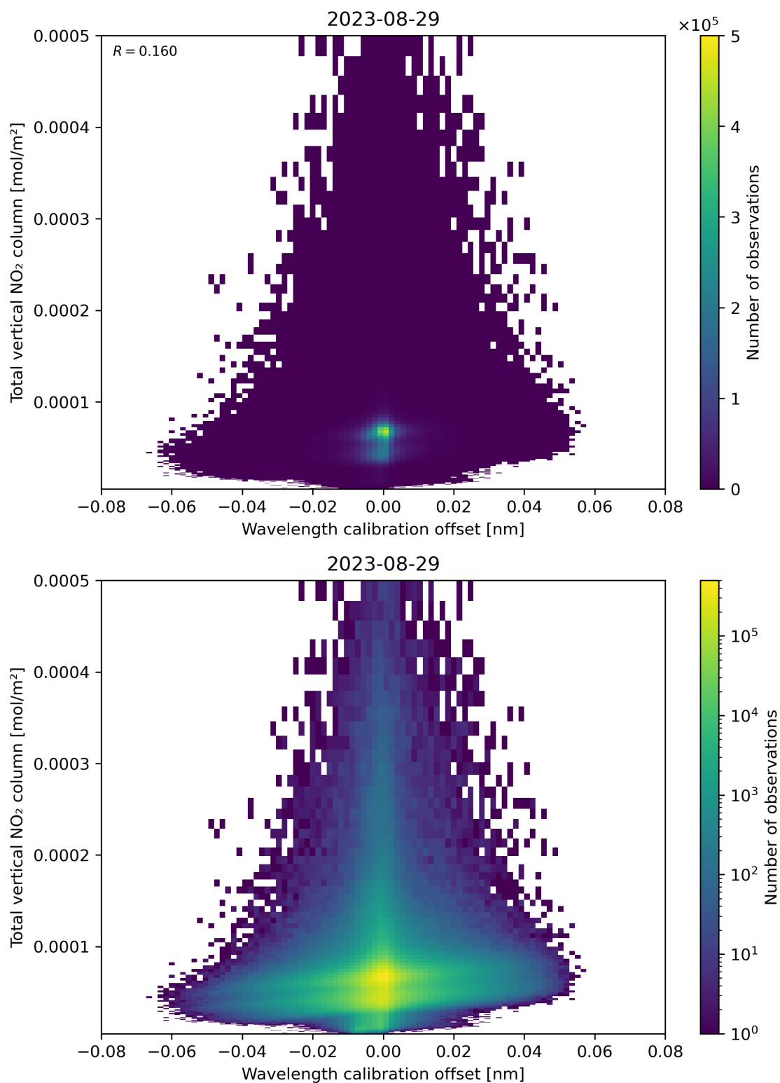
Figure 179: Scatter density plot of “Wavelength calibration offset” against “Total vertical NO 2 column” for 2023-08-28 to 2023-08-30.
