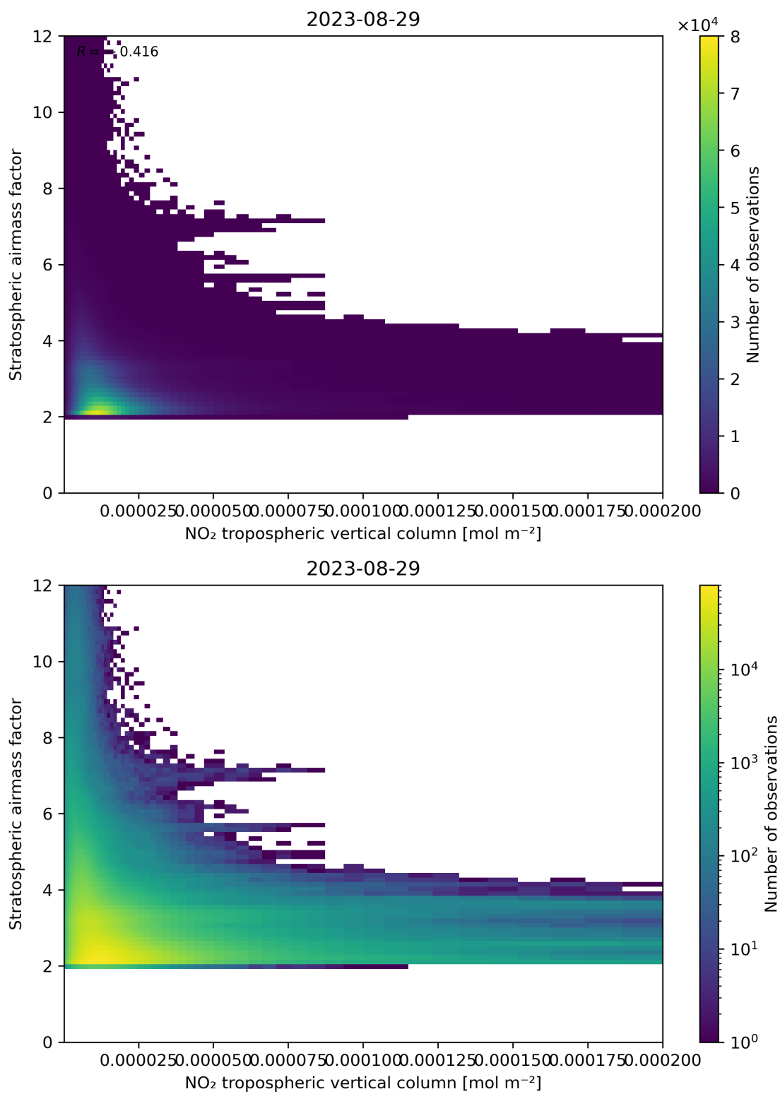
Figure 121: Scatter density plot of “NO 2 tropospheric vertical column” against “Stratospheric air mass factor” for 2023-08-28 to 2023-08-30.
