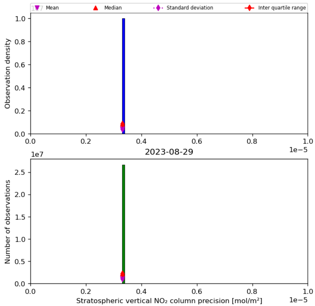
Figure 37: Histogram of “Stratospheric vertical NO 2 column precision” for 2023-08-28 to 2023-08-30
