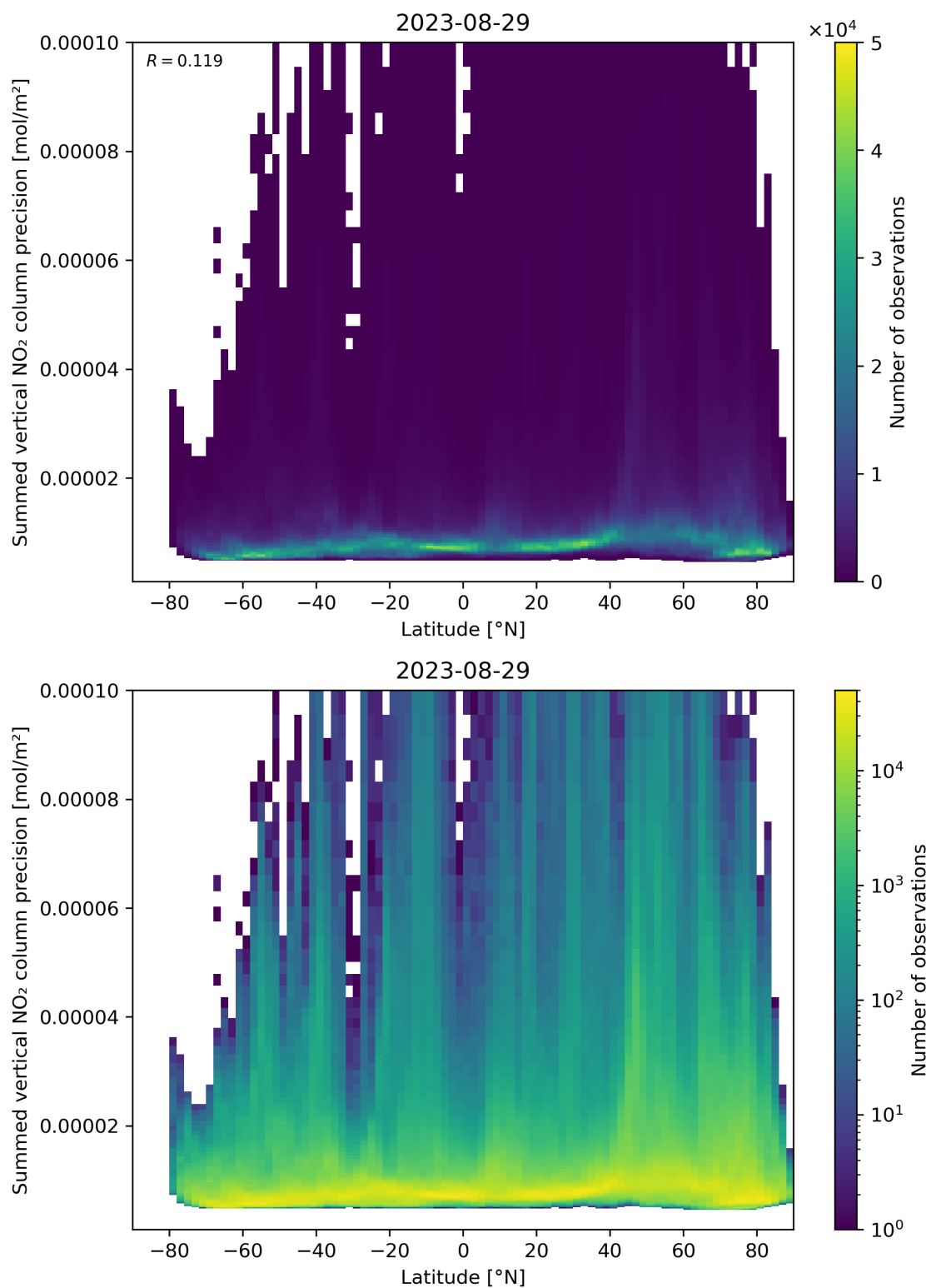
Figure 89: Scatter density plot of “Latitude” against “Summed vertical NO 2 column precision” for 2023-08-28 to 2023-08-30.
