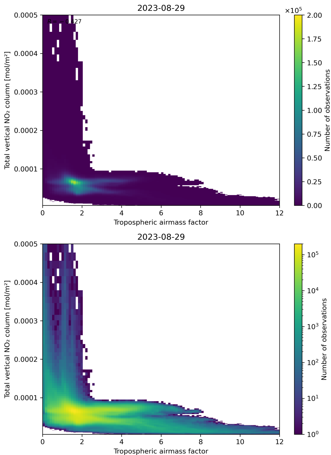
Figure 77: Scatter density plot of “Tropospheric airmass factor” against “Total vertical NO 2 column” for 2023-08-28 to 2023-08-30.
