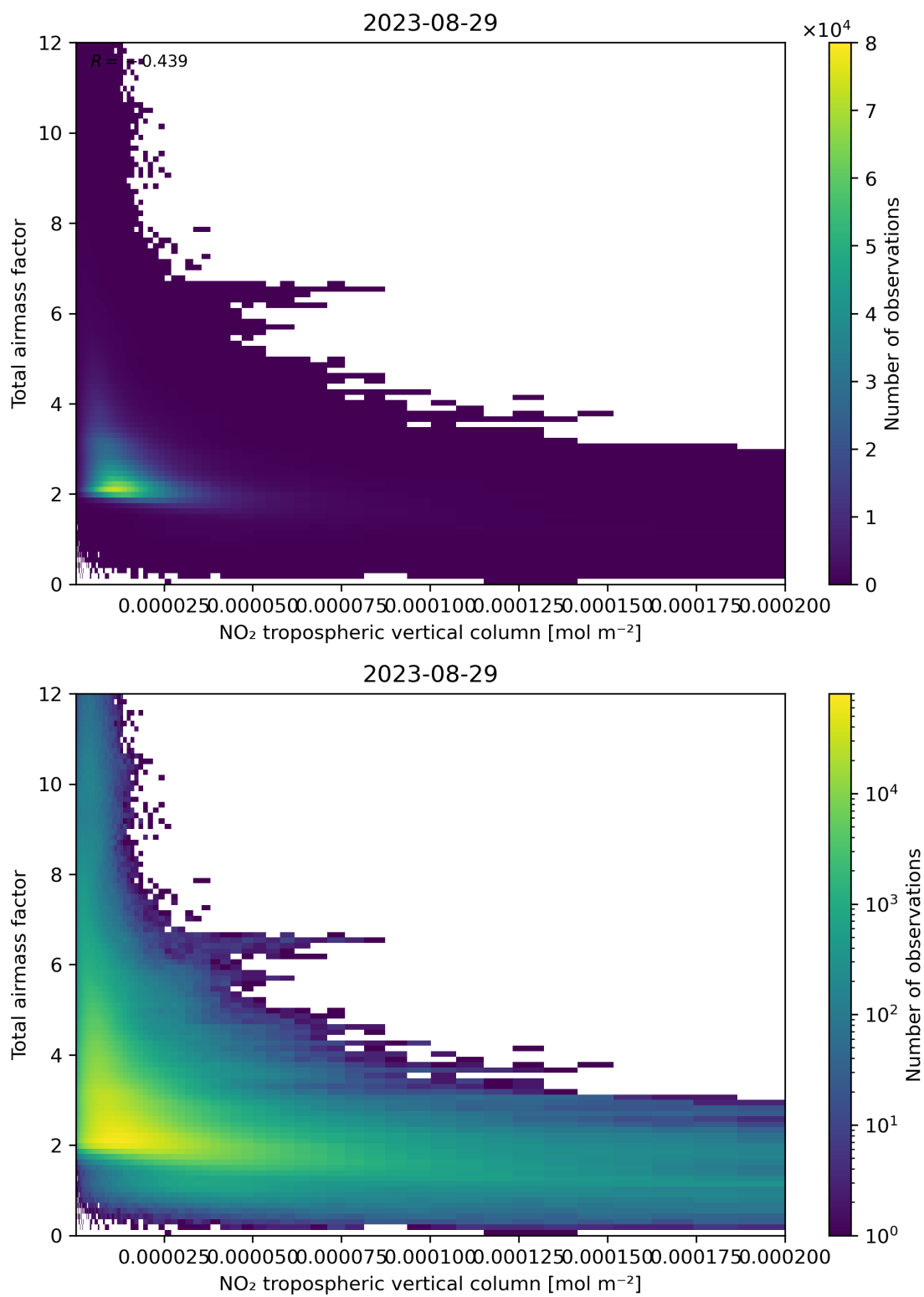
Figure 122: Scatter density plot of “NO 2 tropospheric vertical column” against “Total air mass factor” for 2023-08-28 to 2023-08-30.
