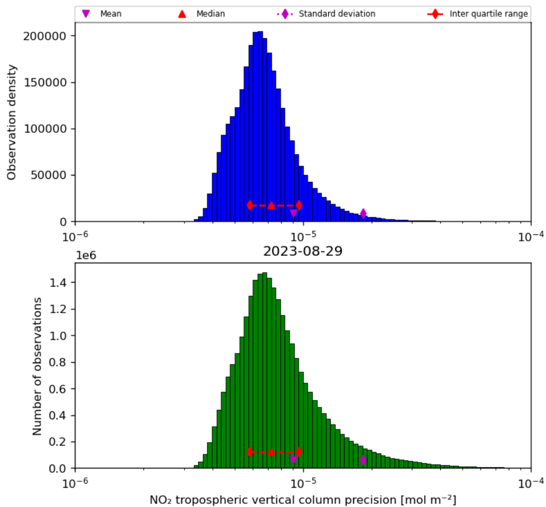
Figure 30: Histogram of “NO 2 tropospheric vertical column precision” for 2023-08-28 to 2023-08-30
