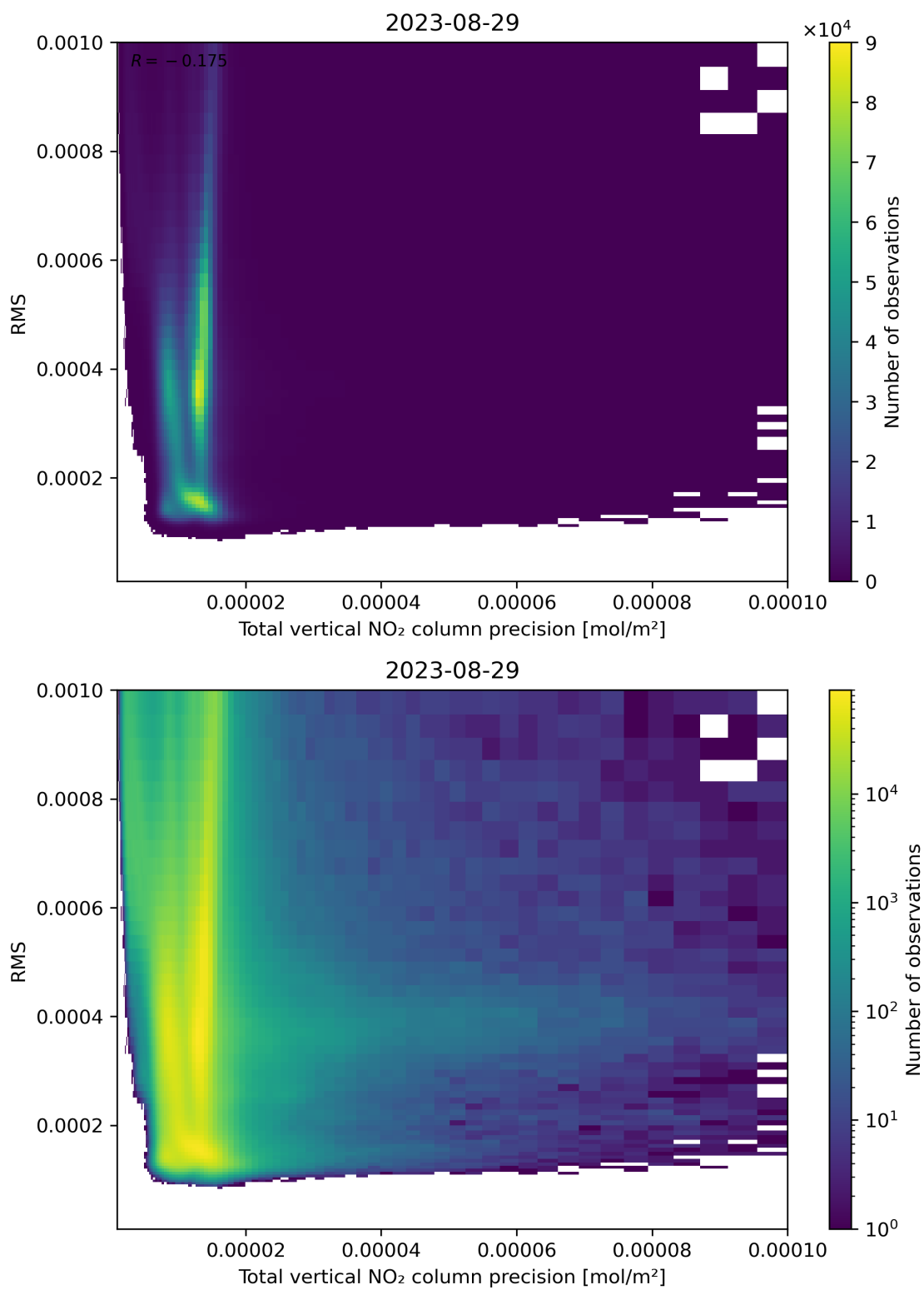
Figure 119: Scatter density plot of “Total vertical NO 2 column precision” against “RMS” for 2023-08-28 to 2023-08-30.
