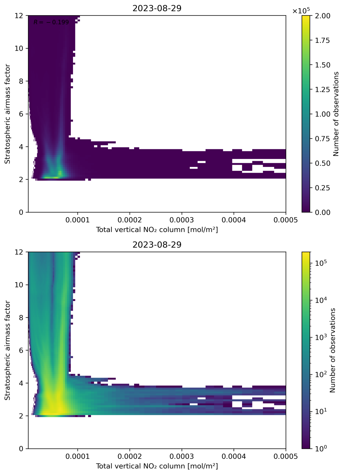
Figure 110: Scatter density plot of “Total vertical NO 2 column” against “Stratospheric airmass factor” for 2023-08-28 to 2023-08-30.
