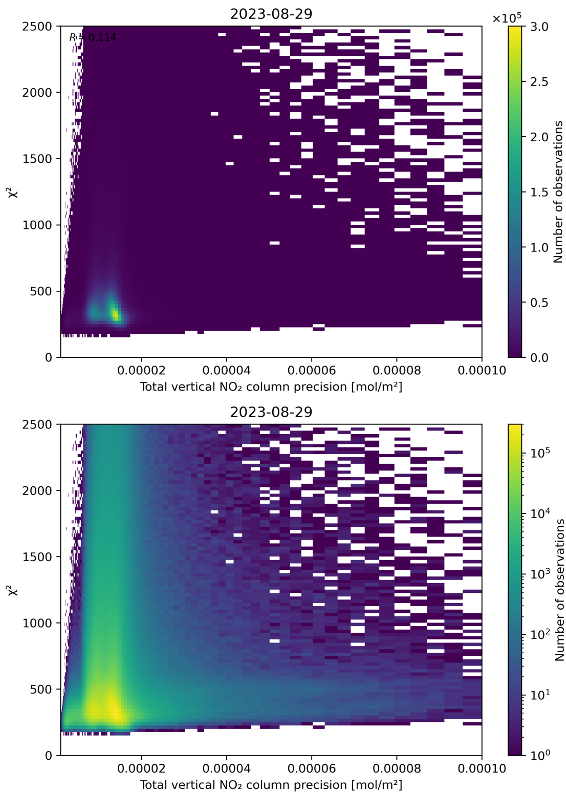
Figure 116: Scatter density plot of “Total vertical NO 2 column precision” against “ \chi^2 ” for 2023-08-28 to 2023-08-30.
