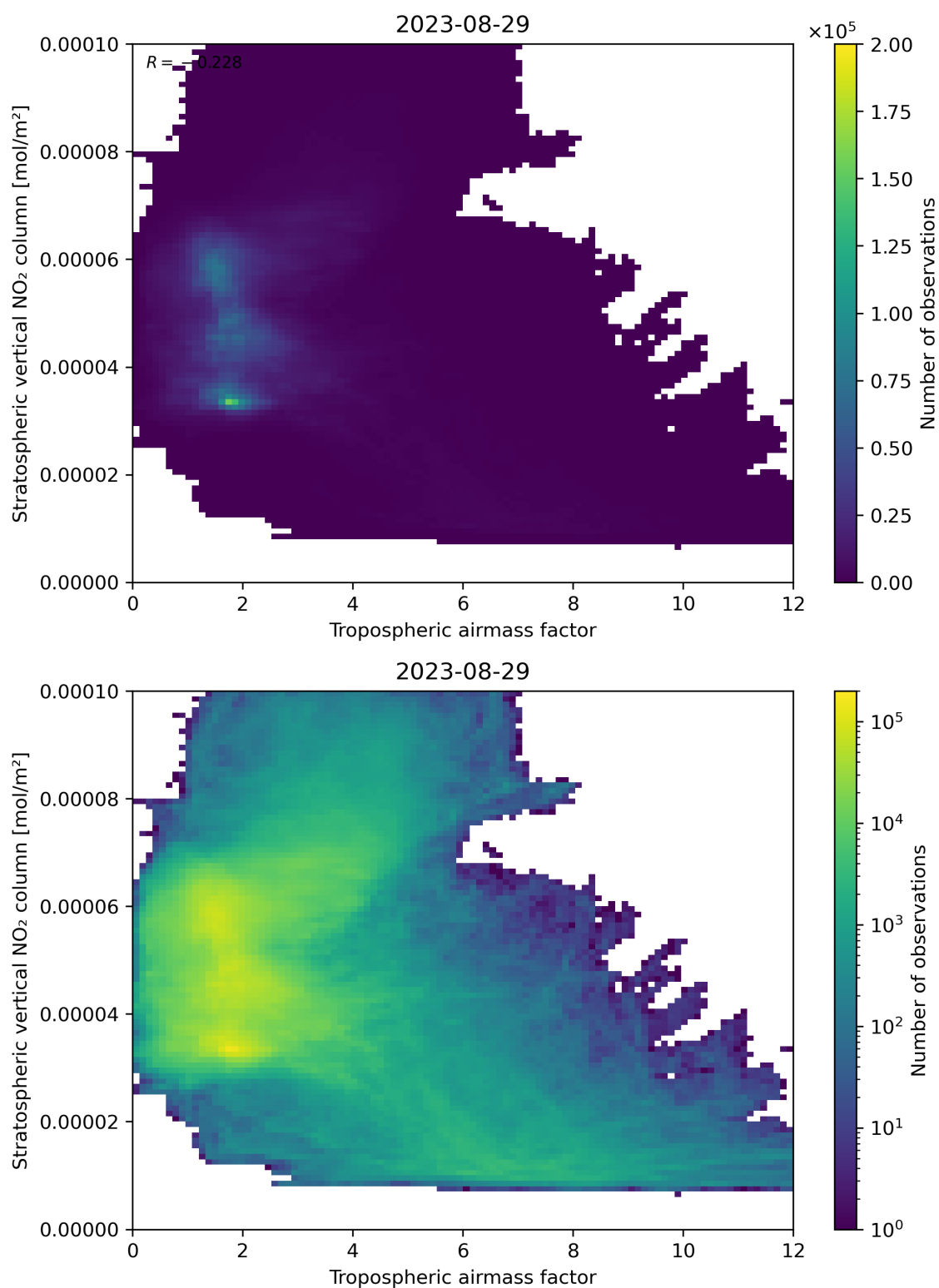
Figure 74: Scatter density plot of “Tropospheric air mass factor” against “Stratospheric vertical NO 2 column” for 2023-08-28 to 2023-08-30.
