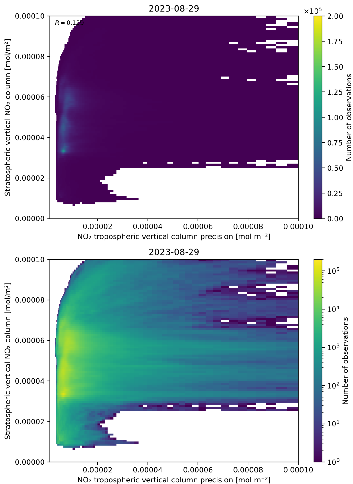
Figure 135: Scatter density plot of “NO 2 tropospheric vertical column precision” against “Stratospheric vertical NO 2 column” for 2023-08-28 to 2023-08-30.
