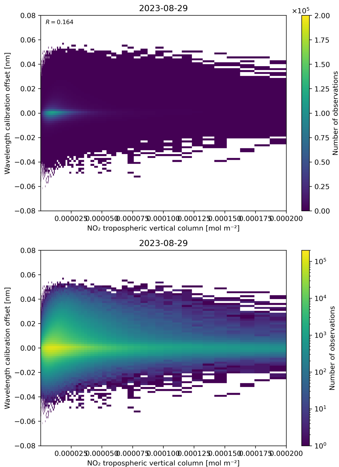
Figure 143: Scatter density plot of “NO 2 tropospheric vertical column” against “Wavelength calibration offset” for 2023-08-28 to 2023-08-30.
