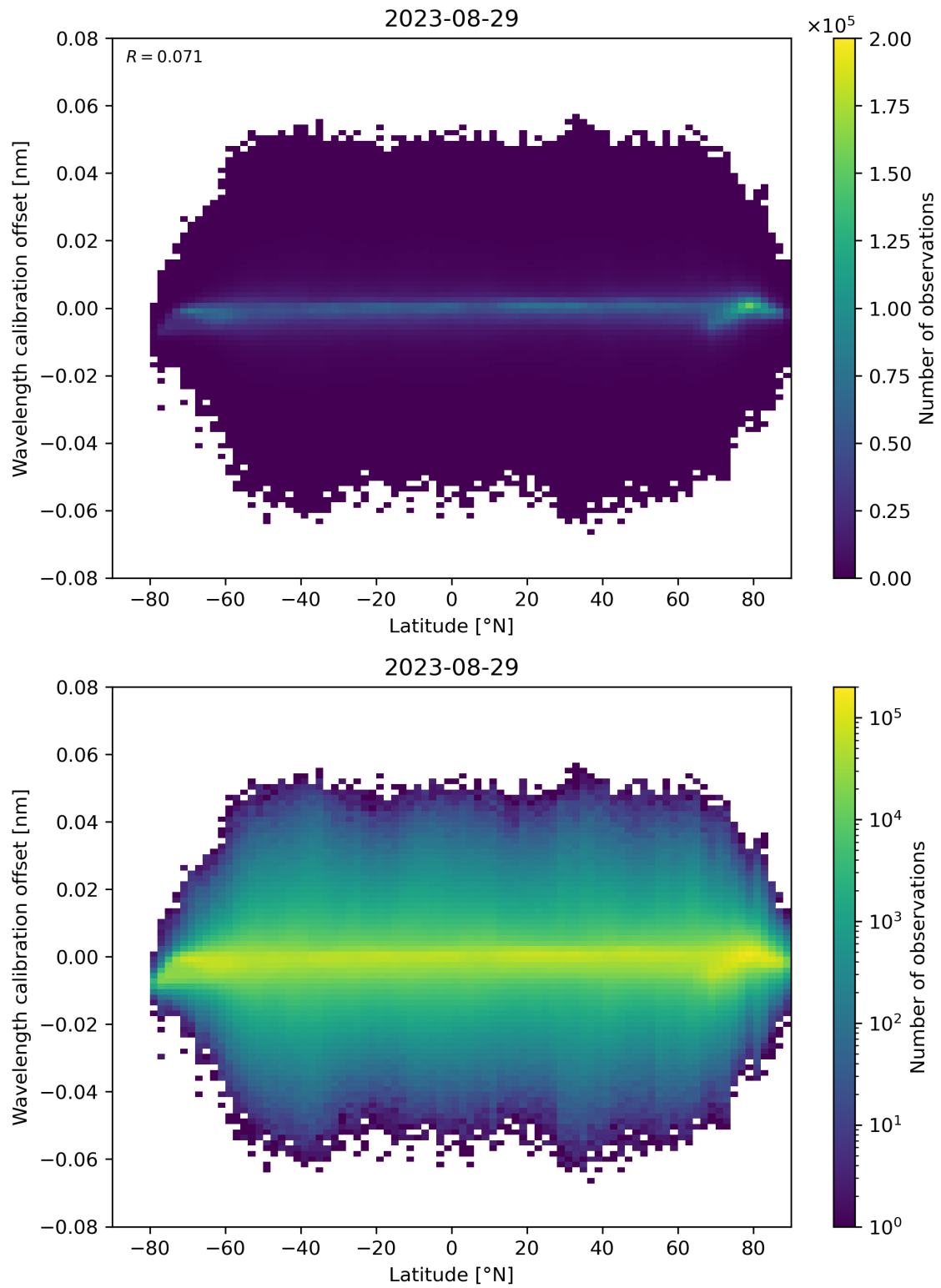
Figure 95: Scatter density plot of “Latitude” against “Wavelength calibration offset” for 2023-08-28 to 2023-08-30.
