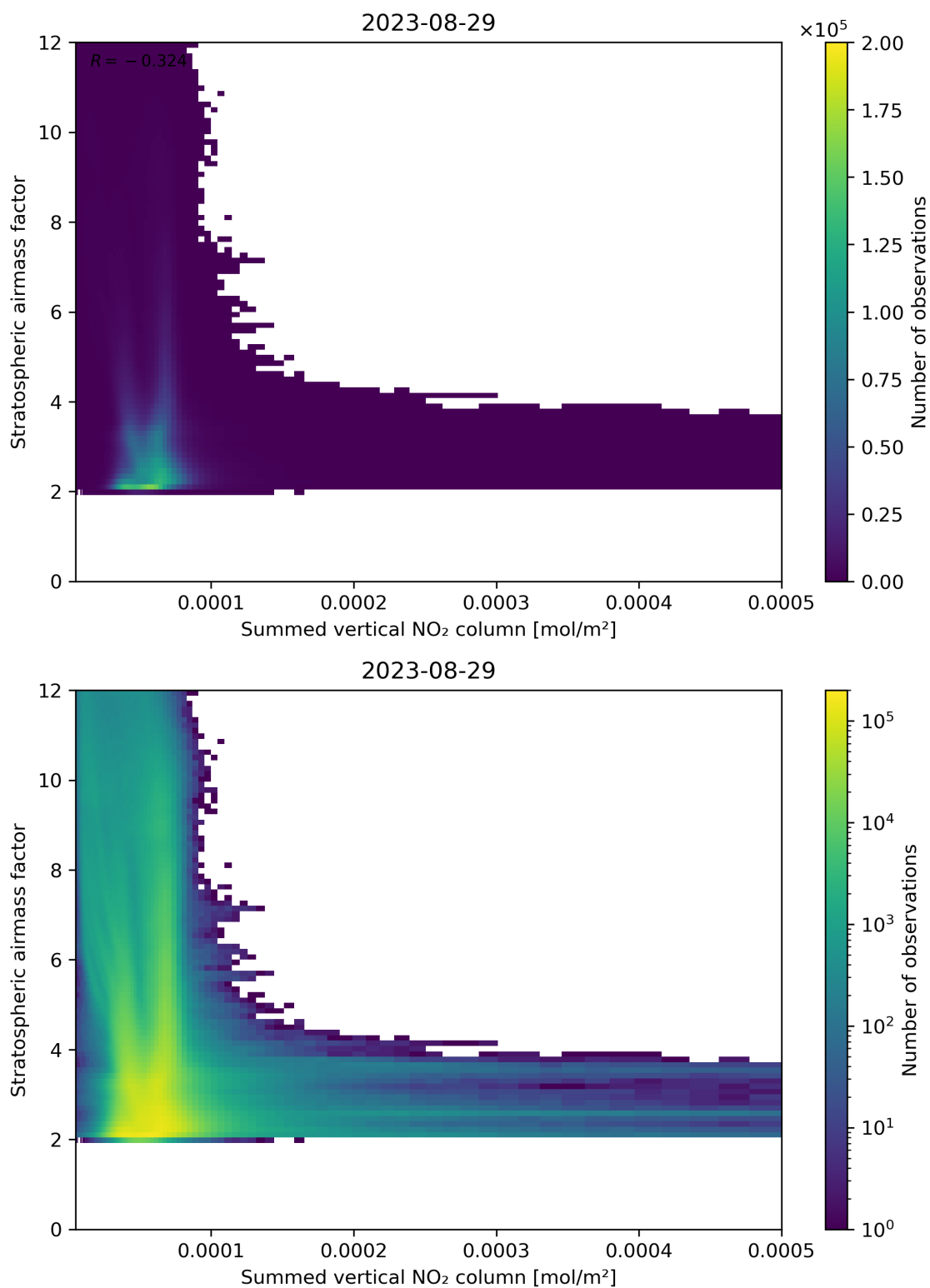
Figure 103: Scatter density plot of “Summed vertical NO 2 column” against “Stratospheric airmass factor” for 2023-08-28 to 2023-08-30.
