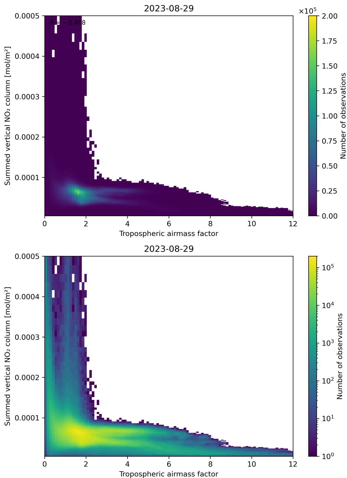
Figure 75: Scatter density plot of “Tropospheric air mass factor” against “Summed vertical NO 2 column” for 2023-08-28 to 2023-08-30.
