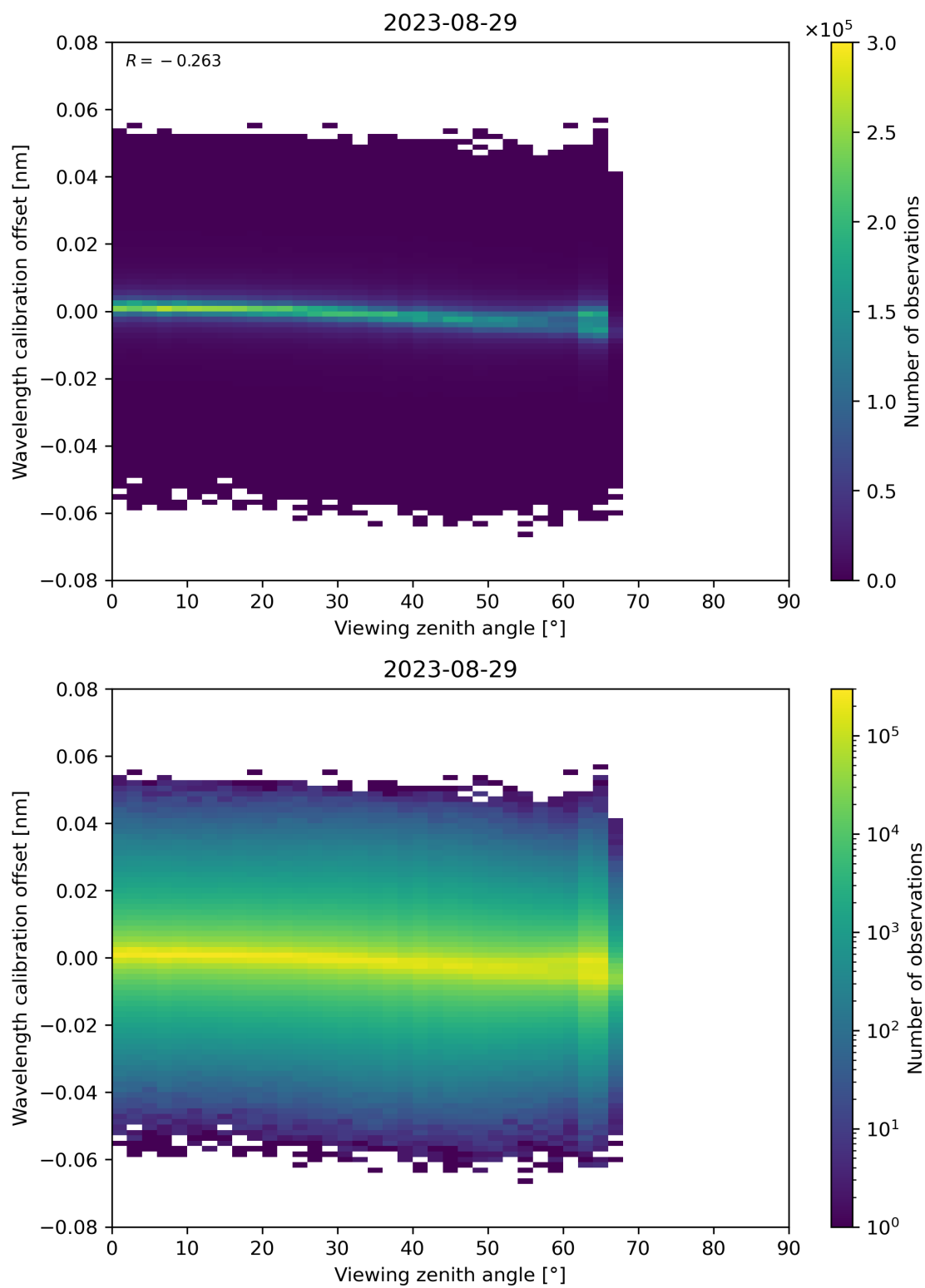
Figure 173: Scatter density plot of “Viewing zenith angle” against “Wavelength calibration offset” for 2023-08-28 to 2023-08-30.
