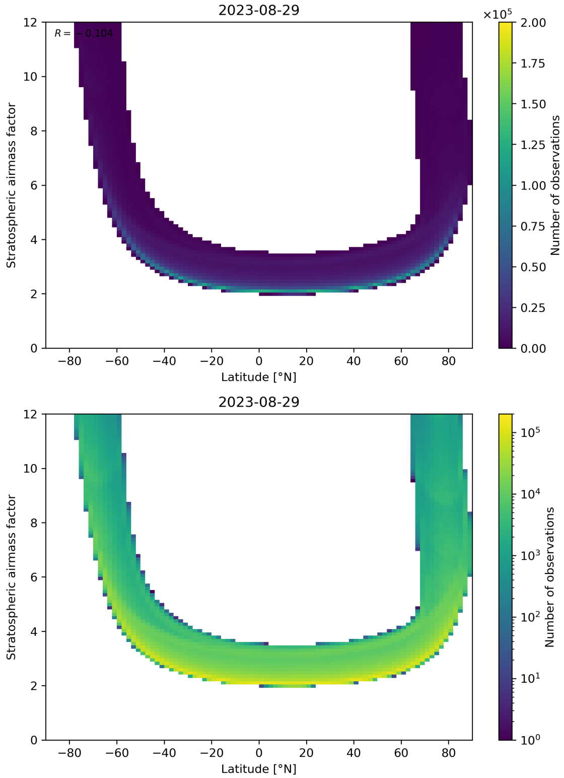
Figure 83: Scatter density plot of “Latitude” against “Stratospheric air mass factor” for 2023-08-28 to 2023-08-30.
