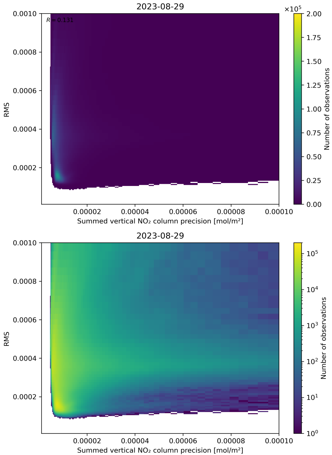
Figure 108: Scatter density plot of “Summed vertical NO 2 column precision” against “RMS” for 2023-08-28 to 2023-08-30.
