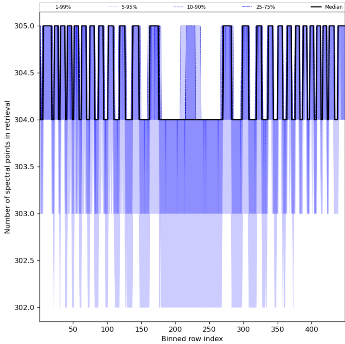
Figure 50: Along track statistics of “Number of spectral points in retrieval” for 2023-08-28 to 2023-08-30
