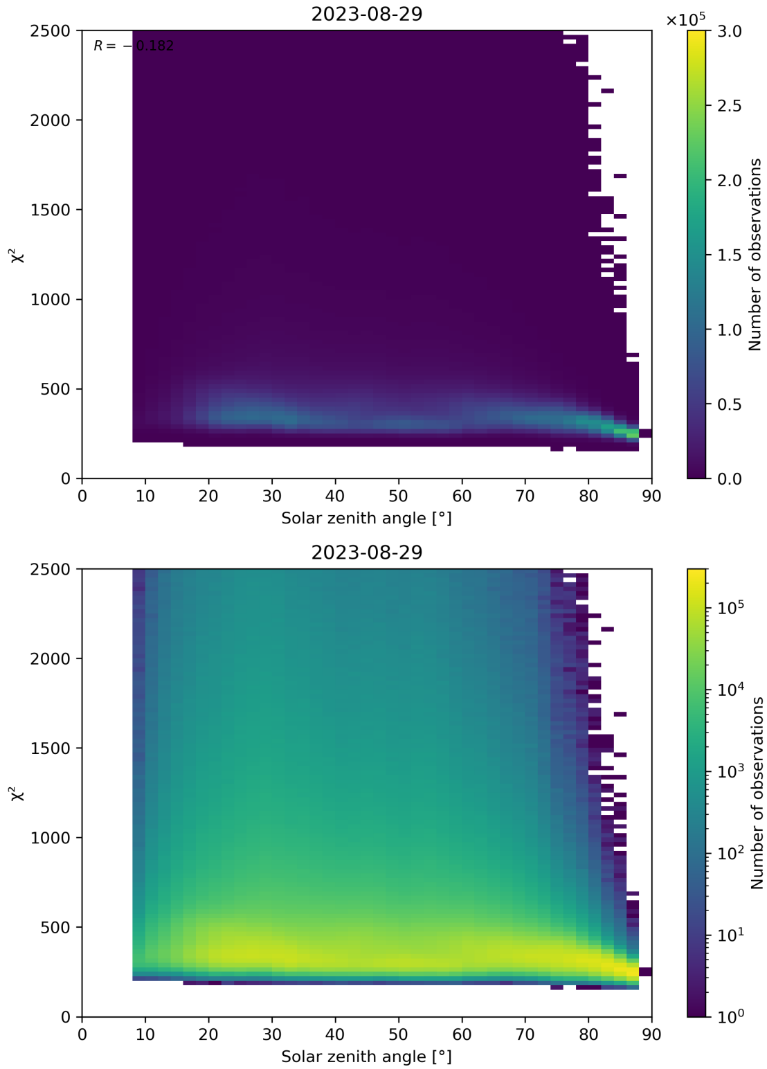
Figure 148: Scatter density plot of “Solar zenith angle” against “ \chi^2 ” for 2023-08-28 to 2023-08-30.
