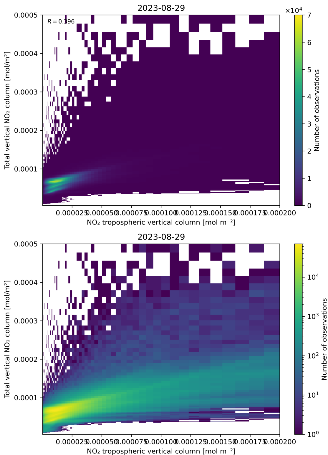
Figure 128: Scatter density plot of “NO 2 tropospheric vertical column” against “Total vertical NO 2 column” for 2023-08-28 to 2023-08-30.
