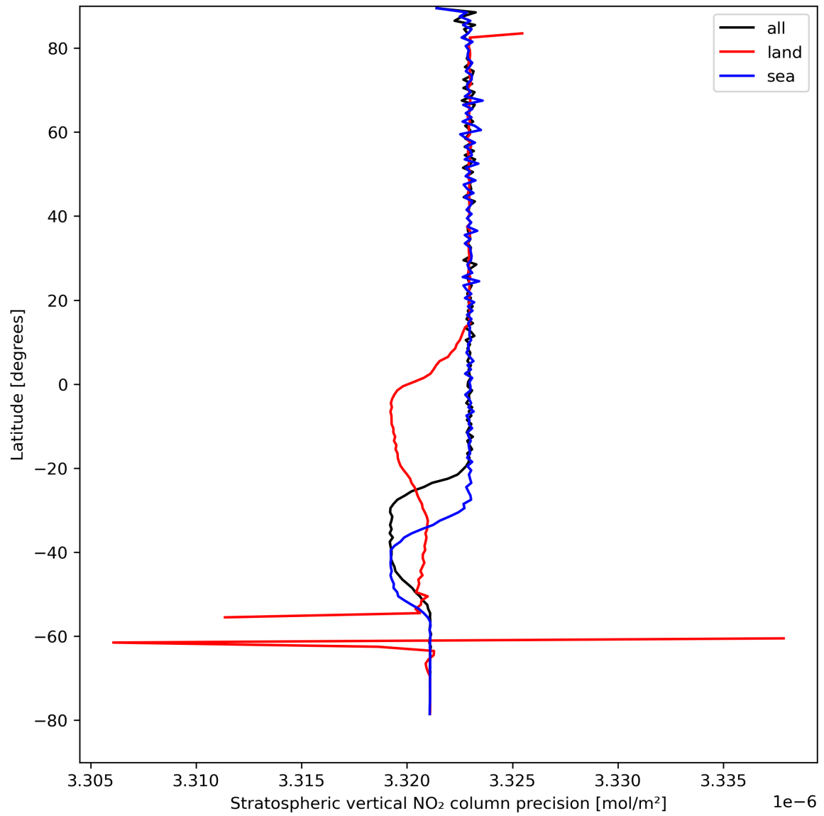
Figure 20: Zonal average of “Stratospheric vertical NO 2 column precision” for 2023-08-28 to 2023-08-30.
