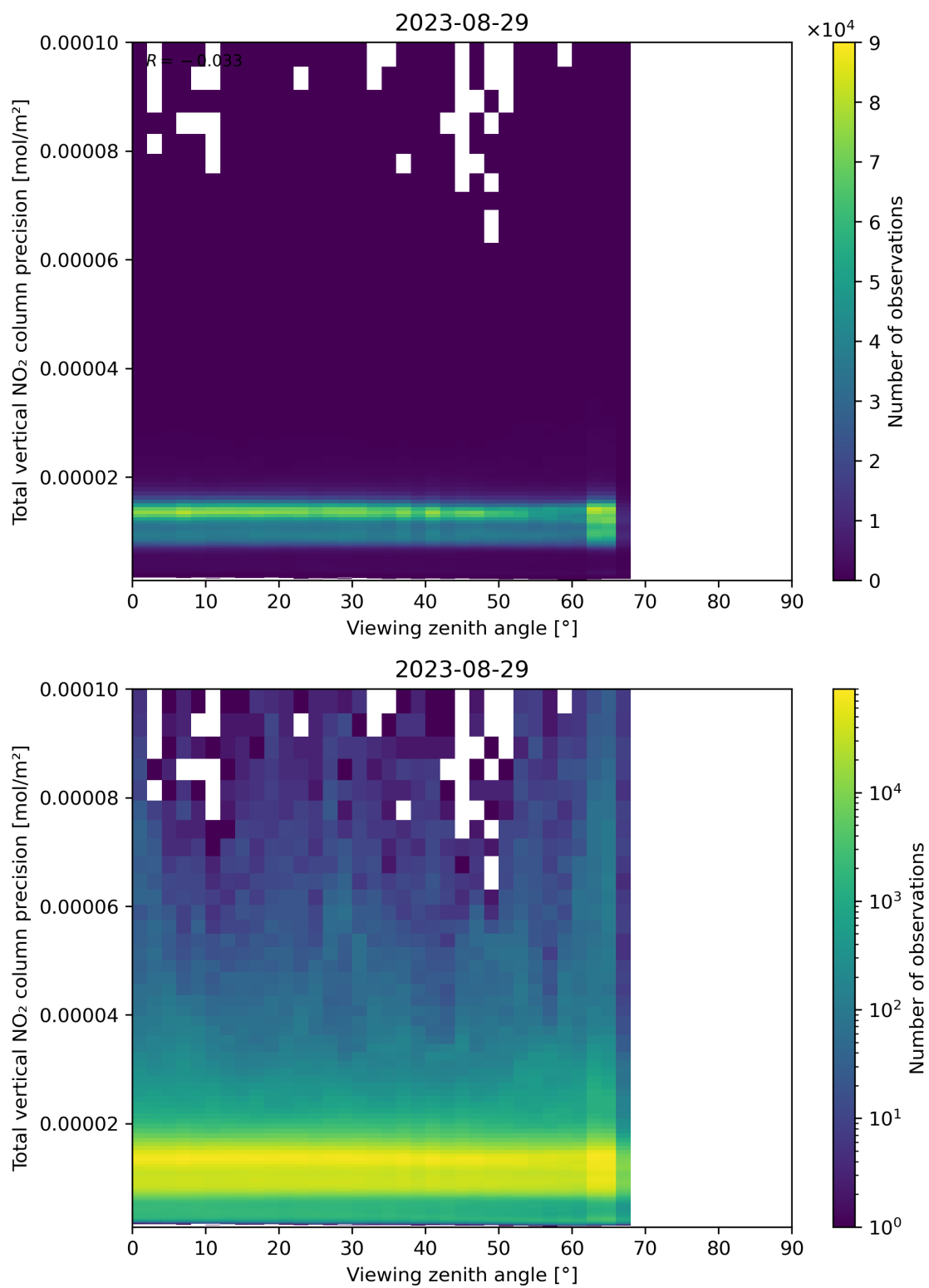
Figure 168: Scatter density plot of “Viewing zenith angle” against “Total vertical NO 2 column precision” for 2023-08-28 to 2023-08-30.
