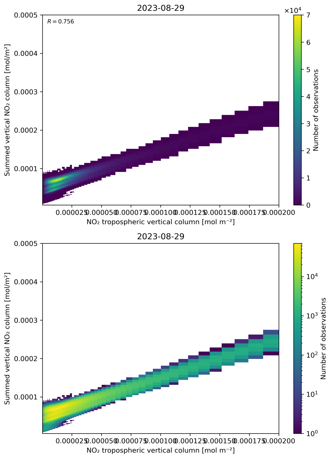
Figure 126: Scatter density plot of “NO 2 tropospheric vertical column” against “Summed vertical NO 2 column” for 2023-08-28 to 2023-08-30.
