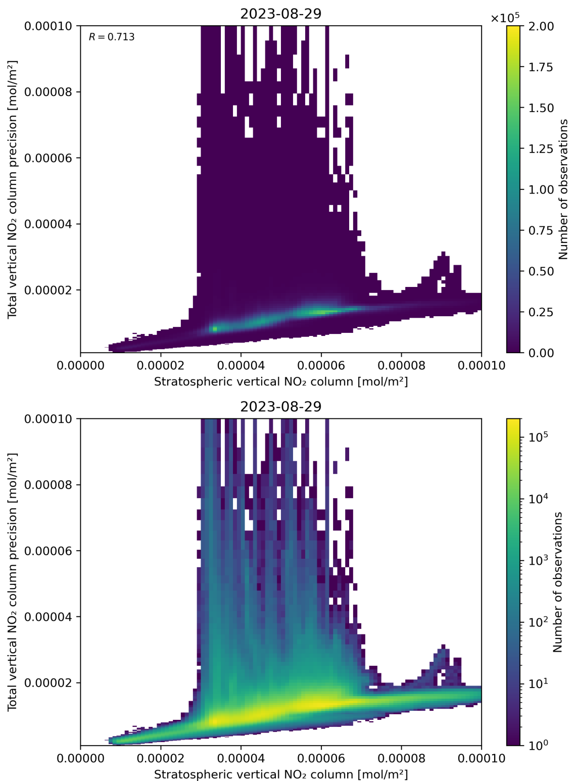
Figure 101: Scatter density plot of “Stratospheric vertical NO 2 column” against “Total vertical NO 2 column precision” for 2023-08-28 to 2023-08-30.
