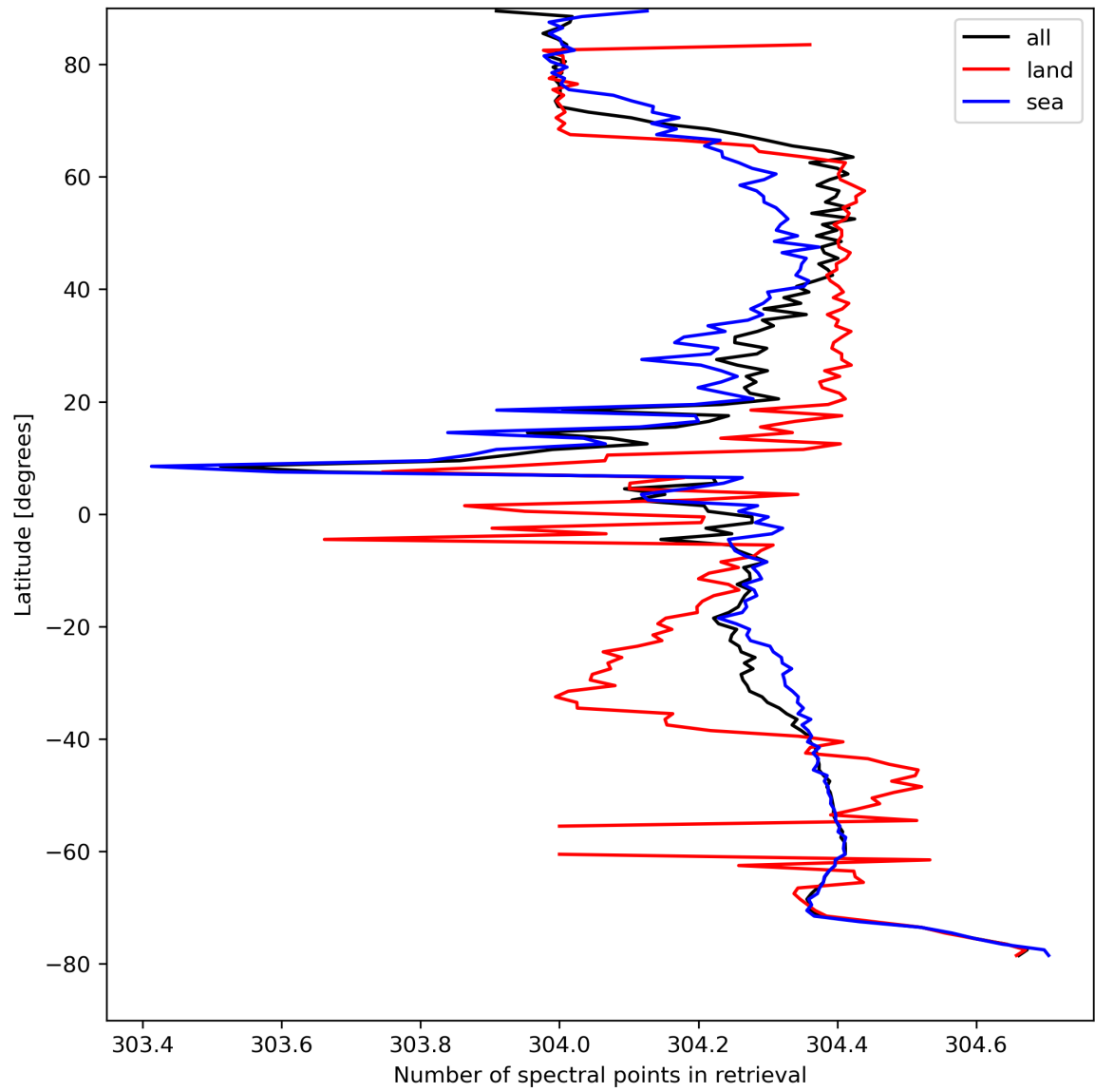
Figure 16: Zonal average of “Number of spectral points in retrieval” for 2023-08-28 to 2023-08-30.
