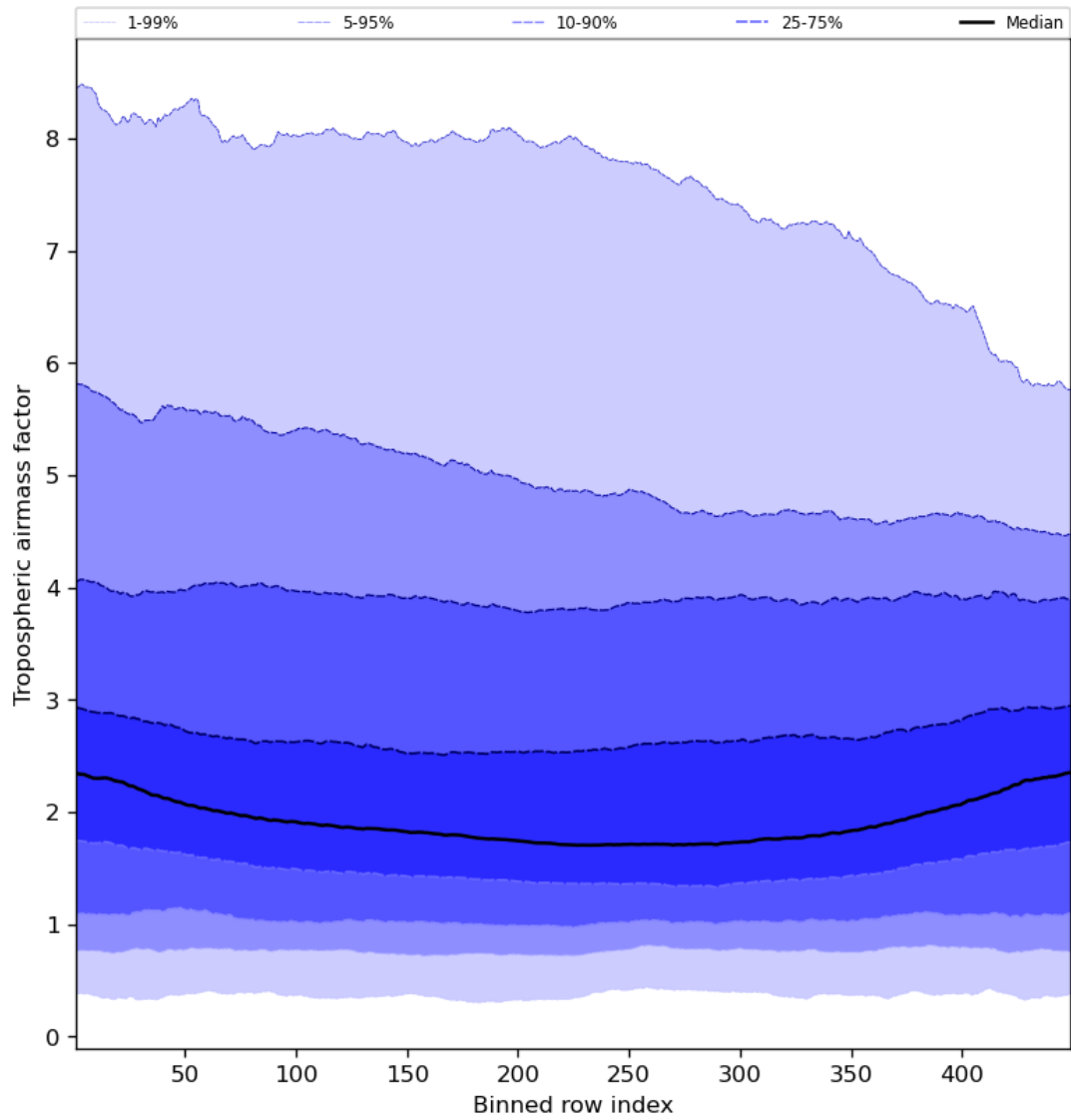
Figure 48: Along track statistics of “Tropospheric airmass factor” for 2023-08-28 to 2023-08-30
