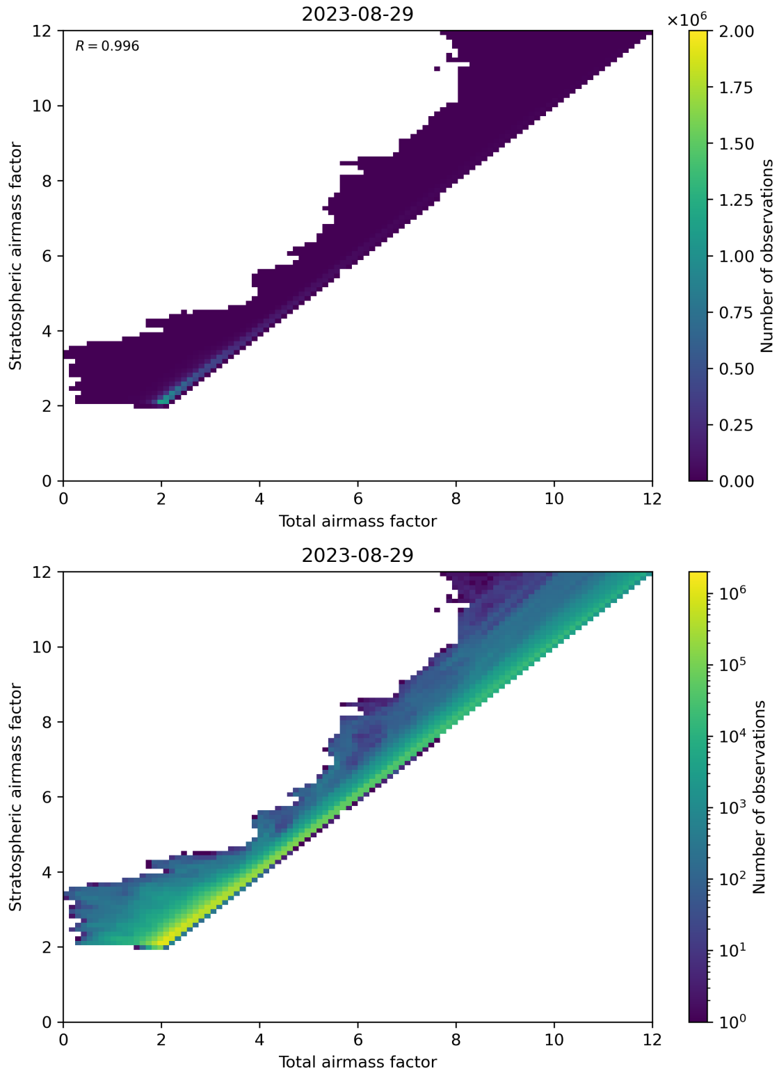
Figure 62: Scatter density plot of “Total airmass factor” against “Stratospheric airmass factor” for 2023-08-28 to 2023-08-30.
