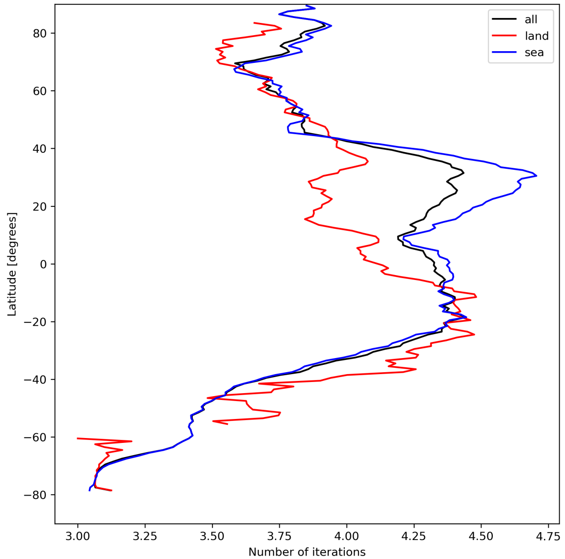
Figure 17: Zonal average of “Number of iterations” for 2023-08-28 to 2023-08-30.
