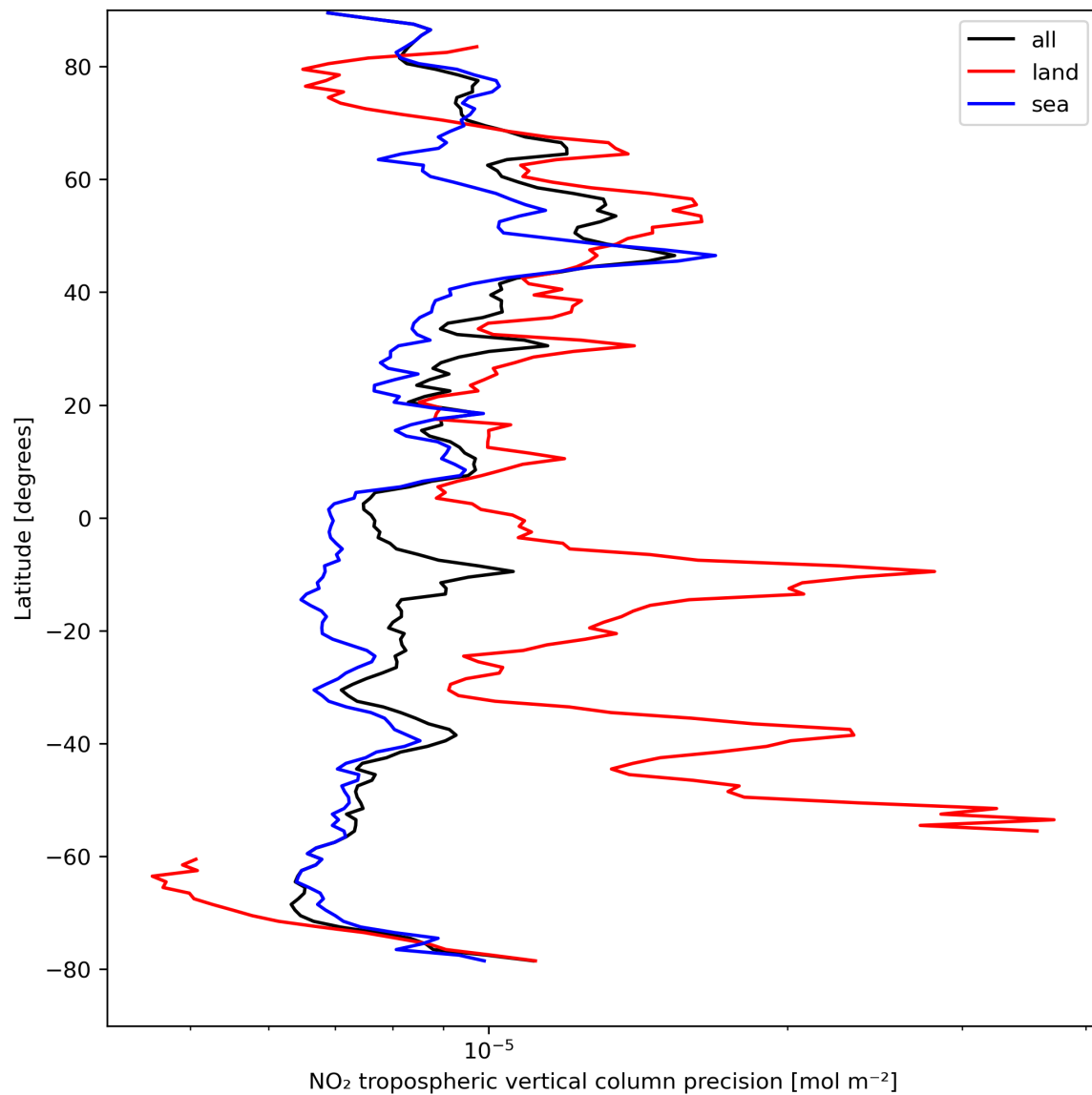
Figure 13: Zonal average of “NO 2 tropospheric vertical column precision” for 2023-08-28 to 2023-08-30.
