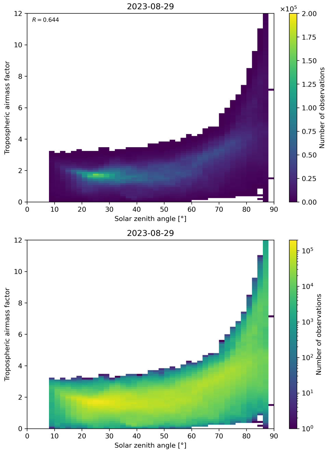
Figure 147: Scatter density plot of “Solar zenith angle” against “Tropospheric airmass factor” for 2023-08-28 to 2023-08-30.
