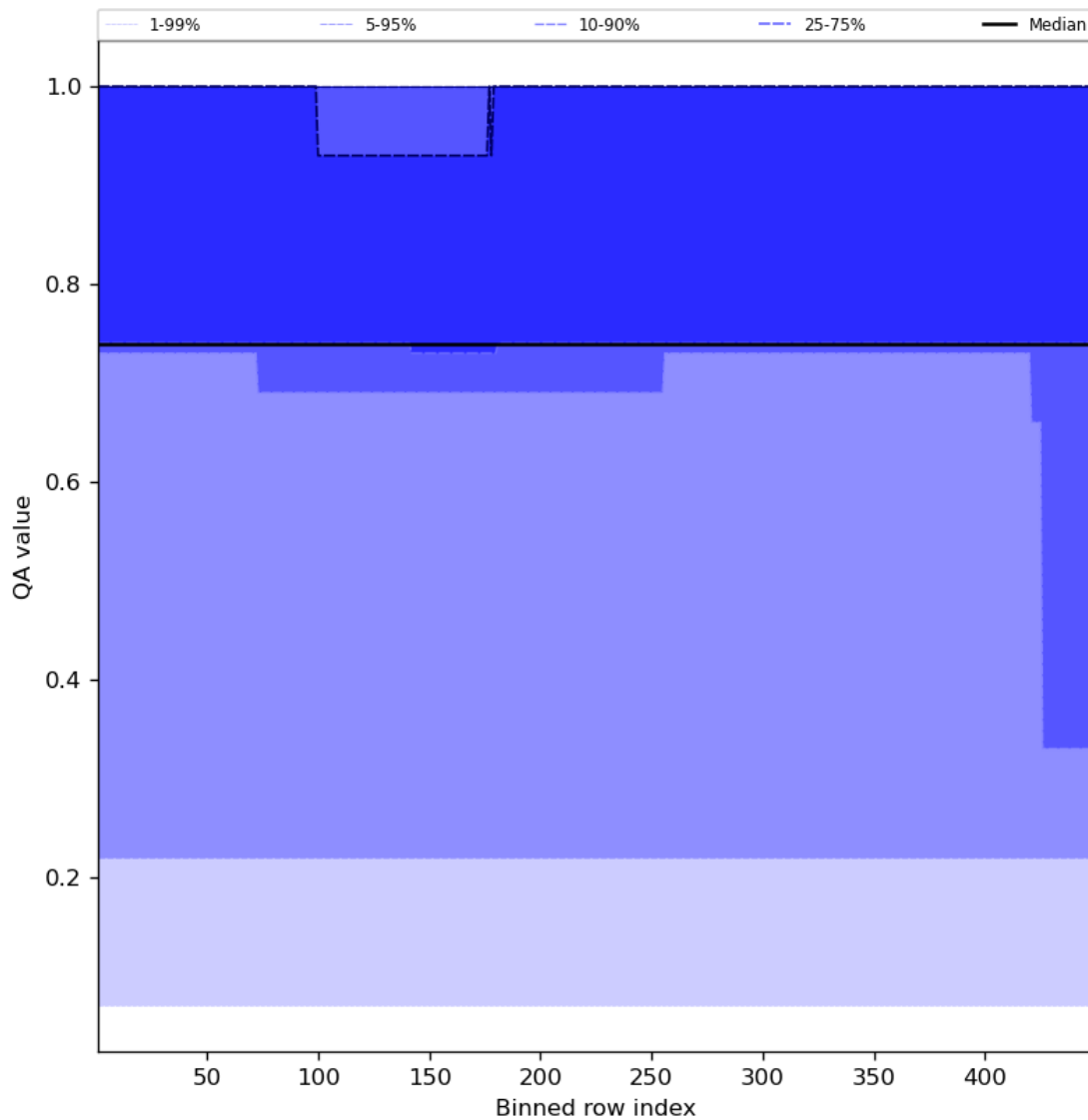
Figure 45: Along track statistics of “QA value” for 2023-08-28 to 2023-08-30
