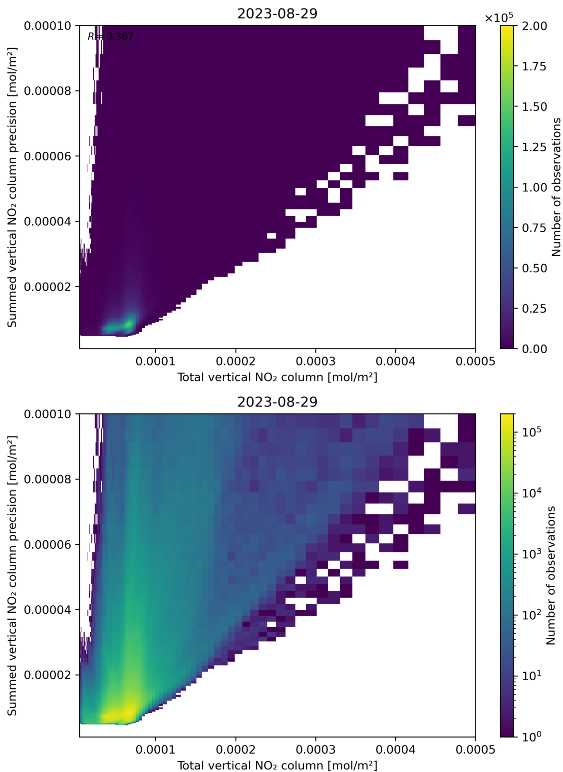
Figure 113: Scatter density plot of “Total vertical NO 2 column” against “Summed vertical NO 2 column precision” for 2023-08-28 to 2023-08-30.
