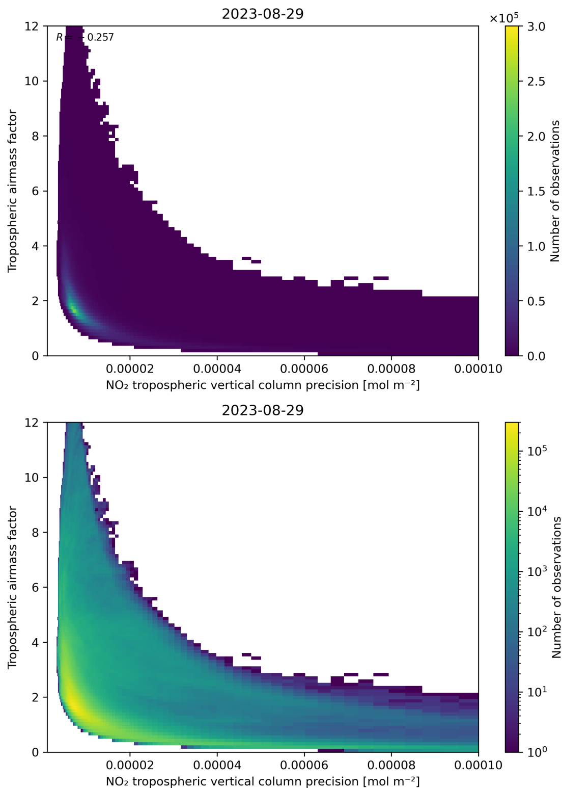
Figure 133: Scatter density plot of “NO 2 tropospheric vertical column precision” against “Tropospheric airmass factor” for 2023-08-28 to 2023-08-30.
