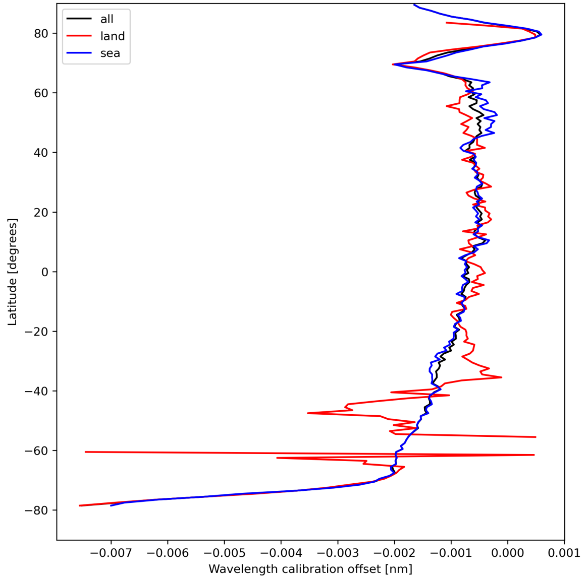
Figure 18: Zonal average of “Wavelength calibration offset” for 2023-08-28 to 2023-08-30.
