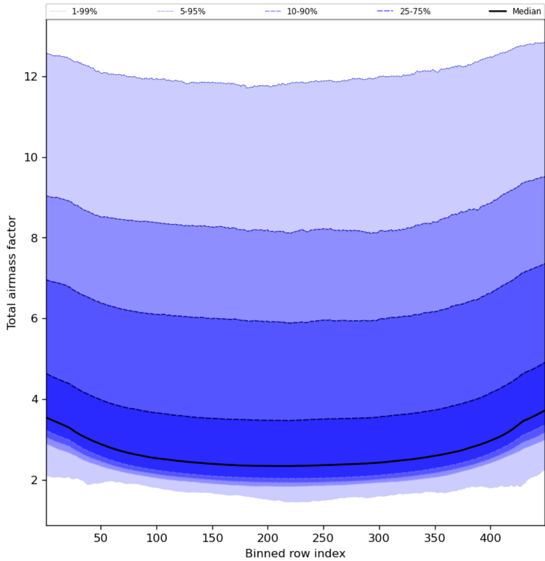
Figure 49: Along track statistics of “Total airmass factor” for 2023-08-28 to 2023-08-30
