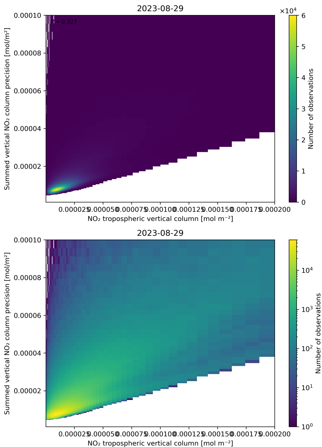
Figure 127: Scatter density plot of “NO 2 tropospheric vertical column” against “Summed vertical NO 2 column precision” for 2023-08-28 to 2023-08-30.
