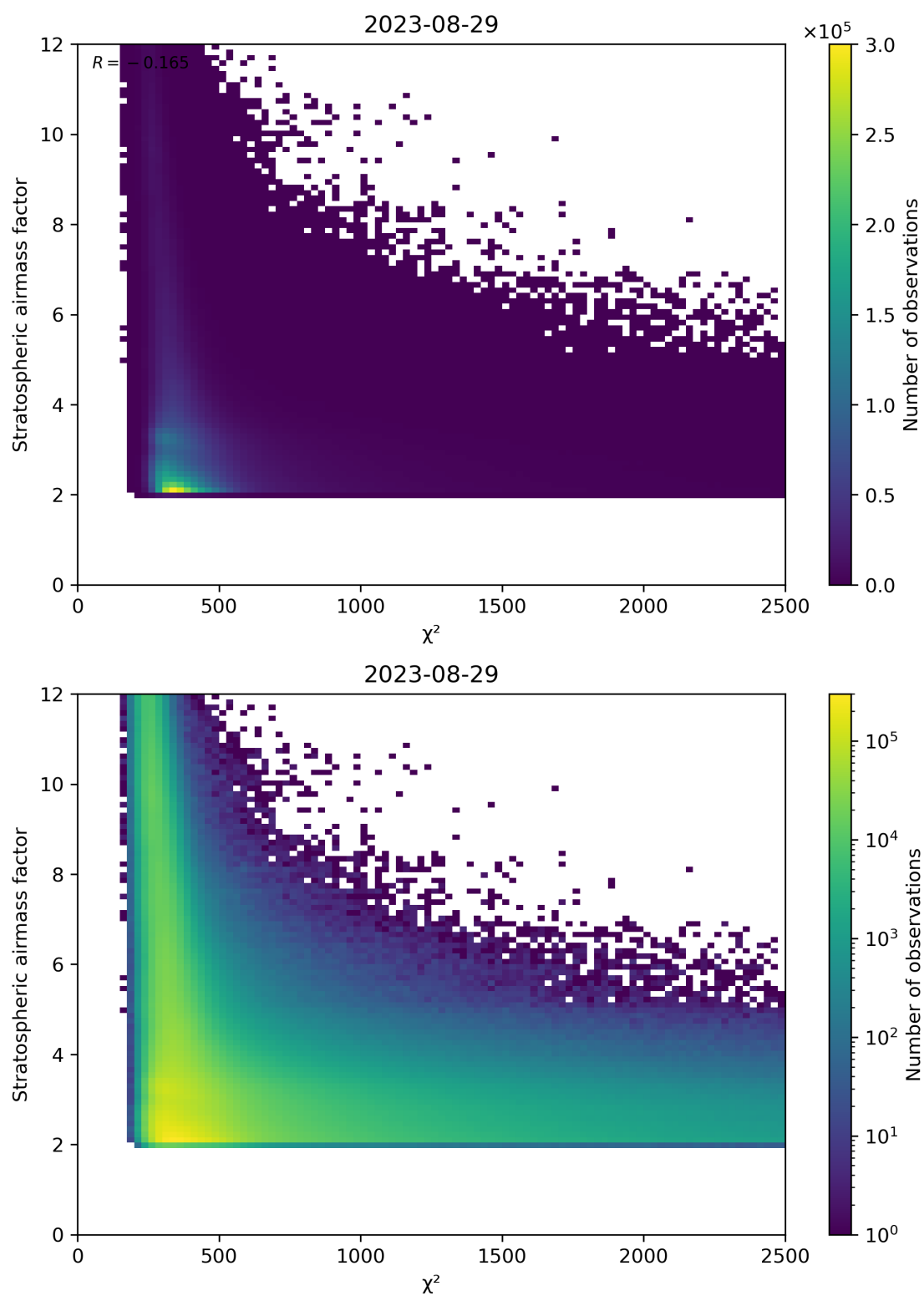
Figure 81: Scatter density plot of “ \chi^2 ” against “Stratospheric airmass factor” for 2023-08-28 to 2023-08-30.
