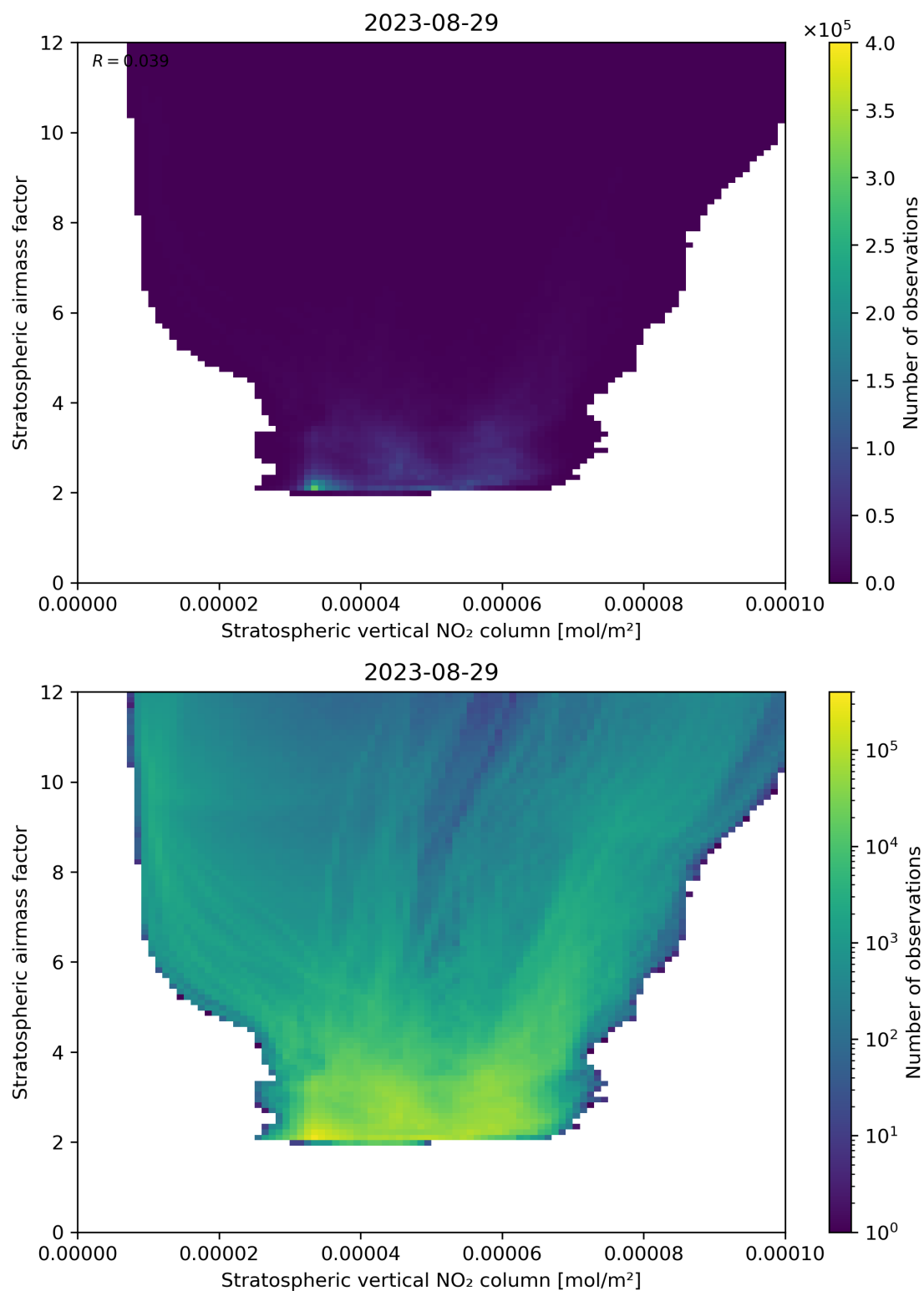
Figure 96: Scatter density plot of “Stratospheric vertical NO 2 column” against “Stratospheric airmass factor” for 2023-08-28 to 2023-08-30.
