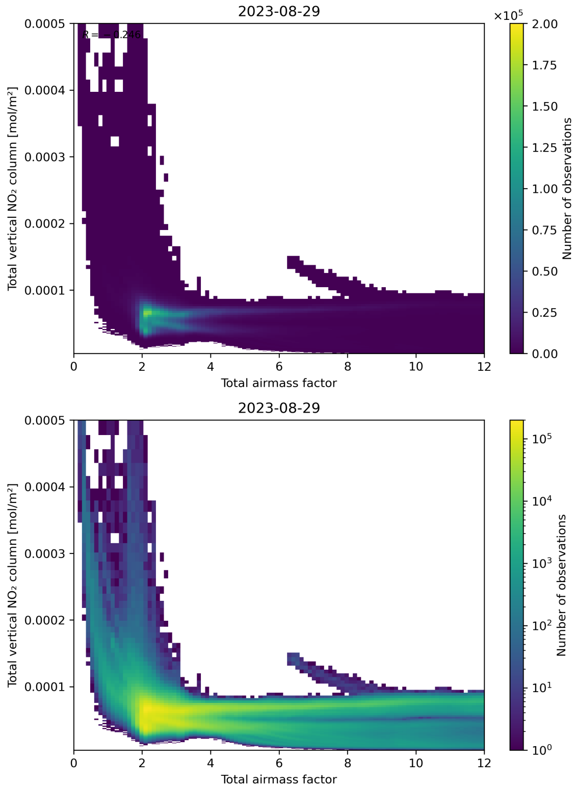
Figure 67: Scatter density plot of “Total airmass factor” against “Total vertical NO 2 column” for 2023-08-28 to 2023-08-30.
