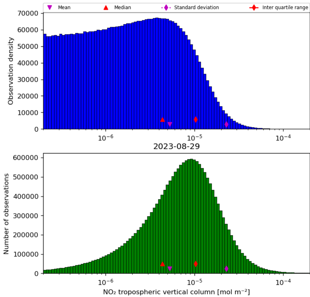
Figure 29: Histogram of “NO 2 tropospheric vertical column” for 2023-08-28 to 2023-08-30
