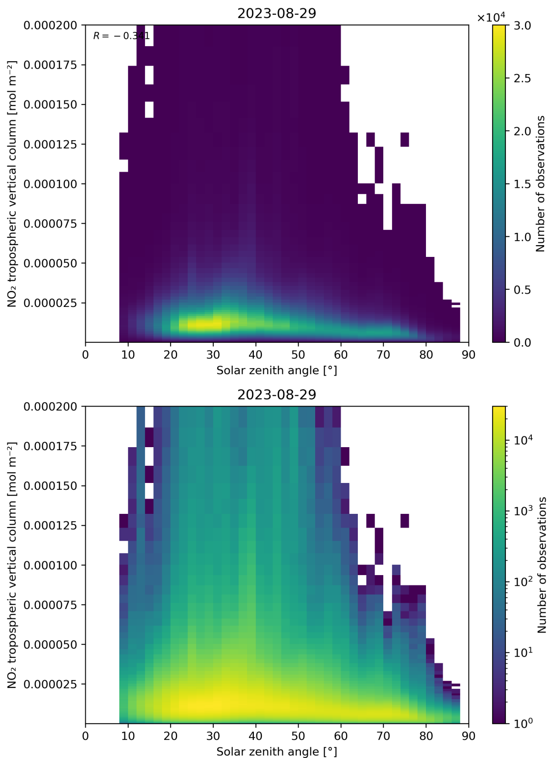
Figure 155: Scatter density plot of “Solar zenith angle” against “NO 2 tropospheric vertical column” for 2023-08-28 to 2023-08-30.
