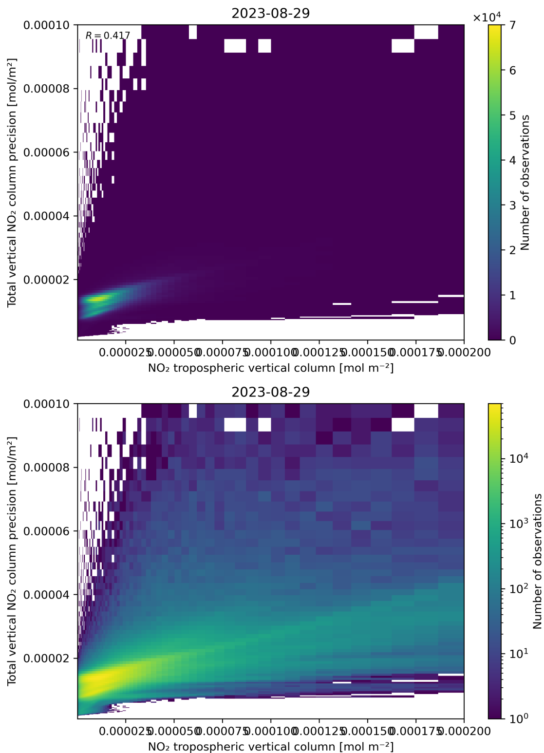
Figure 129: Scatter density plot of “NO 2 tropospheric vertical column” against “Total vertical NO 2 column precision” for 2023-08-28 to 2023-08-30.
