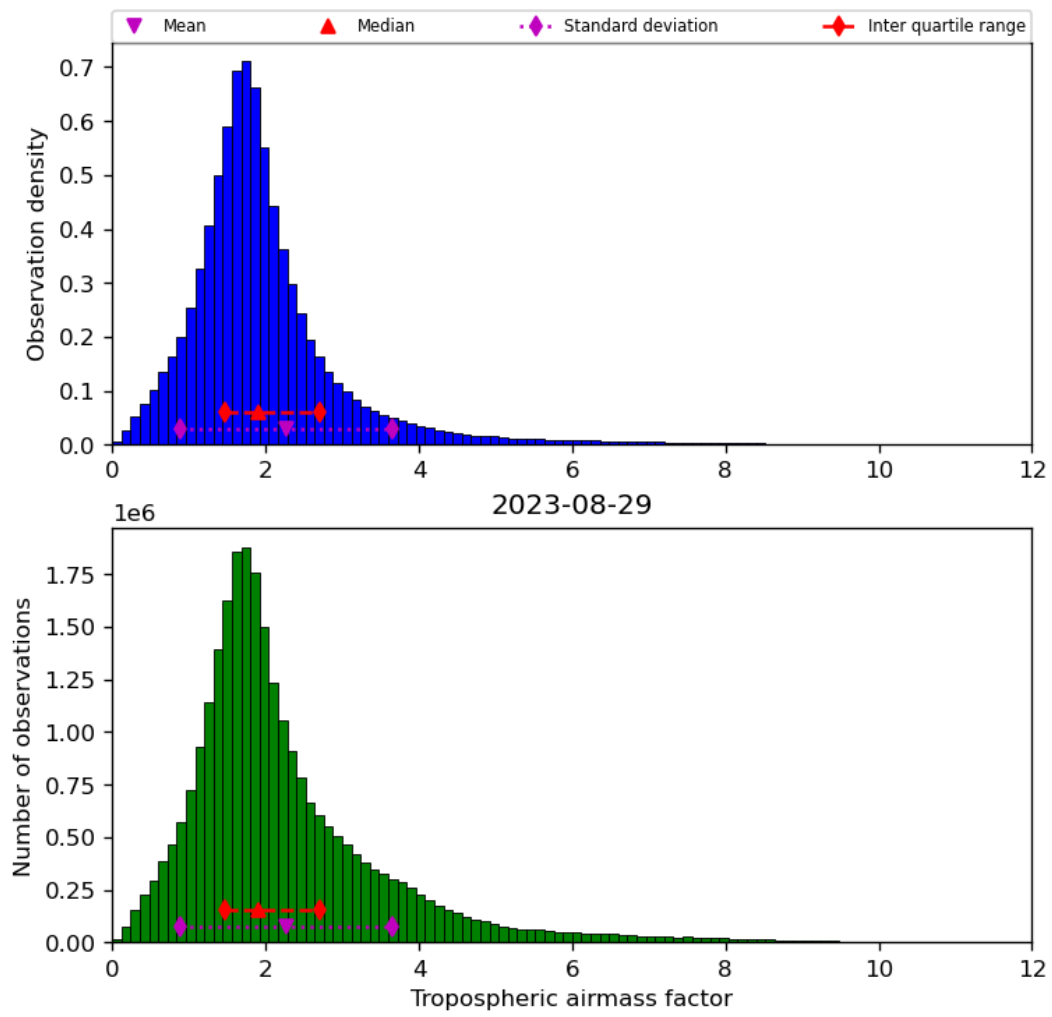
Figure 31: Histogram of “Tropospheric airmass factor” for 2023-08-28 to 2023-08-30
