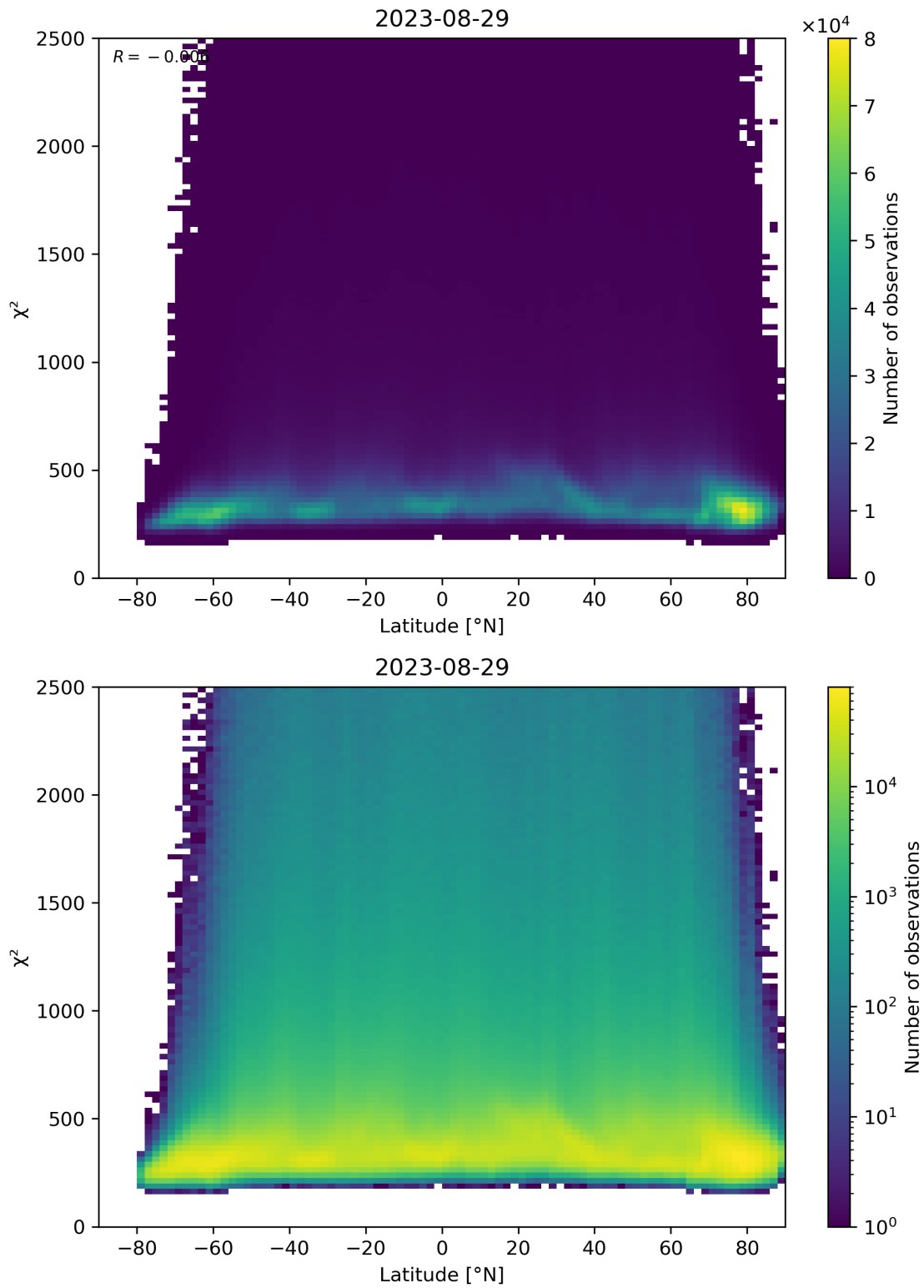
Figure 86: Scatter density plot of “Latitude” against “ \chi^2 ” for 2023-08-28 to 2023-08-30.
