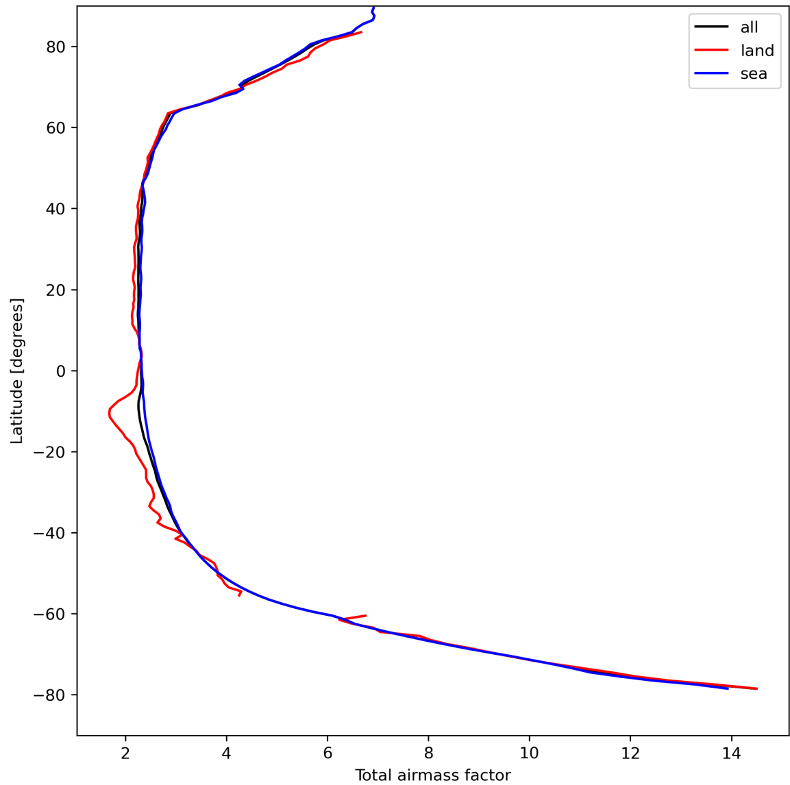
Figure 15: Zonal average of “Total airmass factor” for 2023-08-28 to 2023-08-30.
