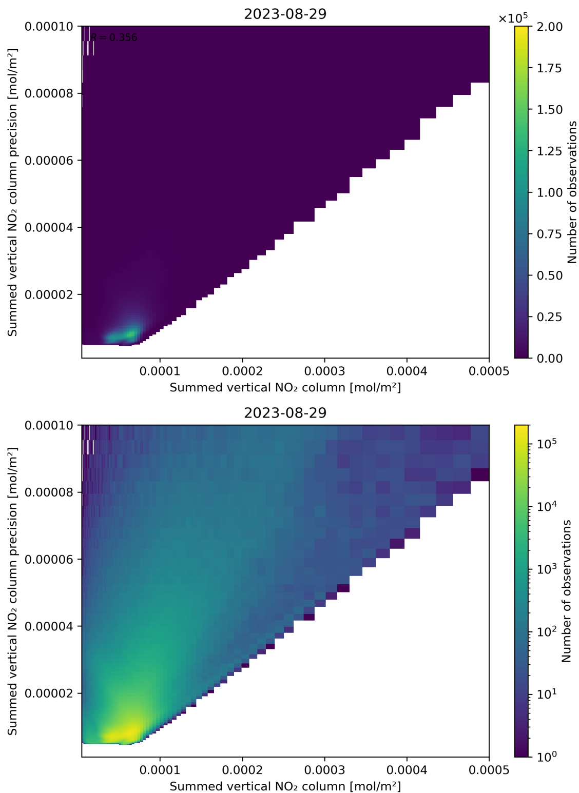
Figure 105: Scatter density plot of “Summed vertical NO 2 column” against “Summed vertical NO 2 column precision” for 2023-08-28 to 2023-08-30.
