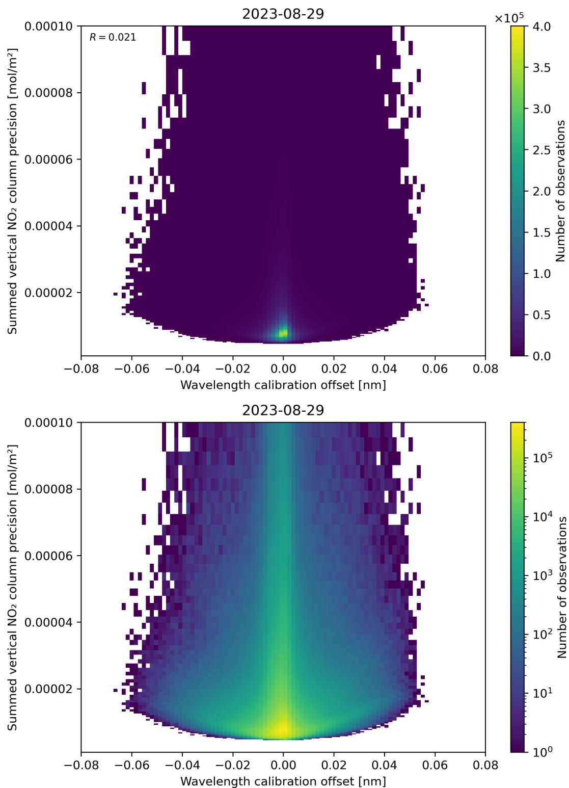
Figure 178: Scatter density plot of “Wavelength calibration offset” against “Summed vertical NO 2 column precision” for 2023-08-28 to 2023-08-30.
