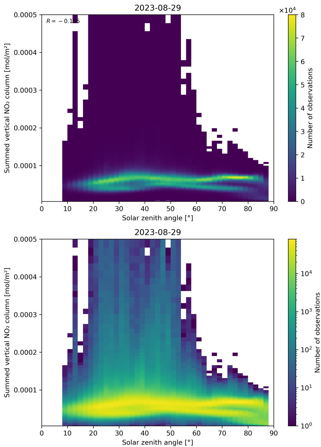
Figure 151: Scatter density plot of “Solar zenith angle” against “Summed vertical NO 2 column” for 2023-08-28 to 2023-08-30.
