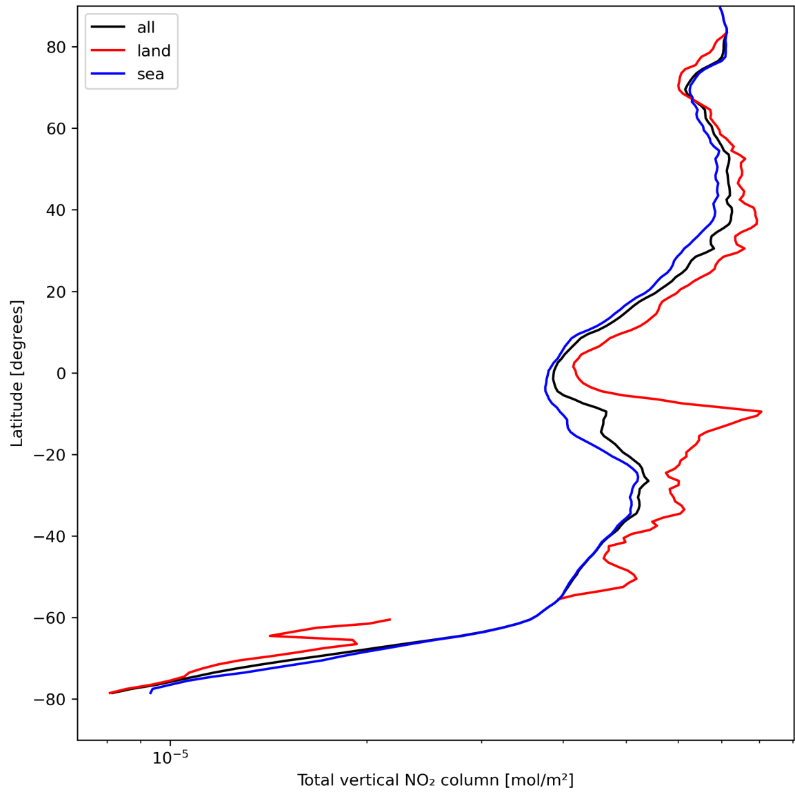
Figure 21: Zonal average of “Total vertical NO 2 column” for 2023-08-28 to 2023-08-30.
