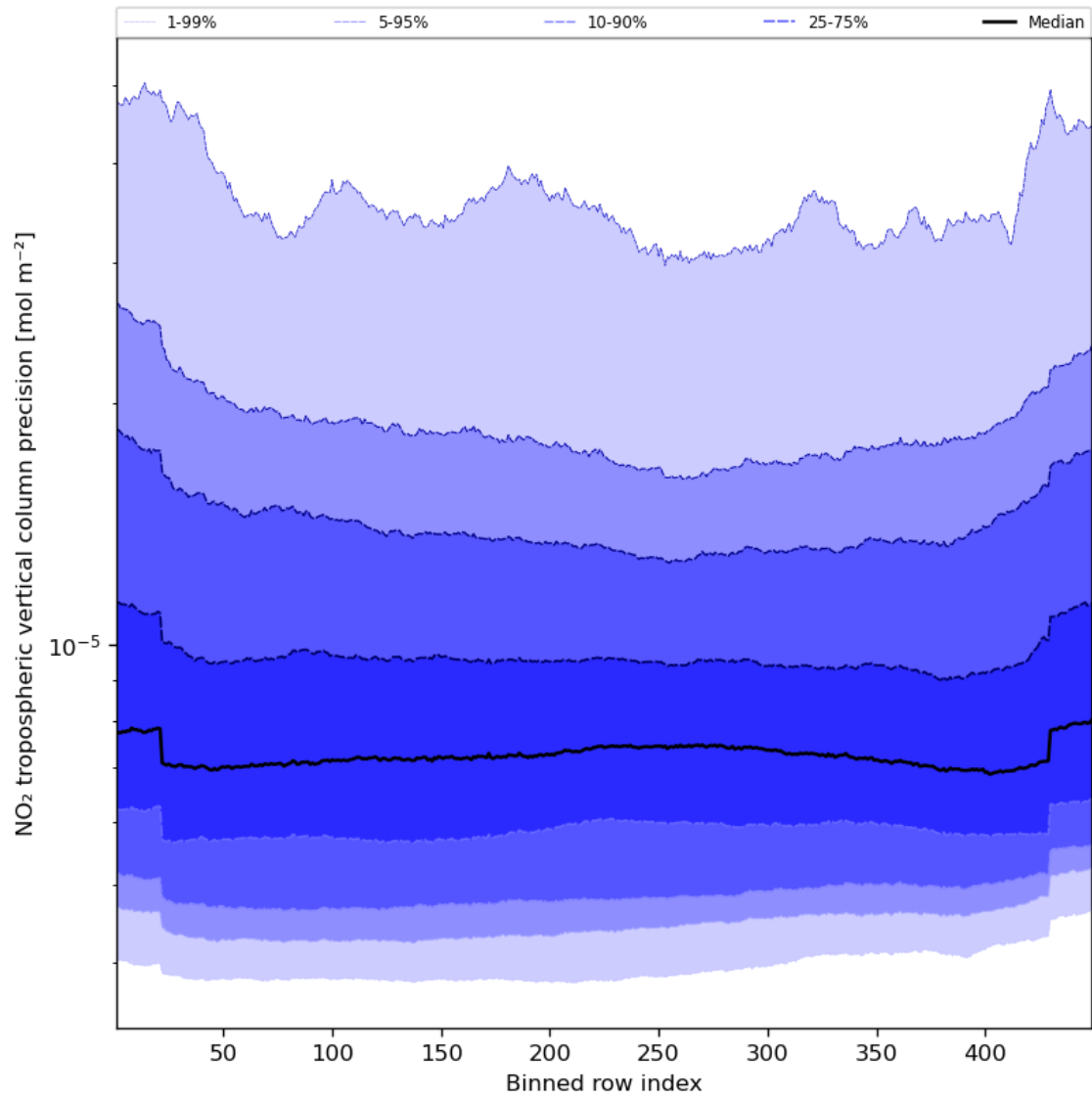
Figure 47: Along track statistics of “NO 2 tropospheric vertical column precision” for 2023-08-28 to 2023-08-30
