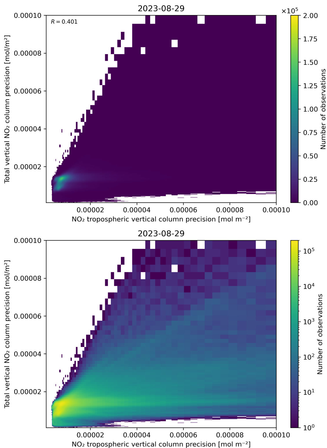
Figure 139: Scatter density plot of “NO 2 tropospheric vertical column precision” against “Total vertical NO 2 column precision” for 2023-08-28 to 2023-08-30.
