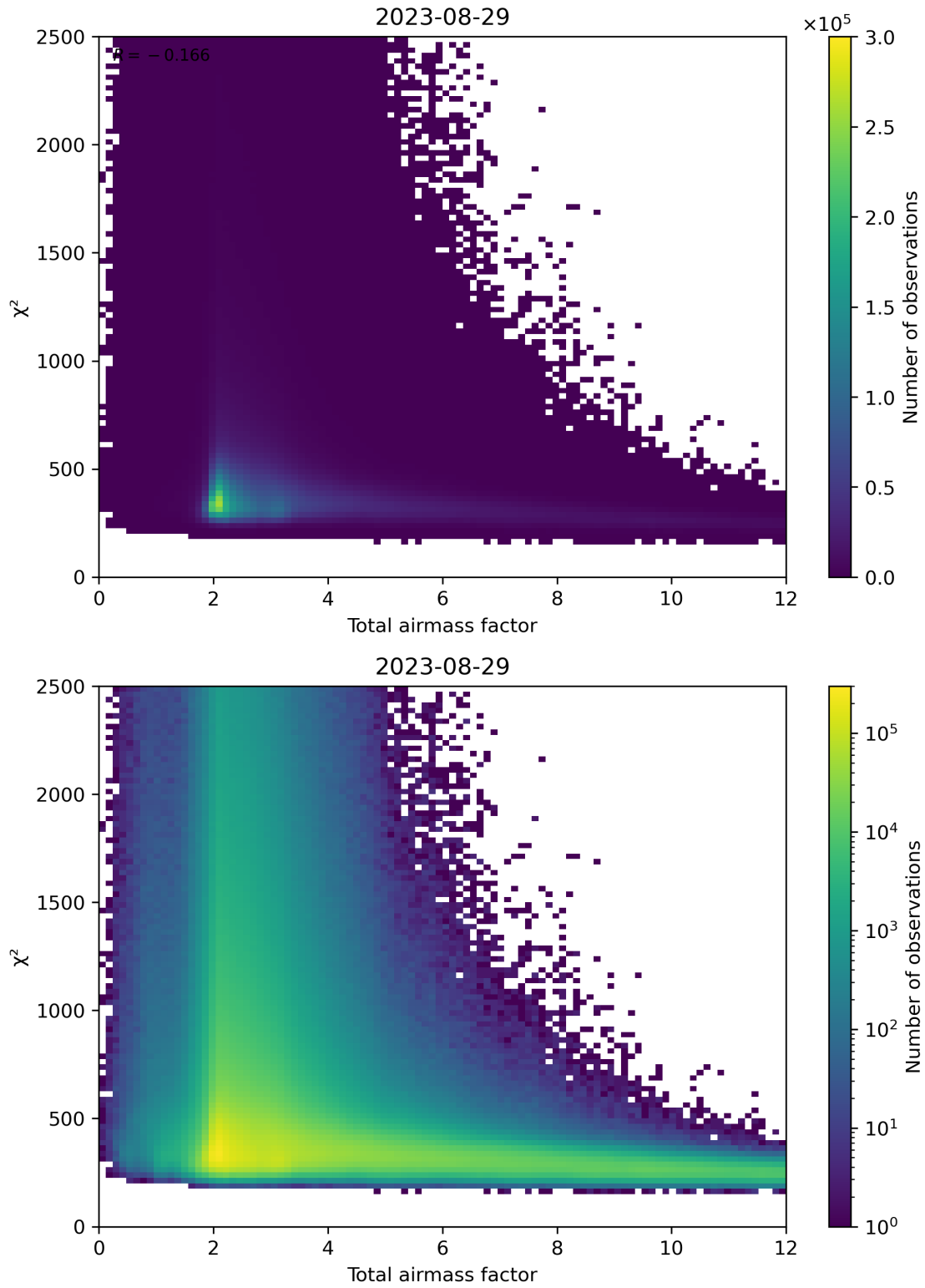
Figure 63: Scatter density plot of “Total airmass factor” against “ \chi^2 ” for 2023-08-28 to 2023-08-30.
