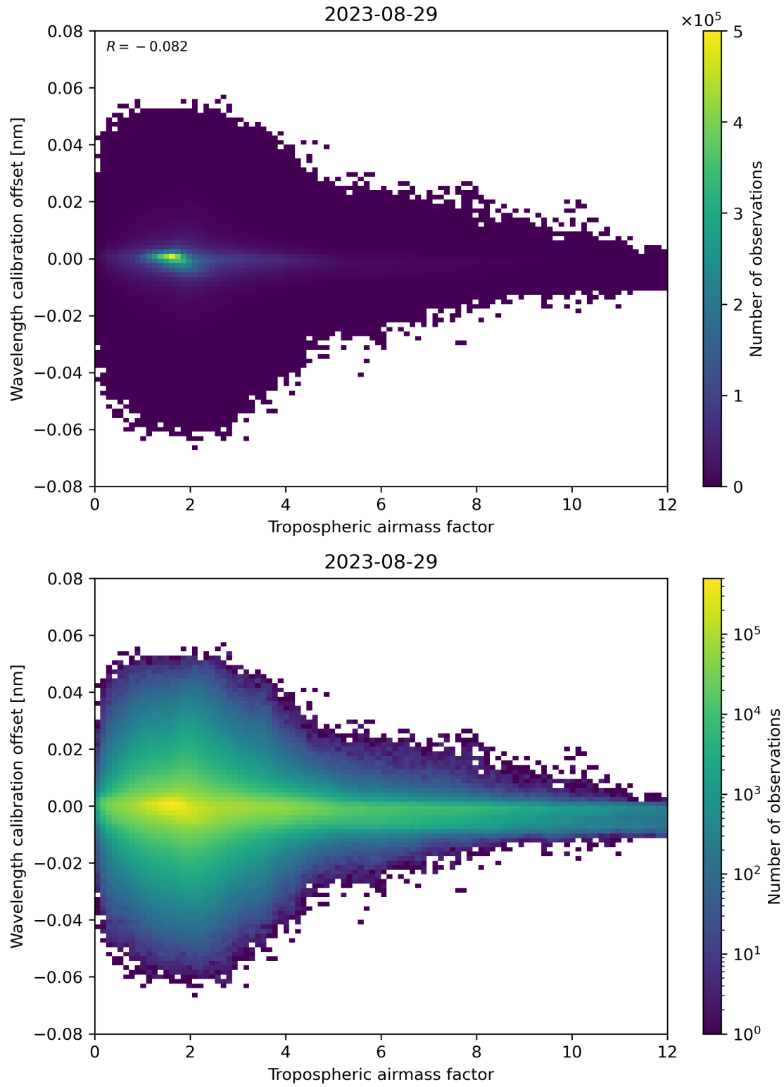
Figure 80: Scatter density plot of “Tropospheric airmass factor” against “Wavelength calibration offset” for 2023-08-28 to 2023-08-30.
