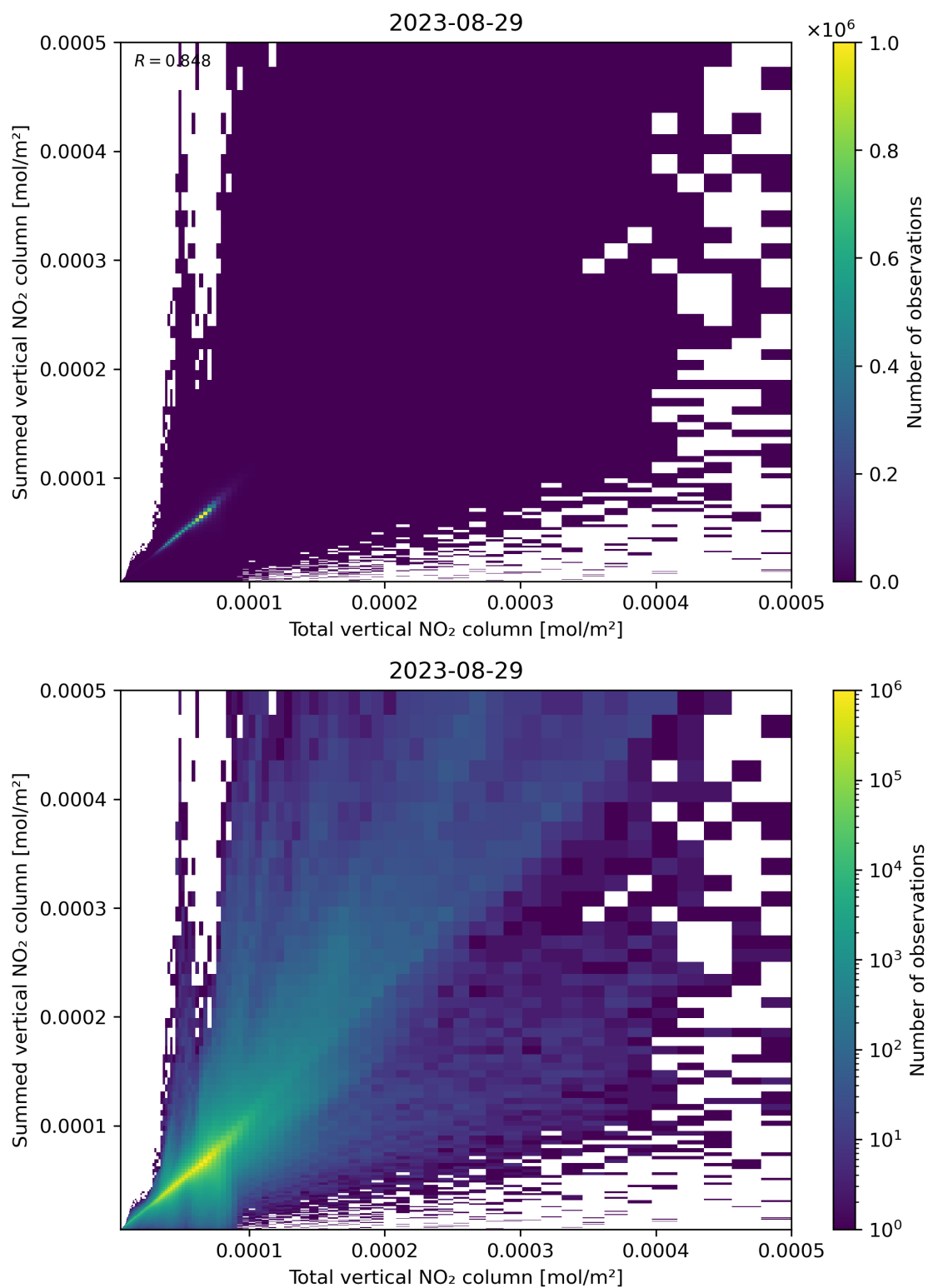
Figure 112: Scatter density plot of “Total vertical NO 2 column” against “Summed vertical NO 2 column” for 2023-08-28 to 2023-08-30.
