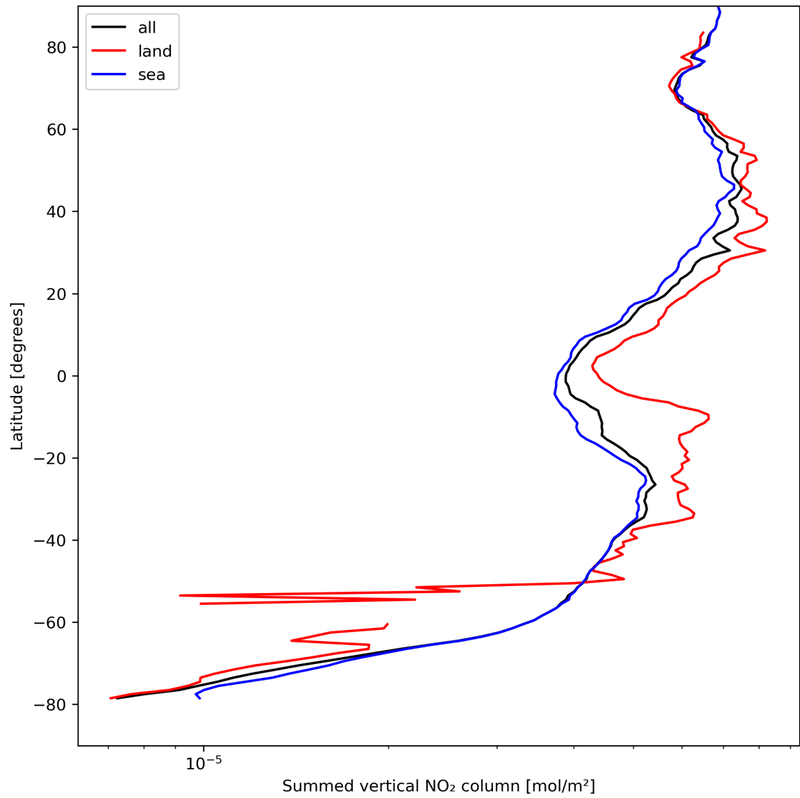
Figure 23: Zonal average of “Summed vertical NO 2 column” for 2023-08-28 to 2023-08-30.
