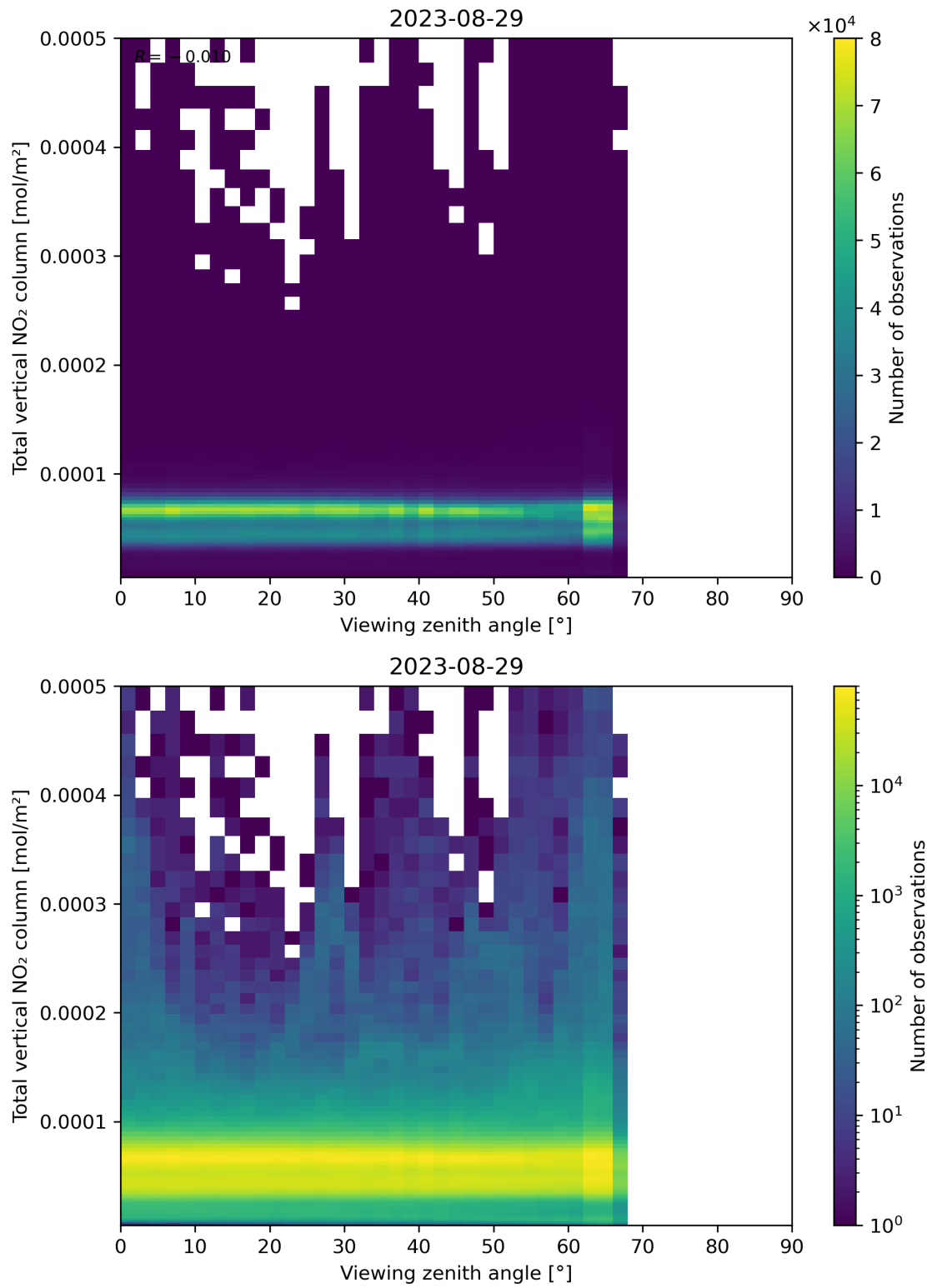
Figure 167: Scatter density plot of “Viewing zenith angle” against “Total vertical NO 2 column” for 2023-08-28 to 2023-08-30.
