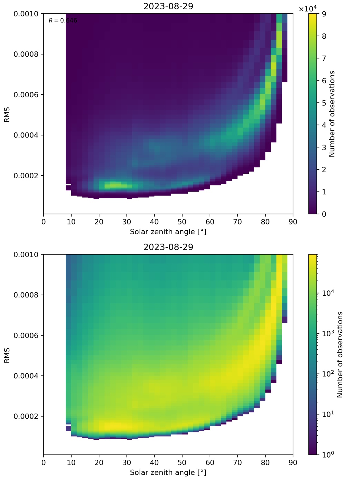
Figure 157: Scatter density plot of “Solar zenith angle” against “RMS” for 2023-08-28 to 2023-08-30.
