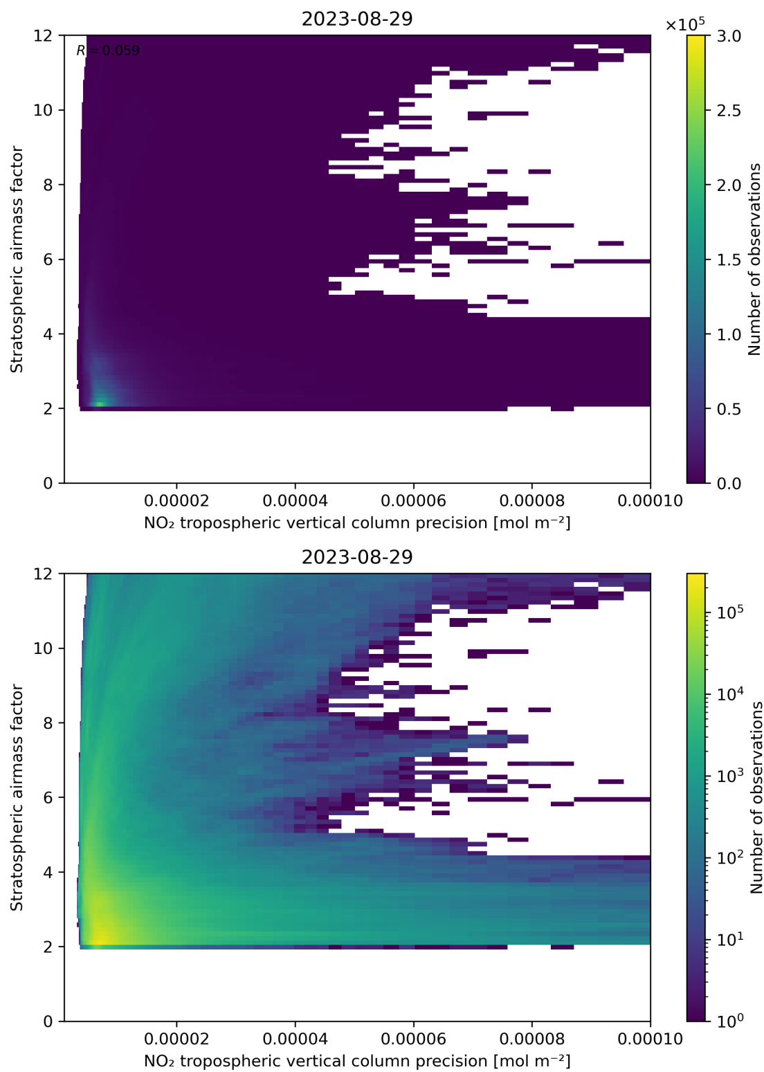
Figure 131: Scatter density plot of “NO 2 tropospheric vertical column precision” against “Stratospheric airmass factor” for 2023-08-28 to 2023-08-30.
