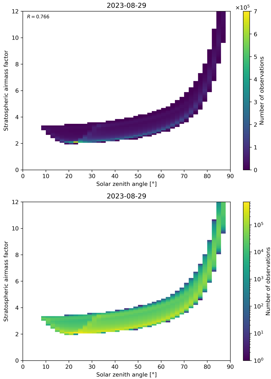
Figure 145: Scatter density plot of “Solar zenith angle” against “Stratospheric airmass factor” for 2023-08-28 to 2023-08-30.
