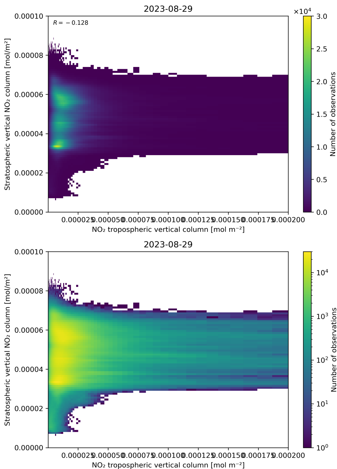
Figure 125: Scatter density plot of “NO 2 tropospheric vertical column” against “Stratospheric vertical NO 2 column” for 2023-08-28 to 2023-08-30.
