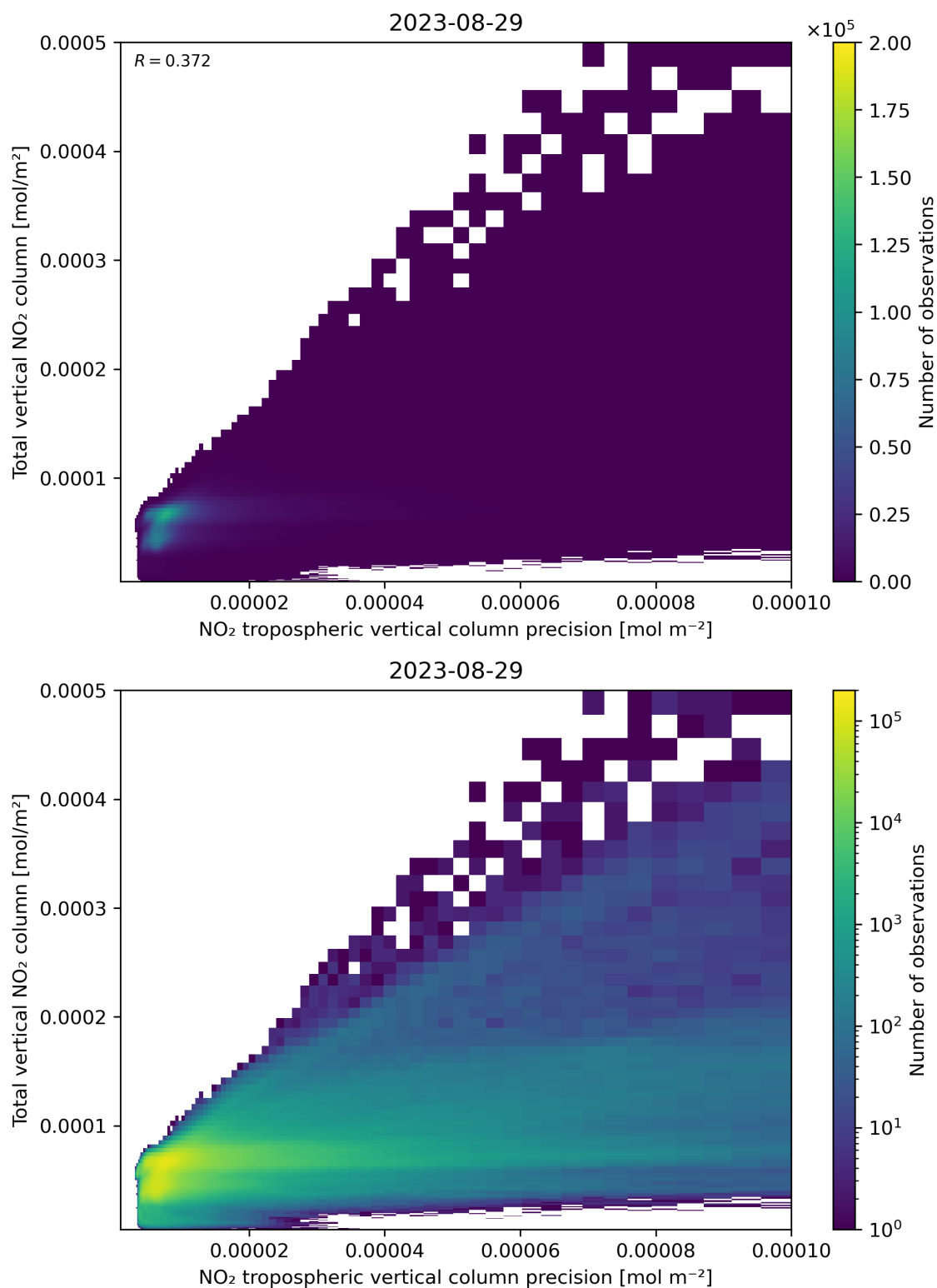
Figure 138: Scatter density plot of “NO 2 tropospheric vertical column precision” against “Total vertical NO 2 column” for 2023-08-28 to 2023-08-30.
