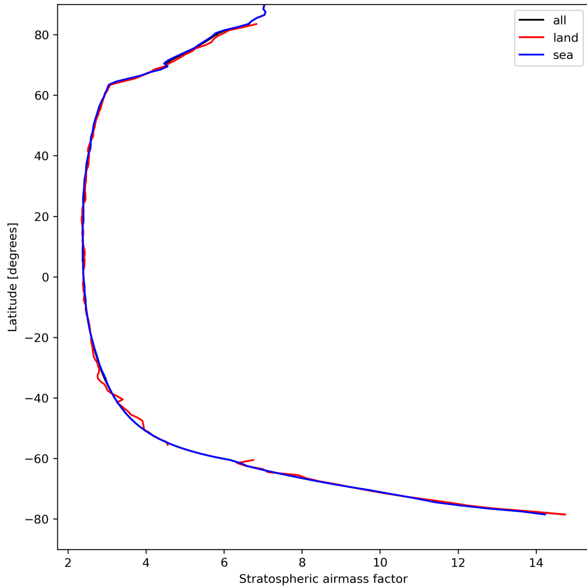
Figure 27: Zonal average of “Stratospheric air mass factor” for 2023-08-28 to 2023-08-30.
