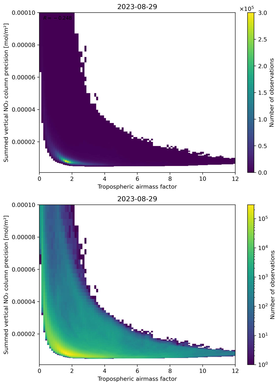
Figure 76: Scatter density plot of “Tropospheric air mass factor” against “Summed vertical NO 2 column precision” for 2023-08-28 to 2023-08-30.
