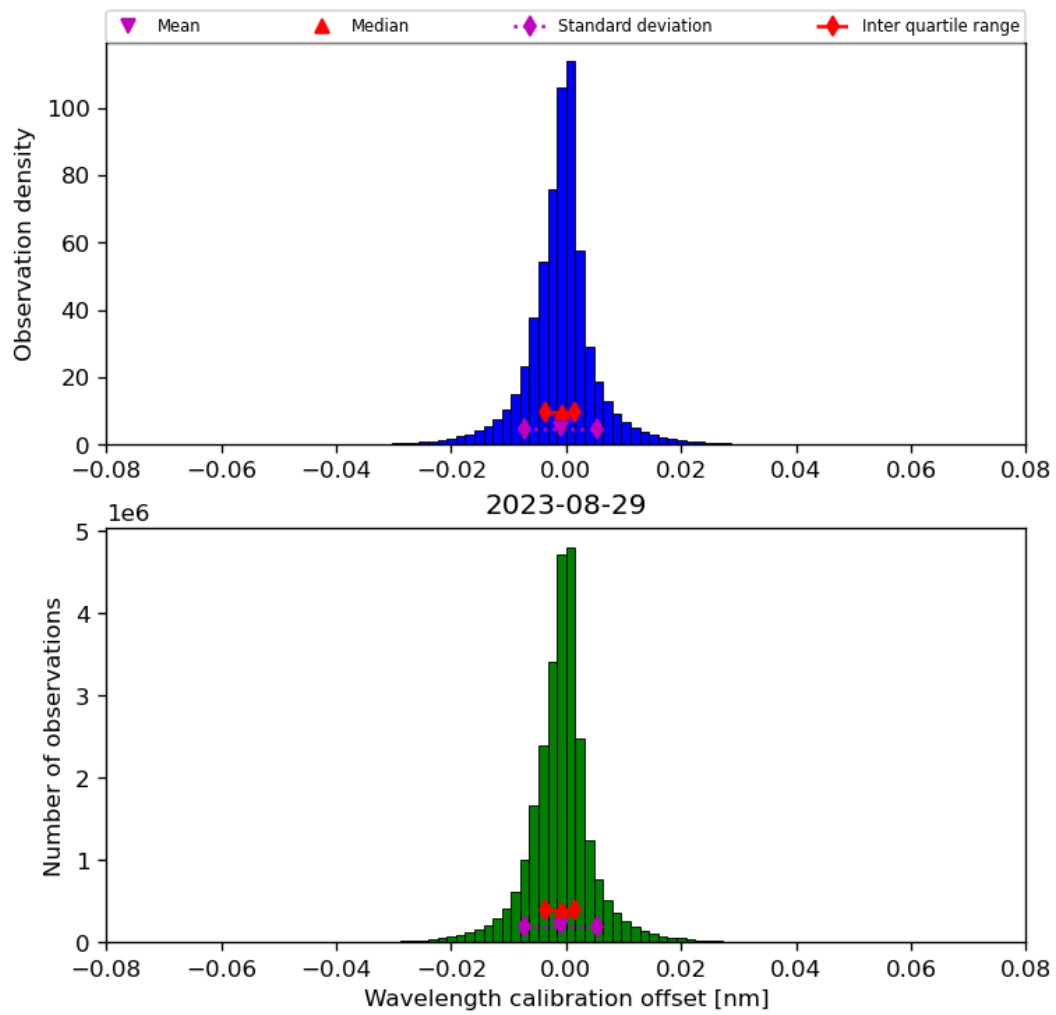
Figure 35: Histogram of “Wavelength calibration offset” for 2023-08-28 to 2023-08-30
