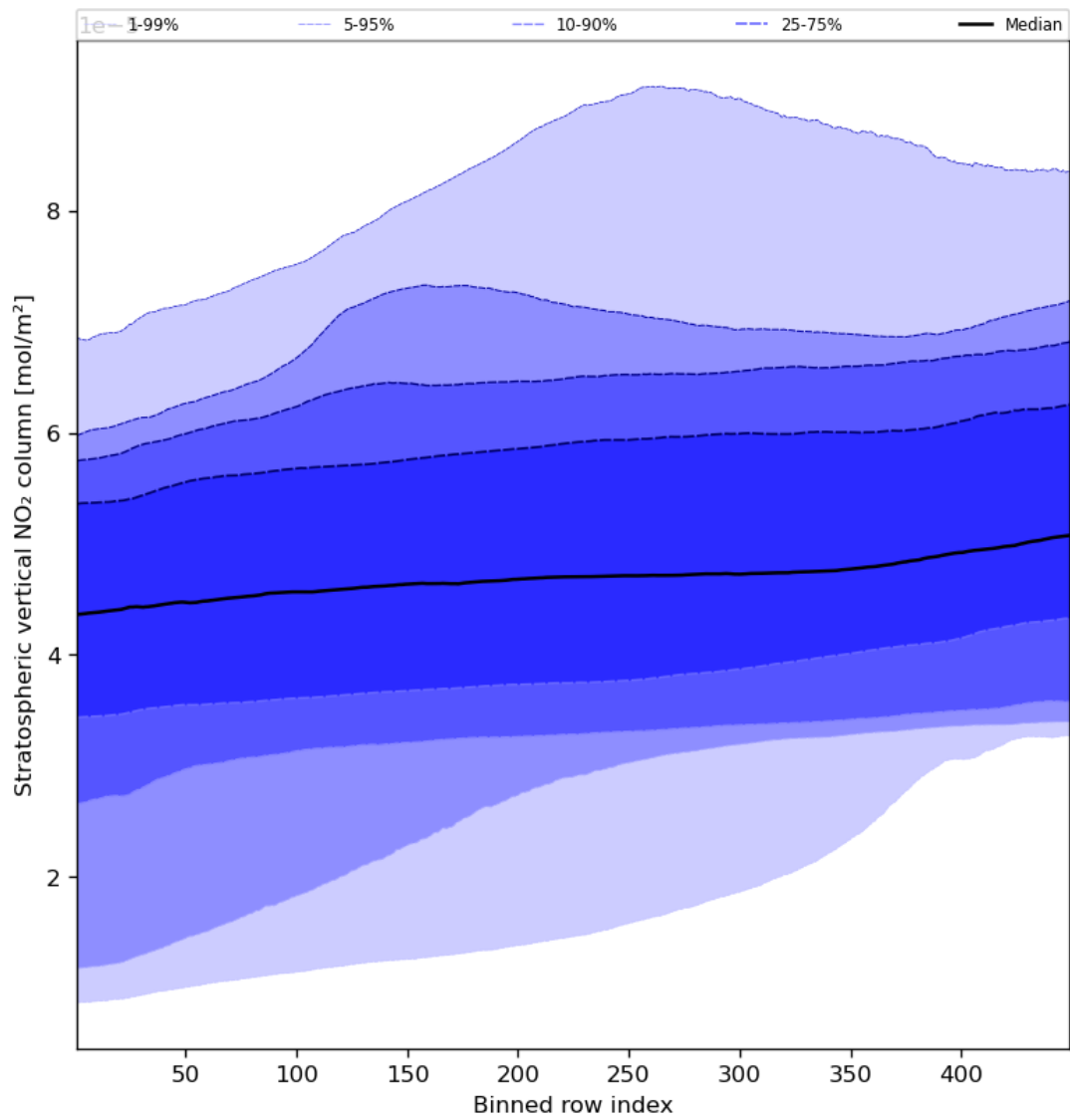
Figure 53: Along track statistics of “Stratospheric vertical NO 2 column” for 2023-08-28 to 2023-08-30
