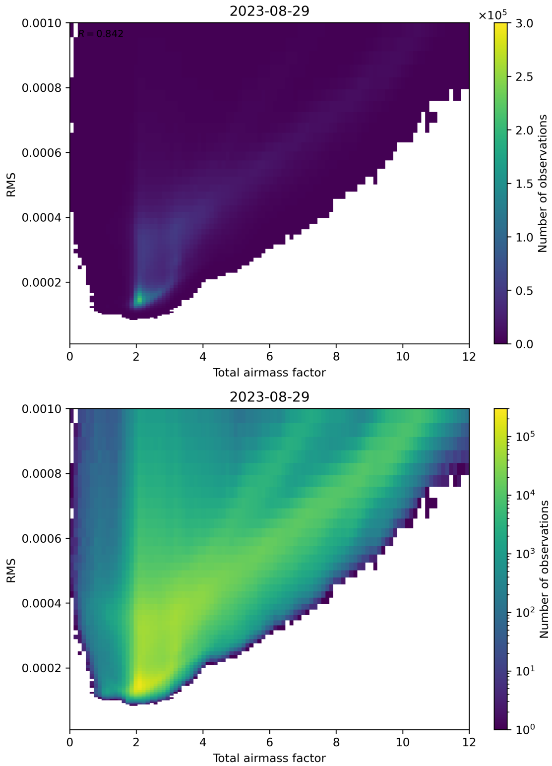
Figure 69: Scatter density plot of “Total airmass factor” against “RMS” for 2023-08-28 to 2023-08-30.
