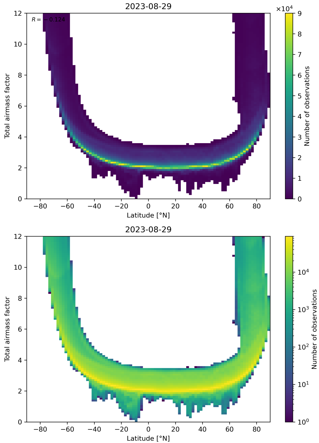
Figure 84: Scatter density plot of “Latitude” against “Total airmass factor” for 2023-08-28 to 2023-08-30.
