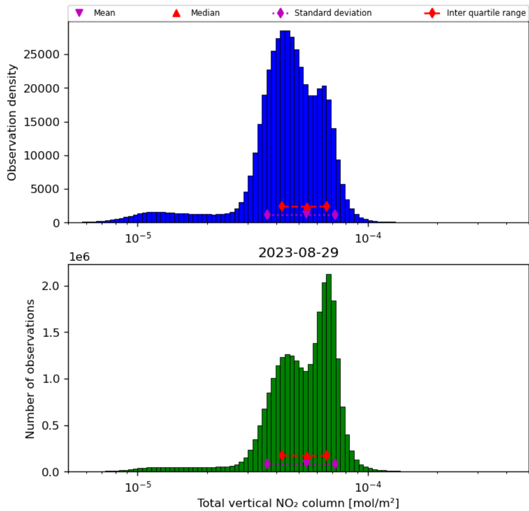
Figure 38: Histogram of “Total vertical NO 2 column” for 2023-08-28 to 2023-08-30
