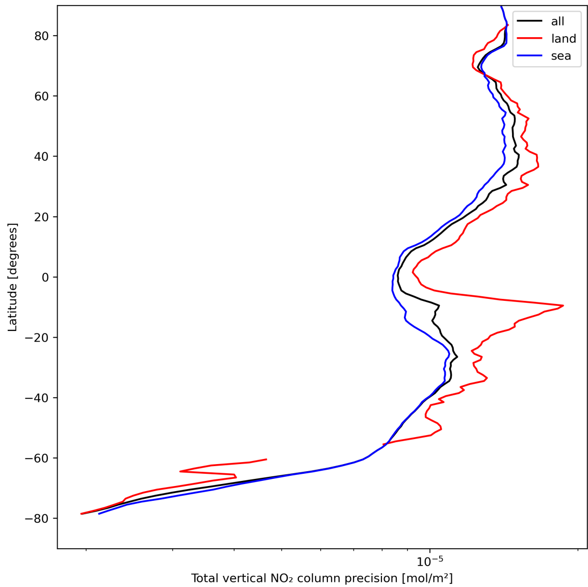
Figure 22: Zonal average of “Total vertical NO 2 column precision” for 2023-08-28 to 2023-08-30.
