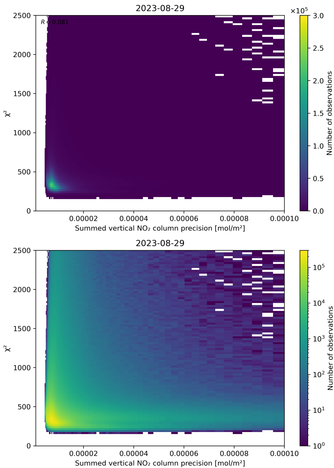
Figure 107: Scatter density plot of “Summed vertical NO 2 column precision” against “ \chi^2 ” for 2023-08-28 to 2023-08-30.
