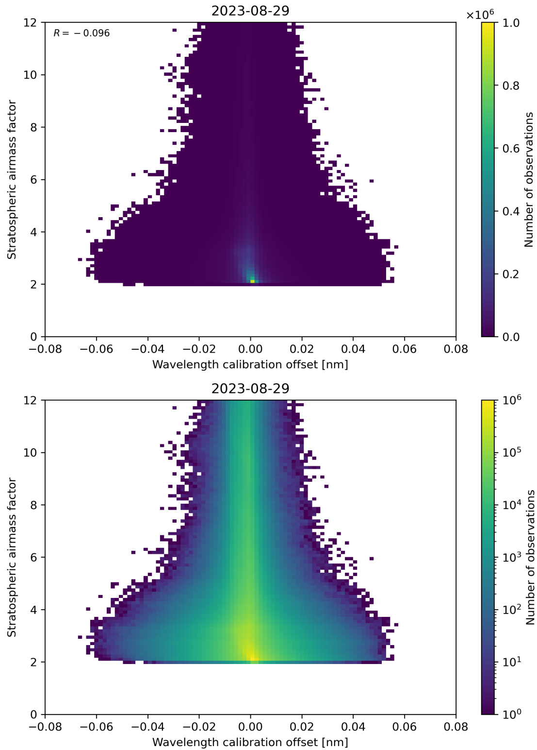
Figure 174: Scatter density plot of “Wavelength calibration offset” against “Stratospheric airmass factor” for 2023-08-28 to 2023-08-30.
