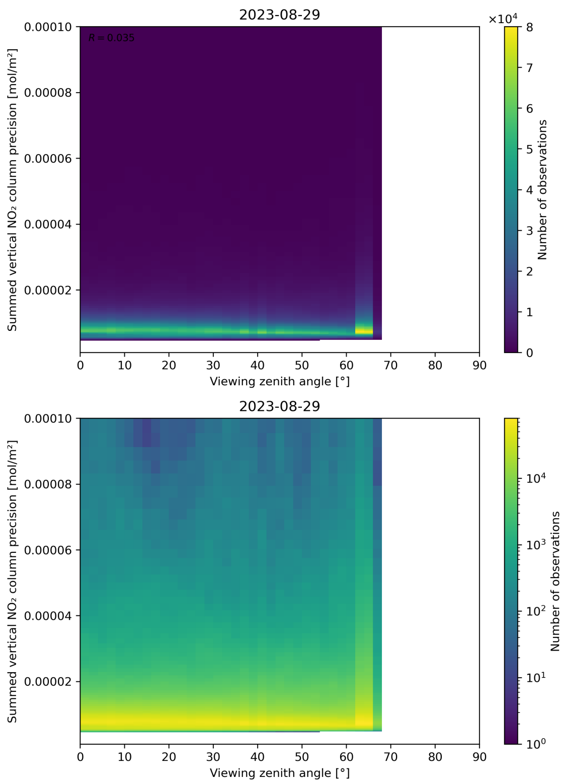
Figure 166: Scatter density plot of “Viewing zenith angle” against “Summed vertical NO 2 column precision” for 2023-08-28 to 2023-08-30.
