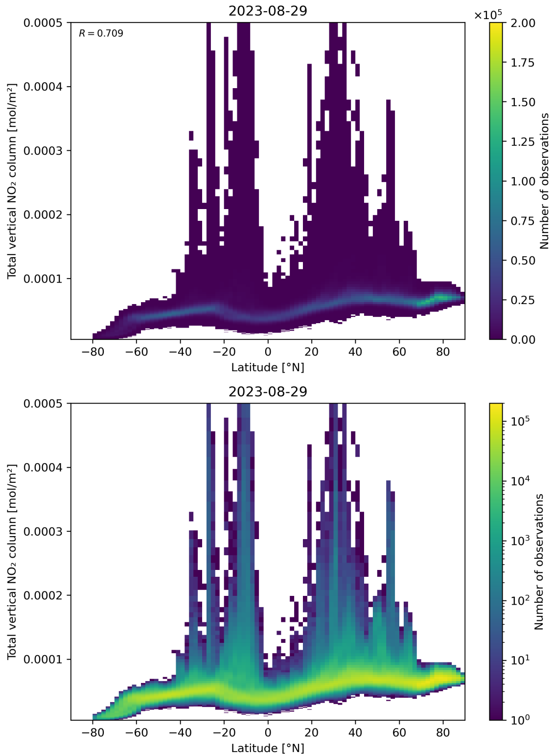
Figure 90: Scatter density plot of “Latitude” against “Total vertical NO 2 column” for 2023-08-28 to 2023-08-30.
