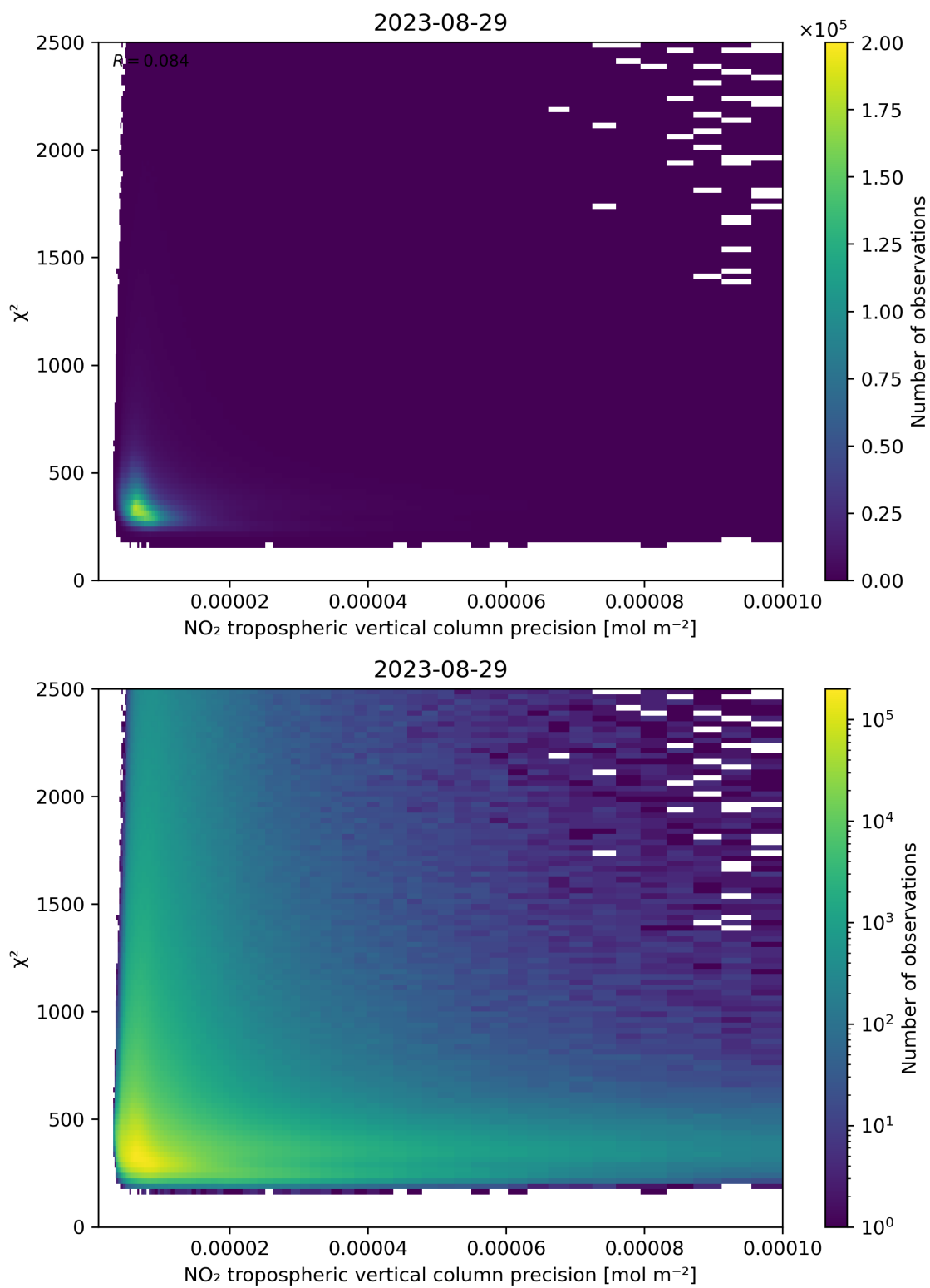
Figure 134: Scatter density plot of “NO 2 tropospheric vertical column precision” against “ \chi^2 ” for 2023-08-28 to 2023-08-30.
