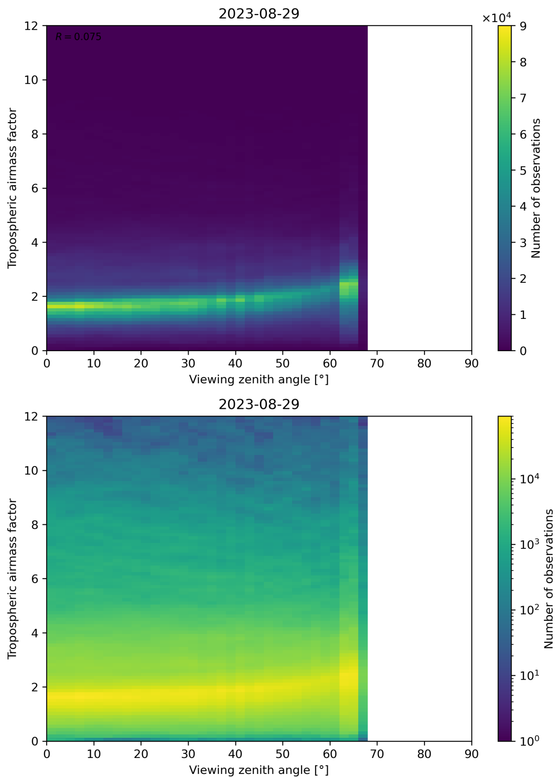
Figure 161: Scatter density plot of “Viewing zenith angle” against “Tropospheric airmass factor” for 2023-08-28 to 2023-08-30.
