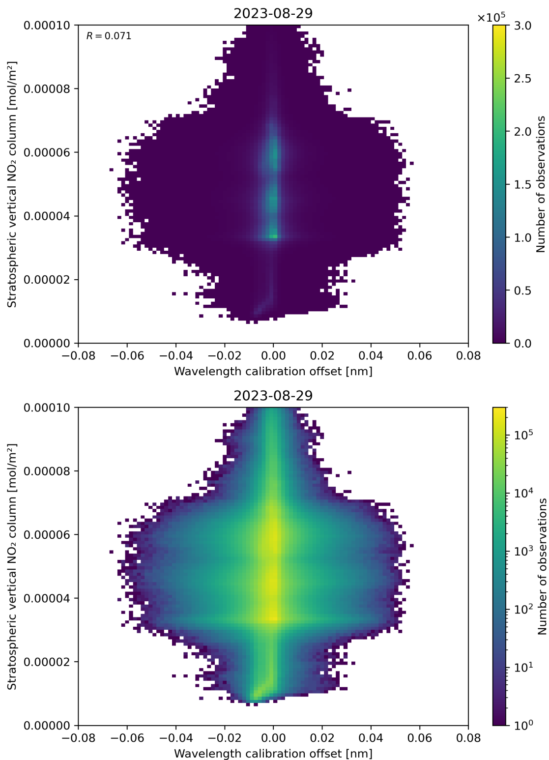
Figure 176: Scatter density plot of “Wavelength calibration offset” against “Stratospheric vertical NO 2 column” for 2023-08-28 to 2023-08-30.
