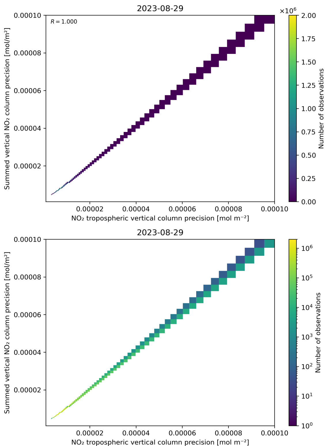
Figure 137: Scatter density plot of “NO 2 tropospheric vertical column precision” against “Summed vertical NO 2 column precision” for 2023-08-28 to 2023-08-30.
