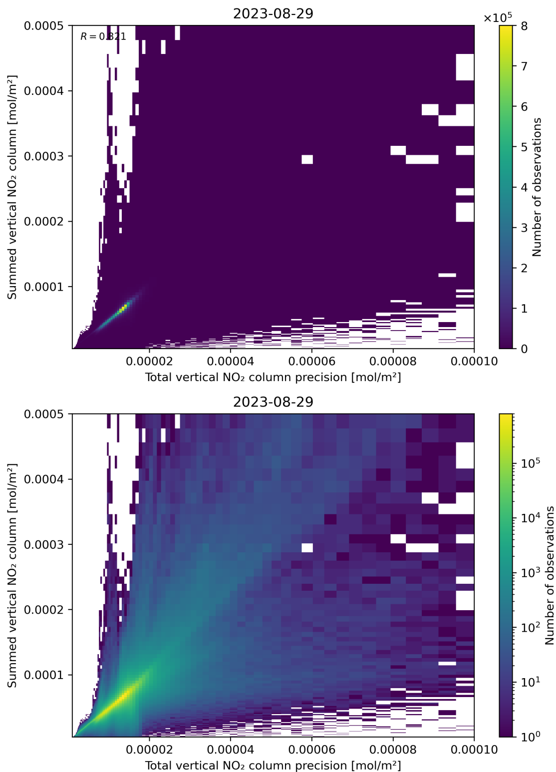
Figure 117: Scatter density plot of “Total vertical NO 2 column precision” against “Summed vertical NO 2 column” for 2023-08-28 to 2023-08-30.
