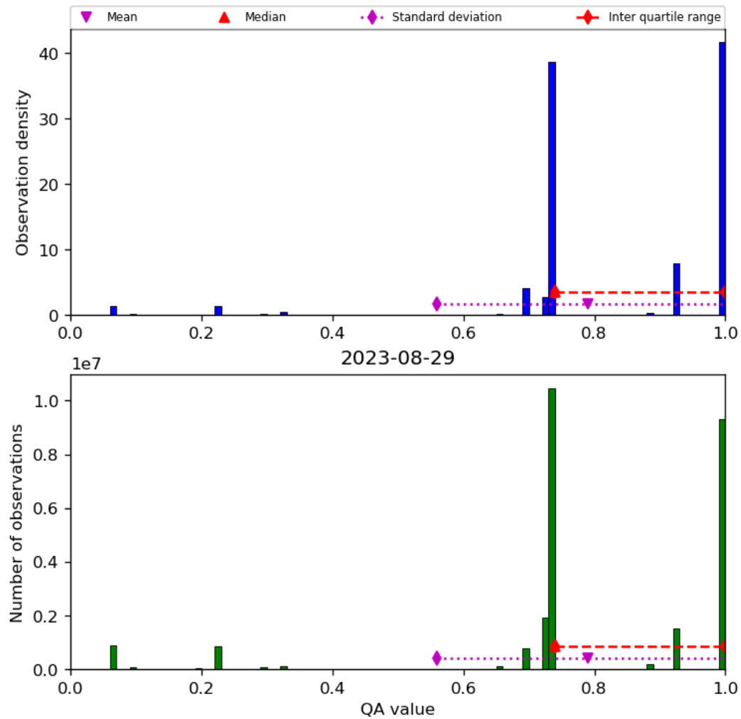
Figure 28: Histogram of “QA value” for 2023-08-28 to 2023-08-30
