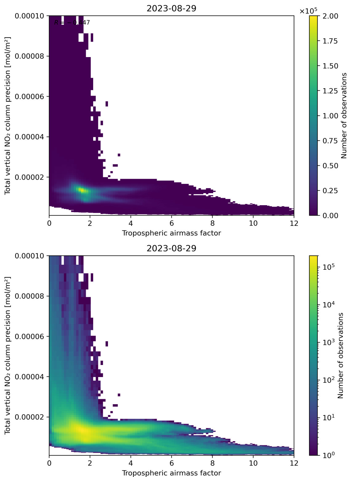
Figure 78: Scatter density plot of “Tropospheric air mass factor” against “Total vertical NO 2 column precision” for 2023-08-28 to 2023-08-30.
