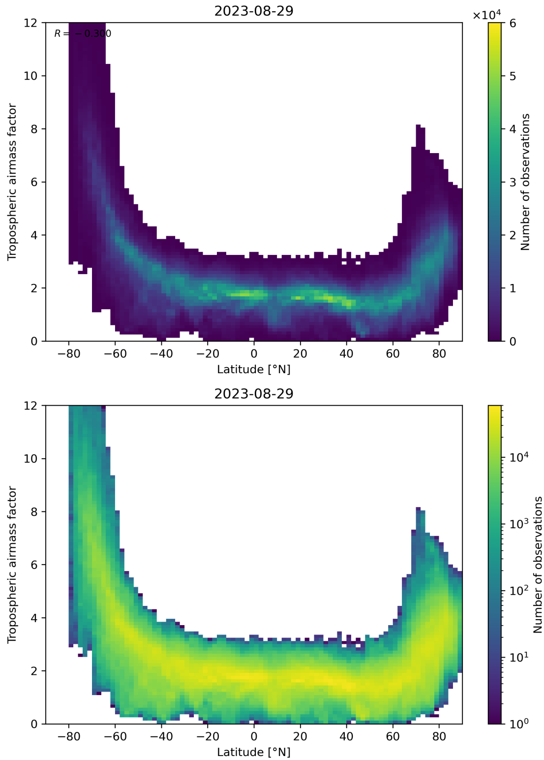
Figure 85: Scatter density plot of “Latitude” against “Tropospheric airmass factor” for 2023-08-28 to 2023-08-30.
