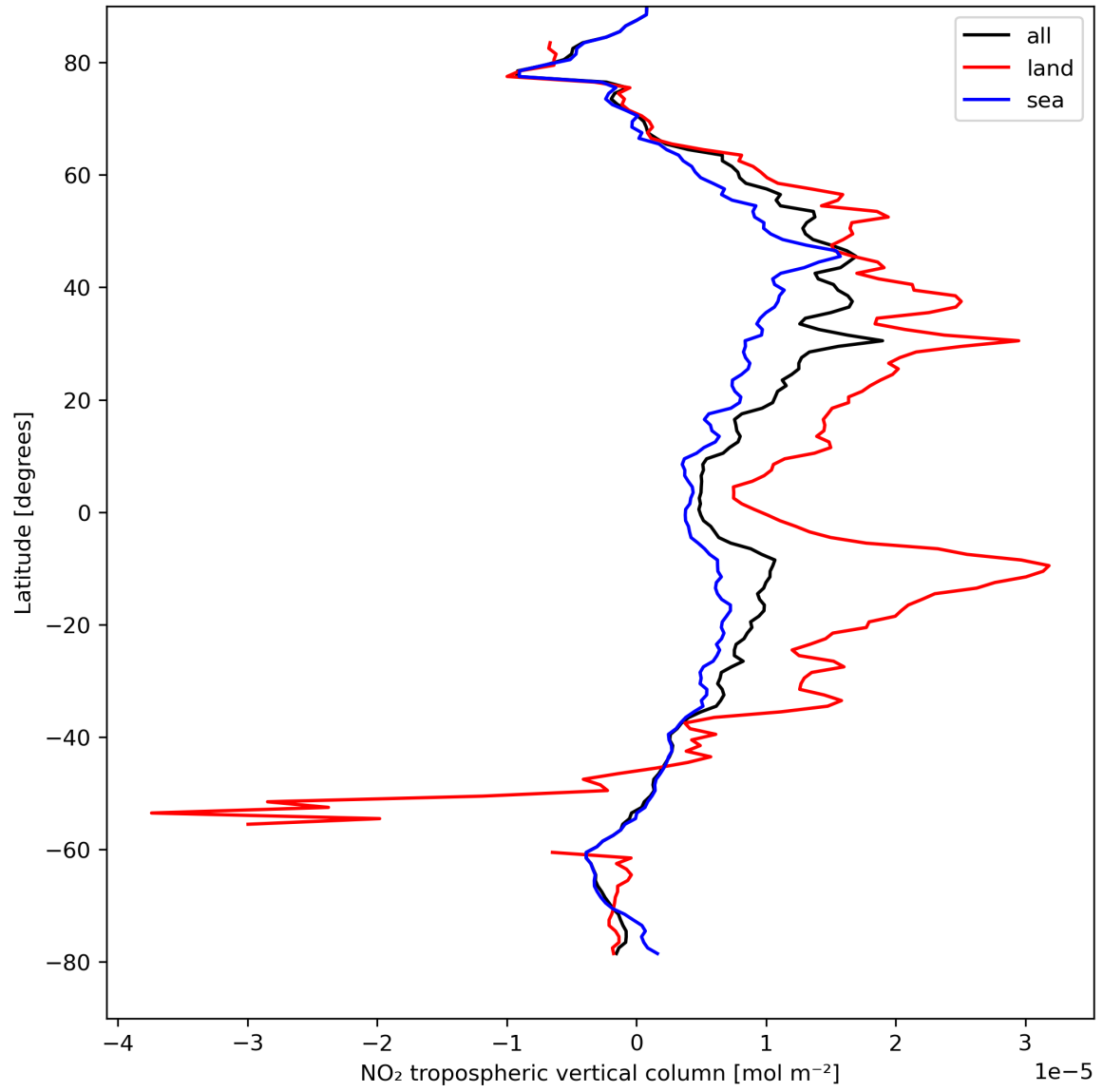
Figure 12: Zonal average of “NO 2 tropospheric vertical column” for 2023-08-28 to 2023-08-30.
