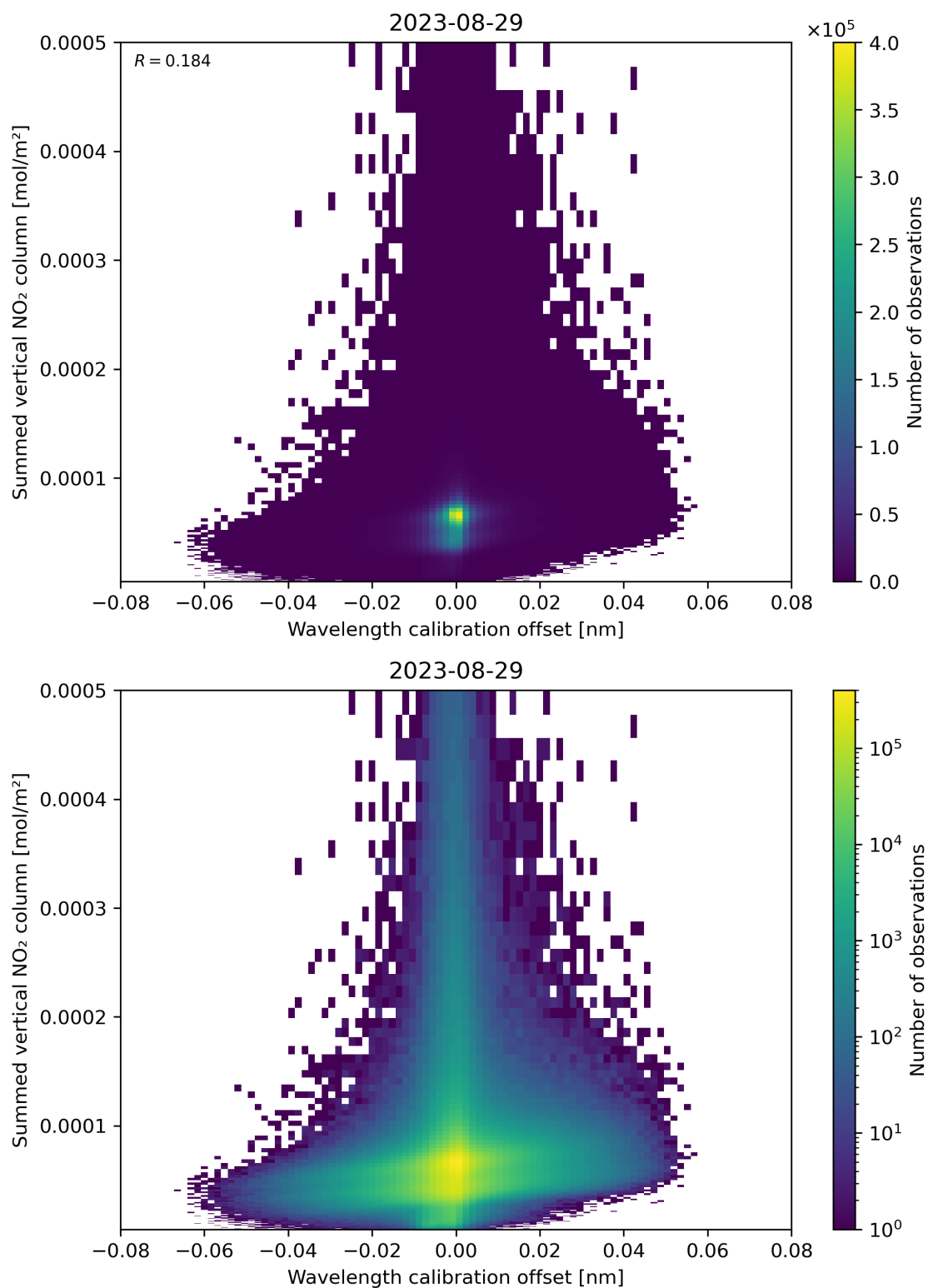
Figure 177: Scatter density plot of “Wavelength calibration offset” against “Summed vertical NO 2 column” for 2023-08-28 to 2023-08-30.
