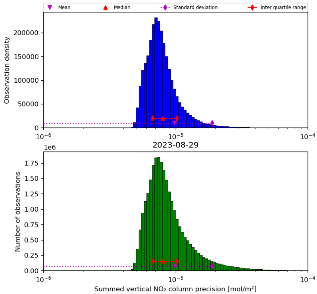
Figure 41: Histogram of “Summed vertical NO 2 column precision” for 2023-08-28 to 2023-08-30
