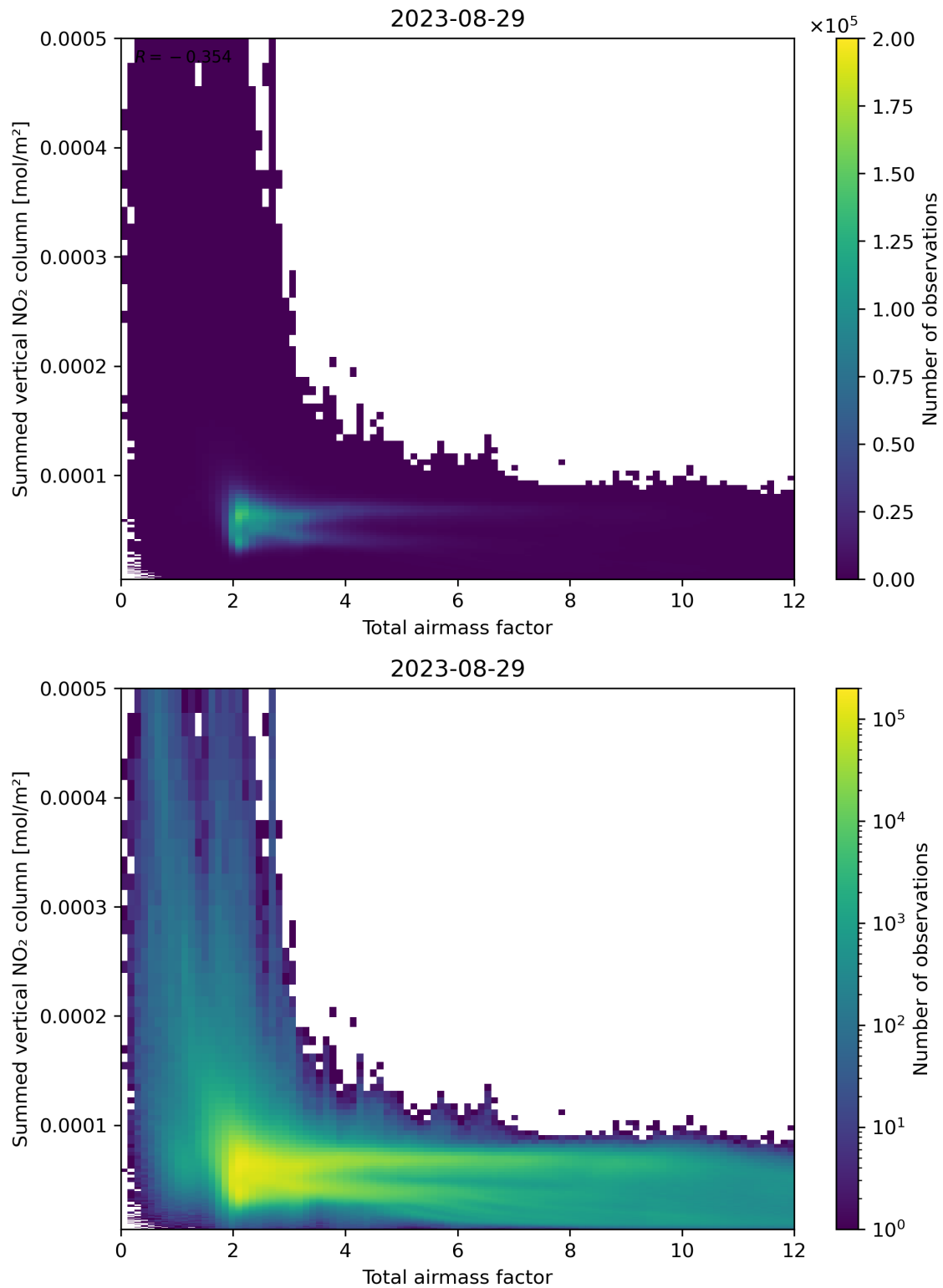
Figure 65: Scatter density plot of “Total air mass factor” against “Summed vertical NO 2 column” for 2023-08-28 to 2023-08-30.
