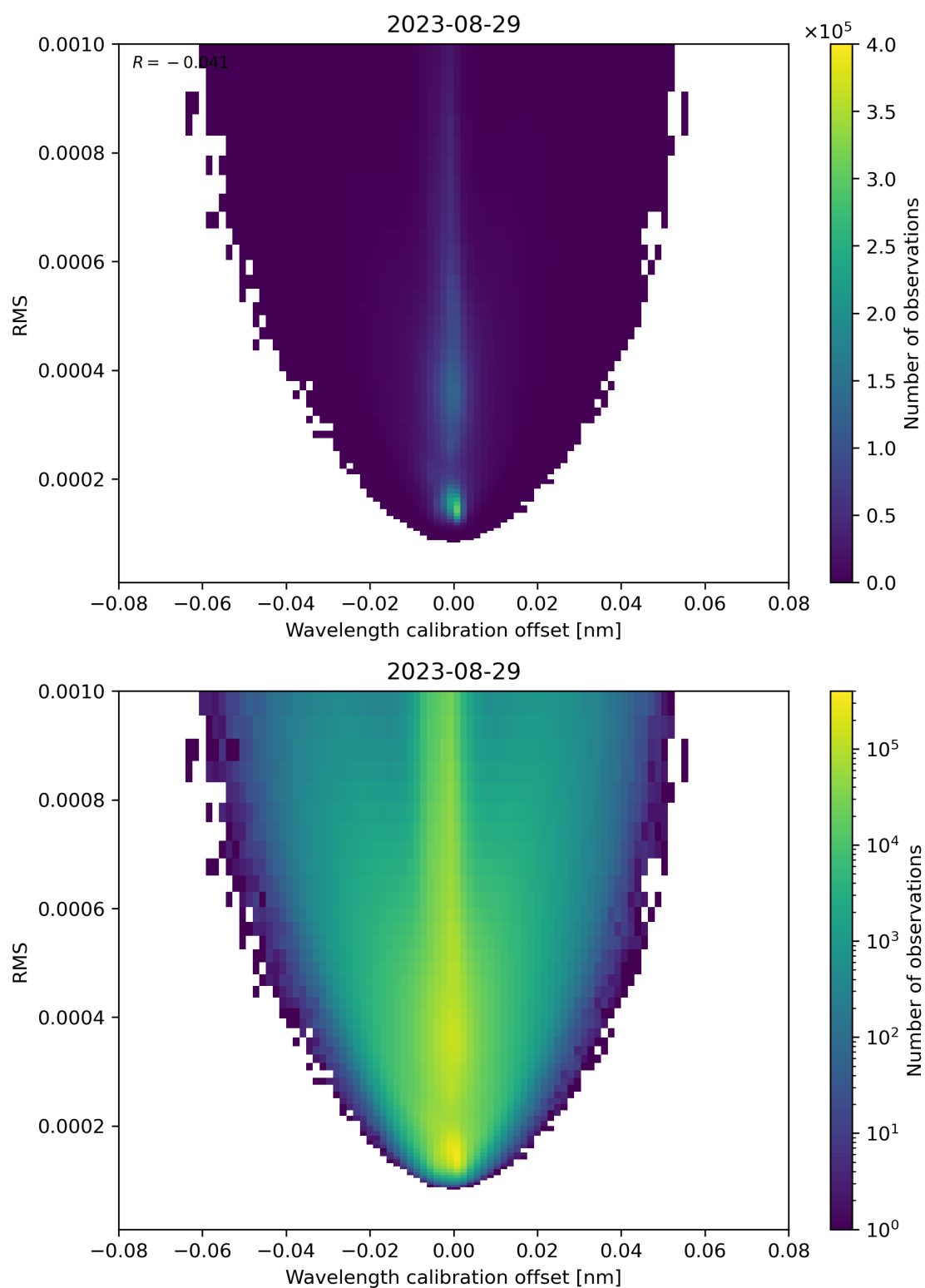
Figure 181: Scatter density plot of “Wavelength calibration offset” against “RMS” for 2023-08-28 to 2023-08-30.
