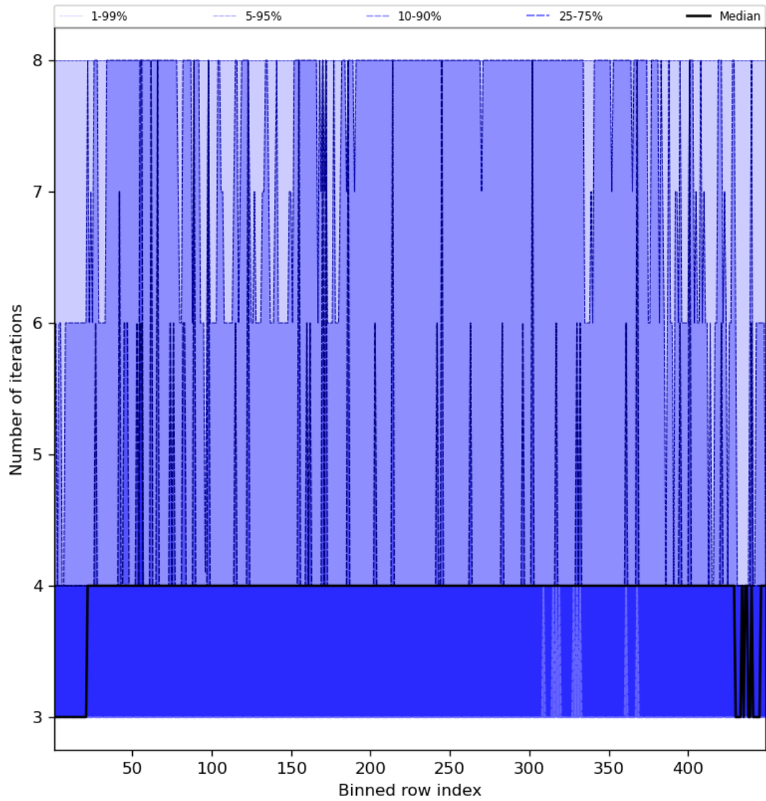
Figure 51: Along track statistics of “Number of iterations” for 2023-08-28 to 2023-08-30
