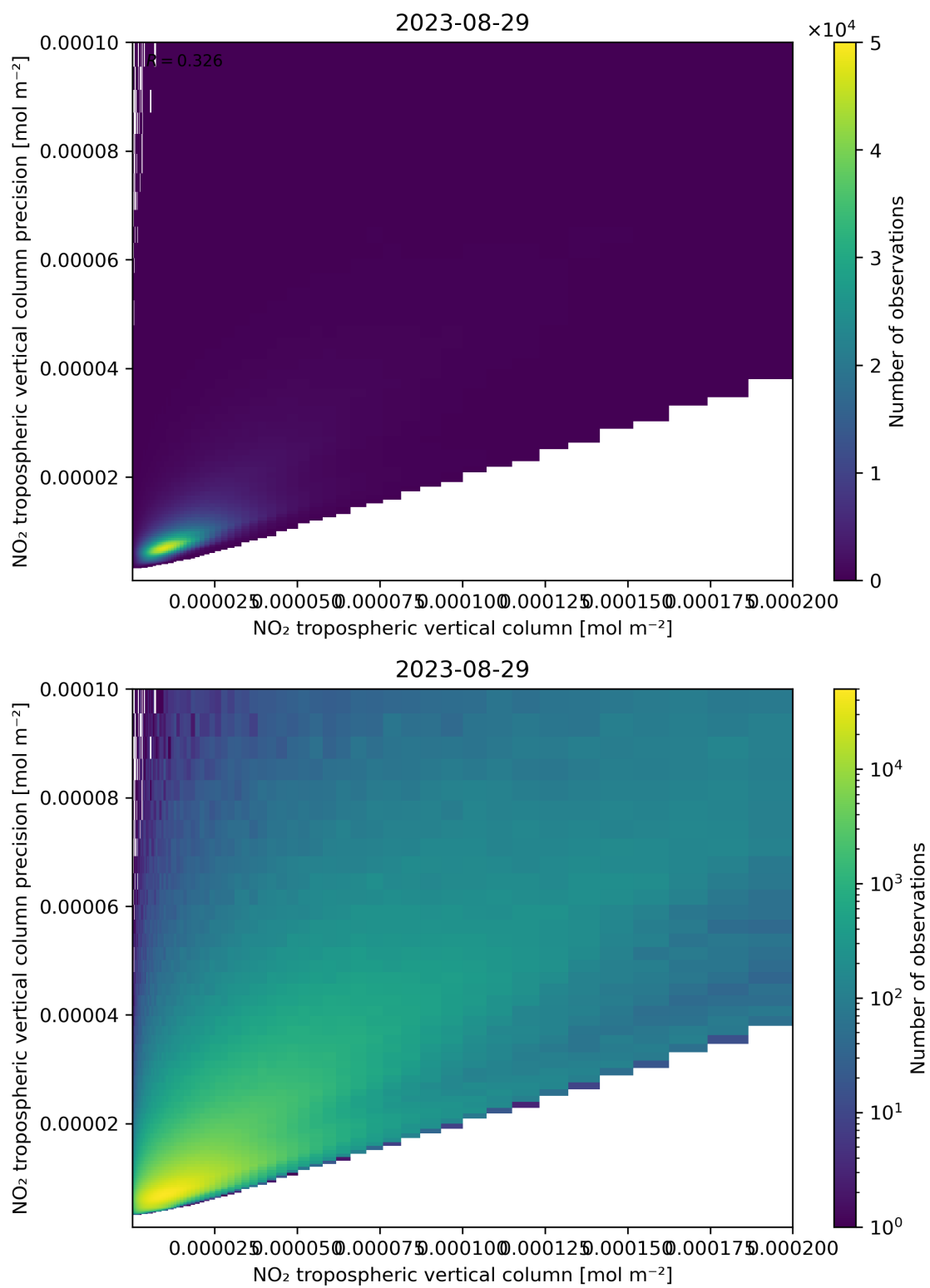
Figure 130: Scatter density plot of “NO 2 tropospheric vertical column” against “NO 2 tropospheric vertical column precision” for 2023-08-28 to 2023-08-30.
