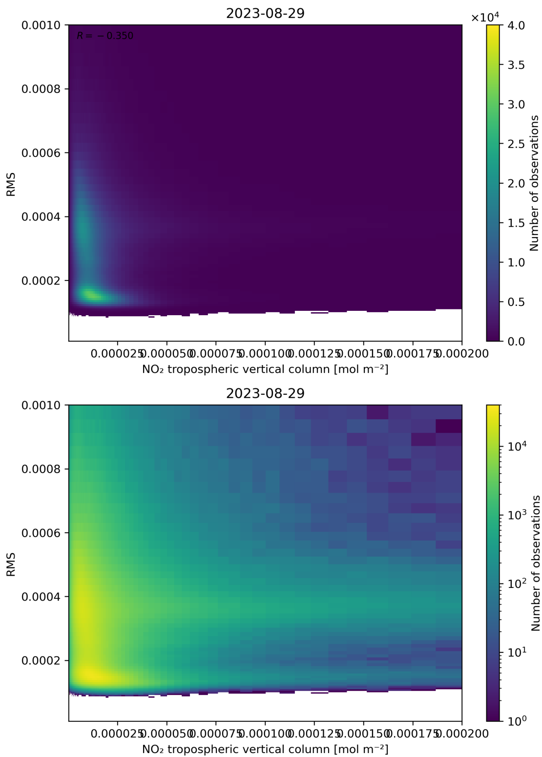
Figure 142: Scatter density plot of “NO 2 tropospheric vertical column” against “RMS” for 2023-08-28 to 2023-08-30.
