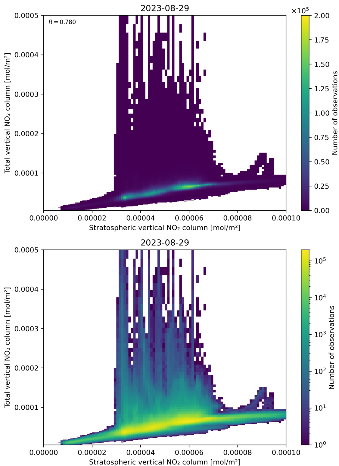
Figure 100: Scatter density plot of “Stratospheric vertical NO 2 column” against “Total vertical NO 2 column” for 2023-08-28 to 2023-08-30.
