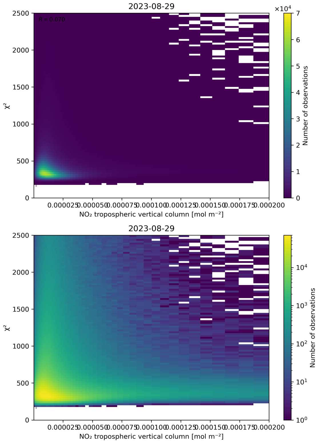
Figure 124: Scatter density plot of “NO 2 tropospheric vertical column” against “ \chi^2 ” for 2023-08-28 to 2023-08-30.
