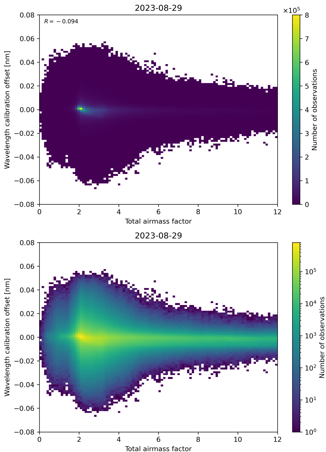
Figure 70: Scatter density plot of “Total airmass factor” against “Wavelength calibration offset” for 2023-08-28 to 2023-08-30.
