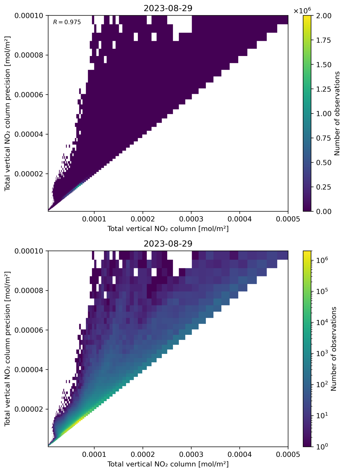
Figure 114: Scatter density plot of “Total vertical NO 2 column” against “Total vertical NO 2 column precision” for 2023-08-28 to 2023-08-30.
