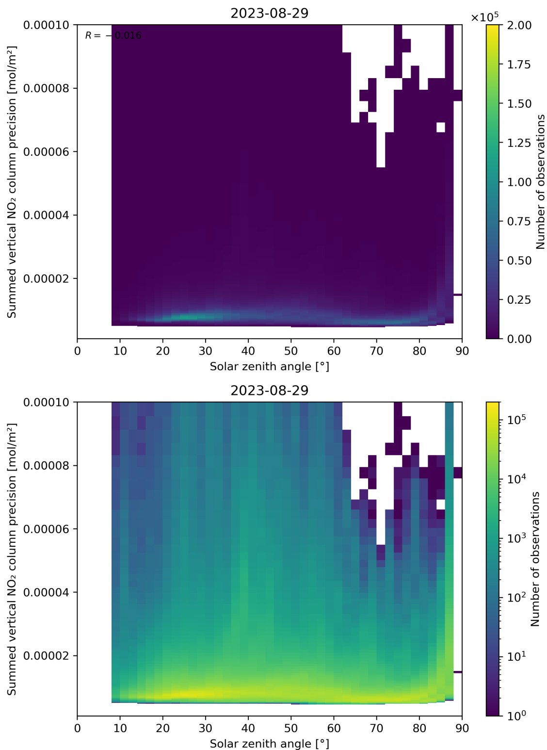
Figure 152: Scatter density plot of “Solar zenith angle” against “Summed vertical NO 2 column precision” for 2023-08-28 to 2023-08-30.
