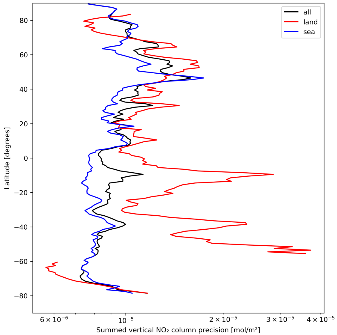
Figure 24: Zonal average of “Summed vertical NO 2 column precision” for 2023-08-28 to 2023-08-30.
