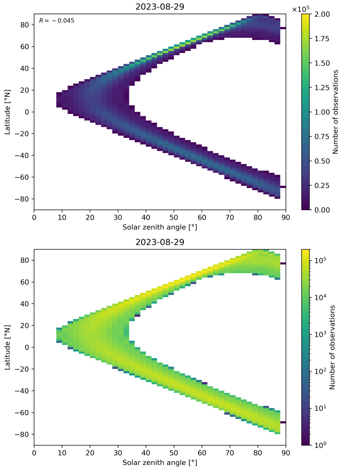
Figure 149: Scatter density plot of “Solar zenith angle” against “Latitude” for 2023-08-28 to 2023-08-30.
