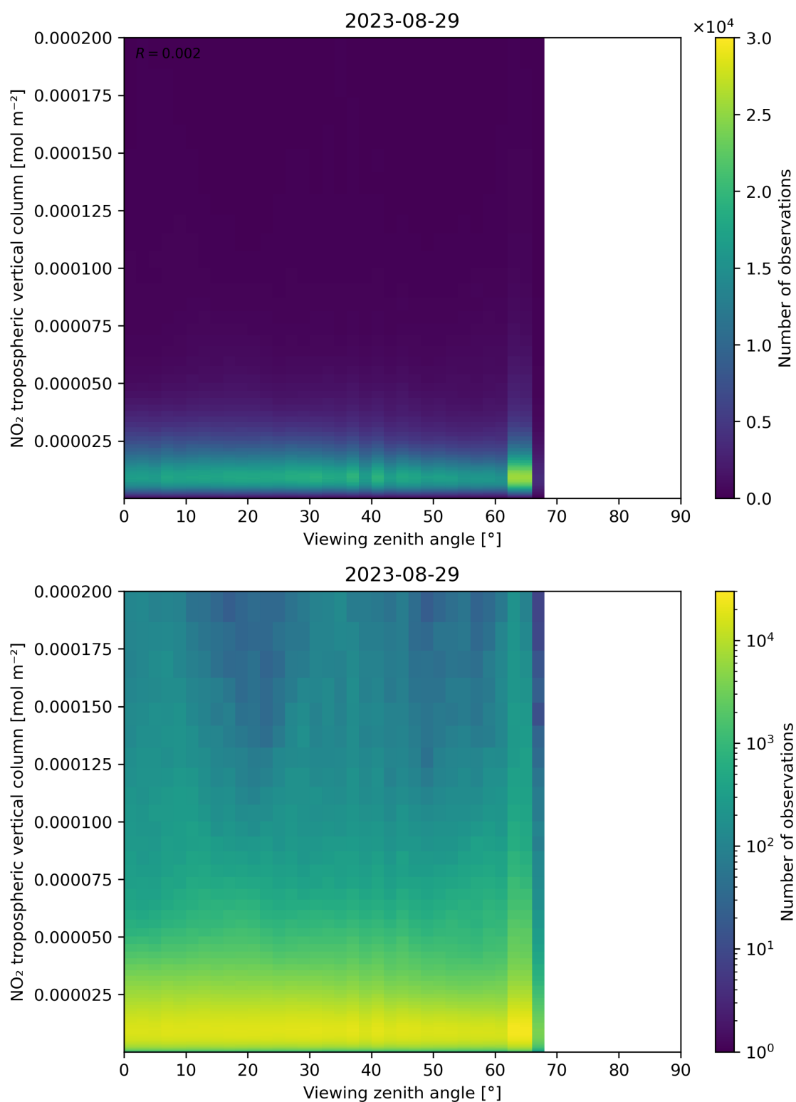
Figure 169: Scatter density plot of “Viewing zenith angle” against “NO 2 tropospheric vertical column” for 2023-08-28 to 2023-08-30.
