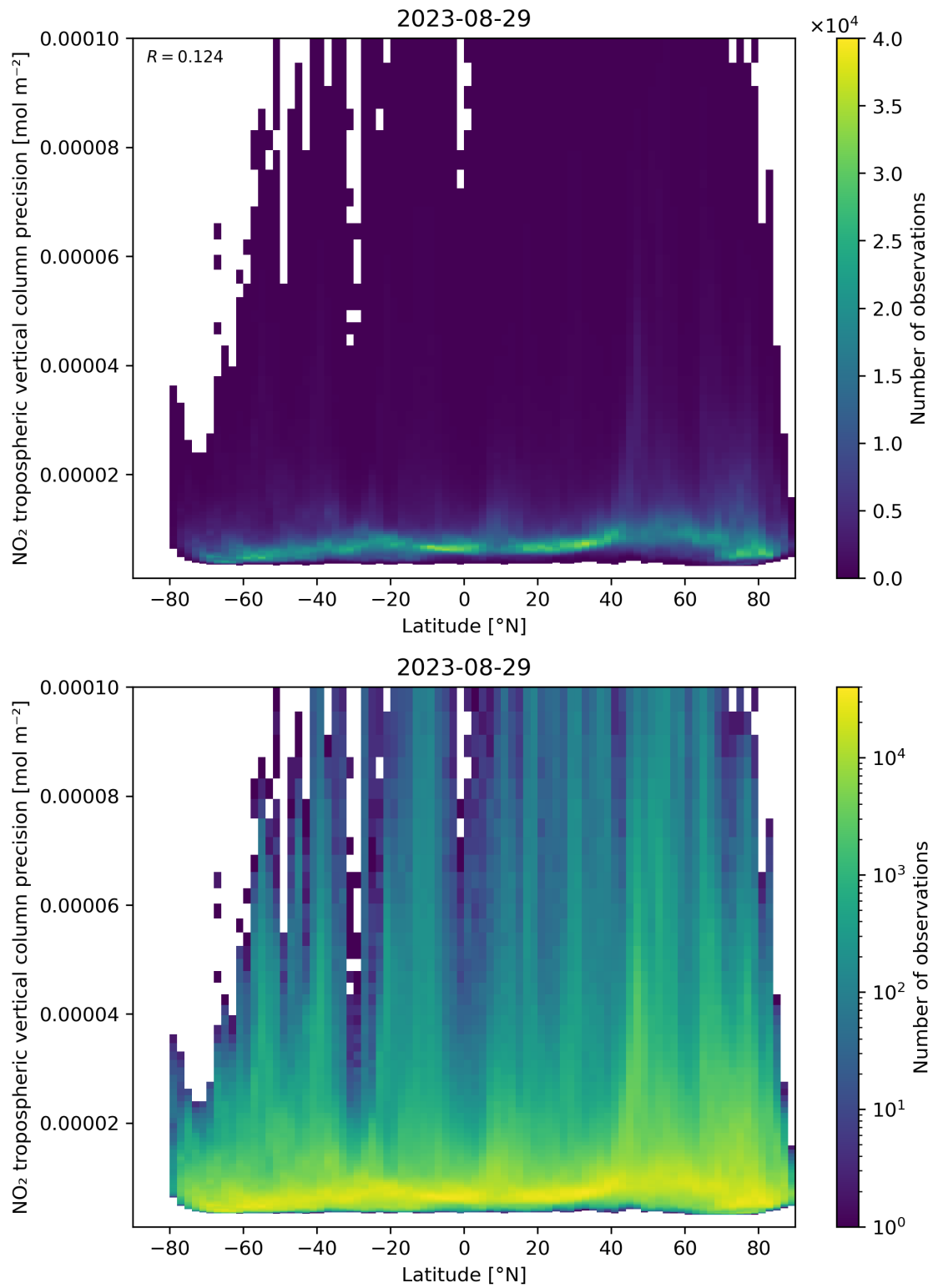
Figure 93: Scatter density plot of “Latitude” against “NO 2 tropospheric vertical column precision” for 2023-08-28 to 2023-08-30.
