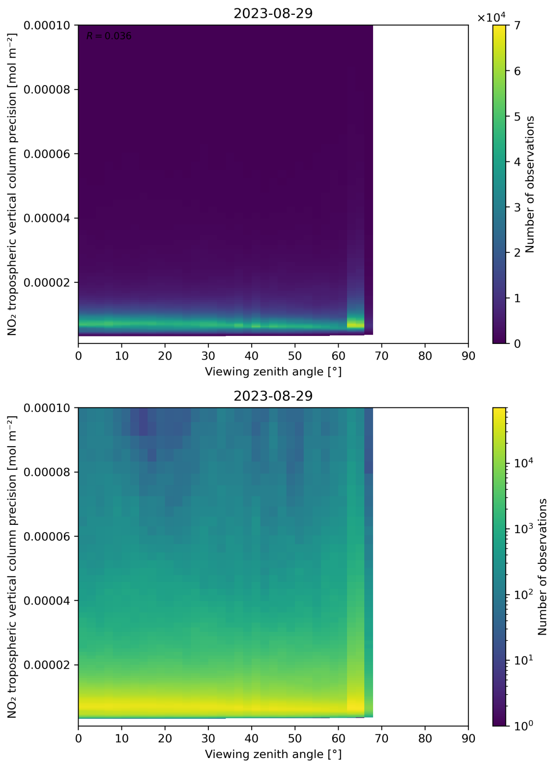
Figure 170: Scatter density plot of “Viewing zenith angle” against “NO 2 tropospheric vertical column precision” for 2023-08-28 to 2023-08-30.
