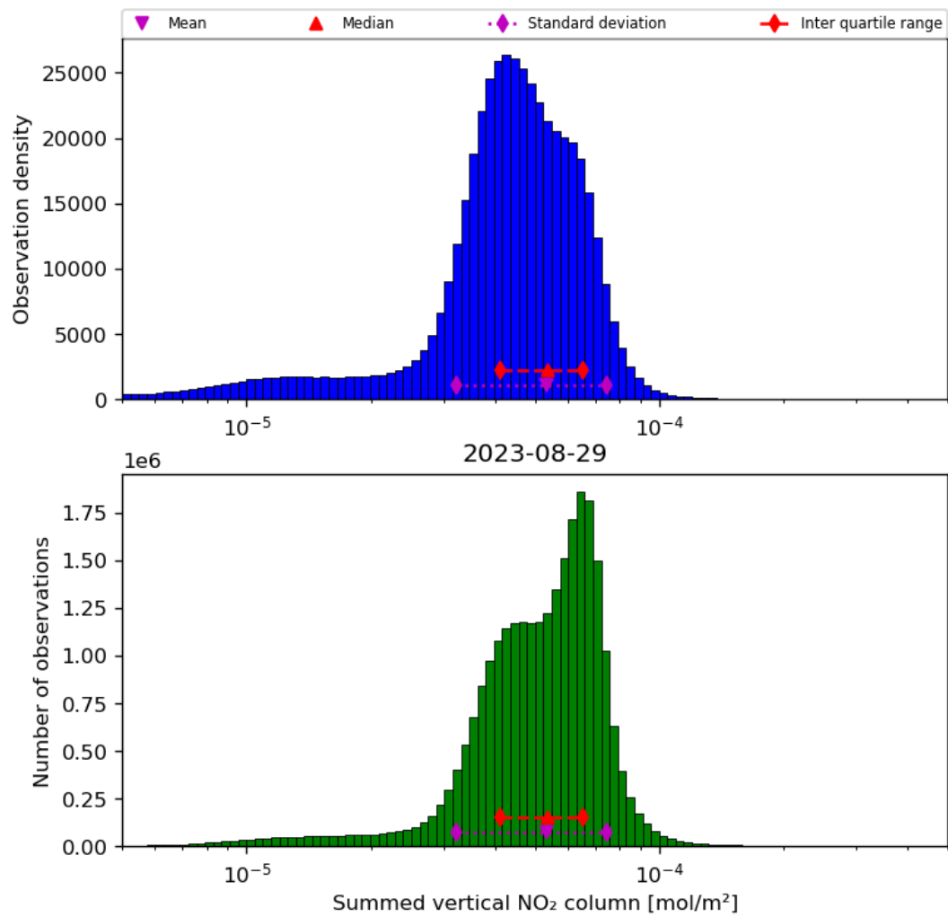
Figure 40: Histogram of “Summed vertical NO 2 column” for 2023-08-28 to 2023-08-30
