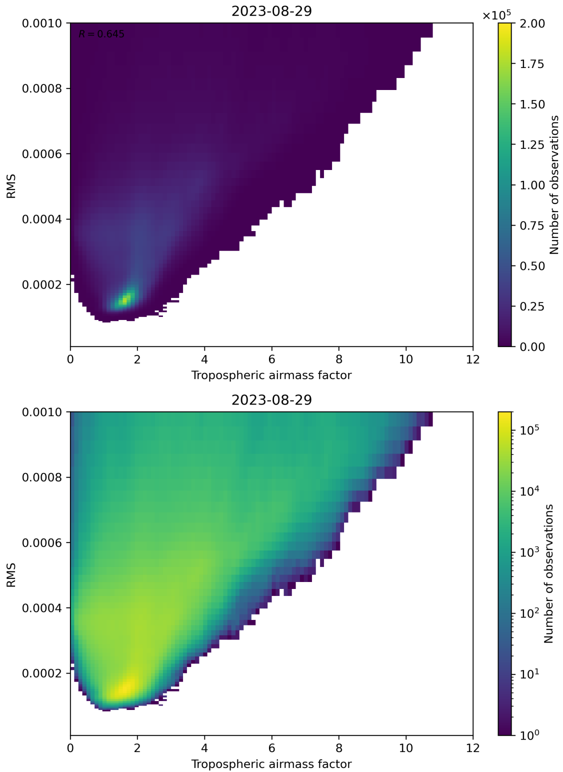
Figure 79: Scatter density plot of “Tropospheric airmass factor” against “RMS” for 2023-08-28 to 2023-08-30.
