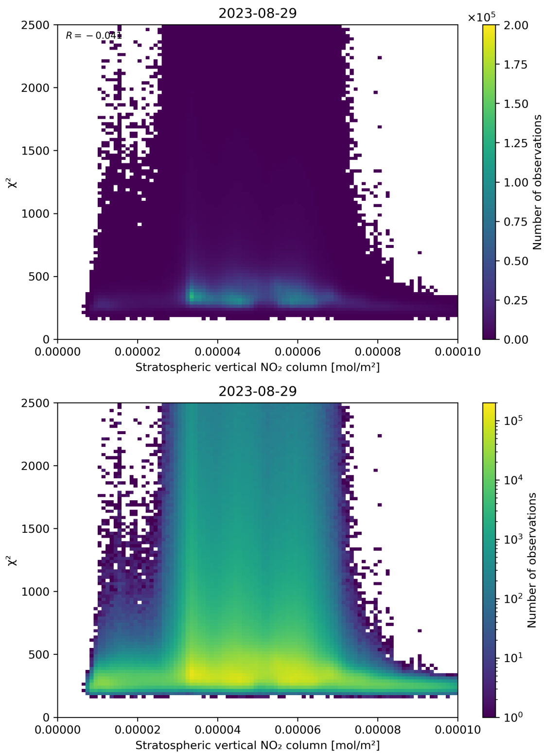
Figure 97: Scatter density plot of “Stratospheric vertical NO 2 column” against “ \chi^2 ” for 2023-08-28 to 2023-08-30.
