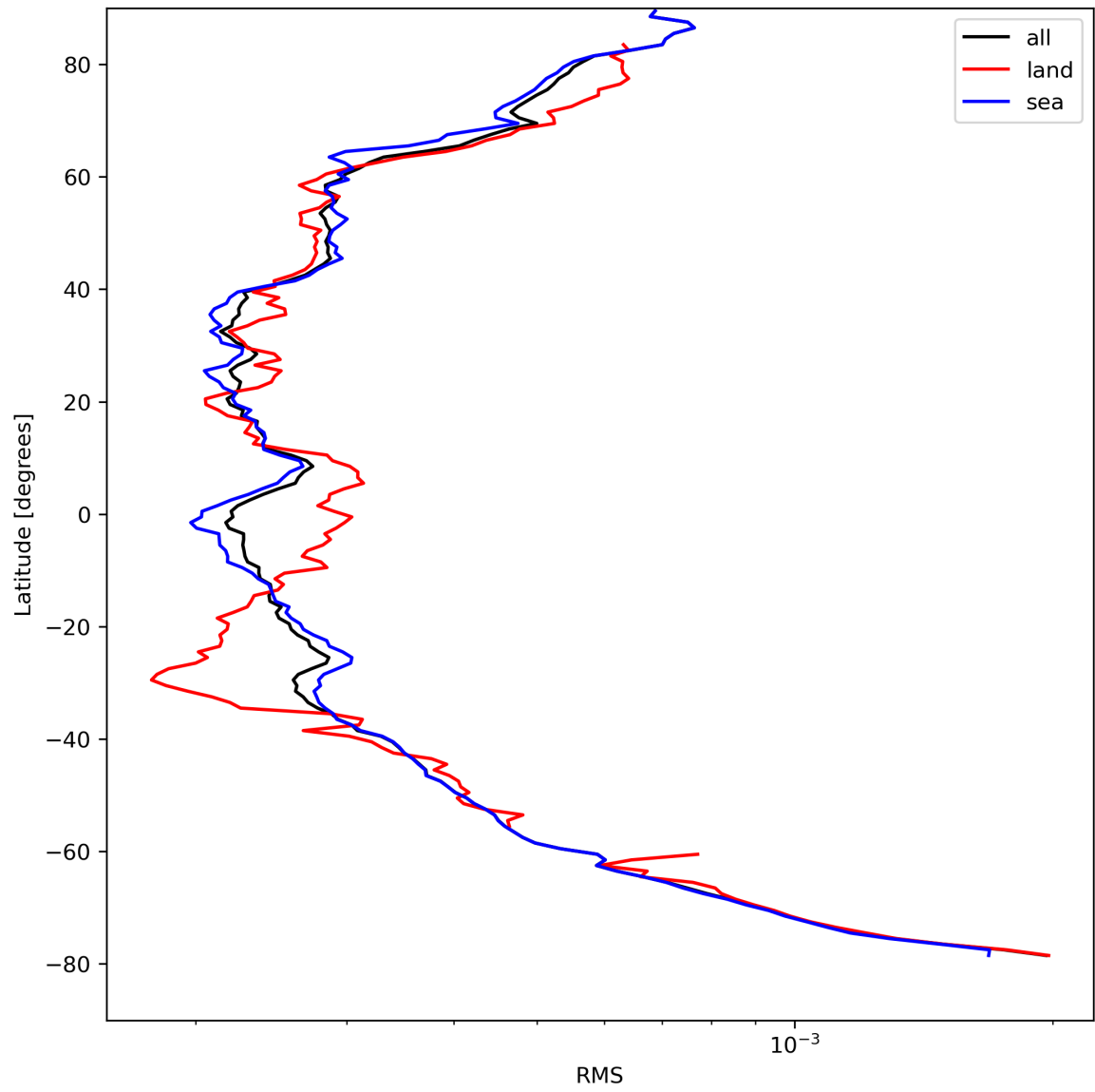
Figure 26: Zonal average of “RMS” for 2023-08-28 to 2023-08-30.
