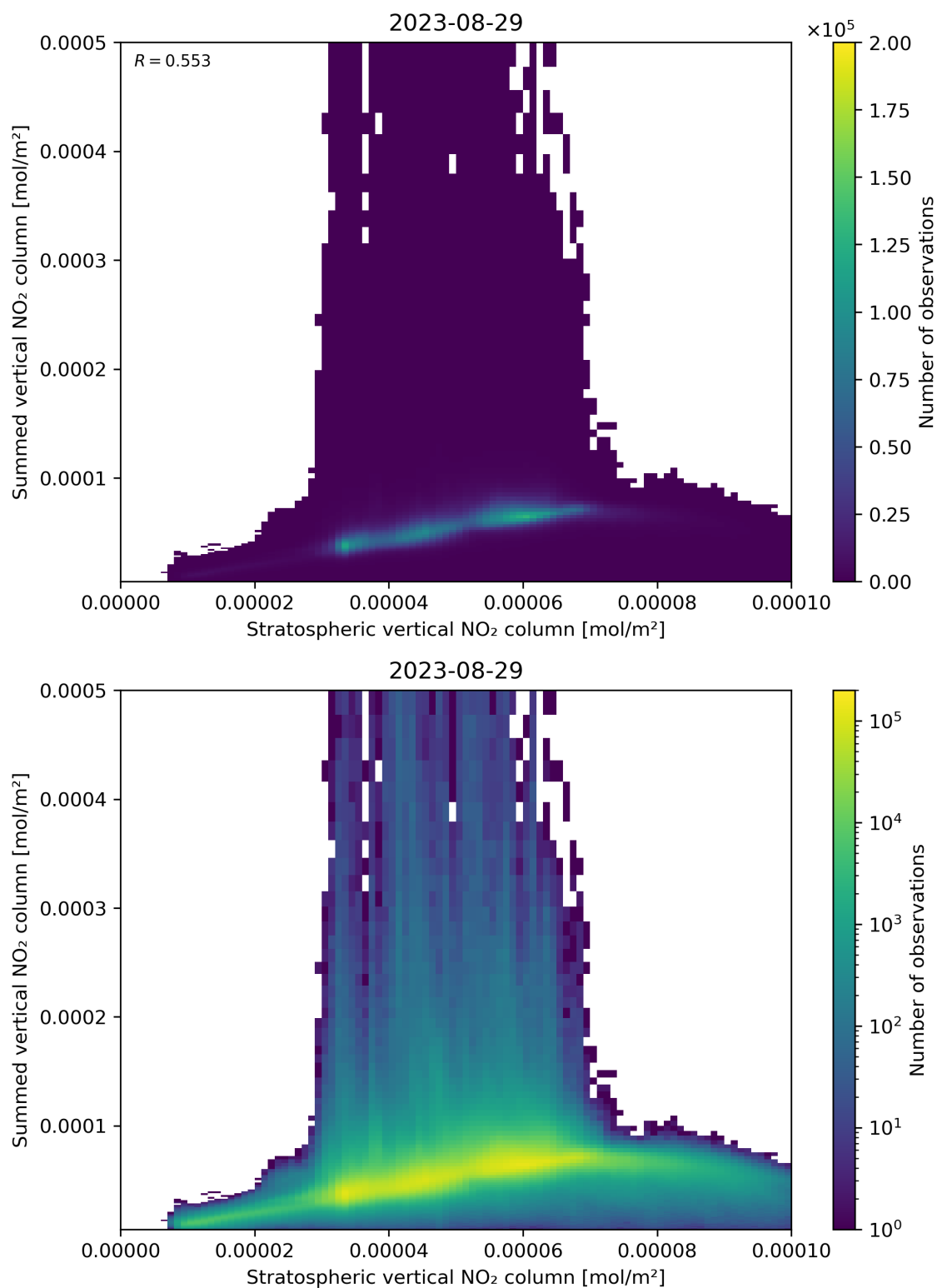
Figure 98: Scatter density plot of “Stratospheric vertical NO 2 column” against “Summed vertical NO 2 column” for 2023-08-28 to 2023-08-30.
