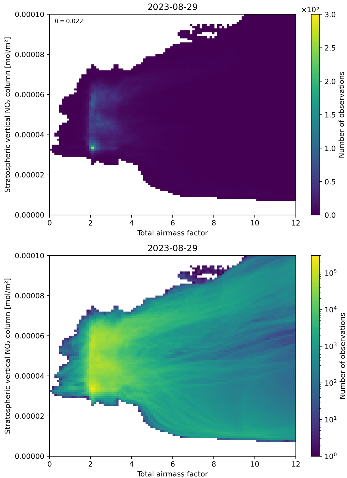
Figure 64: Scatter density plot of “Total airmass factor” against “Stratospheric vertical \text{NO}_2 column” for 2023-08-28 to 2023-08-30.
