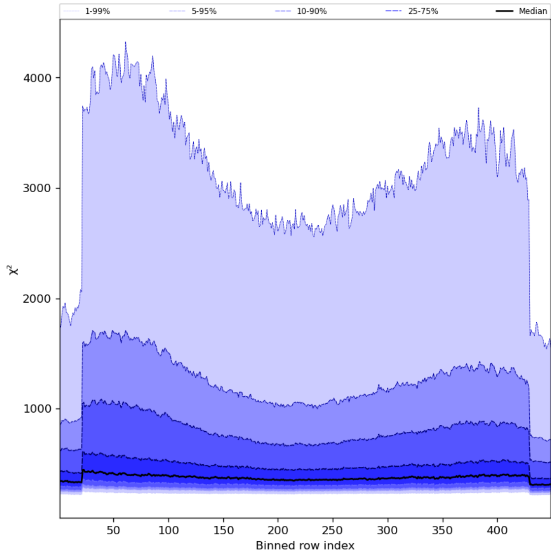
Figure 59: Along track statistics of “ \chi^2 ” for 2023-08-28 to 2023-08-30
