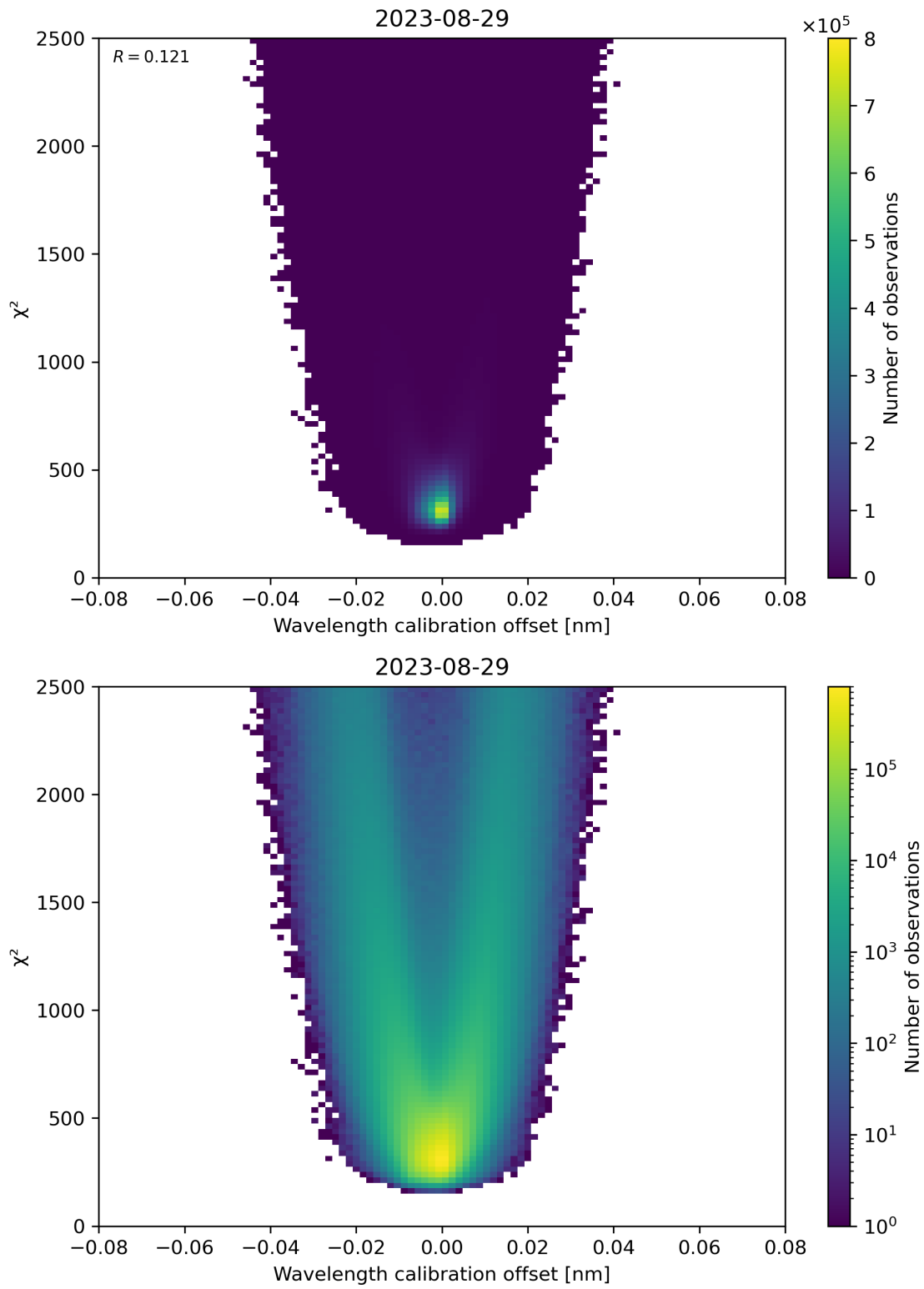
Figure 175: Scatter density plot of “Wavelength calibration offset” against “ \chi^2 ” for 2023-08-28 to 2023-08-30.
