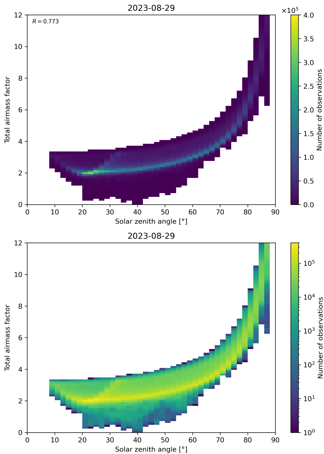
Figure 146: Scatter density plot of “Solar zenith angle” against “Total air mass factor” for 2023-08-28 to 2023-08-30.
