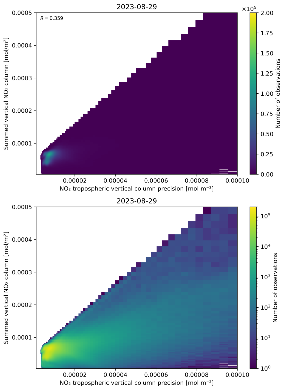
Figure 136: Scatter density plot of “NO 2 tropospheric vertical column precision” against “Summed vertical NO 2 column” for 2023-08-28 to 2023-08-30.
