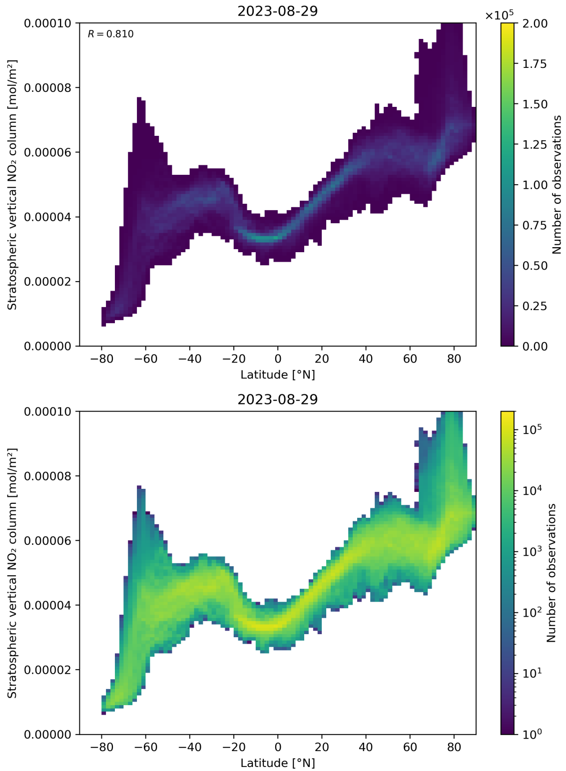
Figure 87: Scatter density plot of “Latitude” against “Stratospheric vertical NO 2 column” for 2023-08-28 to 2023-08-30.
