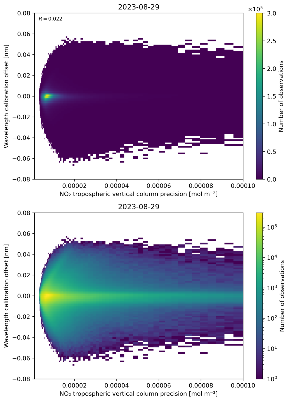
Figure 141: Scatter density plot of “NO 2 tropospheric vertical column precision” against “Wavelength calibration offset” for 2023-08-28 to 2023-08-30.
