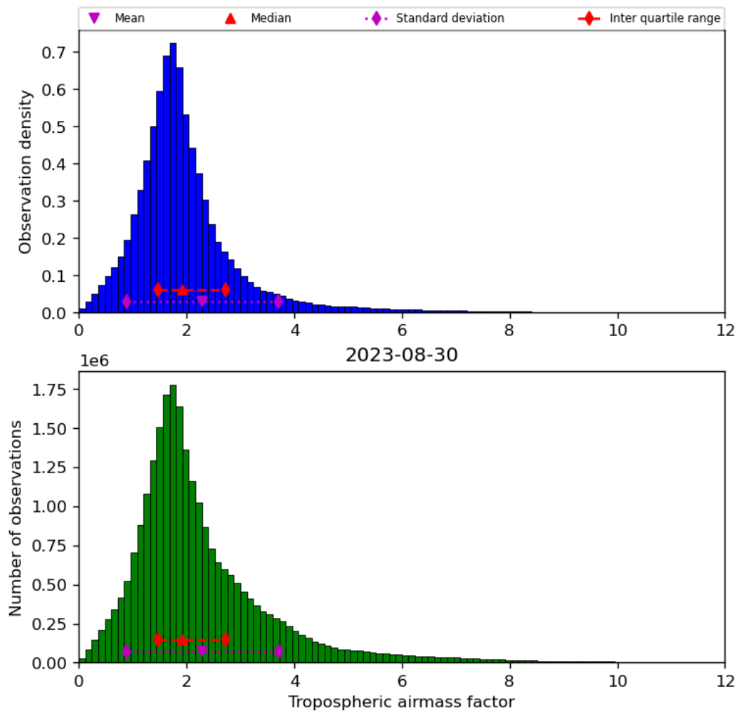
Figure 31: Histogram of “Tropospheric airmass factor” for 2023-08-30 to 2023-08-31
