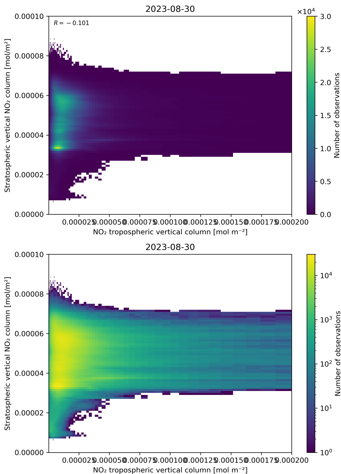
Figure 125: Scatter density plot of “NO 2 tropospheric vertical column” against “Stratospheric vertical NO 2 column” for 2023-08-30 to 2023-08-31.
