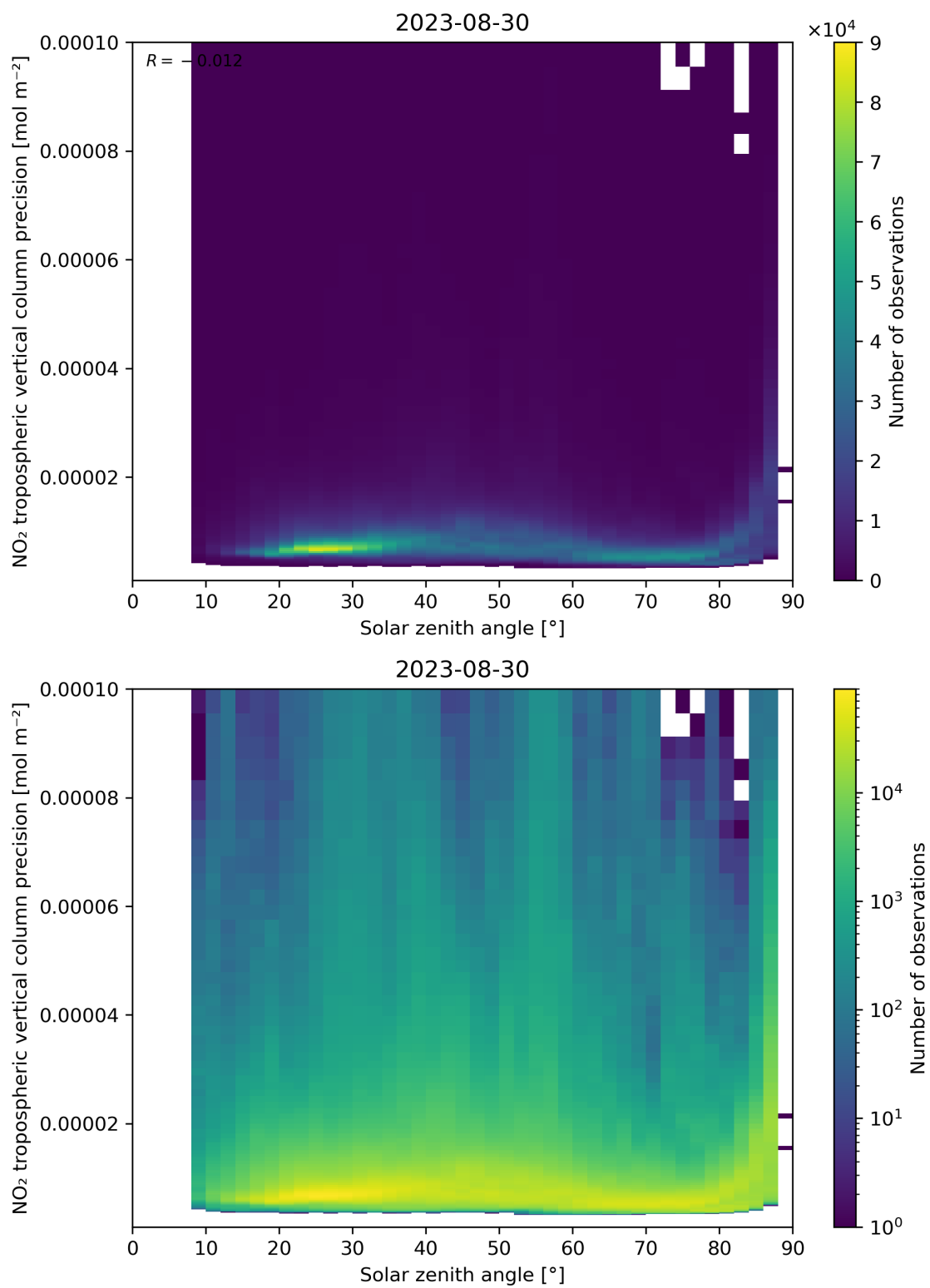
Figure 156: Scatter density plot of “Solar zenith angle” against “NO 2 tropospheric vertical column precision” for 2023-08-30 to 2023-08-31.
