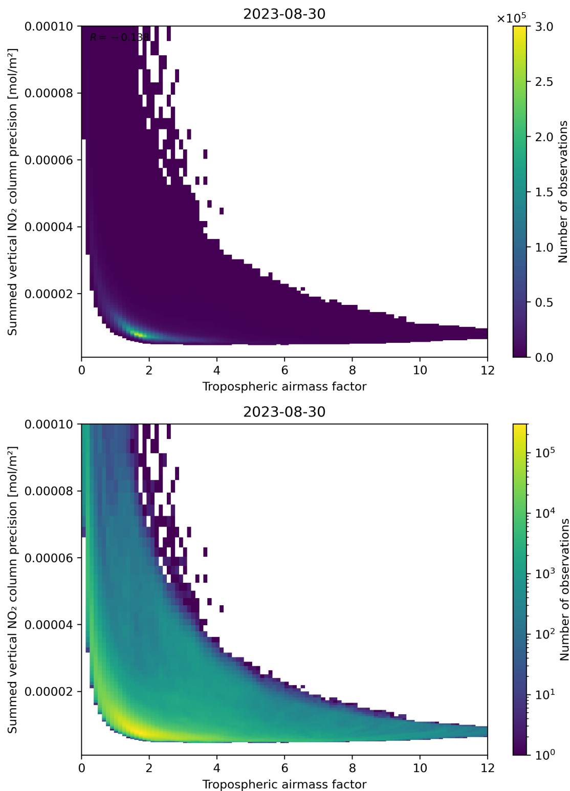
Figure 76: Scatter density plot of “Tropospheric air mass factor” against “Summed vertical NO 2 column precision” for 2023-08-30 to 2023-08-31.
