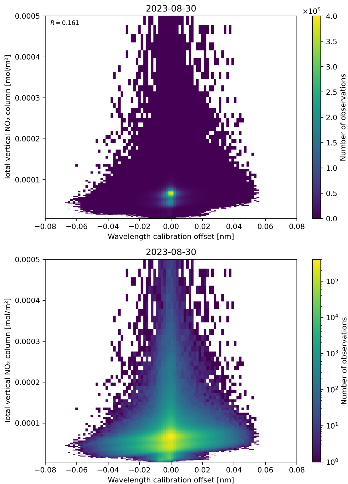
Figure 179: Scatter density plot of “Wavelength calibration offset” against “Total vertical NO 2 column” for 2023-08-30 to 2023-08-31.
