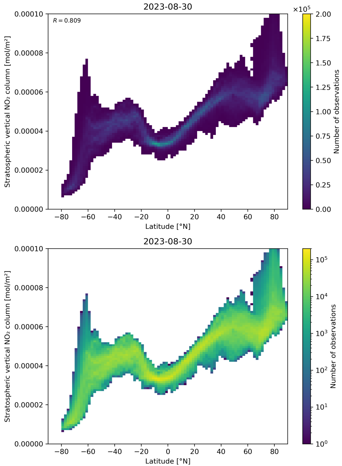
Figure 87: Scatter density plot of “Latitude” against “Stratospheric vertical \text{NO}_2 column” for 2023-08-30 to 2023-08-31.
