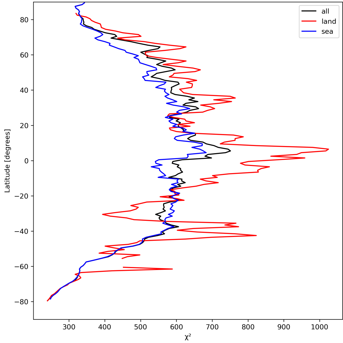
Figure 25: Zonal average of “ \chi^2 ” for 2023-08-30 to 2023-08-31.
