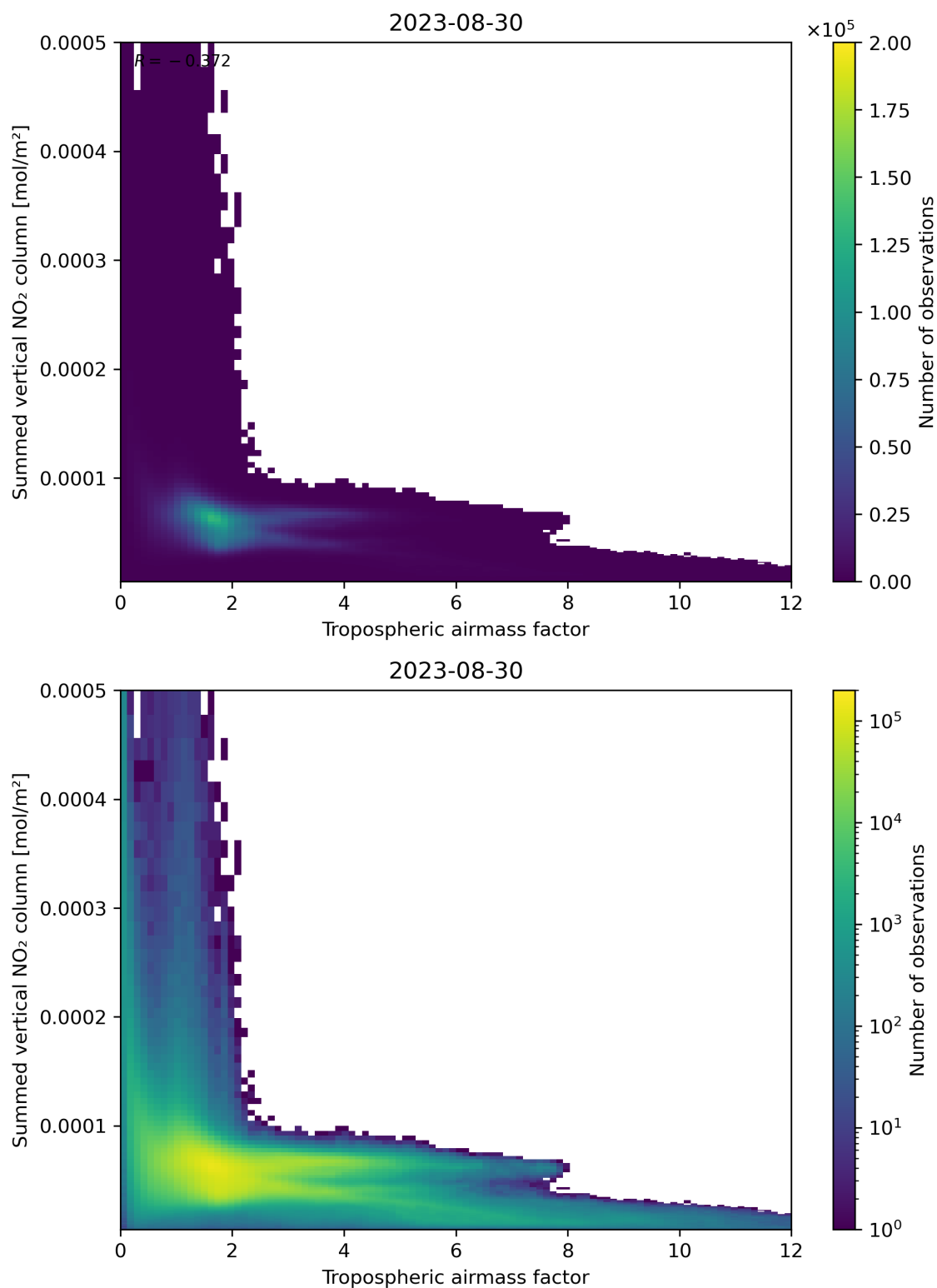
Figure 75: Scatter density plot of “Tropospheric airmass factor” against “Summed vertical NO 2 column” for 2023-08-30 to 2023-08-31.
