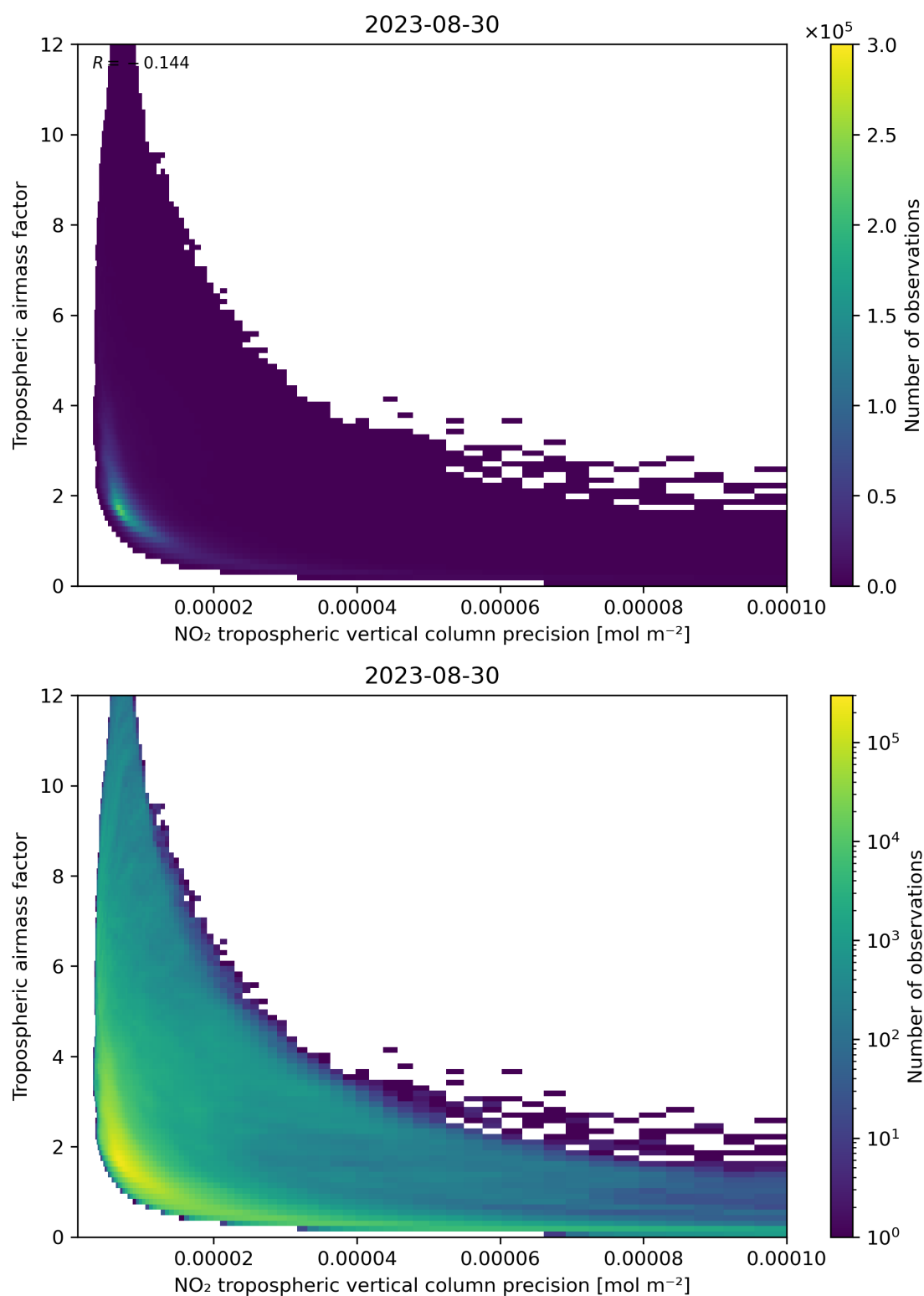
Figure 133: Scatter density plot of “NO 2 tropospheric vertical column precision” against “Tropospheric airmass factor” for 2023-08-30 to 2023-08-31.
