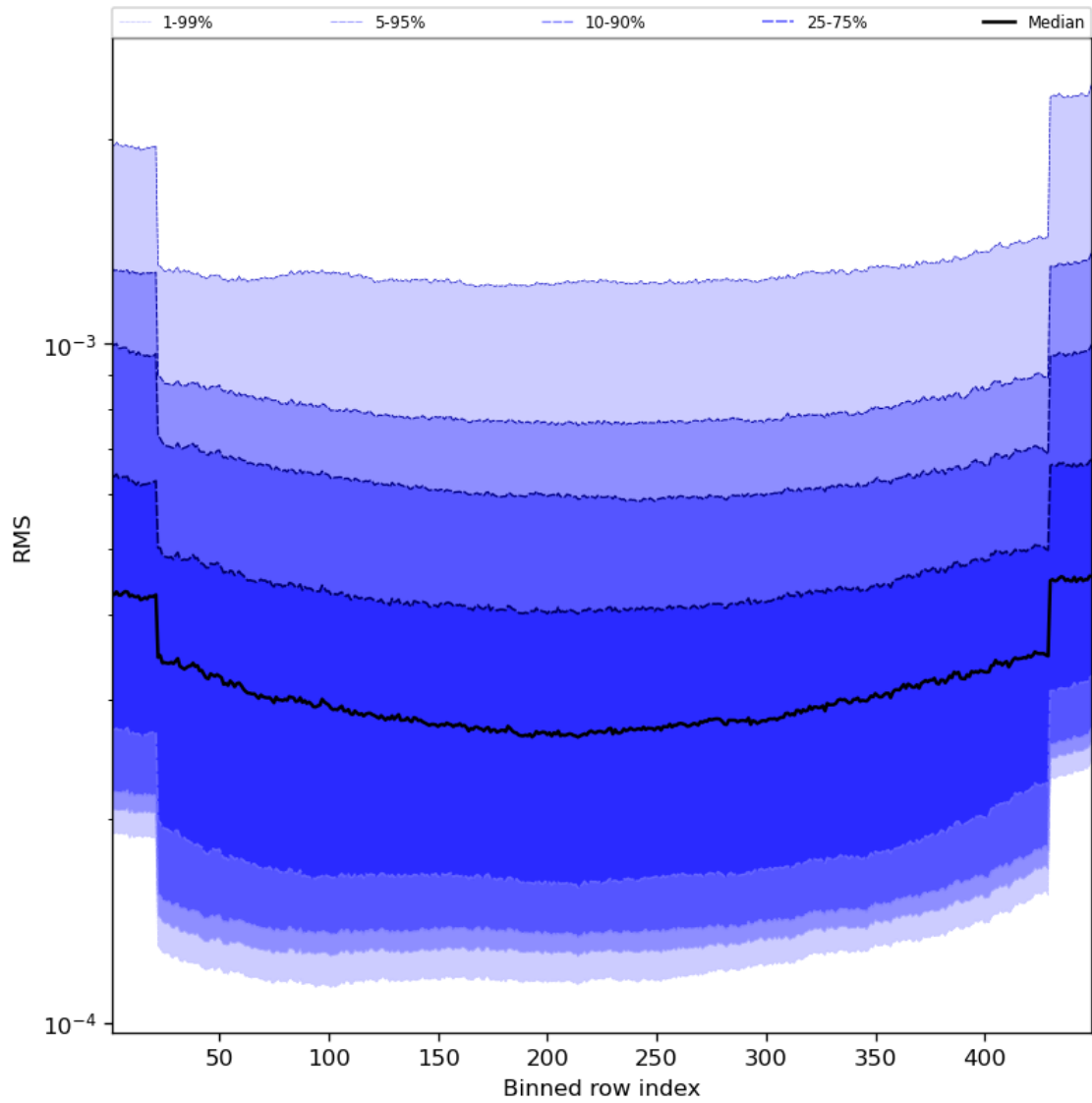
Figure 60: Along track statistics of “RMS” for 2023-08-30 to 2023-08-31
