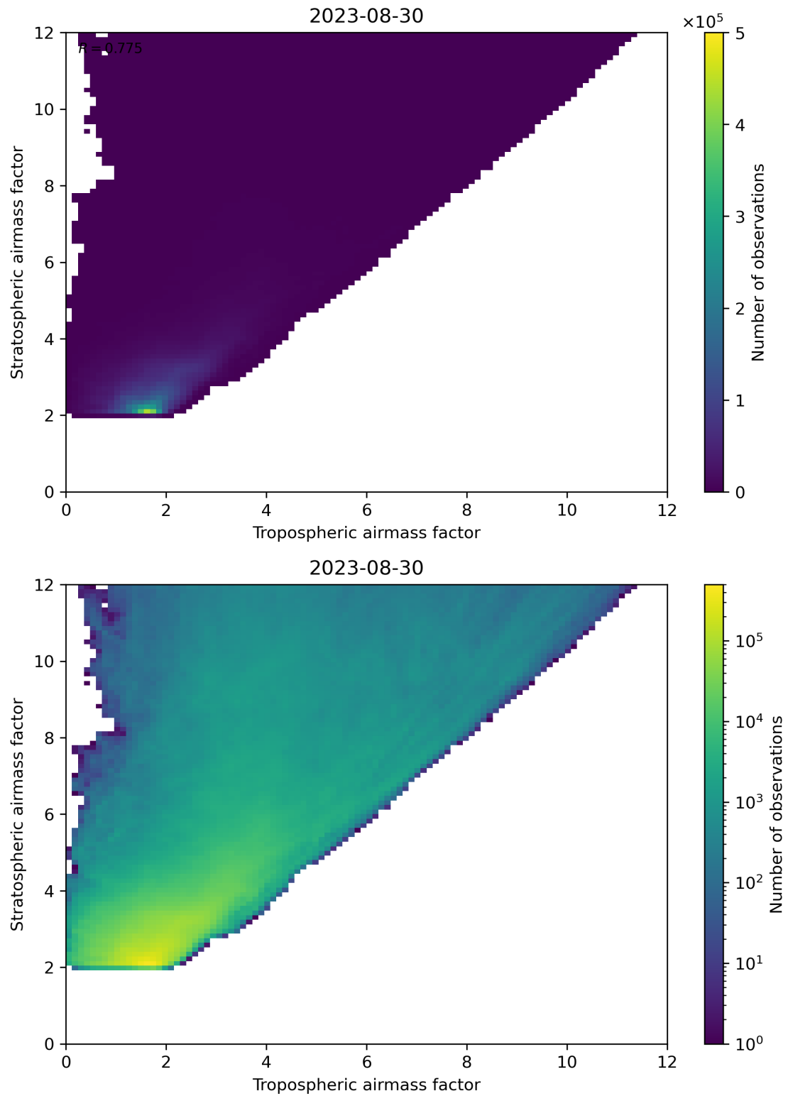
Figure 71: Scatter density plot of “Tropospheric airmass factor” against “Stratospheric airmass factor” for 2023-08-30 to 2023-08-31.
