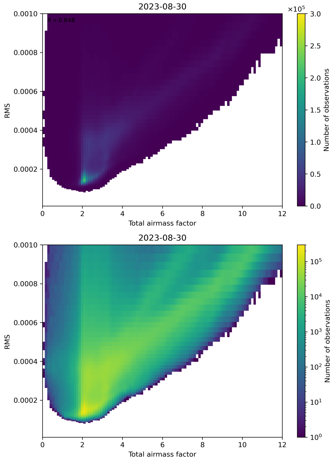
Figure 69: Scatter density plot of “Total airmass factor” against “RMS” for 2023-08-30 to 2023-08-31.
