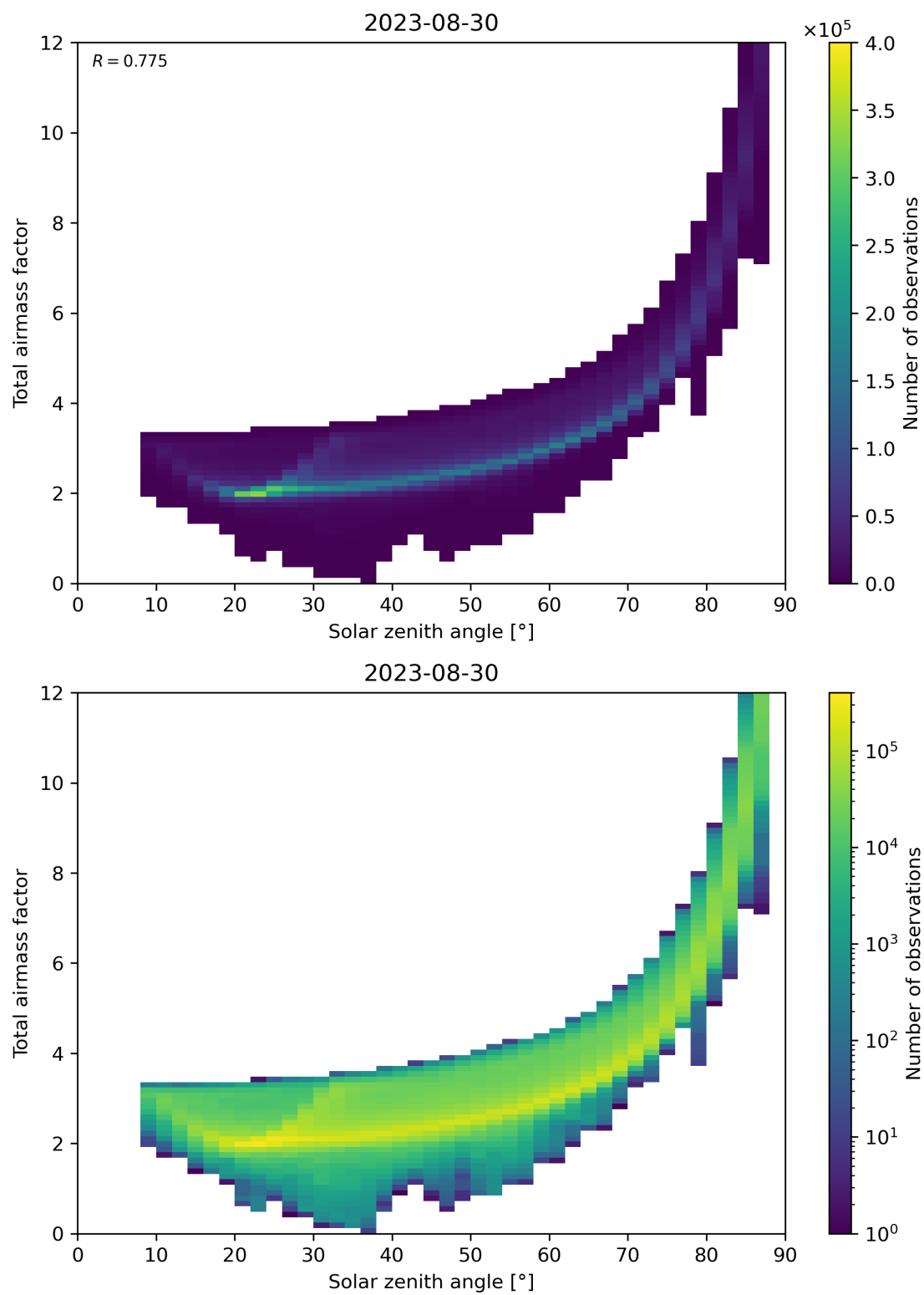
Figure 146: Scatter density plot of “Solar zenith angle” against “Total airmass factor” for 2023-08-30 to 2023-08-31.
