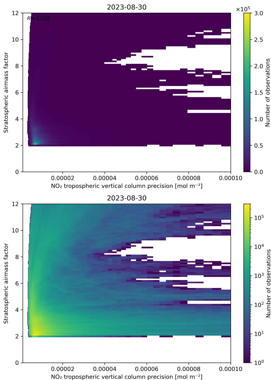
Figure 131: Scatter density plot of “NO 2 tropospheric vertical column precision” against “Stratospheric airmass factor” for 2023-08-30 to 2023-08-31.
