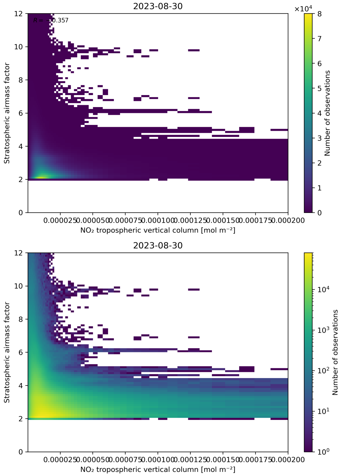
Figure 121: Scatter density plot of “NO 2 tropospheric vertical column” against “Stratospheric air mass factor” for 2023-08-30 to 2023-08-31.
