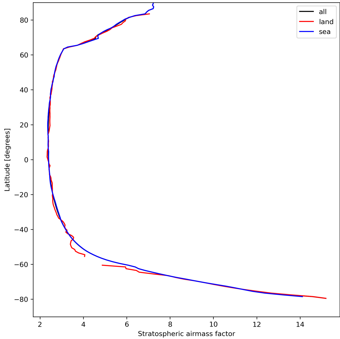
Figure 27: Zonal average of “Stratospheric airmass factor” for 2023-08-30 to 2023-08-31.
