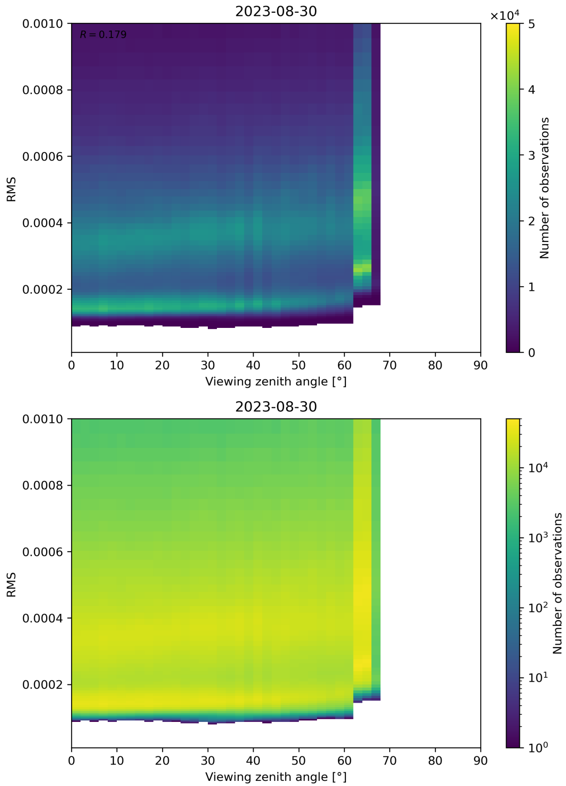
Figure 171: Scatter density plot of “Viewing zenith angle” against “RMS” for 2023-08-30 to 2023-08-31.
