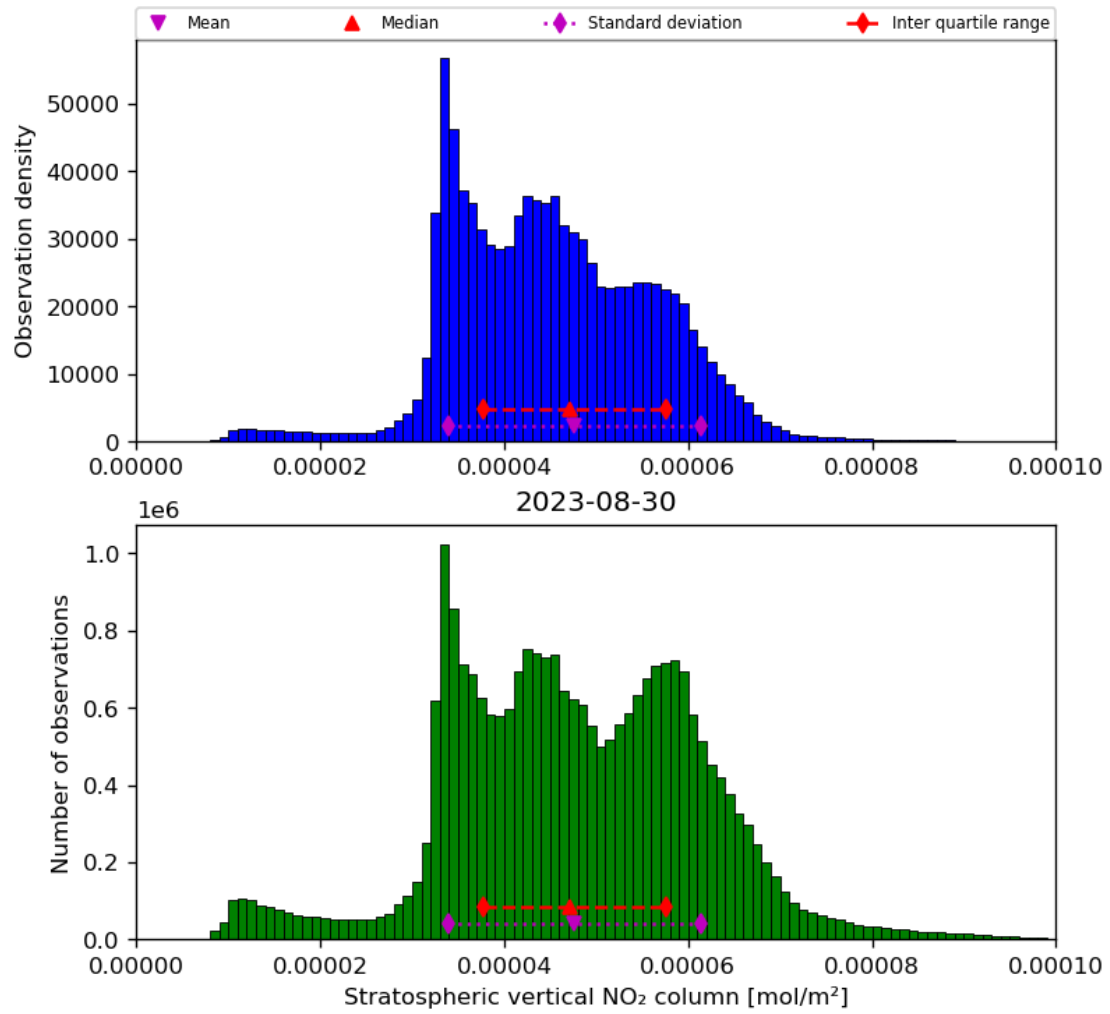
Figure 36: Histogram of “Stratospheric vertical NO 2 column” for 2023-08-30 to 2023-08-31
