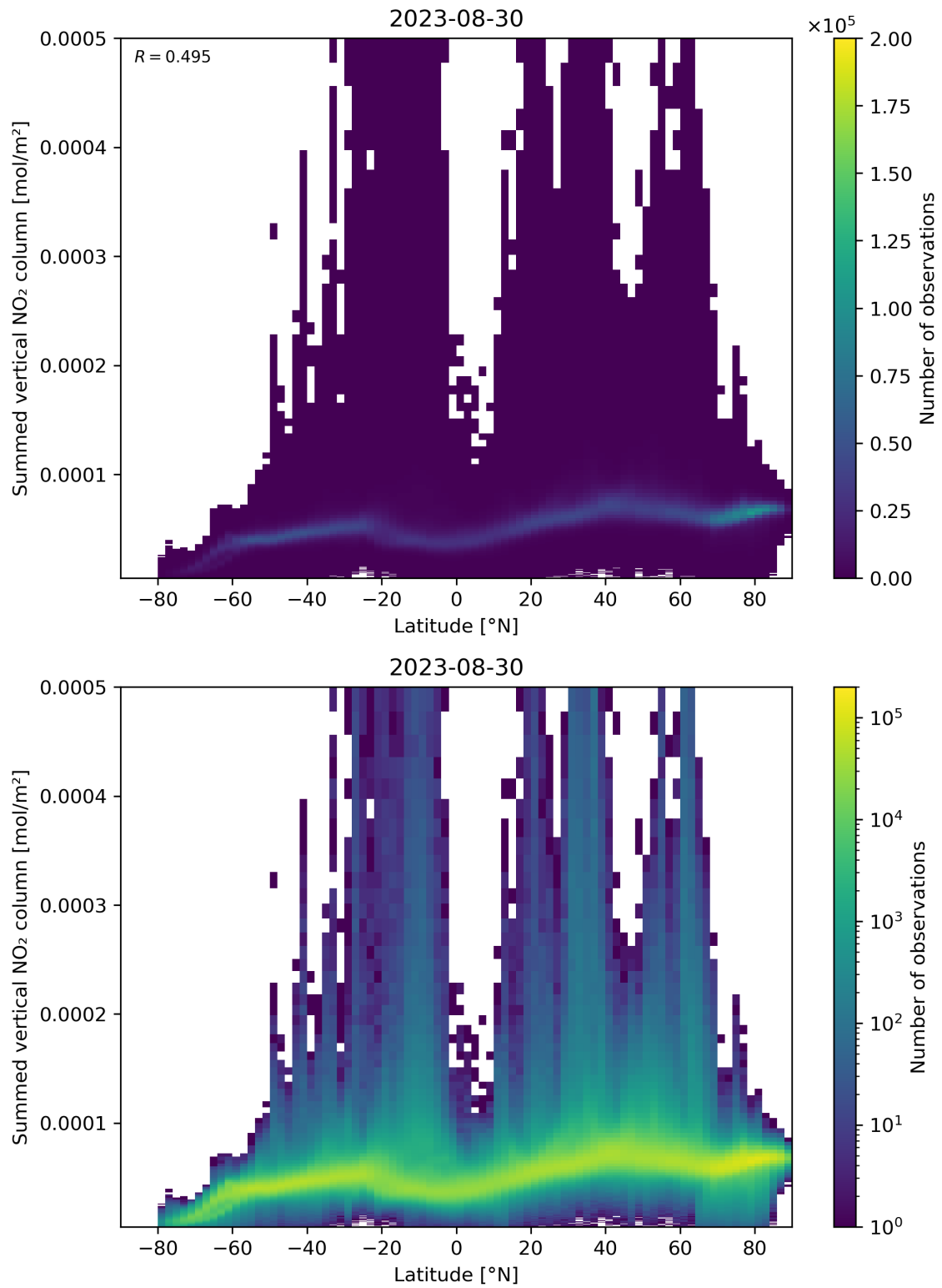
Figure 88: Scatter density plot of “Latitude” against “Summed vertical NO 2 column” for 2023-08-30 to 2023-08-31.
