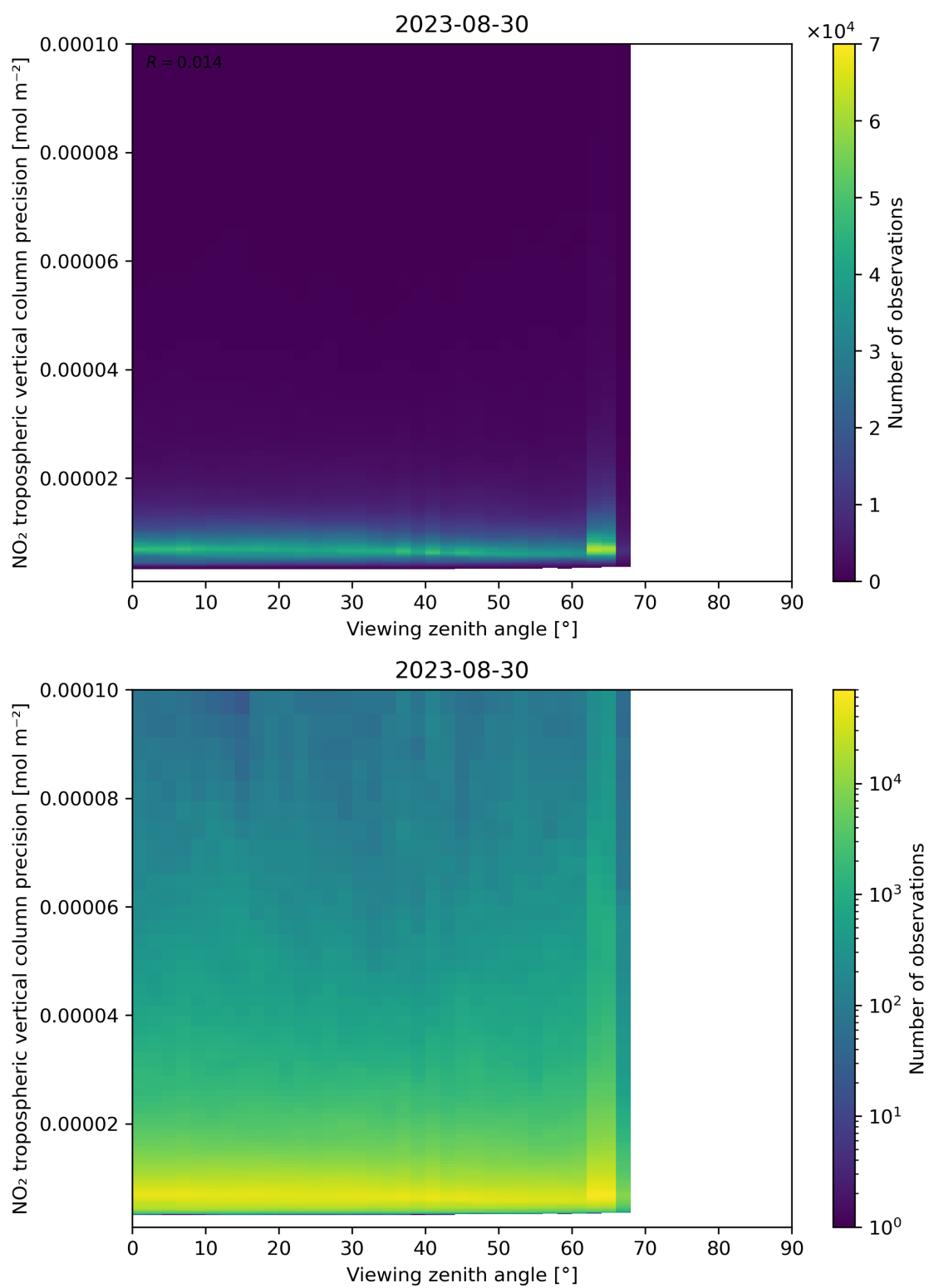
Figure 170: Scatter density plot of “Viewing zenith angle” against “NO 2 tropospheric vertical column precision” for 2023-08-30 to 2023-08-31.
