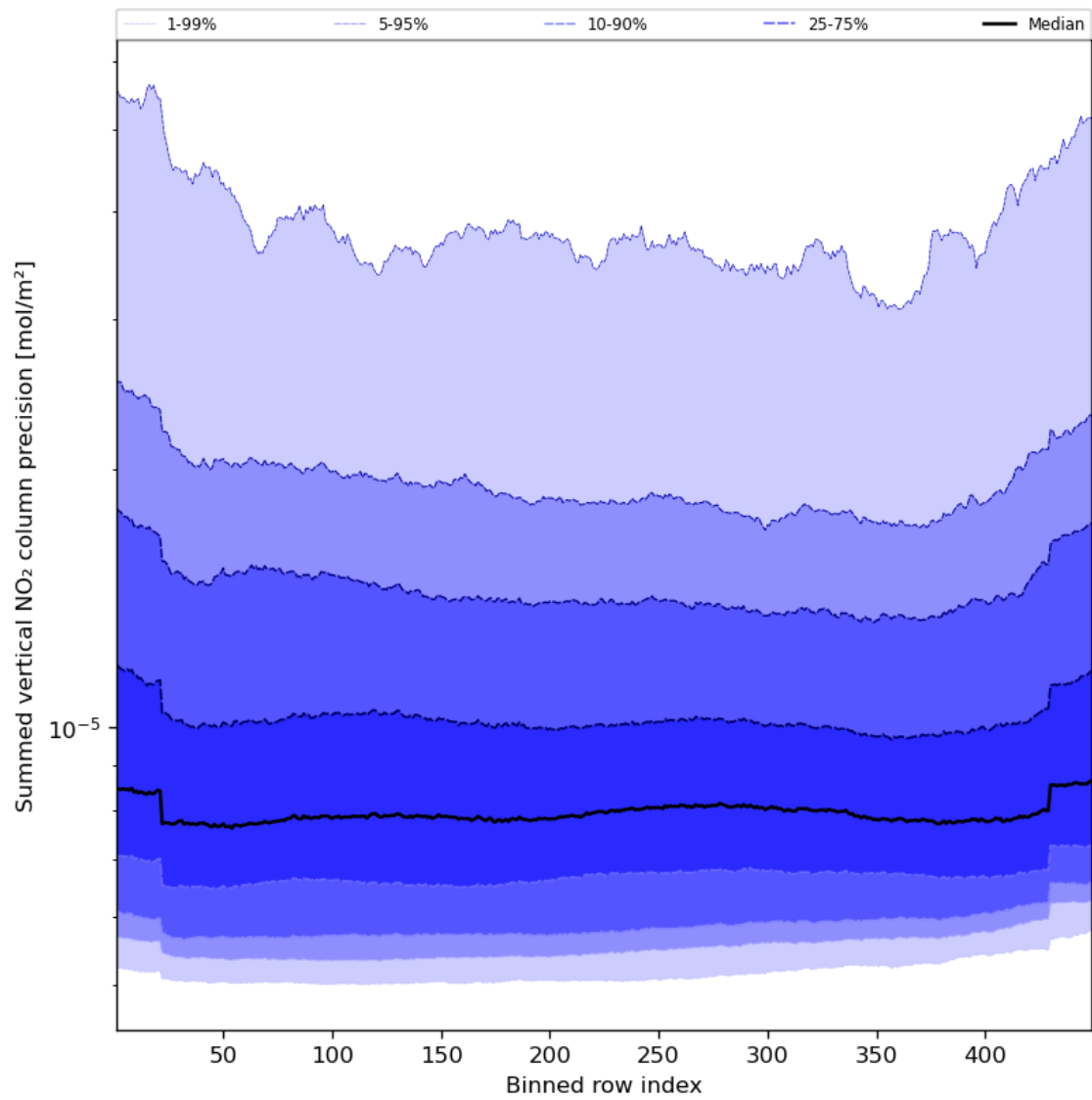
Figure 58: Along track statistics of “Summed vertical NO 2 column precision” for 2023-08-30 to 2023-08-31
