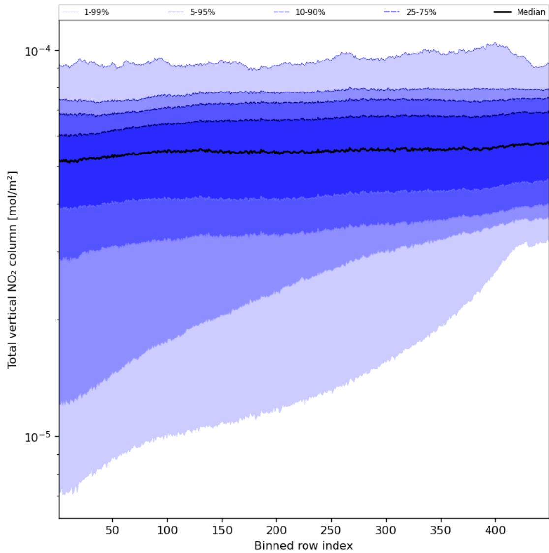
Figure 55: Along track statistics of “Total vertical NO 2 column” for 2023-08-30 to 2023-08-31
