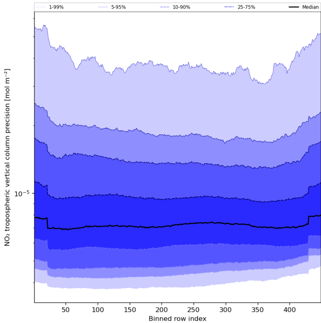
Figure 47: Along track statistics of “NO 2 tropospheric vertical column precision” for 2023-08-30 to 2023-08-31
