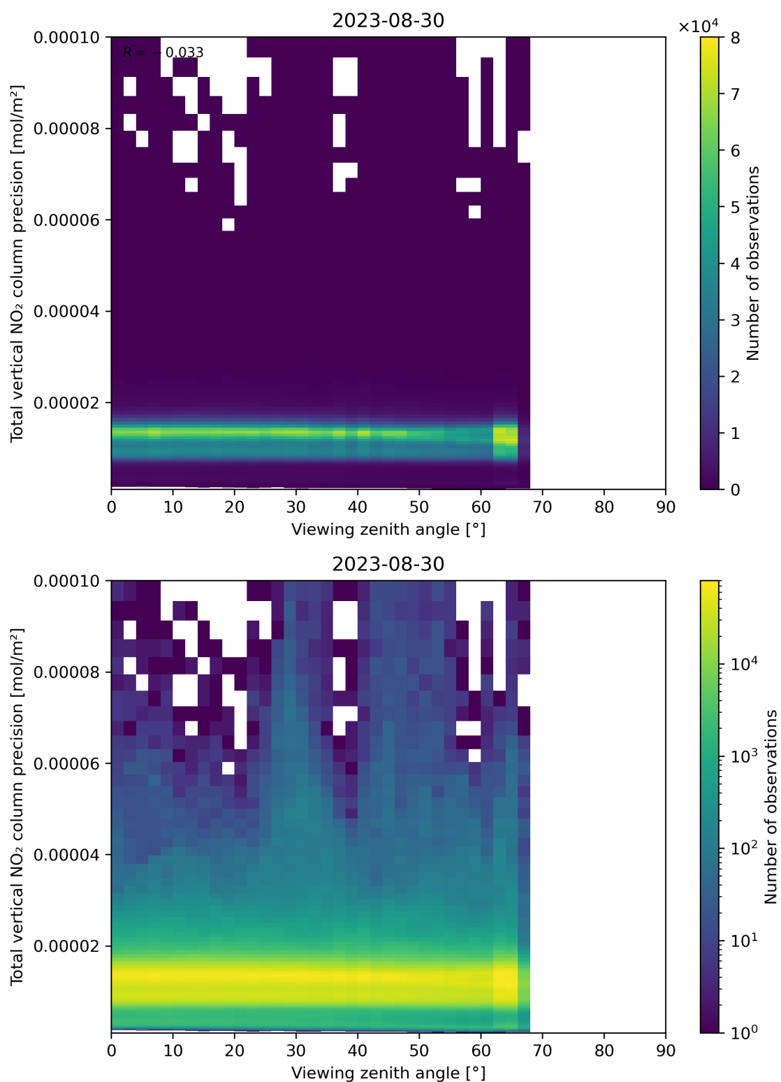
Figure 168: Scatter density plot of “Viewing zenith angle” against “Total vertical NO 2 column precision” for 2023-08-30 to 2023-08-31.
