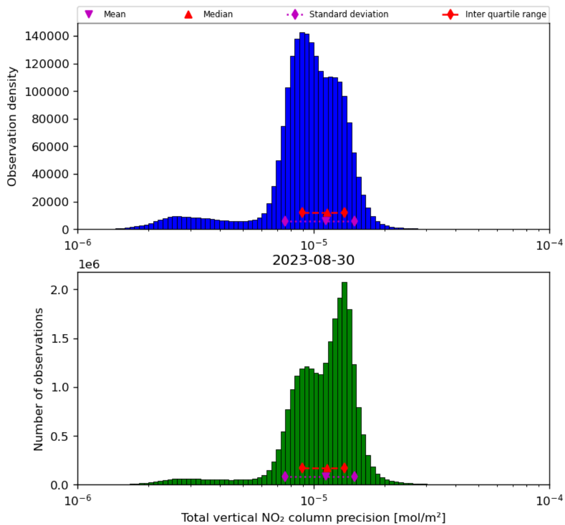
Figure 39: Histogram of "Total vertical NO 2 column precision" for 2023-08-30 to 2023-08-31
