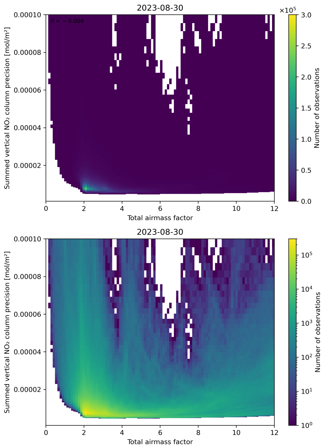
Figure 66: Scatter density plot of “Total airmass factor” against “Summed vertical NO 2 column precision” for 2023-08-30 to 2023-08-31.
