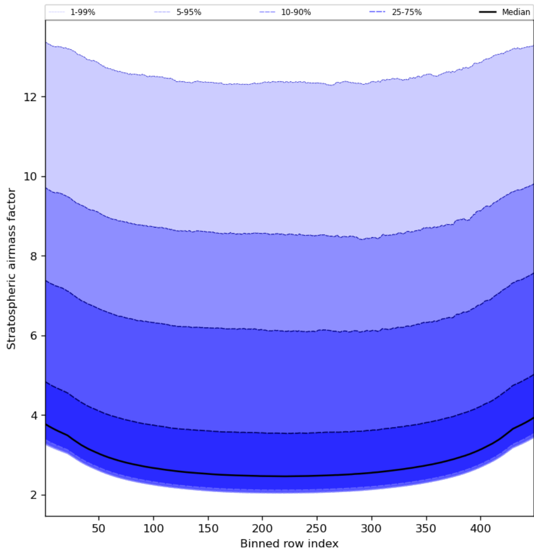
Figure 61: Along track statistics of “Stratospheric air mass factor” for 2023-08-30 to 2023-08-31
