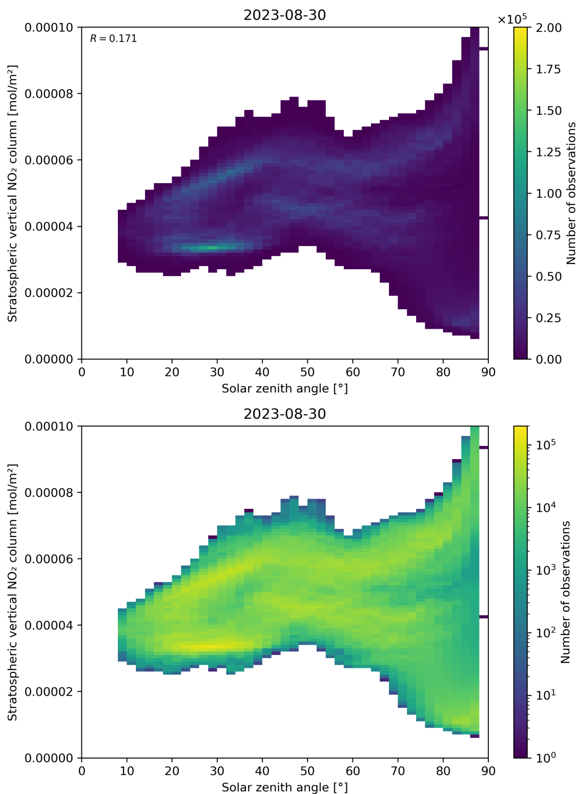
Figure 150: Scatter density plot of “Solar zenith angle” against “Stratospheric vertical NO 2 column” for 2023-08-30 to 2023-08-31.
