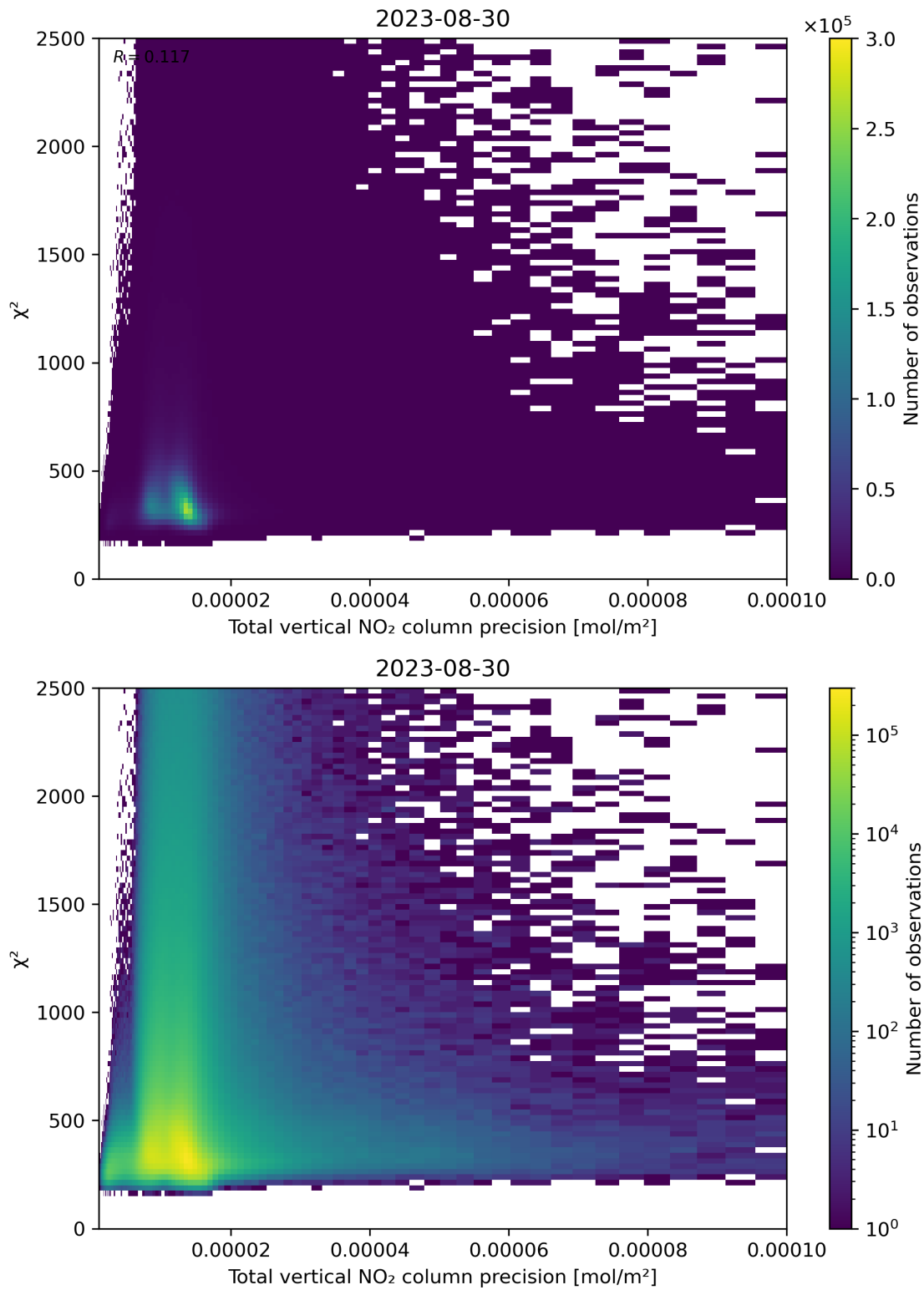
Figure 116: Scatter density plot of “Total vertical NO 2 column precision” against “ \chi^2 ” for 2023-08-30 to 2023-08-31.
