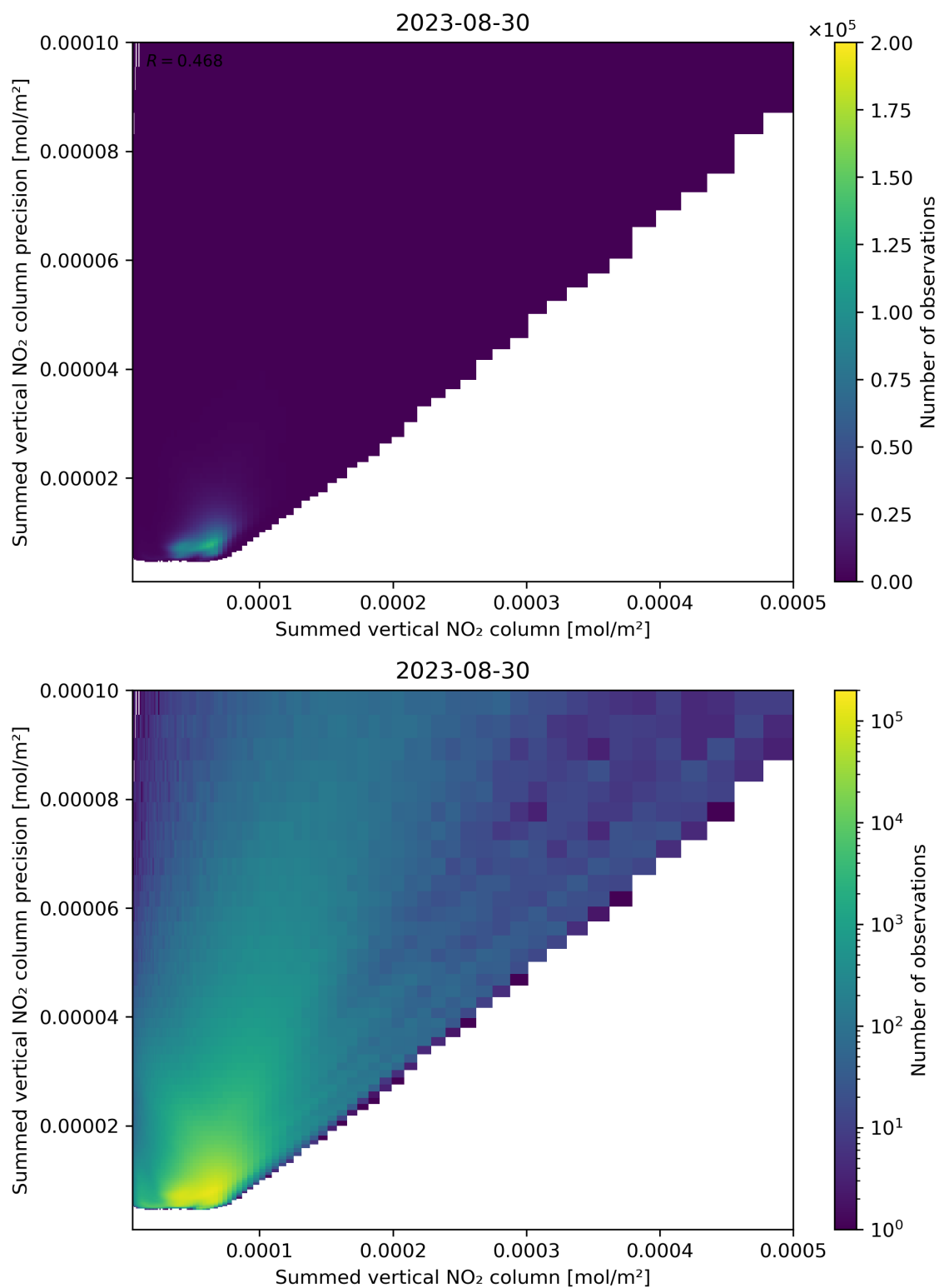
Figure 105: Scatter density plot of “Summed vertical NO 2 column” against “Summed vertical NO 2 column precision” for 2023-08-30 to 2023-08-31.
