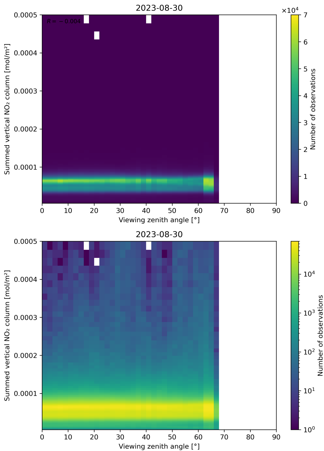
Figure 165: Scatter density plot of “Viewing zenith angle” against “Summed vertical NO 2 column” for 2023-08-30 to 2023-08-31.
