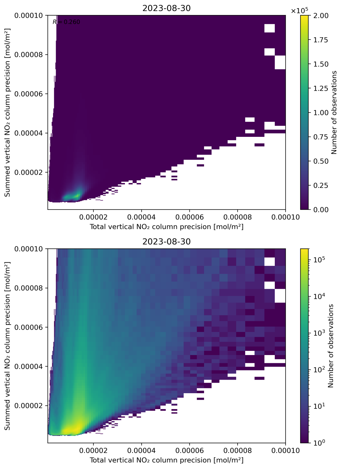
Figure 118: Scatter density plot of “Total vertical NO 2 column precision” against “Summed vertical NO 2 column precision” for 2023-08-30 to 2023-08-31.
