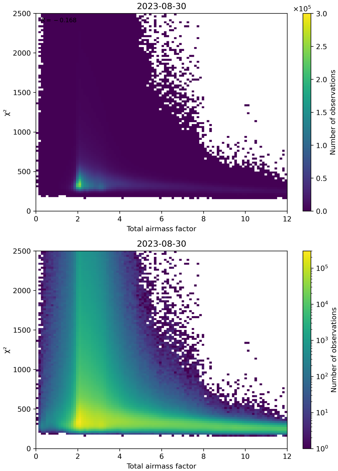
Figure 63: Scatter density plot of “Total airmass factor” against “ \chi^2 ” for 2023-08-30 to 2023-08-31.
