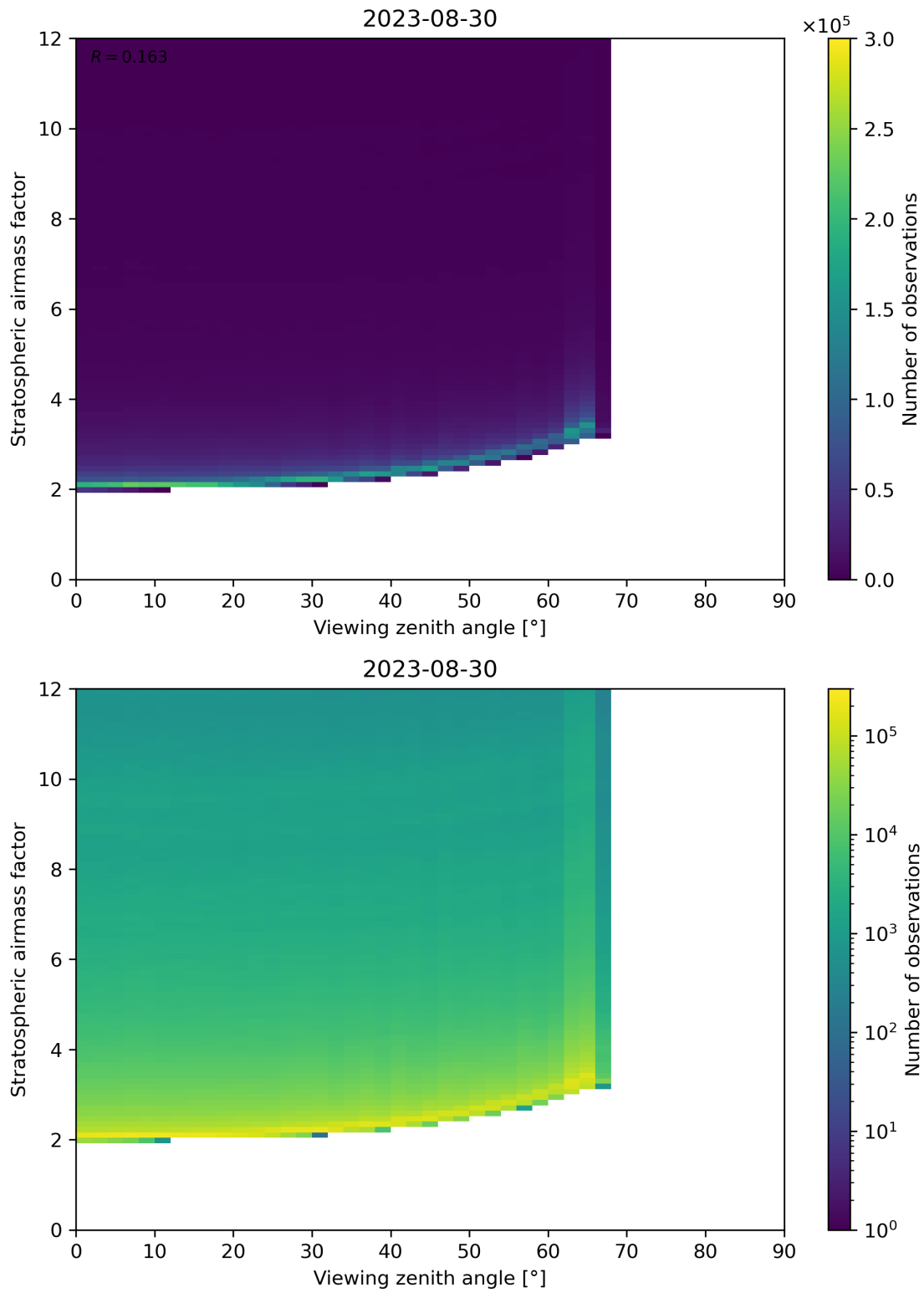
Figure 159: Scatter density plot of “Viewing zenith angle” against “Stratospheric airmass factor” for 2023-08-30 to 2023-08-31.
