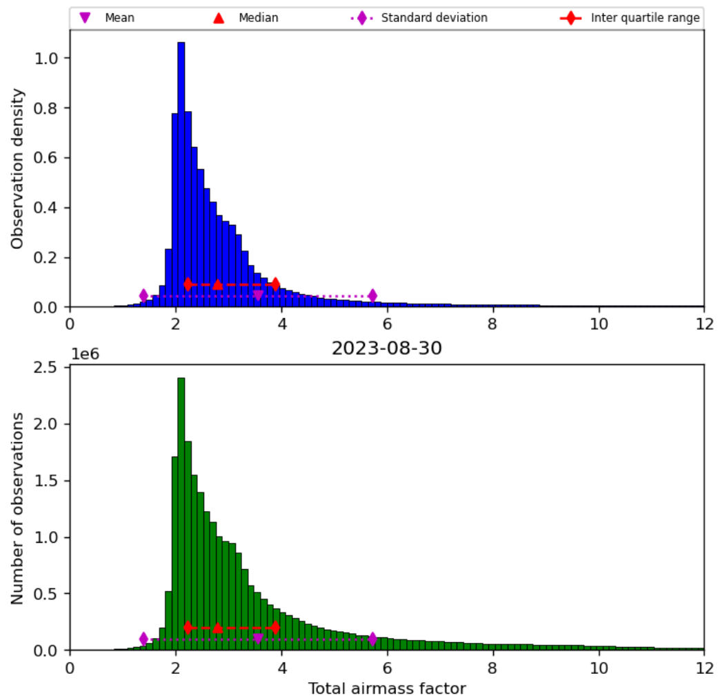
Figure 32: Histogram of “Total airmass factor” for 2023-08-30 to 2023-08-31
