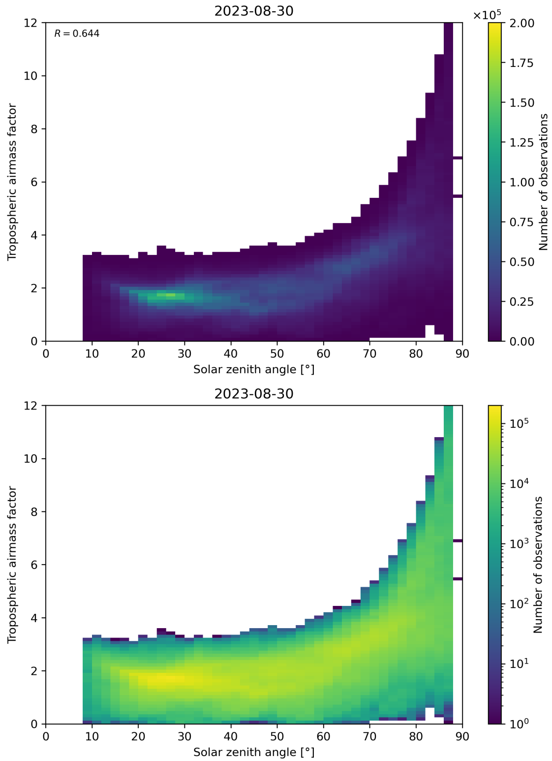
Figure 147: Scatter density plot of “Solar zenith angle” against “Tropospheric airmass factor” for 2023-08-30 to 2023-08-31.
