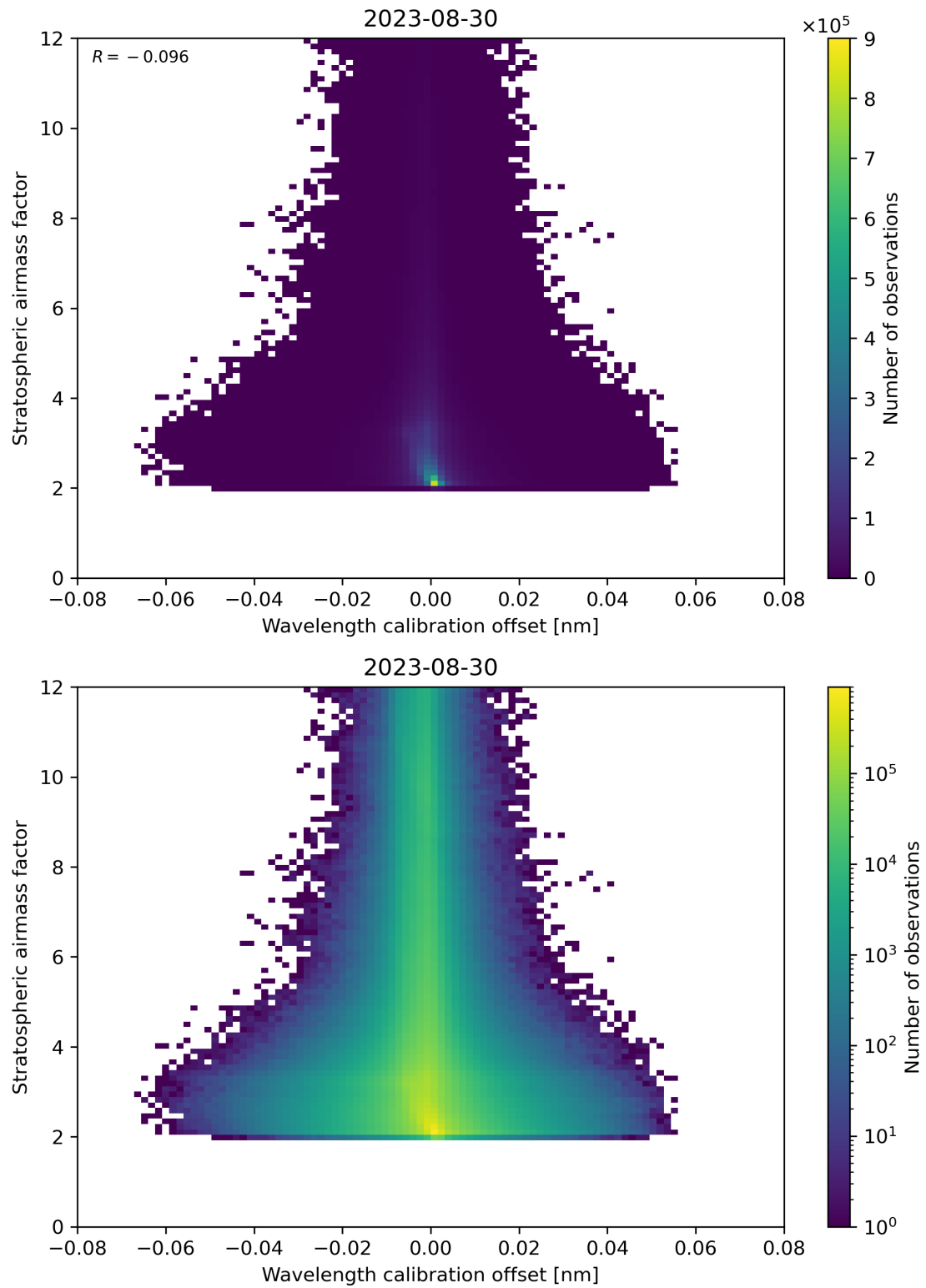
Figure 174: Scatter density plot of “Wavelength calibration offset” against “Stratospheric airmass factor” for 2023-08-30 to 2023-08-31.
