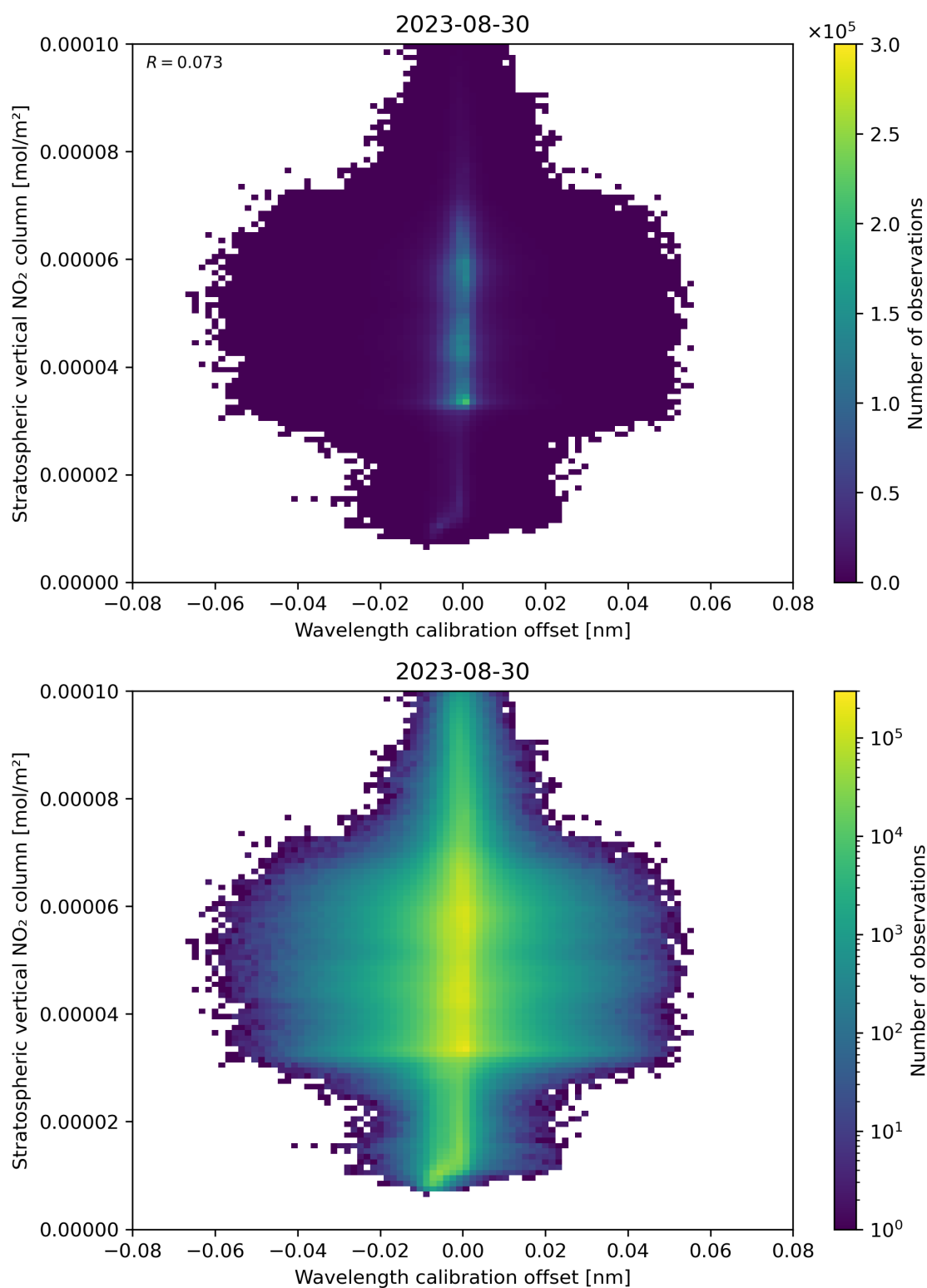
Figure 176: Scatter density plot of “Wavelength calibration offset” against “Stratospheric vertical NO 2 column” for 2023-08-30 to 2023-08-31.
