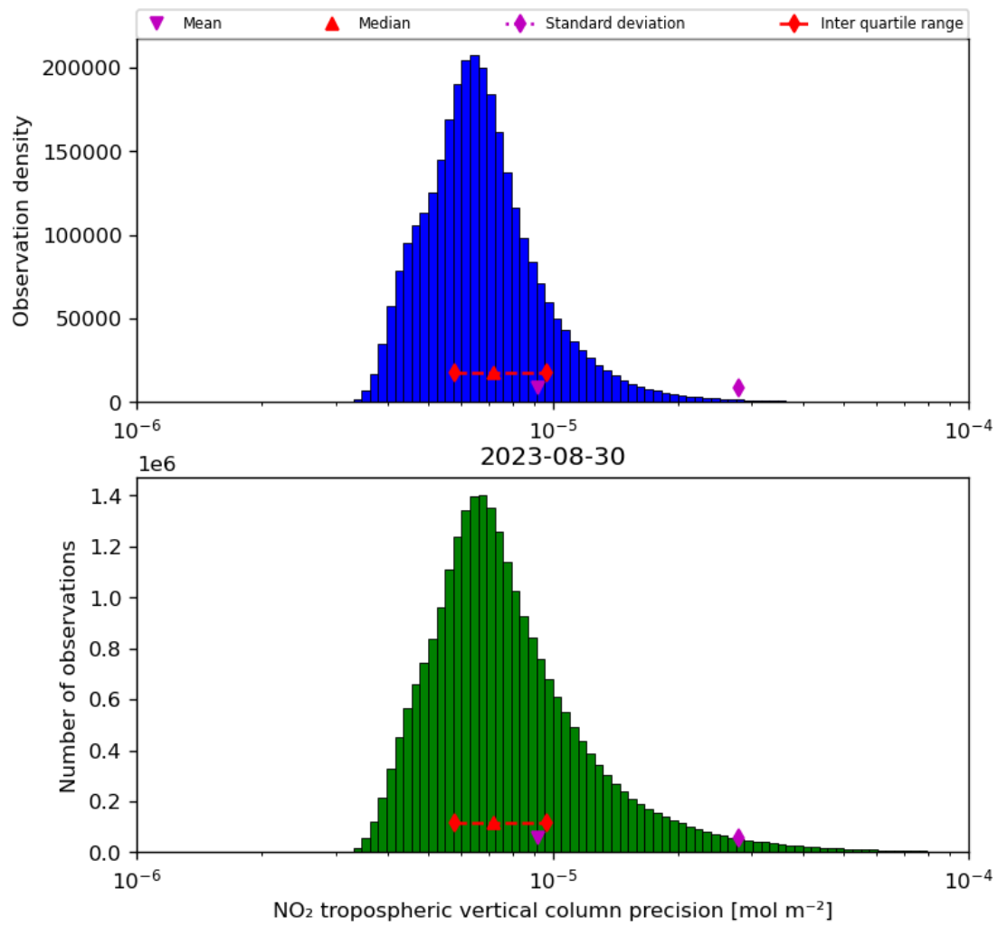
Figure 30: Histogram of “NO 2 tropospheric vertical column precision” for 2023-08-30 to 2023-08-31
