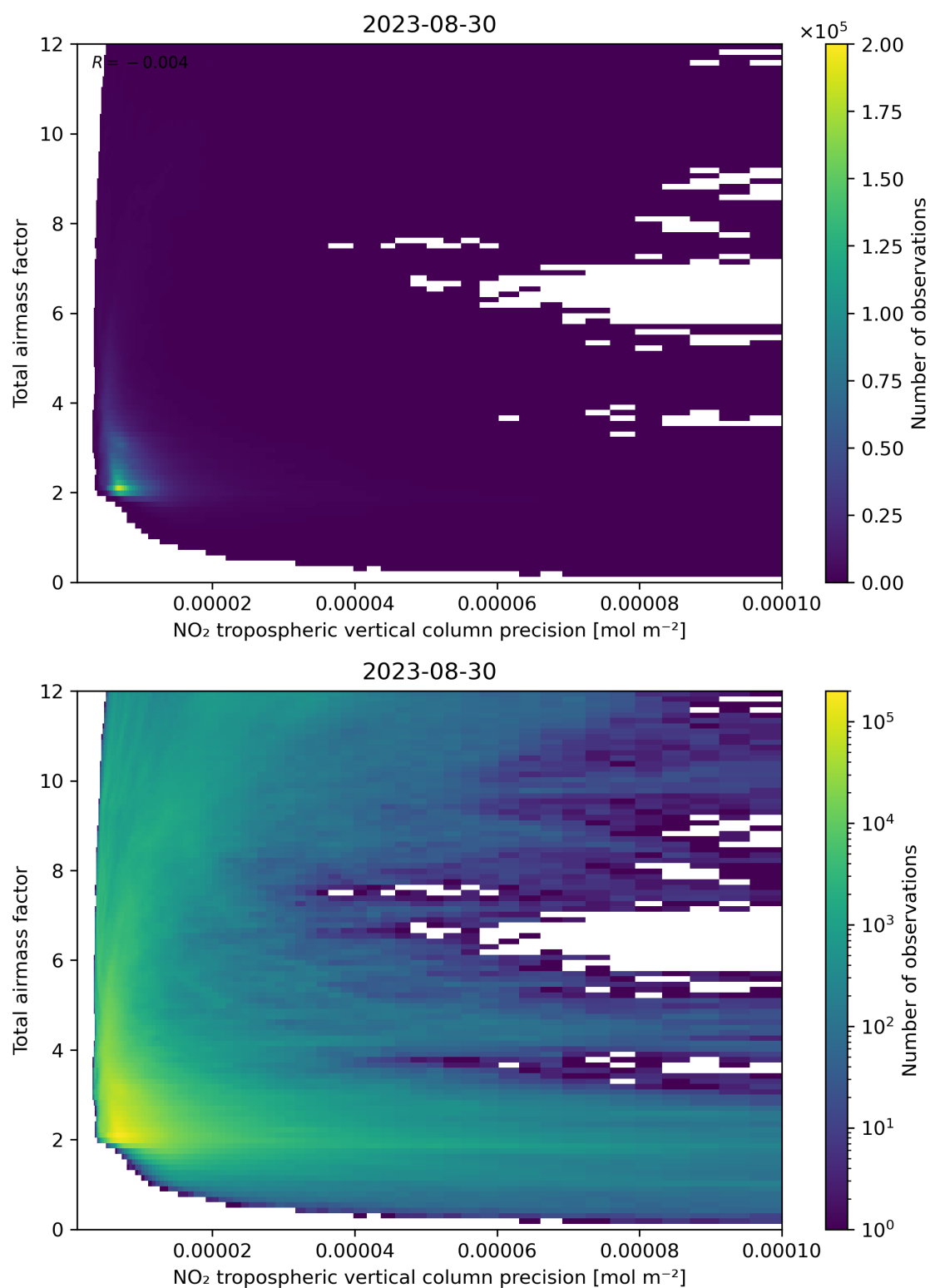
Figure 132: Scatter density plot of “NO 2 tropospheric vertical column precision” against “Total air mass factor” for 2023-08-30 to 2023-08-31.
