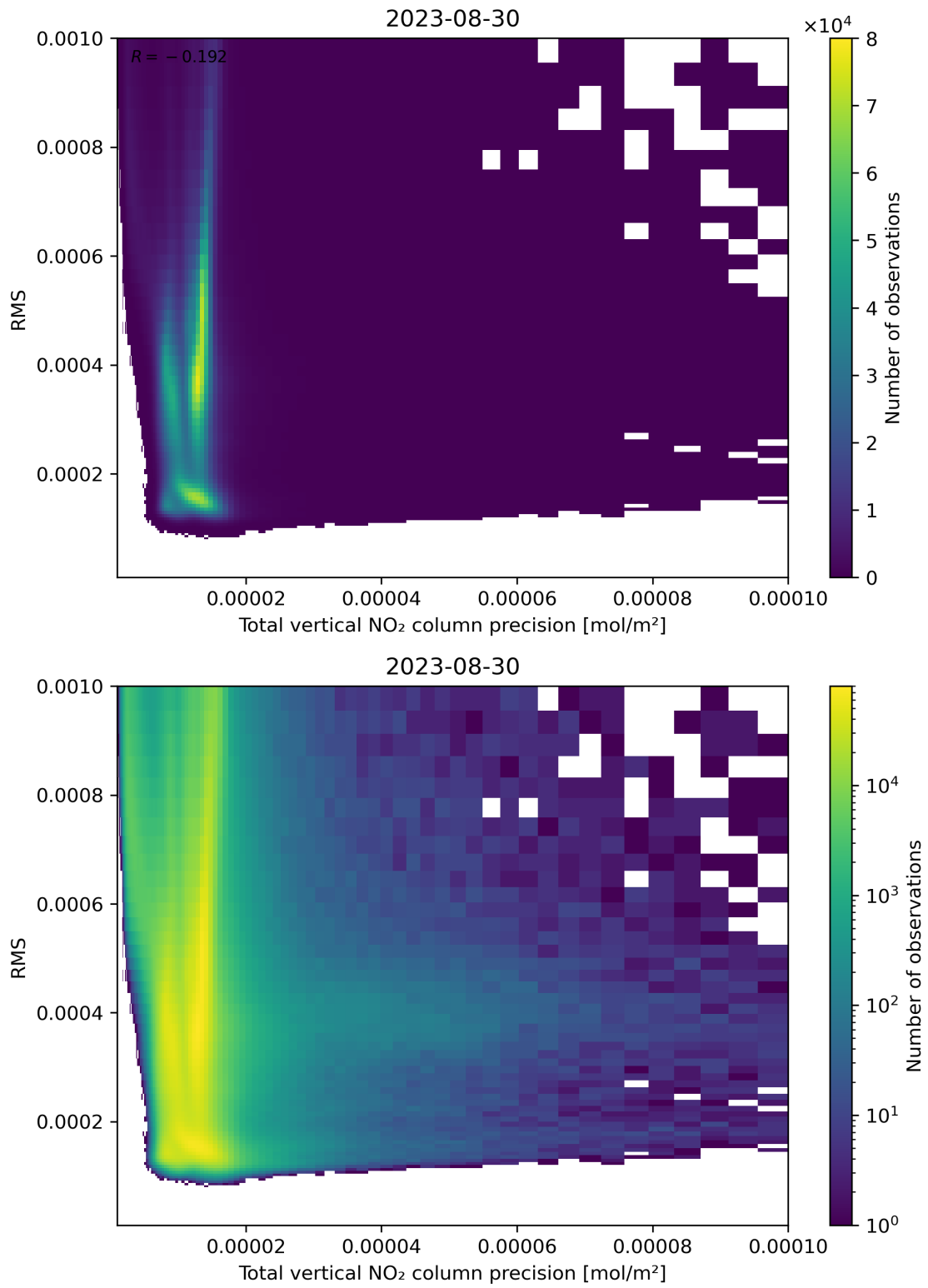
Figure 119: Scatter density plot of “Total vertical NO 2 column precision” against “RMS” for 2023-08-30 to 2023-08-31.
