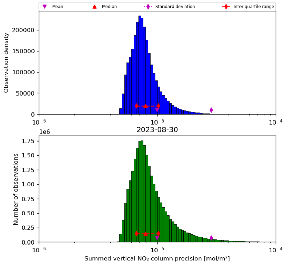
Figure 41: Histogram of "Summed vertical NO 2 column precision" for 2023-08-30 to 2023-08-31
