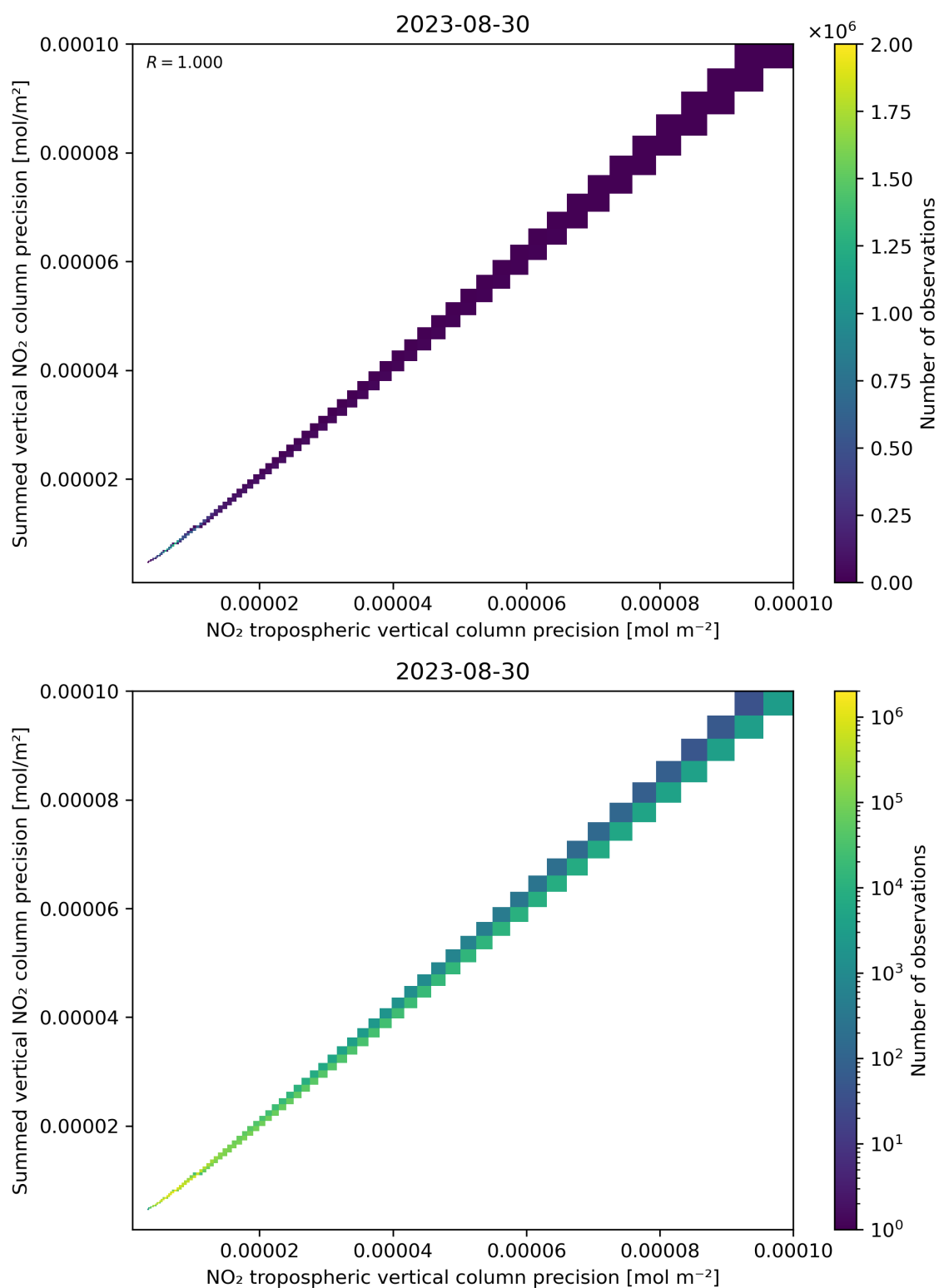
Figure 137: Scatter density plot of “NO 2 tropospheric vertical column precision” against “Summed vertical NO 2 column precision” for 2023-08-30 to 2023-08-31.
