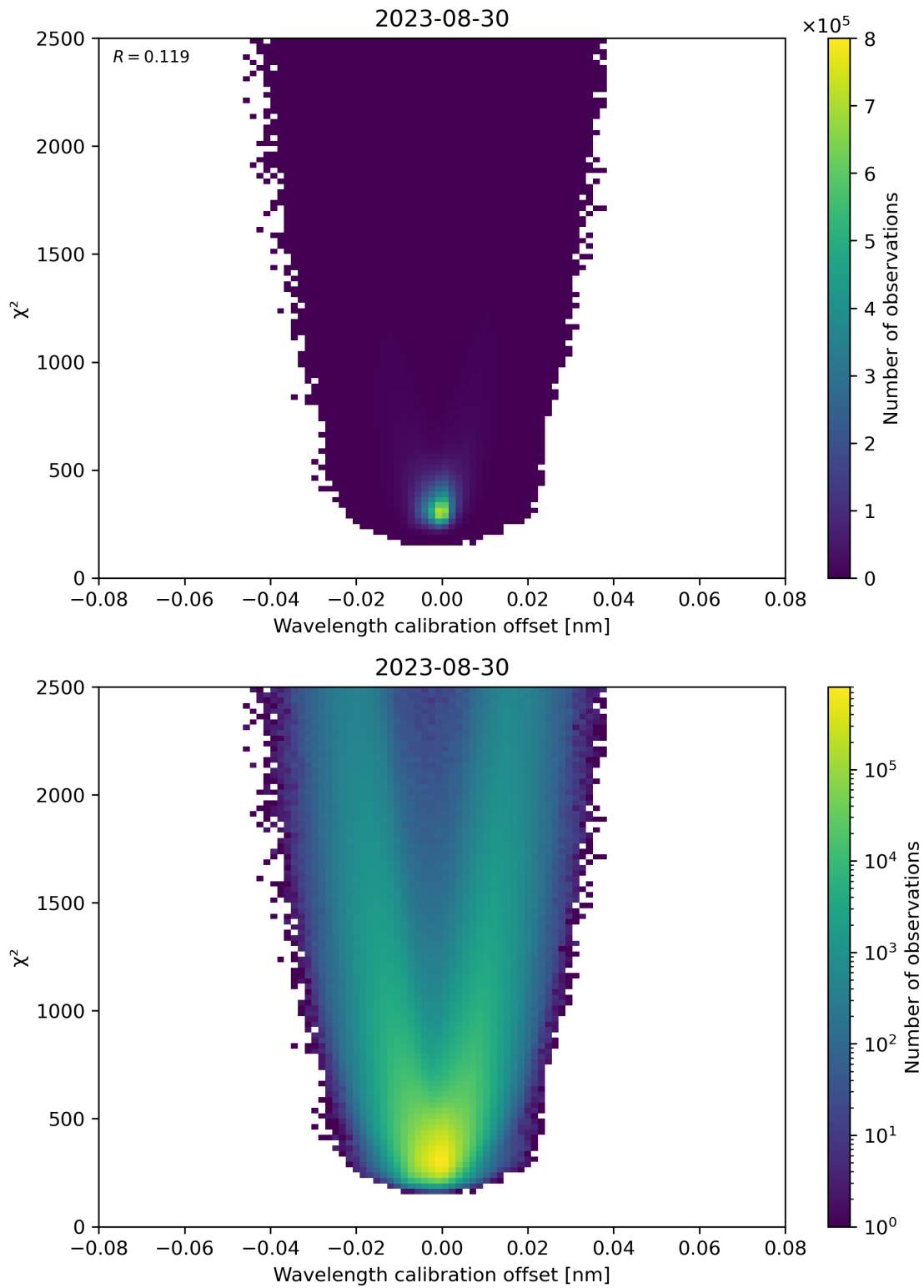
Figure 175: Scatter density plot of “Wavelength calibration offset” against “ \chi^2 ” for 2023-08-30 to 2023-08-31.
