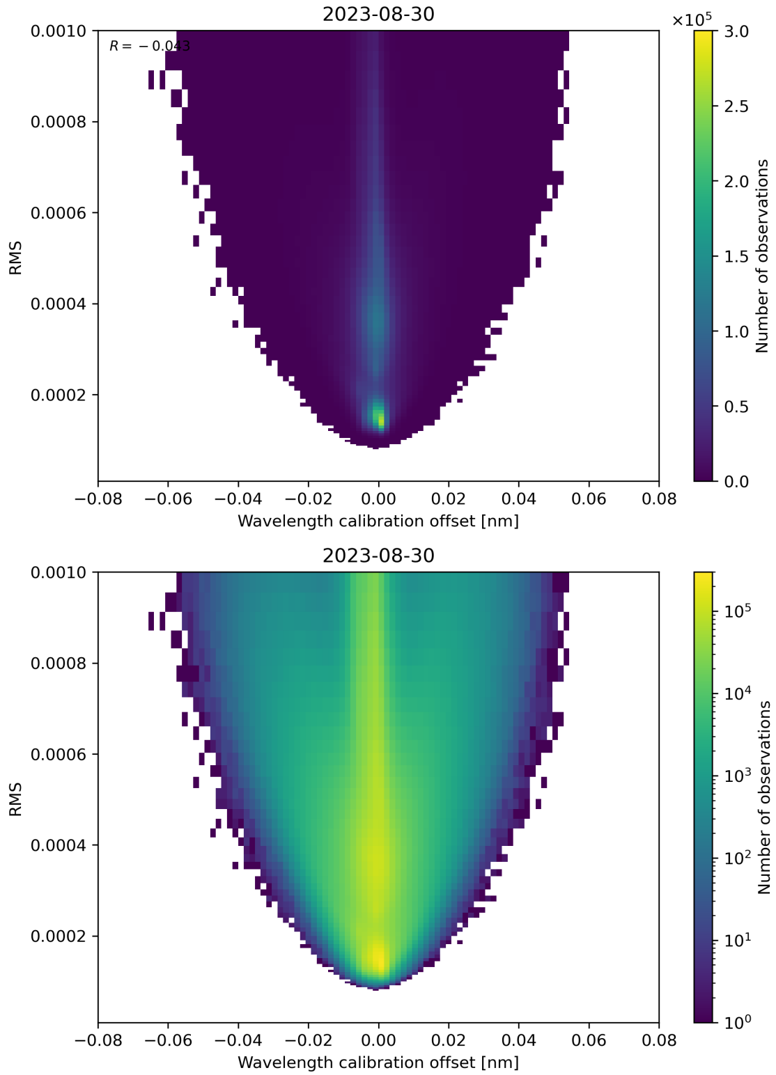
Figure 181: Scatter density plot of “Wavelength calibration offset” against “RMS” for 2023-08-30 to 2023-08-31.
