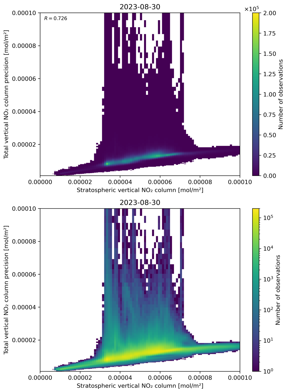
Figure 101: Scatter density plot of “Stratospheric vertical NO 2 column” against “Total vertical NO 2 column precision” for 2023-08-30 to 2023-08-31.
