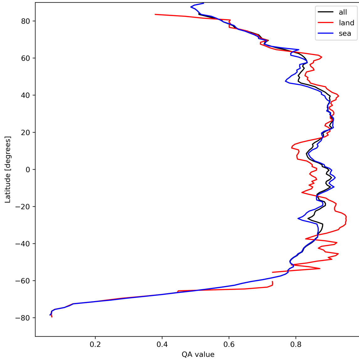
Figure 11: Zonal average of “QA value” for 2023-08-30 to 2023-08-31.
