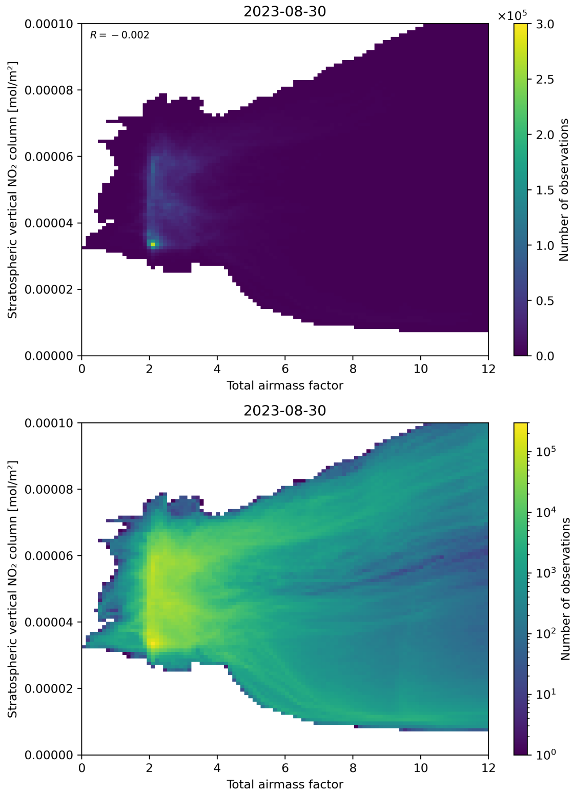
Figure 64: Scatter density plot of “Total airmass factor” against “Stratospheric vertical NO 2 column” for 2023-08-30 to 2023-08-31.
