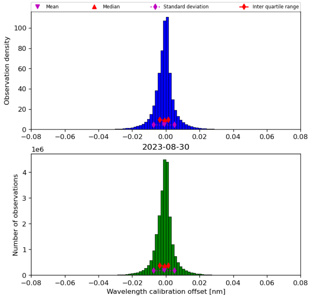
Figure 35: Histogram of “Wavelength calibration offset” for 2023-08-30 to 2023-08-31
