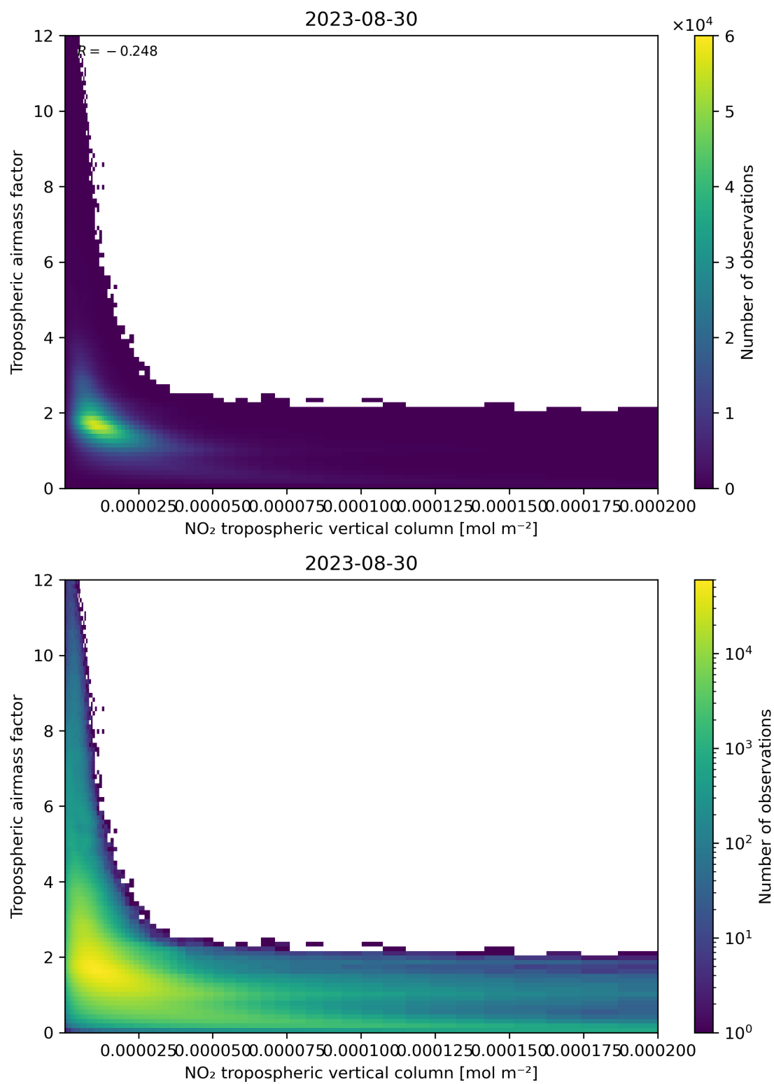
Figure 123: Scatter density plot of “NO 2 tropospheric vertical column” against “Tropospheric air mass factor” for 2023-08-30 to 2023-08-31.
