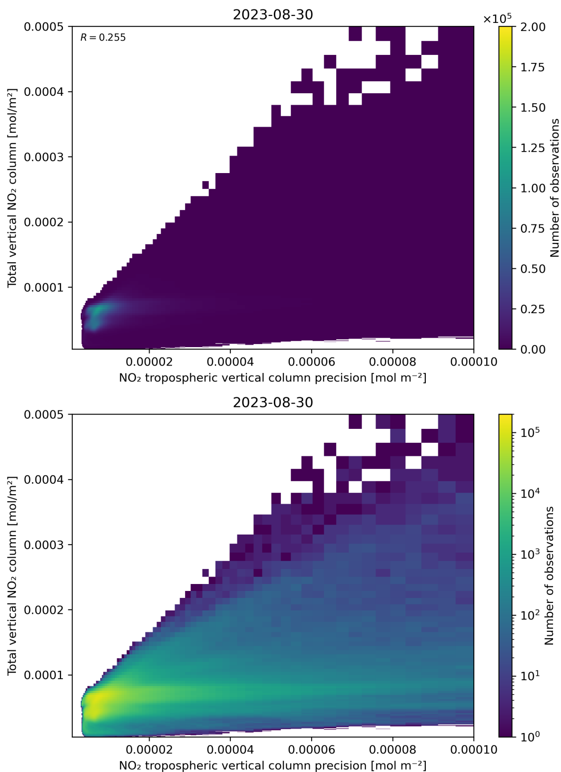
Figure 138: Scatter density plot of “NO 2 tropospheric vertical column precision” against “Total vertical NO 2 column” for 2023-08-30 to 2023-08-31.
