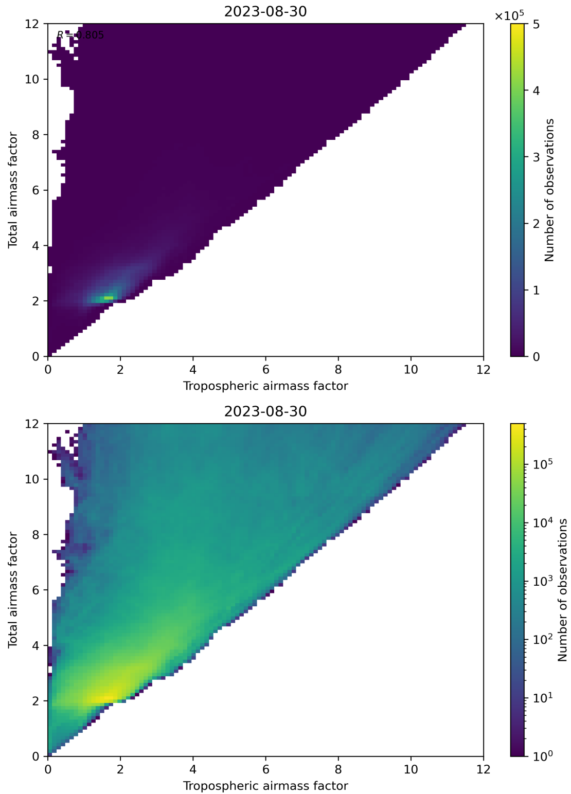
Figure 72: Scatter density plot of “Tropospheric airmass factor” against “Total airmass factor” for 2023-08-30 to 2023-08-31.
