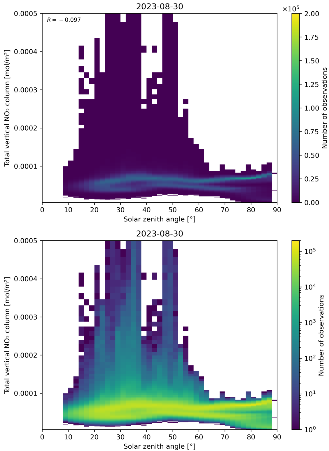
Figure 153: Scatter density plot of “Solar zenith angle” against “Total vertical NO 2 column” for 2023-08-30 to 2023-08-31.
