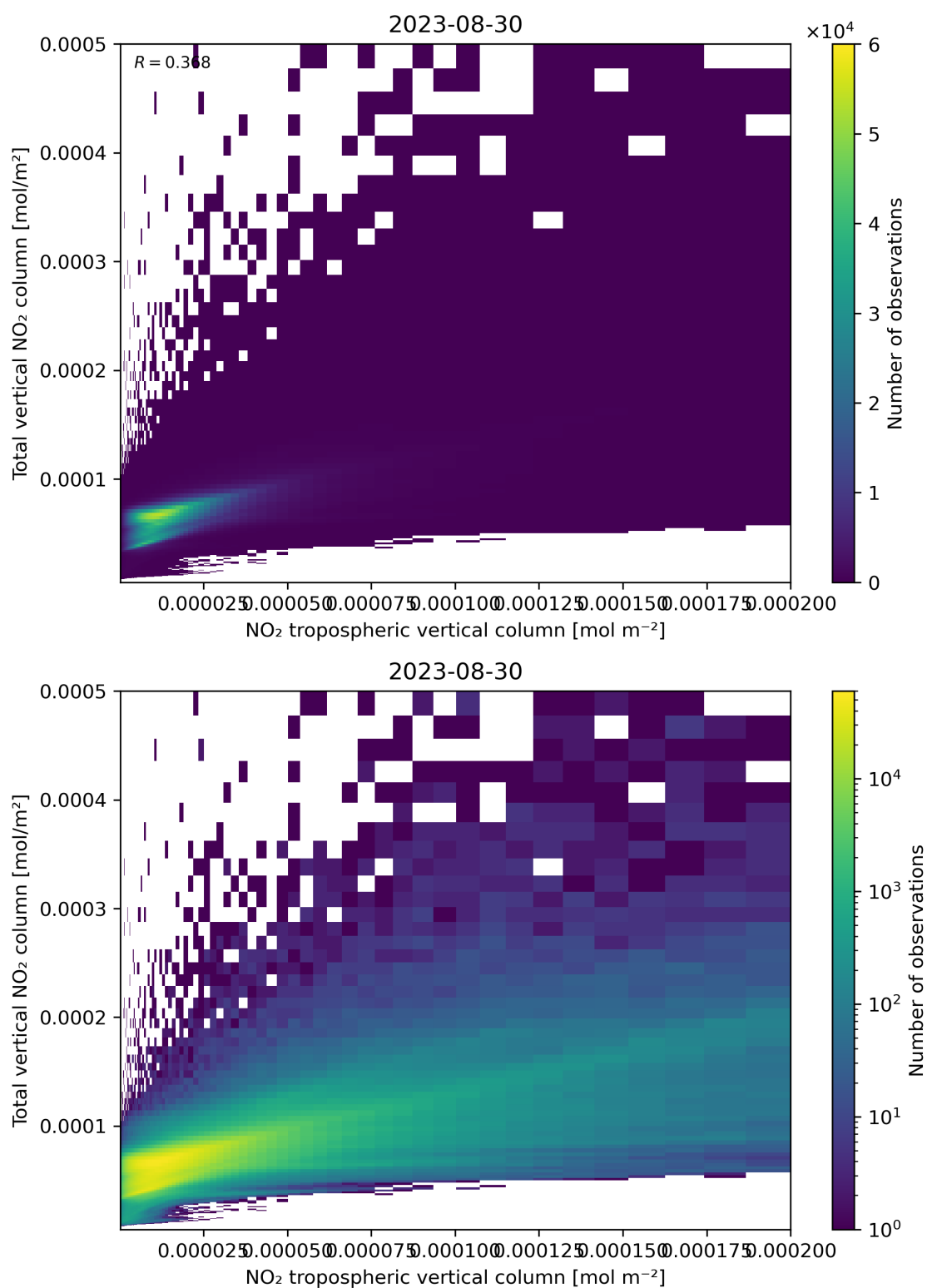
Figure 128: Scatter density plot of “NO 2 tropospheric vertical column” against “Total vertical NO 2 column” for 2023-08-30 to 2023-08-31.
