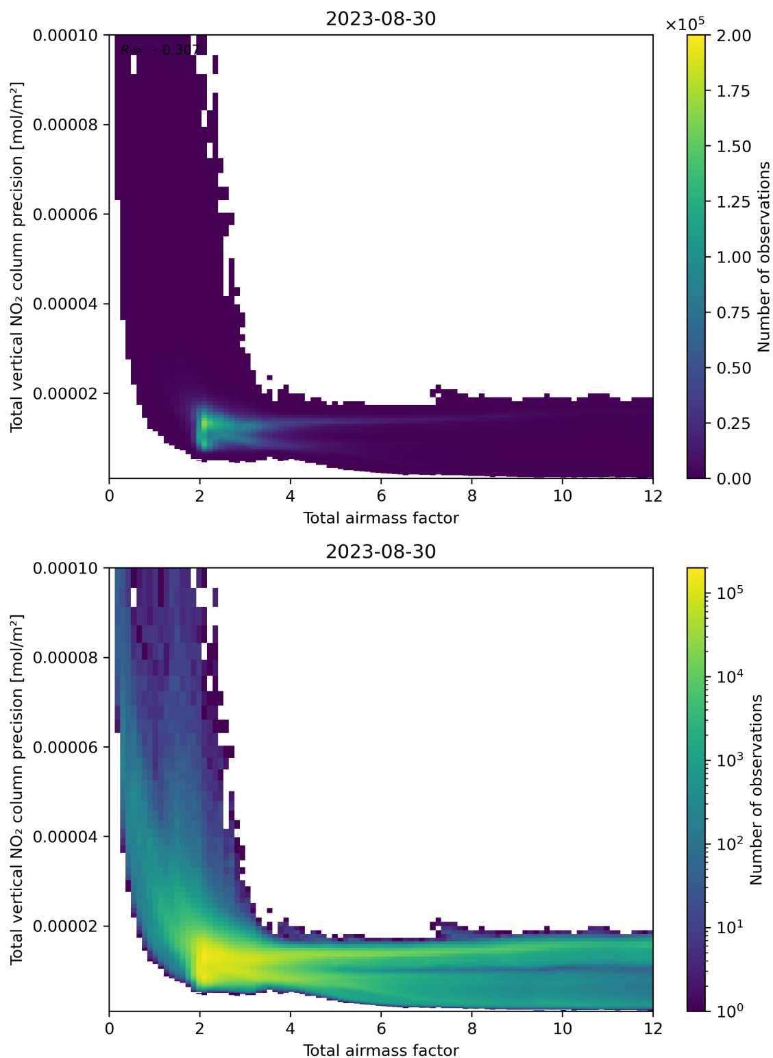
Figure 68: Scatter density plot of “Total airmass factor” against “Total vertical NO 2 column precision” for 2023-08-30 to 2023-08-31.
