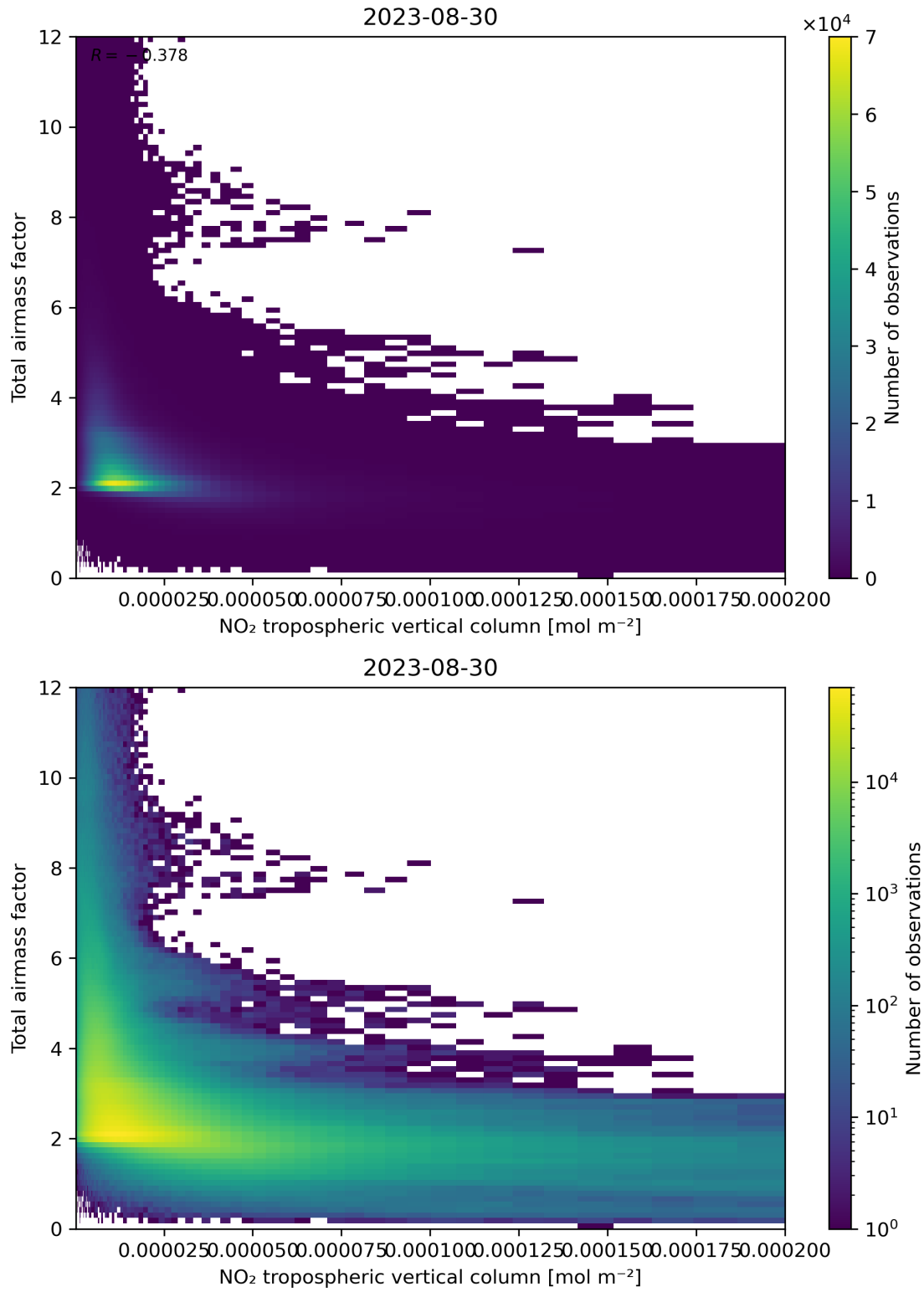
Figure 122: Scatter density plot of “NO 2 tropospheric vertical column” against “Total airmass factor” for 2023-08-30 to 2023-08-31.
