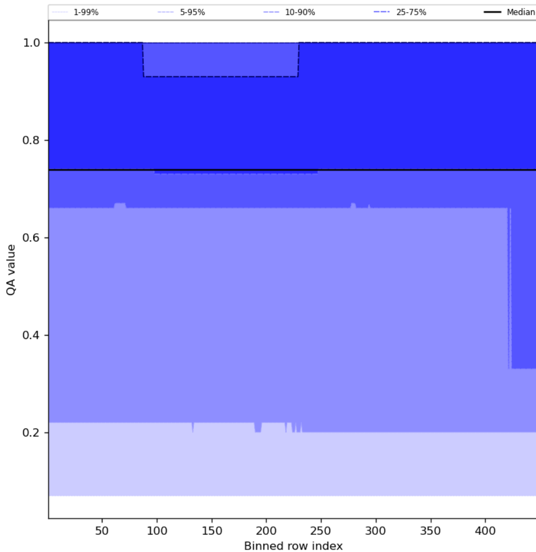
Figure 45: Along track statistics of “QA value” for 2023-08-30 to 2023-08-31
