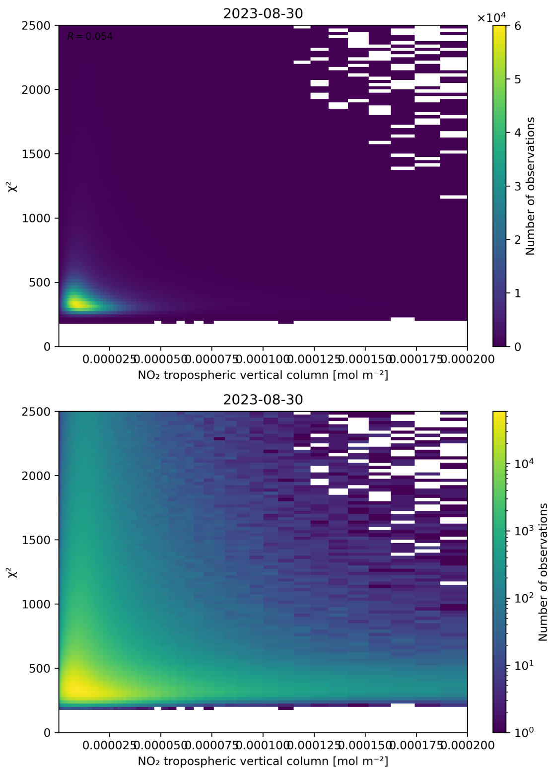
Figure 124: Scatter density plot of “NO 2 tropospheric vertical column” against “ \chi^2 ” for 2023-08-30 to 2023-08-31.
