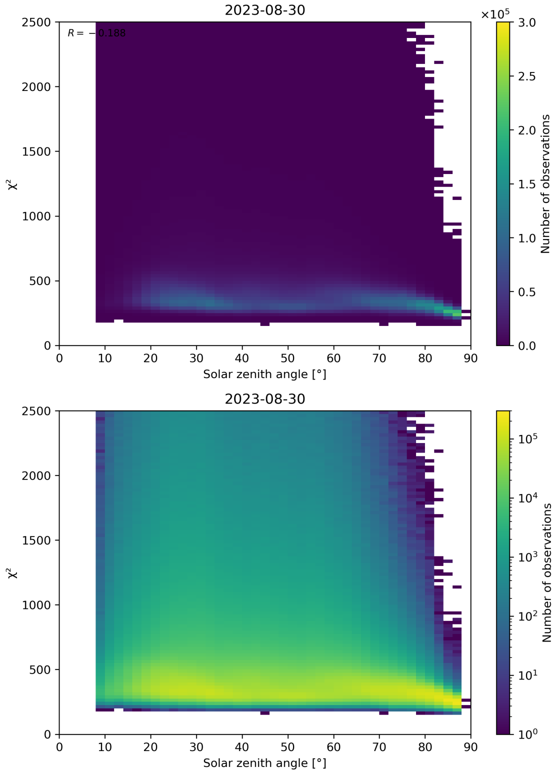
Figure 148: Scatter density plot of “Solar zenith angle” against “ \chi^2 ” for 2023-08-30 to 2023-08-31.
