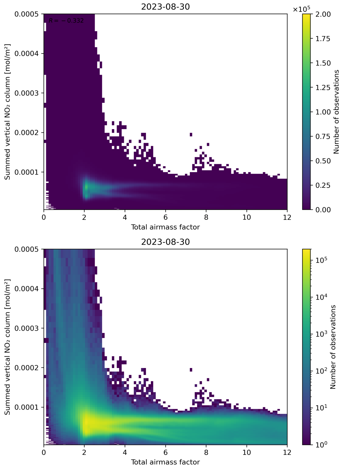
Figure 65: Scatter density plot of “Total airmass factor” against “Summed vertical NO 2 column” for 2023-08-30 to 2023-08-31.
