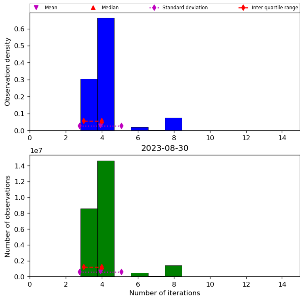
Figure 34: Histogram of “Number of iterations” for 2023-08-30 to 2023-08-31
