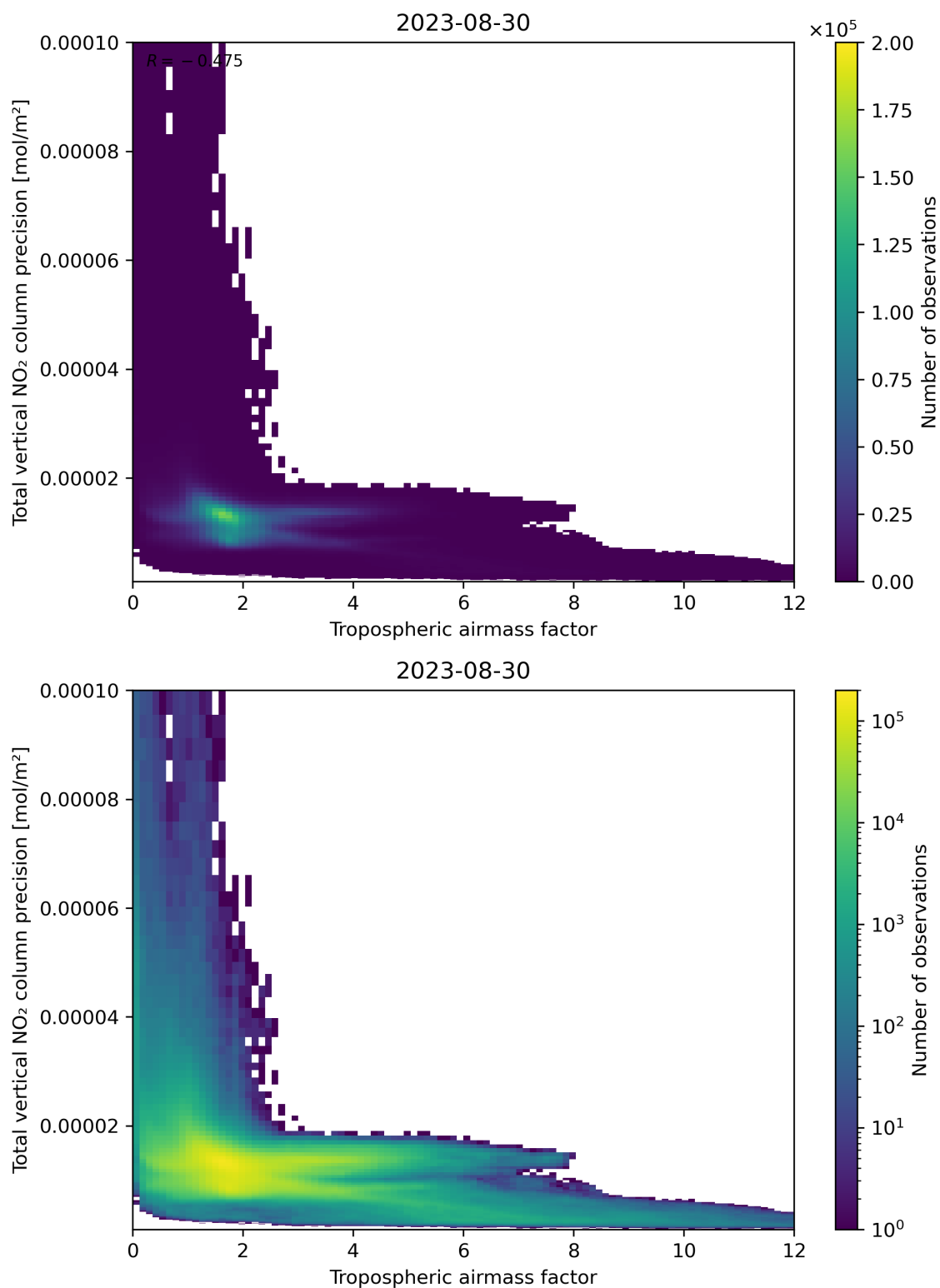
Figure 78: Scatter density plot of “Tropospheric air mass factor” against “Total vertical NO 2 column precision” for 2023-08-30 to 2023-08-31.
