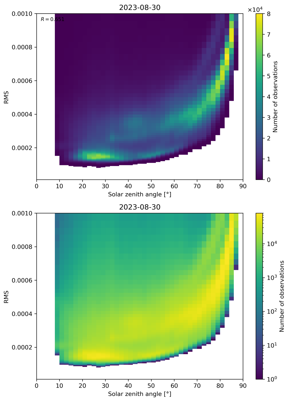
Figure 157: Scatter density plot of “Solar zenith angle” against “RMS” for 2023-08-30 to 2023-08-31.
