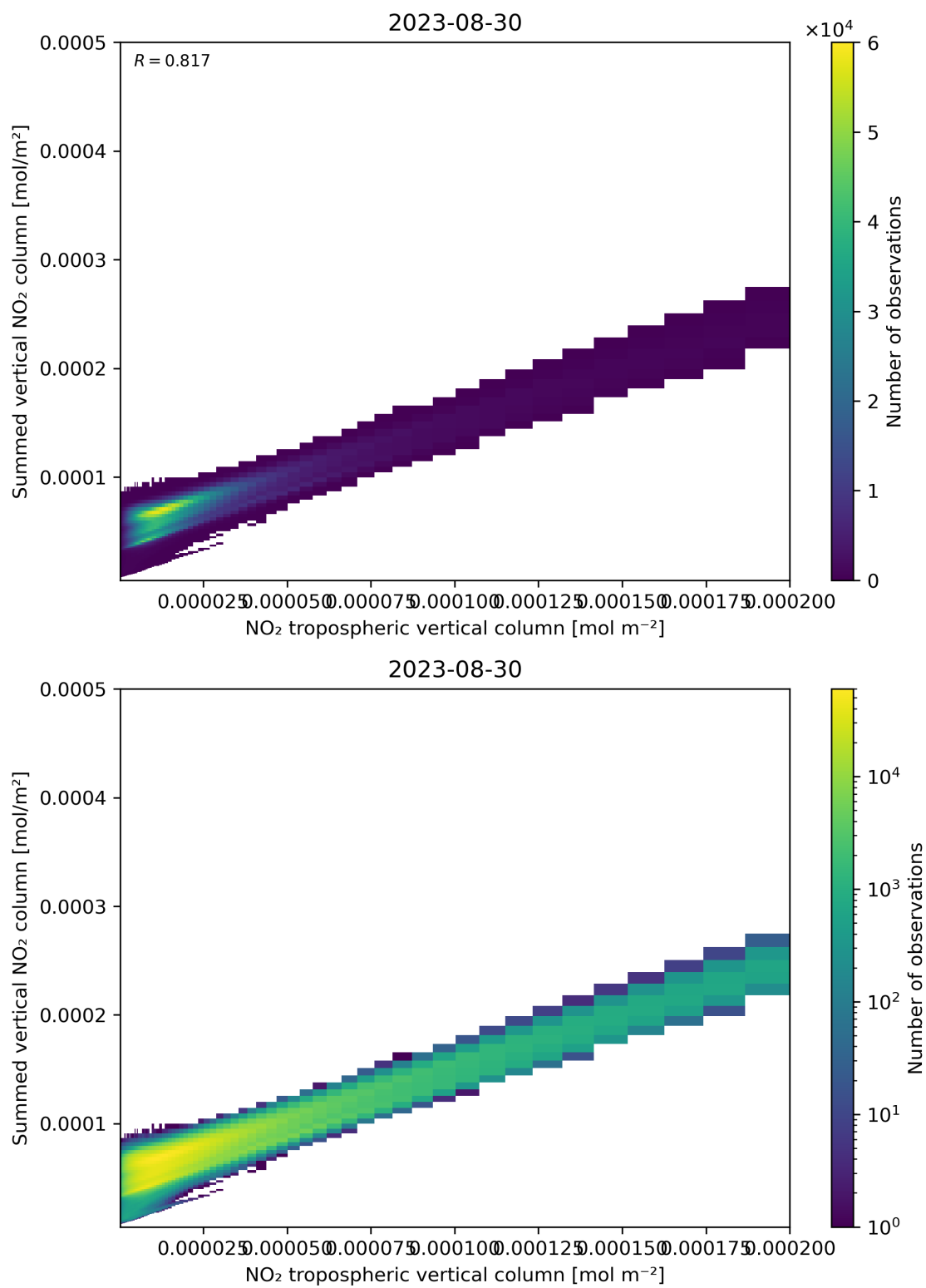
Figure 126: Scatter density plot of “NO 2 tropospheric vertical column” against “Summed vertical NO 2 column” for 2023-08-30 to 2023-08-31.
