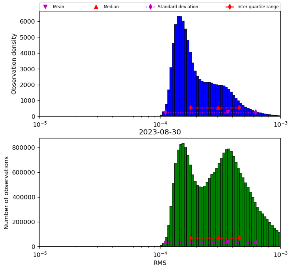
Figure 43: Histogram of “RMS” for 2023-08-30 to 2023-08-31
