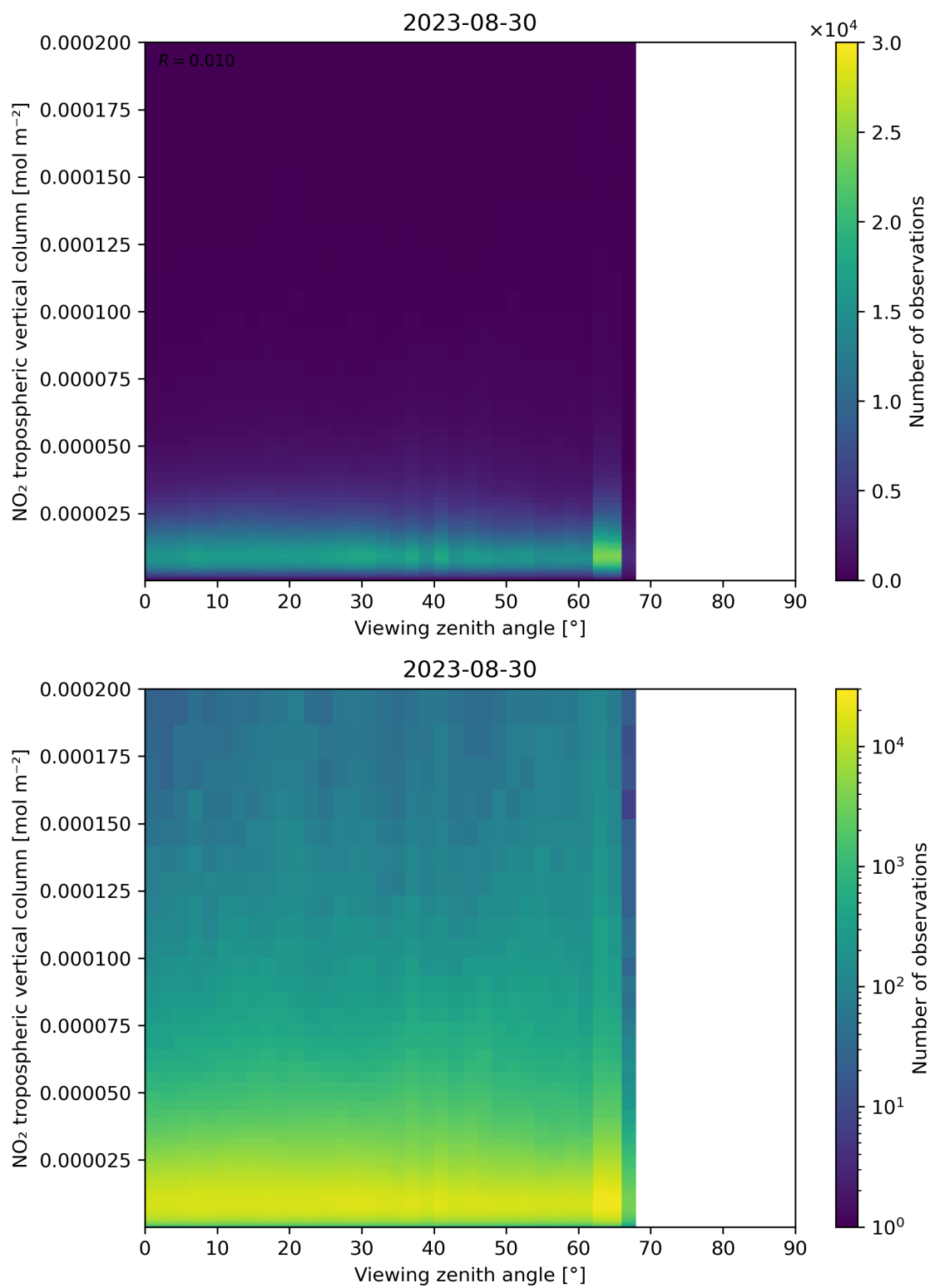
Figure 169: Scatter density plot of “Viewing zenith angle” against “NO 2 tropospheric vertical column” for 2023-08-30 to 2023-08-31.
