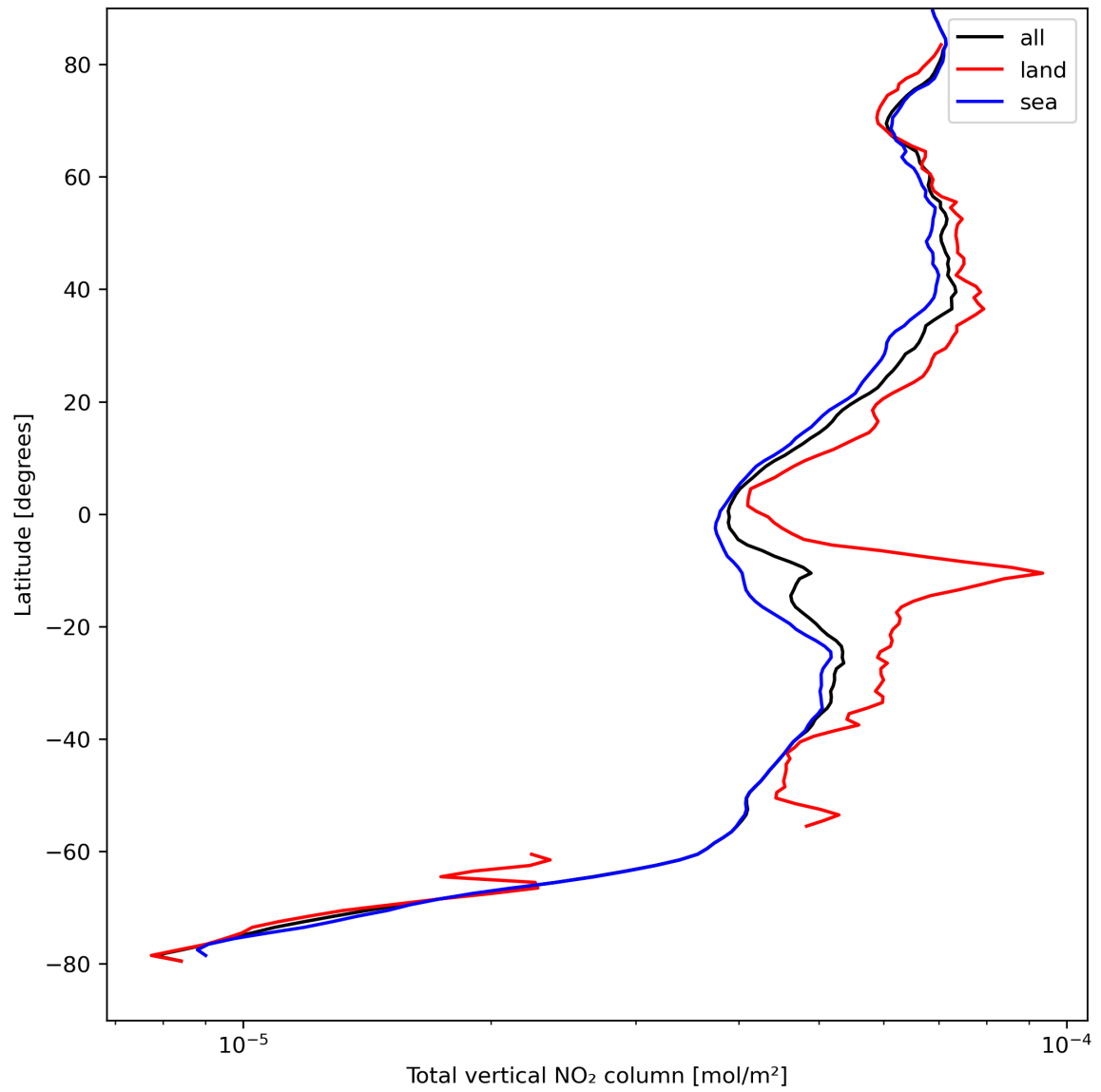
Figure 21: Zonal average of “Total vertical NO 2 column” for 2023-08-30 to 2023-08-31.
