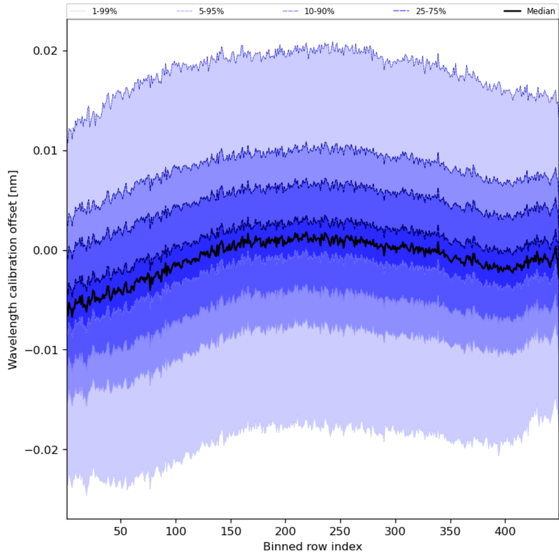
Figure 52: Along track statistics of “Wavelength calibration offset” for 2023-08-30 to 2023-08-31
