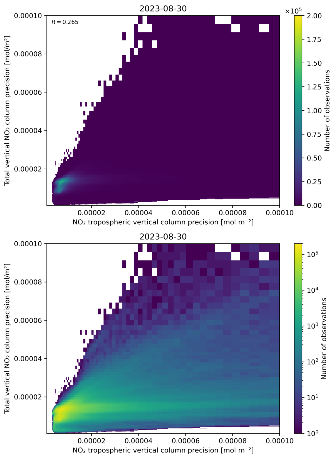
Figure 139: Scatter density plot of “NO 2 tropospheric vertical column precision” against “Total vertical NO 2 column precision” for 2023-08-30 to 2023-08-31.
