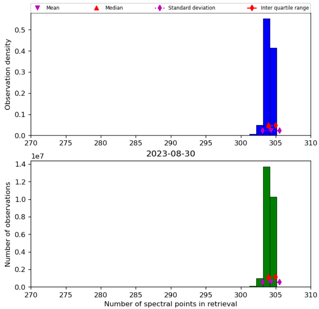
Figure 33: Histogram of “Number of spectral points in retrieval” for 2023-08-30 to 2023-08-31
