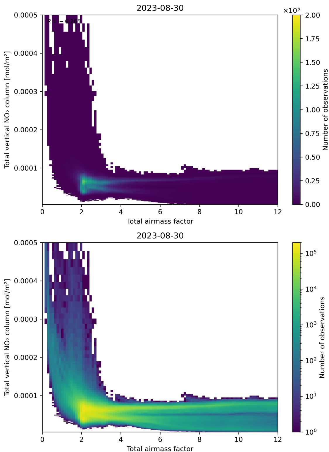
Figure 67: Scatter density plot of “Total airmass factor” against “Total vertical NO 2 column” for 2023-08-30 to 2023-08-31.
