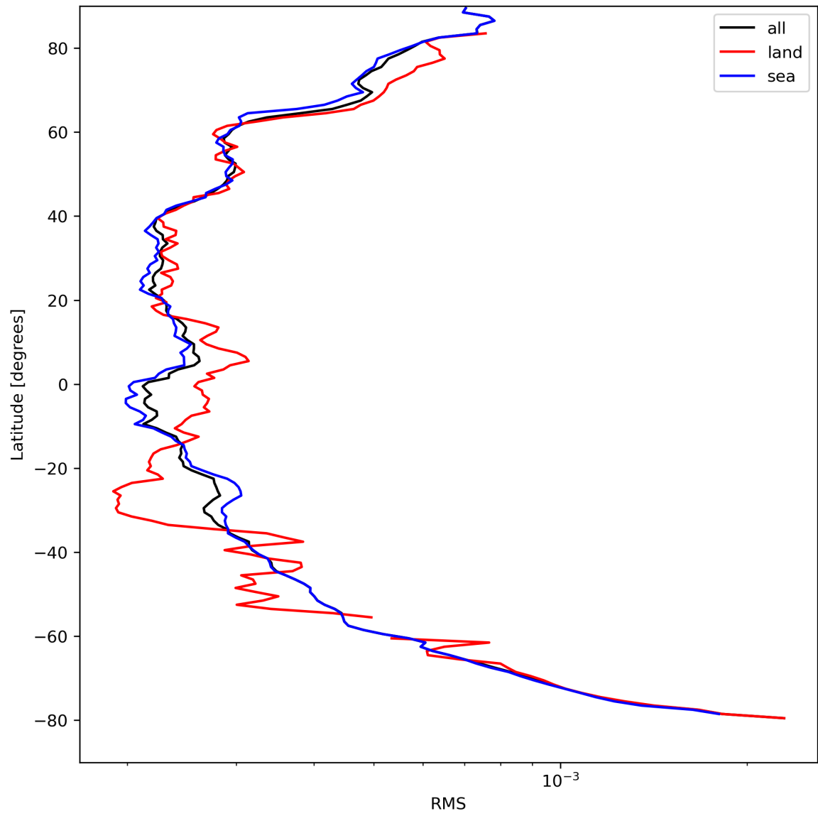
Figure 26: Zonal average of “RMS” for 2023-08-30 to 2023-08-31.
