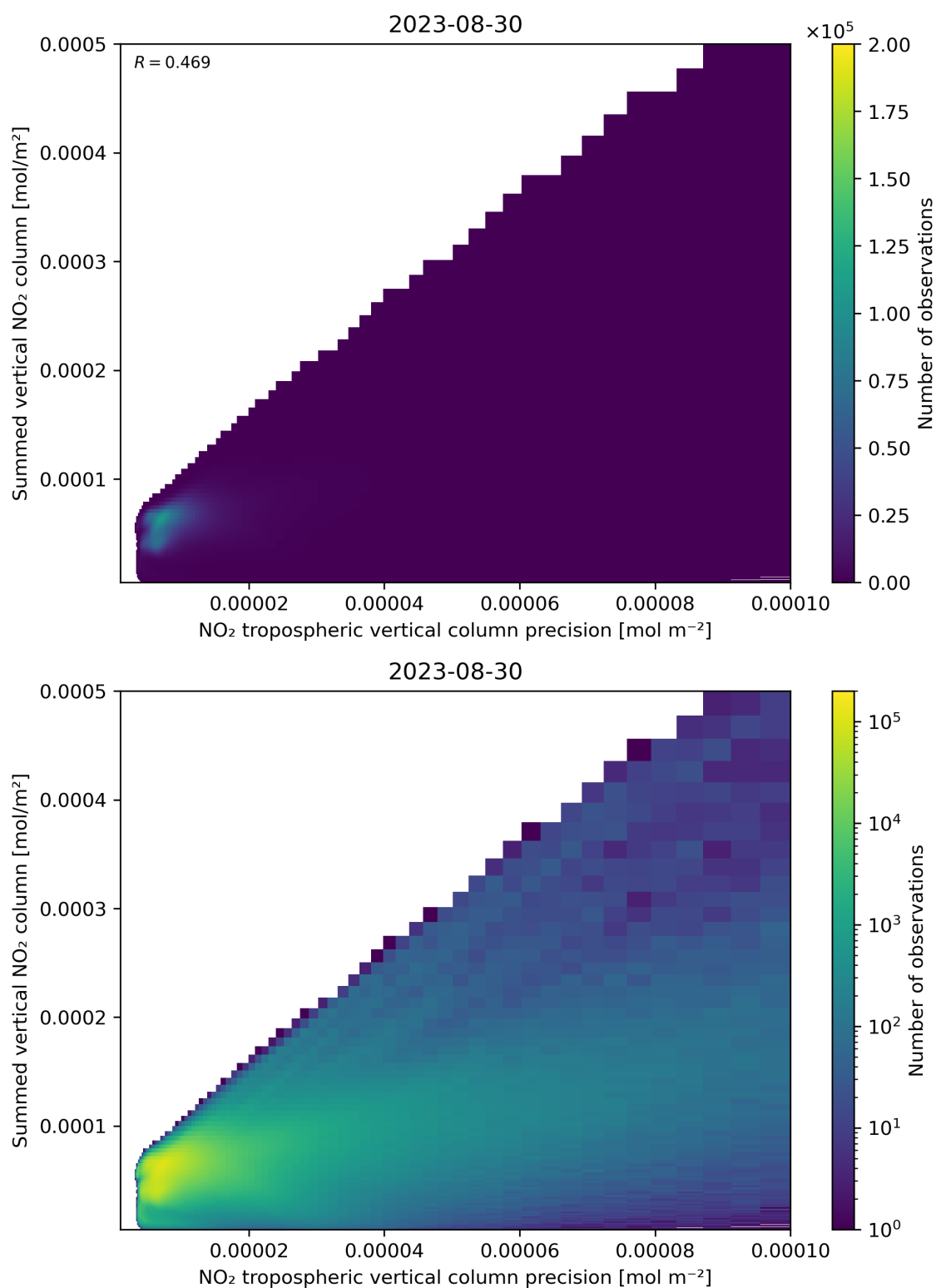
Figure 136: Scatter density plot of “NO 2 tropospheric vertical column precision” against “Summed vertical NO 2 column” for 2023-08-30 to 2023-08-31.
