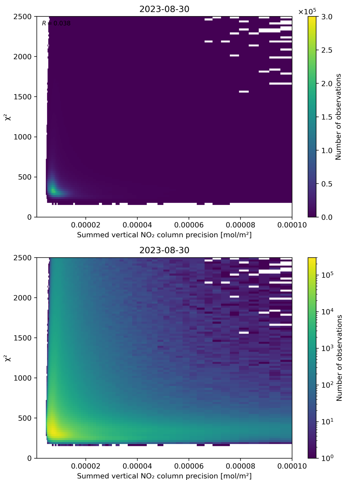
Figure 107: Scatter density plot of “Summed vertical NO 2 column precision” against “ \chi^2 ” for 2023-08-30 to 2023-08-31.
