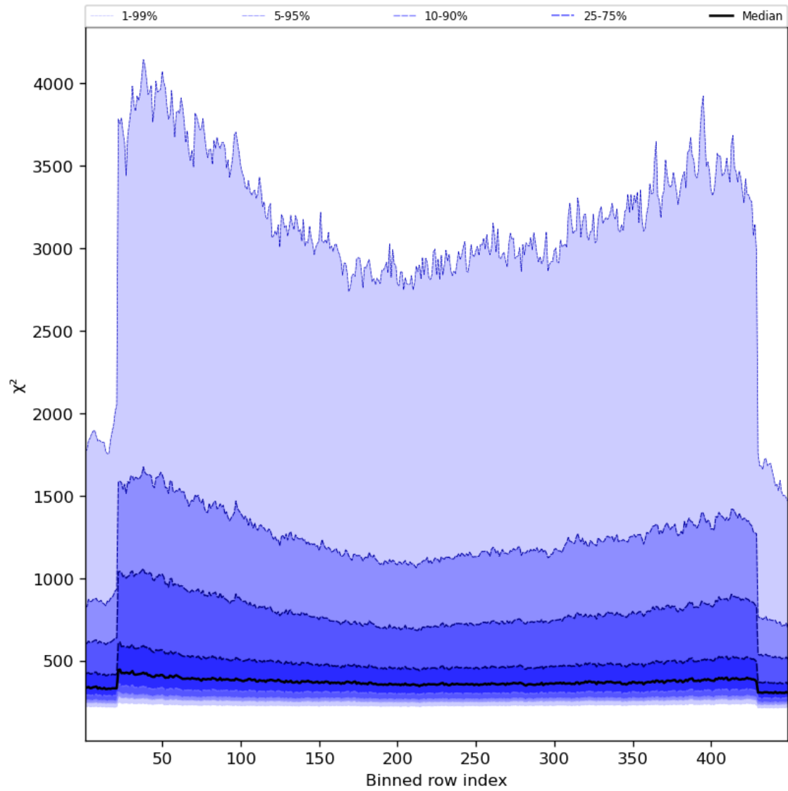
Figure 59: Along track statistics of “ \chi^2 ” for 2023-08-30 to 2023-08-31
