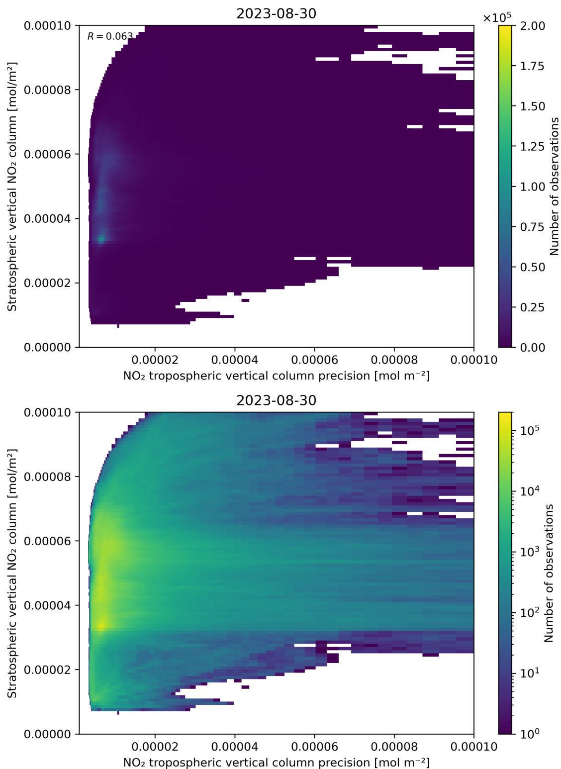
Figure 135: Scatter density plot of “NO 2 tropospheric vertical column precision” against “Stratospheric vertical NO 2 column” for 2023-08-30 to 2023-08-31.
