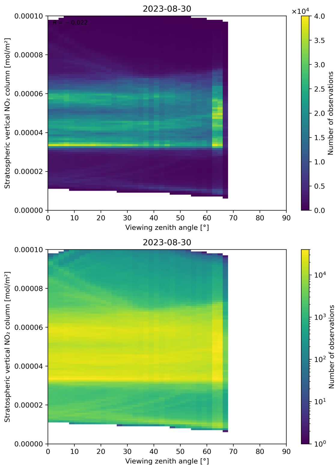
Figure 164: Scatter density plot of “Viewing zenith angle” against “Stratospheric vertical NO 2 column” for 2023-08-30 to 2023-08-31.
