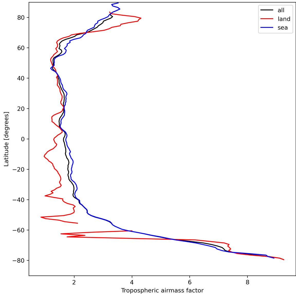
Figure 14: Zonal average of “Tropospheric airmass factor” for 2023-08-30 to 2023-08-31.
