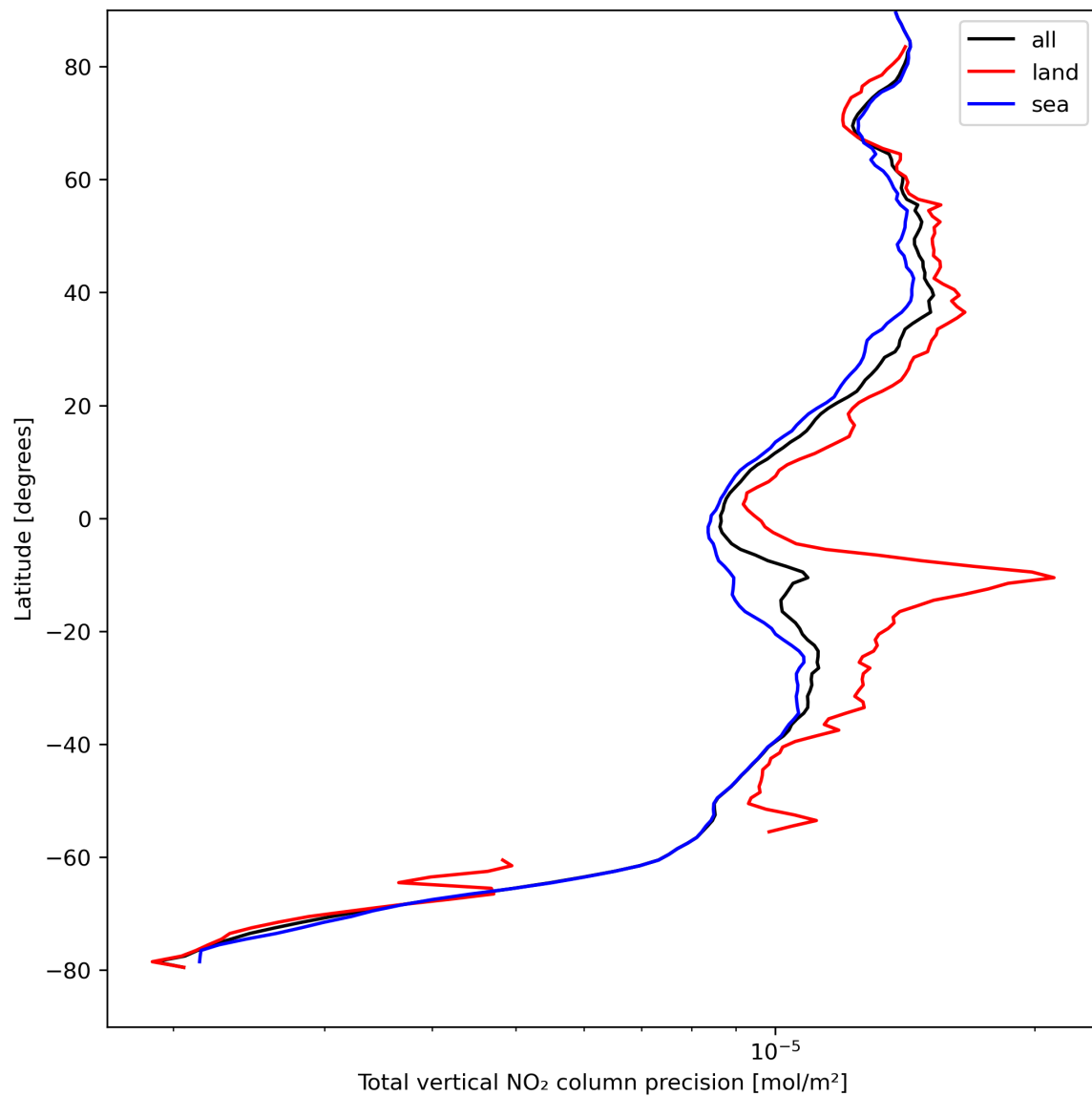
Figure 22: Zonal average of “Total vertical NO 2 column precision” for 2023-08-30 to 2023-08-31.
