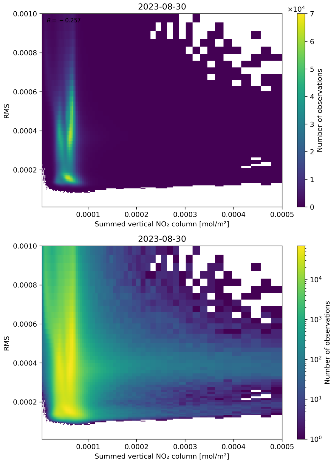
Figure 109: Scatter density plot of “Summed vertical NO 2 column” against “RMS” for 2023-08-30 to 2023-08-31.
