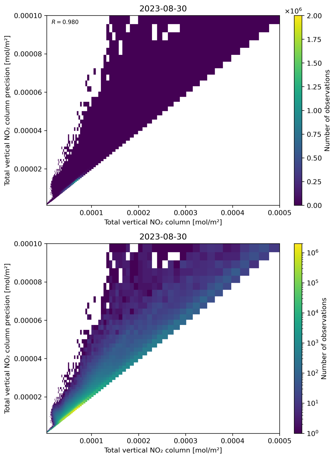
Figure 114: Scatter density plot of “Total vertical NO 2 column” against “Total vertical NO 2 column precision” for 2023-08-30 to 2023-08-31.
