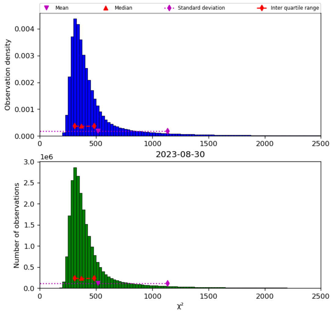
Figure 42: Histogram of “ \chi^2 ” for 2023-08-30 to 2023-08-31
