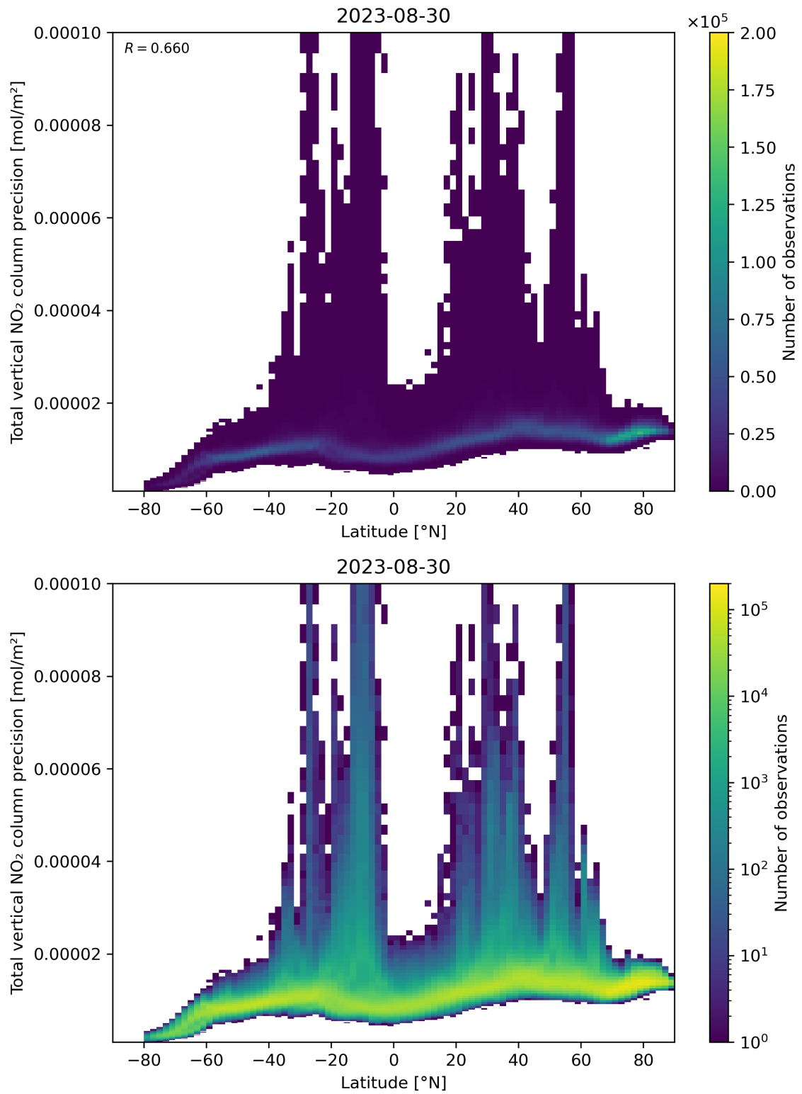
Figure 91: Scatter density plot of “Latitude” against “Total vertical NO 2 column precision” for 2023-08-30 to 2023-08-31.
