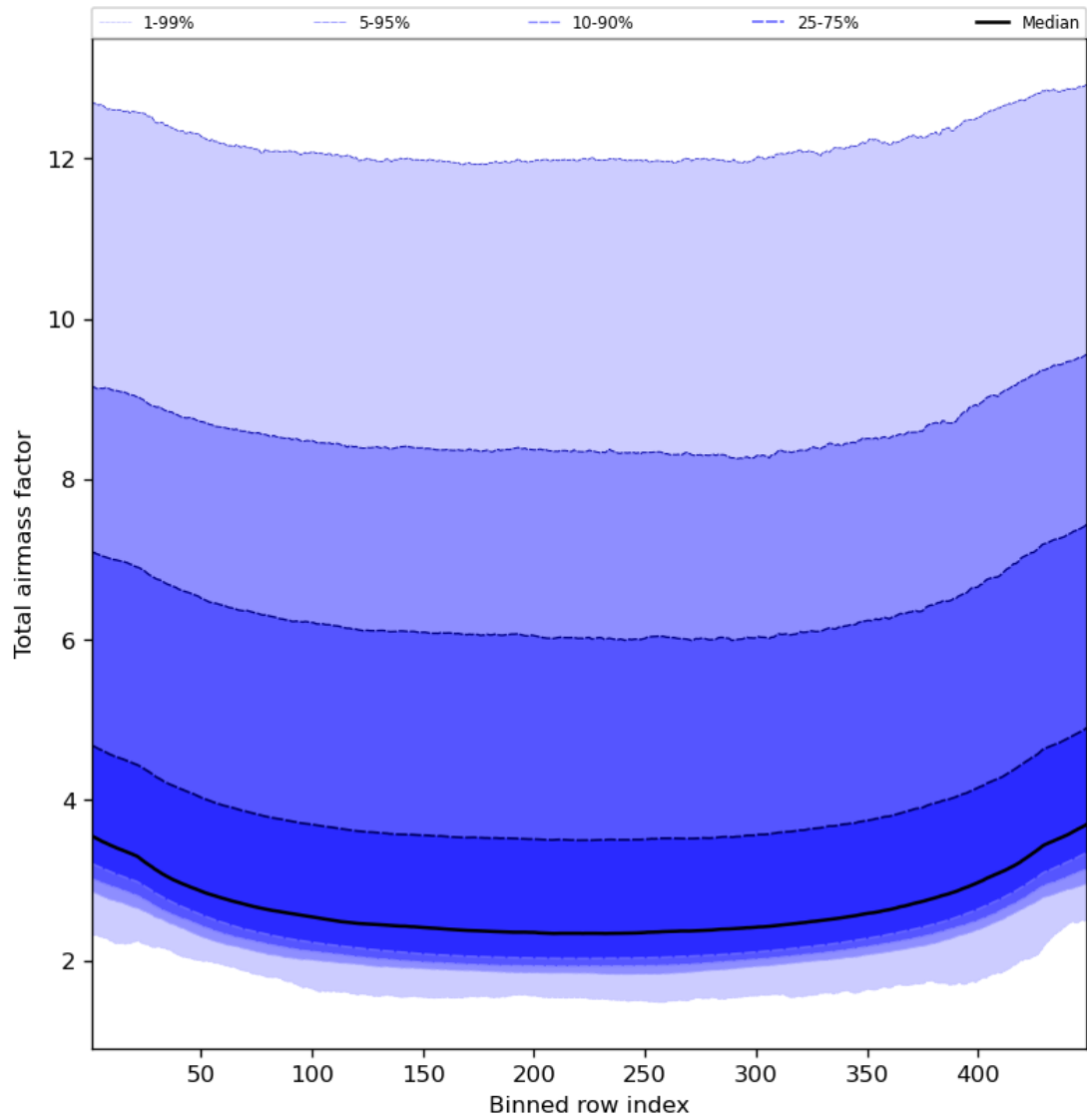
Figure 49: Along track statistics of “Total airmass factor” for 2023-08-30 to 2023-08-31
