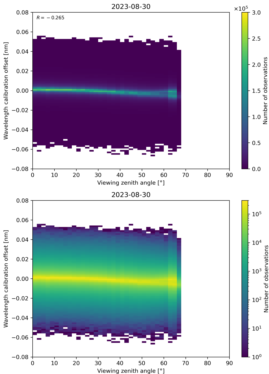
Figure 173: Scatter density plot of “Viewing zenith angle” against “Wavelength calibration offset” for 2023-08-30 to 2023-08-31.
