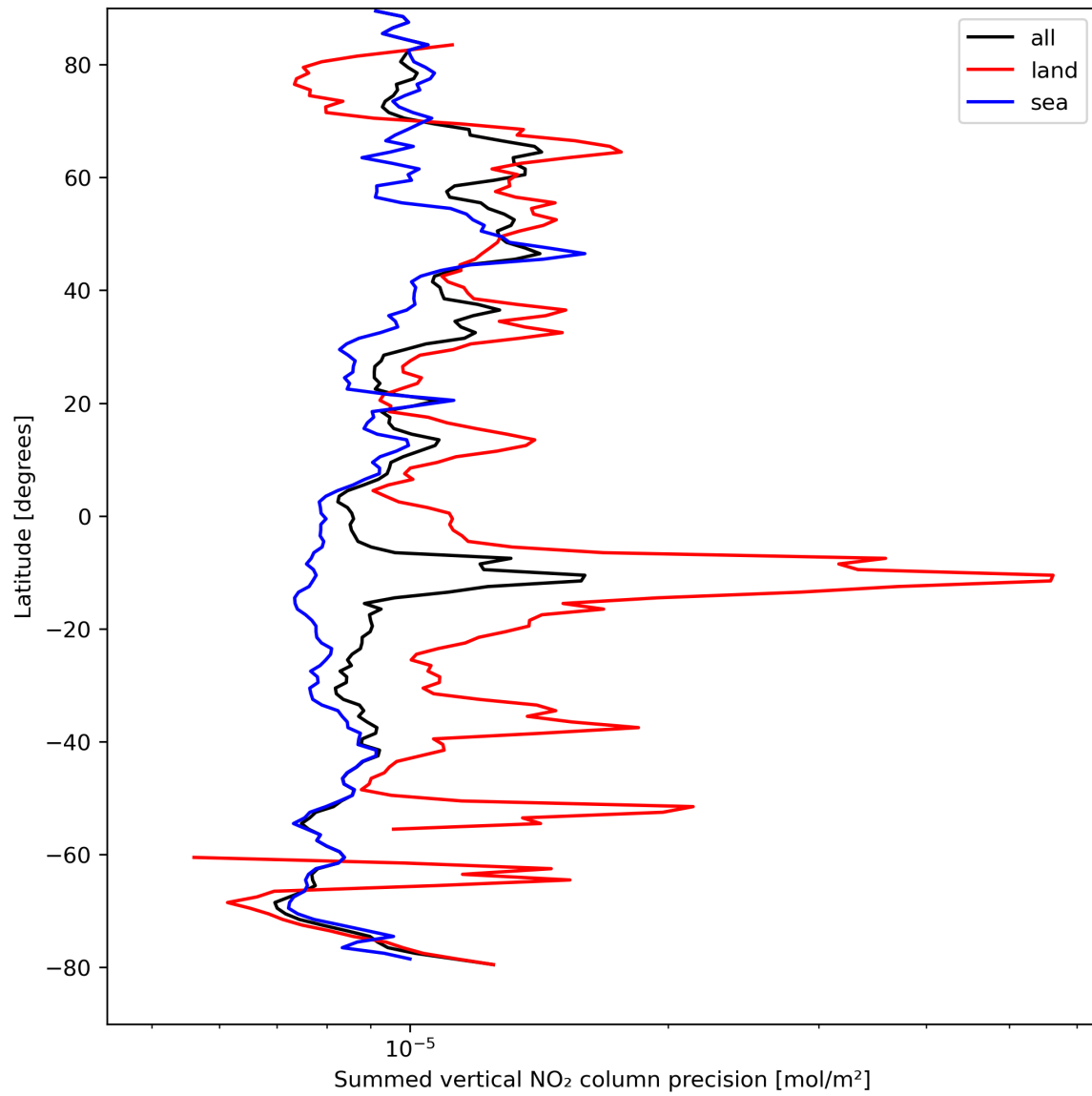
Figure 24: Zonal average of “Summed vertical NO 2 column precision” for 2023-08-30 to 2023-08-31.
