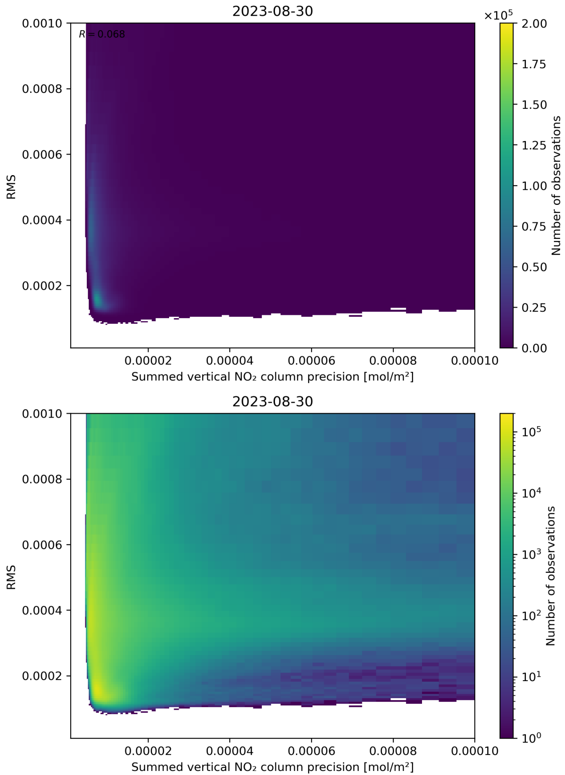
Figure 108: Scatter density plot of “Summed vertical NO 2 column precision” against “RMS” for 2023-08-30 to 2023-08-31.
