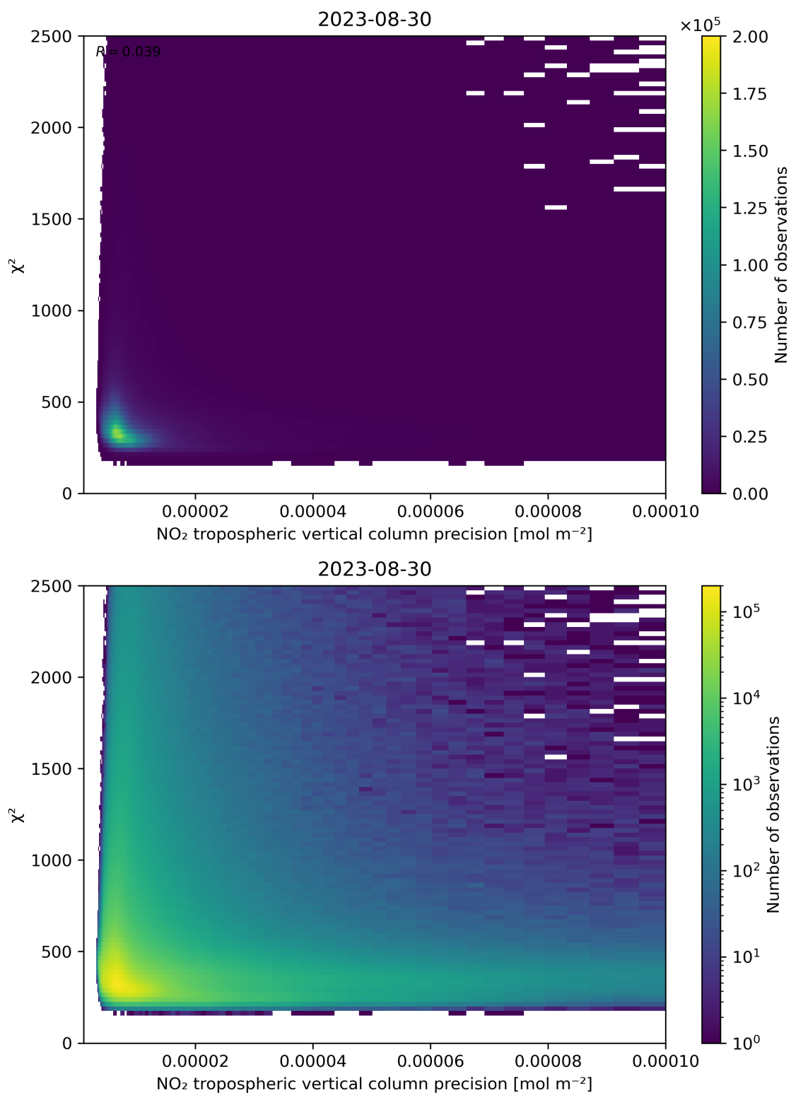
Figure 134: Scatter density plot of “NO 2 tropospheric vertical column precision” against “ \chi^2 ” for 2023-08-30 to 2023-08-31.
