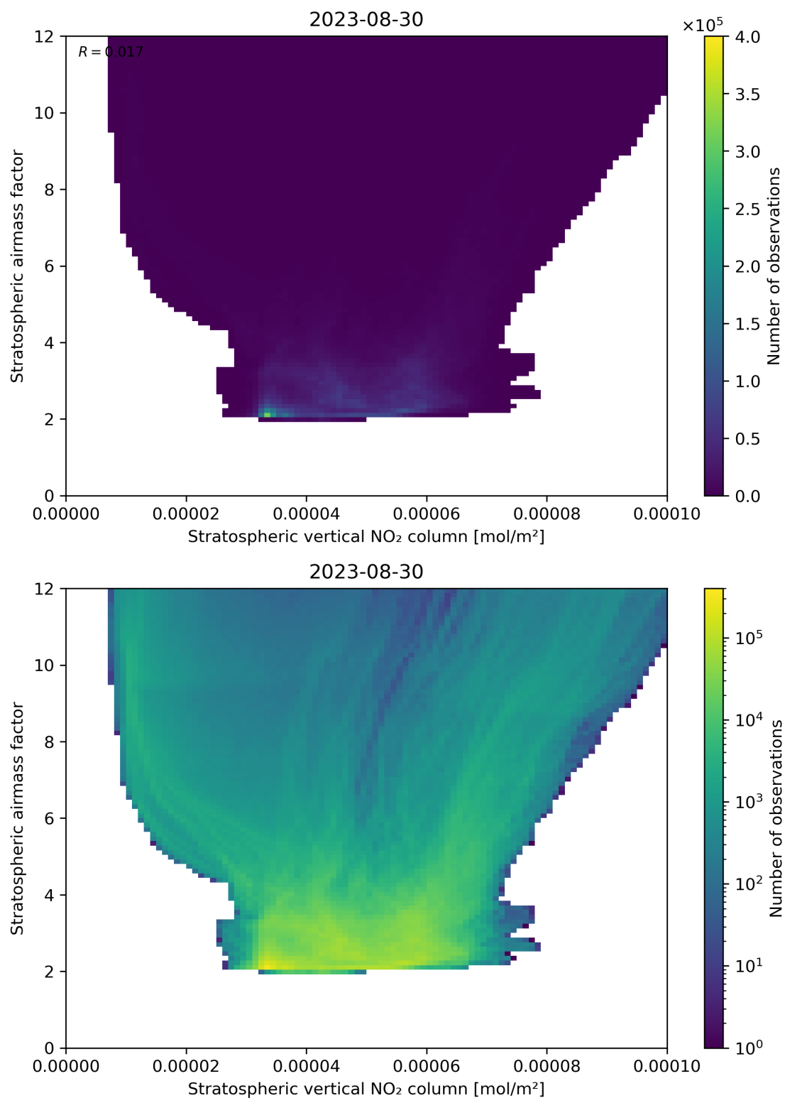
Figure 96: Scatter density plot of “Stratospheric vertical NO 2 column” against “Stratospheric airmass factor” for 2023-08-30 to 2023-08-31.
