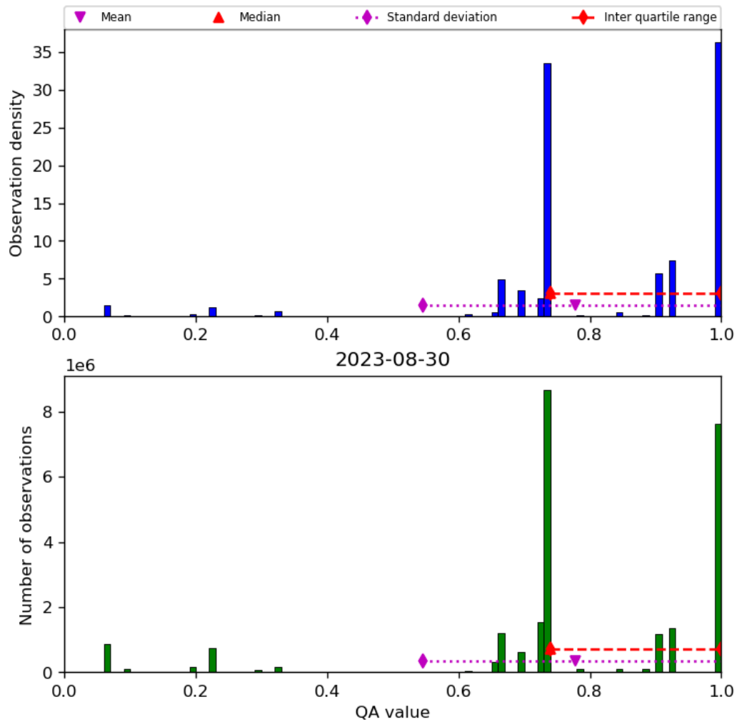
Figure 28: Histogram of “QA value” for 2023-08-30 to 2023-08-31
