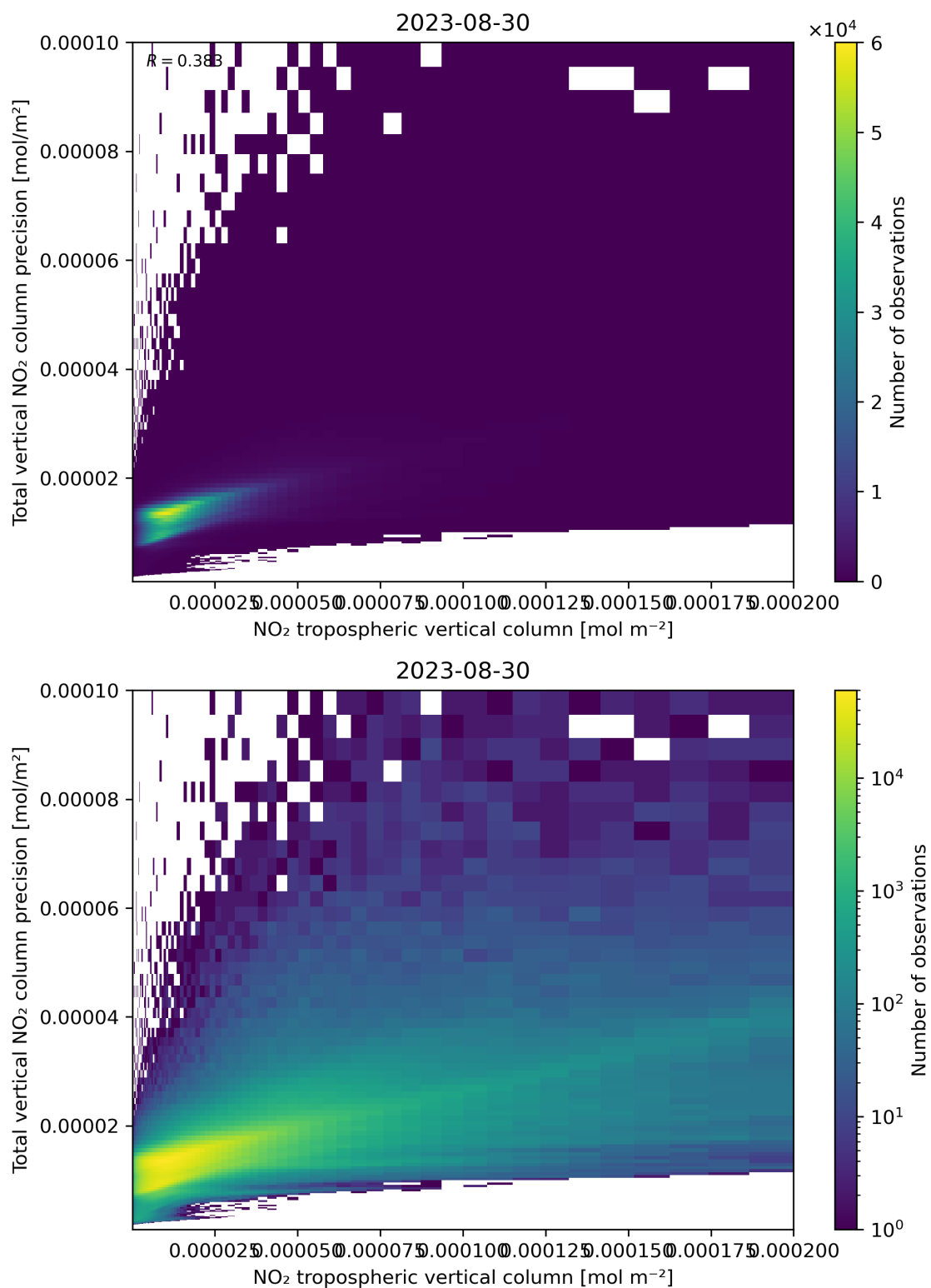
Figure 129: Scatter density plot of “NO 2 tropospheric vertical column” against “Total vertical NO 2 column precision” for 2023-08-30 to 2023-08-31.
