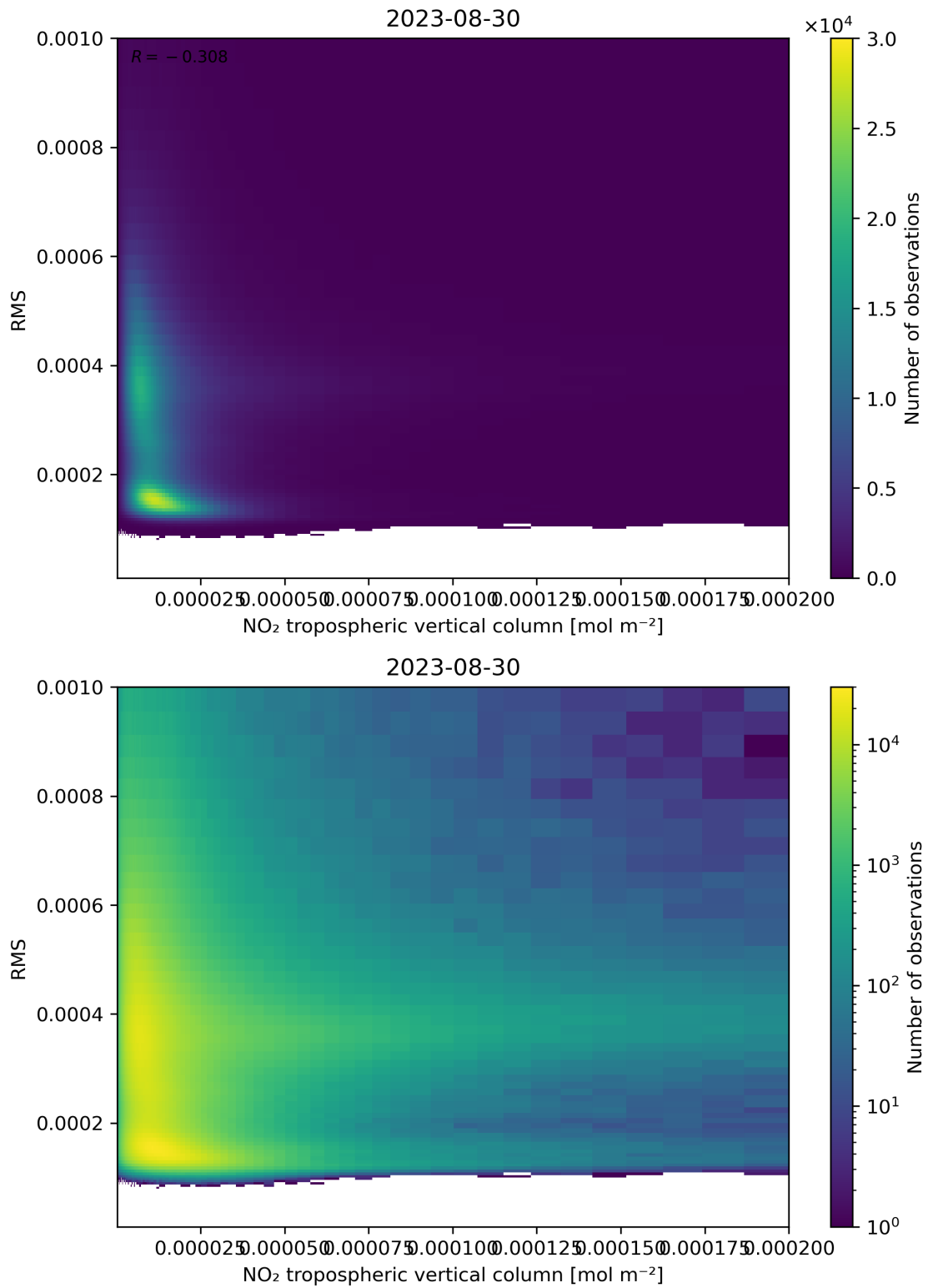
Figure 142: Scatter density plot of “NO 2 tropospheric vertical column” against “RMS” for 2023-08-30 to 2023-08-31.
