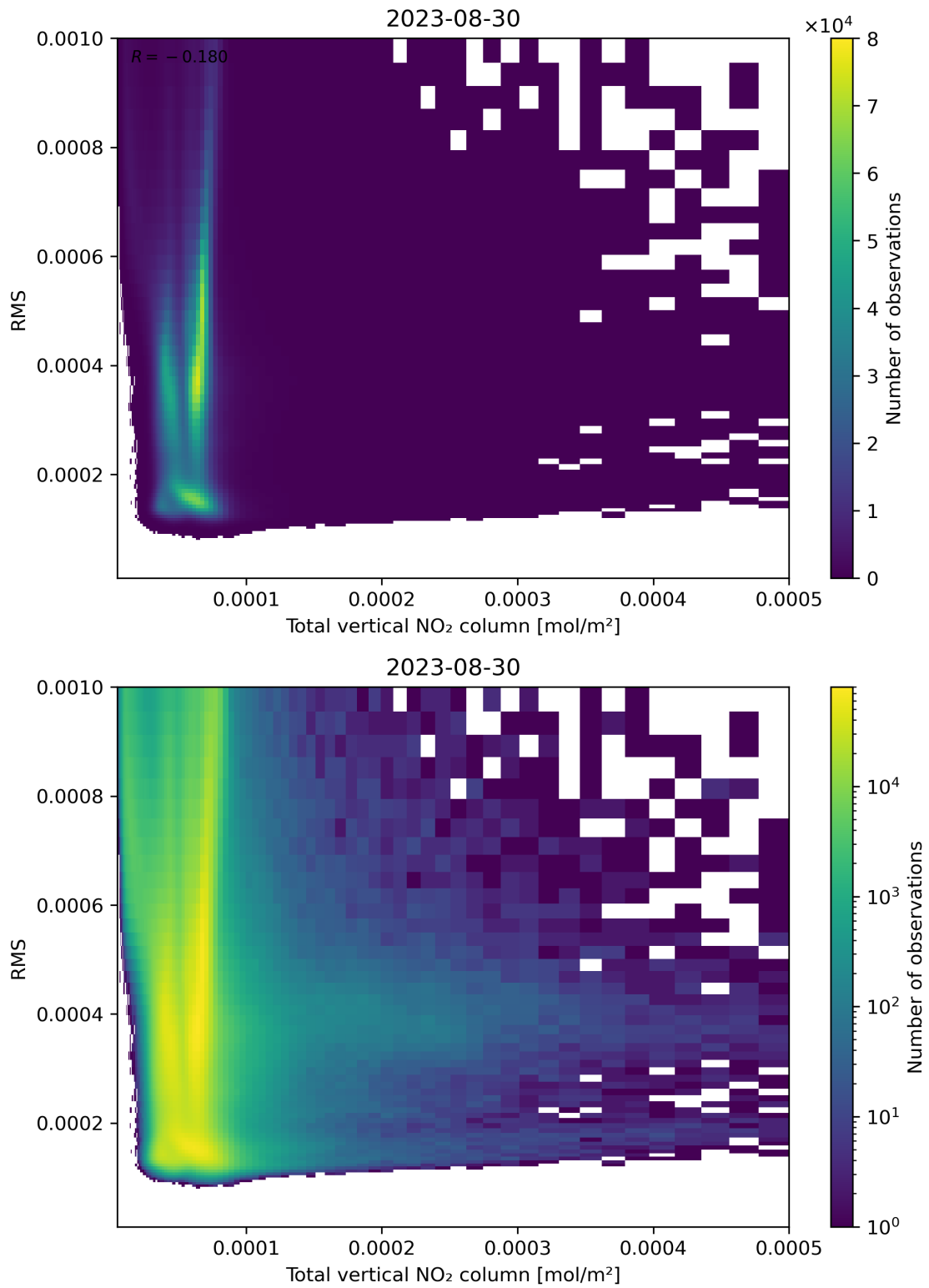
Figure 120: Scatter density plot of “Total vertical NO 2 column” against “RMS” for 2023-08-30 to 2023-08-31.
