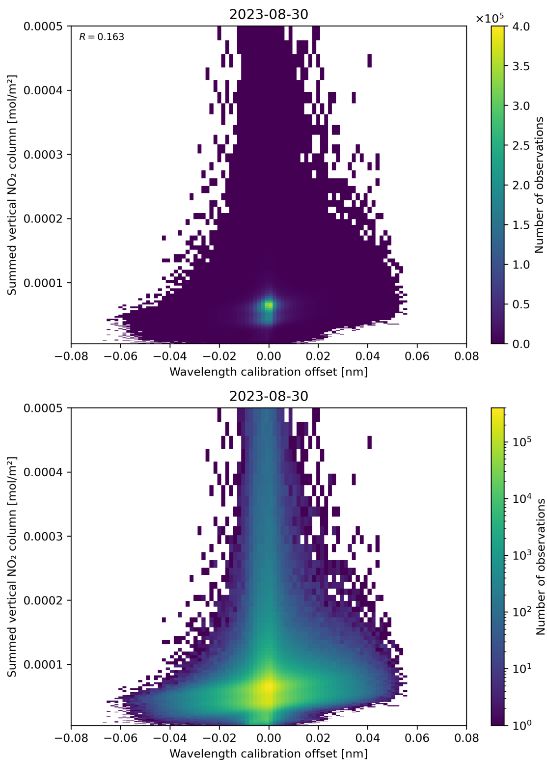
Figure 177: Scatter density plot of “Wavelength calibration offset” against “Summed vertical NO 2 column” for 2023-08-30 to 2023-08-31.
