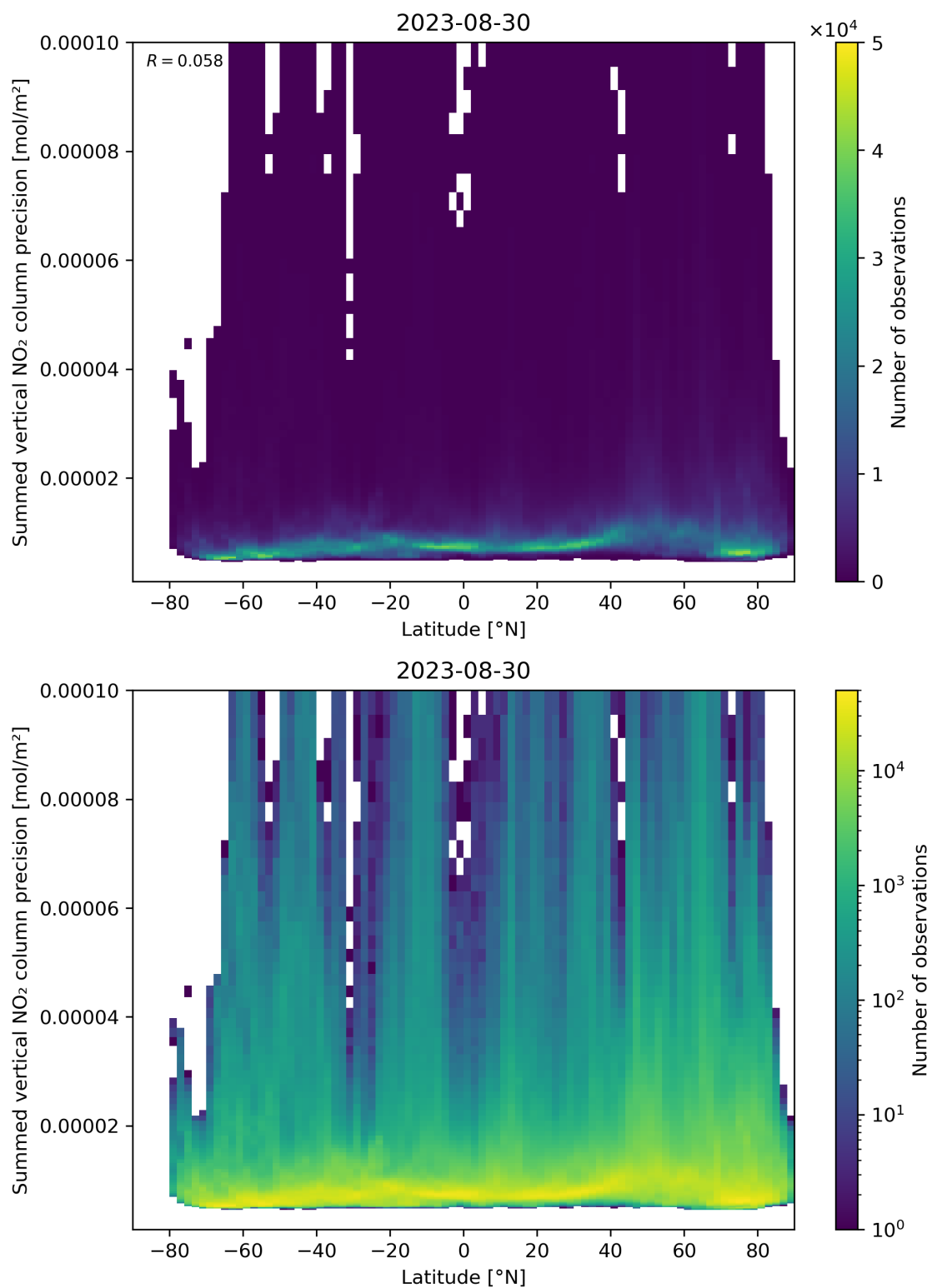
Figure 89: Scatter density plot of “Latitude” against “Summed vertical NO 2 column precision” for 2023-08-30 to 2023-08-31.
