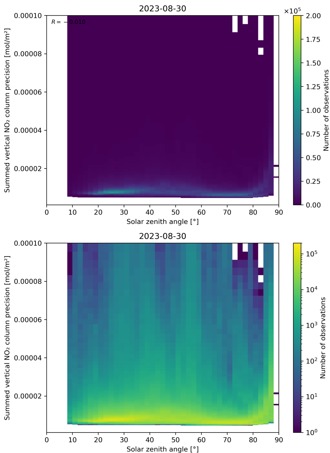
Figure 152: Scatter density plot of “Solar zenith angle” against “Summed vertical NO 2 column precision” for 2023-08-30 to 2023-08-31.
