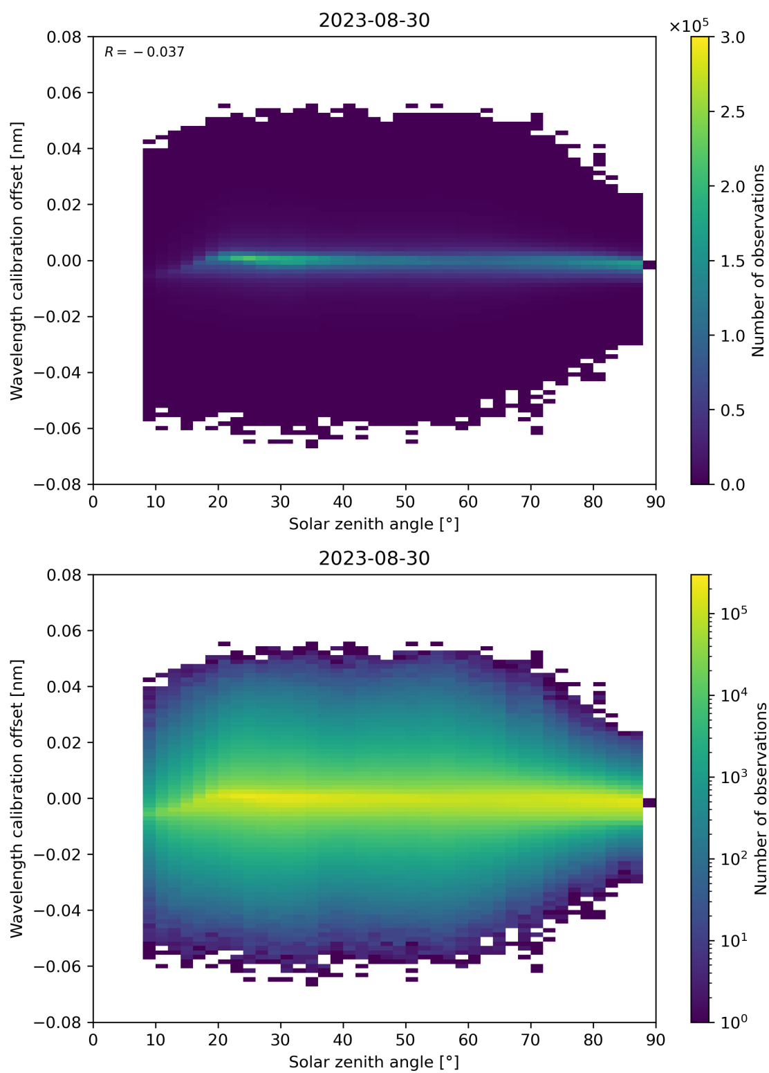
Figure 158: Scatter density plot of “Solar zenith angle” against “Wavelength calibration offset” for 2023-08-30 to 2023-08-31.
