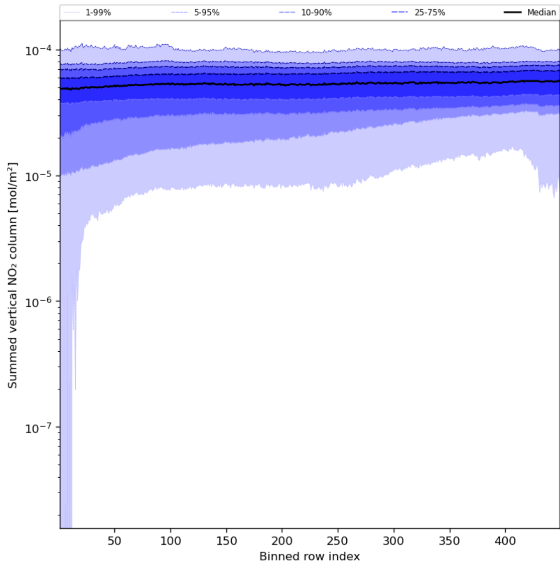
Figure 57: Along track statistics of “Summed vertical NO 2 column” for 2023-08-30 to 2023-08-31
