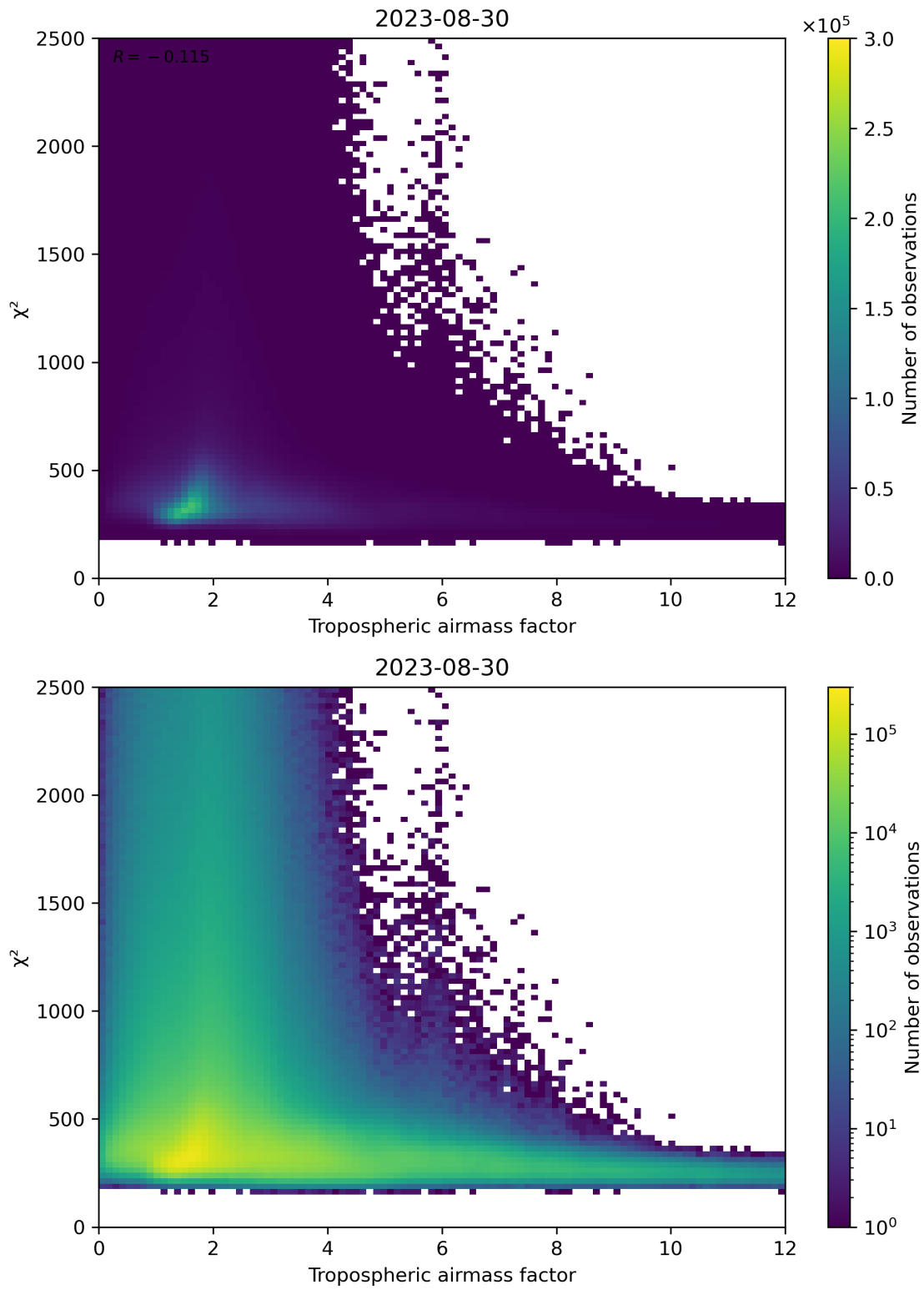
Figure 73: Scatter density plot of “Tropospheric airmass factor” against “ \chi^2 ” for 2023-08-30 to 2023-08-31.
