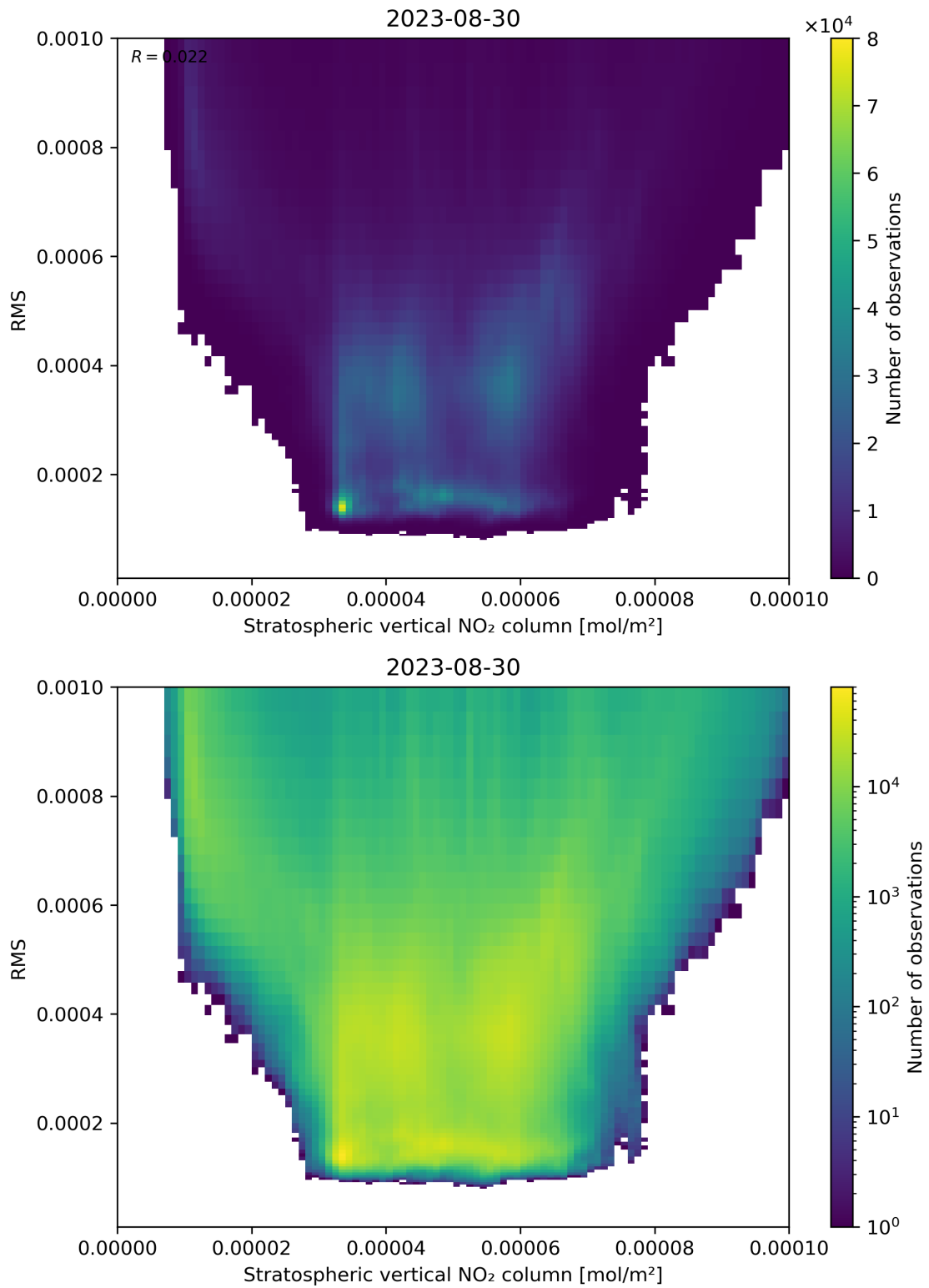
Figure 102: Scatter density plot of “Stratospheric vertical NO 2 column” against “RMS” for 2023-08-30 to 2023-08-31.
