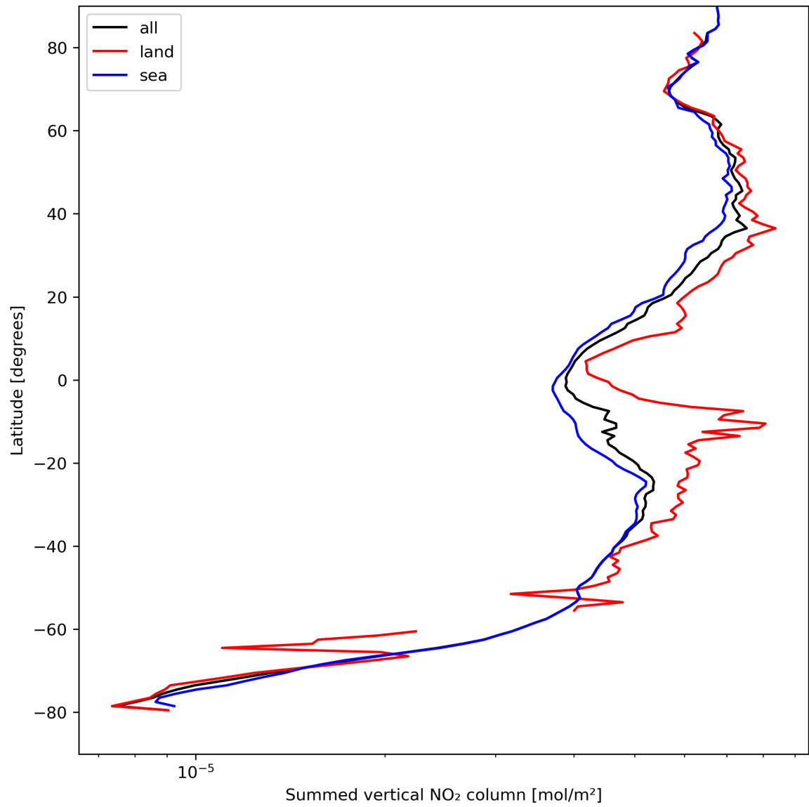
Figure 23: Zonal average of “Summed vertical NO 2 column” for 2023-08-30 to 2023-08-31.
