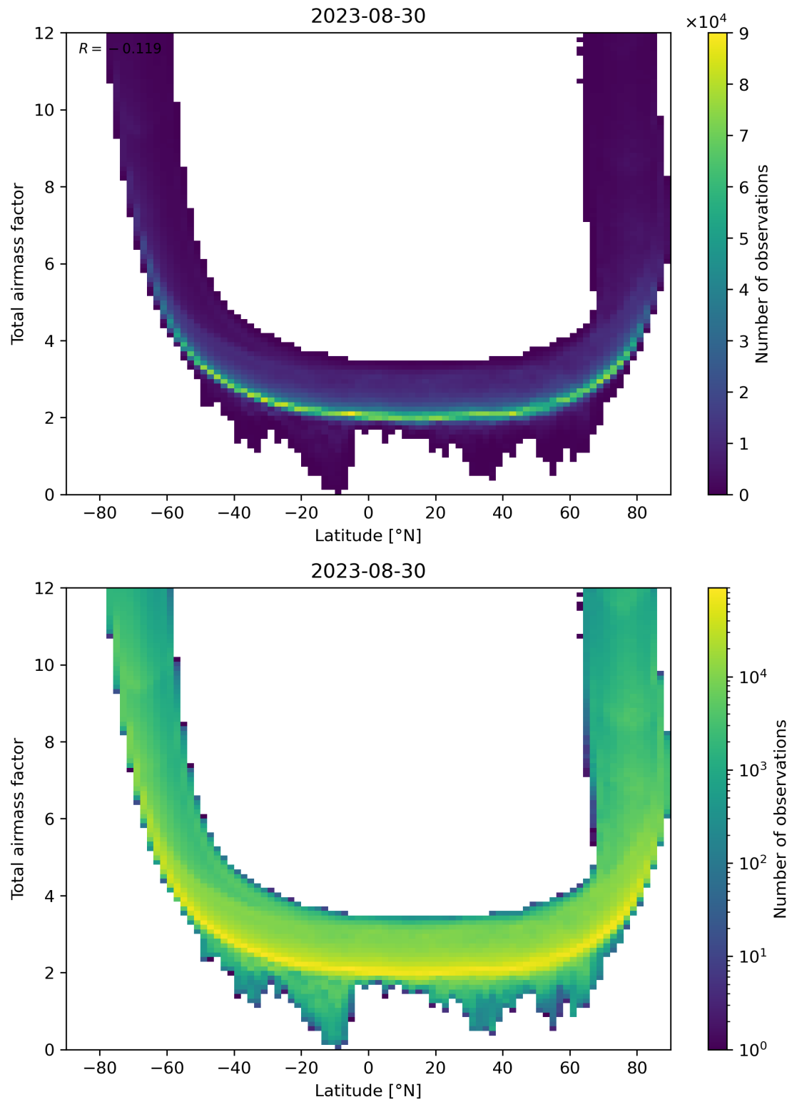
Figure 84: Scatter density plot of “Latitude” against “Total air mass factor” for 2023-08-30 to 2023-08-31.
