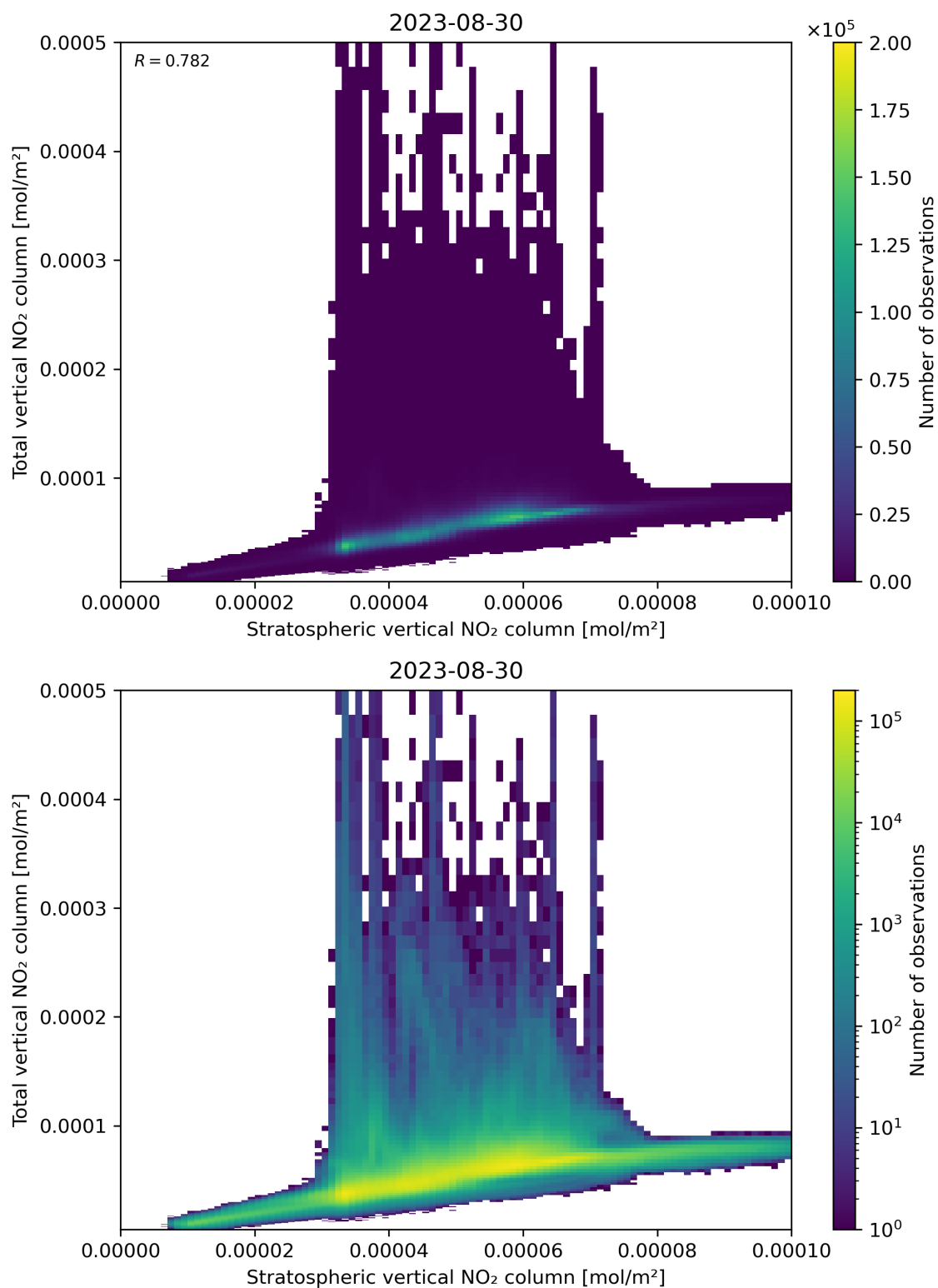
Figure 100: Scatter density plot of “Stratospheric vertical NO 2 column” against “Total vertical NO 2 column” for 2023-08-30 to 2023-08-31.
