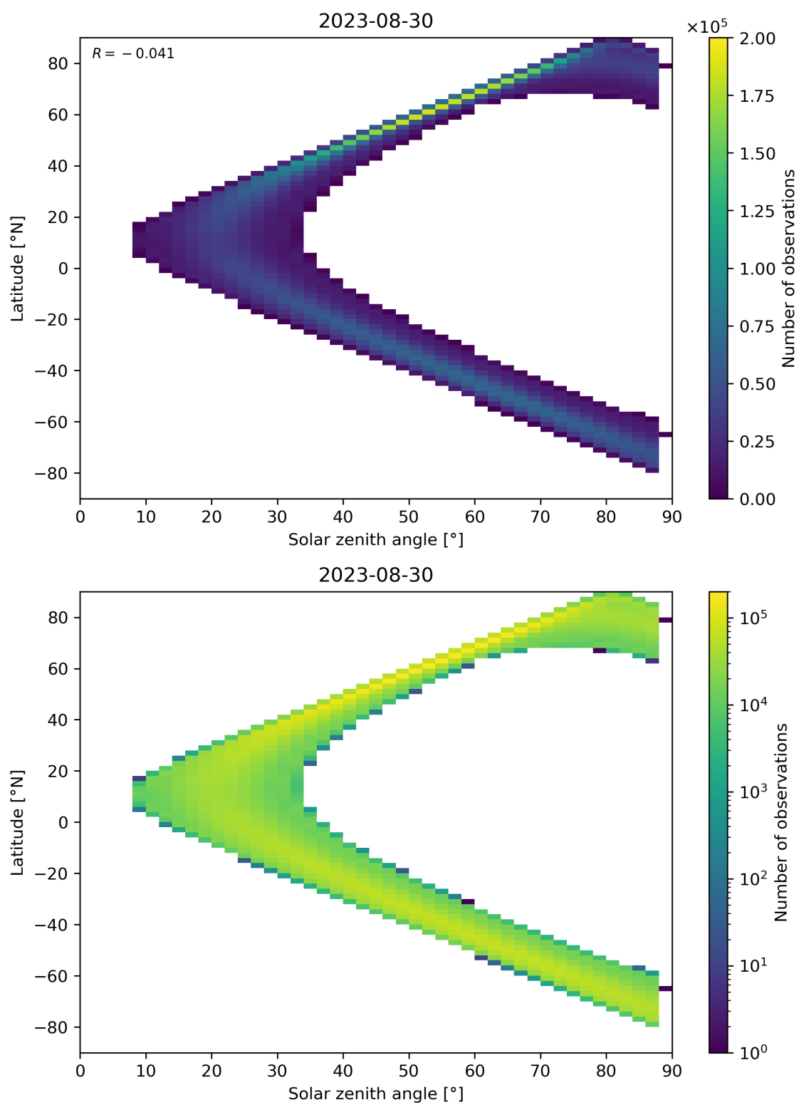
Figure 149: Scatter density plot of “Solar zenith angle” against “Latitude” for 2023-08-30 to 2023-08-31.
