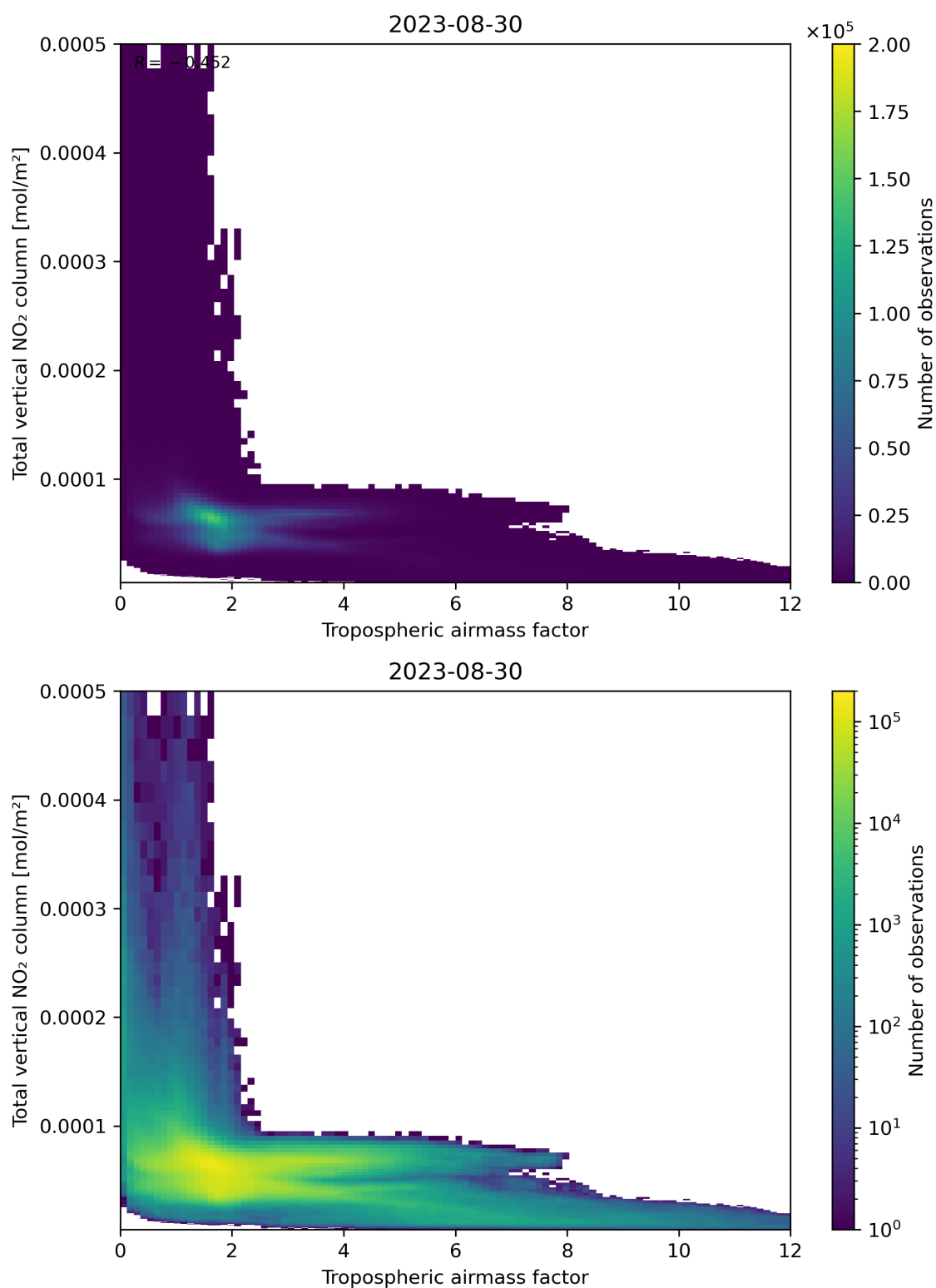
Figure 77: Scatter density plot of “Tropospheric airmass factor” against “Total vertical NO 2 column” for 2023-08-30 to 2023-08-31.
