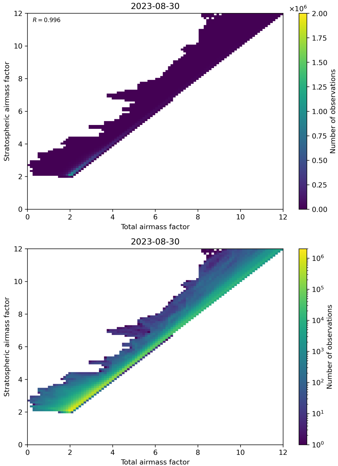
Figure 62: Scatter density plot of “Total airmass factor” against “Stratospheric airmass factor” for 2023-08-30 to 2023-08-31.
