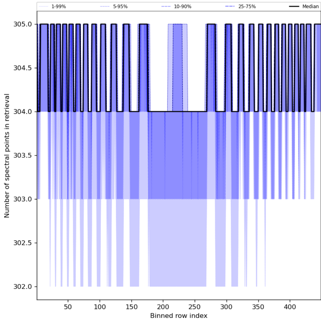
Figure 50: Along track statistics of “Number of spectral points in retrieval” for 2023-08-30 to 2023-08-31
