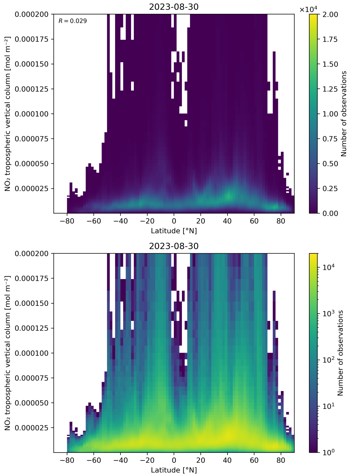
Figure 92: Scatter density plot of “Latitude” against “NO 2 tropospheric vertical column” for 2023-08-30 to 2023-08-31.
