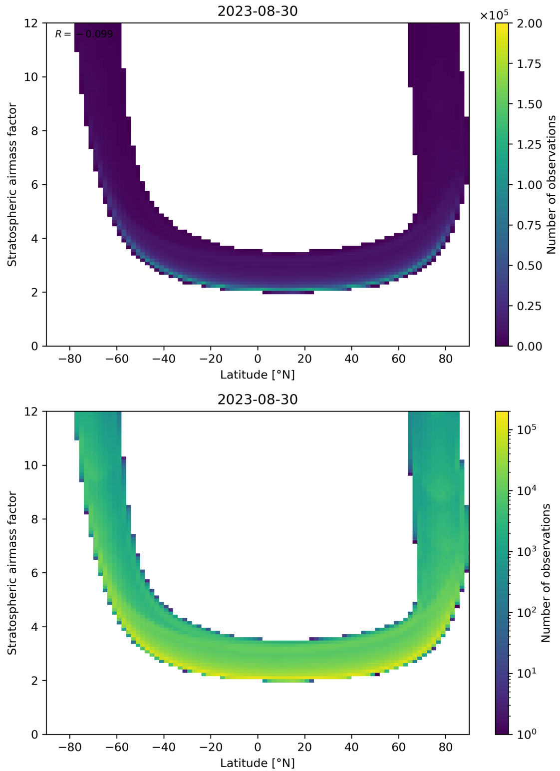
Figure 83: Scatter density plot of “Latitude” against “Stratospheric air mass factor” for 2023-08-30 to 2023-08-31.
