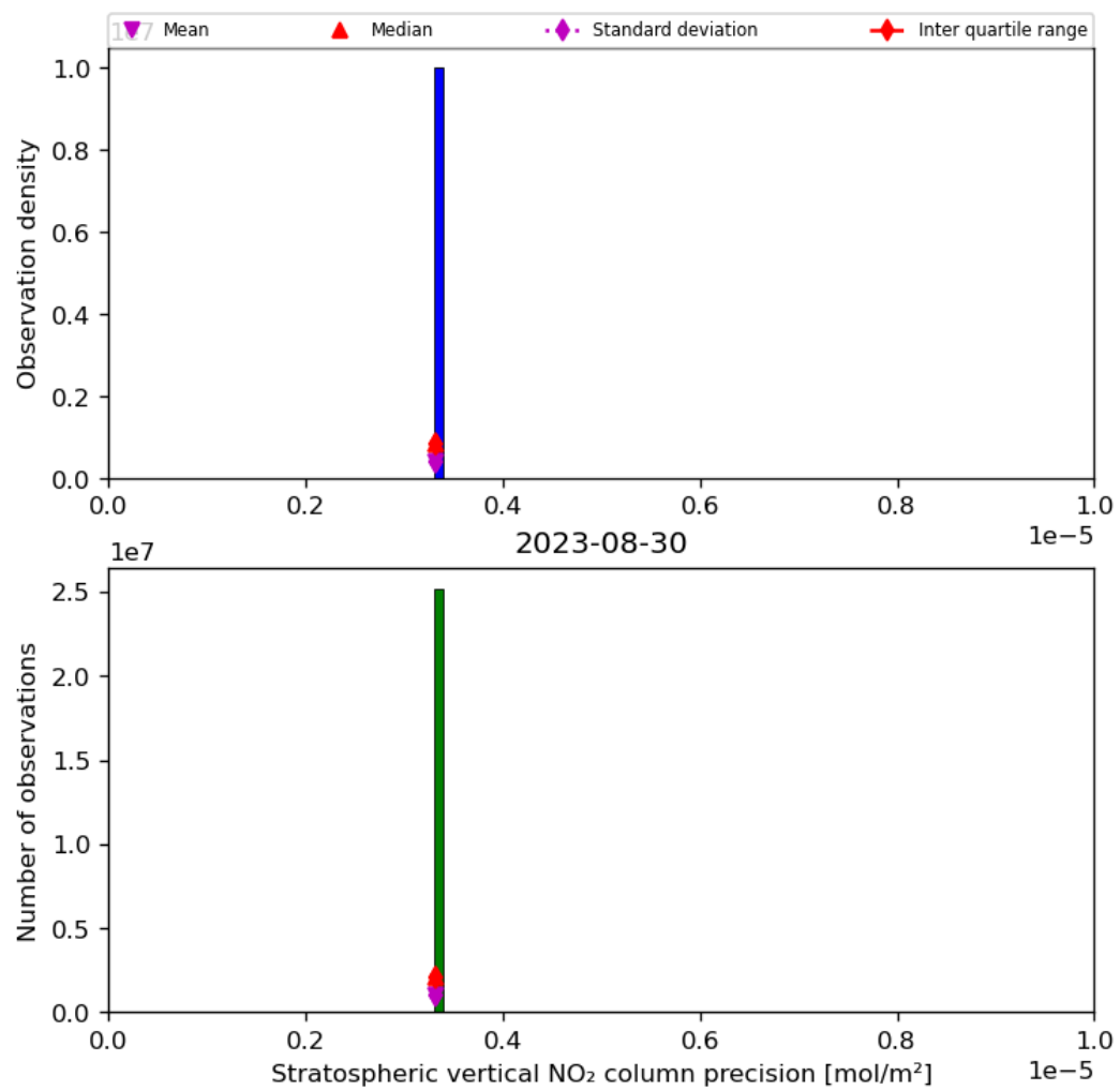
Figure 37: Histogram of “Stratospheric vertical NO 2 column precision” for 2023-08-30 to 2023-08-31
