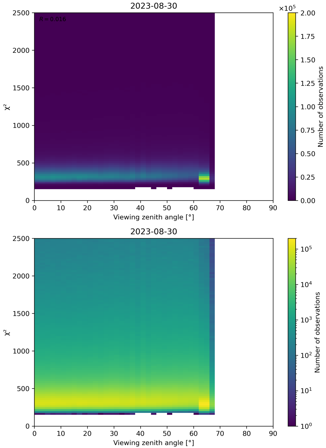
Figure 162: Scatter density plot of “Viewing zenith angle” against “ \chi^2 ” for 2023-08-30 to 2023-08-31.
