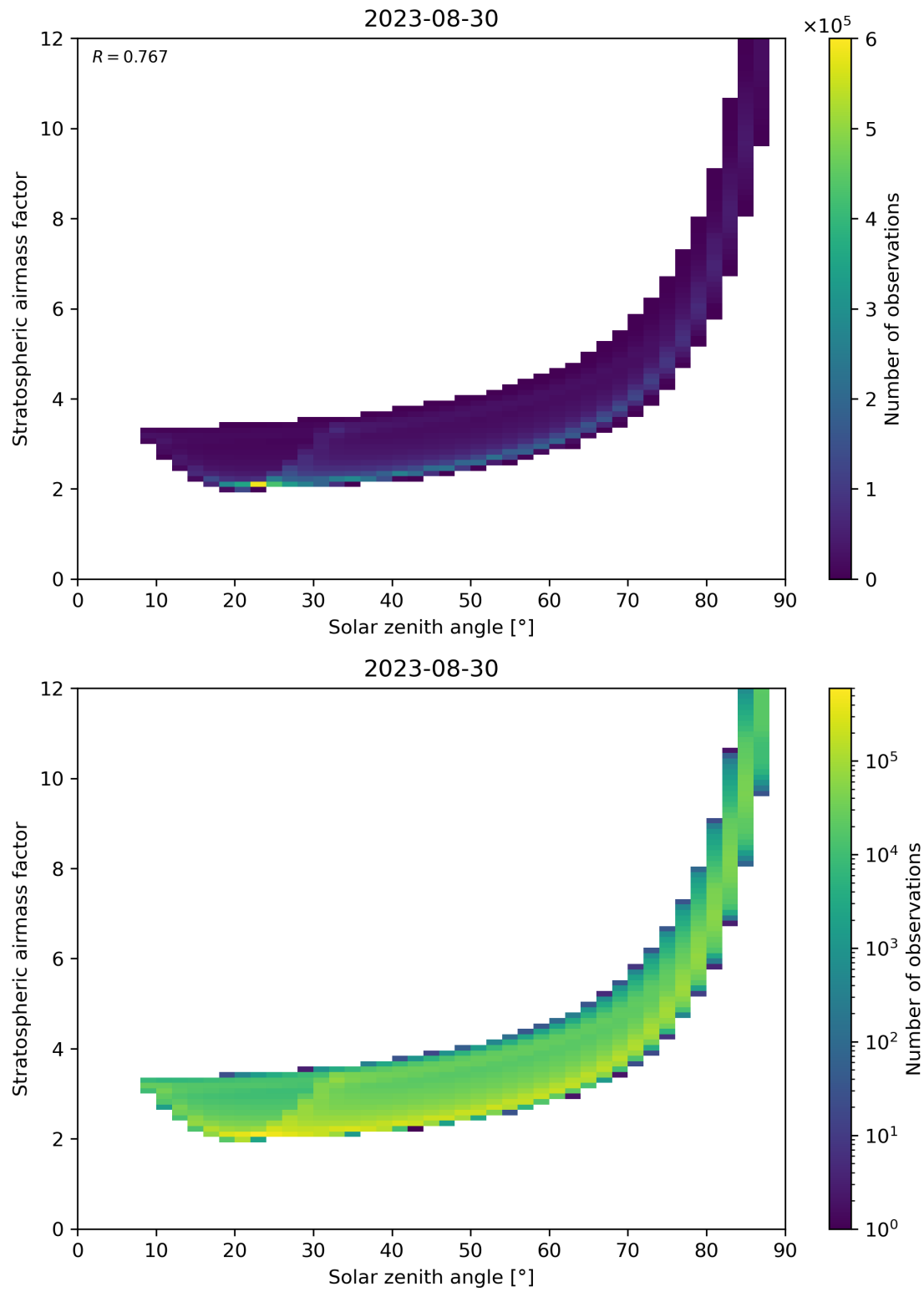
Figure 145: Scatter density plot of “Solar zenith angle” against “Stratospheric airmass factor” for 2023-08-30 to 2023-08-31.
