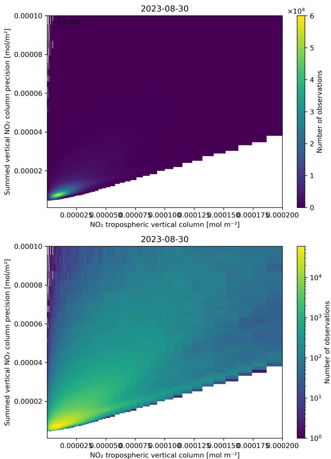
Figure 127: Scatter density plot of “NO 2 tropospheric vertical column” against “Summed vertical NO 2 column precision” for 2023-08-30 to 2023-08-31.
