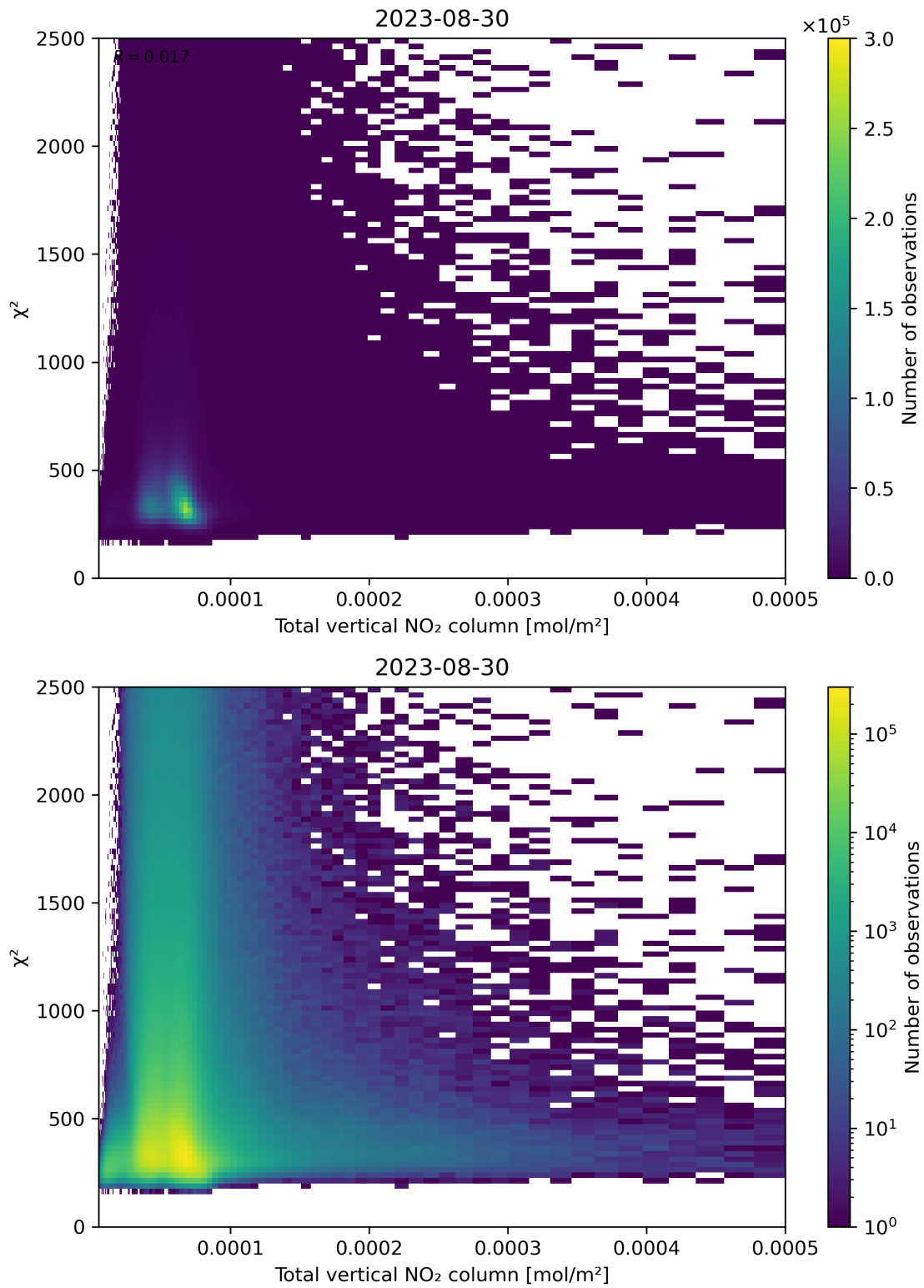
Figure 111: Scatter density plot of “Total vertical NO 2 column” against “ \chi^2 ” for 2023-08-30 to 2023-08-31.
