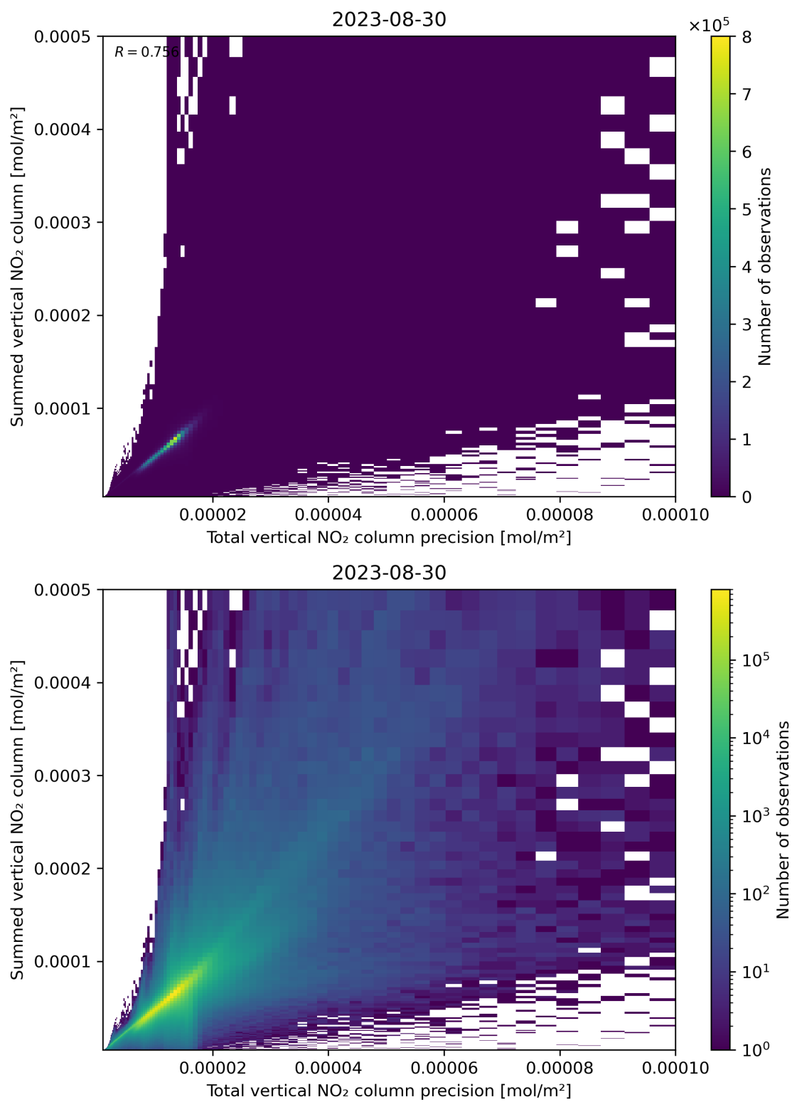
Figure 117: Scatter density plot of “Total vertical NO 2 column precision” against “Summed vertical NO 2 column” for 2023-08-30 to 2023-08-31.
