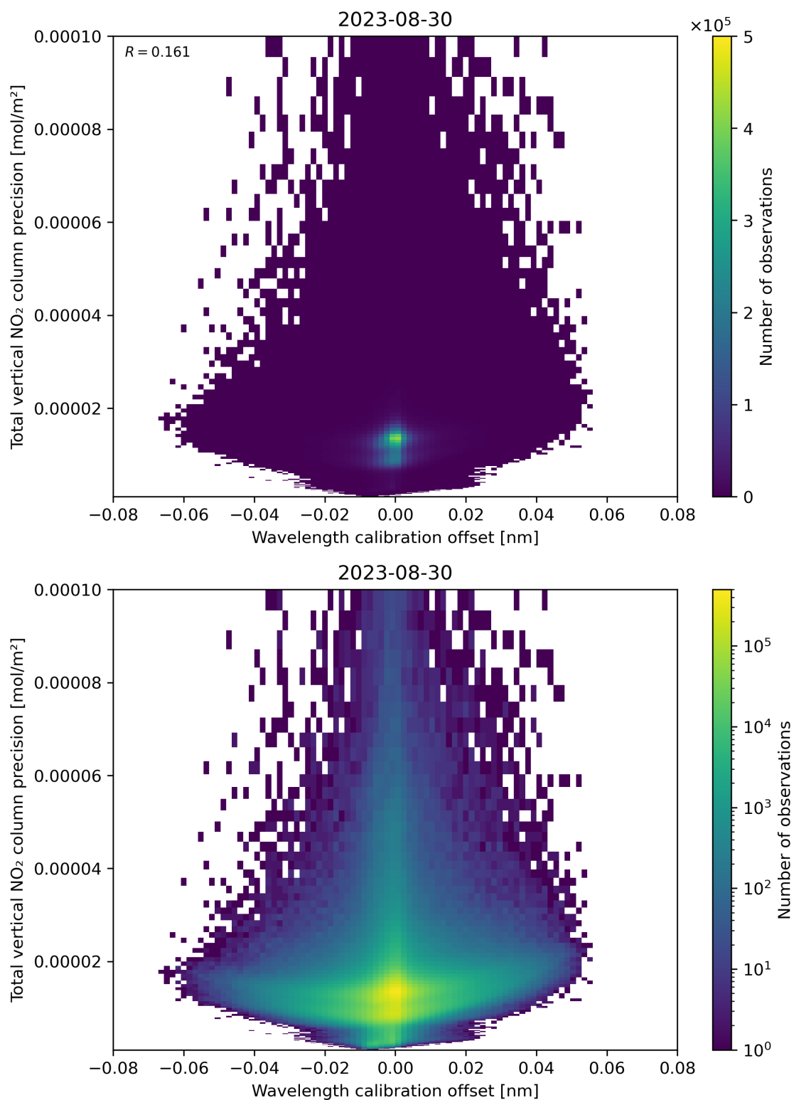
Figure 180: Scatter density plot of “Wavelength calibration offset” against “Total vertical NO 2 column precision” for 2023-08-30 to 2023-08-31.
