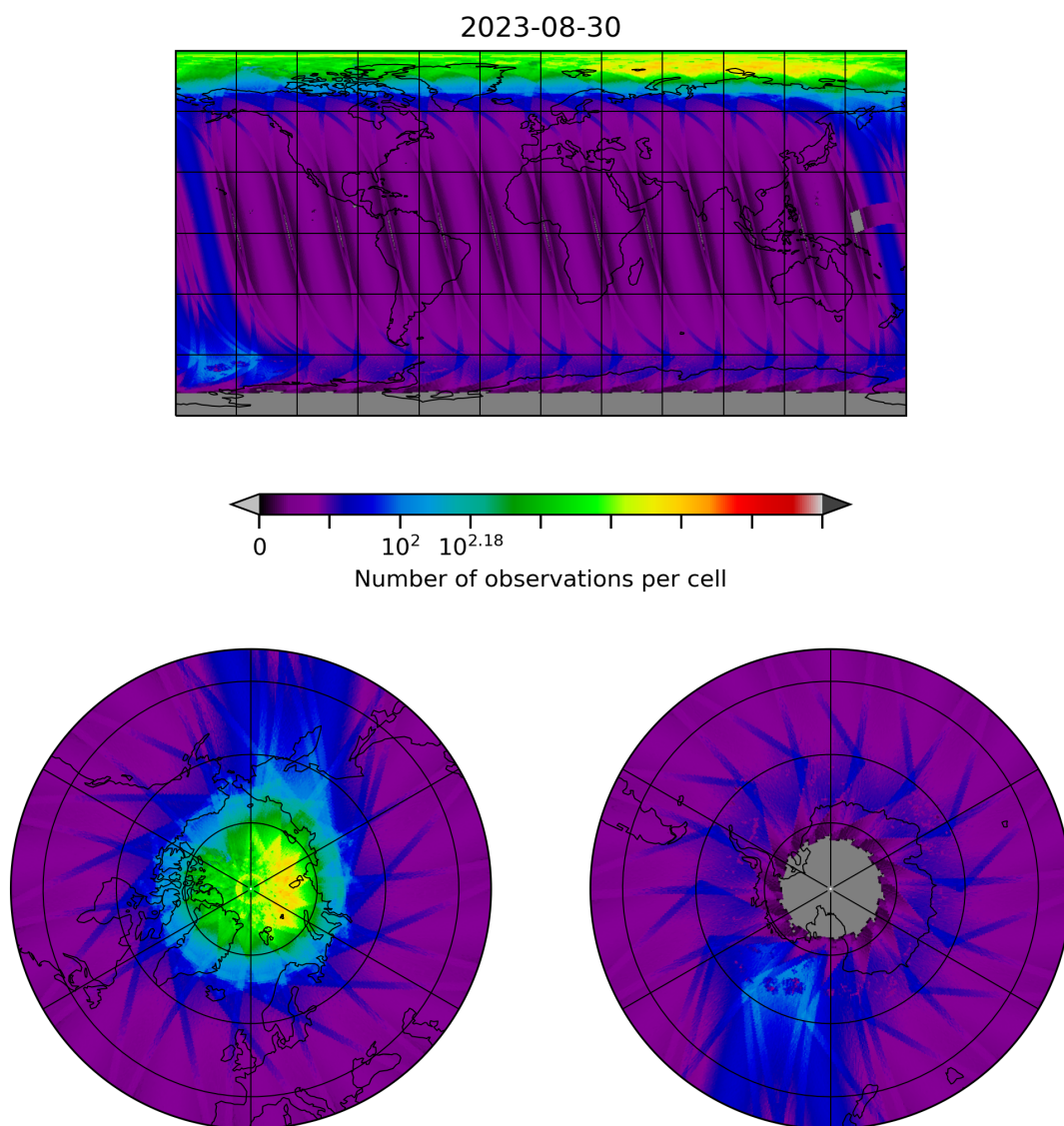
Figure 10: Map of the number of observations for 2023-08-30 to 2023-08-31
