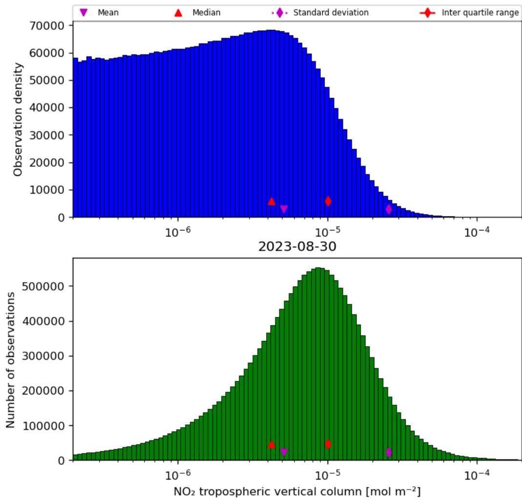
Figure 29: Histogram of “NO 2 tropospheric vertical column” for 2023-08-30 to 2023-08-31
