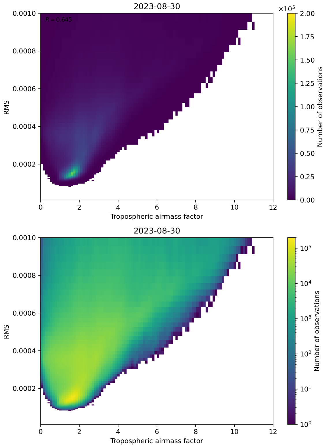
Figure 79: Scatter density plot of “Tropospheric airmass factor” against “RMS” for 2023-08-30 to 2023-08-31.
