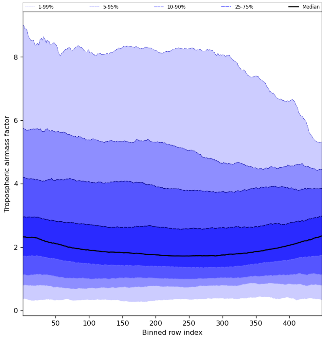
Figure 48: Along track statistics of “Tropospheric airmass factor” for 2023-08-30 to 2023-08-31
