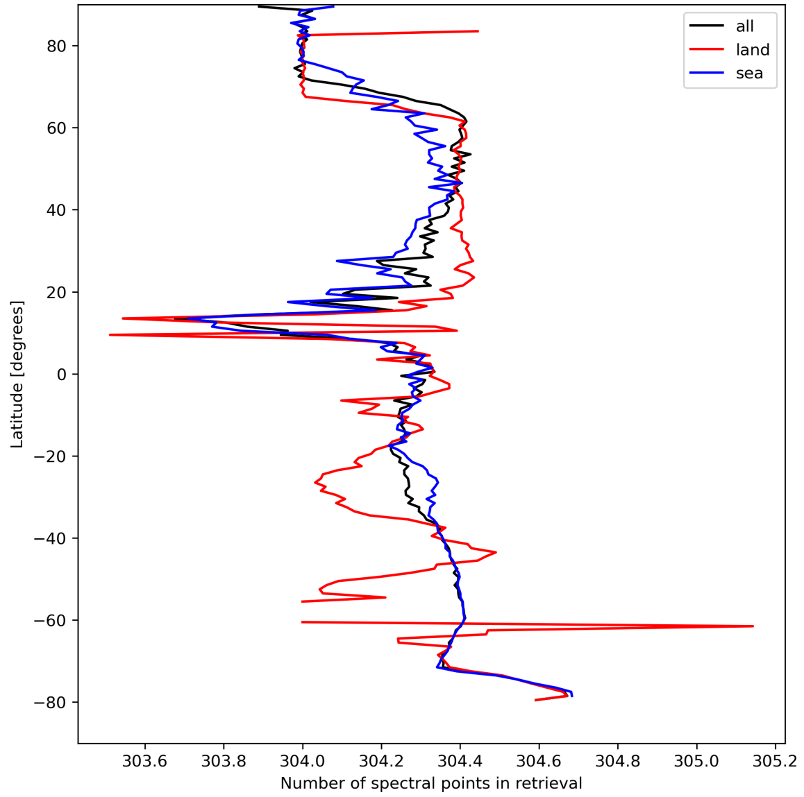
Figure 16: Zonal average of “Number of spectral points in retrieval” for 2023-08-30 to 2023-08-31.
