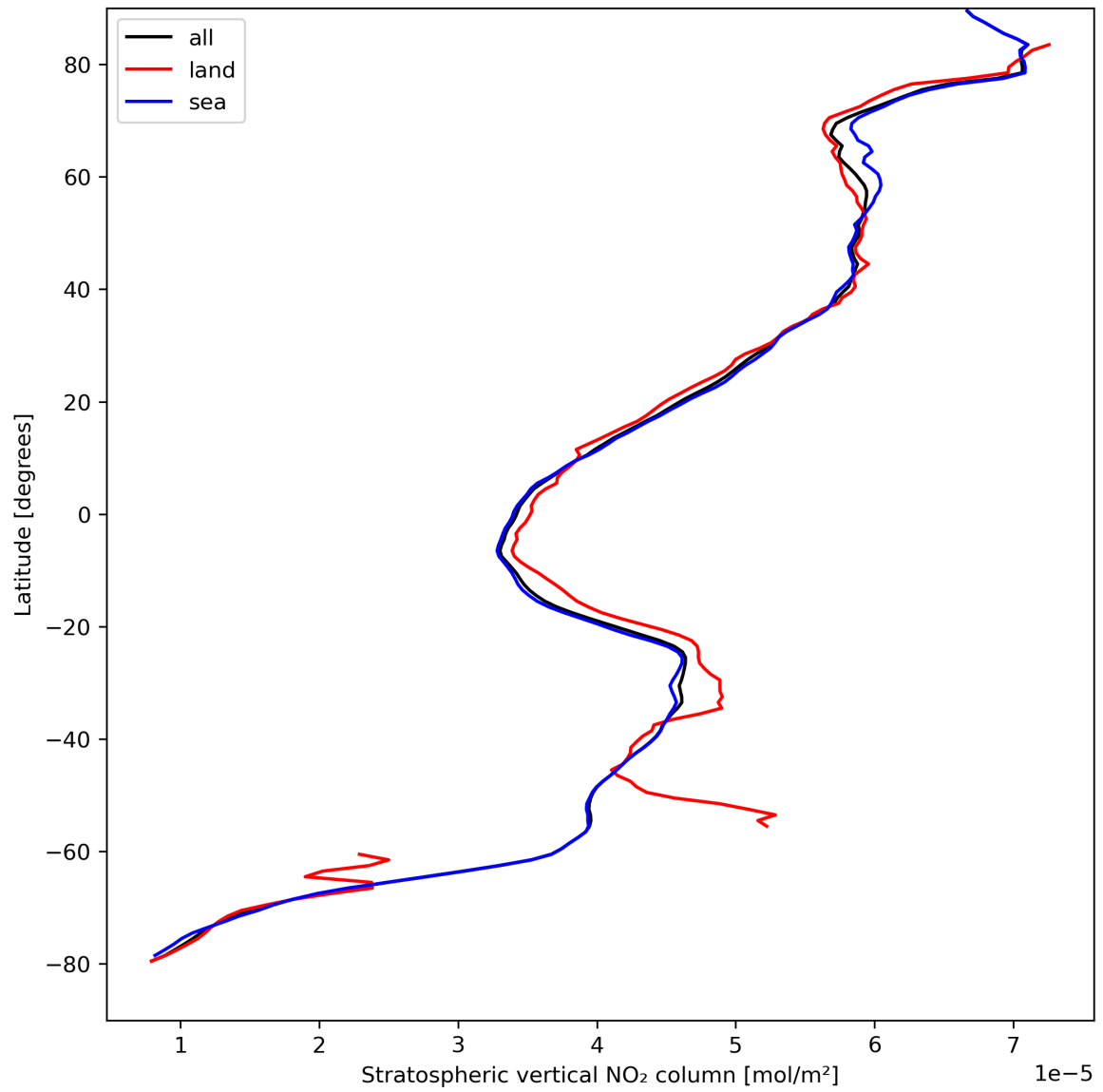
Figure 19: Zonal average of “Stratospheric vertical NO 2 column” for 2023-08-30 to 2023-08-31.
