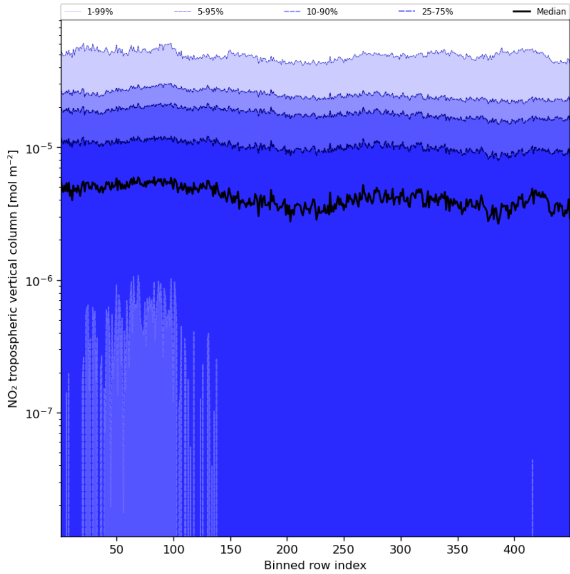
Figure 46: Along track statistics of “NO 2 tropospheric vertical column” for 2023-08-30 to 2023-08-31
