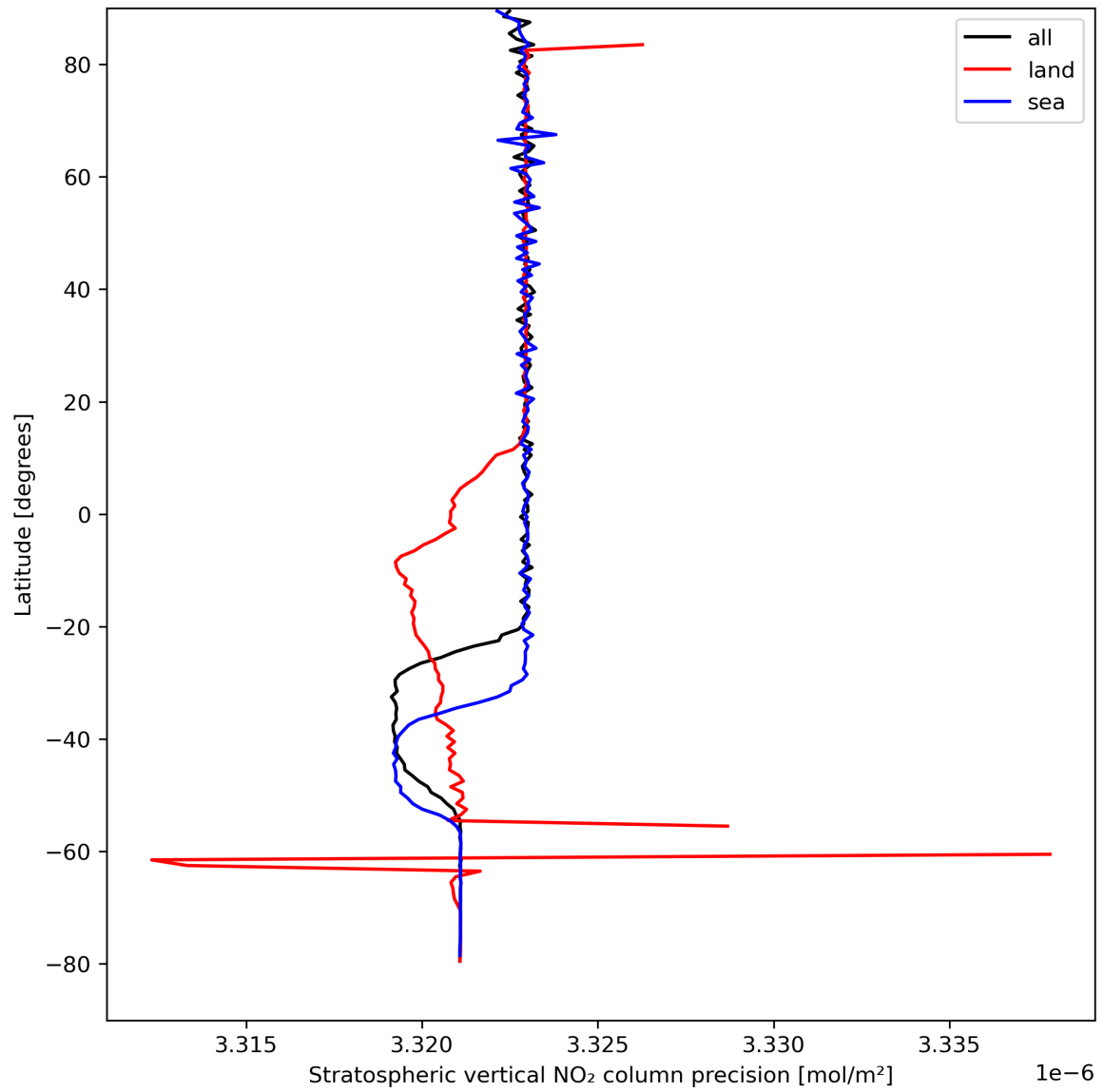
Figure 20: Zonal average of “Stratospheric vertical NO 2 column precision” for 2023-08-30 to 2023-08-31.
