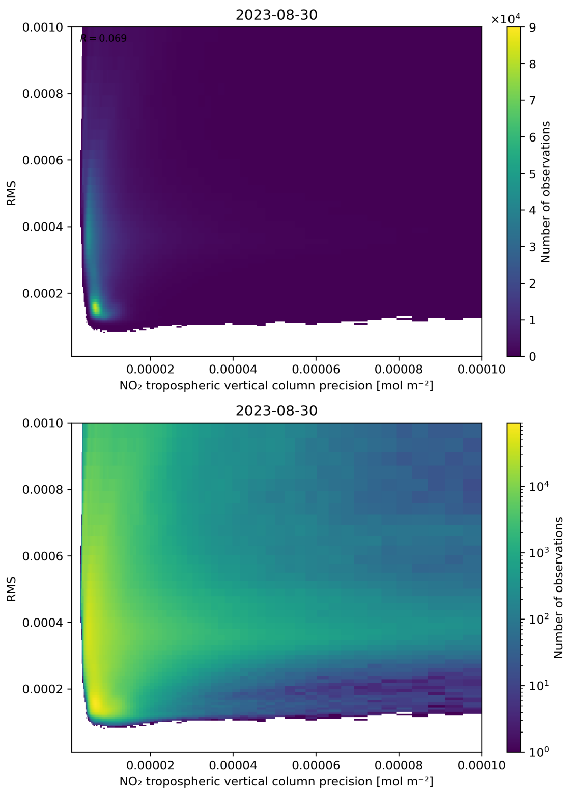
Figure 140: Scatter density plot of “NO 2 tropospheric vertical column precision” against “RMS” for 2023-08-30 to 2023-08-31.
