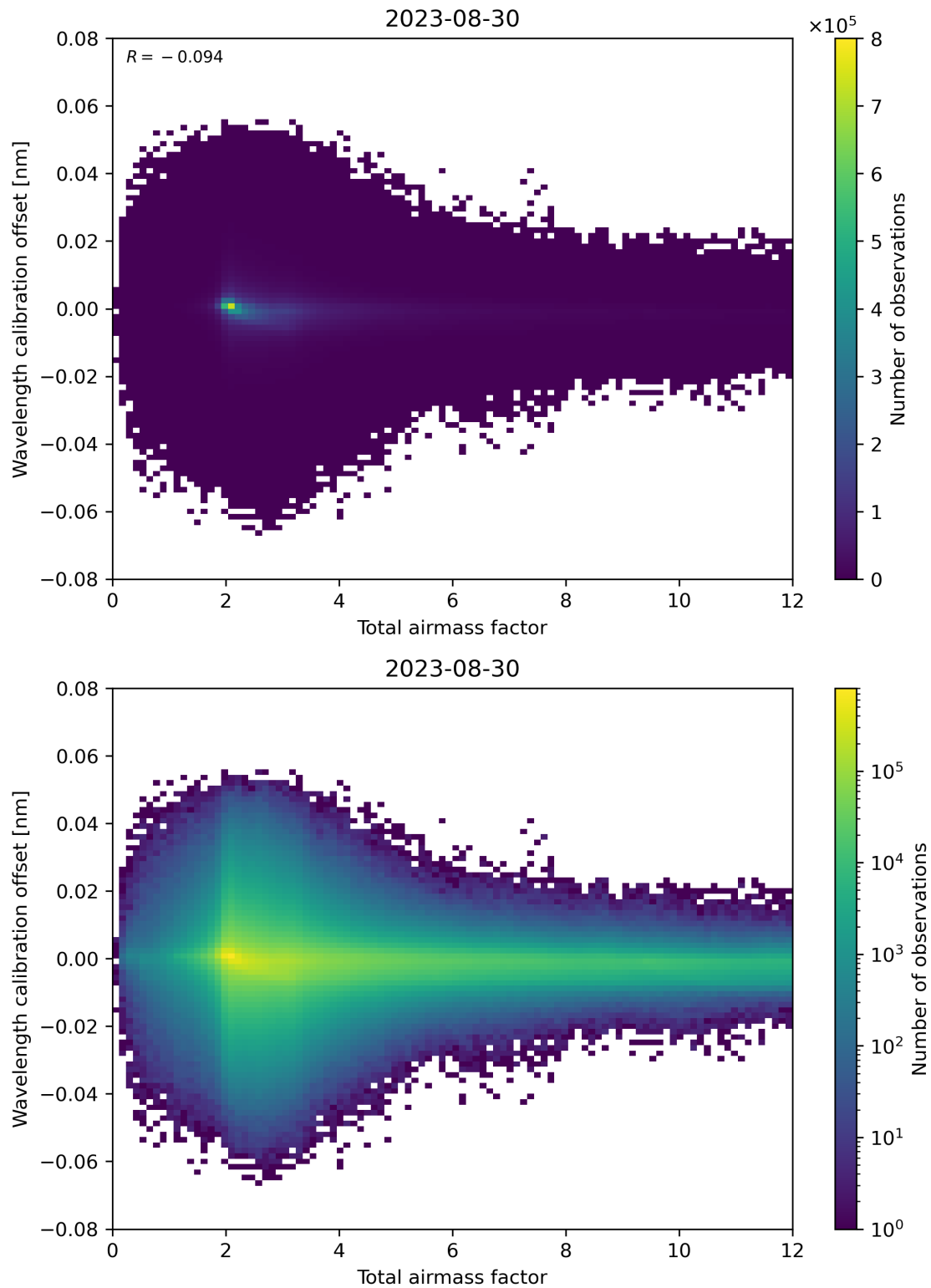
Figure 70: Scatter density plot of “Total airmass factor” against “Wavelength calibration offset” for 2023-08-30 to 2023-08-31.
