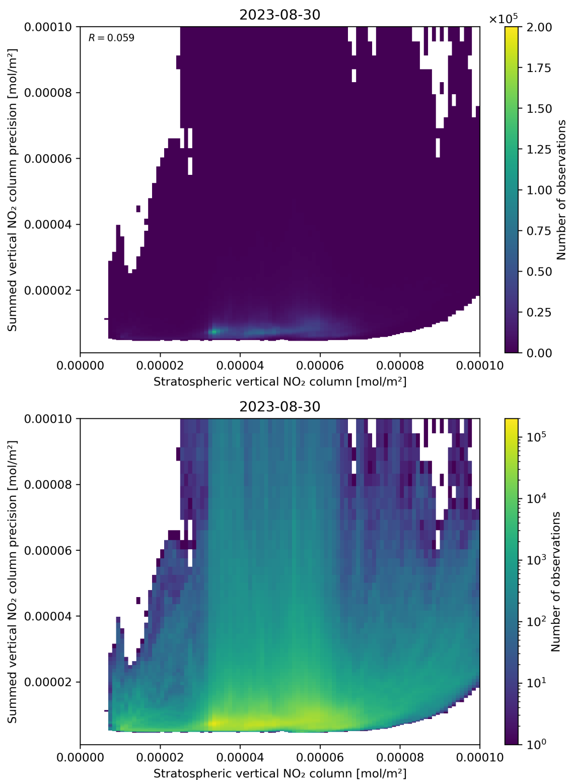
Figure 99: Scatter density plot of “Stratospheric vertical NO 2 column” against “Summed vertical NO 2 column precision” for 2023-08-30 to 2023-08-31.
