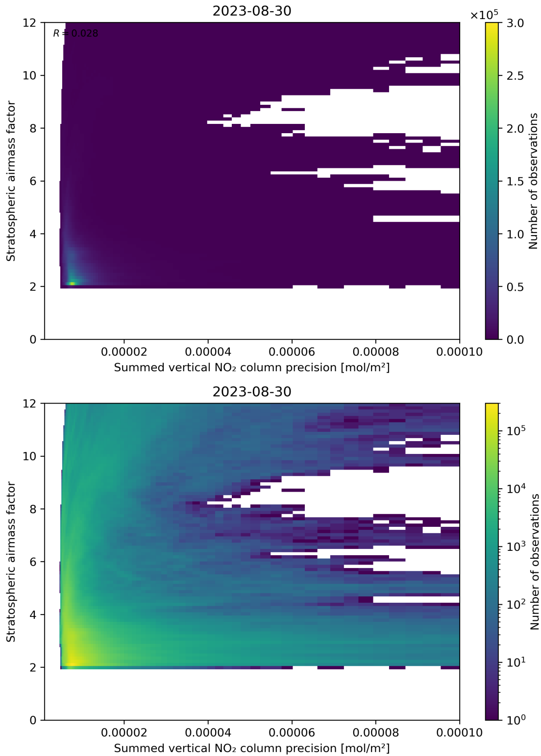
Figure 106: Scatter density plot of “Summed vertical NO 2 column precision” against “Stratospheric airmass factor” for 2023-08-30 to 2023-08-31.
