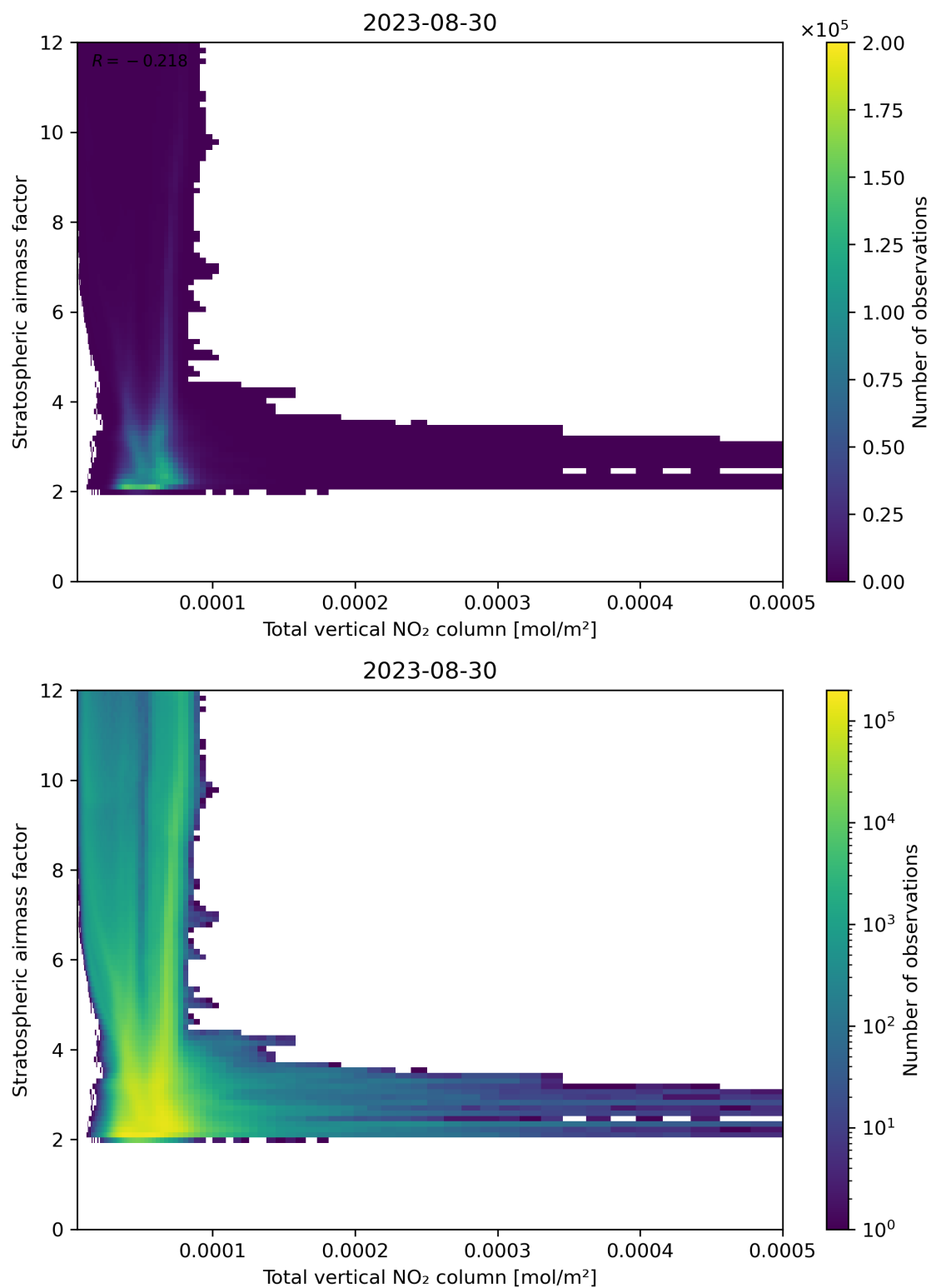
Figure 110: Scatter density plot of “Total vertical NO 2 column” against “Stratospheric airmass factor” for 2023-08-30 to 2023-08-31.
