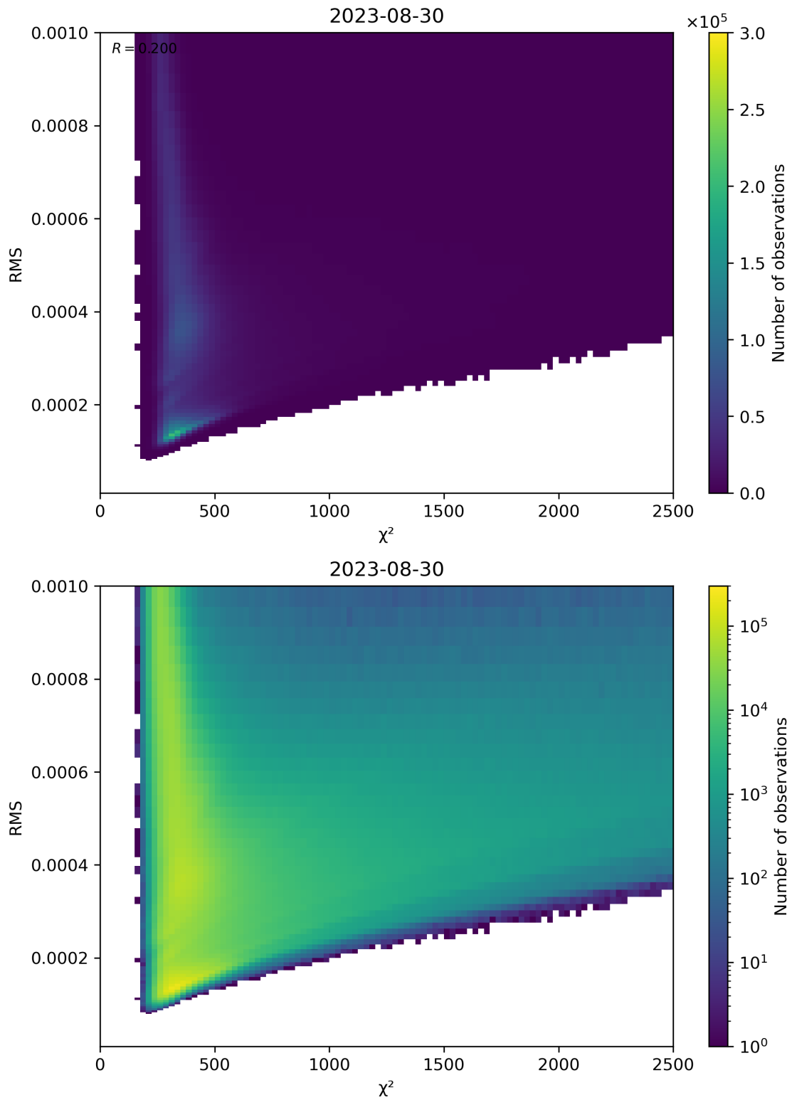
Figure 82: Scatter density plot of “ \chi^2 ” against “RMS” for 2023-08-30 to 2023-08-31.
