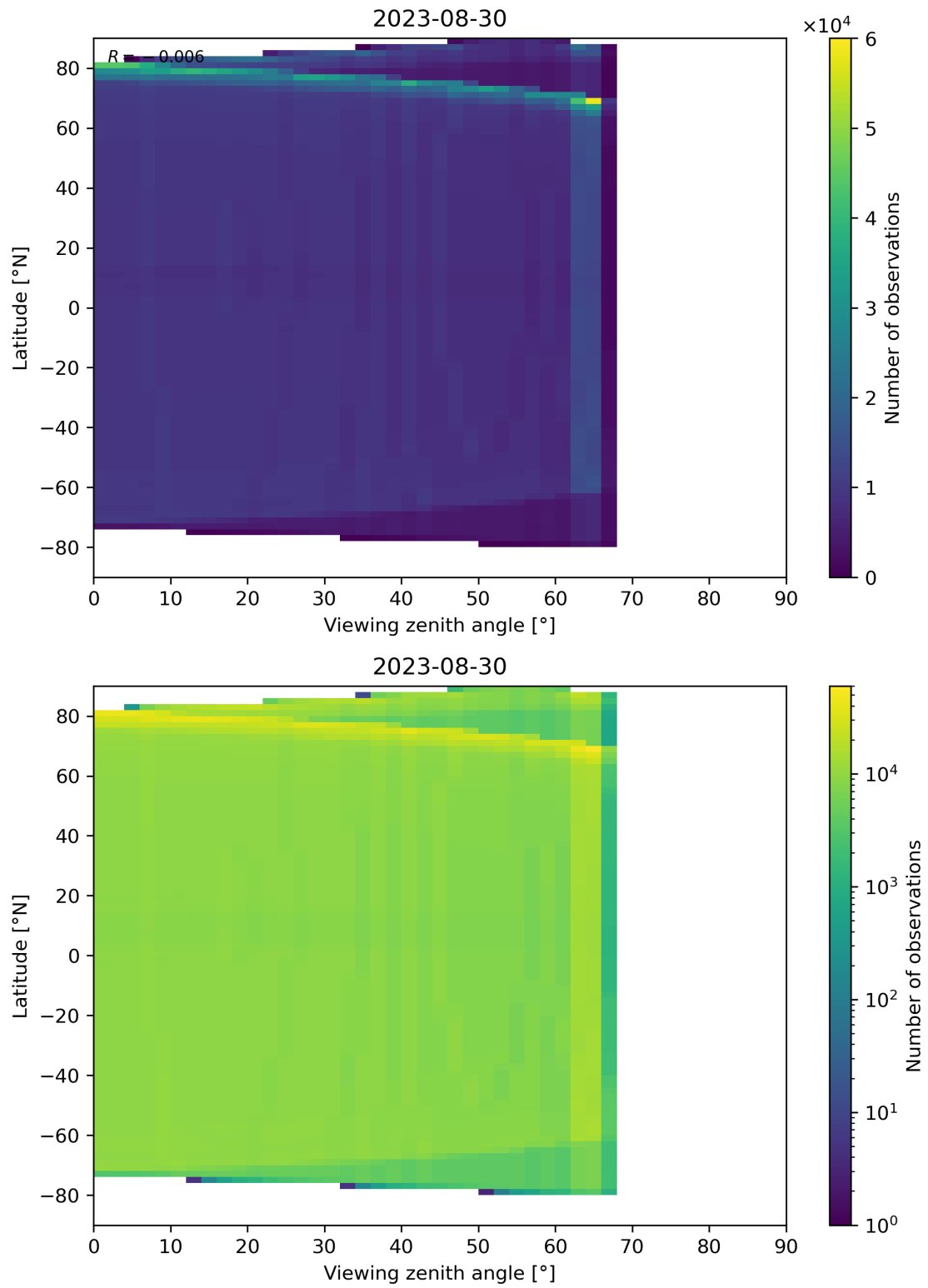
Figure 163: Scatter density plot of “Viewing zenith angle” against “Latitude” for 2023-08-30 to 2023-08-31.
