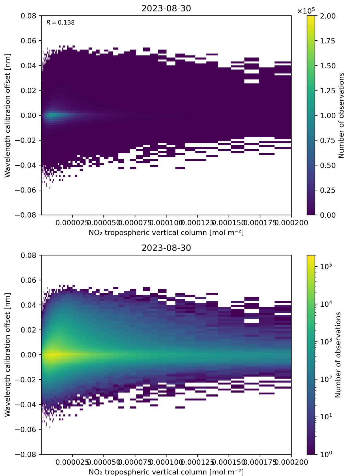
Figure 143: Scatter density plot of “NO 2 tropospheric vertical column” against “Wavelength calibration offset” for 2023-08-30 to 2023-08-31.
