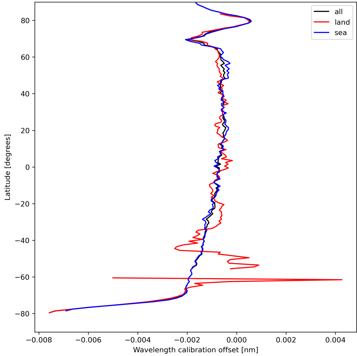
Figure 18: Zonal average of “Wavelength calibration offset” for 2023-08-30 to 2023-08-31.
