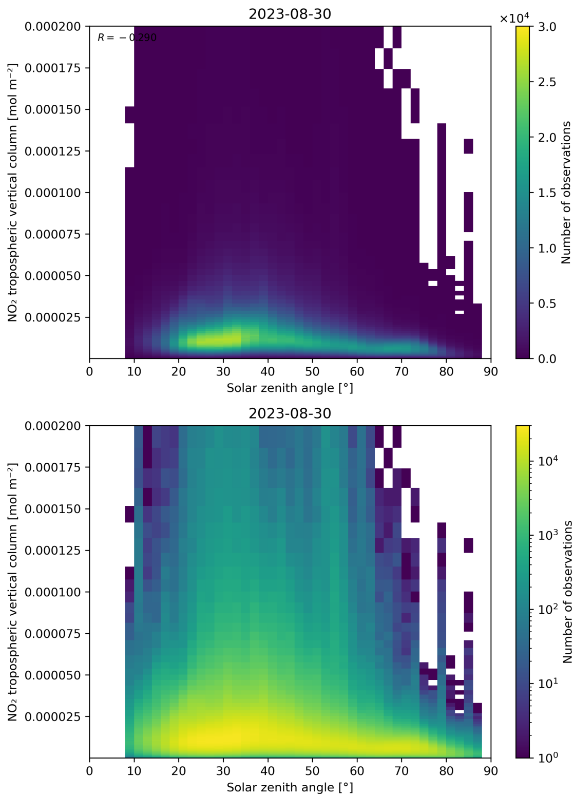
Figure 155: Scatter density plot of “Solar zenith angle” against “NO 2 tropospheric vertical column” for 2023-08-30 to 2023-08-31.
