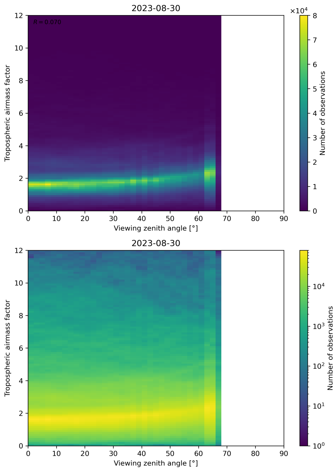
Figure 161: Scatter density plot of “Viewing zenith angle” against “Tropospheric airmass factor” for 2023-08-30 to 2023-08-31.
