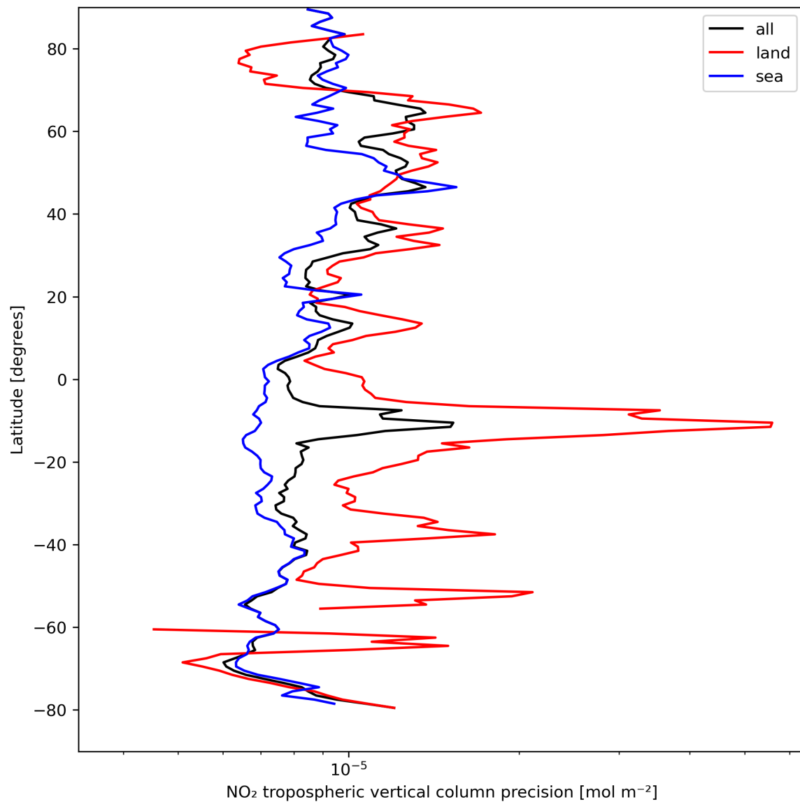
Figure 13: Zonal average of “NO 2 tropospheric vertical column precision” for 2023-08-30 to 2023-08-31.
