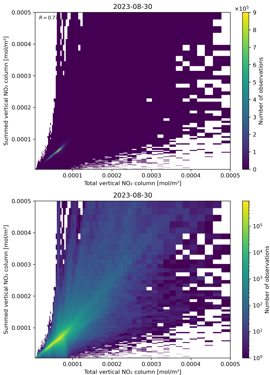
Figure 112: Scatter density plot of “Total vertical NO 2 column” against “Summed vertical NO 2 column” for 2023-08-30 to 2023-08-31.
