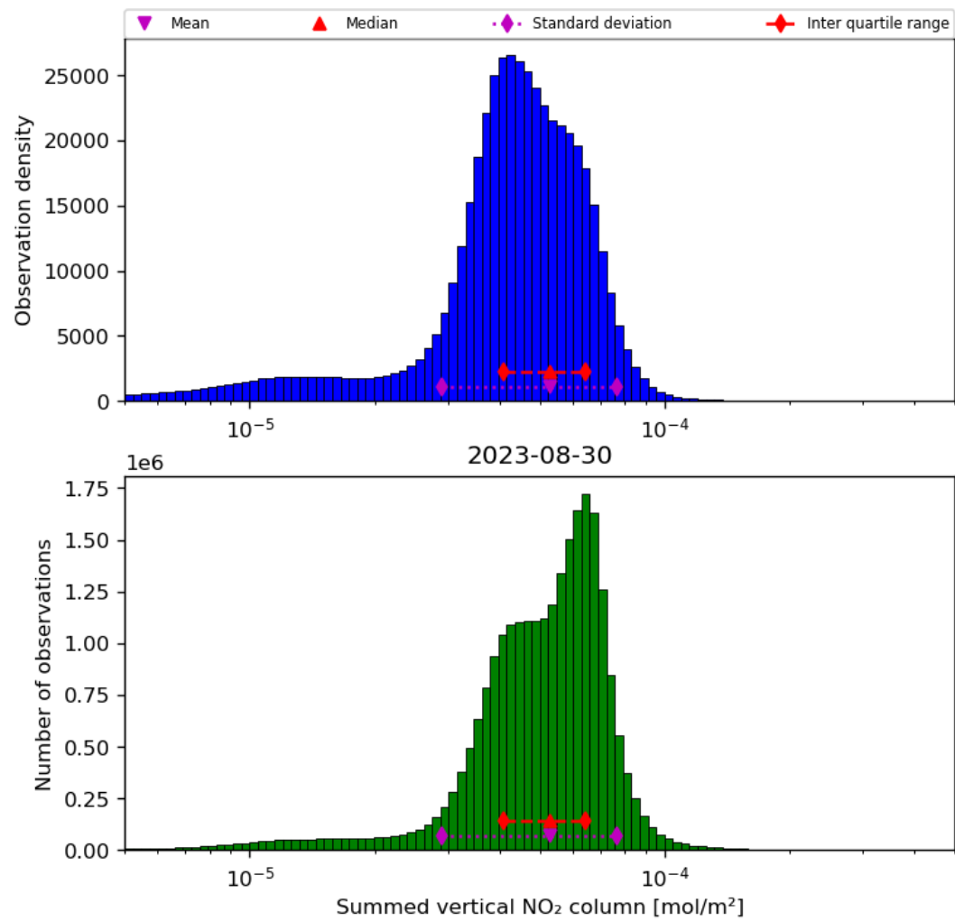
Figure 40: Histogram of “Summed vertical NO 2 column” for 2023-08-30 to 2023-08-31
