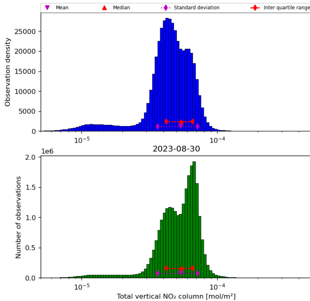
Figure 38: Histogram of “Total vertical NO 2 column” for 2023-08-30 to 2023-08-31
