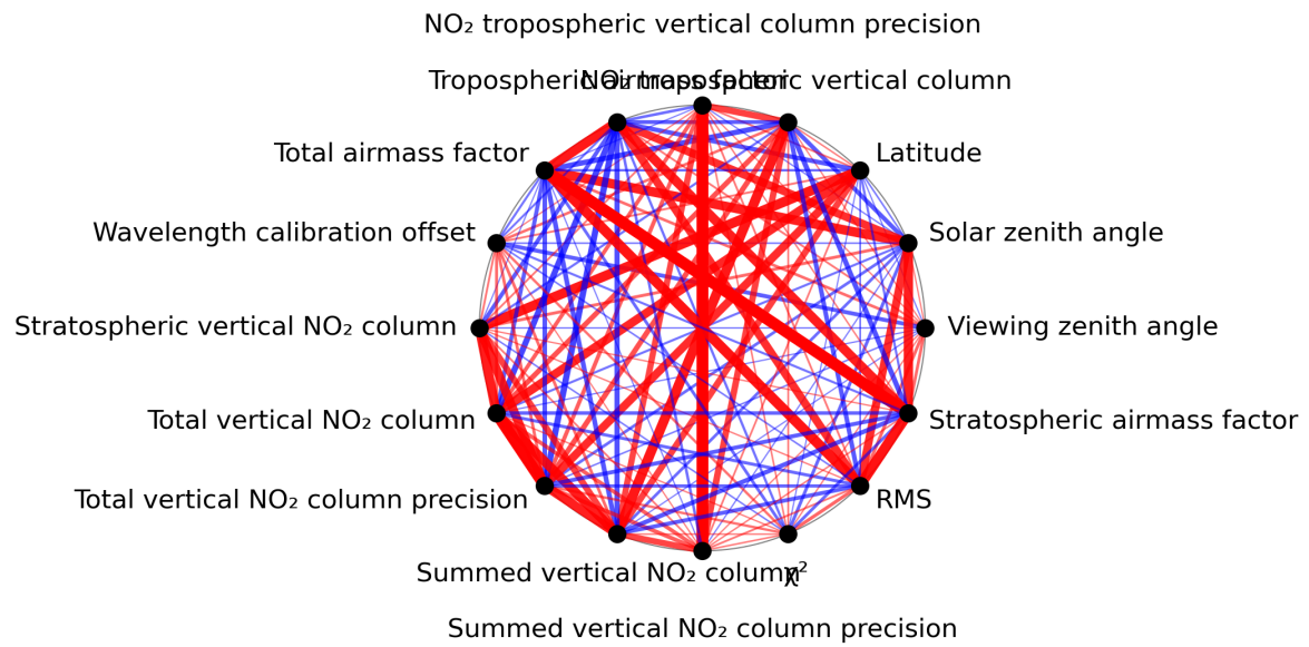
Figure 1: Map of correlation graph for 2023-08-30 to 2023-08-31.
