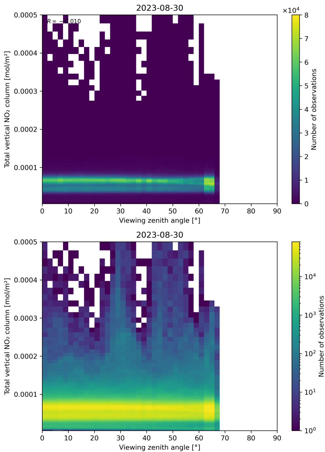
Figure 167: Scatter density plot of “Viewing zenith angle” against “Total vertical NO 2 column” for 2023-08-30 to 2023-08-31.
