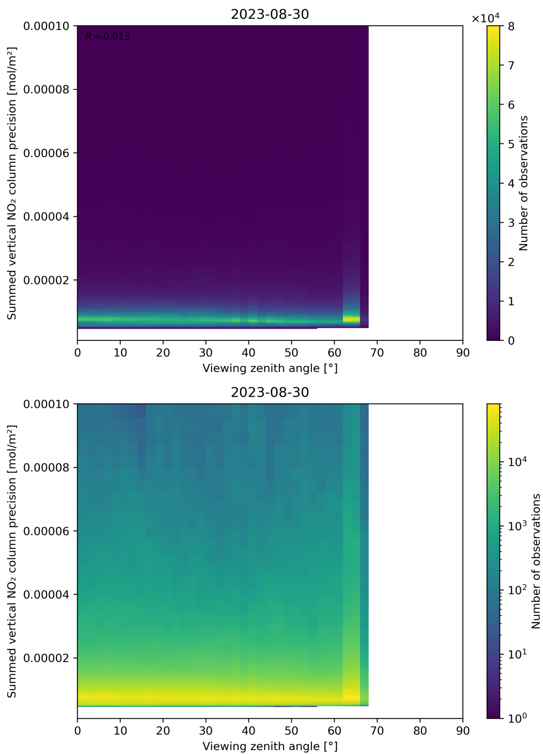
Figure 166: Scatter density plot of “Viewing zenith angle” against “Summed vertical NO 2 column precision” for 2023-08-30 to 2023-08-31.
