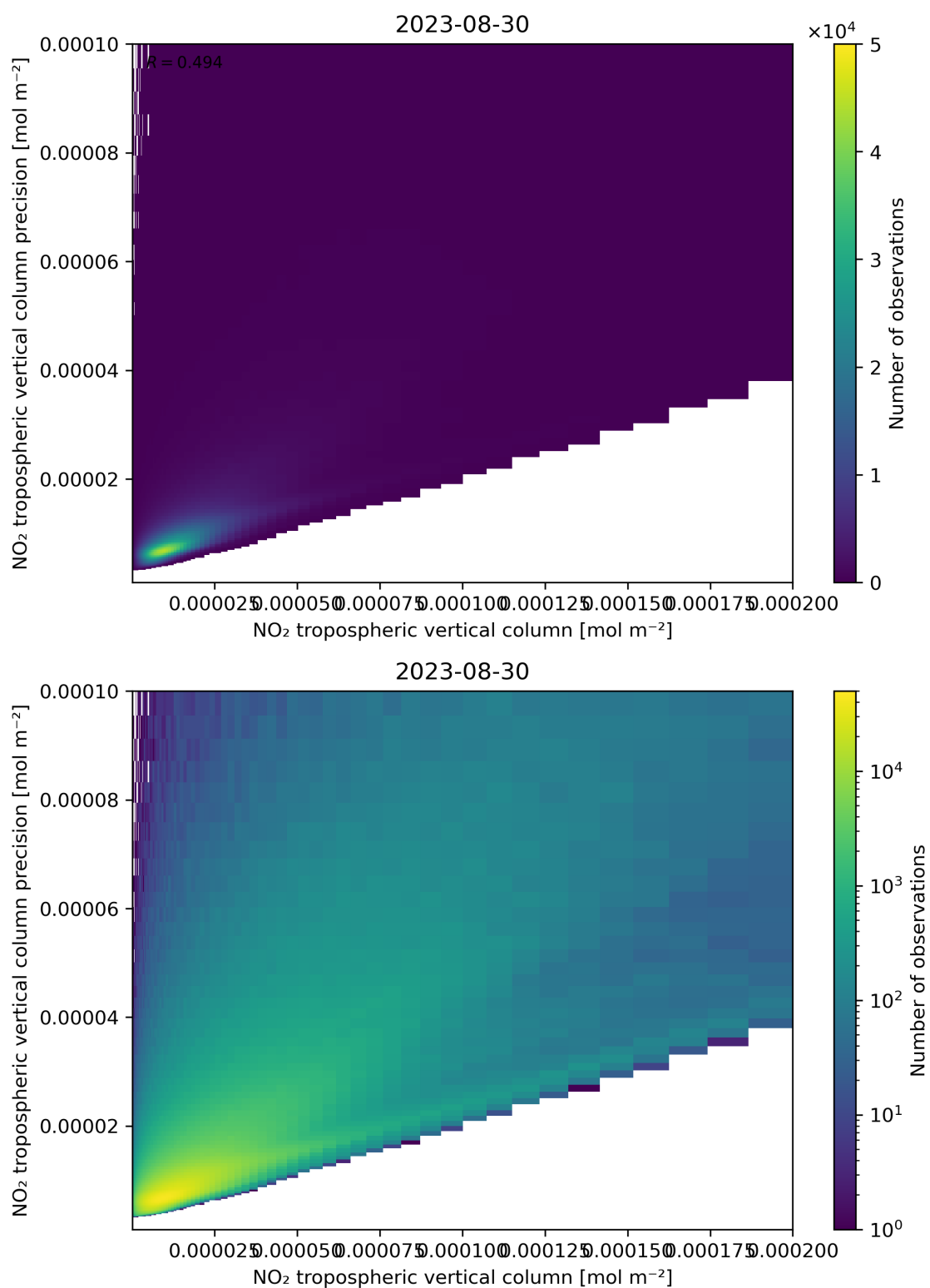
Figure 130: Scatter density plot of “NO 2 tropospheric vertical column” against “NO 2 tropospheric vertical column precision” for 2023-08-30 to 2023-08-31.
