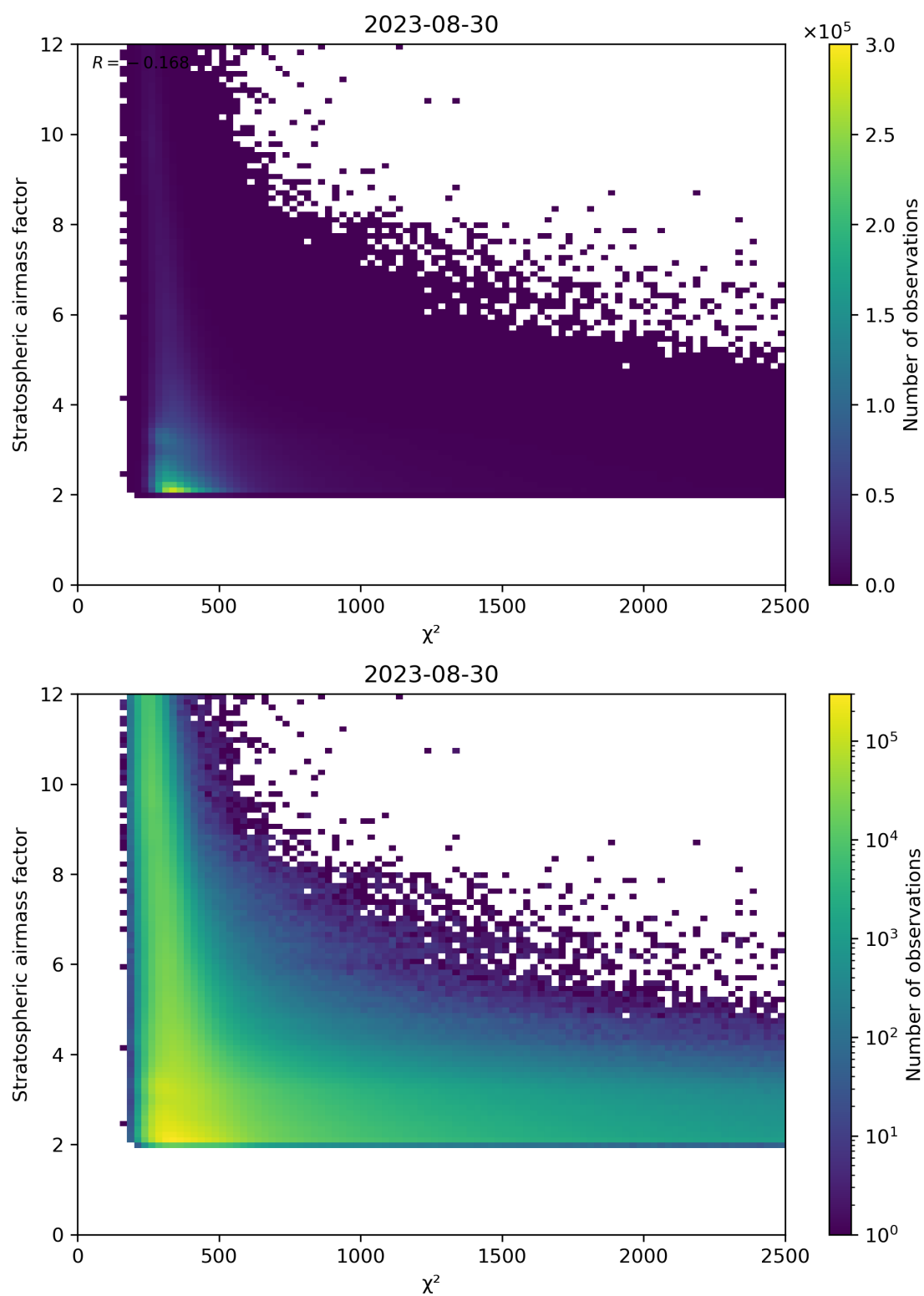
Figure 81: Scatter density plot of “ \chi^2 ” against “Stratospheric airmass factor” for 2023-08-30 to 2023-08-31.
