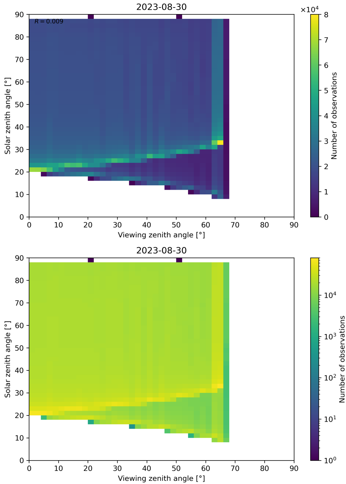
Figure 172: Scatter density plot of “Viewing zenith angle” against “Solar zenith angle” for 2023-08-30 to 2023-08-31.
