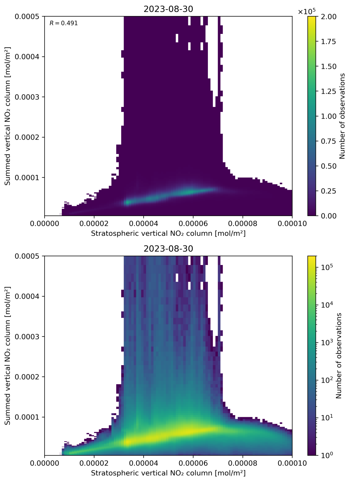
Figure 98: Scatter density plot of “Stratospheric vertical NO 2 column” against “Summed vertical NO 2 column” for 2023-08-30 to 2023-08-31.
