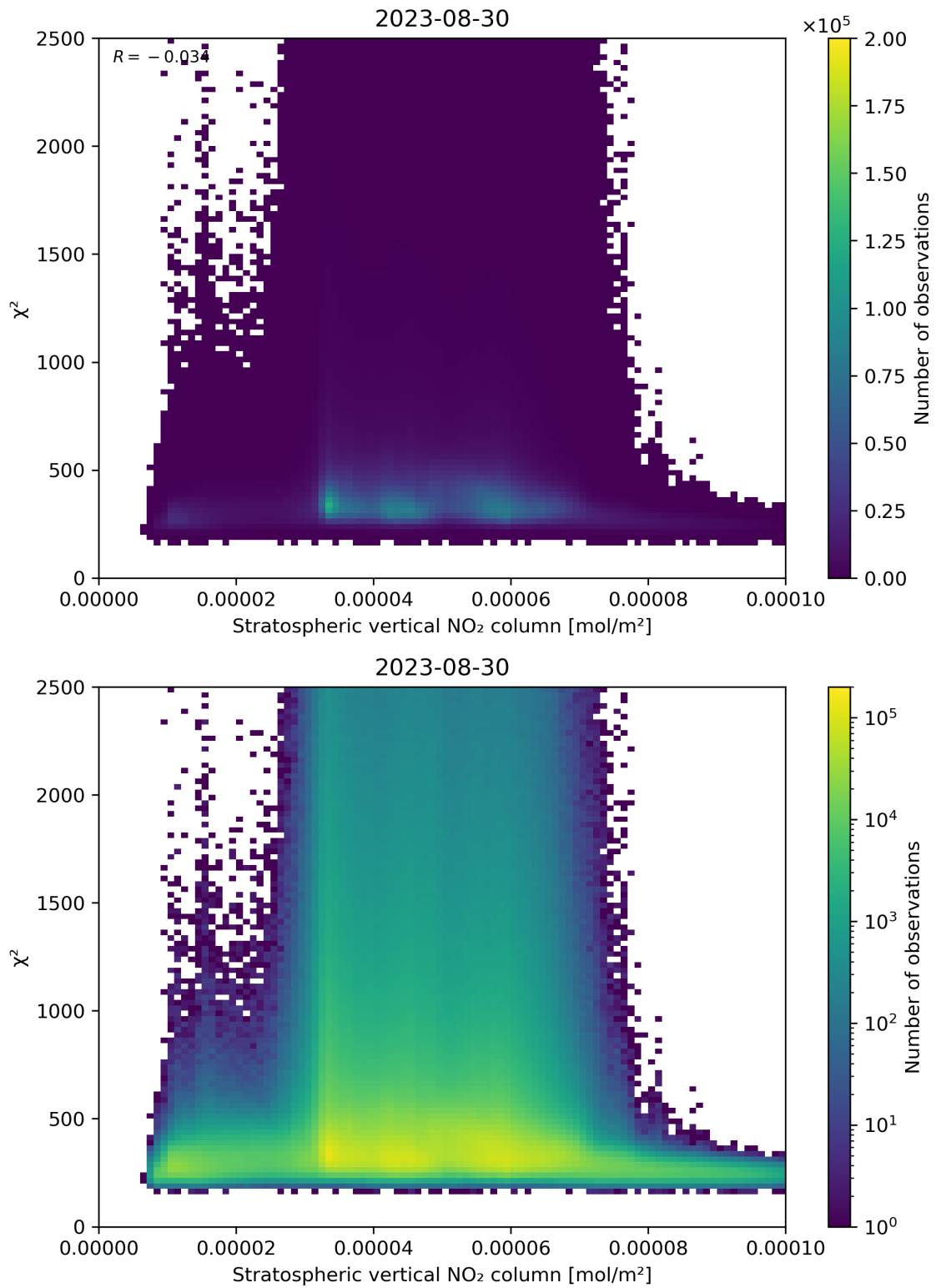
Figure 97: Scatter density plot of “Stratospheric vertical NO 2 column” against “ \chi^2 ” for 2023-08-30 to 2023-08-31.
