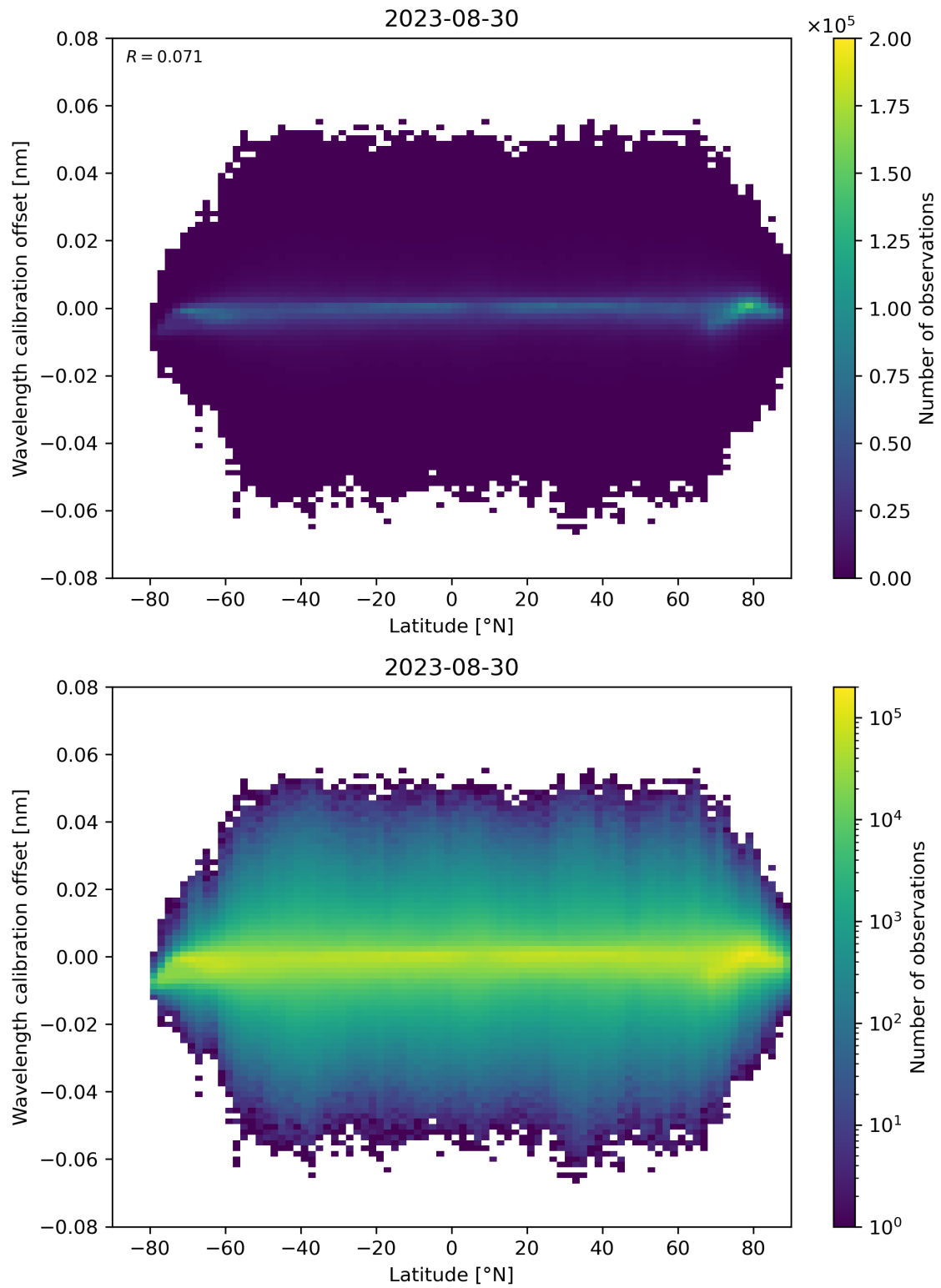
Figure 95: Scatter density plot of “Latitude” against “Wavelength calibration offset” for 2023-08-30 to 2023-08-31.
