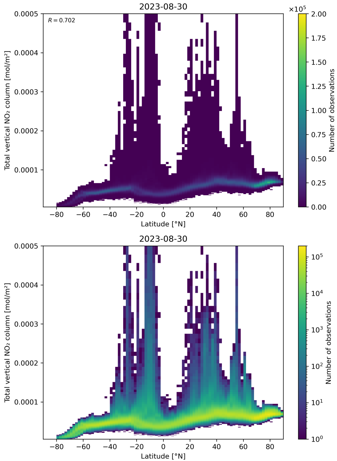
Figure 90: Scatter density plot of “Latitude” against “Total vertical NO 2 column” for 2023-08-30 to 2023-08-31.
