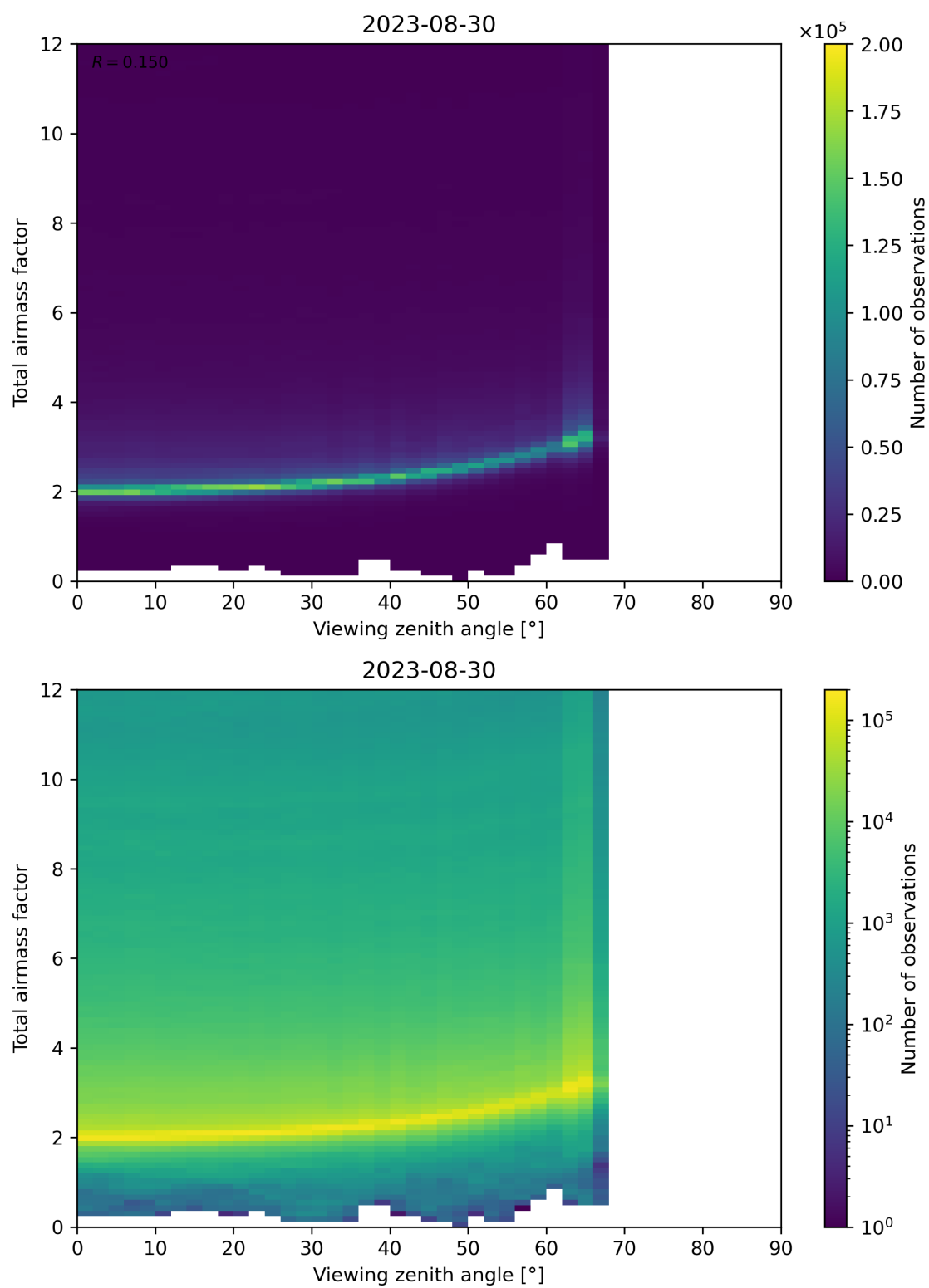
Figure 160: Scatter density plot of “Viewing zenith angle” against “Total airmass factor” for 2023-08-30 to 2023-08-31.
