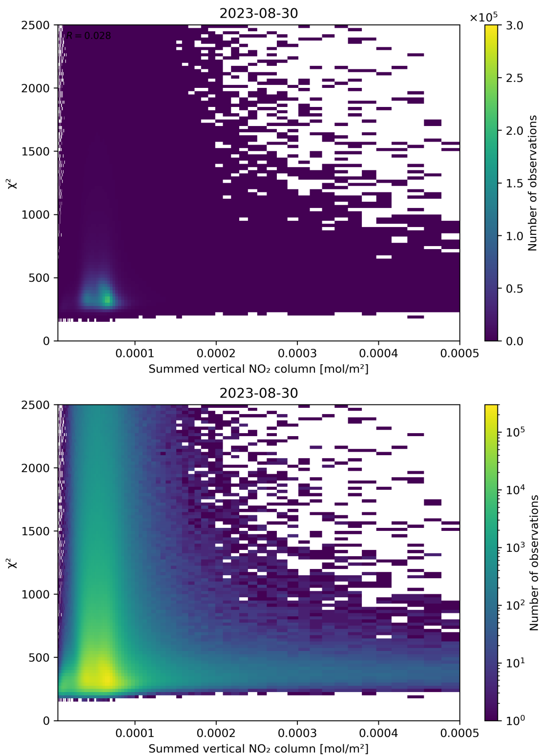
Figure 104: Scatter density plot of “Summed vertical NO 2 column” against “ \chi^2 ” for 2023-08-30 to 2023-08-31.
