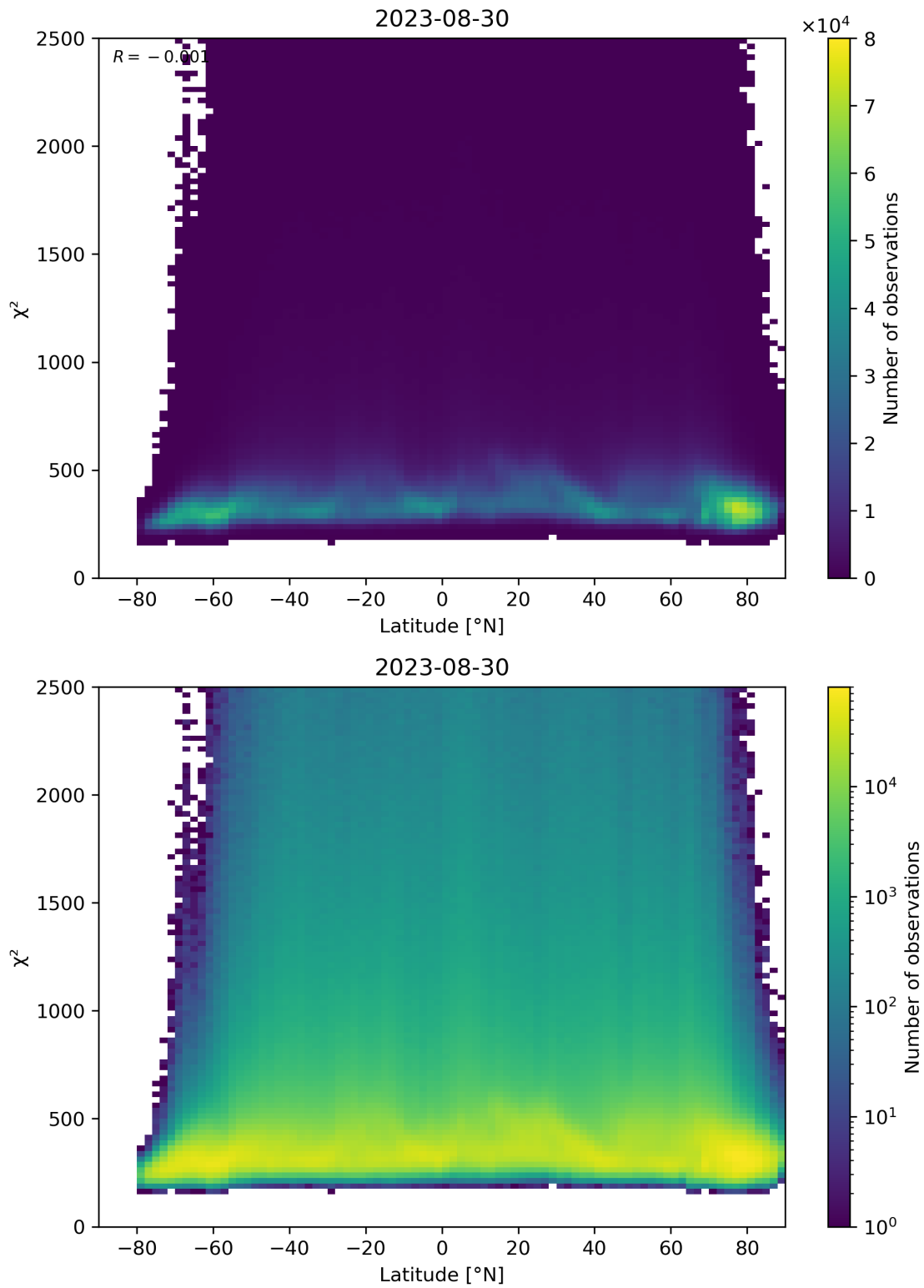
Figure 86: Scatter density plot of “Latitude” against “ \chi^2 ” for 2023-08-30 to 2023-08-31.
