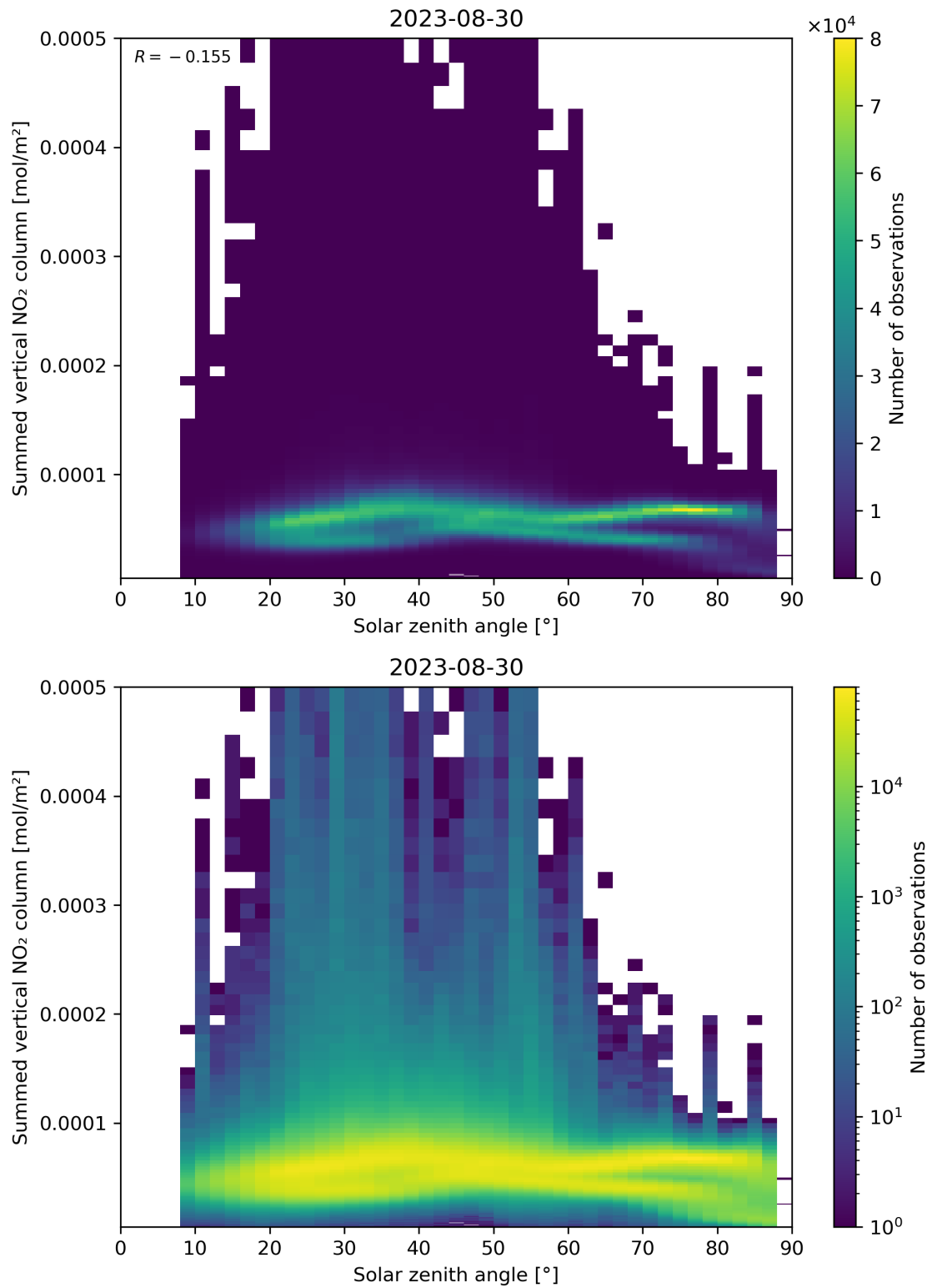
Figure 151: Scatter density plot of “Solar zenith angle” against “Summed vertical NO 2 column” for 2023-08-30 to 2023-08-31.
