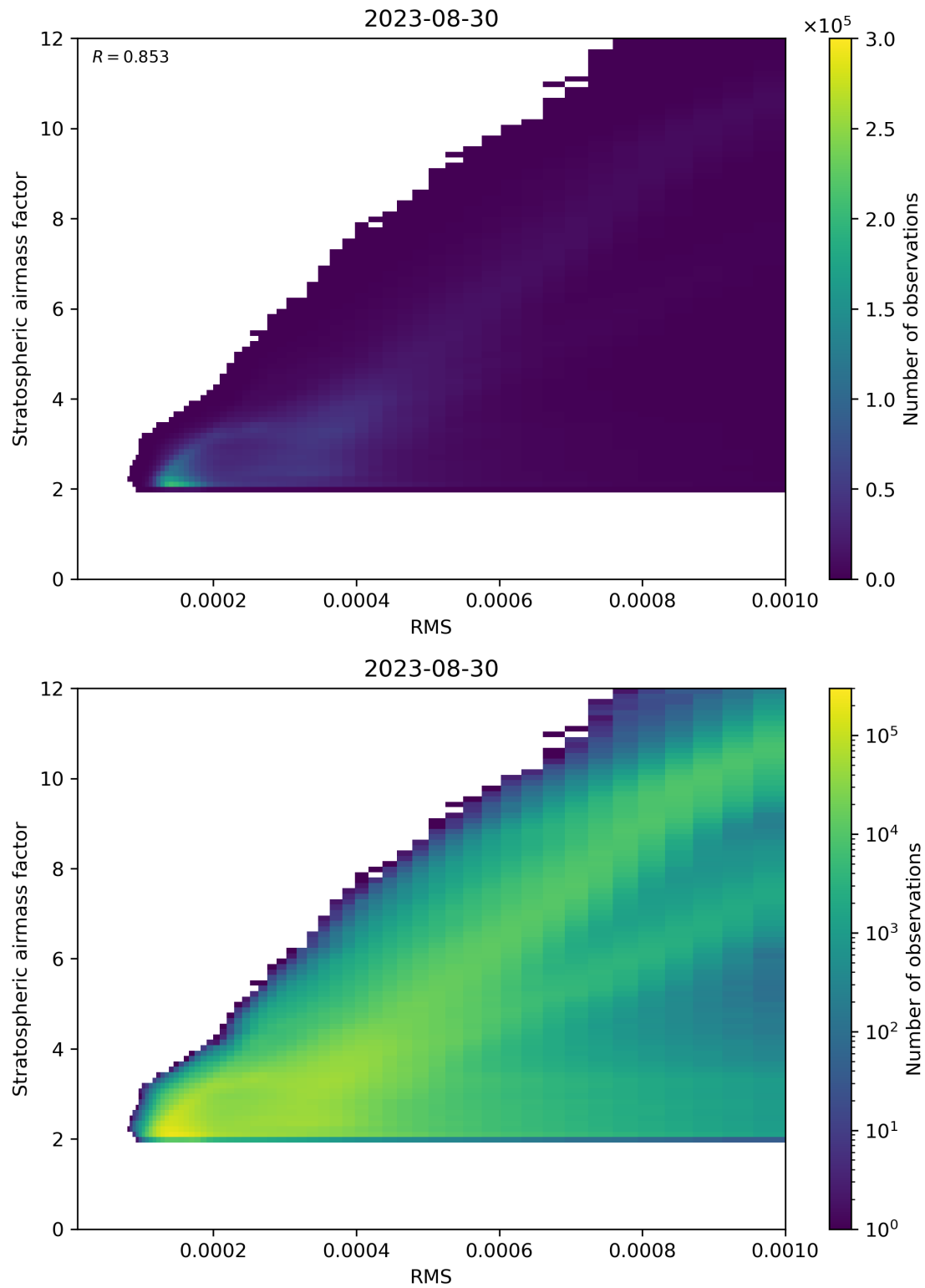
Figure 144: Scatter density plot of “RMS” against “Stratospheric airmass factor” for 2023-08-30 to 2023-08-31.
