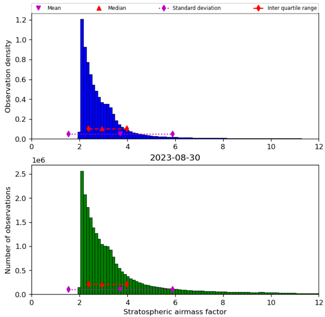
Figure 44: Histogram of “Stratospheric airmass factor” for 2023-08-30 to 2023-08-31
