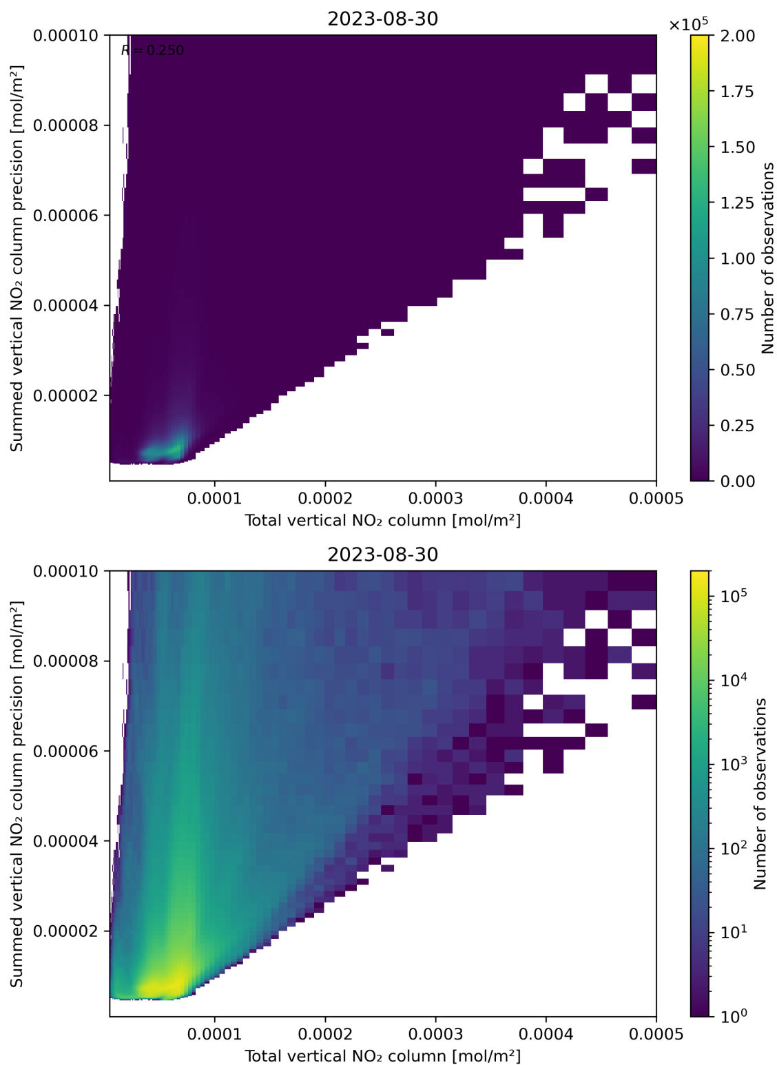
Figure 113: Scatter density plot of “Total vertical NO 2 column” against “Summed vertical NO 2 column precision” for 2023-08-30 to 2023-08-31.
