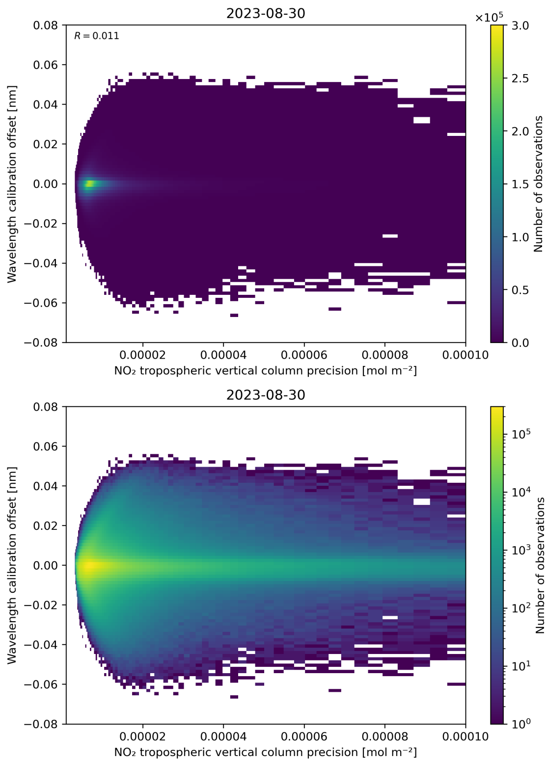
Figure 141: Scatter density plot of “NO 2 tropospheric vertical column precision” against “Wavelength calibration offset” for 2023-08-30 to 2023-08-31.
