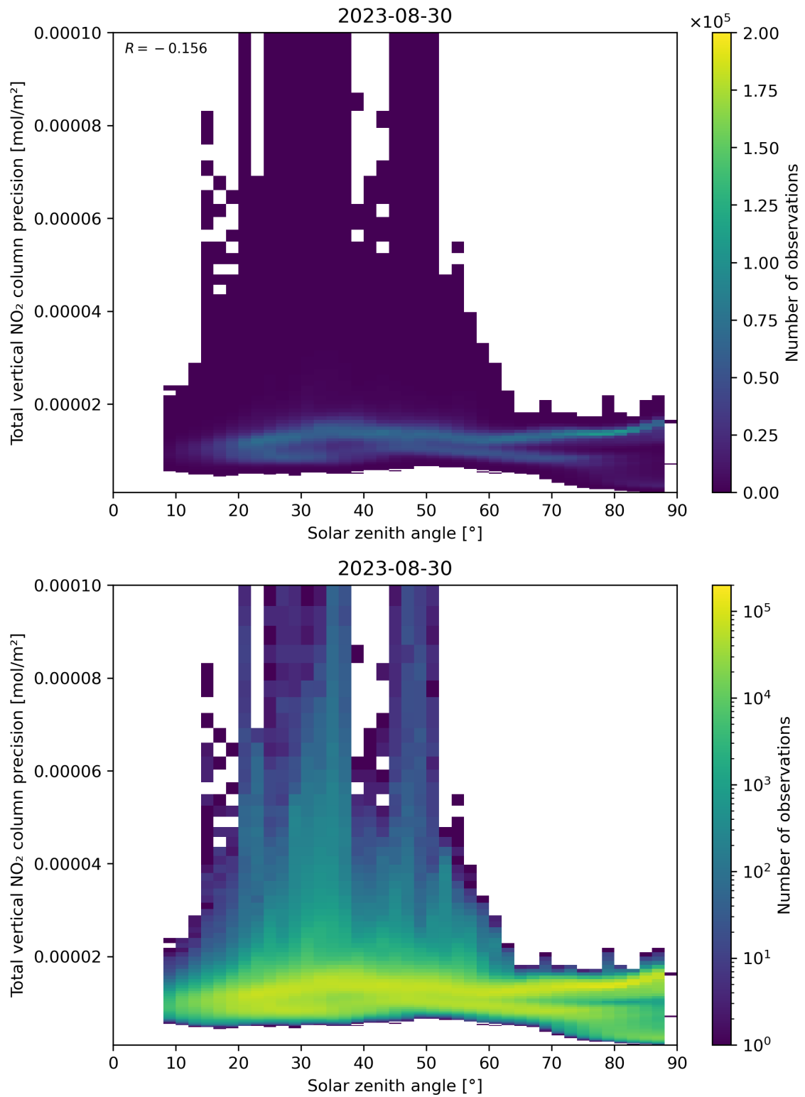
Figure 154: Scatter density plot of “Solar zenith angle” against “Total vertical NO 2 column precision” for 2023-08-30 to 2023-08-31.
