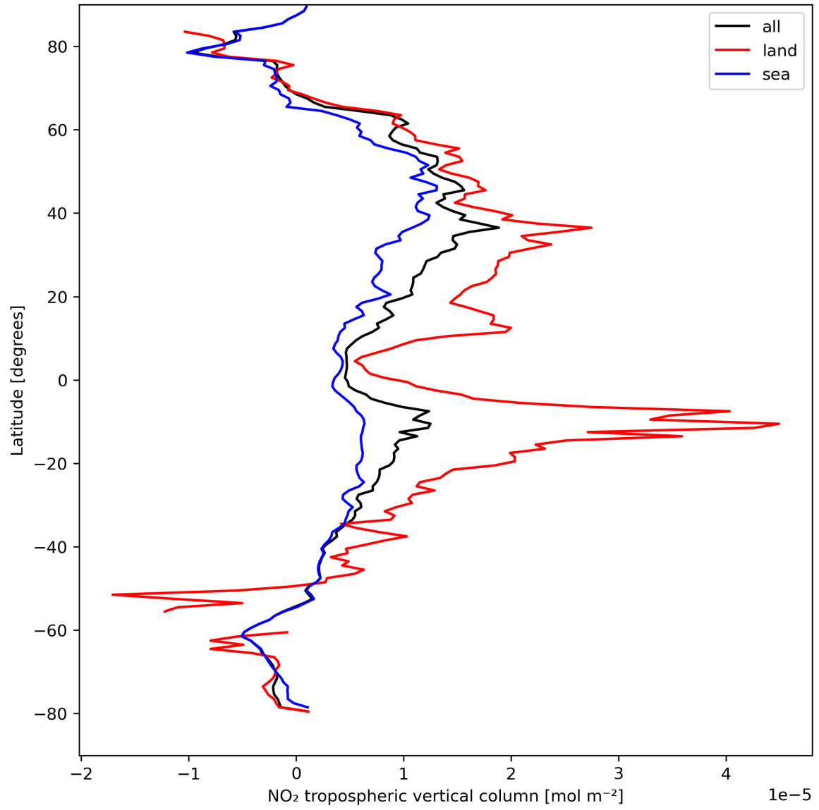
Figure 12: Zonal average of “NO 2 tropospheric vertical column” for 2023-08-30 to 2023-08-31.
