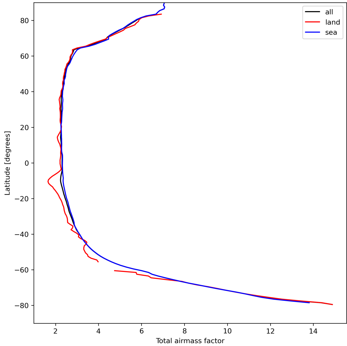
Figure 15: Zonal average of “Total airmass factor” for 2023-08-30 to 2023-08-31.
