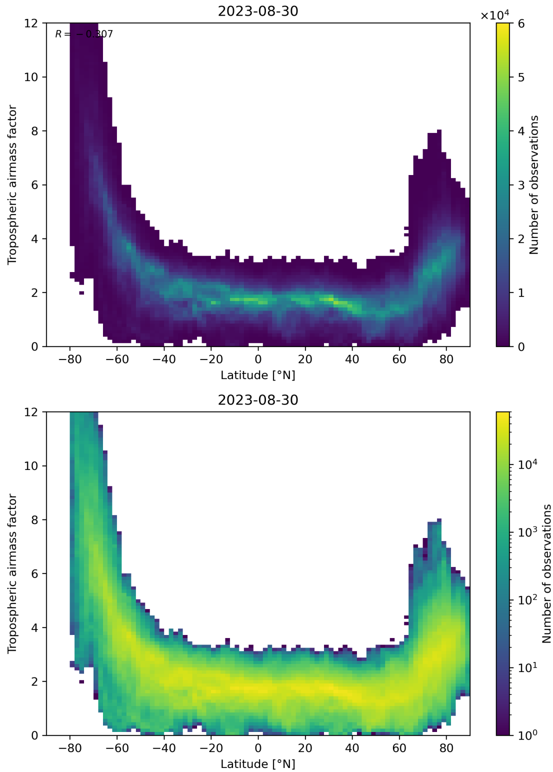
Figure 85: Scatter density plot of “Latitude” against “Tropospheric air mass factor” for 2023-08-30 to 2023-08-31.
