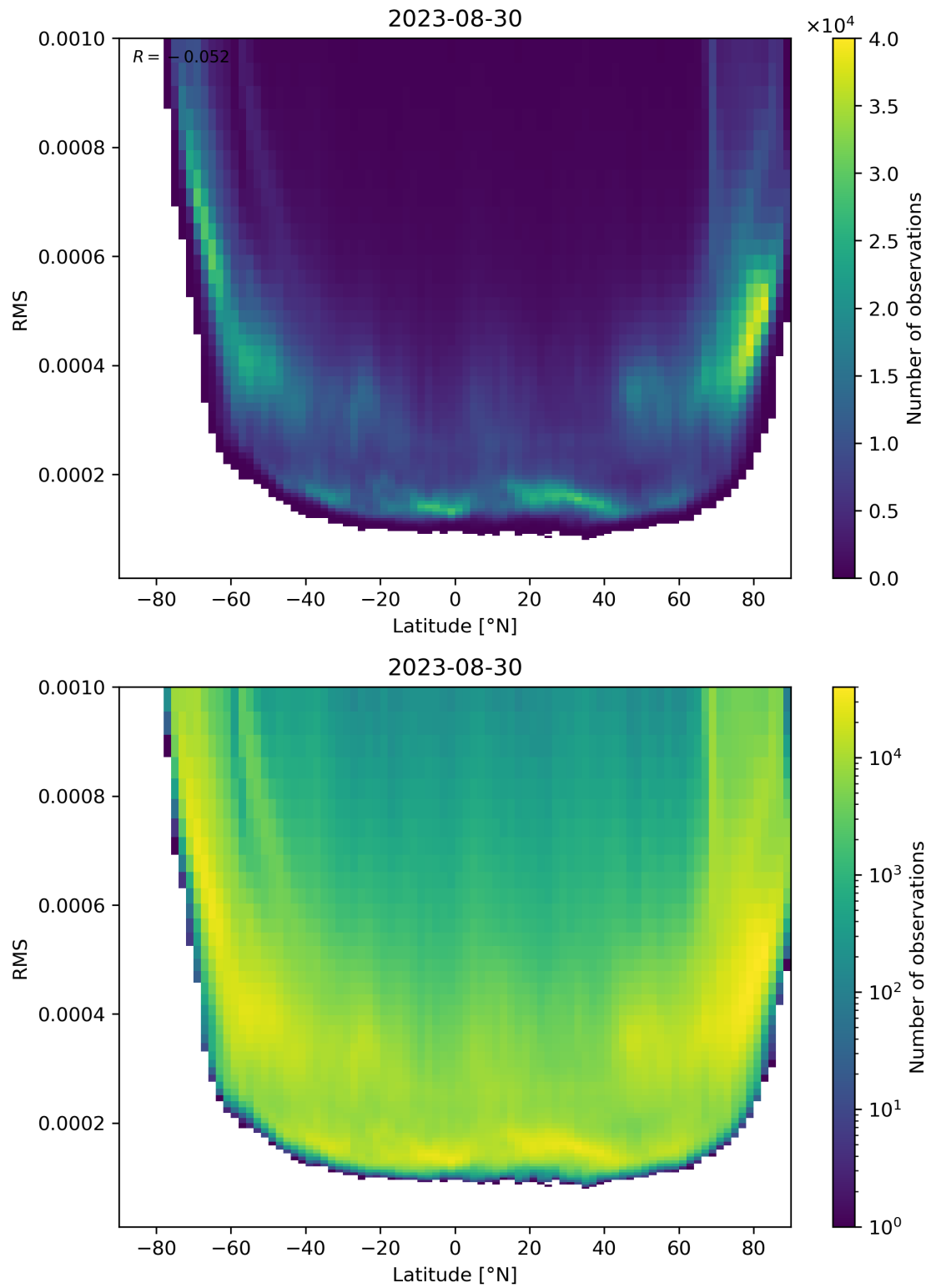
Figure 94: Scatter density plot of “Latitude” against “RMS” for 2023-08-30 to 2023-08-31.
