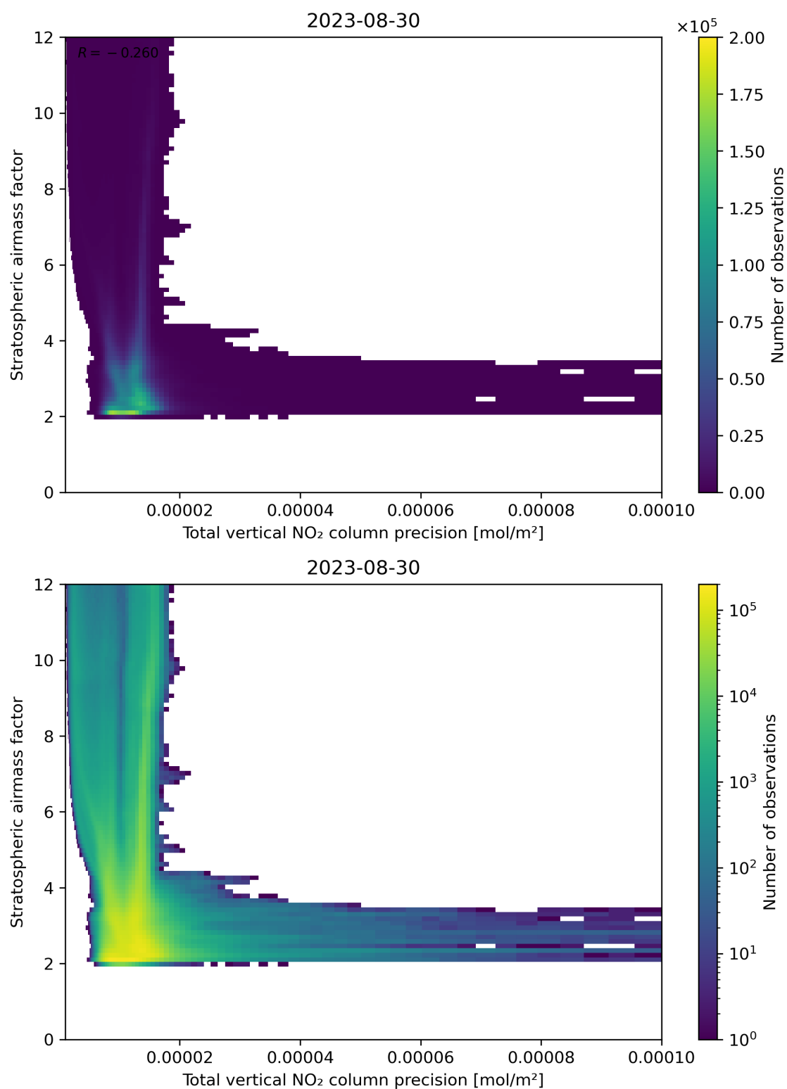
Figure 115: Scatter density plot of “Total vertical NO 2 column precision” against “Stratospheric air mass factor” for 2023-08-30 to 2023-08-31.
