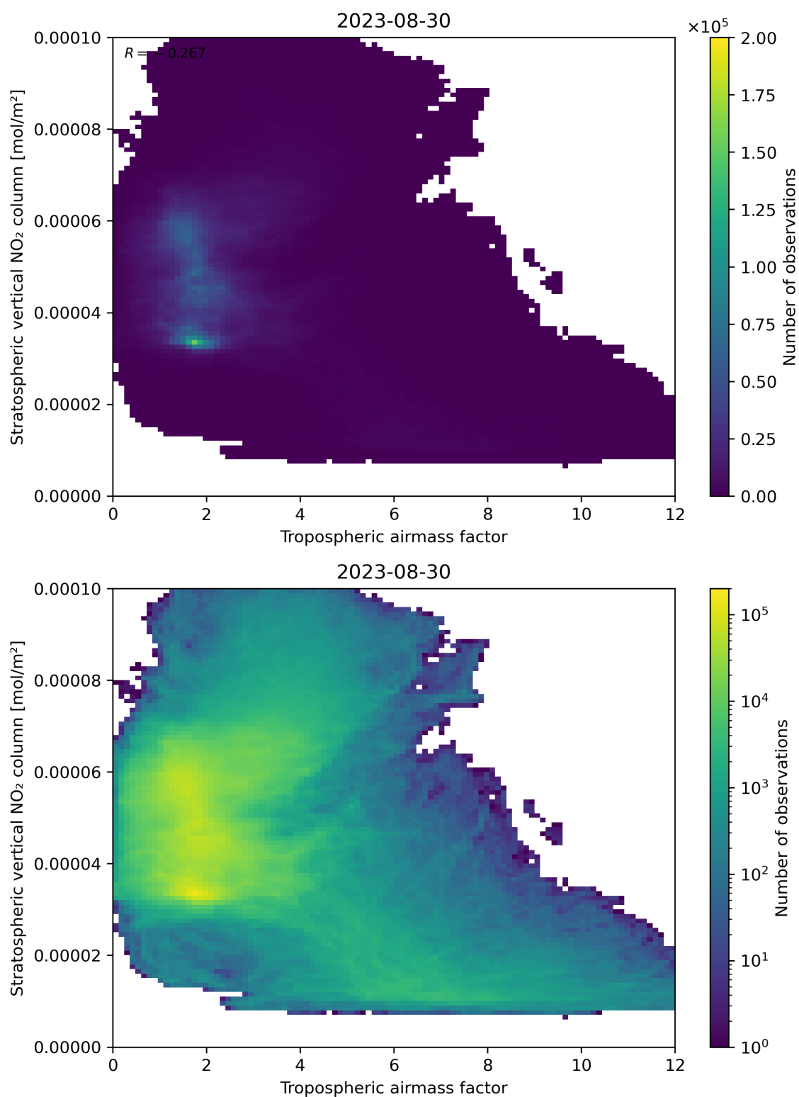
Figure 74: Scatter density plot of “Tropospheric airmass factor” against “Stratospheric vertical NO 2 column” for 2023-08-30 to 2023-08-31.
