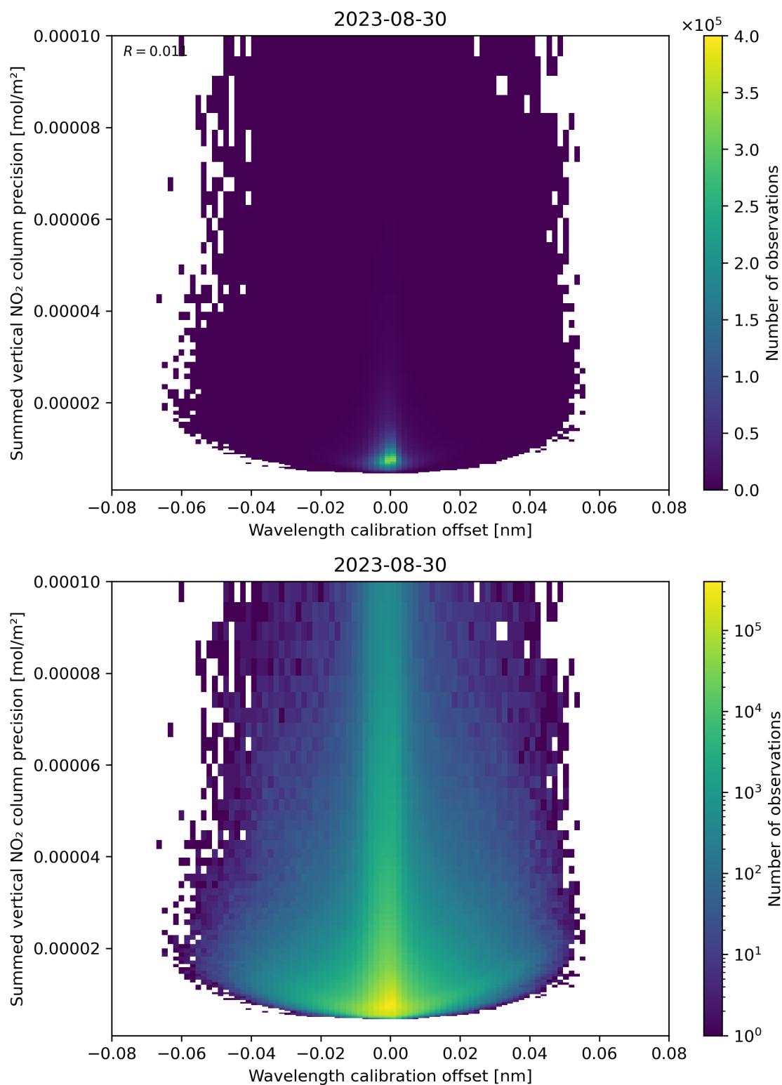
Figure 178: Scatter density plot of “Wavelength calibration offset” against “Summed vertical NO 2 column precision” for 2023-08-30 to 2023-08-31.
