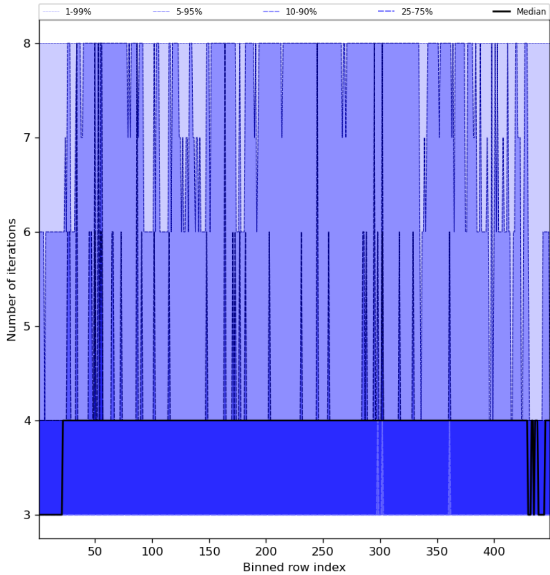
Figure 51: Along track statistics of “Number of iterations” for 2023-08-30 to 2023-08-31
