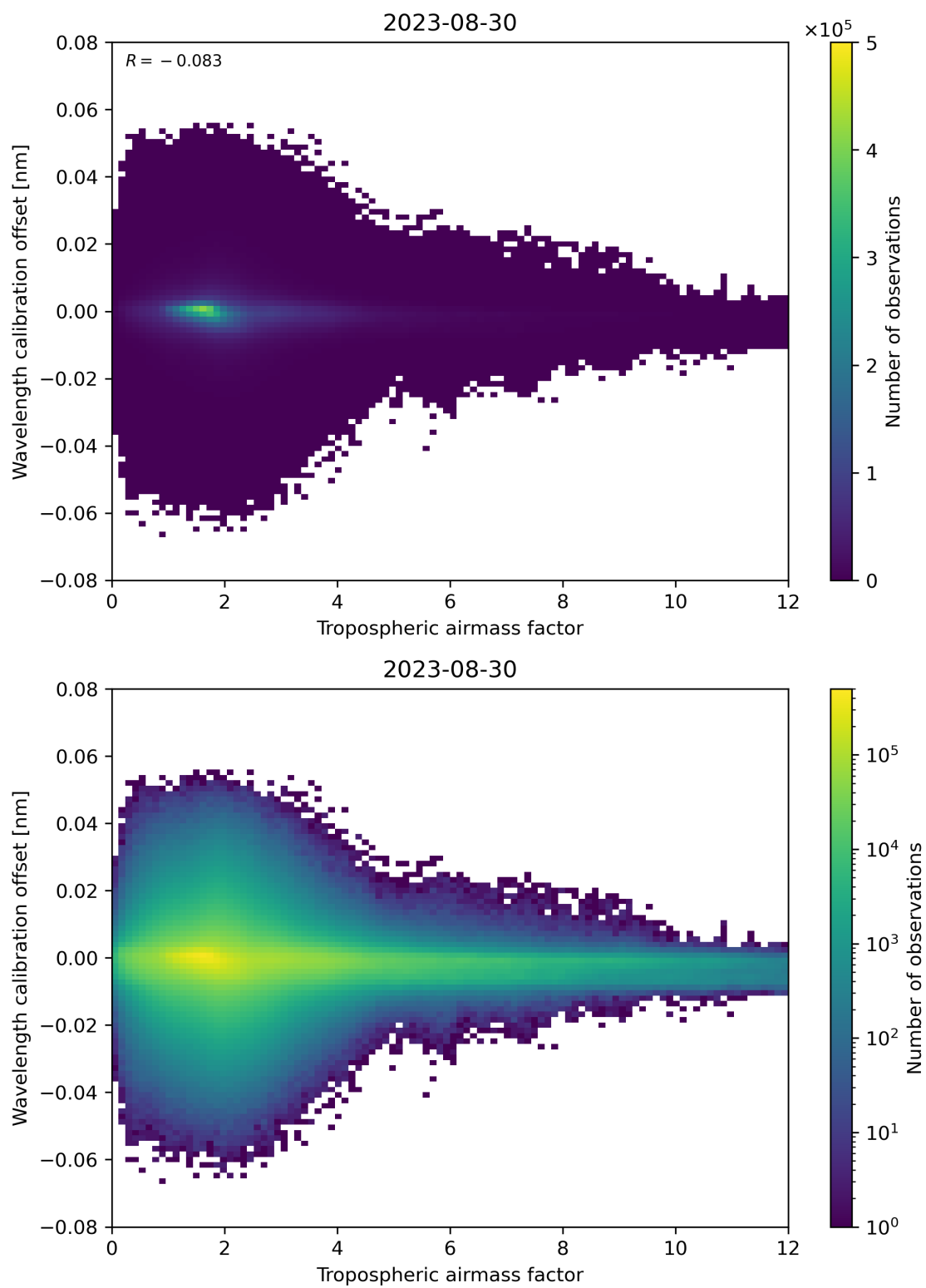
Figure 80: Scatter density plot of “Tropospheric air mass factor” against “Wavelength calibration offset” for 2023-08-30 to 2023-08-31.
