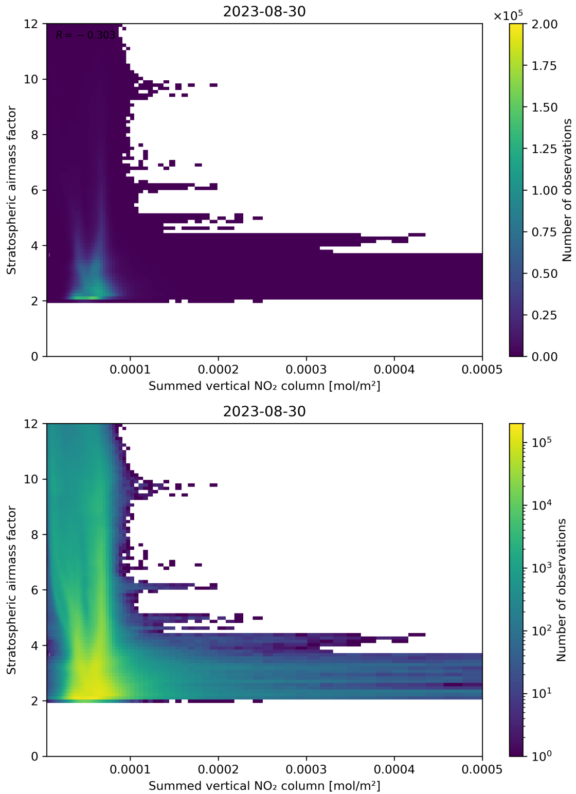
Figure 103: Scatter density plot of “Summed vertical NO 2 column” against “Stratospheric air mass factor” for 2023-08-30 to 2023-08-31.
