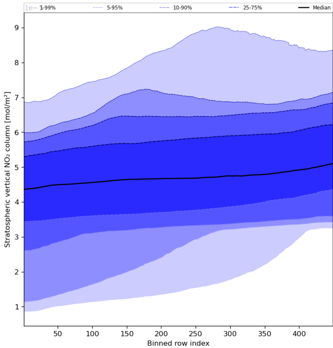
Figure 53: Along track statistics of “Stratospheric vertical NO 2 column” for 2023-08-30 to 2023-08-31
