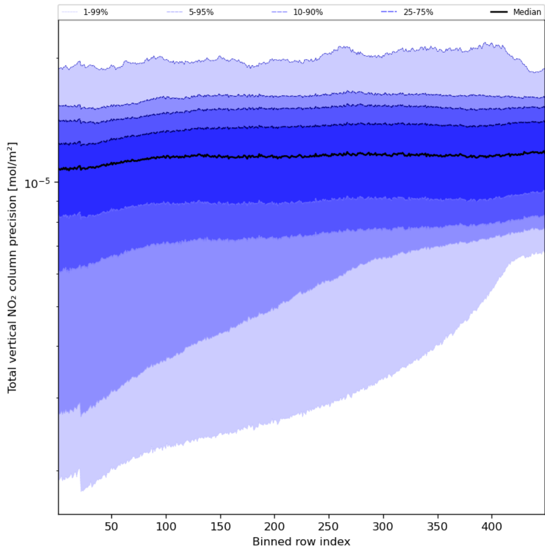
Figure 56: Along track statistics of “Total vertical NO 2 column precision” for 2023-08-30 to 2023-08-31
