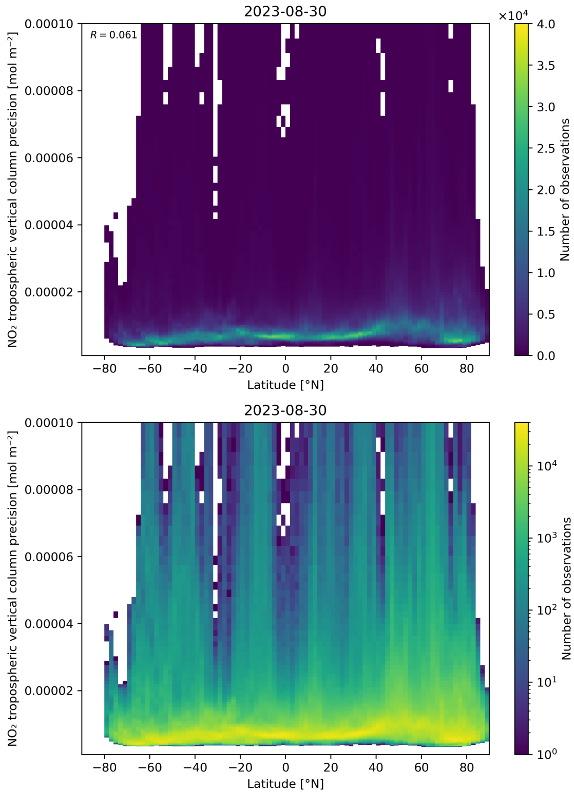
Figure 93: Scatter density plot of “Latitude” against “NO 2 tropospheric vertical column precision” for 2023-08-30 to 2023-08-31.
