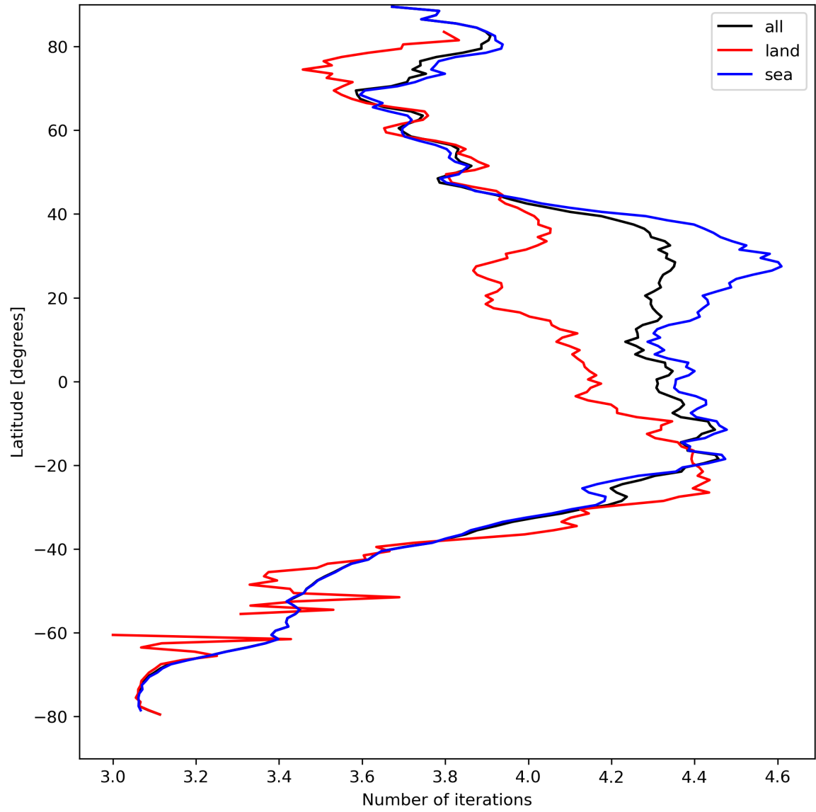
Figure 17: Zonal average of “Number of iterations” for 2023-08-30 to 2023-08-31.
