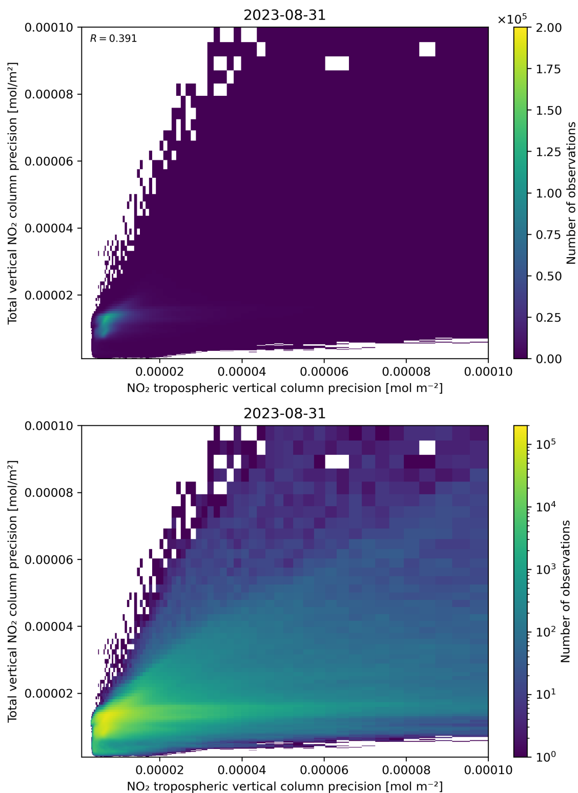
Figure 139: Scatter density plot of “NO 2 tropospheric vertical column precision” against “Total vertical NO 2 column precision” for 2023-08-30 to 2023-09-01.
