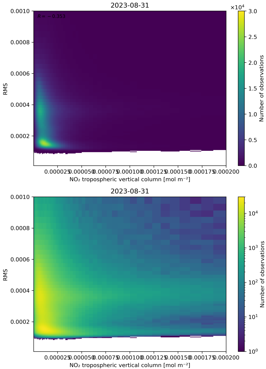
Figure 142: Scatter density plot of “NO 2 tropospheric vertical column” against “RMS” for 2023-08-30 to 2023-09-01.
