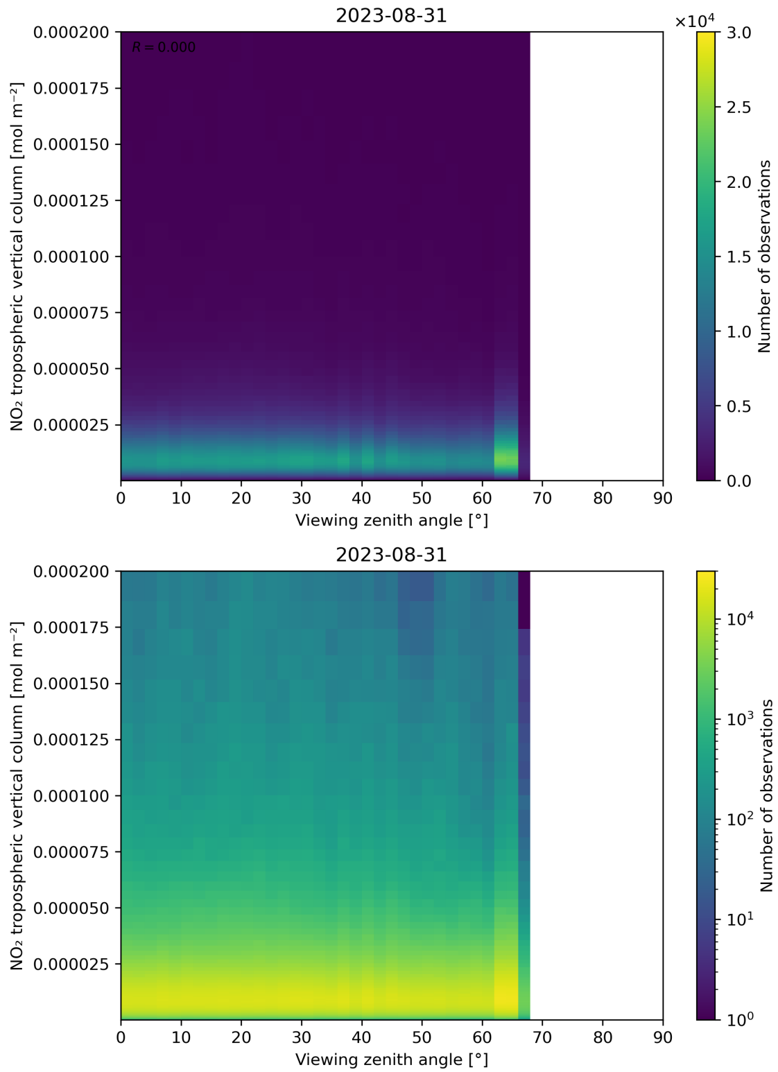
Figure 169: Scatter density plot of “Viewing zenith angle” against “NO 2 tropospheric vertical column” for 2023-08-30 to 2023-09-01.
