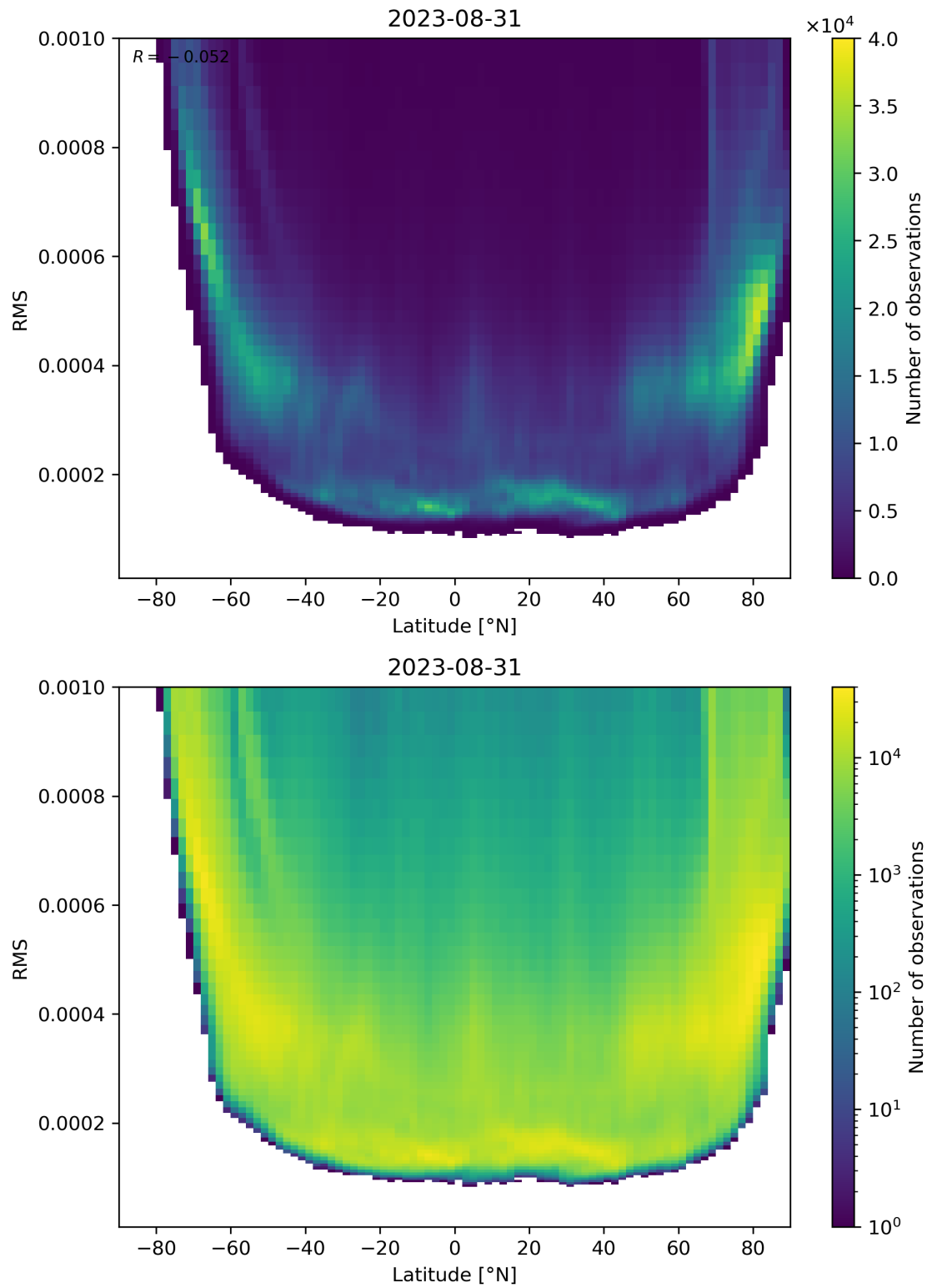
Figure 94: Scatter density plot of “Latitude” against “RMS” for 2023-08-30 to 2023-09-01.
