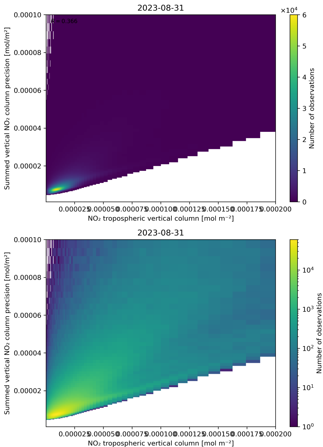
Figure 127: Scatter density plot of “NO 2 tropospheric vertical column” against “Summed vertical NO 2 column precision” for 2023-08-30 to 2023-09-01.
