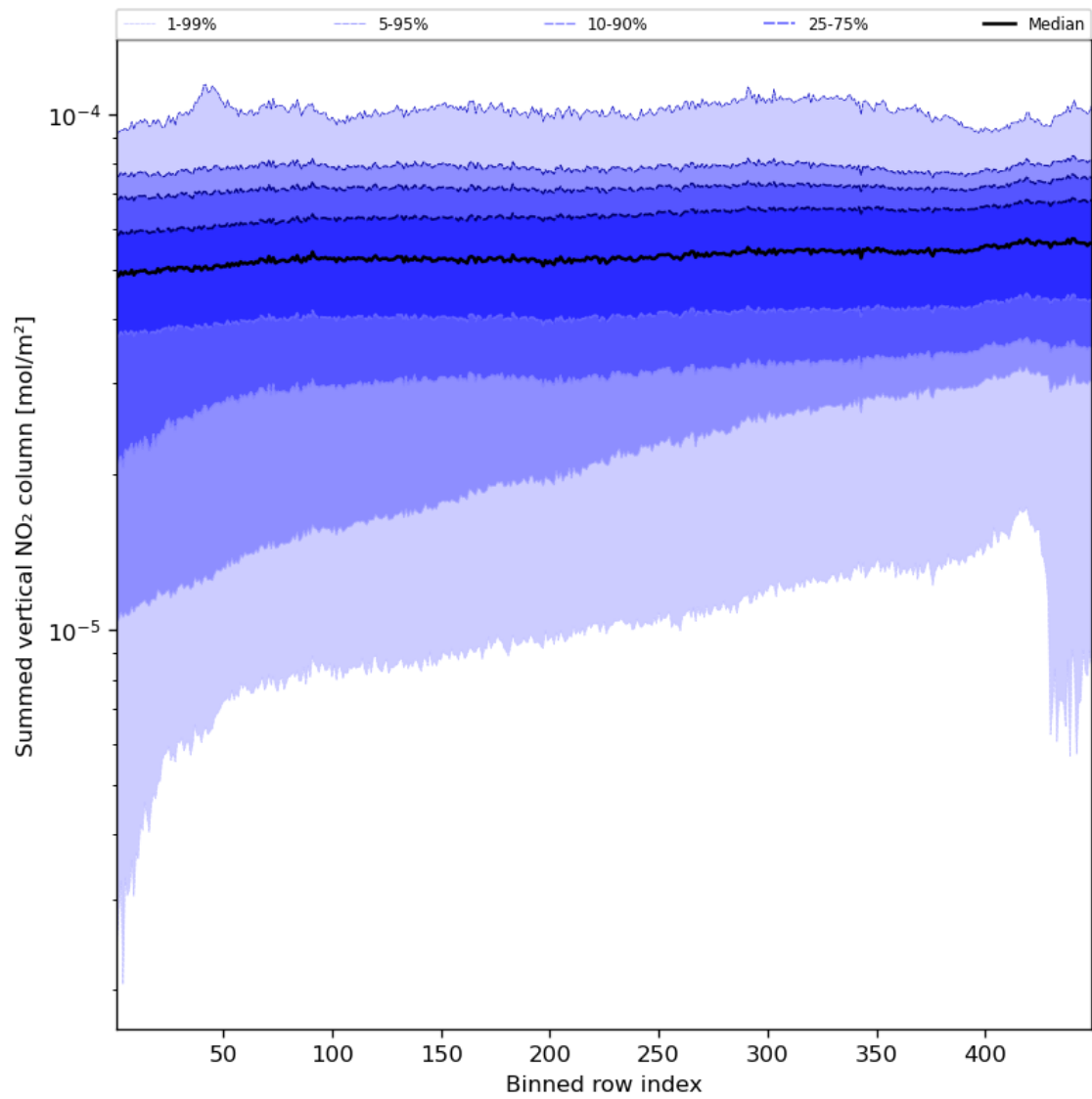
Figure 57: Along track statistics of “Summed vertical NO 2 column” for 2023-08-30 to 2023-09-01
