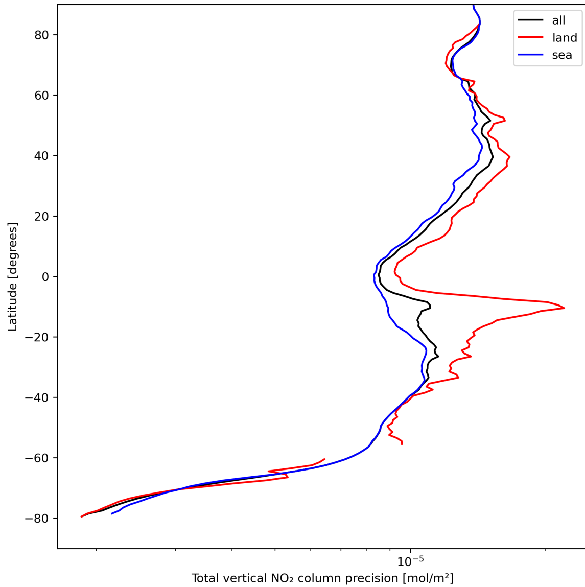
Figure 22: Zonal average of “Total vertical NO 2 column precision” for 2023-08-30 to 2023-09-01.
