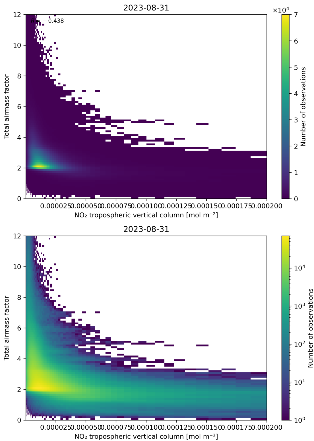
Figure 122: Scatter density plot of “NO 2 tropospheric vertical column” against “Total air mass factor” for 2023-08-30 to 2023-09-01.
