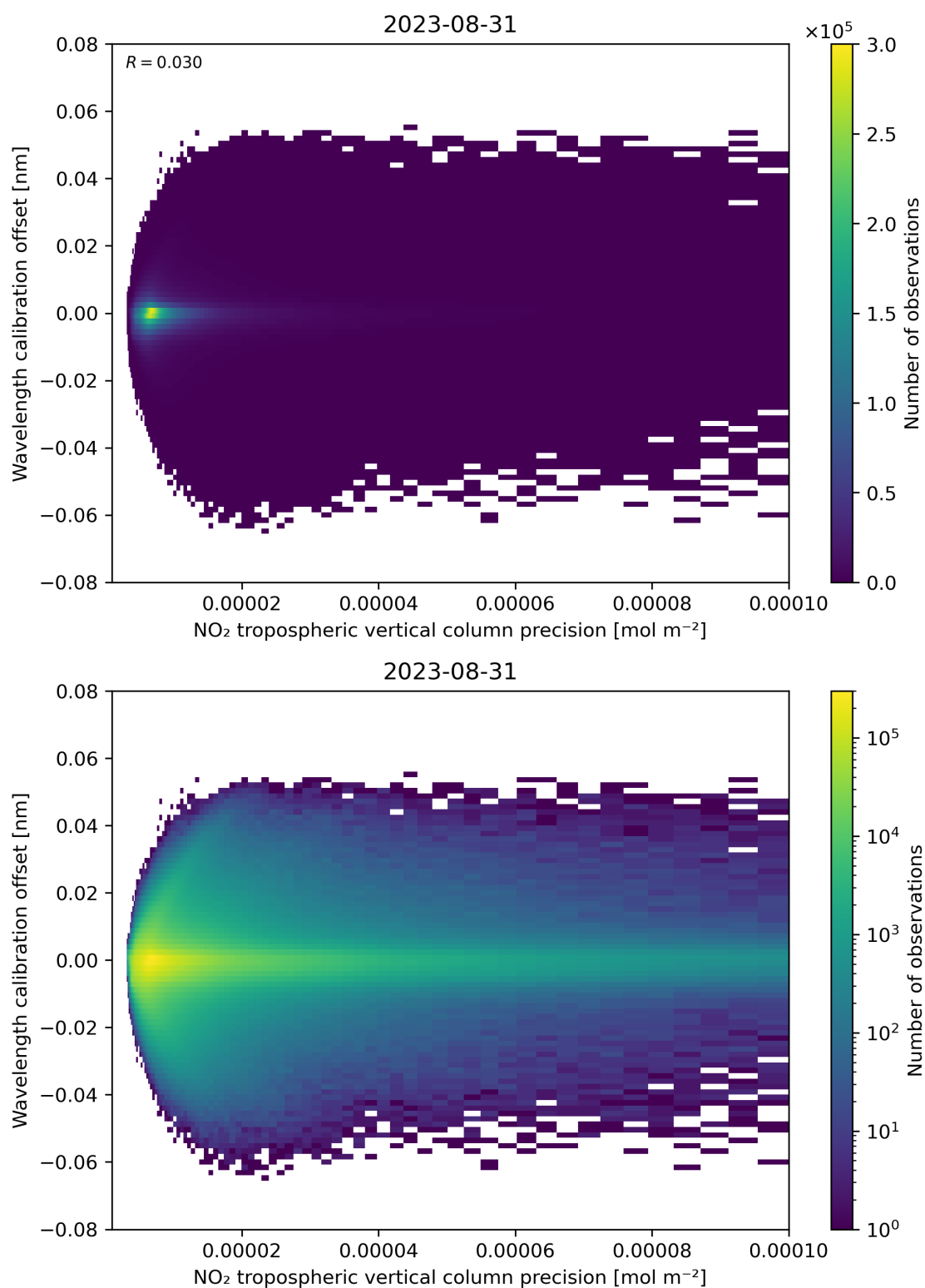
Figure 141: Scatter density plot of “NO 2 tropospheric vertical column precision” against “Wavelength calibration offset” for 2023-08-30 to 2023-09-01.
