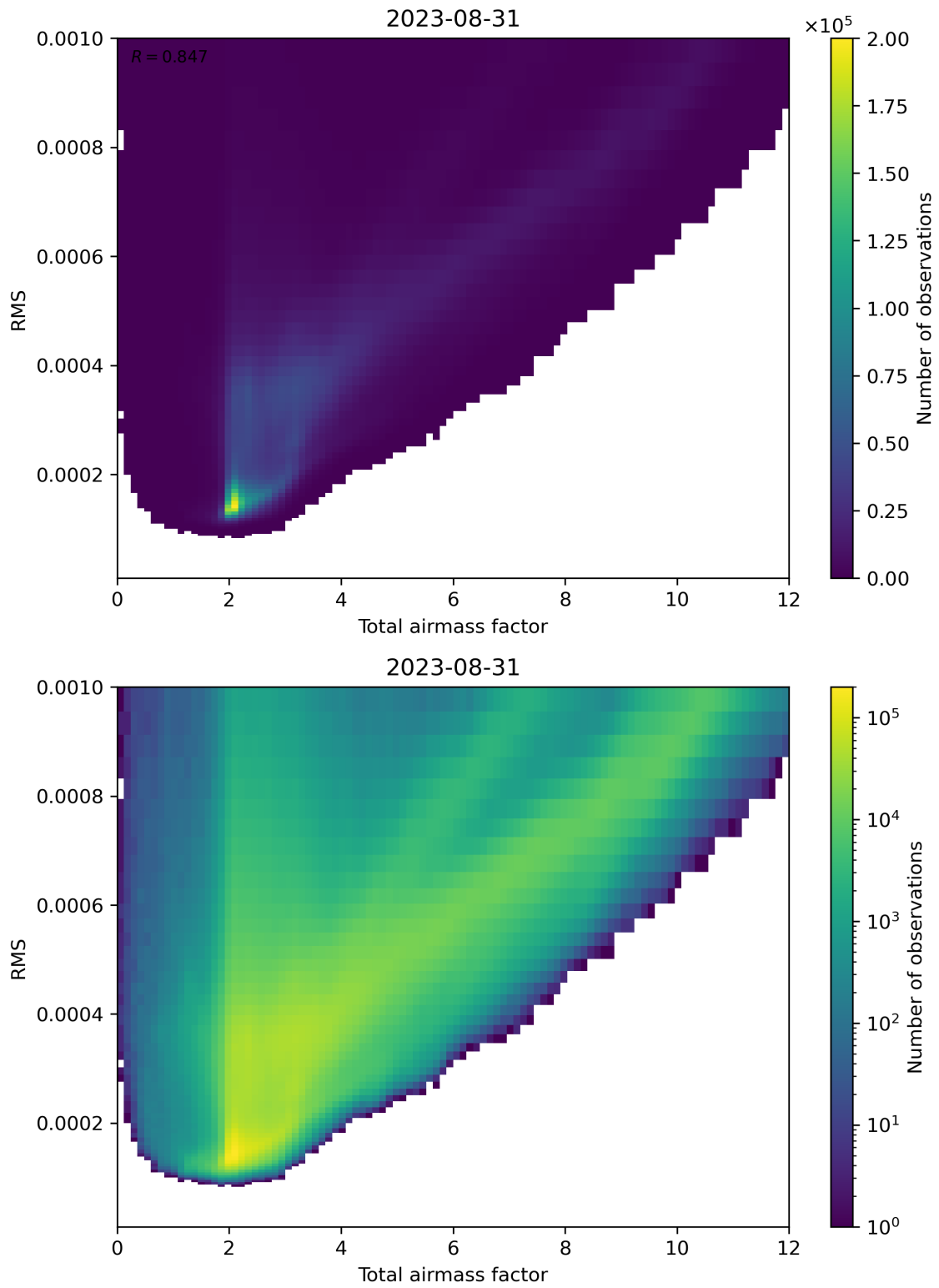
Figure 69: Scatter density plot of “Total airmass factor” against “RMS” for 2023-08-30 to 2023-09-01.
