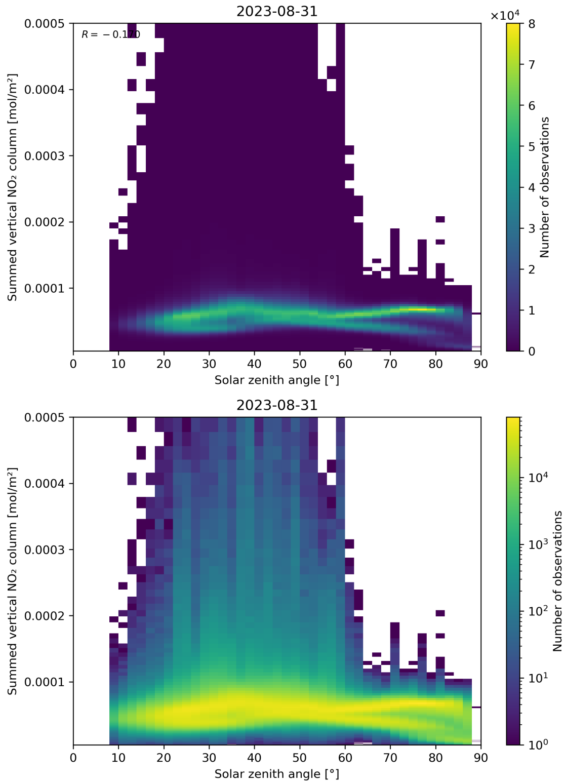
Figure 151: Scatter density plot of “Solar zenith angle” against “Summed vertical NO 2 column” for 2023-08-30 to 2023-09-01.
