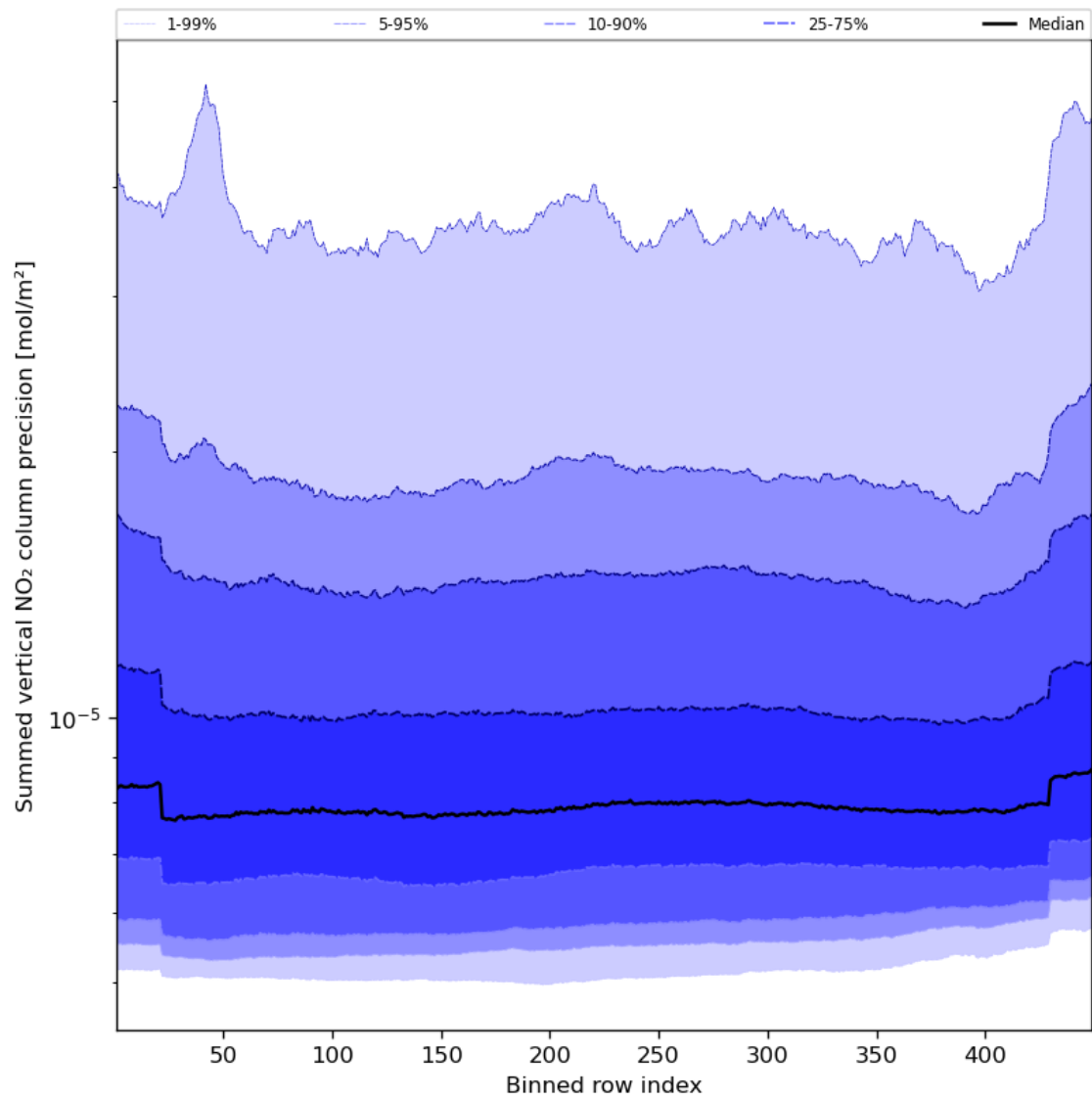
Figure 58: Along track statistics of “Summed vertical NO 2 column precision” for 2023-08-30 to 2023-09-01
