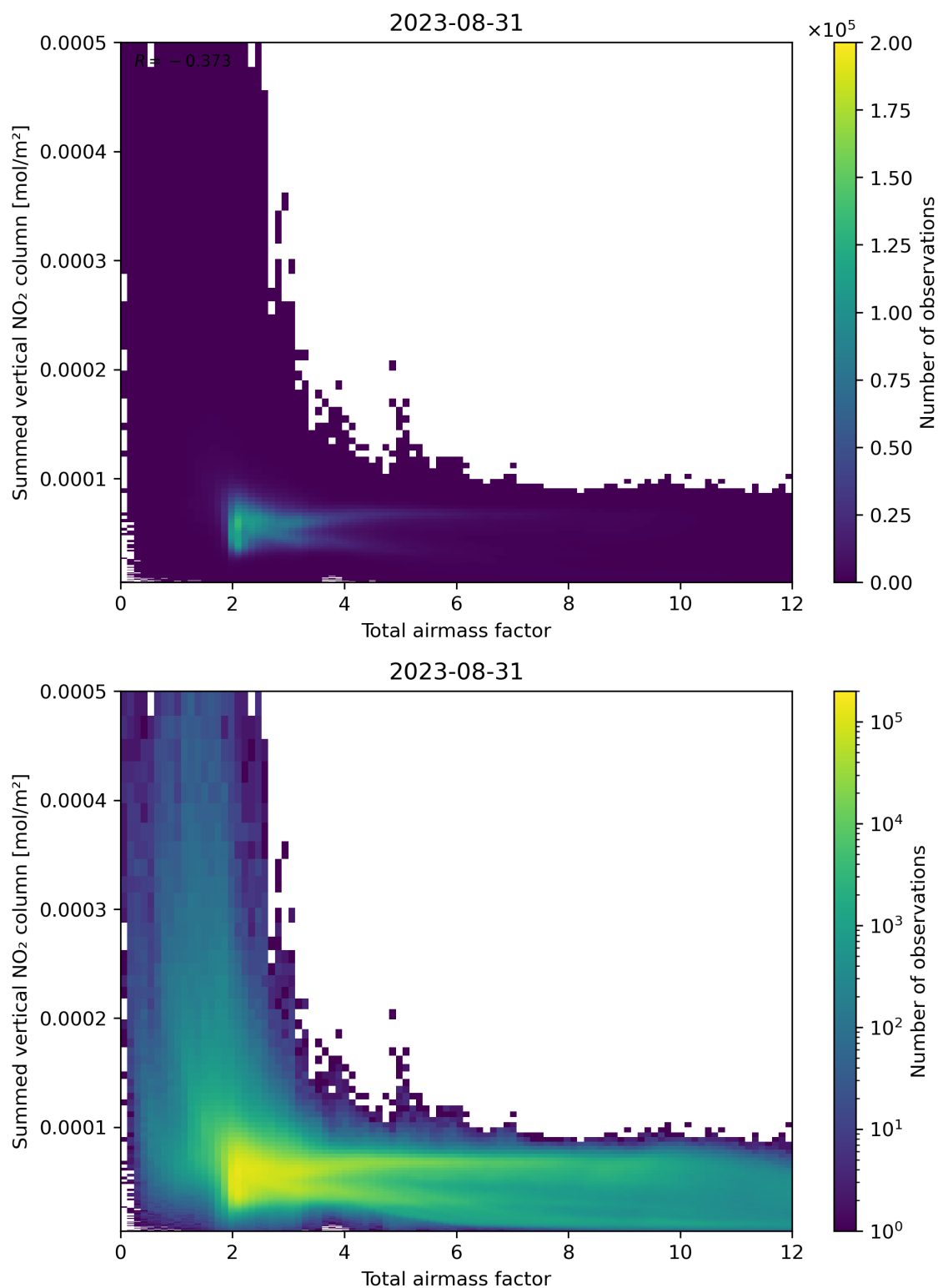
Figure 65: Scatter density plot of “Total airmass factor” against “Summed vertical NO 2 column” for 2023-08-30 to 2023-09-01.
