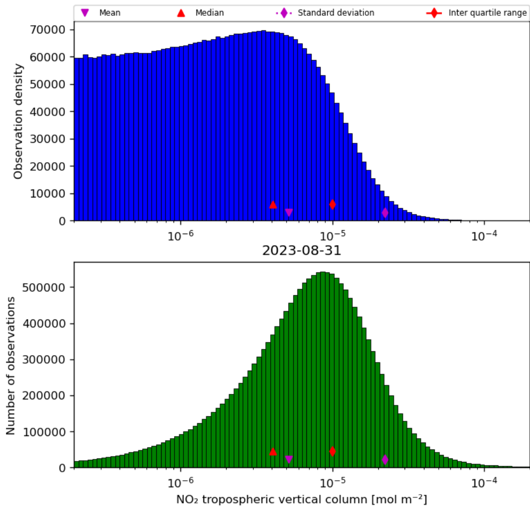
Figure 29: Histogram of “NO 2 tropospheric vertical column” for 2023-08-30 to 2023-09-01
