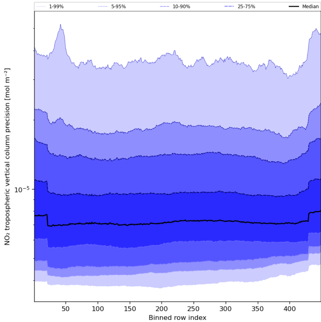
Figure 47: Along track statistics of “NO 2 tropospheric vertical column precision” for 2023-08-30 to 2023-09-01
