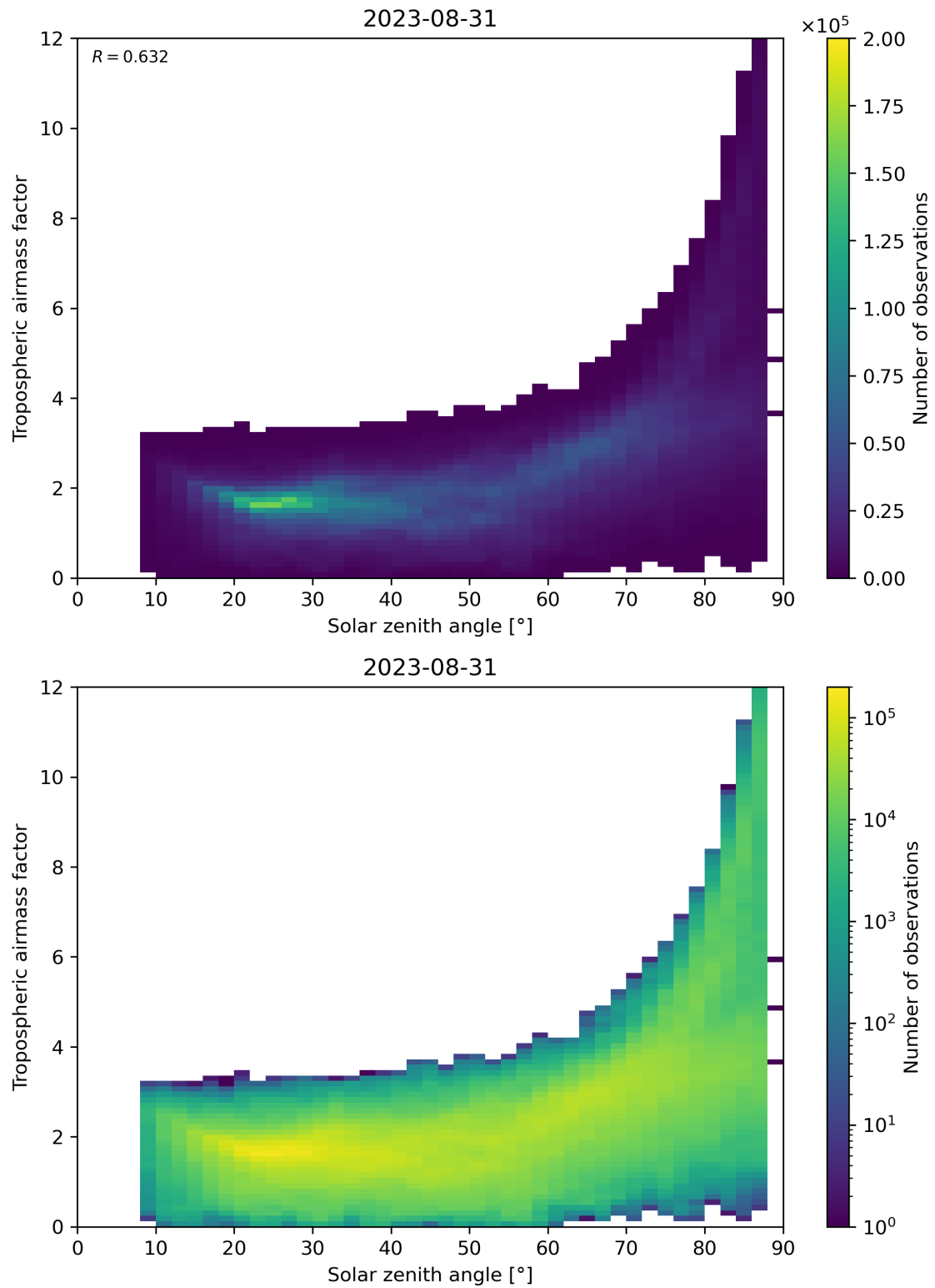
Figure 147: Scatter density plot of “Solar zenith angle” against “Tropospheric airmass factor” for 2023-08-30 to 2023-09-01.
