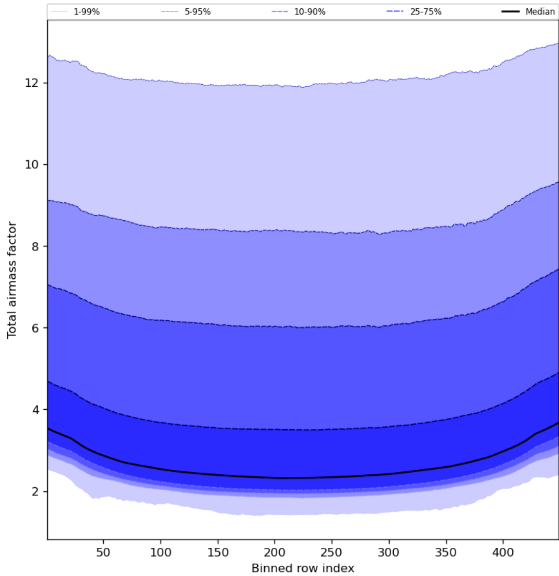
Figure 49: Along track statistics of “Total airmass factor” for 2023-08-30 to 2023-09-01
