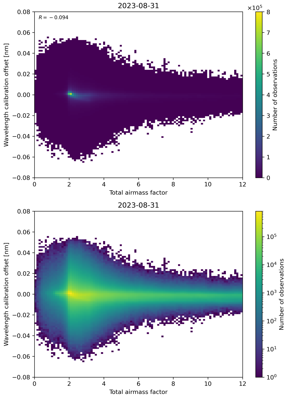
Figure 70: Scatter density plot of “Total airmass factor” against “Wavelength calibration offset” for 2023-08-30 to 2023-09-01.
