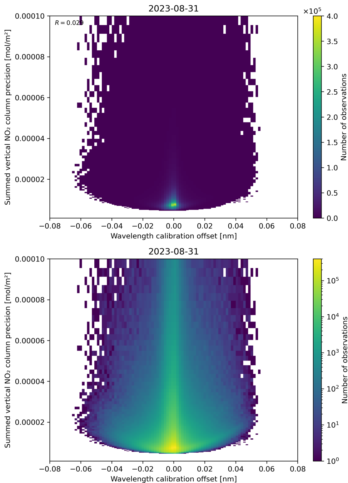
Figure 178: Scatter density plot of “Wavelength calibration offset” against “Summed vertical NO 2 column precision” for 2023-08-30 to 2023-09-01.
