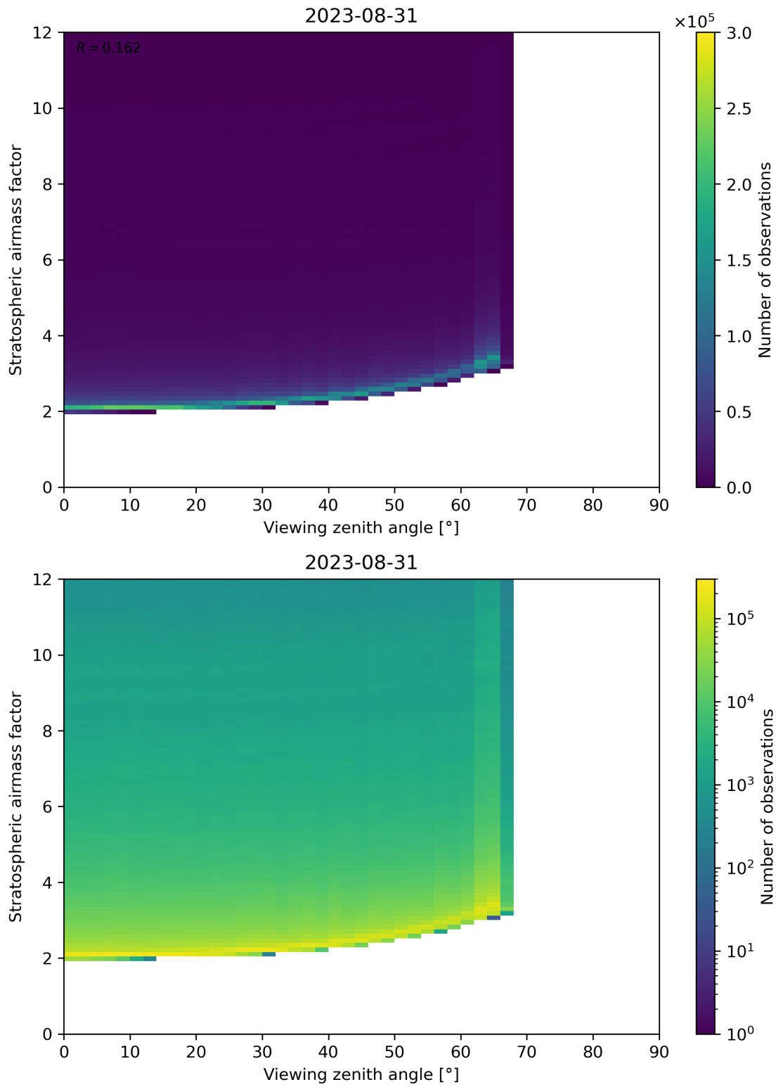
Figure 159: Scatter density plot of “Viewing zenith angle” against “Stratospheric airmass factor” for 2023-08-30 to 2023-09-01.
