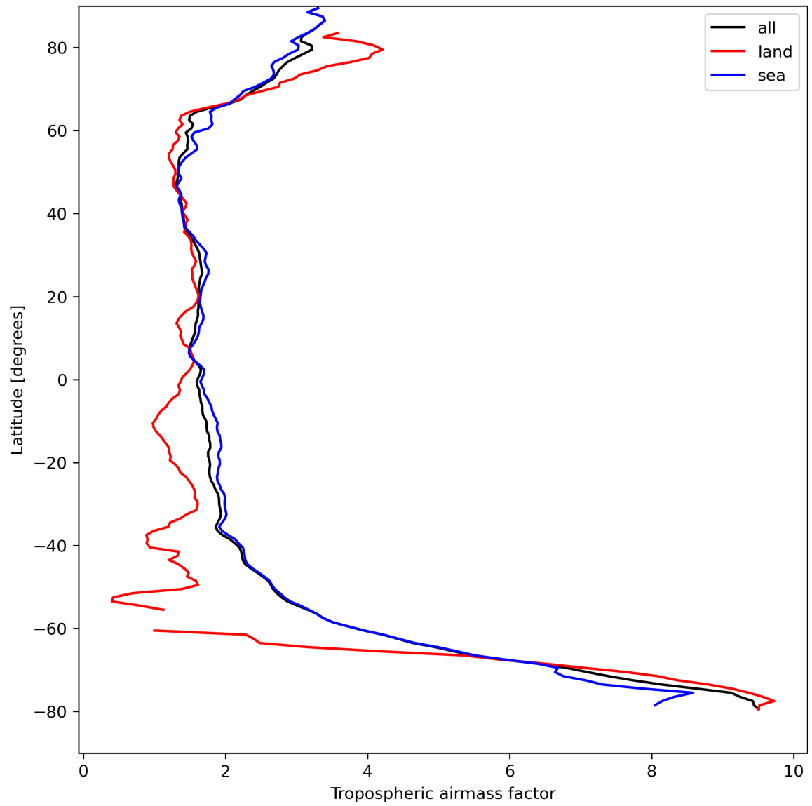
Figure 14: Zonal average of “Tropospheric airmass factor” for 2023-08-30 to 2023-09-01.
