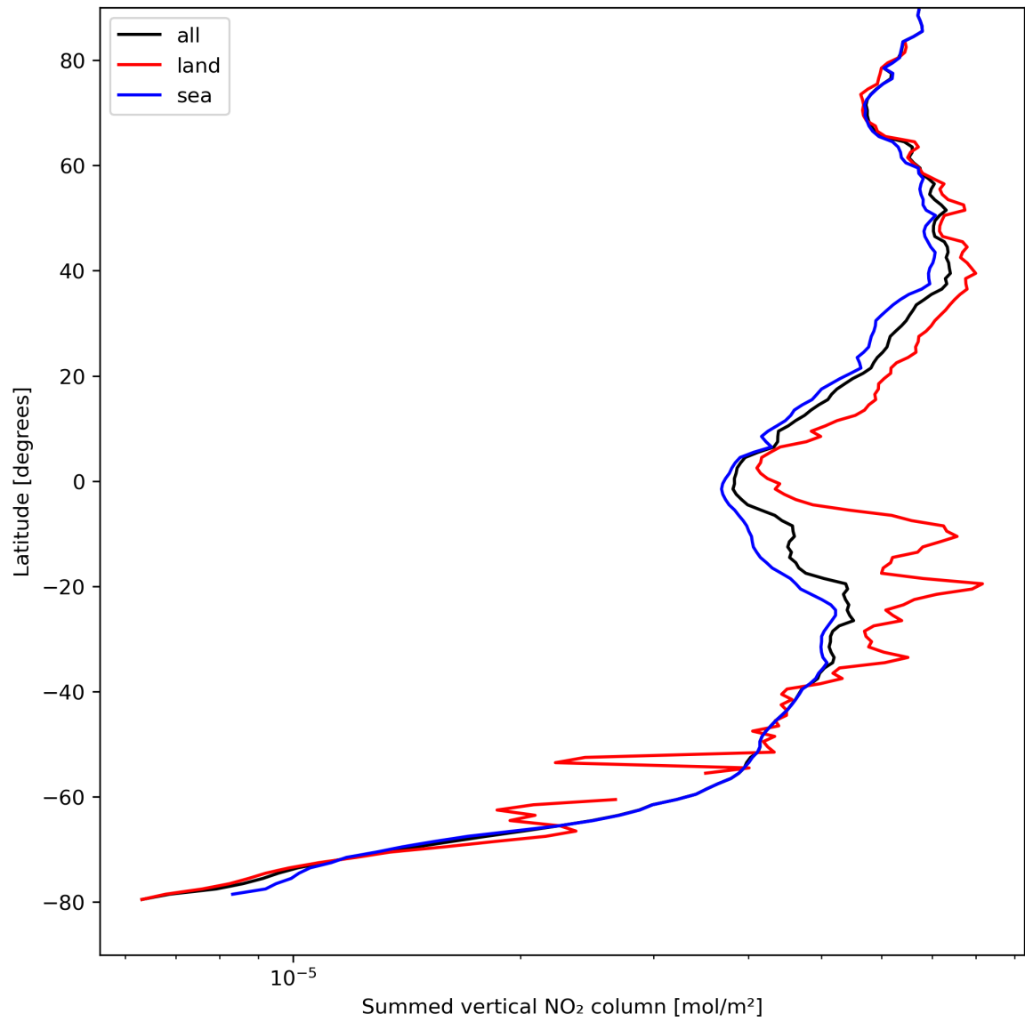
Figure 23: Zonal average of “Summed vertical NO 2 column” for 2023-08-30 to 2023-09-01.
