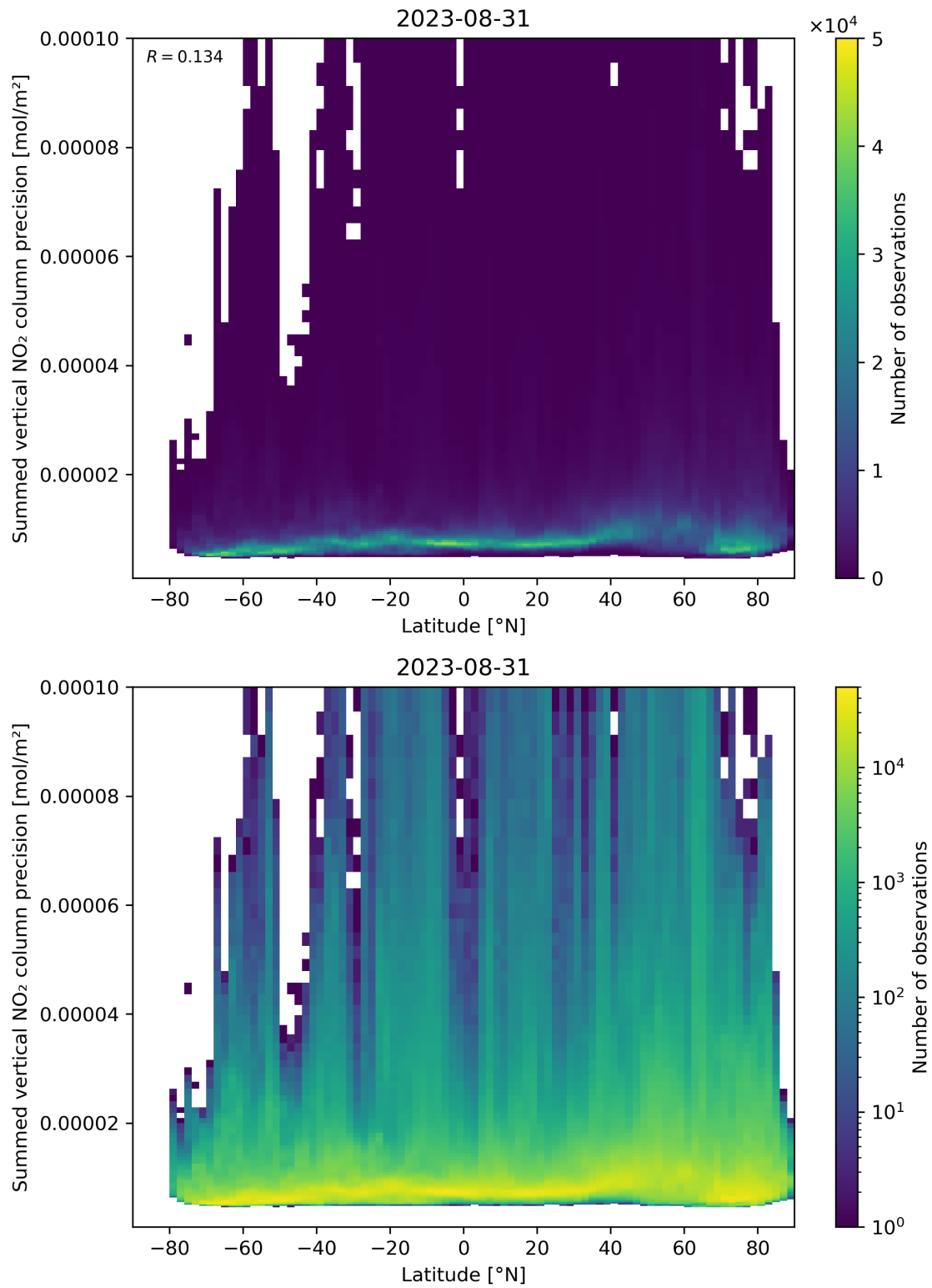
Figure 89: Scatter density plot of “Latitude” against “Summed vertical NO 2 column precision” for 2023-08-30 to 2023-09-01.
