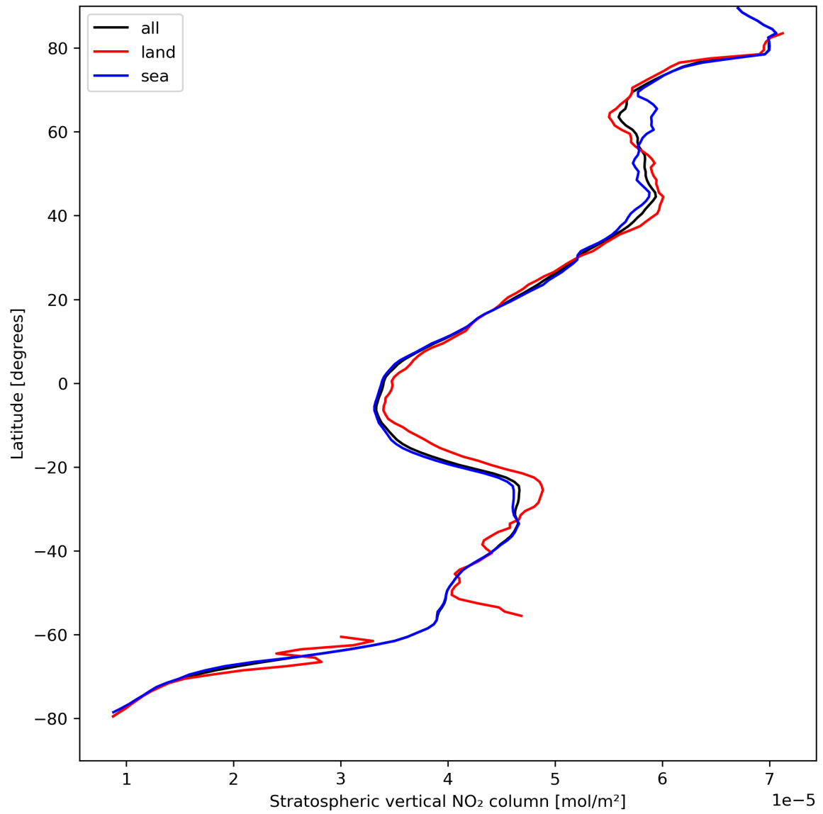
Figure 19: Zonal average of “Stratospheric vertical NO 2 column” for 2023-08-30 to 2023-09-01.
