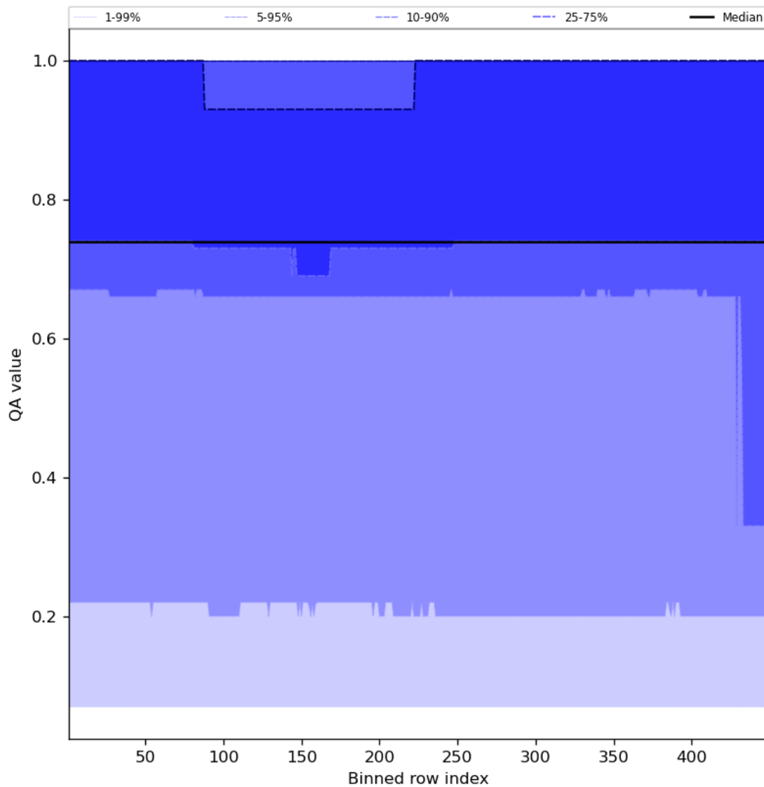
Figure 45: Along track statistics of “QA value” for 2023-08-30 to 2023-09-01
