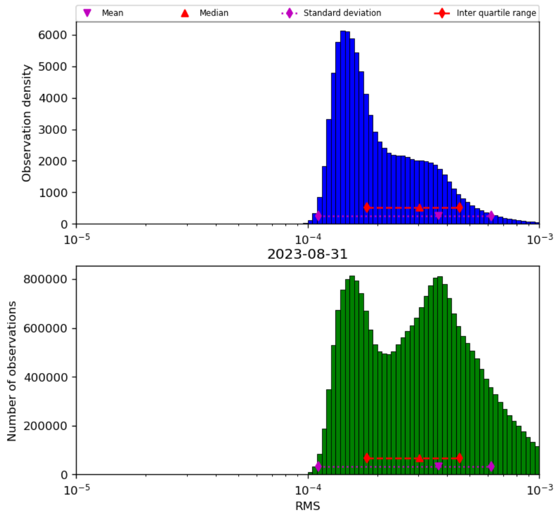
Figure 43: Histogram of “RMS” for 2023-08-30 to 2023-09-01
