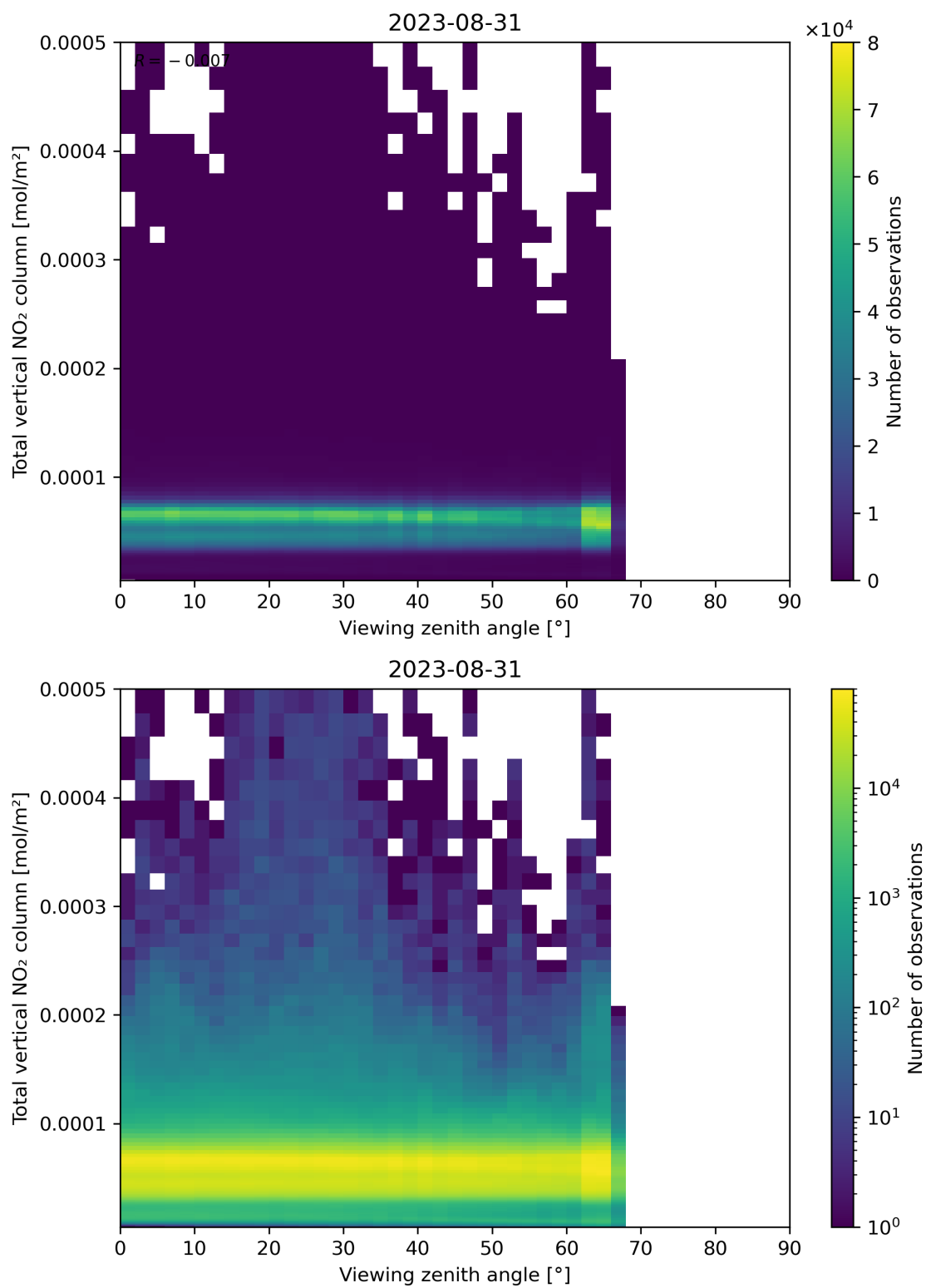
Figure 167: Scatter density plot of “Viewing zenith angle” against “Total vertical NO 2 column” for 2023-08-30 to 2023-09-01.
