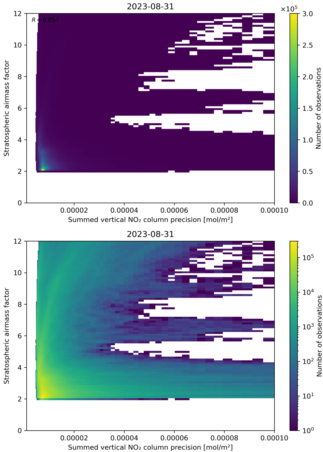
Figure 106: Scatter density plot of “Summed vertical NO 2 column precision” against “Stratospheric airmass factor” for 2023-08-30 to 2023-09-01.
