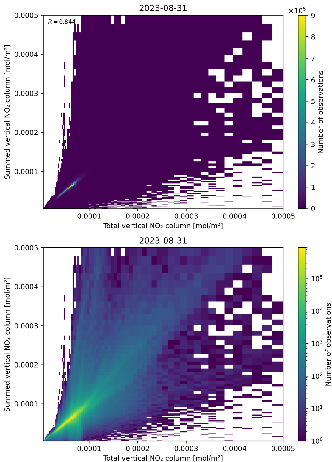
Figure 112: Scatter density plot of “Total vertical NO 2 column” against “Summed vertical NO 2 column” for 2023-08-30 to 2023-09-01.
