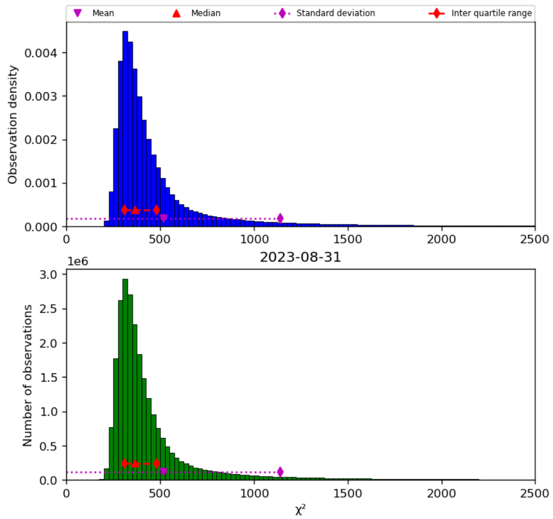
Figure 42: Histogram of “ \chi^2 ” for 2023-08-30 to 2023-09-01
