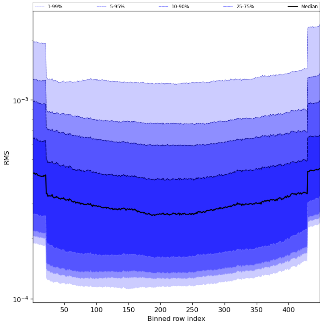
Figure 60: Along track statistics of “RMS” for 2023-08-30 to 2023-09-01
