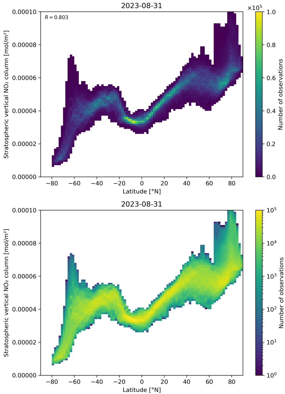
Figure 87: Scatter density plot of “Latitude” against “Stratospheric vertical NO 2 column” for 2023-08-30 to 2023-09-01.
