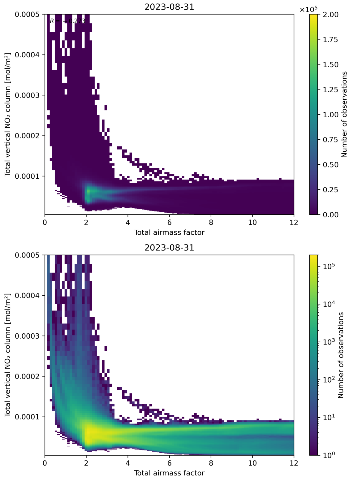
Figure 67: Scatter density plot of “Total air mass factor” against “Total vertical NO 2 column” for 2023-08-30 to 2023-09-01.
