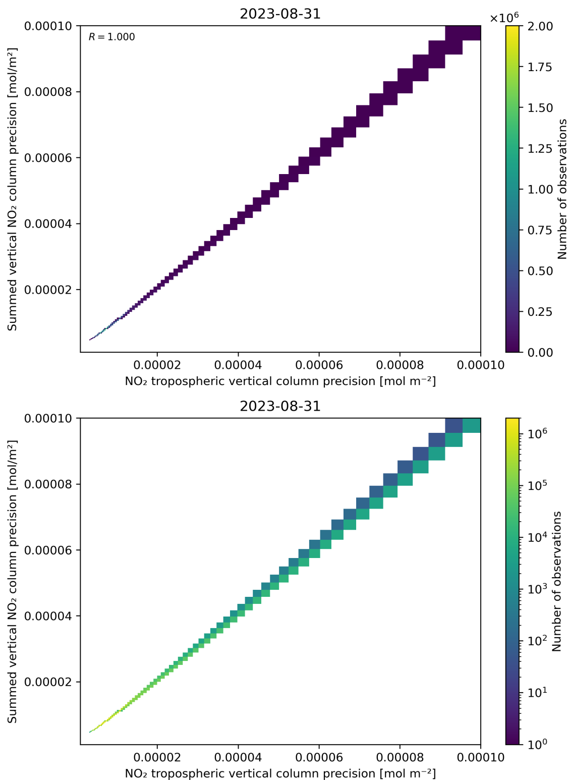
Figure 137: Scatter density plot of “NO 2 tropospheric vertical column precision” against “Summed vertical NO 2 column precision” for 2023-08-30 to 2023-09-01.
