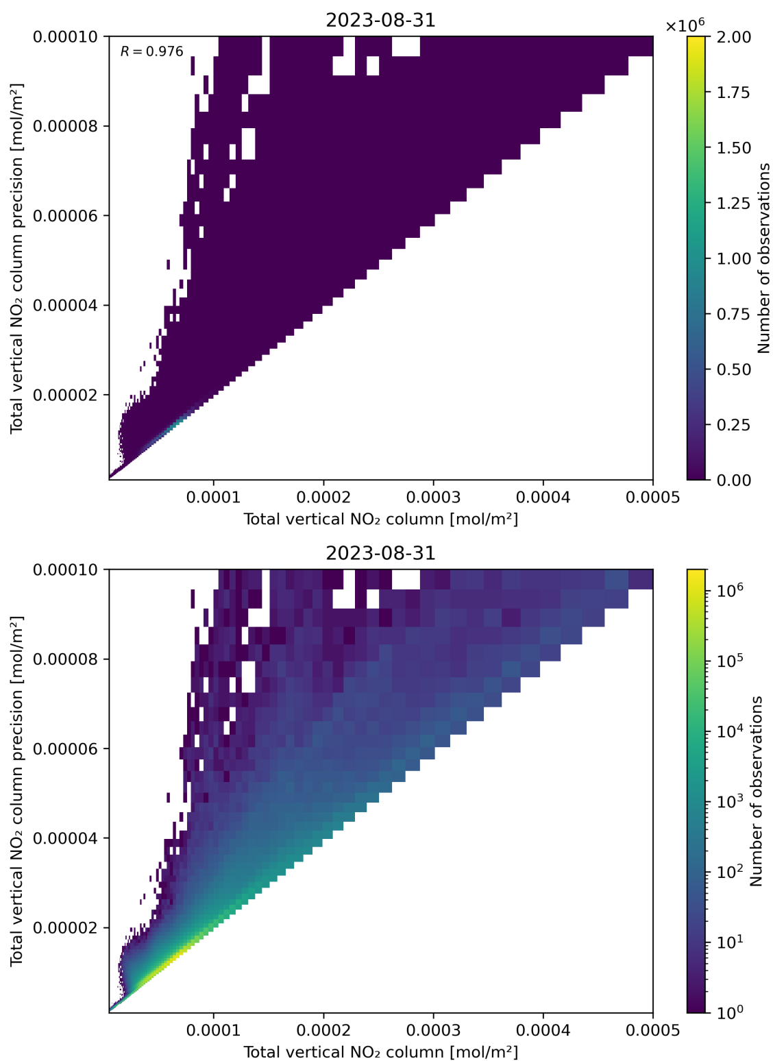
Figure 114: Scatter density plot of “Total vertical NO 2 column” against “Total vertical NO 2 column precision” for 2023-08-30 to 2023-09-01.
