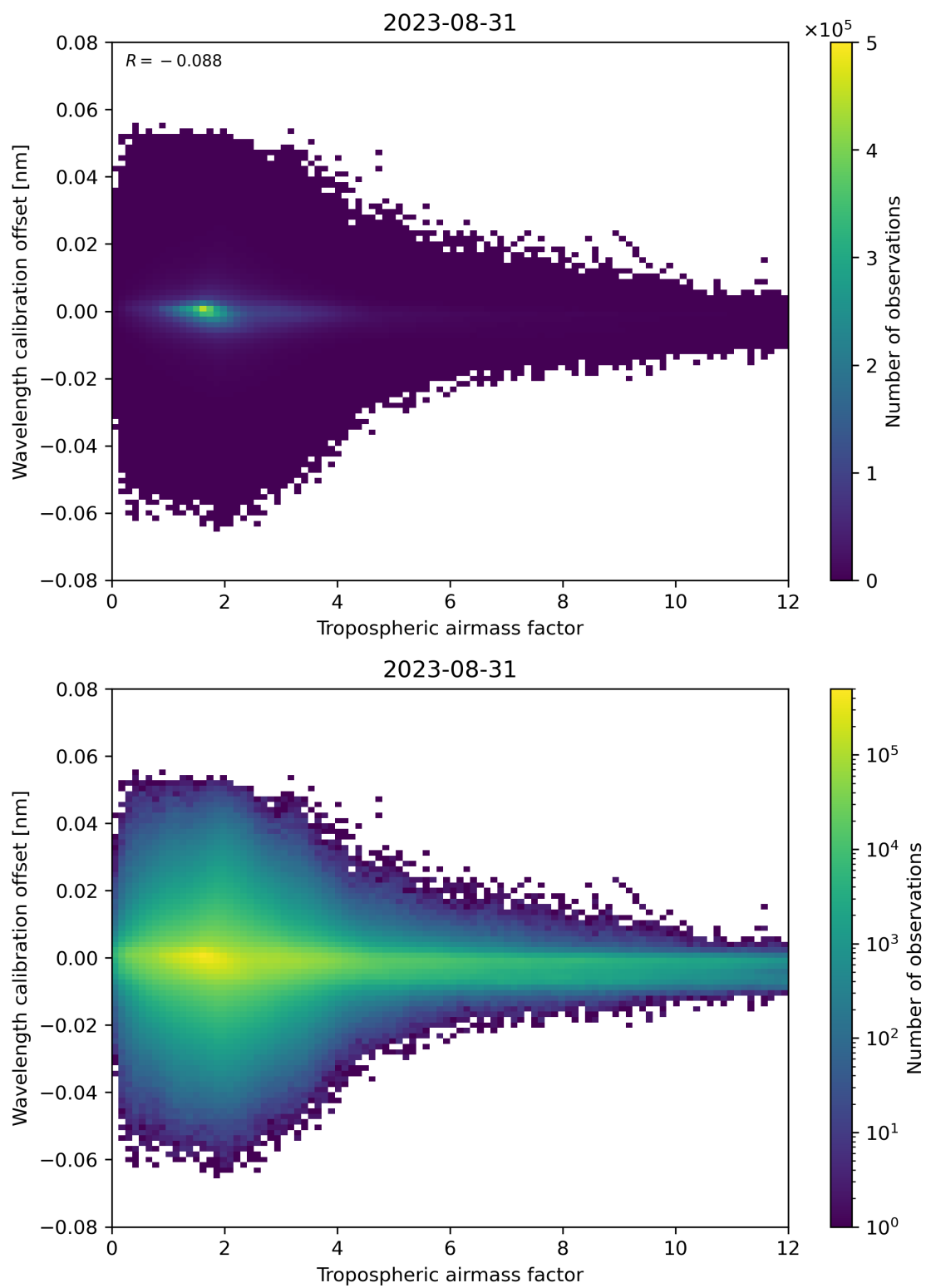
Figure 80: Scatter density plot of “Tropospheric airmass factor” against “Wavelength calibration offset” for 2023-08-30 to 2023-09-01.
