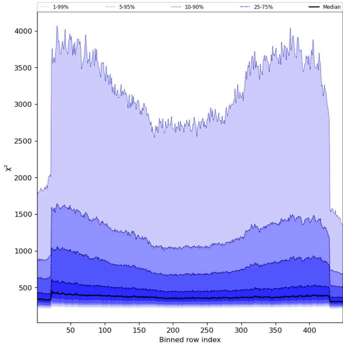
Figure 59: Along track statistics of “ \chi^2 ” for 2023-08-30 to 2023-09-01
