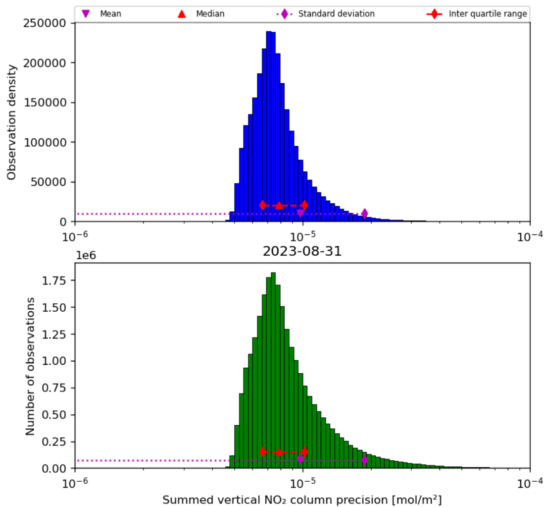
Figure 41: Histogram of “Summed vertical NO 2 column precision” for 2023-08-30 to 2023-09-01
