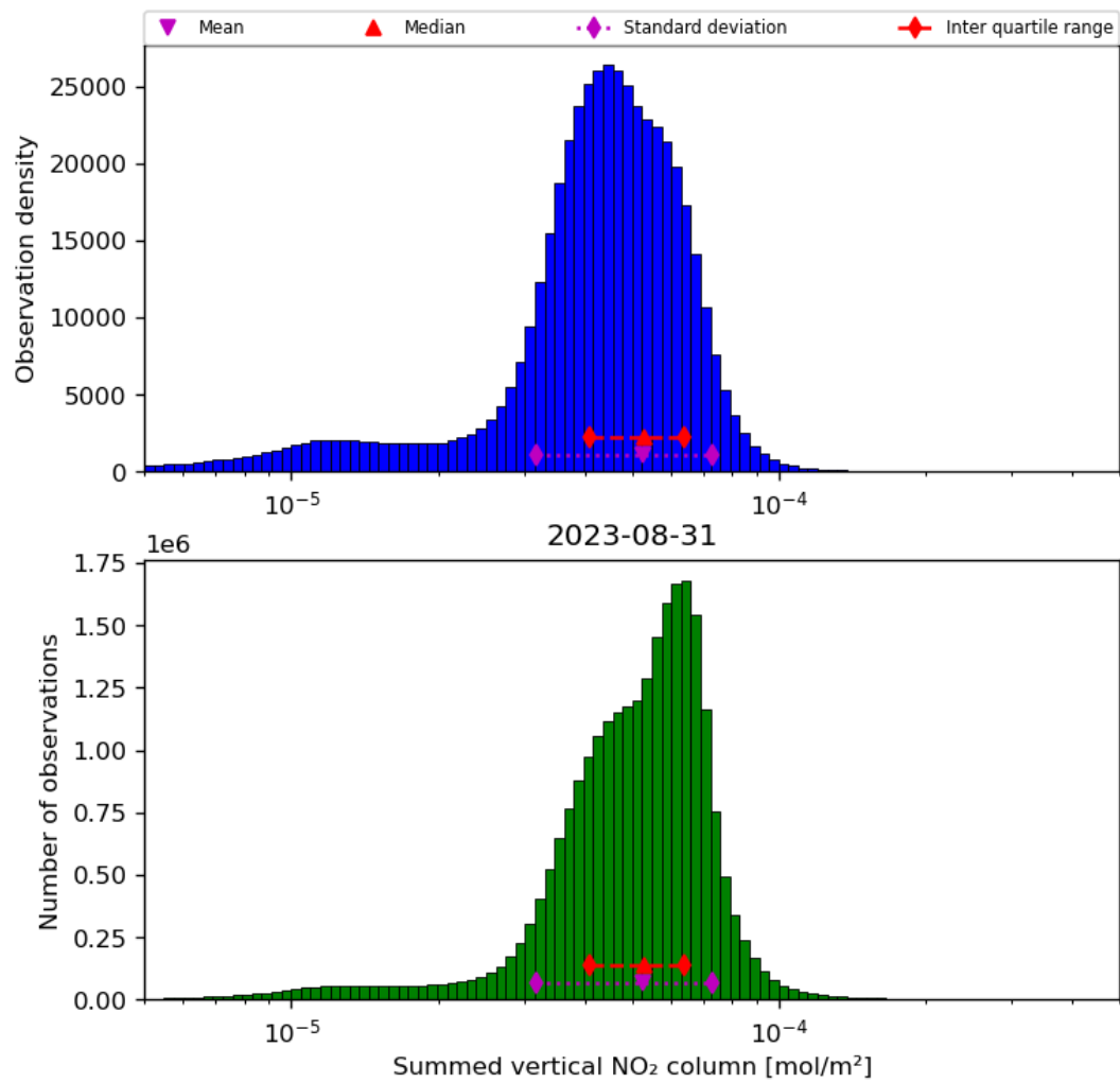
Figure 40: Histogram of "Summed vertical NO 2 column" for 2023-08-30 to 2023-09-01
