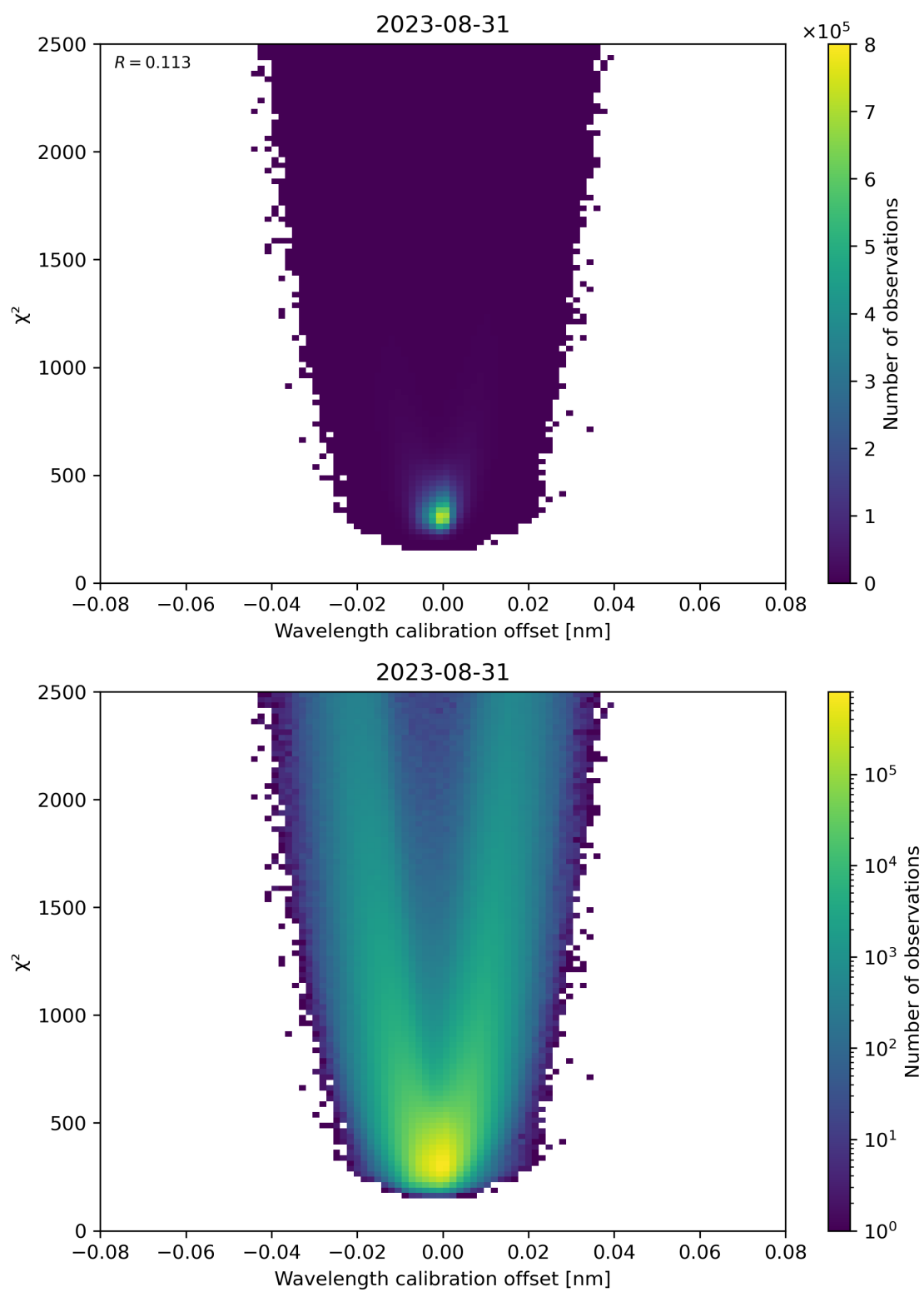
Figure 175: Scatter density plot of “Wavelength calibration offset” against “ \chi^2 ” for 2023-08-30 to 2023-09-01.
