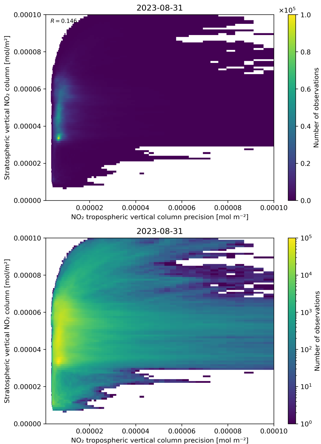
Figure 135: Scatter density plot of “NO 2 tropospheric vertical column precision” against “Stratospheric vertical NO 2 column” for 2023-08-30 to 2023-09-01.
