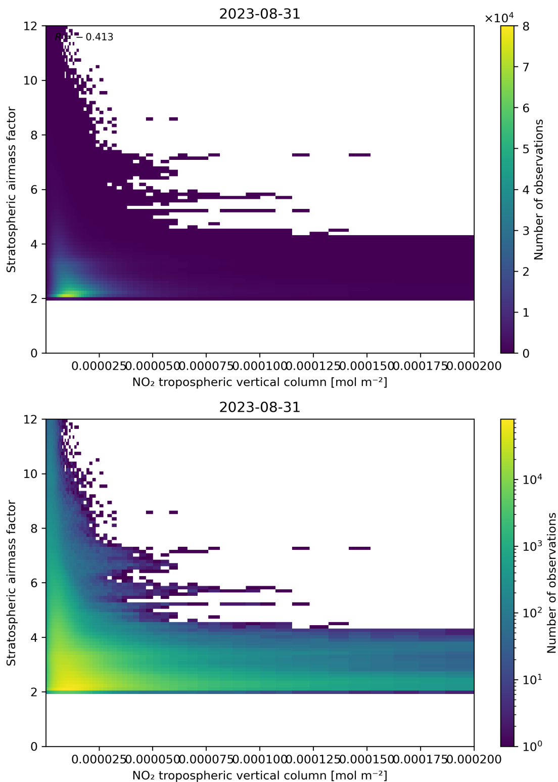
Figure 121: Scatter density plot of “NO 2 tropospheric vertical column” against “Stratospheric air mass factor” for 2023-08-30 to 2023-09-01.
