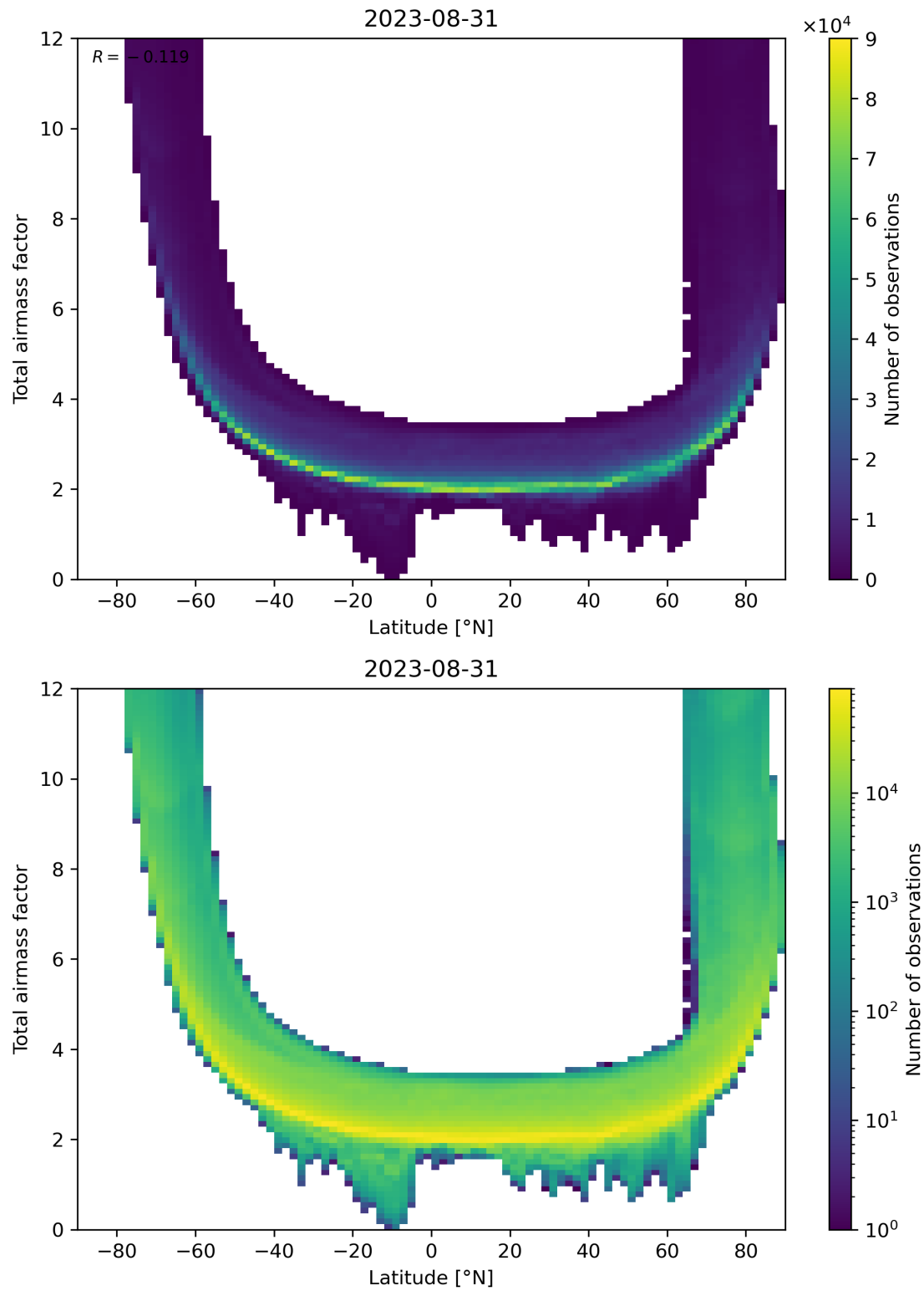
Figure 84: Scatter density plot of “Latitude” against “Total airmass factor” for 2023-08-30 to 2023-09-01.
