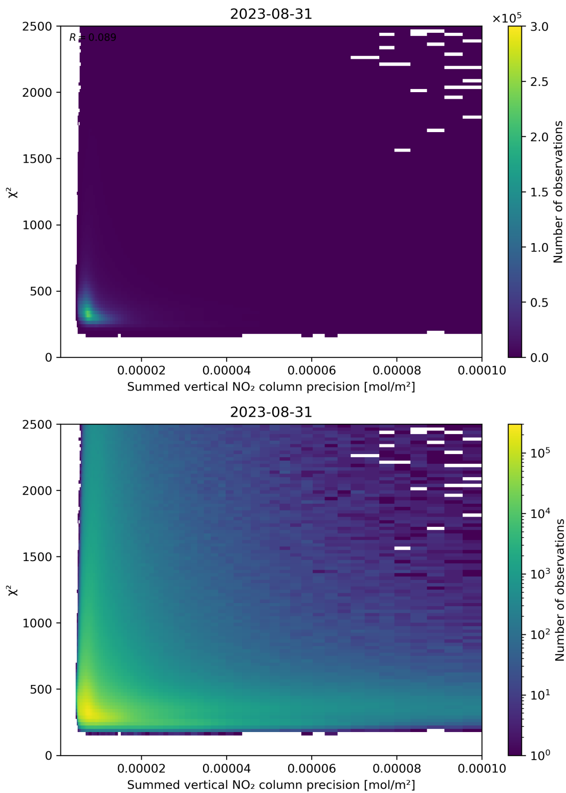
Figure 107: Scatter density plot of “Summed vertical NO 2 column precision” against “ \chi^2 ” for 2023-08-30 to 2023-09-01.
