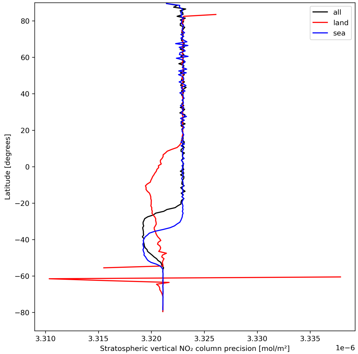
Figure 20: Zonal average of “Stratospheric vertical NO 2 column precision” for 2023-08-30 to 2023-09-01.
