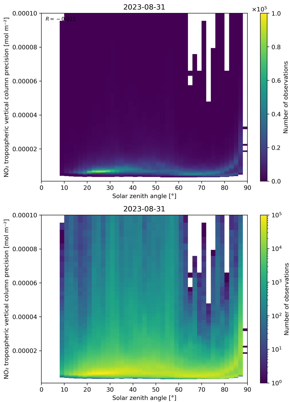
Figure 156: Scatter density plot of “Solar zenith angle” against “NO 2 tropospheric vertical column precision” for 2023-08-30 to 2023-09-01.
