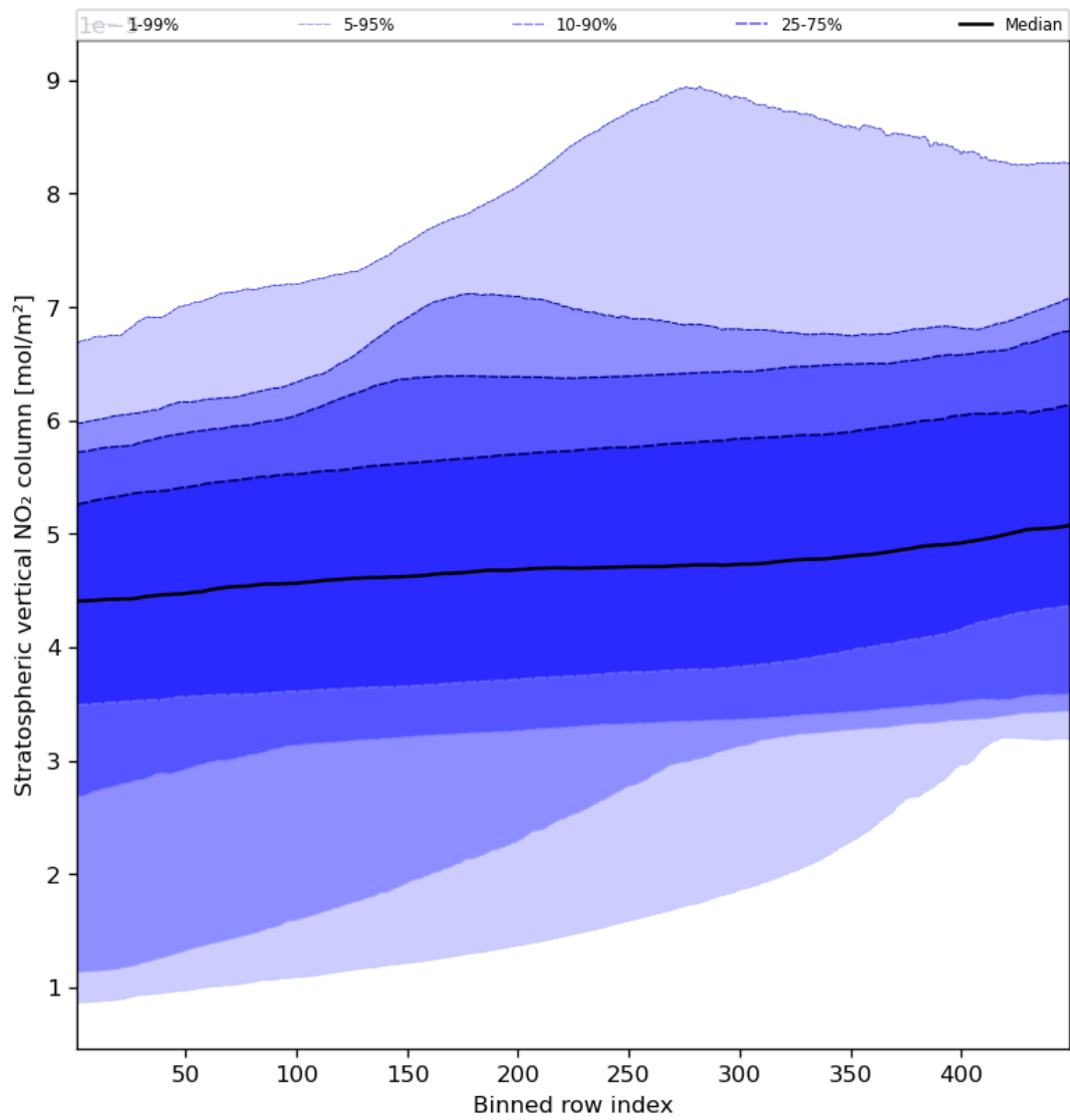
Figure 53: Along track statistics of “Stratospheric vertical NO 2 column” for 2023-08-30 to 2023-09-01
