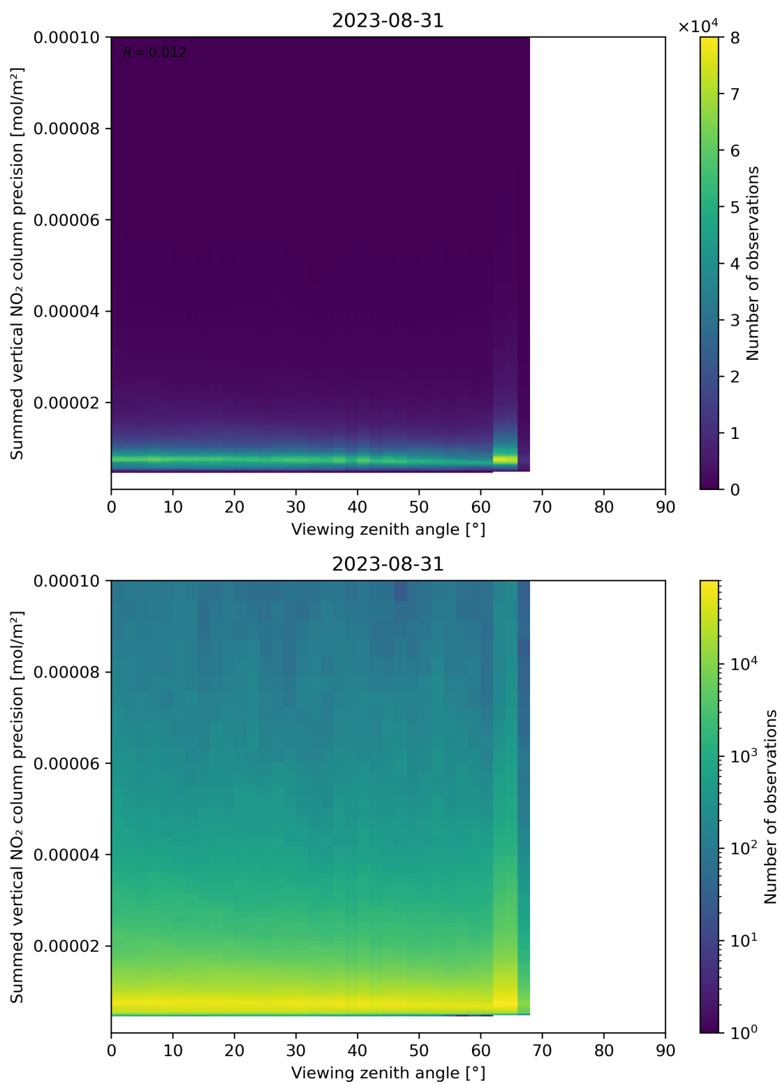
Figure 166: Scatter density plot of “Viewing zenith angle” against “Summed vertical NO 2 column precision” for 2023-08-30 to 2023-09-01.
