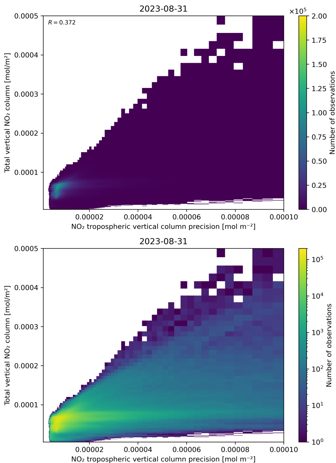
Figure 138: Scatter density plot of “NO 2 tropospheric vertical column precision” against “Total vertical NO 2 column” for 2023-08-30 to 2023-09-01.
