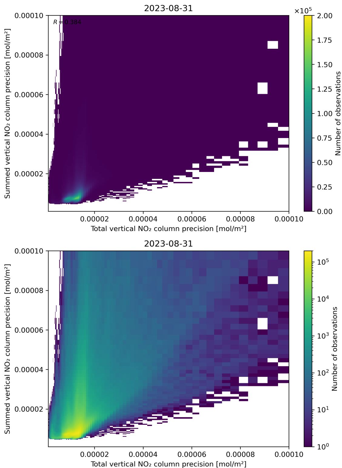
Figure 118: Scatter density plot of “Total vertical NO 2 column precision” against “Summed vertical NO 2 column precision” for 2023-08-30 to 2023-09-01.
