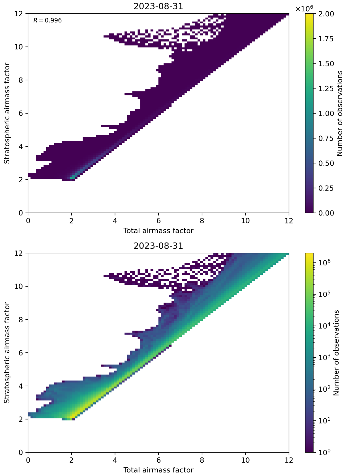
Figure 62: Scatter density plot of “Total airmass factor” against “Stratospheric airmass factor” for 2023-08-30 to 2023-09-01.
