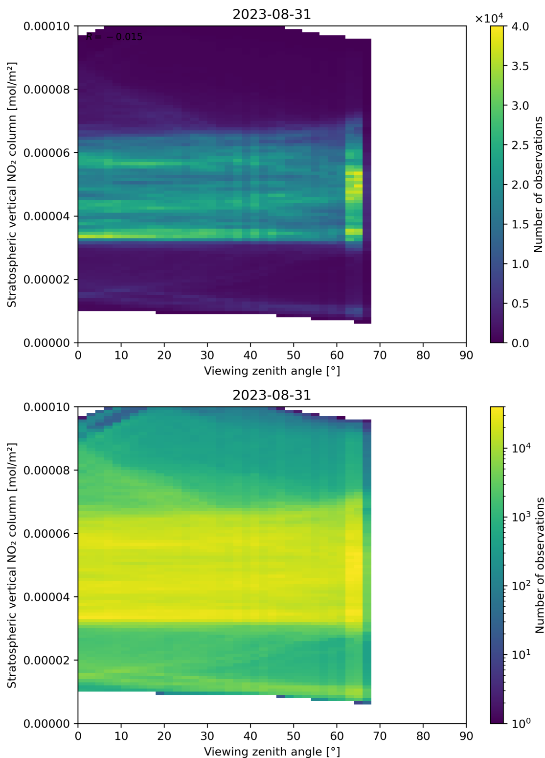
Figure 164: Scatter density plot of “Viewing zenith angle” against “Stratospheric vertical NO 2 column” for 2023-08-30 to 2023-09-01.
