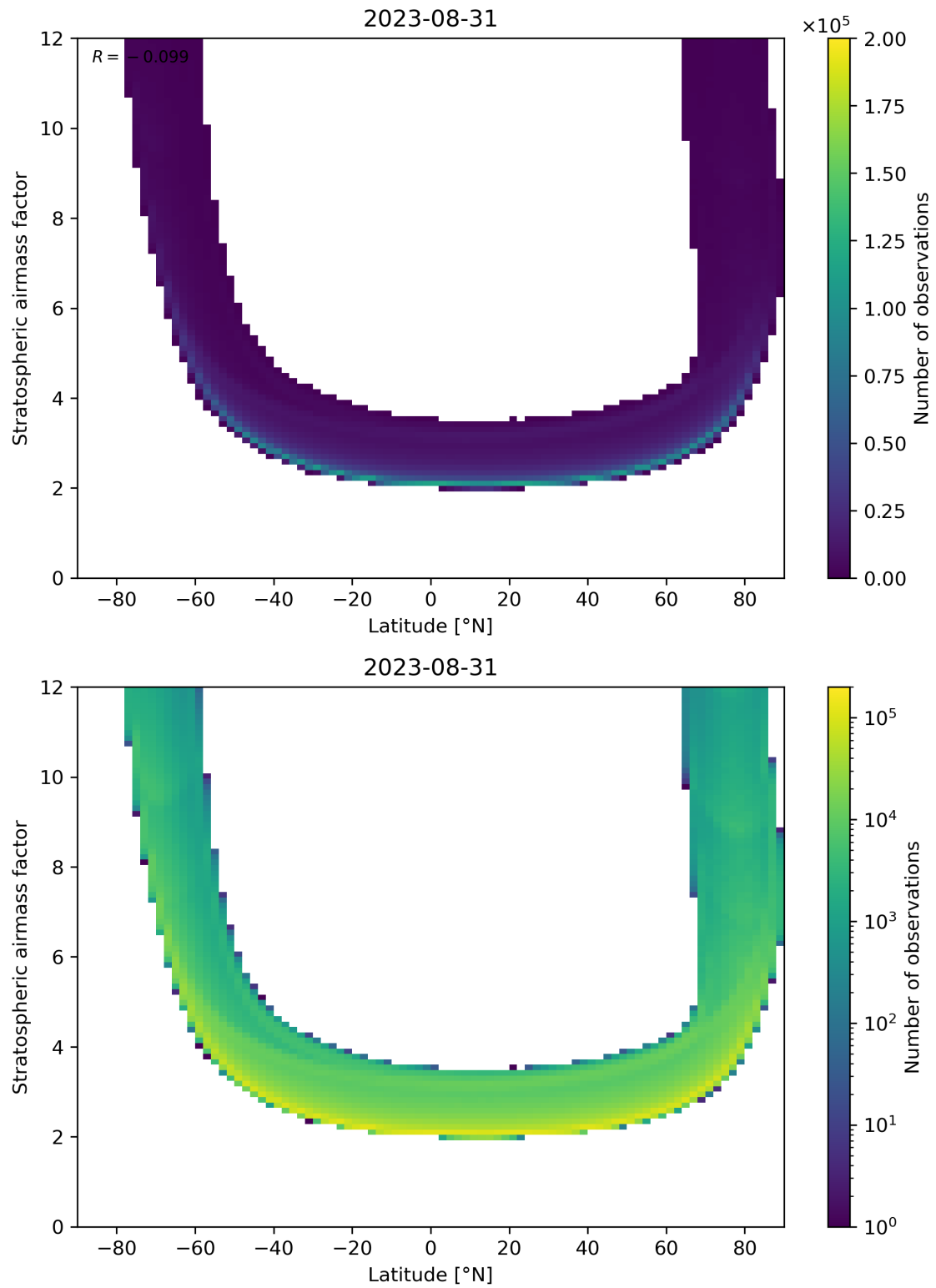
Figure 83: Scatter density plot of “Latitude” against “Stratospheric air mass factor” for 2023-08-30 to 2023-09-01.
