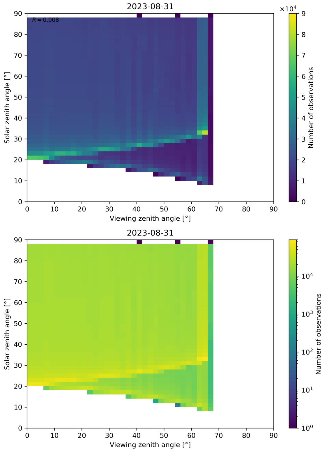
Figure 172: Scatter density plot of “Viewing zenith angle” against “Solar zenith angle” for 2023-08-30 to 2023-09-01.
