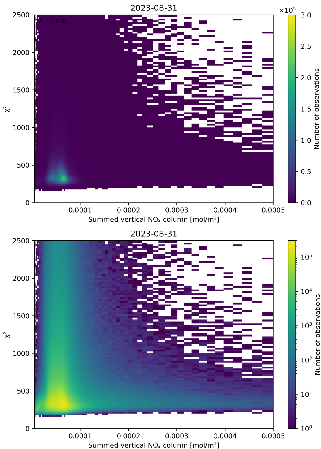
Figure 104: Scatter density plot of “Summed vertical NO 2 column” against “ \chi^2 ” for 2023-08-30 to 2023-09-01.
