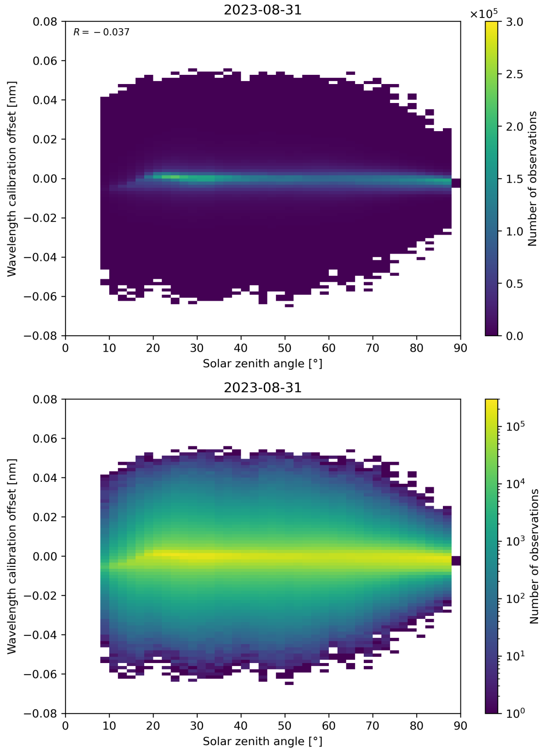
Figure 158: Scatter density plot of “Solar zenith angle” against “Wavelength calibration offset” for 2023-08-30 to 2023-09-01.
