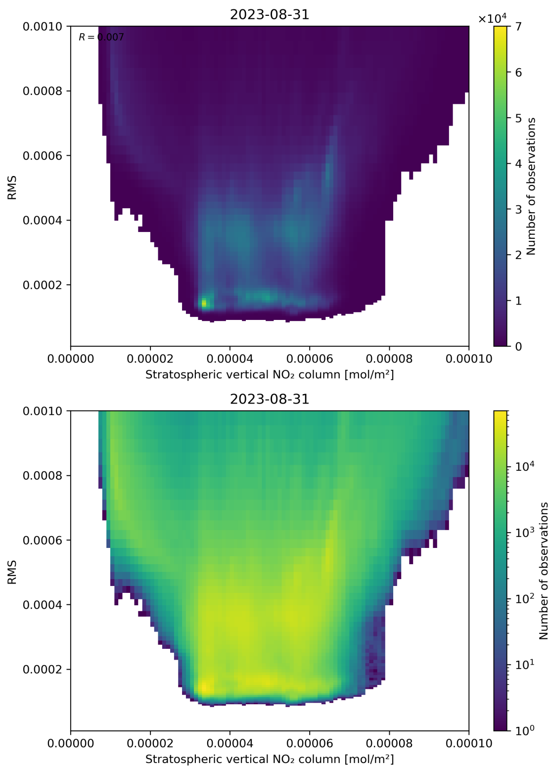
Figure 102: Scatter density plot of “Stratospheric vertical NO 2 column” against “RMS” for 2023-08-30 to 2023-09-01.
