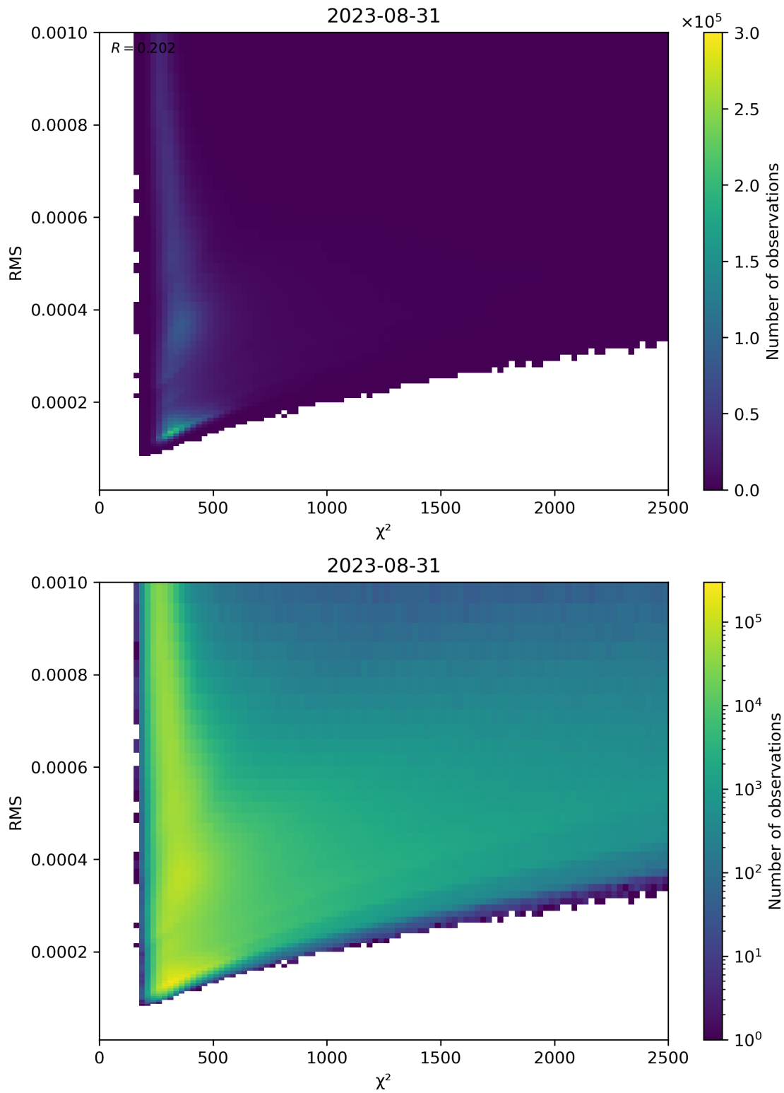
Figure 82: Scatter density plot of “ \chi^2 ” against “RMS” for 2023-08-30 to 2023-09-01.
