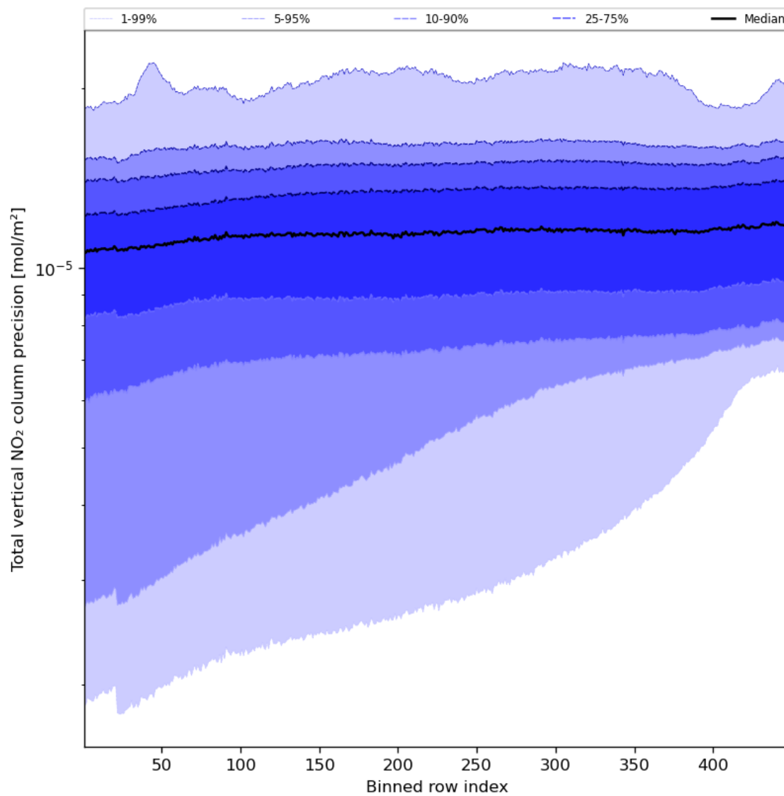
Figure 56: Along track statistics of “Total vertical NO 2 column precision” for 2023-08-30 to 2023-09-01
