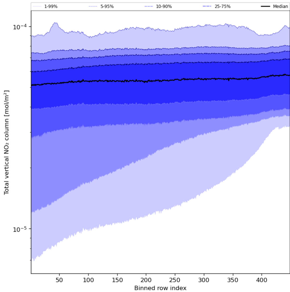
Figure 55: Along track statistics of “Total vertical NO 2 column” for 2023-08-30 to 2023-09-01
