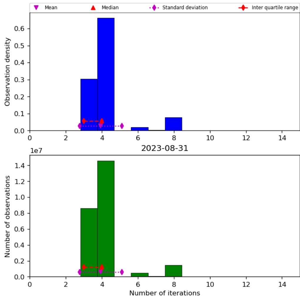
Figure 34: Histogram of “Number of iterations” for 2023-08-30 to 2023-09-01
