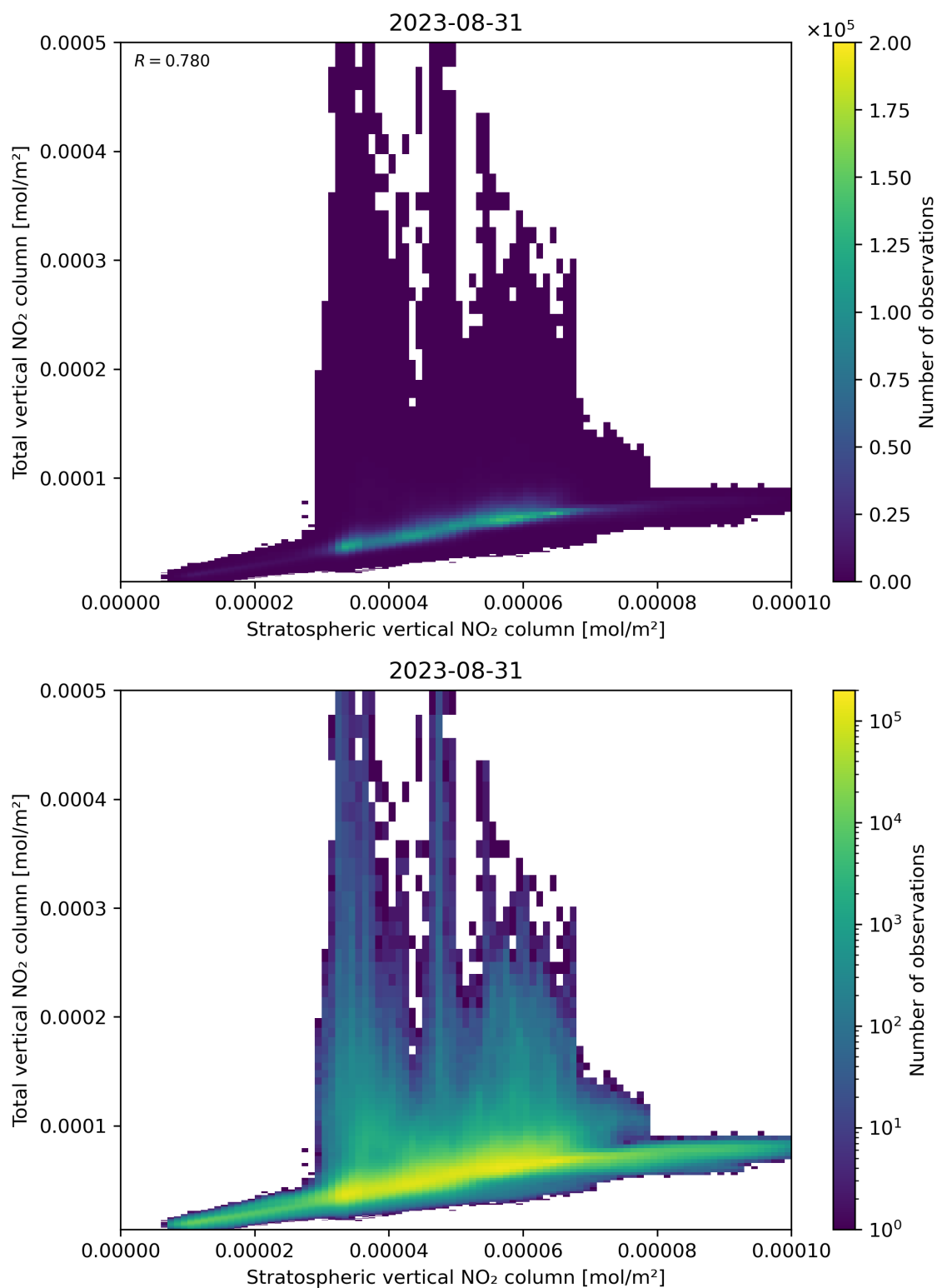
Figure 100: Scatter density plot of “Stratospheric vertical NO 2 column” against “Total vertical NO 2 column” for 2023-08-30 to 2023-09-01.
