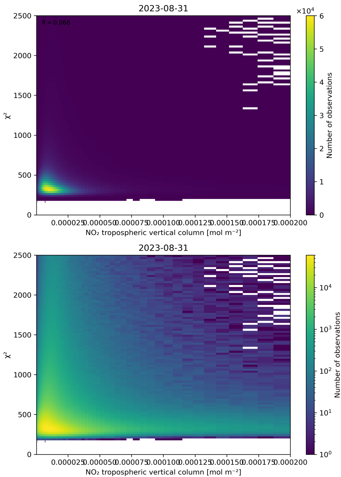
Figure 124: Scatter density plot of “NO 2 tropospheric vertical column” against “ \chi^2 ” for 2023-08-30 to 2023-09-01.
