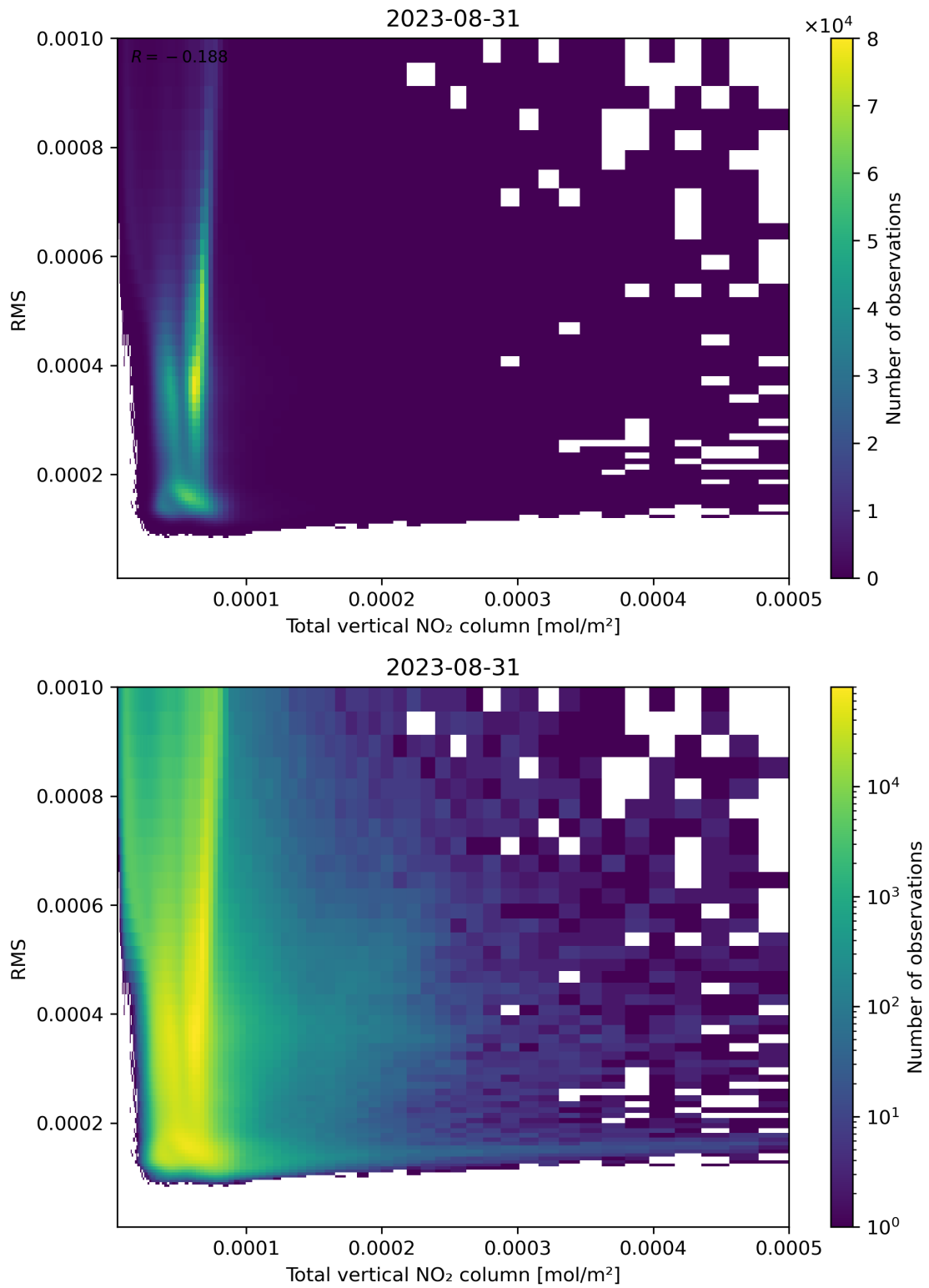
Figure 120: Scatter density plot of “Total vertical NO 2 column” against “RMS” for 2023-08-30 to 2023-09-01.
