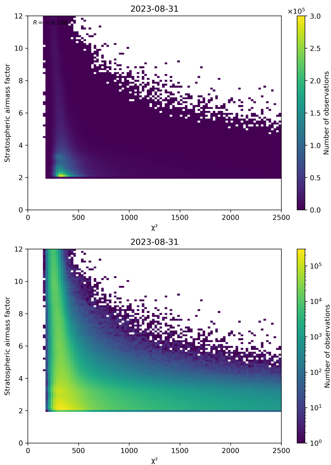
Figure 81: Scatter density plot of “ \chi^2 ” against “Stratospheric airmass factor” for 2023-08-30 to 2023-09-01.
