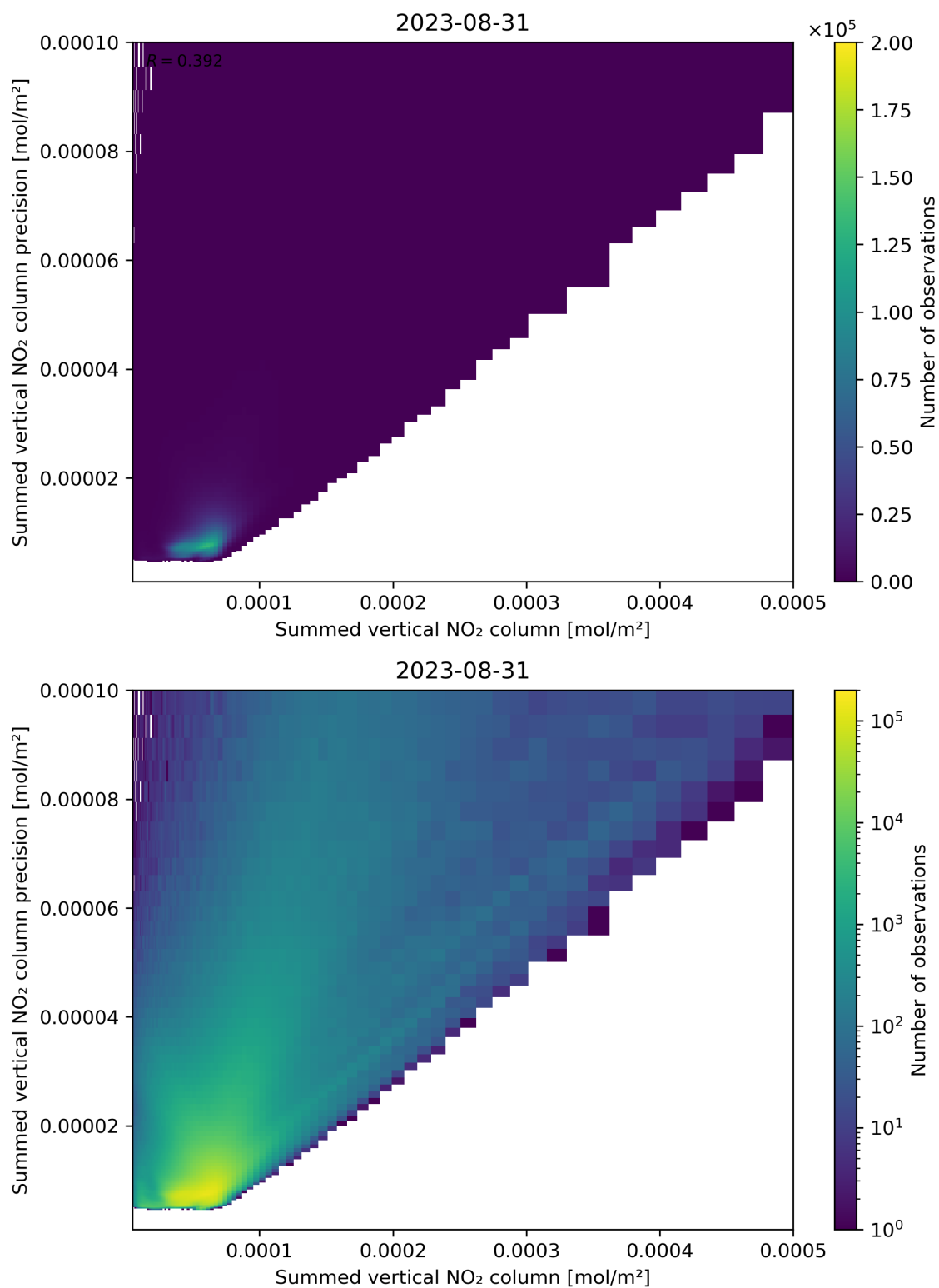
Figure 105: Scatter density plot of “Summed vertical NO 2 column” against “Summed vertical NO 2 column precision” for 2023-08-30 to 2023-09-01.
