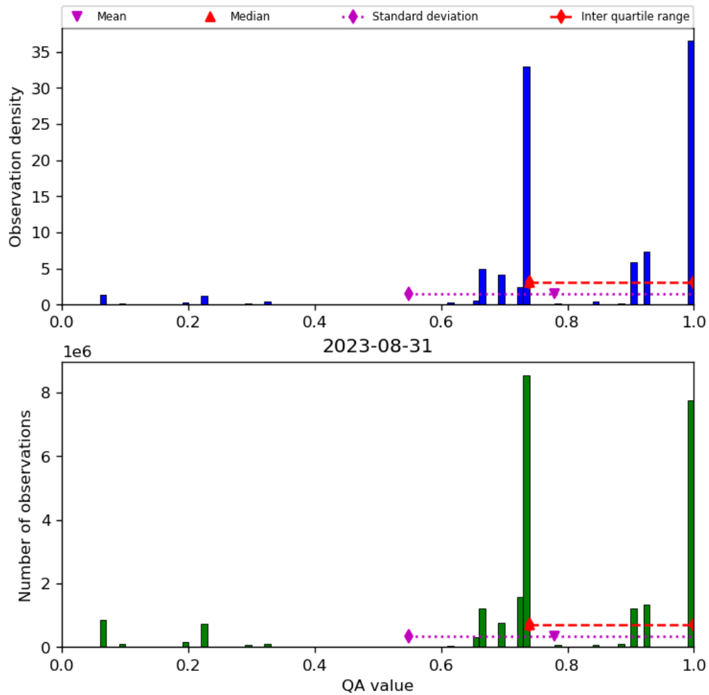
Figure 28: Histogram of “QA value” for 2023-08-30 to 2023-09-01
