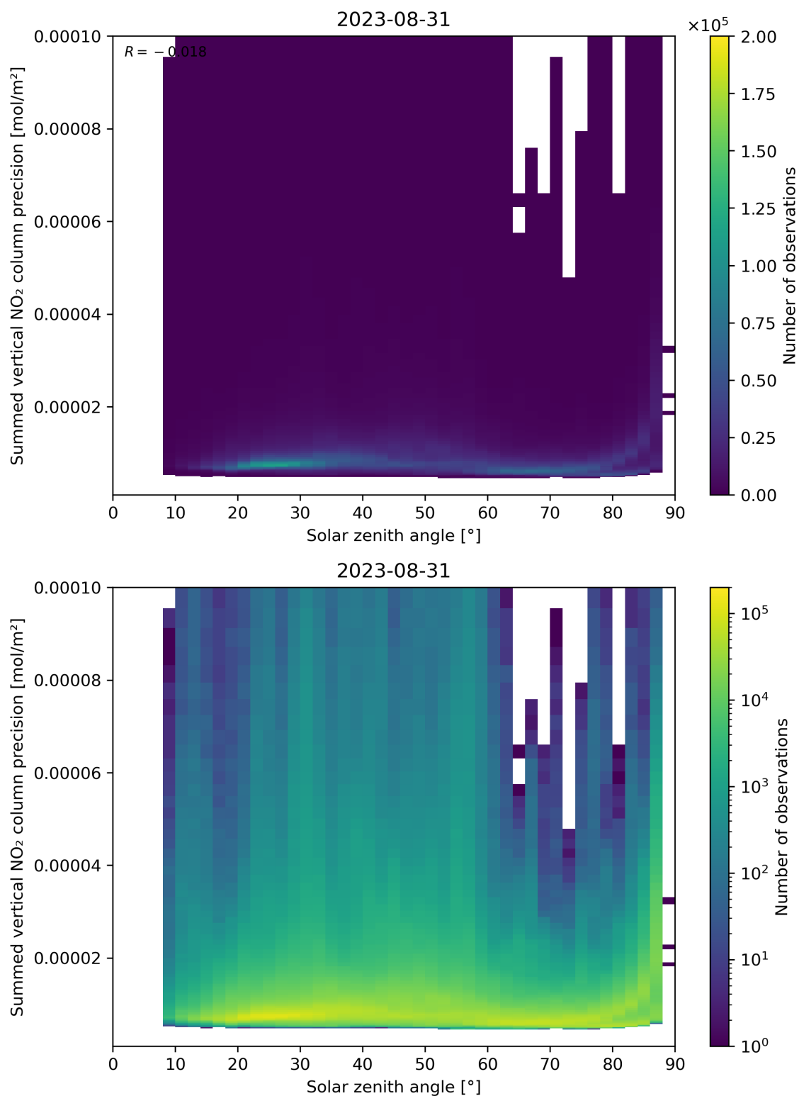
Figure 152: Scatter density plot of “Solar zenith angle” against “Summed vertical NO 2 column precision” for 2023-08-30 to 2023-09-01.
