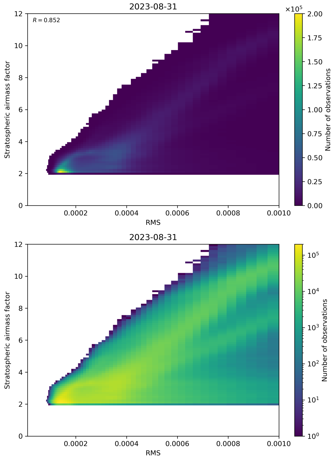
Figure 144: Scatter density plot of “RMS” against “Stratospheric airmass factor” for 2023-08-30 to 2023-09-01.
