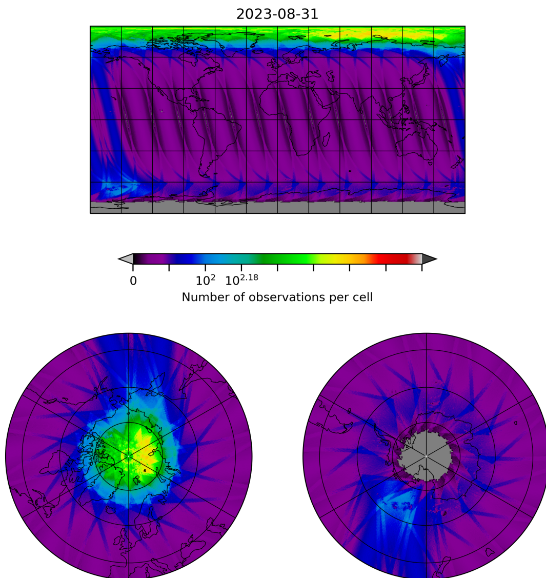
Figure 10: Map of the number of observations for 2023-08-30 to 2023-09-01
