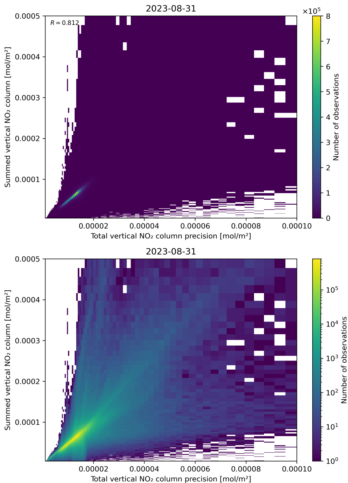
Figure 117: Scatter density plot of “Total vertical NO 2 column precision” against “Summed vertical NO 2 column” for 2023-08-30 to 2023-09-01.
