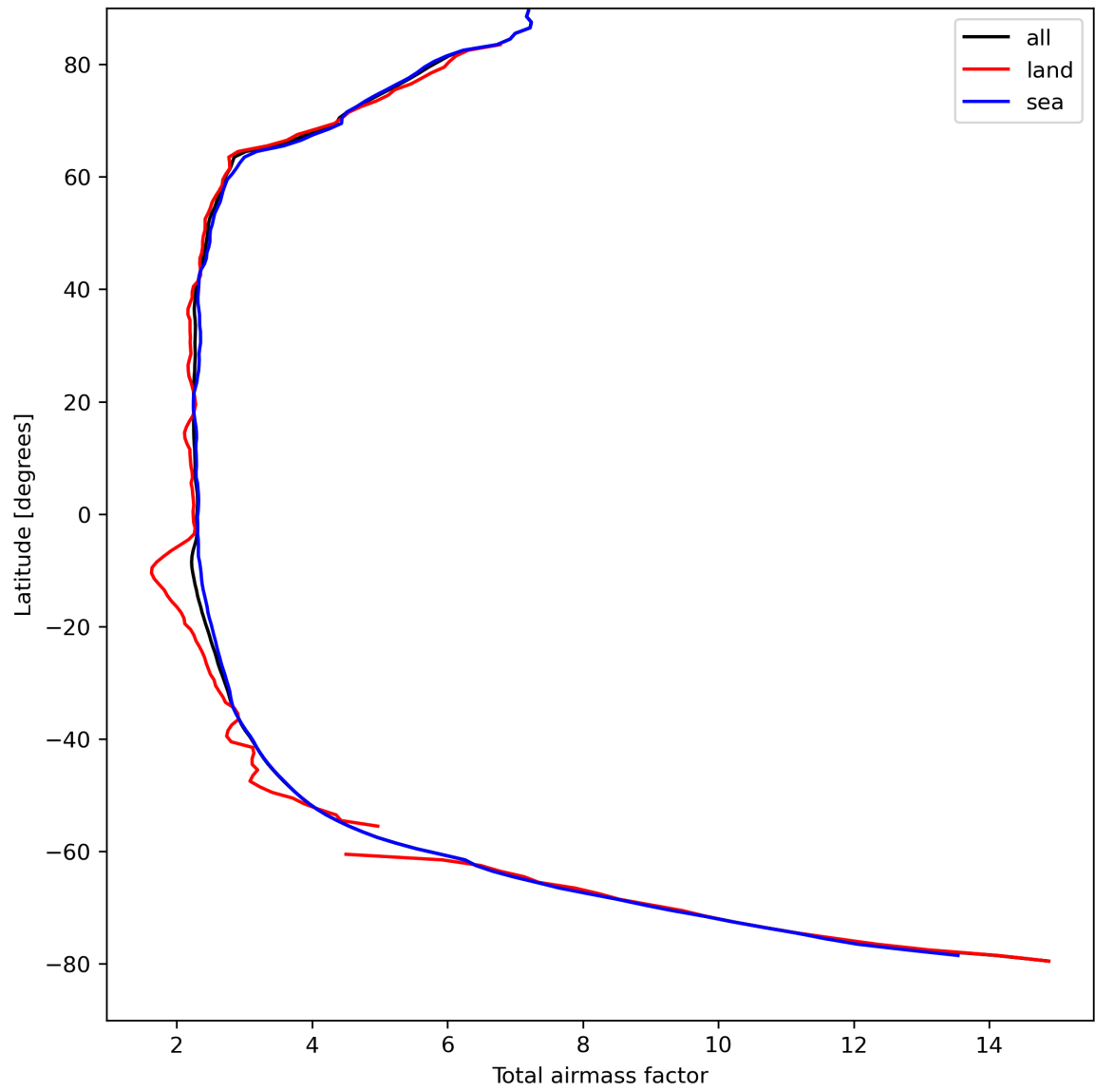
Figure 15: Zonal average of “Total airmass factor” for 2023-08-30 to 2023-09-01.
