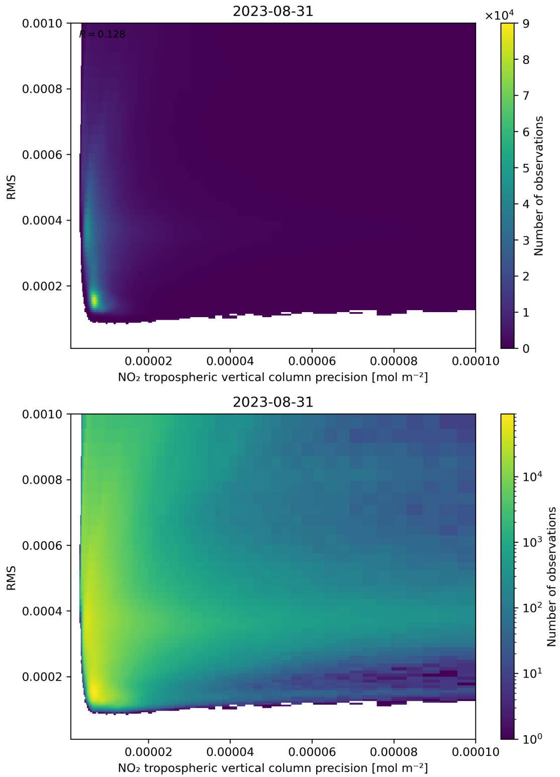
Figure 140: Scatter density plot of “NO 2 tropospheric vertical column precision” against “RMS” for 2023-08-30 to 2023-09-01.
