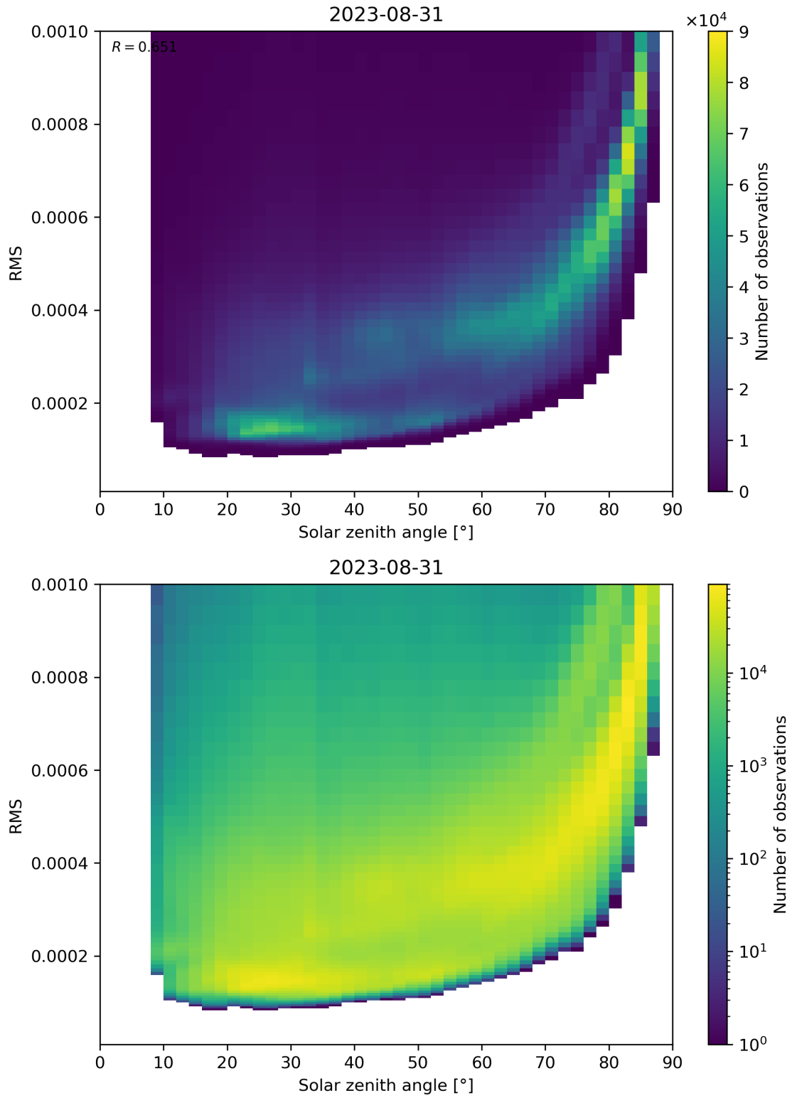
Figure 157: Scatter density plot of “Solar zenith angle” against “RMS” for 2023-08-30 to 2023-09-01.
