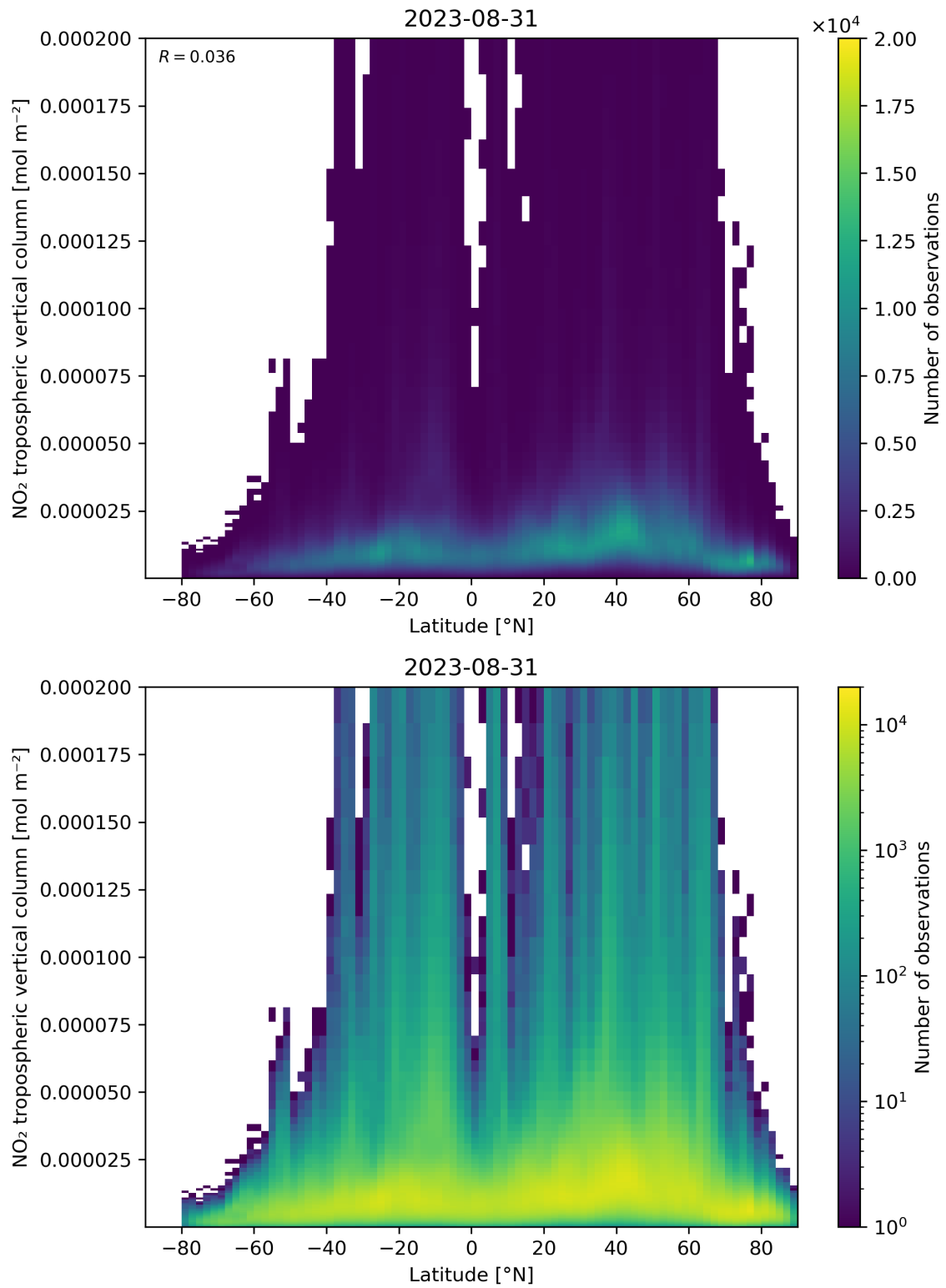
Figure 92: Scatter density plot of “Latitude” against “NO 2 tropospheric vertical column” for 2023-08-30 to 2023-09-01.
