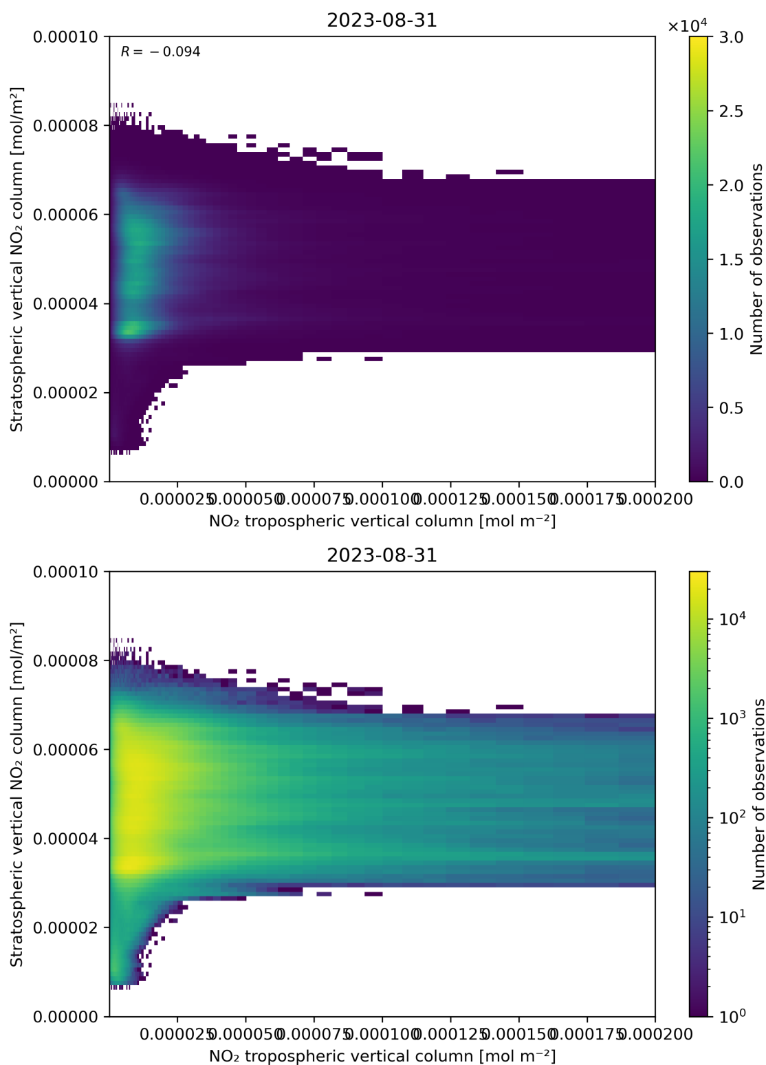
Figure 125: Scatter density plot of “NO 2 tropospheric vertical column” against “Stratospheric vertical NO 2 column” for 2023-08-30 to 2023-09-01.
