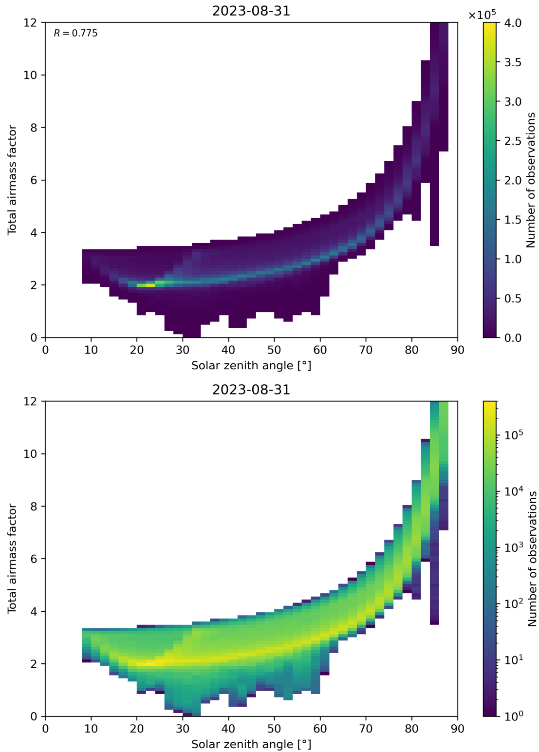
Figure 146: Scatter density plot of “Solar zenith angle” against “Total air mass factor” for 2023-08-30 to 2023-09-01.
