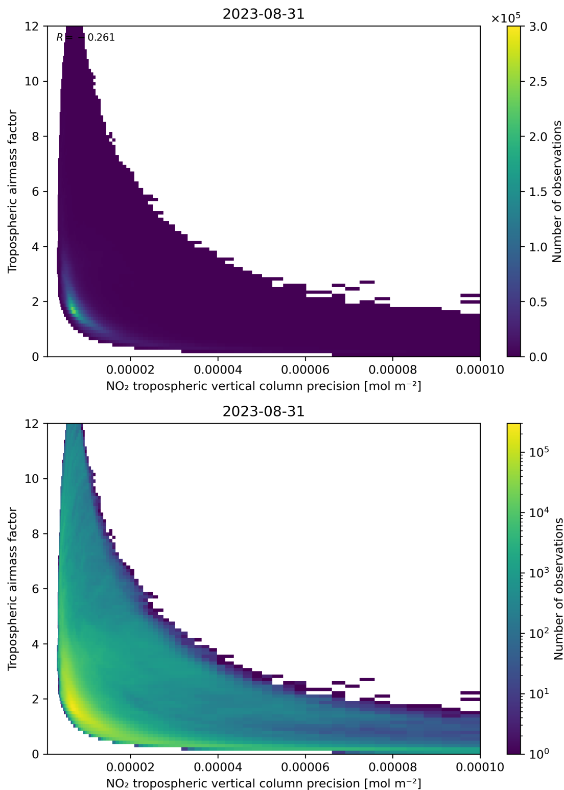
Figure 133: Scatter density plot of “NO 2 tropospheric vertical column precision” against “Tropospheric airmass factor” for 2023-08-30 to 2023-09-01.
