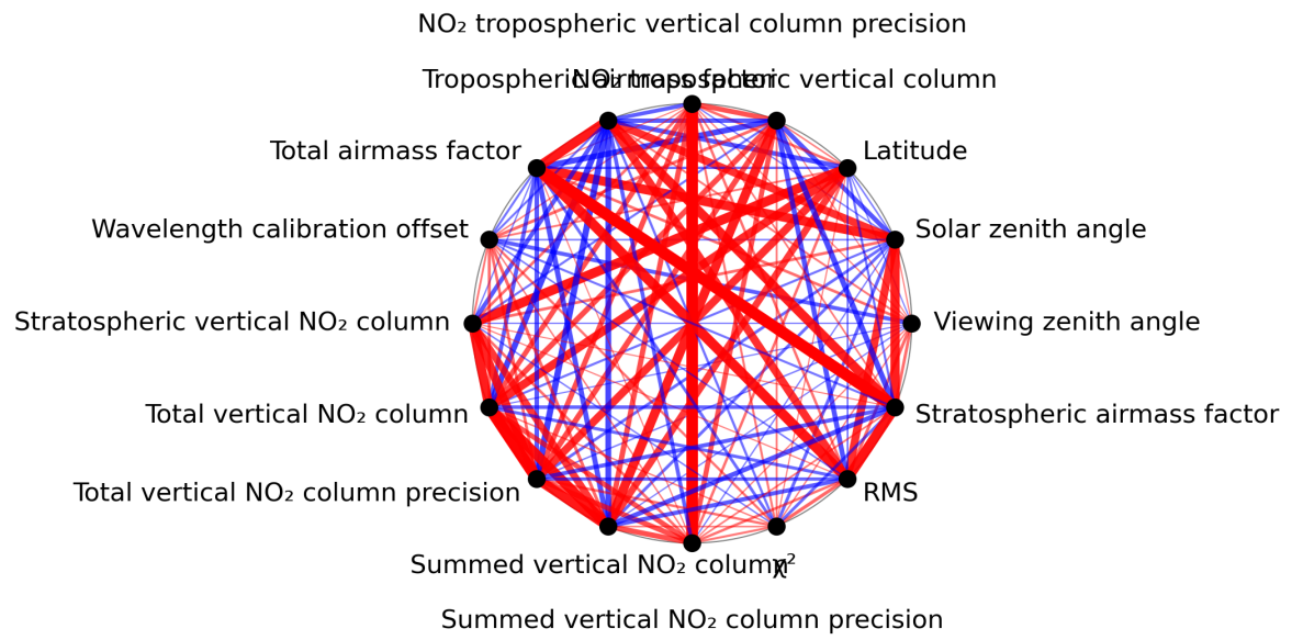
Figure 1: Map of correlation graph for 2023-08-30 to 2023-09-01.
