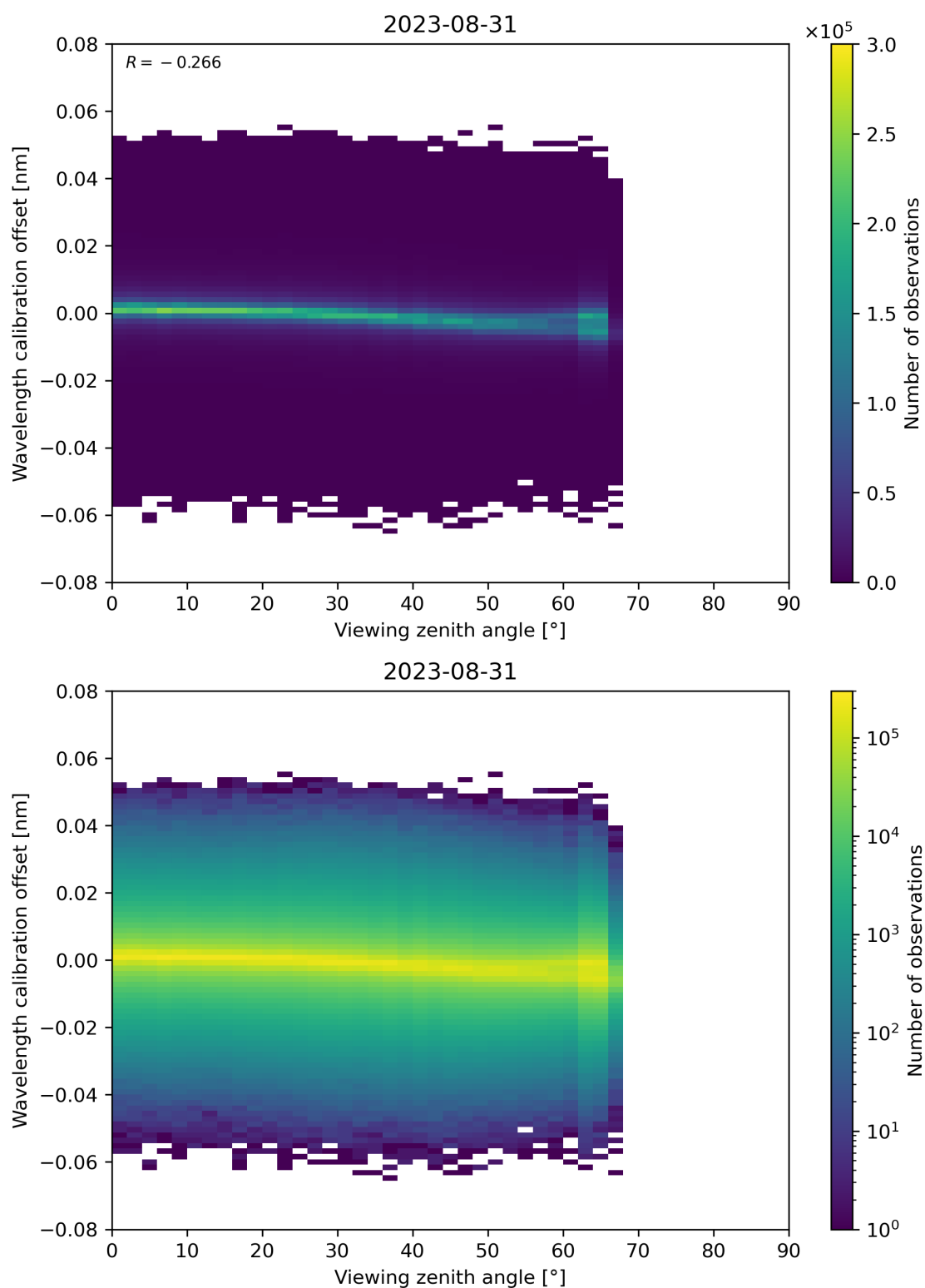
Figure 173: Scatter density plot of “Viewing zenith angle” against “Wavelength calibration offset” for 2023-08-30 to 2023-09-01.
