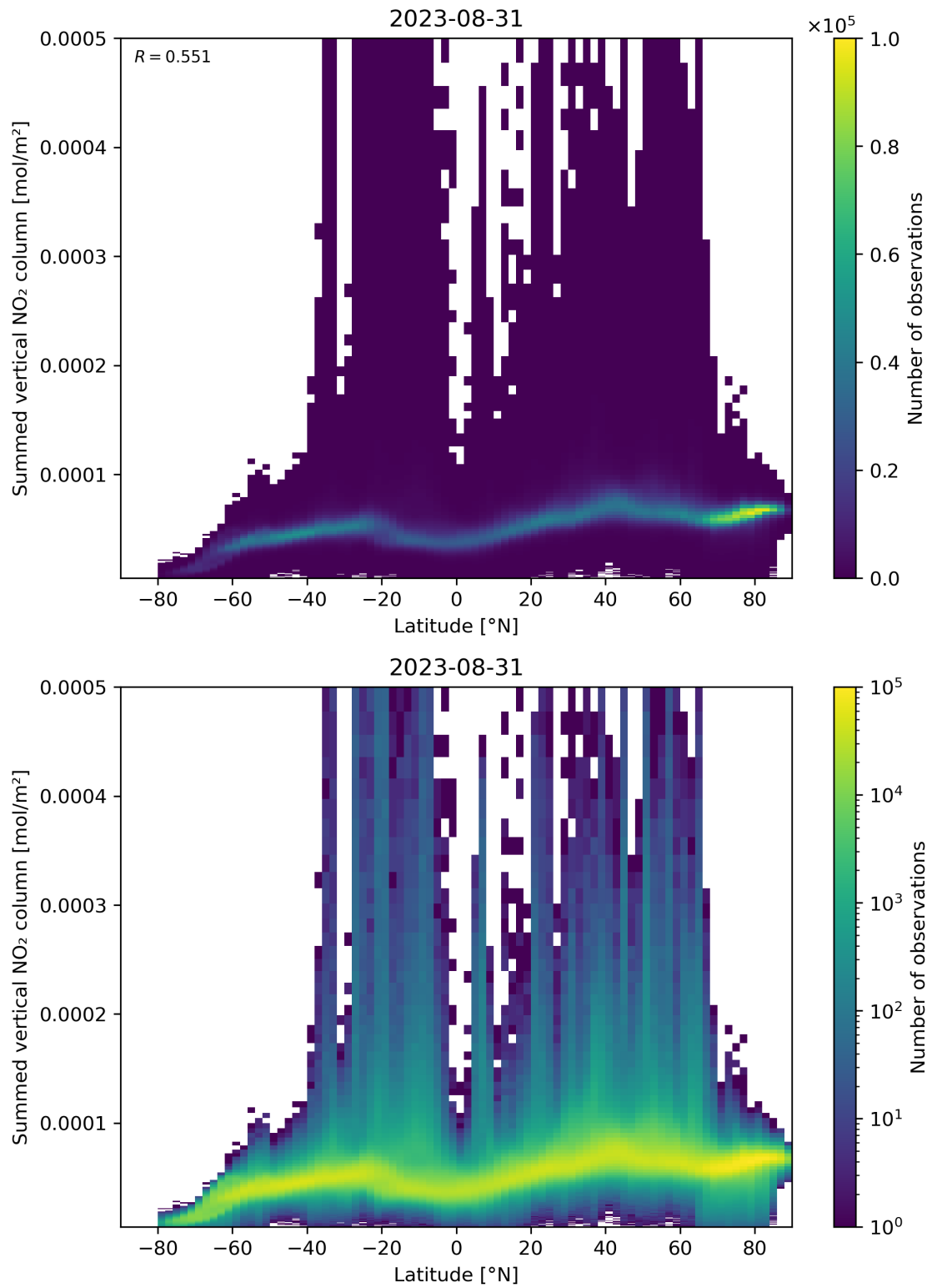
Figure 88: Scatter density plot of “Latitude” against “Summed vertical NO 2 column” for 2023-08-30 to 2023-09-01.
