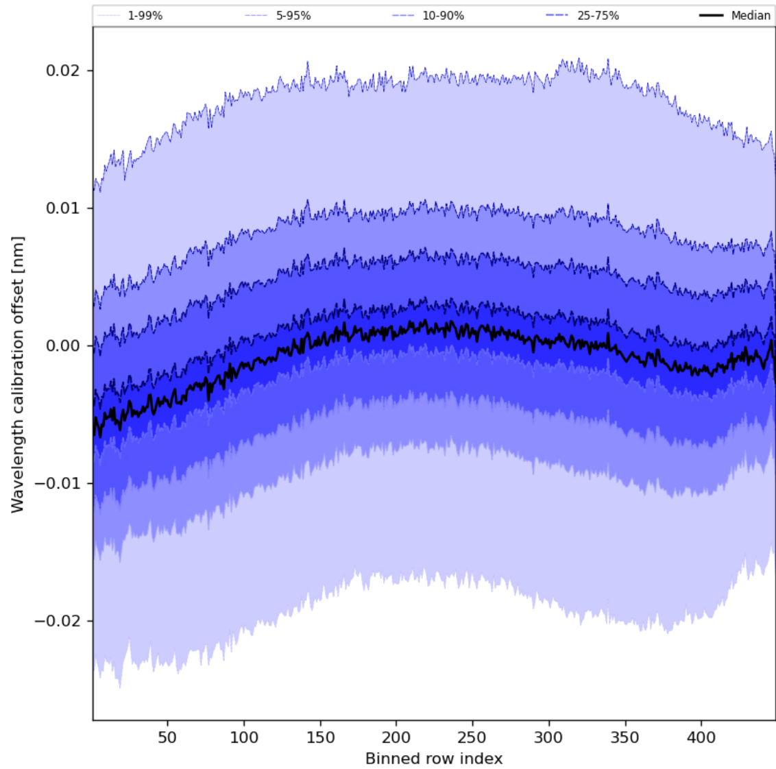
Figure 52: Along track statistics of “Wavelength calibration offset” for 2023-08-30 to 2023-09-01
