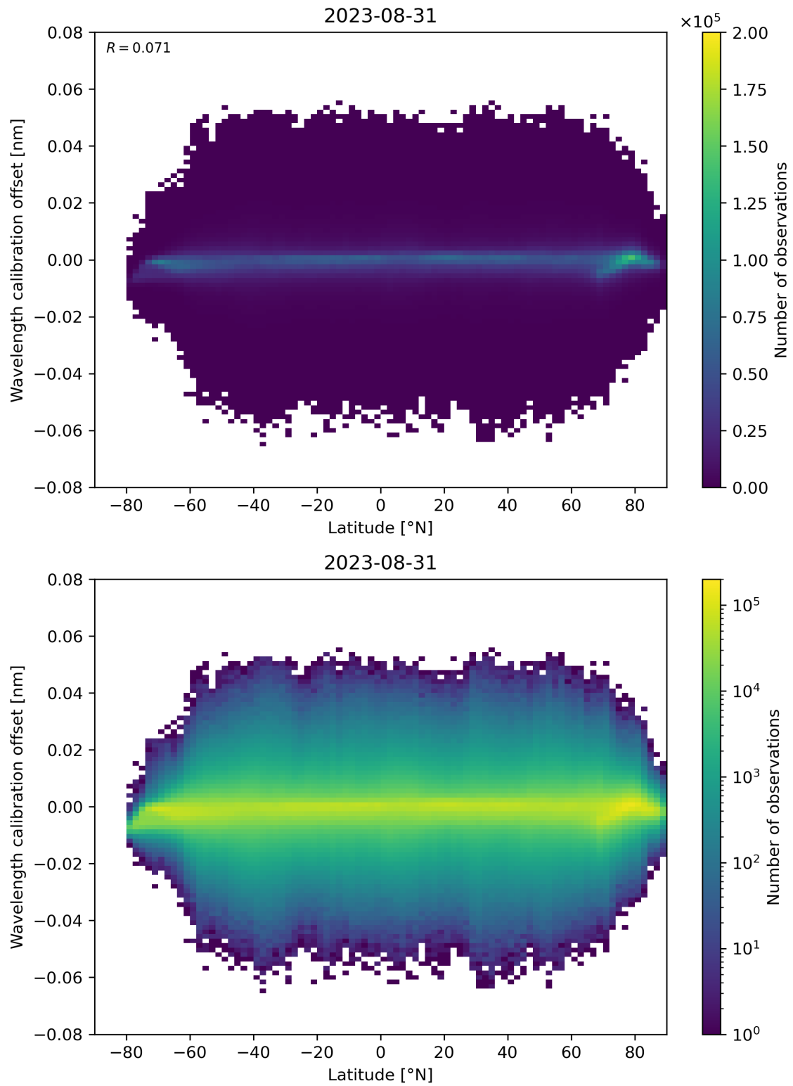
Figure 95: Scatter density plot of “Latitude” against “Wavelength calibration offset” for 2023-08-30 to 2023-09-01.
