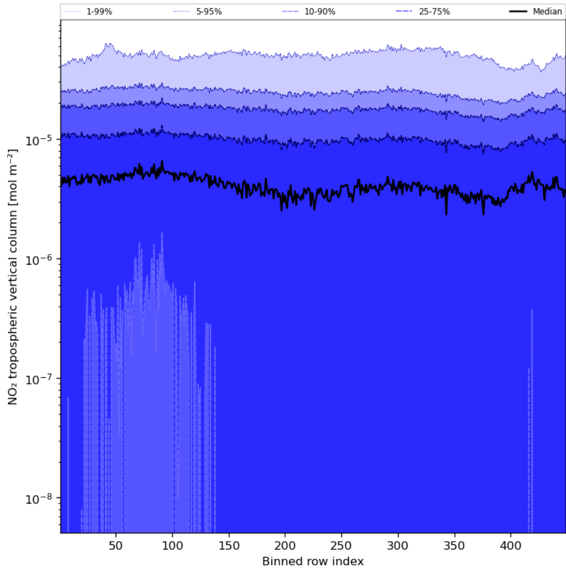
Figure 46: Along track statistics of “NO 2 tropospheric vertical column” for 2023-08-30 to 2023-09-01
