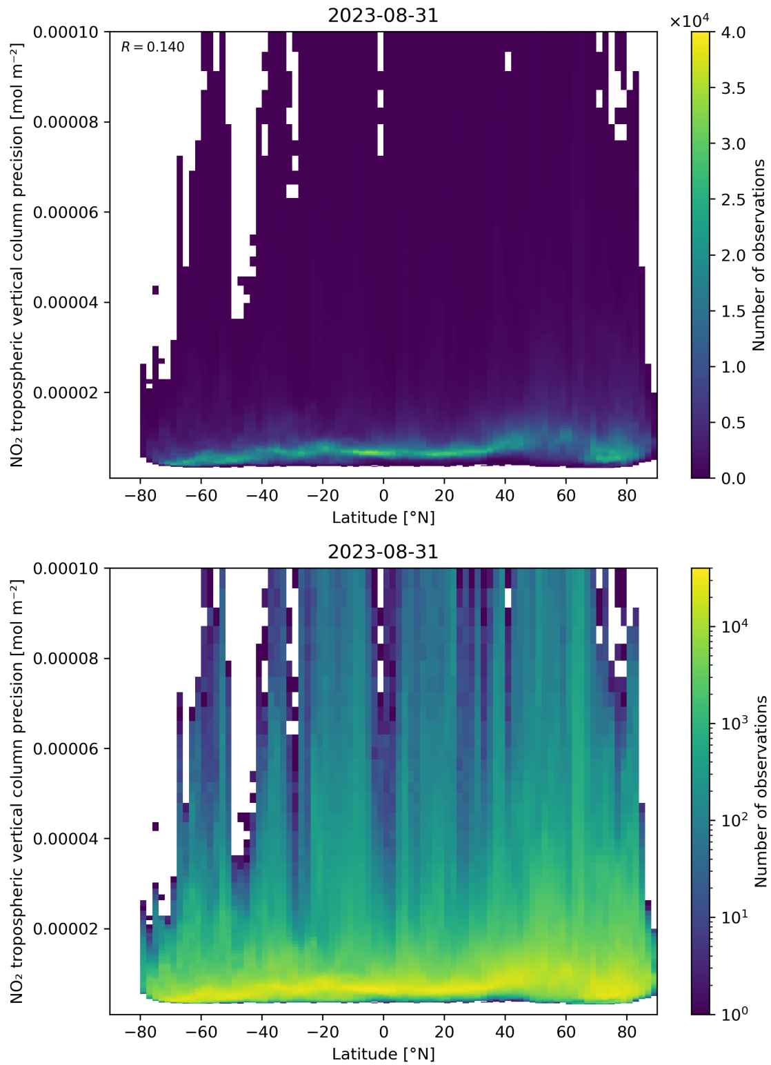
Figure 93: Scatter density plot of “Latitude” against “NO 2 tropospheric vertical column precision” for 2023-08-30 to 2023-09-01.
