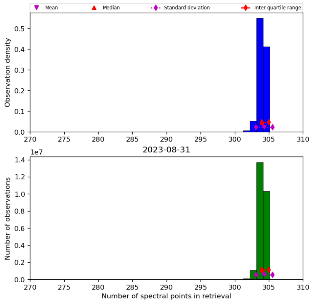
Figure 33: Histogram of “Number of spectral points in retrieval” for 2023-08-30 to 2023-09-01
