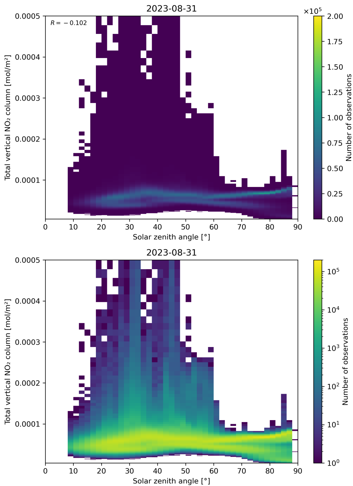
Figure 153: Scatter density plot of “Solar zenith angle” against “Total vertical NO 2 column” for 2023-08-30 to 2023-09-01.
