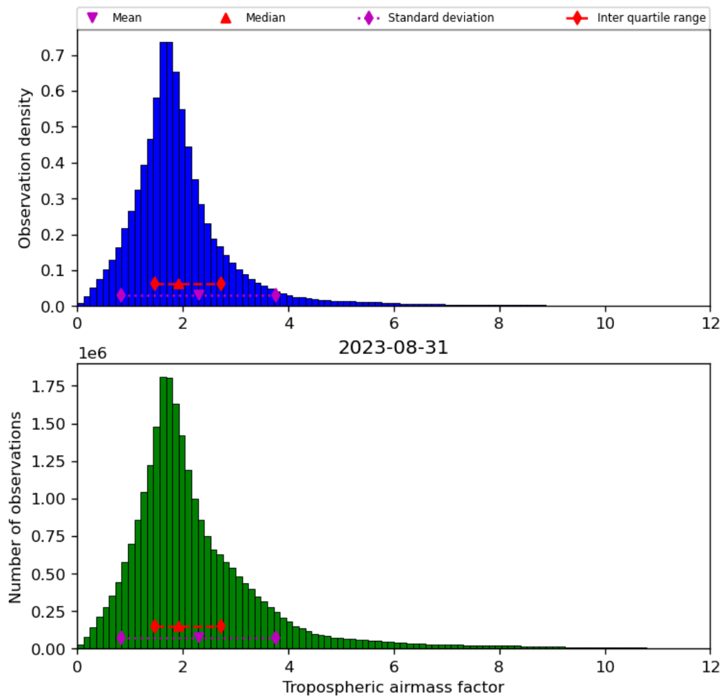
Figure 31: Histogram of “Tropospheric airmass factor” for 2023-08-30 to 2023-09-01
