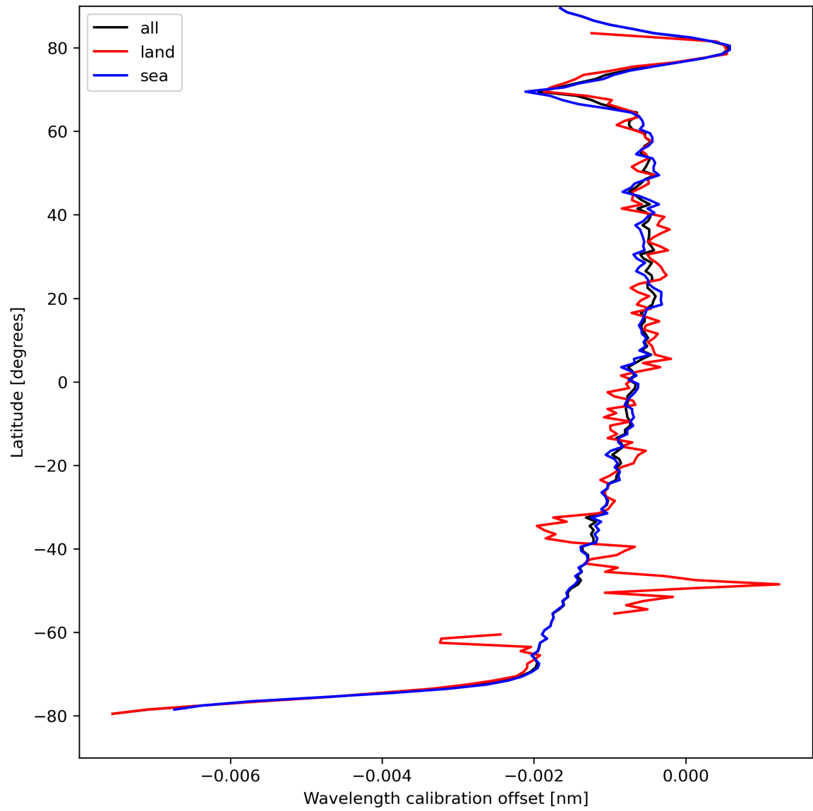
Figure 18: Zonal average of “Wavelength calibration offset” for 2023-08-30 to 2023-09-01.
