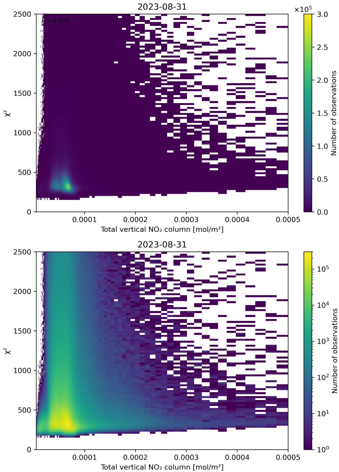
Figure 111: Scatter density plot of “Total vertical NO 2 column” against “ \chi^2 ” for 2023-08-30 to 2023-09-01.
