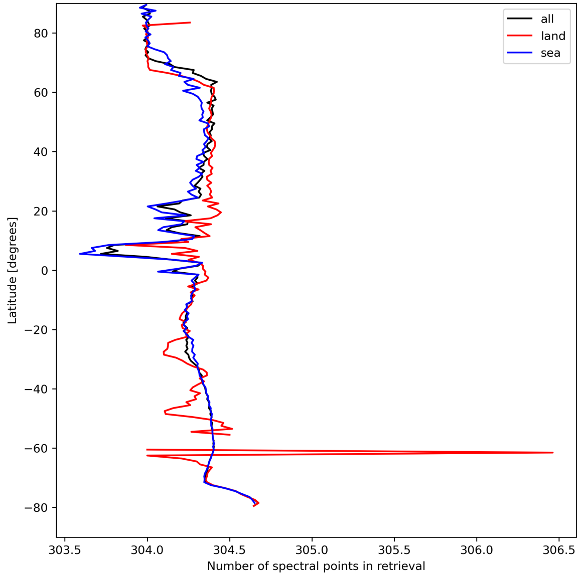
Figure 16: Zonal average of “Number of spectral points in retrieval” for 2023-08-30 to 2023-09-01.
