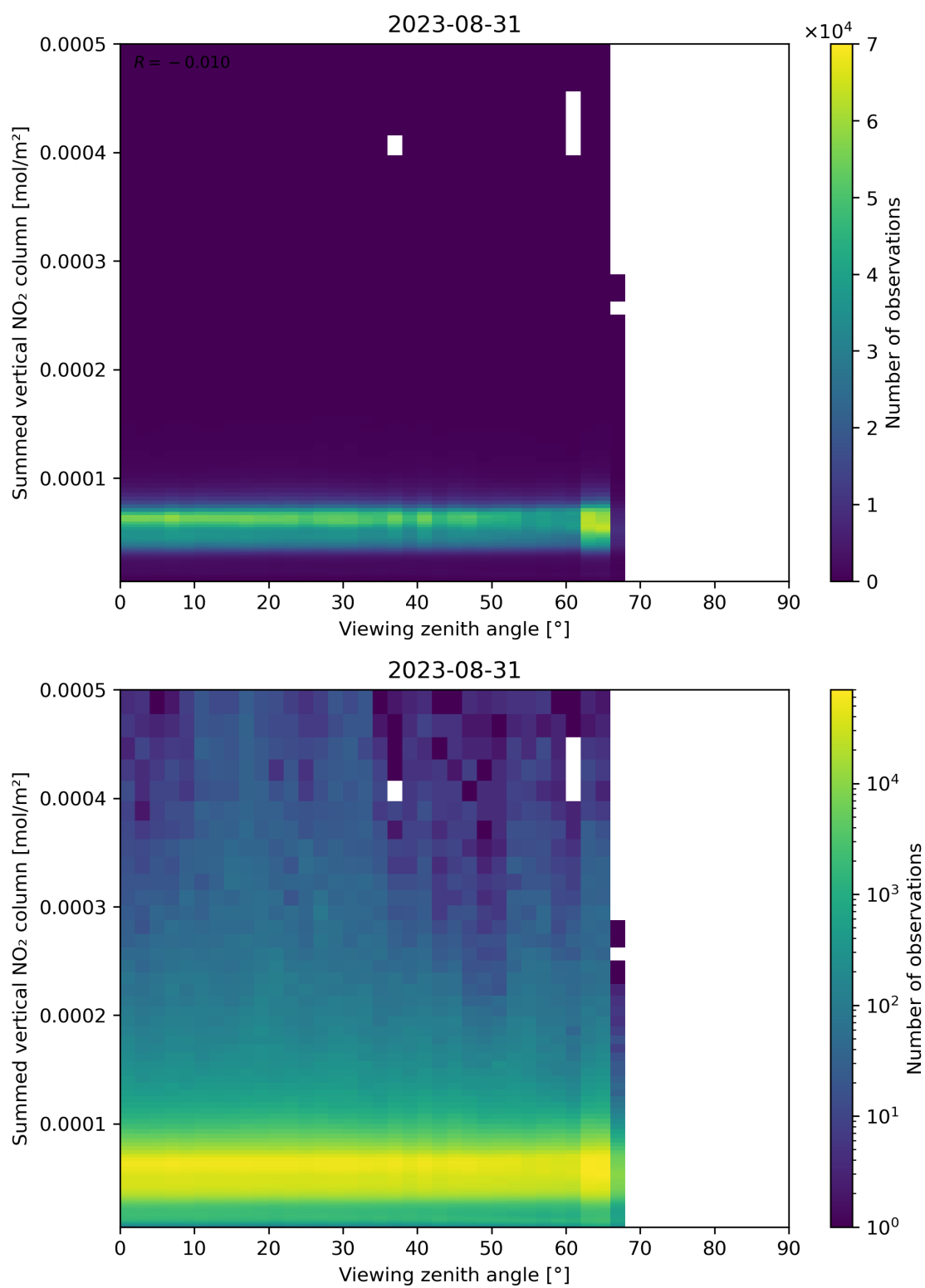
Figure 165: Scatter density plot of “Viewing zenith angle” against “Summed vertical NO 2 column” for 2023-08-30 to 2023-09-01.
