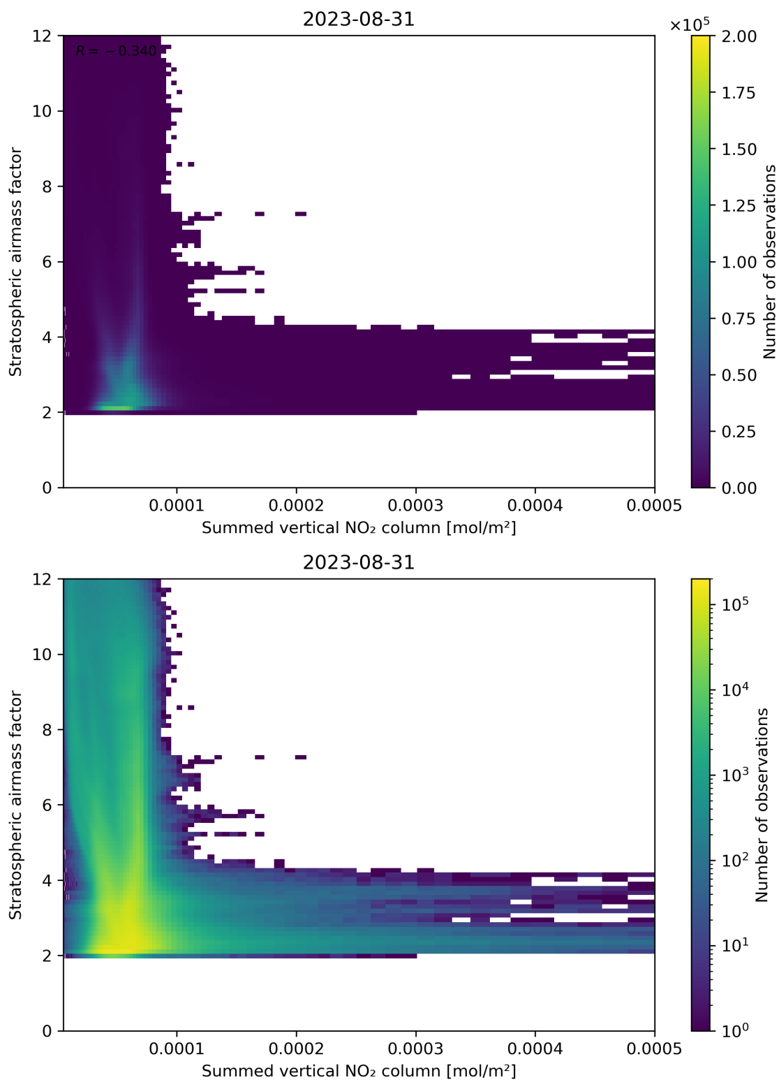
Figure 103: Scatter density plot of “Summed vertical NO 2 column” against “Stratospheric air mass factor” for 2023-08-30 to 2023-09-01.
