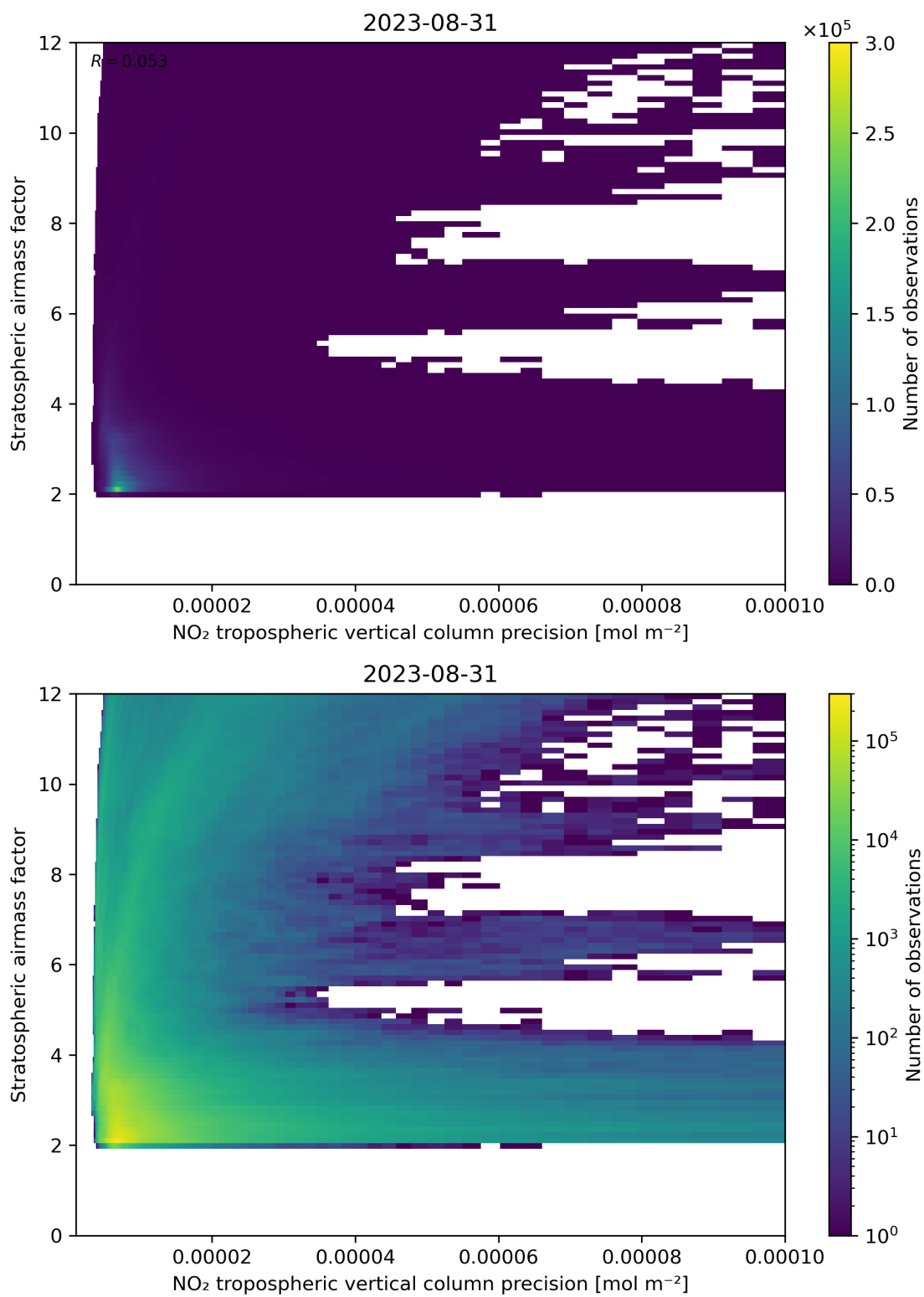
Figure 131: Scatter density plot of “NO 2 tropospheric vertical column precision” against “Stratospheric airmass factor” for 2023-08-30 to 2023-09-01.
