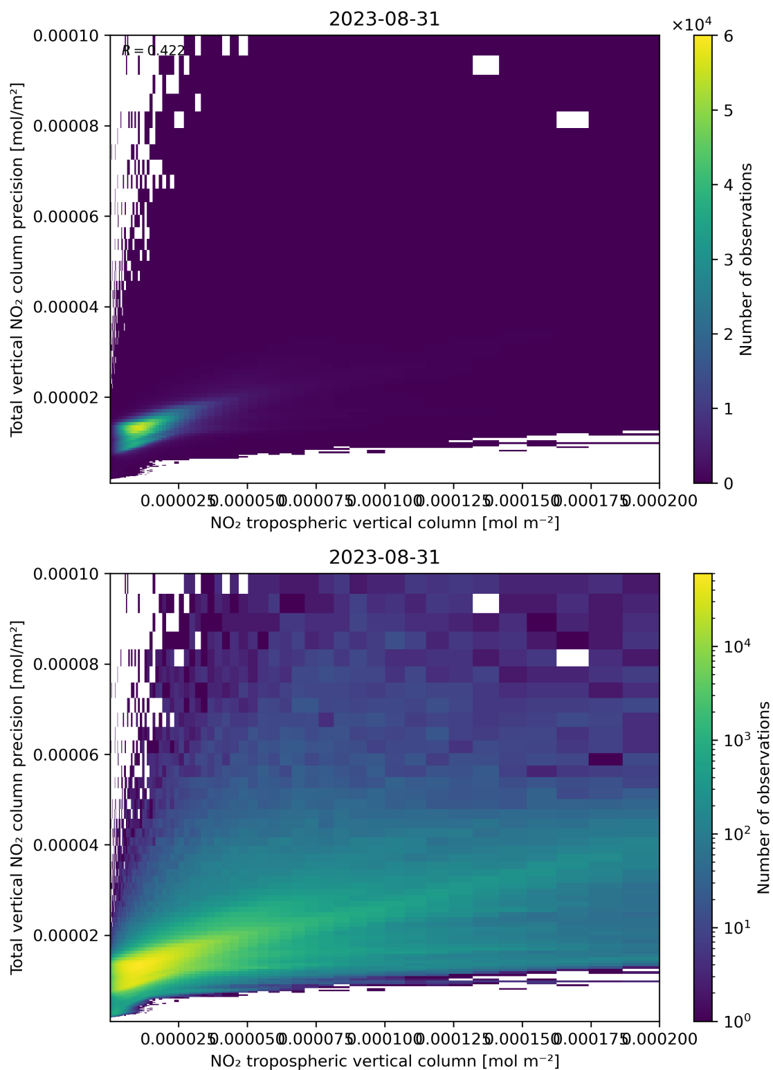
Figure 129: Scatter density plot of “NO 2 tropospheric vertical column” against “Total vertical NO 2 column precision” for 2023-08-30 to 2023-09-01.
