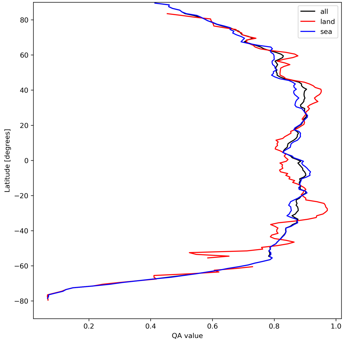
Figure 11: Zonal average of “QA value” for 2023-08-30 to 2023-09-01.
