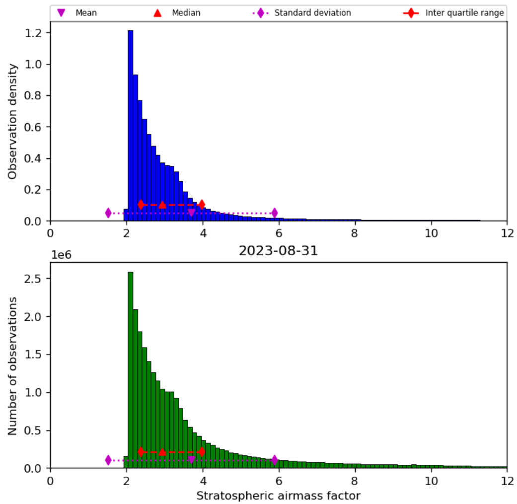
Figure 44: Histogram of “Stratospheric airmass factor” for 2023-08-30 to 2023-09-01
