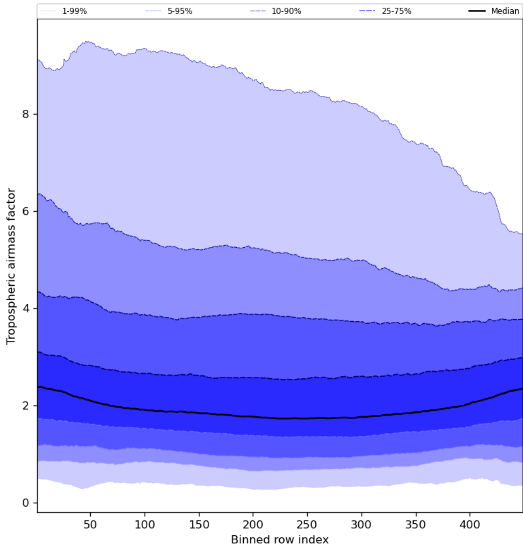
Figure 48: Along track statistics of “Tropospheric airmass factor” for 2023-08-30 to 2023-09-01
