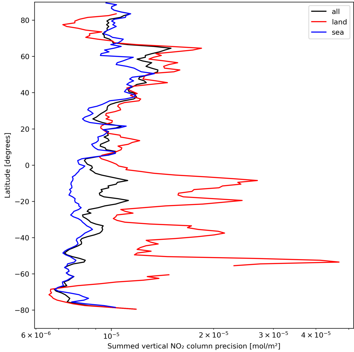
Figure 24: Zonal average of "Summed vertical NO 2 column precision" for 2023-08-30 to 2023-09-01.
