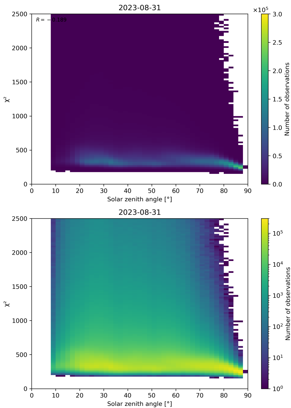
Figure 148: Scatter density plot of “Solar zenith angle” against “ \chi^2 ” for 2023-08-30 to 2023-09-01.
