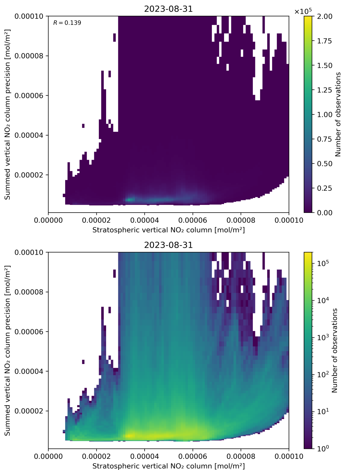
Figure 99: Scatter density plot of “Stratospheric vertical NO 2 column” against “Summed vertical NO 2 column precision” for 2023-08-30 to 2023-09-01.
