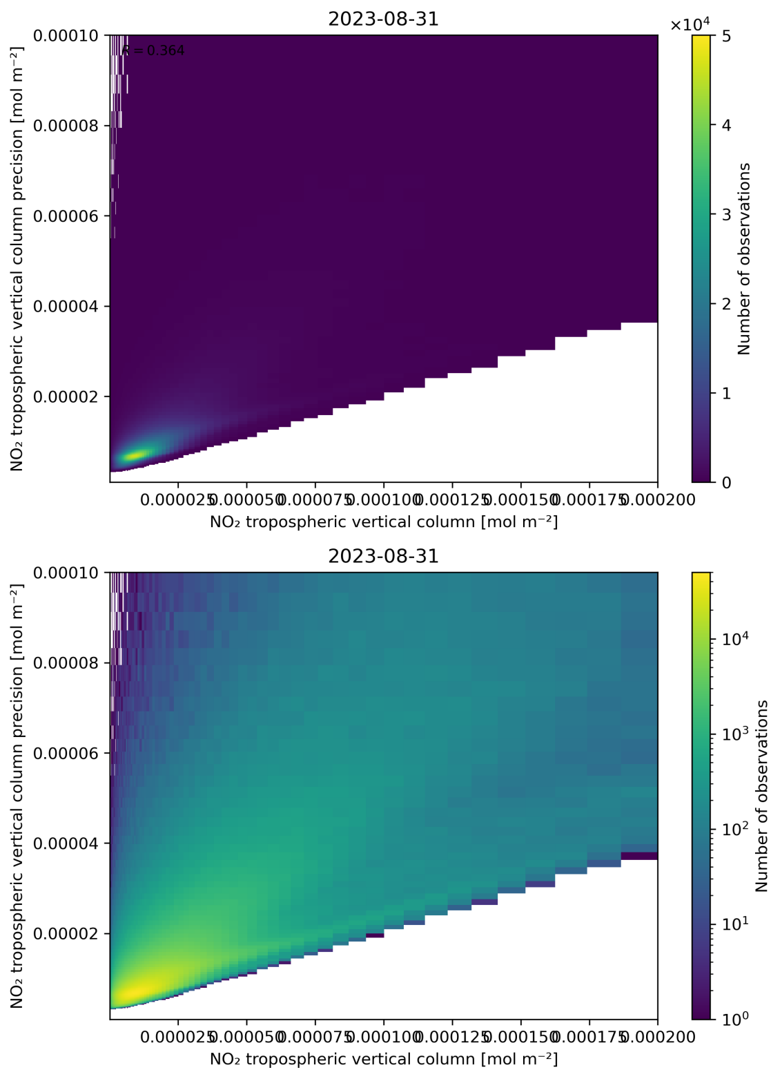
Figure 130: Scatter density plot of “NO 2 tropospheric vertical column” against “NO 2 tropospheric vertical column precision” for 2023-08-30 to 2023-09-01.
