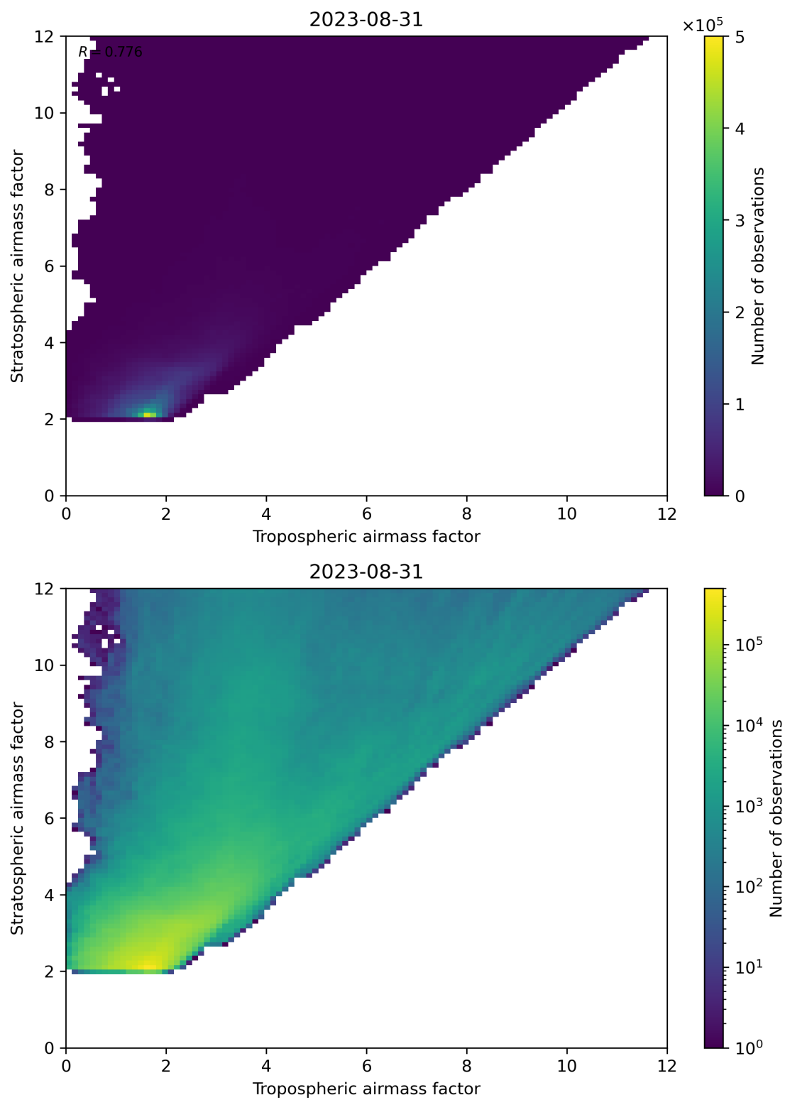
Figure 71: Scatter density plot of “Tropospheric airmass factor” against “Stratospheric airmass factor” for 2023-08-30 to 2023-09-01.
