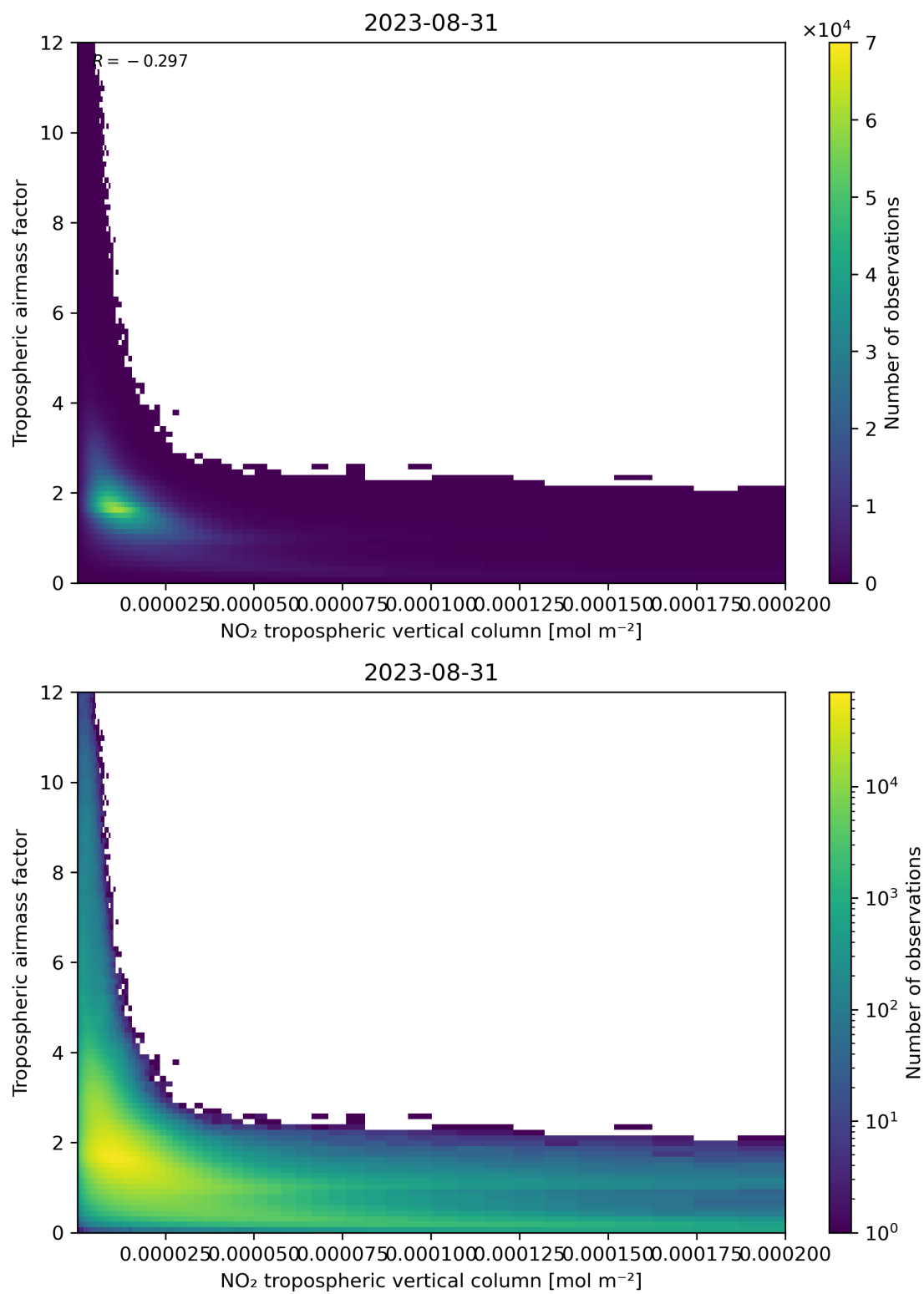
Figure 123: Scatter density plot of “NO 2 tropospheric vertical column” against “Tropospheric air mass factor” for 2023-08-30 to 2023-09-01.
