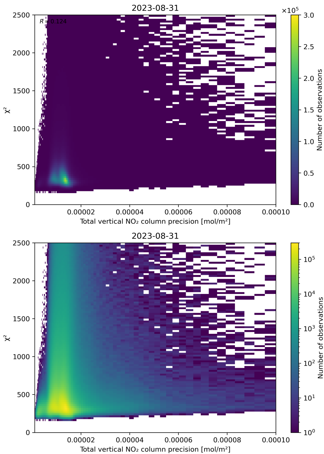
Figure 116: Scatter density plot of “Total vertical NO 2 column precision” against “ \chi^2 ” for 2023-08-30 to 2023-09-01.
