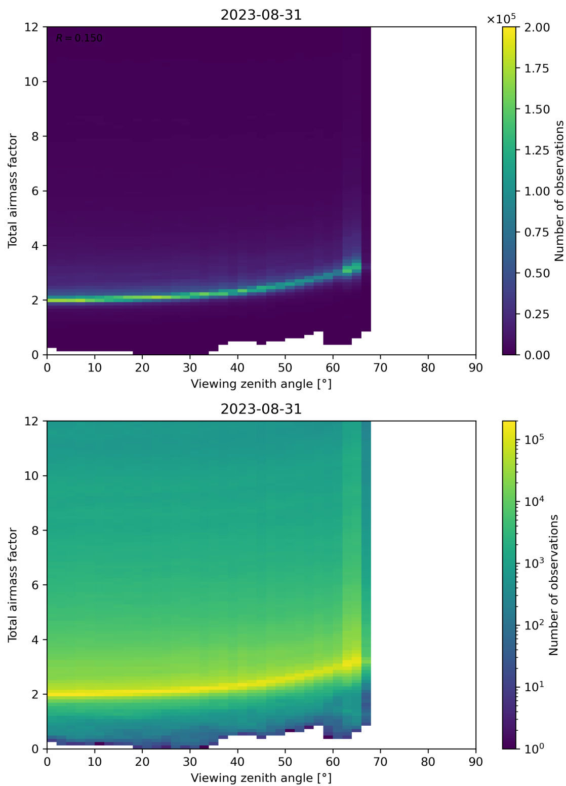
Figure 160: Scatter density plot of “Viewing zenith angle” against “Total airmass factor” for 2023-08-30 to 2023-09-01.
