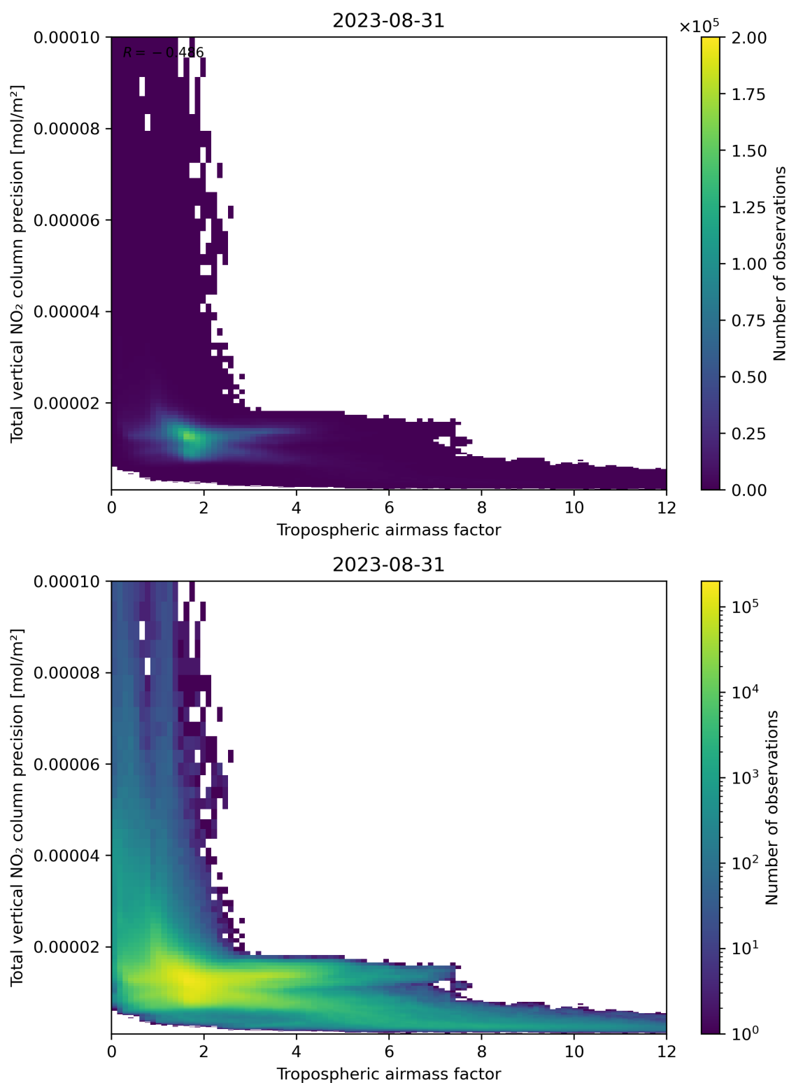
Figure 78: Scatter density plot of “Tropospheric air mass factor” against “Total vertical NO 2 column precision” for 2023-08-30 to 2023-09-01.
