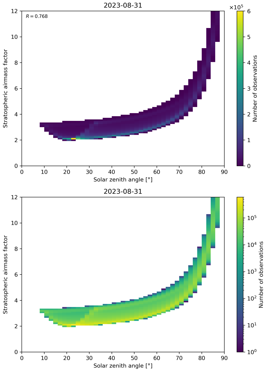
Figure 145: Scatter density plot of “Solar zenith angle” against “Stratospheric airmass factor” for 2023-08-30 to 2023-09-01.
