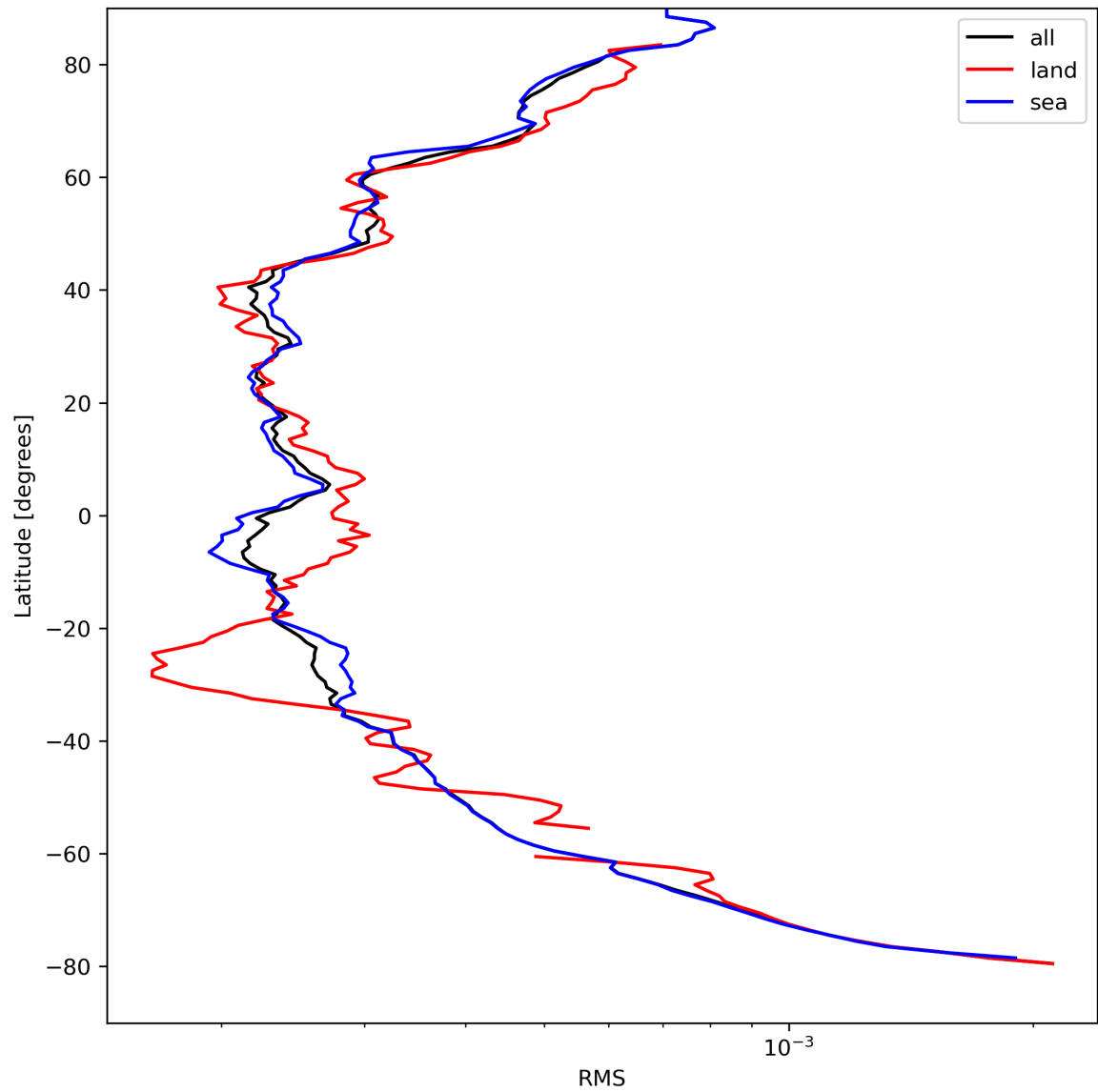
Figure 26: Zonal average of “RMS” for 2023-08-30 to 2023-09-01.
