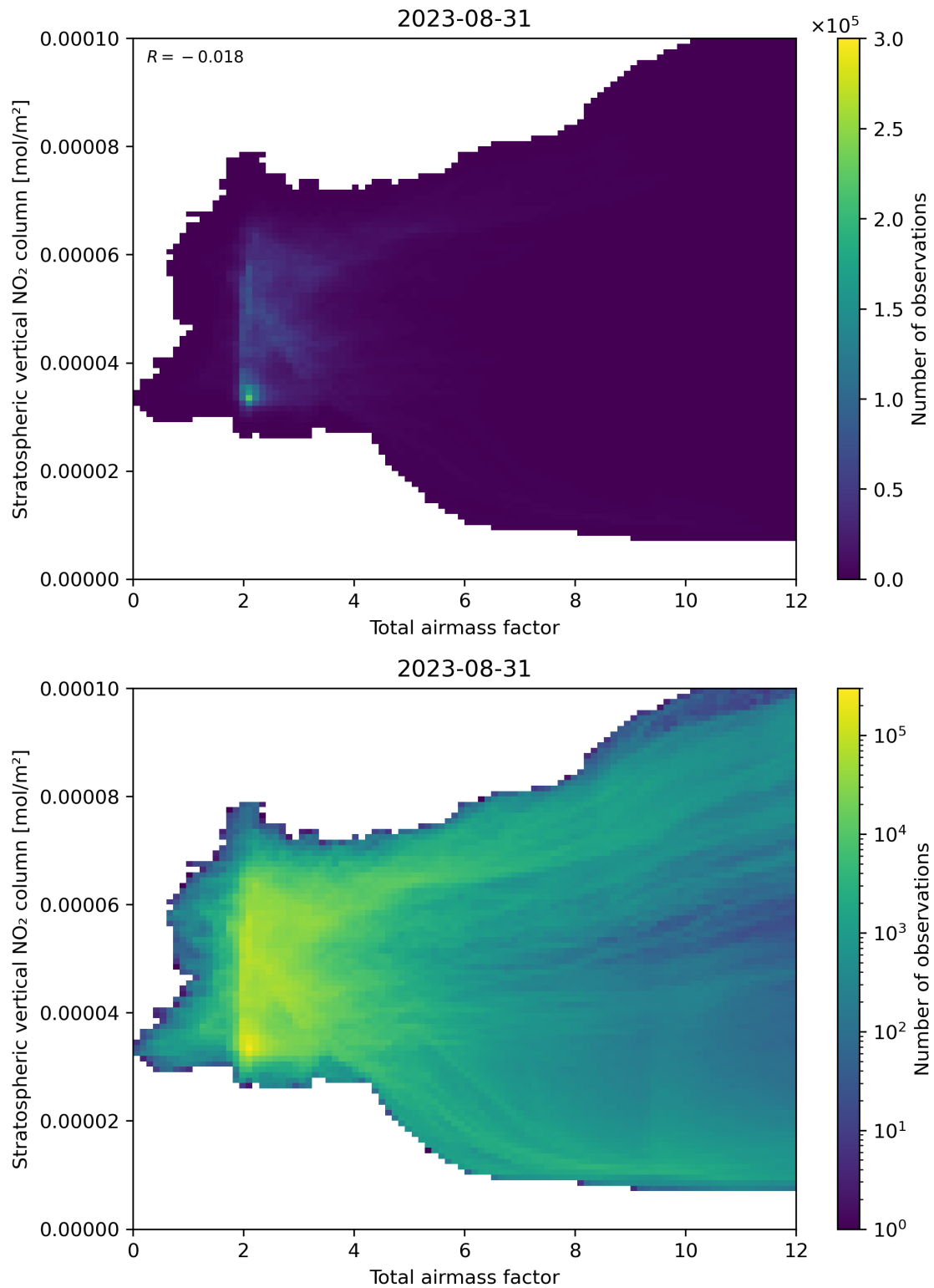
Figure 64: Scatter density plot of “Total airmass factor” against “Stratospheric vertical NO 2 column” for 2023-08-30 to 2023-09-01.
