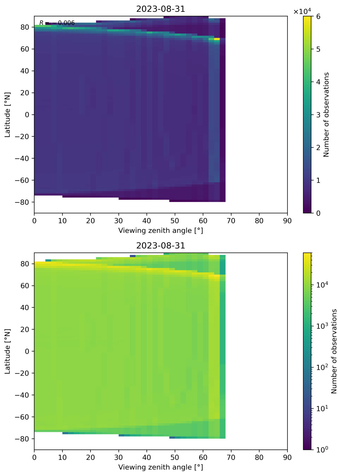
Figure 163: Scatter density plot of “Viewing zenith angle” against “Latitude” for 2023-08-30 to 2023-09-01.
