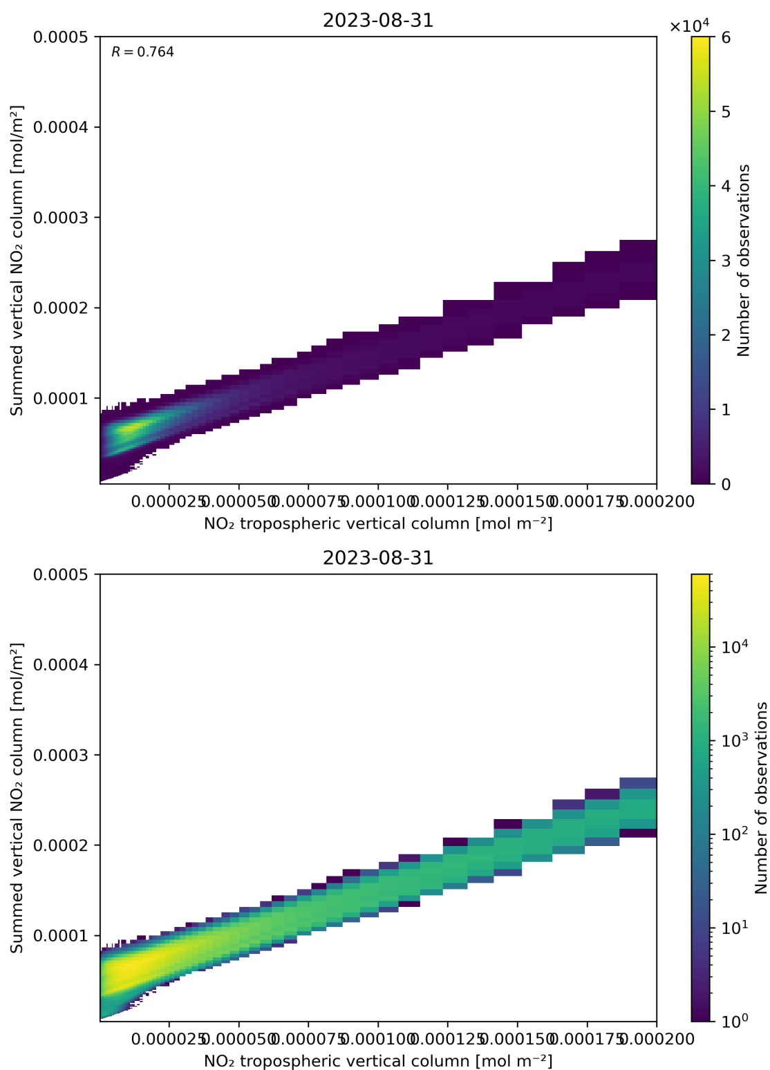
Figure 126: Scatter density plot of “NO 2 tropospheric vertical column” against “Summed vertical NO 2 column” for 2023-08-30 to 2023-09-01.
