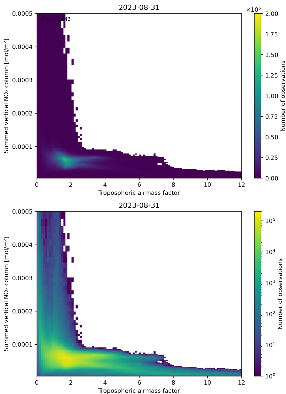
Figure 75: Scatter density plot of “Tropospheric air mass factor” against “Summed vertical NO 2 column” for 2023-08-30 to 2023-09-01.
