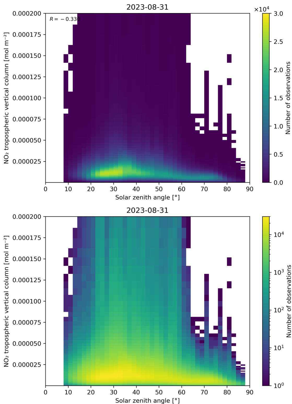
Figure 155: Scatter density plot of “Solar zenith angle” against “NO 2 tropospheric vertical column” for 2023-08-30 to 2023-09-01.
