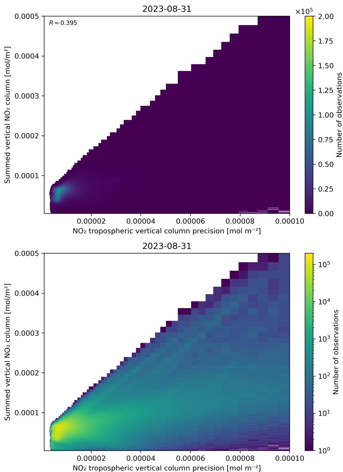
Figure 136: Scatter density plot of “NO 2 tropospheric vertical column precision” against “Summed vertical NO 2 column” for 2023-08-30 to 2023-09-01.
