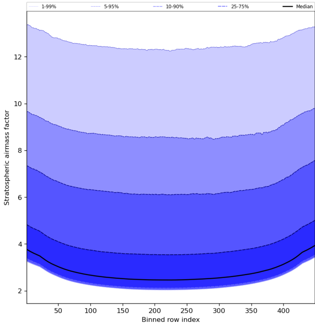
Figure 61: Along track statistics of “Stratospheric airmass factor” for 2023-08-30 to 2023-09-01
