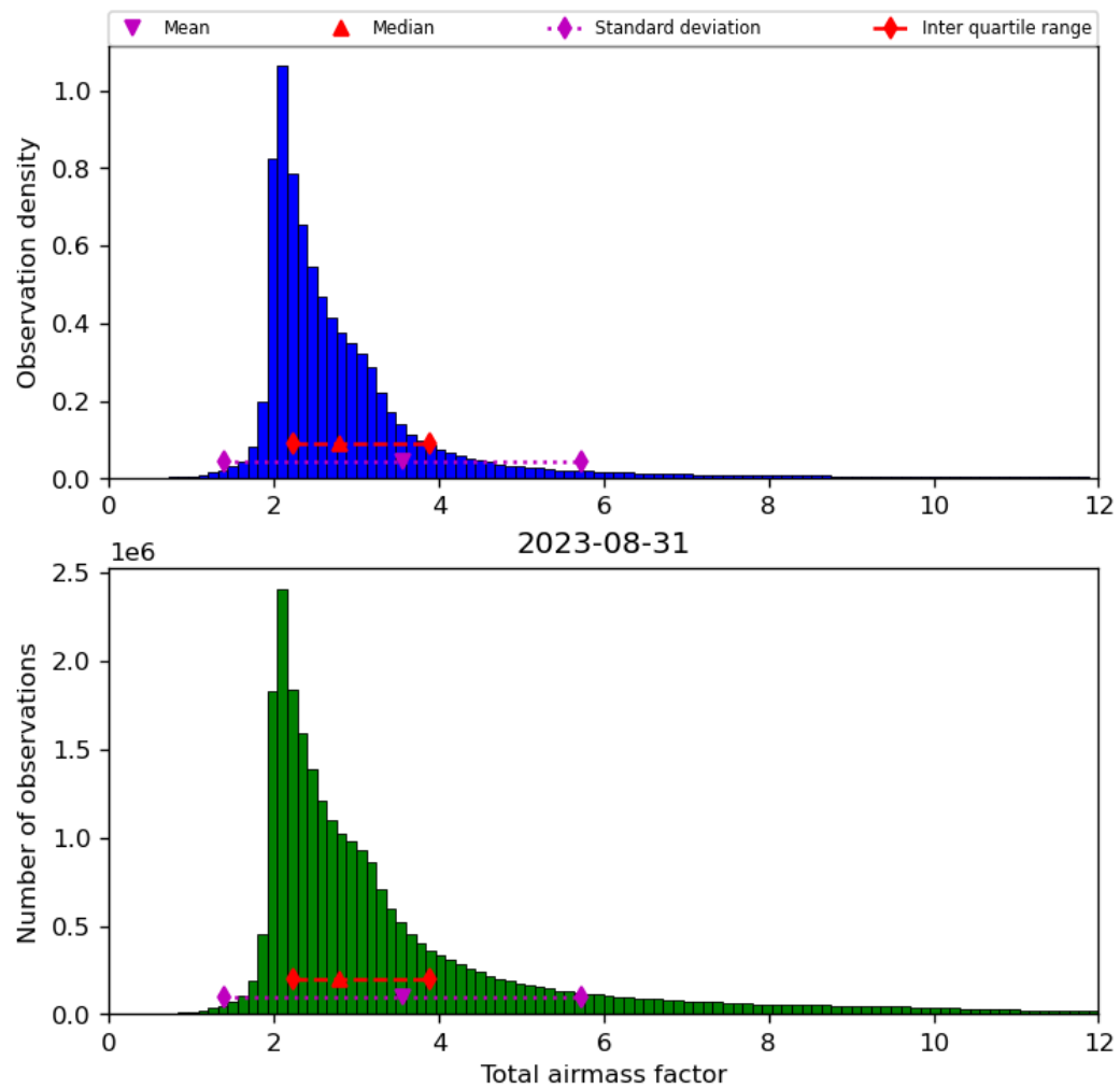
Figure 32: Histogram of “Total airmass factor” for 2023-08-30 to 2023-09-01
