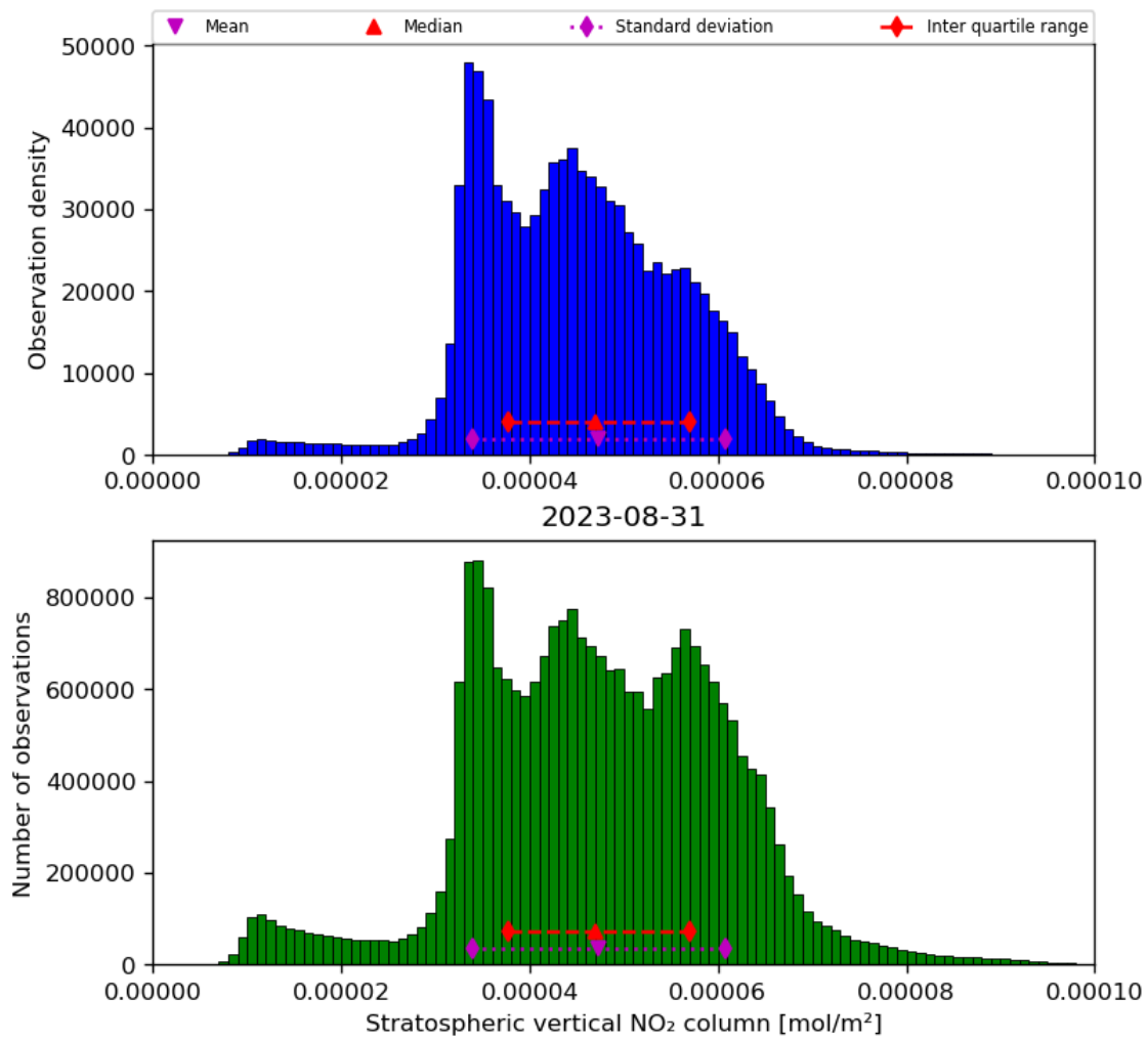
Figure 36: Histogram of “Stratospheric vertical NO 2 column” for 2023-08-30 to 2023-09-01
