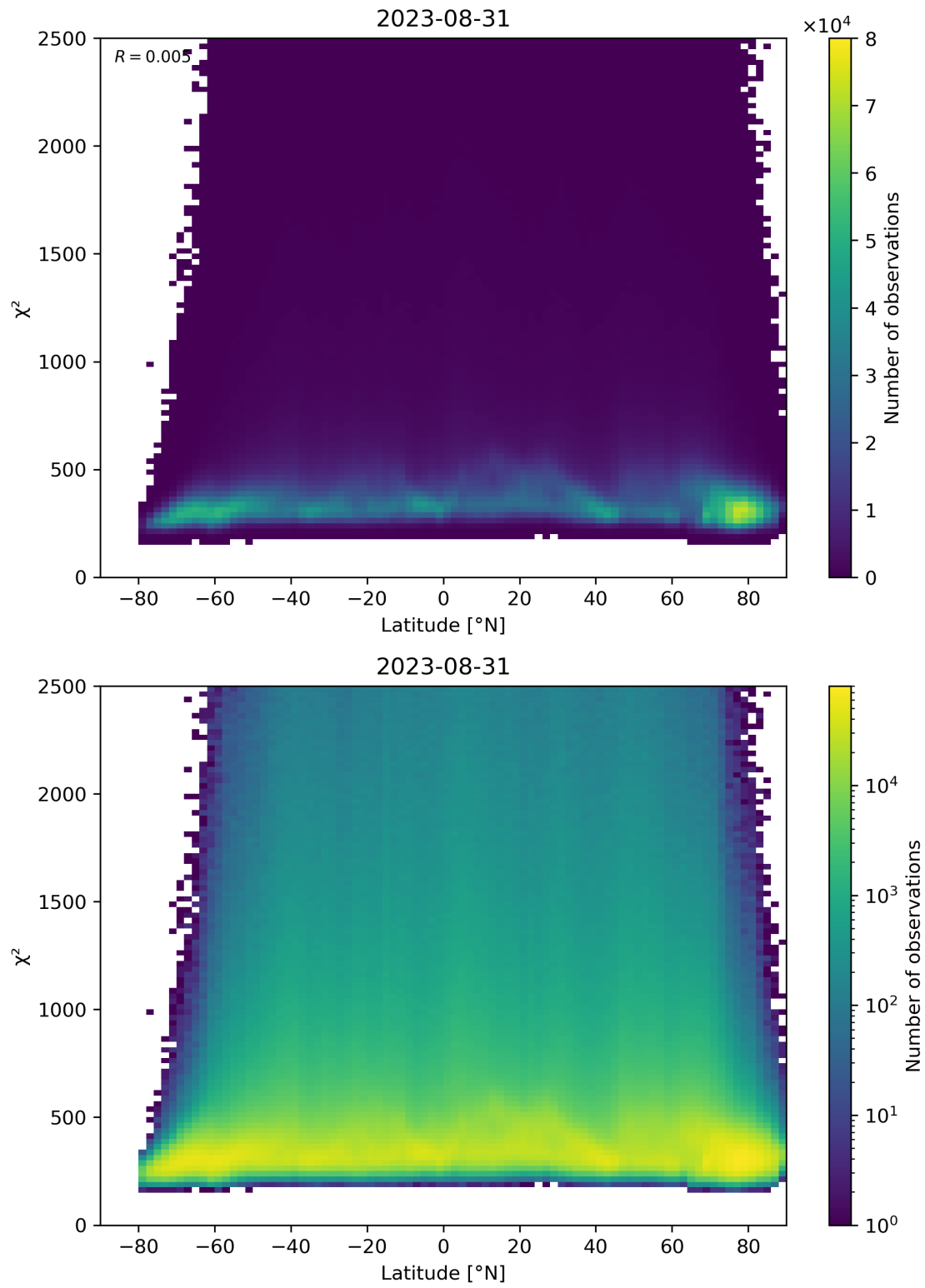
Figure 86: Scatter density plot of “Latitude” against “ \chi^2 ” for 2023-08-30 to 2023-09-01.
