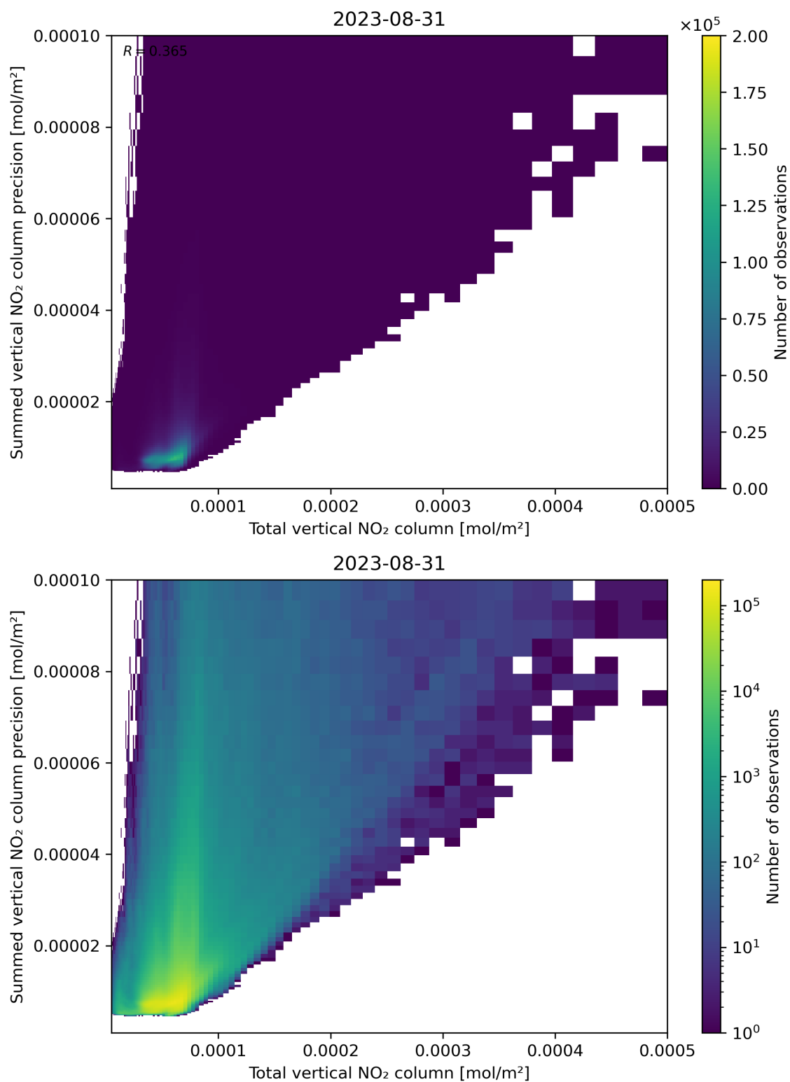
Figure 113: Scatter density plot of “Total vertical NO 2 column” against “Summed vertical NO 2 column precision” for 2023-08-30 to 2023-09-01.
