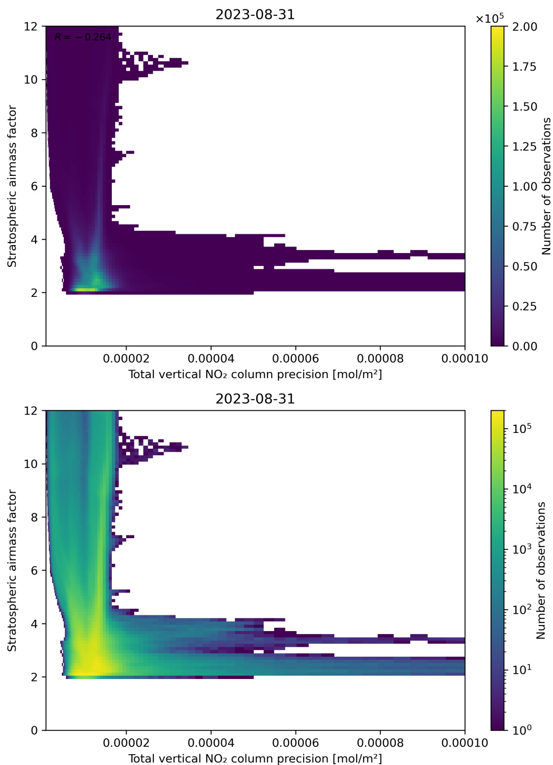
Figure 115: Scatter density plot of “Total vertical NO 2 column precision” against “Stratospheric air mass factor” for 2023-08-30 to 2023-09-01.
