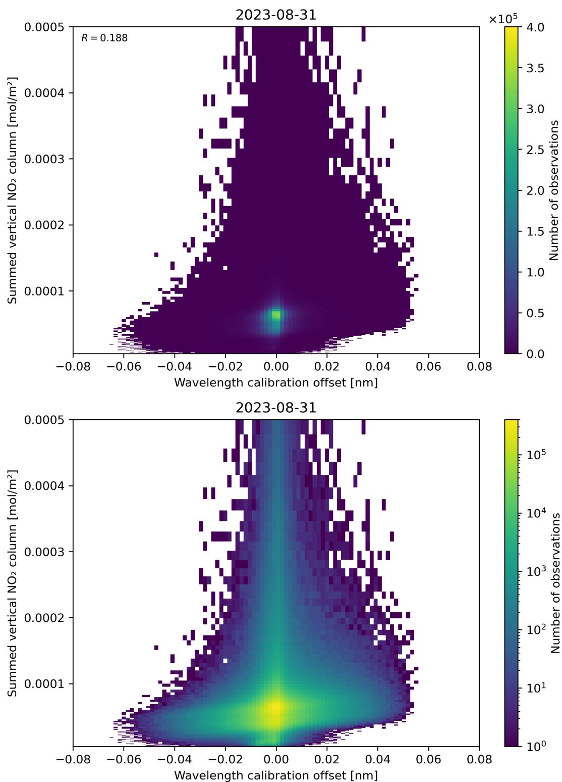
Figure 177: Scatter density plot of “Wavelength calibration offset” against “Summed vertical NO 2 column” for 2023-08-30 to 2023-09-01.
