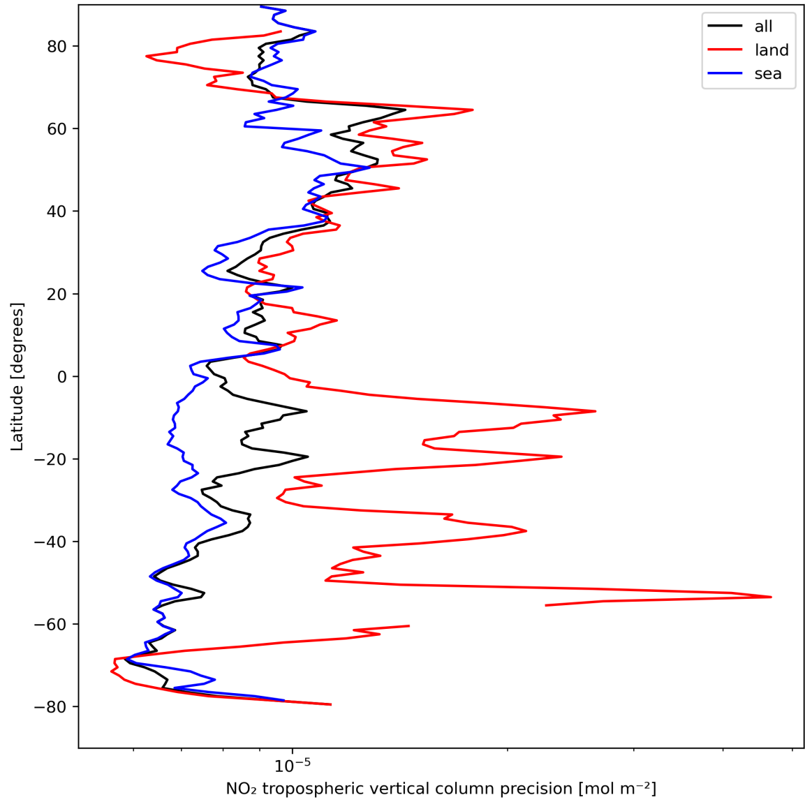
Figure 13: Zonal average of “NO 2 tropospheric vertical column precision” for 2023-08-30 to 2023-09-01.
