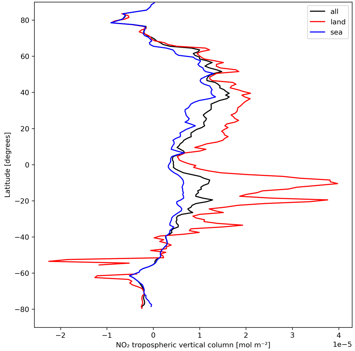
Figure 12: Zonal average of “NO 2 tropospheric vertical column” for 2023-08-30 to 2023-09-01.
