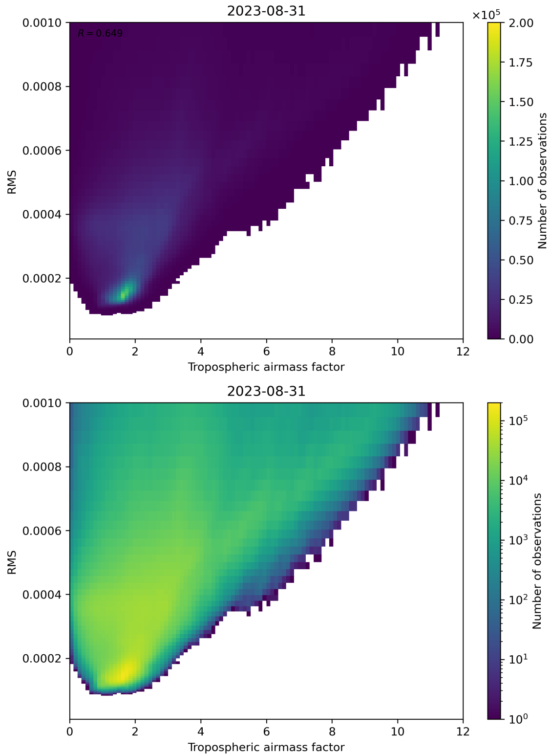
Figure 79: Scatter density plot of “Tropospheric airmass factor” against “RMS” for 2023-08-30 to 2023-09-01.
