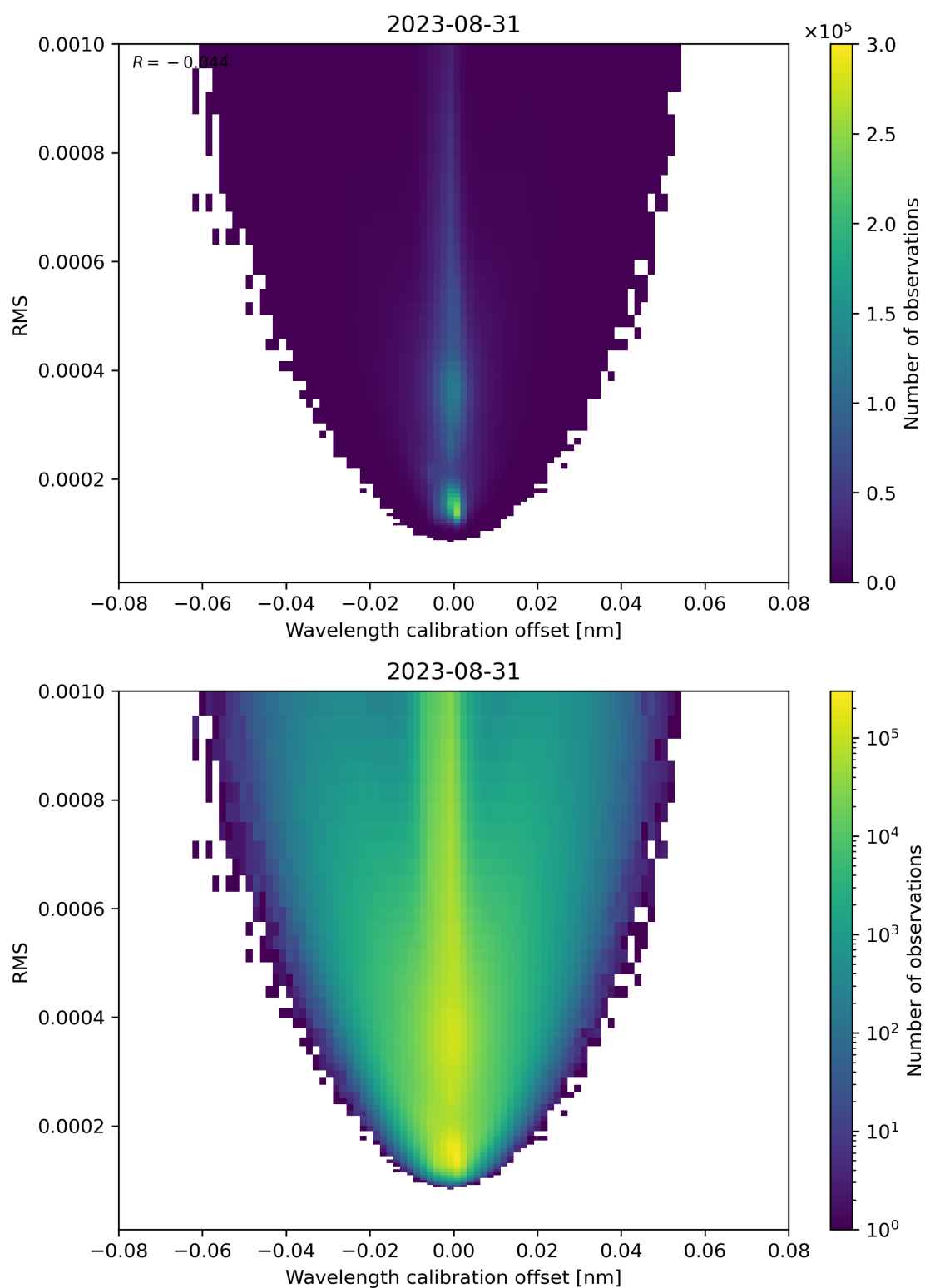
Figure 181: Scatter density plot of “Wavelength calibration offset” against “RMS” for 2023-08-30 to 2023-09-01.
