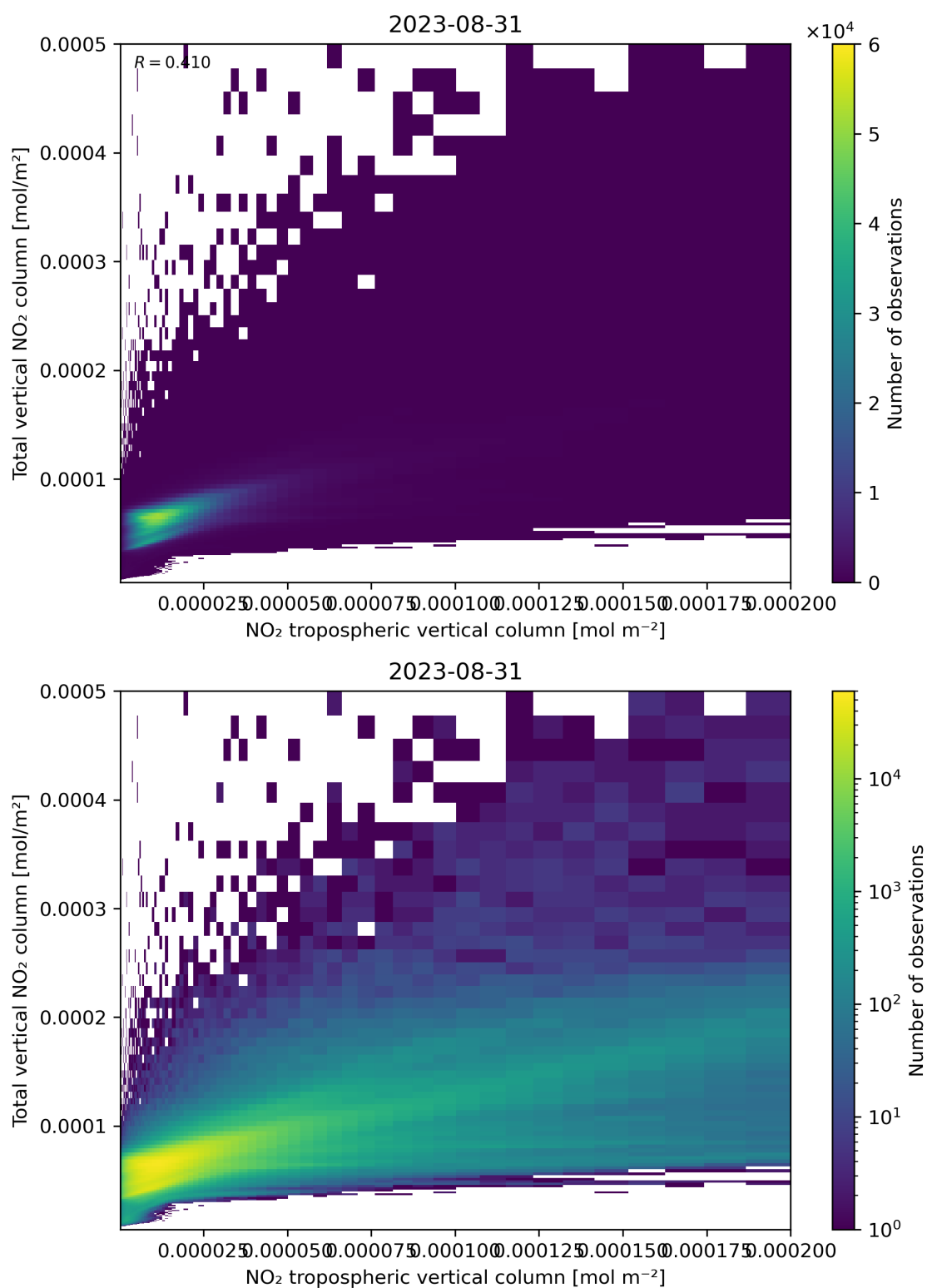
Figure 128: Scatter density plot of “NO 2 tropospheric vertical column” against “Total vertical NO 2 column” for 2023-08-30 to 2023-09-01.
