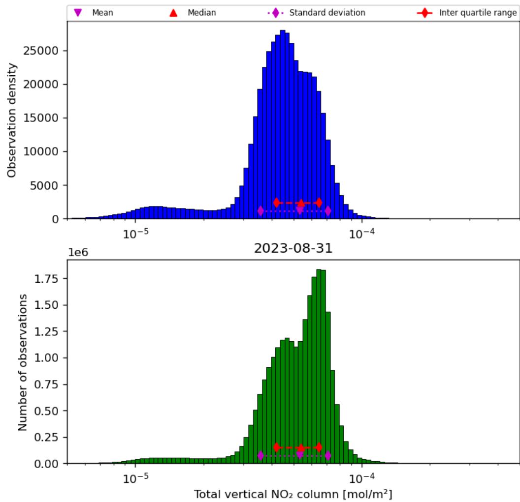
Figure 38: Histogram of “Total vertical NO 2 column” for 2023-08-30 to 2023-09-01
