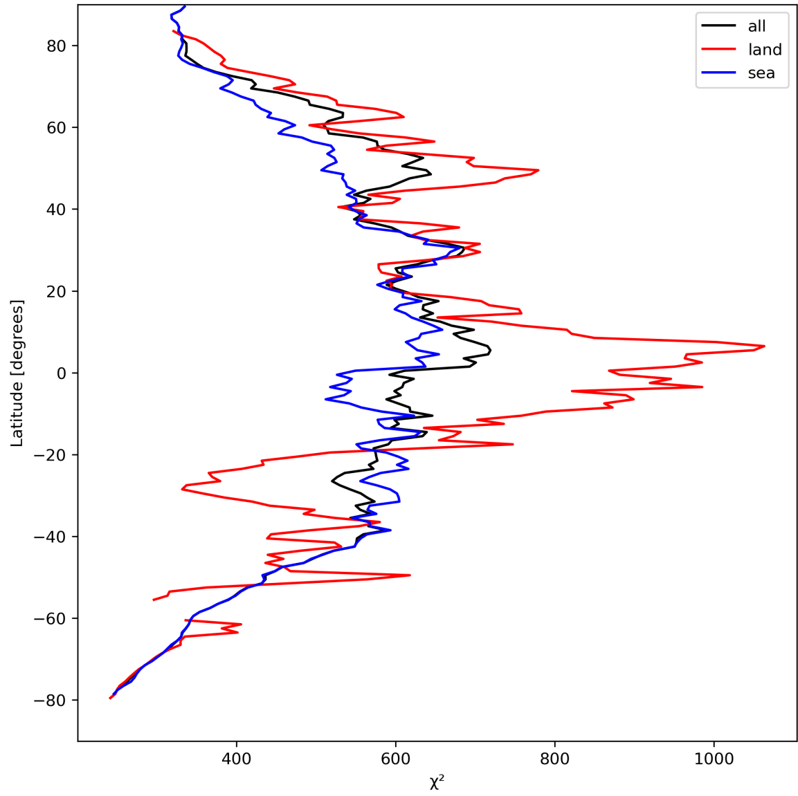
Figure 25: Zonal average of “ \chi^2 ” for 2023-08-30 to 2023-09-01.
