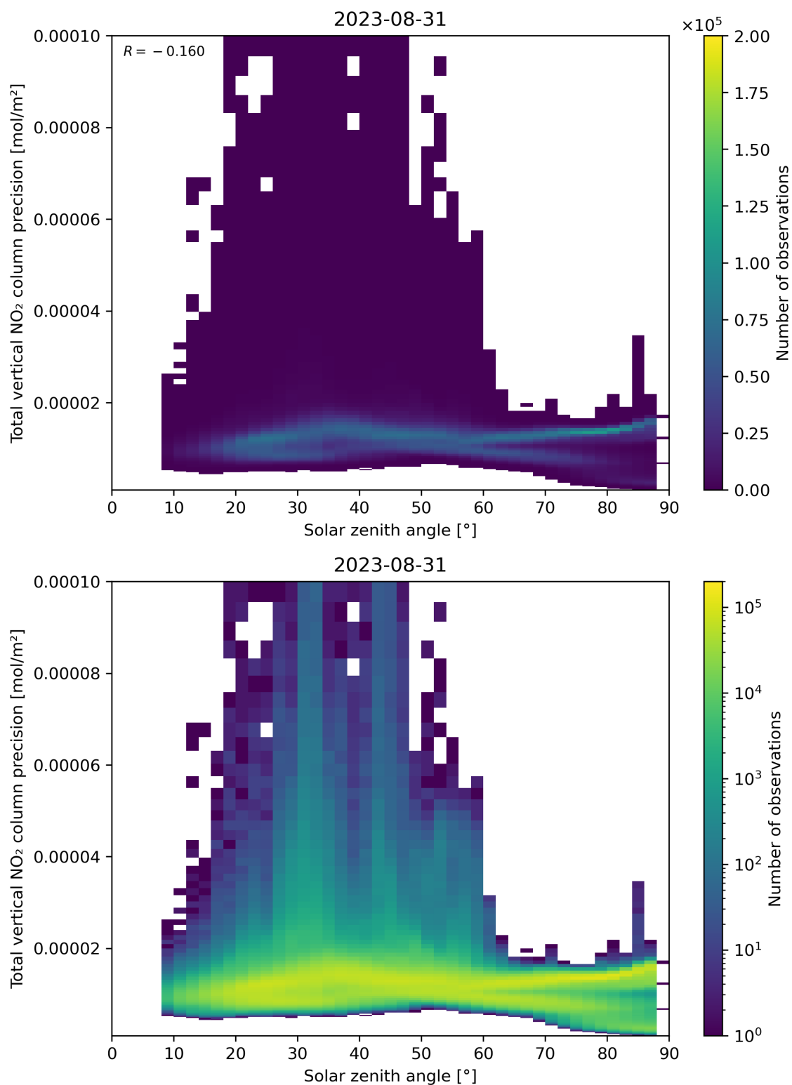
Figure 154: Scatter density plot of “Solar zenith angle” against “Total vertical NO 2 column precision” for 2023-08-30 to 2023-09-01.
