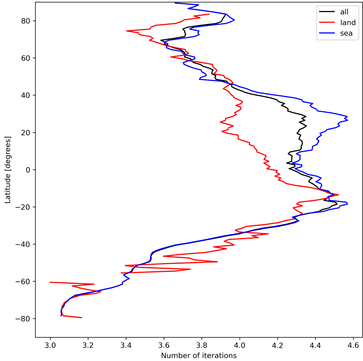
Figure 17: Zonal average of “Number of iterations” for 2023-08-30 to 2023-09-01.
