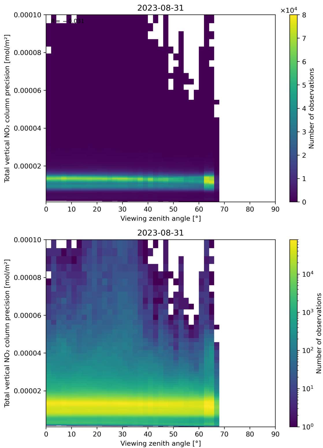
Figure 168: Scatter density plot of “Viewing zenith angle” against “Total vertical NO 2 column precision” for 2023-08-30 to 2023-09-01.
