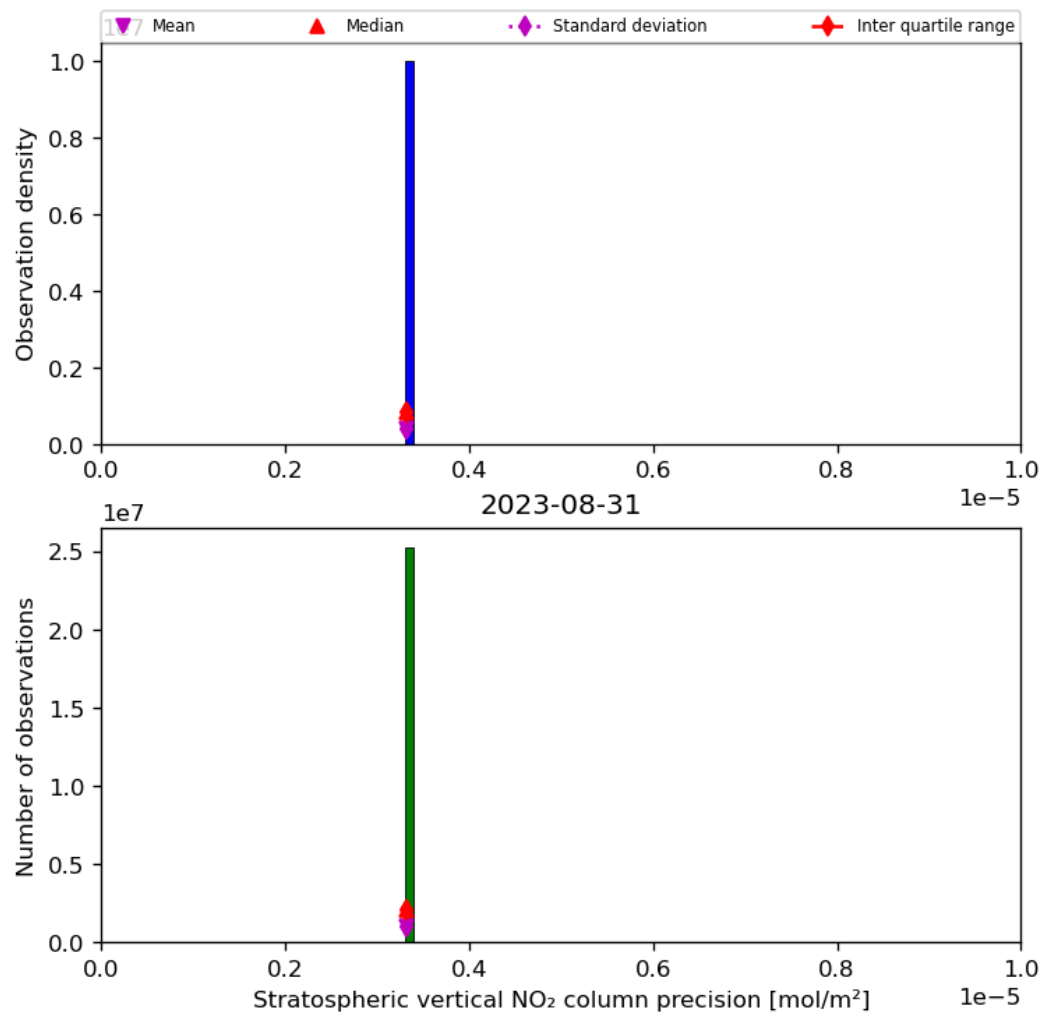
Figure 37: Histogram of “Stratospheric vertical NO 2 column precision” for 2023-08-30 to 2023-09-01
