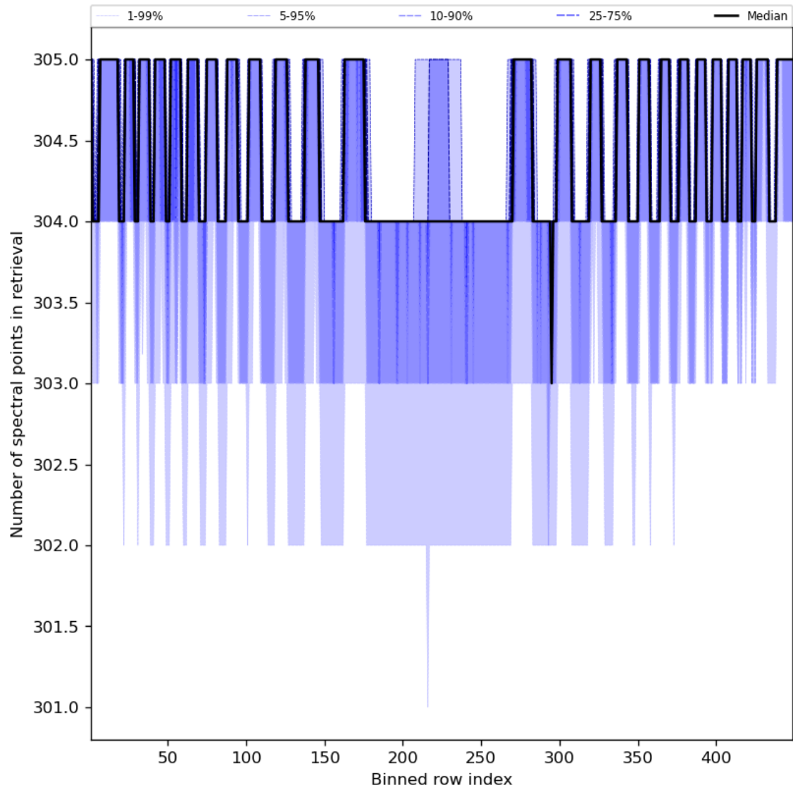
Figure 50: Along track statistics of “Number of spectral points in retrieval” for 2023-08-30 to 2023-09-01
