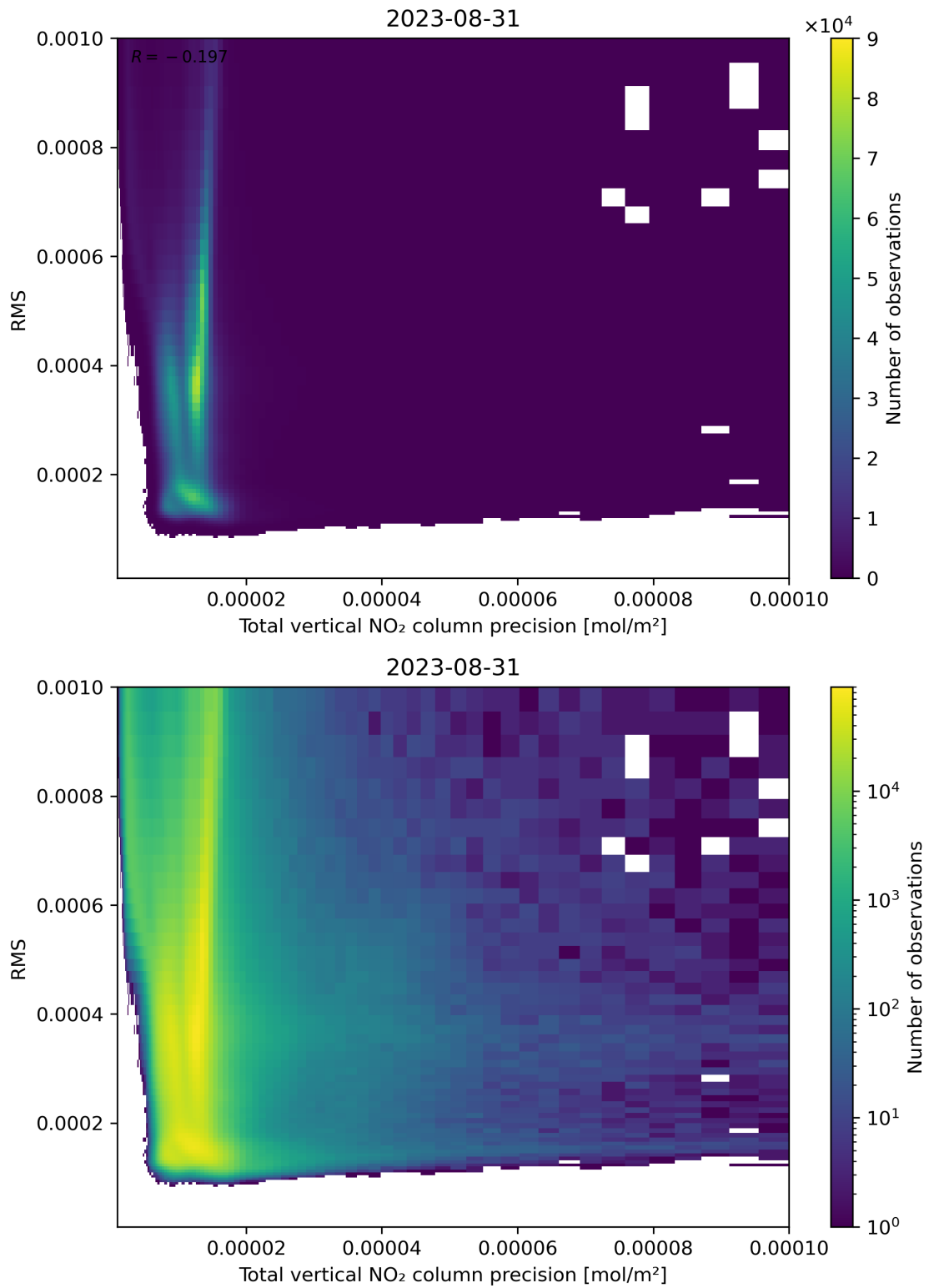
Figure 119: Scatter density plot of “Total vertical NO 2 column precision” against “RMS” for 2023-08-30 to 2023-09-01.
