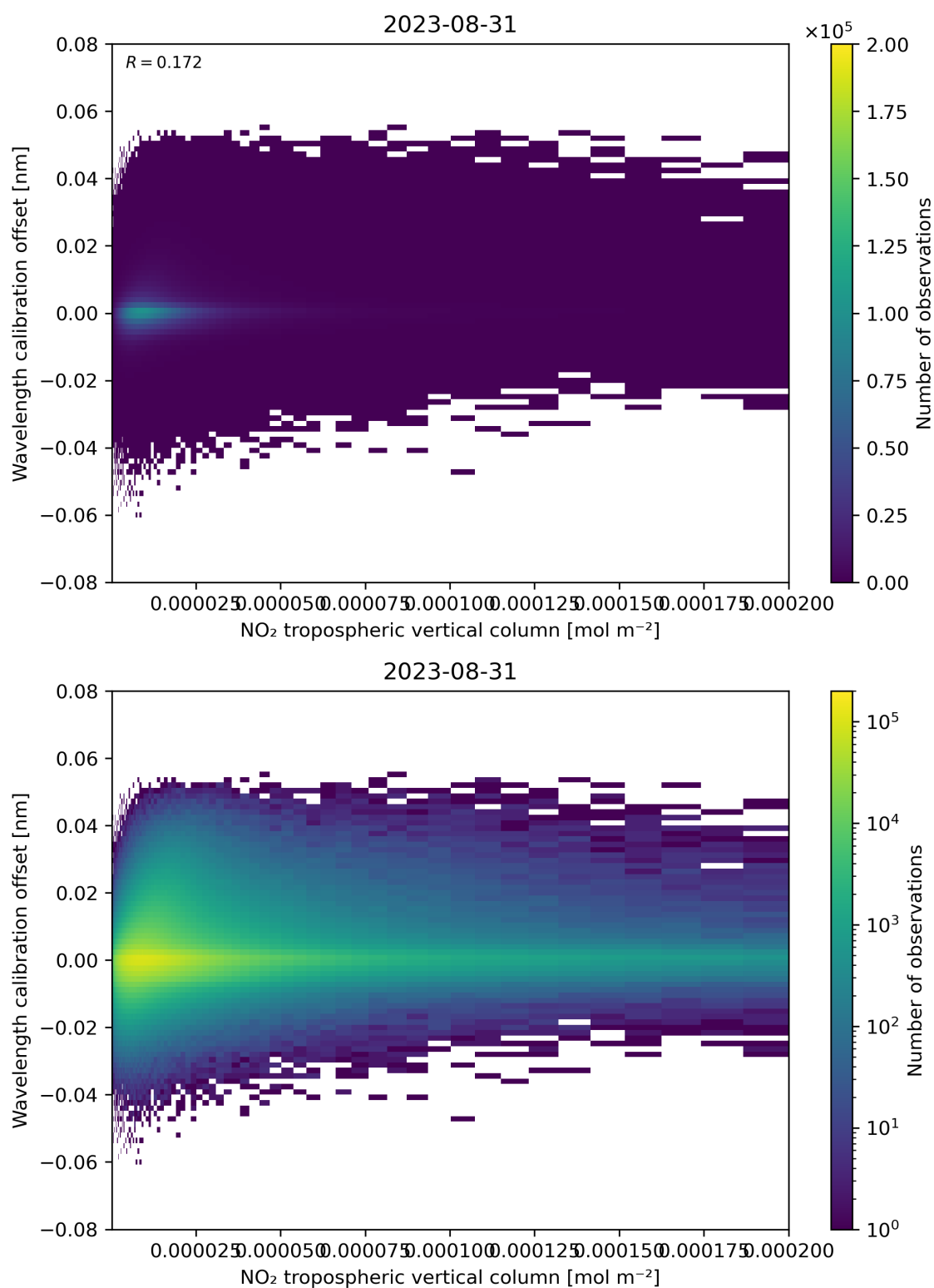
Figure 143: Scatter density plot of “NO 2 tropospheric vertical column” against “Wavelength calibration offset” for 2023-08-30 to 2023-09-01.
