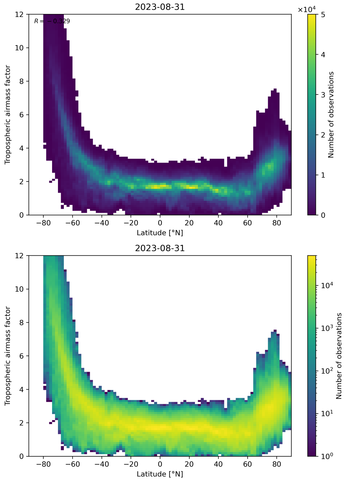
Figure 85: Scatter density plot of “Latitude” against “Tropospheric air mass factor” for 2023-08-30 to 2023-09-01.
