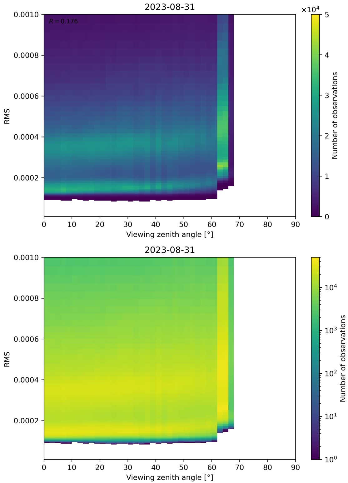
Figure 171: Scatter density plot of “Viewing zenith angle” against “RMS” for 2023-08-30 to 2023-09-01.
