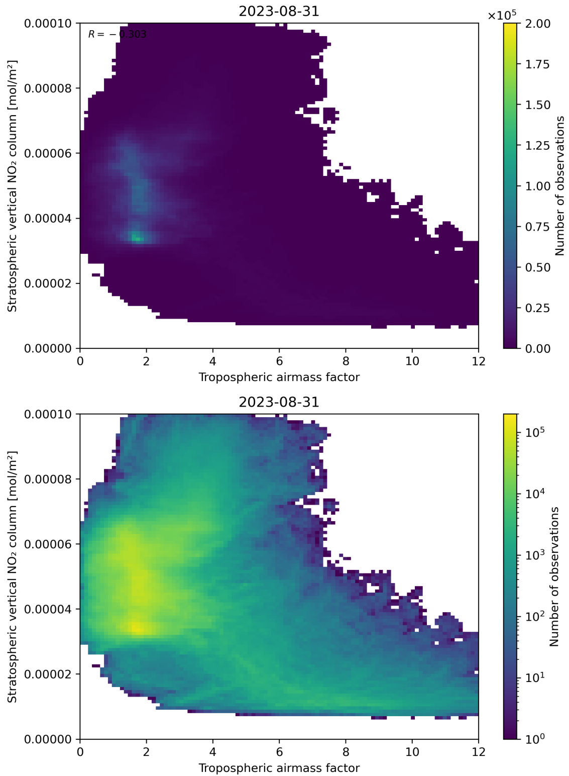
Figure 74: Scatter density plot of “Tropospheric air mass factor” against “Stratospheric vertical NO 2 column” for 2023-08-30 to 2023-09-01.
