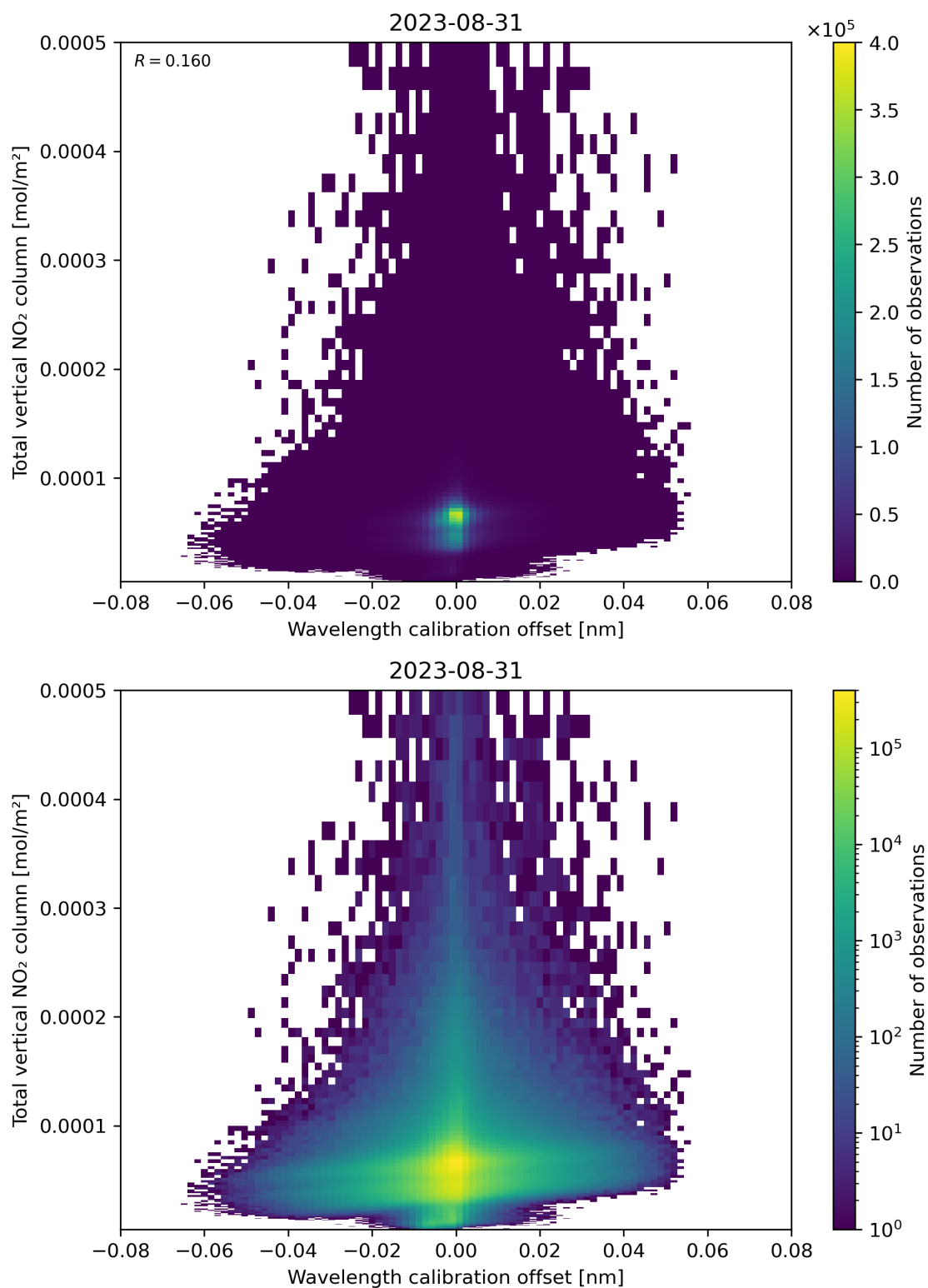
Figure 179: Scatter density plot of “Wavelength calibration offset” against “Total vertical NO 2 column” for 2023-08-30 to 2023-09-01.
