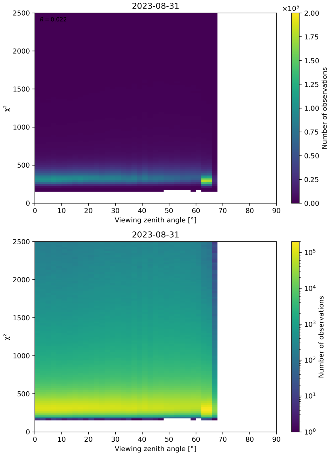
Figure 162: Scatter density plot of “Viewing zenith angle” against “ \chi^2 ” for 2023-08-30 to 2023-09-01.
