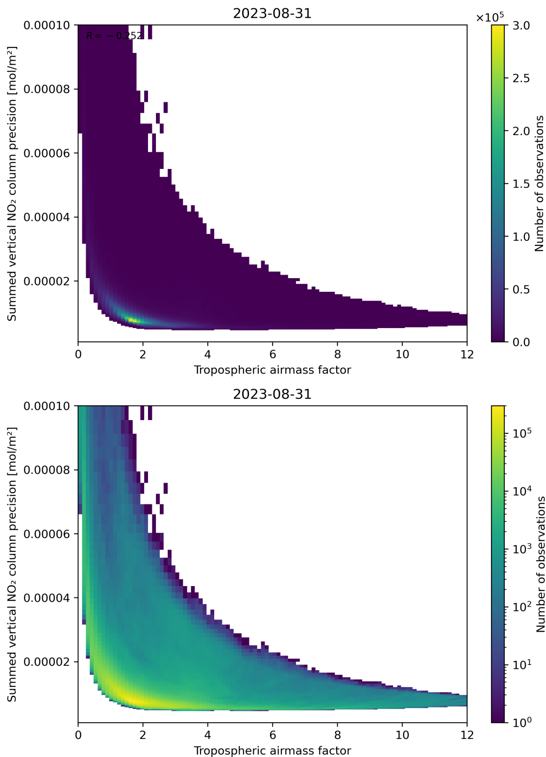
Figure 76: Scatter density plot of “Tropospheric air mass factor” against “Summed vertical NO 2 column precision” for 2023-08-30 to 2023-09-01.
