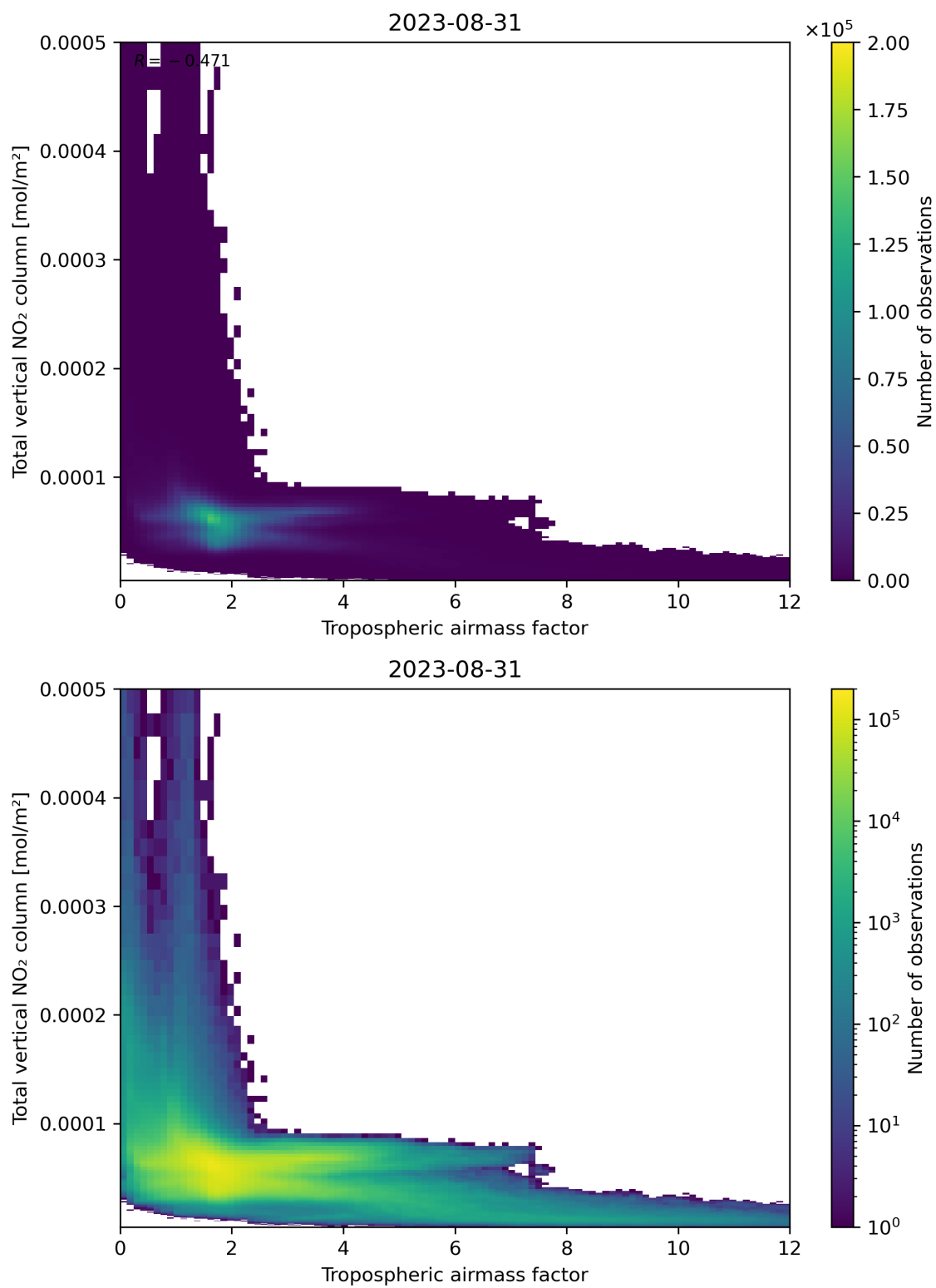
Figure 77: Scatter density plot of “Tropospheric airmass factor” against “Total vertical NO 2 column” for 2023-08-30 to 2023-09-01.
