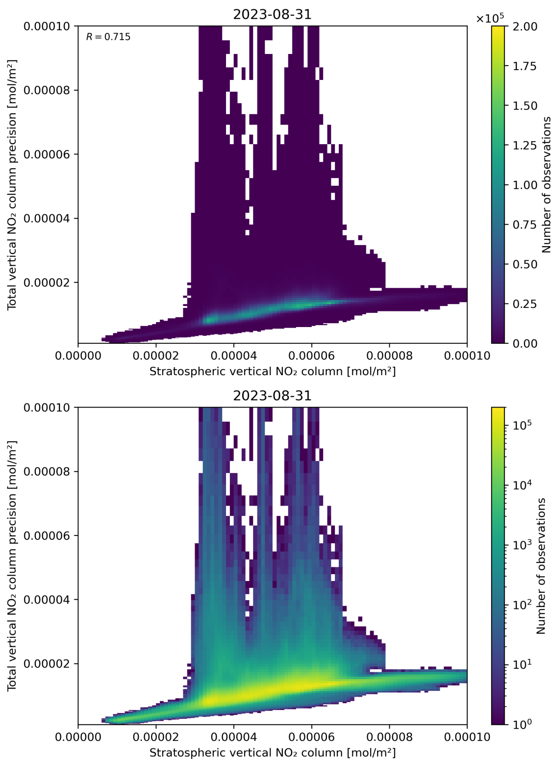
Figure 101: Scatter density plot of “Stratospheric vertical NO 2 column” against “Total vertical NO 2 column precision” for 2023-08-30 to 2023-09-01.
