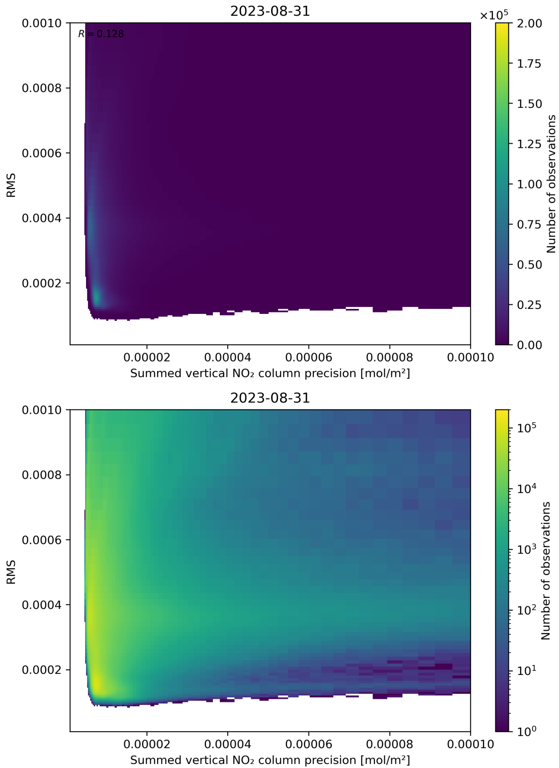
Figure 108: Scatter density plot of “Summed vertical NO 2 column precision” against “RMS” for 2023-08-30 to 2023-09-01.
