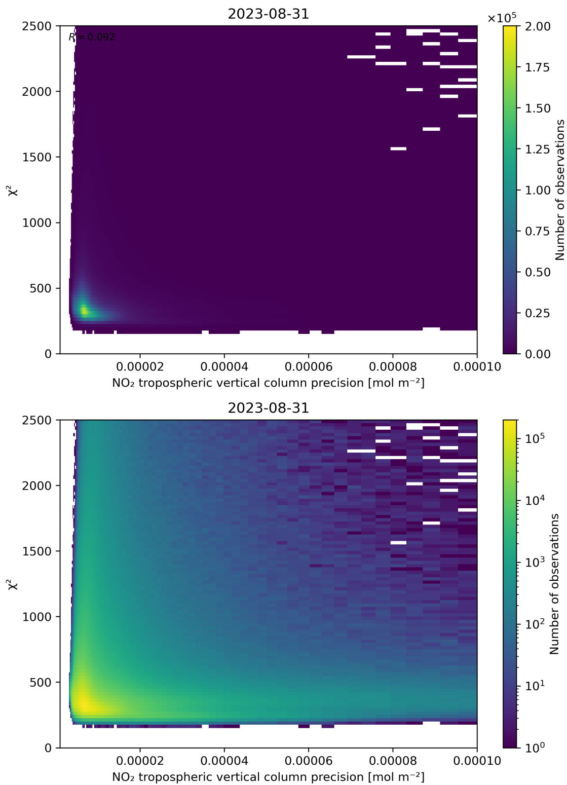
Figure 134: Scatter density plot of “NO 2 tropospheric vertical column precision” against “ \chi^2 ” for 2023-08-30 to 2023-09-01.
