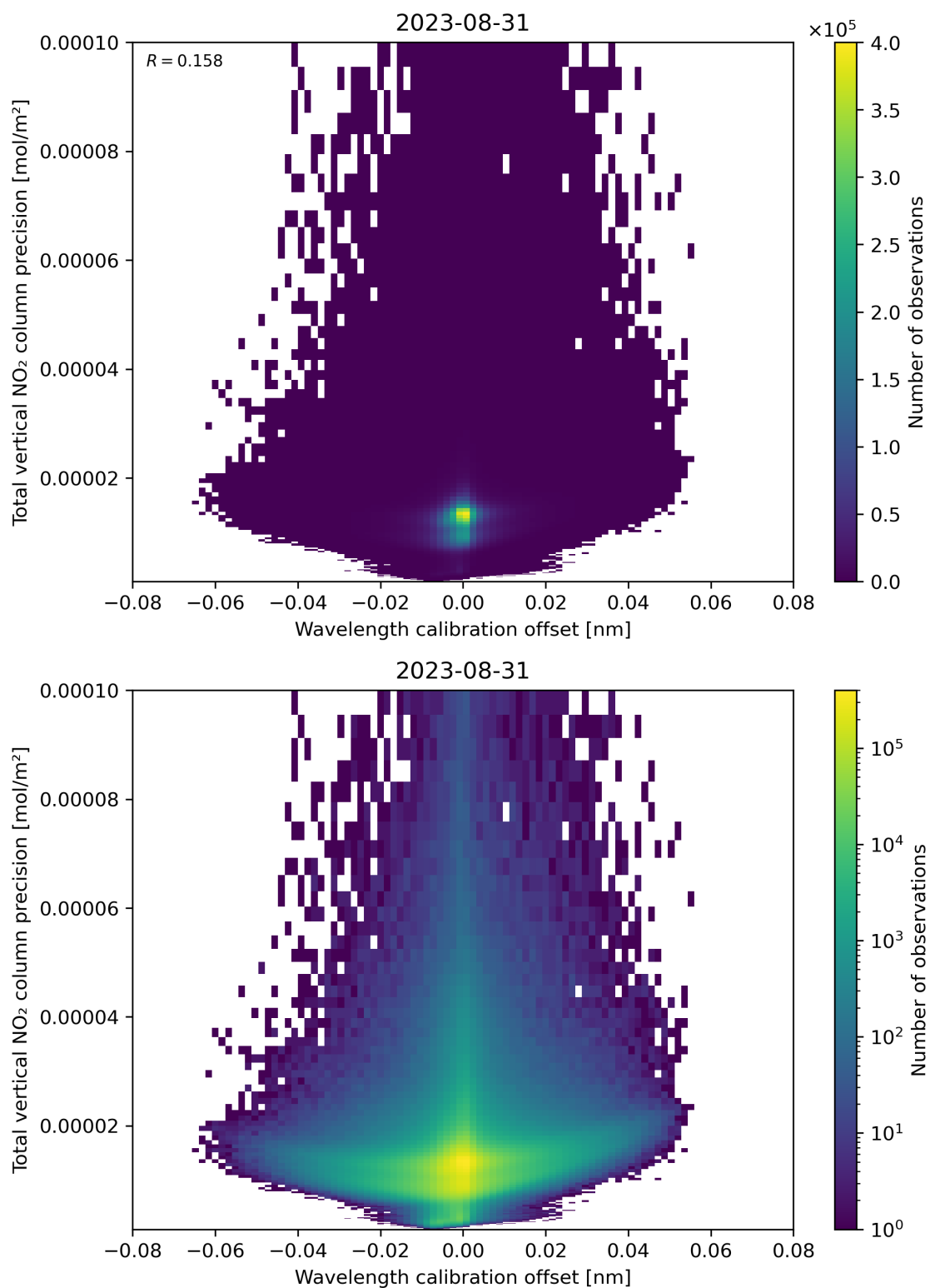
Figure 180: Scatter density plot of “Wavelength calibration offset” against “Total vertical NO 2 column precision” for 2023-08-30 to 2023-09-01.
