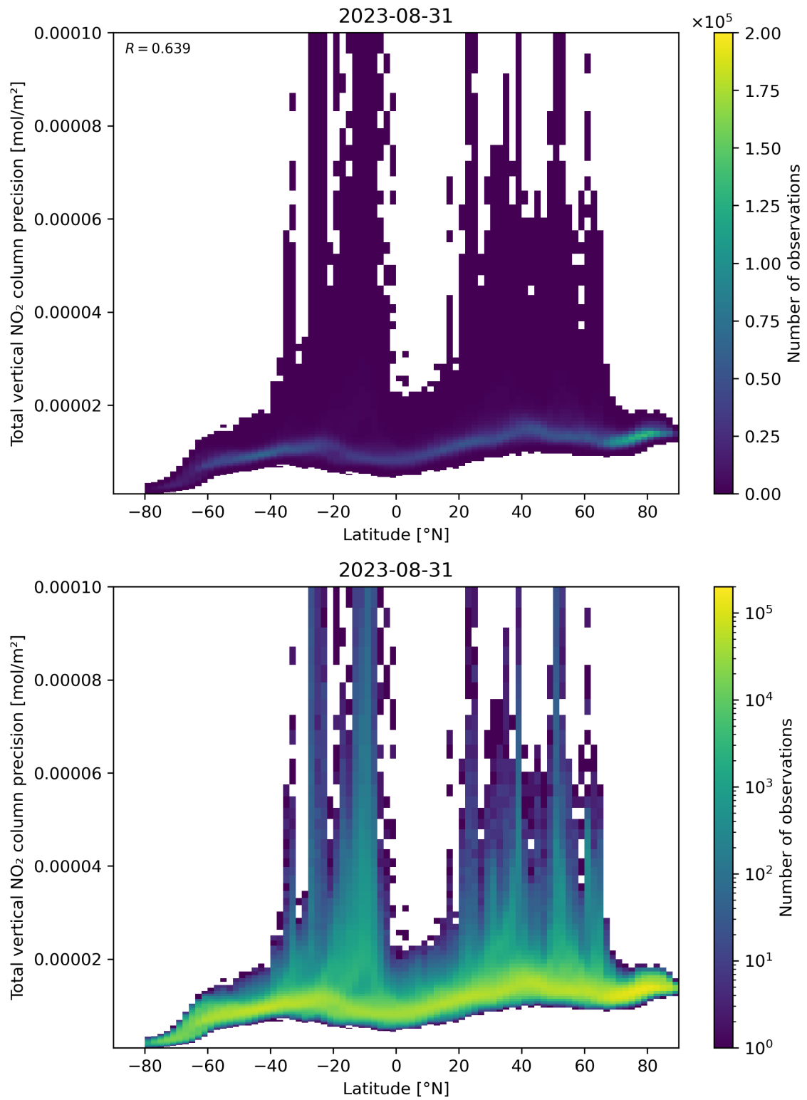
Figure 91: Scatter density plot of “Latitude” against “Total vertical NO 2 column precision” for 2023-08-30 to 2023-09-01.
