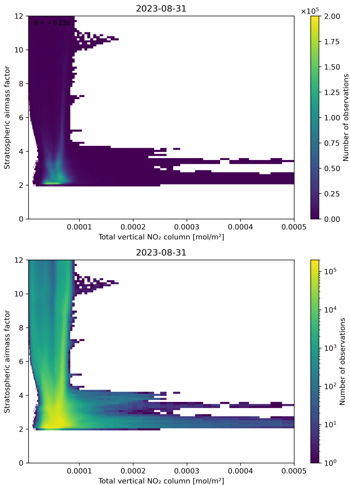
Figure 110: Scatter density plot of “Total vertical NO 2 column” against “Stratospheric airmass factor” for 2023-08-30 to 2023-09-01.
