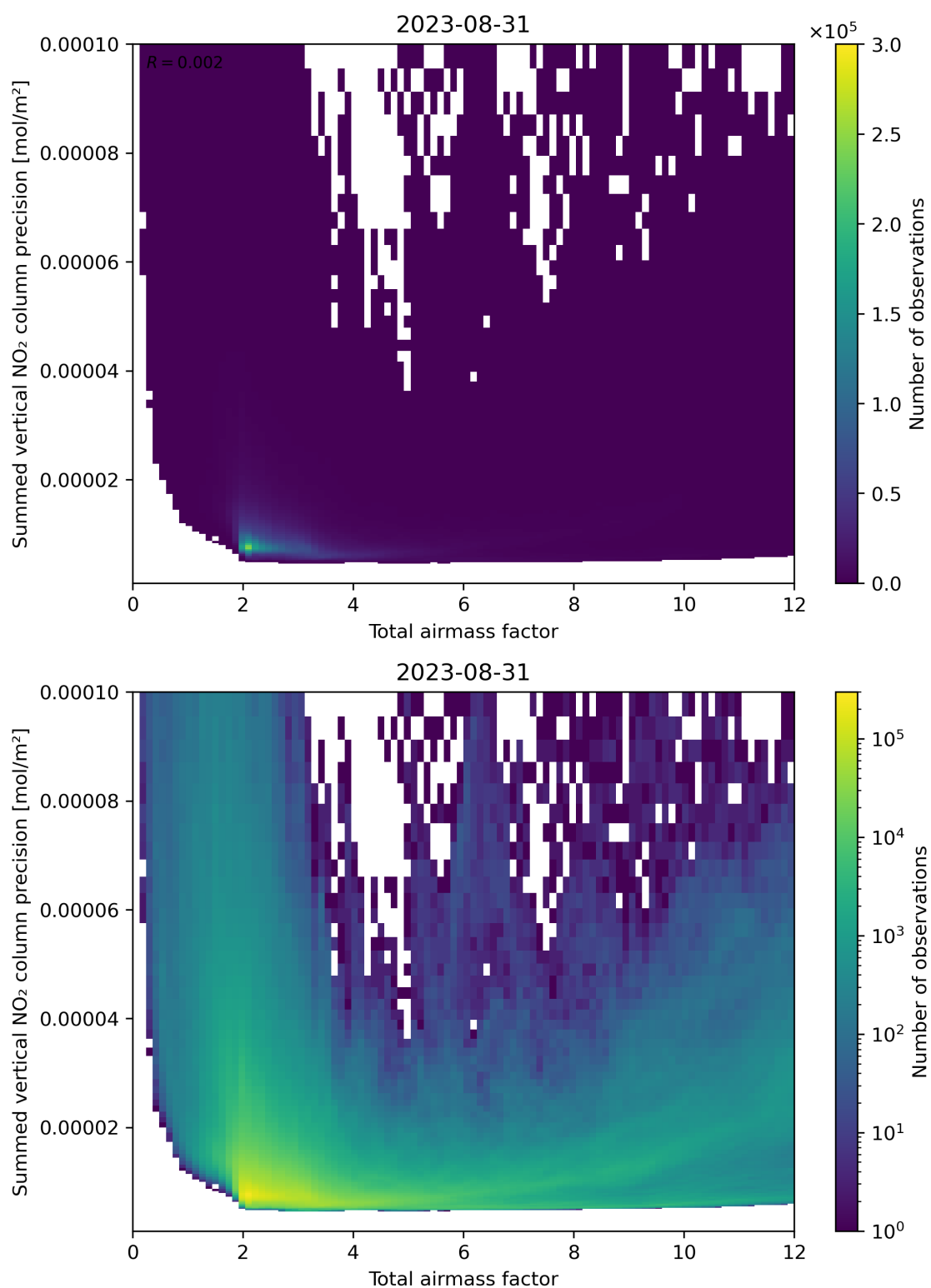
Figure 66: Scatter density plot of “Total airmass factor” against “Summed vertical NO 2 column precision” for 2023-08-30 to 2023-09-01.
