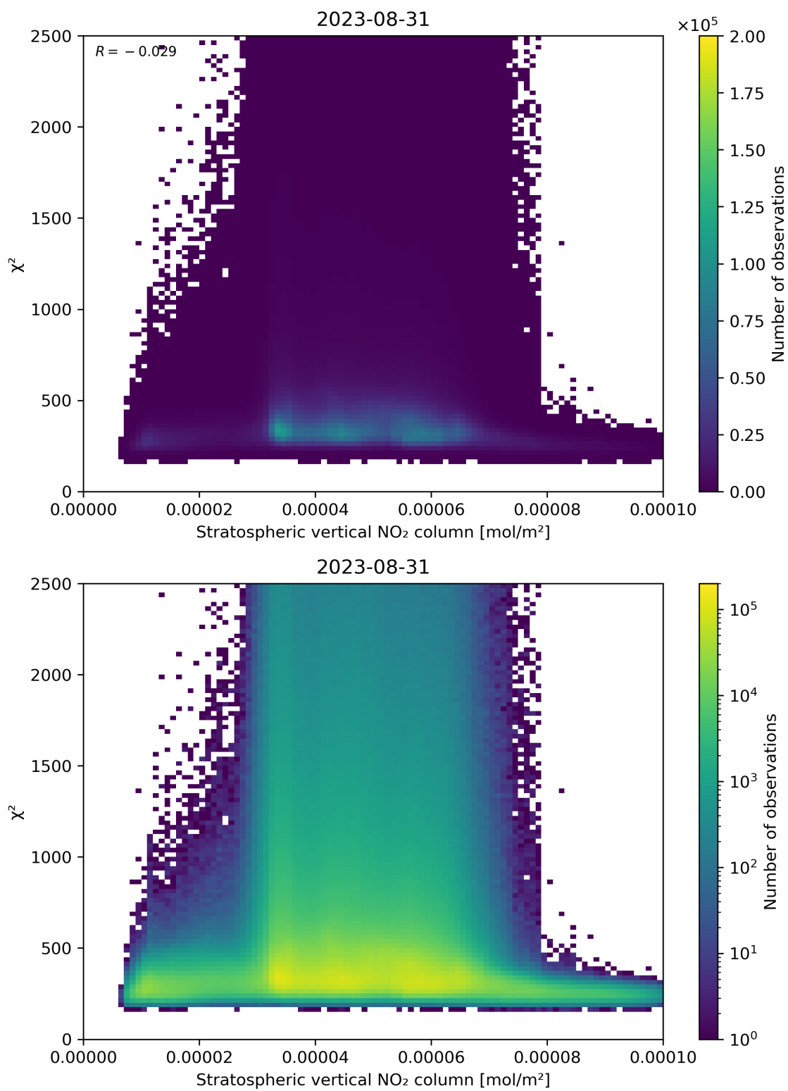
Figure 97: Scatter density plot of “Stratospheric vertical NO 2 column” against “ \chi^2 ” for 2023-08-30 to 2023-09-01.
