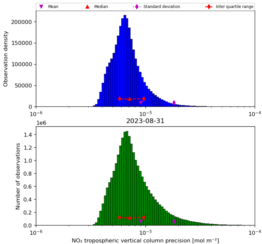
Figure 30: Histogram of “NO 2 tropospheric vertical column precision” for 2023-08-30 to 2023-09-01
