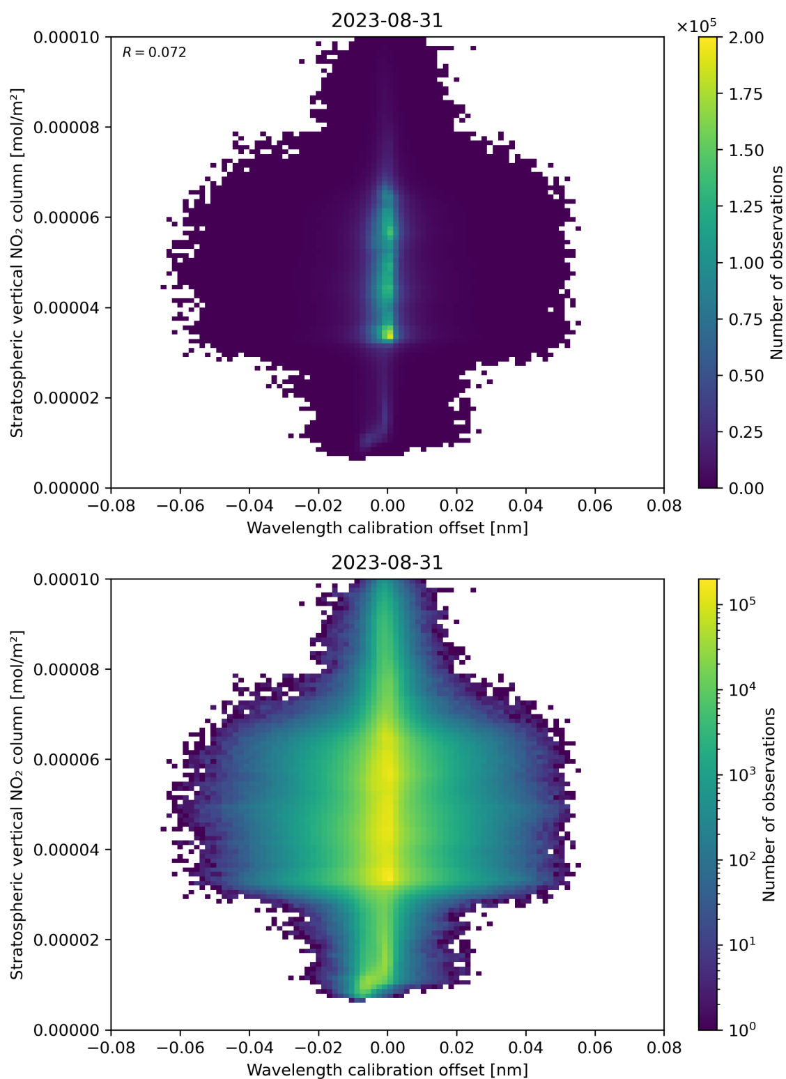
Figure 176: Scatter density plot of “Wavelength calibration offset” against “Stratospheric vertical NO 2 column” for 2023-08-30 to 2023-09-01.
