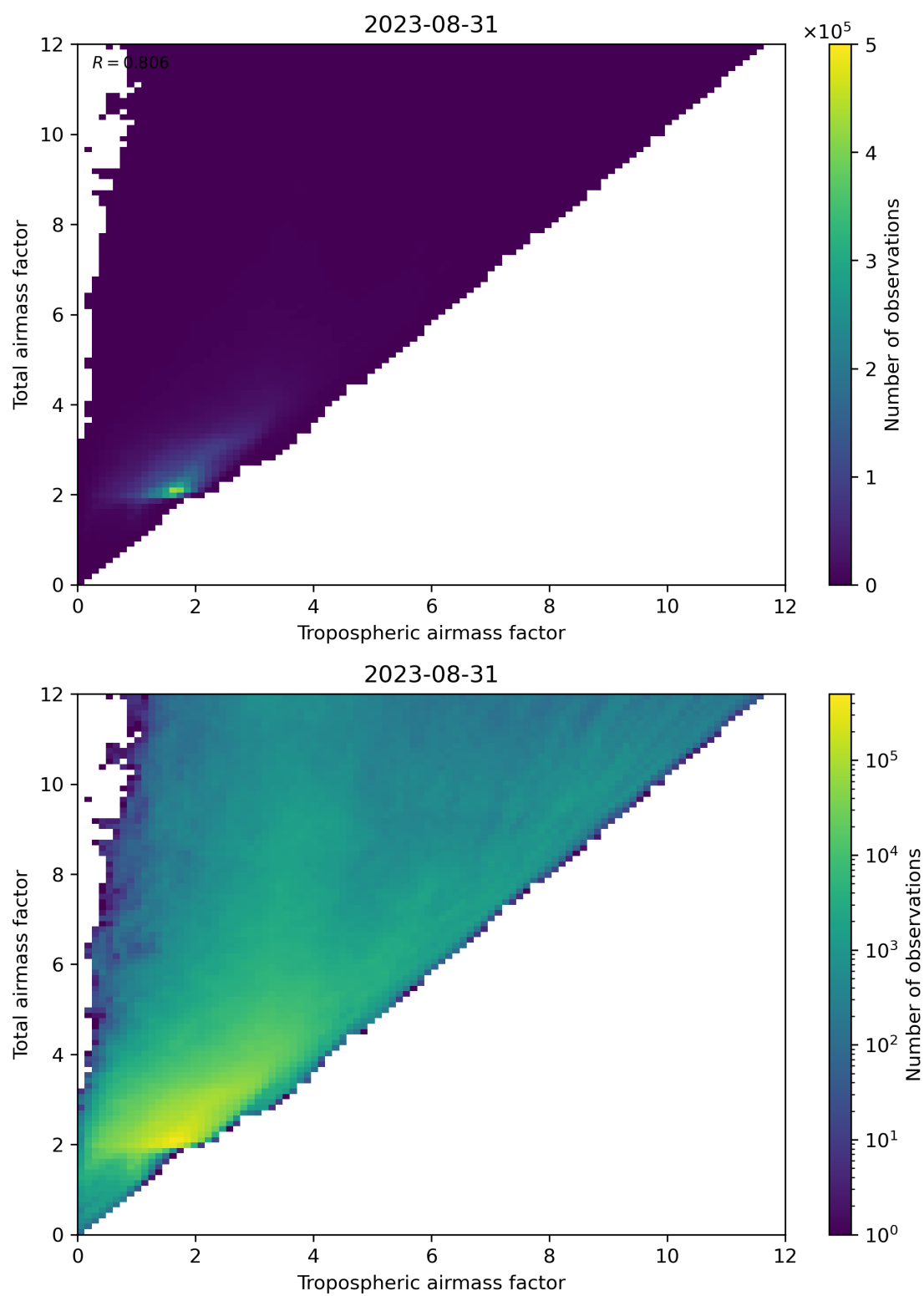
Figure 72: Scatter density plot of “Tropospheric airmass factor” against “Total airmass factor” for 2023-08-30 to 2023-09-01.
