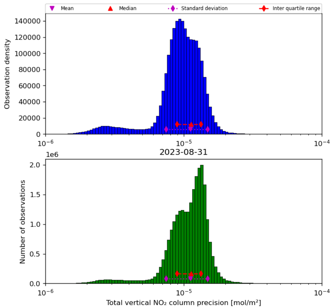
Figure 39: Histogram of “Total vertical NO 2 column precision” for 2023-08-30 to 2023-09-01
