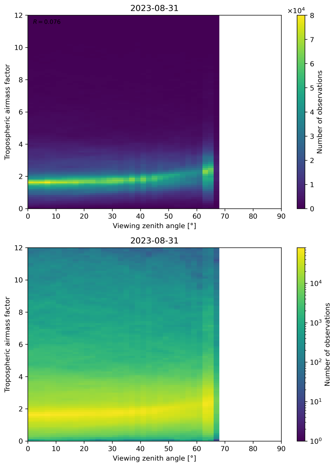
Figure 161: Scatter density plot of “Viewing zenith angle” against “Tropospheric airmass factor” for 2023-08-30 to 2023-09-01.
