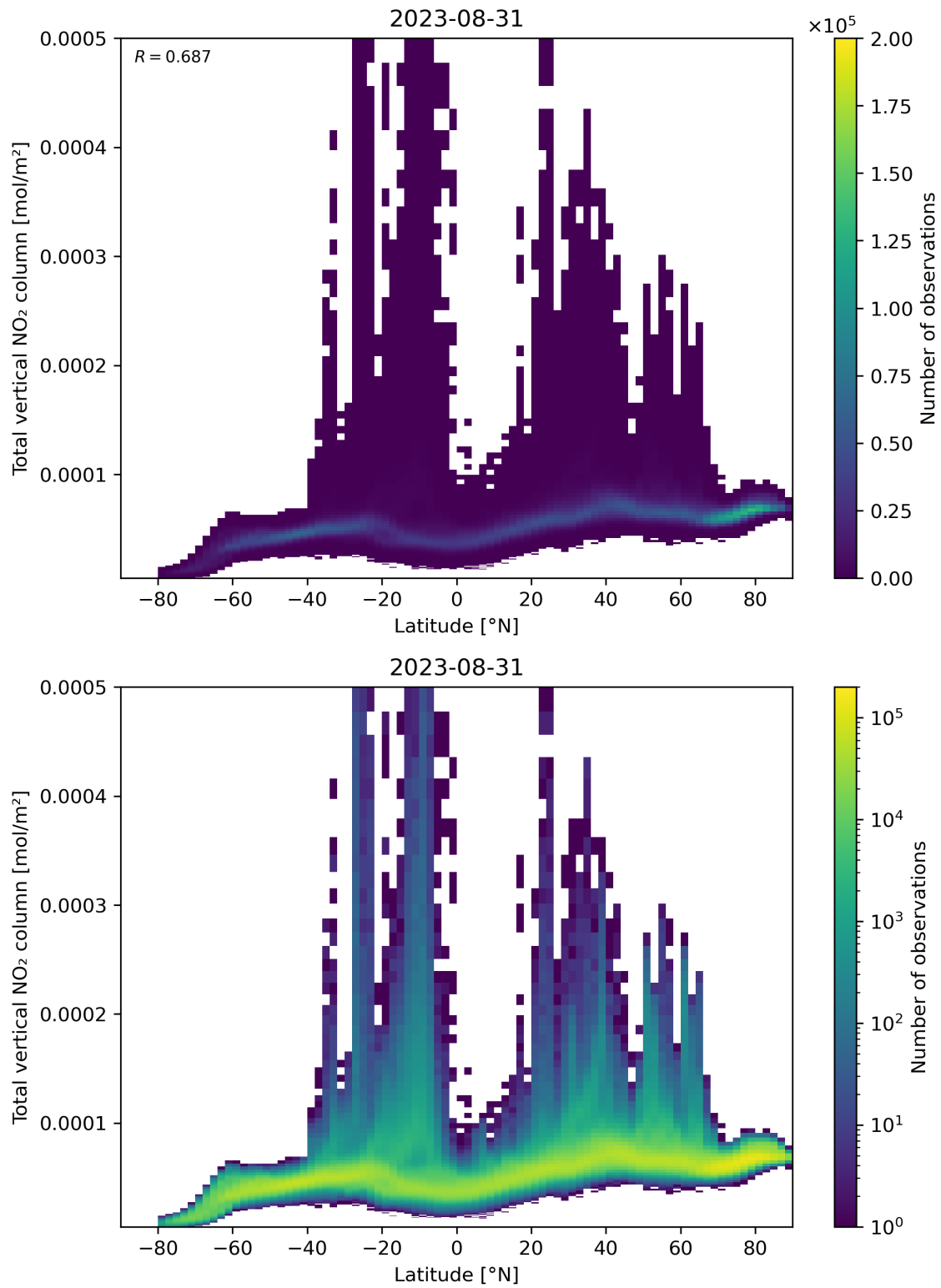
Figure 90: Scatter density plot of “Latitude” against “Total vertical NO 2 column” for 2023-08-30 to 2023-09-01.
