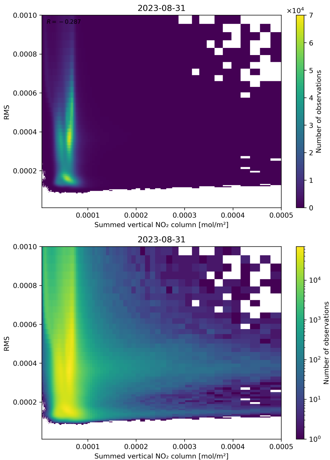
Figure 109: Scatter density plot of “Summed vertical NO 2 column” against “RMS” for 2023-08-30 to 2023-09-01.
