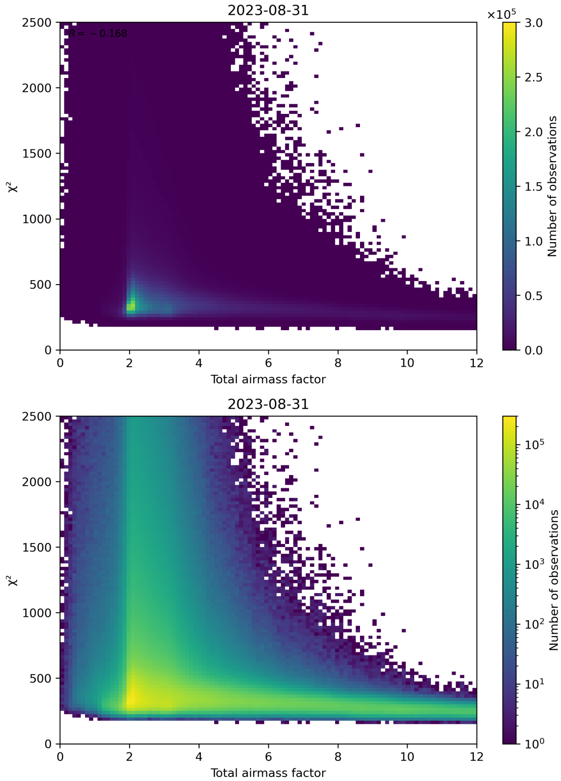
Figure 63: Scatter density plot of “Total airmass factor” against “ \chi^2 ” for 2023-08-30 to 2023-09-01.
