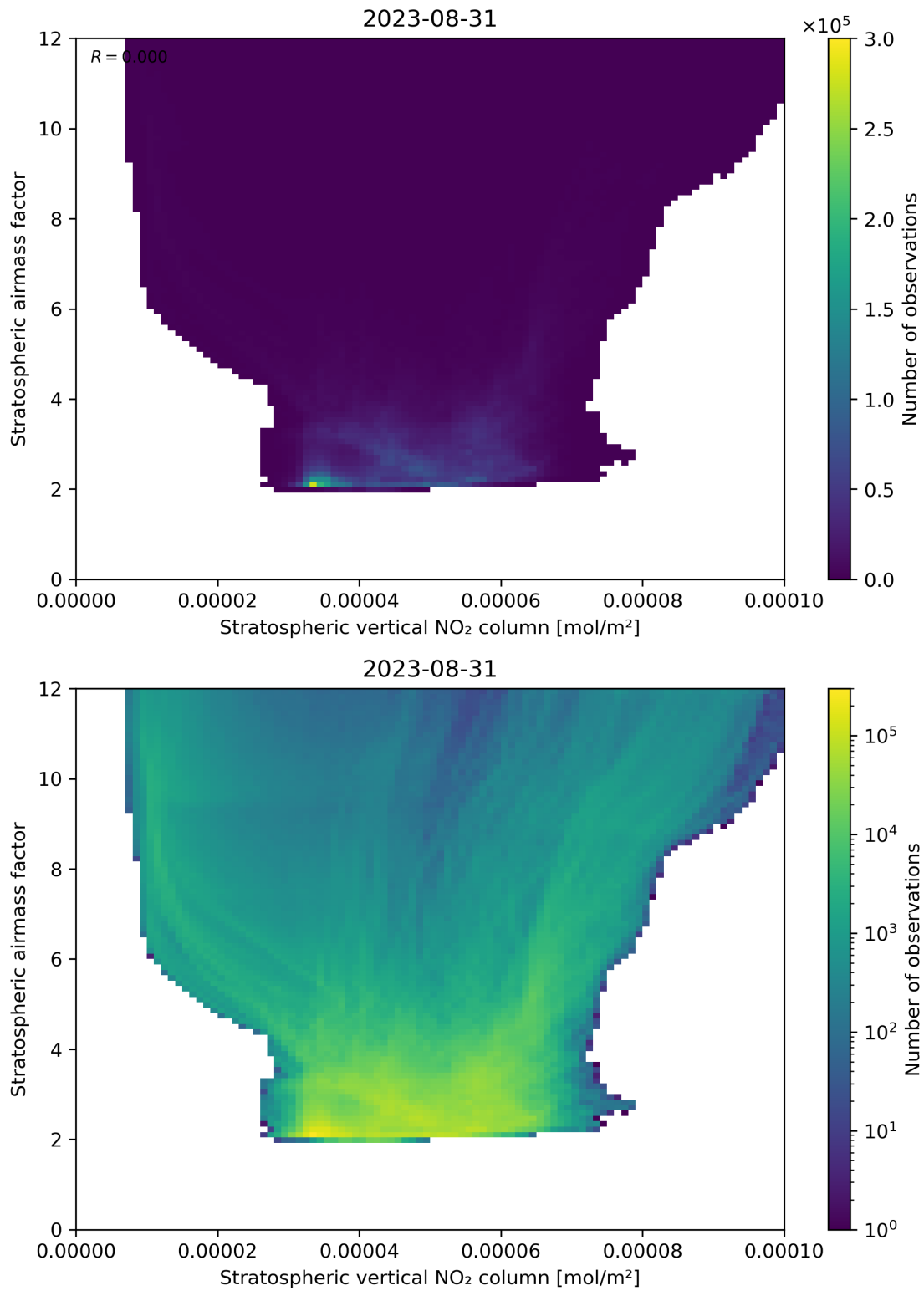
Figure 96: Scatter density plot of “Stratospheric vertical NO 2 column” against “Stratospheric airmass factor” for 2023-08-30 to 2023-09-01.
