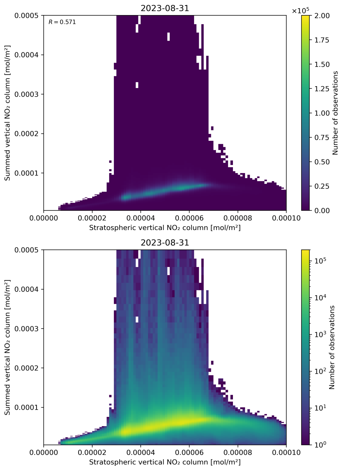
Figure 98: Scatter density plot of “Stratospheric vertical NO 2 column” against “Summed vertical NO 2 column” for 2023-08-30 to 2023-09-01.
