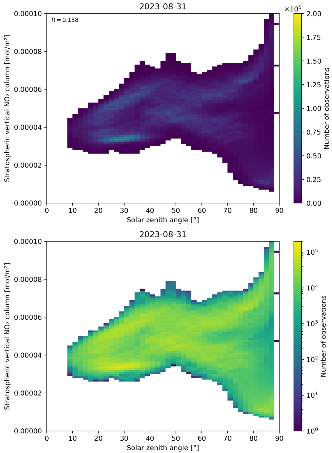
Figure 150: Scatter density plot of “Solar zenith angle” against “Stratospheric vertical NO 2 column” for 2023-08-30 to 2023-09-01.
