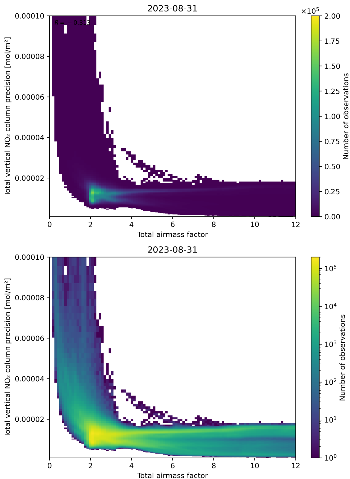
Figure 68: Scatter density plot of “Total airmass factor” against “Total vertical NO 2 column precision” for 2023-08-30 to 2023-09-01.
