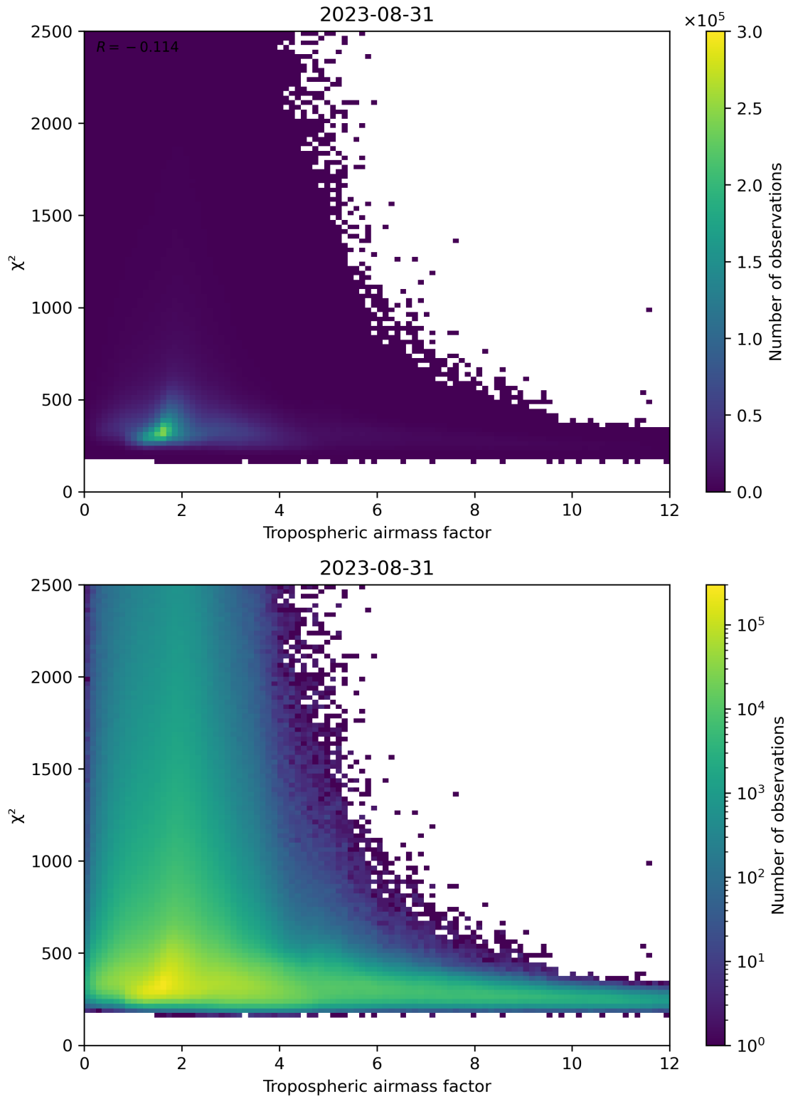
Figure 73: Scatter density plot of “Tropospheric airmass factor” against “ \chi^2 ” for 2023-08-30 to 2023-09-01.
