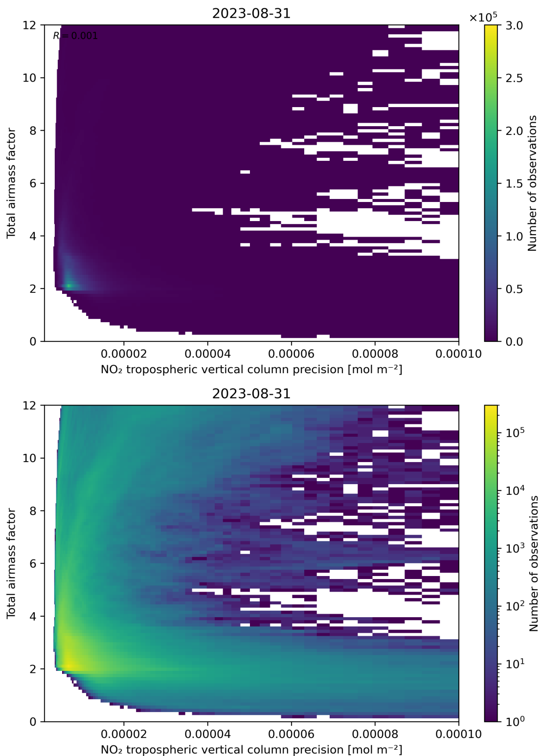
Figure 132: Scatter density plot of “NO 2 tropospheric vertical column precision” against “Total air mass factor” for 2023-08-30 to 2023-09-01.
