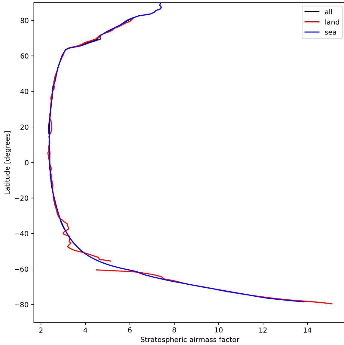
Figure 27: Zonal average of “Stratospheric airmass factor” for 2023-08-30 to 2023-09-01.
