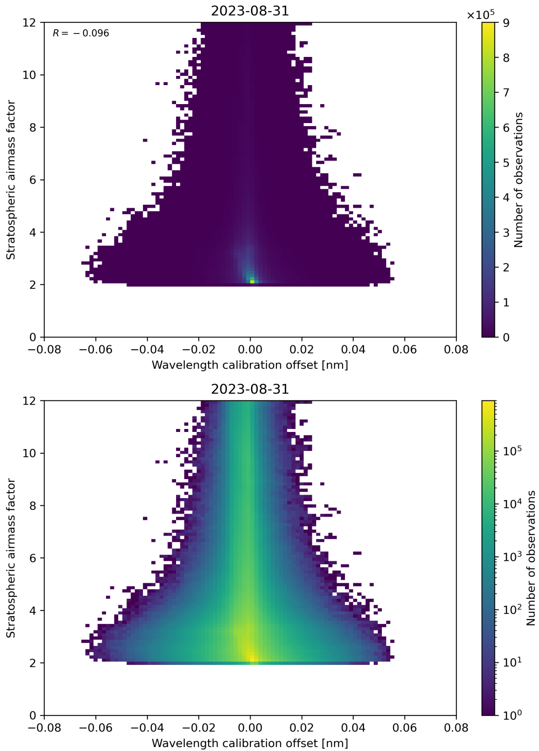
Figure 174: Scatter density plot of “Wavelength calibration offset” against “Stratospheric airmass factor” for 2023-08-30 to 2023-09-01.
