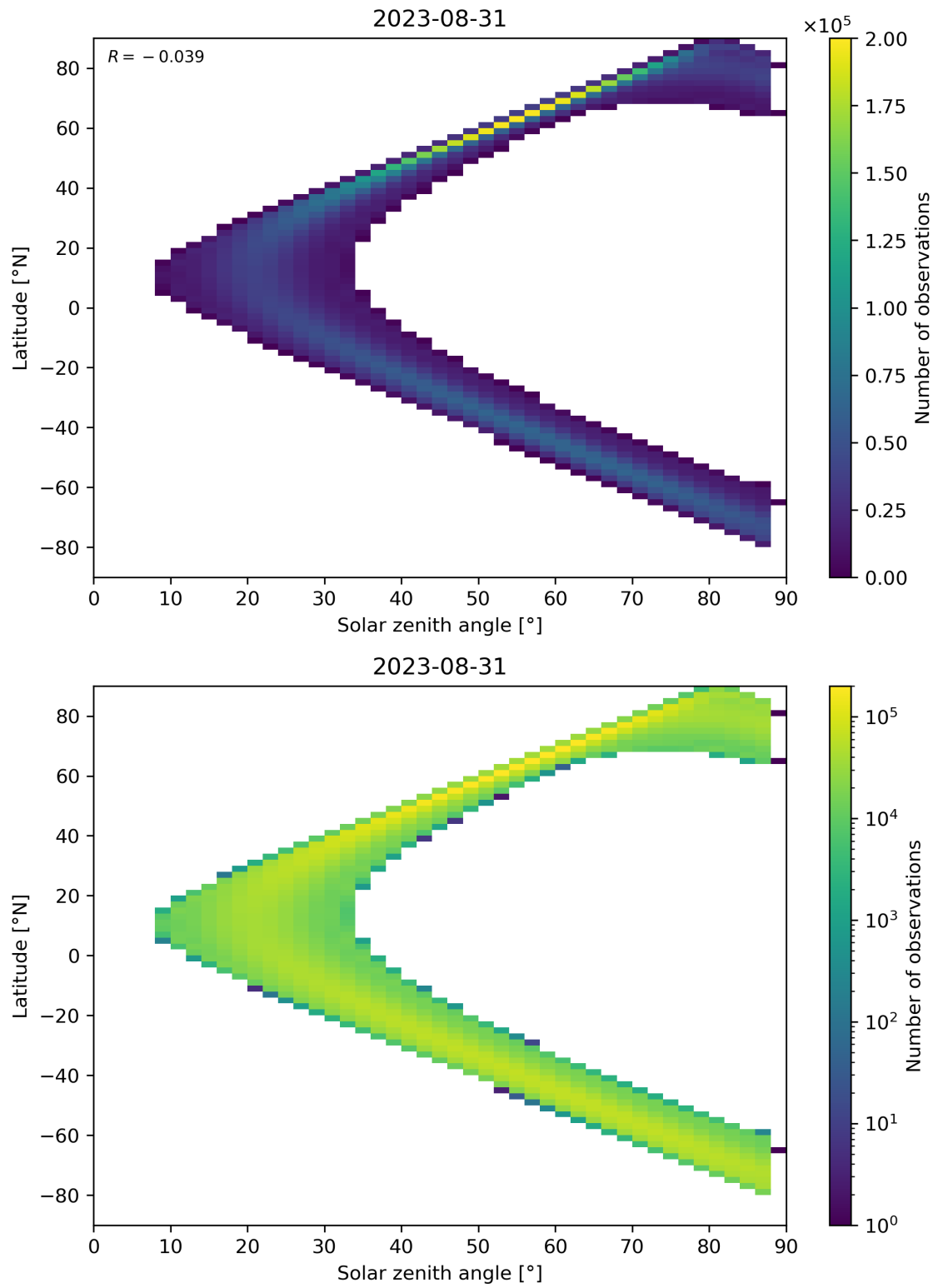
Figure 149: Scatter density plot of “Solar zenith angle” against “Latitude” for 2023-08-30 to 2023-09-01.
