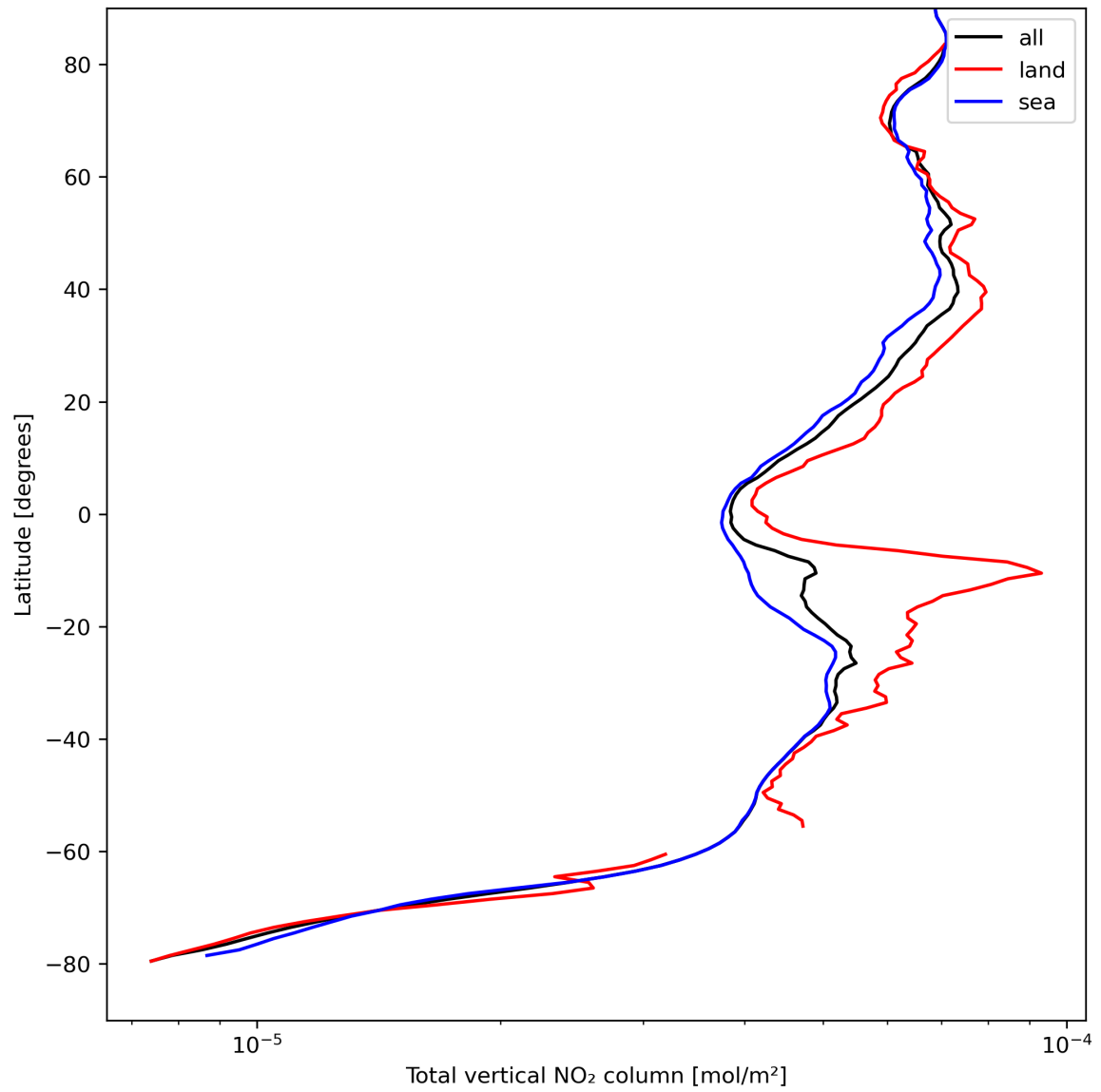
Figure 21: Zonal average of “Total vertical NO 2 column” for 2023-08-30 to 2023-09-01.
