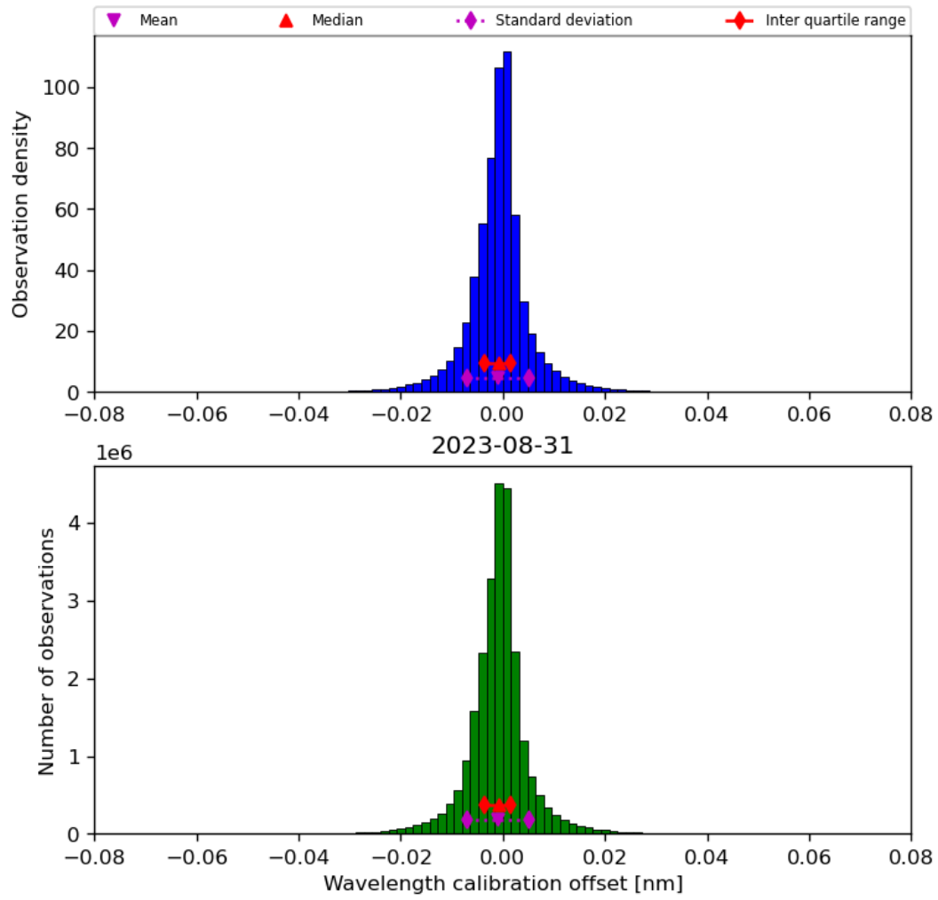
Figure 35: Histogram of “Wavelength calibration offset” for 2023-08-30 to 2023-09-01
