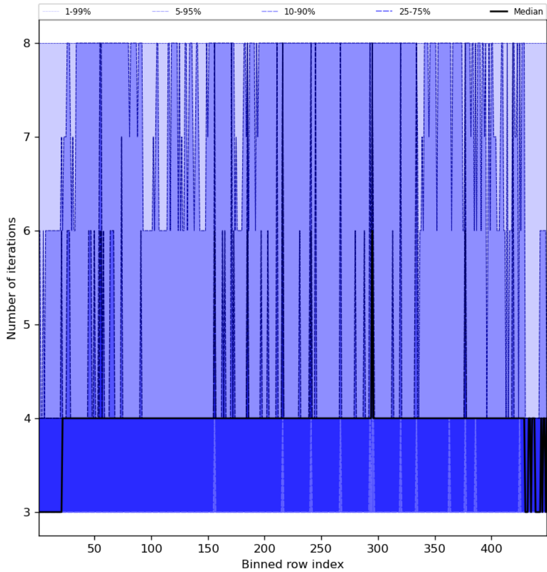
Figure 51: Along track statistics of “Number of iterations” for 2023-08-30 to 2023-09-01
