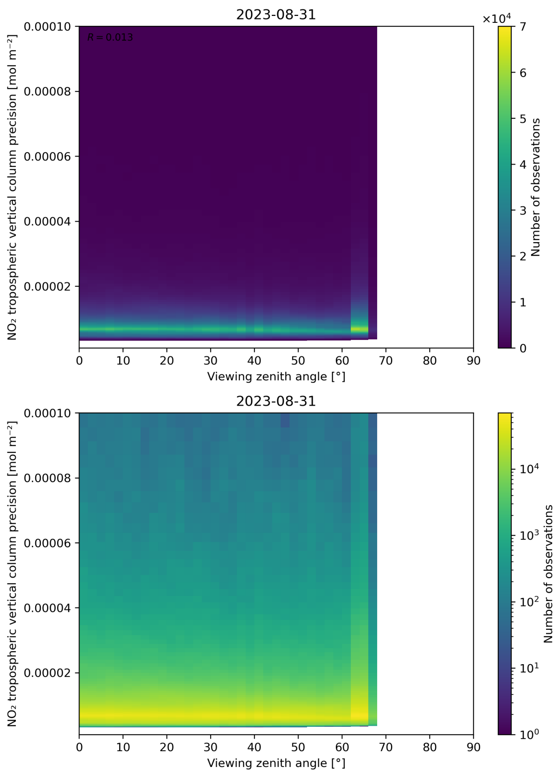
Figure 170: Scatter density plot of “Viewing zenith angle” against “NO 2 tropospheric vertical column precision” for 2023-08-30 to 2023-09-01.
