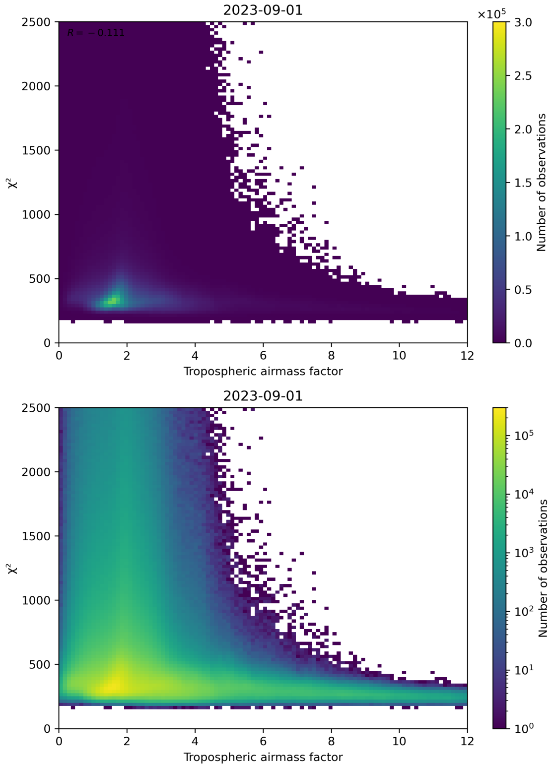
Figure 73: Scatter density plot of “Tropospheric airmass factor” against “ \chi^2 ” for 2023-08-31 to 2023-09-02.
