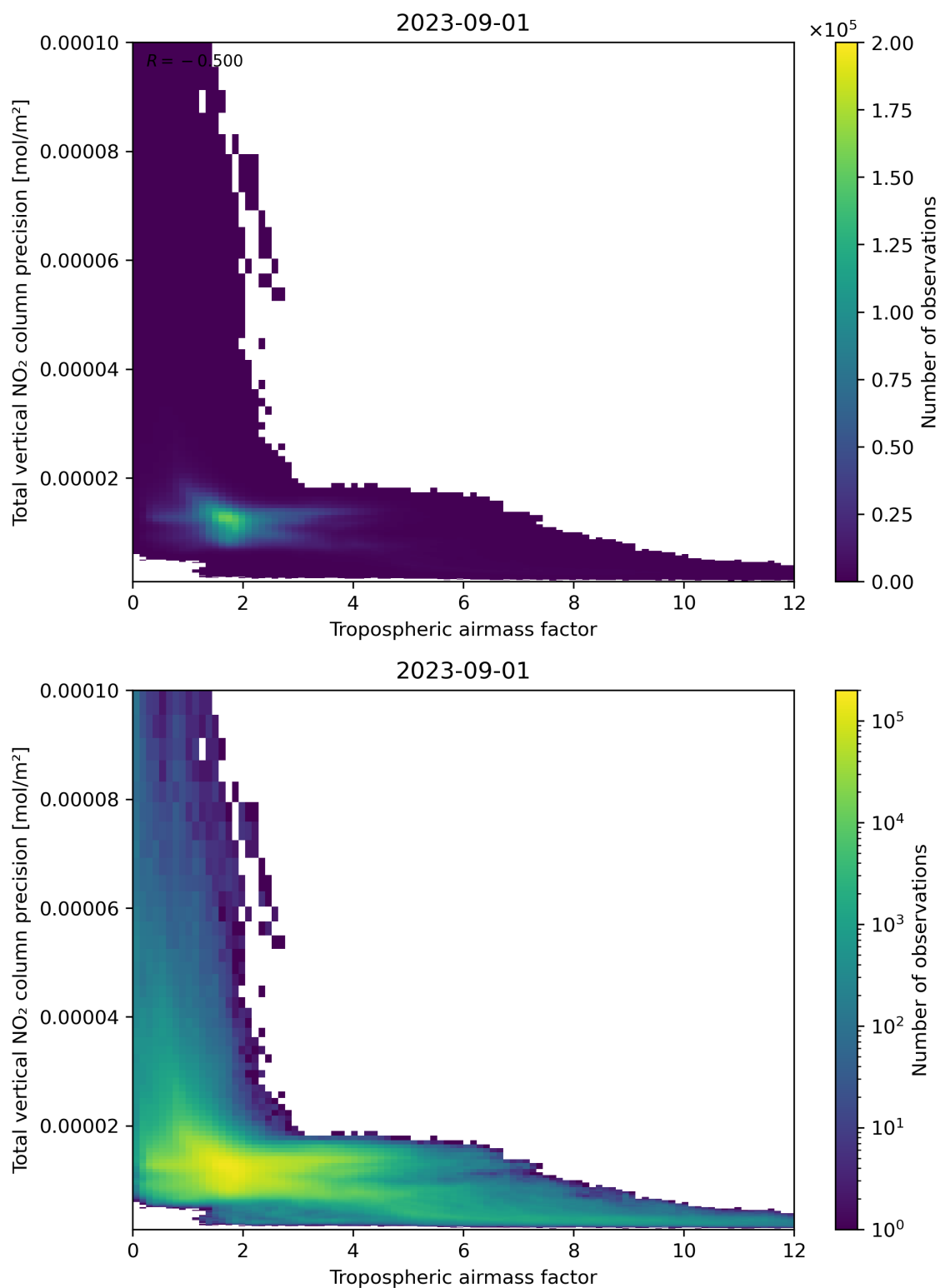
Figure 78: Scatter density plot of “Tropospheric air mass factor” against “Total vertical NO 2 column precision” for 2023-08-31 to 2023-09-02.
