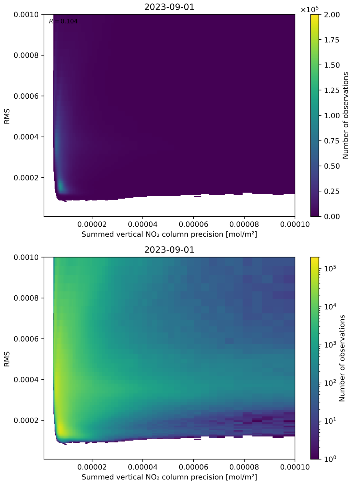
Figure 108: Scatter density plot of “Summed vertical NO 2 column precision” against “RMS” for 2023-08-31 to 2023-09-02.
