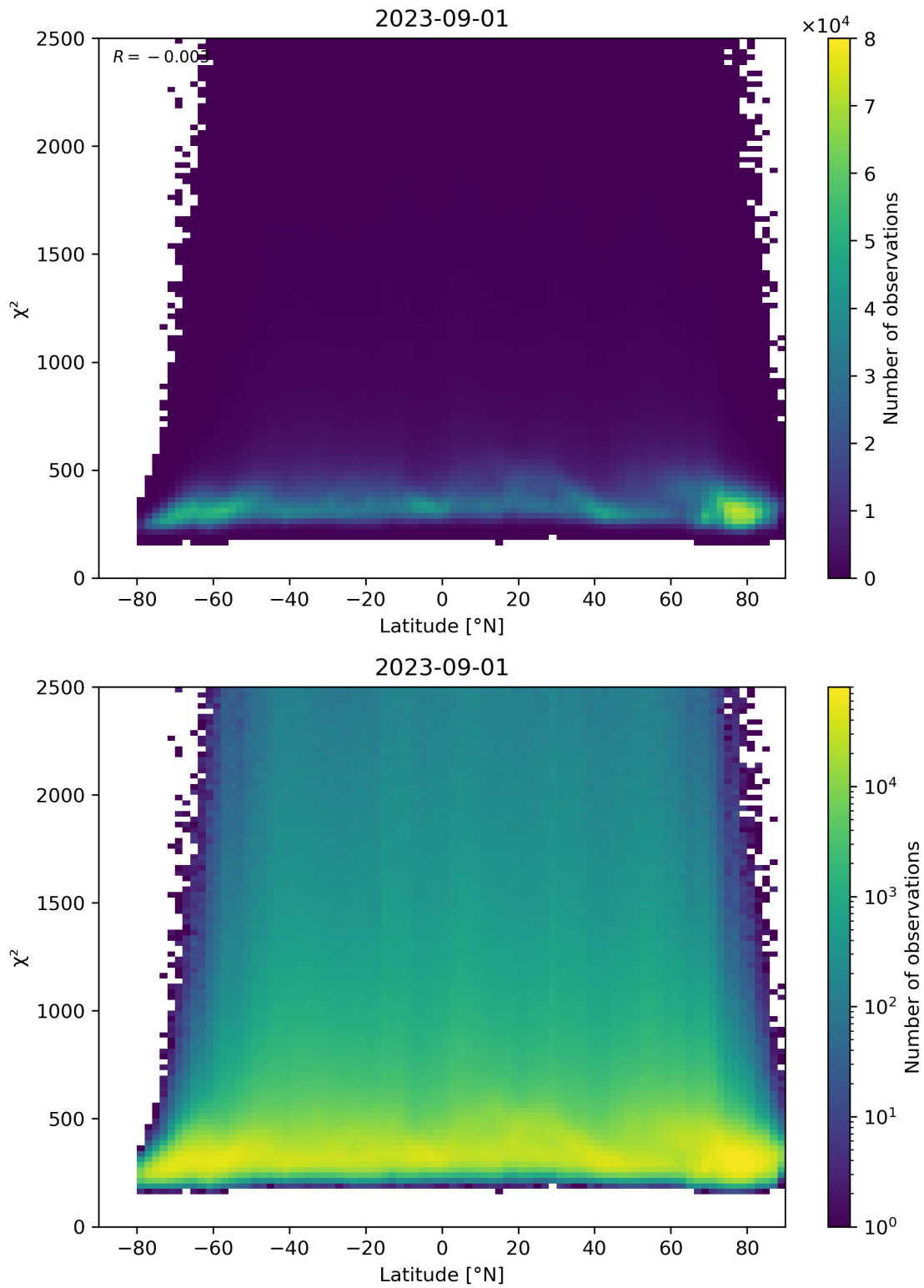
Figure 86: Scatter density plot of “Latitude” against “ \chi^2 ” for 2023-08-31 to 2023-09-02.
