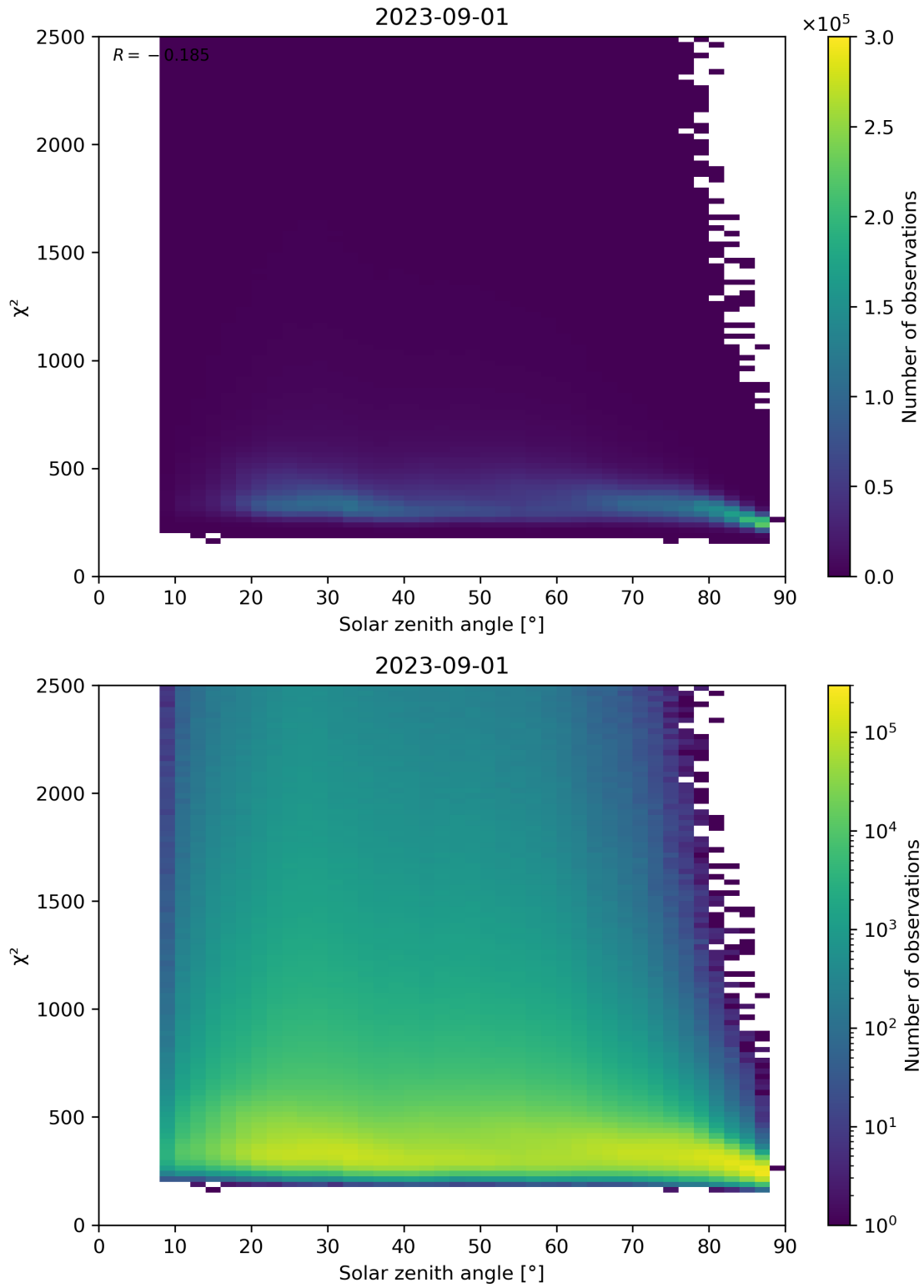
Figure 148: Scatter density plot of “Solar zenith angle” against “ \chi^2 ” for 2023-08-31 to 2023-09-02.
