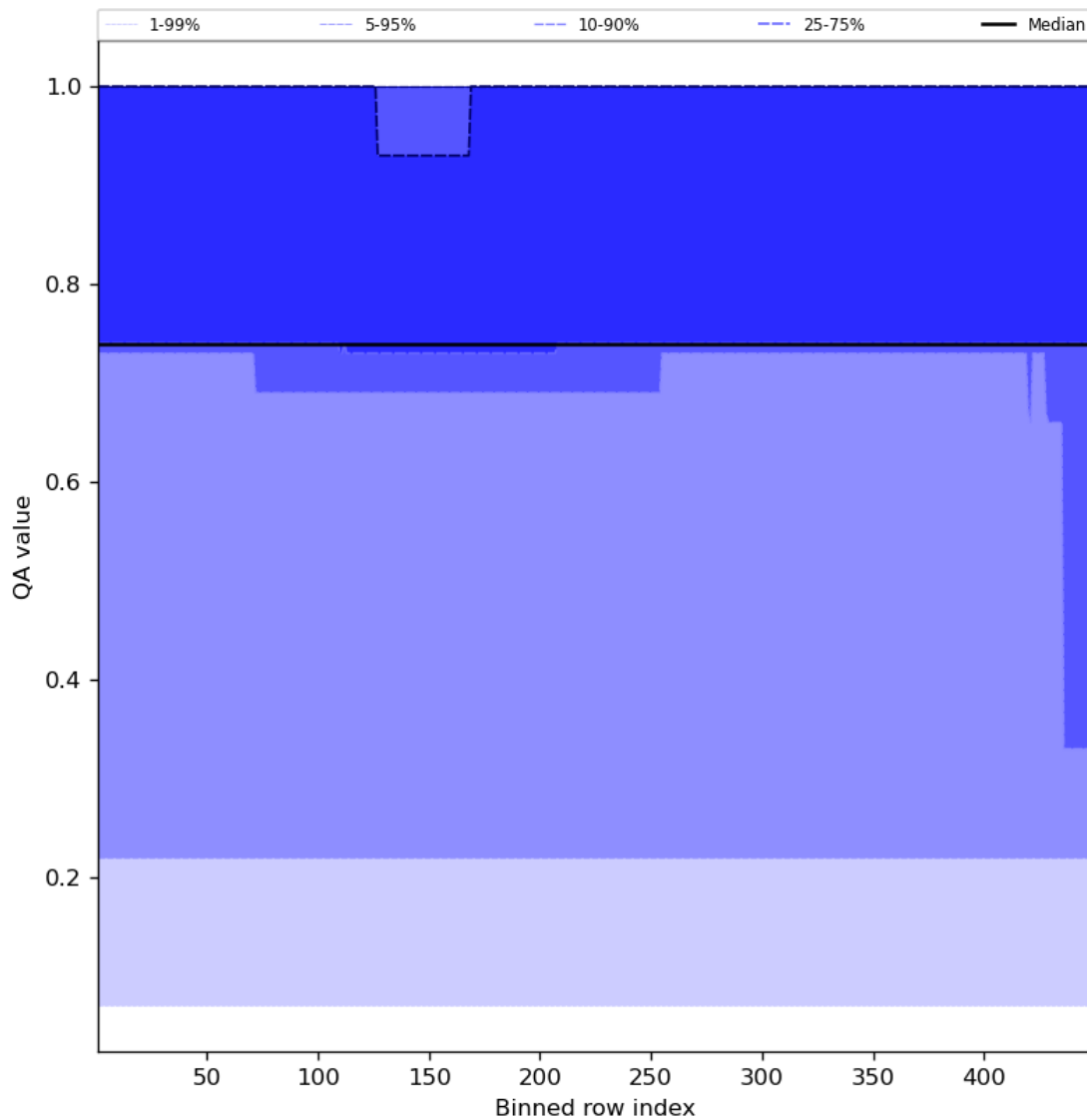
Figure 45: Along track statistics of “QA value” for 2023-08-31 to 2023-09-02
