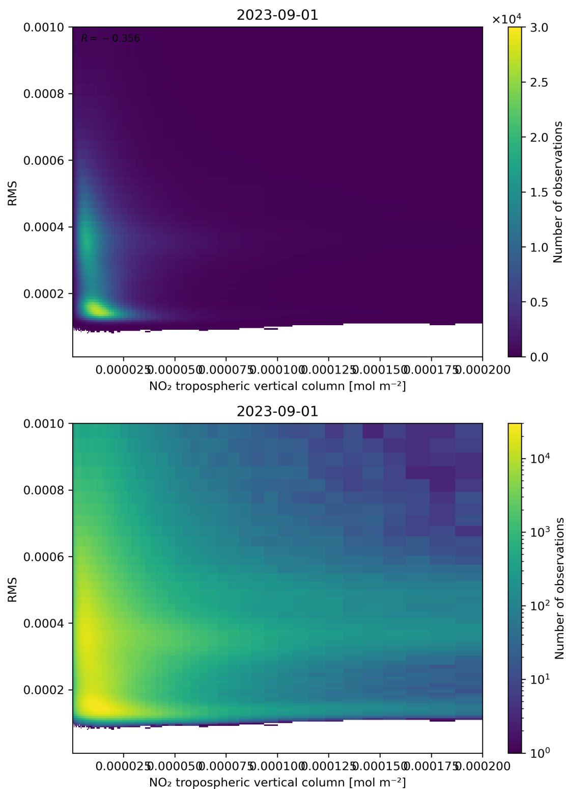
Figure 142: Scatter density plot of “NO 2 tropospheric vertical column” against “RMS” for 2023-08-31 to 2023-09-02.
