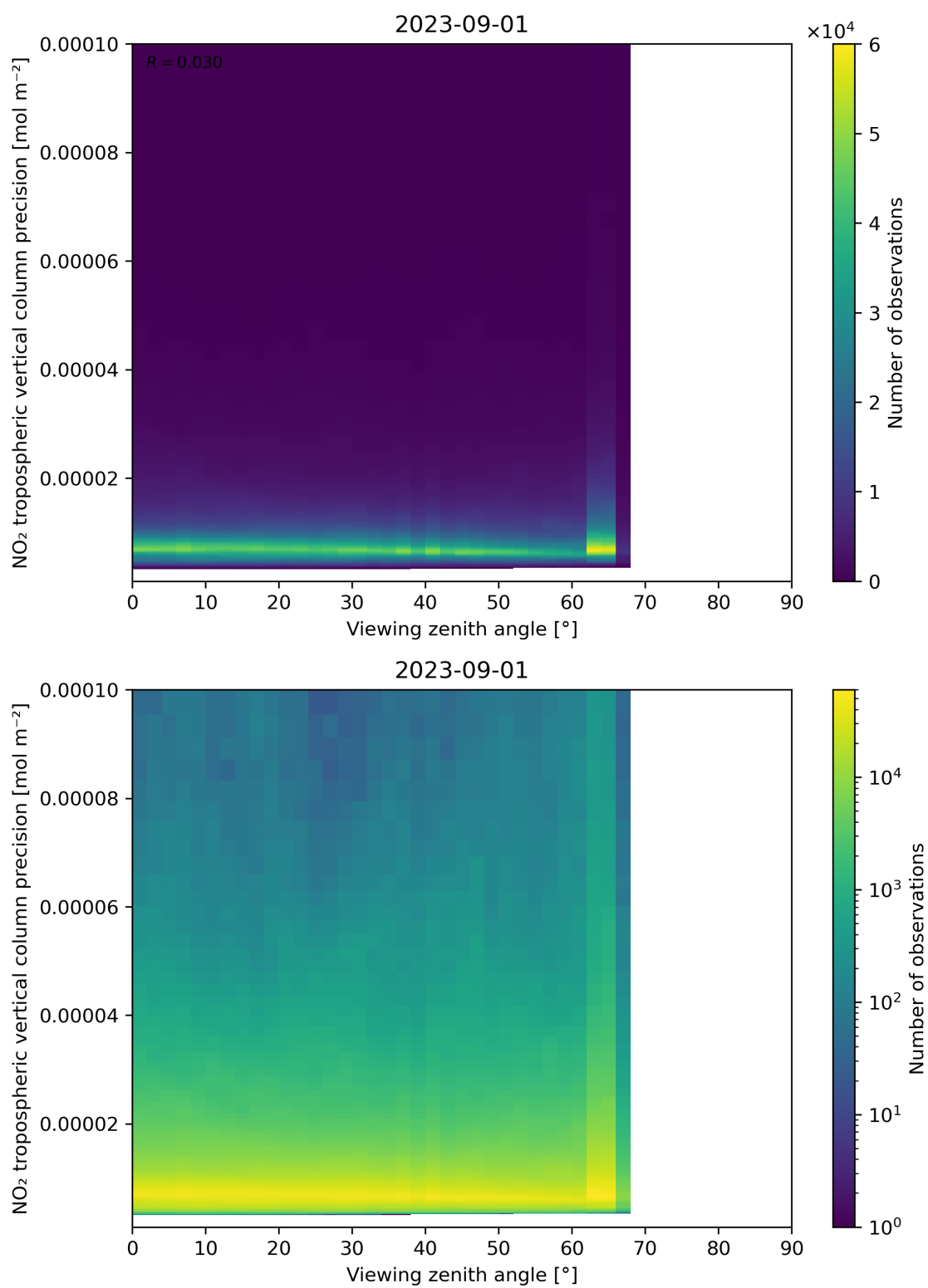
Figure 170: Scatter density plot of “Viewing zenith angle” against “NO 2 tropospheric vertical column precision” for 2023-08-31 to 2023-09-02.
