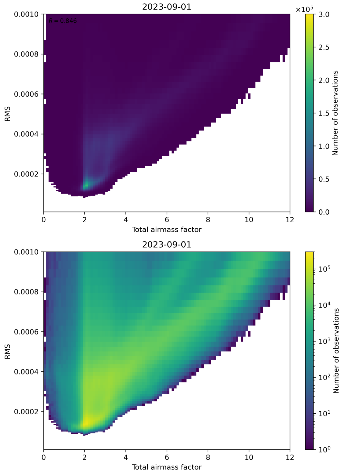
Figure 69: Scatter density plot of “Total airmass factor” against “RMS” for 2023-08-31 to 2023-09-02.
