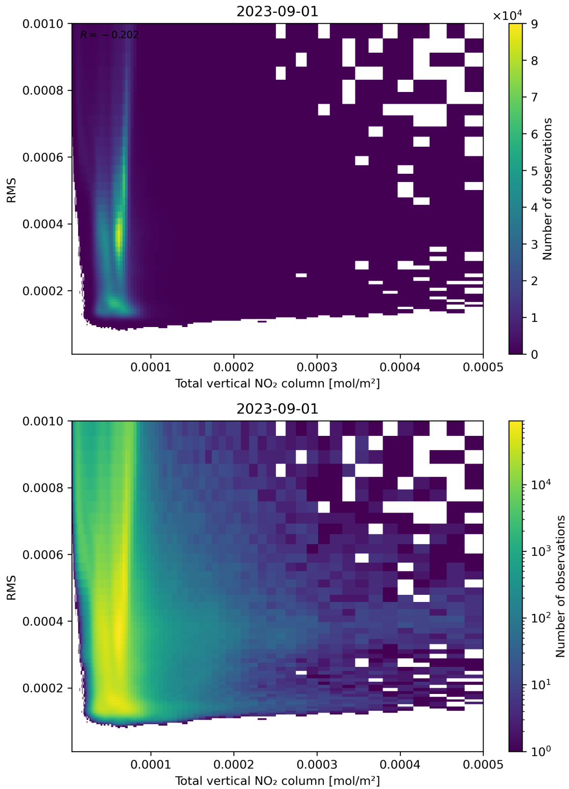
Figure 120: Scatter density plot of “Total vertical NO 2 column” against “RMS” for 2023-08-31 to 2023-09-02.
