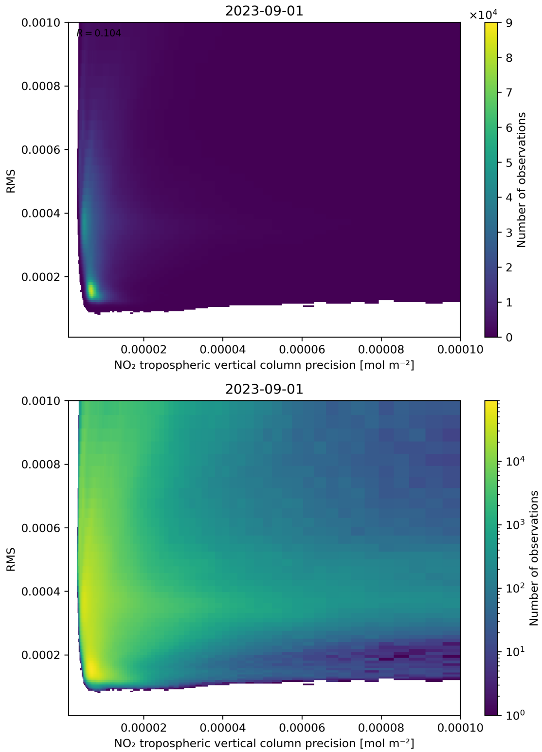
Figure 140: Scatter density plot of “NO 2 tropospheric vertical column precision” against “RMS” for 2023-08-31 to 2023-09-02.
