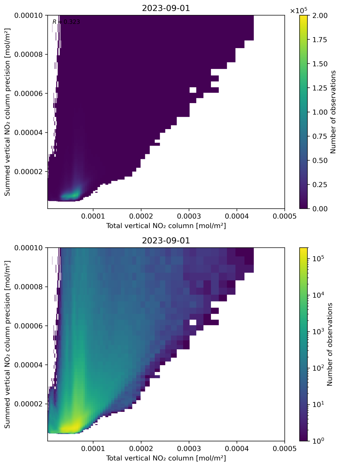
Figure 113: Scatter density plot of “Total vertical NO 2 column” against “Summed vertical NO 2 column precision” for 2023-08-31 to 2023-09-02.
