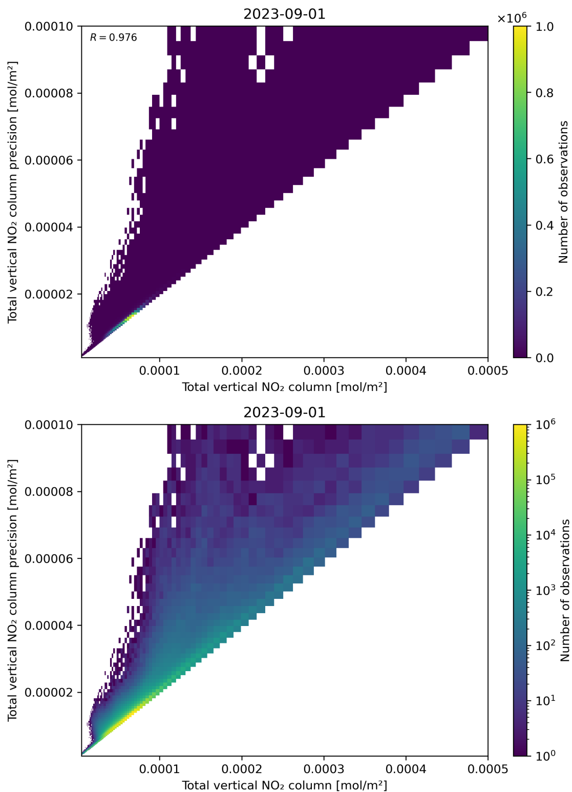
Figure 114: Scatter density plot of “Total vertical NO 2 column” against “Total vertical NO 2 column precision” for 2023-08-31 to 2023-09-02.
