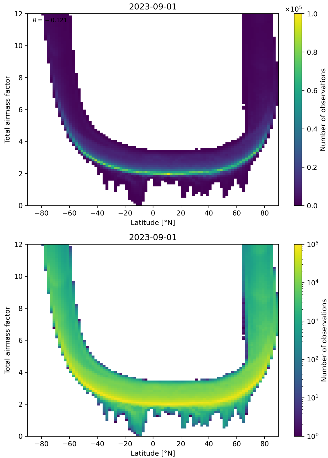
Figure 84: Scatter density plot of “Latitude” against “Total airmass factor” for 2023-08-31 to 2023-09-02.
