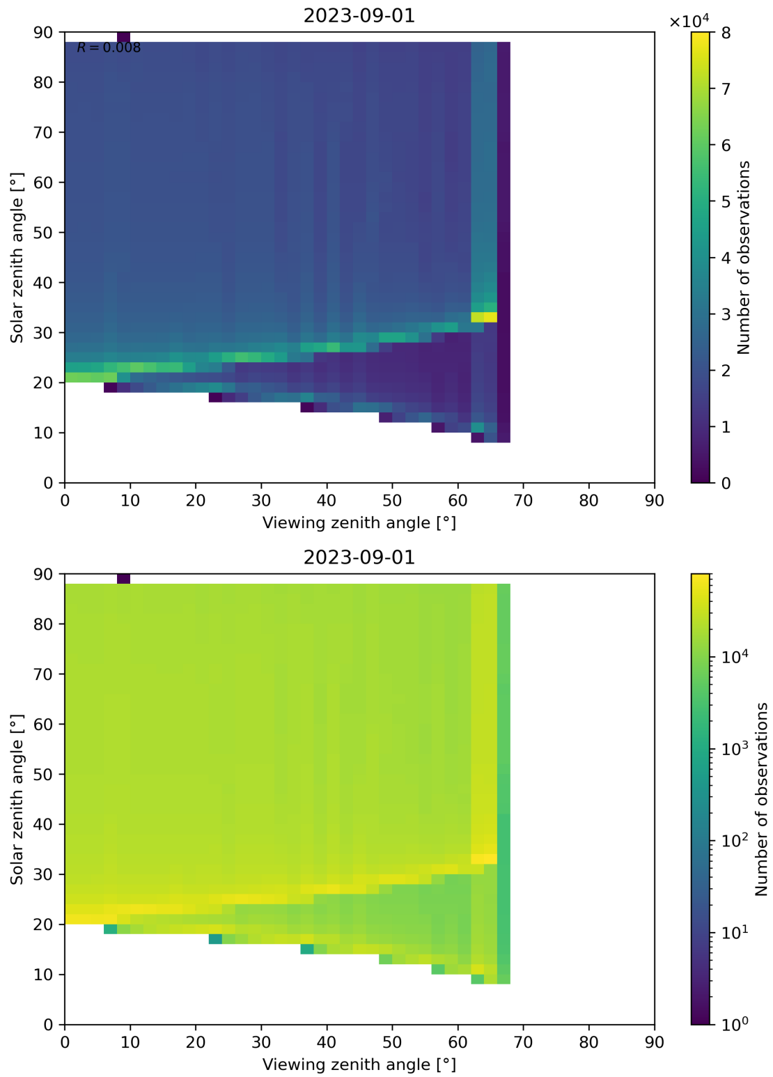
Figure 172: Scatter density plot of “Viewing zenith angle” against “Solar zenith angle” for 2023-08-31 to 2023-09-02.
