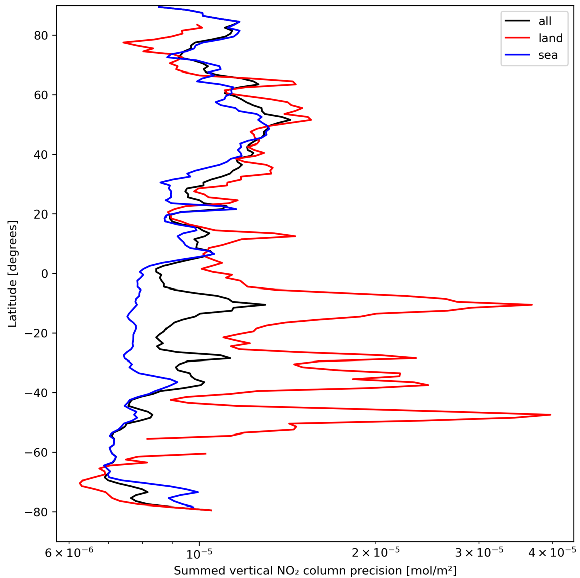
Figure 24: Zonal average of “Summed vertical NO 2 column precision” for 2023-08-31 to 2023-09-02.
