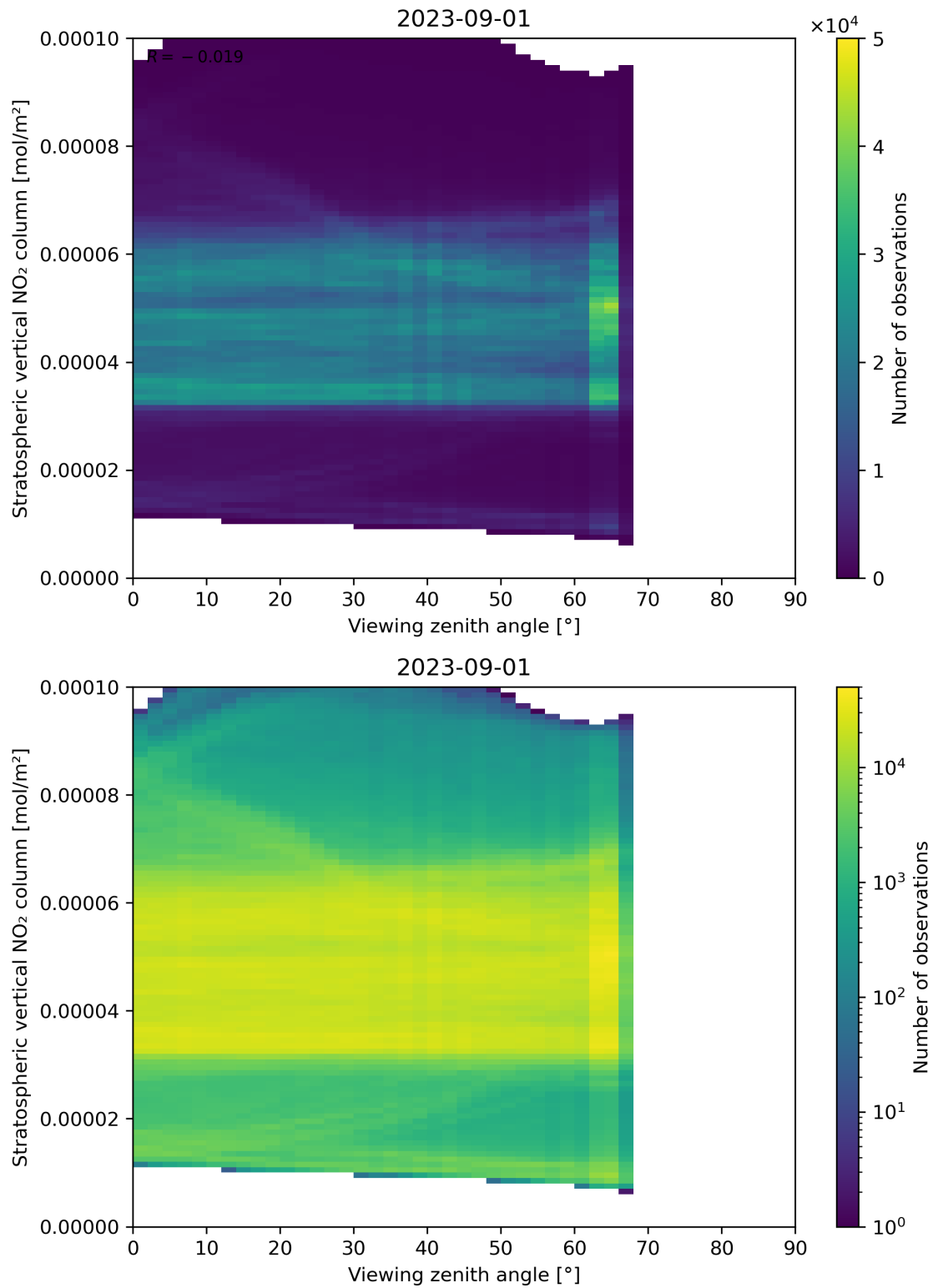
Figure 164: Scatter density plot of “Viewing zenith angle” against “Stratospheric vertical NO 2 column” for 2023-08-31 to 2023-09-02.
