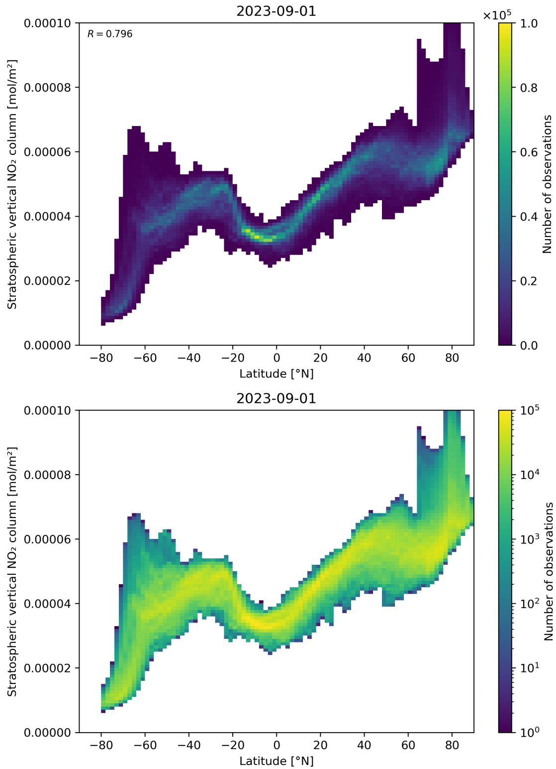
Figure 87: Scatter density plot of “Latitude” against “Stratospheric vertical NO 2 column” for 2023-08-31 to 2023-09-02.
