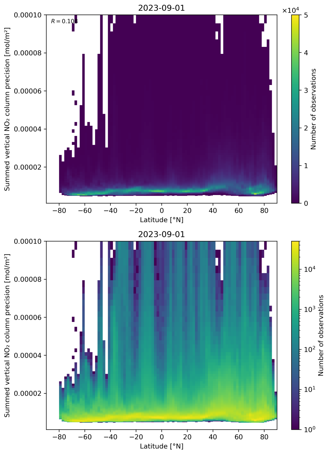
Figure 89: Scatter density plot of “Latitude” against “Summed vertical NO 2 column precision” for 2023-08-31 to 2023-09-02.
