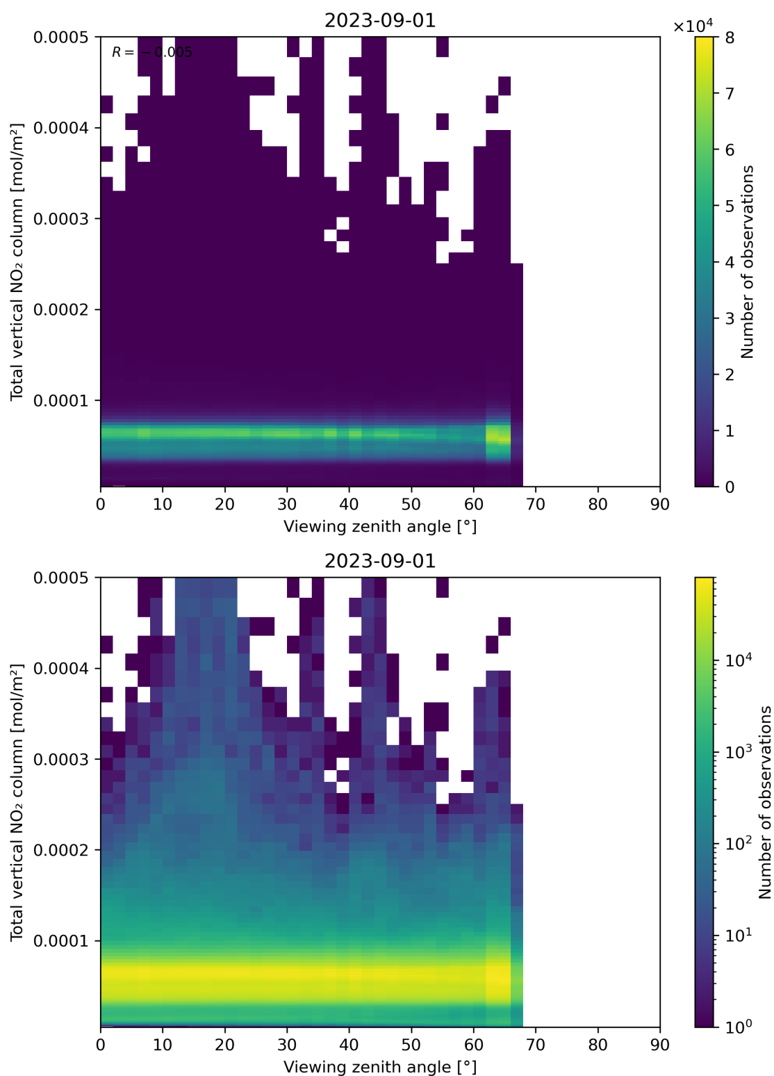
Figure 167: Scatter density plot of “Viewing zenith angle” against “Total vertical NO 2 column” for 2023-08-31 to 2023-09-02.
