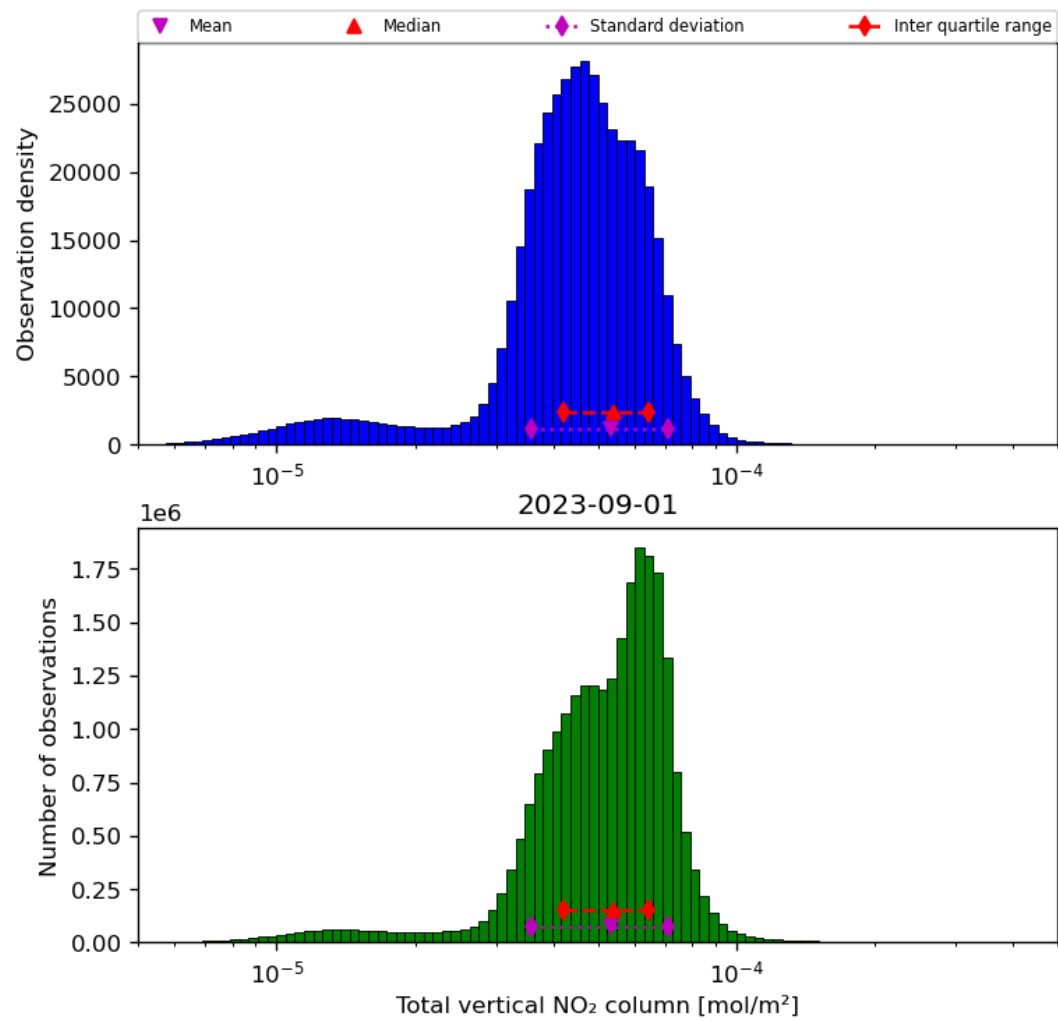
Figure 38: Histogram of “Total vertical NO 2 column” for 2023-08-31 to 2023-09-02
