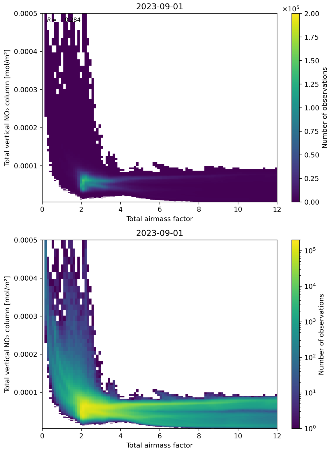
Figure 67: Scatter density plot of “Total airmass factor” against “Total vertical NO 2 column” for 2023-08-31 to 2023-09-02.
