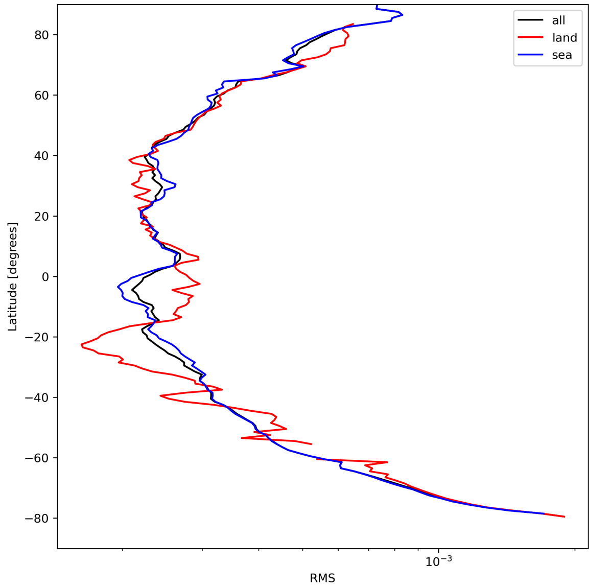
Figure 26: Zonal average of “RMS” for 2023-08-31 to 2023-09-02.
