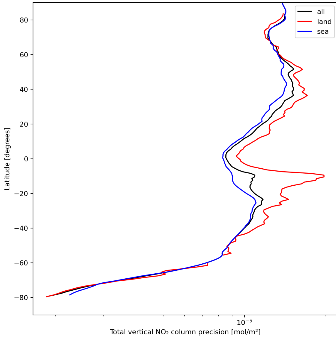
Figure 22: Zonal average of “Total vertical NO 2 column precision” for 2023-08-31 to 2023-09-02.
