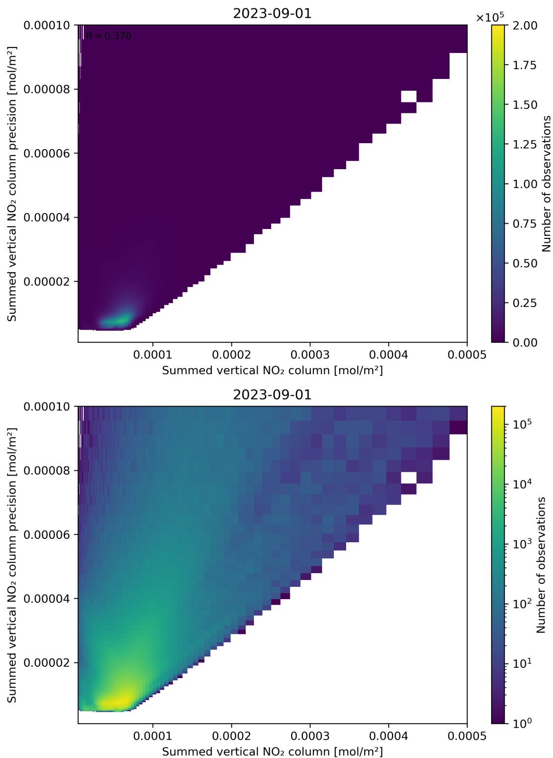
Figure 105: Scatter density plot of “Summed vertical NO 2 column” against “Summed vertical NO 2 column precision” for 2023-08-31 to 2023-09-02.
