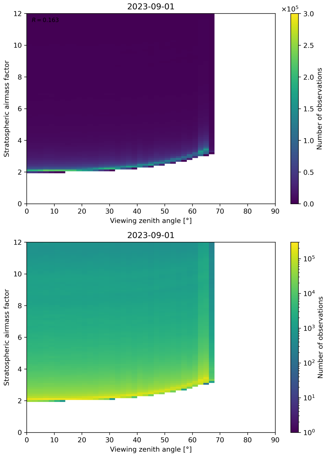
Figure 159: Scatter density plot of “Viewing zenith angle” against “Stratospheric airmass factor” for 2023-08-31 to 2023-09-02.
