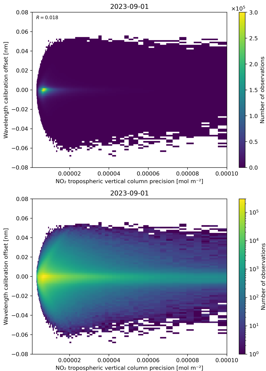
Figure 141: Scatter density plot of “NO 2 tropospheric vertical column precision” against “Wavelength calibration offset” for 2023-08-31 to 2023-09-02.
