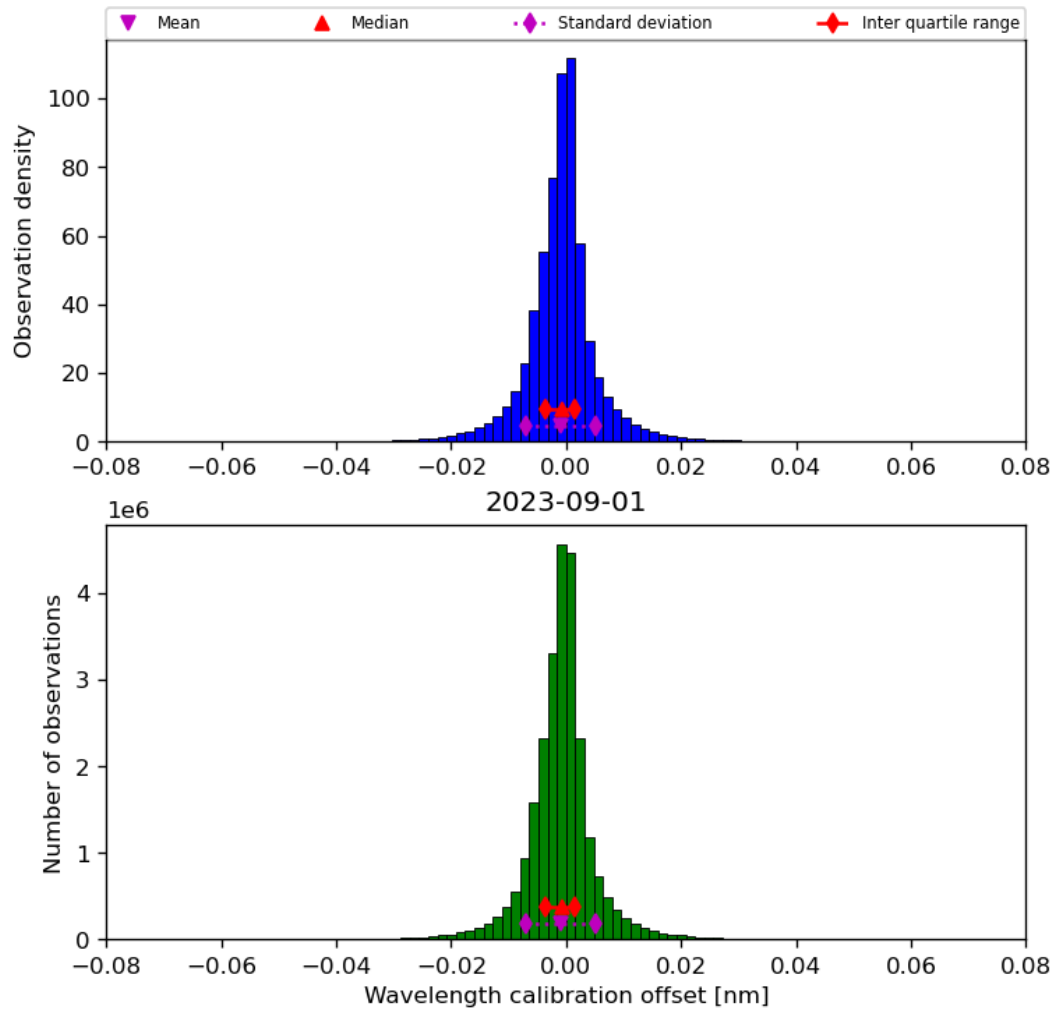
Figure 35: Histogram of “Wavelength calibration offset” for 2023-08-31 to 2023-09-02
