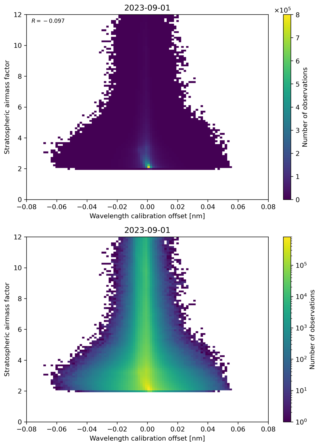
Figure 174: Scatter density plot of “Wavelength calibration offset” against “Stratospheric air mass factor” for 2023-08-31 to 2023-09-02.
