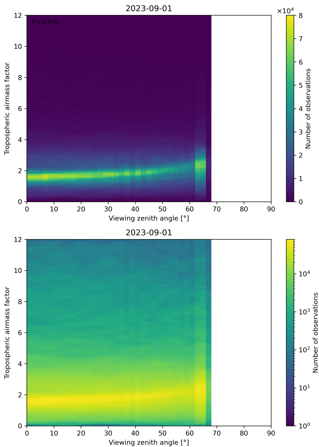
Figure 161: Scatter density plot of “Viewing zenith angle” against “Tropospheric airmass factor” for 2023-08-31 to 2023-09-02.
