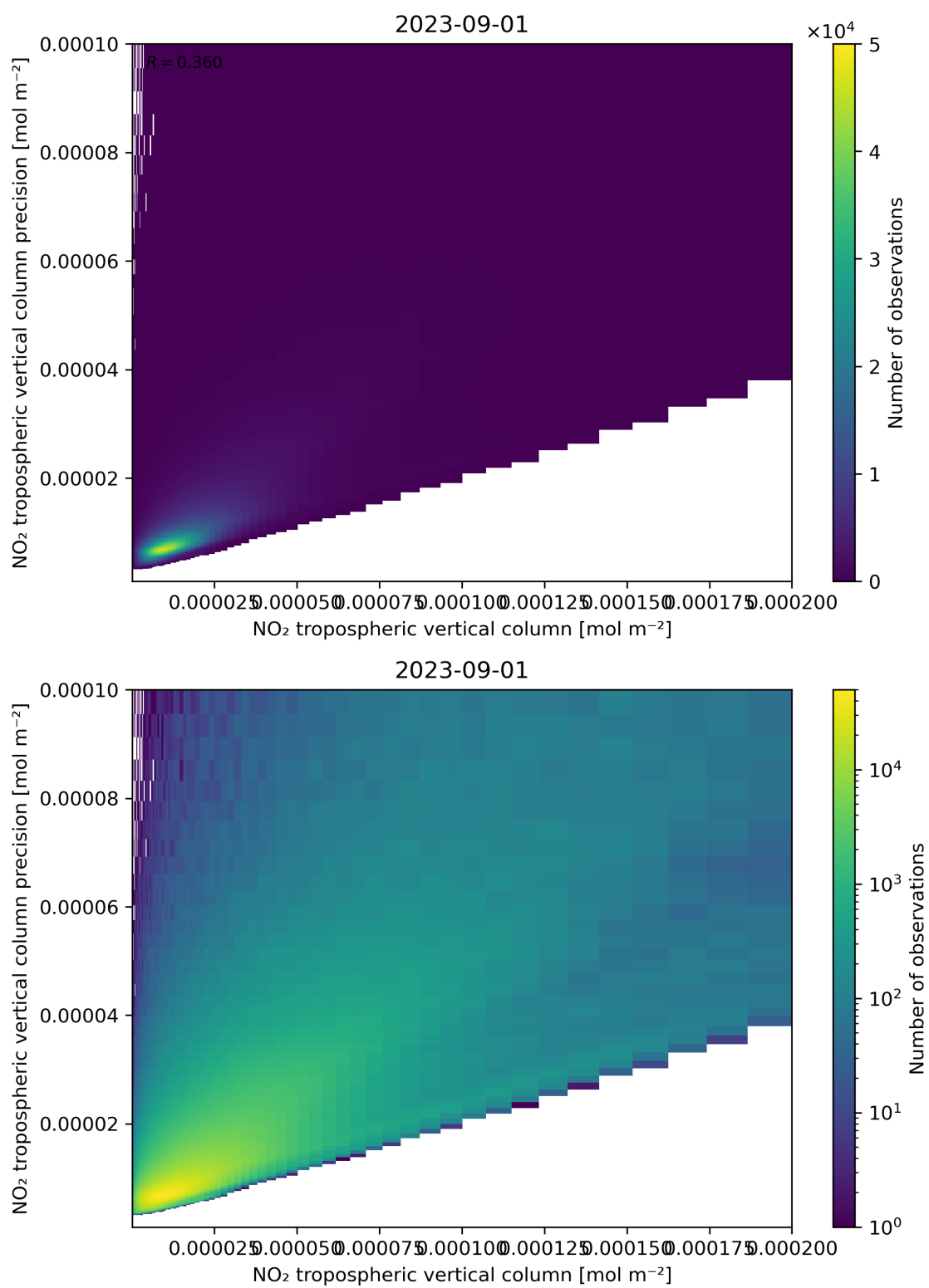
Figure 130: Scatter density plot of “NO 2 tropospheric vertical column” against “NO 2 tropospheric vertical column precision” for 2023-08-31 to 2023-09-02.
