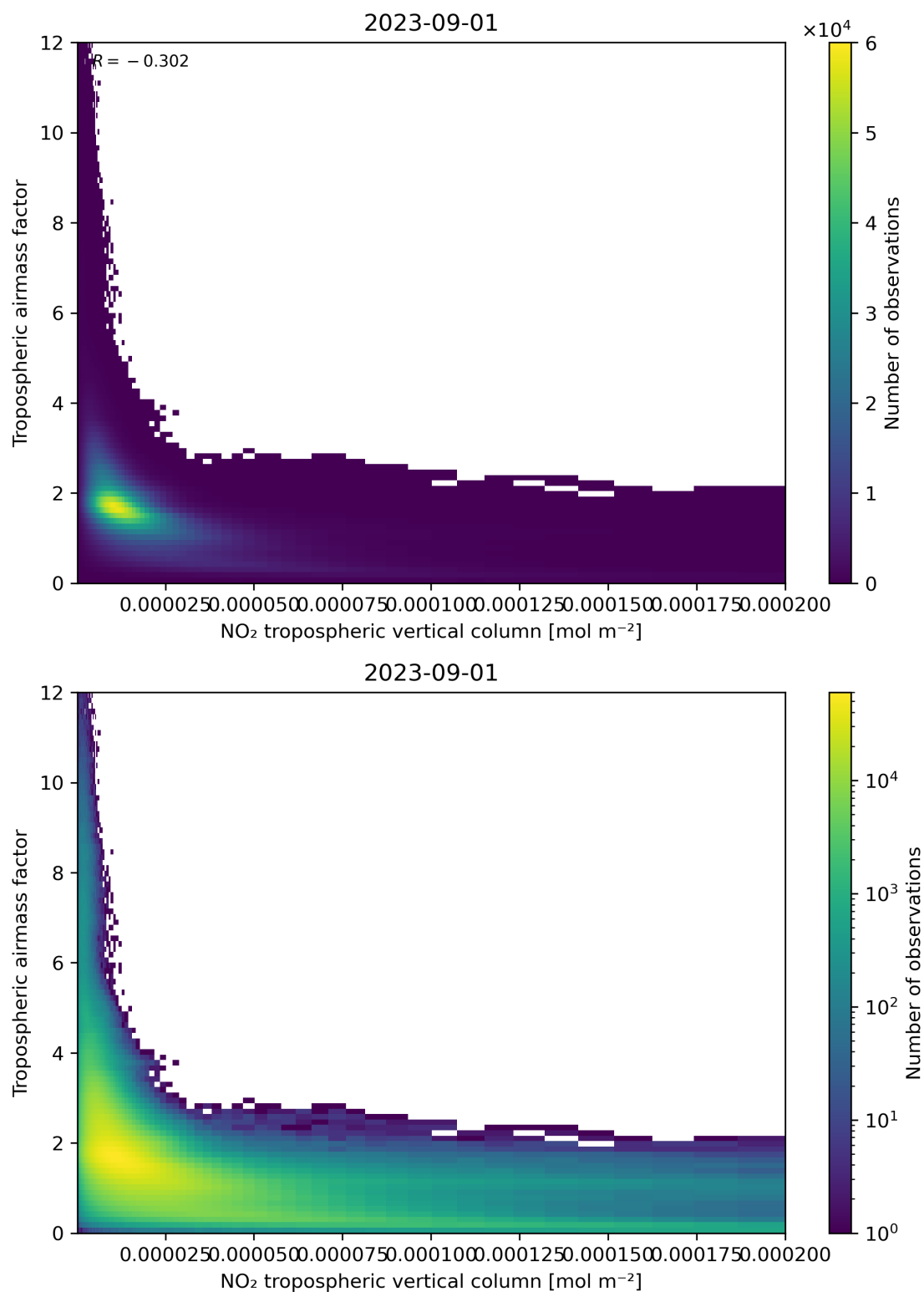
Figure 123: Scatter density plot of “NO 2 tropospheric vertical column” against “Tropospheric air mass factor” for 2023-08-31 to 2023-09-02.
