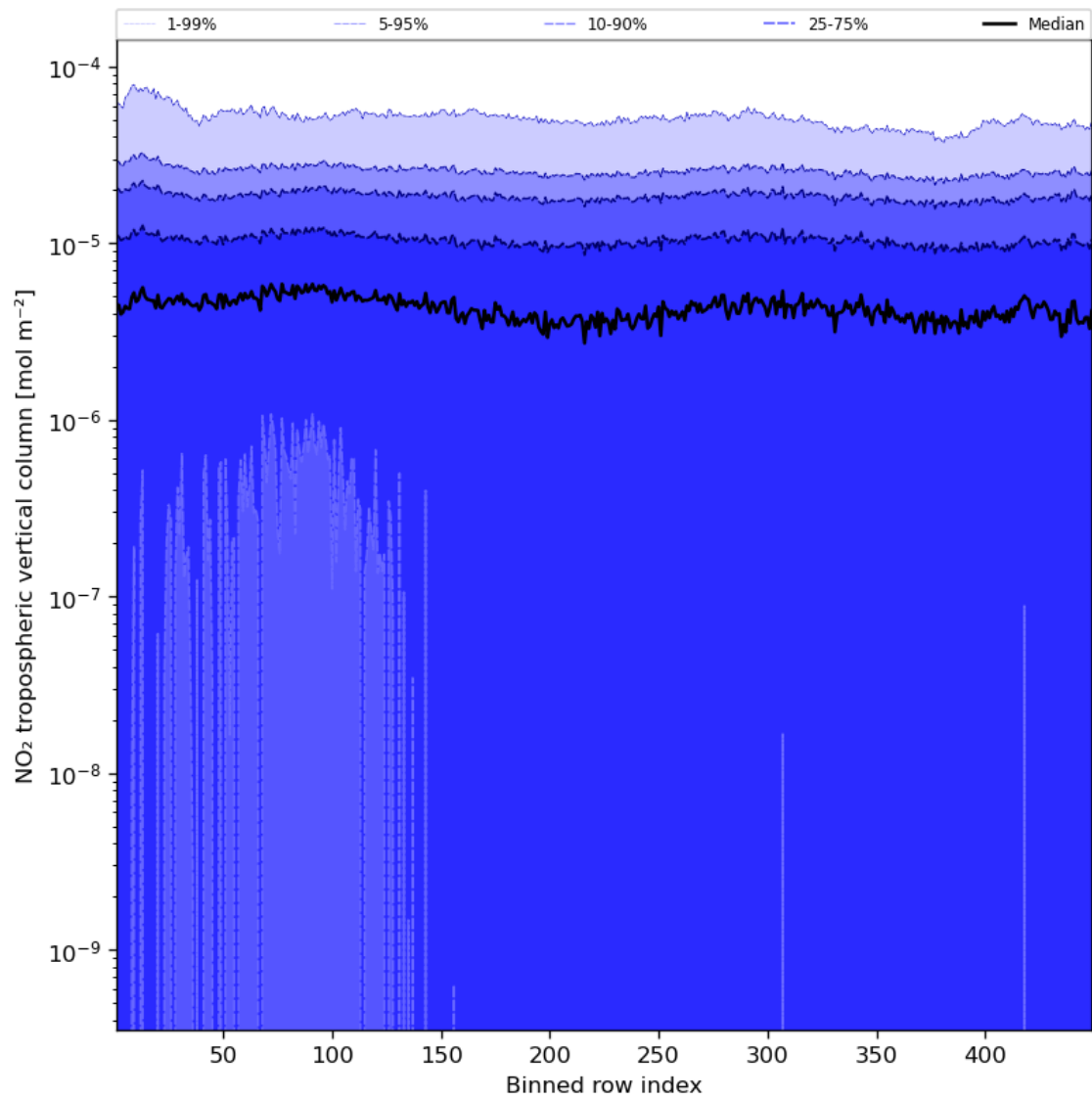
Figure 46: Along track statistics of “NO 2 tropospheric vertical column” for 2023-08-31 to 2023-09-02
