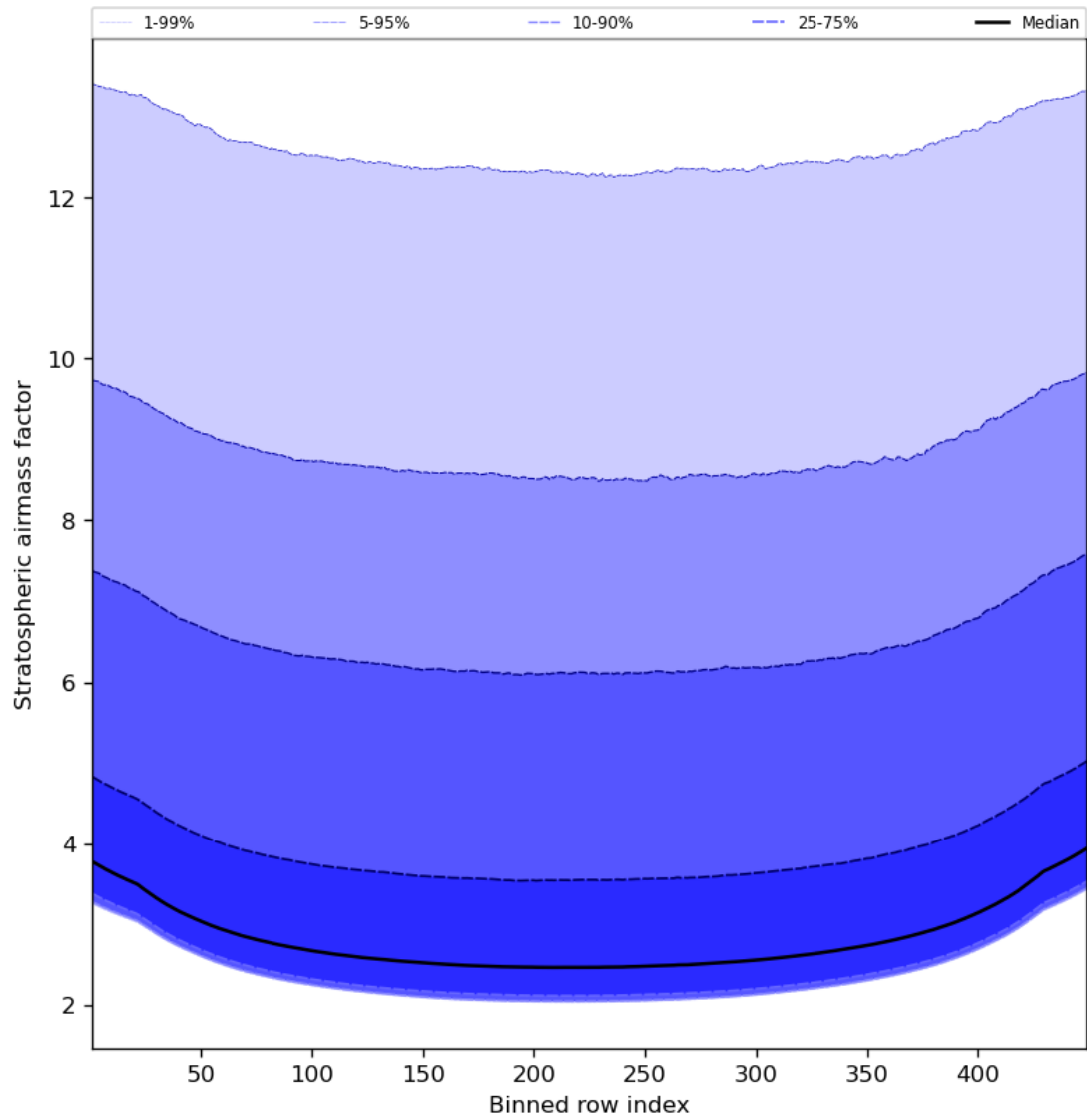
Figure 61: Along track statistics of “Stratospheric airmass factor” for 2023-08-31 to 2023-09-02
