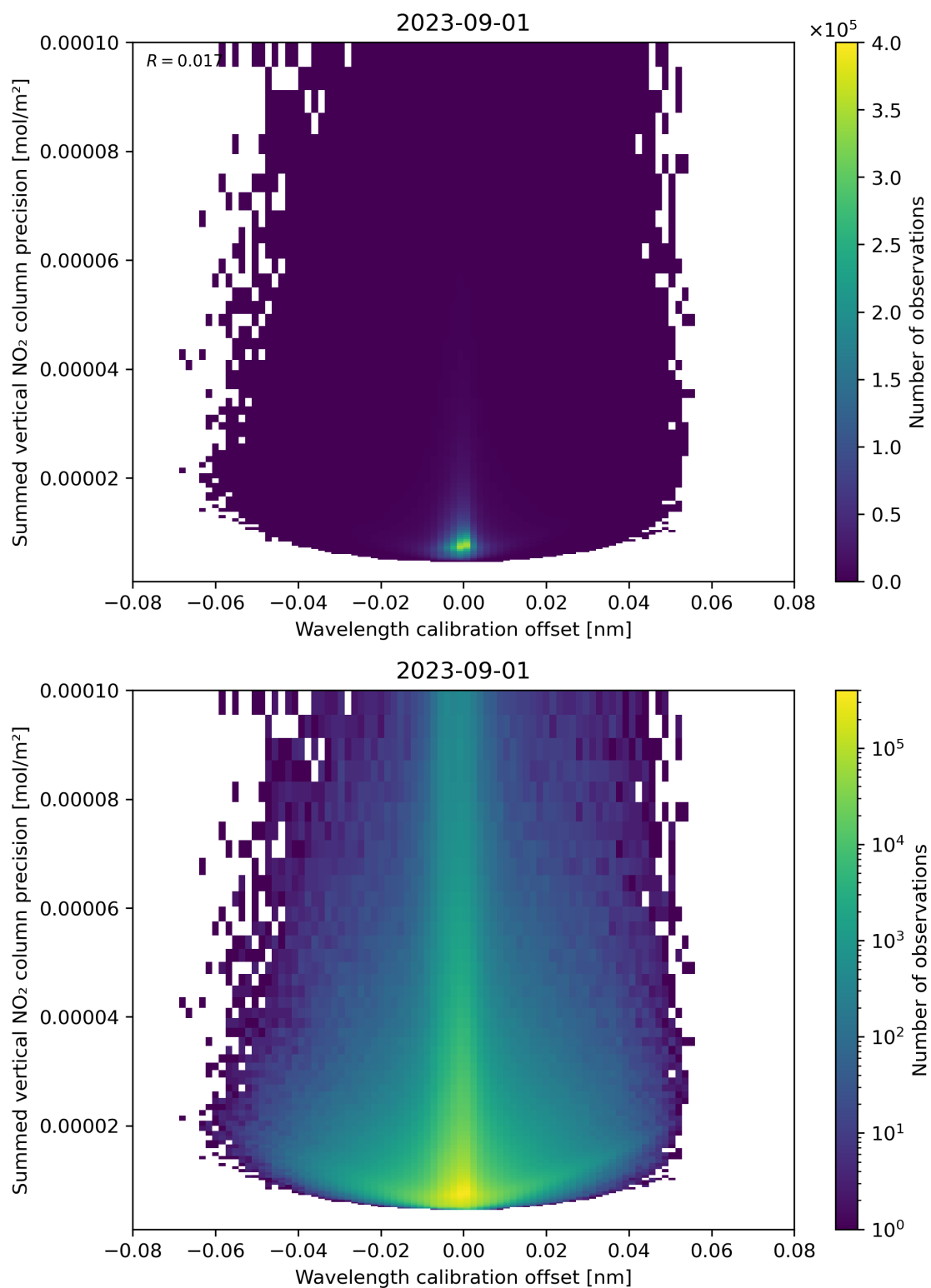
Figure 178: Scatter density plot of “Wavelength calibration offset” against “Summed vertical NO 2 column precision” for 2023-08-31 to 2023-09-02.
