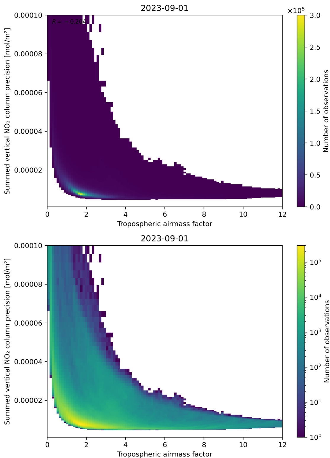
Figure 76: Scatter density plot of “Tropospheric air mass factor” against “Summed vertical NO 2 column precision” for 2023-08-31 to 2023-09-02.
