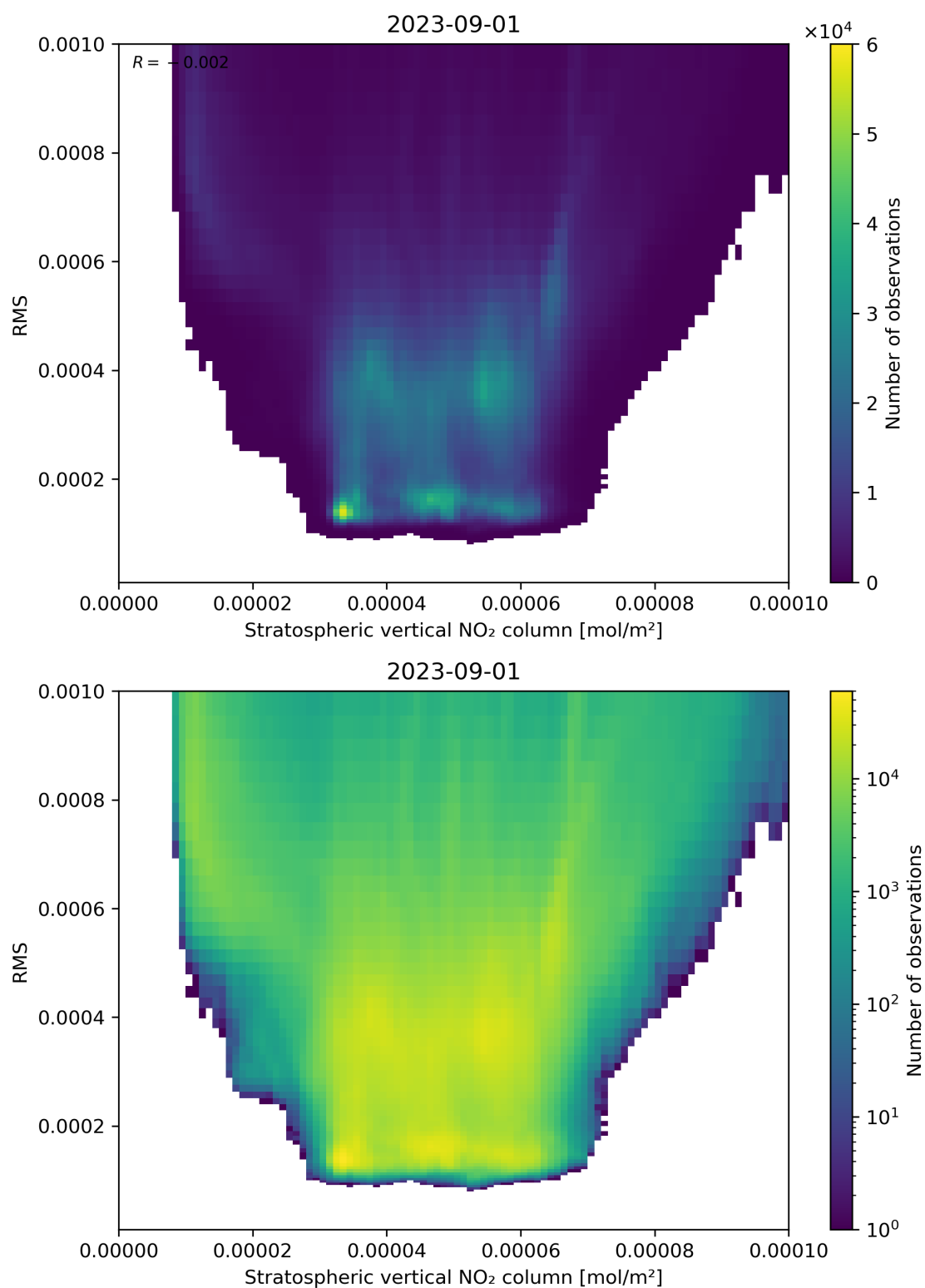
Figure 102: Scatter density plot of “Stratospheric vertical NO 2 column” against “RMS” for 2023-08-31 to 2023-09-02.
