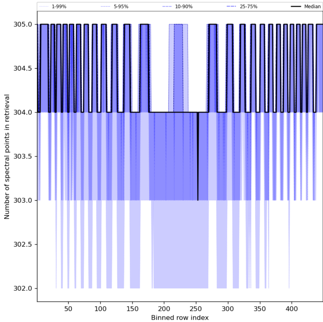
Figure 50: Along track statistics of “Number of spectral points in retrieval” for 2023-08-31 to 2023-09-02
