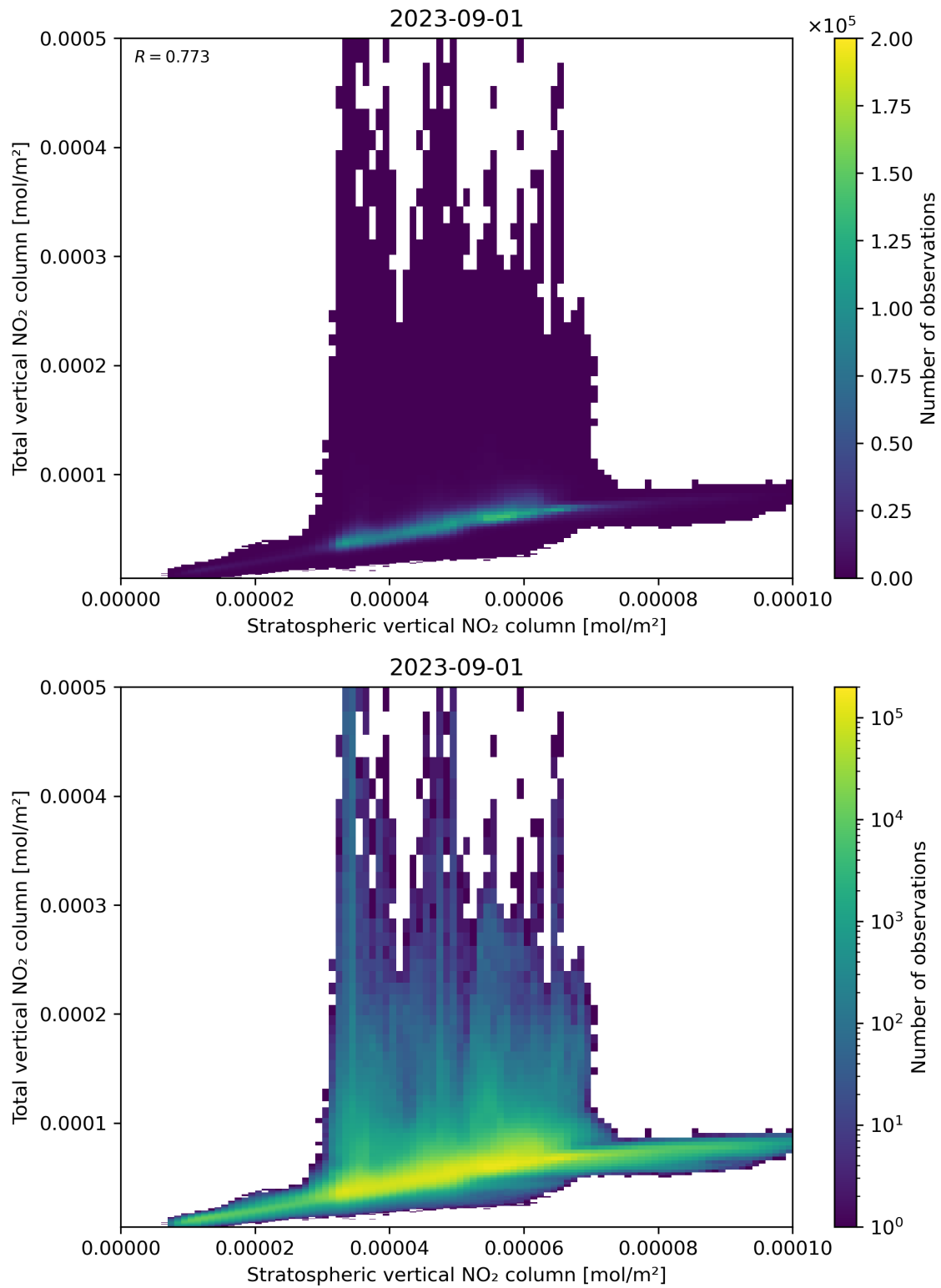
Figure 100: Scatter density plot of “Stratospheric vertical NO 2 column” against “Total vertical NO 2 column” for 2023-08-31 to 2023-09-02.
