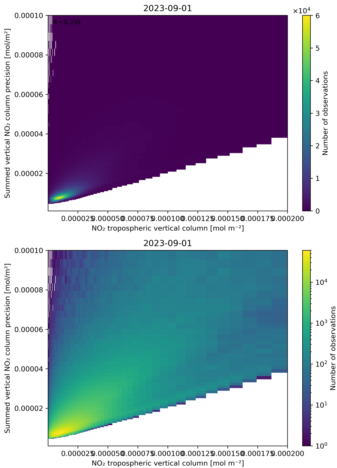
Figure 127: Scatter density plot of “NO 2 tropospheric vertical column” against “Summed vertical NO 2 column precision” for 2023-08-31 to 2023-09-02.
