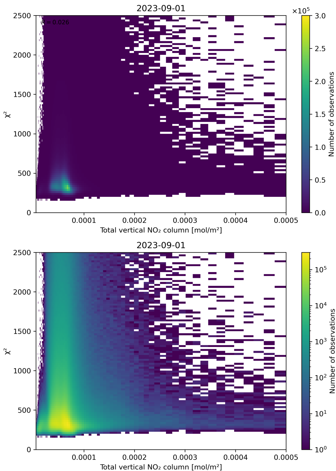
Figure 111: Scatter density plot of “Total vertical NO 2 column” against “ \chi^2 ” for 2023-08-31 to 2023-09-02.
