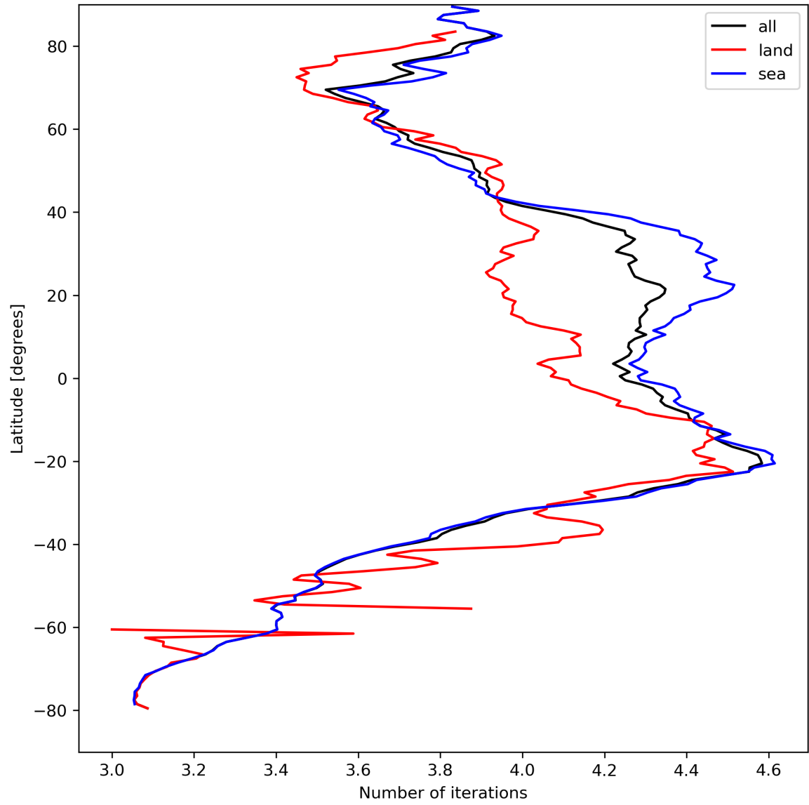
Figure 17: Zonal average of “Number of iterations” for 2023-08-31 to 2023-09-02.
