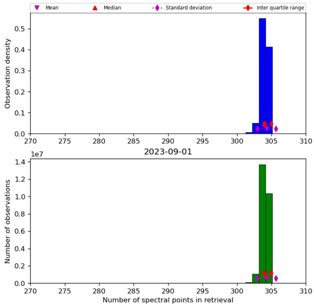
Figure 33: Histogram of “Number of spectral points in retrieval” for 2023-08-31 to 2023-09-02
