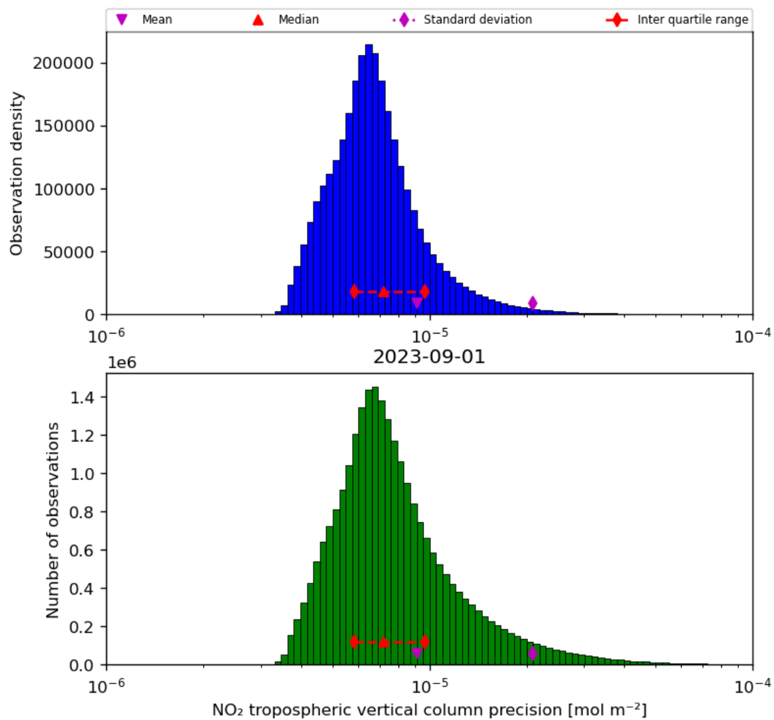
Figure 30: Histogram of “NO 2 tropospheric vertical column precision” for 2023-08-31 to 2023-09-02
