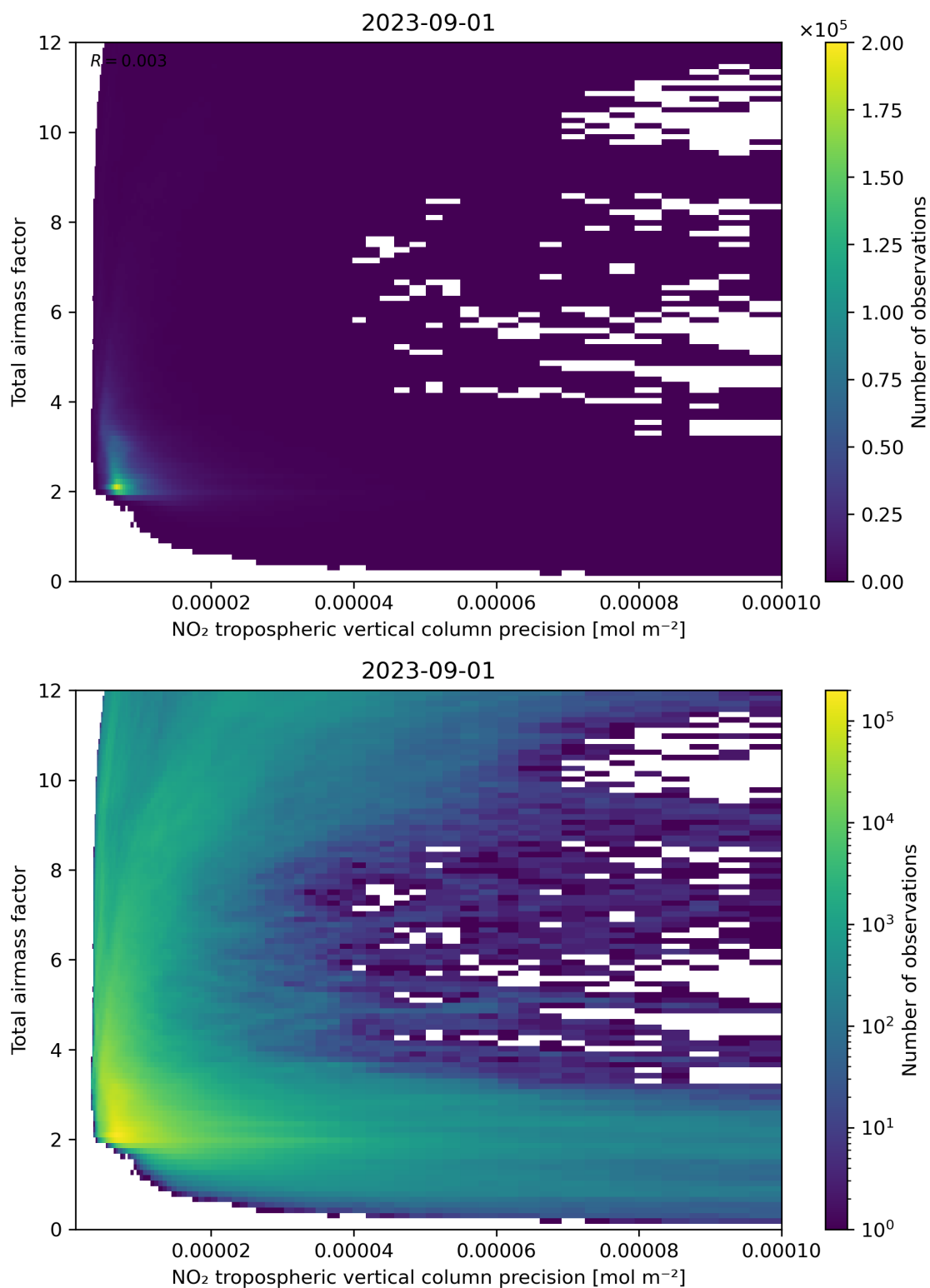
Figure 132: Scatter density plot of “NO 2 tropospheric vertical column precision” against “Total air mass factor” for 2023-08-31 to 2023-09-02.
