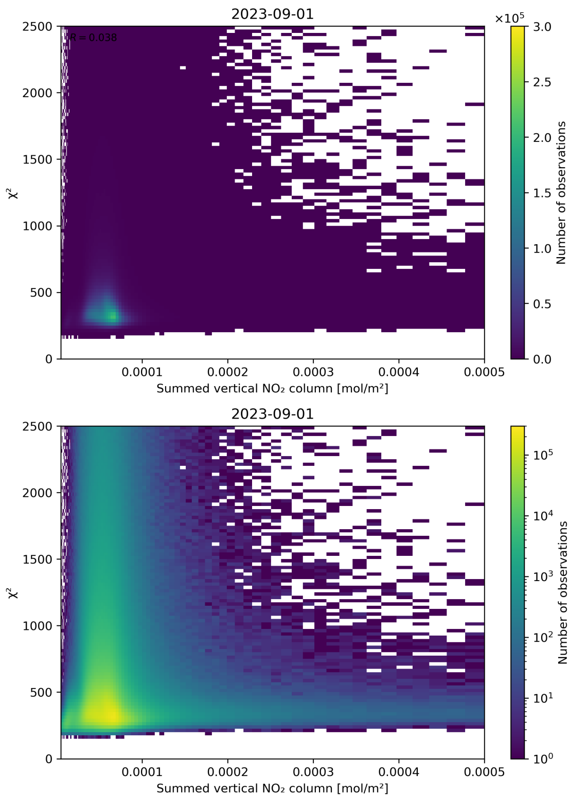
Figure 104: Scatter density plot of “Summed vertical NO 2 column” against “ \chi^2 ” for 2023-08-31 to 2023-09-02.
