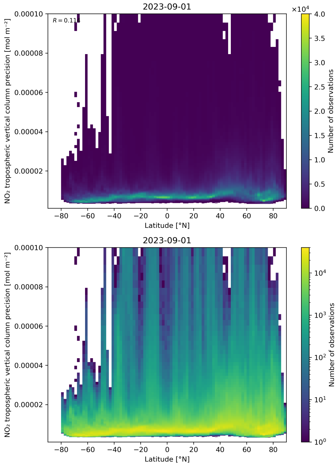
Figure 93: Scatter density plot of “Latitude” against “NO 2 tropospheric vertical column precision” for 2023-08-31 to 2023-09-02.
