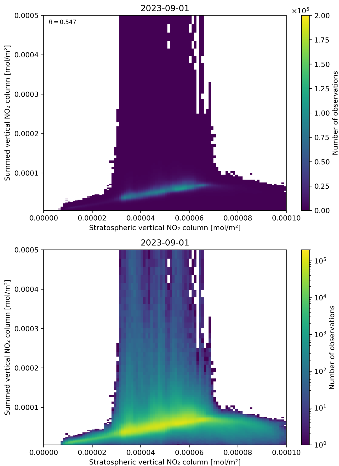
Figure 98: Scatter density plot of “Stratospheric vertical NO 2 column” against “Summed vertical NO 2 column” for 2023-08-31 to 2023-09-02.
