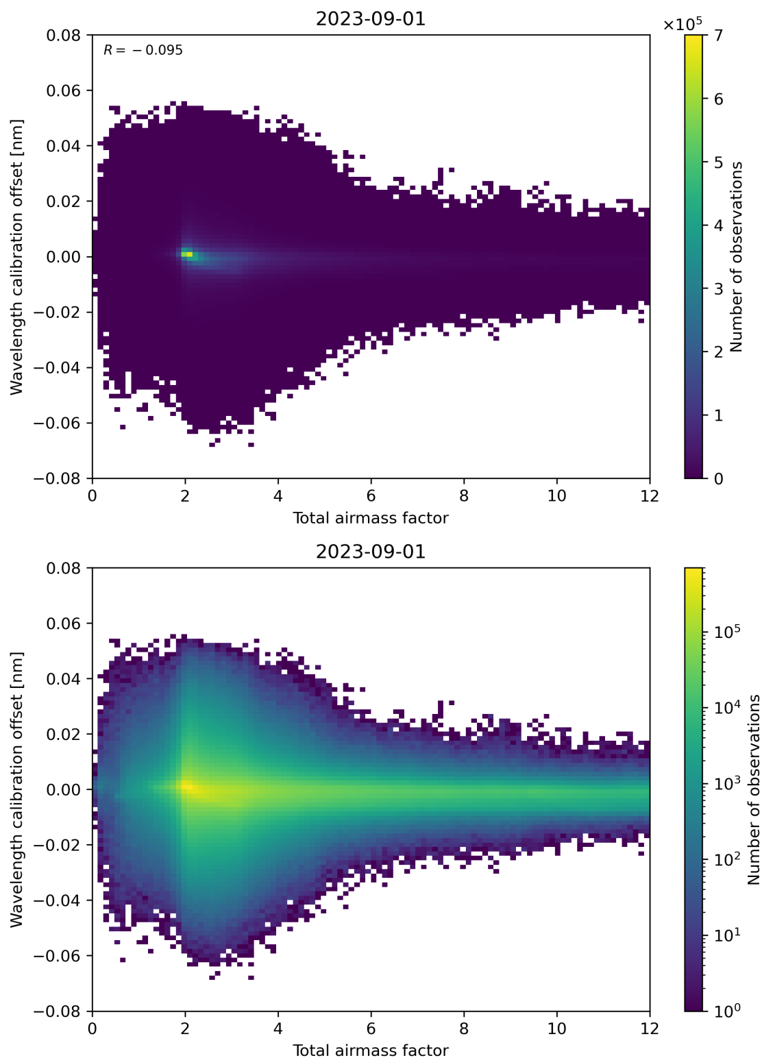
Figure 70: Scatter density plot of “Total airmass factor” against “Wavelength calibration offset” for 2023-08-31 to 2023-09-02.
