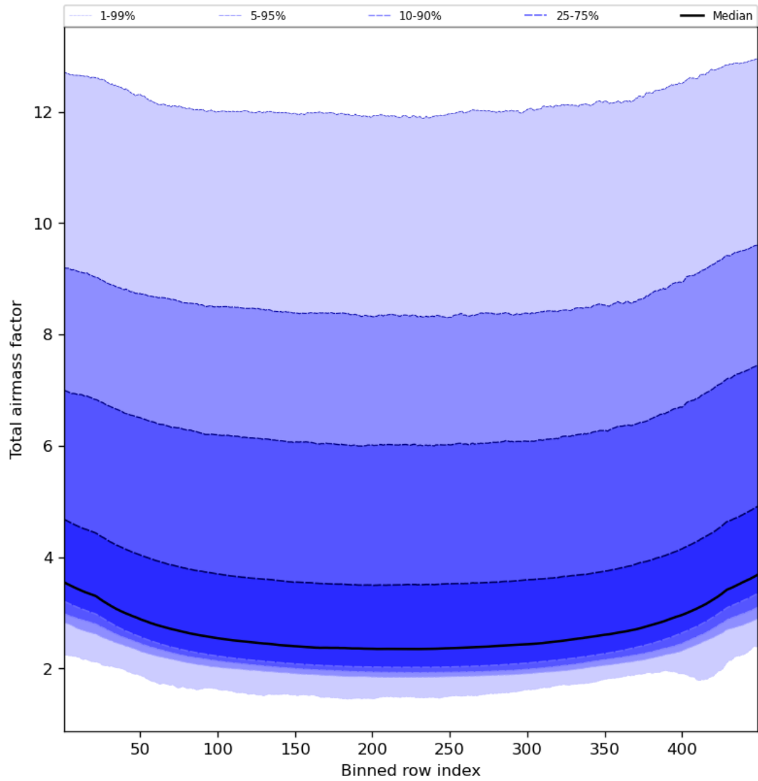
Figure 49: Along track statistics of “Total airmass factor” for 2023-08-31 to 2023-09-02
