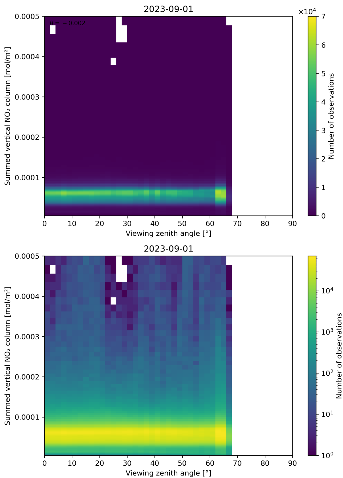
Figure 165: Scatter density plot of “Viewing zenith angle” against “Summed vertical NO 2 column” for 2023-08-31 to 2023-09-02.
