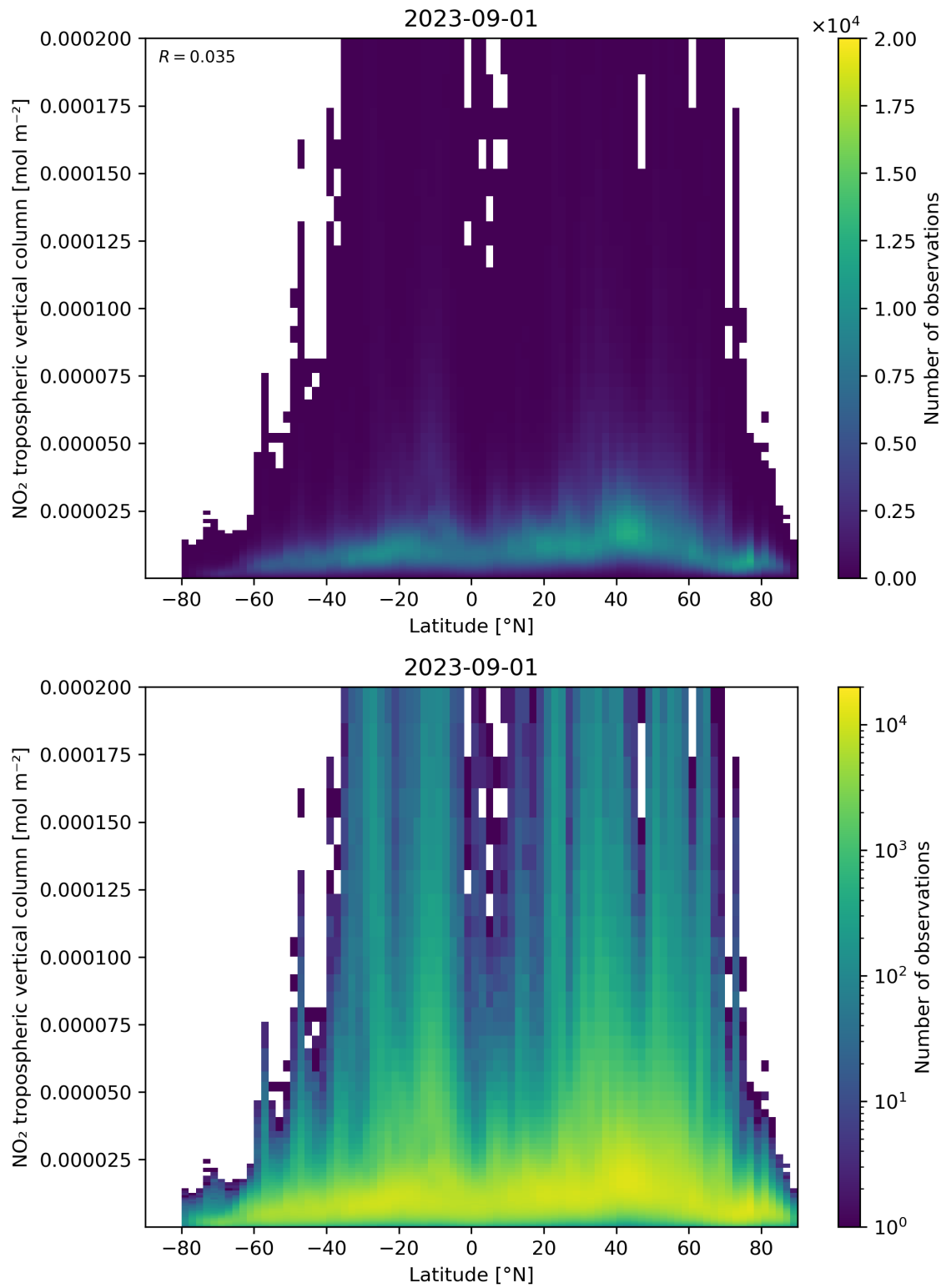
Figure 92: Scatter density plot of “Latitude” against “NO 2 tropospheric vertical column” for 2023-08-31 to 2023-09-02.
