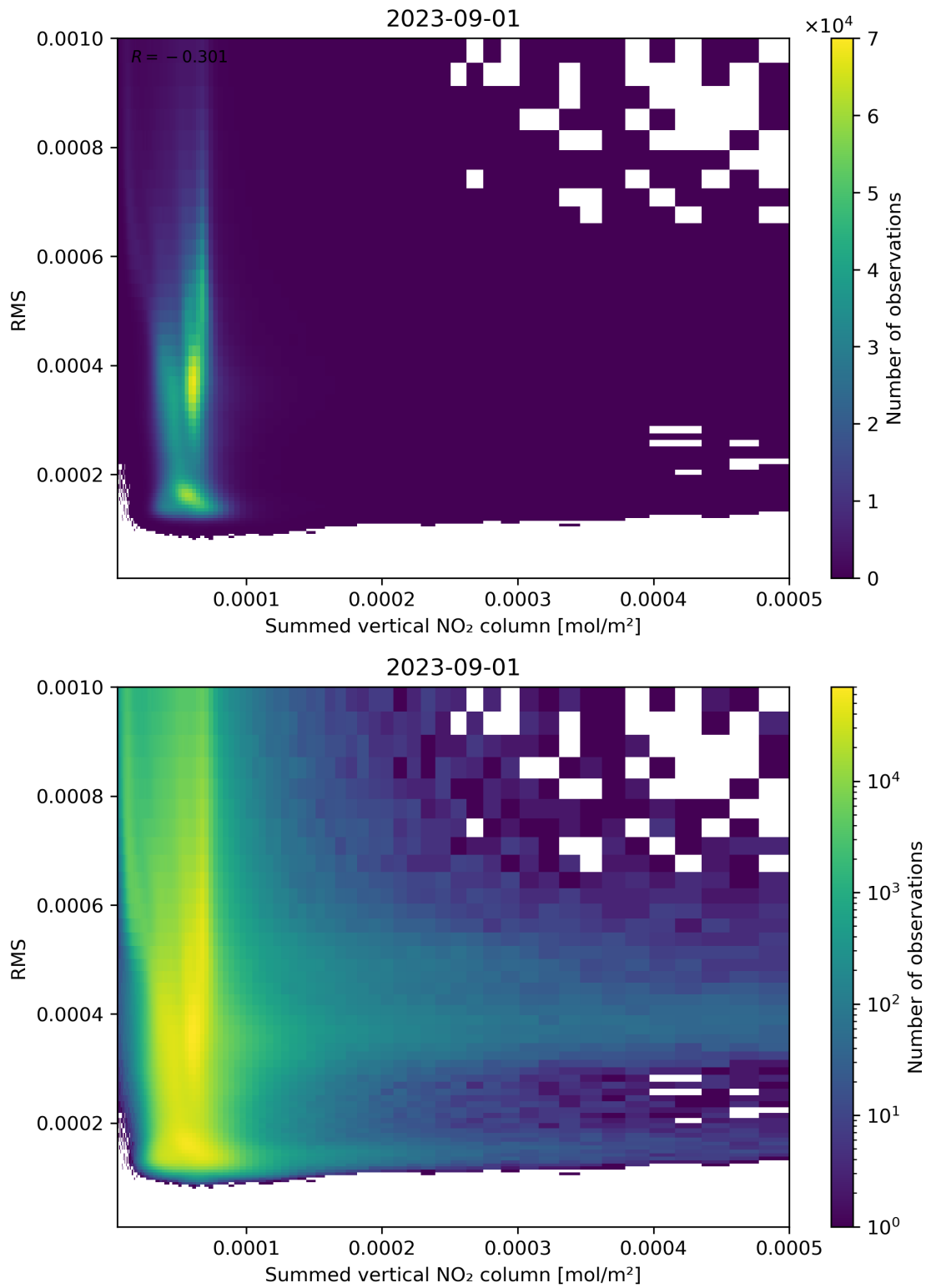
Figure 109: Scatter density plot of “Summed vertical NO 2 column” against “RMS” for 2023-08-31 to 2023-09-02.
