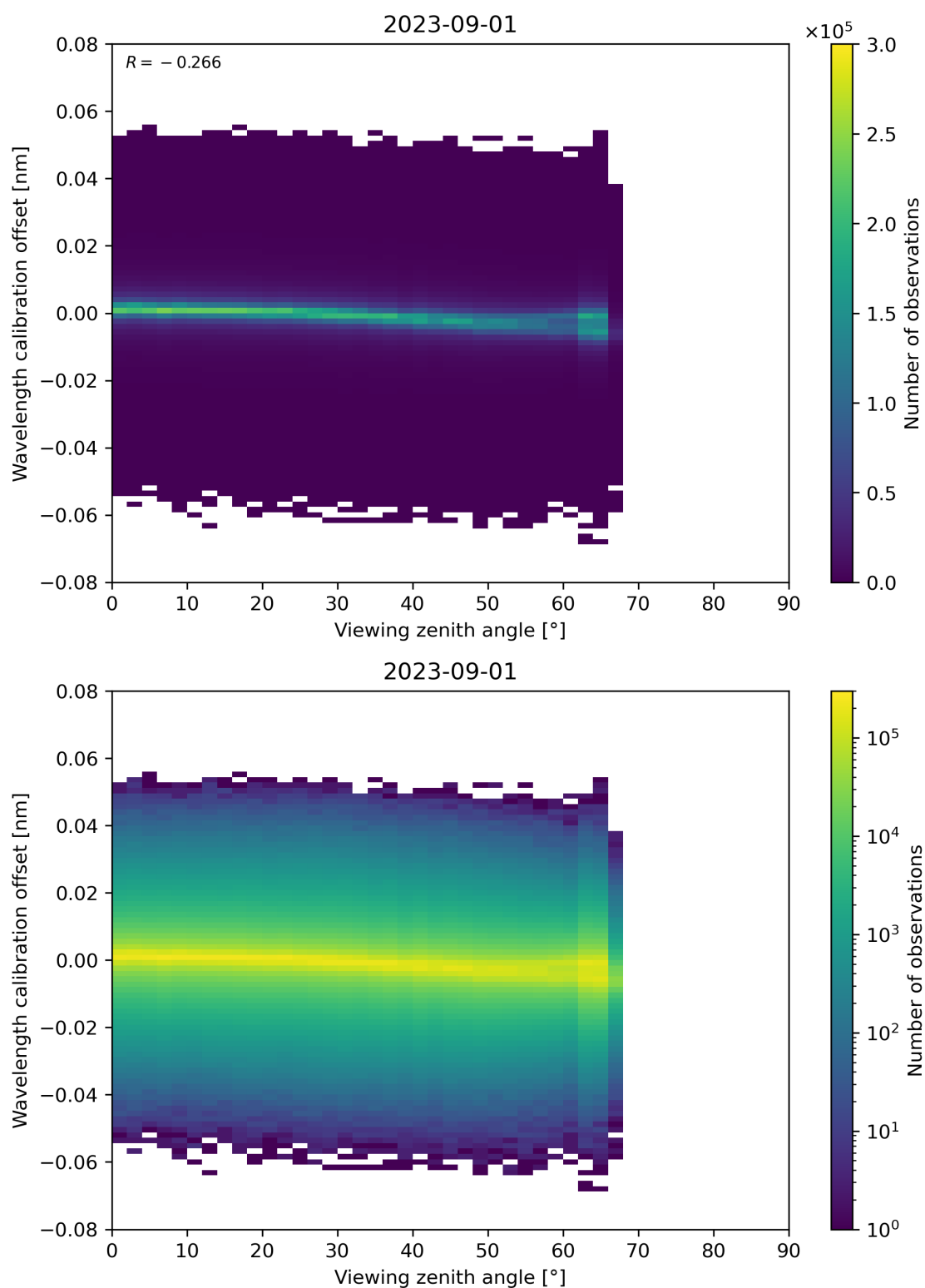
Figure 173: Scatter density plot of “Viewing zenith angle” against “Wavelength calibration offset” for 2023-08-31 to 2023-09-02.
