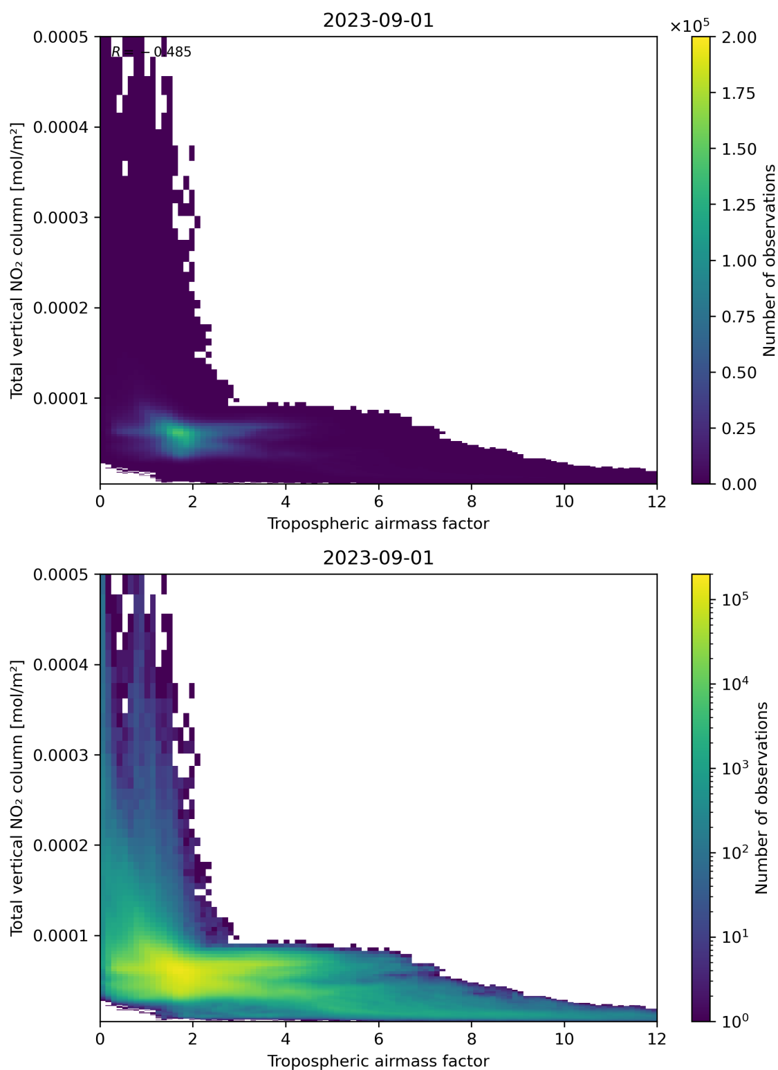
Figure 77: Scatter density plot of “Tropospheric airmass factor” against “Total vertical NO 2 column” for 2023-08-31 to 2023-09-02.
