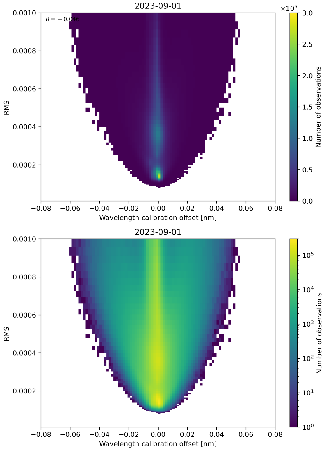
Figure 181: Scatter density plot of “Wavelength calibration offset” against “RMS” for 2023-08-31 to 2023-09-02.
