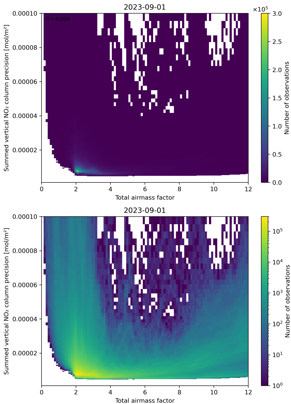
Figure 66: Scatter density plot of “Total airmass factor” against “Summed vertical NO 2 column precision” for 2023-08-31 to 2023-09-02.
