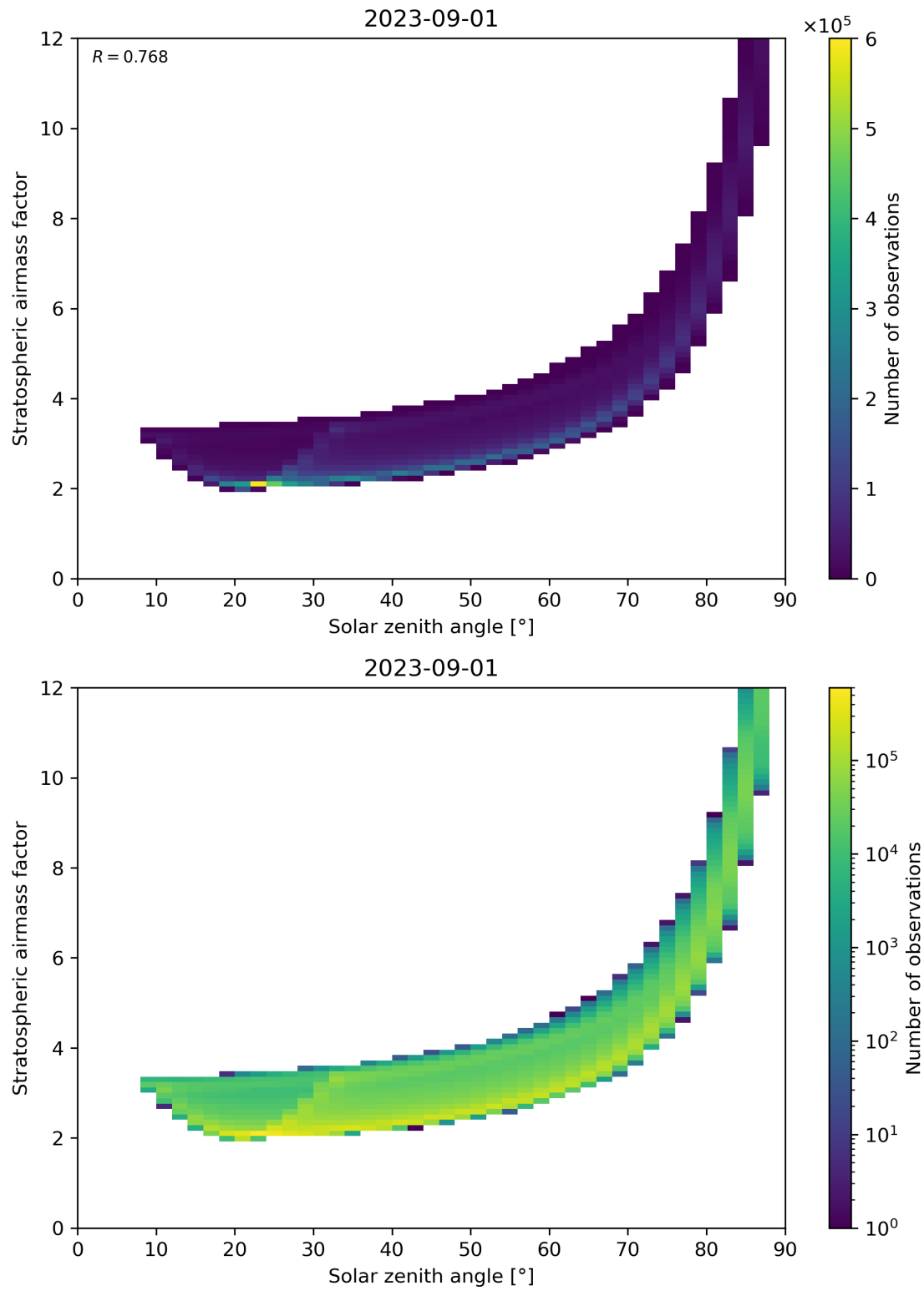
Figure 145: Scatter density plot of “Solar zenith angle” against “Stratospheric airmass factor” for 2023-08-31 to 2023-09-02.
