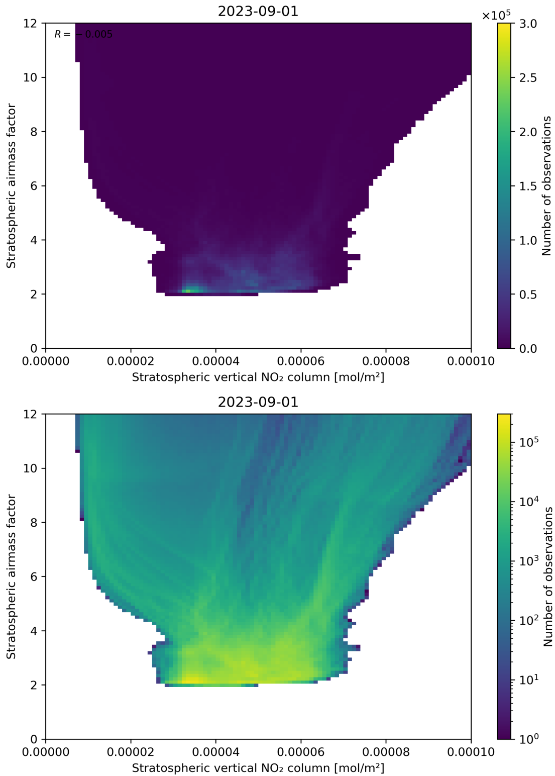
Figure 96: Scatter density plot of “Stratospheric vertical NO 2 column” against “Stratospheric airmass factor” for 2023-08-31 to 2023-09-02.
