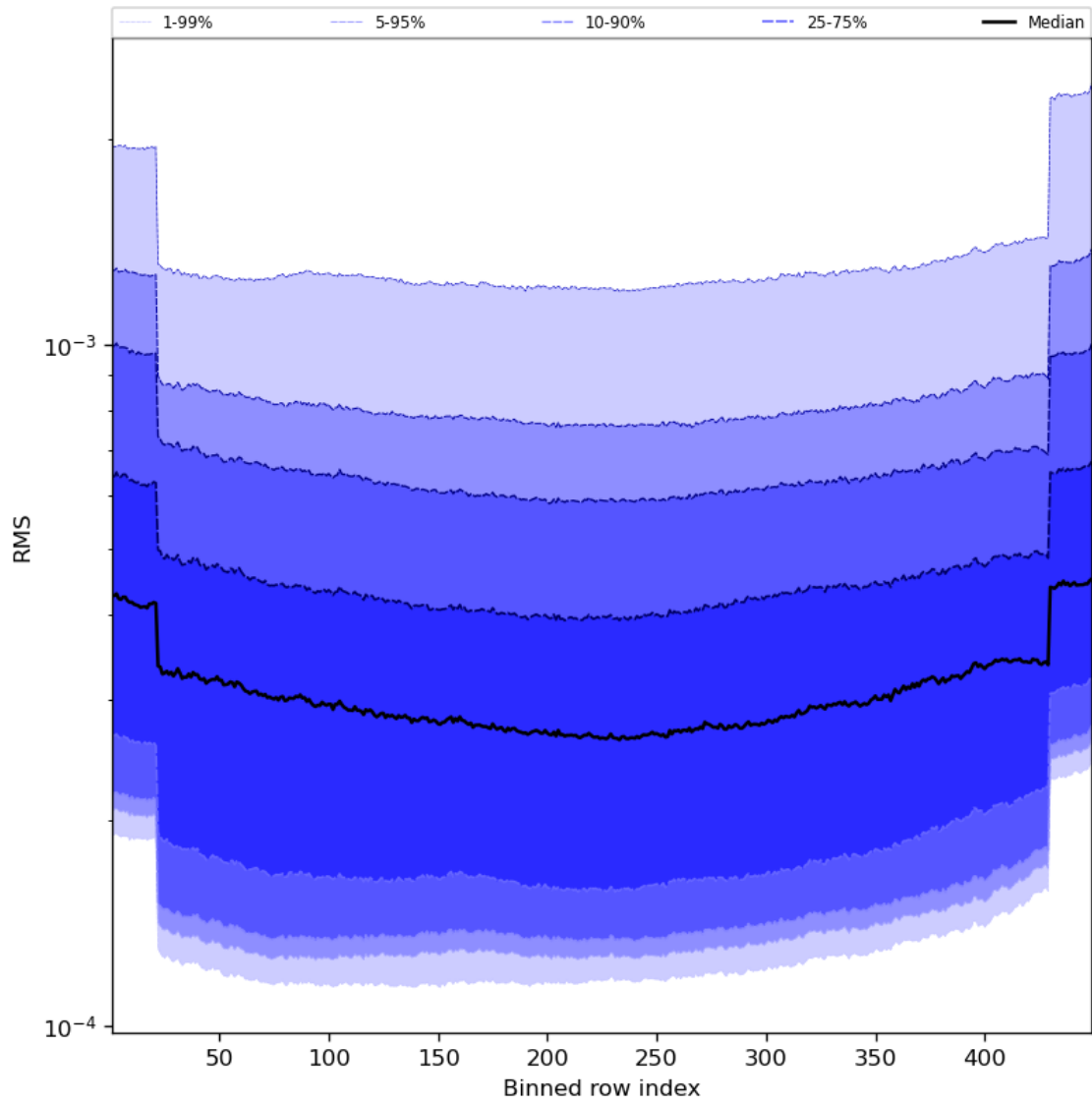
Figure 60: Along track statistics of “RMS” for 2023-08-31 to 2023-09-02
