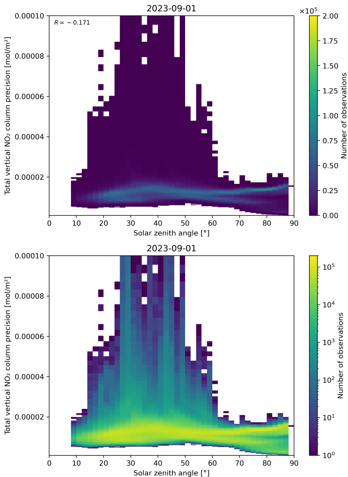
Figure 154: Scatter density plot of “Solar zenith angle” against “Total vertical NO 2 column precision” for 2023-08-31 to 2023-09-02.
