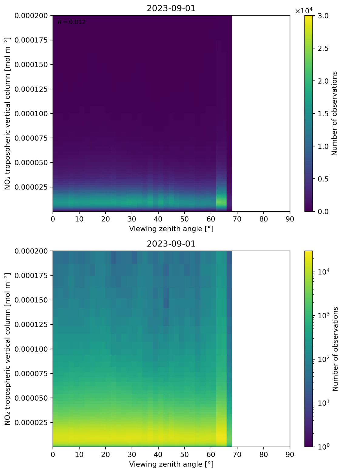
Figure 169: Scatter density plot of “Viewing zenith angle” against “NO 2 tropospheric vertical column” for 2023-08-31 to 2023-09-02.
