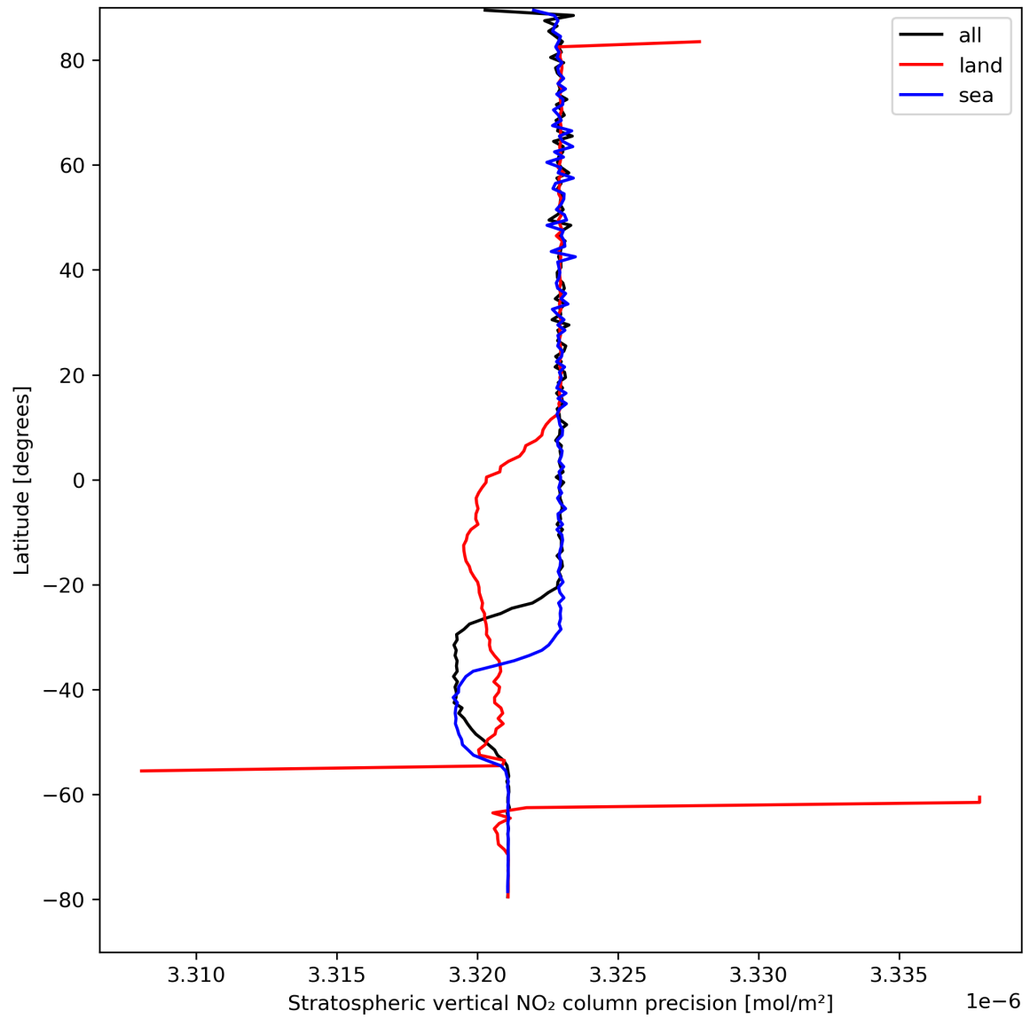
Figure 20: Zonal average of “Stratospheric vertical NO 2 column precision” for 2023-08-31 to 2023-09-02.
