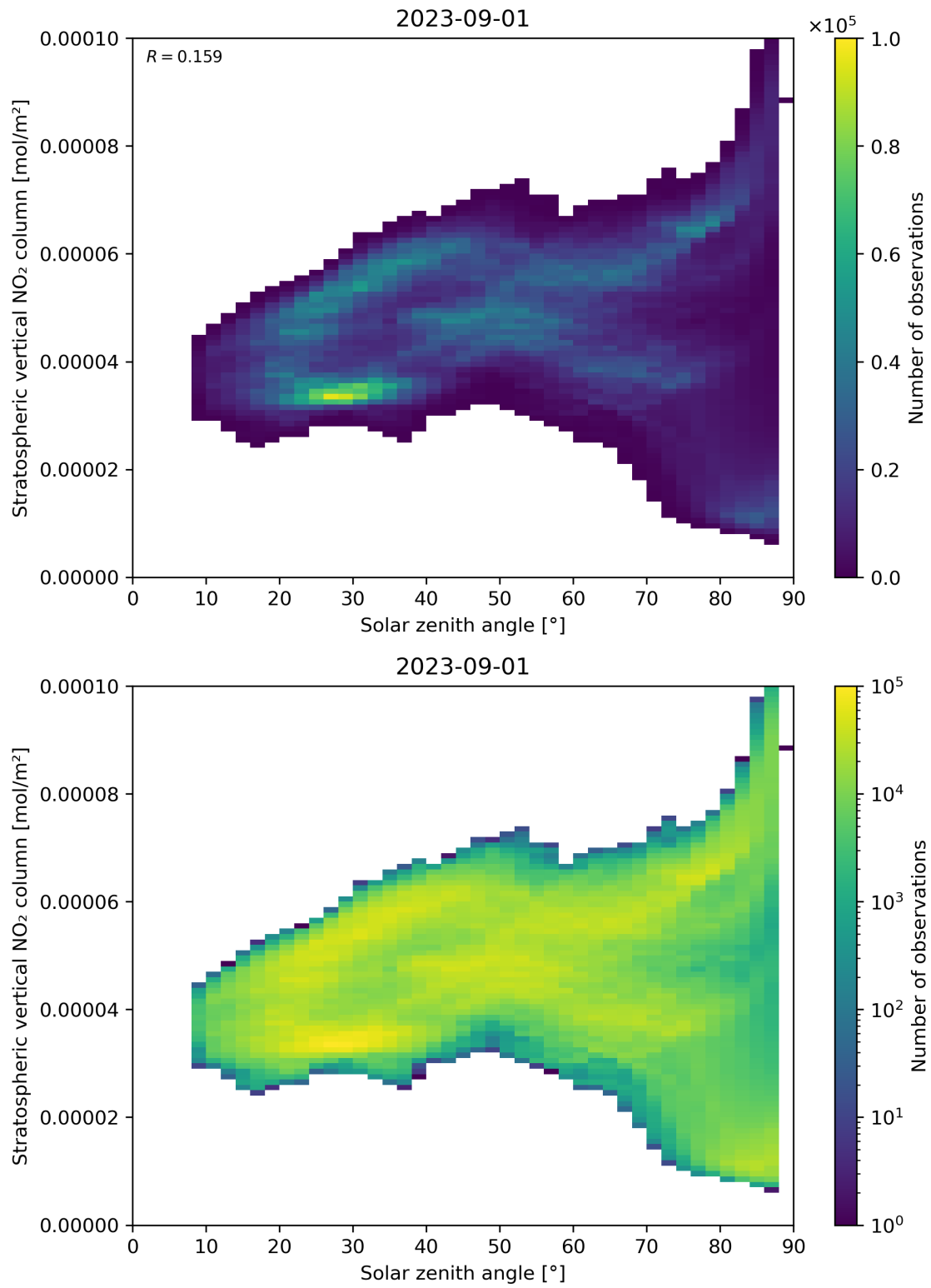
Figure 150: Scatter density plot of “Solar zenith angle” against “Stratospheric vertical NO 2 column” for 2023-08-31 to 2023-09-02.
