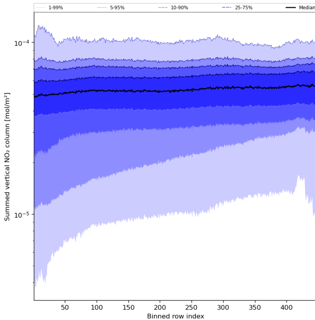
Figure 57: Along track statistics of “Summed vertical NO 2 column” for 2023-08-31 to 2023-09-02
