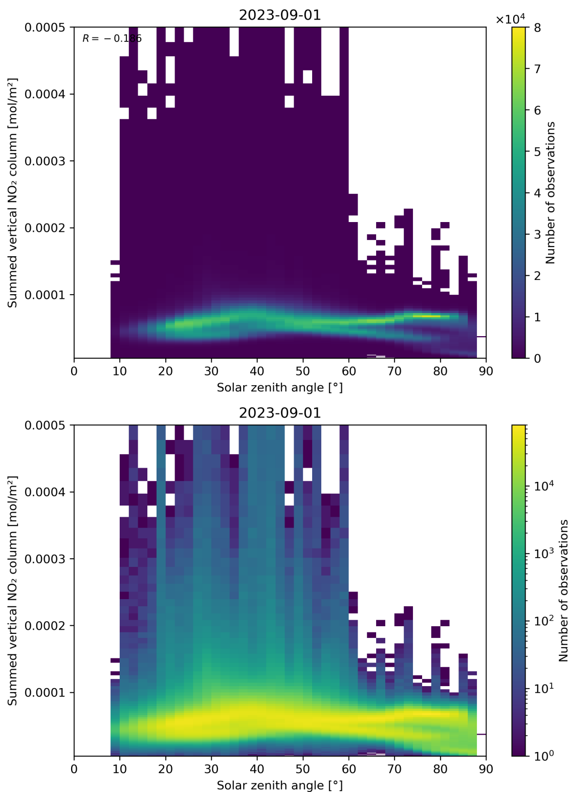
Figure 151: Scatter density plot of “Solar zenith angle” against “Summed vertical NO 2 column” for 2023-08-31 to 2023-09-02.
