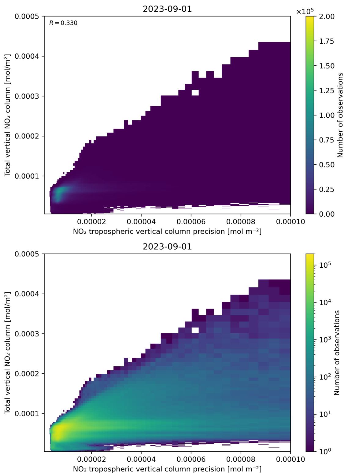
Figure 138: Scatter density plot of “NO 2 tropospheric vertical column precision” against “Total vertical NO 2 column” for 2023-08-31 to 2023-09-02.
