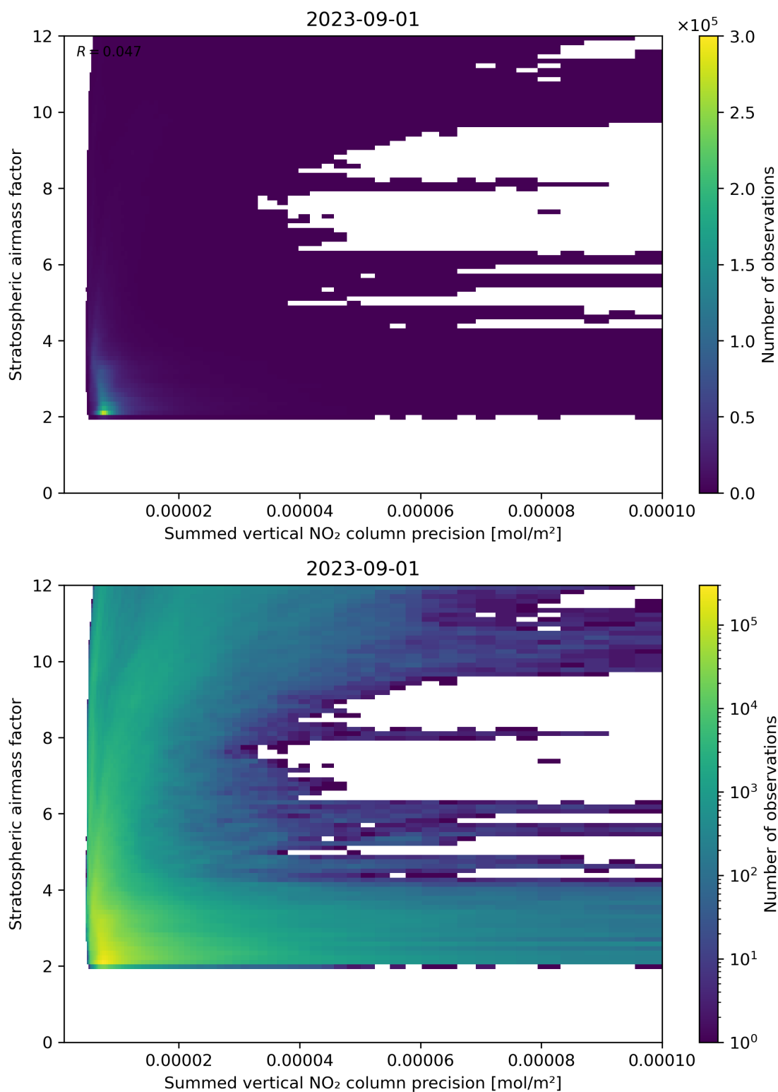
Figure 106: Scatter density plot of “Summed vertical NO 2 column precision” against “Stratospheric airmass factor” for 2023-08-31 to 2023-09-02.
