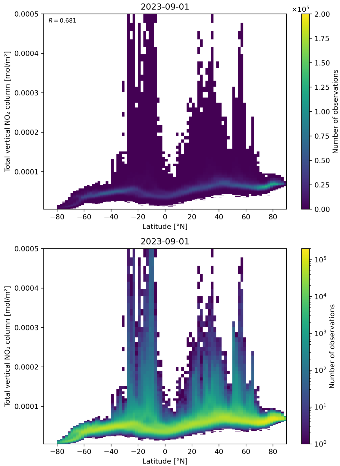
Figure 90: Scatter density plot of “Latitude” against “Total vertical NO 2 column” for 2023-08-31 to 2023-09-02.
