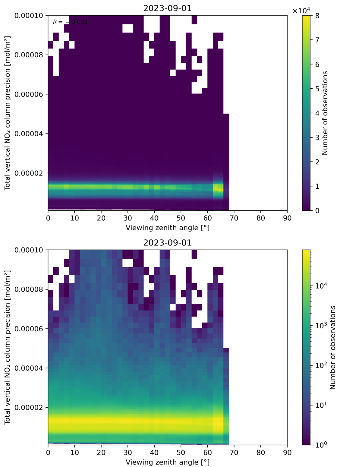
Figure 168: Scatter density plot of “Viewing zenith angle” against “Total vertical NO 2 column precision” for 2023-08-31 to 2023-09-02.
