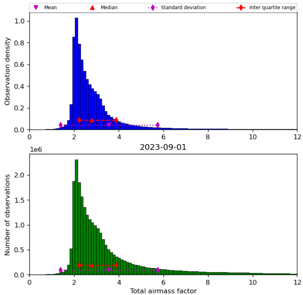
Figure 32: Histogram of “Total airmass factor” for 2023-08-31 to 2023-09-02
