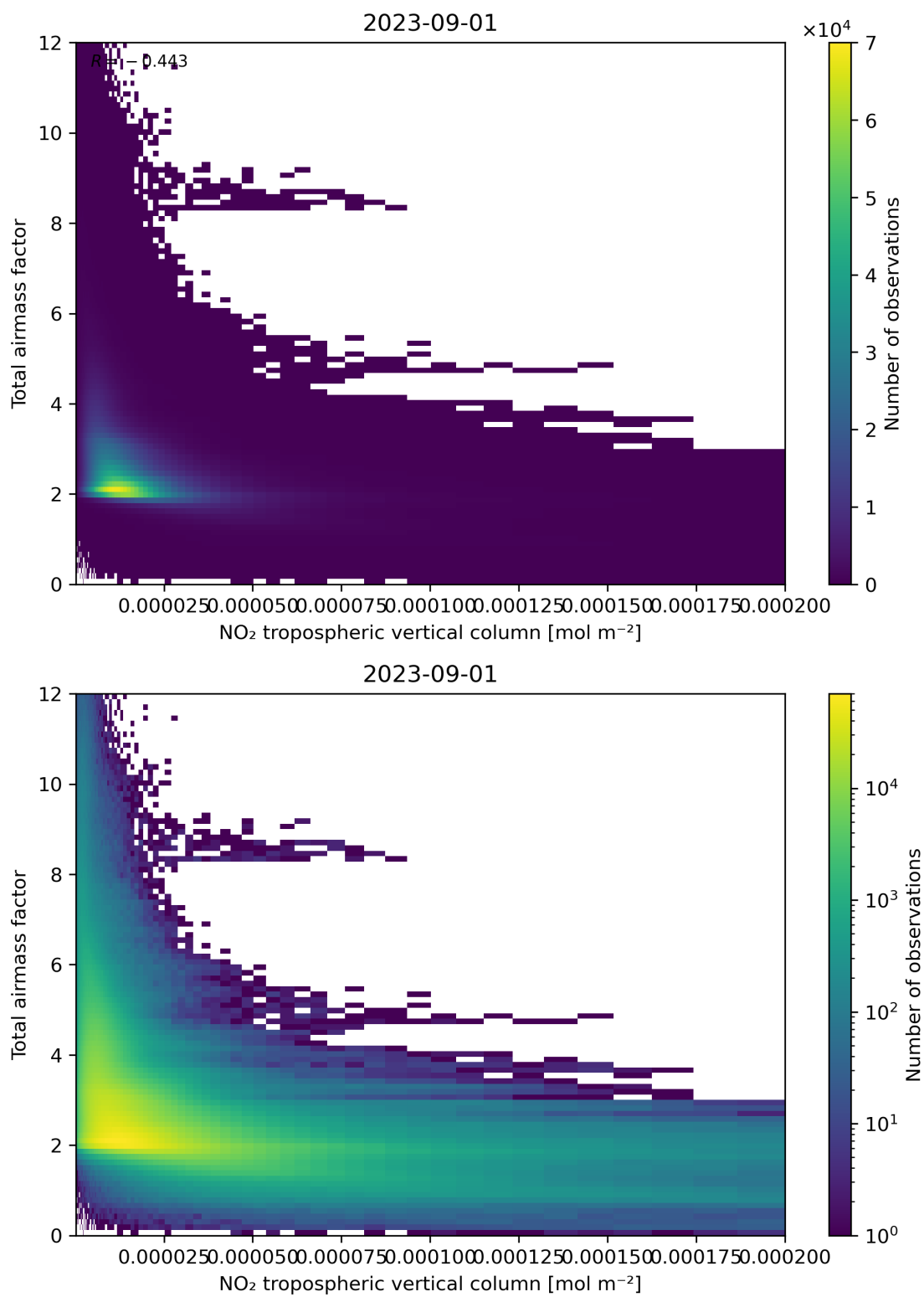
Figure 122: Scatter density plot of “NO 2 tropospheric vertical column” against “Total air mass factor” for 2023-08-31 to 2023-09-02.
