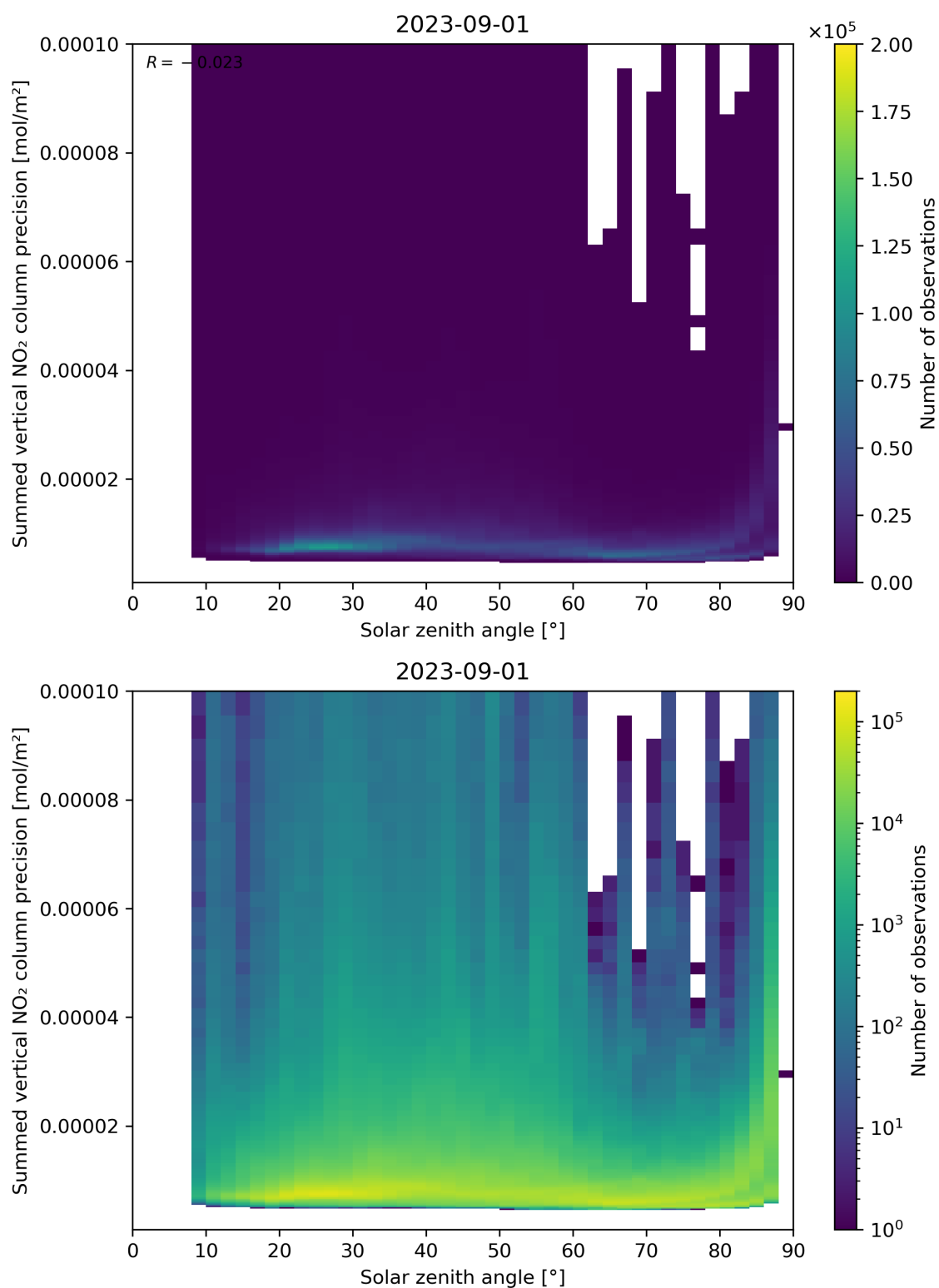
Figure 152: Scatter density plot of “Solar zenith angle” against “Summed vertical NO 2 column precision” for 2023-08-31 to 2023-09-02.
