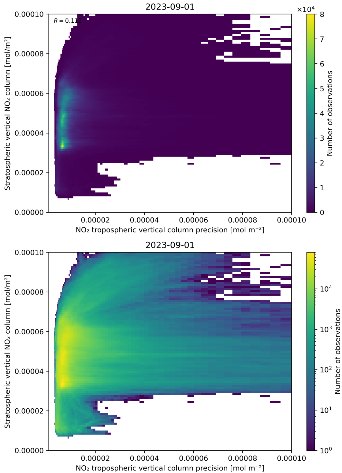
Figure 135: Scatter density plot of “NO 2 tropospheric vertical column precision” against “Stratospheric vertical NO 2 column” for 2023-08-31 to 2023-09-02.
