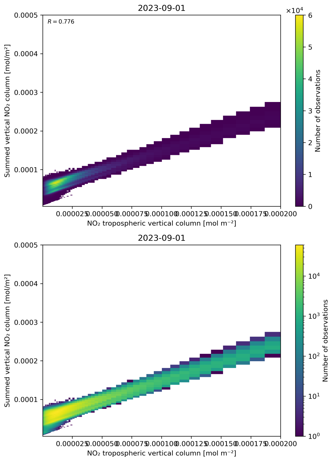
Figure 126: Scatter density plot of “NO 2 tropospheric vertical column” against “Summed vertical NO 2 column” for 2023-08-31 to 2023-09-02.
