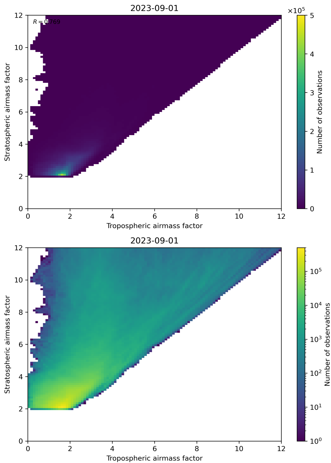
Figure 71: Scatter density plot of “Tropospheric airmass factor” against “Stratospheric airmass factor” for 2023-08-31 to 2023-09-02.
