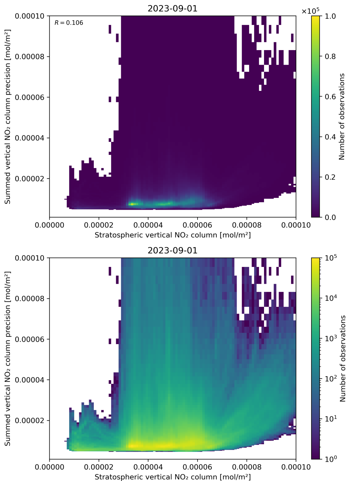
Figure 99: Scatter density plot of “Stratospheric vertical NO 2 column” against “Summed vertical NO 2 column precision” for 2023-08-31 to 2023-09-02.
