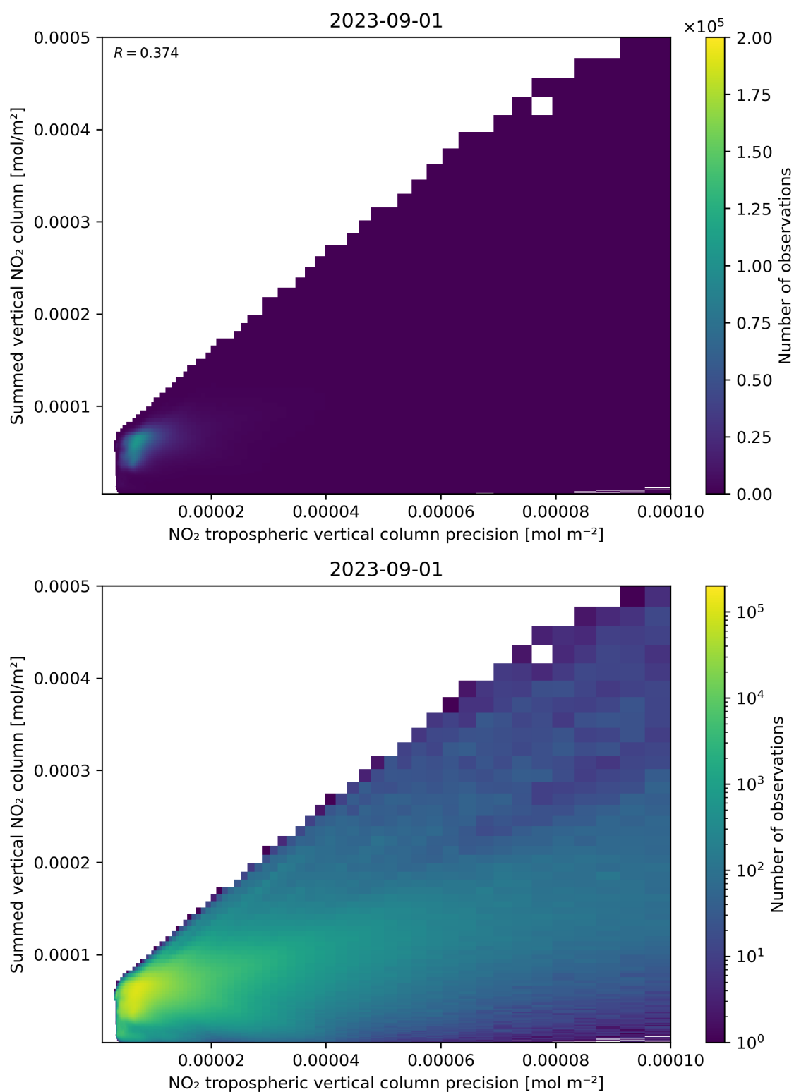
Figure 136: Scatter density plot of “NO 2 tropospheric vertical column precision” against “Summed vertical NO 2 column” for 2023-08-31 to 2023-09-02.
