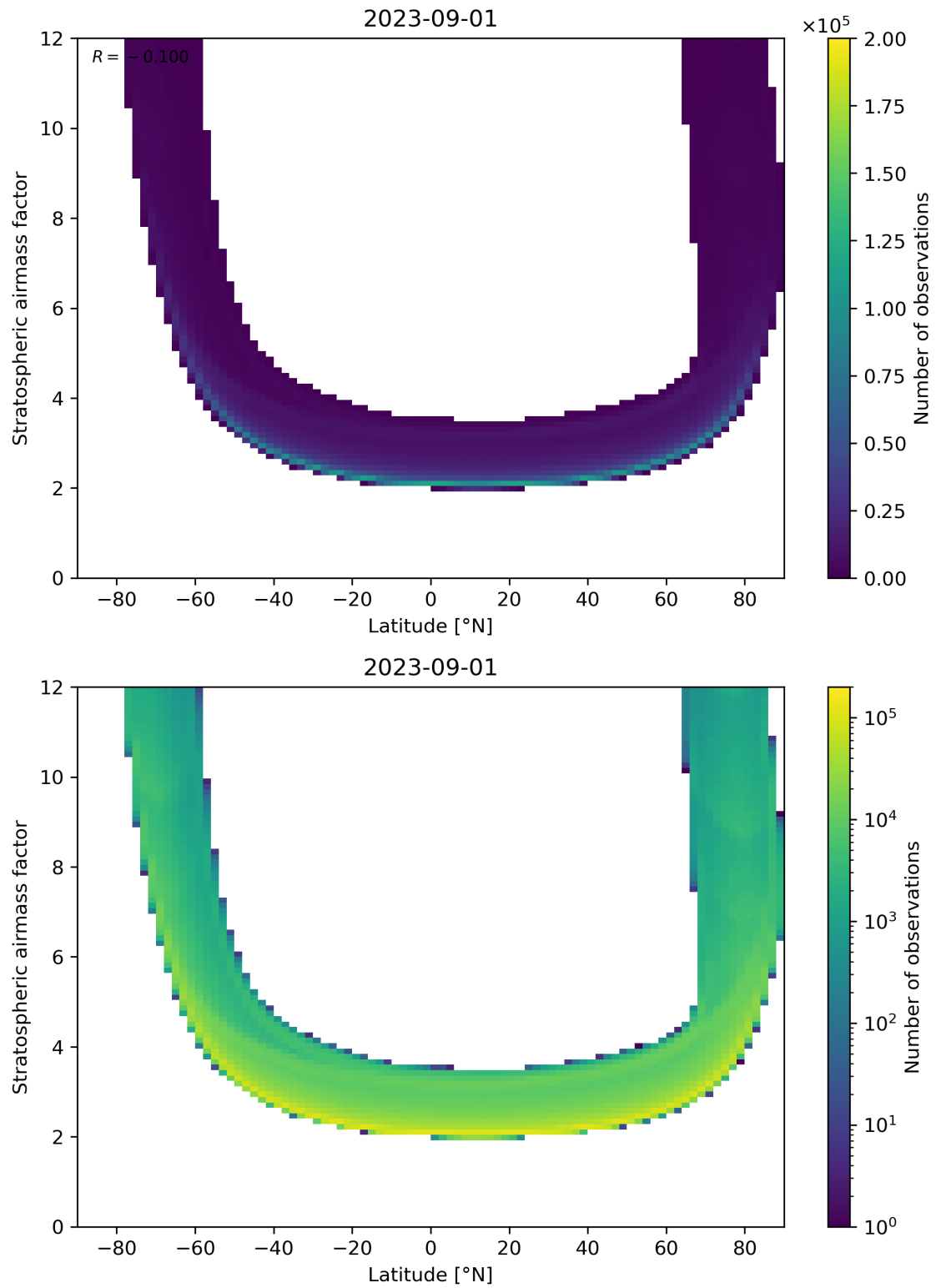
Figure 83: Scatter density plot of “Latitude” against “Stratospheric airmass factor” for 2023-08-31 to 2023-09-02.
