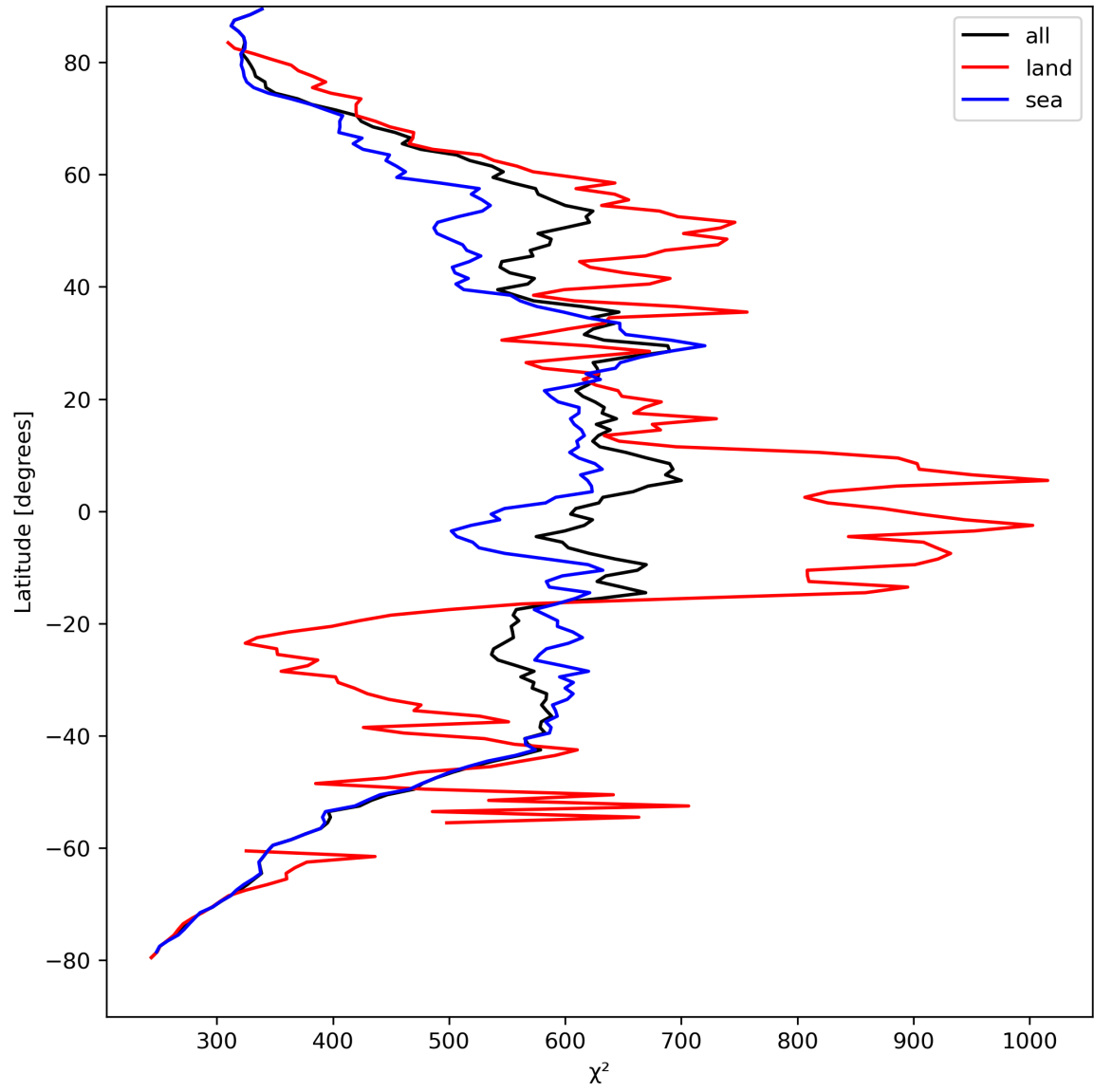
Figure 25: Zonal average of “ \chi^2 ” for 2023-08-31 to 2023-09-02.
