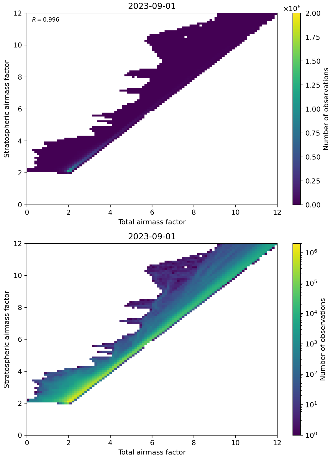
Figure 62: Scatter density plot of “Total airmass factor” against “Stratospheric airmass factor” for 2023-08-31 to 2023-09-02.
