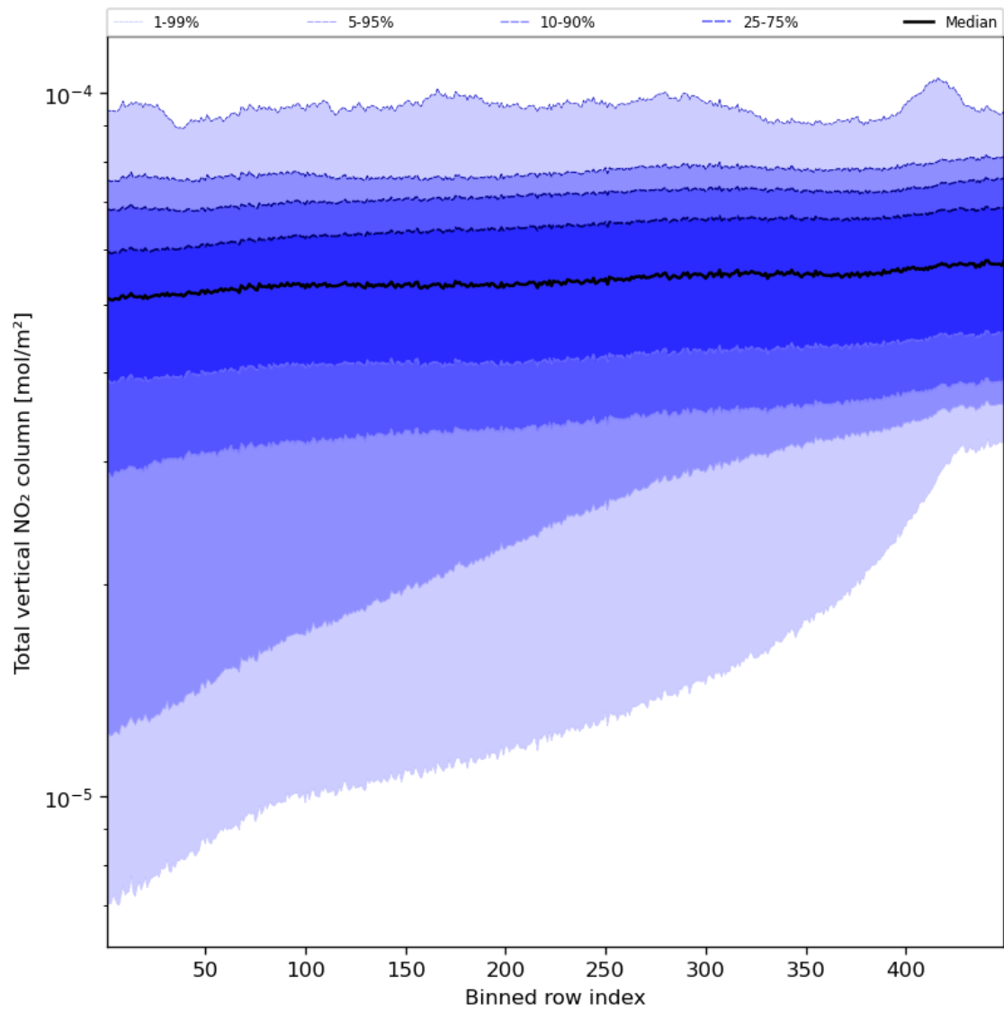
Figure 55: Along track statistics of “Total vertical NO 2 column” for 2023-08-31 to 2023-09-02
