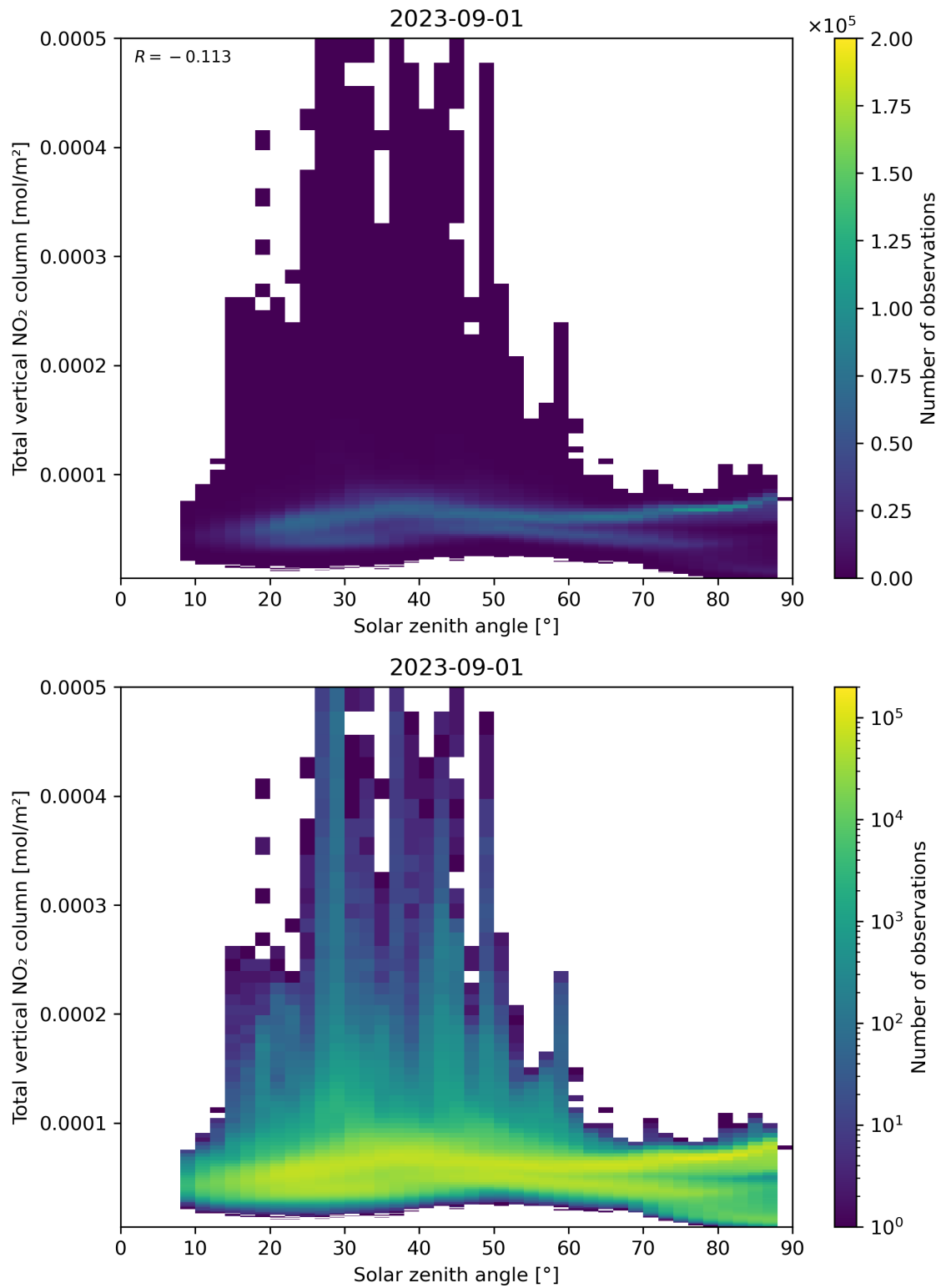
Figure 153: Scatter density plot of “Solar zenith angle” against “Total vertical NO 2 column” for 2023-08-31 to 2023-09-02.
