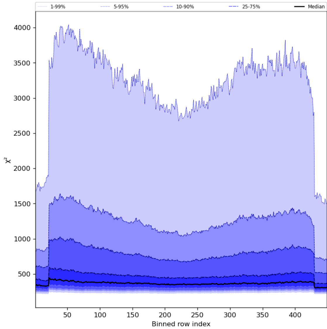
Figure 59: Along track statistics of “ \chi^2 ” for 2023-08-31 to 2023-09-02
