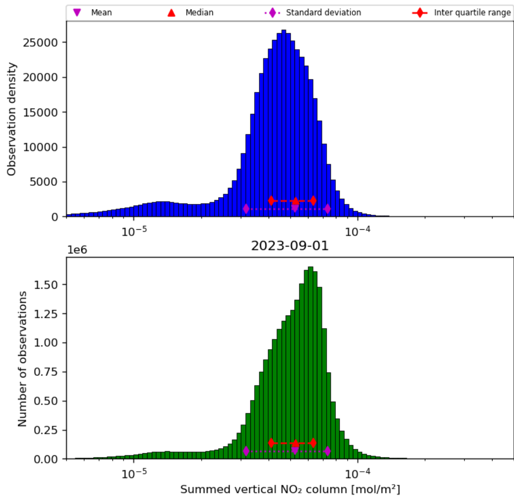
Figure 40: Histogram of “Summed vertical NO 2 column” for 2023-08-31 to 2023-09-02
