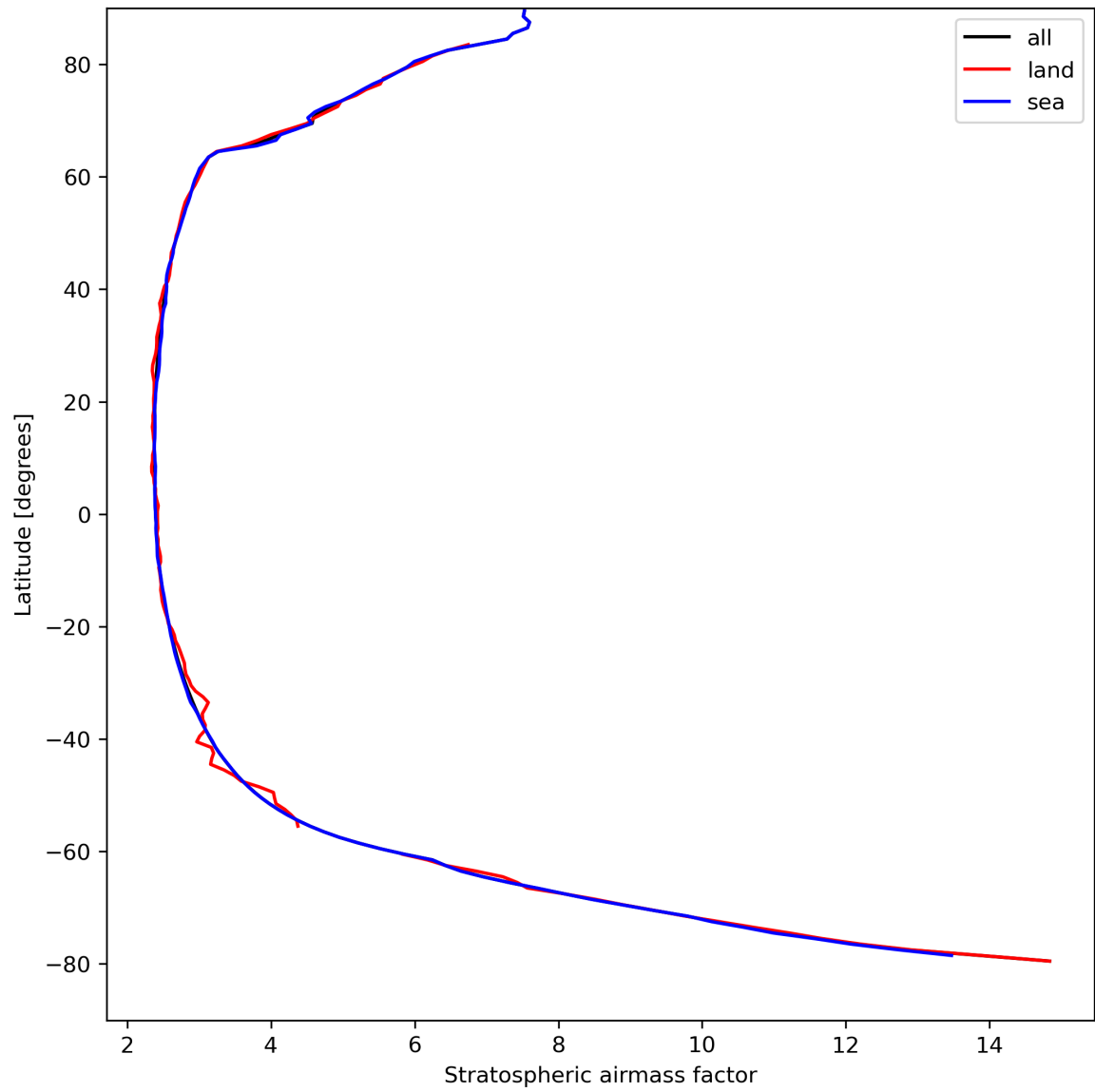
Figure 27: Zonal average of “Stratospheric airmass factor” for 2023-08-31 to 2023-09-02.
