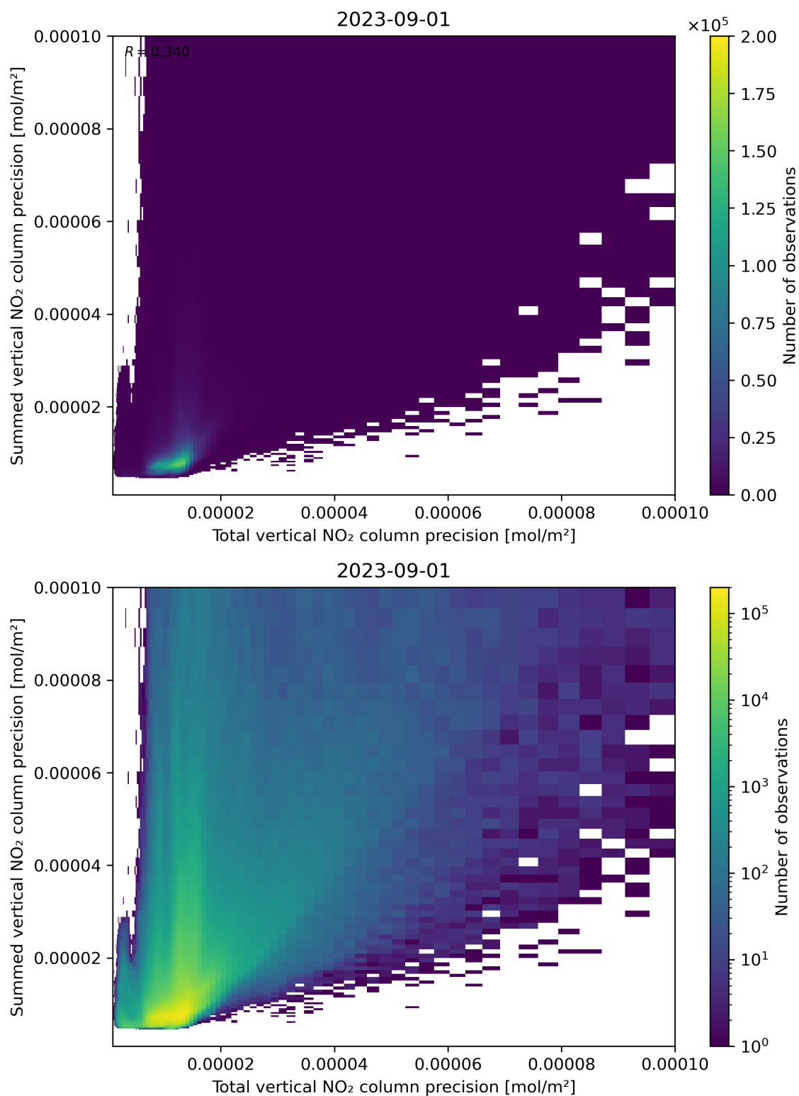
Figure 118: Scatter density plot of “Total vertical NO 2 column precision” against “Summed vertical NO 2 column precision” for 2023-08-31 to 2023-09-02.
