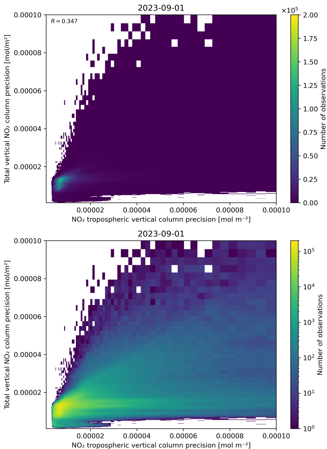
Figure 139: Scatter density plot of “NO 2 tropospheric vertical column precision” against “Total vertical NO 2 column precision” for 2023-08-31 to 2023-09-02.
