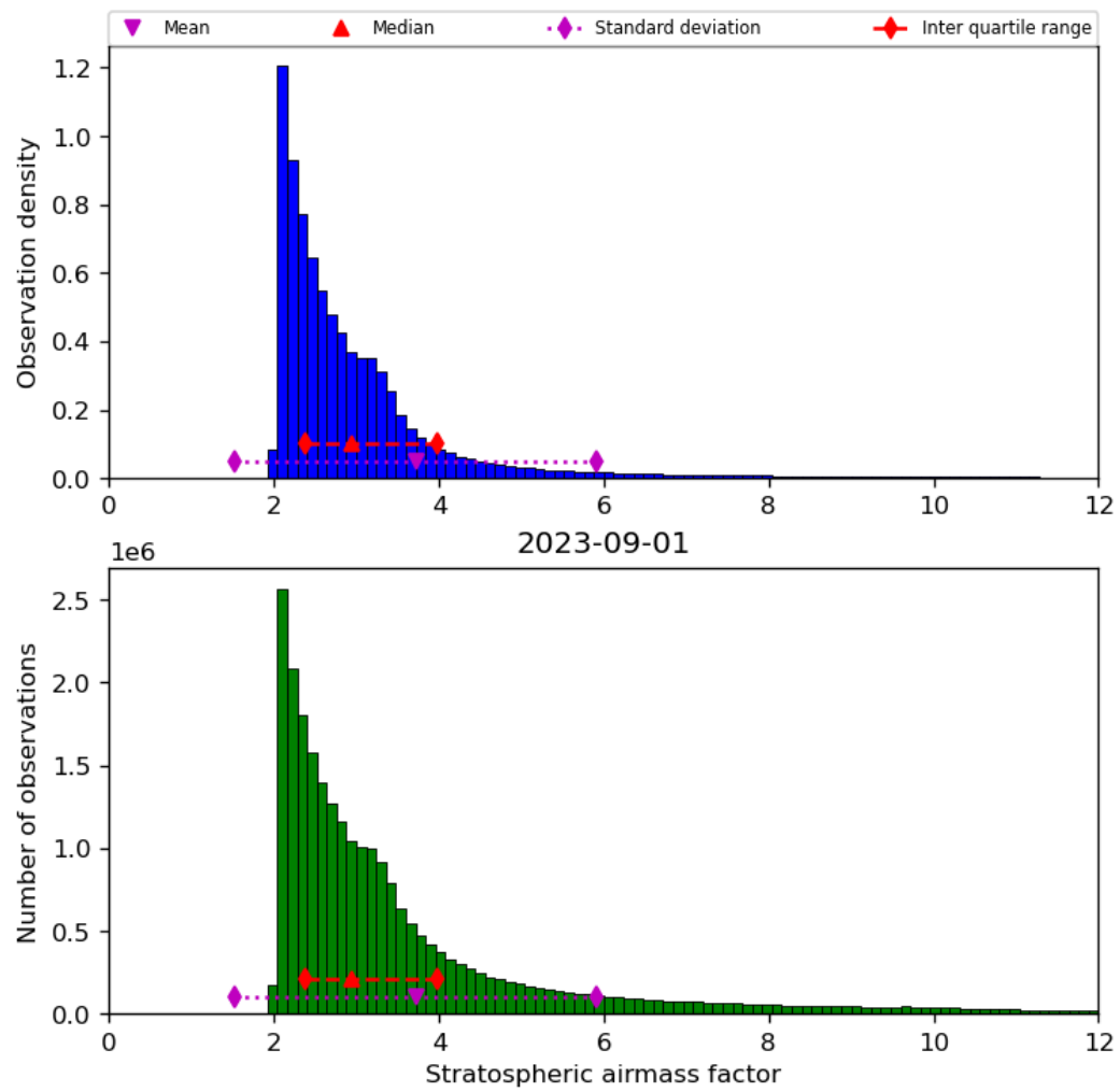
Figure 44: Histogram of “Stratospheric airmass factor” for 2023-08-31 to 2023-09-02
