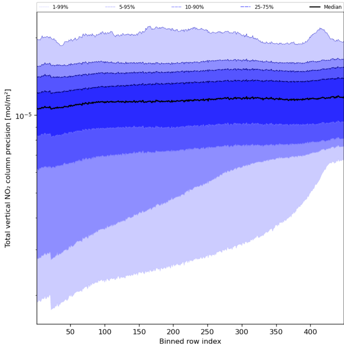
Figure 56: Along track statistics of “Total vertical NO 2 column precision” for 2023-08-31 to 2023-09-02
