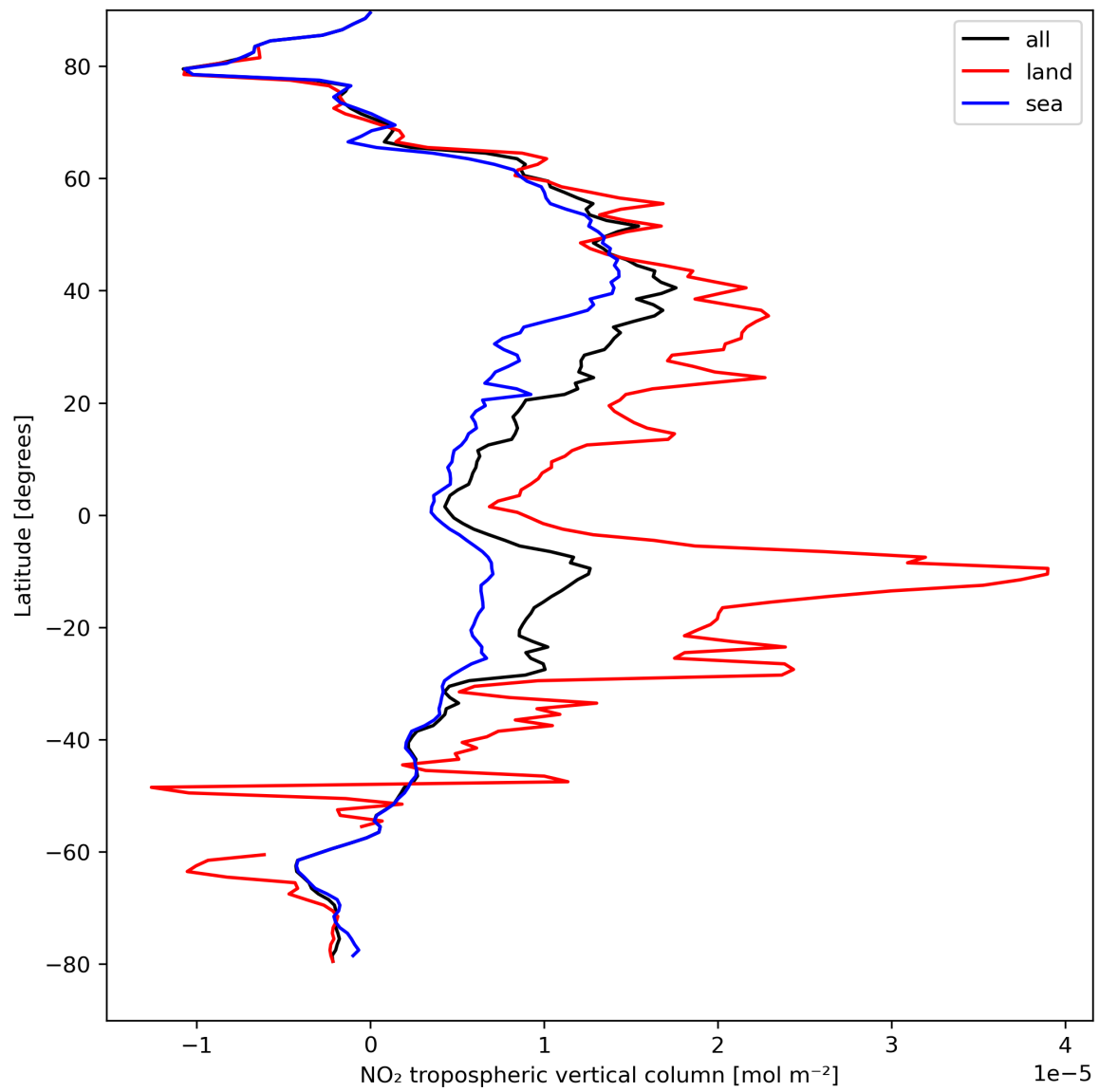
Figure 12: Zonal average of “NO 2 tropospheric vertical column” for 2023-08-31 to 2023-09-02.
