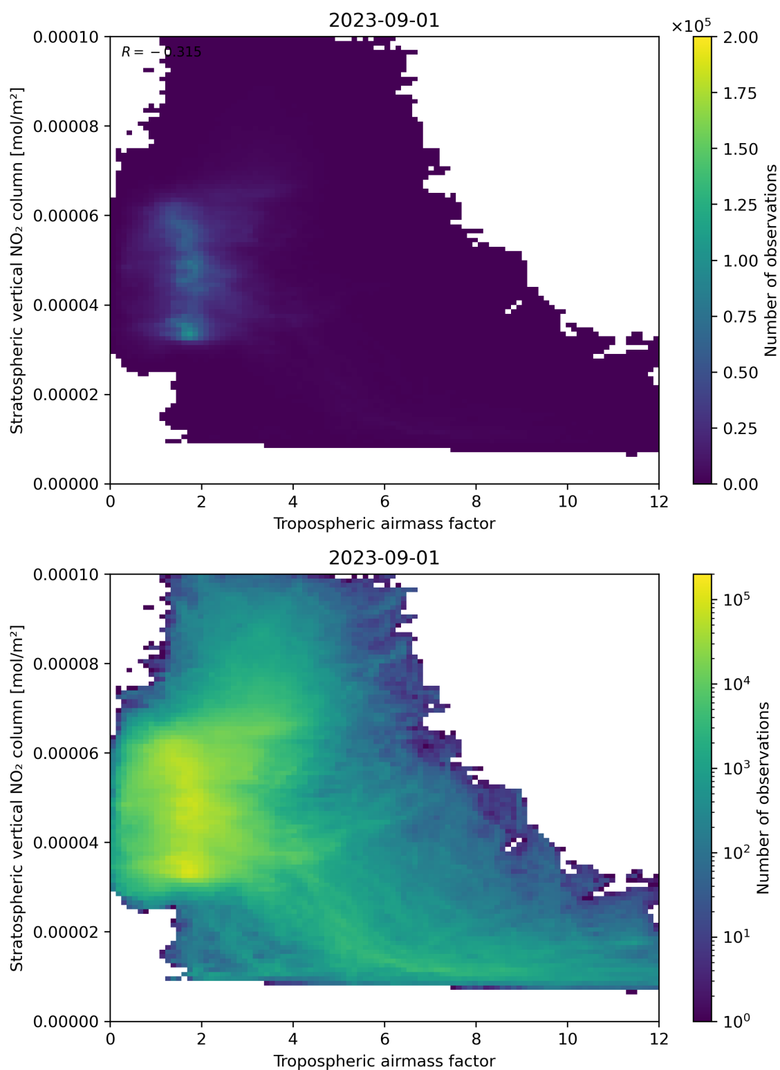
Figure 74: Scatter density plot of “Tropospheric air mass factor” against “Stratospheric vertical NO 2 column” for 2023-08-31 to 2023-09-02.
