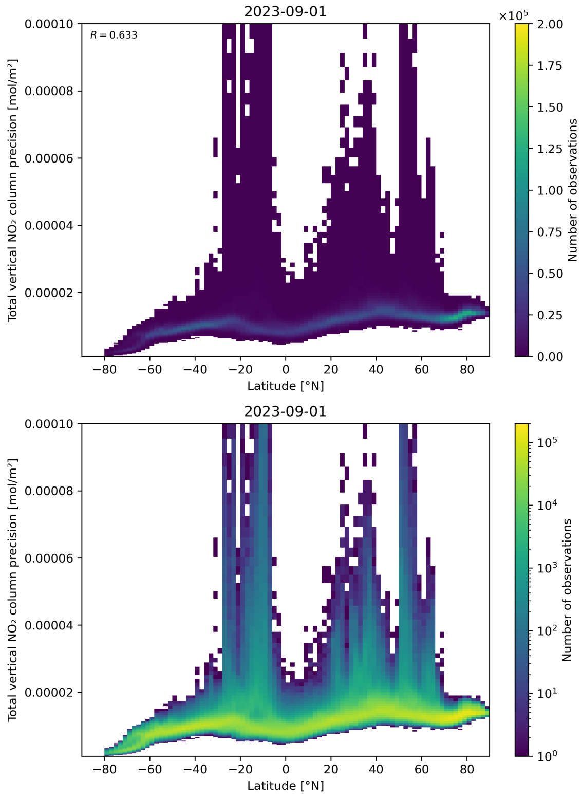
Figure 91: Scatter density plot of “Latitude” against “Total vertical NO 2 column precision” for 2023-08-31 to 2023-09-02.
