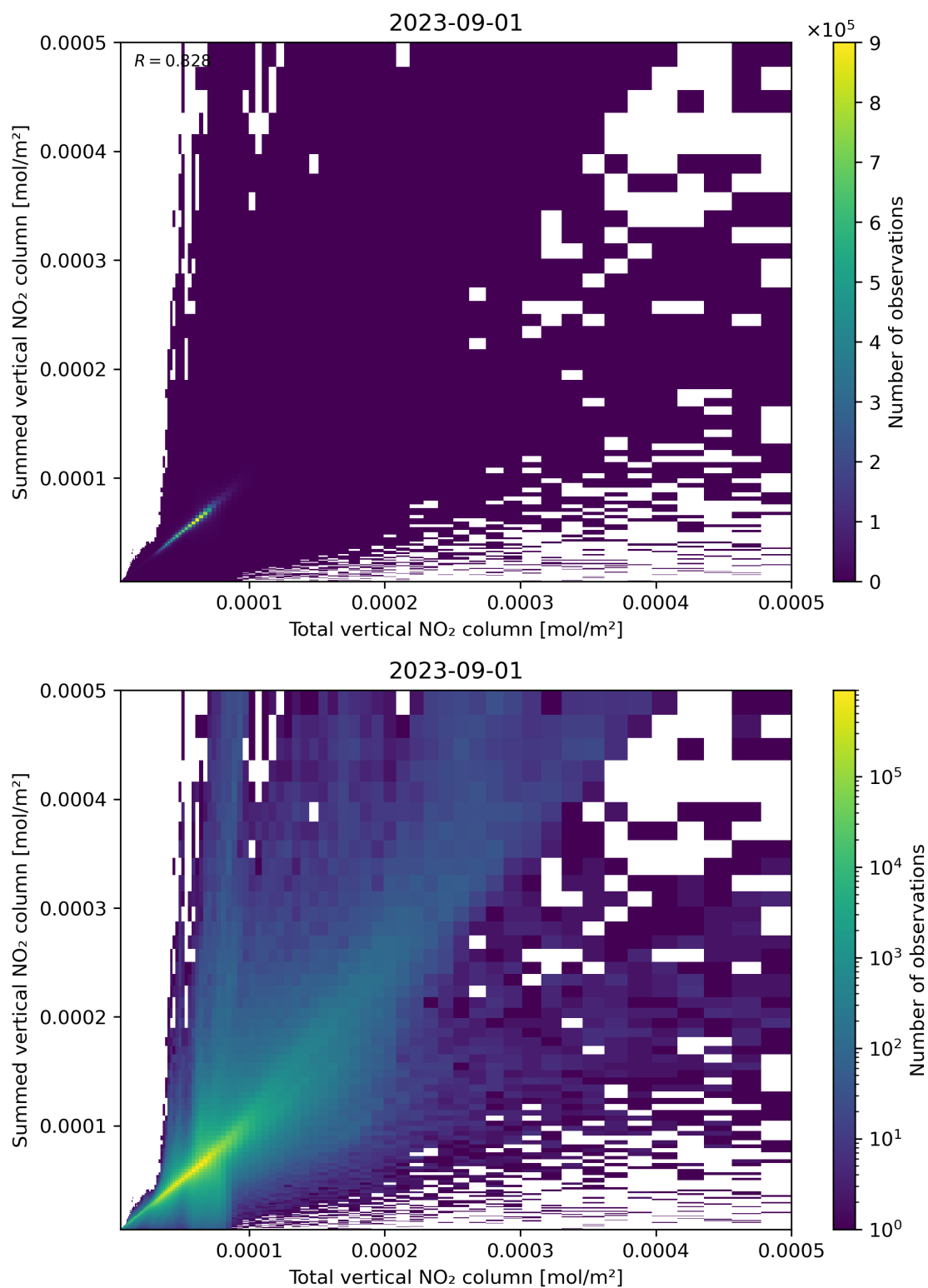
Figure 112: Scatter density plot of “Total vertical NO 2 column” against “Summed vertical NO 2 column” for 2023-08-31 to 2023-09-02.
