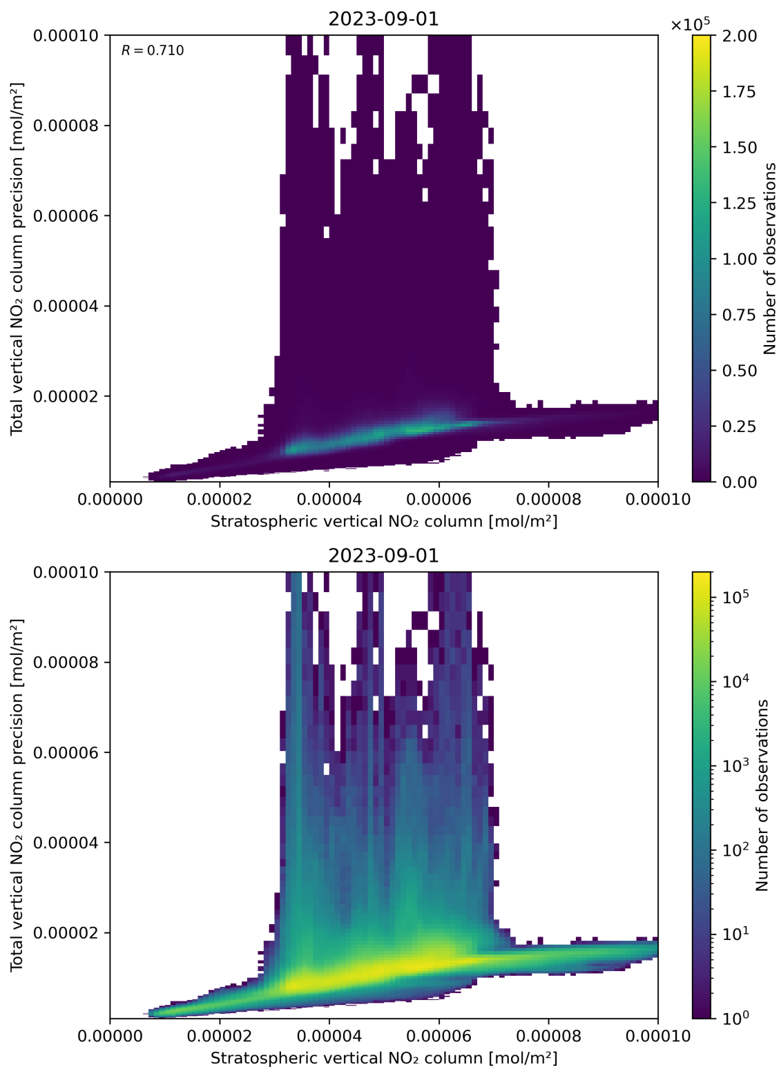
Figure 101: Scatter density plot of “Stratospheric vertical NO 2 column” against “Total vertical NO 2 column precision” for 2023-08-31 to 2023-09-02.
