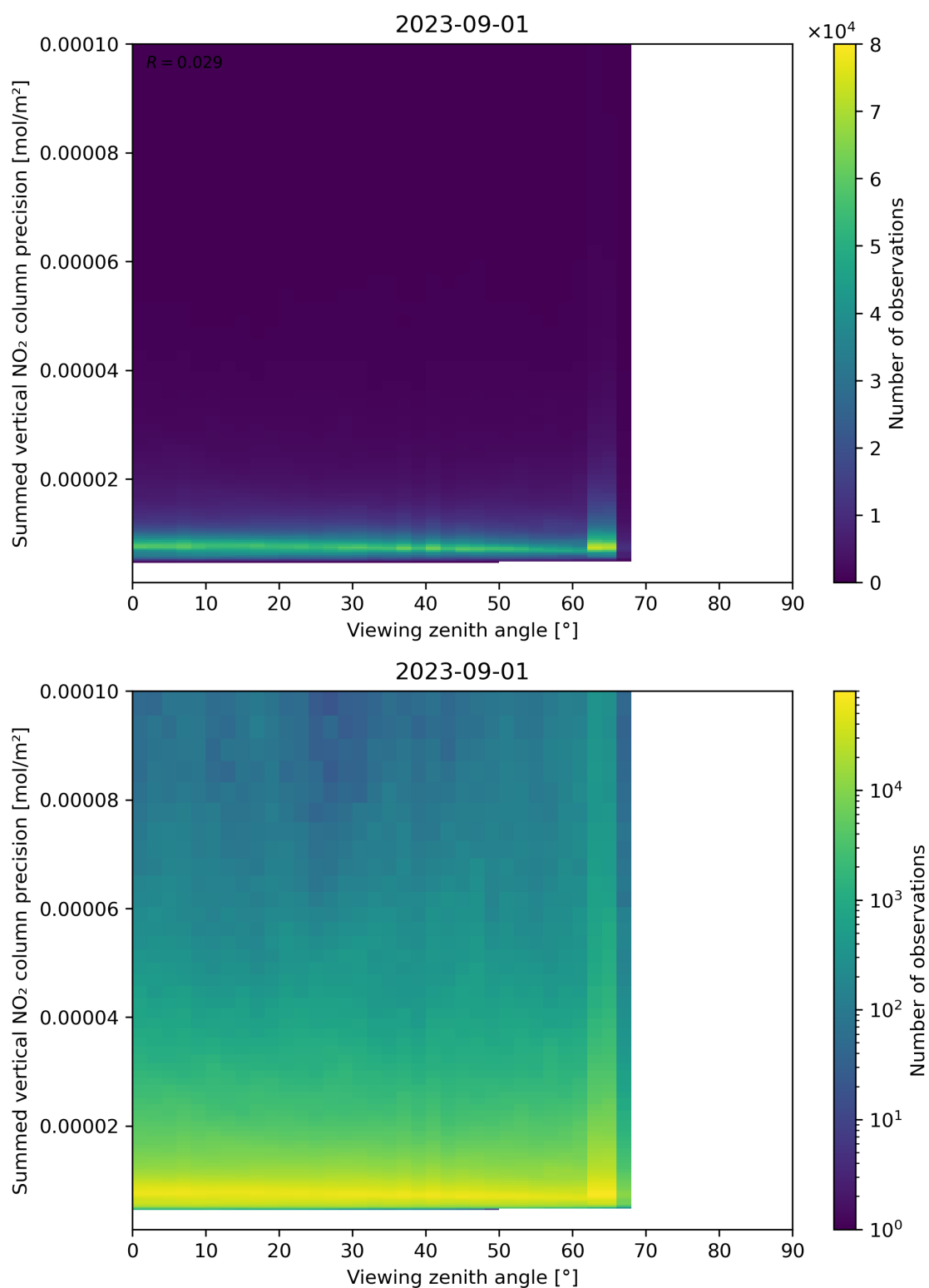
Figure 166: Scatter density plot of “Viewing zenith angle” against “Summed vertical NO 2 column precision” for 2023-08-31 to 2023-09-02.
