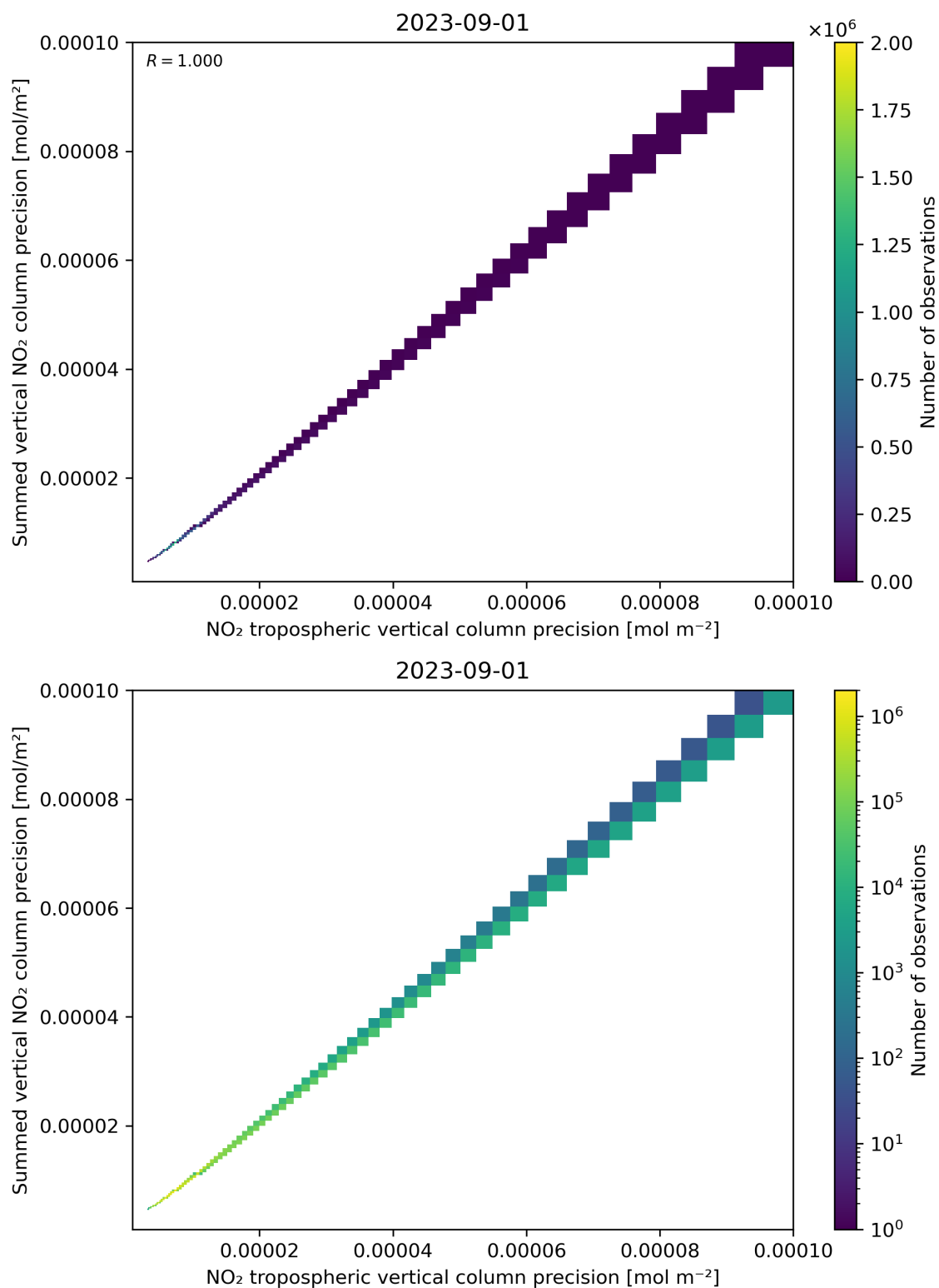
Figure 137: Scatter density plot of “NO 2 tropospheric vertical column precision” against “Summed vertical NO 2 column precision” for 2023-08-31 to 2023-09-02.
