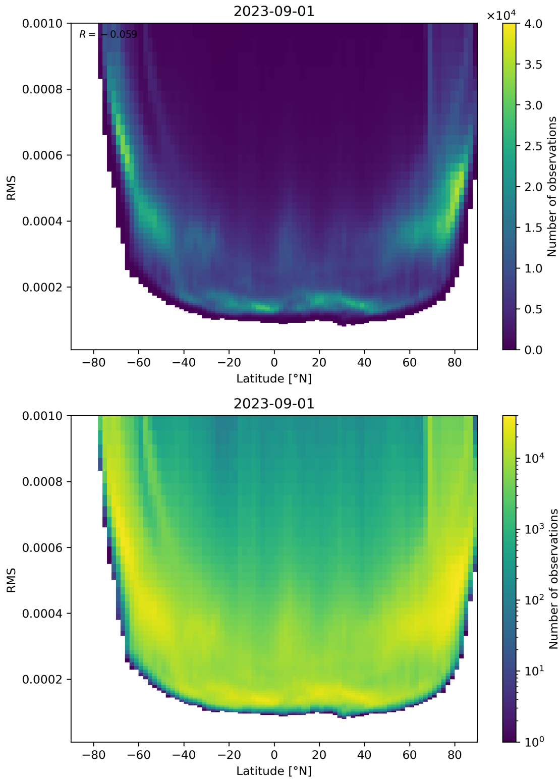
Figure 94: Scatter density plot of “Latitude” against “RMS” for 2023-08-31 to 2023-09-02.
