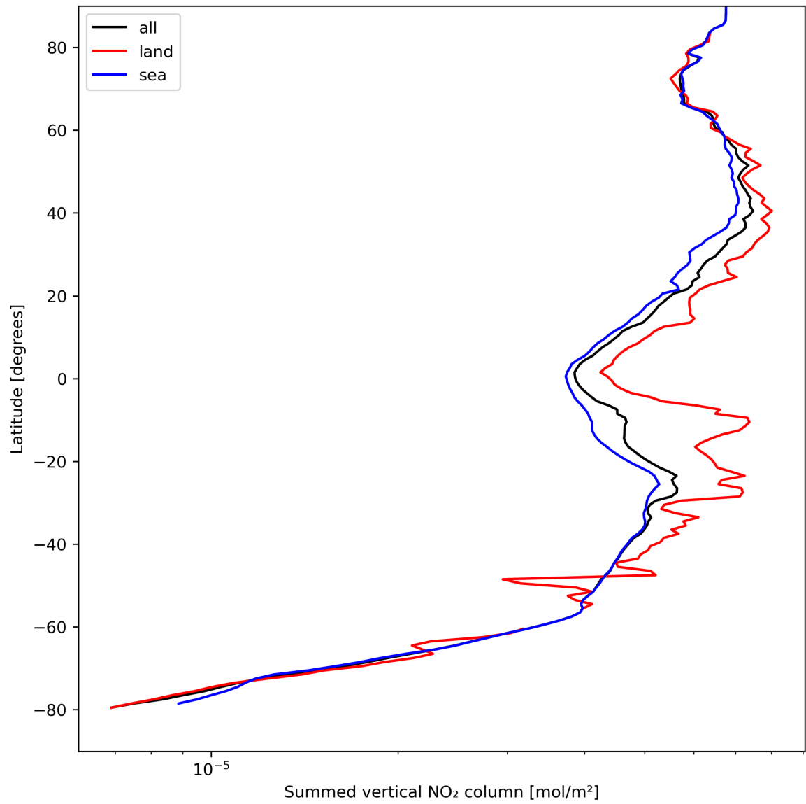
Figure 23: Zonal average of “Summed vertical NO 2 column” for 2023-08-31 to 2023-09-02.
