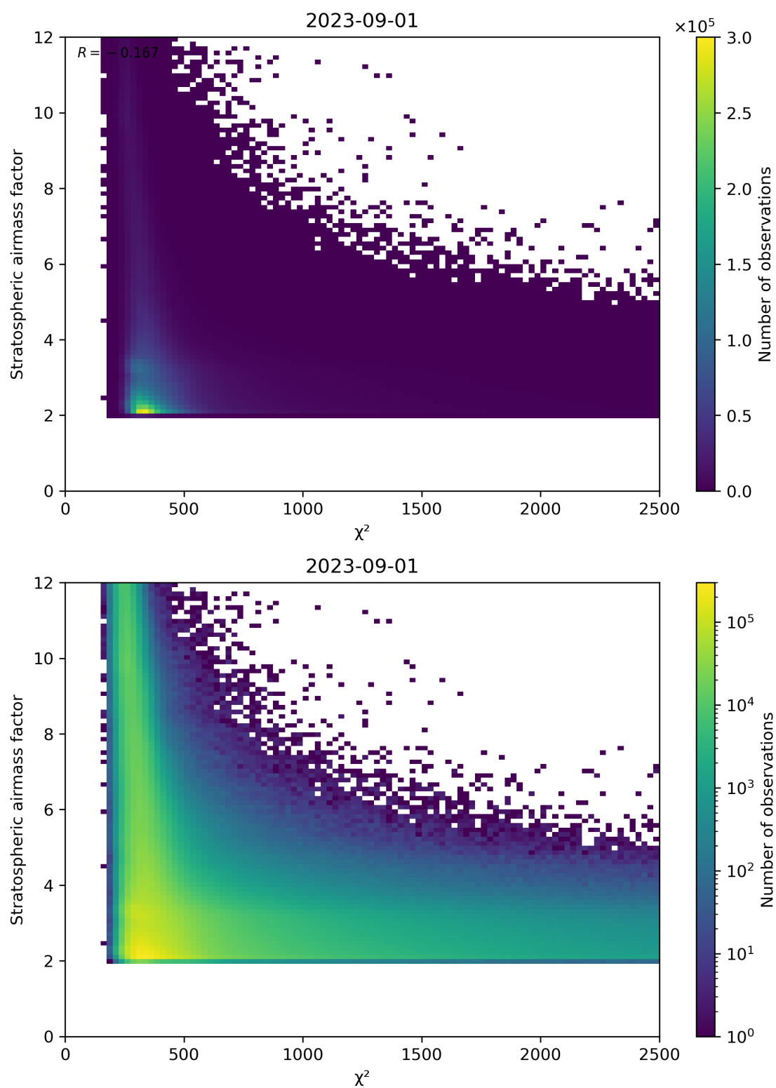
Figure 81: Scatter density plot of “ \chi^2 ” against “Stratospheric airmass factor” for 2023-08-31 to 2023-09-02.
