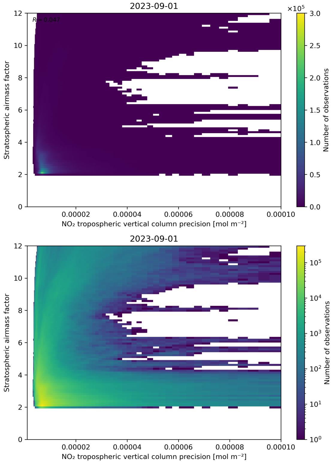
Figure 131: Scatter density plot of “NO 2 tropospheric vertical column precision” against “Stratospheric airmass factor” for 2023-08-31 to 2023-09-02.
