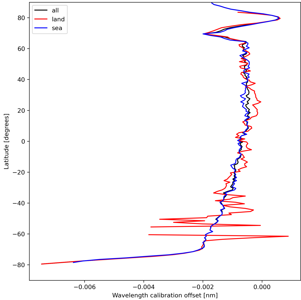
Figure 18: Zonal average of “Wavelength calibration offset” for 2023-08-31 to 2023-09-02.
