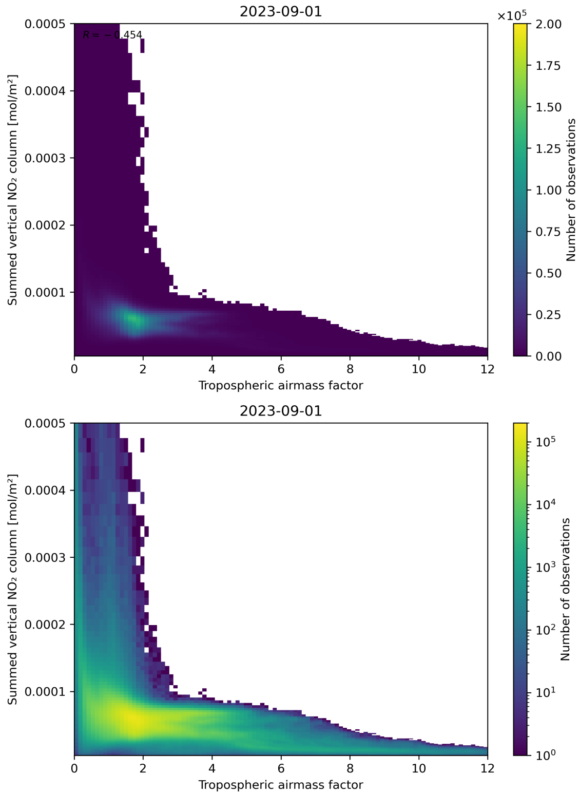
Figure 75: Scatter density plot of “Tropospheric air mass factor” against “Summed vertical NO 2 column” for 2023-08-31 to 2023-09-02.
