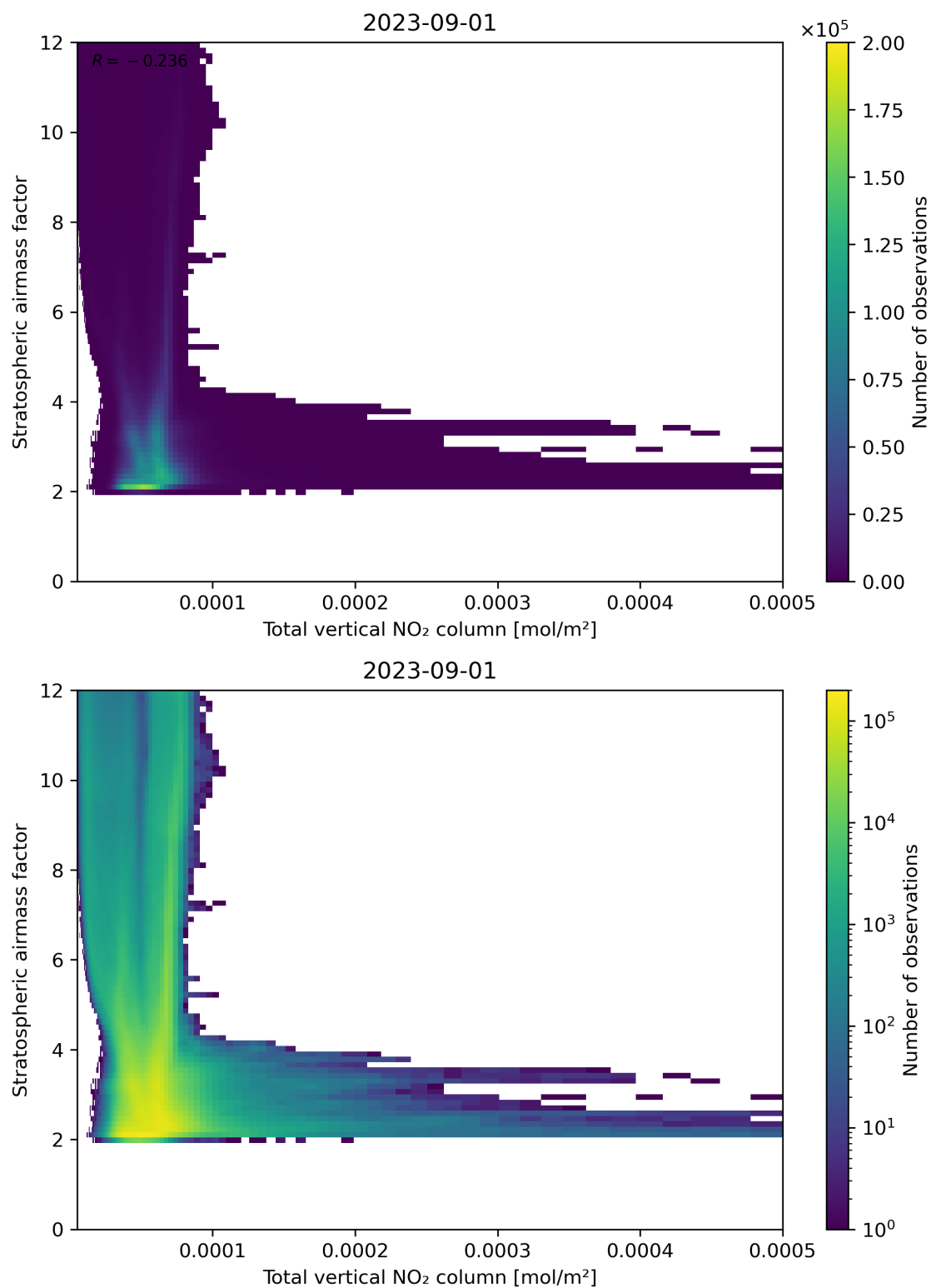
Figure 110: Scatter density plot of “Total vertical NO 2 column” against “Stratospheric airmass factor” for 2023-08-31 to 2023-09-02.
