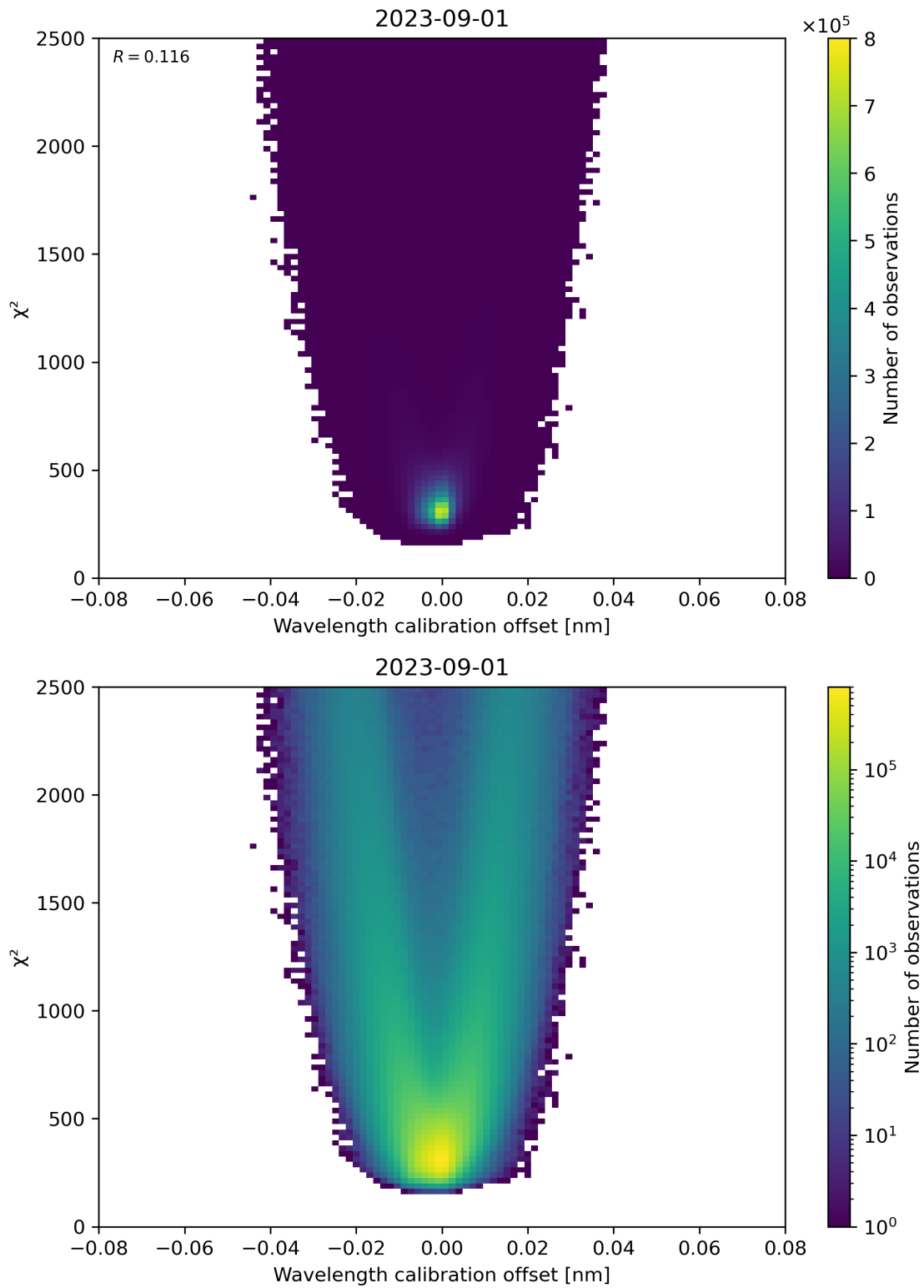
Figure 175: Scatter density plot of “Wavelength calibration offset” against “ \chi^2 ” for 2023-08-31 to 2023-09-02.
