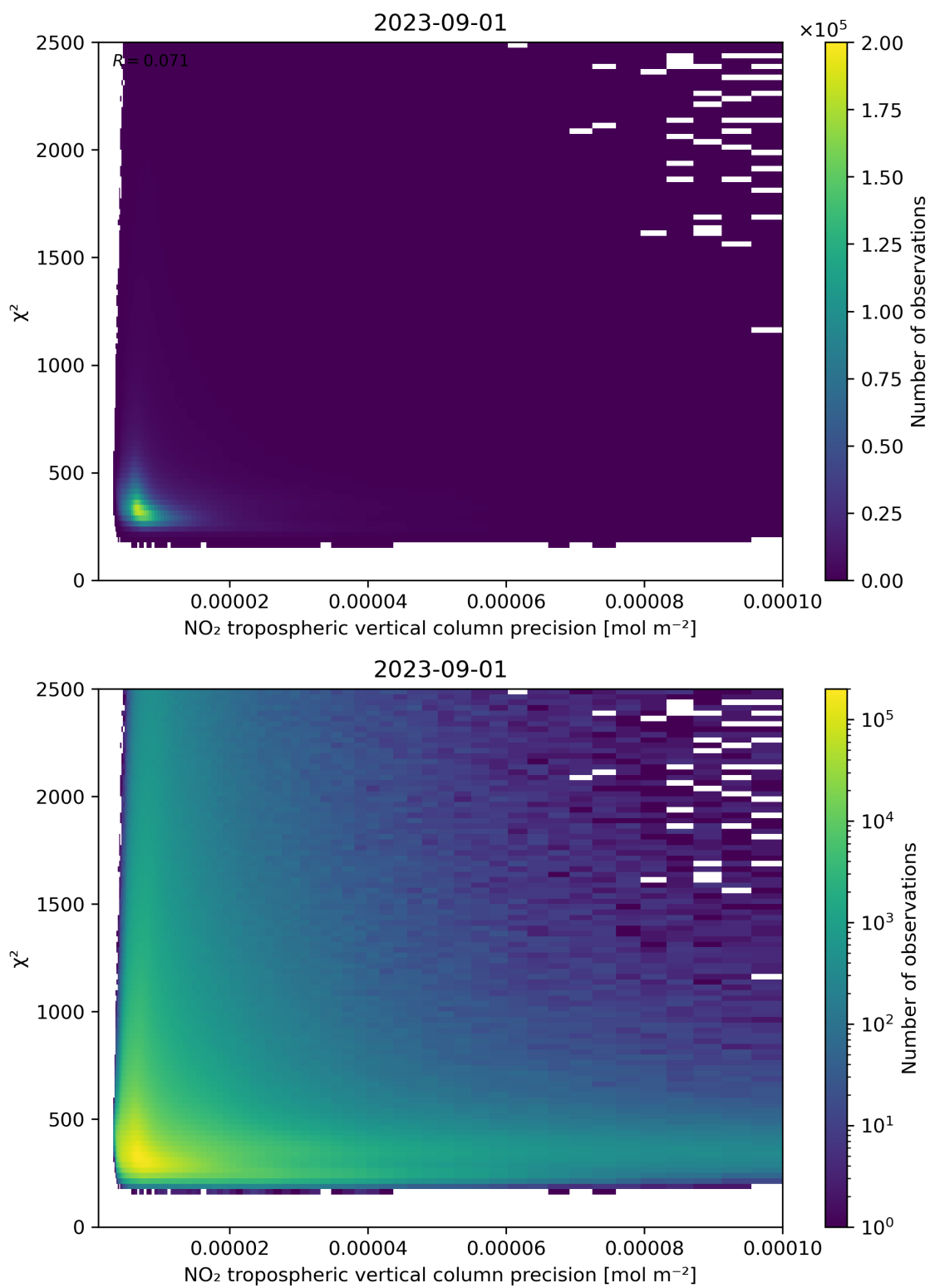
Figure 134: Scatter density plot of “NO 2 tropospheric vertical column precision” against “ \chi^2 ” for 2023-08-31 to 2023-09-02.
