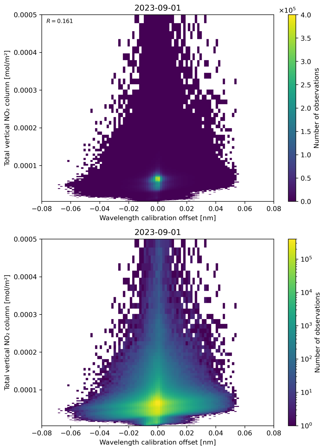
Figure 179: Scatter density plot of “Wavelength calibration offset” against “Total vertical NO 2 column” for 2023-08-31 to 2023-09-02.
