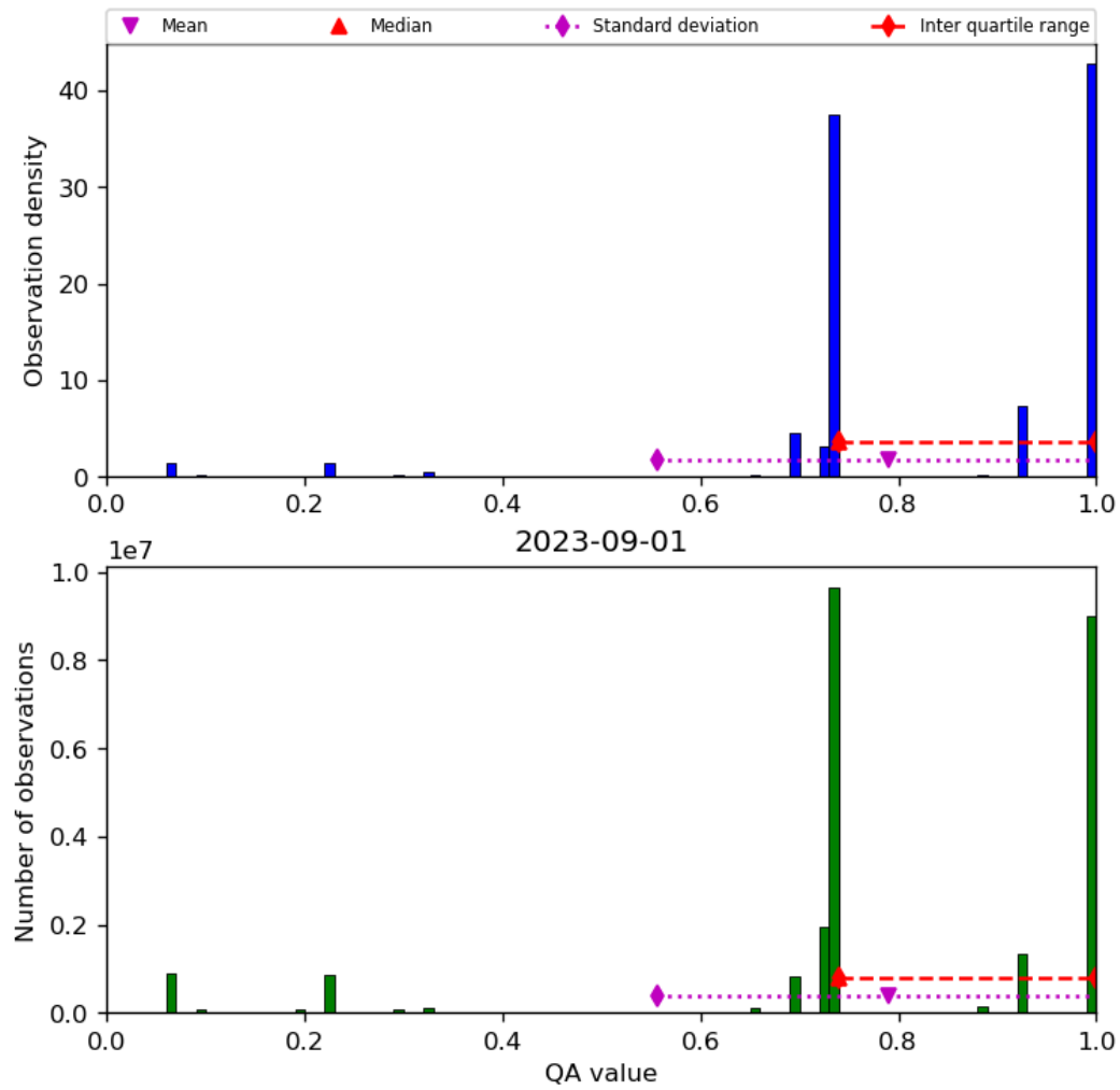
Figure 28: Histogram of “QA value” for 2023-08-31 to 2023-09-02
