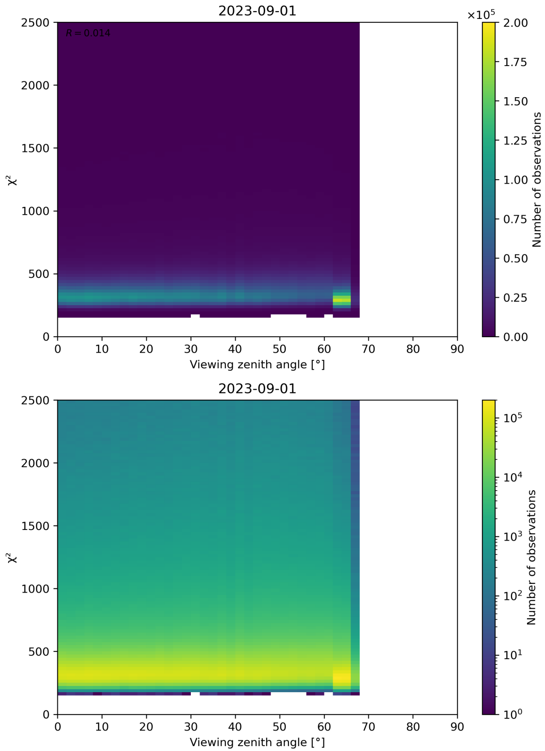
Figure 162: Scatter density plot of “Viewing zenith angle” against “ \chi^2 ” for 2023-08-31 to 2023-09-02.
