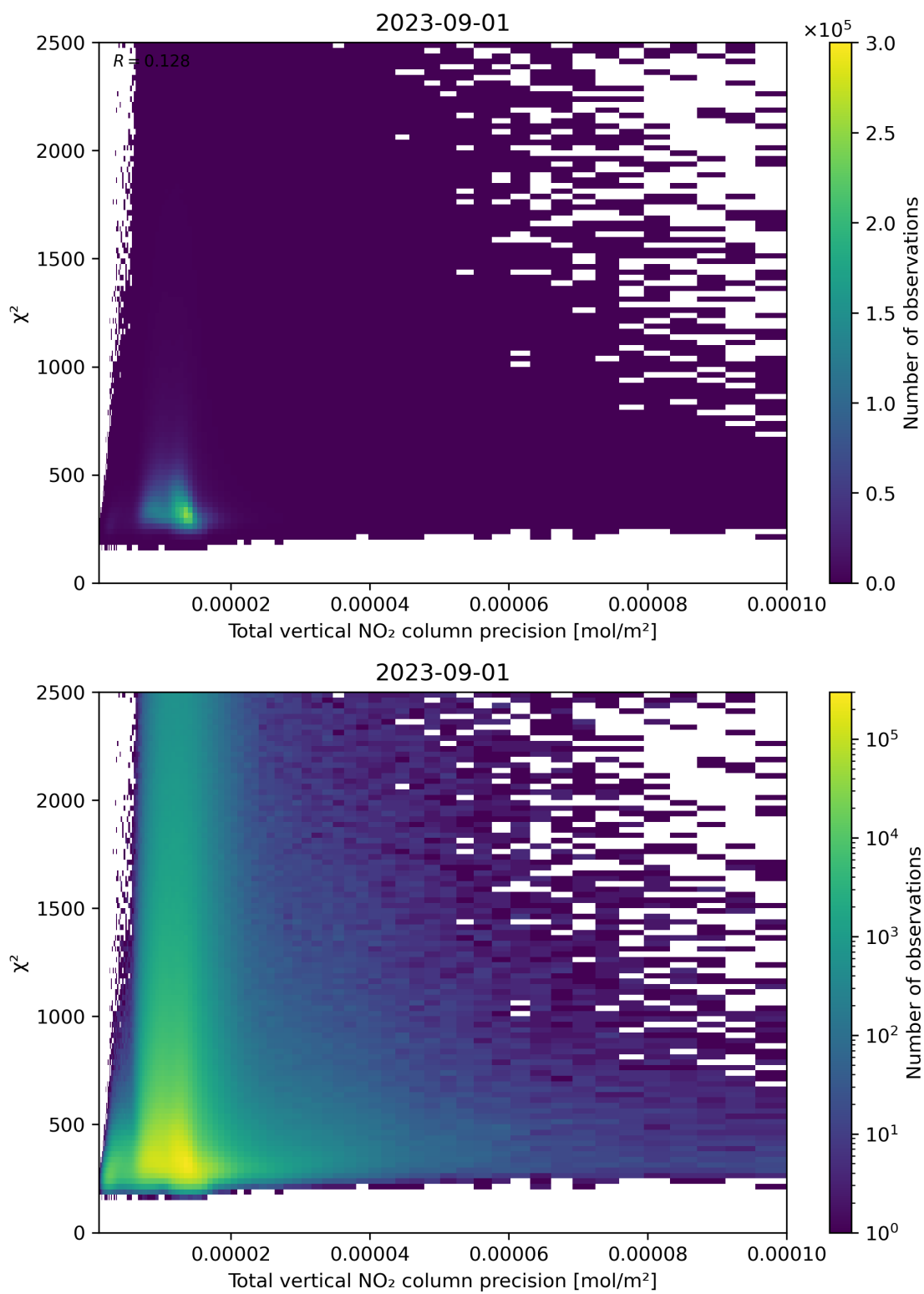
Figure 116: Scatter density plot of “Total vertical NO 2 column precision” against “ \chi^2 ” for 2023-08-31 to 2023-09-02.
