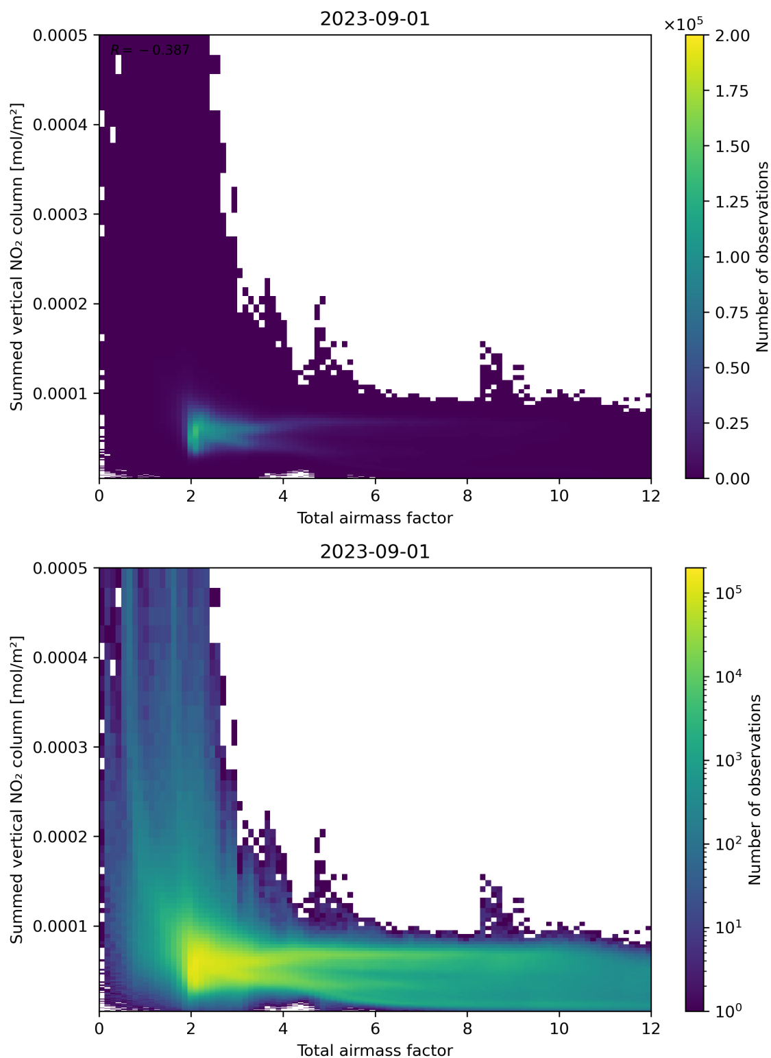
Figure 65: Scatter density plot of “Total airmass factor” against “Summed vertical NO 2 column” for 2023-08-31 to 2023-09-02.
