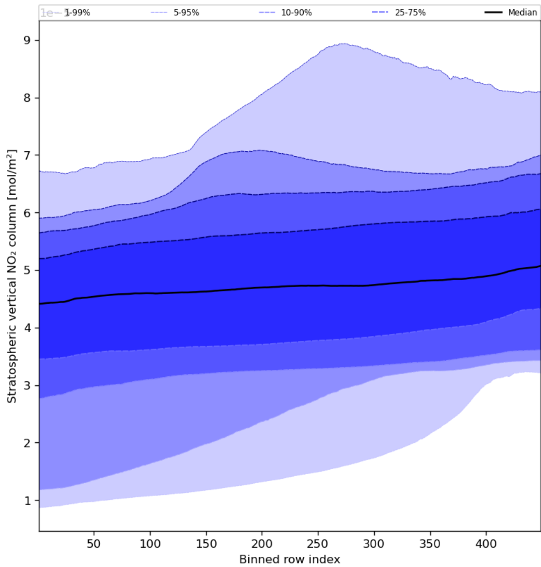
Figure 53: Along track statistics of “Stratospheric vertical NO 2 column” for 2023-08-31 to 2023-09-02
