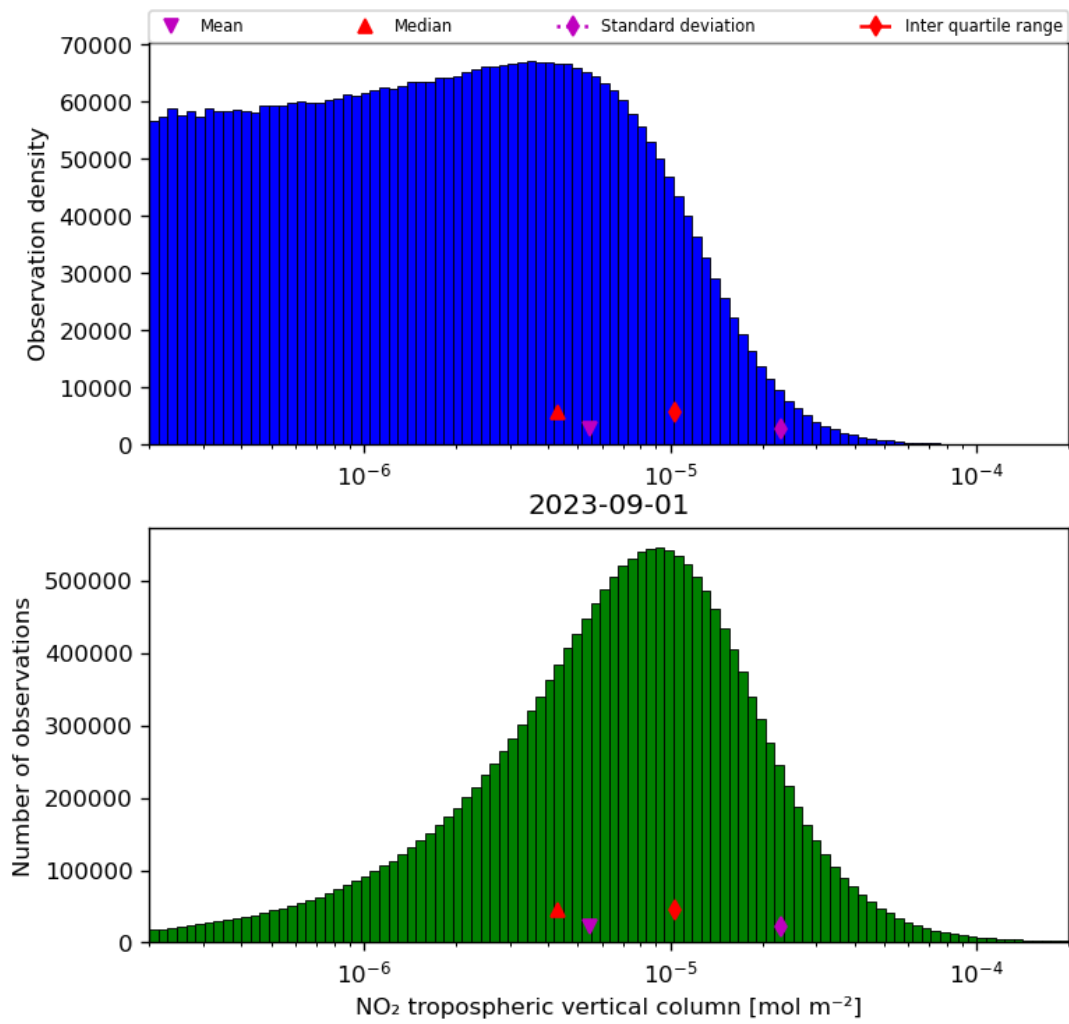
Figure 29: Histogram of “NO 2 tropospheric vertical column” for 2023-08-31 to 2023-09-02
