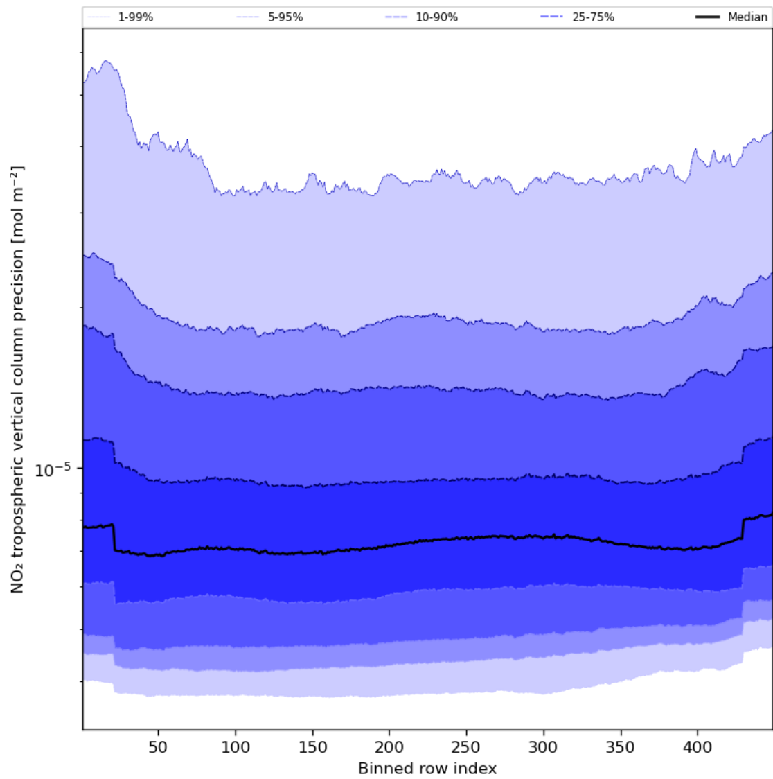
Figure 47: Along track statistics of “NO 2 tropospheric vertical column precision” for 2023-08-31 to 2023-09-02
