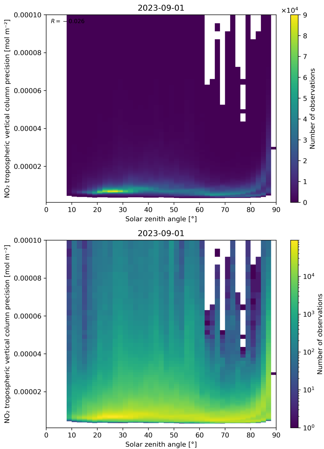
Figure 156: Scatter density plot of “Solar zenith angle” against “NO 2 tropospheric vertical column precision” for 2023-08-31 to 2023-09-02.
