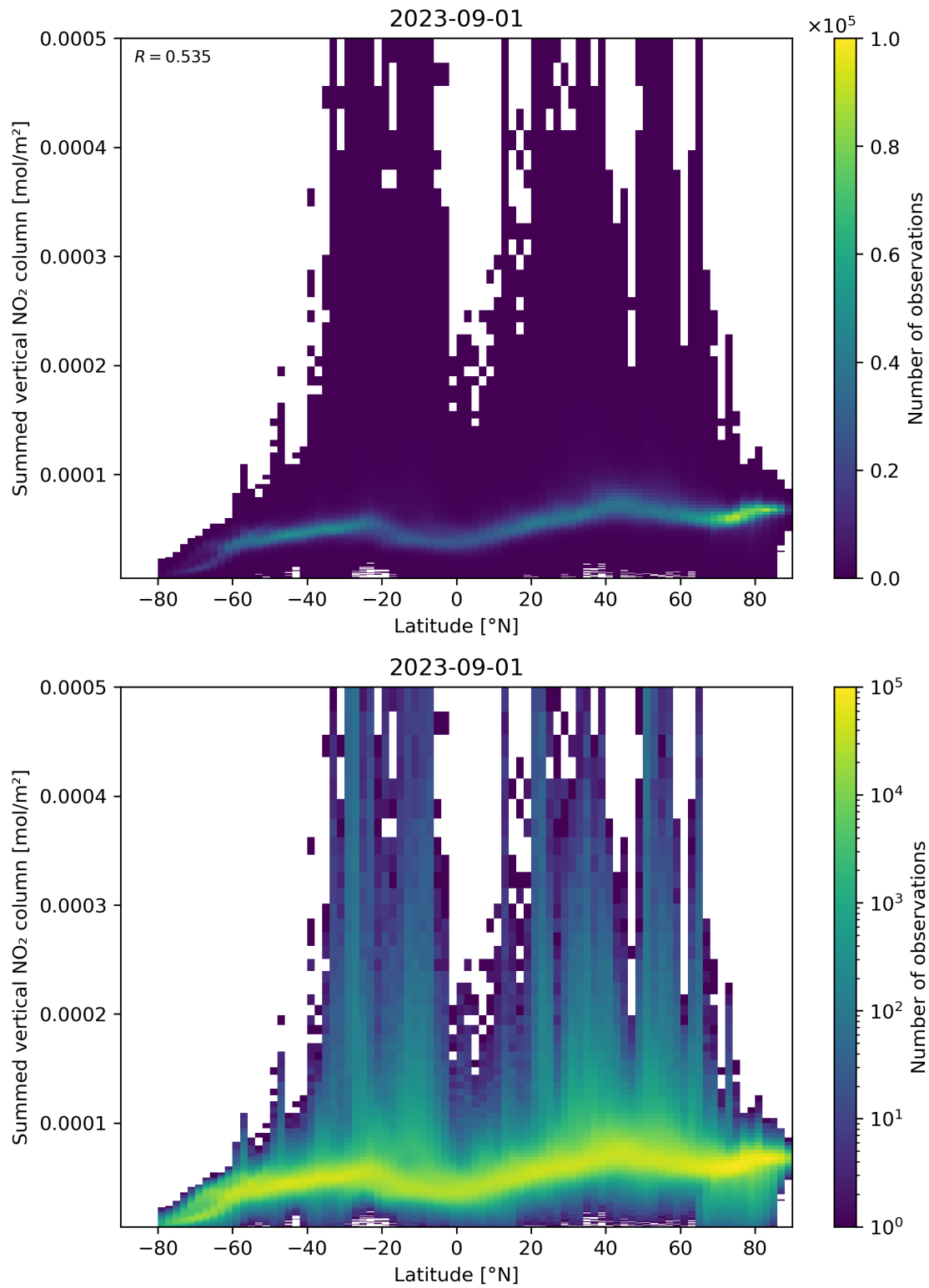
Figure 88: Scatter density plot of “Latitude” against “Summed vertical NO 2 column” for 2023-08-31 to 2023-09-02.
