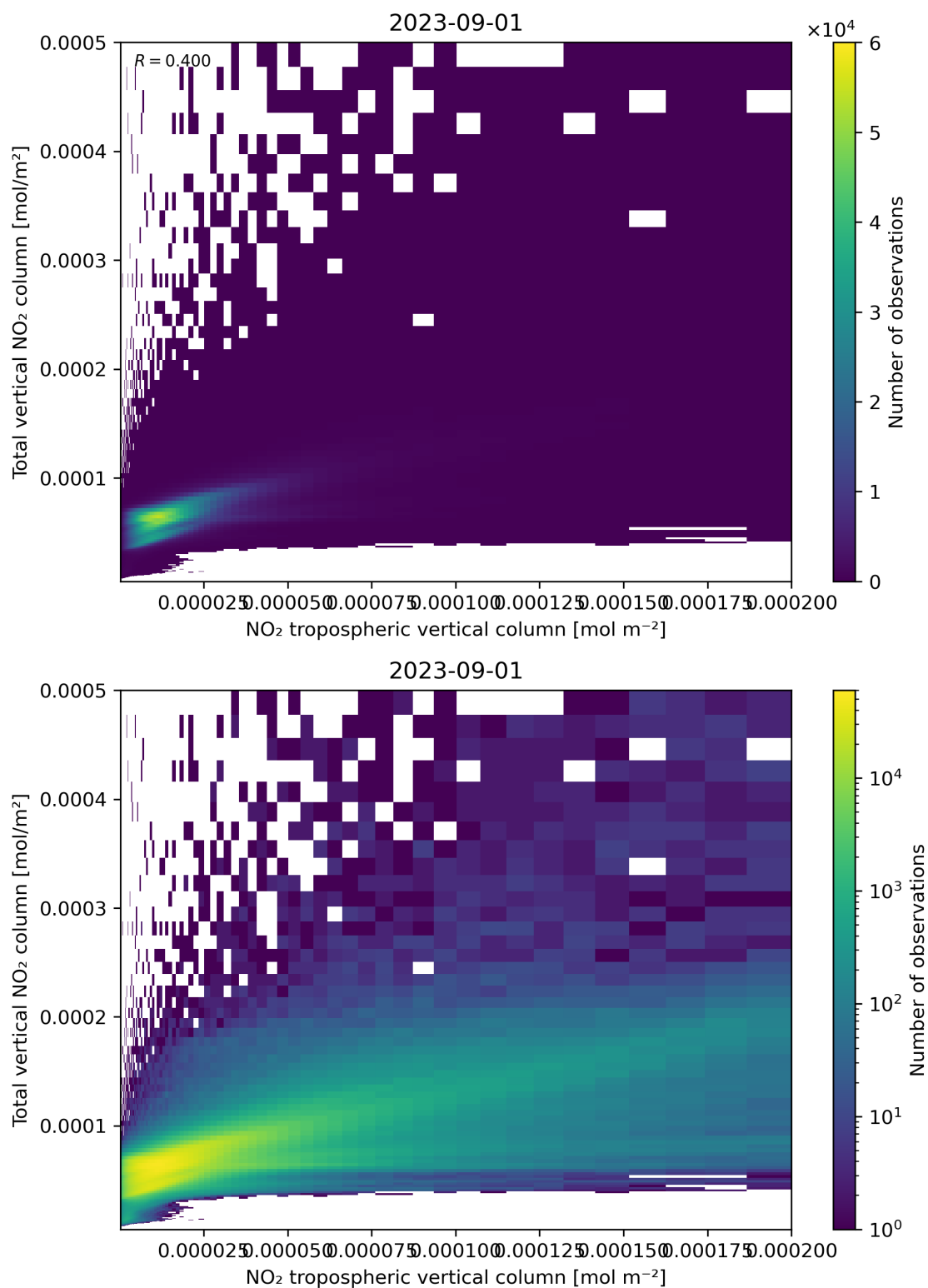
Figure 128: Scatter density plot of “NO 2 tropospheric vertical column” against “Total vertical NO 2 column” for 2023-08-31 to 2023-09-02.
