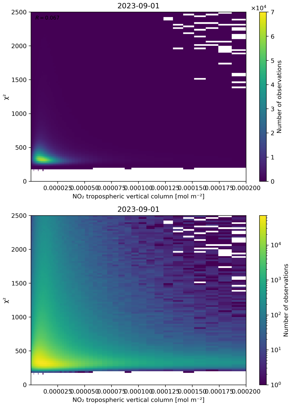
Figure 124: Scatter density plot of “NO 2 tropospheric vertical column” against “ \chi^2 ” for 2023-08-31 to 2023-09-02.
