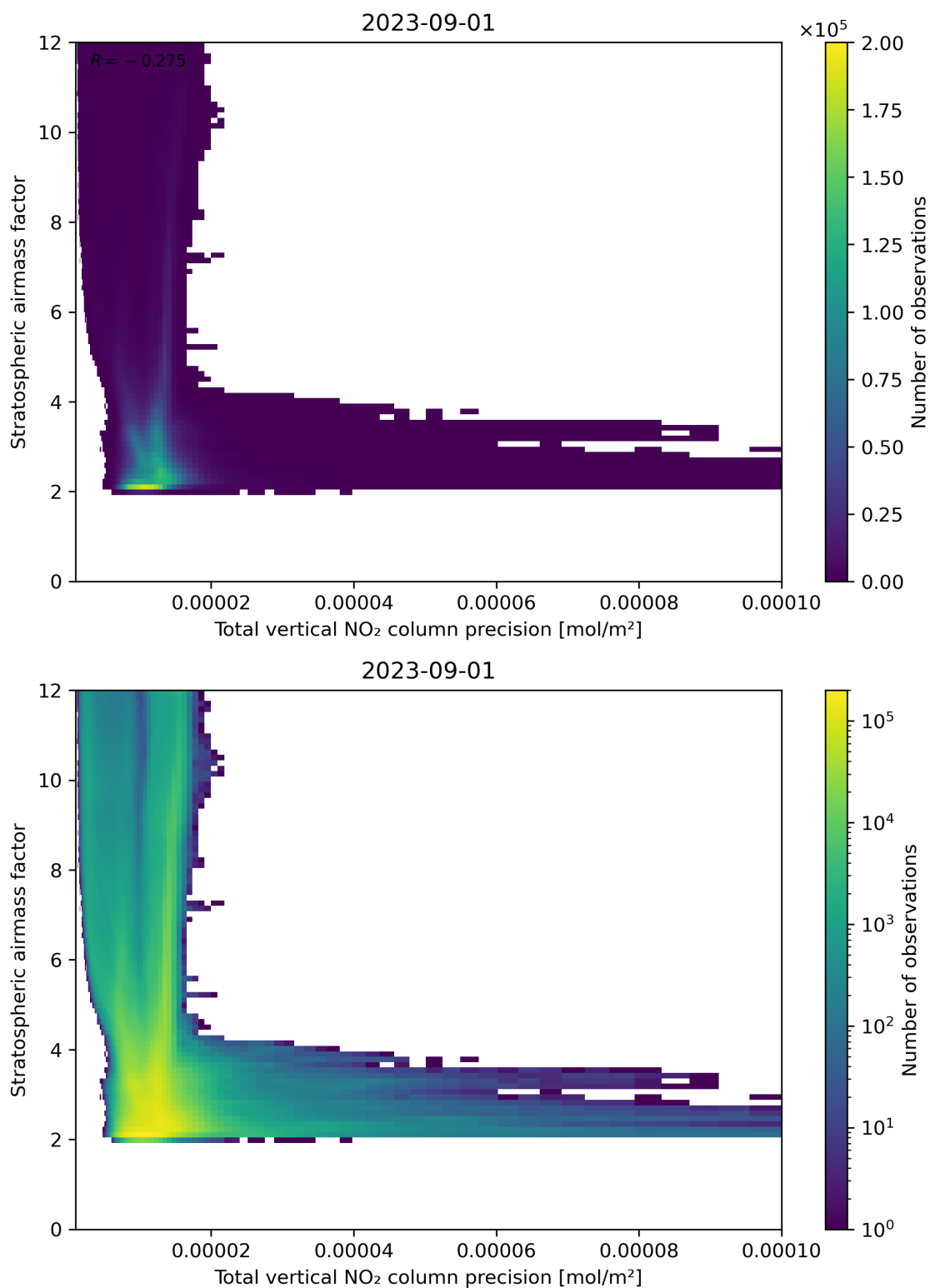
Figure 115: Scatter density plot of “Total vertical NO 2 column precision” against “Stratospheric air mass factor” for 2023-08-31 to 2023-09-02.
