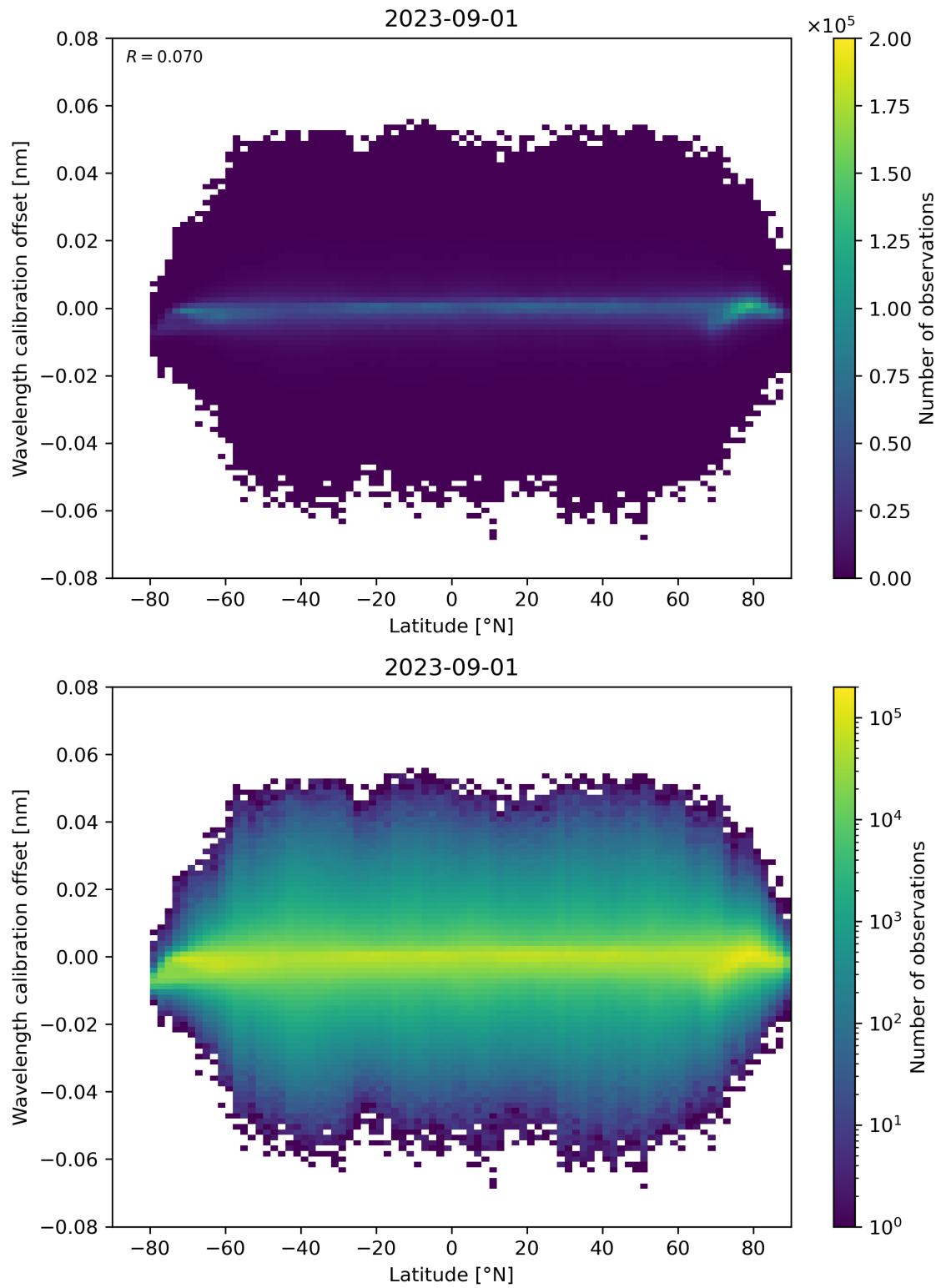
Figure 95: Scatter density plot of “Latitude” against “Wavelength calibration offset” for 2023-08-31 to 2023-09-02.
