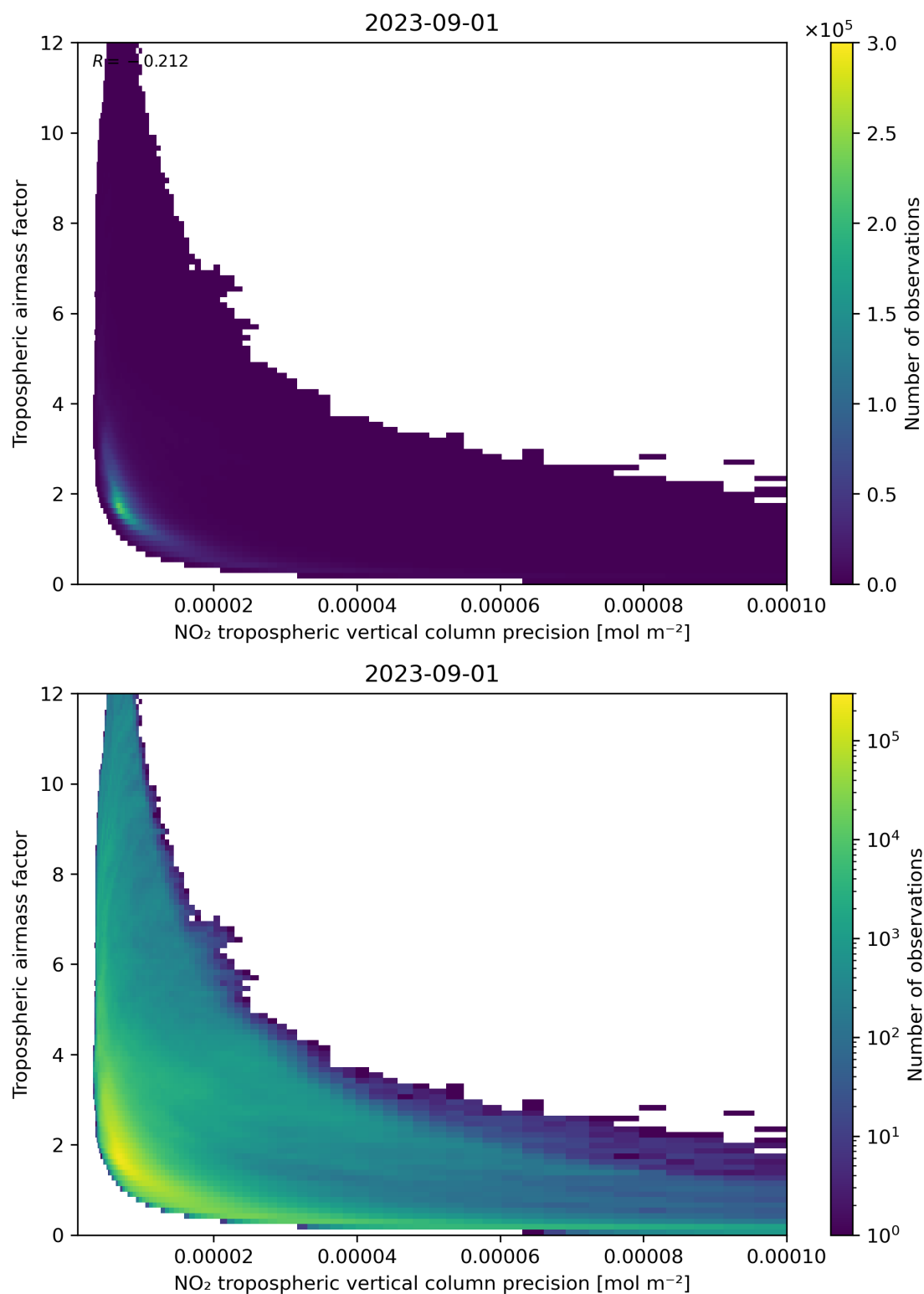
Figure 133: Scatter density plot of “NO 2 tropospheric vertical column precision” against “Tropospheric airmass factor” for 2023-08-31 to 2023-09-02.
