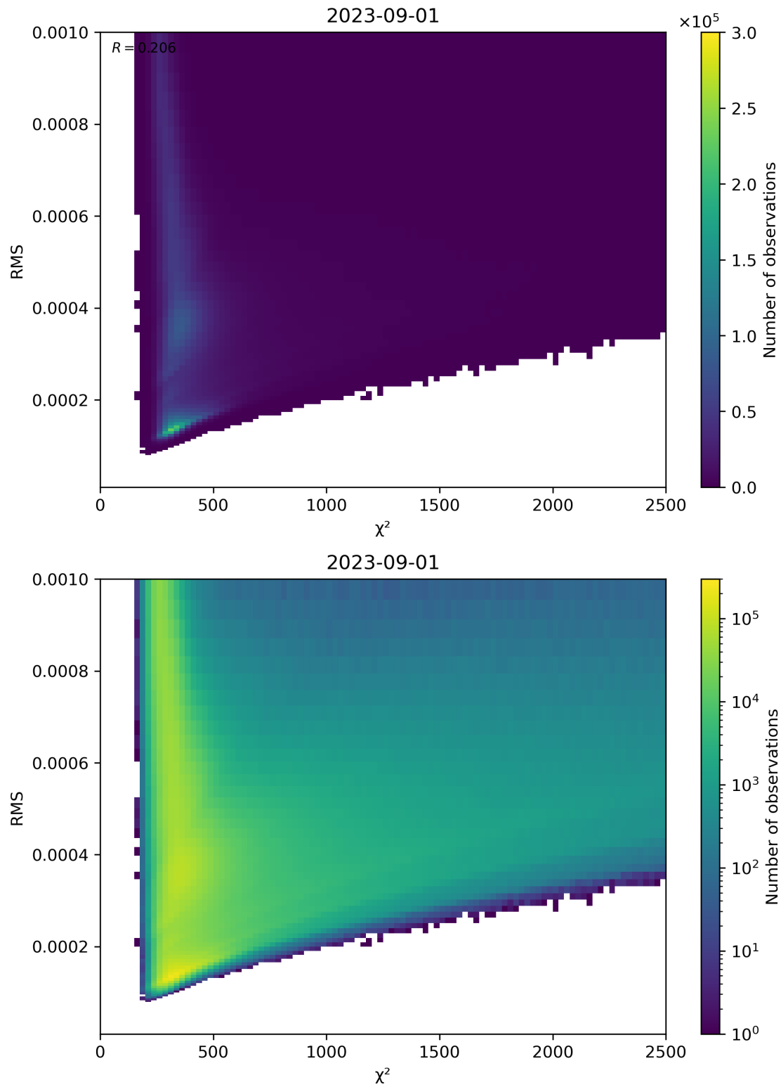
Figure 82: Scatter density plot of “ \chi^2 ” against “RMS” for 2023-08-31 to 2023-09-02.
