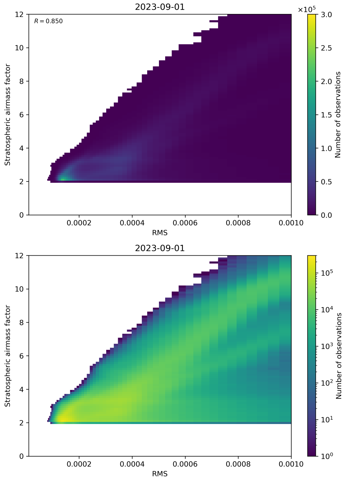
Figure 144: Scatter density plot of “RMS” against “Stratospheric airmass factor” for 2023-08-31 to 2023-09-02.
