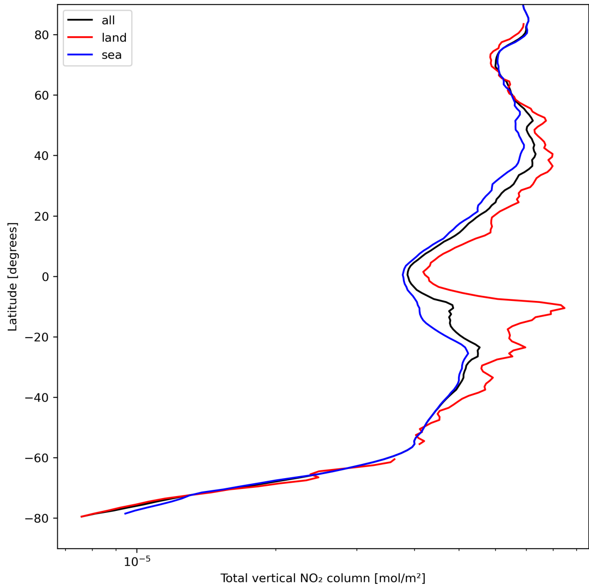
Figure 21: Zonal average of “Total vertical NO 2 column” for 2023-08-31 to 2023-09-02.
