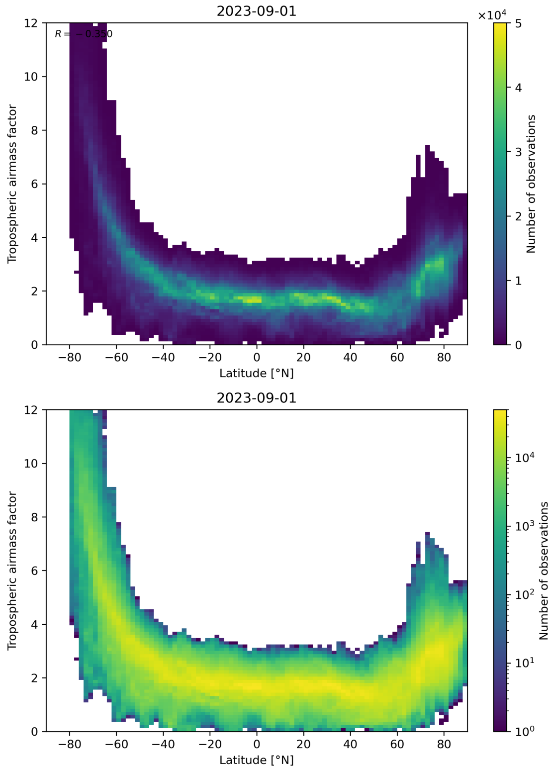
Figure 85: Scatter density plot of “Latitude” against “Tropospheric air mass factor” for 2023-08-31 to 2023-09-02.
