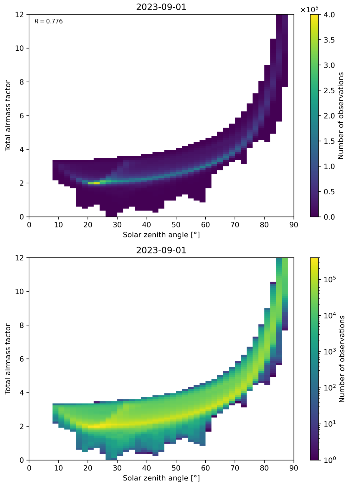
Figure 146: Scatter density plot of “Solar zenith angle” against “Total air mass factor” for 2023-08-31 to 2023-09-02.
