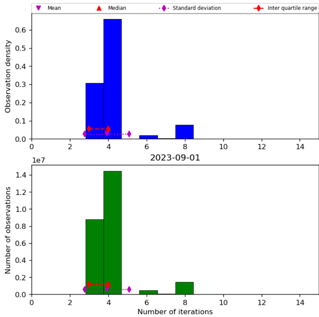
Figure 34: Histogram of “Number of iterations” for 2023-08-31 to 2023-09-02
