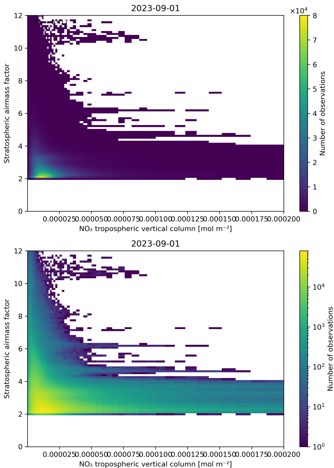
Figure 121: Scatter density plot of “NO 2 tropospheric vertical column” against “Stratospheric air mass factor” for 2023-08-31 to 2023-09-02.
