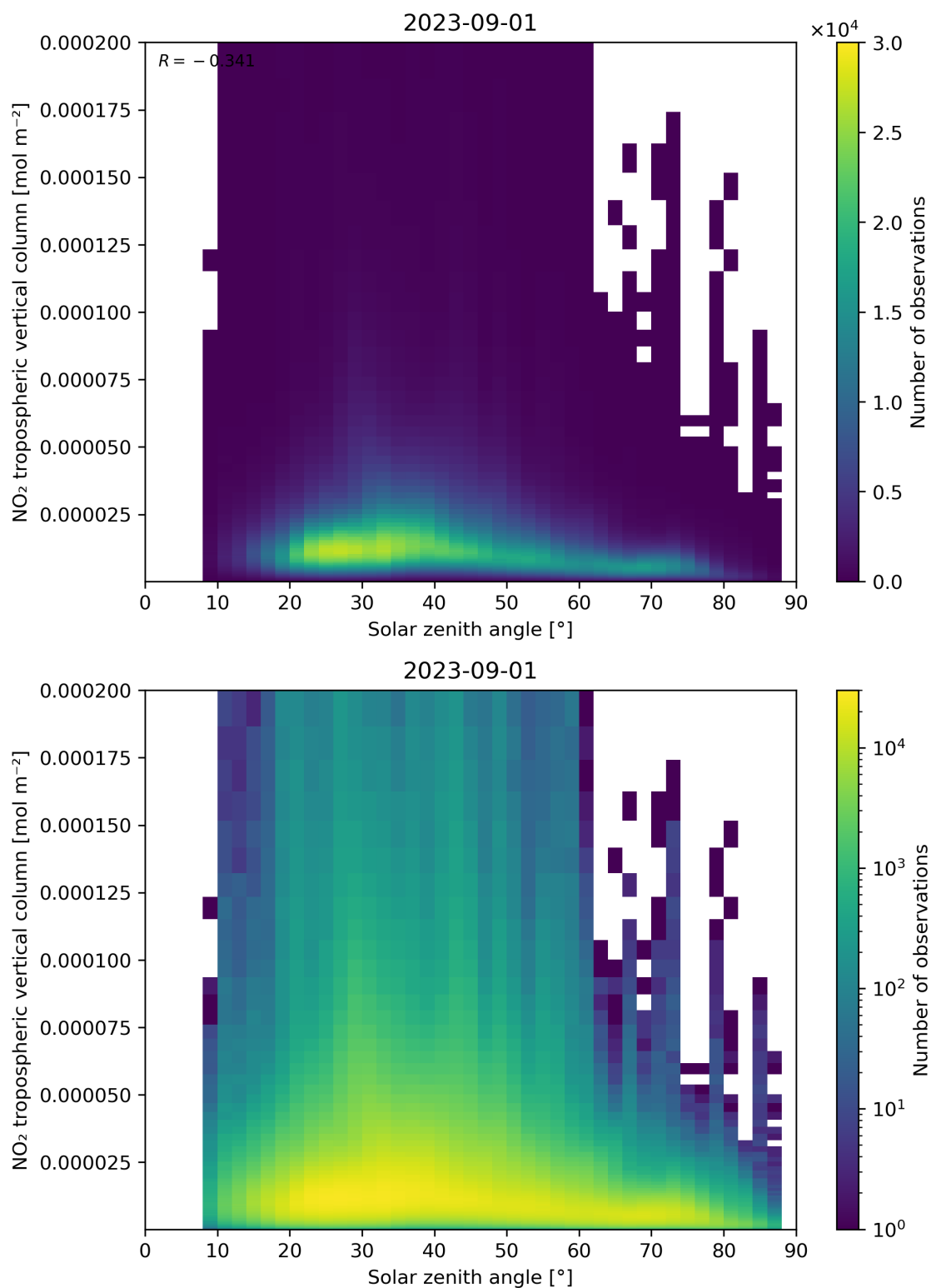
Figure 155: Scatter density plot of “Solar zenith angle” against “NO 2 tropospheric vertical column” for 2023-08-31 to 2023-09-02.
