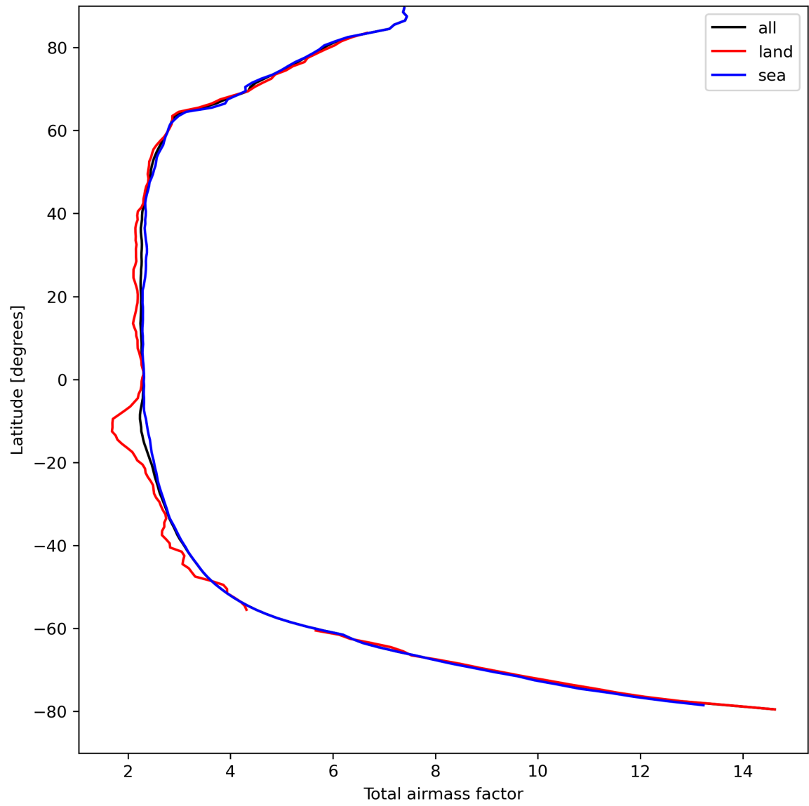
Figure 15: Zonal average of “Total airmass factor” for 2023-08-31 to 2023-09-02.
