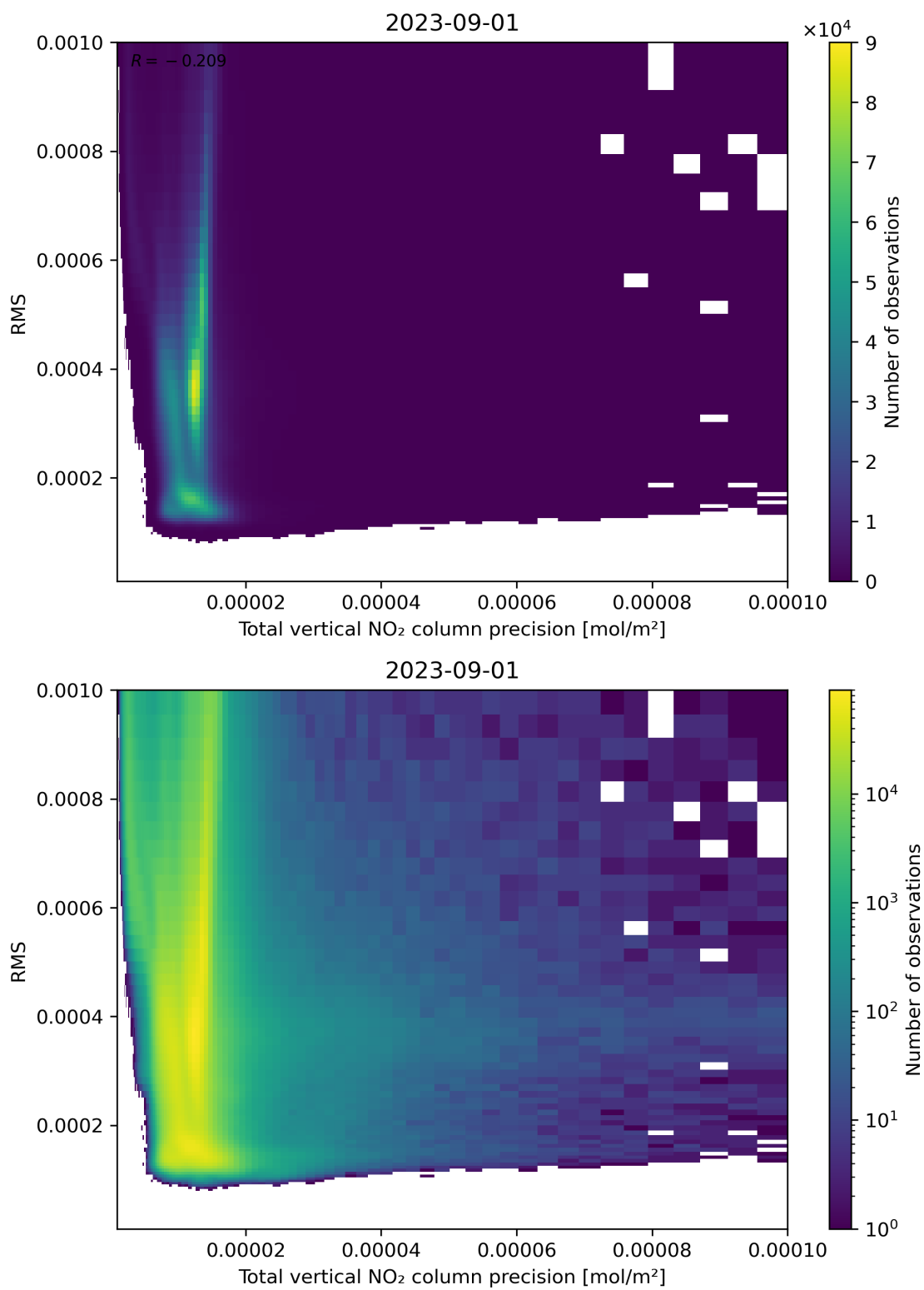
Figure 119: Scatter density plot of “Total vertical NO 2 column precision” against “RMS” for 2023-08-31 to 2023-09-02.
