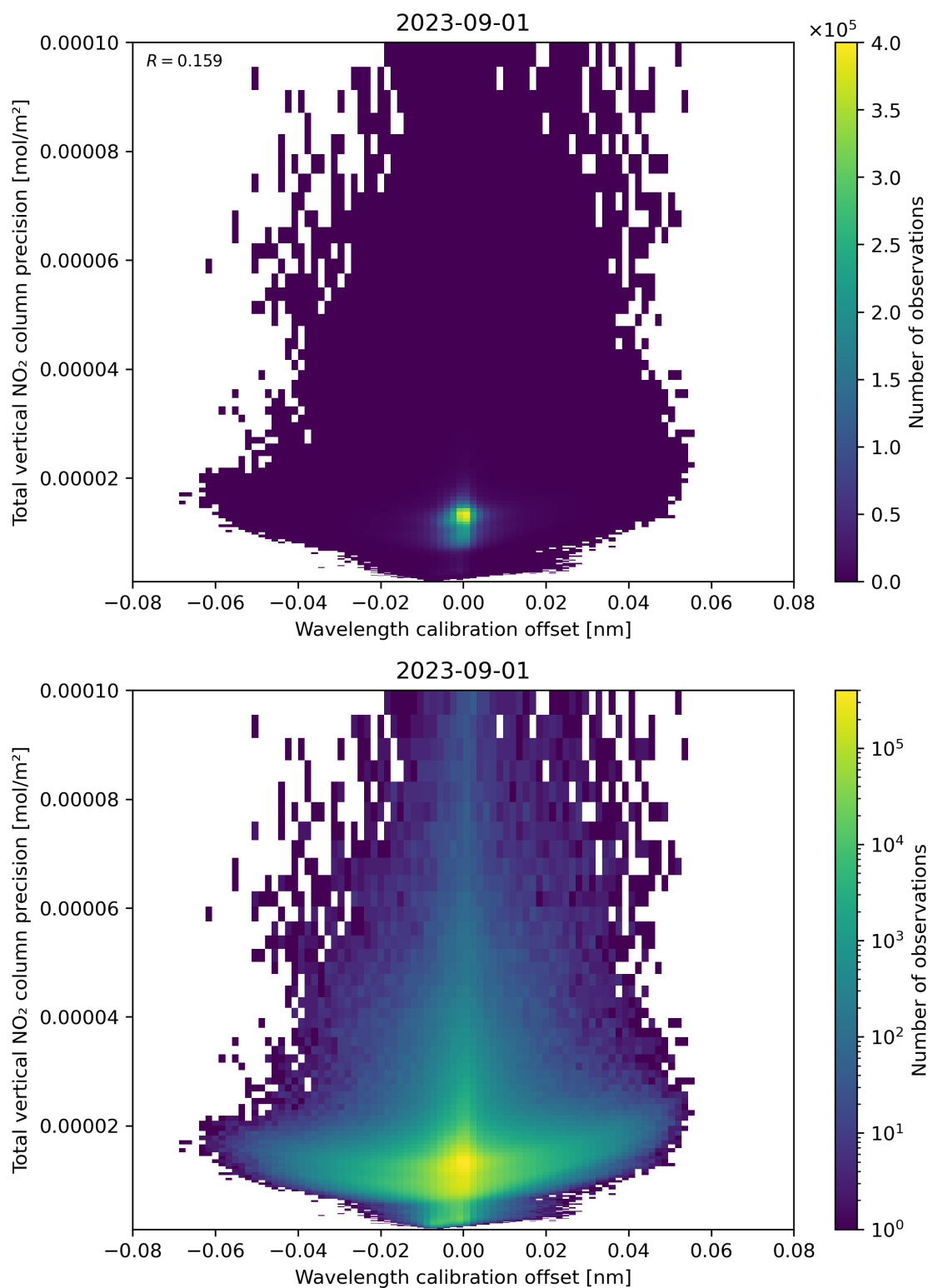
Figure 180: Scatter density plot of “Wavelength calibration offset” against “Total vertical NO 2 column precision” for 2023-08-31 to 2023-09-02.
