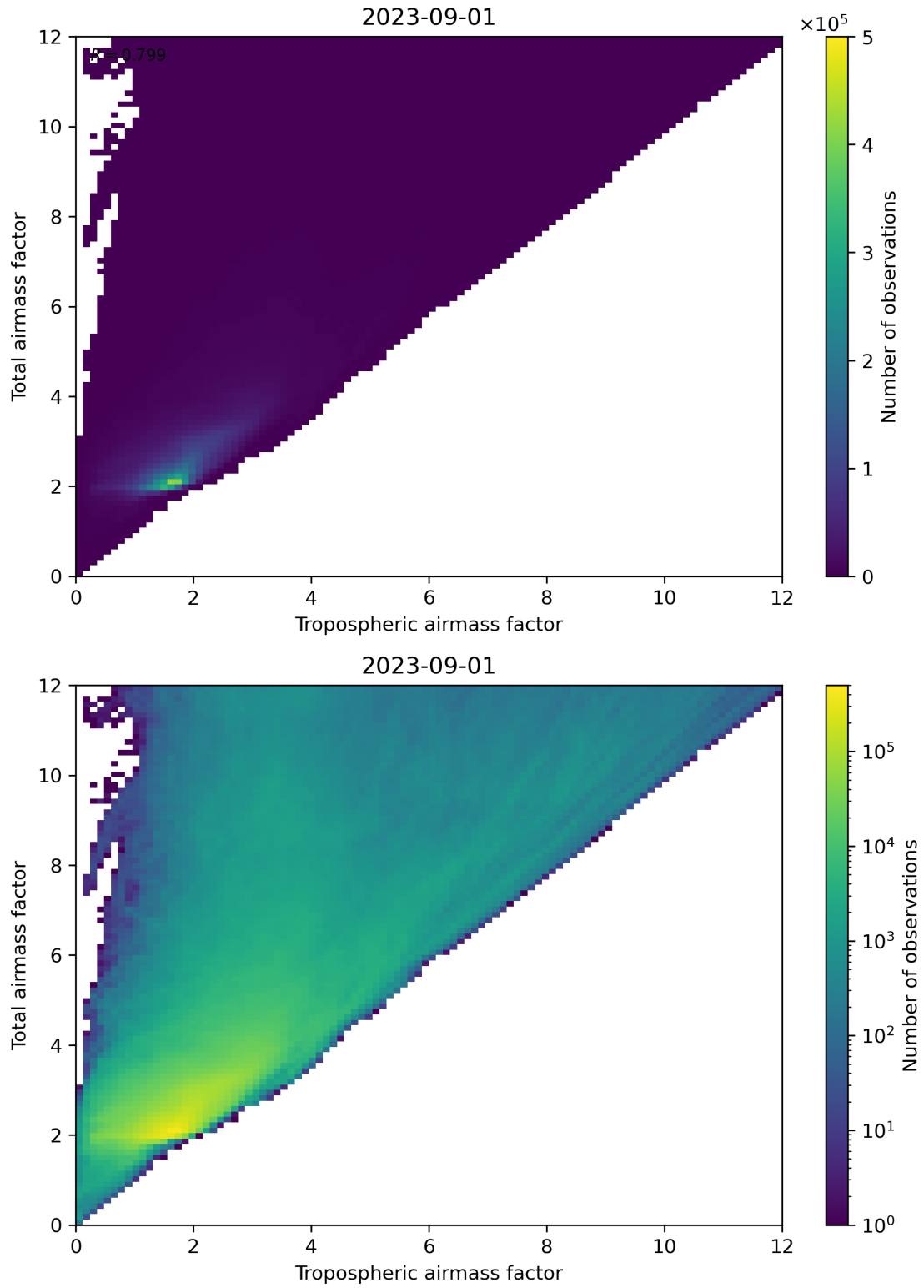
Figure 72: Scatter density plot of “Tropospheric airmass factor” against “Total airmass factor” for 2023-08-31 to 2023-09-02.
