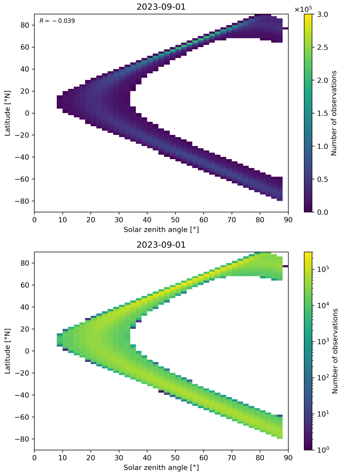
Figure 149: Scatter density plot of “Solar zenith angle” against “Latitude” for 2023-08-31 to 2023-09-02.
