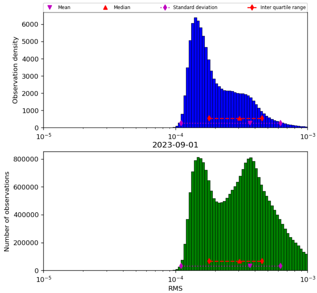
Figure 43: Histogram of “RMS” for 2023-08-31 to 2023-09-02
