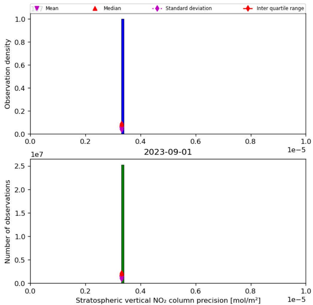
Figure 37: Histogram of “Stratospheric vertical NO 2 column precision” for 2023-08-31 to 2023-09-02
