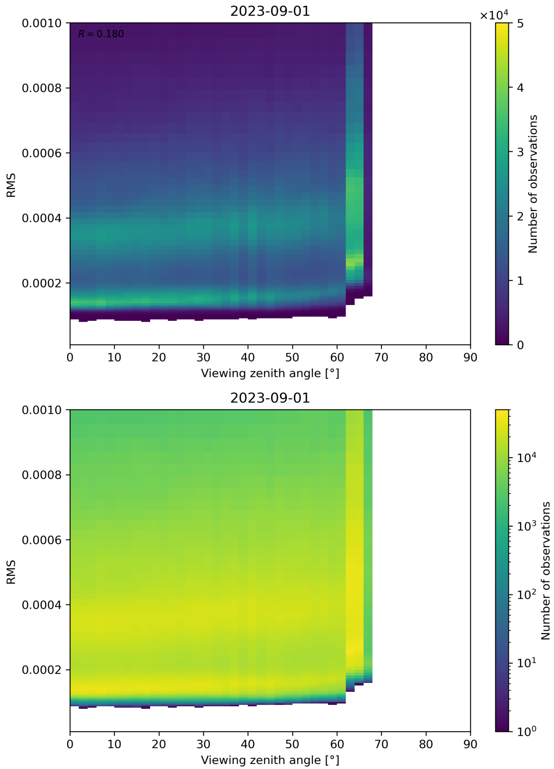
Figure 171: Scatter density plot of “Viewing zenith angle” against “RMS” for 2023-08-31 to 2023-09-02.
