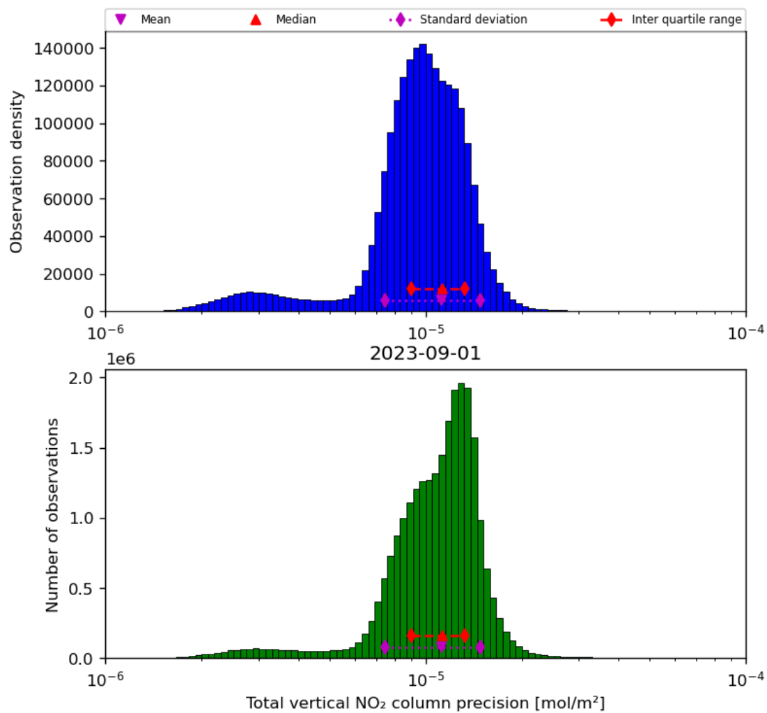
Figure 39: Histogram of “Total vertical NO 2 column precision” for 2023-08-31 to 2023-09-02
