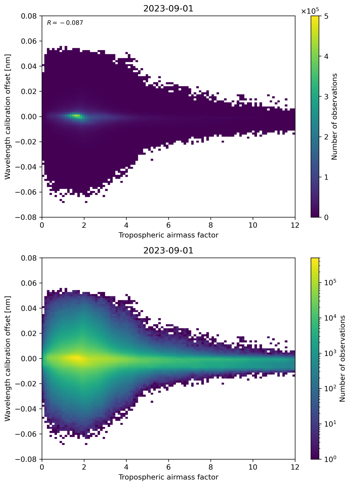
Figure 80: Scatter density plot of “Tropospheric air mass factor” against “Wavelength calibration offset” for 2023-08-31 to 2023-09-02.
