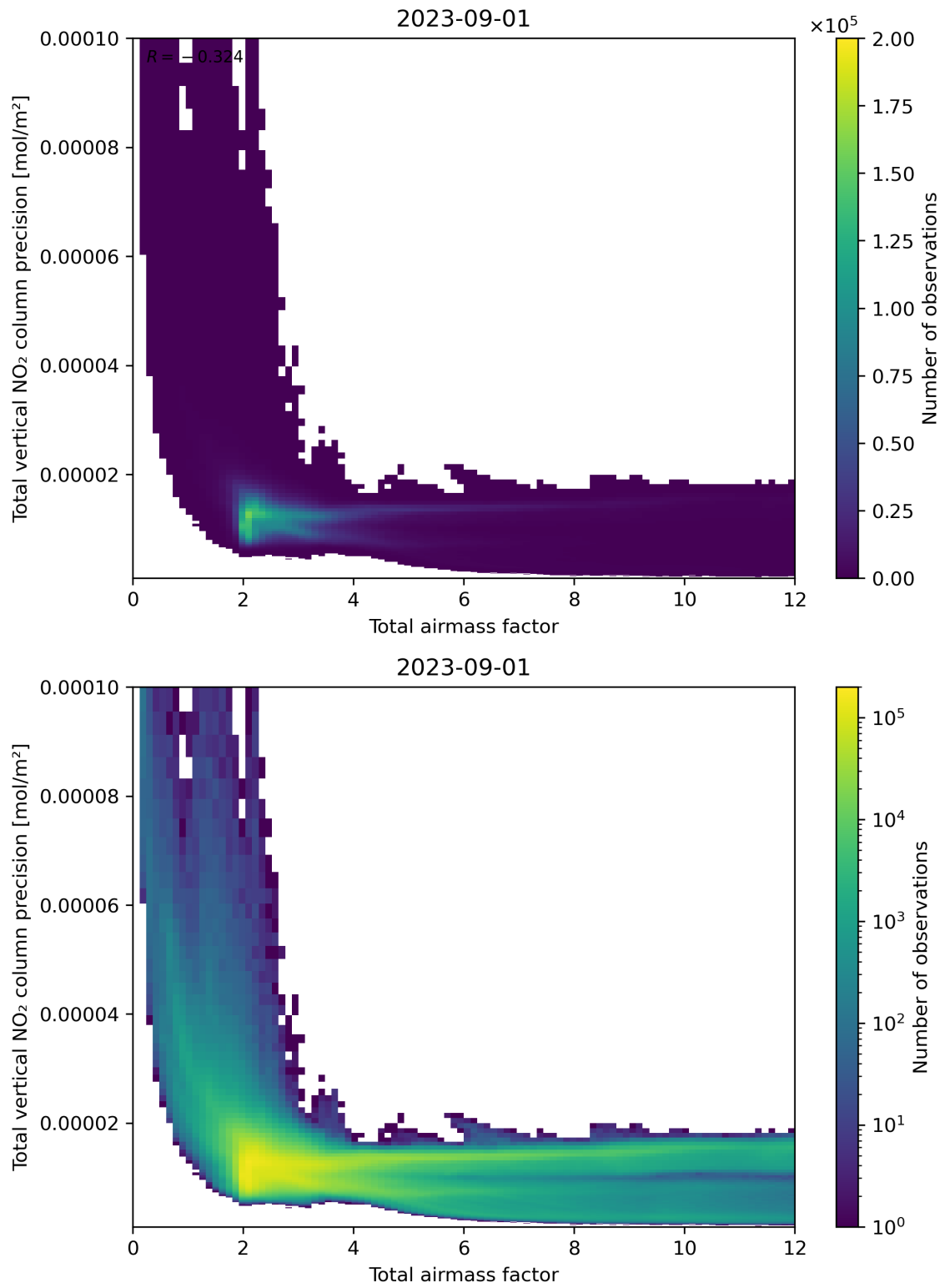
Figure 68: Scatter density plot of “Total airmass factor” against “Total vertical NO 2 column precision” for 2023-08-31 to 2023-09-02.
