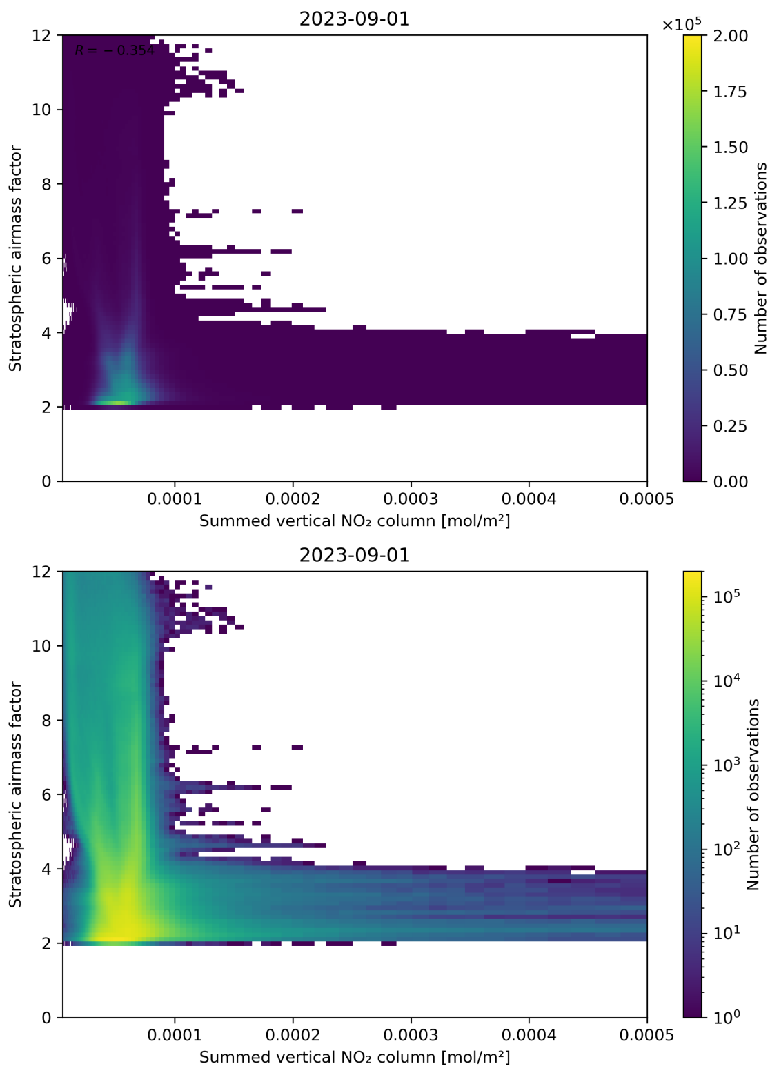
Figure 103: Scatter density plot of “Summed vertical NO 2 column” against “Stratospheric air mass factor” for 2023-08-31 to 2023-09-02.
