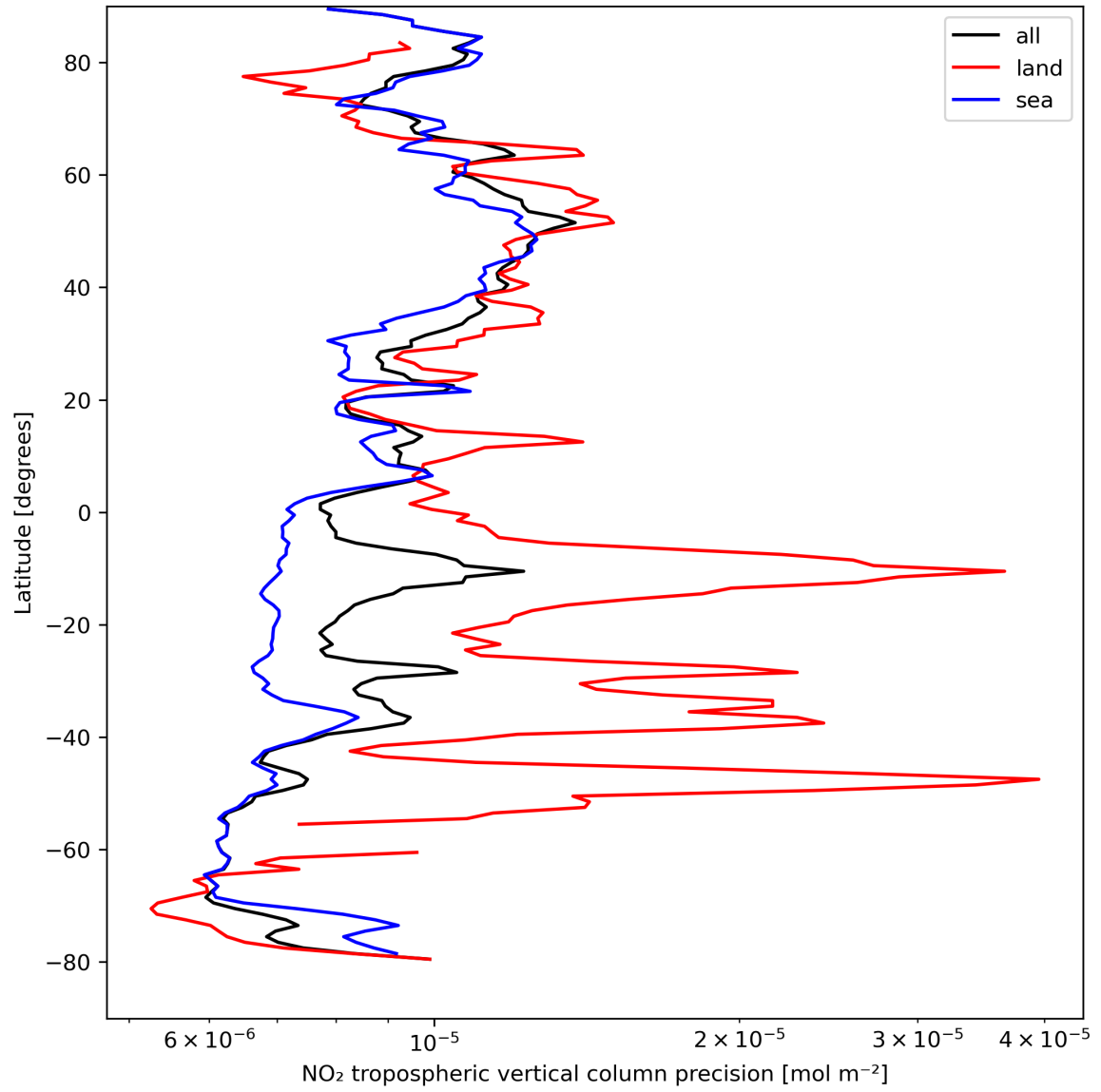
Figure 13: Zonal average of “NO 2 tropospheric vertical column precision” for 2023-08-31 to 2023-09-02.
