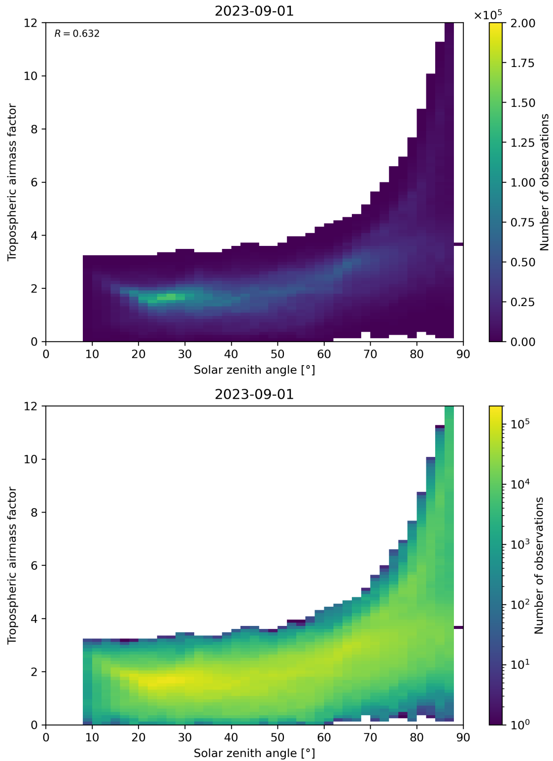
Figure 147: Scatter density plot of “Solar zenith angle” against “Tropospheric airmass factor” for 2023-08-31 to 2023-09-02.
