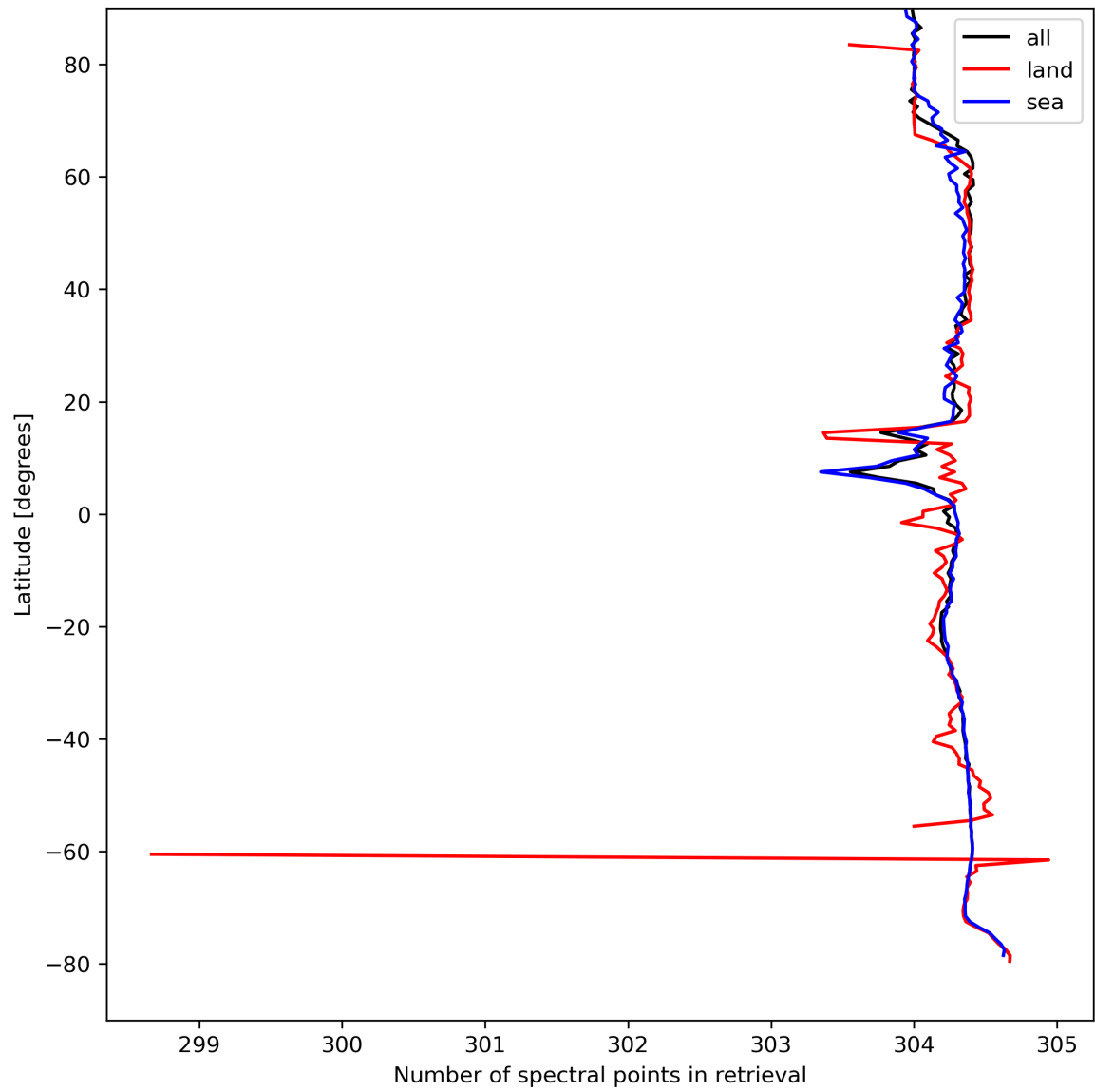
Figure 16: Zonal average of “Number of spectral points in retrieval” for 2023-08-31 to 2023-09-02.
