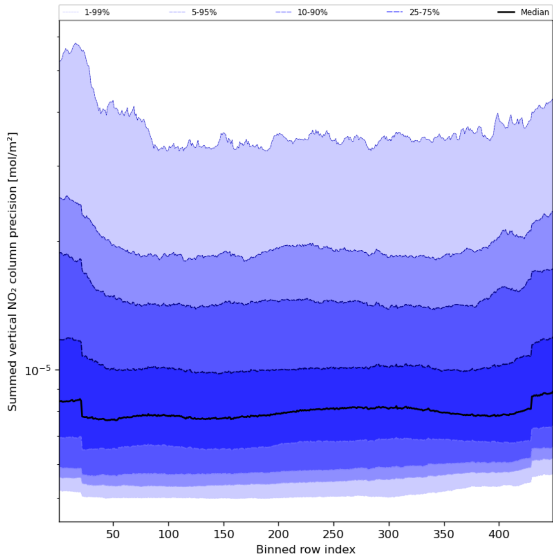
Figure 58: Along track statistics of “Summed vertical NO 2 column precision” for 2023-08-31 to 2023-09-02
