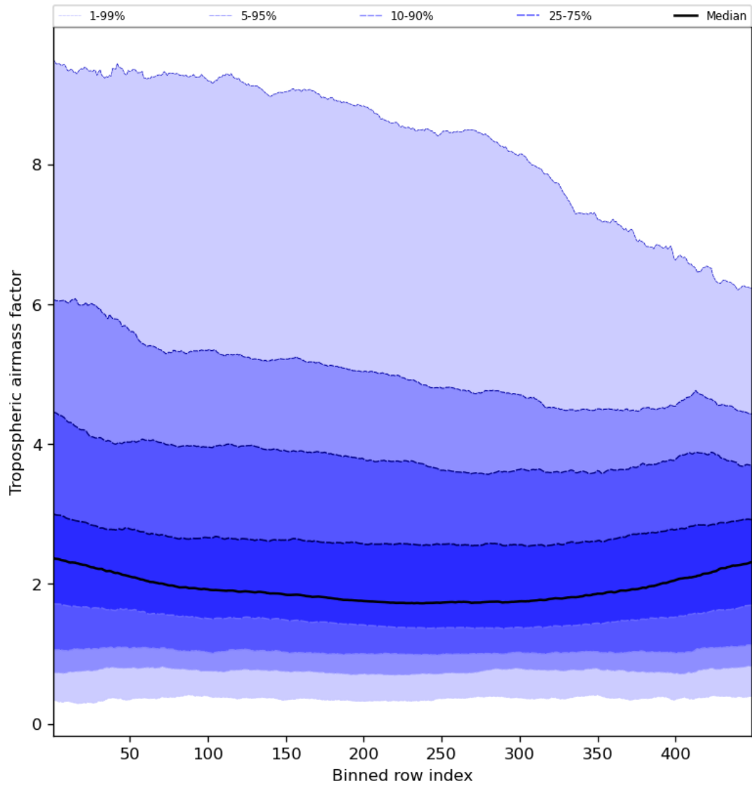
Figure 48: Along track statistics of “Tropospheric airmass factor” for 2023-08-31 to 2023-09-02
