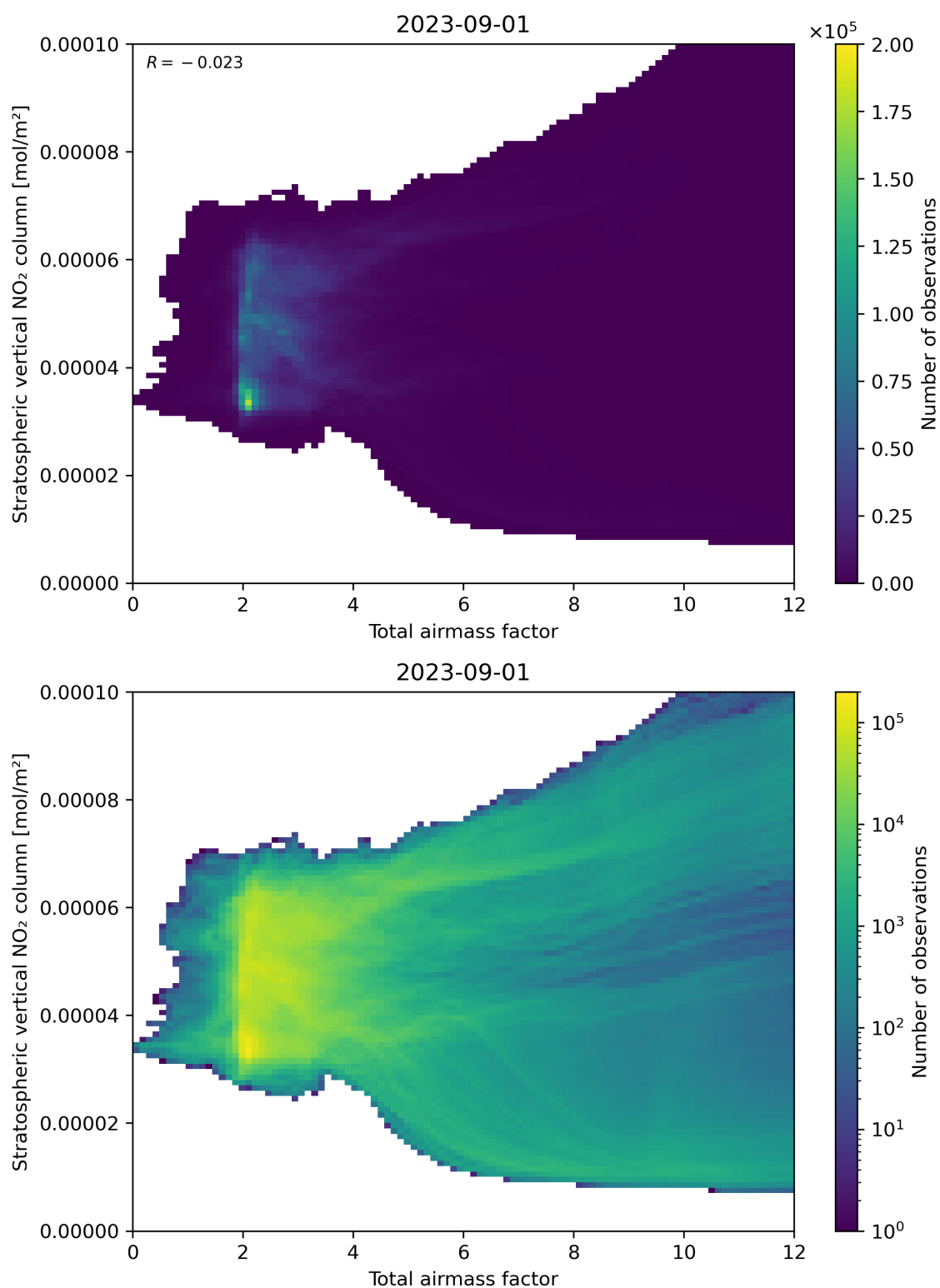
Figure 64: Scatter density plot of “Total airmass factor” against “Stratospheric vertical NO 2 column” for 2023-08-31 to 2023-09-02.
