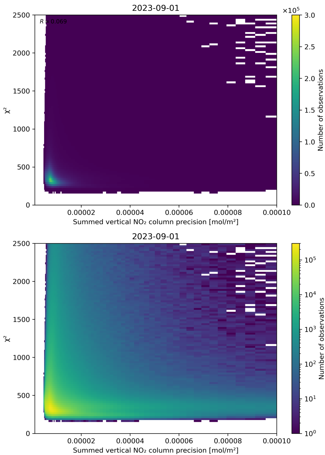
Figure 107: Scatter density plot of “Summed vertical NO 2 column precision” against “ \chi^2 ” for 2023-08-31 to 2023-09-02.
