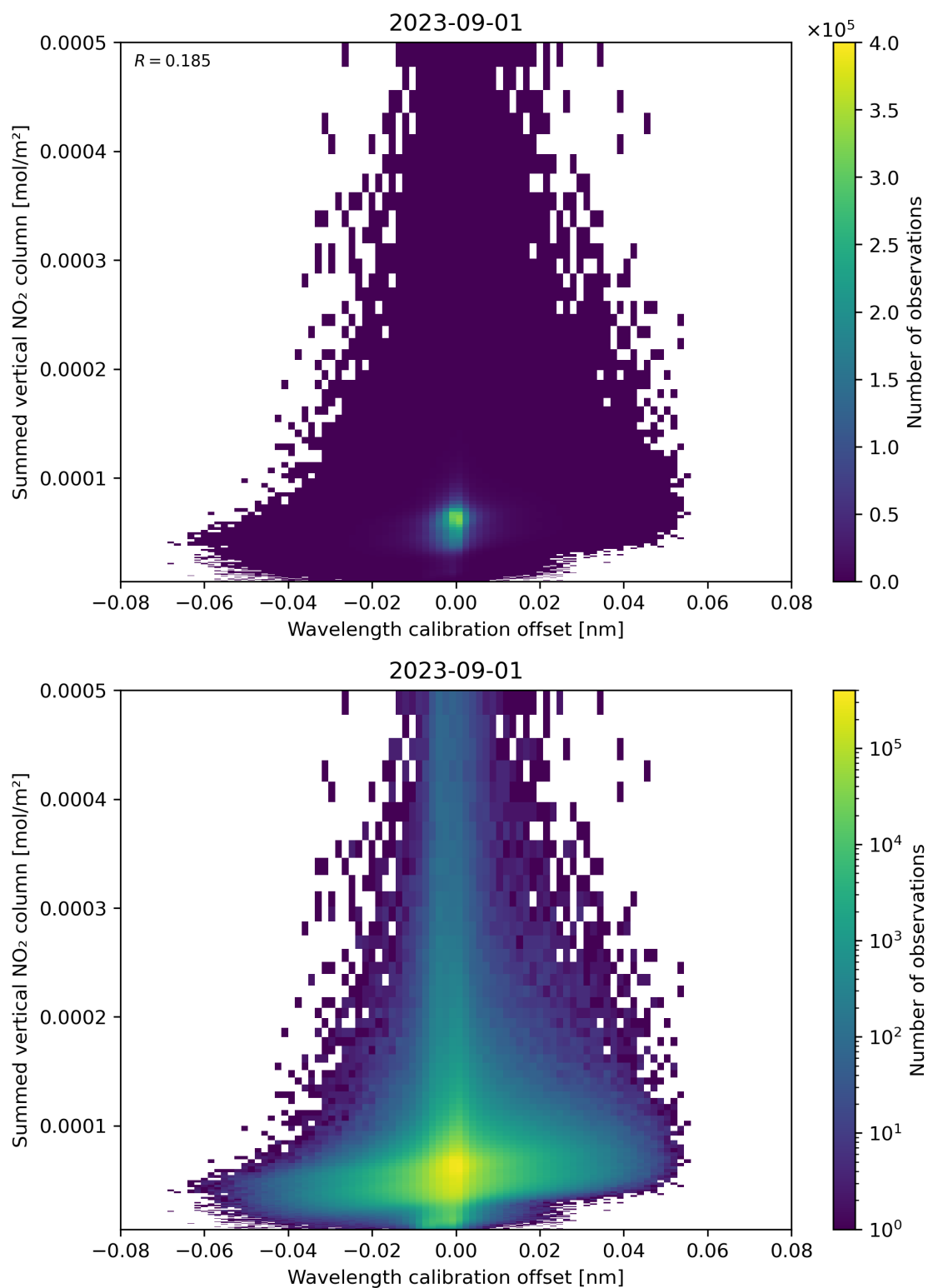
Figure 177: Scatter density plot of “Wavelength calibration offset” against “Summed vertical NO 2 column” for 2023-08-31 to 2023-09-02.
