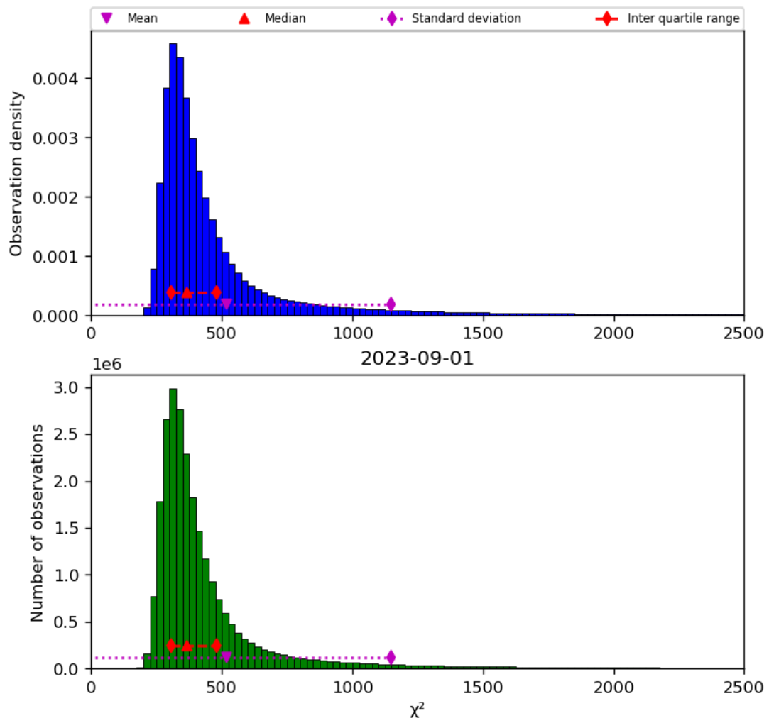
Figure 42: Histogram of “ \chi^2 ” for 2023-08-31 to 2023-09-02
