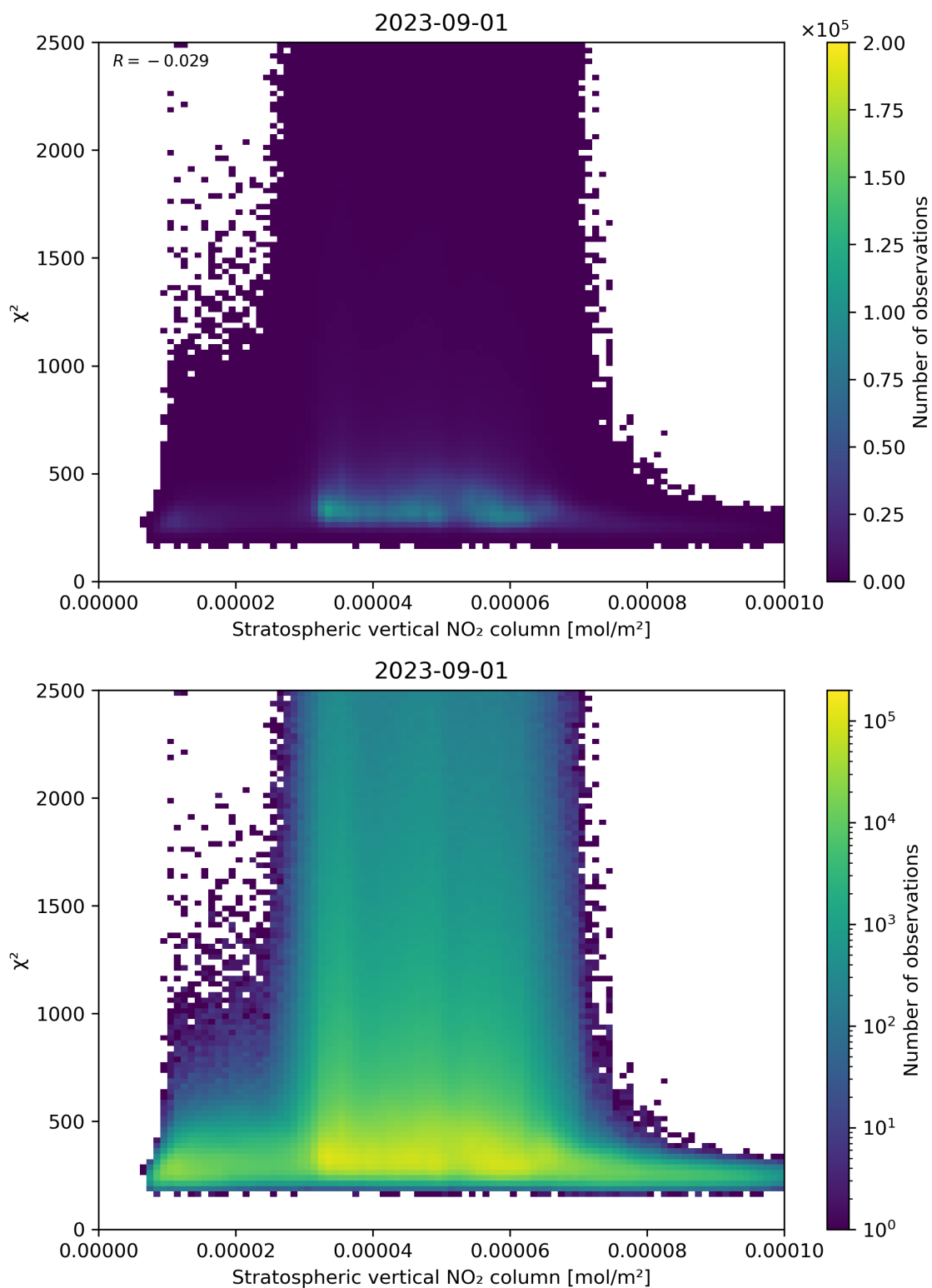
Figure 97: Scatter density plot of “Stratospheric vertical NO 2 column” against “ \chi^2 ” for 2023-08-31 to 2023-09-02.
