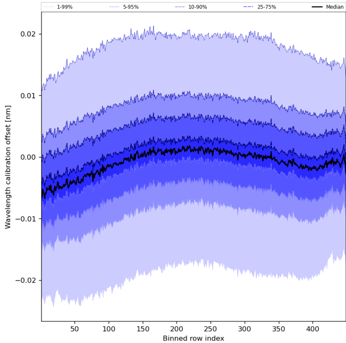
Figure 52: Along track statistics of “Wavelength calibration offset” for 2023-08-31 to 2023-09-02
