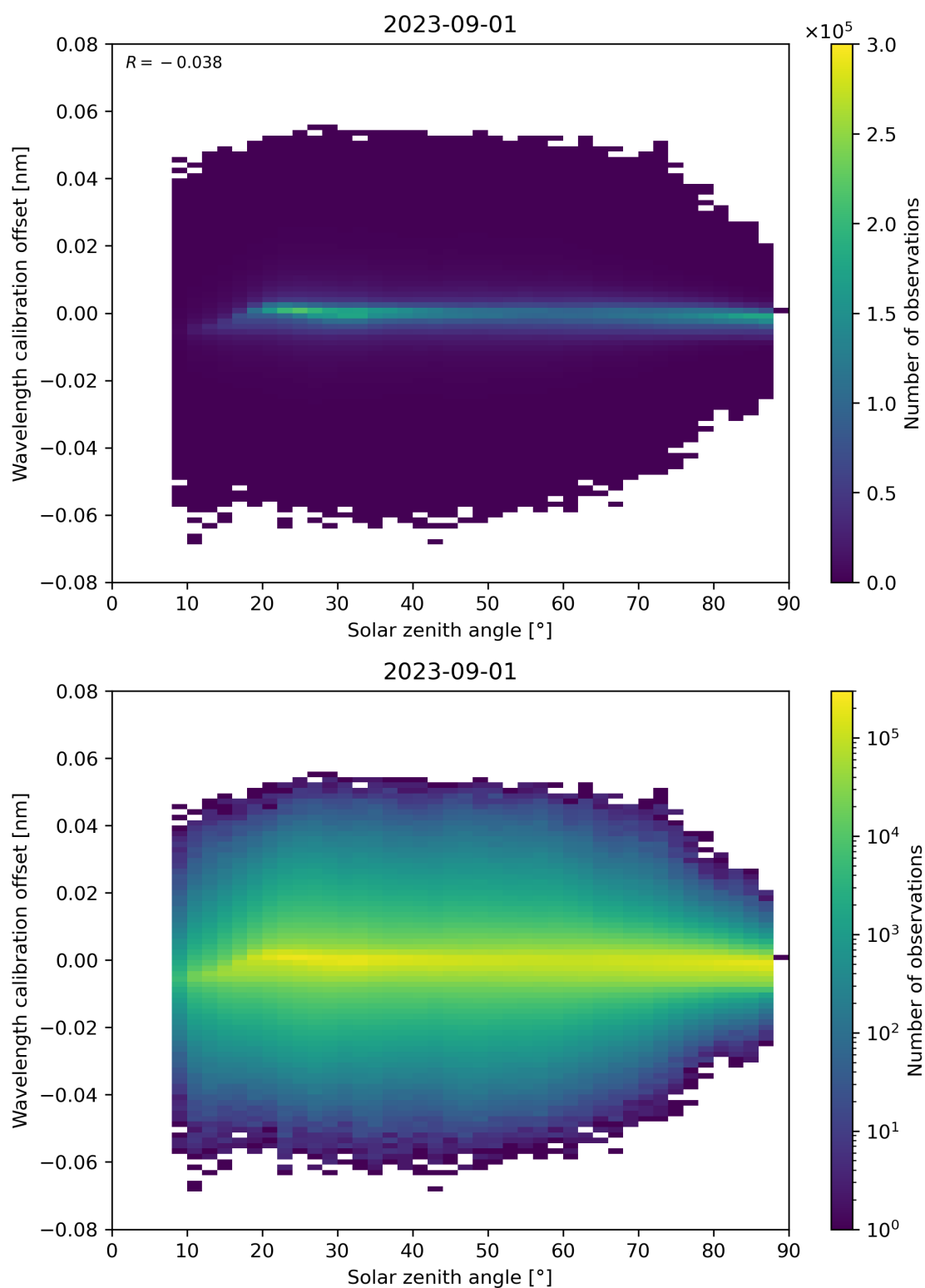
Figure 158: Scatter density plot of “Solar zenith angle” against “Wavelength calibration offset” for 2023-08-31 to 2023-09-02.
