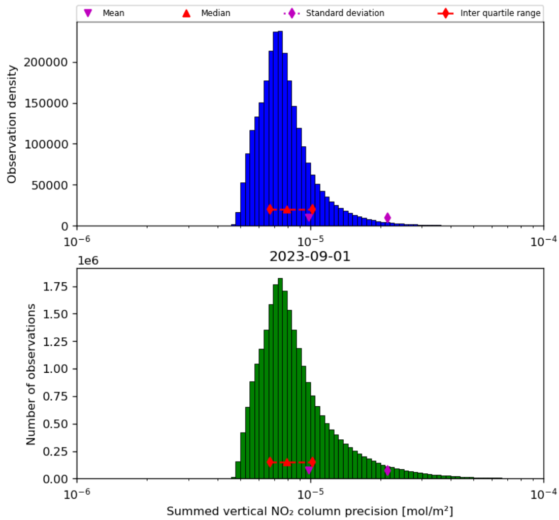
Figure 41: Histogram of "Summed vertical NO 2 column precision" for 2023-08-31 to 2023-09-02
