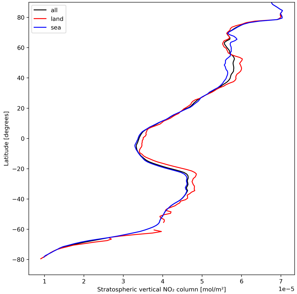
Figure 19: Zonal average of “Stratospheric vertical NO 2 column” for 2023-08-31 to 2023-09-02.
