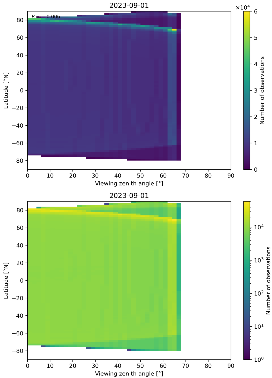
Figure 163: Scatter density plot of “Viewing zenith angle” against “Latitude” for 2023-08-31 to 2023-09-02.
