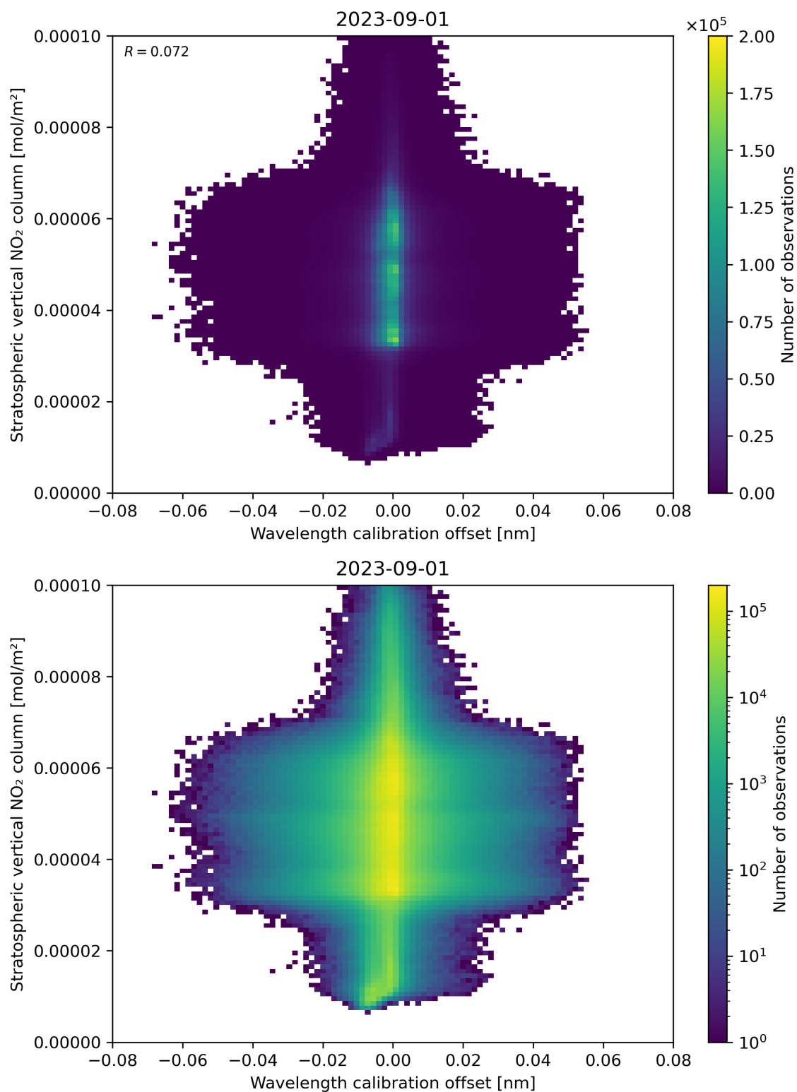
Figure 176: Scatter density plot of “Wavelength calibration offset” against “Stratospheric vertical NO 2 column” for 2023-08-31 to 2023-09-02.
