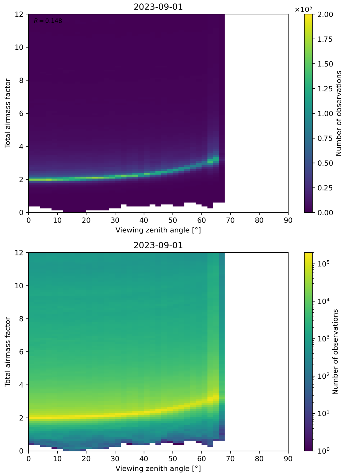
Figure 160: Scatter density plot of “Viewing zenith angle” against “Total airmass factor” for 2023-08-31 to 2023-09-02.
