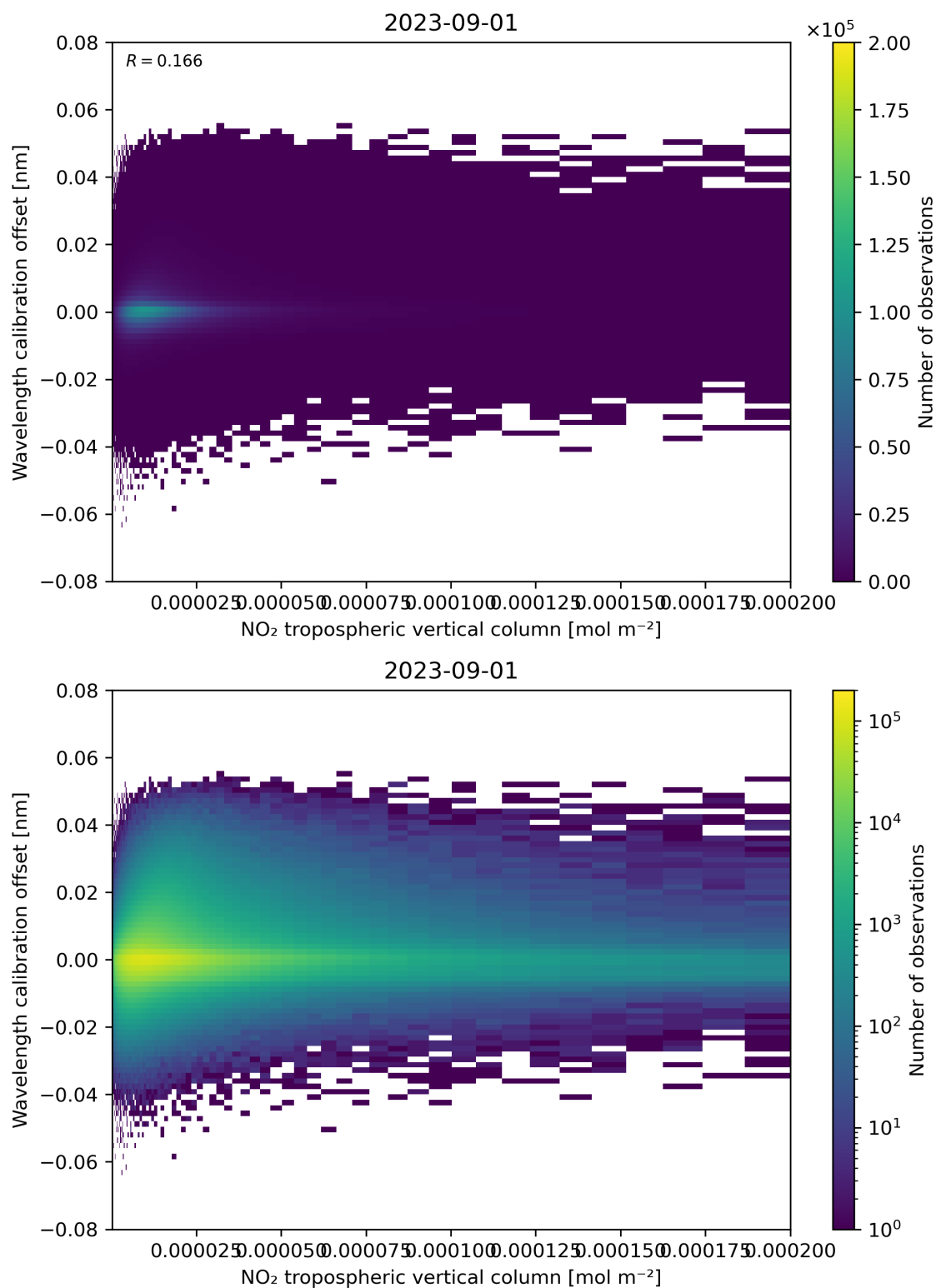
Figure 143: Scatter density plot of “NO 2 tropospheric vertical column” against “Wavelength calibration offset” for 2023-08-31 to 2023-09-02.
