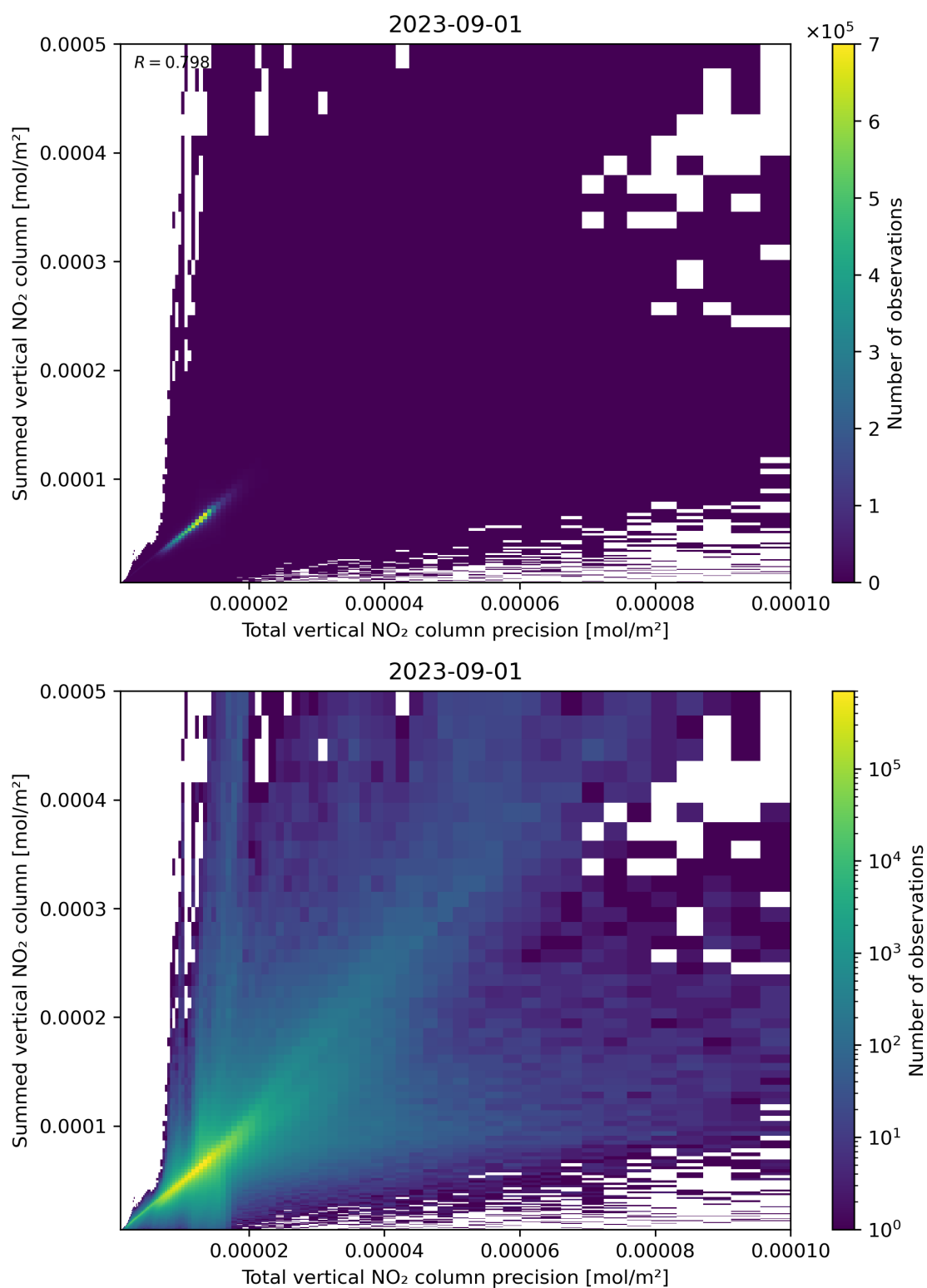
Figure 117: Scatter density plot of “Total vertical NO 2 column precision” against “Summed vertical NO 2 column” for 2023-08-31 to 2023-09-02.
