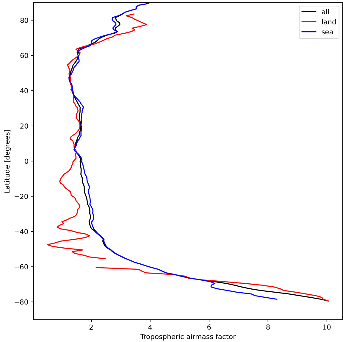
Figure 14: Zonal average of “Tropospheric airmass factor” for 2023-08-31 to 2023-09-02.
