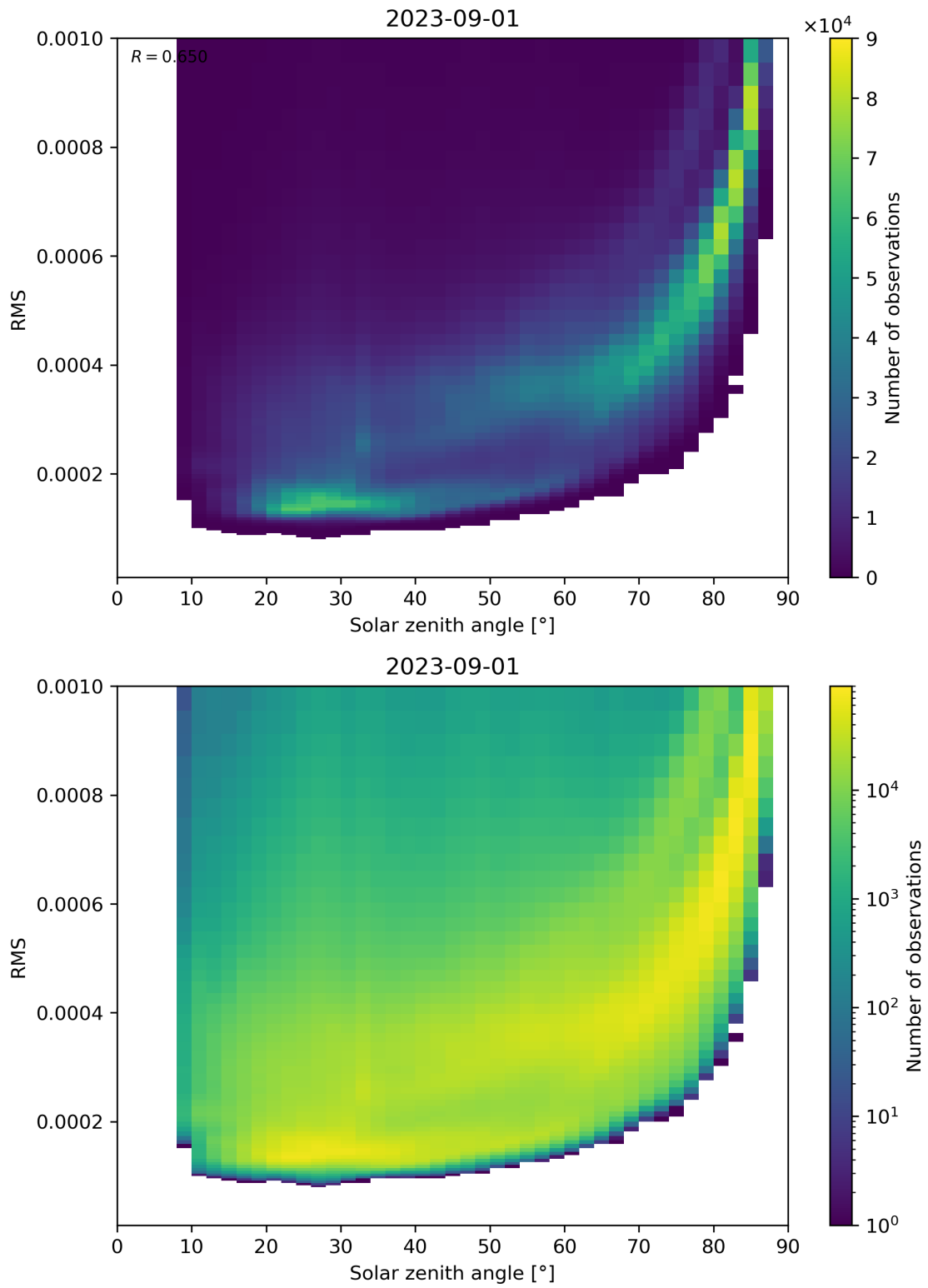
Figure 157: Scatter density plot of “Solar zenith angle” against “RMS” for 2023-08-31 to 2023-09-02.
