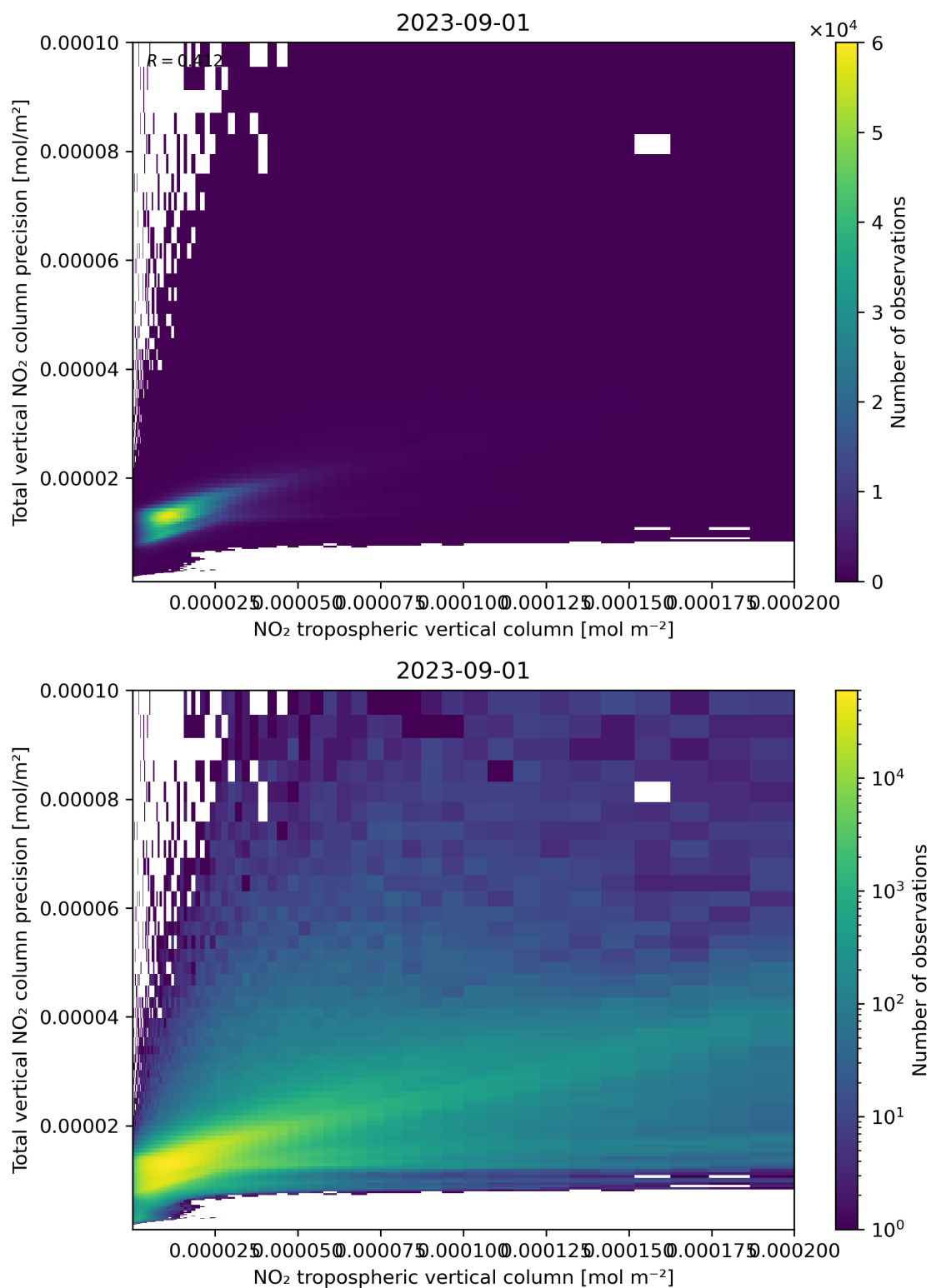
Figure 129: Scatter density plot of “NO 2 tropospheric vertical column” against “Total vertical NO 2 column precision” for 2023-08-31 to 2023-09-02.
