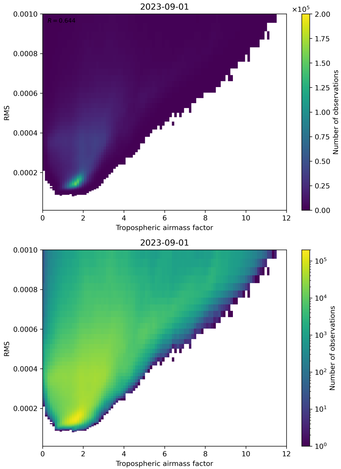
Figure 79: Scatter density plot of “Tropospheric airmass factor” against “RMS” for 2023-08-31 to 2023-09-02.
