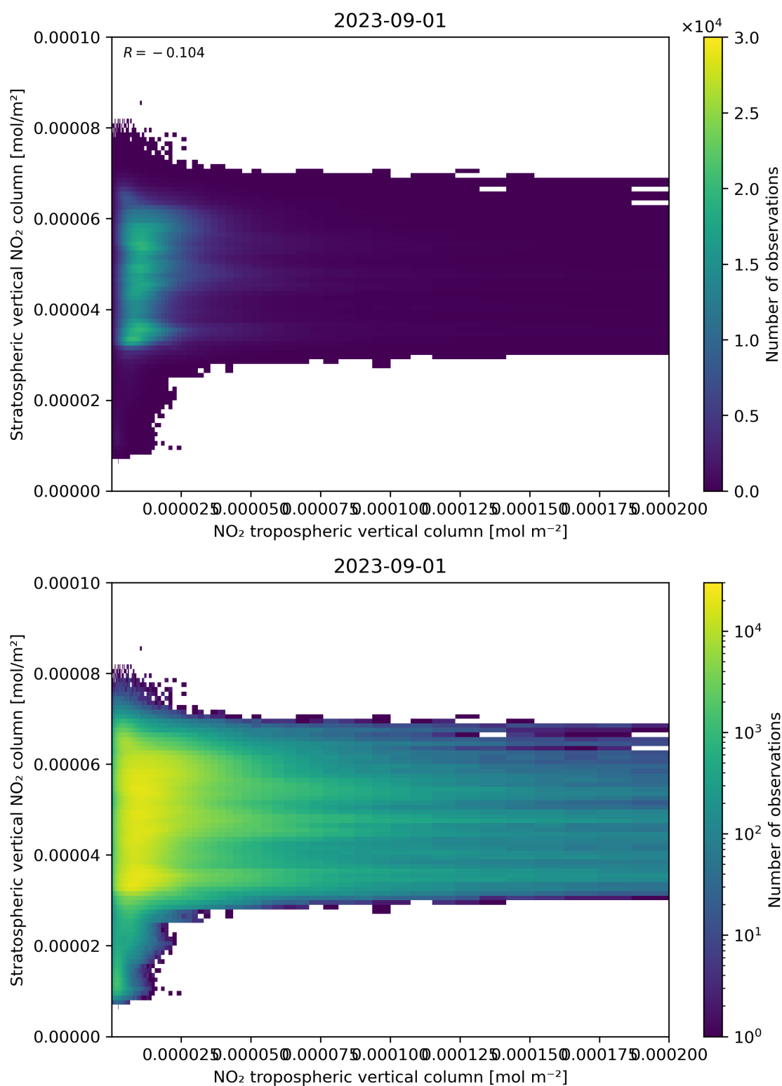
Figure 125: Scatter density plot of “NO 2 tropospheric vertical column” against “Stratospheric vertical NO 2 column” for 2023-08-31 to 2023-09-02.
