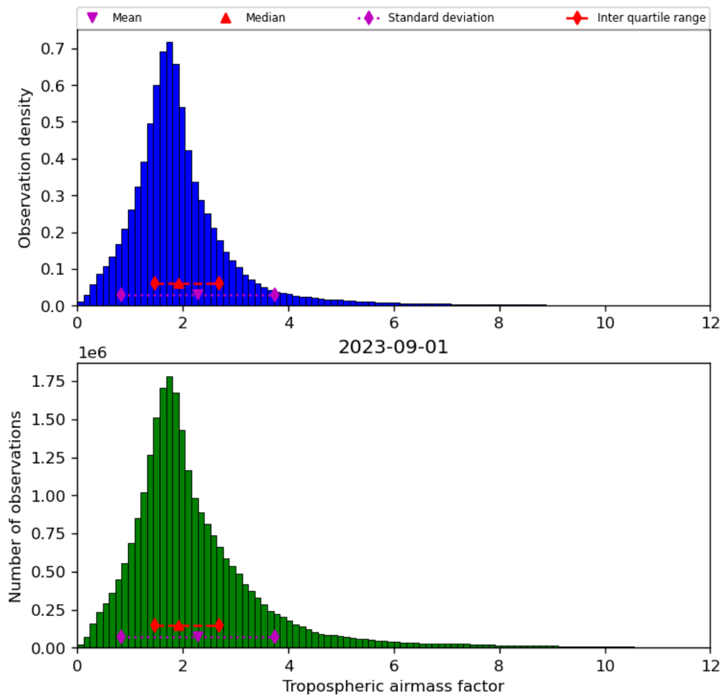
Figure 31: Histogram of “Tropospheric airmass factor” for 2023-08-31 to 2023-09-02
