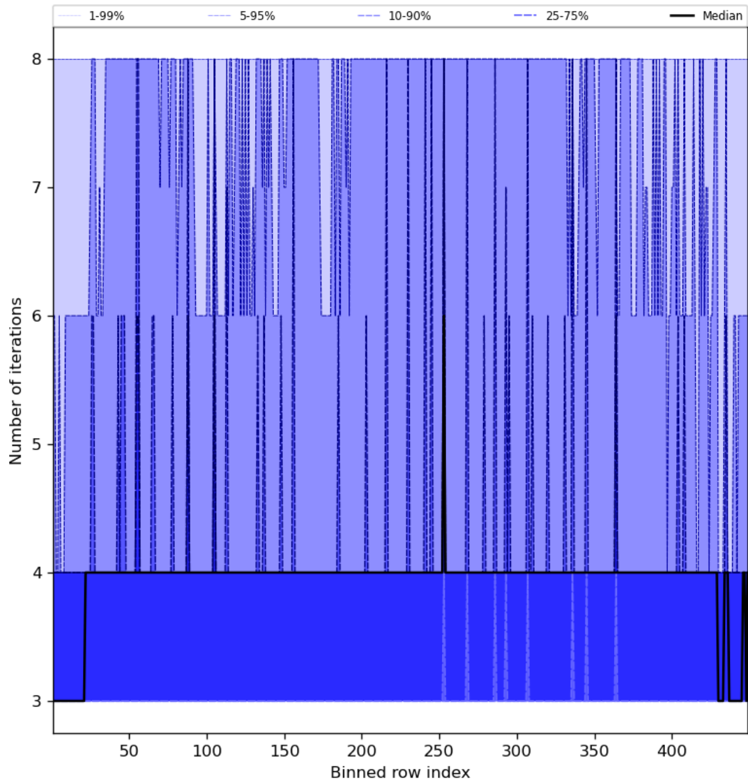
Figure 51: Along track statistics of “Number of iterations” for 2023-08-31 to 2023-09-02
