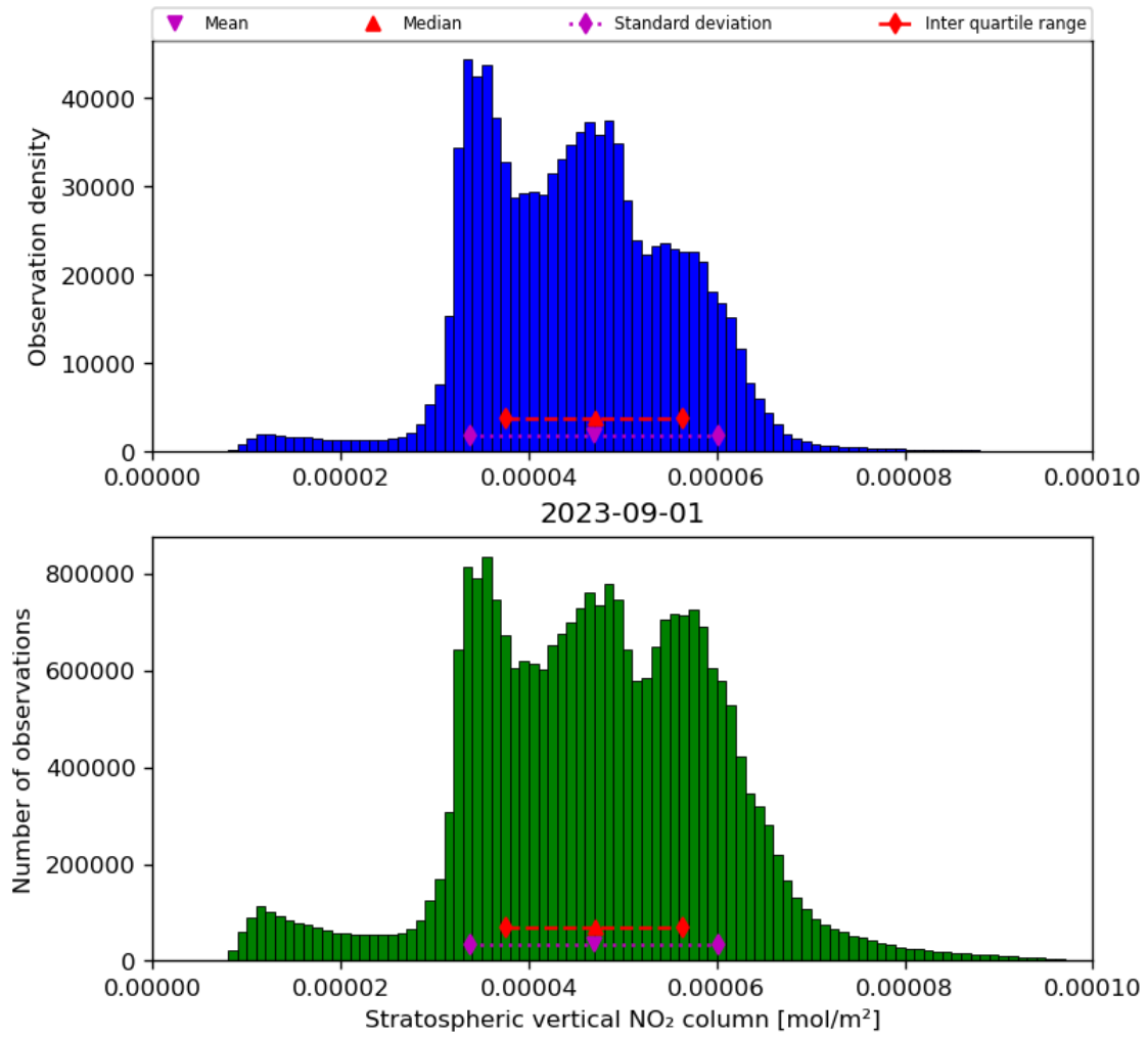
Figure 36: Histogram of “Stratospheric vertical NO 2 column” for 2023-08-31 to 2023-09-02
