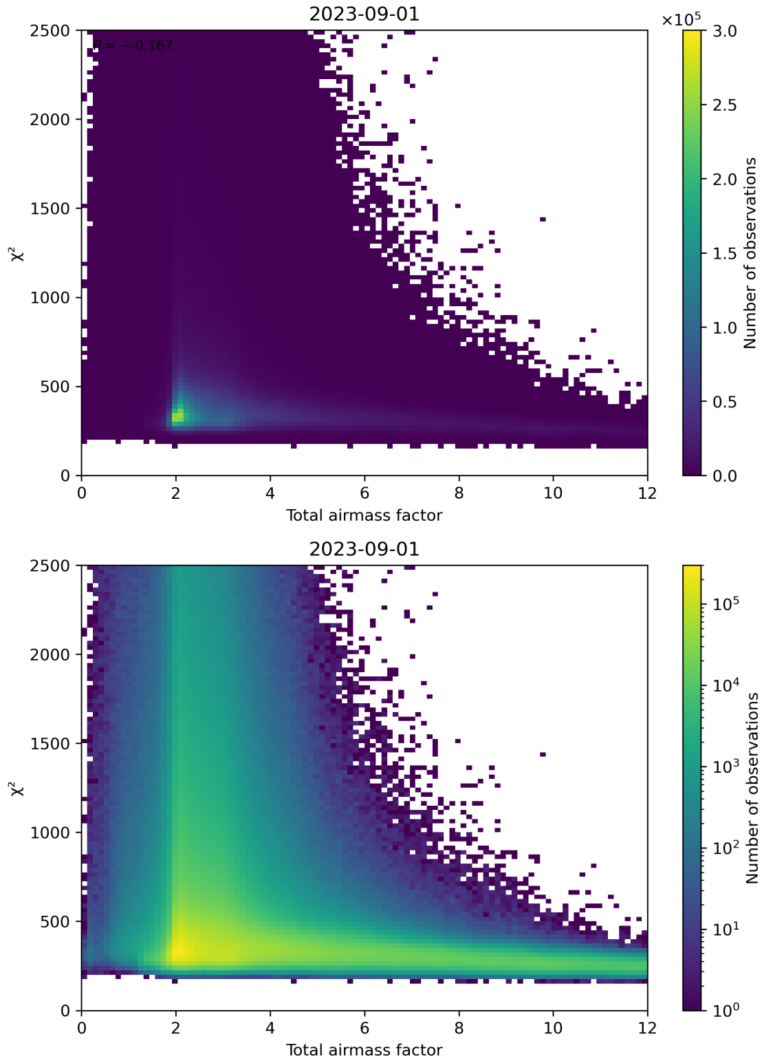
Figure 63: Scatter density plot of “Total airmass factor” against “ \chi^2 ” for 2023-08-31 to 2023-09-02.
