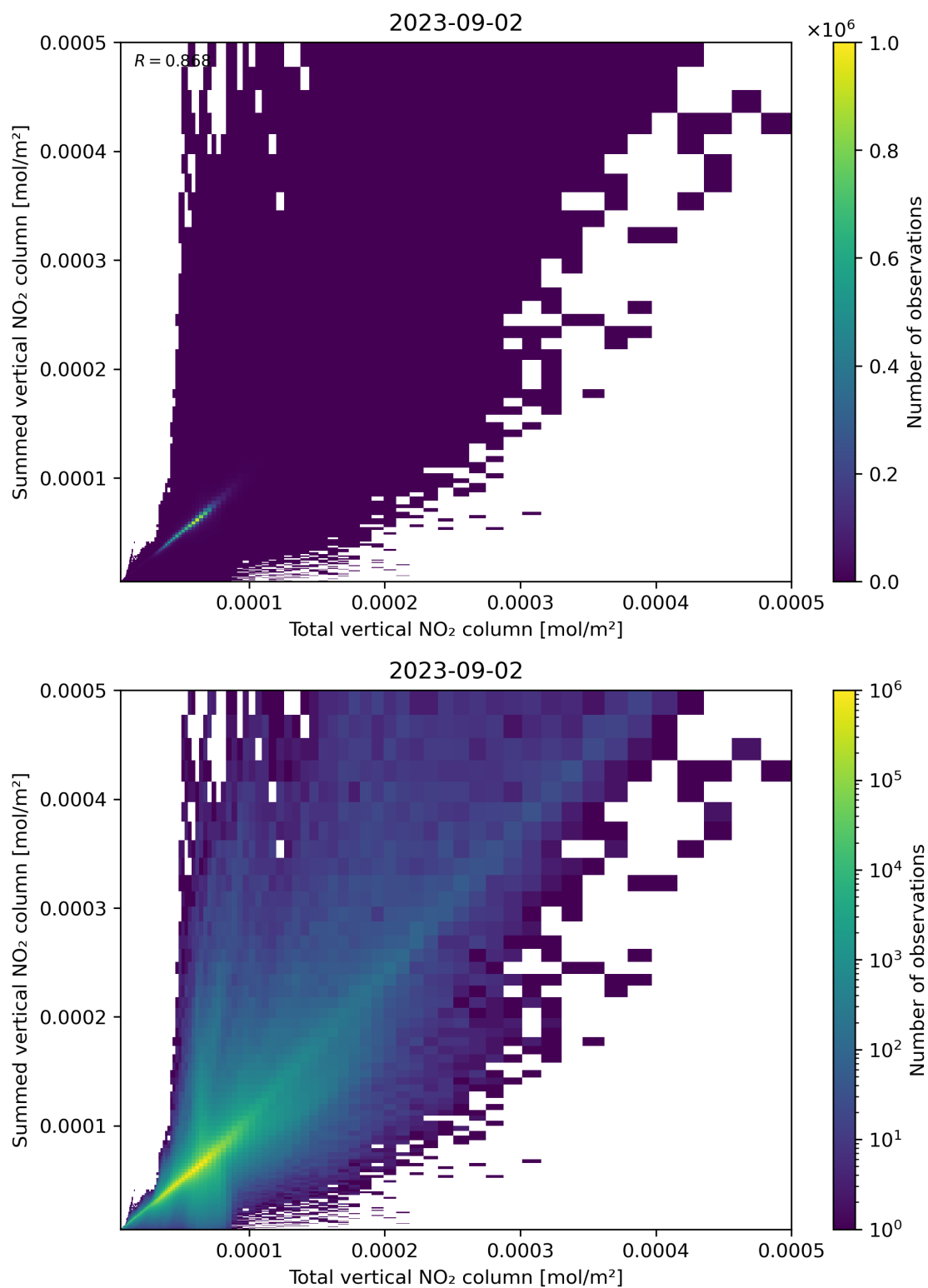
Figure 112: Scatter density plot of “Total vertical NO 2 column” against “Summed vertical NO 2 column” for 2023-09-01 to 2023-09-03.
