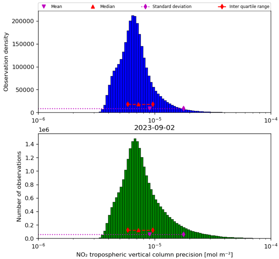
Figure 30: Histogram of “NO 2 tropospheric vertical column precision” for 2023-09-01 to 2023-09-03
