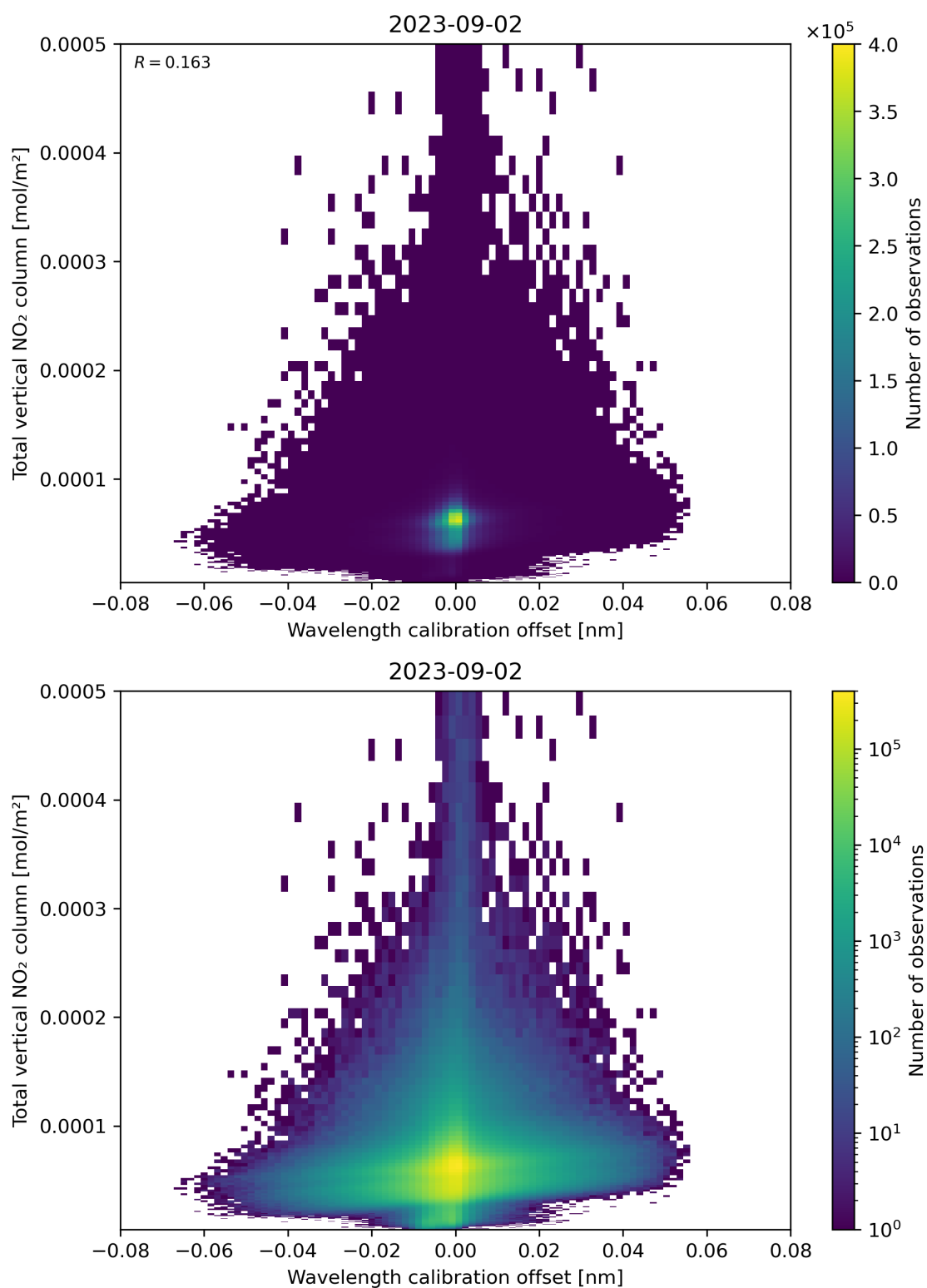
Figure 179: Scatter density plot of “Wavelength calibration offset” against “Total vertical NO 2 column” for 2023-09-01 to 2023-09-03.
