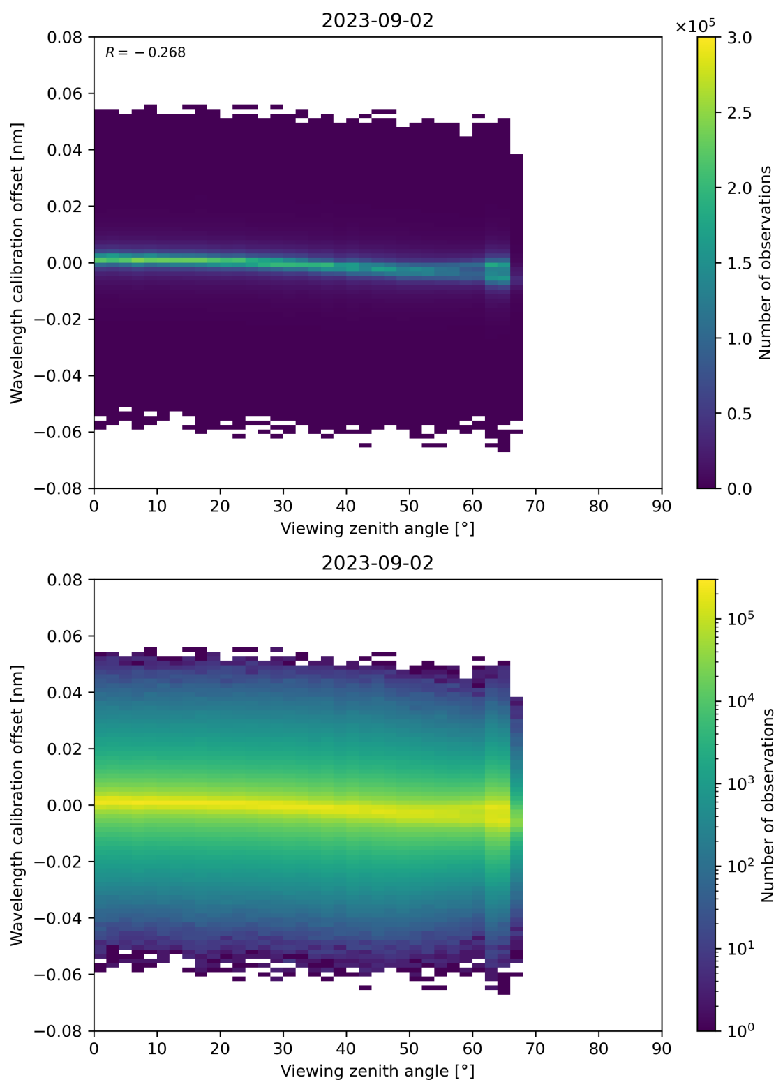
Figure 173: Scatter density plot of “Viewing zenith angle” against “Wavelength calibration offset” for 2023-09-01 to 2023-09-03.
