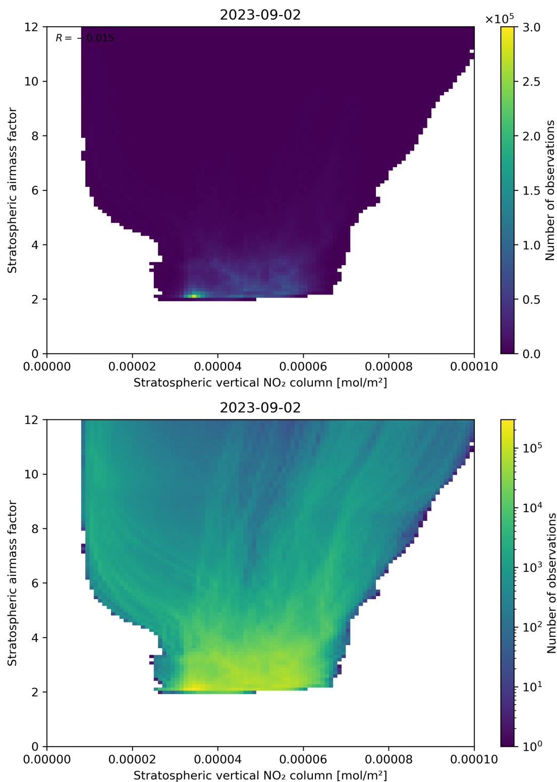
Figure 96: Scatter density plot of “Stratospheric vertical NO 2 column” against “Stratospheric airmass factor” for 2023-09-01 to 2023-09-03.
