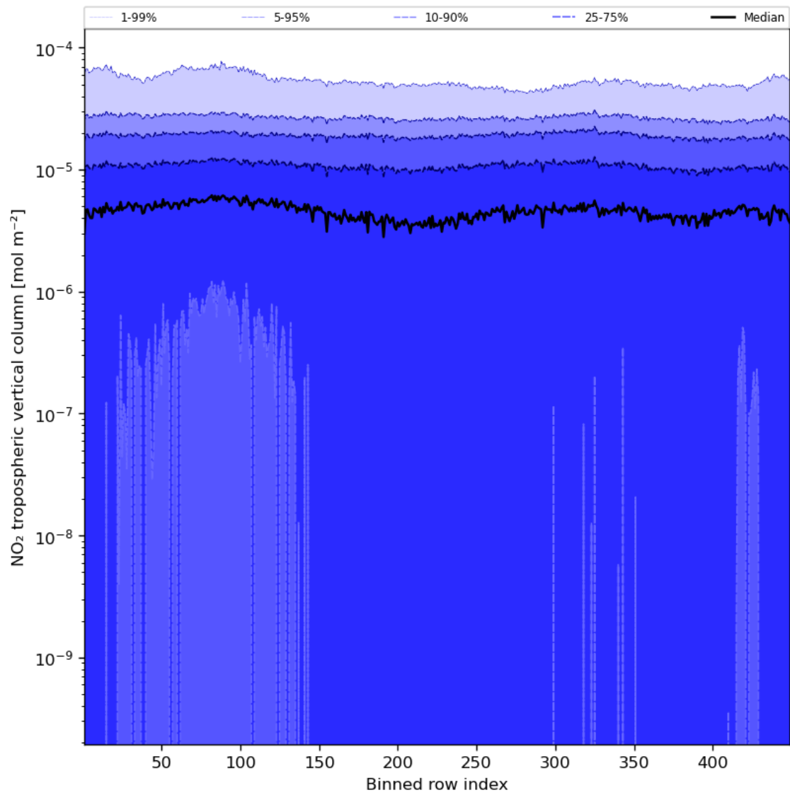
Figure 46: Along track statistics of “NO 2 tropospheric vertical column” for 2023-09-01 to 2023-09-03
