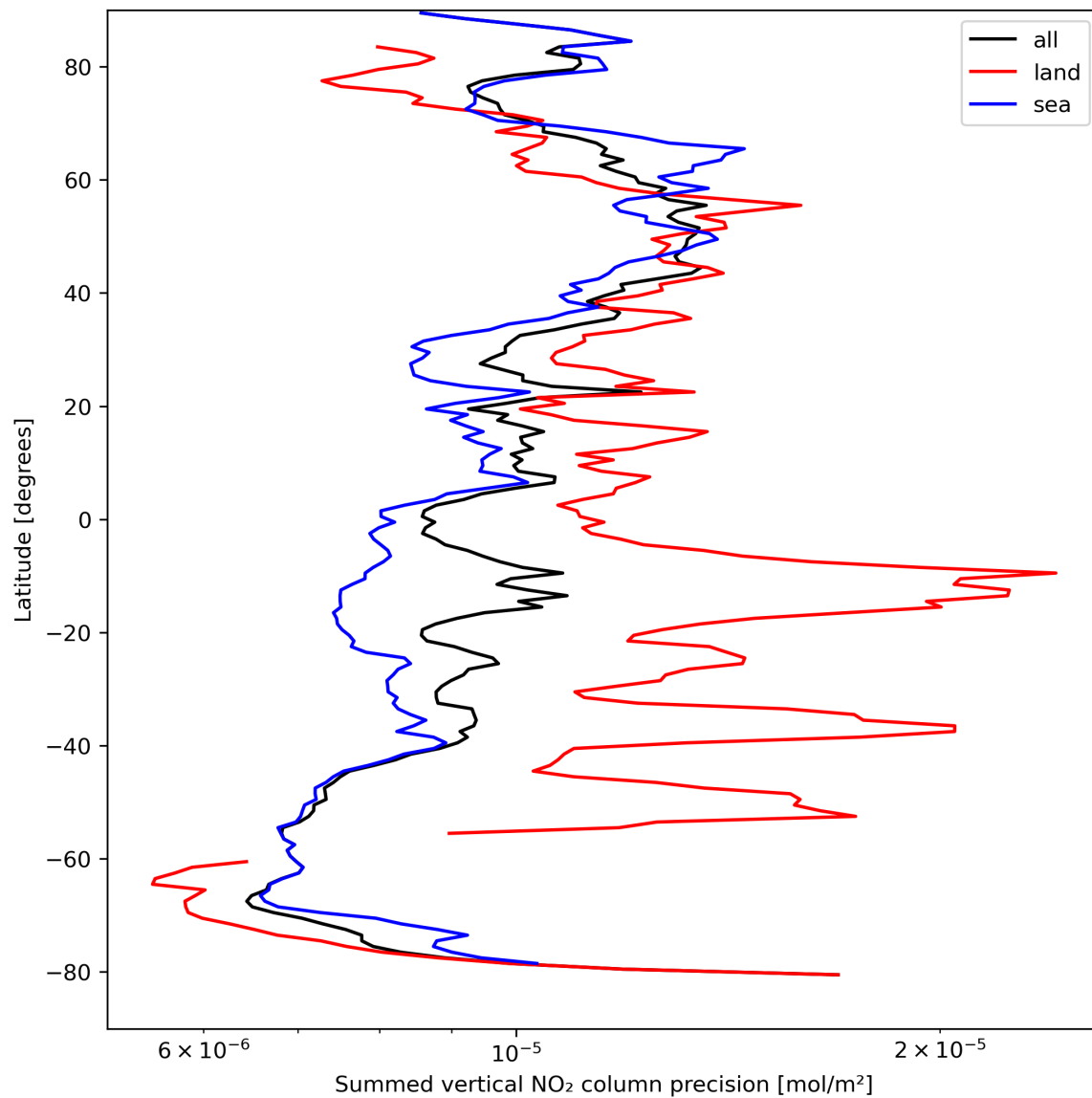
Figure 24: Zonal average of “Summed vertical NO 2 column precision” for 2023-09-01 to 2023-09-03.
