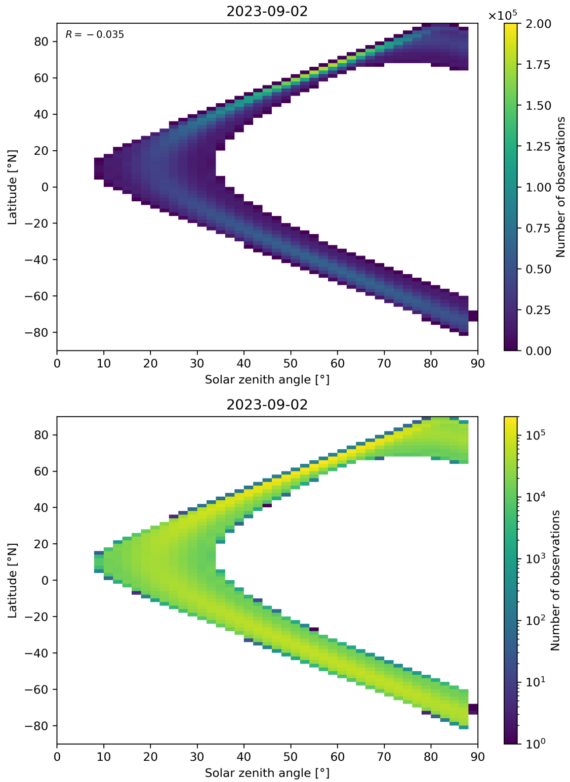
Figure 149: Scatter density plot of “Solar zenith angle” against “Latitude” for 2023-09-01 to 2023-09-03.
