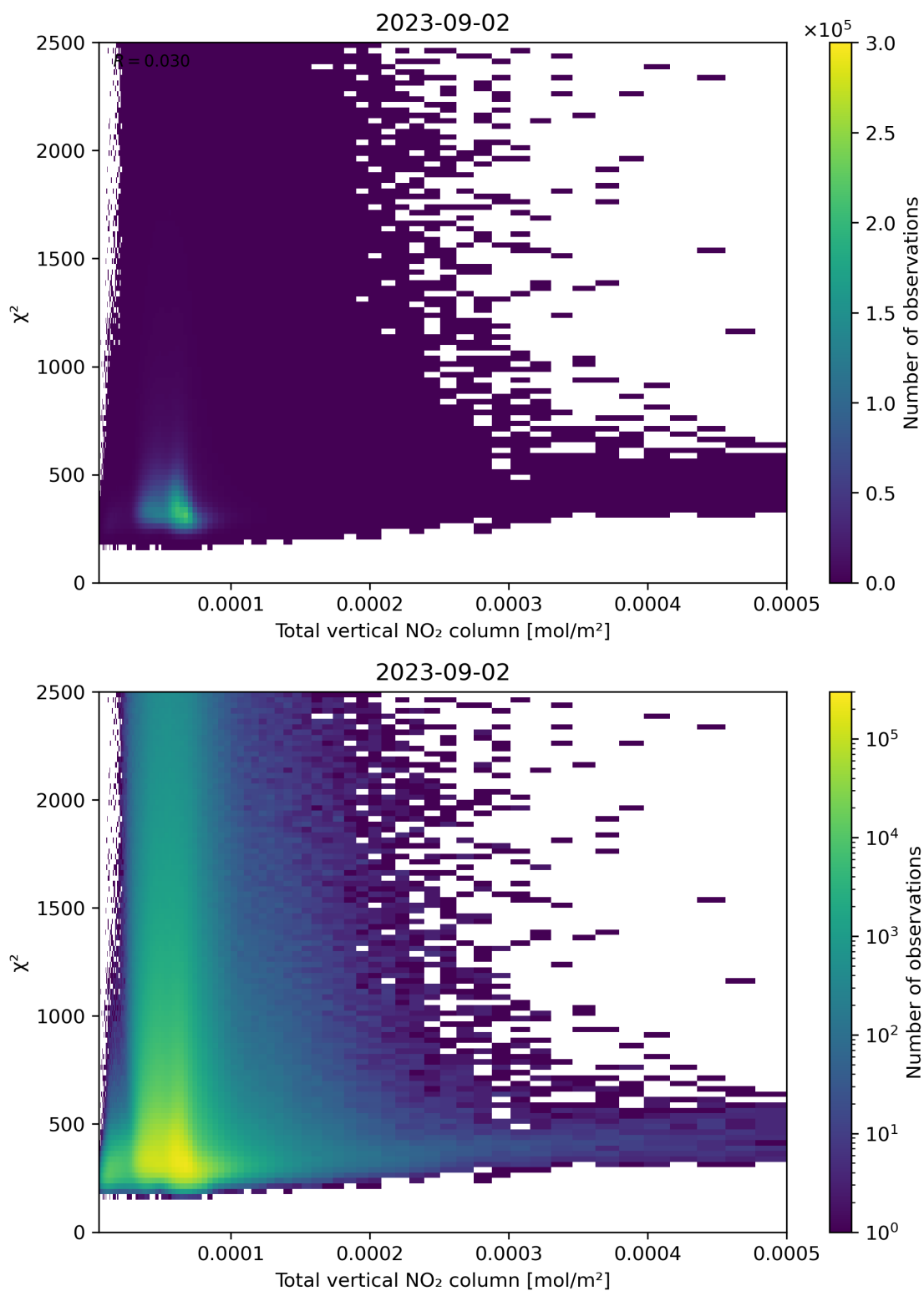
Figure 111: Scatter density plot of “Total vertical NO 2 column” against “ \chi^2 ” for 2023-09-01 to 2023-09-03.
