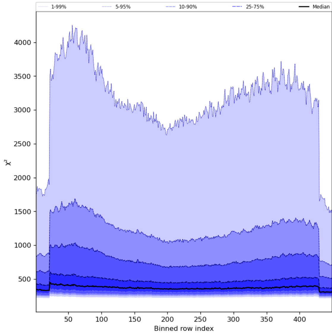
Figure 59: Along track statistics of “ \chi^2 ” for 2023-09-01 to 2023-09-03
