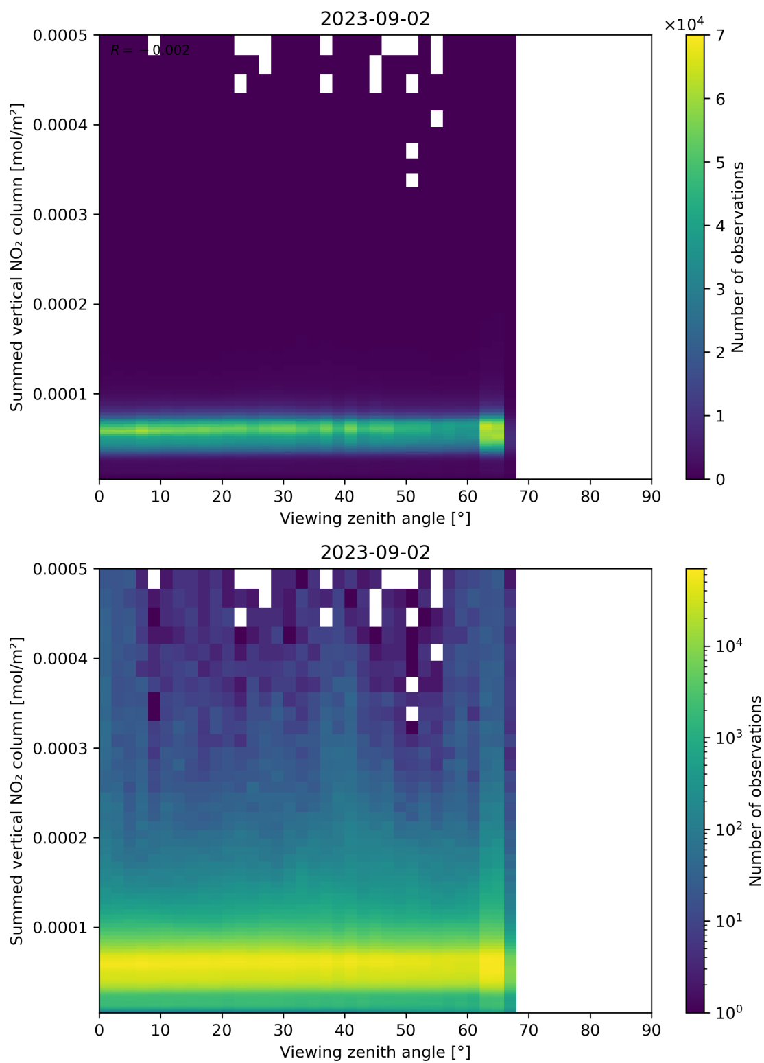
Figure 165: Scatter density plot of “Viewing zenith angle” against “Summed vertical NO 2 column” for 2023-09-01 to 2023-09-03.
