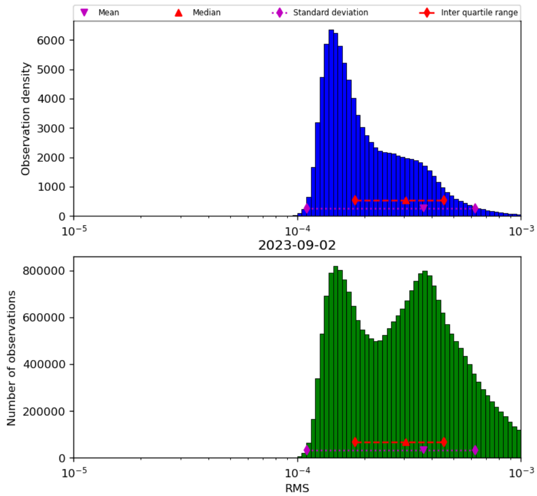
Figure 43: Histogram of “RMS” for 2023-09-01 to 2023-09-03
