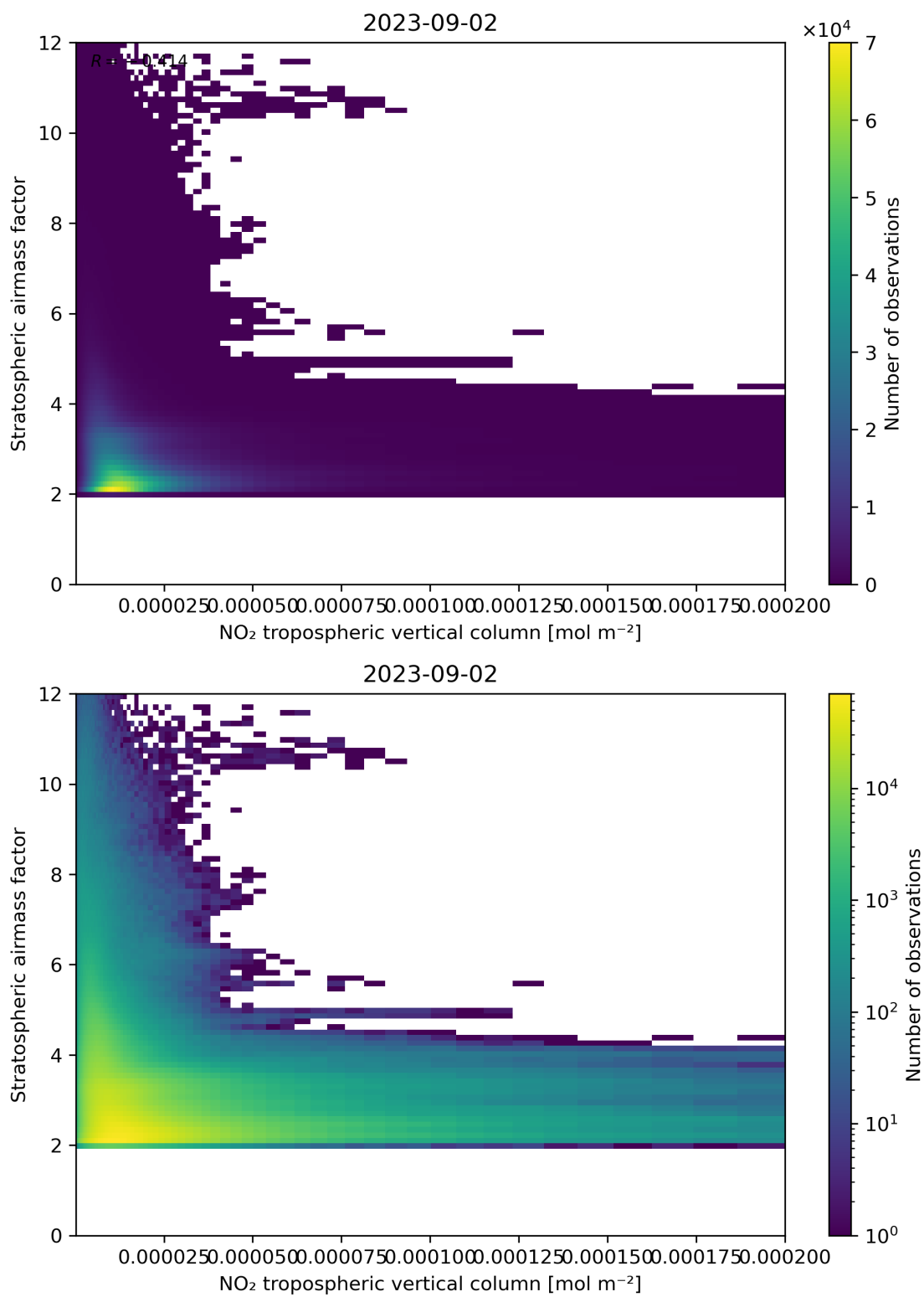
Figure 121: Scatter density plot of “NO 2 tropospheric vertical column” against “Stratospheric air mass factor” for 2023-09-01 to 2023-09-03.
