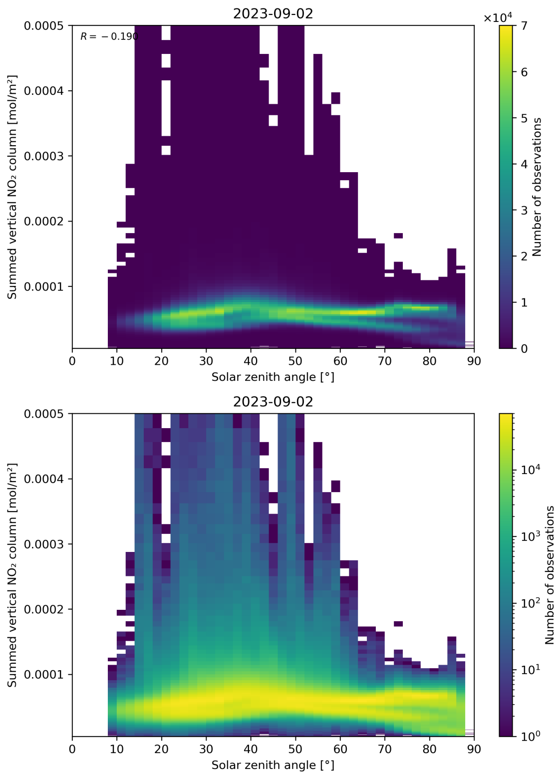
Figure 151: Scatter density plot of “Solar zenith angle” against “Summed vertical NO 2 column” for 2023-09-01 to 2023-09-03.
