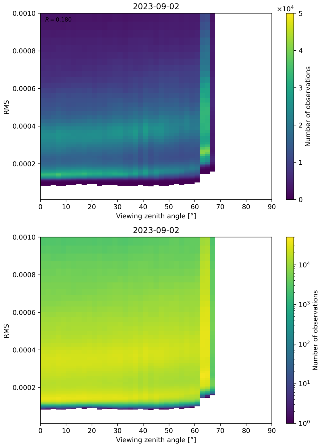
Figure 171: Scatter density plot of “Viewing zenith angle” against “RMS” for 2023-09-01 to 2023-09-03.
