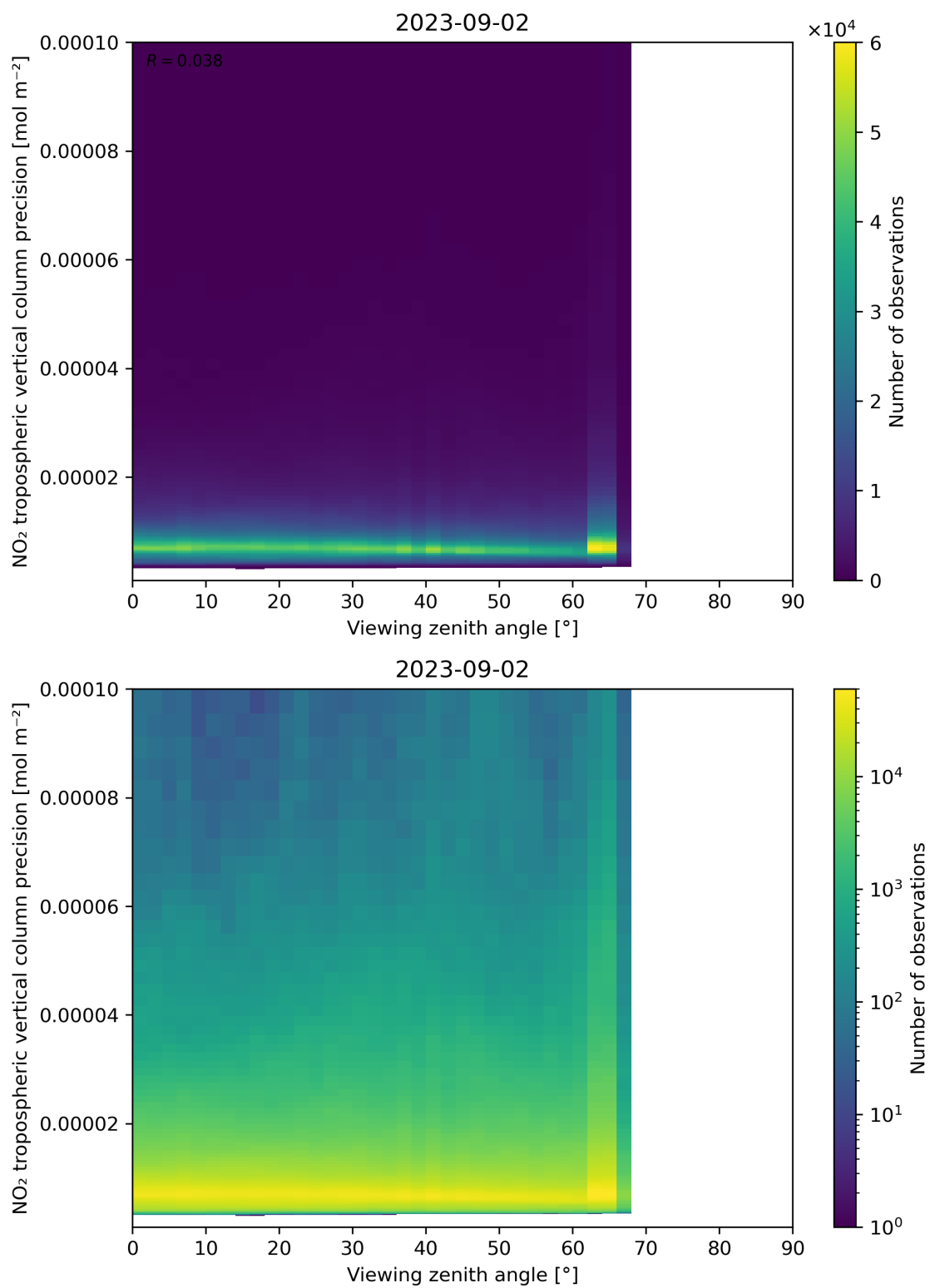
Figure 170: Scatter density plot of “Viewing zenith angle” against “NO 2 tropospheric vertical column precision” for 2023-09-01 to 2023-09-03.
