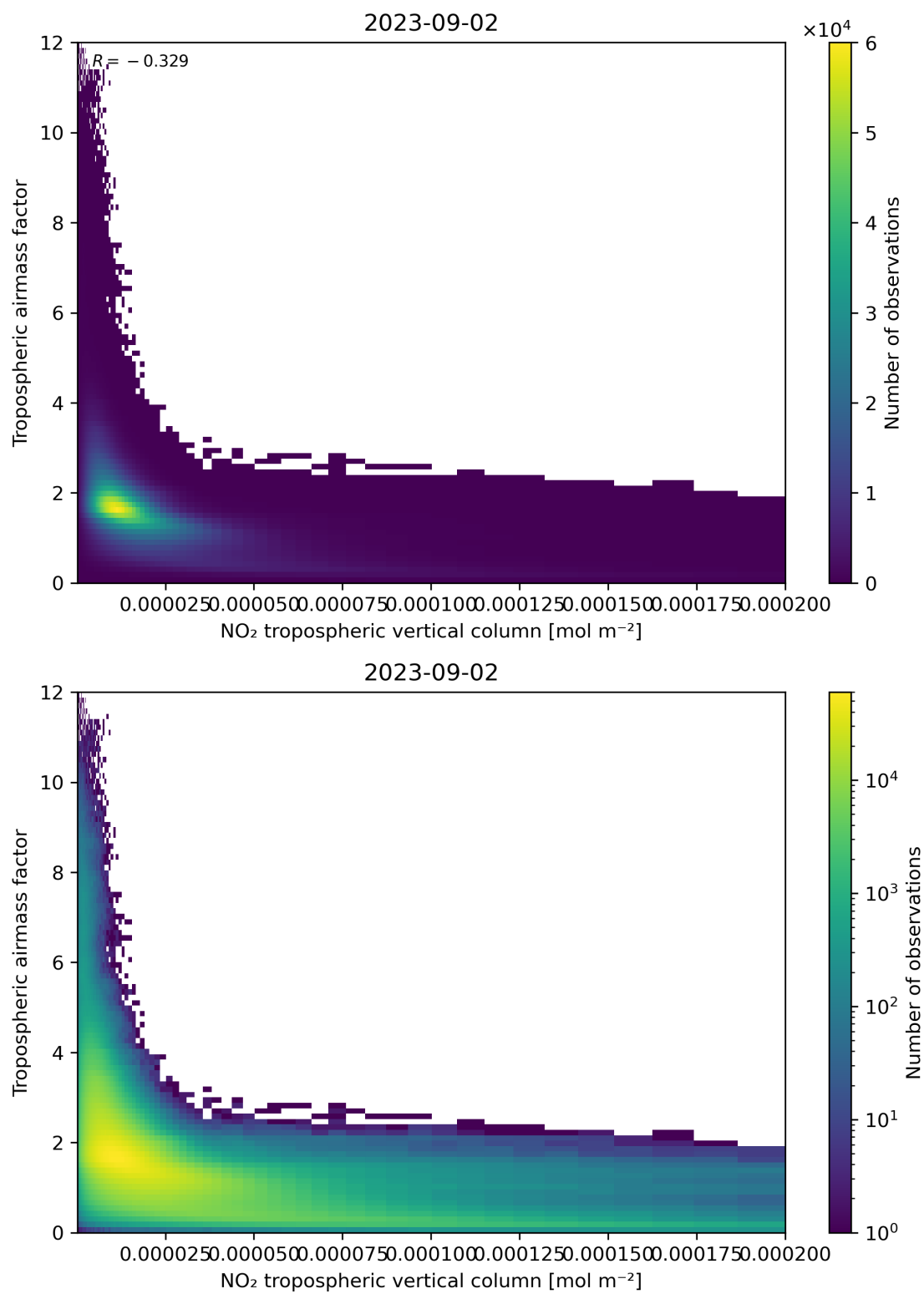
Figure 123: Scatter density plot of “NO 2 tropospheric vertical column” against “Tropospheric air mass factor” for 2023-09-01 to 2023-09-03.
