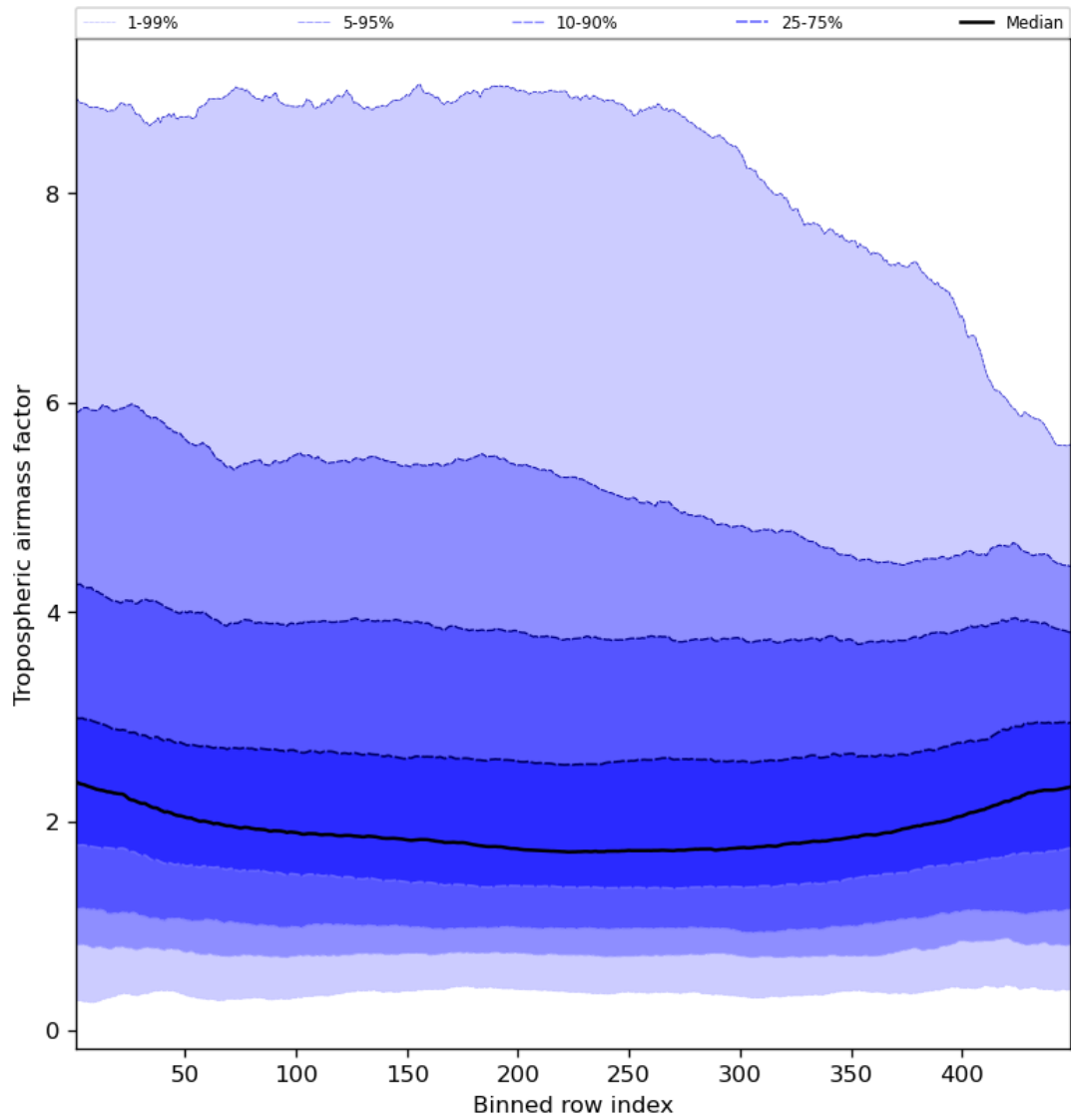
Figure 48: Along track statistics of “Tropospheric air mass factor” for 2023-09-01 to 2023-09-03
