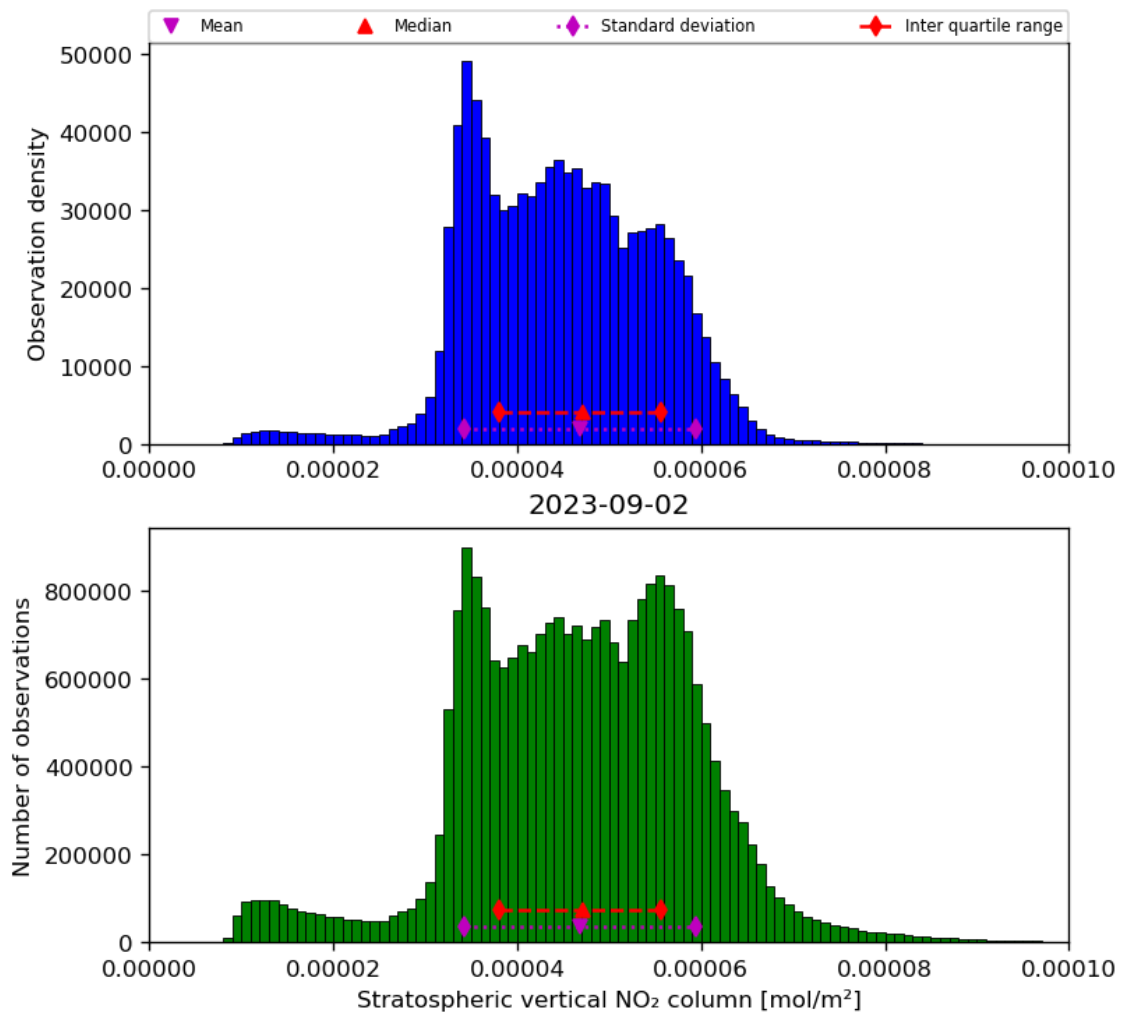
Figure 36: Histogram of “Stratospheric vertical NO 2 column” for 2023-09-01 to 2023-09-03
