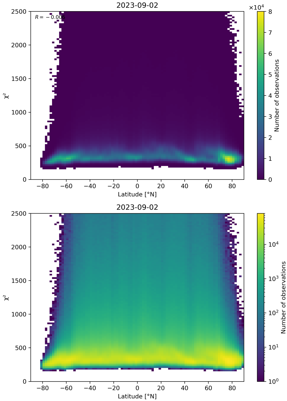
Figure 86: Scatter density plot of “Latitude” against “ \chi^2 ” for 2023-09-01 to 2023-09-03.
