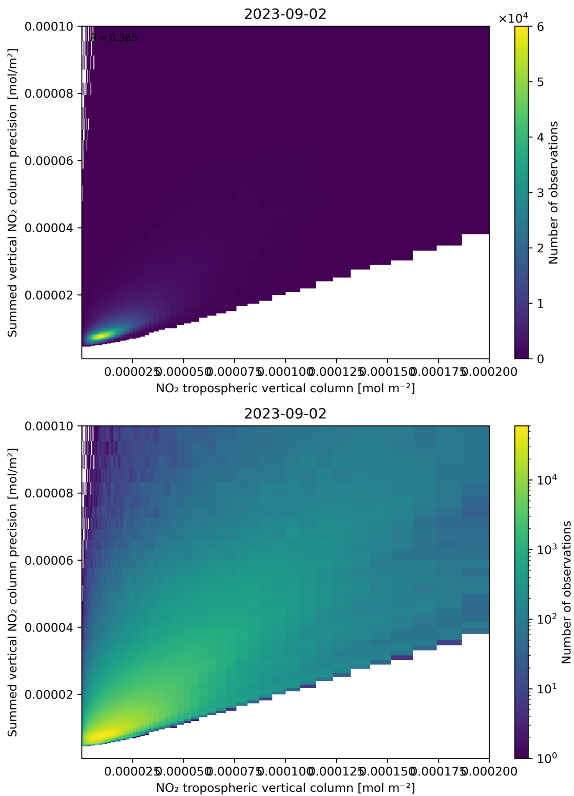
Figure 127: Scatter density plot of “NO 2 tropospheric vertical column” against “Summed vertical NO 2 column precision” for 2023-09-01 to 2023-09-03.
