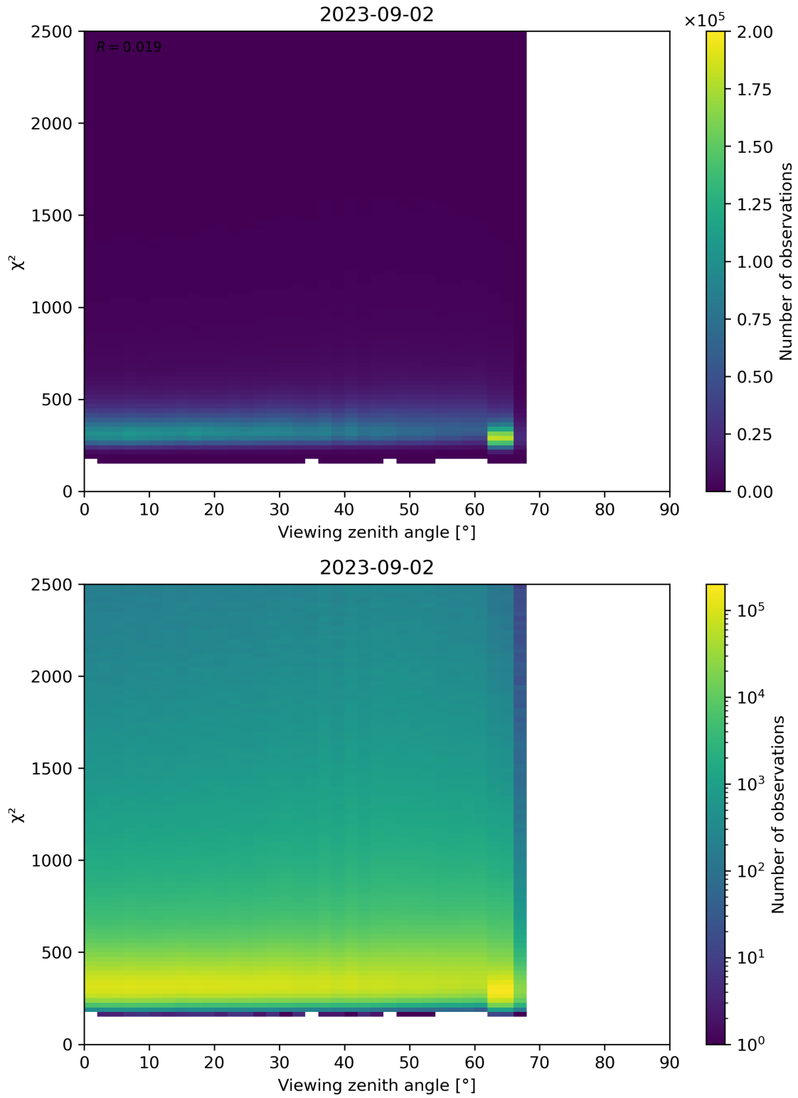
Figure 162: Scatter density plot of “Viewing zenith angle” against “ \chi^2 ” for 2023-09-01 to 2023-09-03.
