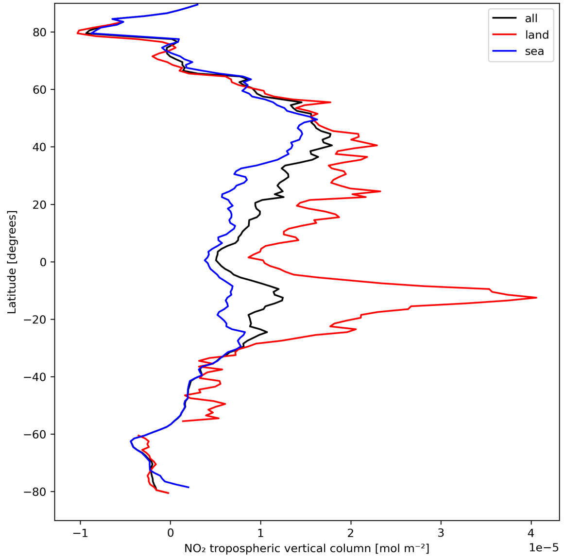
Figure 12: Zonal average of “NO 2 tropospheric vertical column” for 2023-09-01 to 2023-09-03.
