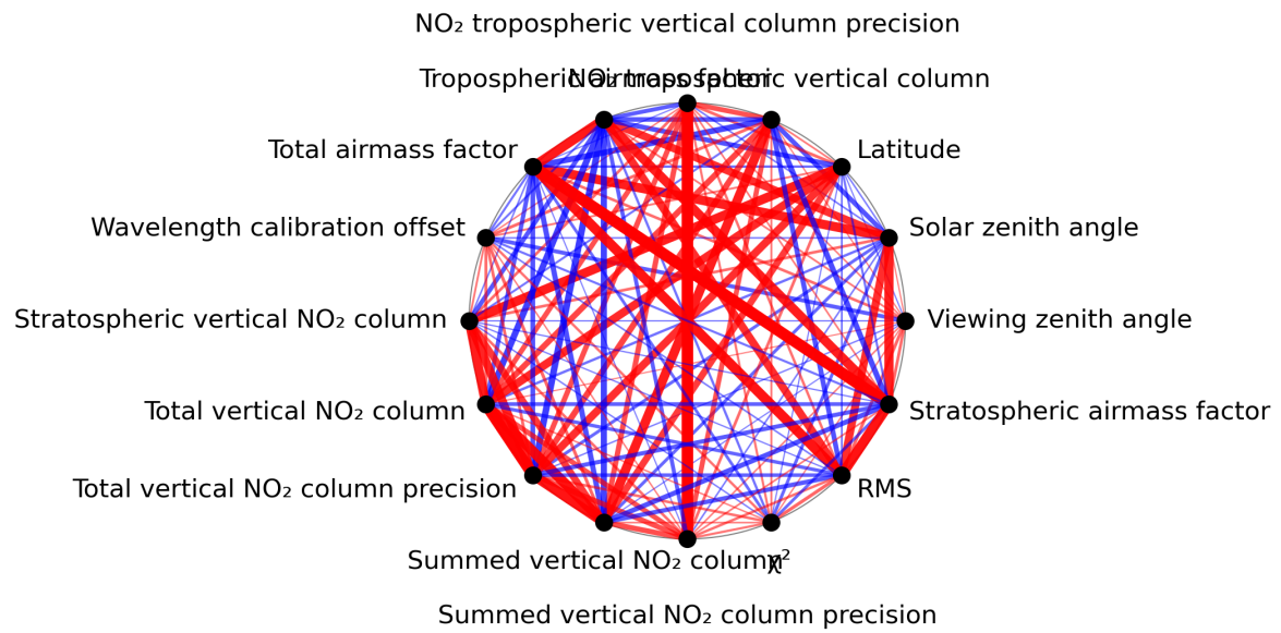
Figure 1: Map of correlation graph for 2023-09-01 to 2023-09-03.
