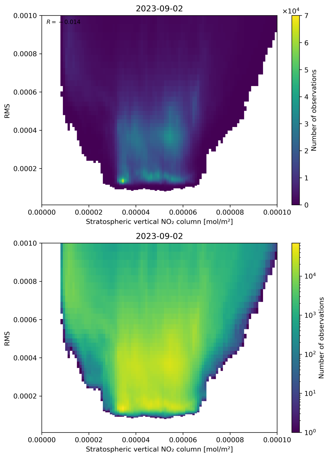
Figure 102: Scatter density plot of “Stratospheric vertical NO 2 column” against “RMS” for 2023-09-01 to 2023-09-03.
