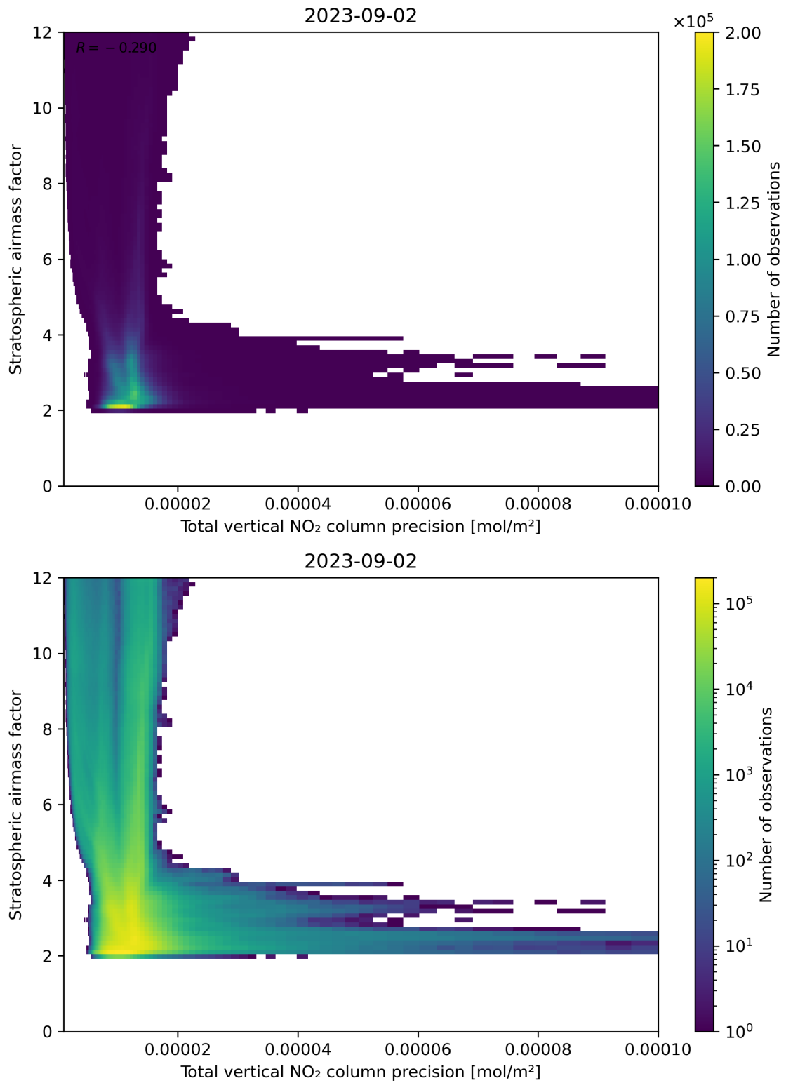
Figure 115: Scatter density plot of “Total vertical NO 2 column precision” against “Stratospheric air mass factor” for 2023-09-01 to 2023-09-03.
