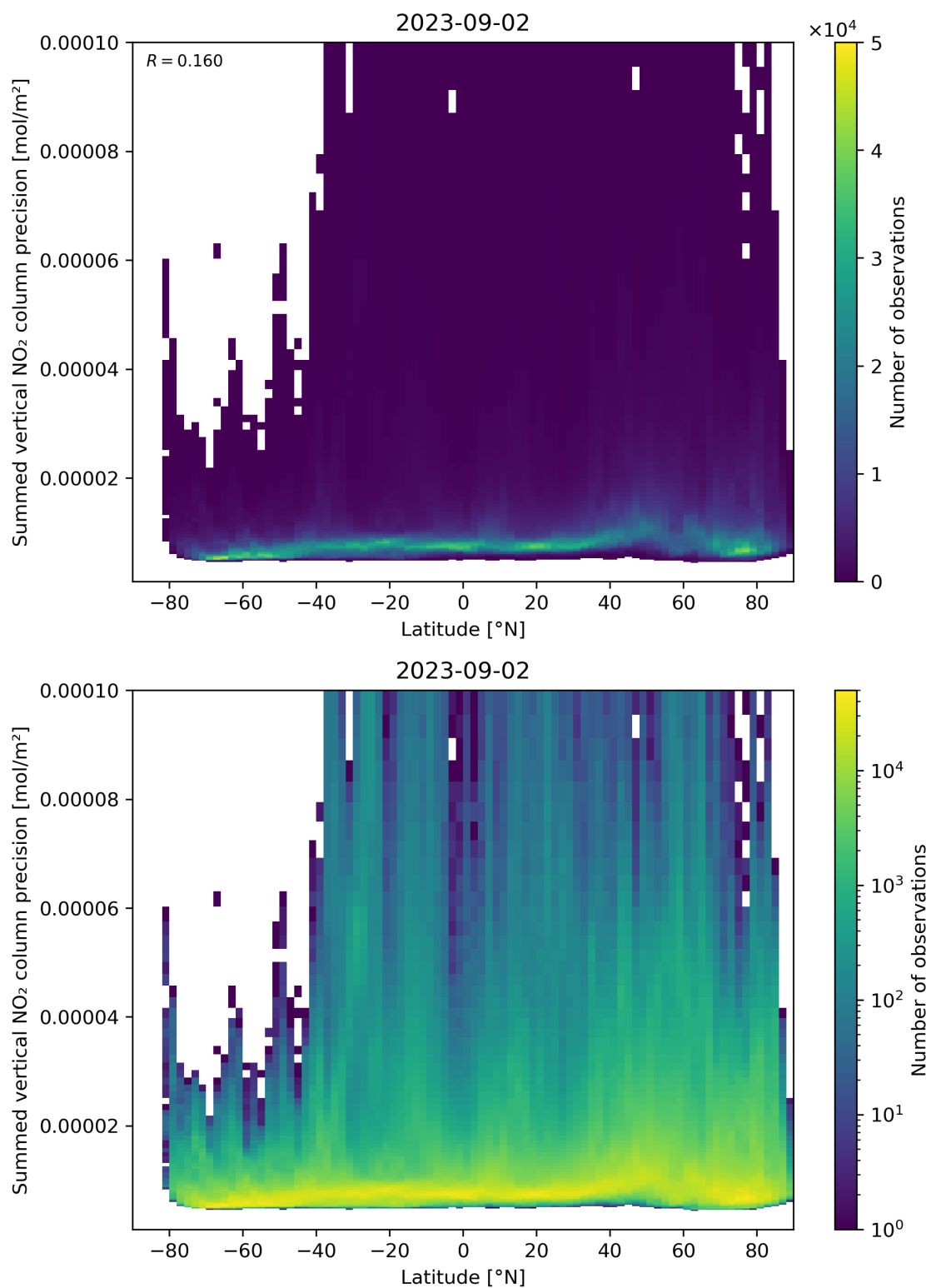
Figure 89: Scatter density plot of “Latitude” against “Summed vertical NO 2 column precision” for 2023-09-01 to 2023-09-03.
