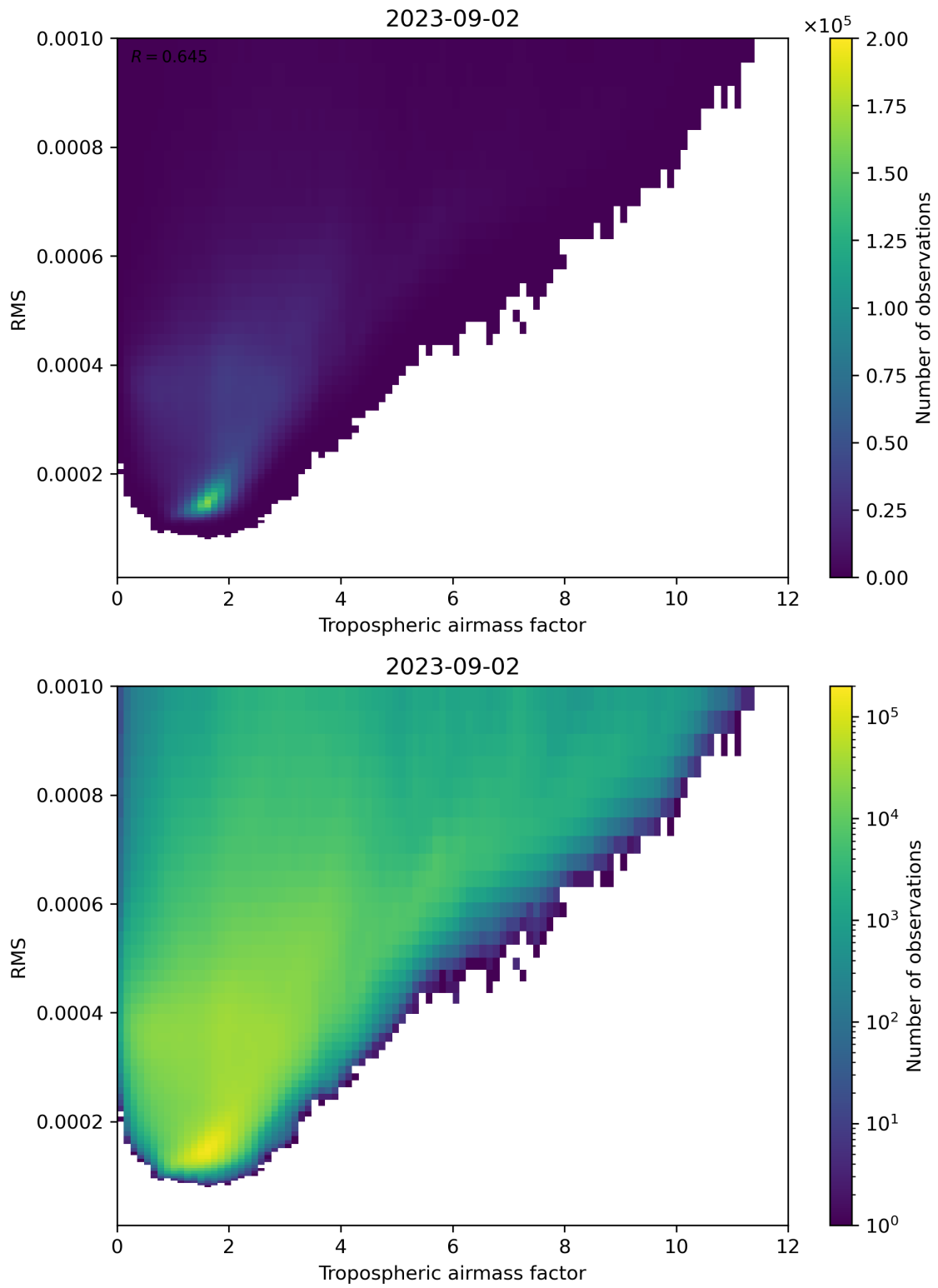
Figure 79: Scatter density plot of “Tropospheric airmass factor” against “RMS” for 2023-09-01 to 2023-09-03.
