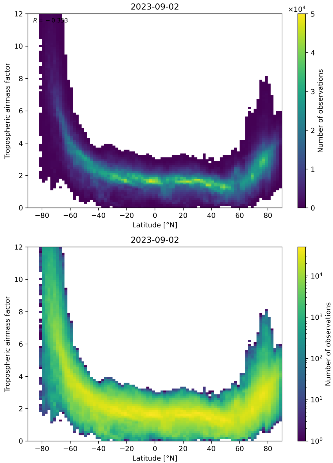
Figure 85: Scatter density plot of “Latitude” against “Tropospheric airmass factor” for 2023-09-01 to 2023-09-03.
