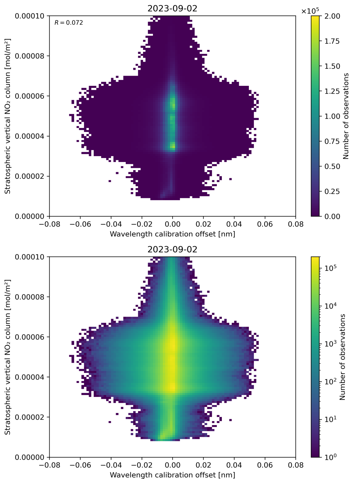
Figure 176: Scatter density plot of “Wavelength calibration offset” against “Stratospheric vertical NO 2 column” for 2023-09-01 to 2023-09-03.
