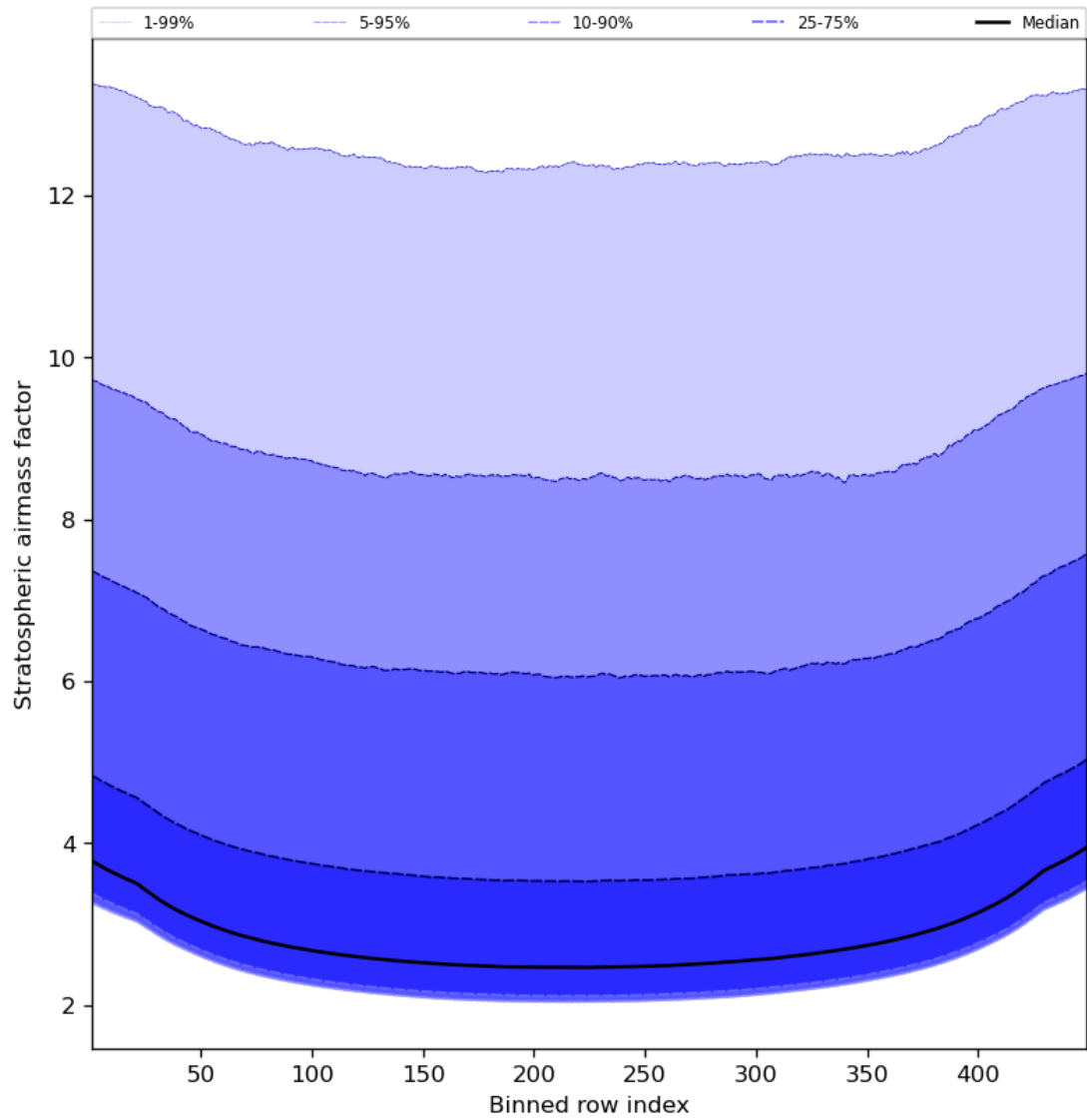
Figure 61: Along track statistics of “Stratospheric airmass factor” for 2023-09-01 to 2023-09-03
