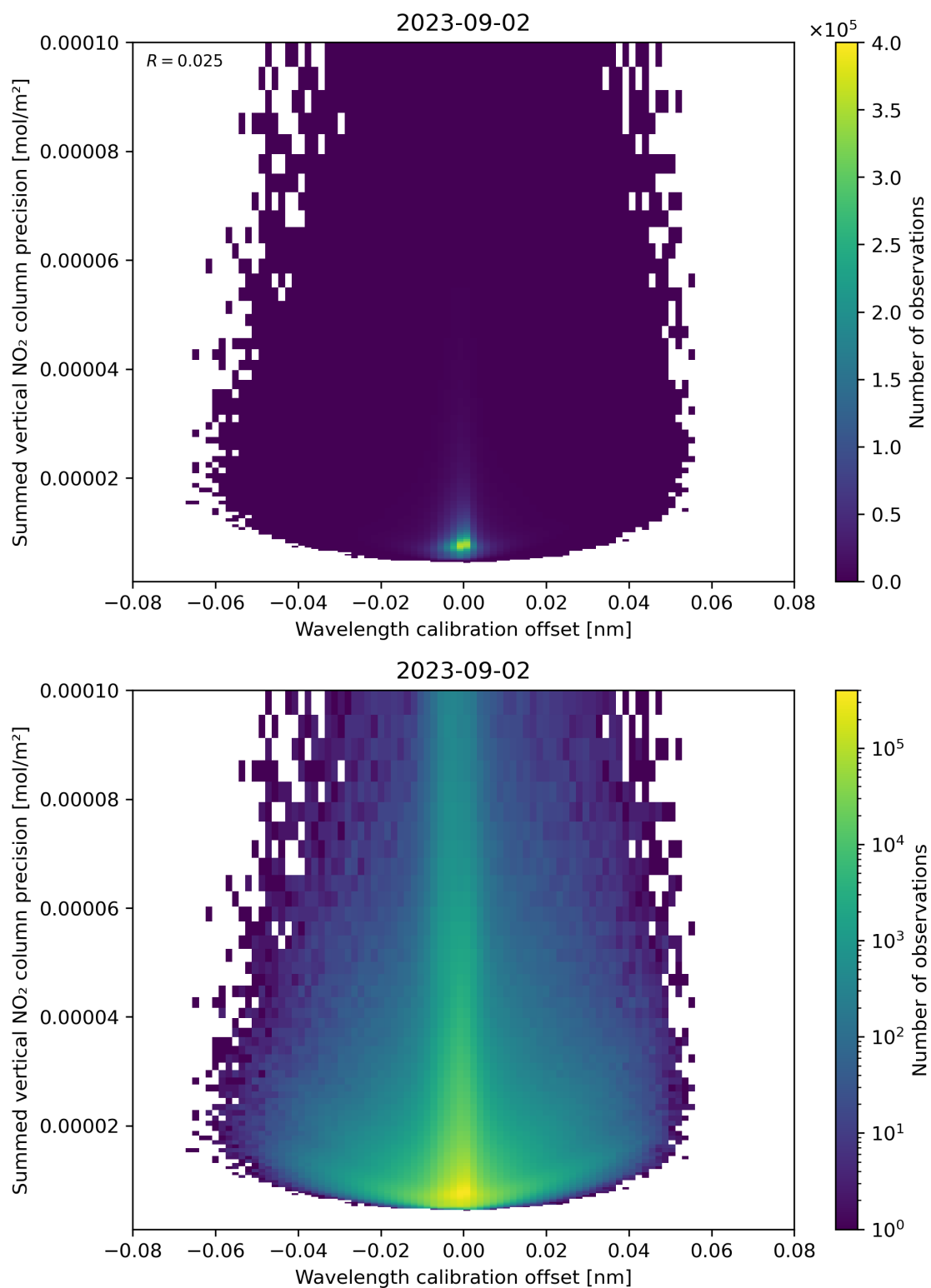
Figure 178: Scatter density plot of “Wavelength calibration offset” against “Summed vertical NO 2 column precision” for 2023-09-01 to 2023-09-03.
