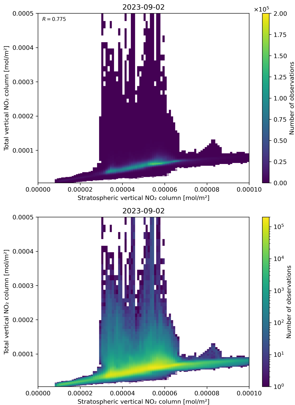
Figure 100: Scatter density plot of “Stratospheric vertical NO 2 column” against “Total vertical NO 2 column” for 2023-09-01 to 2023-09-03.
