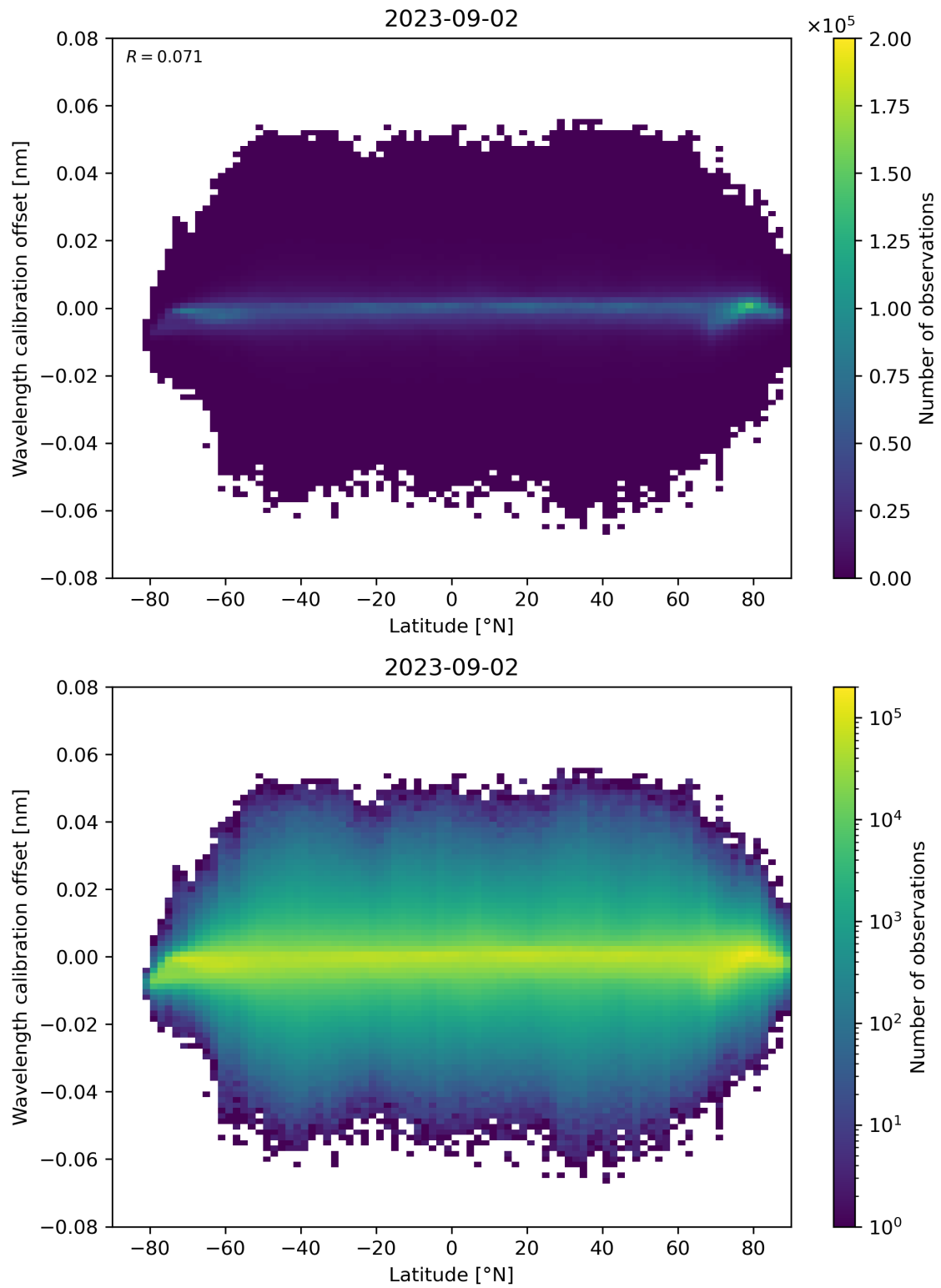
Figure 95: Scatter density plot of “Latitude” against “Wavelength calibration offset” for 2023-09-01 to 2023-09-03.
