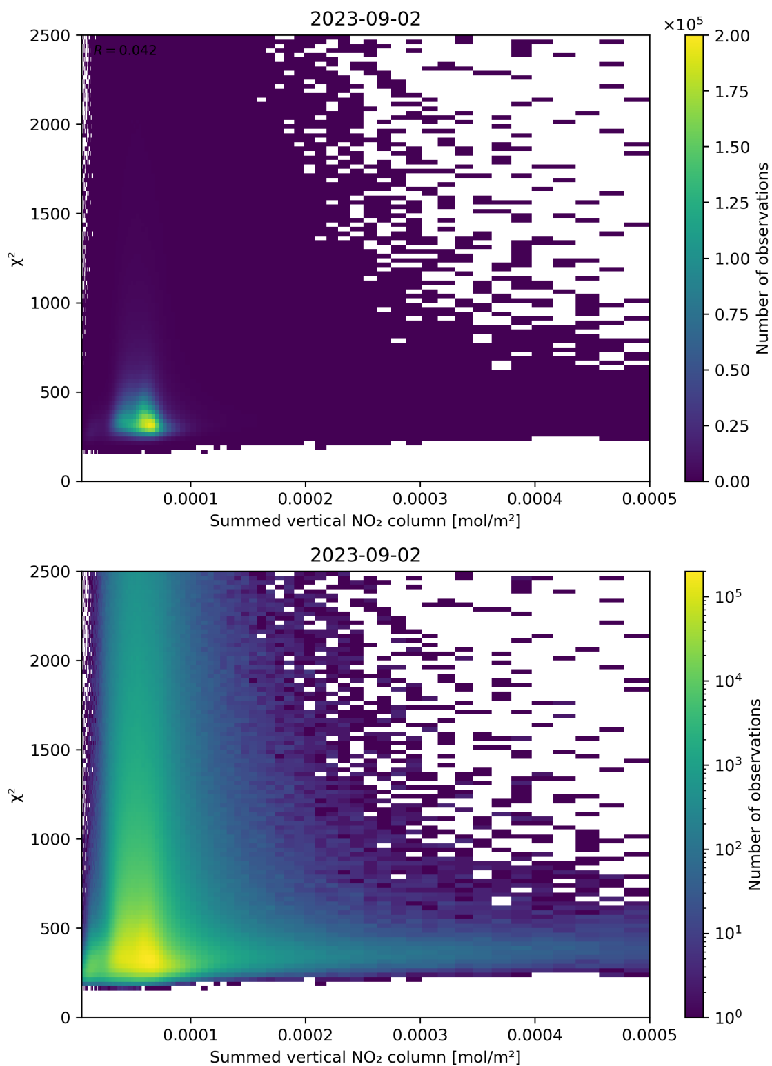
Figure 104: Scatter density plot of “Summed vertical NO 2 column” against “ \chi^2 ” for 2023-09-01 to 2023-09-03.
