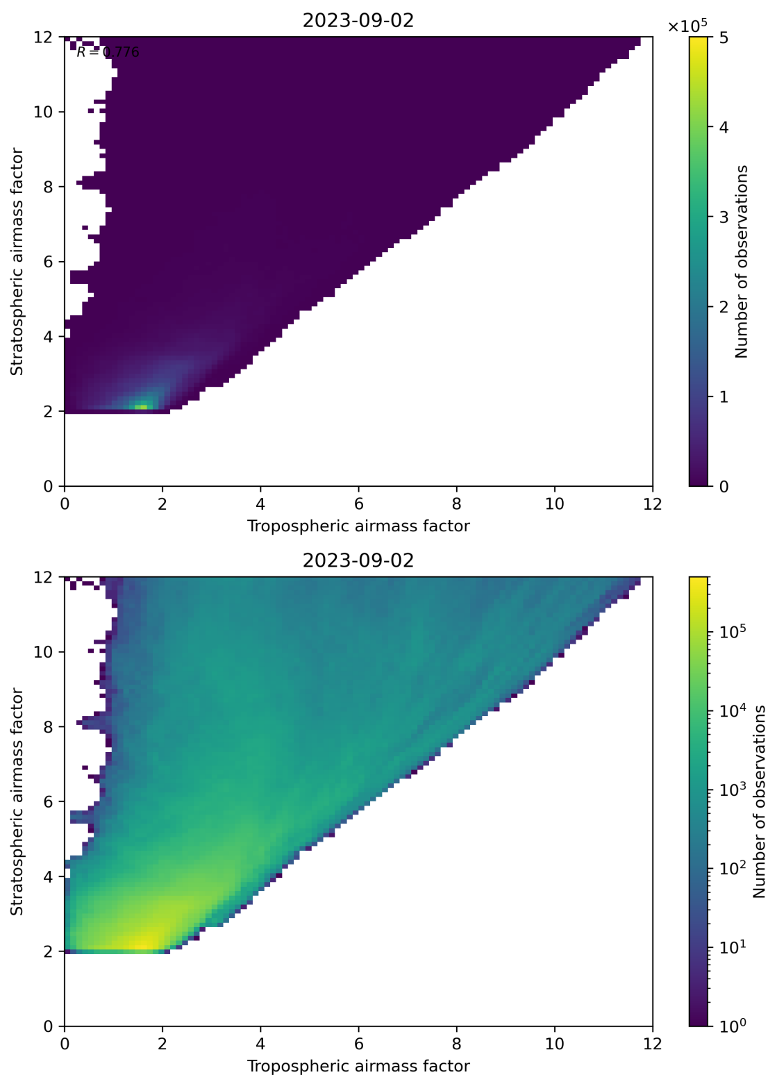
Figure 71: Scatter density plot of “Tropospheric airmass factor” against “Stratospheric airmass factor” for 2023-09-01 to 2023-09-03.
