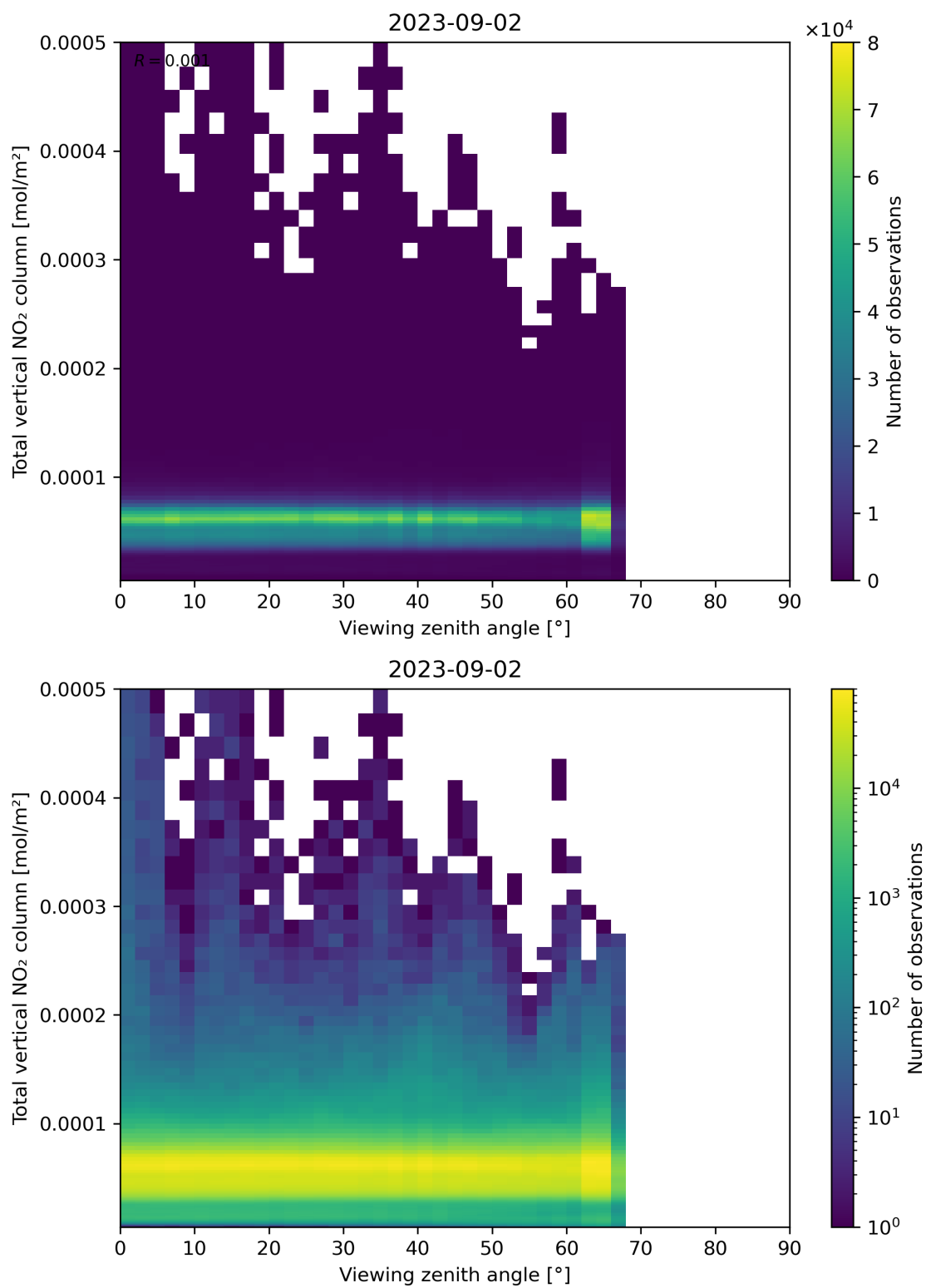
Figure 167: Scatter density plot of “Viewing zenith angle” against “Total vertical NO 2 column” for 2023-09-01 to 2023-09-03.
