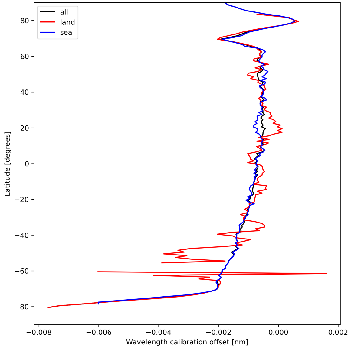
Figure 18: Zonal average of “Wavelength calibration offset” for 2023-09-01 to 2023-09-03.
