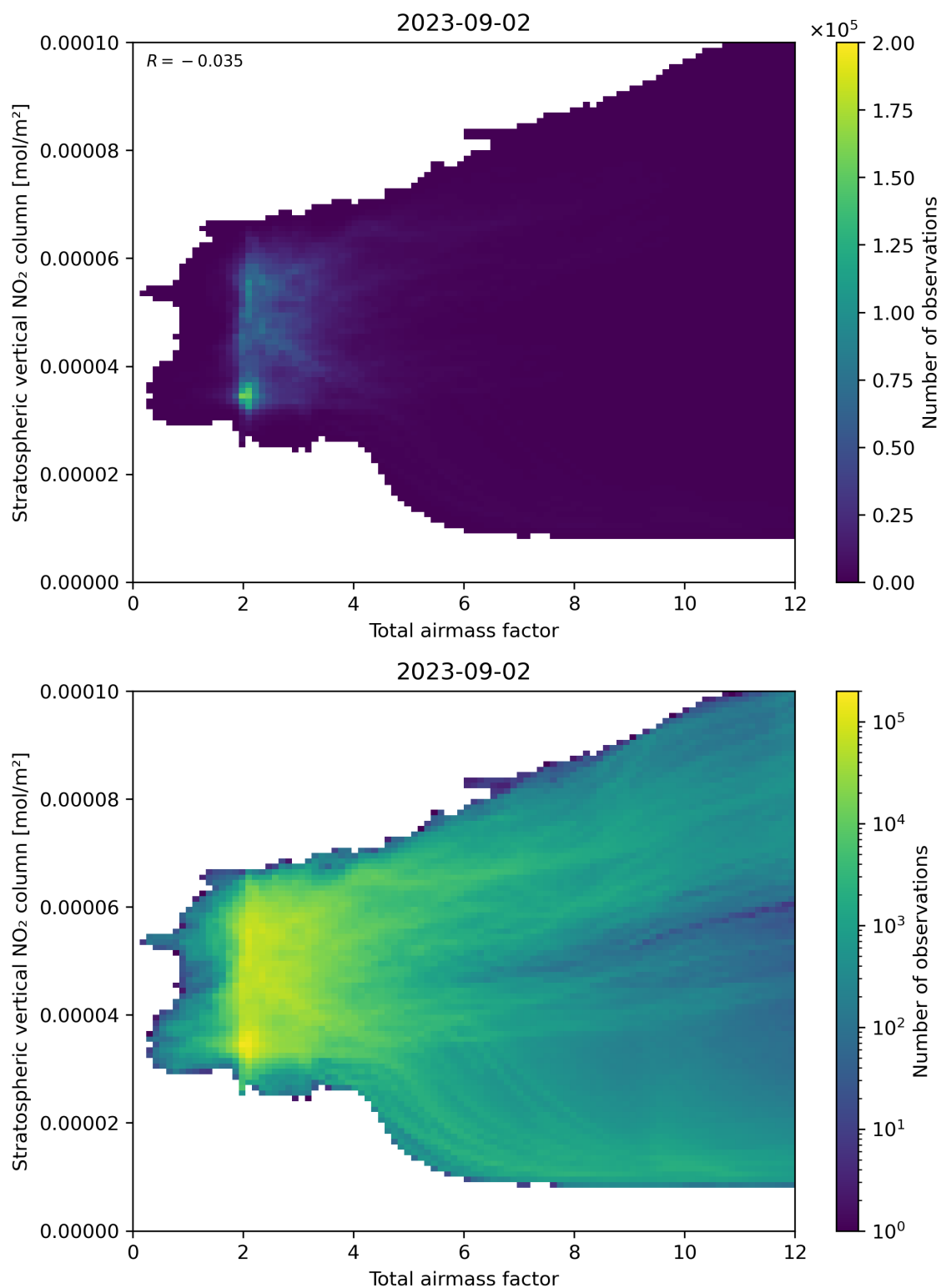
Figure 64: Scatter density plot of “Total airmass factor” against “Stratospheric vertical NO 2 column” for 2023-09-01 to 2023-09-03.
