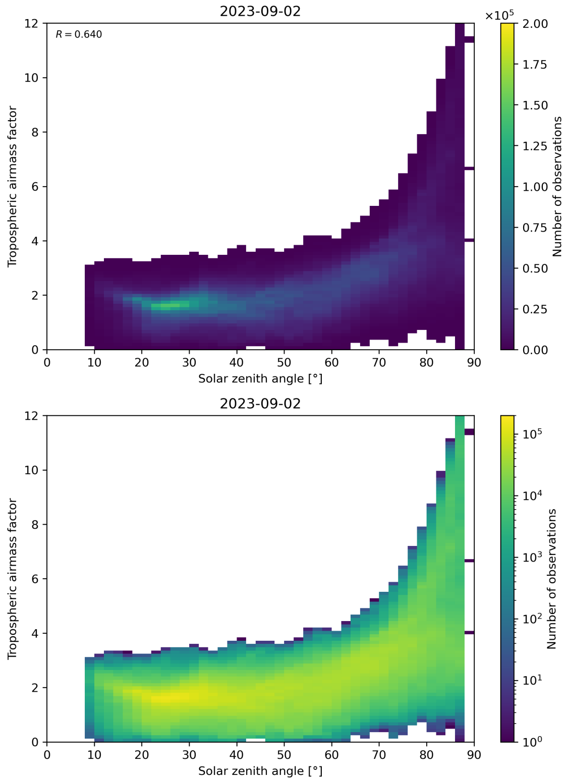
Figure 147: Scatter density plot of “Solar zenith angle” against “Tropospheric airmass factor” for 2023-09-01 to 2023-09-03.
