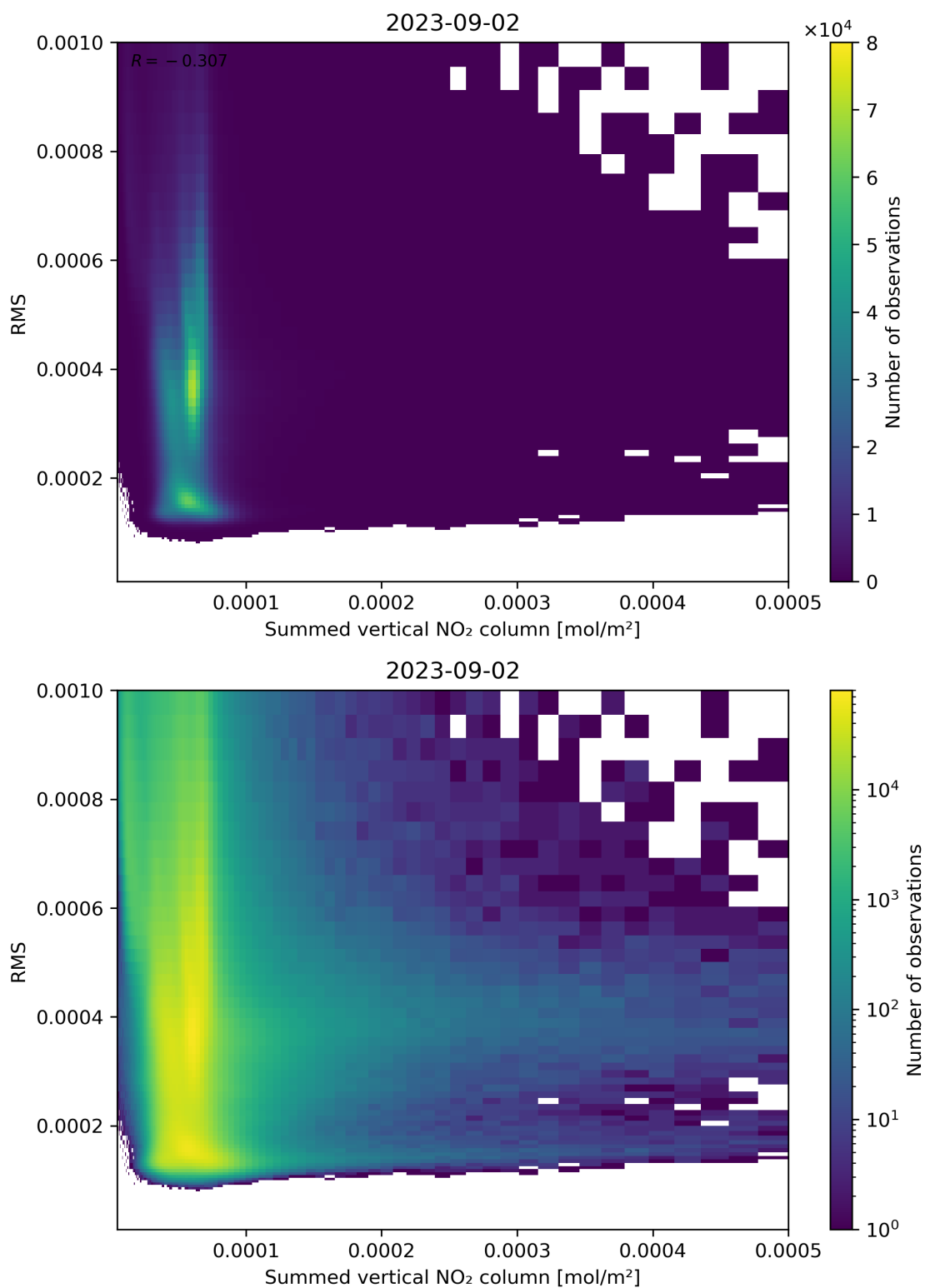
Figure 109: Scatter density plot of “Summed vertical NO 2 column” against “RMS” for 2023-09-01 to 2023-09-03.
