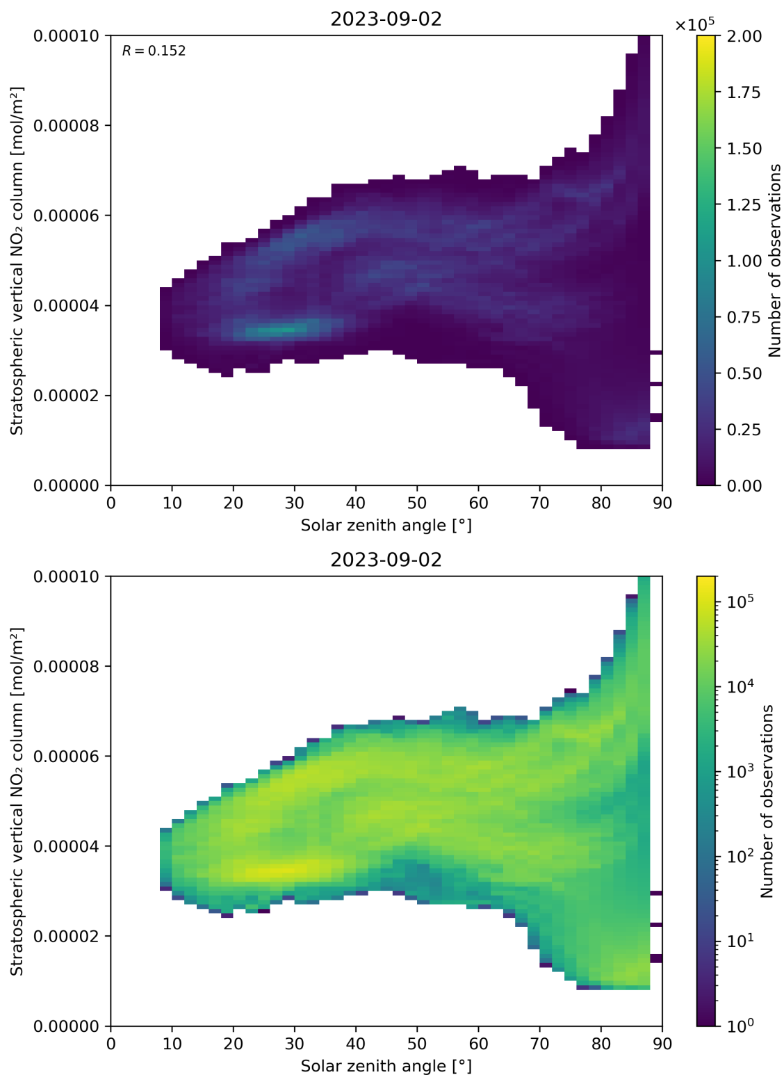
Figure 150: Scatter density plot of “Solar zenith angle” against “Stratospheric vertical NO 2 column” for 2023-09-01 to 2023-09-03.
