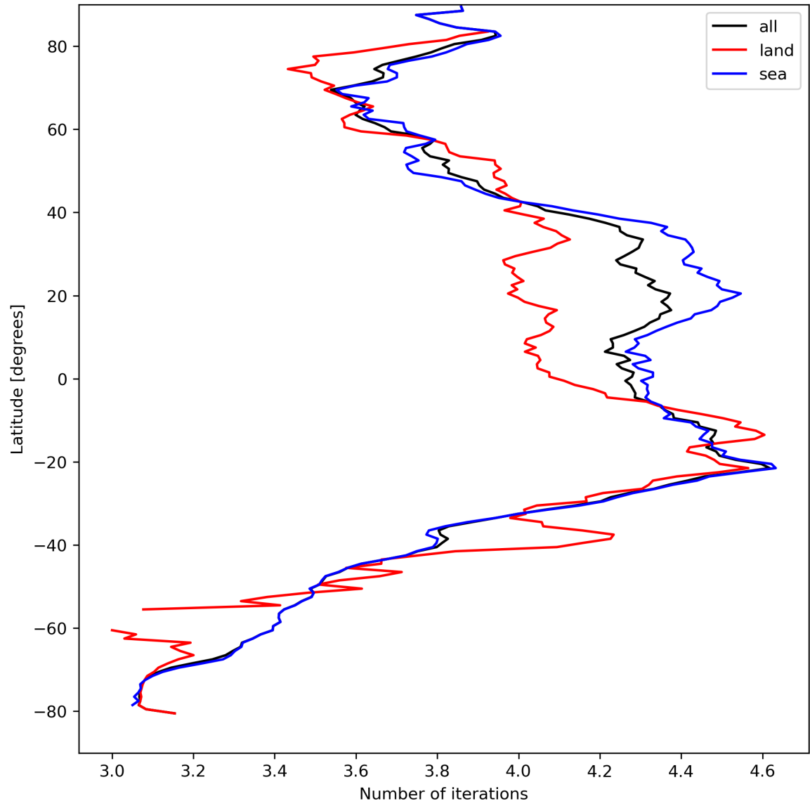
Figure 17: Zonal average of “Number of iterations” for 2023-09-01 to 2023-09-03.
