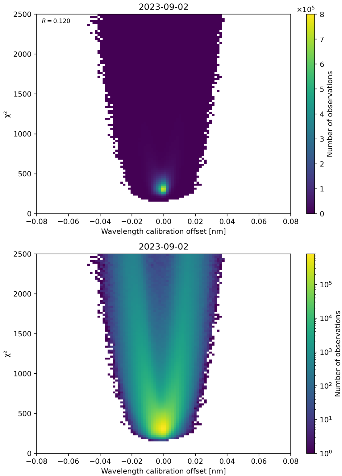
Figure 175: Scatter density plot of “Wavelength calibration offset” against “ \chi^2 ” for 2023-09-01 to 2023-09-03.
