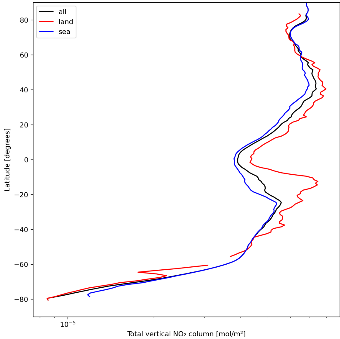
Figure 21: Zonal average of “Total vertical NO 2 column” for 2023-09-01 to 2023-09-03.
