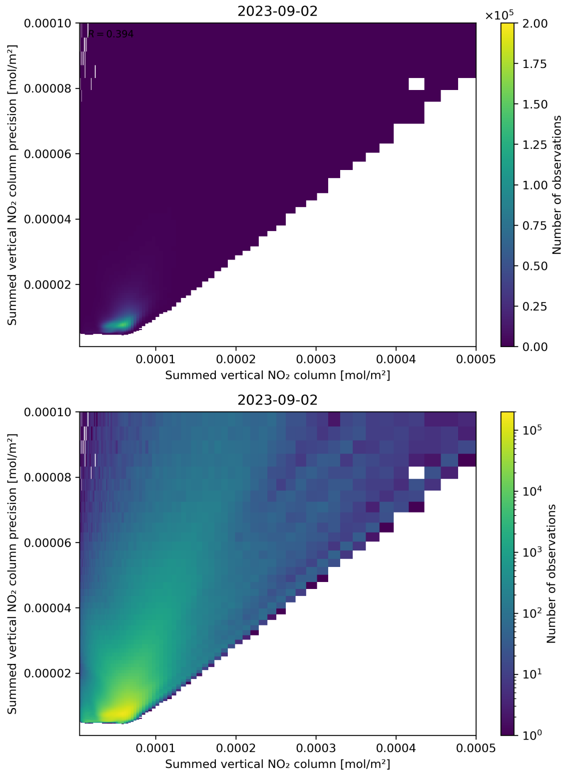
Figure 105: Scatter density plot of “Summed vertical NO 2 column” against “Summed vertical NO 2 column precision” for 2023-09-01 to 2023-09-03.
