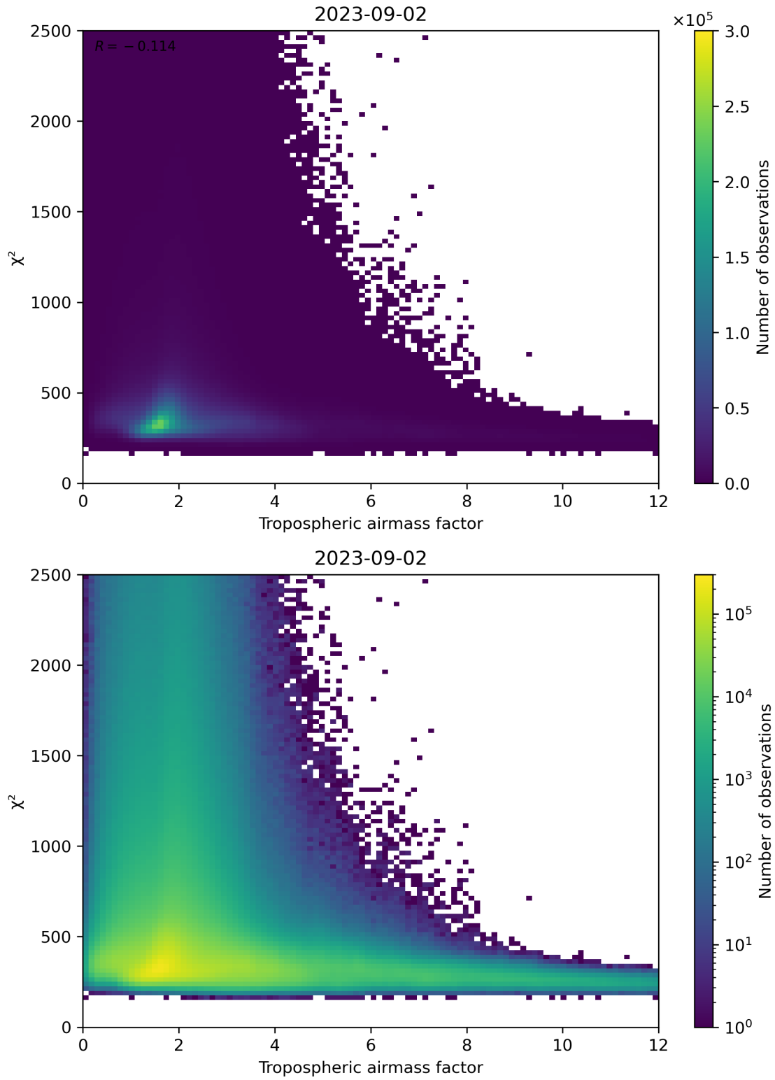
Figure 73: Scatter density plot of “Tropospheric airmass factor” against “ \chi^2 ” for 2023-09-01 to 2023-09-03.
