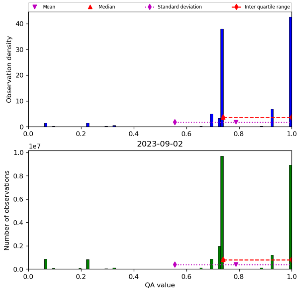
Figure 28: Histogram of “QA value” for 2023-09-01 to 2023-09-03
