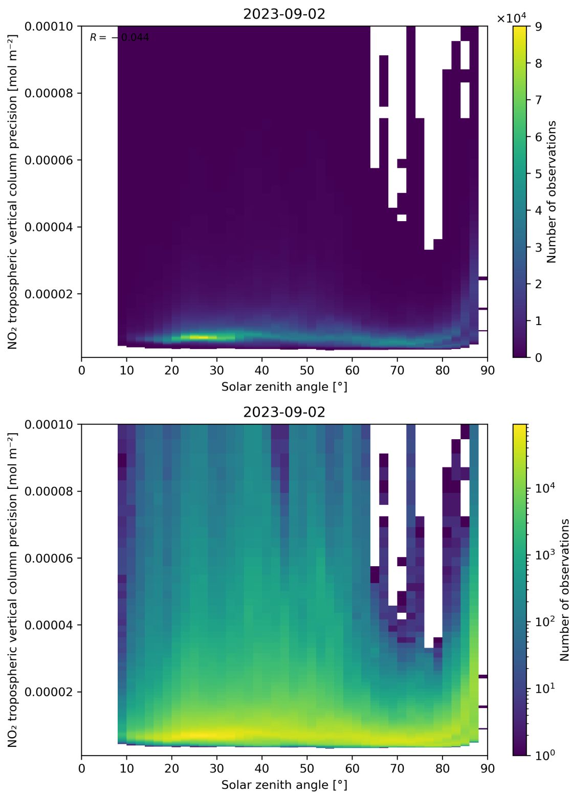
Figure 156: Scatter density plot of “Solar zenith angle” against “NO 2 tropospheric vertical column precision” for 2023-09-01 to 2023-09-03.
