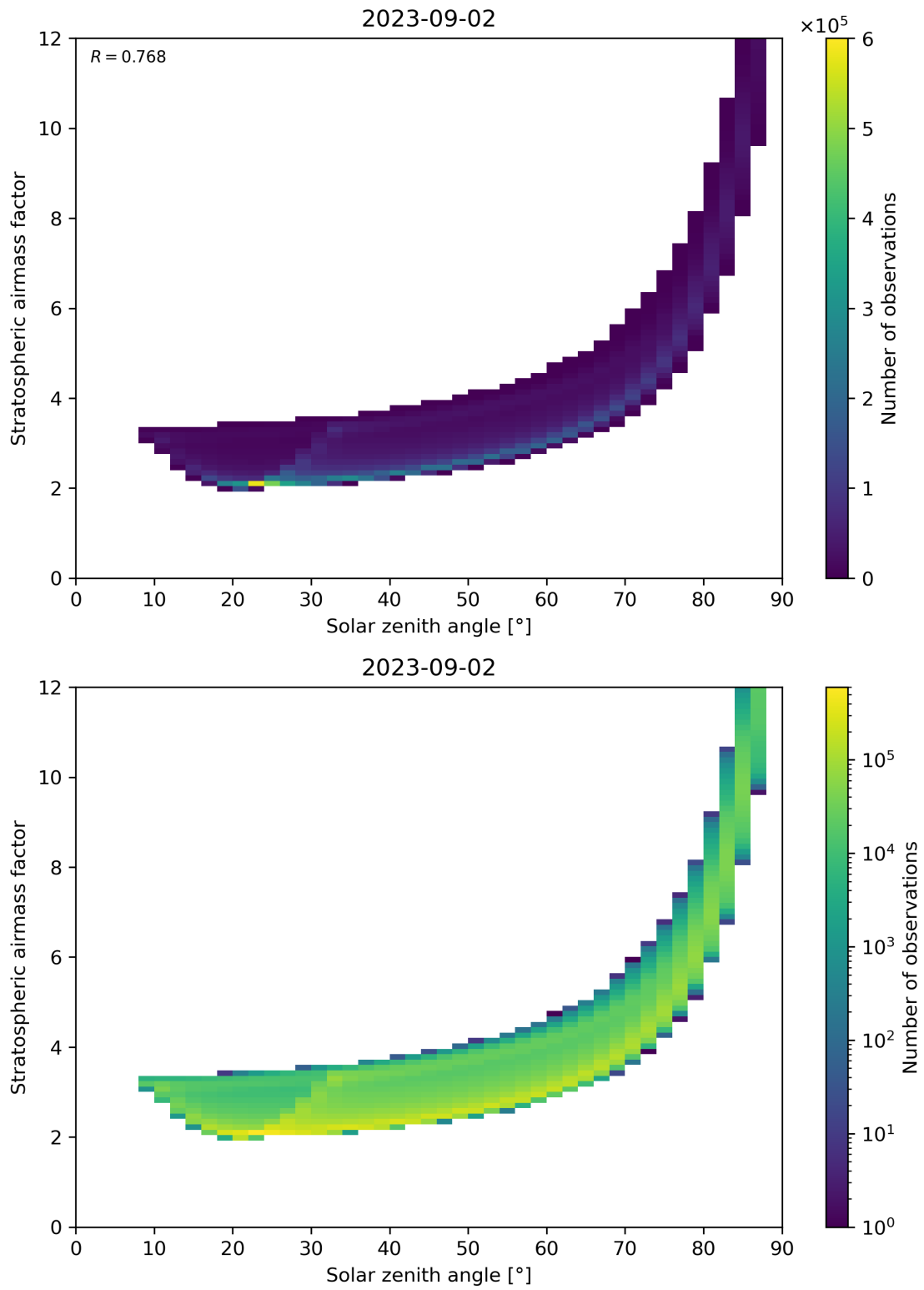
Figure 145: Scatter density plot of “Solar zenith angle” against “Stratospheric airmass factor” for 2023-09-01 to 2023-09-03.
