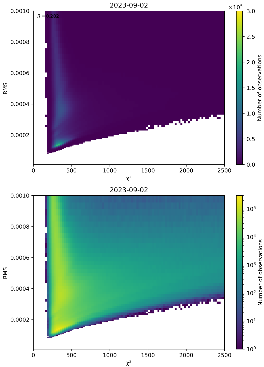
Figure 82: Scatter density plot of “ \chi^2 ” against “RMS” for 2023-09-01 to 2023-09-03.
