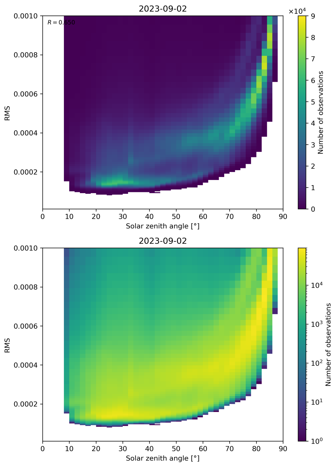
Figure 157: Scatter density plot of “Solar zenith angle” against “RMS” for 2023-09-01 to 2023-09-03.
