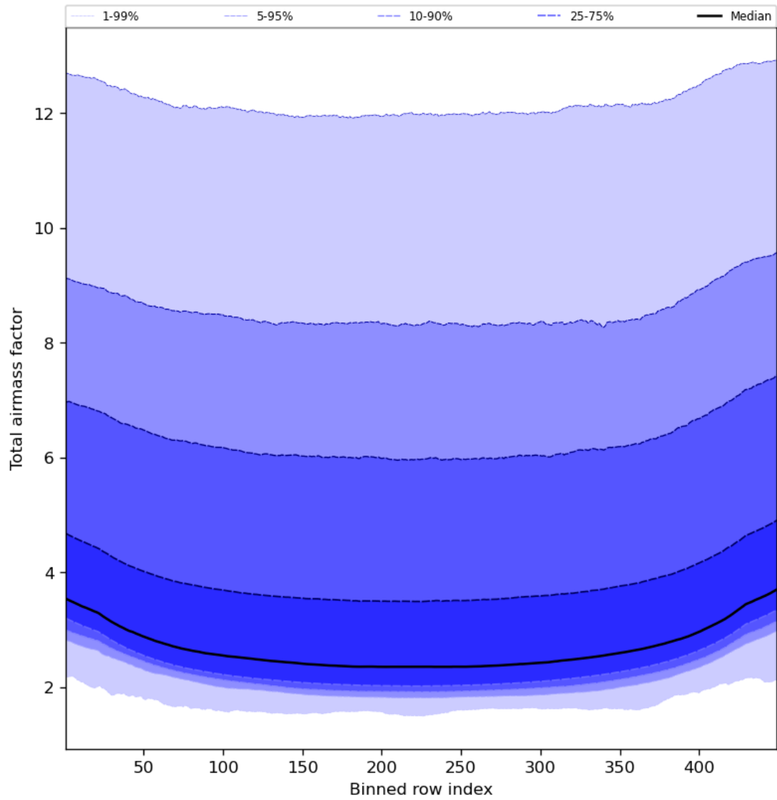
Figure 49: Along track statistics of “Total airmass factor” for 2023-09-01 to 2023-09-03
