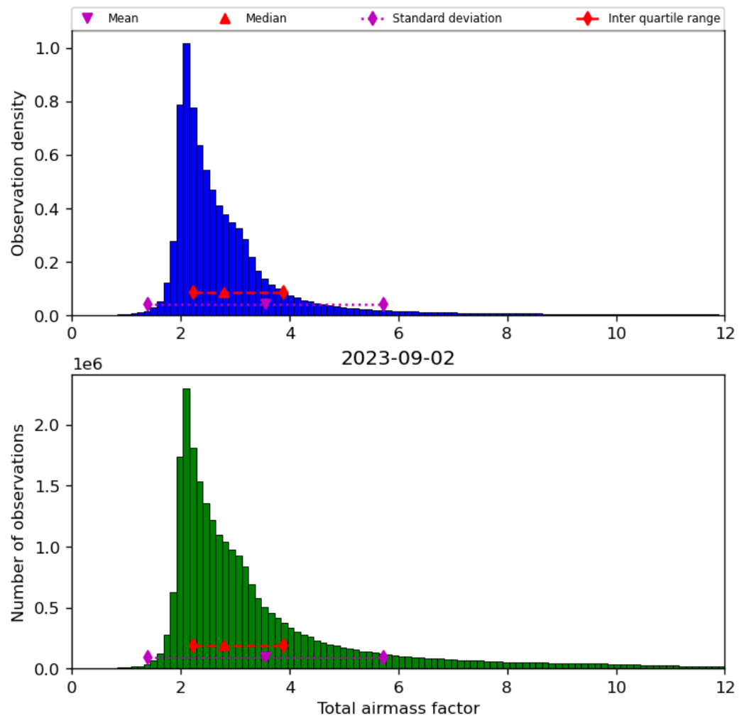
Figure 32: Histogram of “Total airmass factor” for 2023-09-01 to 2023-09-03
