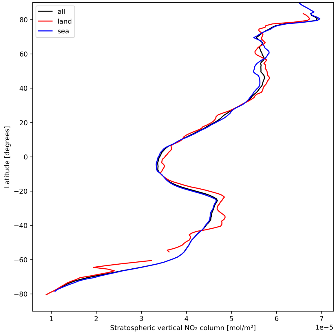
Figure 19: Zonal average of “Stratospheric vertical NO 2 column” for 2023-09-01 to 2023-09-03.
