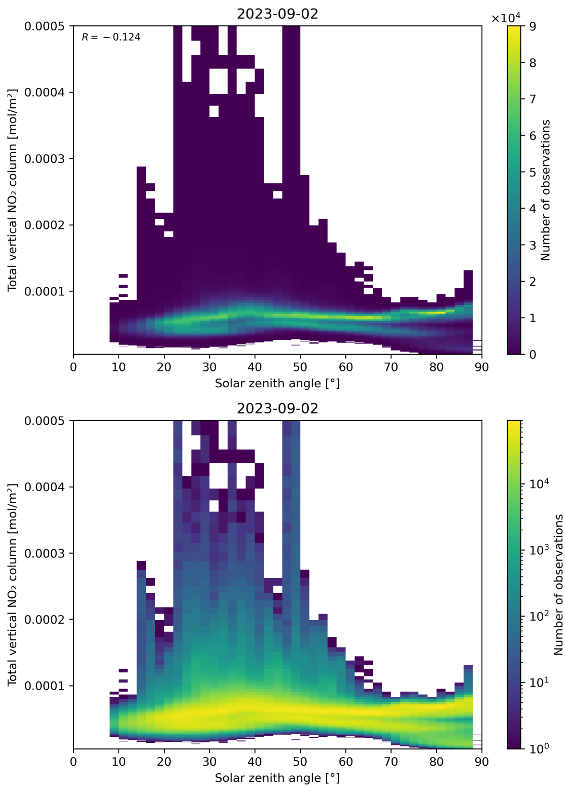
Figure 153: Scatter density plot of “Solar zenith angle” against “Total vertical NO 2 column” for 2023-09-01 to 2023-09-03.
