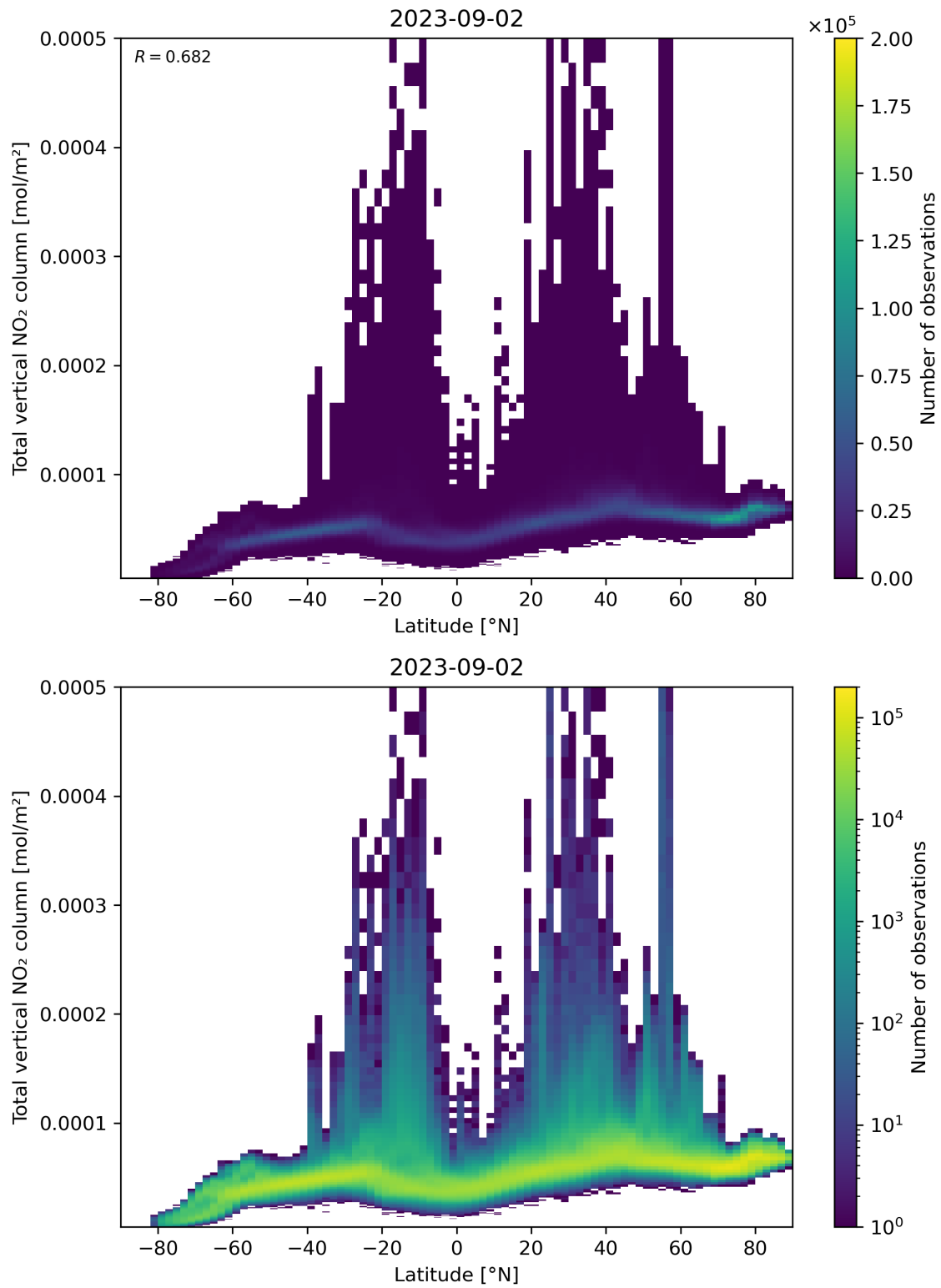
Figure 90: Scatter density plot of “Latitude” against “Total vertical NO 2 column” for 2023-09-01 to 2023-09-03.
