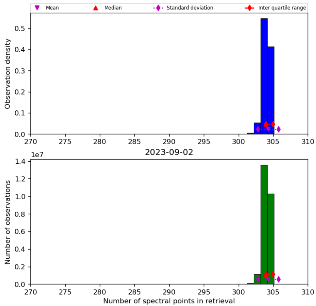
Figure 33: Histogram of “Number of spectral points in retrieval” for 2023-09-01 to 2023-09-03
