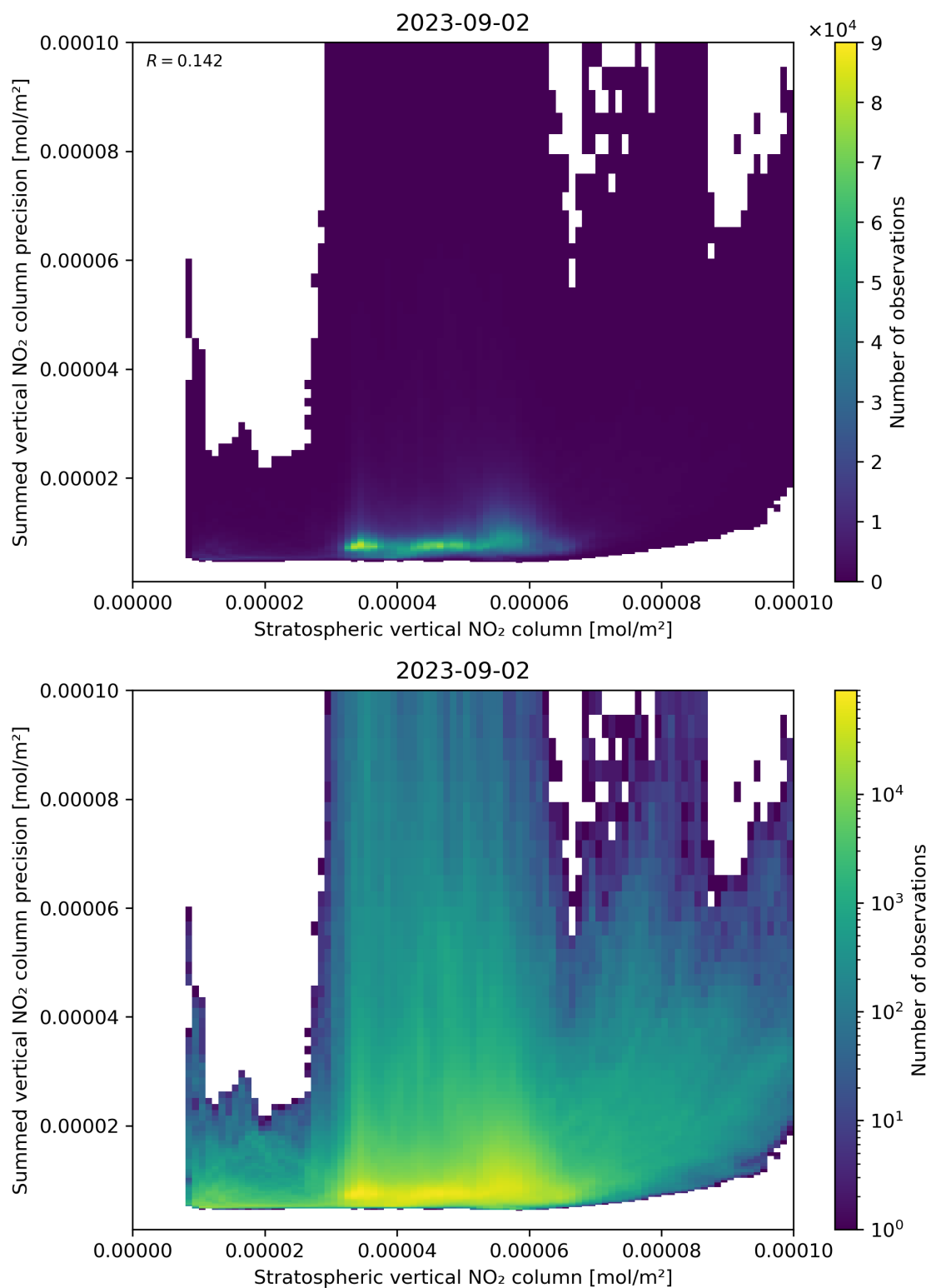
Figure 99: Scatter density plot of “Stratospheric vertical NO 2 column” against “Summed vertical NO 2 column precision” for 2023-09-01 to 2023-09-03.
