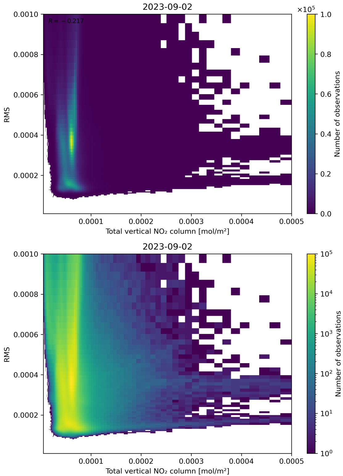
Figure 120: Scatter density plot of “Total vertical NO 2 column” against “RMS” for 2023-09-01 to 2023-09-03.
