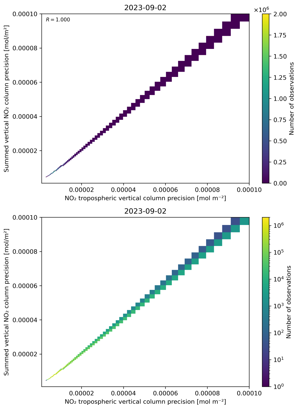
Figure 137: Scatter density plot of “NO 2 tropospheric vertical column precision” against “Summed vertical NO 2 column precision” for 2023-09-01 to 2023-09-03.
