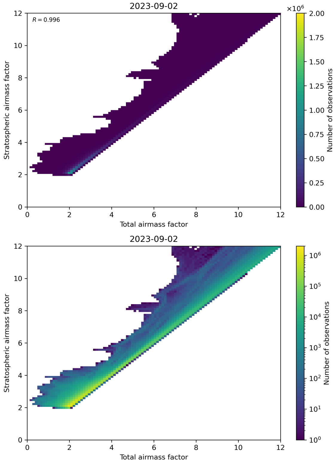
Figure 62: Scatter density plot of “Total airmass factor” against “Stratospheric airmass factor” for 2023-09-01 to 2023-09-03.
