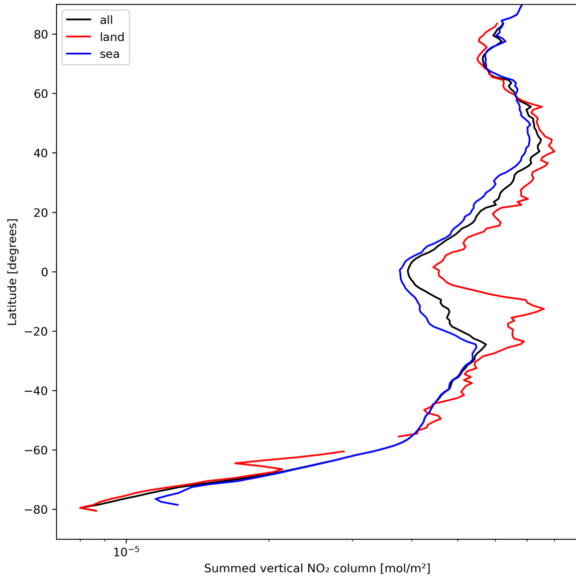
Figure 23: Zonal average of “Summed vertical NO 2 column” for 2023-09-01 to 2023-09-03.
