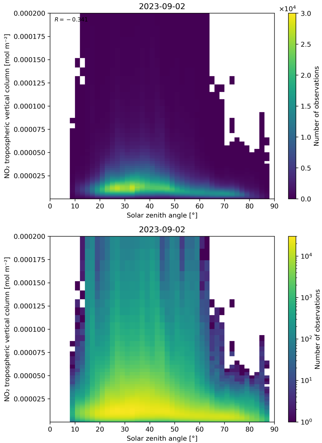
Figure 155: Scatter density plot of “Solar zenith angle” against “NO 2 tropospheric vertical column” for 2023-09-01 to 2023-09-03.
