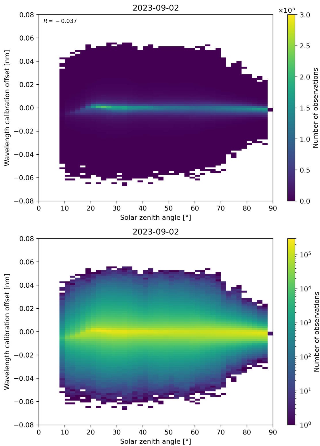
Figure 158: Scatter density plot of “Solar zenith angle” against “Wavelength calibration offset” for 2023-09-01 to 2023-09-03.
