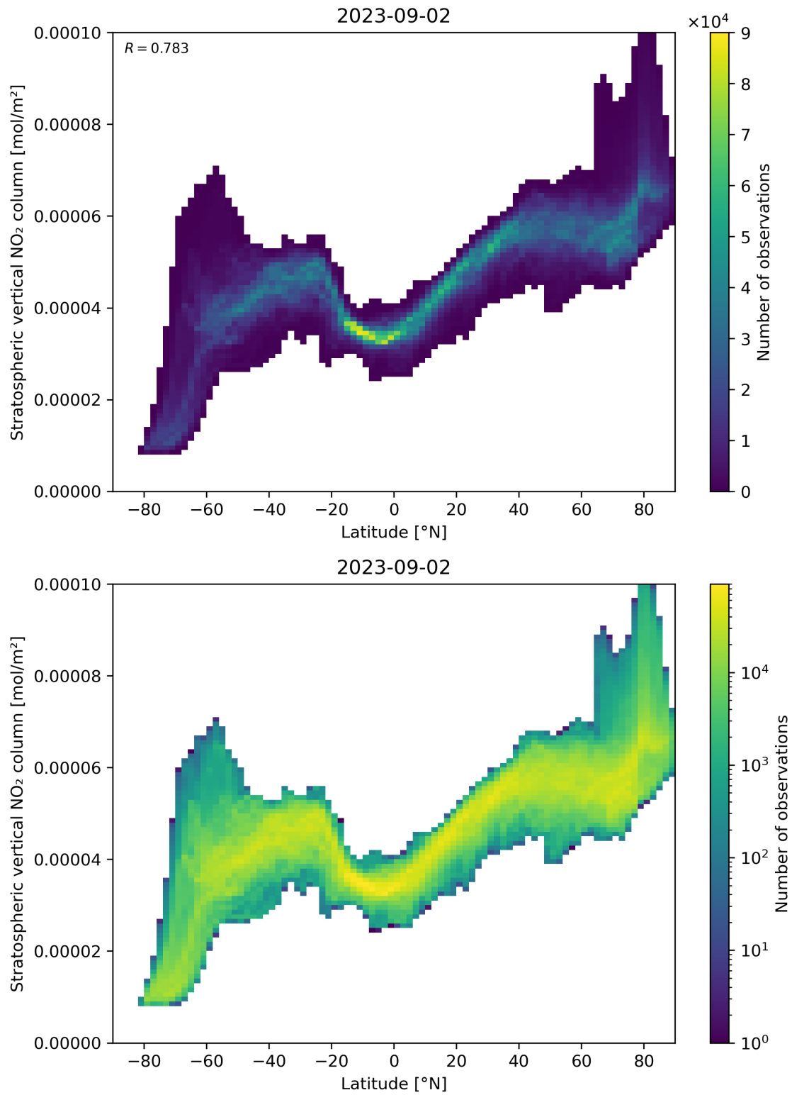
Figure 87: Scatter density plot of “Latitude” against “Stratospheric vertical NO 2 column” for 2023-09-01 to 2023-09-03.
