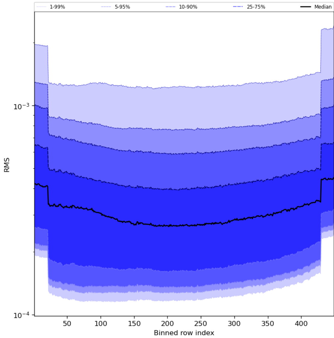
Figure 60: Along track statistics of “RMS” for 2023-09-01 to 2023-09-03
