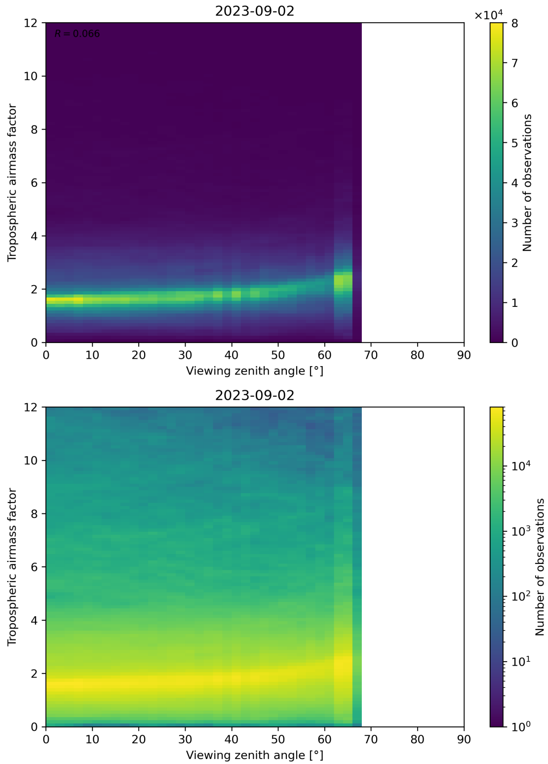
Figure 161: Scatter density plot of “Viewing zenith angle” against “Tropospheric airmass factor” for 2023-09-01 to 2023-09-03.
