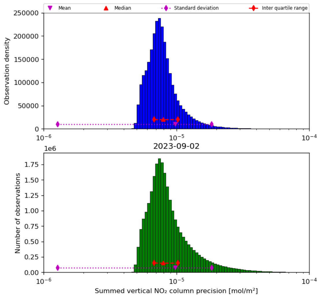
Figure 41: Histogram of “Summed vertical NO 2 column precision” for 2023-09-01 to 2023-09-03
