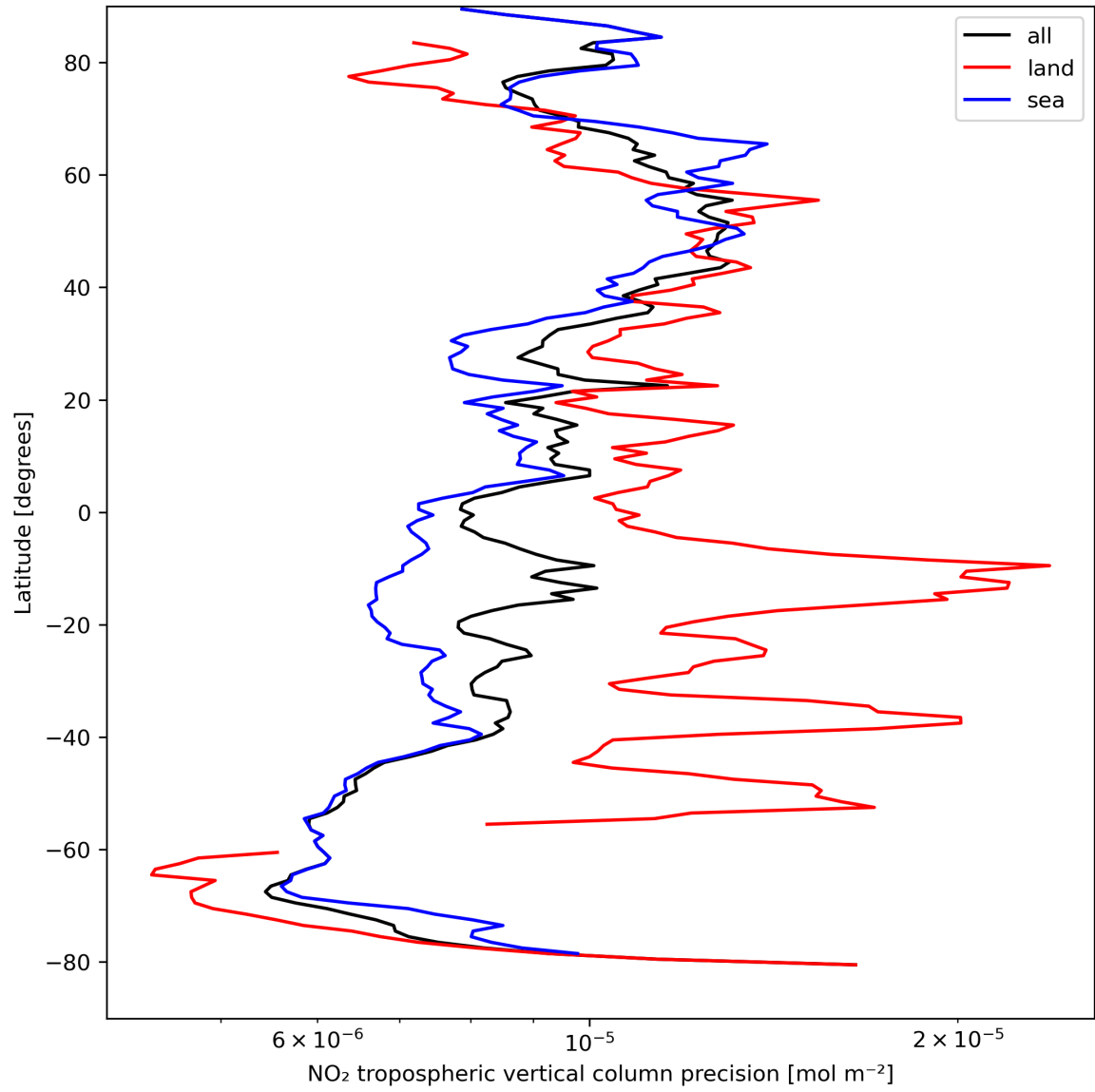
Figure 13: Zonal average of “NO 2 tropospheric vertical column precision” for 2023-09-01 to 2023-09-03.
