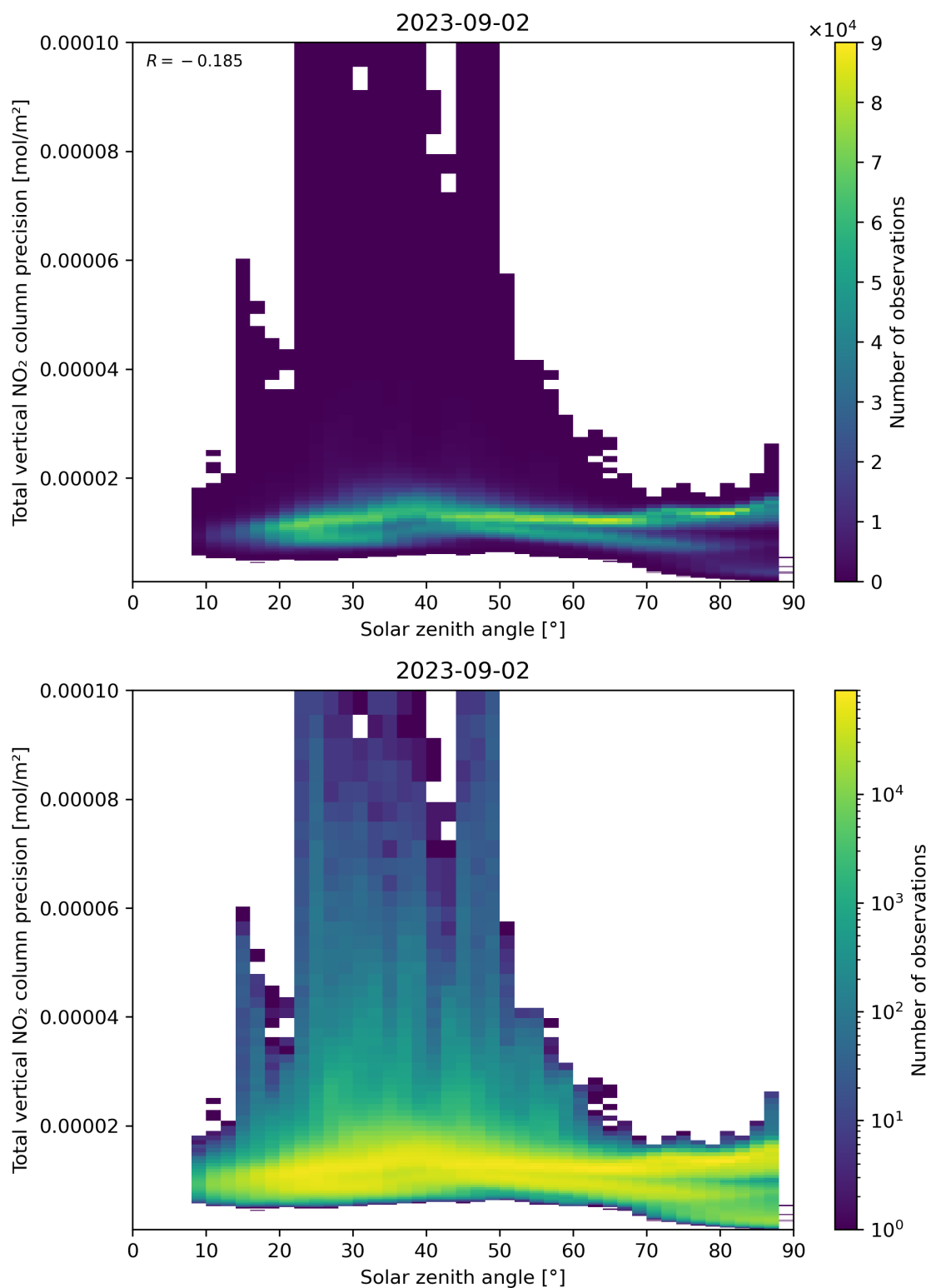
Figure 154: Scatter density plot of “Solar zenith angle” against “Total vertical NO 2 column precision” for 2023-09-01 to 2023-09-03.
