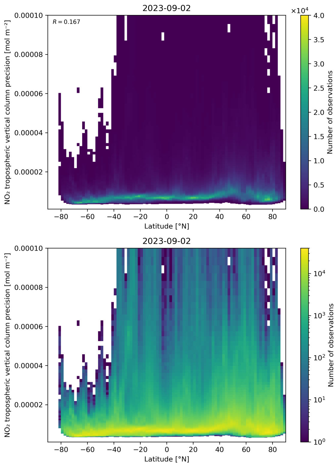
Figure 93: Scatter density plot of “Latitude” against “NO 2 tropospheric vertical column precision” for 2023-09-01 to 2023-09-03.
