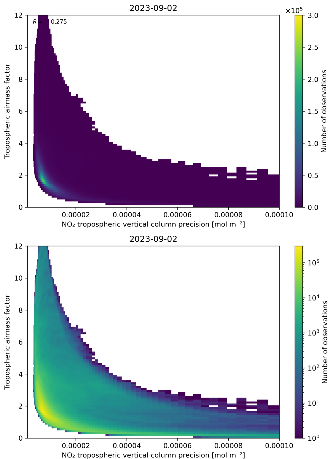
Figure 133: Scatter density plot of “NO 2 tropospheric vertical column precision” against “Tropospheric airmass factor” for 2023-09-01 to 2023-09-03.
