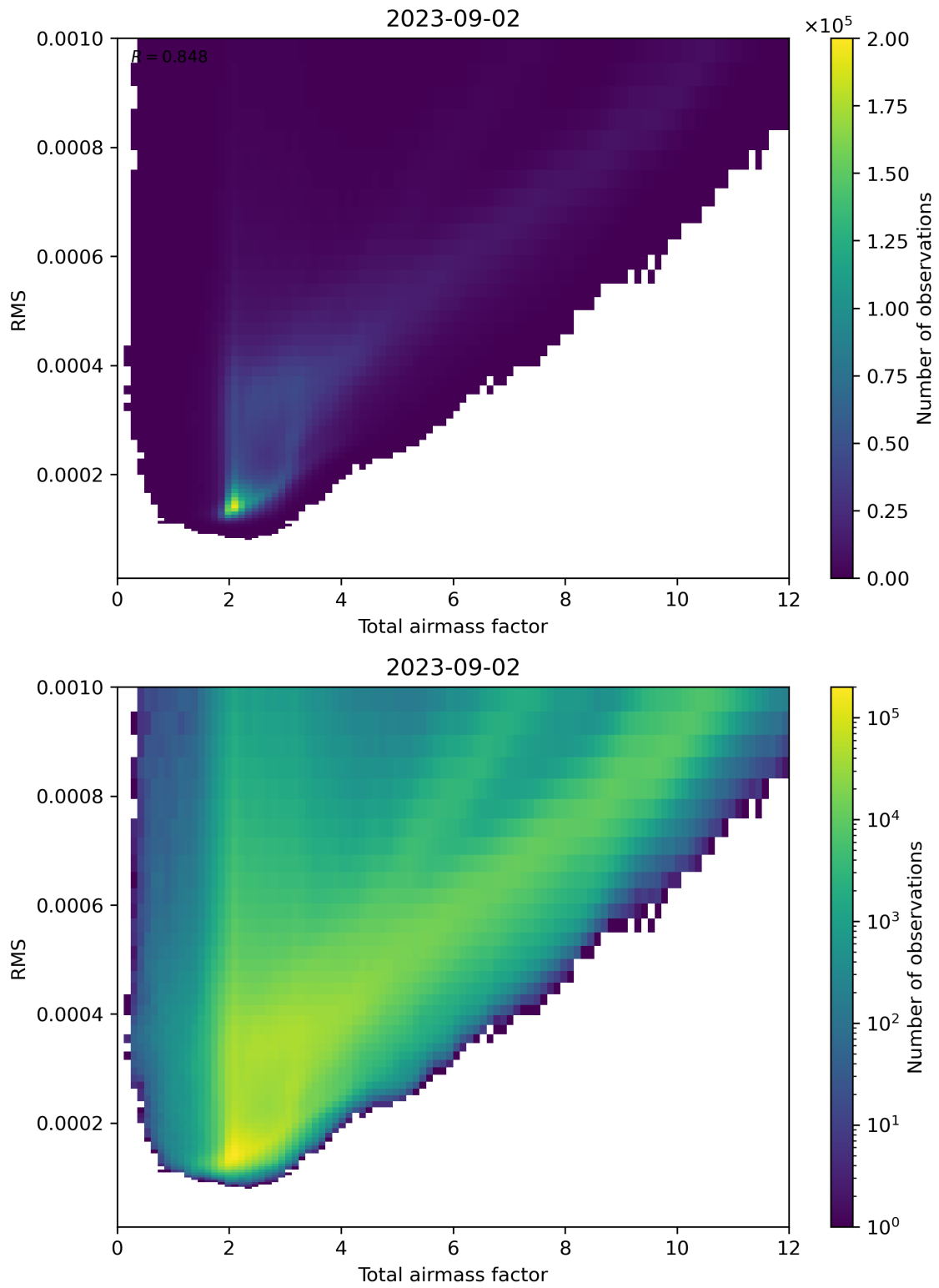
Figure 69: Scatter density plot of “Total airmass factor” against “RMS” for 2023-09-01 to 2023-09-03.
