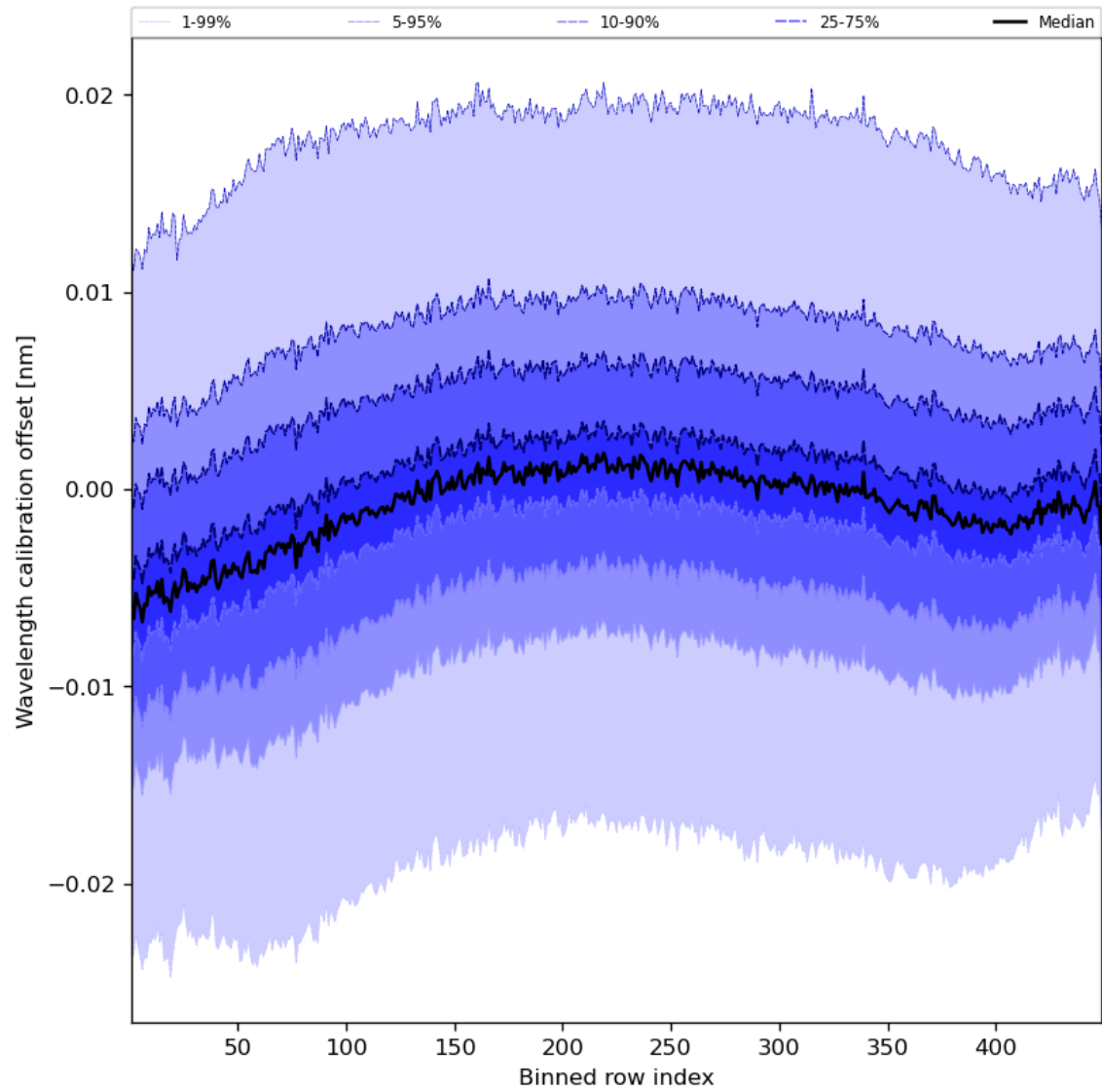
Figure 52: Along track statistics of “Wavelength calibration offset” for 2023-09-01 to 2023-09-03
