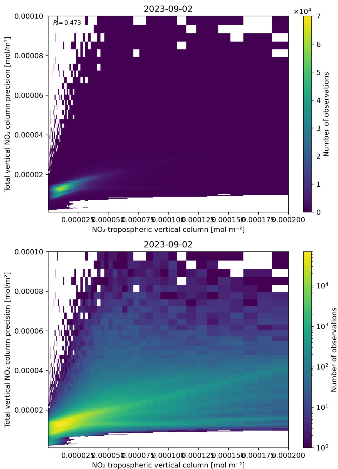
Figure 129: Scatter density plot of “NO 2 tropospheric vertical column” against “Total vertical NO 2 column precision” for 2023-09-01 to 2023-09-03.
