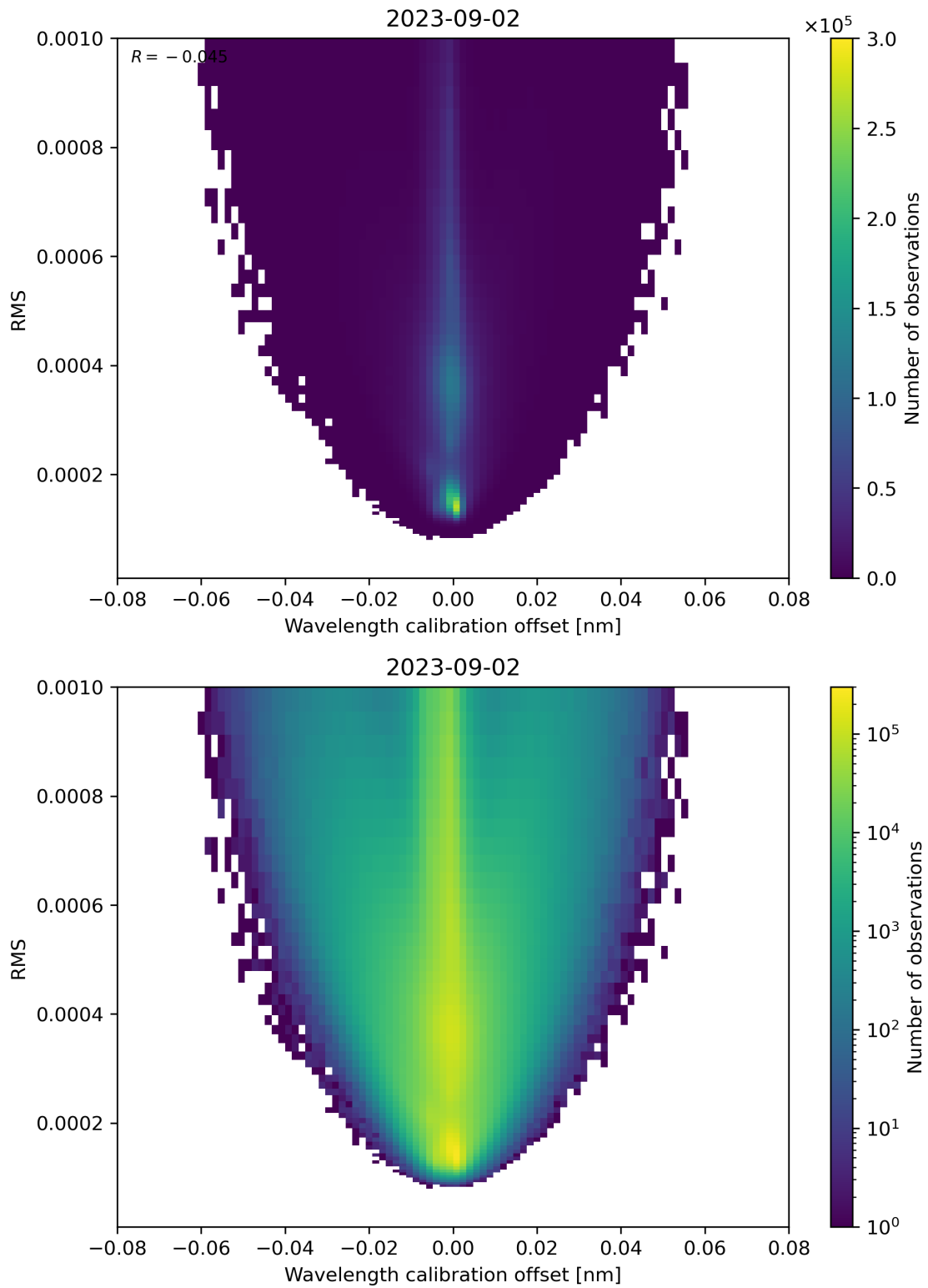
Figure 181: Scatter density plot of “Wavelength calibration offset” against “RMS” for 2023-09-01 to 2023-09-03.
