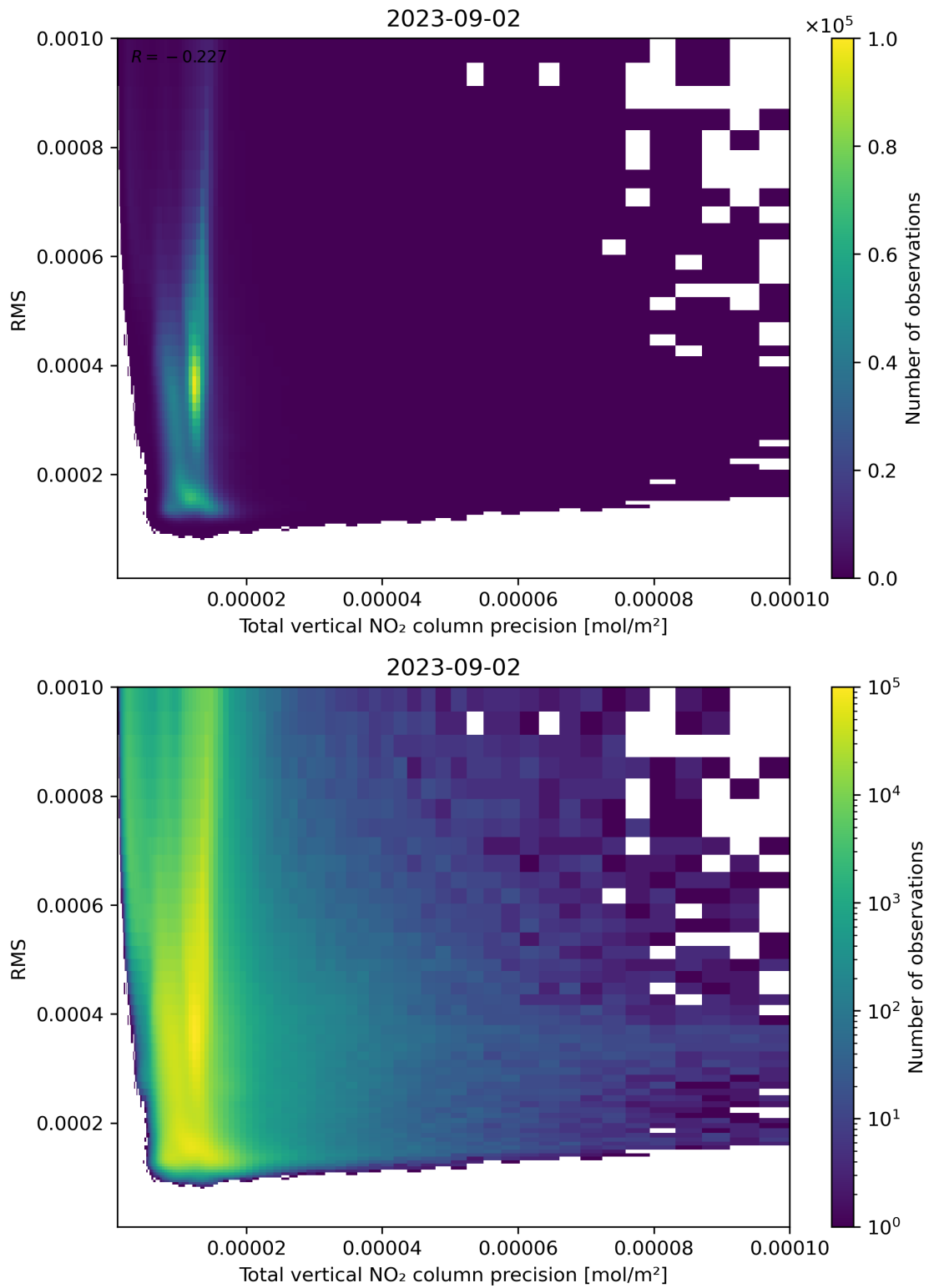
Figure 119: Scatter density plot of “Total vertical NO 2 column precision” against “RMS” for 2023-09-01 to 2023-09-03.
