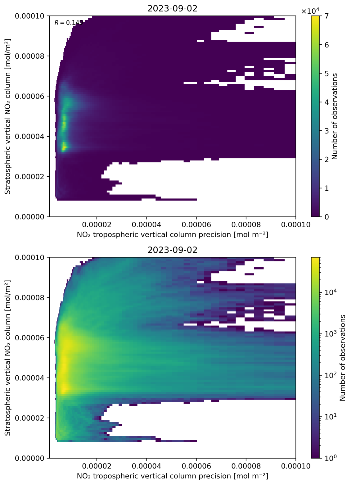
Figure 135: Scatter density plot of “NO 2 tropospheric vertical column precision” against “Stratospheric vertical NO 2 column” for 2023-09-01 to 2023-09-03.
