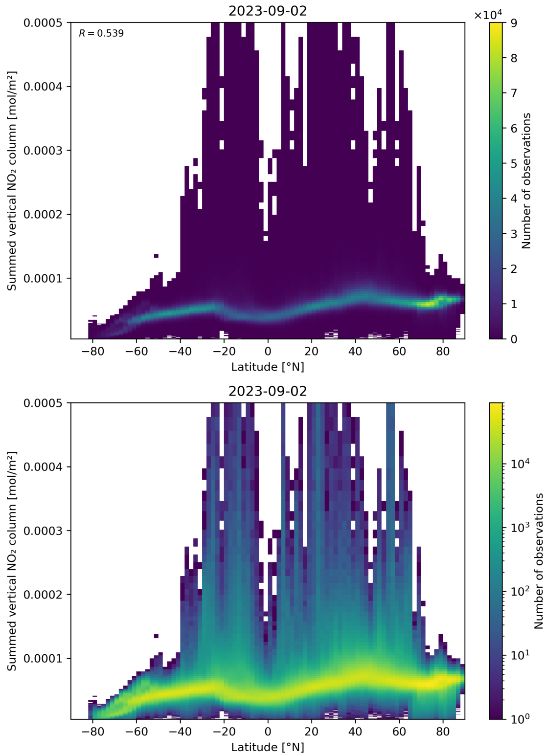
Figure 88: Scatter density plot of “Latitude” against “Summed vertical NO 2 column” for 2023-09-01 to 2023-09-03.
