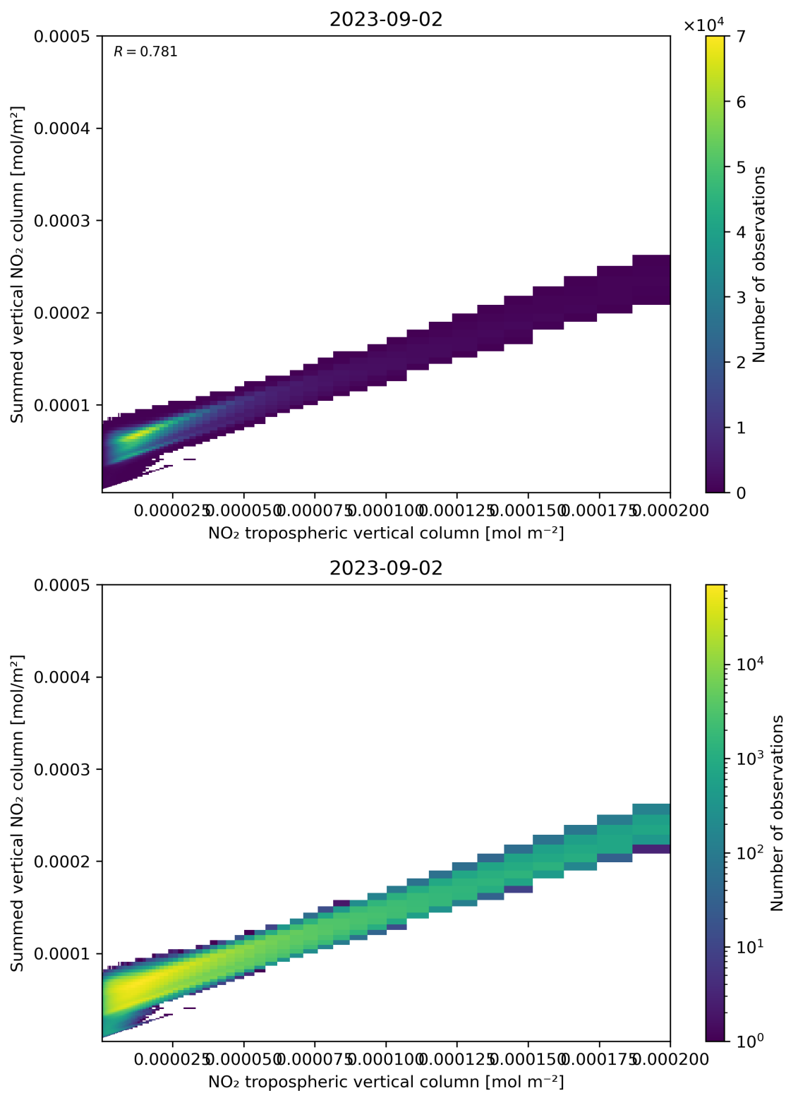
Figure 126: Scatter density plot of “NO 2 tropospheric vertical column” against “Summed vertical NO 2 column” for 2023-09-01 to 2023-09-03.
