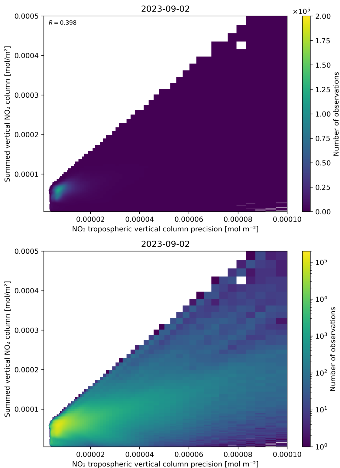
Figure 136: Scatter density plot of “NO 2 tropospheric vertical column precision” against “Summed vertical NO 2 column” for 2023-09-01 to 2023-09-03.
