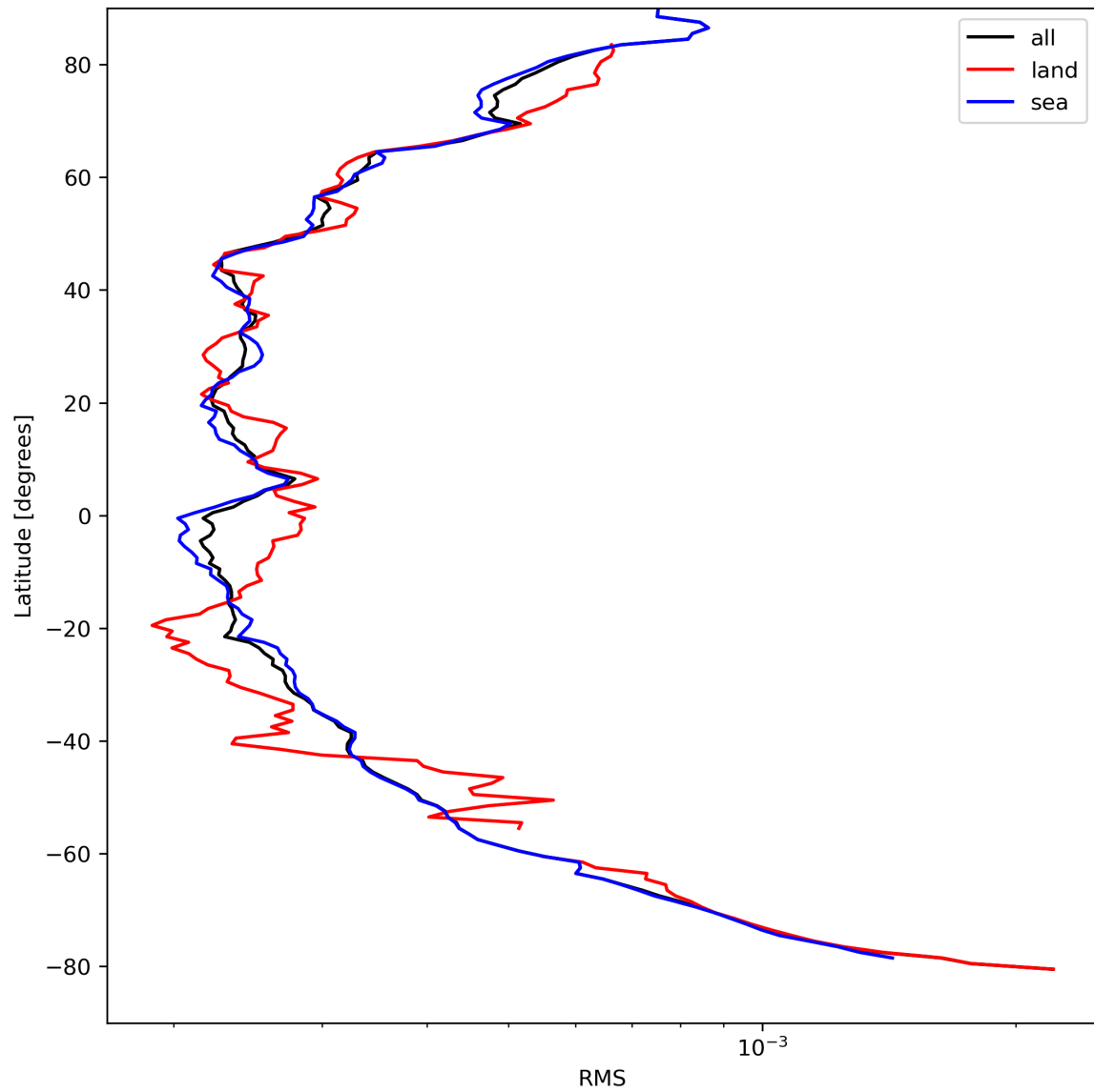
Figure 26: Zonal average of “RMS” for 2023-09-01 to 2023-09-03.
