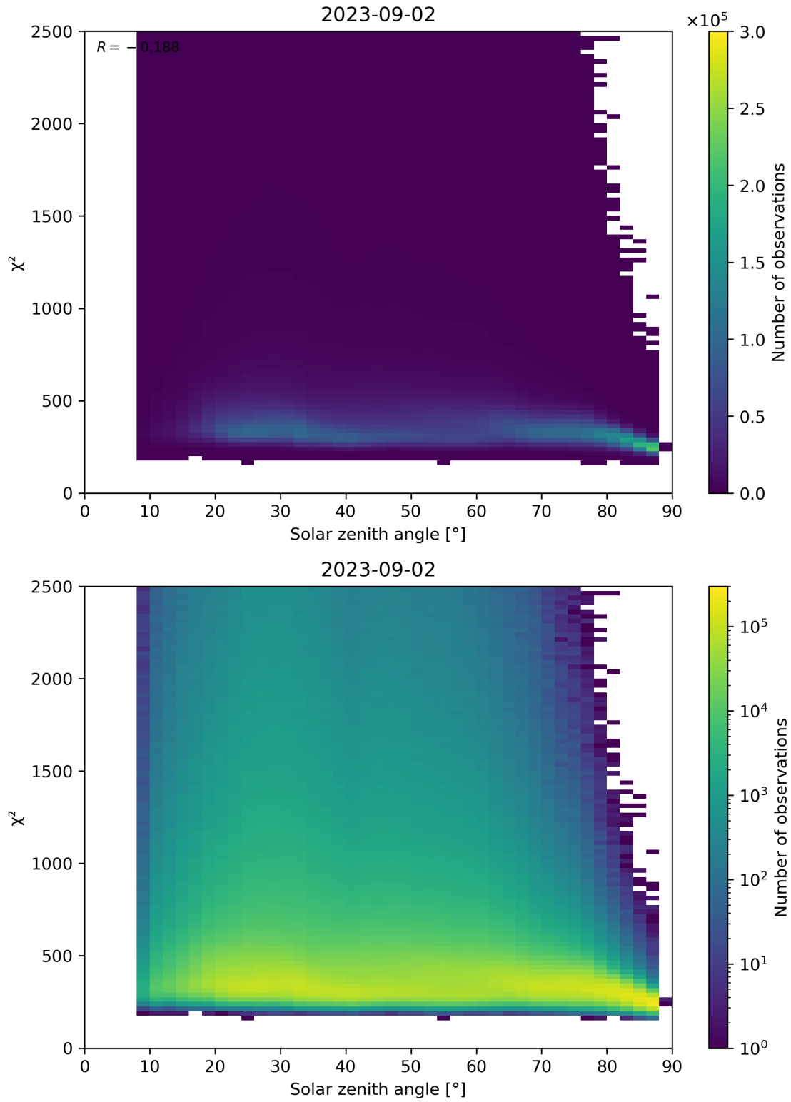
Figure 148: Scatter density plot of “Solar zenith angle” against “ \chi^2 ” for 2023-09-01 to 2023-09-03.
