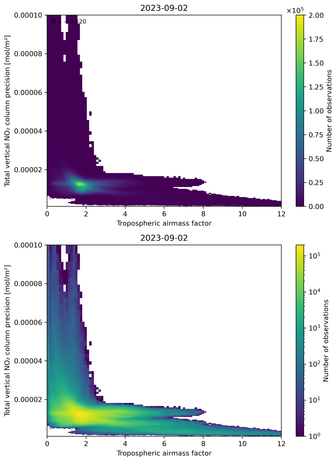
Figure 78: Scatter density plot of “Tropospheric air mass factor” against “Total vertical NO 2 column precision” for 2023-09-01 to 2023-09-03.
