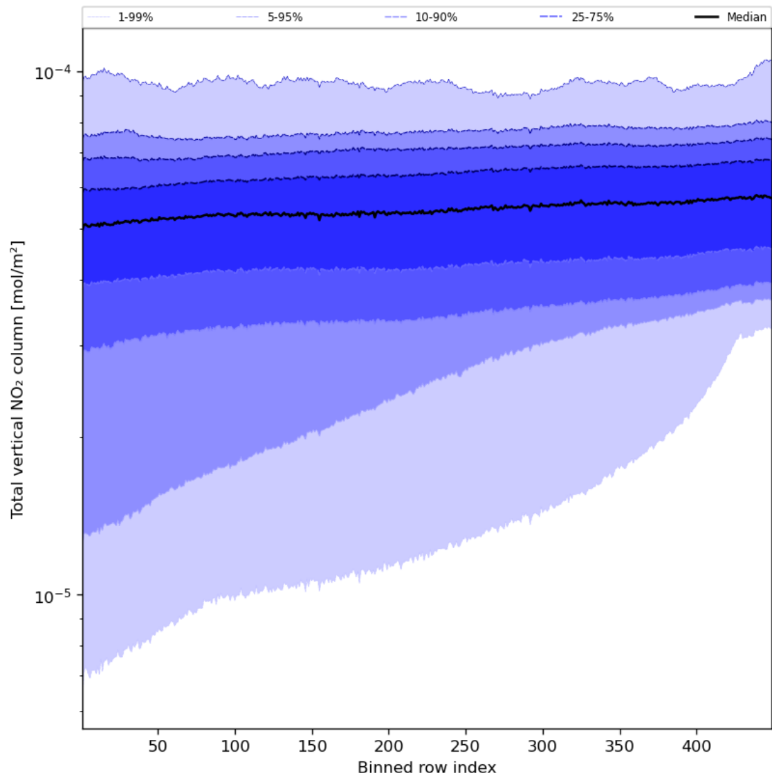
Figure 55: Along track statistics of “Total vertical NO 2 column” for 2023-09-01 to 2023-09-03
