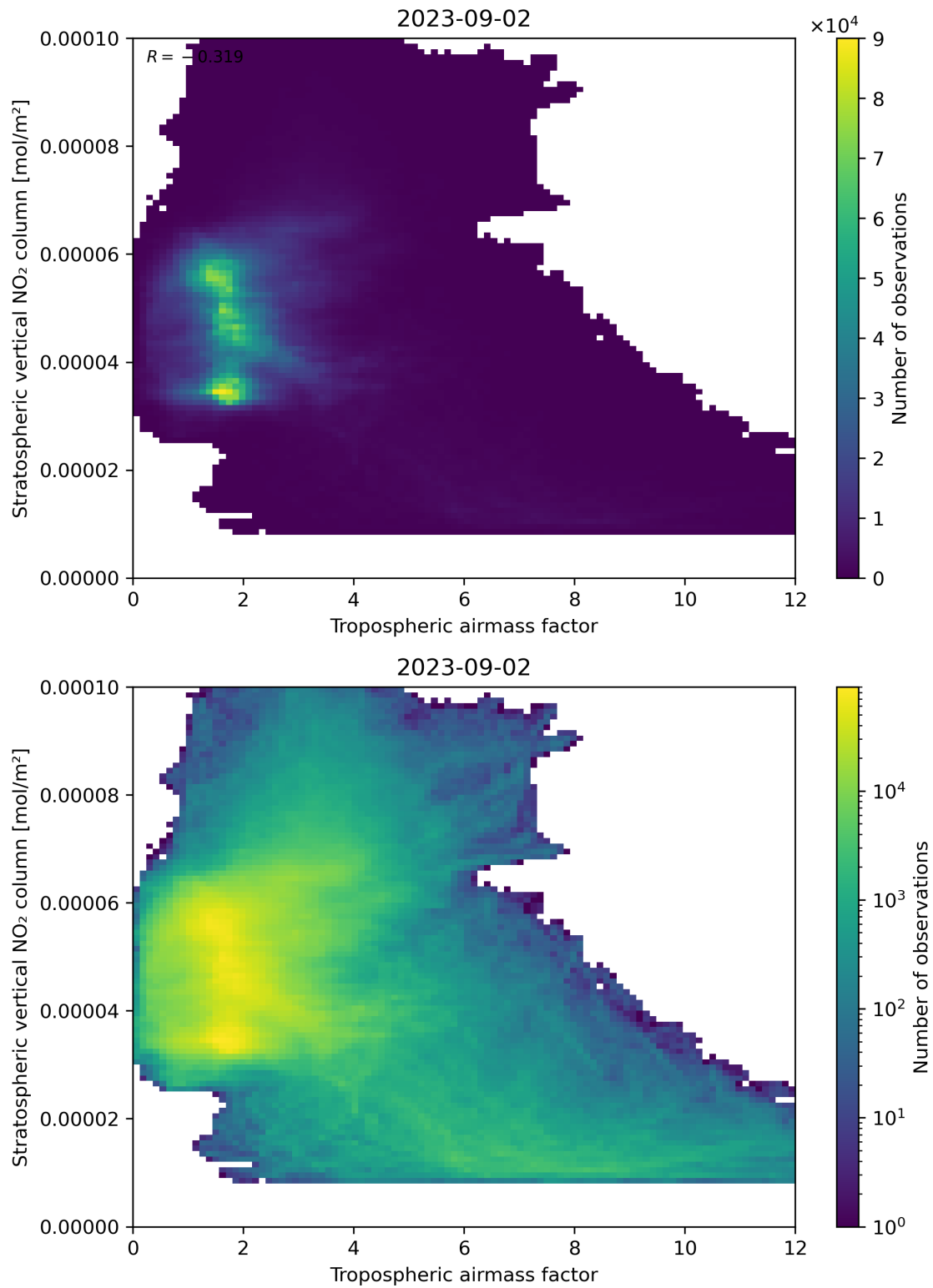
Figure 74: Scatter density plot of “Tropospheric air mass factor” against “Stratospheric vertical NO 2 column” for 2023-09-01 to 2023-09-03.
