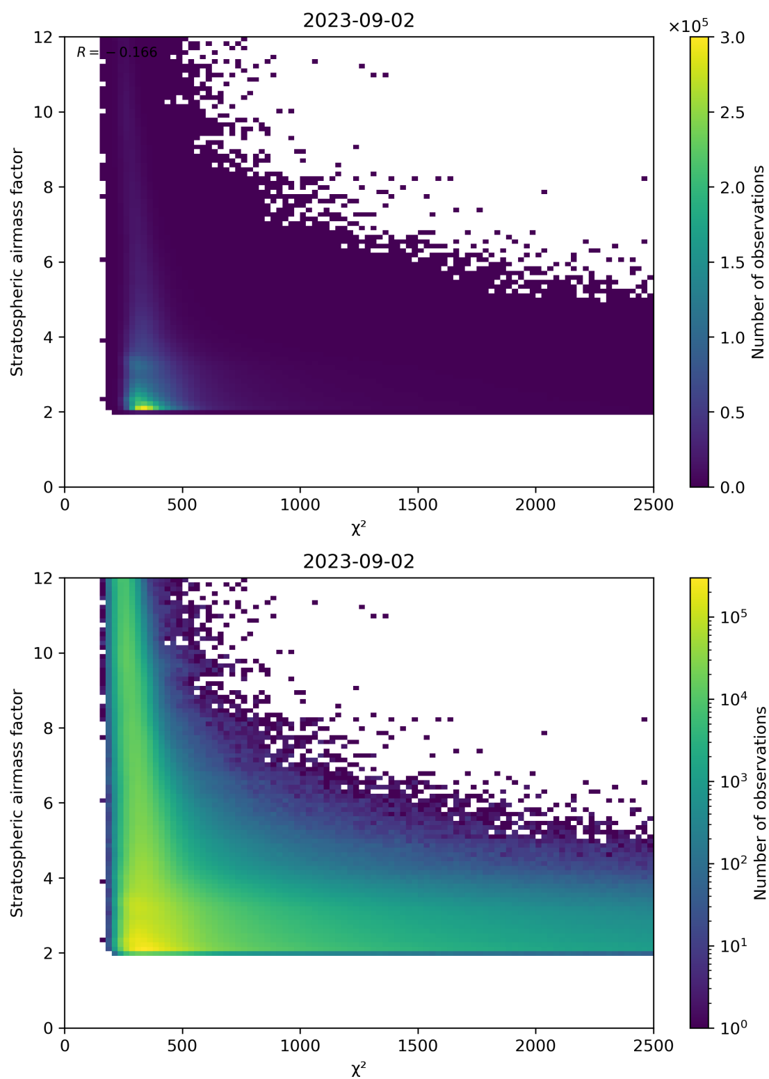
Figure 81: Scatter density plot of “ \chi^2 ” against “Stratospheric airmass factor” for 2023-09-01 to 2023-09-03.
