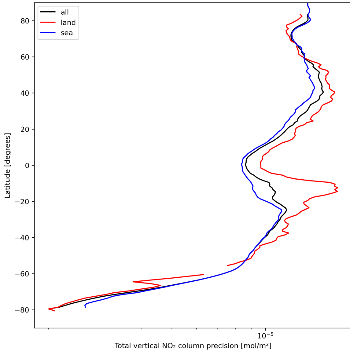
Figure 22: Zonal average of “Total vertical NO 2 column precision” for 2023-09-01 to 2023-09-03.
