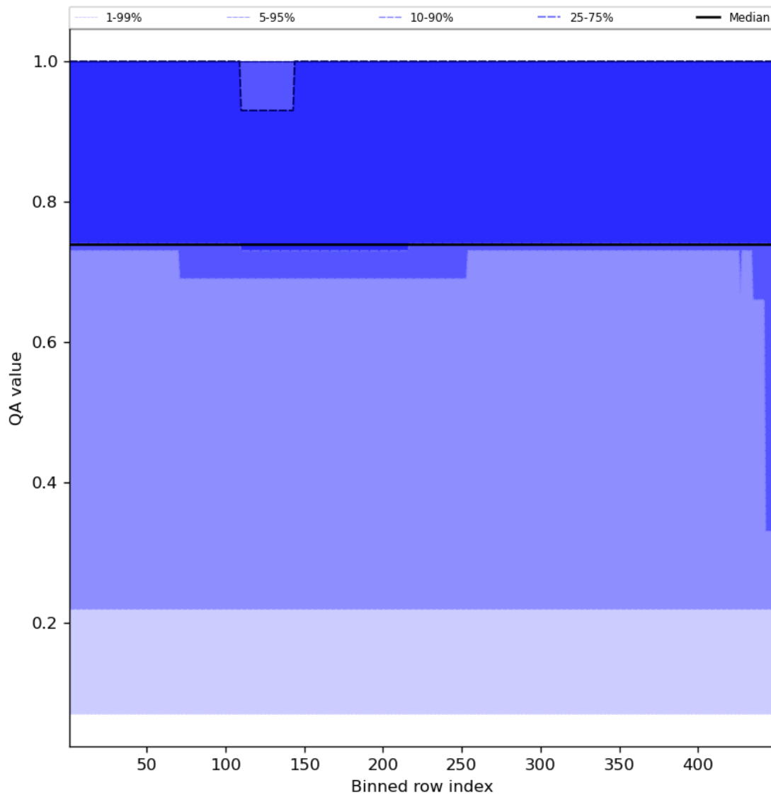
Figure 45: Along track statistics of “QA value” for 2023-09-01 to 2023-09-03
