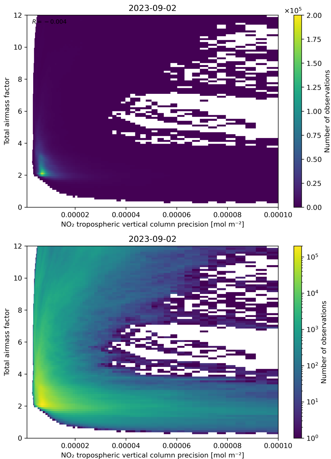
Figure 132: Scatter density plot of “NO 2 tropospheric vertical column precision” against “Total air mass factor” for 2023-09-01 to 2023-09-03.
