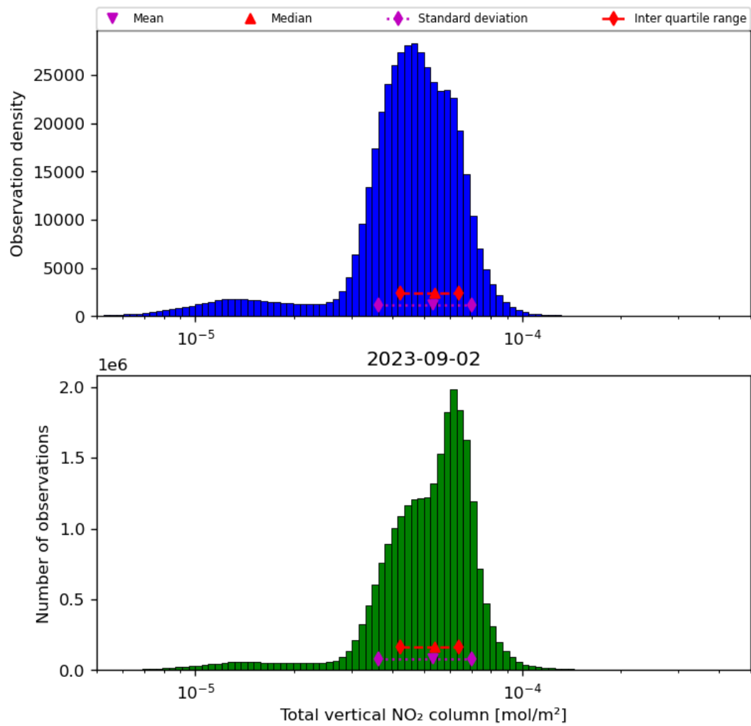
Figure 38: Histogram of “Total vertical NO 2 column” for 2023-09-01 to 2023-09-03
