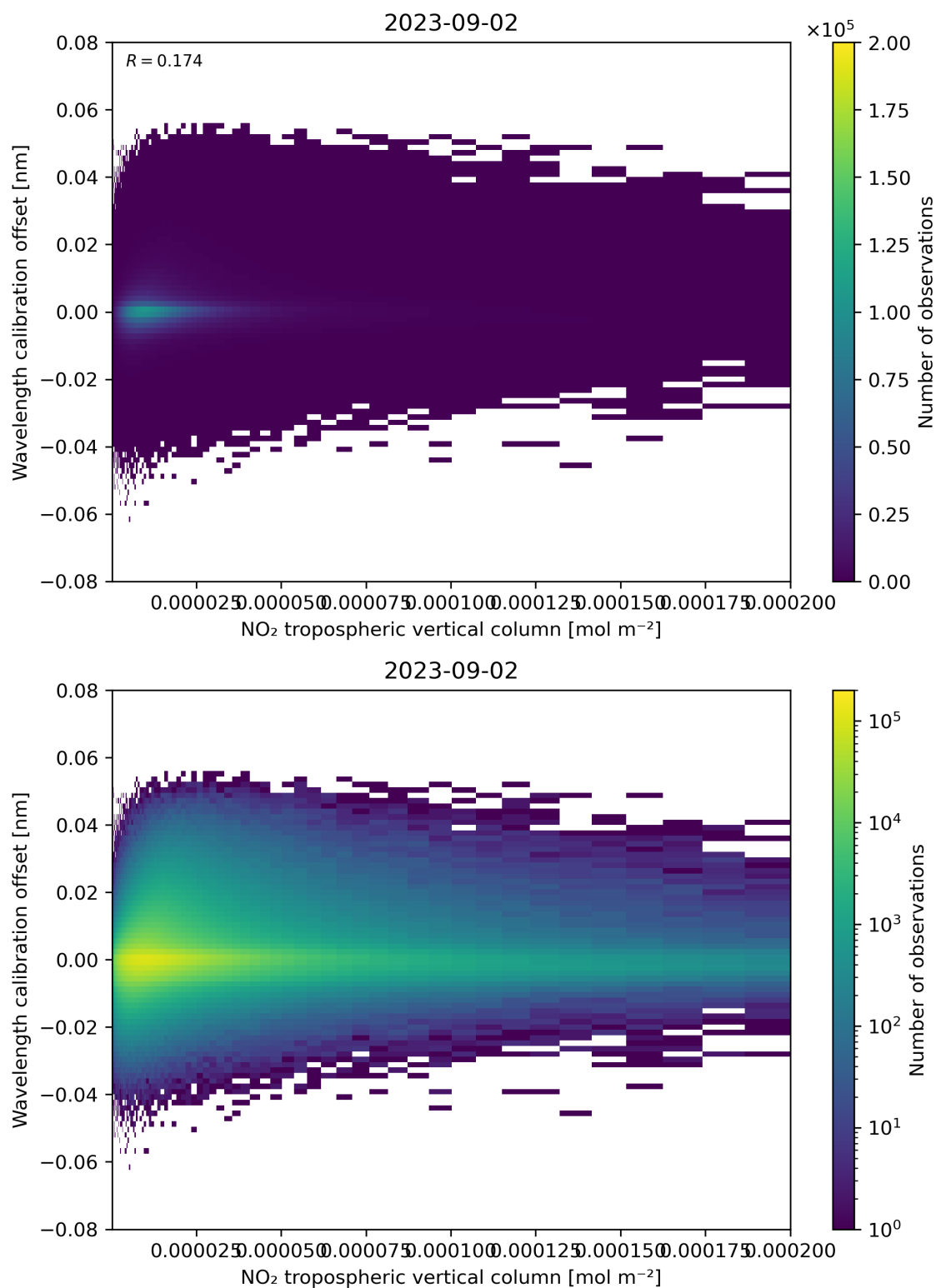
Figure 143: Scatter density plot of “NO 2 tropospheric vertical column” against “Wavelength calibration offset” for 2023-09-01 to 2023-09-03.
