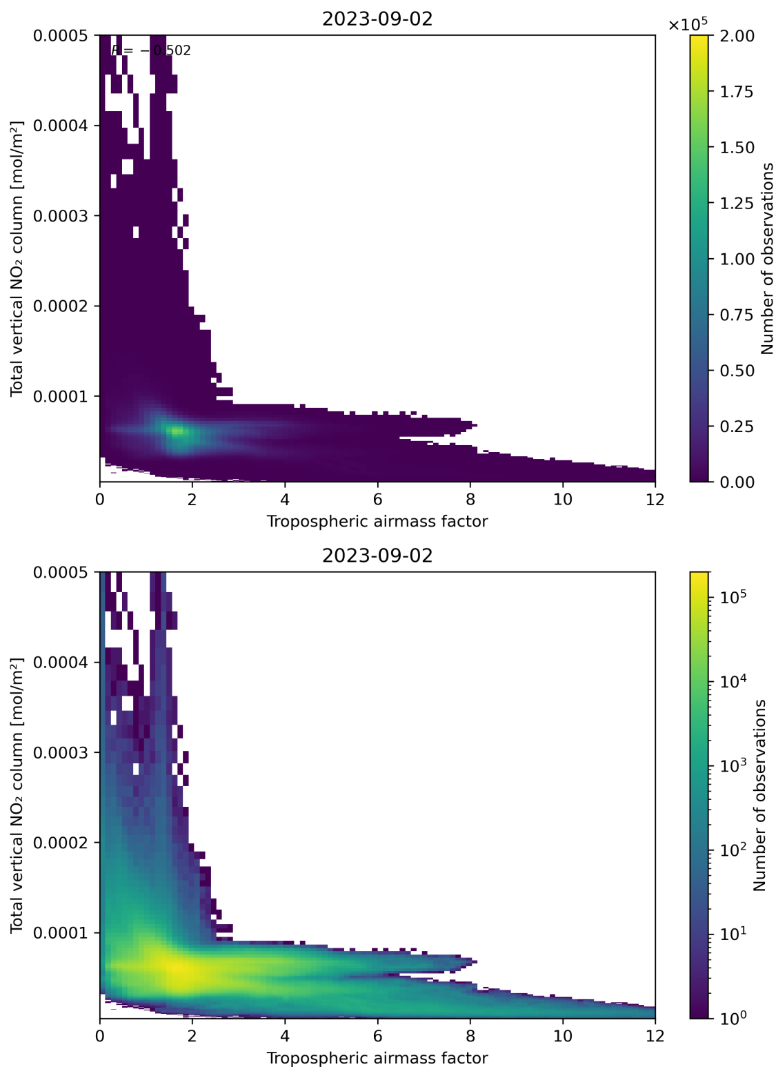
Figure 77: Scatter density plot of “Tropospheric airmass factor” against “Total vertical NO 2 column” for 2023-09-01 to 2023-09-03.
