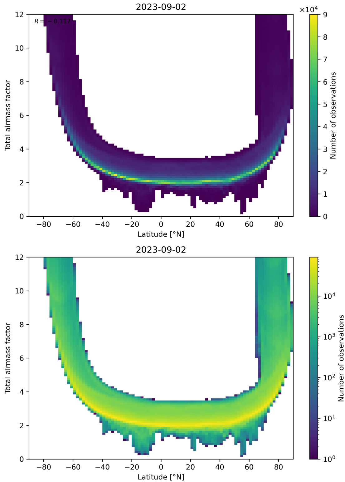
Figure 84: Scatter density plot of “Latitude” against “Total airmass factor” for 2023-09-01 to 2023-09-03.
