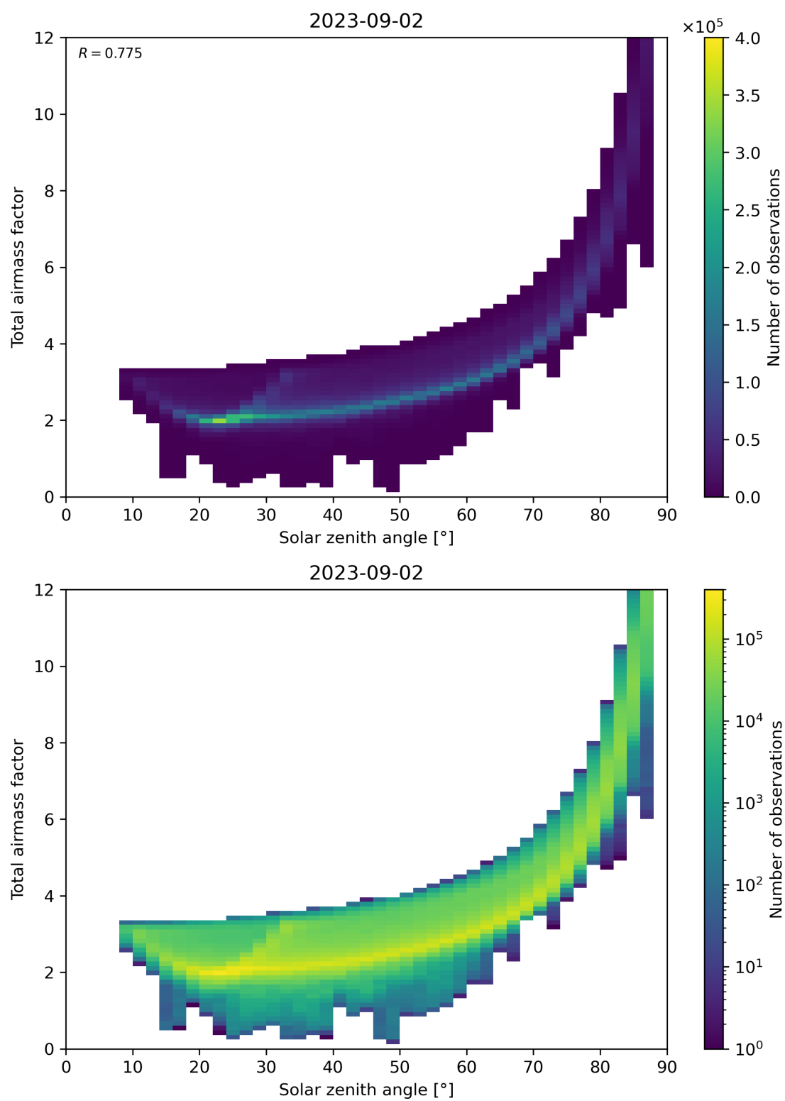
Figure 146: Scatter density plot of “Solar zenith angle” against “Total airmass factor” for 2023-09-01 to 2023-09-03.
