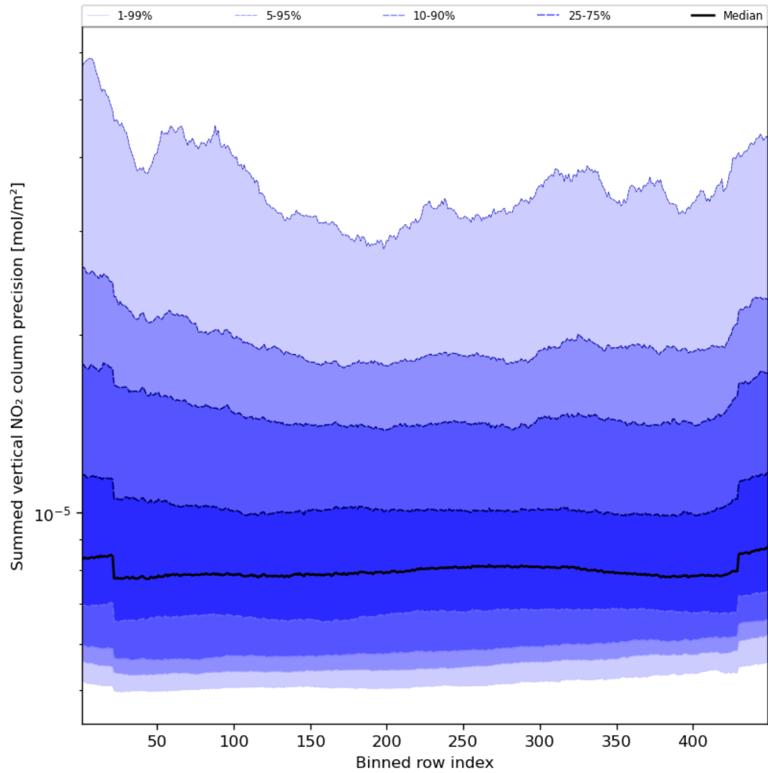
Figure 58: Along track statistics of “Summed vertical NO 2 column precision” for 2023-09-01 to 2023-09-03
