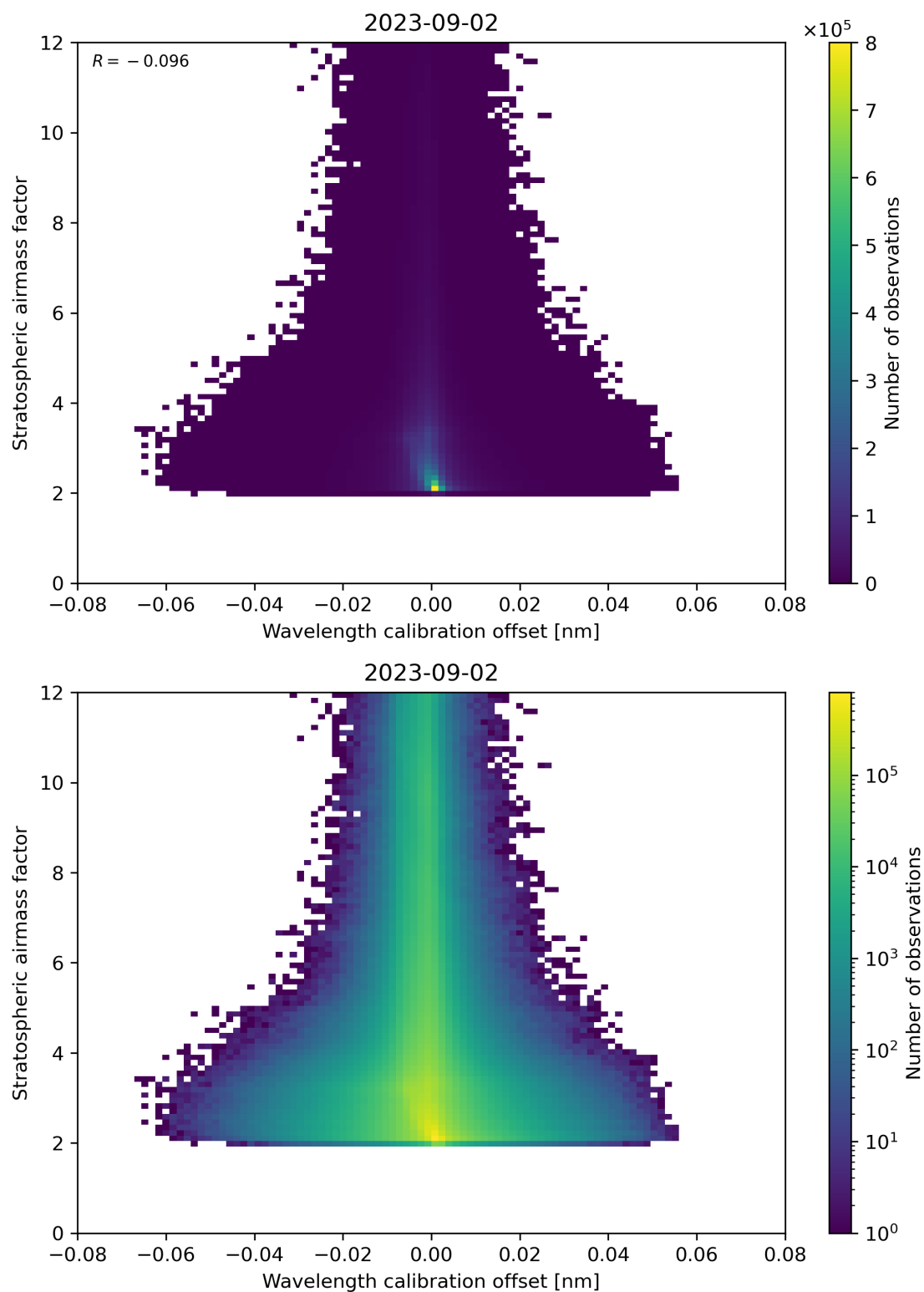
Figure 174: Scatter density plot of “Wavelength calibration offset” against “Stratospheric airmass factor” for 2023-09-01 to 2023-09-03.
