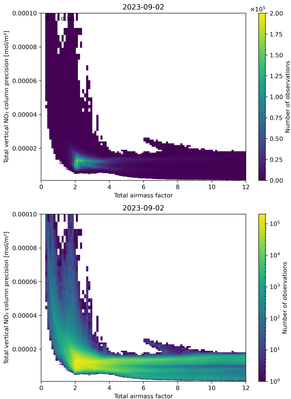
Figure 68: Scatter density plot of “Total airmass factor” against “Total vertical NO 2 column precision” for 2023-09-01 to 2023-09-03.
