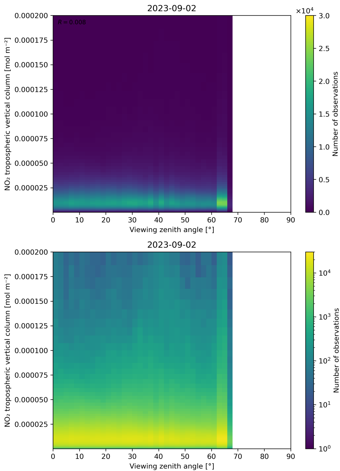
Figure 169: Scatter density plot of “Viewing zenith angle” against “NO 2 tropospheric vertical column” for 2023-09-01 to 2023-09-03.
