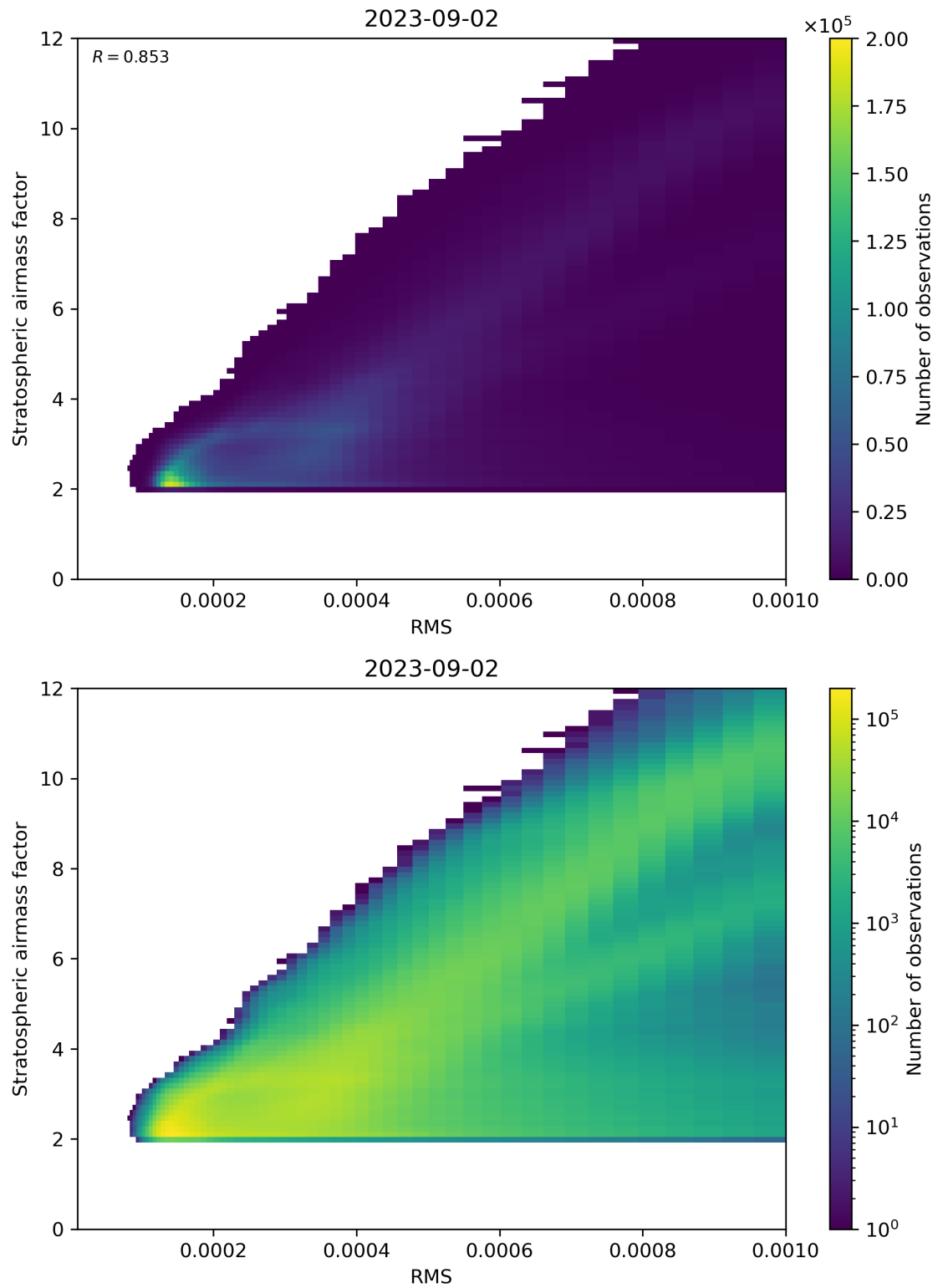
Figure 144: Scatter density plot of “RMS” against “Stratospheric airmass factor” for 2023-09-01 to 2023-09-03.
