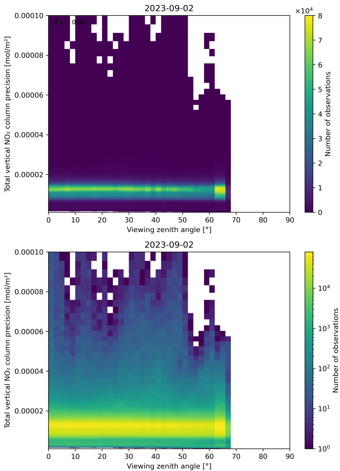
Figure 168: Scatter density plot of “Viewing zenith angle” against “Total vertical NO 2 column precision” for 2023-09-01 to 2023-09-03.
