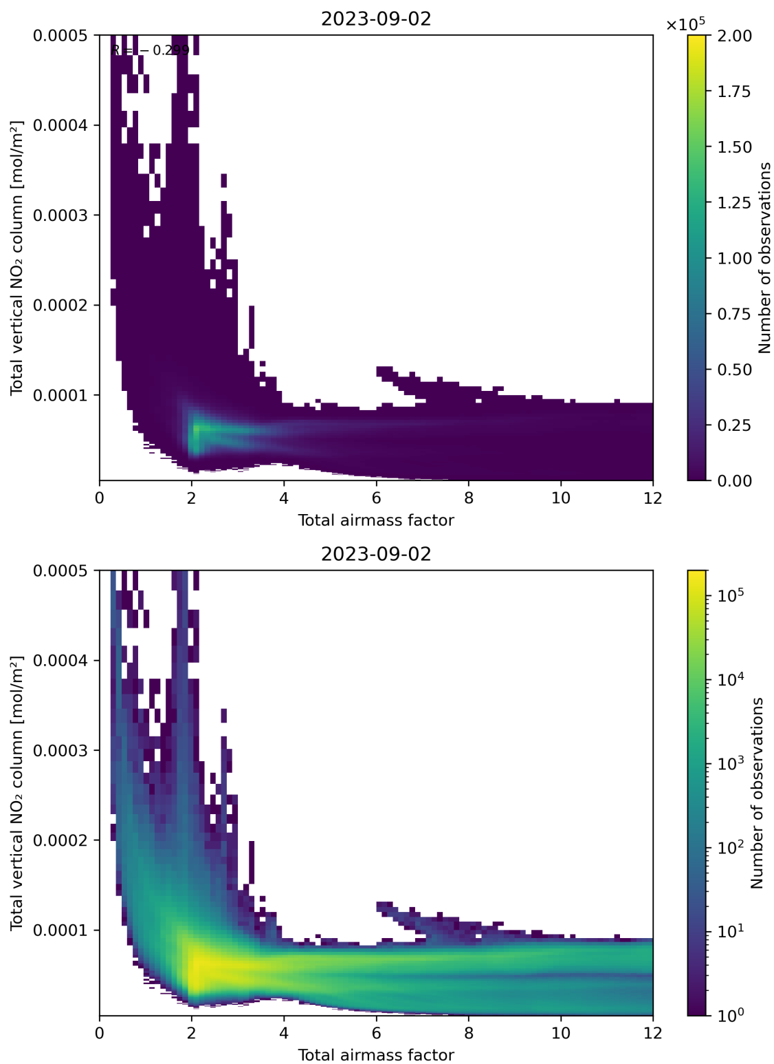
Figure 67: Scatter density plot of “Total airmass factor” against “Total vertical NO 2 column” for 2023-09-01 to 2023-09-03.
