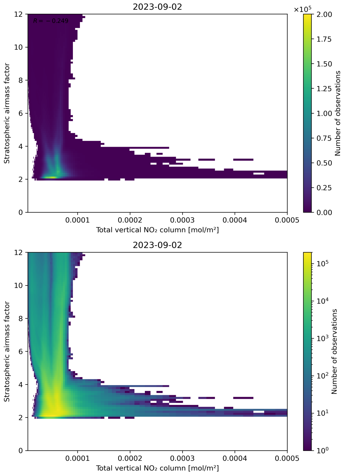
Figure 110: Scatter density plot of “Total vertical NO 2 column” against “Stratospheric airmass factor” for 2023-09-01 to 2023-09-03.
