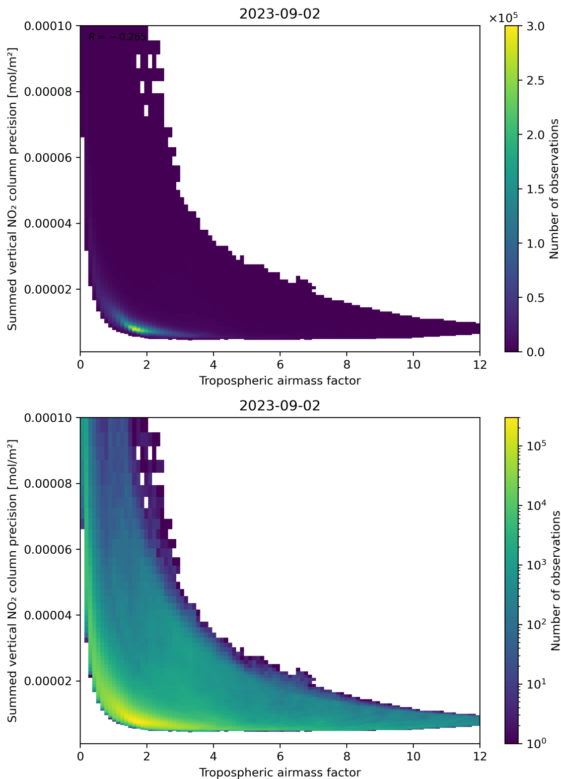
Figure 76: Scatter density plot of “Tropospheric air mass factor” against “Summed vertical NO 2 column precision” for 2023-09-01 to 2023-09-03.
