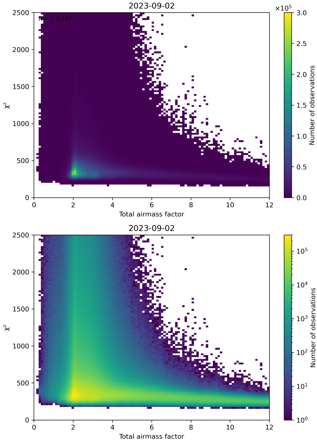
Figure 63: Scatter density plot of “Total airmass factor” against “ \chi^2 ” for 2023-09-01 to 2023-09-03.
