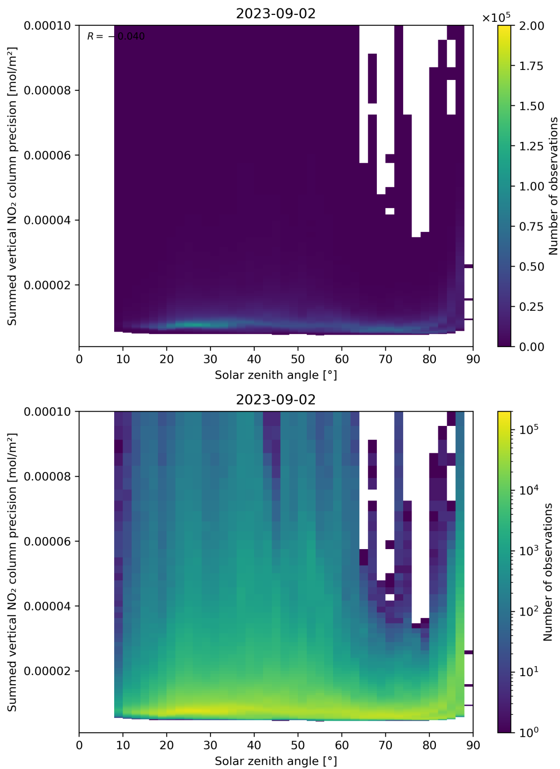
Figure 152: Scatter density plot of “Solar zenith angle” against “Summed vertical NO 2 column precision” for 2023-09-01 to 2023-09-03.
