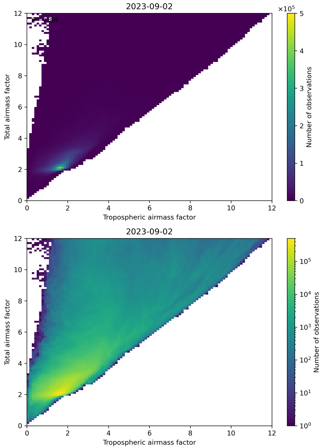
Figure 72: Scatter density plot of “Tropospheric airmass factor” against “Total airmass factor” for 2023-09-01 to 2023-09-03.
