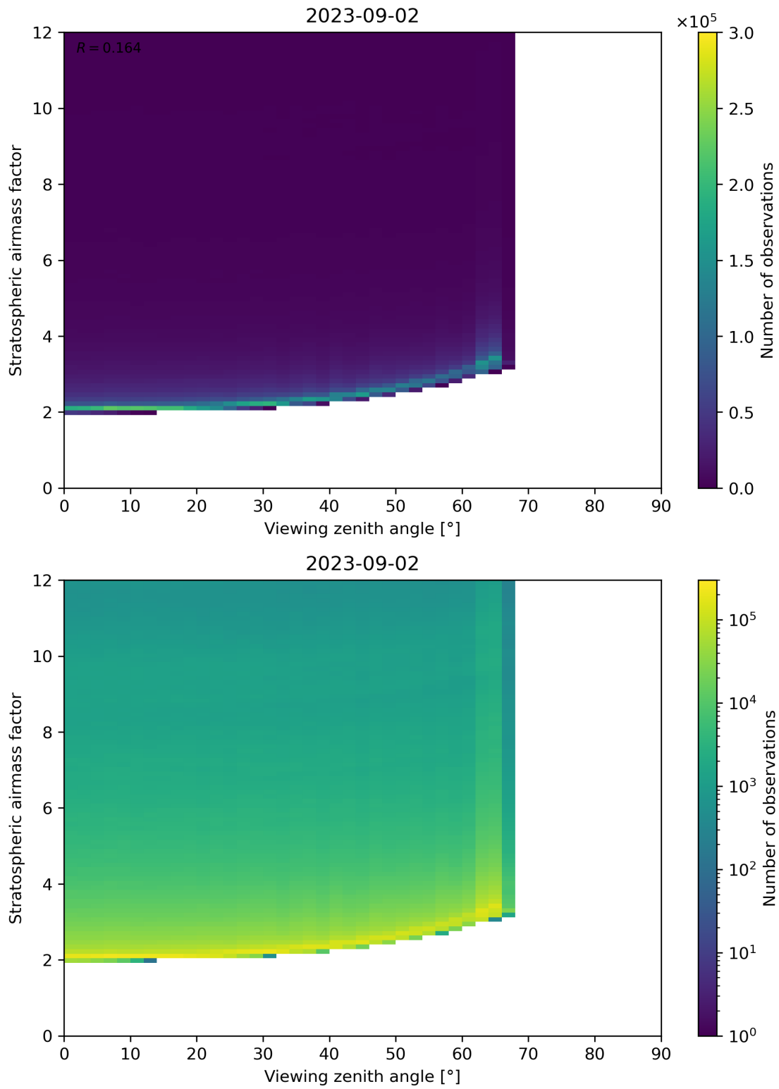
Figure 159: Scatter density plot of “Viewing zenith angle” against “Stratospheric airmass factor” for 2023-09-01 to 2023-09-03.
