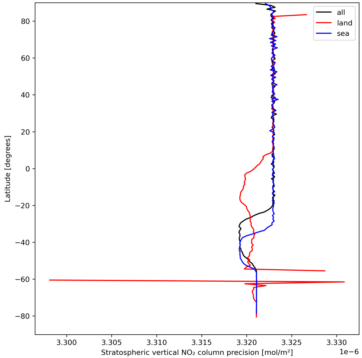
Figure 20: Zonal average of “Stratospheric vertical NO 2 column precision” for 2023-09-01 to 2023-09-03.
