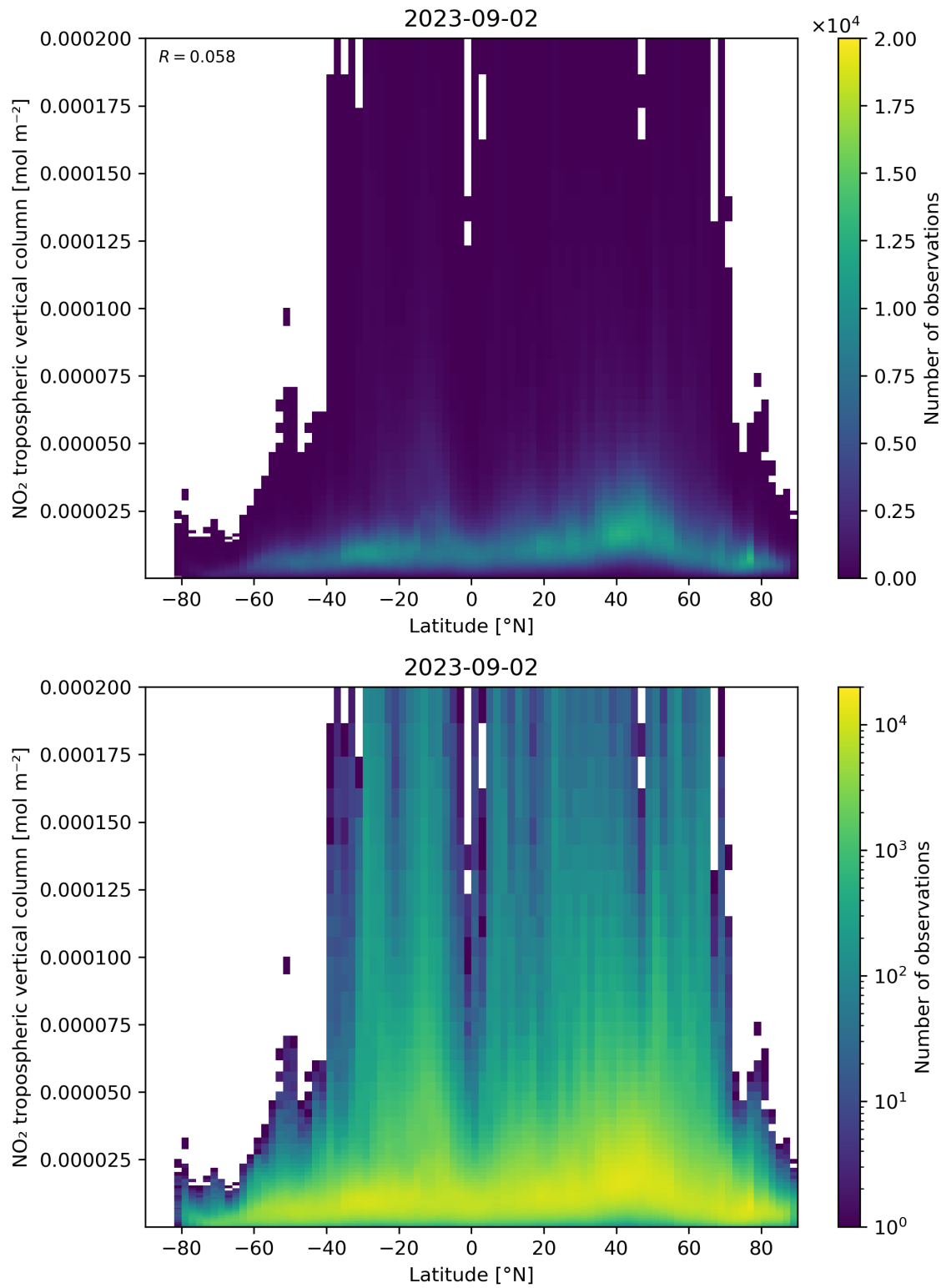
Figure 92: Scatter density plot of “Latitude” against “NO 2 tropospheric vertical column” for 2023-09-01 to 2023-09-03.
