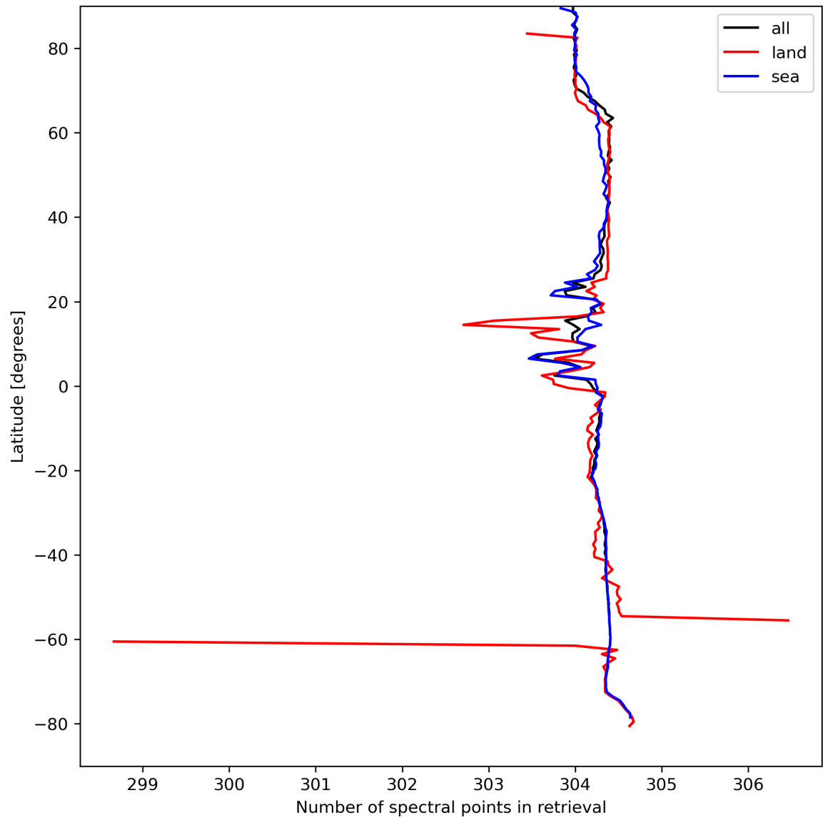
Figure 16: Zonal average of “Number of spectral points in retrieval” for 2023-09-01 to 2023-09-03.
