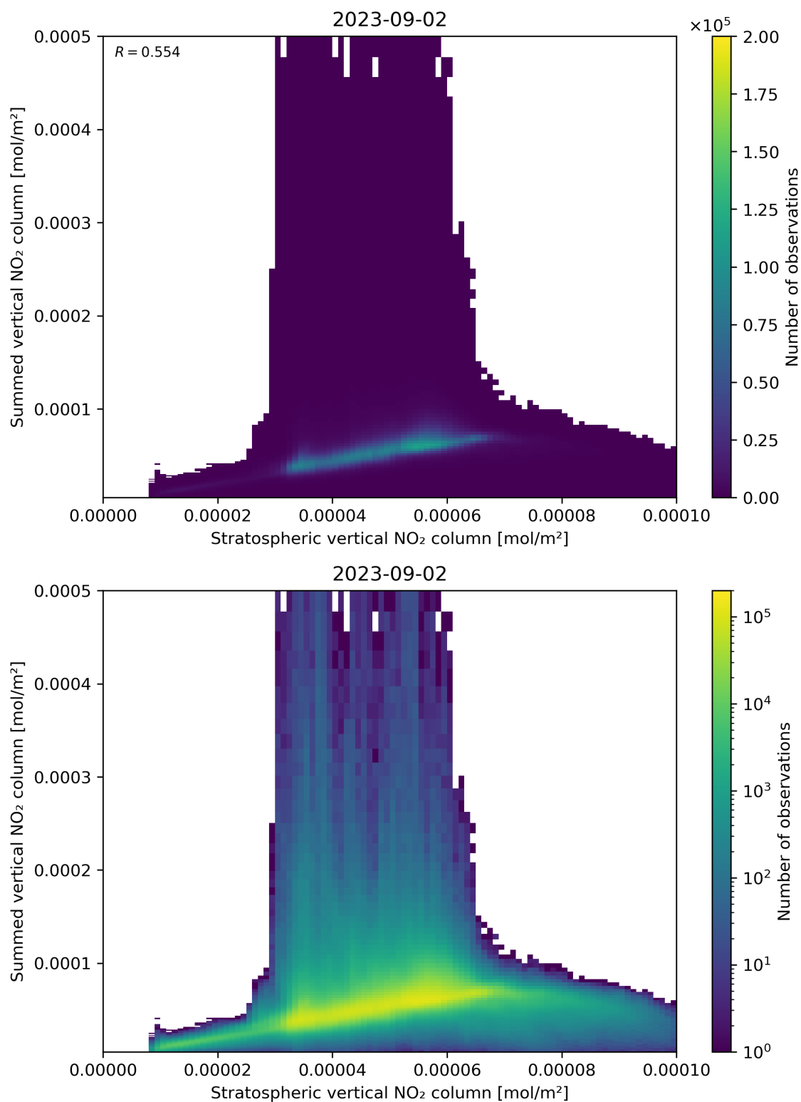
Figure 98: Scatter density plot of “Stratospheric vertical NO 2 column” against “Summed vertical NO 2 column” for 2023-09-01 to 2023-09-03.
