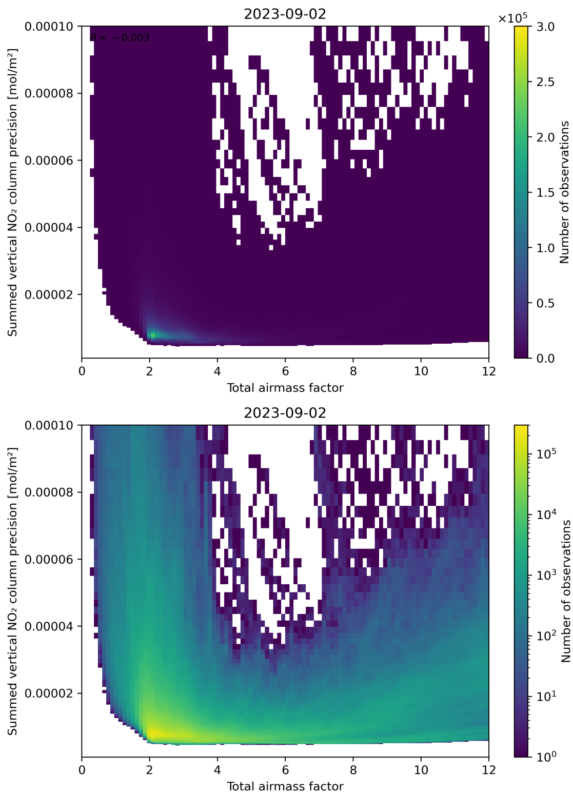
Figure 66: Scatter density plot of “Total airmass factor” against “Summed vertical NO 2 column precision” for 2023-09-01 to 2023-09-03.
