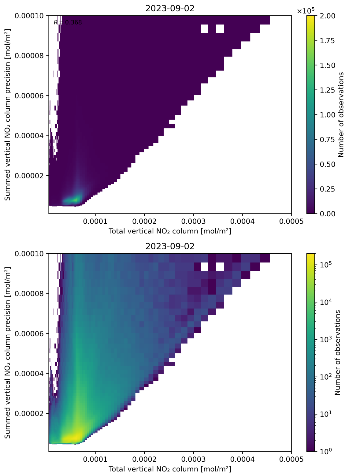
Figure 113: Scatter density plot of “Total vertical NO 2 column” against “Summed vertical NO 2 column precision” for 2023-09-01 to 2023-09-03.
