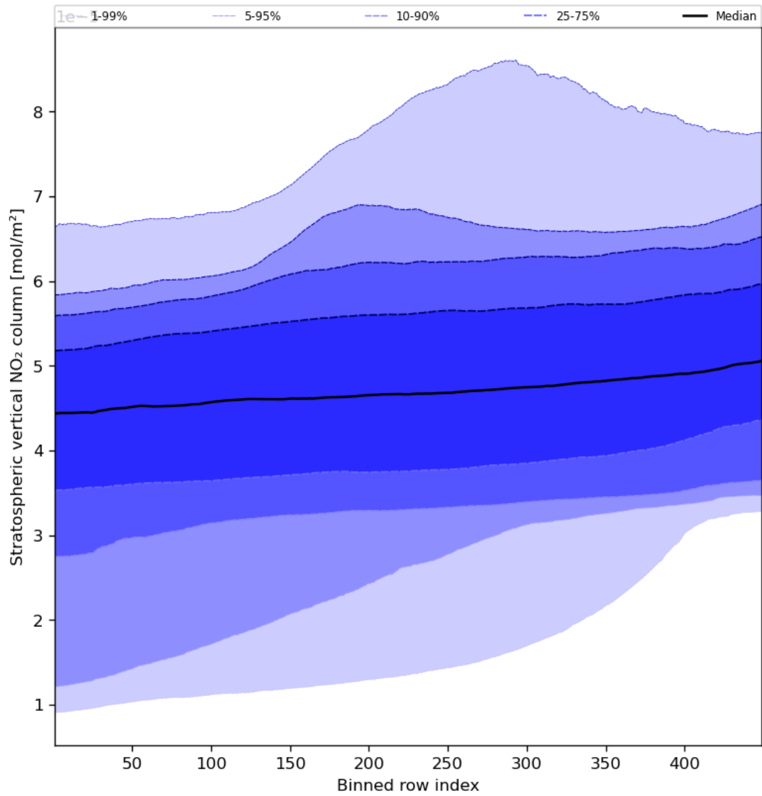
Figure 53: Along track statistics of “Stratospheric vertical NO 2 column” for 2023-09-01 to 2023-09-03
