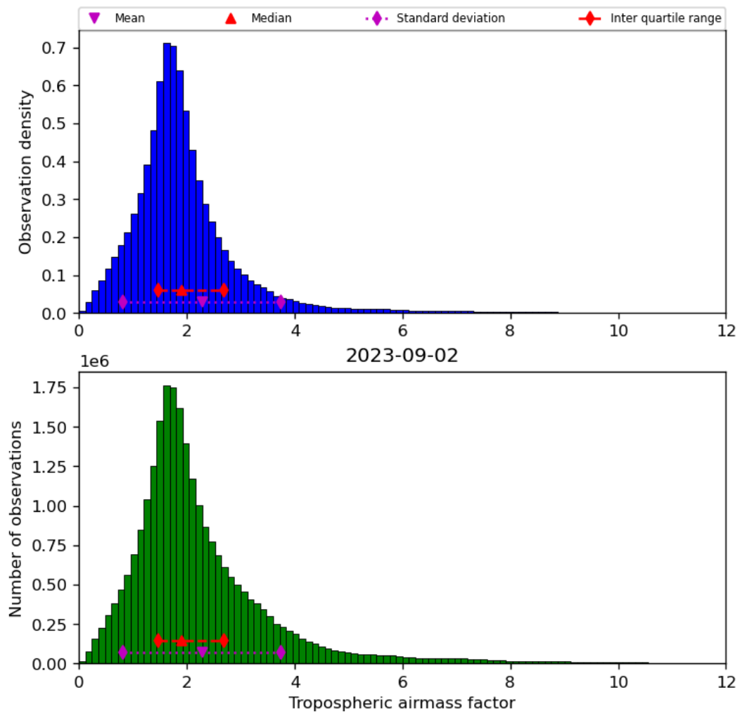
Figure 31: Histogram of “Tropospheric airmass factor” for 2023-09-01 to 2023-09-03
