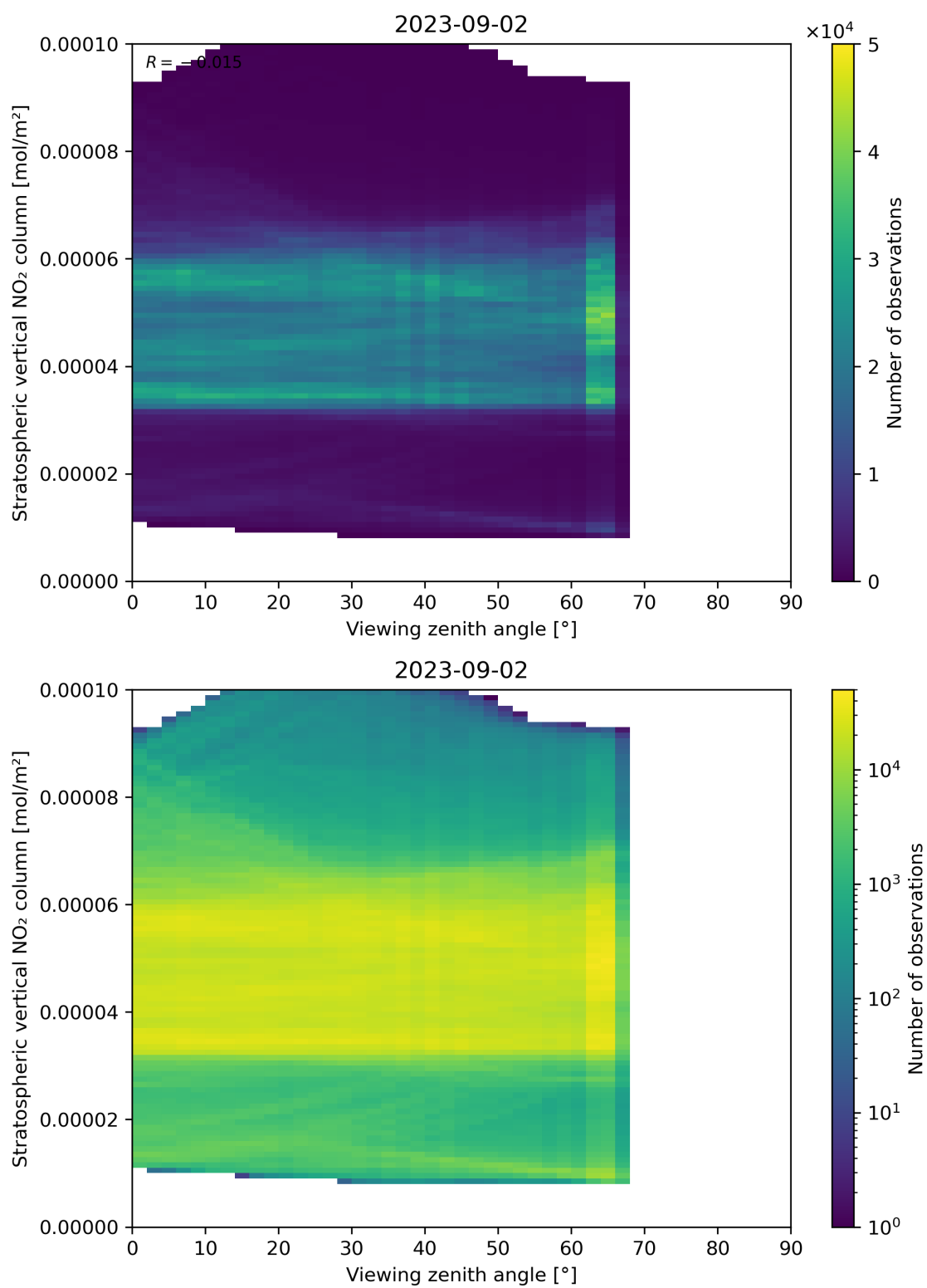
Figure 164: Scatter density plot of “Viewing zenith angle” against “Stratospheric vertical NO 2 column” for 2023-09-01 to 2023-09-03.
