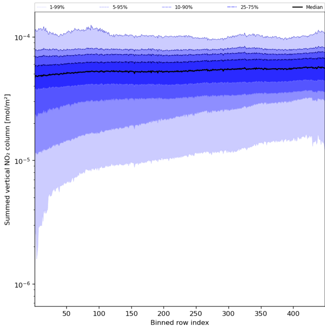
Figure 57: Along track statistics of “Summed vertical NO 2 column” for 2023-09-01 to 2023-09-03
