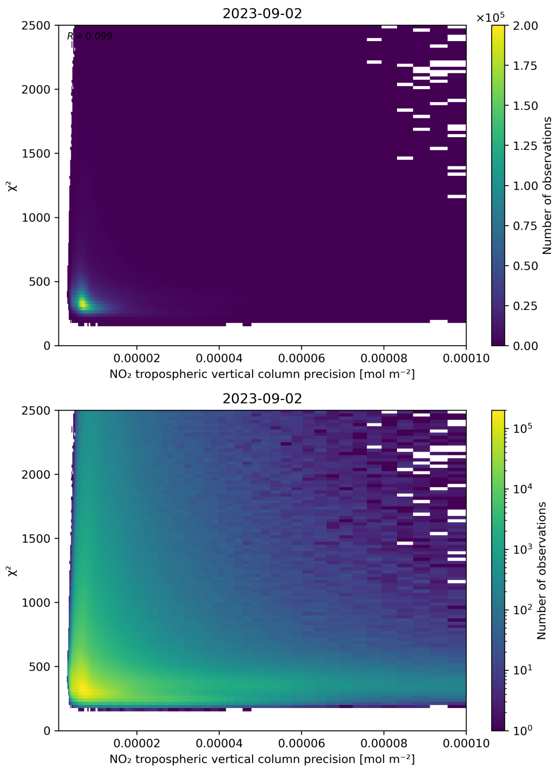
Figure 134: Scatter density plot of “NO 2 tropospheric vertical column precision” against “ \chi^2 ” for 2023-09-01 to 2023-09-03.
