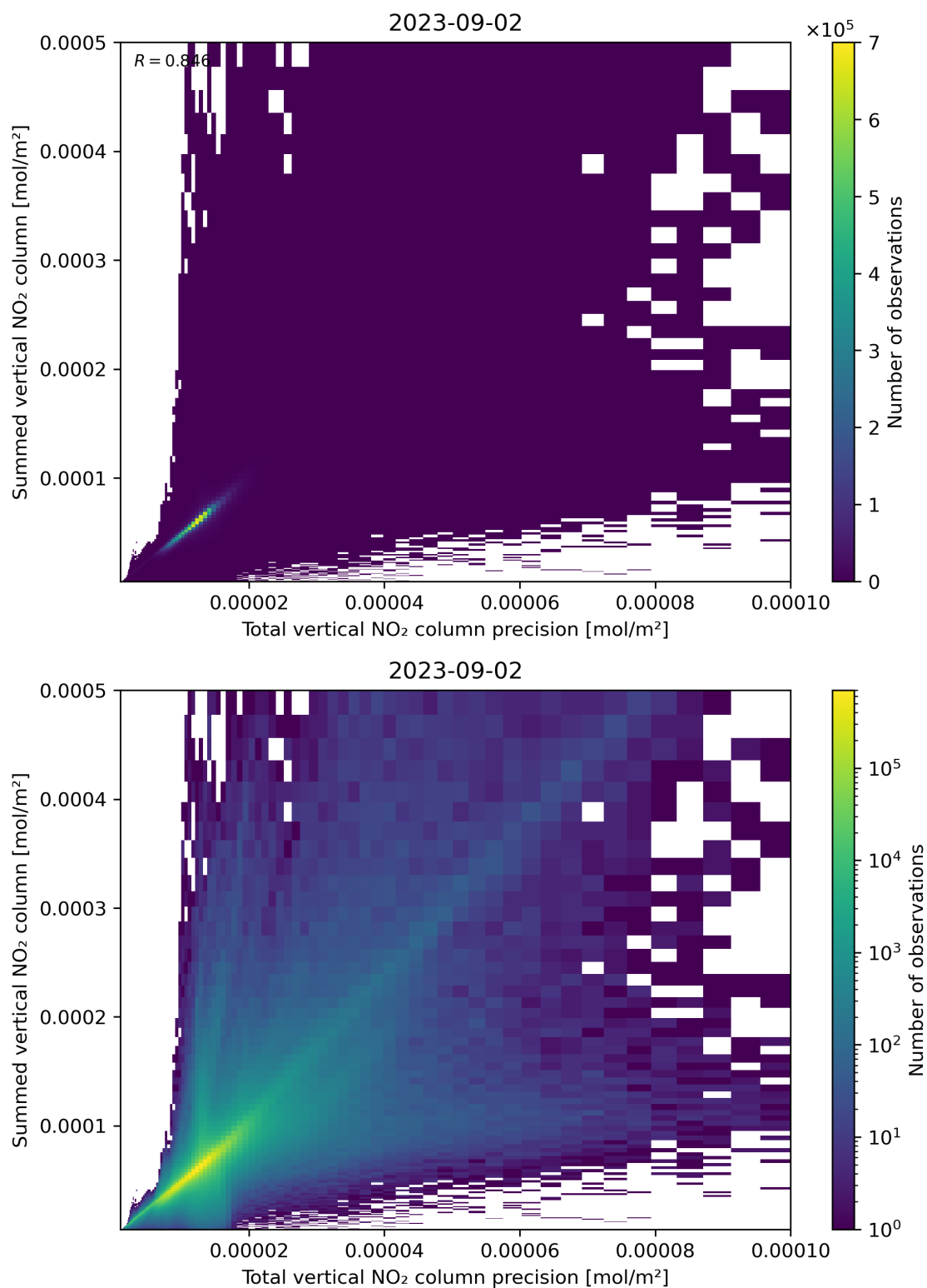
Figure 117: Scatter density plot of “Total vertical NO 2 column precision” against “Summed vertical NO 2 column” for 2023-09-01 to 2023-09-03.
