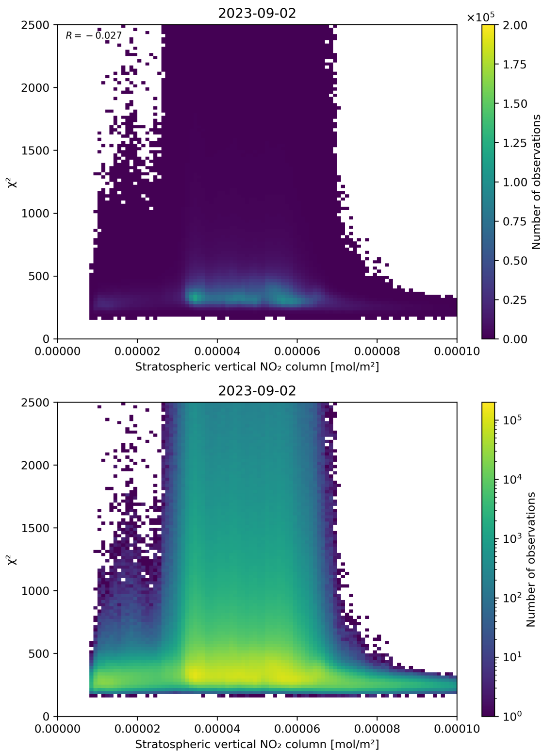
Figure 97: Scatter density plot of “Stratospheric vertical NO 2 column” against “ \chi^2 ” for 2023-09-01 to 2023-09-03.
