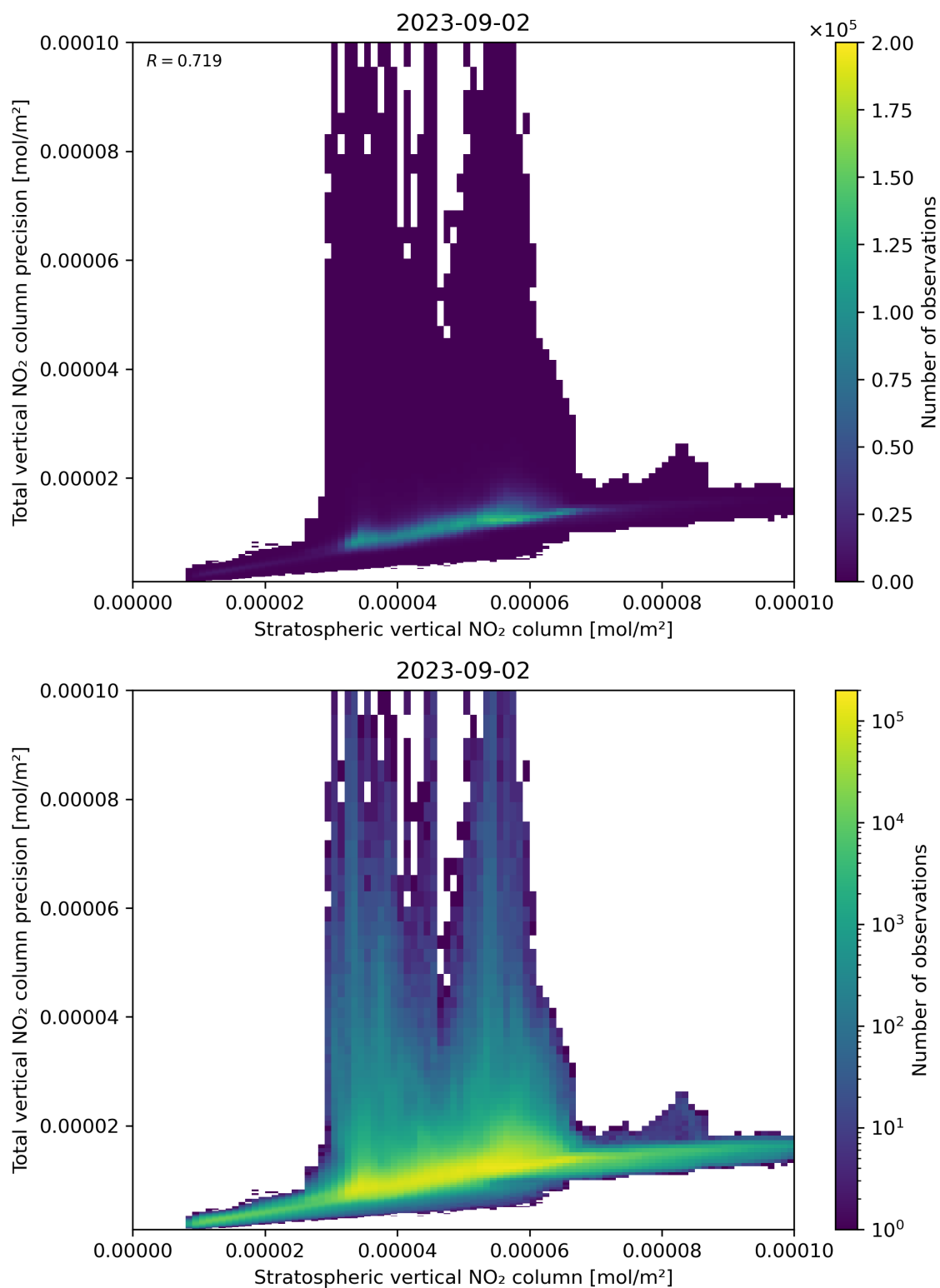
Figure 101: Scatter density plot of “Stratospheric vertical NO 2 column” against “Total vertical NO 2 column precision” for 2023-09-01 to 2023-09-03.
