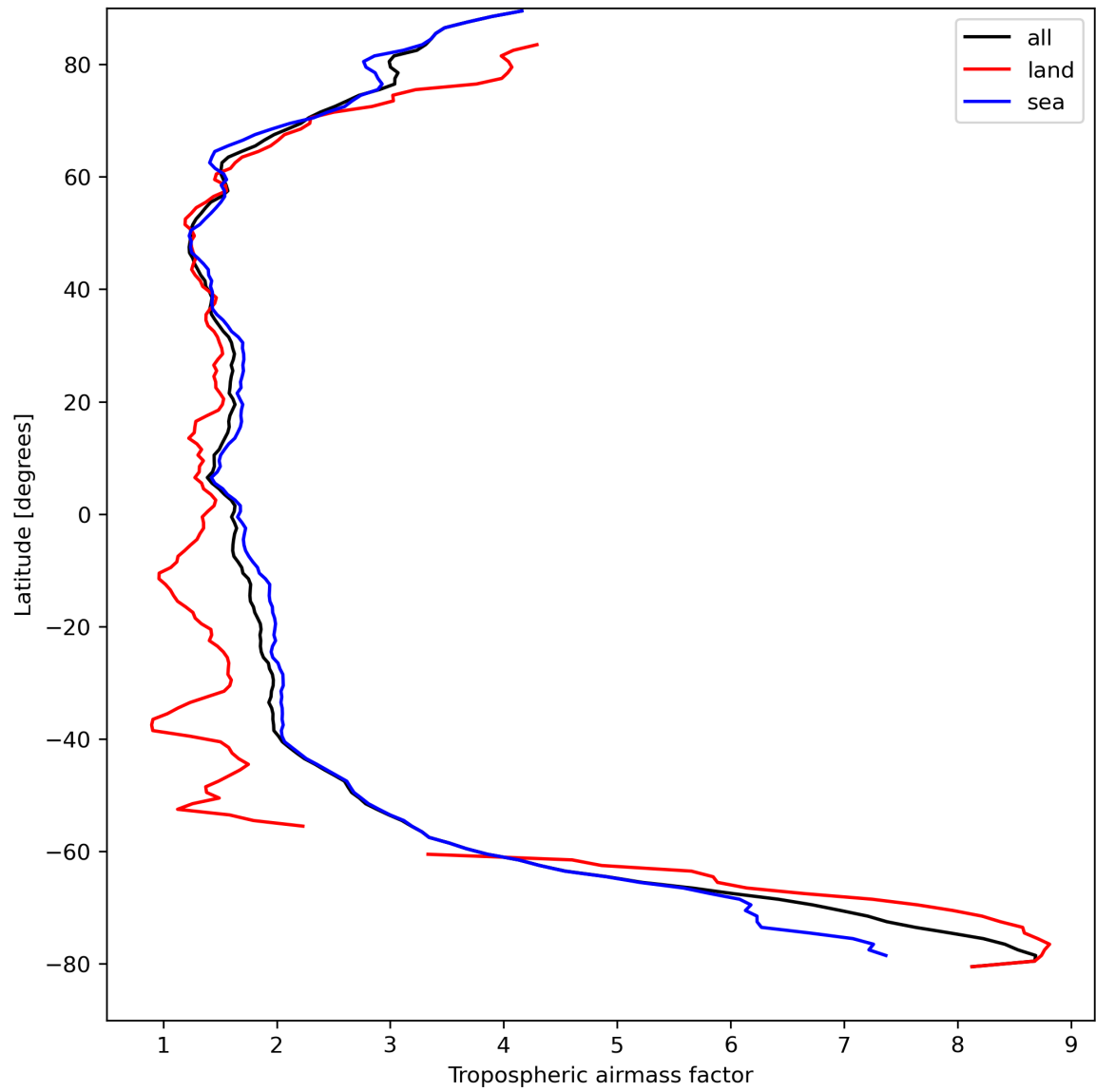
Figure 14: Zonal average of “Tropospheric airmass factor” for 2023-09-01 to 2023-09-03.
