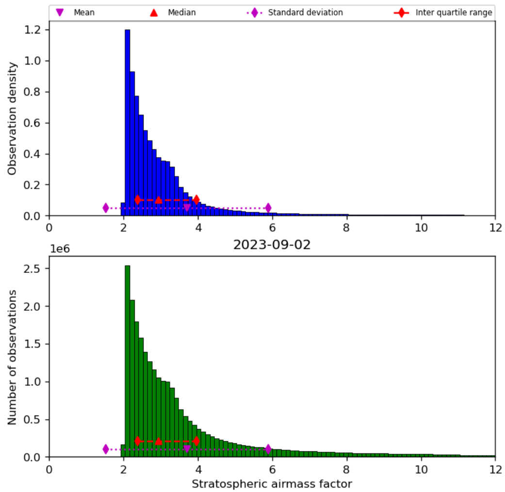
Figure 44: Histogram of “Stratospheric airmass factor” for 2023-09-01 to 2023-09-03
