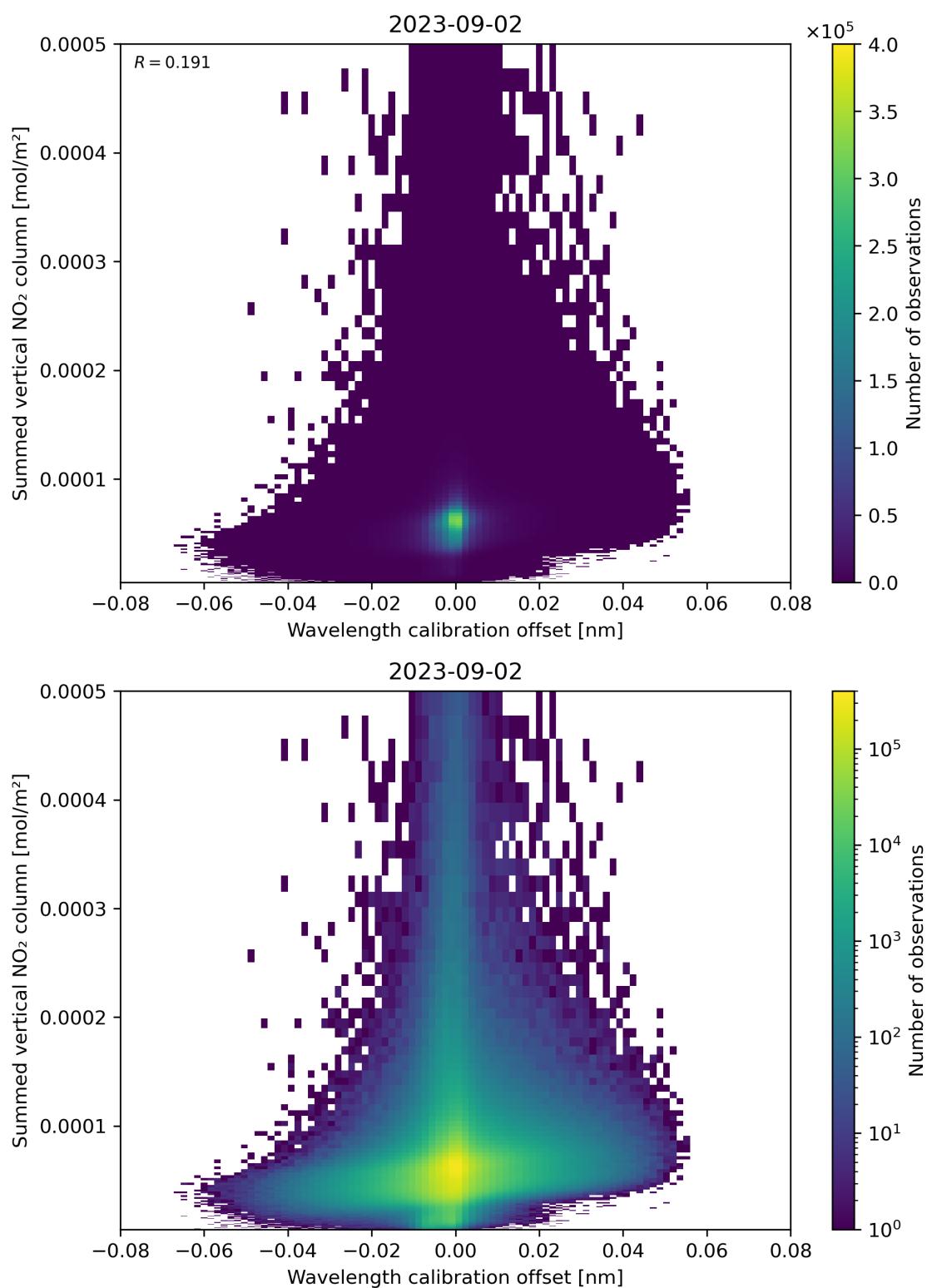
Figure 177: Scatter density plot of “Wavelength calibration offset” against “Summed vertical NO 2 column” for 2023-09-01 to 2023-09-03.
