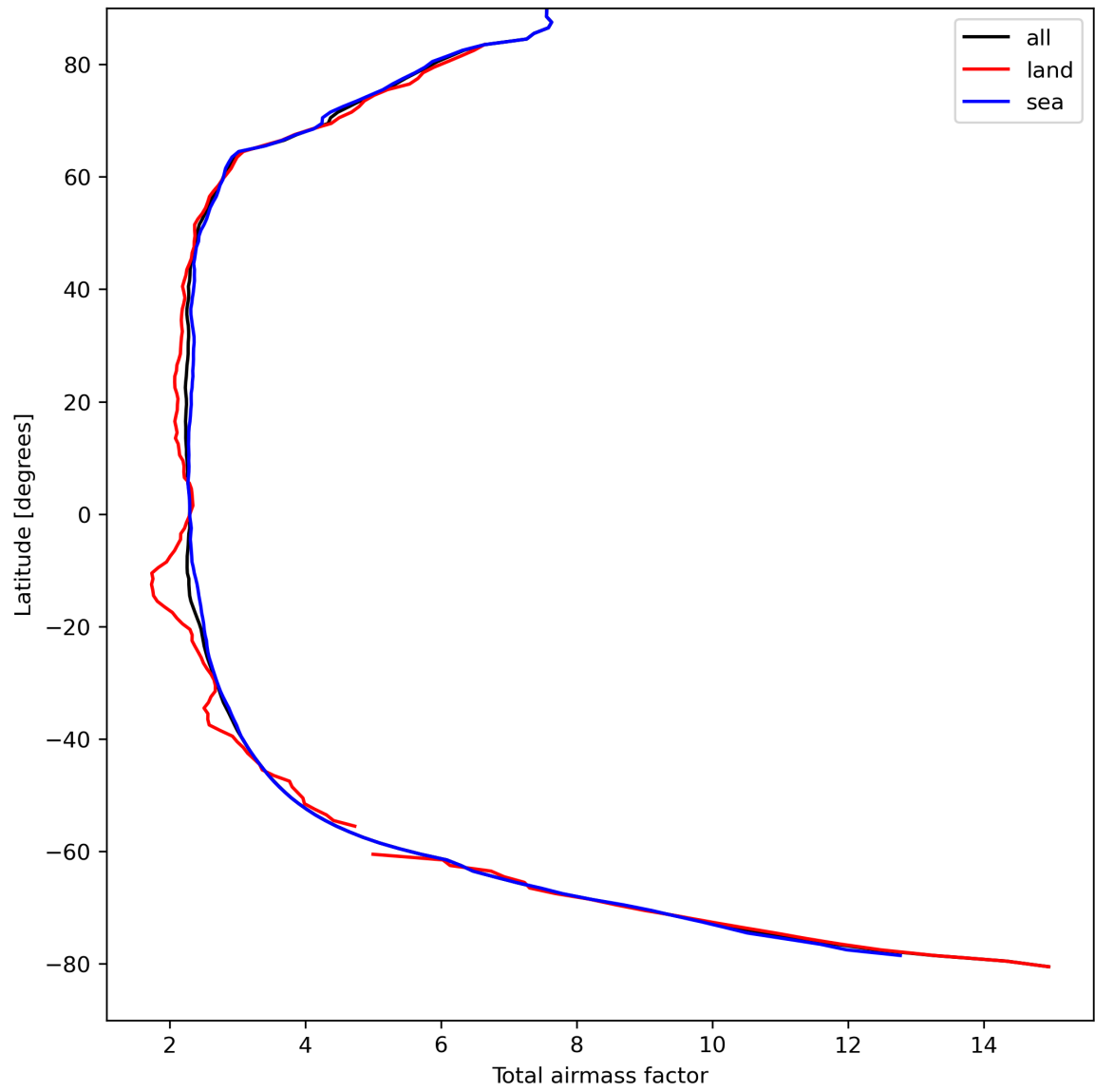
Figure 15: Zonal average of “Total airmass factor” for 2023-09-01 to 2023-09-03.
