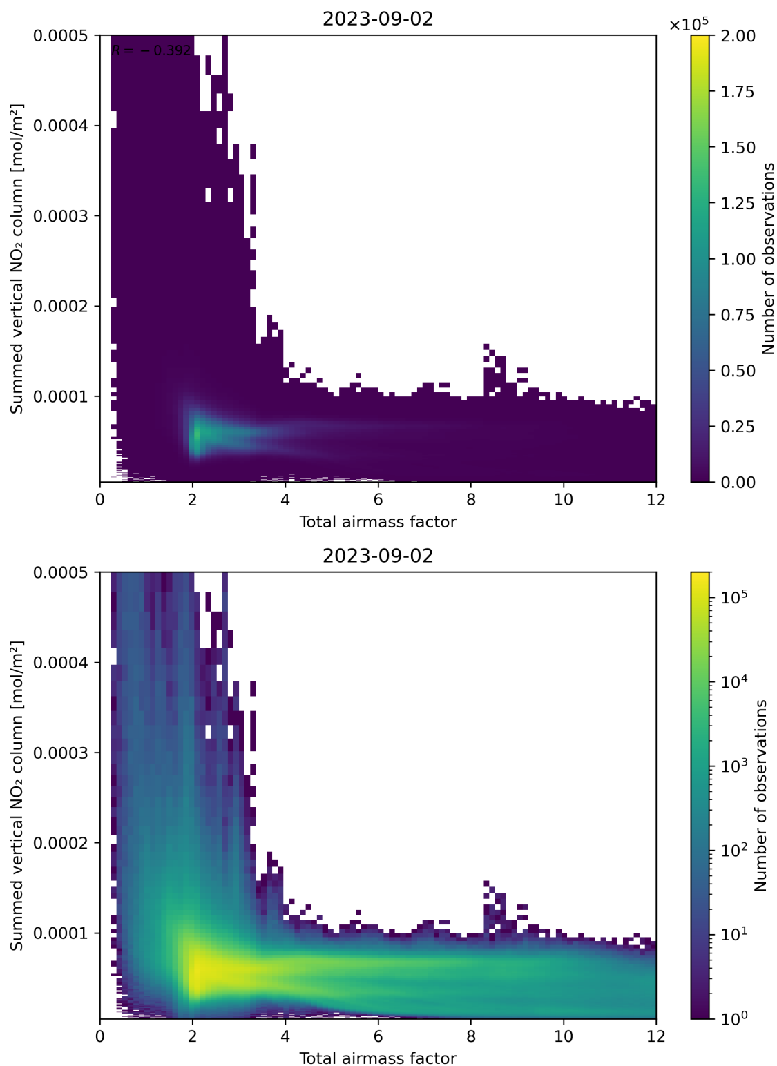
Figure 65: Scatter density plot of “Total airmass factor” against “Summed vertical NO 2 column” for 2023-09-01 to 2023-09-03.
