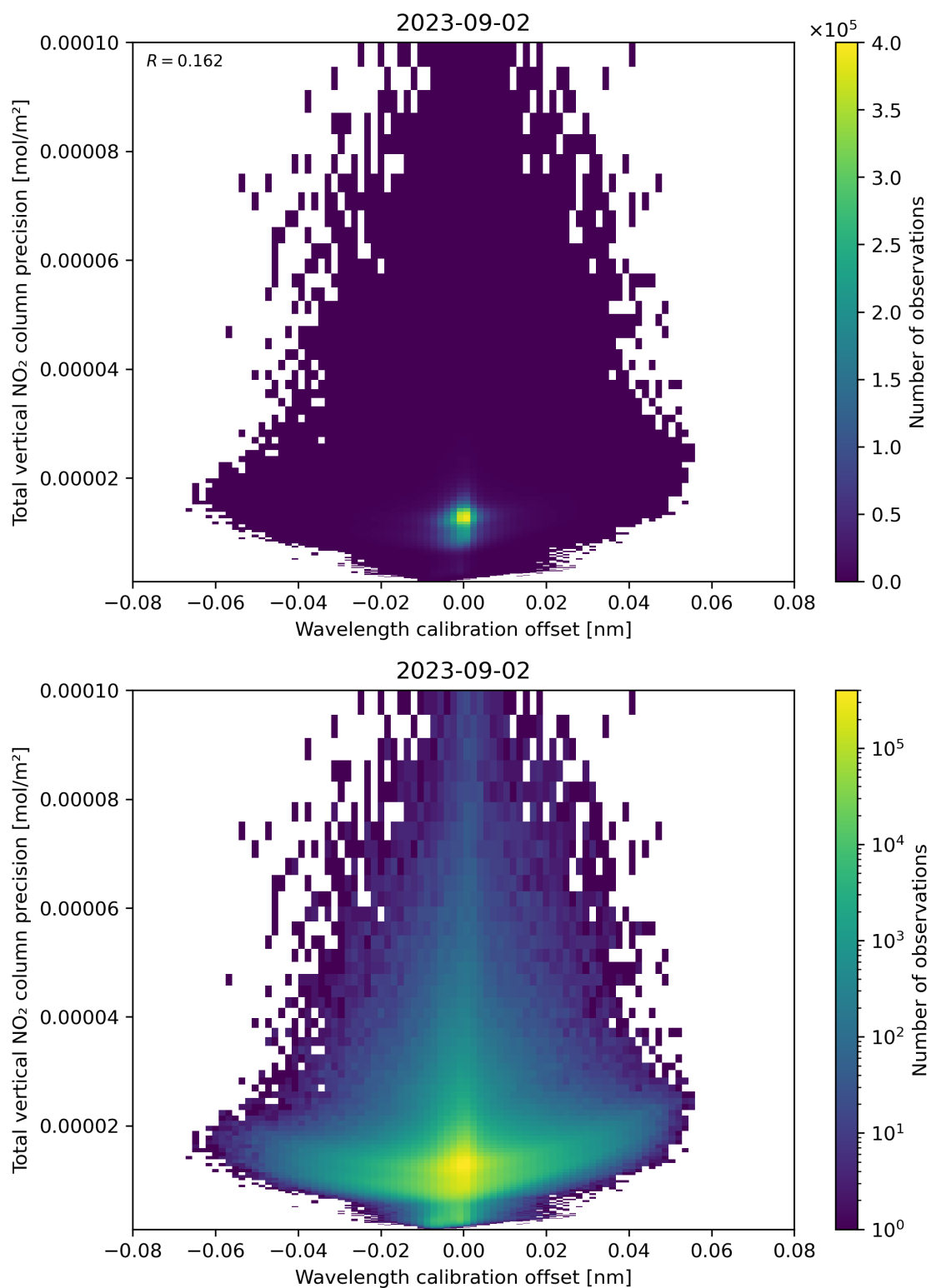
Figure 180: Scatter density plot of “Wavelength calibration offset” against “Total vertical NO 2 column precision” for 2023-09-01 to 2023-09-03.
