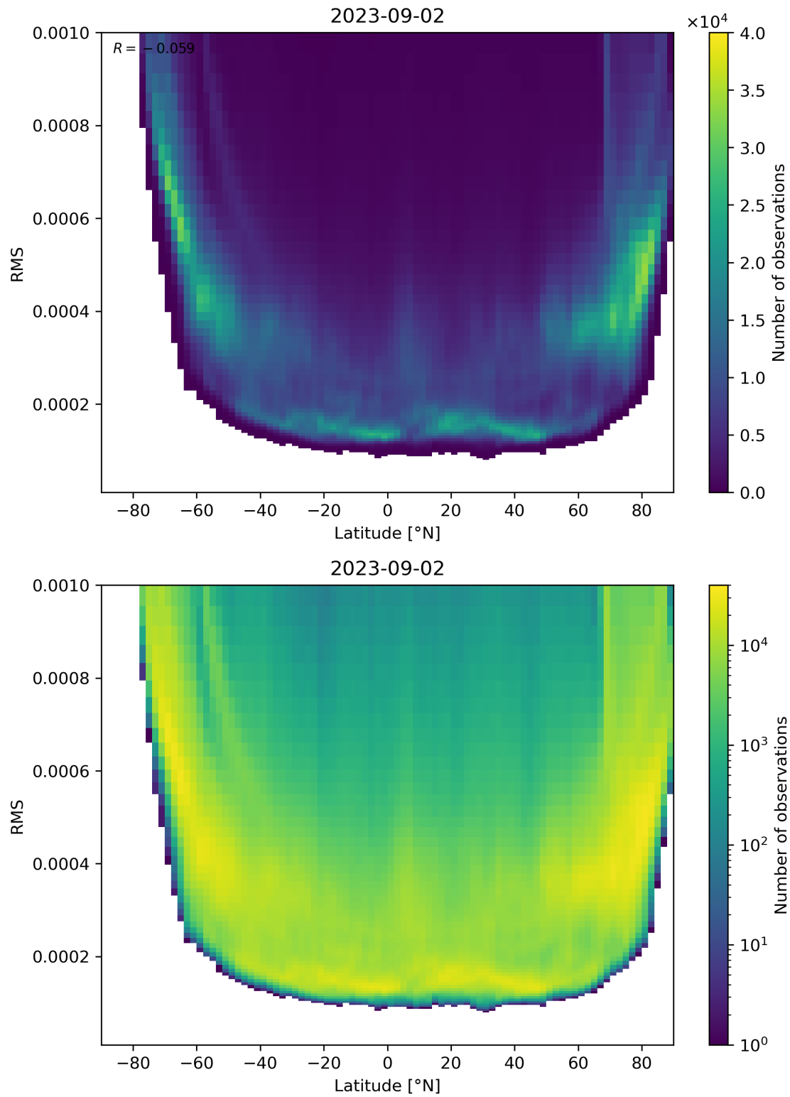
Figure 94: Scatter density plot of “Latitude” against “RMS” for 2023-09-01 to 2023-09-03.
