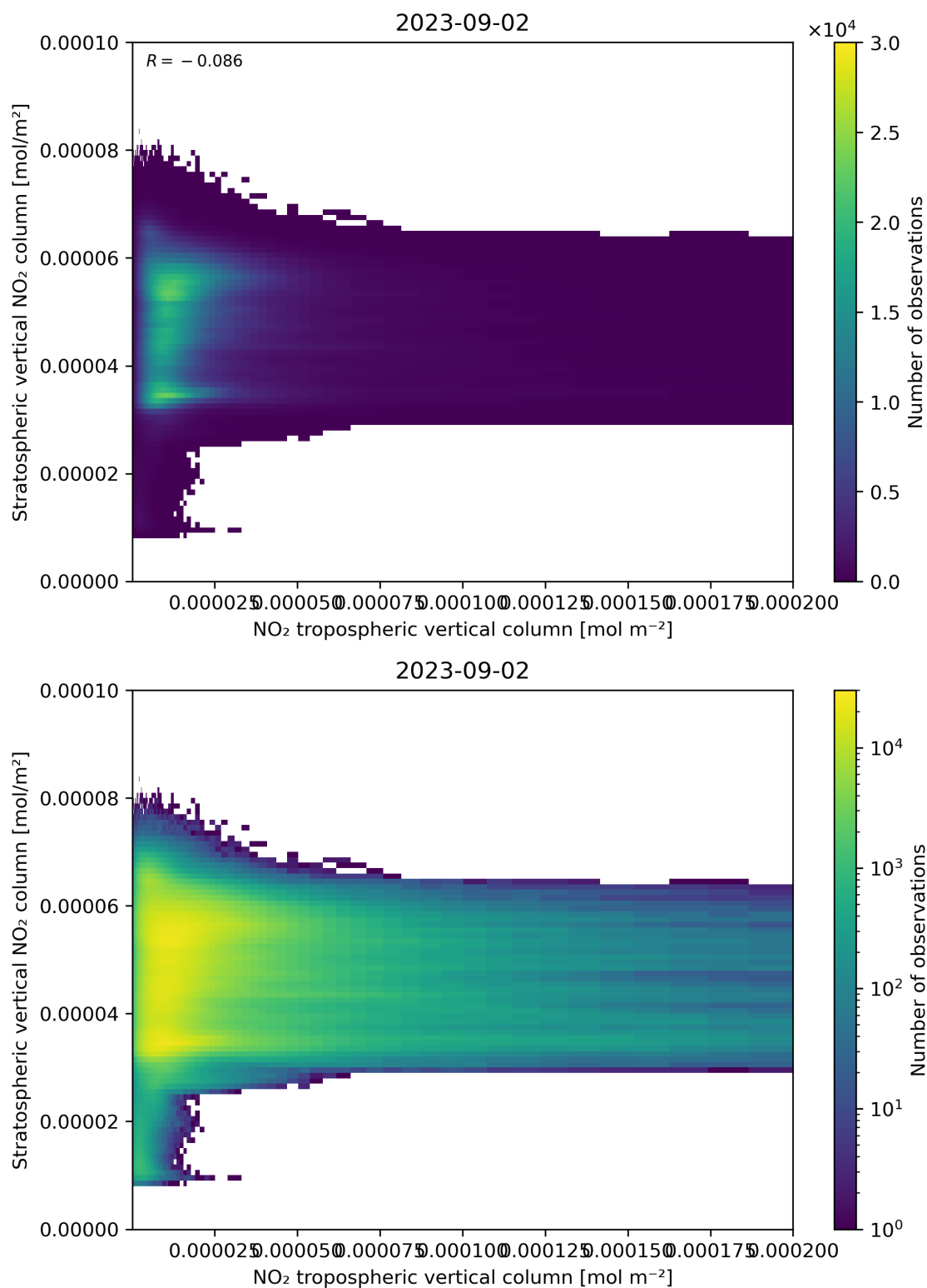
Figure 125: Scatter density plot of “NO 2 tropospheric vertical column” against “Stratospheric vertical NO 2 column” for 2023-09-01 to 2023-09-03.
