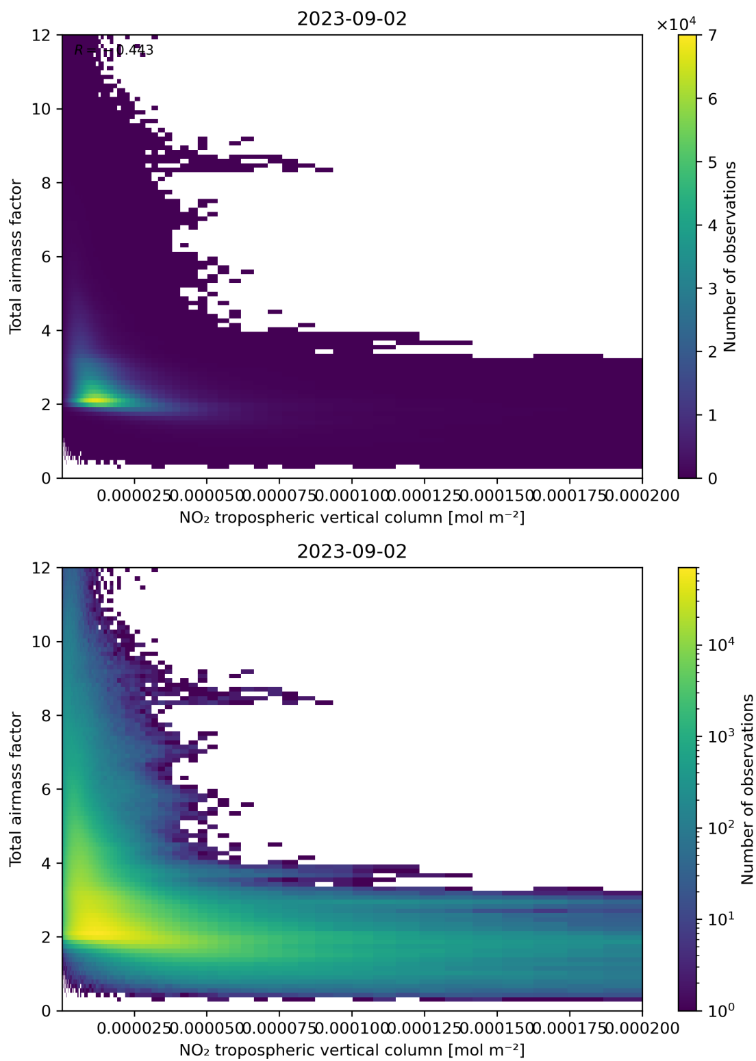
Figure 122: Scatter density plot of “NO 2 tropospheric vertical column” against “Total air mass factor” for 2023-09-01 to 2023-09-03.
