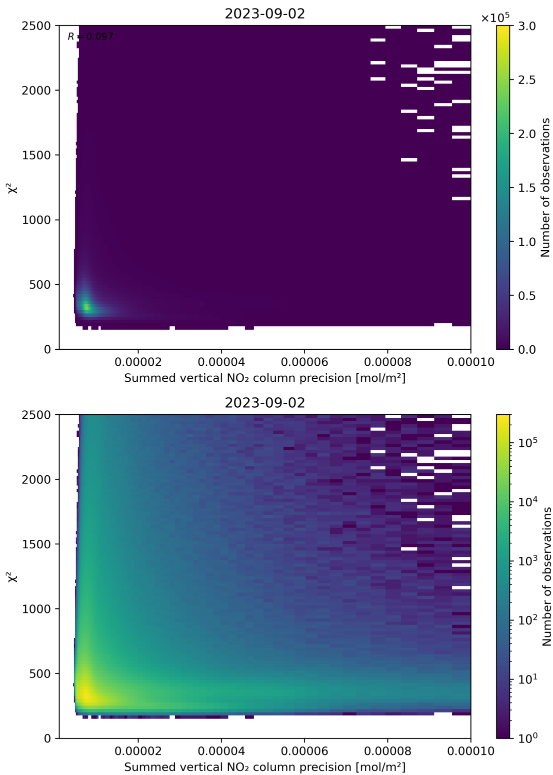
Figure 107: Scatter density plot of “Summed vertical NO 2 column precision” against “ \chi^2 ” for 2023-09-01 to 2023-09-03.
