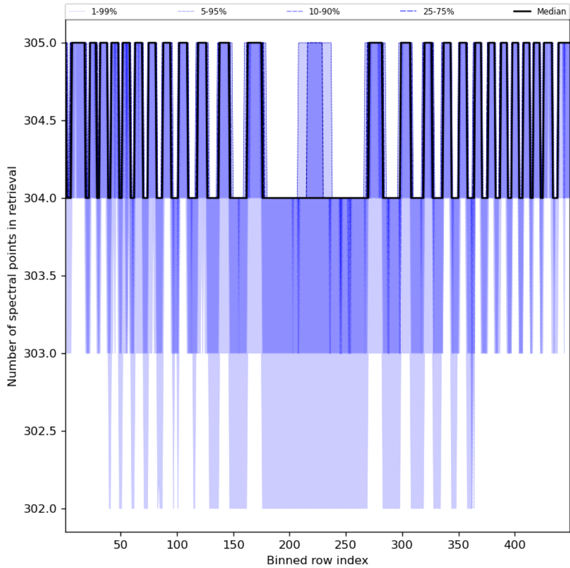
Figure 50: Along track statistics of “Number of spectral points in retrieval” for 2023-09-01 to 2023-09-03
