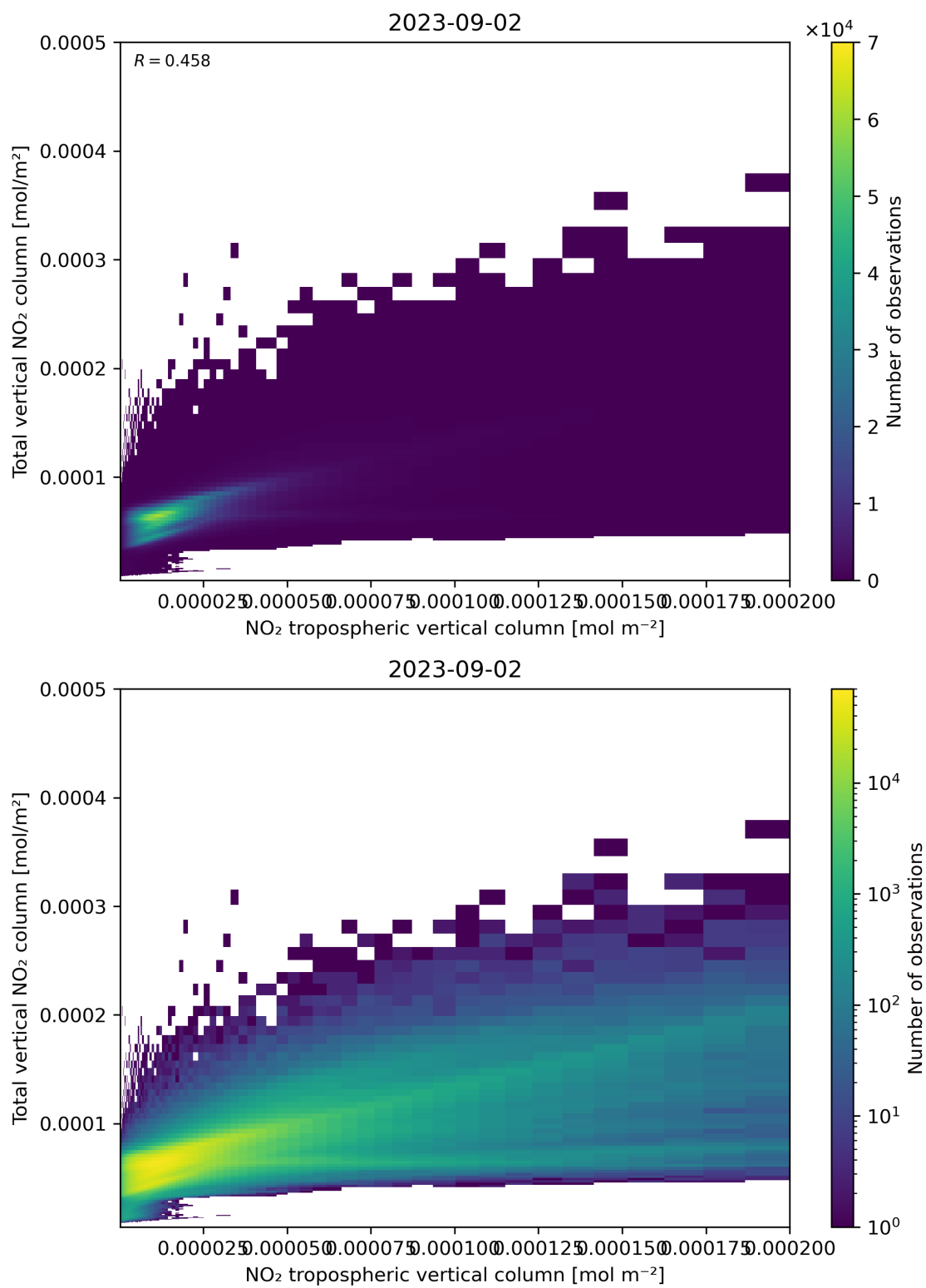
Figure 128: Scatter density plot of “NO 2 tropospheric vertical column” against “Total vertical NO 2 column” for 2023-09-01 to 2023-09-03.
