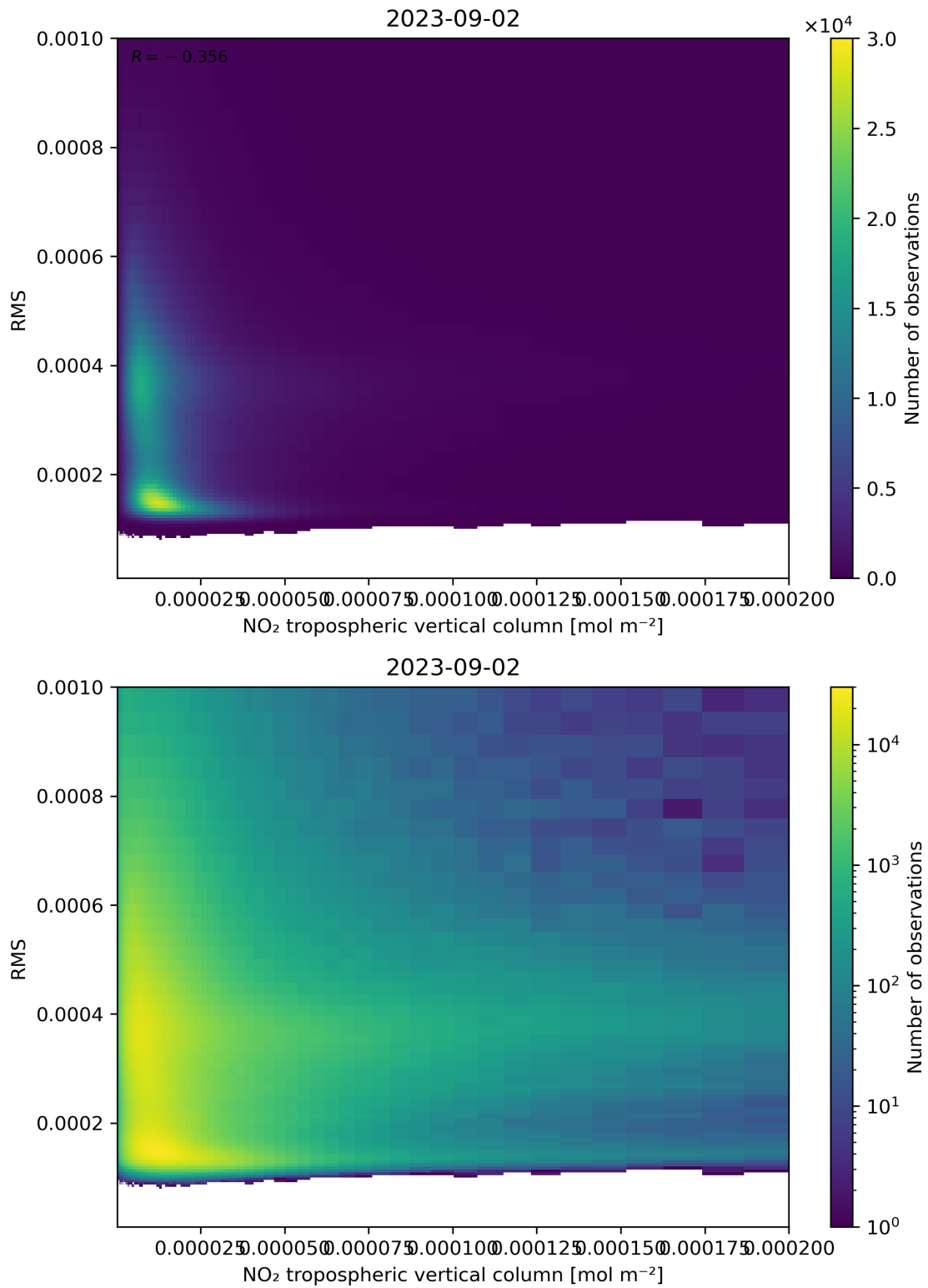
Figure 142: Scatter density plot of “NO 2 tropospheric vertical column” against “RMS” for 2023-09-01 to 2023-09-03.
