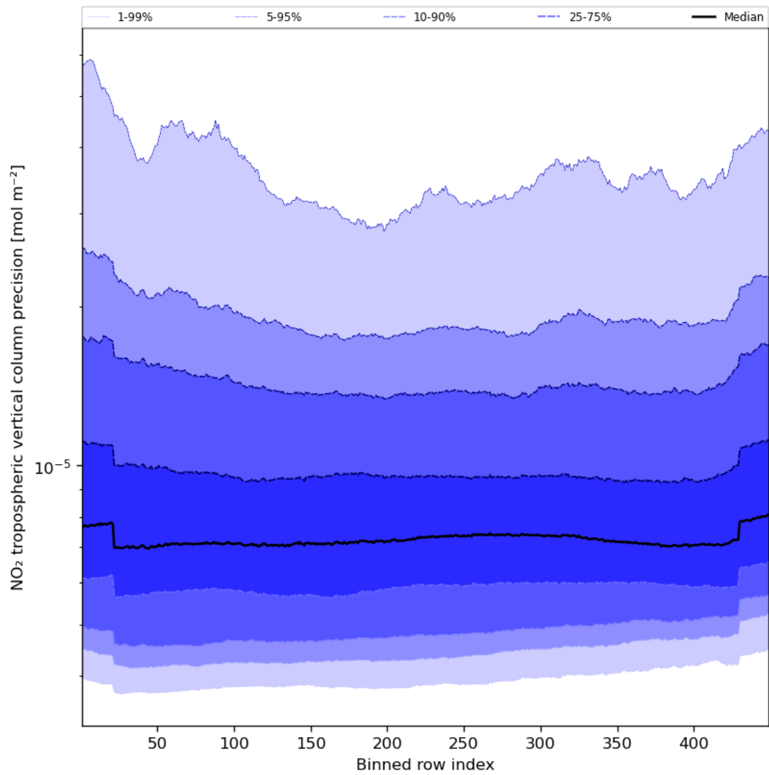
Figure 47: Along track statistics of “NO 2 tropospheric vertical column precision” for 2023-09-01 to 2023-09-03
