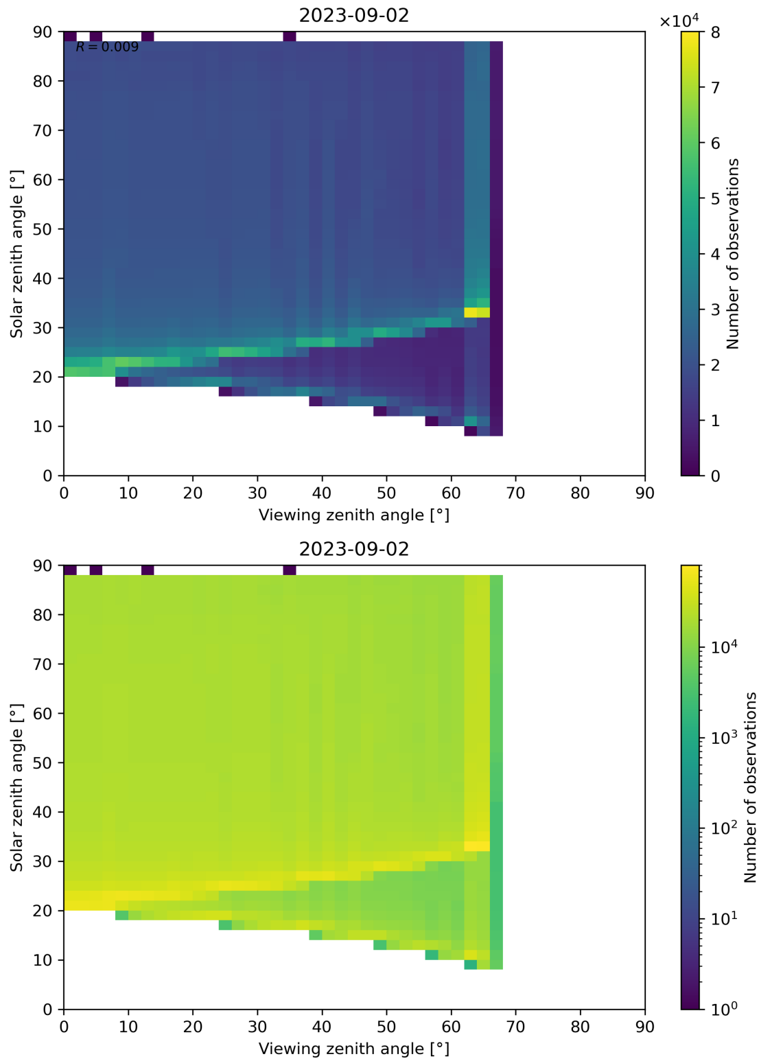
Figure 172: Scatter density plot of “Viewing zenith angle” against “Solar zenith angle” for 2023-09-01 to 2023-09-03.
