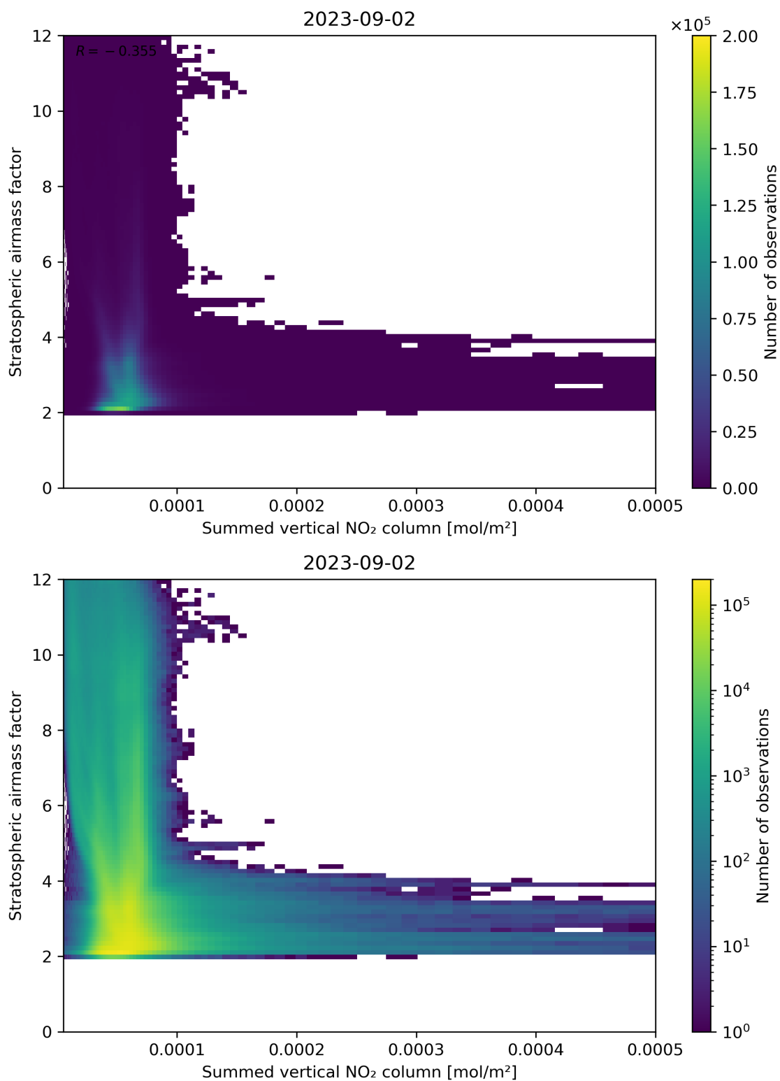
Figure 103: Scatter density plot of “Summed vertical NO 2 column” against “Stratospheric air mass factor” for 2023-09-01 to 2023-09-03.
