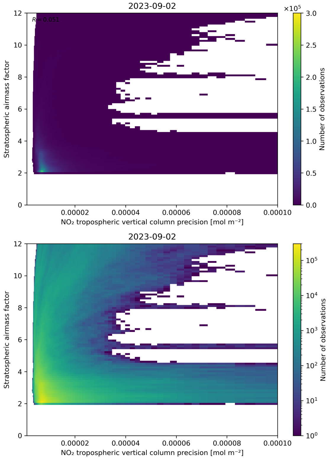
Figure 131: Scatter density plot of “NO 2 tropospheric vertical column precision” against “Stratospheric airmass factor” for 2023-09-01 to 2023-09-03.
