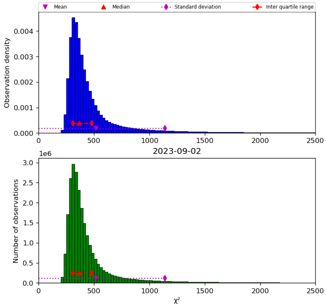
Figure 42: Histogram of “ \chi^2 ” for 2023-09-01 to 2023-09-03
