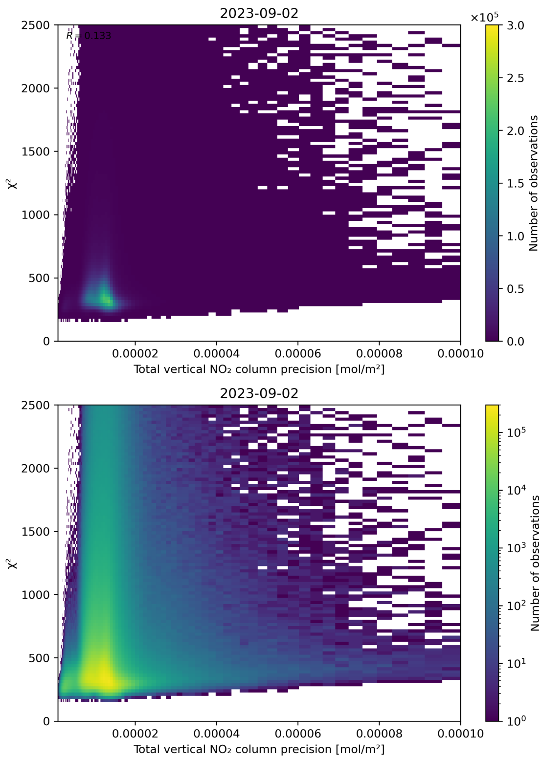
Figure 116: Scatter density plot of “Total vertical NO 2 column precision” against “ \chi^2 ” for 2023-09-01 to 2023-09-03.
