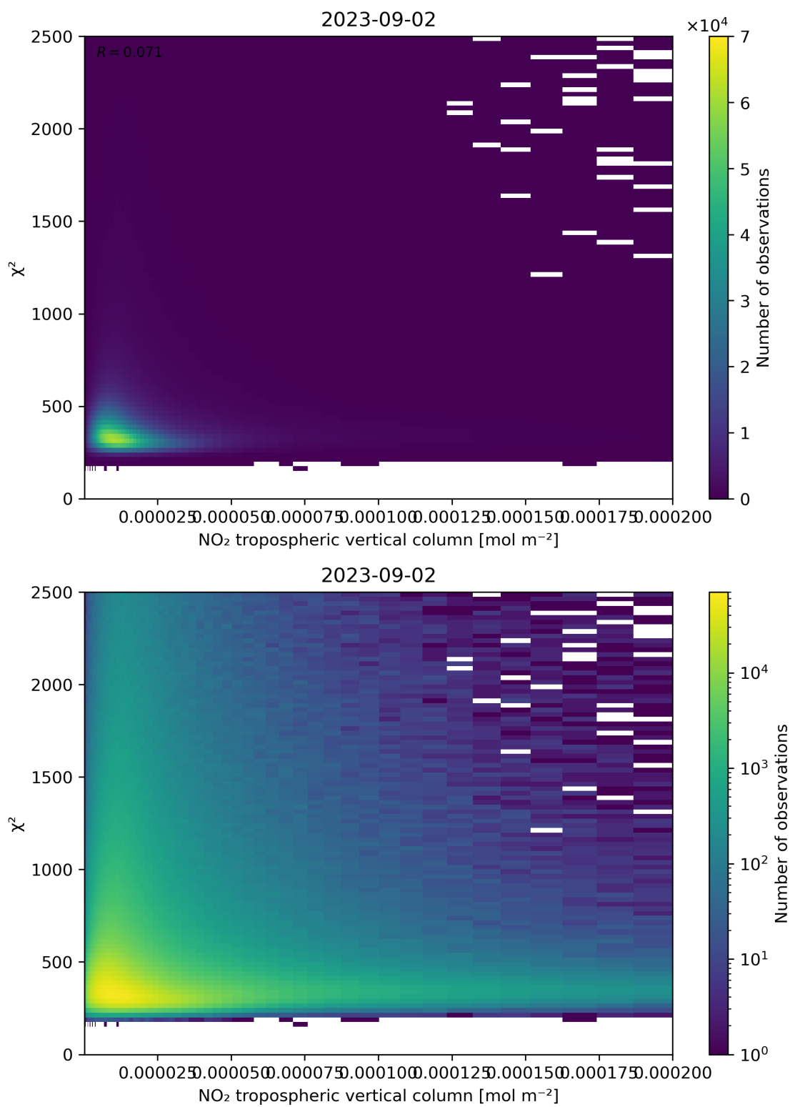
Figure 124: Scatter density plot of “NO 2 tropospheric vertical column” against “ \chi^2 ” for 2023-09-01 to 2023-09-03.
