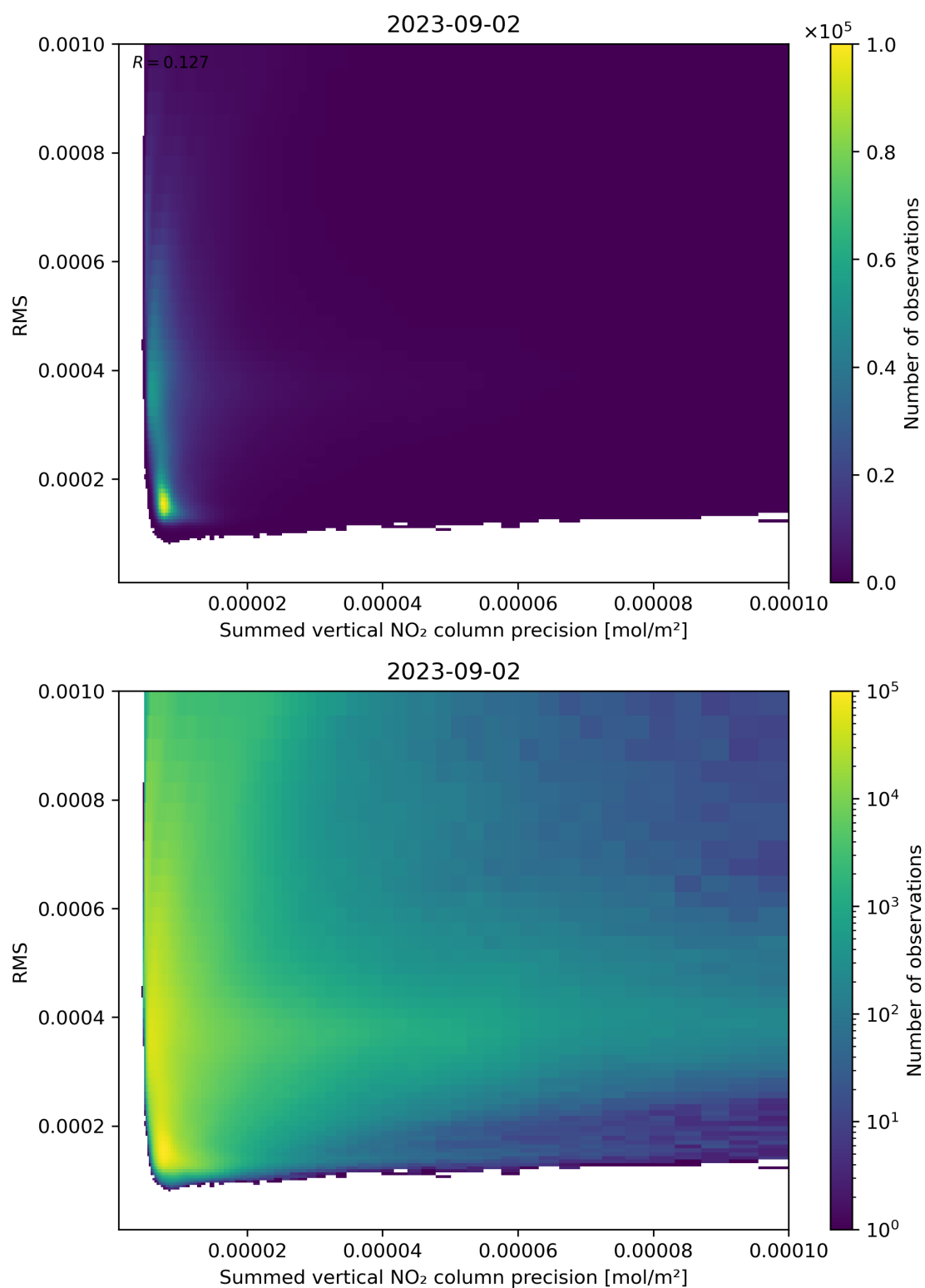
Figure 108: Scatter density plot of “Summed vertical NO 2 column precision” against “RMS” for 2023-09-01 to 2023-09-03.
