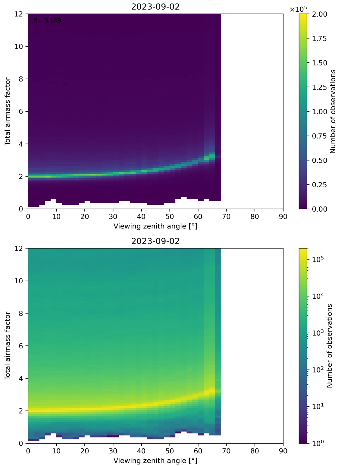
Figure 160: Scatter density plot of “Viewing zenith angle” against “Total airmass factor” for 2023-09-01 to 2023-09-03.
