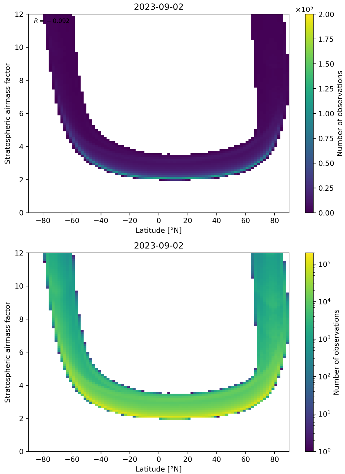
Figure 83: Scatter density plot of “Latitude” against “Stratospheric air mass factor” for 2023-09-01 to 2023-09-03.
