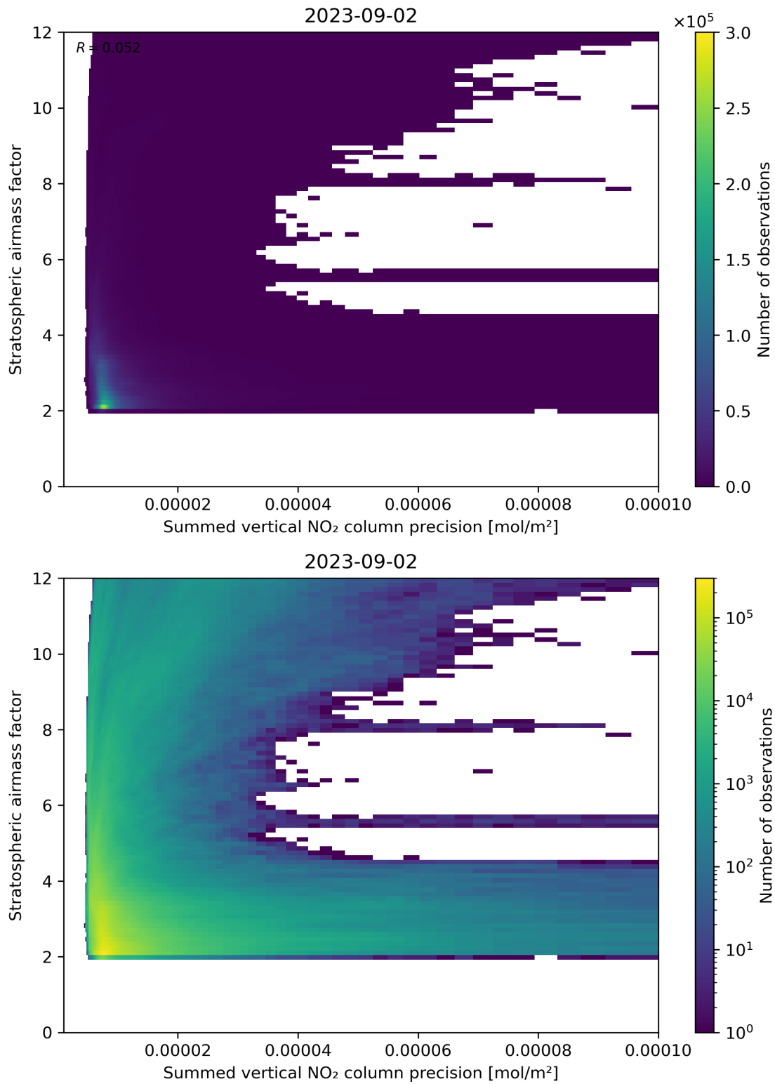
Figure 106: Scatter density plot of “Summed vertical NO 2 column precision” against “Stratospheric airmass factor” for 2023-09-01 to 2023-09-03.
