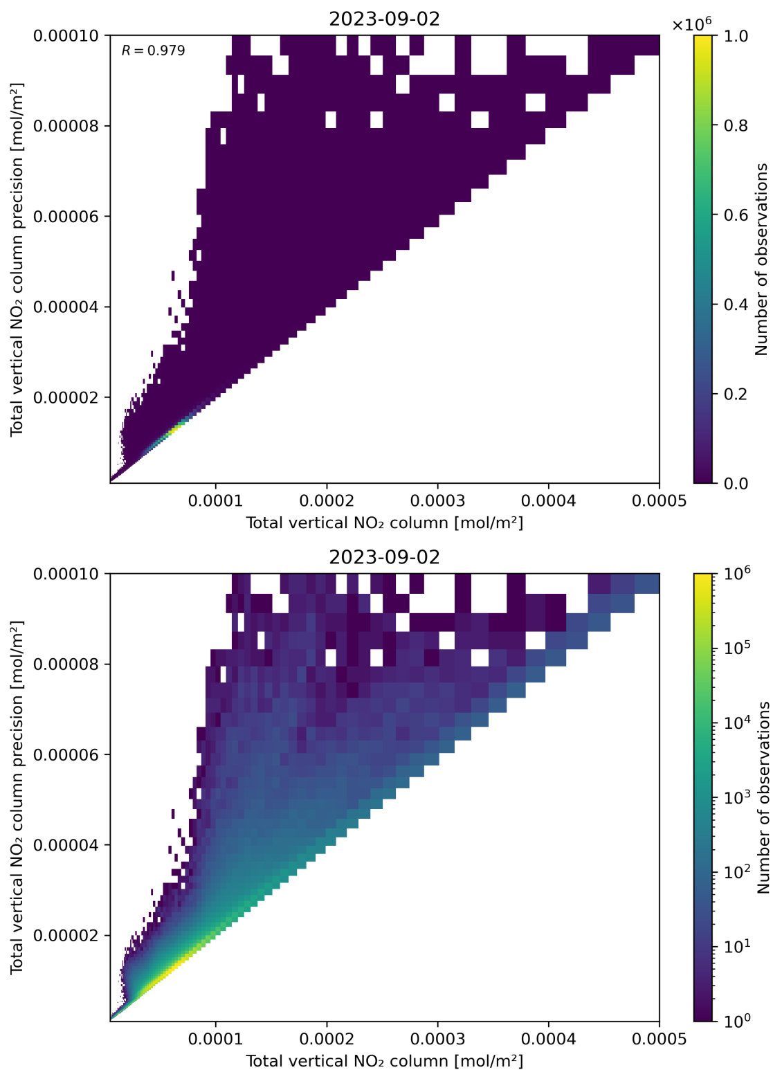
Figure 114: Scatter density plot of “Total vertical NO 2 column” against “Total vertical NO 2 column precision” for 2023-09-01 to 2023-09-03.
