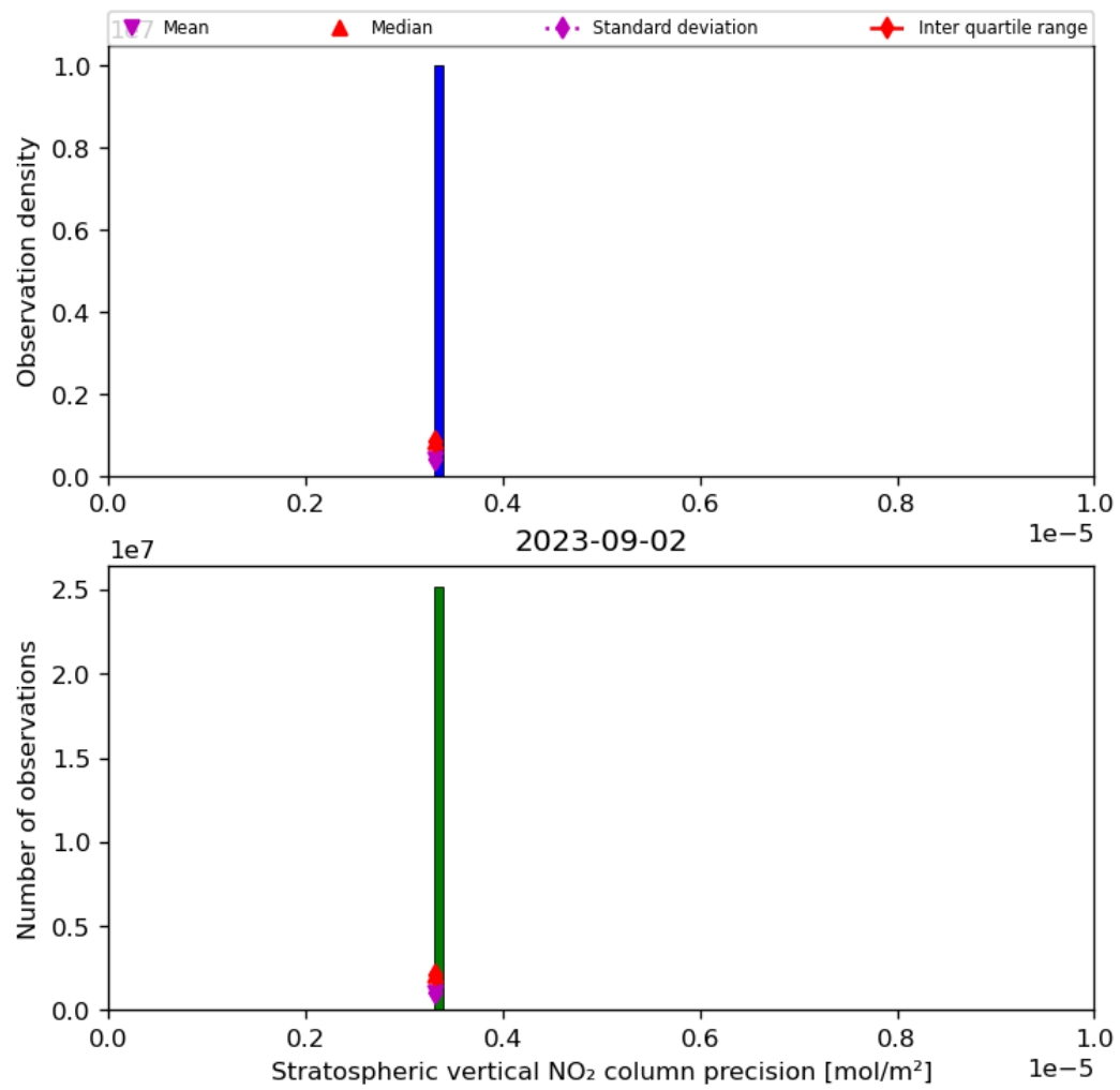
Figure 37: Histogram of “Stratospheric vertical NO 2 column precision” for 2023-09-01 to 2023-09-03
