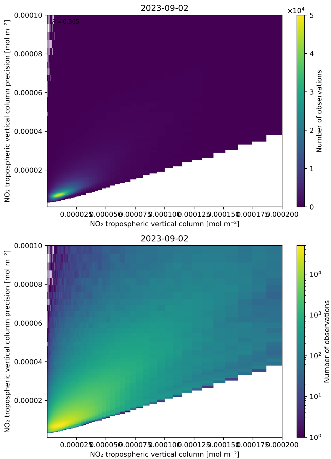
Figure 130: Scatter density plot of “NO 2 tropospheric vertical column” against “NO 2 tropospheric vertical column precision” for 2023-09-01 to 2023-09-03.
