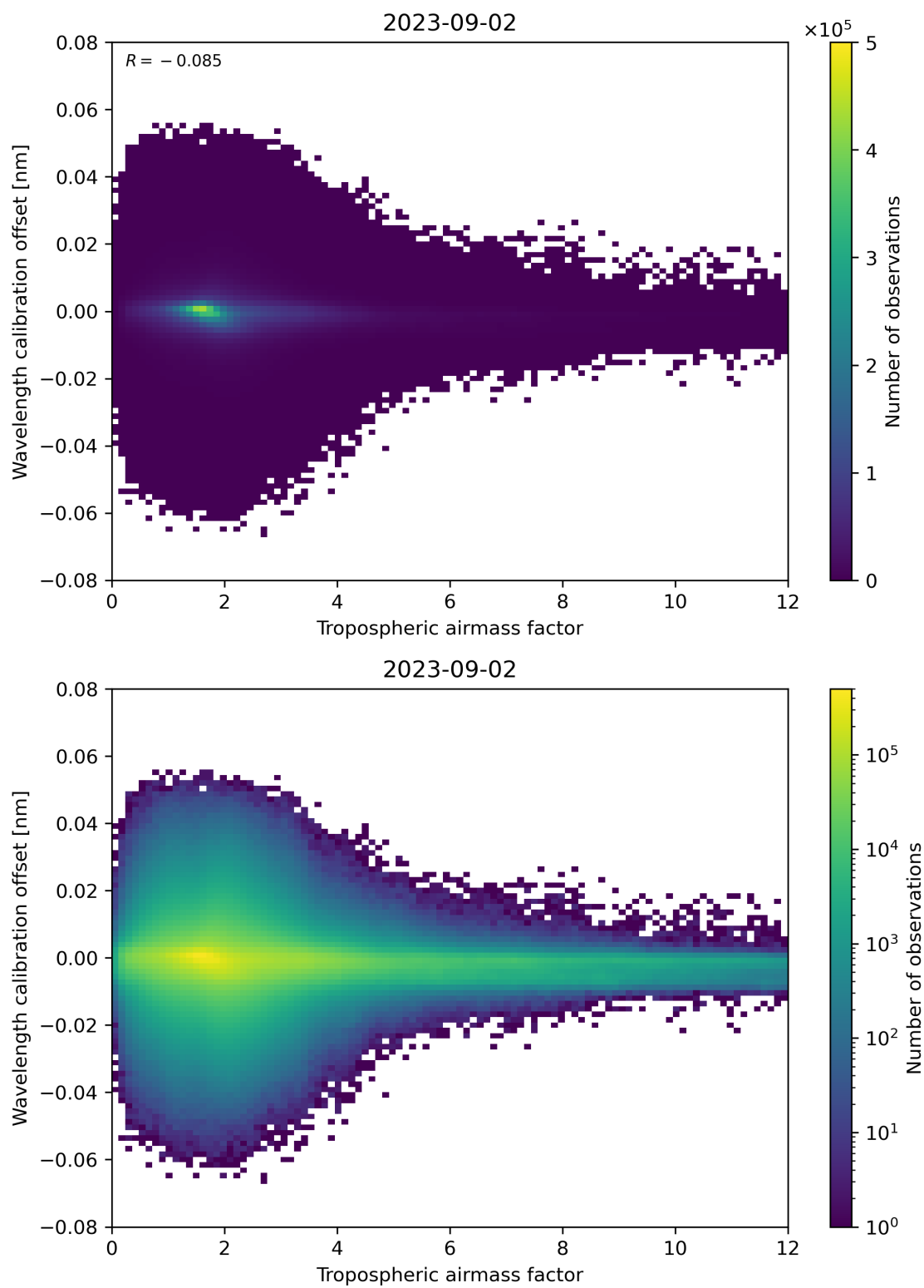
Figure 80: Scatter density plot of “Tropospheric airmass factor” against “Wavelength calibration offset” for 2023-09-01 to 2023-09-03.
