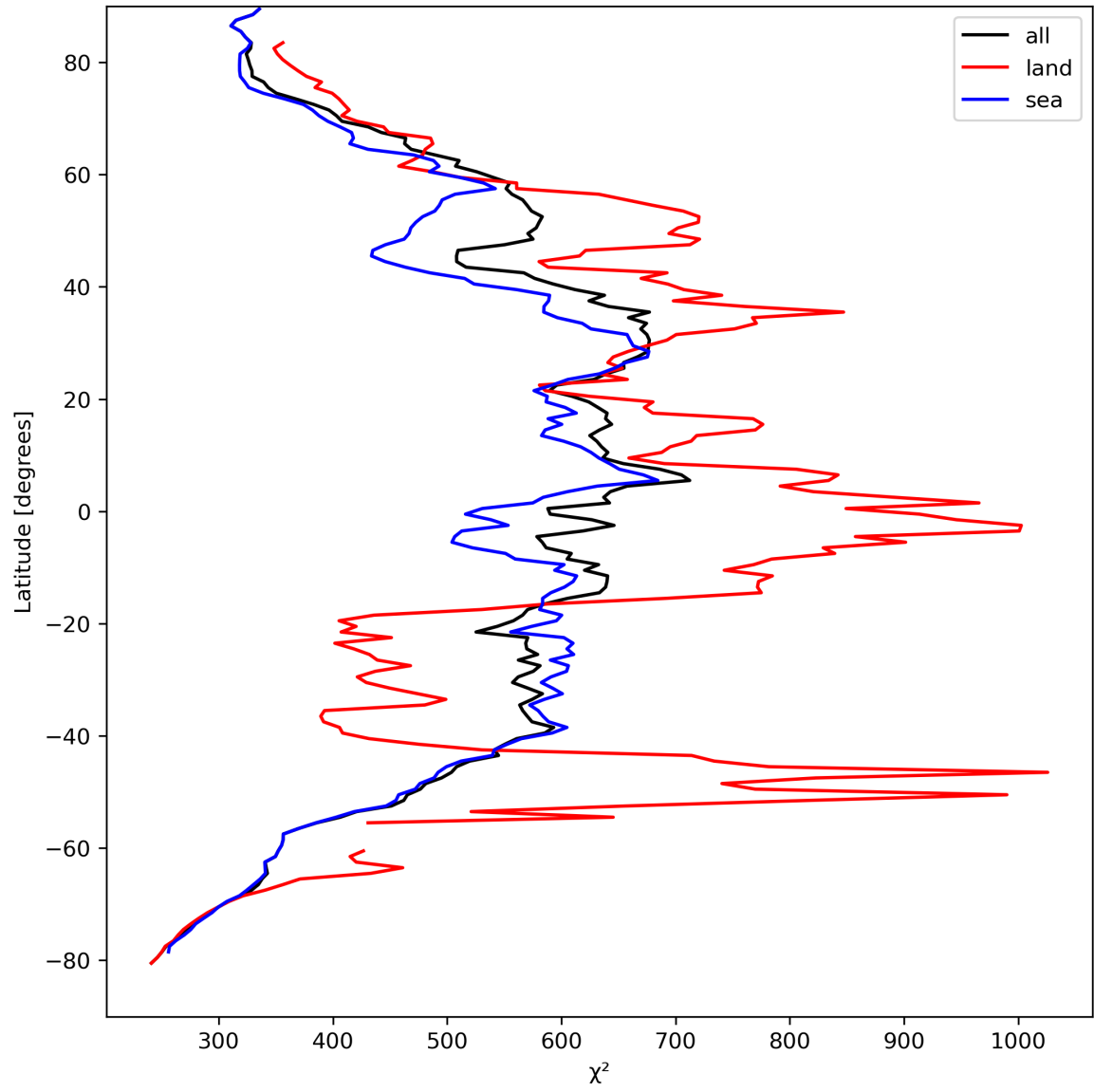
Figure 25: Zonal average of “ \chi^2 ” for 2023-09-01 to 2023-09-03.
