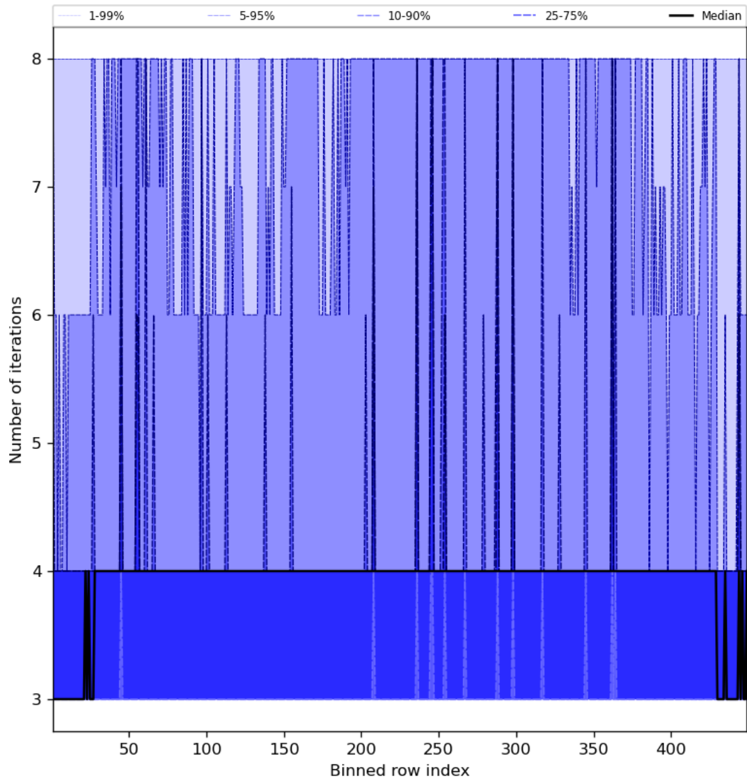
Figure 51: Along track statistics of “Number of iterations” for 2023-09-01 to 2023-09-03
