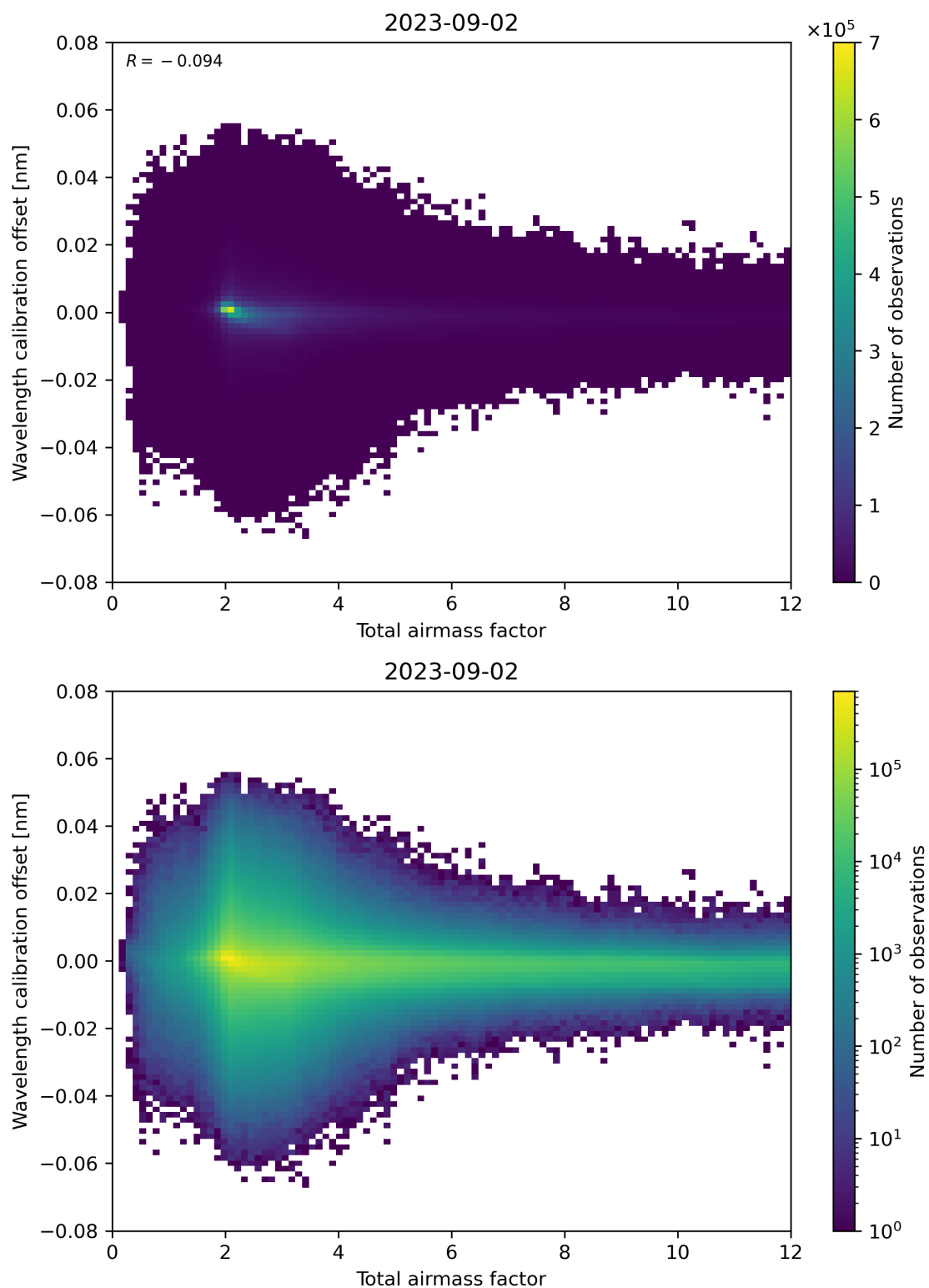
Figure 70: Scatter density plot of “Total airmass factor” against “Wavelength calibration offset” for 2023-09-01 to 2023-09-03.
