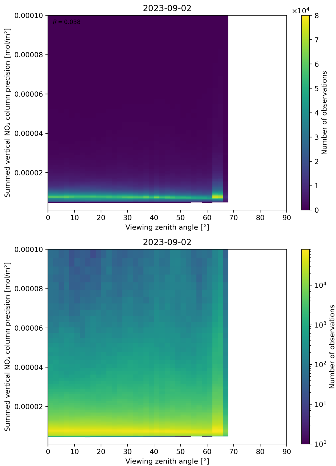
Figure 166: Scatter density plot of “Viewing zenith angle” against “Summed vertical NO 2 column precision” for 2023-09-01 to 2023-09-03.
