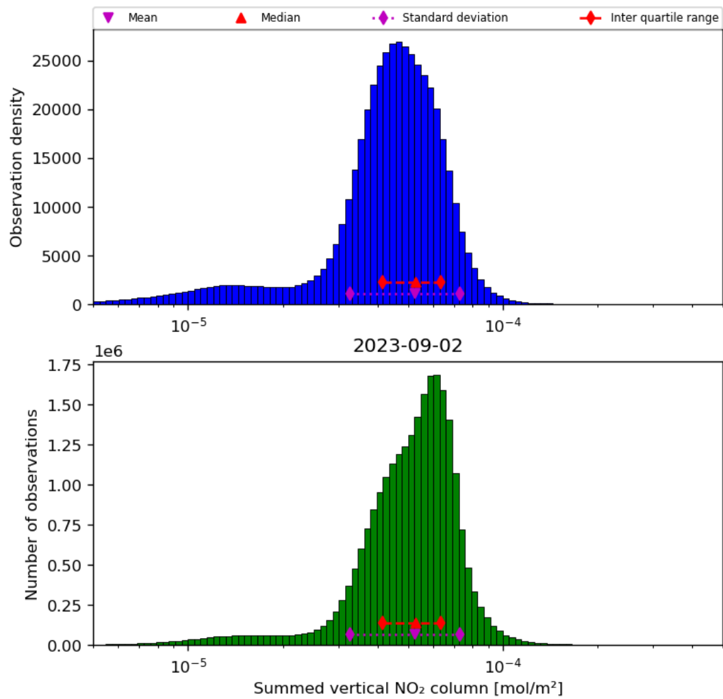
Figure 40: Histogram of “Summed vertical NO 2 column” for 2023-09-01 to 2023-09-03
