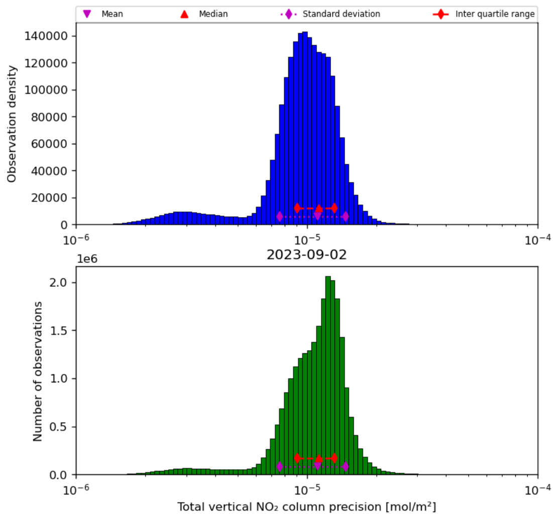
Figure 39: Histogram of “Total vertical NO 2 column precision” for 2023-09-01 to 2023-09-03
