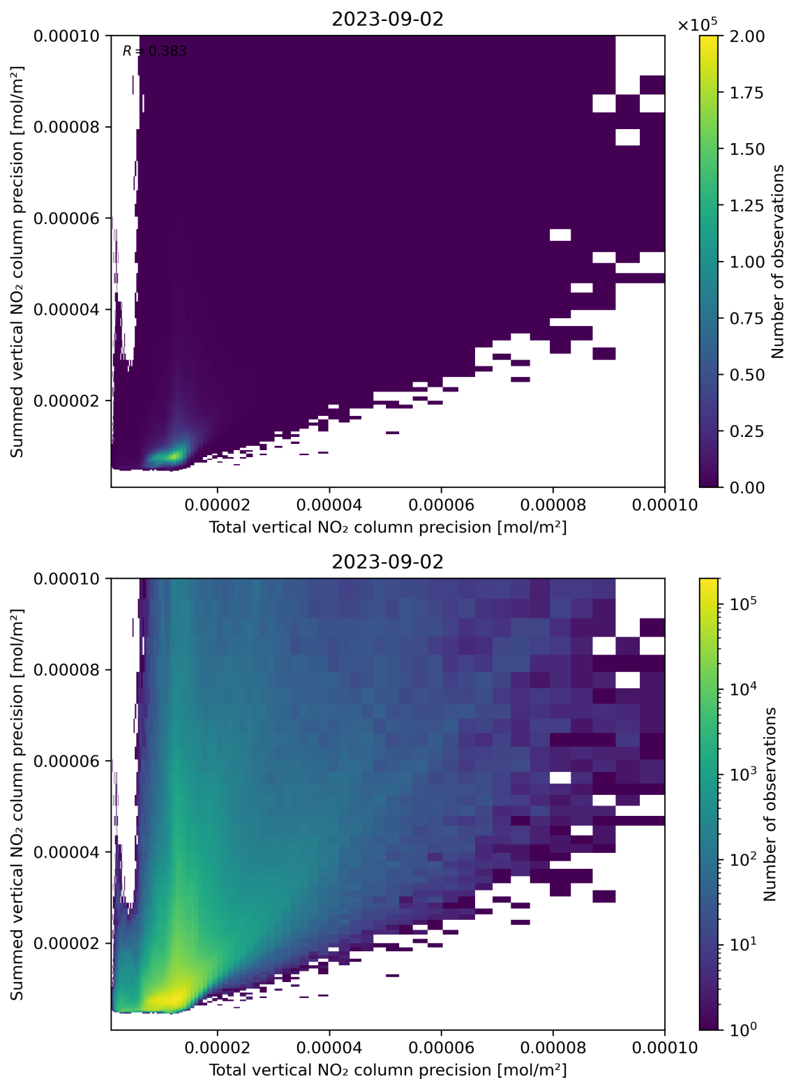
Figure 118: Scatter density plot of “Total vertical NO 2 column precision” against “Summed vertical NO 2 column precision” for 2023-09-01 to 2023-09-03.
