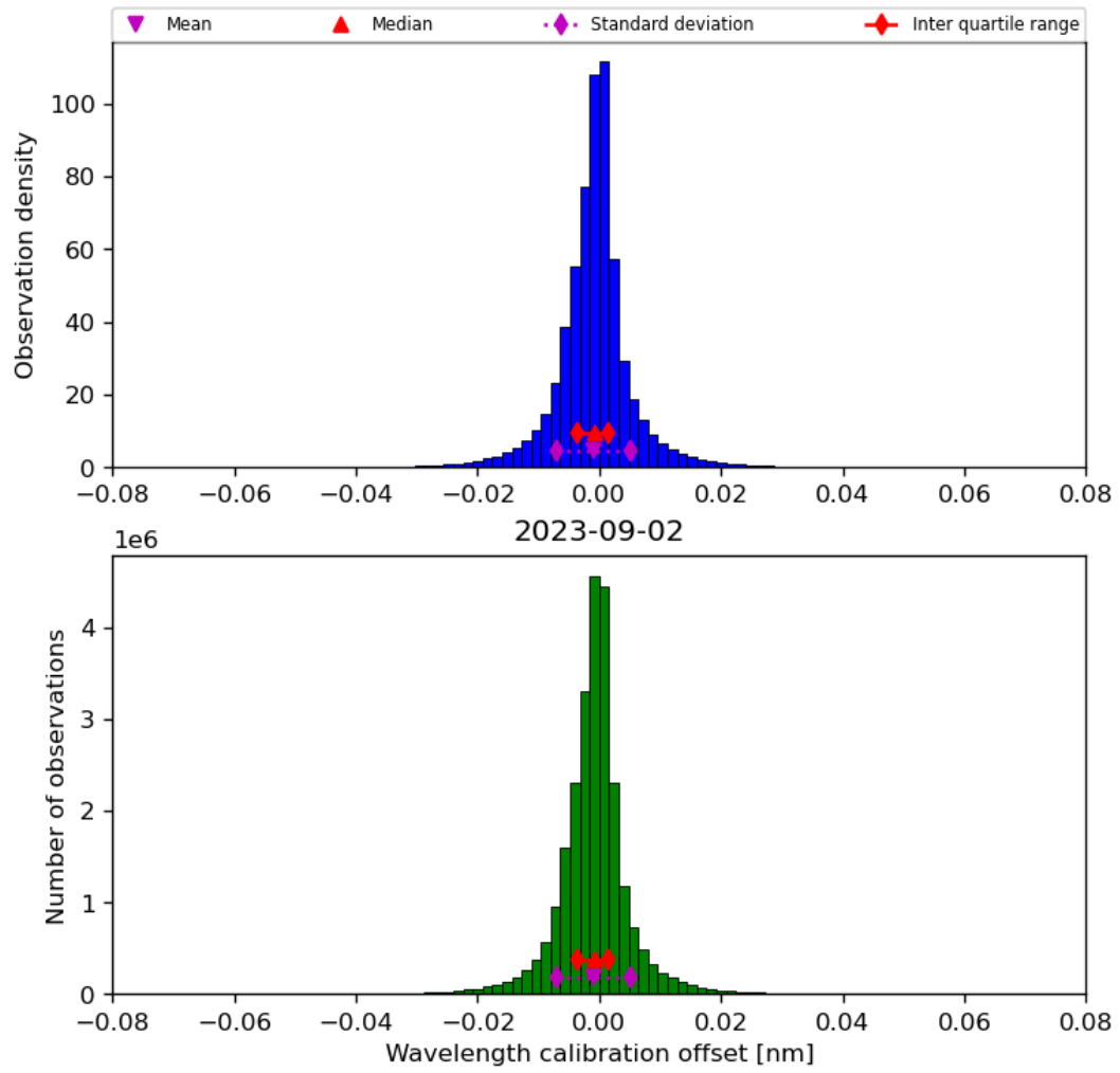
Figure 35: Histogram of “Wavelength calibration offset” for 2023-09-01 to 2023-09-03
