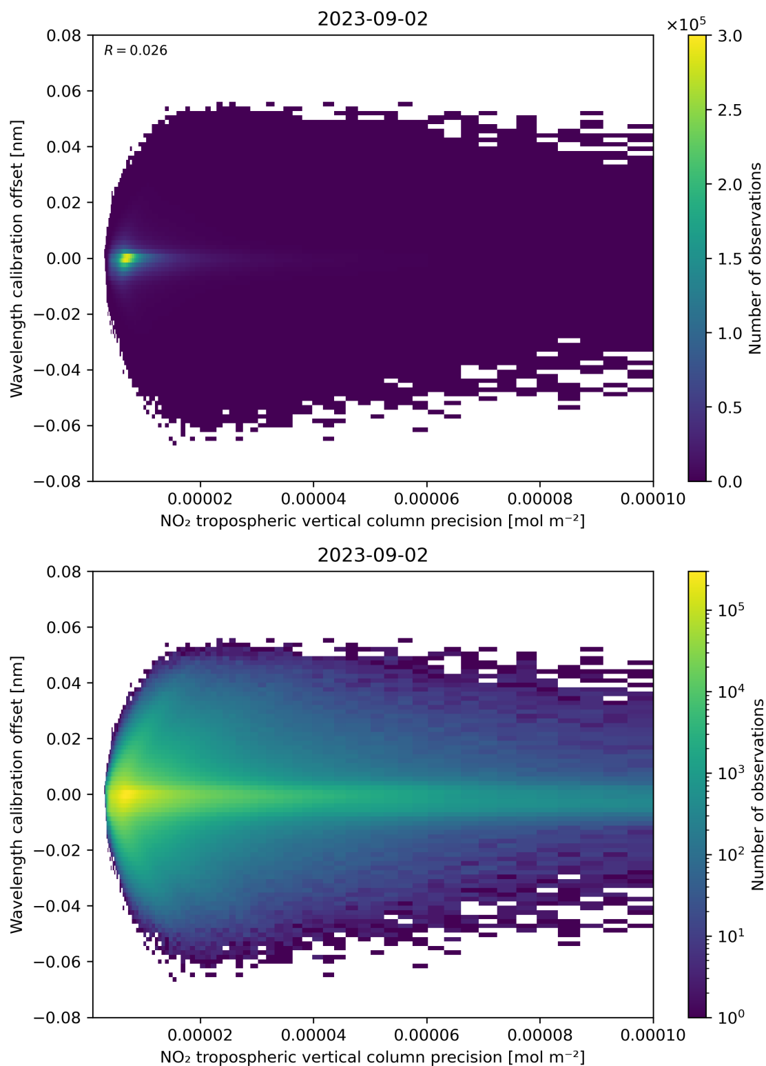
Figure 141: Scatter density plot of “NO 2 tropospheric vertical column precision” against “Wavelength calibration offset” for 2023-09-01 to 2023-09-03.
