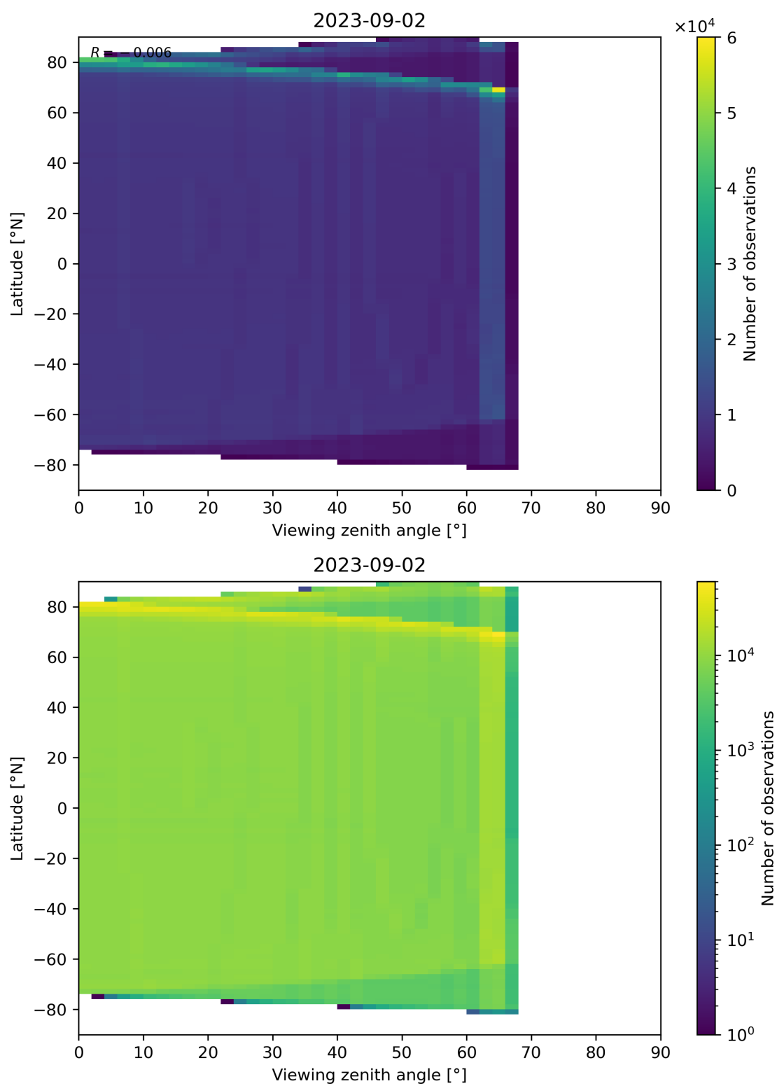
Figure 163: Scatter density plot of “Viewing zenith angle” against “Latitude” for 2023-09-01 to 2023-09-03.
