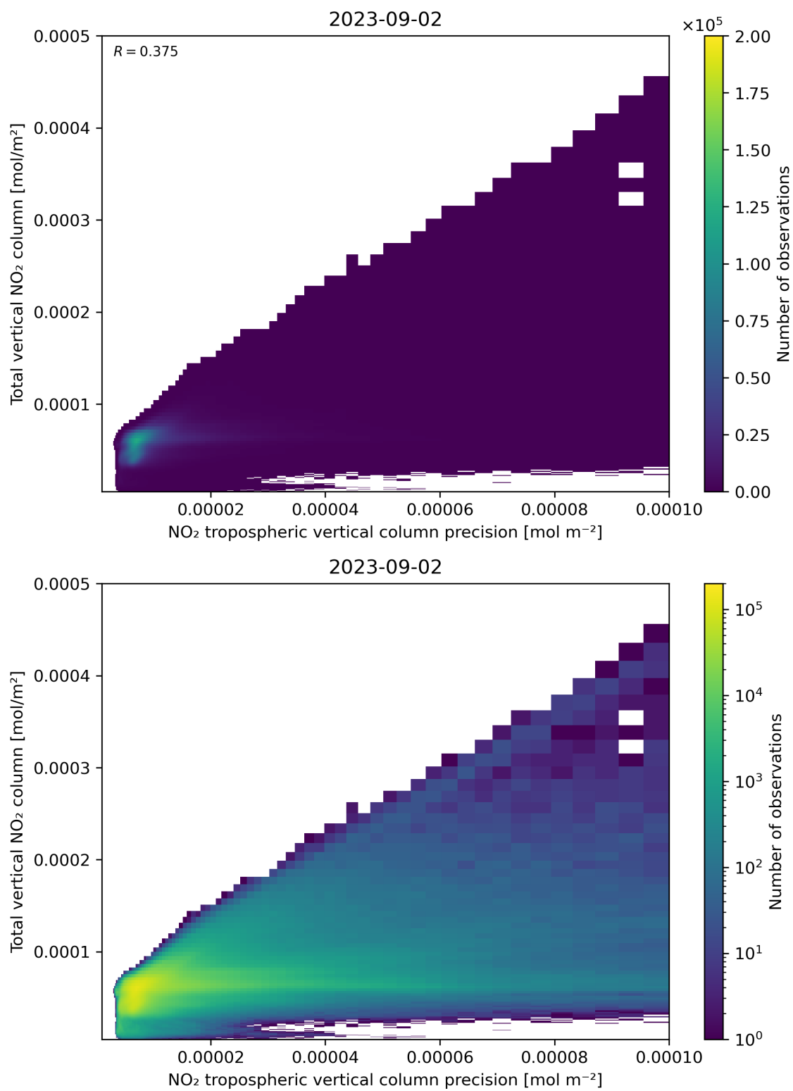
Figure 138: Scatter density plot of “NO 2 tropospheric vertical column precision” against “Total vertical NO 2 column” for 2023-09-01 to 2023-09-03.
