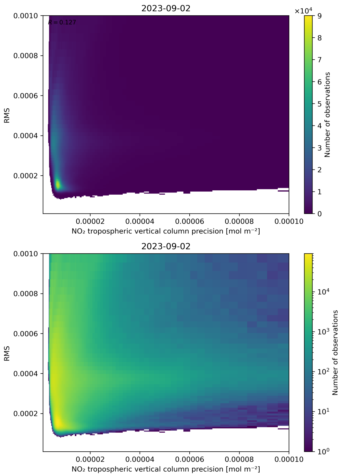
Figure 140: Scatter density plot of “NO 2 tropospheric vertical column precision” against “RMS” for 2023-09-01 to 2023-09-03.
