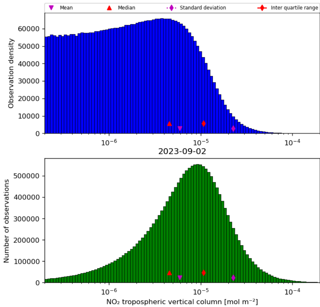
Figure 29: Histogram of “NO 2 tropospheric vertical column” for 2023-09-01 to 2023-09-03
