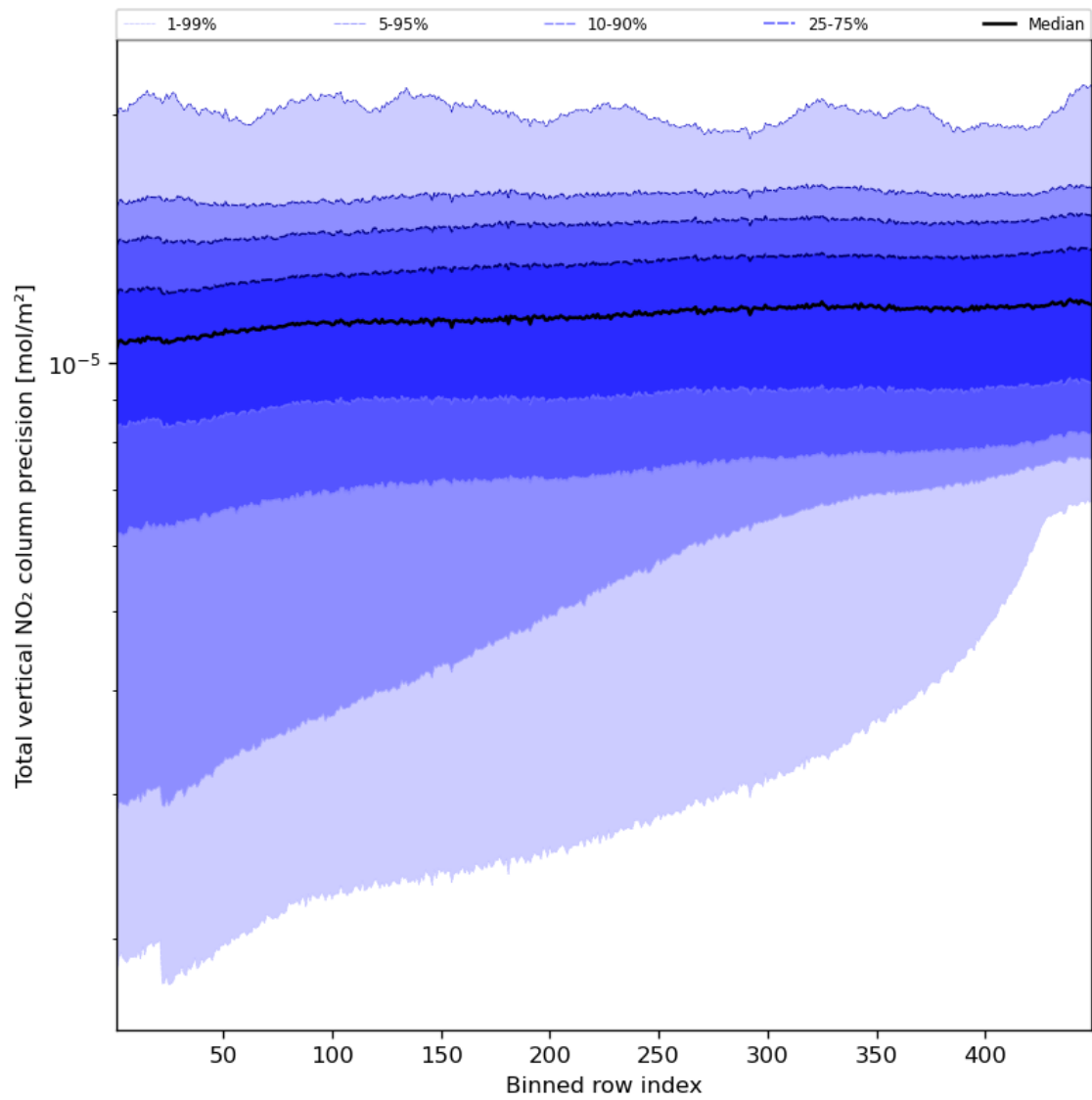
Figure 56: Along track statistics of “Total vertical NO 2 column precision” for 2023-09-01 to 2023-09-03
