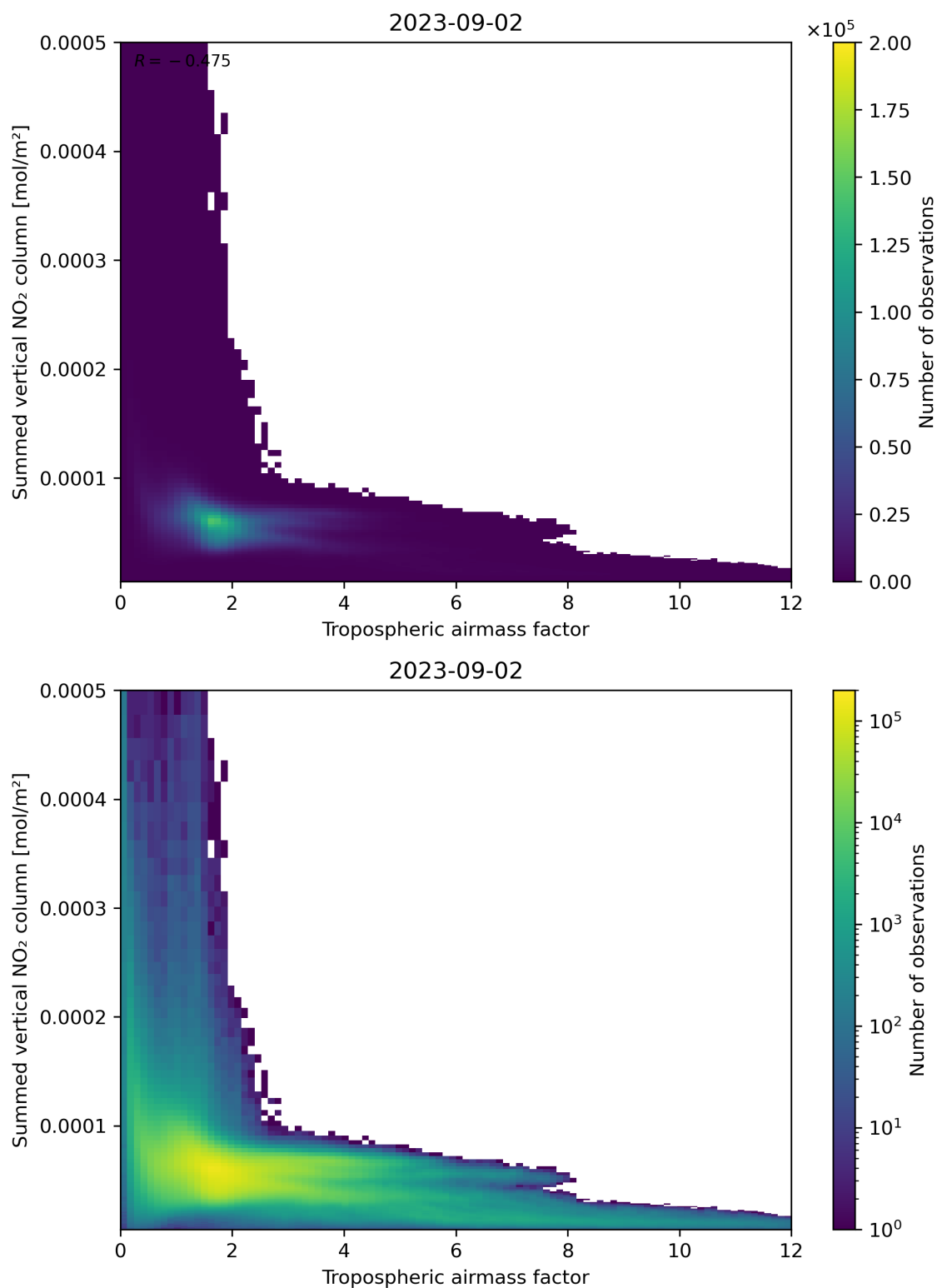
Figure 75: Scatter density plot of “Tropospheric airmass factor” against “Summed vertical NO 2 column” for 2023-09-01 to 2023-09-03.
