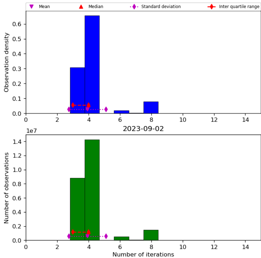
Figure 34: Histogram of “Number of iterations” for 2023-09-01 to 2023-09-03
