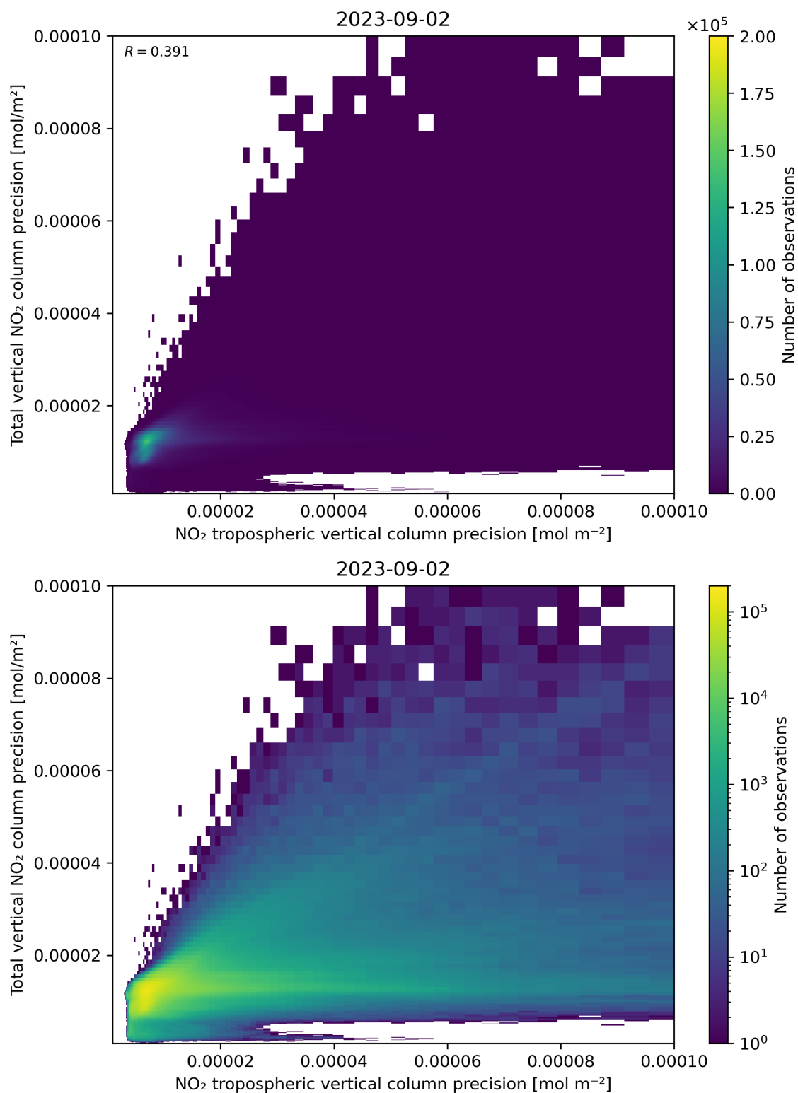
Figure 139: Scatter density plot of “NO 2 tropospheric vertical column precision” against “Total vertical NO 2 column precision” for 2023-09-01 to 2023-09-03.
