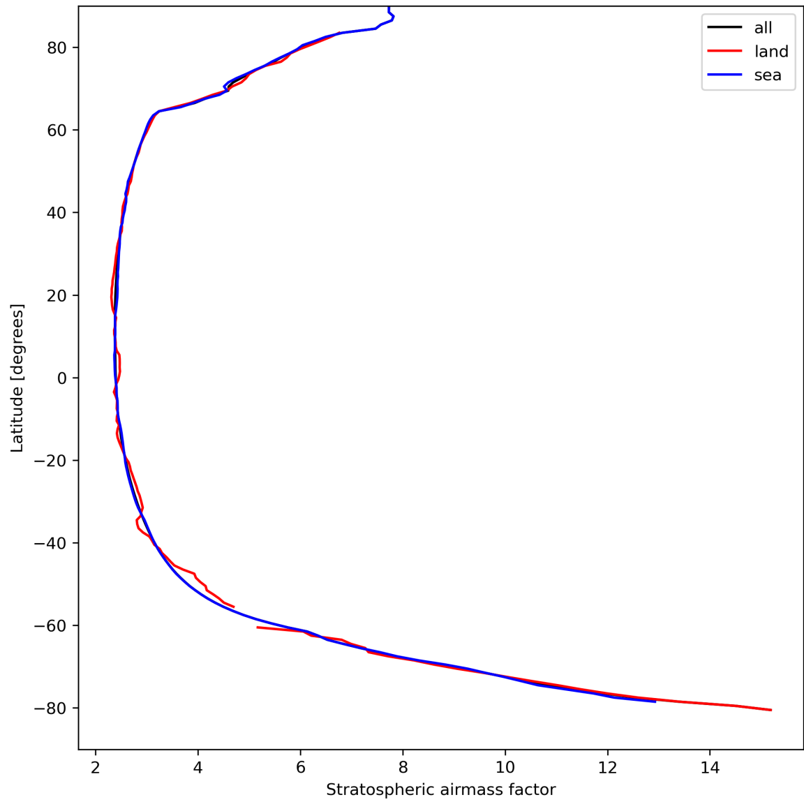
Figure 27: Zonal average of “Stratospheric air mass factor” for 2023-09-01 to 2023-09-03.
