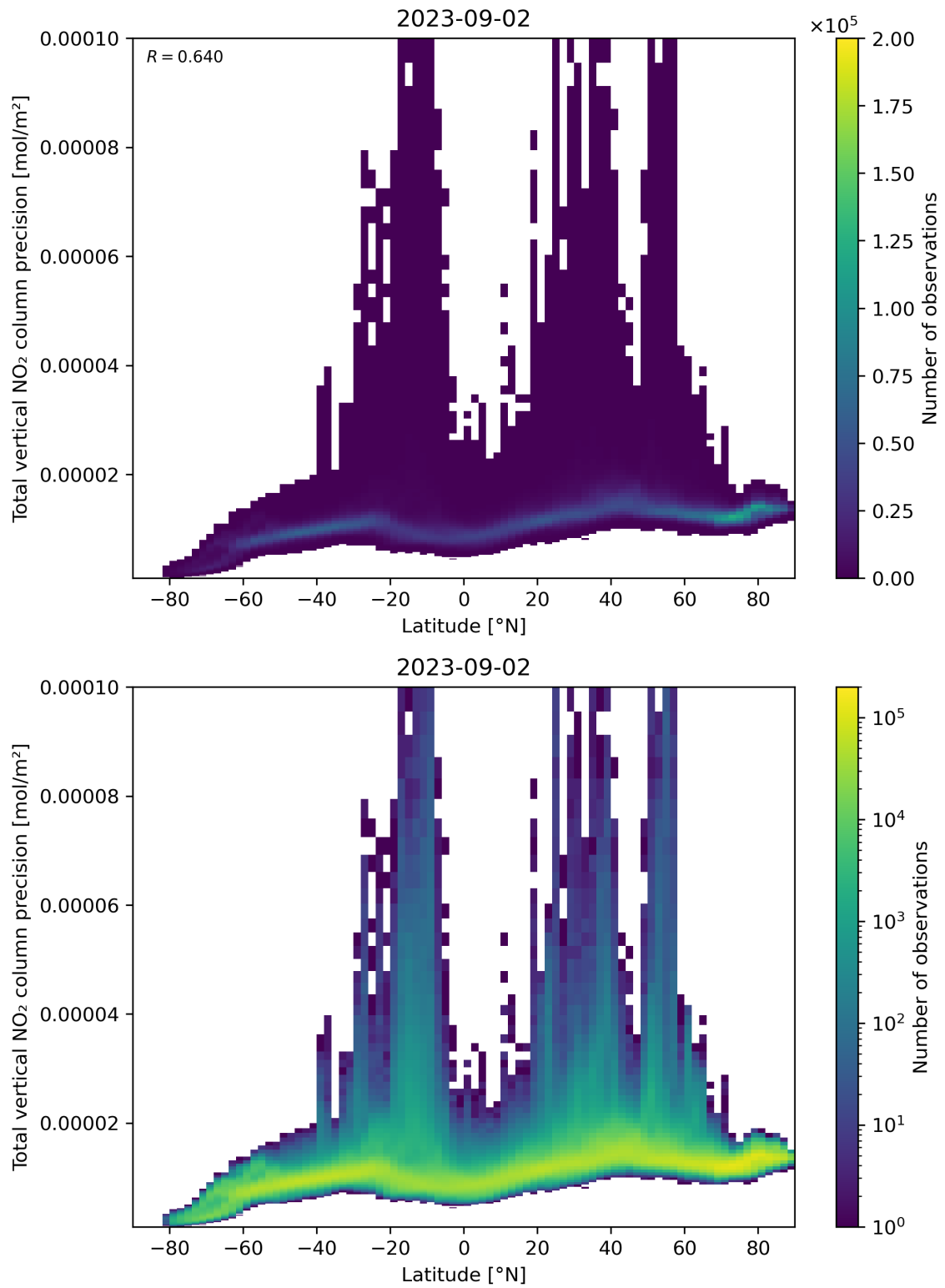
Figure 91: Scatter density plot of “Latitude” against “Total vertical NO 2 column precision” for 2023-09-01 to 2023-09-03.
