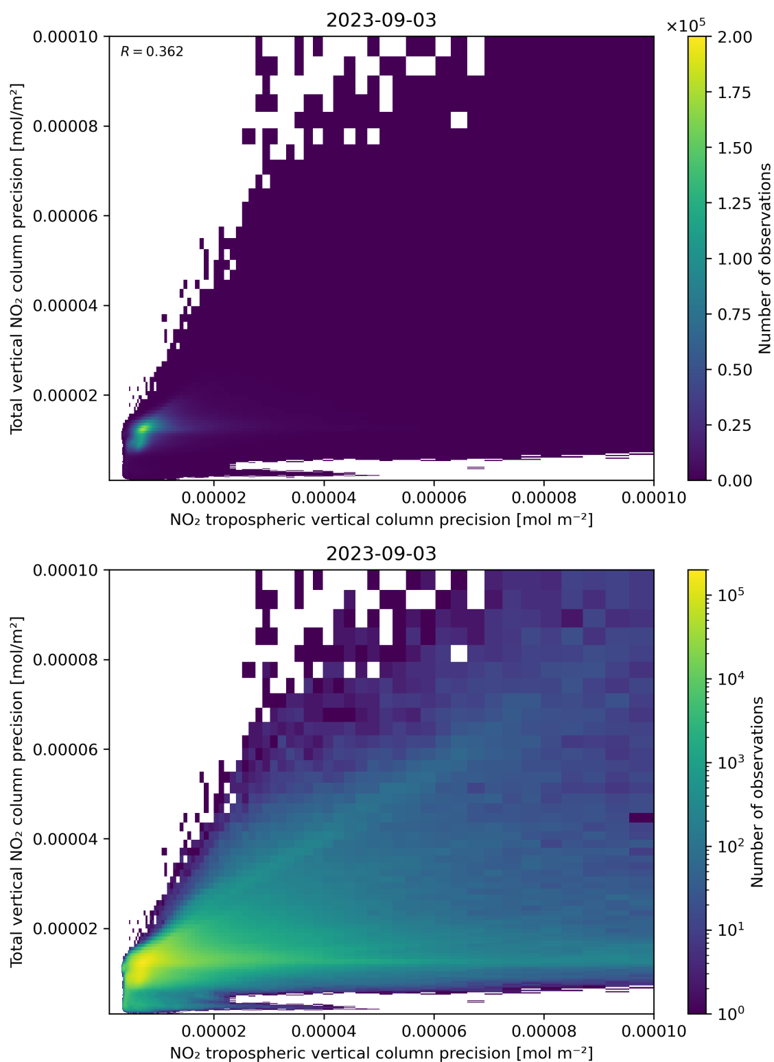
Figure 139: Scatter density plot of “NO 2 tropospheric vertical column precision” against “Total vertical NO 2 column precision” for 2023-09-02 to 2023-09-04.
