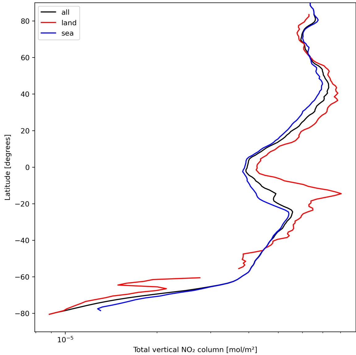
Figure 21: Zonal average of “Total vertical NO 2 column” for 2023-09-02 to 2023-09-04.
