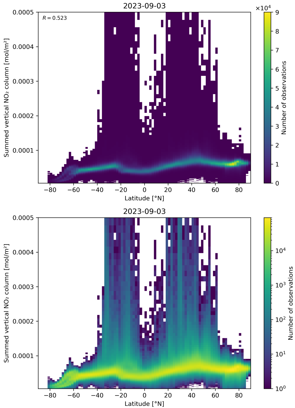
Figure 88: Scatter density plot of “Latitude” against “Summed vertical NO 2 column” for 2023-09-02 to 2023-09-04.
