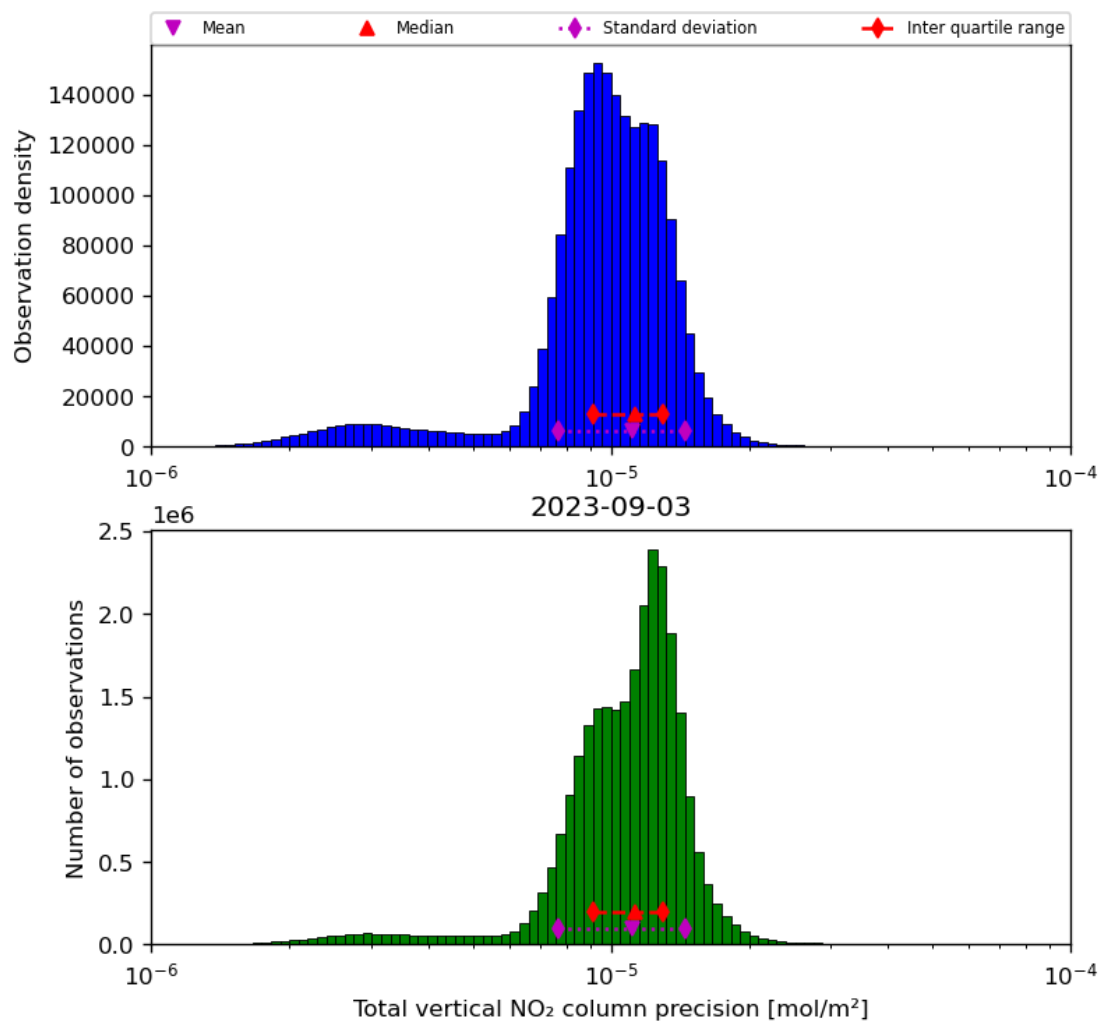
Figure 39: Histogram of "Total vertical NO 2 column precision" for 2023-09-02 to 2023-09-04
