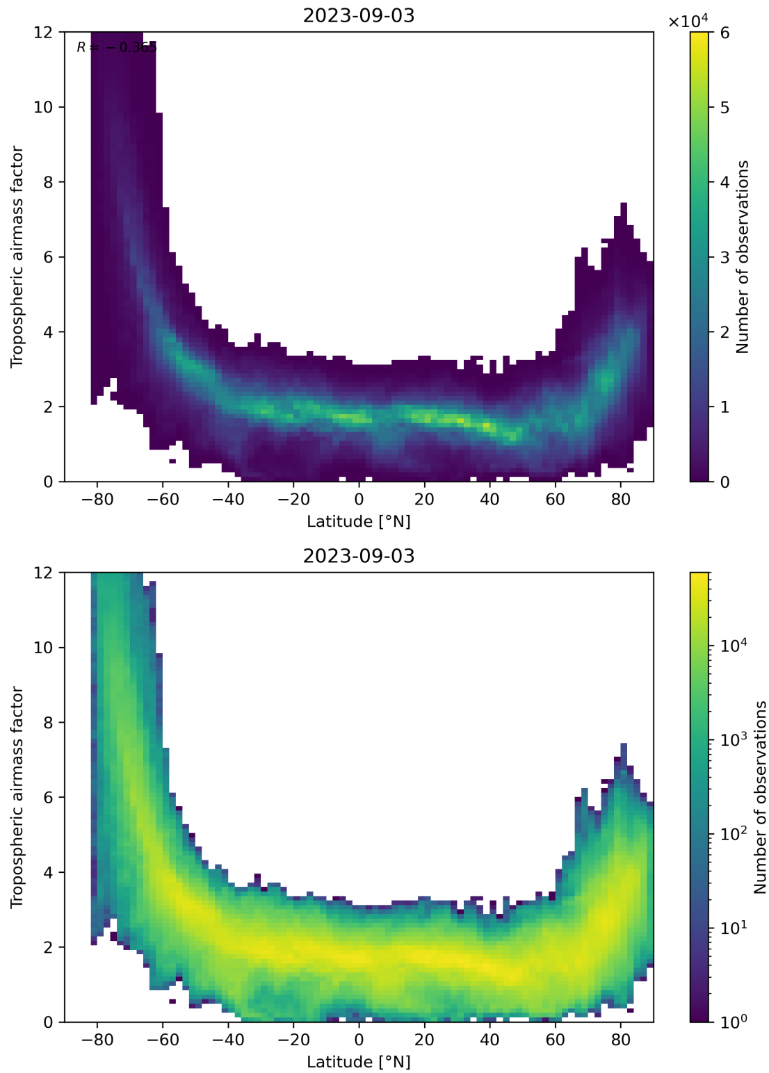
Figure 85: Scatter density plot of “Latitude” against “Tropospheric airmass factor” for 2023-09-02 to 2023-09-04.
