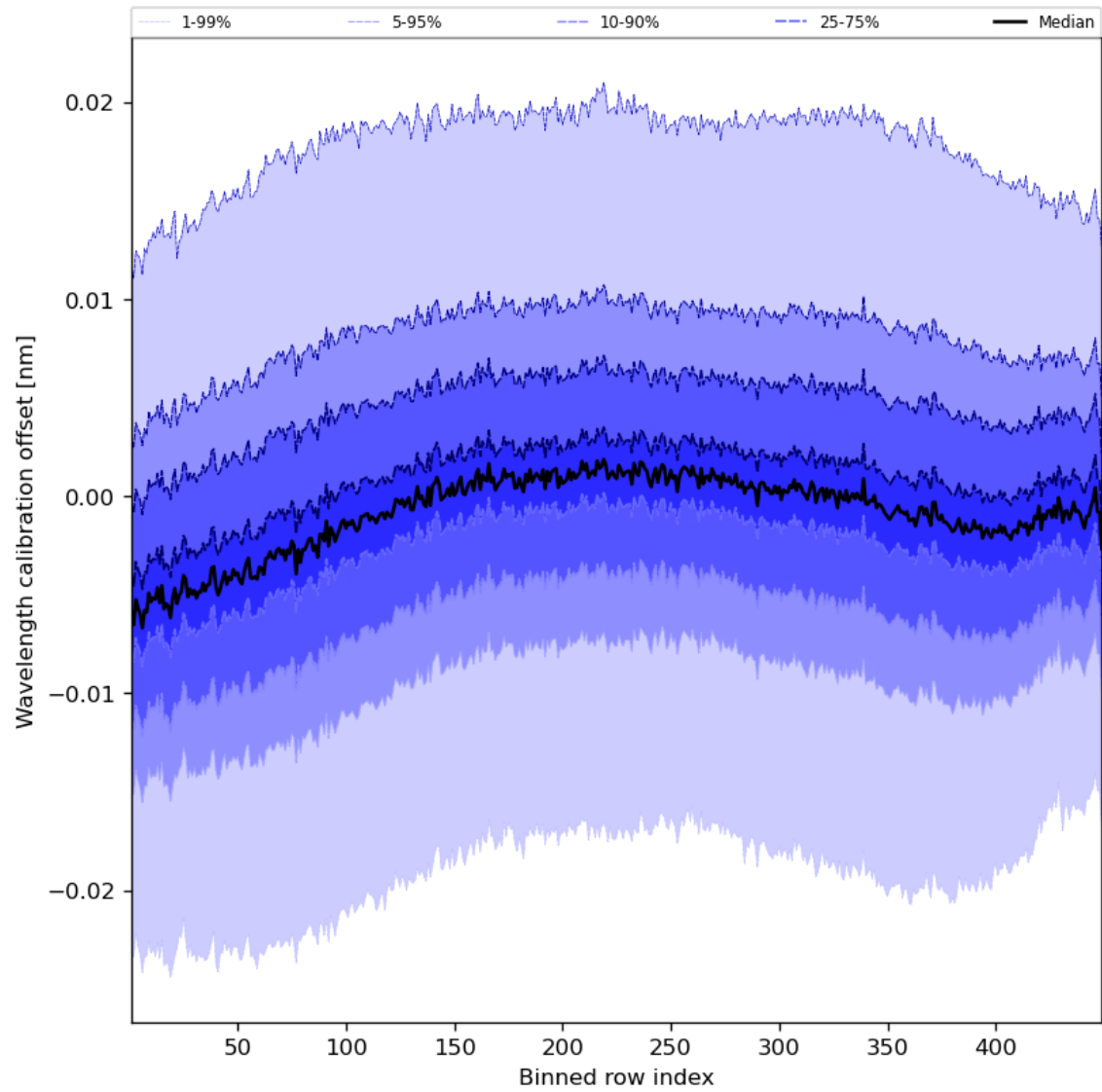
Figure 52: Along track statistics of “Wavelength calibration offset” for 2023-09-02 to 2023-09-04
