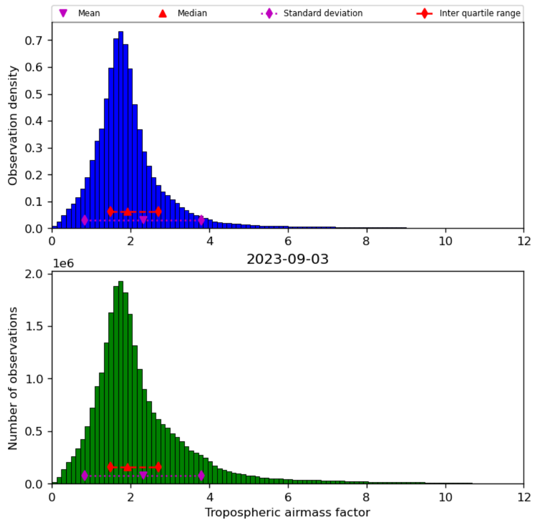
Figure 31: Histogram of “Tropospheric airmass factor” for 2023-09-02 to 2023-09-04
