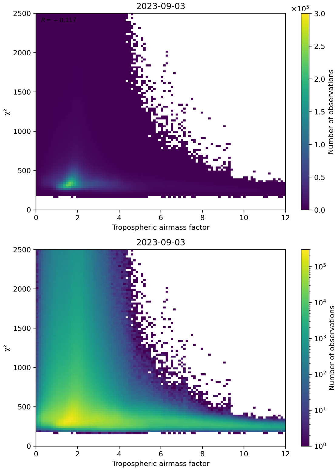
Figure 73: Scatter density plot of “Tropospheric airmass factor” against “ \chi^2 ” for 2023-09-02 to 2023-09-04.
