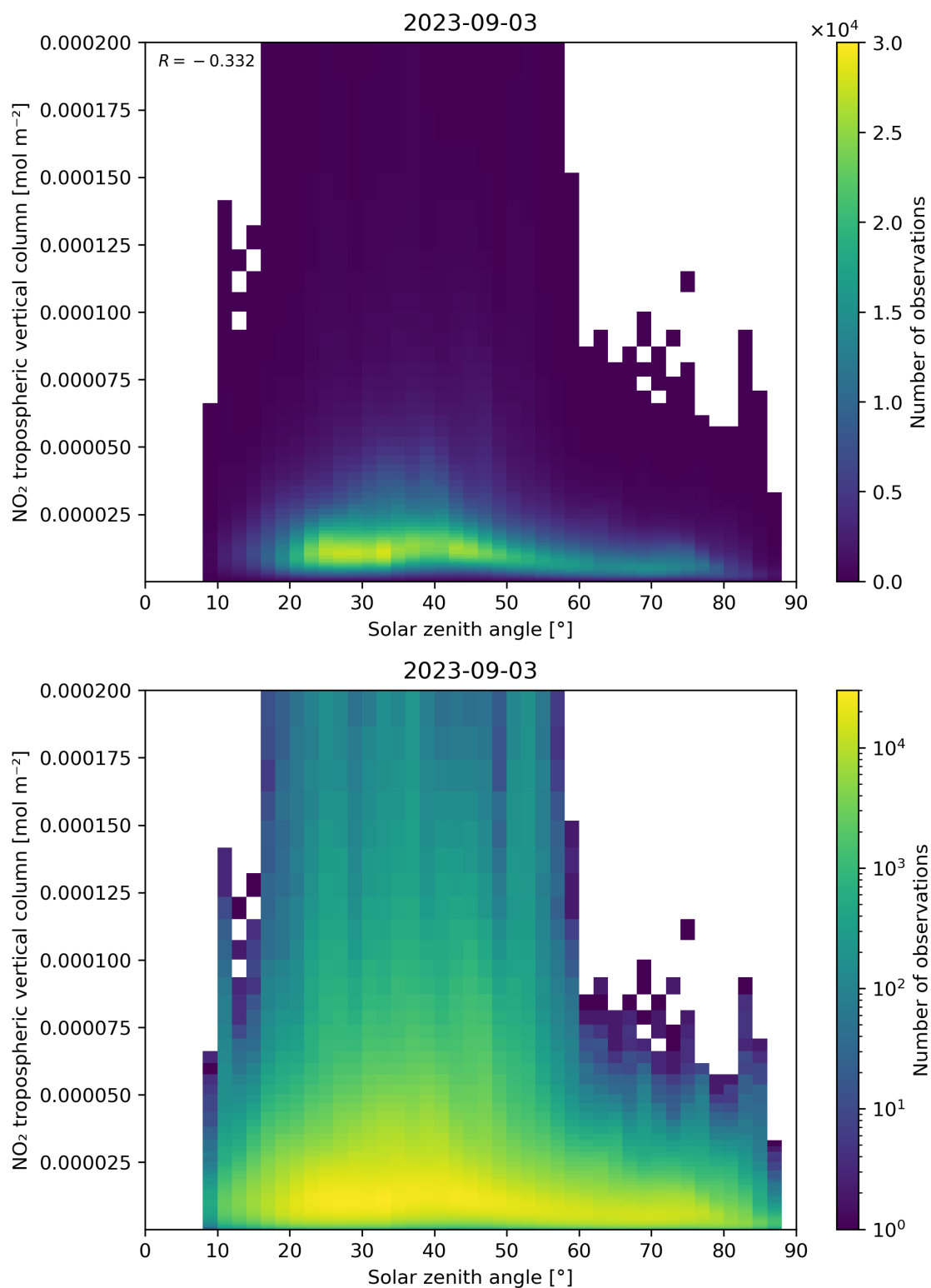
Figure 155: Scatter density plot of “Solar zenith angle” against “NO 2 tropospheric vertical column” for 2023-09-02 to 2023-09-04.
