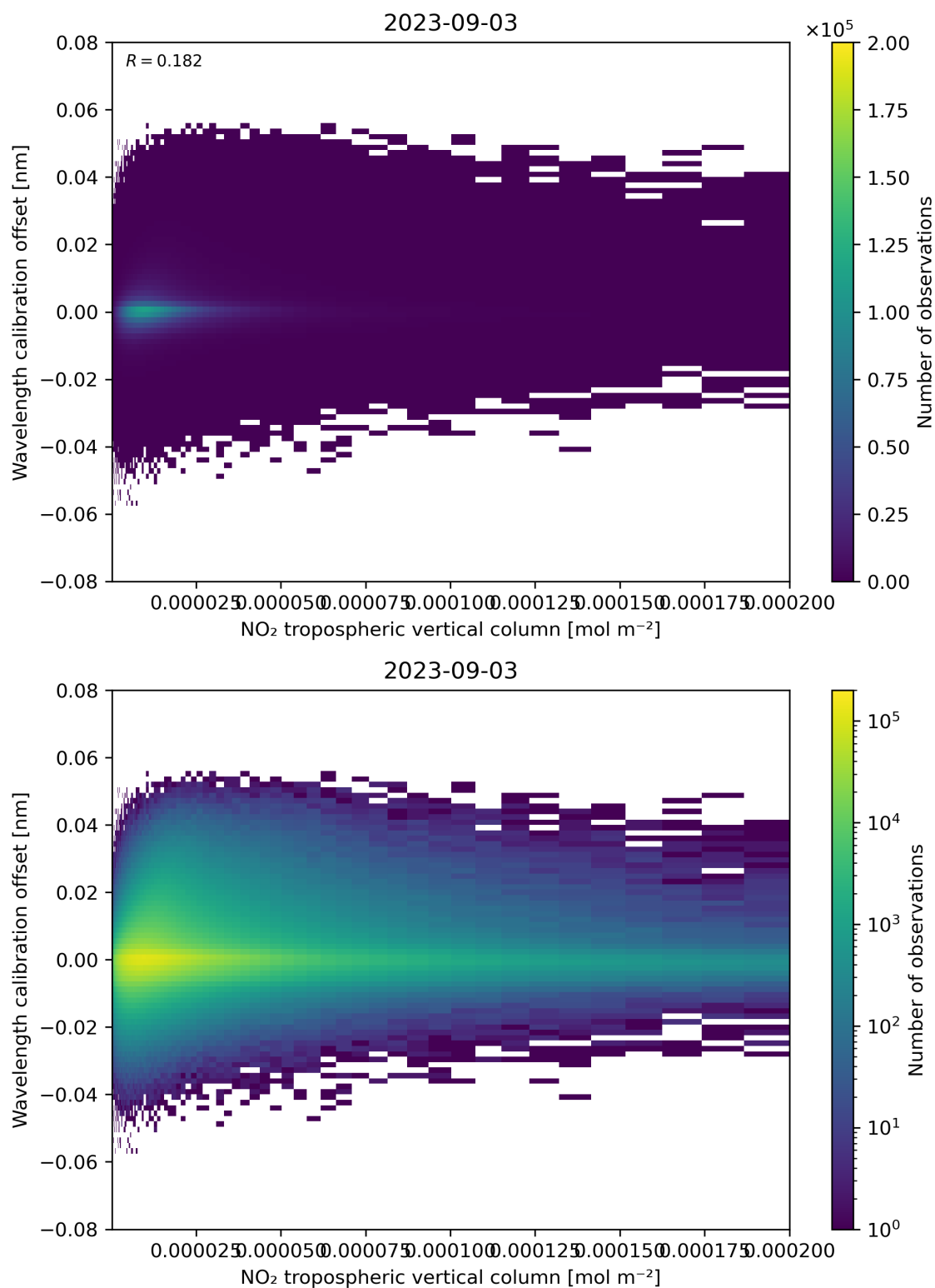
Figure 143: Scatter density plot of “NO 2 tropospheric vertical column” against “Wavelength calibration offset” for 2023-09-02 to 2023-09-04.
