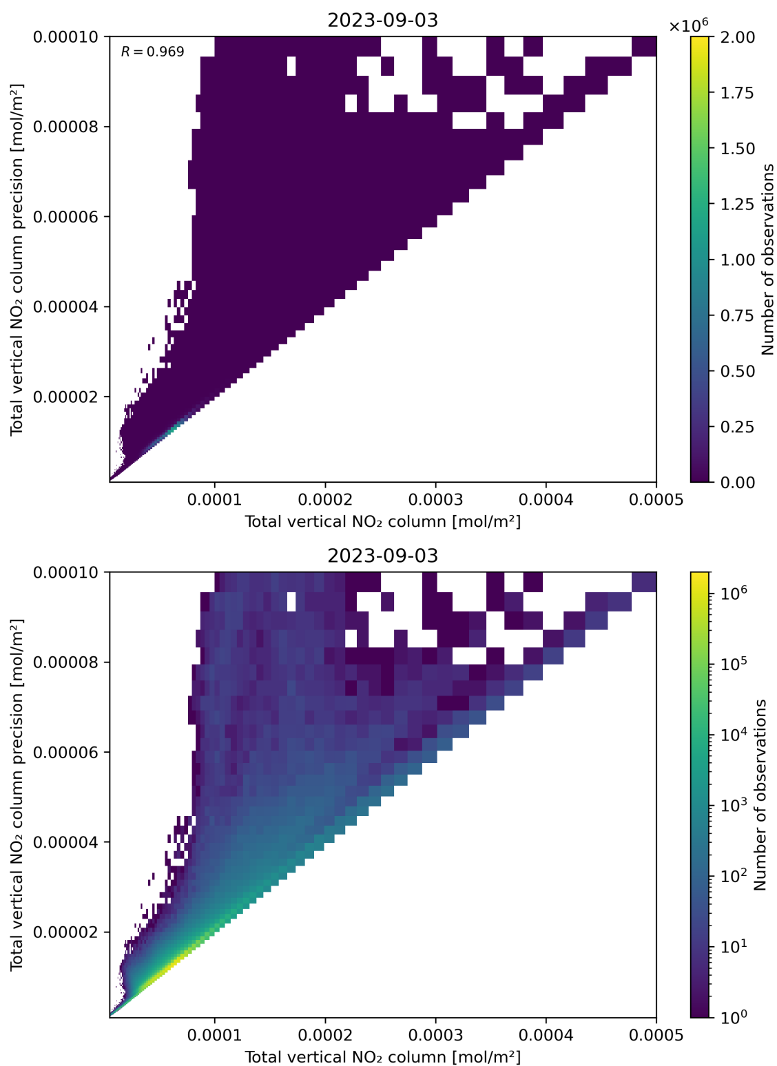
Figure 114: Scatter density plot of “Total vertical NO 2 column” against “Total vertical NO 2 column precision” for 2023-09-02 to 2023-09-04.
