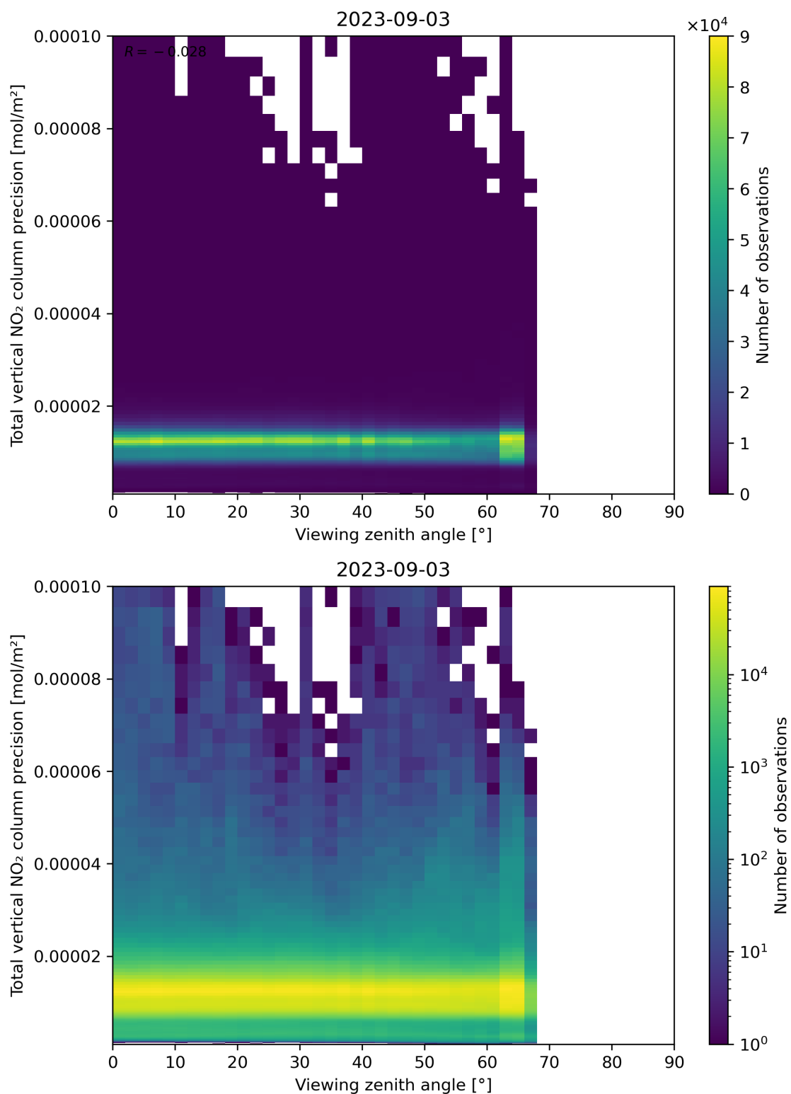
Figure 168: Scatter density plot of “Viewing zenith angle” against “Total vertical NO 2 column precision” for 2023-09-02 to 2023-09-04.
