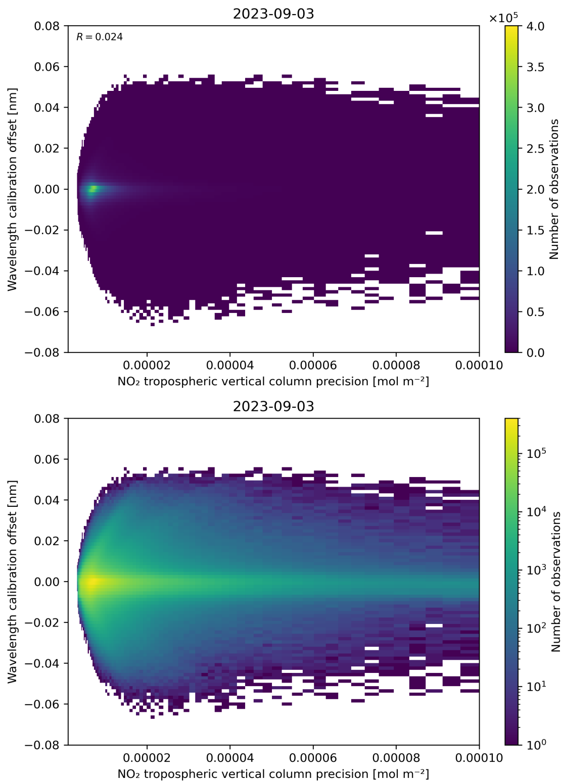
Figure 141: Scatter density plot of “NO 2 tropospheric vertical column precision” against “Wavelength calibration offset” for 2023-09-02 to 2023-09-04.
