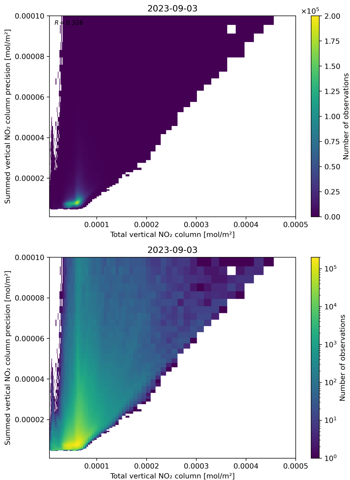
Figure 113: Scatter density plot of “Total vertical NO 2 column” against “Summed vertical NO 2 column precision” for 2023-09-02 to 2023-09-04.
