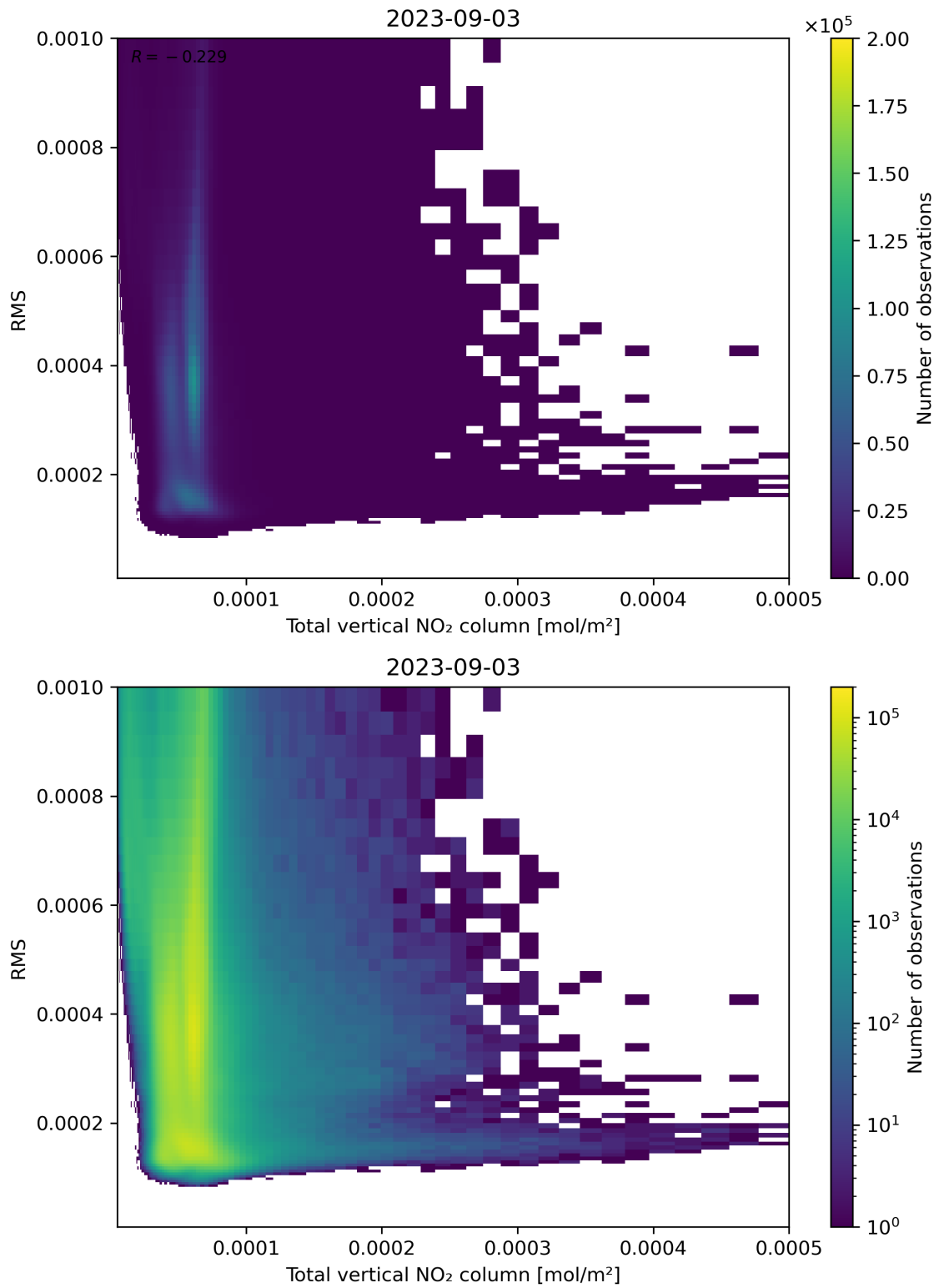
Figure 120: Scatter density plot of “Total vertical NO 2 column” against “RMS” for 2023-09-02 to 2023-09-04.
