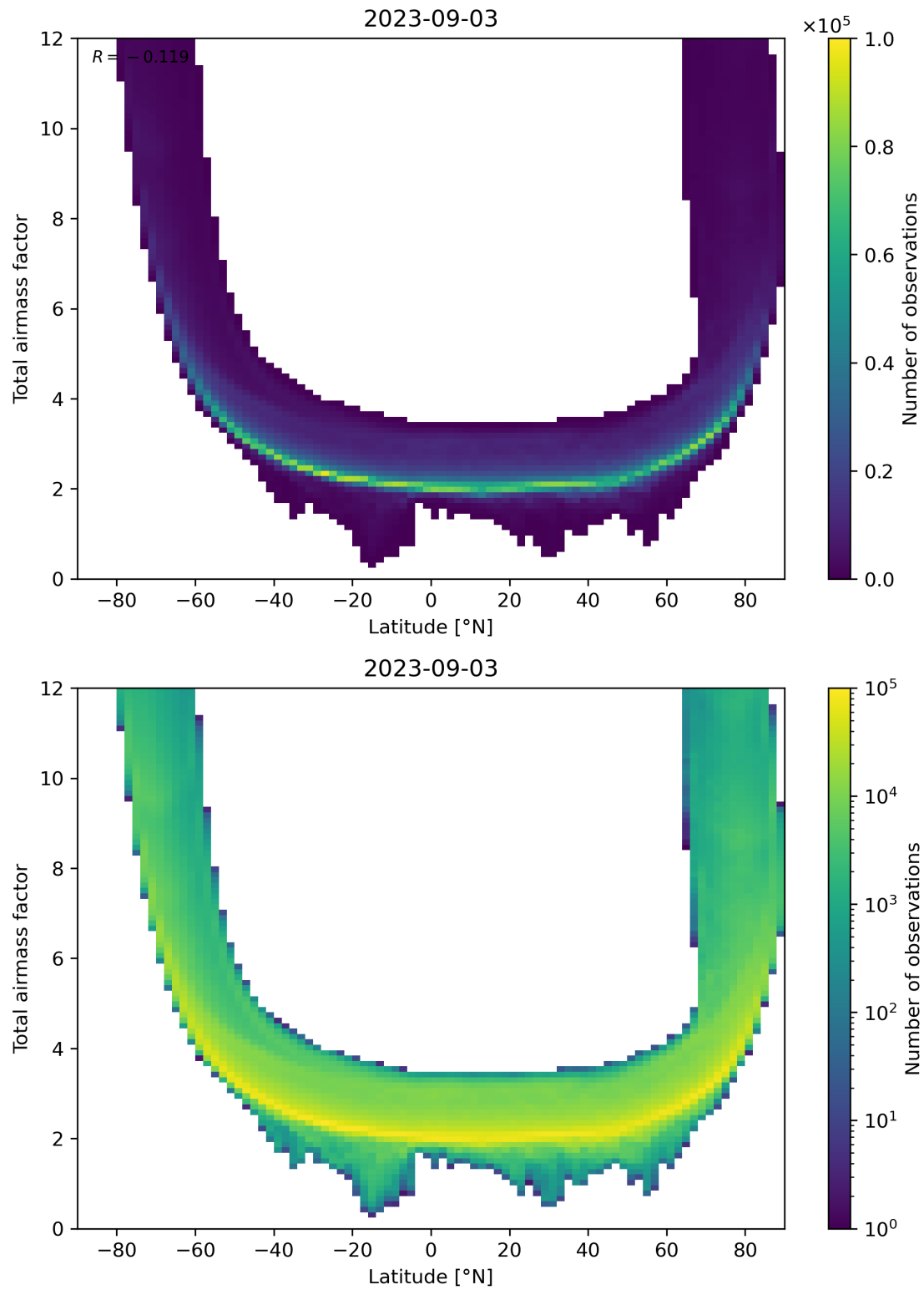
Figure 84: Scatter density plot of “Latitude” against “Total airmass factor” for 2023-09-02 to 2023-09-04.
