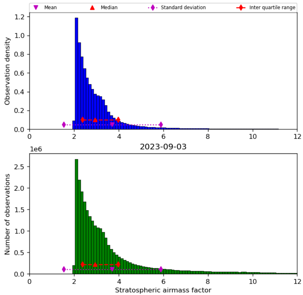
Figure 44: Histogram of “Stratospheric airmass factor” for 2023-09-02 to 2023-09-04
