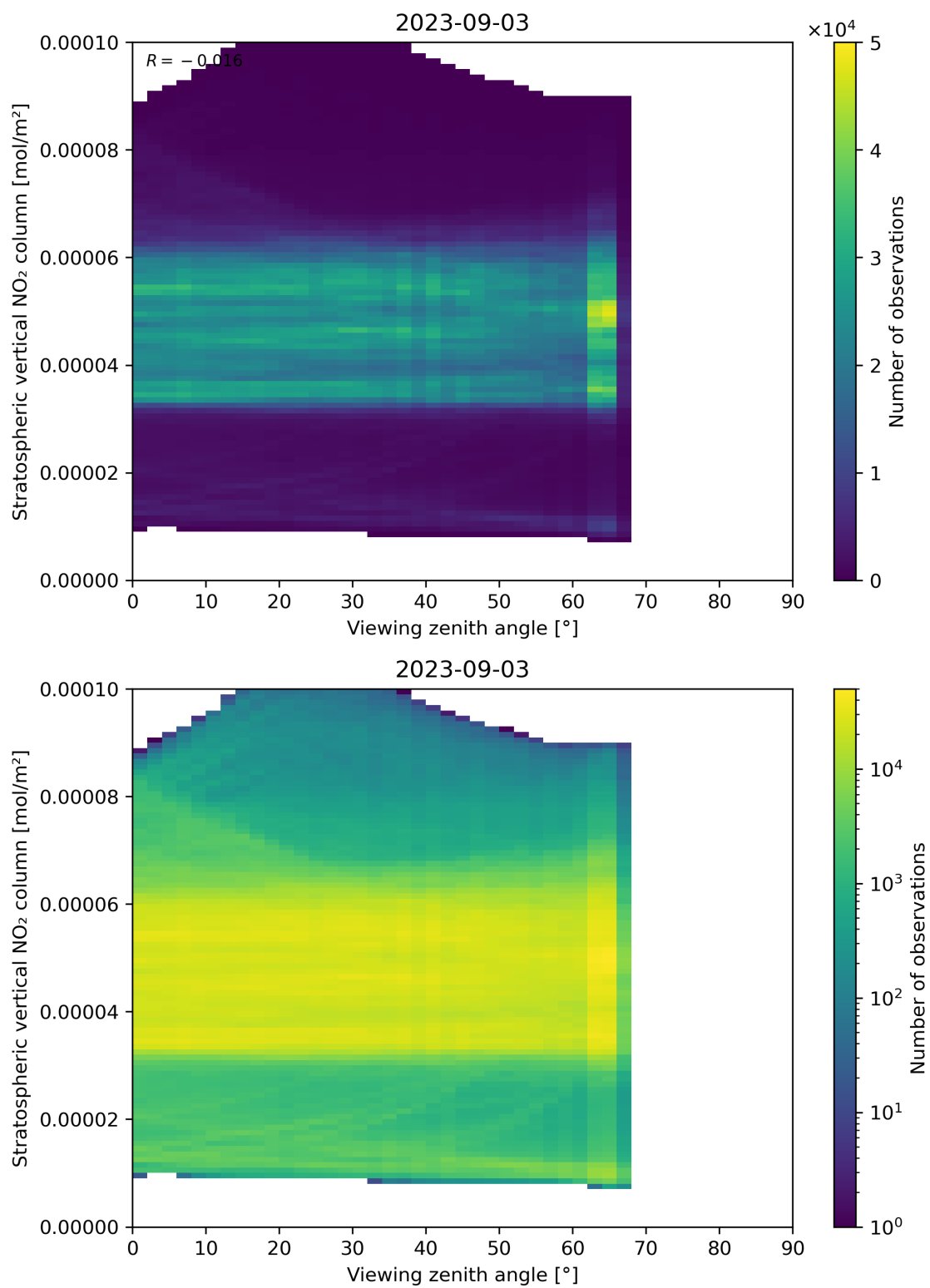
Figure 164: Scatter density plot of “Viewing zenith angle” against “Stratospheric vertical NO 2 column” for 2023-09-02 to 2023-09-04.
