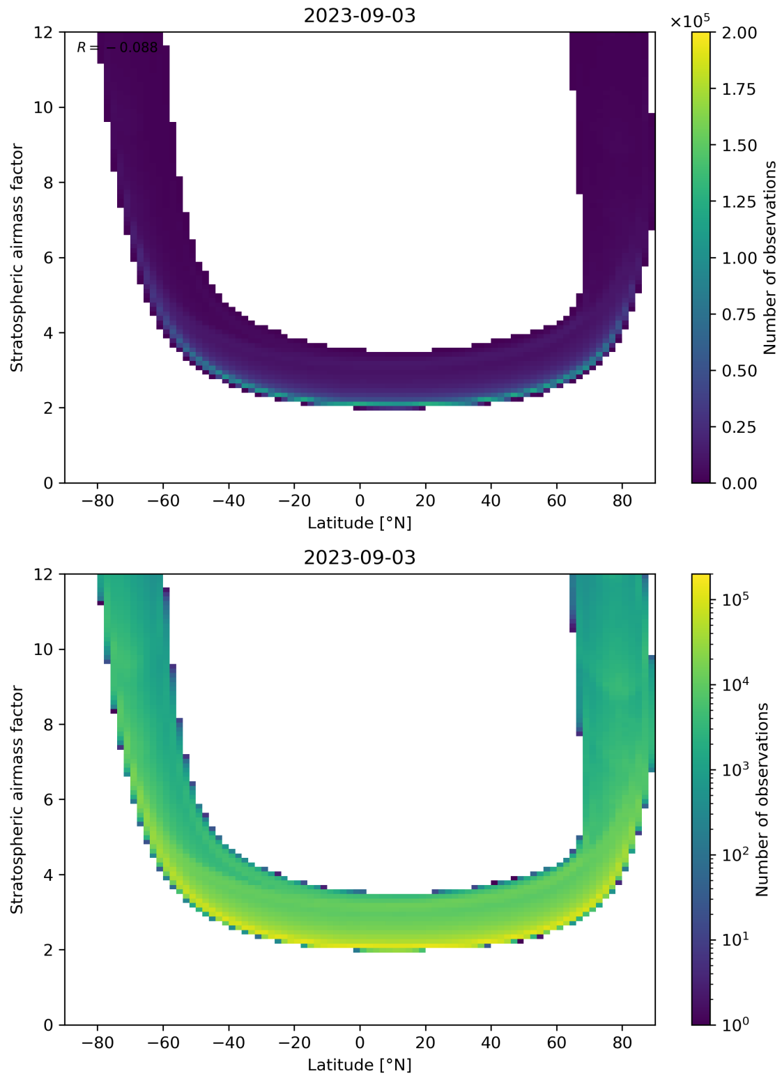
Figure 83: Scatter density plot of “Latitude” against “Stratospheric air mass factor” for 2023-09-02 to 2023-09-04.
