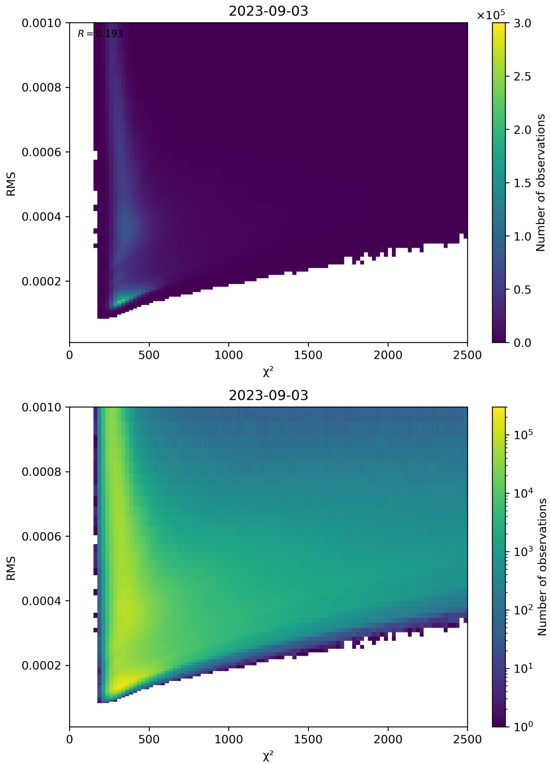
Figure 82: Scatter density plot of “ \chi^2 ” against “RMS” for 2023-09-02 to 2023-09-04.
