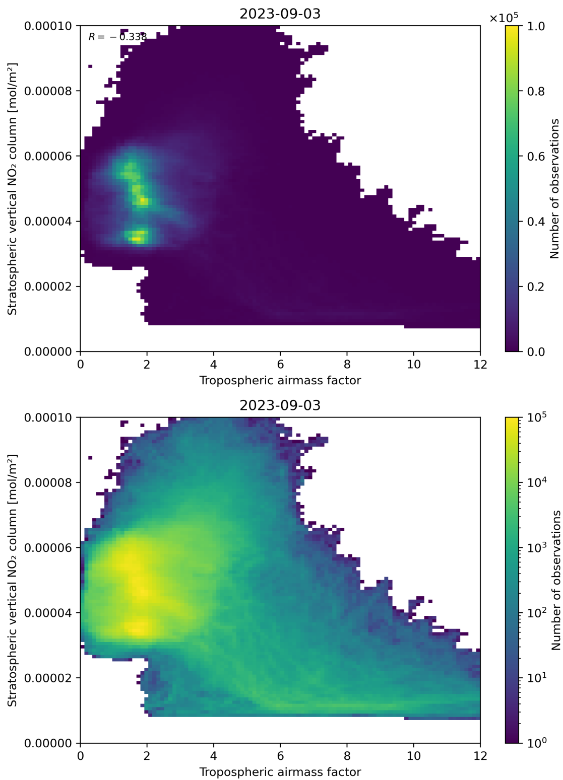
Figure 74: Scatter density plot of “Tropospheric air mass factor” against “Stratospheric vertical NO 2 column” for 2023-09-02 to 2023-09-04.
