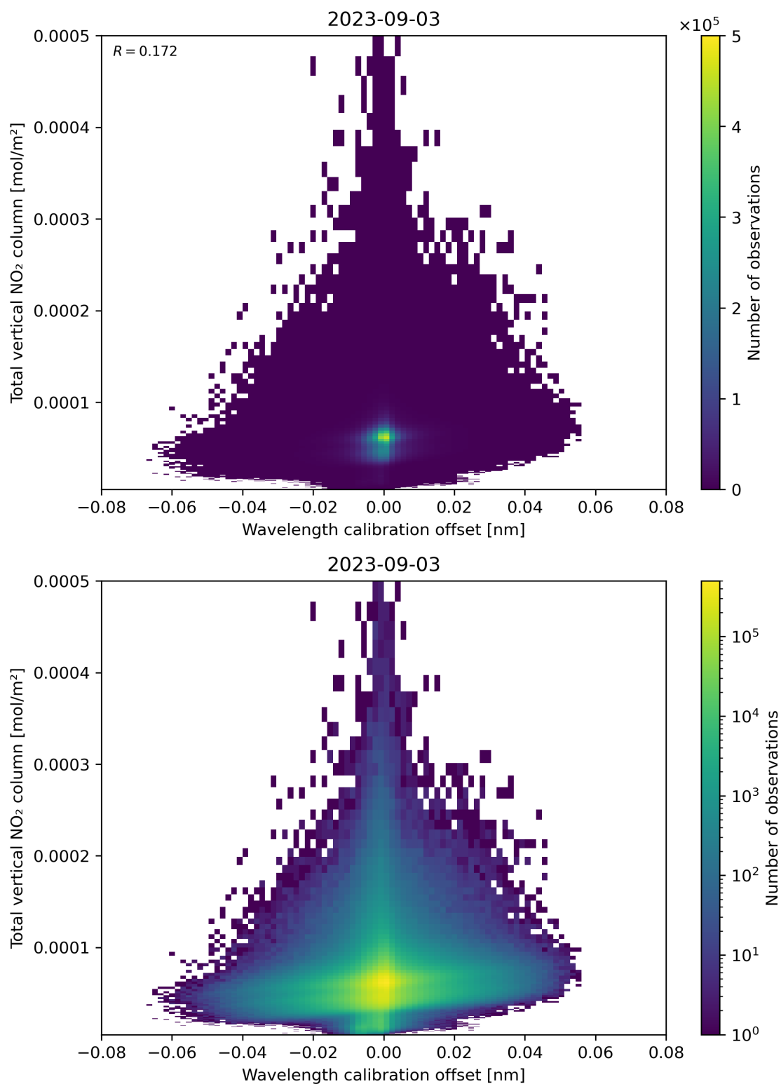
Figure 179: Scatter density plot of “Wavelength calibration offset” against “Total vertical NO 2 column” for 2023-09-02 to 2023-09-04.
