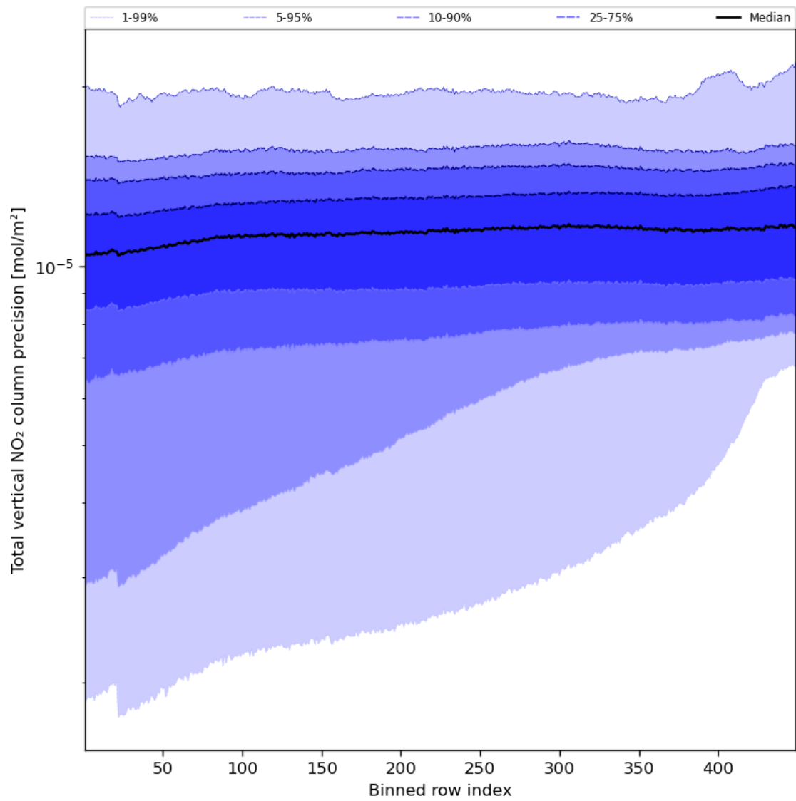
Figure 56: Along track statistics of “Total vertical NO 2 column precision” for 2023-09-02 to 2023-09-04
