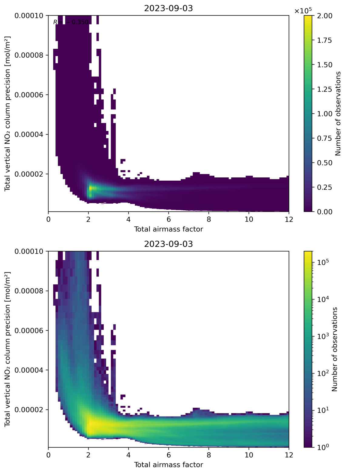
Figure 68: Scatter density plot of “Total airmass factor” against “Total vertical NO 2 column precision” for 2023-09-02 to 2023-09-04.
