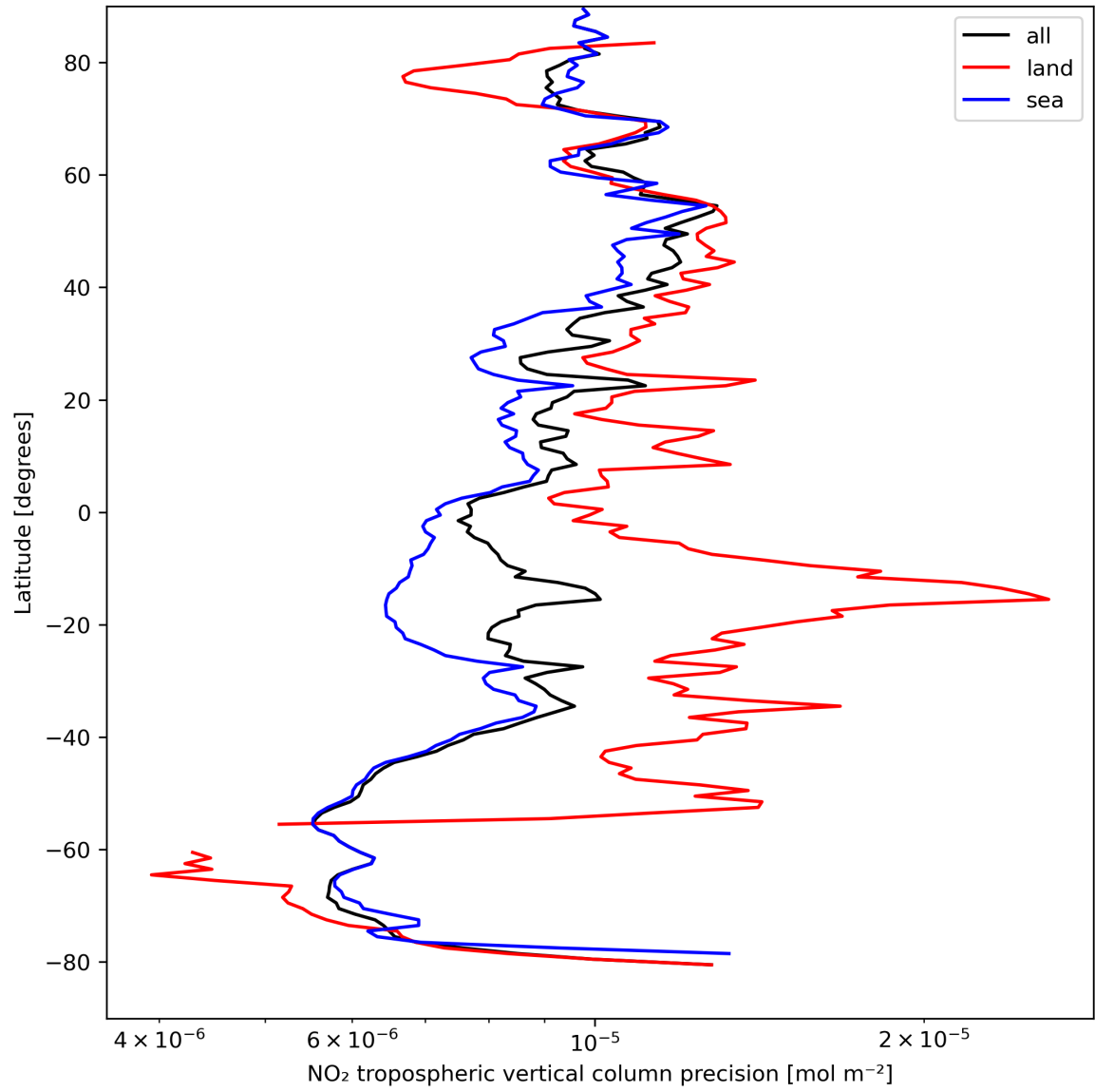
Figure 13: Zonal average of “NO 2 tropospheric vertical column precision” for 2023-09-02 to 2023-09-04.
