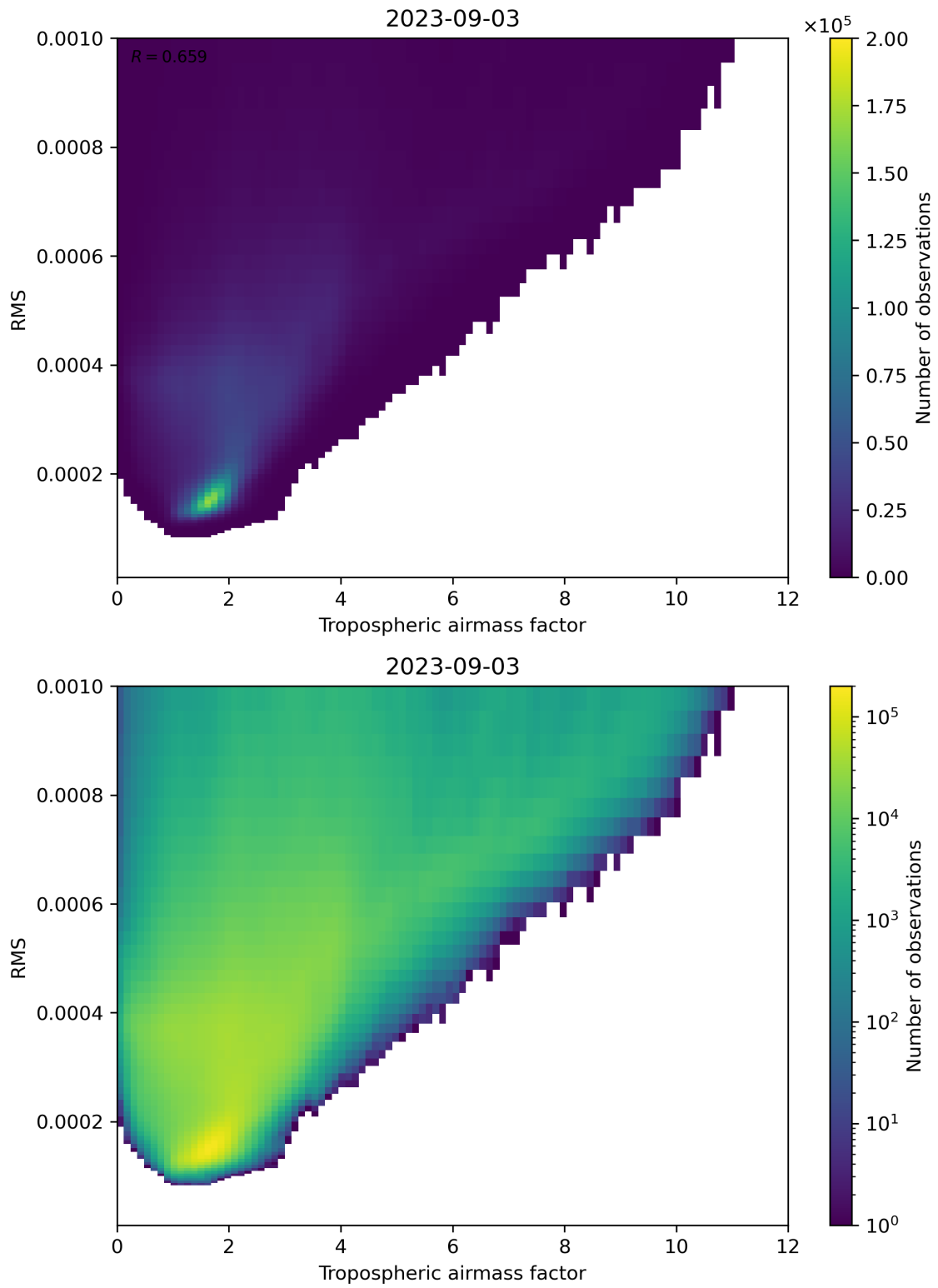
Figure 79: Scatter density plot of “Tropospheric airmass factor” against “RMS” for 2023-09-02 to 2023-09-04.
