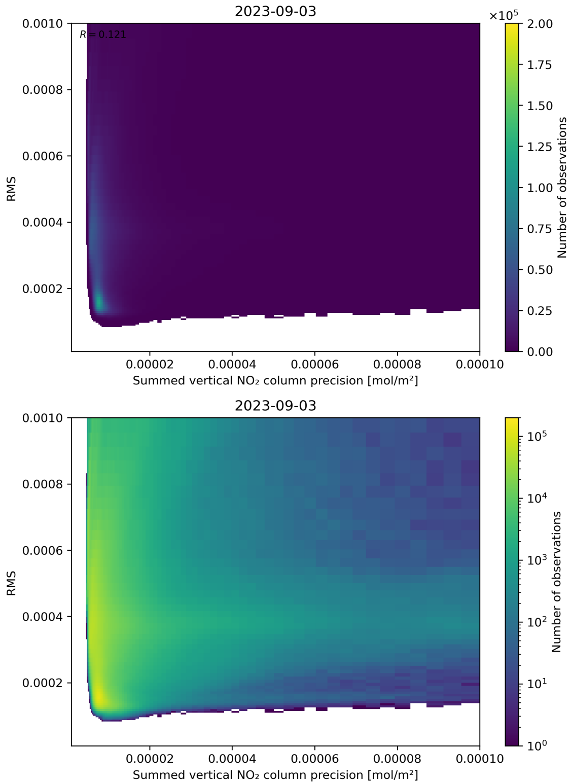
Figure 108: Scatter density plot of “Summed vertical NO 2 column precision” against “RMS” for 2023-09-02 to 2023-09-04.
