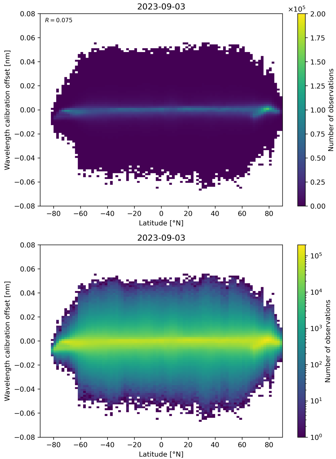
Figure 95: Scatter density plot of “Latitude” against “Wavelength calibration offset” for 2023-09-02 to 2023-09-04.
