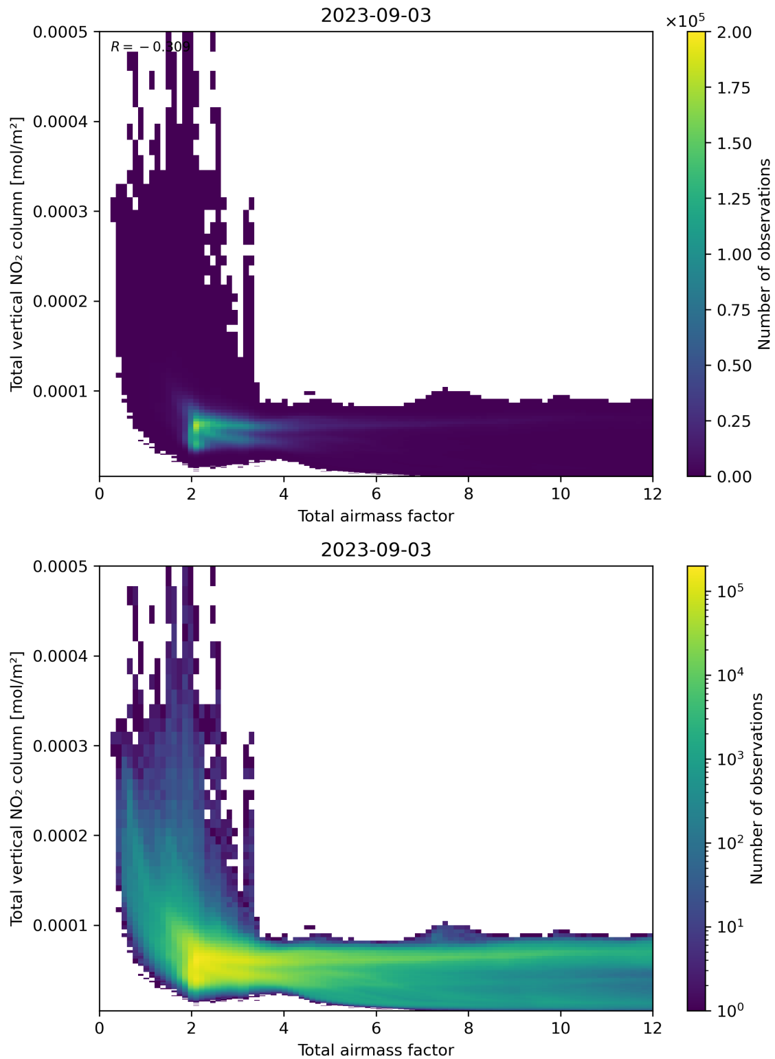
Figure 67: Scatter density plot of “Total airmass factor” against “Total vertical NO 2 column” for 2023-09-02 to 2023-09-04.
