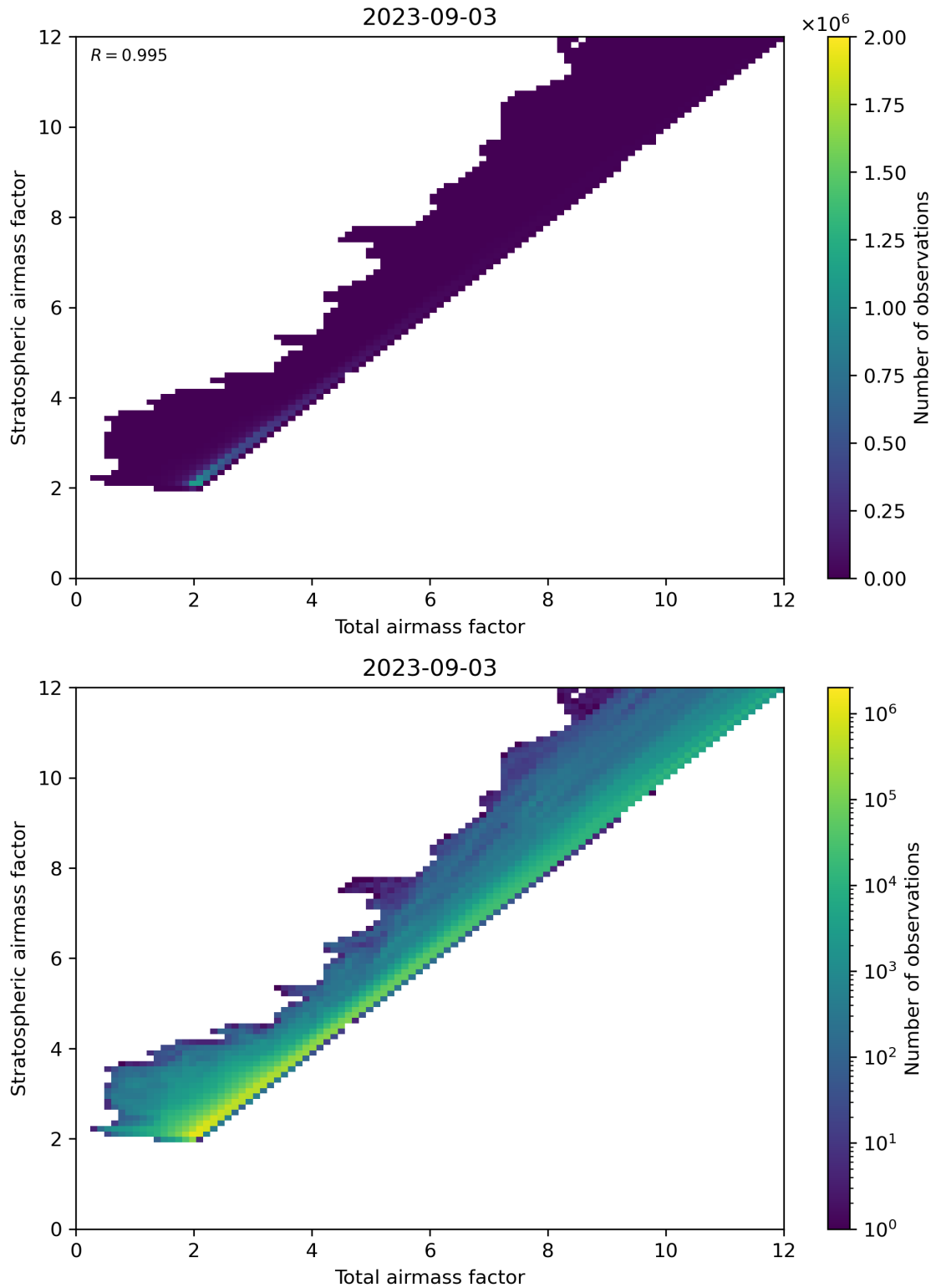
Figure 62: Scatter density plot of “Total airmass factor” against “Stratospheric airmass factor” for 2023-09-02 to 2023-09-04.
