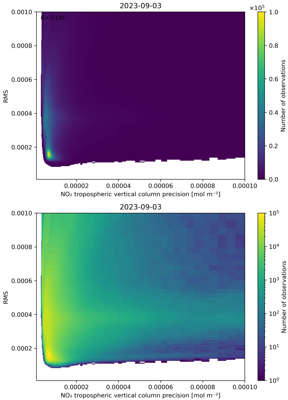
Figure 140: Scatter density plot of “NO 2 tropospheric vertical column precision” against “RMS” for 2023-09-02 to 2023-09-04.
