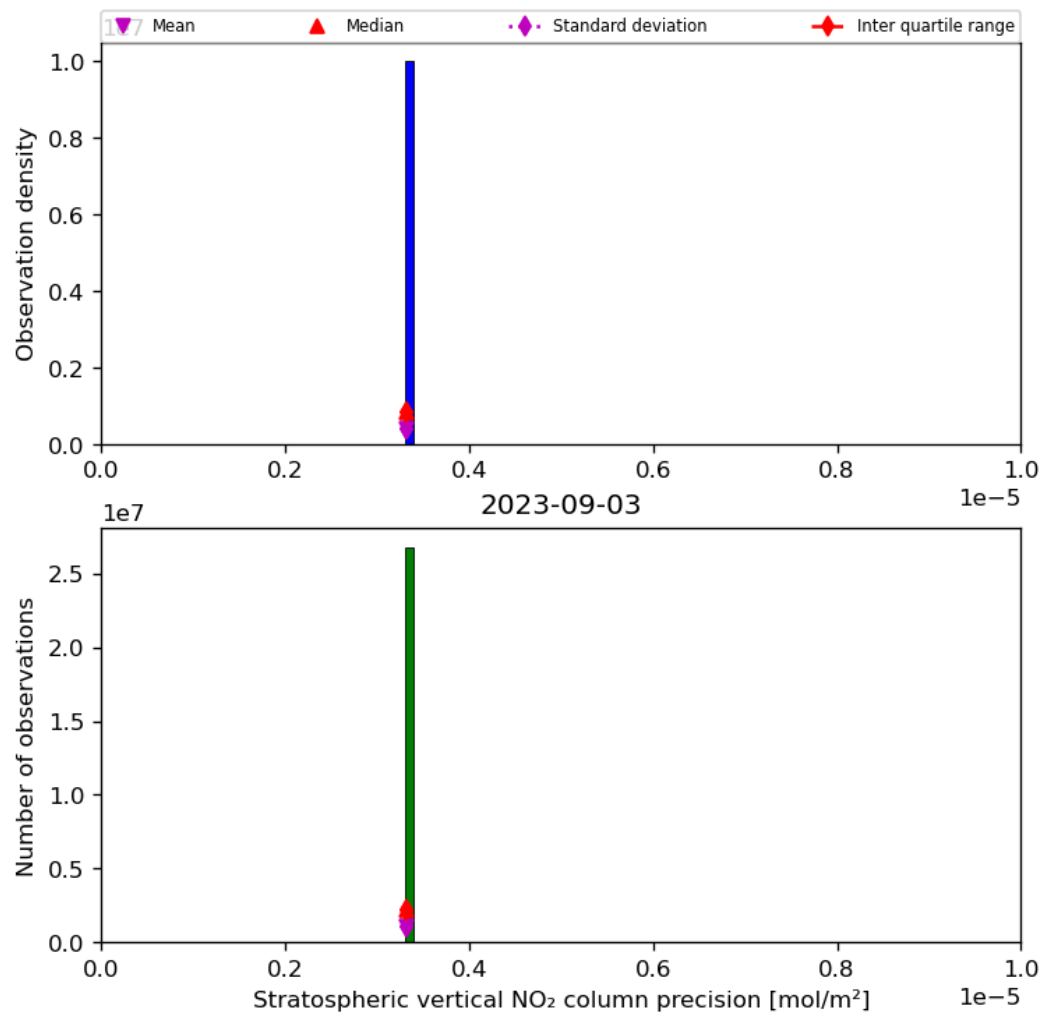
Figure 37: Histogram of “Stratospheric vertical NO 2 column precision” for 2023-09-02 to 2023-09-04
