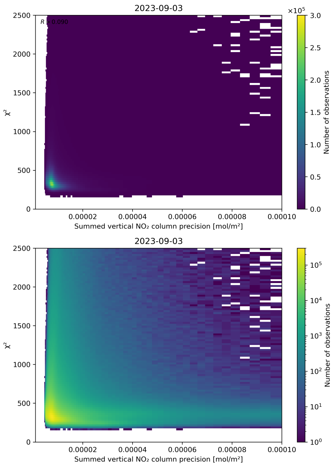
Figure 107: Scatter density plot of “Summed vertical NO 2 column precision” against “ \chi^2 ” for 2023-09-02 to 2023-09-04.
