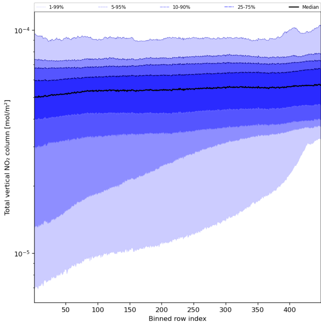
Figure 55: Along track statistics of “Total vertical NO 2 column” for 2023-09-02 to 2023-09-04
