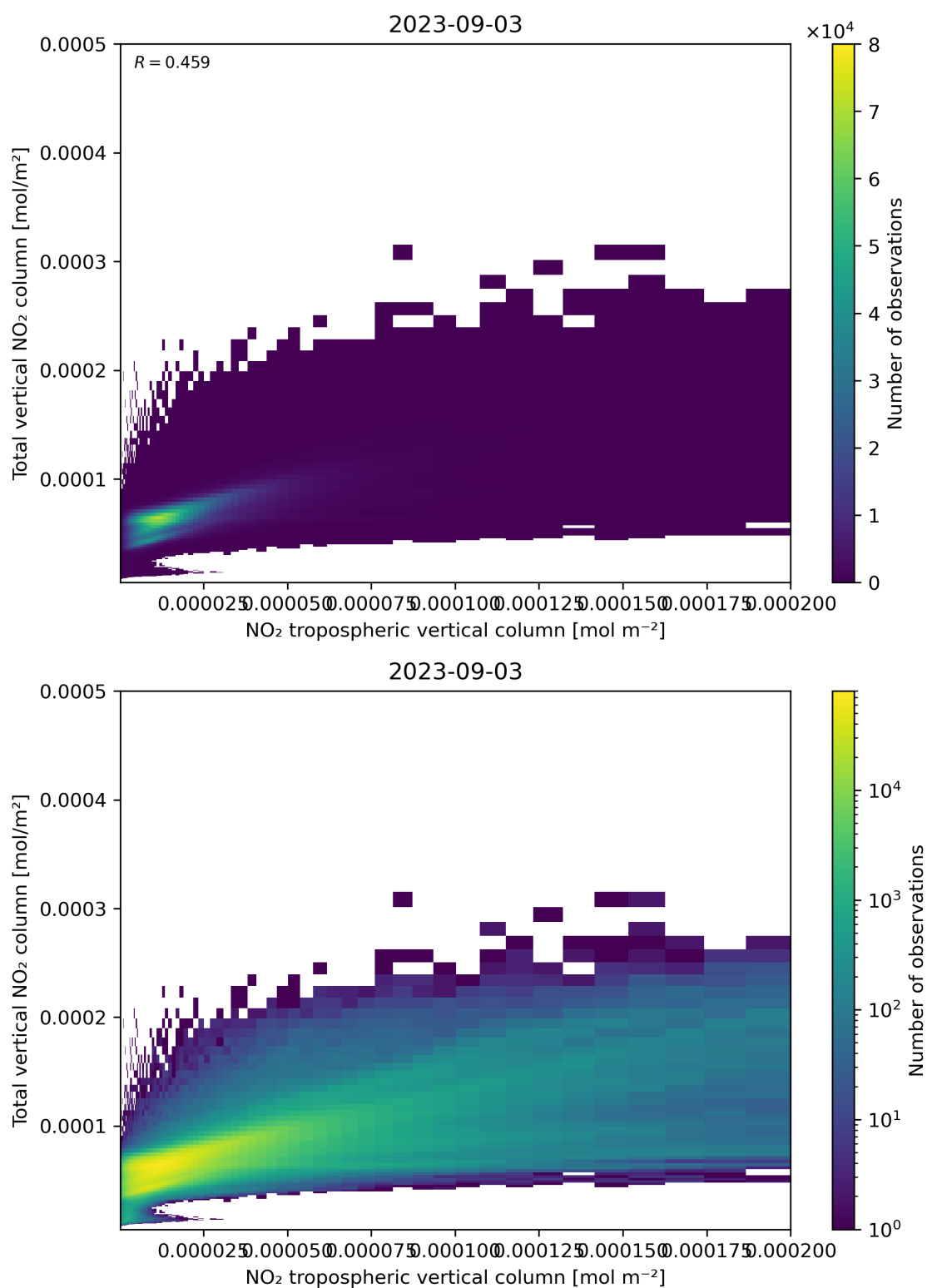
Figure 128: Scatter density plot of “NO 2 tropospheric vertical column” against “Total vertical NO 2 column” for 2023-09-02 to 2023-09-04.
