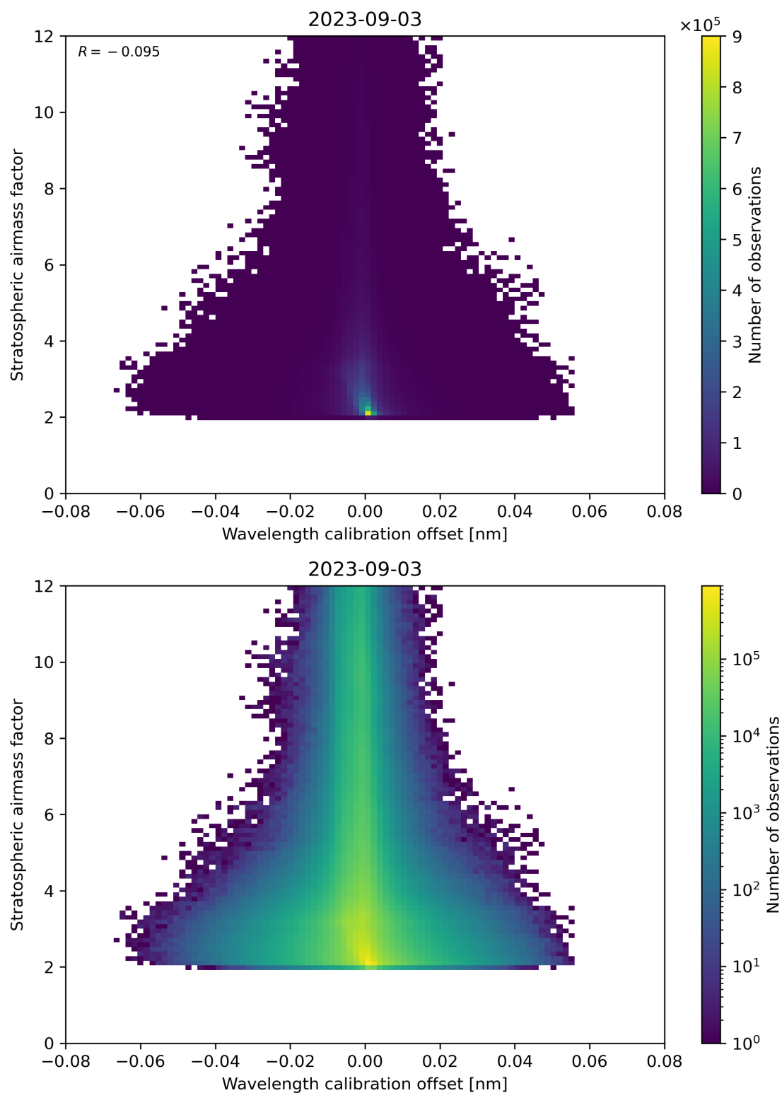
Figure 174: Scatter density plot of “Wavelength calibration offset” against “Stratospheric air mass factor” for 2023-09-02 to 2023-09-04.
