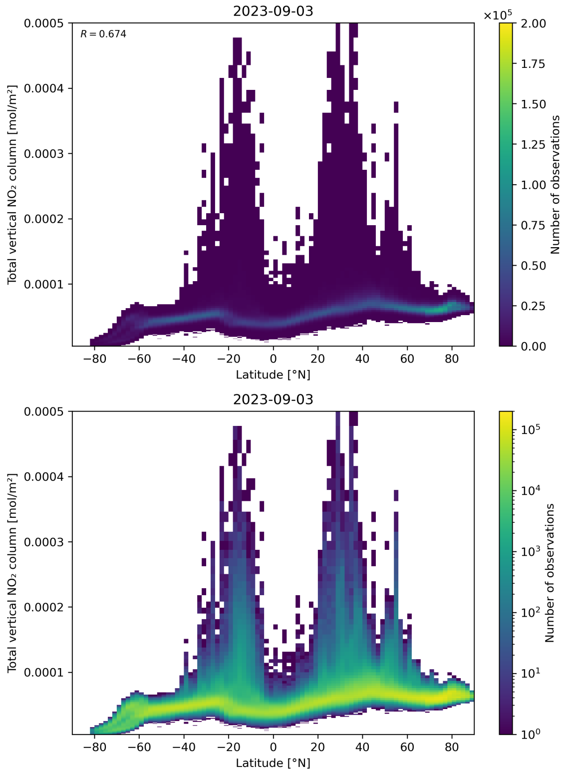
Figure 90: Scatter density plot of “Latitude” against “Total vertical NO 2 column” for 2023-09-02 to 2023-09-04.
