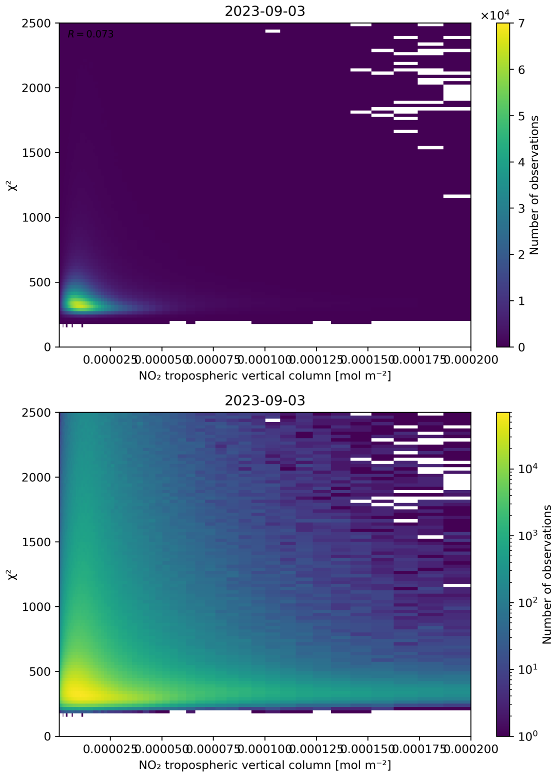
Figure 124: Scatter density plot of “NO 2 tropospheric vertical column” against “ \chi^2 ” for 2023-09-02 to 2023-09-04.
