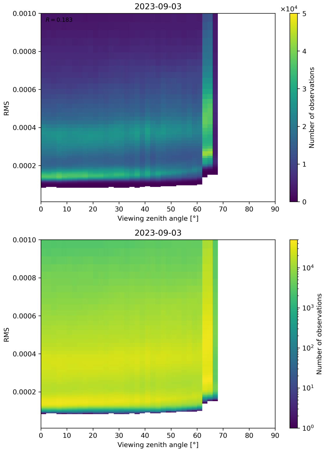
Figure 171: Scatter density plot of “Viewing zenith angle” against “RMS” for 2023-09-02 to 2023-09-04.
