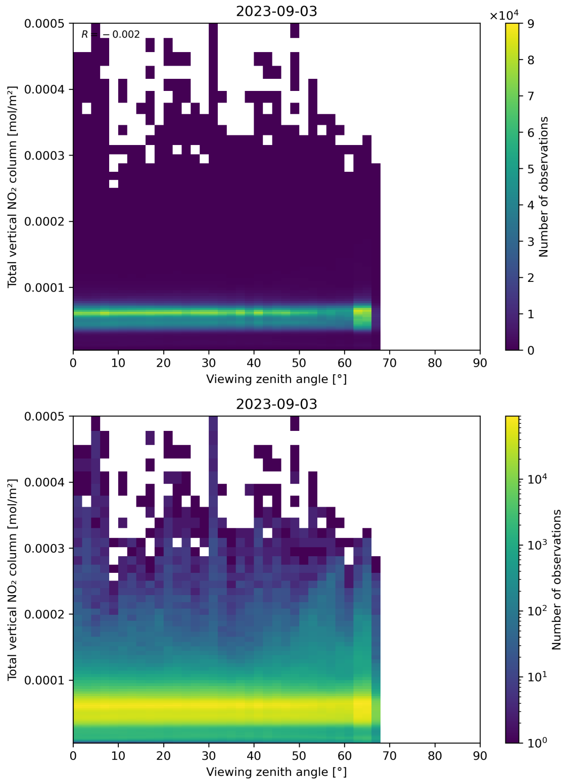
Figure 167: Scatter density plot of “Viewing zenith angle” against “Total vertical NO 2 column” for 2023-09-02 to 2023-09-04.
