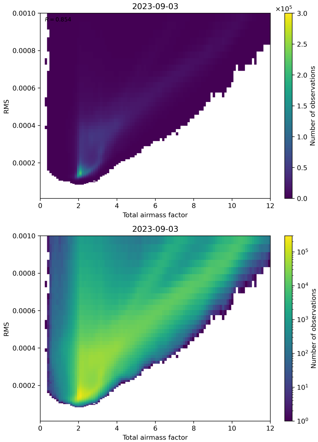
Figure 69: Scatter density plot of “Total airmass factor” against “RMS” for 2023-09-02 to 2023-09-04.
