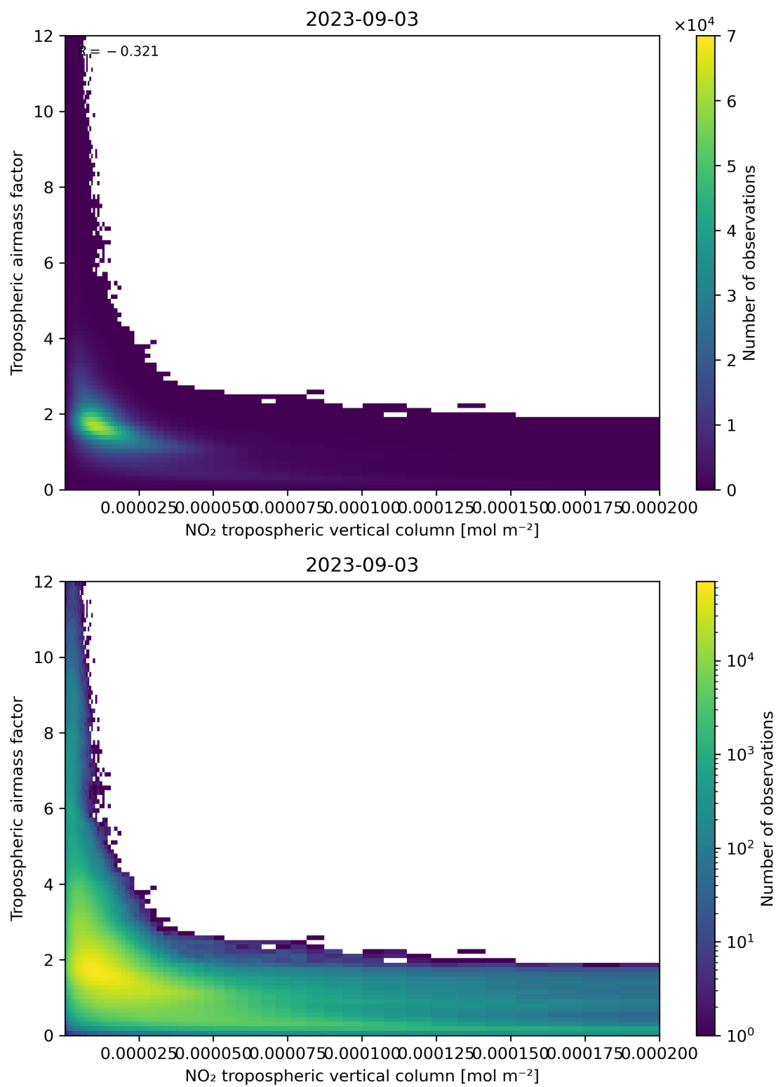
Figure 123: Scatter density plot of “NO 2 tropospheric vertical column” against “Tropospheric air mass factor” for 2023-09-02 to 2023-09-04.
