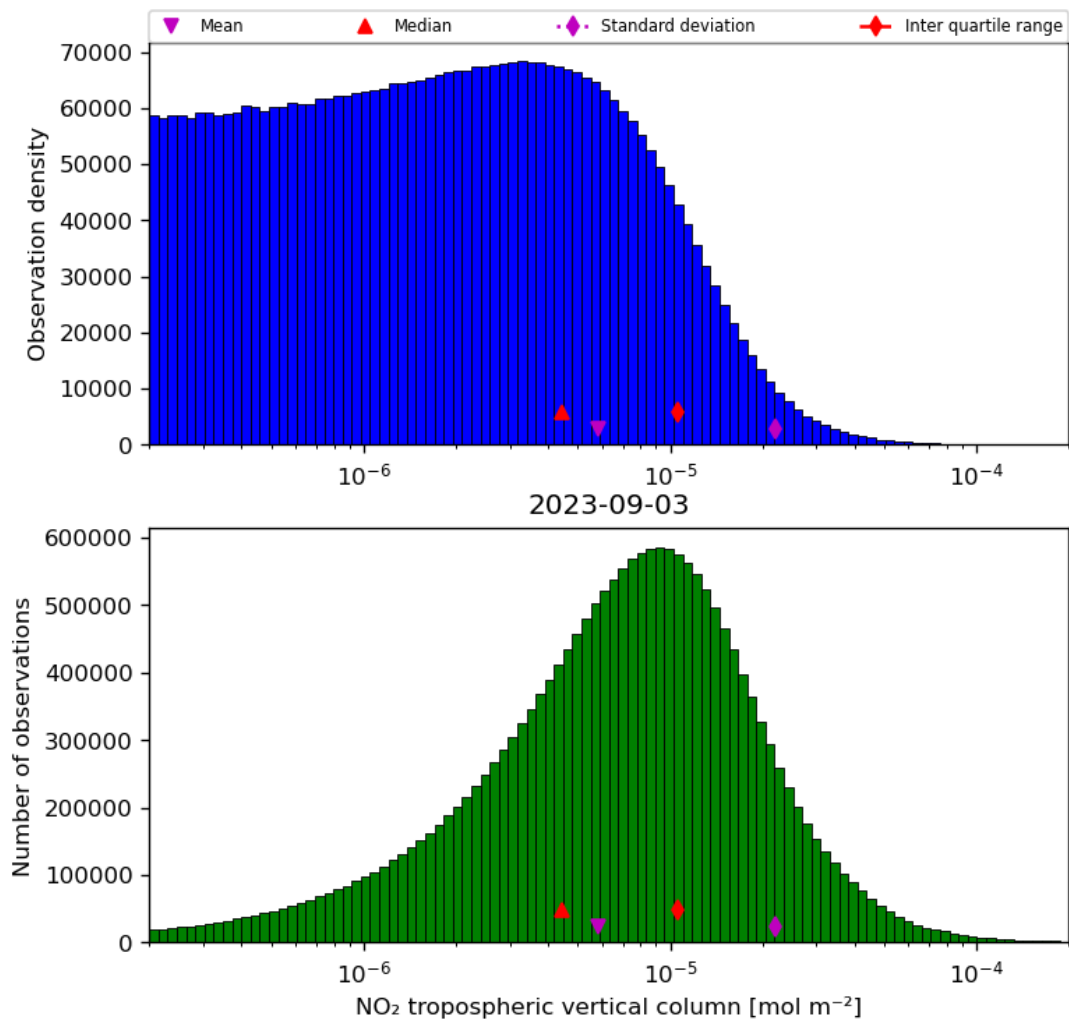
Figure 29: Histogram of “ \text{NO}_2 tropospheric vertical column” for 2023-09-02 to 2023-09-04
