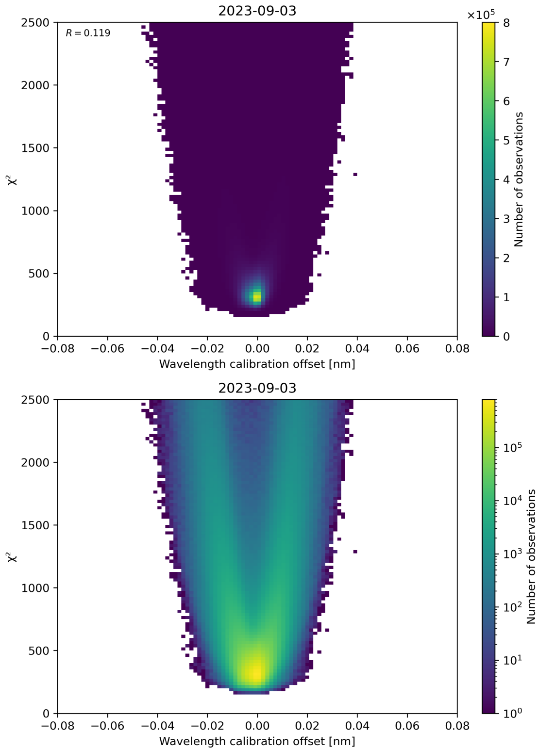
Figure 175: Scatter density plot of “Wavelength calibration offset” against “ \chi^2 ” for 2023-09-02 to 2023-09-04.
