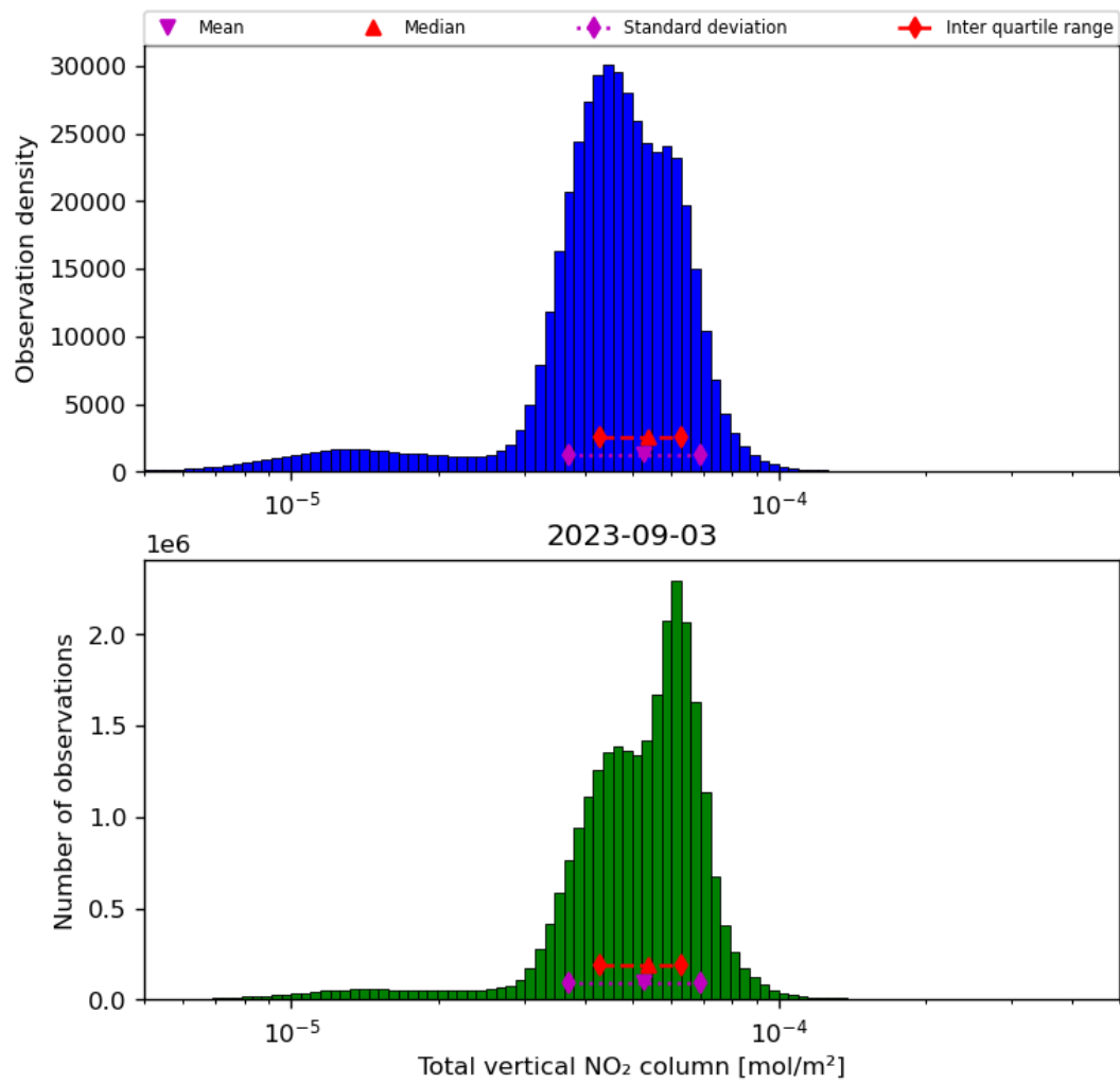
Figure 38: Histogram of “Total vertical NO 2 column” for 2023-09-02 to 2023-09-04
