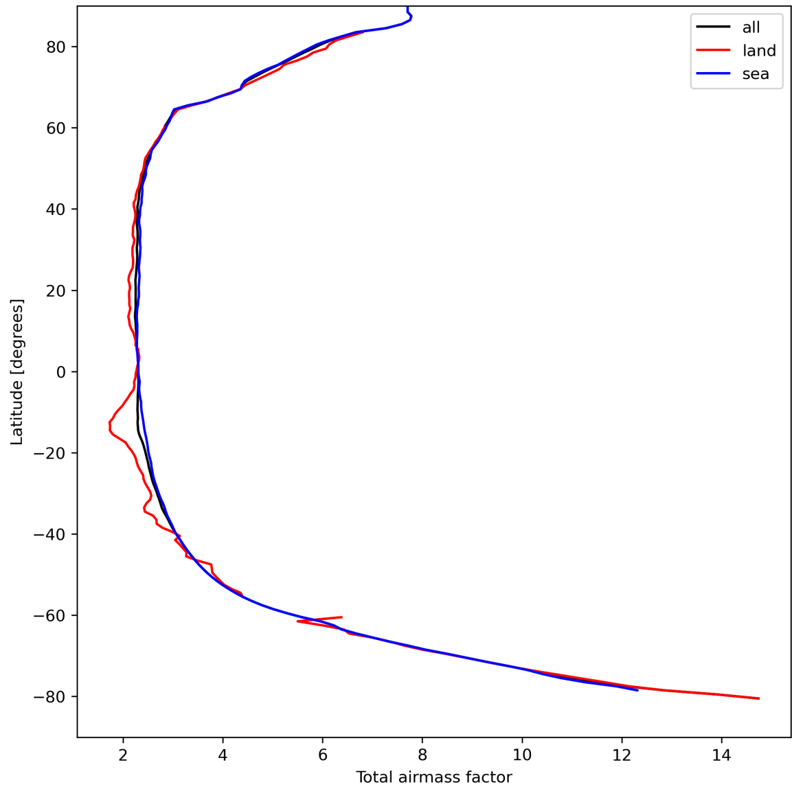
Figure 15: Zonal average of “Total airmass factor” for 2023-09-02 to 2023-09-04.
