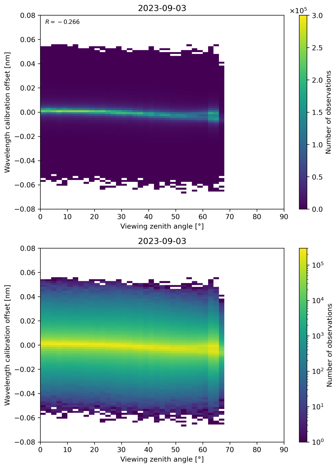
Figure 173: Scatter density plot of “Viewing zenith angle” against “Wavelength calibration offset” for 2023-09-02 to 2023-09-04.
