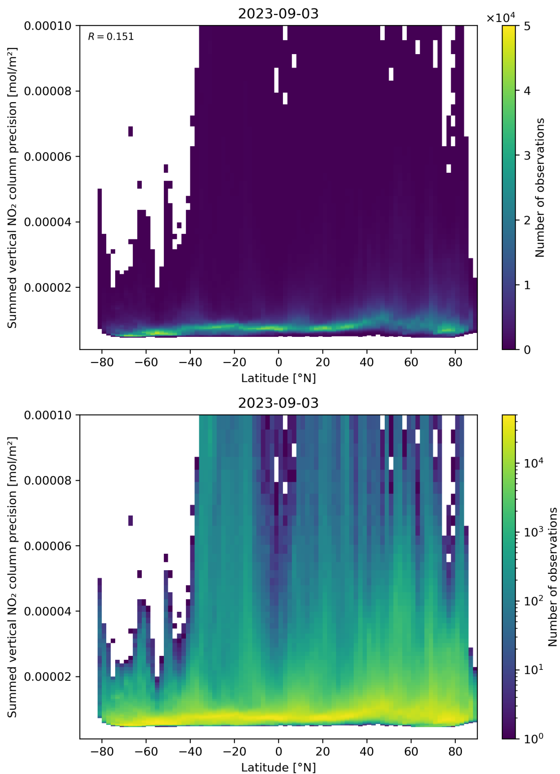
Figure 89: Scatter density plot of “Latitude” against “Summed vertical NO 2 column precision” for 2023-09-02 to 2023-09-04.
