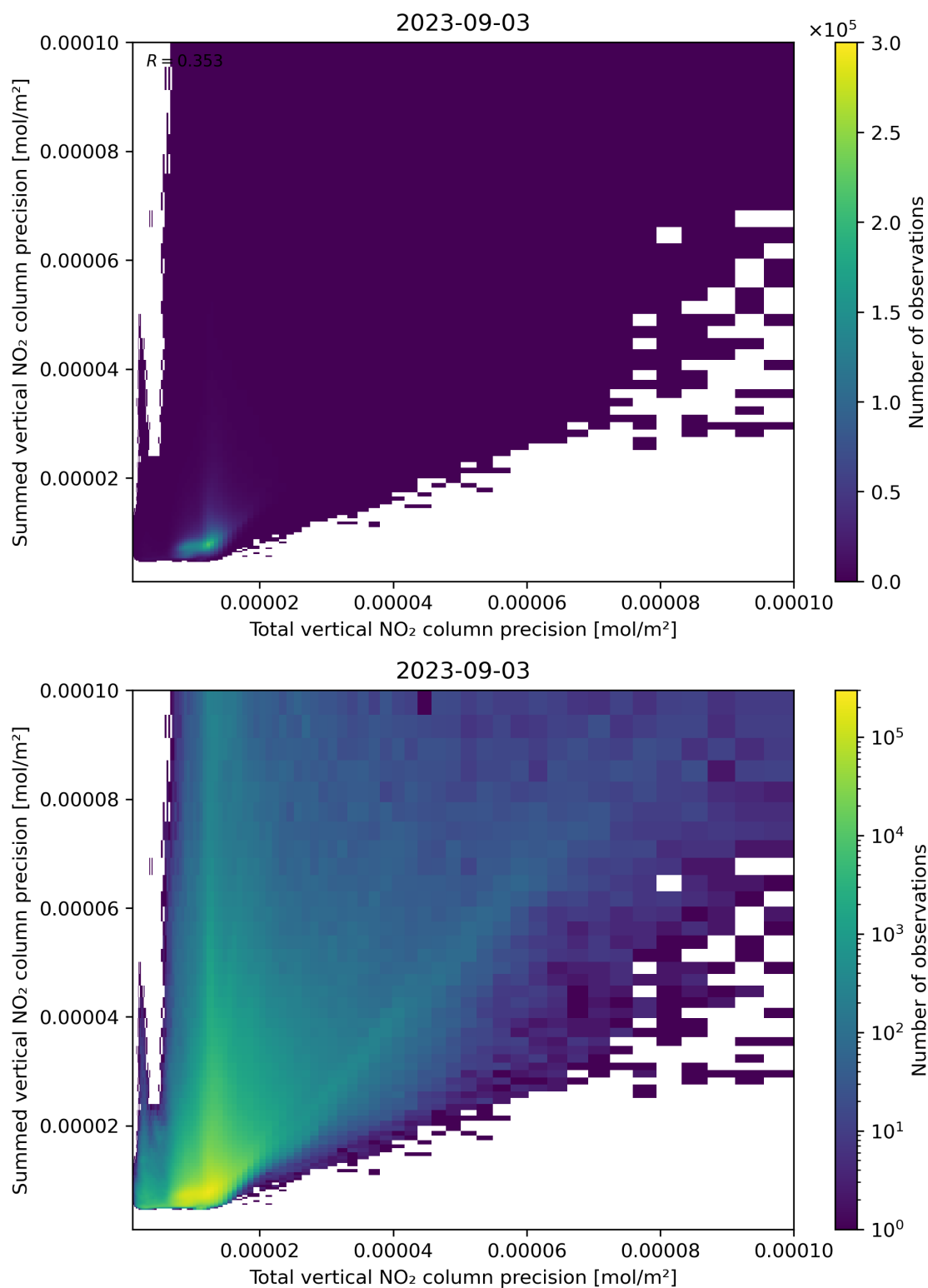
Figure 118: Scatter density plot of “Total vertical NO 2 column precision” against “Summed vertical NO 2 column precision” for 2023-09-02 to 2023-09-04.
