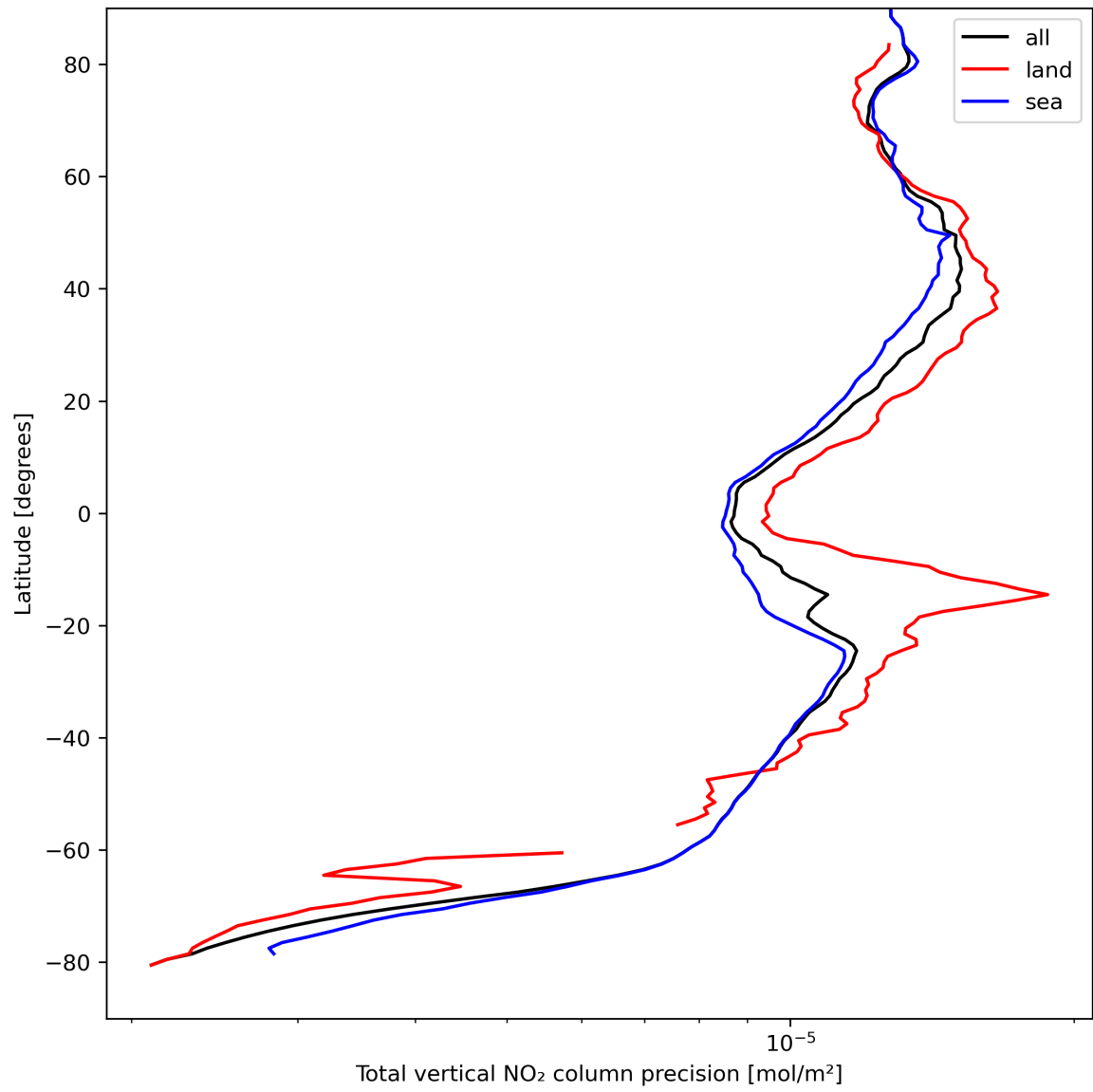
Figure 22: Zonal average of “Total vertical NO 2 column precision” for 2023-09-02 to 2023-09-04.
