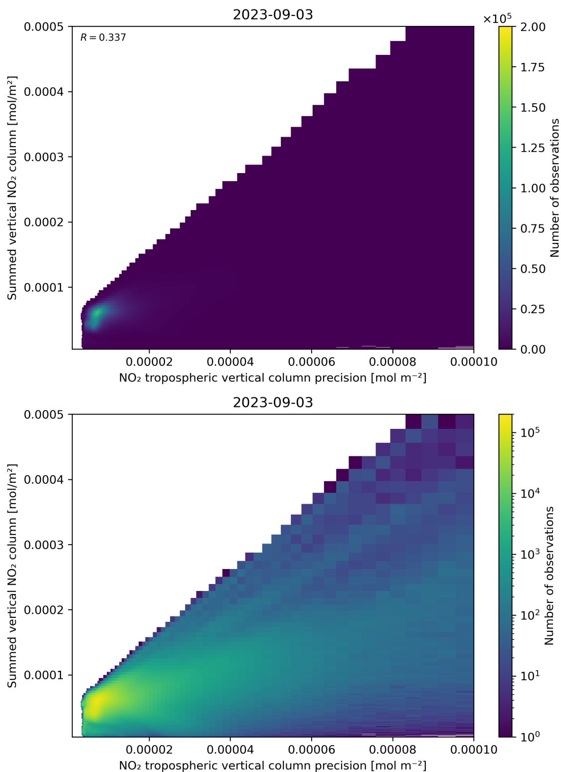
Figure 136: Scatter density plot of “NO 2 tropospheric vertical column precision” against “Summed vertical NO 2 column” for 2023-09-02 to 2023-09-04.
