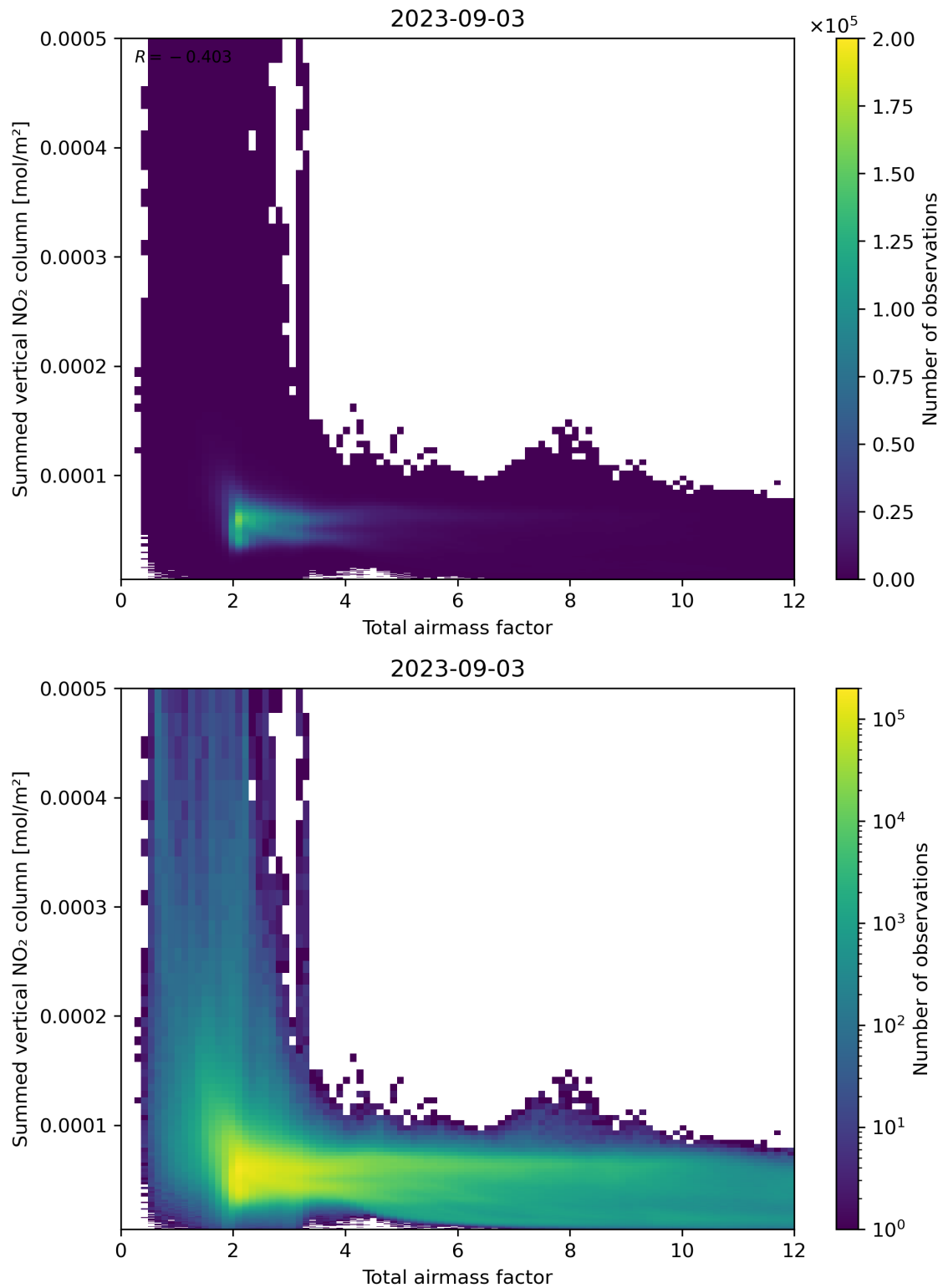
Figure 65: Scatter density plot of “Total airmass factor” against “Summed vertical NO 2 column” for 2023-09-02 to 2023-09-04.
