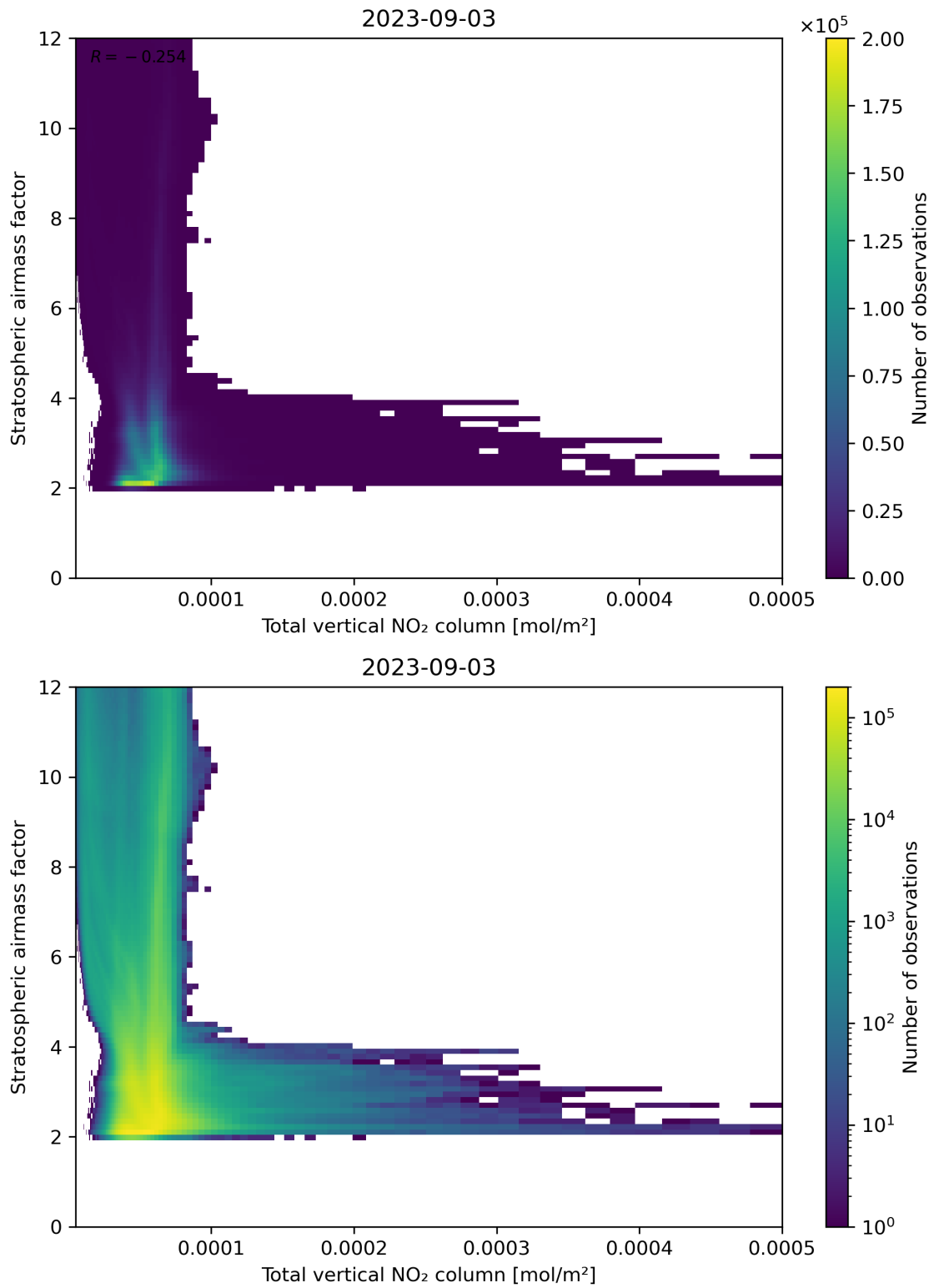
Figure 110: Scatter density plot of “Total vertical NO 2 column” against “Stratospheric airmass factor” for 2023-09-02 to 2023-09-04.
