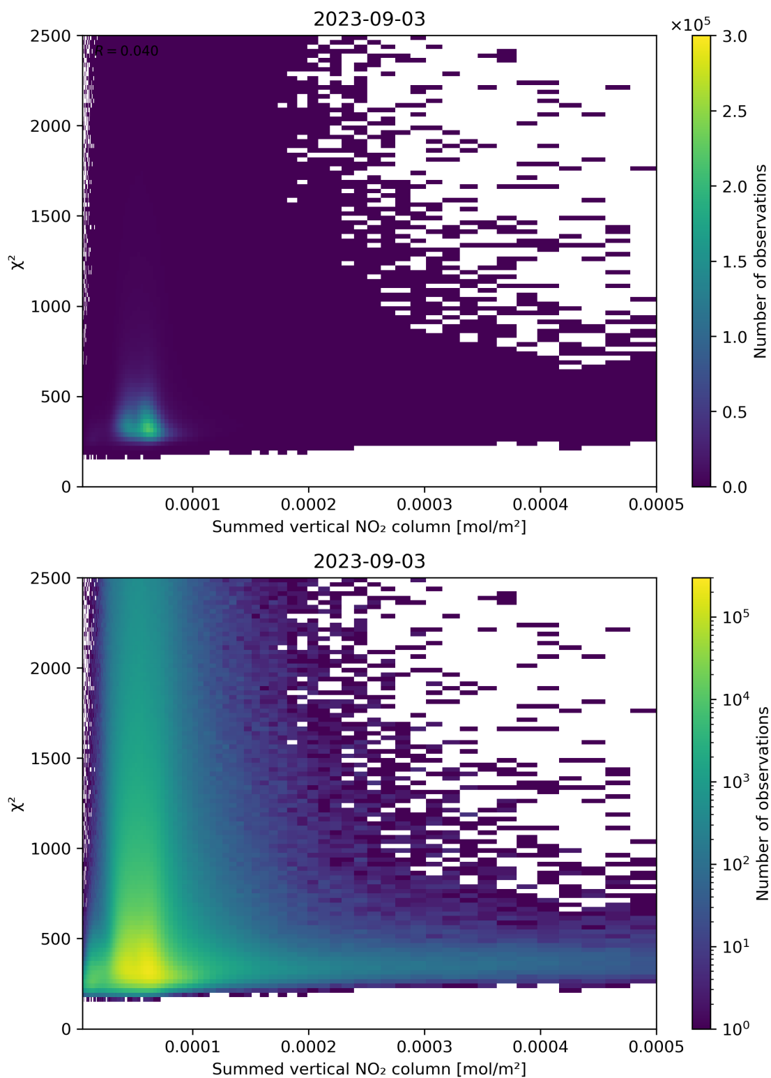
Figure 104: Scatter density plot of “Summed vertical NO 2 column” against “ \chi^2 ” for 2023-09-02 to 2023-09-04.
