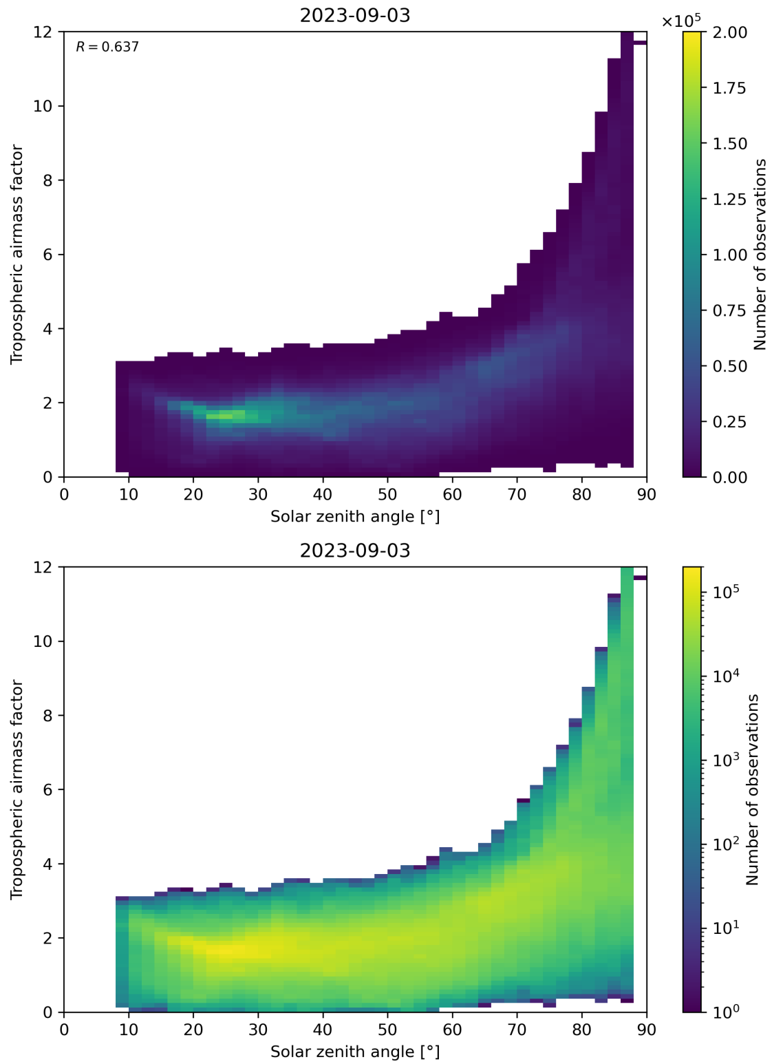
Figure 147: Scatter density plot of “Solar zenith angle” against “Tropospheric airmass factor” for 2023-09-02 to 2023-09-04.
