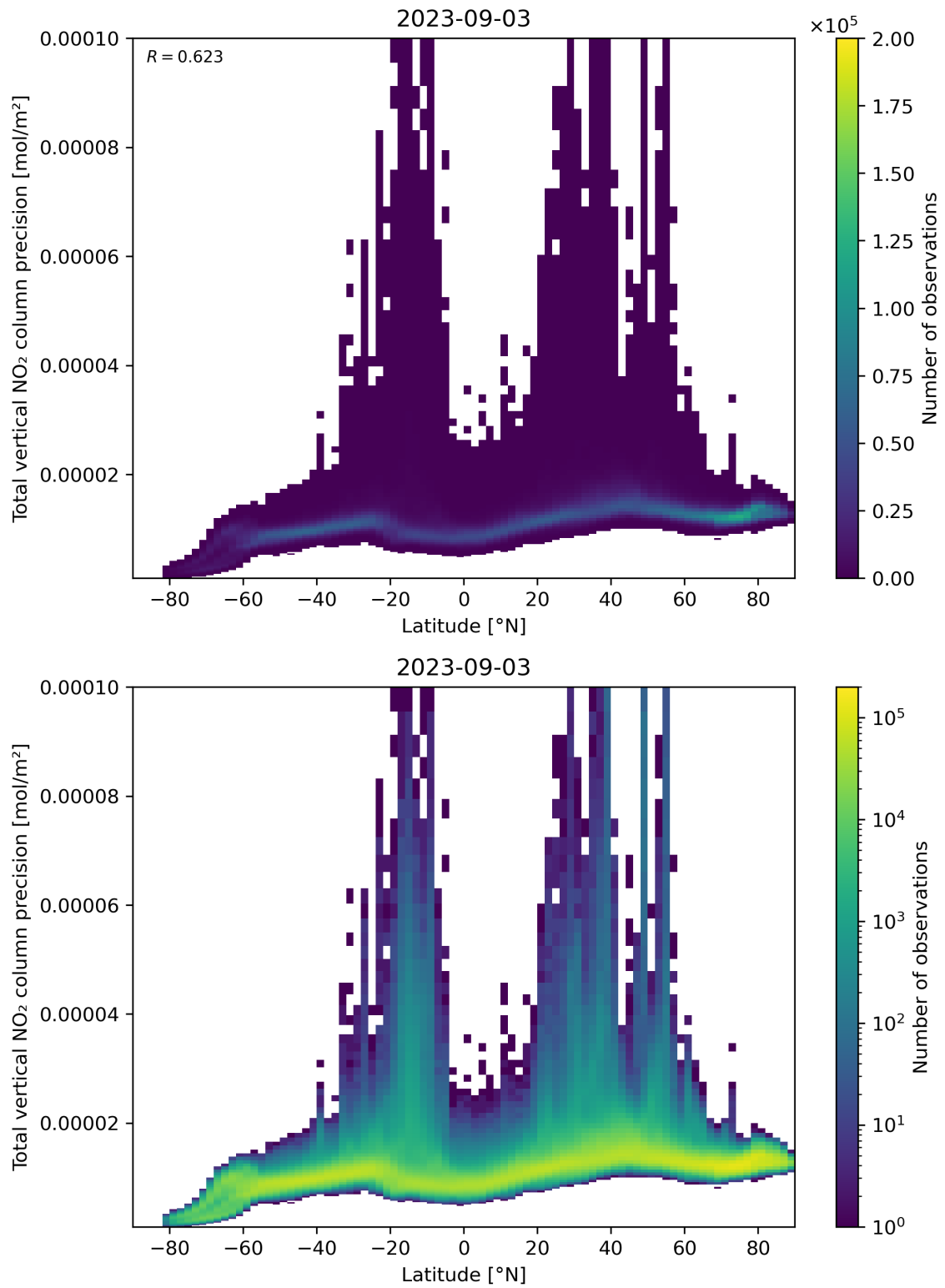
Figure 91: Scatter density plot of “Latitude” against “Total vertical NO 2 column precision” for 2023-09-02 to 2023-09-04.
