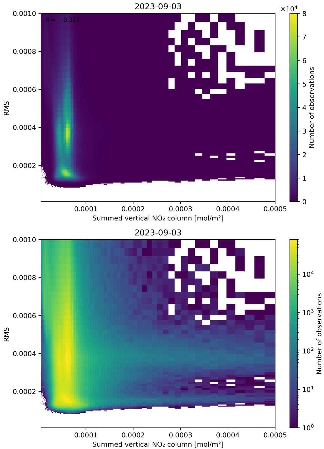
Figure 109: Scatter density plot of “Summed vertical NO 2 column” against “RMS” for 2023-09-02 to 2023-09-04.
