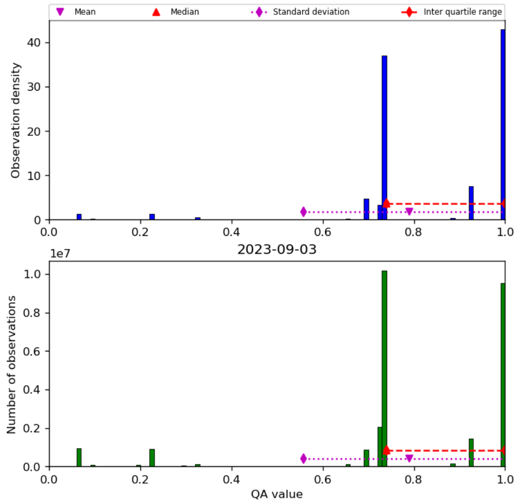
Figure 28: Histogram of “QA value” for 2023-09-02 to 2023-09-04
