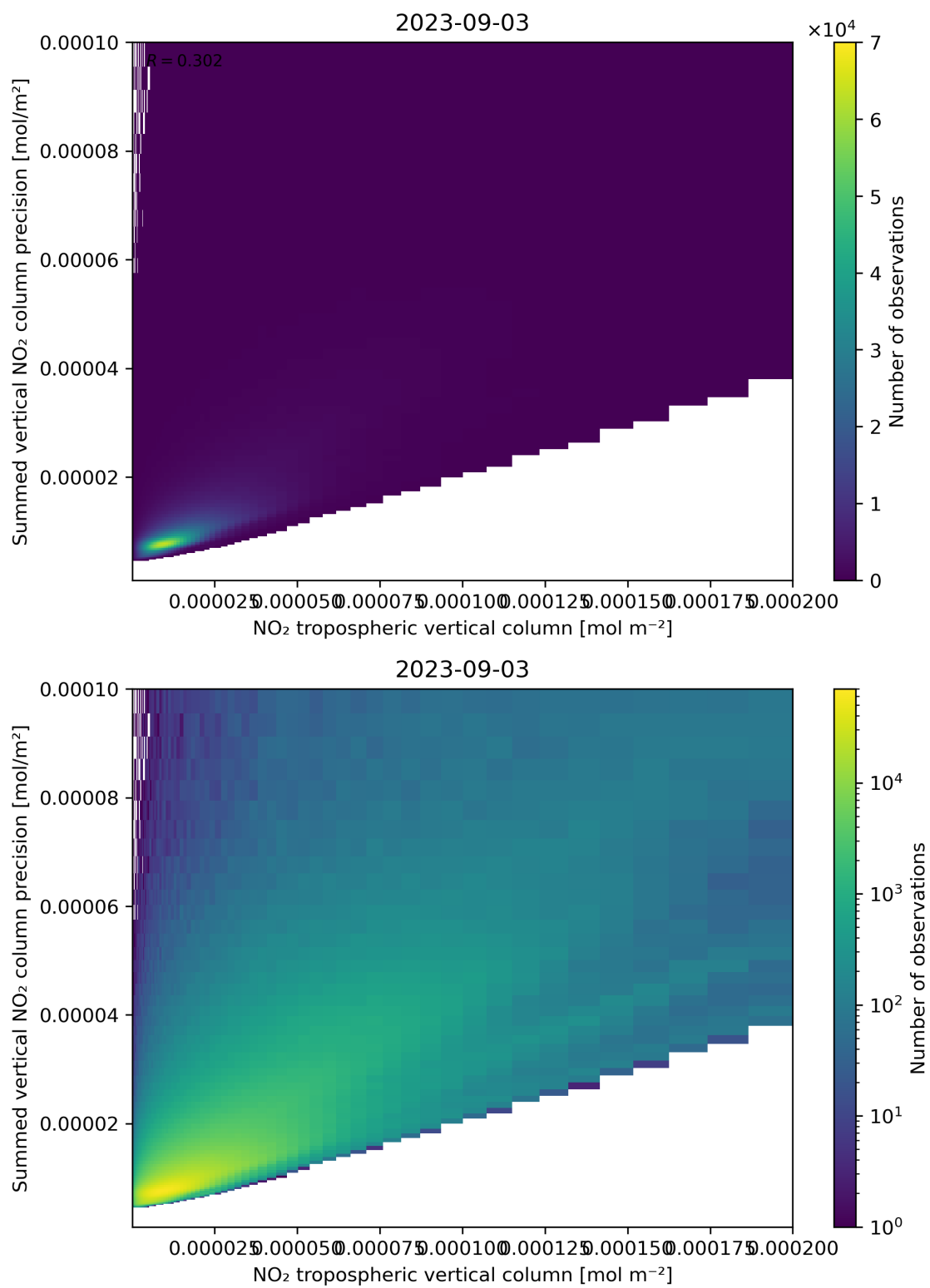
Figure 127: Scatter density plot of “NO 2 tropospheric vertical column” against “Summed vertical NO 2 column precision” for 2023-09-02 to 2023-09-04.
