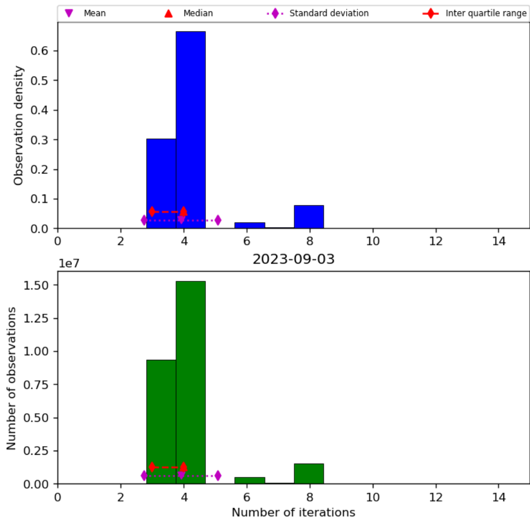
Figure 34: Histogram of “Number of iterations” for 2023-09-02 to 2023-09-04
