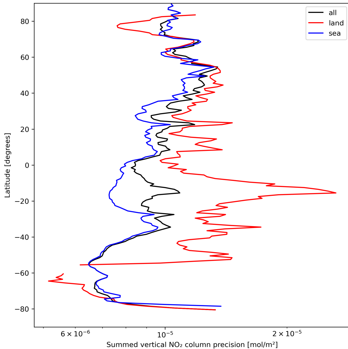
Figure 24: Zonal average of “Summed vertical NO 2 column precision” for 2023-09-02 to 2023-09-04.
