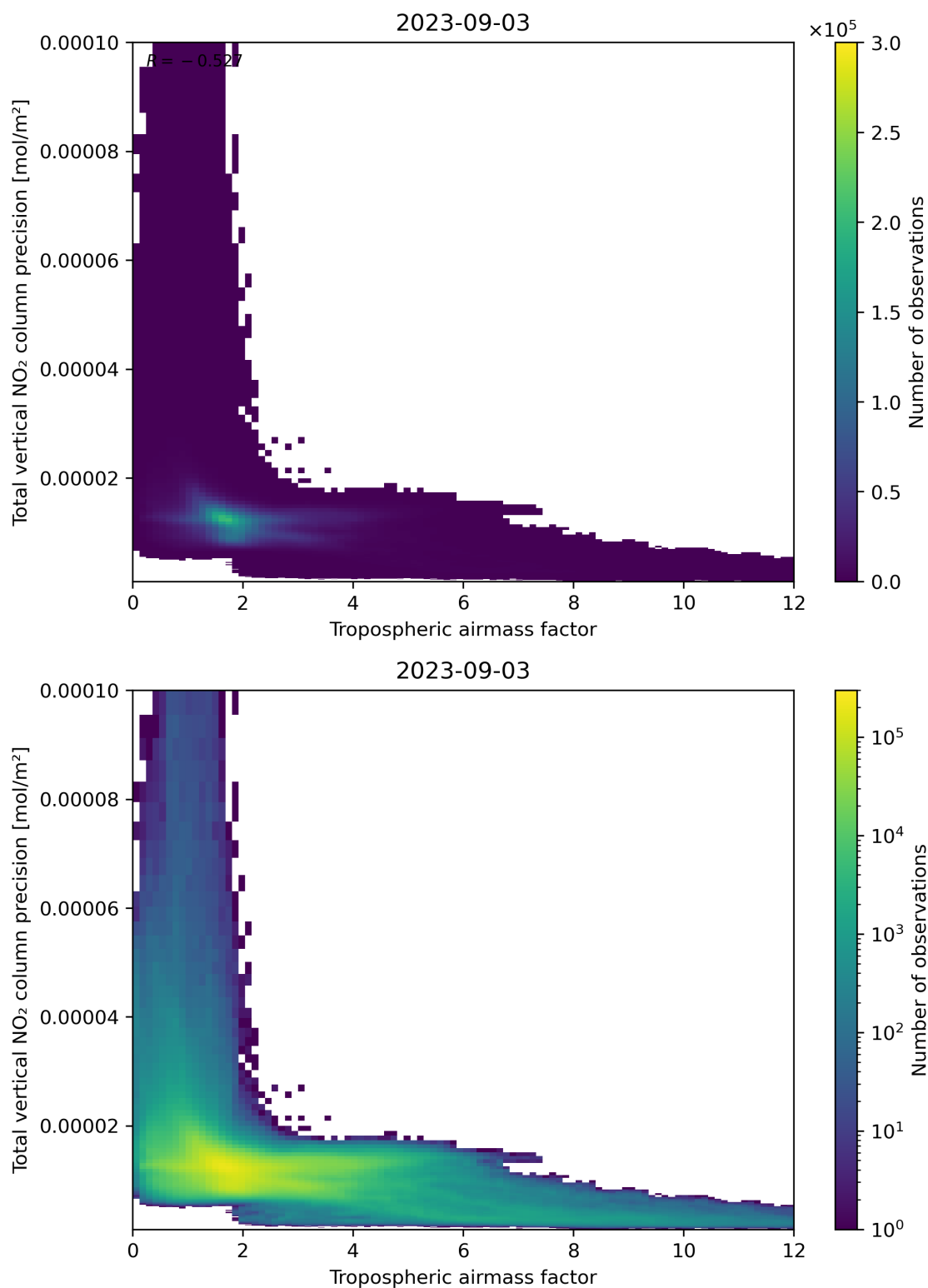
Figure 78: Scatter density plot of “Tropospheric air mass factor” against “Total vertical NO 2 column precision” for 2023-09-02 to 2023-09-04.
