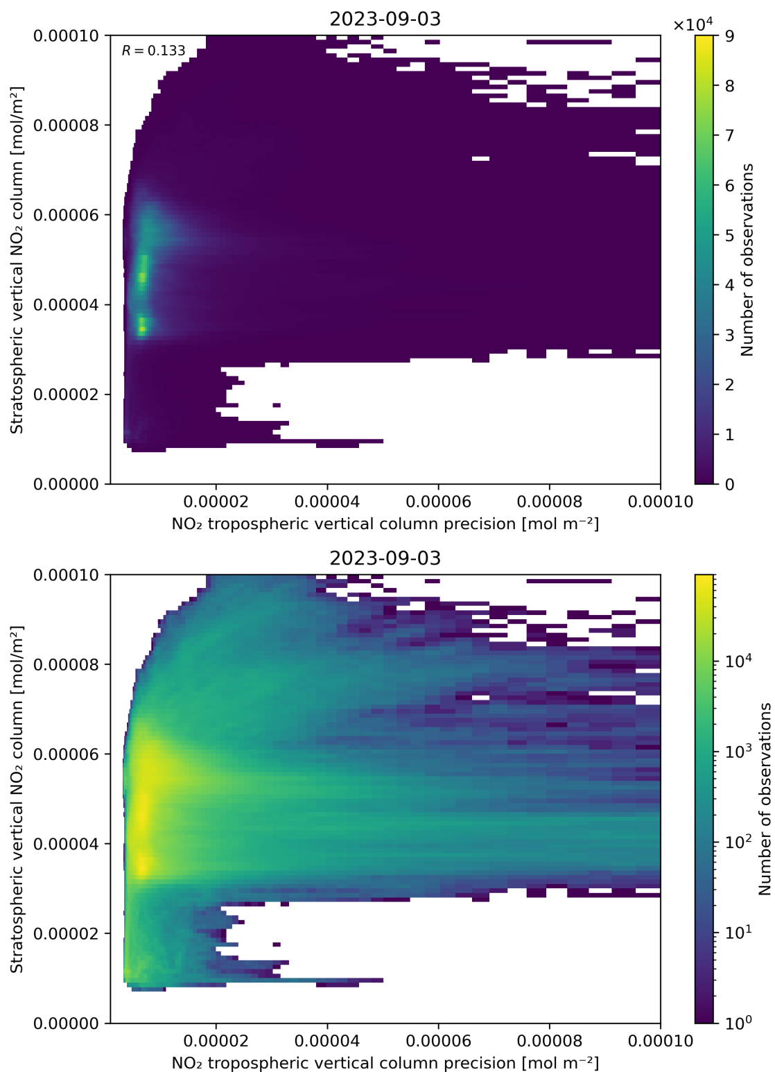
Figure 135: Scatter density plot of “NO 2 tropospheric vertical column precision” against “Stratospheric vertical NO 2 column” for 2023-09-02 to 2023-09-04.
