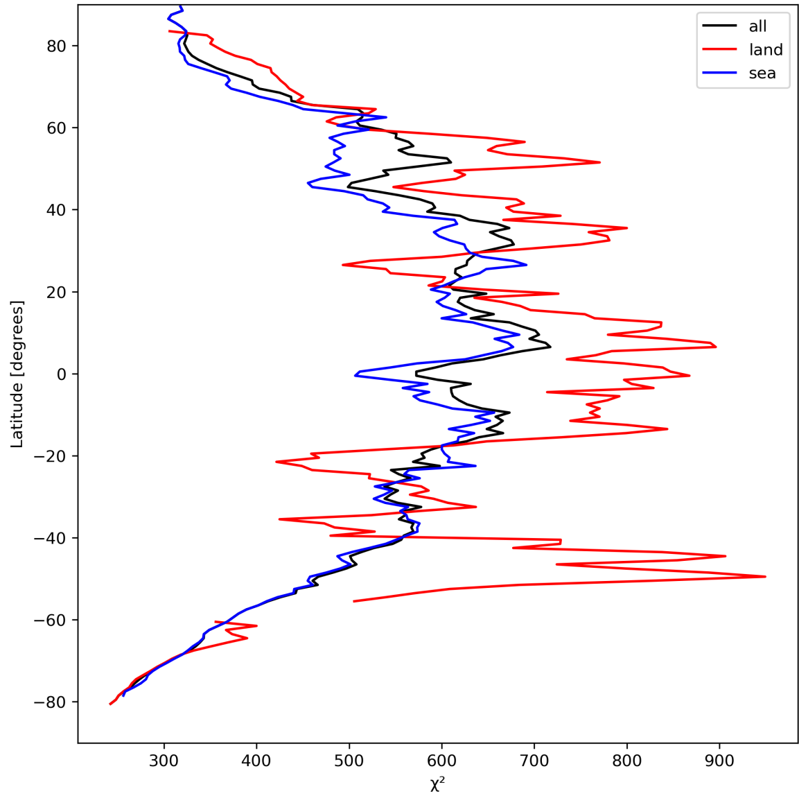
Figure 25: Zonal average of “ \chi^2 ” for 2023-09-02 to 2023-09-04.
