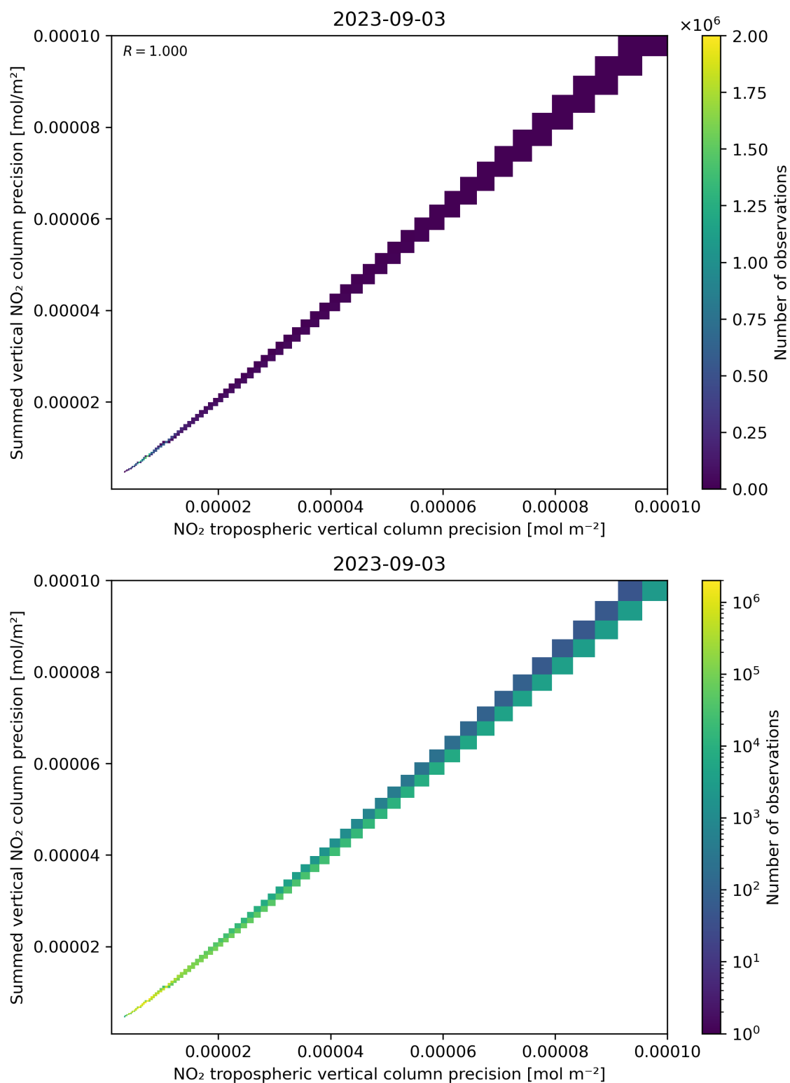
Figure 137: Scatter density plot of “NO 2 tropospheric vertical column precision” against “Summed vertical NO 2 column precision” for 2023-09-02 to 2023-09-04.
