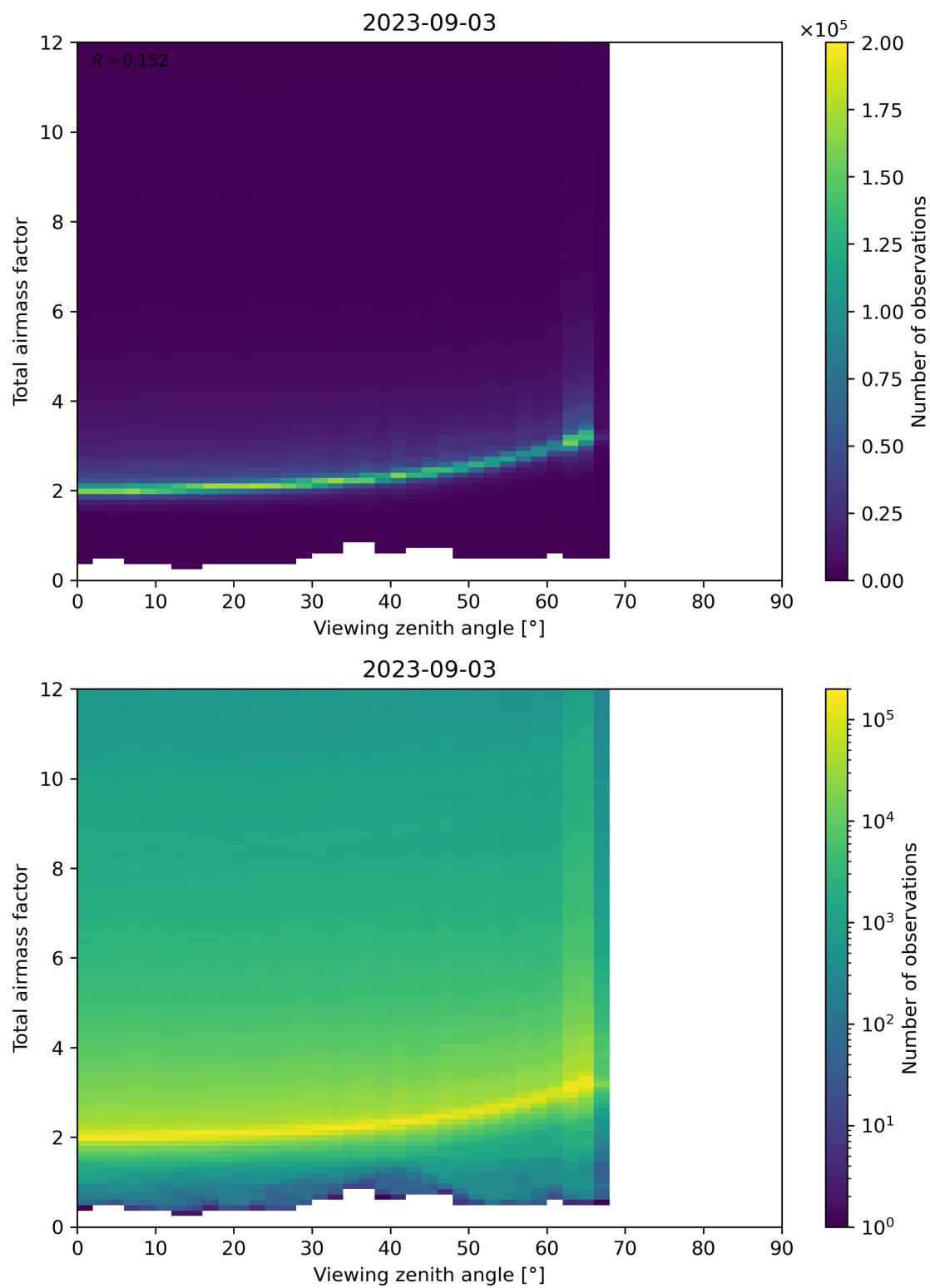
Figure 160: Scatter density plot of “Viewing zenith angle” against “Total airmass factor” for 2023-09-02 to 2023-09-04.
