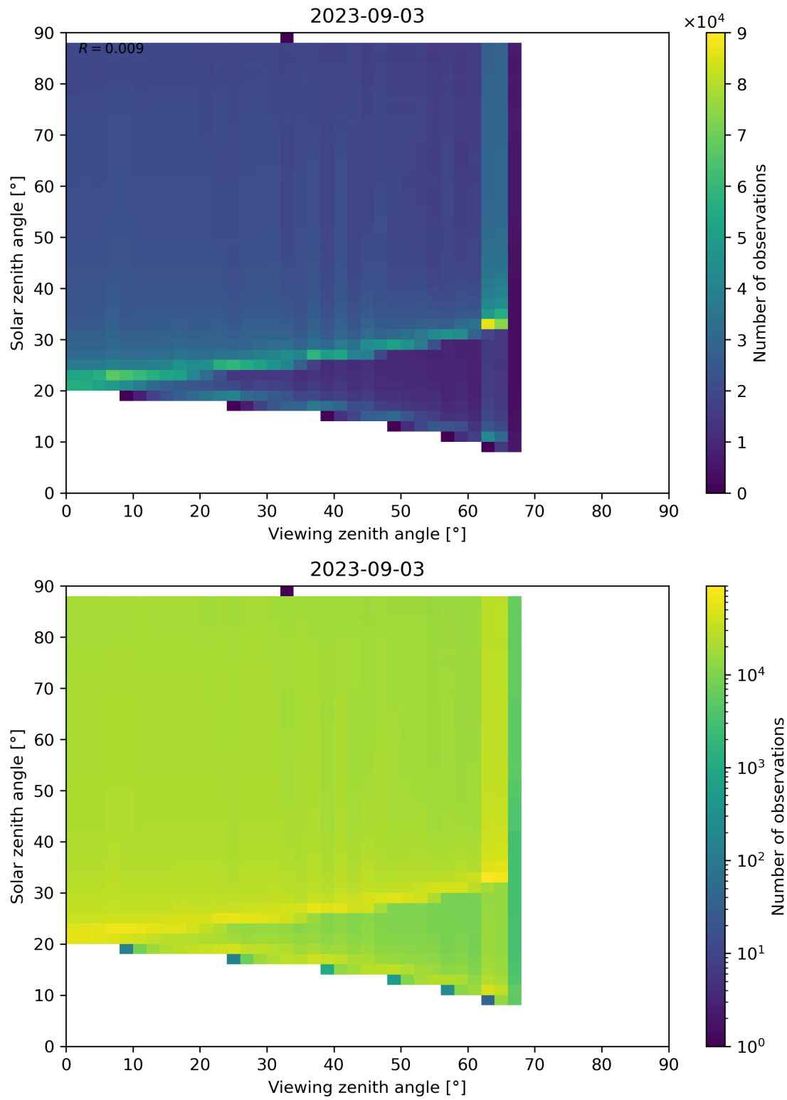
Figure 172: Scatter density plot of “Viewing zenith angle” against “Solar zenith angle” for 2023-09-02 to 2023-09-04.
