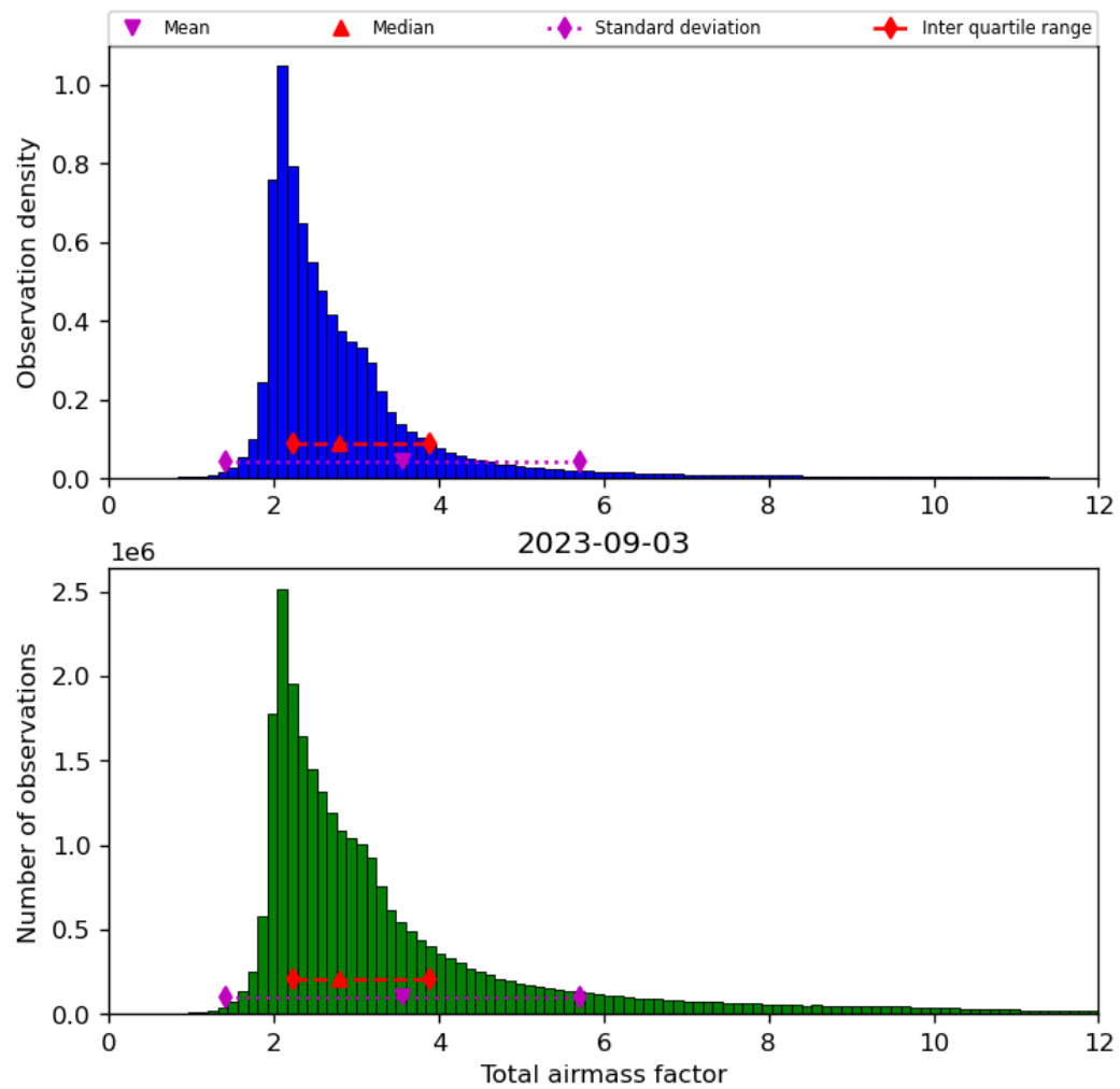
Figure 32: Histogram of “Total airmass factor” for 2023-09-02 to 2023-09-04
