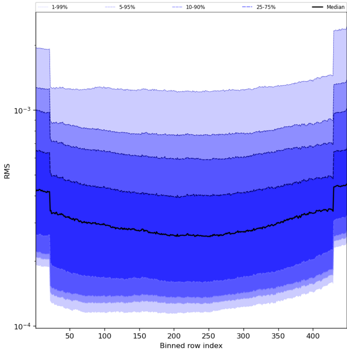
Figure 60: Along track statistics of “RMS” for 2023-09-02 to 2023-09-04
