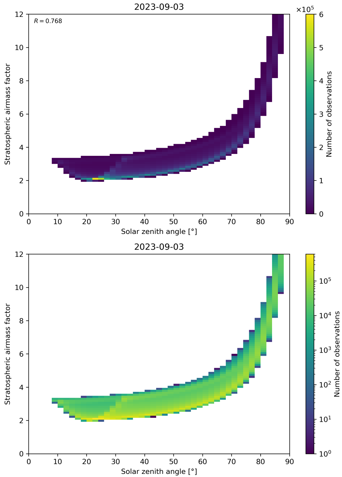
Figure 145: Scatter density plot of “Solar zenith angle” against “Stratospheric airmass factor” for 2023-09-02 to 2023-09-04.
