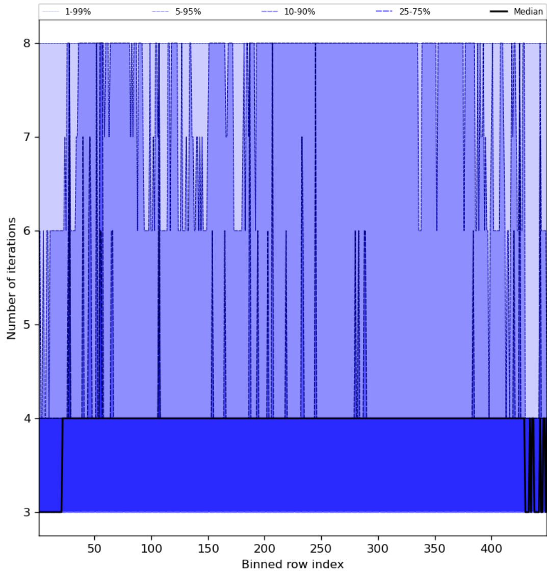
Figure 51: Along track statistics of “Number of iterations” for 2023-09-02 to 2023-09-04
