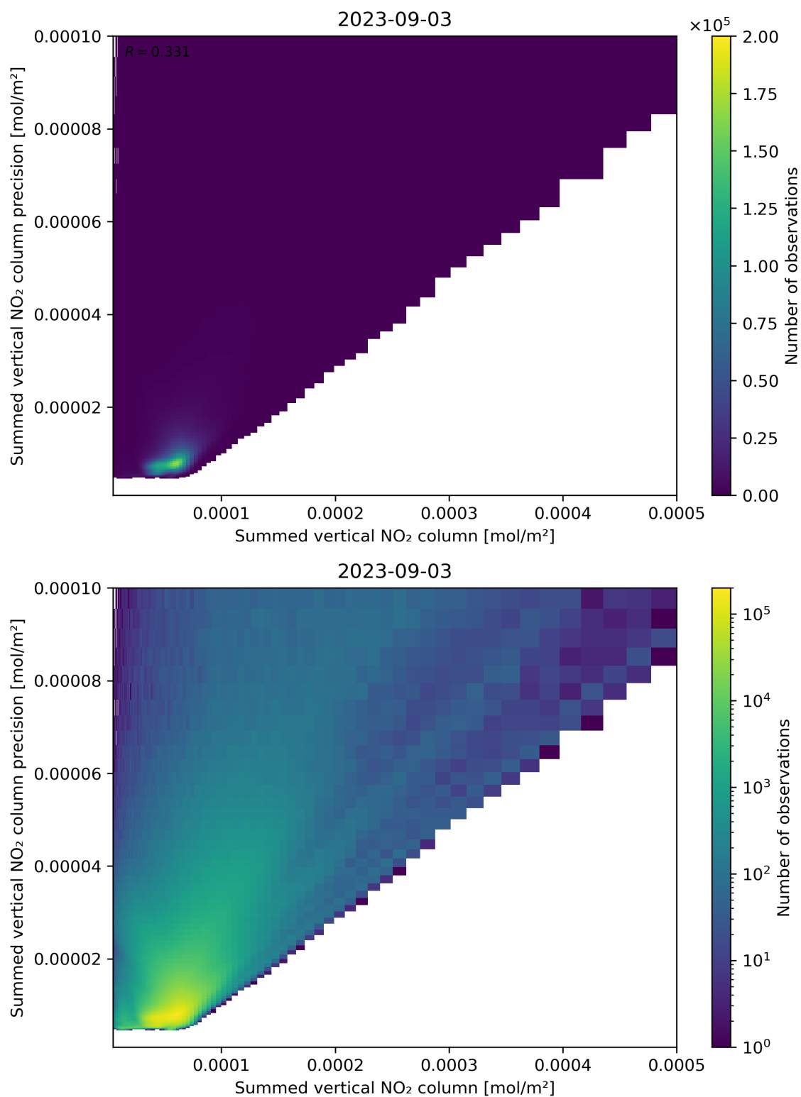
Figure 105: Scatter density plot of “Summed vertical NO 2 column” against “Summed vertical NO 2 column precision” for 2023-09-02 to 2023-09-04.
