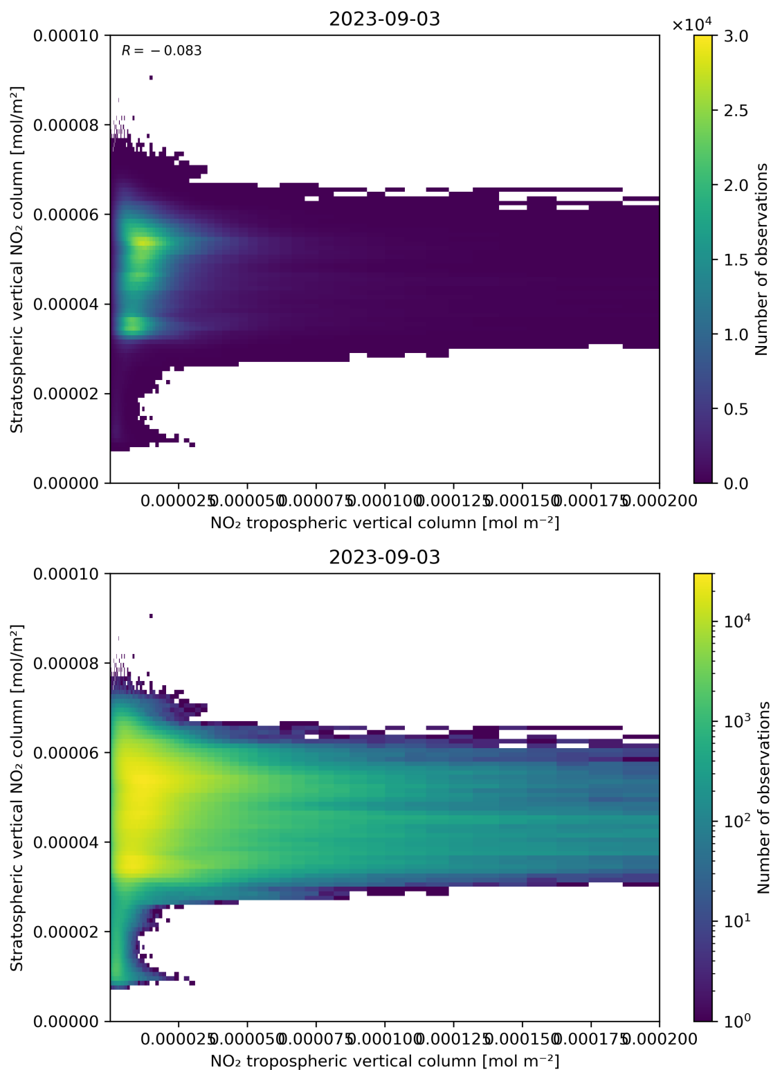
Figure 125: Scatter density plot of “NO 2 tropospheric vertical column” against “Stratospheric vertical NO 2 column” for 2023-09-02 to 2023-09-04.
