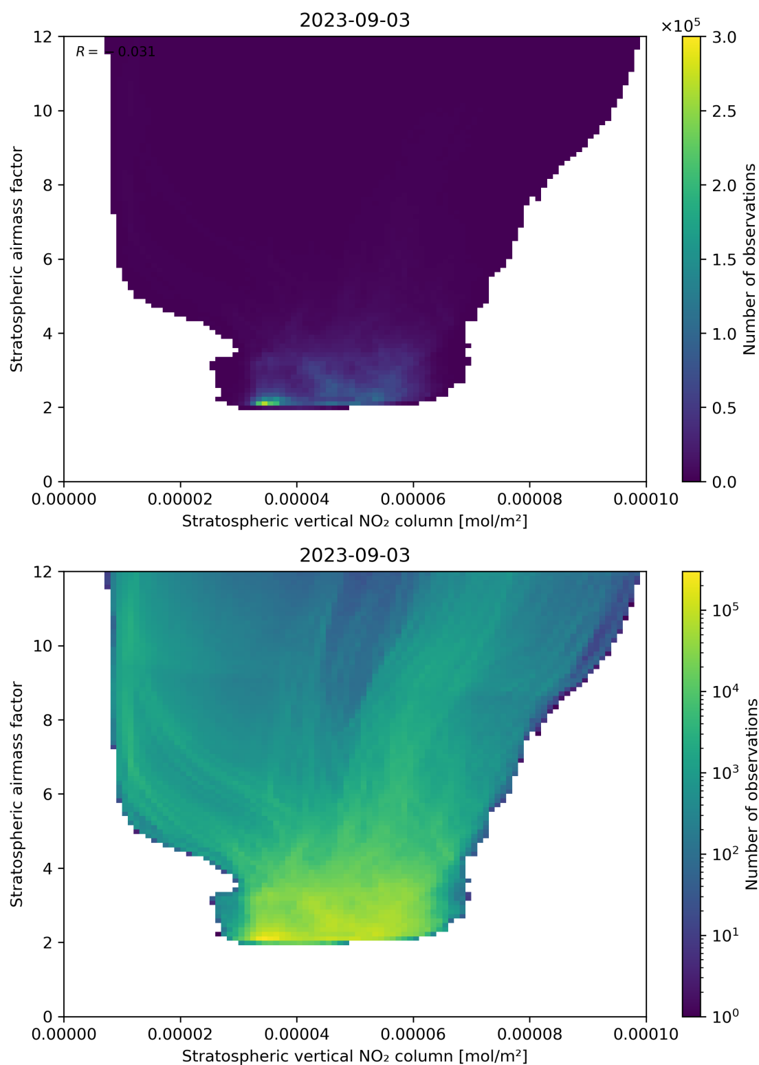
Figure 96: Scatter density plot of “Stratospheric vertical NO 2 column” against “Stratospheric airmass factor” for 2023-09-02 to 2023-09-04.
