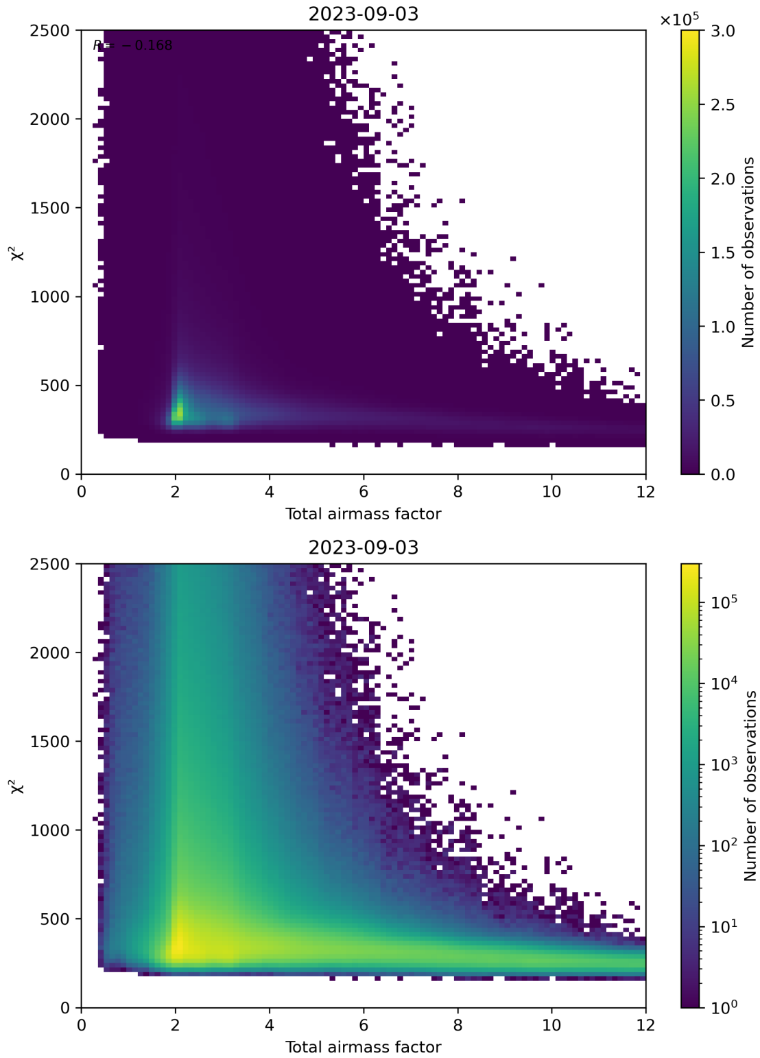
Figure 63: Scatter density plot of “Total airmass factor” against “ \chi^2 ” for 2023-09-02 to 2023-09-04.
