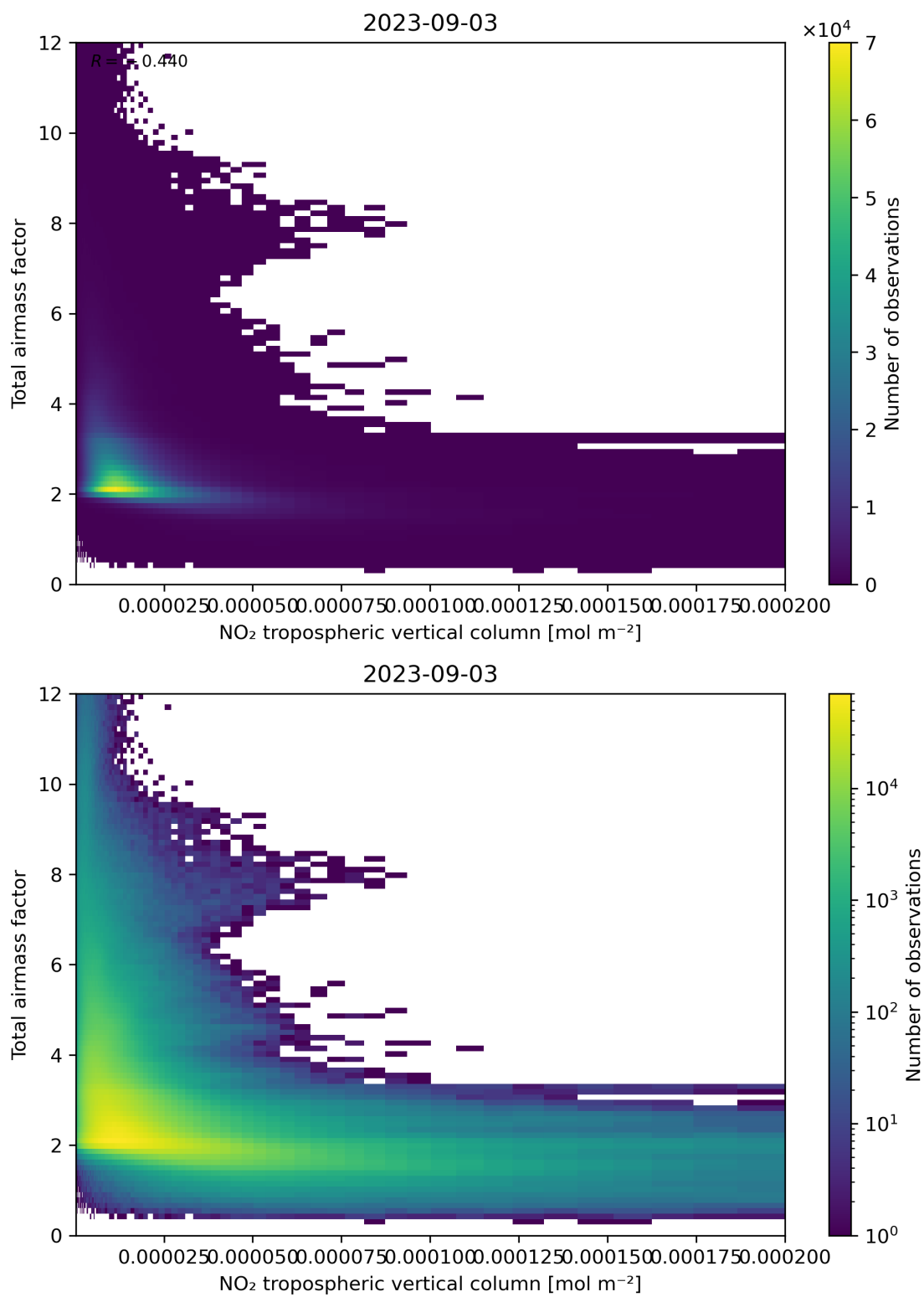
Figure 122: Scatter density plot of “NO 2 tropospheric vertical column” against “Total air mass factor” for 2023-09-02 to 2023-09-04.
