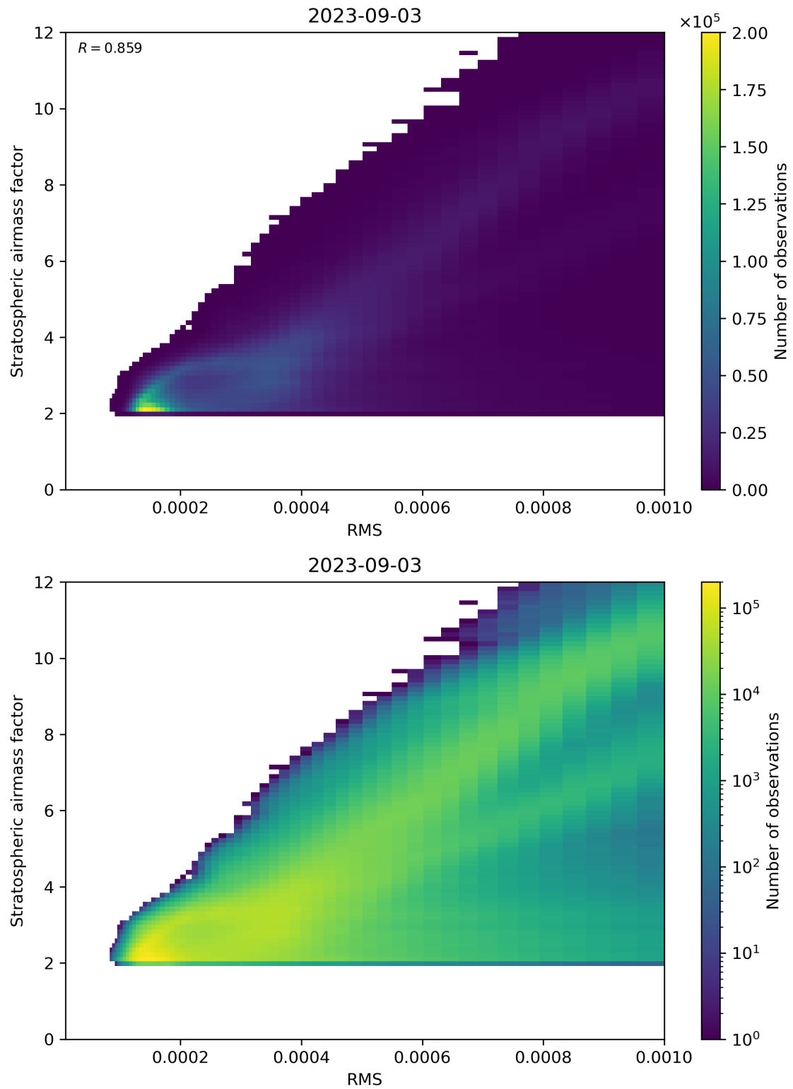
Figure 144: Scatter density plot of “RMS” against “Stratospheric airmass factor” for 2023-09-02 to 2023-09-04.
