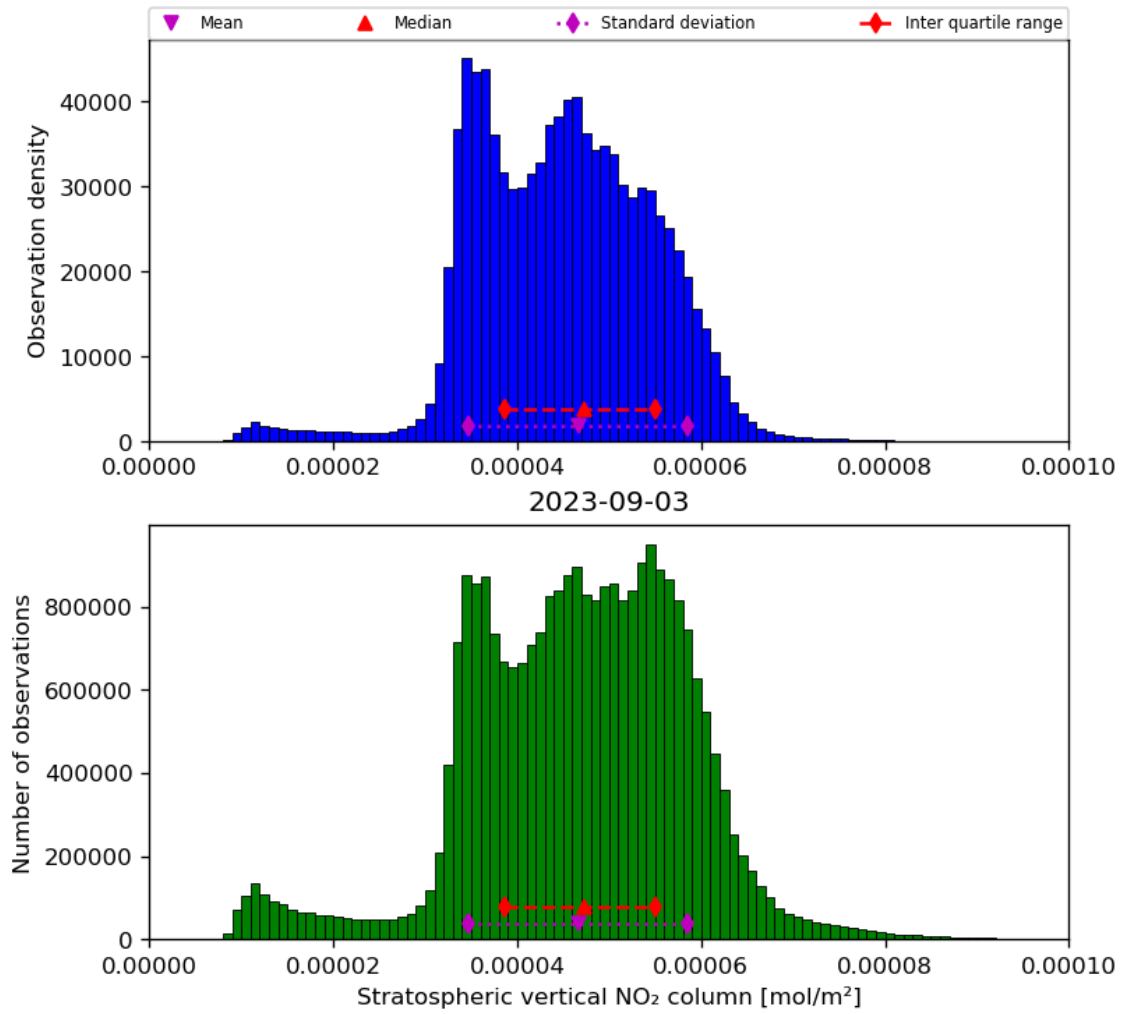
Figure 36: Histogram of “Stratospheric vertical NO 2 column” for 2023-09-02 to 2023-09-04
