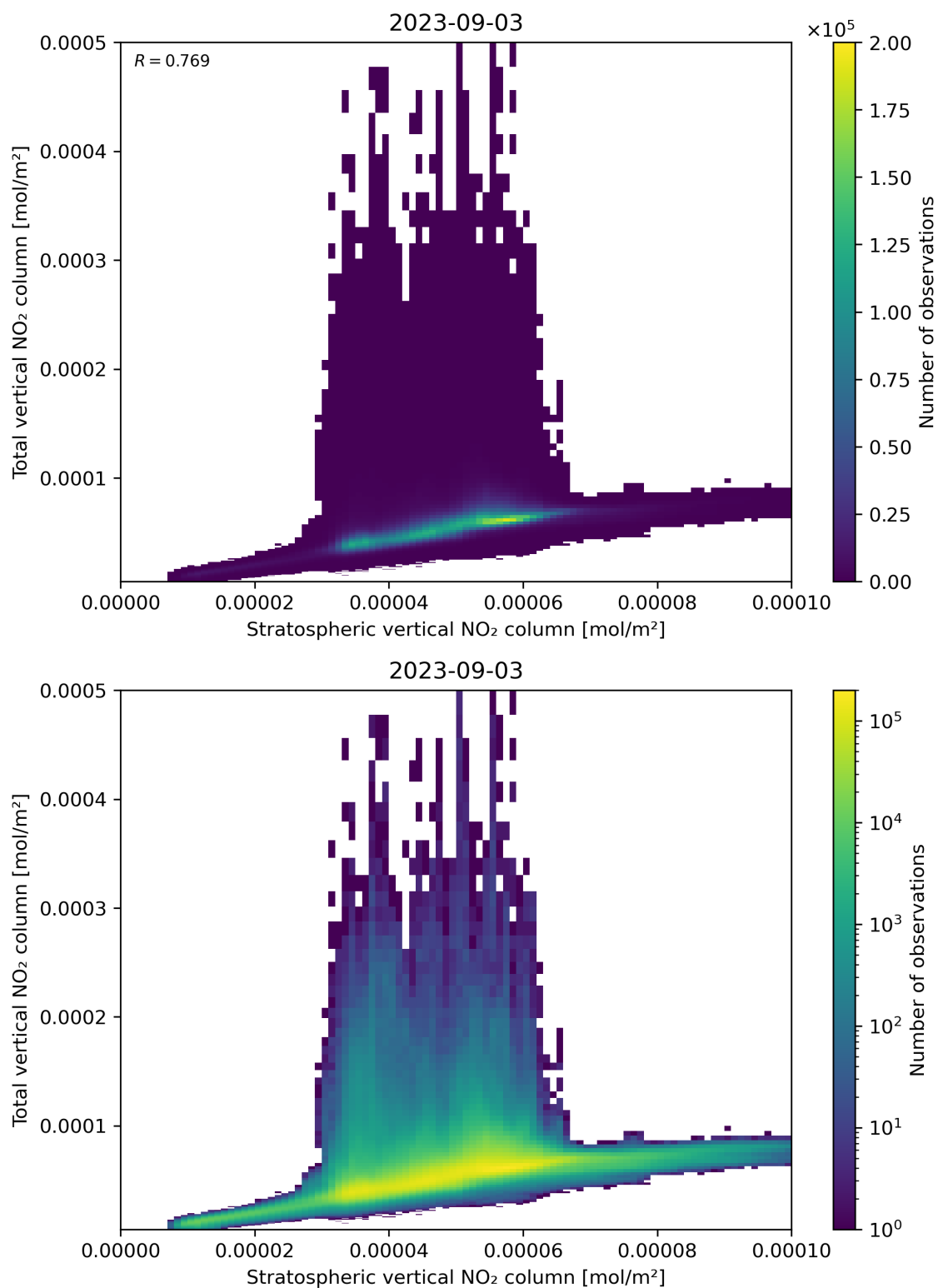
Figure 100: Scatter density plot of “Stratospheric vertical NO 2 column” against “Total vertical NO 2 column” for 2023-09-02 to 2023-09-04.
