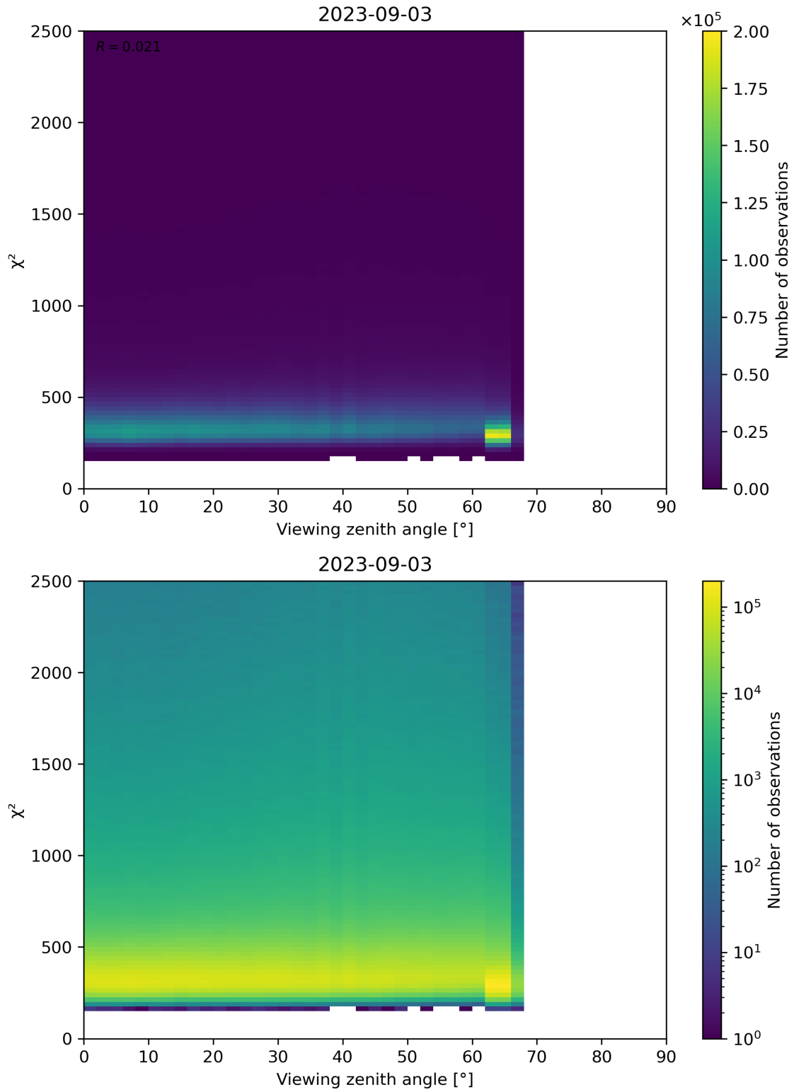
Figure 162: Scatter density plot of “Viewing zenith angle” against “ \chi^2 ” for 2023-09-02 to 2023-09-04.
