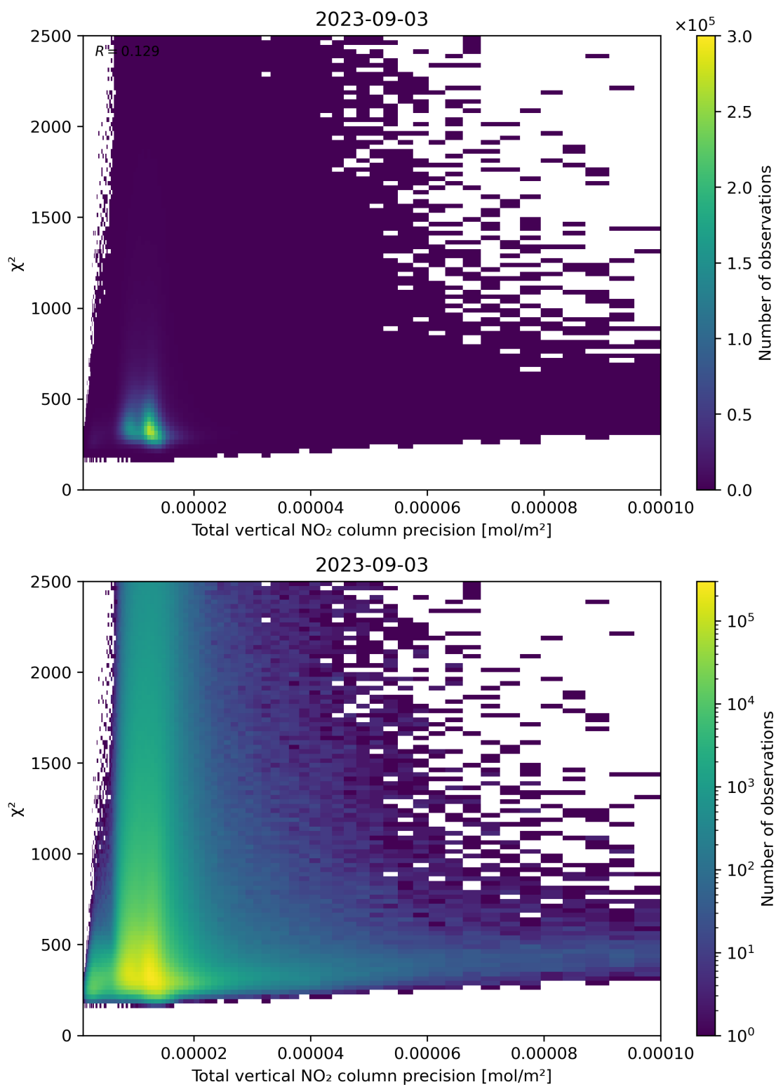
Figure 116: Scatter density plot of “Total vertical NO 2 column precision” against “ \chi^2 ” for 2023-09-02 to 2023-09-04.
