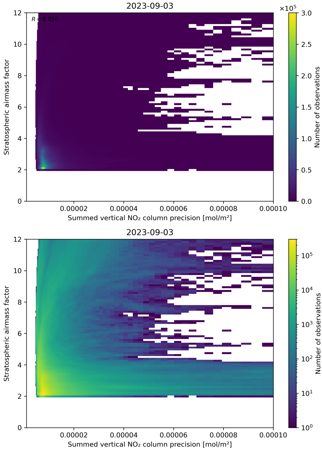
Figure 106: Scatter density plot of “Summed vertical NO 2 column precision” against “Stratospheric airmass factor” for 2023-09-02 to 2023-09-04.
