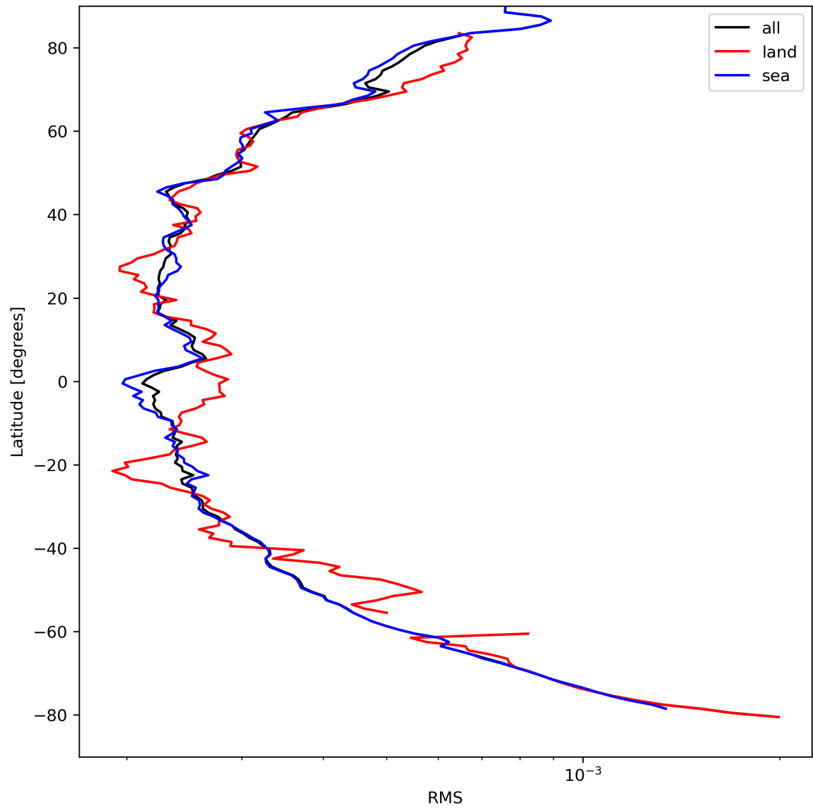
Figure 26: Zonal average of “RMS” for 2023-09-02 to 2023-09-04.
