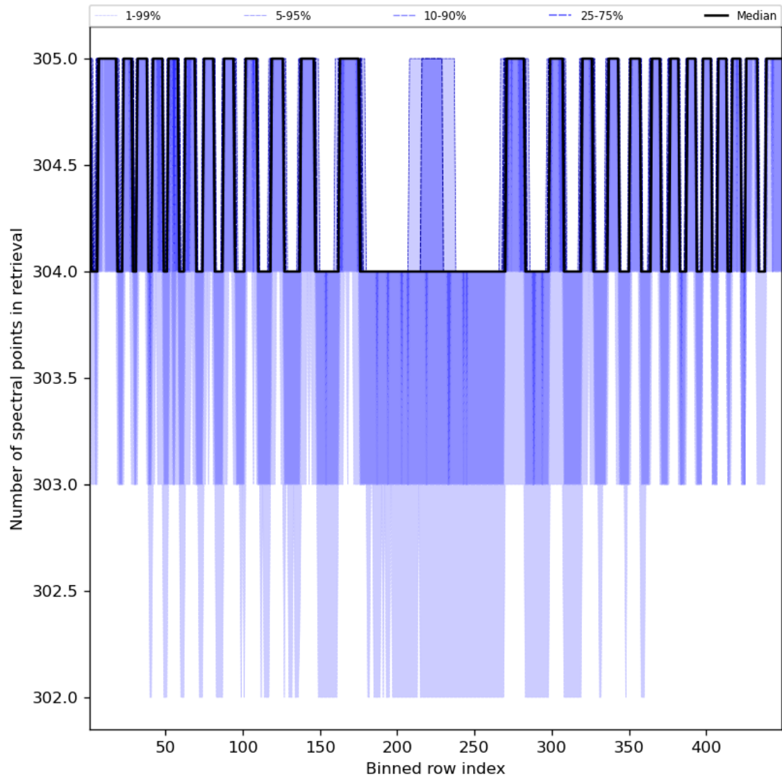
Figure 50: Along track statistics of “Number of spectral points in retrieval” for 2023-09-02 to 2023-09-04
