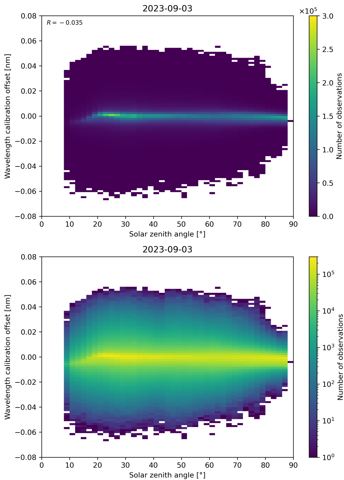
Figure 158: Scatter density plot of “Solar zenith angle” against “Wavelength calibration offset” for 2023-09-02 to 2023-09-04.
