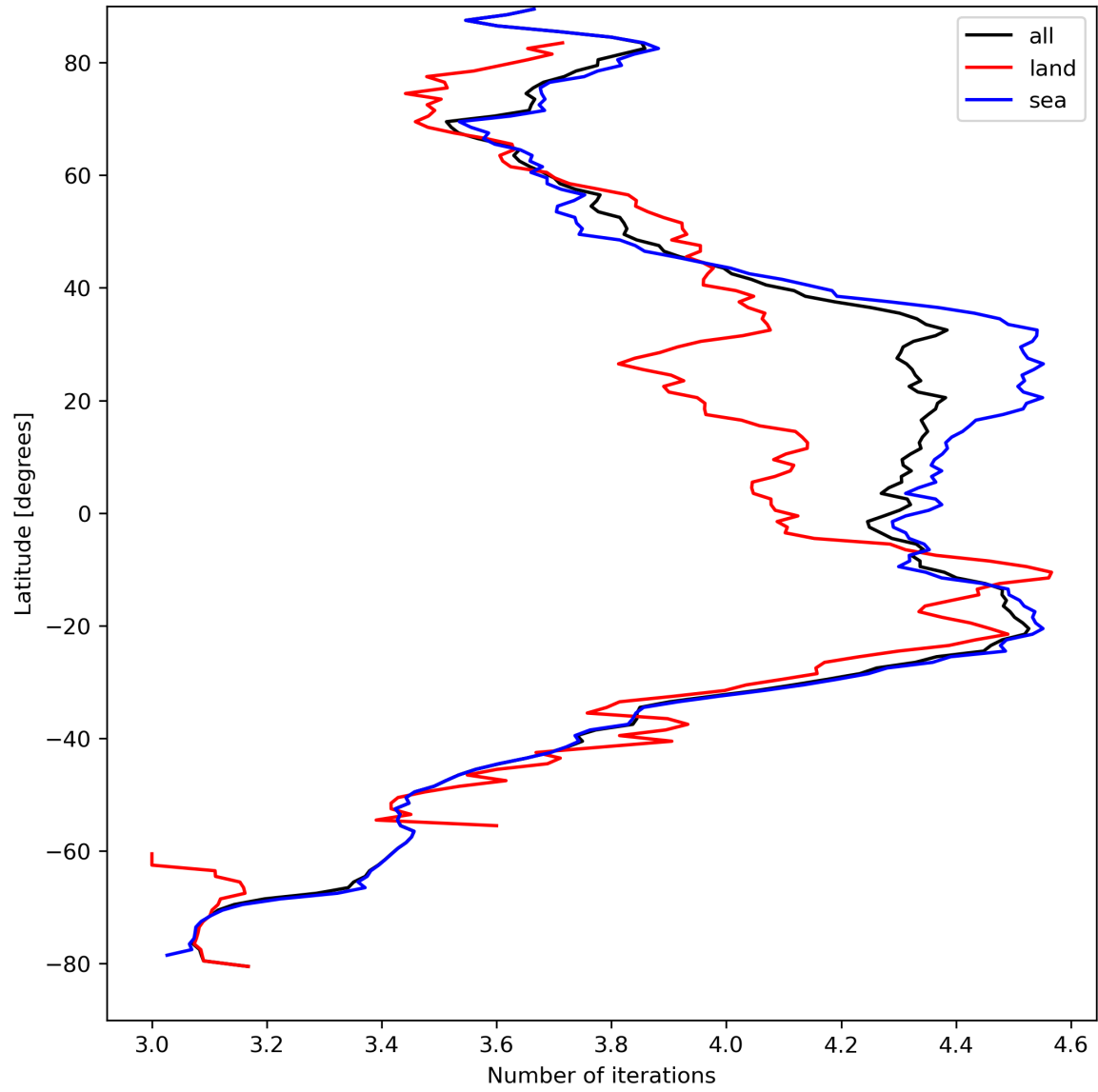
Figure 17: Zonal average of “Number of iterations” for 2023-09-02 to 2023-09-04.
