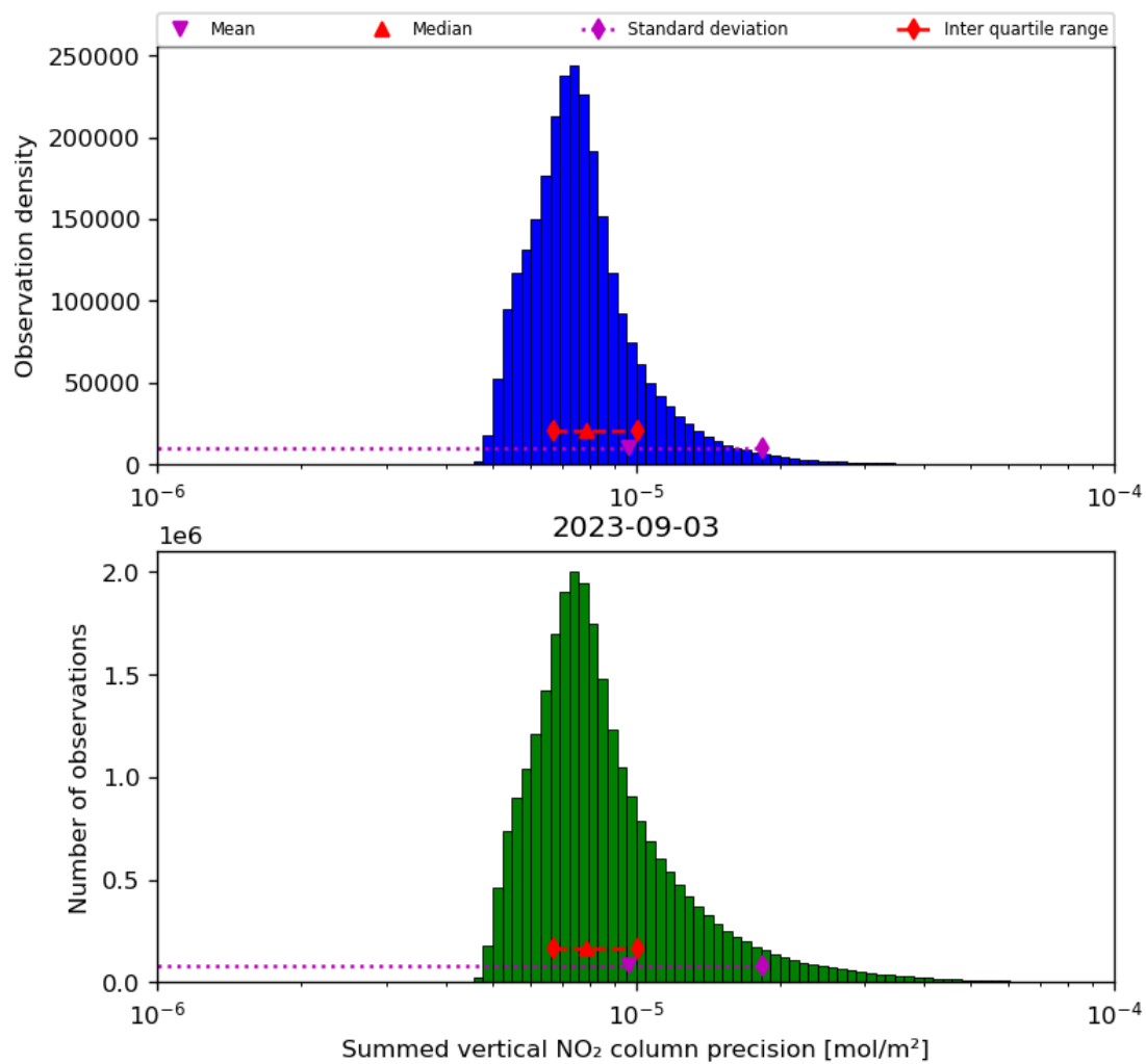
Figure 41: Histogram of "Summed vertical NO 2 column precision" for 2023-09-02 to 2023-09-04
