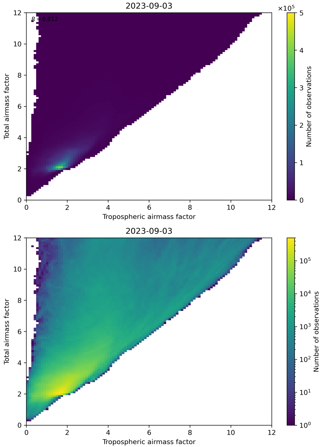
Figure 72: Scatter density plot of “Tropospheric airmass factor” against “Total airmass factor” for 2023-09-02 to 2023-09-04.
