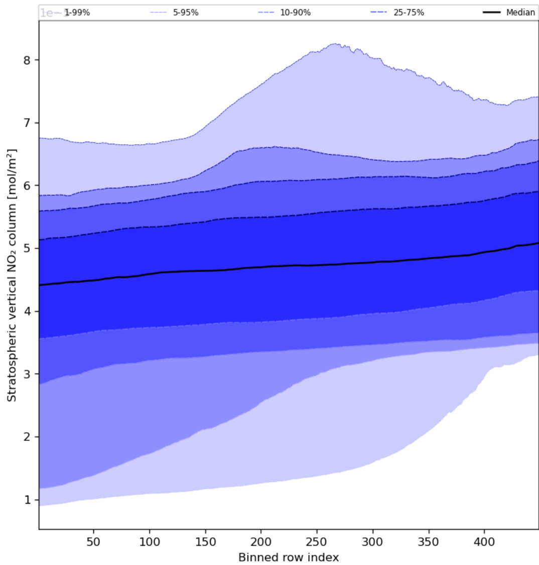
Figure 53: Along track statistics of “Stratospheric vertical NO 2 column” for 2023-09-02 to 2023-09-04
