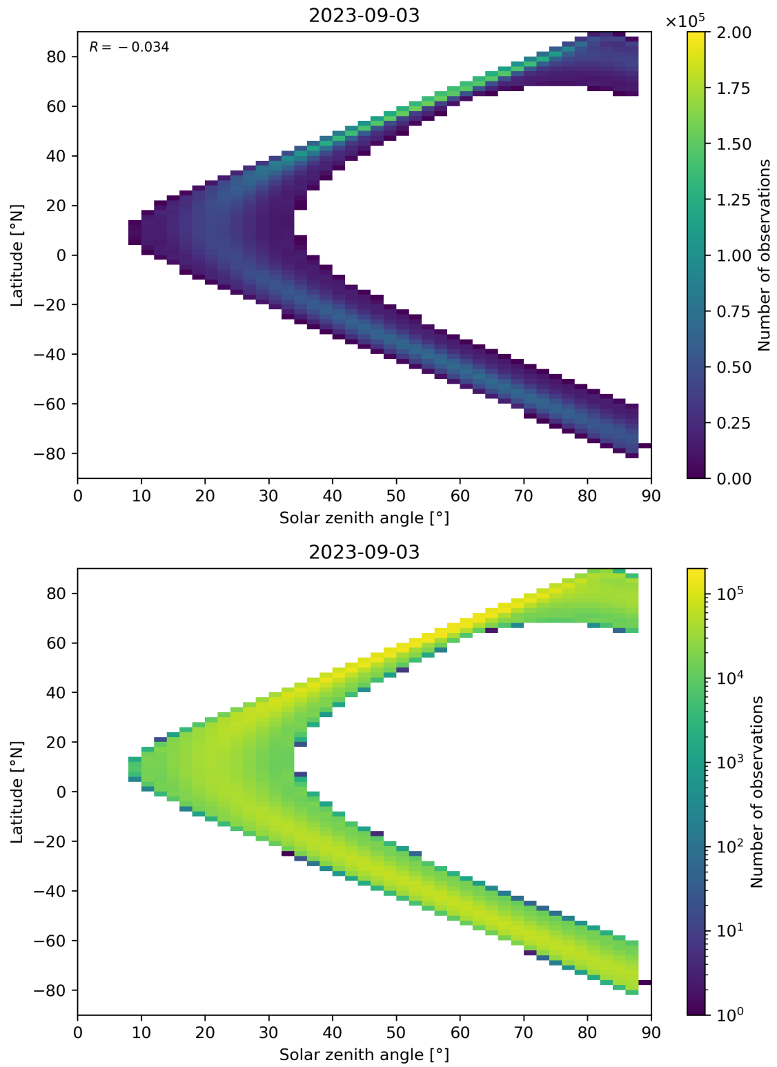
Figure 149: Scatter density plot of “Solar zenith angle” against “Latitude” for 2023-09-02 to 2023-09-04.
