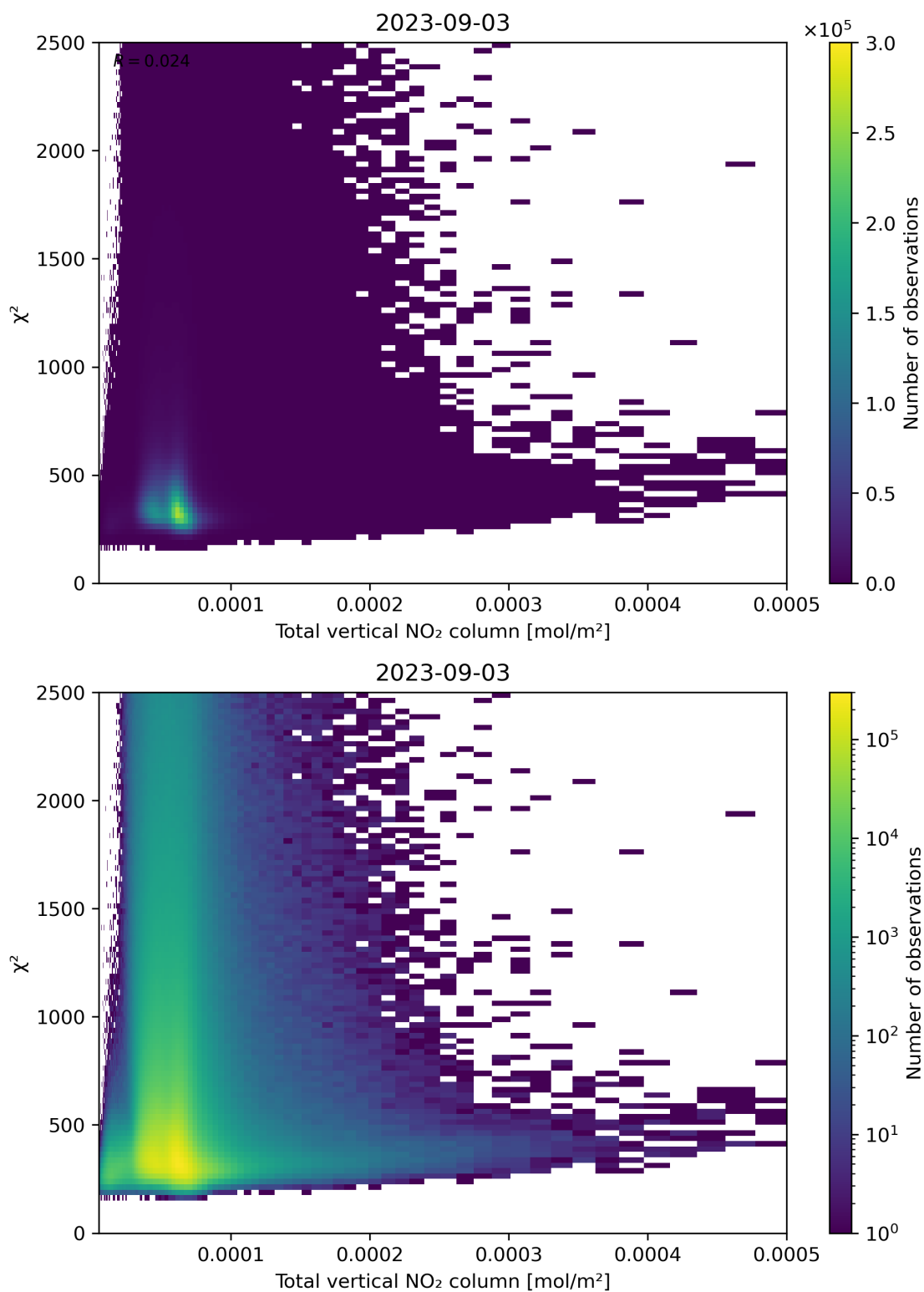
Figure 111: Scatter density plot of “Total vertical NO 2 column” against “ \chi^2 ” for 2023-09-02 to 2023-09-04.
