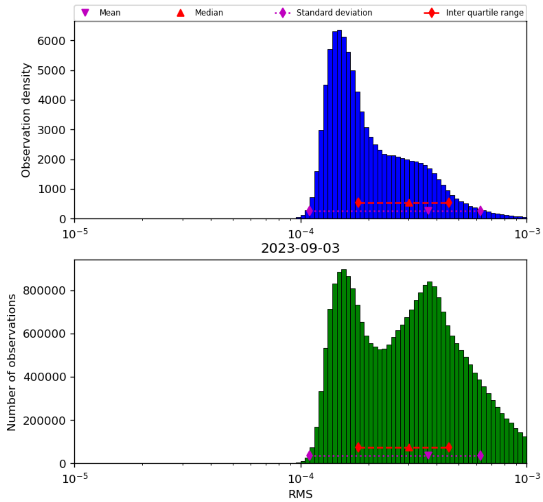
Figure 43: Histogram of “RMS” for 2023-09-02 to 2023-09-04
