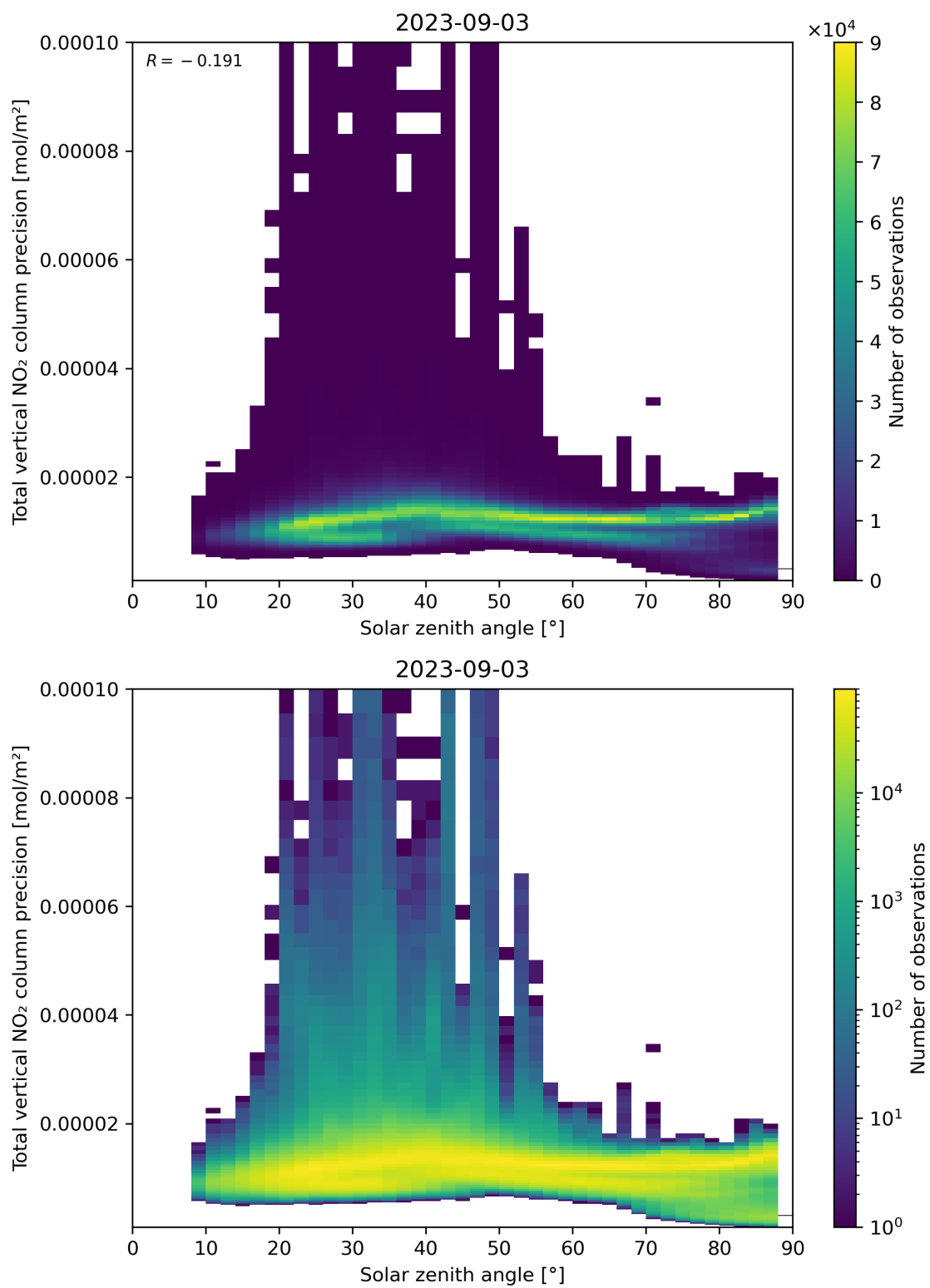
Figure 154: Scatter density plot of “Solar zenith angle” against “Total vertical NO 2 column precision” for 2023-09-02 to 2023-09-04.
