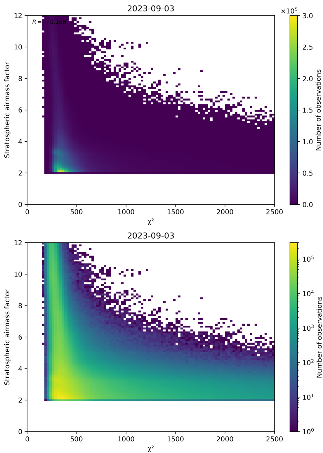
Figure 81: Scatter density plot of “ \chi^2 ” against “Stratospheric airmass factor” for 2023-09-02 to 2023-09-04.
