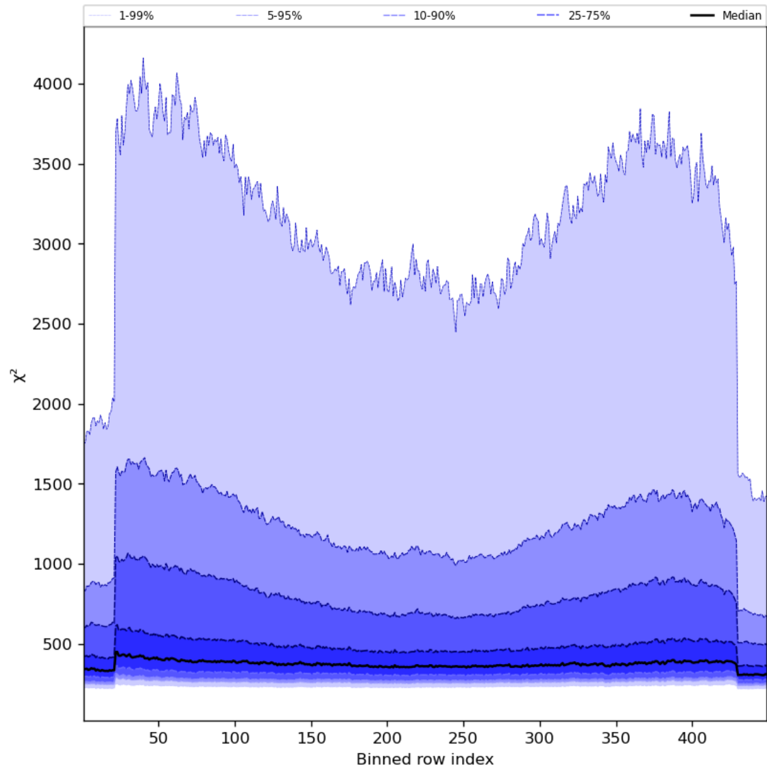
Figure 59: Along track statistics of “ \chi^2 ” for 2023-09-02 to 2023-09-04
