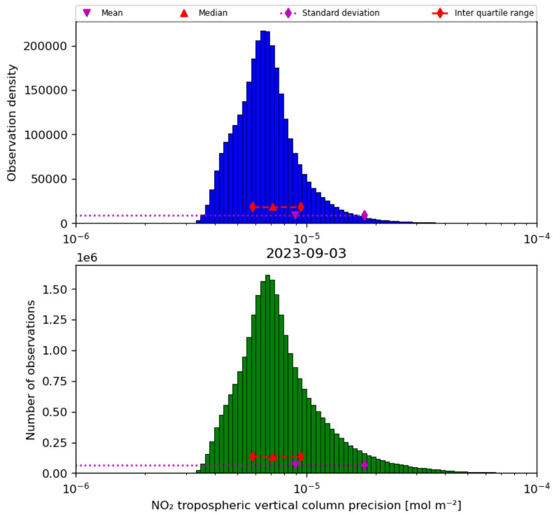
Figure 30: Histogram of “NO 2 tropospheric vertical column precision” for 2023-09-02 to 2023-09-04
