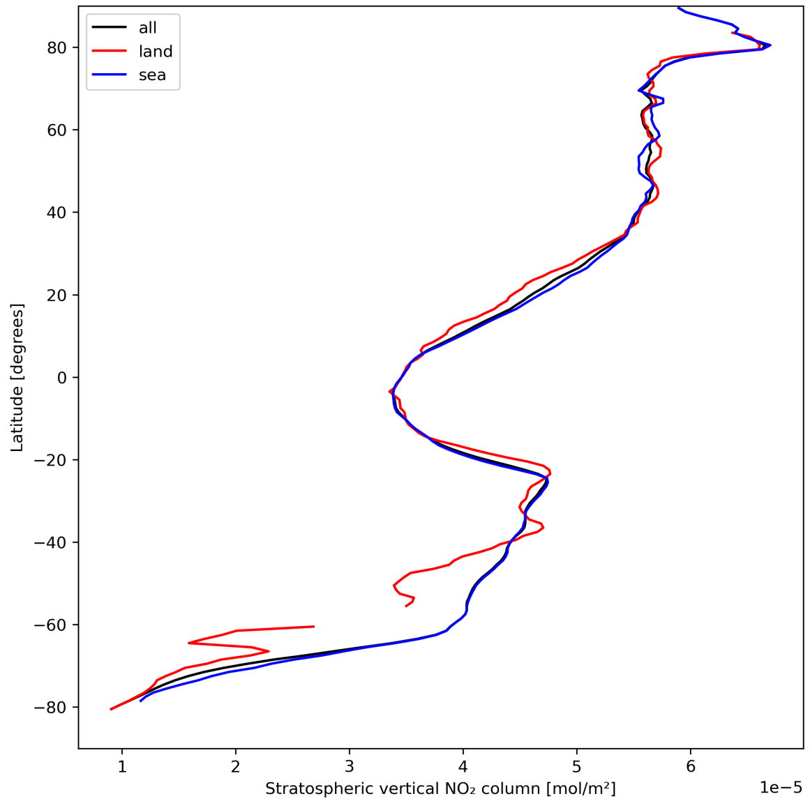
Figure 19: Zonal average of “Stratospheric vertical NO 2 column” for 2023-09-02 to 2023-09-04.
