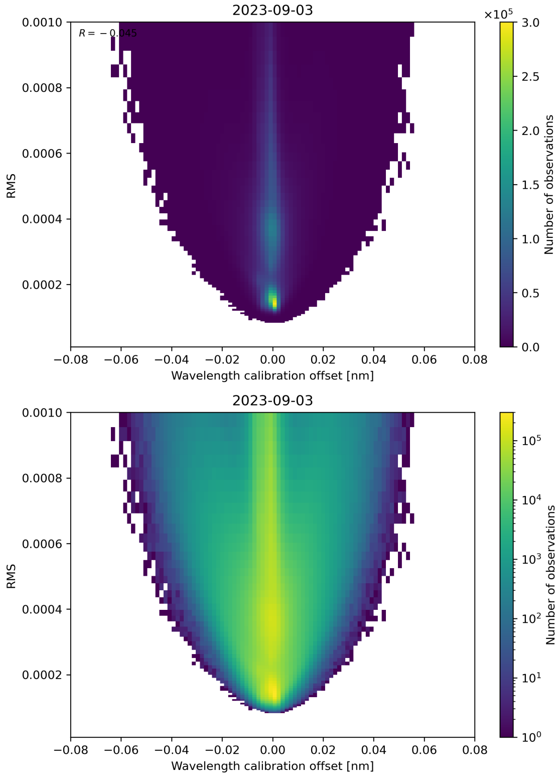
Figure 181: Scatter density plot of “Wavelength calibration offset” against “RMS” for 2023-09-02 to 2023-09-04.
