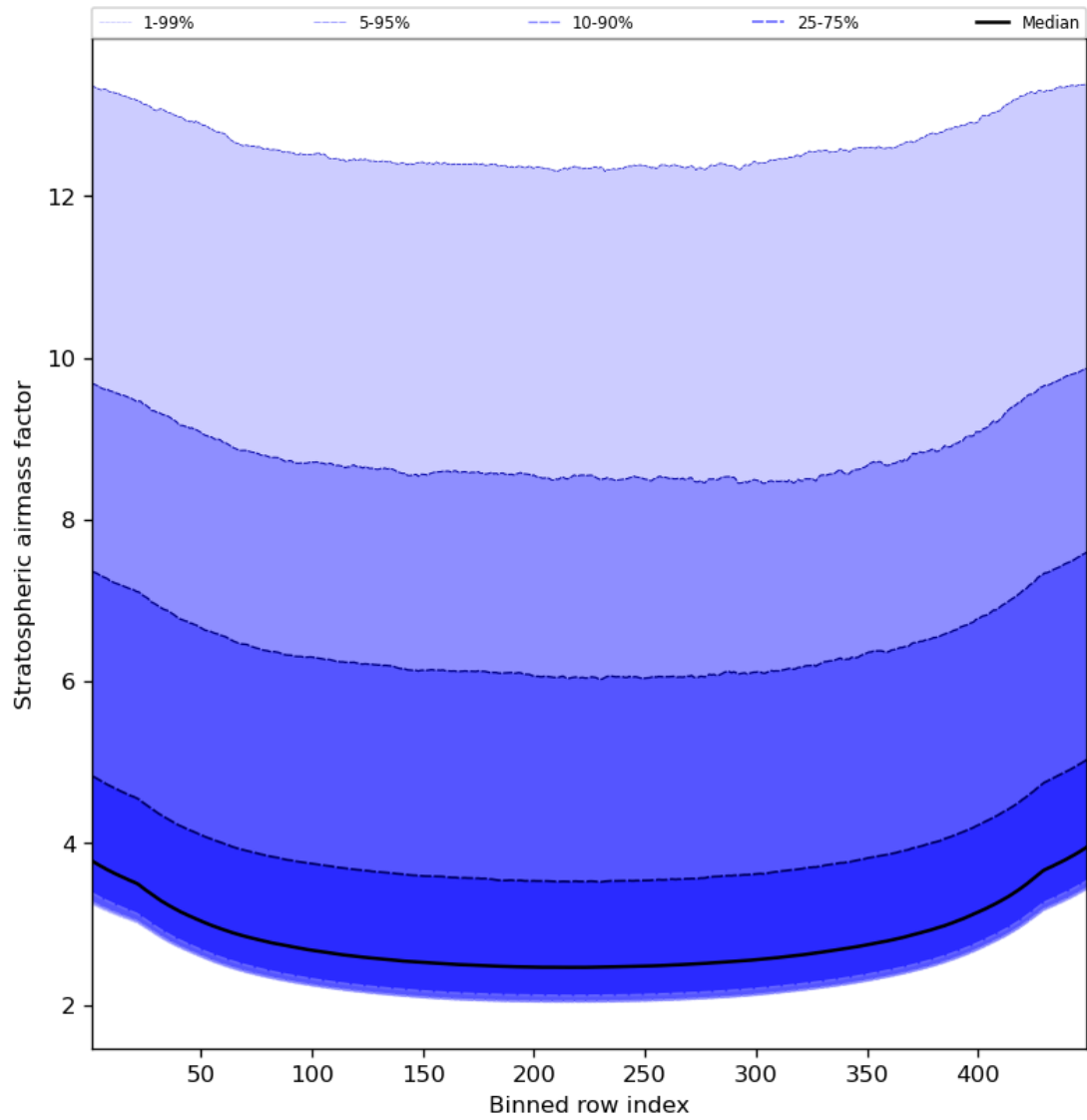
Figure 61: Along track statistics of “Stratospheric airmass factor” for 2023-09-02 to 2023-09-04
