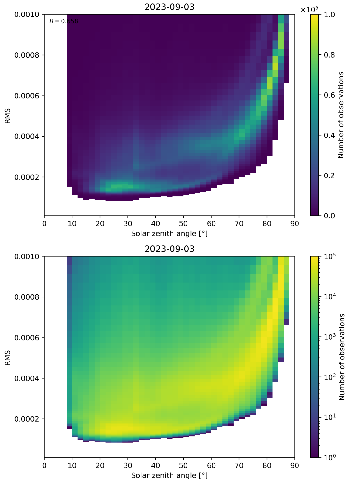
Figure 157: Scatter density plot of “Solar zenith angle” against “RMS” for 2023-09-02 to 2023-09-04.
