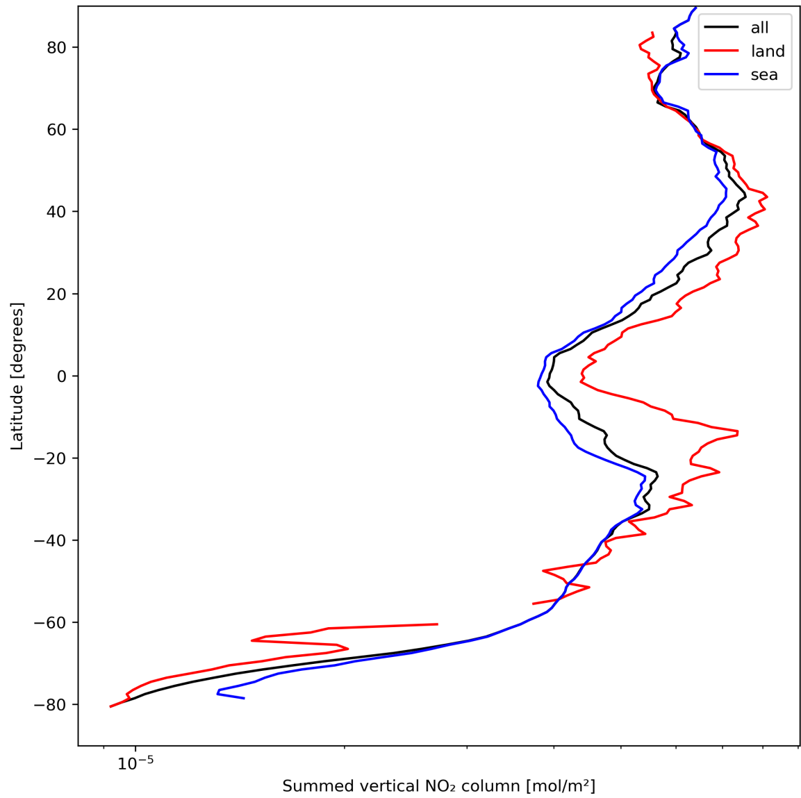
Figure 23: Zonal average of “Summed vertical NO 2 column” for 2023-09-02 to 2023-09-04.
