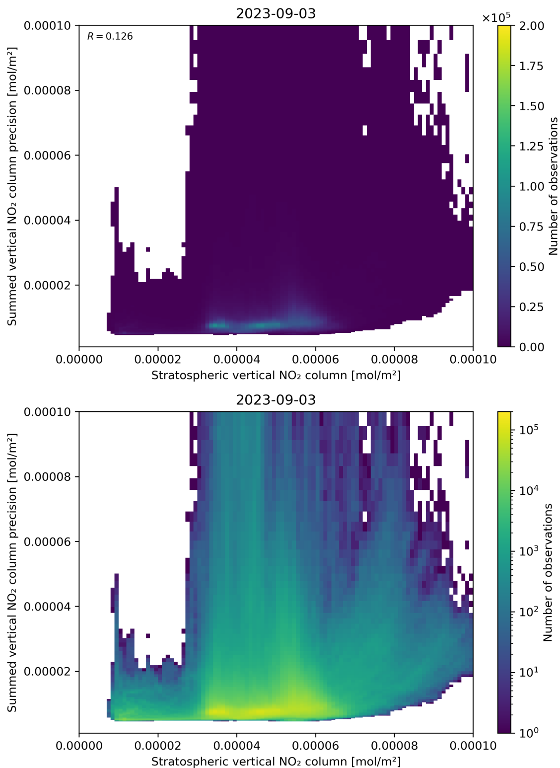
Figure 99: Scatter density plot of “Stratospheric vertical NO 2 column” against “Summed vertical NO 2 column precision” for 2023-09-02 to 2023-09-04.
