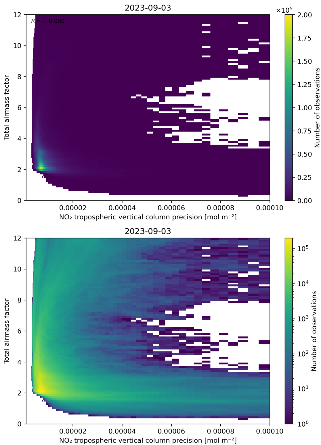
Figure 132: Scatter density plot of “NO 2 tropospheric vertical column precision” against “Total air mass factor” for 2023-09-02 to 2023-09-04.
