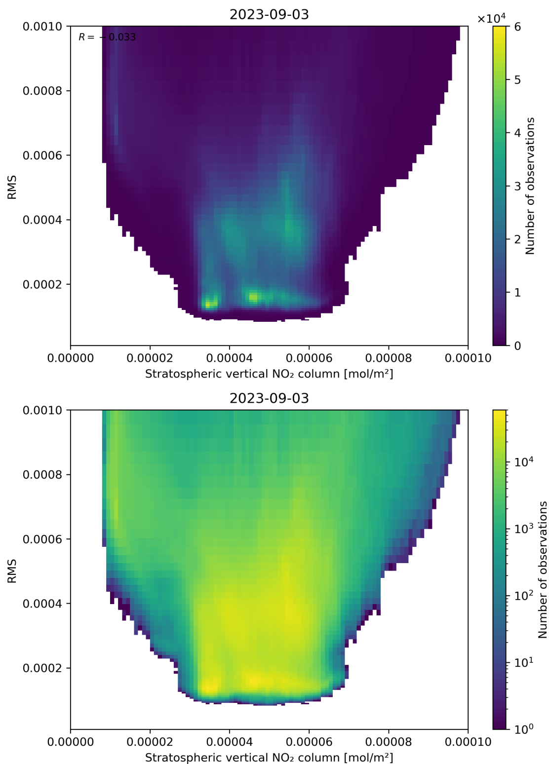
Figure 102: Scatter density plot of “Stratospheric vertical NO 2 column” against “RMS” for 2023-09-02 to 2023-09-04.
