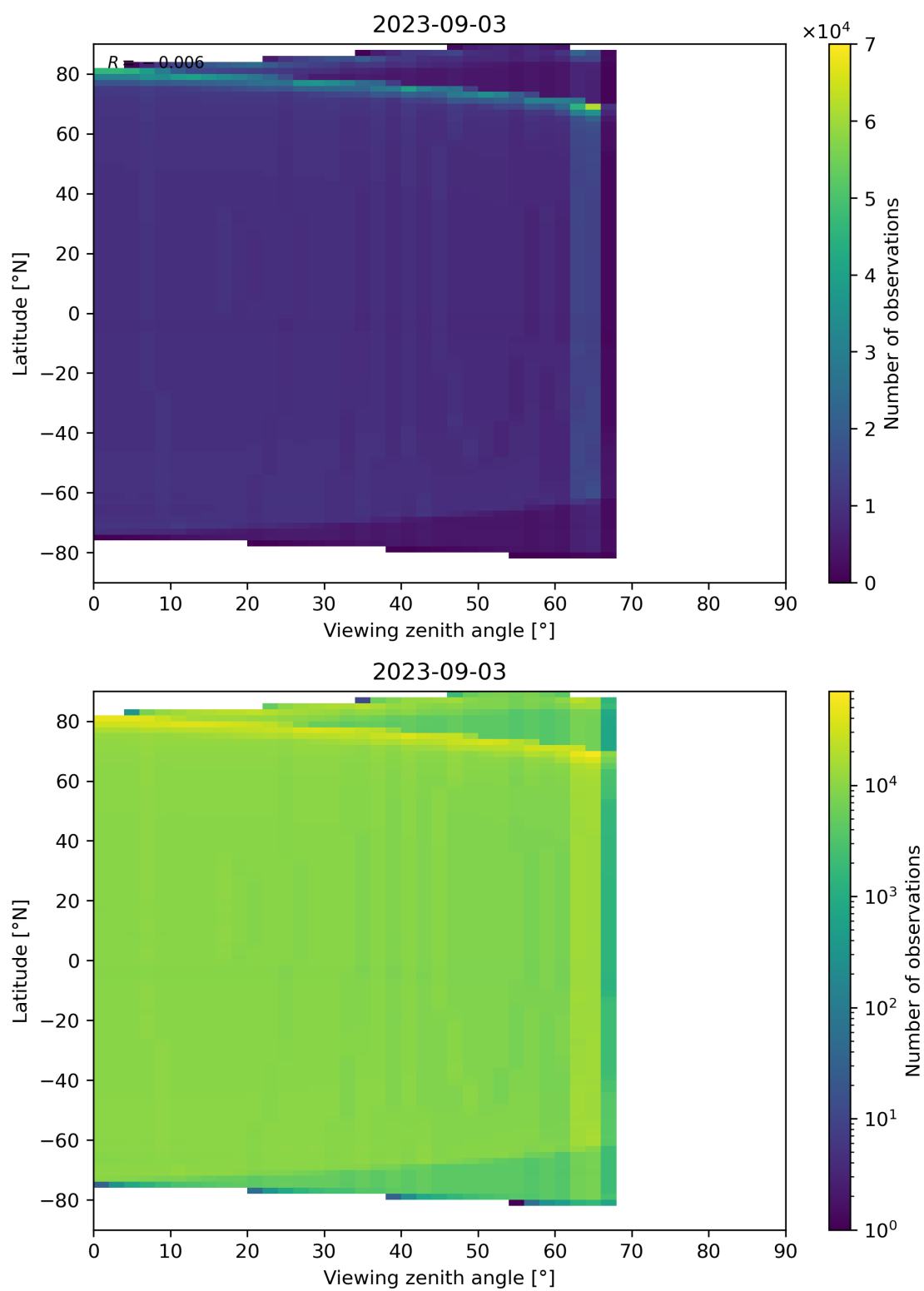
Figure 163: Scatter density plot of “Viewing zenith angle” against “Latitude” for 2023-09-02 to 2023-09-04.
