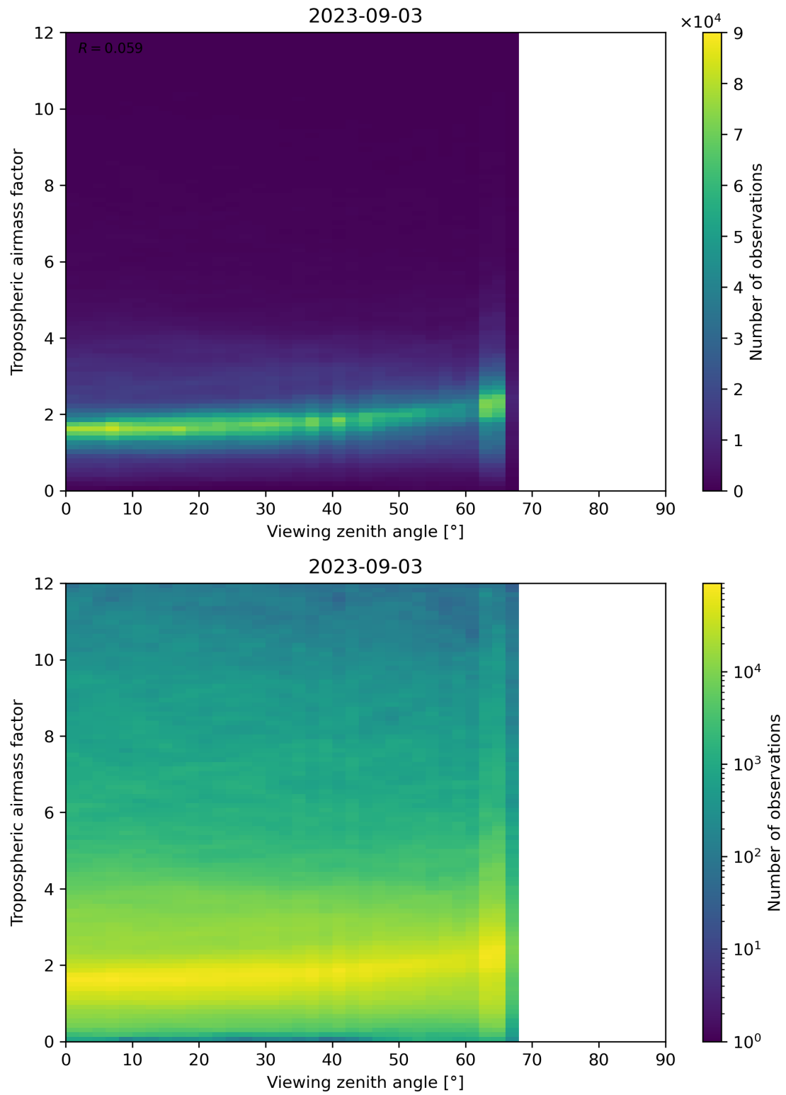
Figure 161: Scatter density plot of “Viewing zenith angle” against “Tropospheric airmass factor” for 2023-09-02 to 2023-09-04.
