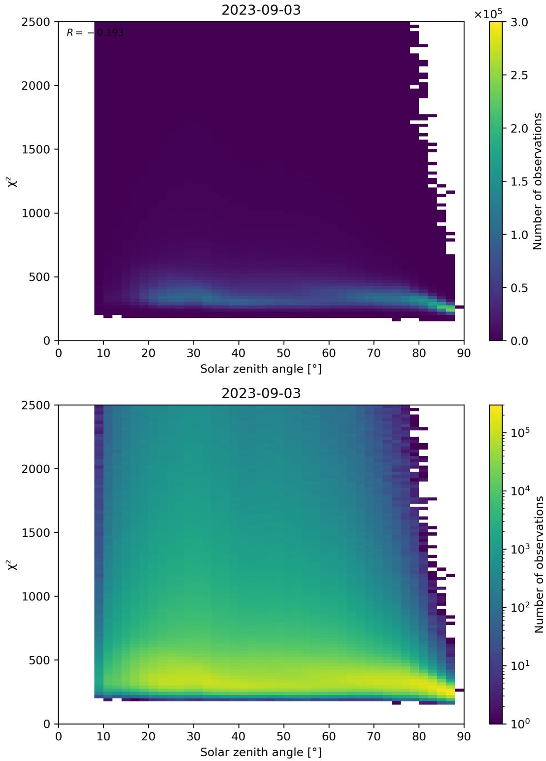
Figure 148: Scatter density plot of “Solar zenith angle” against “ \chi^2 ” for 2023-09-02 to 2023-09-04.
