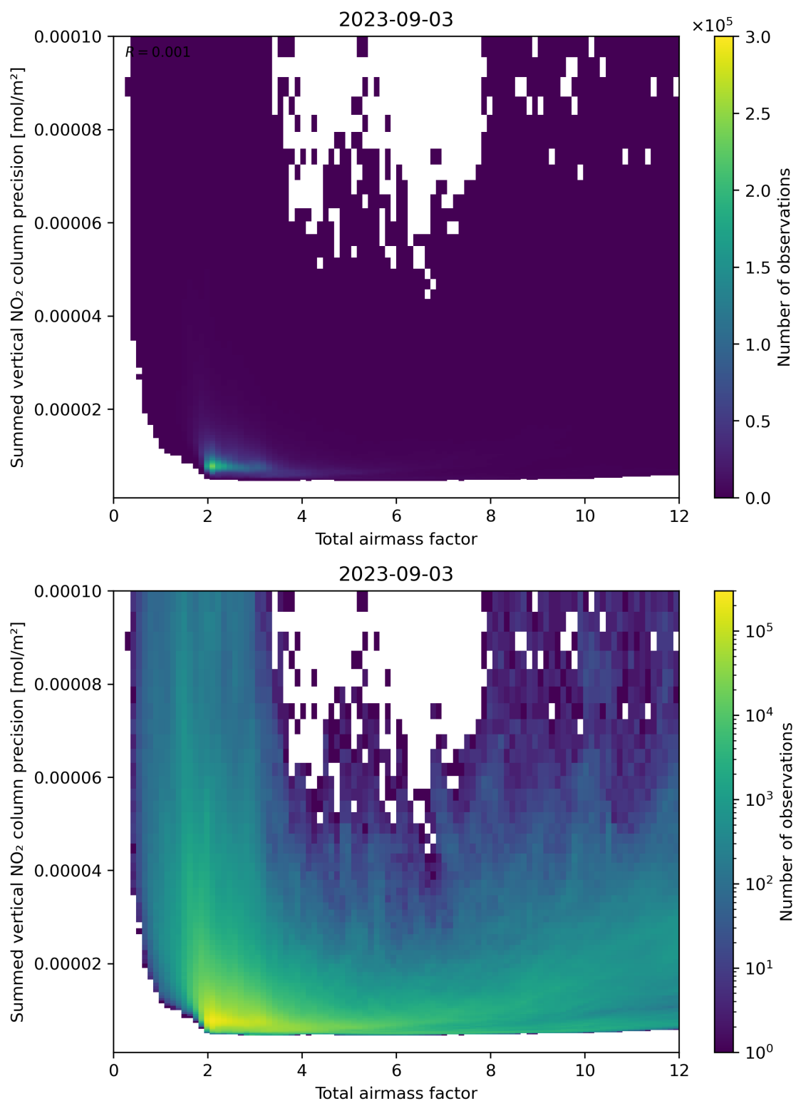
Figure 66: Scatter density plot of “Total airmass factor” against “Summed vertical NO 2 column precision” for 2023-09-02 to 2023-09-04.
