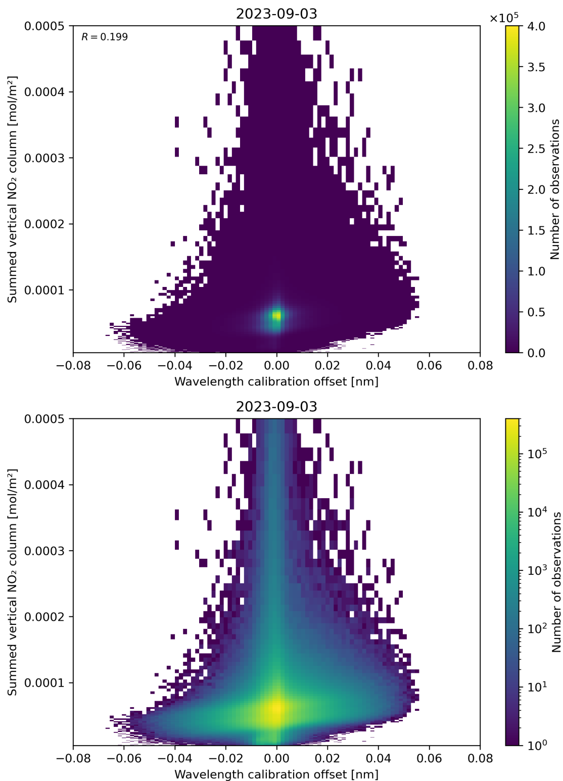
Figure 177: Scatter density plot of “Wavelength calibration offset” against “Summed vertical NO 2 column” for 2023-09-02 to 2023-09-04.
