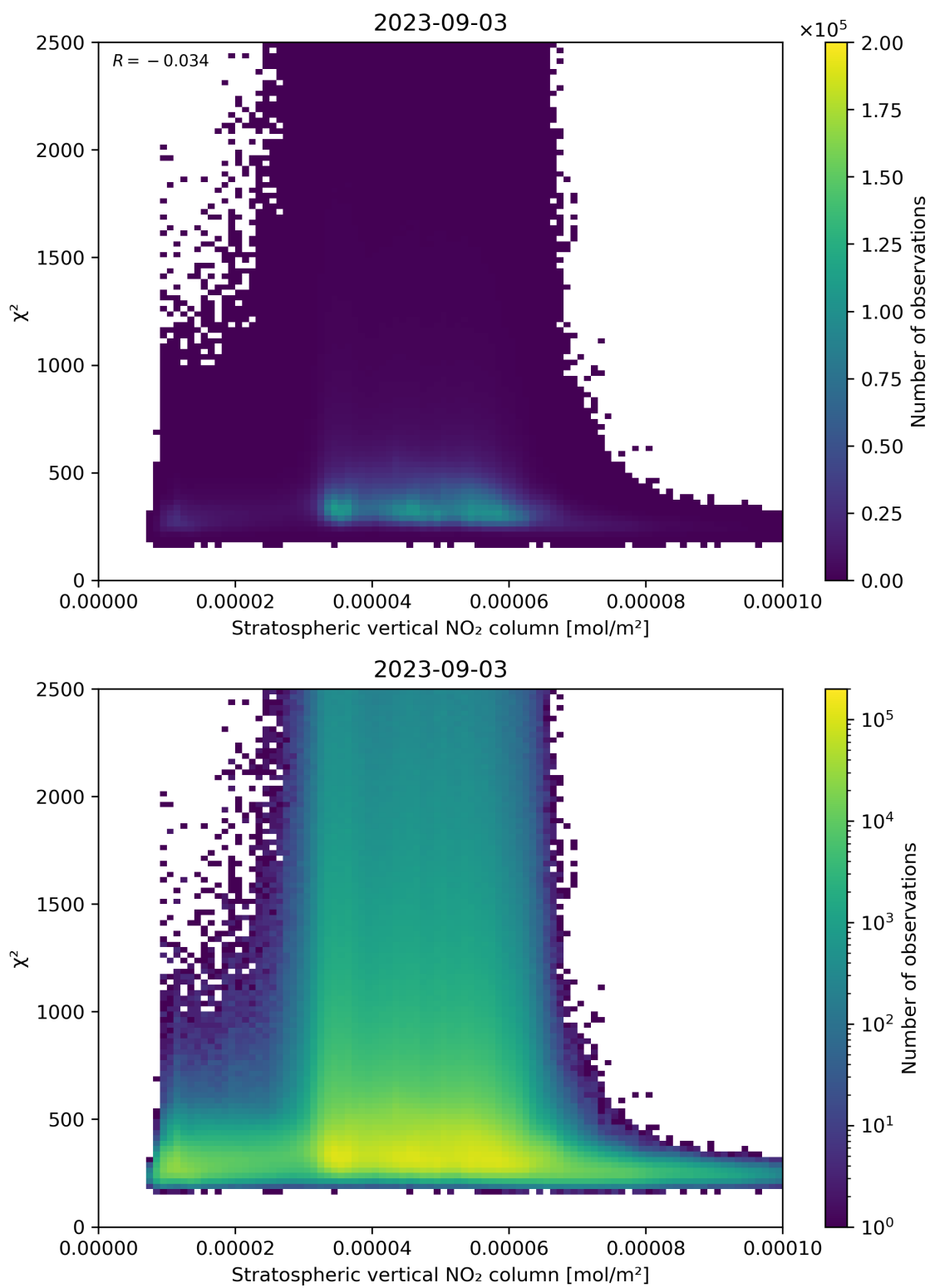
Figure 97: Scatter density plot of “Stratospheric vertical NO 2 column” against “ \chi^2 ” for 2023-09-02 to 2023-09-04.
