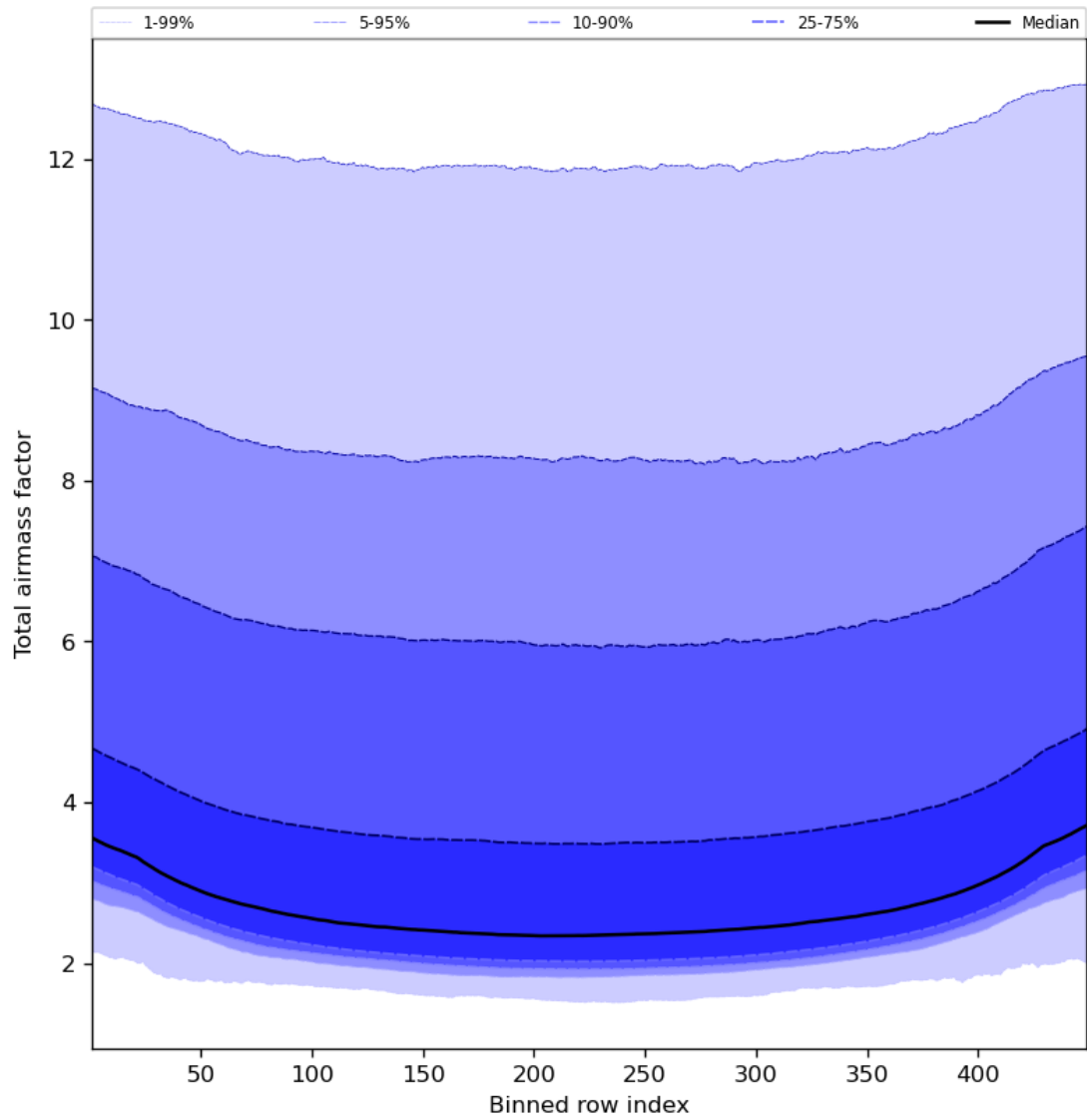
Figure 49: Along track statistics of “Total airmass factor” for 2023-09-02 to 2023-09-04
