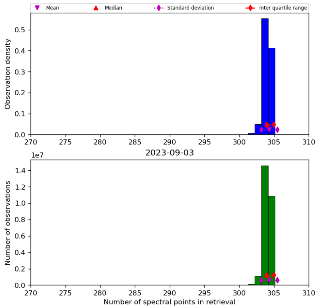
Figure 33: Histogram of “Number of spectral points in retrieval” for 2023-09-02 to 2023-09-04
