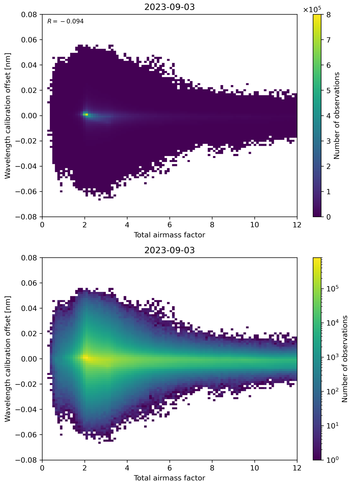
Figure 70: Scatter density plot of “Total airmass factor” against “Wavelength calibration offset” for 2023-09-02 to 2023-09-04.
