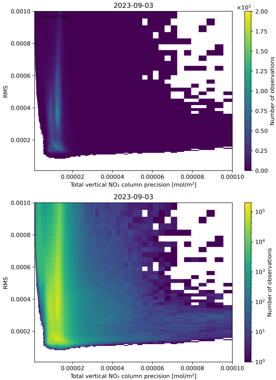
Figure 119: Scatter density plot of “Total vertical NO 2 column precision” against “RMS” for 2023-09-02 to 2023-09-04.
