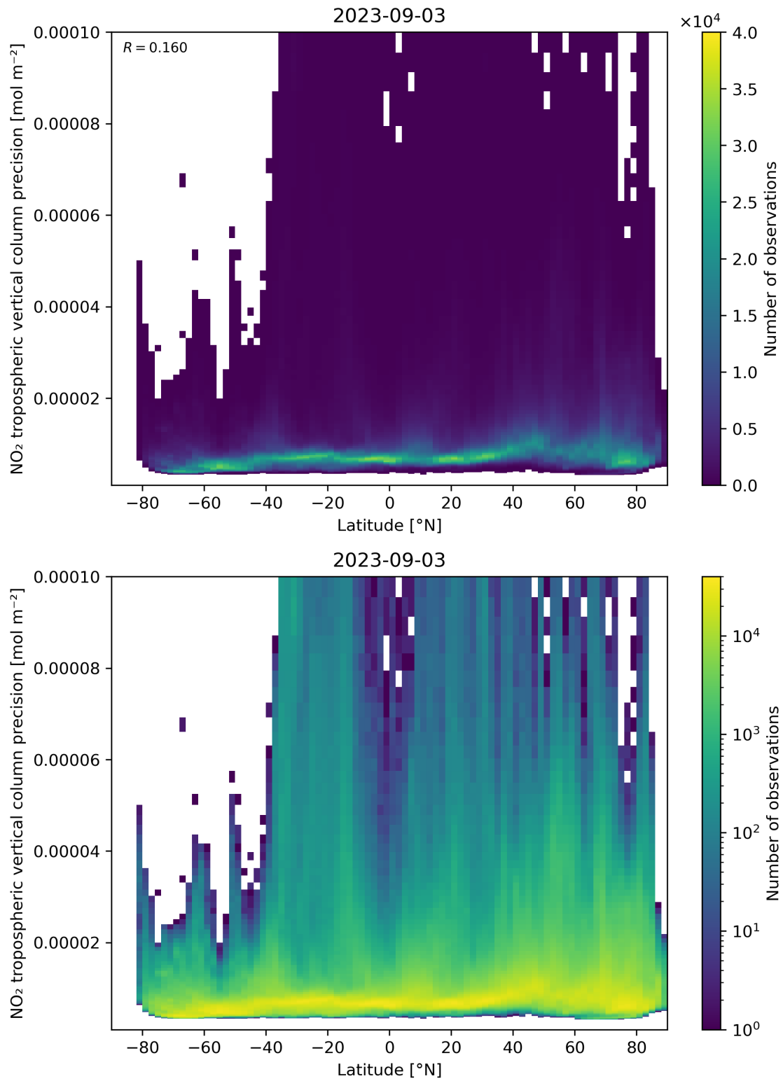
Figure 93: Scatter density plot of “Latitude” against “NO 2 tropospheric vertical column precision” for 2023-09-02 to 2023-09-04.
