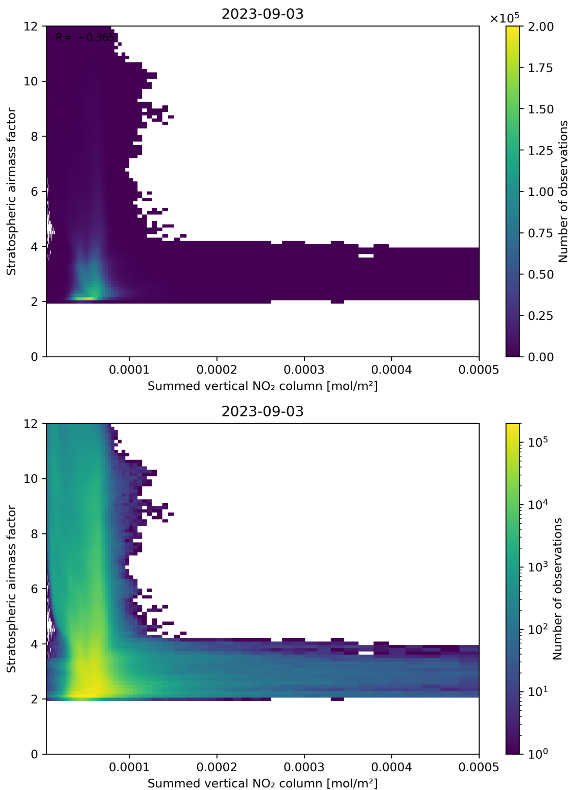
Figure 103: Scatter density plot of “Summed vertical NO 2 column” against “Stratospheric air mass factor” for 2023-09-02 to 2023-09-04.
