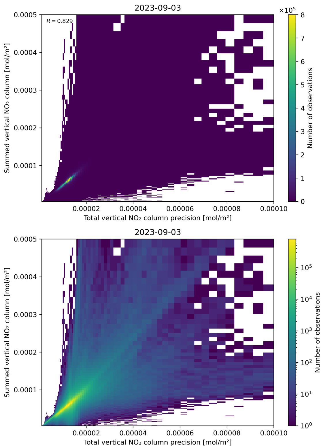
Figure 117: Scatter density plot of “Total vertical NO 2 column precision” against “Summed vertical NO 2 column” for 2023-09-02 to 2023-09-04.
