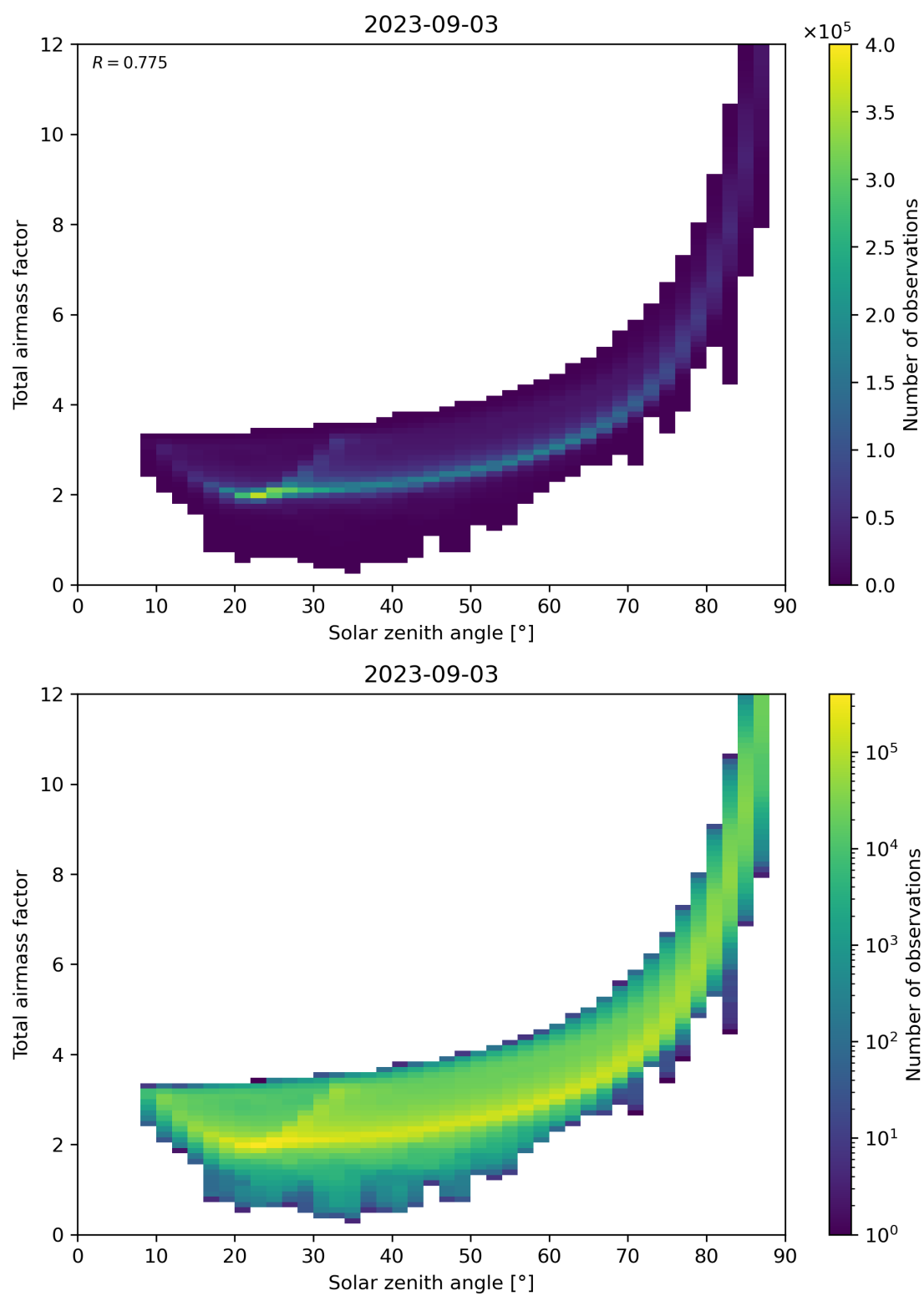
Figure 146: Scatter density plot of “Solar zenith angle” against “Total air mass factor” for 2023-09-02 to 2023-09-04.
