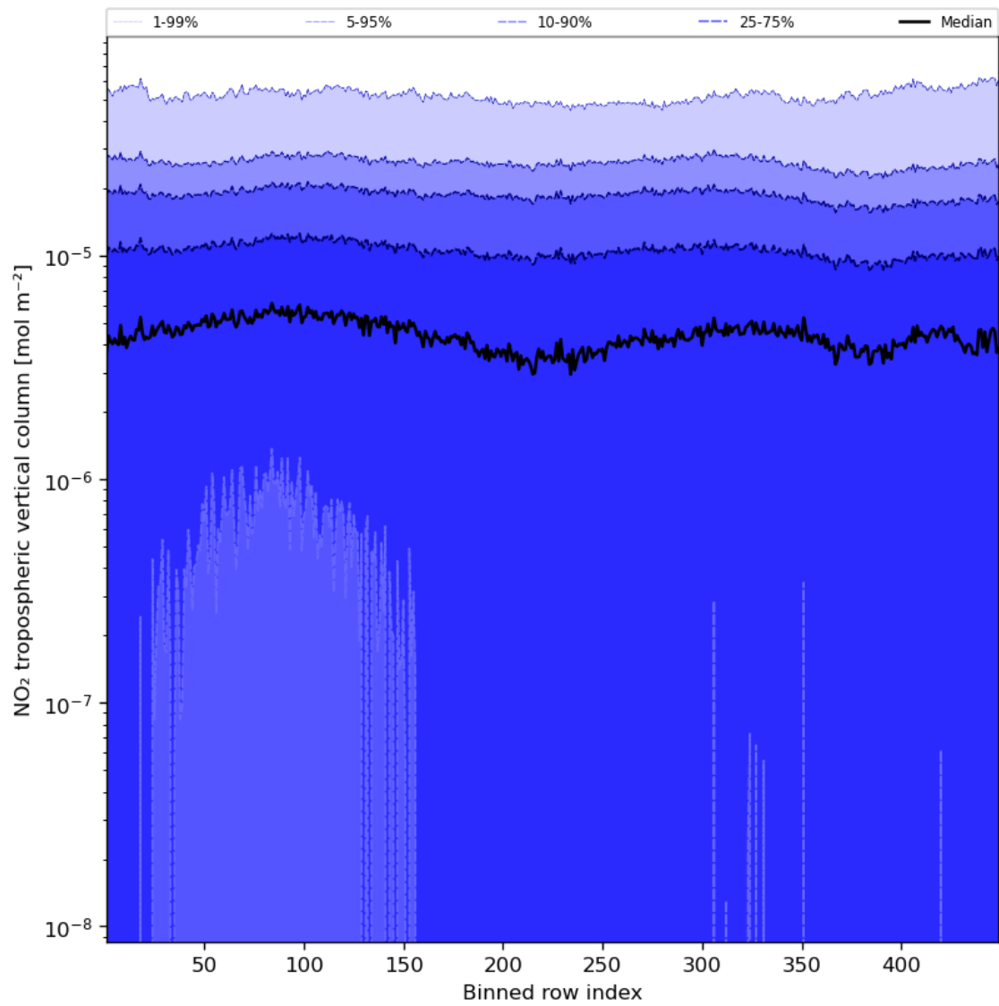
Figure 46: Along track statistics of “NO 2 tropospheric vertical column” for 2023-09-02 to 2023-09-04
