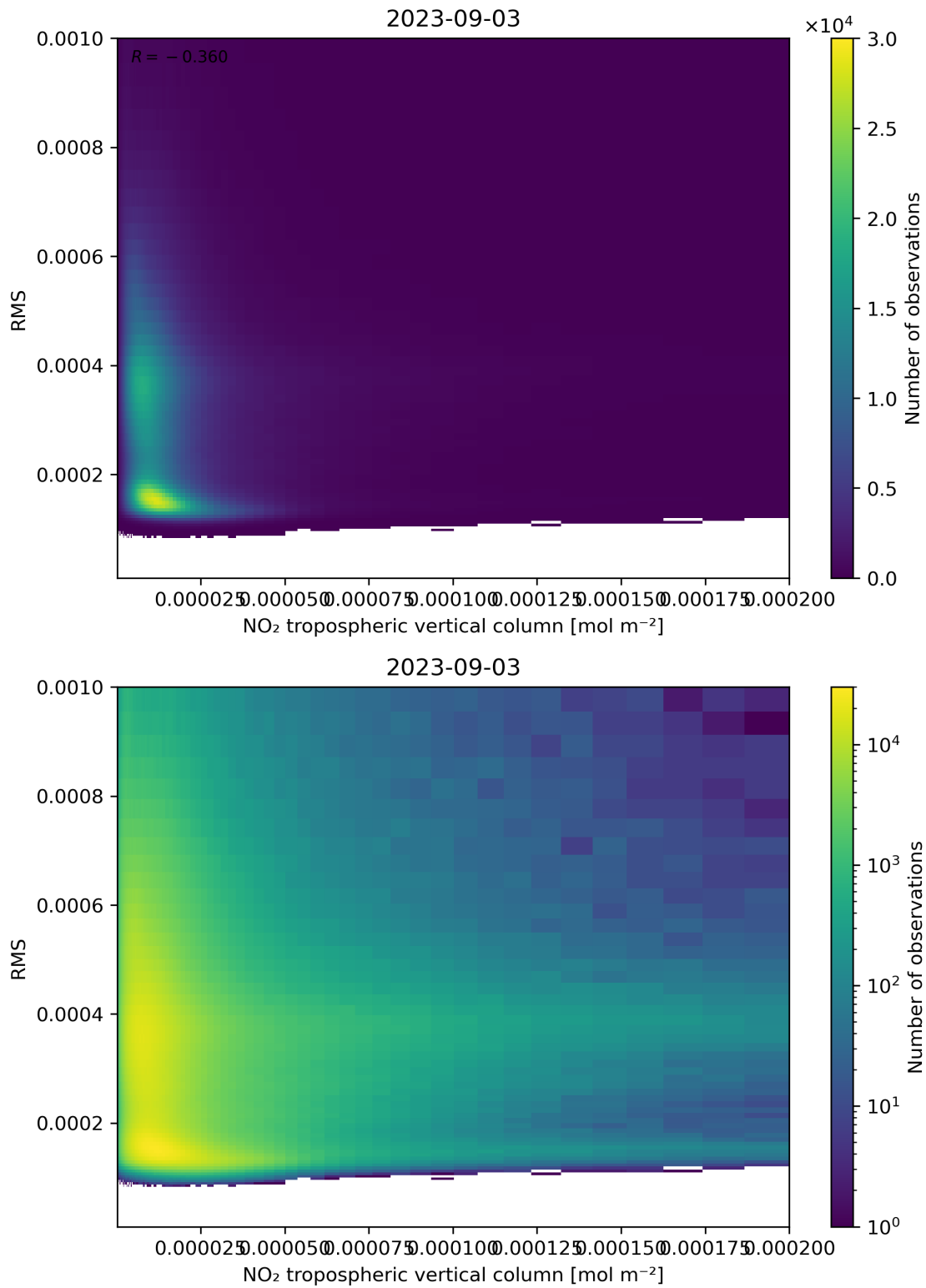
Figure 142: Scatter density plot of “NO 2 tropospheric vertical column” against “RMS” for 2023-09-02 to 2023-09-04.
