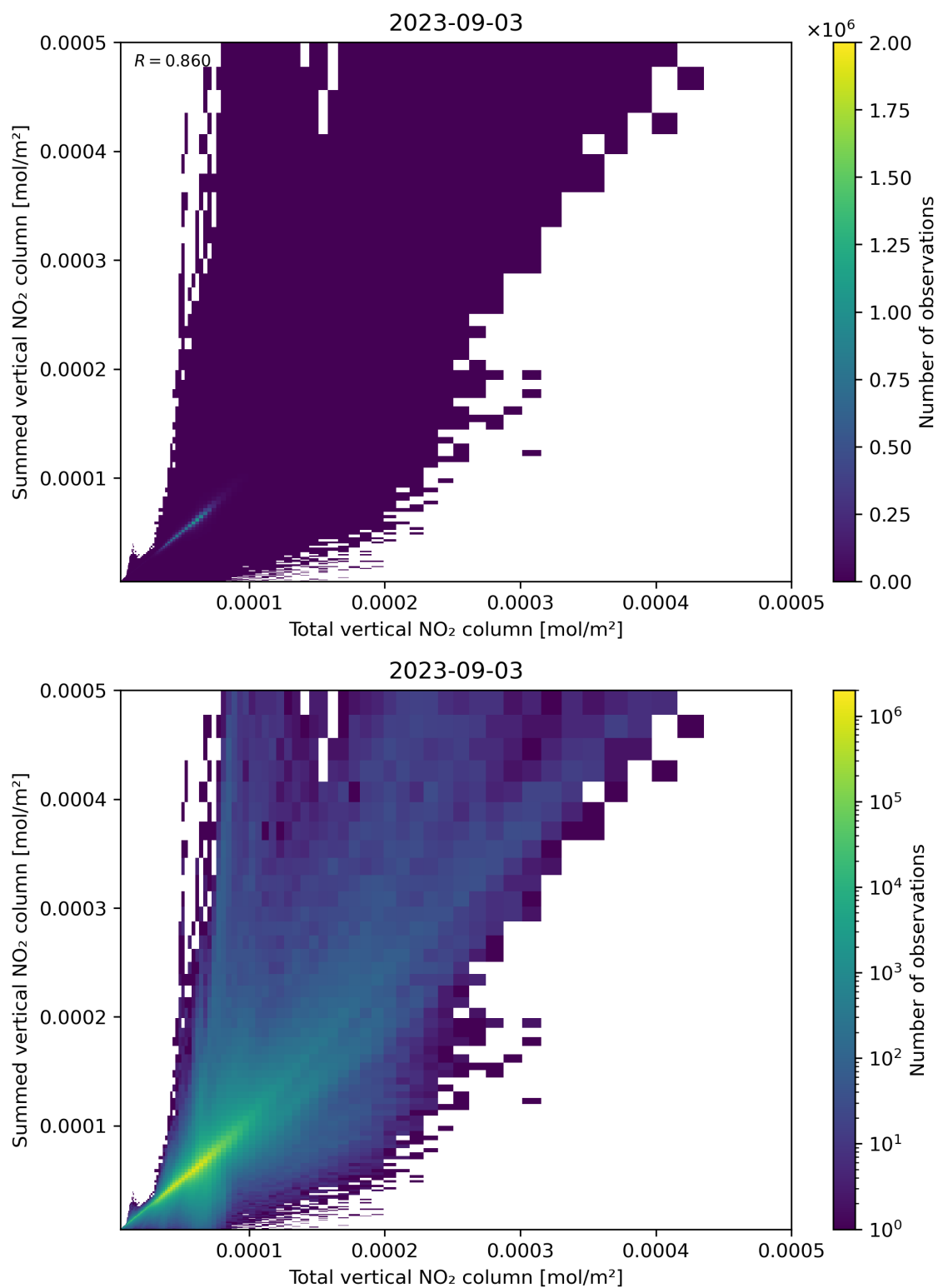
Figure 112: Scatter density plot of “Total vertical NO 2 column” against “Summed vertical NO 2 column” for 2023-09-02 to 2023-09-04.
