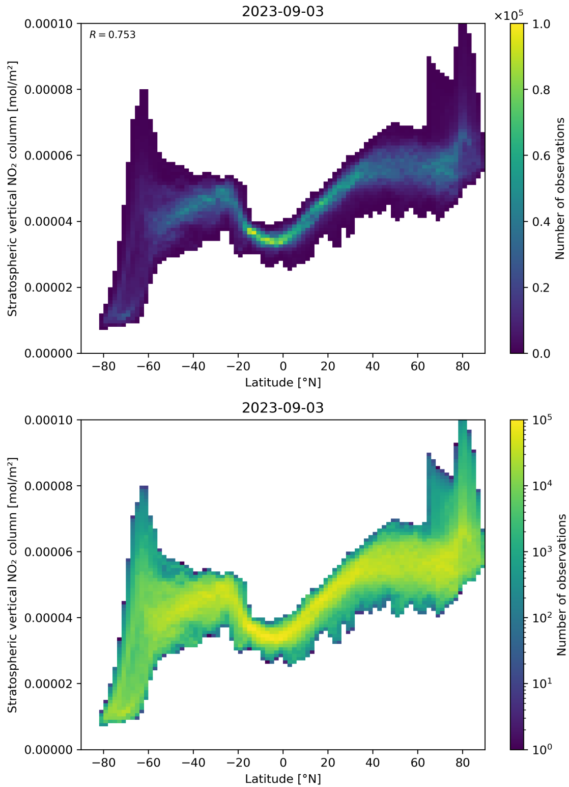
Figure 87: Scatter density plot of “Latitude” against “Stratospheric vertical NO 2 column” for 2023-09-02 to 2023-09-04.
