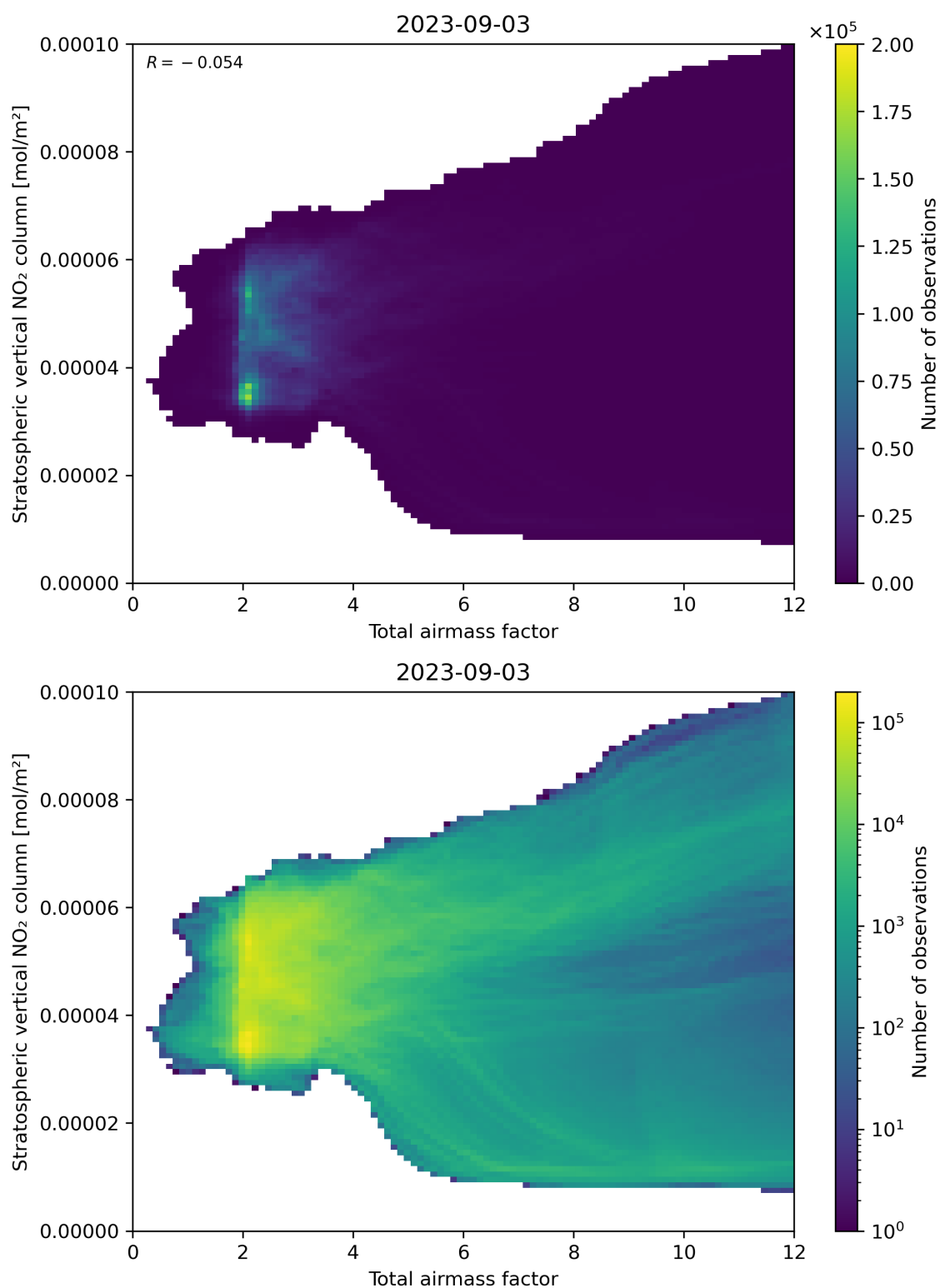
Figure 64: Scatter density plot of “Total airmass factor” against “Stratospheric vertical NO 2 column” for 2023-09-02 to 2023-09-04.
