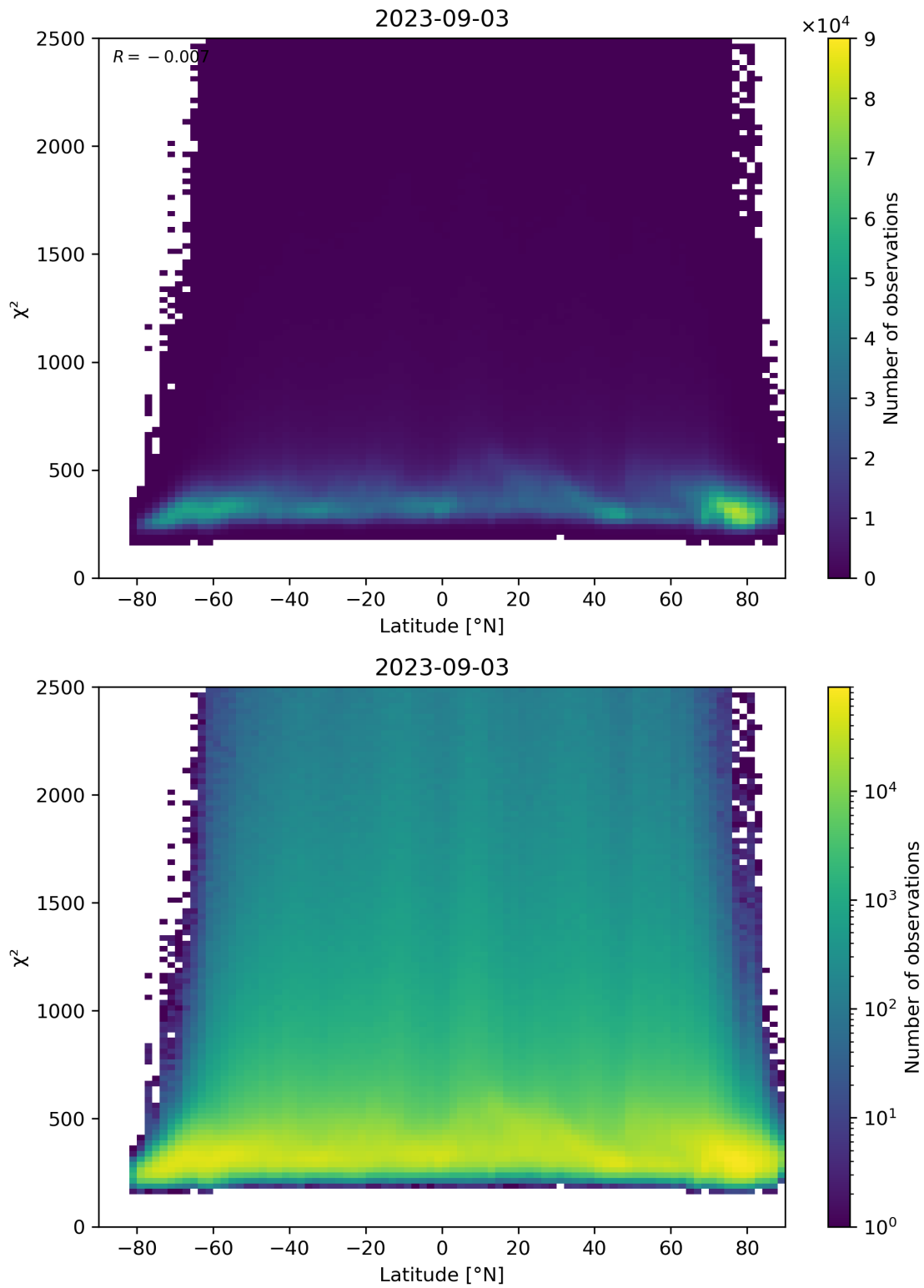
Figure 86: Scatter density plot of “Latitude” against “ \chi^2 ” for 2023-09-02 to 2023-09-04.
