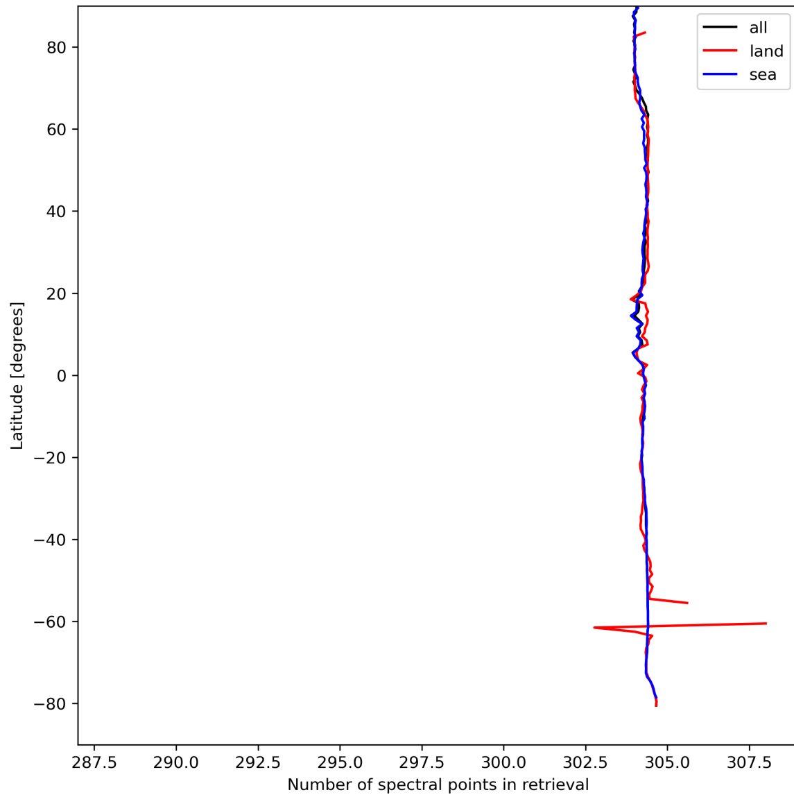
Figure 16: Zonal average of “Number of spectral points in retrieval” for 2023-09-02 to 2023-09-04.
