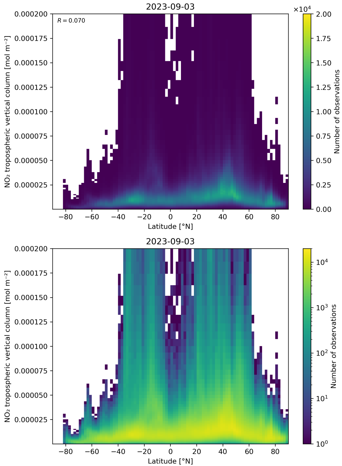
Figure 92: Scatter density plot of “Latitude” against “NO 2 tropospheric vertical column” for 2023-09-02 to 2023-09-04.
