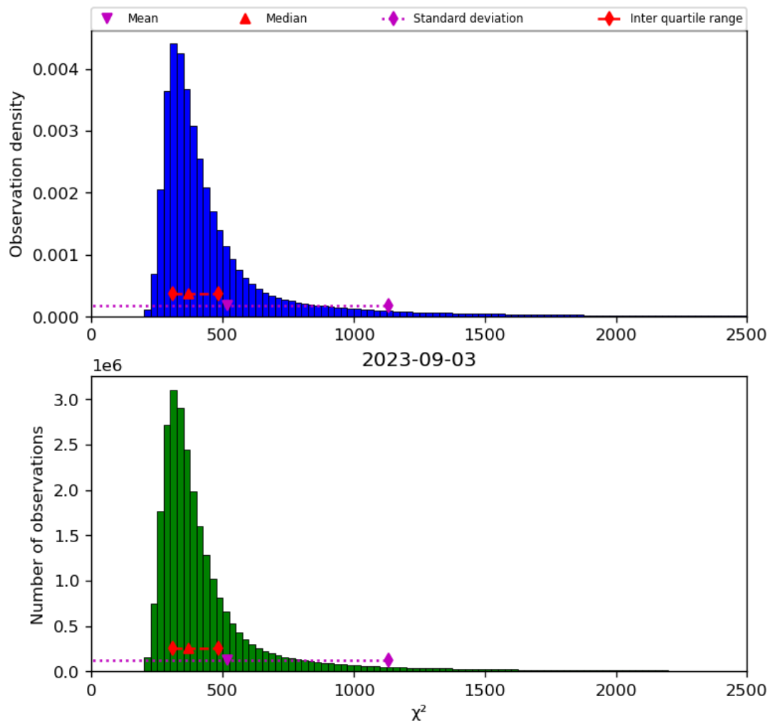
Figure 42: Histogram of “ \chi^2 ” for 2023-09-02 to 2023-09-04
