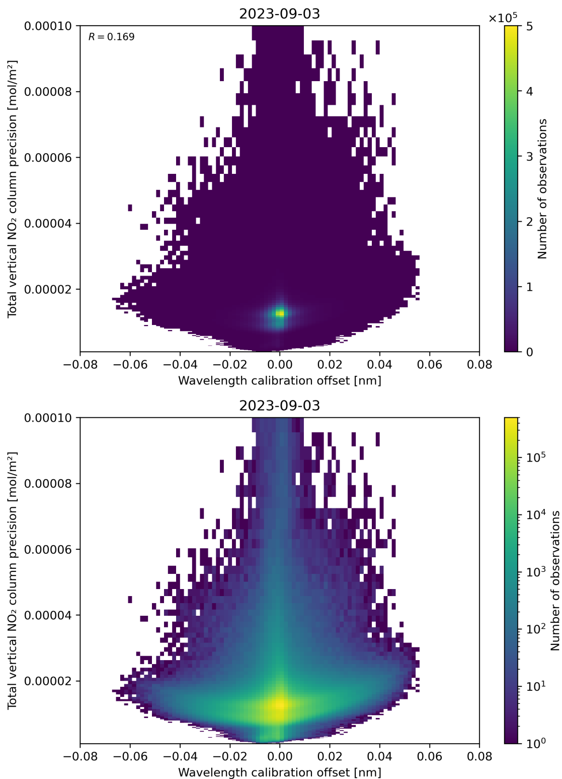
Figure 180: Scatter density plot of “Wavelength calibration offset” against “Total vertical NO 2 column precision” for 2023-09-02 to 2023-09-04.
