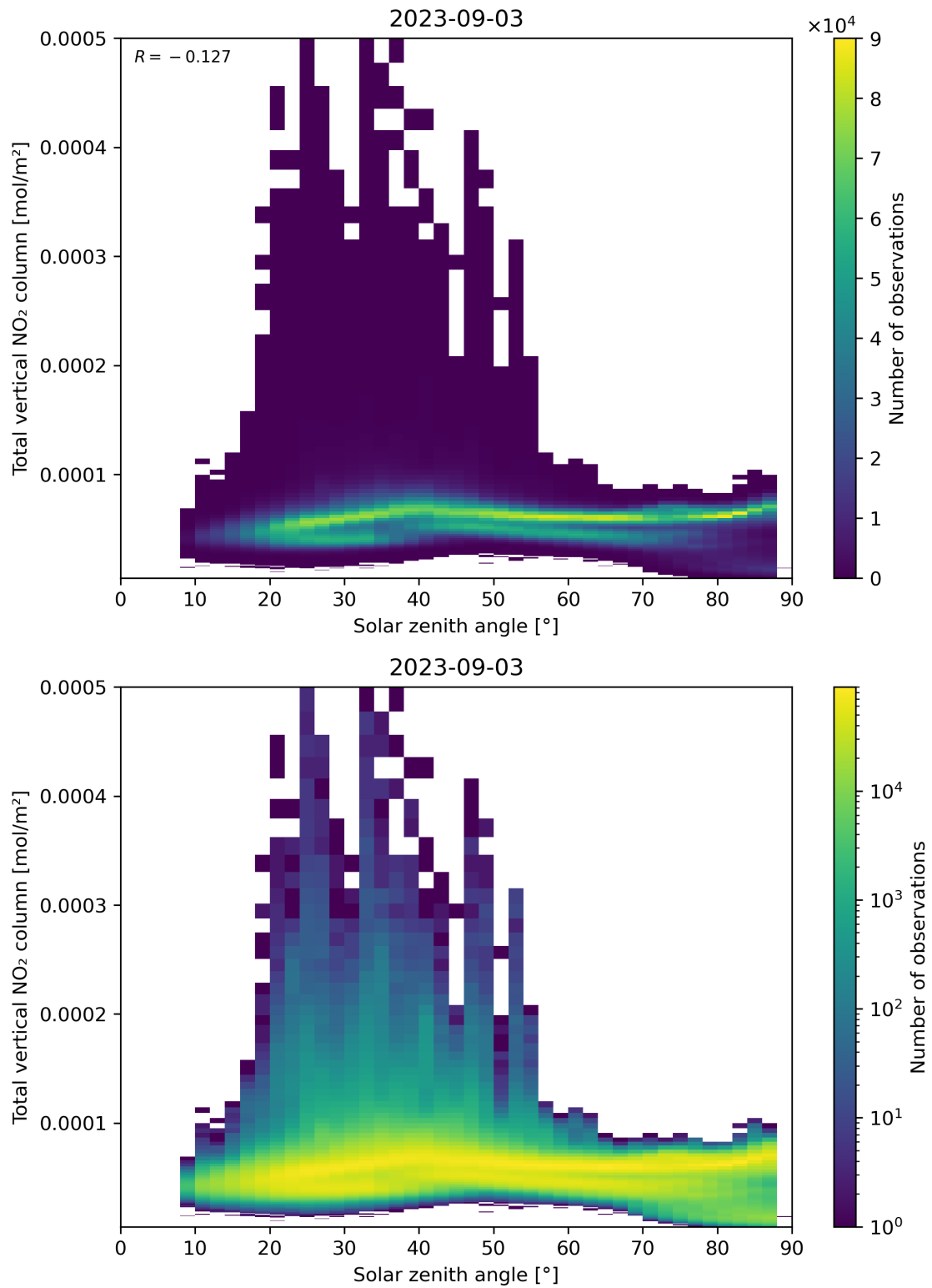
Figure 153: Scatter density plot of “Solar zenith angle” against “Total vertical NO 2 column” for 2023-09-02 to 2023-09-04.
