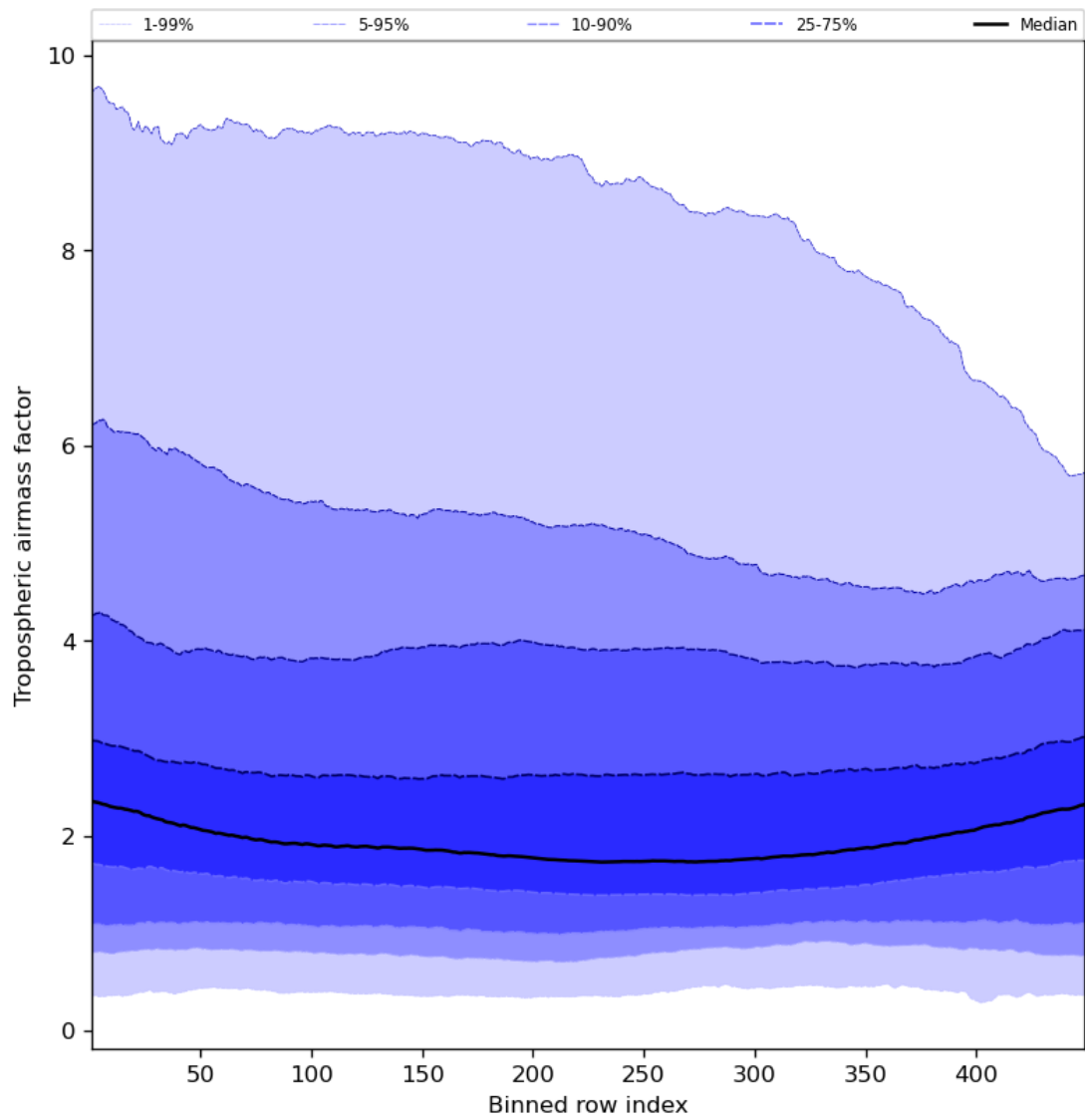
Figure 48: Along track statistics of “Tropospheric air mass factor” for 2023-09-02 to 2023-09-04
