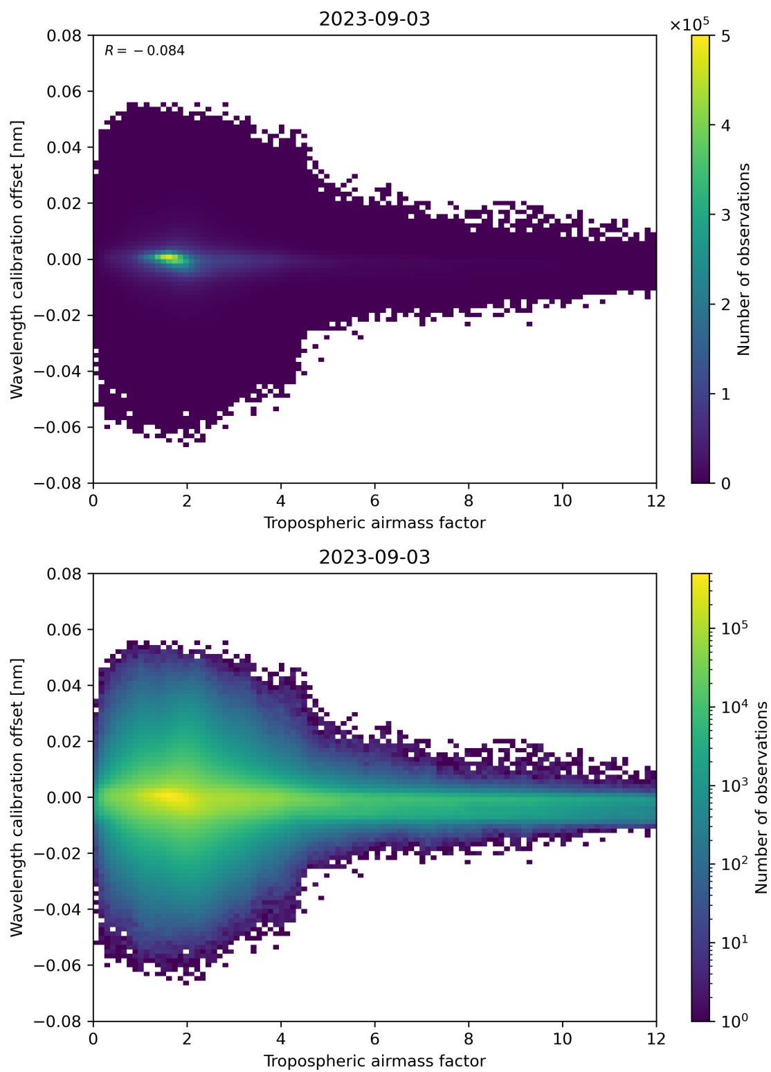
Figure 80: Scatter density plot of “Tropospheric airmass factor” against “Wavelength calibration offset” for 2023-09-02 to 2023-09-04.
