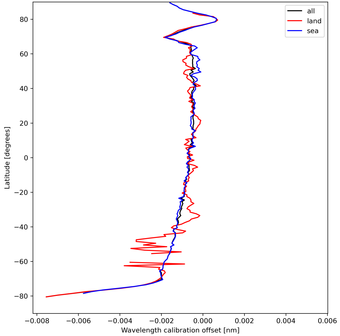
Figure 18: Zonal average of “Wavelength calibration offset” for 2023-09-02 to 2023-09-04.
