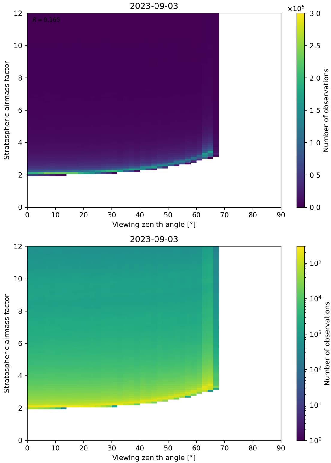
Figure 159: Scatter density plot of “Viewing zenith angle” against “Stratospheric airmass factor” for 2023-09-02 to 2023-09-04.
