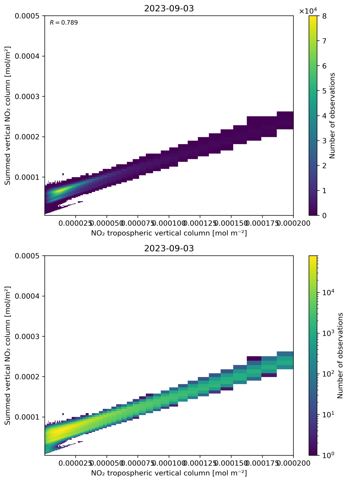
Figure 126: Scatter density plot of “NO 2 tropospheric vertical column” against “Summed vertical NO 2 column” for 2023-09-02 to 2023-09-04.
