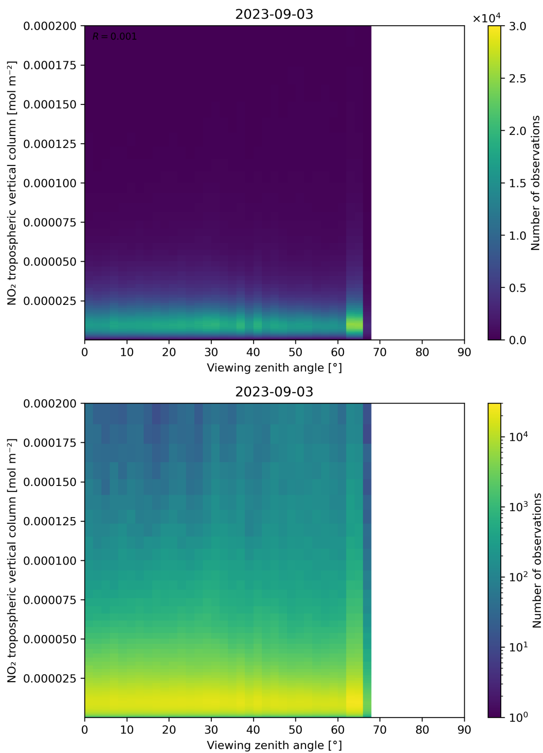
Figure 169: Scatter density plot of “Viewing zenith angle” against “NO 2 tropospheric vertical column” for 2023-09-02 to 2023-09-04.
