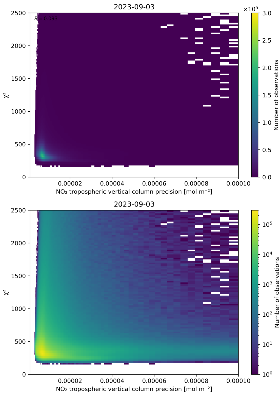
Figure 134: Scatter density plot of “NO 2 tropospheric vertical column precision” against “ \chi^2 ” for 2023-09-02 to 2023-09-04.
