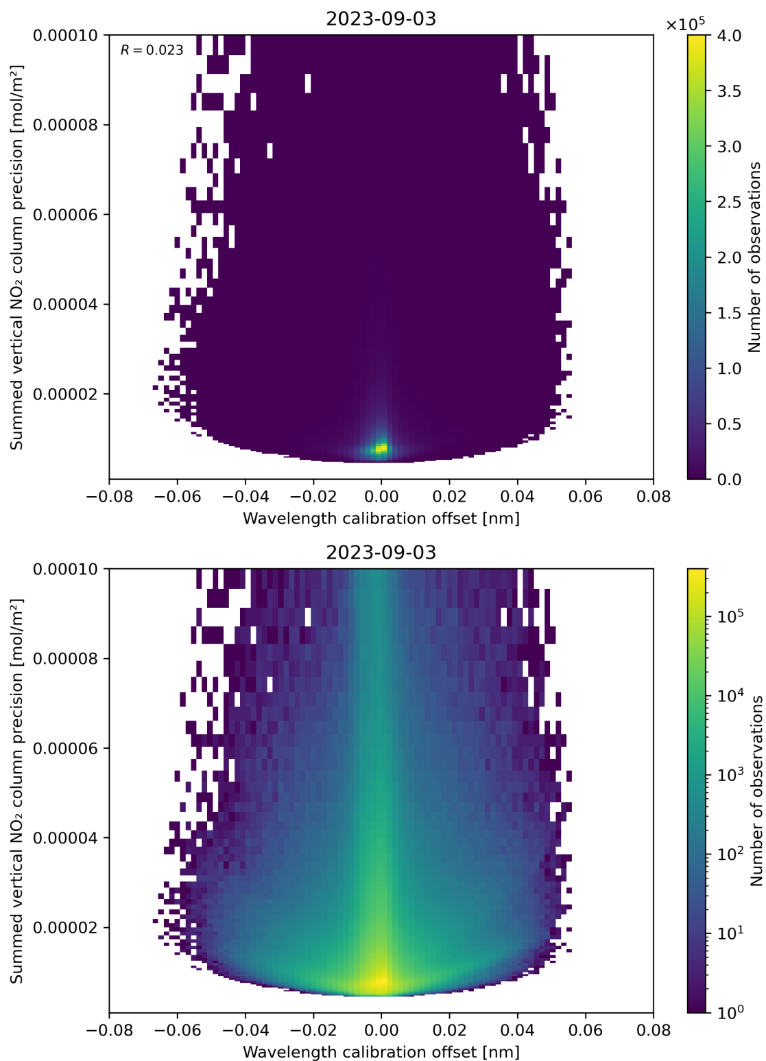
Figure 178: Scatter density plot of “Wavelength calibration offset” against “Summed vertical NO 2 column precision” for 2023-09-02 to 2023-09-04.
