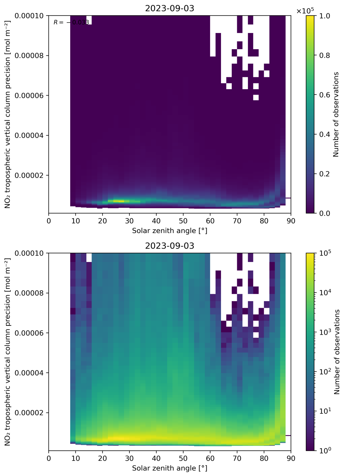
Figure 156: Scatter density plot of “Solar zenith angle” against “NO 2 tropospheric vertical column precision” for 2023-09-02 to 2023-09-04.
