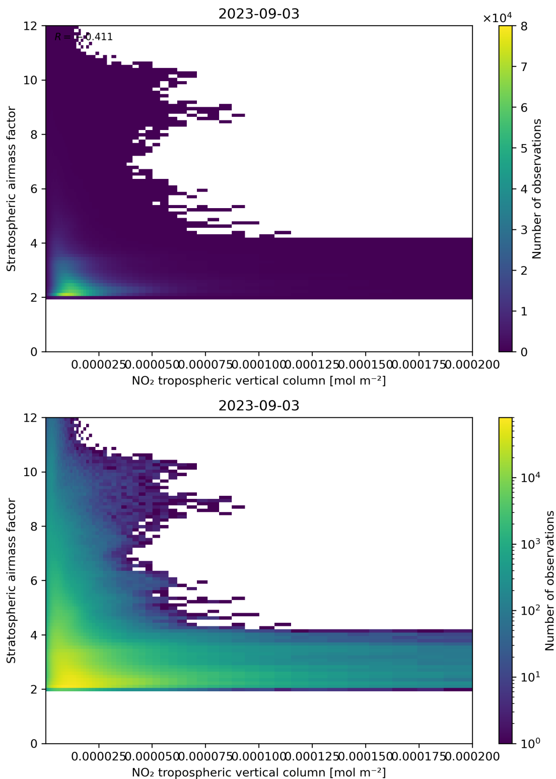
Figure 121: Scatter density plot of “NO 2 tropospheric vertical column” against “Stratospheric air mass factor” for 2023-09-02 to 2023-09-04.
