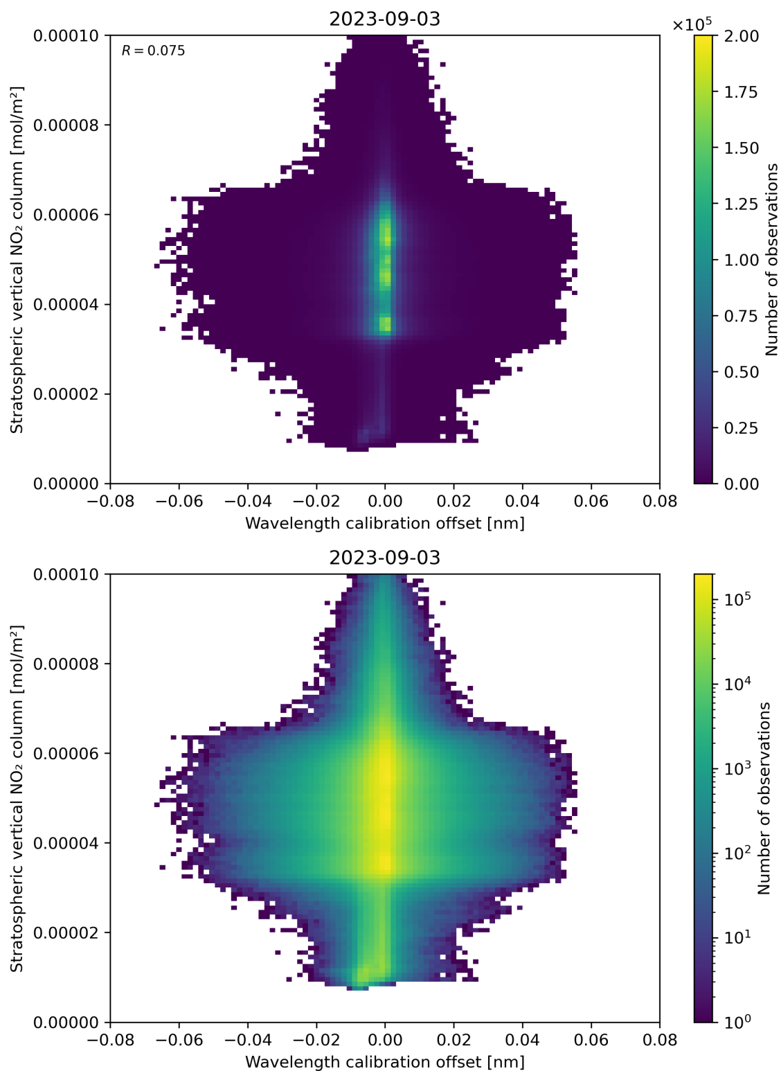
Figure 176: Scatter density plot of “Wavelength calibration offset” against “Stratospheric vertical NO 2 column” for 2023-09-02 to 2023-09-04.
