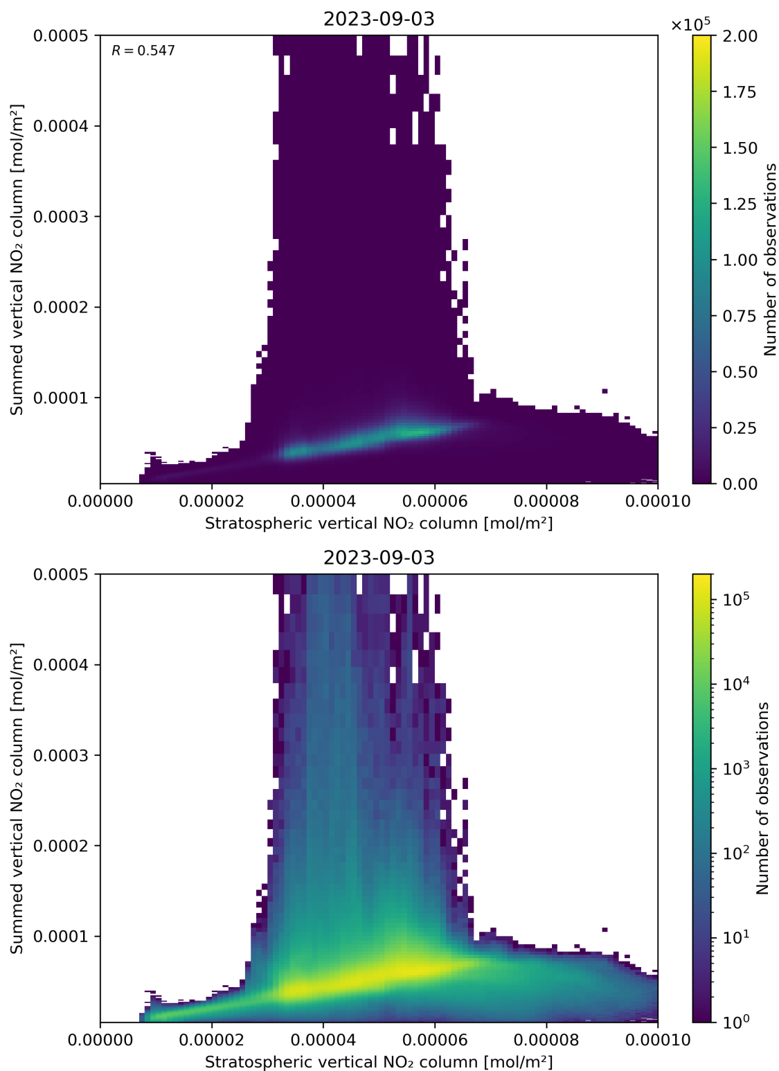
Figure 98: Scatter density plot of “Stratospheric vertical NO 2 column” against “Summed vertical NO 2 column” for 2023-09-02 to 2023-09-04.
