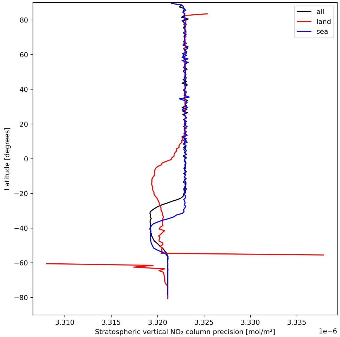
Figure 20: Zonal average of “Stratospheric vertical NO 2 column precision” for 2023-09-02 to 2023-09-04.
