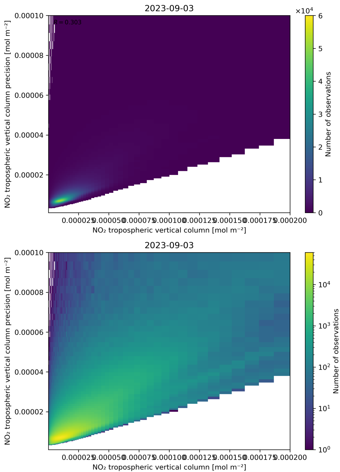
Figure 130: Scatter density plot of “NO 2 tropospheric vertical column” against “NO 2 tropospheric vertical column precision” for 2023-09-02 to 2023-09-04.
