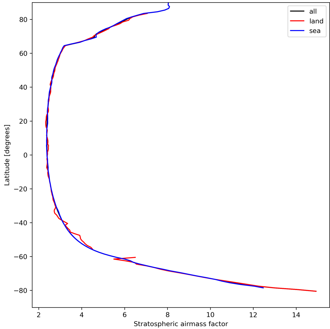
Figure 27: Zonal average of “Stratospheric air mass factor” for 2023-09-02 to 2023-09-04.
