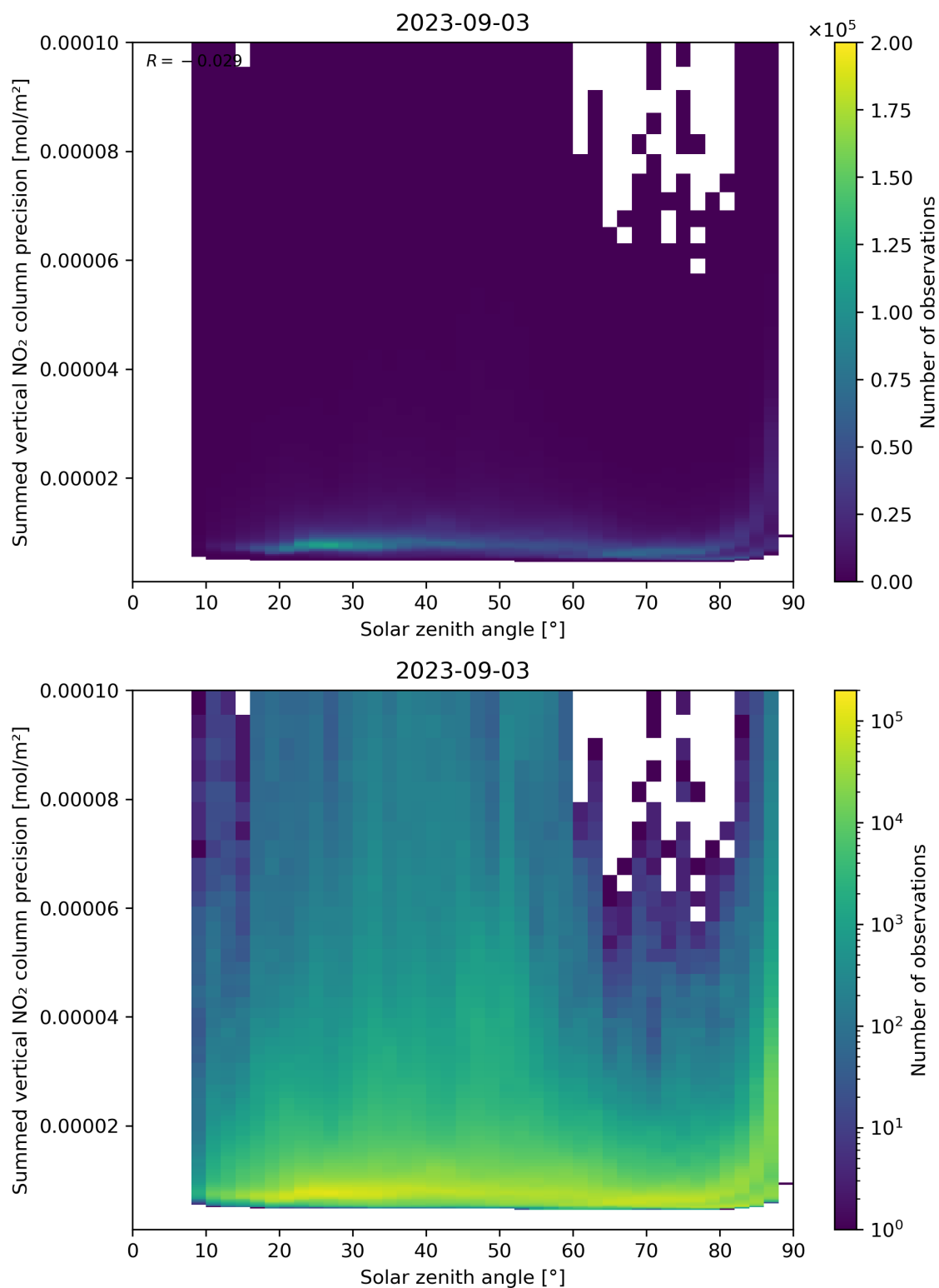
Figure 152: Scatter density plot of “Solar zenith angle” against “Summed vertical NO 2 column precision” for 2023-09-02 to 2023-09-04.
