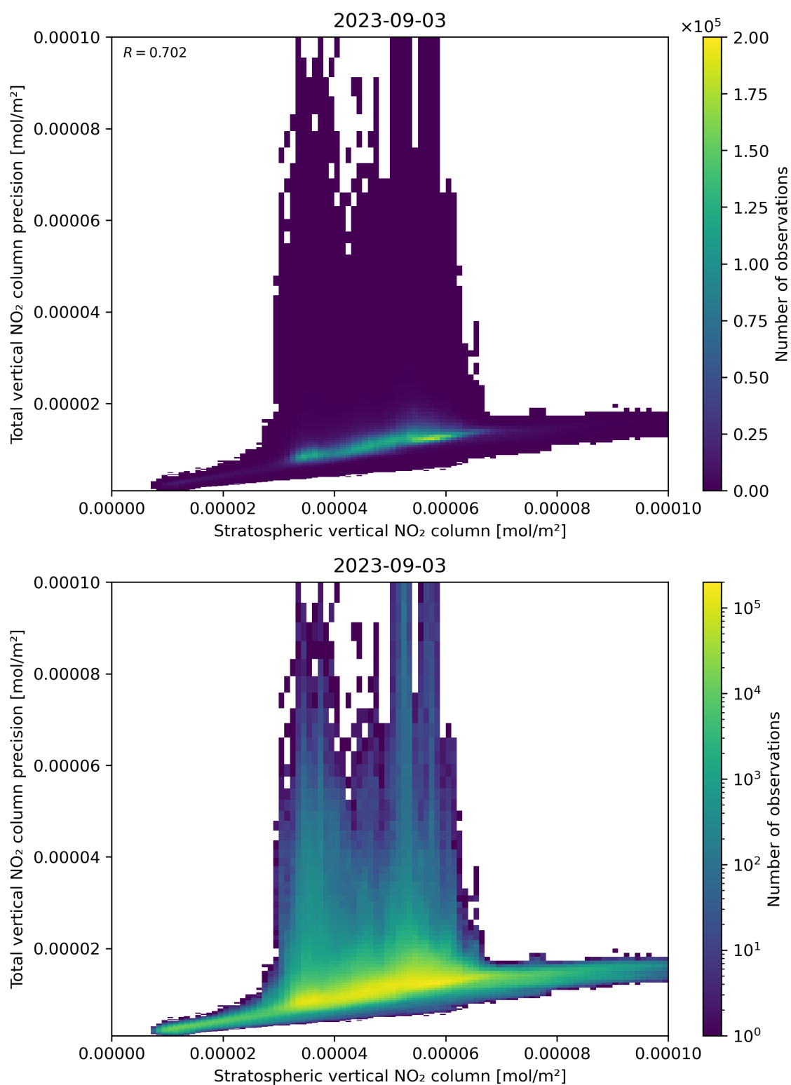
Figure 101: Scatter density plot of “Stratospheric vertical NO 2 column” against “Total vertical NO 2 column precision” for 2023-09-02 to 2023-09-04.
