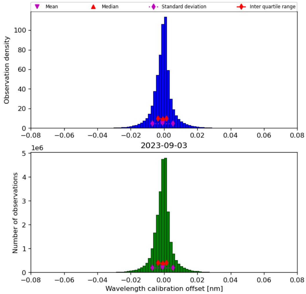
Figure 35: Histogram of “Wavelength calibration offset” for 2023-09-02 to 2023-09-04
