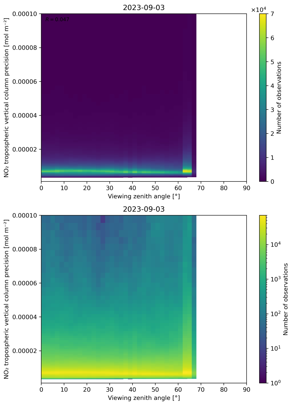
Figure 170: Scatter density plot of “Viewing zenith angle” against “NO 2 tropospheric vertical column precision” for 2023-09-02 to 2023-09-04.
