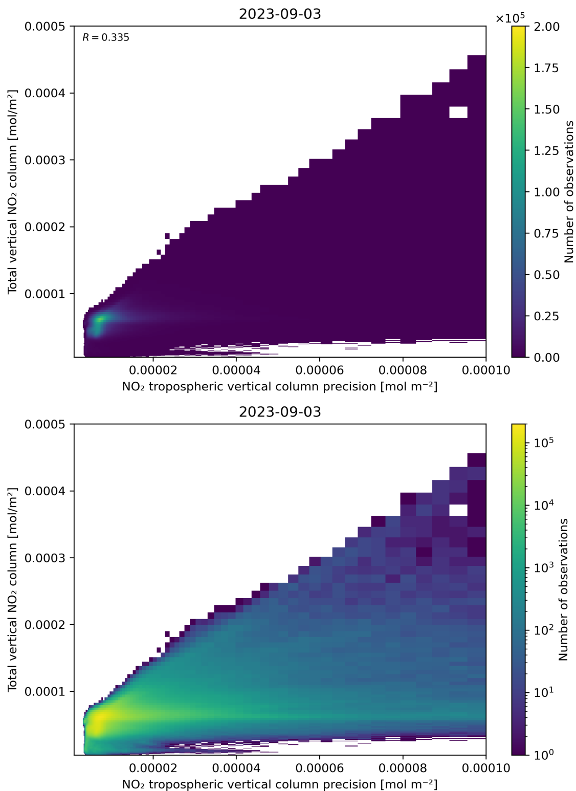
Figure 138: Scatter density plot of “NO 2 tropospheric vertical column precision” against “Total vertical NO 2 column” for 2023-09-02 to 2023-09-04.
