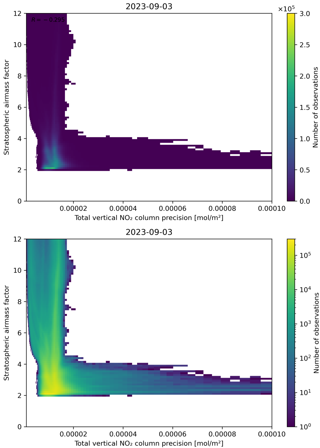
Figure 115: Scatter density plot of “Total vertical NO 2 column precision” against “Stratospheric air mass factor” for 2023-09-02 to 2023-09-04.
