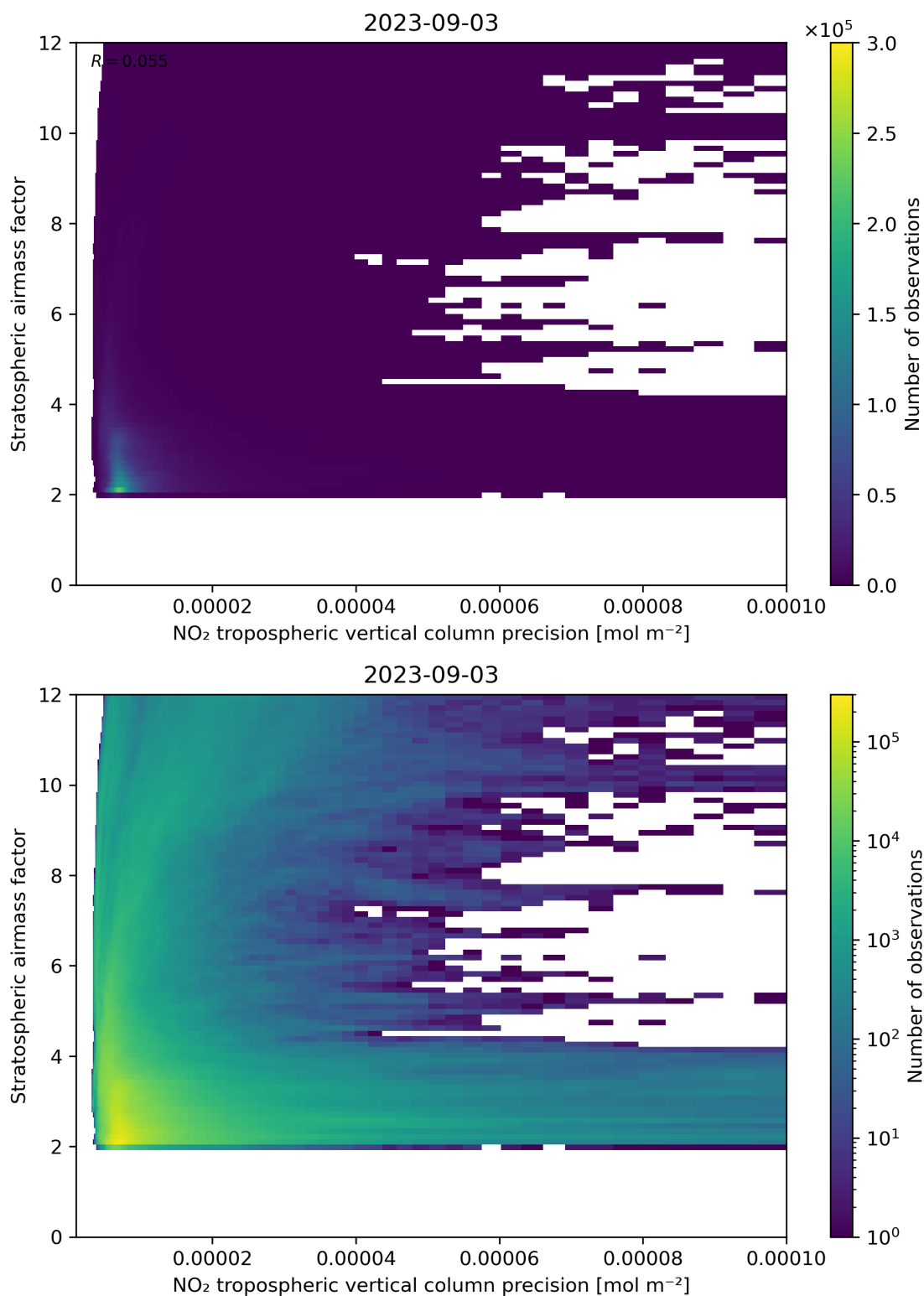
Figure 131: Scatter density plot of “NO 2 tropospheric vertical column precision” against “Stratospheric airmass factor” for 2023-09-02 to 2023-09-04.
