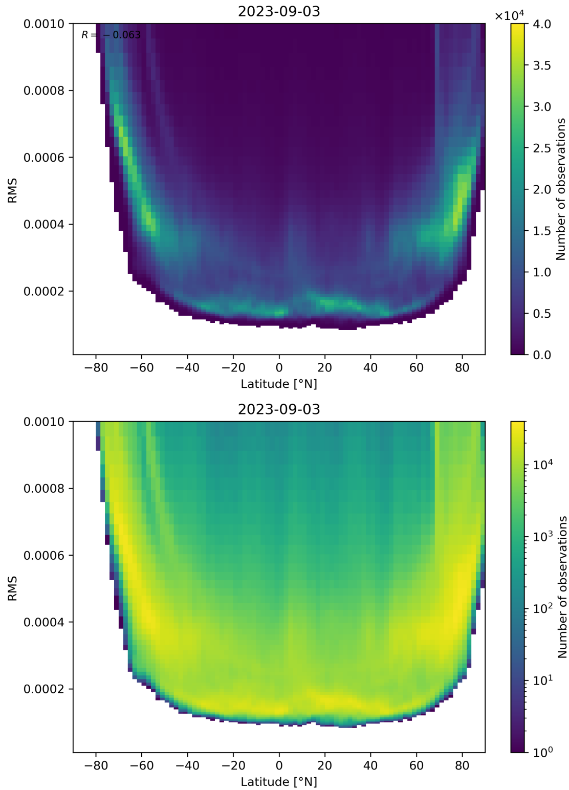
Figure 94: Scatter density plot of “Latitude” against “RMS” for 2023-09-02 to 2023-09-04.
