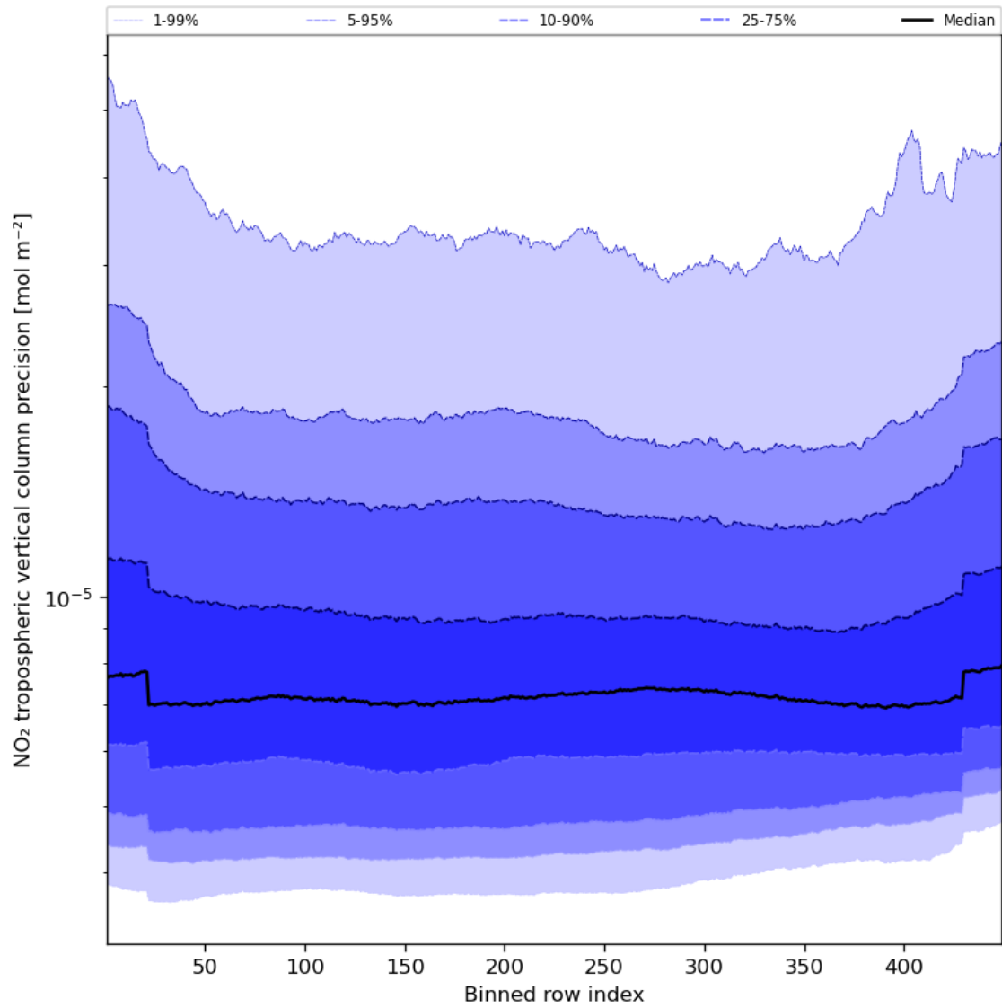
Figure 47: Along track statistics of “NO 2 tropospheric vertical column precision” for 2023-09-02 to 2023-09-04
