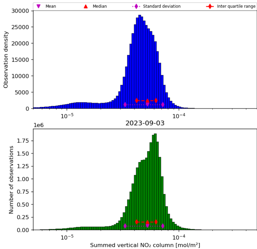
Figure 40: Histogram of “Summed vertical NO 2 column” for 2023-09-02 to 2023-09-04
