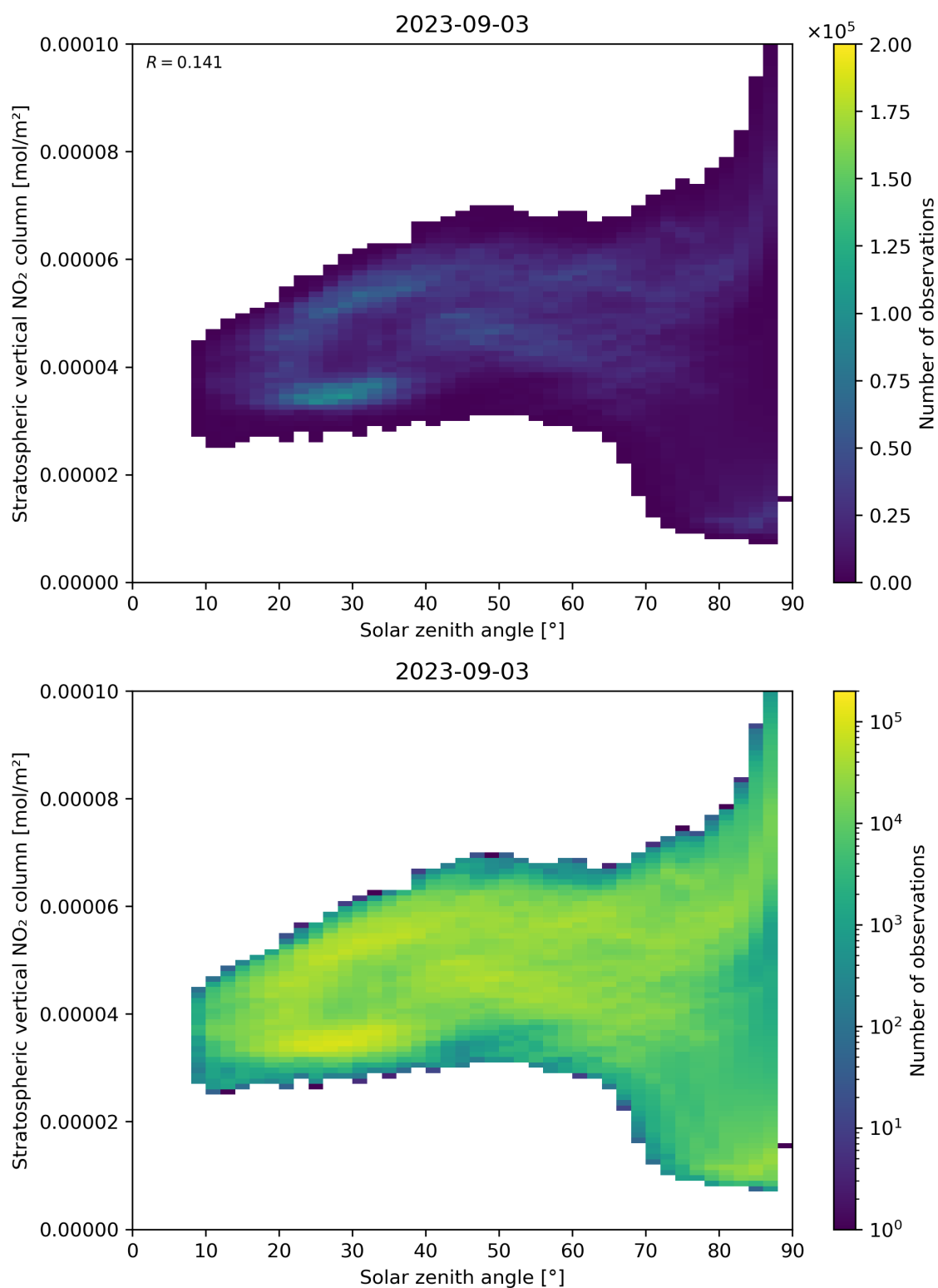
Figure 150: Scatter density plot of “Solar zenith angle” against “Stratospheric vertical NO 2 column” for 2023-09-02 to 2023-09-04.
