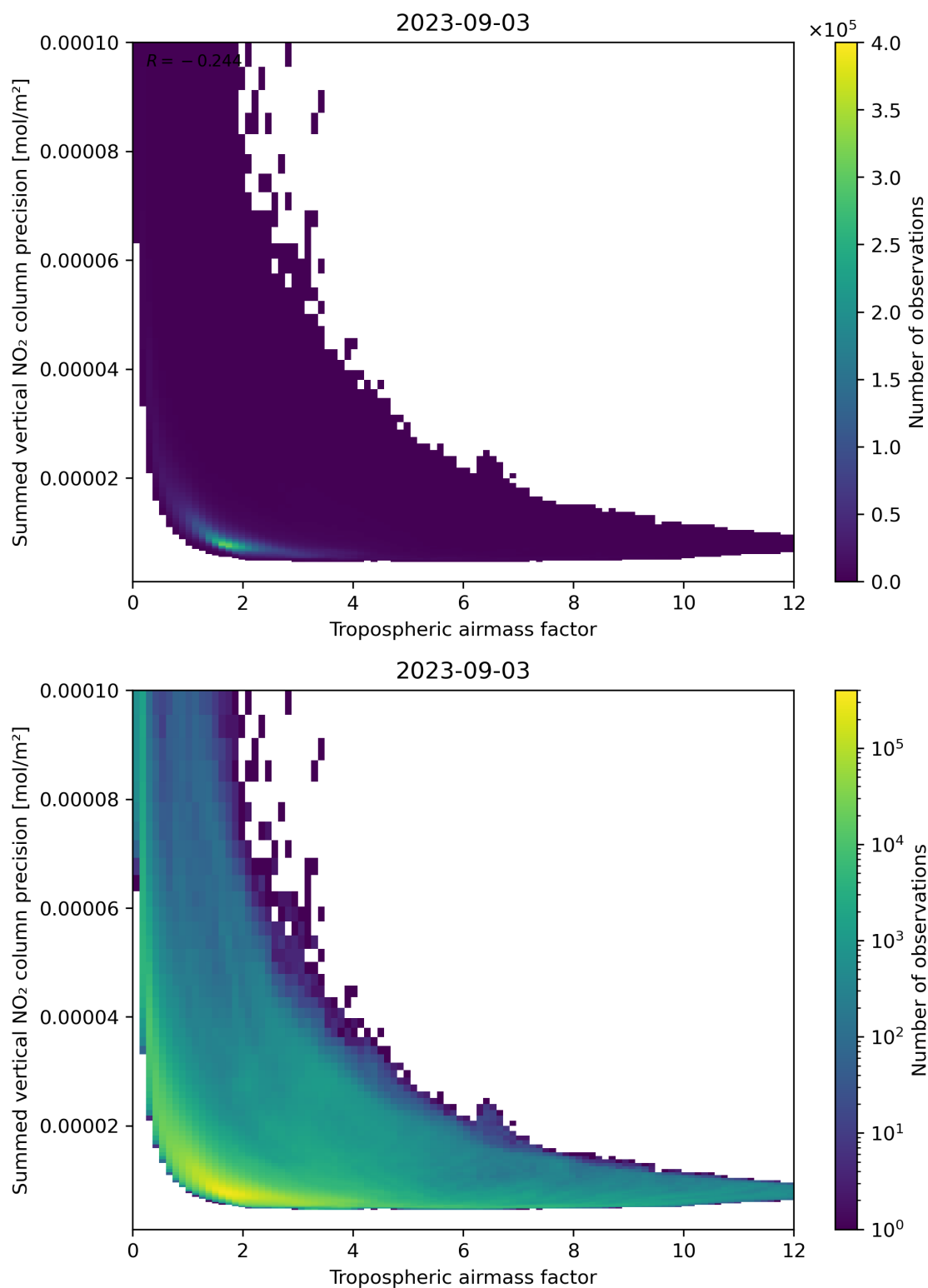
Figure 76: Scatter density plot of “Tropospheric air mass factor” against “Summed vertical NO 2 column precision” for 2023-09-02 to 2023-09-04.
