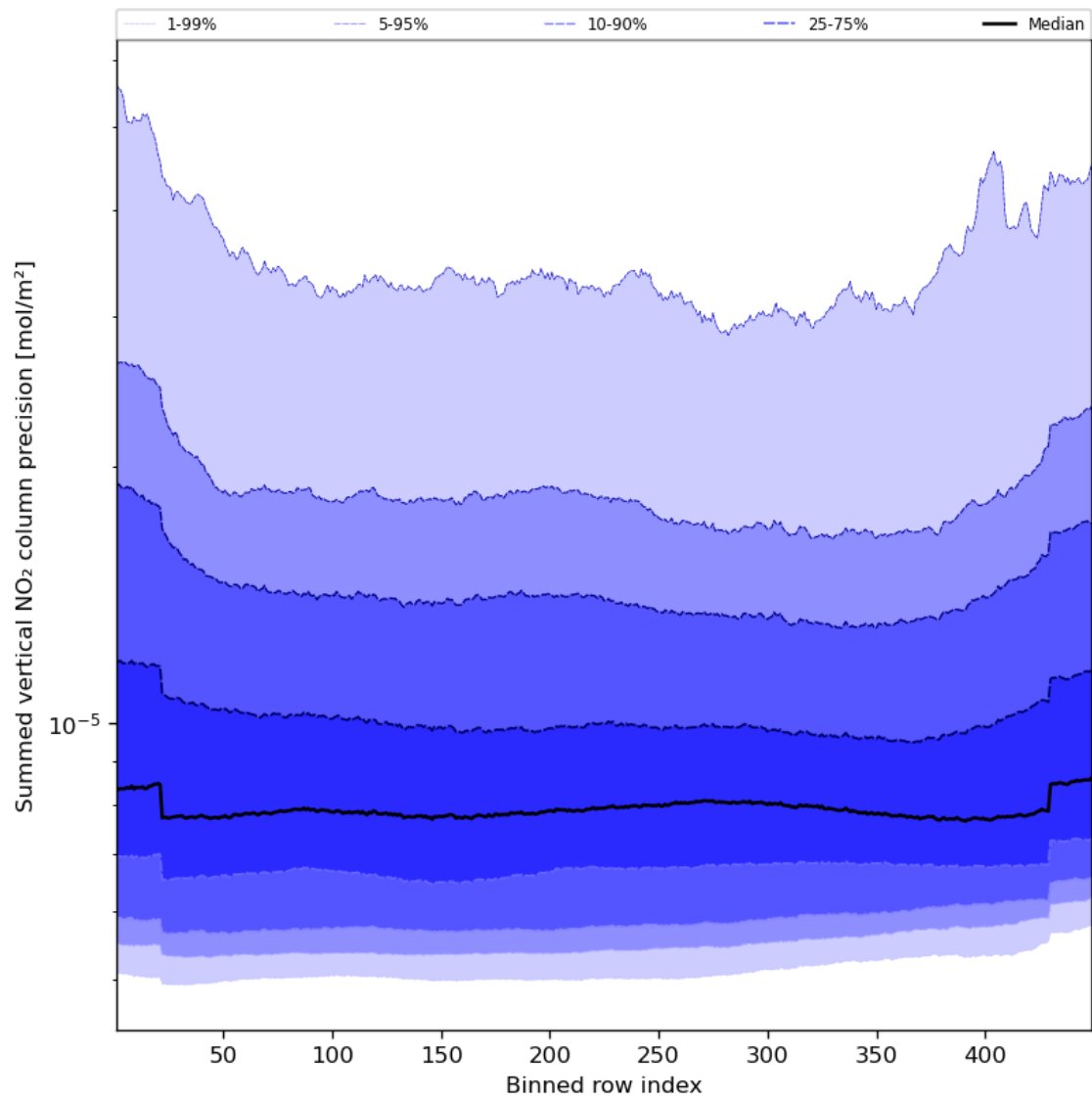
Figure 58: Along track statistics of “Summed vertical NO 2 column precision” for 2023-09-02 to 2023-09-04
