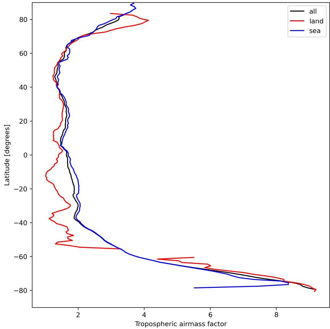
Figure 14: Zonal average of “Tropospheric air mass factor” for 2023-09-02 to 2023-09-04.
