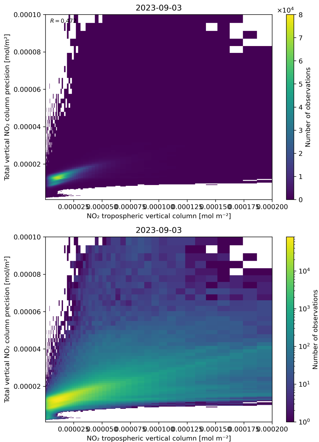
Figure 129: Scatter density plot of “NO 2 tropospheric vertical column” against “Total vertical NO 2 column precision” for 2023-09-02 to 2023-09-04.
