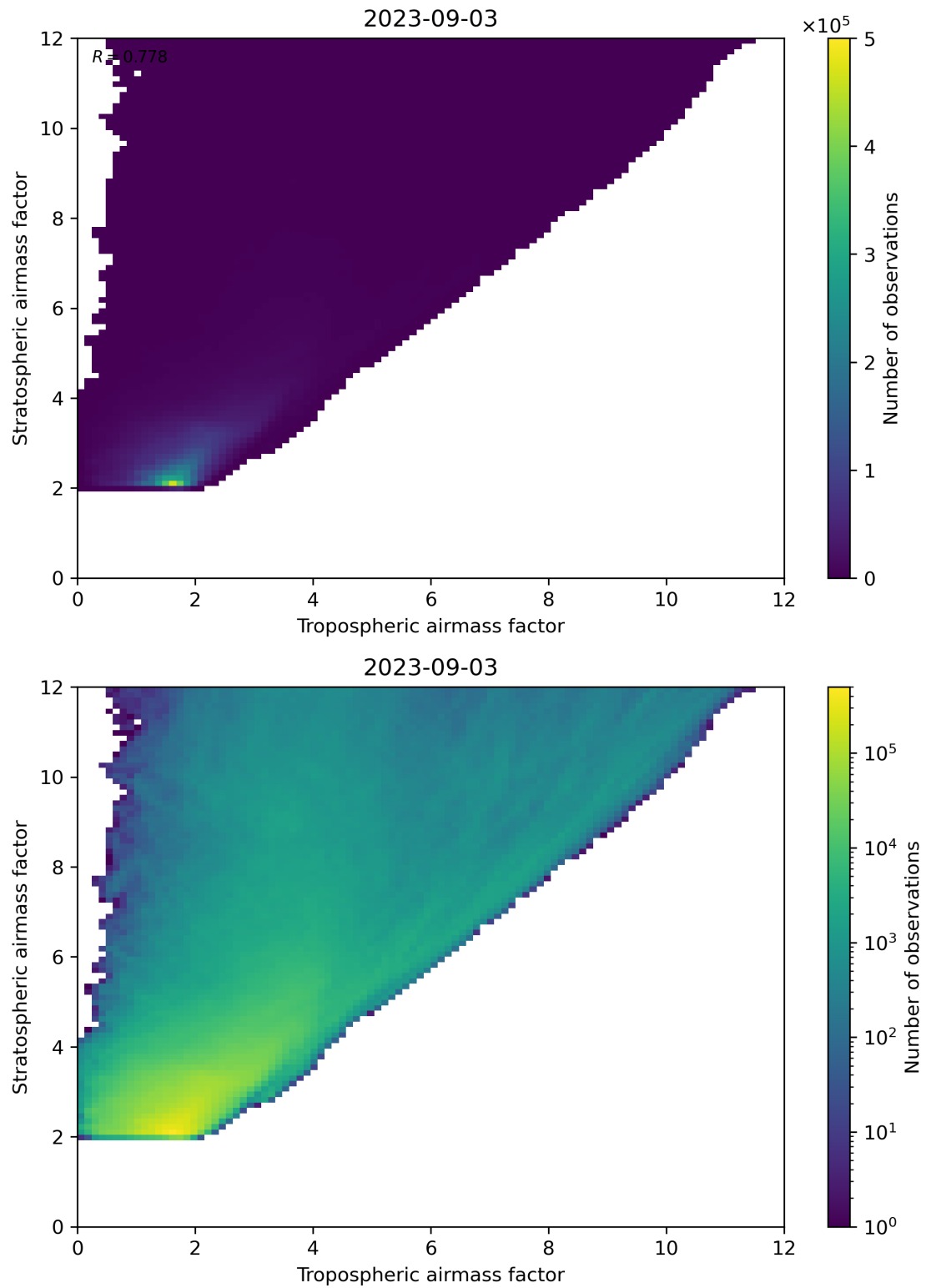
Figure 71: Scatter density plot of “Tropospheric airmass factor” against “Stratospheric airmass factor” for 2023-09-02 to 2023-09-04.
