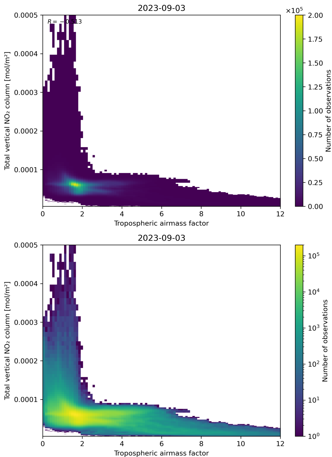
Figure 77: Scatter density plot of “Tropospheric airmass factor” against “Total vertical NO 2 column” for 2023-09-02 to 2023-09-04.
