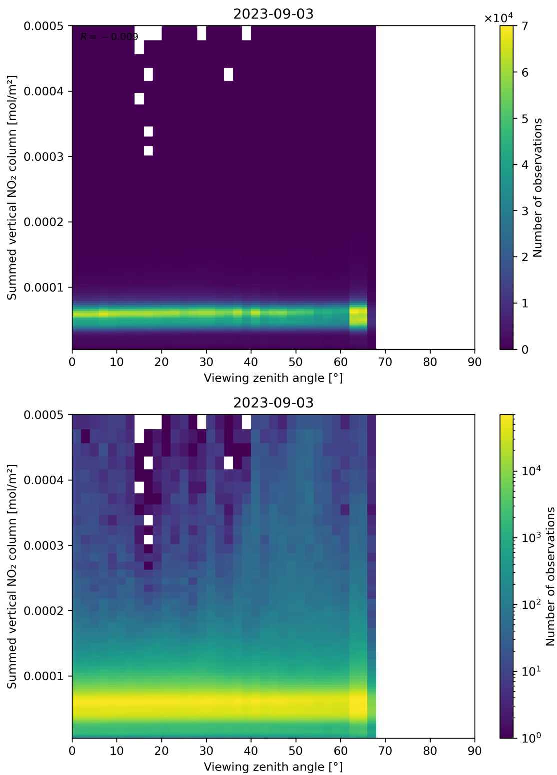
Figure 165: Scatter density plot of “Viewing zenith angle” against “Summed vertical NO 2 column” for 2023-09-02 to 2023-09-04.
