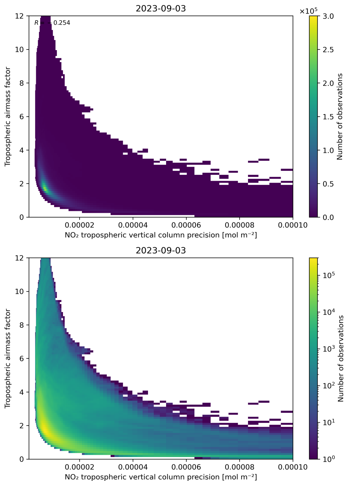
Figure 133: Scatter density plot of “NO 2 tropospheric vertical column precision” against “Tropospheric airmass factor” for 2023-09-02 to 2023-09-04.
