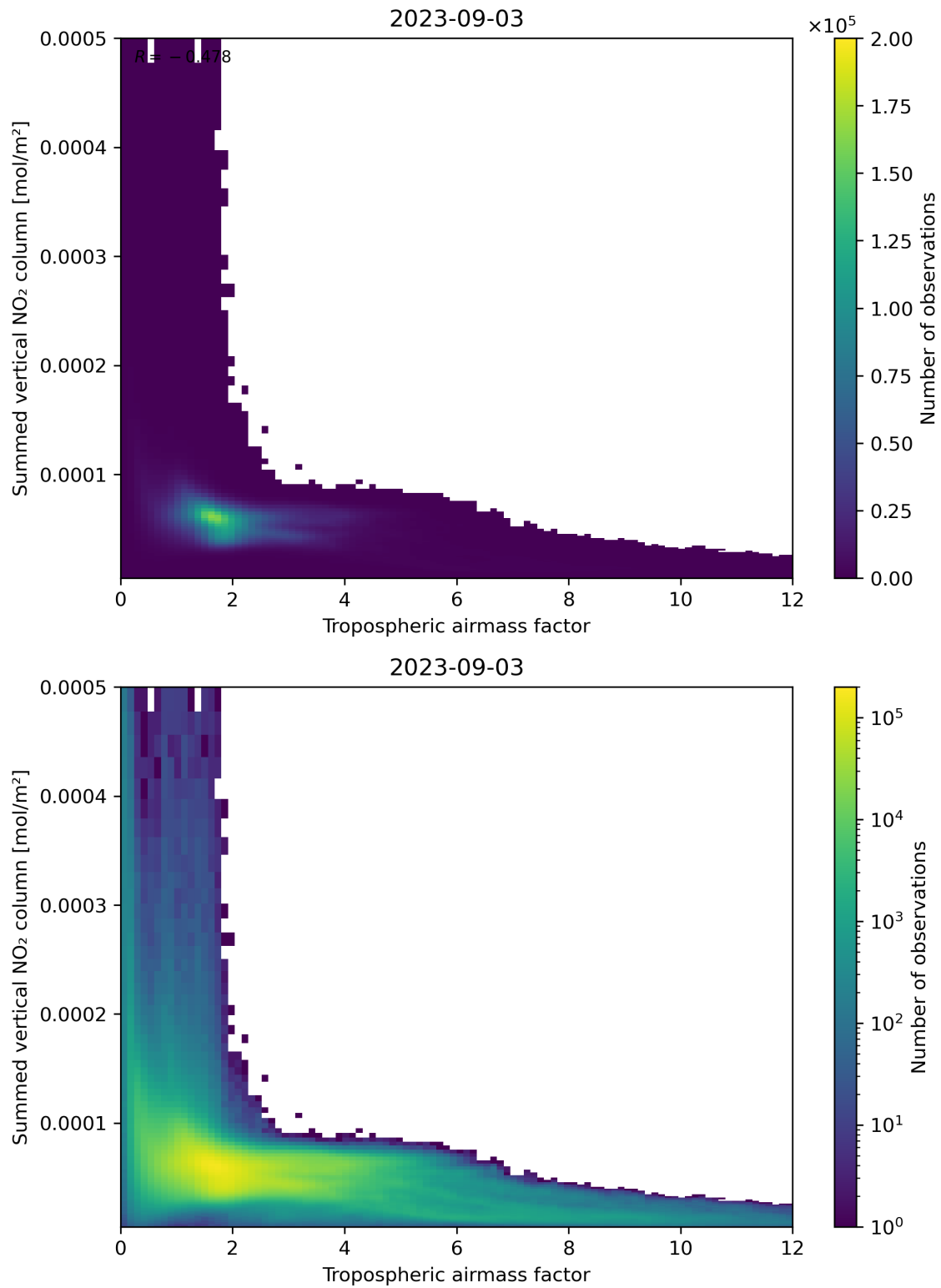
Figure 75: Scatter density plot of “Tropospheric airmass factor” against “Summed vertical NO 2 column” for 2023-09-02 to 2023-09-04.
