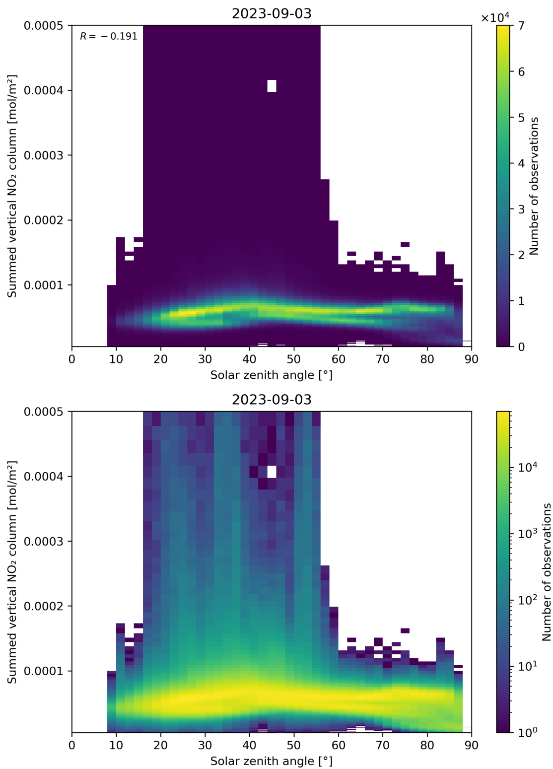
Figure 151: Scatter density plot of “Solar zenith angle” against “Summed vertical NO 2 column” for 2023-09-02 to 2023-09-04.
