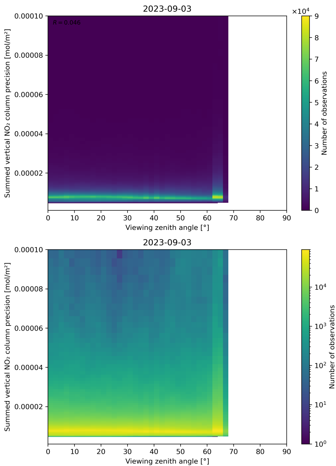
Figure 166: Scatter density plot of “Viewing zenith angle” against “Summed vertical NO 2 column precision” for 2023-09-02 to 2023-09-04.
