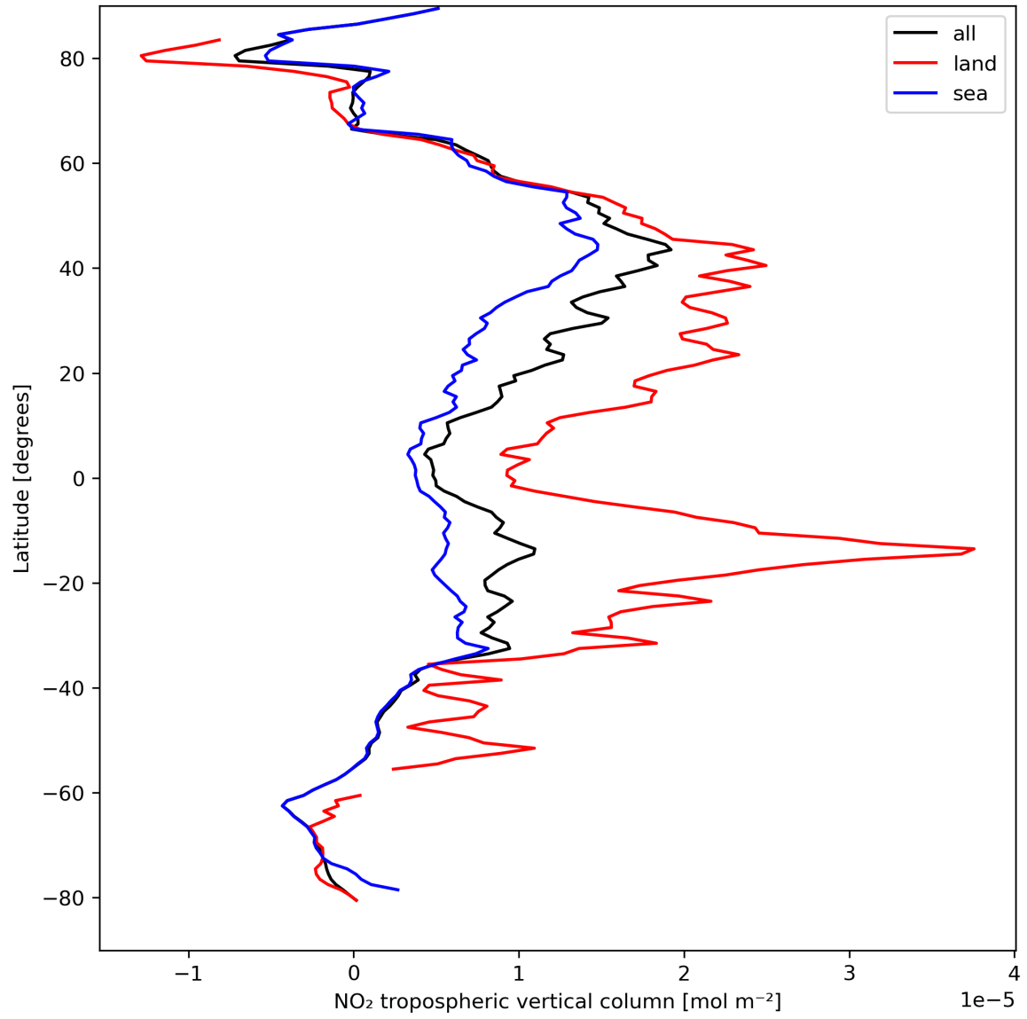
Figure 12: Zonal average of “NO 2 tropospheric vertical column” for 2023-09-02 to 2023-09-04.
