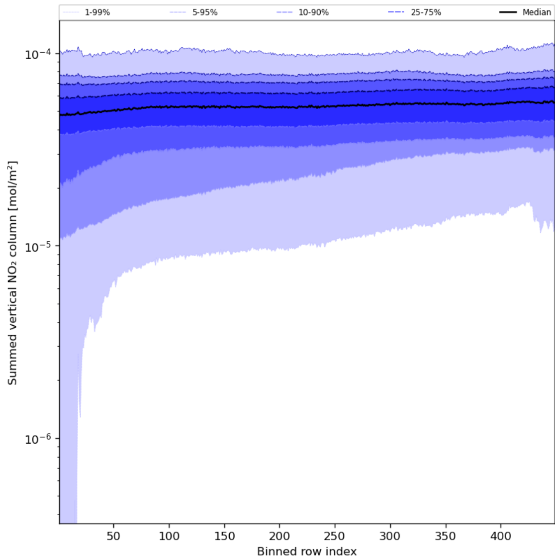
Figure 57: Along track statistics of “Summed vertical NO 2 column” for 2023-09-02 to 2023-09-04
