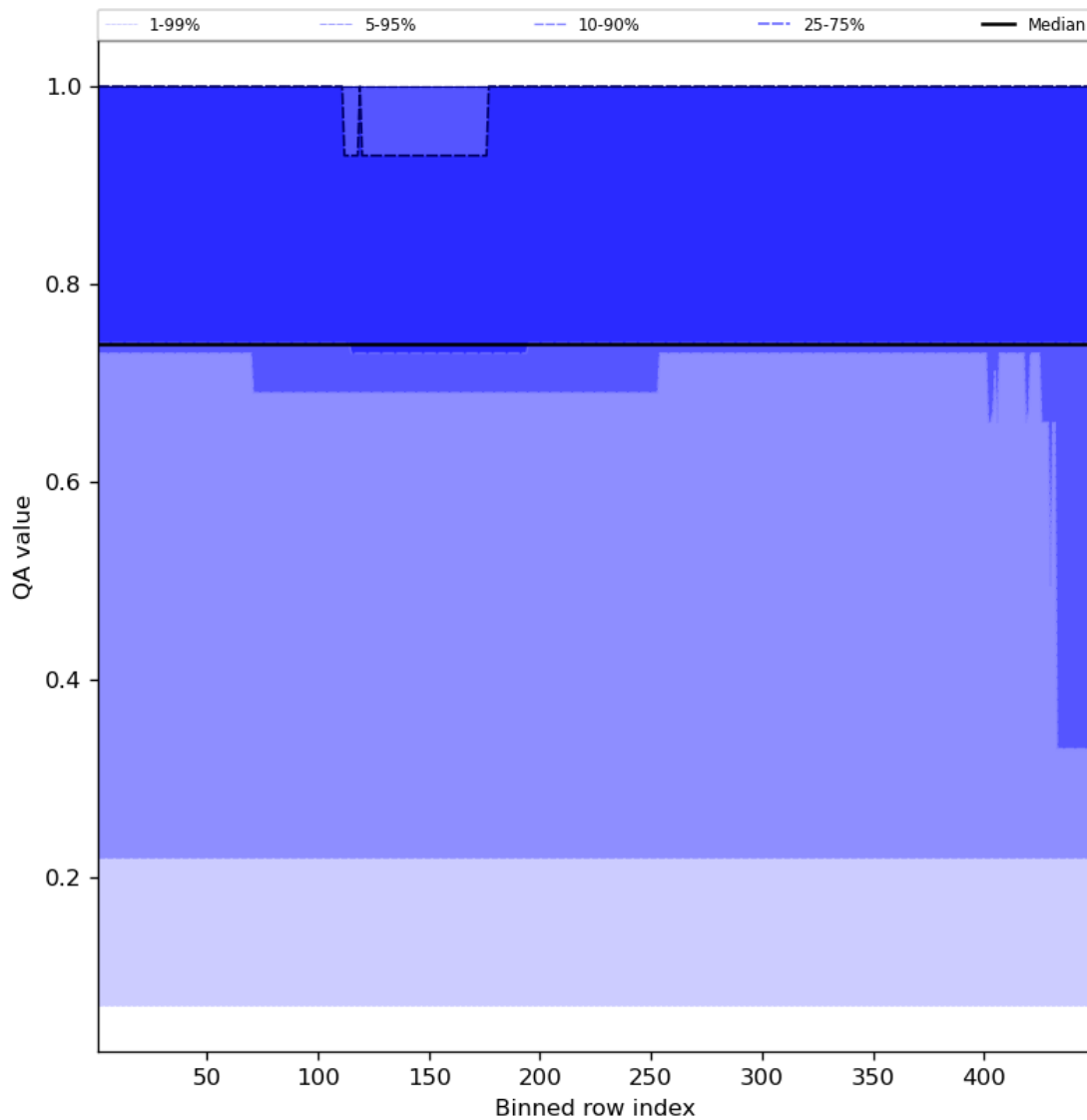
Figure 45: Along track statistics of “QA value” for 2023-09-02 to 2023-09-04
