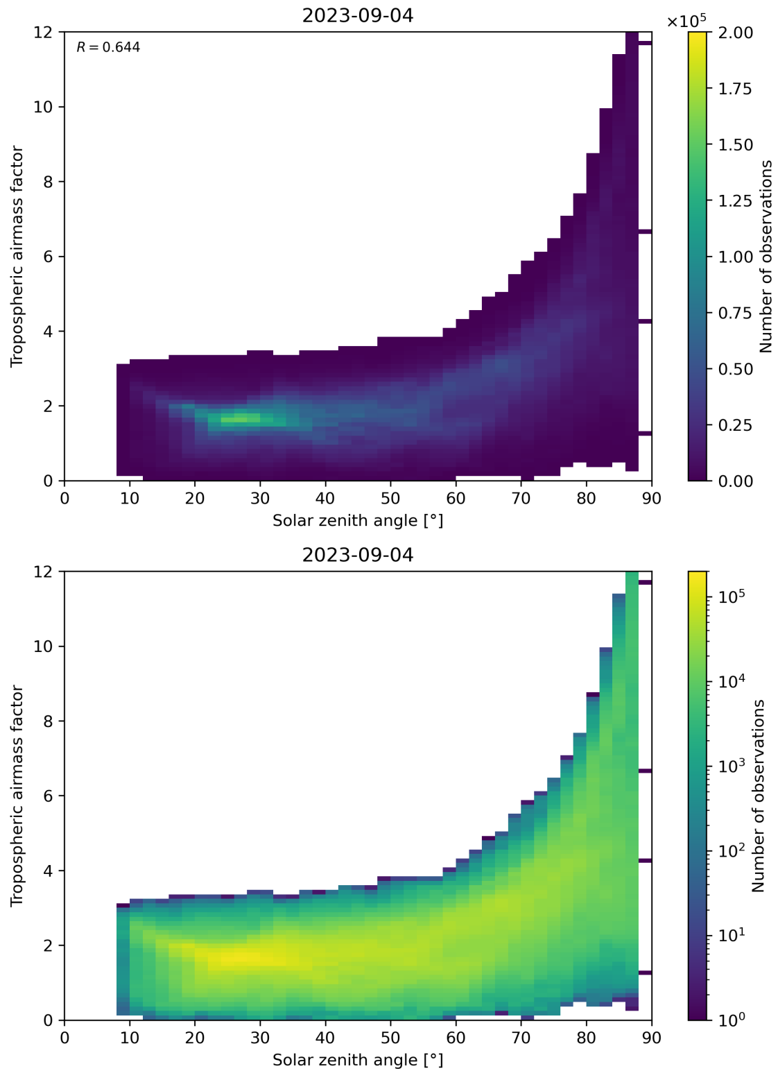
Figure 147: Scatter density plot of “Solar zenith angle” against “Tropospheric airmass factor” for 2023-09-04 to 2023-09-05.
