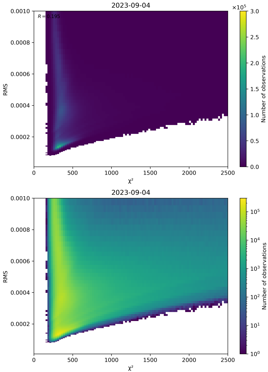
Figure 82: Scatter density plot of “ \chi^2 ” against “RMS” for 2023-09-04 to 2023-09-05.
