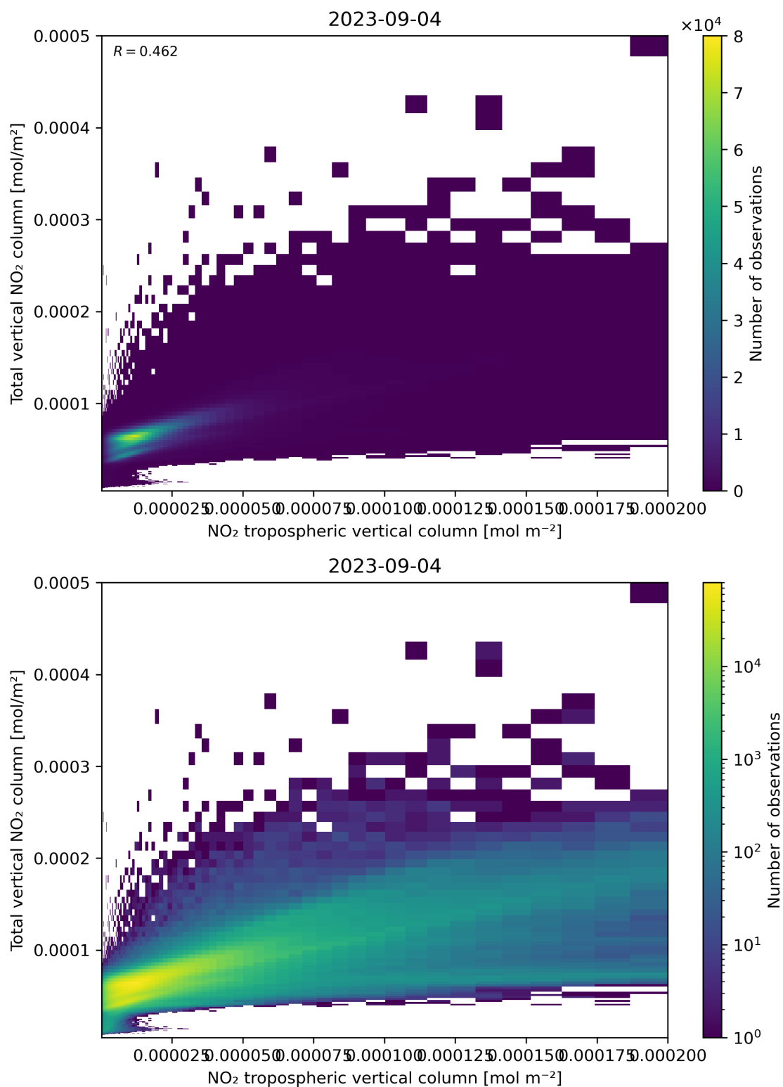
Figure 128: Scatter density plot of “NO 2 tropospheric vertical column” against “Total vertical NO 2 column” for 2023-09-04 to 2023-09-05.
