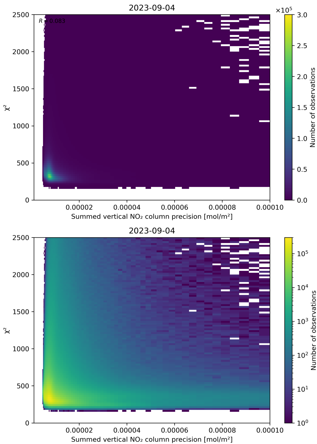
Figure 107: Scatter density plot of “Summed vertical NO 2 column precision” against “ \chi^2 ” for 2023-09-04 to 2023-09-05.
