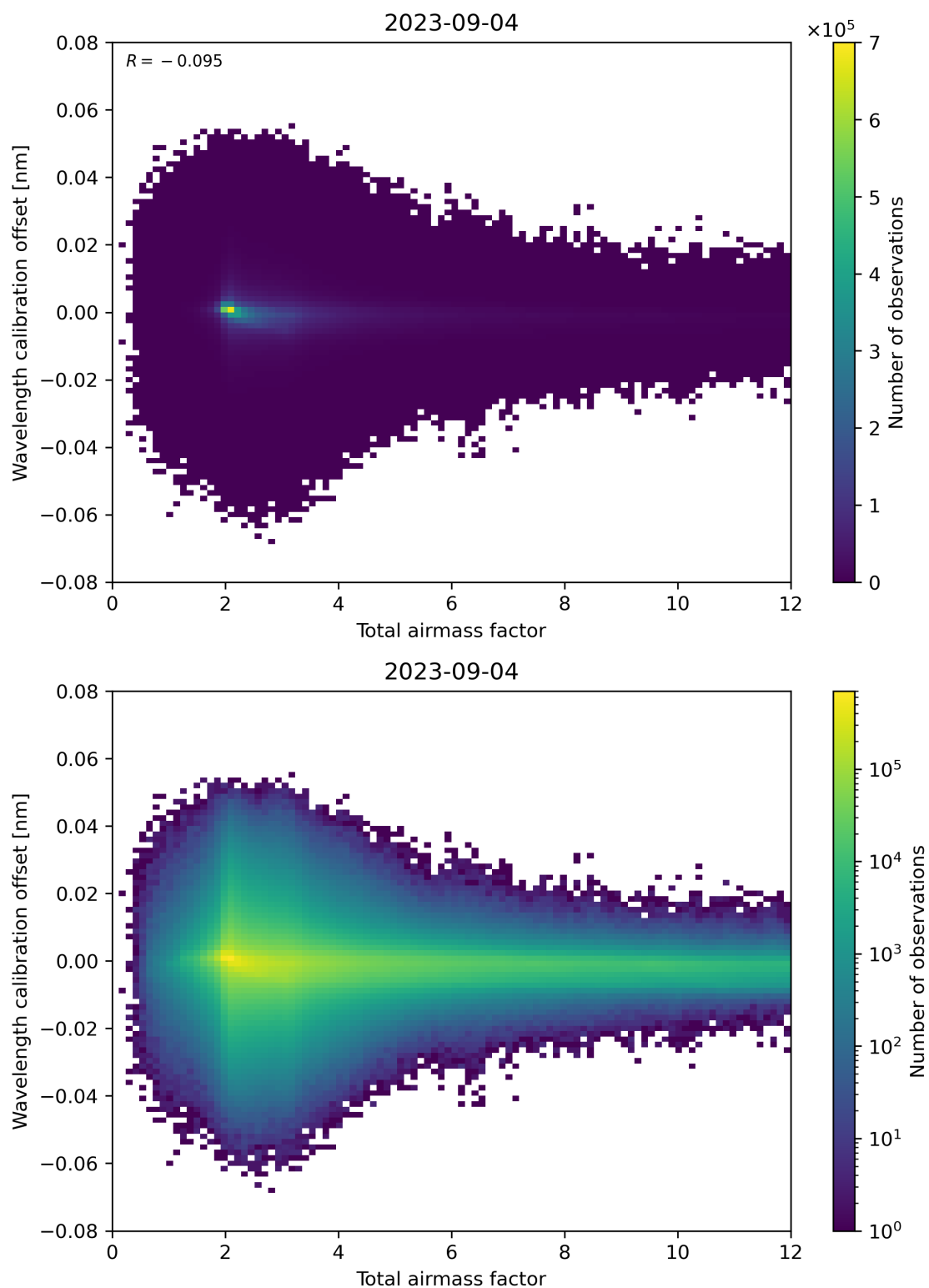
Figure 70: Scatter density plot of “Total airmass factor” against “Wavelength calibration offset” for 2023-09-04 to 2023-09-05.
