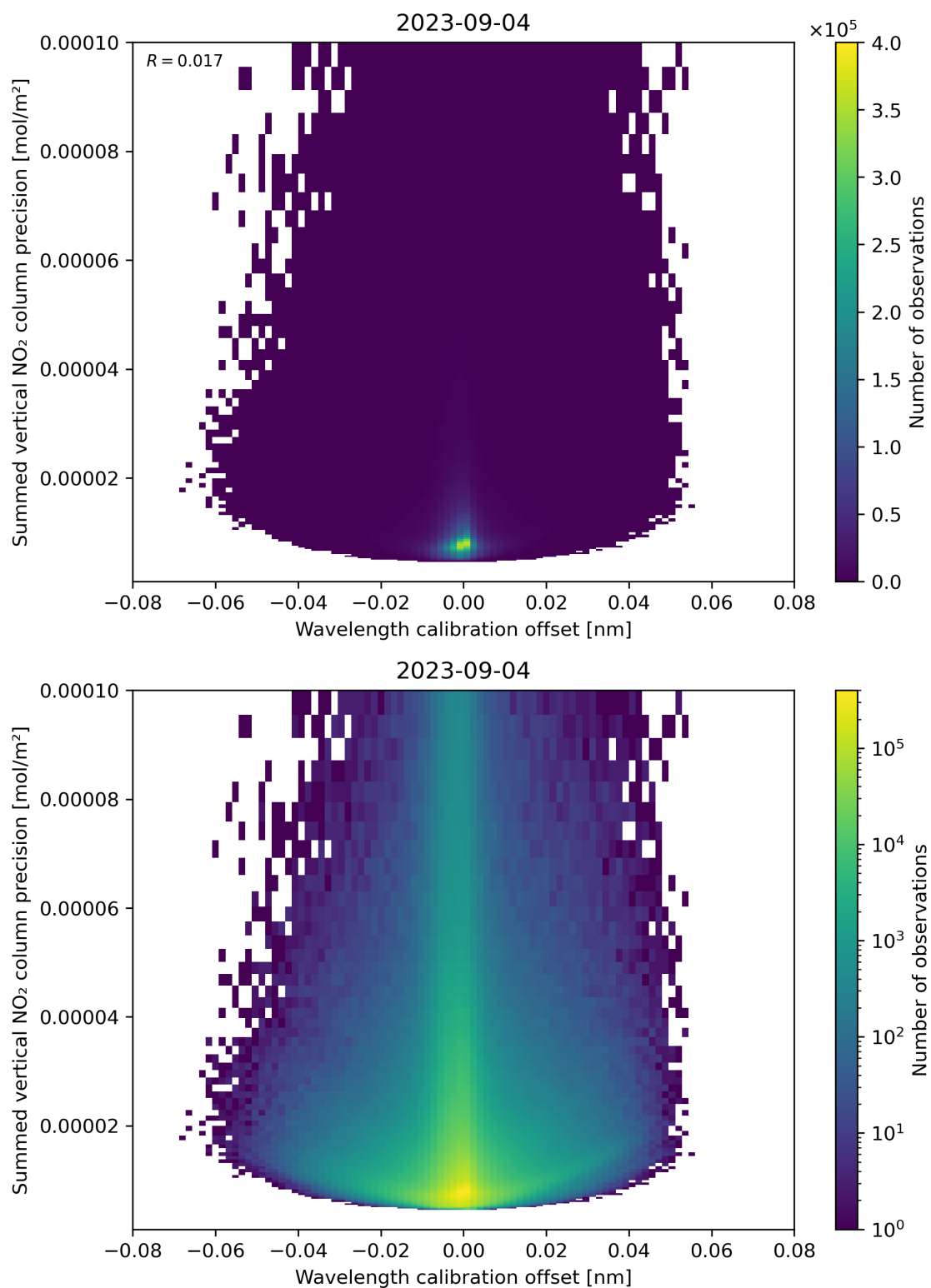
Figure 178: Scatter density plot of “Wavelength calibration offset” against “Summed vertical NO 2 column precision” for 2023-09-04 to 2023-09-05.
