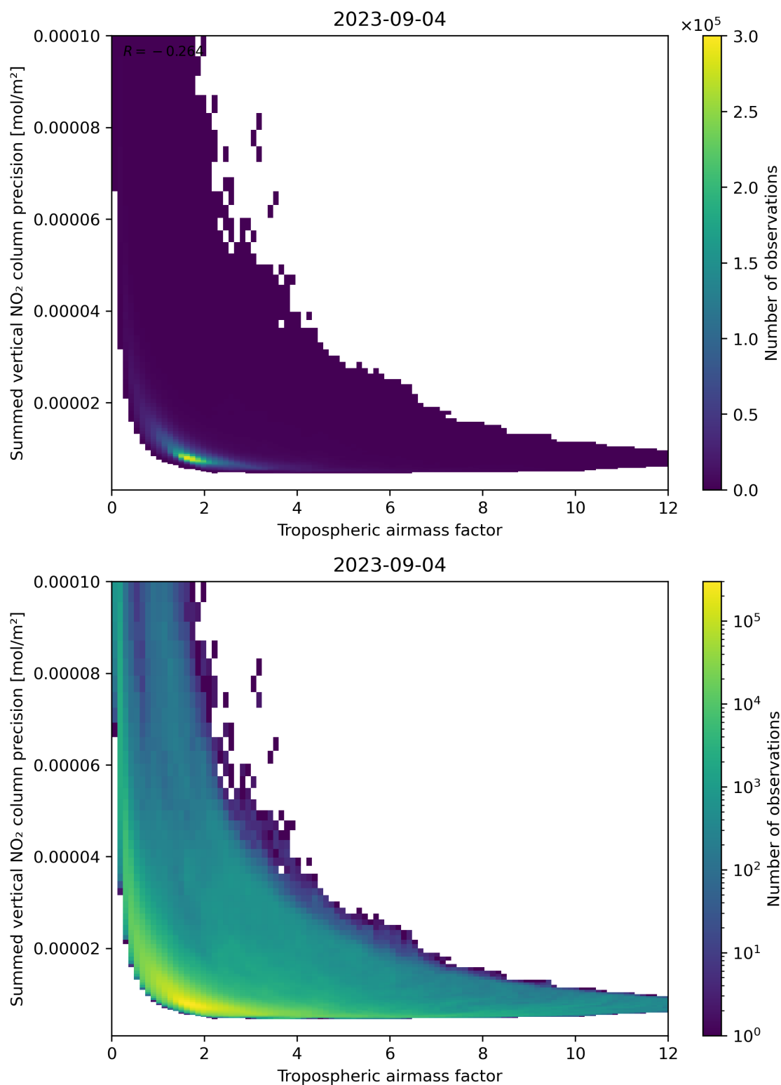
Figure 76: Scatter density plot of “Tropospheric air mass factor” against “Summed vertical NO 2 column precision” for 2023-09-04 to 2023-09-05.
