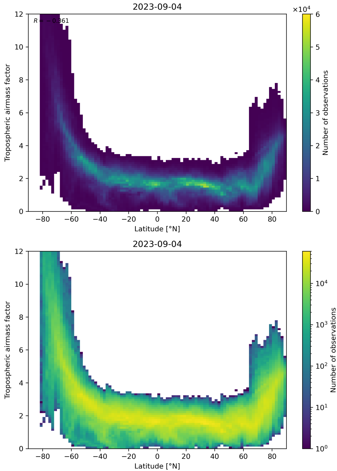
Figure 85: Scatter density plot of “Latitude” against “Tropospheric airmass factor” for 2023-09-04 to 2023-09-05.
