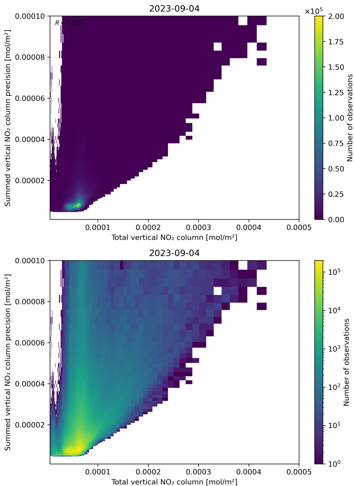
Figure 113: Scatter density plot of “Total vertical NO 2 column” against “Summed vertical NO 2 column precision” for 2023-09-04 to 2023-09-05.
