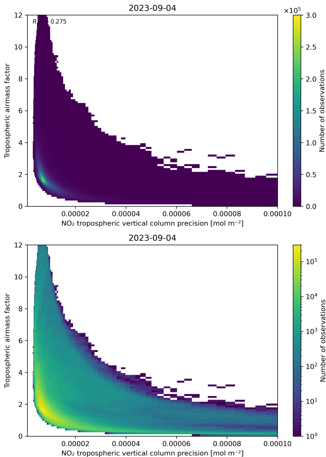
Figure 133: Scatter density plot of “NO 2 tropospheric vertical column precision” against “Tropospheric airmass factor” for 2023-09-04 to 2023-09-05.
