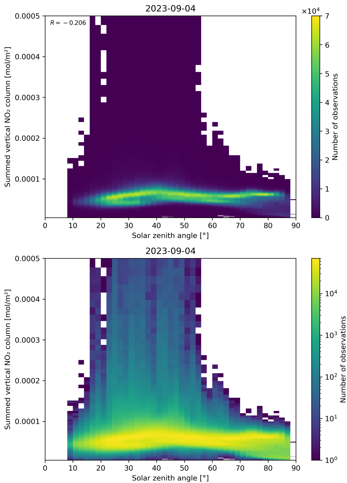
Figure 151: Scatter density plot of “Solar zenith angle” against “Summed vertical NO 2 column” for 2023-09-04 to 2023-09-05.
