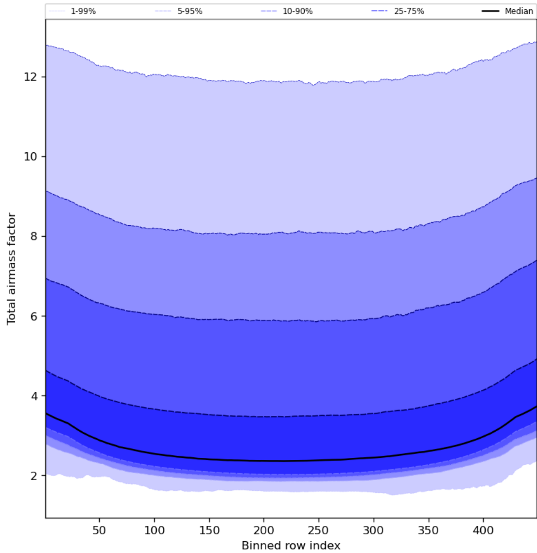
Figure 49: Along track statistics of “Total airmass factor” for 2023-09-04 to 2023-09-05
