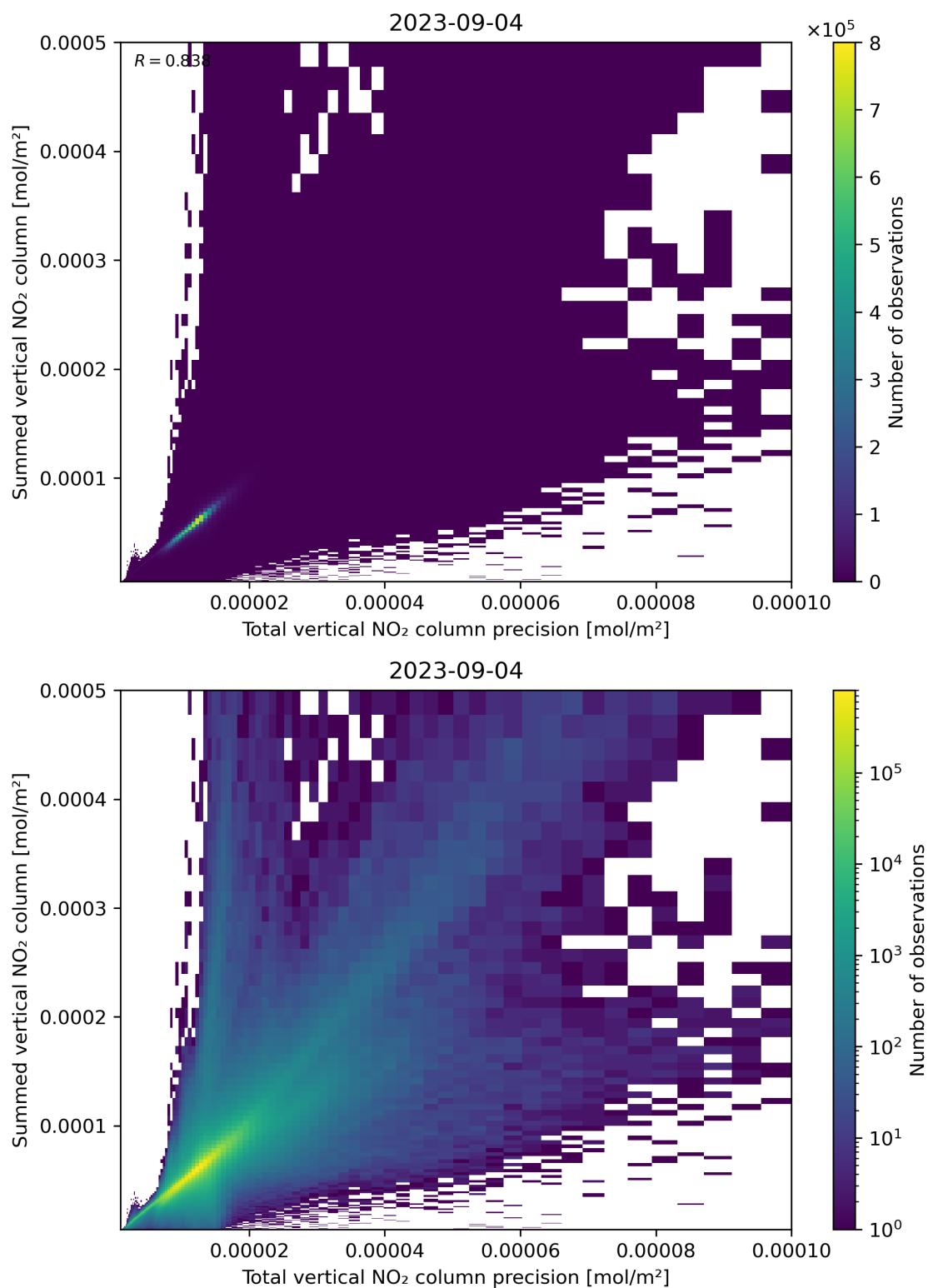
Figure 117: Scatter density plot of “Total vertical NO 2 column precision” against “Summed vertical NO 2 column” for 2023-09-04 to 2023-09-05.
