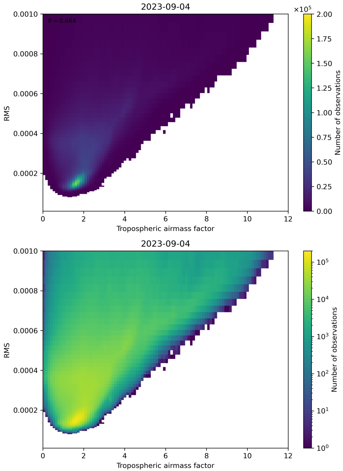
Figure 79: Scatter density plot of “Tropospheric airmass factor” against “RMS” for 2023-09-04 to 2023-09-05.
