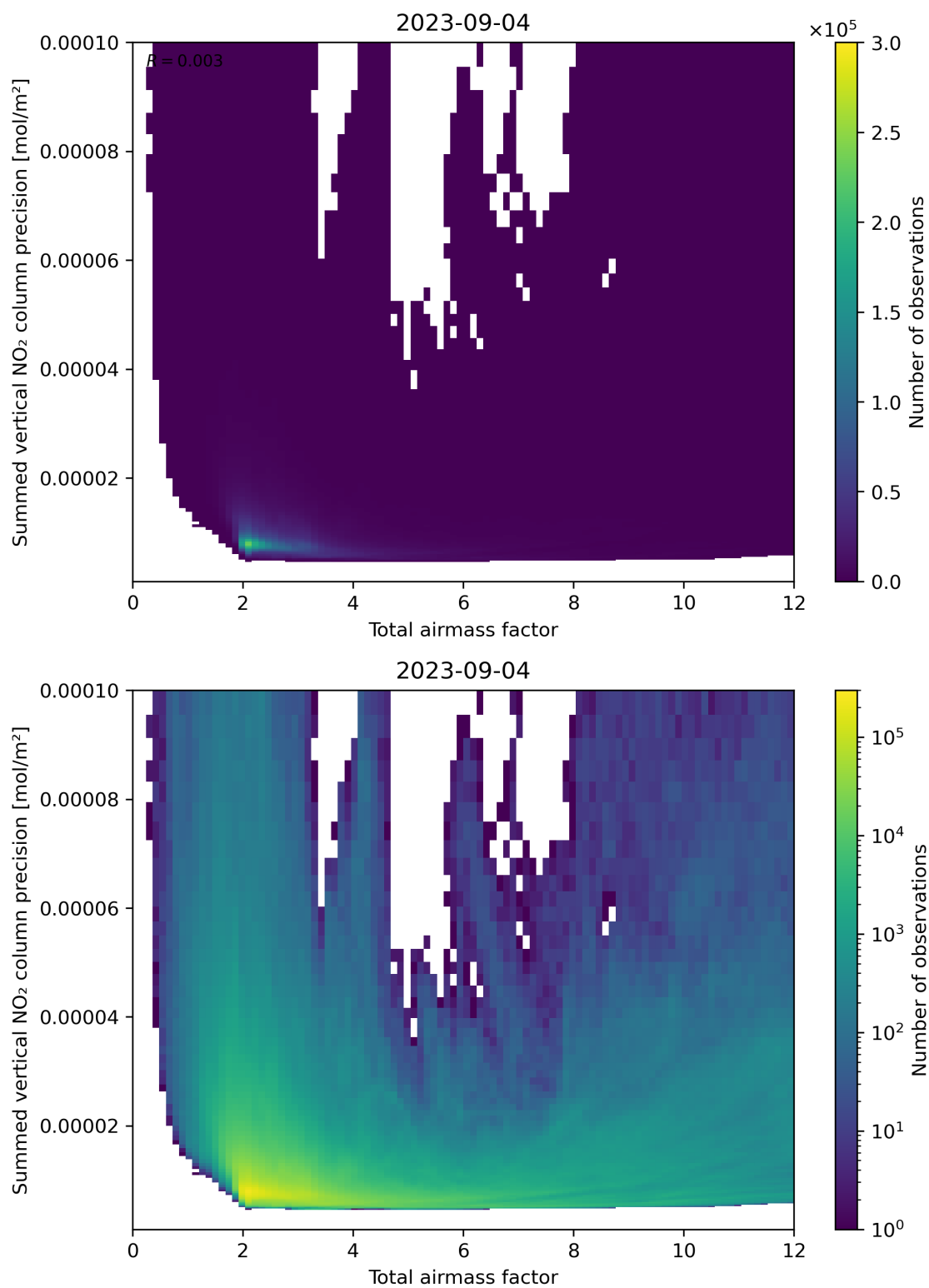
Figure 66: Scatter density plot of “Total airmass factor” against “Summed vertical NO 2 column precision” for 2023-09-04 to 2023-09-05.
