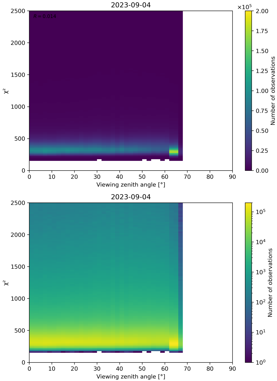
Figure 162: Scatter density plot of “Viewing zenith angle” against “ \chi^2 ” for 2023-09-04 to 2023-09-05.
