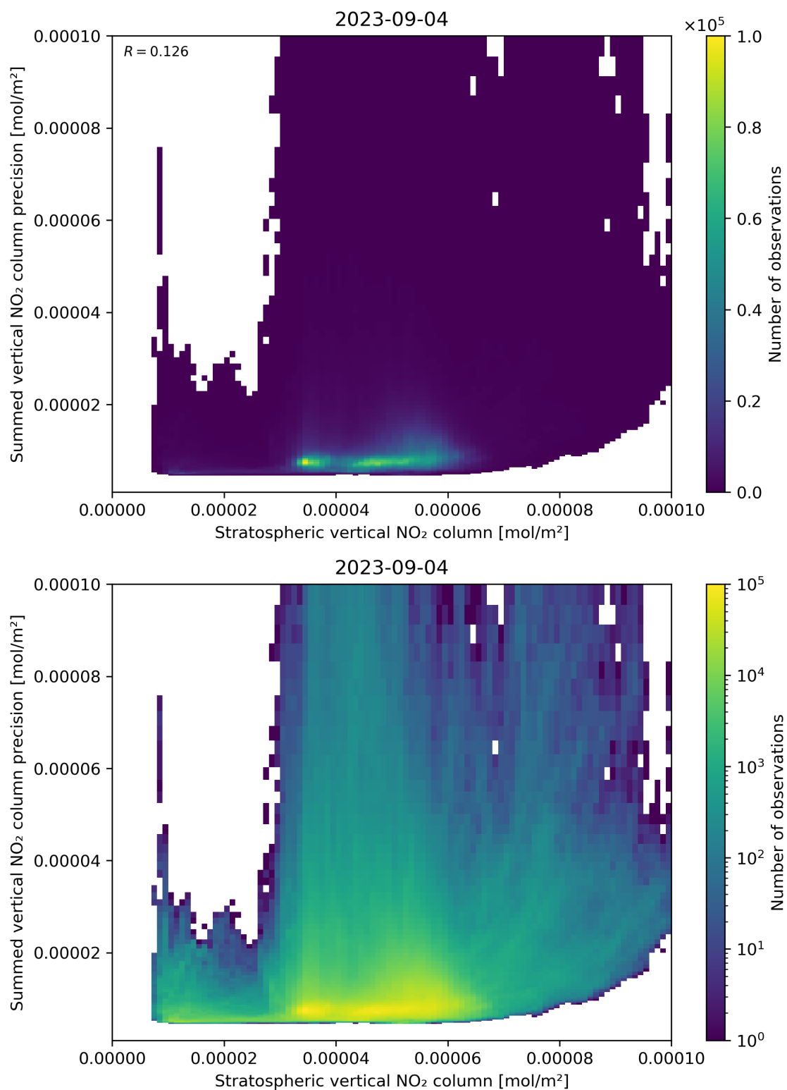
Figure 99: Scatter density plot of “Stratospheric vertical NO 2 column” against “Summed vertical NO 2 column precision” for 2023-09-04 to 2023-09-05.
