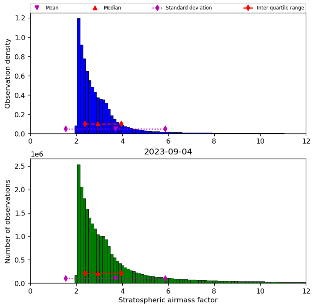
Figure 44: Histogram of “Stratospheric airmass factor” for 2023-09-04 to 2023-09-05
