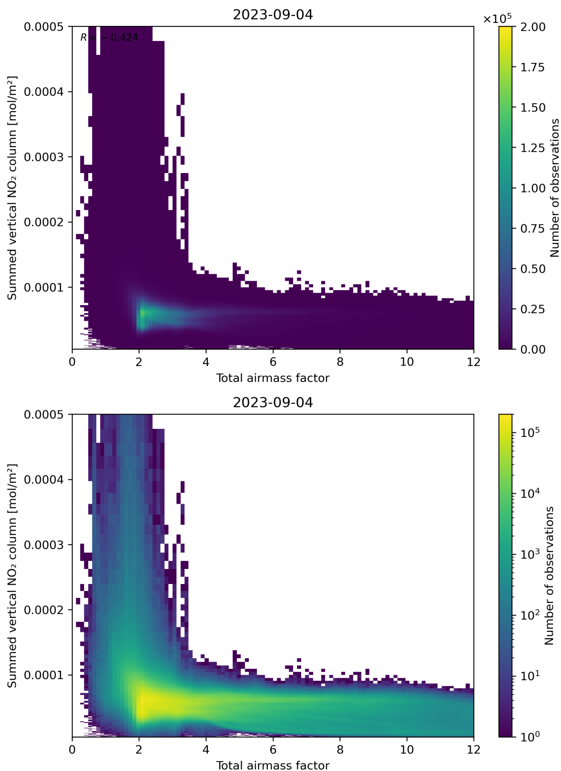
Figure 65: Scatter density plot of “Total airmass factor” against “Summed vertical NO 2 column” for 2023-09-04 to 2023-09-05.
