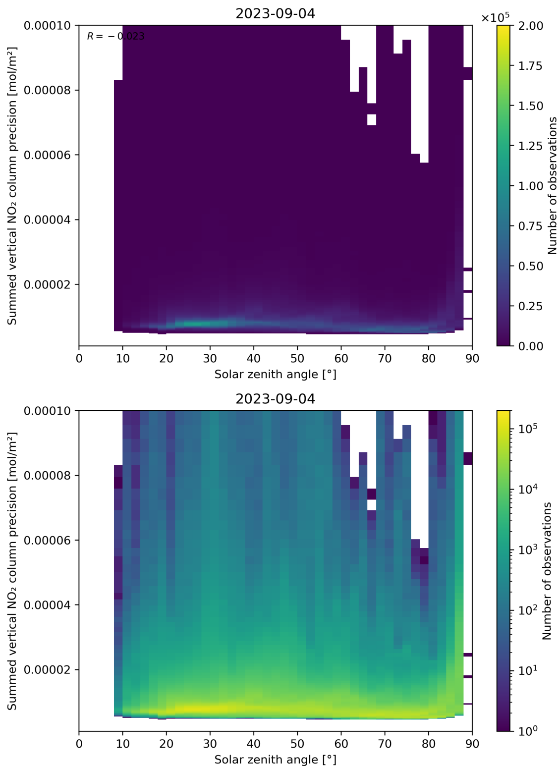
Figure 152: Scatter density plot of “Solar zenith angle” against “Summed vertical NO 2 column precision” for 2023-09-04 to 2023-09-05.
