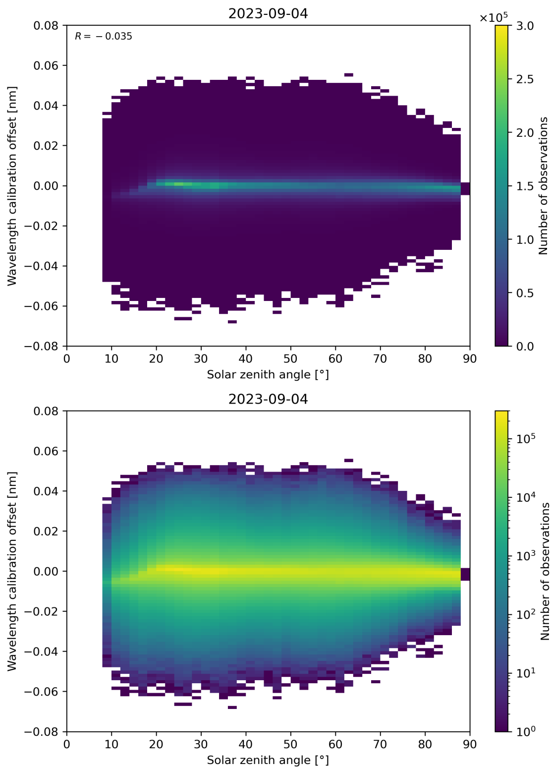
Figure 158: Scatter density plot of “Solar zenith angle” against “Wavelength calibration offset” for 2023-09-04 to 2023-09-05.
