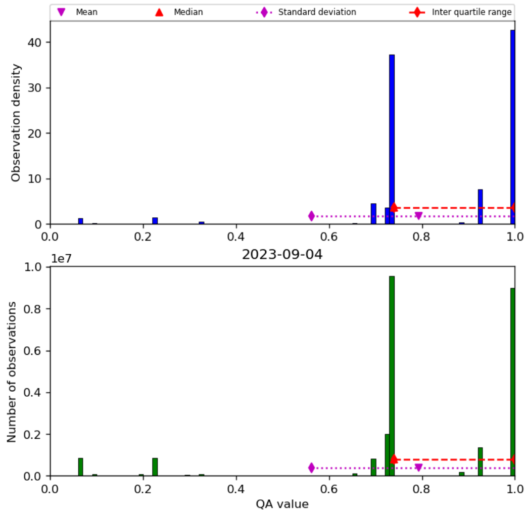
Figure 28: Histogram of “QA value” for 2023-09-04 to 2023-09-05
