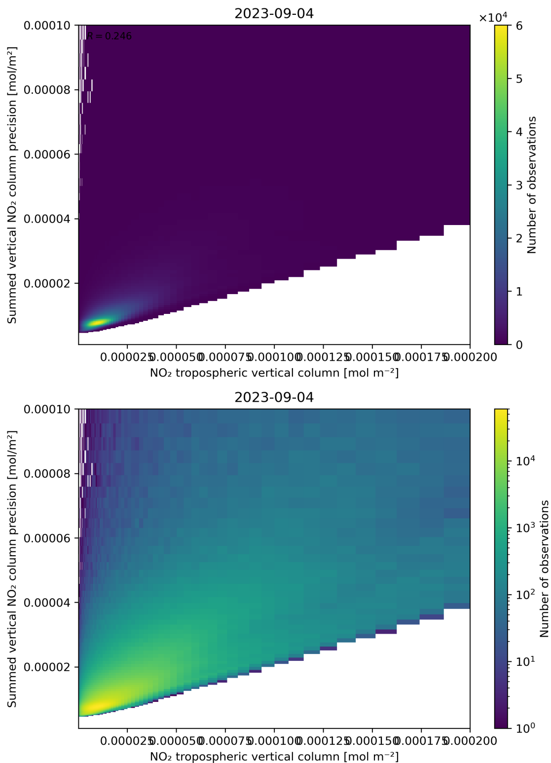
Figure 127: Scatter density plot of “NO 2 tropospheric vertical column” against “Summed vertical NO 2 column precision” for 2023-09-04 to 2023-09-05.
