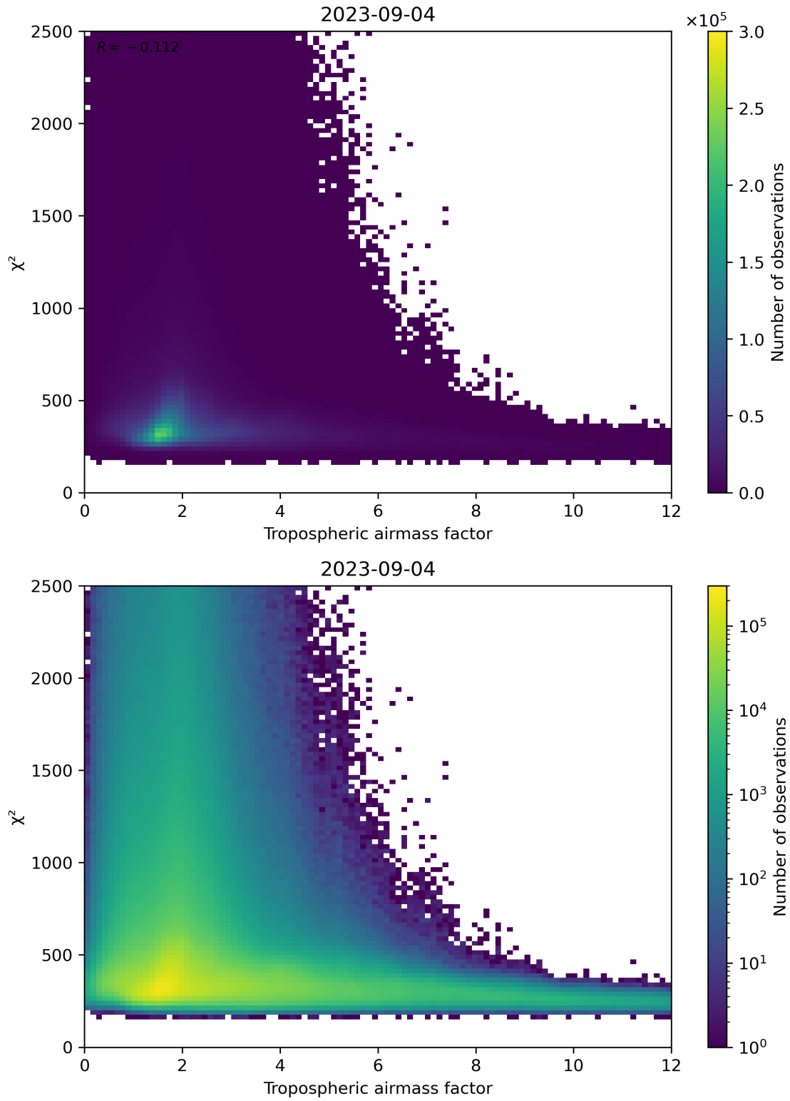
Figure 73: Scatter density plot of “Tropospheric airmass factor” against “ \chi^2 ” for 2023-09-04 to 2023-09-05.
