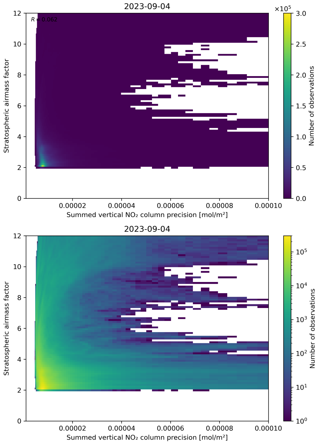
Figure 106: Scatter density plot of “Summed vertical NO 2 column precision” against “Stratospheric airmass factor” for 2023-09-04 to 2023-09-05.
