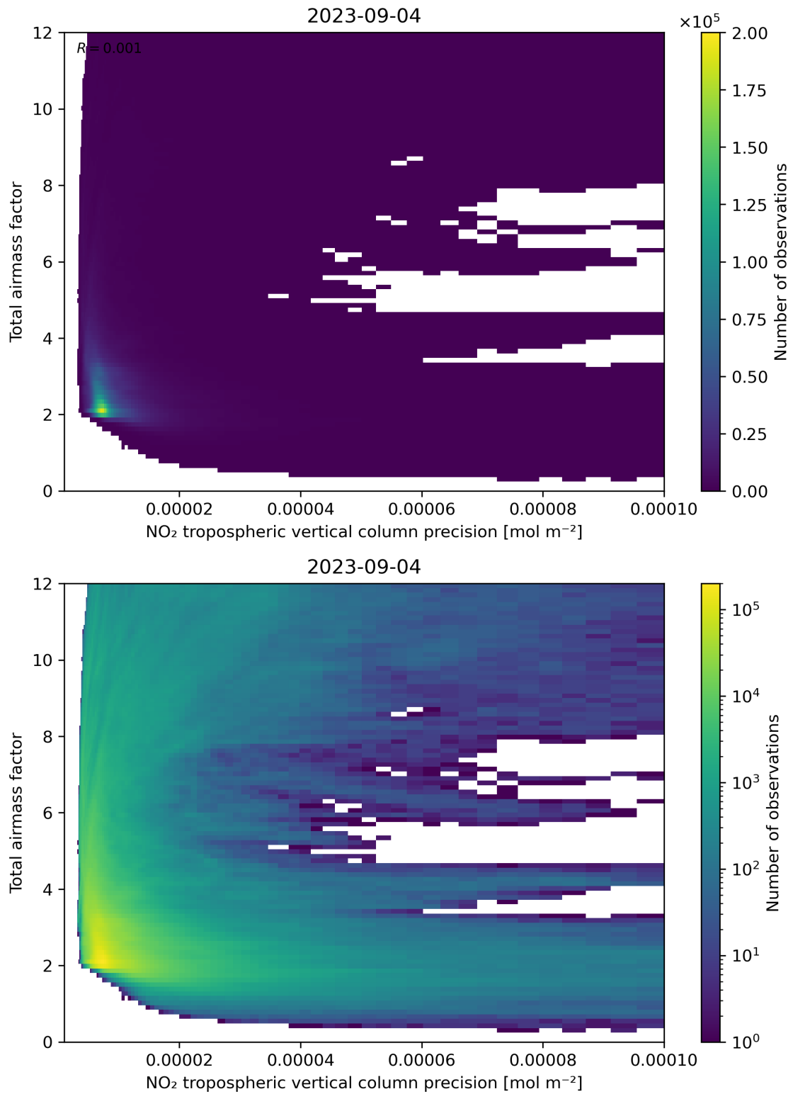
Figure 132: Scatter density plot of “NO 2 tropospheric vertical column precision” against “Total air mass factor” for 2023-09-04 to 2023-09-05.
