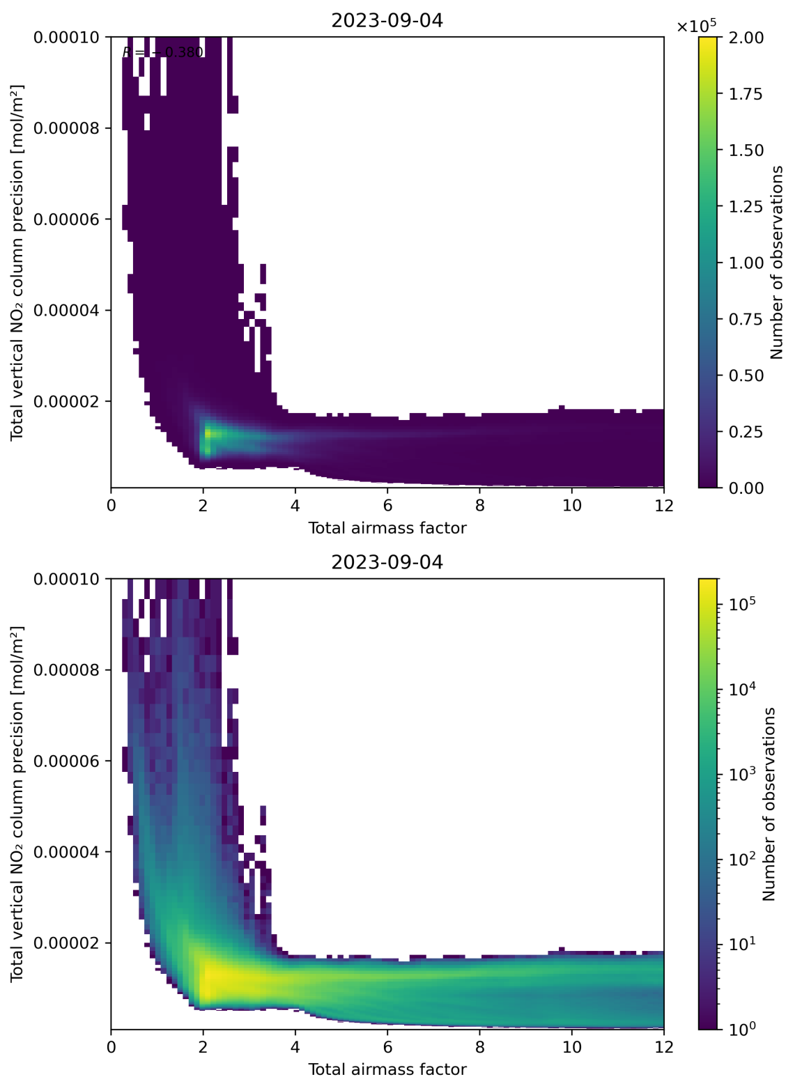
Figure 68: Scatter density plot of “Total airmass factor” against “Total vertical NO 2 column precision” for 2023-09-04 to 2023-09-05.
