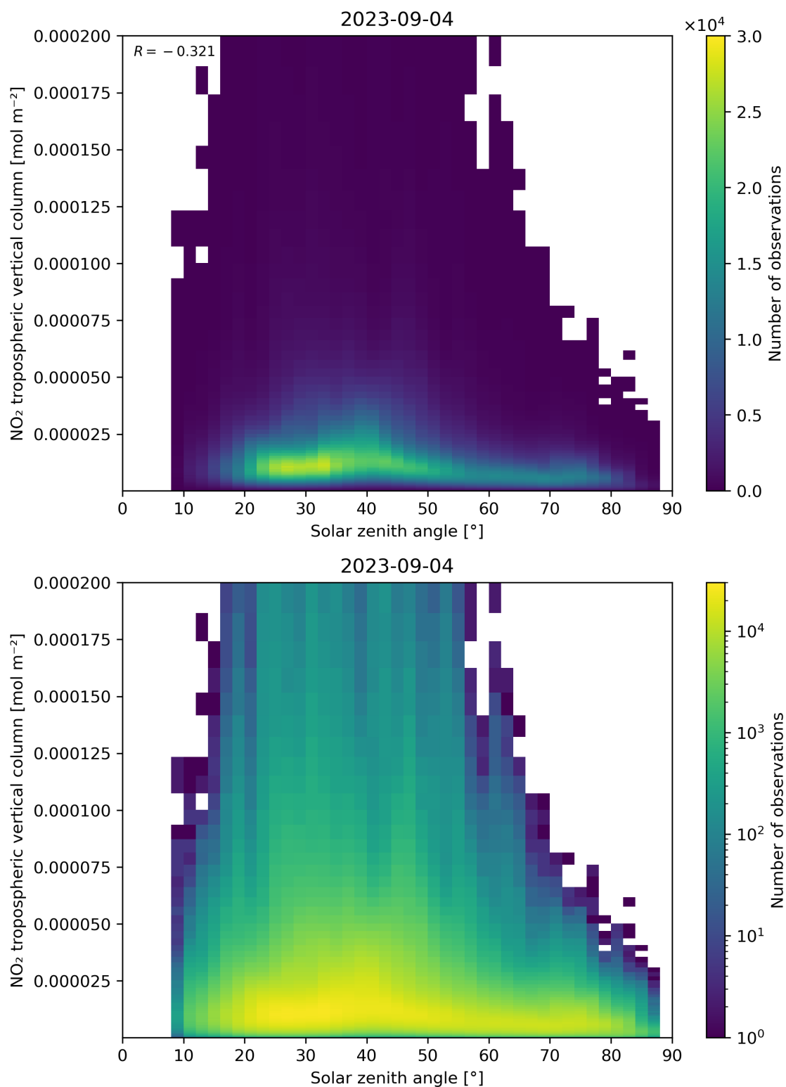
Figure 155: Scatter density plot of “Solar zenith angle” against “NO 2 tropospheric vertical column” for 2023-09-04 to 2023-09-05.
