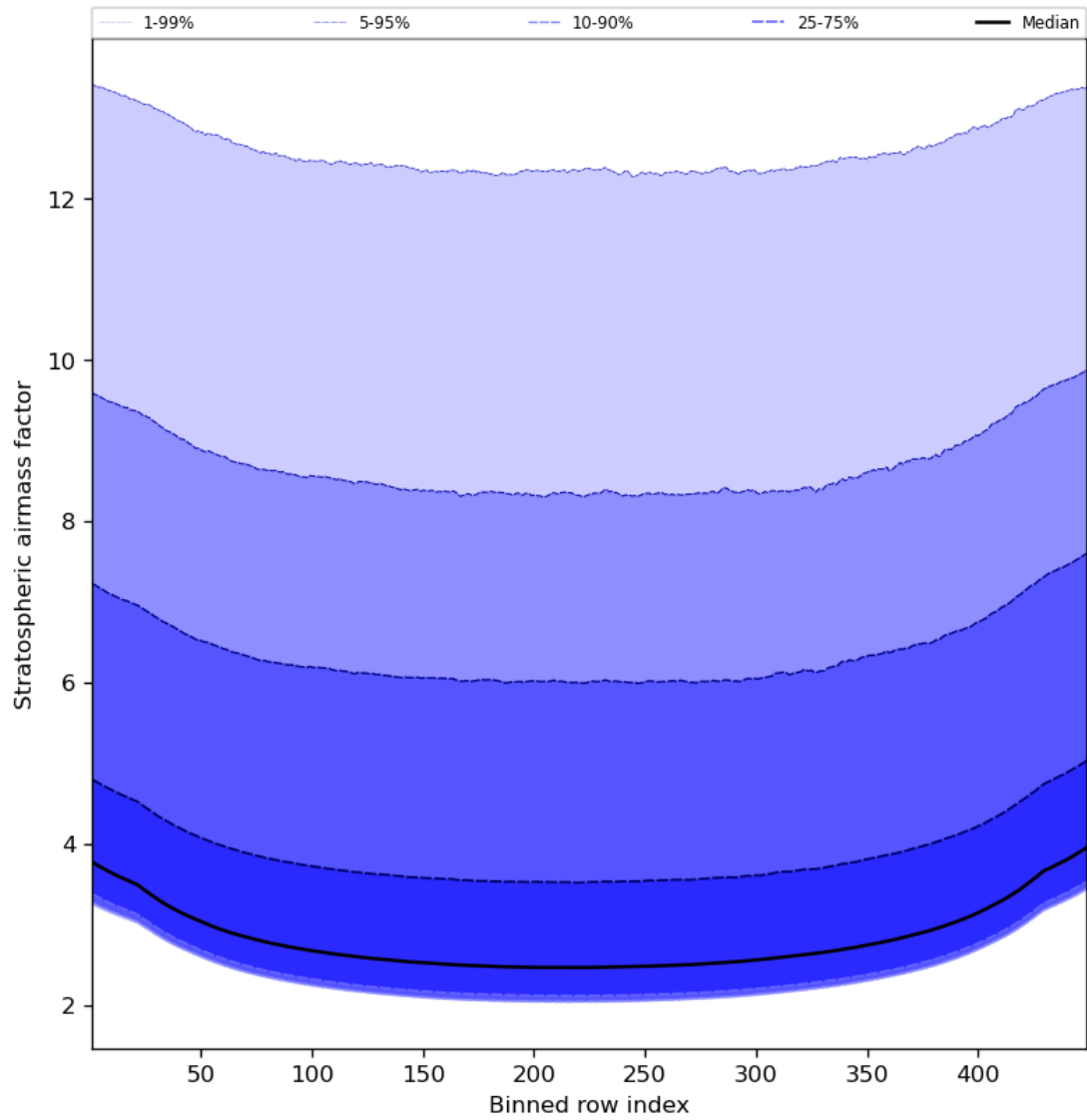
Figure 61: Along track statistics of “Stratospheric airmass factor” for 2023-09-04 to 2023-09-05
