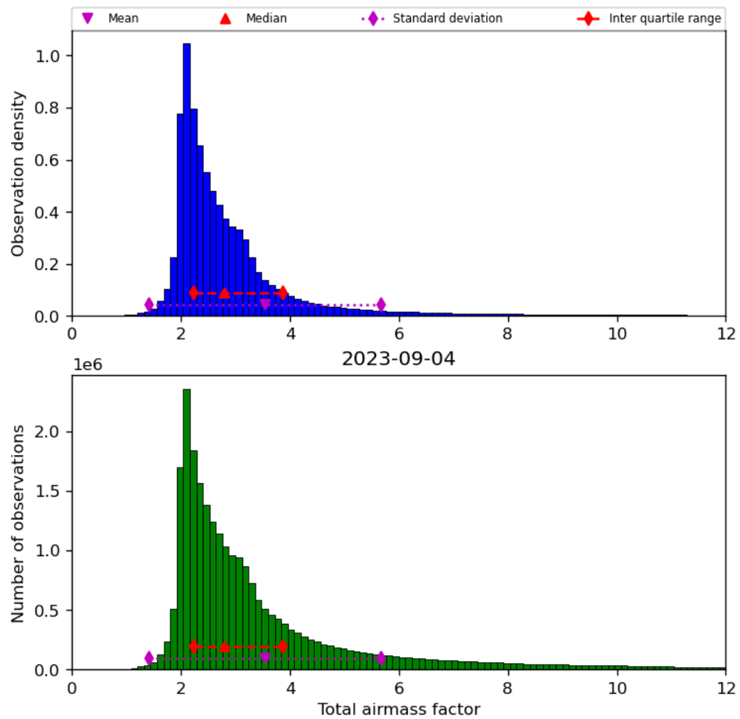
Figure 32: Histogram of “Total airmass factor” for 2023-09-04 to 2023-09-05
