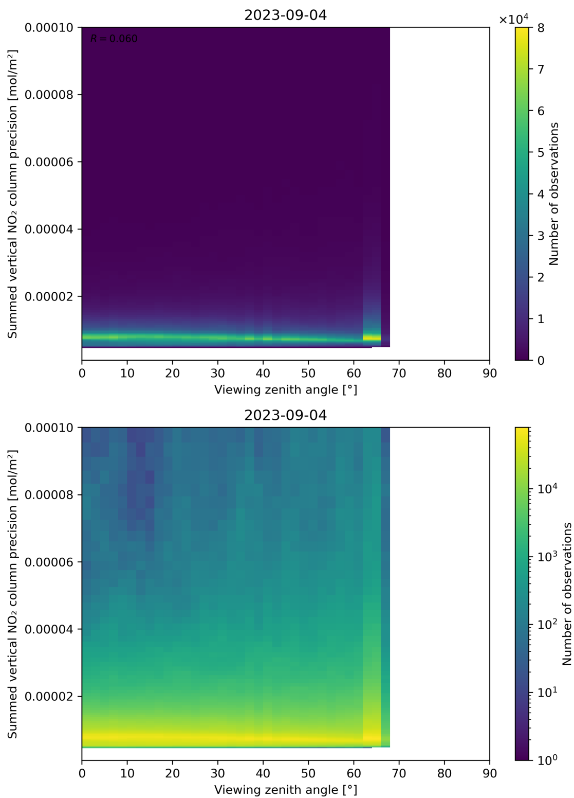
Figure 166: Scatter density plot of “Viewing zenith angle” against “Summed vertical NO 2 column precision” for 2023-09-04 to 2023-09-05.
