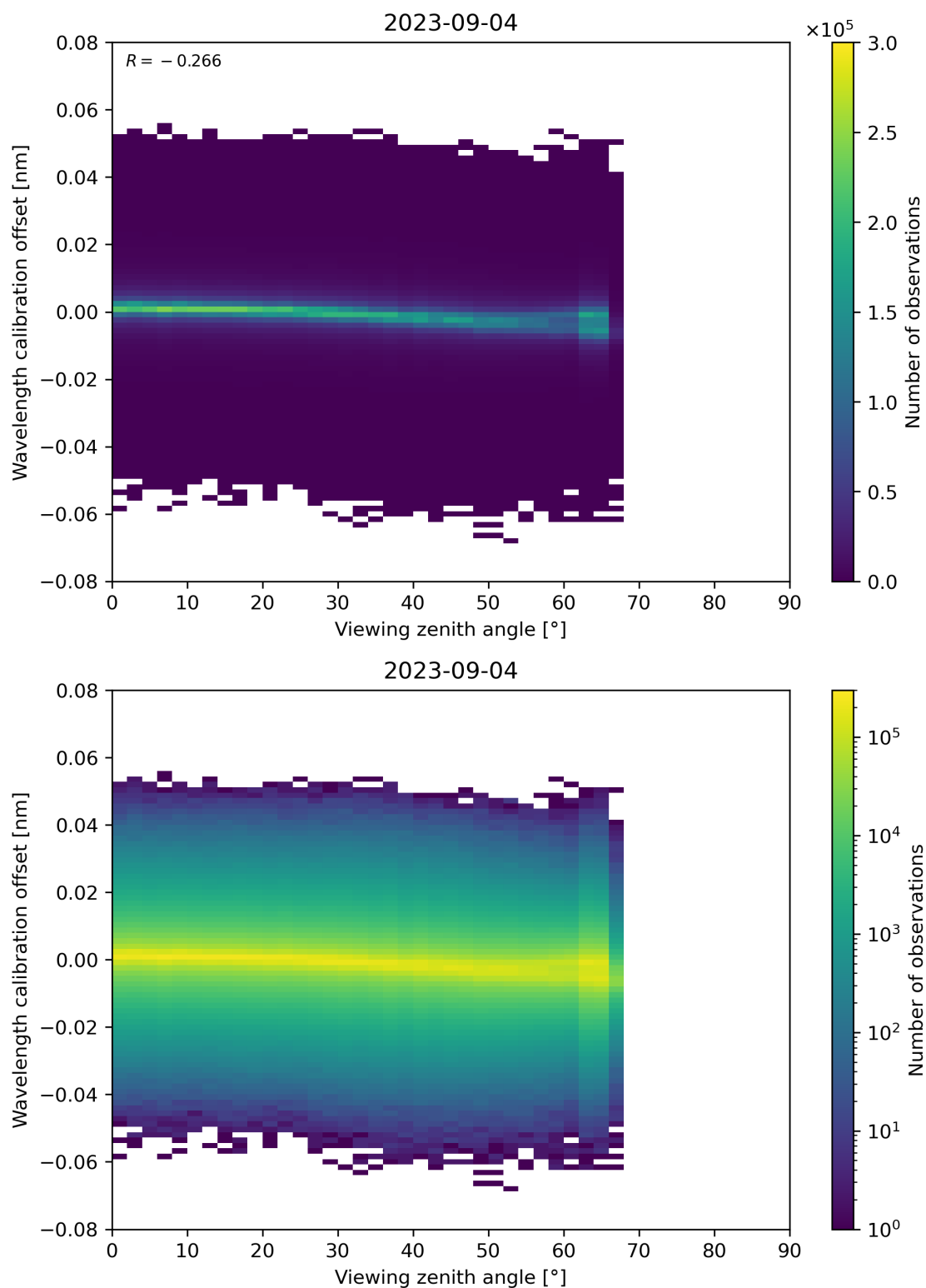
Figure 173: Scatter density plot of “Viewing zenith angle” against “Wavelength calibration offset” for 2023-09-04 to 2023-09-05.
