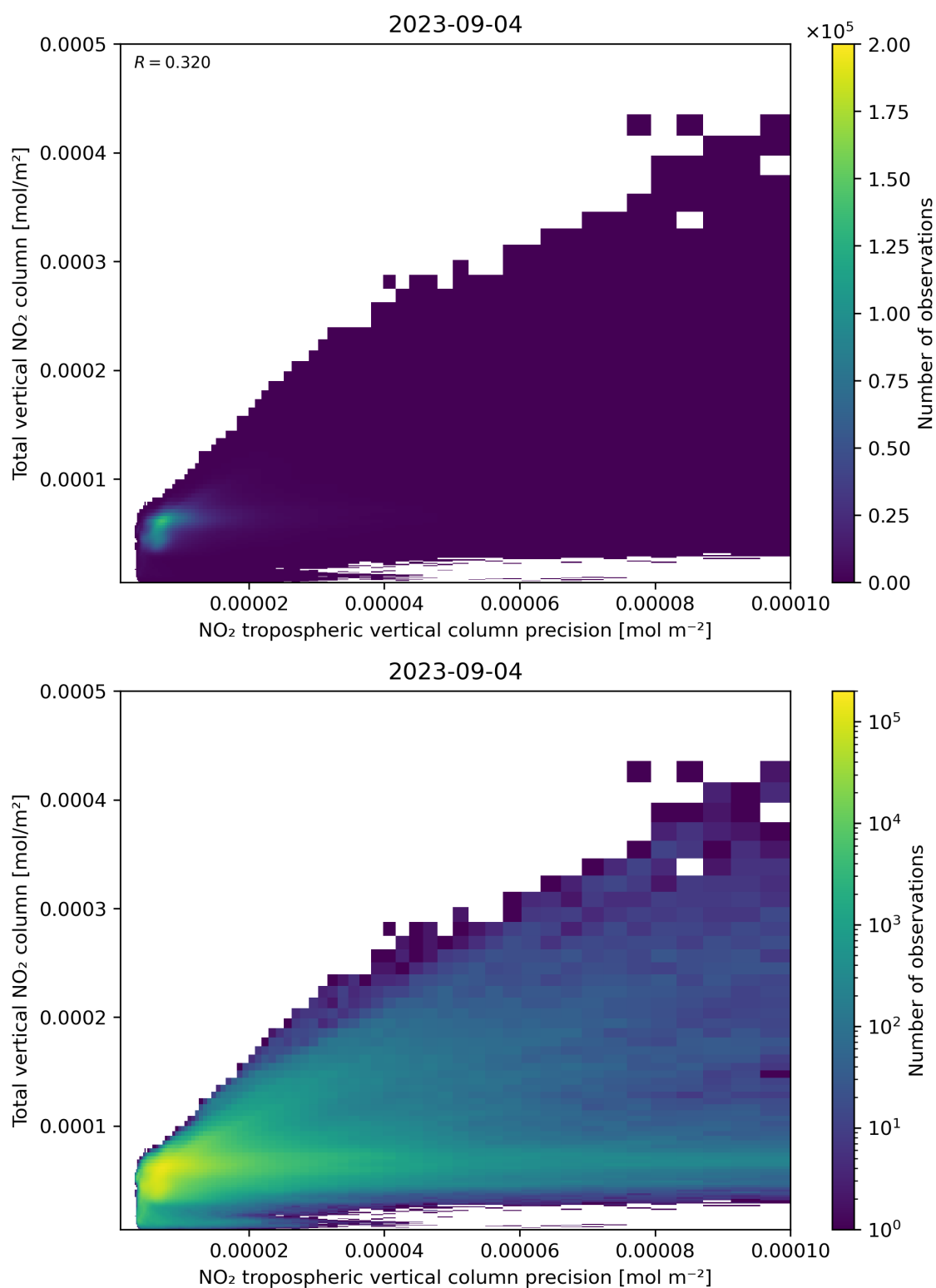
Figure 138: Scatter density plot of “NO 2 tropospheric vertical column precision” against “Total vertical NO 2 column” for 2023-09-04 to 2023-09-05.
