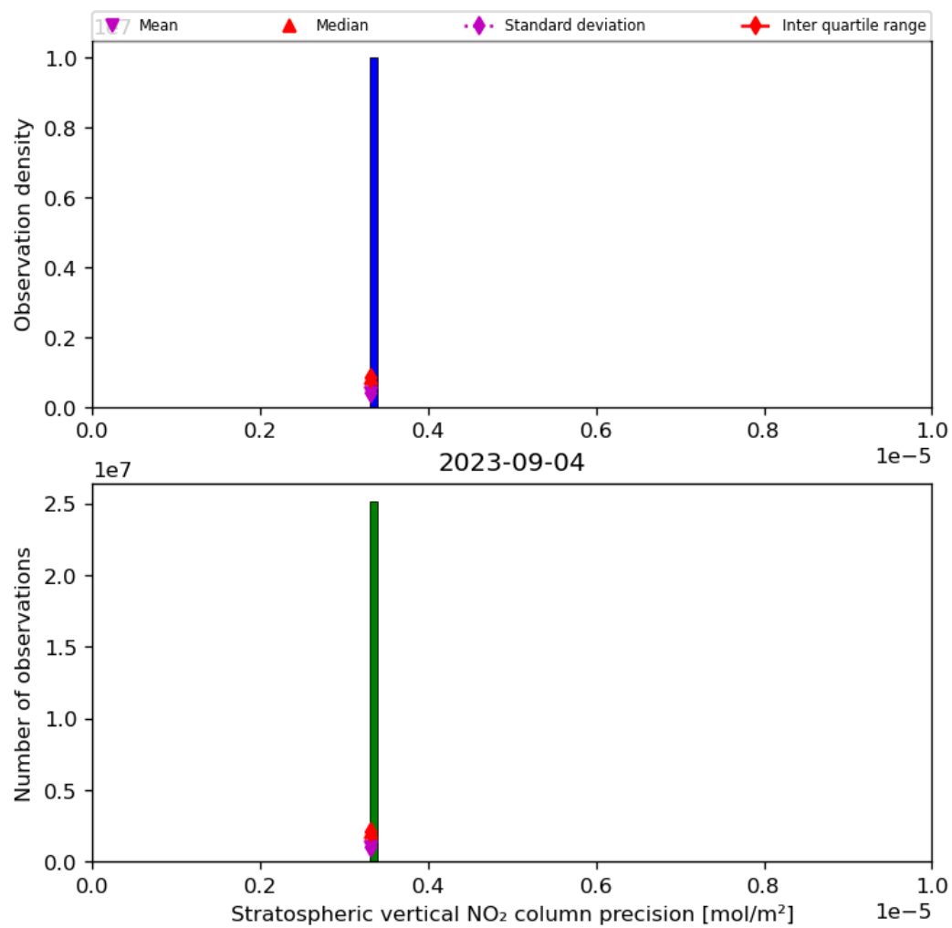
Figure 37: Histogram of “Stratospheric vertical NO 2 column precision” for 2023-09-04 to 2023-09-05
