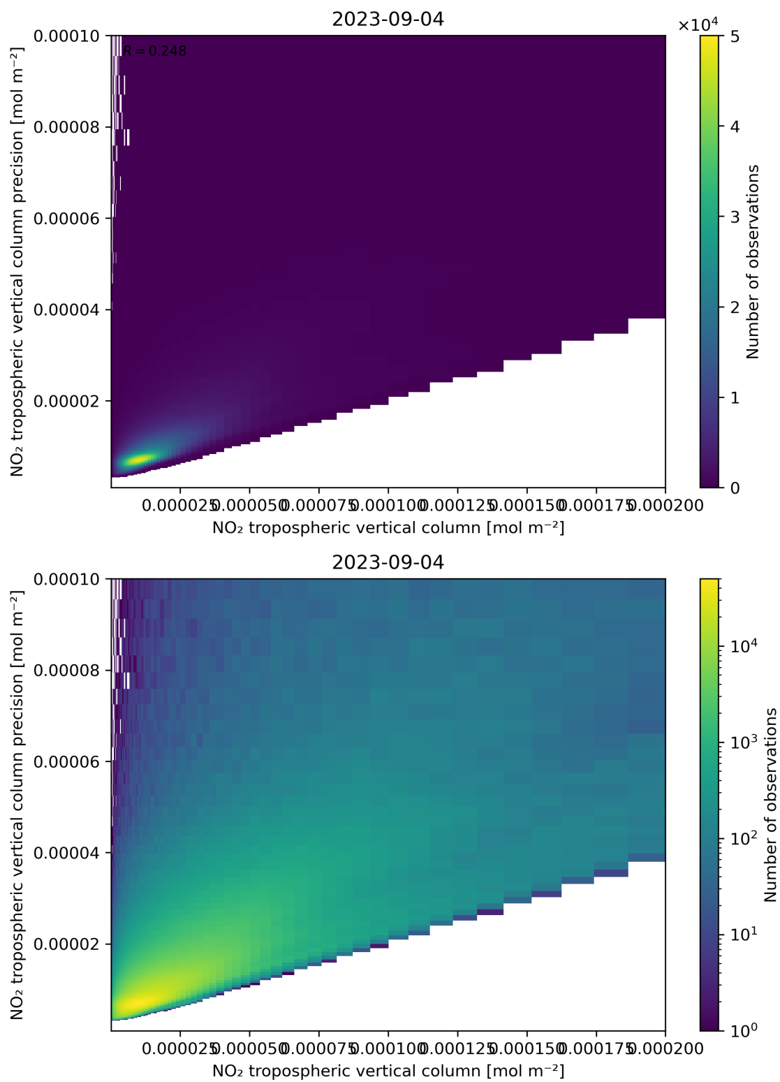
Figure 130: Scatter density plot of “NO 2 tropospheric vertical column” against “NO 2 tropospheric vertical column precision” for 2023-09-04 to 2023-09-05.
