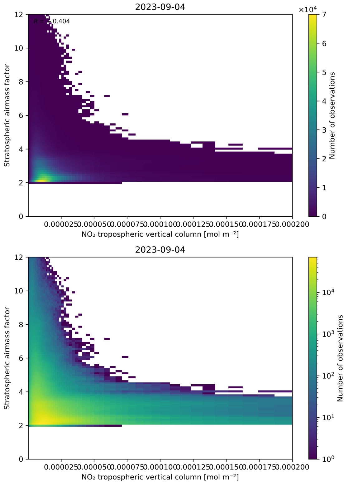
Figure 121: Scatter density plot of “NO 2 tropospheric vertical column” against “Stratospheric air mass factor” for 2023-09-04 to 2023-09-05.
