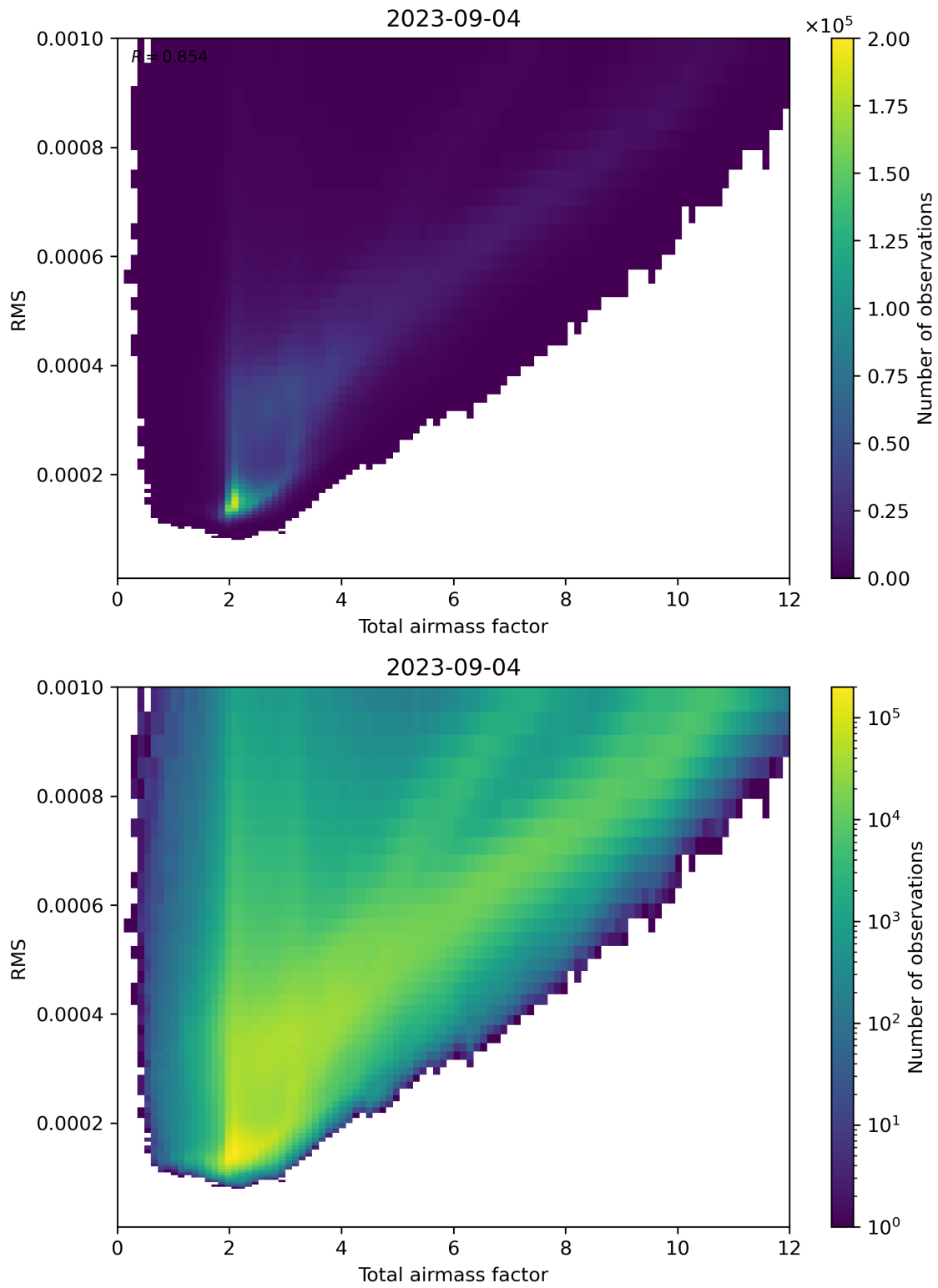
Figure 69: Scatter density plot of “Total airmass factor” against “RMS” for 2023-09-04 to 2023-09-05.
