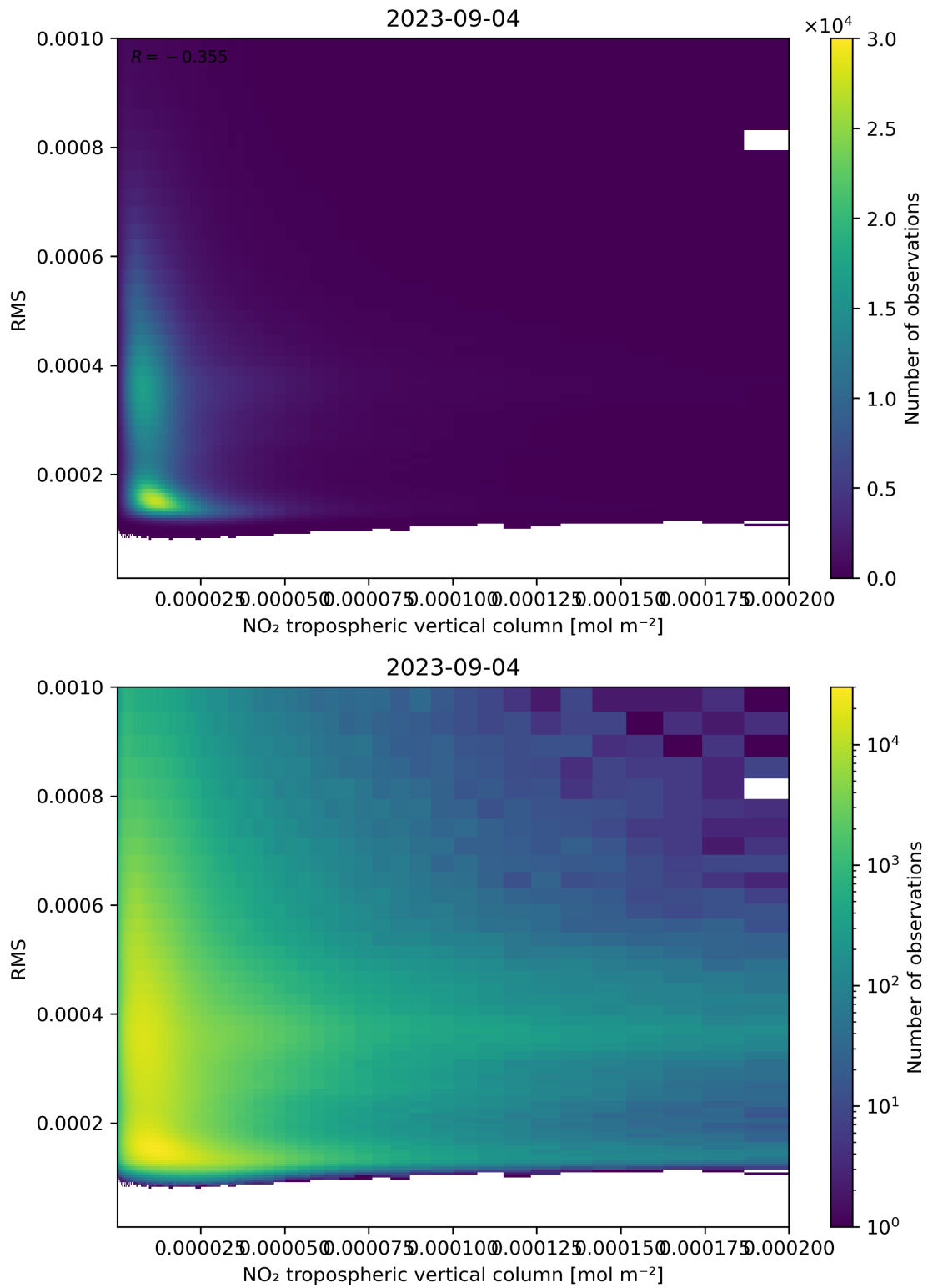
Figure 142: Scatter density plot of “NO 2 tropospheric vertical column” against “RMS” for 2023-09-04 to 2023-09-05.
