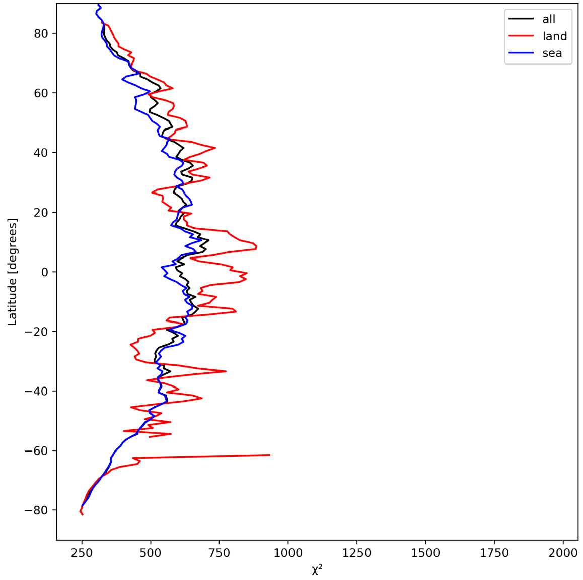
Figure 25: Zonal average of “ \chi^2 ” for 2023-09-04 to 2023-09-05.
