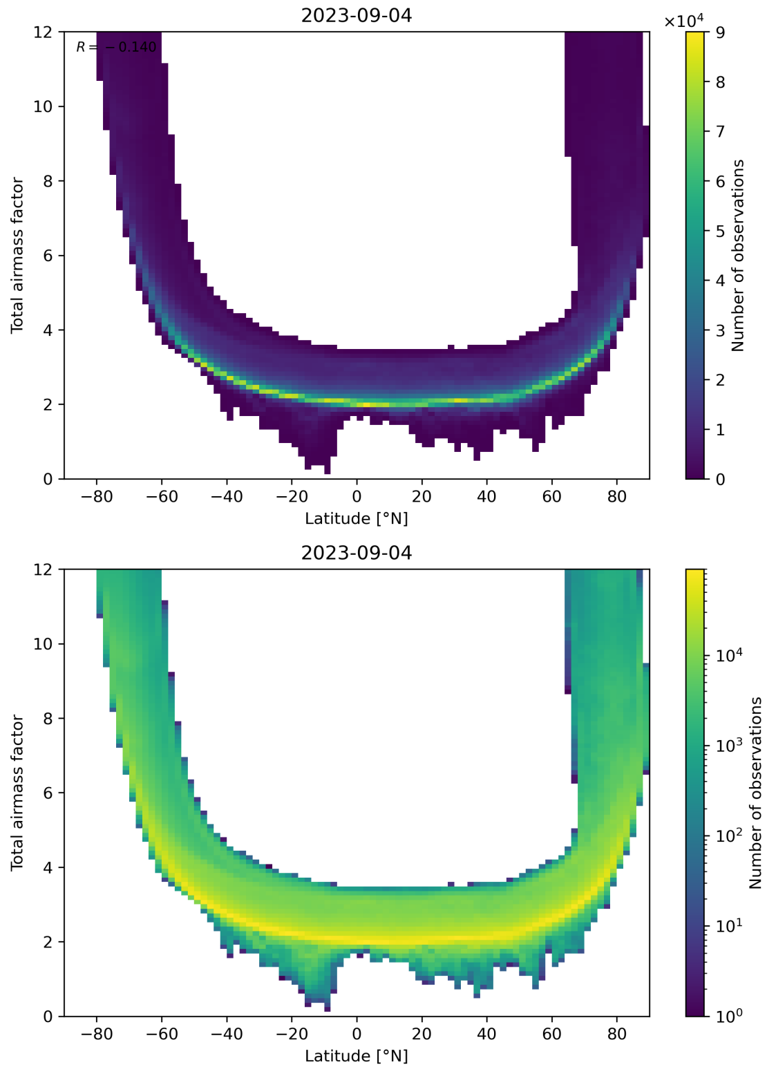
Figure 84: Scatter density plot of “Latitude” against “Total airmass factor” for 2023-09-04 to 2023-09-05.
