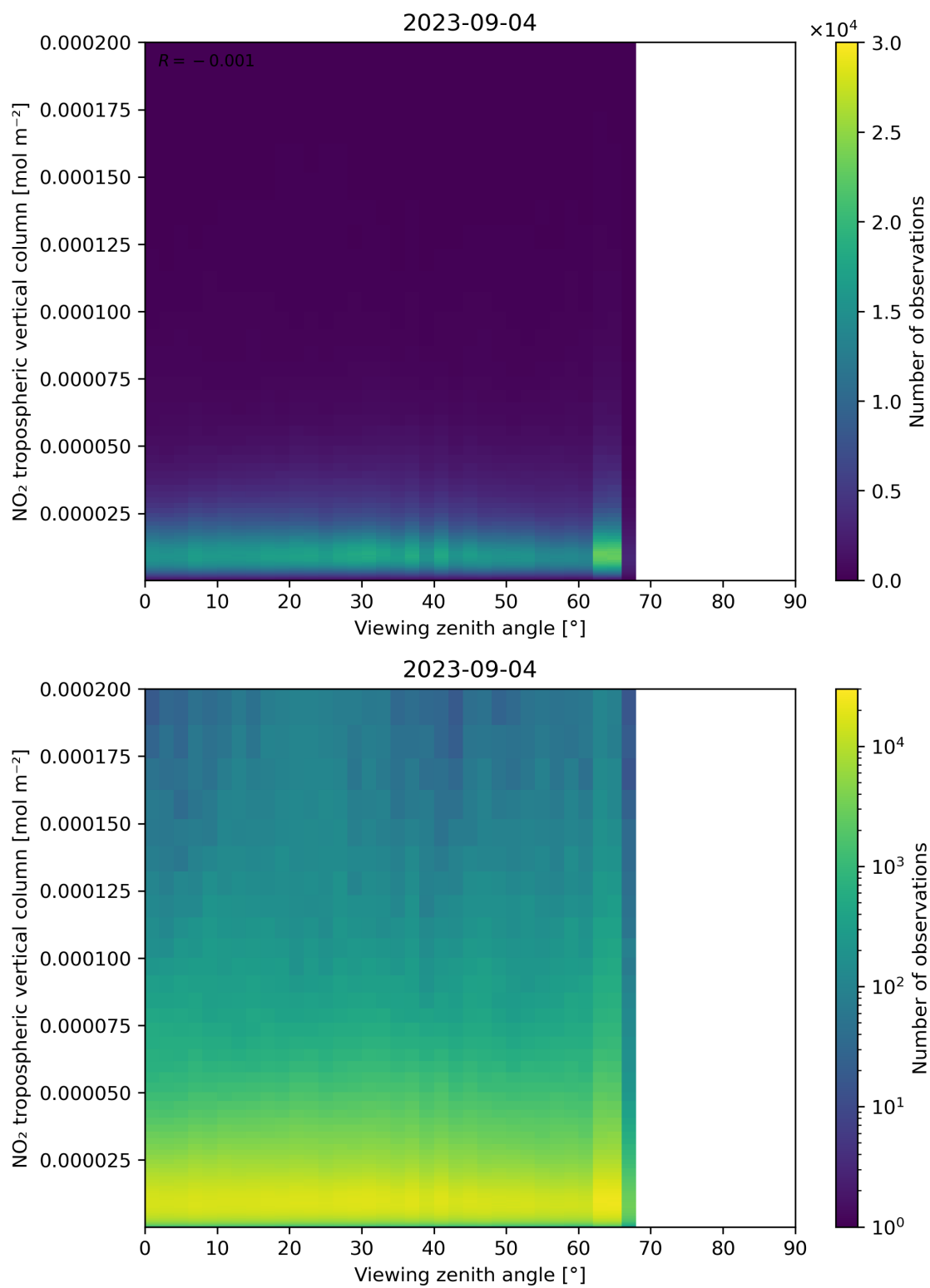
Figure 169: Scatter density plot of “Viewing zenith angle” against “NO 2 tropospheric vertical column” for 2023-09-04 to 2023-09-05.
