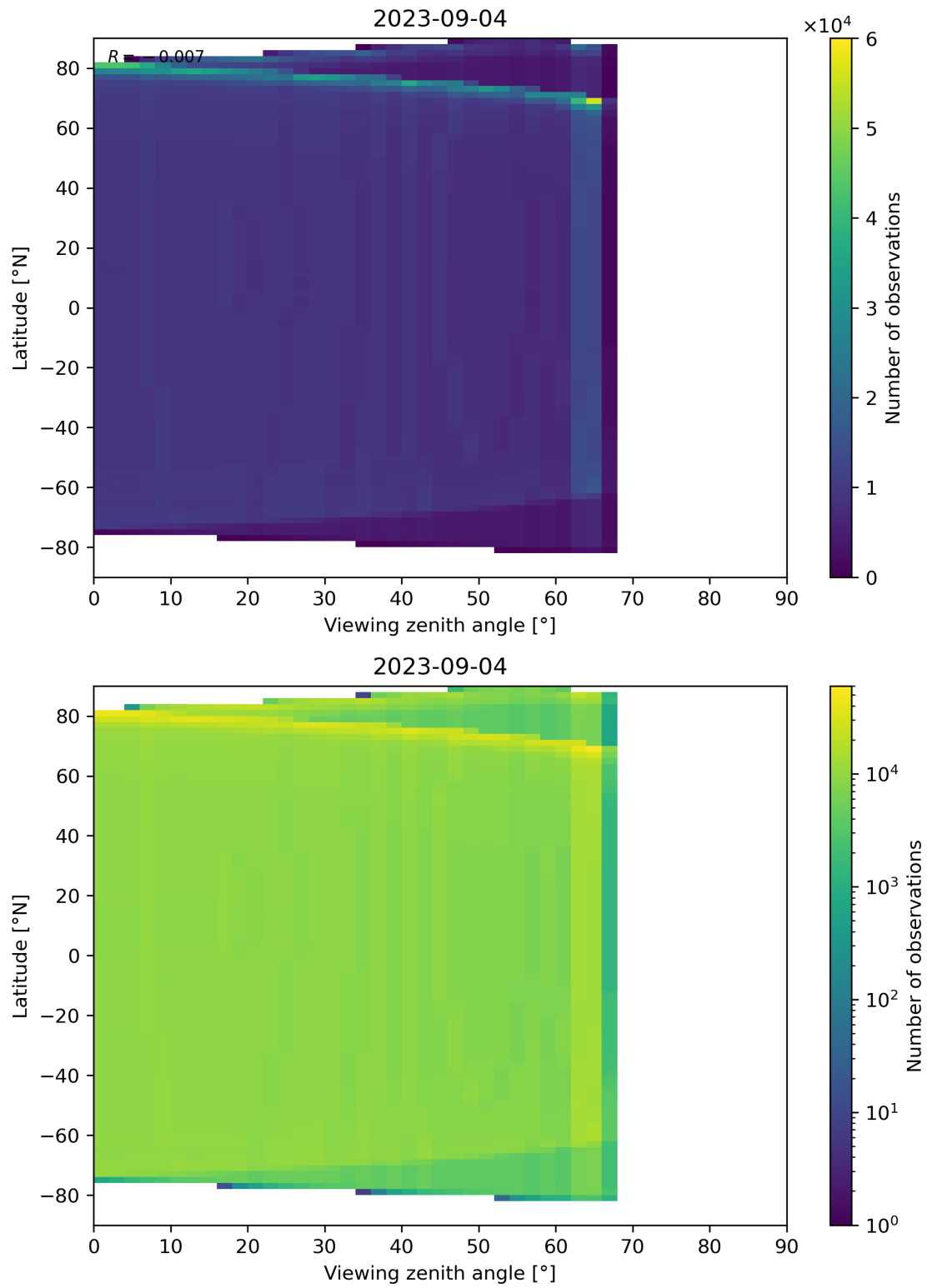
Figure 163: Scatter density plot of “Viewing zenith angle” against “Latitude” for 2023-09-04 to 2023-09-05.
