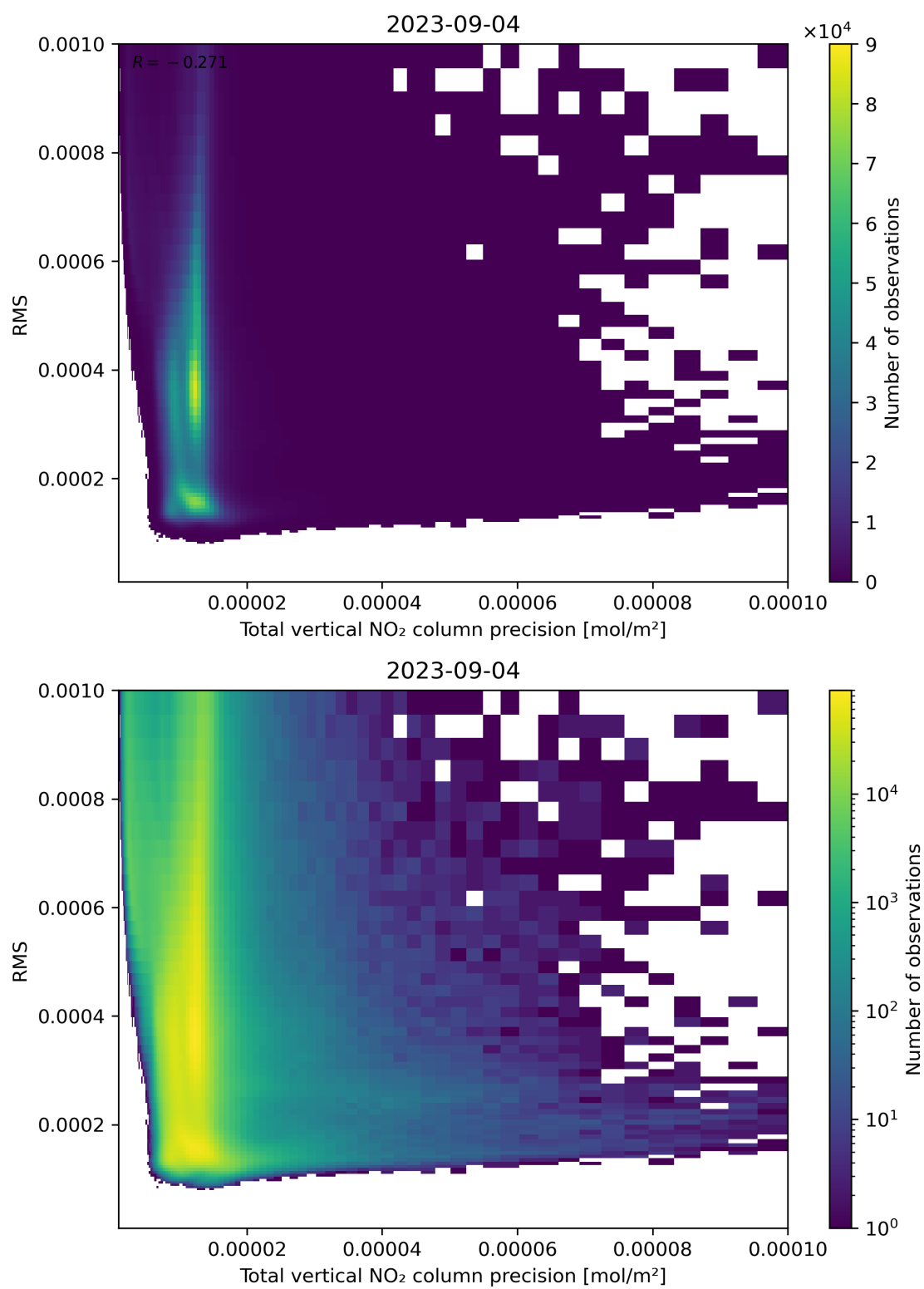
Figure 119: Scatter density plot of “Total vertical NO 2 column precision” against “RMS” for 2023-09-04 to 2023-09-05.
