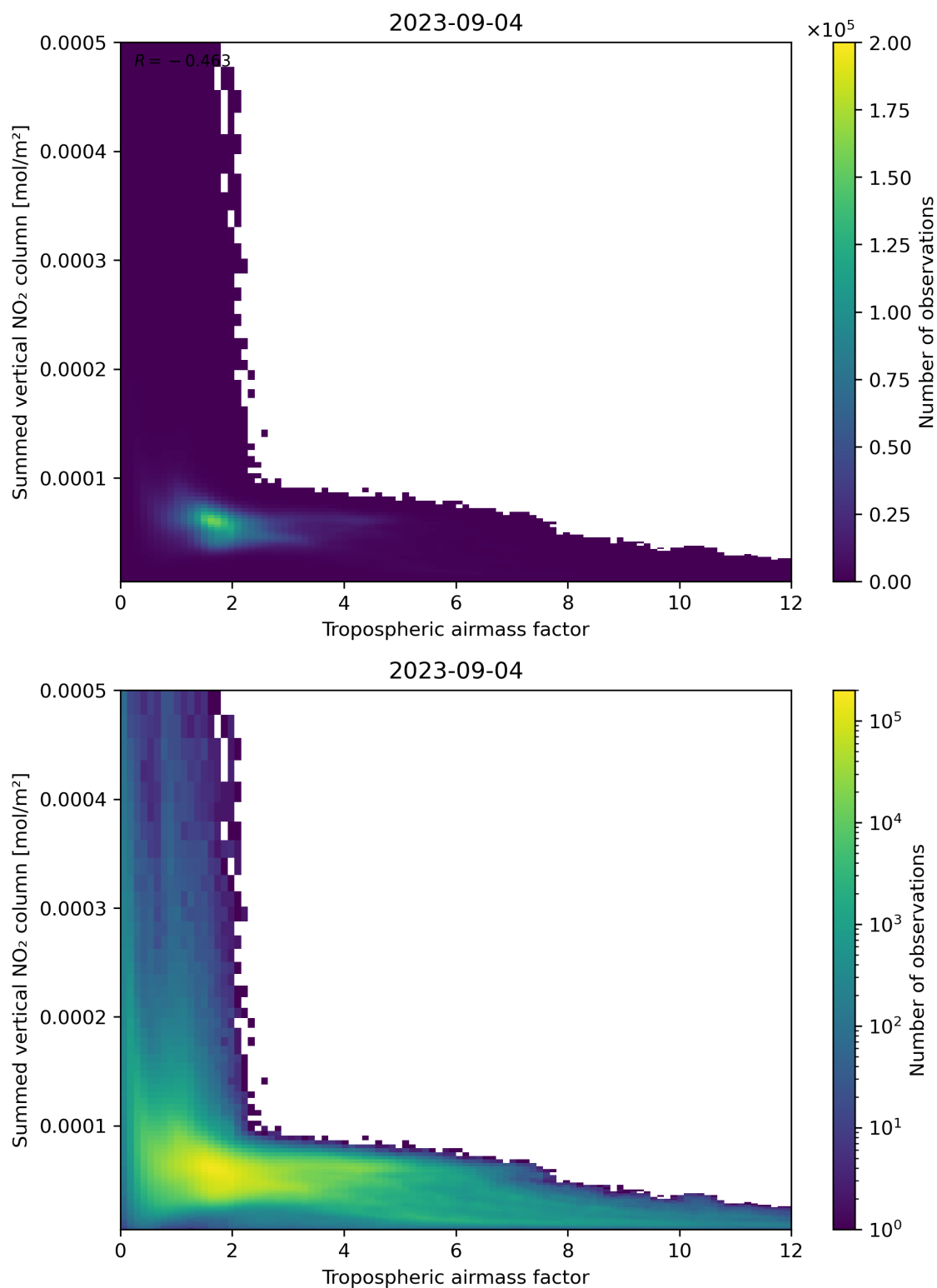
Figure 75: Scatter density plot of “Tropospheric air mass factor” against “Summed vertical NO 2 column” for 2023-09-04 to 2023-09-05.
