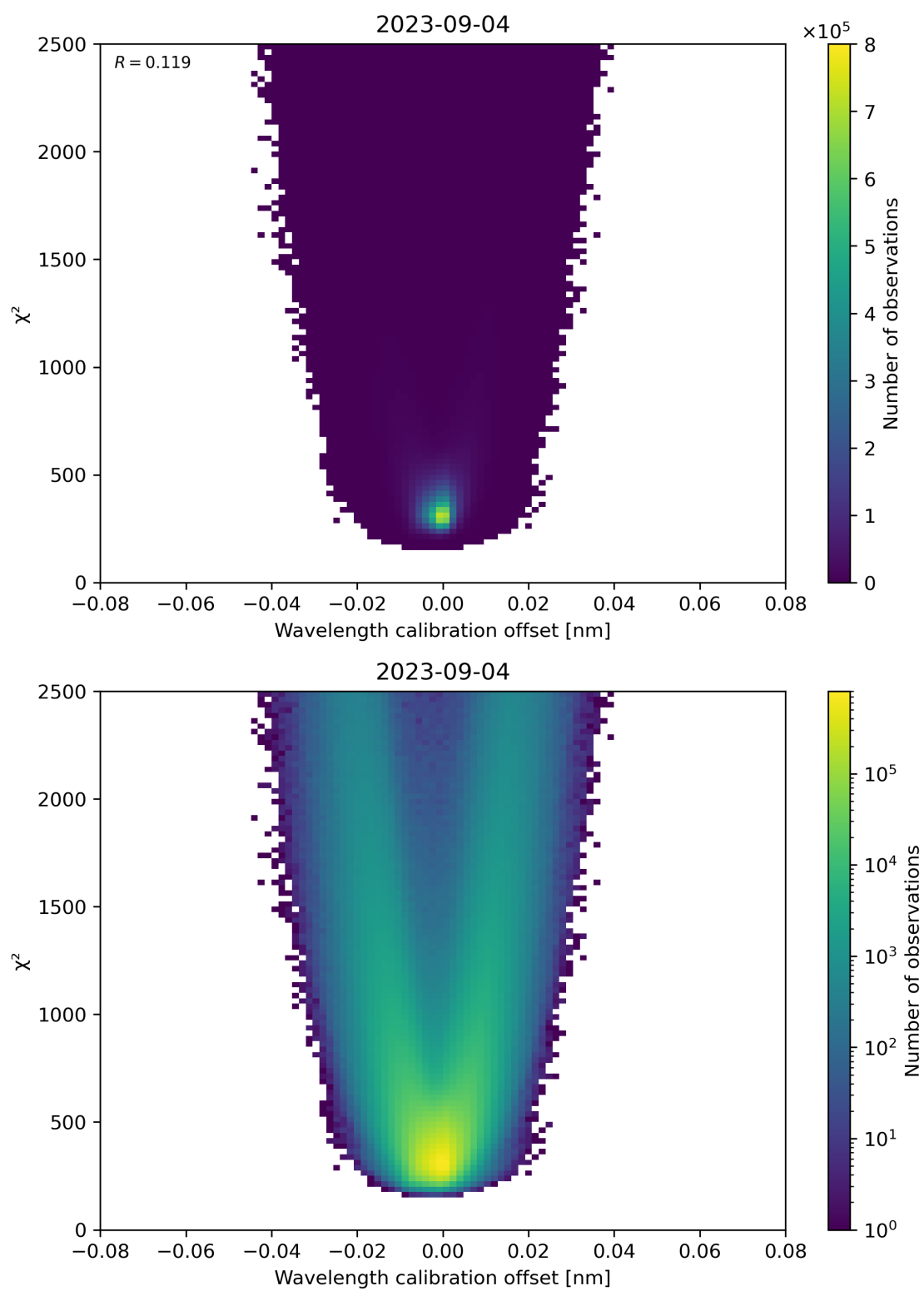
Figure 175: Scatter density plot of “Wavelength calibration offset” against “ \chi^2 ” for 2023-09-04 to 2023-09-05.
