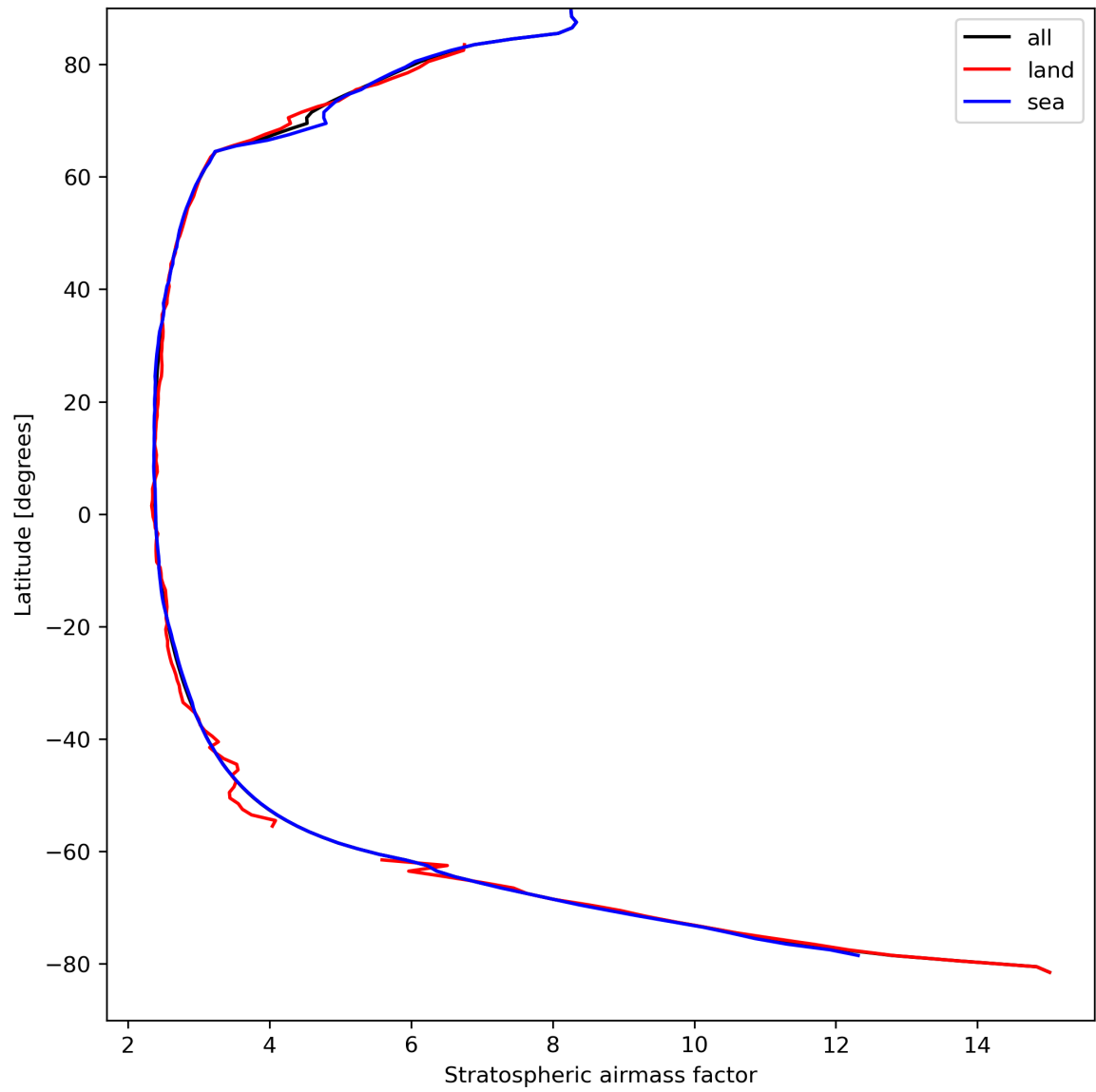
Figure 27: Zonal average of “Stratospheric air mass factor” for 2023-09-04 to 2023-09-05.
