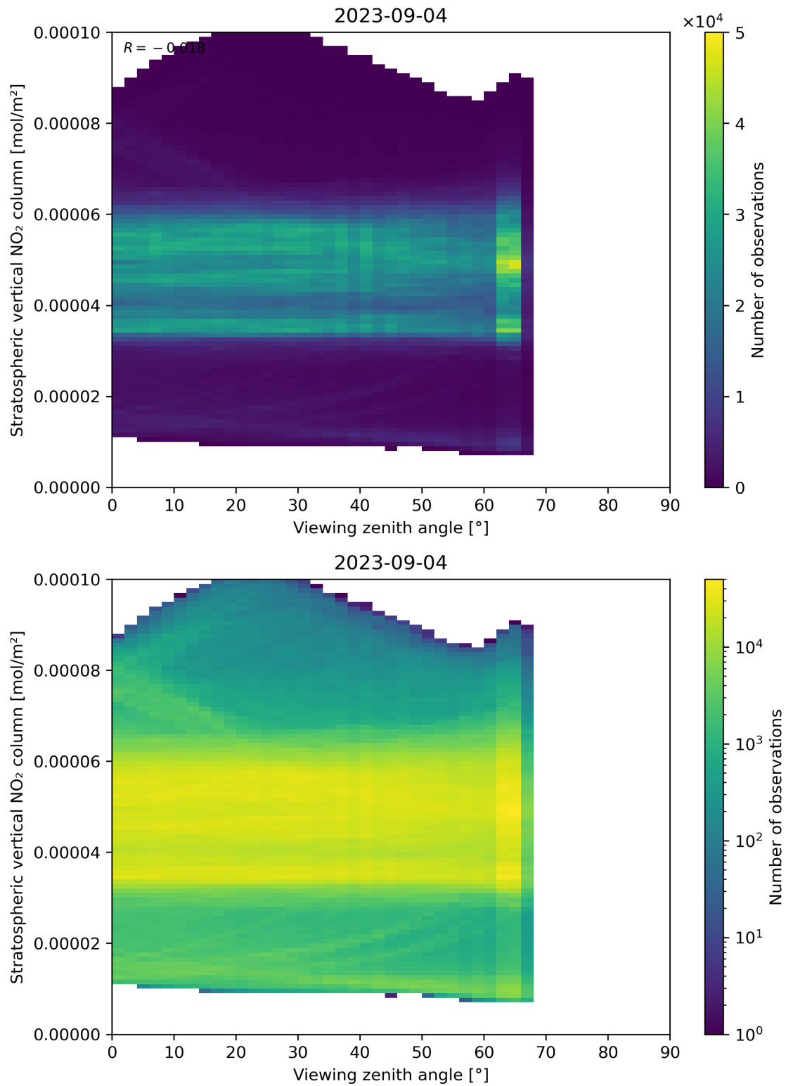
Figure 164: Scatter density plot of “Viewing zenith angle” against “Stratospheric vertical NO 2 column” for 2023-09-04 to 2023-09-05.
