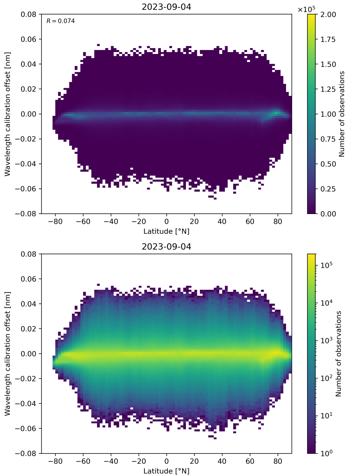
Figure 95: Scatter density plot of “Latitude” against “Wavelength calibration offset” for 2023-09-04 to 2023-09-05.
