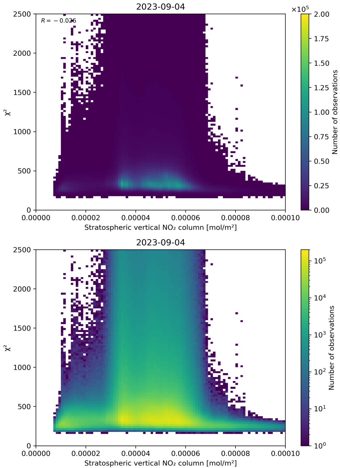
Figure 97: Scatter density plot of “Stratospheric vertical NO 2 column” against “ \chi^2 ” for 2023-09-04 to 2023-09-05.
