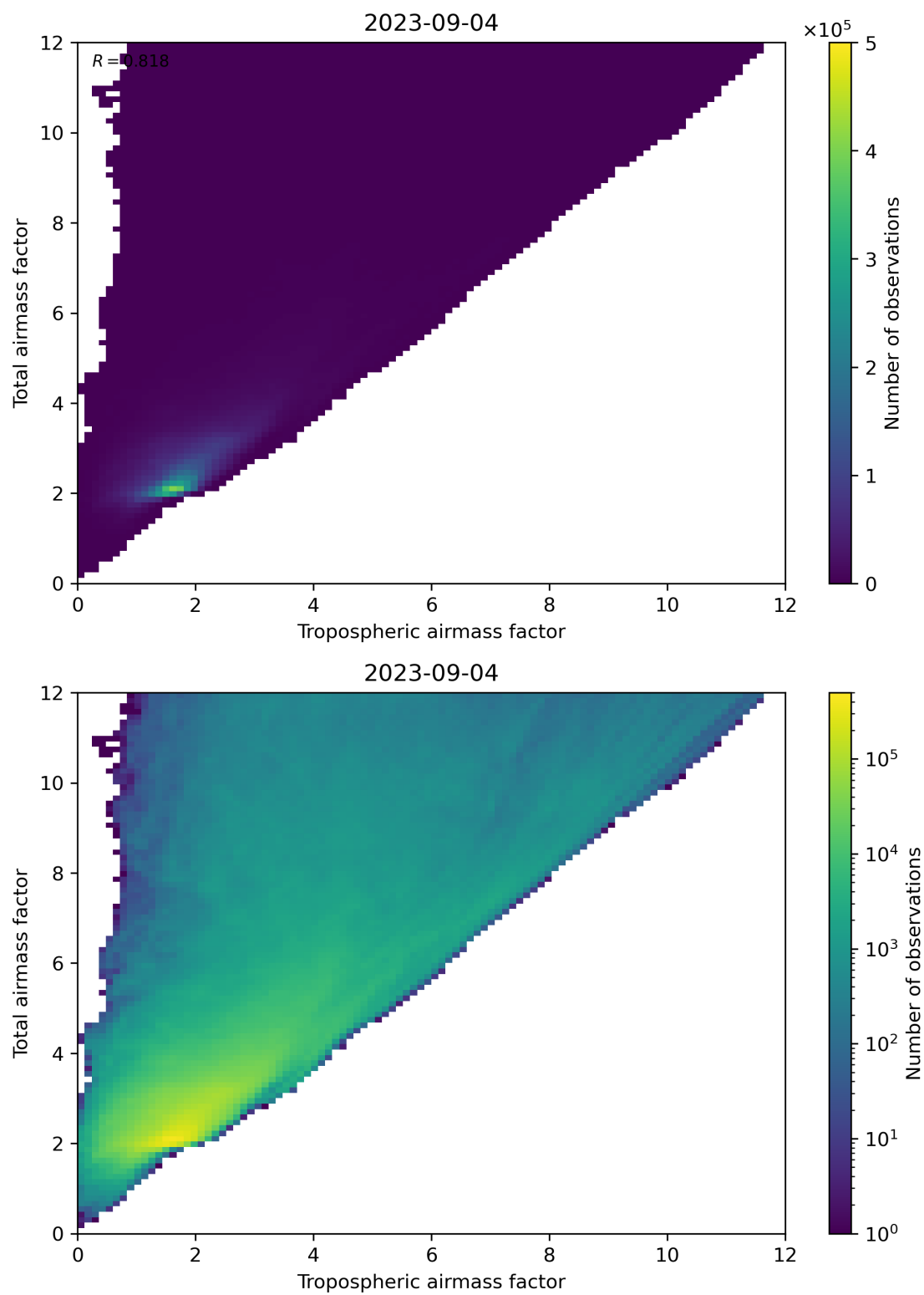
Figure 72: Scatter density plot of “Tropospheric airmass factor” against “Total airmass factor” for 2023-09-04 to 2023-09-05.
