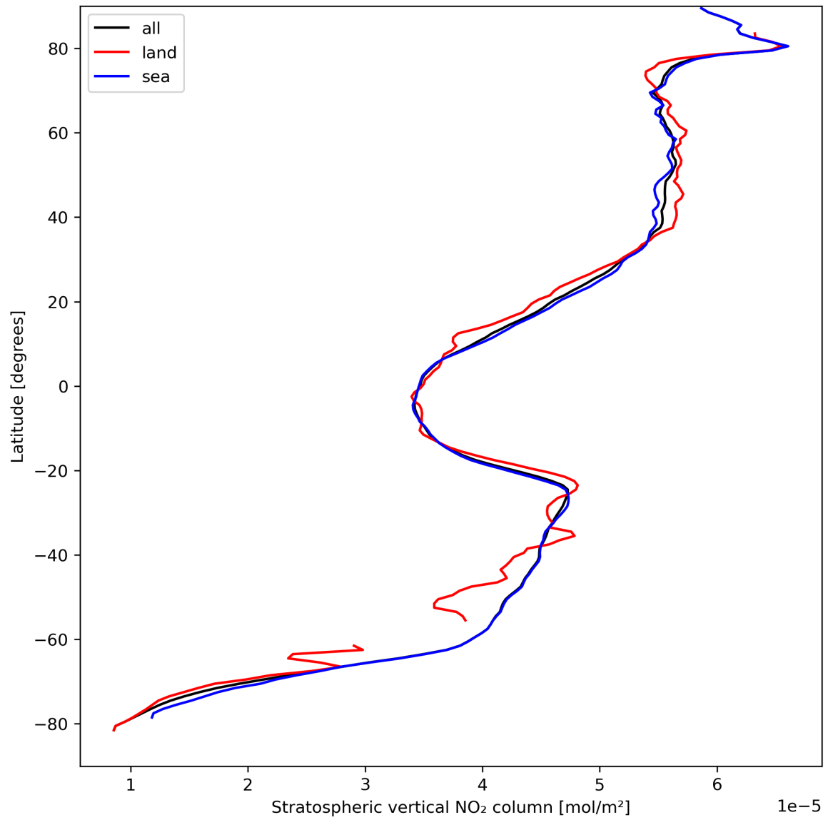
Figure 19: Zonal average of “Stratospheric vertical NO 2 column” for 2023-09-04 to 2023-09-05.
