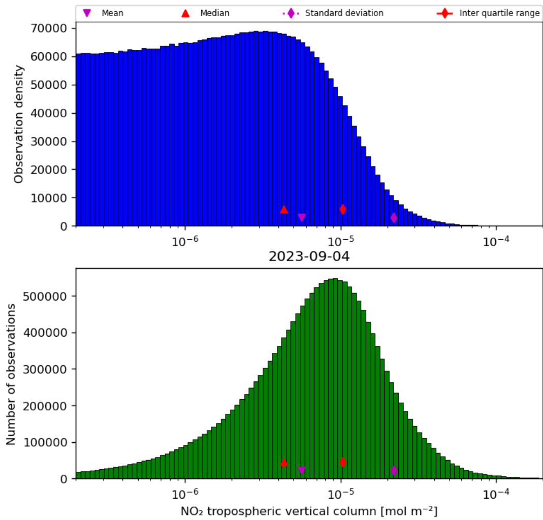
Figure 29: Histogram of “NO 2 tropospheric vertical column” for 2023-09-04 to 2023-09-05
