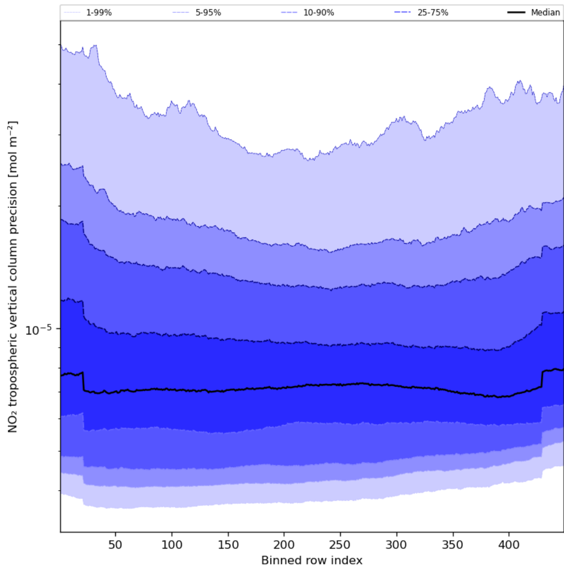
Figure 47: Along track statistics of “NO 2 tropospheric vertical column precision” for 2023-09-04 to 2023-09-05
