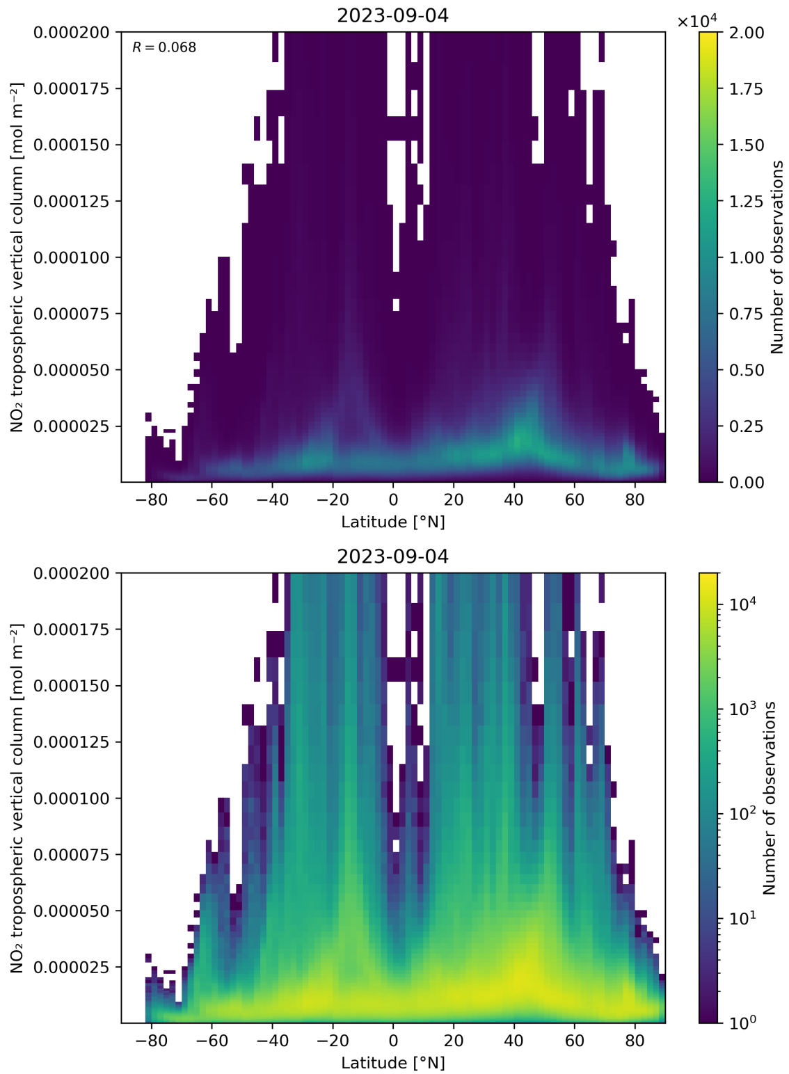
Figure 92: Scatter density plot of “Latitude” against “NO 2 tropospheric vertical column” for 2023-09-04 to 2023-09-05.
