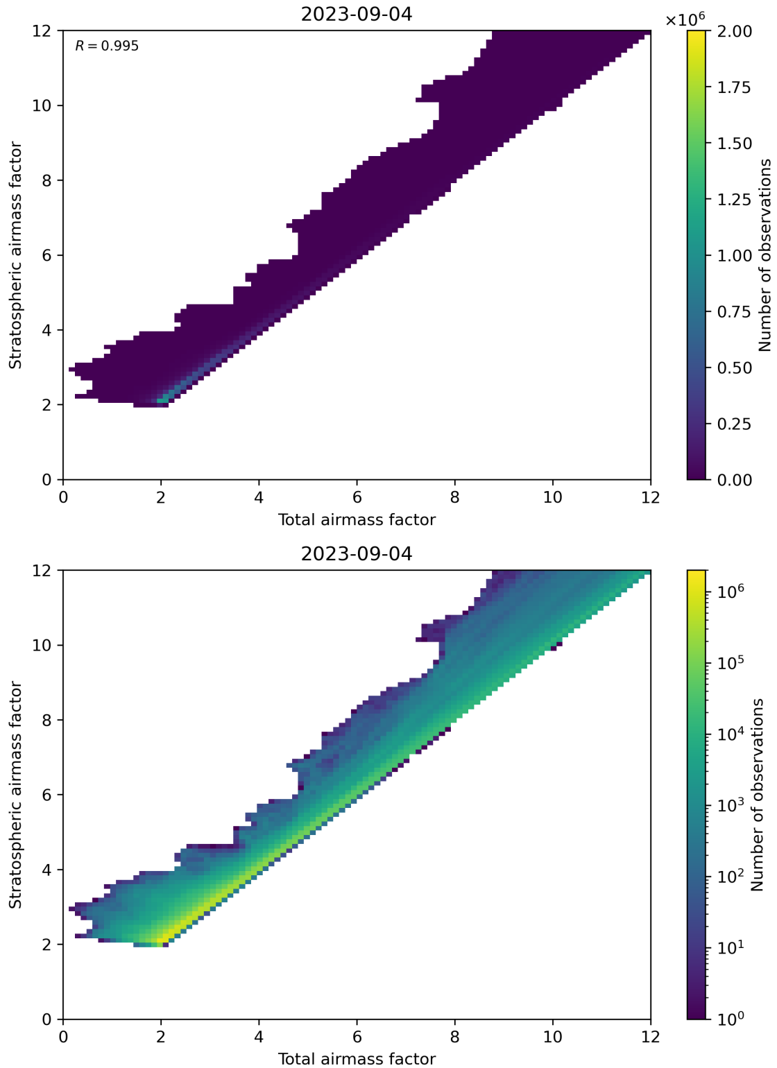
Figure 62: Scatter density plot of “Total airmass factor” against “Stratospheric airmass factor” for 2023-09-04 to 2023-09-05.
