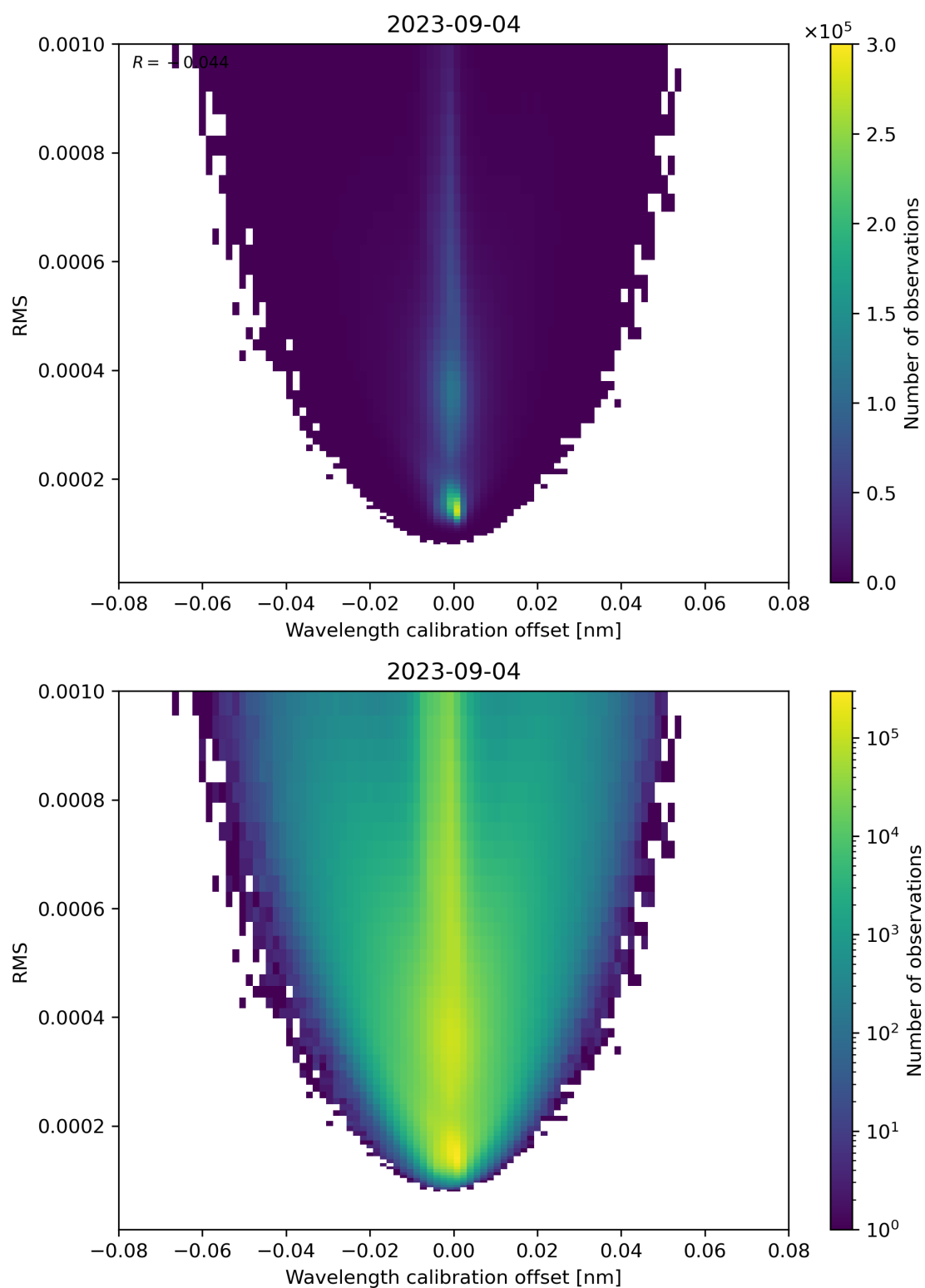
Figure 181: Scatter density plot of “Wavelength calibration offset” against “RMS” for 2023-09-04 to 2023-09-05.
