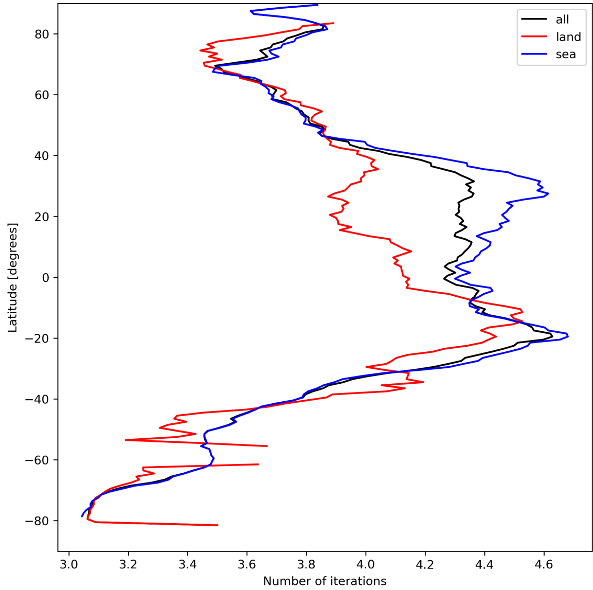
Figure 17: Zonal average of “Number of iterations” for 2023-09-04 to 2023-09-05.
