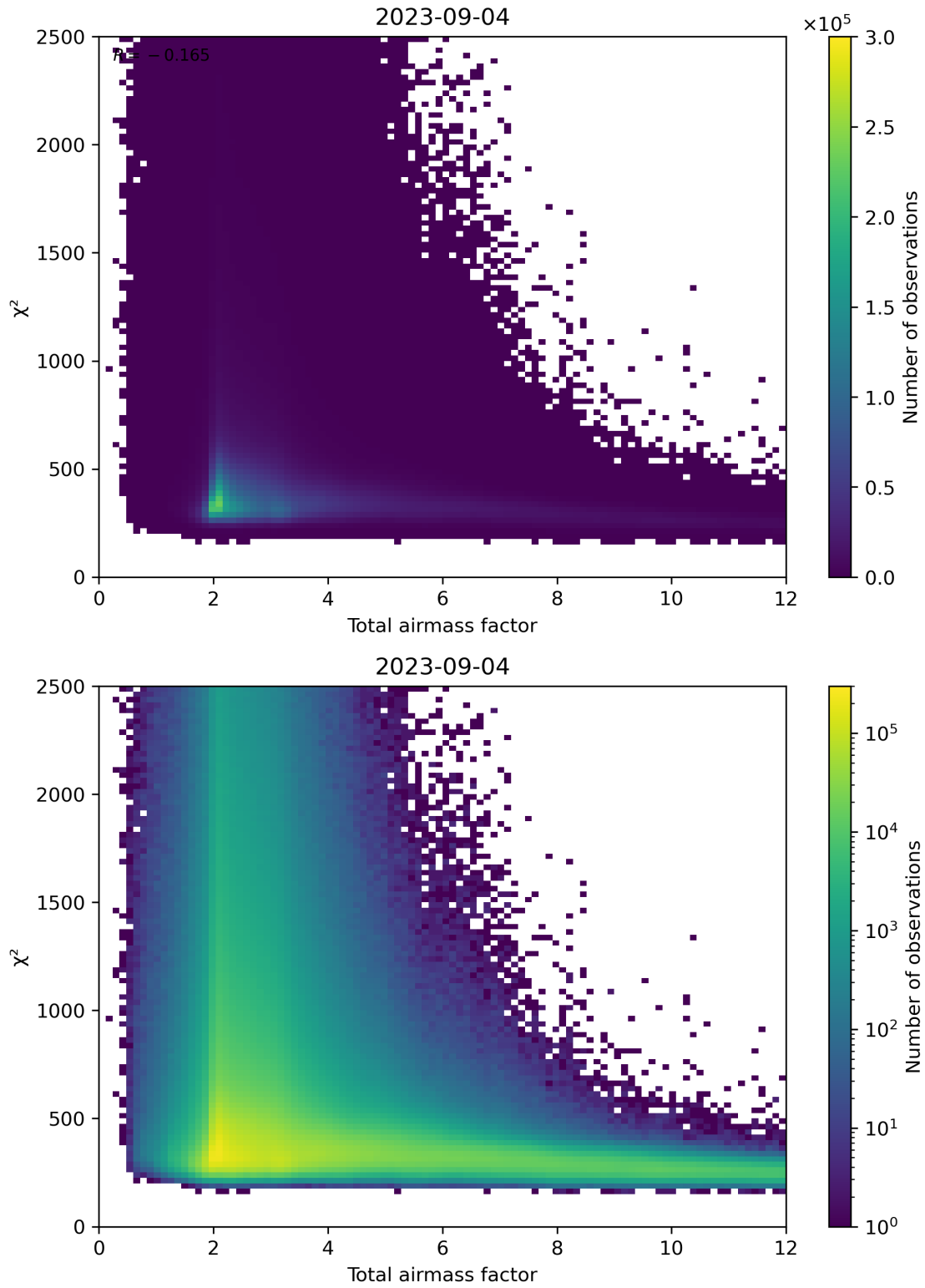
Figure 63: Scatter density plot of “Total airmass factor” against “ \chi^2 ” for 2023-09-04 to 2023-09-05.
