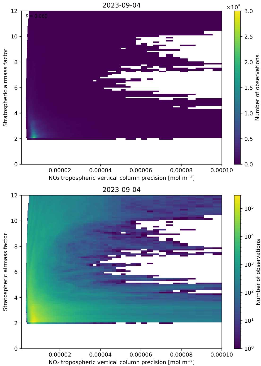
Figure 131: Scatter density plot of “NO 2 tropospheric vertical column precision” against “Stratospheric airmass factor” for 2023-09-04 to 2023-09-05.
