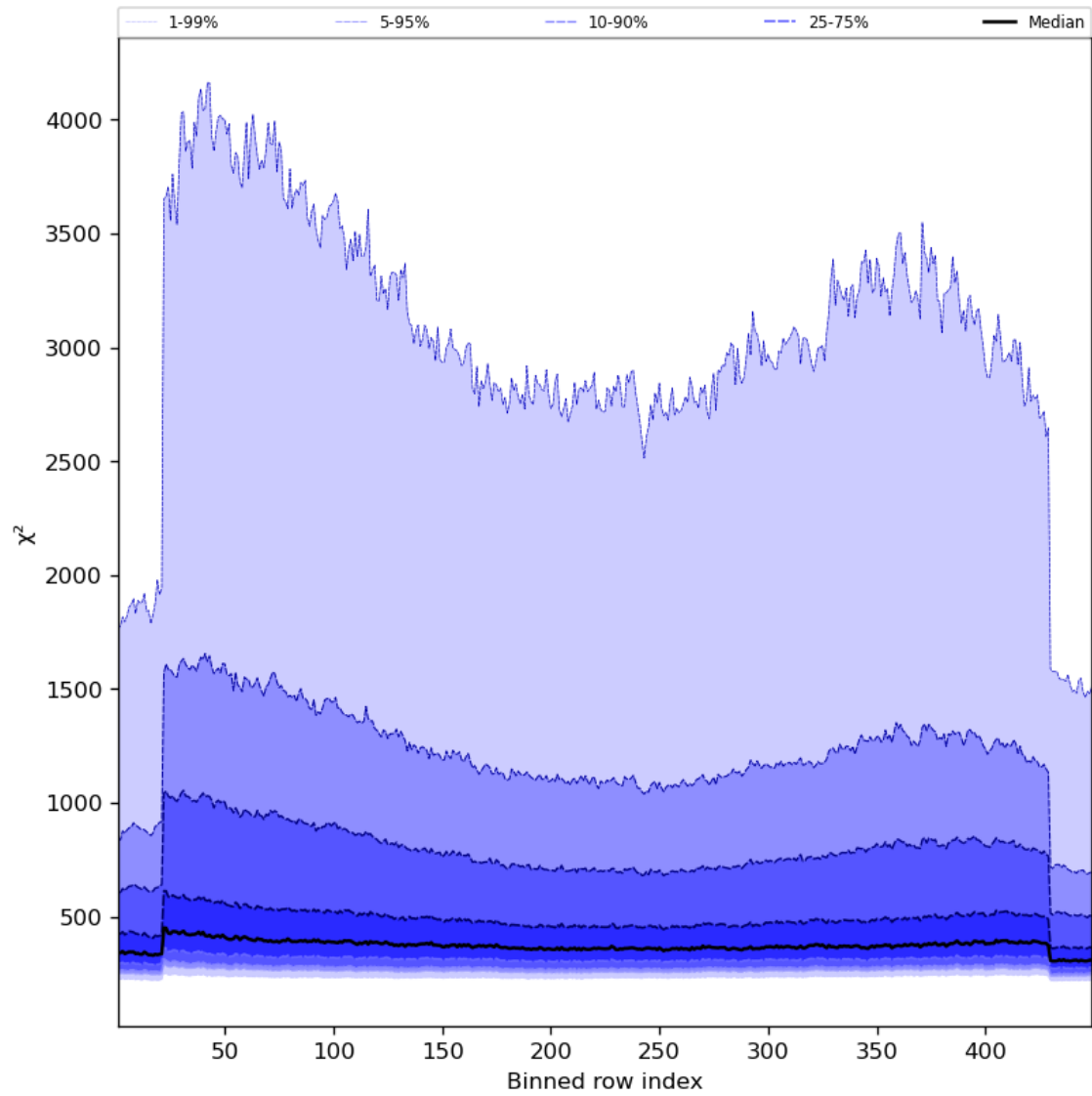
Figure 59: Along track statistics of “ \chi^2 ” for 2023-09-04 to 2023-09-05
