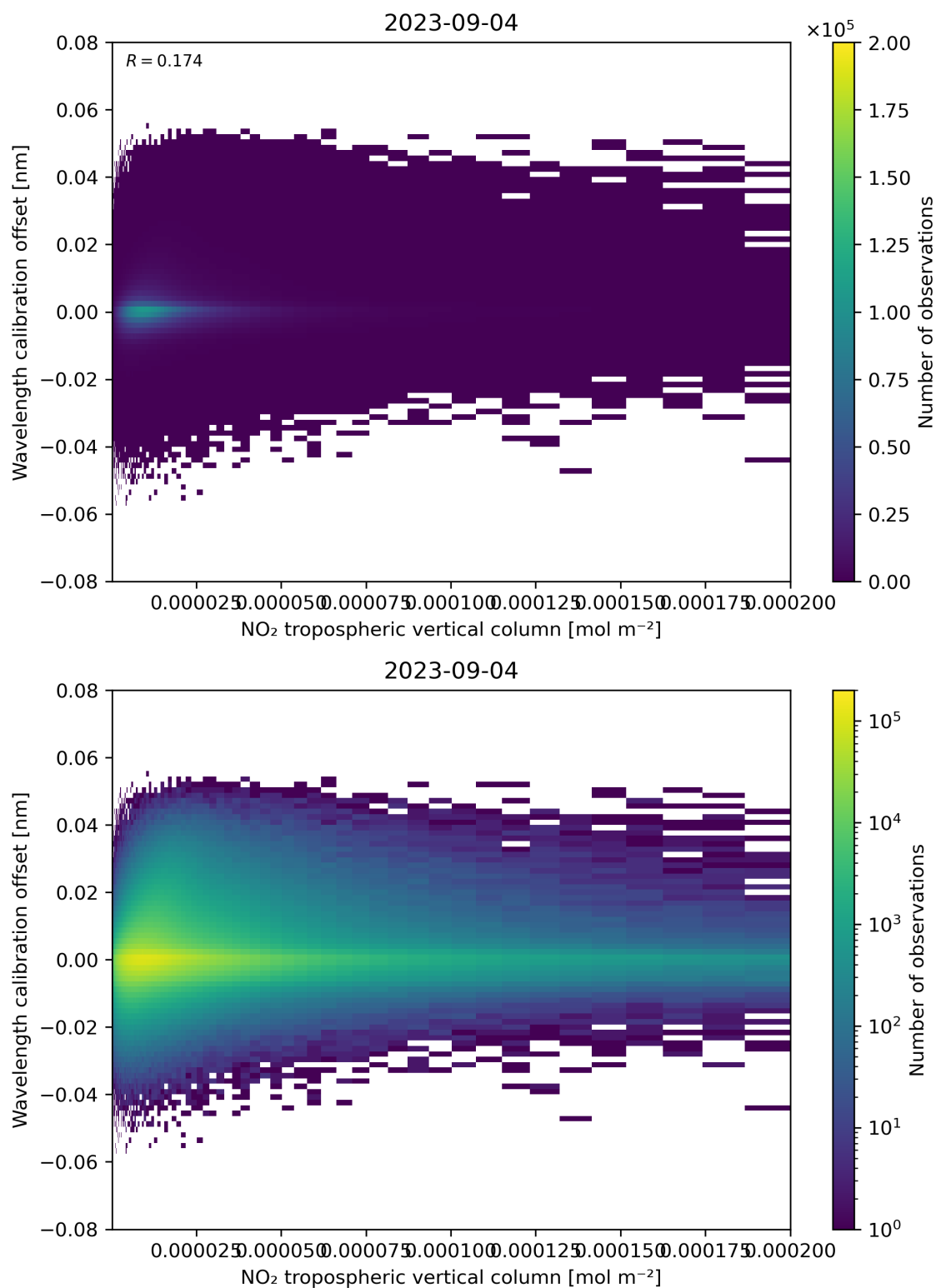
Figure 143: Scatter density plot of “NO 2 tropospheric vertical column” against “Wavelength calibration offset” for 2023-09-04 to 2023-09-05.
