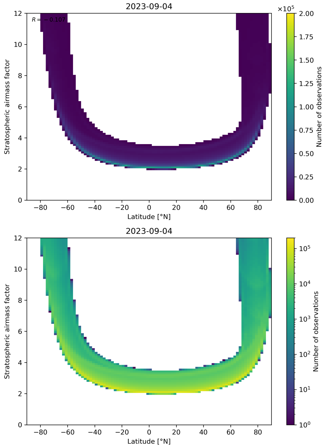
Figure 83: Scatter density plot of “Latitude” against “Stratospheric airmass factor” for 2023-09-04 to 2023-09-05.
