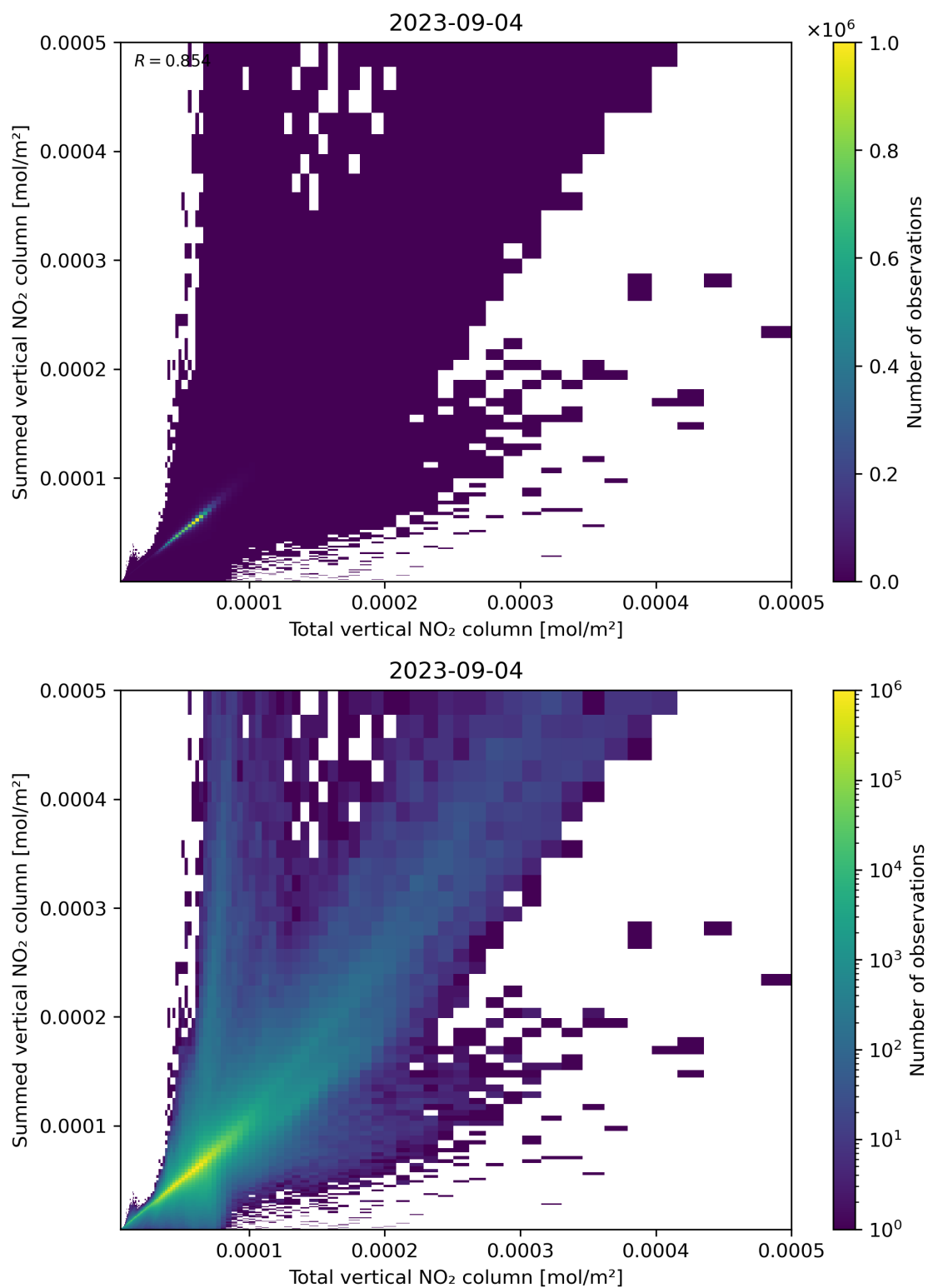
Figure 112: Scatter density plot of “Total vertical NO 2 column” against “Summed vertical NO 2 column” for 2023-09-04 to 2023-09-05.
