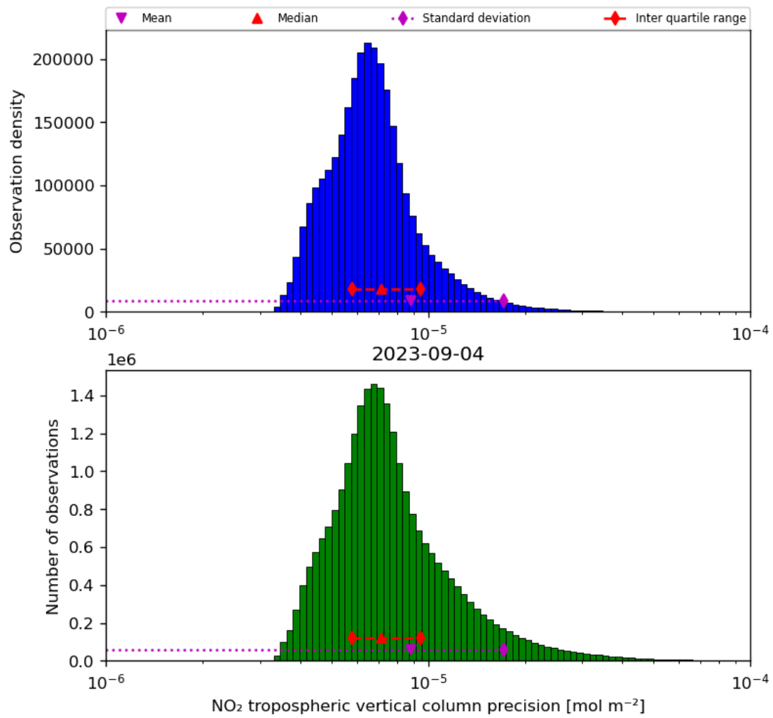
Figure 30: Histogram of “NO 2 tropospheric vertical column precision” for 2023-09-04 to 2023-09-05
