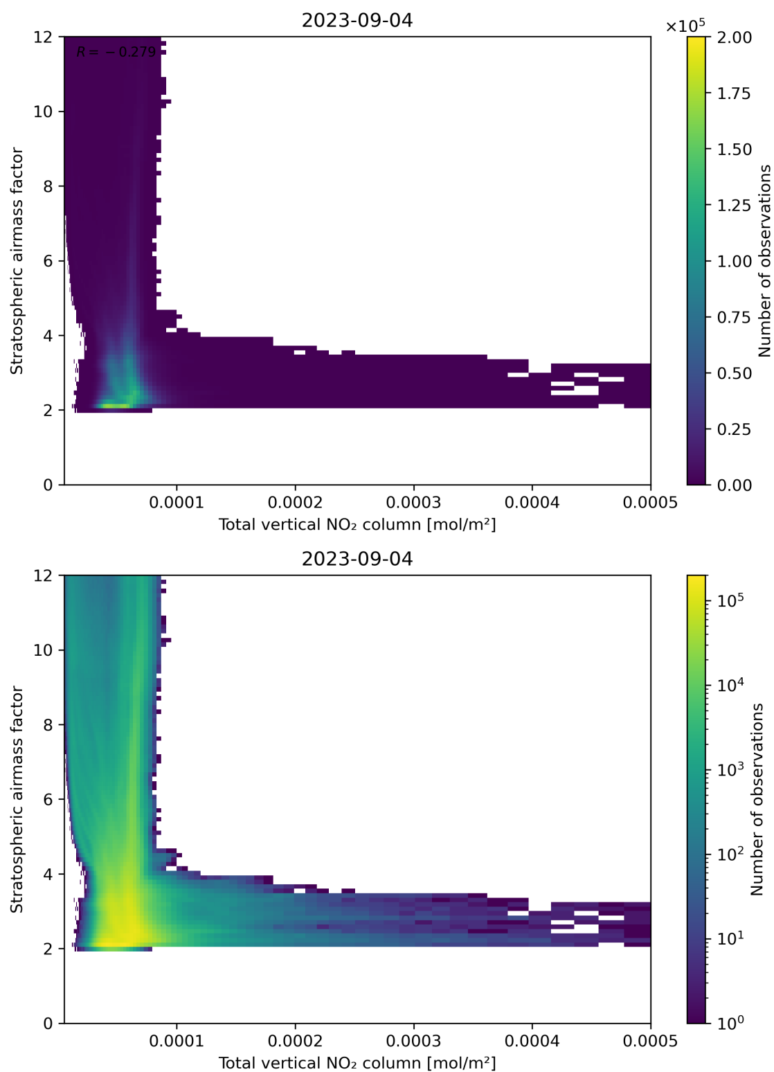
Figure 110: Scatter density plot of “Total vertical NO 2 column” against “Stratospheric air mass factor” for 2023-09-04 to 2023-09-05.
