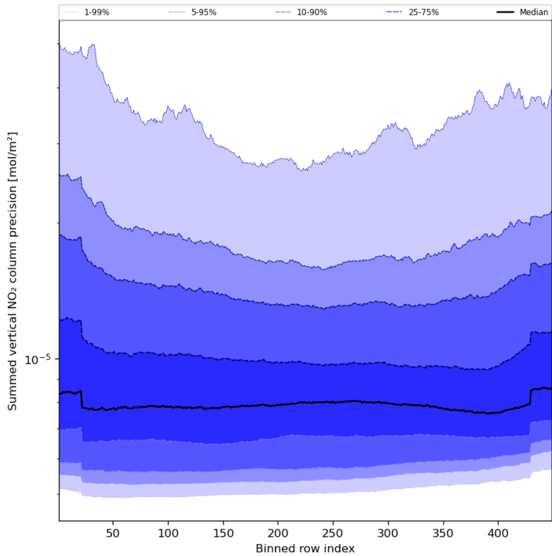
Figure 58: Along track statistics of “Summed vertical NO 2 column precision” for 2023-09-04 to 2023-09-05
