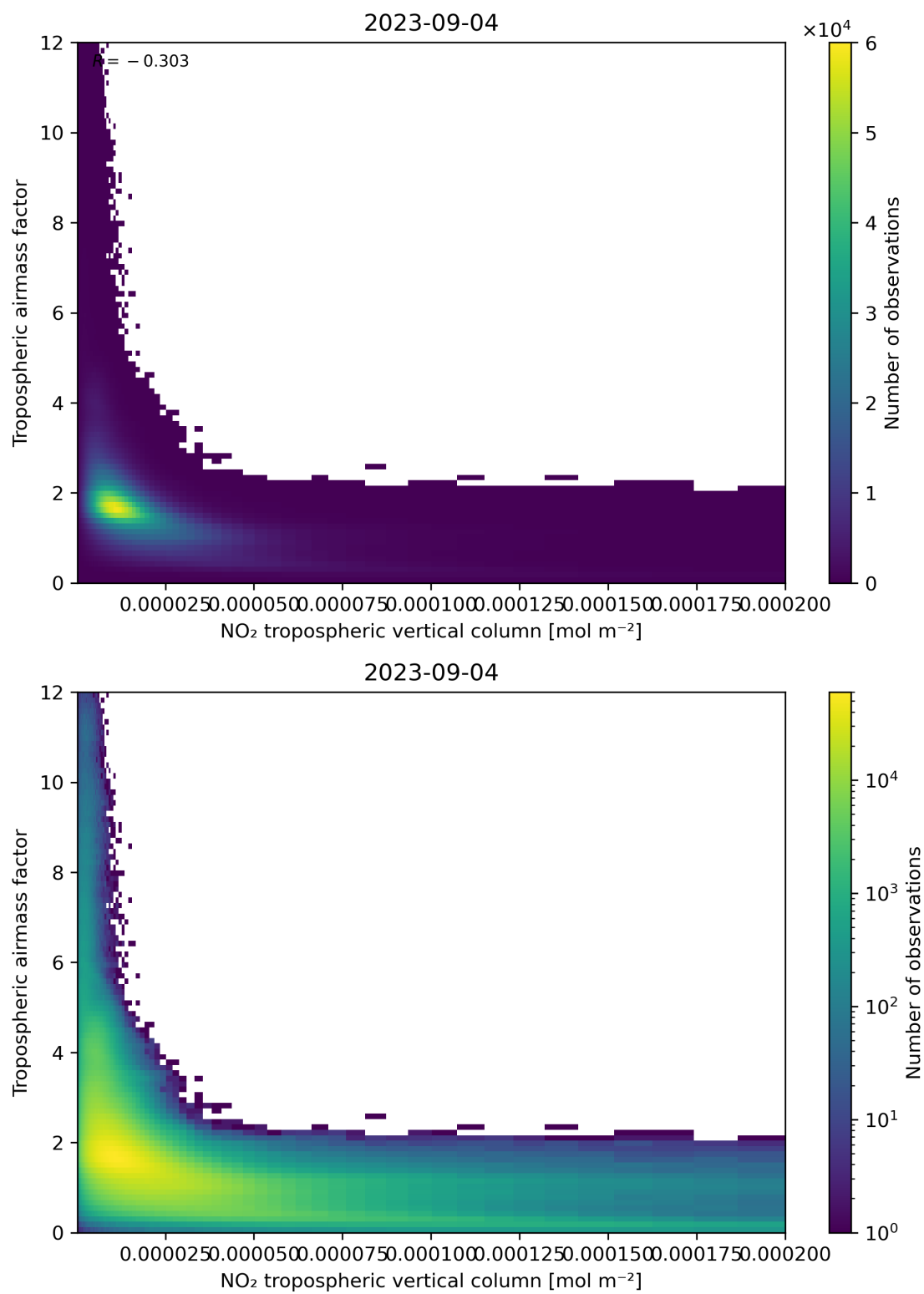
Figure 123: Scatter density plot of “NO 2 tropospheric vertical column” against “Tropospheric air mass factor” for 2023-09-04 to 2023-09-05.
