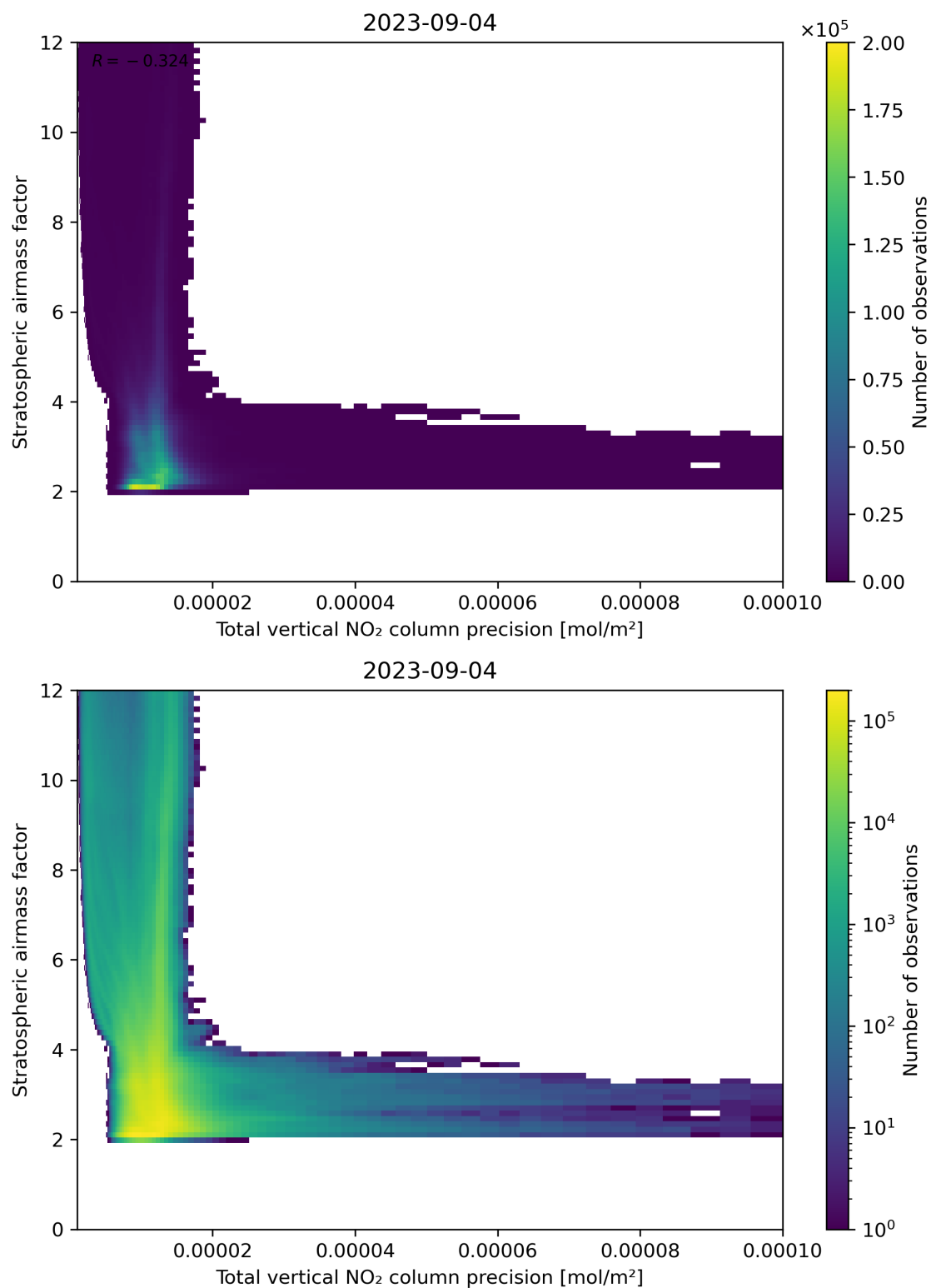
Figure 115: Scatter density plot of “Total vertical NO 2 column precision” against “Stratospheric air mass factor” for 2023-09-04 to 2023-09-05.
