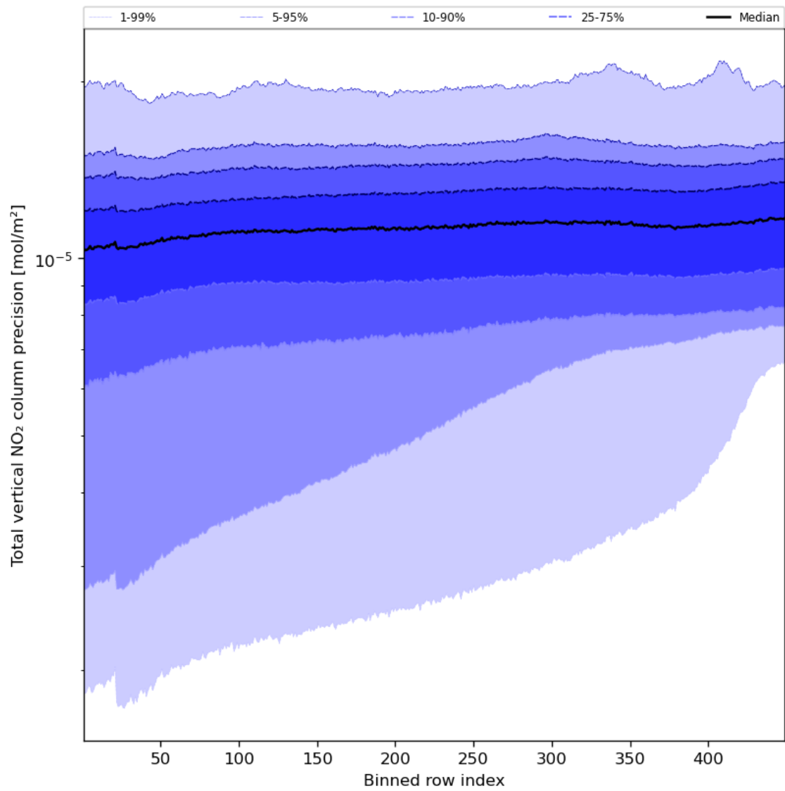
Figure 56: Along track statistics of “Total vertical NO 2 column precision” for 2023-09-04 to 2023-09-05
