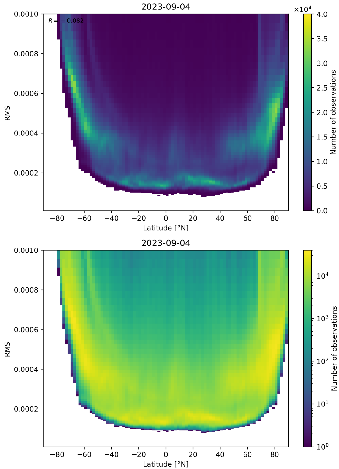
Figure 94: Scatter density plot of “Latitude” against “RMS” for 2023-09-04 to 2023-09-05.
