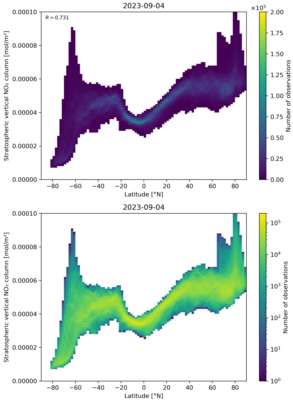
Figure 87: Scatter density plot of “Latitude” against “Stratospheric vertical NO 2 column” for 2023-09-04 to 2023-09-05.
