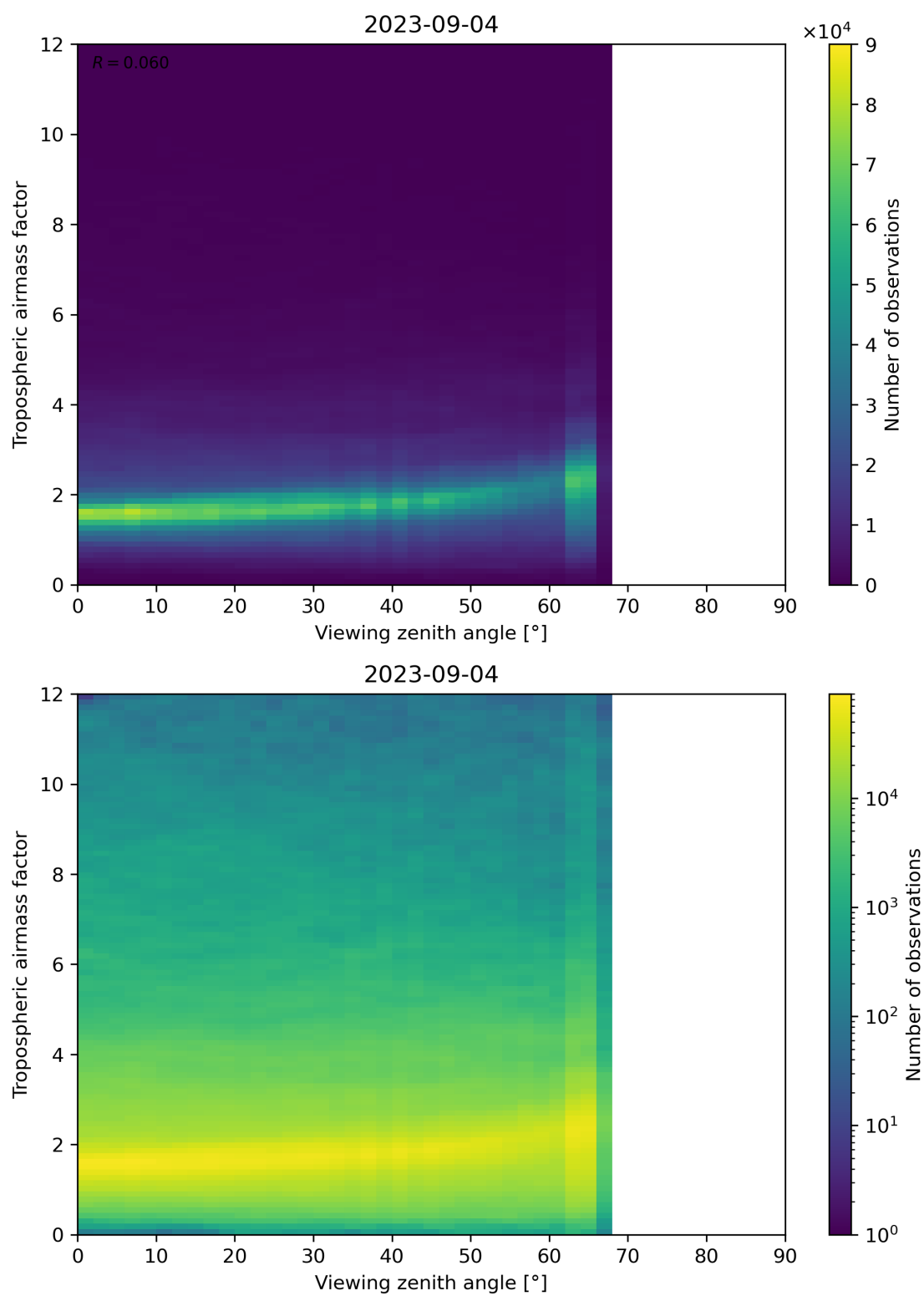
Figure 161: Scatter density plot of “Viewing zenith angle” against “Tropospheric airmass factor” for 2023-09-04 to 2023-09-05.
