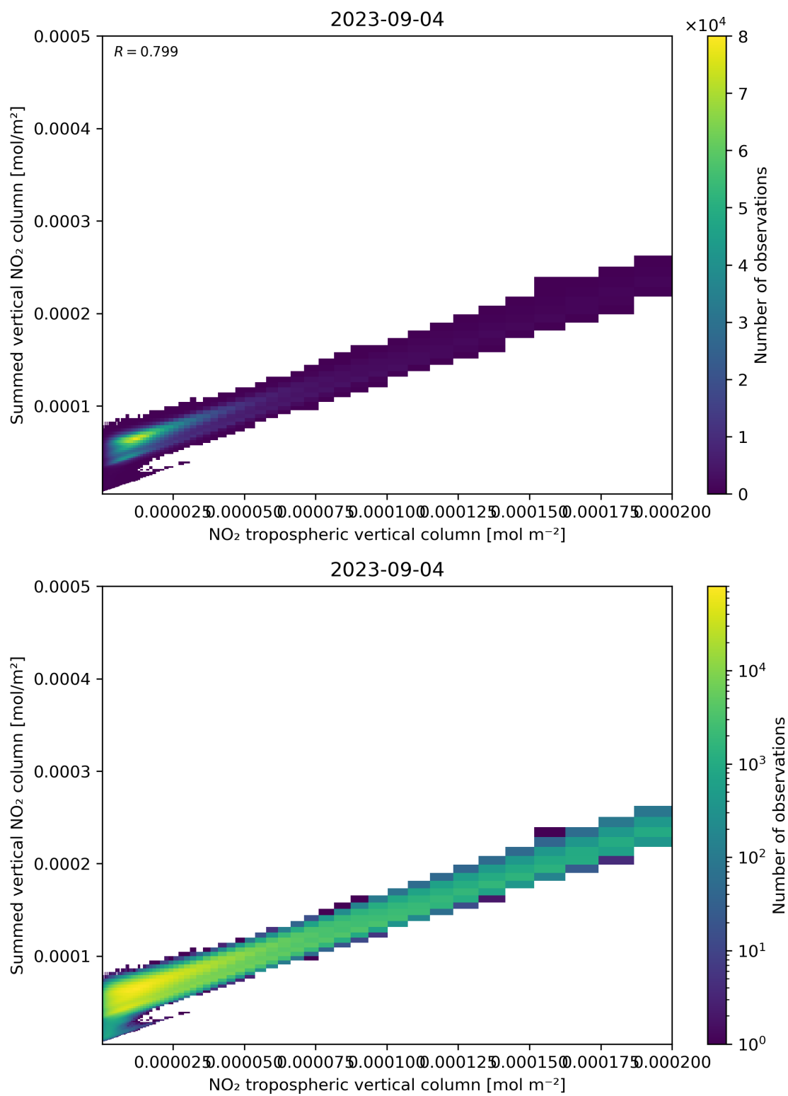
Figure 126: Scatter density plot of “NO 2 tropospheric vertical column” against “Summed vertical NO 2 column” for 2023-09-04 to 2023-09-05.
