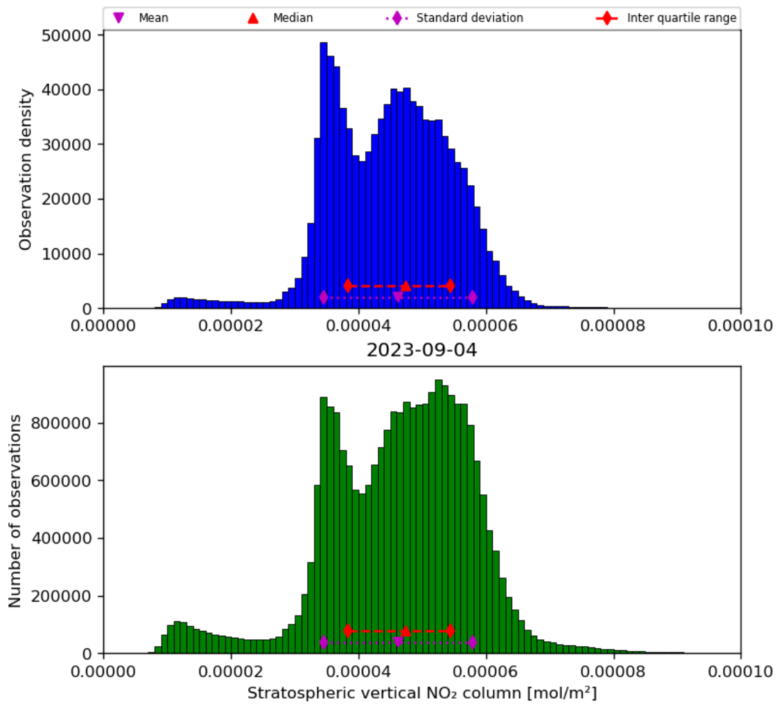
Figure 36: Histogram of “Stratospheric vertical NO 2 column” for 2023-09-04 to 2023-09-05
