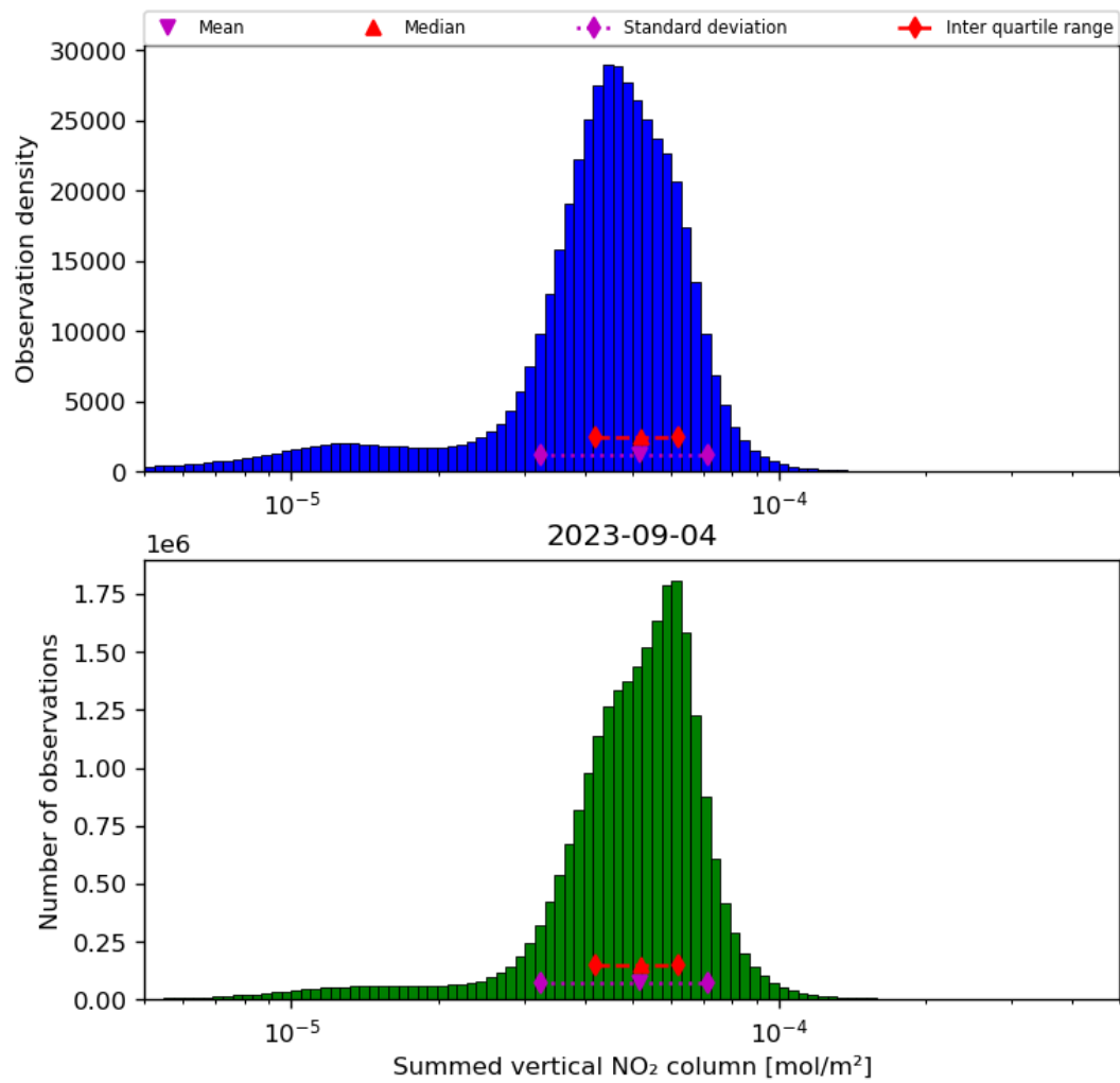
Figure 40: Histogram of “Summed vertical NO 2 column” for 2023-09-04 to 2023-09-05
