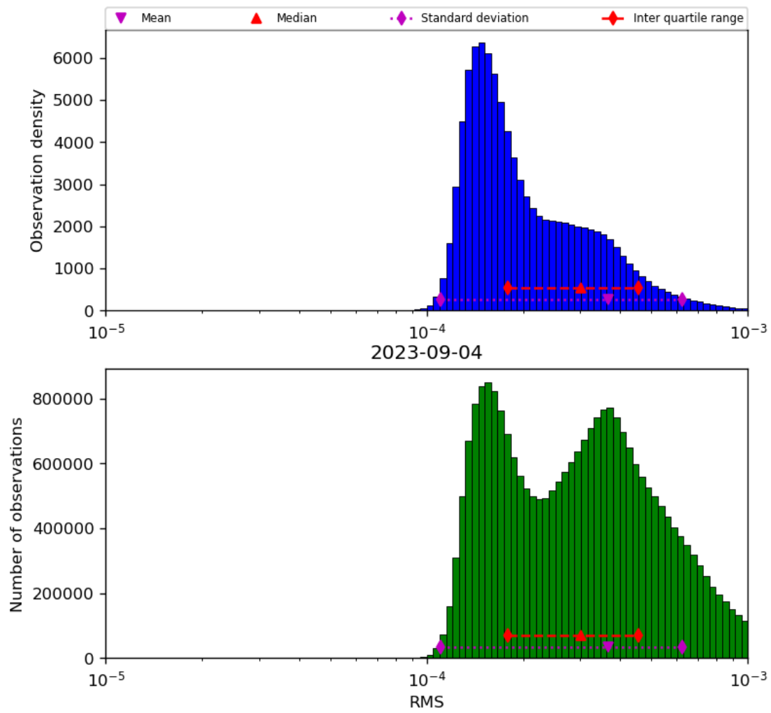
Figure 43: Histogram of “RMS” for 2023-09-04 to 2023-09-05
