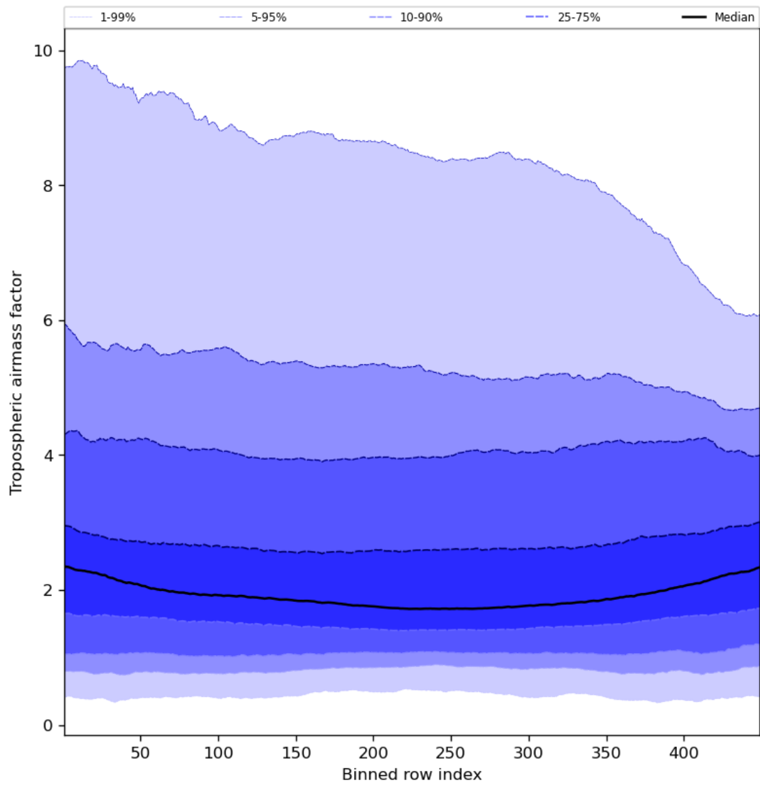
Figure 48: Along track statistics of “Tropospheric airmass factor” for 2023-09-04 to 2023-09-05
