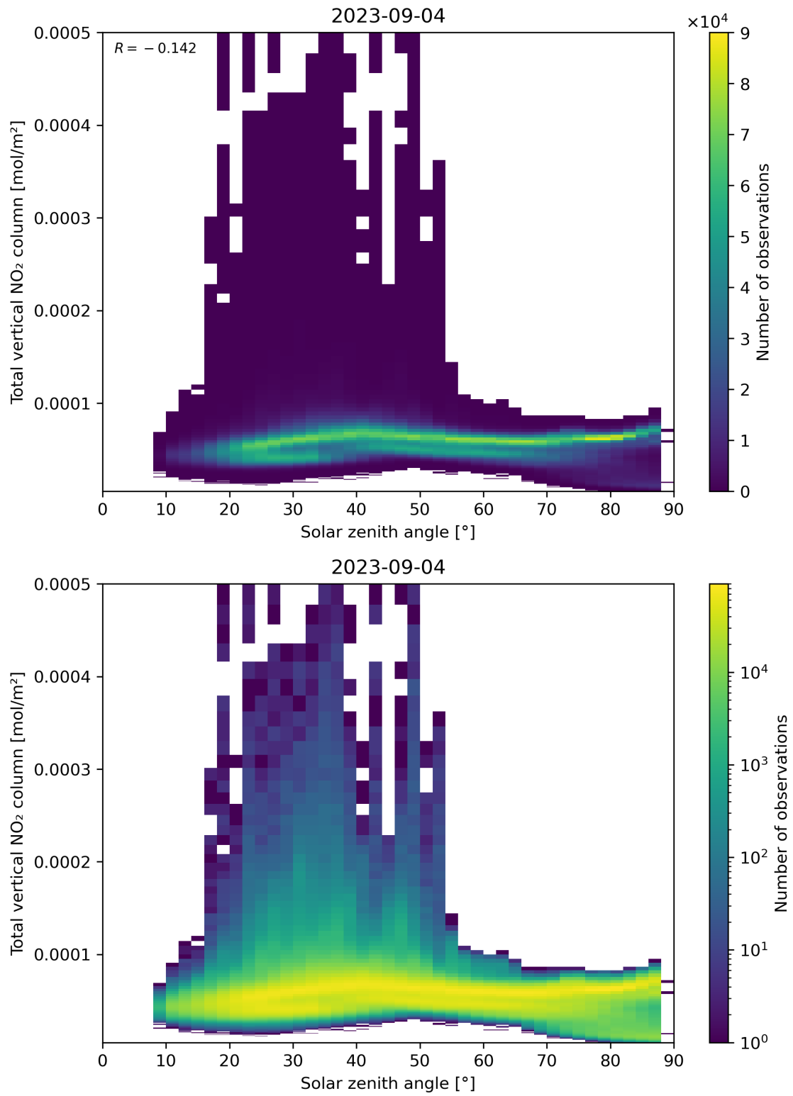
Figure 153: Scatter density plot of “Solar zenith angle” against “Total vertical NO 2 column” for 2023-09-04 to 2023-09-05.
