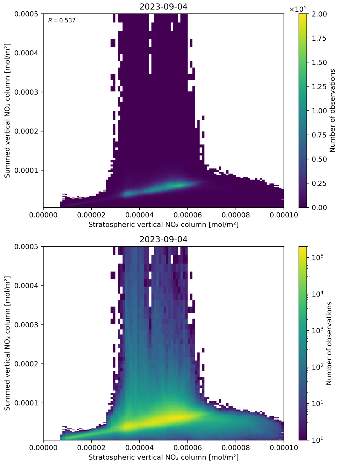
Figure 98: Scatter density plot of “Stratospheric vertical NO 2 column” against “Summed vertical NO 2 column” for 2023-09-04 to 2023-09-05.
