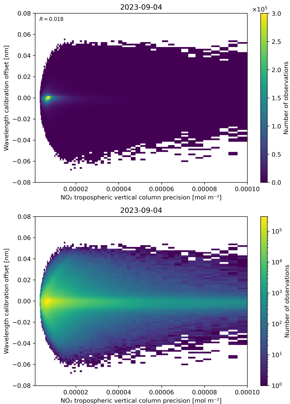
Figure 141: Scatter density plot of “NO 2 tropospheric vertical column precision” against “Wavelength calibration offset” for 2023-09-04 to 2023-09-05.
