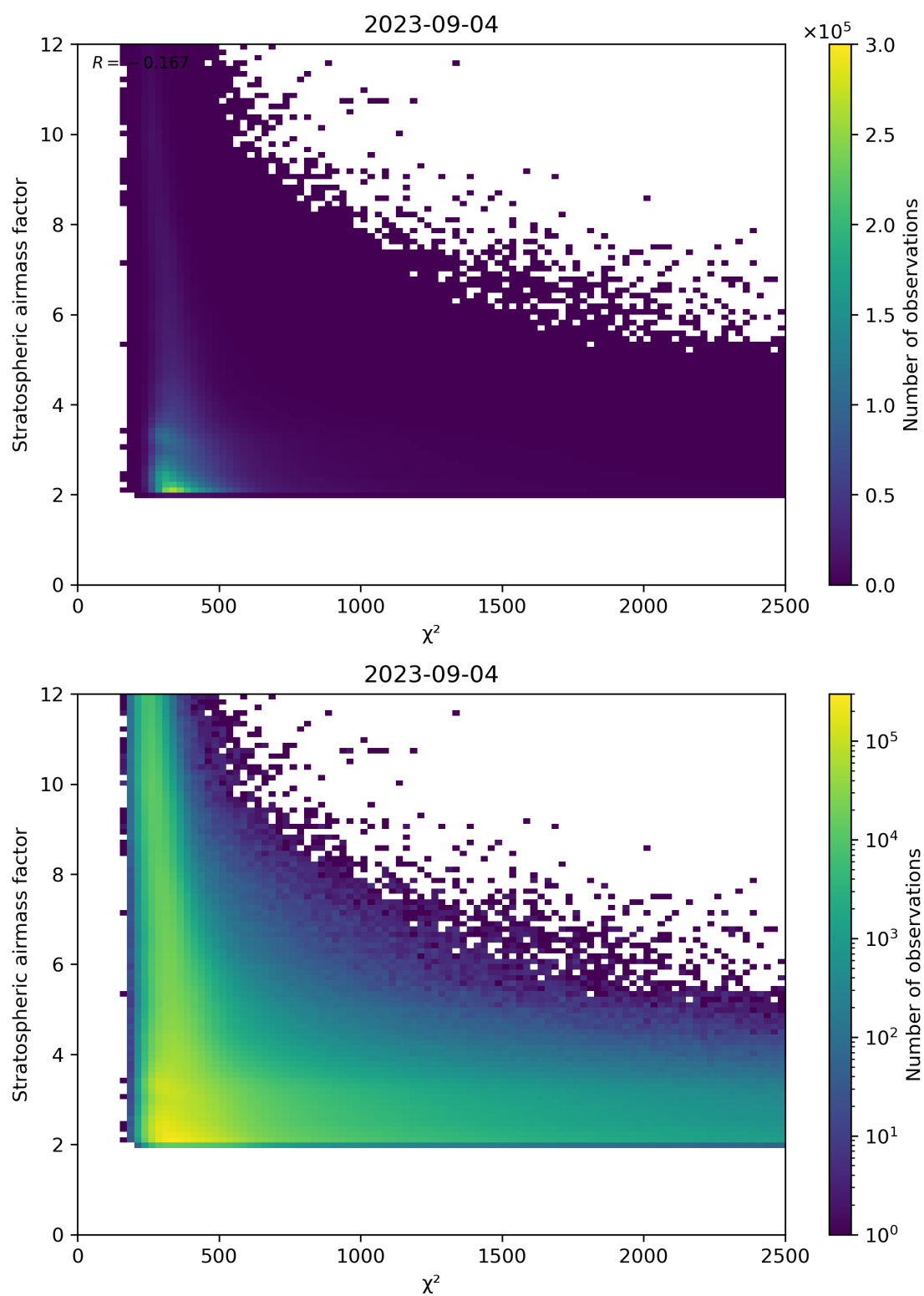
Figure 81: Scatter density plot of “ \chi^2 ” against “Stratospheric airmass factor” for 2023-09-04 to 2023-09-05.
