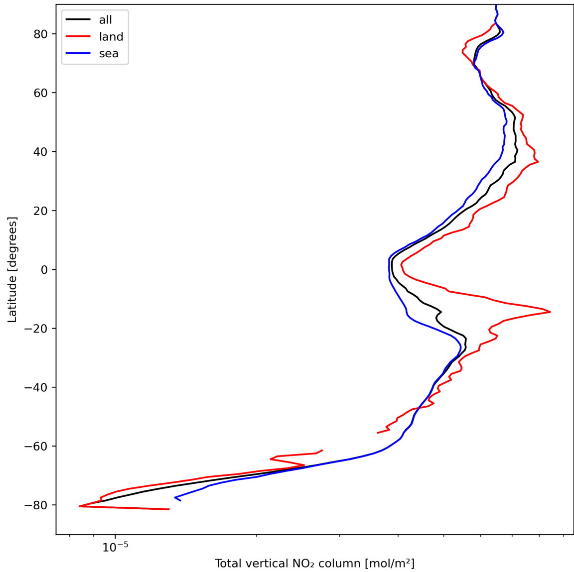
Figure 21: Zonal average of “Total vertical NO 2 column” for 2023-09-04 to 2023-09-05.
