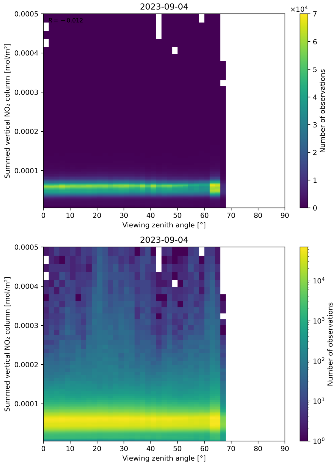
Figure 165: Scatter density plot of “Viewing zenith angle” against “Summed vertical NO 2 column” for 2023-09-04 to 2023-09-05.
