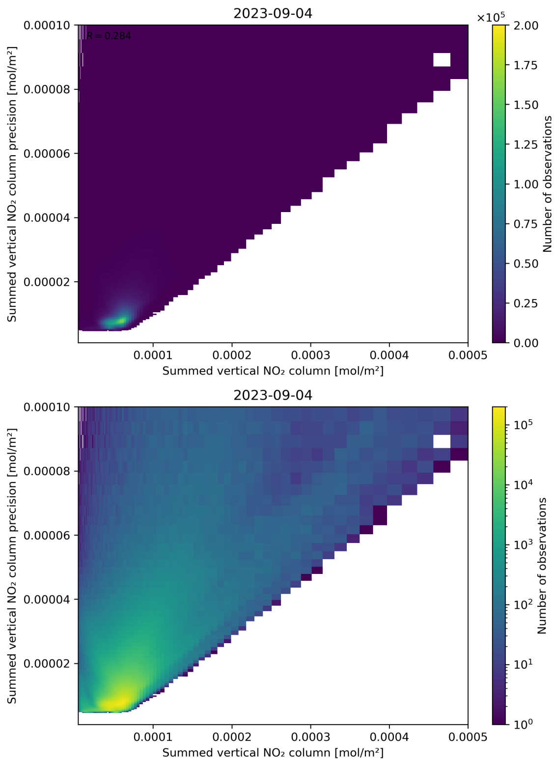
Figure 105: Scatter density plot of “Summed vertical NO 2 column” against “Summed vertical NO 2 column precision” for 2023-09-04 to 2023-09-05.
