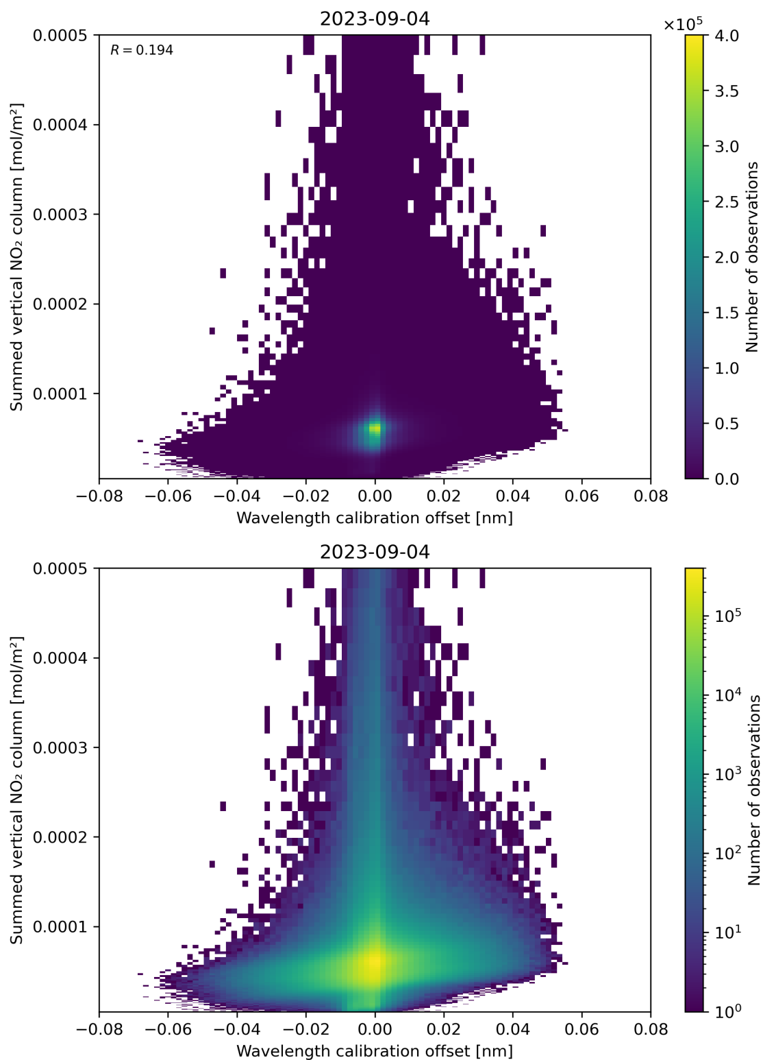
Figure 177: Scatter density plot of “Wavelength calibration offset” against “Summed vertical NO 2 column” for 2023-09-04 to 2023-09-05.
