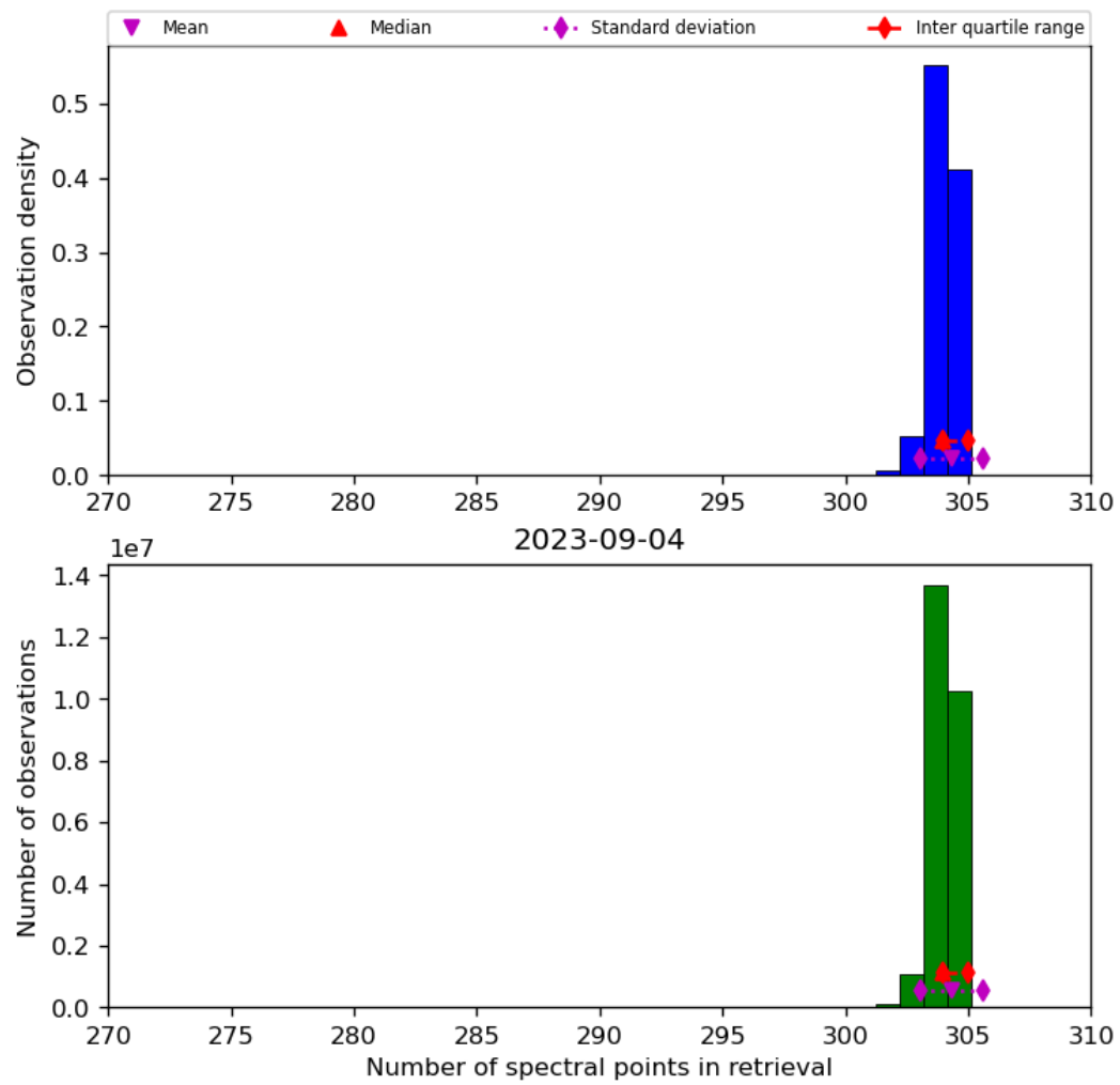
Figure 33: Histogram of “Number of spectral points in retrieval” for 2023-09-04 to 2023-09-05
