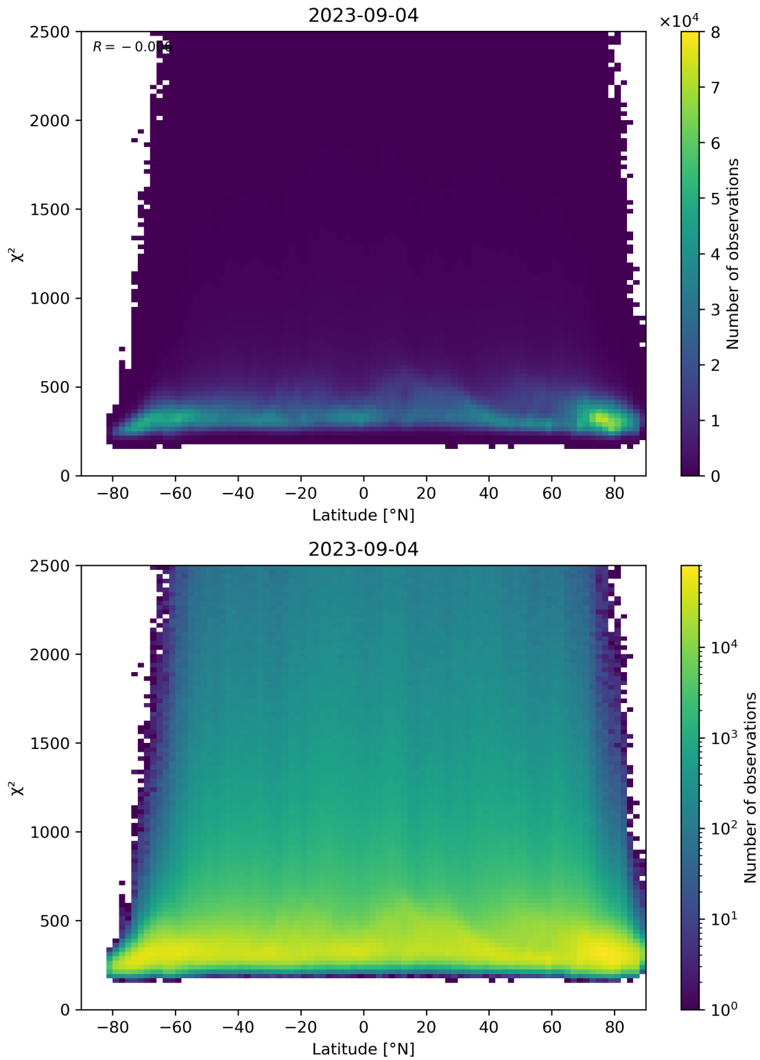
Figure 86: Scatter density plot of “Latitude” against “ \chi^2 ” for 2023-09-04 to 2023-09-05.
