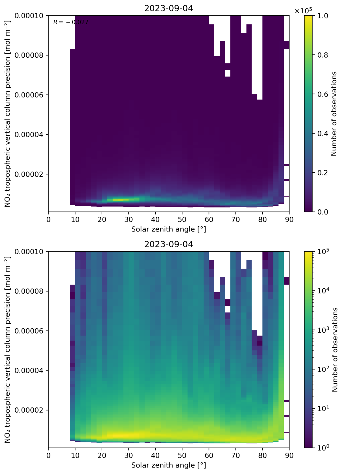
Figure 156: Scatter density plot of “Solar zenith angle” against “NO 2 tropospheric vertical column precision” for 2023-09-04 to 2023-09-05.
