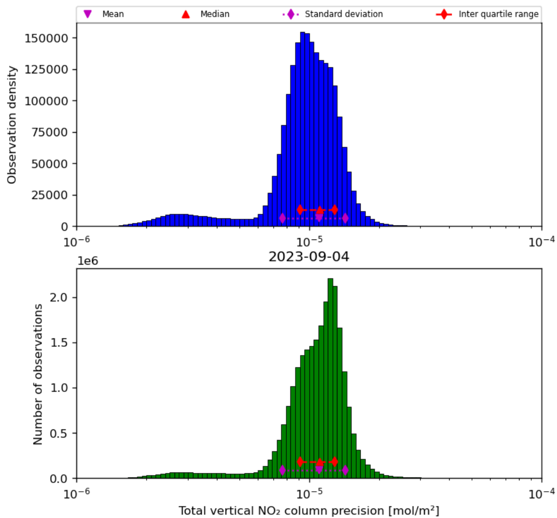
Figure 39: Histogram of “Total vertical NO 2 column precision” for 2023-09-04 to 2023-09-05
