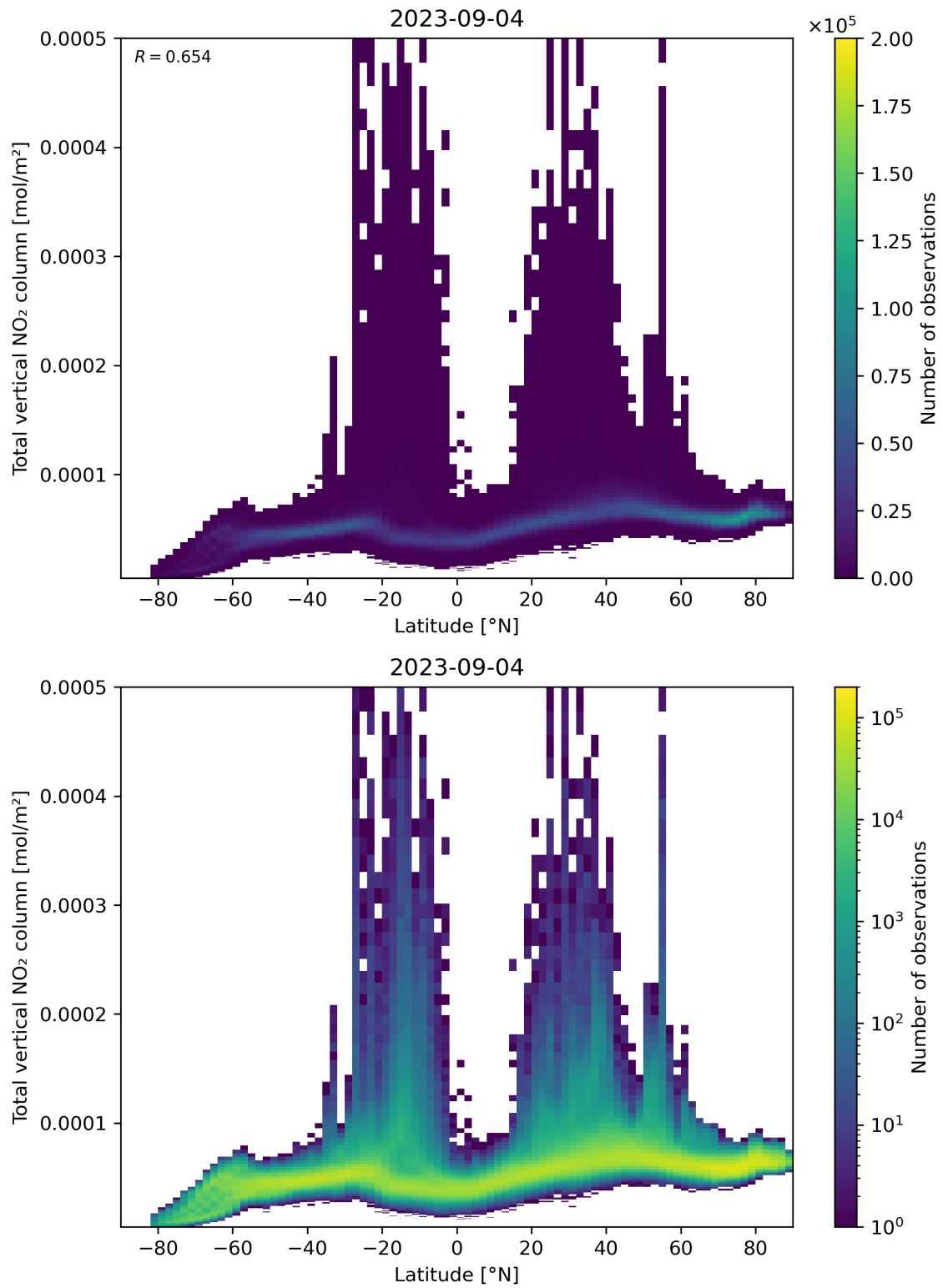
Figure 90: Scatter density plot of “Latitude” against “Total vertical NO 2 column” for 2023-09-04 to 2023-09-05.
