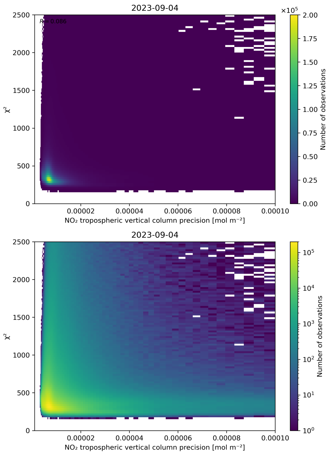
Figure 134: Scatter density plot of “NO 2 tropospheric vertical column precision” against “ \chi^2 ” for 2023-09-04 to 2023-09-05.
