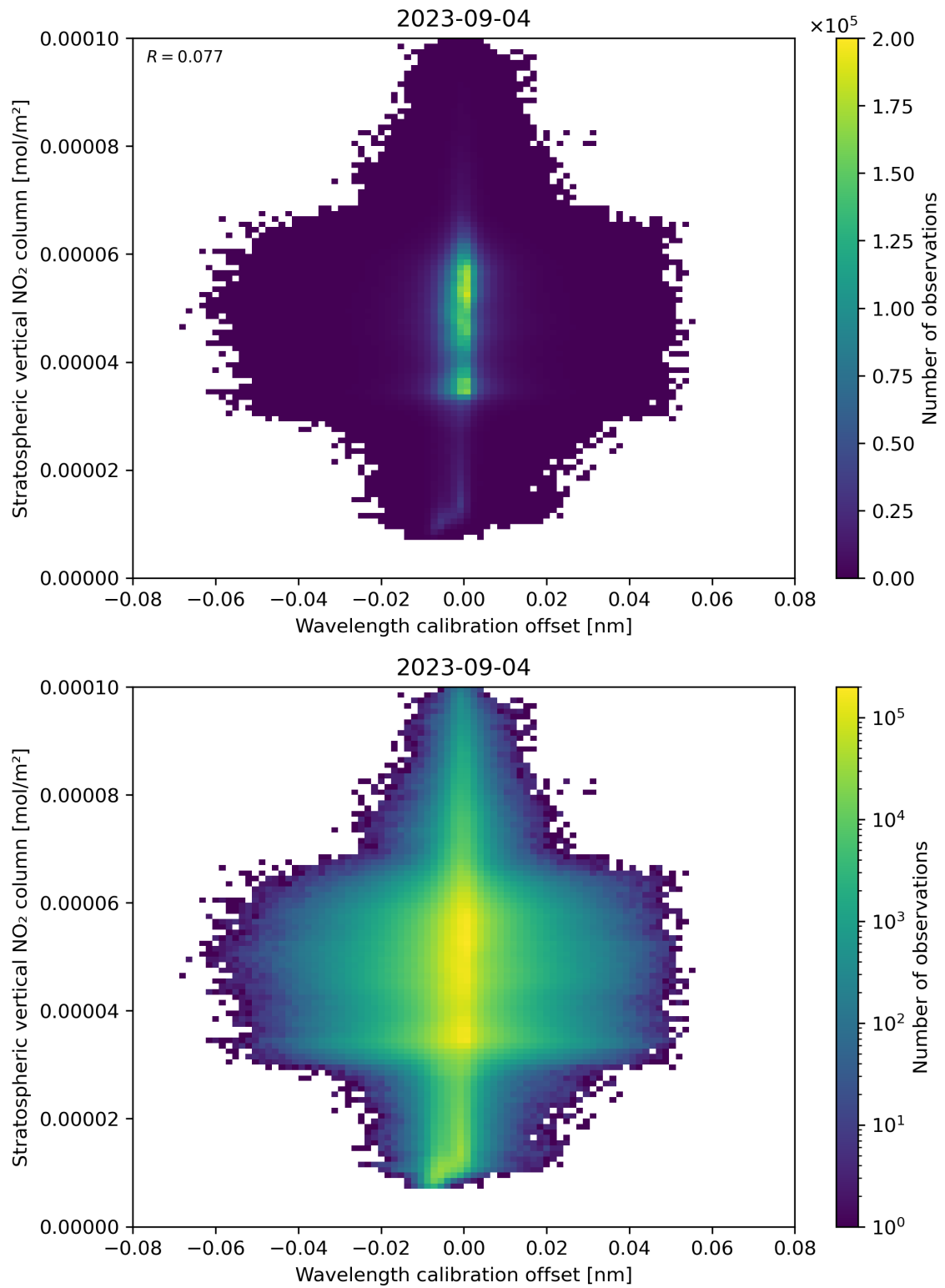
Figure 176: Scatter density plot of “Wavelength calibration offset” against “Stratospheric vertical NO 2 column” for 2023-09-04 to 2023-09-05.
