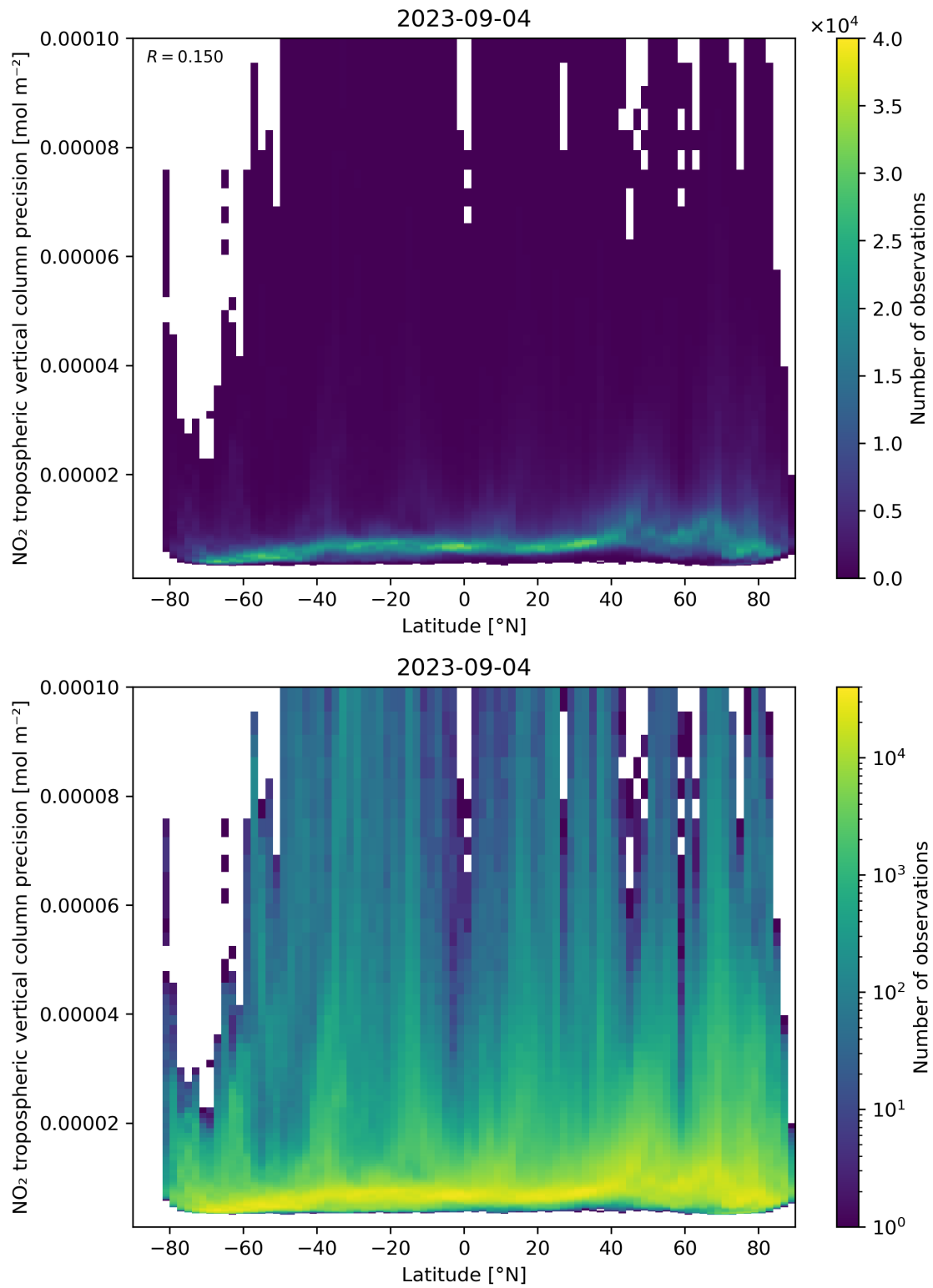
Figure 93: Scatter density plot of “Latitude” against “NO 2 tropospheric vertical column precision” for 2023-09-04 to 2023-09-05.
