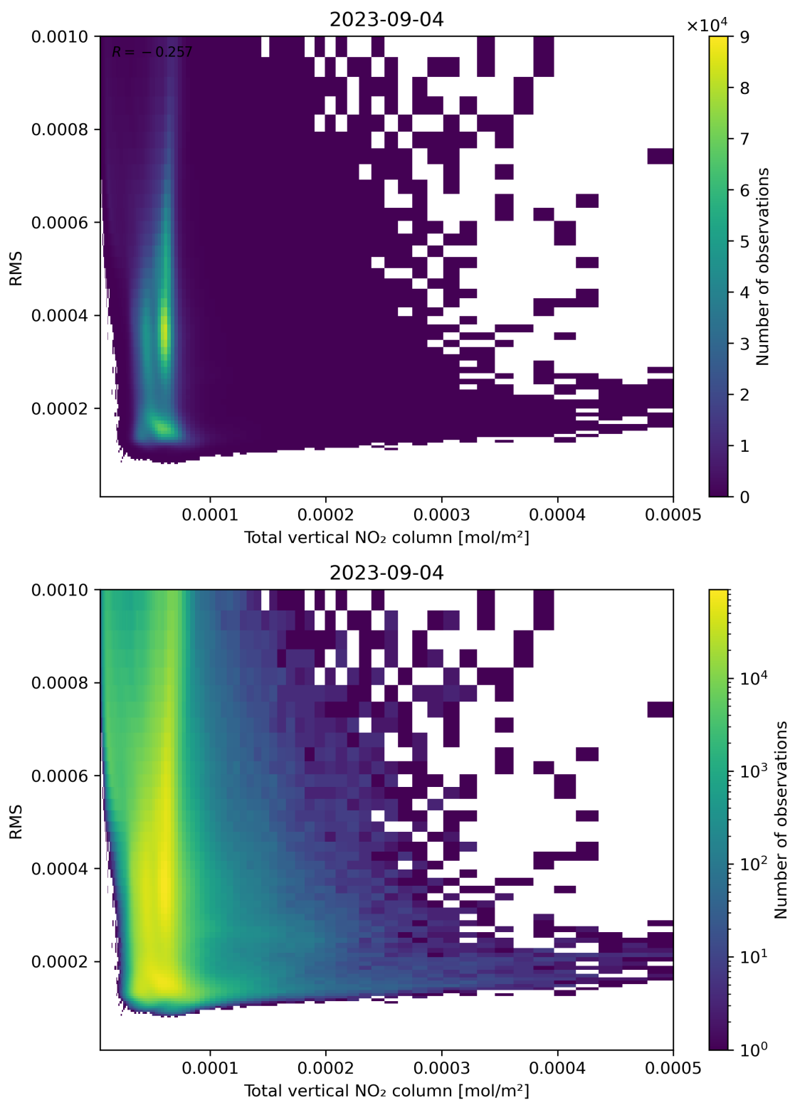
Figure 120: Scatter density plot of “Total vertical NO 2 column” against “RMS” for 2023-09-04 to 2023-09-05.
