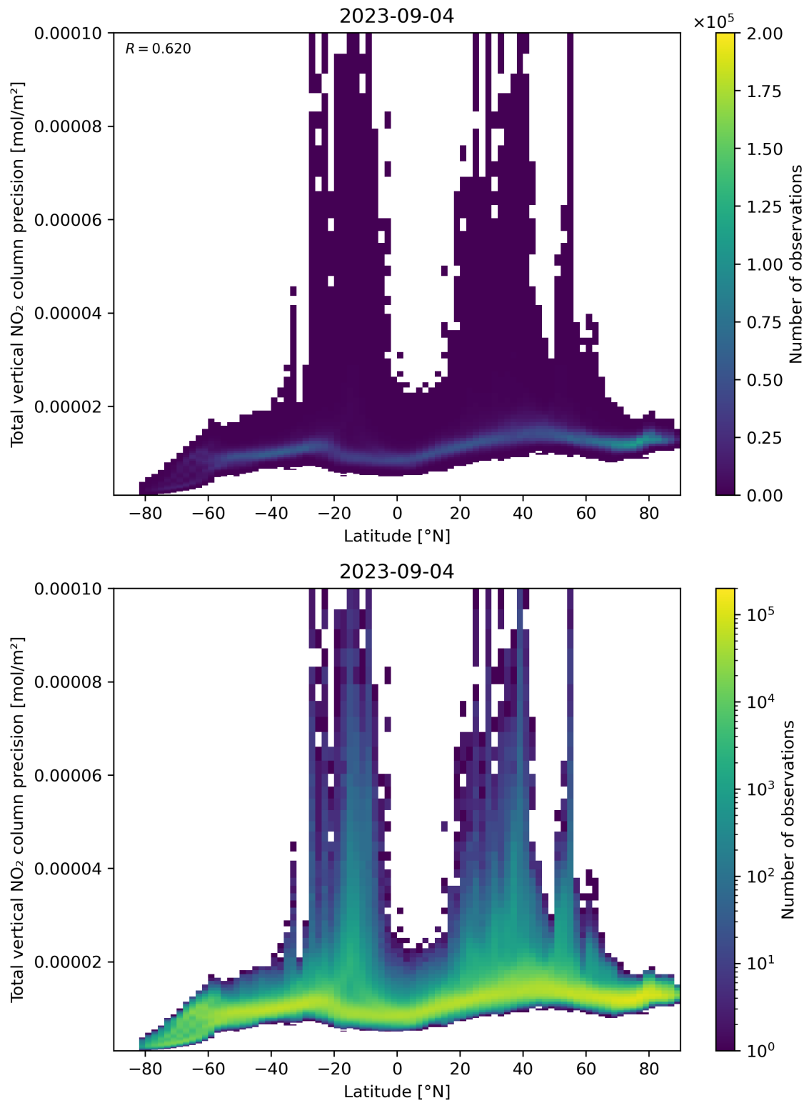
Figure 91: Scatter density plot of “Latitude” against “Total vertical NO 2 column precision” for 2023-09-04 to 2023-09-05.
