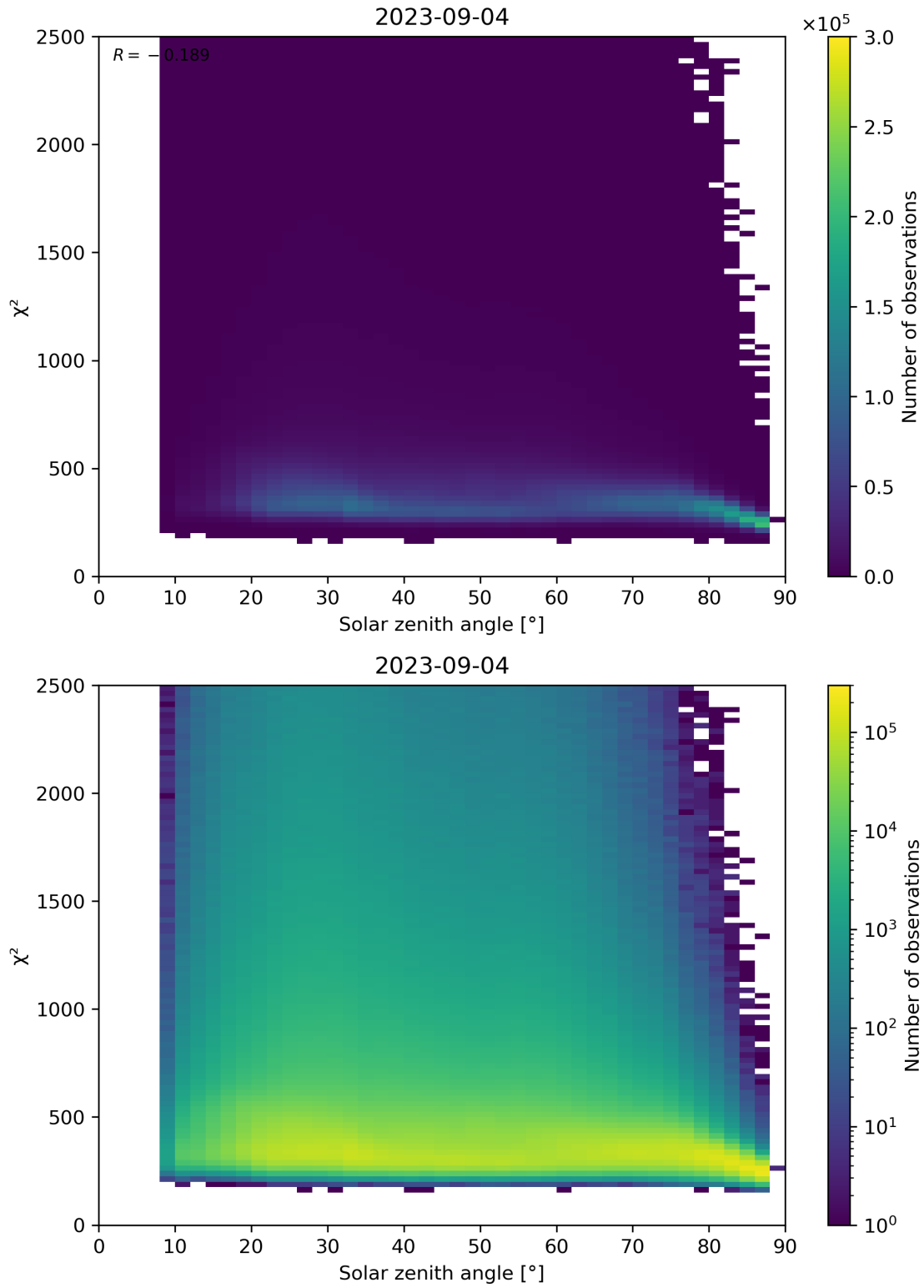
Figure 148: Scatter density plot of “Solar zenith angle” against “ \chi^2 ” for 2023-09-04 to 2023-09-05.
