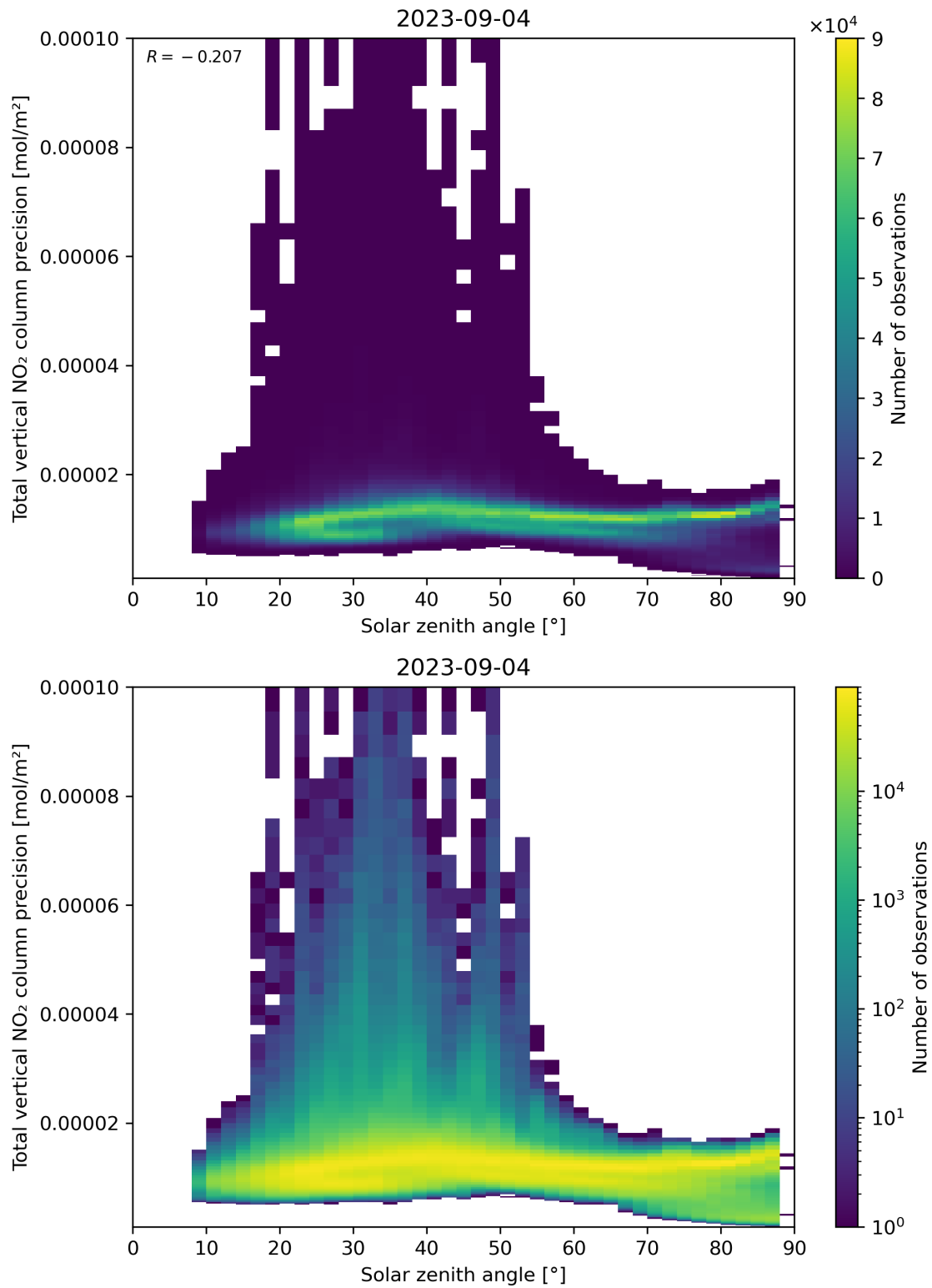
Figure 154: Scatter density plot of “Solar zenith angle” against “Total vertical NO 2 column precision” for 2023-09-04 to 2023-09-05.
