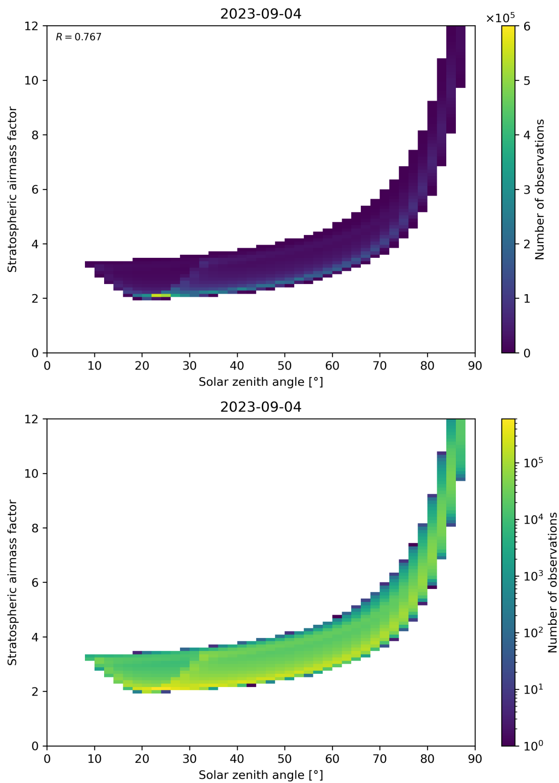
Figure 145: Scatter density plot of “Solar zenith angle” against “Stratospheric airmass factor” for 2023-09-04 to 2023-09-05.
