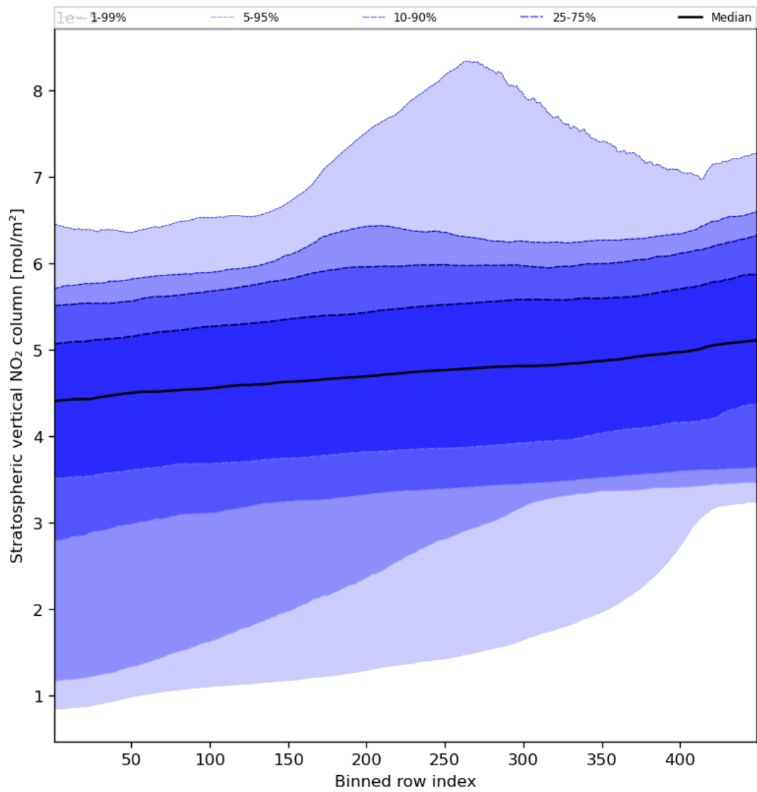
Figure 53: Along track statistics of “Stratospheric vertical NO 2 column” for 2023-09-04 to 2023-09-05
