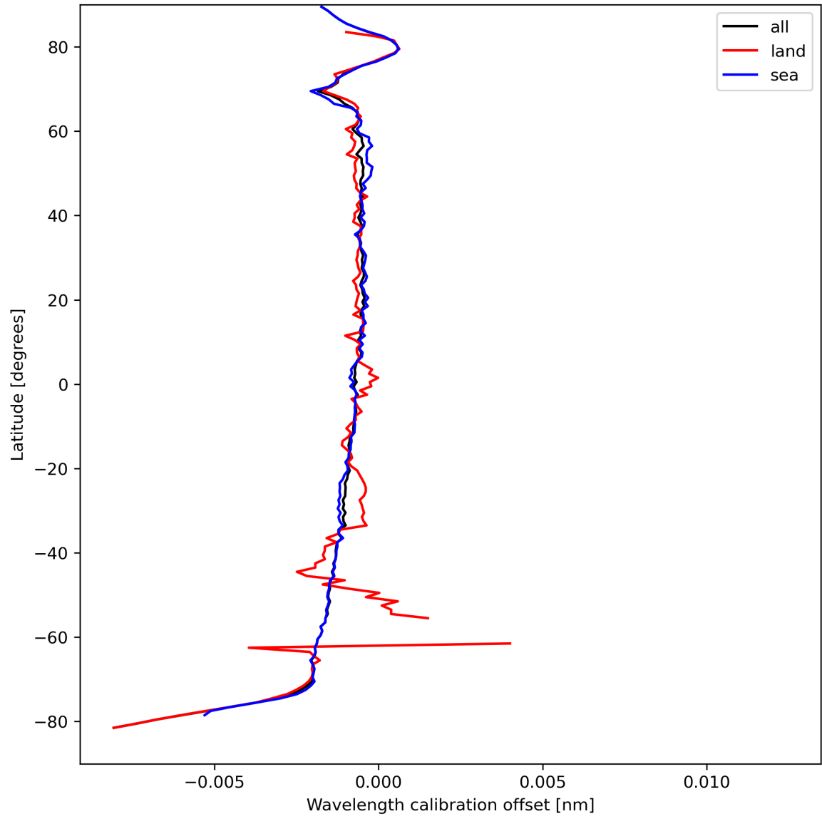
Figure 18: Zonal average of “Wavelength calibration offset” for 2023-09-04 to 2023-09-05.
