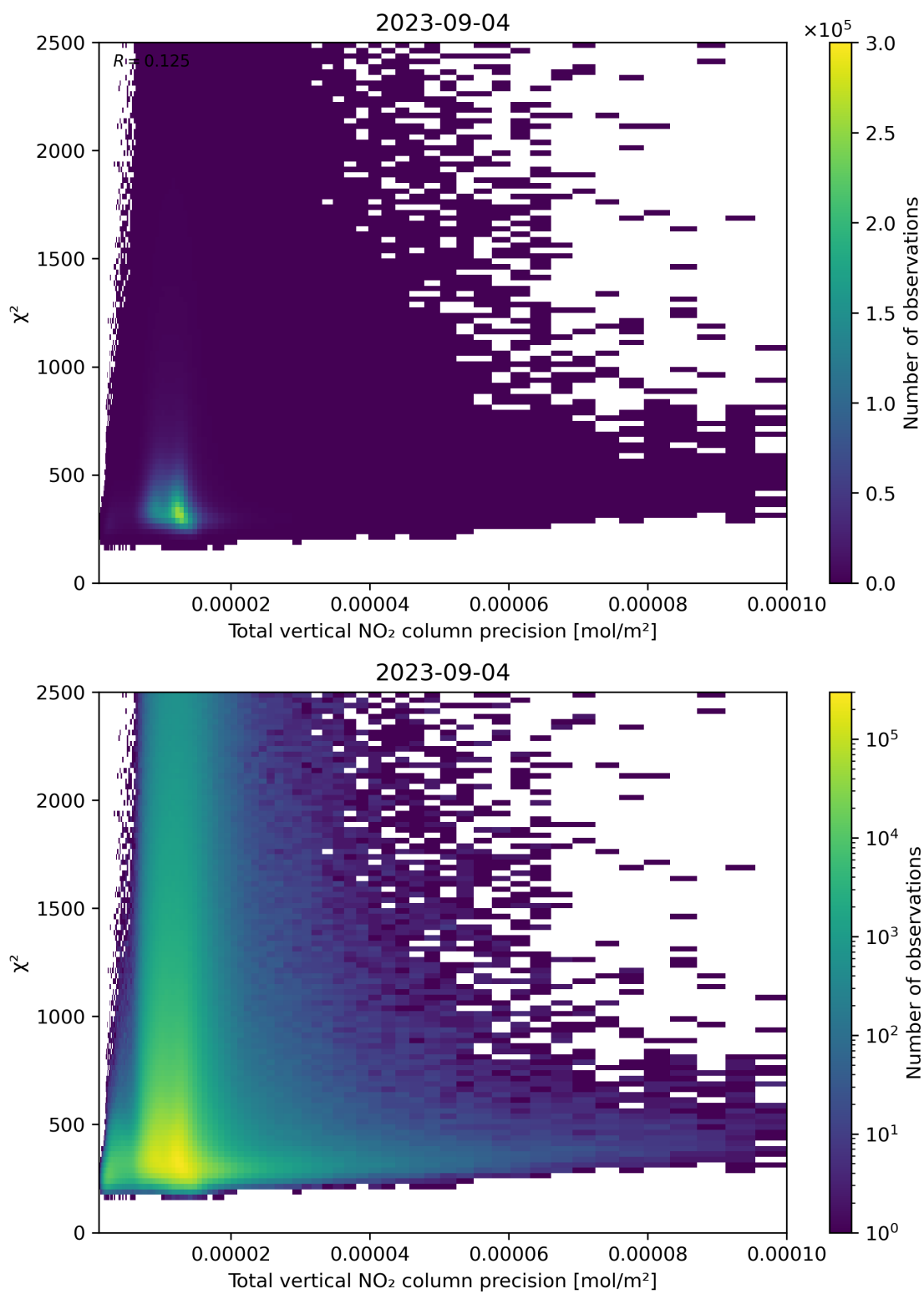
Figure 116: Scatter density plot of “Total vertical NO 2 column precision” against “ \chi^2 ” for 2023-09-04 to 2023-09-05.
