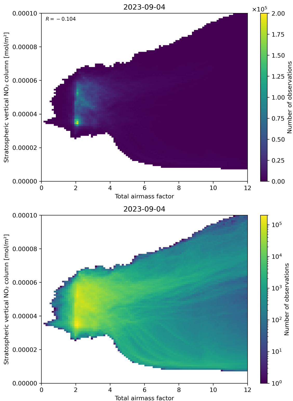
Figure 64: Scatter density plot of “Total airmass factor” against “Stratospheric vertical NO 2 column” for 2023-09-04 to 2023-09-05.
