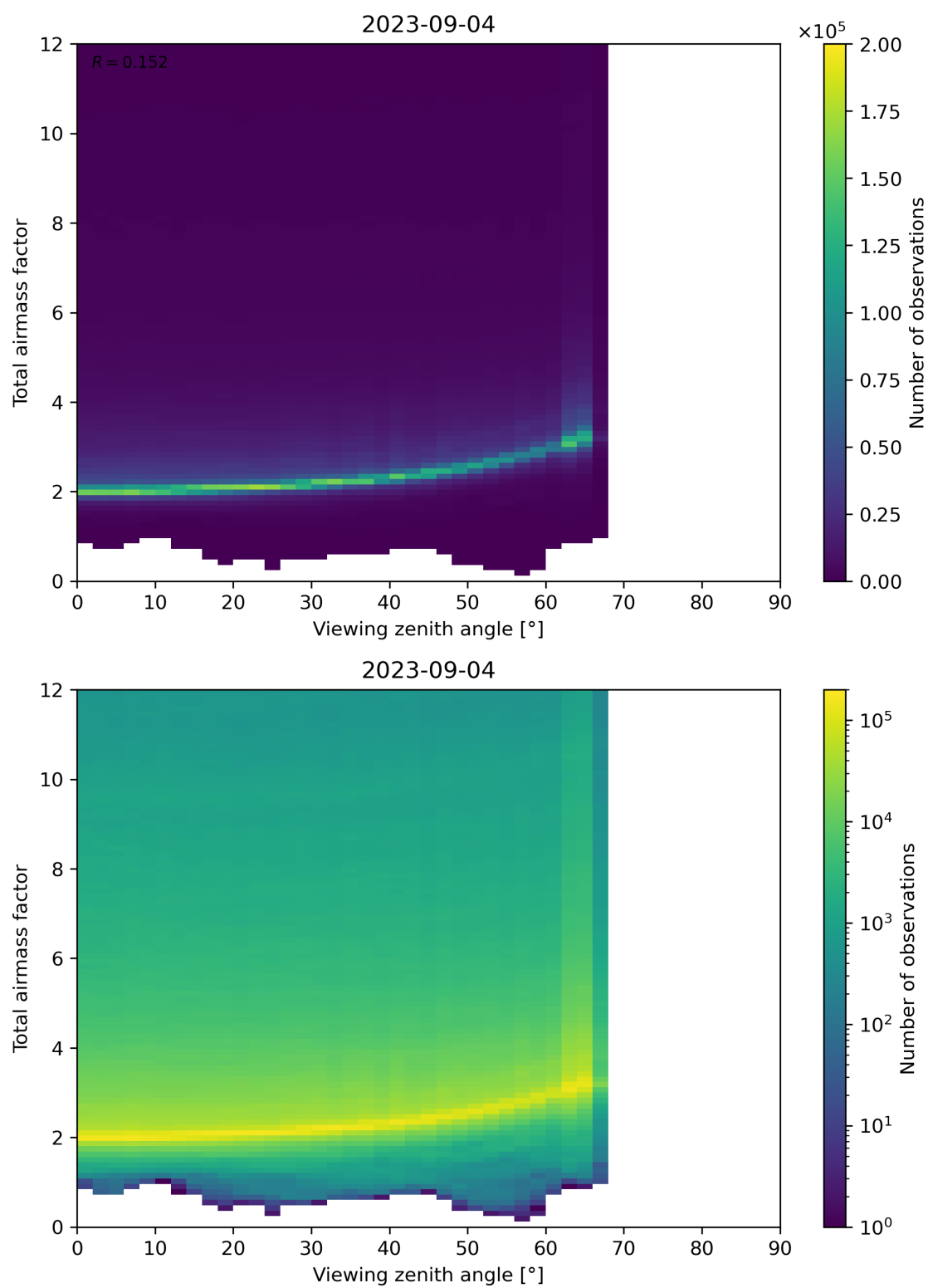
Figure 160: Scatter density plot of “Viewing zenith angle” against “Total airmass factor” for 2023-09-04 to 2023-09-05.
