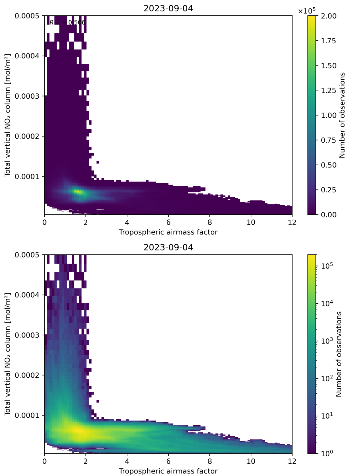
Figure 77: Scatter density plot of “Tropospheric airmass factor” against “Total vertical NO 2 column” for 2023-09-04 to 2023-09-05.
