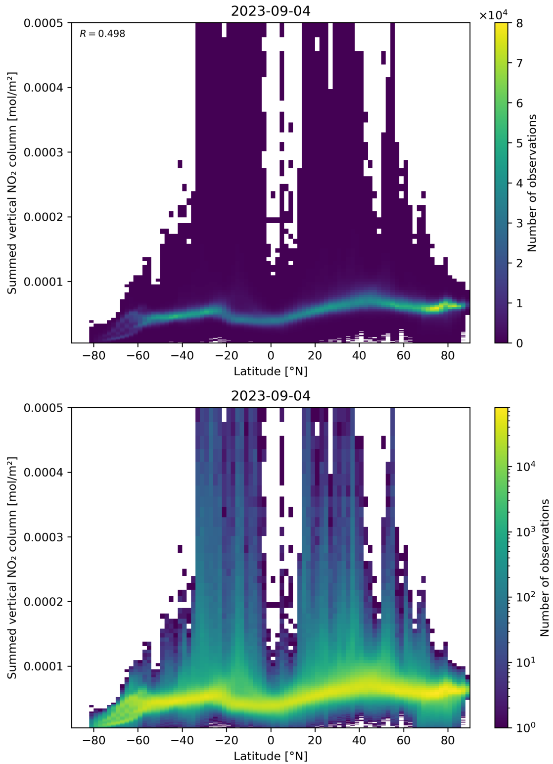
Figure 88: Scatter density plot of “Latitude” against “Summed vertical NO 2 column” for 2023-09-04 to 2023-09-05.
