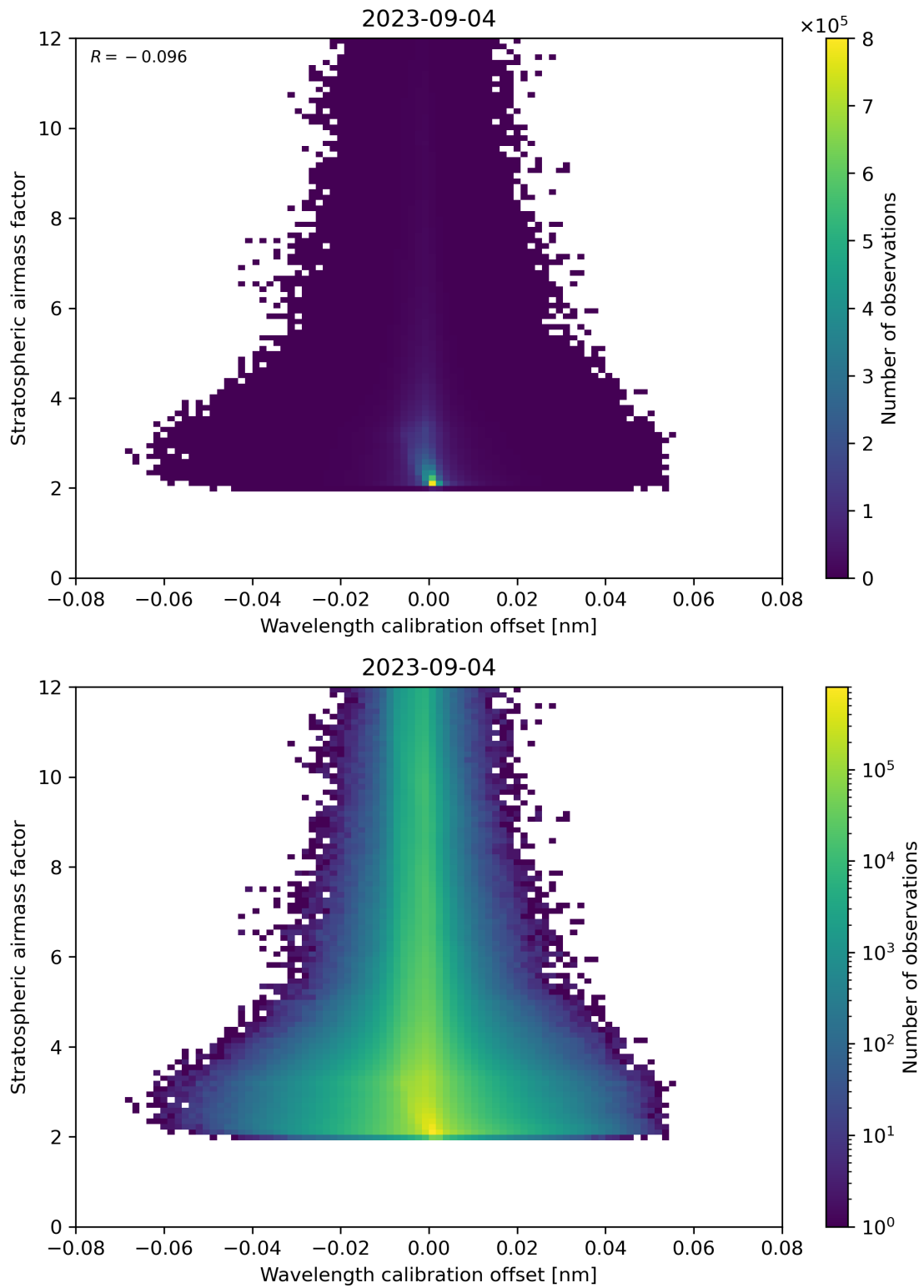
Figure 174: Scatter density plot of “Wavelength calibration offset” against “Stratospheric air mass factor” for 2023-09-04 to 2023-09-05.
