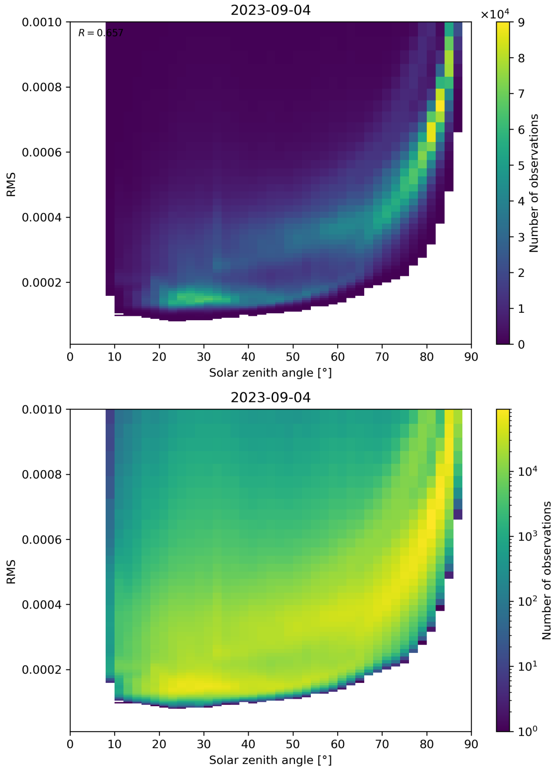
Figure 157: Scatter density plot of “Solar zenith angle” against “RMS” for 2023-09-04 to 2023-09-05.
