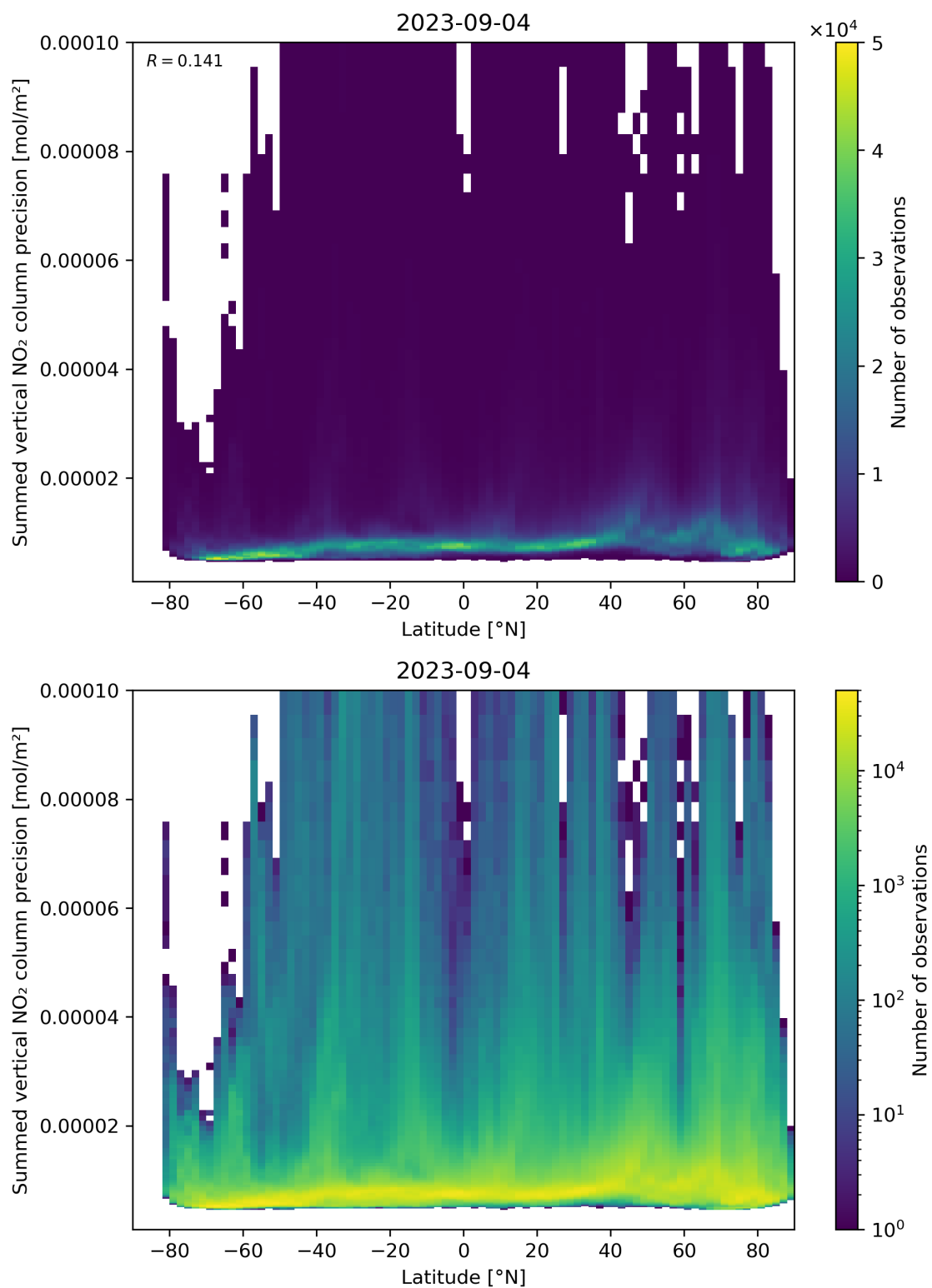
Figure 89: Scatter density plot of “Latitude” against “Summed vertical NO 2 column precision” for 2023-09-04 to 2023-09-05.
