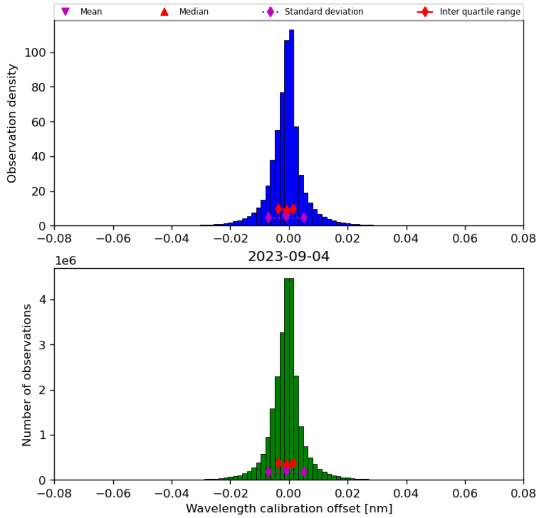
Figure 35: Histogram of “Wavelength calibration offset” for 2023-09-04 to 2023-09-05
