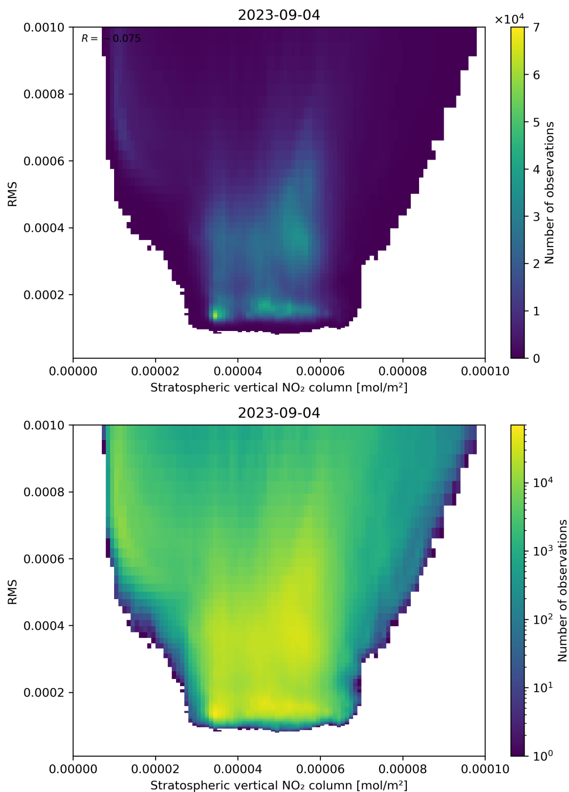
Figure 102: Scatter density plot of “Stratospheric vertical NO 2 column” against “RMS” for 2023-09-04 to 2023-09-05.
