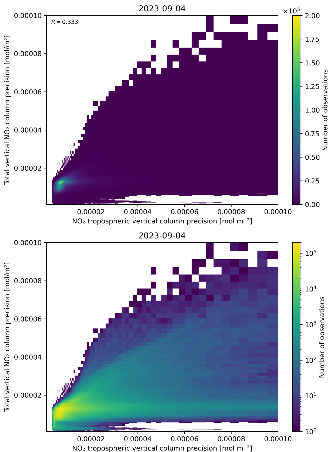
Figure 139: Scatter density plot of “NO 2 tropospheric vertical column precision” against “Total vertical NO 2 column precision” for 2023-09-04 to 2023-09-05.
