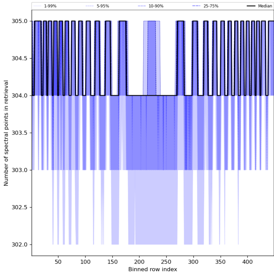
Figure 50: Along track statistics of “Number of spectral points in retrieval” for 2023-09-04 to 2023-09-05
