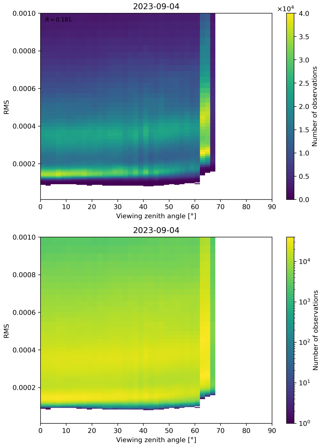
Figure 171: Scatter density plot of “Viewing zenith angle” against “RMS” for 2023-09-04 to 2023-09-05.
