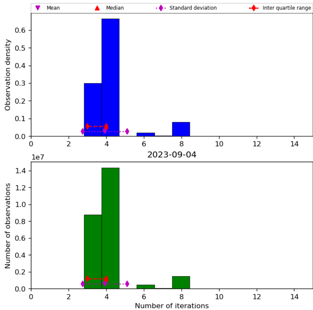
Figure 34: Histogram of “Number of iterations” for 2023-09-04 to 2023-09-05
