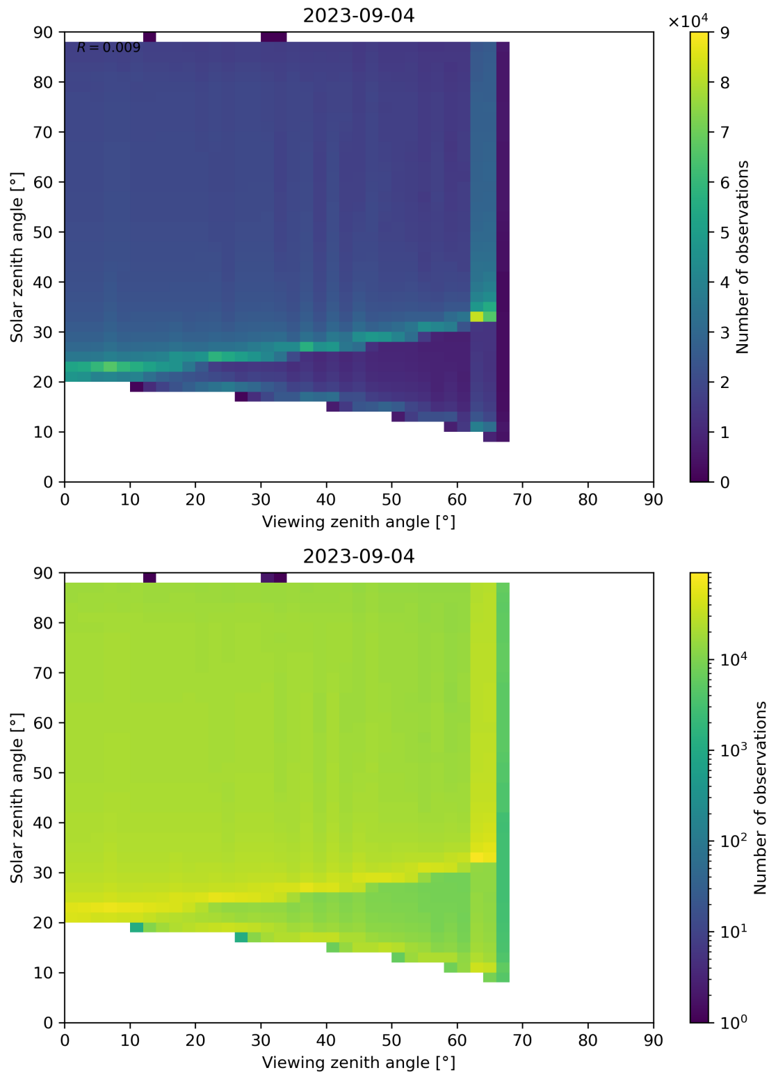
Figure 172: Scatter density plot of “Viewing zenith angle” against “Solar zenith angle” for 2023-09-04 to 2023-09-05.
