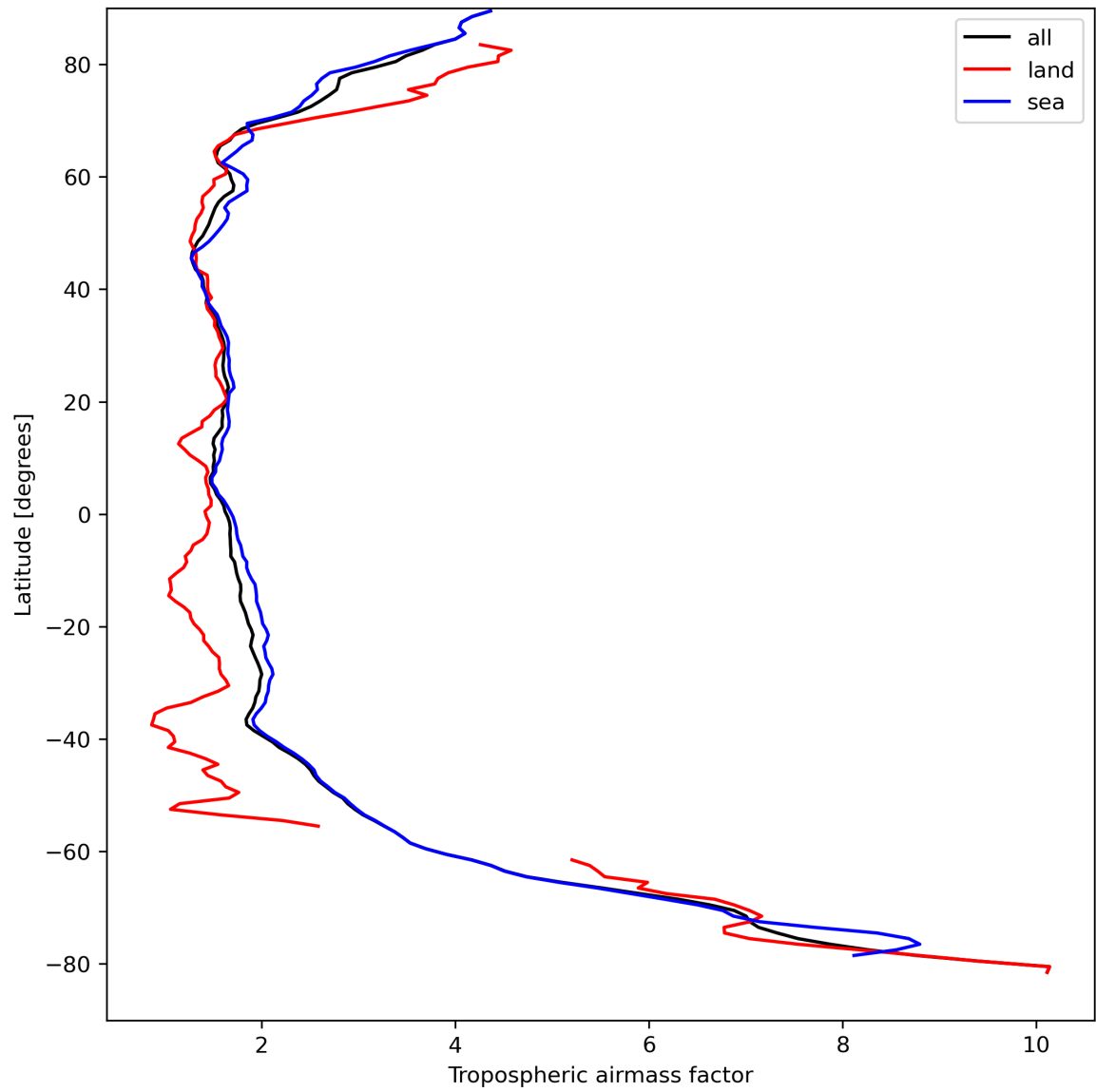
Figure 14: Zonal average of “Tropospheric airmass factor” for 2023-09-04 to 2023-09-05.
