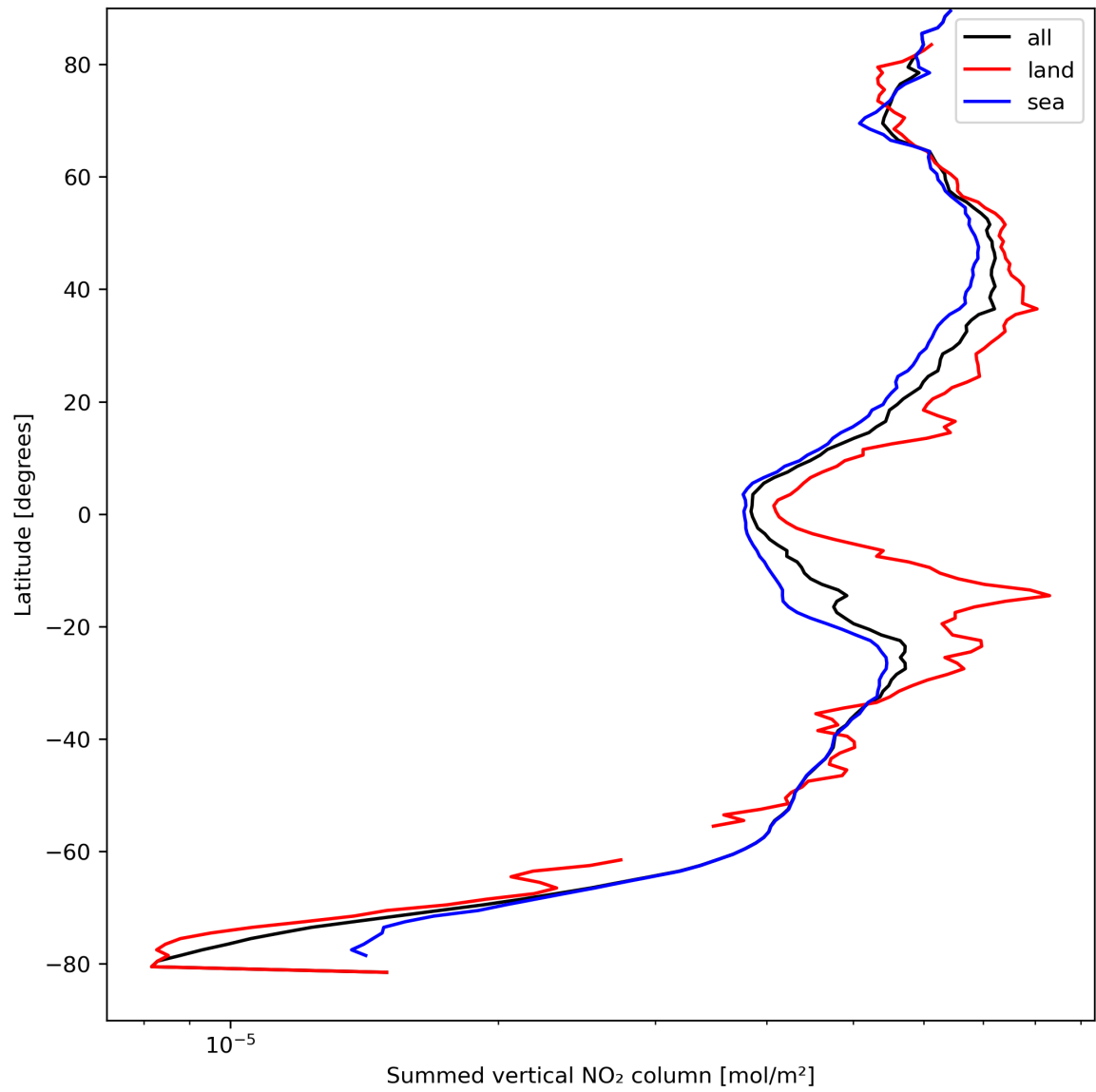
Figure 23: Zonal average of “Summed vertical NO 2 column” for 2023-09-04 to 2023-09-05.
