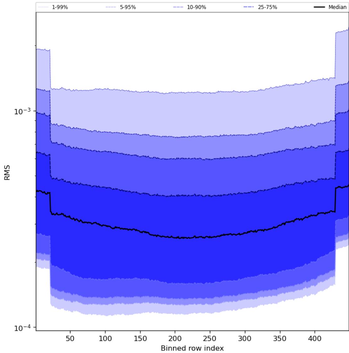
Figure 60: Along track statistics of “RMS” for 2023-09-04 to 2023-09-05
