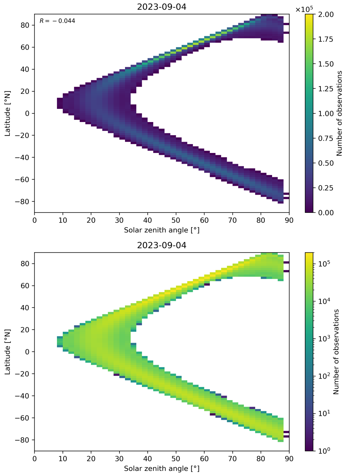
Figure 149: Scatter density plot of “Solar zenith angle” against “Latitude” for 2023-09-04 to 2023-09-05.
