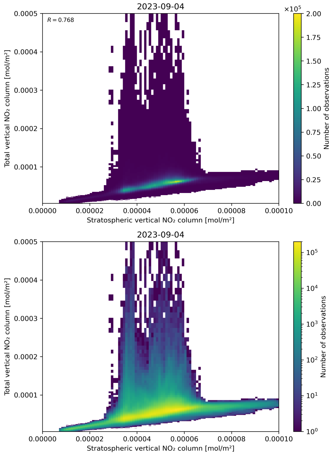
Figure 100: Scatter density plot of “Stratospheric vertical NO 2 column” against “Total vertical NO 2 column” for 2023-09-04 to 2023-09-05.
