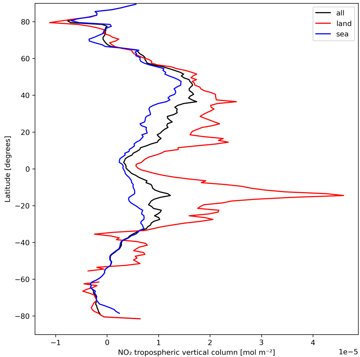
Figure 12: Zonal average of “NO 2 tropospheric vertical column” for 2023-09-04 to 2023-09-05.
