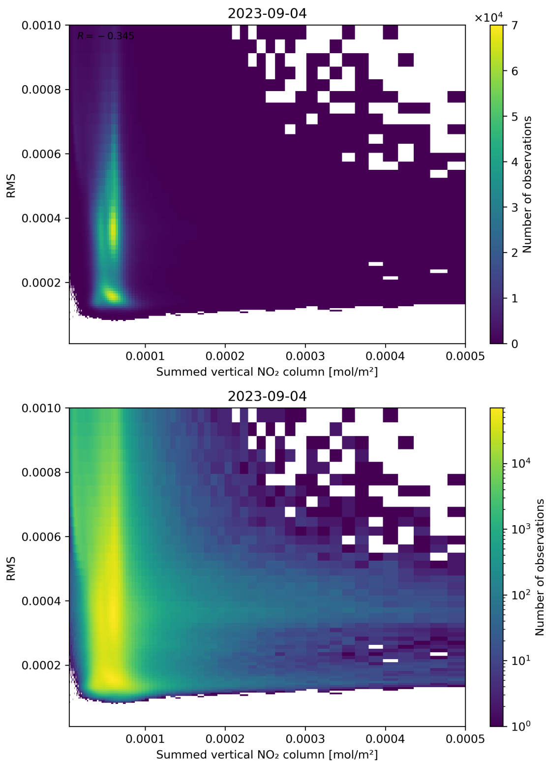
Figure 109: Scatter density plot of “Summed vertical NO 2 column” against “RMS” for 2023-09-04 to 2023-09-05.
