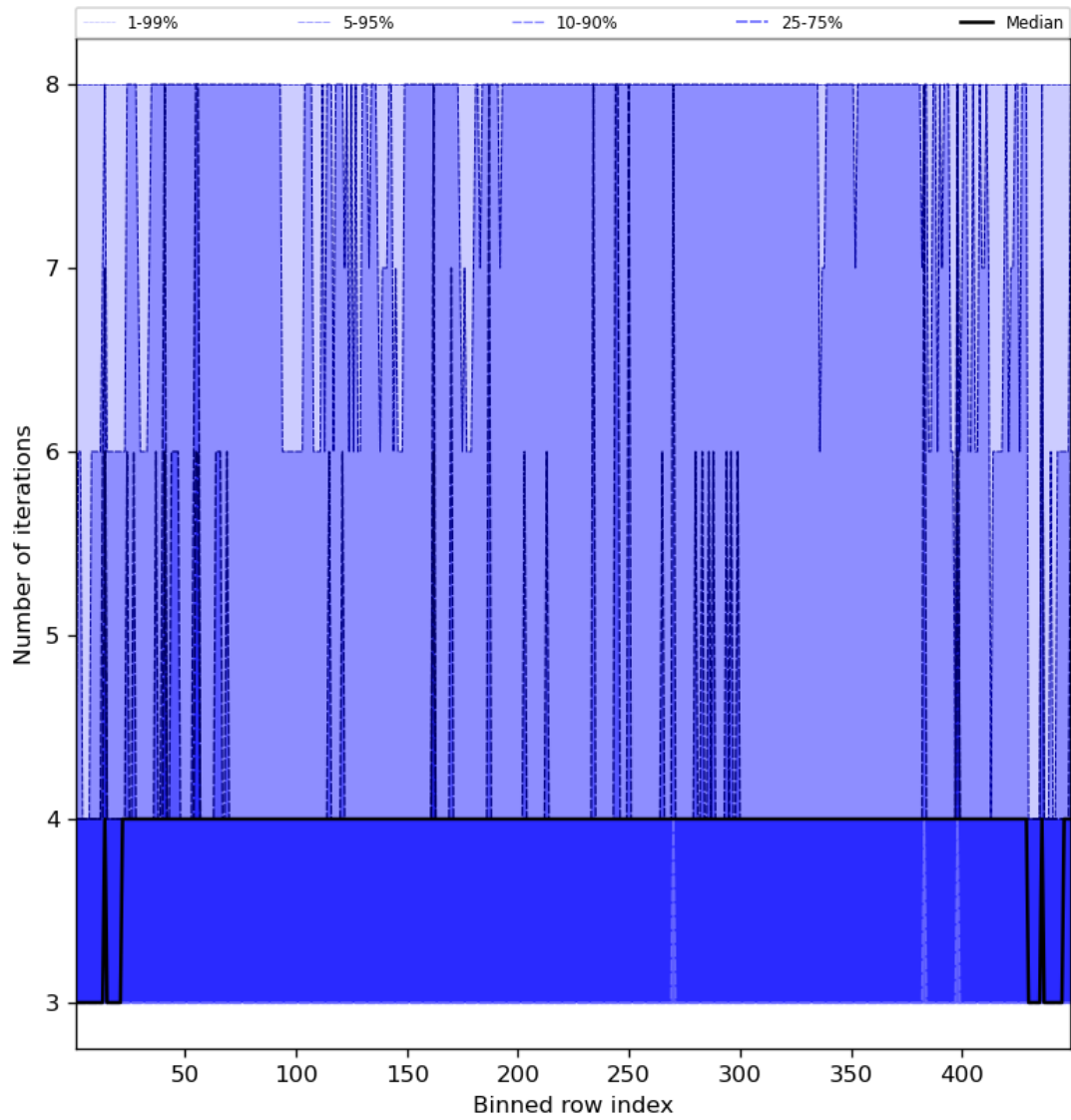
Figure 51: Along track statistics of “Number of iterations” for 2023-09-04 to 2023-09-05
