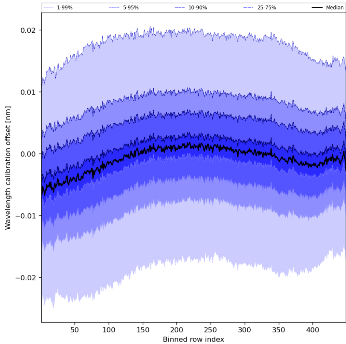
Figure 52: Along track statistics of “Wavelength calibration offset” for 2023-09-04 to 2023-09-05
