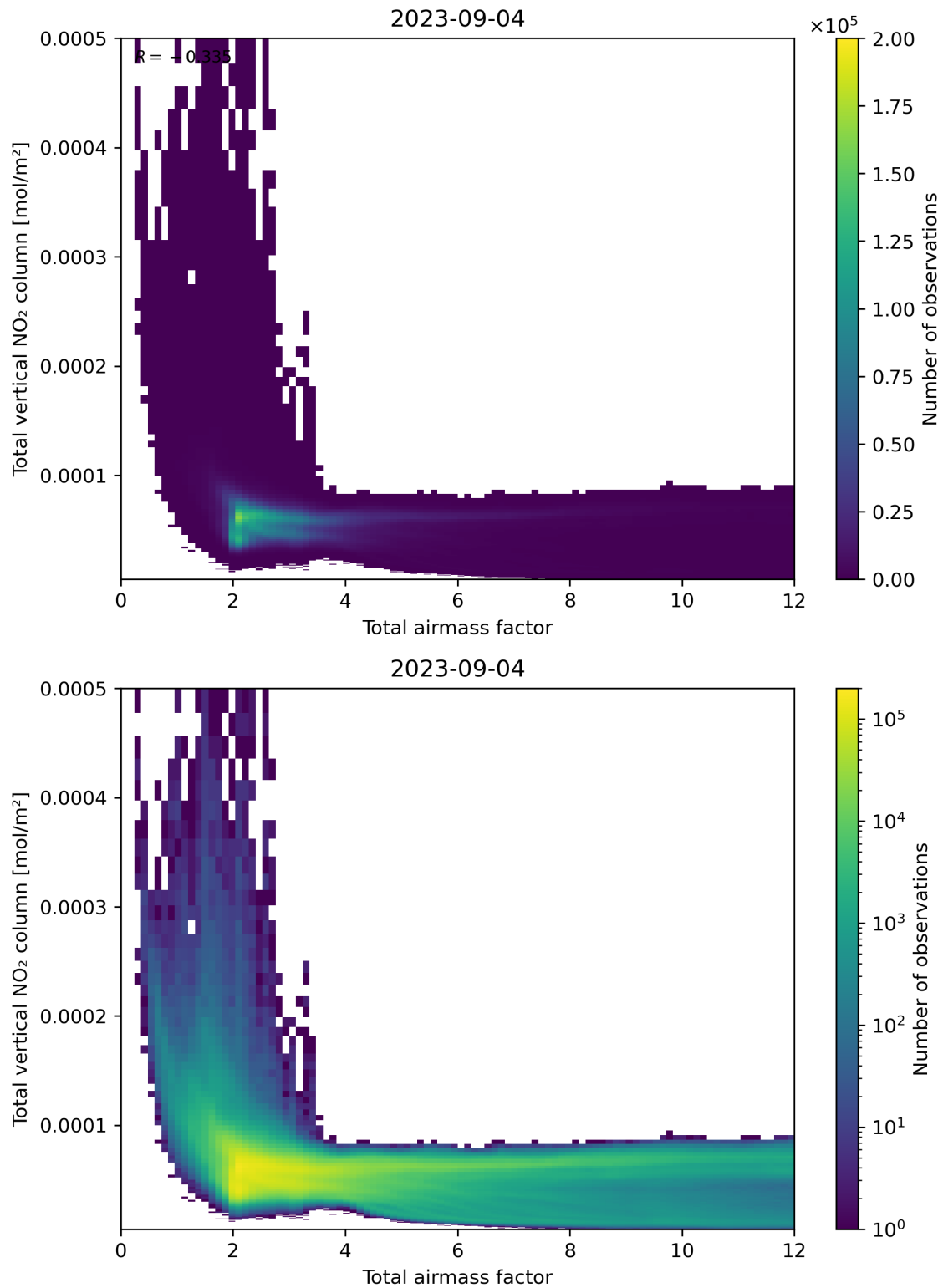
Figure 67: Scatter density plot of “Total airmass factor” against “Total vertical NO 2 column” for 2023-09-04 to 2023-09-05.
