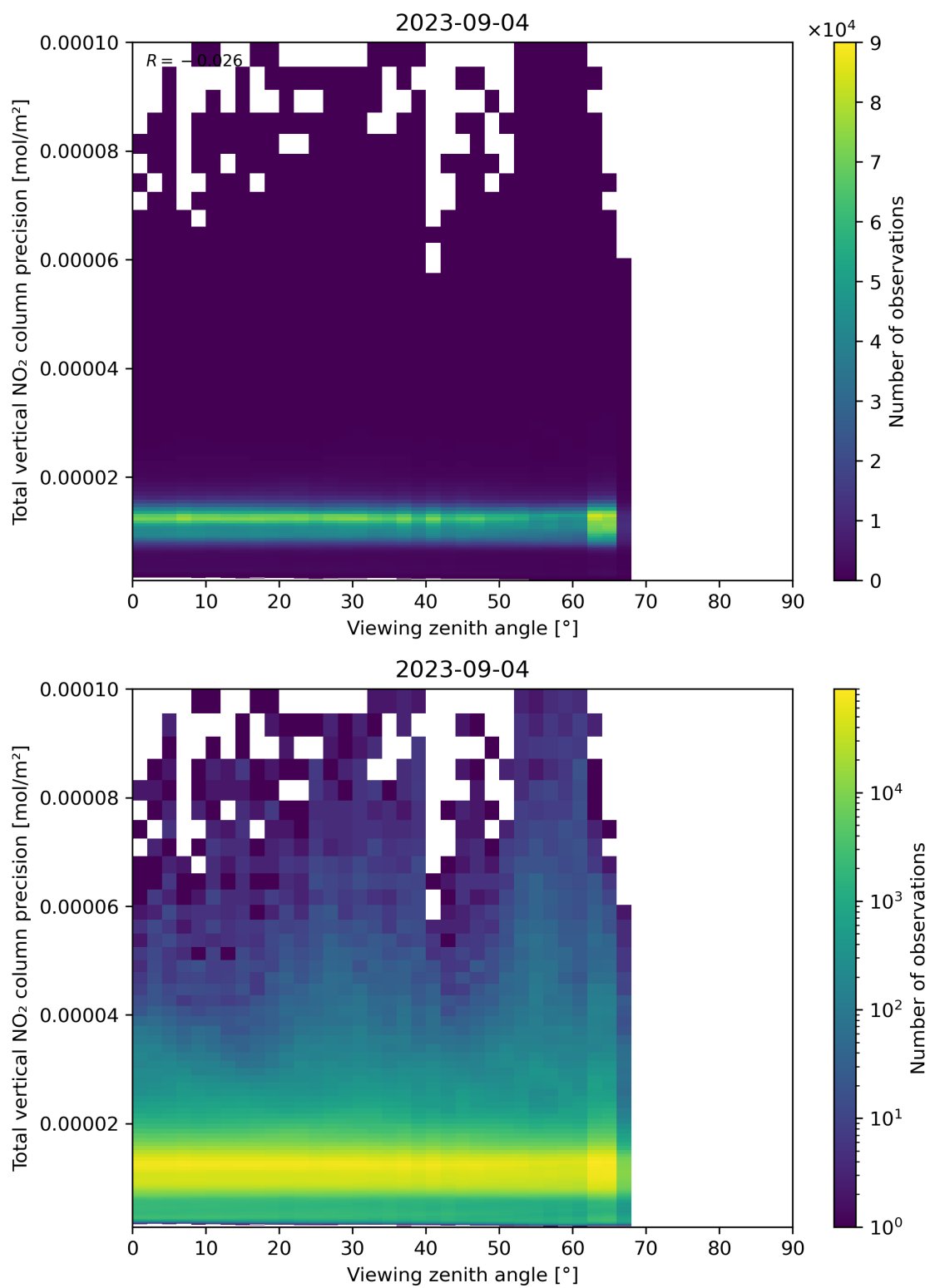
Figure 168: Scatter density plot of “Viewing zenith angle” against “Total vertical NO 2 column precision” for 2023-09-04 to 2023-09-05.
