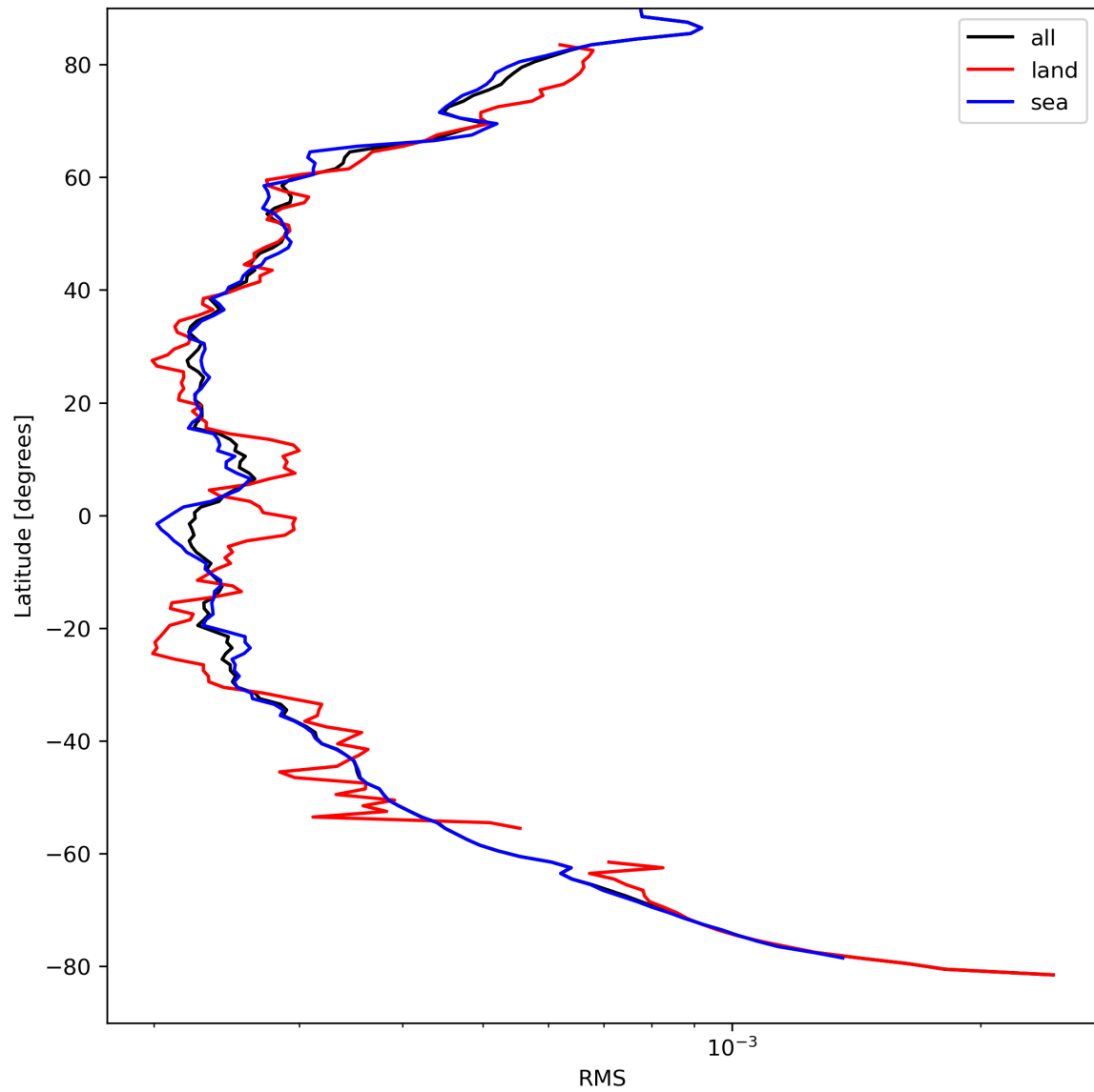
Figure 26: Zonal average of “RMS” for 2023-09-04 to 2023-09-05.
