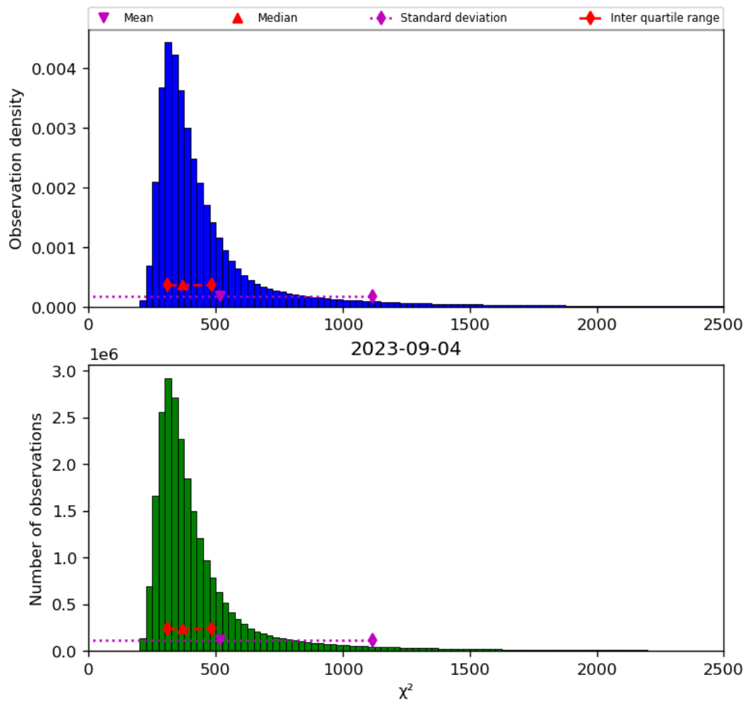
Figure 42: Histogram of “ \chi^2 ” for 2023-09-04 to 2023-09-05
