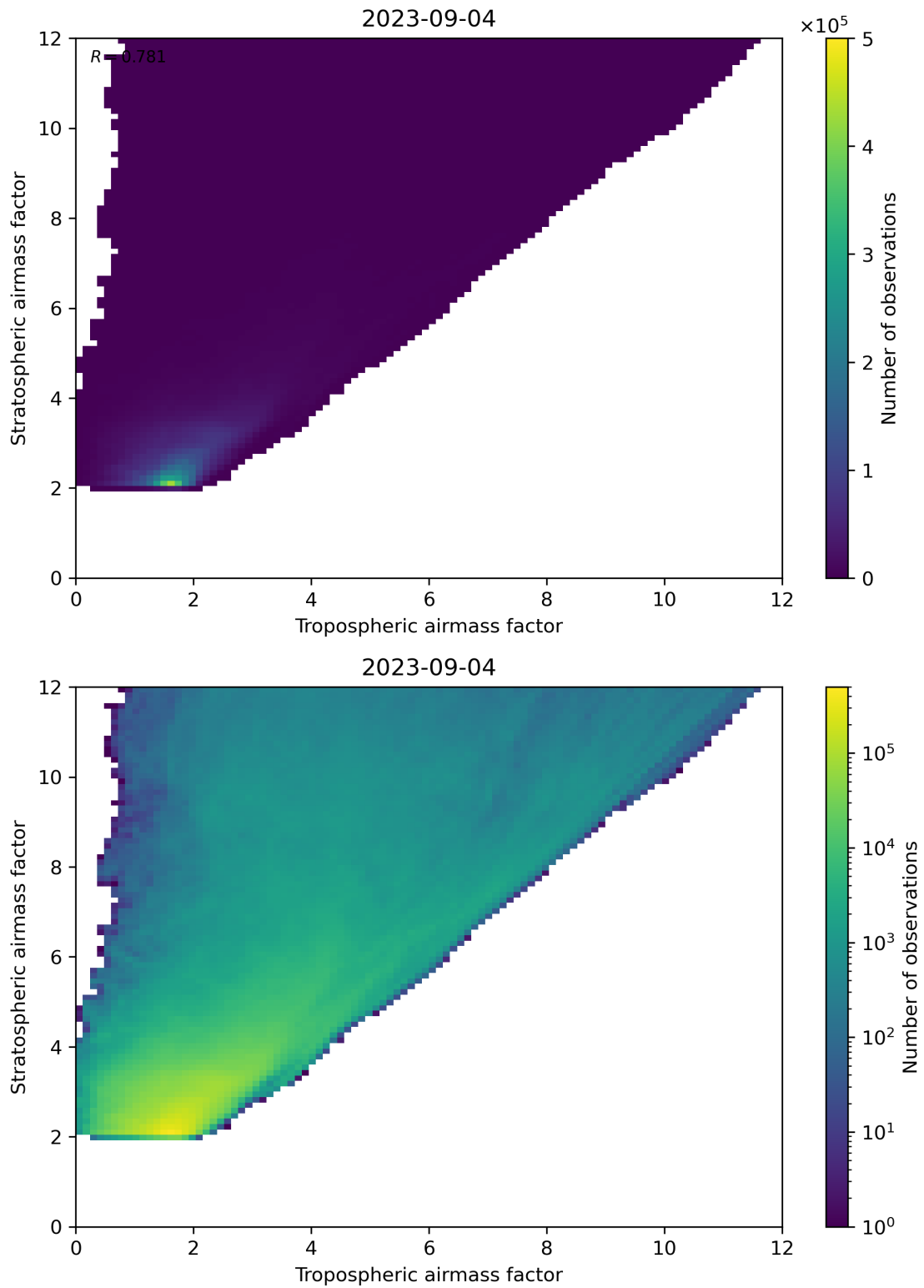
Figure 71: Scatter density plot of “Tropospheric airmass factor” against “Stratospheric airmass factor” for 2023-09-04 to 2023-09-05.
