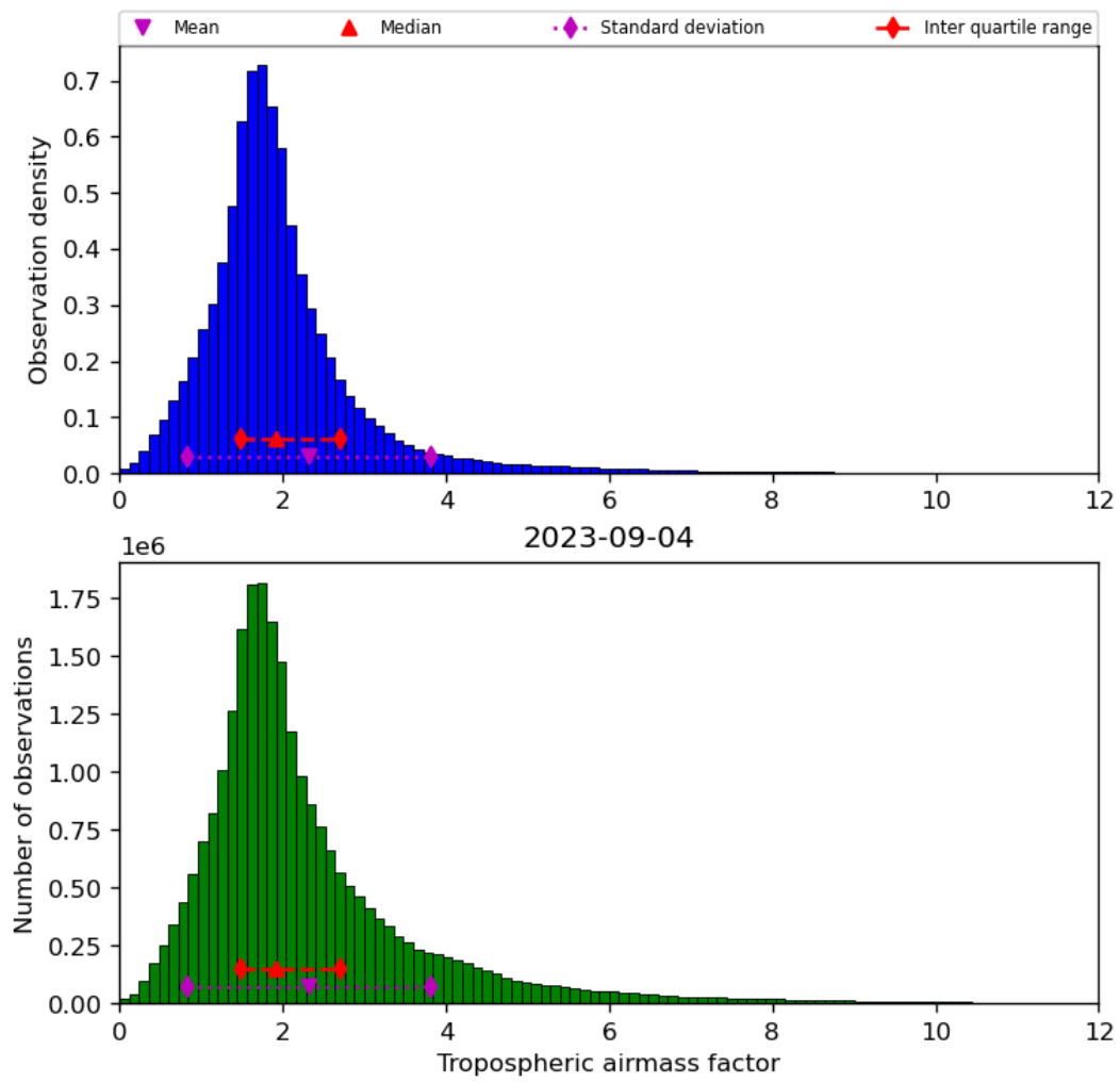
Figure 31: Histogram of “Tropospheric airmass factor” for 2023-09-04 to 2023-09-05
