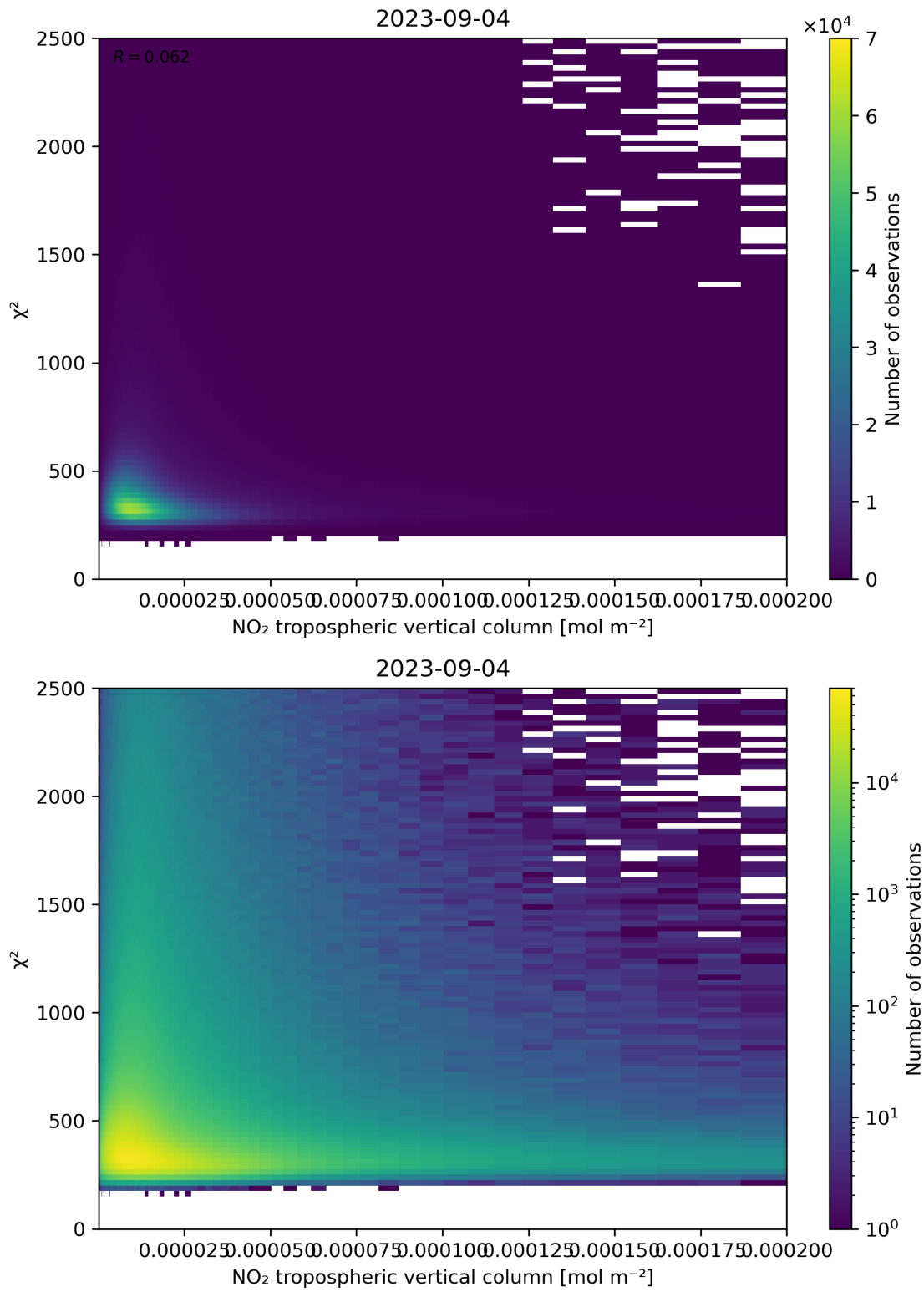
Figure 124: Scatter density plot of “NO 2 tropospheric vertical column” against “ \chi^2 ” for 2023-09-04 to 2023-09-05.
