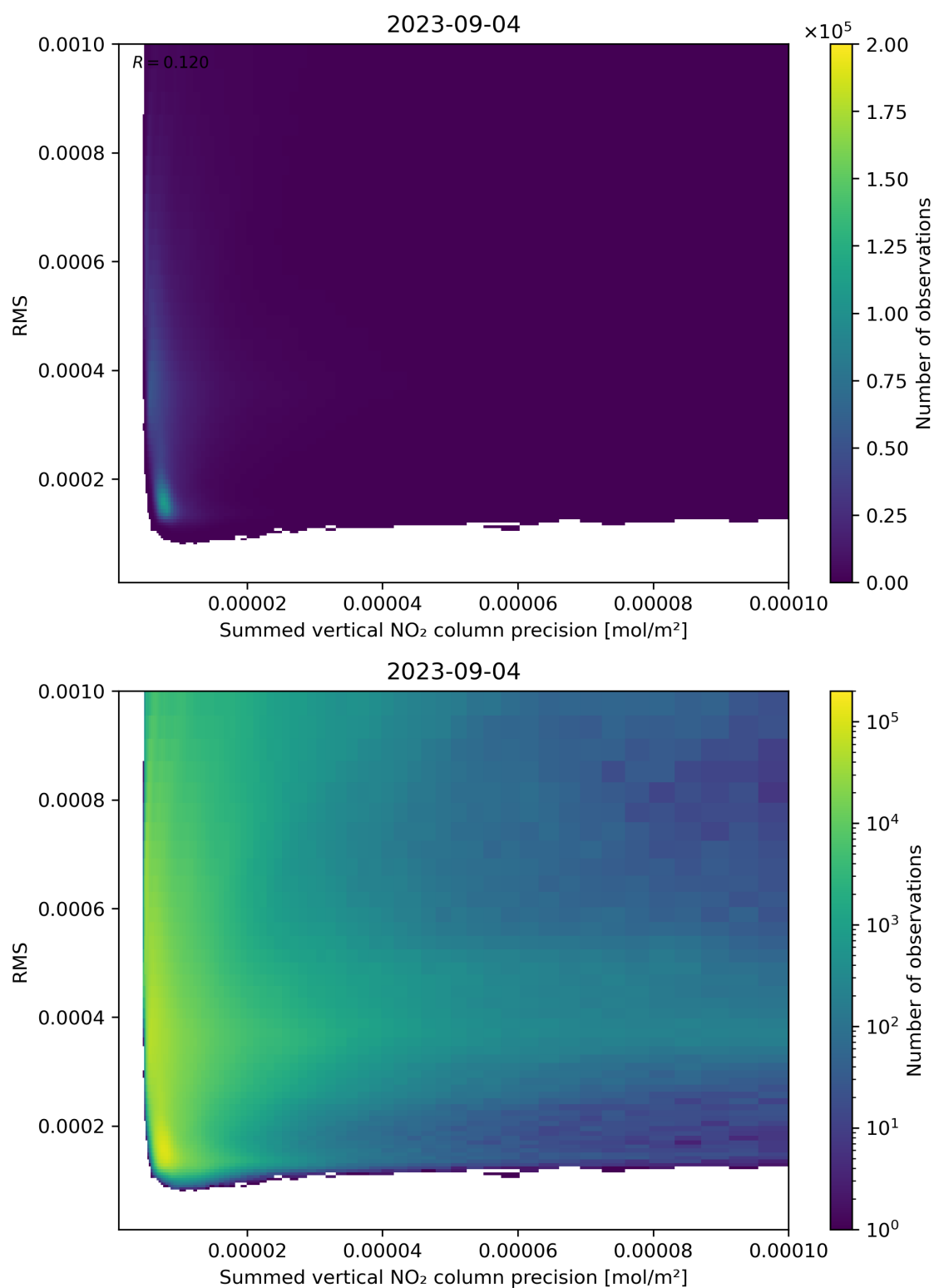
Figure 108: Scatter density plot of “Summed vertical NO 2 column precision” against “RMS” for 2023-09-04 to 2023-09-05.
