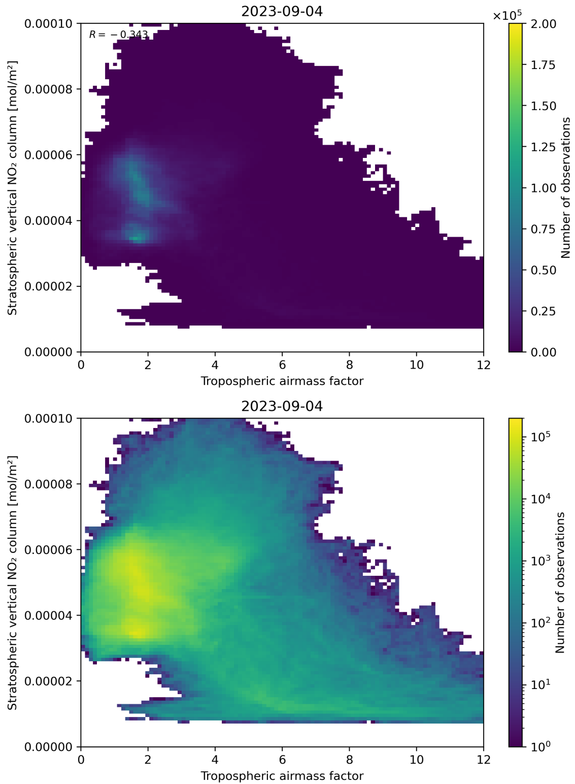
Figure 74: Scatter density plot of “Tropospheric air mass factor” against “Stratospheric vertical NO 2 column” for 2023-09-04 to 2023-09-05.
