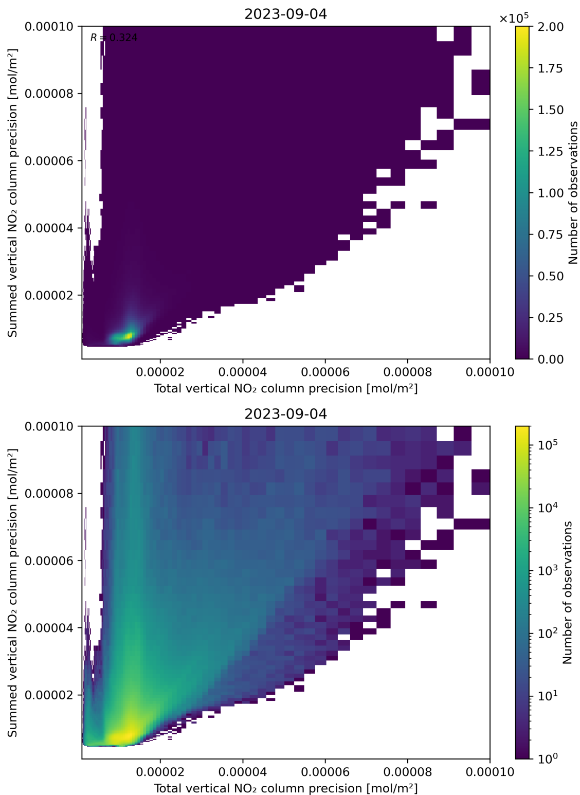
Figure 118: Scatter density plot of “Total vertical NO 2 column precision” against “Summed vertical NO 2 column precision” for 2023-09-04 to 2023-09-05.
