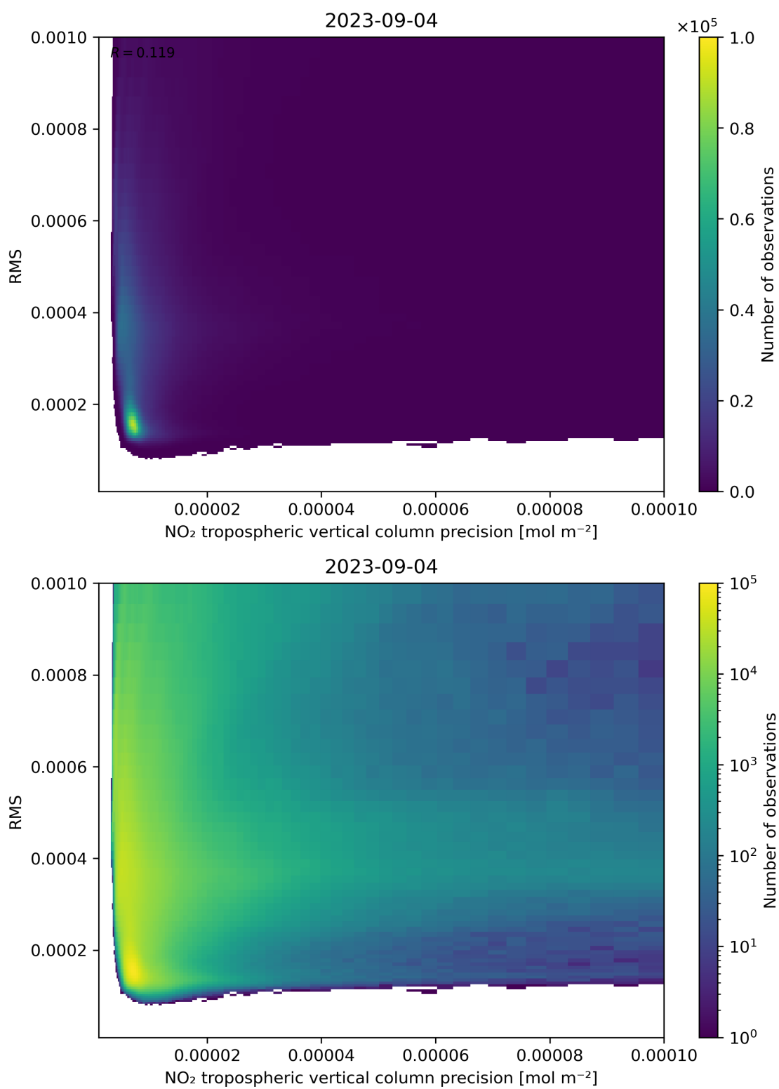
Figure 140: Scatter density plot of “NO 2 tropospheric vertical column precision” against “RMS” for 2023-09-04 to 2023-09-05.
