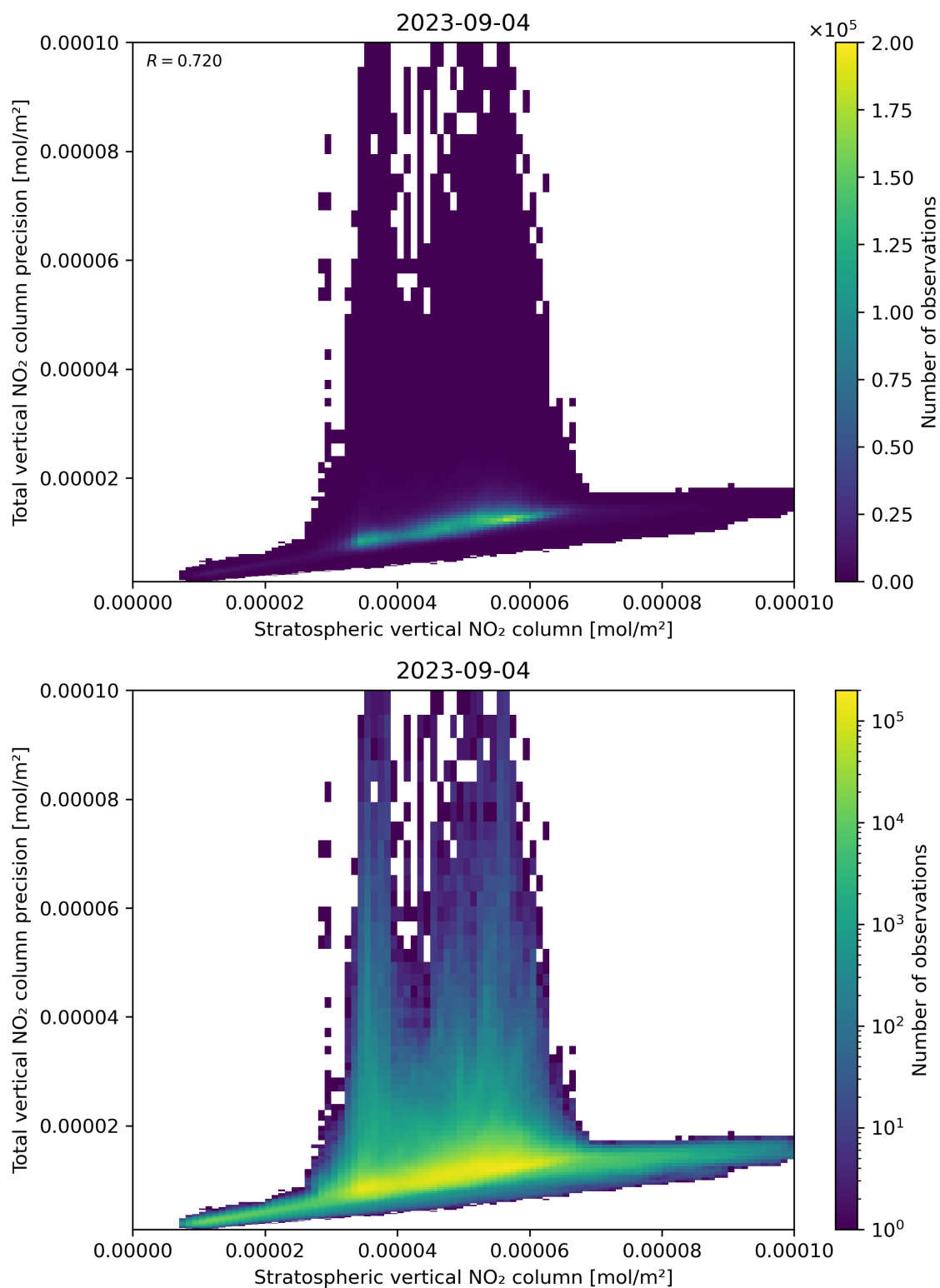
Figure 101: Scatter density plot of “Stratospheric vertical NO 2 column” against “Total vertical NO 2 column precision” for 2023-09-04 to 2023-09-05.
