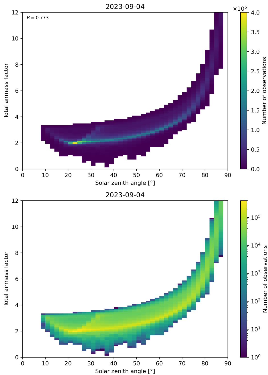
Figure 146: Scatter density plot of “Solar zenith angle” against “Total air mass factor” for 2023-09-04 to 2023-09-05.
