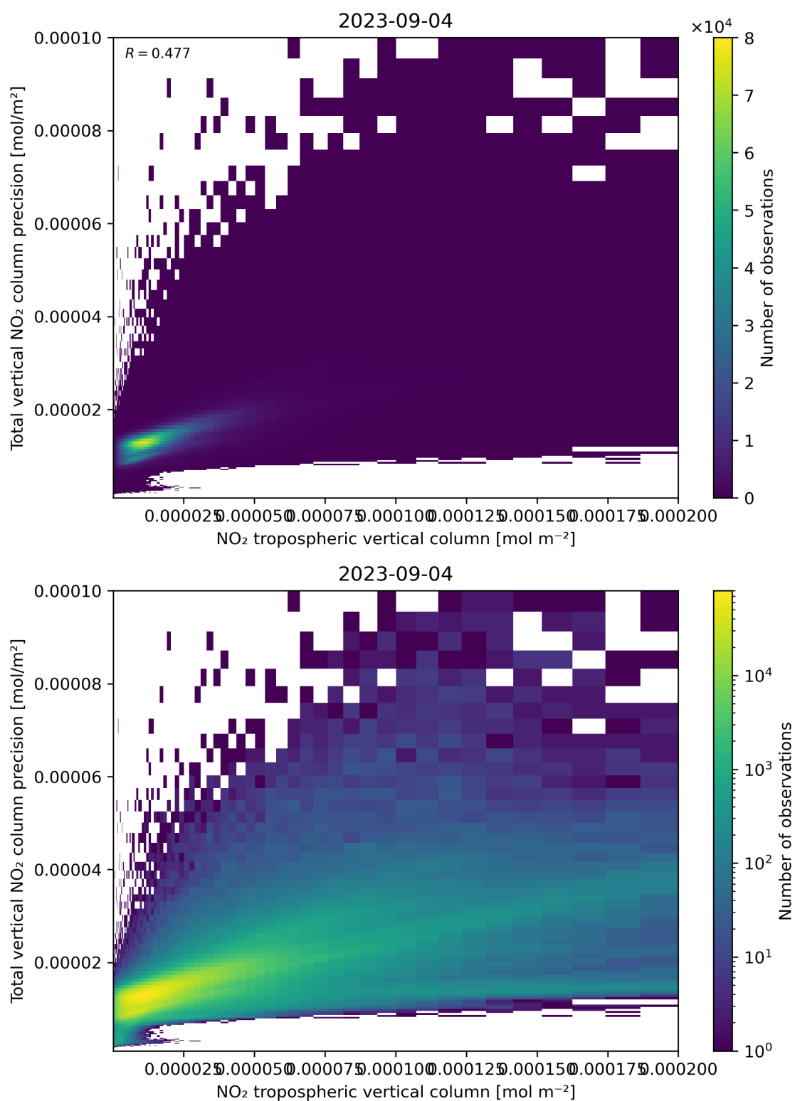
Figure 129: Scatter density plot of “NO 2 tropospheric vertical column” against “Total vertical NO 2 column precision” for 2023-09-04 to 2023-09-05.
