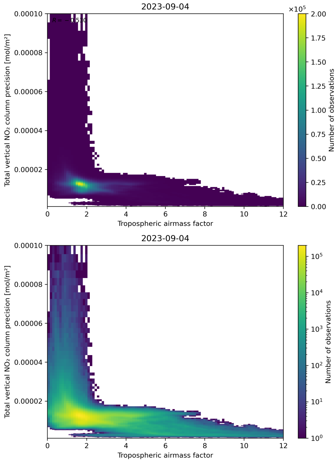
Figure 78: Scatter density plot of “Tropospheric air mass factor” against “Total vertical NO 2 column precision” for 2023-09-04 to 2023-09-05.
