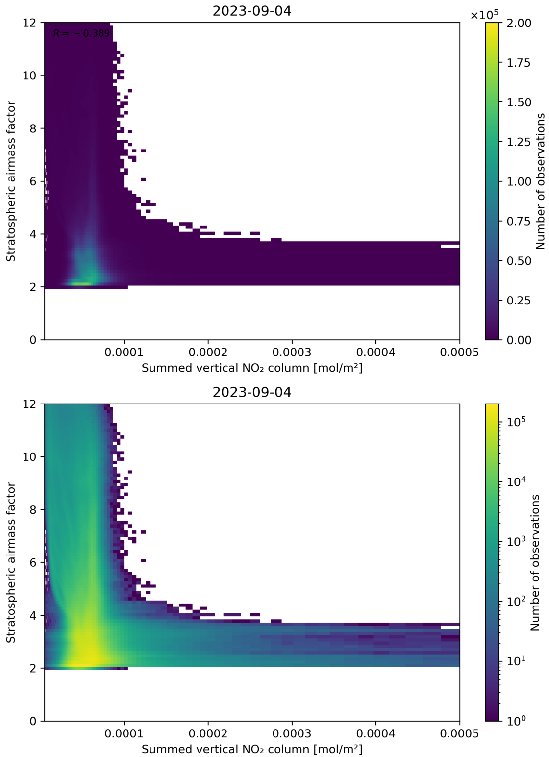
Figure 103: Scatter density plot of “Summed vertical NO 2 column” against “Stratospheric airmass factor” for 2023-09-04 to 2023-09-05.
