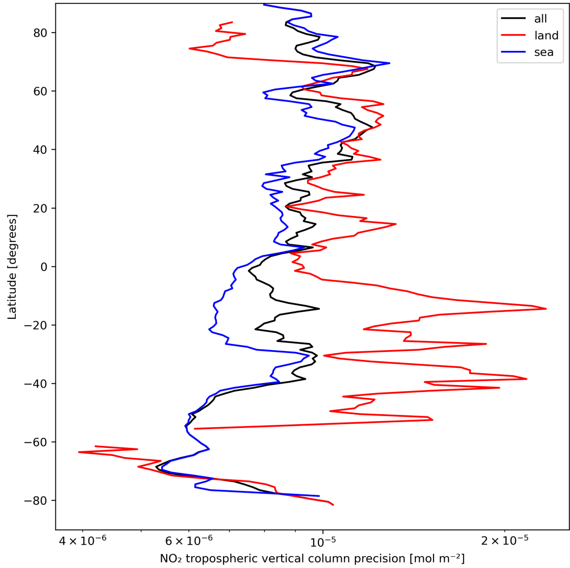
Figure 13: Zonal average of “NO 2 tropospheric vertical column precision” for 2023-09-04 to 2023-09-05.
