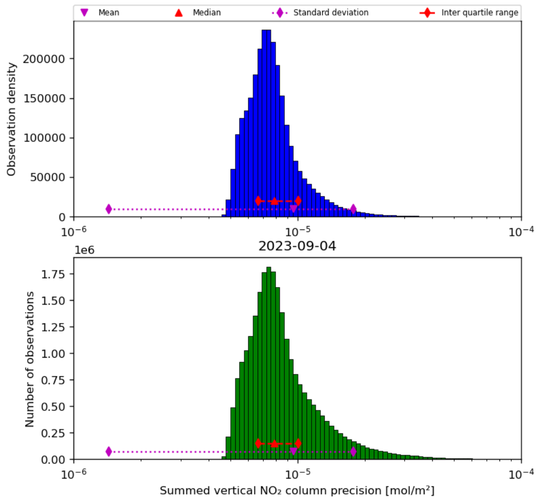
Figure 41: Histogram of “Summed vertical NO 2 column precision” for 2023-09-04 to 2023-09-05
