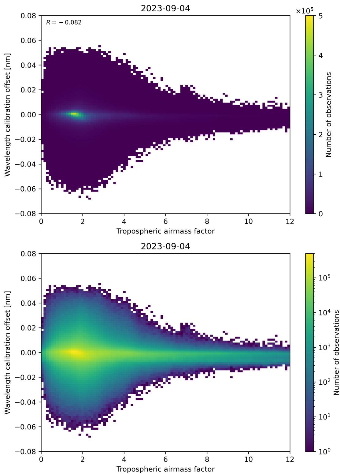
Figure 80: Scatter density plot of “Tropospheric airmass factor” against “Wavelength calibration offset” for 2023-09-04 to 2023-09-05.
