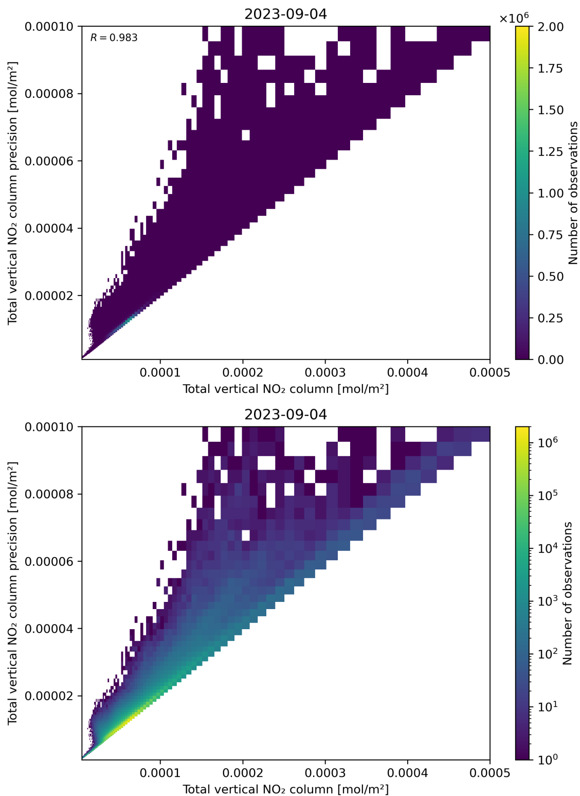
Figure 114: Scatter density plot of “Total vertical NO 2 column” against “Total vertical NO 2 column precision” for 2023-09-04 to 2023-09-05.
