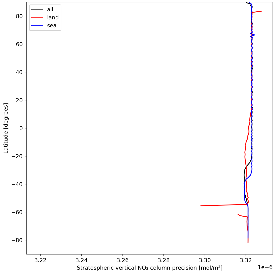
Figure 20: Zonal average of “Stratospheric vertical NO 2 column precision” for 2023-09-04 to 2023-09-05.
