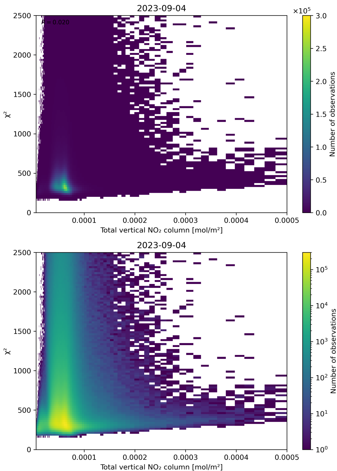
Figure 111: Scatter density plot of “Total vertical NO 2 column” against “ \chi^2 ” for 2023-09-04 to 2023-09-05.
