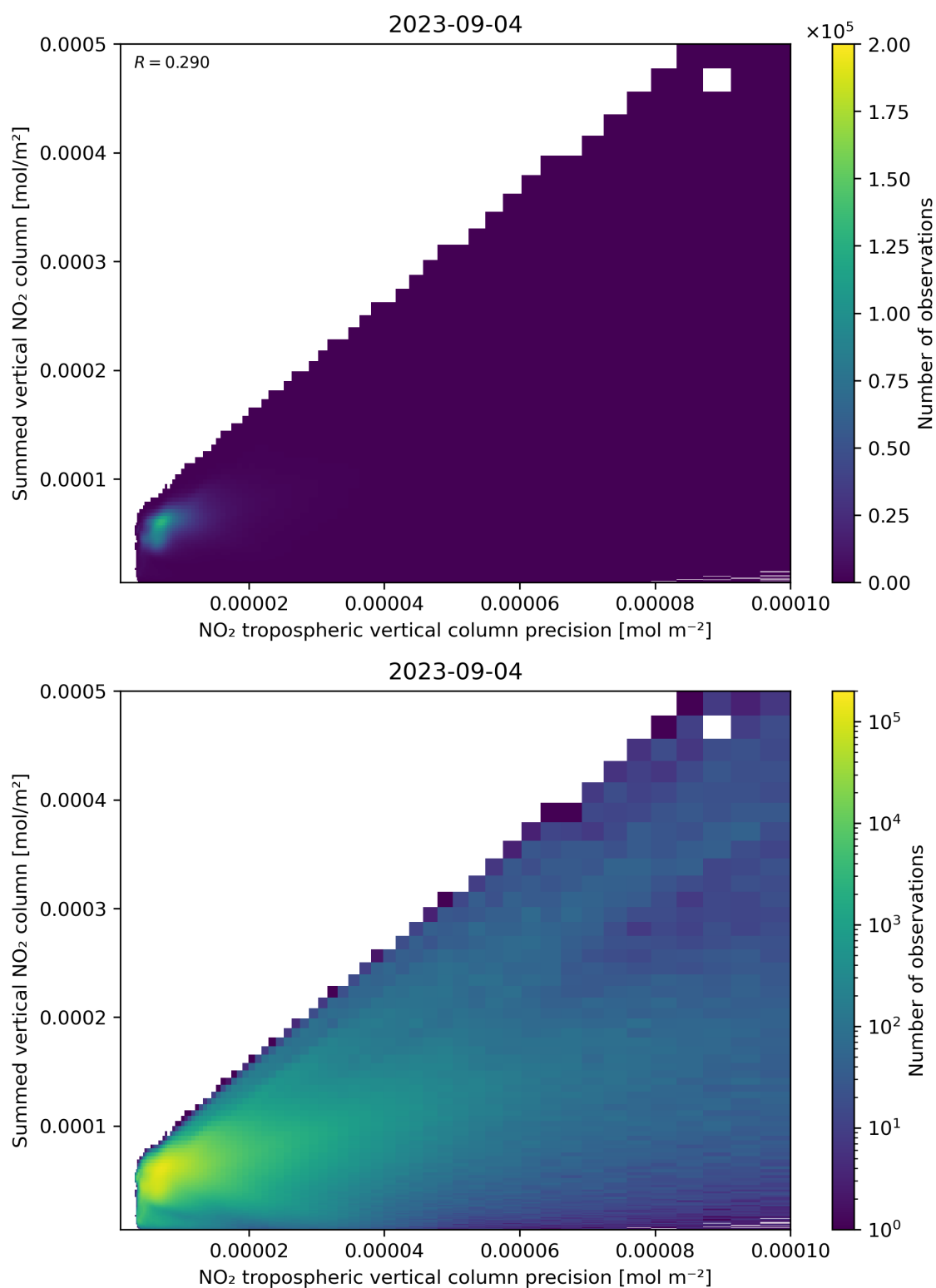
Figure 136: Scatter density plot of “NO 2 tropospheric vertical column precision” against “Summed vertical NO 2 column” for 2023-09-04 to 2023-09-05.
