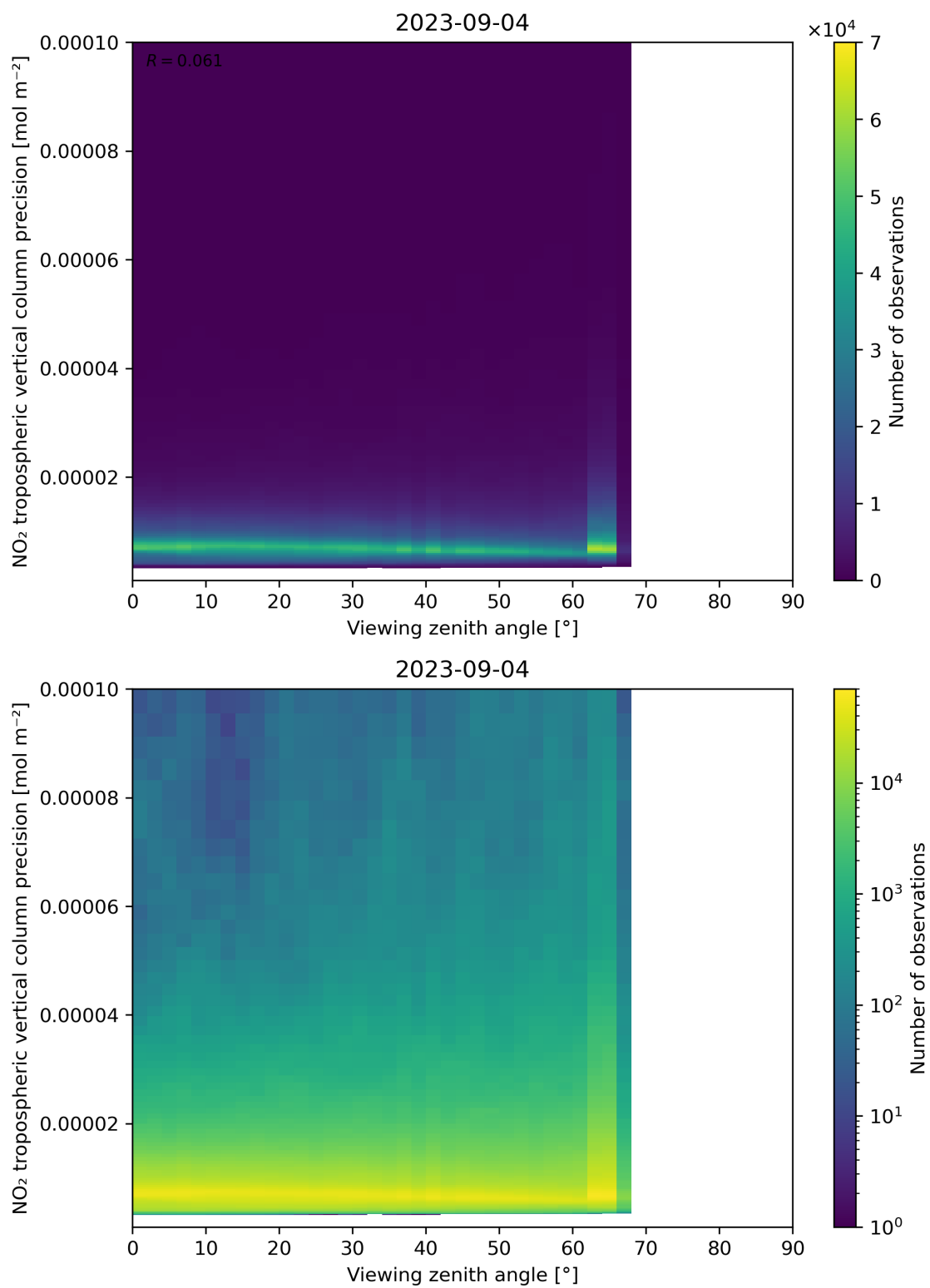
Figure 170: Scatter density plot of “Viewing zenith angle” against “NO 2 tropospheric vertical column precision” for 2023-09-04 to 2023-09-05.
