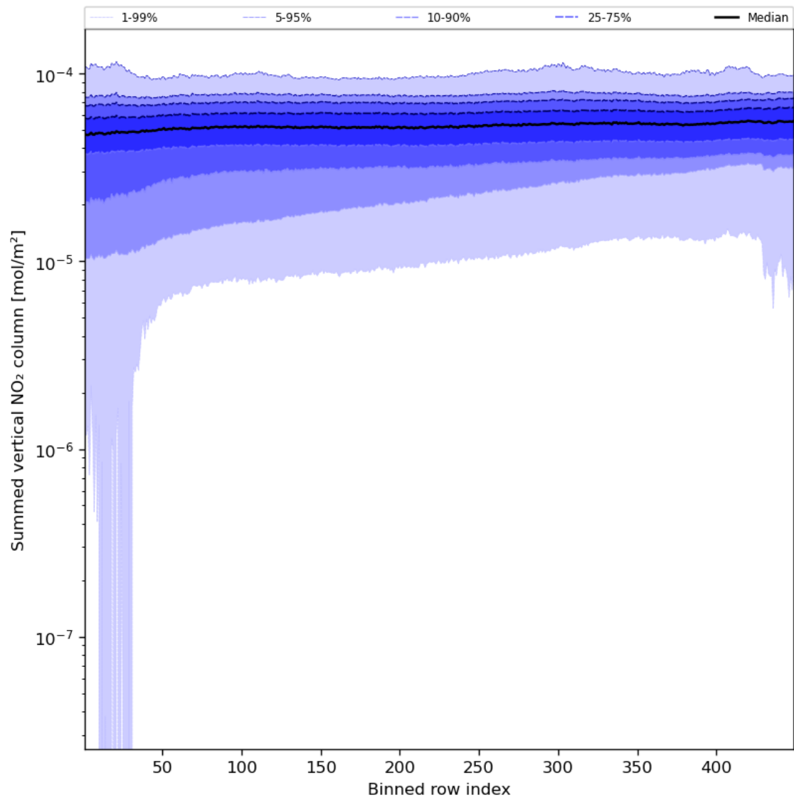
Figure 57: Along track statistics of “Summed vertical NO 2 column” for 2023-09-04 to 2023-09-05
