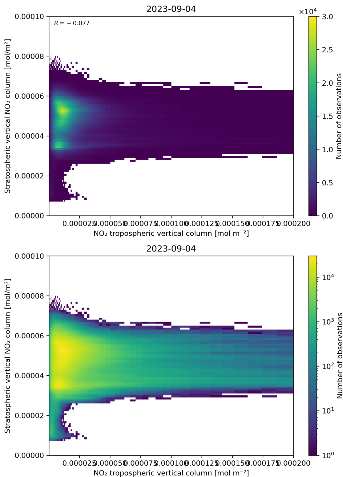
Figure 125: Scatter density plot of “NO 2 tropospheric vertical column” against “Stratospheric vertical NO 2 column” for 2023-09-04 to 2023-09-05.
