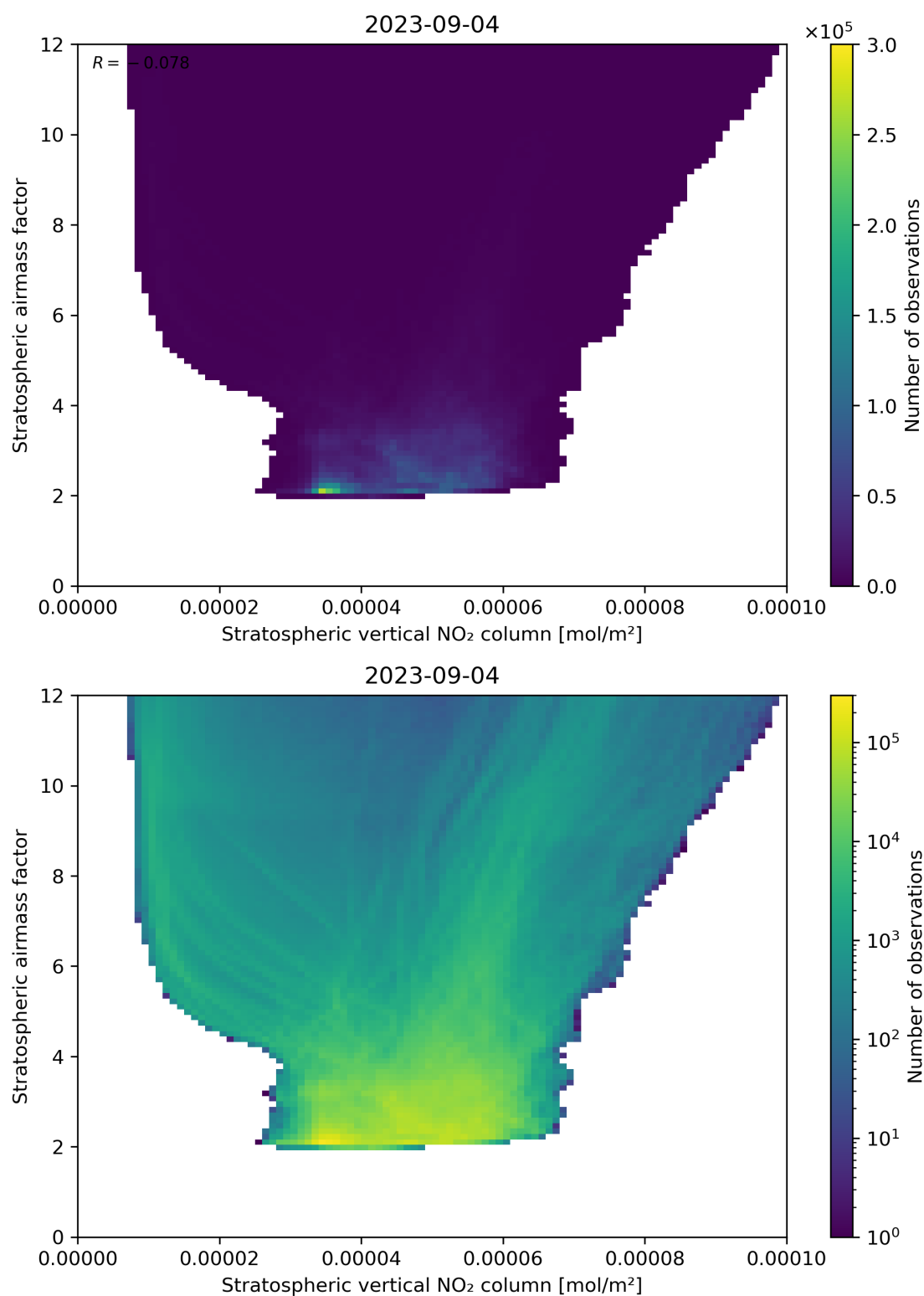
Figure 96: Scatter density plot of “Stratospheric vertical NO 2 column” against “Stratospheric airmass factor” for 2023-09-04 to 2023-09-05.
