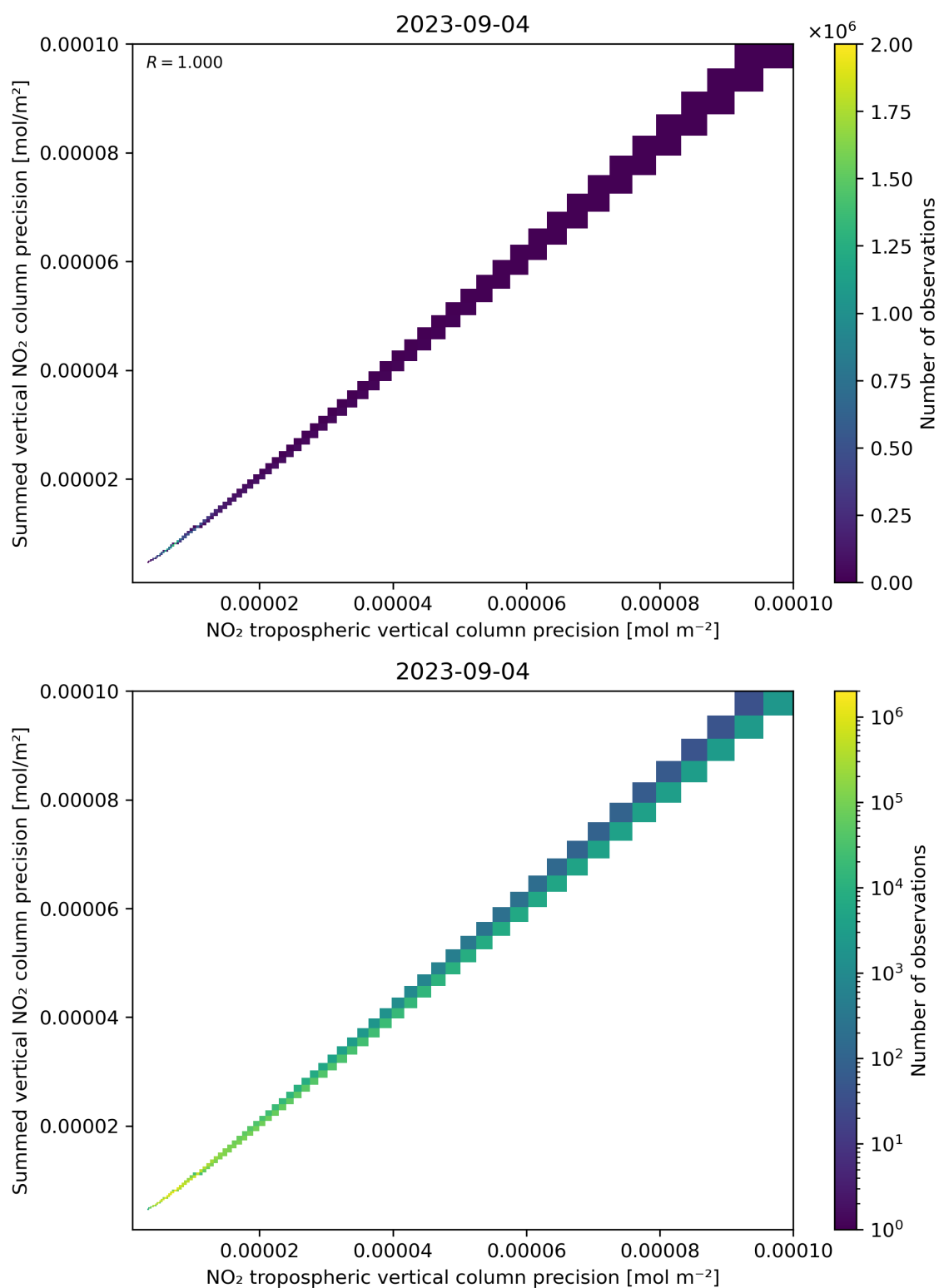
Figure 137: Scatter density plot of “NO 2 tropospheric vertical column precision” against “Summed vertical NO 2 column precision” for 2023-09-04 to 2023-09-05.
