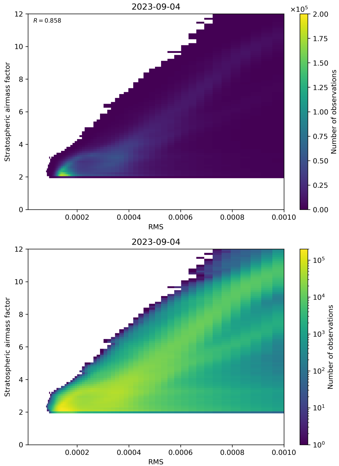
Figure 144: Scatter density plot of “RMS” against “Stratospheric airmass factor” for 2023-09-04 to 2023-09-05.
