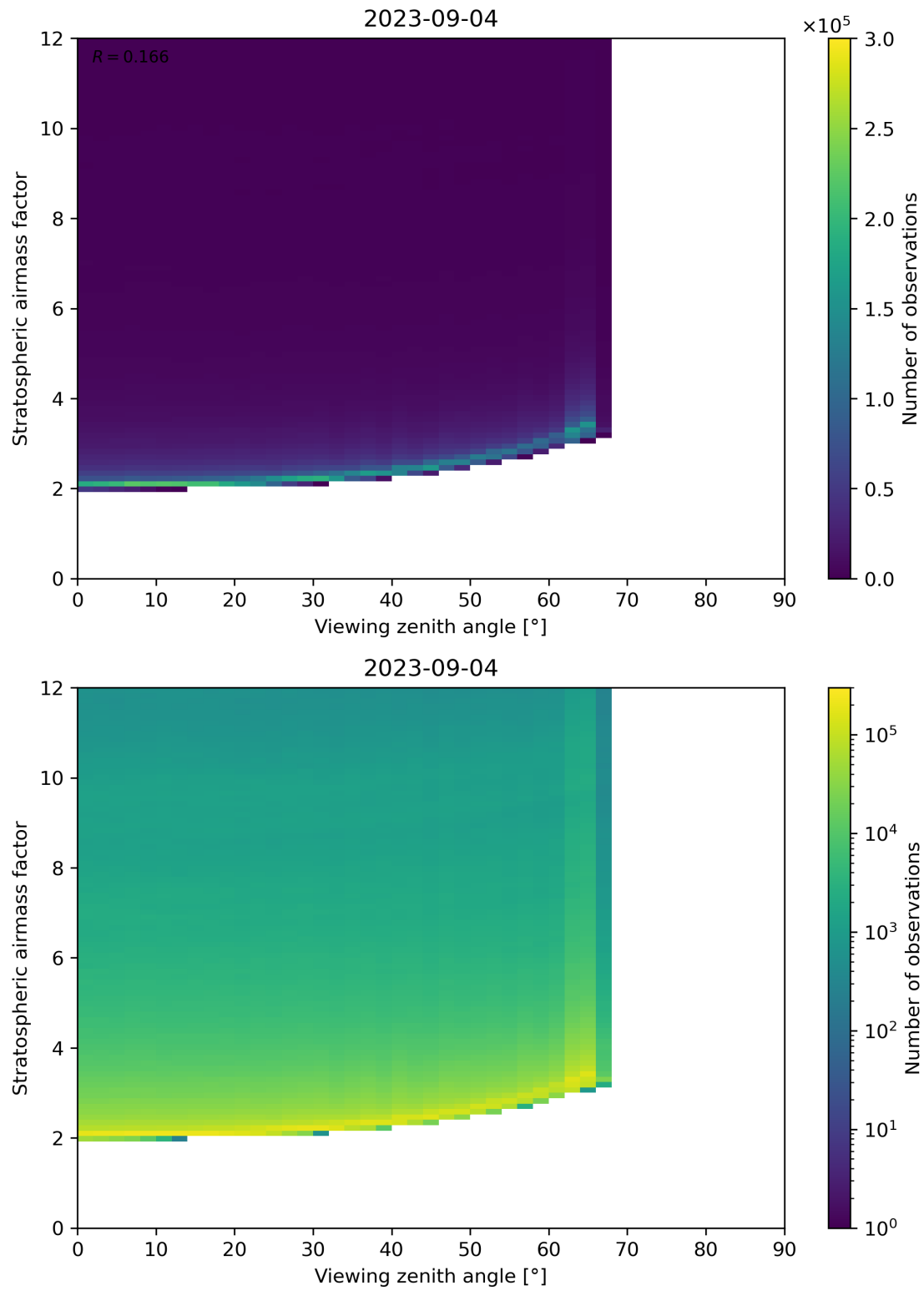
Figure 159: Scatter density plot of “Viewing zenith angle” against “Stratospheric airmass factor” for 2023-09-04 to 2023-09-05.
