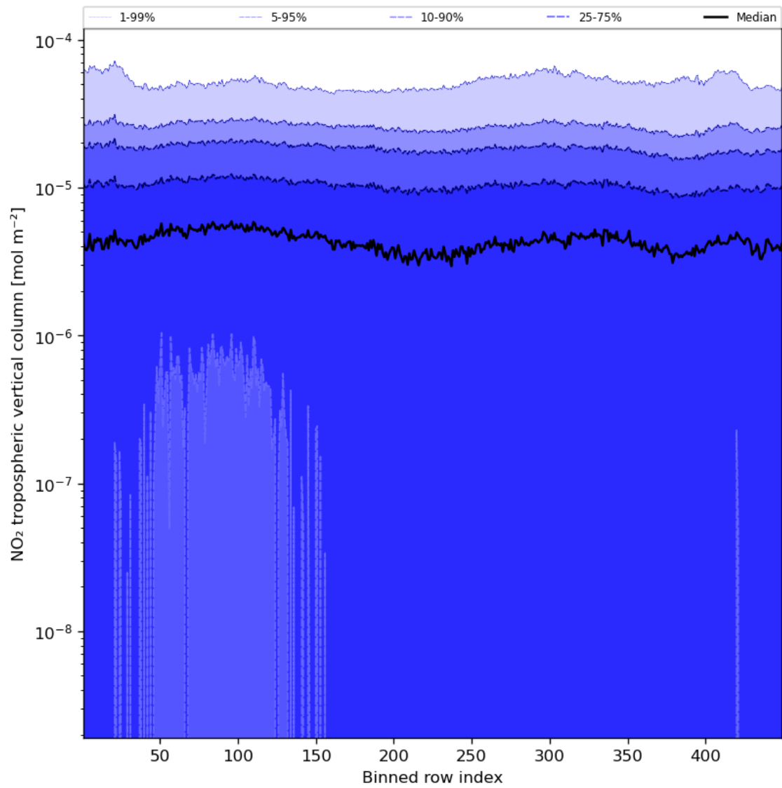
Figure 46: Along track statistics of “NO 2 tropospheric vertical column” for 2023-09-04 to 2023-09-05
