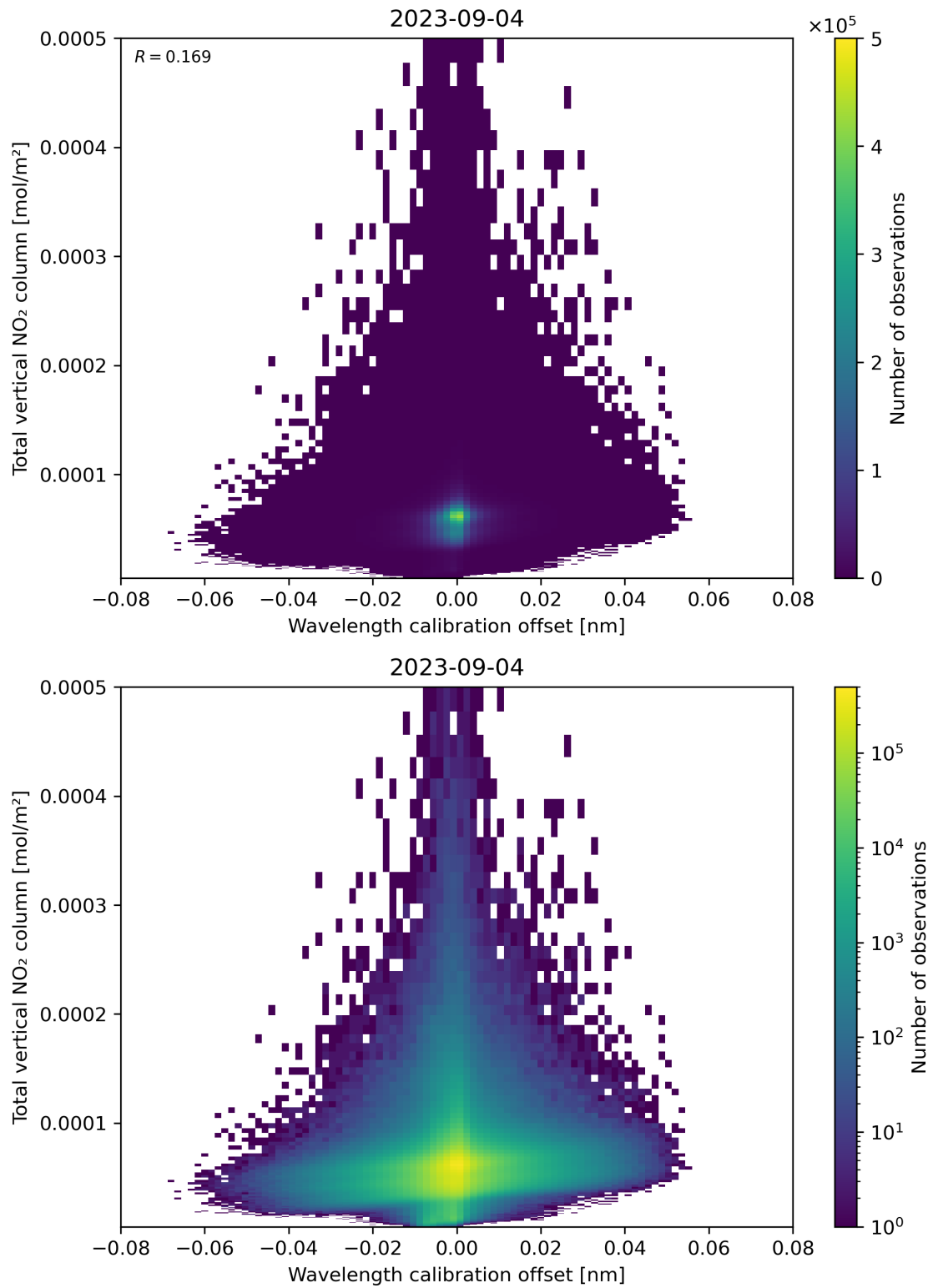
Figure 179: Scatter density plot of “Wavelength calibration offset” against “Total vertical NO 2 column” for 2023-09-04 to 2023-09-05.
