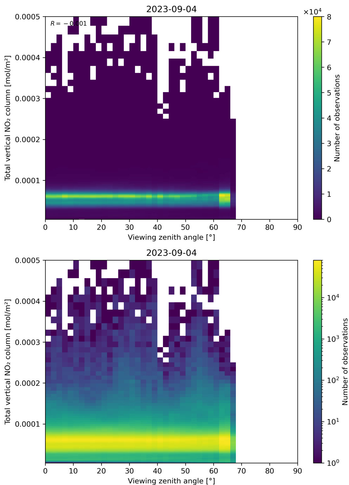
Figure 167: Scatter density plot of “Viewing zenith angle” against “Total vertical NO 2 column” for 2023-09-04 to 2023-09-05.
