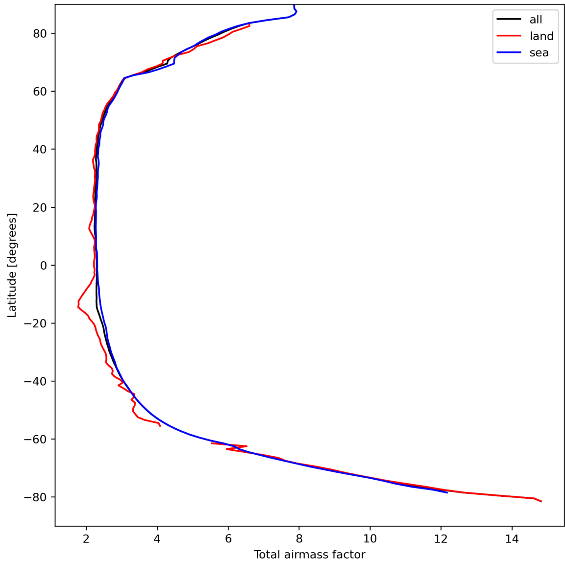
Figure 15: Zonal average of “Total airmass factor” for 2023-09-04 to 2023-09-05.
