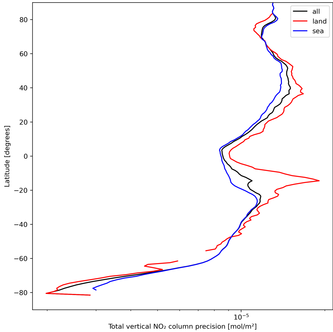
Figure 22: Zonal average of “Total vertical NO 2 column precision” for 2023-09-04 to 2023-09-05.
