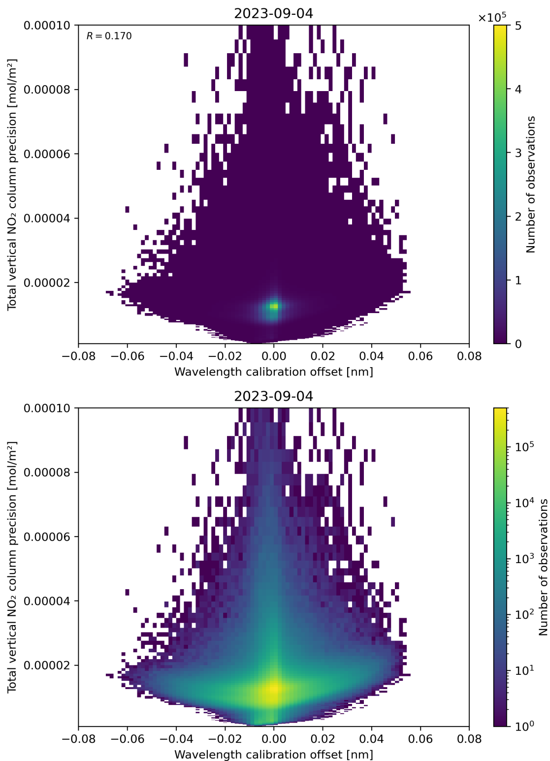
Figure 180: Scatter density plot of “Wavelength calibration offset” against “Total vertical NO 2 column precision” for 2023-09-04 to 2023-09-05.
