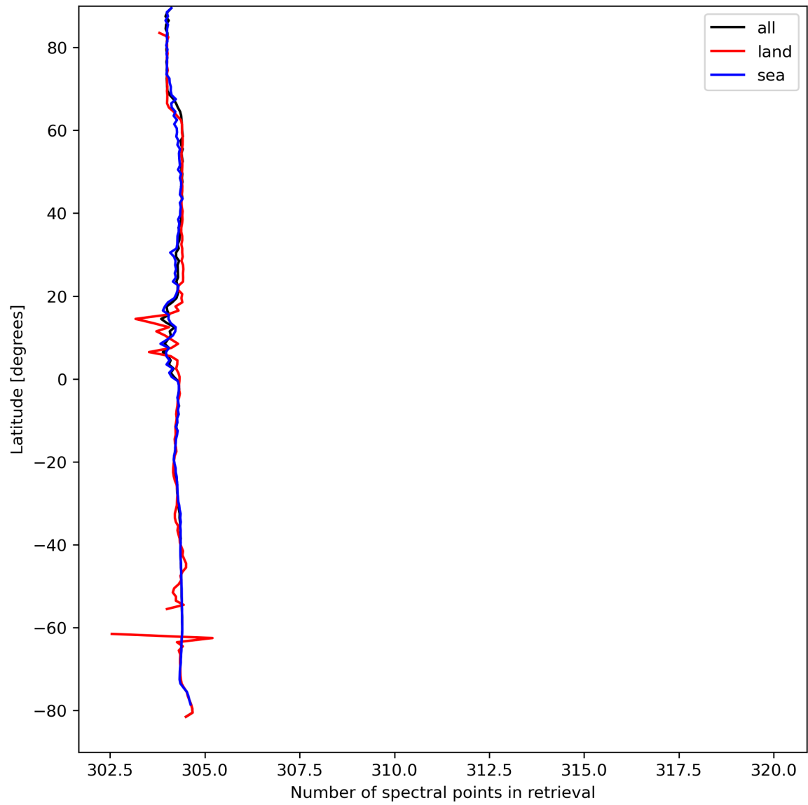
Figure 16: Zonal average of “Number of spectral points in retrieval” for 2023-09-04 to 2023-09-05.
