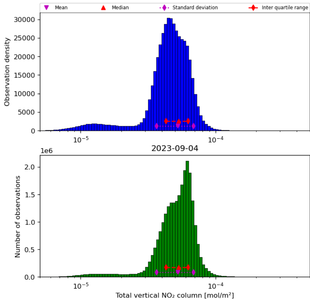
Figure 38: Histogram of “Total vertical NO 2 column” for 2023-09-04 to 2023-09-05
