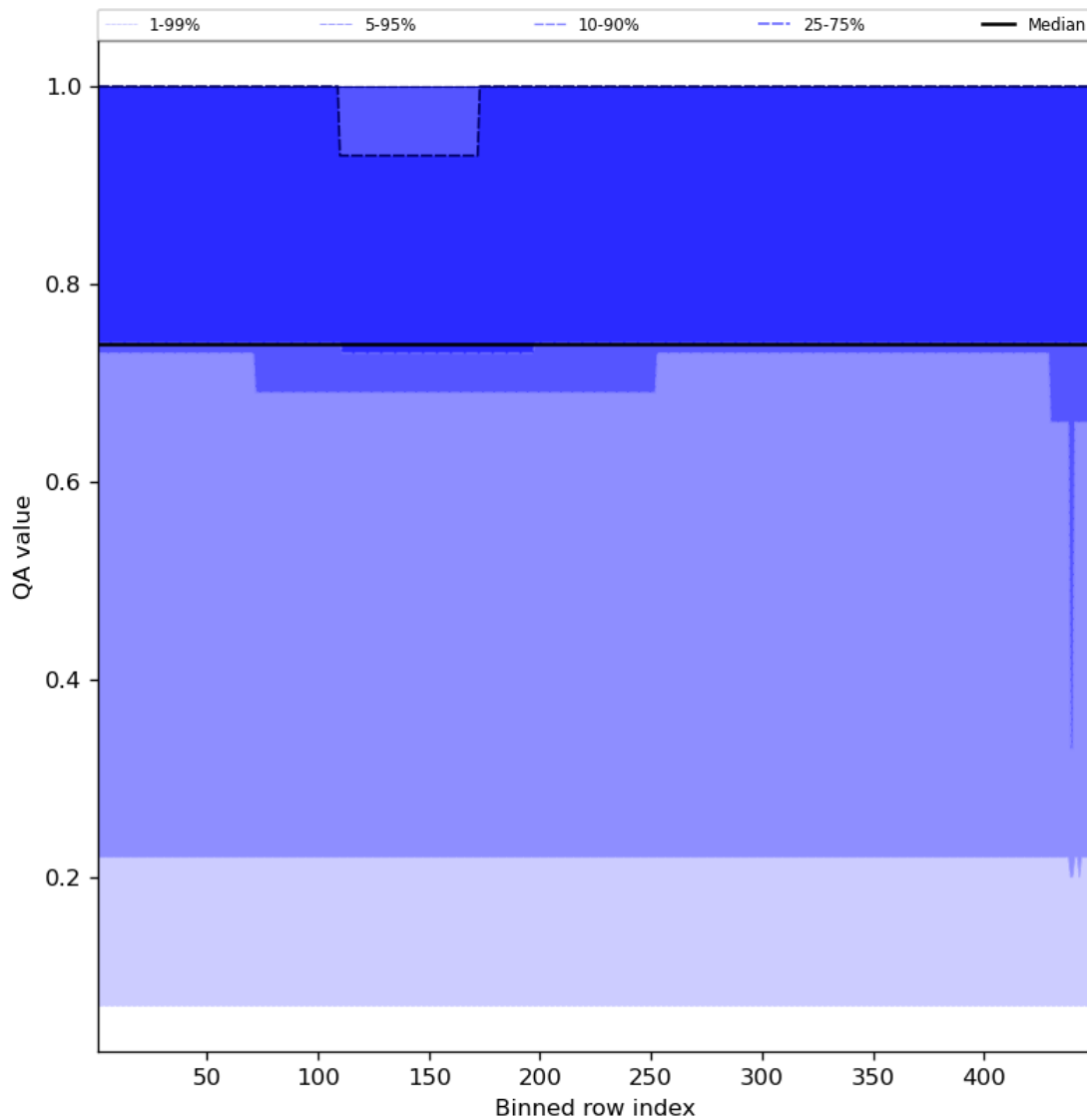
Figure 45: Along track statistics of “QA value” for 2023-09-04 to 2023-09-05
