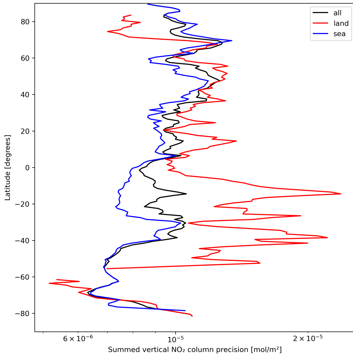
Figure 24: Zonal average of “Summed vertical NO 2 column precision” for 2023-09-04 to 2023-09-05.
