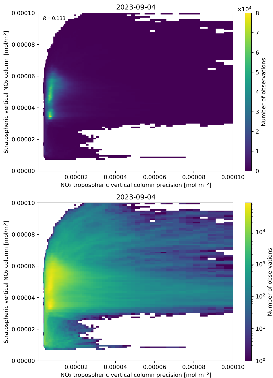
Figure 135: Scatter density plot of “NO 2 tropospheric vertical column precision” against “Stratospheric vertical NO 2 column” for 2023-09-04 to 2023-09-05.
