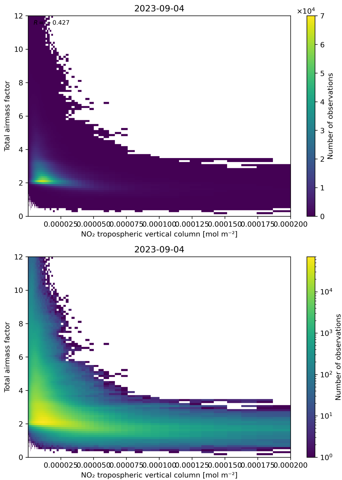
Figure 122: Scatter density plot of “NO 2 tropospheric vertical column” against “Total airmass factor” for 2023-09-04 to 2023-09-05.
