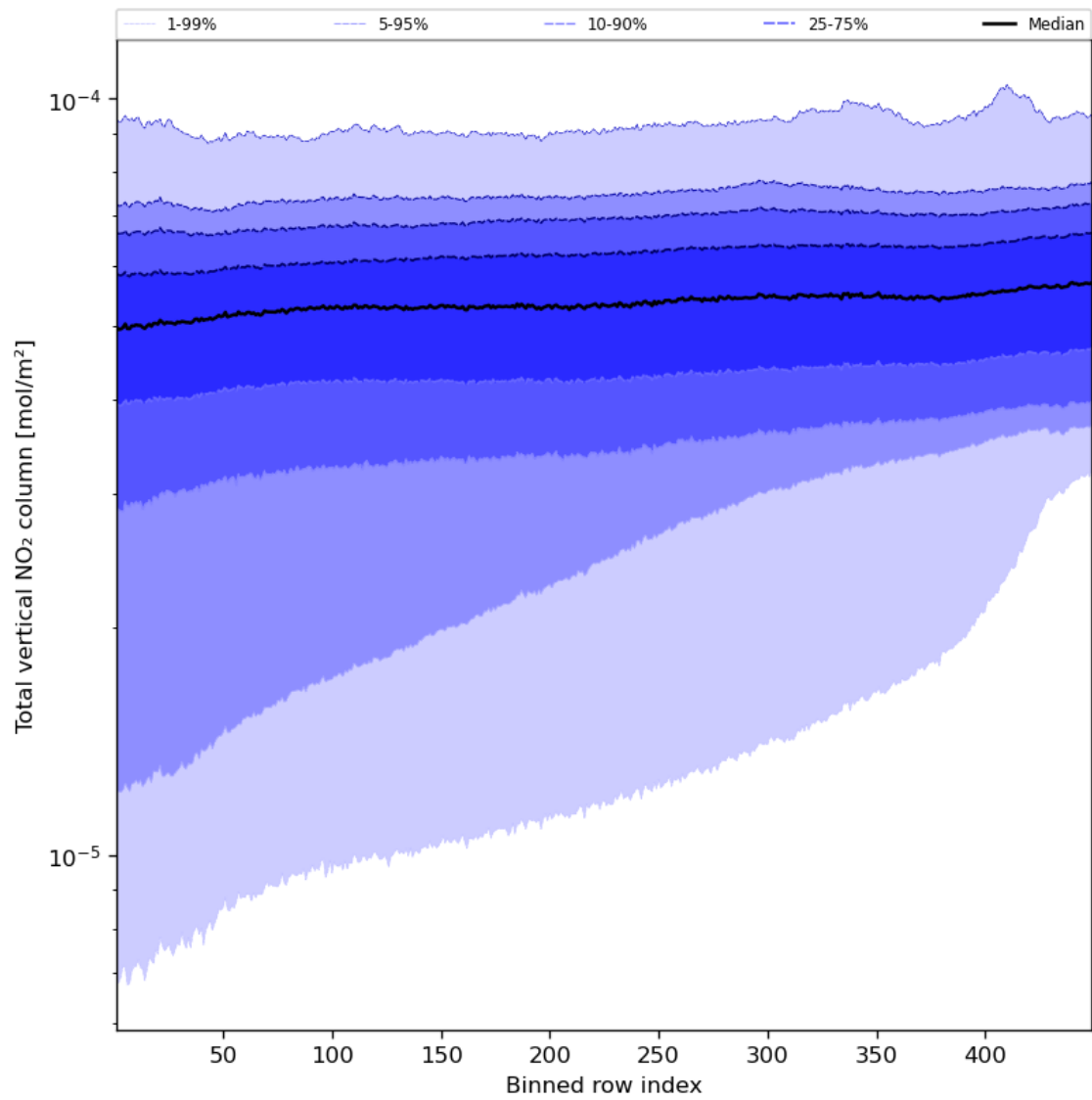
Figure 55: Along track statistics of “Total vertical NO 2 column” for 2023-09-04 to 2023-09-05
