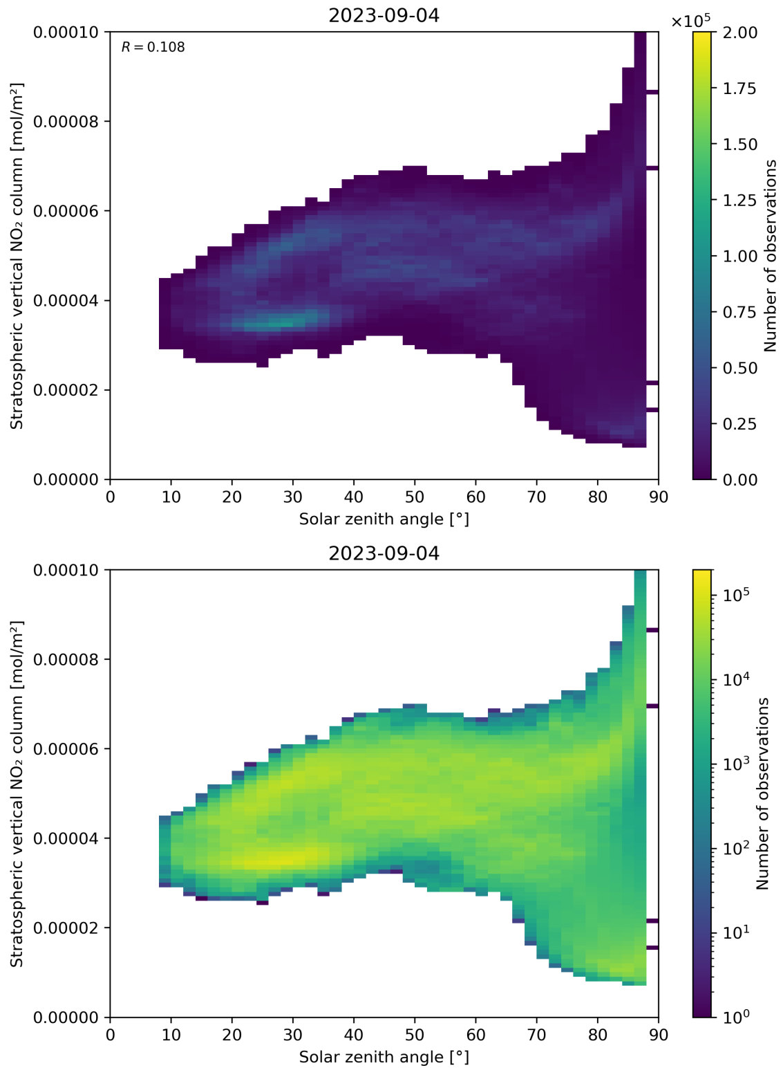
Figure 150: Scatter density plot of “Solar zenith angle” against “Stratospheric vertical NO 2 column” for 2023-09-04 to 2023-09-05.
