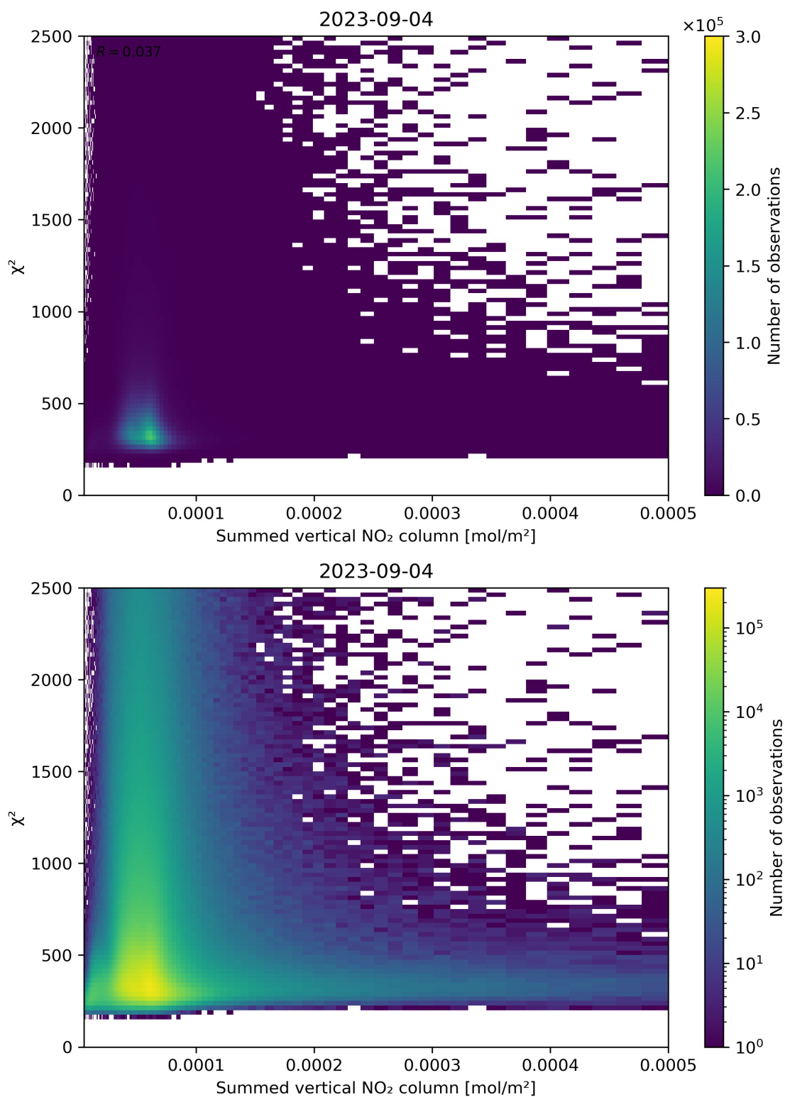
Figure 104: Scatter density plot of “Summed vertical NO 2 column” against “ \chi^2 ” for 2023-09-04 to 2023-09-05.
