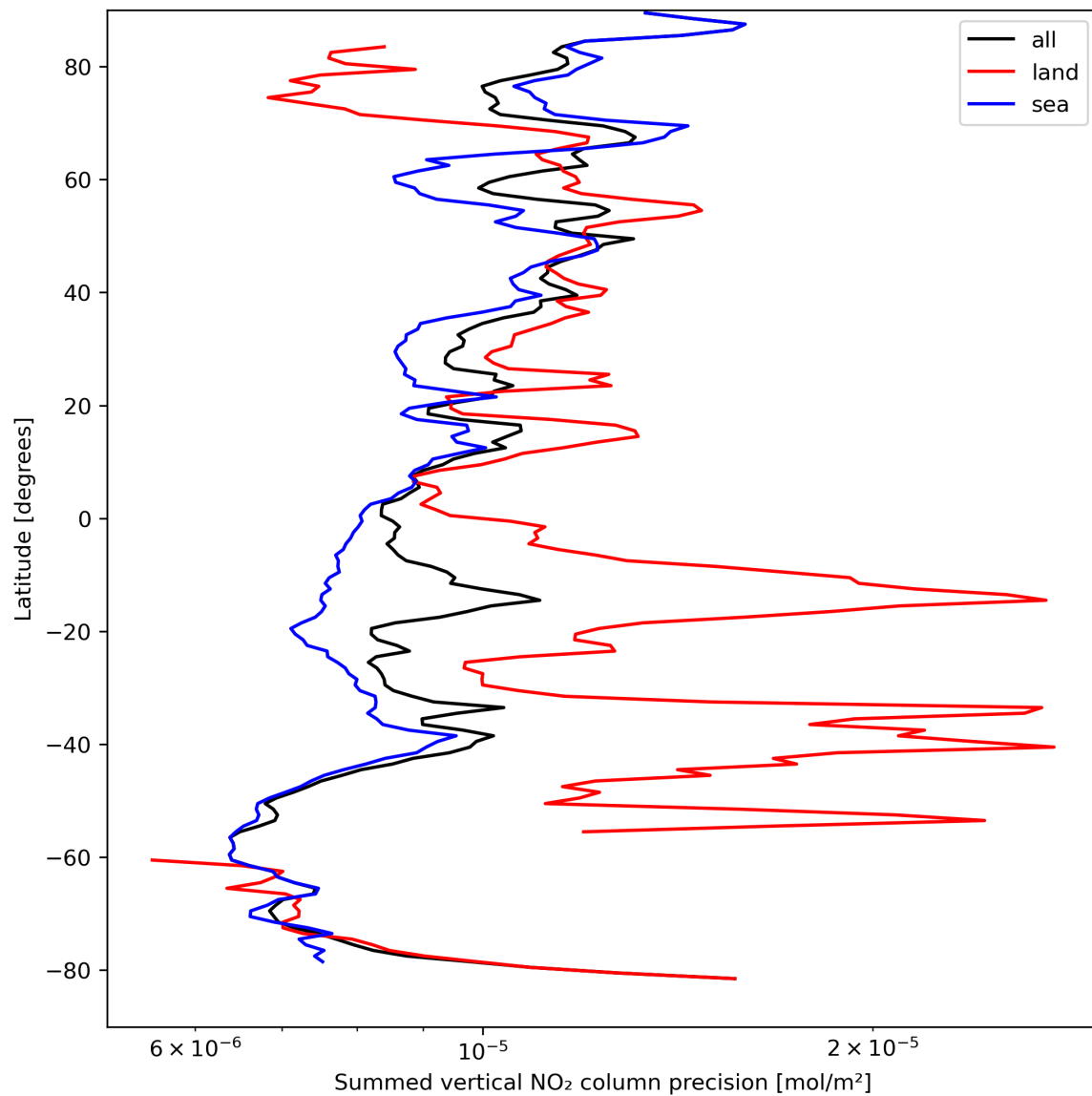
Figure 24: Zonal average of “Summed vertical NO 2 column precision” for 2023-09-05 to 2023-09-06.
