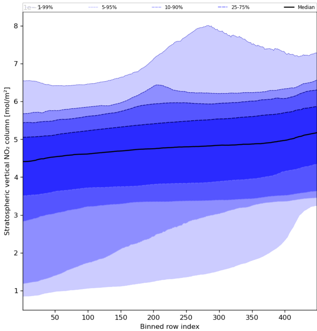
Figure 53: Along track statistics of “Stratospheric vertical NO 2 column” for 2023-09-05 to 2023-09-06
