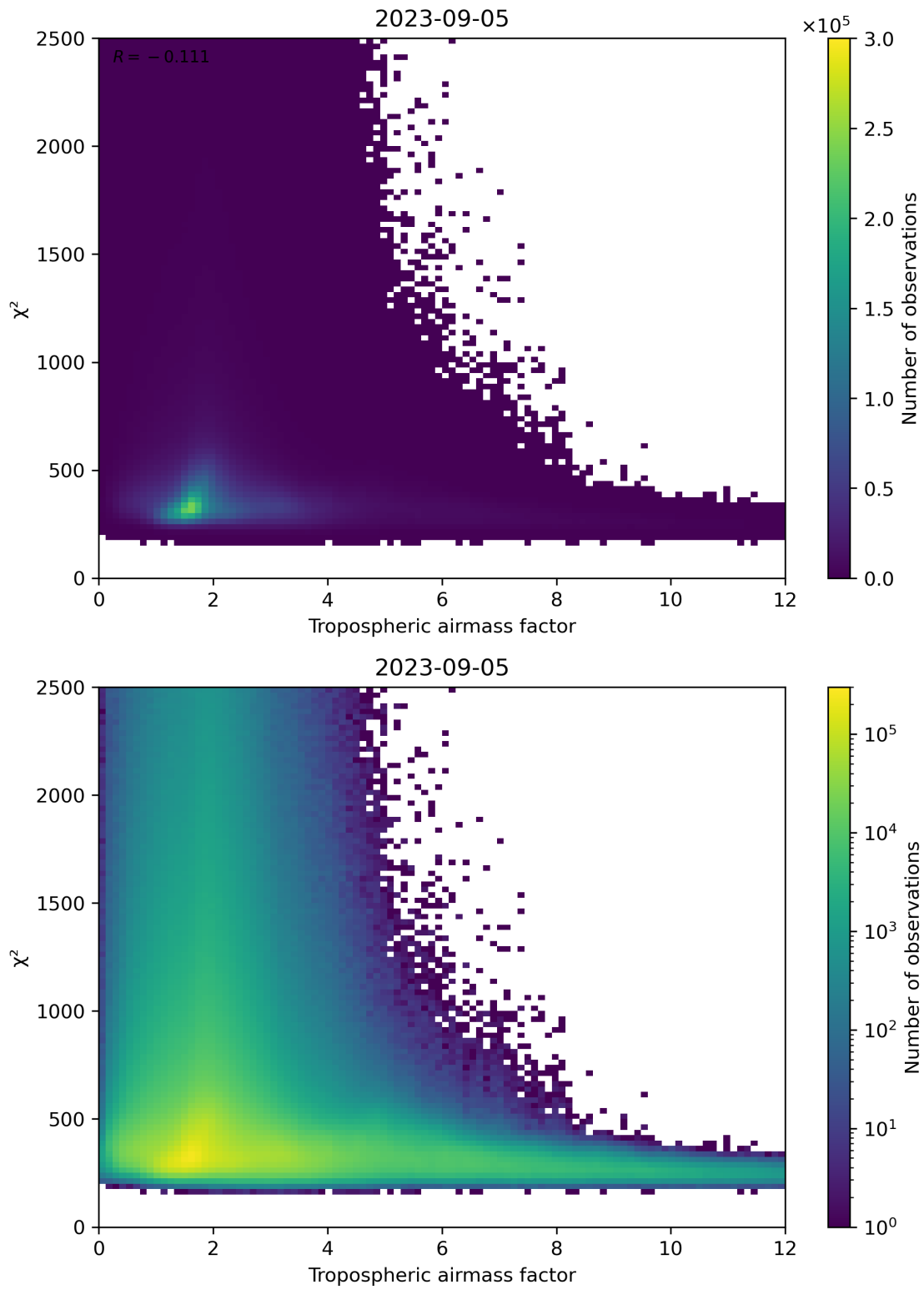
Figure 73: Scatter density plot of “Tropospheric airmass factor” against “ \chi^2 ” for 2023-09-05 to 2023-09-06.
