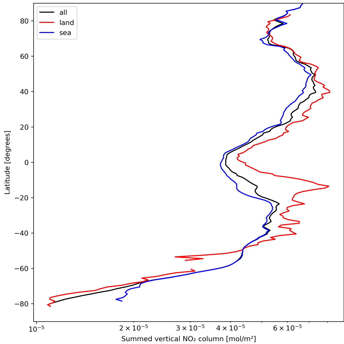
Figure 23: Zonal average of “Summed vertical NO 2 column” for 2023-09-05 to 2023-09-06.
