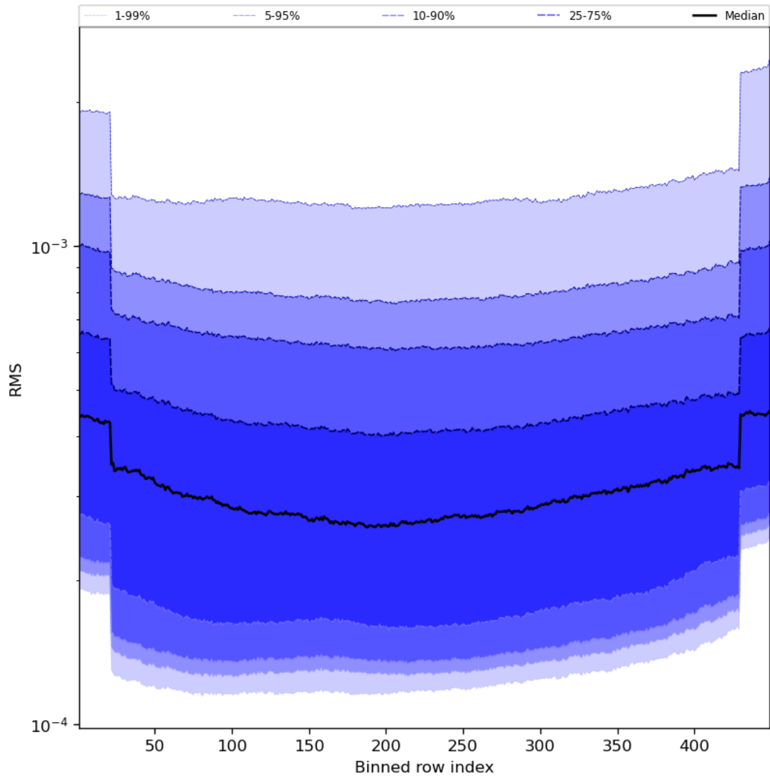
Figure 60: Along track statistics of “RMS” for 2023-09-05 to 2023-09-06
