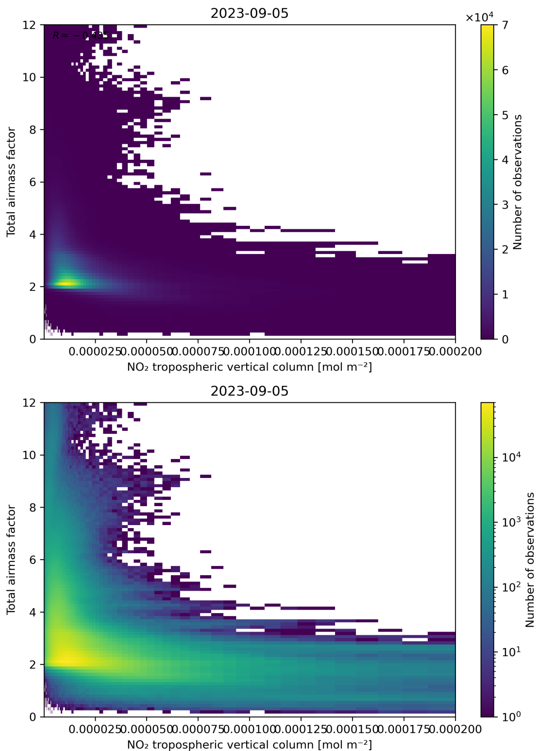
Figure 122: Scatter density plot of “NO 2 tropospheric vertical column” against “Total air mass factor” for 2023-09-05 to 2023-09-06.
