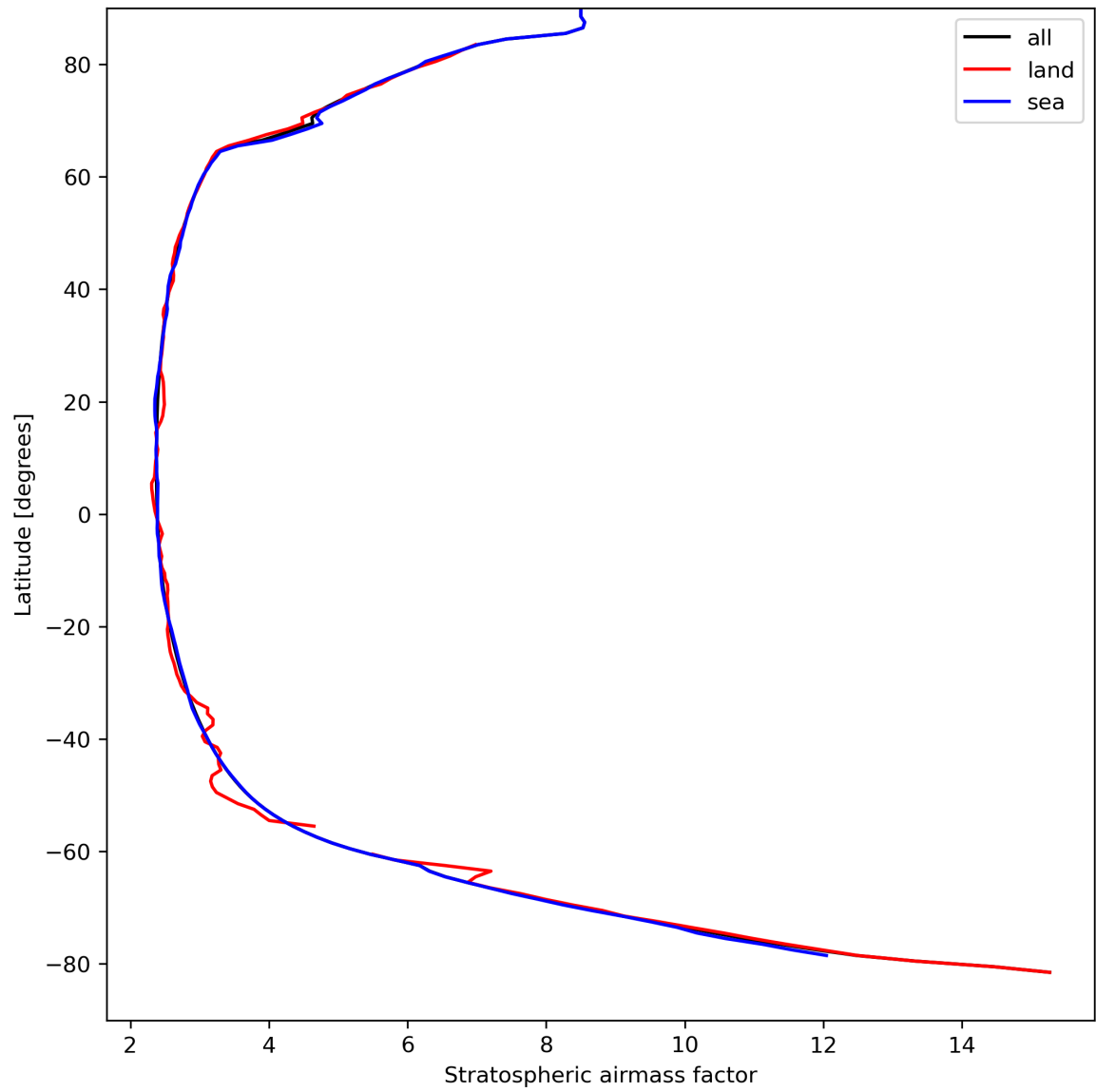
Figure 27: Zonal average of “Stratospheric airmass factor” for 2023-09-05 to 2023-09-06.
