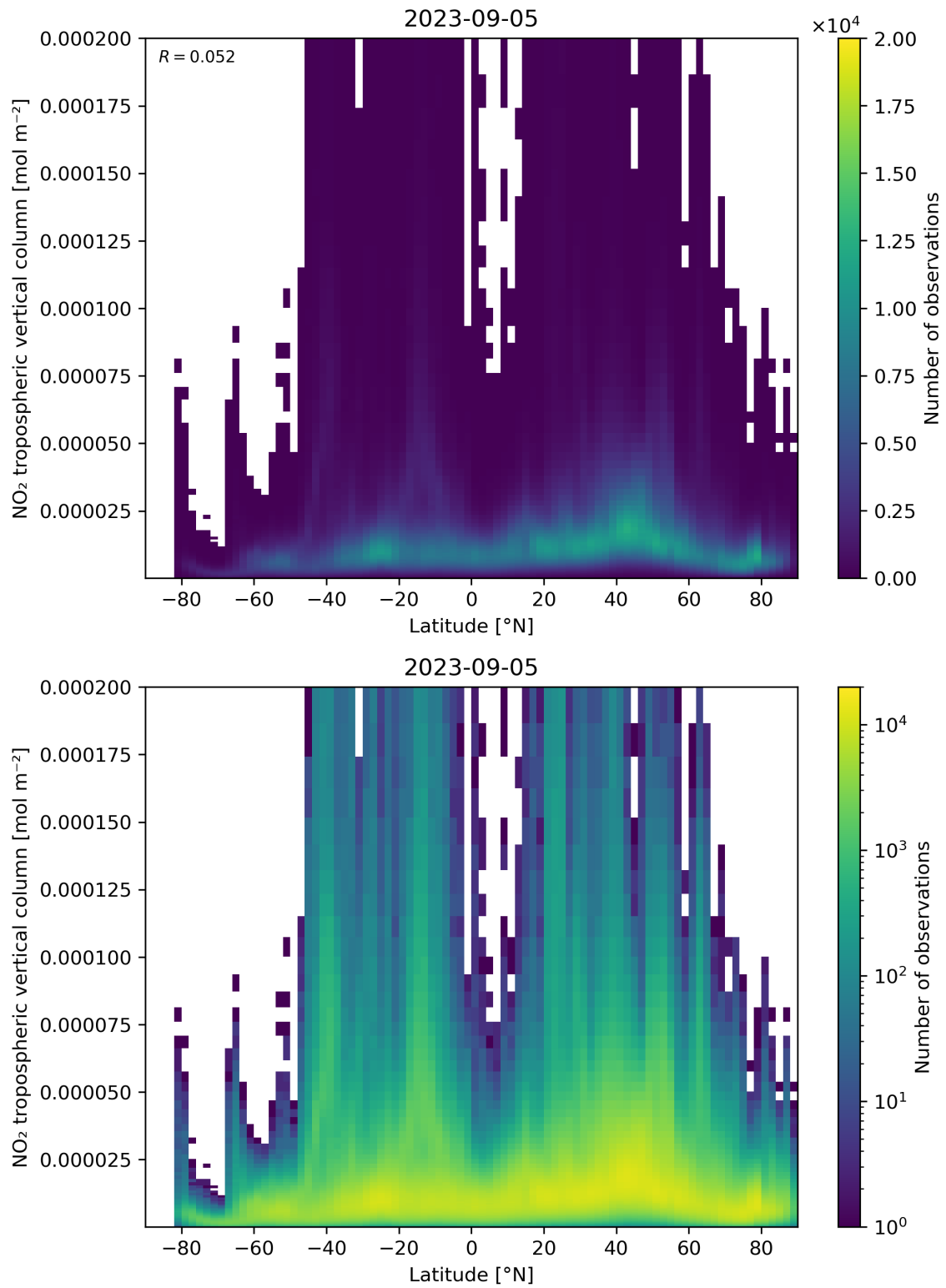
Figure 92: Scatter density plot of “Latitude” against “NO 2 tropospheric vertical column” for 2023-09-05 to 2023-09-06.
