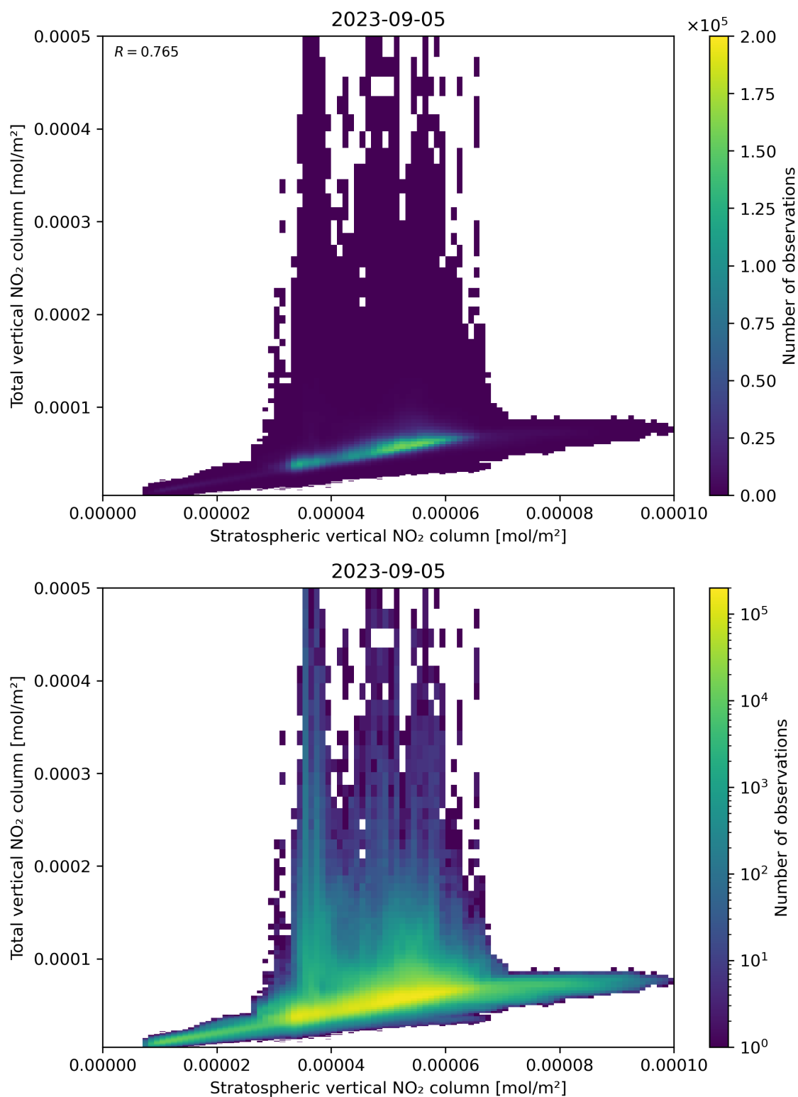
Figure 100: Scatter density plot of “Stratospheric vertical NO 2 column” against “Total vertical NO 2 column” for 2023-09-05 to 2023-09-06.
