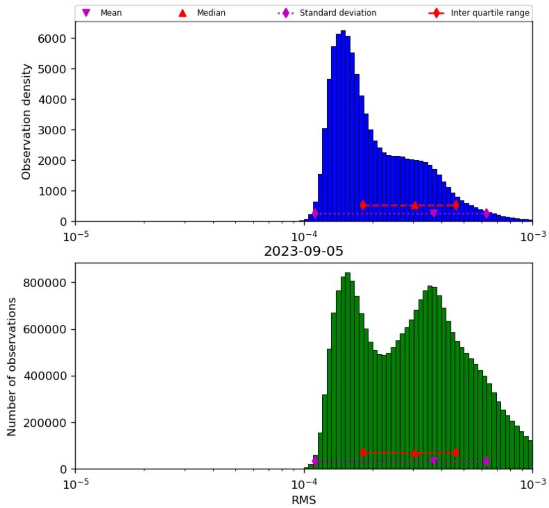
Figure 43: Histogram of “RMS” for 2023-09-05 to 2023-09-06
