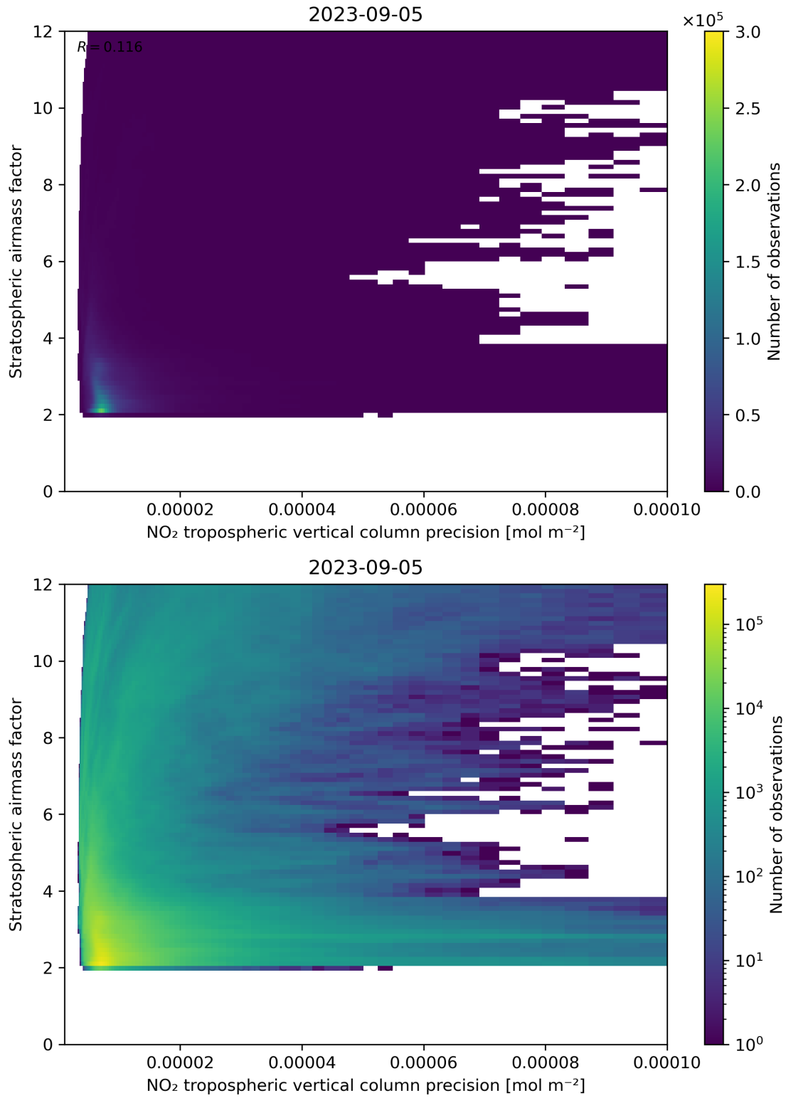
Figure 131: Scatter density plot of “NO 2 tropospheric vertical column precision” against “Stratospheric airmass factor” for 2023-09-05 to 2023-09-06.
