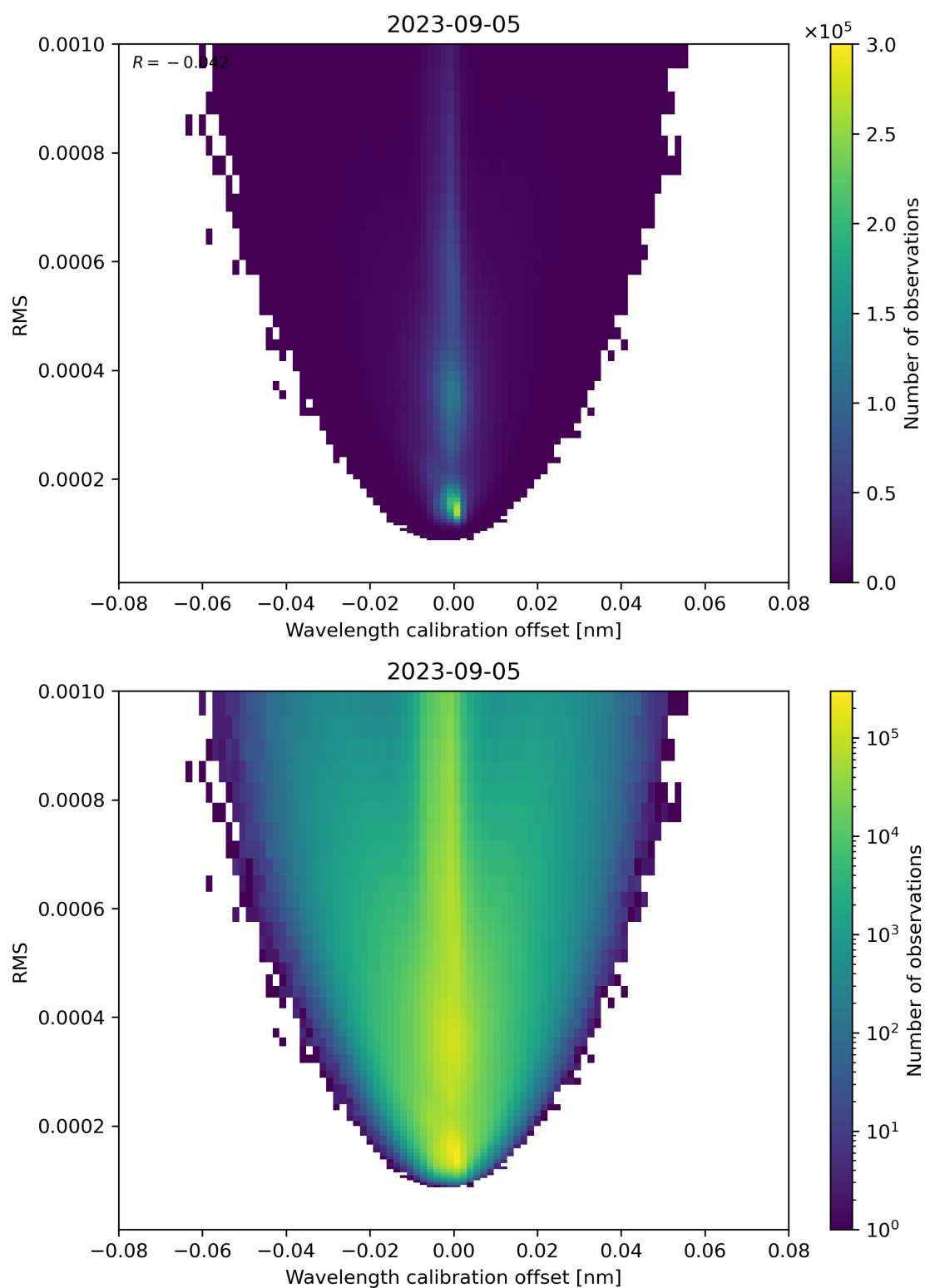
Figure 181: Scatter density plot of “Wavelength calibration offset” against “RMS” for 2023-09-05 to 2023-09-06.
