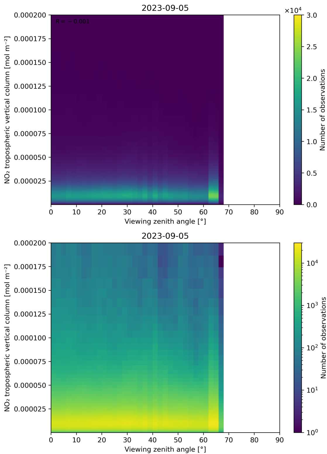
Figure 169: Scatter density plot of “Viewing zenith angle” against “NO 2 tropospheric vertical column” for 2023-09-05 to 2023-09-06.
