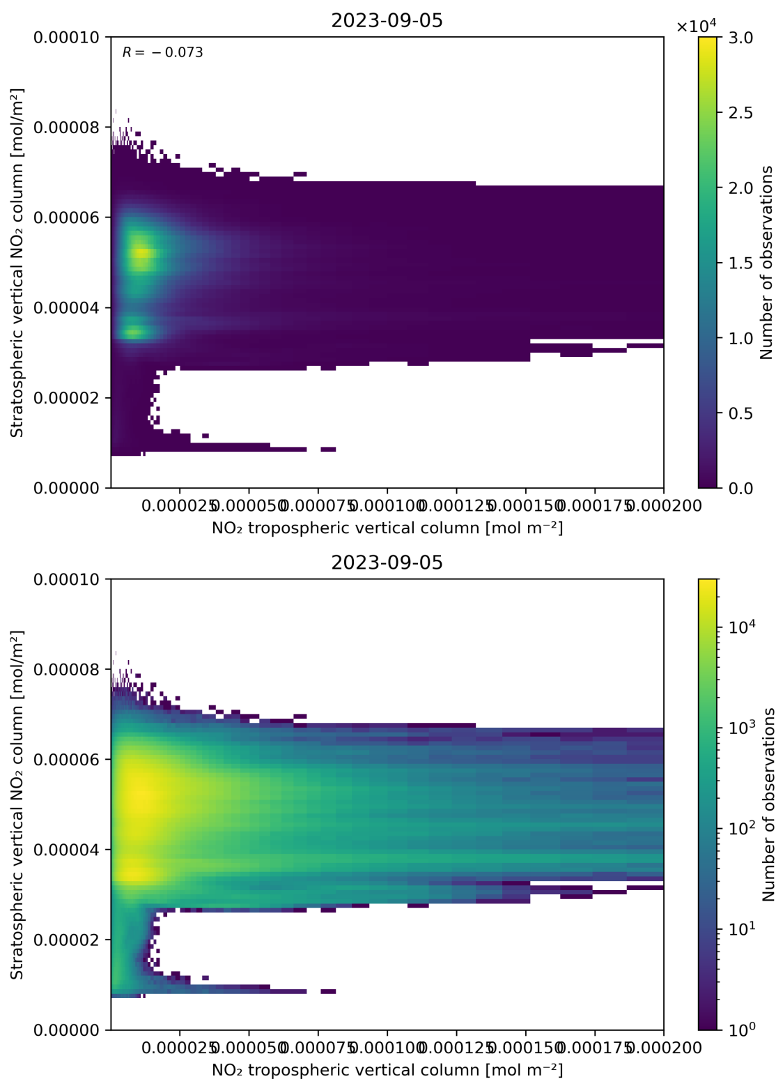
Figure 125: Scatter density plot of “NO 2 tropospheric vertical column” against “Stratospheric vertical NO 2 column” for 2023-09-05 to 2023-09-06.
