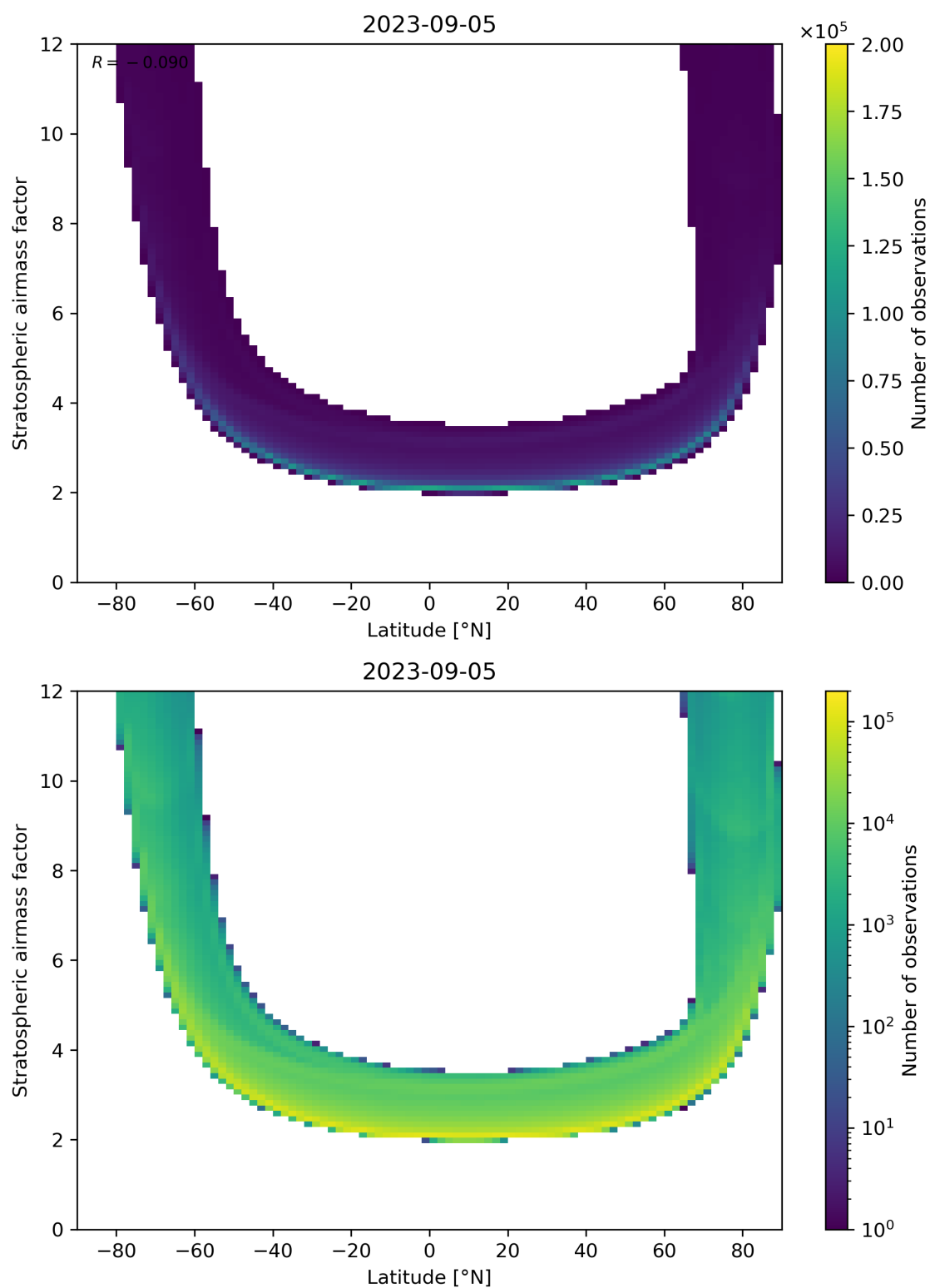
Figure 83: Scatter density plot of “Latitude” against “Stratospheric air mass factor” for 2023-09-05 to 2023-09-06.
