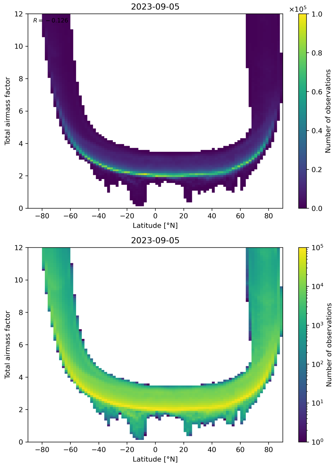
Figure 84: Scatter density plot of “Latitude” against “Total airmass factor” for 2023-09-05 to 2023-09-06.
