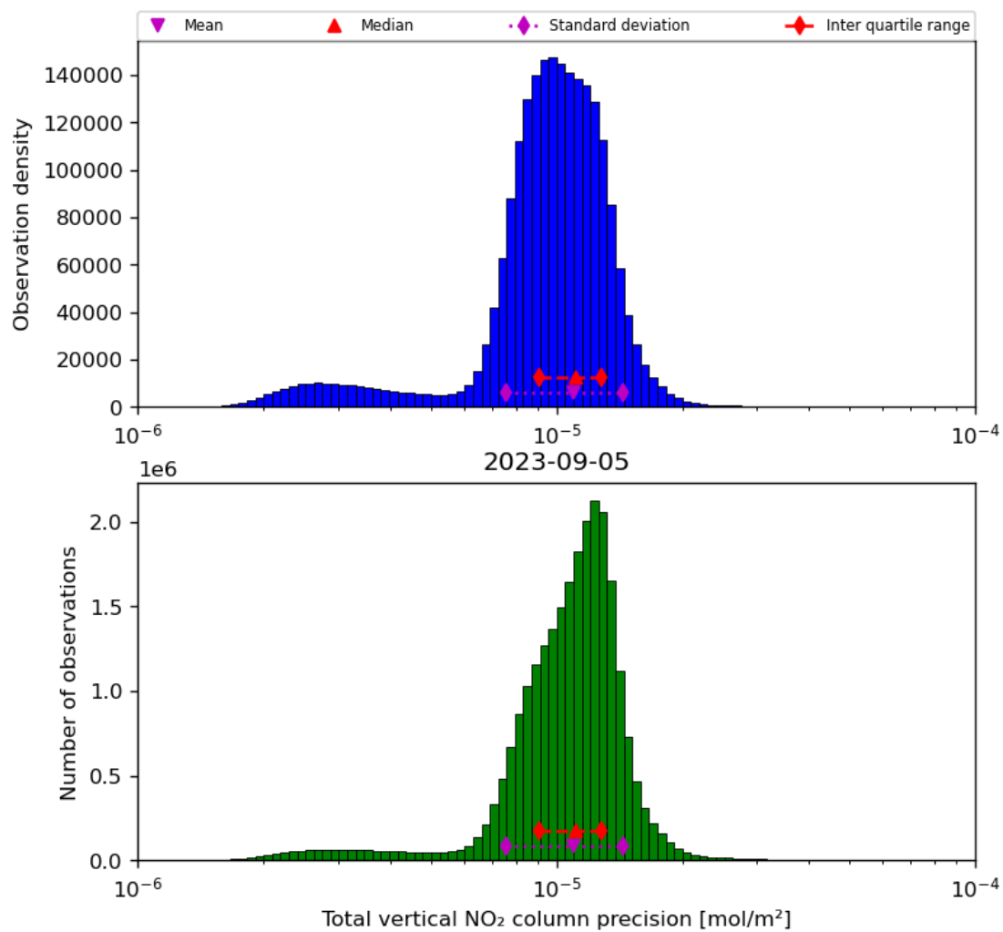
Figure 39: Histogram of “Total vertical NO 2 column precision” for 2023-09-05 to 2023-09-06
