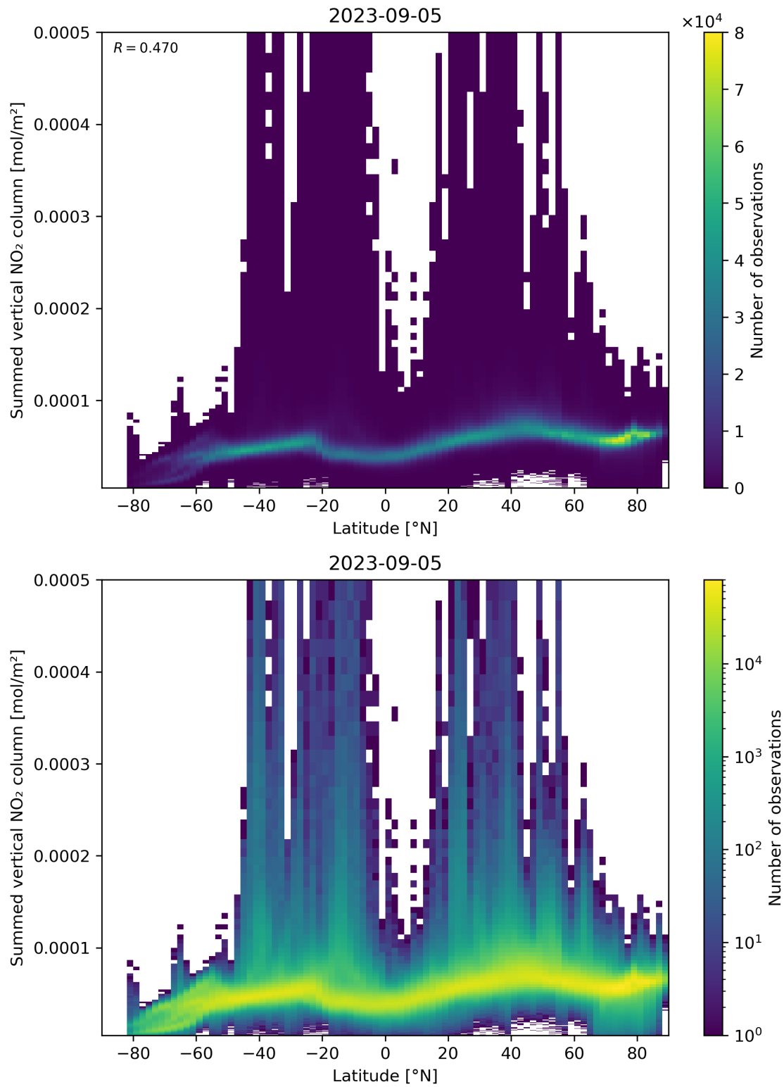
Figure 88: Scatter density plot of “Latitude” against “Summed vertical NO 2 column” for 2023-09-05 to 2023-09-06.
