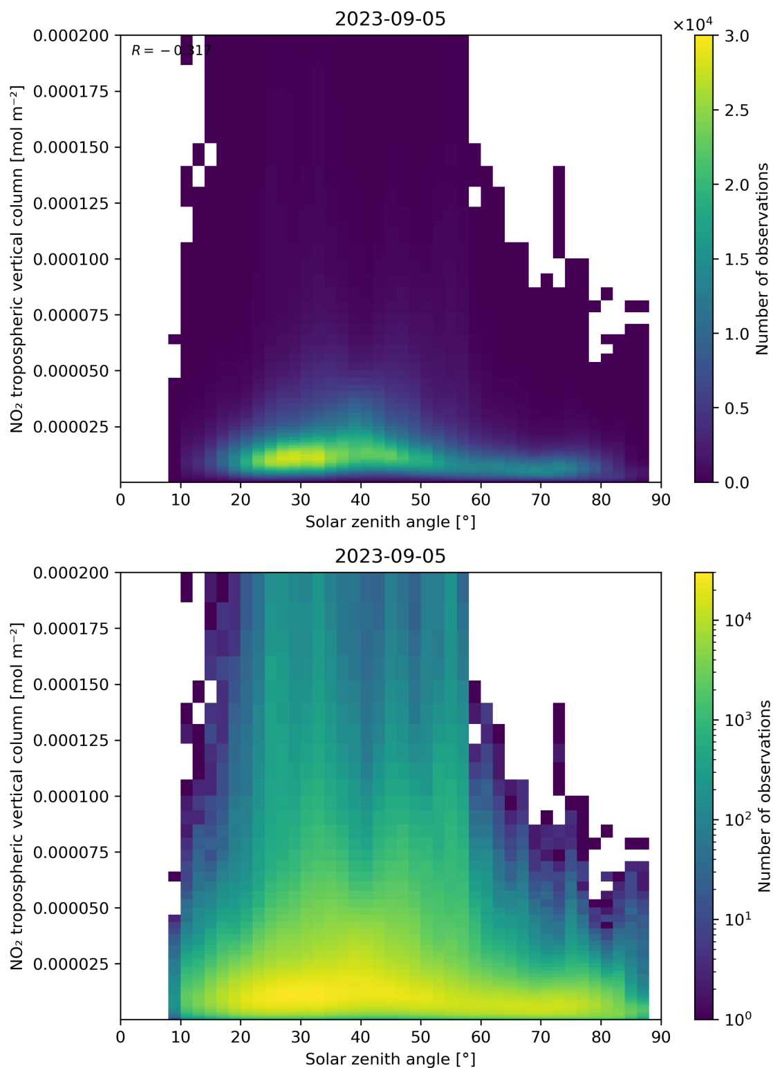
Figure 155: Scatter density plot of “Solar zenith angle” against “NO 2 tropospheric vertical column” for 2023-09-05 to 2023-09-06.
