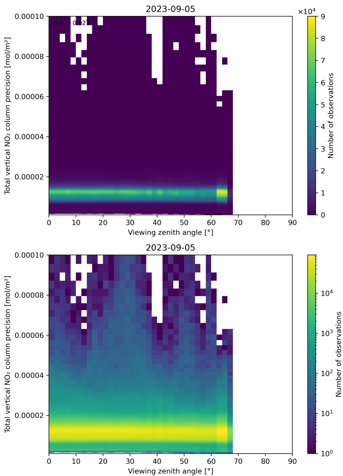
Figure 168: Scatter density plot of “Viewing zenith angle” against “Total vertical NO 2 column precision” for 2023-09-05 to 2023-09-06.
