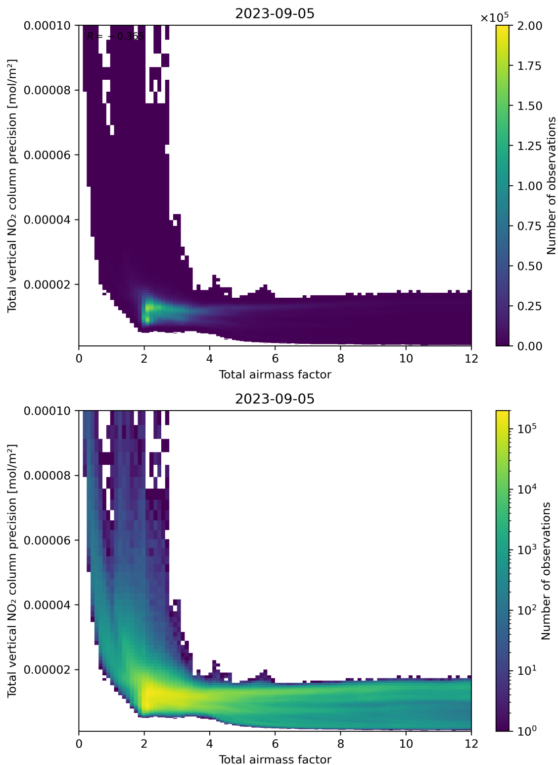
Figure 68: Scatter density plot of “Total airmass factor” against “Total vertical NO 2 column precision” for 2023-09-05 to 2023-09-06.
