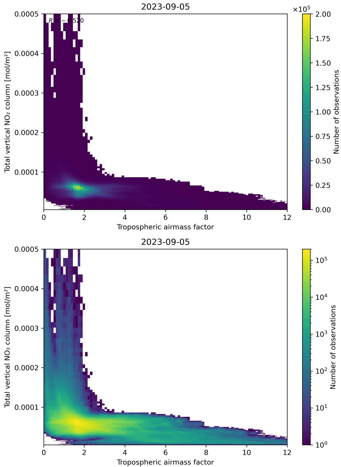
Figure 77: Scatter density plot of “Tropospheric airmass factor” against “Total vertical NO 2 column” for 2023-09-05 to 2023-09-06.
