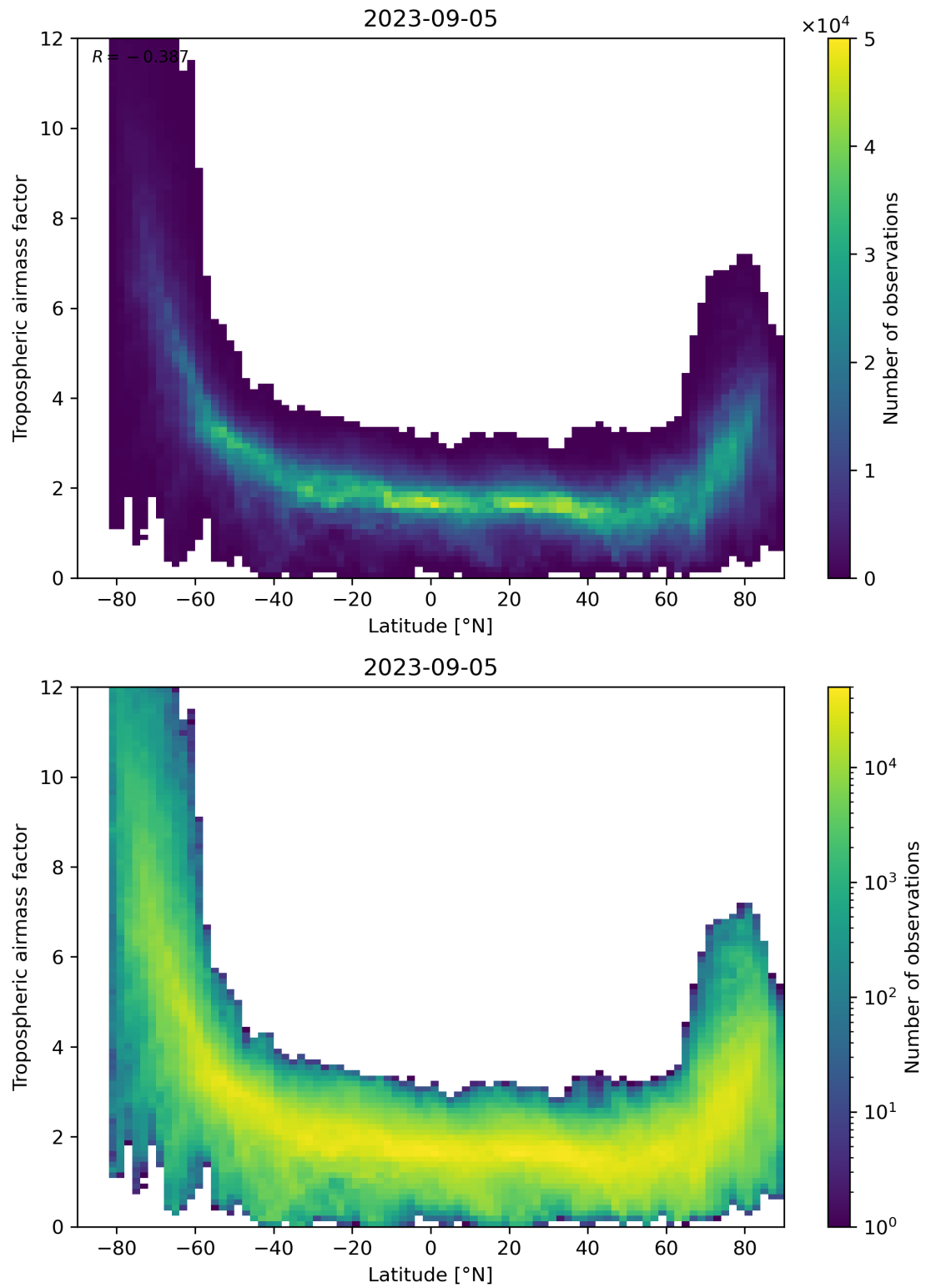
Figure 85: Scatter density plot of “Latitude” against “Tropospheric airmass factor” for 2023-09-05 to 2023-09-06.
