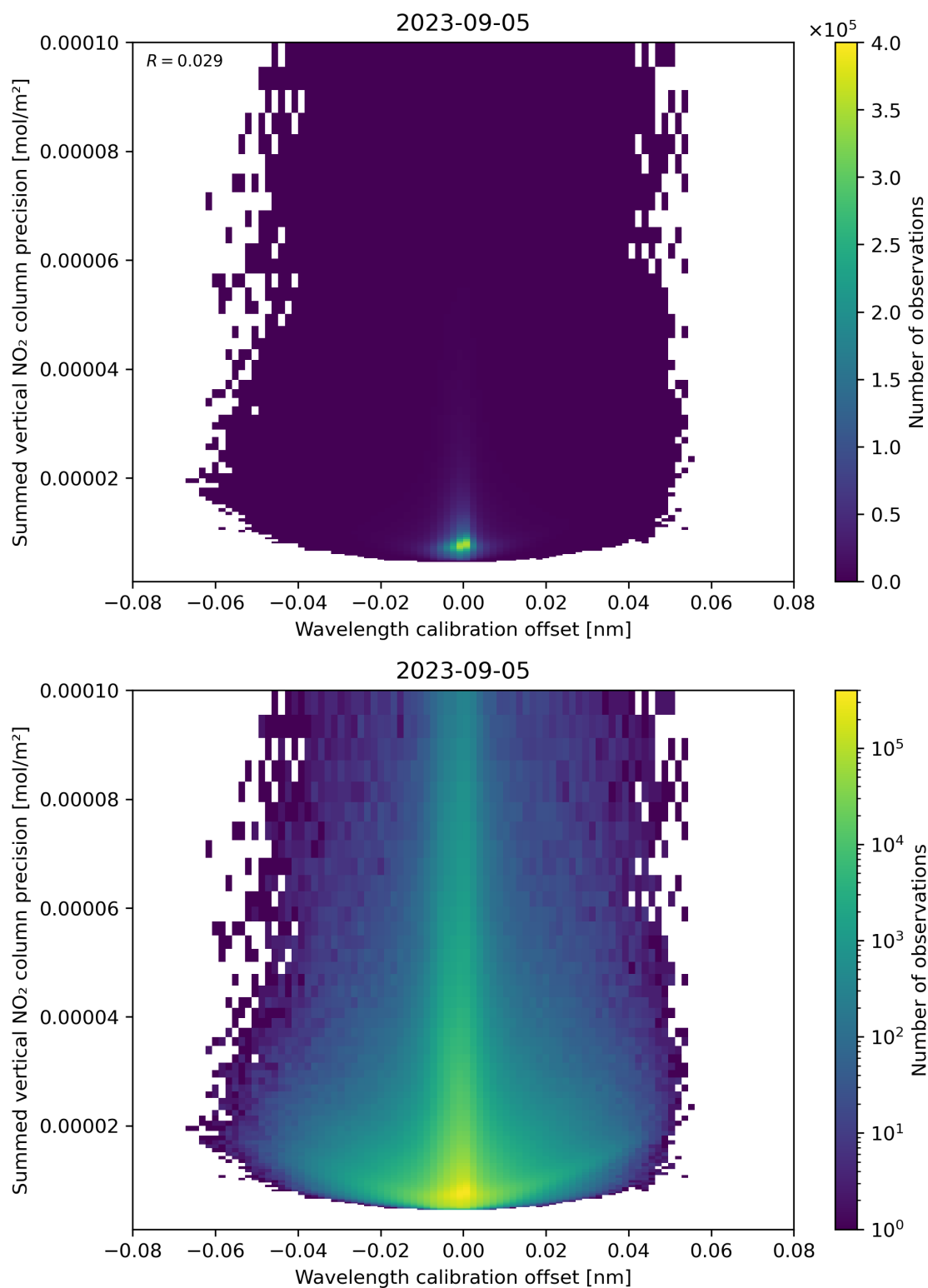
Figure 178: Scatter density plot of “Wavelength calibration offset” against “Summed vertical NO 2 column precision” for 2023-09-05 to 2023-09-06.
