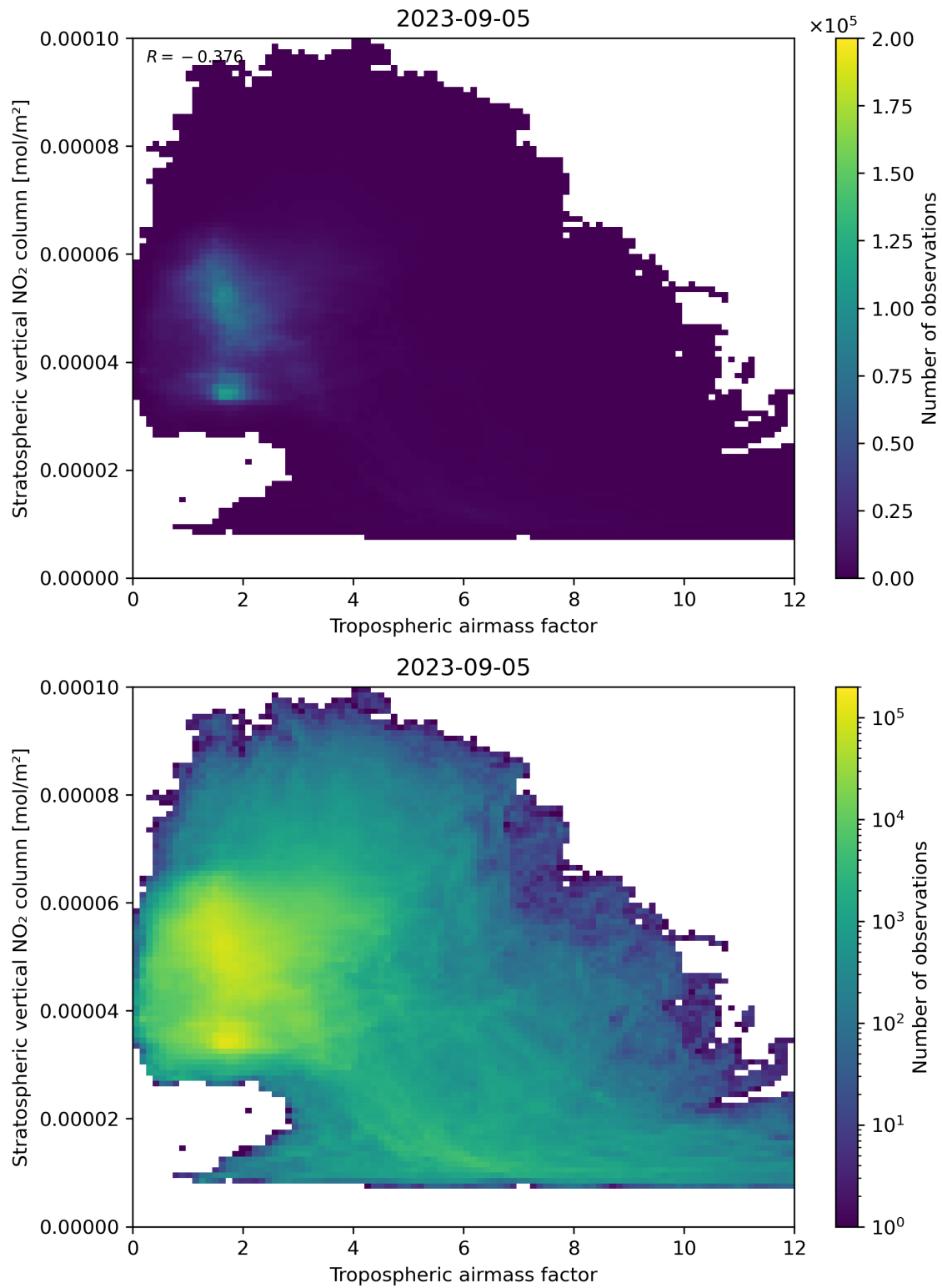
Figure 74: Scatter density plot of “Tropospheric air mass factor” against “Stratospheric vertical NO 2 column” for 2023-09-05 to 2023-09-06.
