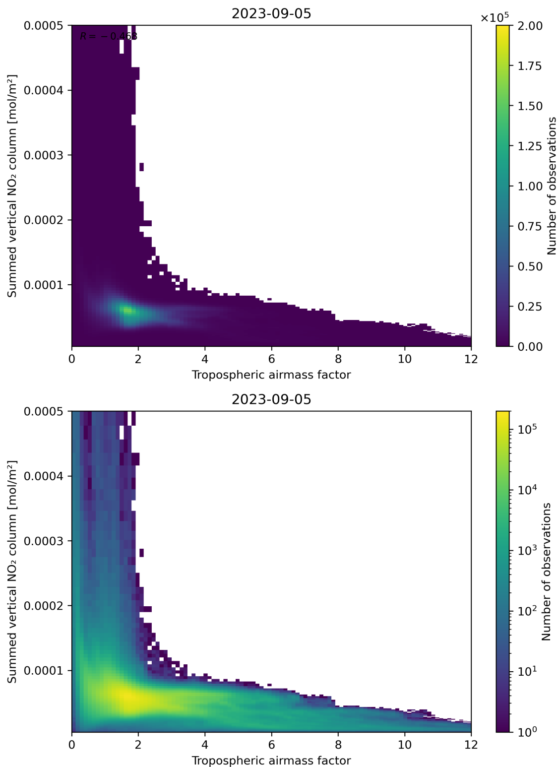
Figure 75: Scatter density plot of “Tropospheric airmass factor” against “Summed vertical NO 2 column” for 2023-09-05 to 2023-09-06.
