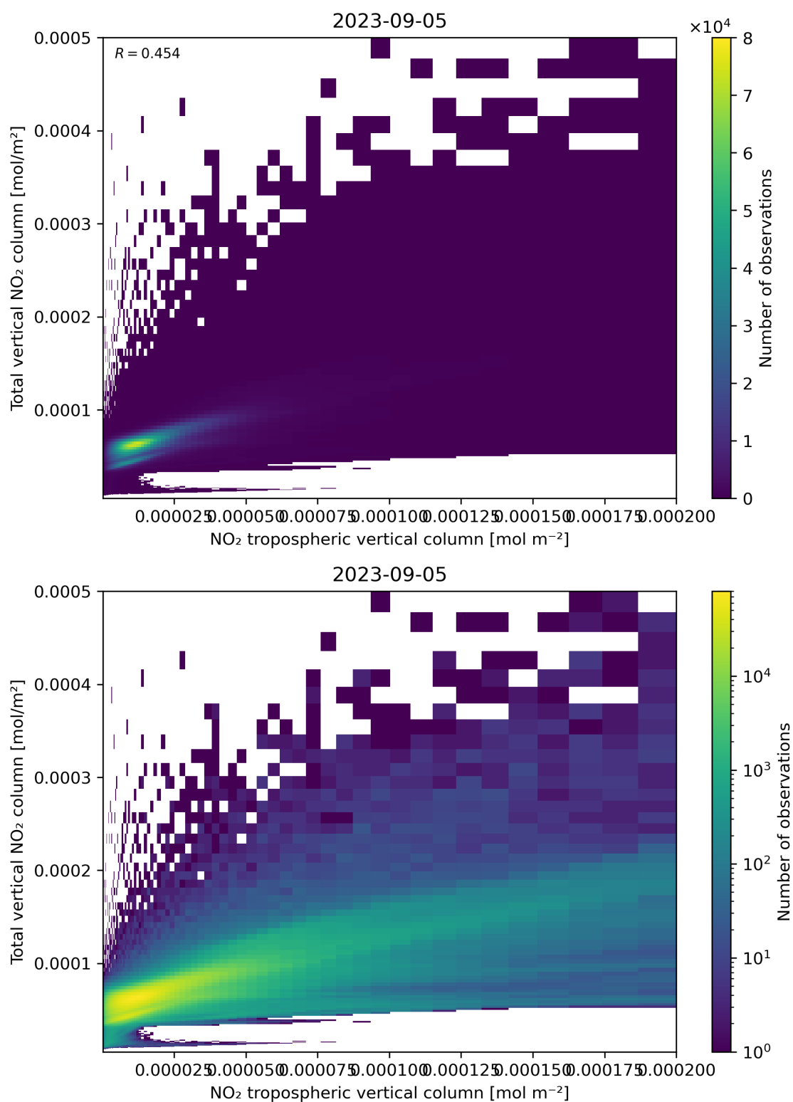
Figure 128: Scatter density plot of “NO 2 tropospheric vertical column” against “Total vertical NO 2 column” for 2023-09-05 to 2023-09-06.
