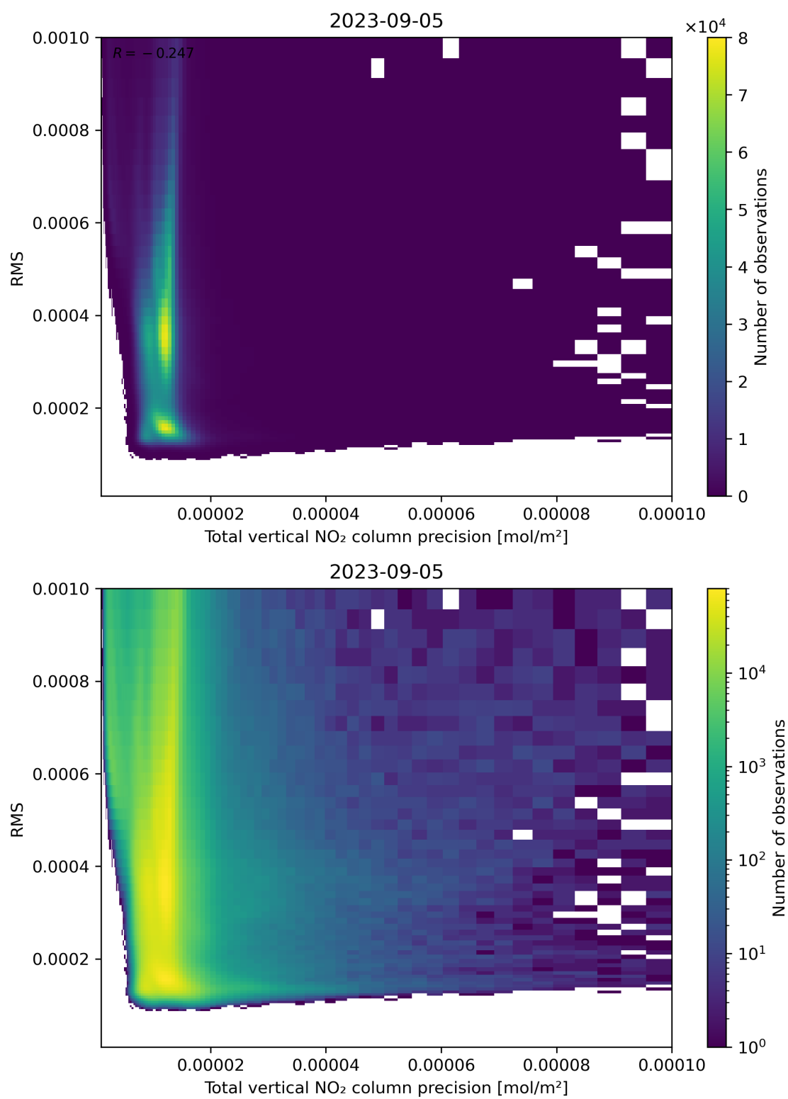
Figure 119: Scatter density plot of “Total vertical NO 2 column precision” against “RMS” for 2023-09-05 to 2023-09-06.
