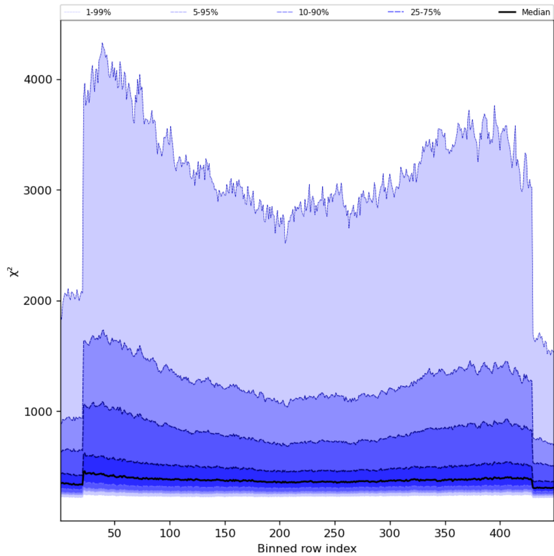
Figure 59: Along track statistics of “ \chi^2 ” for 2023-09-05 to 2023-09-06
