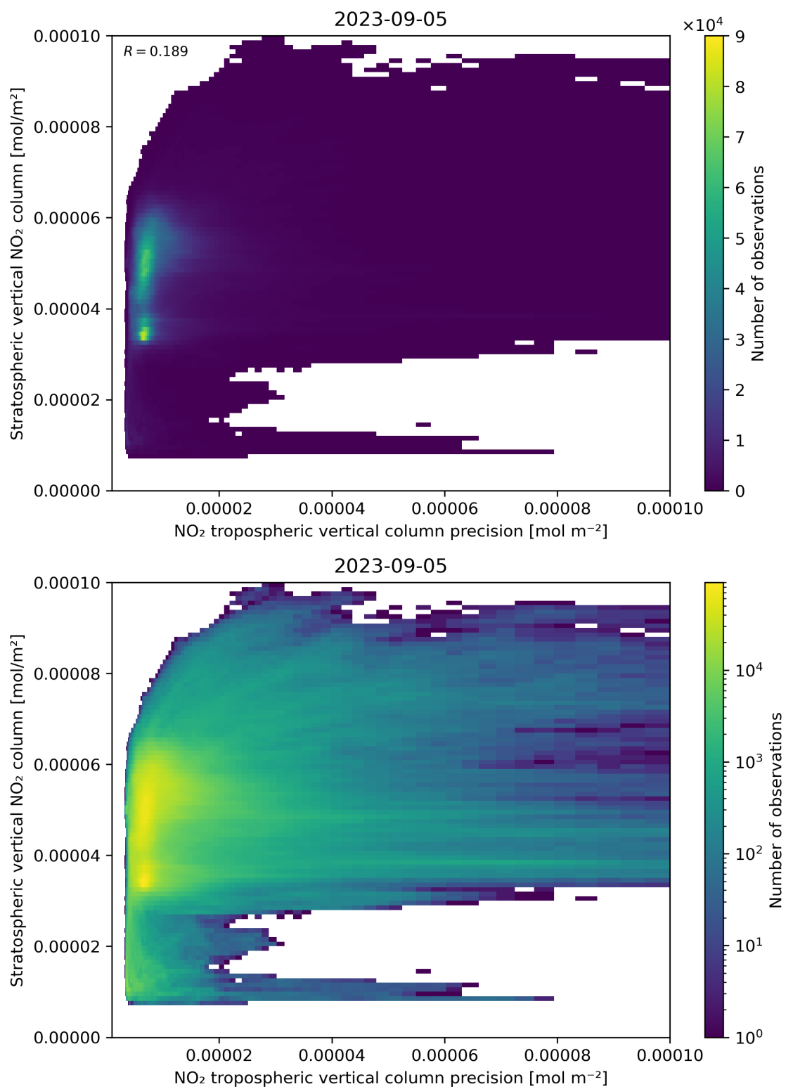
Figure 135: Scatter density plot of “NO 2 tropospheric vertical column precision” against “Stratospheric vertical NO 2 column” for 2023-09-05 to 2023-09-06.
