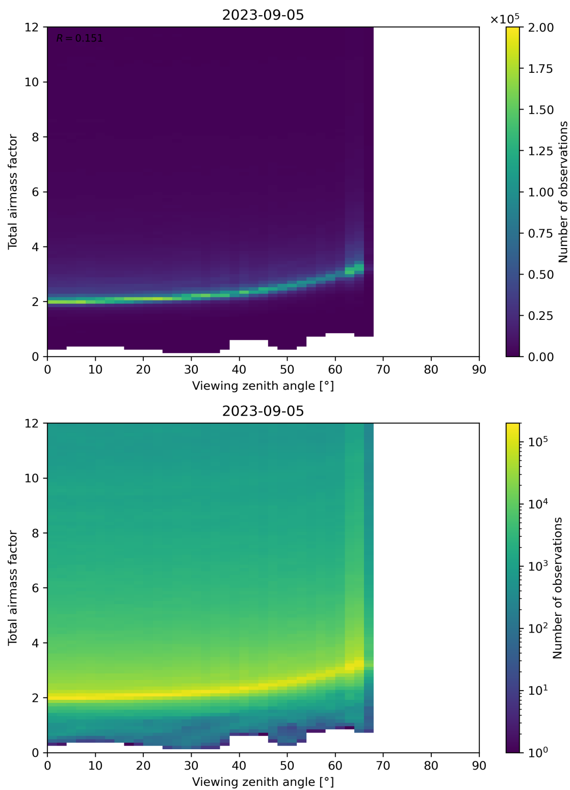
Figure 160: Scatter density plot of “Viewing zenith angle” against “Total airmass factor” for 2023-09-05 to 2023-09-06.
