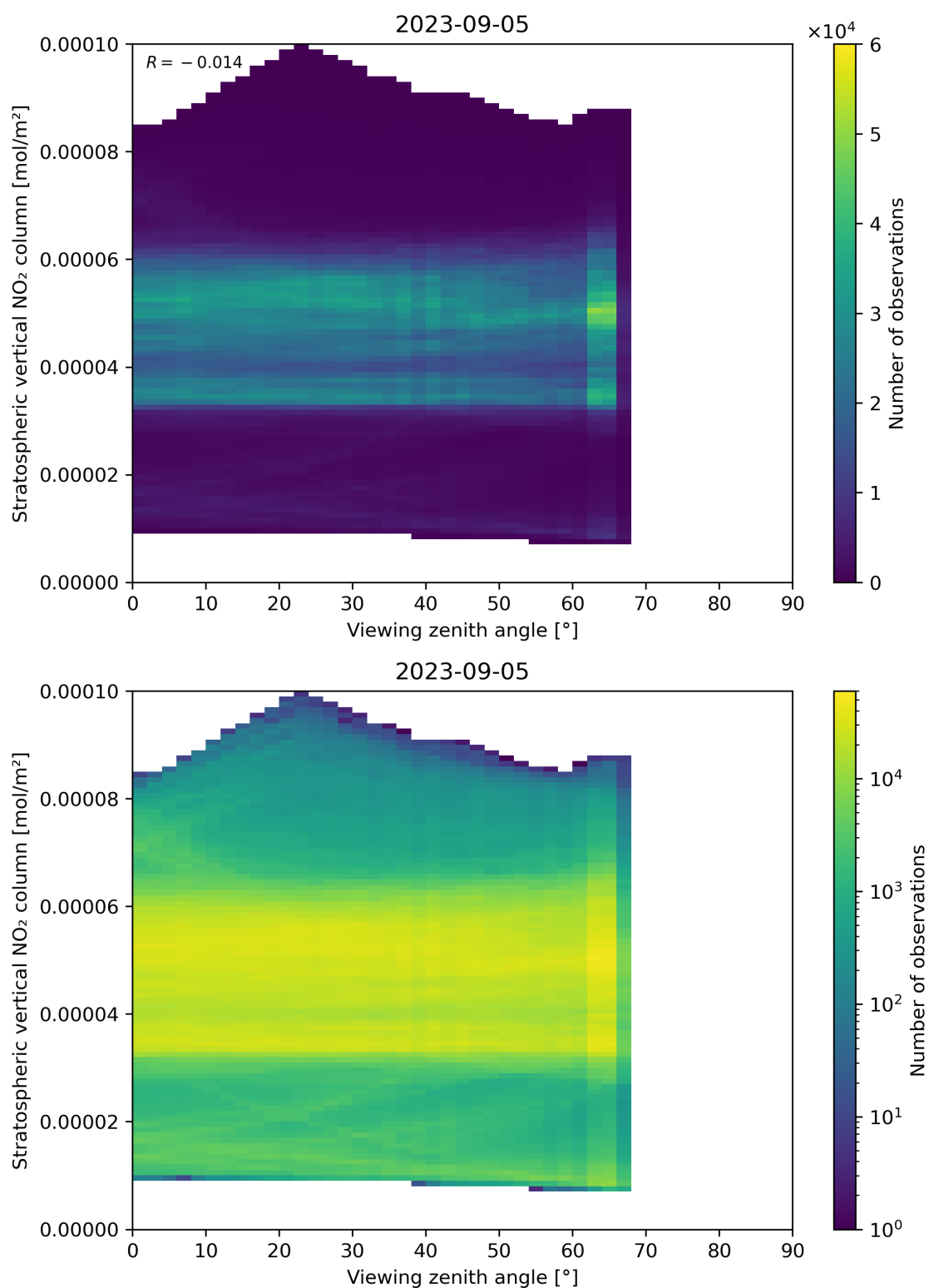
Figure 164: Scatter density plot of “Viewing zenith angle” against “Stratospheric vertical NO 2 column” for 2023-09-05 to 2023-09-06.
