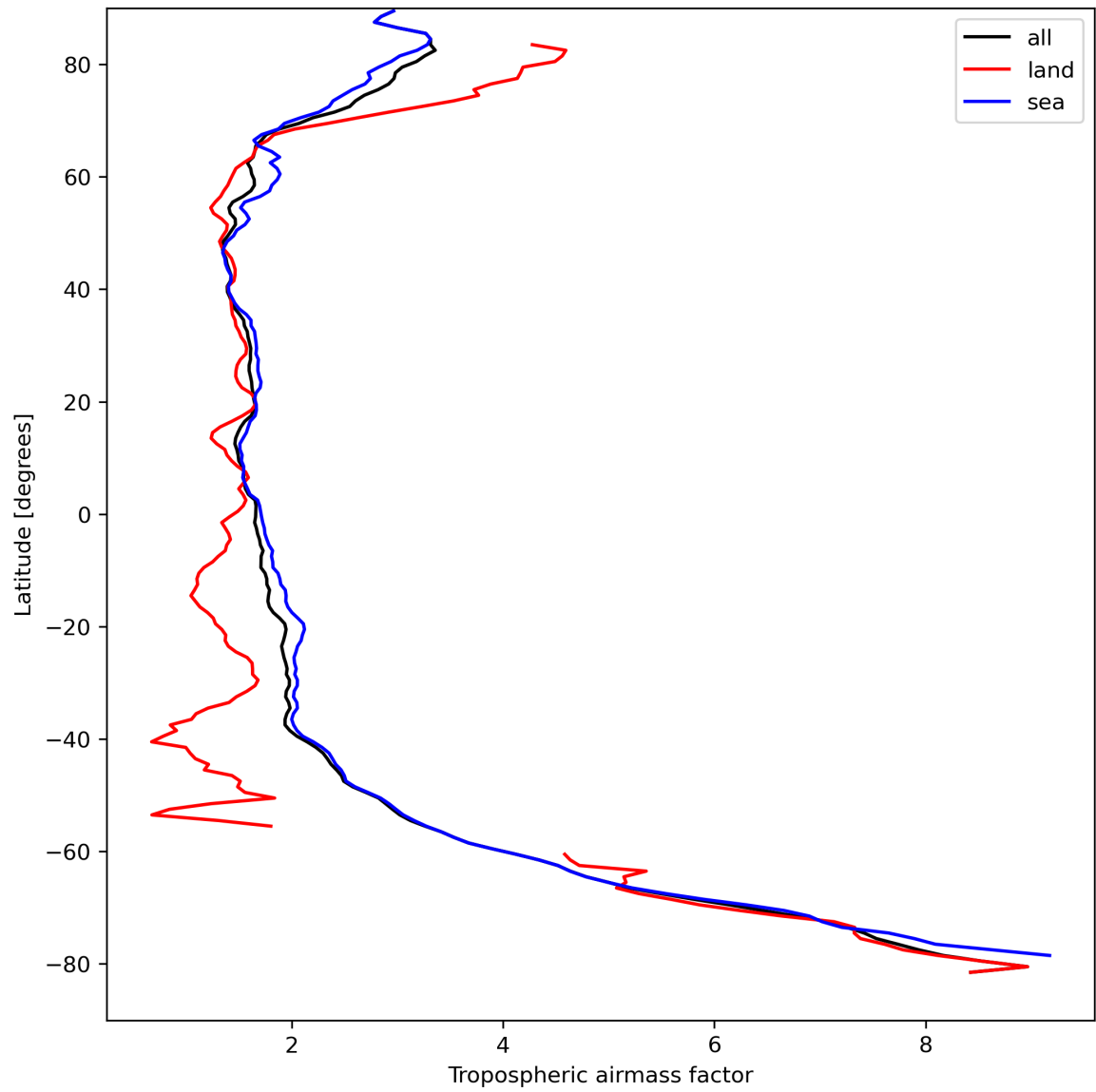
Figure 14: Zonal average of “Tropospheric airmass factor” for 2023-09-05 to 2023-09-06.
