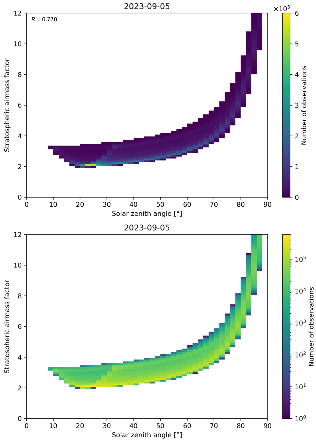
Figure 145: Scatter density plot of “Solar zenith angle” against “Stratospheric airmass factor” for 2023-09-05 to 2023-09-06.
