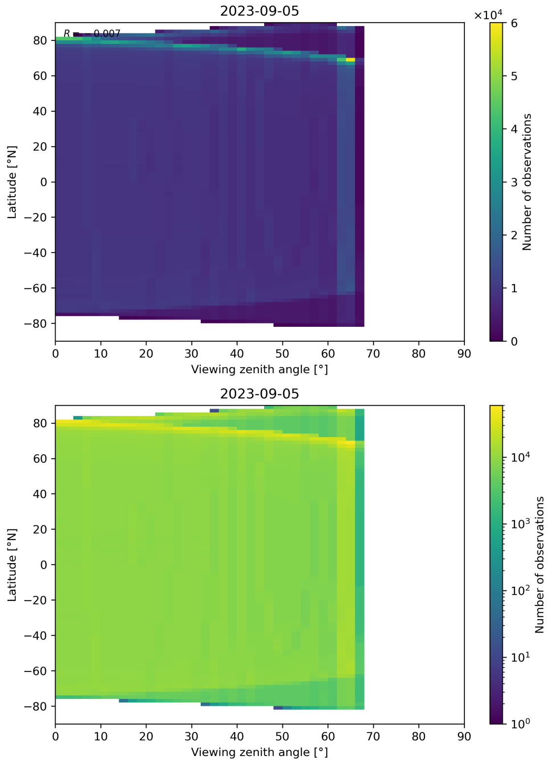
Figure 163: Scatter density plot of “Viewing zenith angle” against “Latitude” for 2023-09-05 to 2023-09-06.
