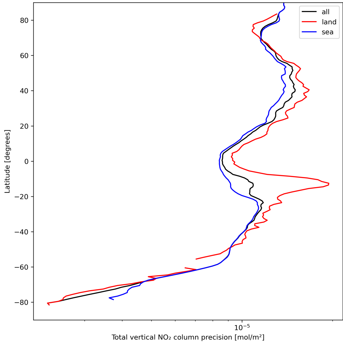
Figure 22: Zonal average of “Total vertical NO 2 column precision” for 2023-09-05 to 2023-09-06.
