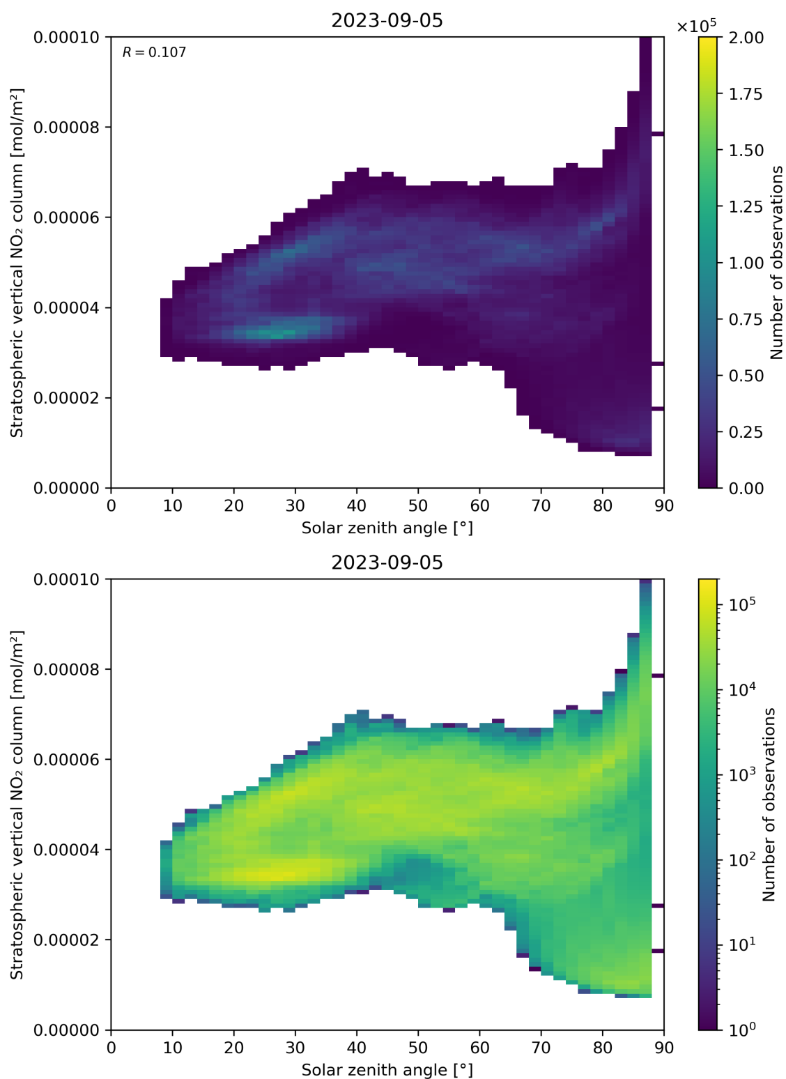
Figure 150: Scatter density plot of “Solar zenith angle” against “Stratospheric vertical NO 2 column” for 2023-09-05 to 2023-09-06.
