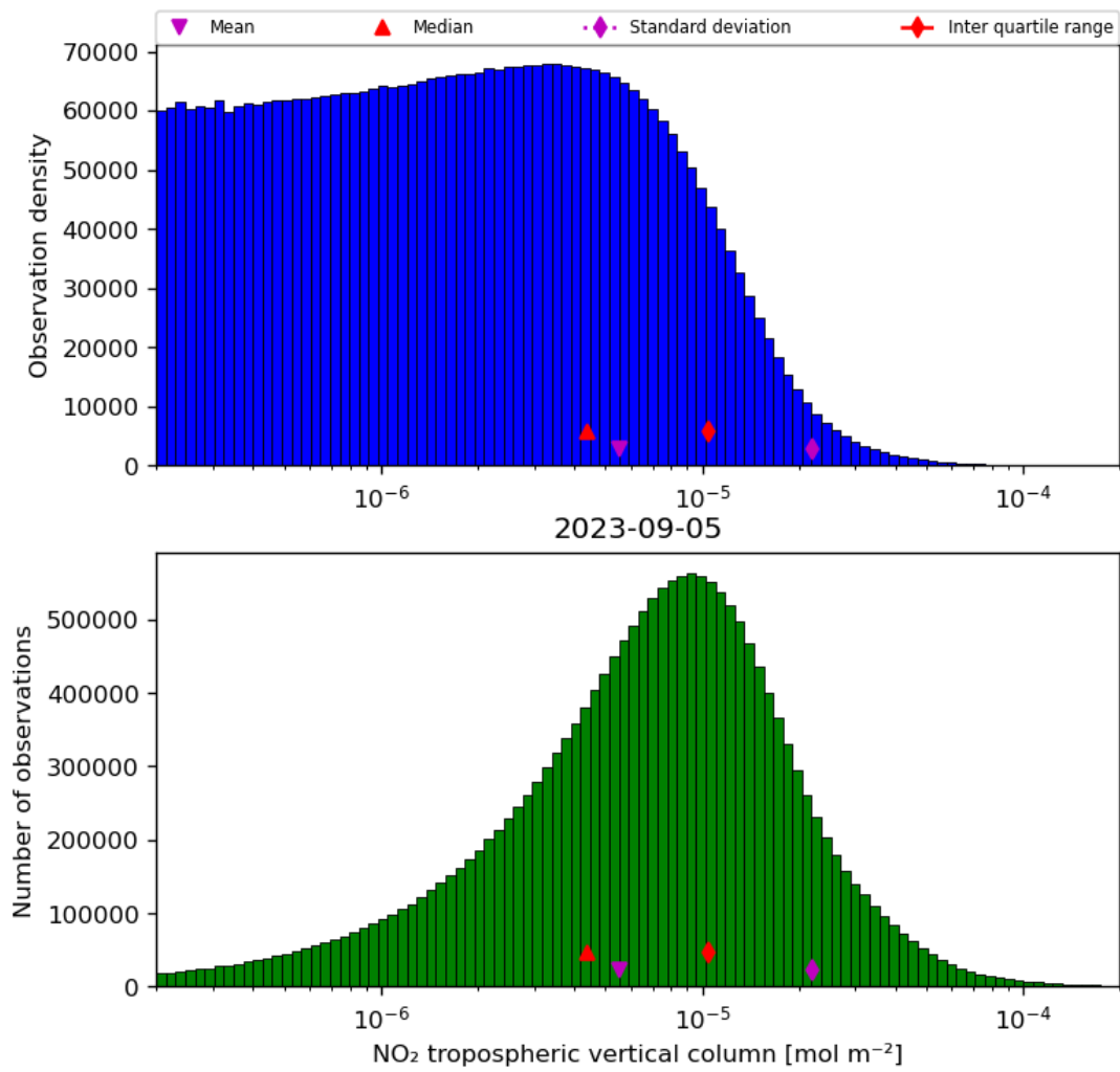
Figure 29: Histogram of “NO 2 tropospheric vertical column” for 2023-09-05 to 2023-09-06
