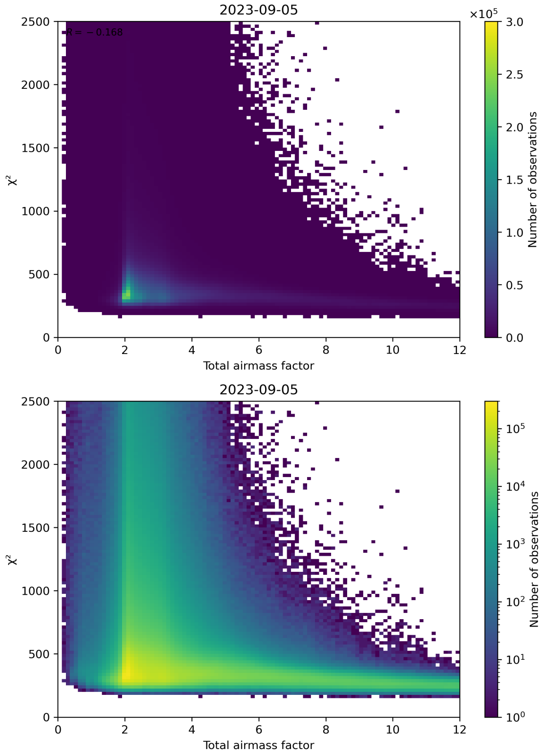
Figure 63: Scatter density plot of “Total airmass factor” against “ \chi^2 ” for 2023-09-05 to 2023-09-06.
