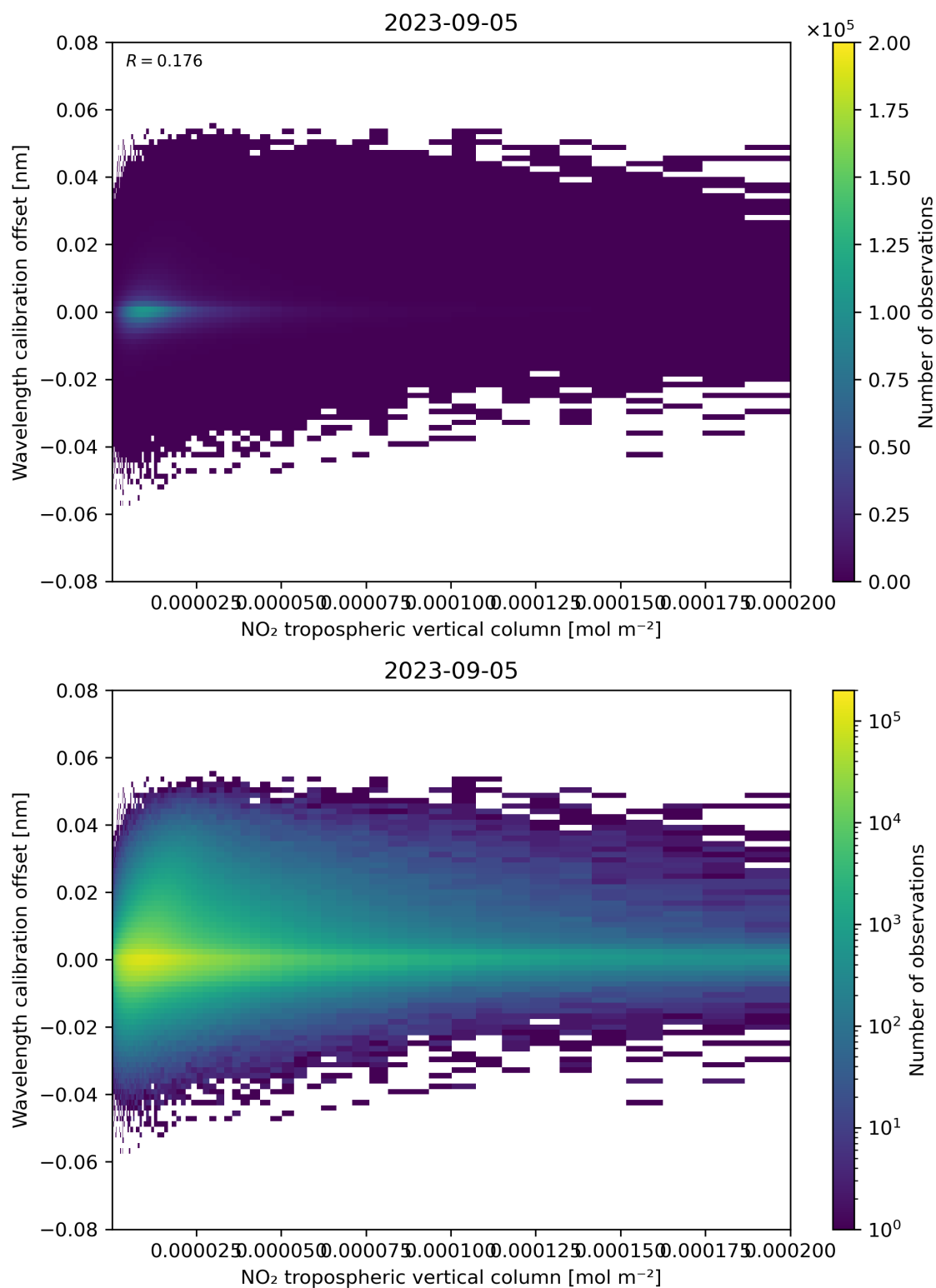
Figure 143: Scatter density plot of “NO 2 tropospheric vertical column” against “Wavelength calibration offset” for 2023-09-05 to 2023-09-06.
