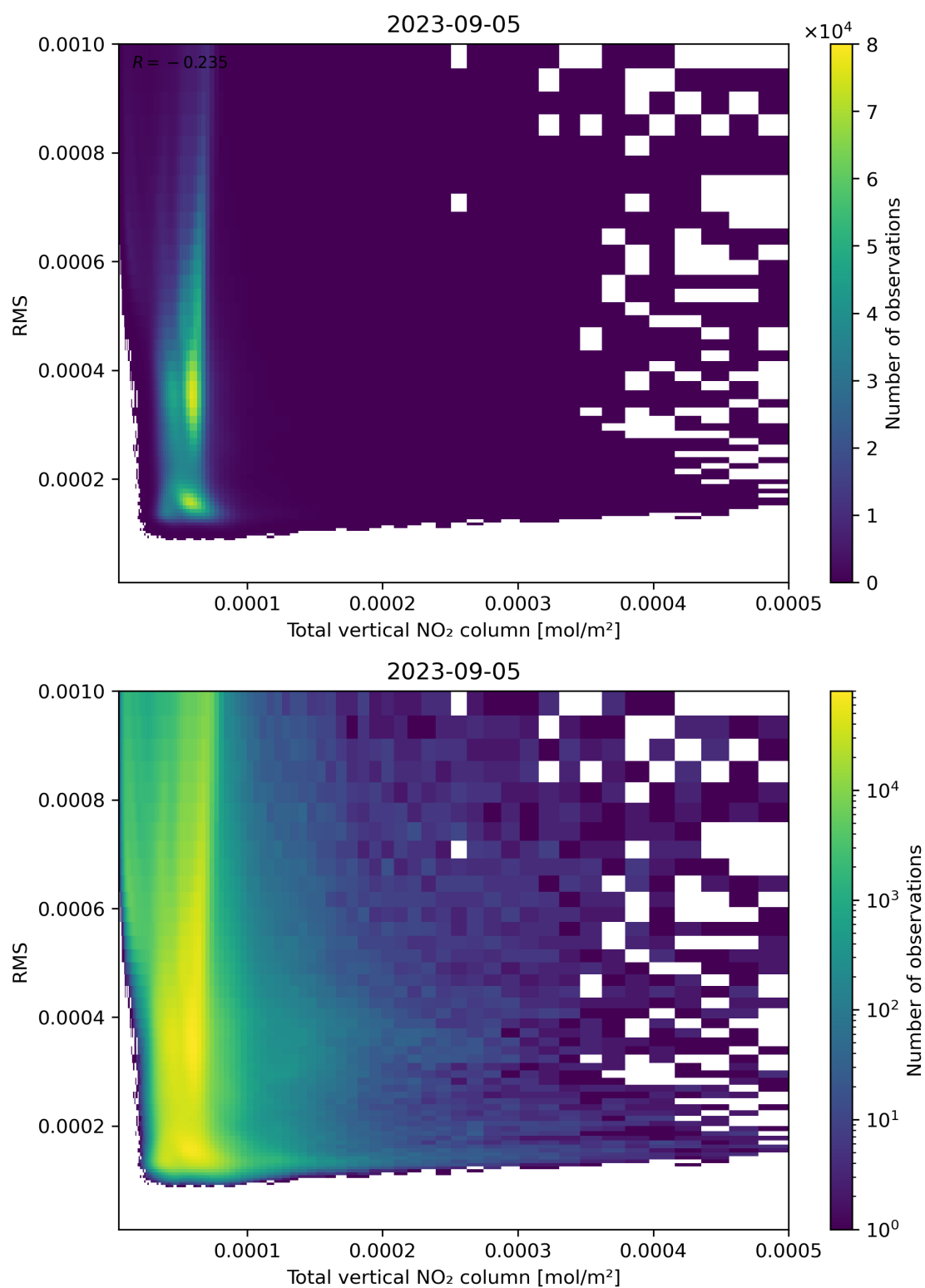
Figure 120: Scatter density plot of “Total vertical NO 2 column” against “RMS” for 2023-09-05 to 2023-09-06.
