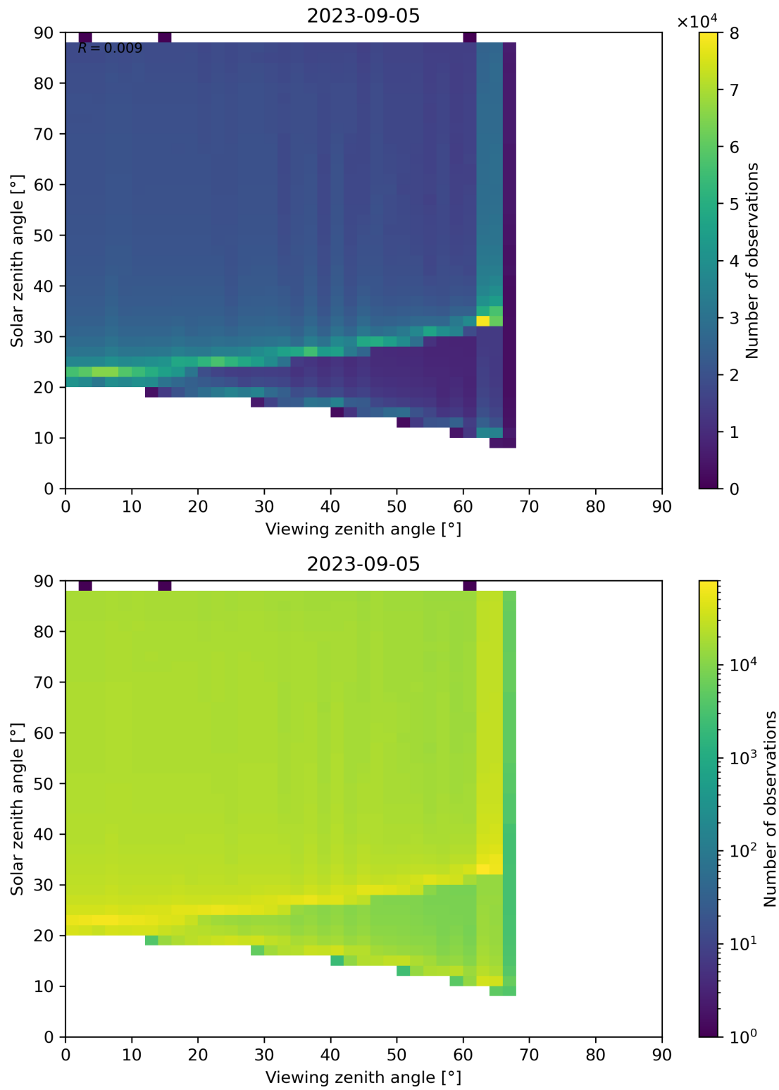
Figure 172: Scatter density plot of “Viewing zenith angle” against “Solar zenith angle” for 2023-09-05 to 2023-09-06.
