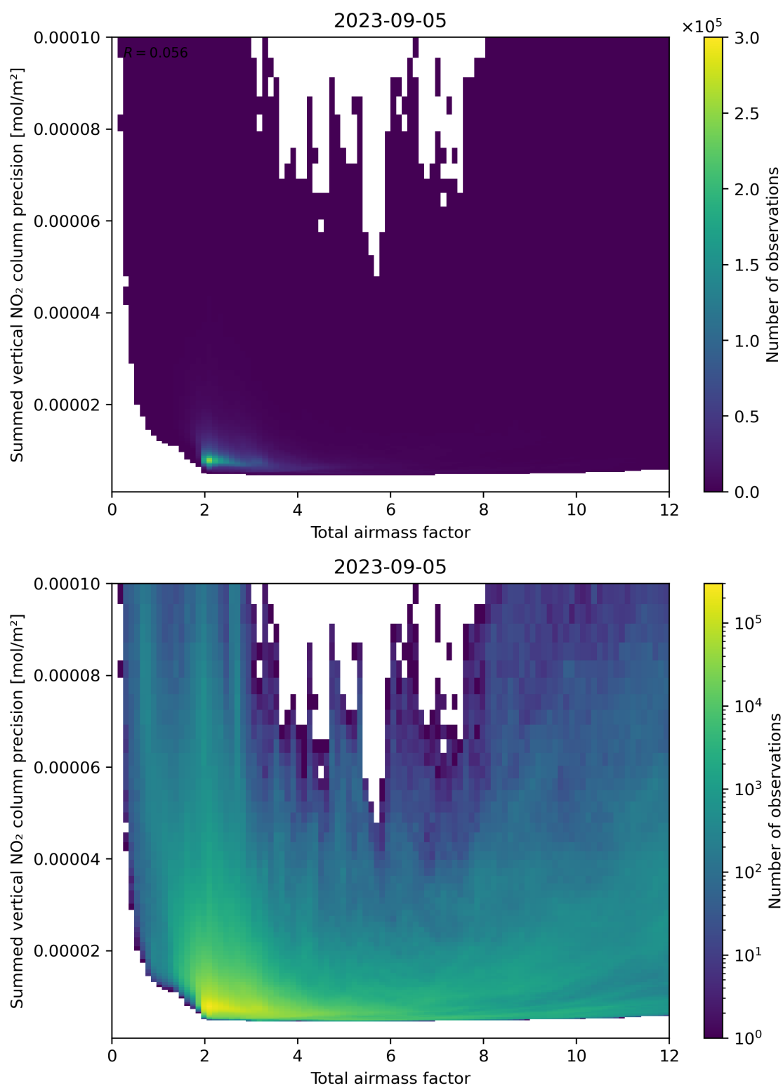
Figure 66: Scatter density plot of “Total airmass factor” against “Summed vertical NO 2 column precision” for 2023-09-05 to 2023-09-06.
