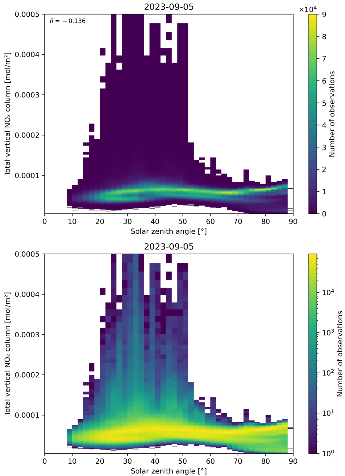
Figure 153: Scatter density plot of “Solar zenith angle” against “Total vertical NO 2 column” for 2023-09-05 to 2023-09-06.
