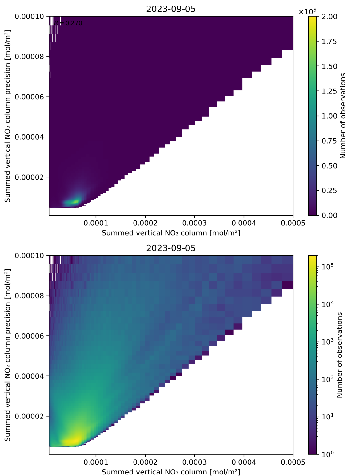
Figure 105: Scatter density plot of “Summed vertical NO 2 column” against “Summed vertical NO 2 column precision” for 2023-09-05 to 2023-09-06.
