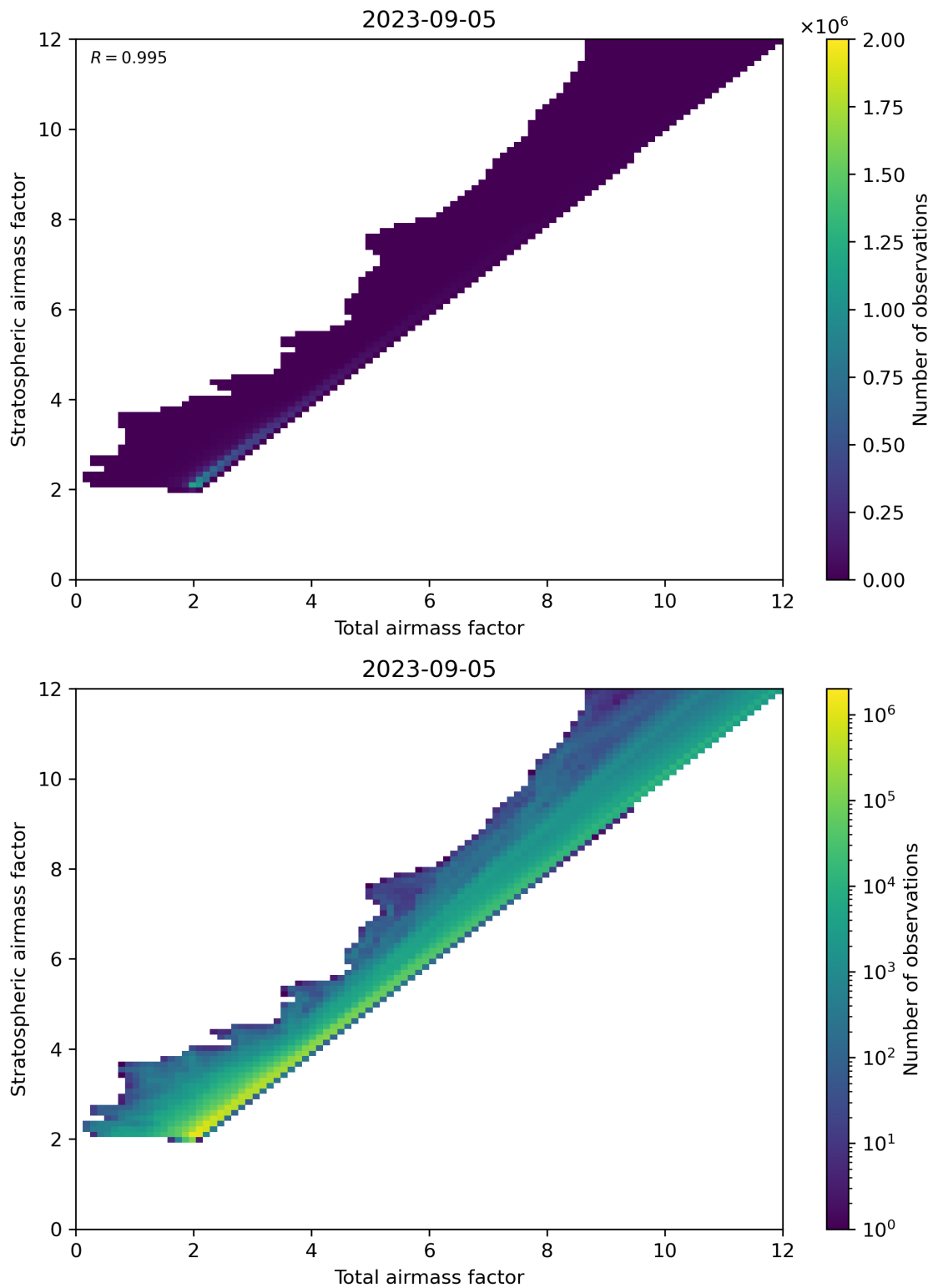
Figure 62: Scatter density plot of “Total airmass factor” against “Stratospheric airmass factor” for 2023-09-05 to 2023-09-06.
