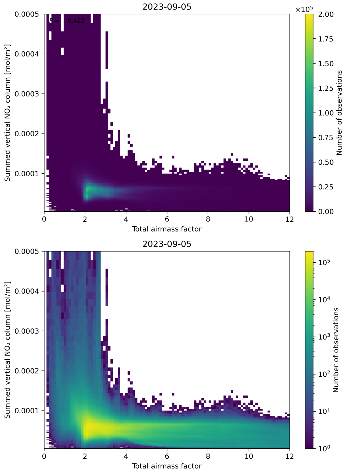
Figure 65: Scatter density plot of “Total airmass factor” against “Summed vertical NO 2 column” for 2023-09-05 to 2023-09-06.
