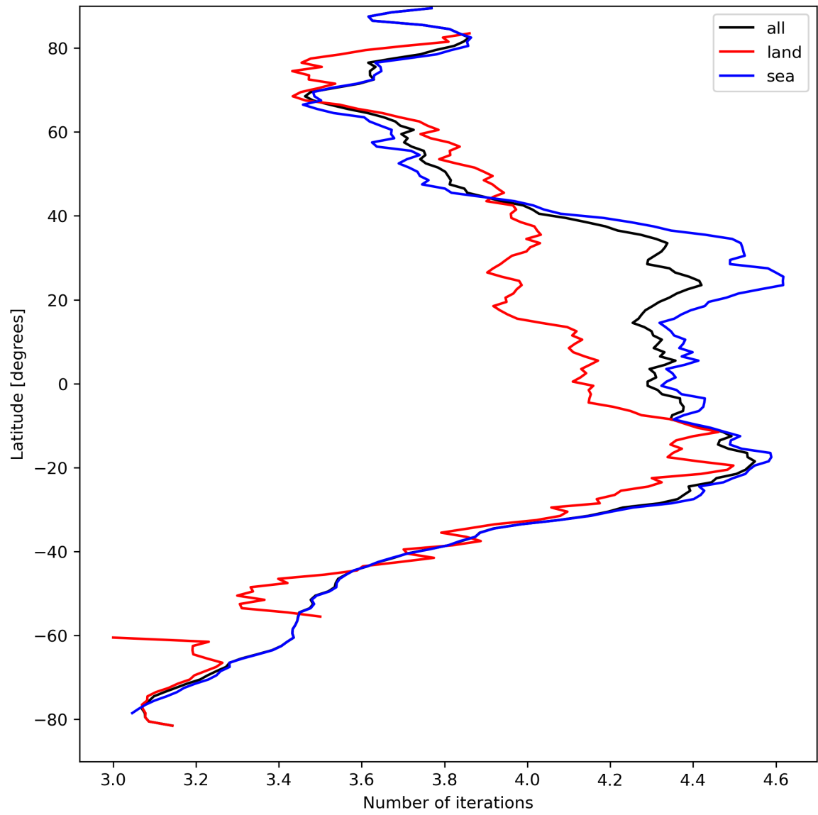
Figure 17: Zonal average of “Number of iterations” for 2023-09-05 to 2023-09-06.
