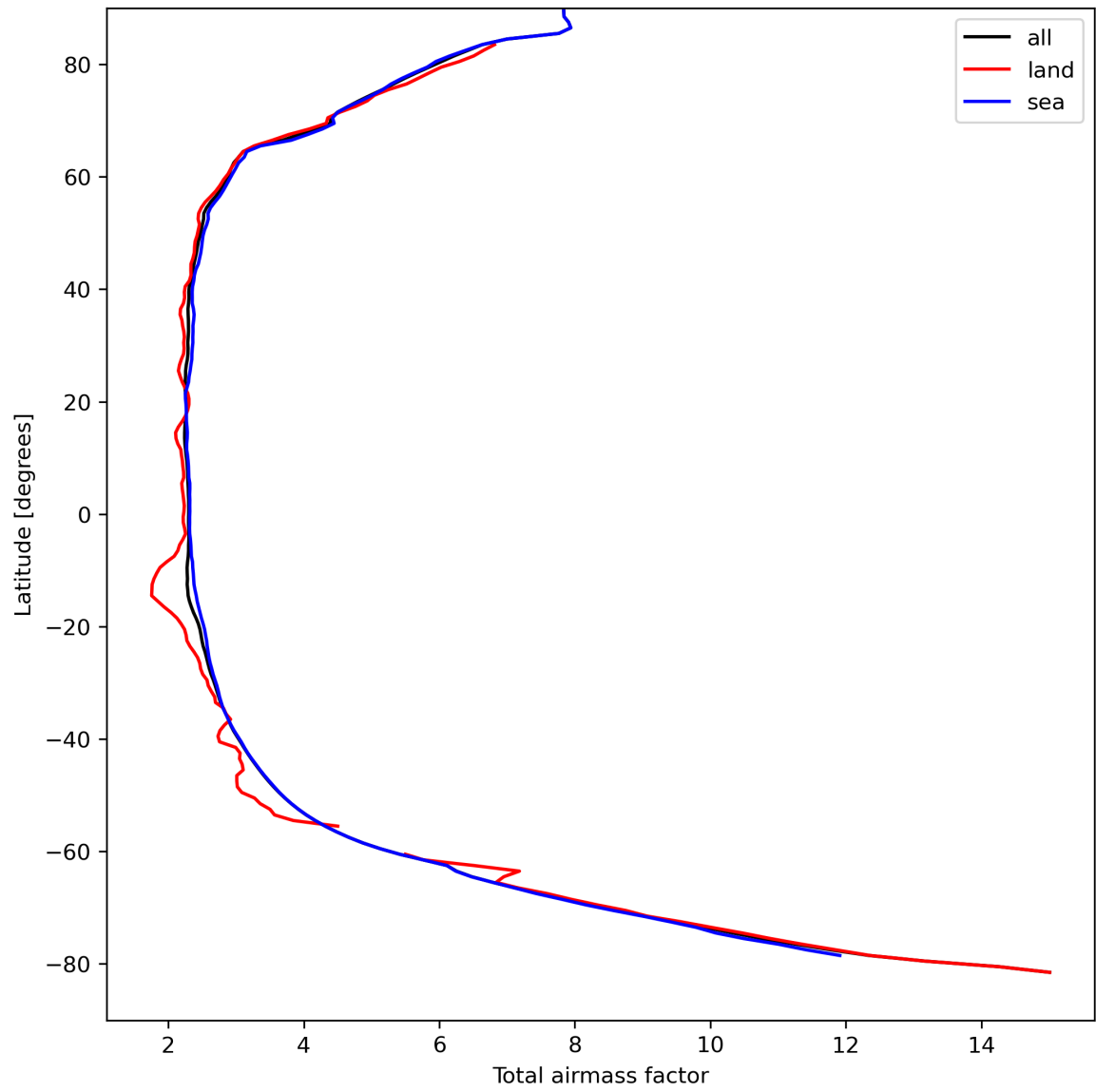
Figure 15: Zonal average of “Total airmass factor” for 2023-09-05 to 2023-09-06.
