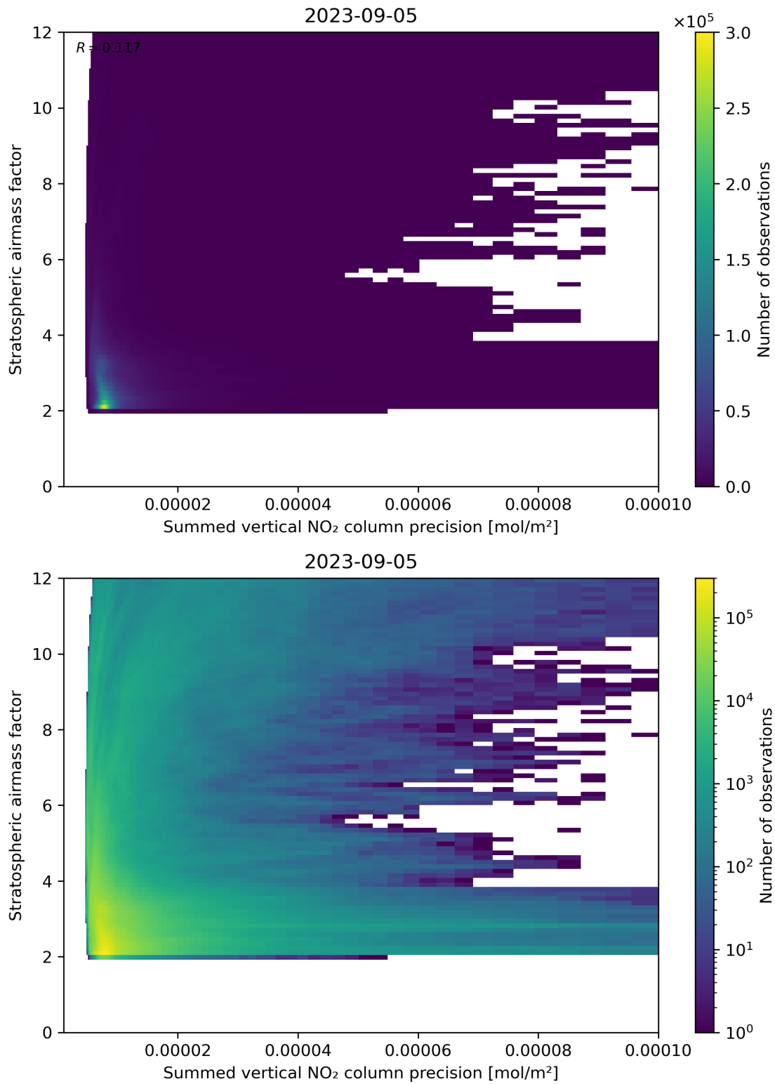
Figure 106: Scatter density plot of “Summed vertical NO 2 column precision” against “Stratospheric airmass factor” for 2023-09-05 to 2023-09-06.
