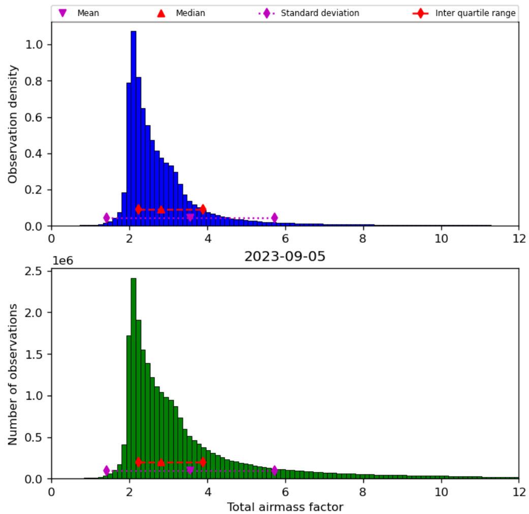
Figure 32: Histogram of “Total airmass factor” for 2023-09-05 to 2023-09-06
