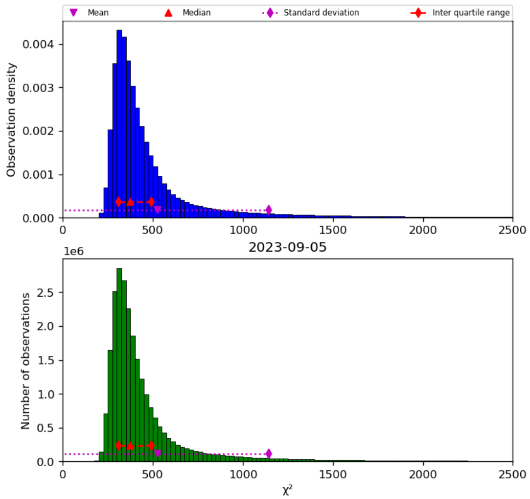
Figure 42: Histogram of “ \chi^2 ” for 2023-09-05 to 2023-09-06
