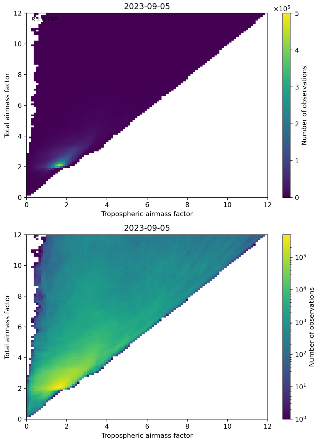
Figure 72: Scatter density plot of “Tropospheric airmass factor” against “Total airmass factor” for 2023-09-05 to 2023-09-06.
