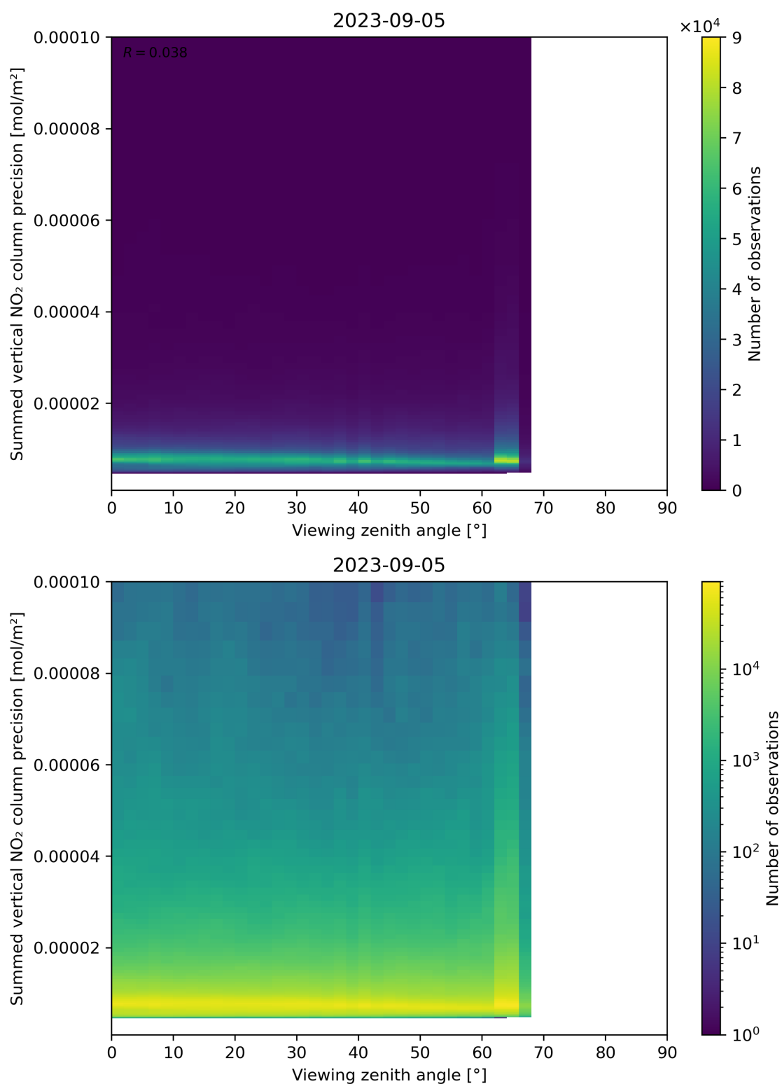
Figure 166: Scatter density plot of “Viewing zenith angle” against “Summed vertical NO 2 column precision” for 2023-09-05 to 2023-09-06.
