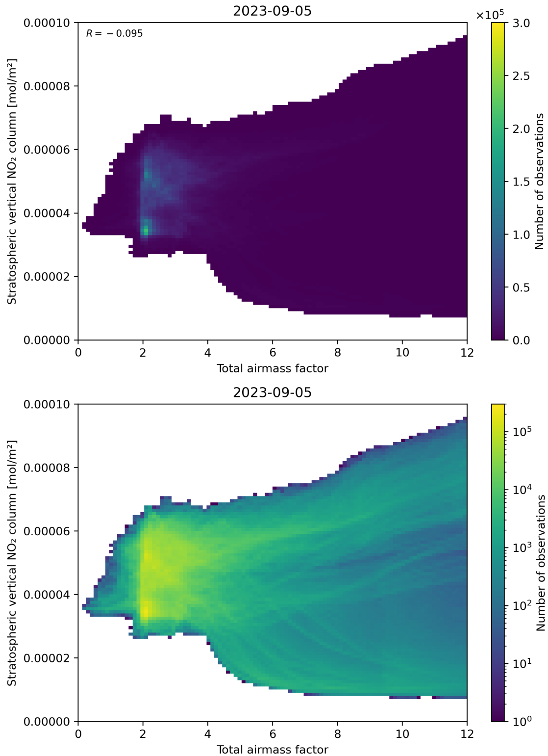
Figure 64: Scatter density plot of “Total airmass factor” against “Stratospheric vertical NO 2 column” for 2023-09-05 to 2023-09-06.
