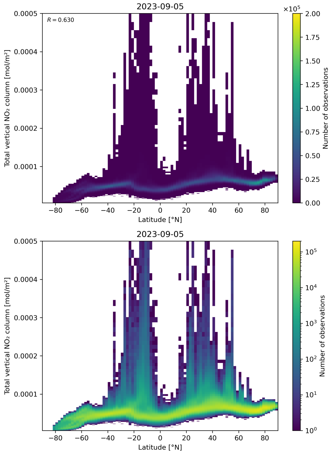
Figure 90: Scatter density plot of “Latitude” against “Total vertical NO 2 column” for 2023-09-05 to 2023-09-06.
