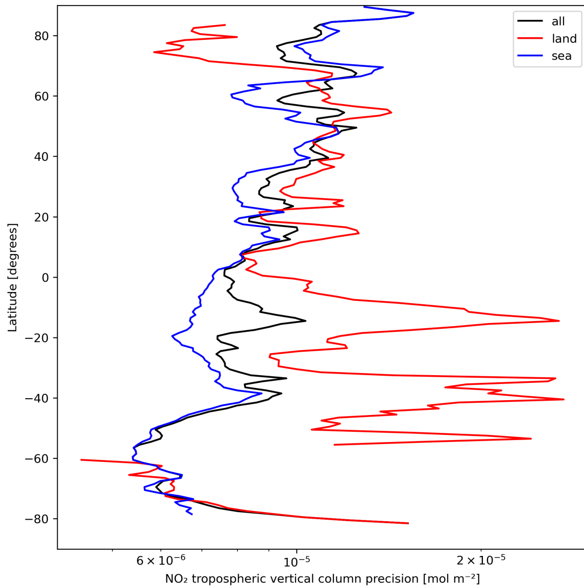
Figure 13: Zonal average of “NO 2 tropospheric vertical column precision” for 2023-09-05 to 2023-09-06.
