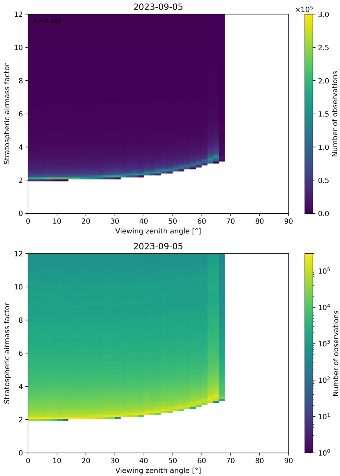
Figure 159: Scatter density plot of “Viewing zenith angle” against “Stratospheric airmass factor” for 2023-09-05 to 2023-09-06.
