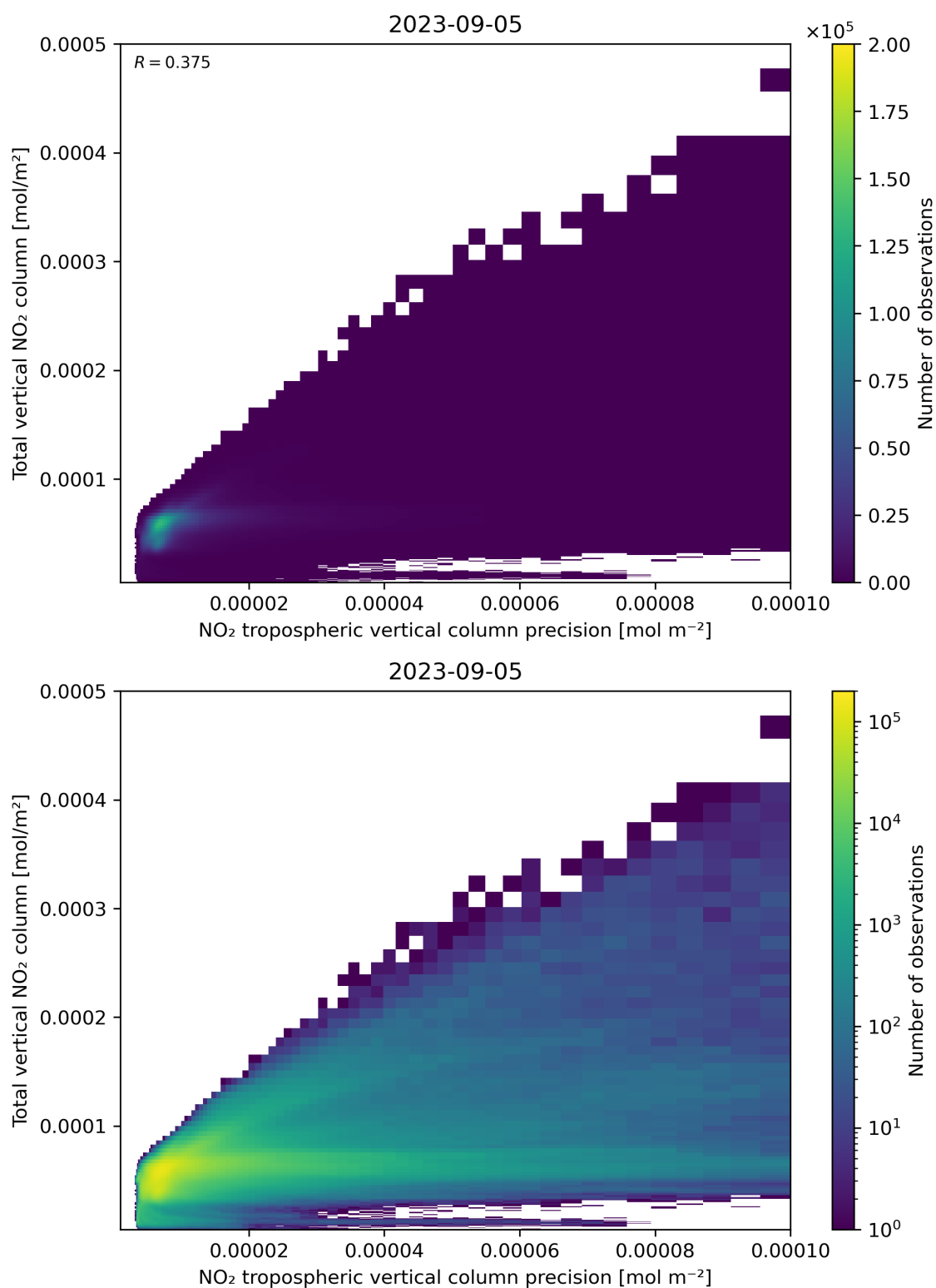
Figure 138: Scatter density plot of “NO 2 tropospheric vertical column precision” against “Total vertical NO 2 column” for 2023-09-05 to 2023-09-06.
