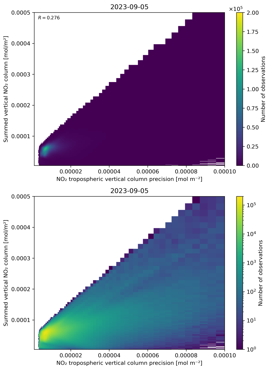
Figure 136: Scatter density plot of “NO 2 tropospheric vertical column precision” against “Summed vertical NO 2 column” for 2023-09-05 to 2023-09-06.
