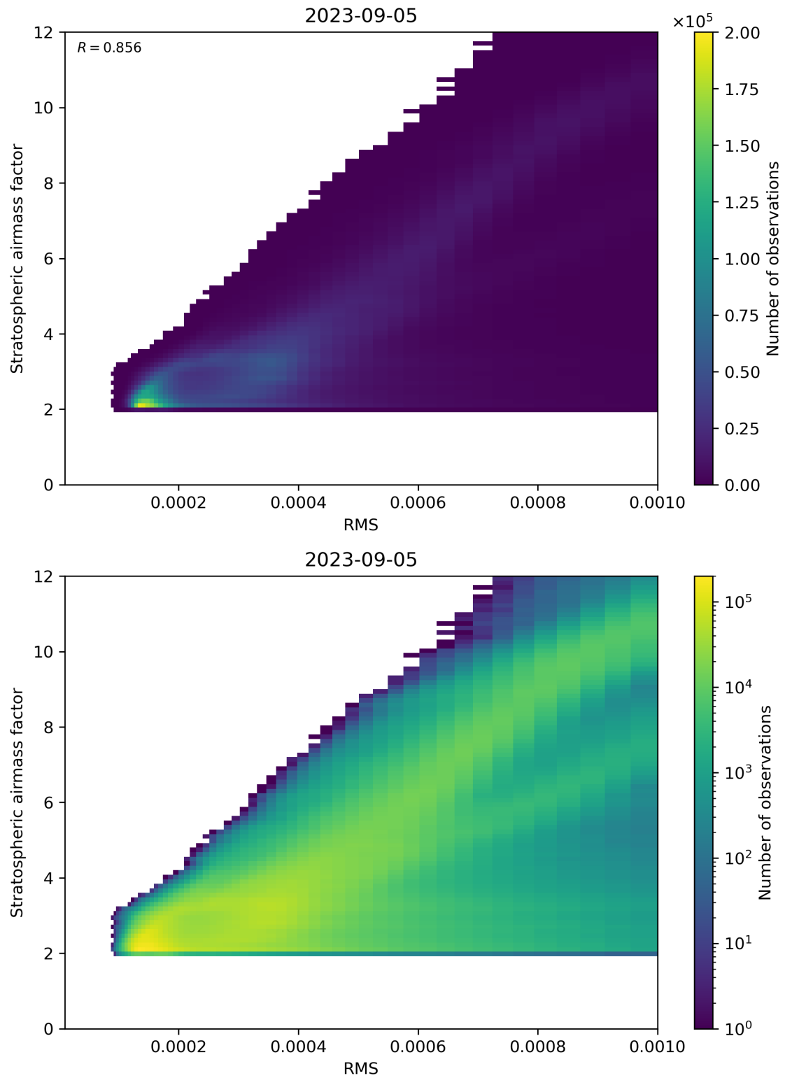
Figure 144: Scatter density plot of “RMS” against “Stratospheric airmass factor” for 2023-09-05 to 2023-09-06.
