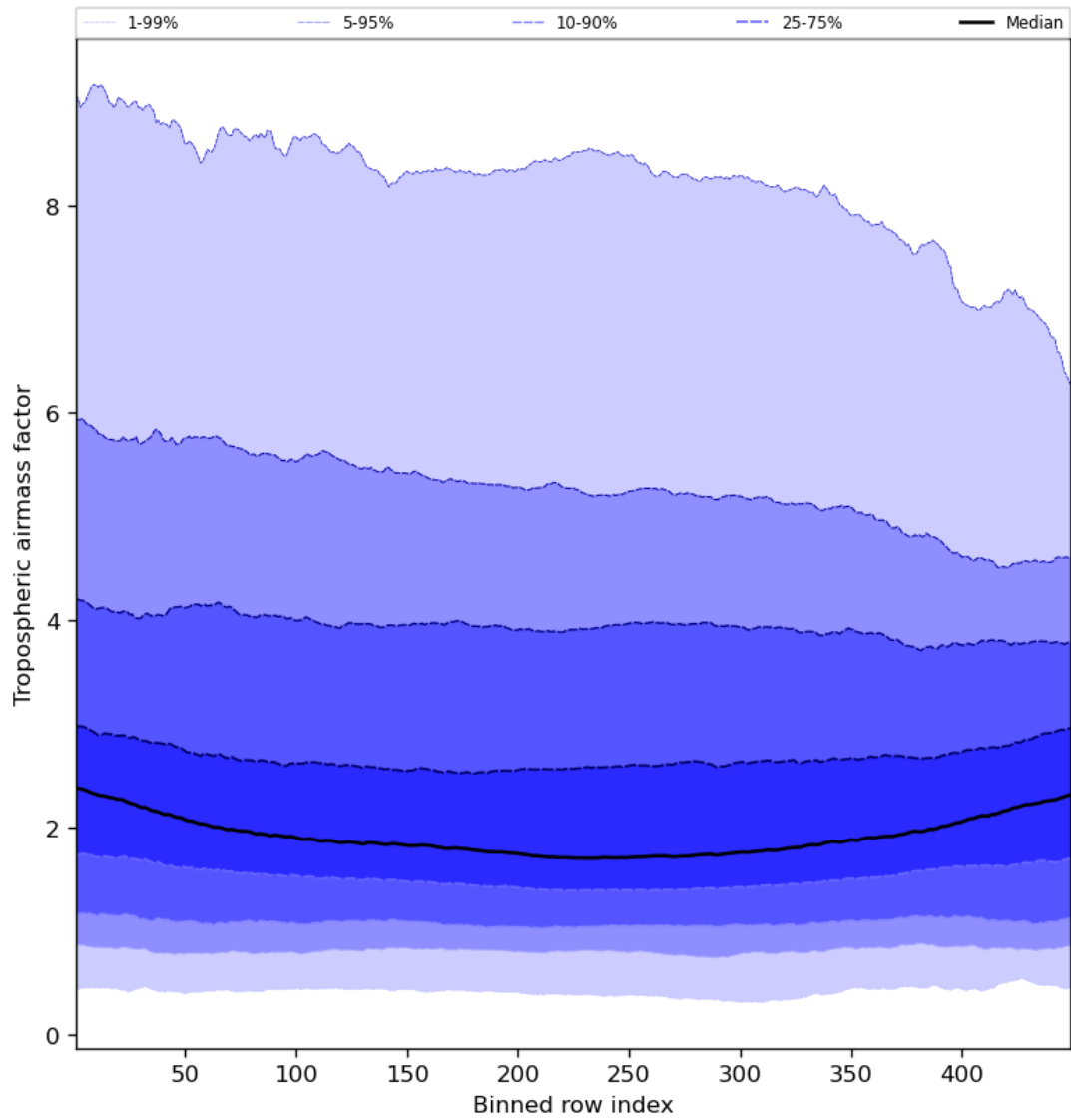
Figure 48: Along track statistics of “Tropospheric air mass factor” for 2023-09-05 to 2023-09-06
