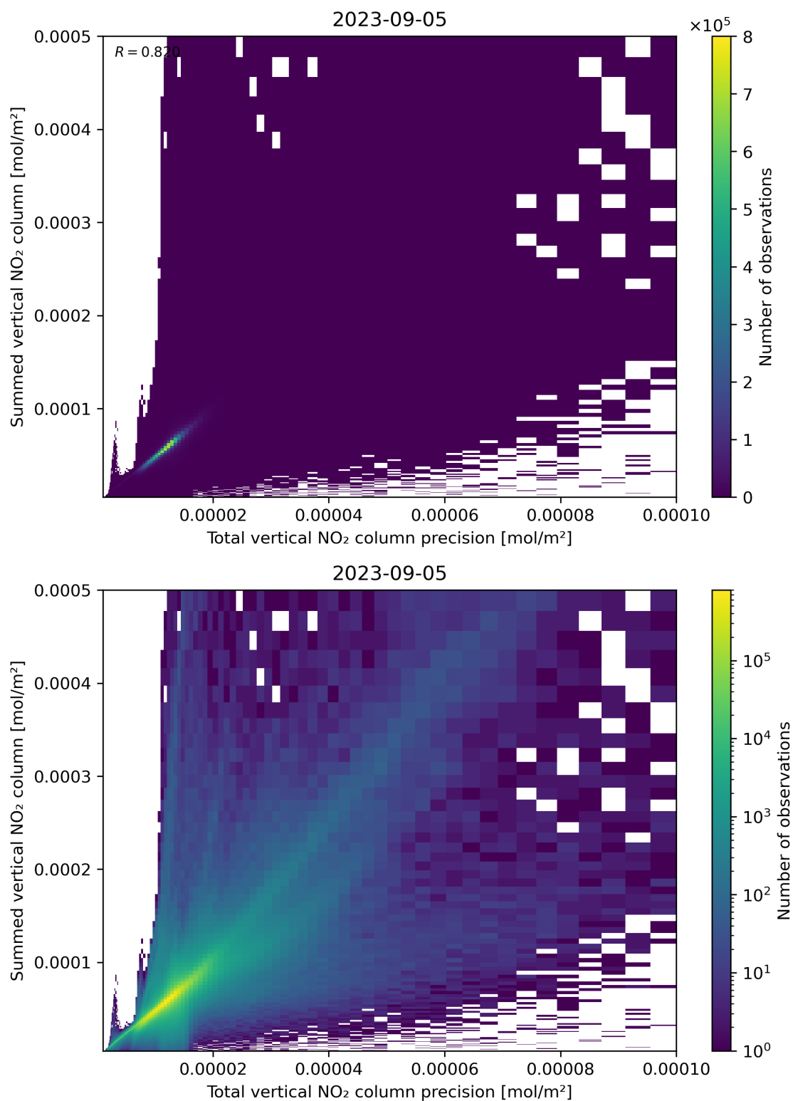
Figure 117: Scatter density plot of “Total vertical NO 2 column precision” against “Summed vertical NO 2 column” for 2023-09-05 to 2023-09-06.
