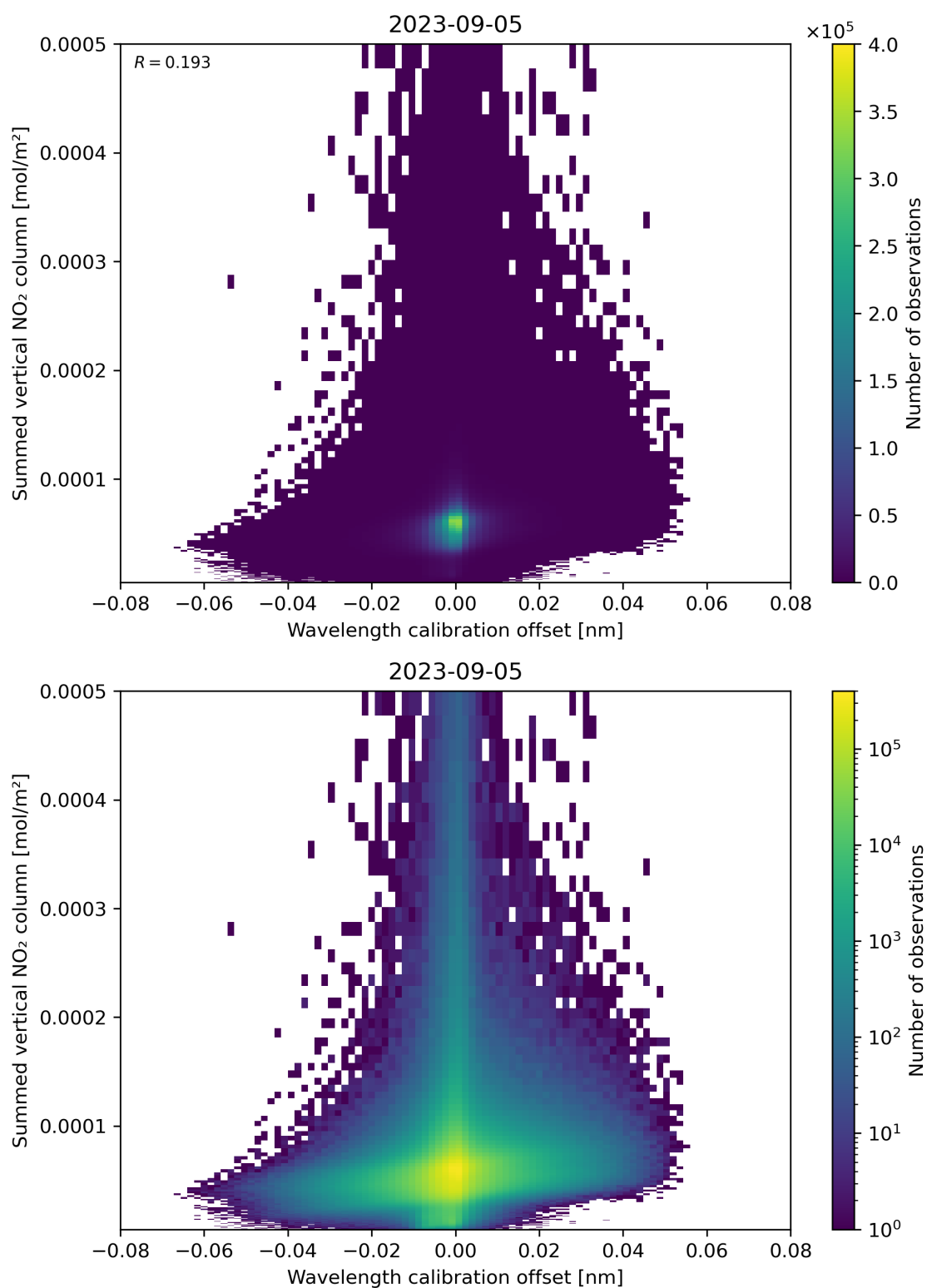
Figure 177: Scatter density plot of “Wavelength calibration offset” against “Summed vertical NO 2 column” for 2023-09-05 to 2023-09-06.
