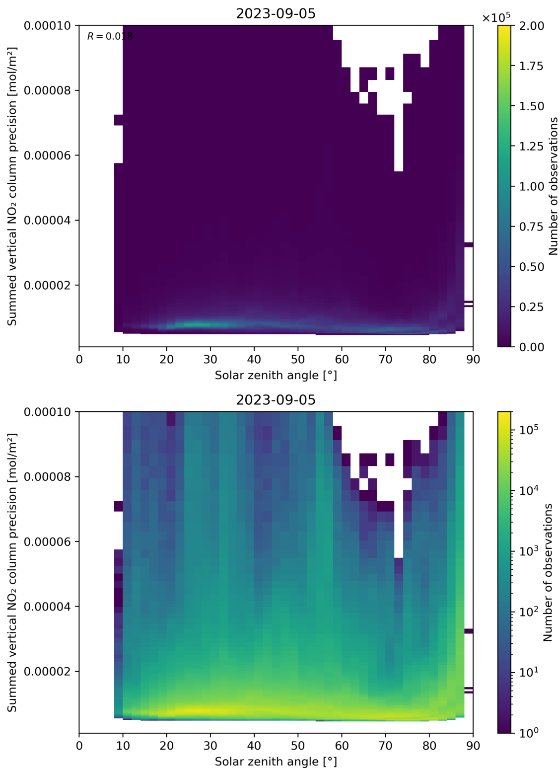
Figure 152: Scatter density plot of “Solar zenith angle” against “Summed vertical NO 2 column precision” for 2023-09-05 to 2023-09-06.
