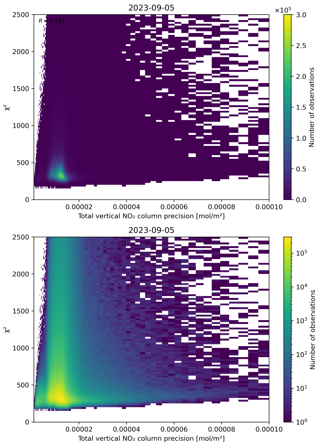
Figure 116: Scatter density plot of “Total vertical NO 2 column precision” against “ \chi^2 ” for 2023-09-05 to 2023-09-06.
