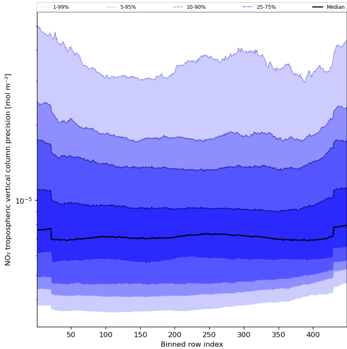
Figure 47: Along track statistics of “NO 2 tropospheric vertical column precision” for 2023-09-05 to 2023-09-06
