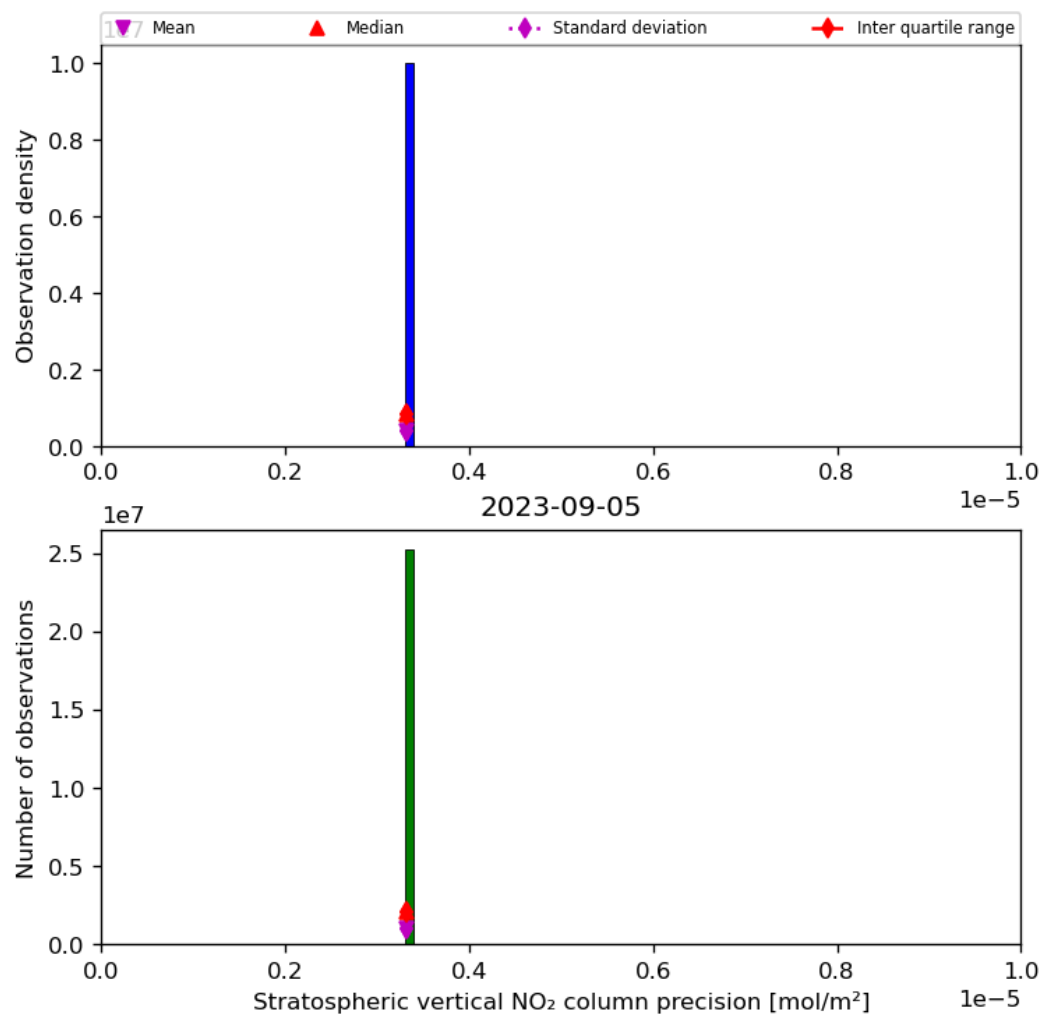
Figure 37: Histogram of “Stratospheric vertical NO 2 column precision” for 2023-09-05 to 2023-09-06
