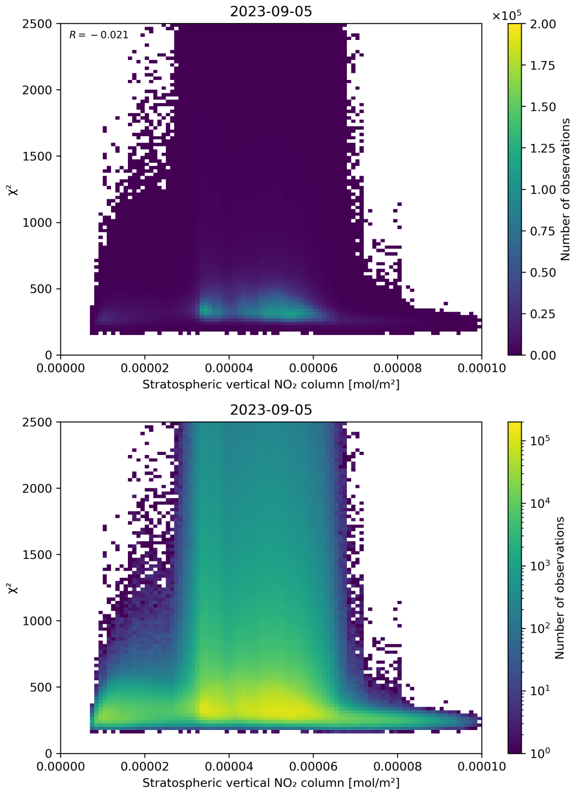
Figure 97: Scatter density plot of “Stratospheric vertical NO 2 column” against “ \chi^2 ” for 2023-09-05 to 2023-09-06.
