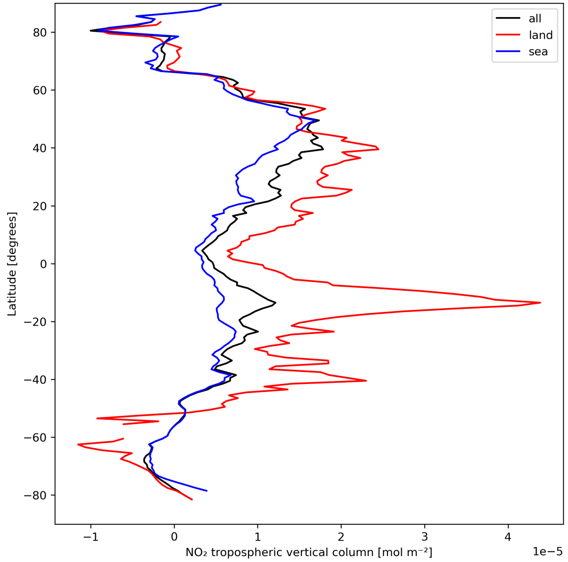
Figure 12: Zonal average of “NO 2 tropospheric vertical column” for 2023-09-05 to 2023-09-06.
