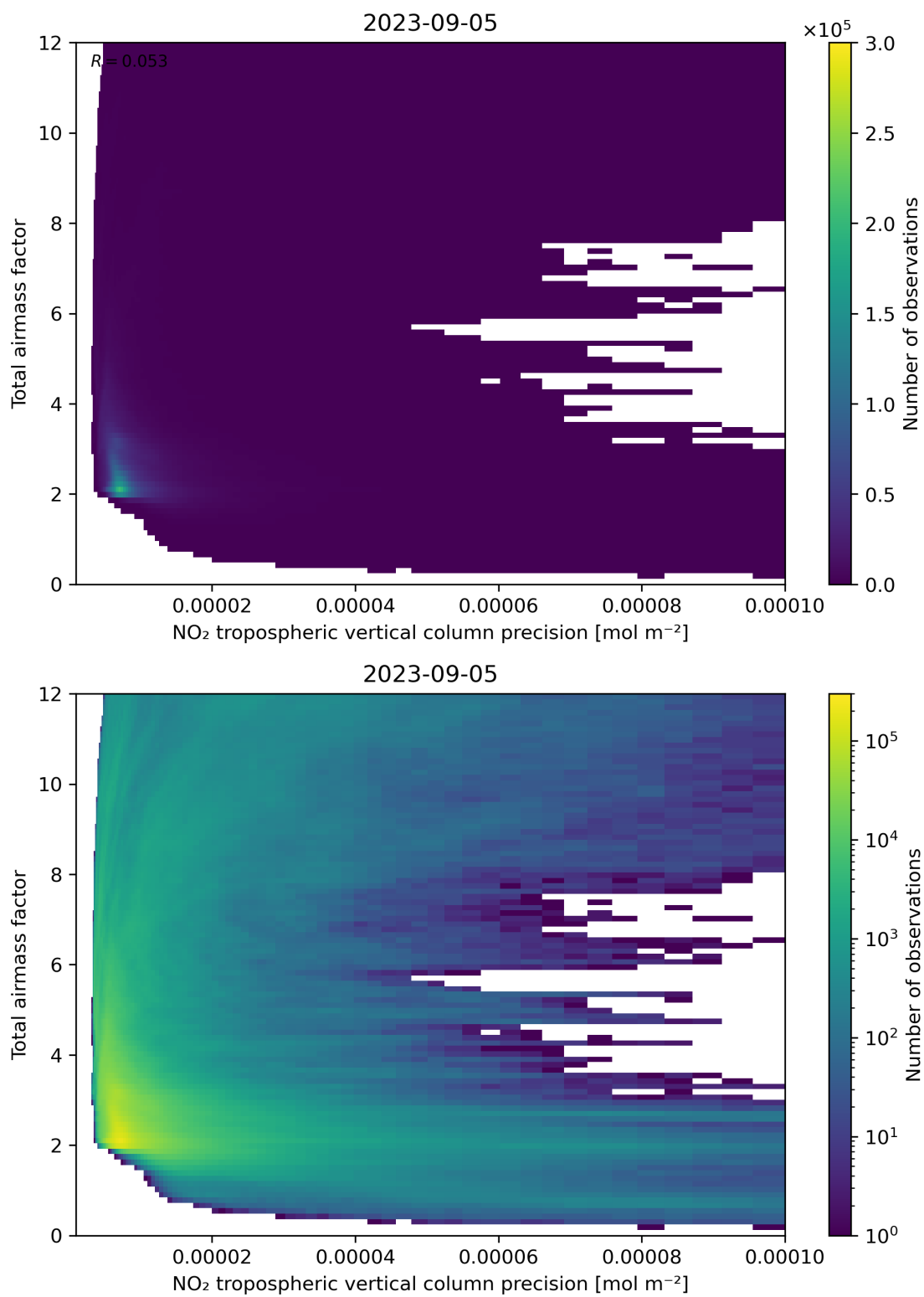
Figure 132: Scatter density plot of “NO 2 tropospheric vertical column precision” against “Total air mass factor” for 2023-09-05 to 2023-09-06.
