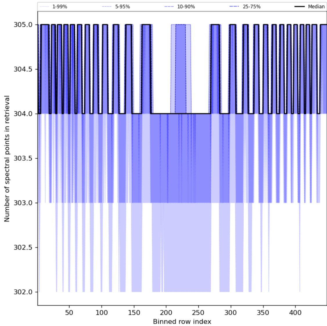
Figure 50: Along track statistics of “Number of spectral points in retrieval” for 2023-09-05 to 2023-09-06
