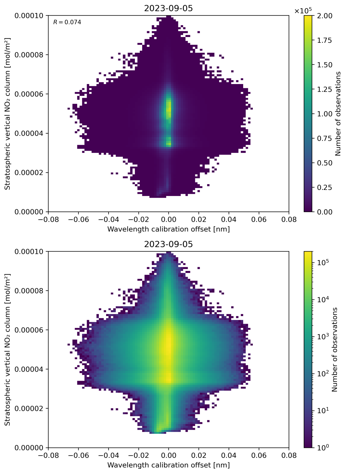
Figure 176: Scatter density plot of “Wavelength calibration offset” against “Stratospheric vertical NO 2 column” for 2023-09-05 to 2023-09-06.
