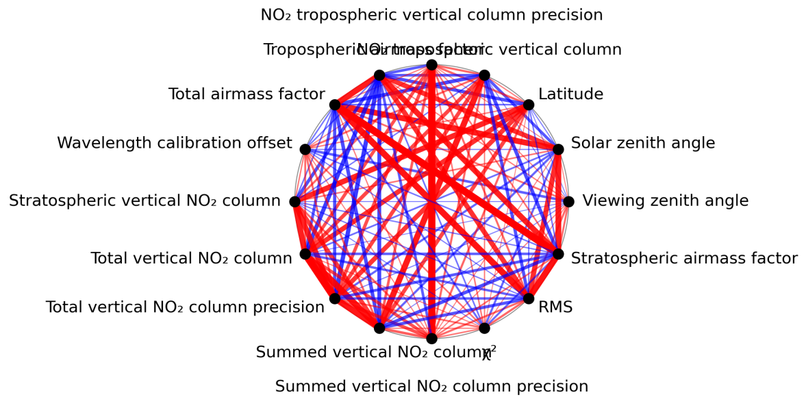
Figure 1: Map of correlation graph for 2023-09-05 to 2023-09-06.
