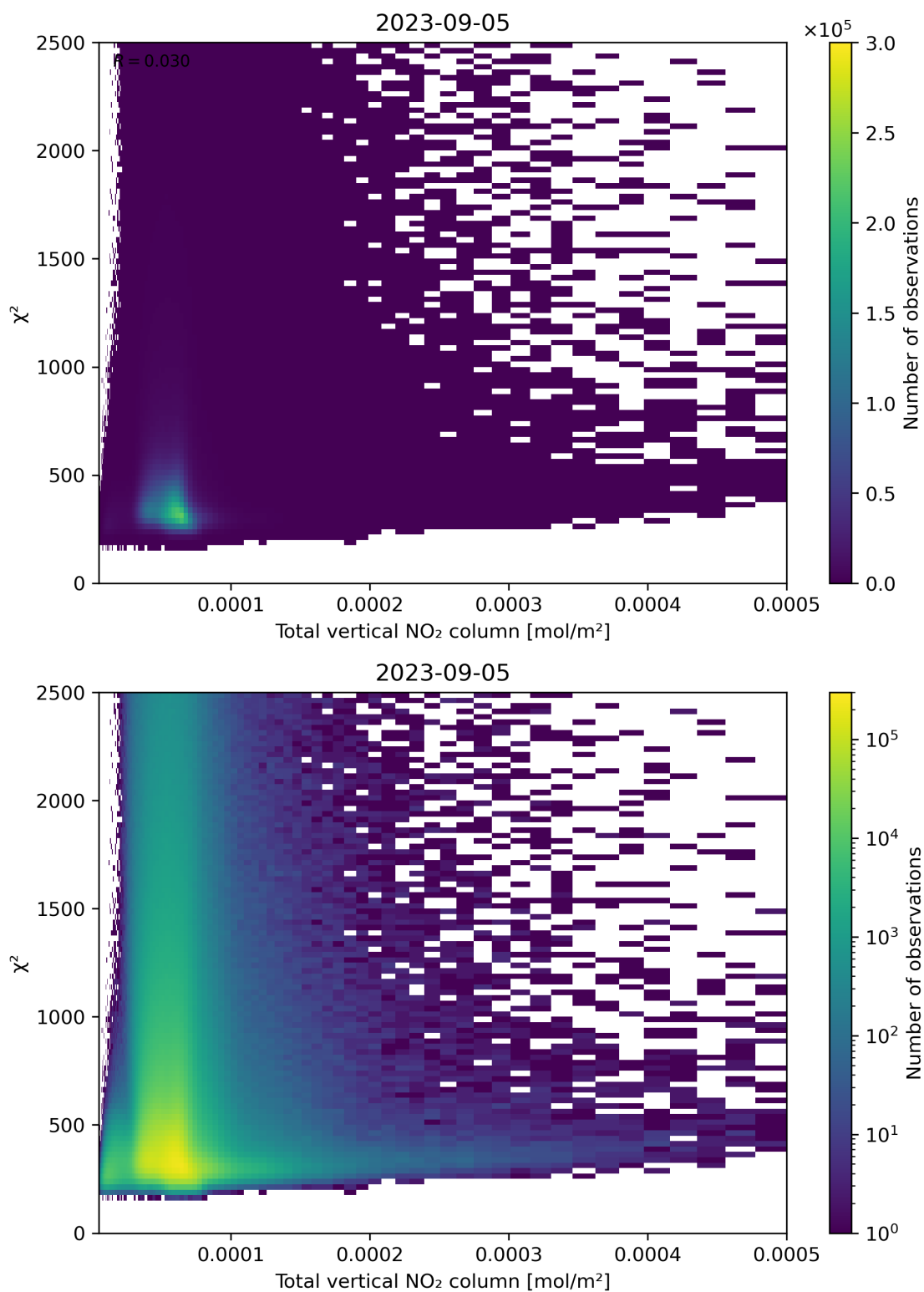
Figure 111: Scatter density plot of “Total vertical NO 2 column” against “ \chi^2 ” for 2023-09-05 to 2023-09-06.
