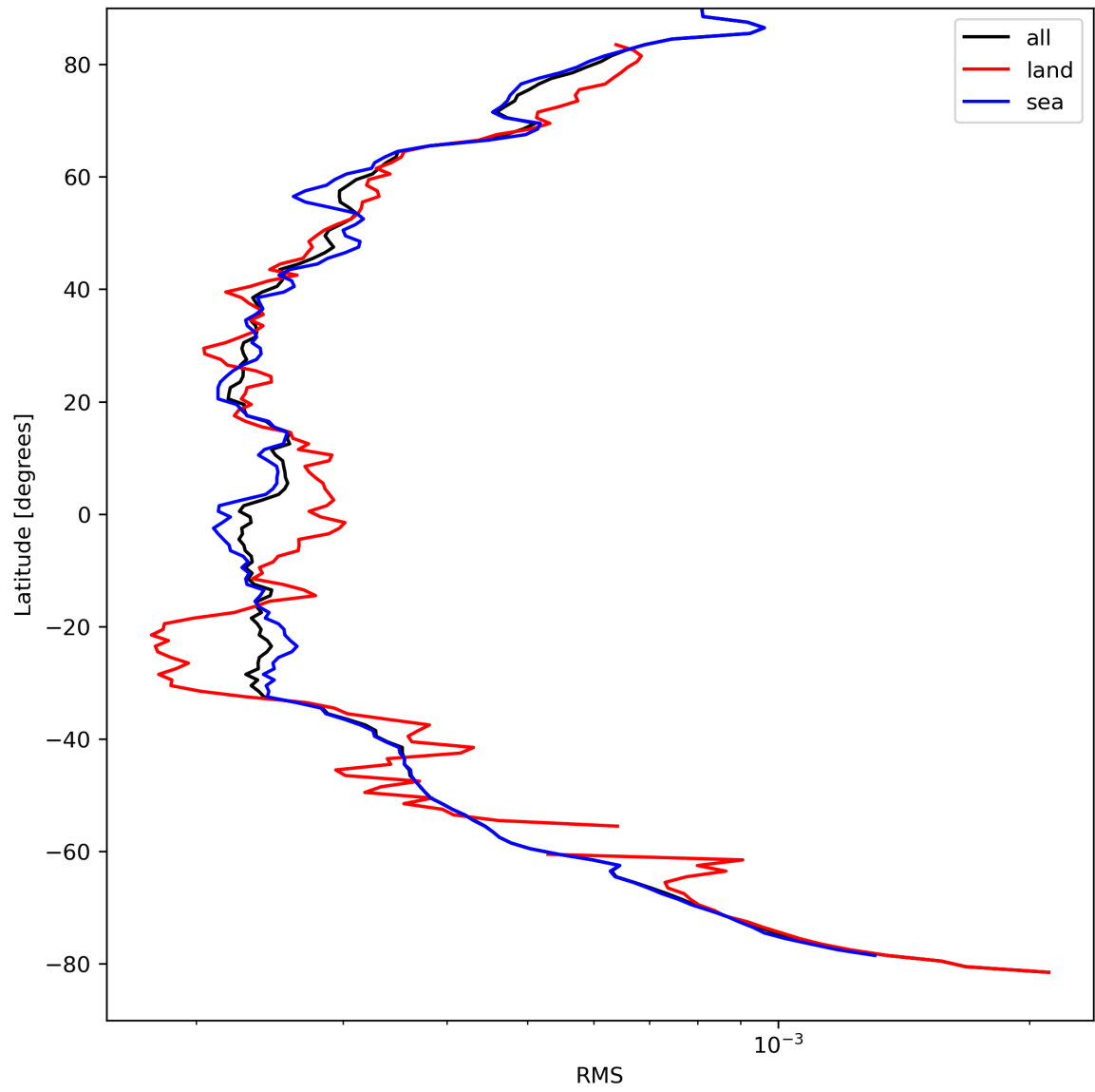
Figure 26: Zonal average of “RMS” for 2023-09-05 to 2023-09-06.
