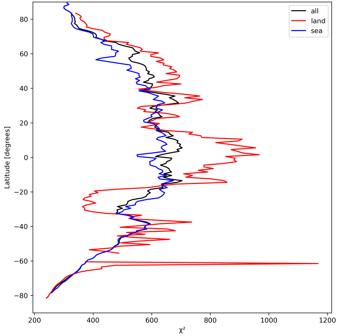
Figure 25: Zonal average of “ \chi^2 ” for 2023-09-05 to 2023-09-06.
