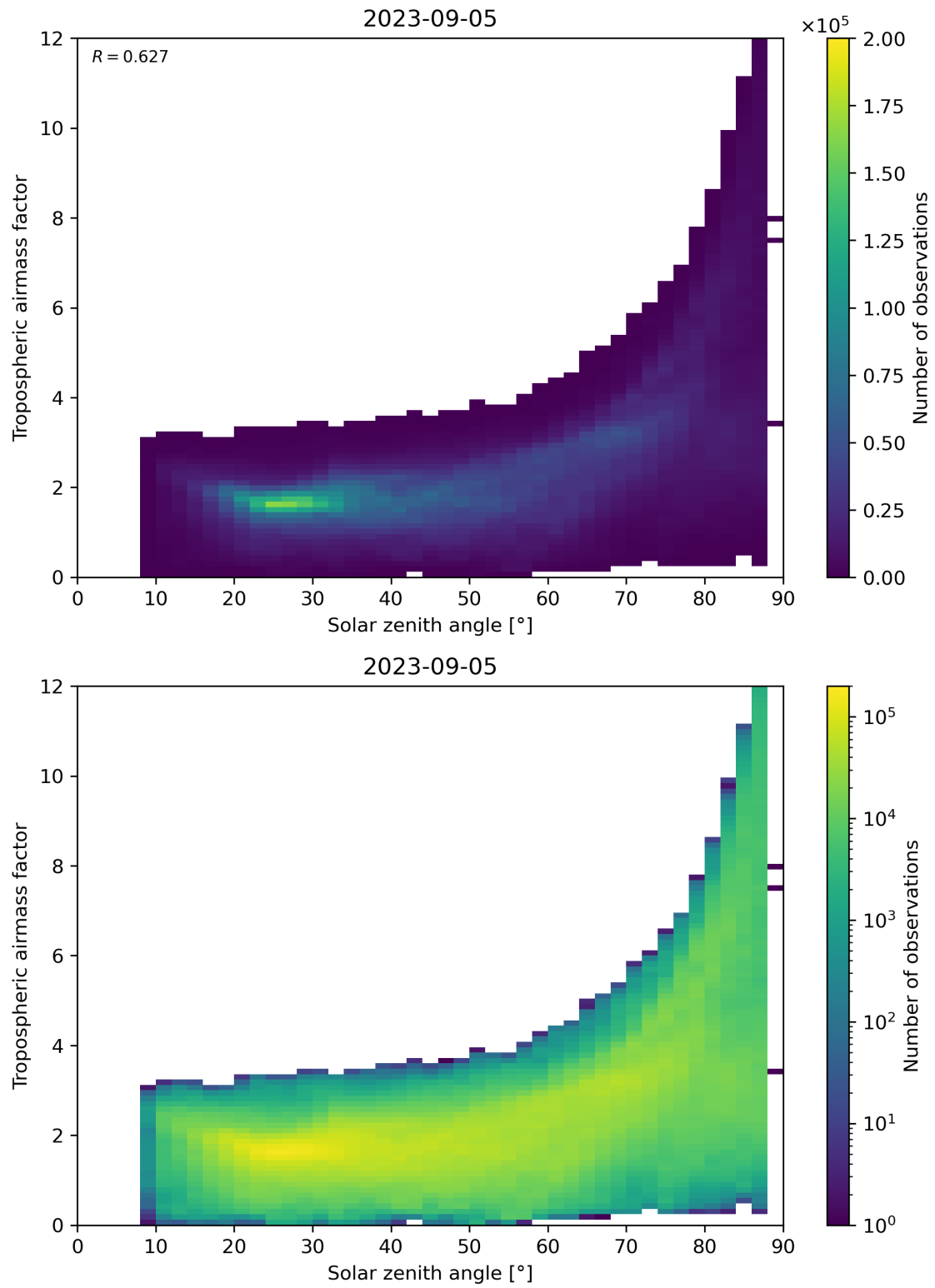
Figure 147: Scatter density plot of “Solar zenith angle” against “Tropospheric airmass factor” for 2023-09-05 to 2023-09-06.
