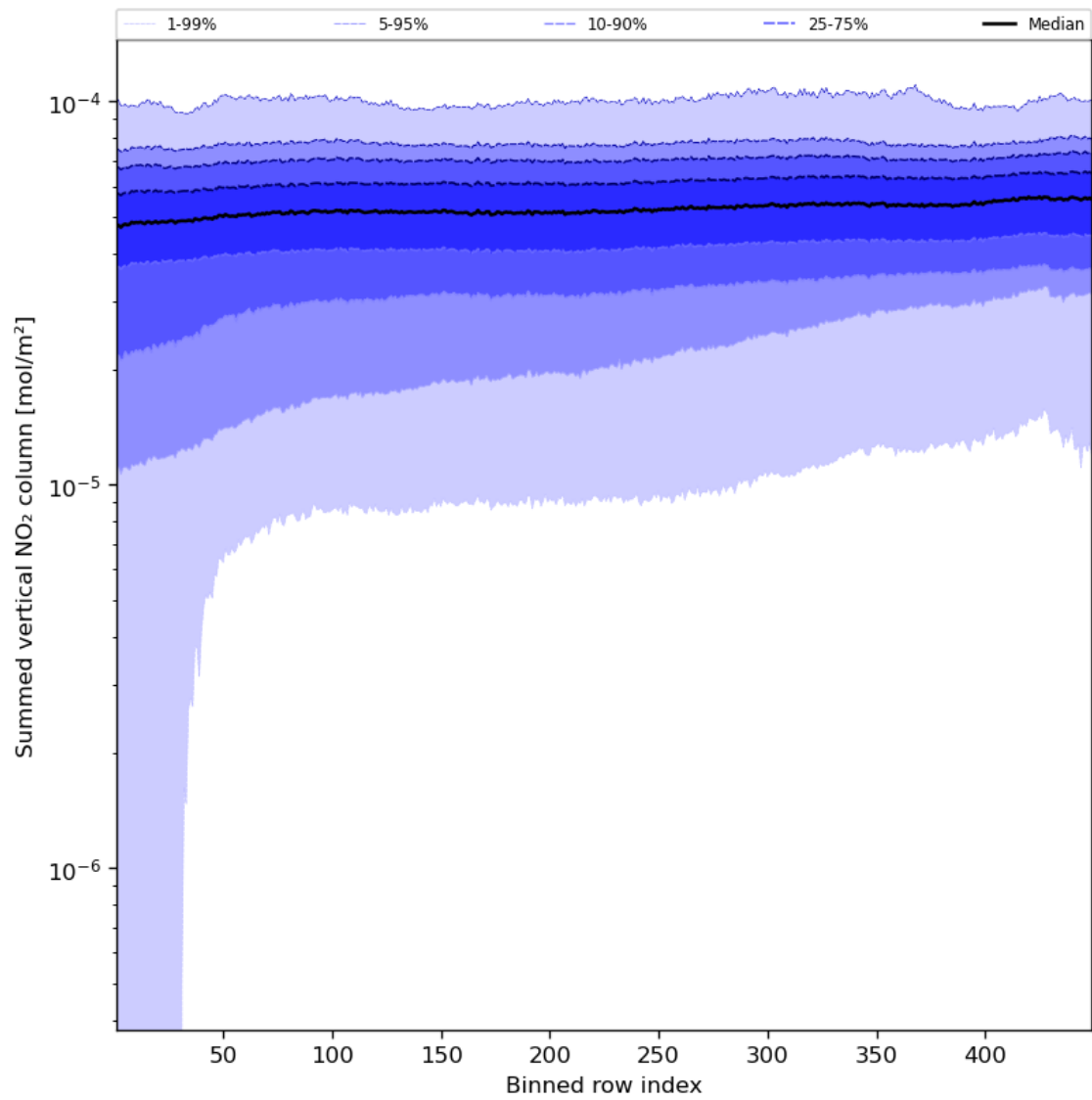
Figure 57: Along track statistics of “Summed vertical NO 2 column” for 2023-09-05 to 2023-09-06
