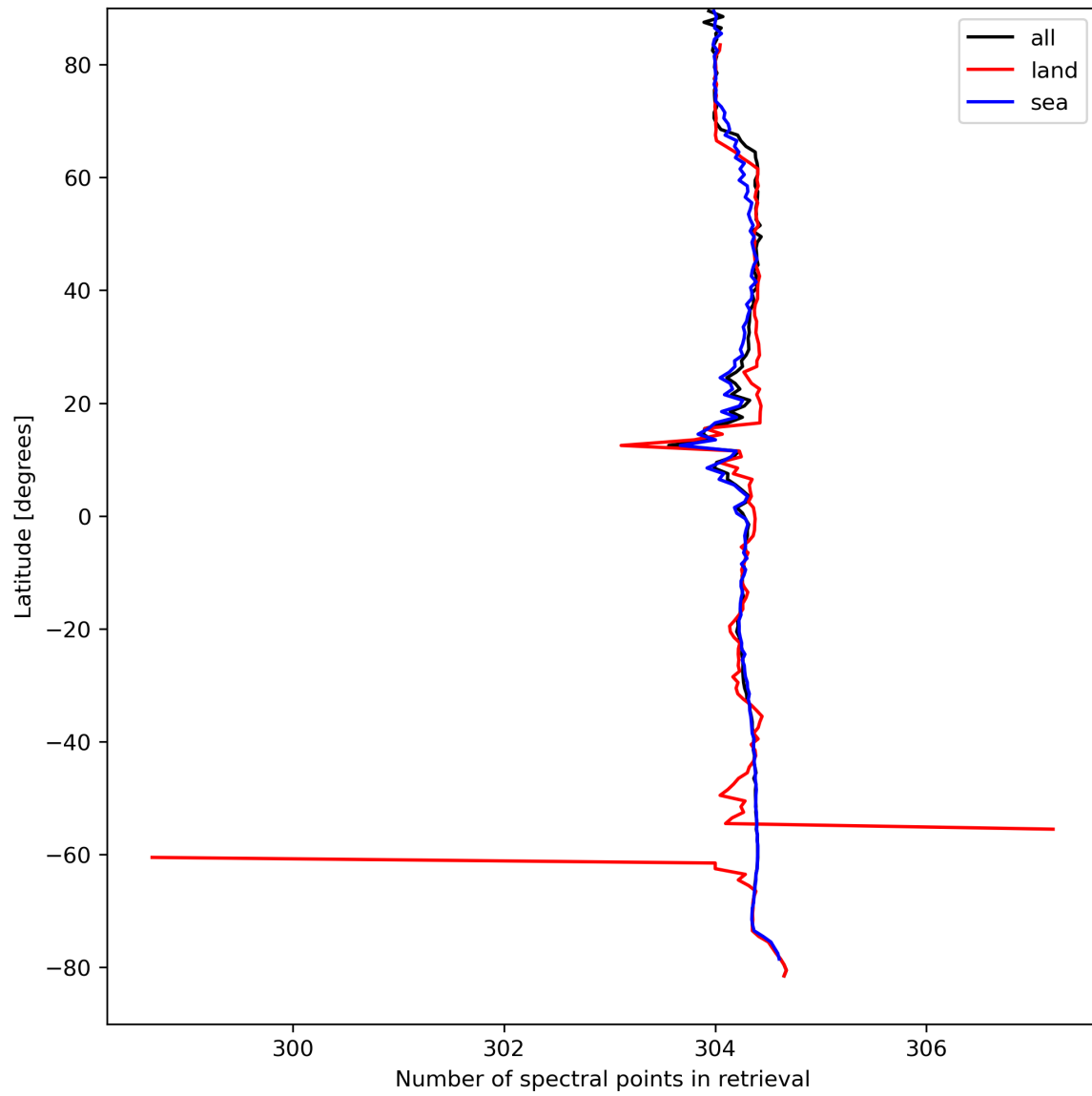
Figure 16: Zonal average of “Number of spectral points in retrieval” for 2023-09-05 to 2023-09-06.
