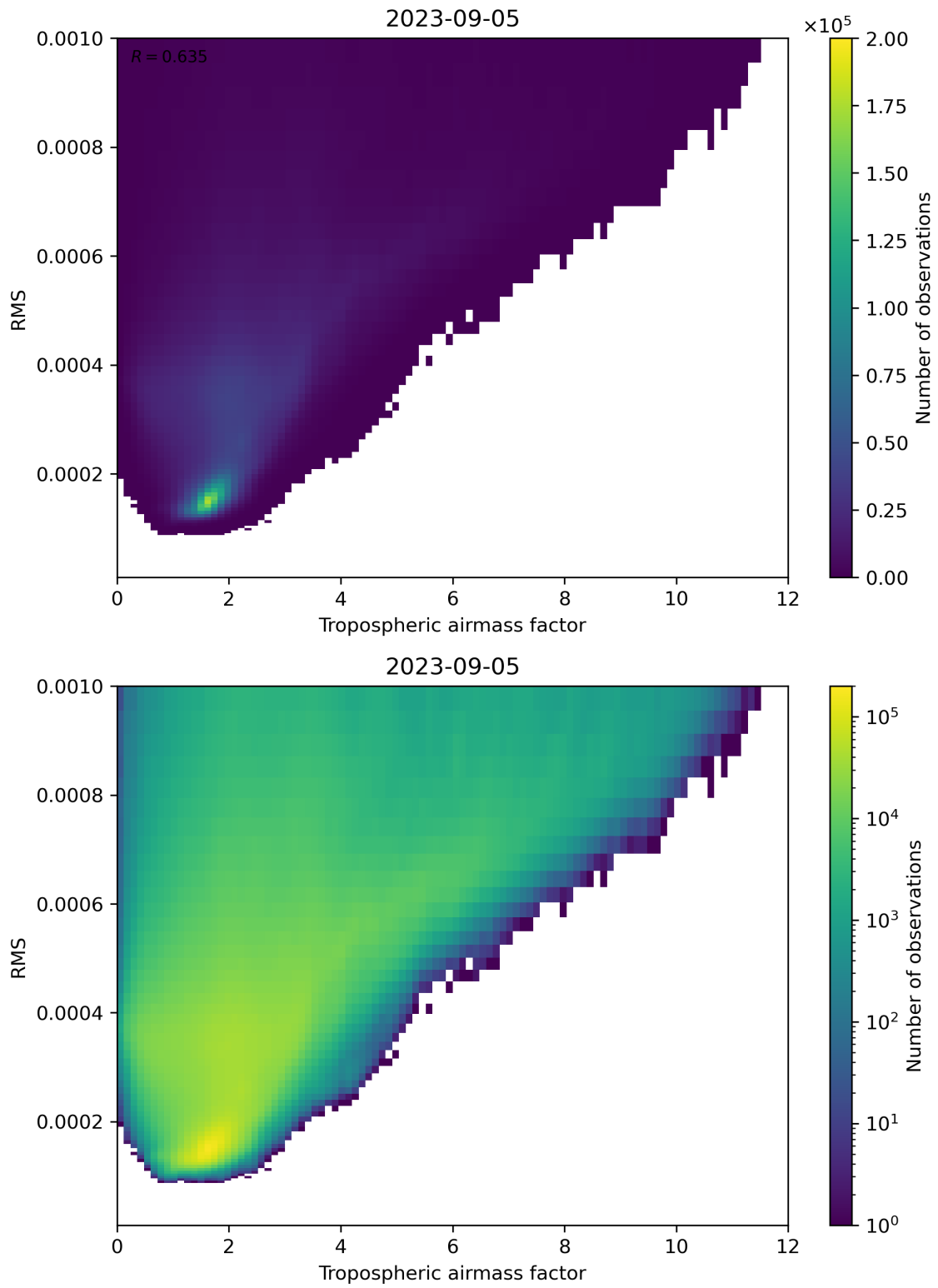
Figure 79: Scatter density plot of “Tropospheric airmass factor” against “RMS” for 2023-09-05 to 2023-09-06.
