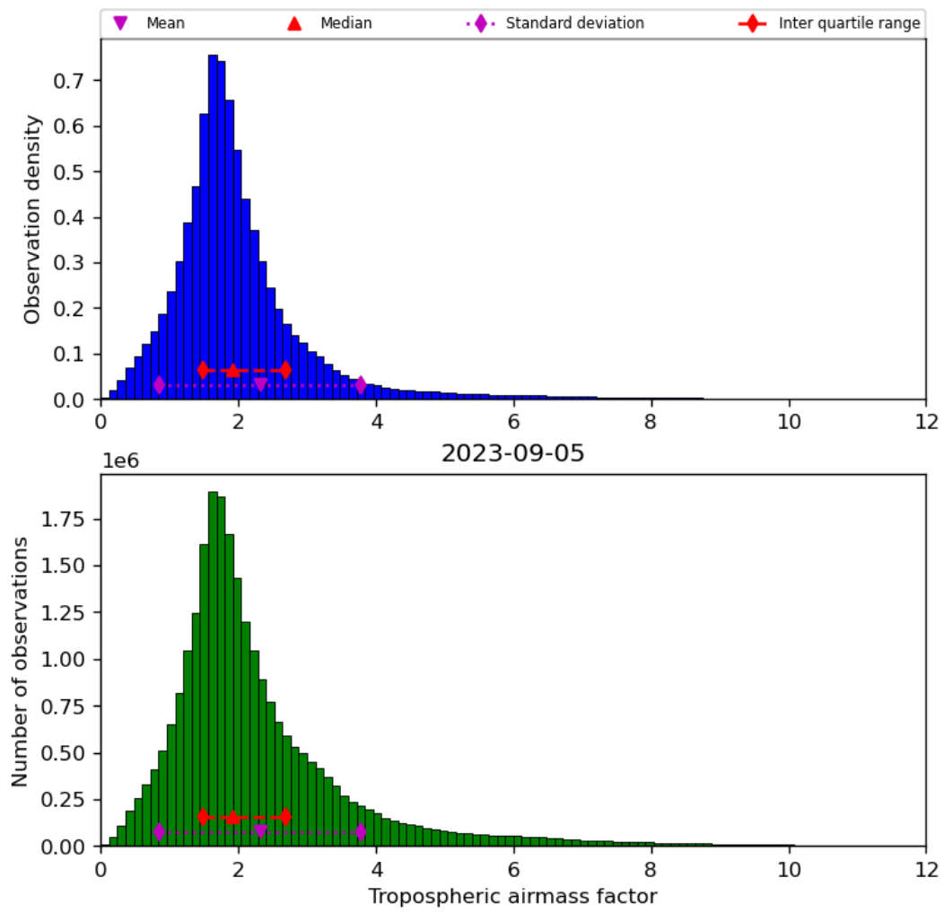
Figure 31: Histogram of “Tropospheric airmass factor” for 2023-09-05 to 2023-09-06
