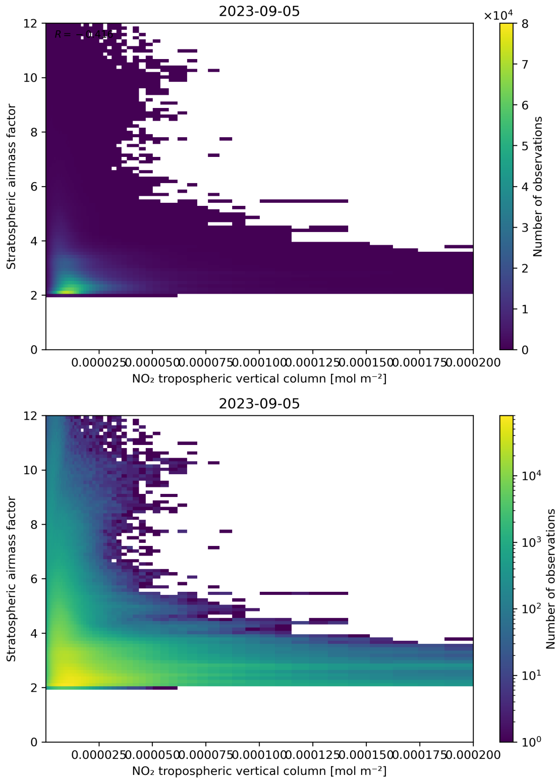
Figure 121: Scatter density plot of “NO 2 tropospheric vertical column” against “Stratospheric air mass factor” for 2023-09-05 to 2023-09-06.
