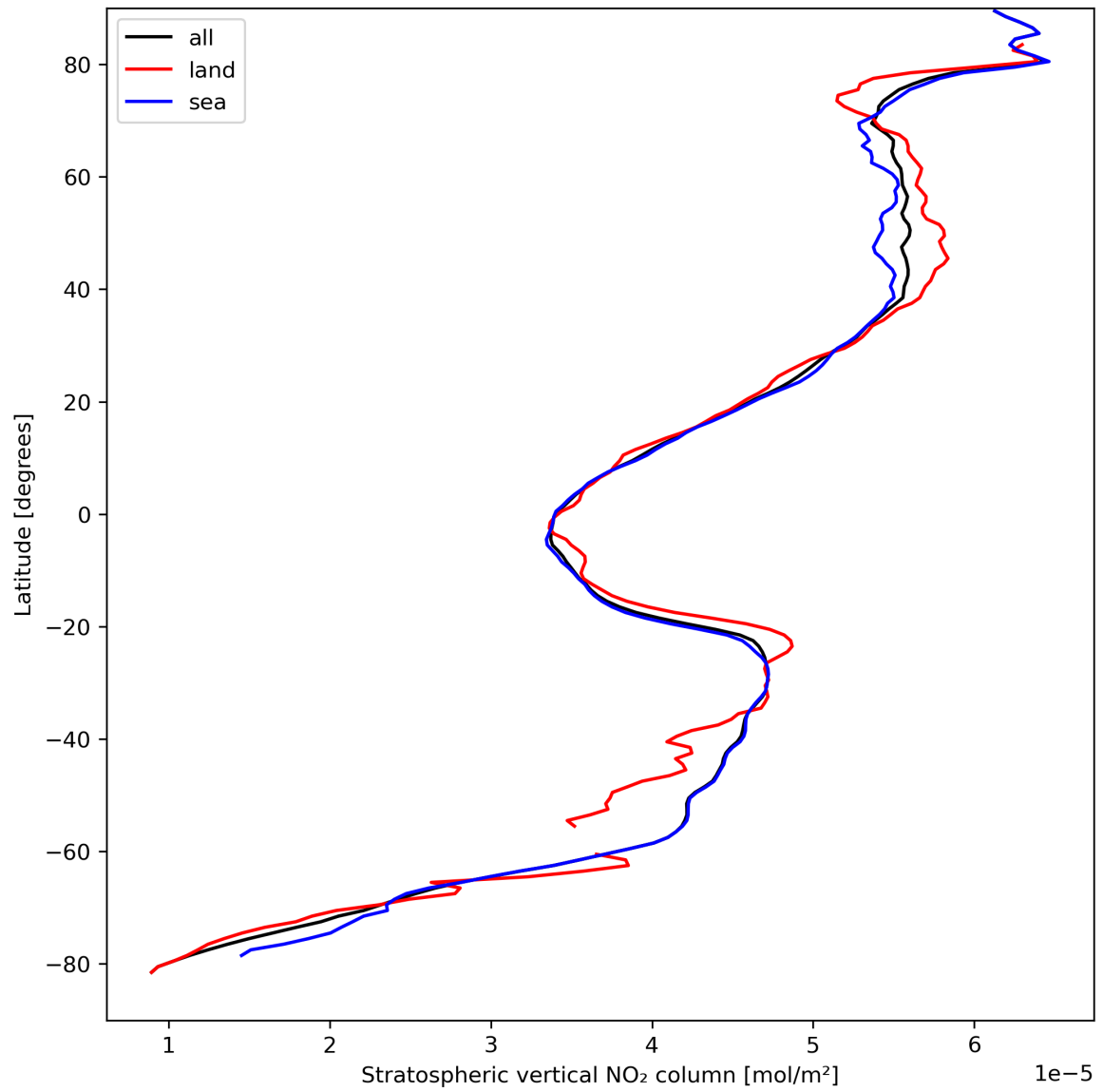
Figure 19: Zonal average of “Stratospheric vertical NO 2 column” for 2023-09-05 to 2023-09-06.
