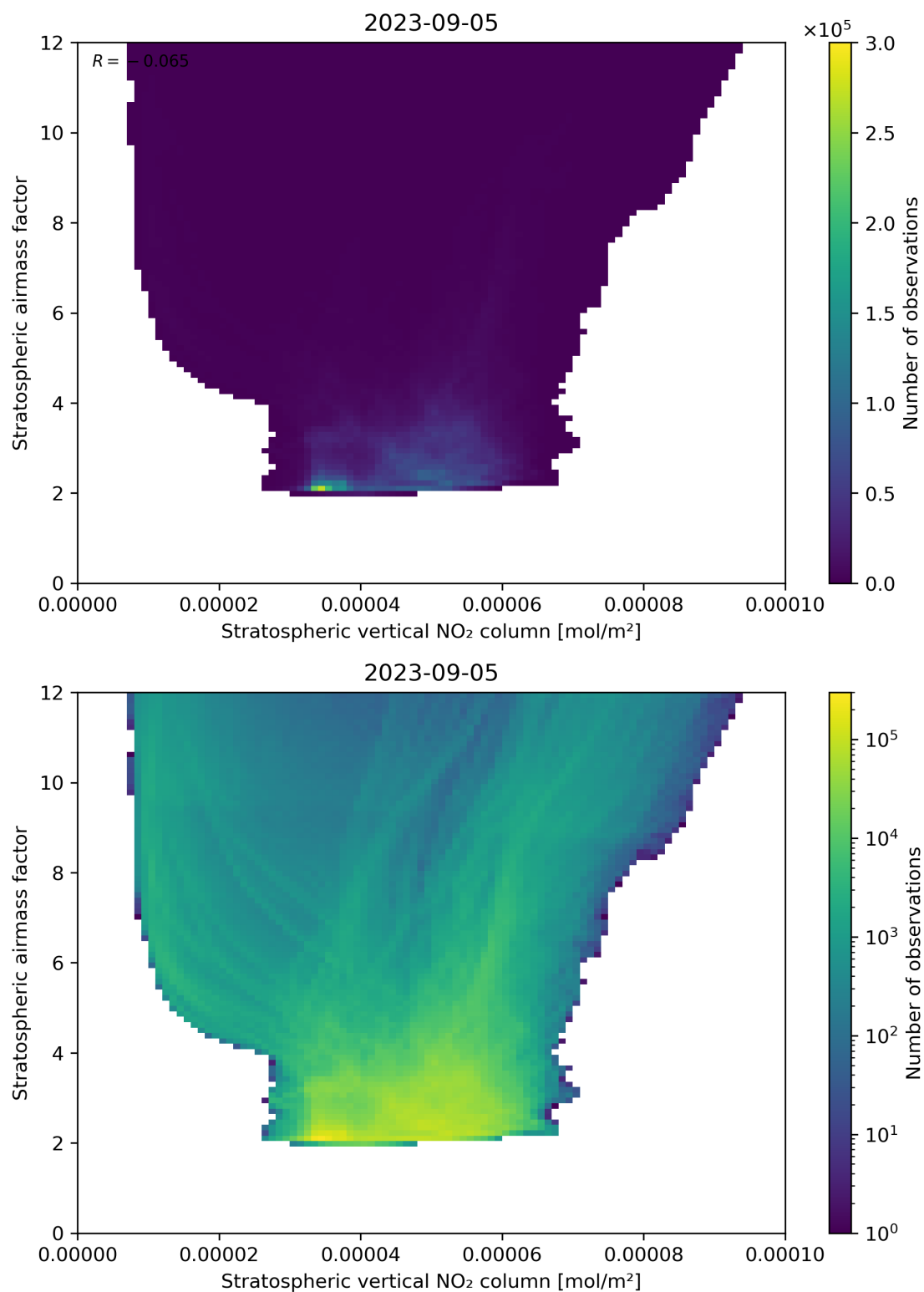
Figure 96: Scatter density plot of “Stratospheric vertical NO 2 column” against “Stratospheric airmass factor” for 2023-09-05 to 2023-09-06.
