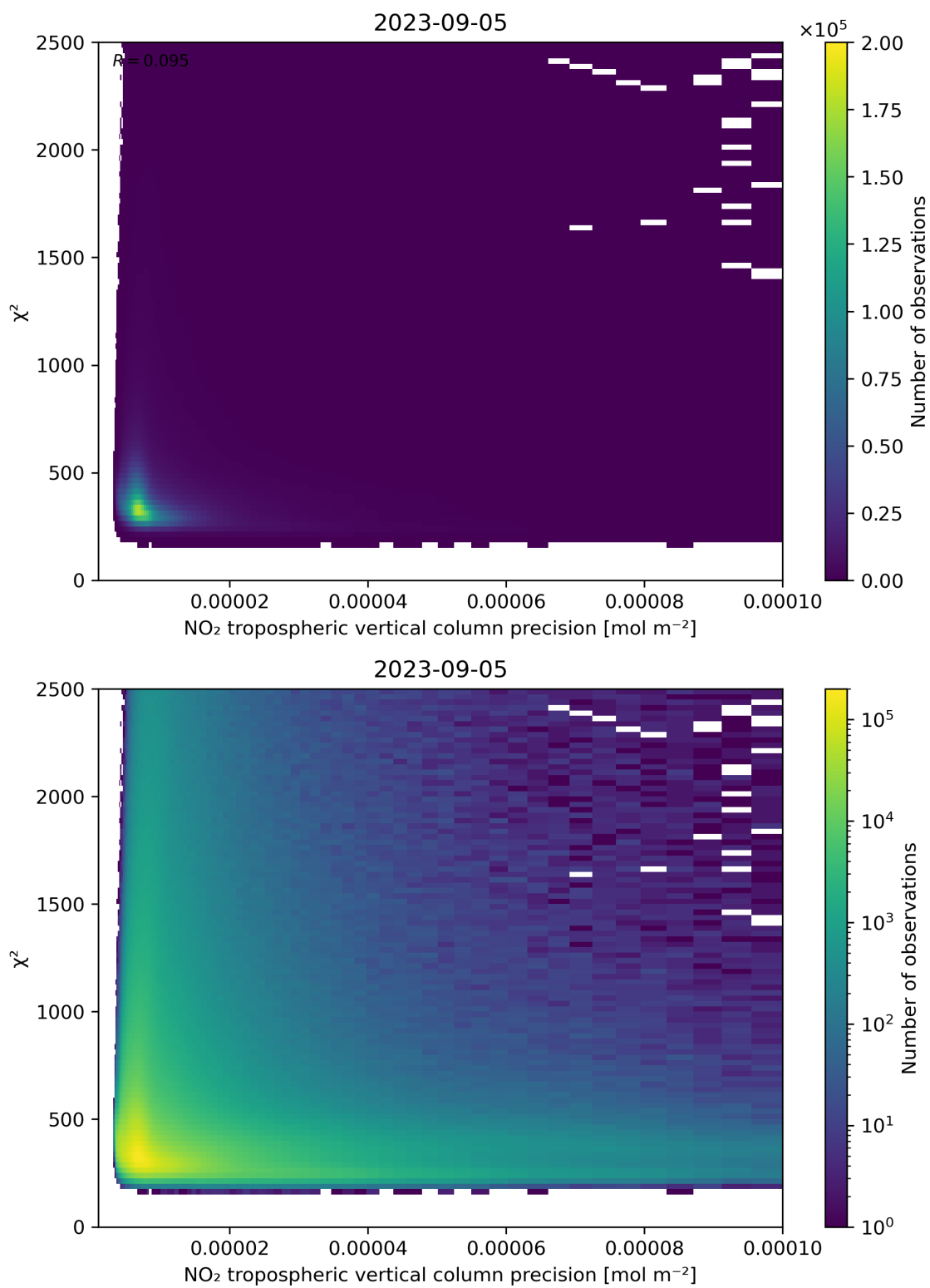
Figure 134: Scatter density plot of “NO 2 tropospheric vertical column precision” against “ \chi^2 ” for 2023-09-05 to 2023-09-06.
