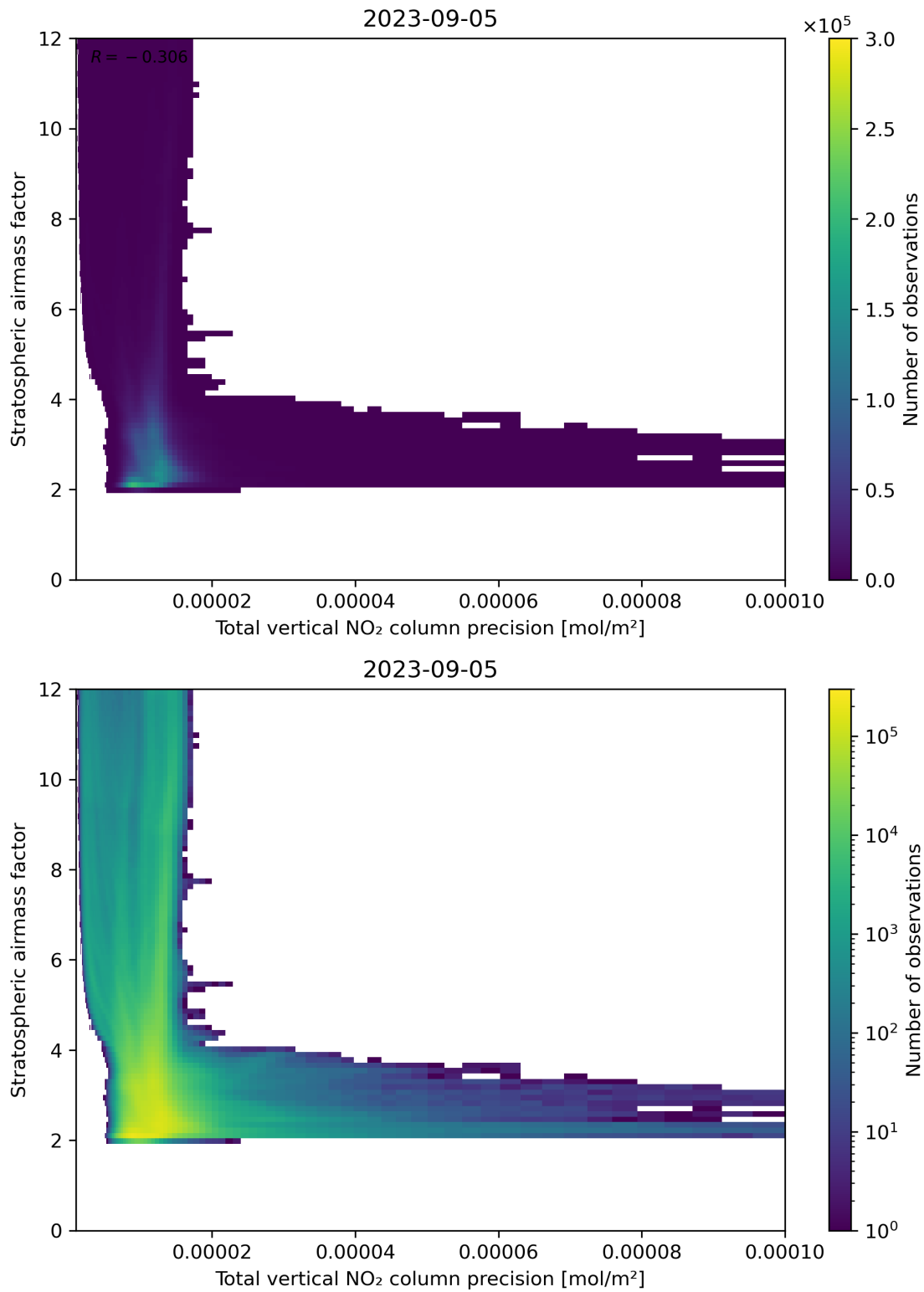
Figure 115: Scatter density plot of “Total vertical NO 2 column precision” against “Stratospheric airmass factor” for 2023-09-05 to 2023-09-06.
