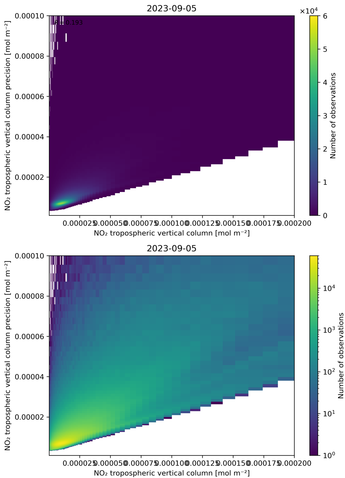
Figure 130: Scatter density plot of “NO 2 tropospheric vertical column” against “NO 2 tropospheric vertical column precision” for 2023-09-05 to 2023-09-06.
