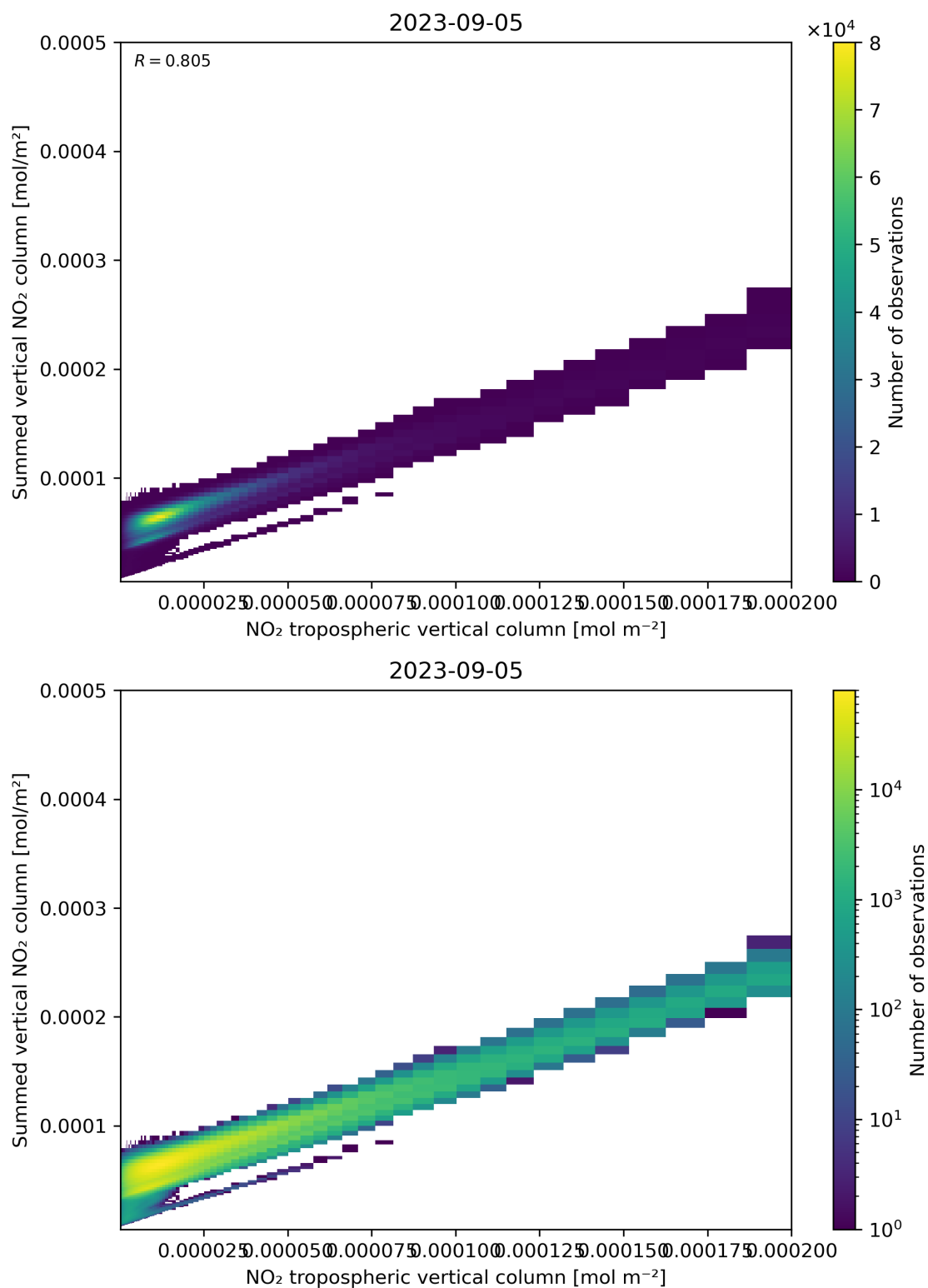
Figure 126: Scatter density plot of “NO 2 tropospheric vertical column” against “Summed vertical NO 2 column” for 2023-09-05 to 2023-09-06.
