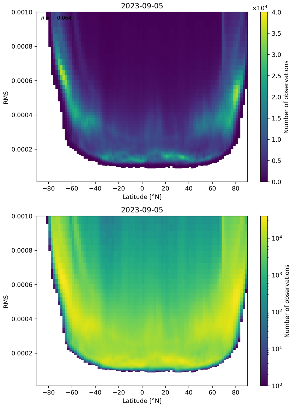
Figure 94: Scatter density plot of “Latitude” against “RMS” for 2023-09-05 to 2023-09-06.
