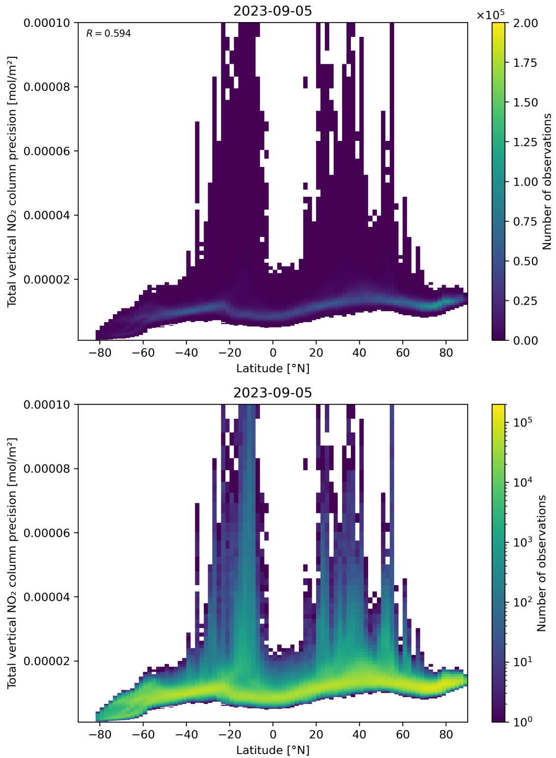
Figure 91: Scatter density plot of “Latitude” against “Total vertical NO 2 column precision” for 2023-09-05 to 2023-09-06.
