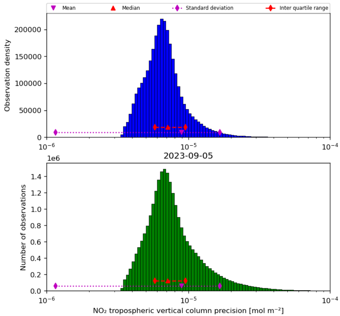
Figure 30: Histogram of “NO 2 tropospheric vertical column precision” for 2023-09-05 to 2023-09-06
