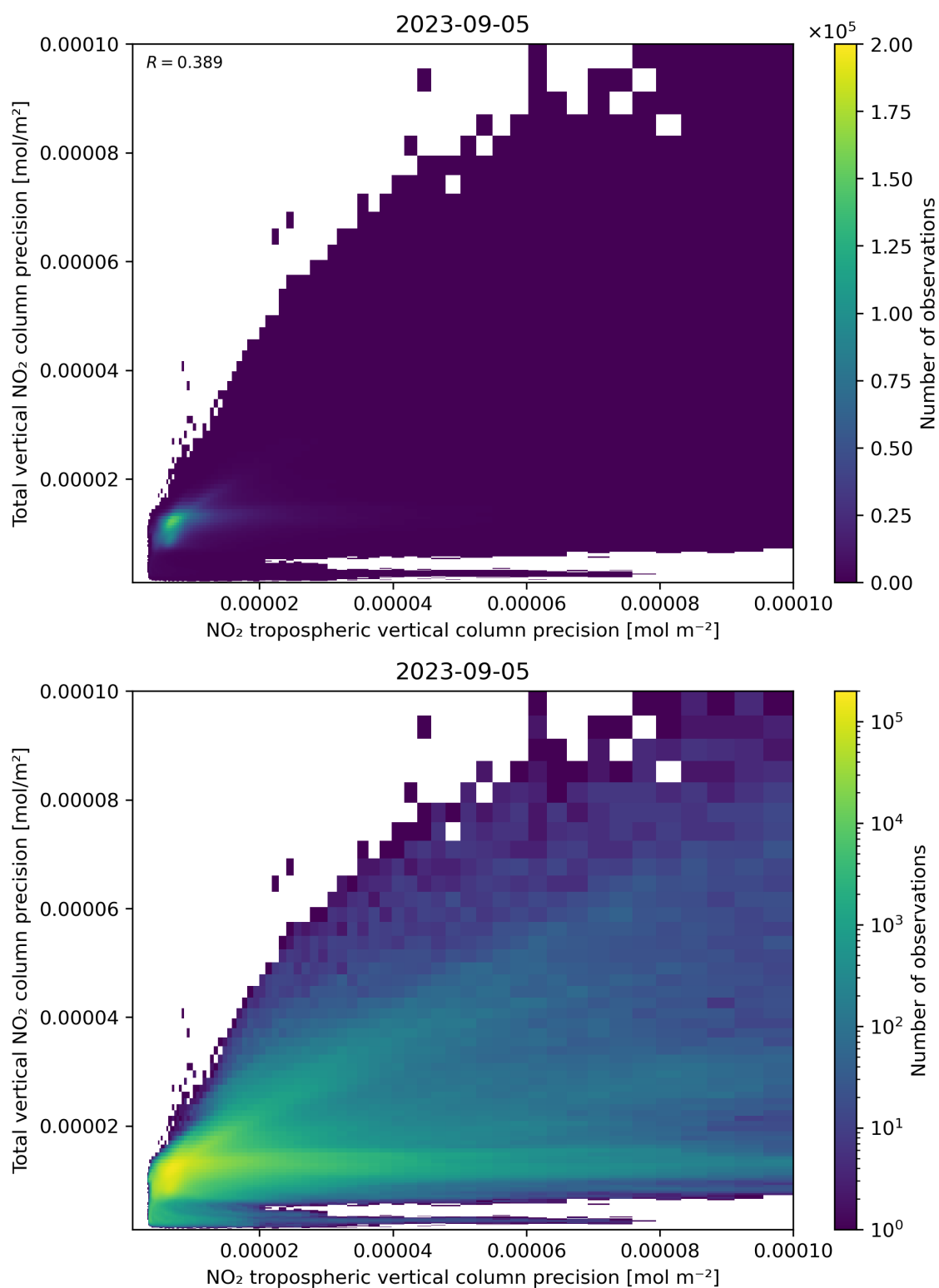
Figure 139: Scatter density plot of “NO 2 tropospheric vertical column precision” against “Total vertical NO 2 column precision” for 2023-09-05 to 2023-09-06.
