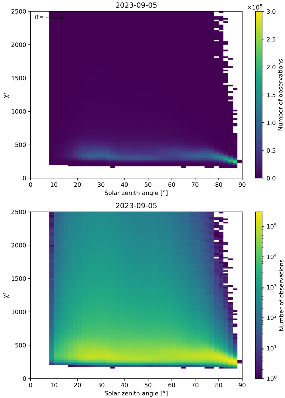
Figure 148: Scatter density plot of “Solar zenith angle” against “ \chi^2 ” for 2023-09-05 to 2023-09-06.
