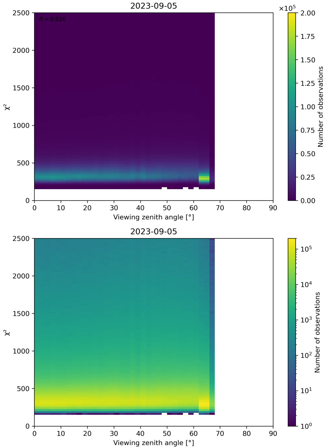
Figure 162: Scatter density plot of “Viewing zenith angle” against “ \chi^2 ” for 2023-09-05 to 2023-09-06.
