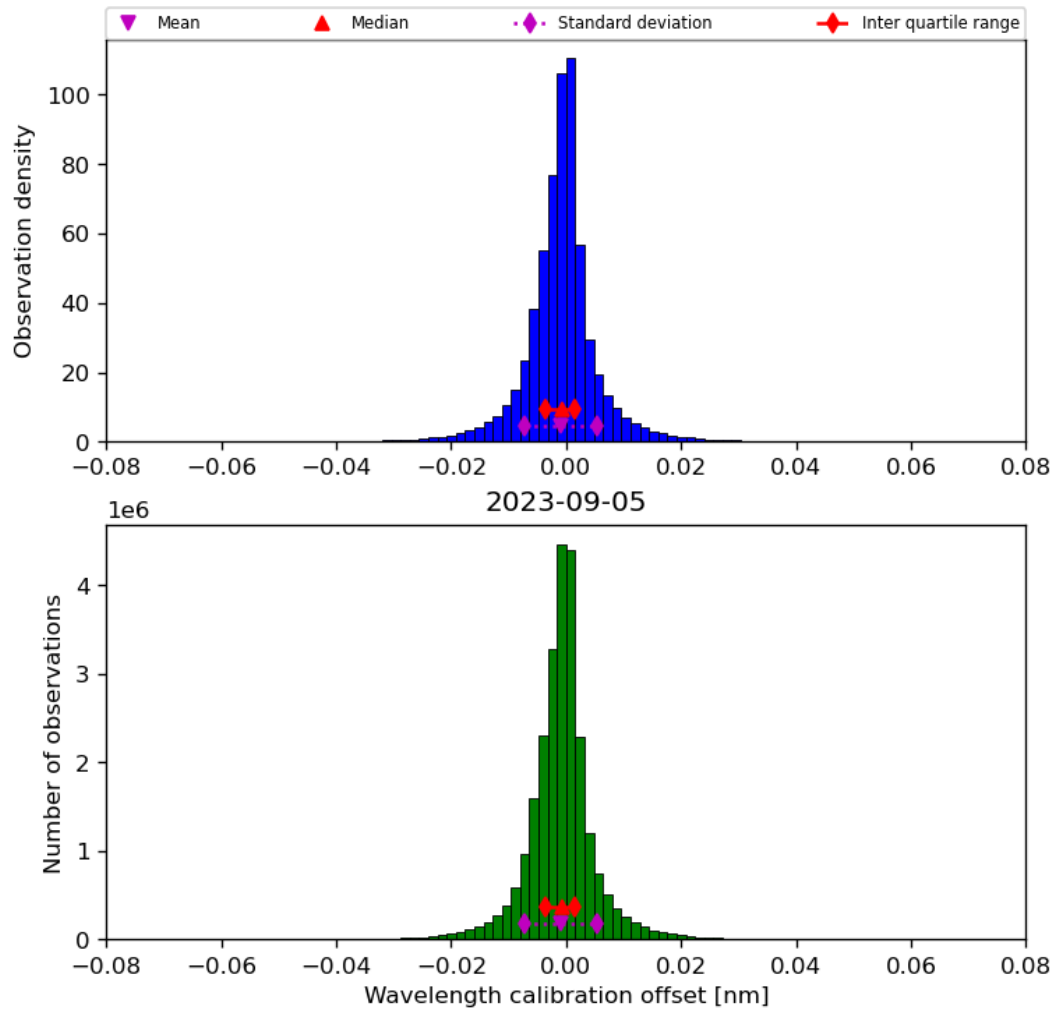
Figure 35: Histogram of “Wavelength calibration offset” for 2023-09-05 to 2023-09-06
