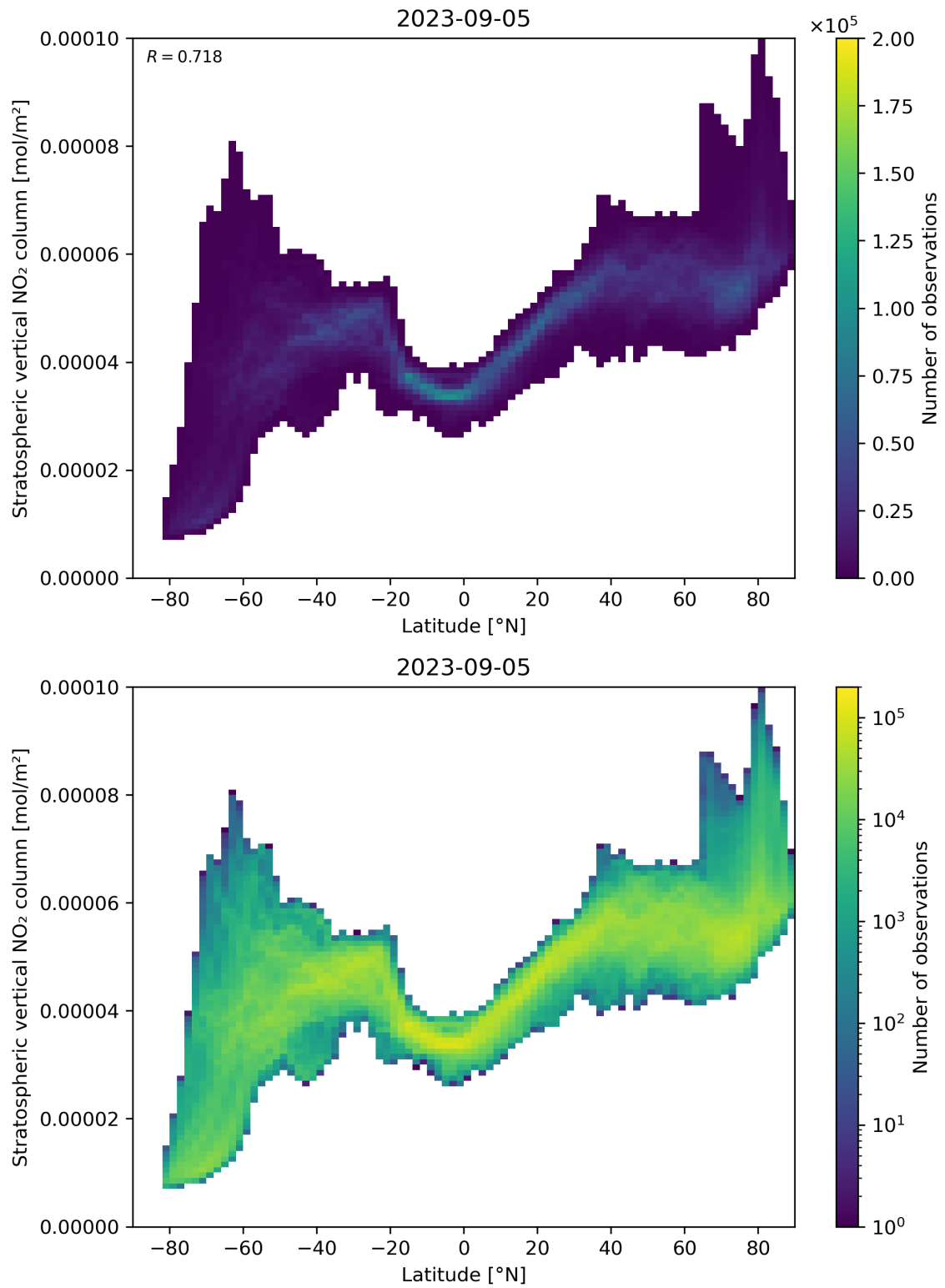
Figure 87: Scatter density plot of “Latitude” against “Stratospheric vertical NO 2 column” for 2023-09-05 to 2023-09-06.
