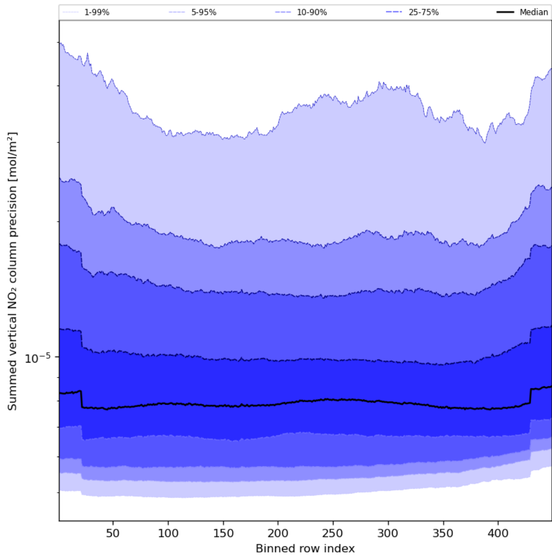
Figure 58: Along track statistics of “Summed vertical NO 2 column precision” for 2023-09-05 to 2023-09-06
