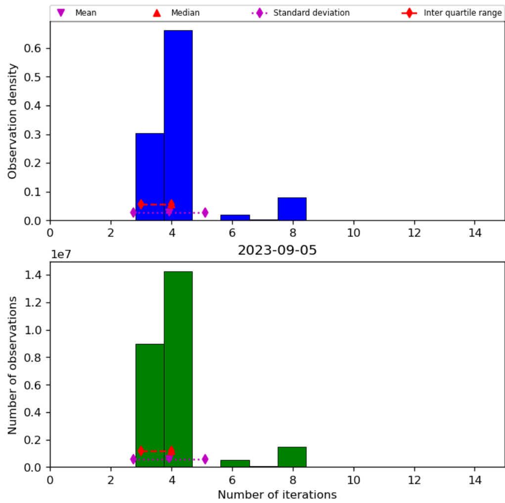
Figure 34: Histogram of “Number of iterations” for 2023-09-05 to 2023-09-06
