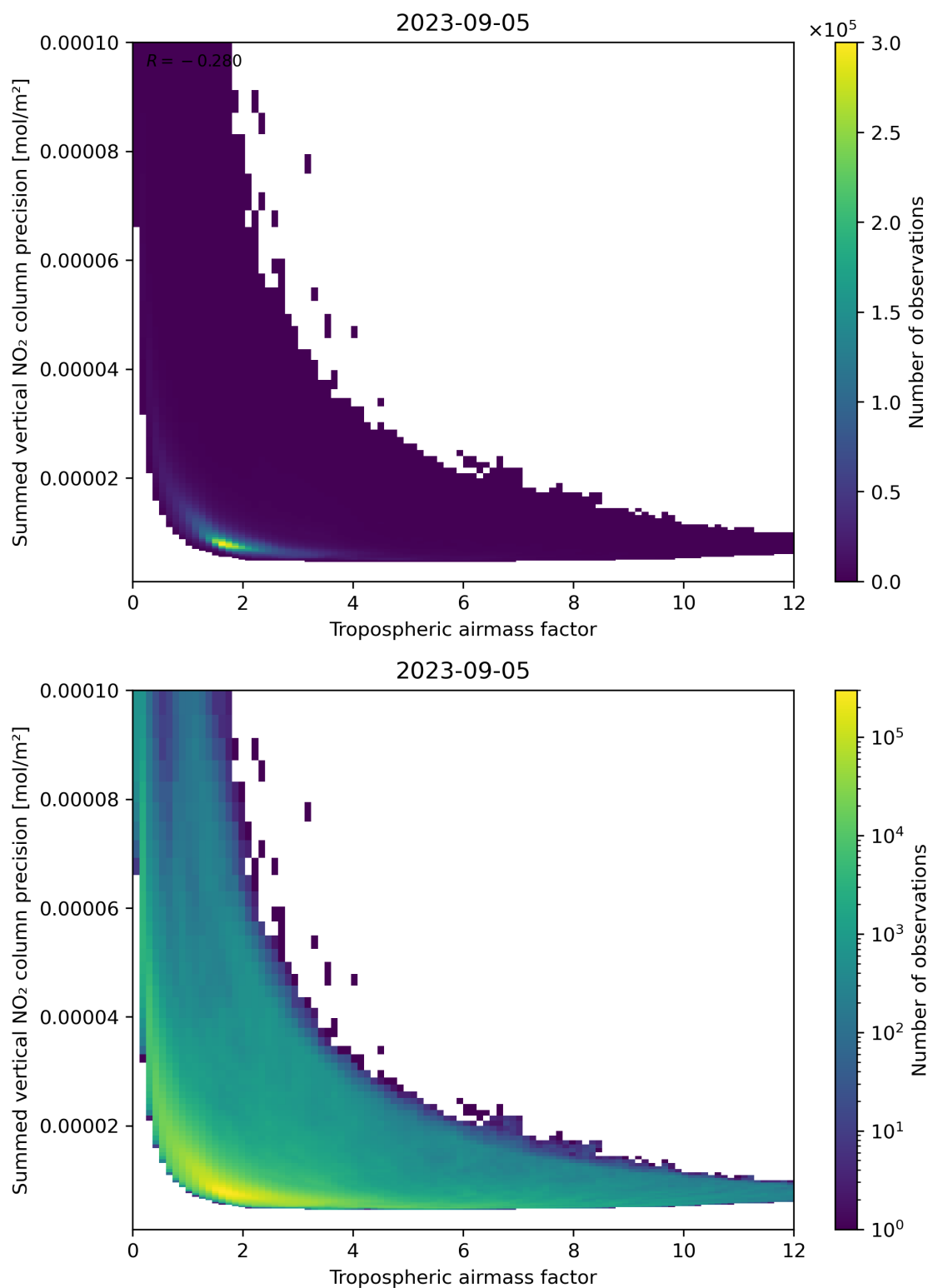
Figure 76: Scatter density plot of “Tropospheric air mass factor” against “Summed vertical NO 2 column precision” for 2023-09-05 to 2023-09-06.
