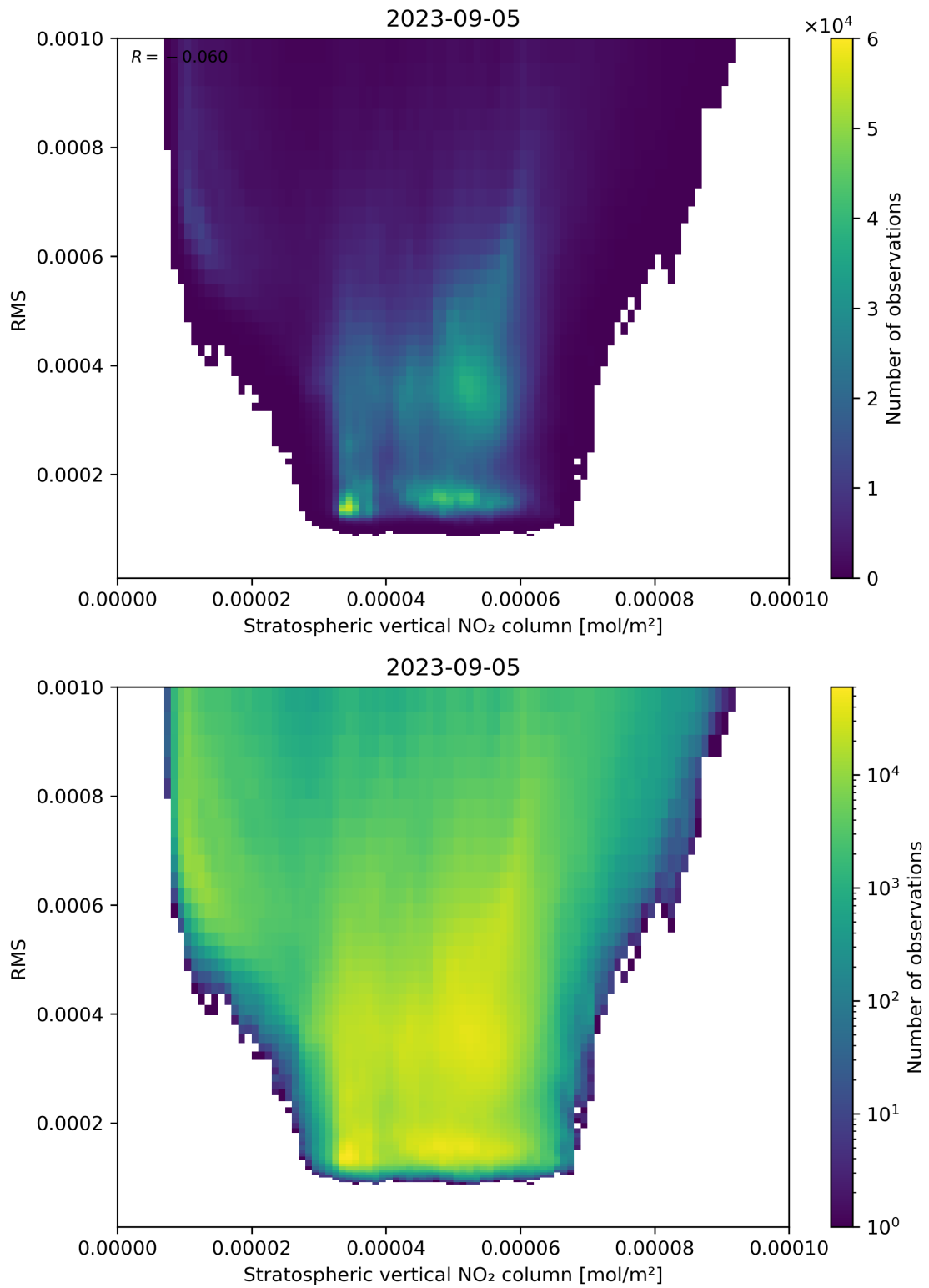
Figure 102: Scatter density plot of “Stratospheric vertical NO 2 column” against “RMS” for 2023-09-05 to 2023-09-06.
