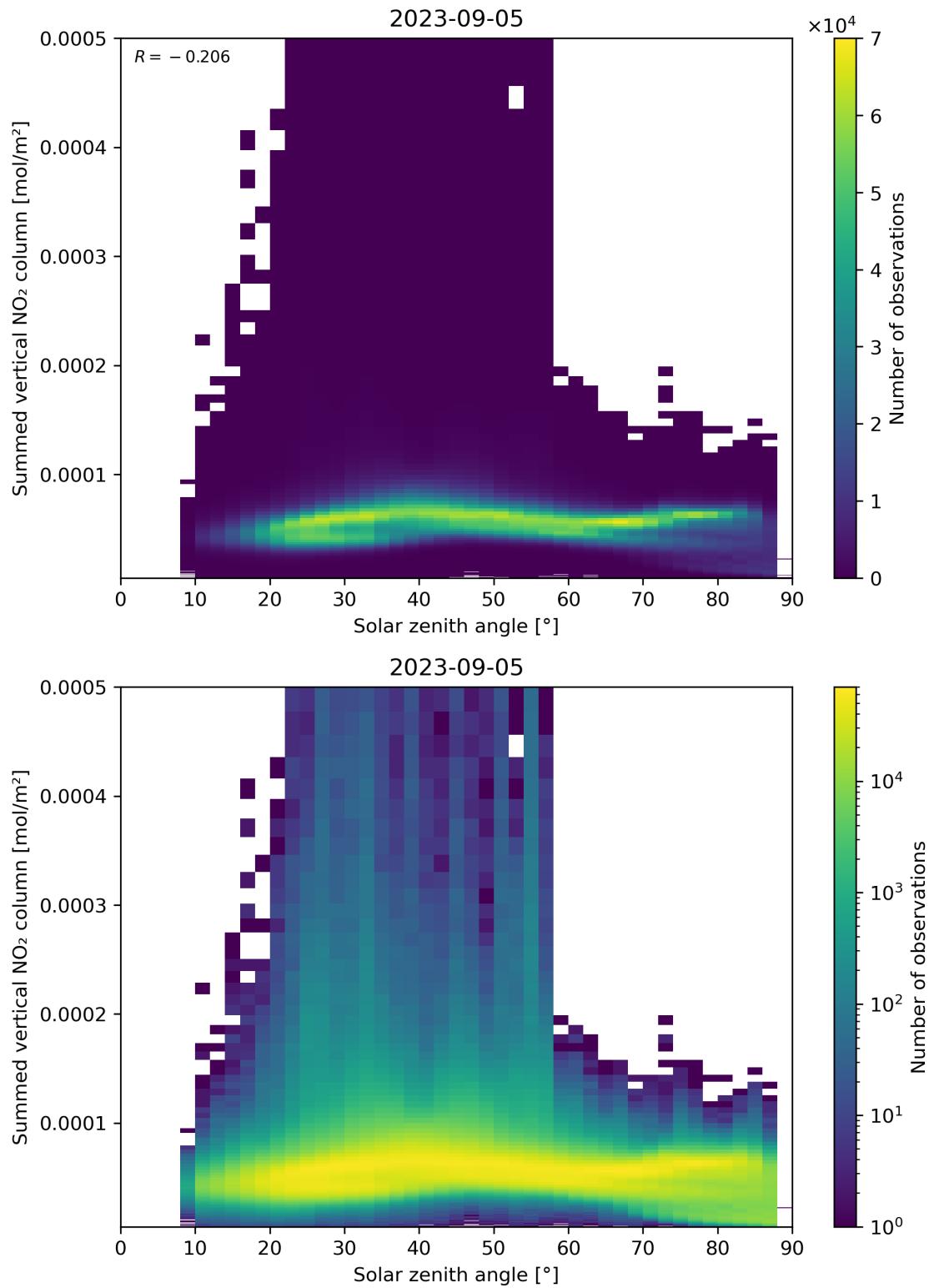
Figure 151: Scatter density plot of “Solar zenith angle” against “Summed vertical NO 2 column” for 2023-09-05 to 2023-09-06.
