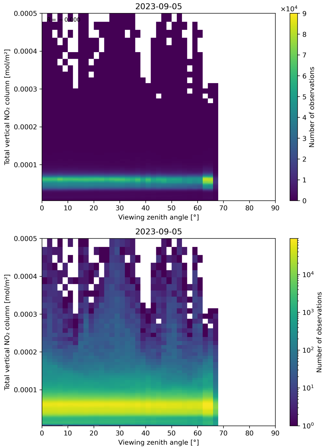
Figure 167: Scatter density plot of “Viewing zenith angle” against “Total vertical NO 2 column” for 2023-09-05 to 2023-09-06.
