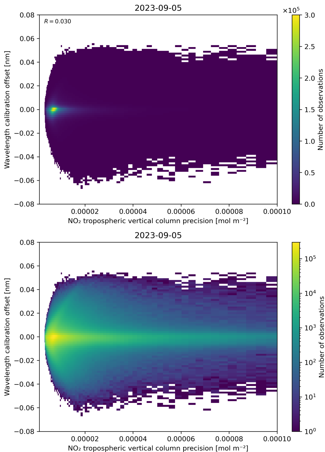
Figure 141: Scatter density plot of “NO 2 tropospheric vertical column precision” against “Wavelength calibration offset” for 2023-09-05 to 2023-09-06.
