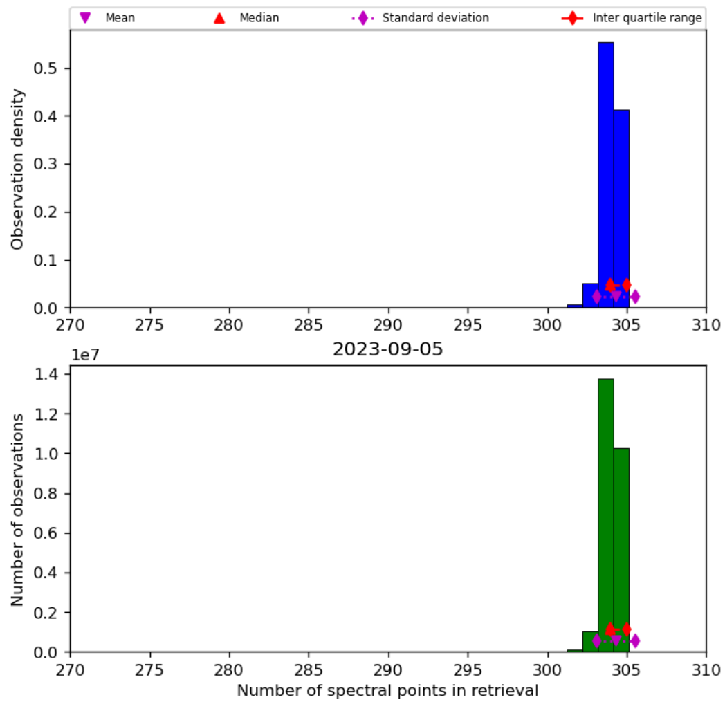
Figure 33: Histogram of “Number of spectral points in retrieval” for 2023-09-05 to 2023-09-06
