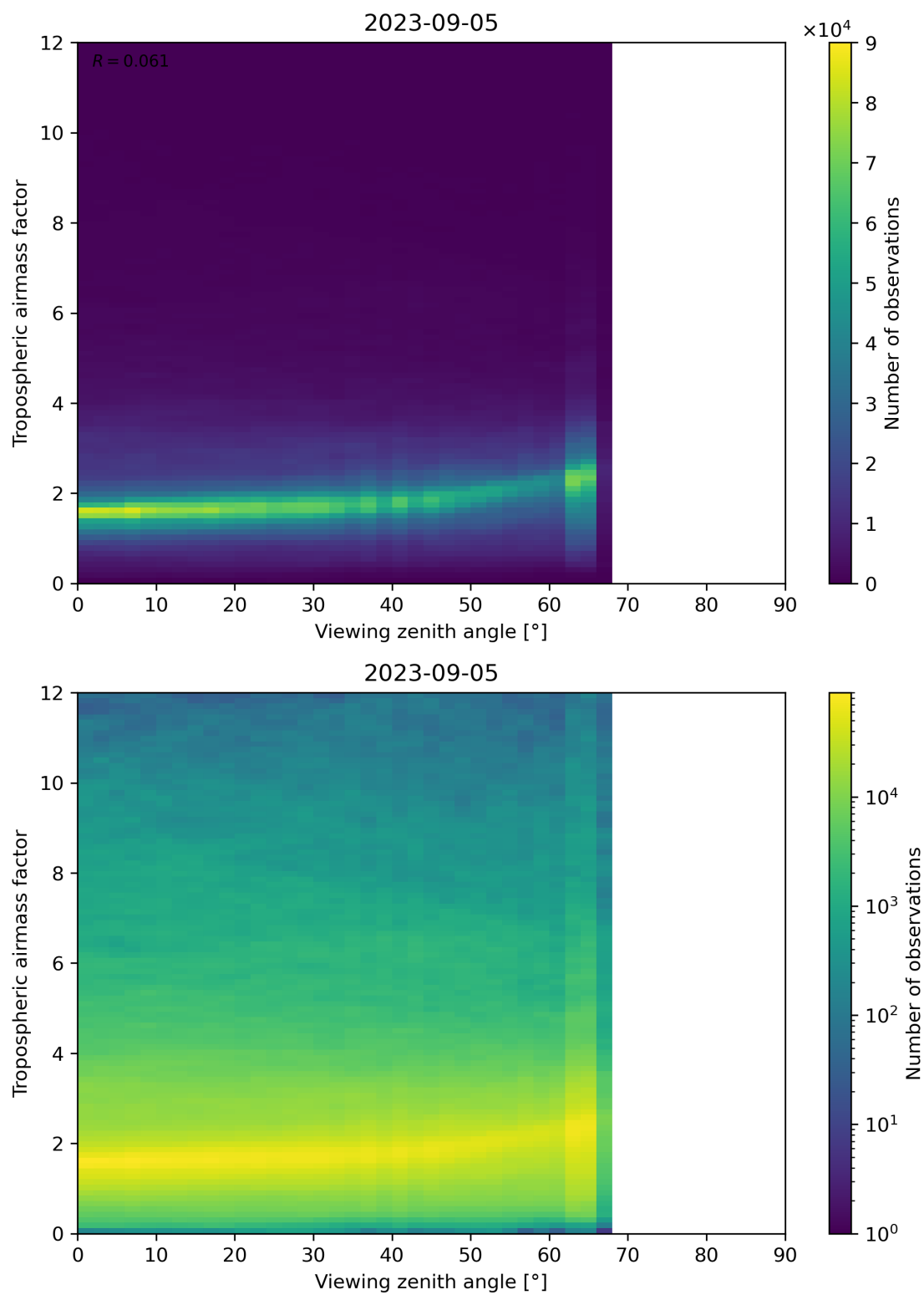
Figure 161: Scatter density plot of “Viewing zenith angle” against “Tropospheric airmass factor” for 2023-09-05 to 2023-09-06.
