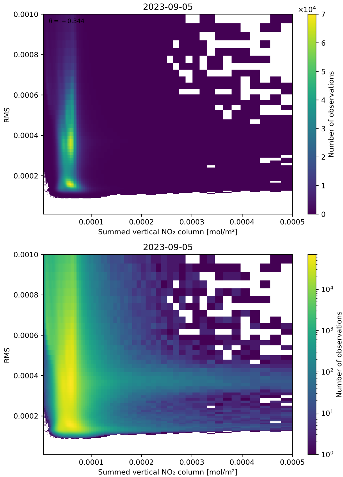
Figure 109: Scatter density plot of “Summed vertical NO 2 column” against “RMS” for 2023-09-05 to 2023-09-06.
