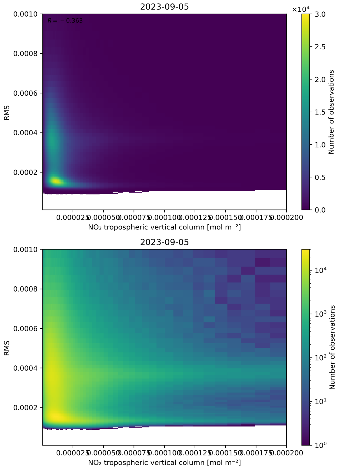
Figure 142: Scatter density plot of “NO 2 tropospheric vertical column” against “RMS” for 2023-09-05 to 2023-09-06.
