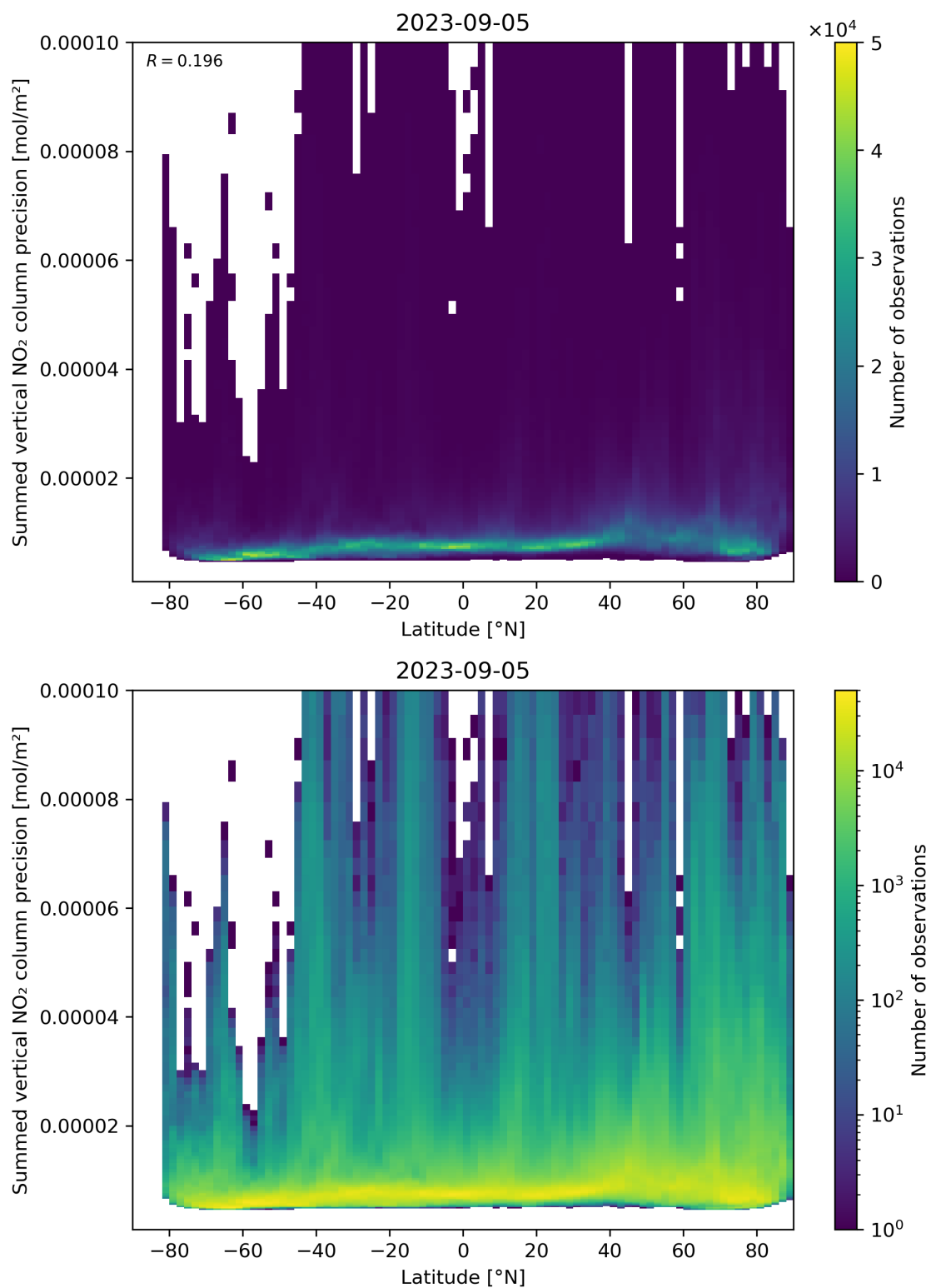
Figure 89: Scatter density plot of “Latitude” against “Summed vertical NO 2 column precision” for 2023-09-05 to 2023-09-06.
