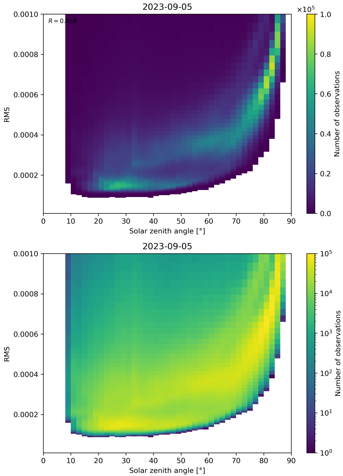
Figure 157: Scatter density plot of “Solar zenith angle” against “RMS” for 2023-09-05 to 2023-09-06.
