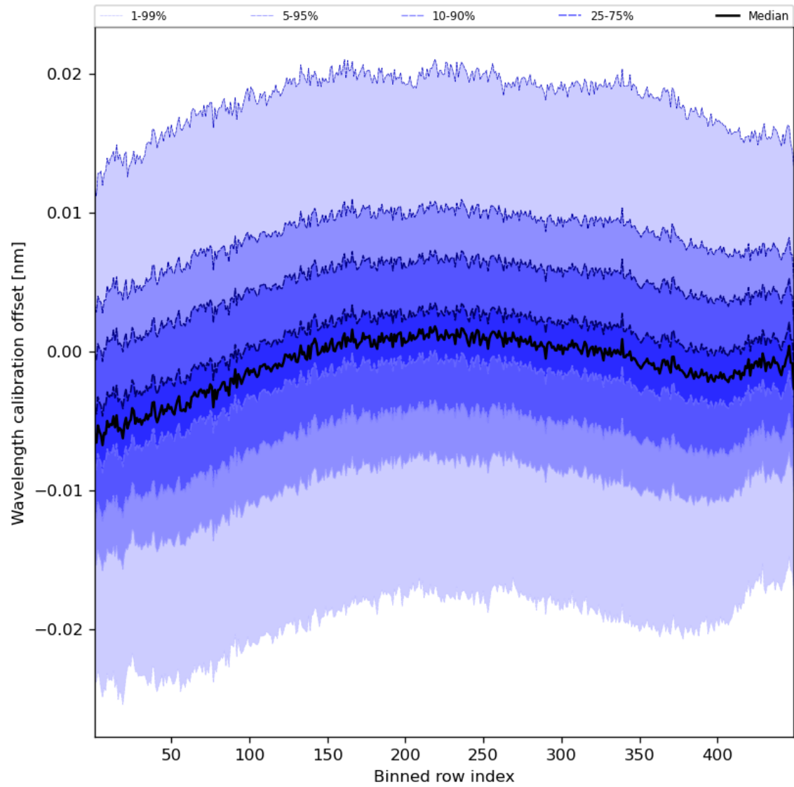
Figure 52: Along track statistics of “Wavelength calibration offset” for 2023-09-05 to 2023-09-06
