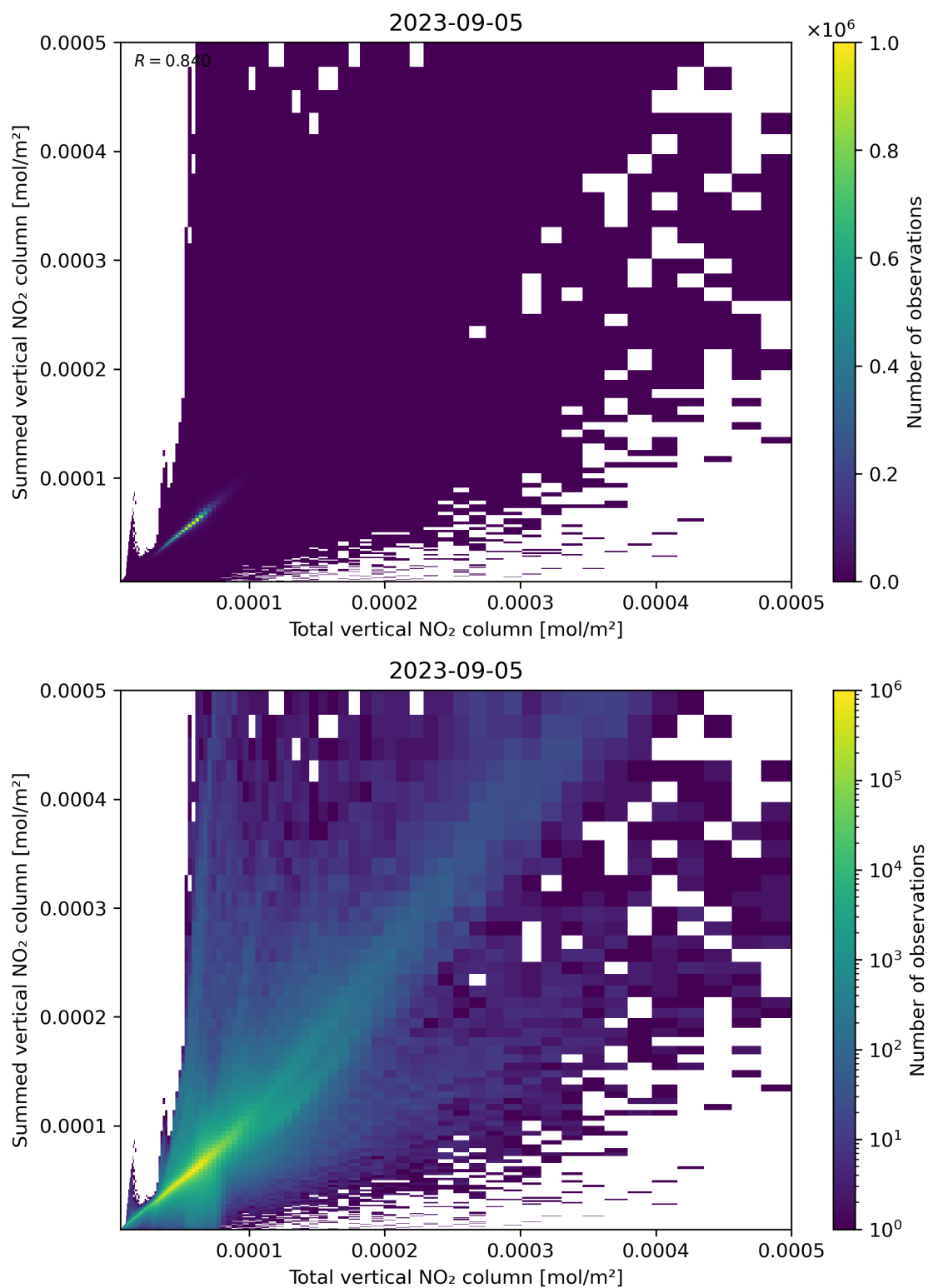
Figure 112: Scatter density plot of “Total vertical NO 2 column” against “Summed vertical NO 2 column” for 2023-09-05 to 2023-09-06.
