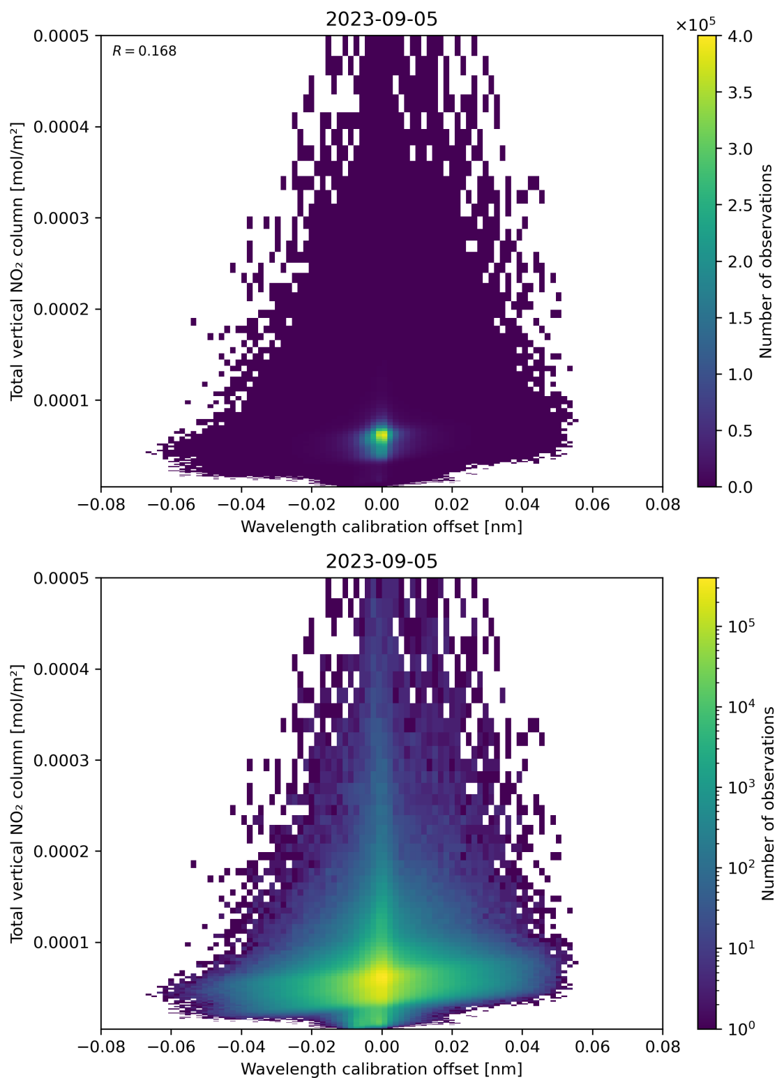
Figure 179: Scatter density plot of “Wavelength calibration offset” against “Total vertical NO 2 column” for 2023-09-05 to 2023-09-06.
