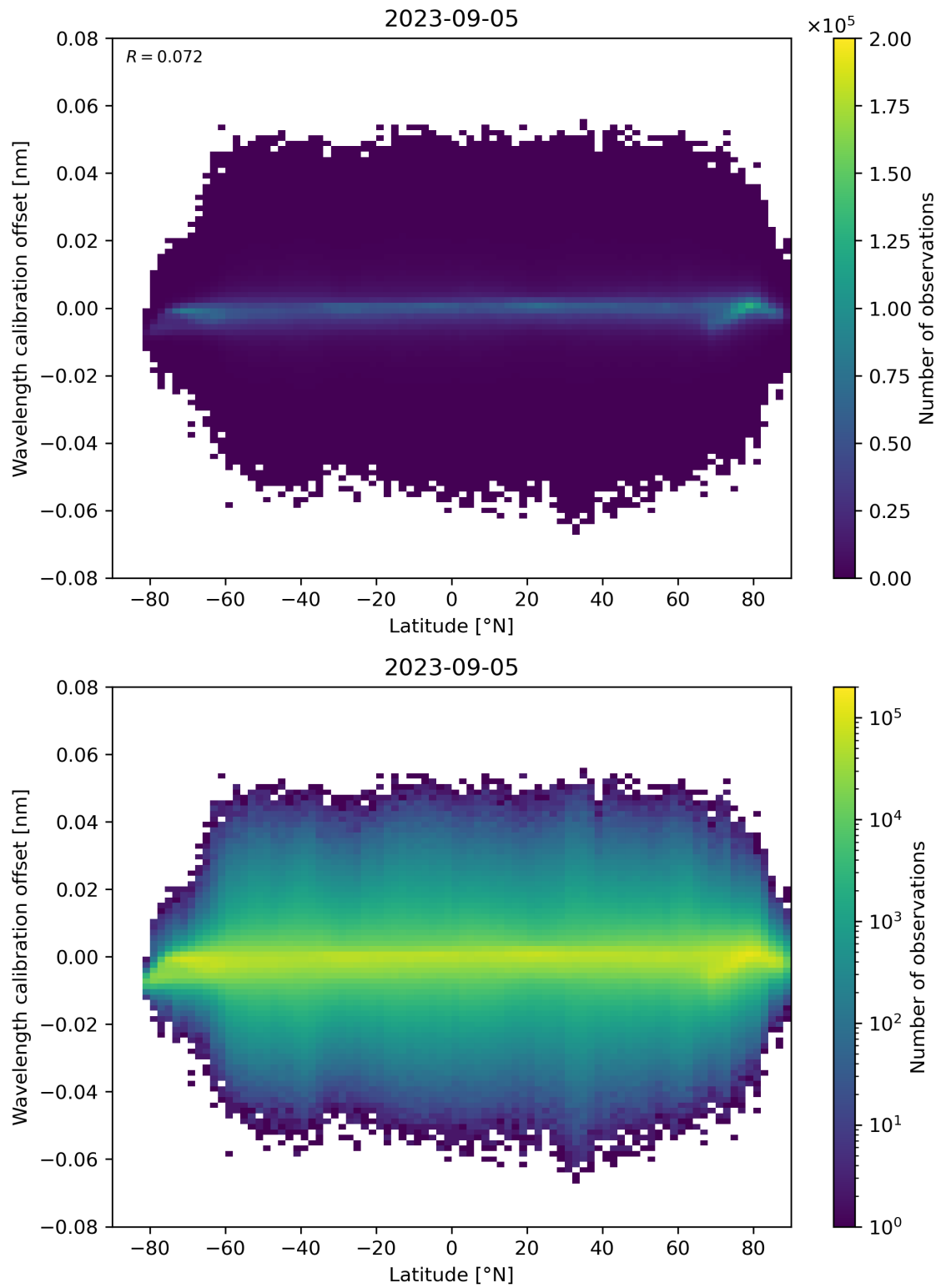
Figure 95: Scatter density plot of “Latitude” against “Wavelength calibration offset” for 2023-09-05 to 2023-09-06.
