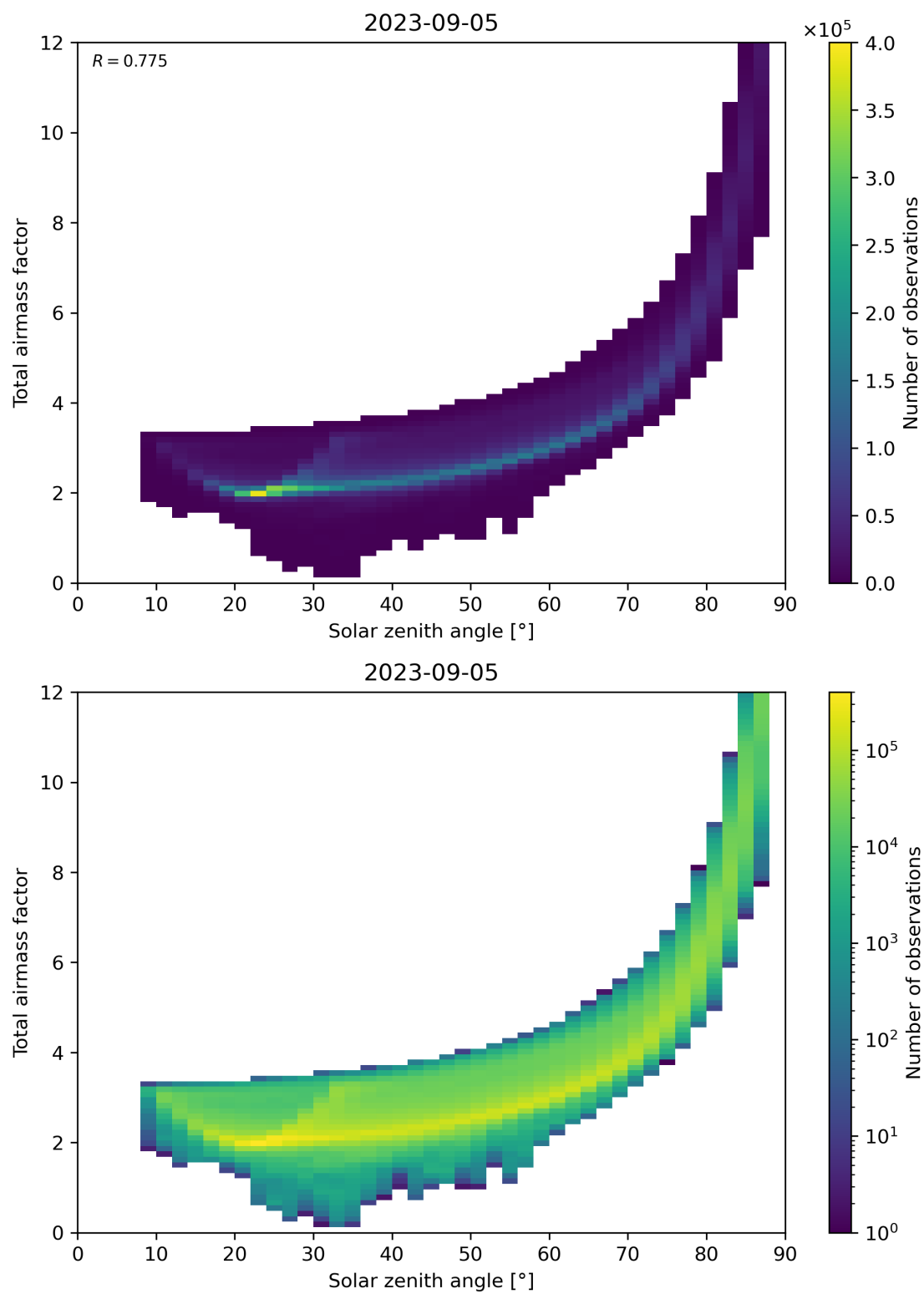
Figure 146: Scatter density plot of “Solar zenith angle” against “Total air mass factor” for 2023-09-05 to 2023-09-06.
