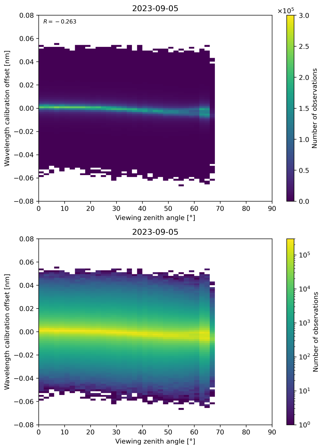
Figure 173: Scatter density plot of “Viewing zenith angle” against “Wavelength calibration offset” for 2023-09-05 to 2023-09-06.
