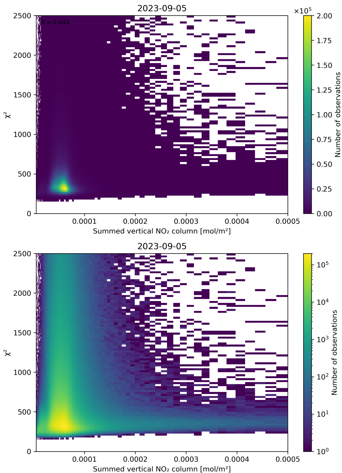
Figure 104: Scatter density plot of “Summed vertical NO 2 column” against “ \chi^2 ” for 2023-09-05 to 2023-09-06.
