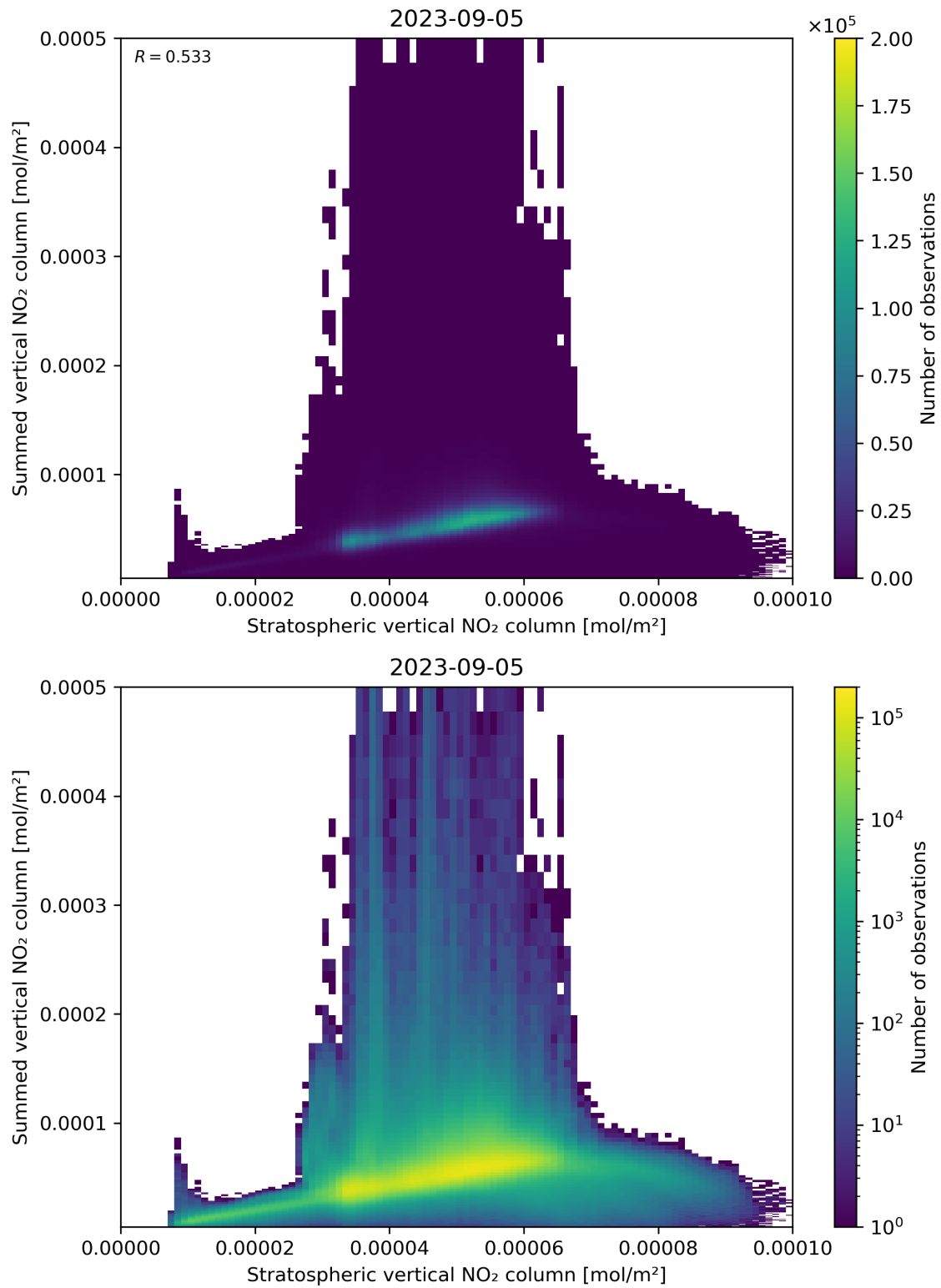
Figure 98: Scatter density plot of “Stratospheric vertical NO 2 column” against “Summed vertical NO 2 column” for 2023-09-05 to 2023-09-06.
