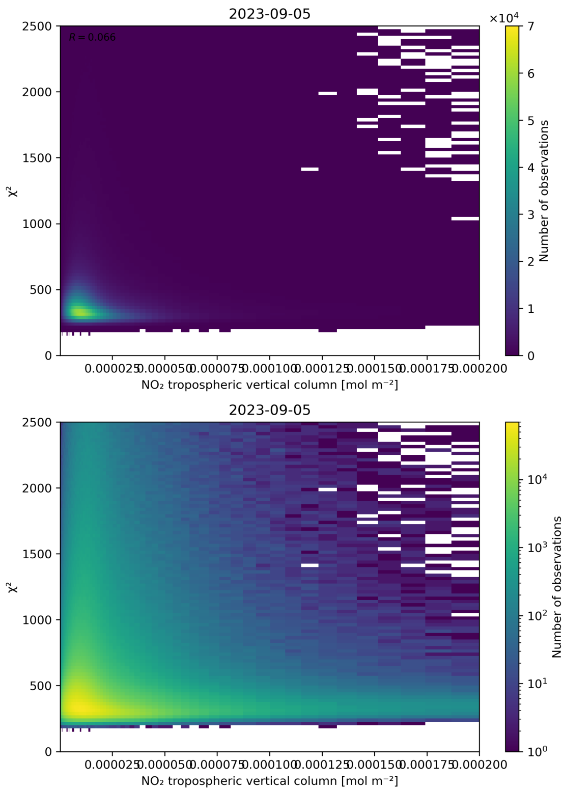
Figure 124: Scatter density plot of “NO 2 tropospheric vertical column” against “ \chi^2 ” for 2023-09-05 to 2023-09-06.
