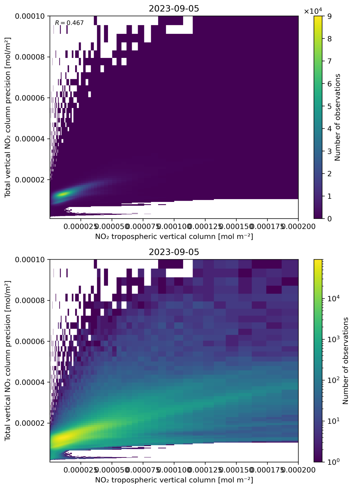
Figure 129: Scatter density plot of “NO 2 tropospheric vertical column” against “Total vertical NO 2 column precision” for 2023-09-05 to 2023-09-06.
