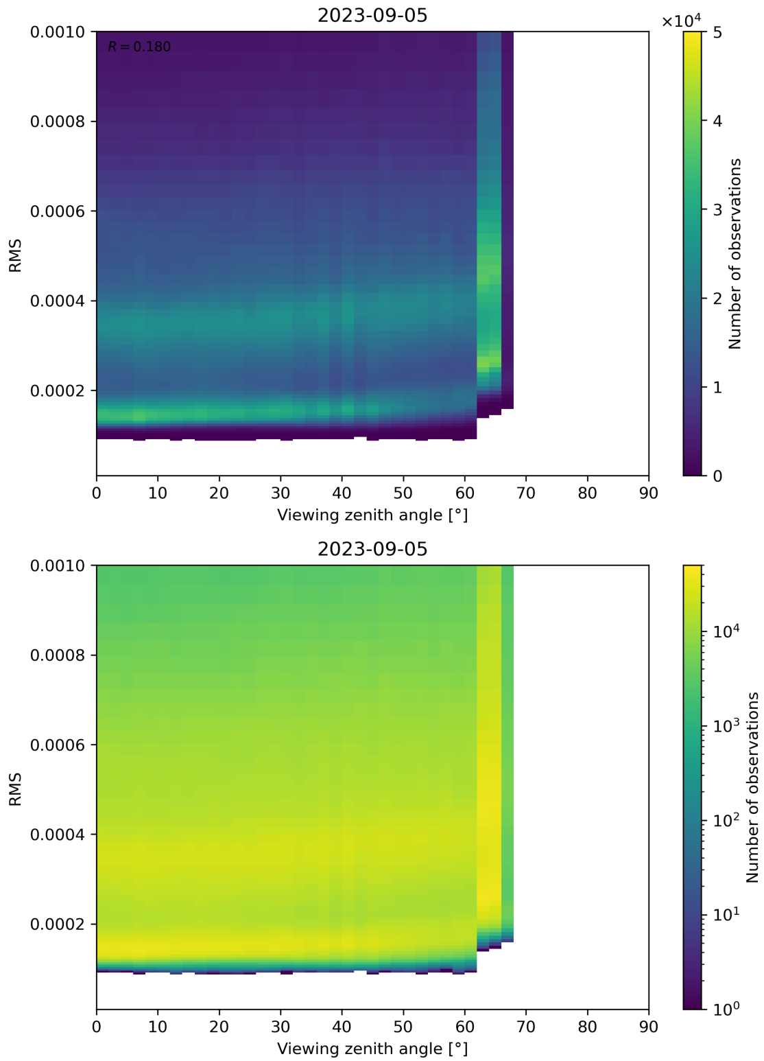
Figure 171: Scatter density plot of “Viewing zenith angle” against “RMS” for 2023-09-05 to 2023-09-06.
