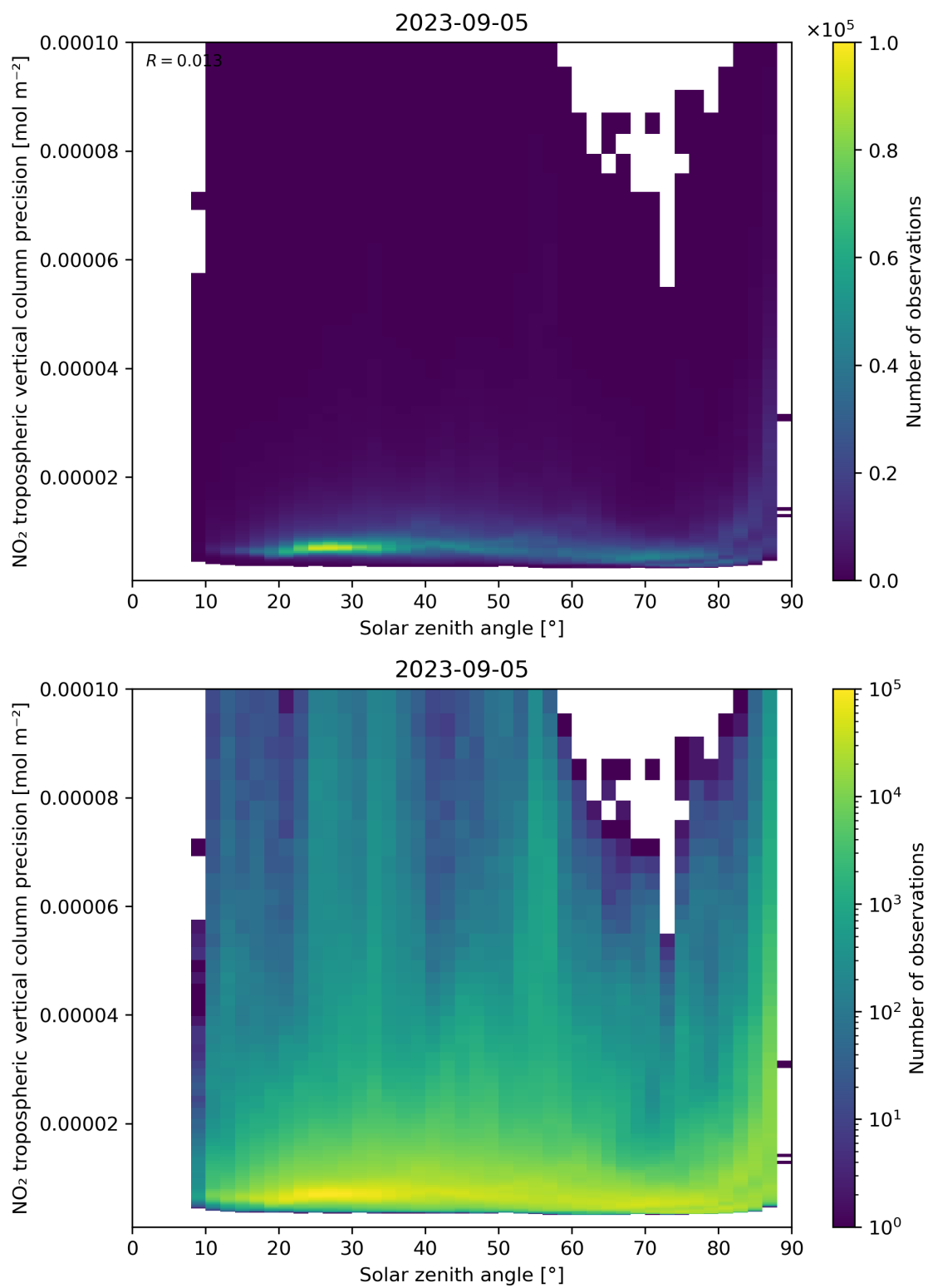
Figure 156: Scatter density plot of “Solar zenith angle” against “NO 2 tropospheric vertical column precision” for 2023-09-05 to 2023-09-06.
