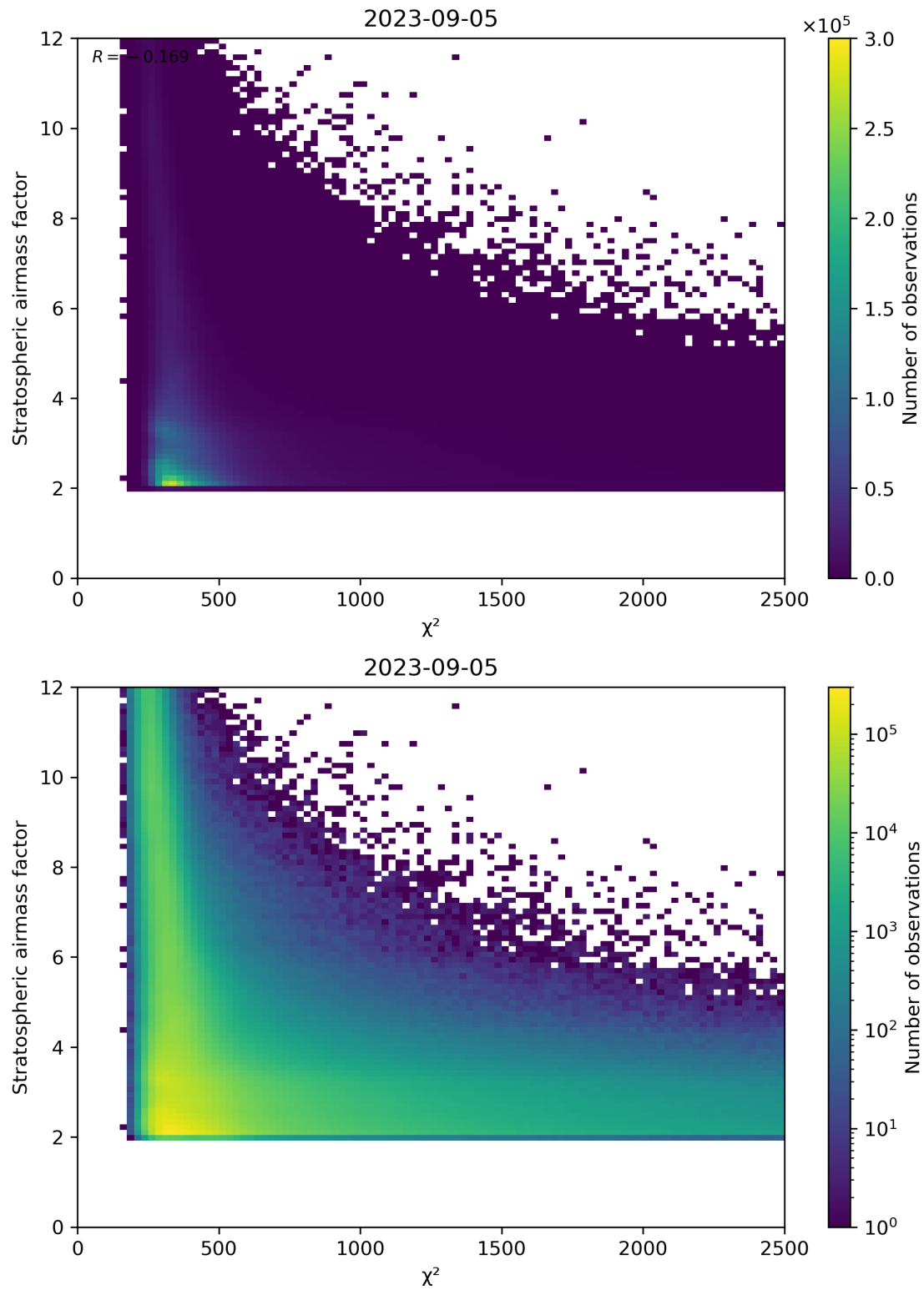
Figure 81: Scatter density plot of “ \chi^2 ” against “Stratospheric airmass factor” for 2023-09-05 to 2023-09-06.
