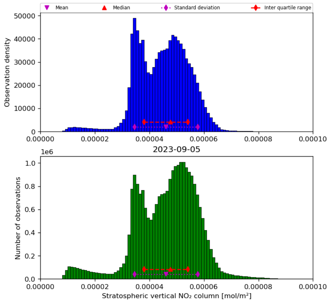
Figure 36: Histogram of “Stratospheric vertical NO 2 column” for 2023-09-05 to 2023-09-06
