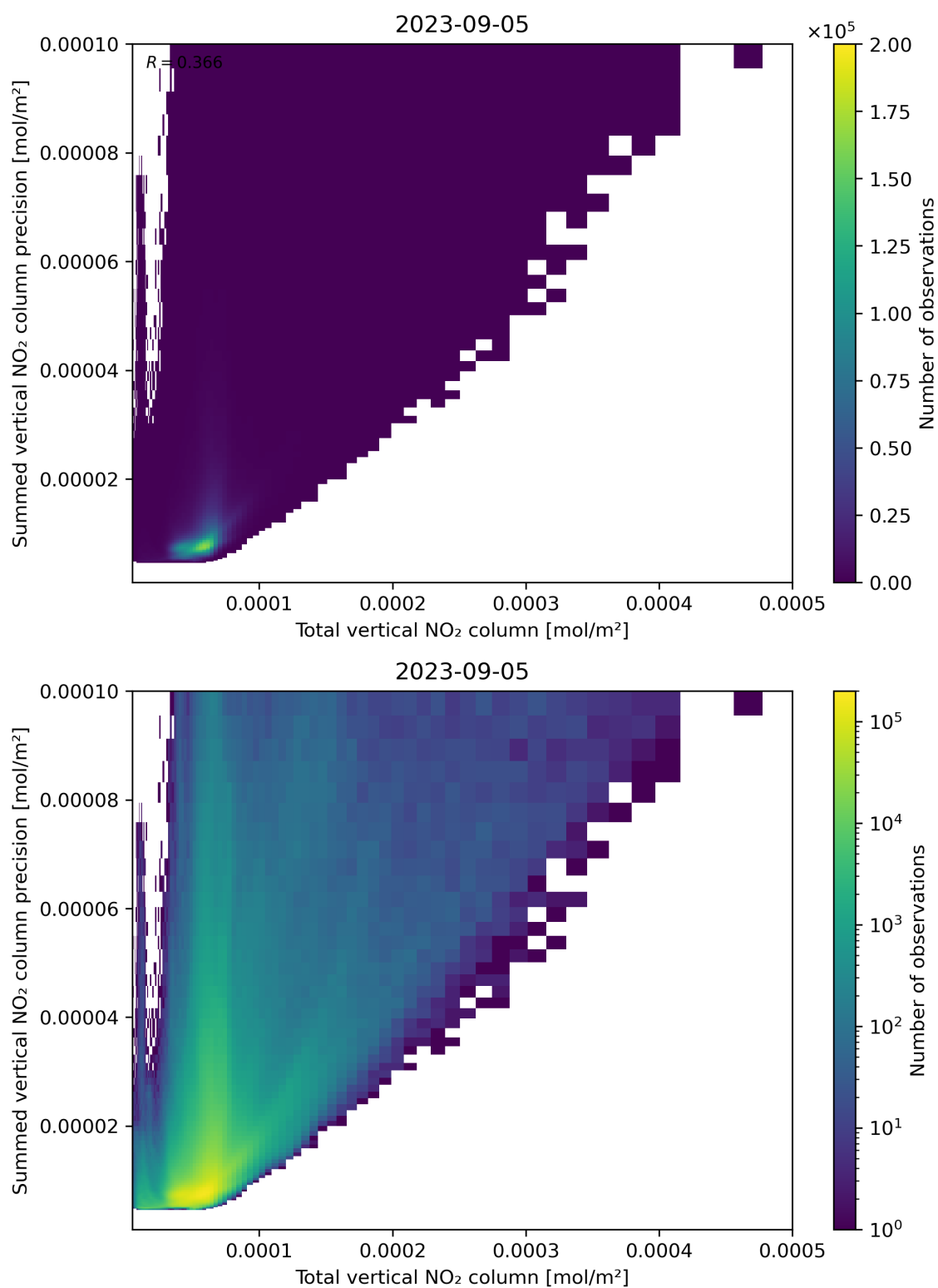
Figure 113: Scatter density plot of “Total vertical NO 2 column” against “Summed vertical NO 2 column precision” for 2023-09-05 to 2023-09-06.
