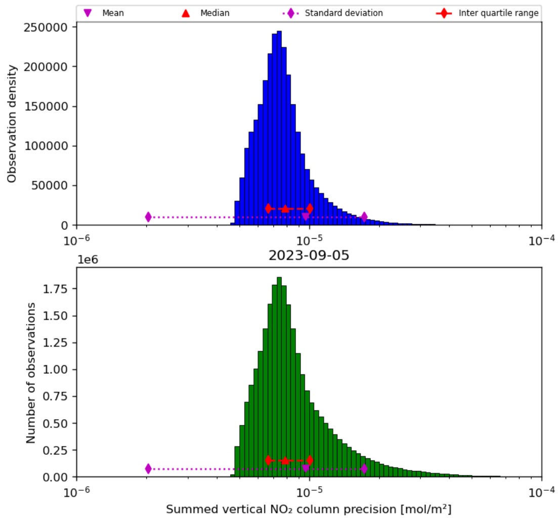
Figure 41: Histogram of “Summed vertical NO 2 column precision” for 2023-09-05 to 2023-09-06
