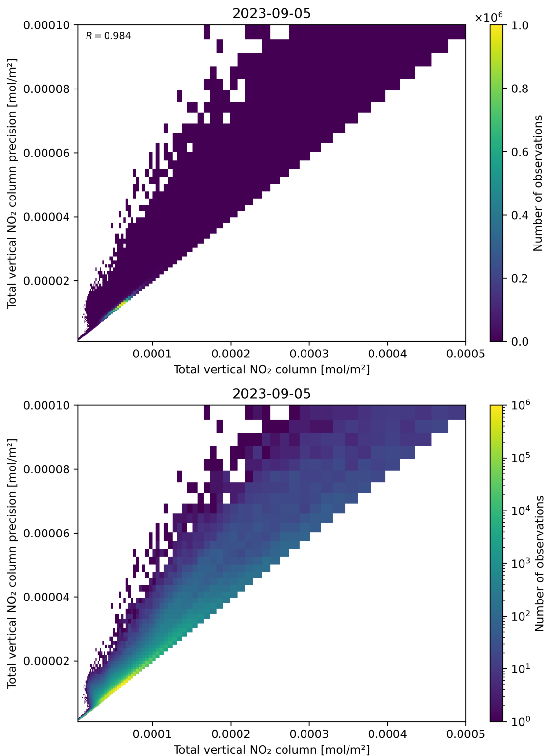
Figure 114: Scatter density plot of “Total vertical NO 2 column” against “Total vertical NO 2 column precision” for 2023-09-05 to 2023-09-06.
