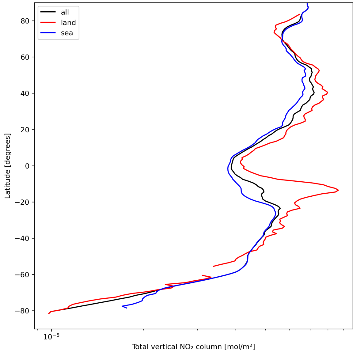
Figure 21: Zonal average of “Total vertical NO 2 column” for 2023-09-05 to 2023-09-06.
