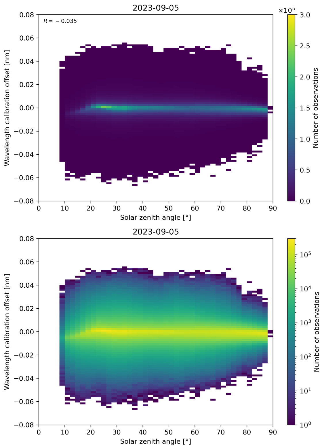
Figure 158: Scatter density plot of “Solar zenith angle” against “Wavelength calibration offset” for 2023-09-05 to 2023-09-06.
