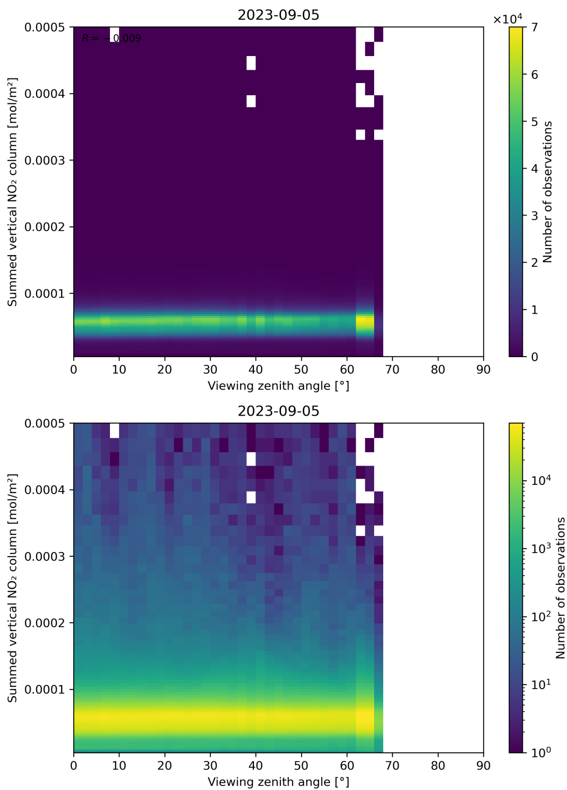
Figure 165: Scatter density plot of “Viewing zenith angle” against “Summed vertical NO 2 column” for 2023-09-05 to 2023-09-06.
