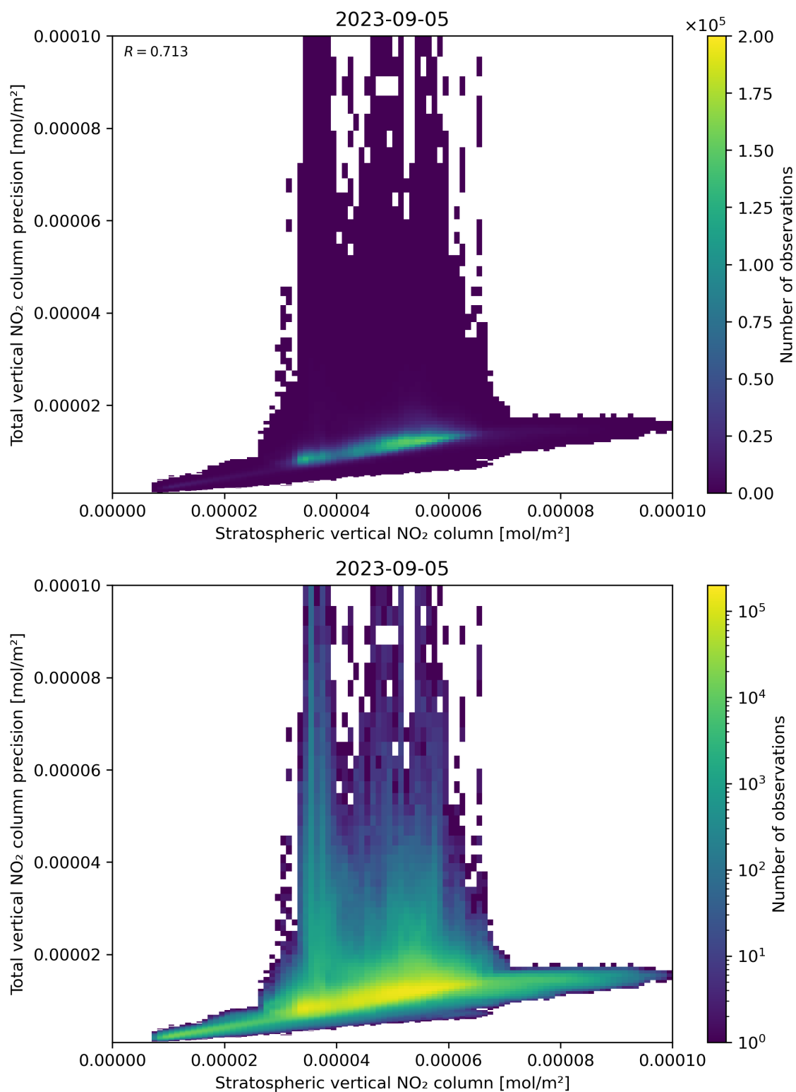
Figure 101: Scatter density plot of “Stratospheric vertical NO 2 column” against “Total vertical NO 2 column precision” for 2023-09-05 to 2023-09-06.
