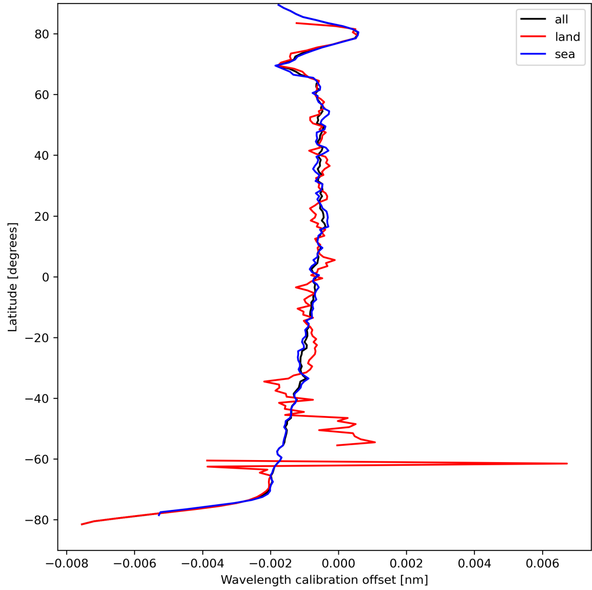
Figure 18: Zonal average of “Wavelength calibration offset” for 2023-09-05 to 2023-09-06.
