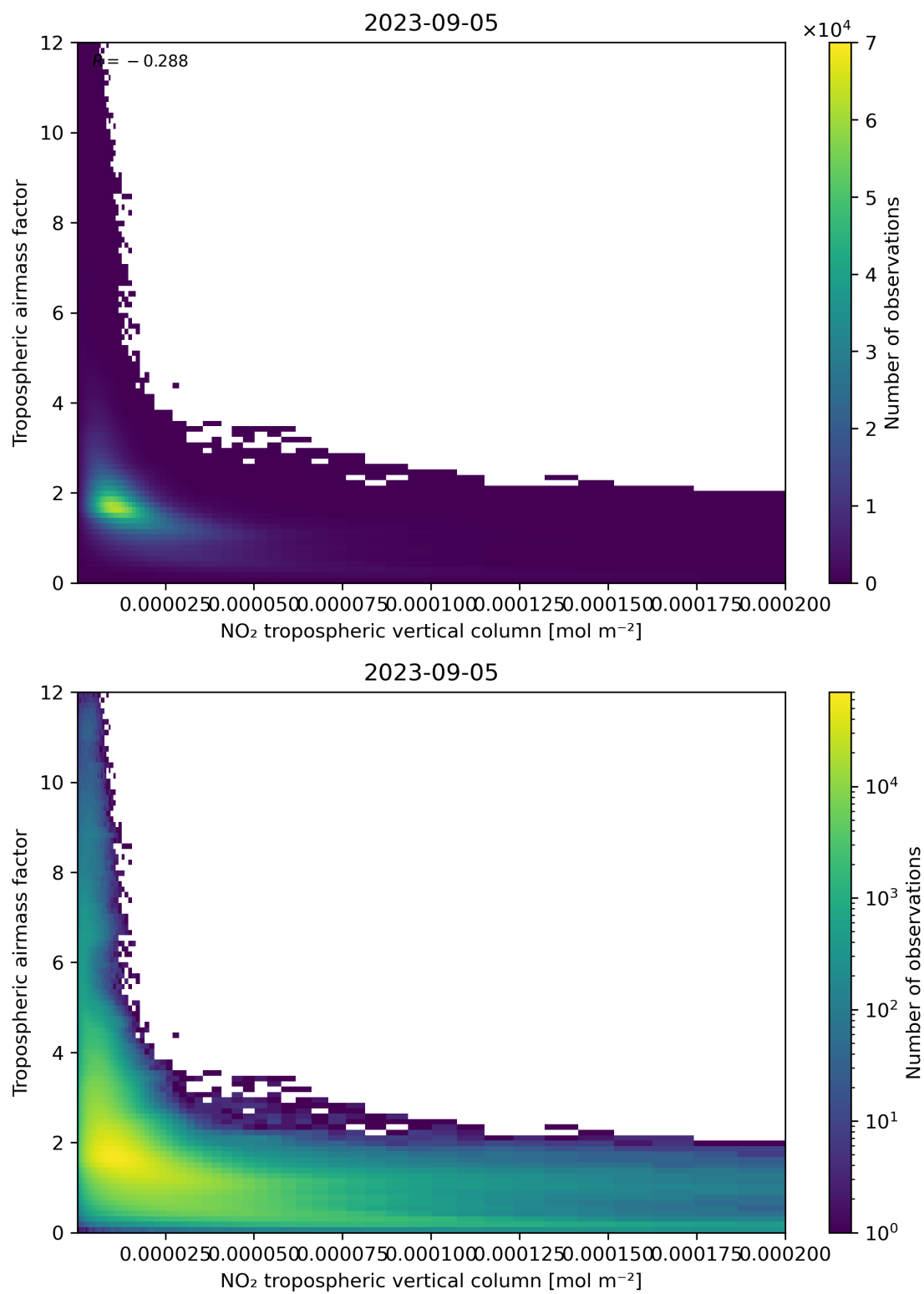
Figure 123: Scatter density plot of “NO 2 tropospheric vertical column” against “Tropospheric air mass factor” for 2023-09-05 to 2023-09-06.
