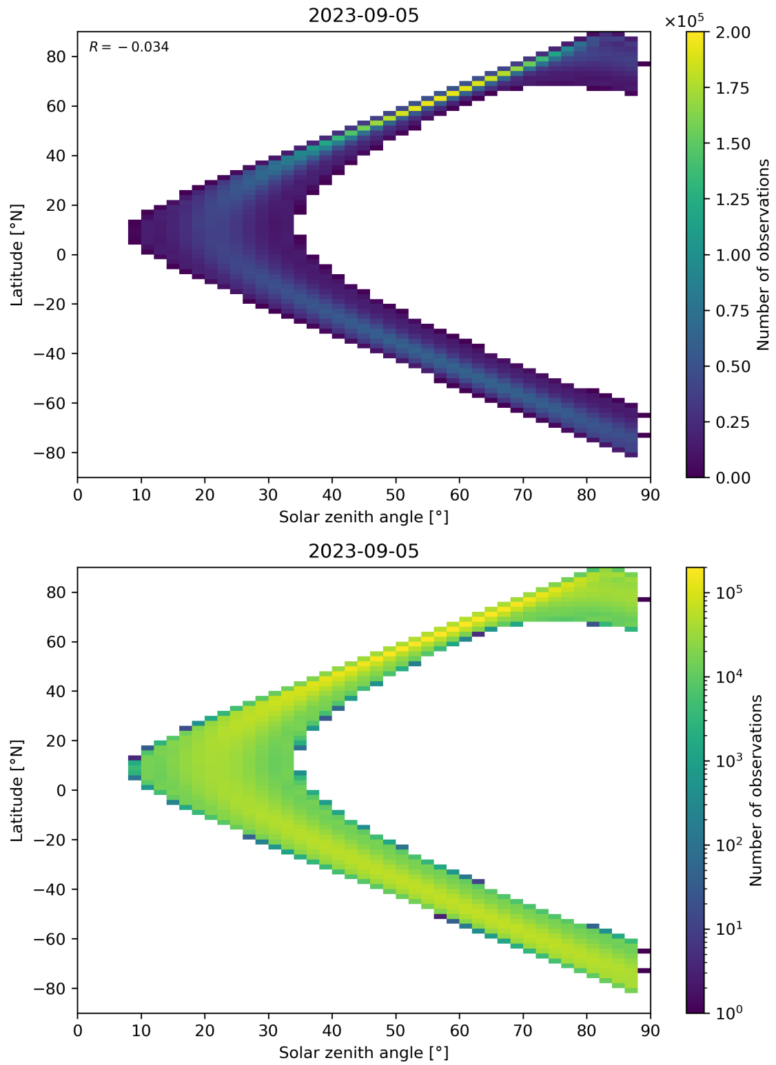
Figure 149: Scatter density plot of “Solar zenith angle” against “Latitude” for 2023-09-05 to 2023-09-06.
