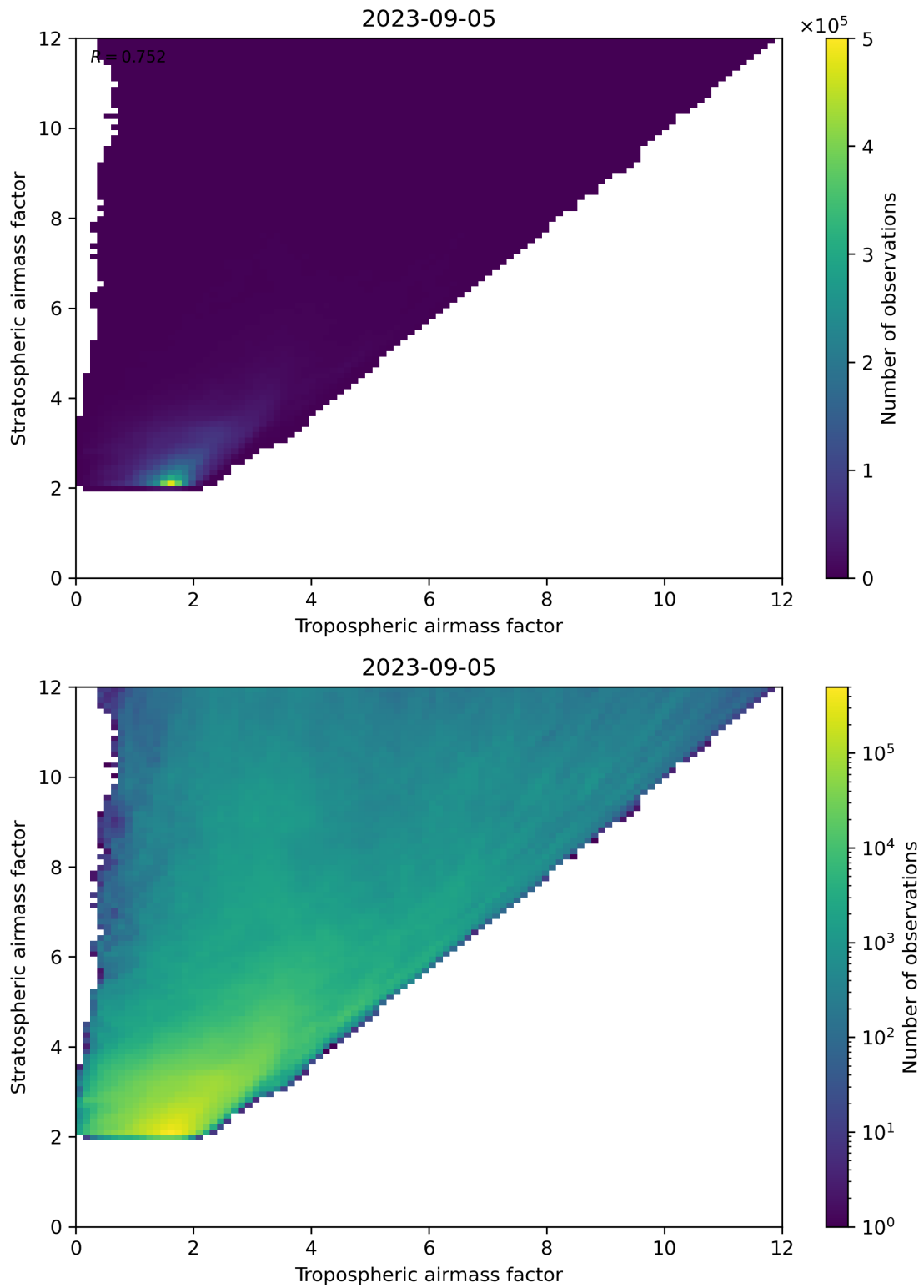
Figure 71: Scatter density plot of “Tropospheric airmass factor” against “Stratospheric airmass factor” for 2023-09-05 to 2023-09-06.
