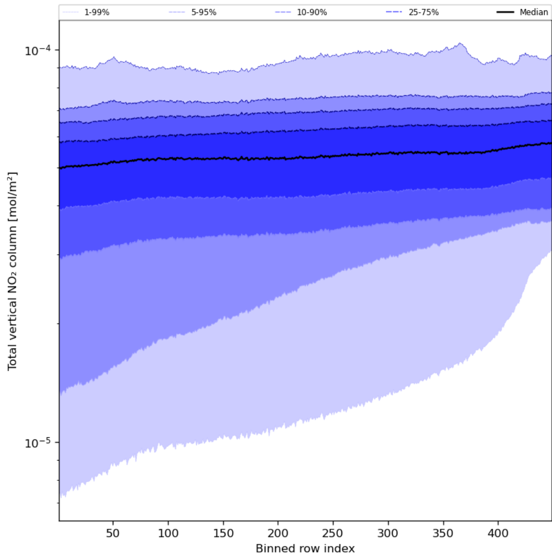
Figure 55: Along track statistics of “Total vertical NO 2 column” for 2023-09-05 to 2023-09-06
