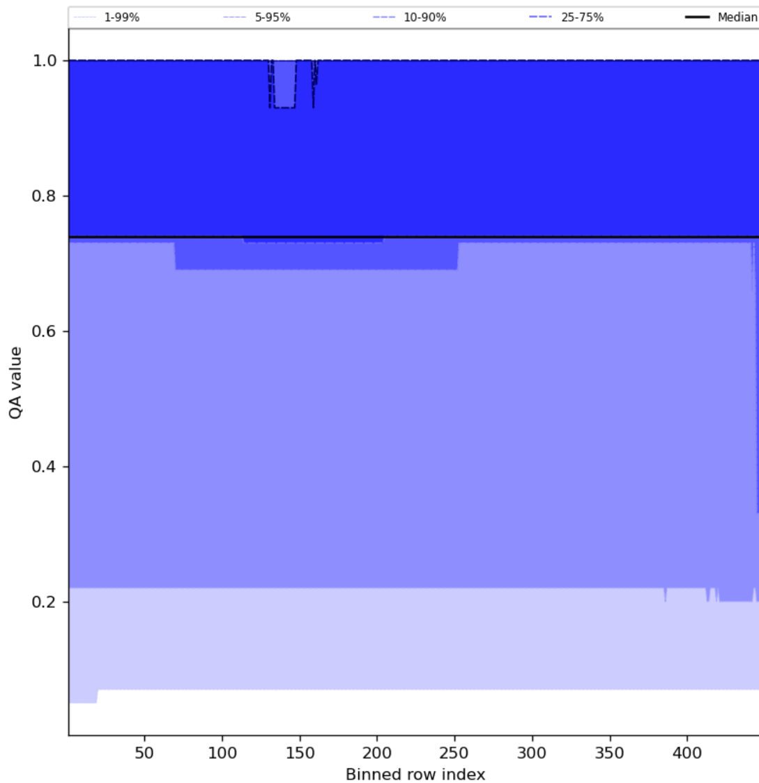
Figure 45: Along track statistics of “QA value” for 2023-09-05 to 2023-09-06
