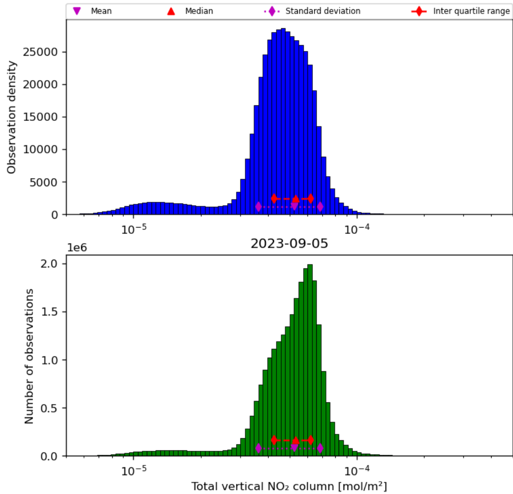
Figure 38: Histogram of “Total vertical NO 2 column” for 2023-09-05 to 2023-09-06
