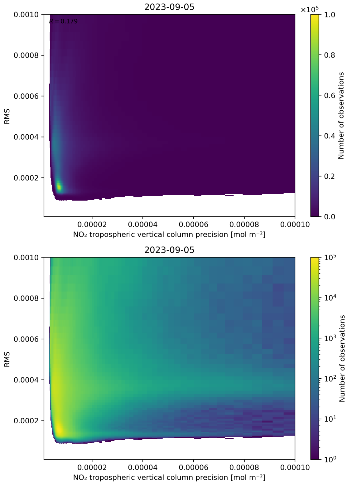
Figure 140: Scatter density plot of “NO 2 tropospheric vertical column precision” against “RMS” for 2023-09-05 to 2023-09-06.
