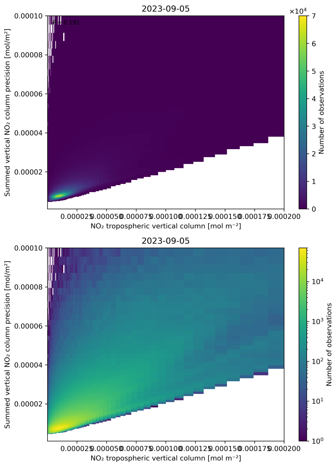
Figure 127: Scatter density plot of “NO 2 tropospheric vertical column” against “Summed vertical NO 2 column precision” for 2023-09-05 to 2023-09-06.
