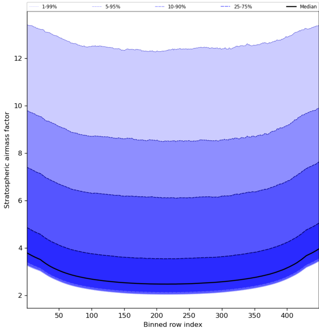
Figure 61: Along track statistics of “Stratospheric airmass factor” for 2023-09-05 to 2023-09-06
