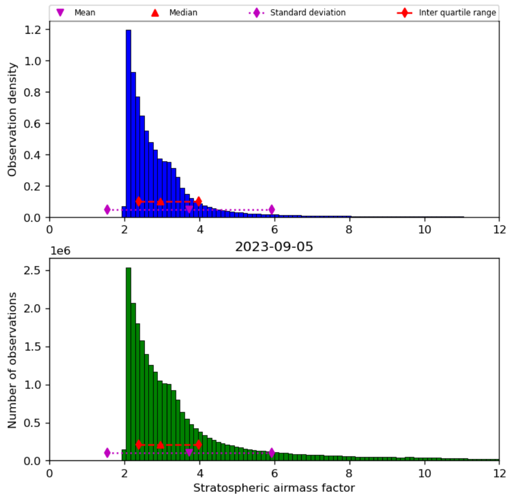
Figure 44: Histogram of “Stratospheric airmass factor” for 2023-09-05 to 2023-09-06
