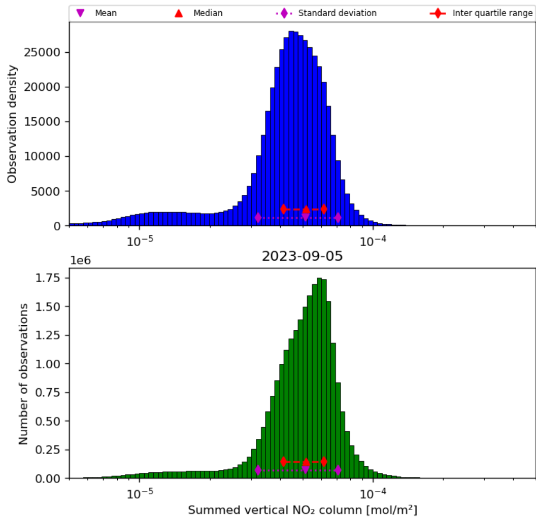
Figure 40: Histogram of "Summed vertical NO 2 column" for 2023-09-05 to 2023-09-06
