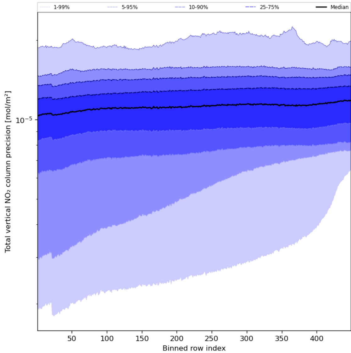
Figure 56: Along track statistics of “Total vertical NO 2 column precision” for 2023-09-05 to 2023-09-06
