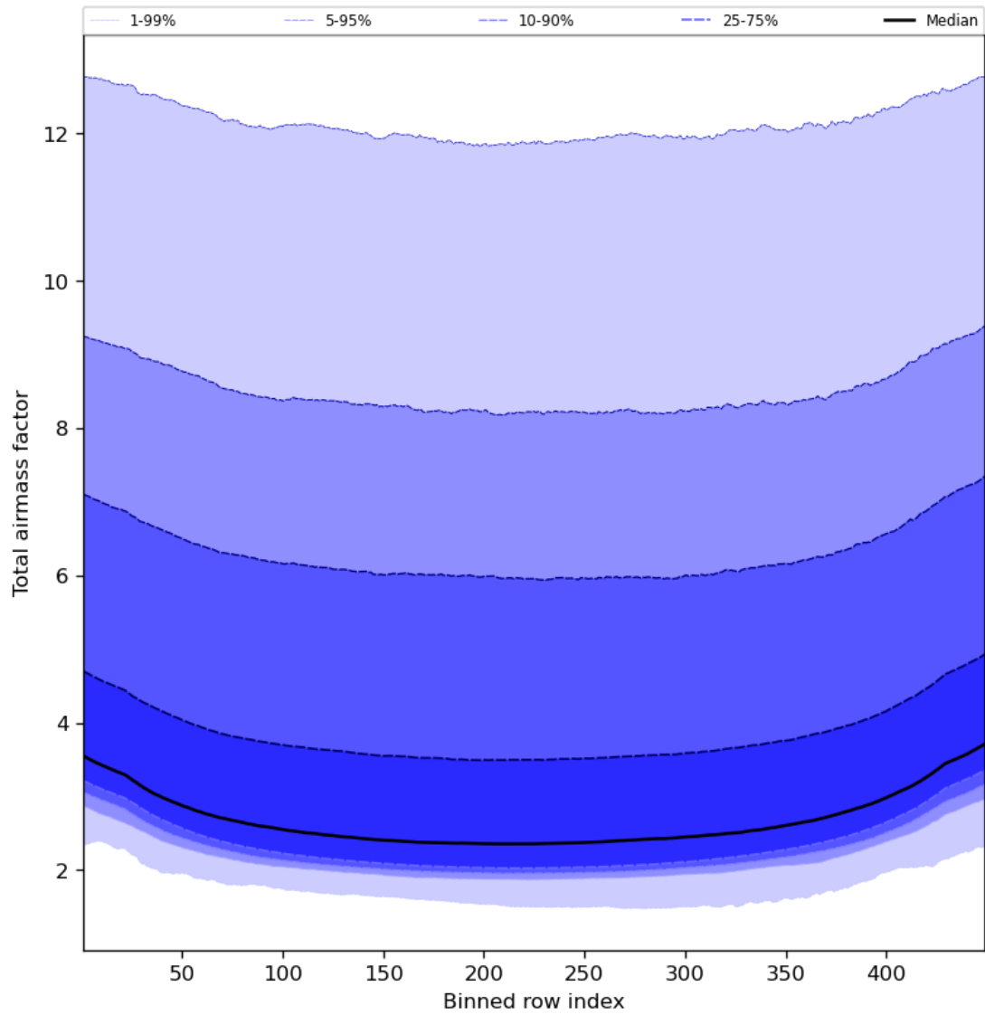
Figure 49: Along track statistics of “Total airmass factor” for 2023-09-05 to 2023-09-06
