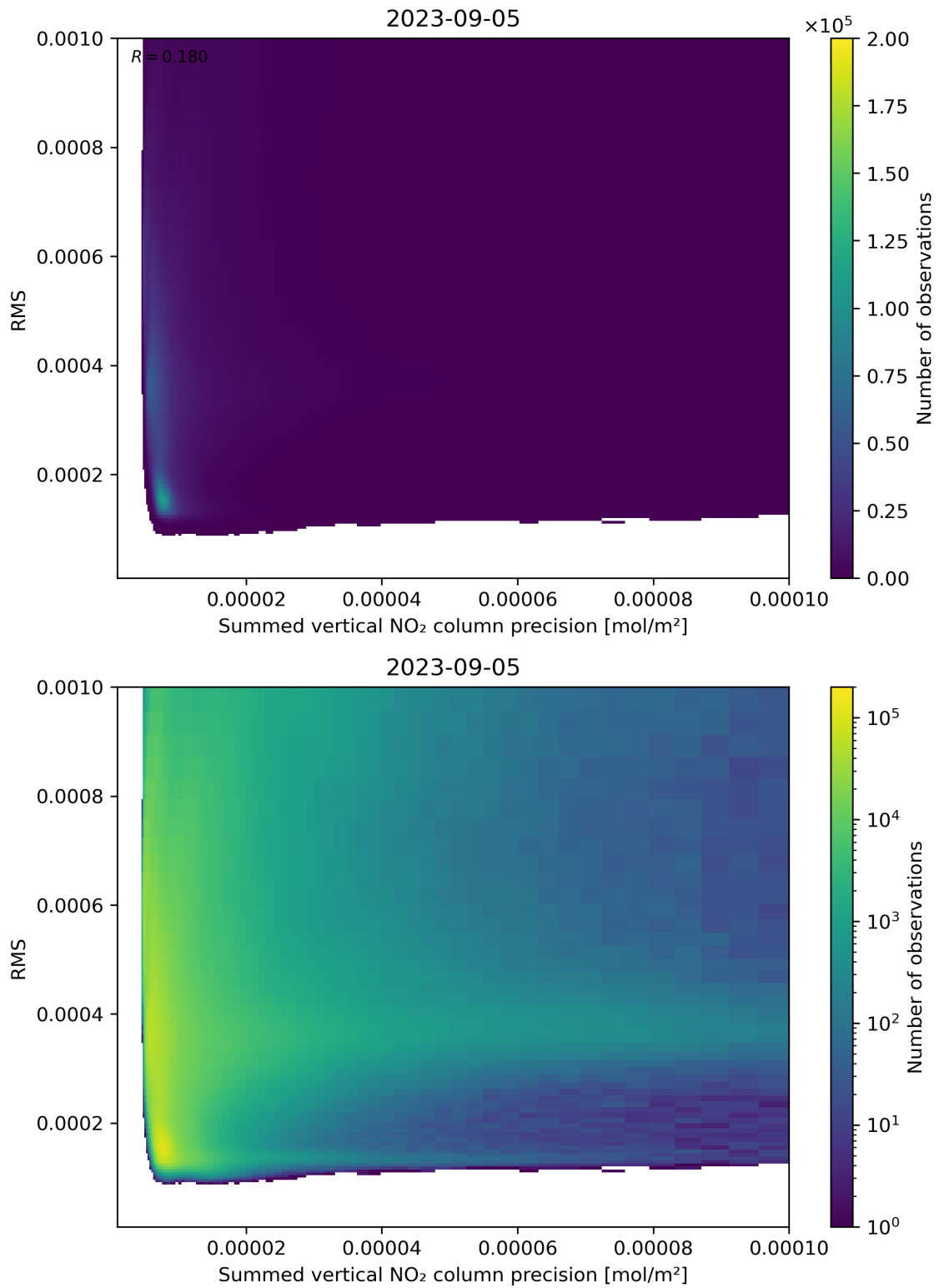
Figure 108: Scatter density plot of “Summed vertical NO 2 column precision” against “RMS” for 2023-09-05 to 2023-09-06.
