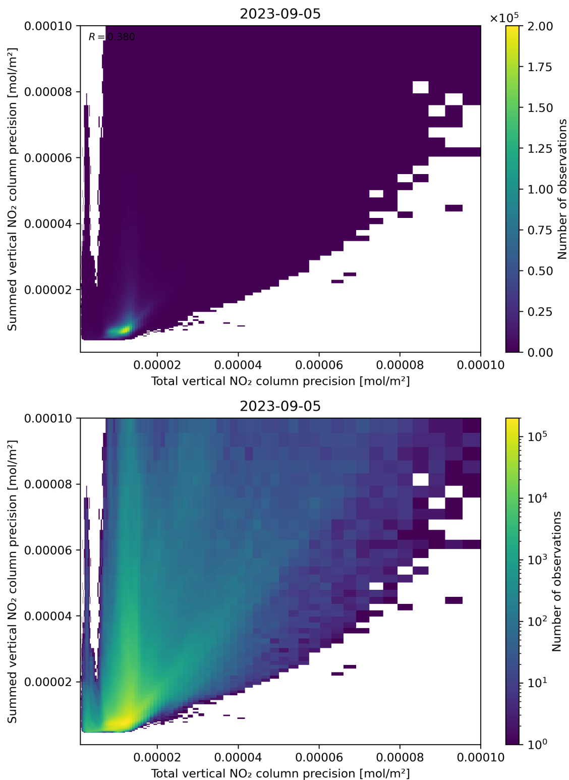
Figure 118: Scatter density plot of “Total vertical NO 2 column precision” against “Summed vertical NO 2 column precision” for 2023-09-05 to 2023-09-06.
