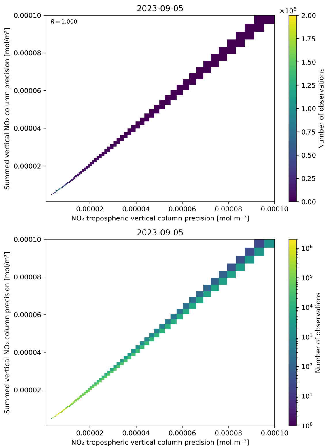
Figure 137: Scatter density plot of “NO 2 tropospheric vertical column precision” against “Summed vertical NO 2 column precision” for 2023-09-05 to 2023-09-06.
