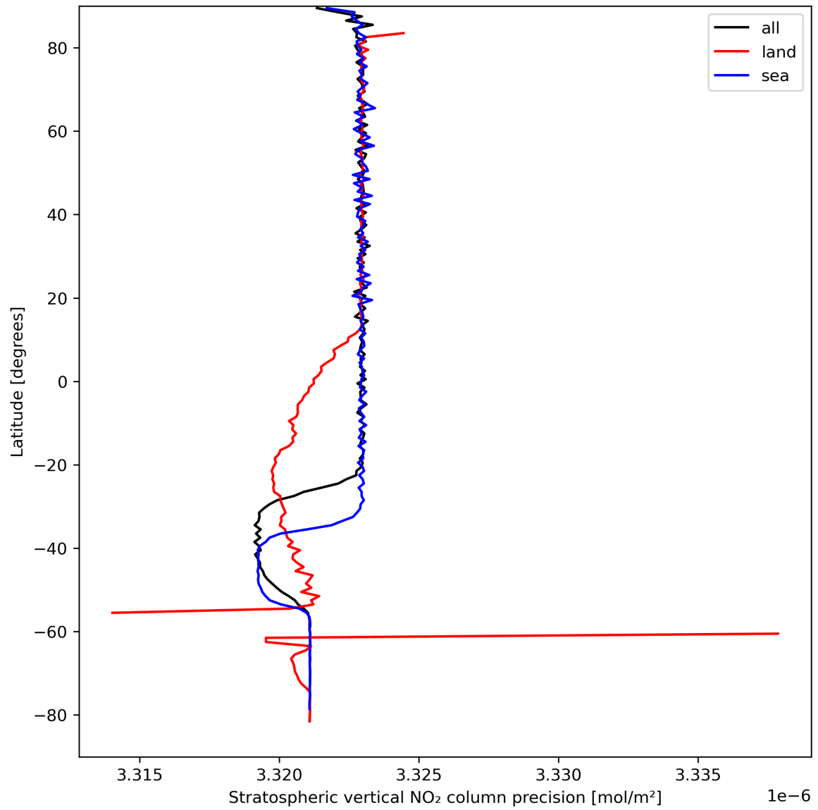
Figure 20: Zonal average of “Stratospheric vertical NO 2 column precision” for 2023-09-05 to 2023-09-06.
