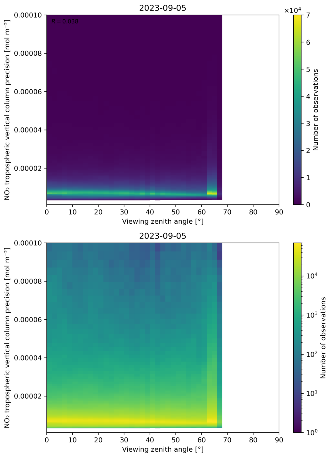
Figure 170: Scatter density plot of “Viewing zenith angle” against “NO 2 tropospheric vertical column precision” for 2023-09-05 to 2023-09-06.
