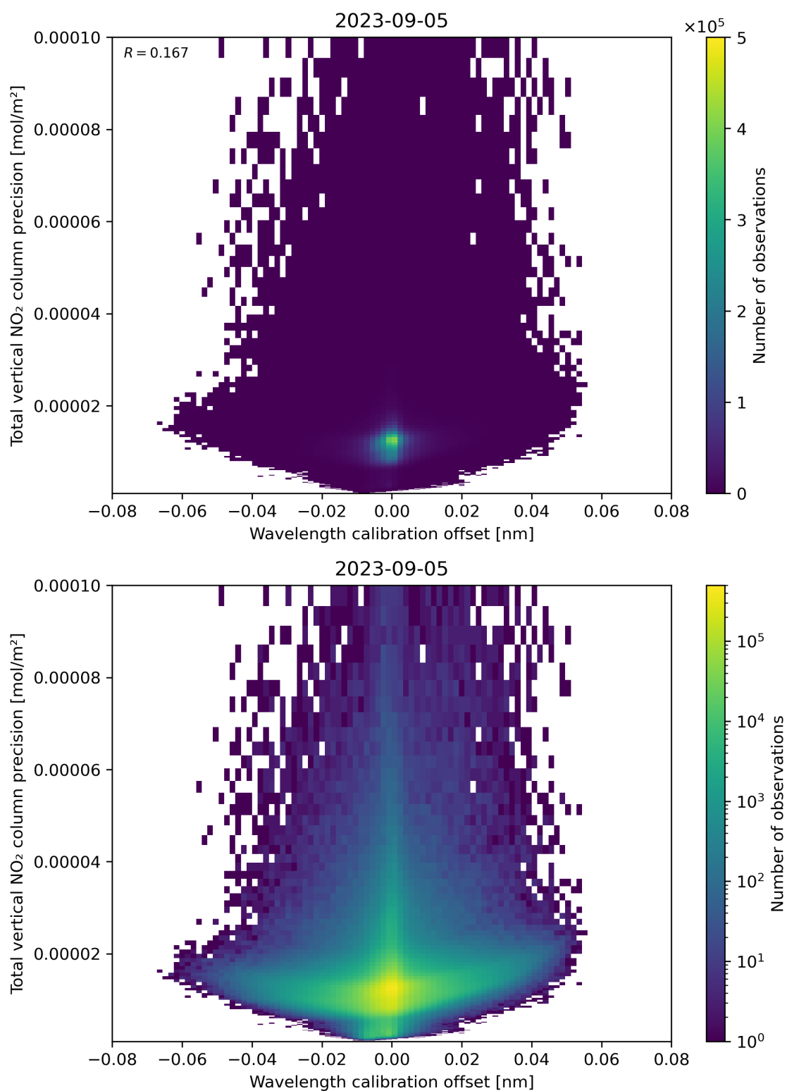
Figure 180: Scatter density plot of “Wavelength calibration offset” against “Total vertical NO 2 column precision” for 2023-09-05 to 2023-09-06.
