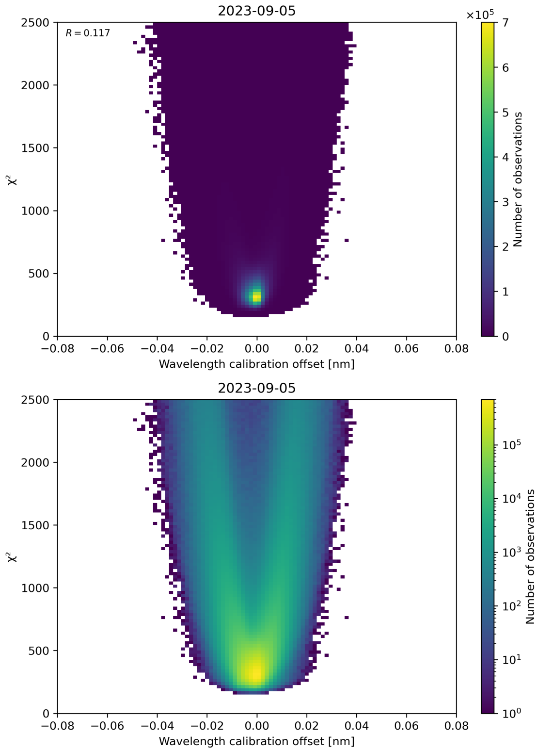
Figure 175: Scatter density plot of “Wavelength calibration offset” against “ \chi^2 ” for 2023-09-05 to 2023-09-06.
