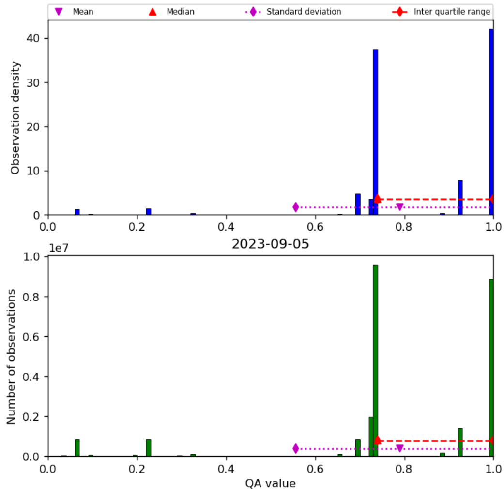
Figure 28: Histogram of “QA value” for 2023-09-05 to 2023-09-06
