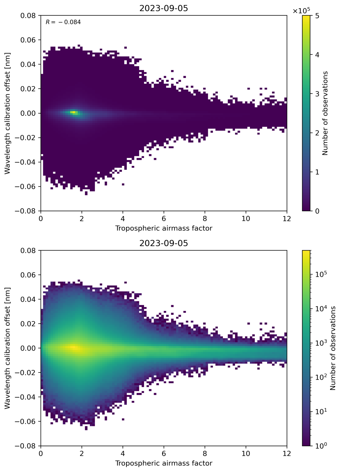
Figure 80: Scatter density plot of “Tropospheric airmass factor” against “Wavelength calibration offset” for 2023-09-05 to 2023-09-06.
