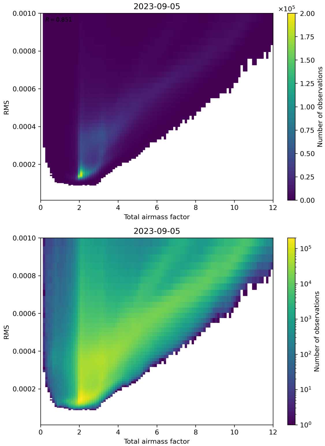
Figure 69: Scatter density plot of “Total airmass factor” against “RMS” for 2023-09-05 to 2023-09-06.
