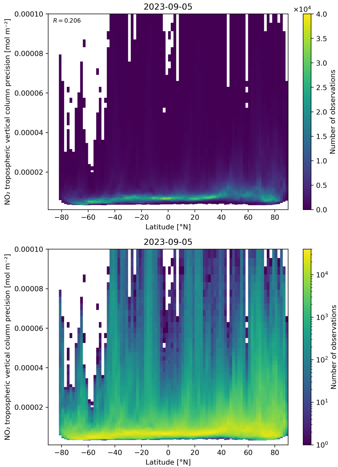
Figure 93: Scatter density plot of “Latitude” against “NO 2 tropospheric vertical column precision” for 2023-09-05 to 2023-09-06.
