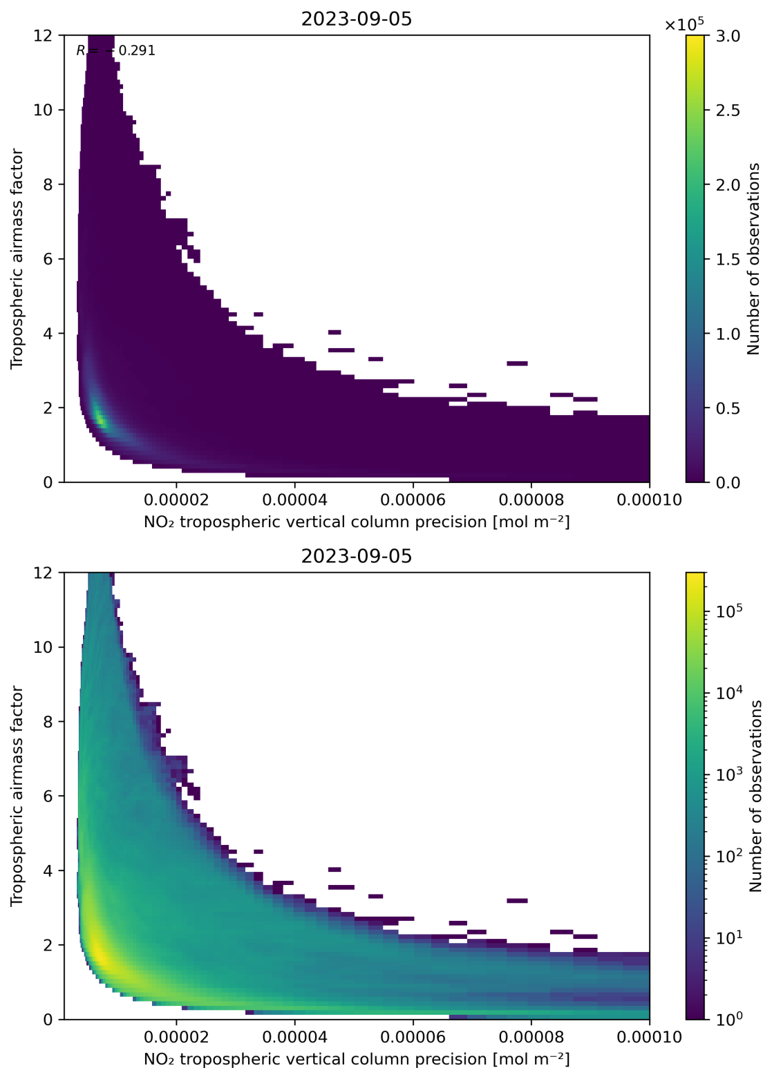
Figure 133: Scatter density plot of “NO 2 tropospheric vertical column precision” against “Tropospheric airmass factor” for 2023-09-05 to 2023-09-06.
