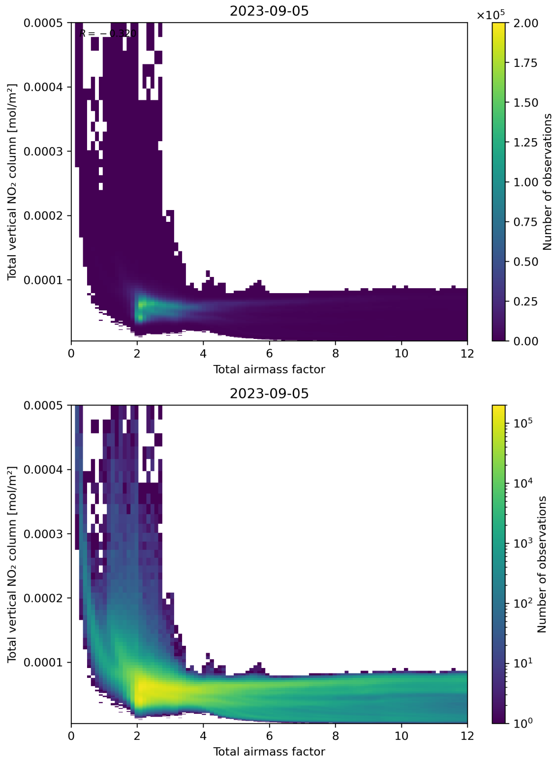
Figure 67: Scatter density plot of “Total airmass factor” against “Total vertical NO 2 column” for 2023-09-05 to 2023-09-06.
