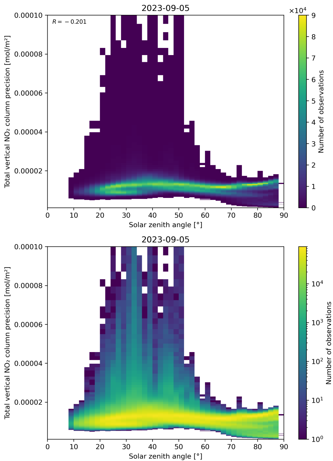
Figure 154: Scatter density plot of “Solar zenith angle” against “Total vertical NO 2 column precision” for 2023-09-05 to 2023-09-06.
