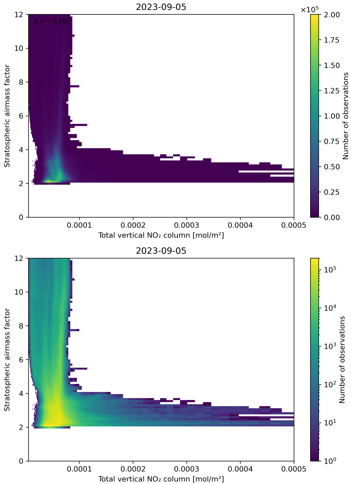
Figure 110: Scatter density plot of “Total vertical NO 2 column” against “Stratospheric airmass factor” for 2023-09-05 to 2023-09-06.
