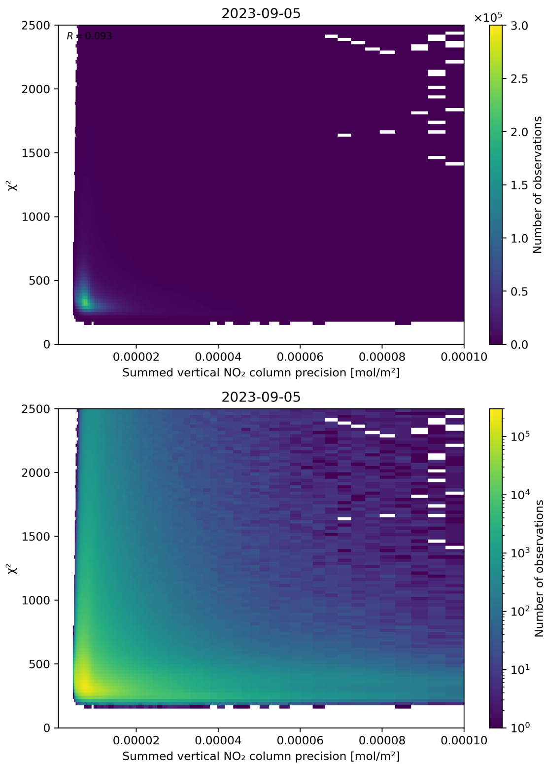
Figure 107: Scatter density plot of “Summed vertical NO 2 column precision” against “ \chi^2 ” for 2023-09-05 to 2023-09-06.
