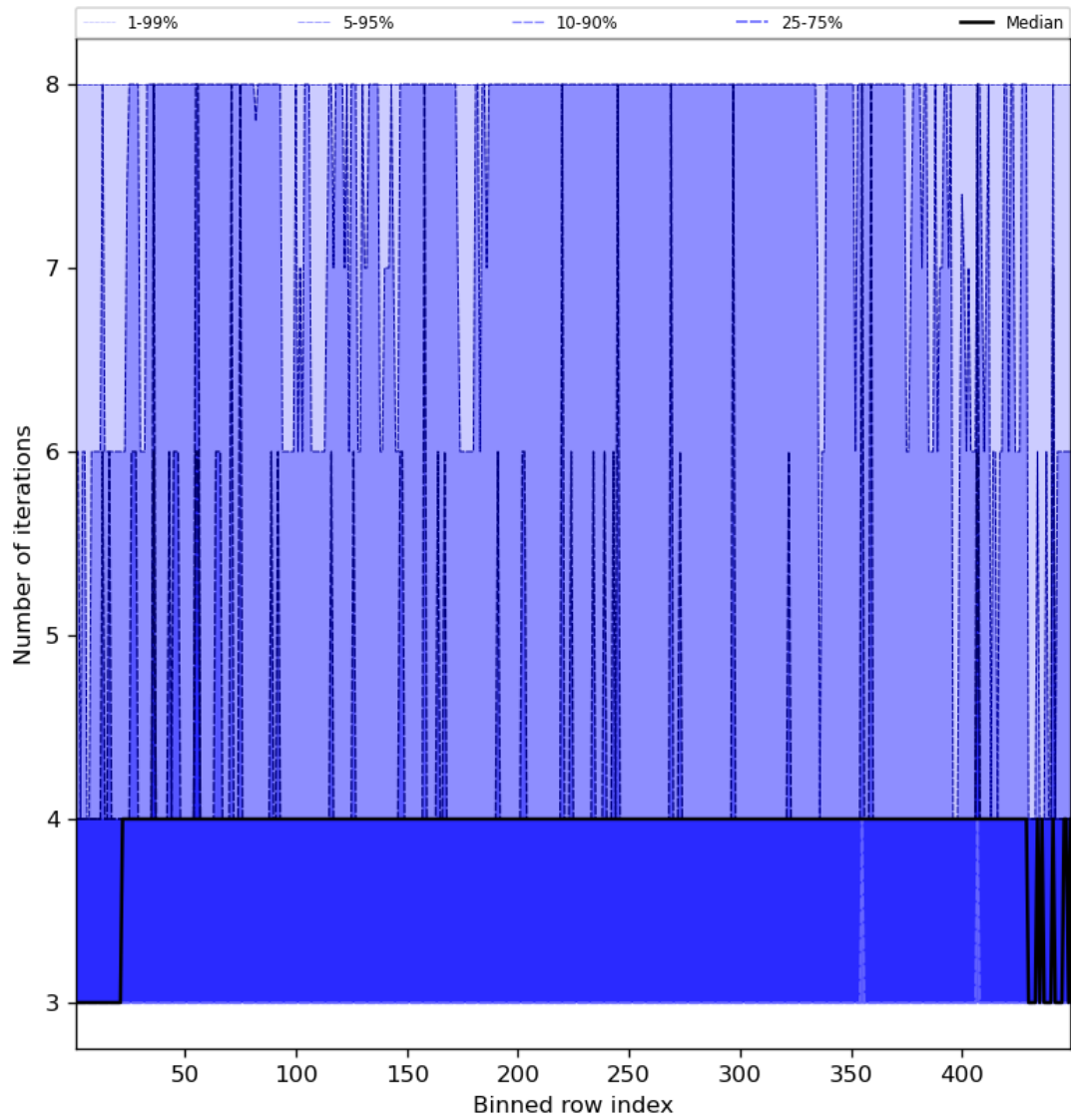
Figure 51: Along track statistics of “Number of iterations” for 2023-09-05 to 2023-09-06
