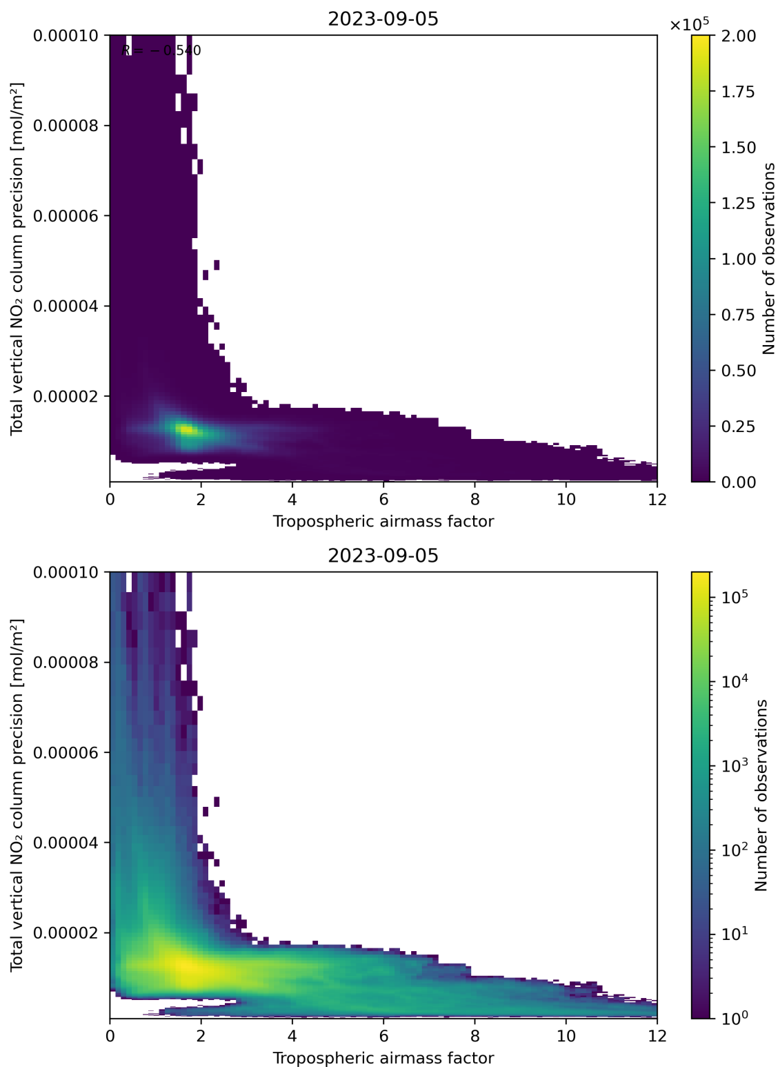
Figure 78: Scatter density plot of “Tropospheric air mass factor” against “Total vertical NO 2 column precision” for 2023-09-05 to 2023-09-06.
