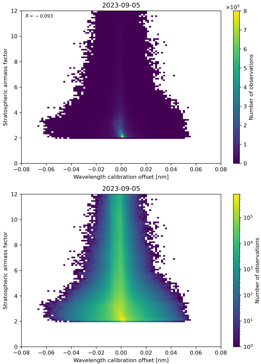
Figure 174: Scatter density plot of “Wavelength calibration offset” against “Stratospheric airmass factor” for 2023-09-05 to 2023-09-06.
