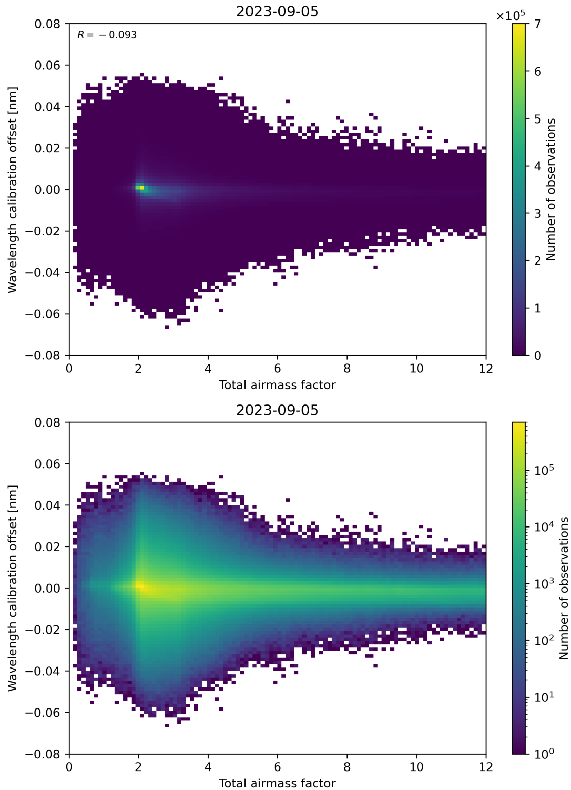
Figure 70: Scatter density plot of “Total airmass factor” against “Wavelength calibration offset” for 2023-09-05 to 2023-09-06.
