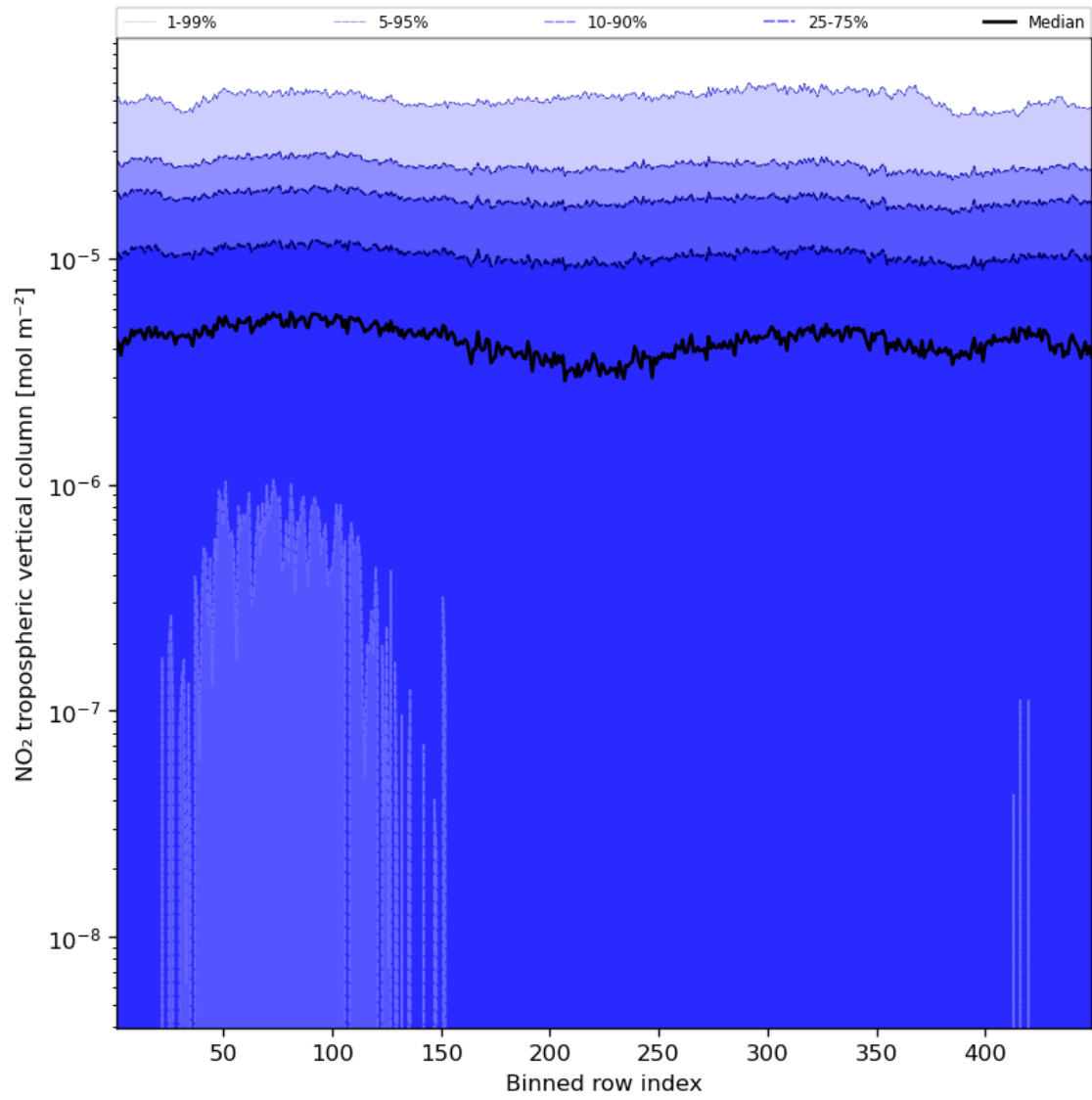
Figure 46: Along track statistics of “NO 2 tropospheric vertical column” for 2023-09-05 to 2023-09-06
