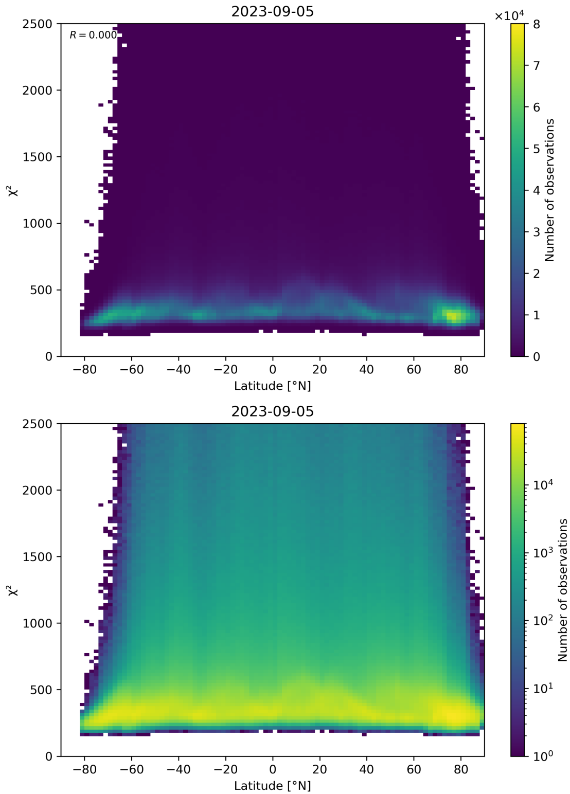
Figure 86: Scatter density plot of “Latitude” against “ \chi^2 ” for 2023-09-05 to 2023-09-06.
