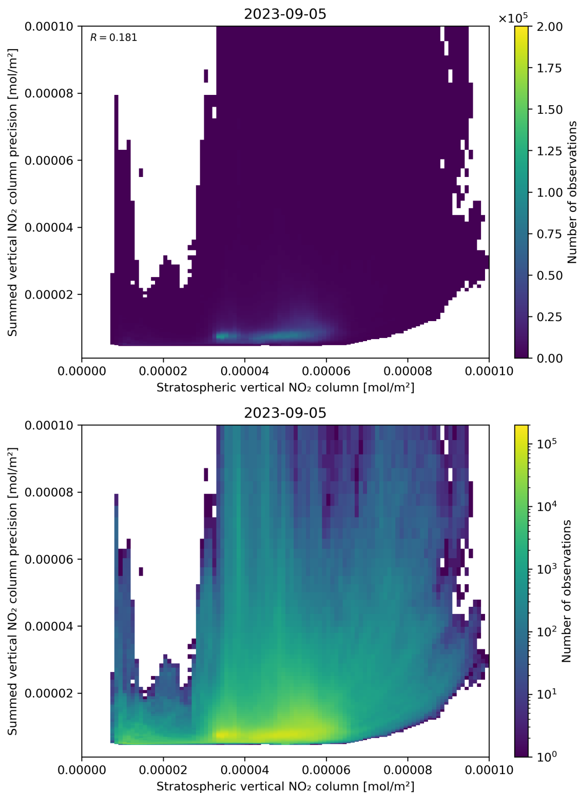
Figure 99: Scatter density plot of “Stratospheric vertical NO 2 column” against “Summed vertical NO 2 column precision” for 2023-09-05 to 2023-09-06.
