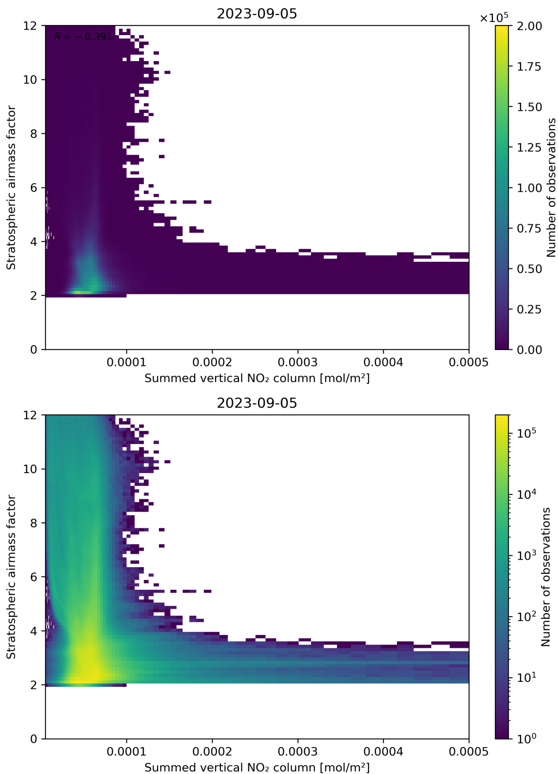
Figure 103: Scatter density plot of “Summed vertical NO 2 column” against “Stratospheric airmass factor” for 2023-09-05 to 2023-09-06.
