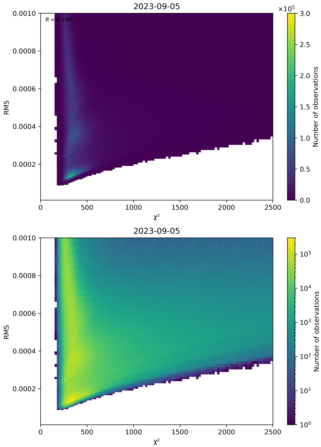
Figure 82: Scatter density plot of “ \chi^2 ” against “RMS” for 2023-09-05 to 2023-09-06.
