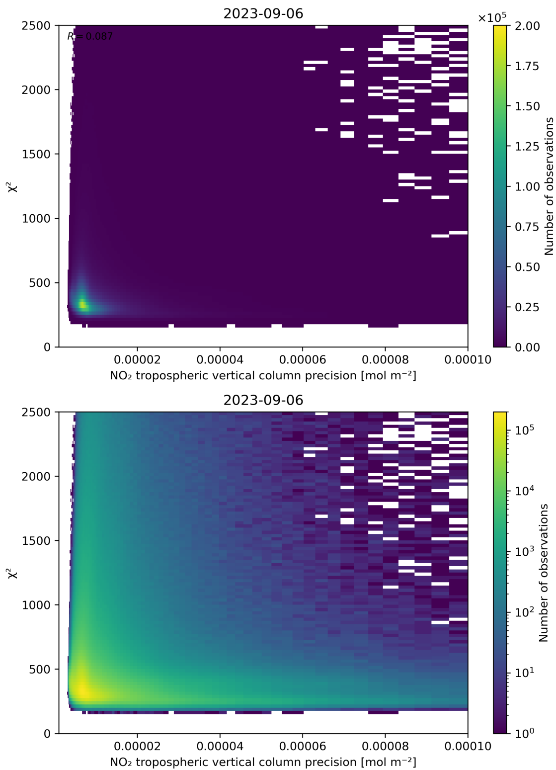
Figure 134: Scatter density plot of “NO 2 tropospheric vertical column precision” against “ \chi^2 ” for 2023-09-05 to 2023-09-07.
