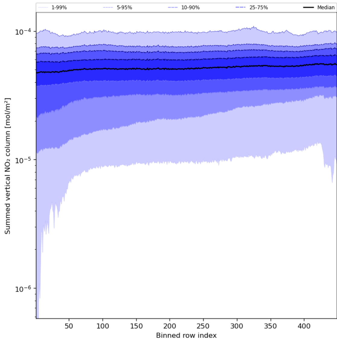
Figure 57: Along track statistics of “Summed vertical NO 2 column” for 2023-09-05 to 2023-09-07
