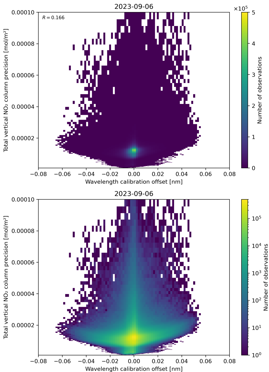
Figure 180: Scatter density plot of “Wavelength calibration offset” against “Total vertical NO 2 column precision” for 2023-09-05 to 2023-09-07.
