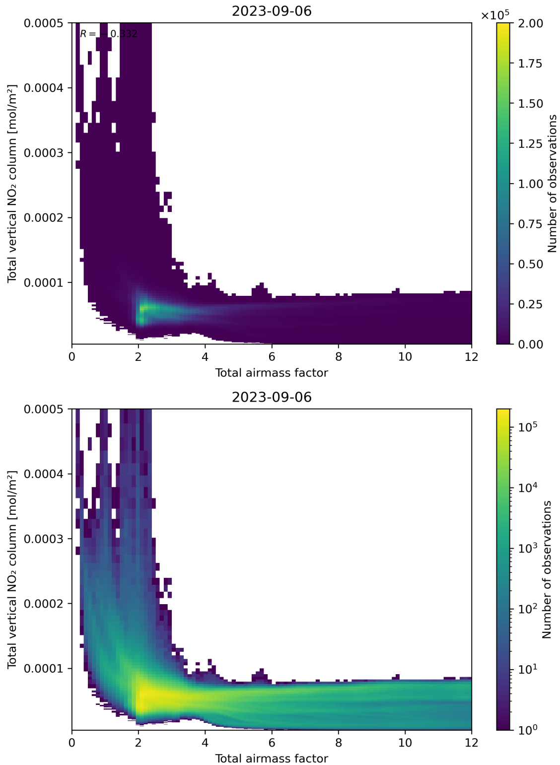
Figure 67: Scatter density plot of “Total airmass factor” against “Total vertical NO 2 column” for 2023-09-05 to 2023-09-07.
