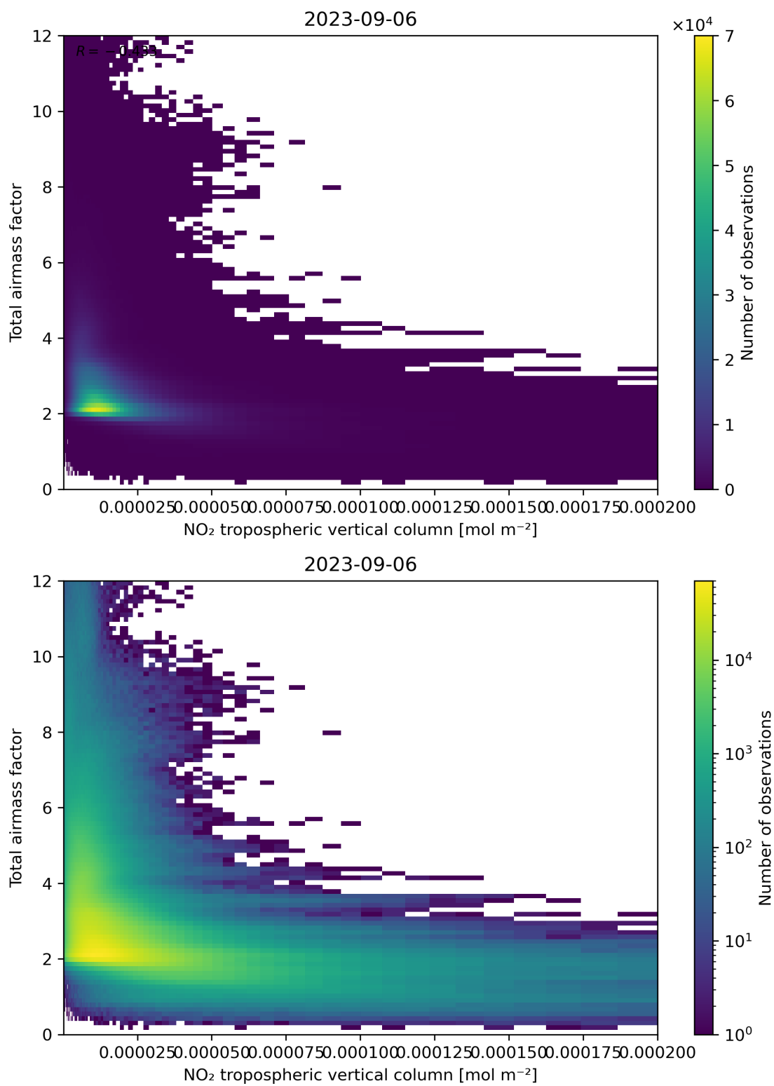
Figure 122: Scatter density plot of “NO 2 tropospheric vertical column” against “Total air mass factor” for 2023-09-05 to 2023-09-07.
