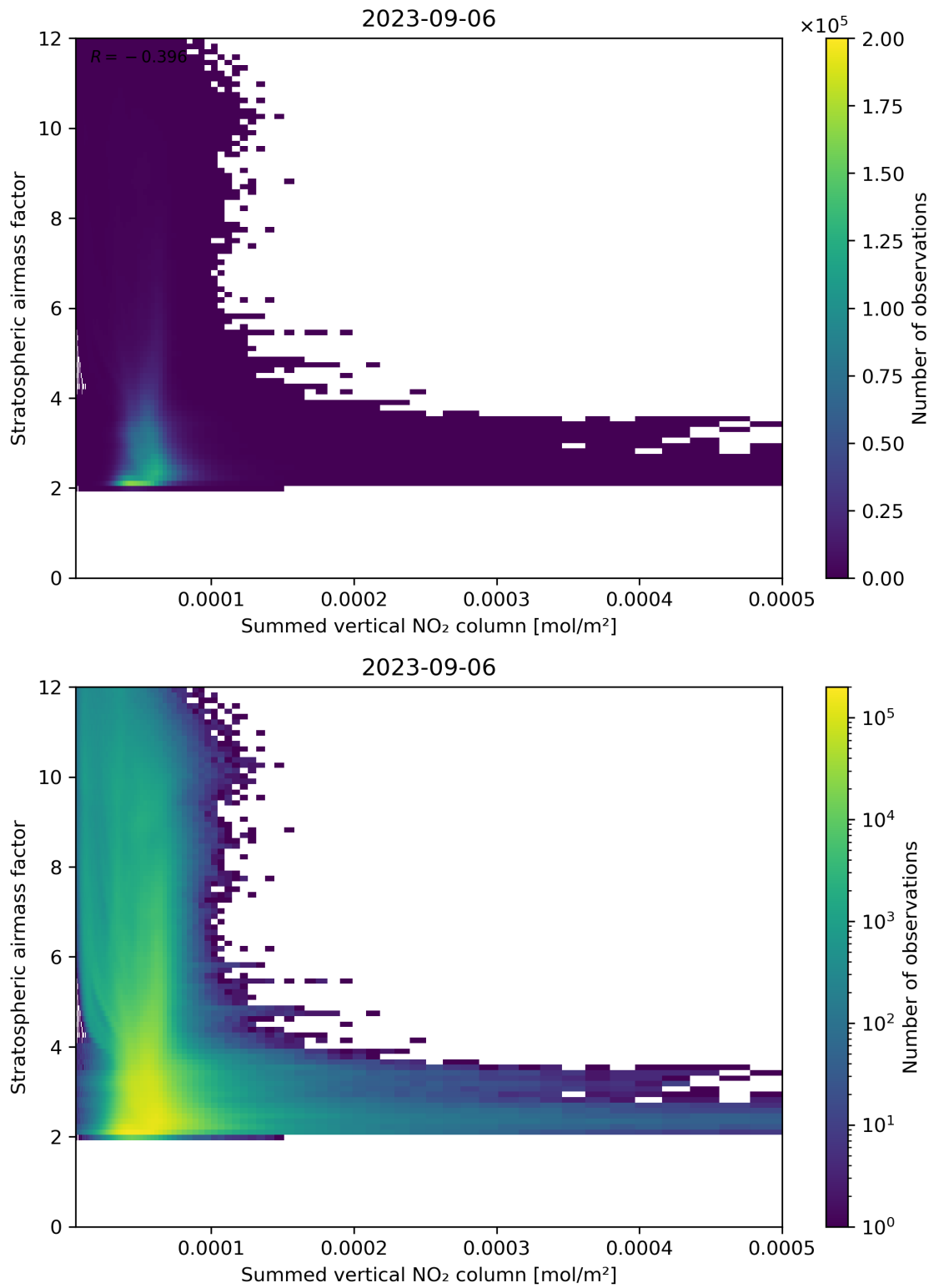
Figure 103: Scatter density plot of “Summed vertical NO 2 column” against “Stratospheric airmass factor” for 2023-09-05 to 2023-09-07.
