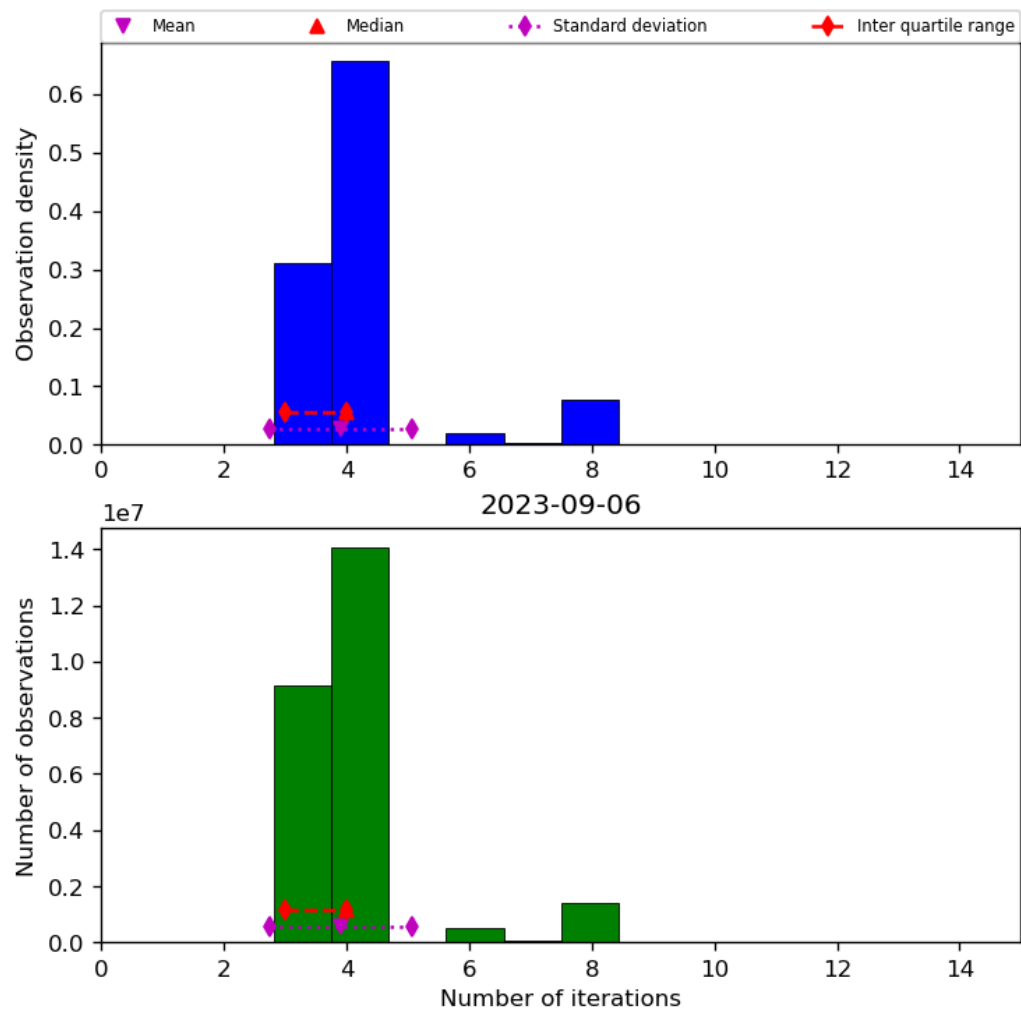
Figure 34: Histogram of “Number of iterations” for 2023-09-05 to 2023-09-07
