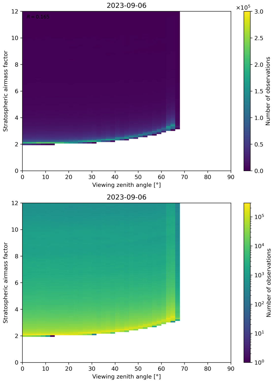
Figure 159: Scatter density plot of “Viewing zenith angle” against “Stratospheric airmass factor” for 2023-09-05 to 2023-09-07.
