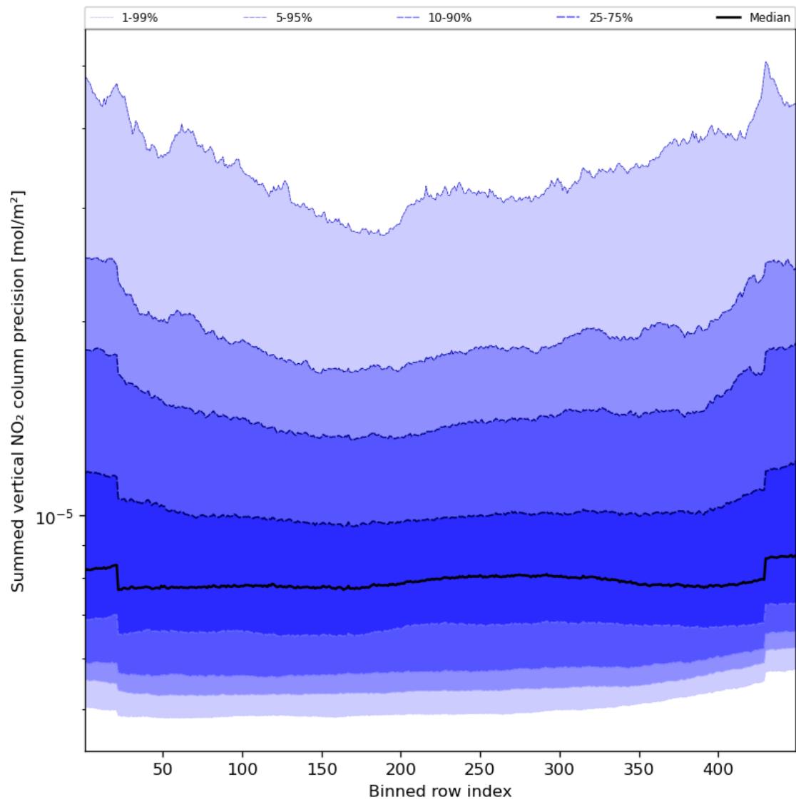
Figure 58: Along track statistics of “Summed vertical NO 2 column precision” for 2023-09-05 to 2023-09-07
