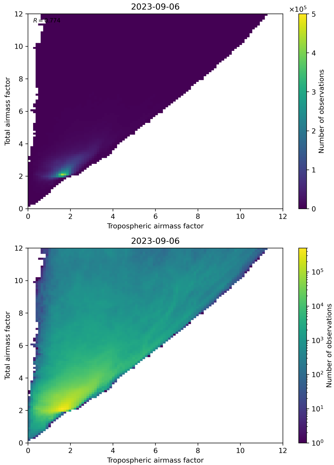
Figure 72: Scatter density plot of “Tropospheric airmass factor” against “Total airmass factor” for 2023-09-05 to 2023-09-07.
