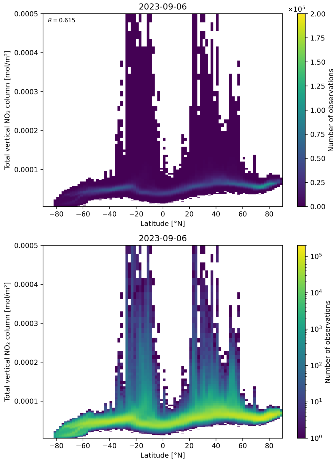
Figure 90: Scatter density plot of “Latitude” against “Total vertical NO 2 column” for 2023-09-05 to 2023-09-07.
