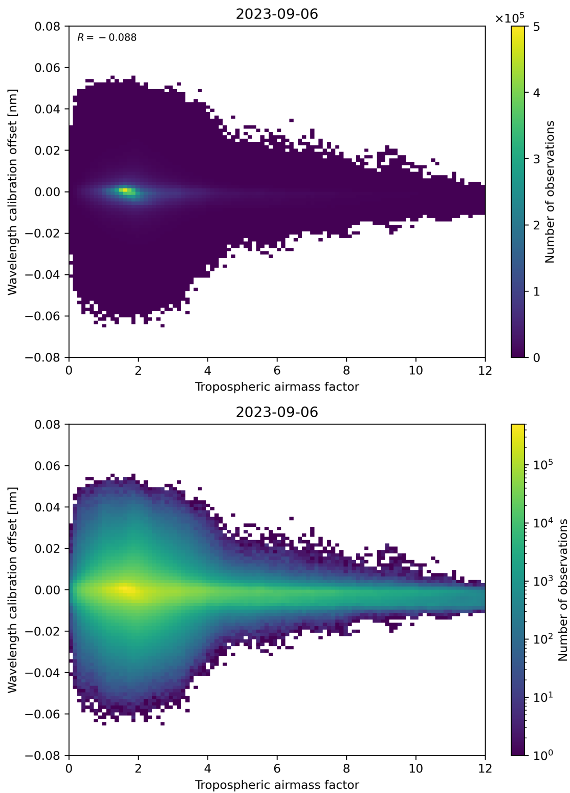
Figure 80: Scatter density plot of “Tropospheric airmass factor” against “Wavelength calibration offset” for 2023-09-05 to 2023-09-07.
