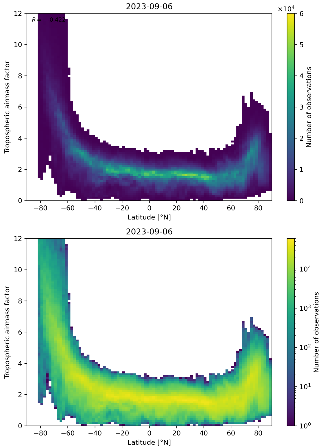
Figure 85: Scatter density plot of “Latitude” against “Tropospheric airmass factor” for 2023-09-05 to 2023-09-07.
