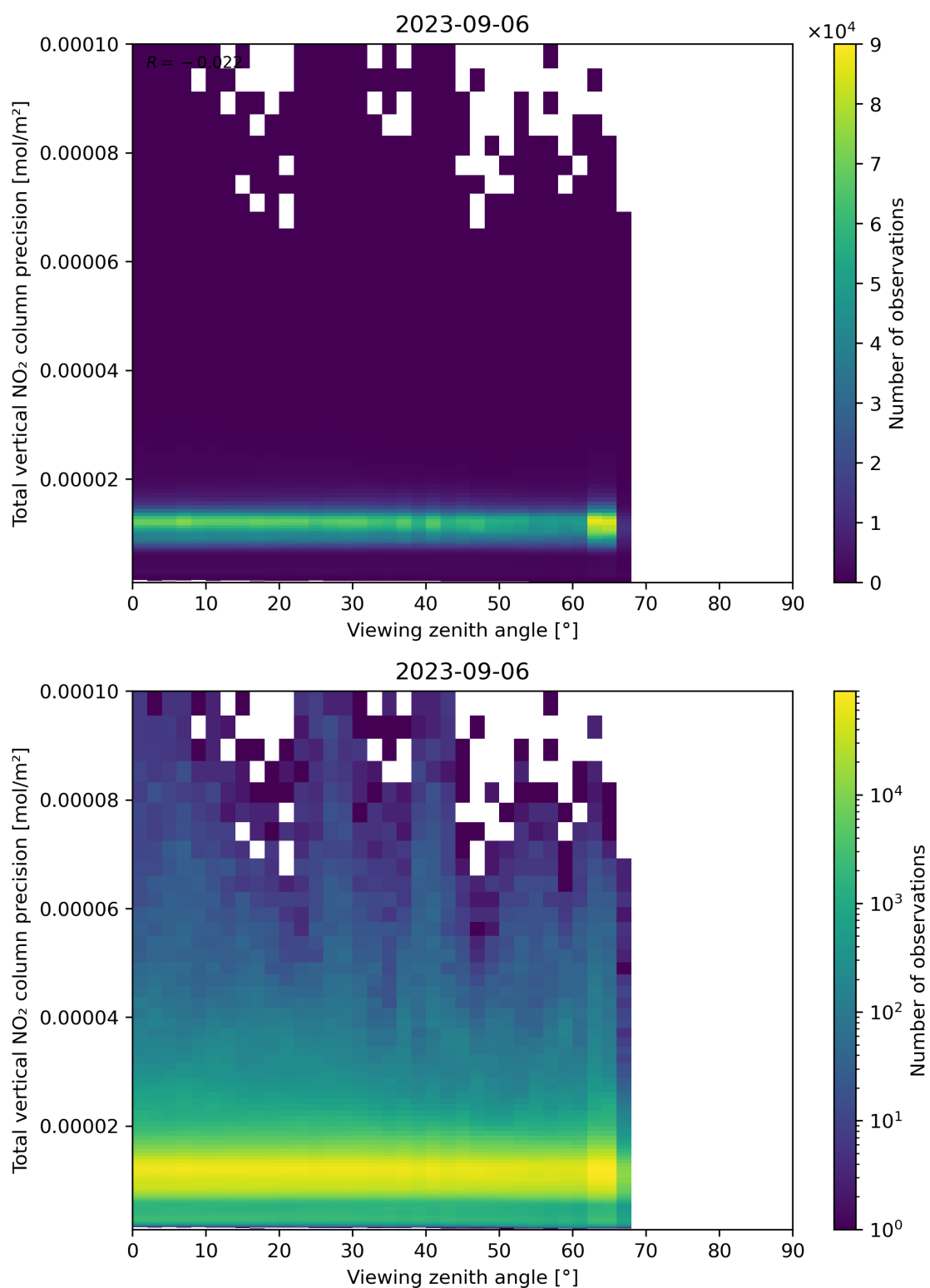
Figure 168: Scatter density plot of “Viewing zenith angle” against “Total vertical NO 2 column precision” for 2023-09-05 to 2023-09-07.
