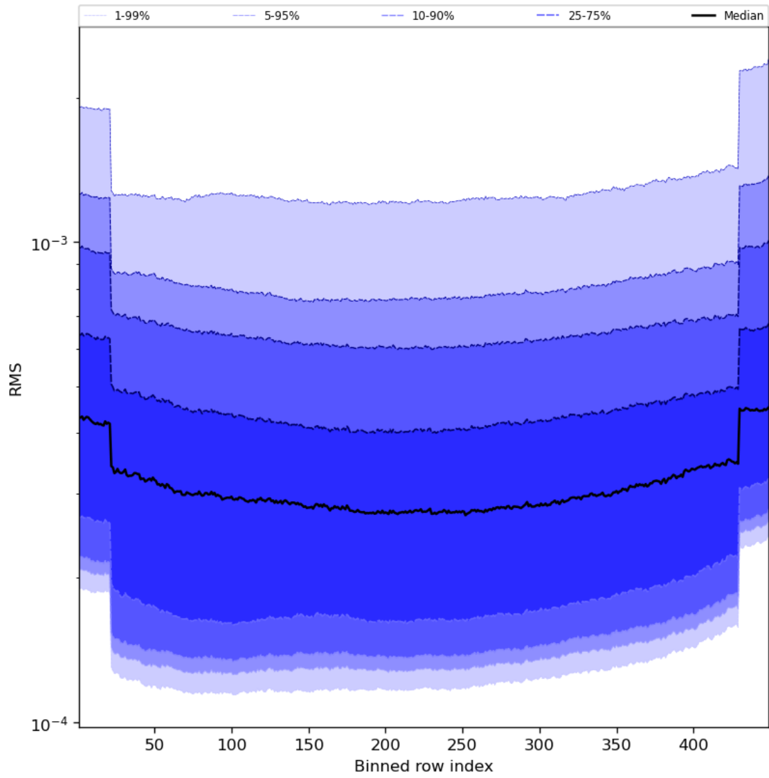
Figure 60: Along track statistics of “RMS” for 2023-09-05 to 2023-09-07
