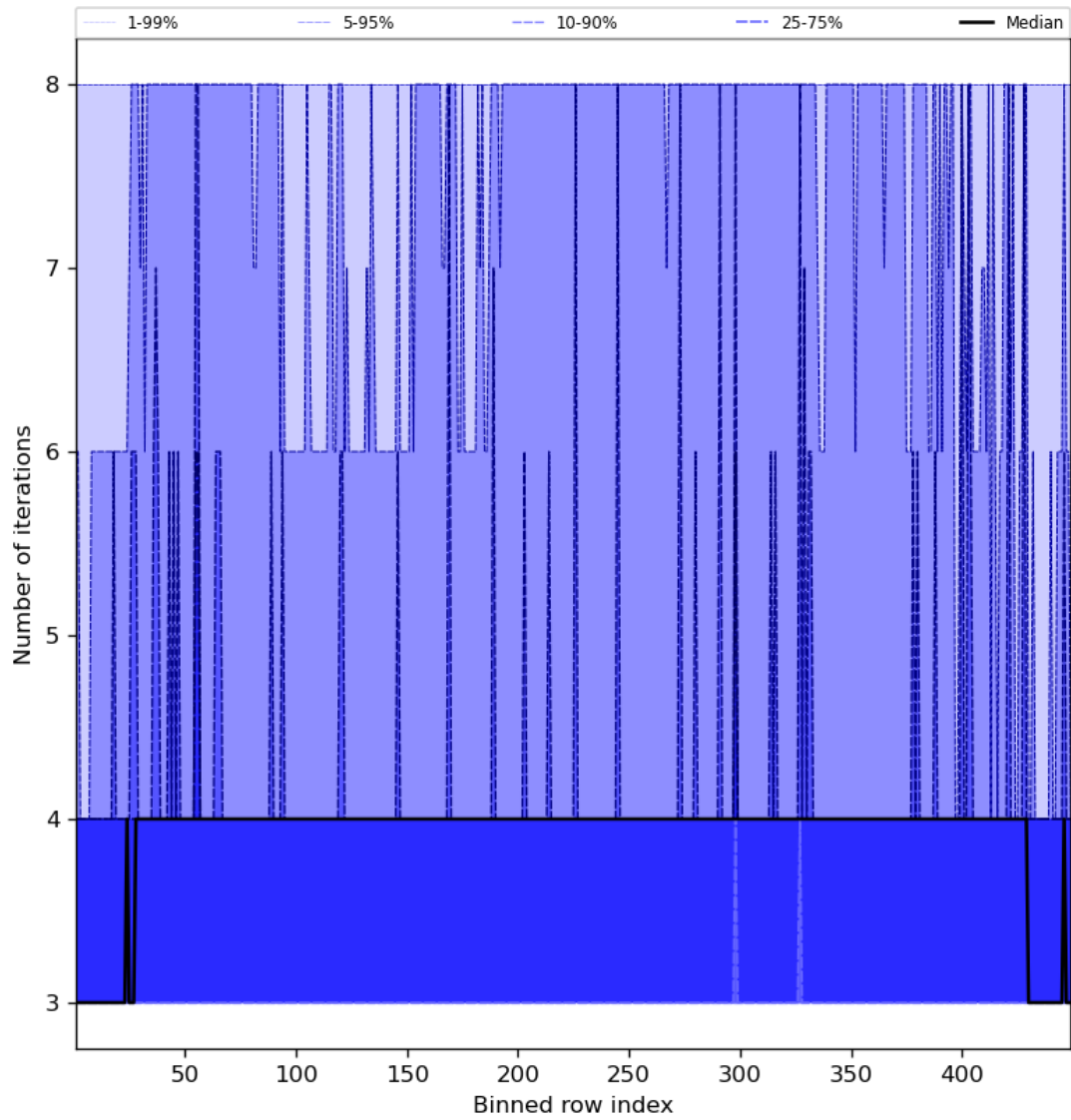
Figure 51: Along track statistics of “Number of iterations” for 2023-09-05 to 2023-09-07
