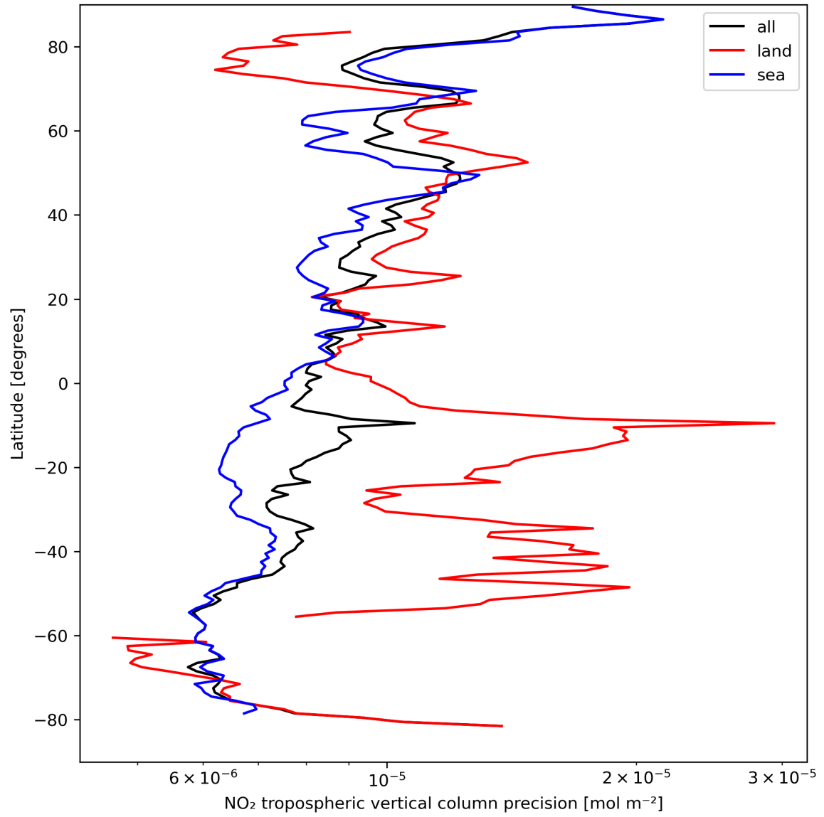
Figure 13: Zonal average of "NO 2 tropospheric vertical column precision" for 2023-09-05 to 2023-09-07.
