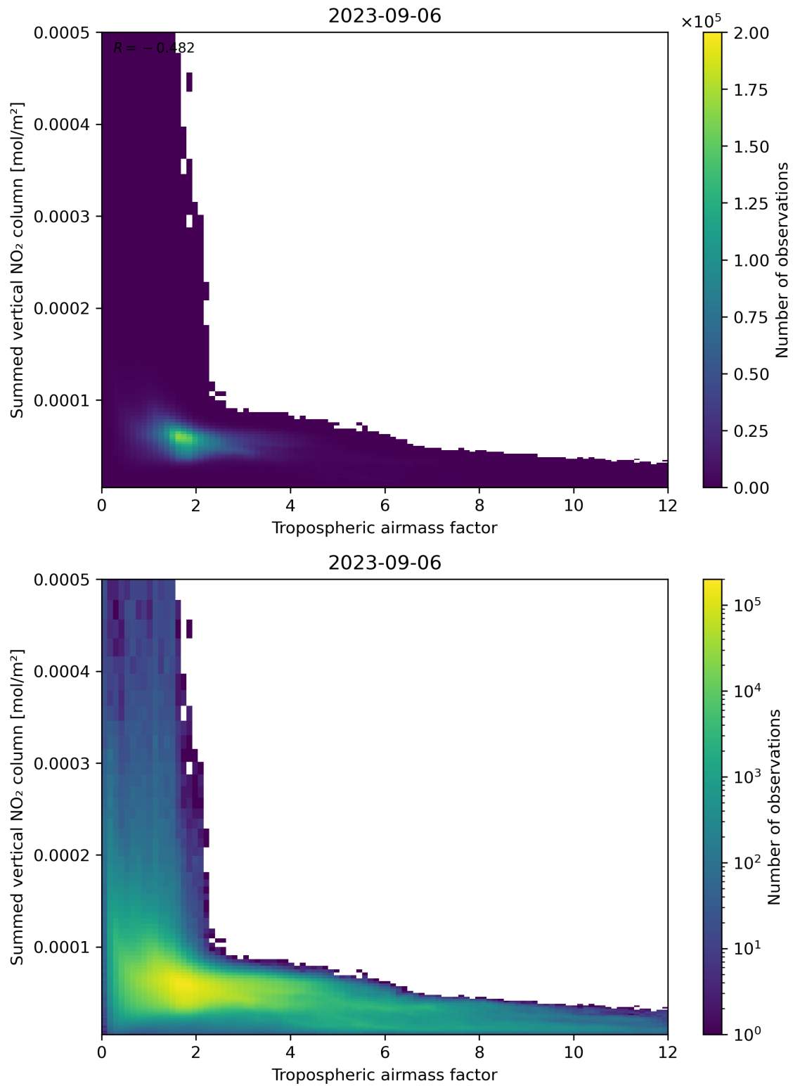
Figure 75: Scatter density plot of “Tropospheric airmass factor” against “Summed vertical NO 2 column” for 2023-09-05 to 2023-09-07.
