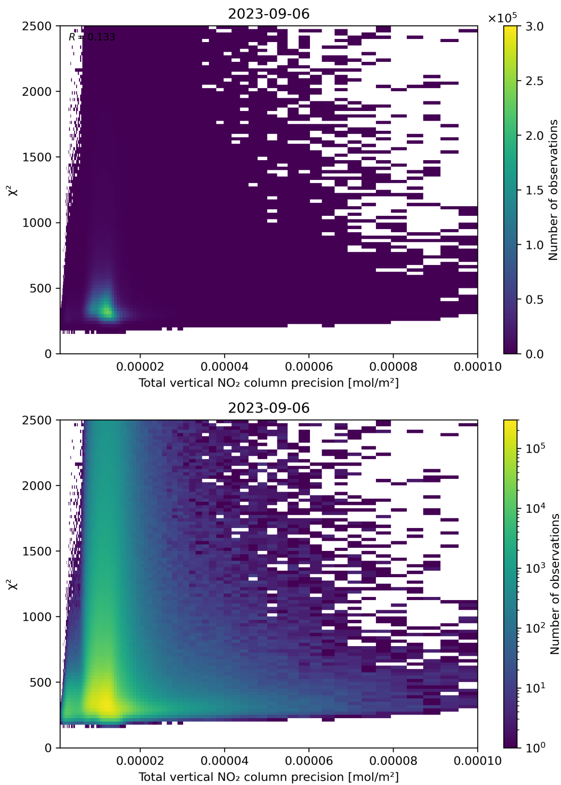
Figure 116: Scatter density plot of “Total vertical NO 2 column precision” against “ \chi^2 ” for 2023-09-05 to 2023-09-07.
