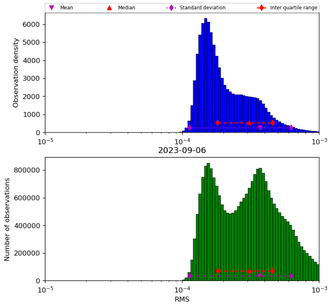
Figure 43: Histogram of “RMS” for 2023-09-05 to 2023-09-07
