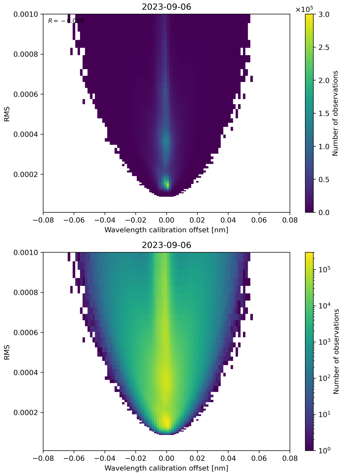
Figure 181: Scatter density plot of “Wavelength calibration offset” against “RMS” for 2023-09-05 to 2023-09-07.
