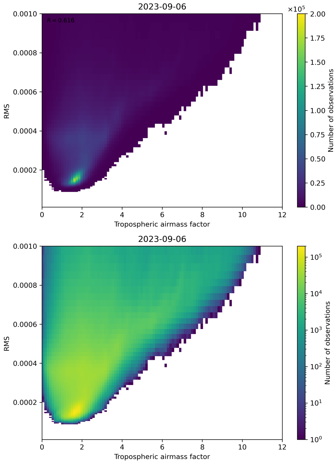
Figure 79: Scatter density plot of “Tropospheric airmass factor” against “RMS” for 2023-09-05 to 2023-09-07.
