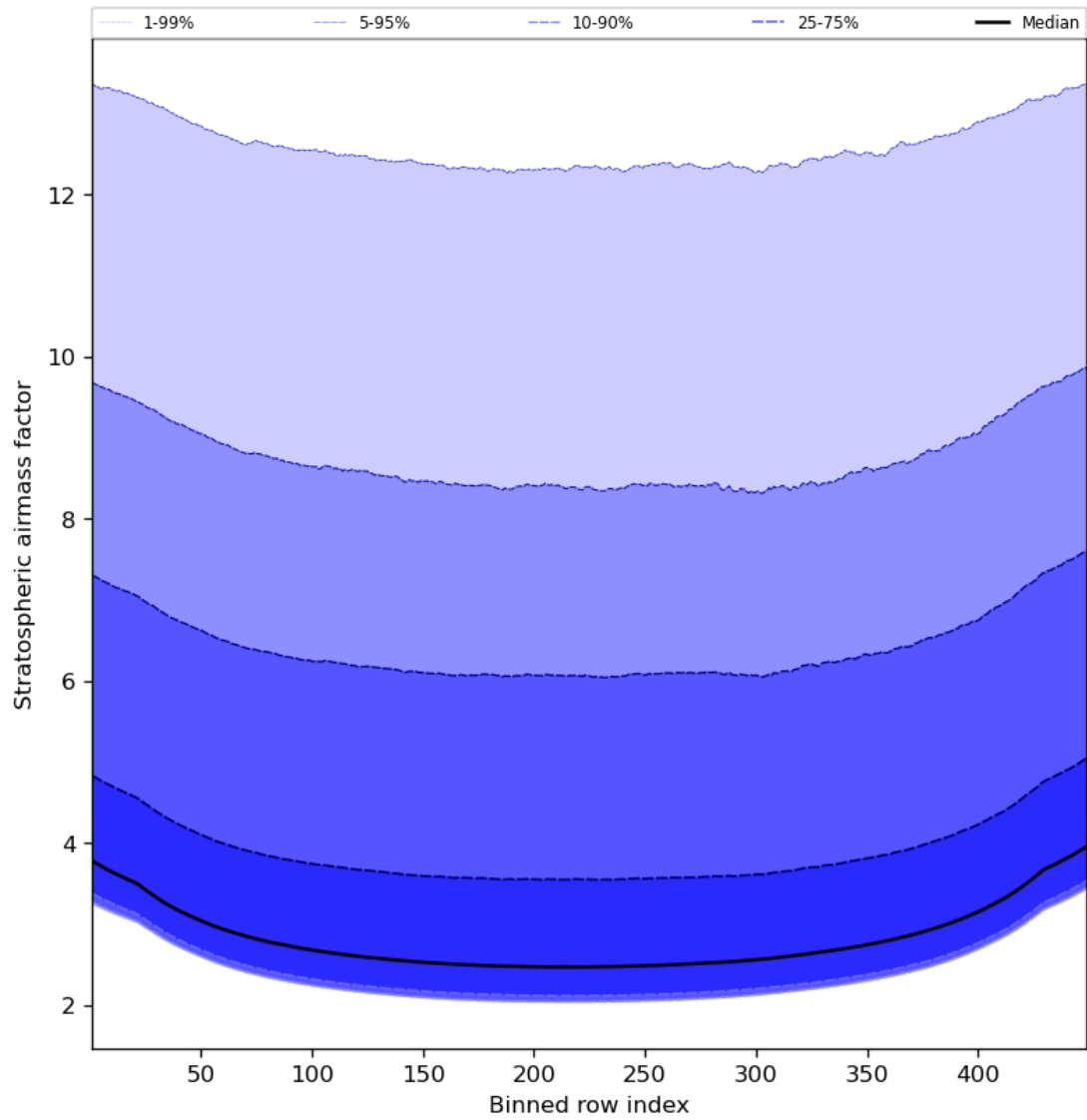
Figure 61: Along track statistics of “Stratospheric airmass factor” for 2023-09-05 to 2023-09-07
