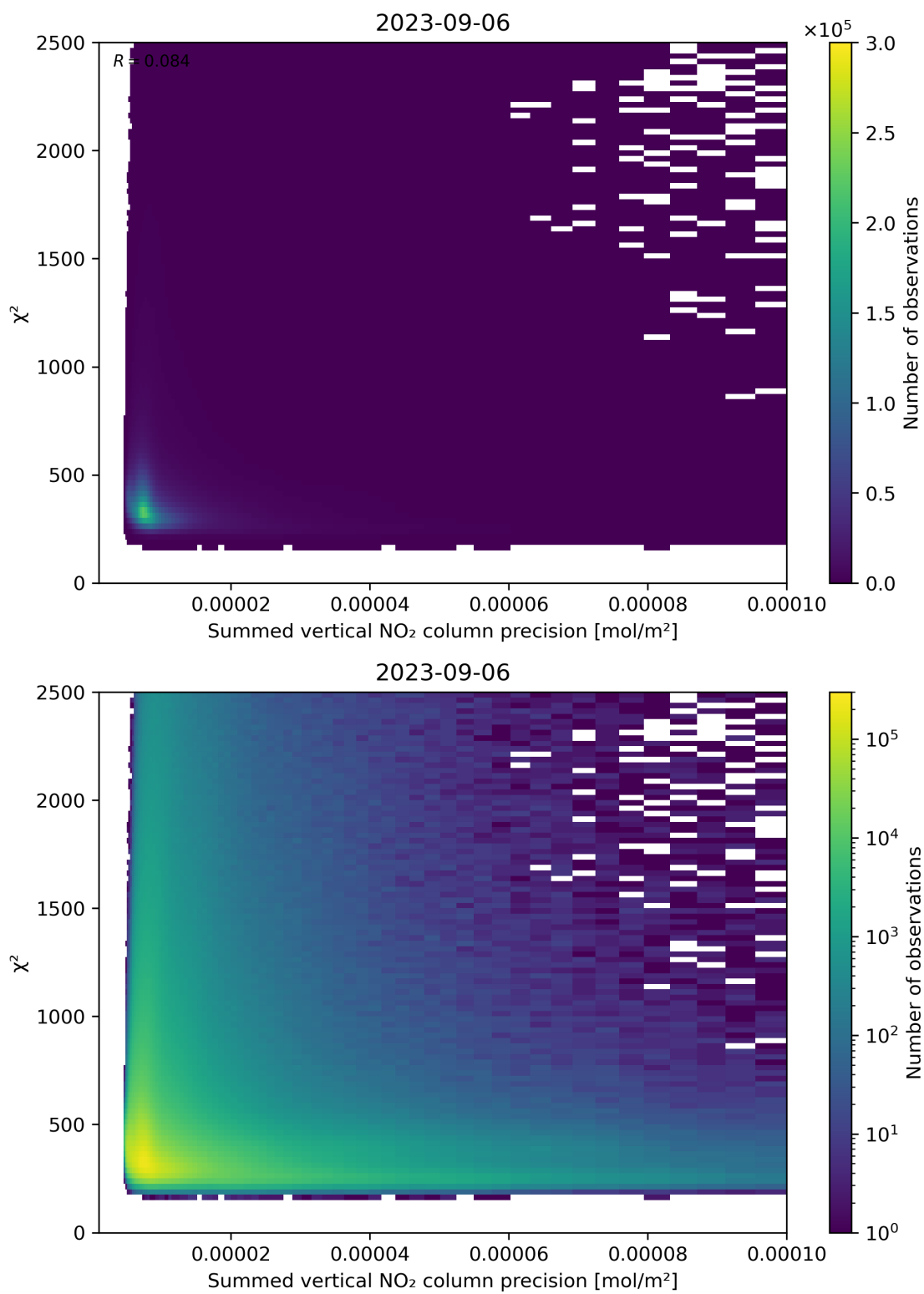
Figure 107: Scatter density plot of “Summed vertical NO 2 column precision” against “ \chi^2 ” for 2023-09-05 to 2023-09-07.
