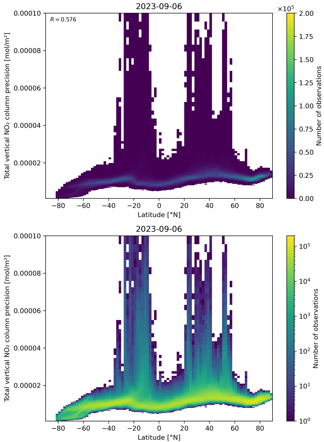
Figure 91: Scatter density plot of “Latitude” against “Total vertical NO 2 column precision” for 2023-09-05 to 2023-09-07.
