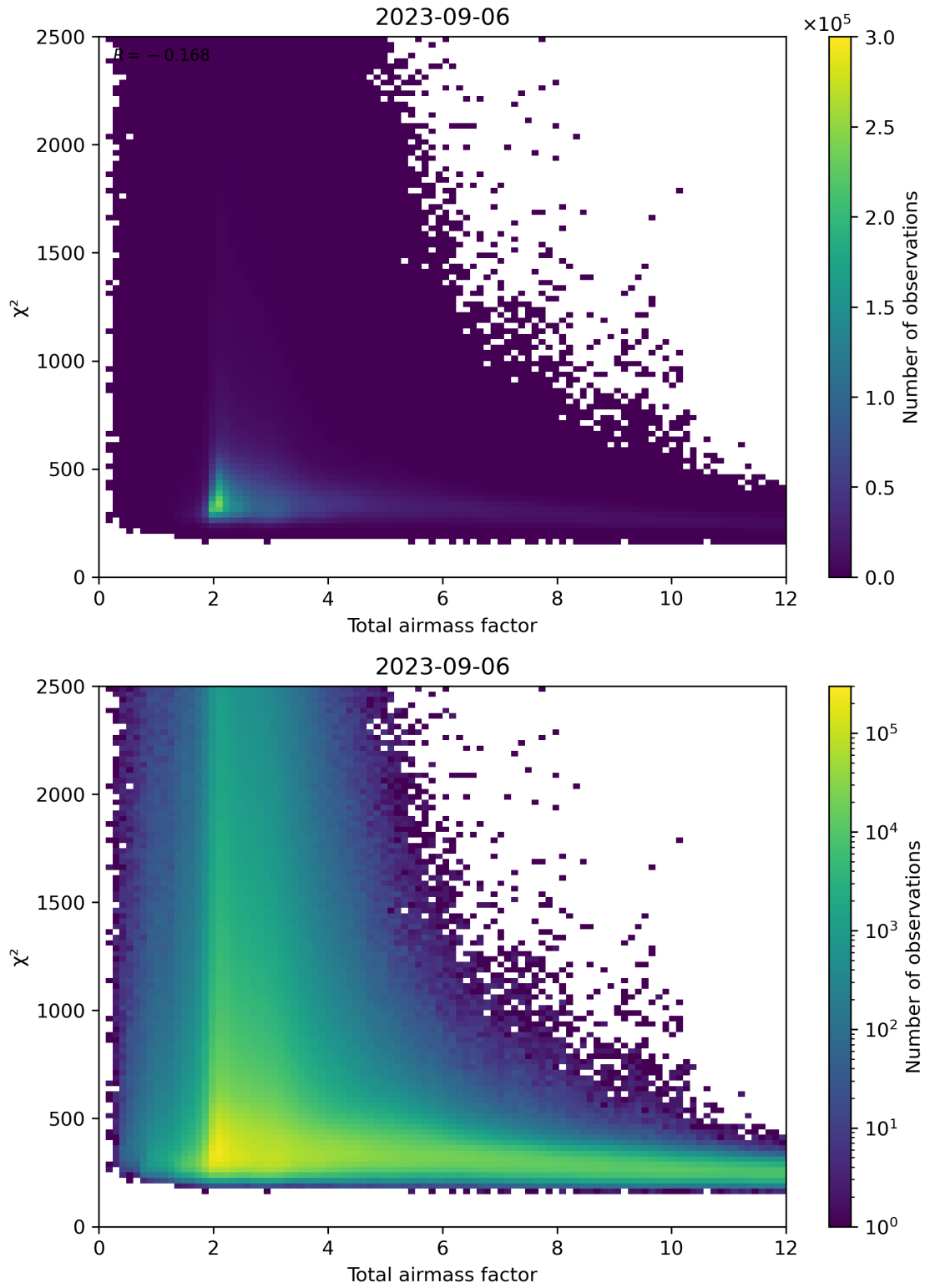
Figure 63: Scatter density plot of “Total airmass factor” against “ \chi^2 ” for 2023-09-05 to 2023-09-07.
