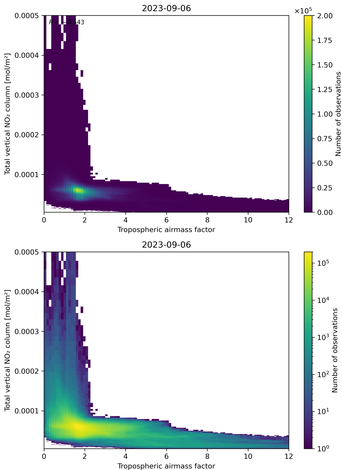
Figure 77: Scatter density plot of “Tropospheric airmass factor” against “Total vertical NO 2 column” for 2023-09-05 to 2023-09-07.
