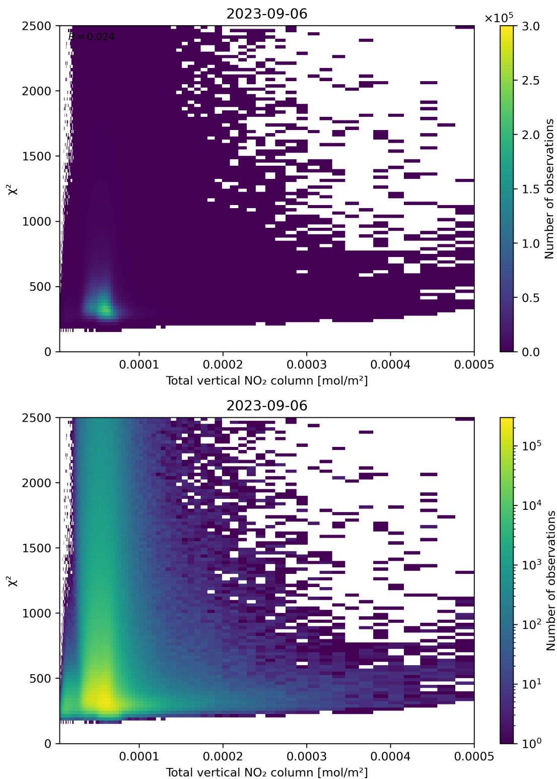
Figure 111: Scatter density plot of “Total vertical NO 2 column” against “ \chi^2 ” for 2023-09-05 to 2023-09-07.
