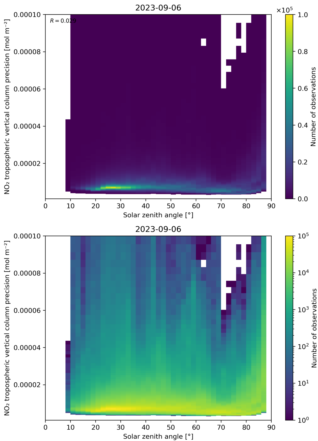
Figure 156: Scatter density plot of “Solar zenith angle” against “NO 2 tropospheric vertical column precision” for 2023-09-05 to 2023-09-07.
