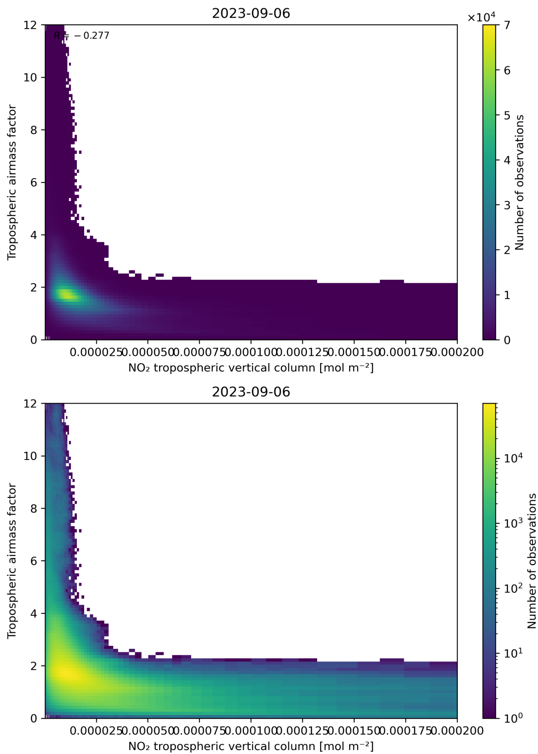
Figure 123: Scatter density plot of “NO 2 tropospheric vertical column” against “Tropospheric air mass factor” for 2023-09-05 to 2023-09-07.
