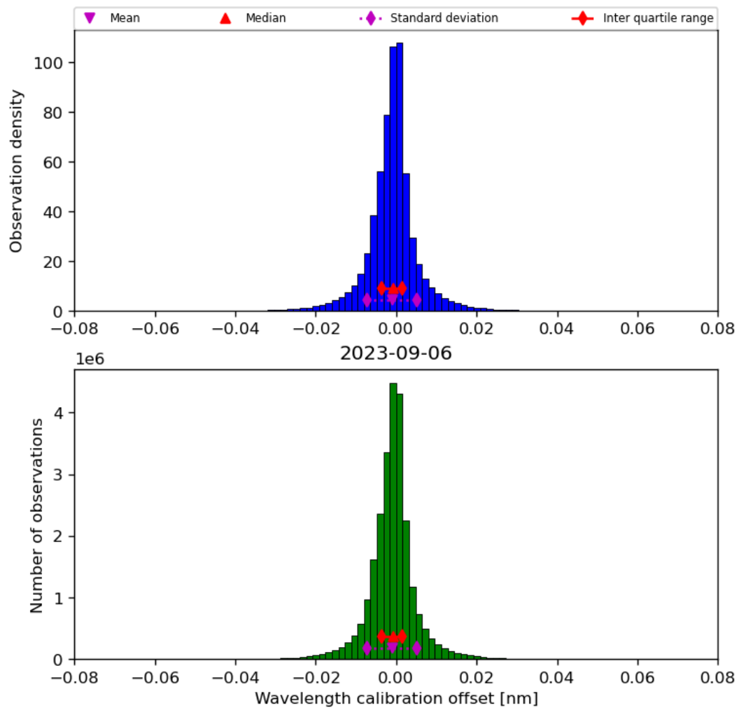
Figure 35: Histogram of “Wavelength calibration offset” for 2023-09-05 to 2023-09-07
