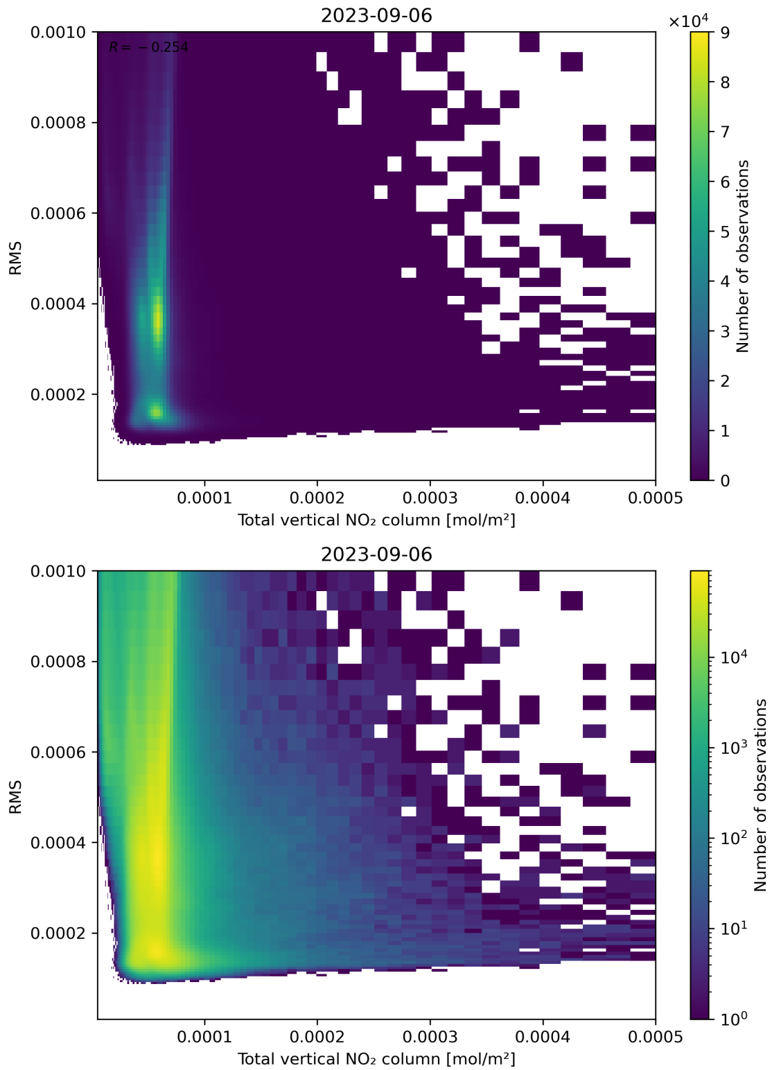
Figure 120: Scatter density plot of “Total vertical NO 2 column” against “RMS” for 2023-09-05 to 2023-09-07.
