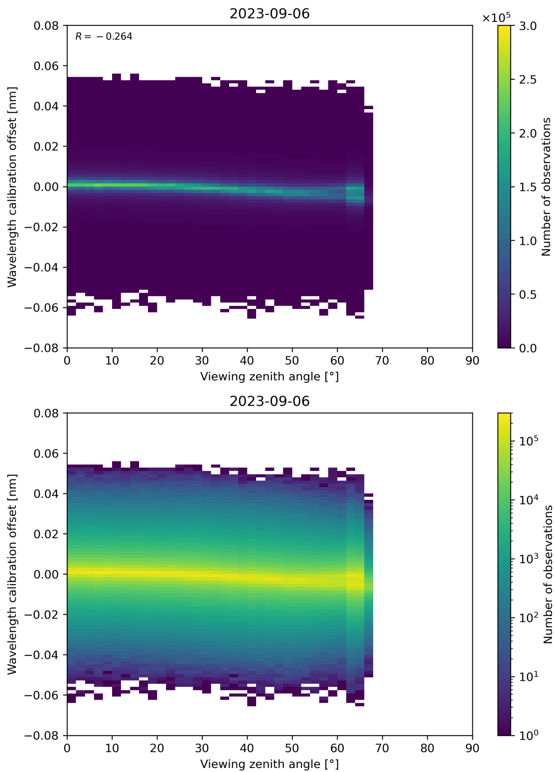
Figure 173: Scatter density plot of “Viewing zenith angle” against “Wavelength calibration offset” for 2023-09-05 to 2023-09-07.
