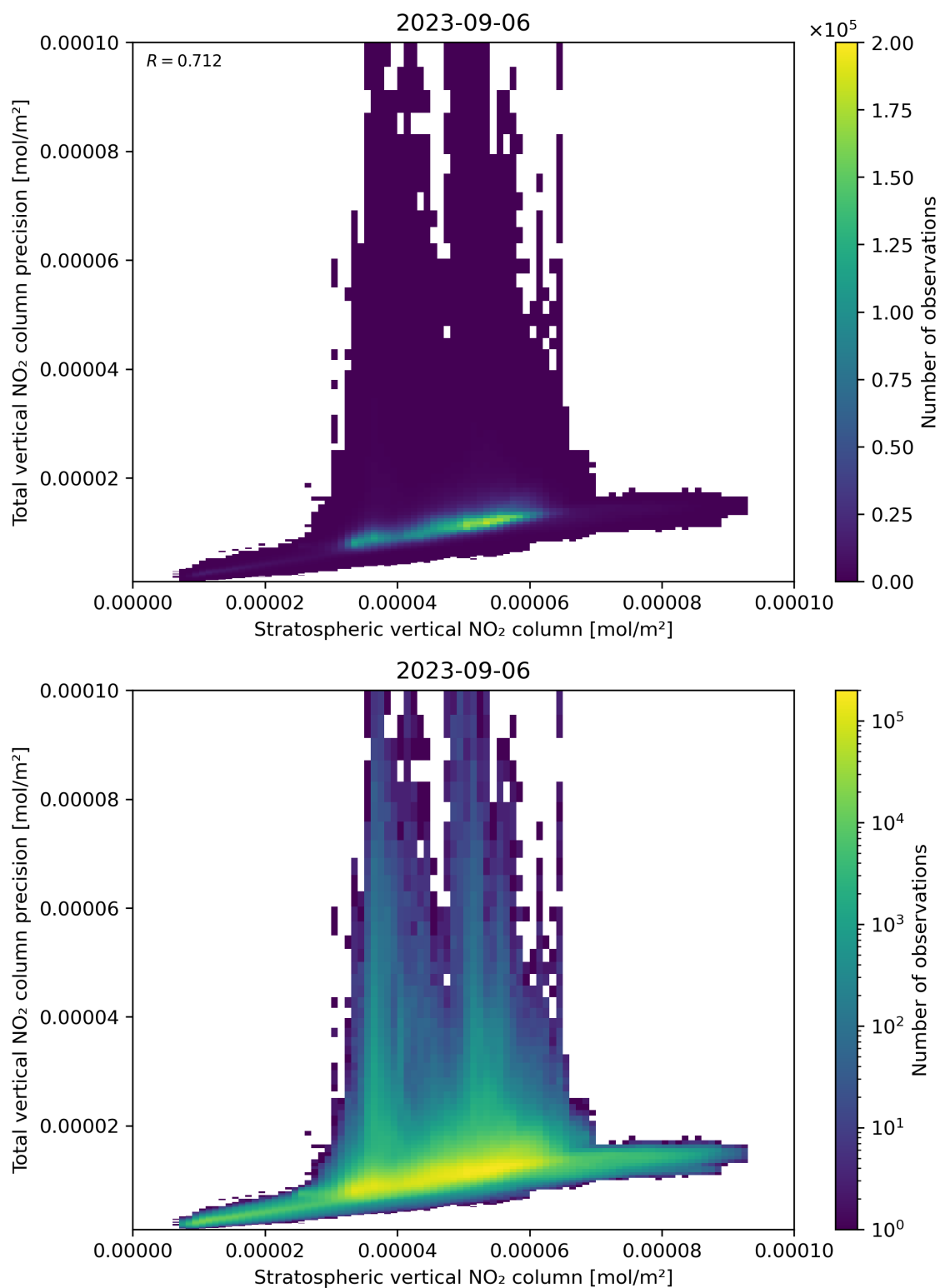
Figure 101: Scatter density plot of “Stratospheric vertical NO 2 column” against “Total vertical NO 2 column precision” for 2023-09-05 to 2023-09-07.
