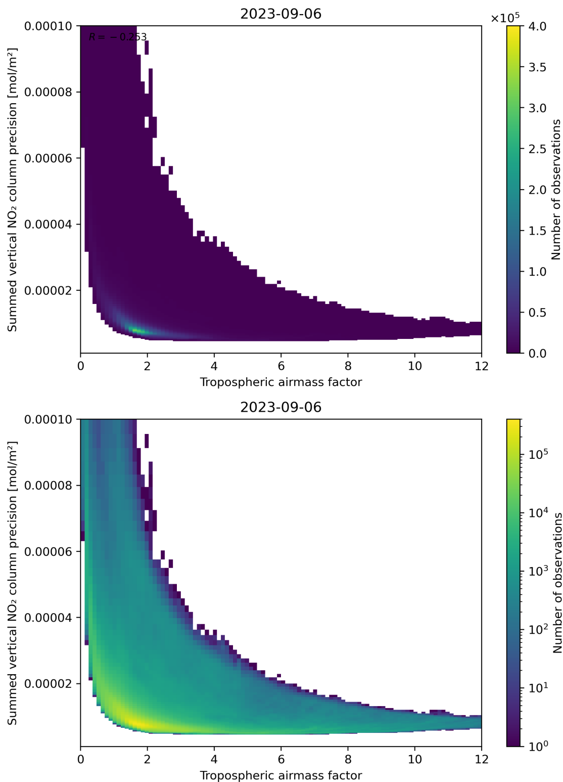
Figure 76: Scatter density plot of “Tropospheric air mass factor” against “Summed vertical NO 2 column precision” for 2023-09-05 to 2023-09-07.
