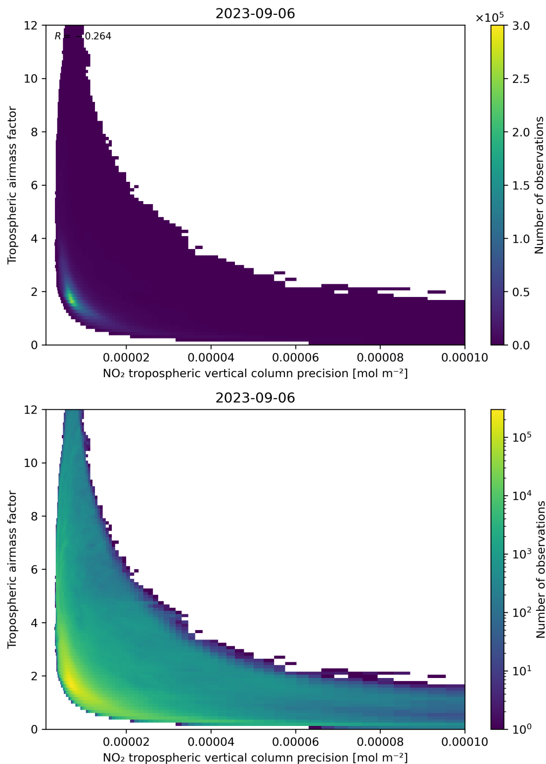
Figure 133: Scatter density plot of “NO 2 tropospheric vertical column precision” against “Tropospheric air mass factor” for 2023-09-05 to 2023-09-07.
