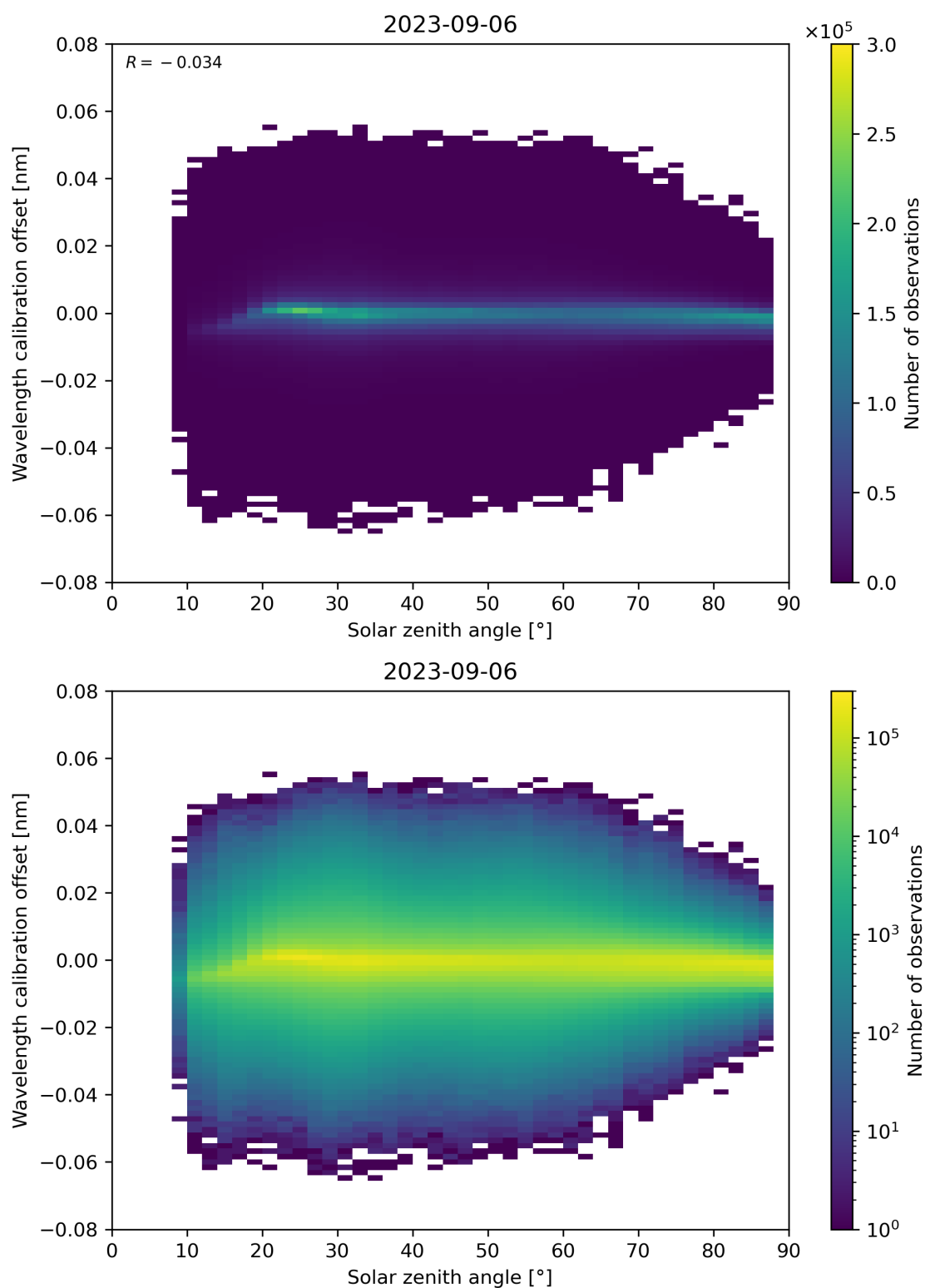
Figure 158: Scatter density plot of “Solar zenith angle” against “Wavelength calibration offset” for 2023-09-05 to 2023-09-07.
