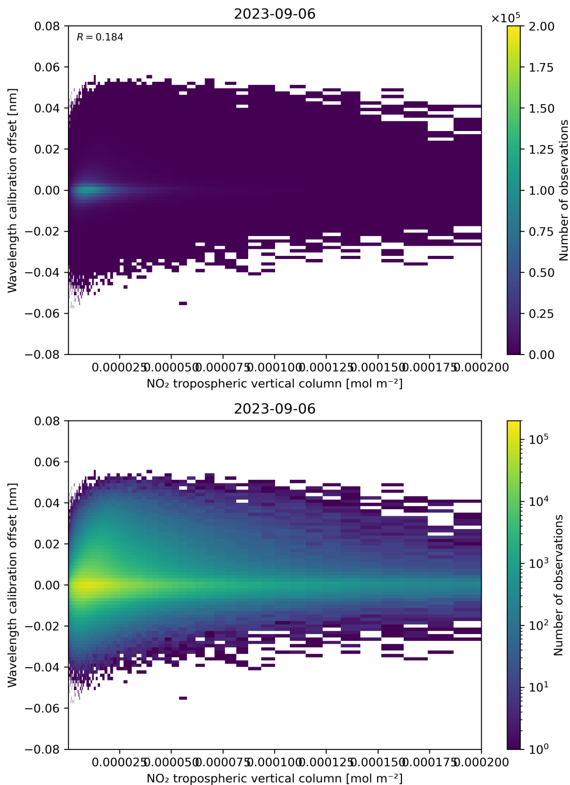
Figure 143: Scatter density plot of “NO 2 tropospheric vertical column” against “Wavelength calibration offset” for 2023-09-05 to 2023-09-07.
