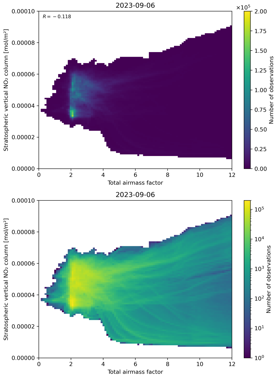
Figure 64: Scatter density plot of “Total airmass factor” against “Stratospheric vertical NO 2 column” for 2023-09-05 to 2023-09-07.
