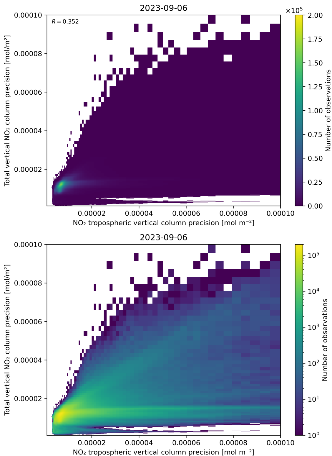
Figure 139: Scatter density plot of “NO 2 tropospheric vertical column precision” against “Total vertical NO 2 column precision” for 2023-09-05 to 2023-09-07.
