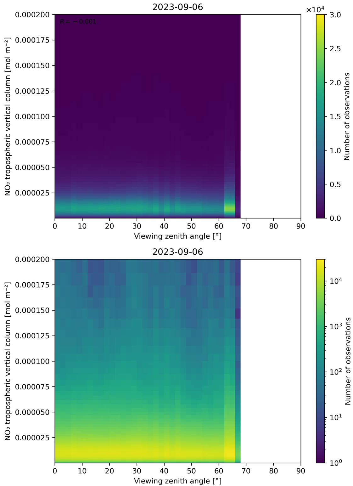
Figure 169: Scatter density plot of “Viewing zenith angle” against “NO 2 tropospheric vertical column” for 2023-09-05 to 2023-09-07.
