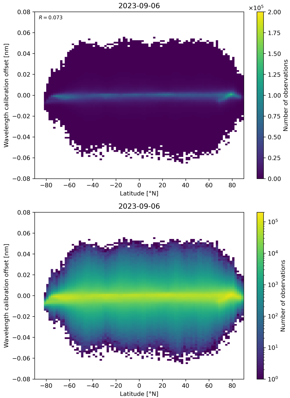
Figure 95: Scatter density plot of “Latitude” against “Wavelength calibration offset” for 2023-09-05 to 2023-09-07.
