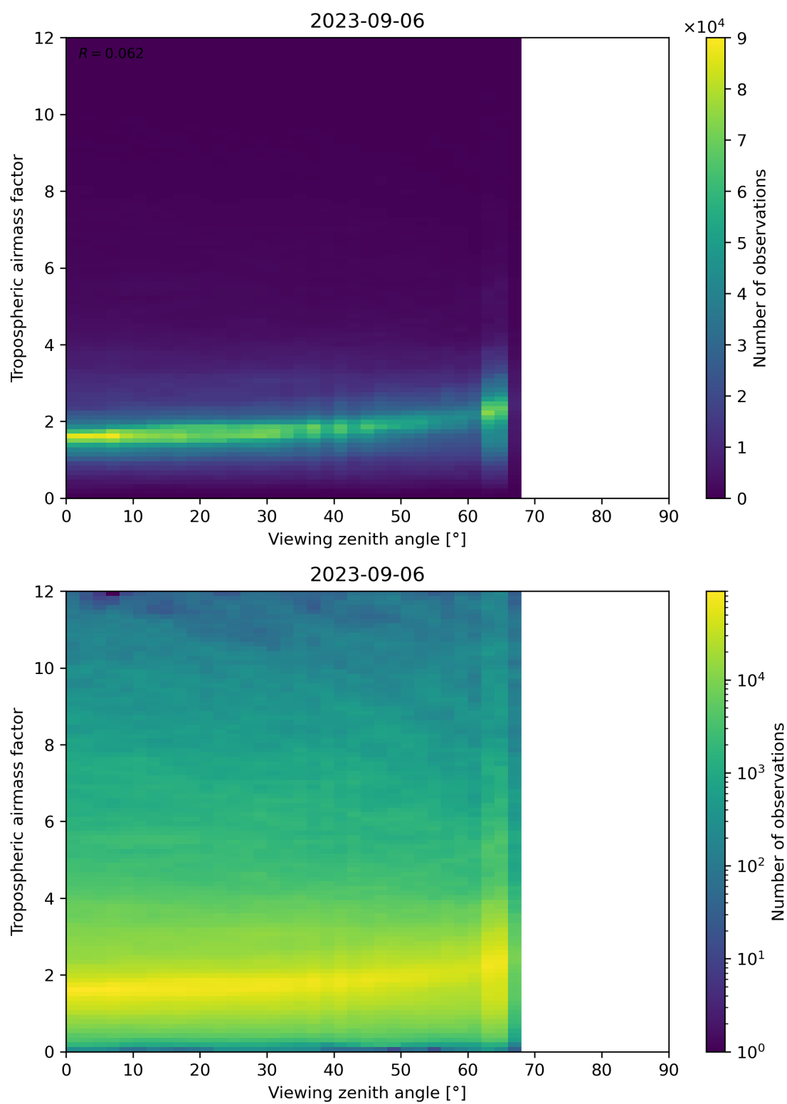
Figure 161: Scatter density plot of “Viewing zenith angle” against “Tropospheric airmass factor” for 2023-09-05 to 2023-09-07.
