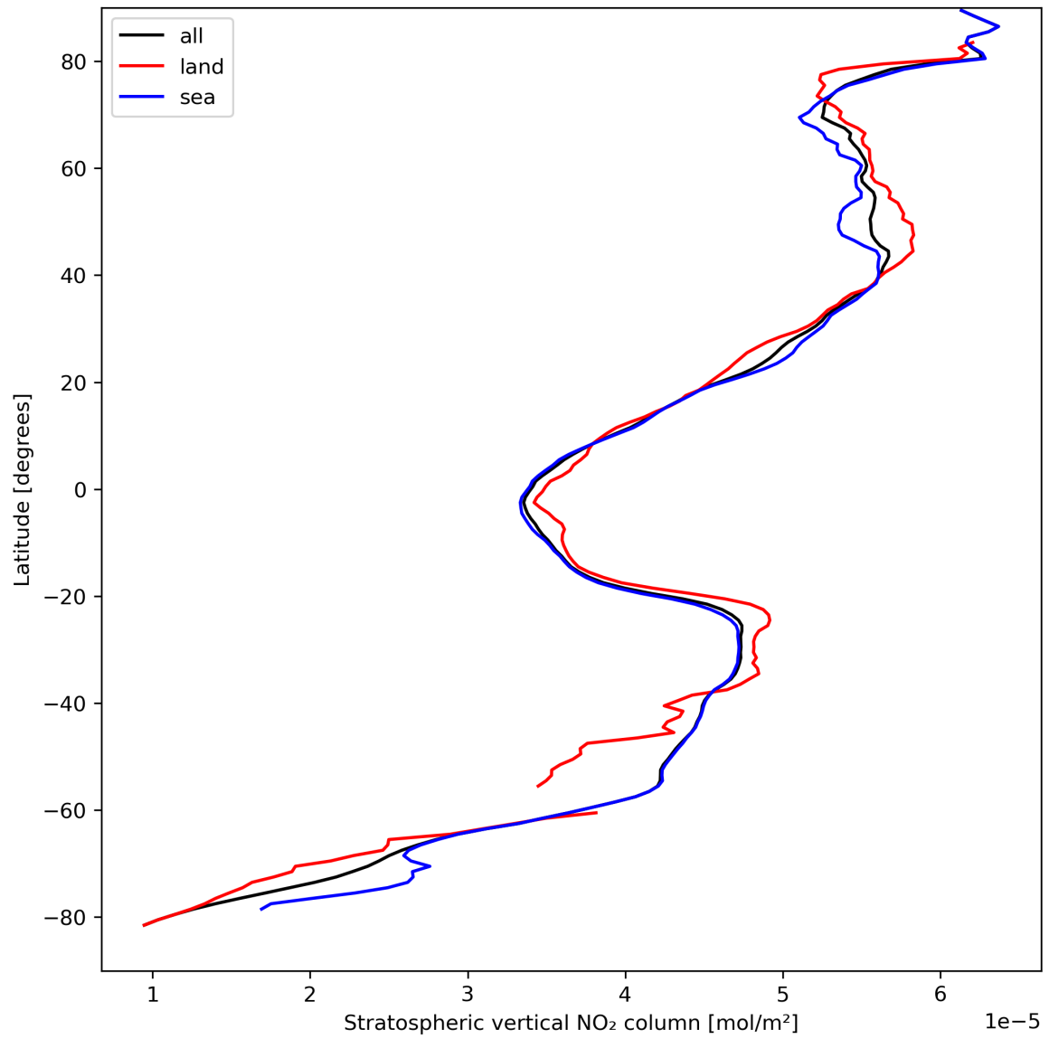
Figure 19: Zonal average of “Stratospheric vertical NO 2 column” for 2023-09-05 to 2023-09-07.
