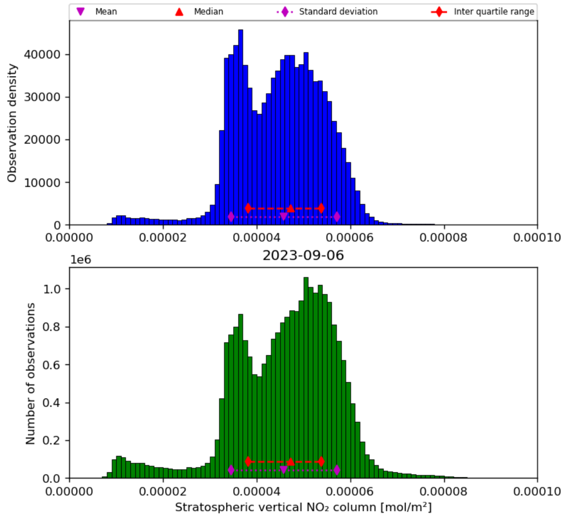
Figure 36: Histogram of “Stratospheric vertical NO 2 column” for 2023-09-05 to 2023-09-07
