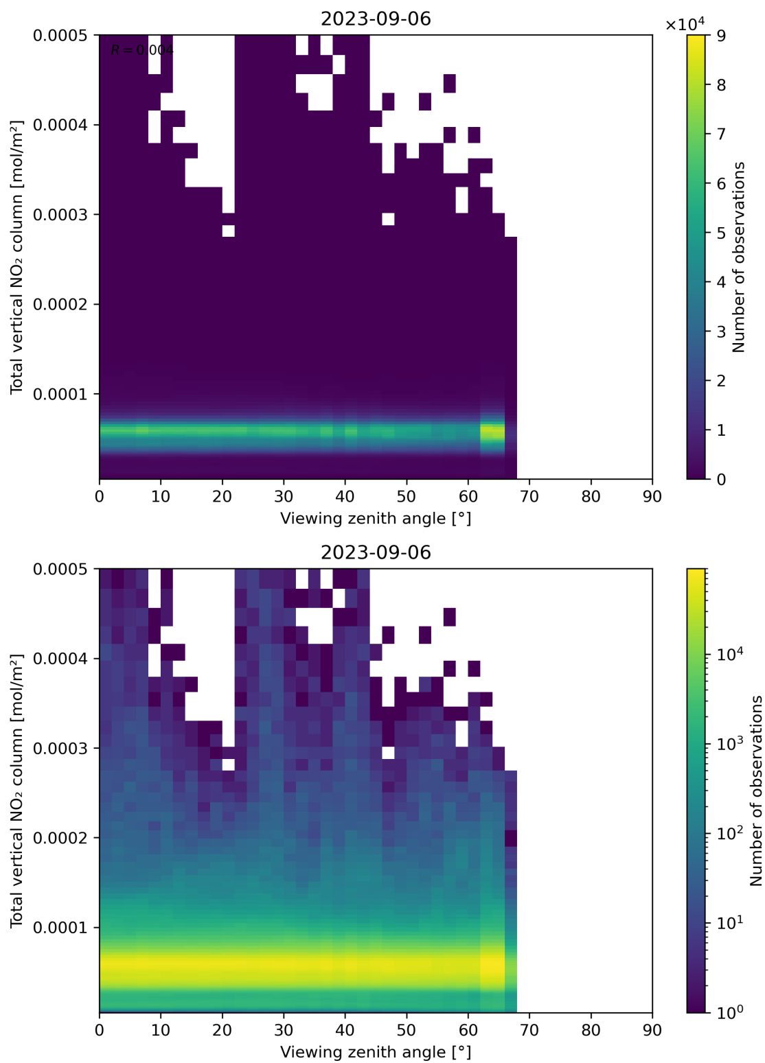
Figure 167: Scatter density plot of “Viewing zenith angle” against “Total vertical NO 2 column” for 2023-09-05 to 2023-09-07.
