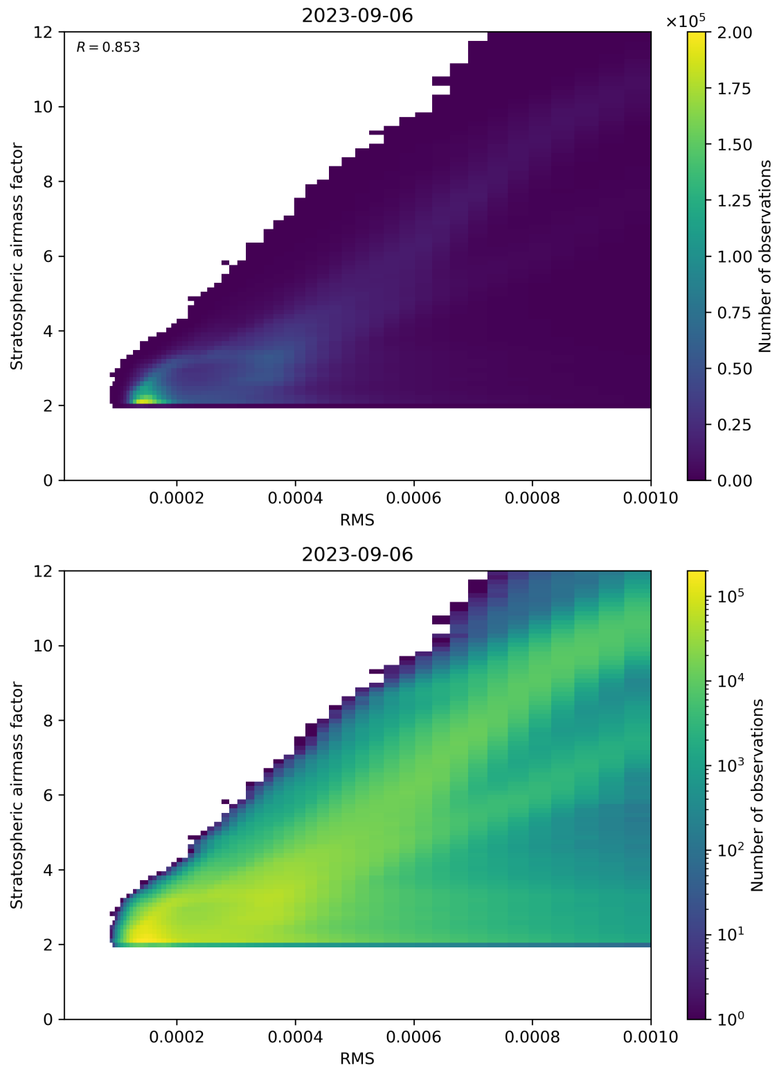
Figure 144: Scatter density plot of “RMS” against “Stratospheric airmass factor” for 2023-09-05 to 2023-09-07.
