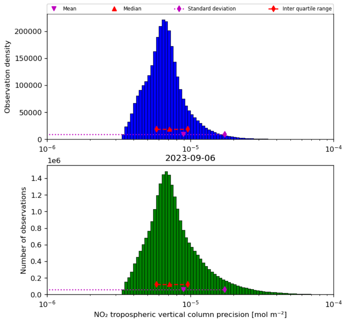
Figure 30: Histogram of “NO 2 tropospheric vertical column precision” for 2023-09-05 to 2023-09-07
