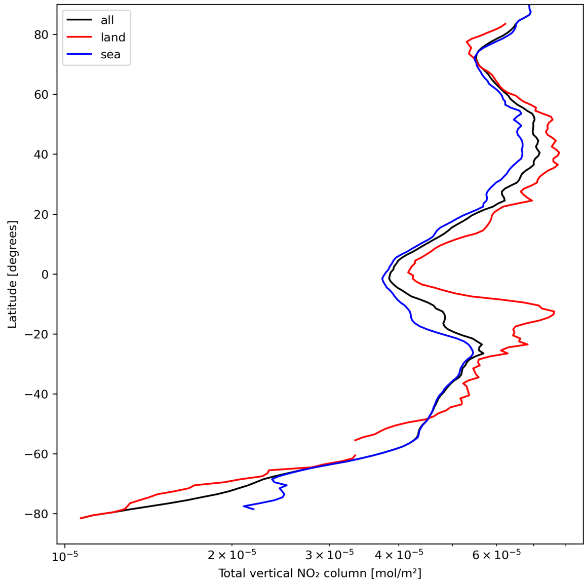
Figure 21: Zonal average of “Total vertical NO 2 column” for 2023-09-05 to 2023-09-07.
