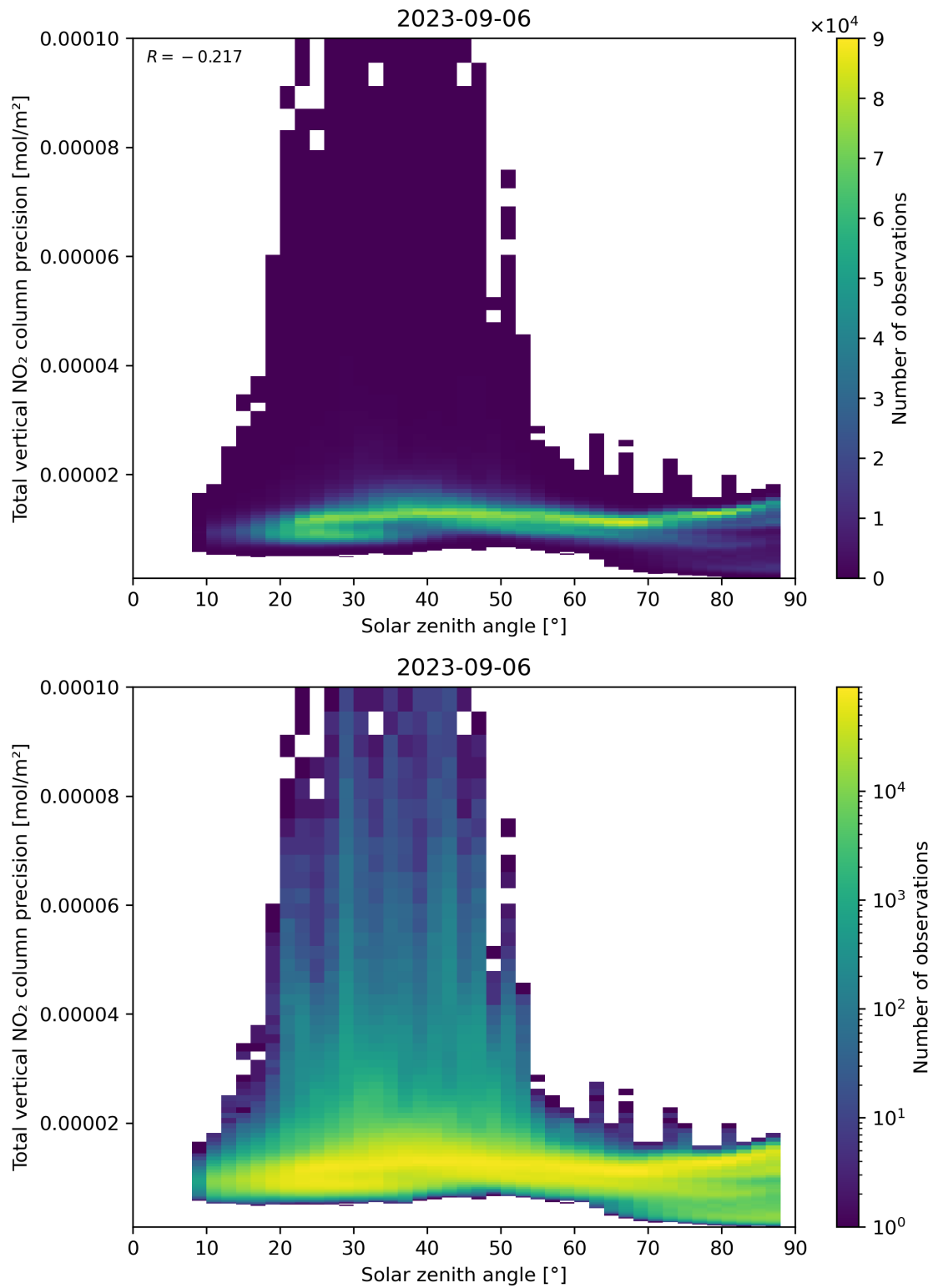
Figure 154: Scatter density plot of “Solar zenith angle” against “Total vertical NO 2 column precision” for 2023-09-05 to 2023-09-07.
