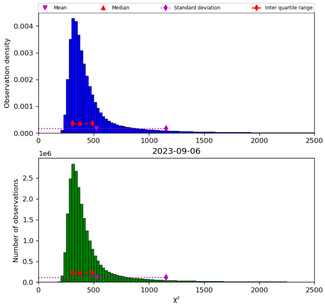
Figure 42: Histogram of “ \chi^2 ” for 2023-09-05 to 2023-09-07
