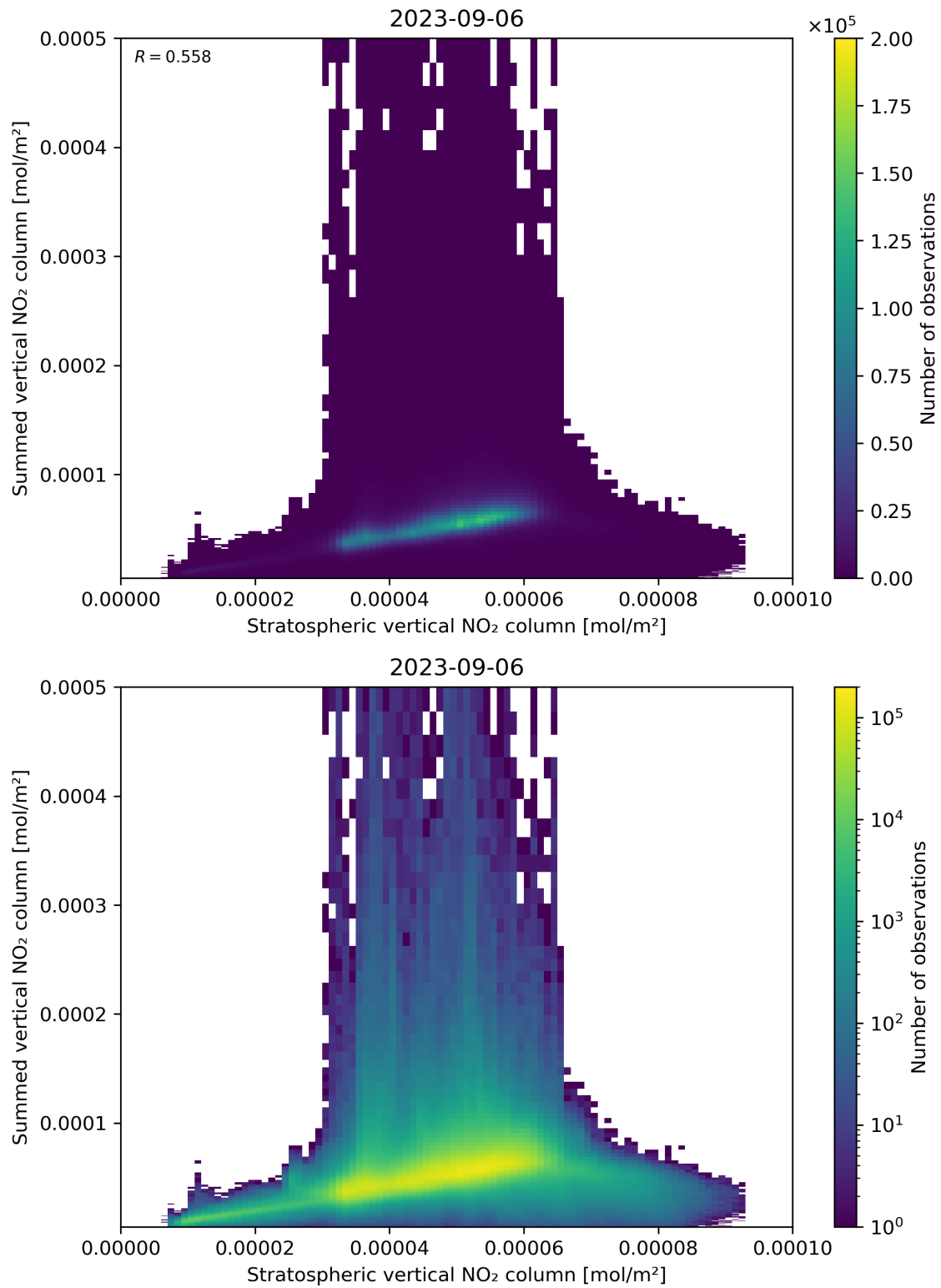
Figure 98: Scatter density plot of “Stratospheric vertical NO 2 column” against “Summed vertical NO 2 column” for 2023-09-05 to 2023-09-07.
