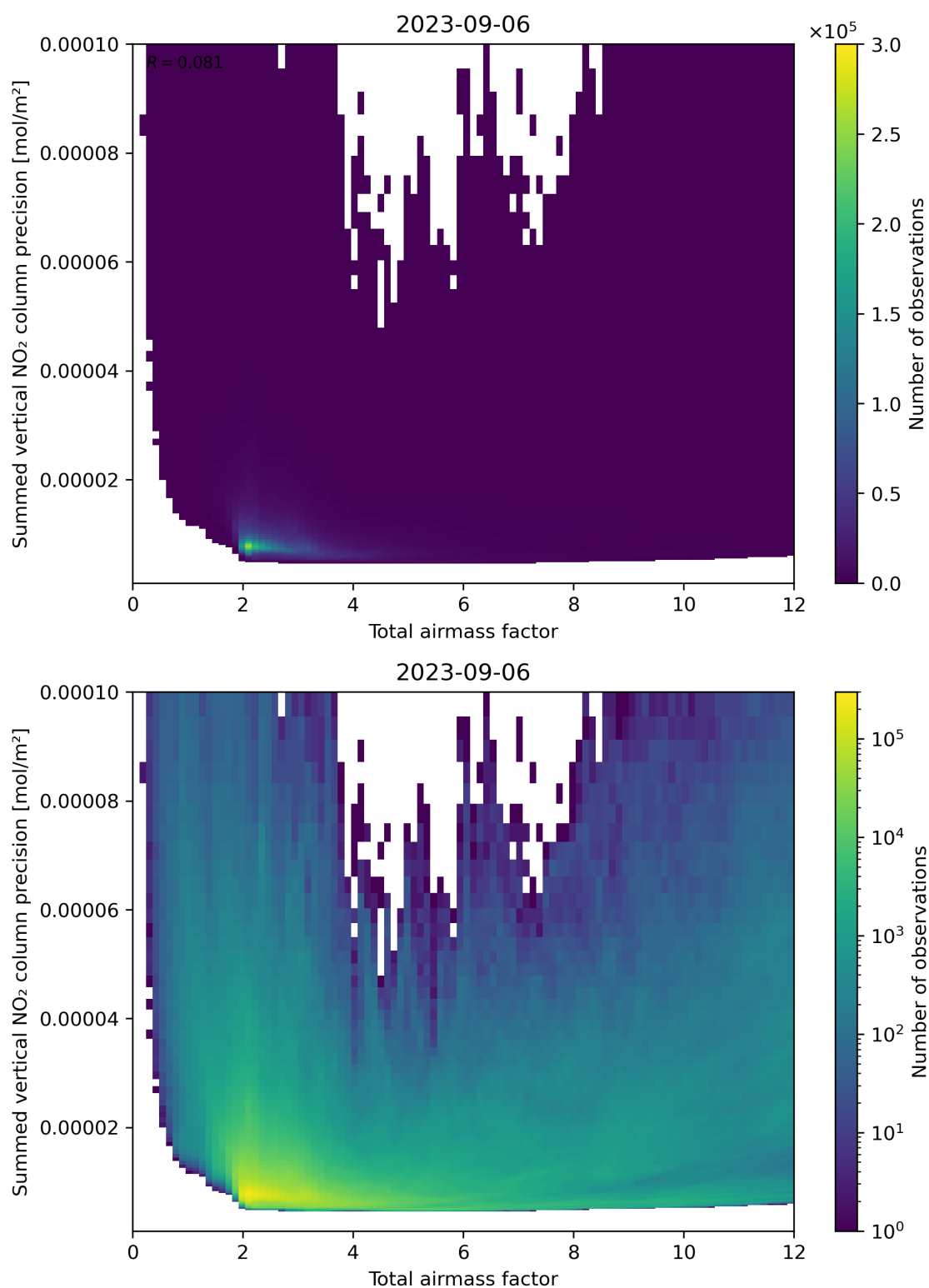
Figure 66: Scatter density plot of “Total airmass factor” against “Summed vertical NO 2 column precision” for 2023-09-05 to 2023-09-07.
