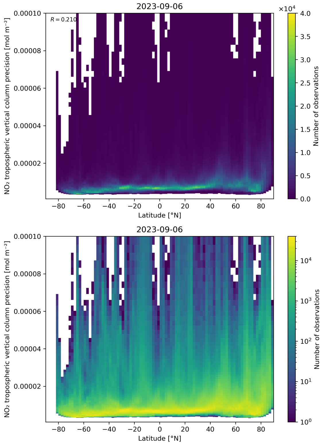
Figure 93: Scatter density plot of “Latitude” against “NO 2 tropospheric vertical column precision” for 2023-09-05 to 2023-09-07.
