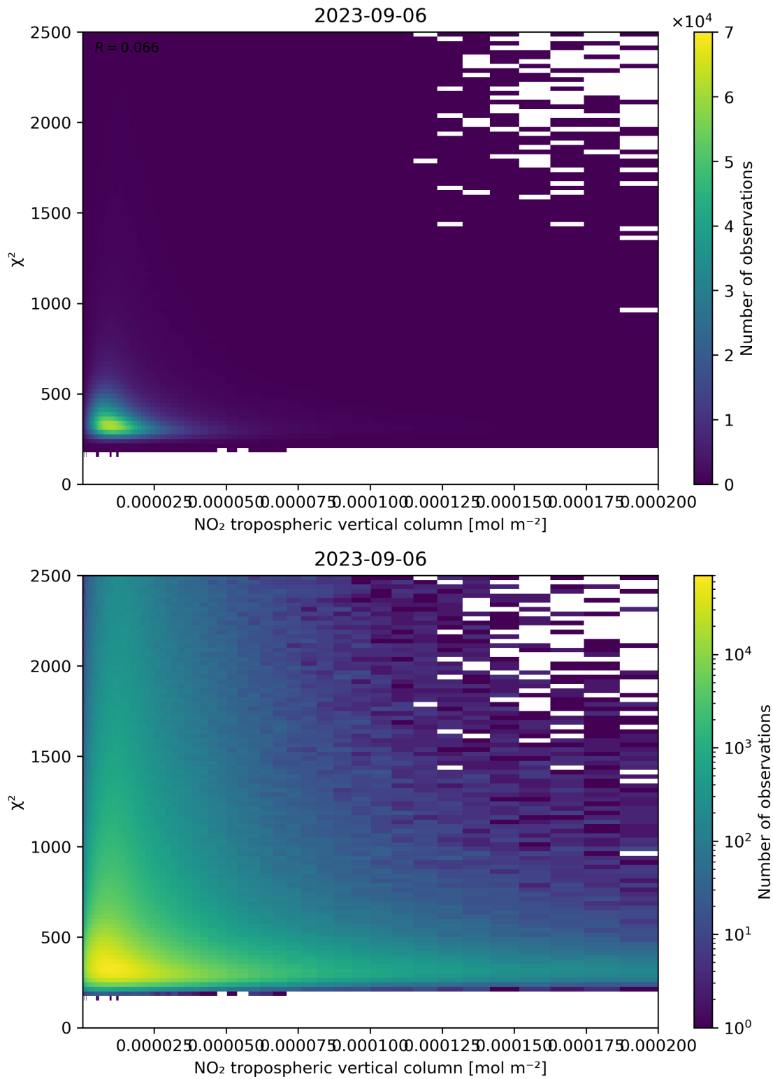
Figure 124: Scatter density plot of “NO 2 tropospheric vertical column” against “ \chi^2 ” for 2023-09-05 to 2023-09-07.
