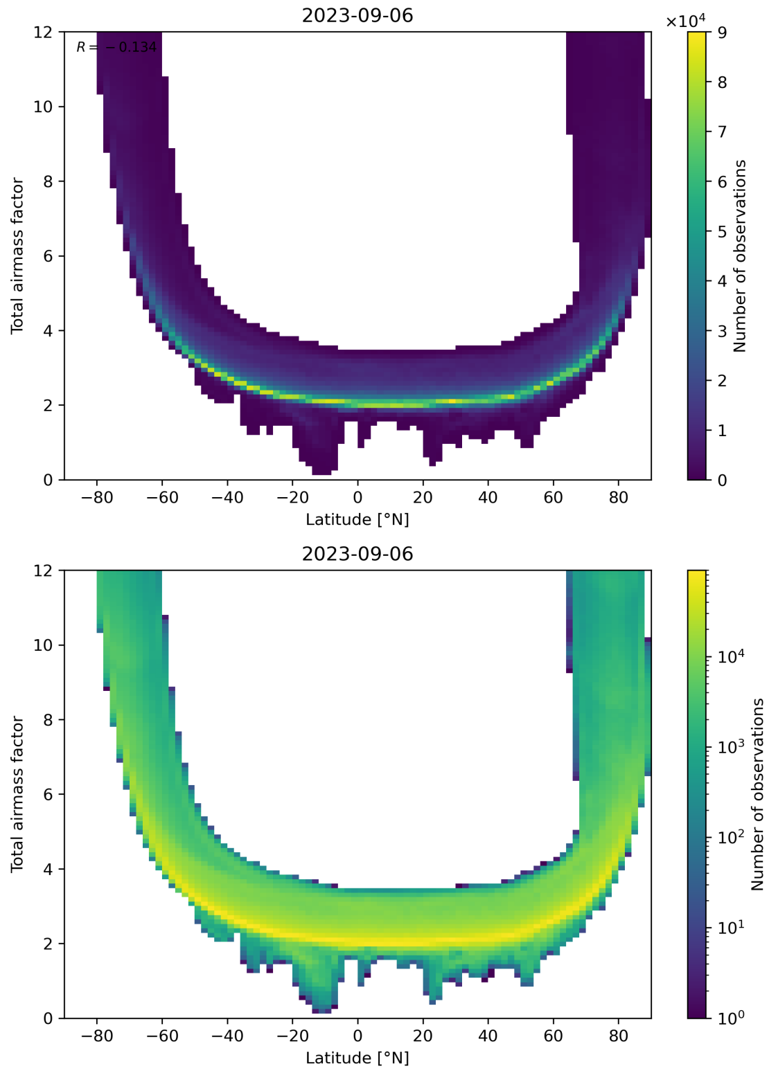
Figure 84: Scatter density plot of “Latitude” against “Total airmass factor” for 2023-09-05 to 2023-09-07.
