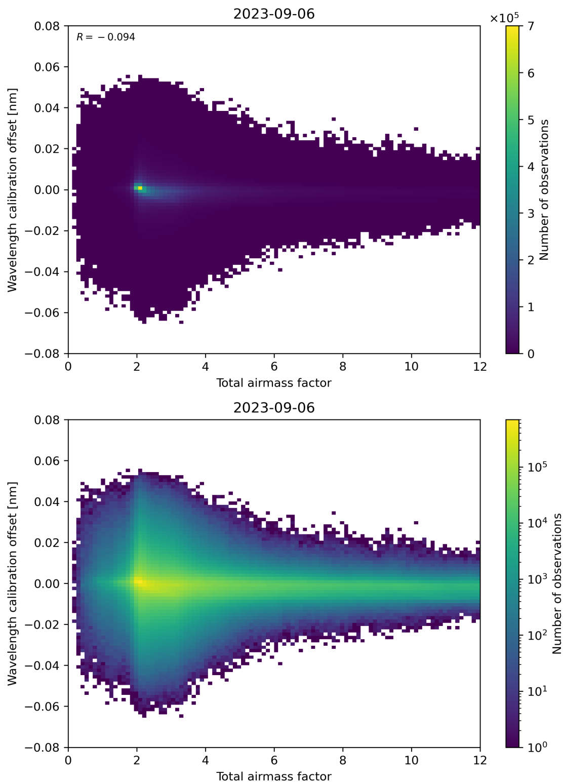
Figure 70: Scatter density plot of “Total airmass factor” against “Wavelength calibration offset” for 2023-09-05 to 2023-09-07.
