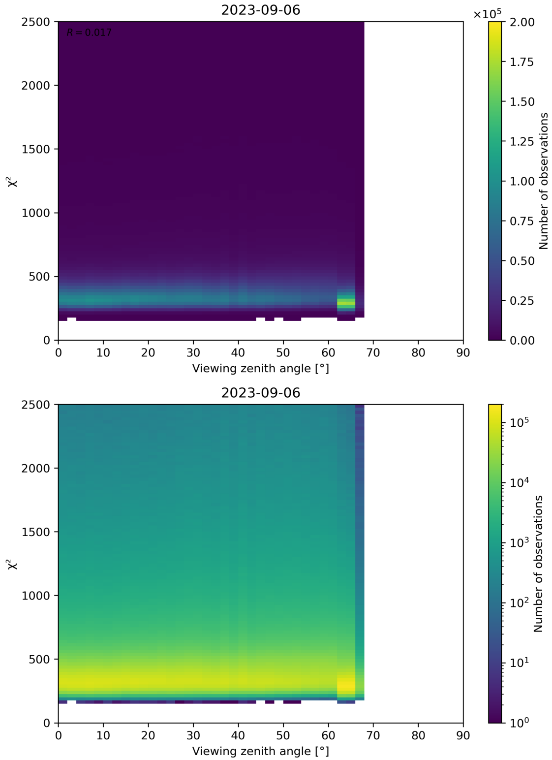
Figure 162: Scatter density plot of “Viewing zenith angle” against “ \chi^2 ” for 2023-09-05 to 2023-09-07.
