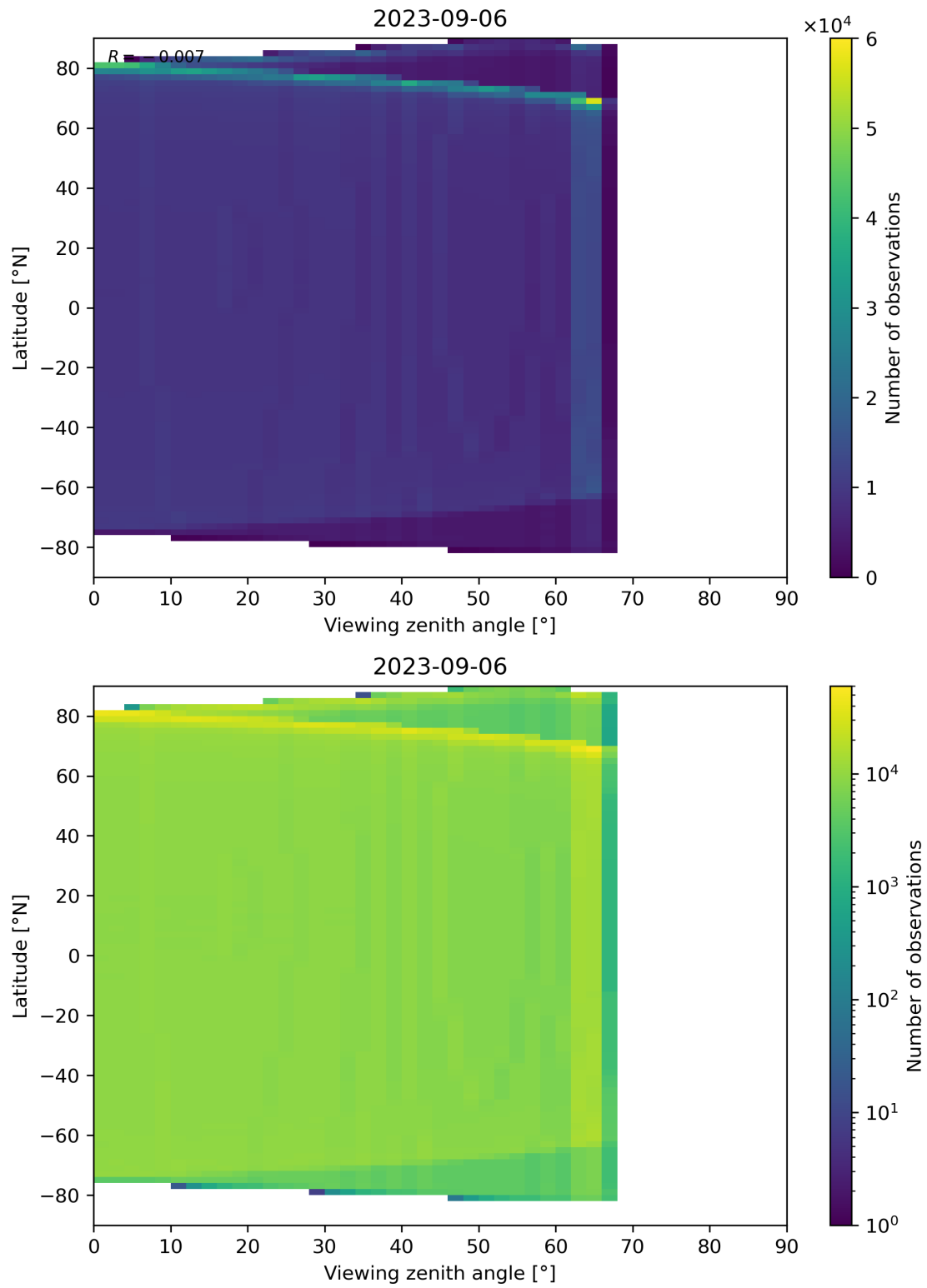
Figure 163: Scatter density plot of “Viewing zenith angle” against “Latitude” for 2023-09-05 to 2023-09-07.
