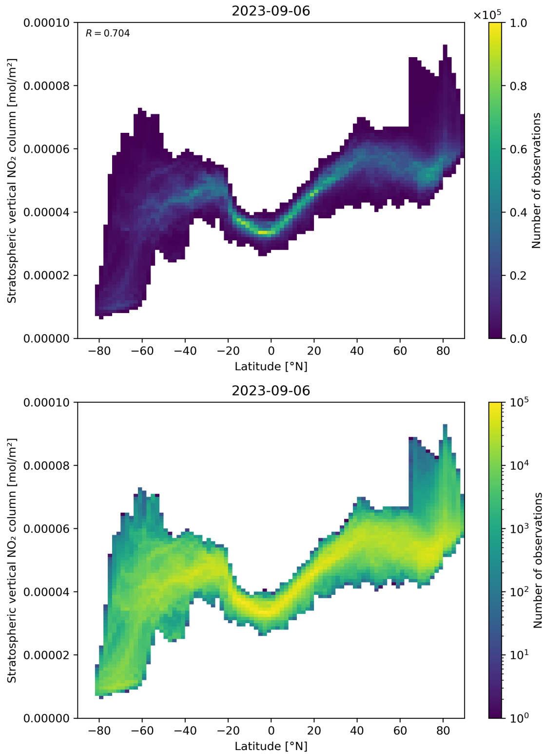
Figure 87: Scatter density plot of “Latitude” against “Stratospheric vertical \text{NO}_2 column” for 2023-09-05 to 2023-09-07.
