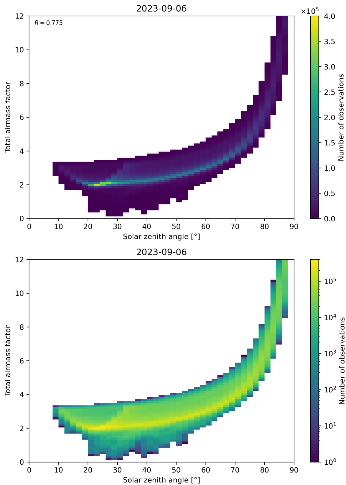
Figure 146: Scatter density plot of “Solar zenith angle” against “Total air mass factor” for 2023-09-05 to 2023-09-07.
