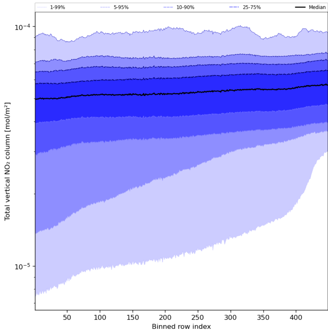
Figure 55: Along track statistics of “Total vertical NO 2 column” for 2023-09-05 to 2023-09-07
