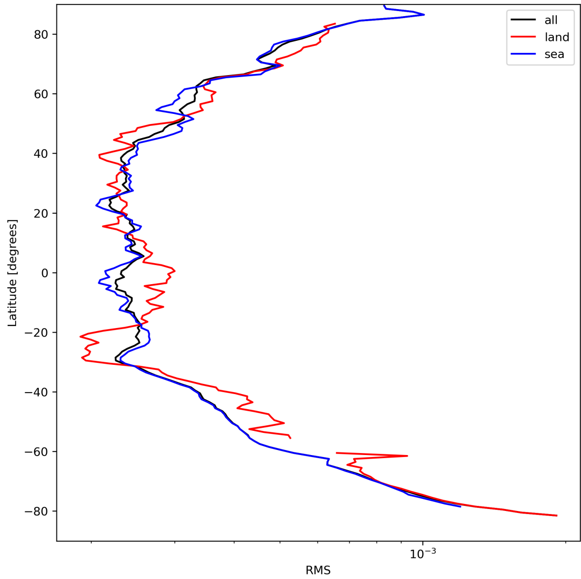
Figure 26: Zonal average of “RMS” for 2023-09-05 to 2023-09-07.
