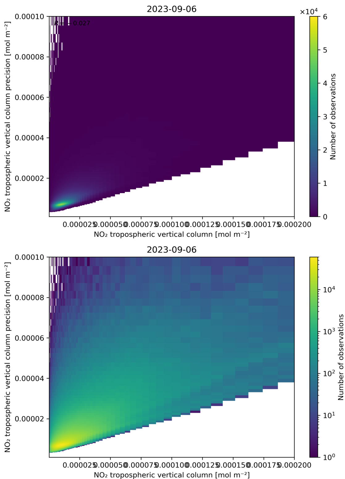
Figure 130: Scatter density plot of “NO 2 tropospheric vertical column” against “NO 2 tropospheric vertical column precision” for 2023-09-05 to 2023-09-07.
