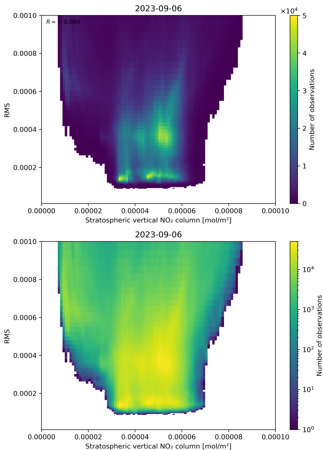
Figure 102: Scatter density plot of “Stratospheric vertical NO 2 column” against “RMS” for 2023-09-05 to 2023-09-07.
