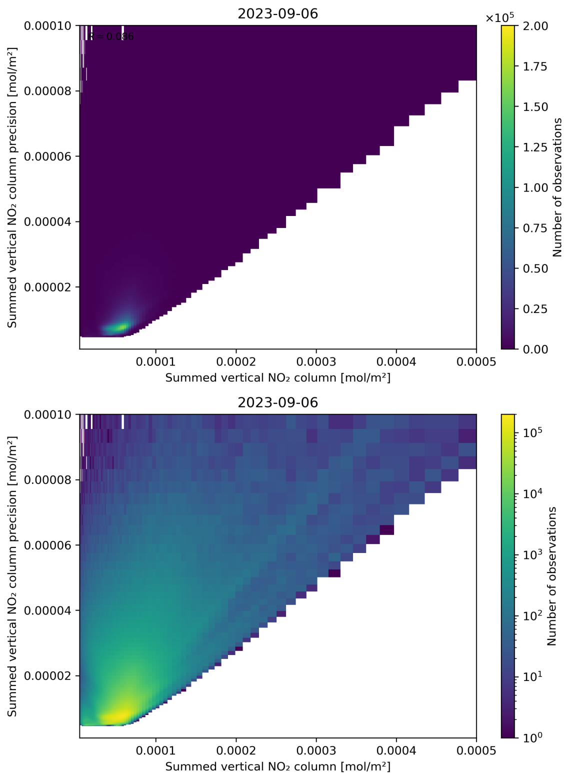
Figure 105: Scatter density plot of “Summed vertical NO 2 column” against “Summed vertical NO 2 column precision” for 2023-09-05 to 2023-09-07.
