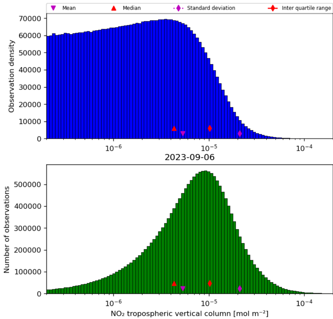
Figure 29: Histogram of “NO 2 tropospheric vertical column” for 2023-09-05 to 2023-09-07
