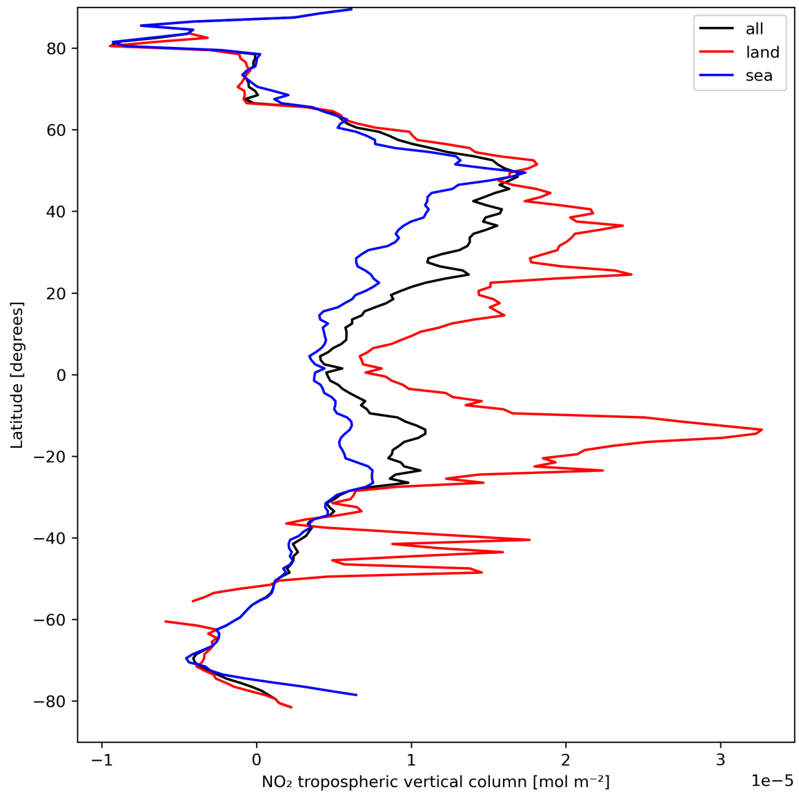
Figure 12: Zonal average of “NO 2 tropospheric vertical column” for 2023-09-05 to 2023-09-07.
