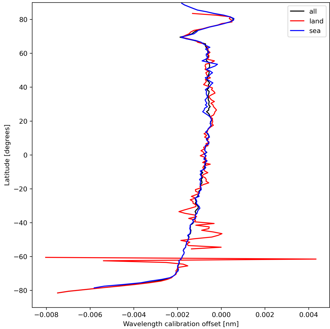
Figure 18: Zonal average of “Wavelength calibration offset” for 2023-09-05 to 2023-09-07.
