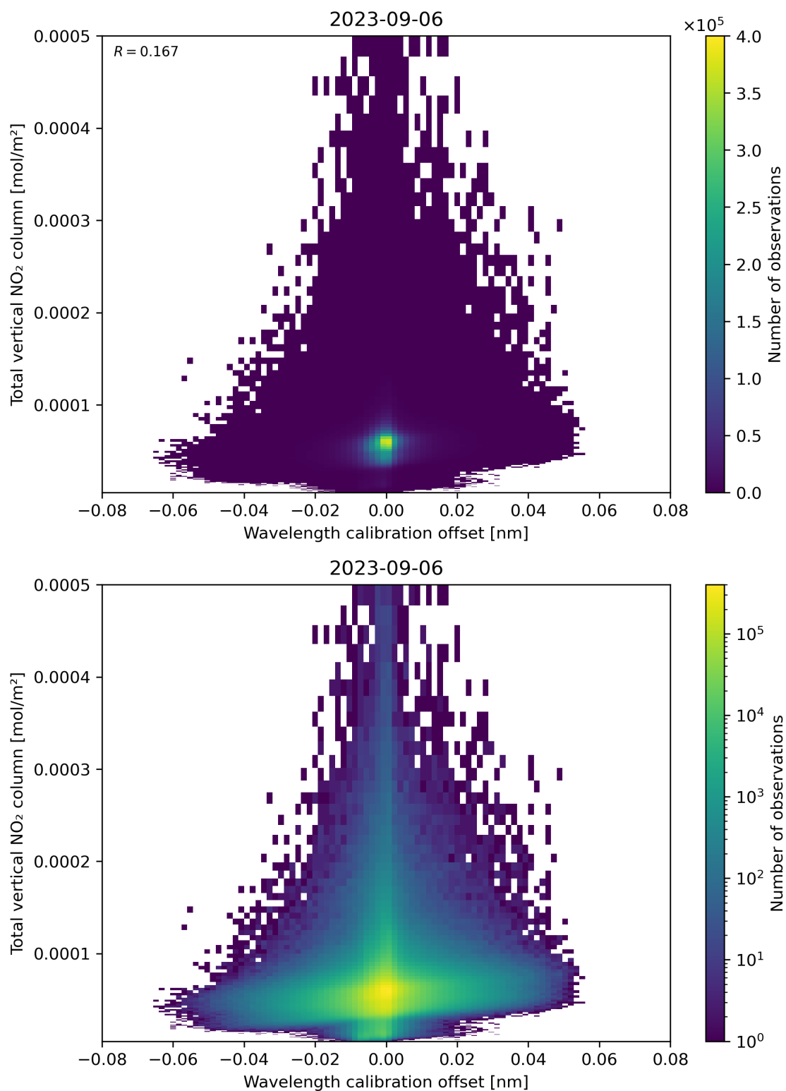
Figure 179: Scatter density plot of “Wavelength calibration offset” against “Total vertical NO 2 column” for 2023-09-05 to 2023-09-07.
