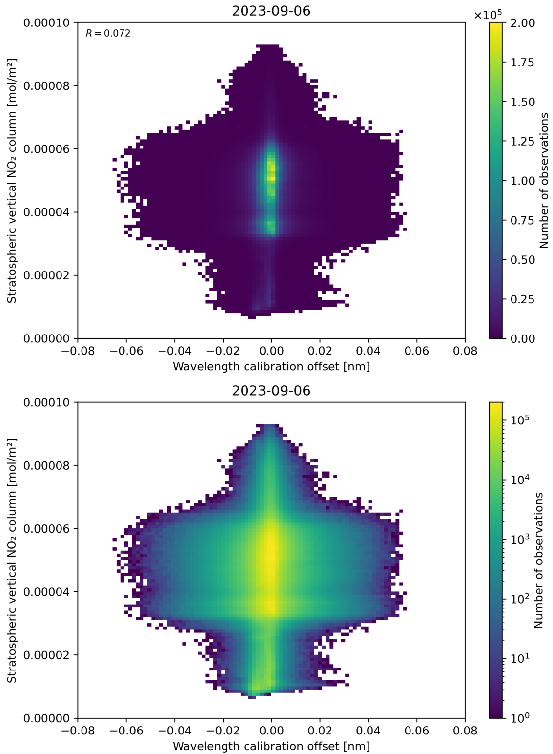
Figure 176: Scatter density plot of “Wavelength calibration offset” against “Stratospheric vertical NO 2 column” for 2023-09-05 to 2023-09-07.
