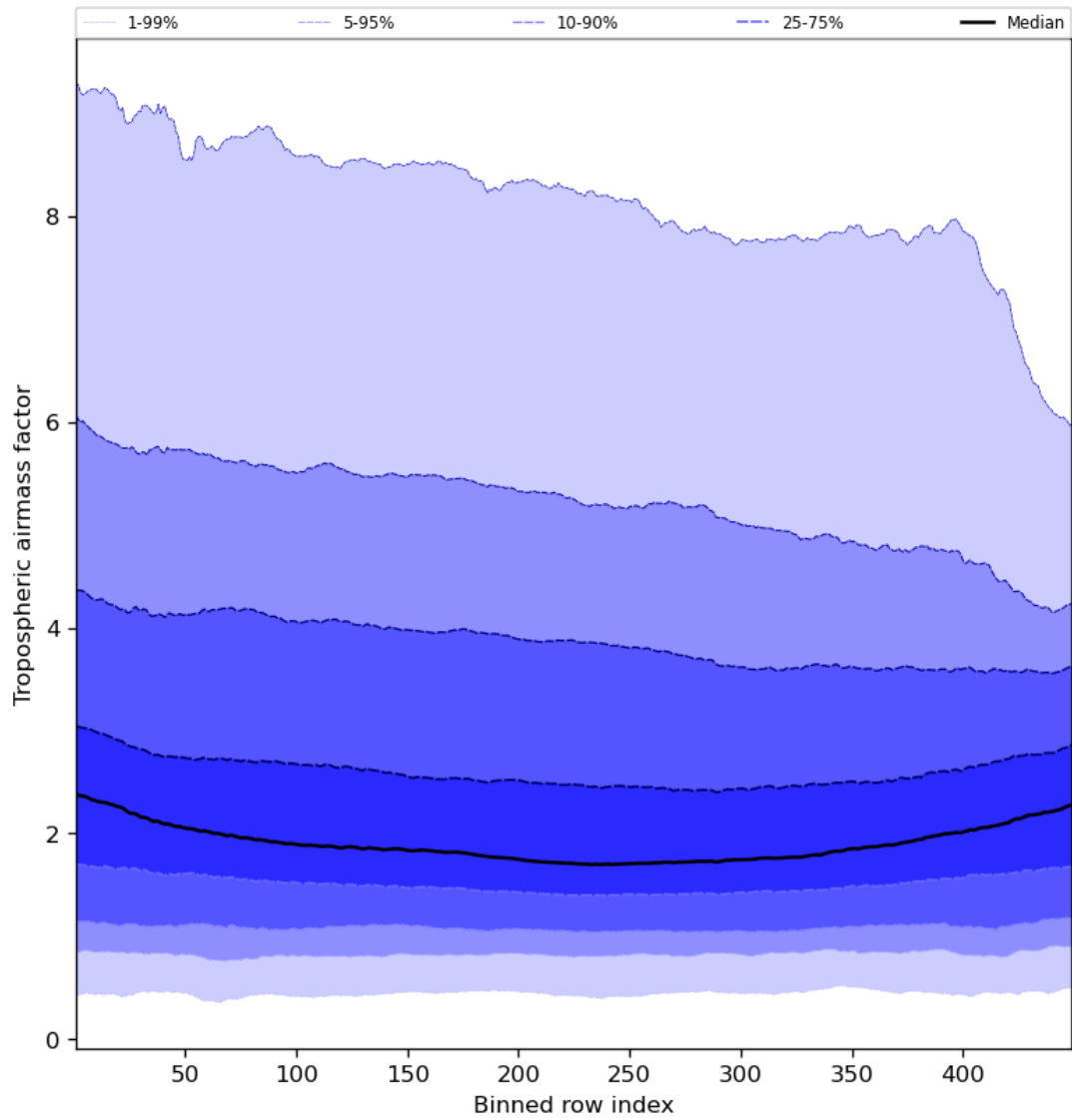
Figure 48: Along track statistics of “Tropospheric air mass factor” for 2023-09-05 to 2023-09-07
