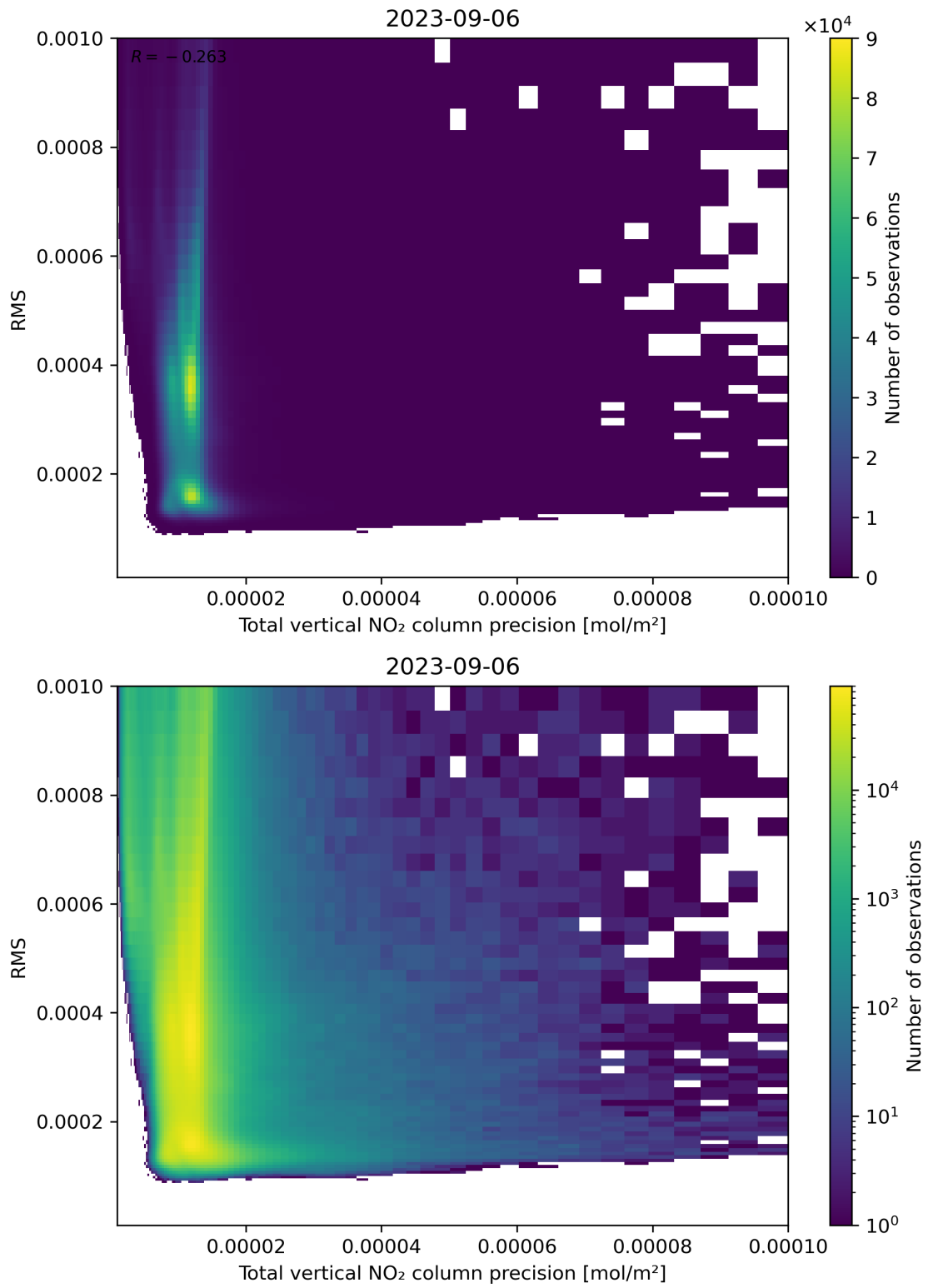
Figure 119: Scatter density plot of “Total vertical NO 2 column precision” against “RMS” for 2023-09-05 to 2023-09-07.
