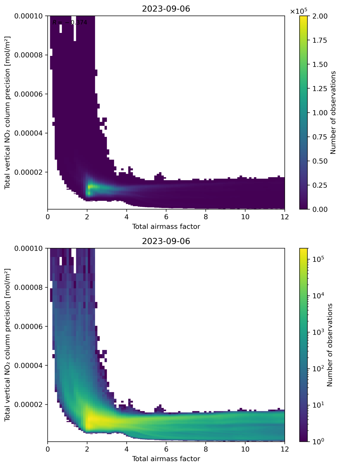
Figure 68: Scatter density plot of “Total airmass factor” against “Total vertical NO 2 column precision” for 2023-09-05 to 2023-09-07.
