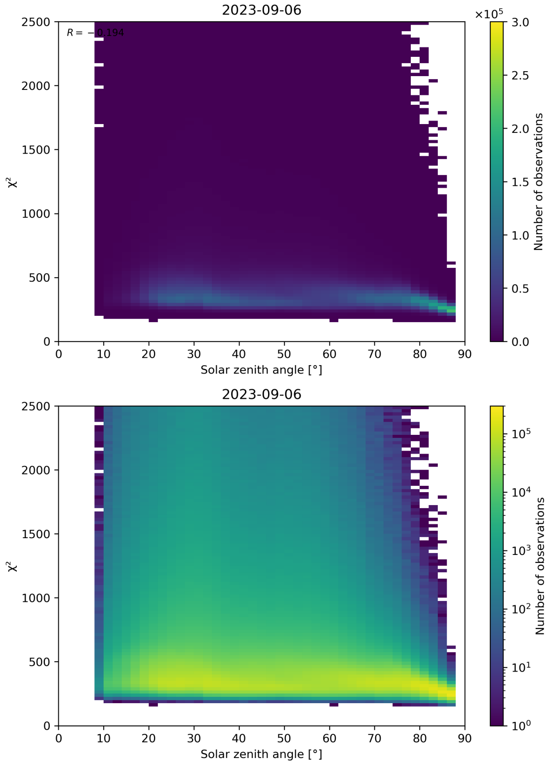
Figure 148: Scatter density plot of “Solar zenith angle” against “ \chi^2 ” for 2023-09-05 to 2023-09-07.
