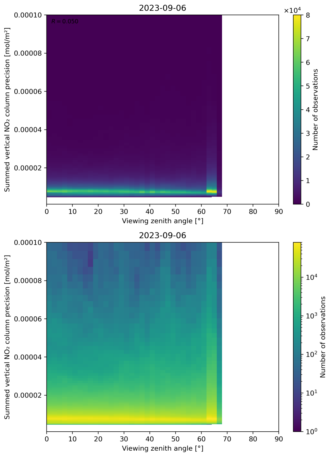
Figure 166: Scatter density plot of “Viewing zenith angle” against “Summed vertical NO 2 column precision” for 2023-09-05 to 2023-09-07.
