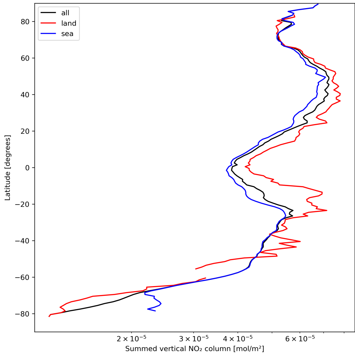
Figure 23: Zonal average of “Summed vertical NO 2 column” for 2023-09-05 to 2023-09-07.
