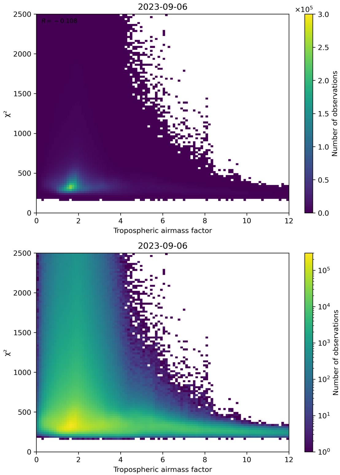
Figure 73: Scatter density plot of “Tropospheric airmass factor” against “ \chi^2 ” for 2023-09-05 to 2023-09-07.
