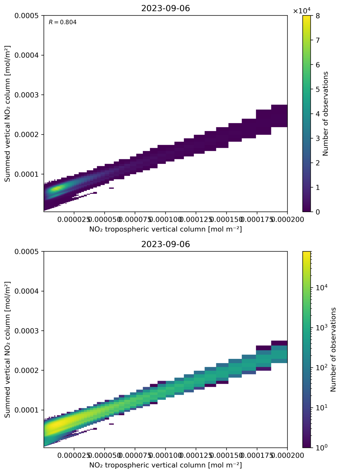
Figure 126: Scatter density plot of “NO 2 tropospheric vertical column” against “Summed vertical NO 2 column” for 2023-09-05 to 2023-09-07.
