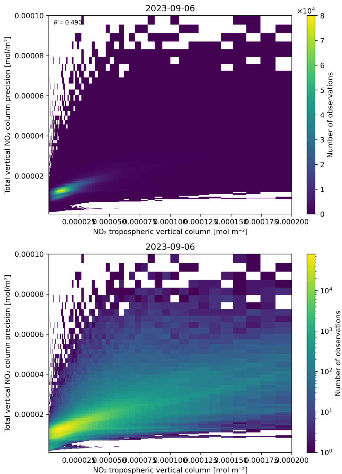
Figure 129: Scatter density plot of “NO 2 tropospheric vertical column” against “Total vertical NO 2 column precision” for 2023-09-05 to 2023-09-07.
