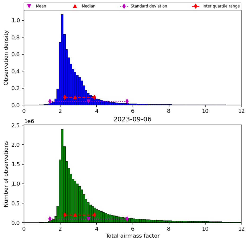
Figure 32: Histogram of “Total airmass factor” for 2023-09-05 to 2023-09-07
