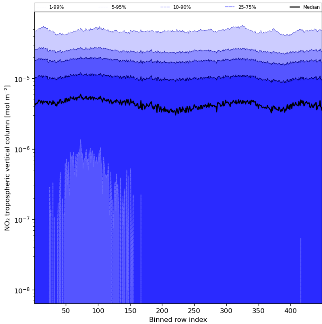
Figure 46: Along track statistics of “NO 2 tropospheric vertical column” for 2023-09-05 to 2023-09-07
