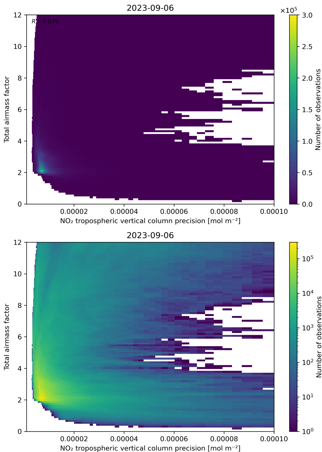
Figure 132: Scatter density plot of “NO 2 tropospheric vertical column precision” against “Total air mass factor” for 2023-09-05 to 2023-09-07.
