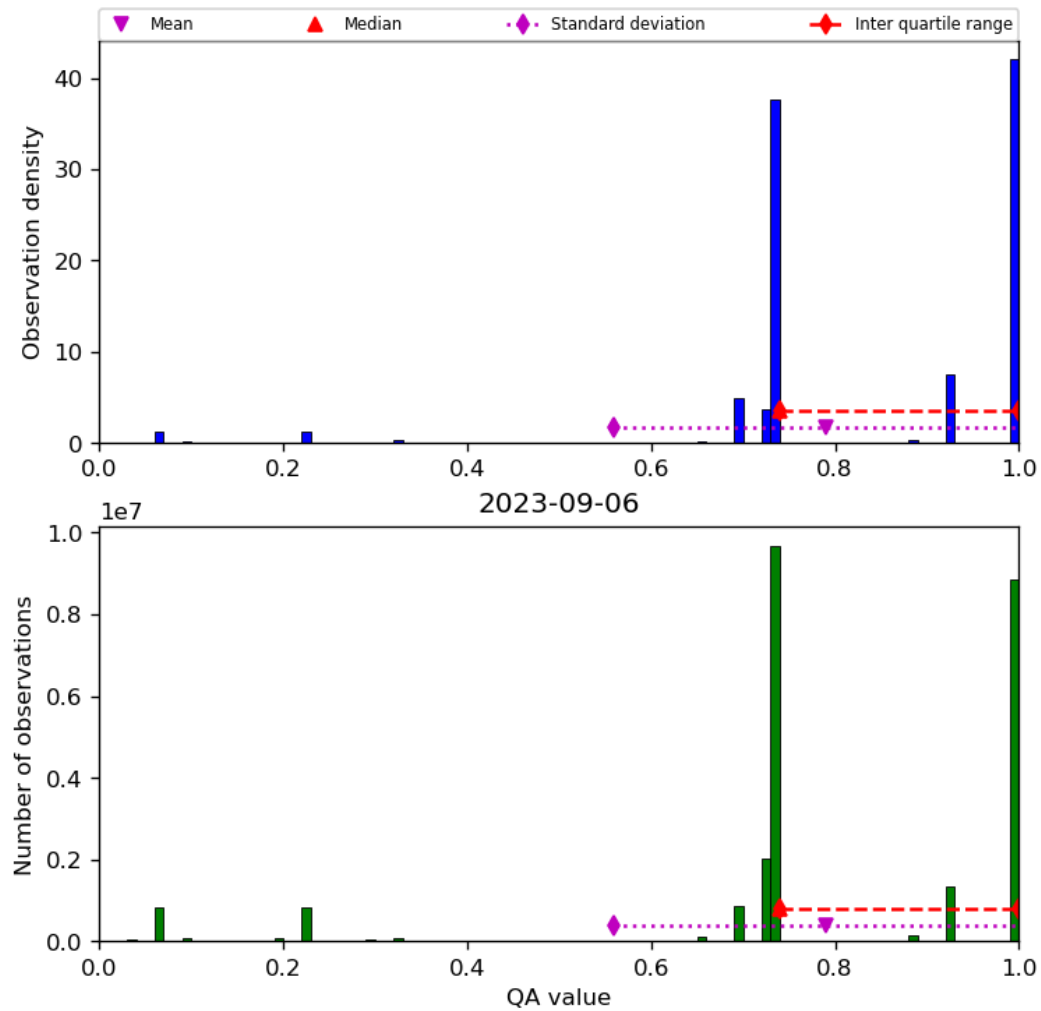
Figure 28: Histogram of “QA value” for 2023-09-05 to 2023-09-07
