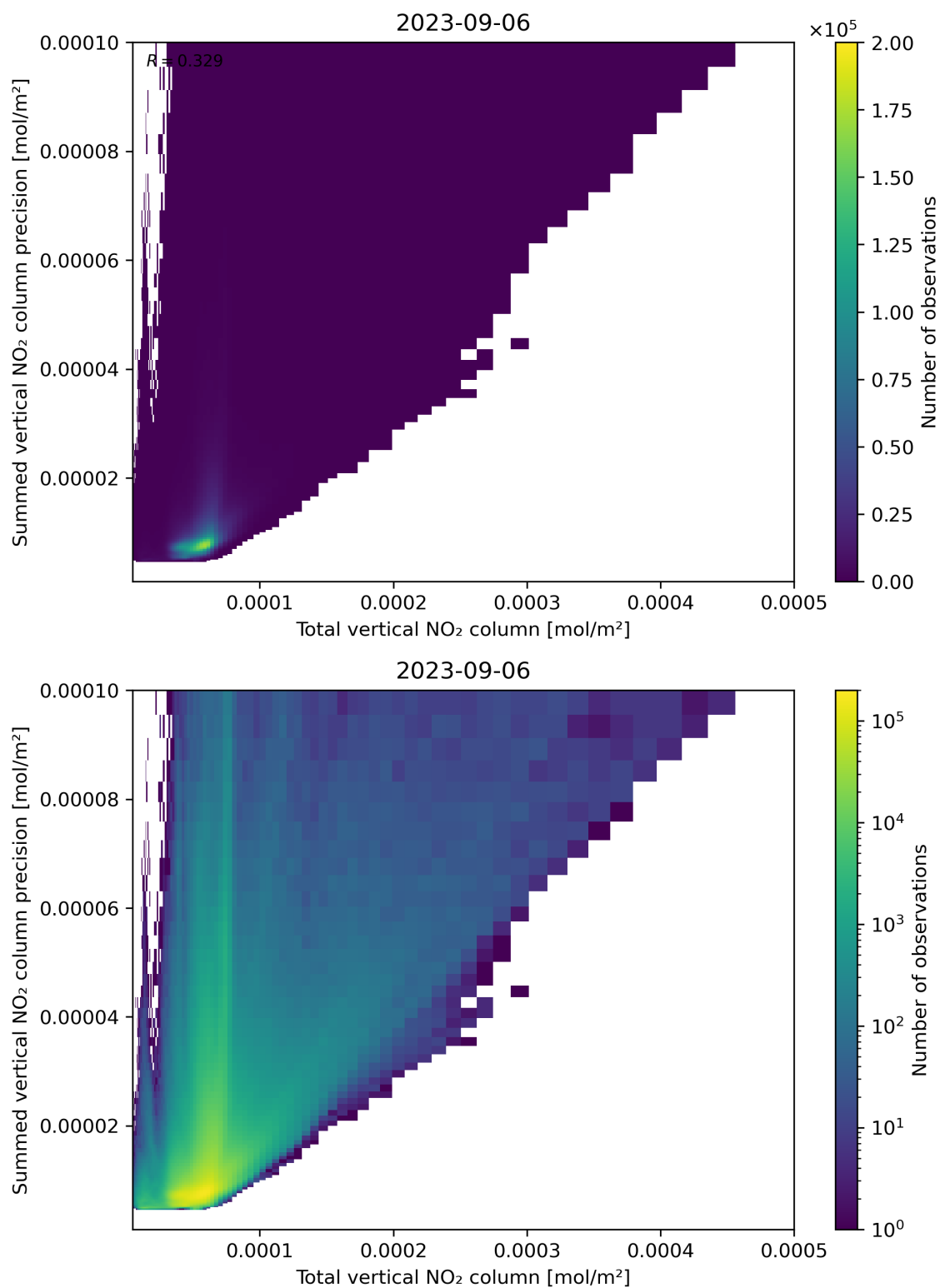
Figure 113: Scatter density plot of “Total vertical NO 2 column” against “Summed vertical NO 2 column precision” for 2023-09-05 to 2023-09-07.
