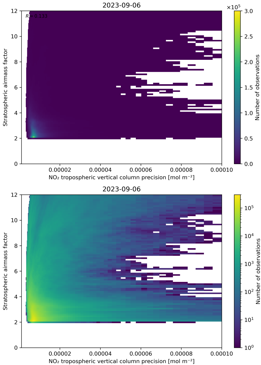
Figure 131: Scatter density plot of “NO 2 tropospheric vertical column precision” against “Stratospheric airmass factor” for 2023-09-05 to 2023-09-07.
