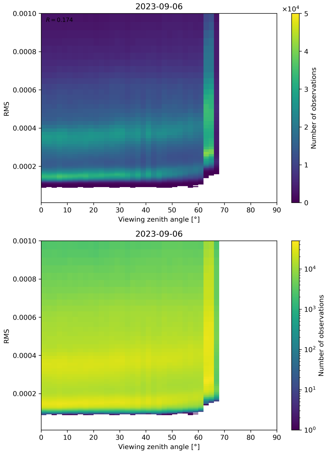
Figure 171: Scatter density plot of “Viewing zenith angle” against “RMS” for 2023-09-05 to 2023-09-07.
