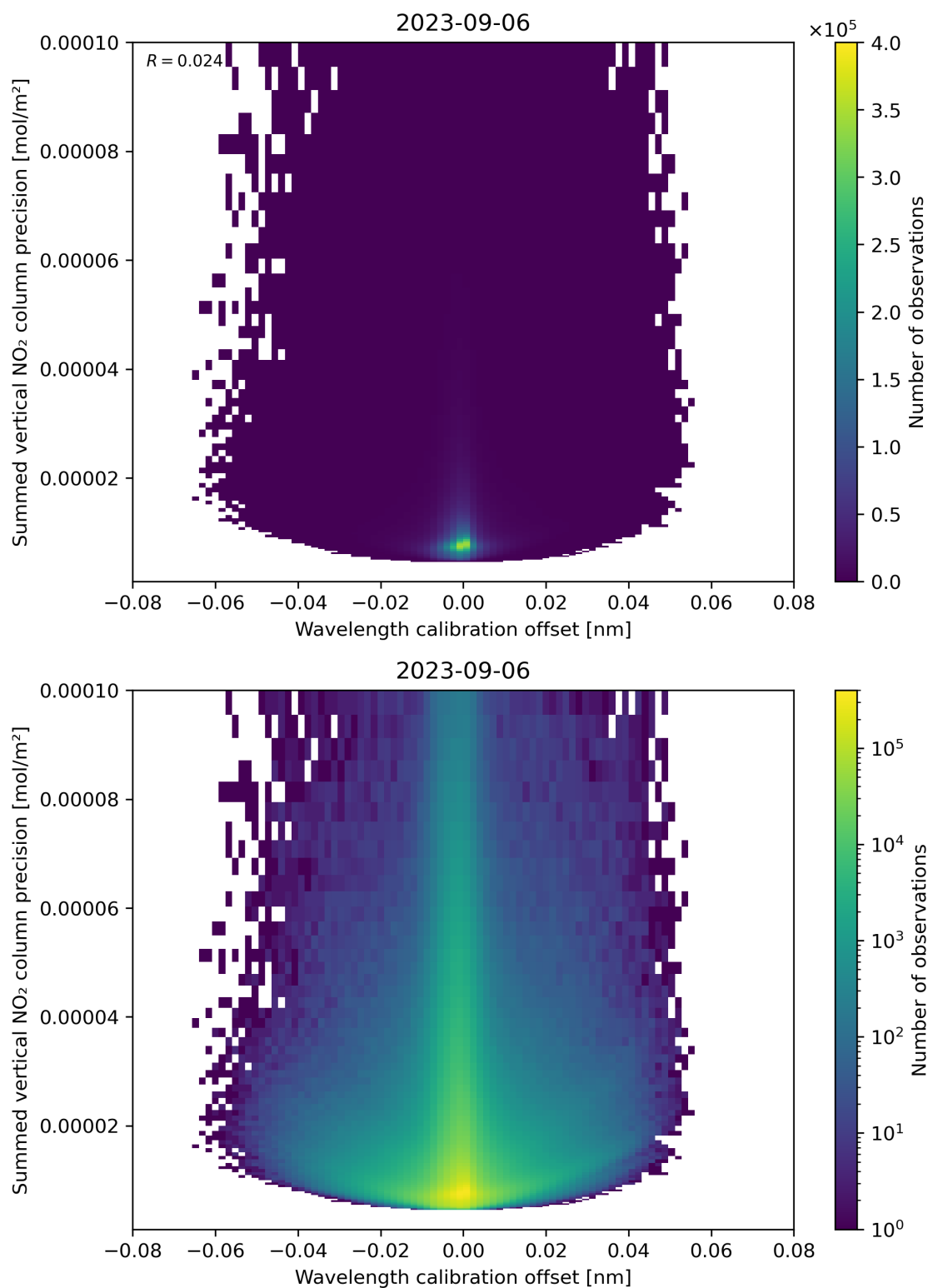
Figure 178: Scatter density plot of “Wavelength calibration offset” against “Summed vertical NO 2 column precision” for 2023-09-05 to 2023-09-07.
