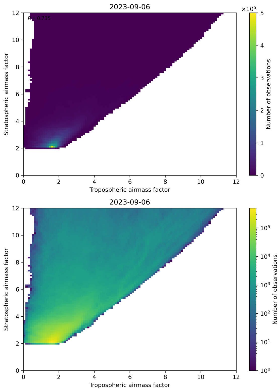
Figure 71: Scatter density plot of “Tropospheric airmass factor” against “Stratospheric airmass factor” for 2023-09-05 to 2023-09-07.
