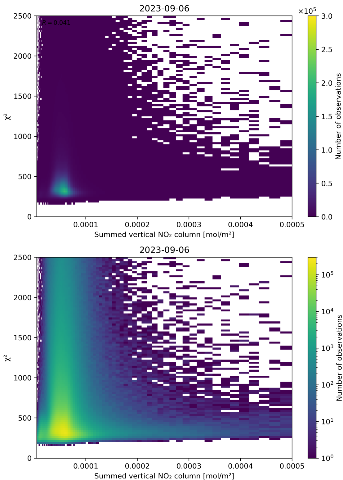
Figure 104: Scatter density plot of “Summed vertical NO 2 column” against “ \chi^2 ” for 2023-09-05 to 2023-09-07.
