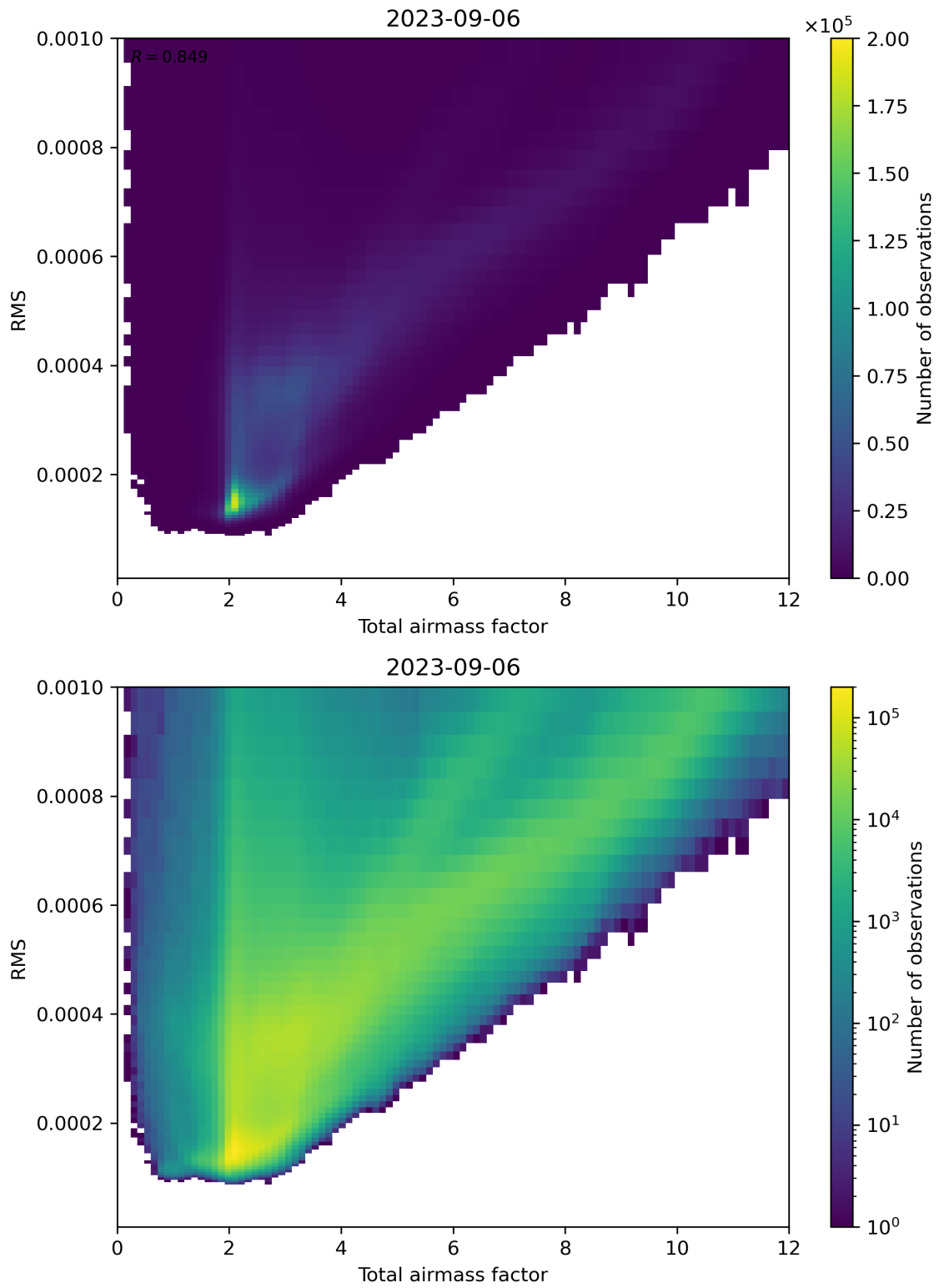
Figure 69: Scatter density plot of “Total airmass factor” against “RMS” for 2023-09-05 to 2023-09-07.
