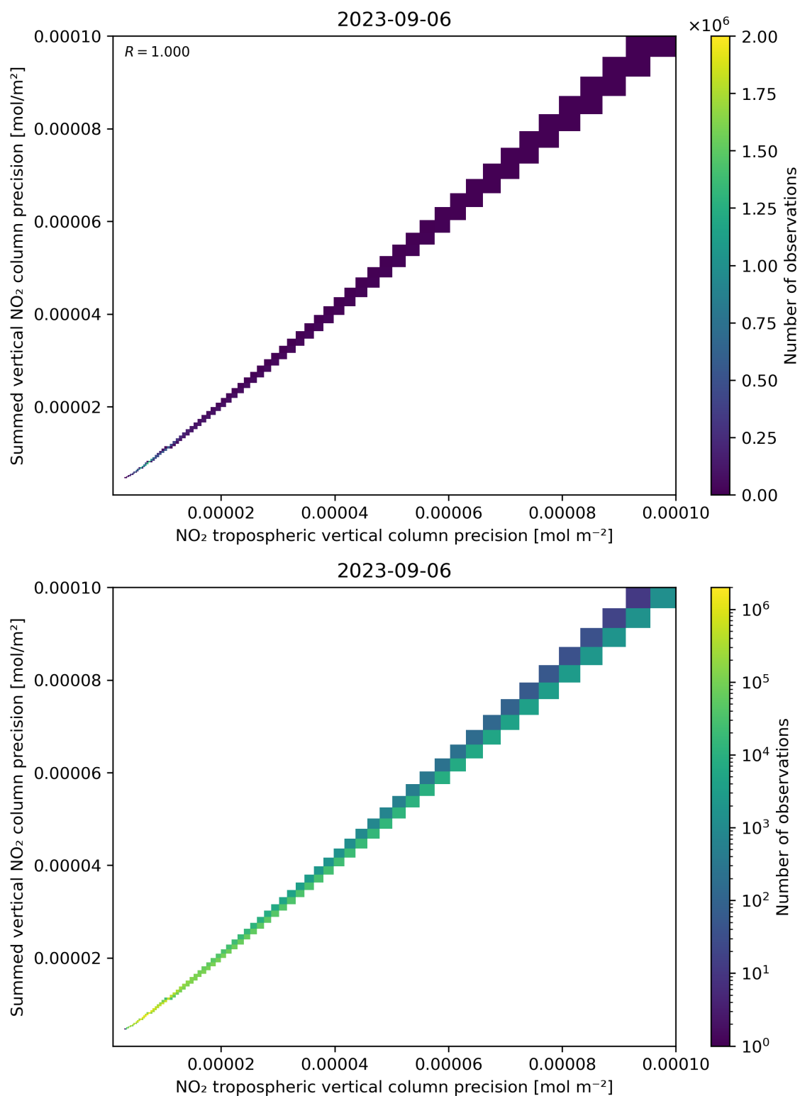
Figure 137: Scatter density plot of “NO 2 tropospheric vertical column precision” against “Summed vertical NO 2 column precision” for 2023-09-05 to 2023-09-07.
