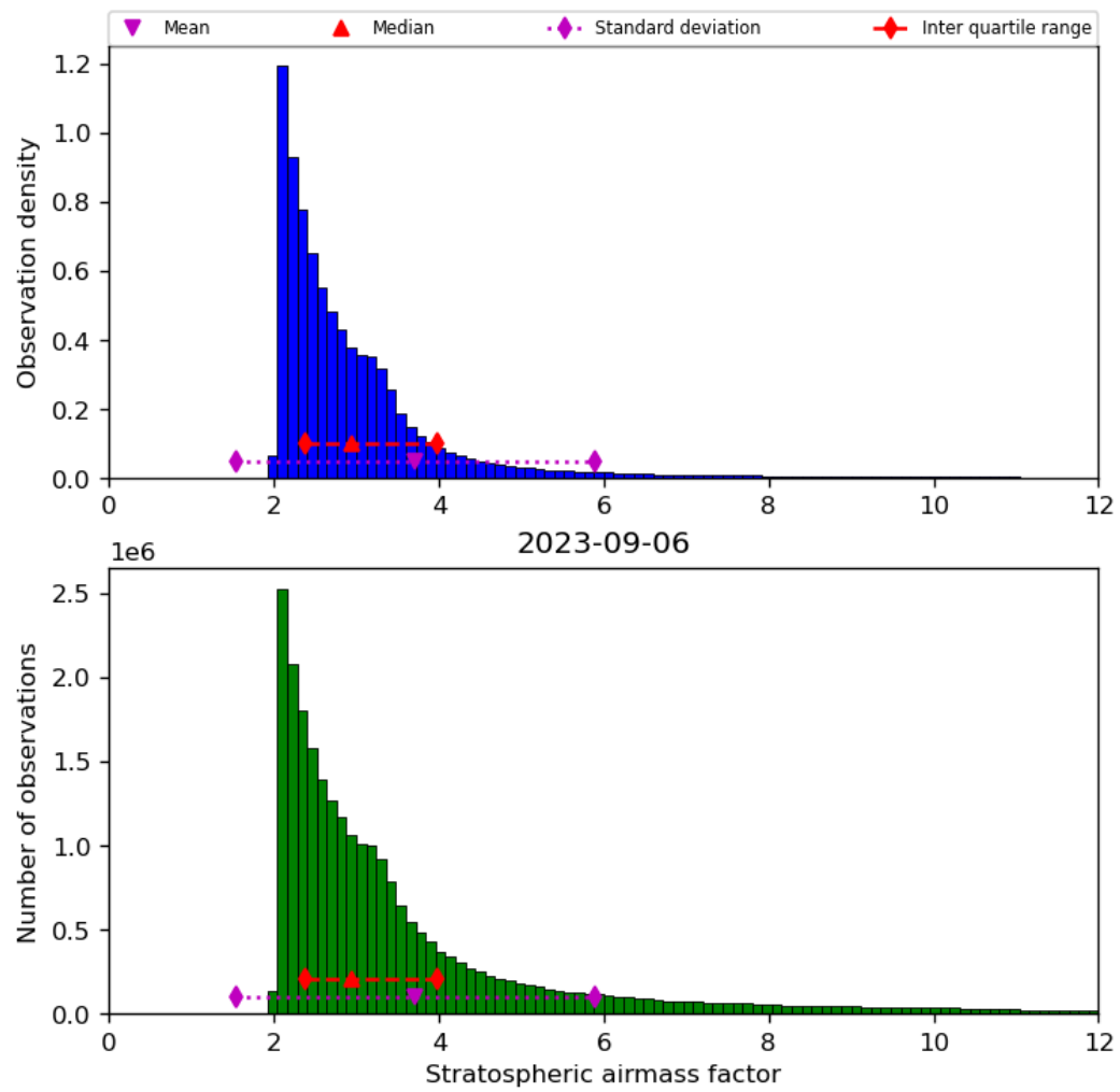
Figure 44: Histogram of “Stratospheric airmass factor” for 2023-09-05 to 2023-09-07
