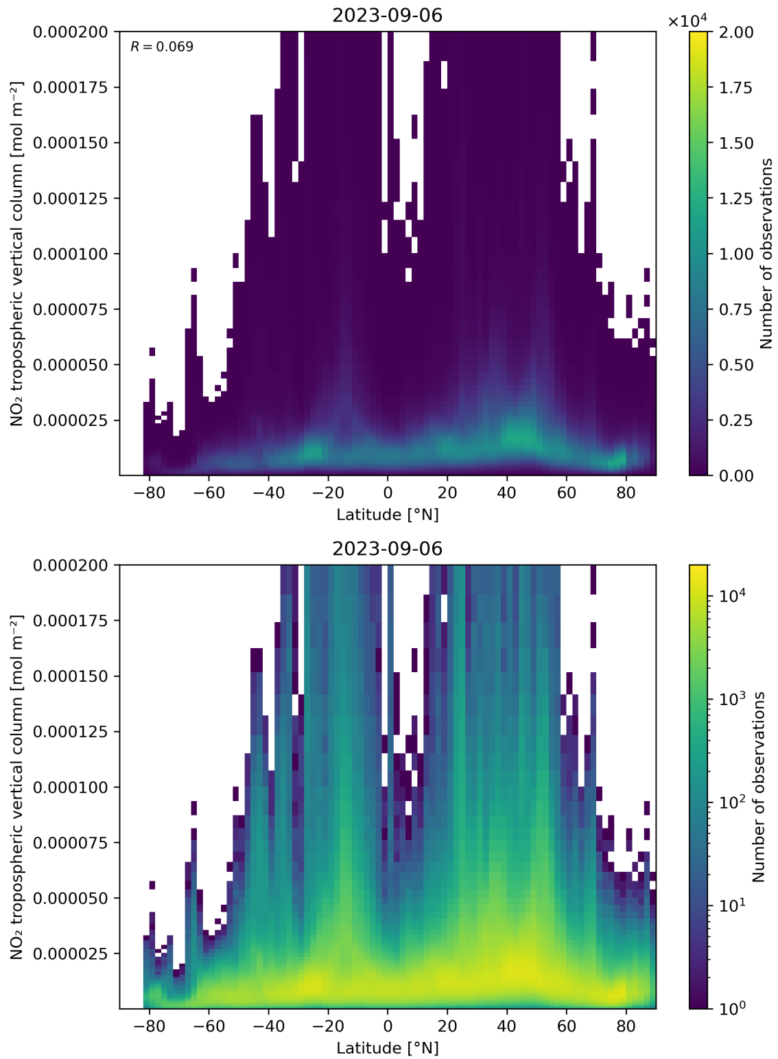
Figure 92: Scatter density plot of “Latitude” against “NO 2 tropospheric vertical column” for 2023-09-05 to 2023-09-07.
