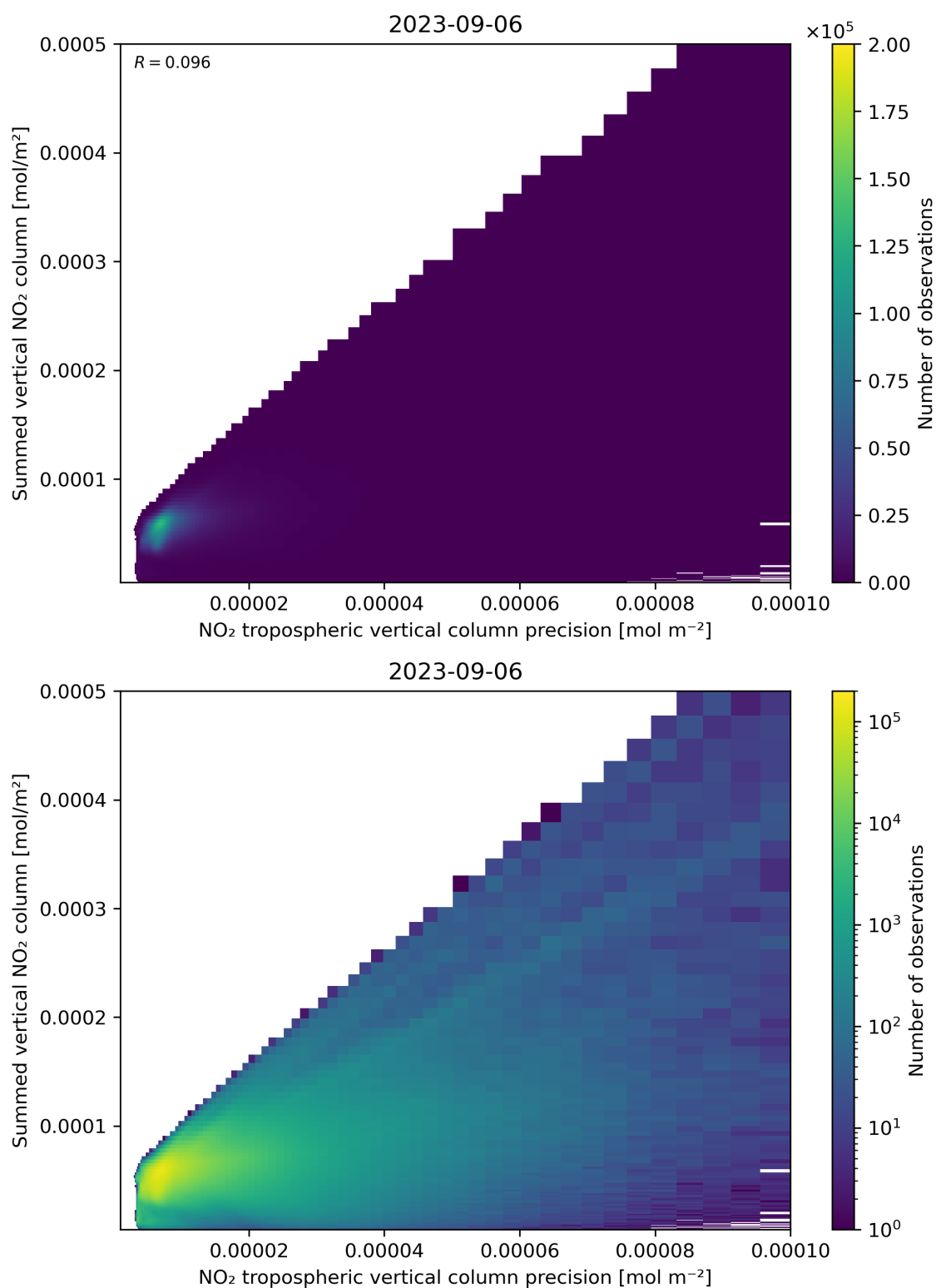
Figure 136: Scatter density plot of “NO 2 tropospheric vertical column precision” against “Summed vertical NO 2 column” for 2023-09-05 to 2023-09-07.
