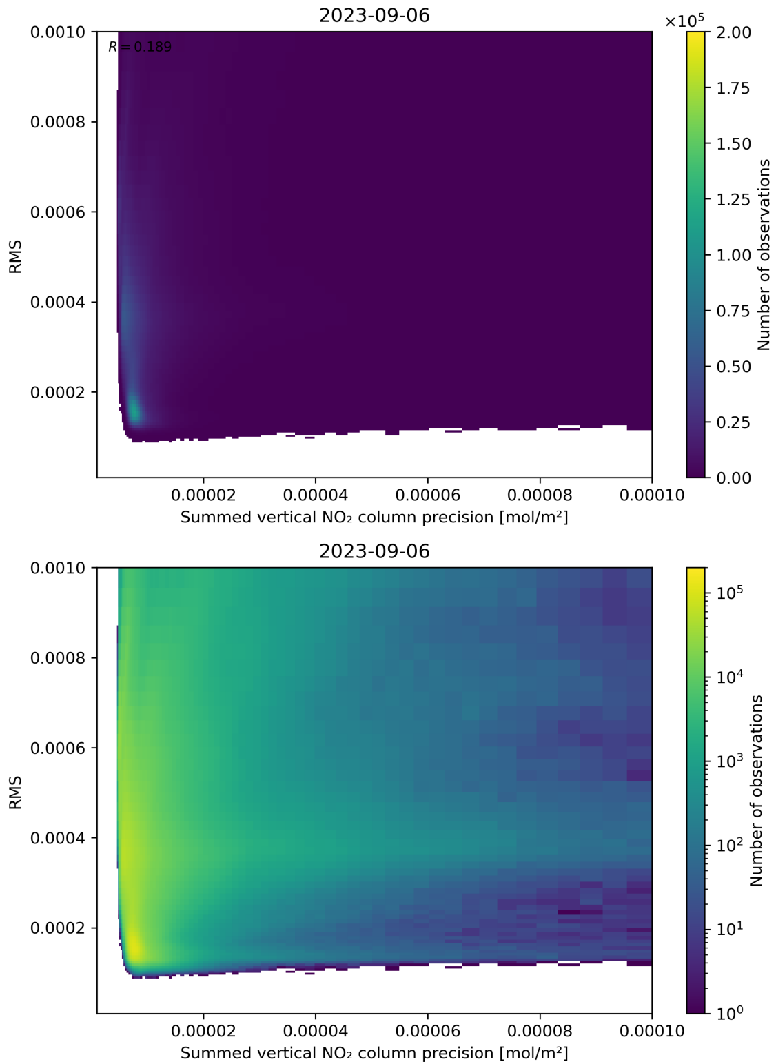
Figure 108: Scatter density plot of “Summed vertical NO 2 column precision” against “RMS” for 2023-09-05 to 2023-09-07.
