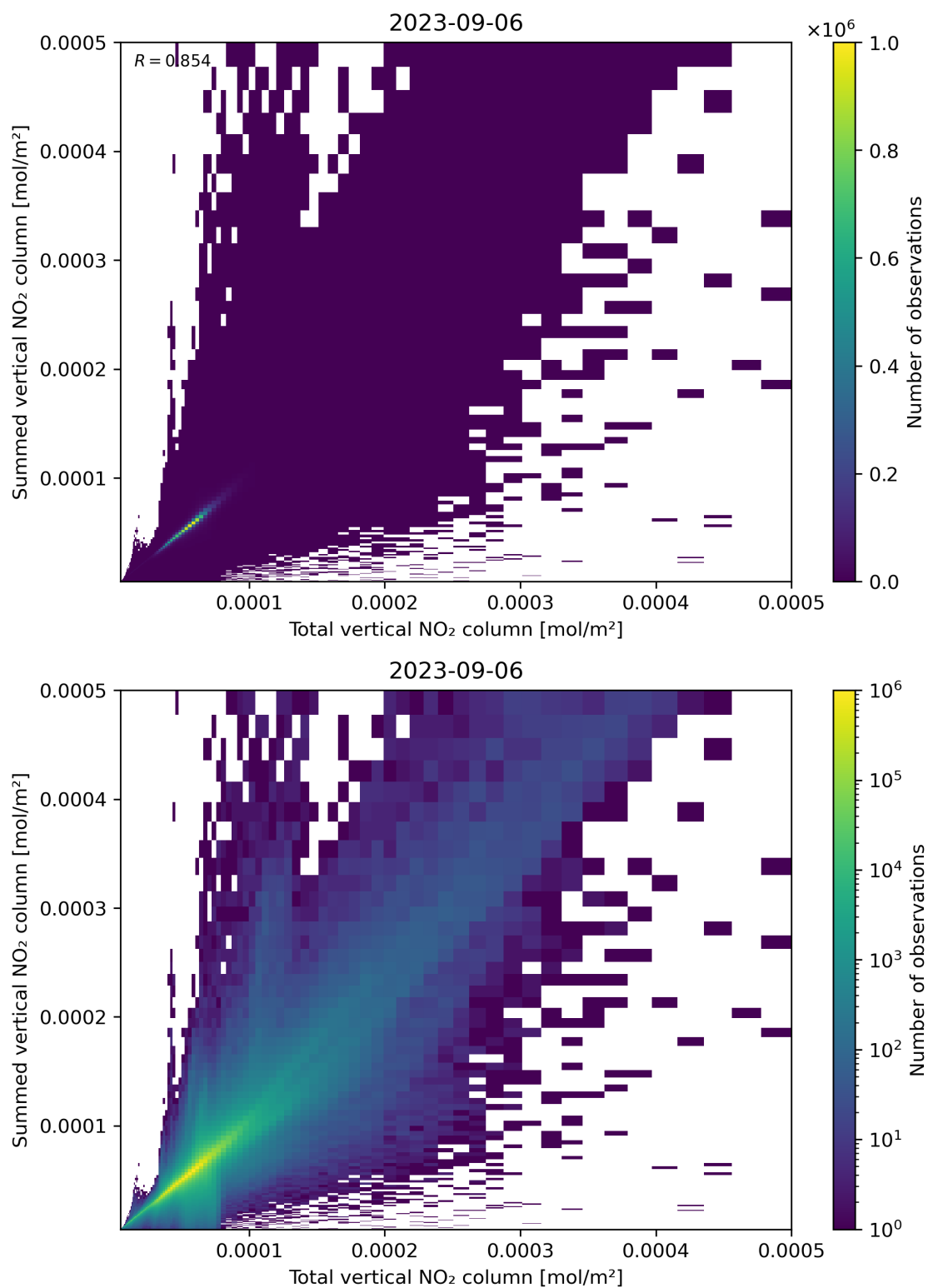
Figure 112: Scatter density plot of “Total vertical NO 2 column” against “Summed vertical NO 2 column” for 2023-09-05 to 2023-09-07.
