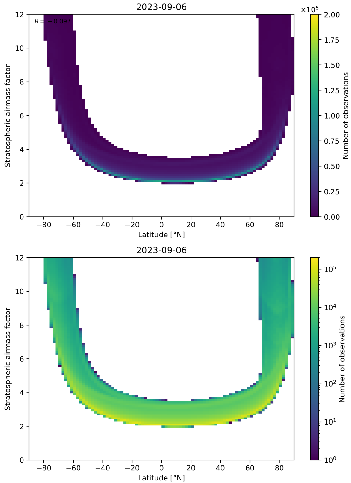
Figure 83: Scatter density plot of “Latitude” against “Stratospheric airmass factor” for 2023-09-05 to 2023-09-07.
