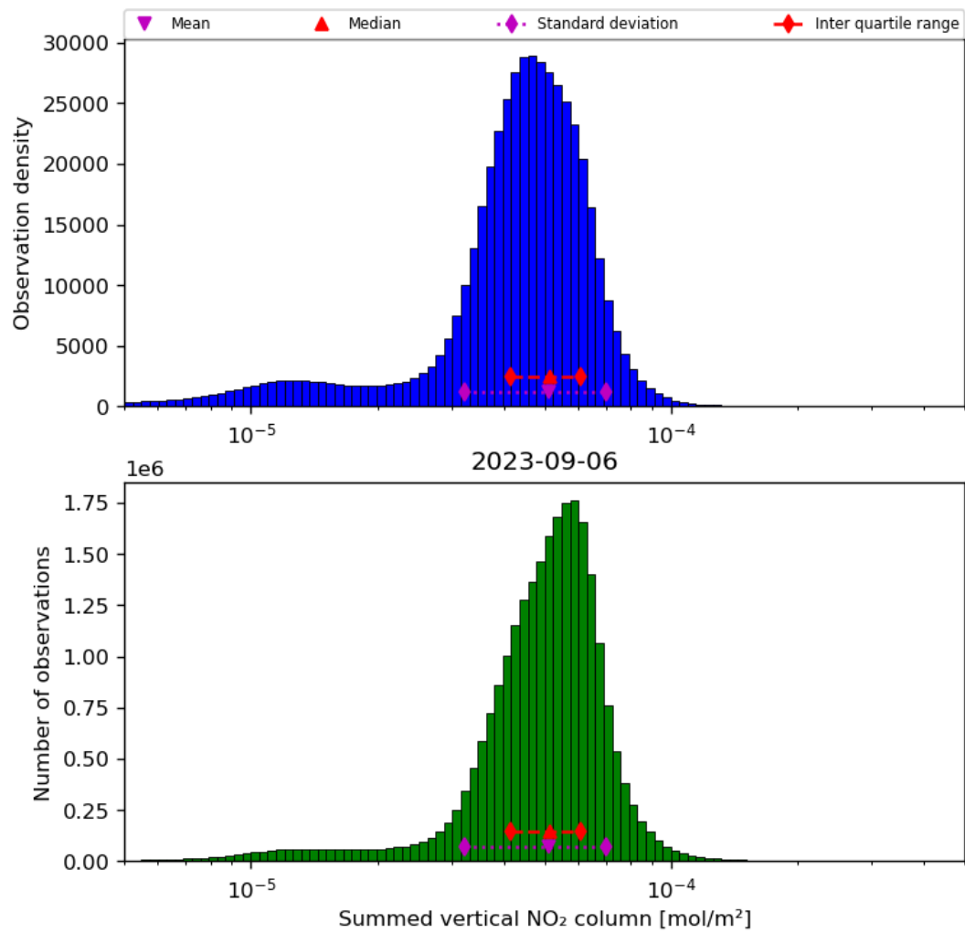
Figure 40: Histogram of “Summed vertical NO 2 column” for 2023-09-05 to 2023-09-07
