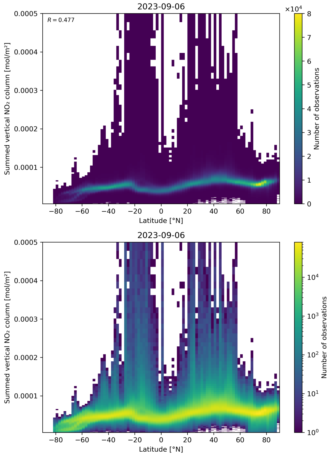
Figure 88: Scatter density plot of “Latitude” against “Summed vertical NO 2 column” for 2023-09-05 to 2023-09-07.
