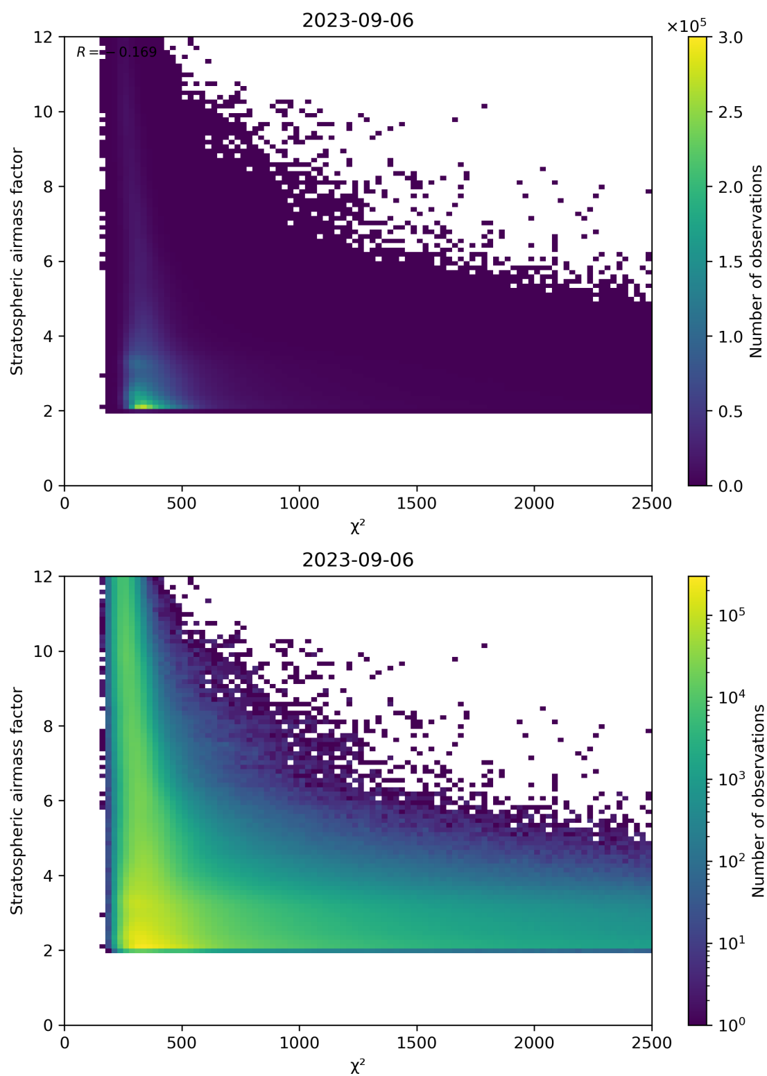
Figure 81: Scatter density plot of “ \chi^2 ” against “Stratospheric airmass factor” for 2023-09-05 to 2023-09-07.
