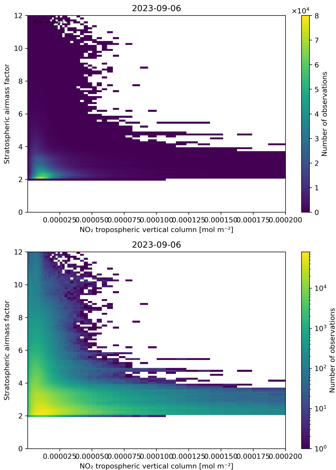
Figure 121: Scatter density plot of “NO 2 tropospheric vertical column” against “Stratospheric air mass factor” for 2023-09-05 to 2023-09-07.
