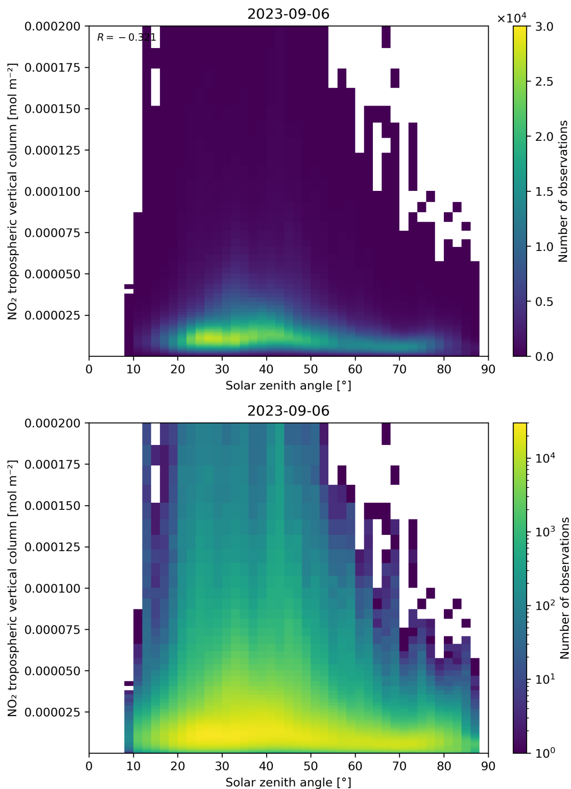
Figure 155: Scatter density plot of “Solar zenith angle” against “NO 2 tropospheric vertical column” for 2023-09-05 to 2023-09-07.
