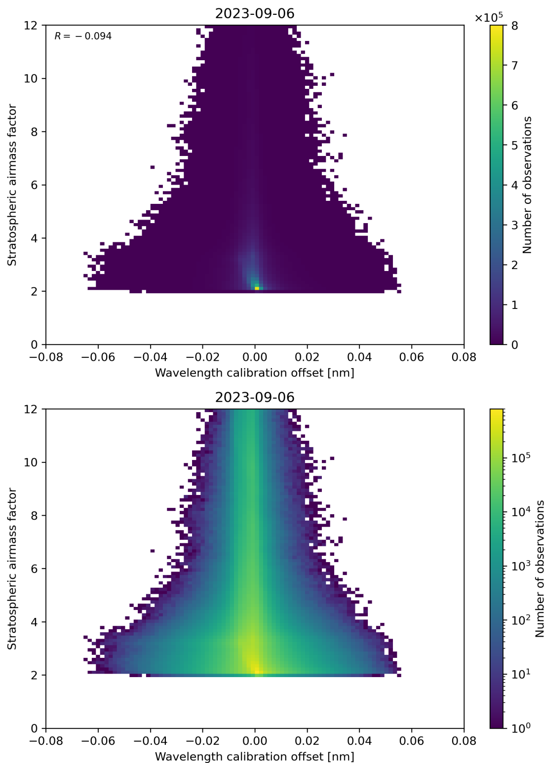
Figure 174: Scatter density plot of “Wavelength calibration offset” against “Stratospheric air mass factor” for 2023-09-05 to 2023-09-07.
