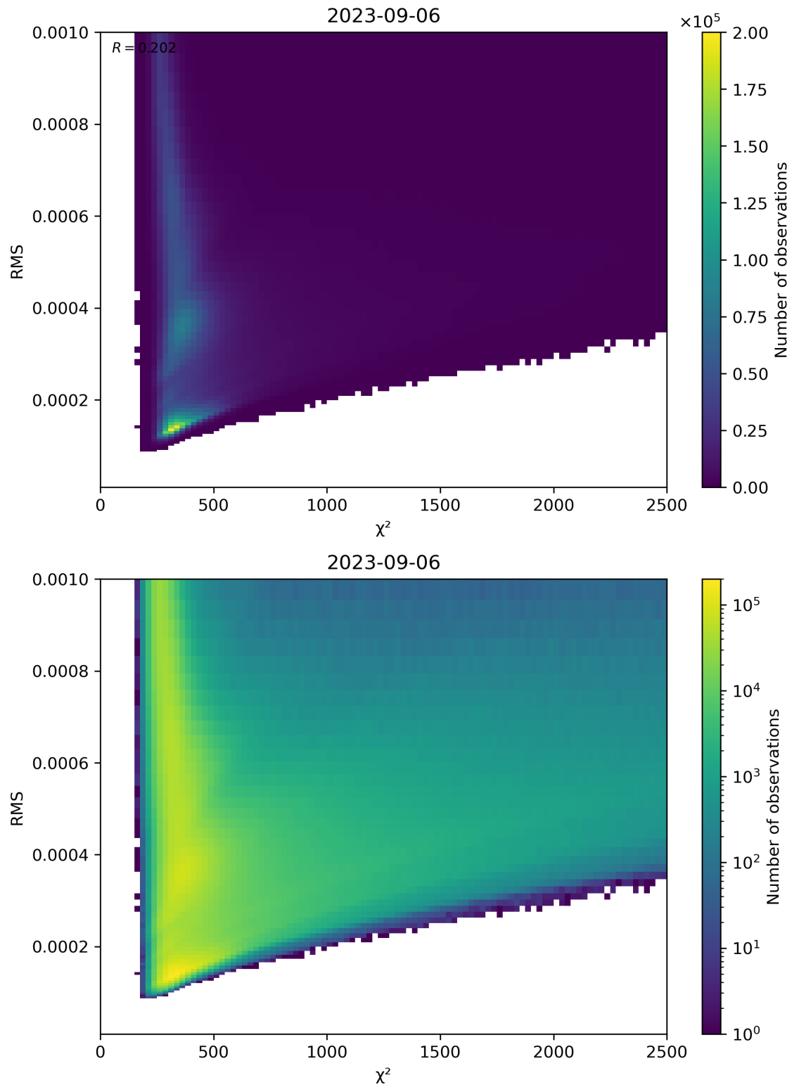
Figure 82: Scatter density plot of “ \chi^2 ” against “RMS” for 2023-09-05 to 2023-09-07.
