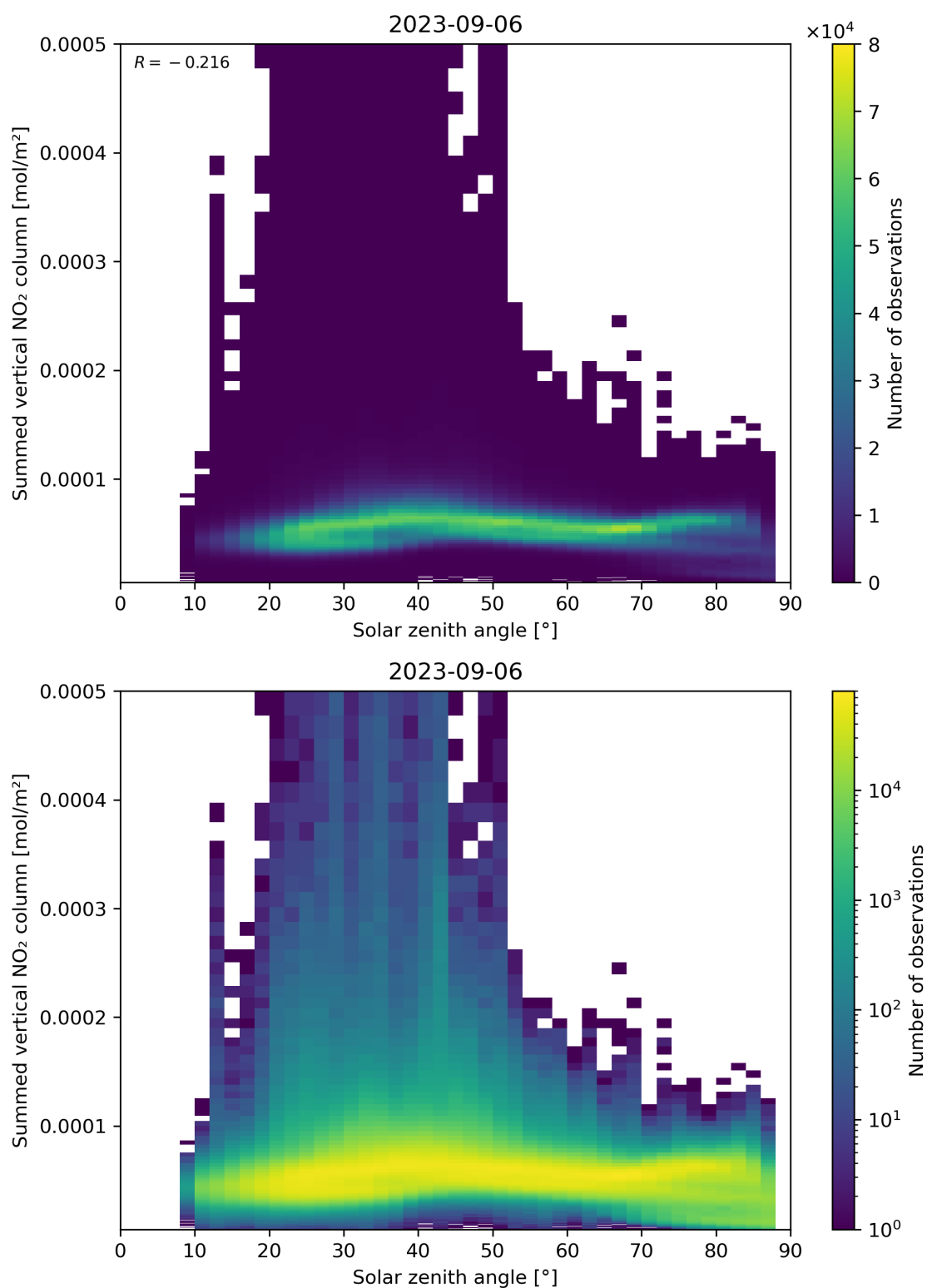
Figure 151: Scatter density plot of “Solar zenith angle” against “Summed vertical NO 2 column” for 2023-09-05 to 2023-09-07.
