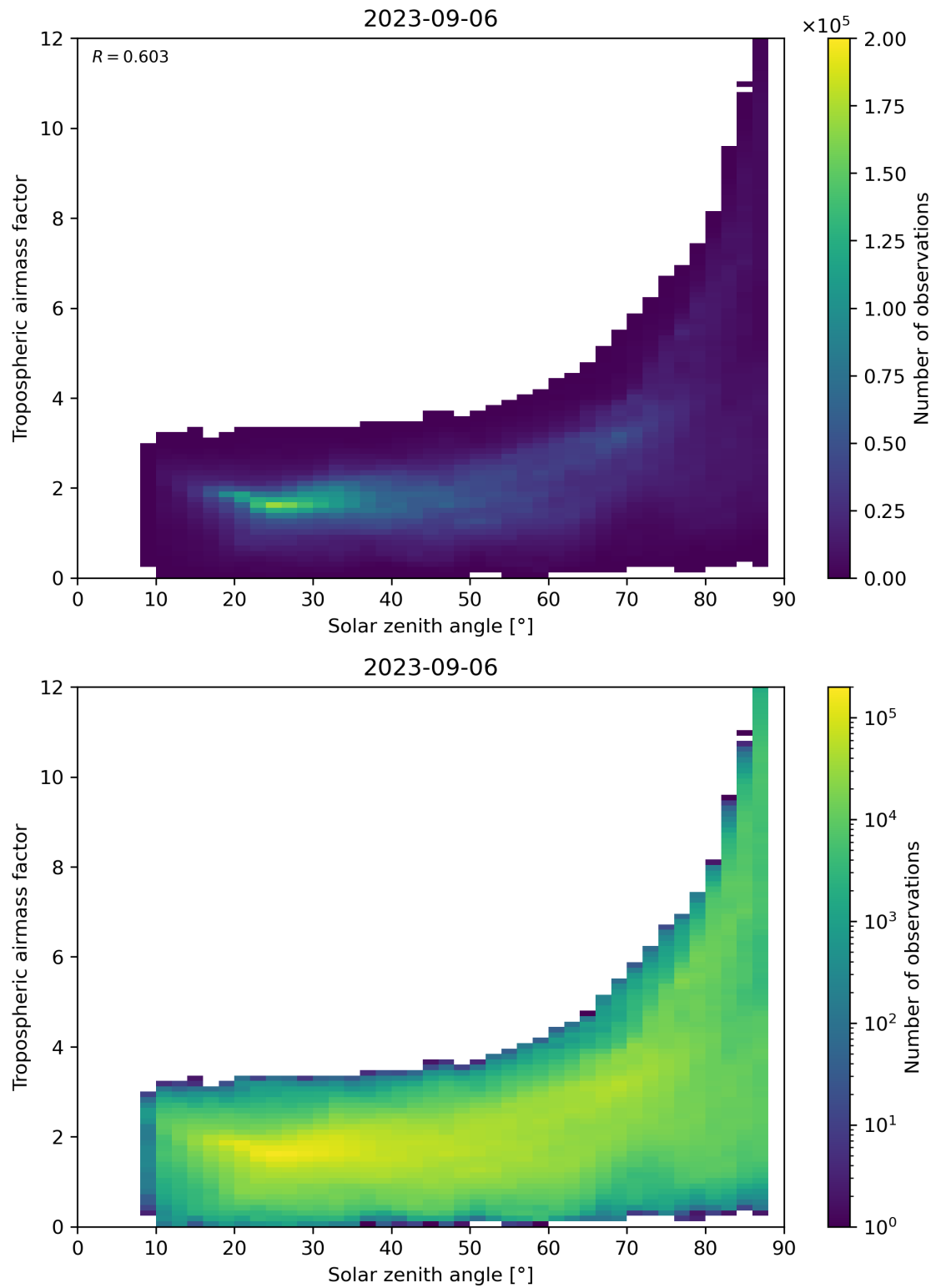
Figure 147: Scatter density plot of “Solar zenith angle” against “Tropospheric airmass factor” for 2023-09-05 to 2023-09-07.
