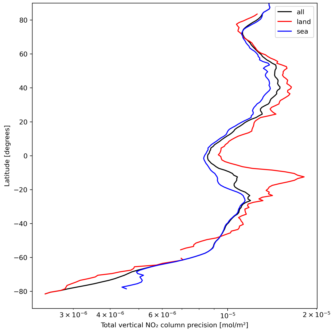
Figure 22: Zonal average of “Total vertical NO 2 column precision” for 2023-09-05 to 2023-09-07.
