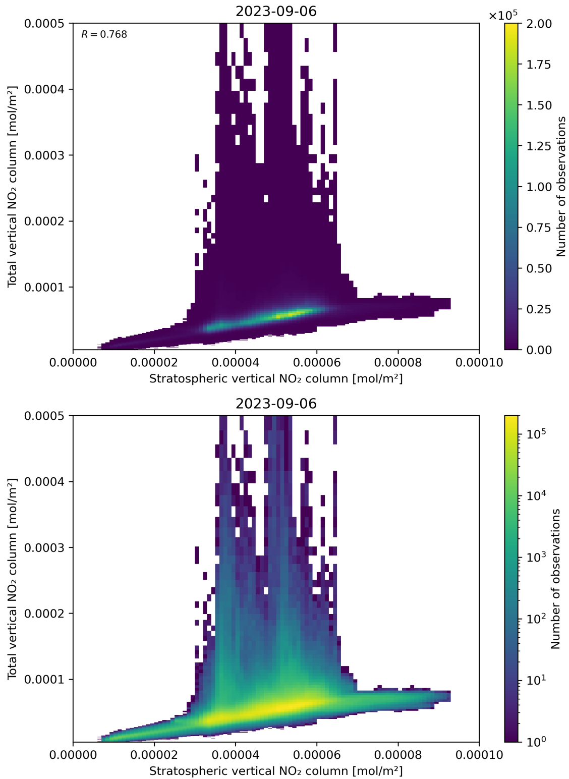
Figure 100: Scatter density plot of “Stratospheric vertical NO 2 column” against “Total vertical NO 2 column” for 2023-09-05 to 2023-09-07.
