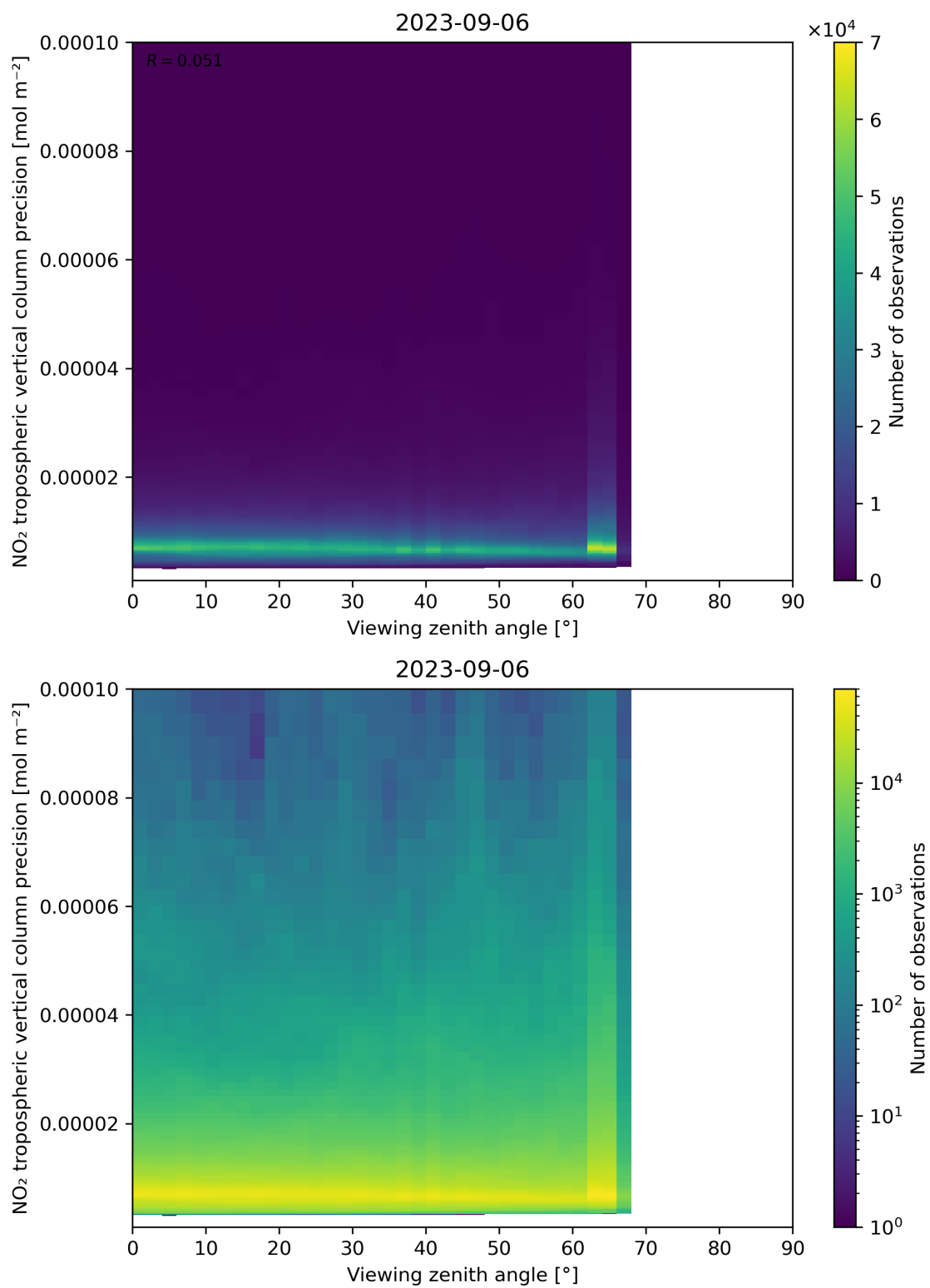
Figure 170: Scatter density plot of “Viewing zenith angle” against “NO 2 tropospheric vertical column precision” for 2023-09-05 to 2023-09-07.
