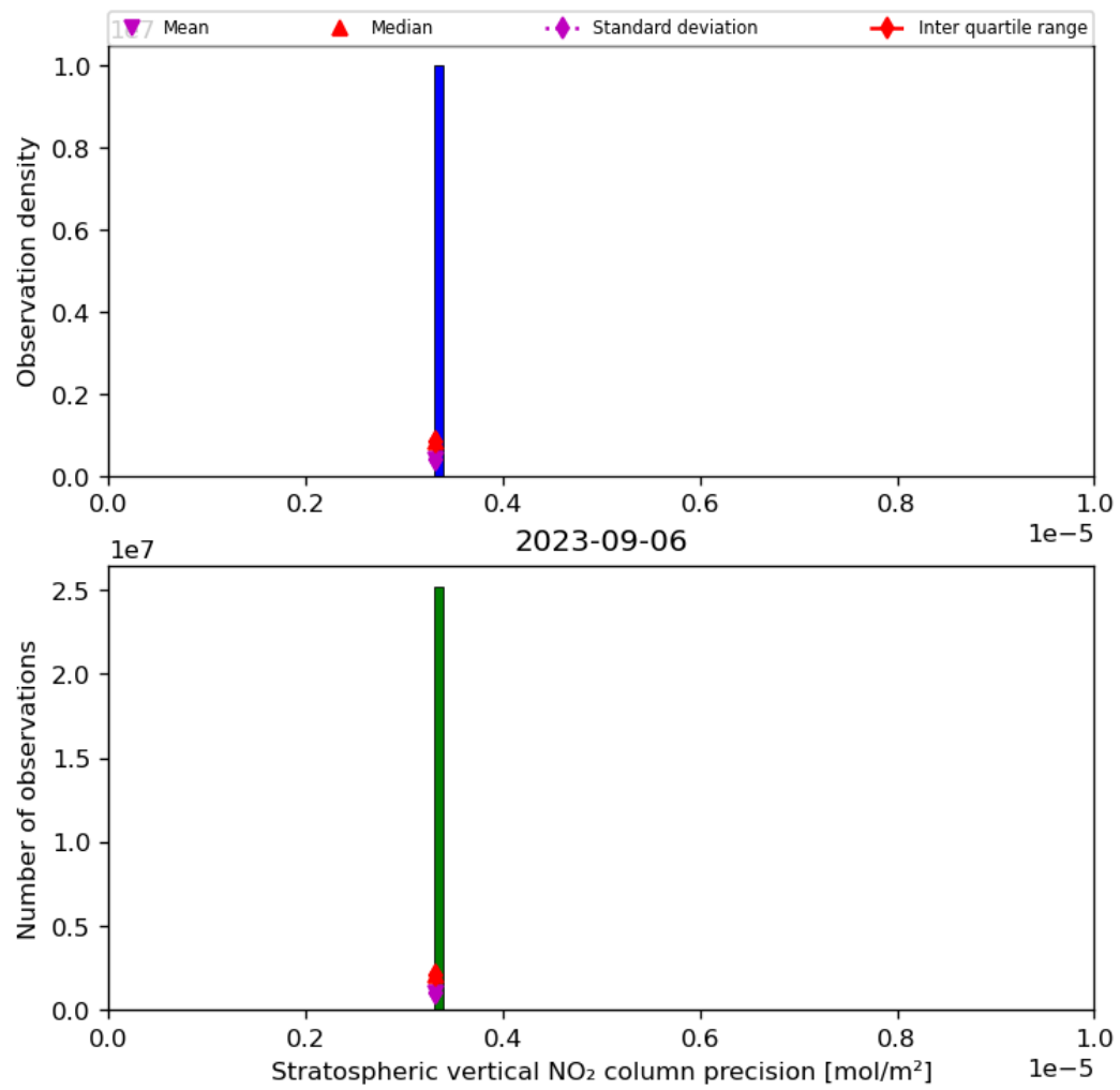
Figure 37: Histogram of “Stratospheric vertical NO 2 column precision” for 2023-09-05 to 2023-09-07
