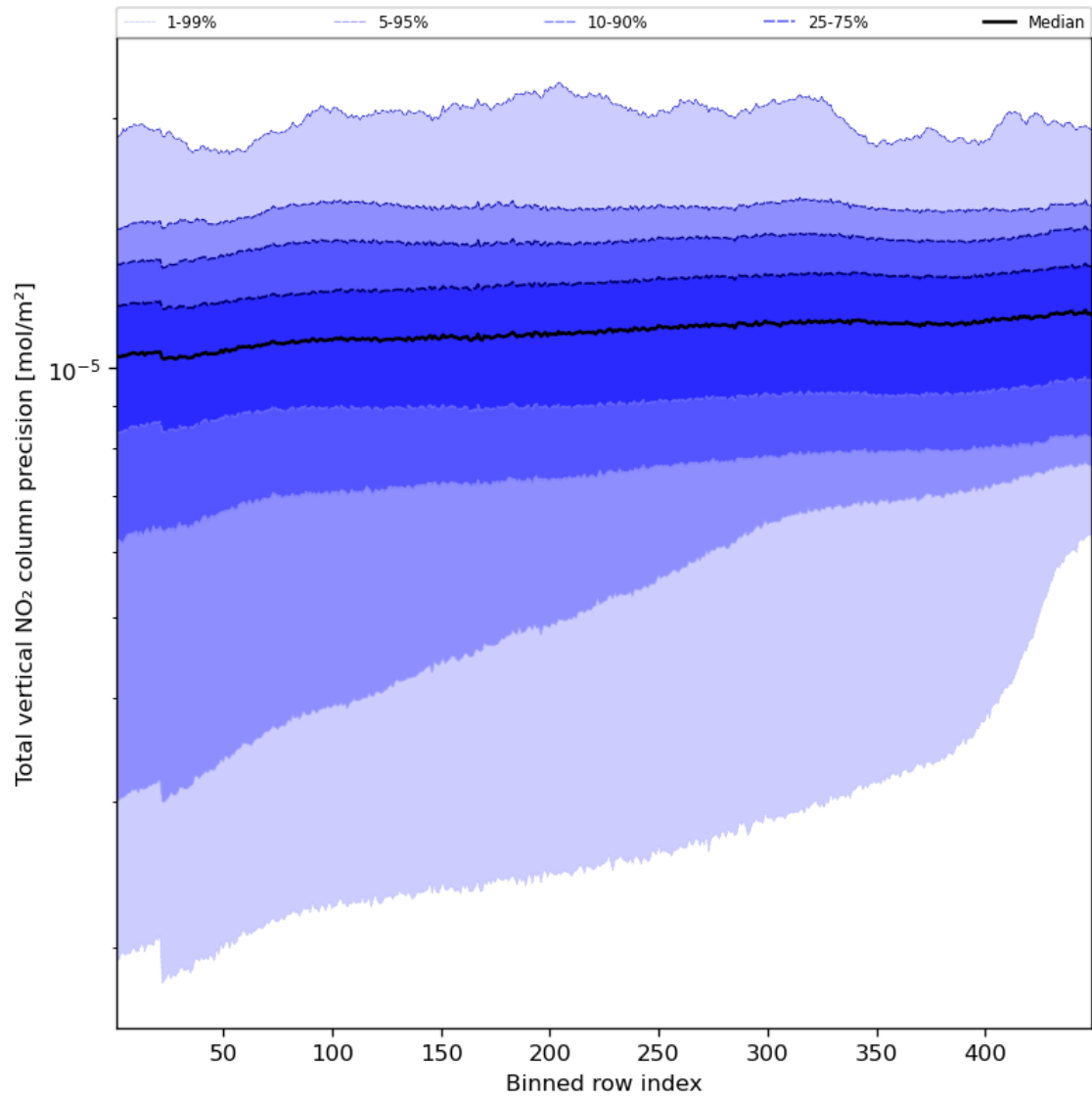
Figure 56: Along track statistics of “Total vertical NO 2 column precision” for 2023-09-05 to 2023-09-07
