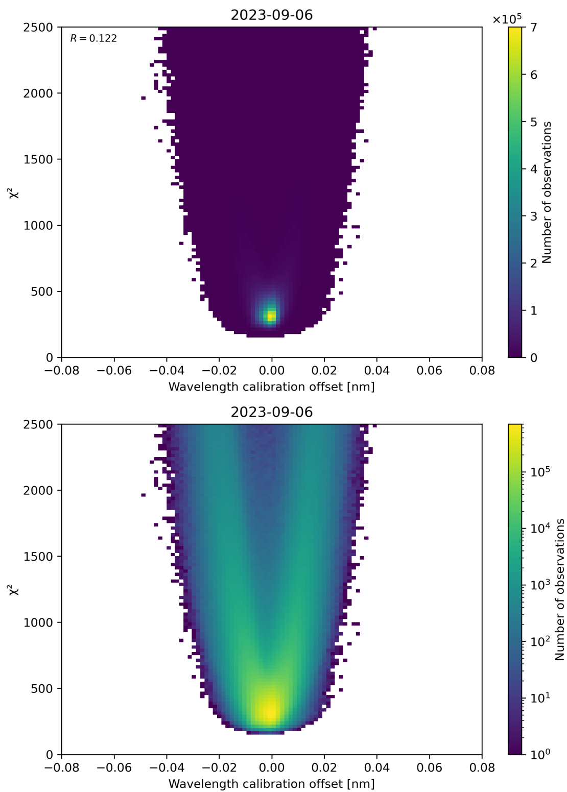
Figure 175: Scatter density plot of “Wavelength calibration offset” against “ \chi^2 ” for 2023-09-05 to 2023-09-07.
