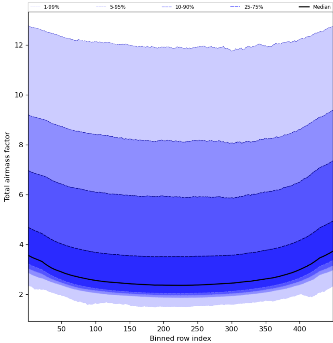
Figure 49: Along track statistics of “Total airmass factor” for 2023-09-05 to 2023-09-07
