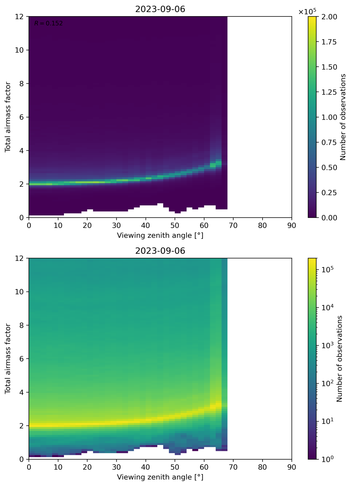
Figure 160: Scatter density plot of “Viewing zenith angle” against “Total airmass factor” for 2023-09-05 to 2023-09-07.
