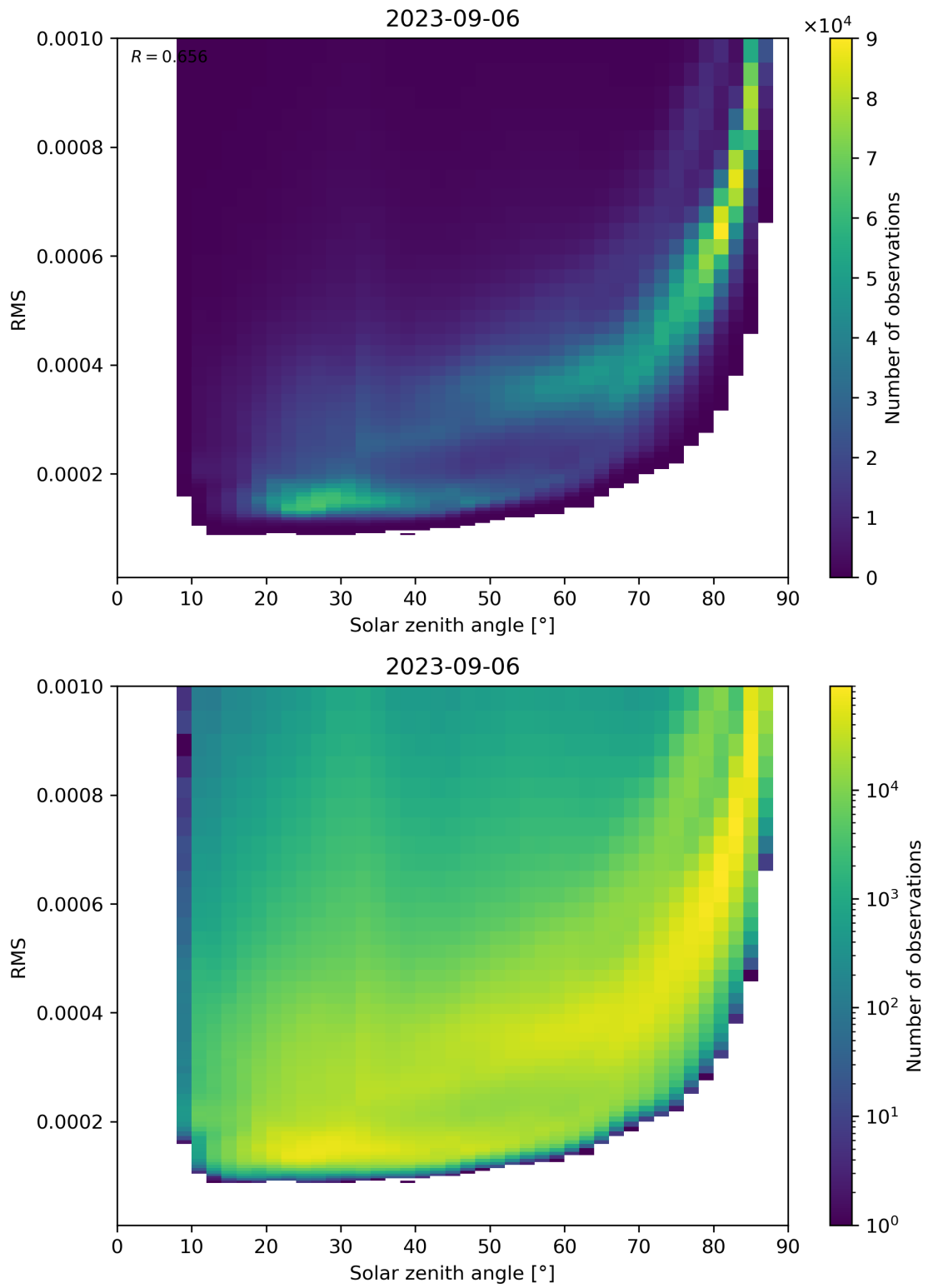
Figure 157: Scatter density plot of “Solar zenith angle” against “RMS” for 2023-09-05 to 2023-09-07.
