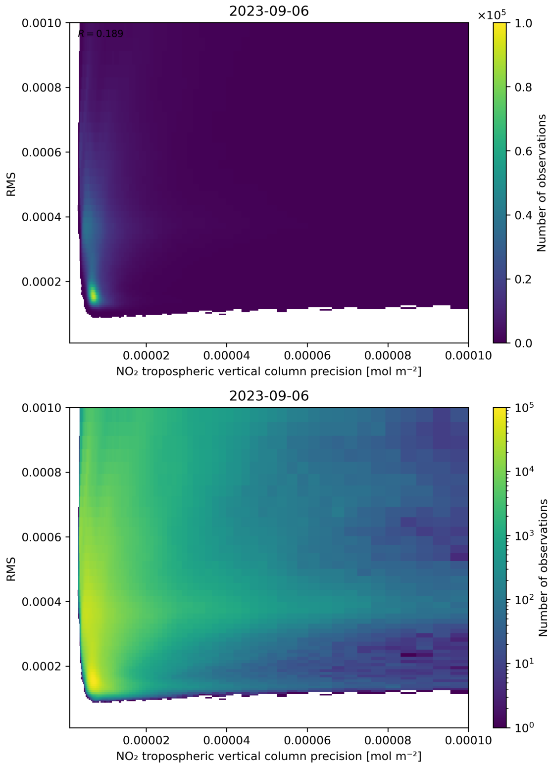
Figure 140: Scatter density plot of “NO 2 tropospheric vertical column precision” against “RMS” for 2023-09-05 to 2023-09-07.
