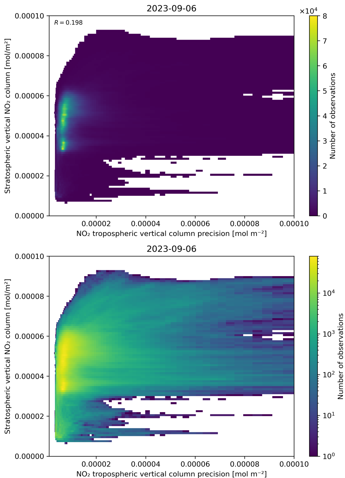
Figure 135: Scatter density plot of “NO 2 tropospheric vertical column precision” against “Stratospheric vertical NO 2 column” for 2023-09-05 to 2023-09-07.
