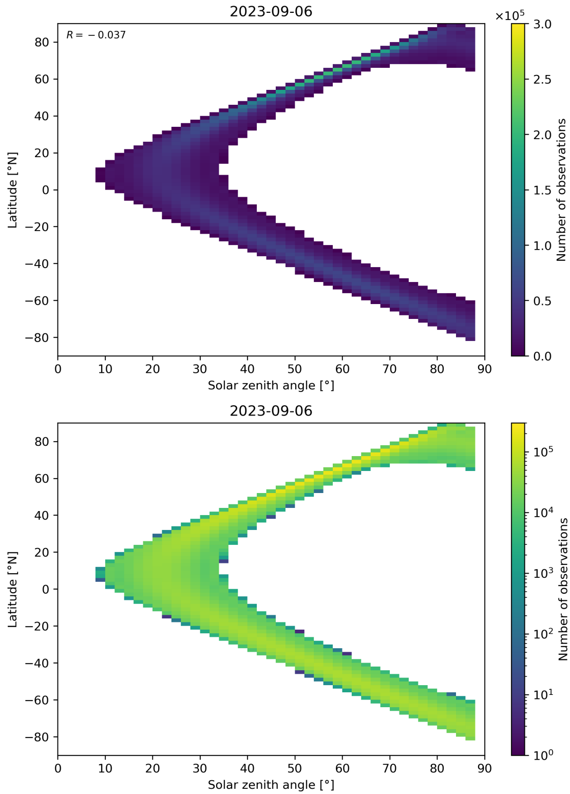
Figure 149: Scatter density plot of “Solar zenith angle” against “Latitude” for 2023-09-05 to 2023-09-07.
