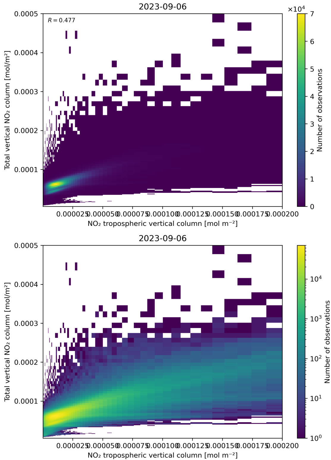
Figure 128: Scatter density plot of “NO 2 tropospheric vertical column” against “Total vertical NO 2 column” for 2023-09-05 to 2023-09-07.
