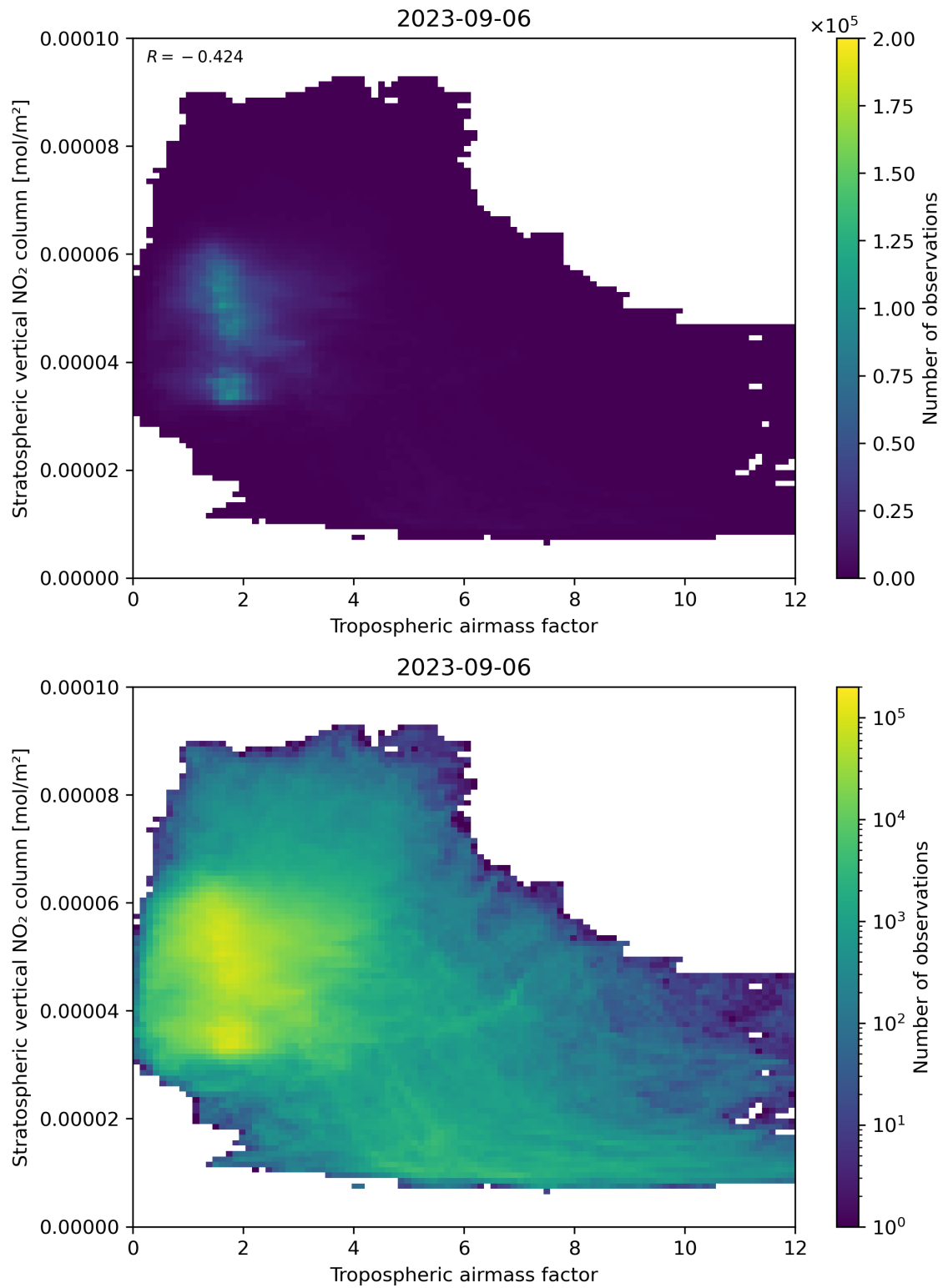
Figure 74: Scatter density plot of “Tropospheric air mass factor” against “Stratospheric vertical NO 2 column” for 2023-09-05 to 2023-09-07.
