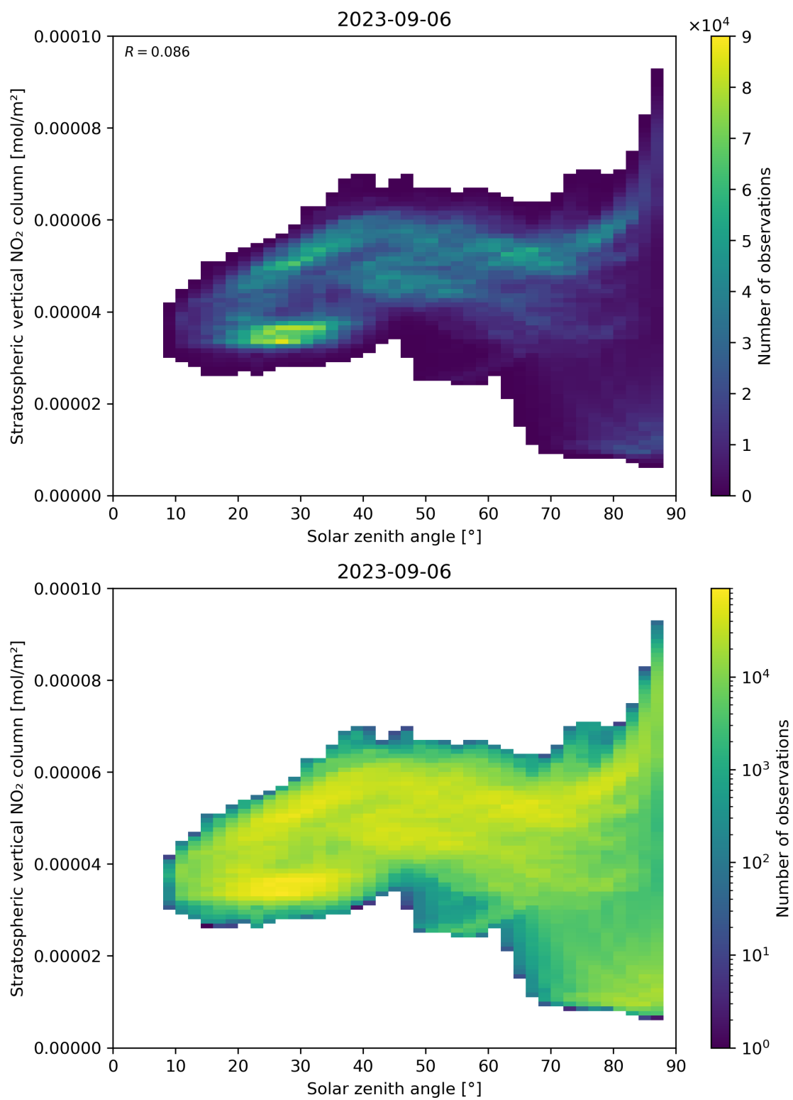
Figure 150: Scatter density plot of “Solar zenith angle” against “Stratospheric vertical NO 2 column” for 2023-09-05 to 2023-09-07.
