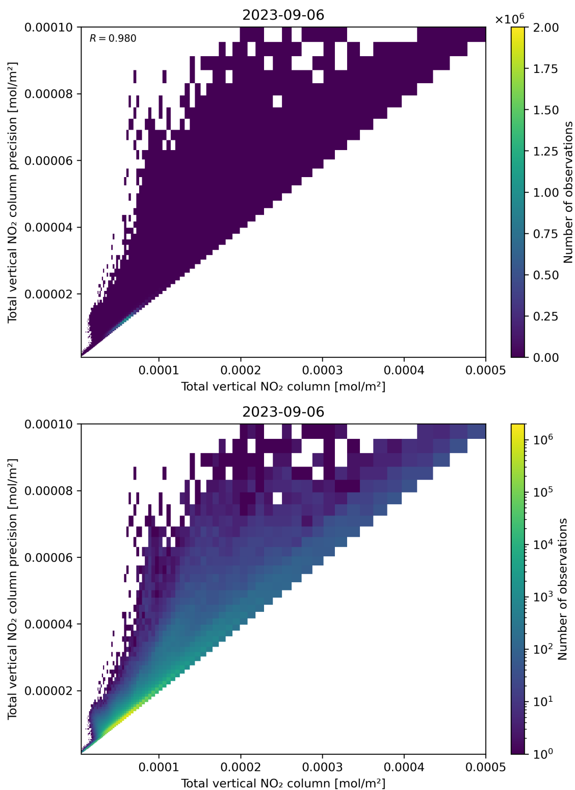
Figure 114: Scatter density plot of “Total vertical NO 2 column” against “Total vertical NO 2 column precision” for 2023-09-05 to 2023-09-07.
