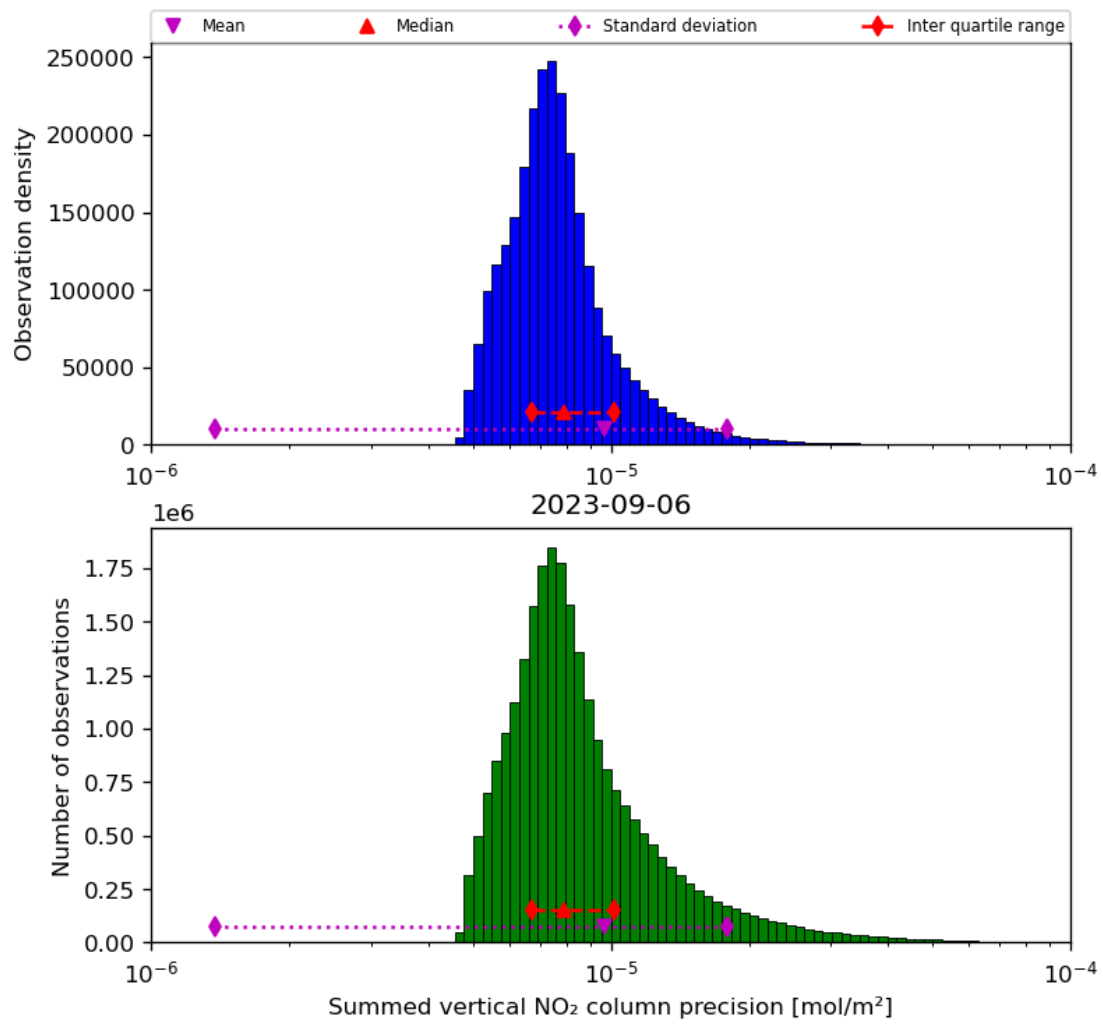
Figure 41: Histogram of "Summed vertical NO 2 column precision" for 2023-09-05 to 2023-09-07
