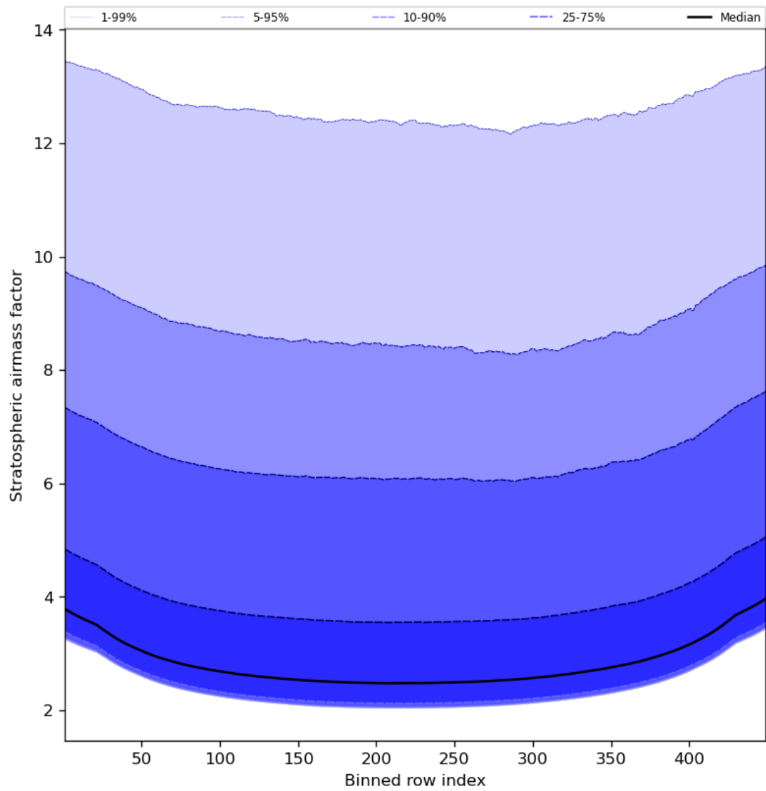
Figure 61: Along track statistics of “Stratospheric airmass factor” for 2023-09-06 to 2023-09-08
