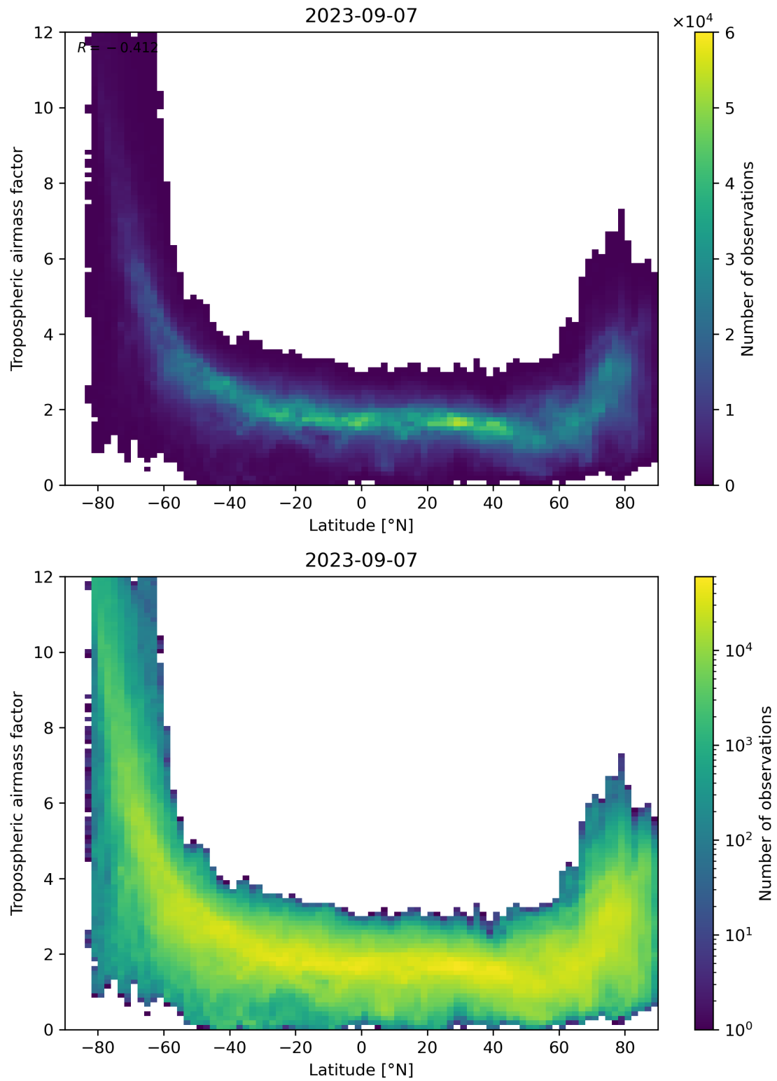
Figure 85: Scatter density plot of “Latitude” against “Tropospheric airmass factor” for 2023-09-06 to 2023-09-08.
