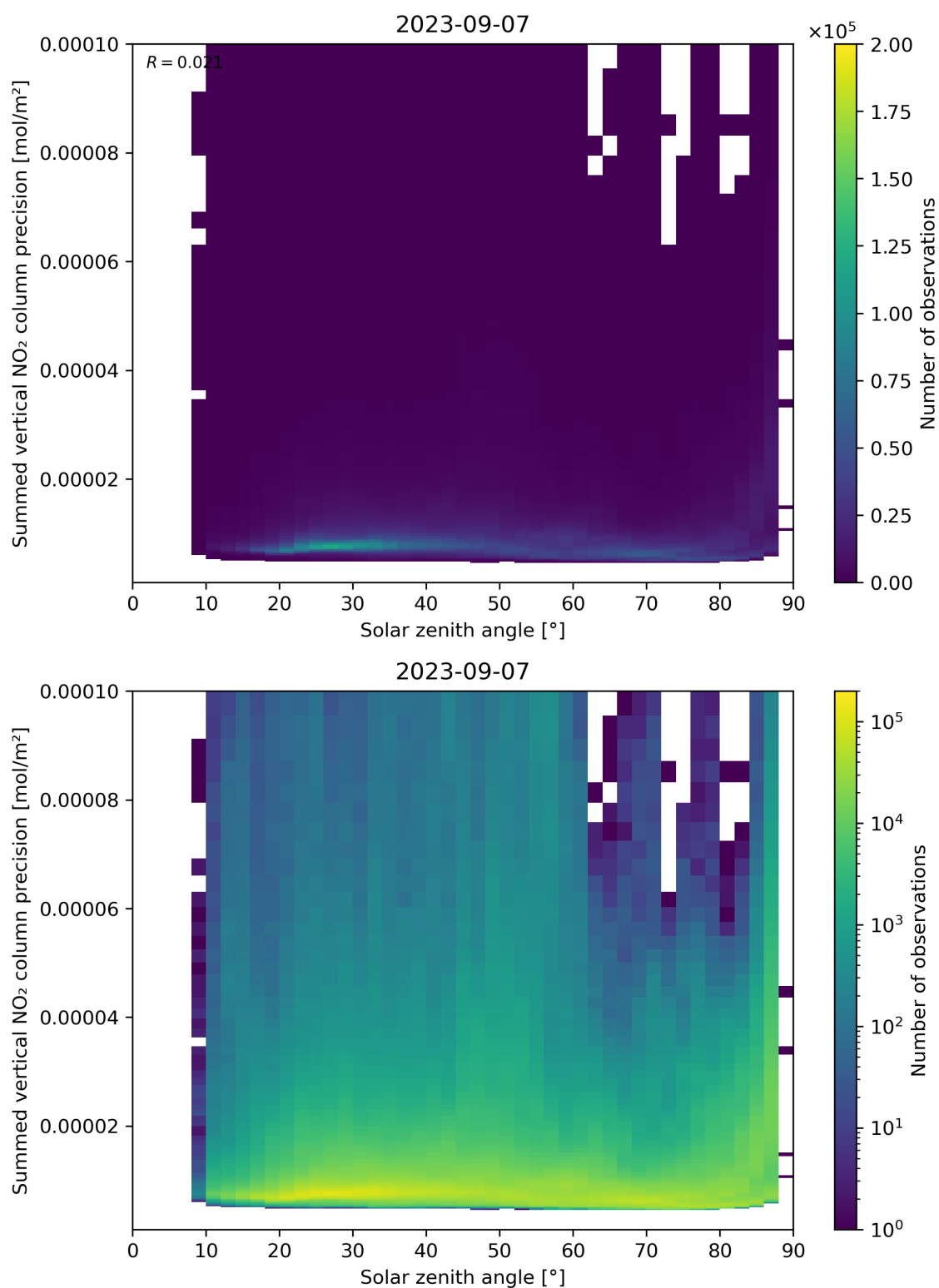
Figure 152: Scatter density plot of “Solar zenith angle” against “Summed vertical NO 2 column precision” for 2023-09-06 to 2023-09-08.
