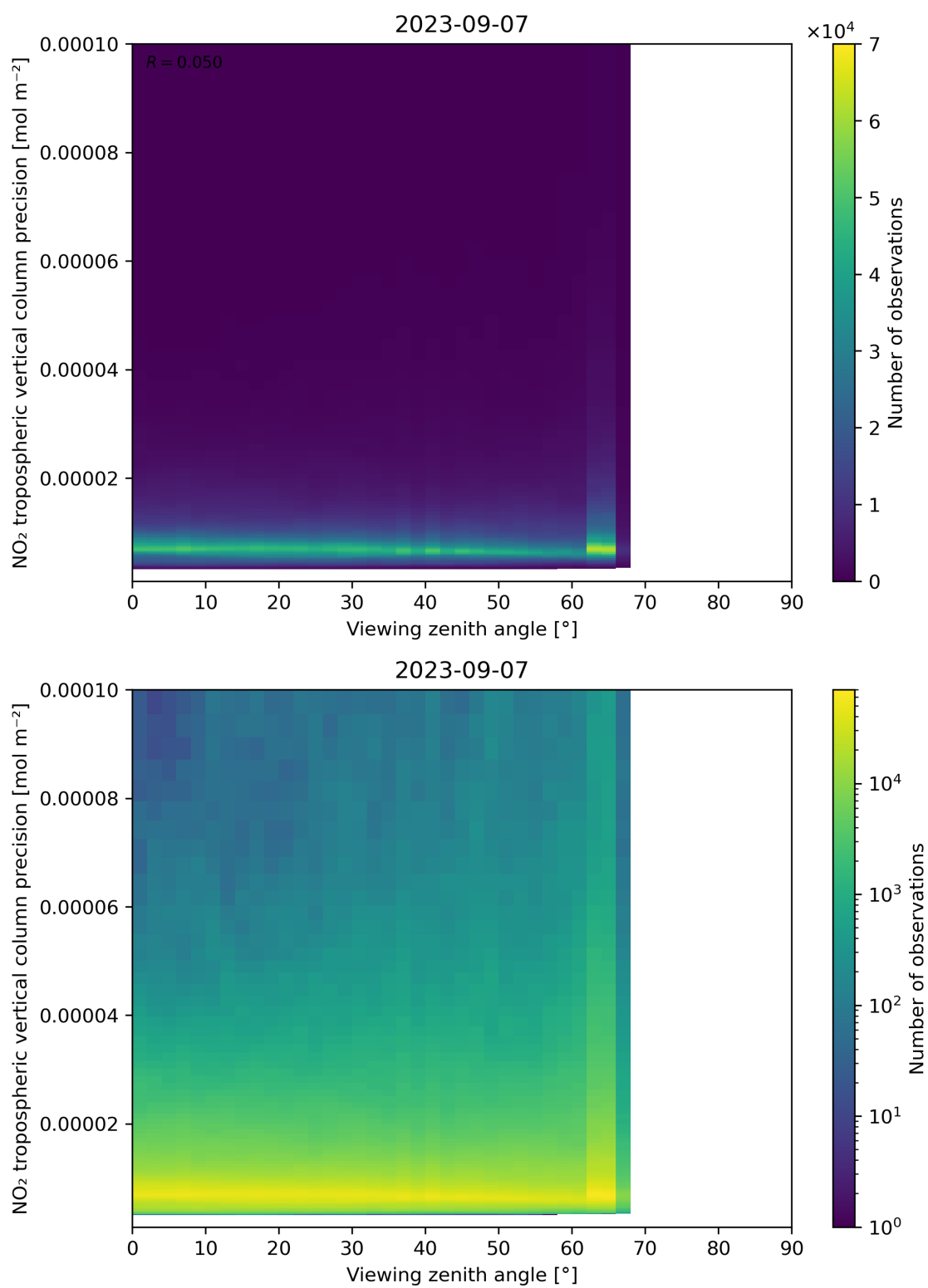
Figure 170: Scatter density plot of “Viewing zenith angle” against “NO 2 tropospheric vertical column precision” for 2023-09-06 to 2023-09-08.
