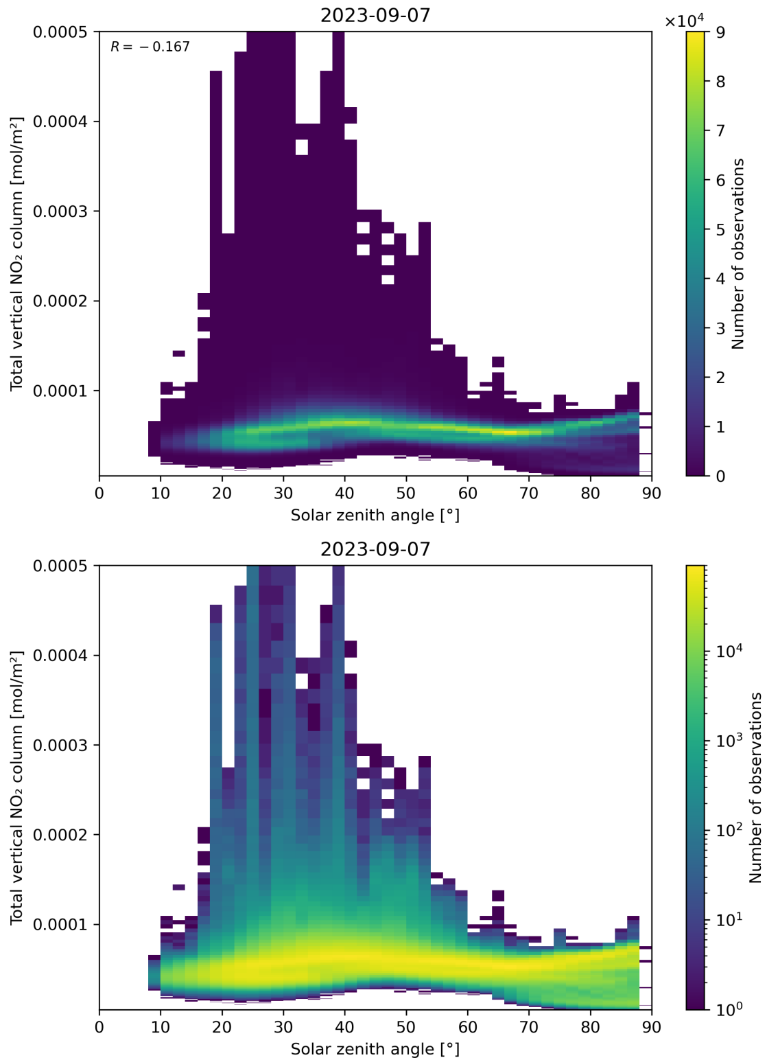
Figure 153: Scatter density plot of “Solar zenith angle” against “Total vertical NO 2 column” for 2023-09-06 to 2023-09-08.
