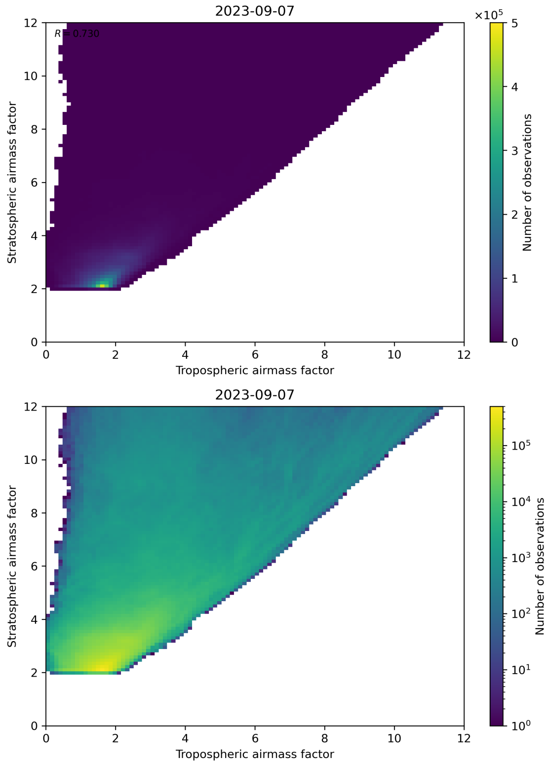
Figure 71: Scatter density plot of “Tropospheric airmass factor” against “Stratospheric airmass factor” for 2023-09-06 to 2023-09-08.
