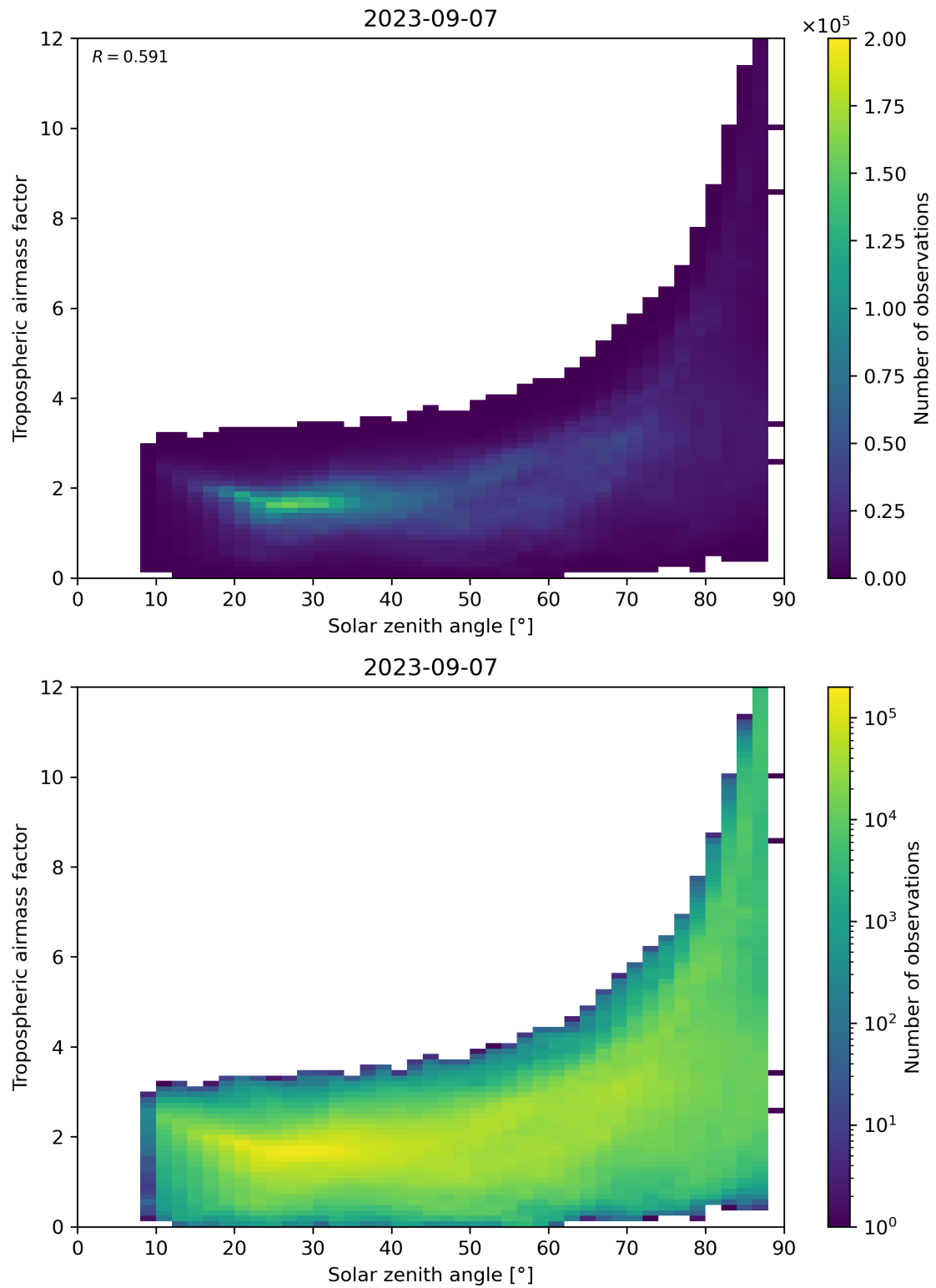
Figure 147: Scatter density plot of “Solar zenith angle” against “Tropospheric airmass factor” for 2023-09-06 to 2023-09-08.
