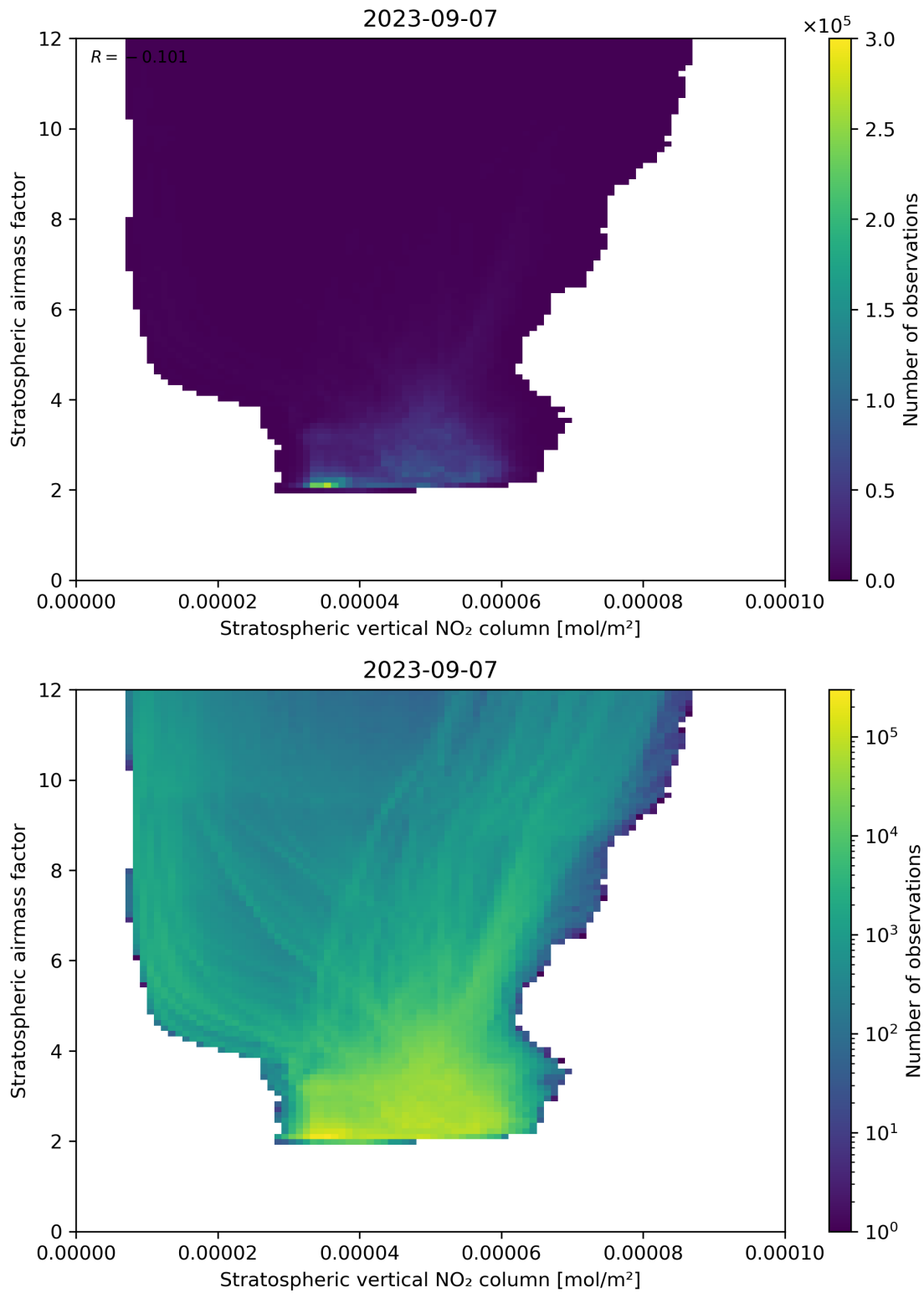
Figure 96: Scatter density plot of “Stratospheric vertical NO 2 column” against “Stratospheric airmass factor” for 2023-09-06 to 2023-09-08.
