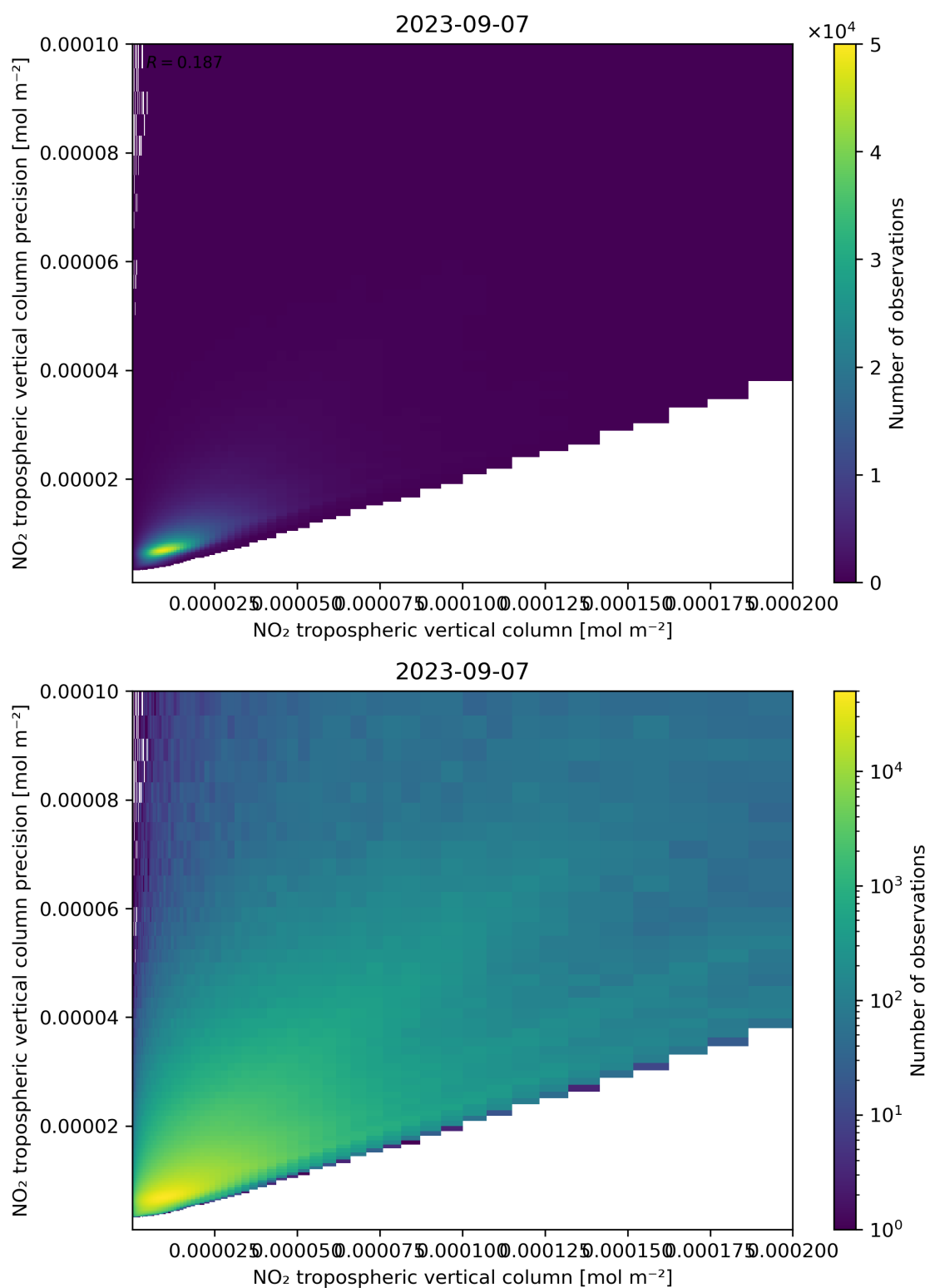
Figure 130: Scatter density plot of “NO 2 tropospheric vertical column” against “NO 2 tropospheric vertical column precision” for 2023-09-06 to 2023-09-08.
