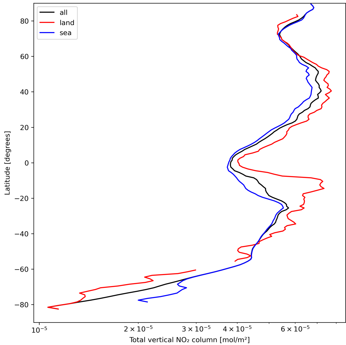
Figure 21: Zonal average of “Total vertical NO 2 column” for 2023-09-06 to 2023-09-08.
