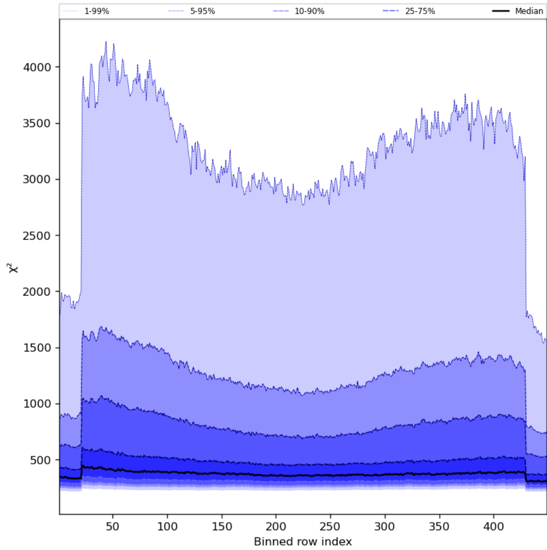
Figure 59: Along track statistics of “ \chi^2 ” for 2023-09-06 to 2023-09-08
