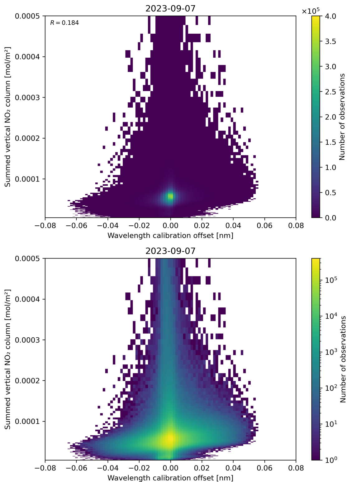
Figure 177: Scatter density plot of “Wavelength calibration offset” against “Summed vertical NO 2 column” for 2023-09-06 to 2023-09-08.
