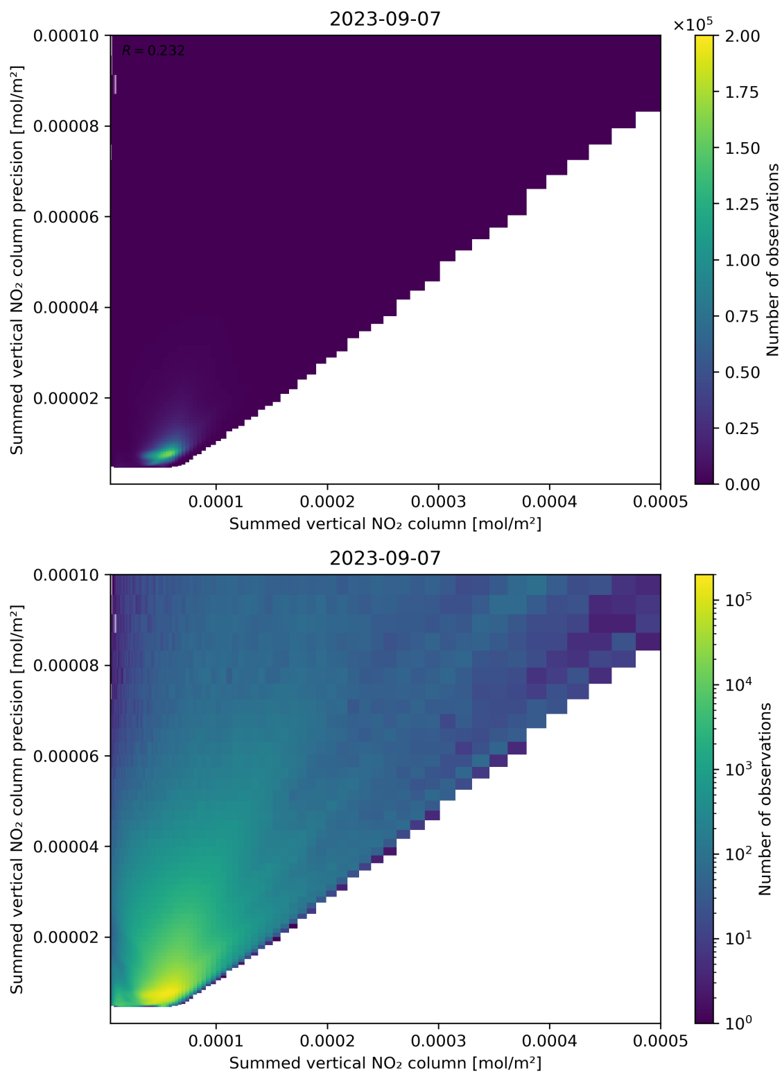
Figure 105: Scatter density plot of “Summed vertical NO 2 column” against “Summed vertical NO 2 column precision” for 2023-09-06 to 2023-09-08.
