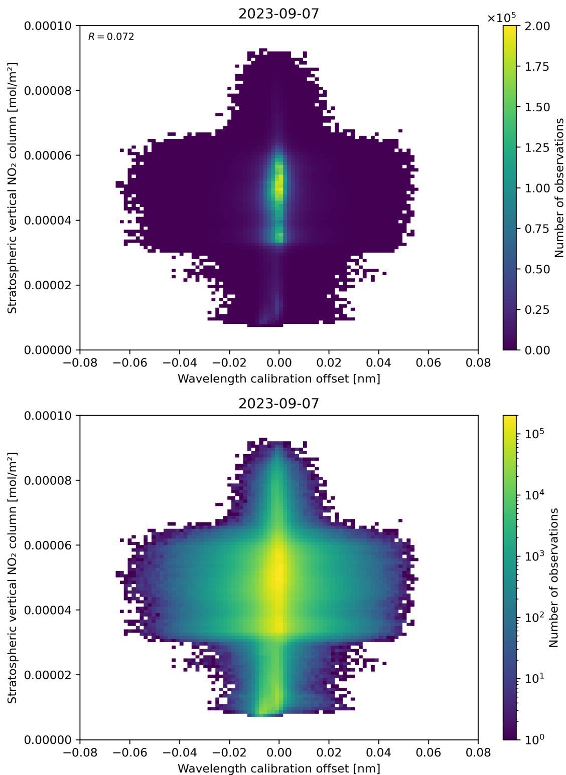
Figure 176: Scatter density plot of “Wavelength calibration offset” against “Stratospheric vertical NO 2 column” for 2023-09-06 to 2023-09-08.
