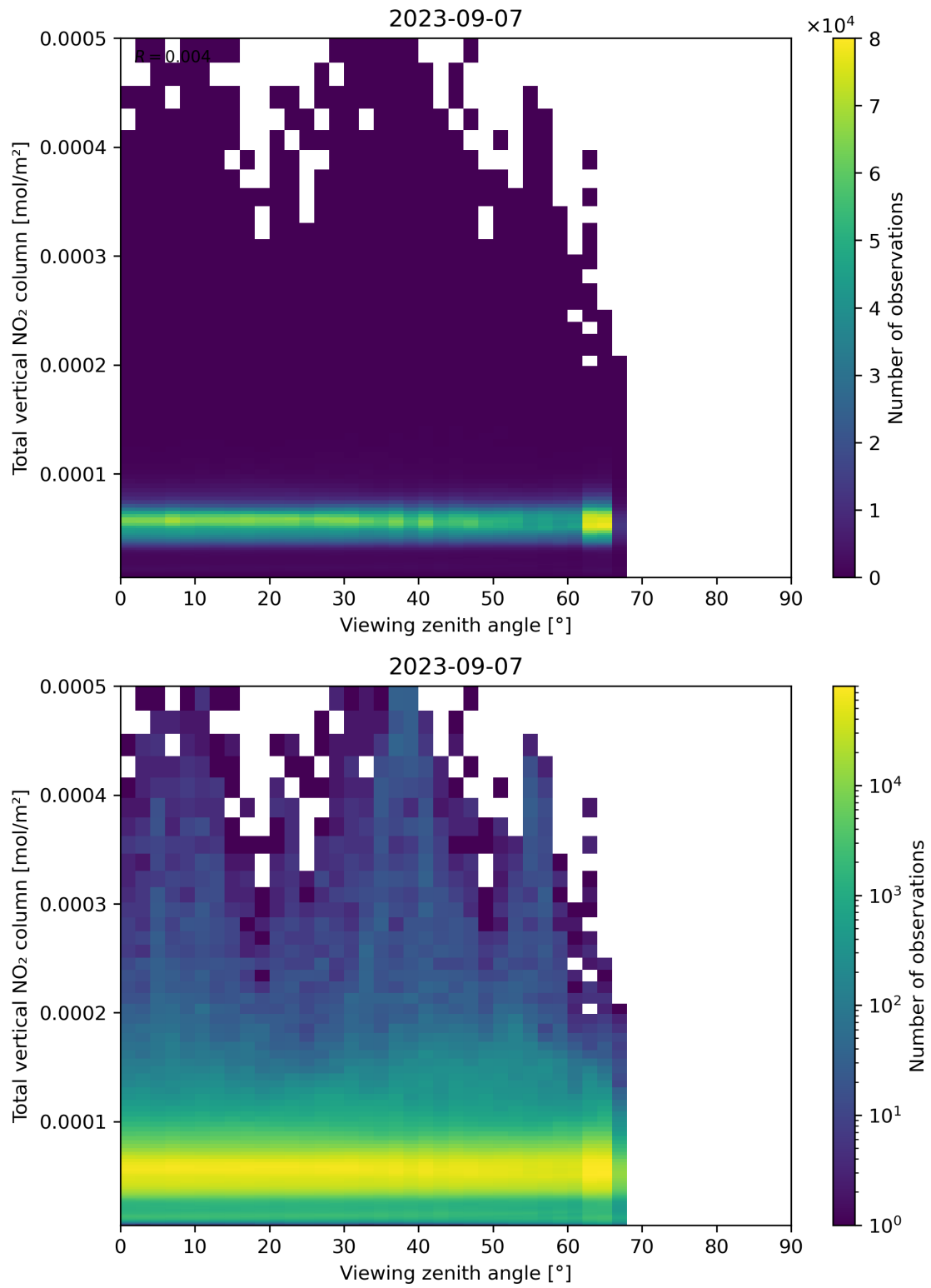
Figure 167: Scatter density plot of “Viewing zenith angle” against “Total vertical NO 2 column” for 2023-09-06 to 2023-09-08.
