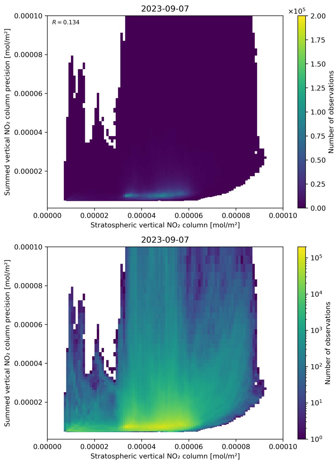
Figure 99: Scatter density plot of “Stratospheric vertical NO 2 column” against “Summed vertical NO 2 column precision” for 2023-09-06 to 2023-09-08.
