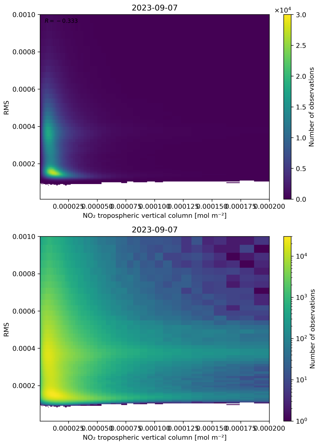
Figure 142: Scatter density plot of “NO 2 tropospheric vertical column” against “RMS” for 2023-09-06 to 2023-09-08.
