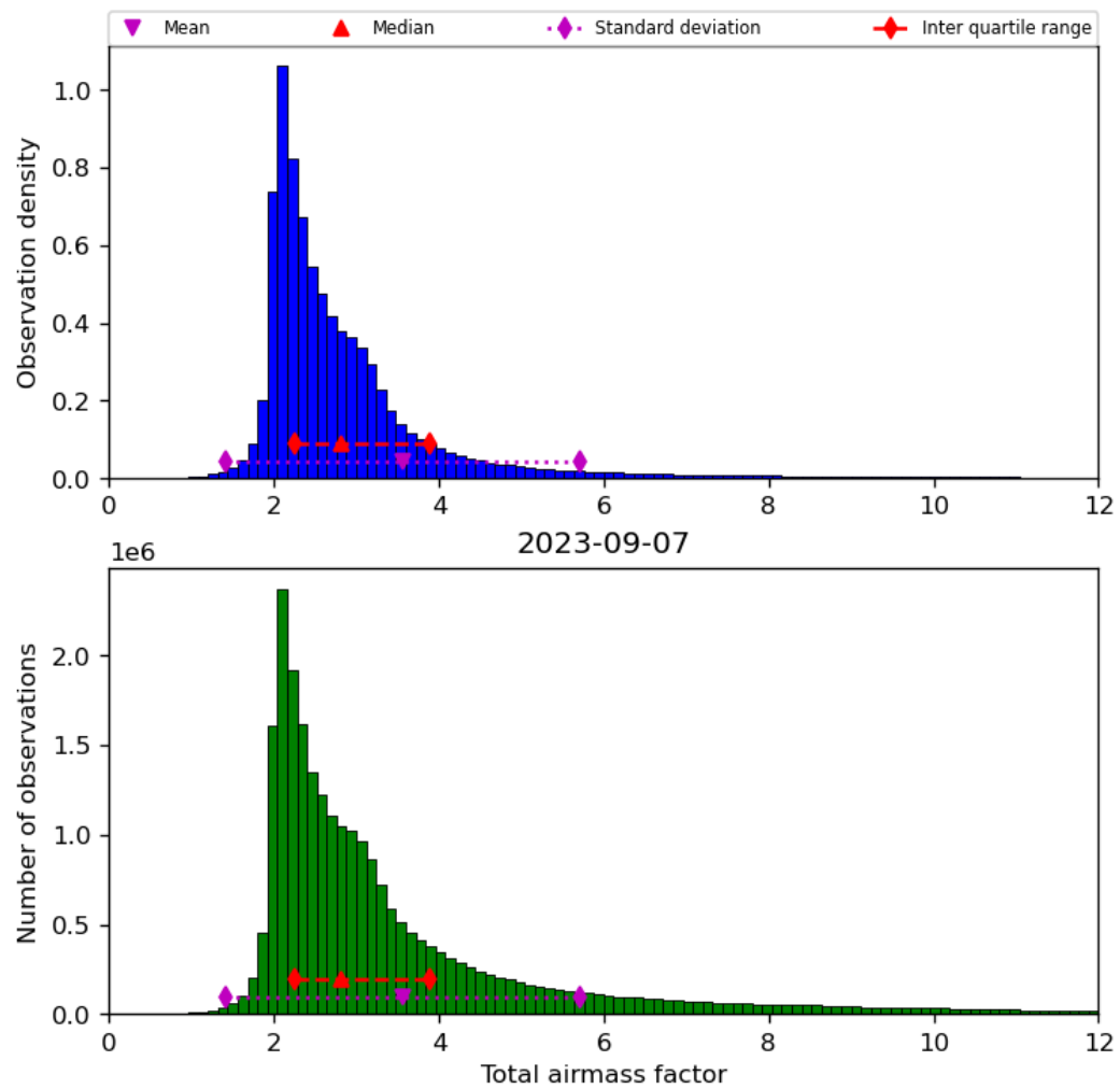
Figure 32: Histogram of “Total airmass factor” for 2023-09-06 to 2023-09-08
