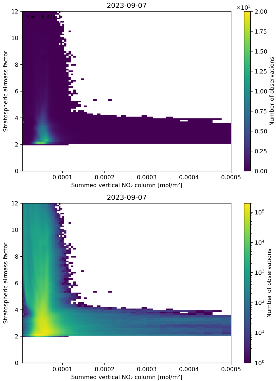
Figure 103: Scatter density plot of “Summed vertical NO 2 column” against “Stratospheric airmass factor” for 2023-09-06 to 2023-09-08.
