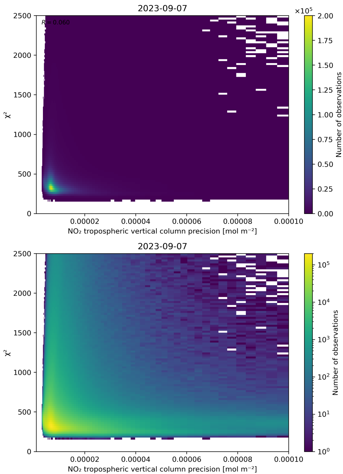
Figure 134: Scatter density plot of “NO 2 tropospheric vertical column precision” against “ \chi^2 ” for 2023-09-06 to 2023-09-08.
