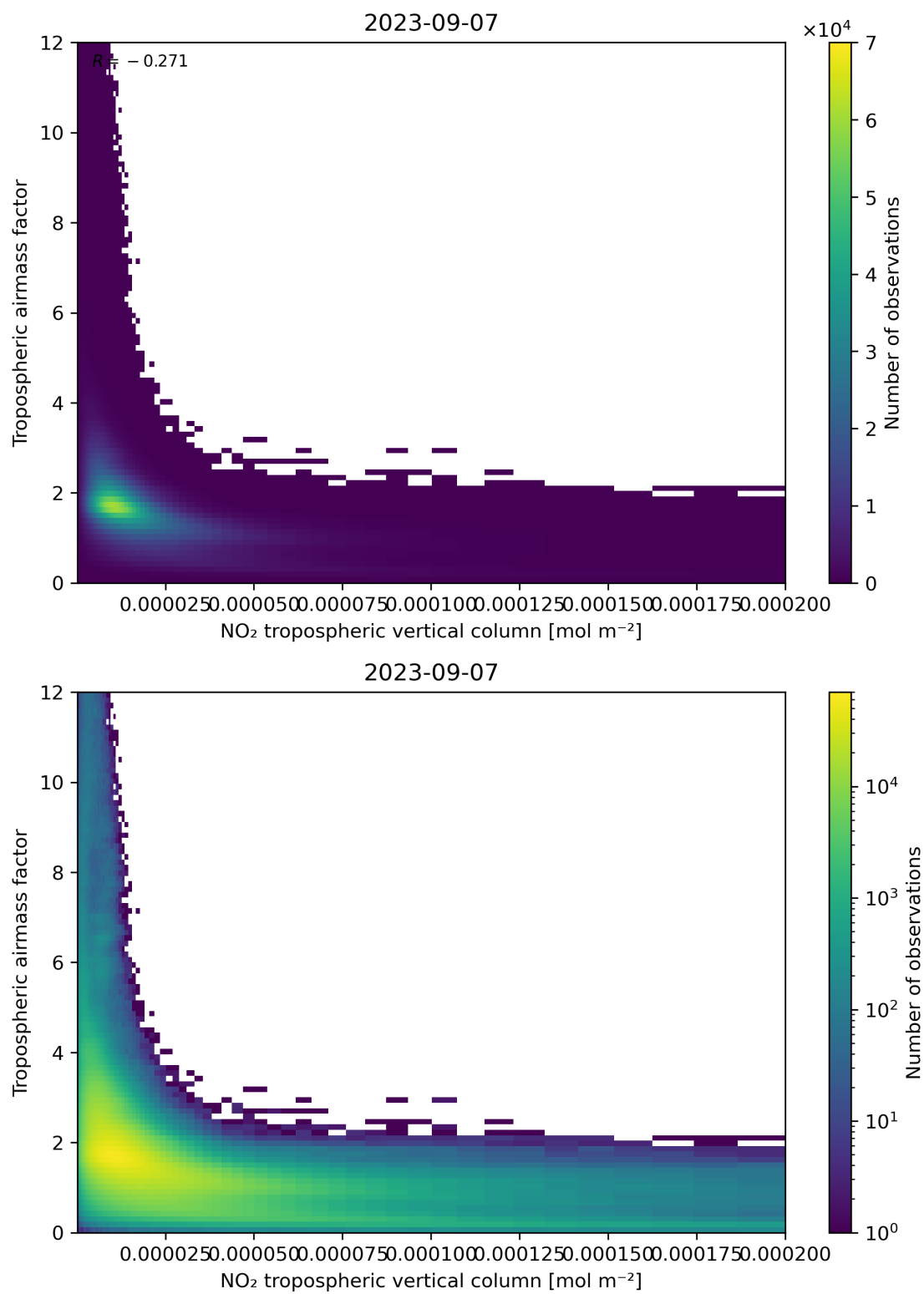
Figure 123: Scatter density plot of “NO 2 tropospheric vertical column” against “Tropospheric air mass factor” for 2023-09-06 to 2023-09-08.
