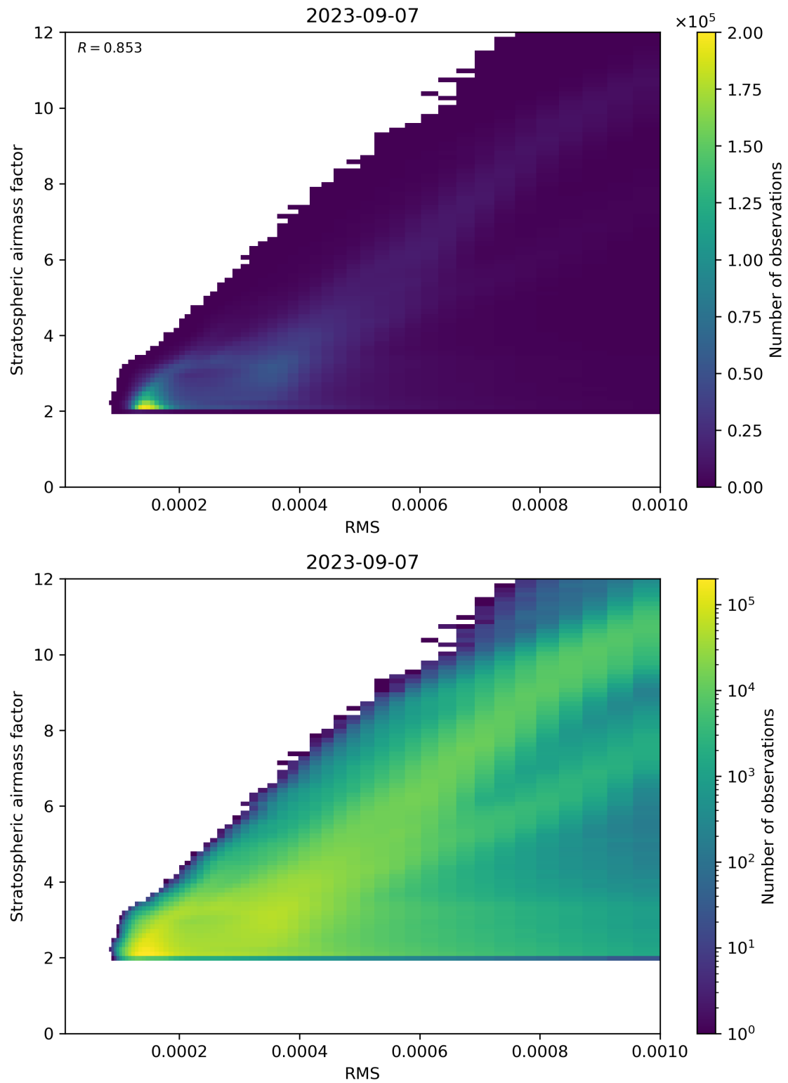
Figure 144: Scatter density plot of “RMS” against “Stratospheric airmass factor” for 2023-09-06 to 2023-09-08.
