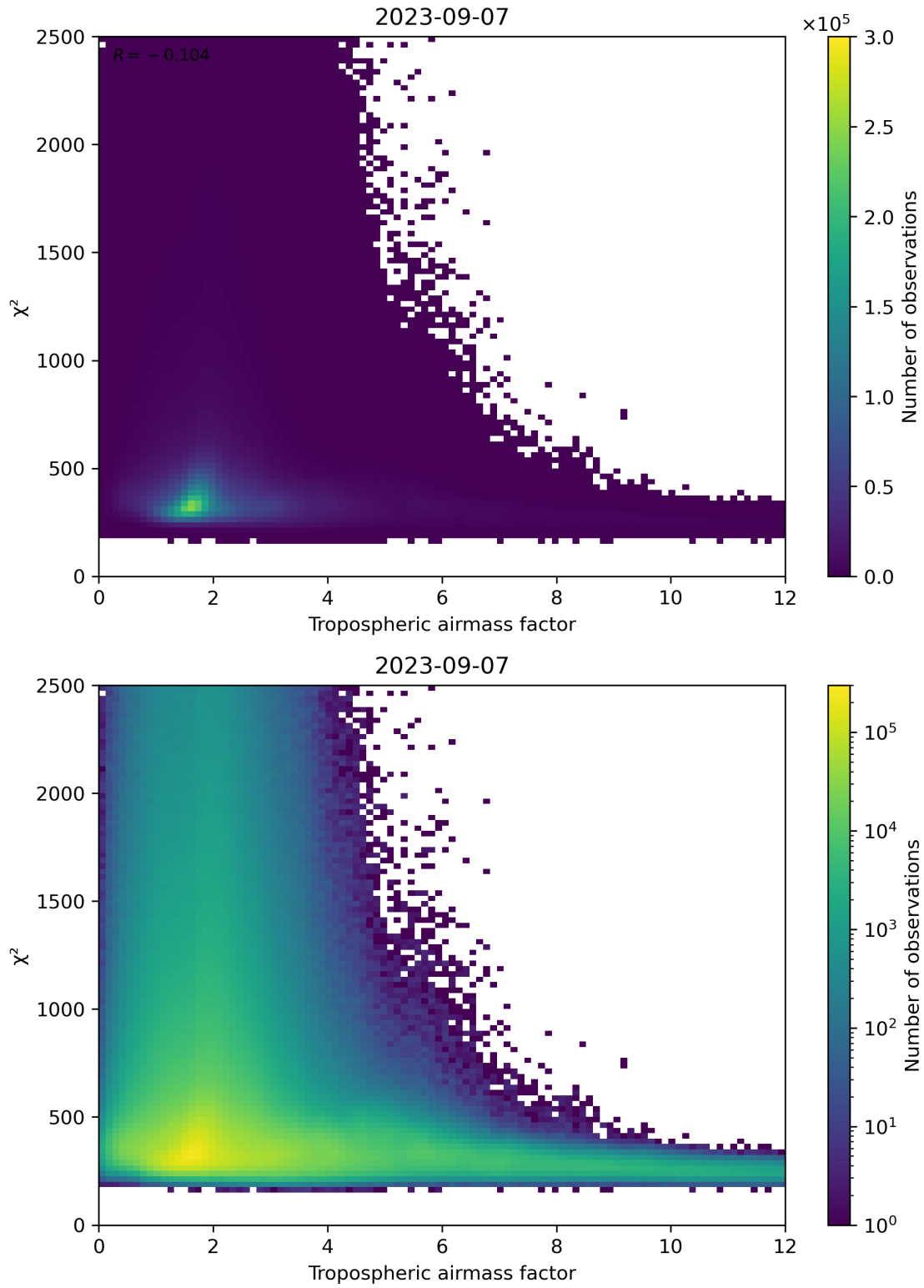
Figure 73: Scatter density plot of “Tropospheric airmass factor” against “ \chi^2 ” for 2023-09-06 to 2023-09-08.
