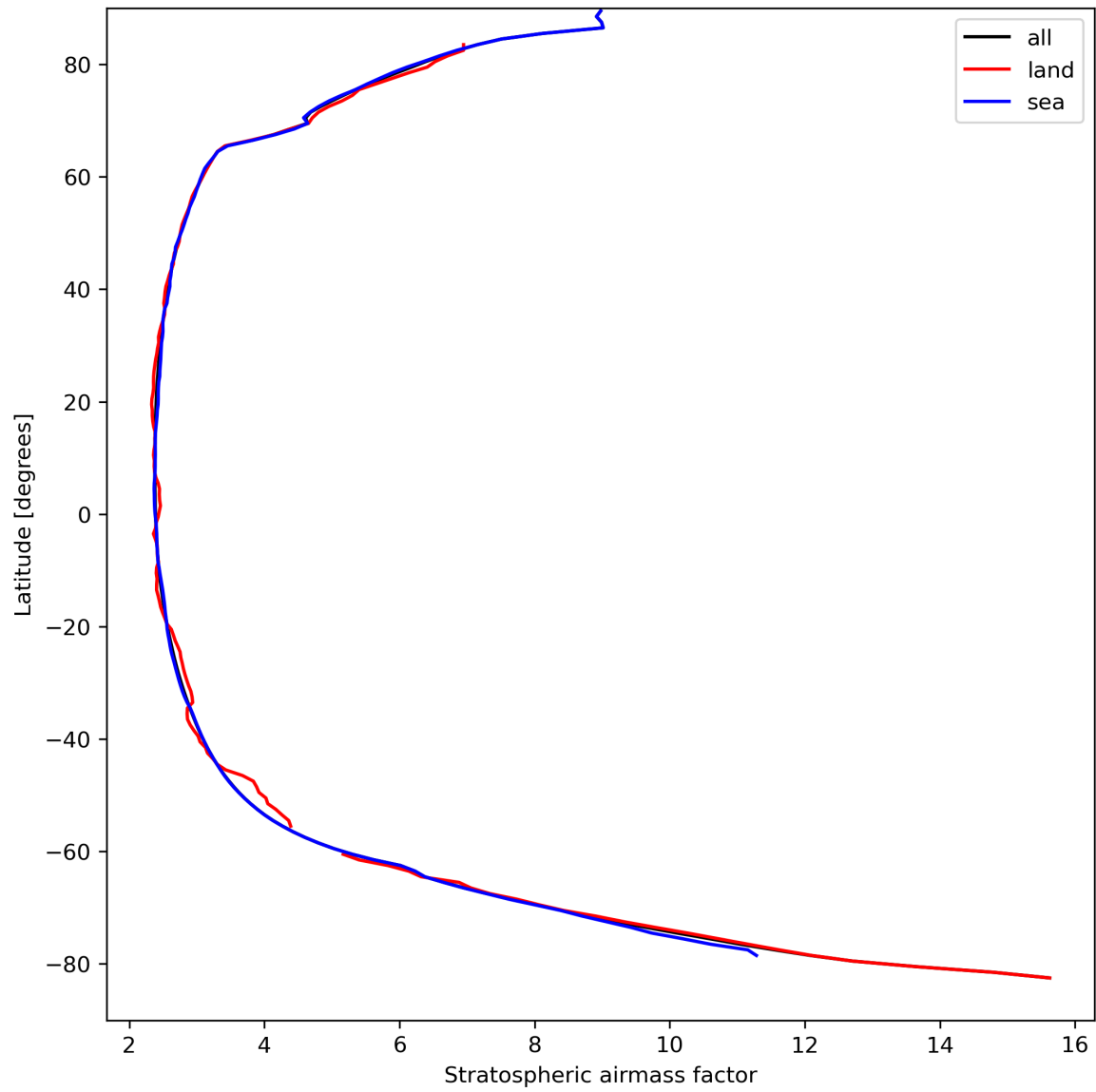
Figure 27: Zonal average of “Stratospheric air mass factor” for 2023-09-06 to 2023-09-08.
