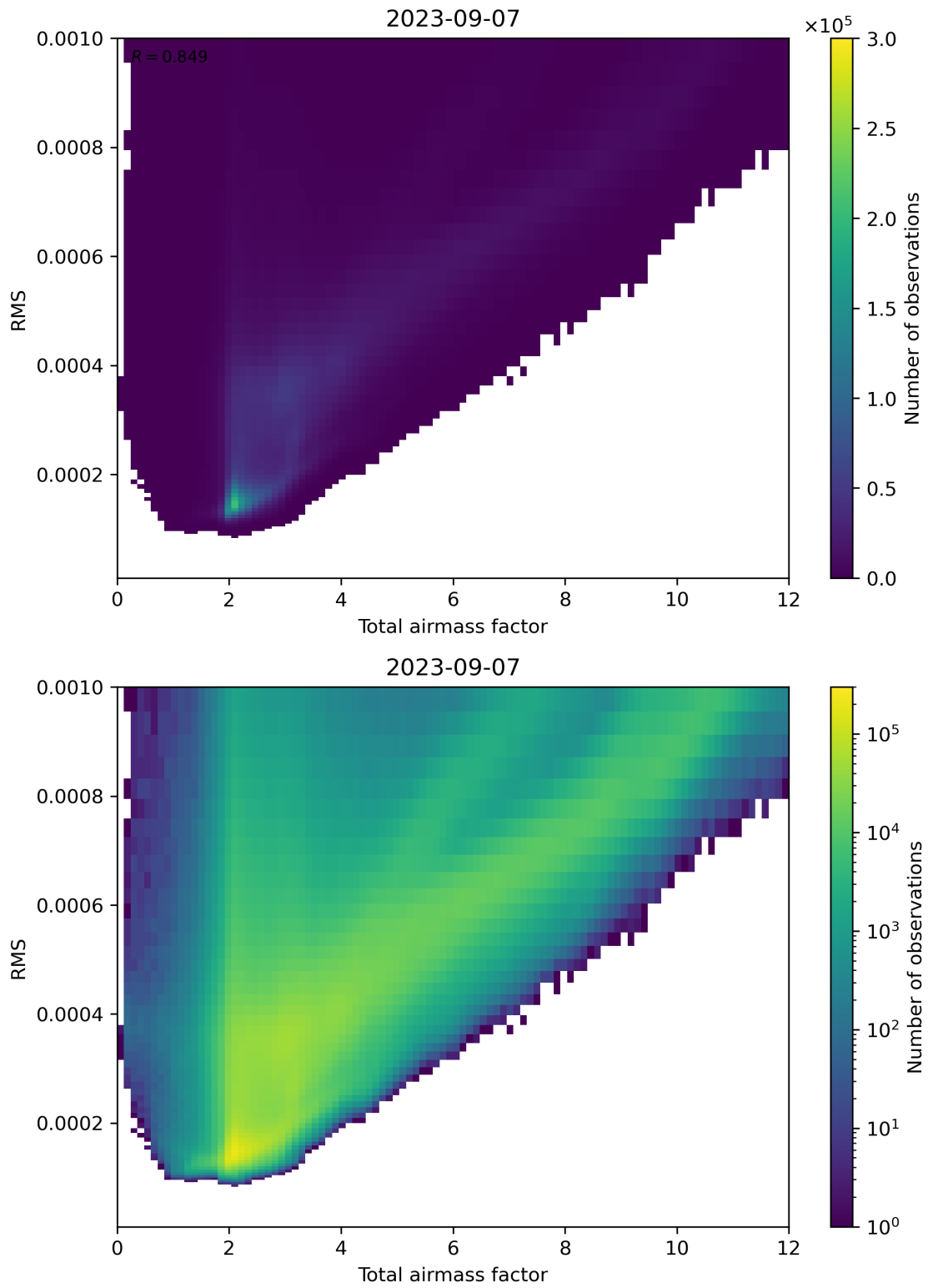
Figure 69: Scatter density plot of “Total airmass factor” against “RMS” for 2023-09-06 to 2023-09-08.
