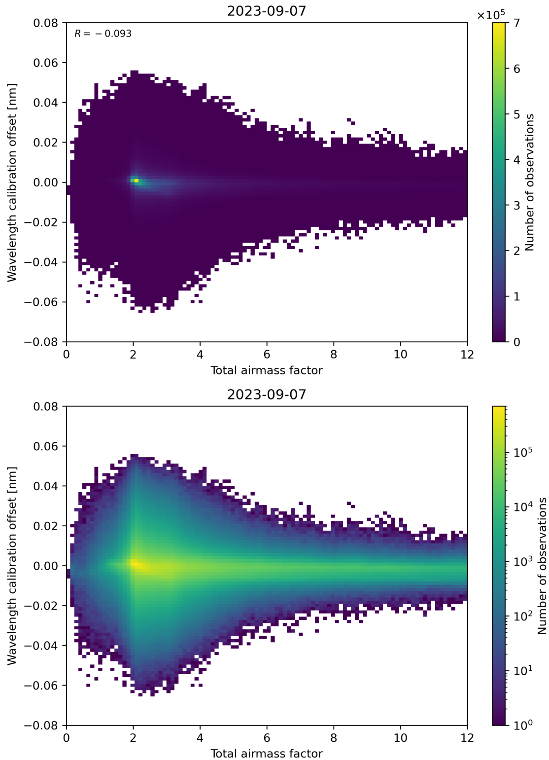
Figure 70: Scatter density plot of “Total airmass factor” against “Wavelength calibration offset” for 2023-09-06 to 2023-09-08.
