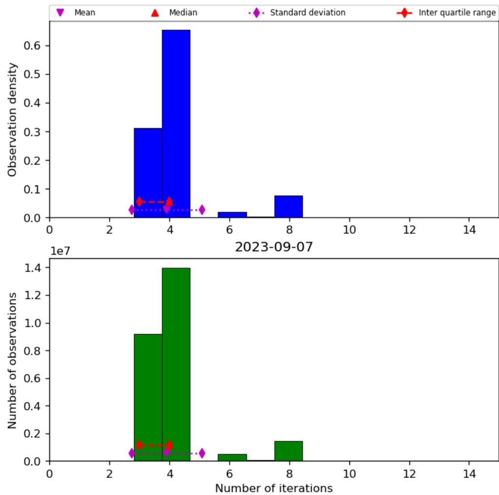
Figure 34: Histogram of “Number of iterations” for 2023-09-06 to 2023-09-08
