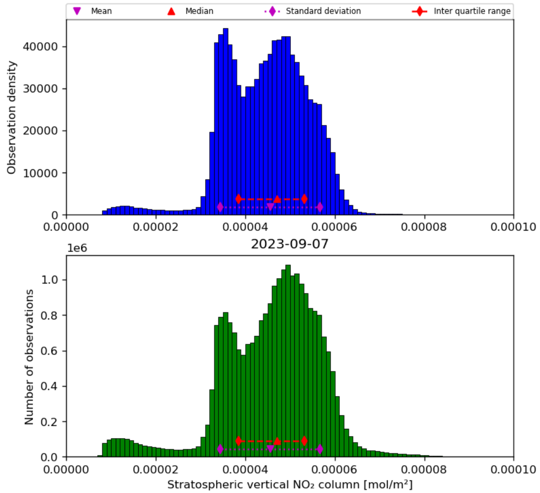
Figure 36: Histogram of “Stratospheric vertical NO 2 column” for 2023-09-06 to 2023-09-08
