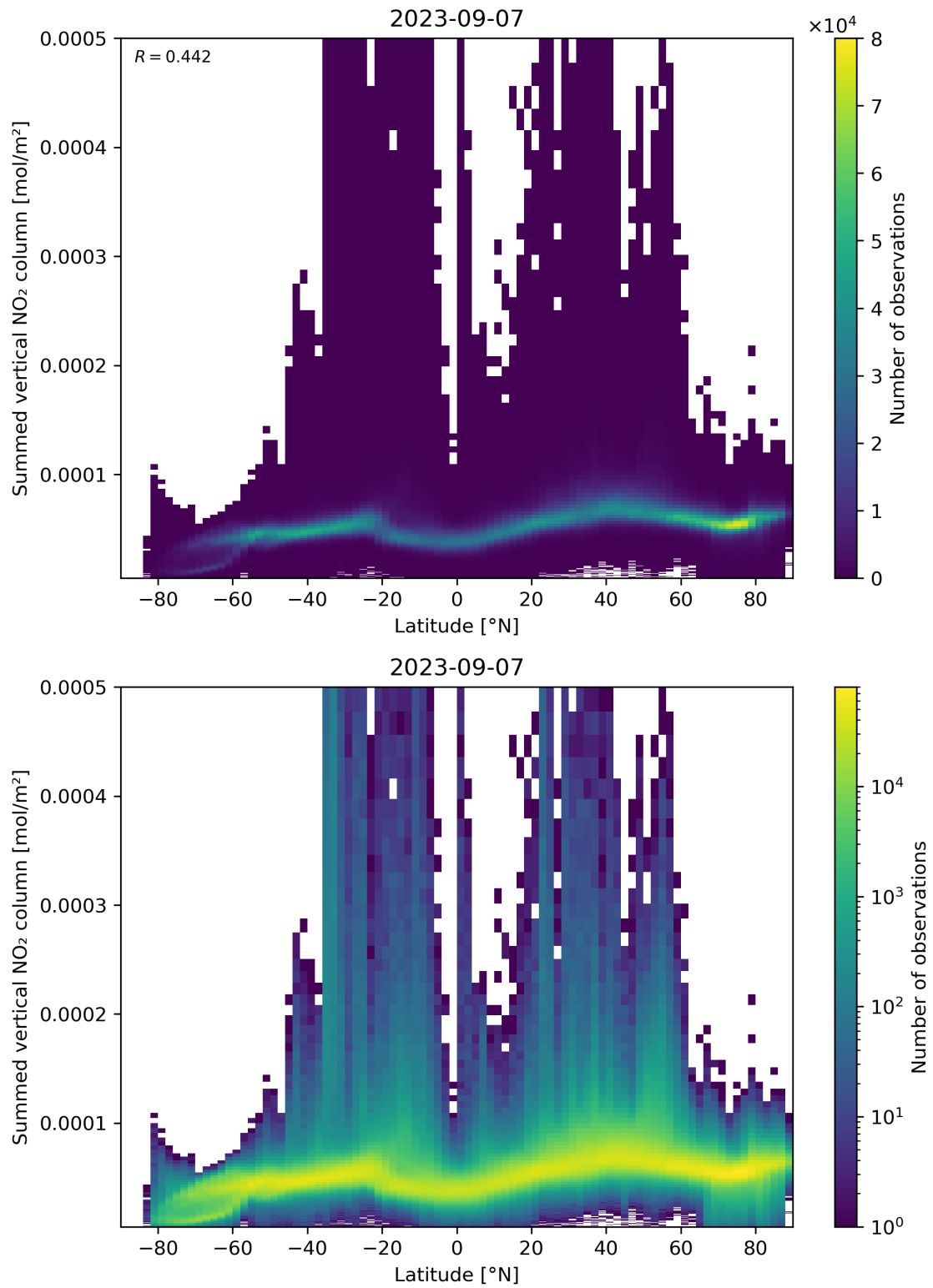
Figure 88: Scatter density plot of “Latitude” against “Summed vertical NO 2 column” for 2023-09-06 to 2023-09-08.
