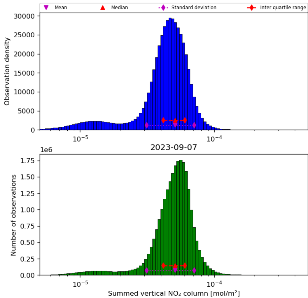
Figure 40: Histogram of “Summed vertical NO 2 column” for 2023-09-06 to 2023-09-08
