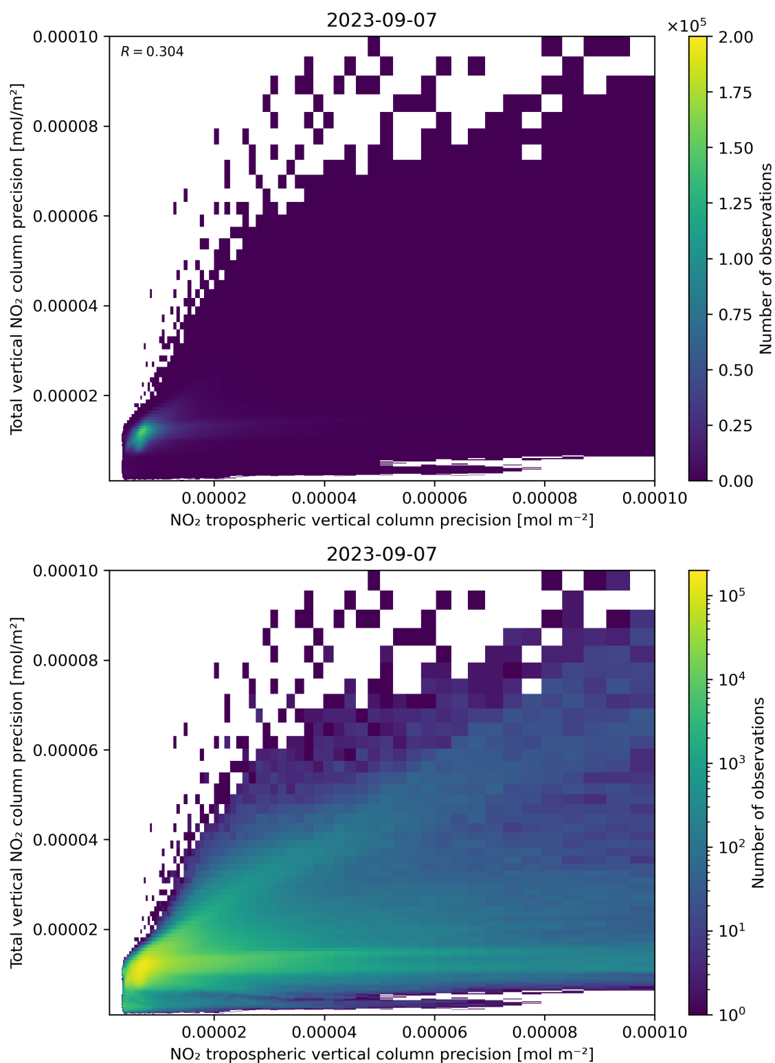
Figure 139: Scatter density plot of “NO 2 tropospheric vertical column precision” against “Total vertical NO 2 column precision” for 2023-09-06 to 2023-09-08.
