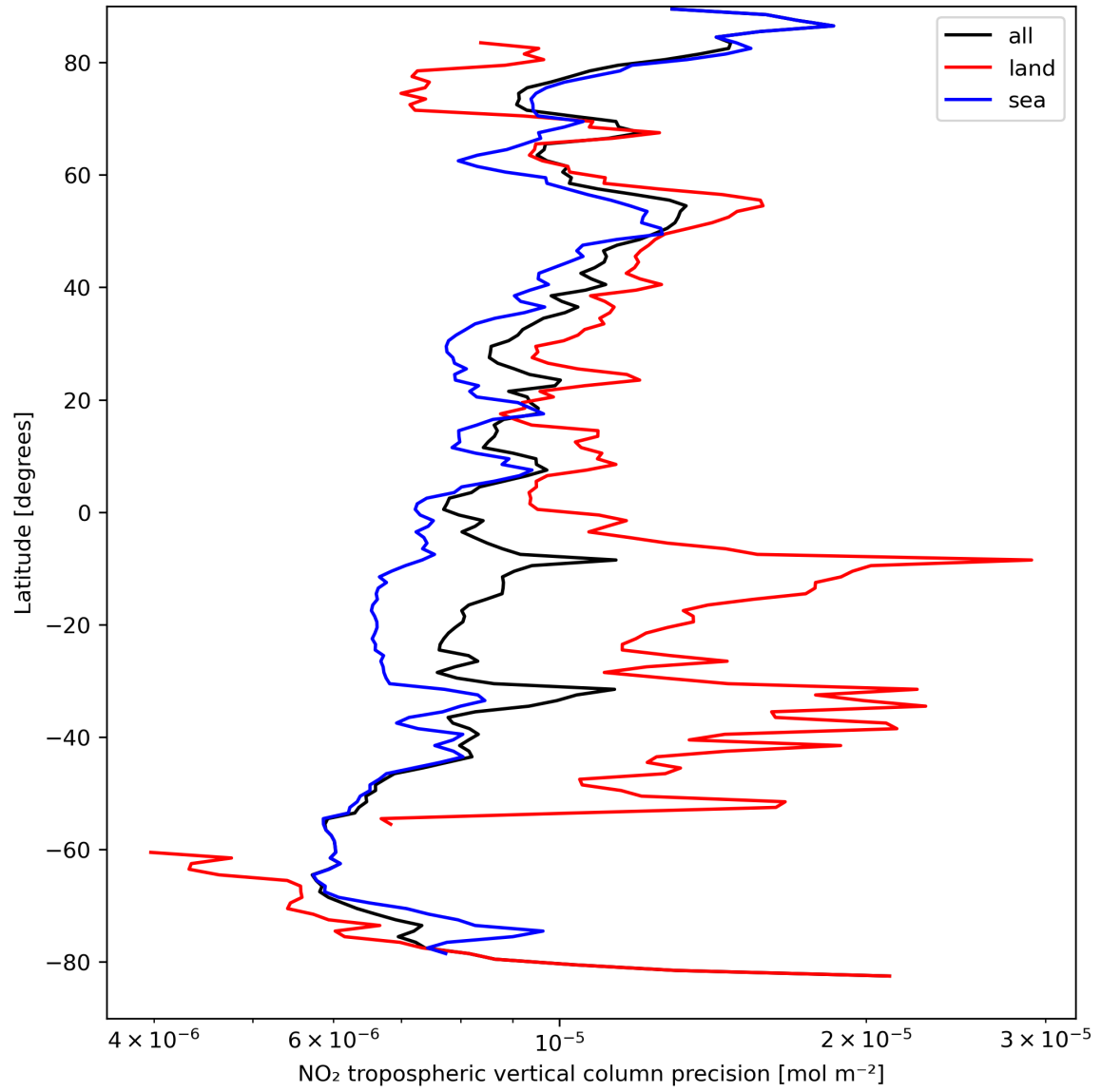
Figure 13: Zonal average of “NO 2 tropospheric vertical column precision” for 2023-09-06 to 2023-09-08.
