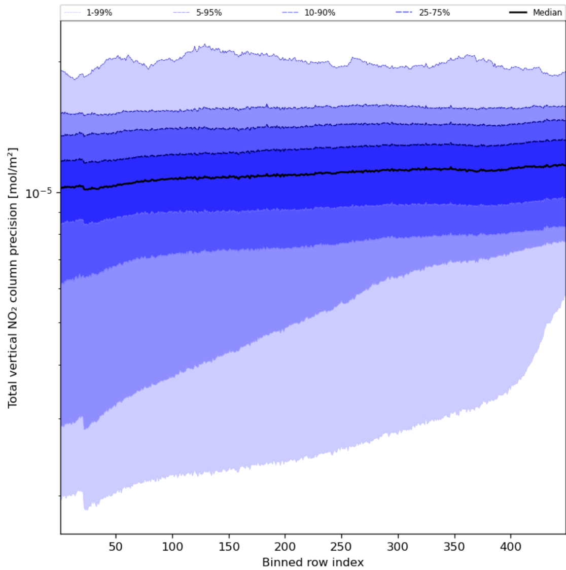
Figure 56: Along track statistics of “Total vertical NO 2 column precision” for 2023-09-06 to 2023-09-08
