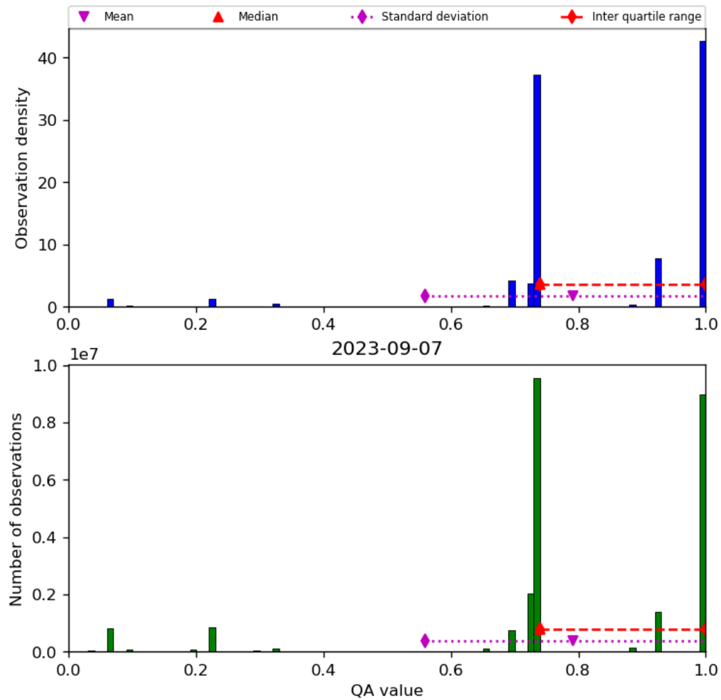
Figure 28: Histogram of “QA value” for 2023-09-06 to 2023-09-08
