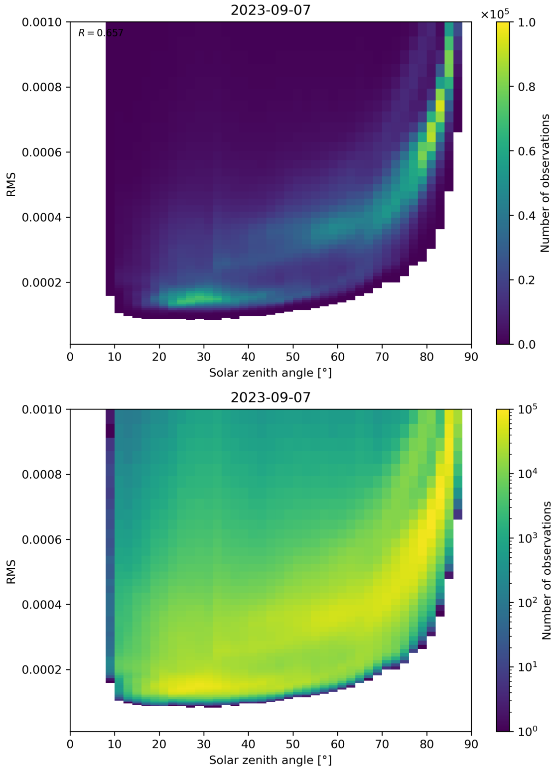
Figure 157: Scatter density plot of “Solar zenith angle” against “RMS” for 2023-09-06 to 2023-09-08.
