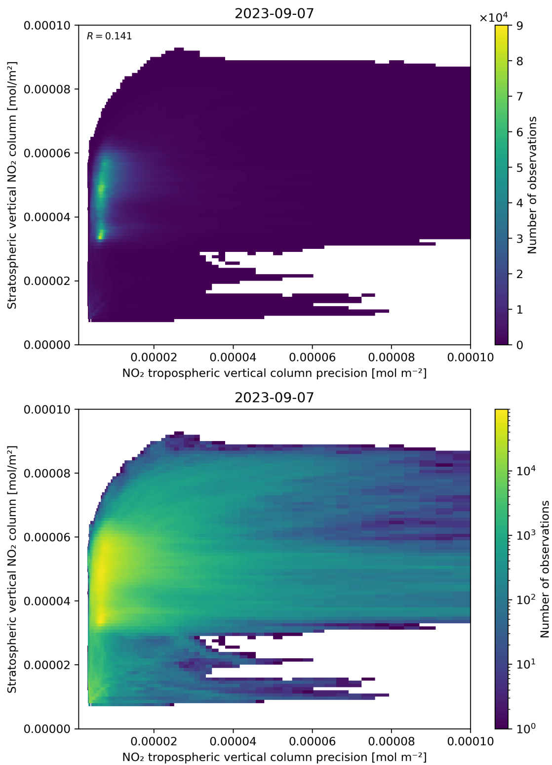
Figure 135: Scatter density plot of “NO 2 tropospheric vertical column precision” against “Stratospheric vertical NO 2 column” for 2023-09-06 to 2023-09-08.
