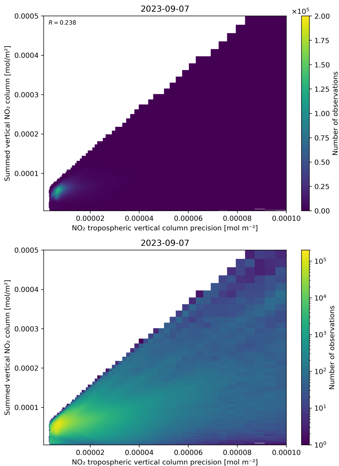
Figure 136: Scatter density plot of “NO 2 tropospheric vertical column precision” against “Summed vertical NO 2 column” for 2023-09-06 to 2023-09-08.
