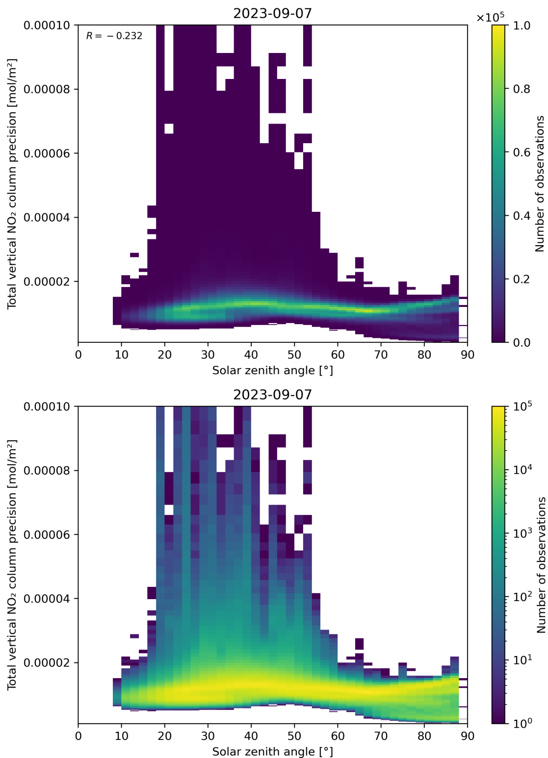
Figure 154: Scatter density plot of “Solar zenith angle” against “Total vertical NO 2 column precision” for 2023-09-06 to 2023-09-08.
