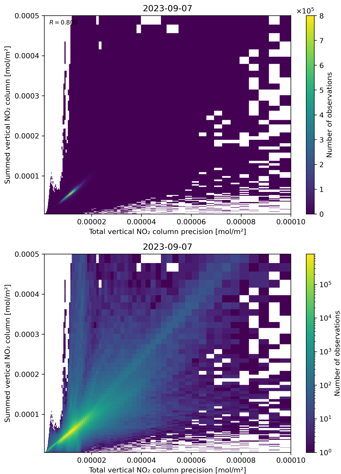
Figure 117: Scatter density plot of “Total vertical NO 2 column precision” against “Summed vertical NO 2 column” for 2023-09-06 to 2023-09-08.
