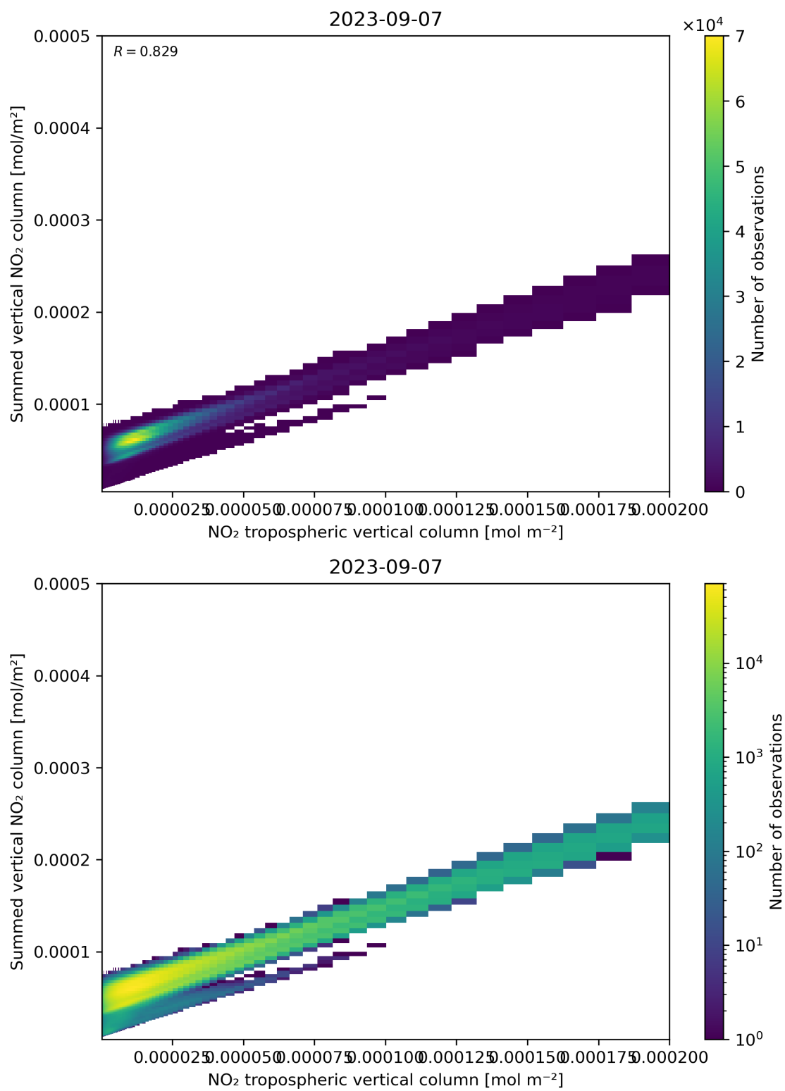
Figure 126: Scatter density plot of “NO 2 tropospheric vertical column” against “Summed vertical NO 2 column” for 2023-09-06 to 2023-09-08.
