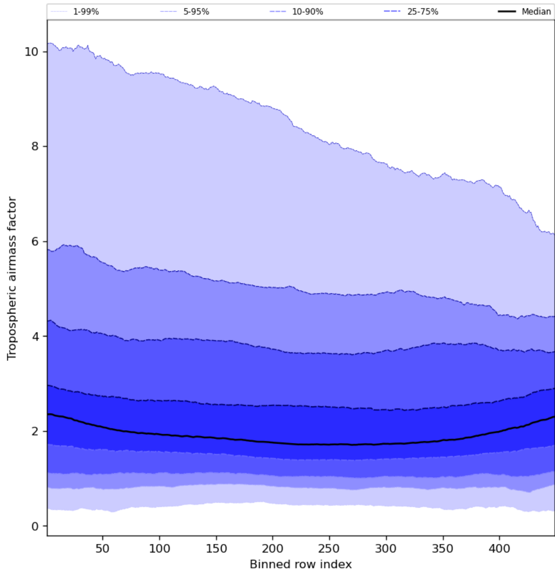
Figure 48: Along track statistics of “Tropospheric airmass factor” for 2023-09-06 to 2023-09-08
