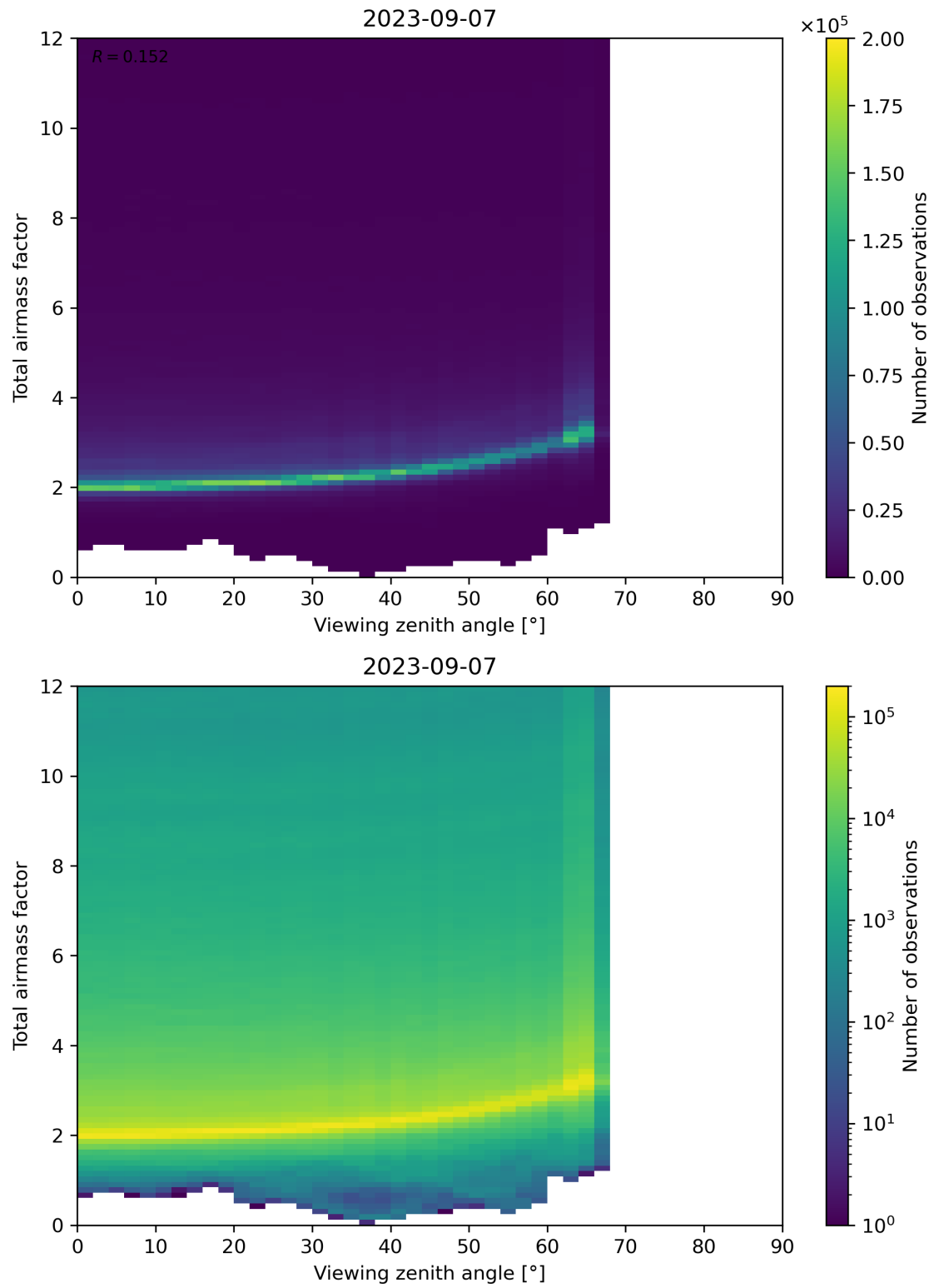
Figure 160: Scatter density plot of “Viewing zenith angle” against “Total airmass factor” for 2023-09-06 to 2023-09-08.
