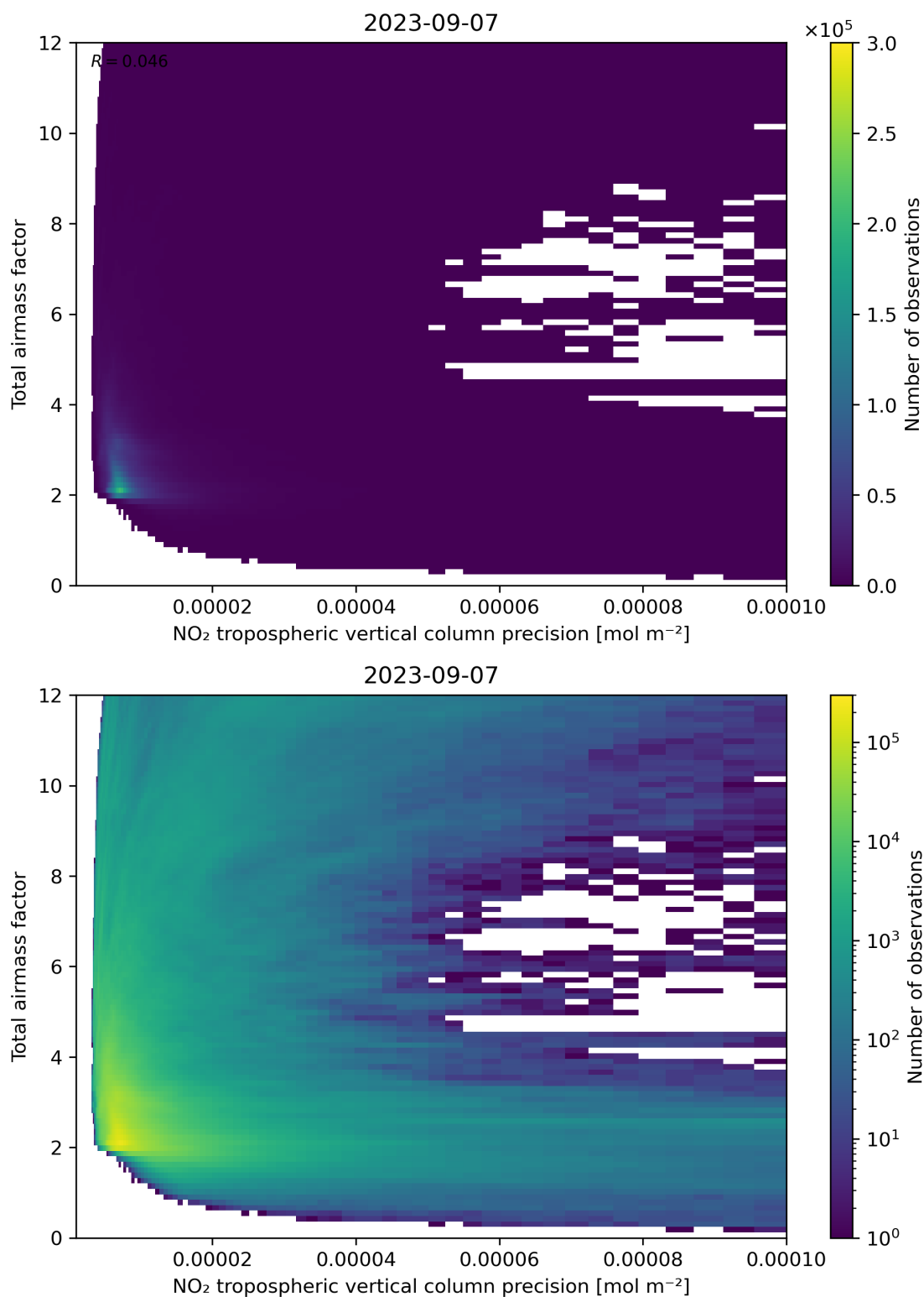
Figure 132: Scatter density plot of “NO 2 tropospheric vertical column precision” against “Total airmass factor” for 2023-09-06 to 2023-09-08.
