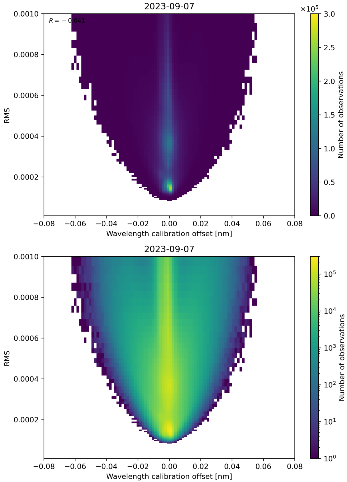
Figure 181: Scatter density plot of “Wavelength calibration offset” against “RMS” for 2023-09-06 to 2023-09-08.
