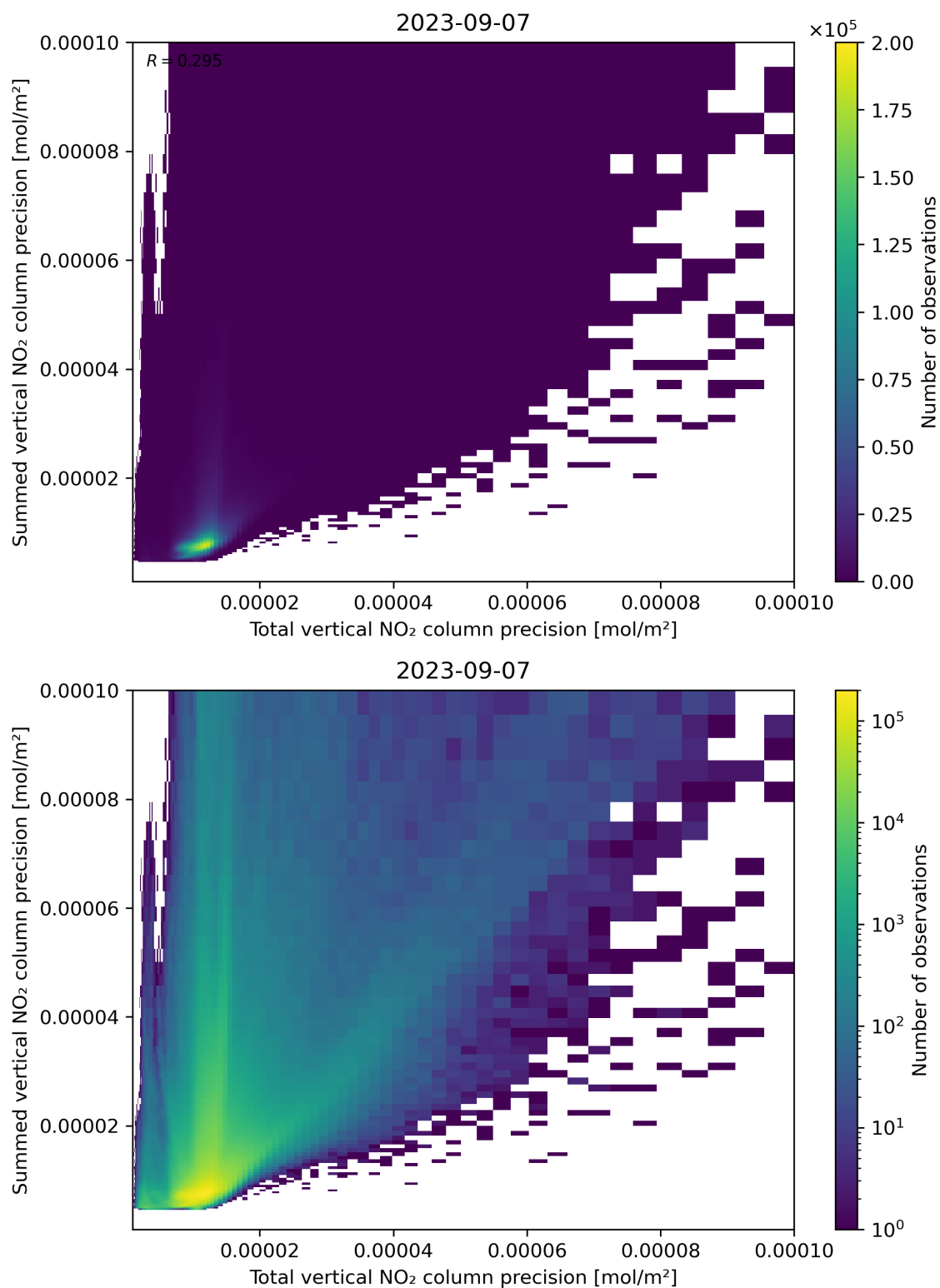
Figure 118: Scatter density plot of “Total vertical NO 2 column precision” against “Summed vertical NO 2 column precision” for 2023-09-06 to 2023-09-08.
