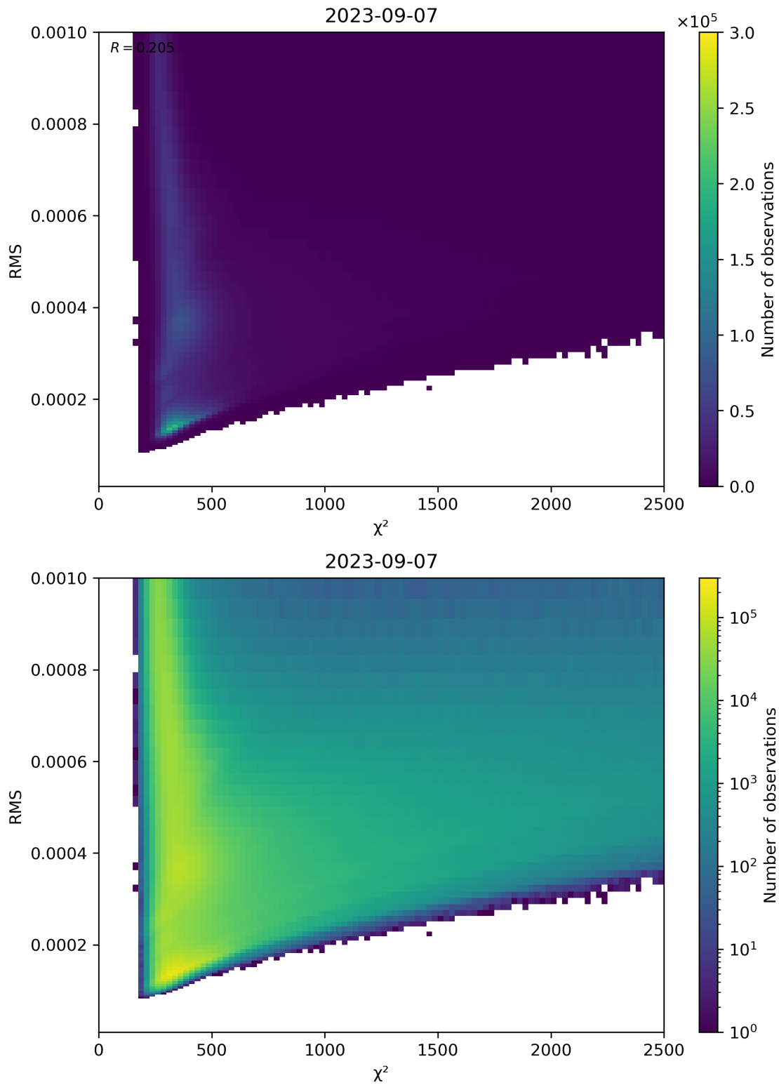
Figure 82: Scatter density plot of “ \chi^2 ” against “RMS” for 2023-09-06 to 2023-09-08.
