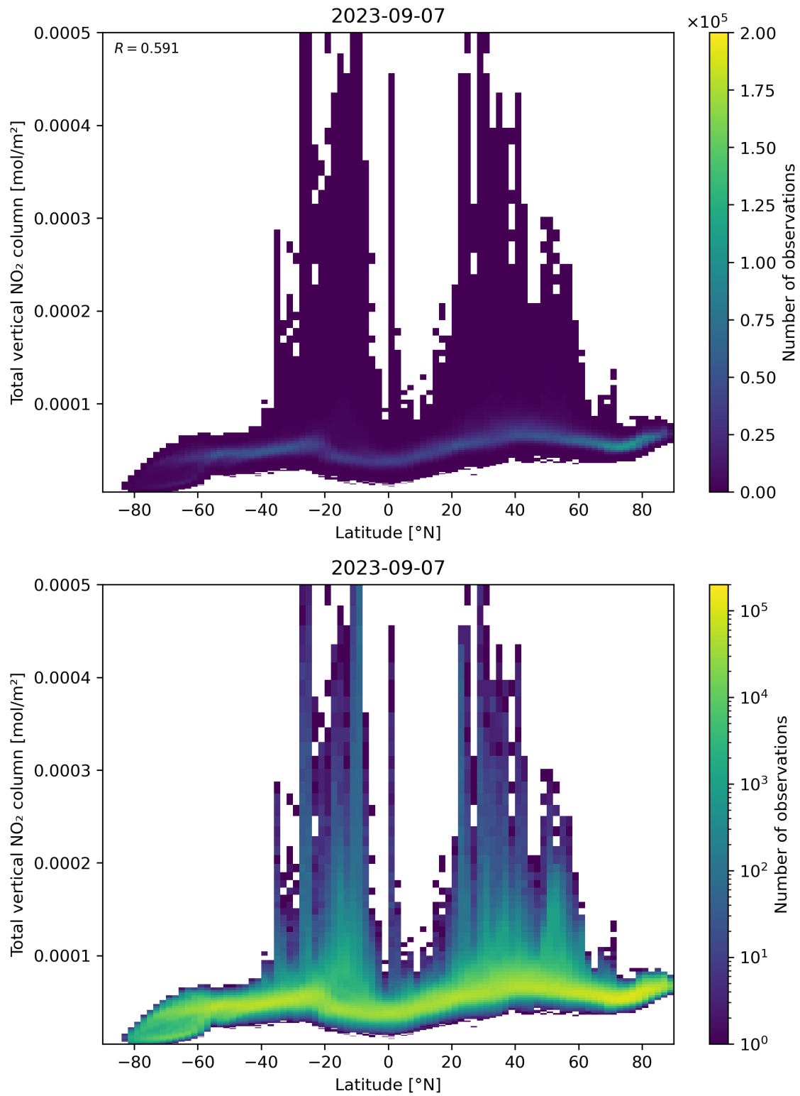
Figure 90: Scatter density plot of “Latitude” against “Total vertical NO 2 column” for 2023-09-06 to 2023-09-08.
