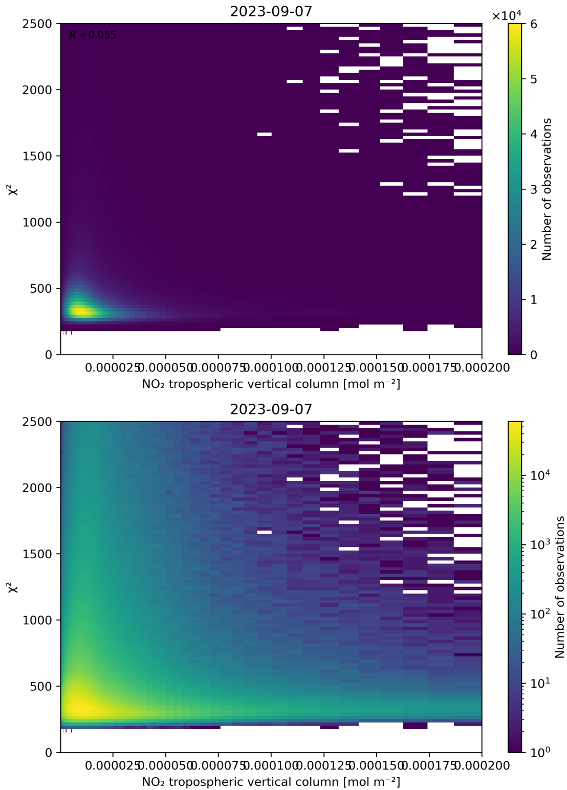
Figure 124: Scatter density plot of “NO 2 tropospheric vertical column” against “ \chi^2 ” for 2023-09-06 to 2023-09-08.
