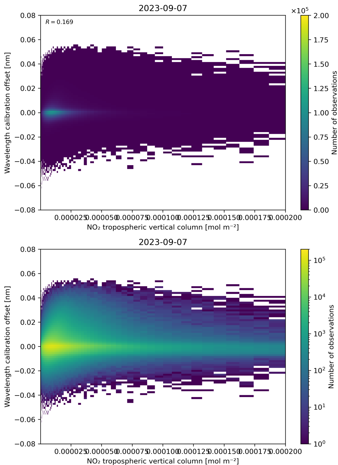
Figure 143: Scatter density plot of “NO 2 tropospheric vertical column” against “Wavelength calibration offset” for 2023-09-06 to 2023-09-08.
