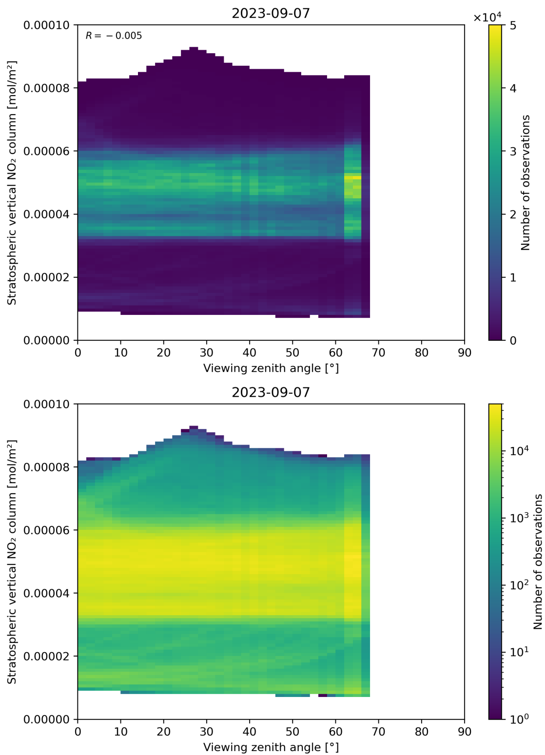
Figure 164: Scatter density plot of “Viewing zenith angle” against “Stratospheric vertical NO 2 column” for 2023-09-06 to 2023-09-08.
