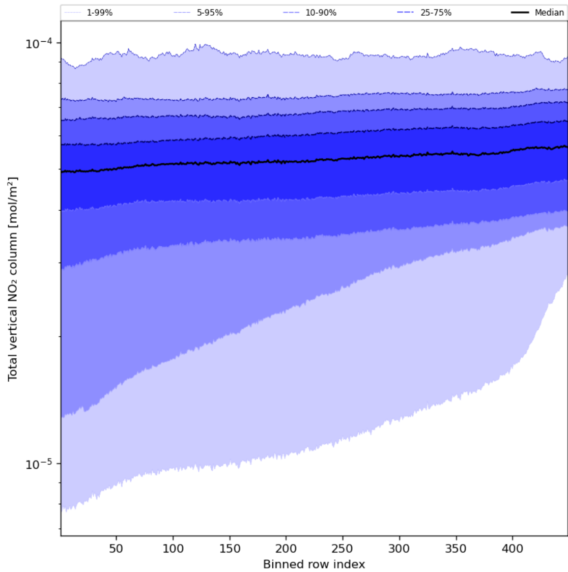
Figure 55: Along track statistics of “Total vertical NO 2 column” for 2023-09-06 to 2023-09-08
