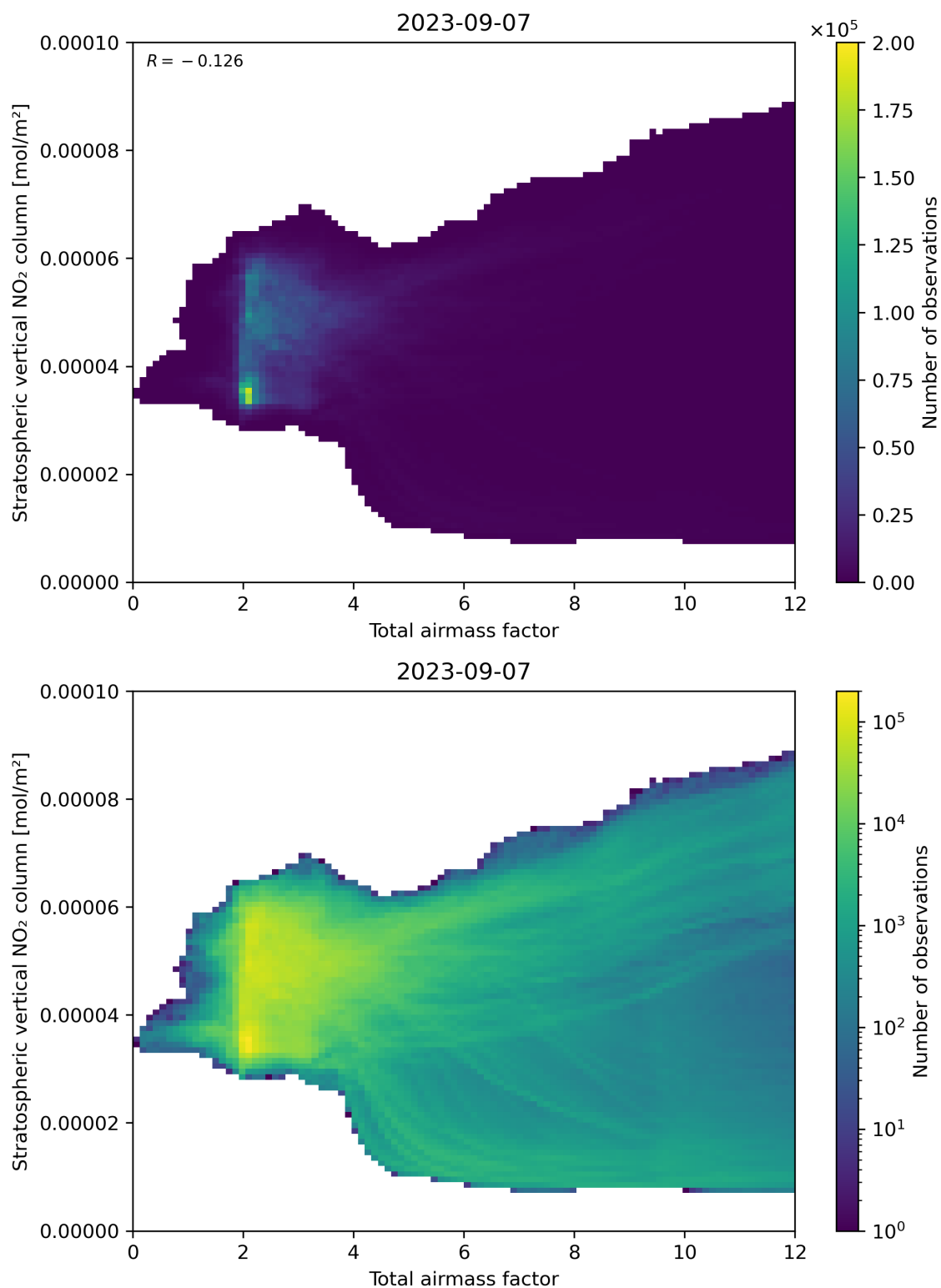
Figure 64: Scatter density plot of “Total airmass factor” against “Stratospheric vertical \text{NO}_2 column” for 2023-09-06 to 2023-09-08.
