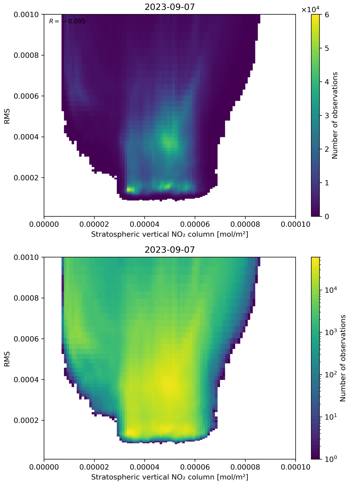
Figure 102: Scatter density plot of “Stratospheric vertical NO 2 column” against “RMS” for 2023-09-06 to 2023-09-08.
