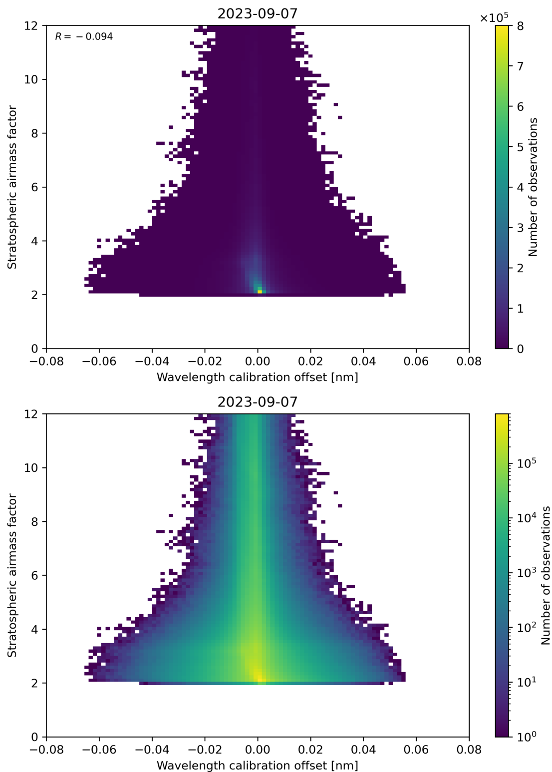
Figure 174: Scatter density plot of “Wavelength calibration offset” against “Stratospheric air mass factor” for 2023-09-06 to 2023-09-08.
