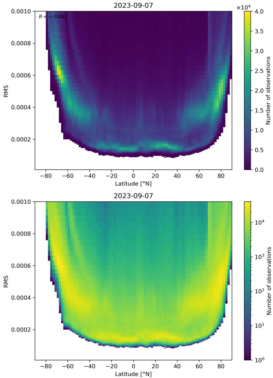
Figure 94: Scatter density plot of “Latitude” against “RMS” for 2023-09-06 to 2023-09-08.
