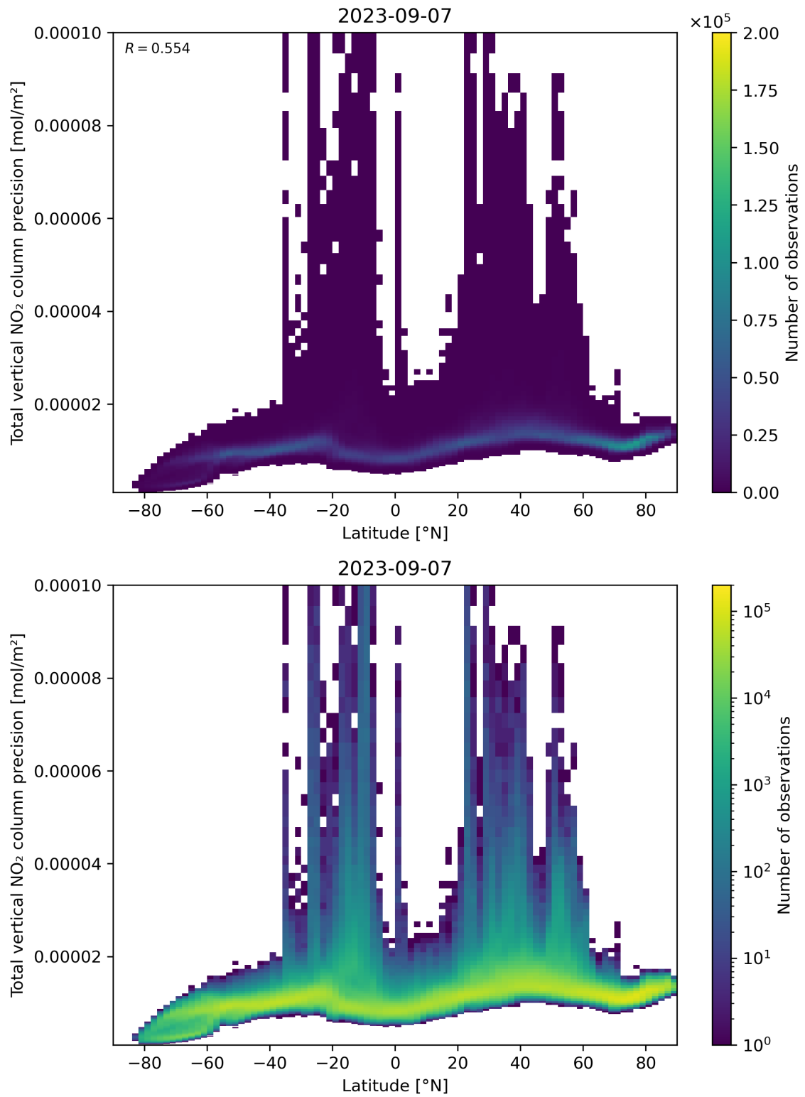
Figure 91: Scatter density plot of “Latitude” against “Total vertical NO 2 column precision” for 2023-09-06 to 2023-09-08.
