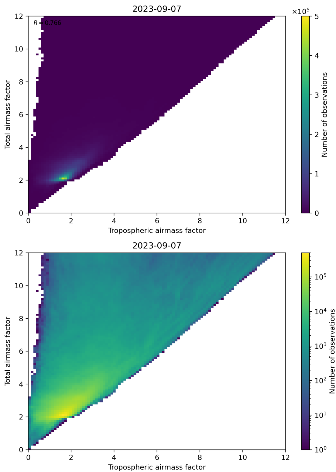
Figure 72: Scatter density plot of “Tropospheric airmass factor” against “Total airmass factor” for 2023-09-06 to 2023-09-08.
