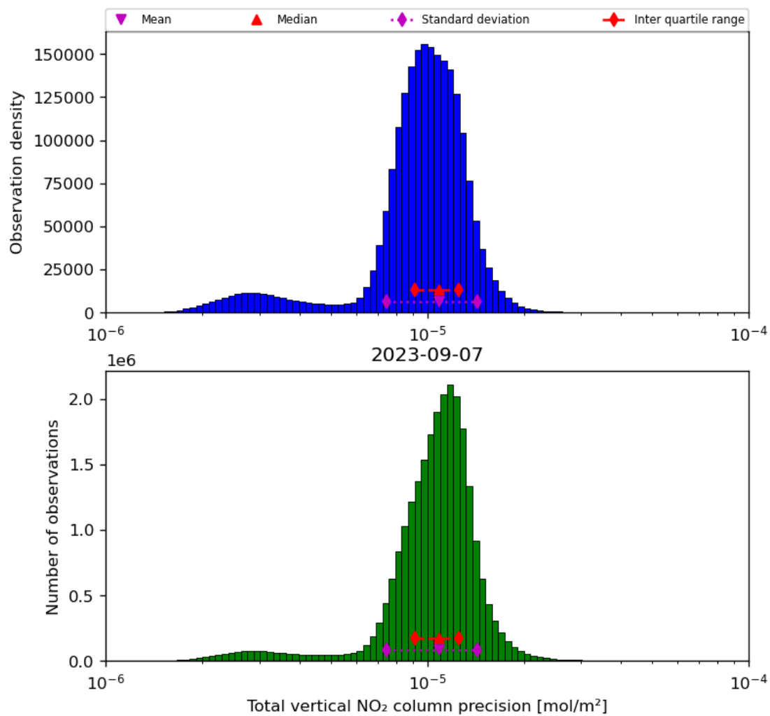
Figure 39: Histogram of "Total vertical NO 2 column precision" for 2023-09-06 to 2023-09-08
