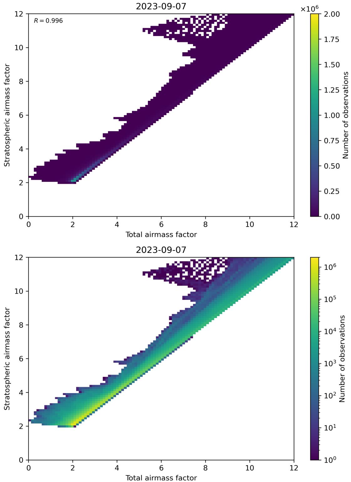
Figure 62: Scatter density plot of “Total airmass factor” against “Stratospheric airmass factor” for 2023-09-06 to 2023-09-08.
