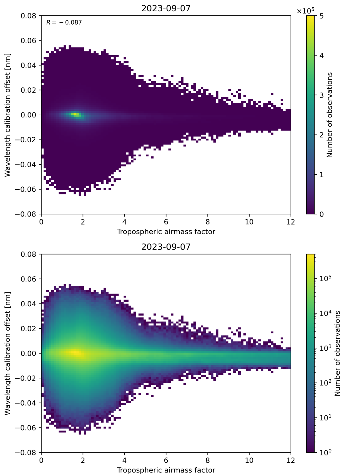
Figure 80: Scatter density plot of “Tropospheric airmass factor” against “Wavelength calibration offset” for 2023-09-06 to 2023-09-08.
