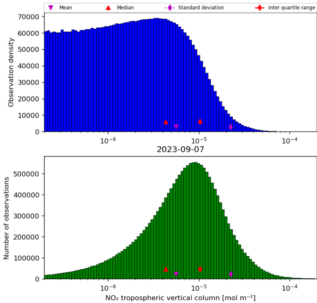
Figure 29: Histogram of “NO 2 tropospheric vertical column” for 2023-09-06 to 2023-09-08
