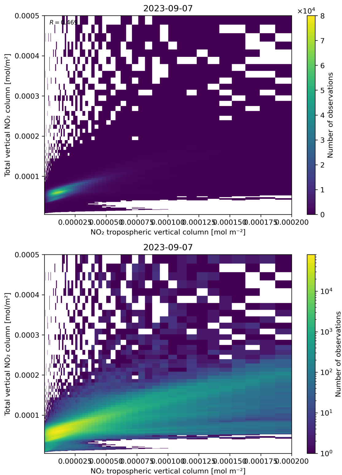
Figure 128: Scatter density plot of “NO 2 tropospheric vertical column” against “Total vertical NO 2 column” for 2023-09-06 to 2023-09-08.
