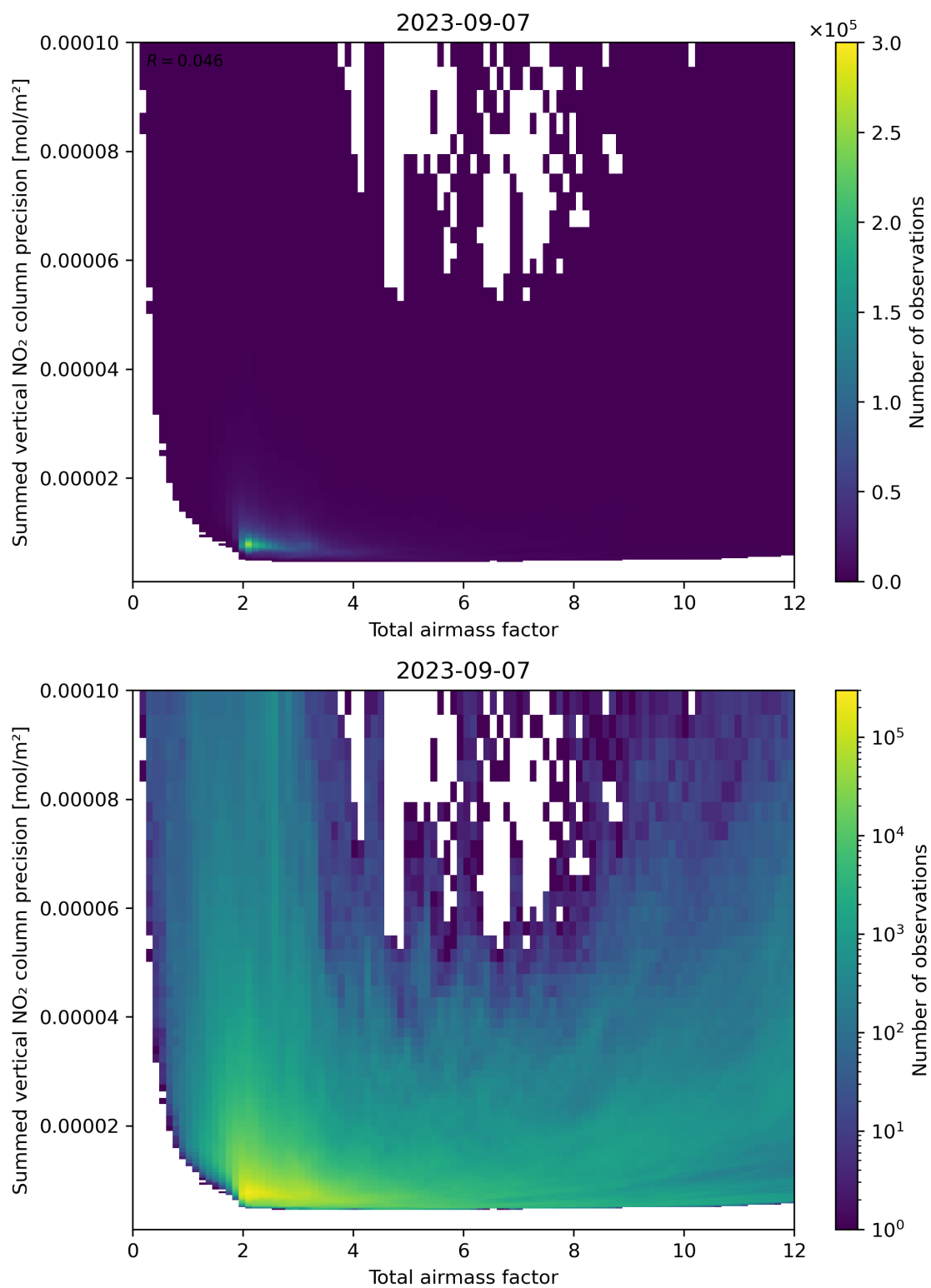
Figure 66: Scatter density plot of “Total airmass factor” against “Summed vertical NO 2 column precision” for 2023-09-06 to 2023-09-08.
