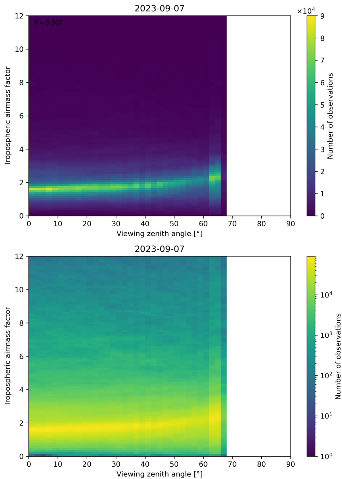
Figure 161: Scatter density plot of “Viewing zenith angle” against “Tropospheric airmass factor” for 2023-09-06 to 2023-09-08.
