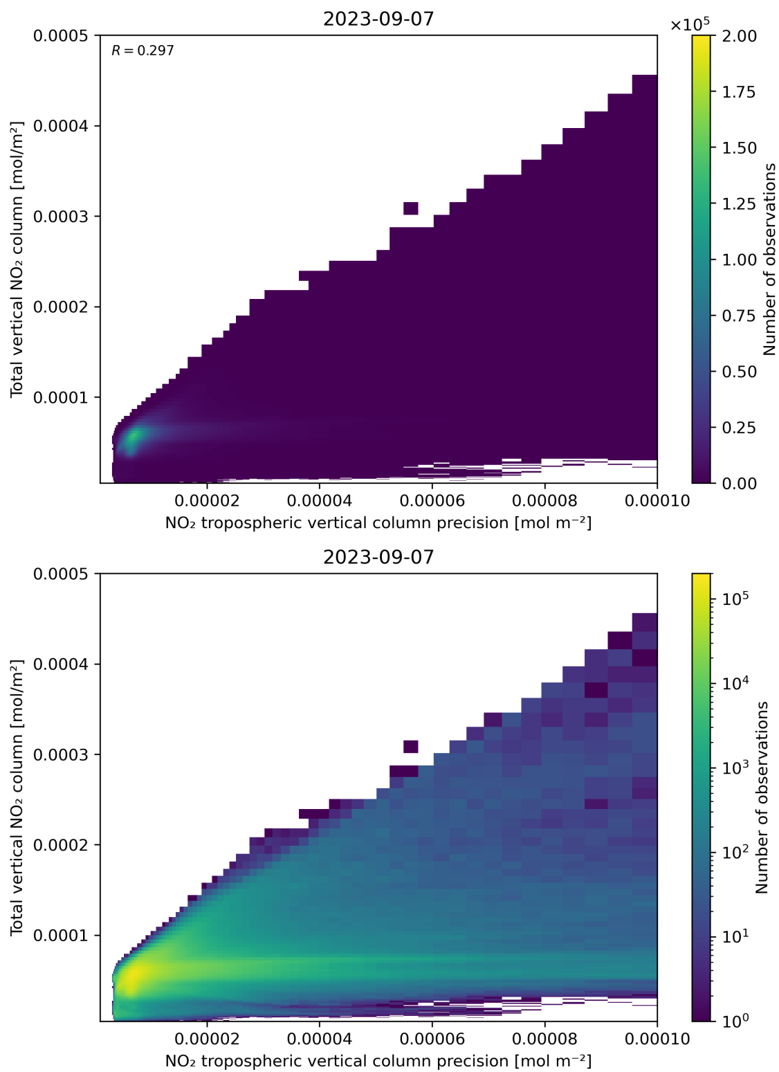
Figure 138: Scatter density plot of “NO 2 tropospheric vertical column precision” against “Total vertical NO 2 column” for 2023-09-06 to 2023-09-08.
