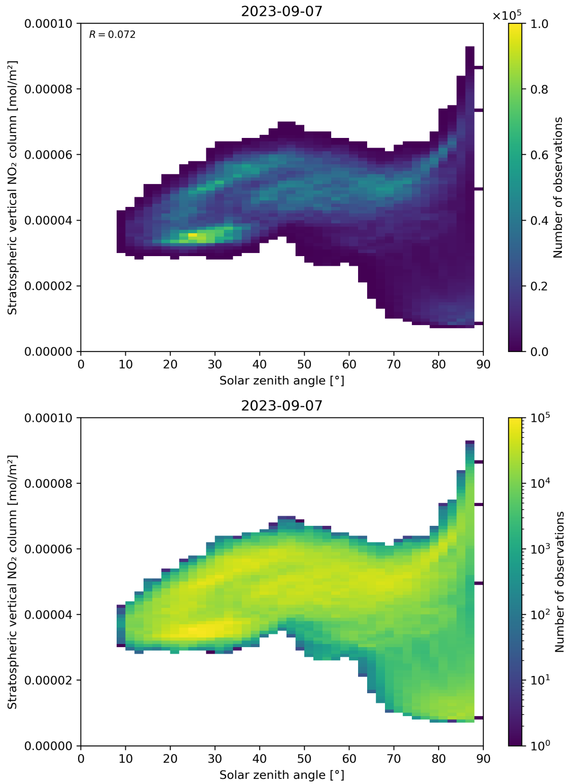
Figure 150: Scatter density plot of “Solar zenith angle” against “Stratospheric vertical NO 2 column” for 2023-09-06 to 2023-09-08.
