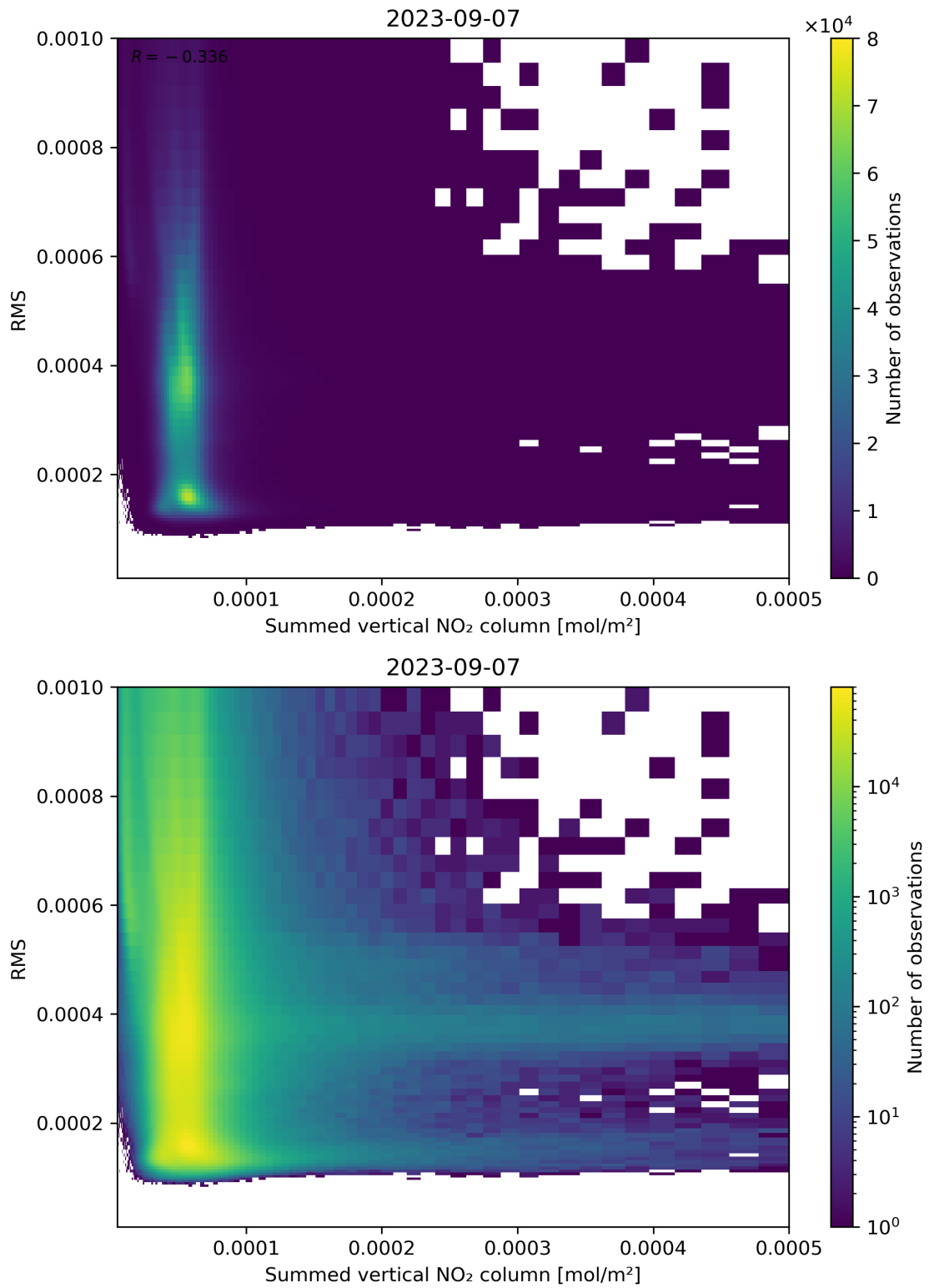
Figure 109: Scatter density plot of “Summed vertical NO 2 column” against “RMS” for 2023-09-06 to 2023-09-08.
