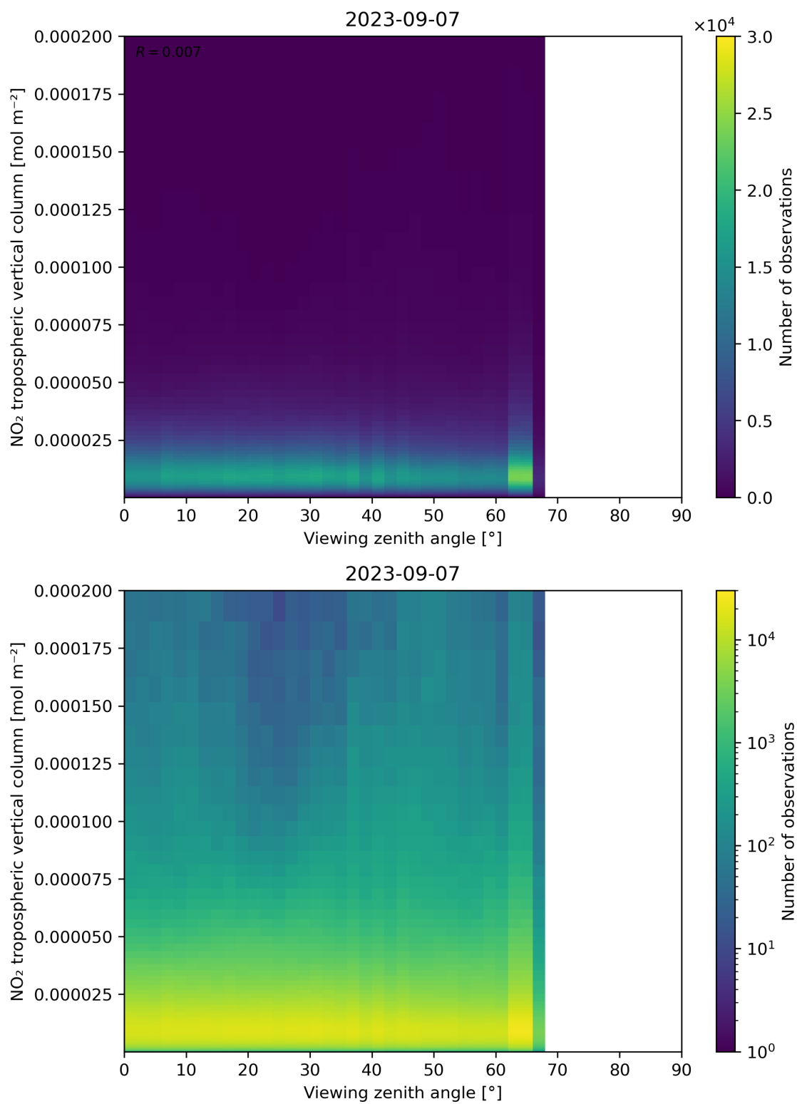
Figure 169: Scatter density plot of “Viewing zenith angle” against “NO 2 tropospheric vertical column” for 2023-09-06 to 2023-09-08.
