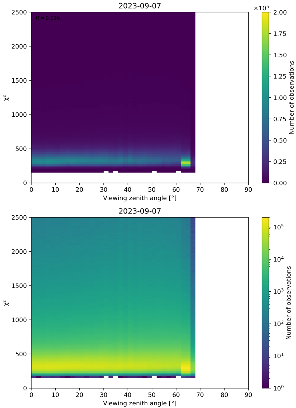
Figure 162: Scatter density plot of “Viewing zenith angle” against “ \chi^2 ” for 2023-09-06 to 2023-09-08.
