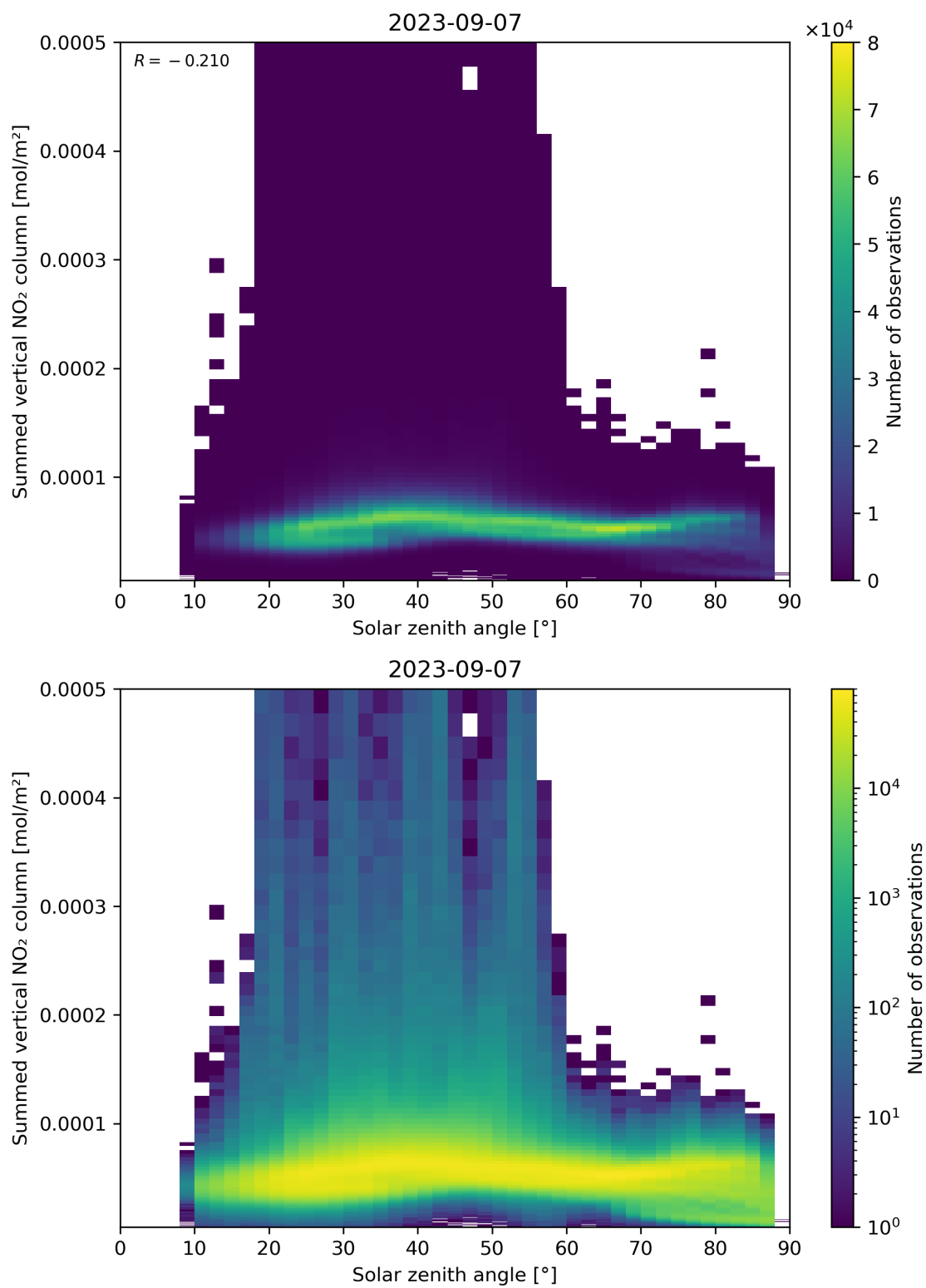
Figure 151: Scatter density plot of “Solar zenith angle” against “Summed vertical NO 2 column” for 2023-09-06 to 2023-09-08.
