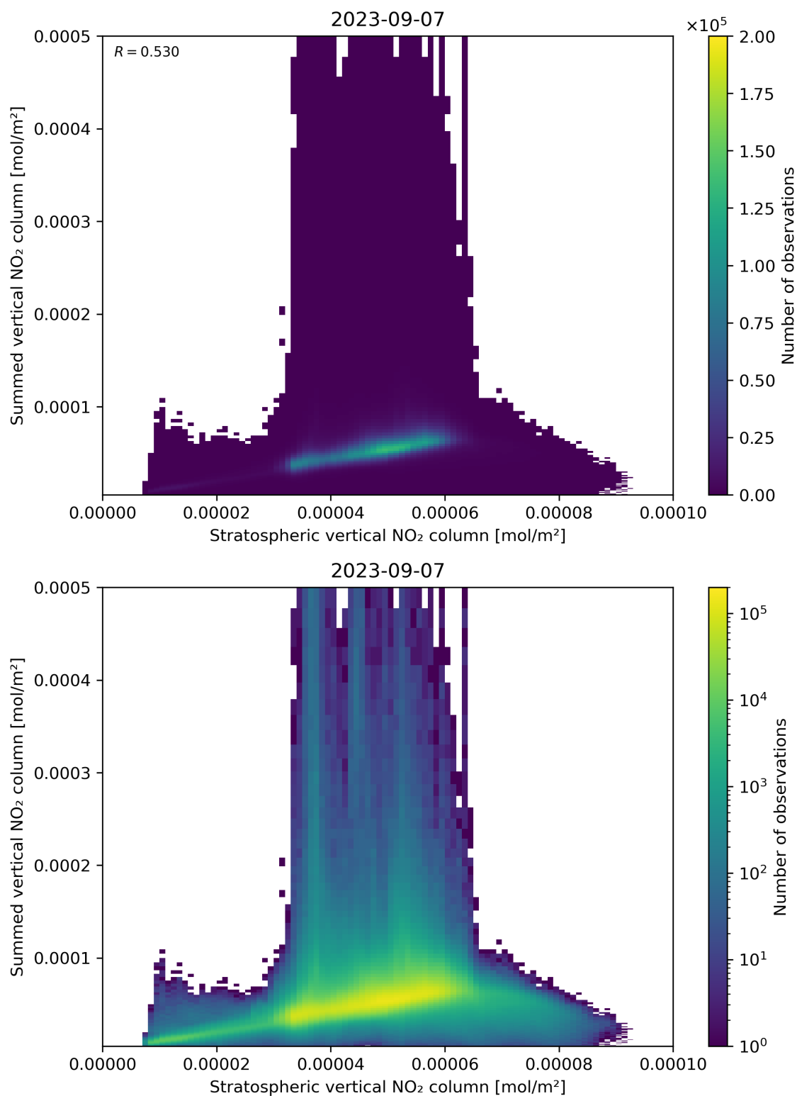
Figure 98: Scatter density plot of “Stratospheric vertical NO 2 column” against “Summed vertical NO 2 column” for 2023-09-06 to 2023-09-08.
