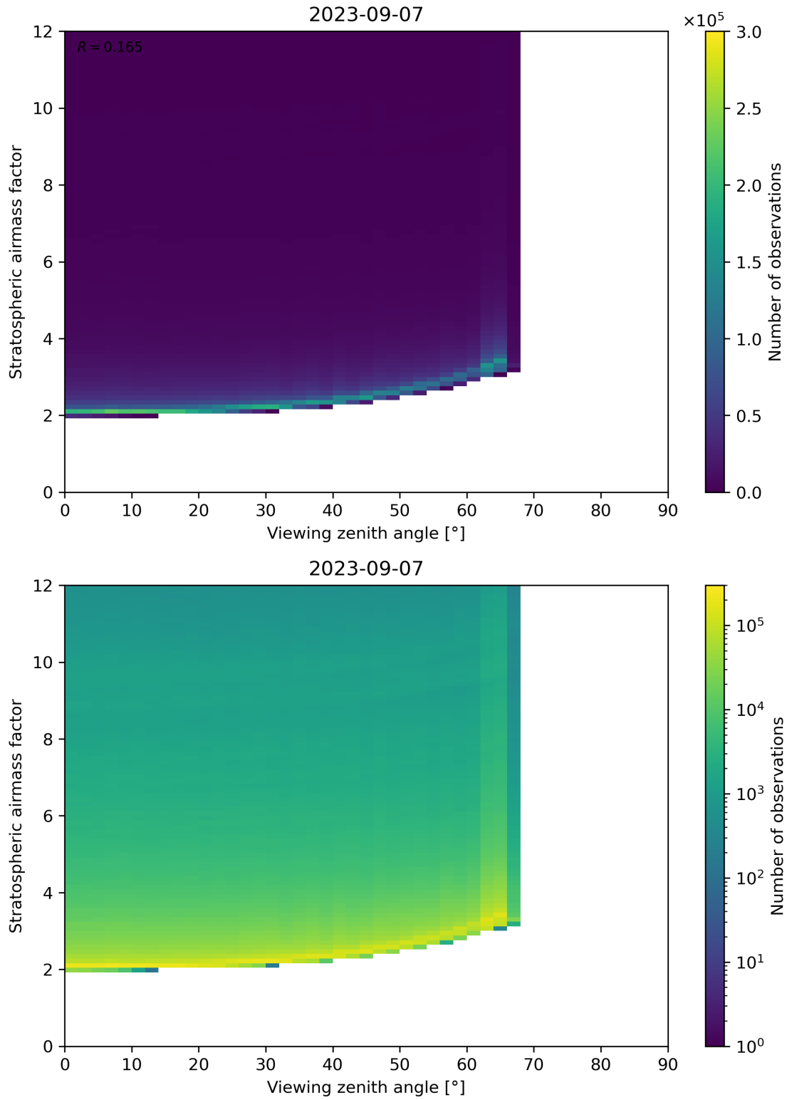
Figure 159: Scatter density plot of “Viewing zenith angle” against “Stratospheric airmass factor” for 2023-09-06 to 2023-09-08.
