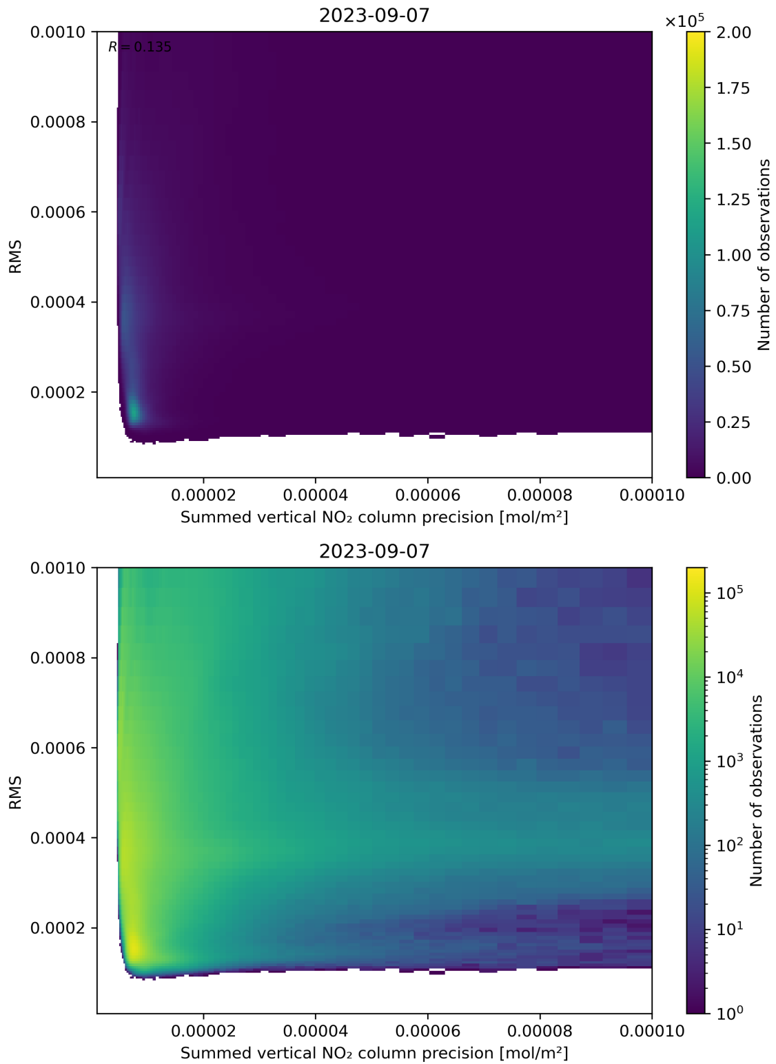
Figure 108: Scatter density plot of “Summed vertical NO 2 column precision” against “RMS” for 2023-09-06 to 2023-09-08.
