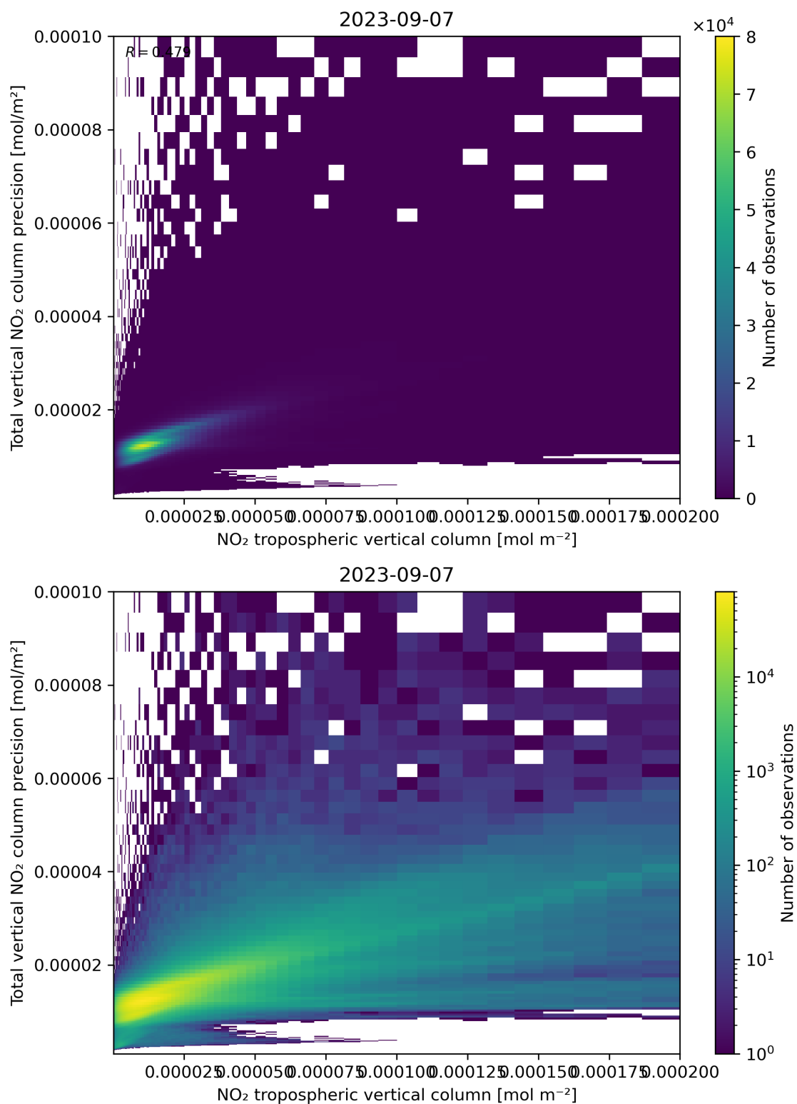
Figure 129: Scatter density plot of “NO 2 tropospheric vertical column” against “Total vertical NO 2 column precision” for 2023-09-06 to 2023-09-08.
