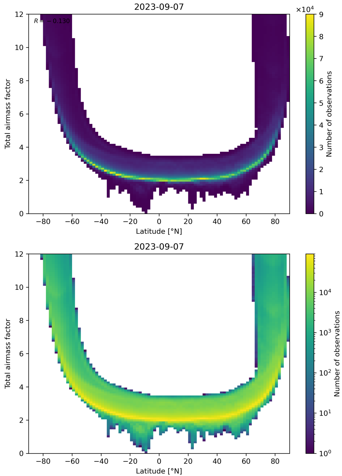
Figure 84: Scatter density plot of “Latitude” against “Total airmass factor” for 2023-09-06 to 2023-09-08.
