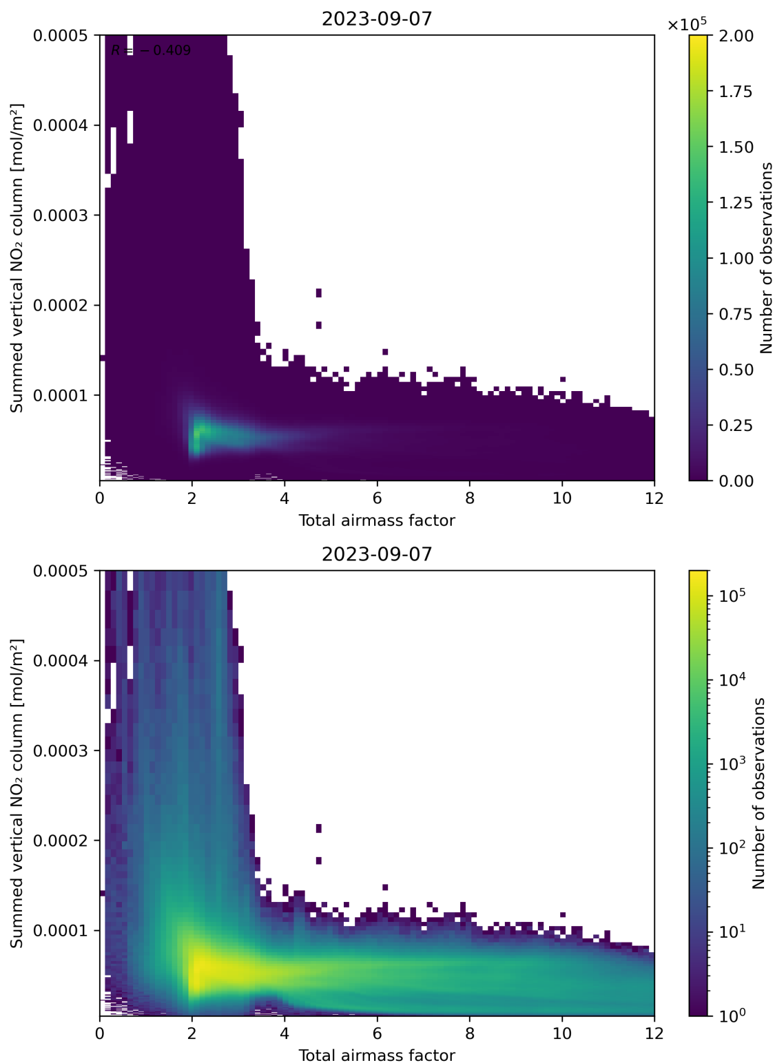
Figure 65: Scatter density plot of “Total airmass factor” against “Summed vertical NO 2 column” for 2023-09-06 to 2023-09-08.
