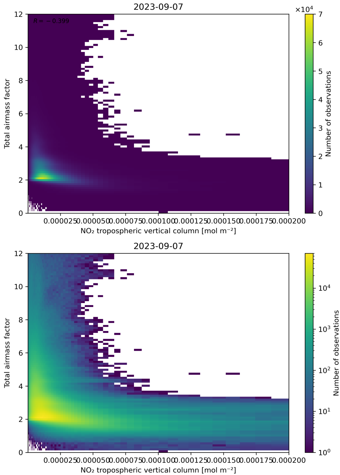
Figure 122: Scatter density plot of “NO 2 tropospheric vertical column” against “Total airmass factor” for 2023-09-06 to 2023-09-08.
