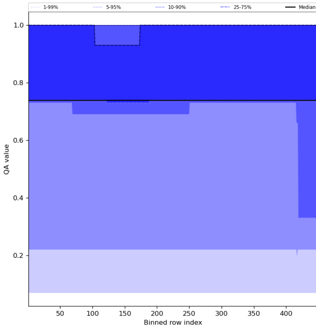
Figure 45: Along track statistics of “QA value” for 2023-09-06 to 2023-09-08
