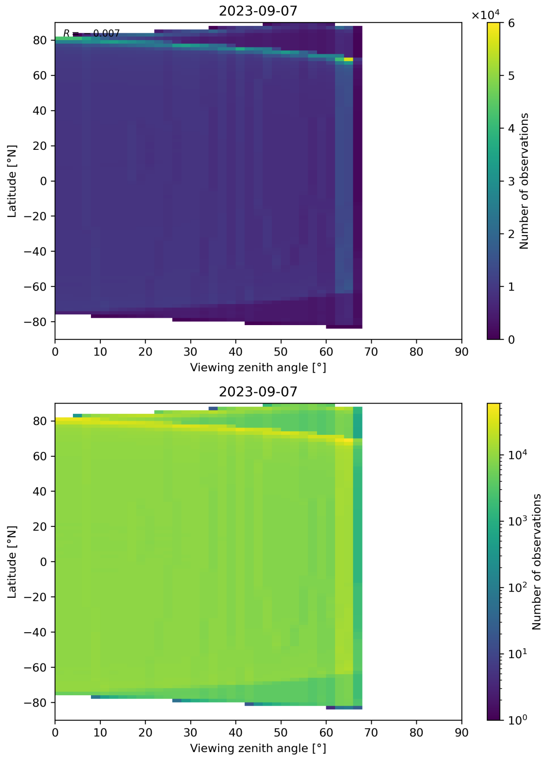
Figure 163: Scatter density plot of “Viewing zenith angle” against “Latitude” for 2023-09-06 to 2023-09-08.
