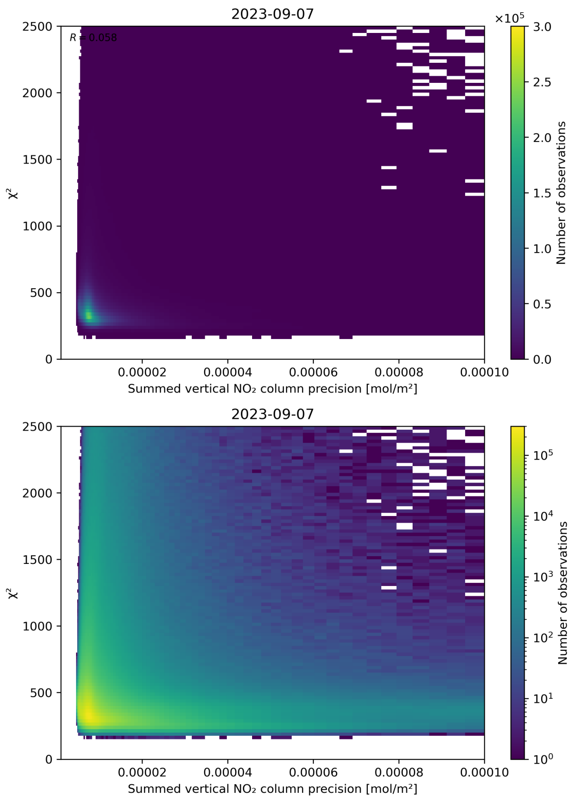
Figure 107: Scatter density plot of “Summed vertical NO 2 column precision” against “ \chi^2 ” for 2023-09-06 to 2023-09-08.
