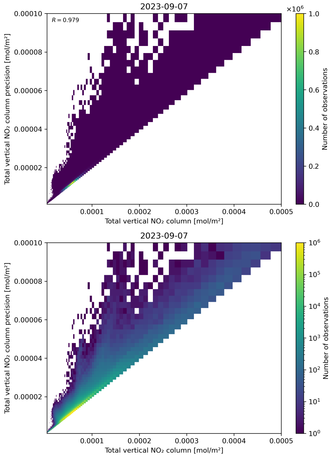
Figure 114: Scatter density plot of “Total vertical NO 2 column” against “Total vertical NO 2 column precision” for 2023-09-06 to 2023-09-08.
