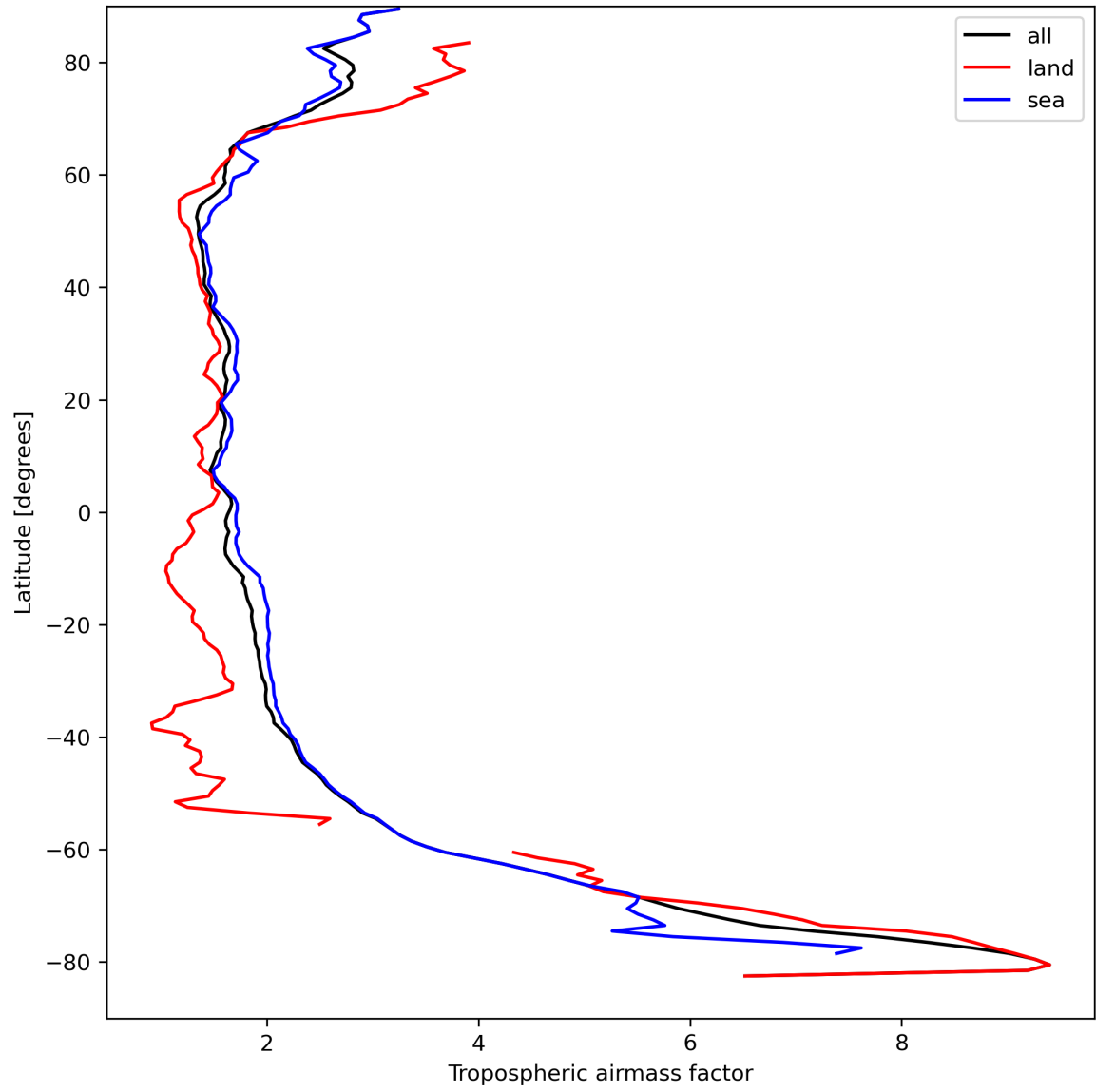
Figure 14: Zonal average of “Tropospheric airmass factor” for 2023-09-06 to 2023-09-08.
