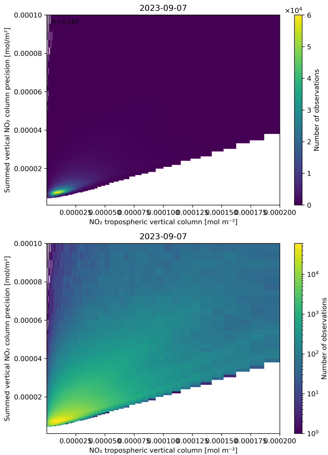
Figure 127: Scatter density plot of “NO 2 tropospheric vertical column” against “Summed vertical NO 2 column precision” for 2023-09-06 to 2023-09-08.
