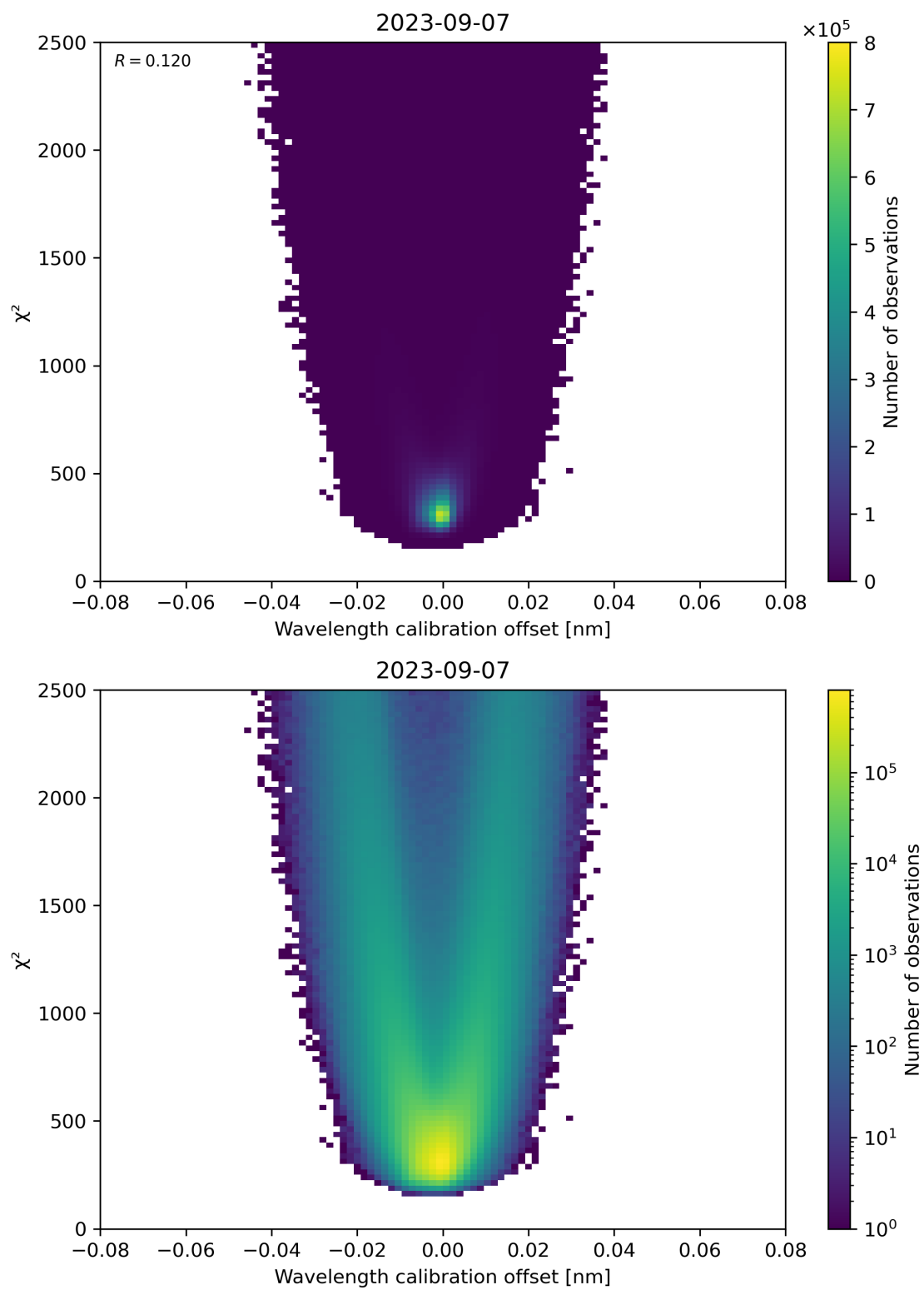
Figure 175: Scatter density plot of “Wavelength calibration offset” against “ \chi^2 ” for 2023-09-06 to 2023-09-08.
