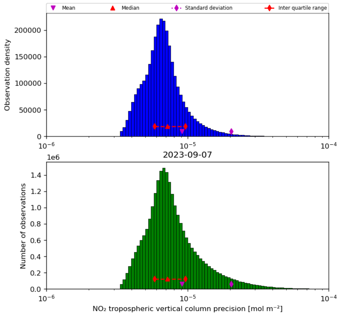
Figure 30: Histogram of “NO 2 tropospheric vertical column precision” for 2023-09-06 to 2023-09-08
