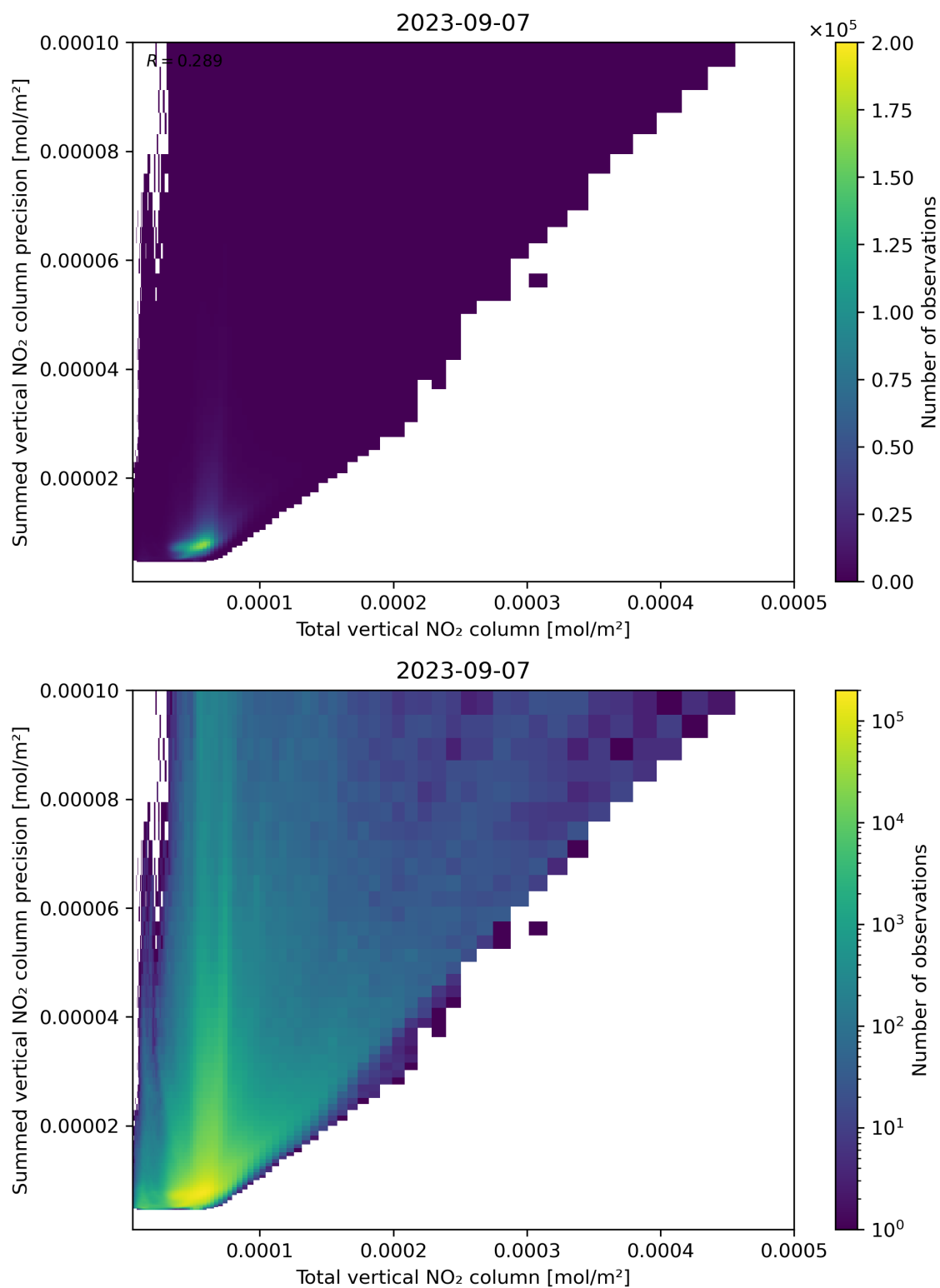
Figure 113: Scatter density plot of “Total vertical NO 2 column” against “Summed vertical NO 2 column precision” for 2023-09-06 to 2023-09-08.
