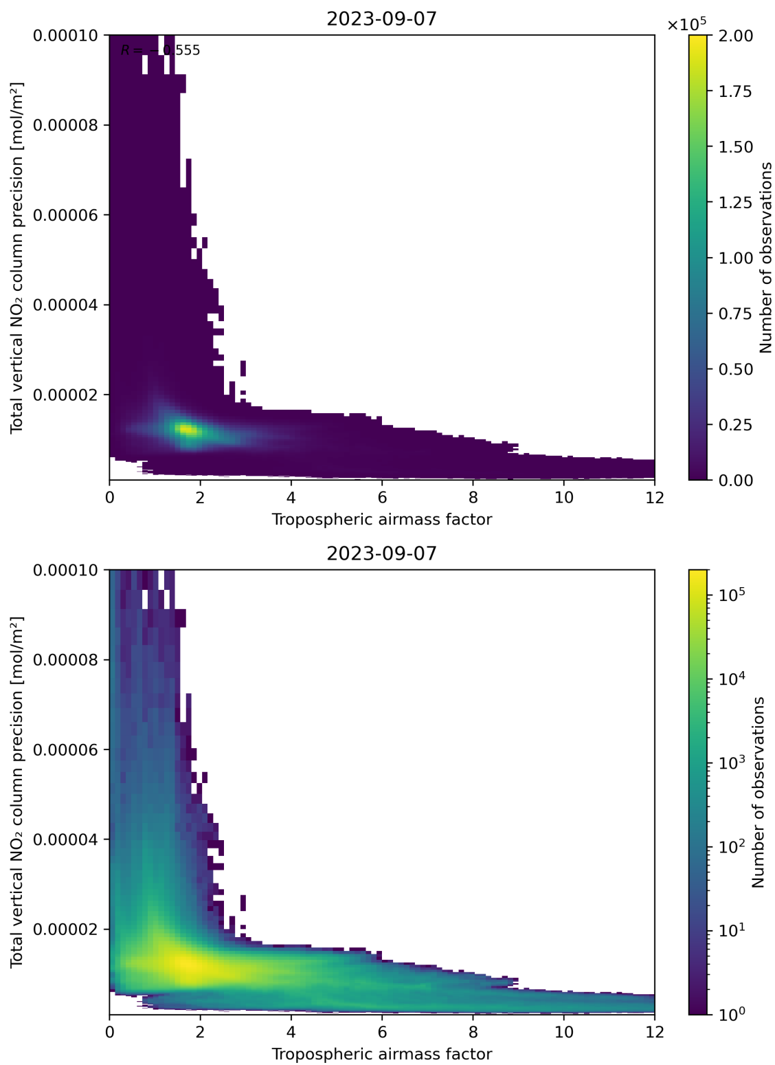
Figure 78: Scatter density plot of “Tropospheric air mass factor” against “Total vertical NO 2 column precision” for 2023-09-06 to 2023-09-08.
