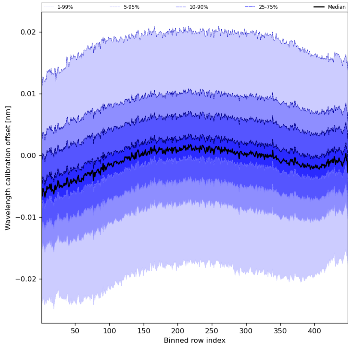
Figure 52: Along track statistics of “Wavelength calibration offset” for 2023-09-06 to 2023-09-08
