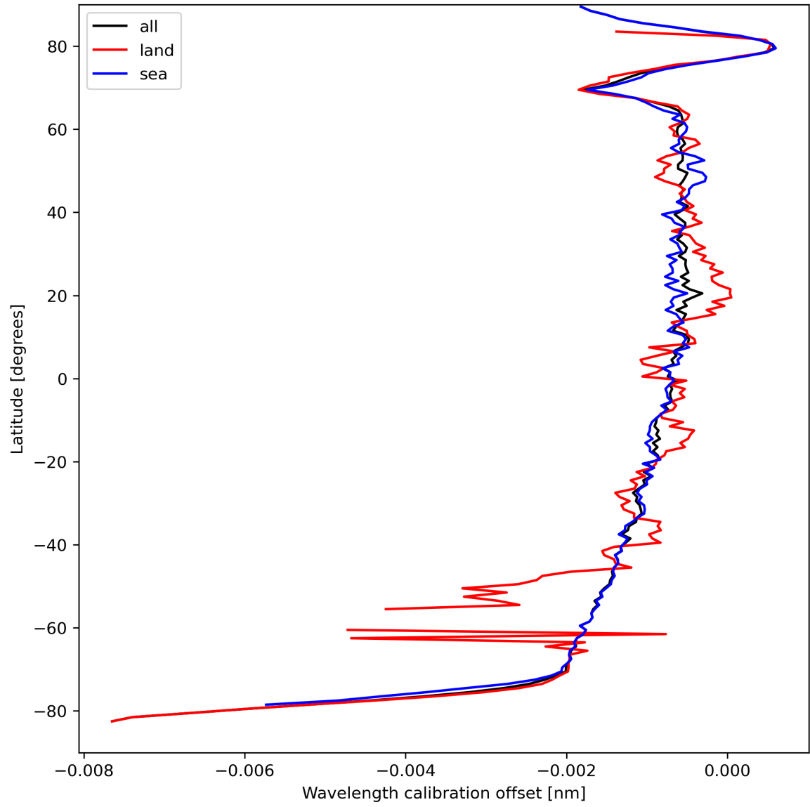
Figure 18: Zonal average of “Wavelength calibration offset” for 2023-09-06 to 2023-09-08.
