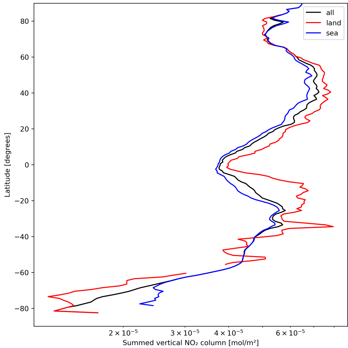
Figure 23: Zonal average of “Summed vertical NO 2 column” for 2023-09-06 to 2023-09-08.
