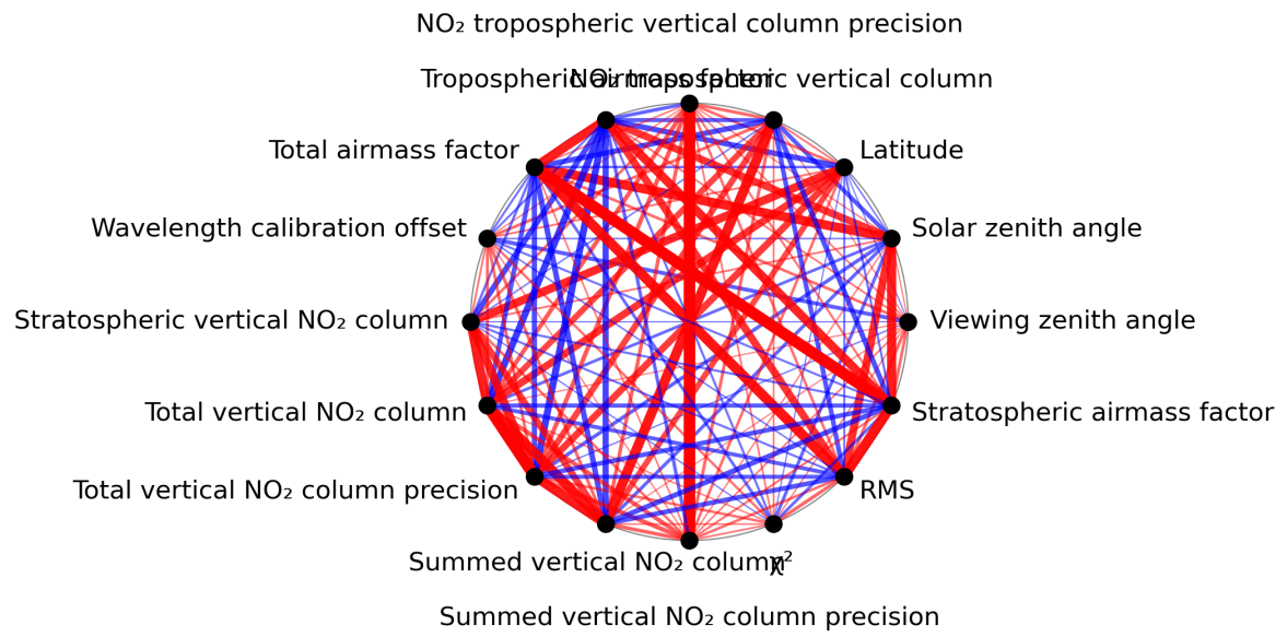
Figure 1: Map of correlation graph for 2023-09-06 to 2023-09-08.
