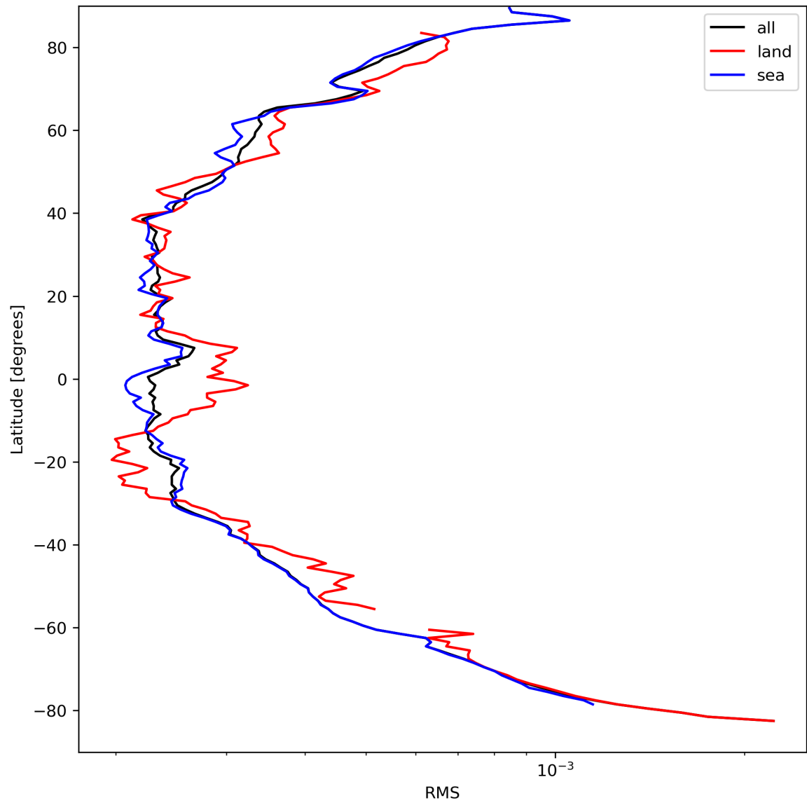
Figure 26: Zonal average of “RMS” for 2023-09-06 to 2023-09-08.
