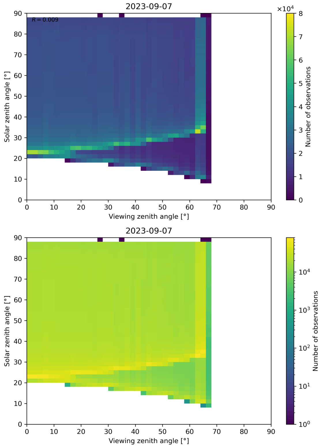
Figure 172: Scatter density plot of “Viewing zenith angle” against “Solar zenith angle” for 2023-09-06 to 2023-09-08.
