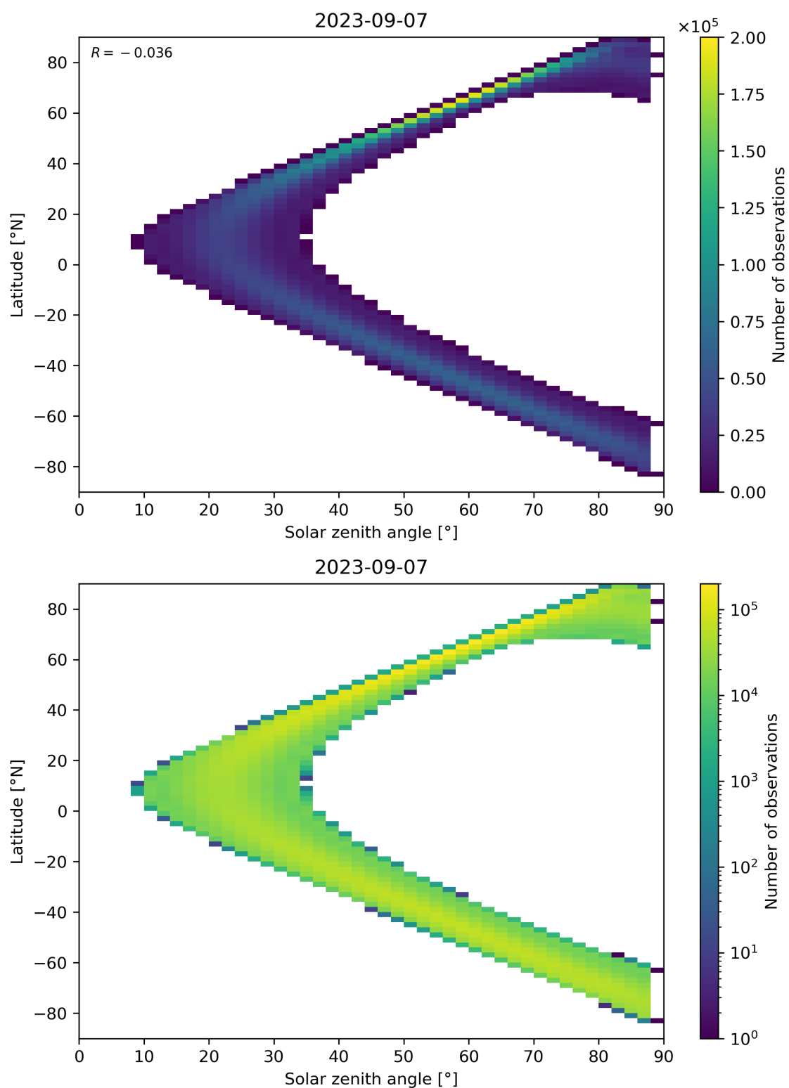
Figure 149: Scatter density plot of “Solar zenith angle” against “Latitude” for 2023-09-06 to 2023-09-08.
