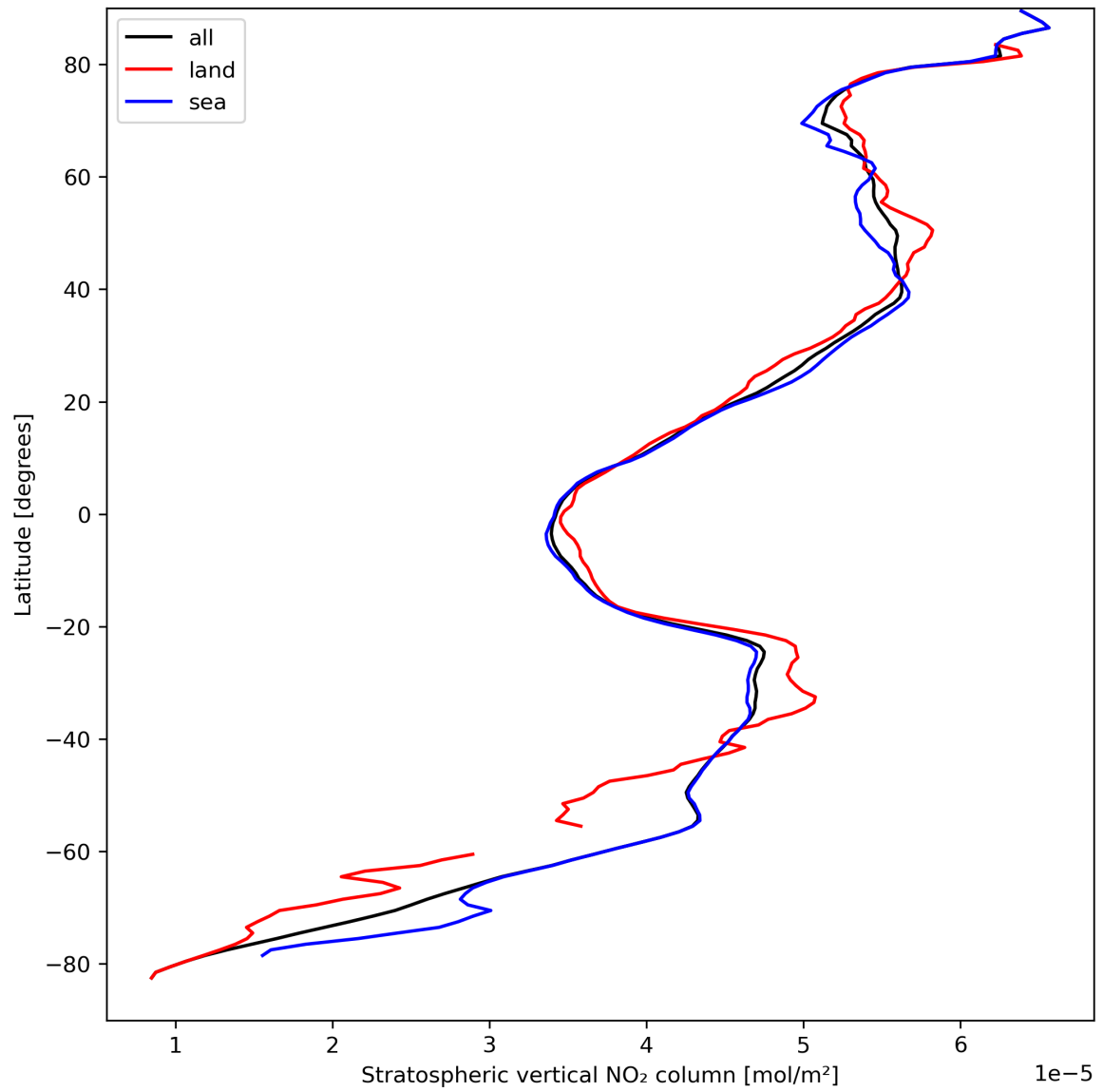
Figure 19: Zonal average of “Stratospheric vertical NO 2 column” for 2023-09-06 to 2023-09-08.
