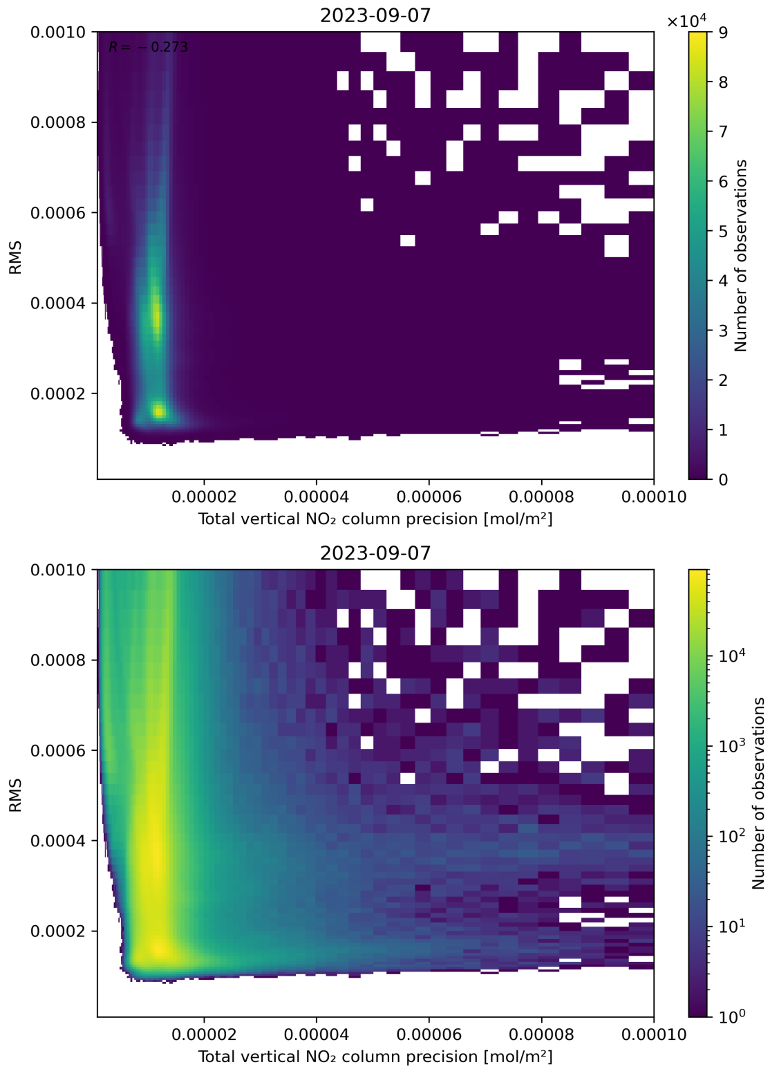
Figure 119: Scatter density plot of “Total vertical NO 2 column precision” against “RMS” for 2023-09-06 to 2023-09-08.
