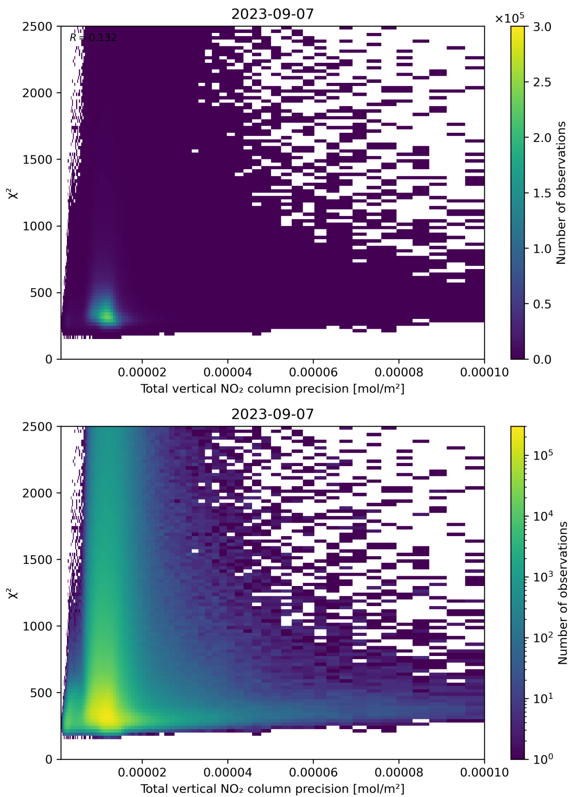
Figure 116: Scatter density plot of “Total vertical NO 2 column precision” against “ \chi^2 ” for 2023-09-06 to 2023-09-08.
