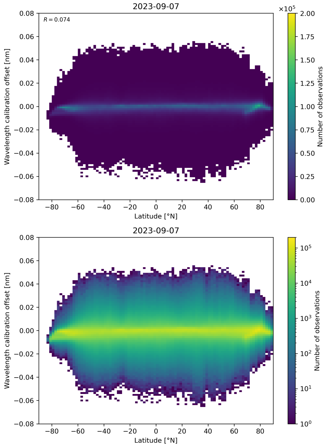
Figure 95: Scatter density plot of “Latitude” against “Wavelength calibration offset” for 2023-09-06 to 2023-09-08.
