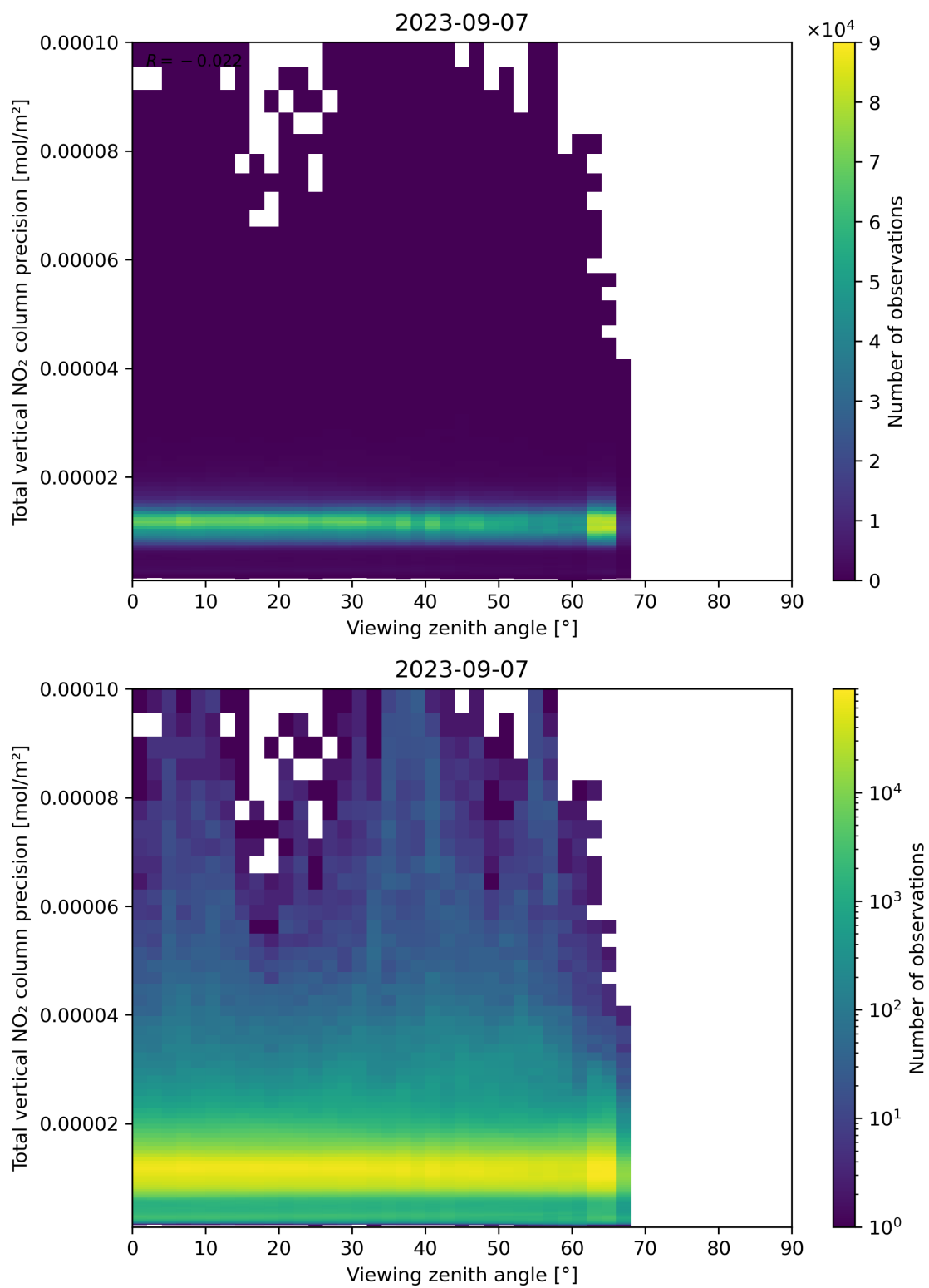
Figure 168: Scatter density plot of “Viewing zenith angle” against “Total vertical NO 2 column precision” for 2023-09-06 to 2023-09-08.
