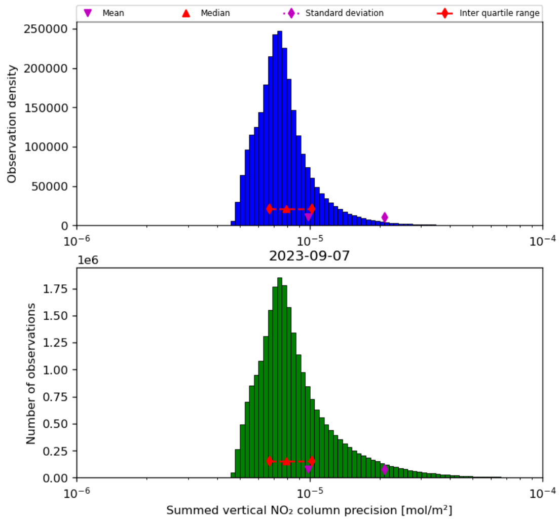
Figure 41: Histogram of "Summed vertical NO 2 column precision" for 2023-09-06 to 2023-09-08
