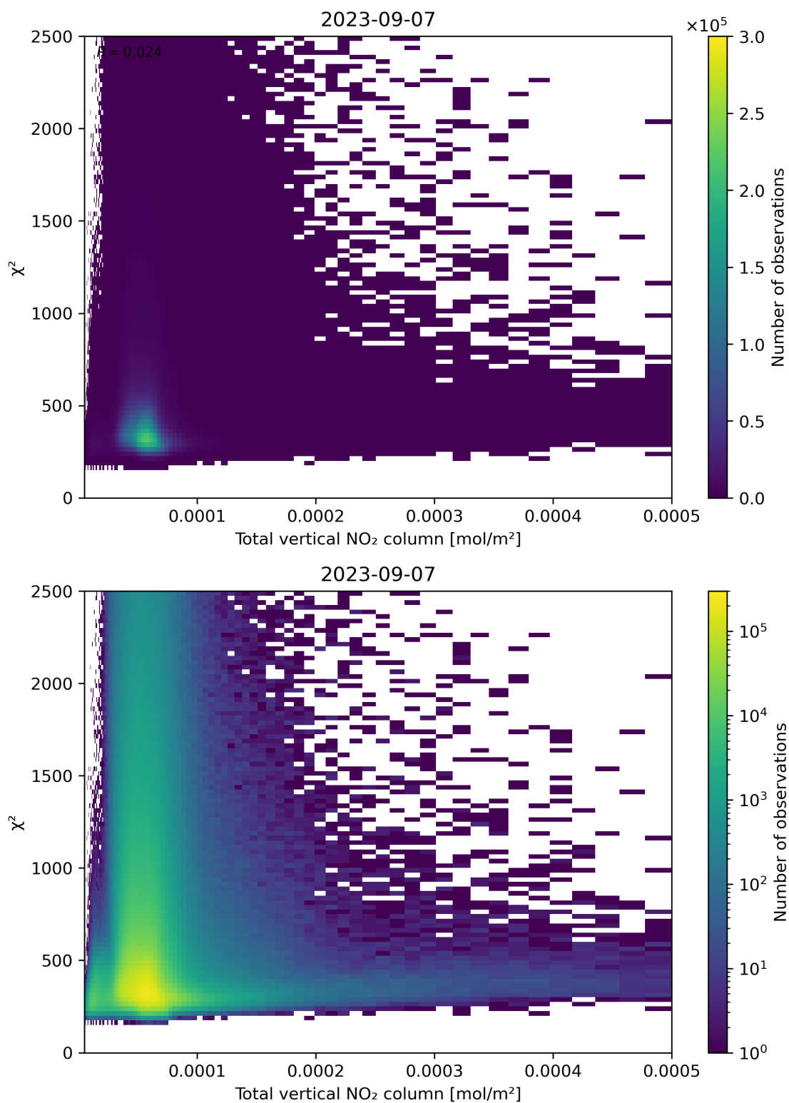
Figure 111: Scatter density plot of “Total vertical NO 2 column” against “ \chi^2 ” for 2023-09-06 to 2023-09-08.
