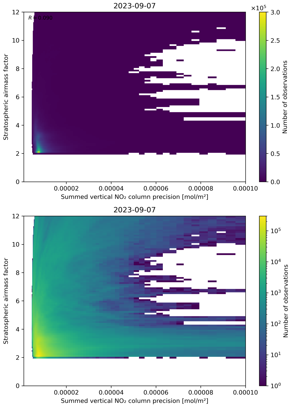
Figure 106: Scatter density plot of “Summed vertical NO 2 column precision” against “Stratospheric airmass factor” for 2023-09-06 to 2023-09-08.
