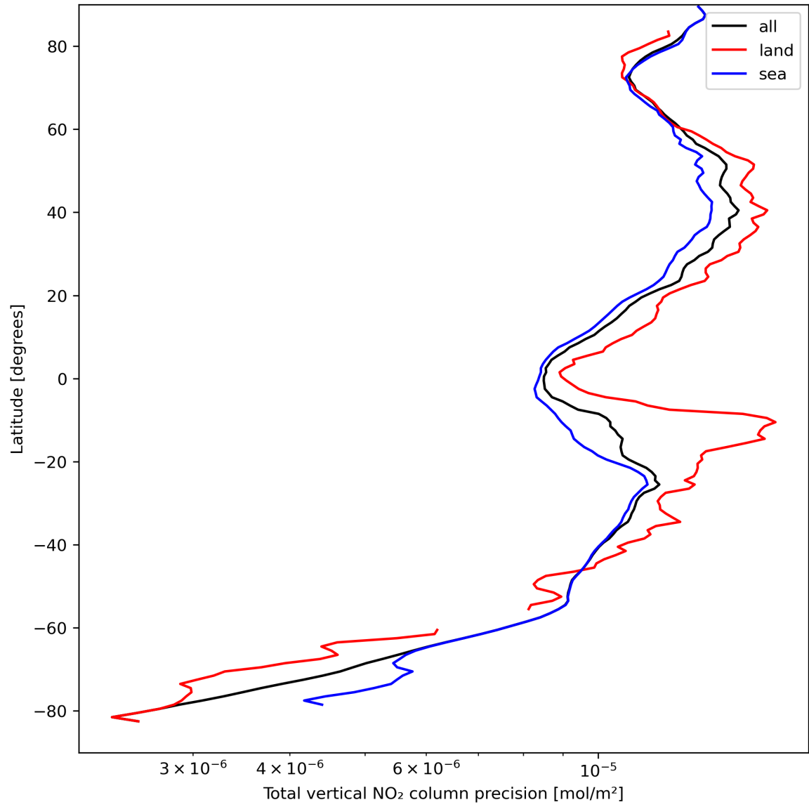
Figure 22: Zonal average of “Total vertical NO 2 column precision” for 2023-09-06 to 2023-09-08.
