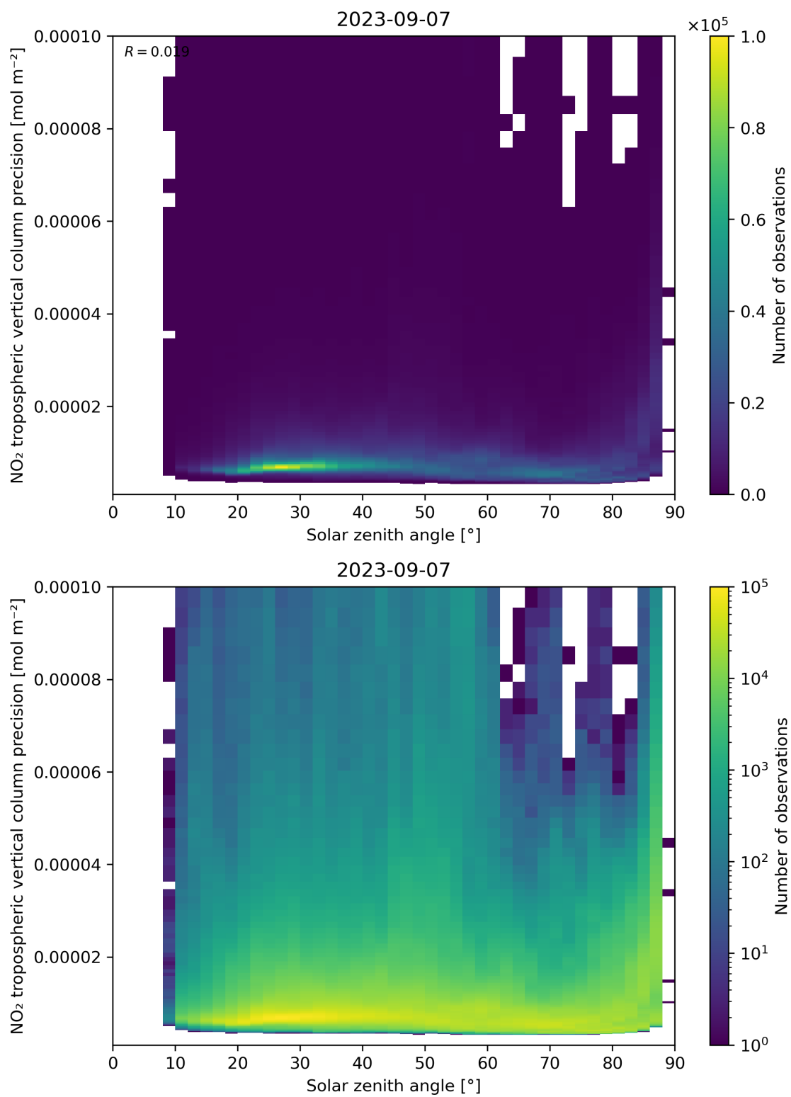
Figure 156: Scatter density plot of “Solar zenith angle” against “NO 2 tropospheric vertical column precision” for 2023-09-06 to 2023-09-08.
