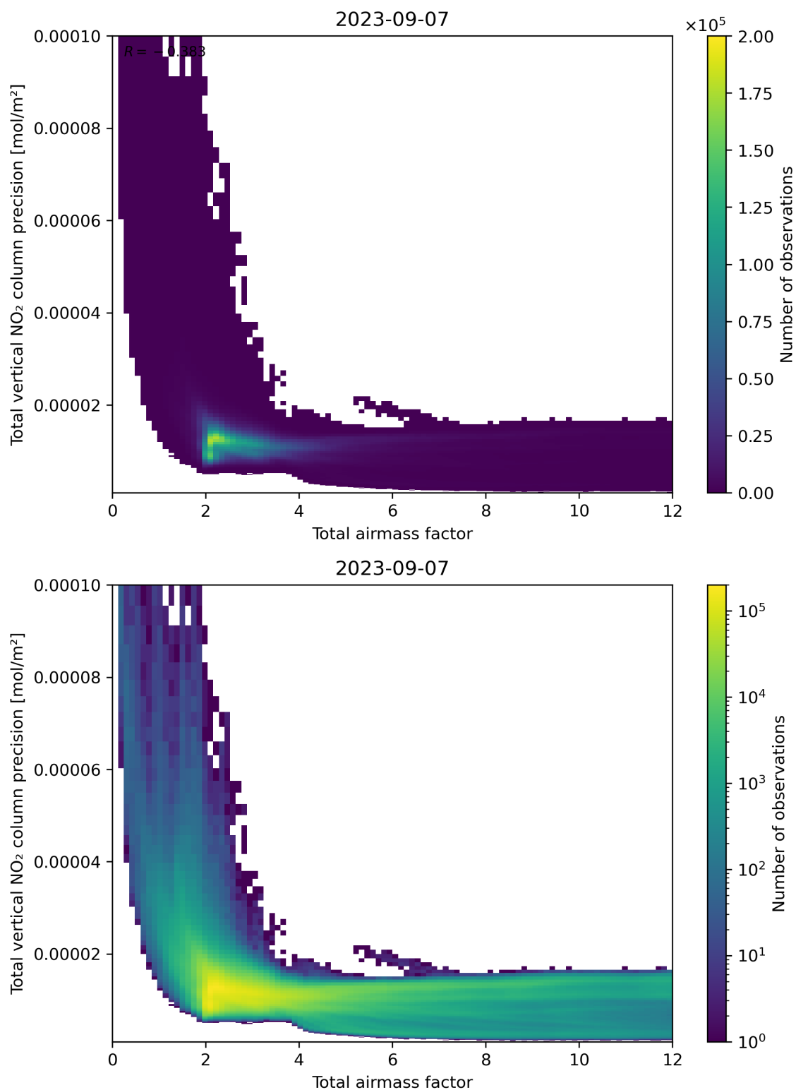
Figure 68: Scatter density plot of “Total airmass factor” against “Total vertical NO 2 column precision” for 2023-09-06 to 2023-09-08.
