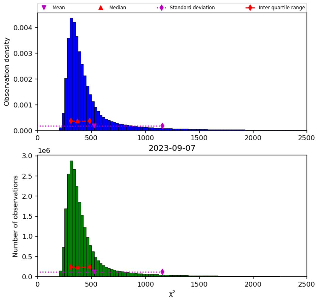
Figure 42: Histogram of “ \chi^2 ” for 2023-09-06 to 2023-09-08
