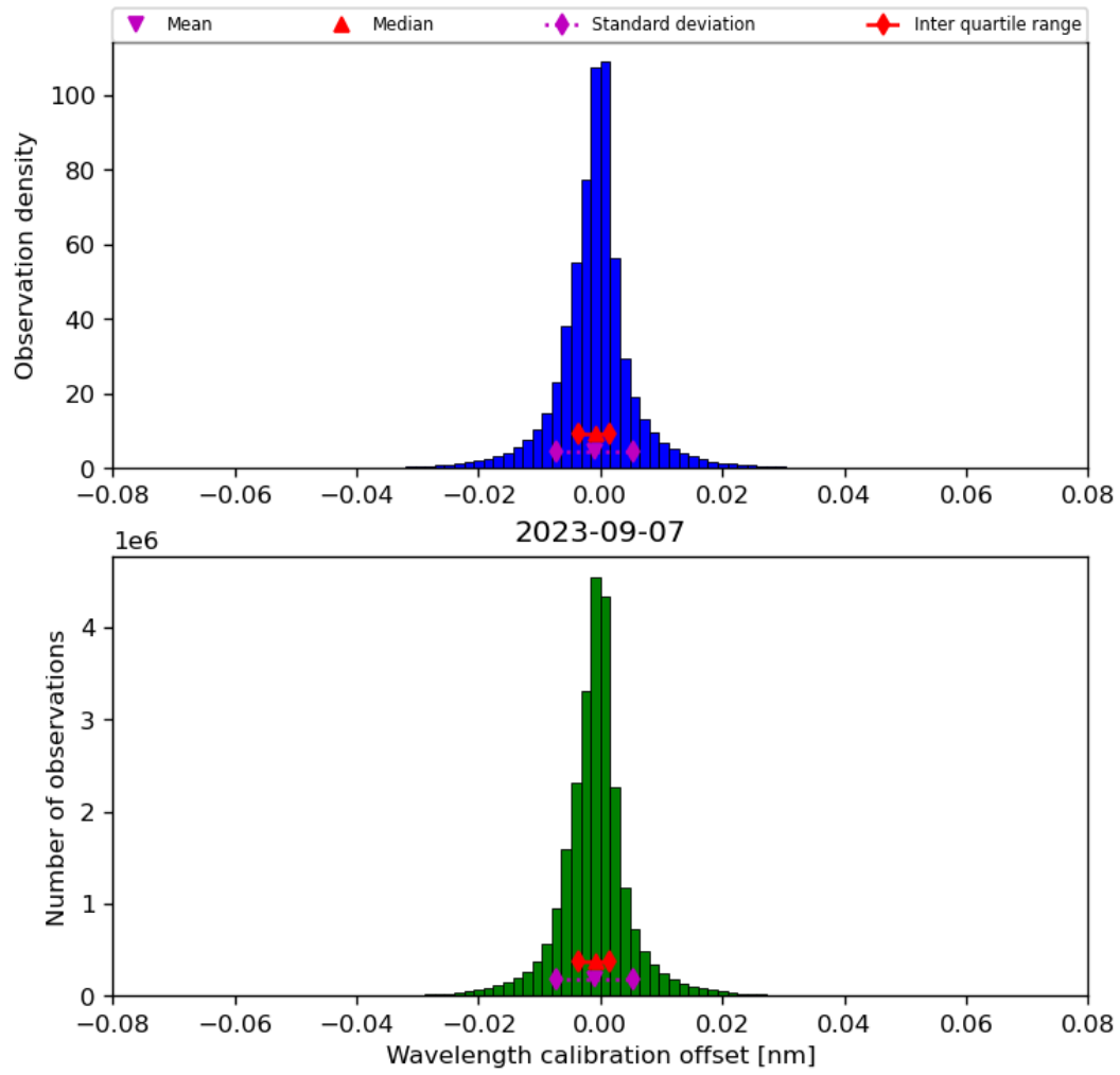
Figure 35: Histogram of “Wavelength calibration offset” for 2023-09-06 to 2023-09-08
