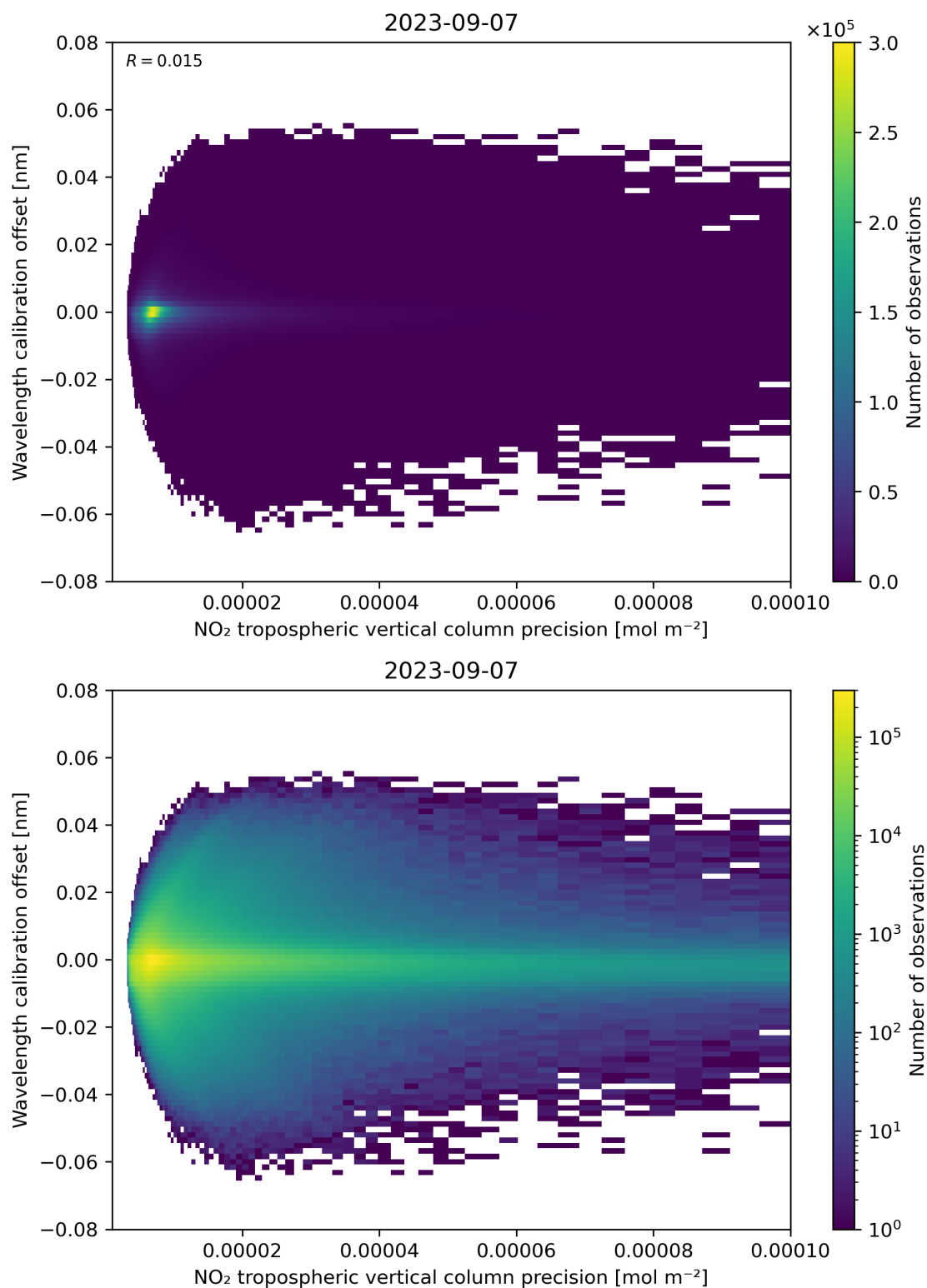
Figure 141: Scatter density plot of “NO 2 tropospheric vertical column precision” against “Wavelength calibration offset” for 2023-09-06 to 2023-09-08.
