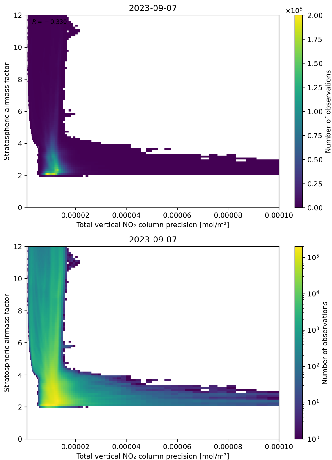
Figure 115: Scatter density plot of “Total vertical NO 2 column precision” against “Stratospheric airmass factor” for 2023-09-06 to 2023-09-08.
