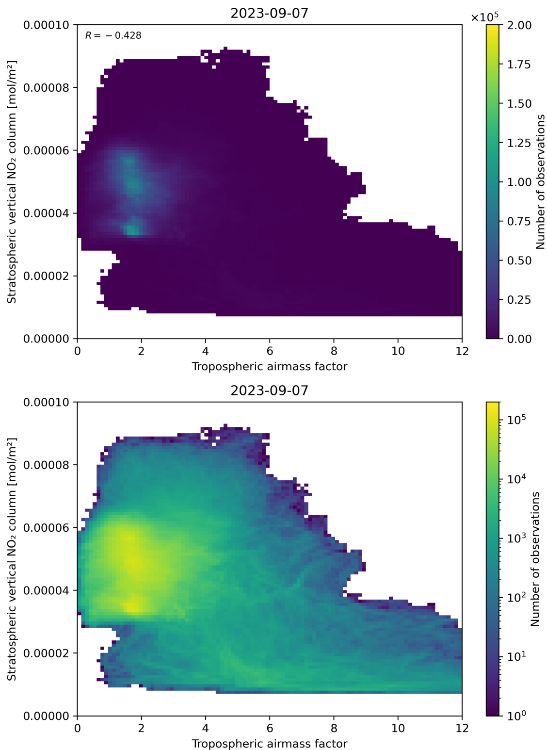
Figure 74: Scatter density plot of “Tropospheric air mass factor” against “Stratospheric vertical NO 2 column” for 2023-09-06 to 2023-09-08.
