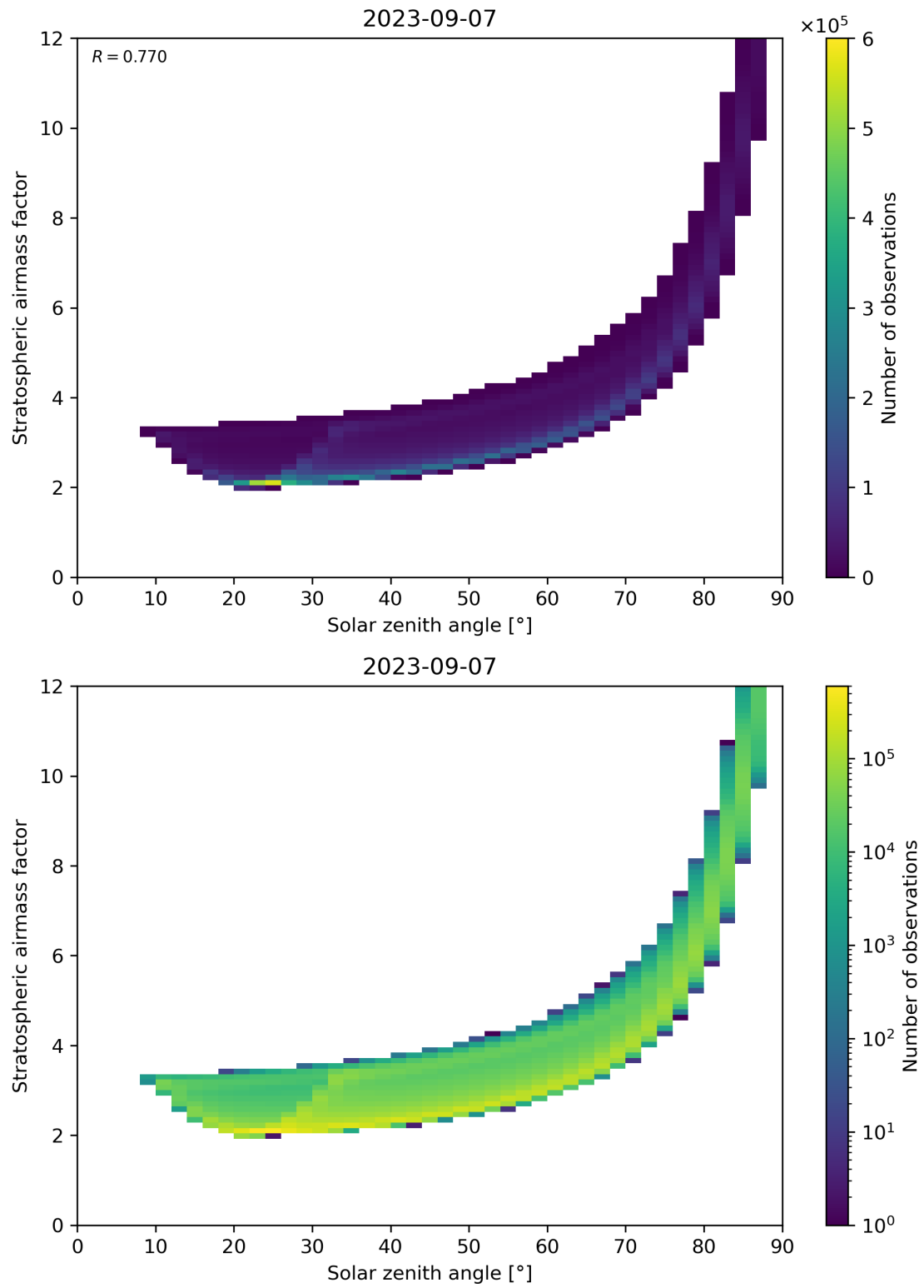
Figure 145: Scatter density plot of “Solar zenith angle” against “Stratospheric airmass factor” for 2023-09-06 to 2023-09-08.
