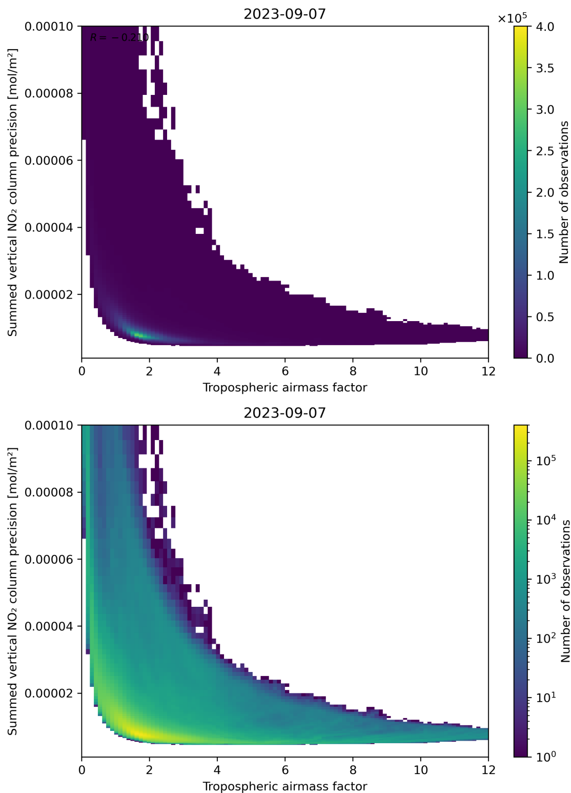
Figure 76: Scatter density plot of “Tropospheric air mass factor” against “Summed vertical NO 2 column precision” for 2023-09-06 to 2023-09-08.
