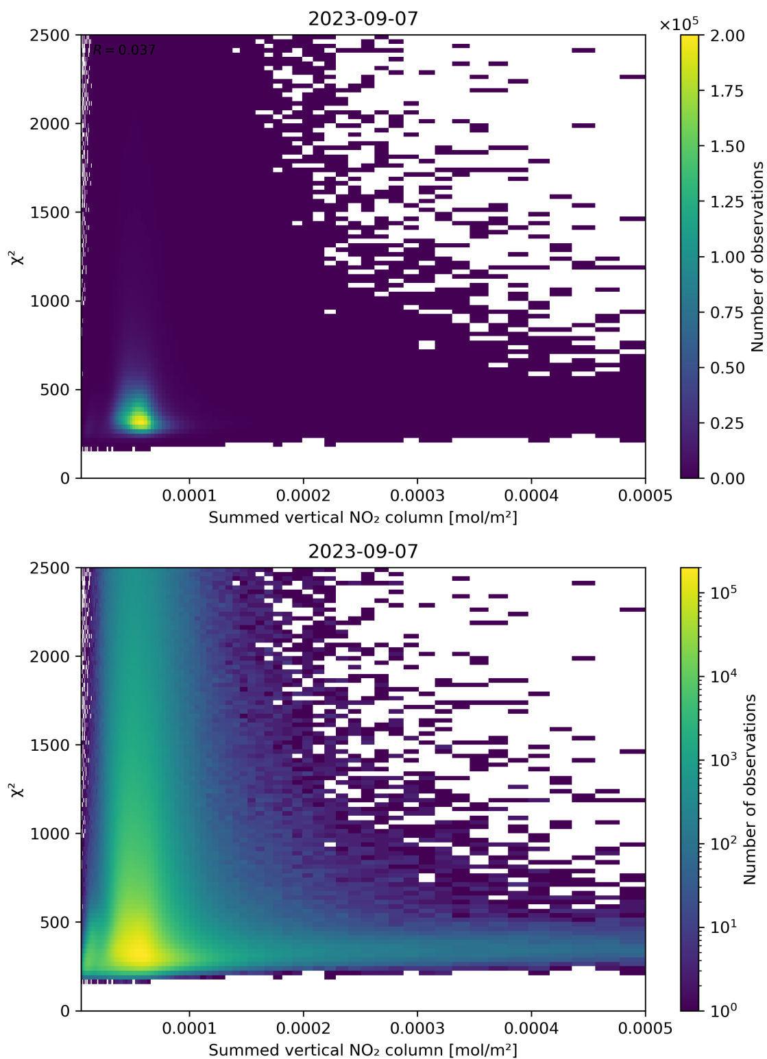
Figure 104: Scatter density plot of “Summed vertical NO 2 column” against “ \chi^2 ” for 2023-09-06 to 2023-09-08.
