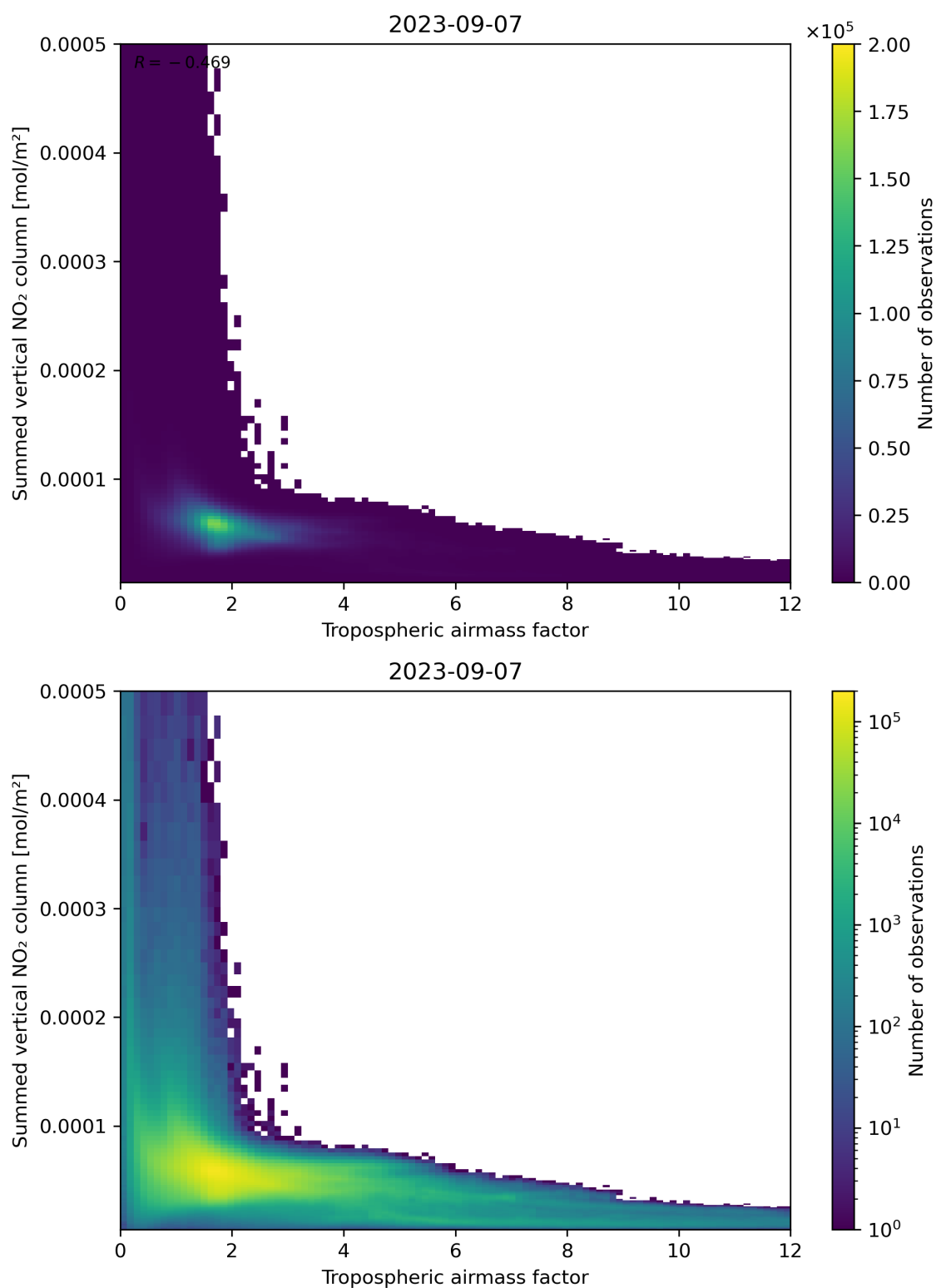
Figure 75: Scatter density plot of “Tropospheric airmass factor” against “Summed vertical NO 2 column” for 2023-09-06 to 2023-09-08.
