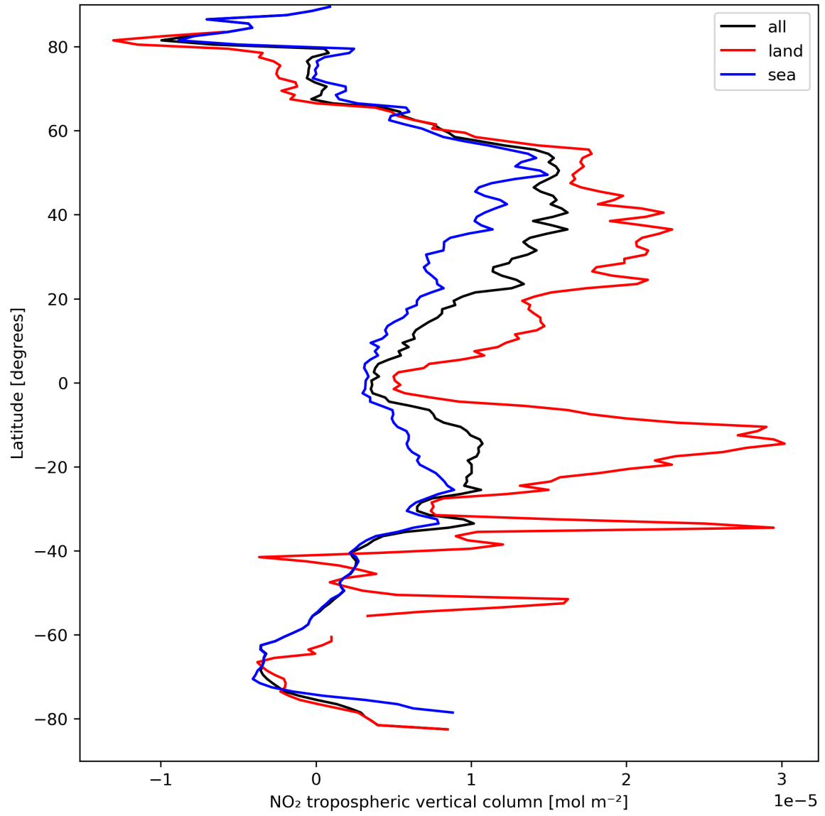
Figure 12: Zonal average of “NO 2 tropospheric vertical column” for 2023-09-06 to 2023-09-08.
