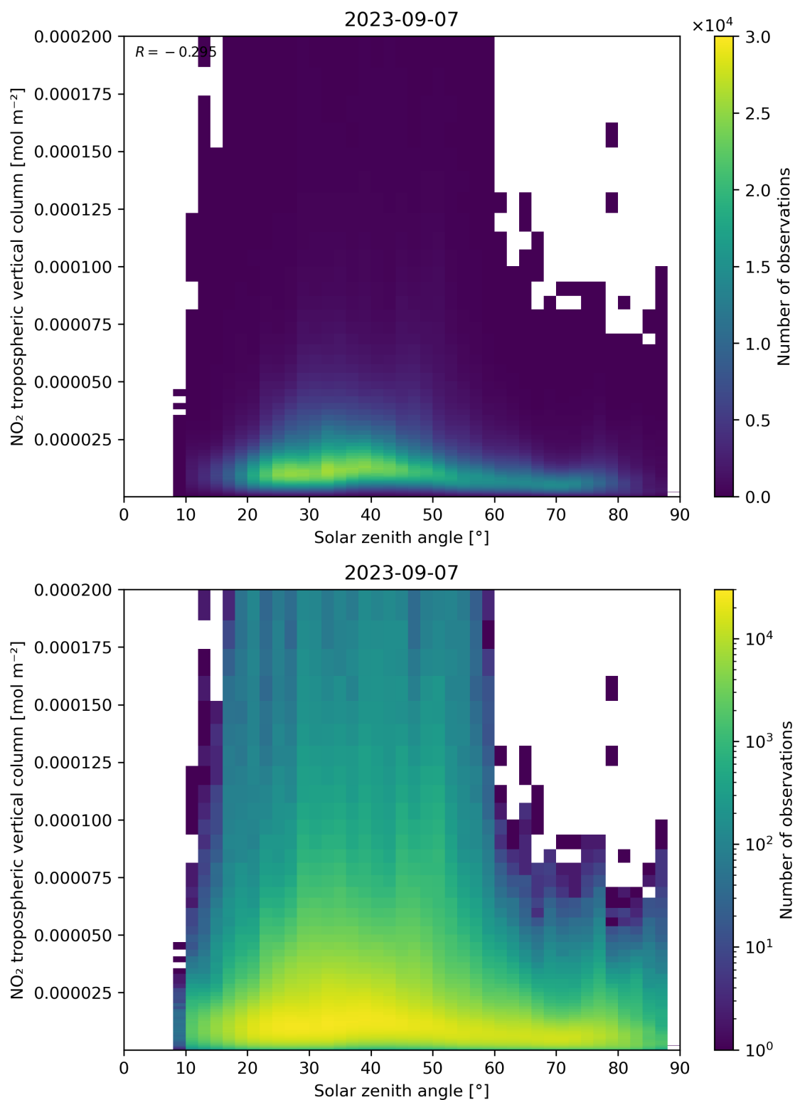
Figure 155: Scatter density plot of “Solar zenith angle” against “NO 2 tropospheric vertical column” for 2023-09-06 to 2023-09-08.
