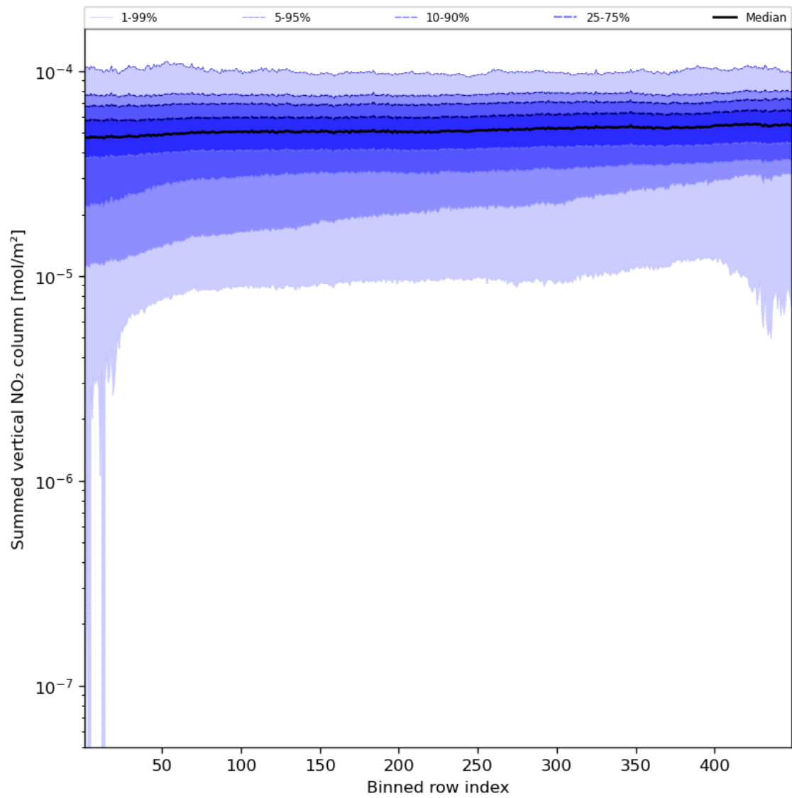
Figure 57: Along track statistics of “Summed vertical NO 2 column” for 2023-09-06 to 2023-09-08
