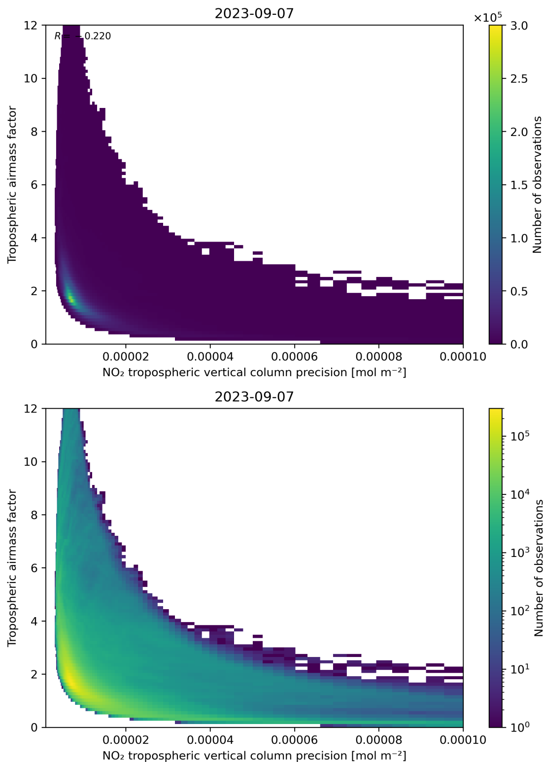
Figure 133: Scatter density plot of “NO 2 tropospheric vertical column precision” against “Tropospheric airmass factor” for 2023-09-06 to 2023-09-08.
