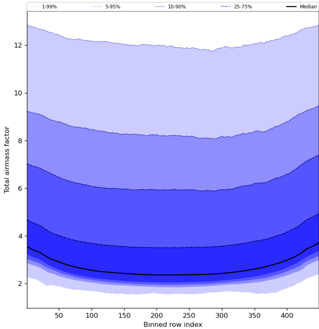
Figure 49: Along track statistics of “Total airmass factor” for 2023-09-06 to 2023-09-08
