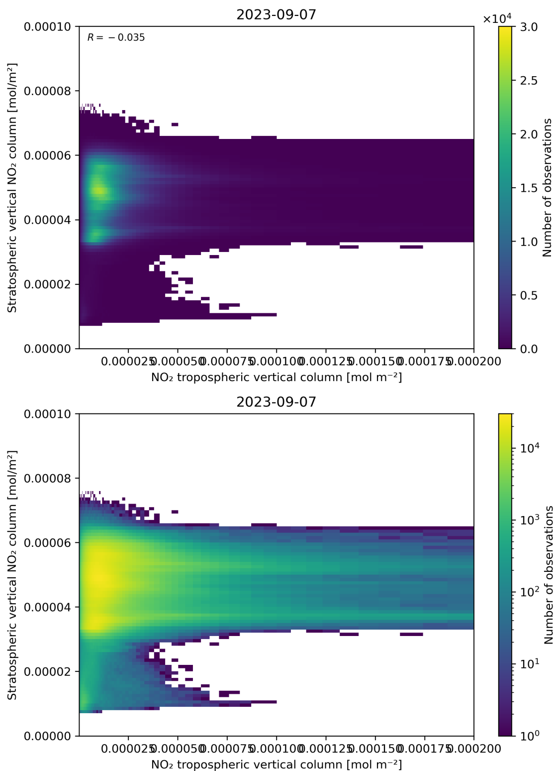
Figure 125: Scatter density plot of “NO 2 tropospheric vertical column” against “Stratospheric vertical NO 2 column” for 2023-09-06 to 2023-09-08.
