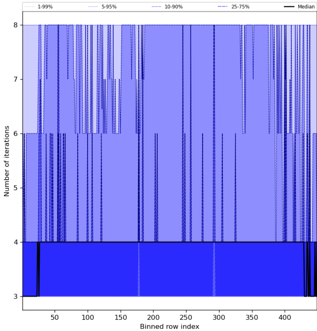
Figure 51: Along track statistics of “Number of iterations” for 2023-09-06 to 2023-09-08
