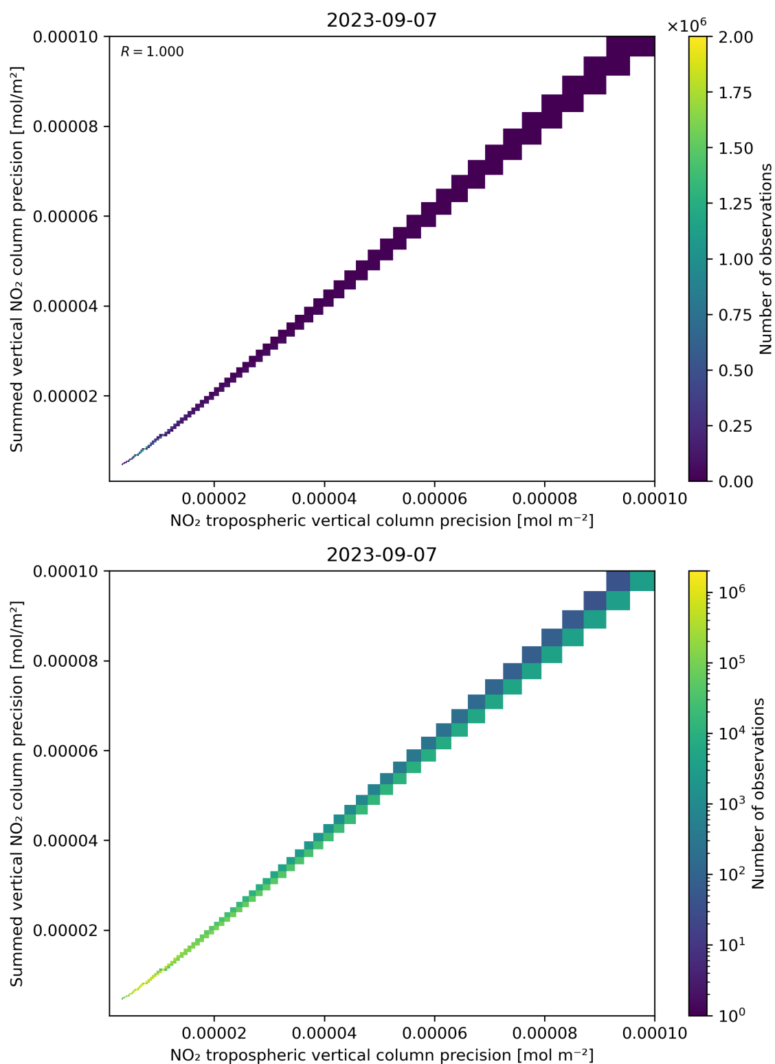
Figure 137: Scatter density plot of “NO 2 tropospheric vertical column precision” against “Summed vertical NO 2 column precision” for 2023-09-06 to 2023-09-08.
