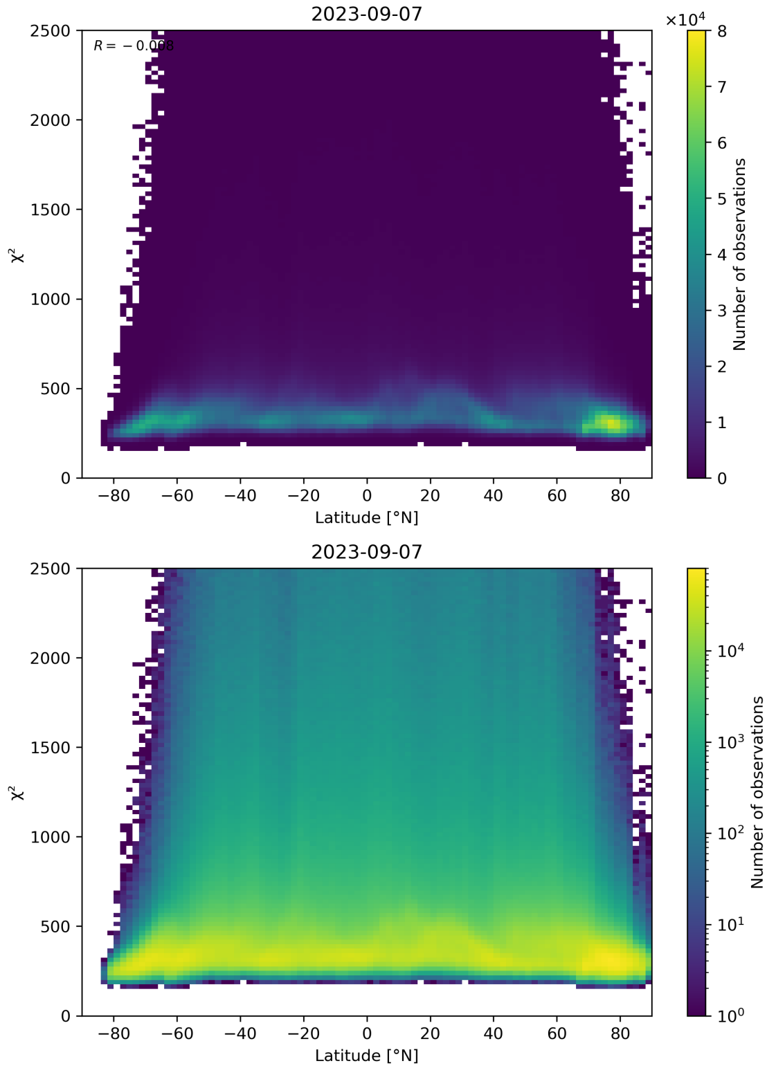
Figure 86: Scatter density plot of “Latitude” against “ \chi^2 ” for 2023-09-06 to 2023-09-08.
