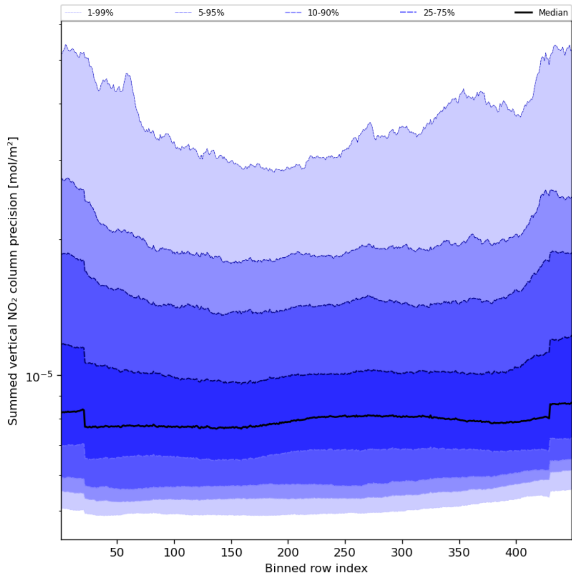
Figure 58: Along track statistics of “Summed vertical NO 2 column precision” for 2023-09-06 to 2023-09-08
