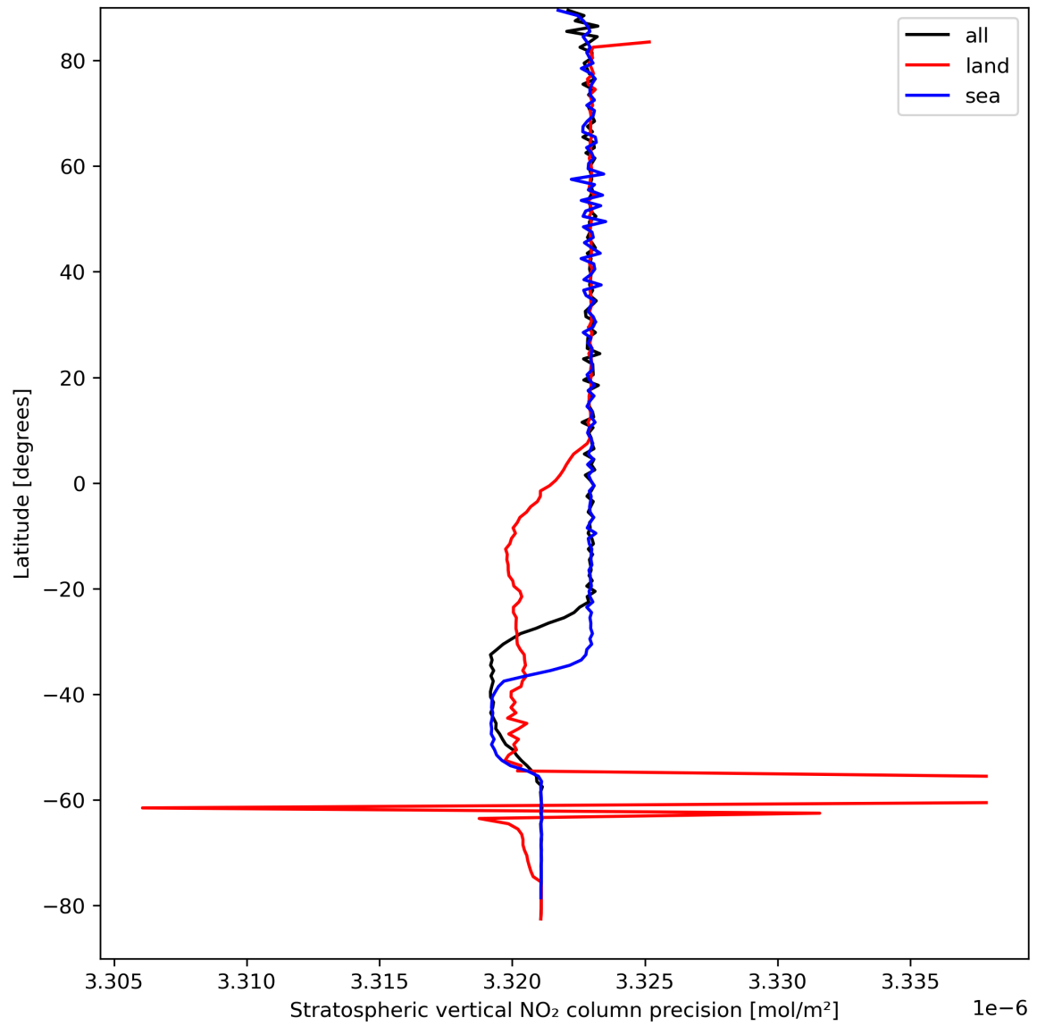
Figure 20: Zonal average of “Stratospheric vertical NO 2 column precision” for 2023-09-06 to 2023-09-08.
