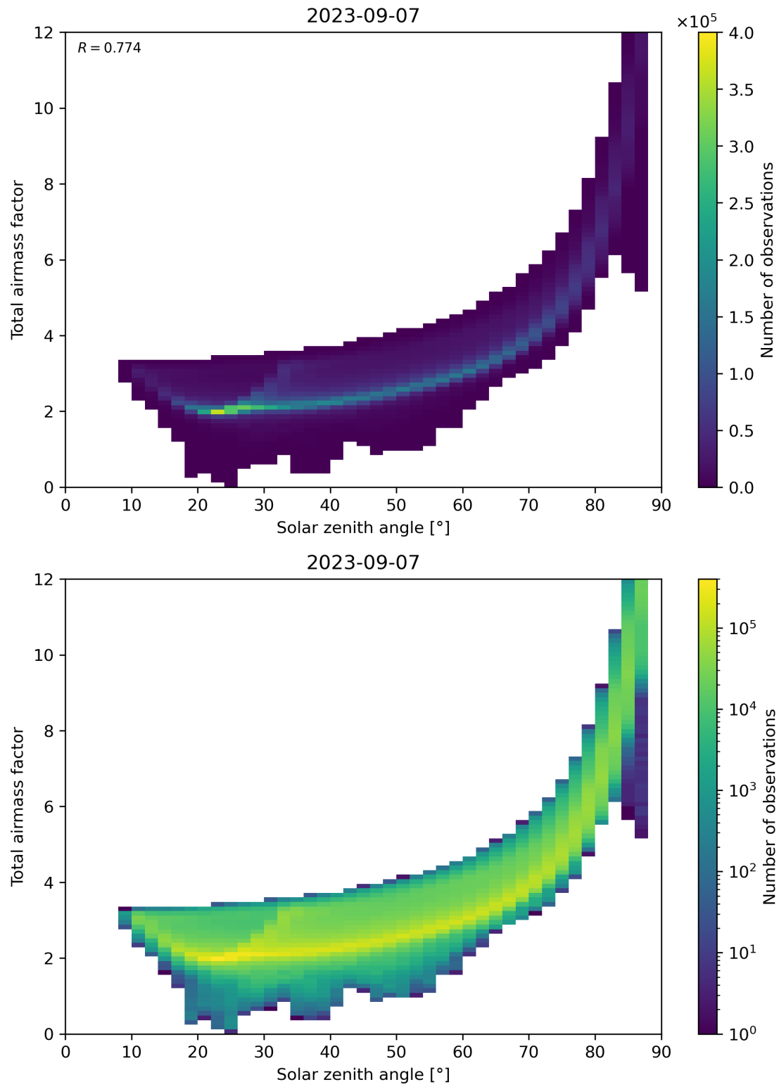
Figure 146: Scatter density plot of “Solar zenith angle” against “Total airmass factor” for 2023-09-06 to 2023-09-08.
