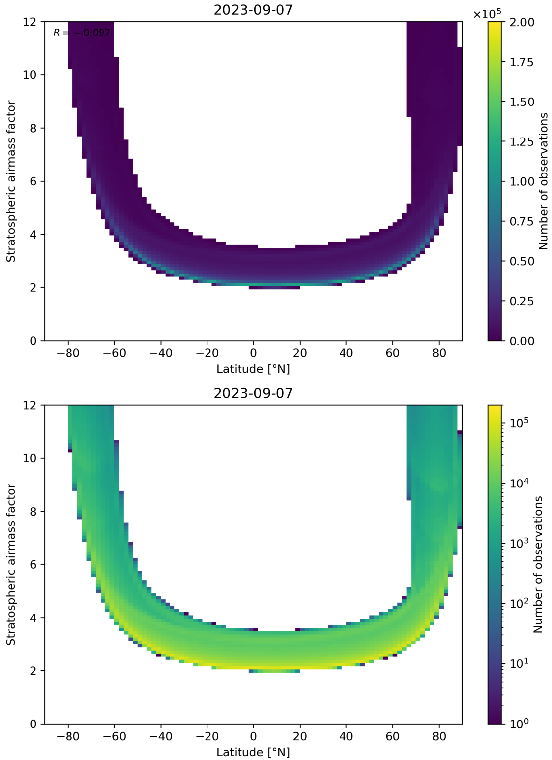
Figure 83: Scatter density plot of “Latitude” against “Stratospheric airmass factor” for 2023-09-06 to 2023-09-08.
