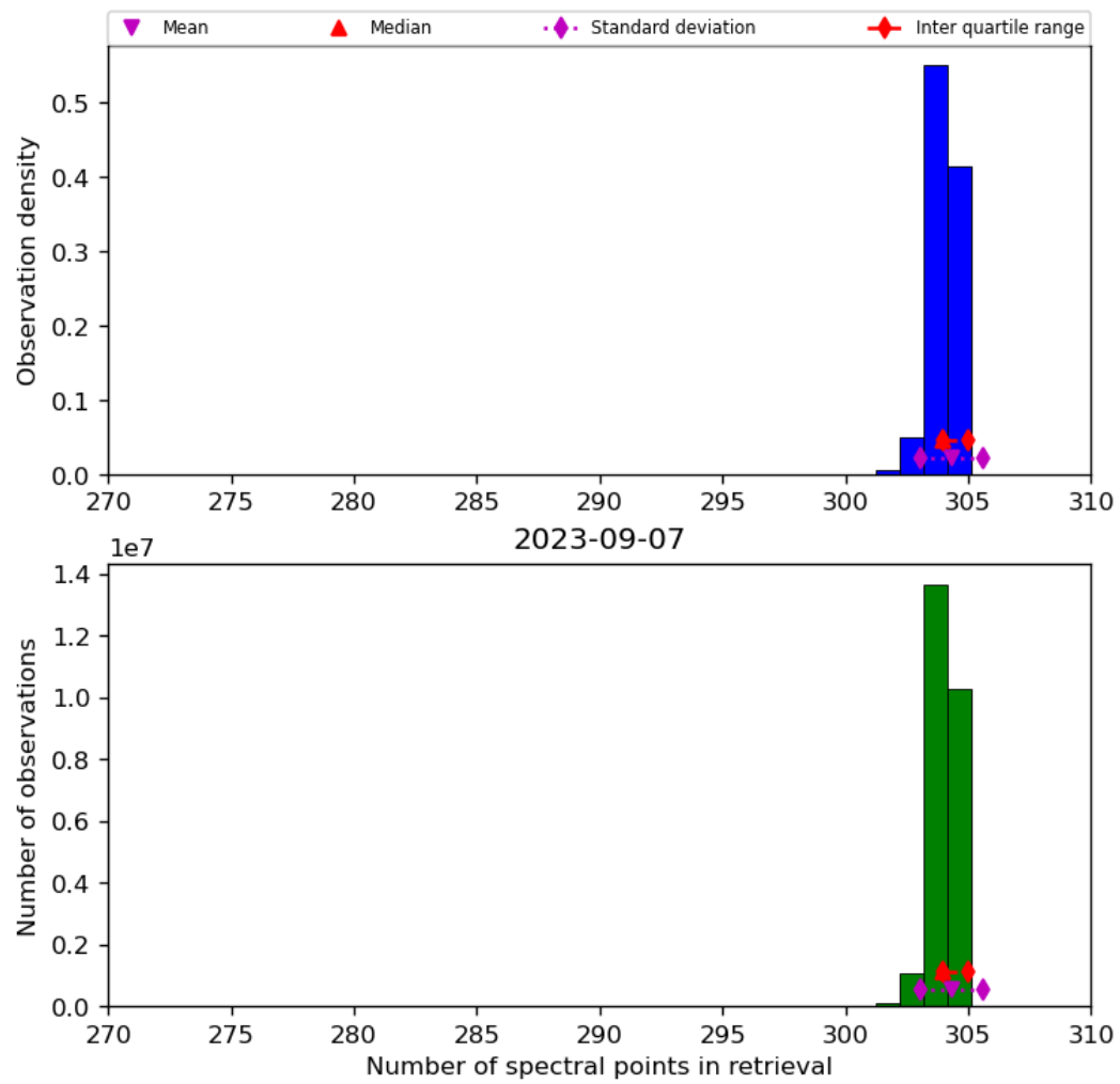
Figure 33: Histogram of “Number of spectral points in retrieval” for 2023-09-06 to 2023-09-08
