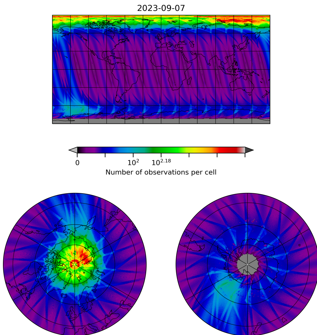
Figure 10: Map of the number of observations for 2023-09-06 to 2023-09-08
