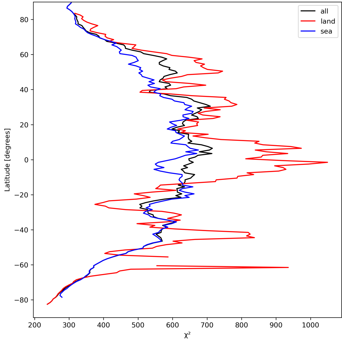
Figure 25: Zonal average of “ \chi^2 ” for 2023-09-06 to 2023-09-08.
