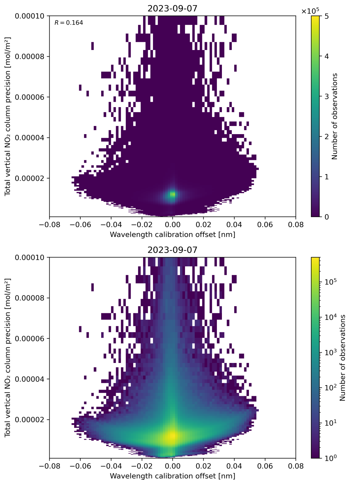
Figure 180: Scatter density plot of “Wavelength calibration offset” against “Total vertical NO 2 column precision” for 2023-09-06 to 2023-09-08.
