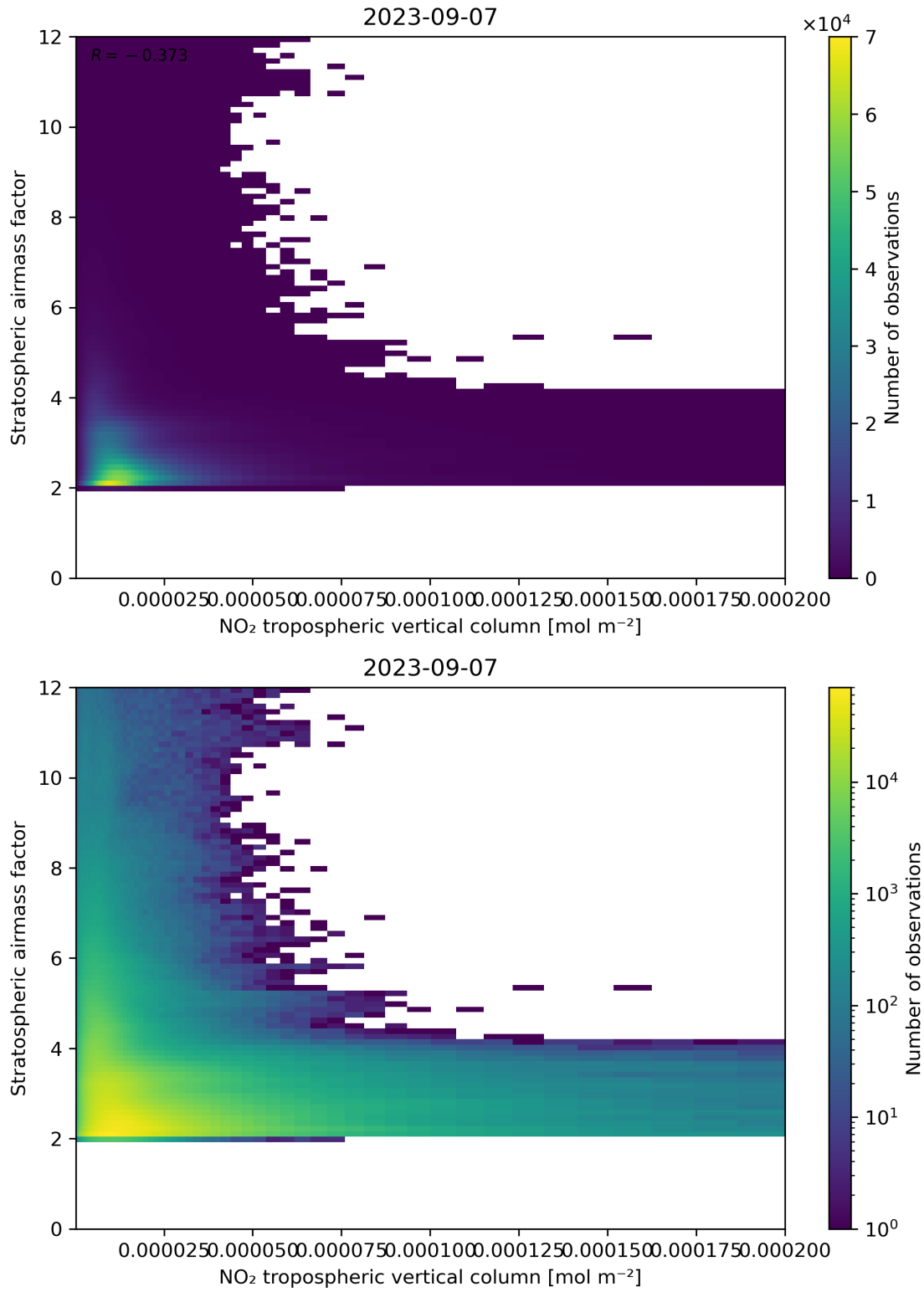
Figure 121: Scatter density plot of “NO 2 tropospheric vertical column” against “Stratospheric air mass factor” for 2023-09-06 to 2023-09-08.
