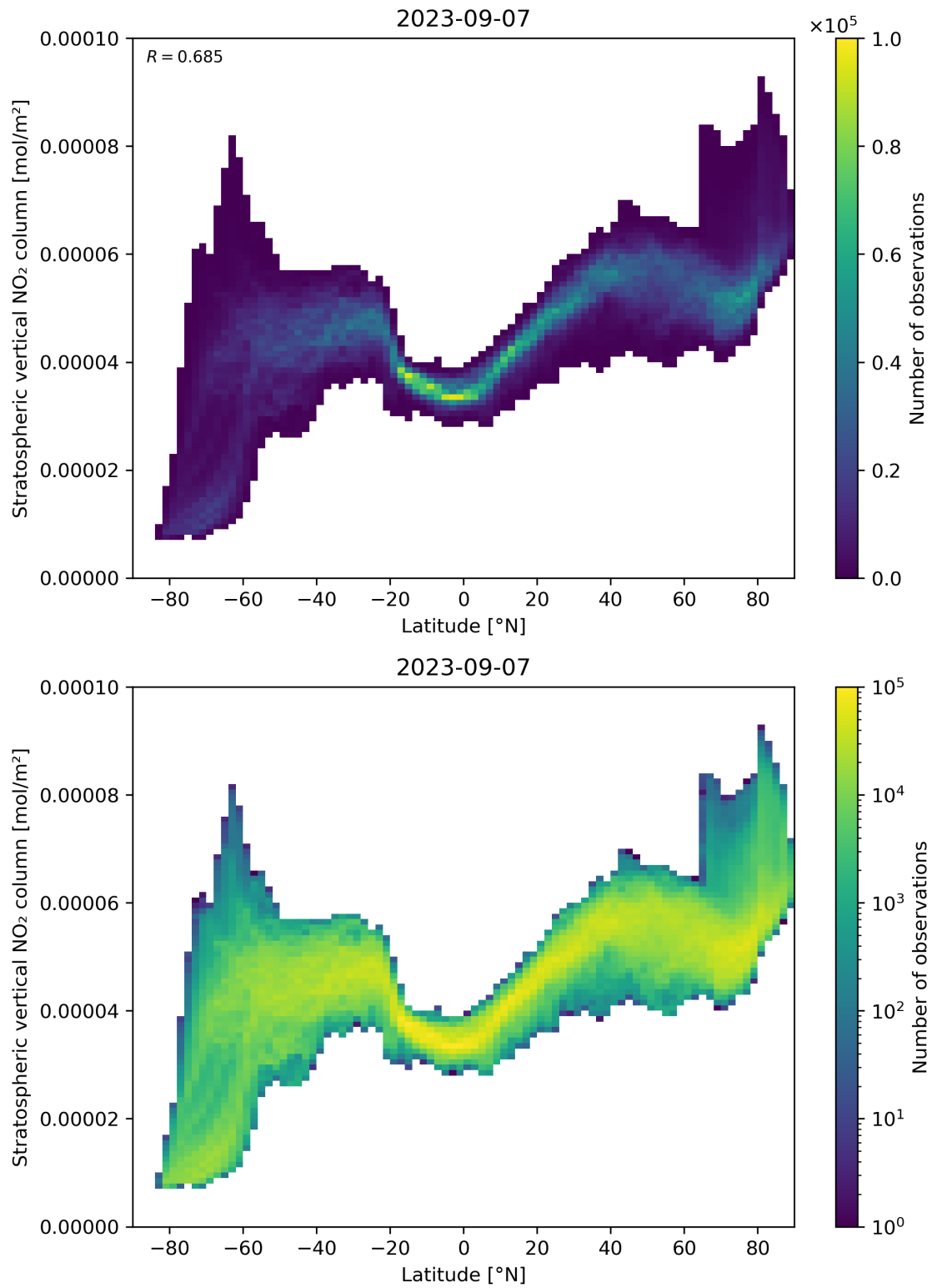
Figure 87: Scatter density plot of “Latitude” against “Stratospheric vertical \text{NO}_2 column” for 2023-09-06 to 2023-09-08.
