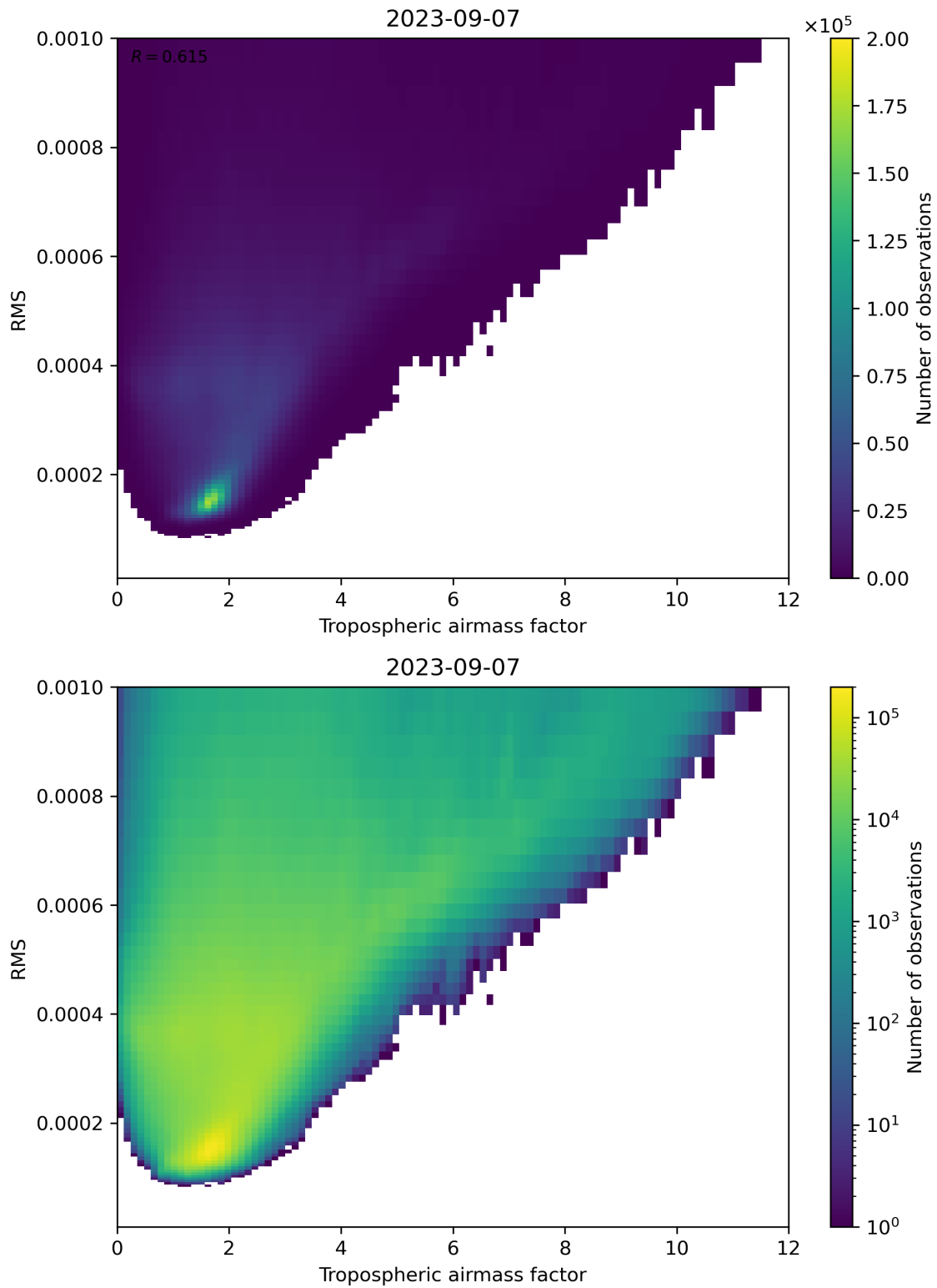
Figure 79: Scatter density plot of “Tropospheric airmass factor” against “RMS” for 2023-09-06 to 2023-09-08.
