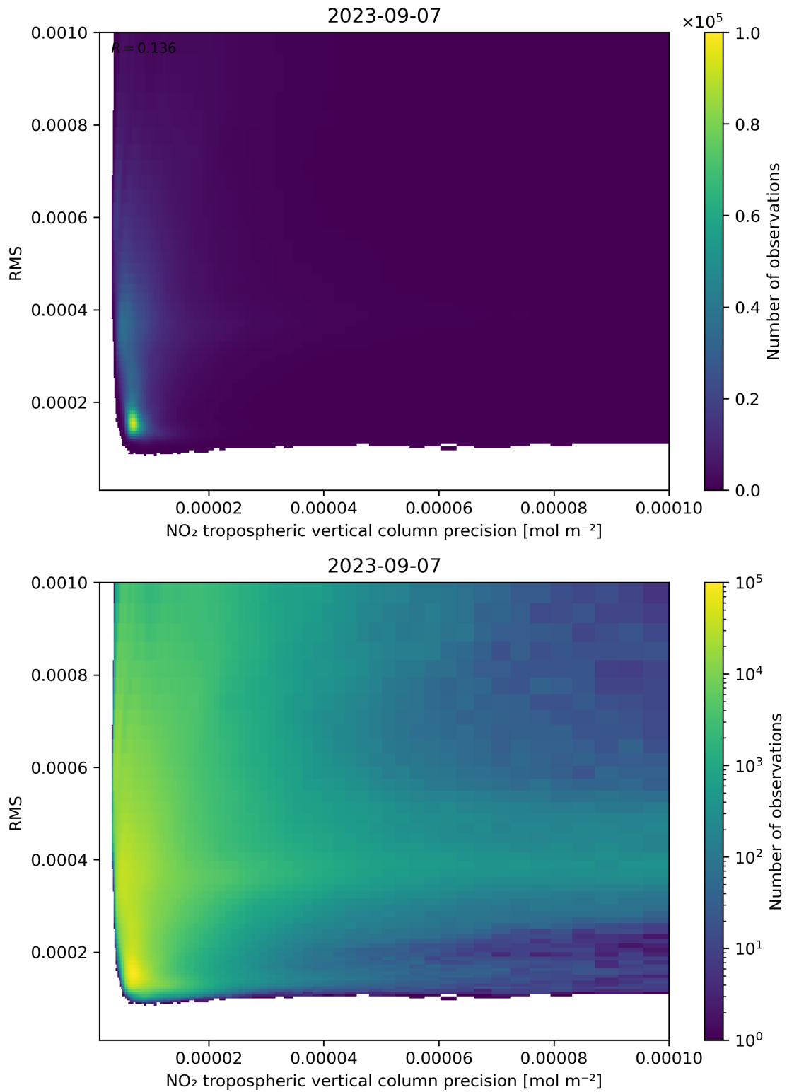
Figure 140: Scatter density plot of “NO 2 tropospheric vertical column precision” against “RMS” for 2023-09-06 to 2023-09-08.
