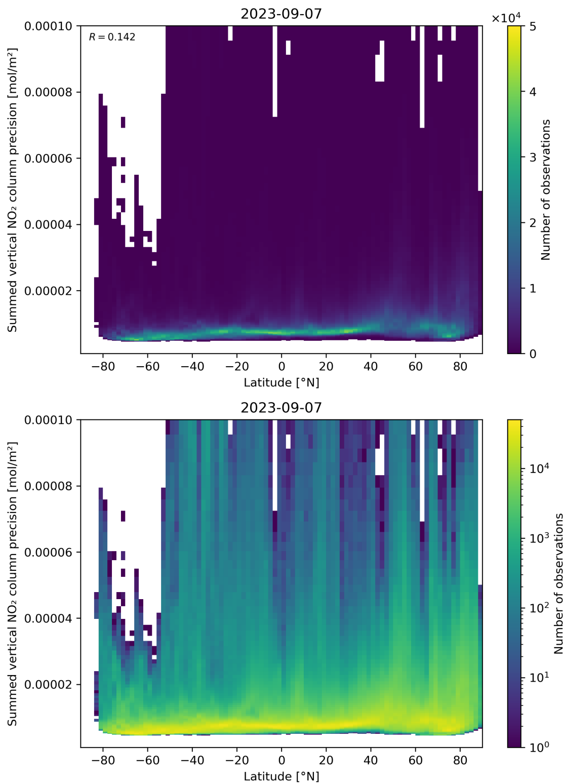
Figure 89: Scatter density plot of “Latitude” against “Summed vertical NO 2 column precision” for 2023-09-06 to 2023-09-08.
