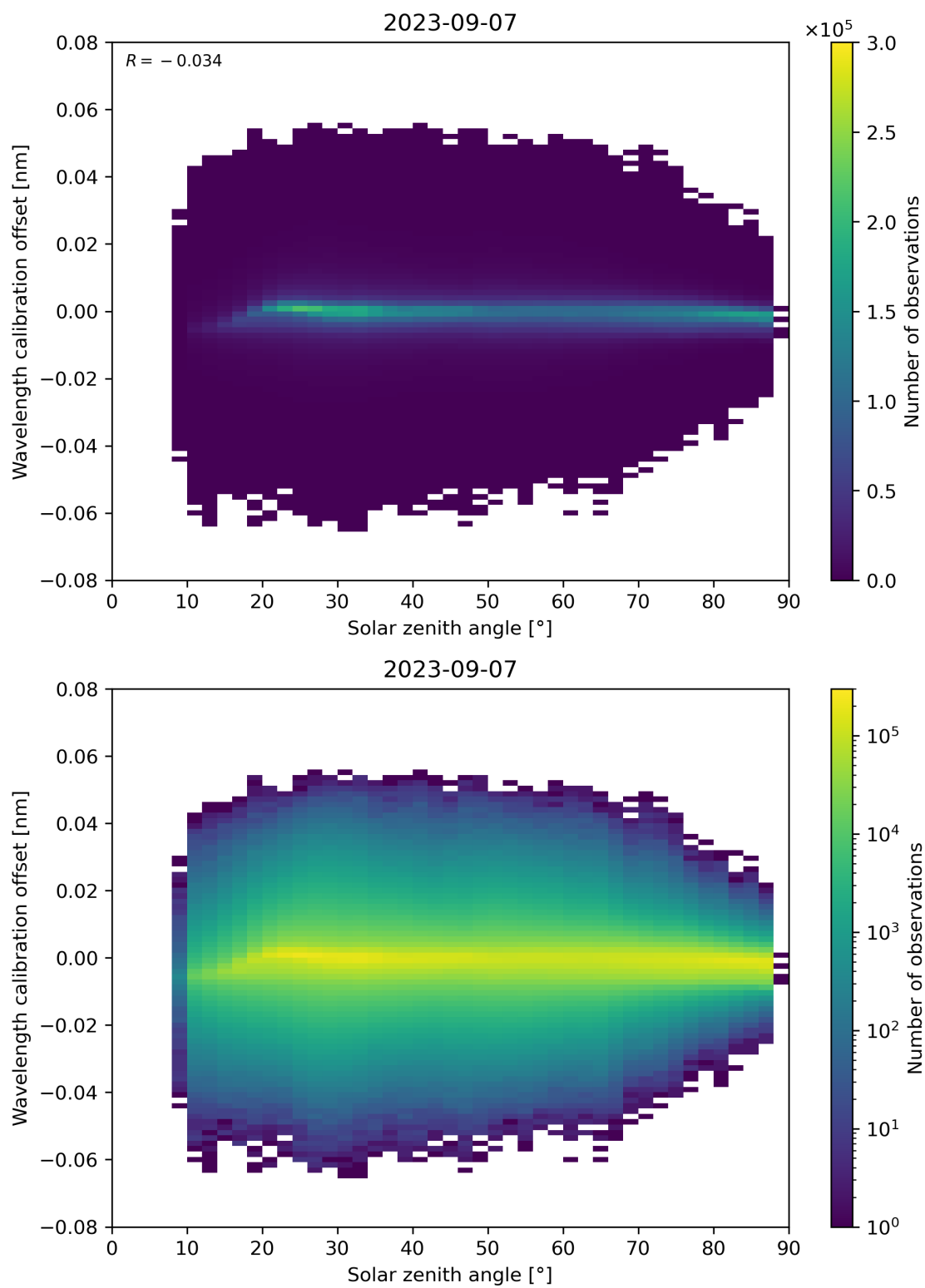
Figure 158: Scatter density plot of “Solar zenith angle” against “Wavelength calibration offset” for 2023-09-06 to 2023-09-08.
