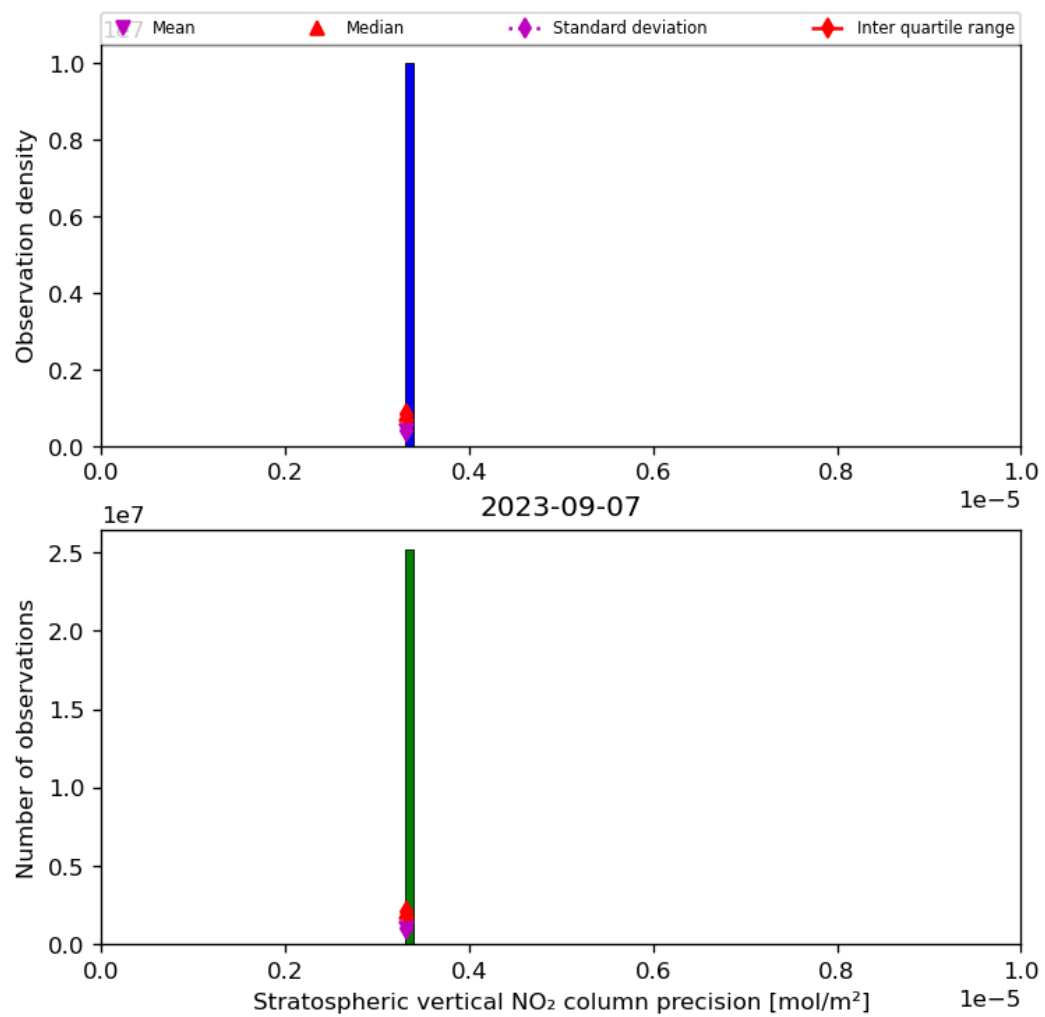
Figure 37: Histogram of “Stratospheric vertical NO 2 column precision” for 2023-09-06 to 2023-09-08
