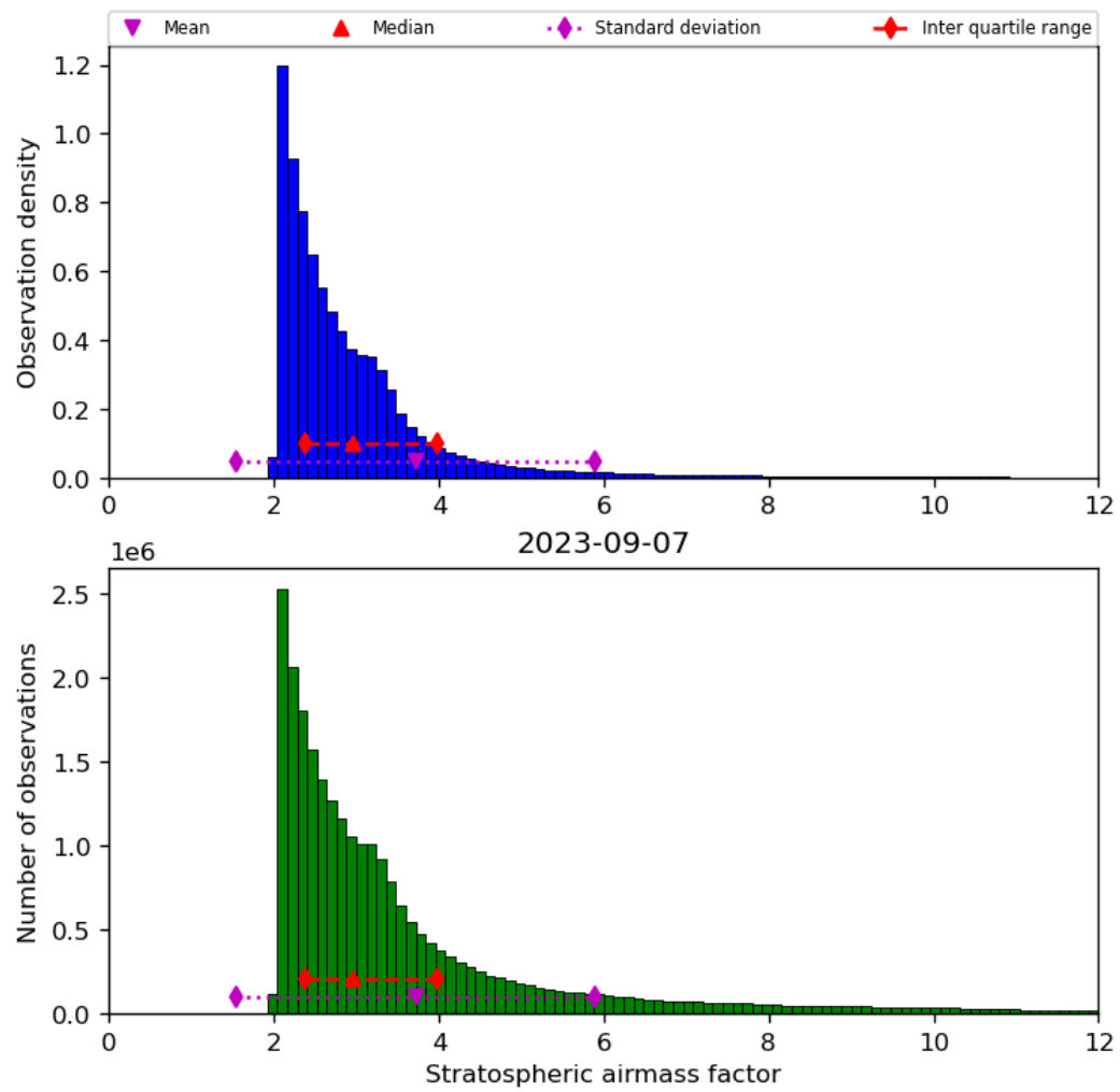
Figure 44: Histogram of “Stratospheric airmass factor” for 2023-09-06 to 2023-09-08
