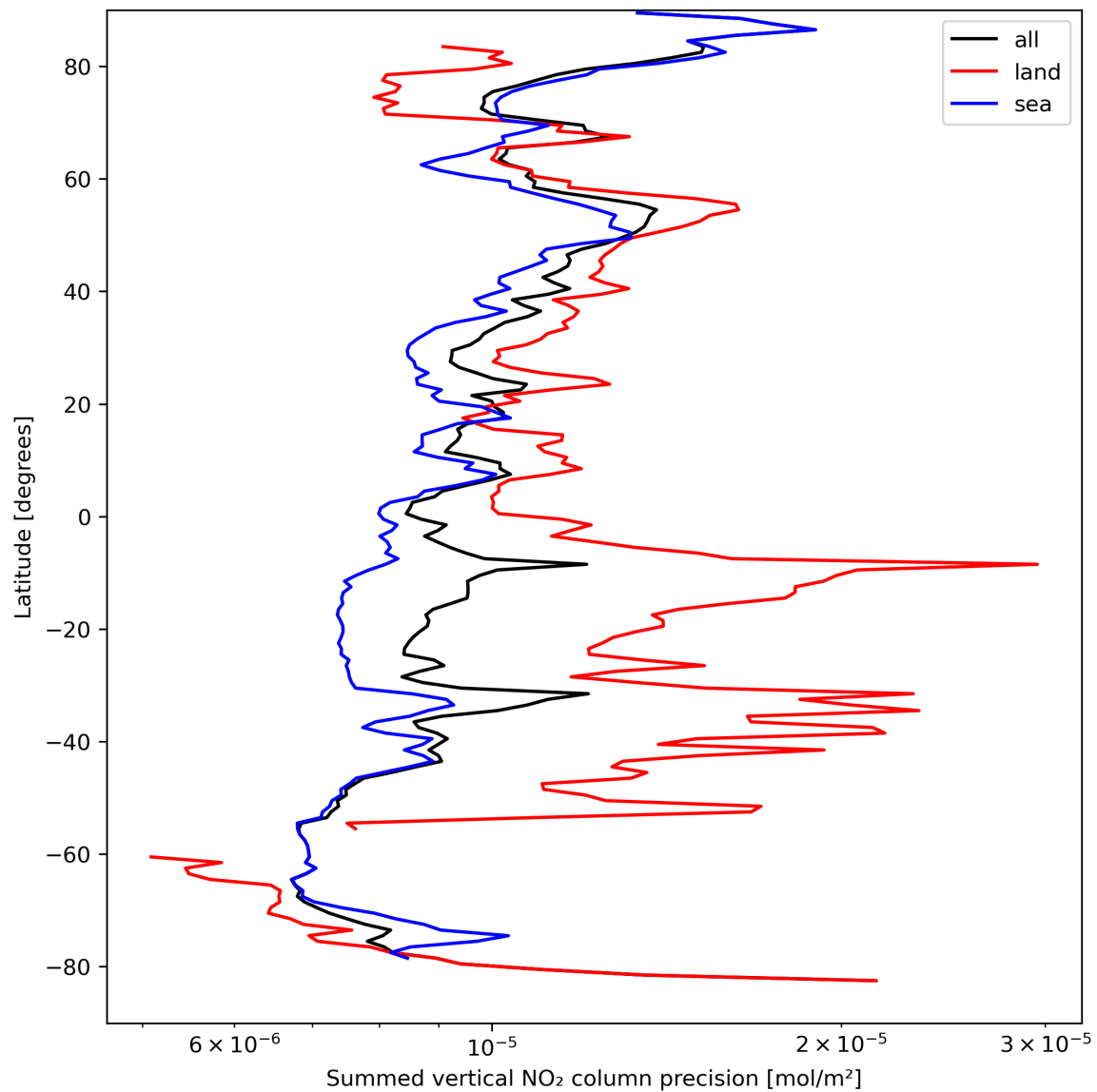
Figure 24: Zonal average of “Summed vertical NO 2 column precision” for 2023-09-06 to 2023-09-08.
