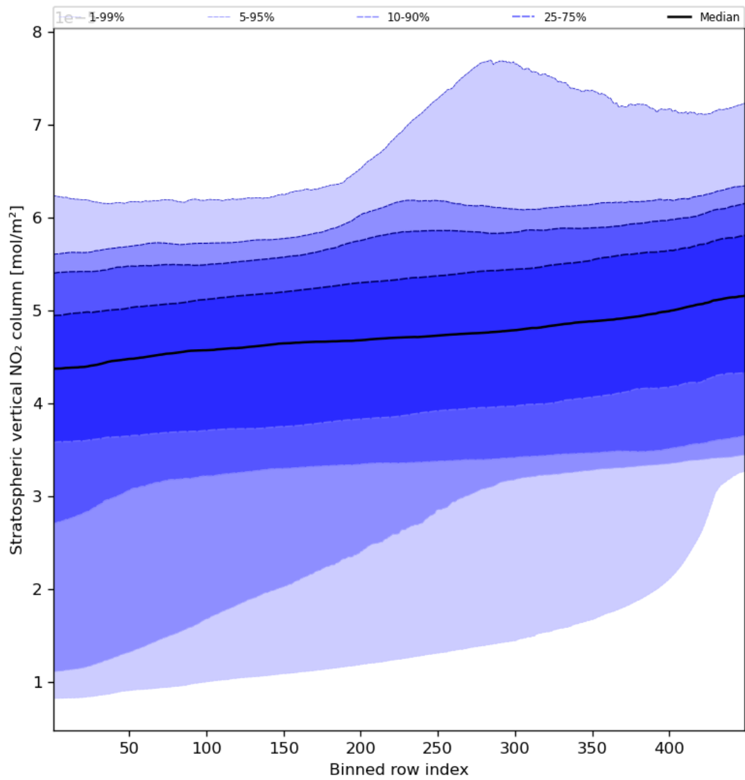
Figure 53: Along track statistics of “Stratospheric vertical NO 2 column” for 2023-09-06 to 2023-09-08
