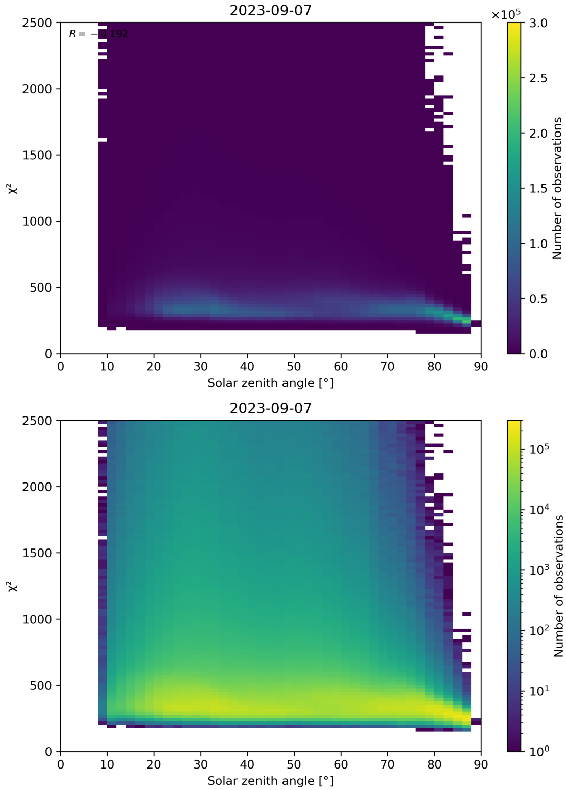
Figure 148: Scatter density plot of “Solar zenith angle” against “ \chi^2 ” for 2023-09-06 to 2023-09-08.
