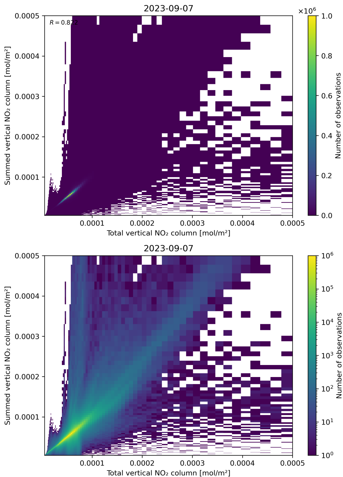
Figure 112: Scatter density plot of “Total vertical NO 2 column” against “Summed vertical NO 2 column” for 2023-09-06 to 2023-09-08.
