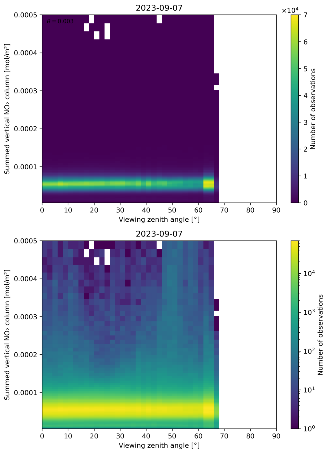
Figure 165: Scatter density plot of “Viewing zenith angle” against “Summed vertical NO 2 column” for 2023-09-06 to 2023-09-08.
