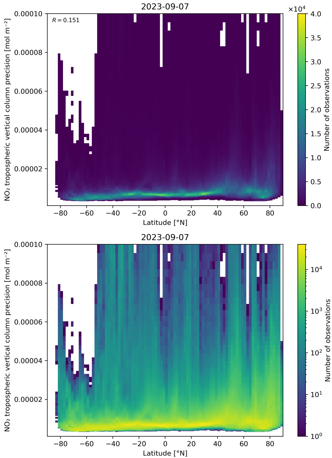
Figure 93: Scatter density plot of “Latitude” against “NO 2 tropospheric vertical column precision” for 2023-09-06 to 2023-09-08.
