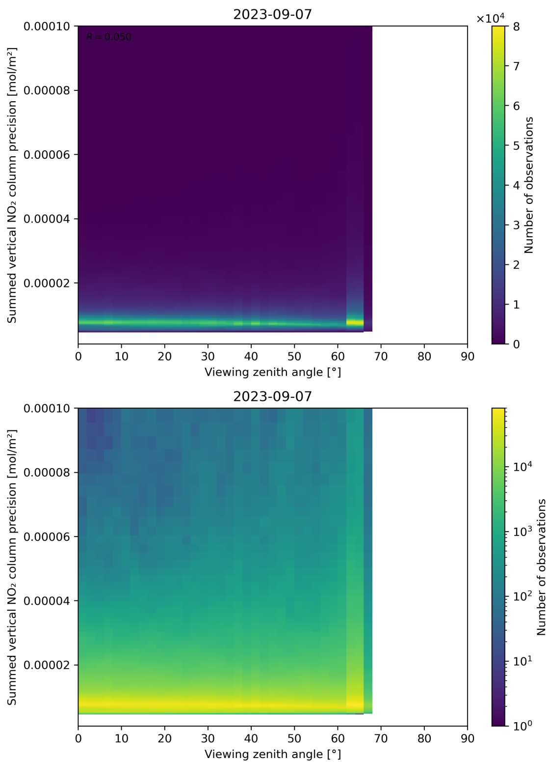
Figure 166: Scatter density plot of “Viewing zenith angle” against “Summed vertical NO 2 column precision” for 2023-09-06 to 2023-09-08.
