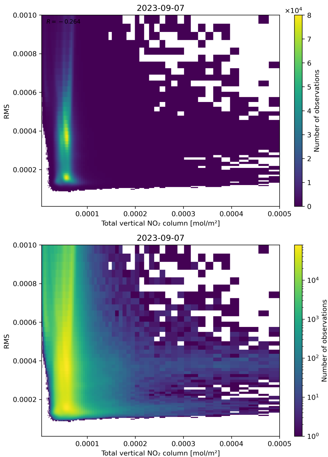
Figure 120: Scatter density plot of “Total vertical NO 2 column” against “RMS” for 2023-09-06 to 2023-09-08.
