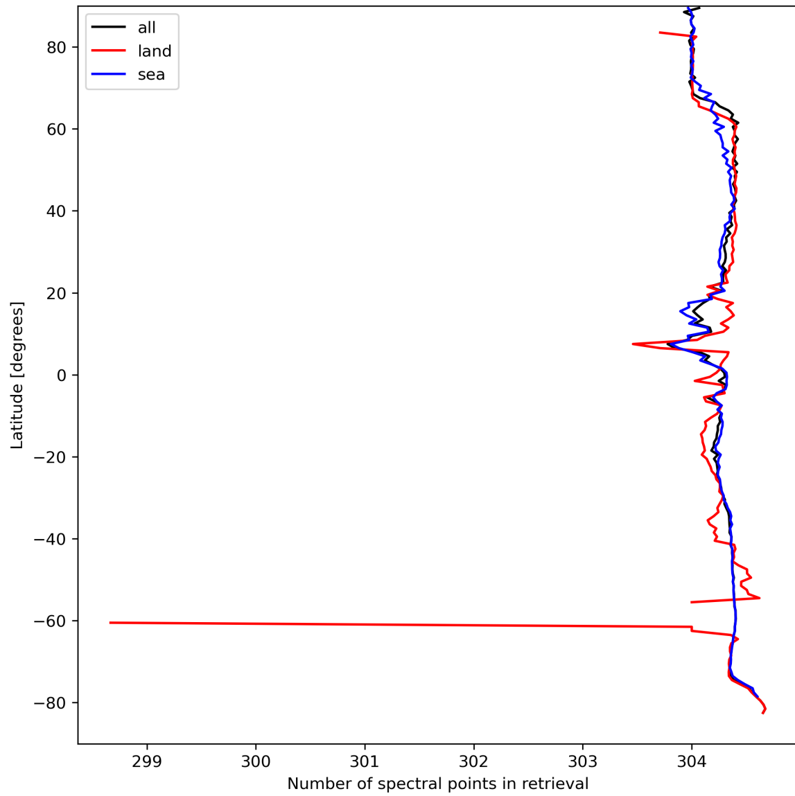
Figure 16: Zonal average of “Number of spectral points in retrieval” for 2023-09-06 to 2023-09-08.
