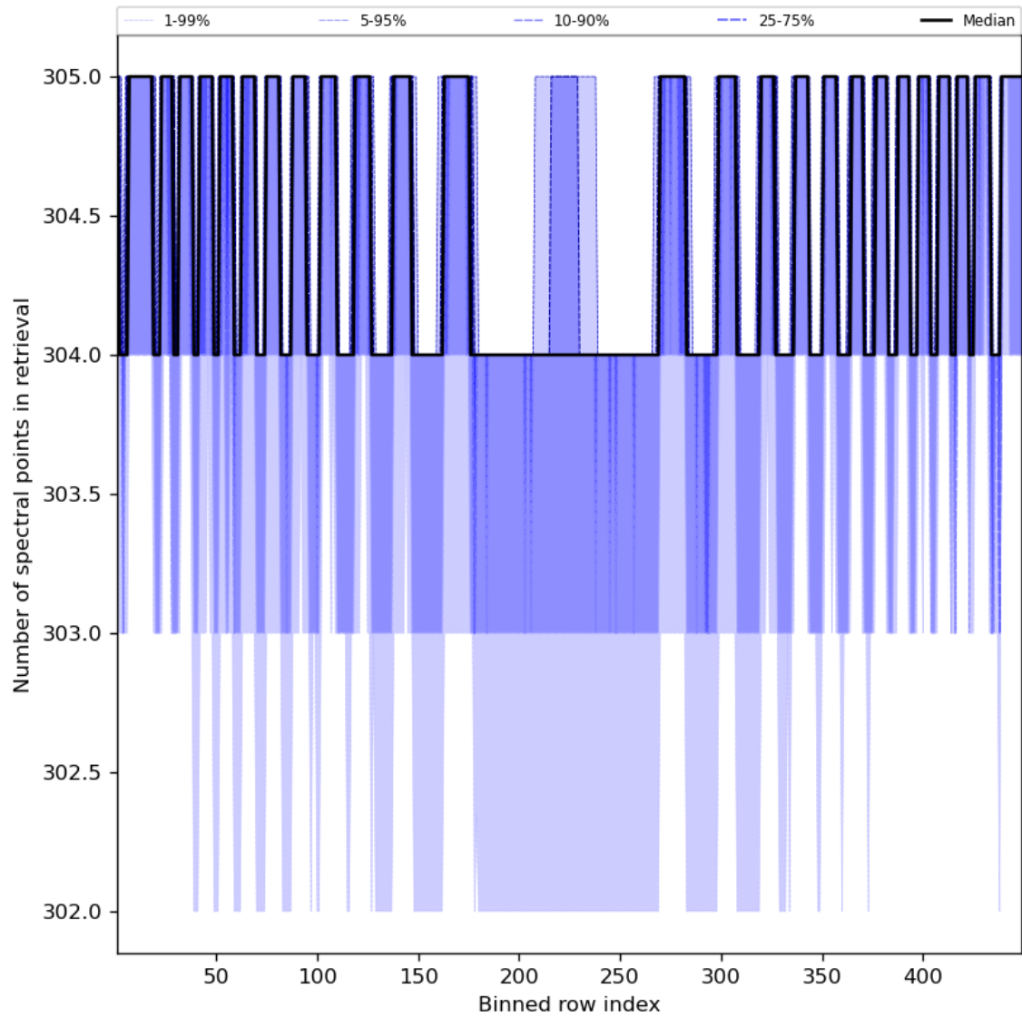
Figure 50: Along track statistics of “Number of spectral points in retrieval” for 2023-09-06 to 2023-09-08
