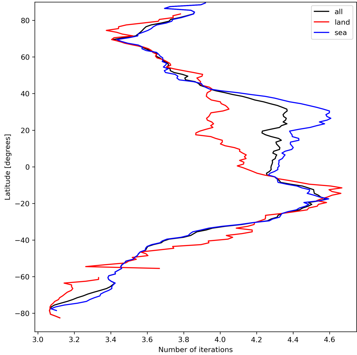
Figure 17: Zonal average of “Number of iterations” for 2023-09-06 to 2023-09-08.
