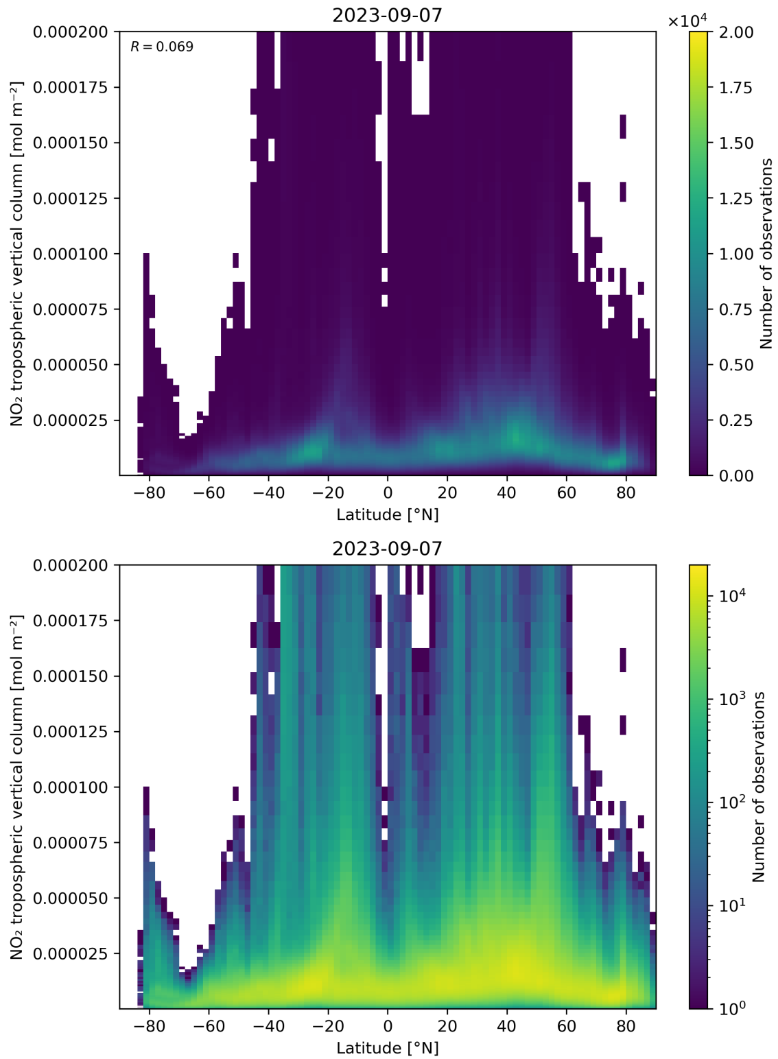
Figure 92: Scatter density plot of “Latitude” against “NO 2 tropospheric vertical column” for 2023-09-06 to 2023-09-08.
