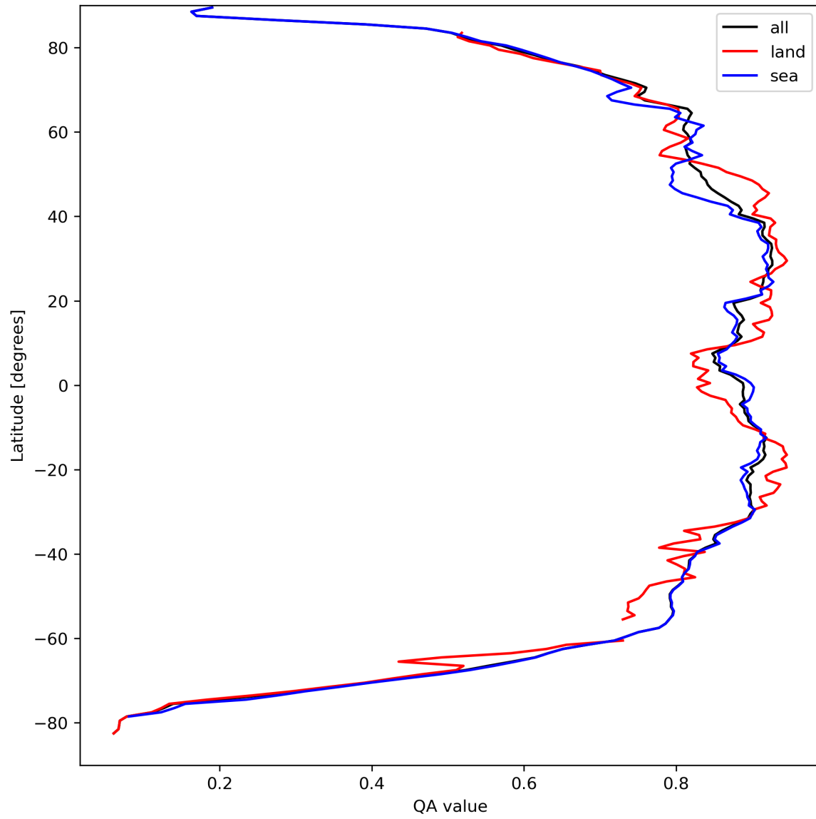
Figure 11: Zonal average of “QA value” for 2023-09-06 to 2023-09-08.
