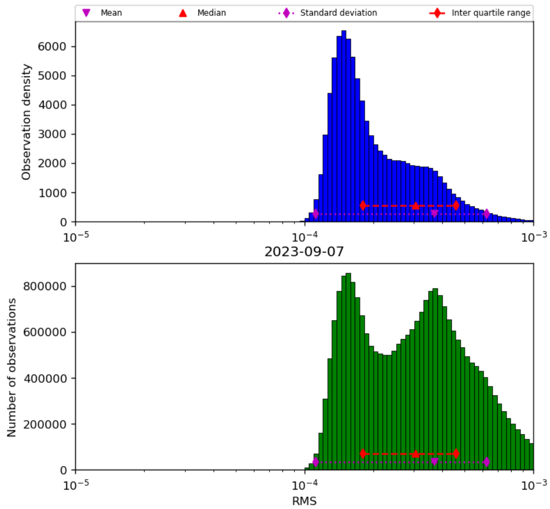
Figure 43: Histogram of “RMS” for 2023-09-06 to 2023-09-08
