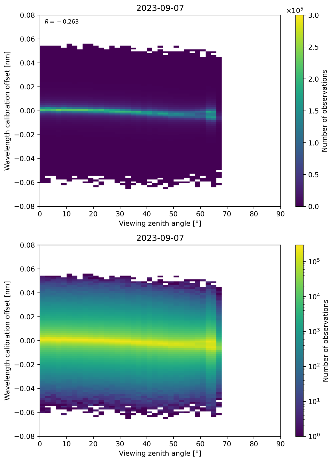
Figure 173: Scatter density plot of “Viewing zenith angle” against “Wavelength calibration offset” for 2023-09-06 to 2023-09-08.
