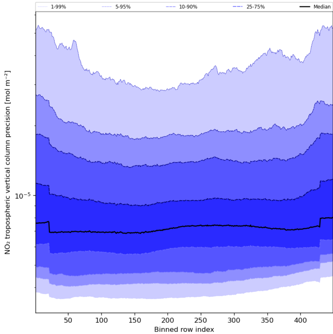
Figure 47: Along track statistics of “NO 2 tropospheric vertical column precision” for 2023-09-06 to 2023-09-08
