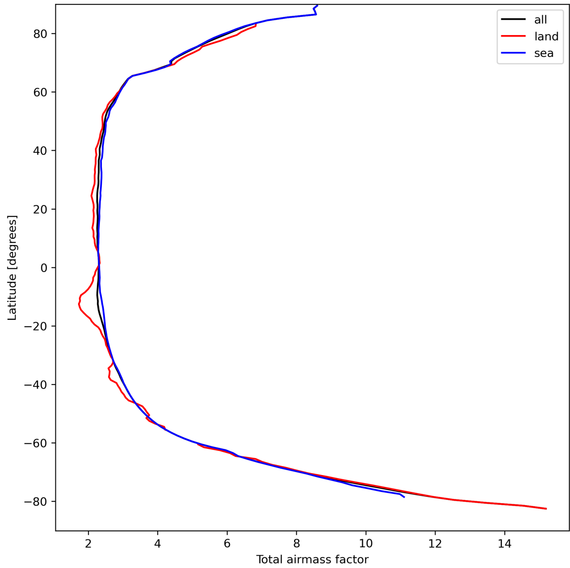
Figure 15: Zonal average of “Total airmass factor” for 2023-09-06 to 2023-09-08.
