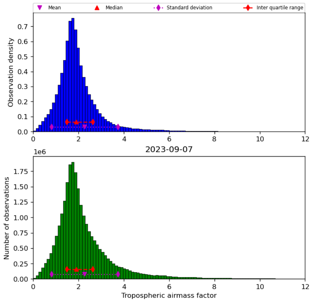
Figure 31: Histogram of “Tropospheric airmass factor” for 2023-09-06 to 2023-09-08
