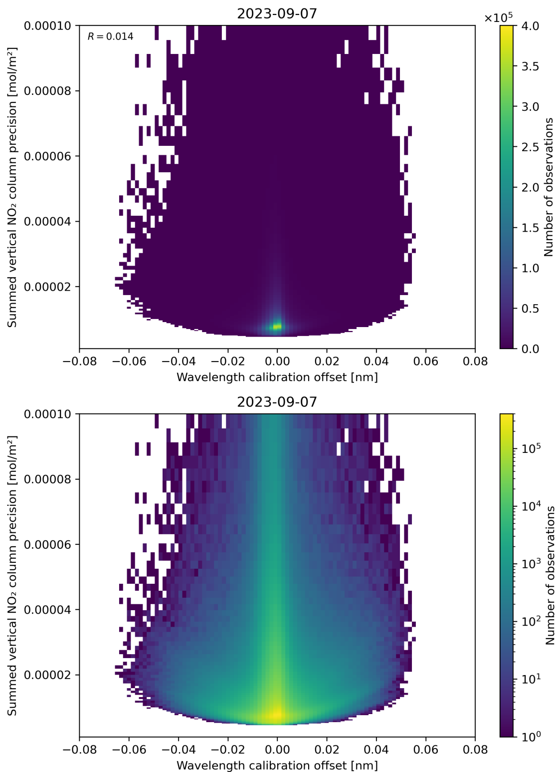
Figure 178: Scatter density plot of “Wavelength calibration offset” against “Summed vertical NO 2 column precision” for 2023-09-06 to 2023-09-08.
