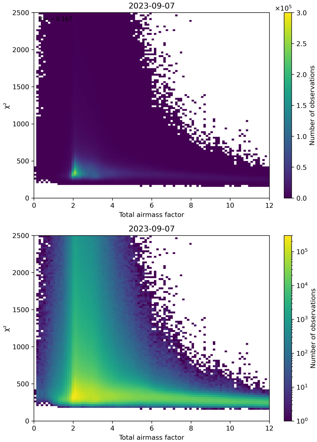
Figure 63: Scatter density plot of “Total airmass factor” against “ \chi^2 ” for 2023-09-06 to 2023-09-08.
