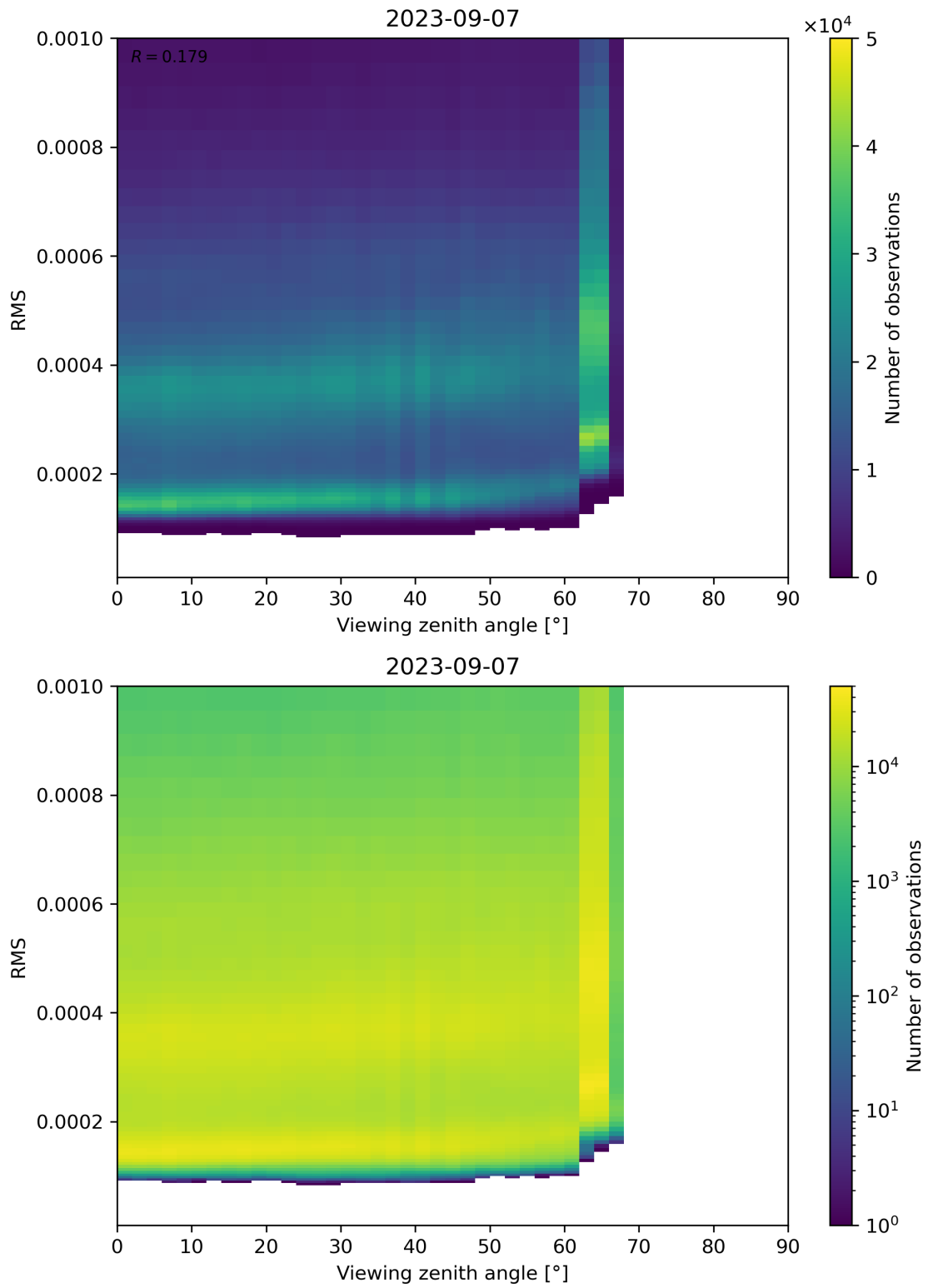
Figure 171: Scatter density plot of “Viewing zenith angle” against “RMS” for 2023-09-06 to 2023-09-08.
