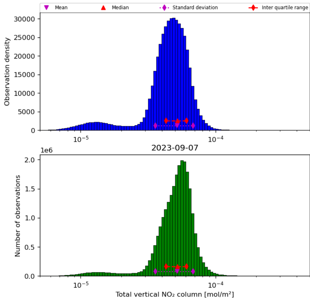
Figure 38: Histogram of "Total vertical NO 2 column" for 2023-09-06 to 2023-09-08
