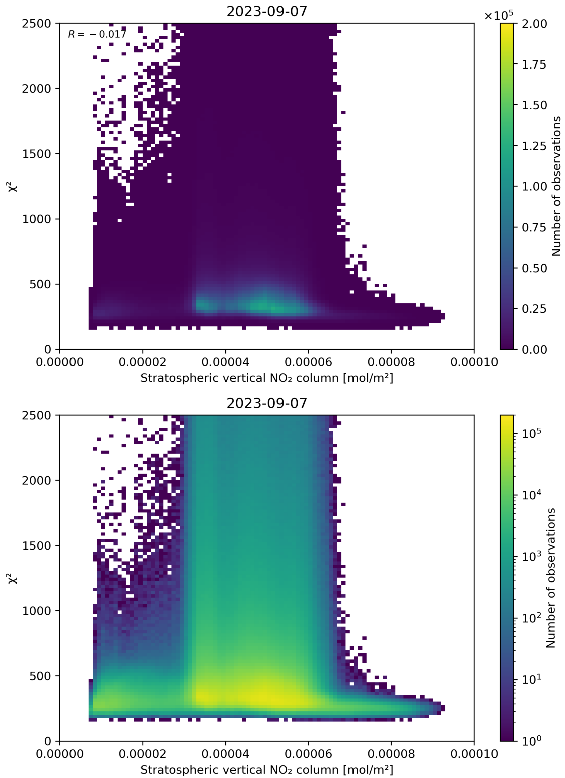
Figure 97: Scatter density plot of “Stratospheric vertical NO 2 column” against “ \chi^2 ” for 2023-09-06 to 2023-09-08.
