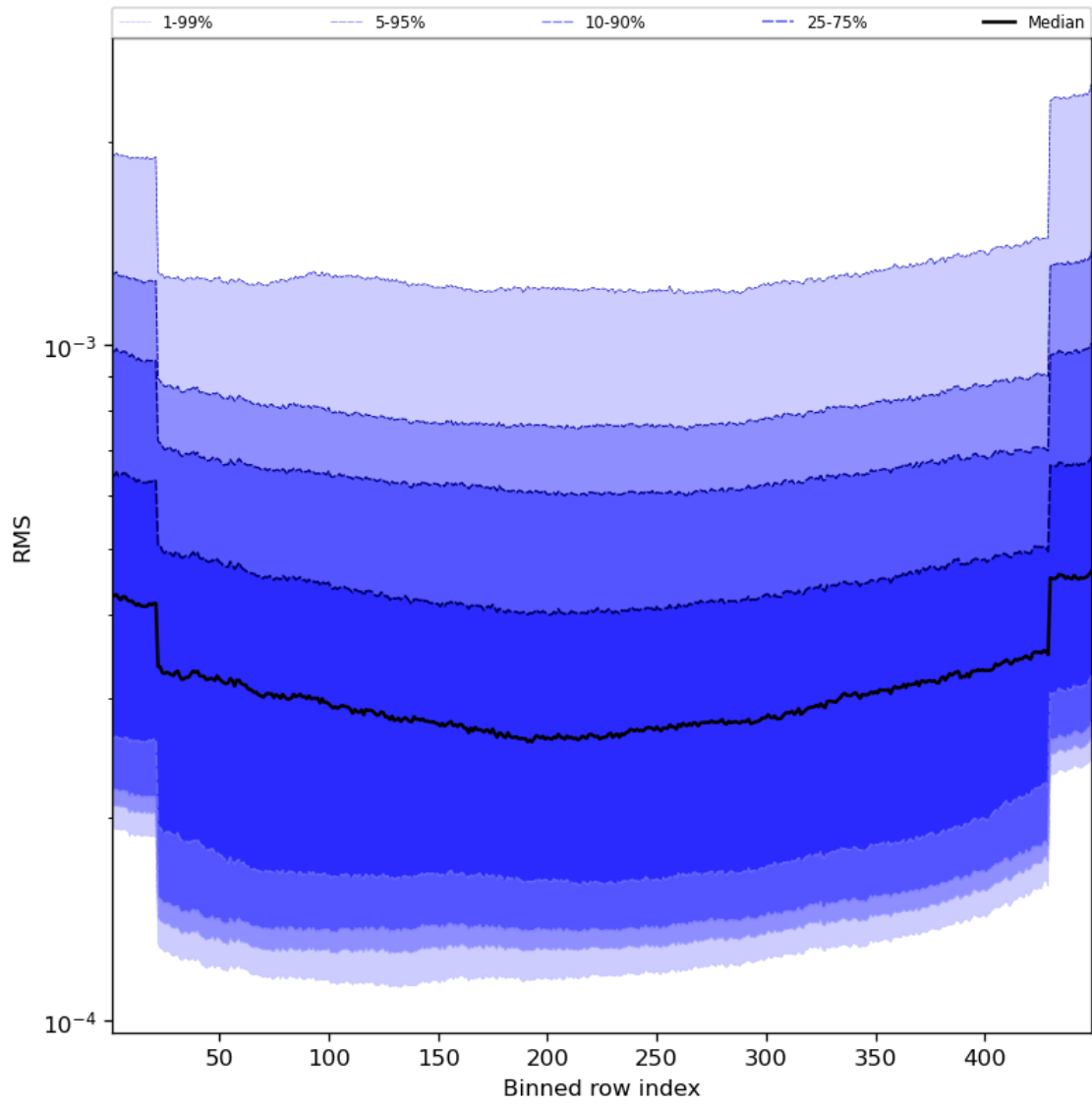
Figure 60: Along track statistics of “RMS” for 2023-09-06 to 2023-09-08
