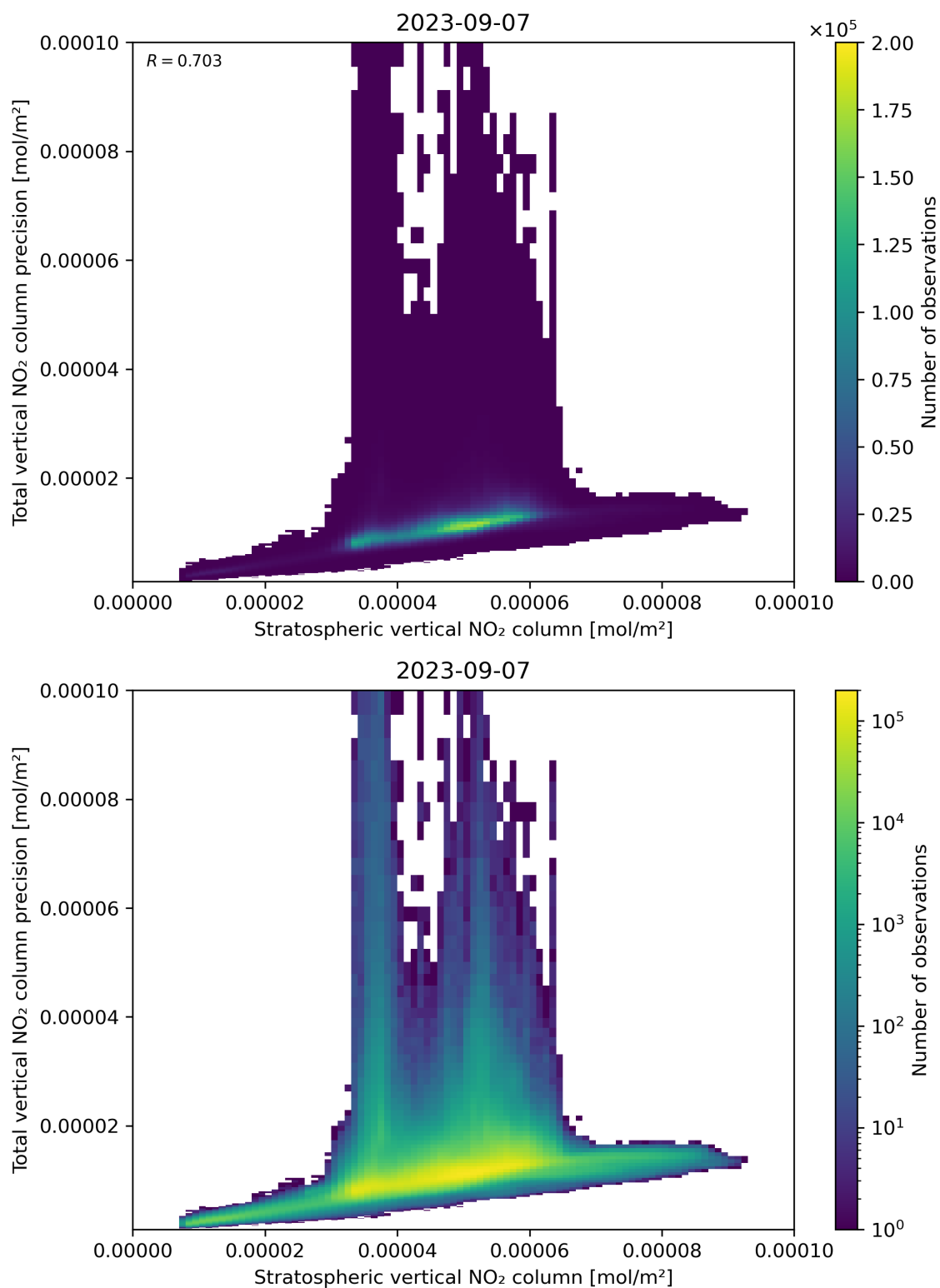
Figure 101: Scatter density plot of “Stratospheric vertical NO 2 column” against “Total vertical NO 2 column precision” for 2023-09-06 to 2023-09-08.
