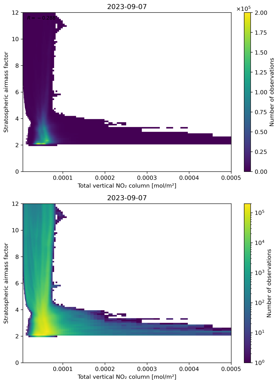
Figure 110: Scatter density plot of “Total vertical NO 2 column” against “Stratospheric airmass factor” for 2023-09-06 to 2023-09-08.
