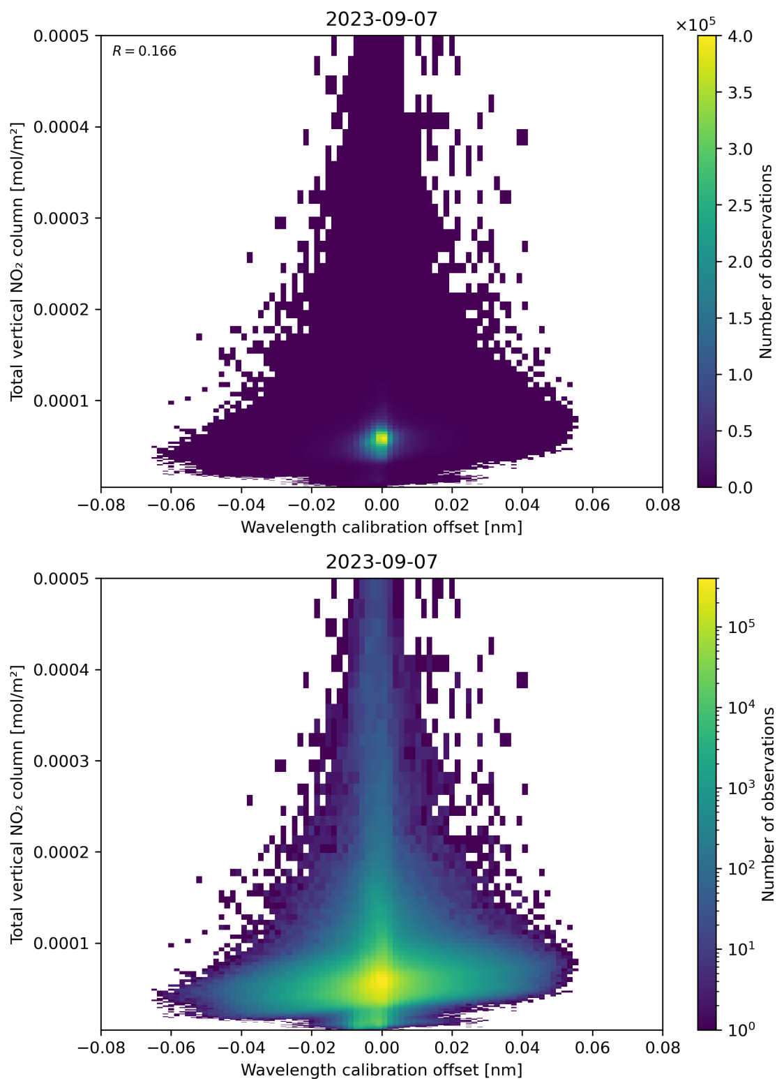
Figure 179: Scatter density plot of “Wavelength calibration offset” against “Total vertical NO 2 column” for 2023-09-06 to 2023-09-08.
