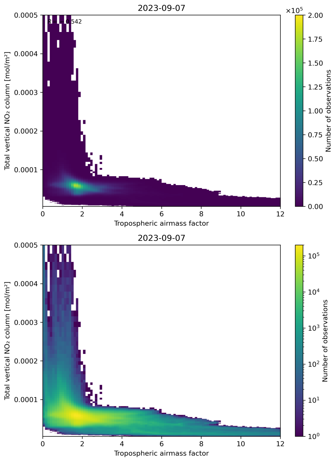
Figure 77: Scatter density plot of “Tropospheric airmass factor” against “Total vertical NO 2 column” for 2023-09-06 to 2023-09-08.
