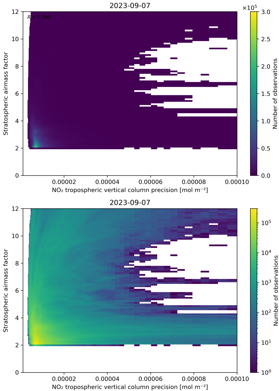
Figure 131: Scatter density plot of “NO 2 tropospheric vertical column precision” against “Stratospheric airmass factor” for 2023-09-06 to 2023-09-08.
