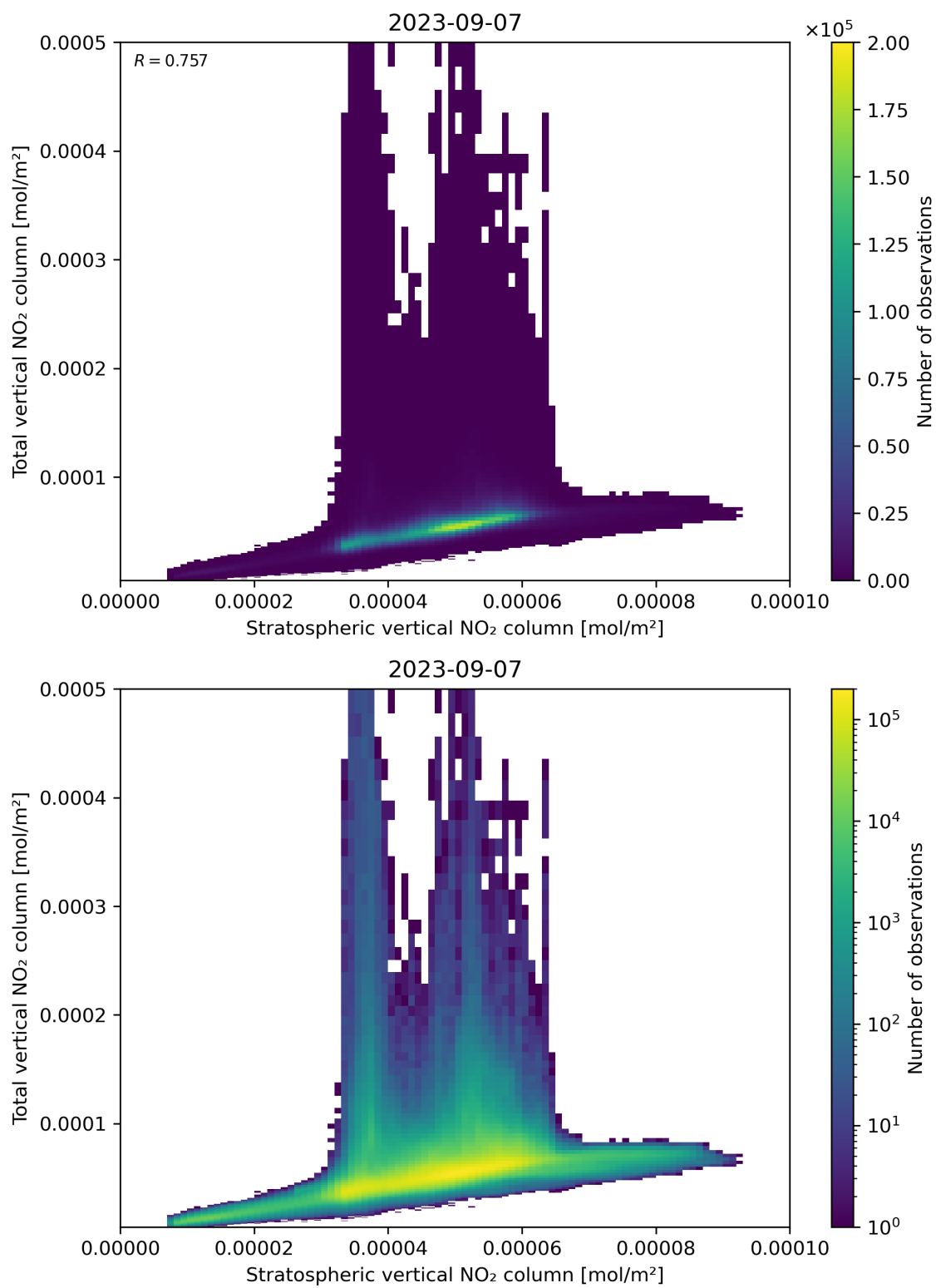
Figure 100: Scatter density plot of “Stratospheric vertical NO 2 column” against “Total vertical NO 2 column” for 2023-09-06 to 2023-09-08.
