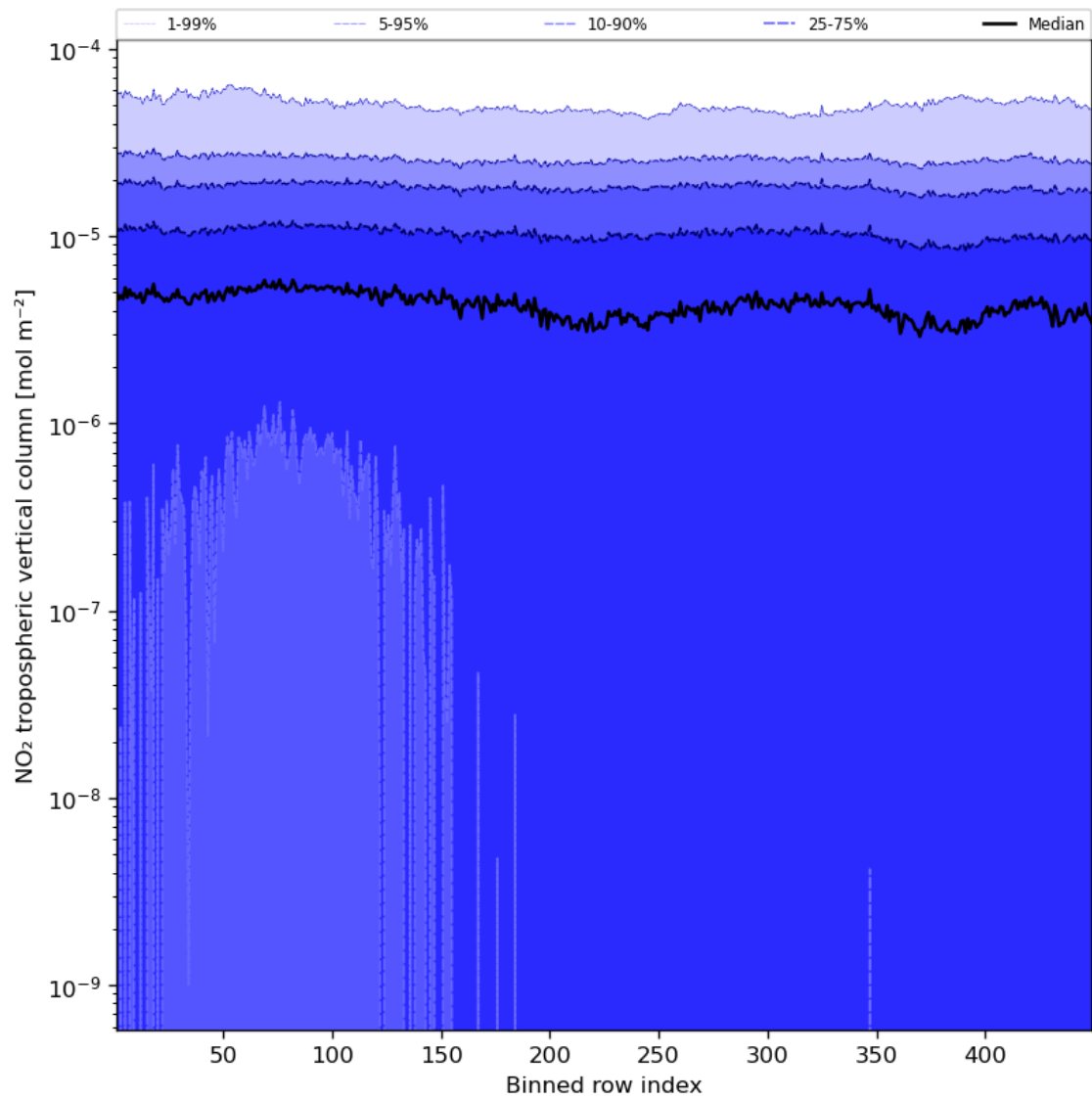
Figure 46: Along track statistics of “ \text{NO}_2 tropospheric vertical column” for 2023-09-06 to 2023-09-08
