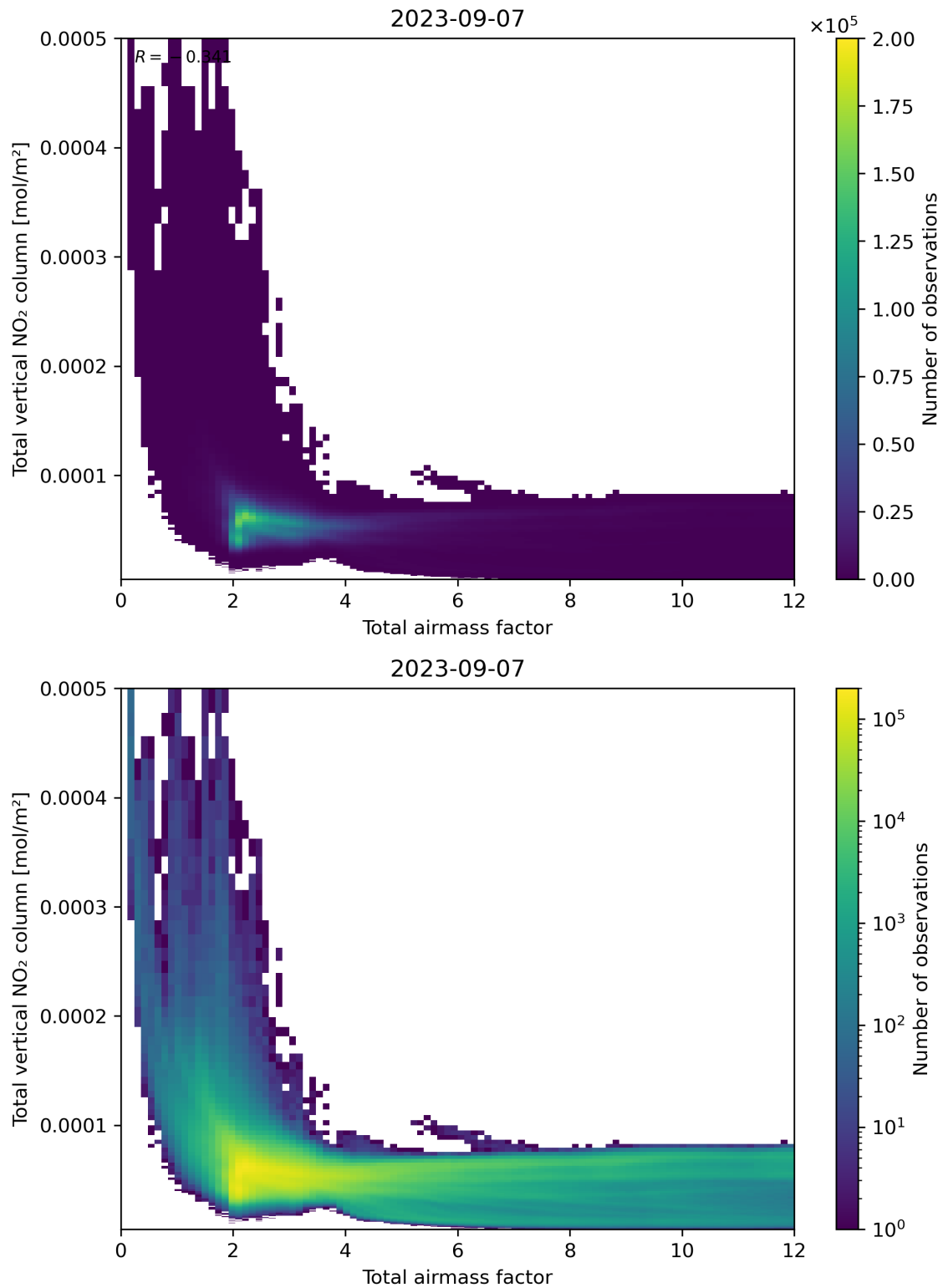
Figure 67: Scatter density plot of “Total airmass factor” against “Total vertical NO 2 column” for 2023-09-06 to 2023-09-08.
