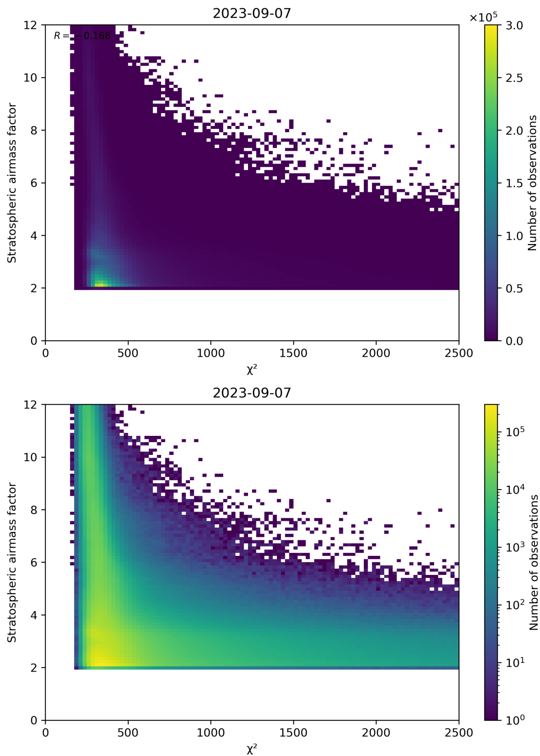
Figure 81: Scatter density plot of “ \chi^2 ” against “Stratospheric airmass factor” for 2023-09-06 to 2023-09-08.
