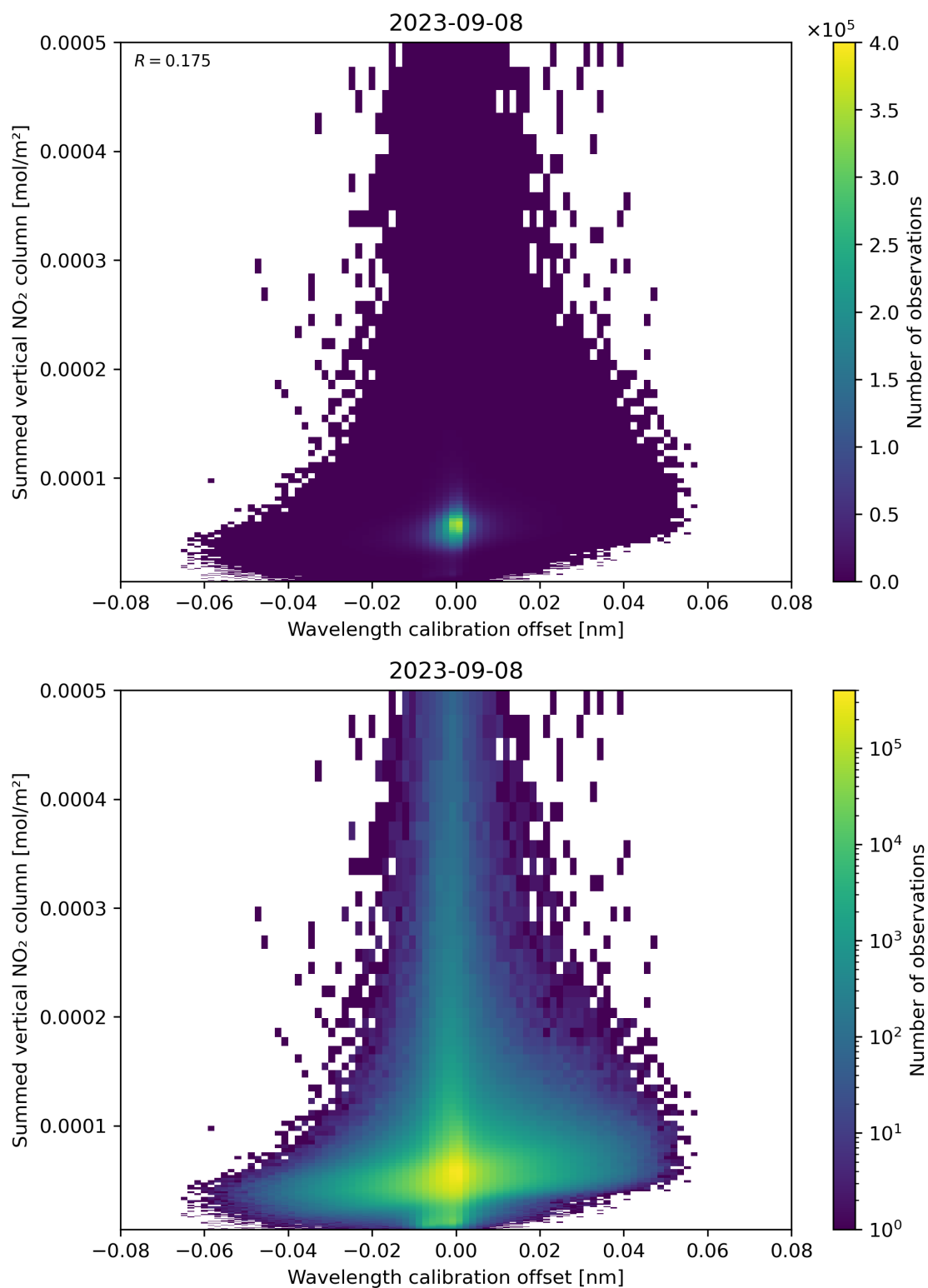
Figure 177: Scatter density plot of “Wavelength calibration offset” against “Summed vertical NO 2 column” for 2023-09-07 to 2023-09-09.
