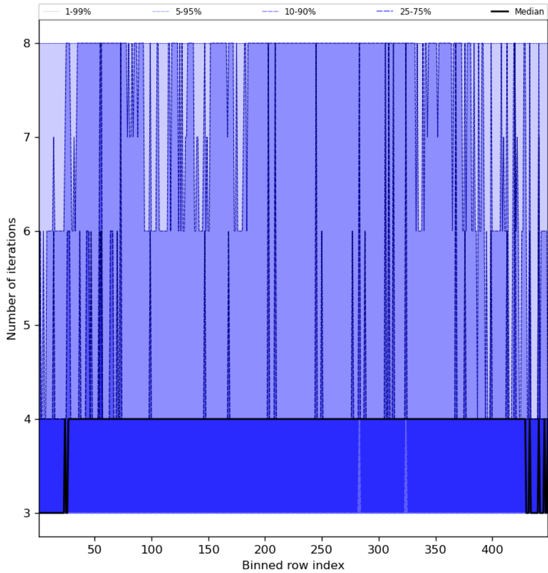
Figure 51: Along track statistics of “Number of iterations” for 2023-09-07 to 2023-09-09
