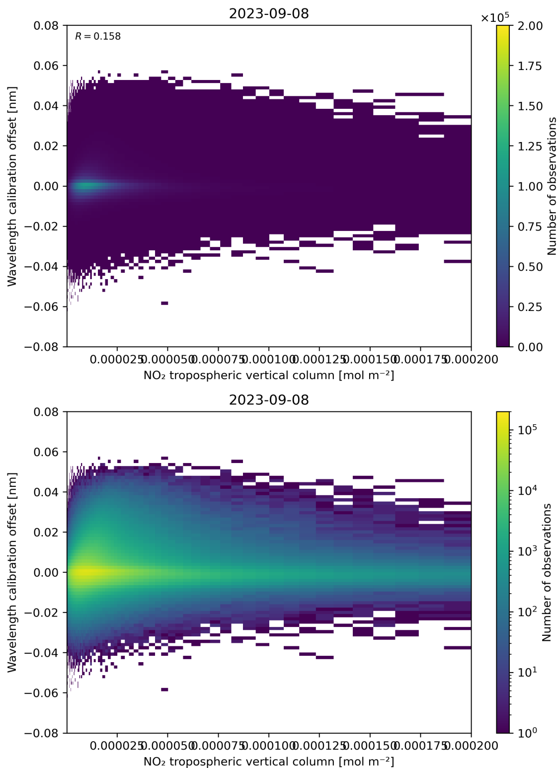
Figure 143: Scatter density plot of “NO 2 tropospheric vertical column” against “Wavelength calibration offset” for 2023-09-07 to 2023-09-09.
