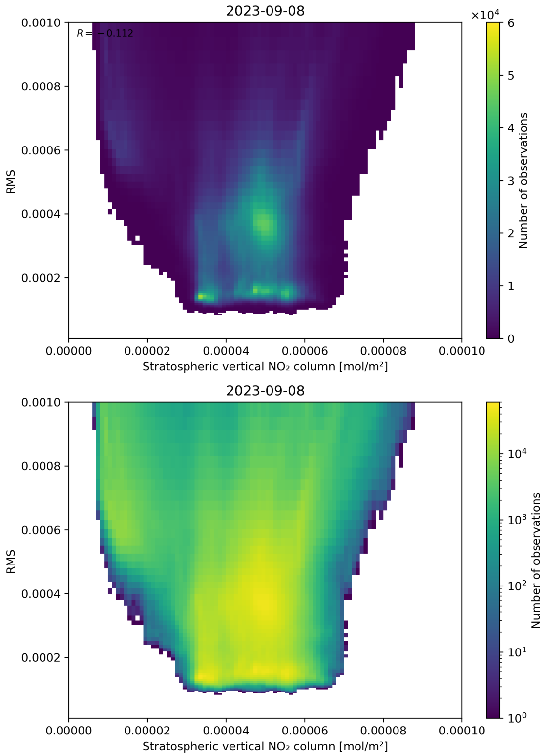
Figure 102: Scatter density plot of “Stratospheric vertical NO 2 column” against “RMS” for 2023-09-07 to 2023-09-09.
