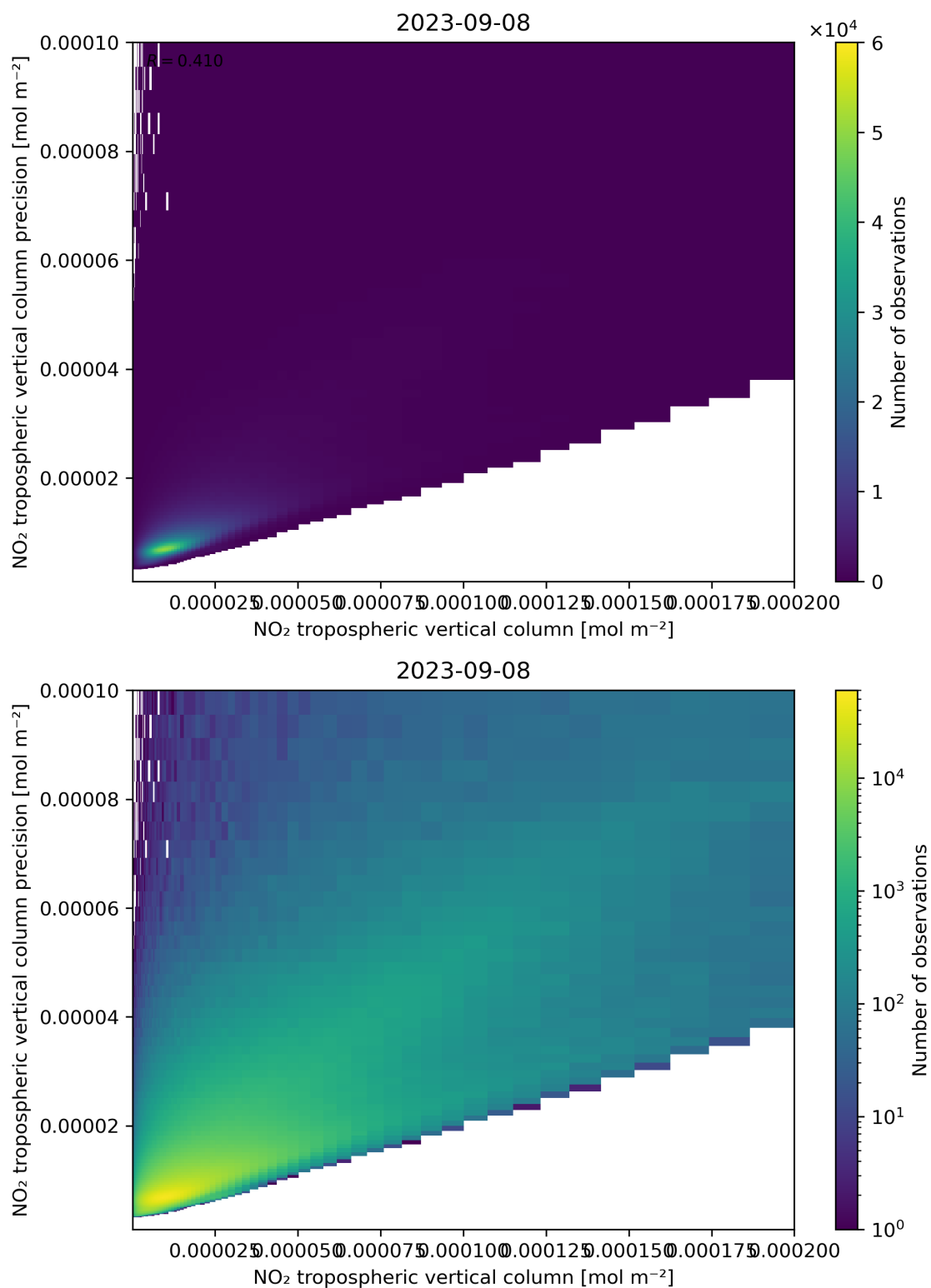
Figure 130: Scatter density plot of “NO 2 tropospheric vertical column” against “NO 2 tropospheric vertical column precision” for 2023-09-07 to 2023-09-09.
