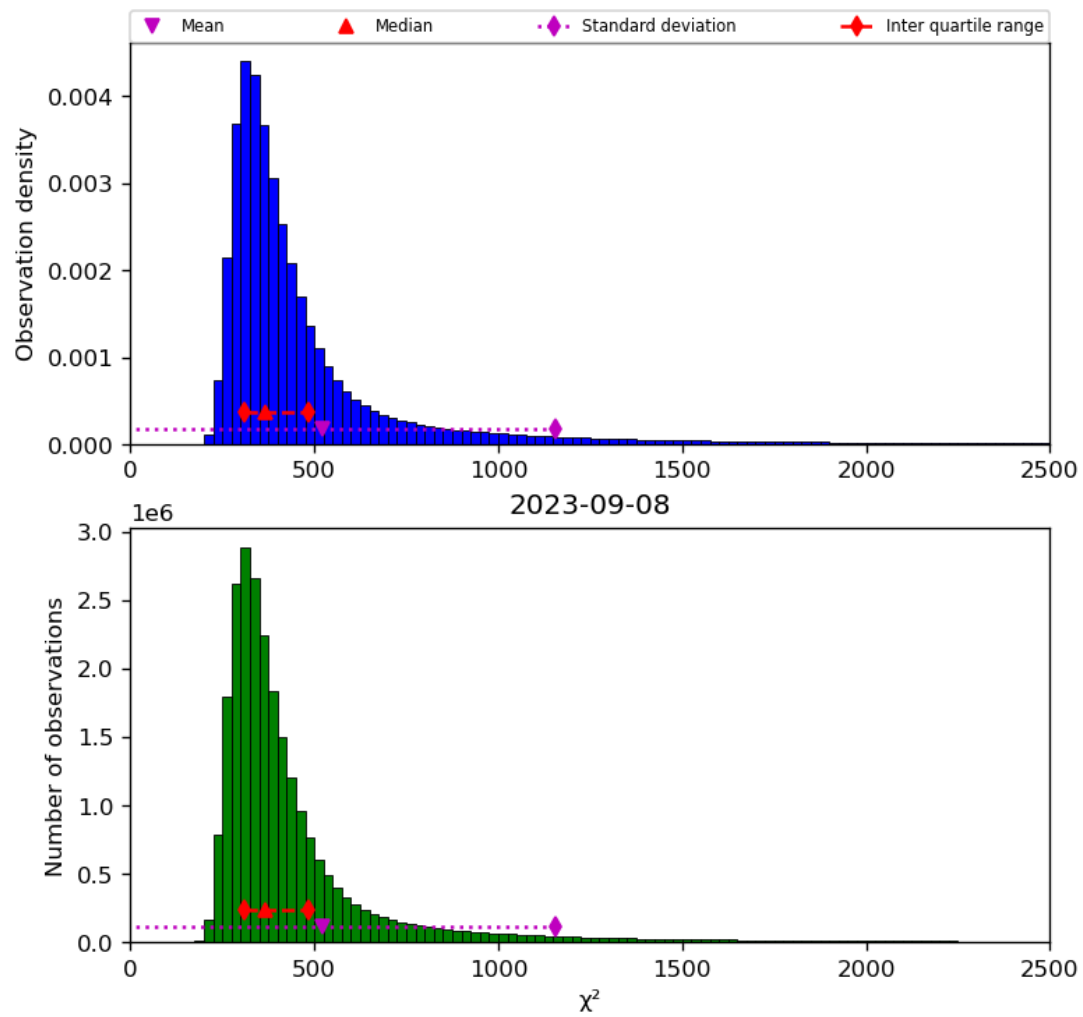
Figure 42: Histogram of “ \chi^2 ” for 2023-09-07 to 2023-09-09
