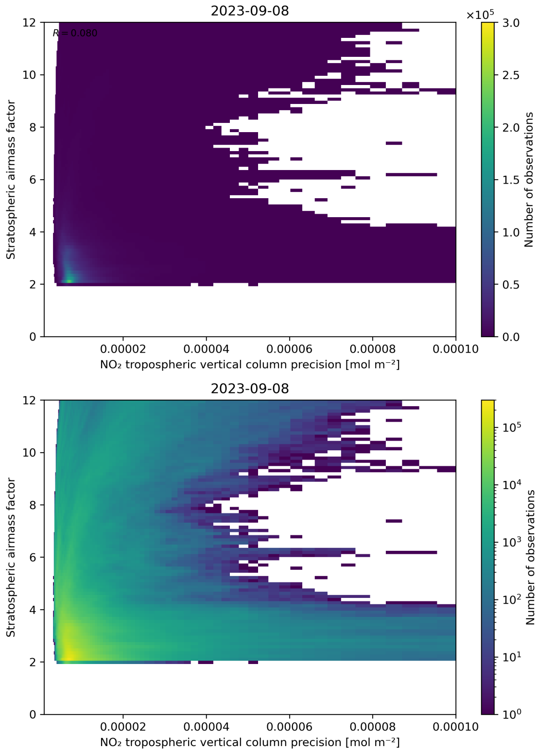
Figure 131: Scatter density plot of “NO 2 tropospheric vertical column precision” against “Stratospheric airmass factor” for 2023-09-07 to 2023-09-09.
