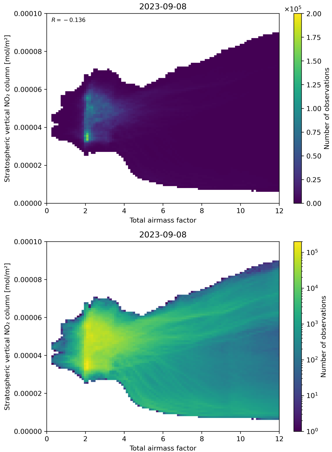
Figure 64: Scatter density plot of “Total airmass factor” against “Stratospheric vertical NO 2 column” for 2023-09-07 to 2023-09-09.
