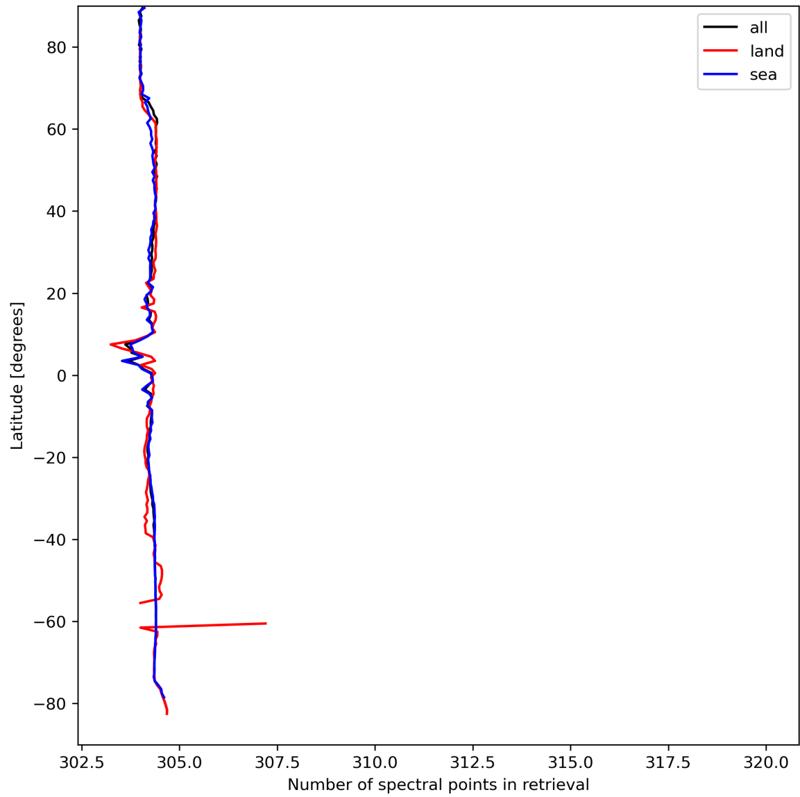
Figure 16: Zonal average of “Number of spectral points in retrieval” for 2023-09-07 to 2023-09-09.
