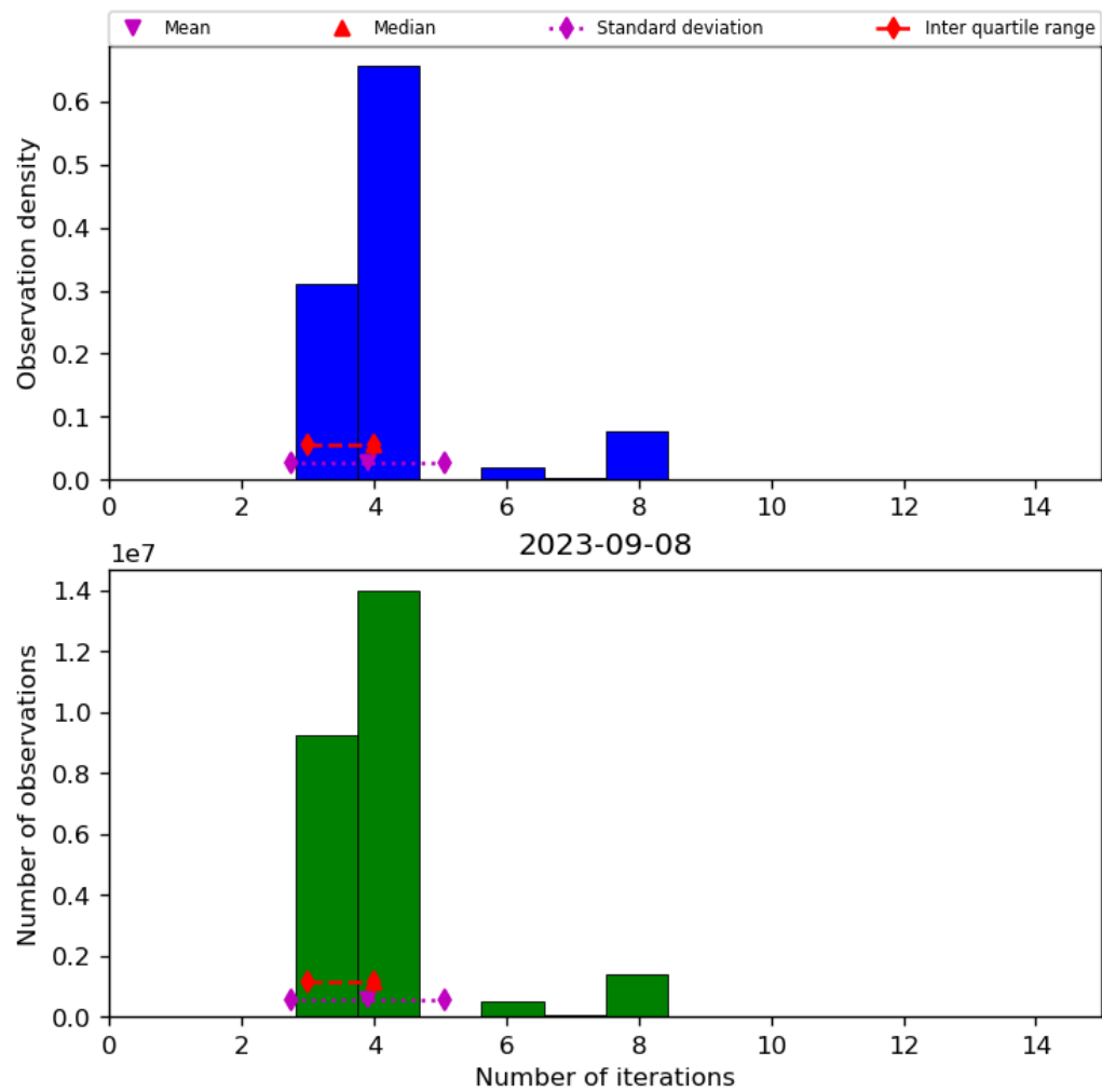
Figure 34: Histogram of “Number of iterations” for 2023-09-07 to 2023-09-09
