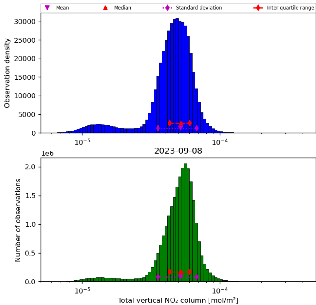
Figure 38: Histogram of "Total vertical NO 2 column" for 2023-09-07 to 2023-09-09
