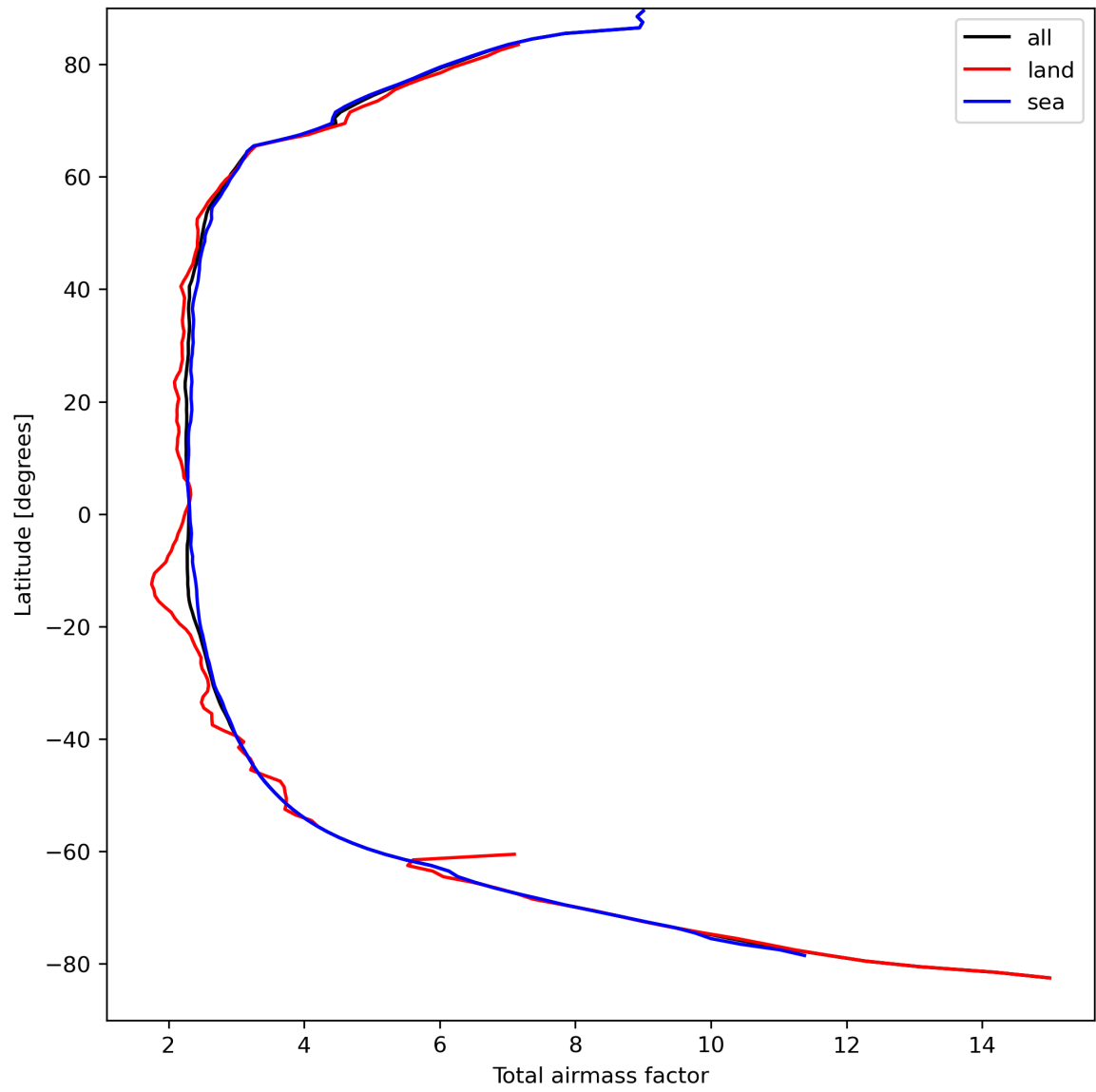
Figure 15: Zonal average of “Total airmass factor” for 2023-09-07 to 2023-09-09.
