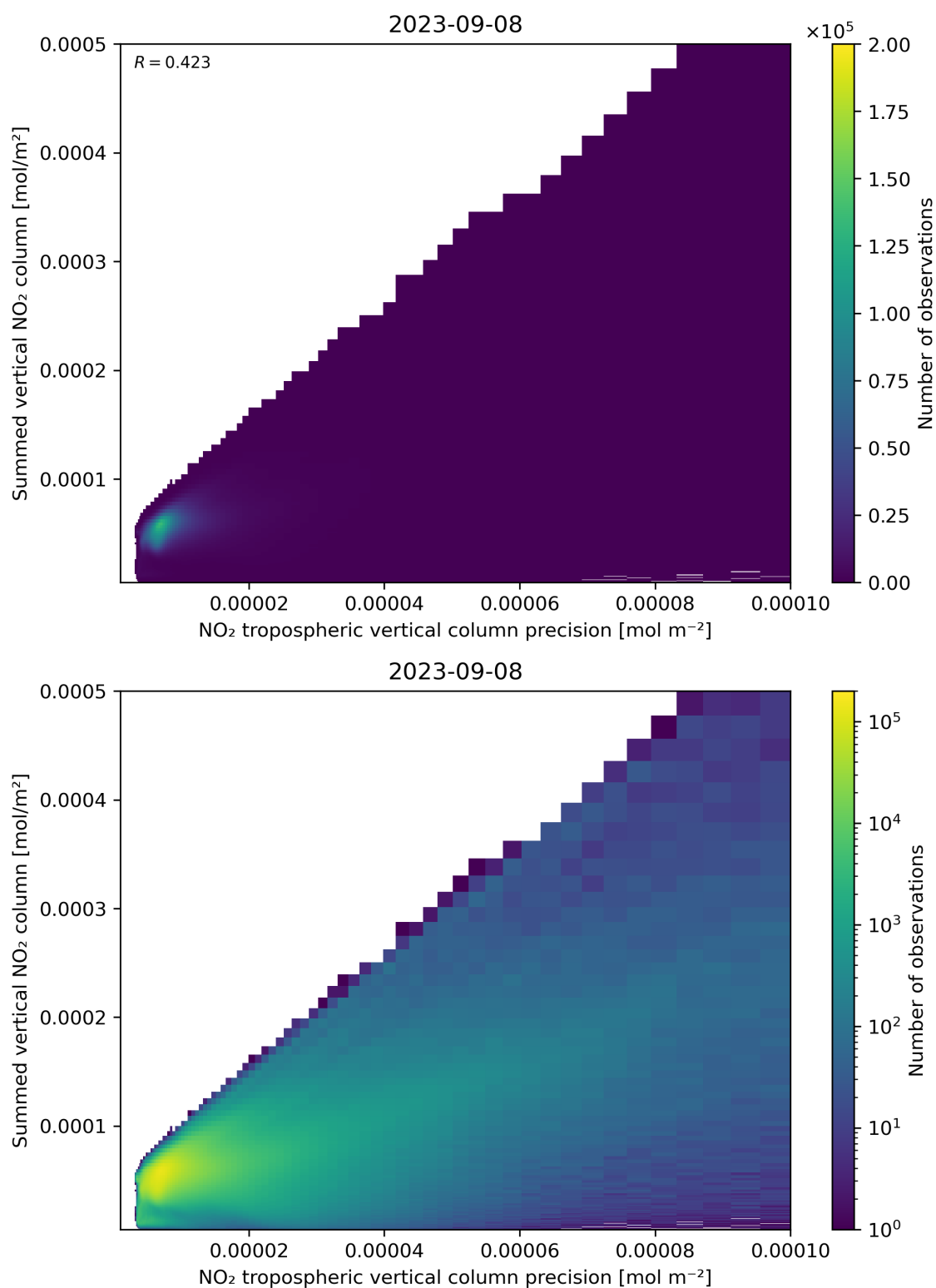
Figure 136: Scatter density plot of “NO 2 tropospheric vertical column precision” against “Summed vertical NO 2 column” for 2023-09-07 to 2023-09-09.
