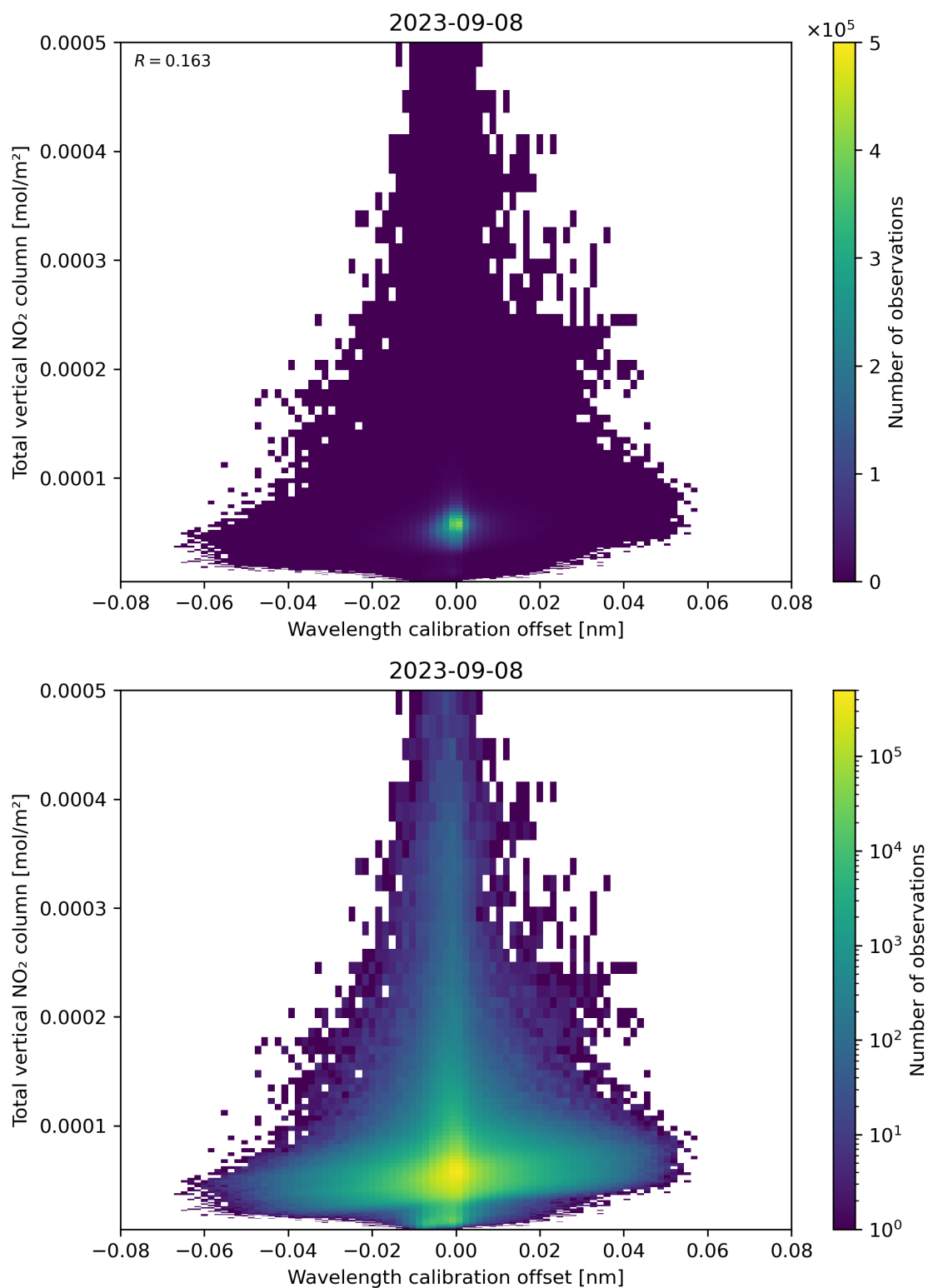
Figure 179: Scatter density plot of “Wavelength calibration offset” against “Total vertical NO 2 column” for 2023-09-07 to 2023-09-09.
