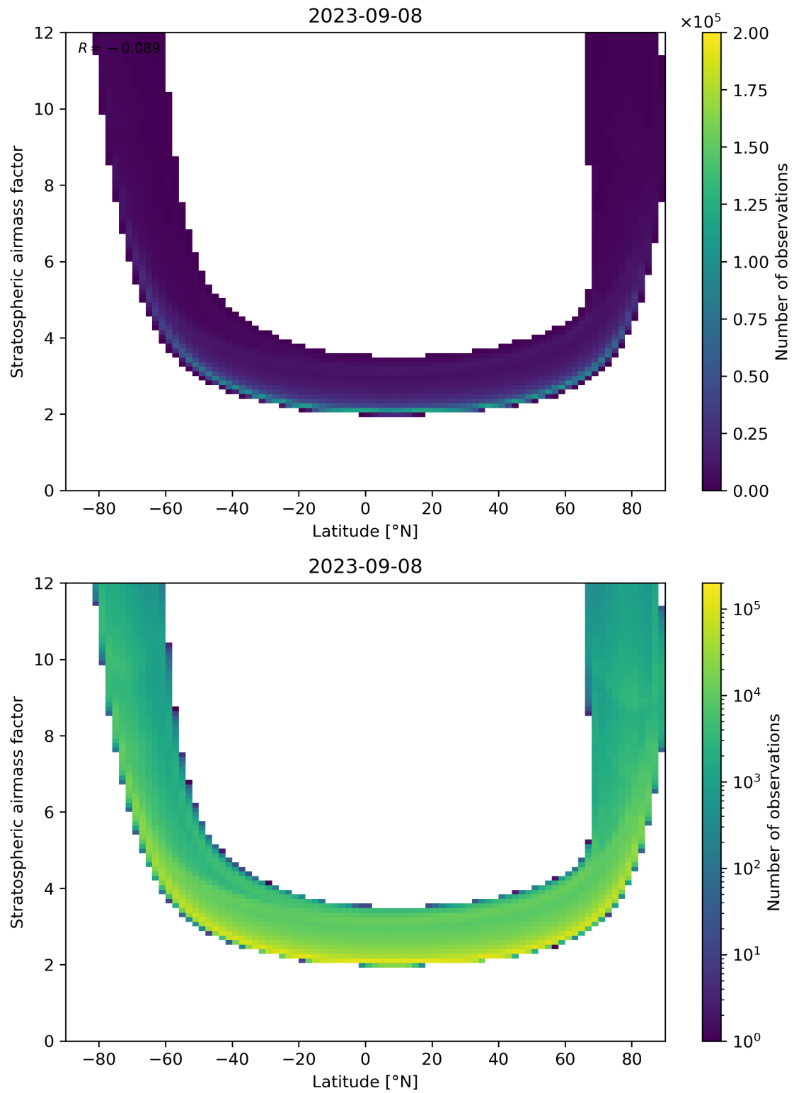
Figure 83: Scatter density plot of “Latitude” against “Stratospheric airmass factor” for 2023-09-07 to 2023-09-09.
