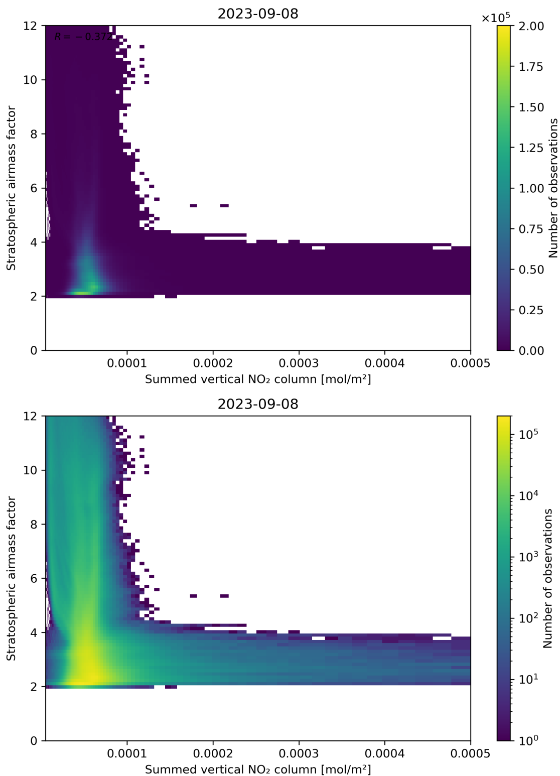
Figure 103: Scatter density plot of “Summed vertical NO 2 column” against “Stratospheric air mass factor” for 2023-09-07 to 2023-09-09.
