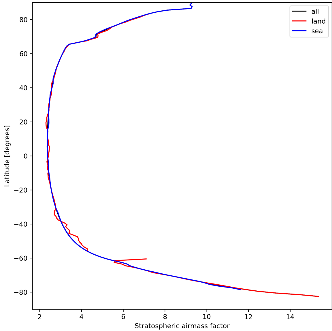
Figure 27: Zonal average of “Stratospheric airmass factor” for 2023-09-07 to 2023-09-09.
