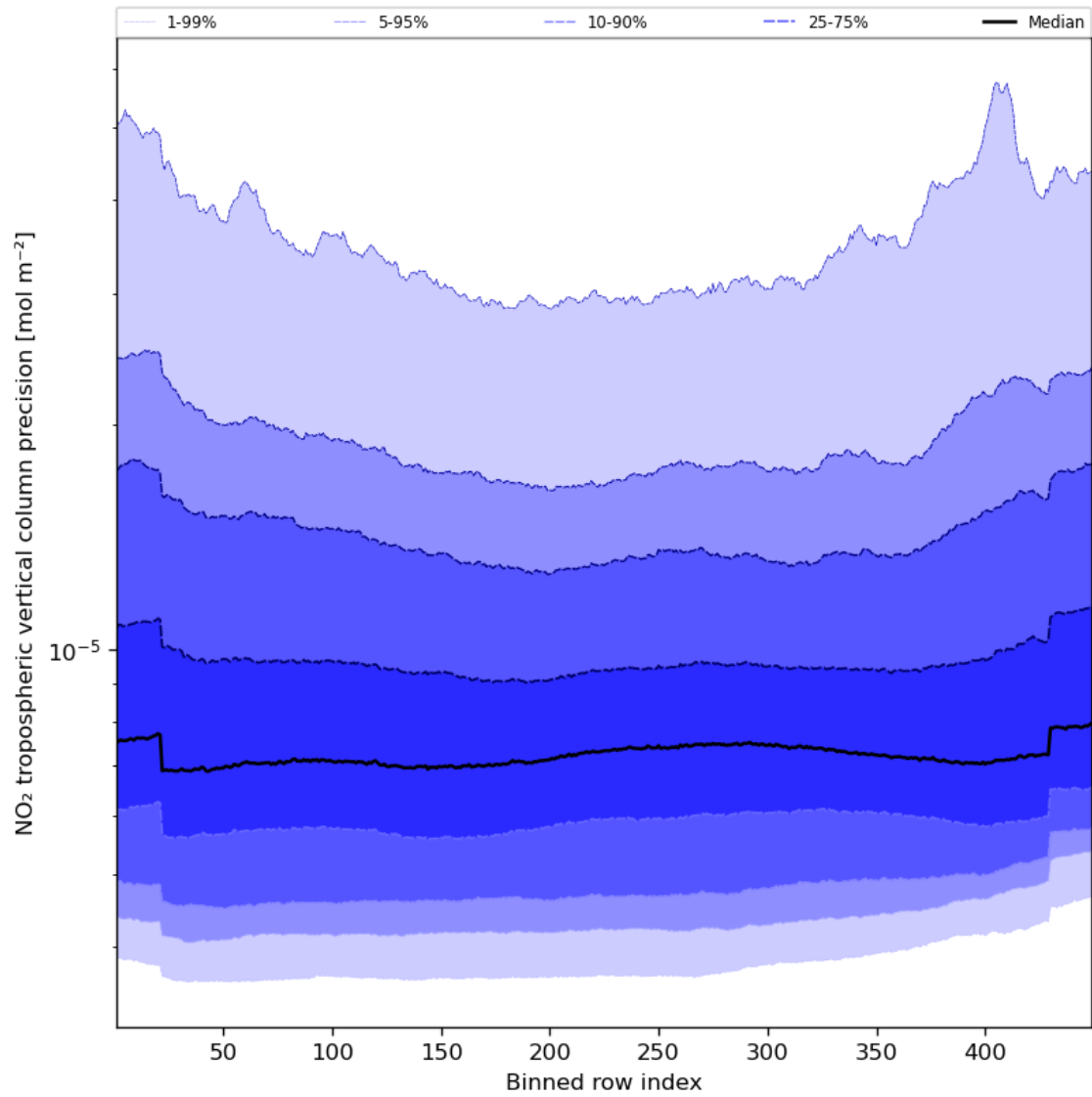
Figure 47: Along track statistics of “NO 2 tropospheric vertical column precision” for 2023-09-07 to 2023-09-09
