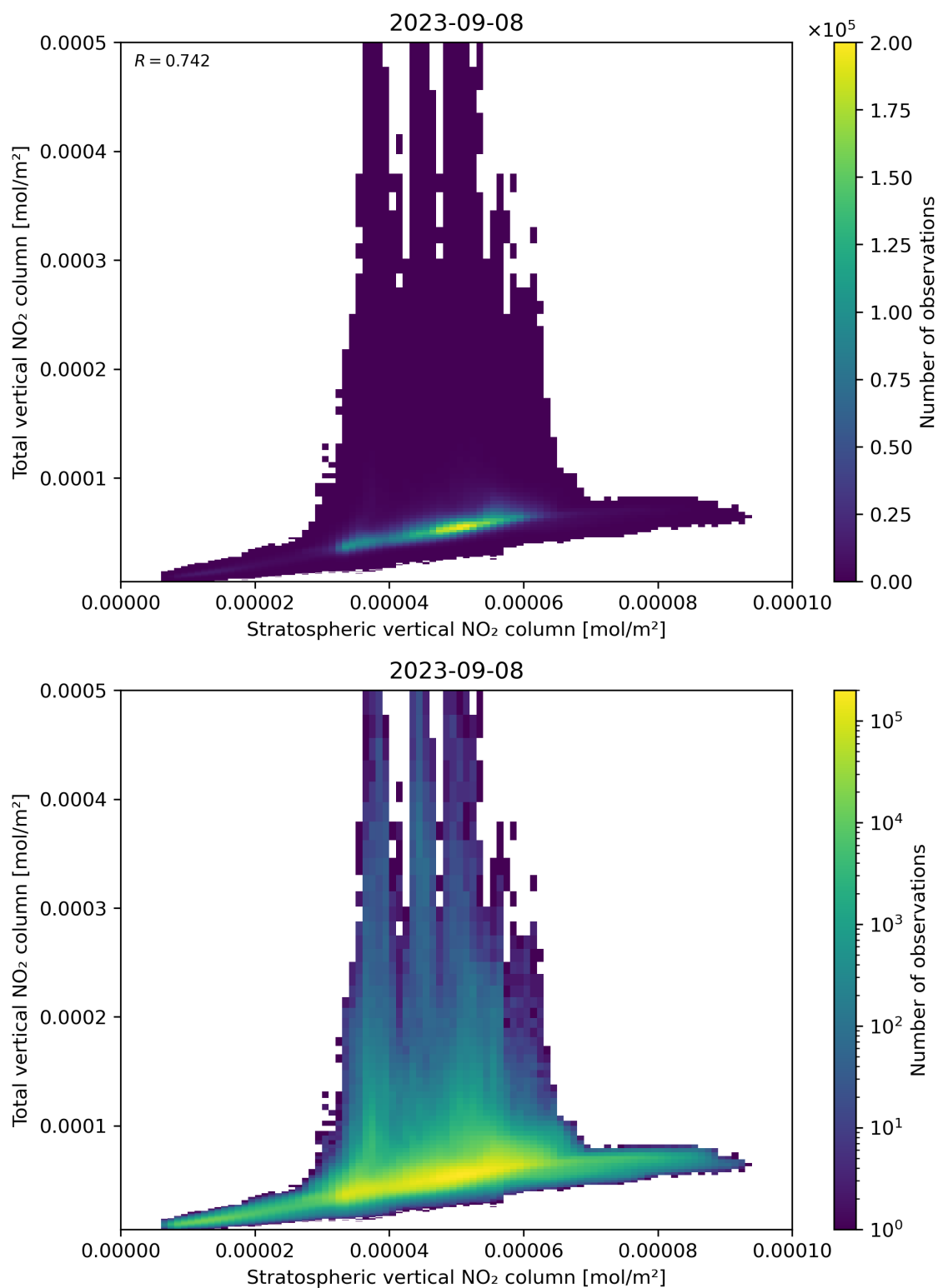
Figure 100: Scatter density plot of “Stratospheric vertical NO 2 column” against “Total vertical NO 2 column” for 2023-09-07 to 2023-09-09.
