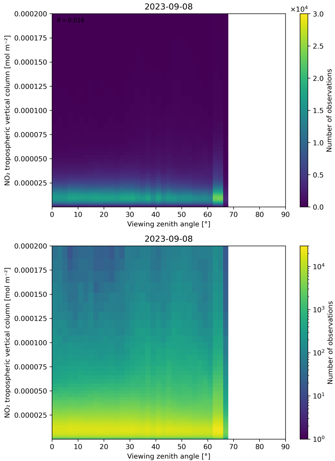
Figure 169: Scatter density plot of “Viewing zenith angle” against “NO 2 tropospheric vertical column” for 2023-09-07 to 2023-09-09.
