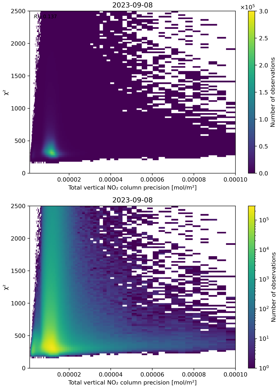
Figure 116: Scatter density plot of “Total vertical NO 2 column precision” against “ \chi^2 ” for 2023-09-07 to 2023-09-09.
