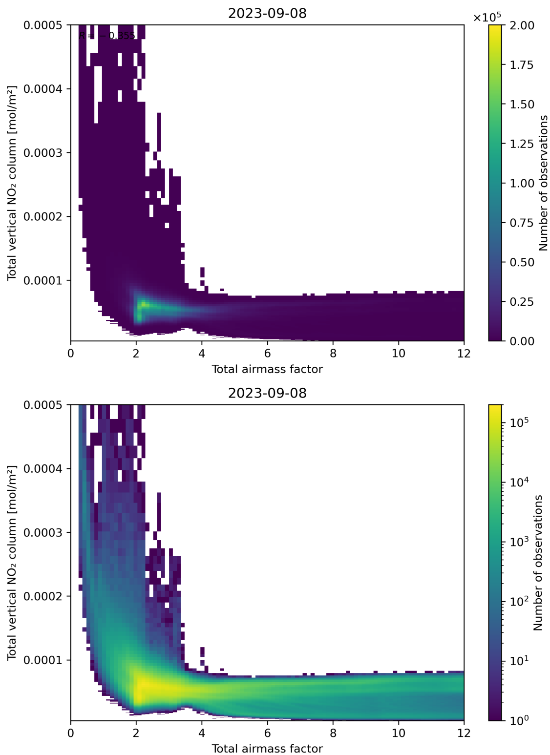
Figure 67: Scatter density plot of “Total airmass factor” against “Total vertical NO 2 column” for 2023-09-07 to 2023-09-09.
