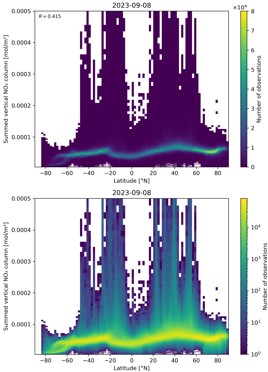
Figure 88: Scatter density plot of “Latitude” against “Summed vertical NO 2 column” for 2023-09-07 to 2023-09-09.
