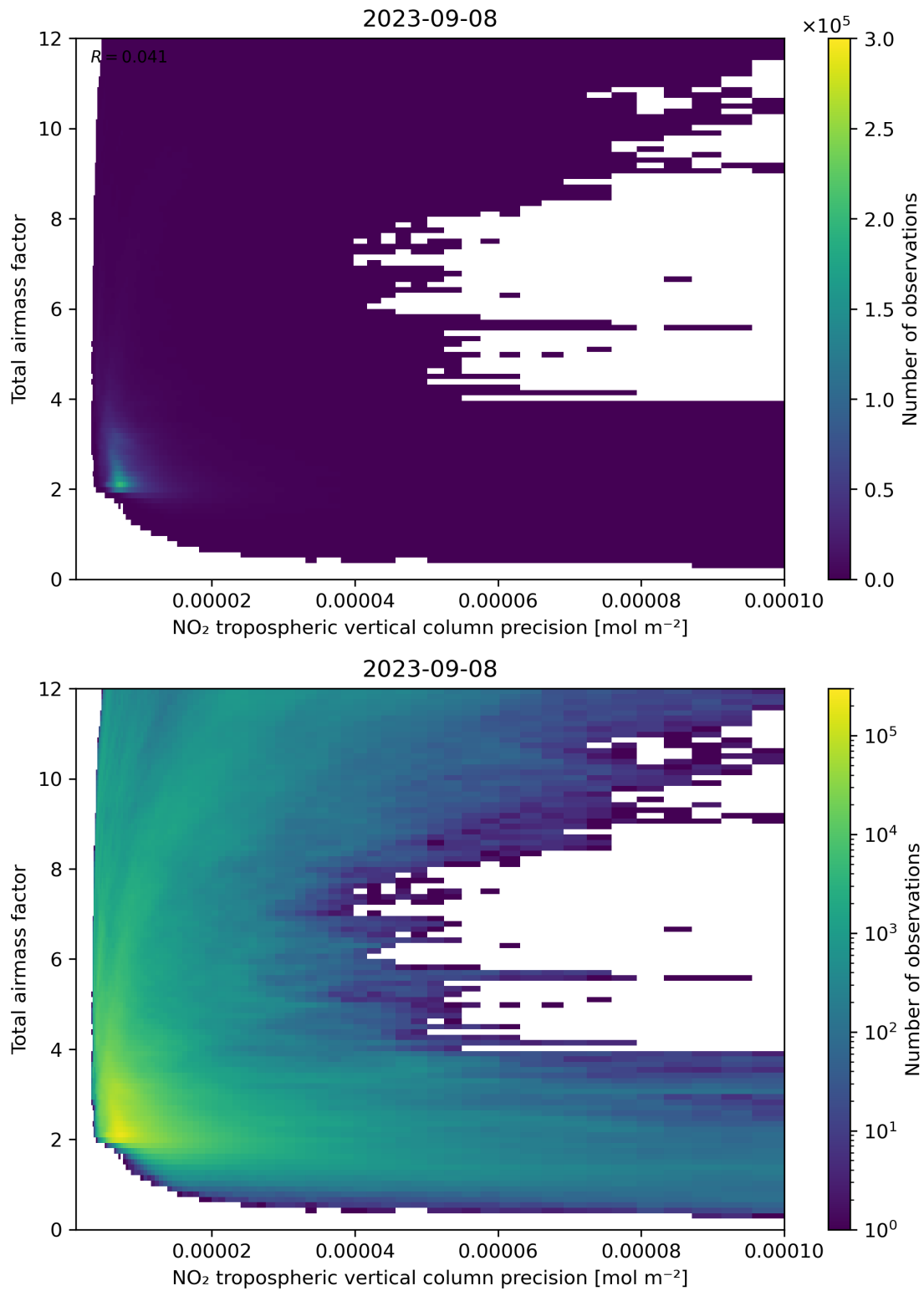
Figure 132: Scatter density plot of “NO 2 tropospheric vertical column precision” against “Total air mass factor” for 2023-09-07 to 2023-09-09.
