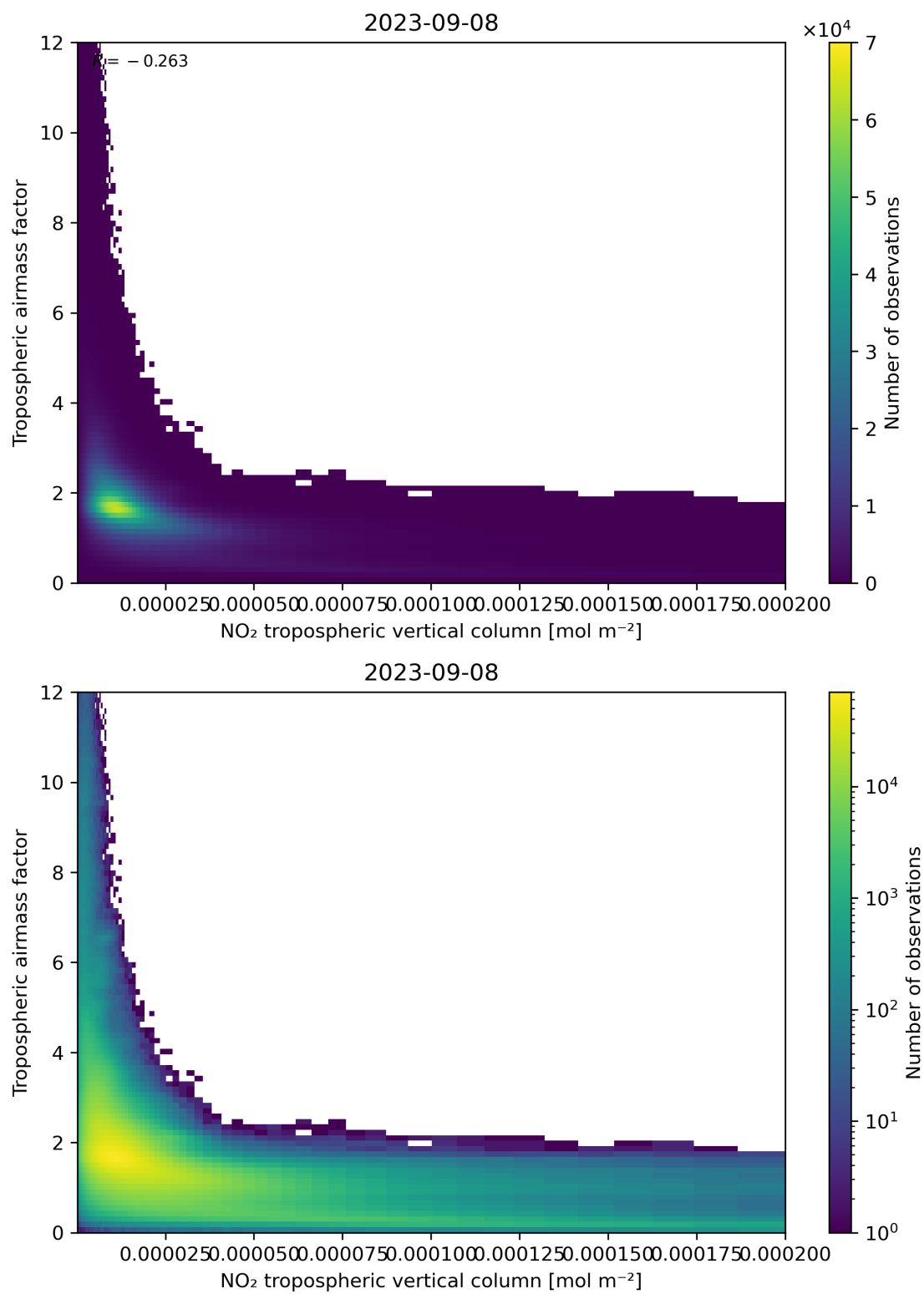
Figure 123: Scatter density plot of “NO 2 tropospheric vertical column” against “Tropospheric air mass factor” for 2023-09-07 to 2023-09-09.
