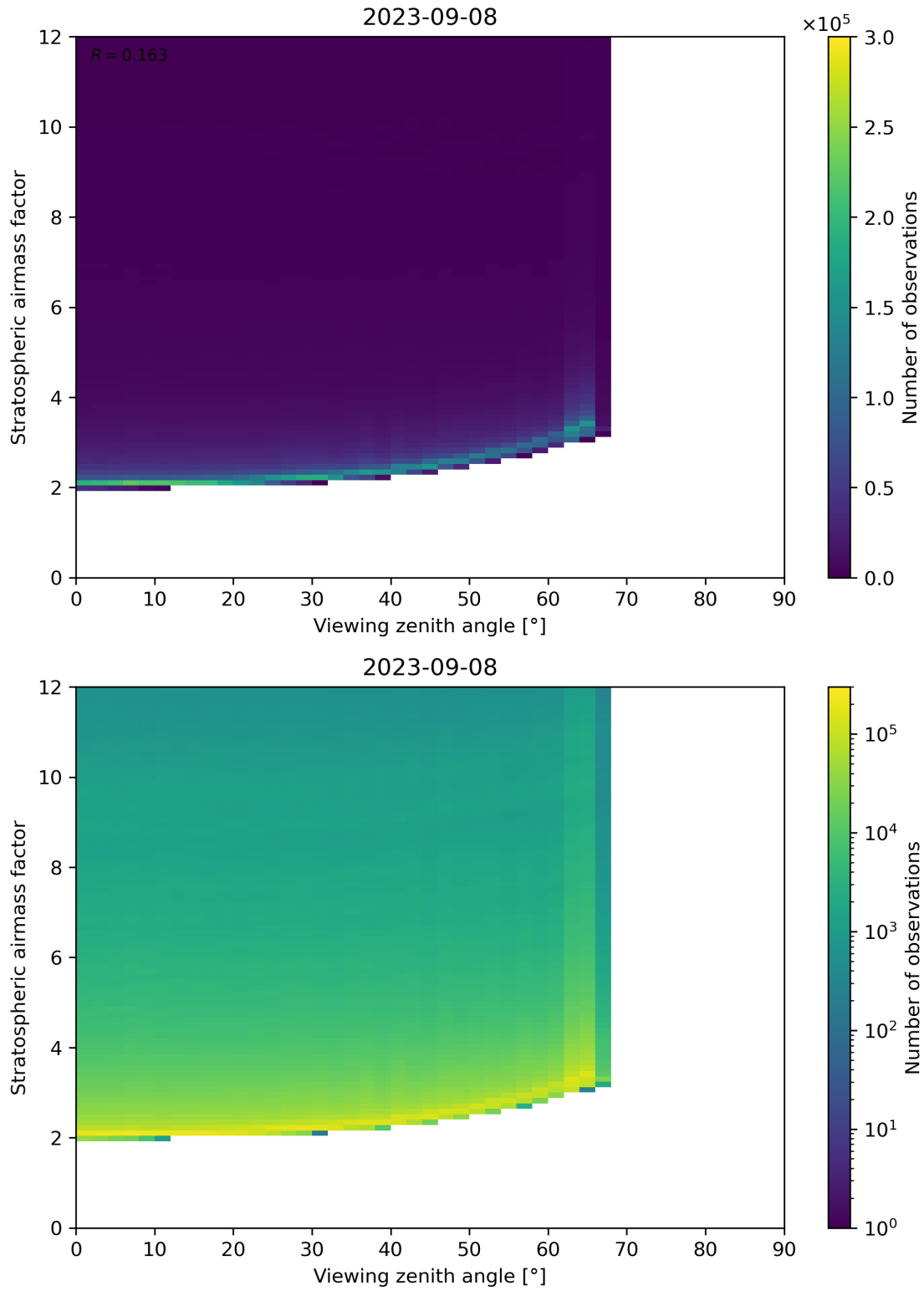
Figure 159: Scatter density plot of “Viewing zenith angle” against “Stratospheric airmass factor” for 2023-09-07 to 2023-09-09.
