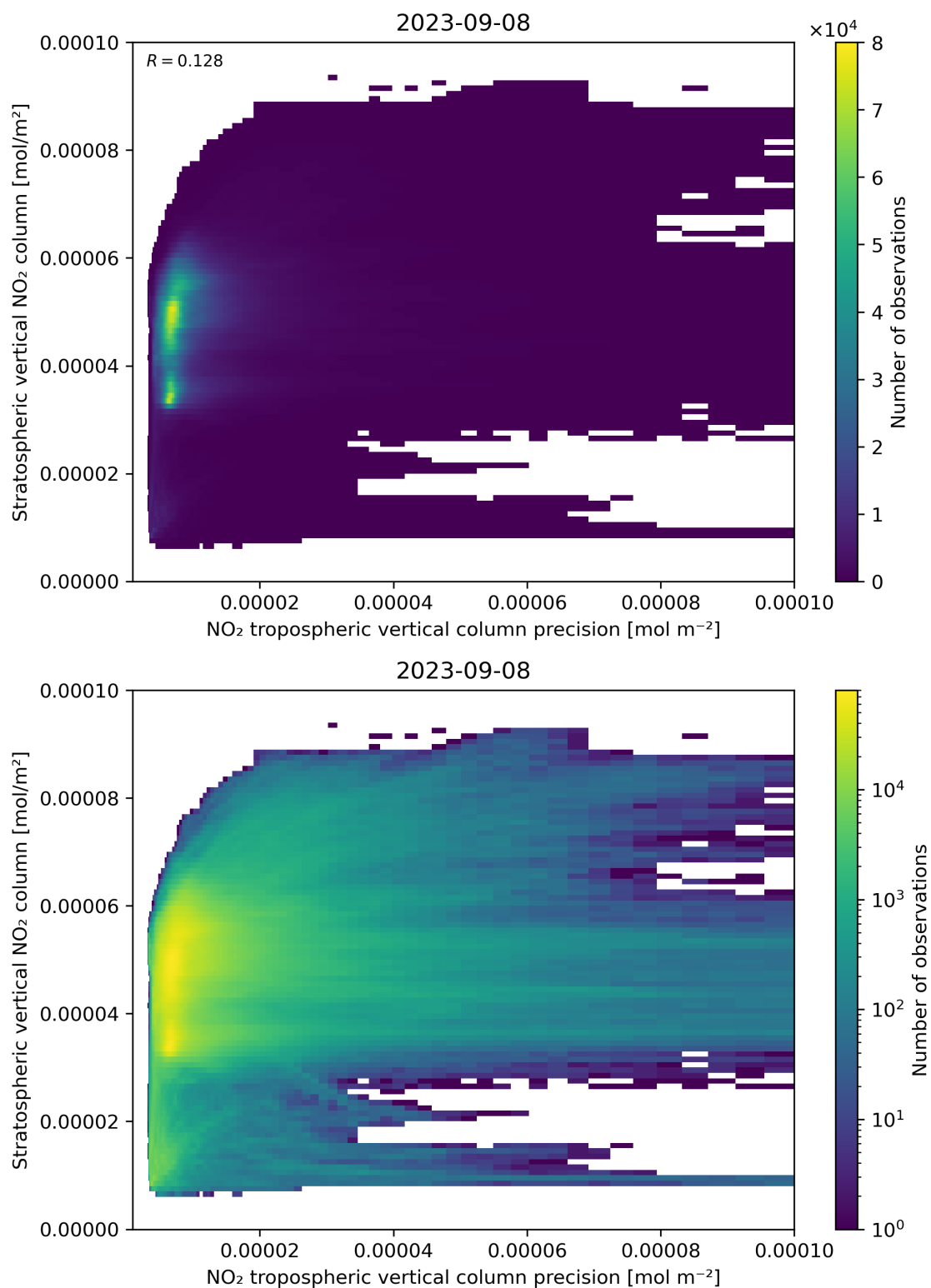
Figure 135: Scatter density plot of “NO 2 tropospheric vertical column precision” against “Stratospheric vertical NO 2 column” for 2023-09-07 to 2023-09-09.
