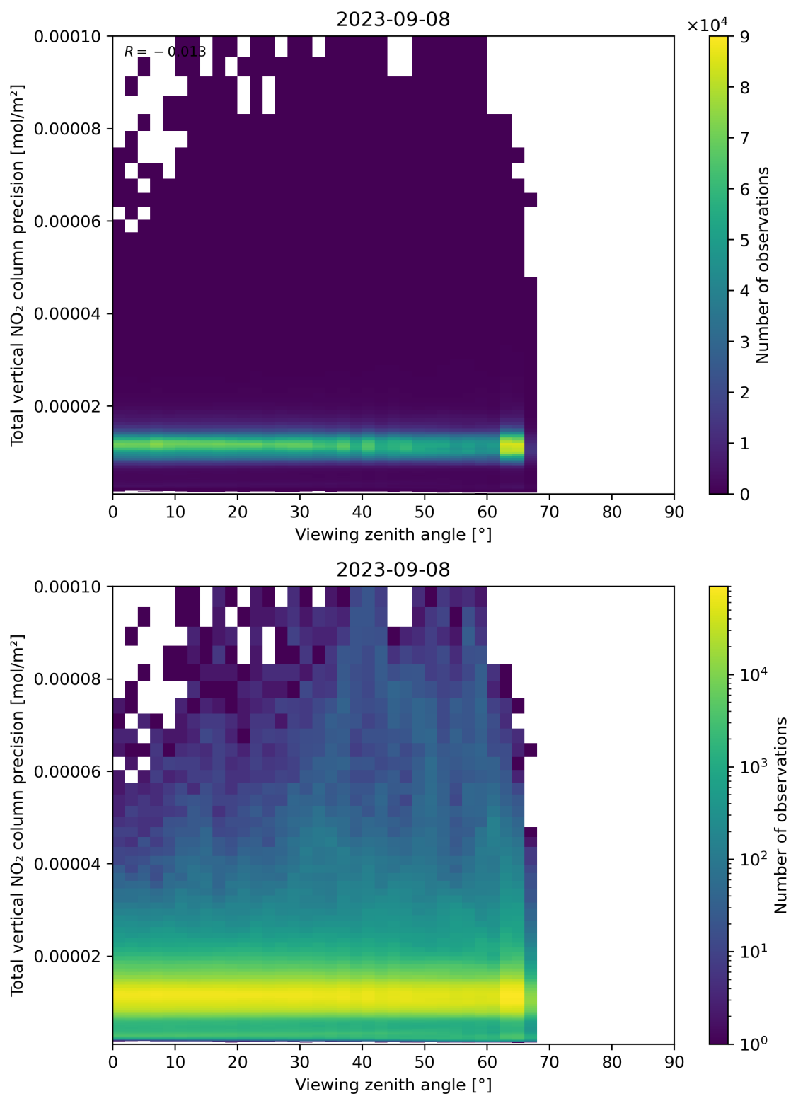
Figure 168: Scatter density plot of “Viewing zenith angle” against “Total vertical NO 2 column precision” for 2023-09-07 to 2023-09-09.
