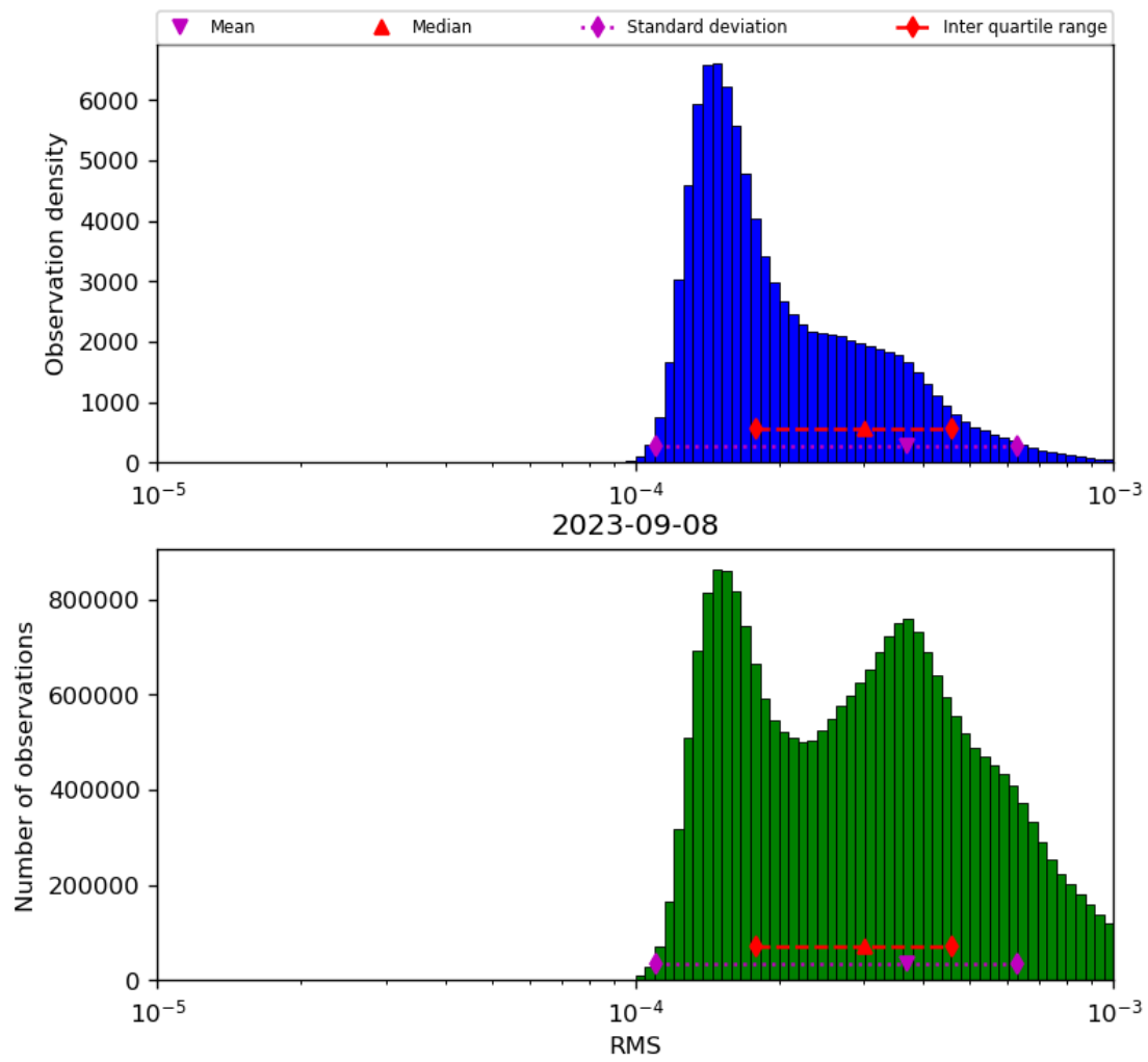
Figure 43: Histogram of “RMS” for 2023-09-07 to 2023-09-09
