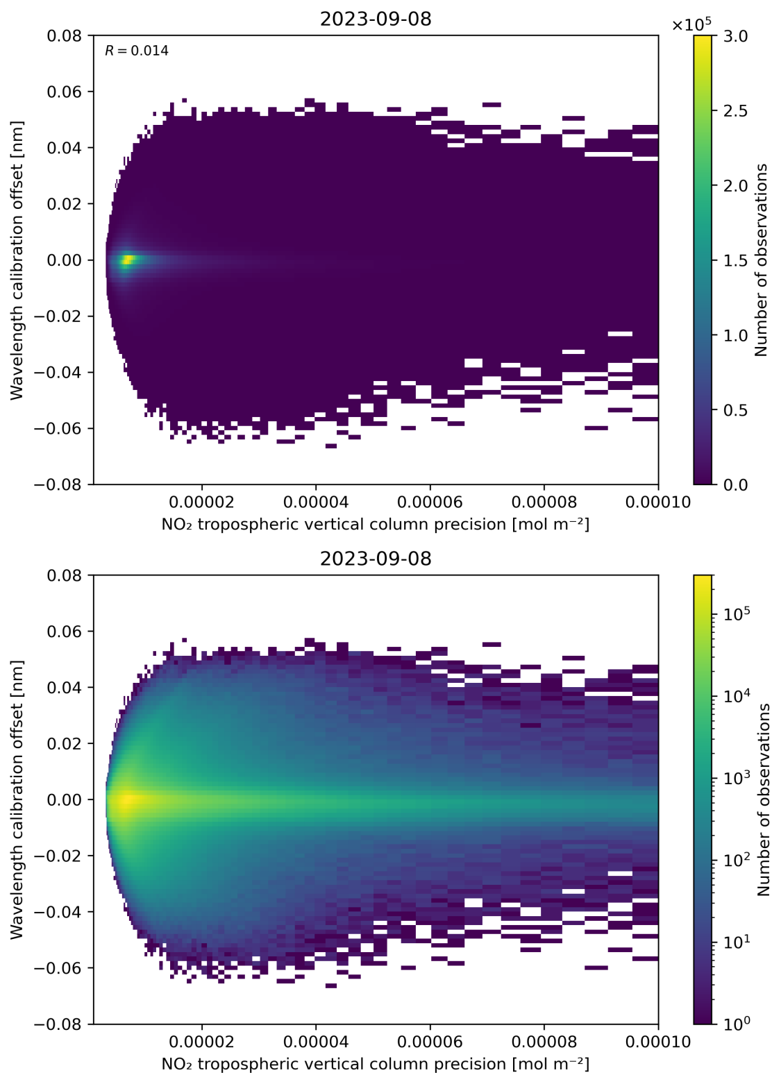
Figure 141: Scatter density plot of “NO 2 tropospheric vertical column precision” against “Wavelength calibration offset” for 2023-09-07 to 2023-09-09.
