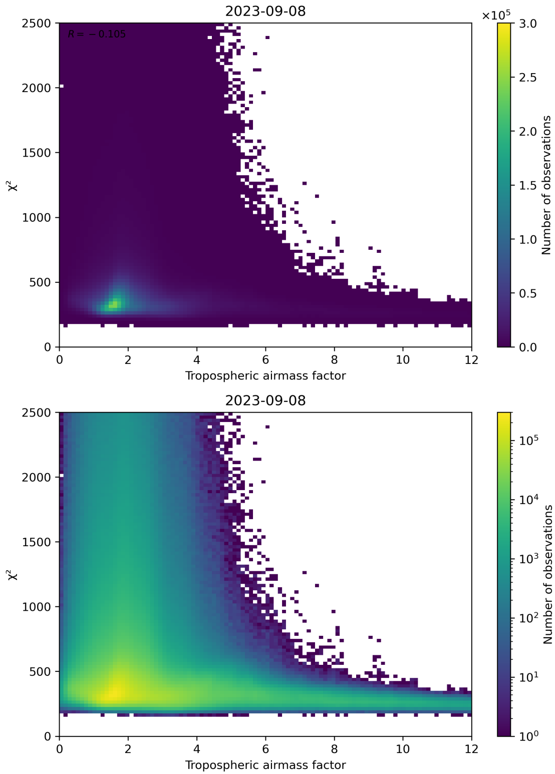
Figure 73: Scatter density plot of “Tropospheric airmass factor” against “ \chi^2 ” for 2023-09-07 to 2023-09-09.
