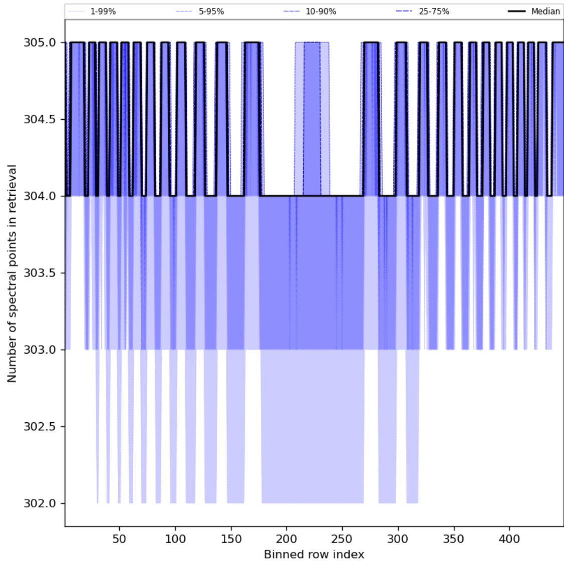
Figure 50: Along track statistics of “Number of spectral points in retrieval” for 2023-09-07 to 2023-09-09
