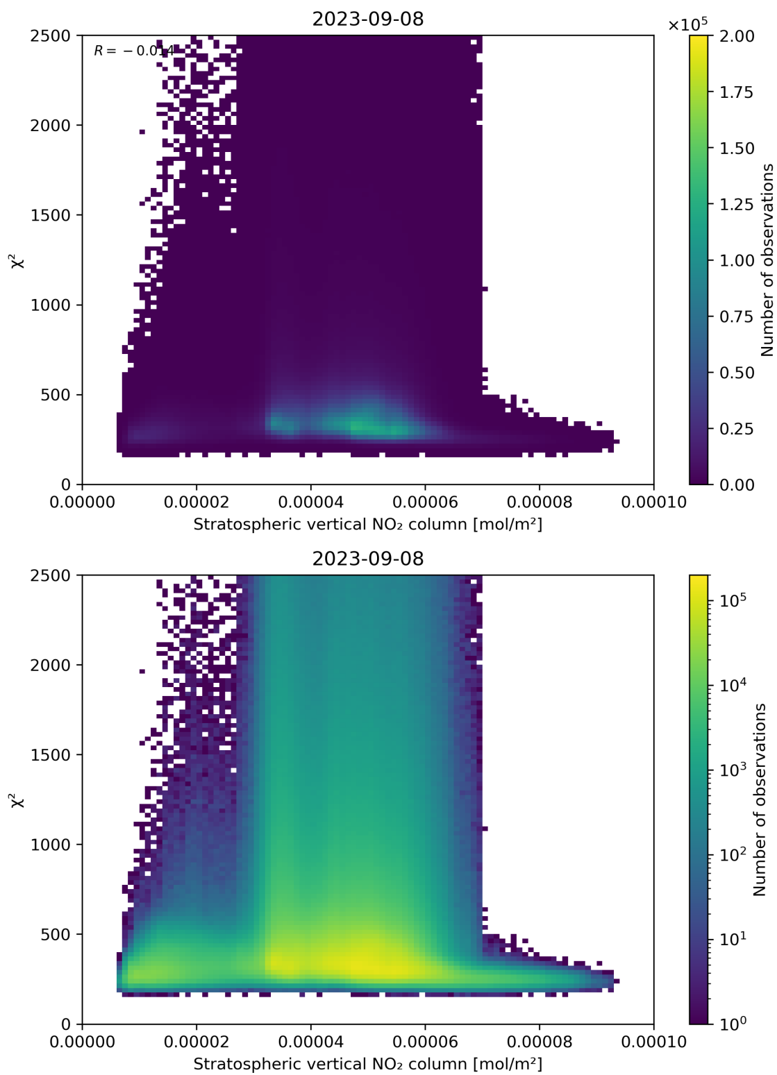
Figure 97: Scatter density plot of “Stratospheric vertical NO 2 column” against “ \chi^2 ” for 2023-09-07 to 2023-09-09.
