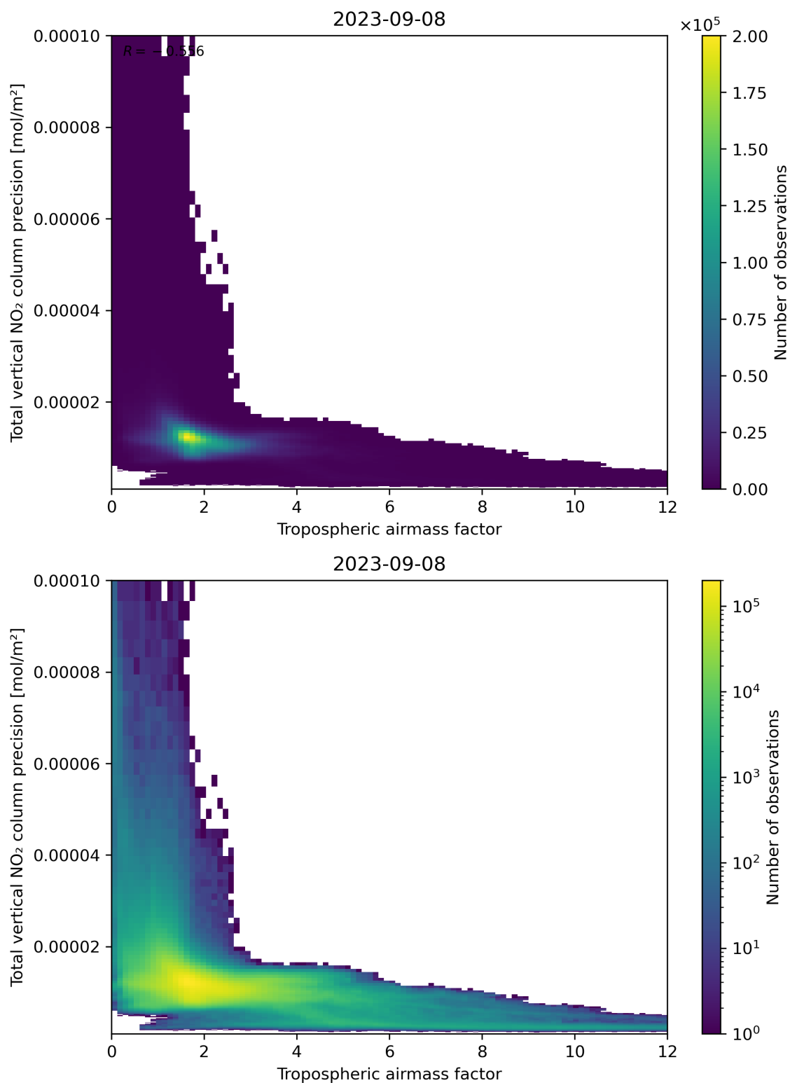
Figure 78: Scatter density plot of “Tropospheric air mass factor” against “Total vertical NO 2 column precision” for 2023-09-07 to 2023-09-09.
