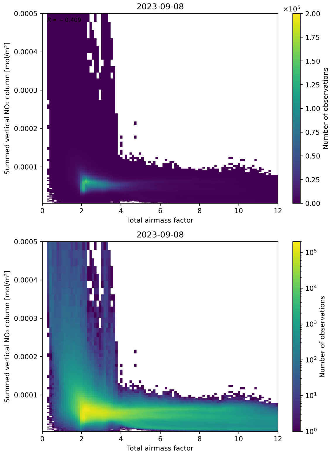
Figure 65: Scatter density plot of “Total airmass factor” against “Summed vertical NO 2 column” for 2023-09-07 to 2023-09-09.
