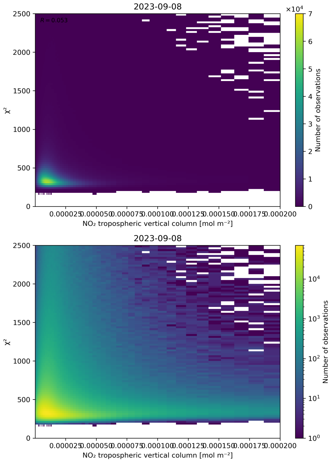
Figure 124: Scatter density plot of “NO 2 tropospheric vertical column” against “ \chi^2 ” for 2023-09-07 to 2023-09-09.
