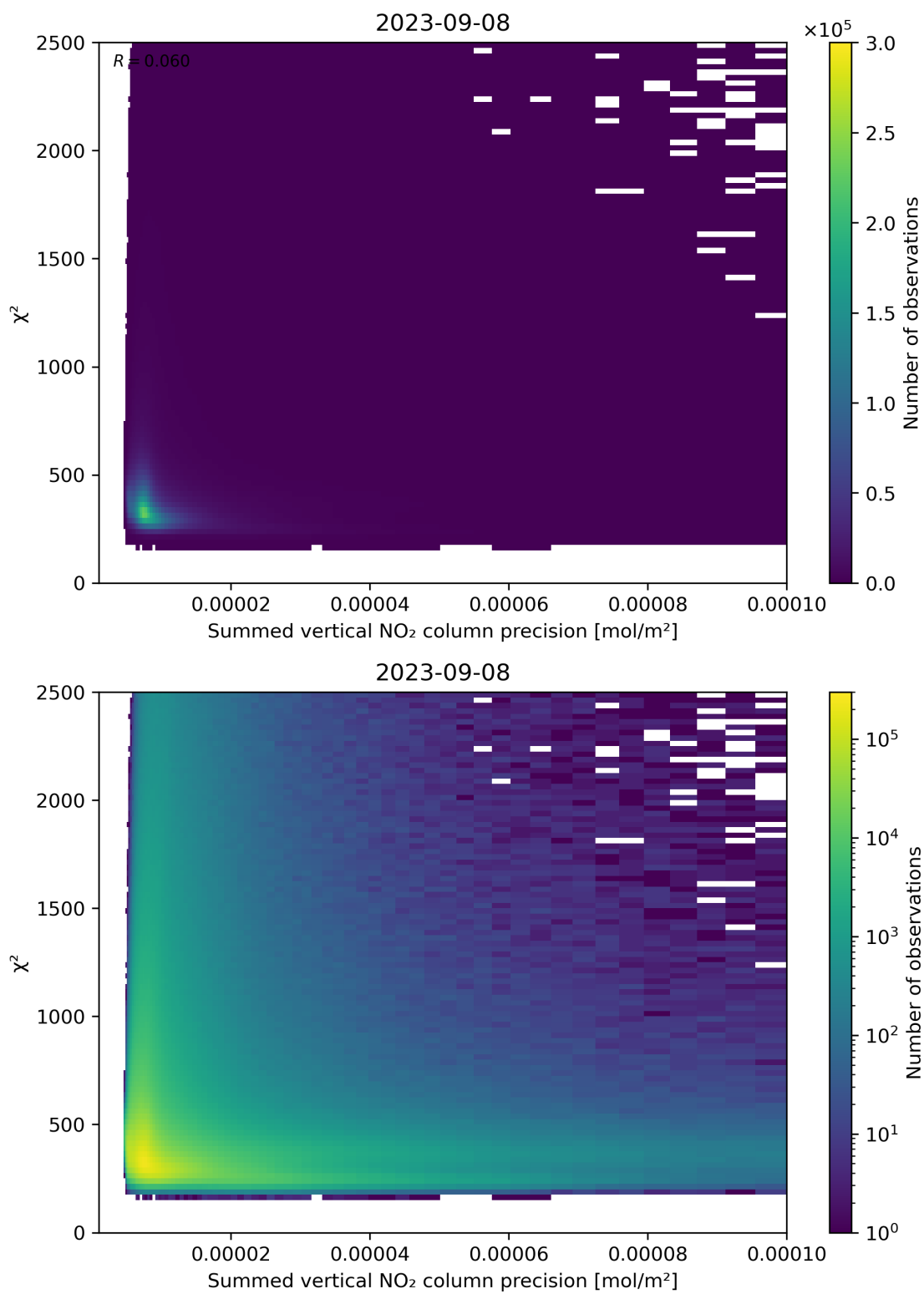
Figure 107: Scatter density plot of “Summed vertical NO 2 column precision” against “ \chi^2 ” for 2023-09-07 to 2023-09-09.
