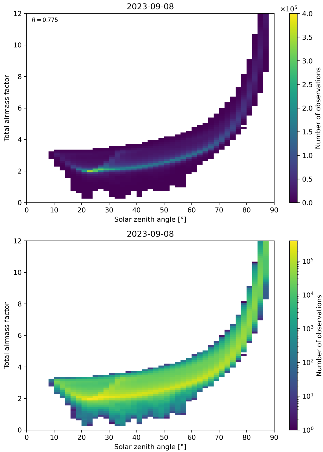
Figure 146: Scatter density plot of “Solar zenith angle” against “Total air mass factor” for 2023-09-07 to 2023-09-09.
