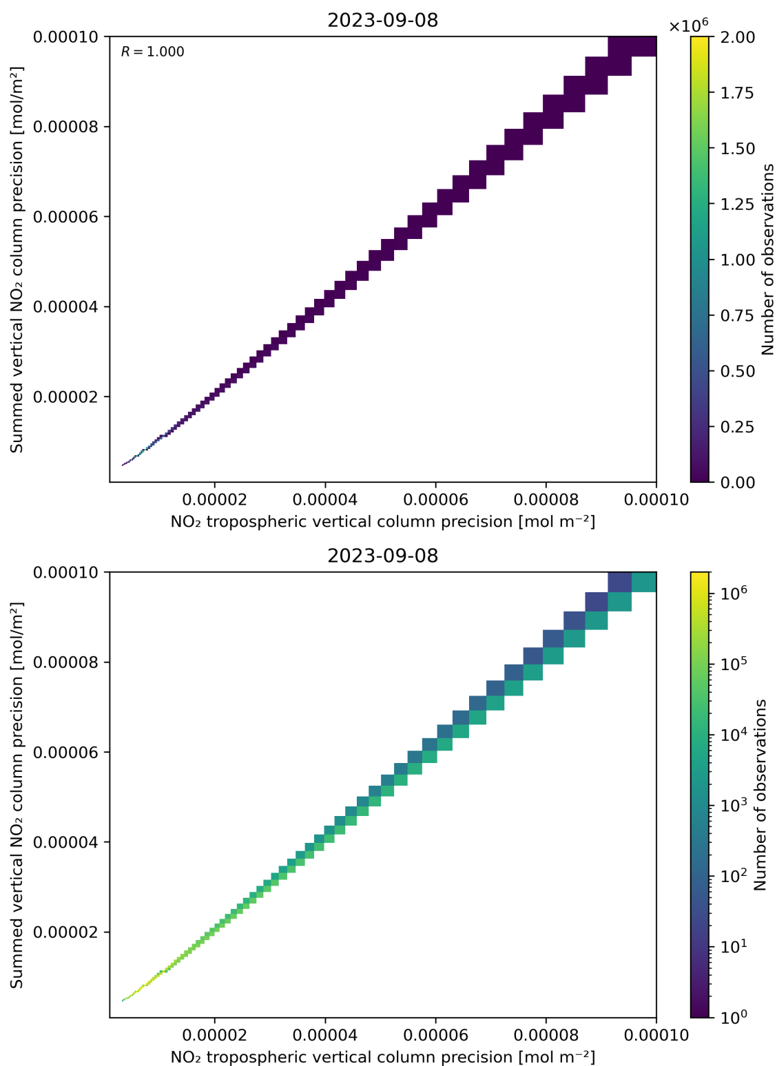
Figure 137: Scatter density plot of “NO 2 tropospheric vertical column precision” against “Summed vertical NO 2 column precision” for 2023-09-07 to 2023-09-09.
