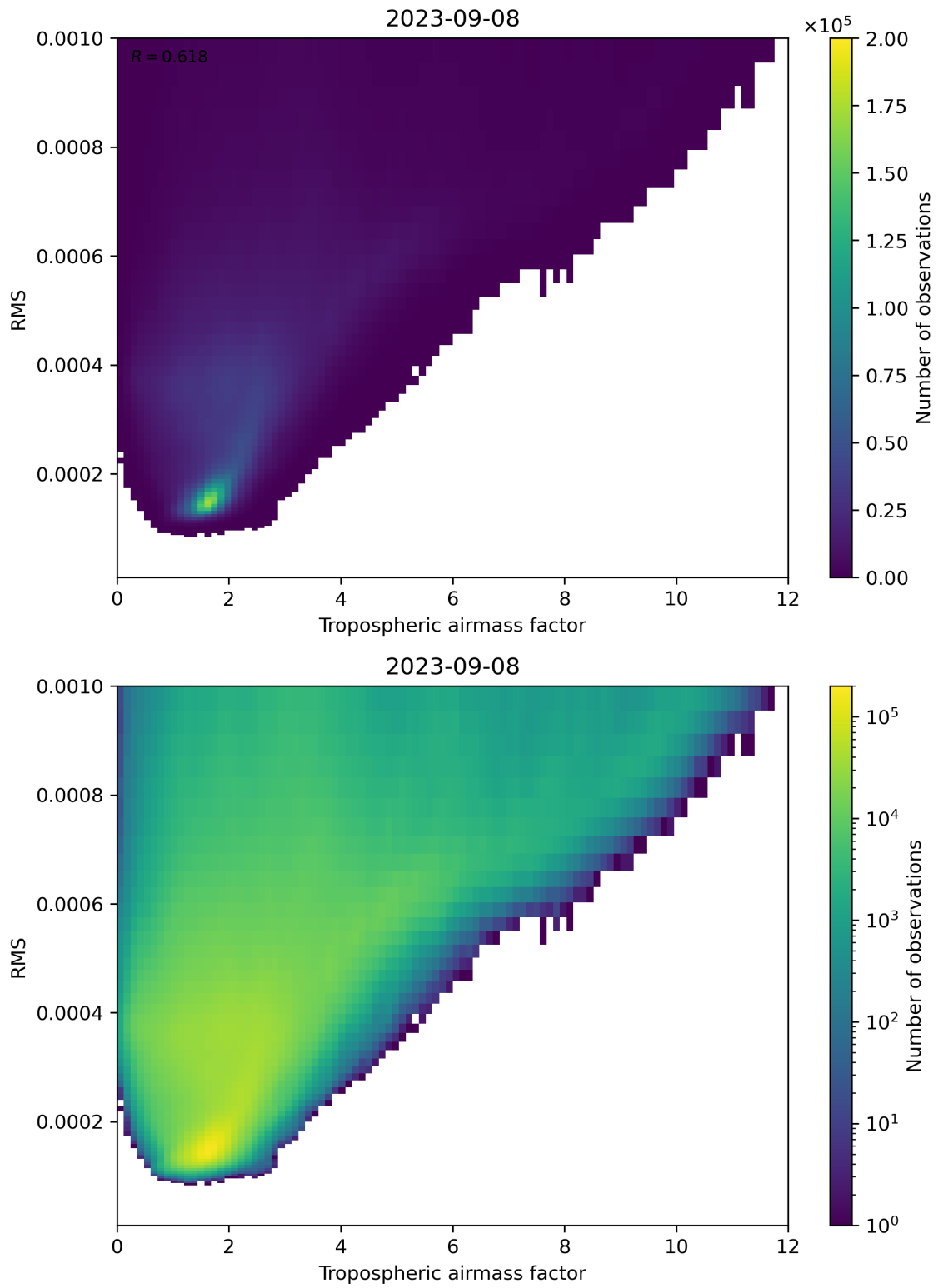
Figure 79: Scatter density plot of “Tropospheric airmass factor” against “RMS” for 2023-09-07 to 2023-09-09.
