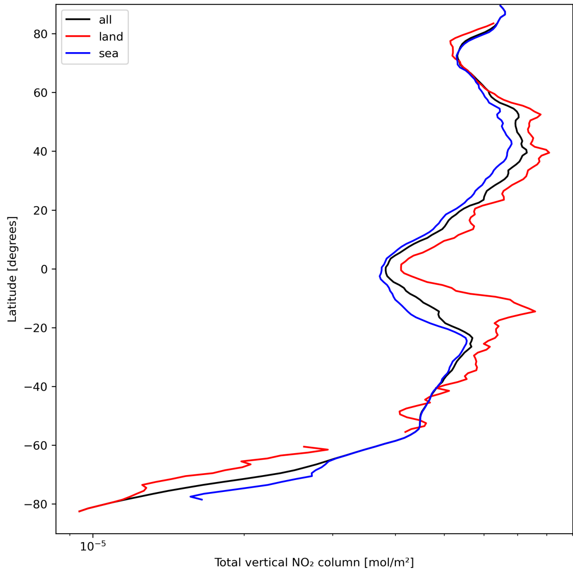
Figure 21: Zonal average of “Total vertical NO 2 column” for 2023-09-07 to 2023-09-09.
