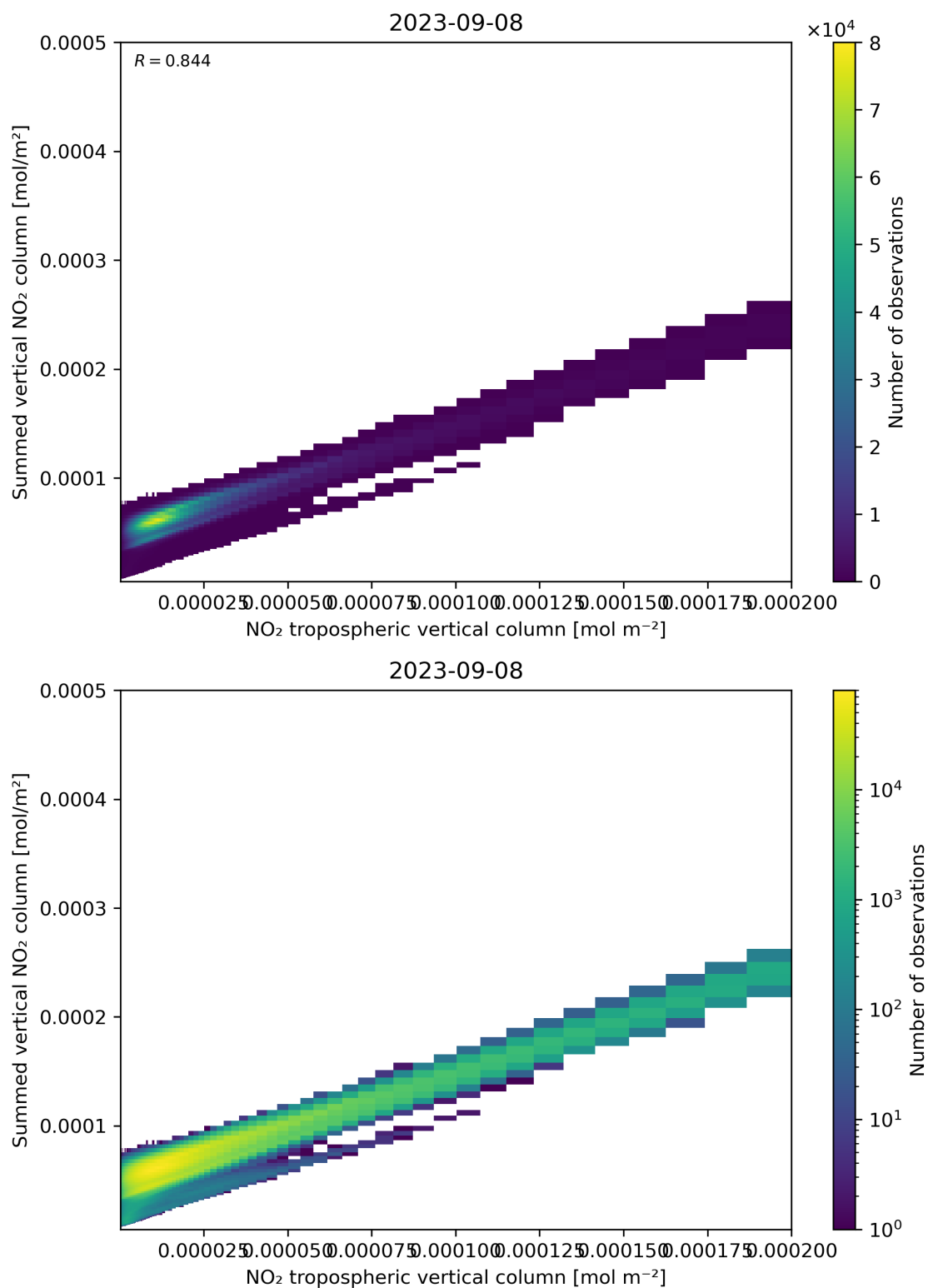
Figure 126: Scatter density plot of “NO 2 tropospheric vertical column” against “Summed vertical NO 2 column” for 2023-09-07 to 2023-09-09.
