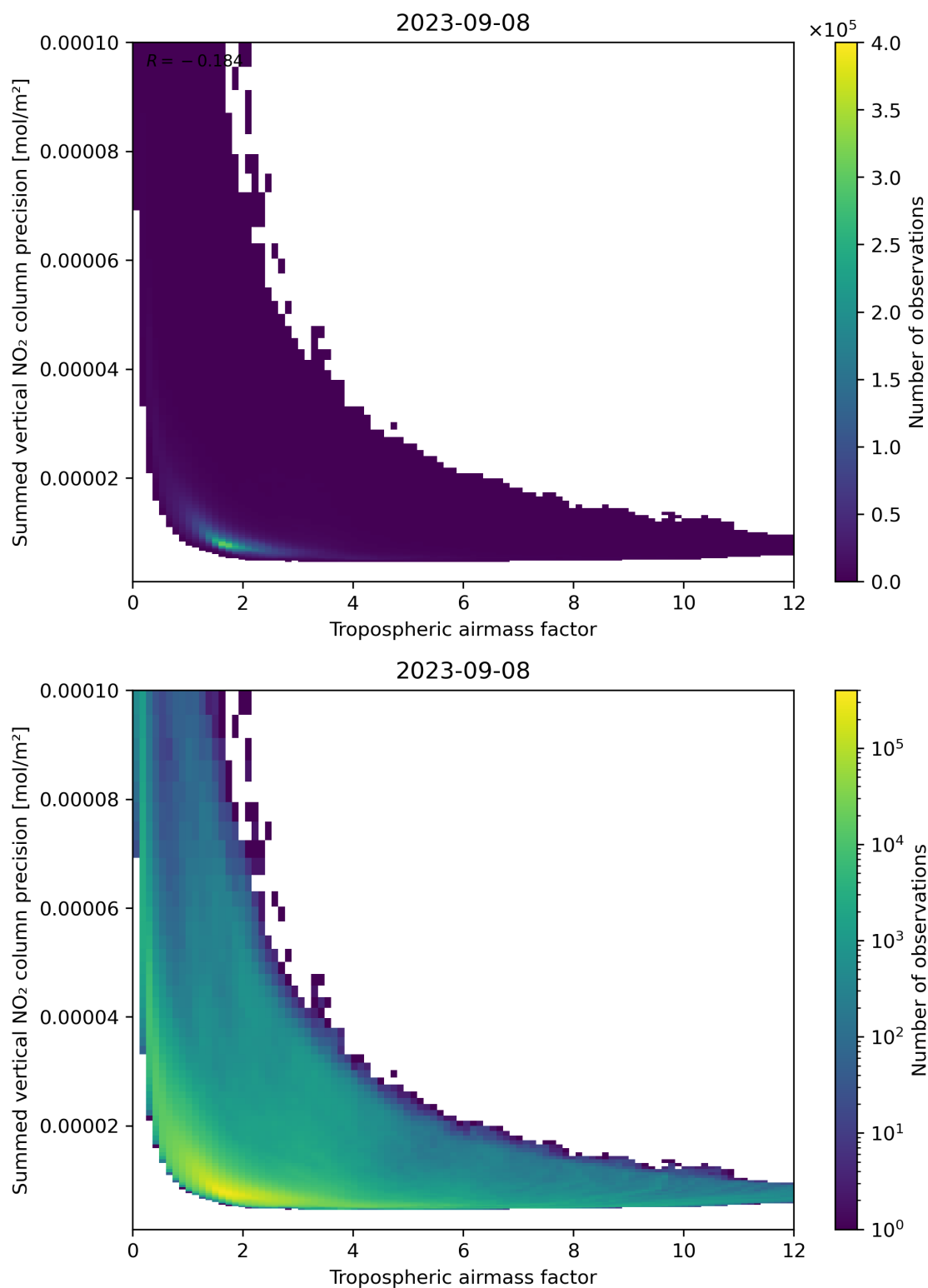
Figure 76: Scatter density plot of “Tropospheric air mass factor” against “Summed vertical NO 2 column precision” for 2023-09-07 to 2023-09-09.
