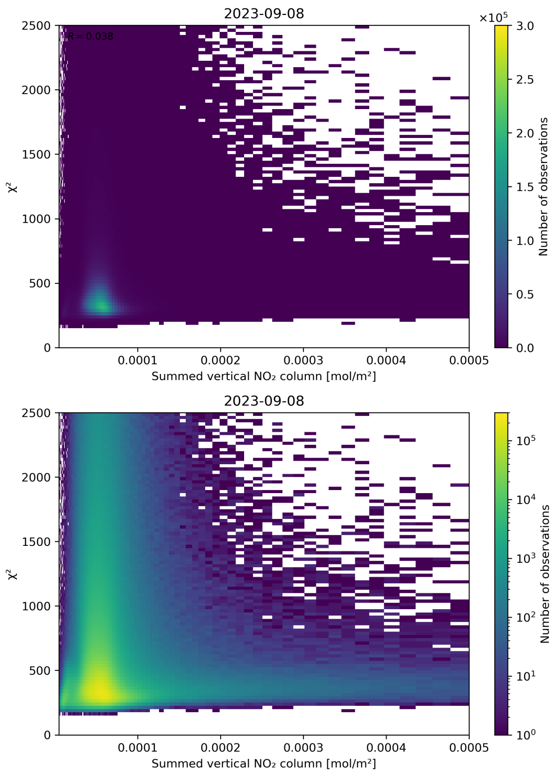
Figure 104: Scatter density plot of “Summed vertical NO 2 column” against “ \chi^2 ” for 2023-09-07 to 2023-09-09.
