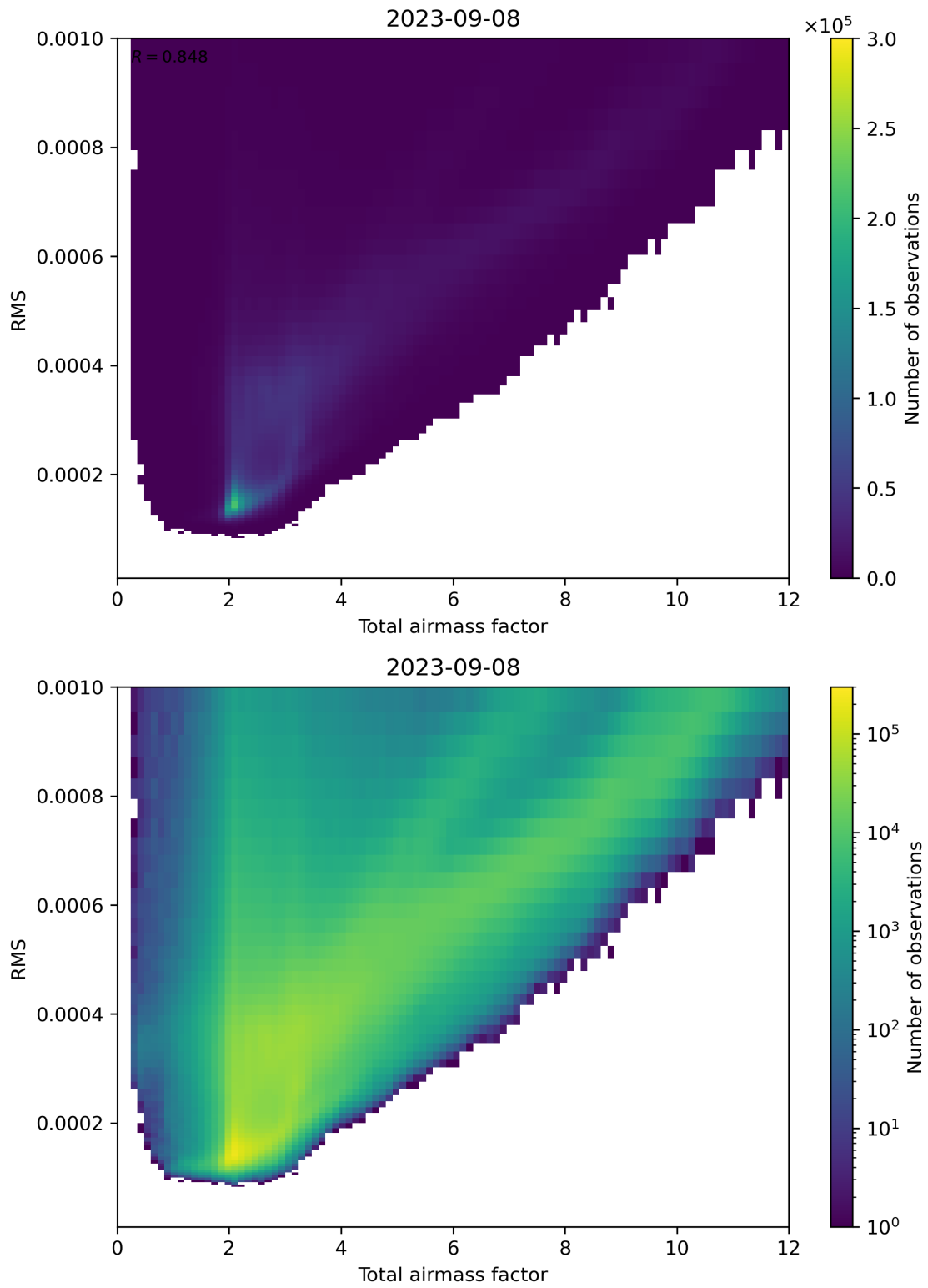
Figure 69: Scatter density plot of “Total airmass factor” against “RMS” for 2023-09-07 to 2023-09-09.
