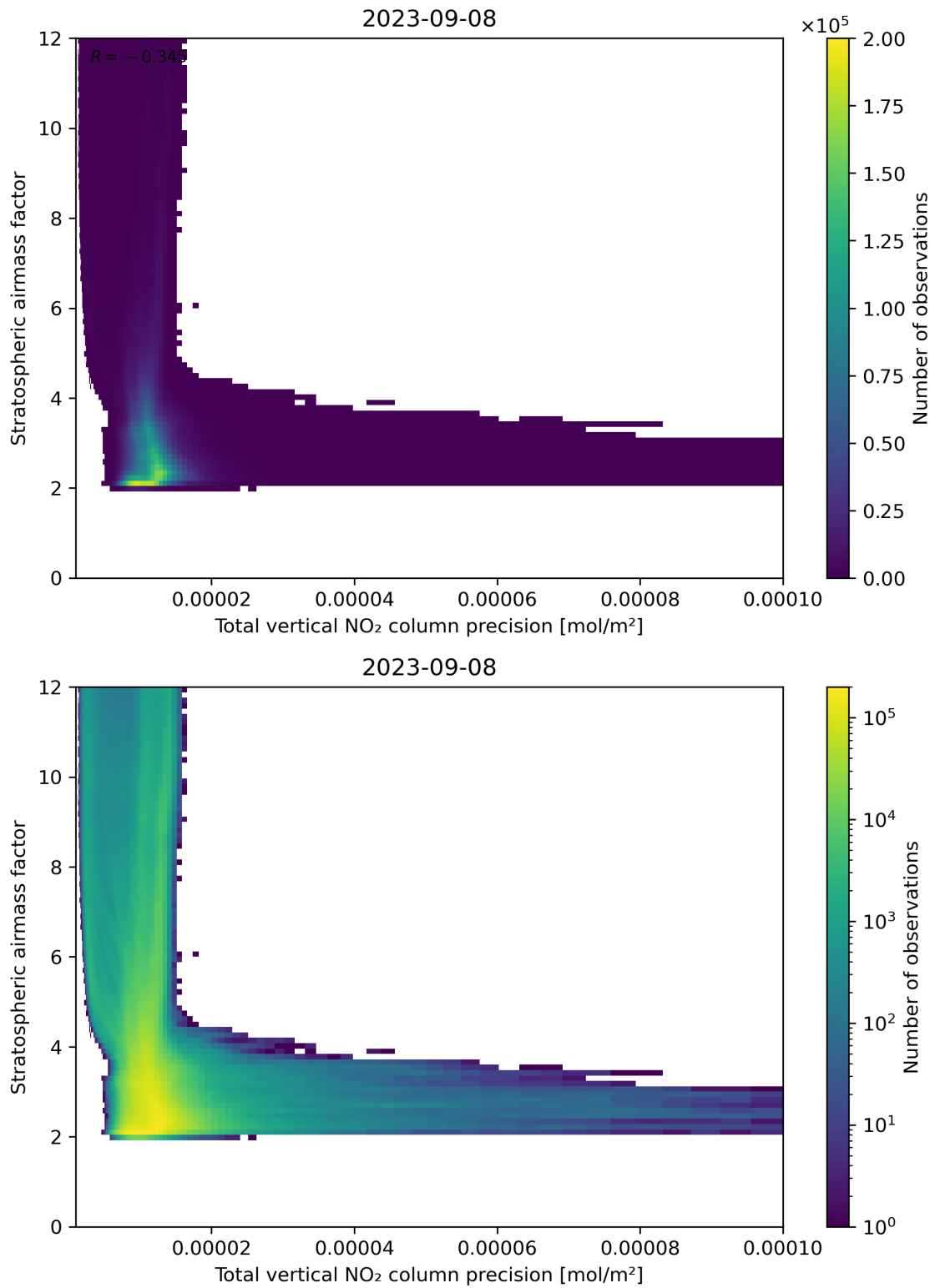
Figure 115: Scatter density plot of “Total vertical NO 2 column precision” against “Stratospheric air mass factor” for 2023-09-07 to 2023-09-09.
