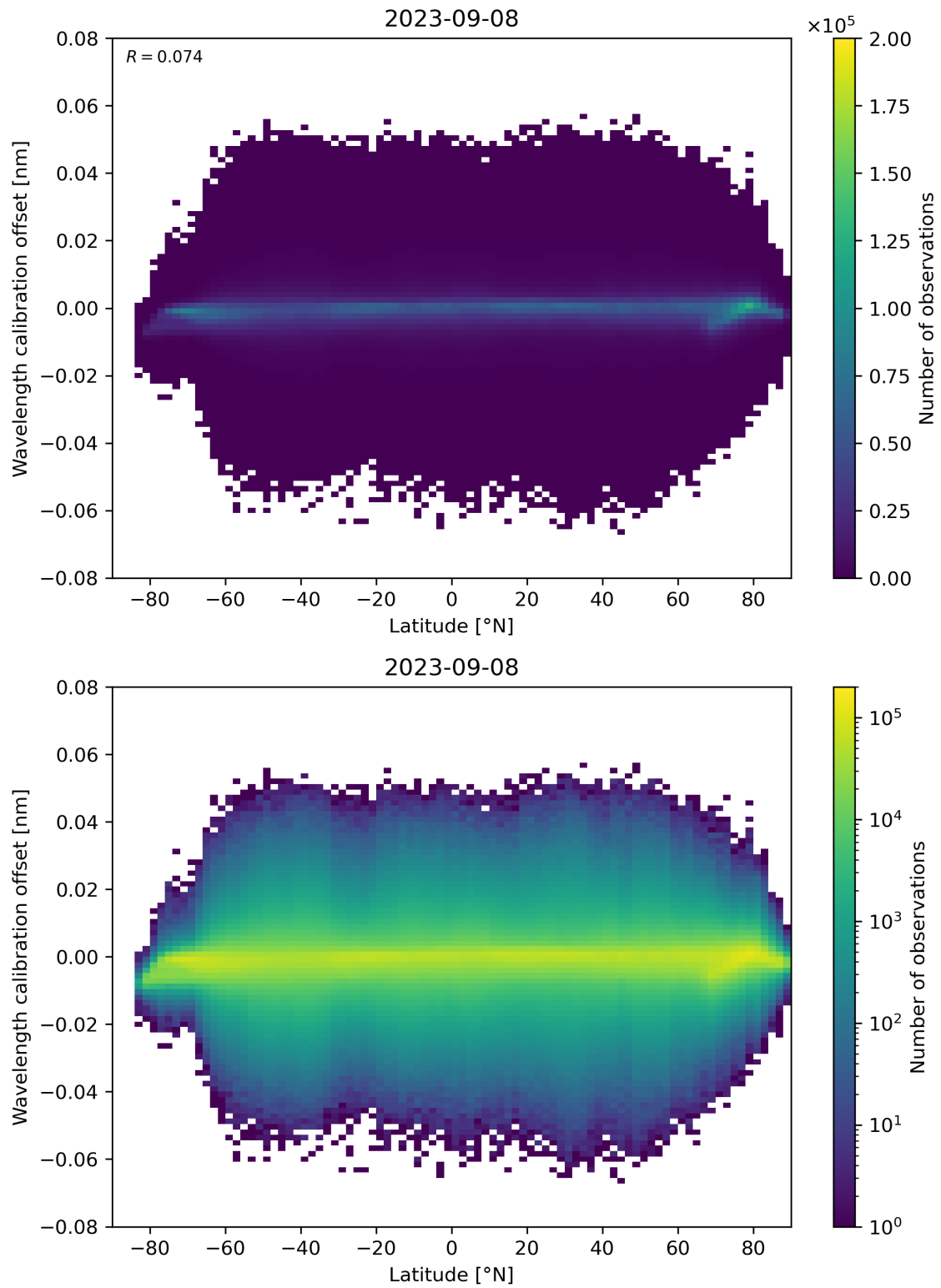
Figure 95: Scatter density plot of “Latitude” against “Wavelength calibration offset” for 2023-09-07 to 2023-09-09.
