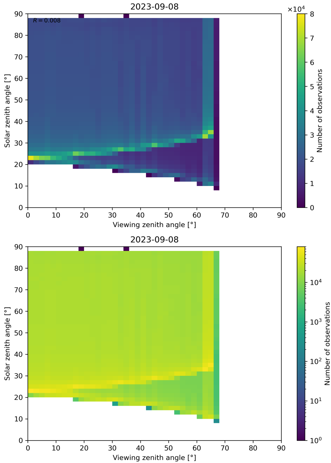
Figure 172: Scatter density plot of “Viewing zenith angle” against “Solar zenith angle” for 2023-09-07 to 2023-09-09.
