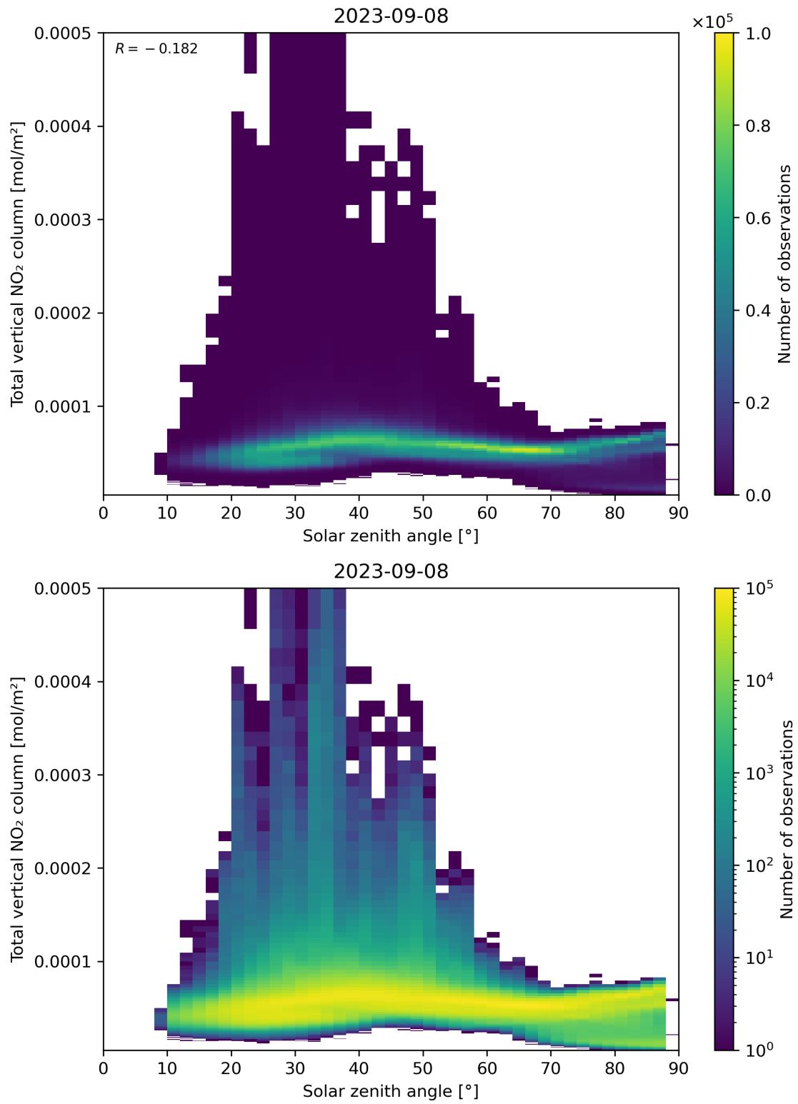
Figure 153: Scatter density plot of “Solar zenith angle” against “Total vertical NO 2 column” for 2023-09-07 to 2023-09-09.
