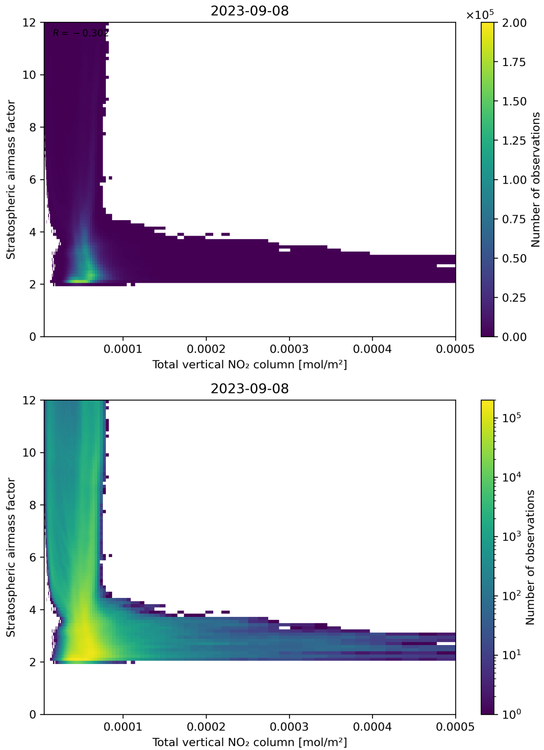
Figure 110: Scatter density plot of “Total vertical NO 2 column” against “Stratospheric airmass factor” for 2023-09-07 to 2023-09-09.
