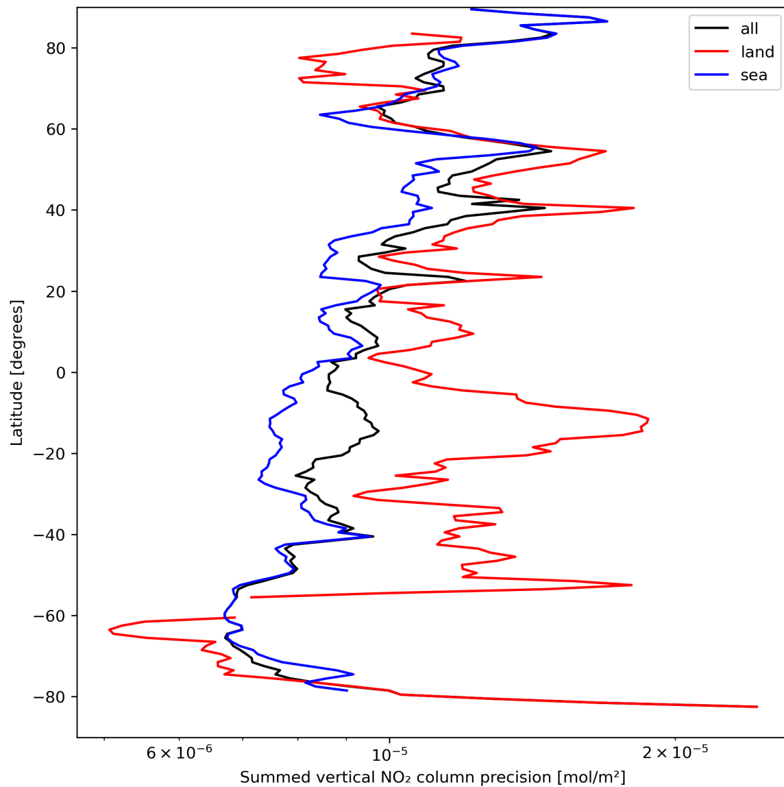
Figure 24: Zonal average of “Summed vertical NO 2 column precision” for 2023-09-07 to 2023-09-09.
