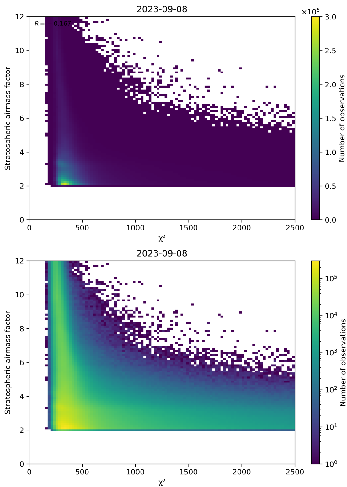
Figure 81: Scatter density plot of “ \chi^2 ” against “Stratospheric airmass factor” for 2023-09-07 to 2023-09-09.
