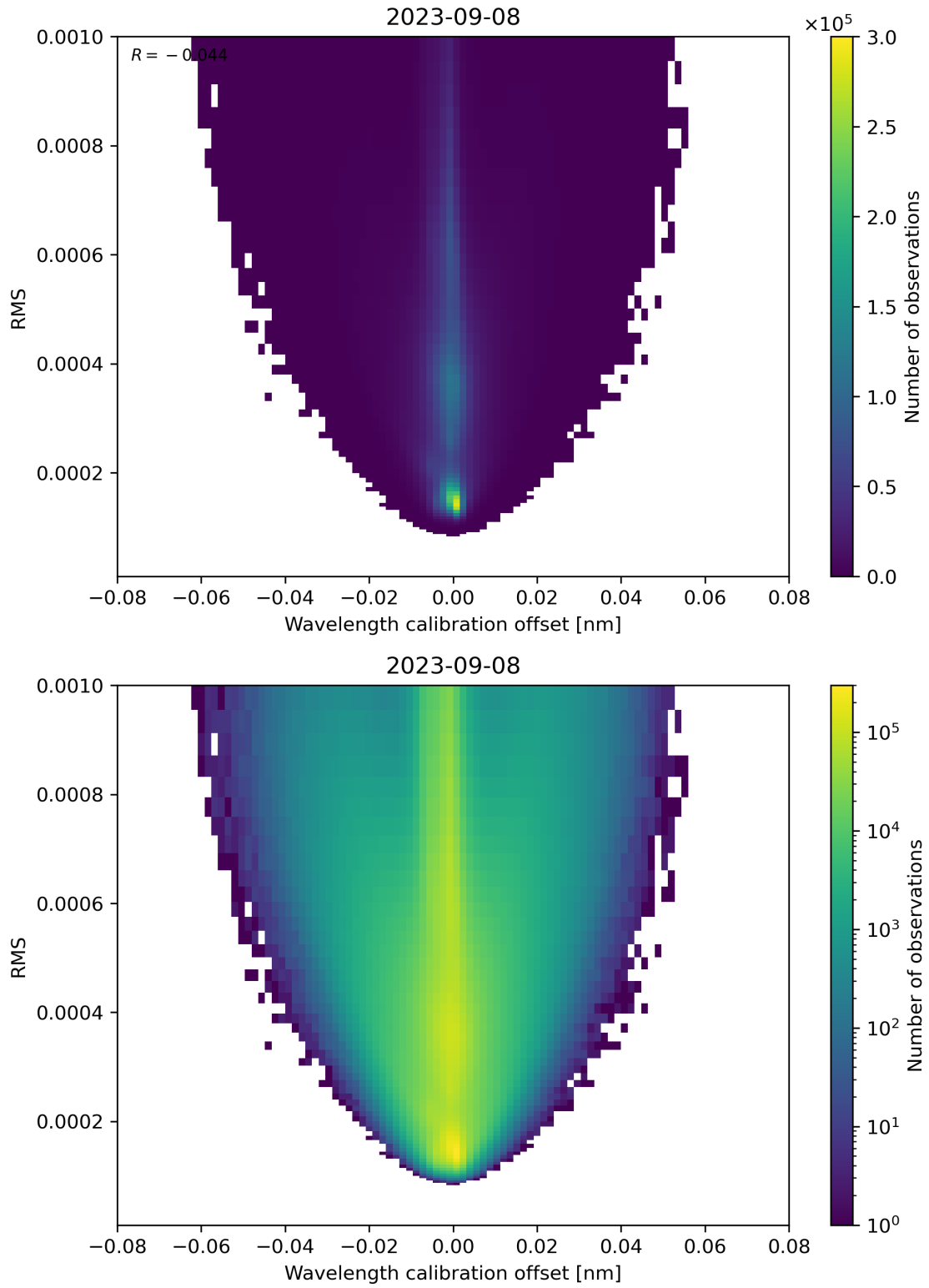
Figure 181: Scatter density plot of “Wavelength calibration offset” against “RMS” for 2023-09-07 to 2023-09-09.
