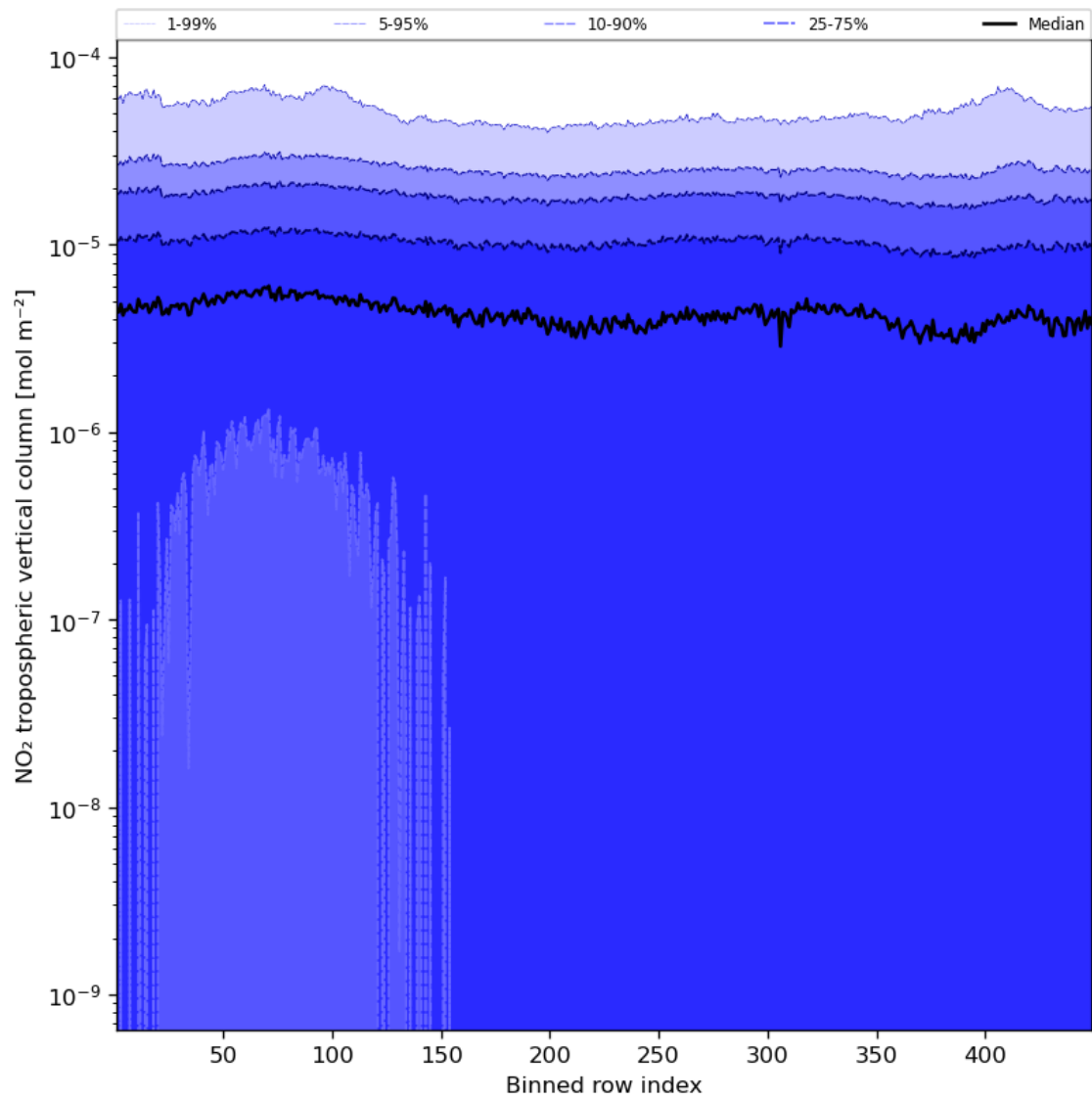
Figure 46: Along track statistics of “NO 2 tropospheric vertical column” for 2023-09-07 to 2023-09-09
