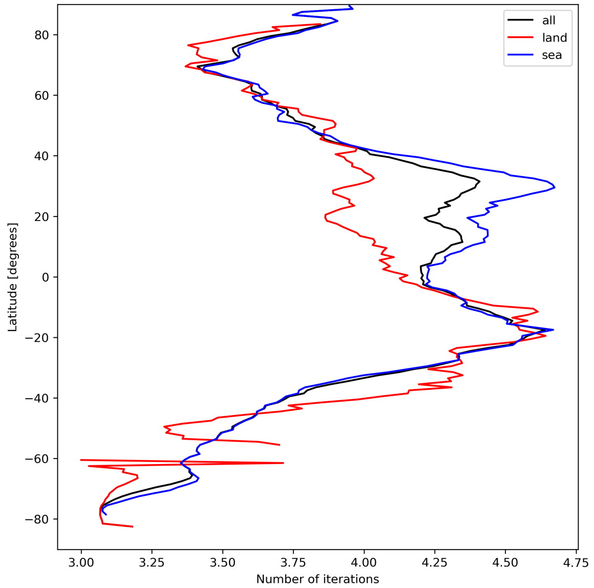
Figure 17: Zonal average of “Number of iterations” for 2023-09-07 to 2023-09-09.
