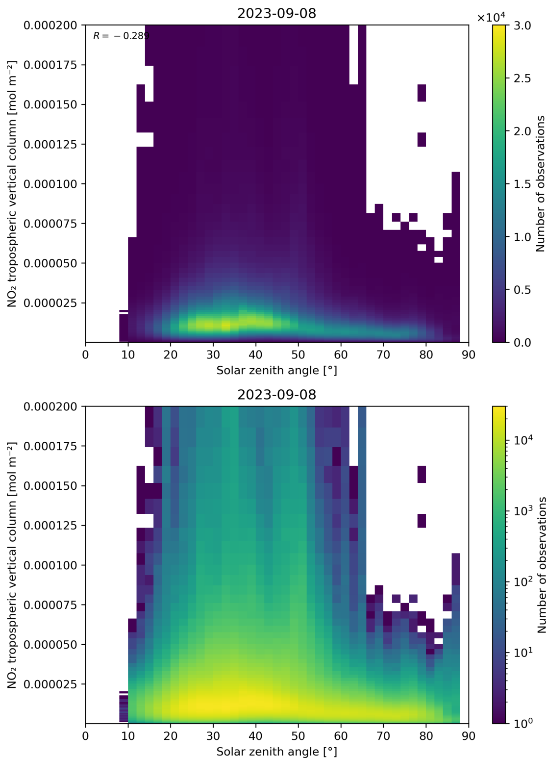
Figure 155: Scatter density plot of “Solar zenith angle” against “NO 2 tropospheric vertical column” for 2023-09-07 to 2023-09-09.
