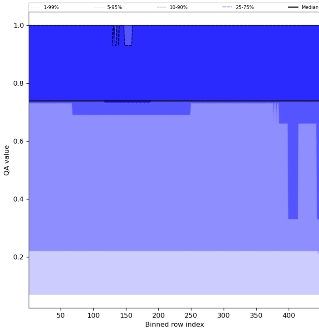
Figure 45: Along track statistics of “QA value” for 2023-09-07 to 2023-09-09
