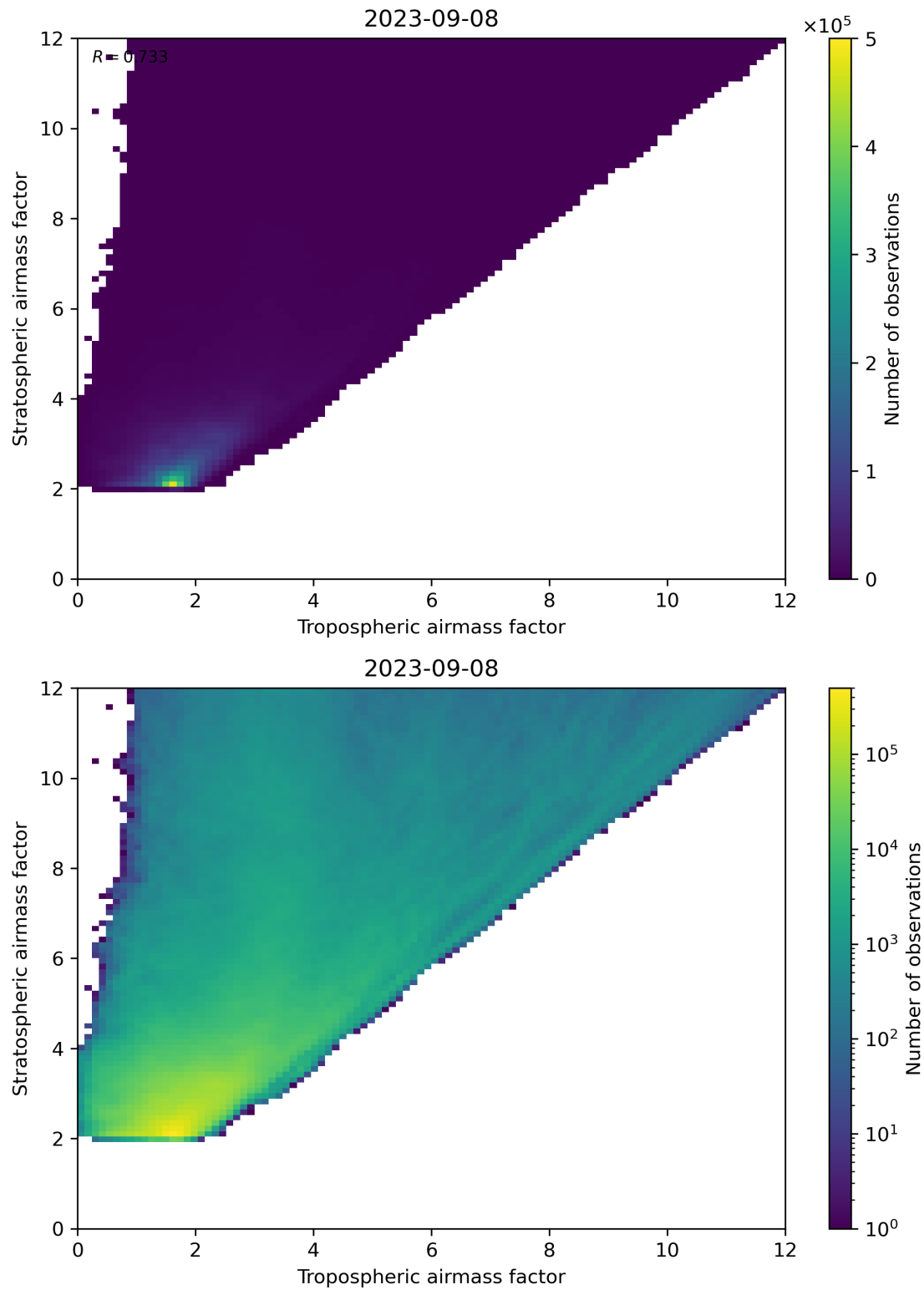
Figure 71: Scatter density plot of “Tropospheric airmass factor” against “Stratospheric airmass factor” for 2023-09-07 to 2023-09-09.
