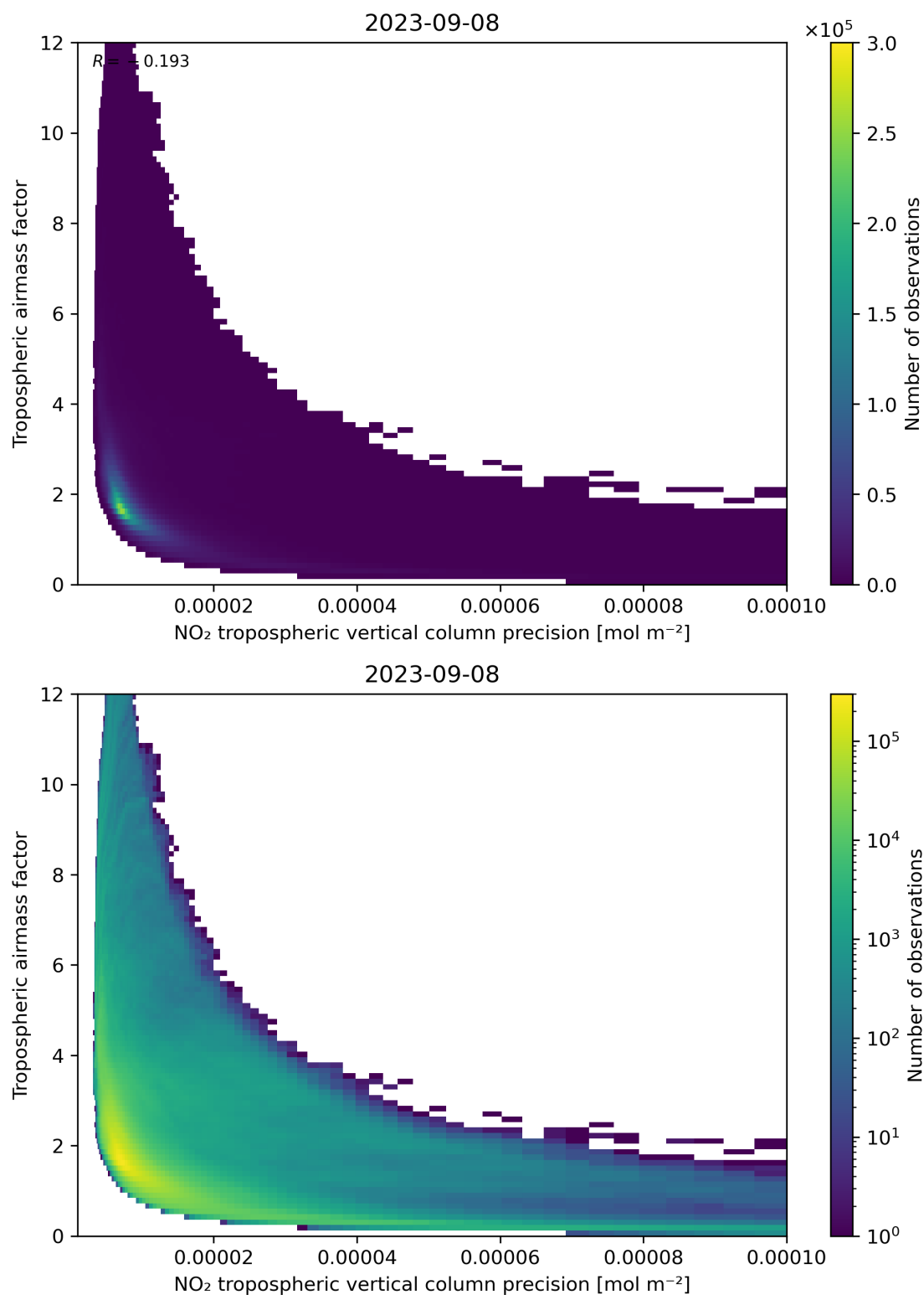
Figure 133: Scatter density plot of “NO 2 tropospheric vertical column precision” against “Tropospheric air mass factor” for 2023-09-07 to 2023-09-09.
