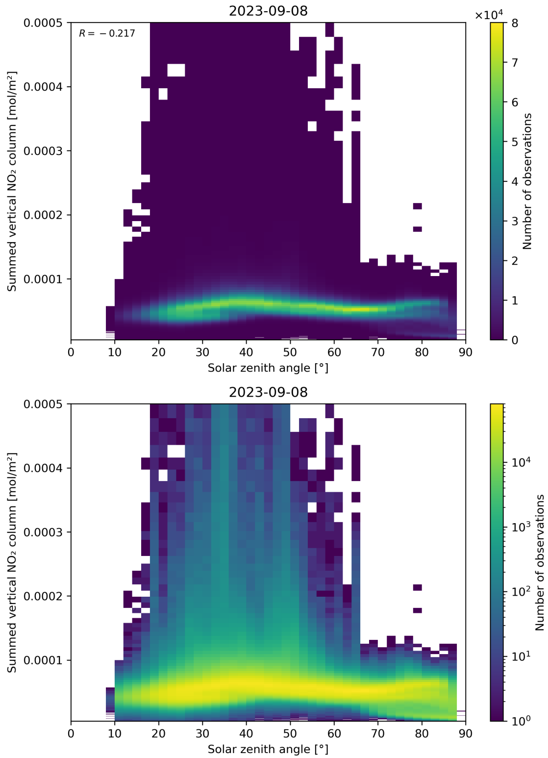
Figure 151: Scatter density plot of “Solar zenith angle” against “Summed vertical NO 2 column” for 2023-09-07 to 2023-09-09.
