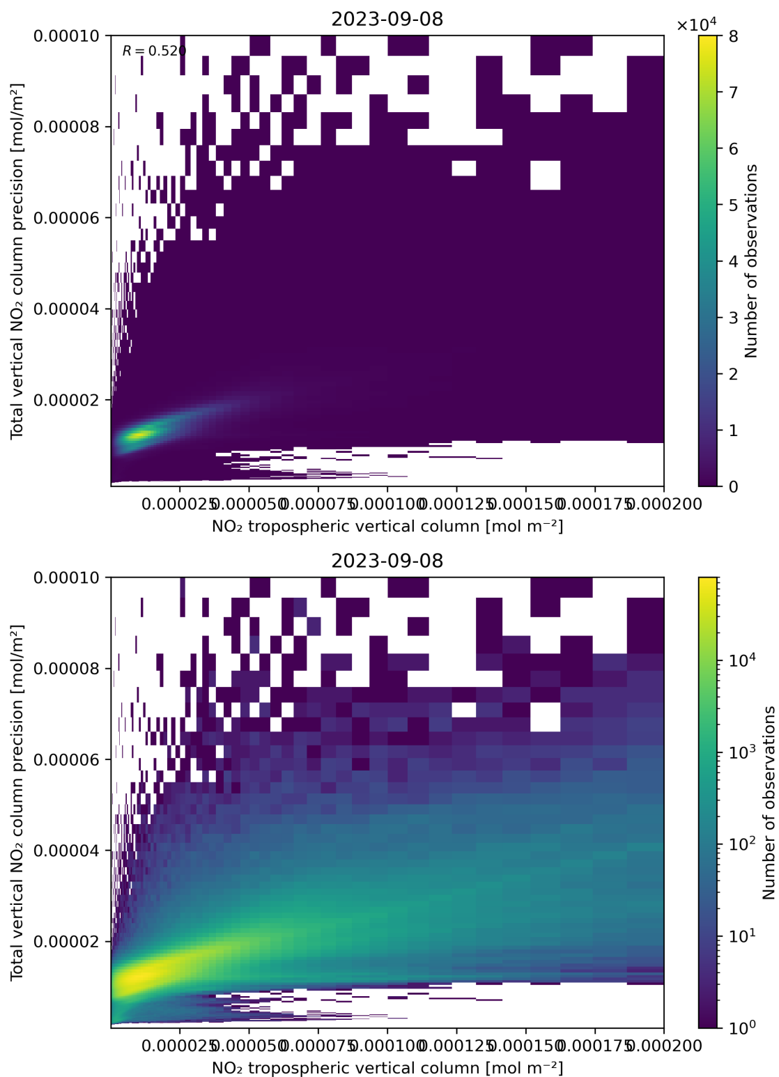
Figure 129: Scatter density plot of “NO 2 tropospheric vertical column” against “Total vertical NO 2 column precision” for 2023-09-07 to 2023-09-09.
