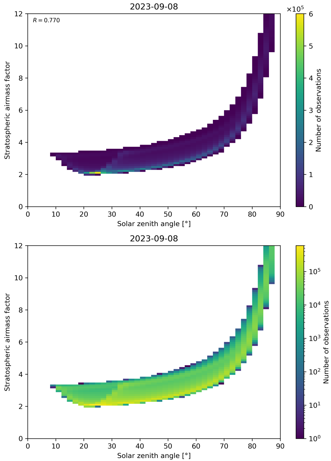
Figure 145: Scatter density plot of “Solar zenith angle” against “Stratospheric airmass factor” for 2023-09-07 to 2023-09-09.
