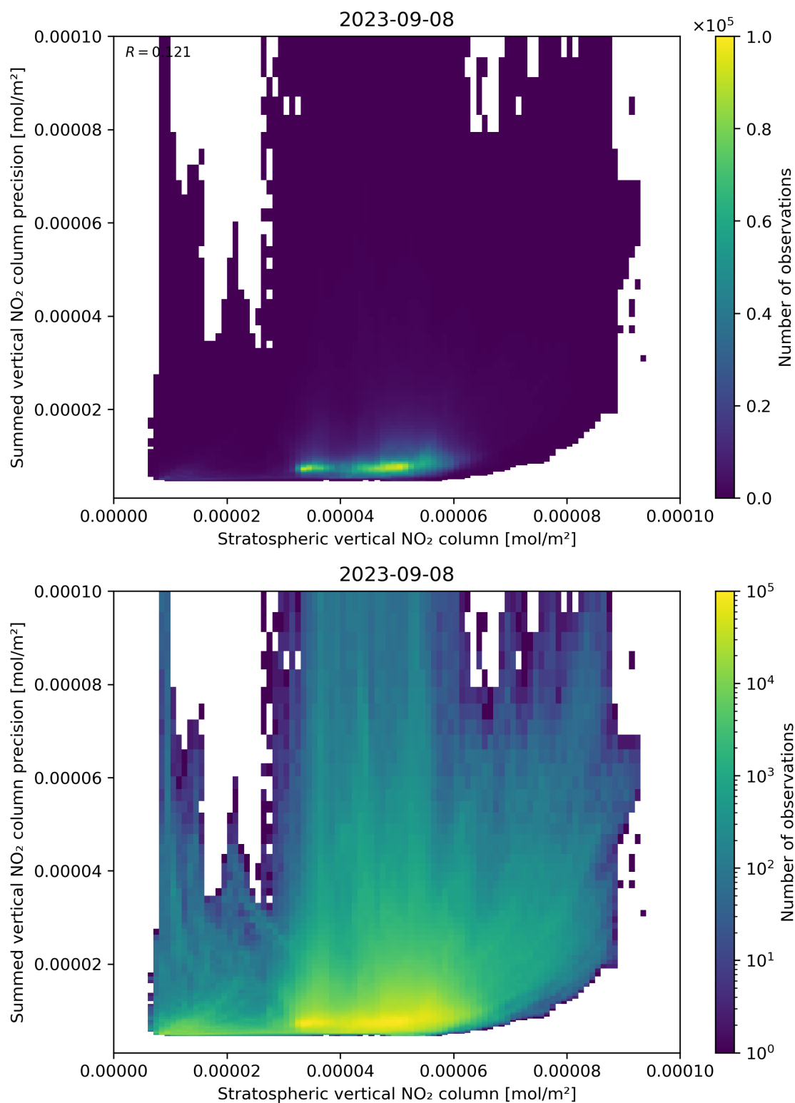
Figure 99: Scatter density plot of “Stratospheric vertical NO 2 column” against “Summed vertical NO 2 column precision” for 2023-09-07 to 2023-09-09.
