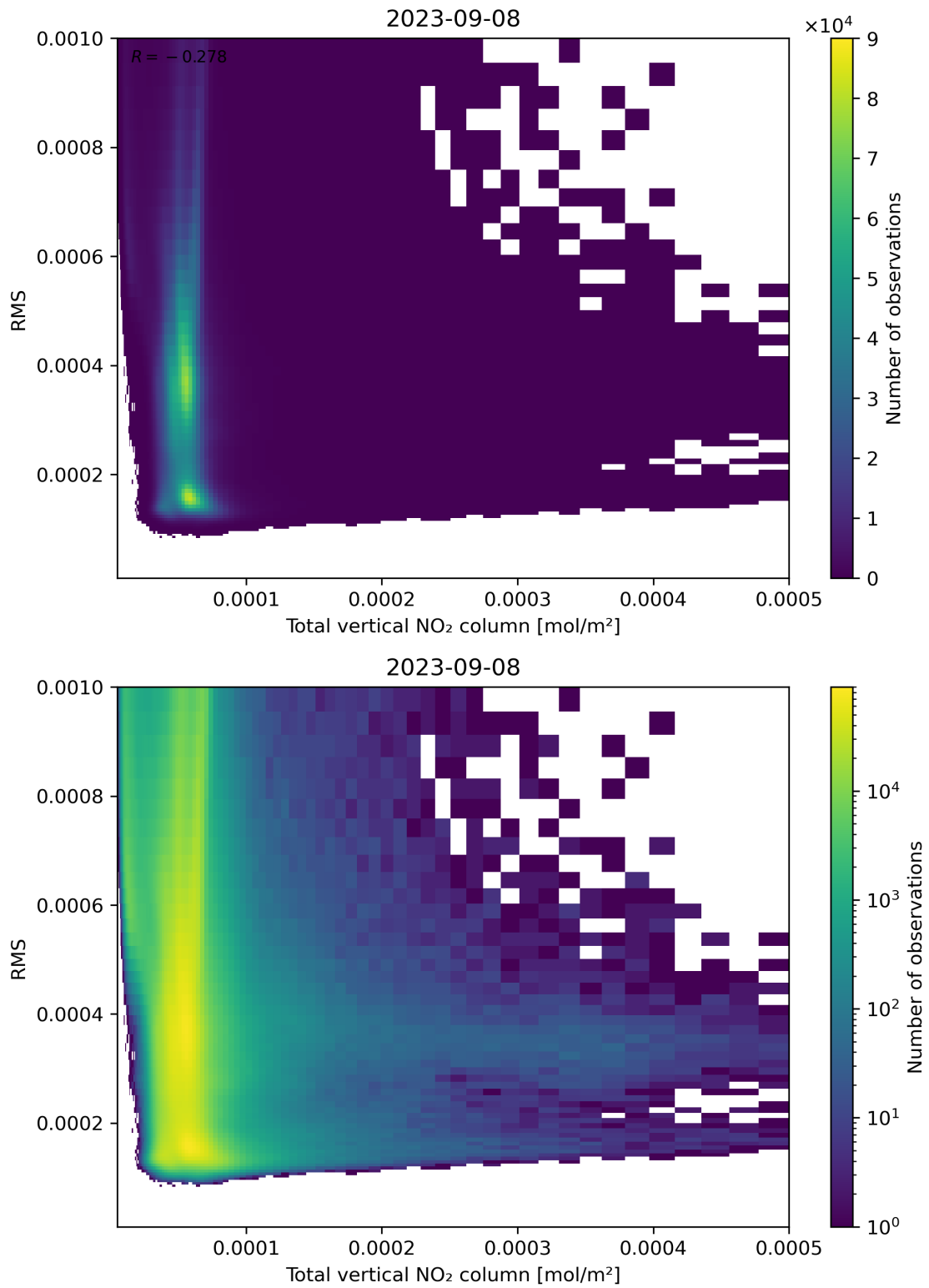
Figure 120: Scatter density plot of “Total vertical NO 2 column” against “RMS” for 2023-09-07 to 2023-09-09.
