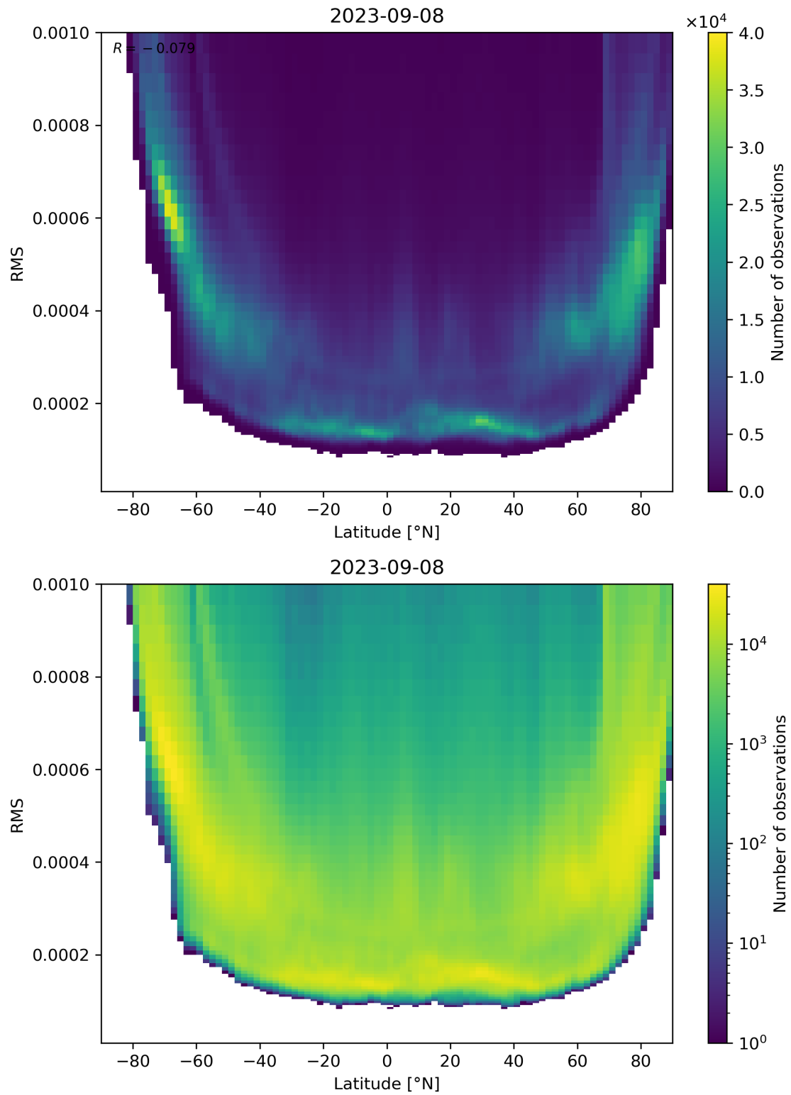
Figure 94: Scatter density plot of “Latitude” against “RMS” for 2023-09-07 to 2023-09-09.
