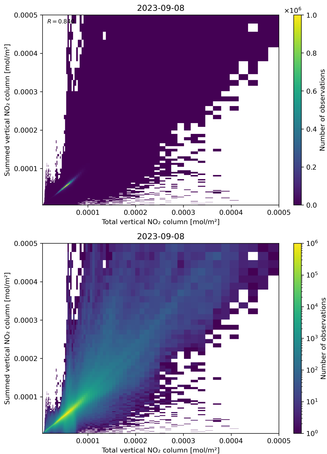
Figure 112: Scatter density plot of “Total vertical NO 2 column” against “Summed vertical NO 2 column” for 2023-09-07 to 2023-09-09.
