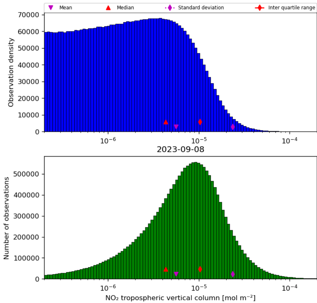
Figure 29: Histogram of “NO 2 tropospheric vertical column” for 2023-09-07 to 2023-09-09
