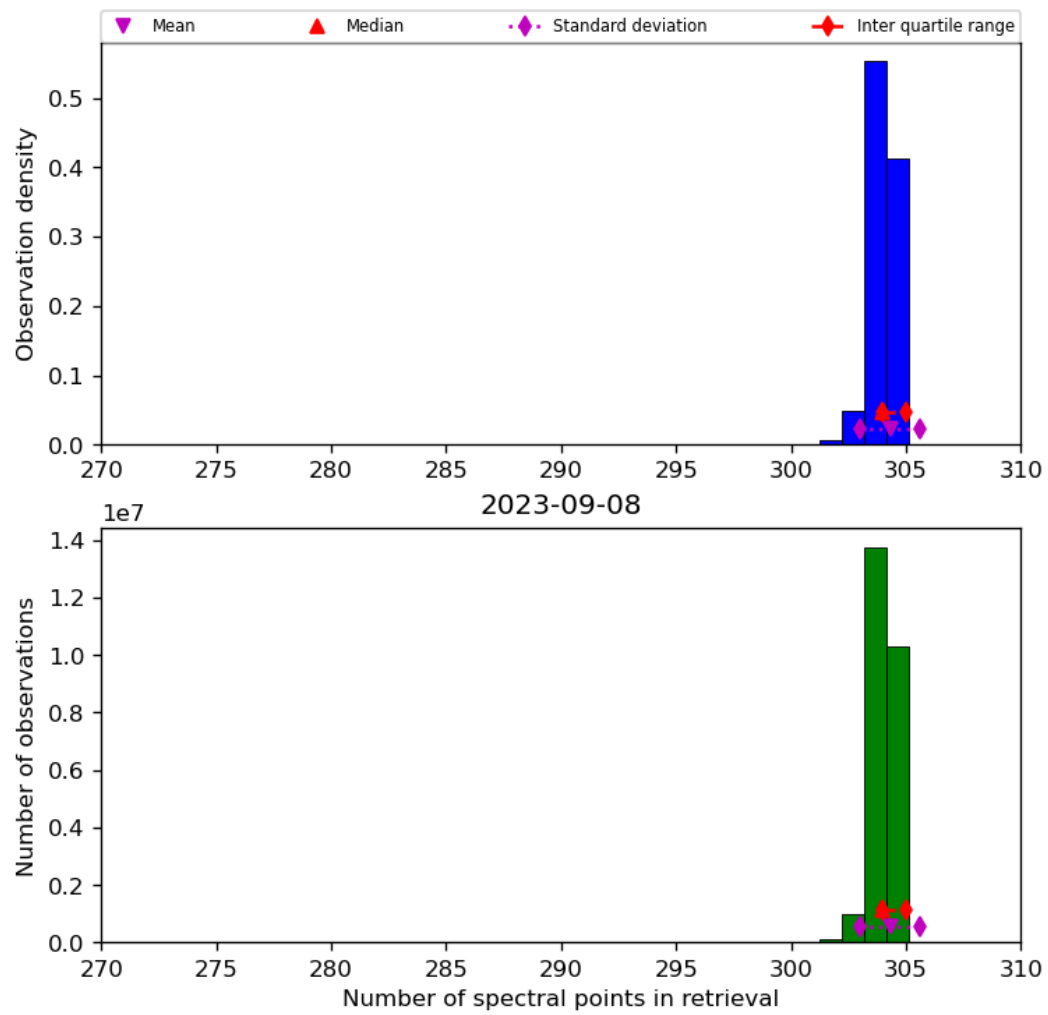
Figure 33: Histogram of “Number of spectral points in retrieval” for 2023-09-07 to 2023-09-09
