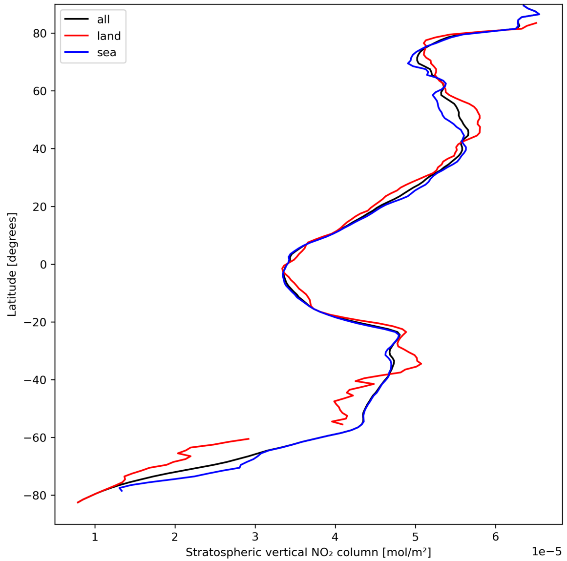
Figure 19: Zonal average of “Stratospheric vertical NO 2 column” for 2023-09-07 to 2023-09-09.
