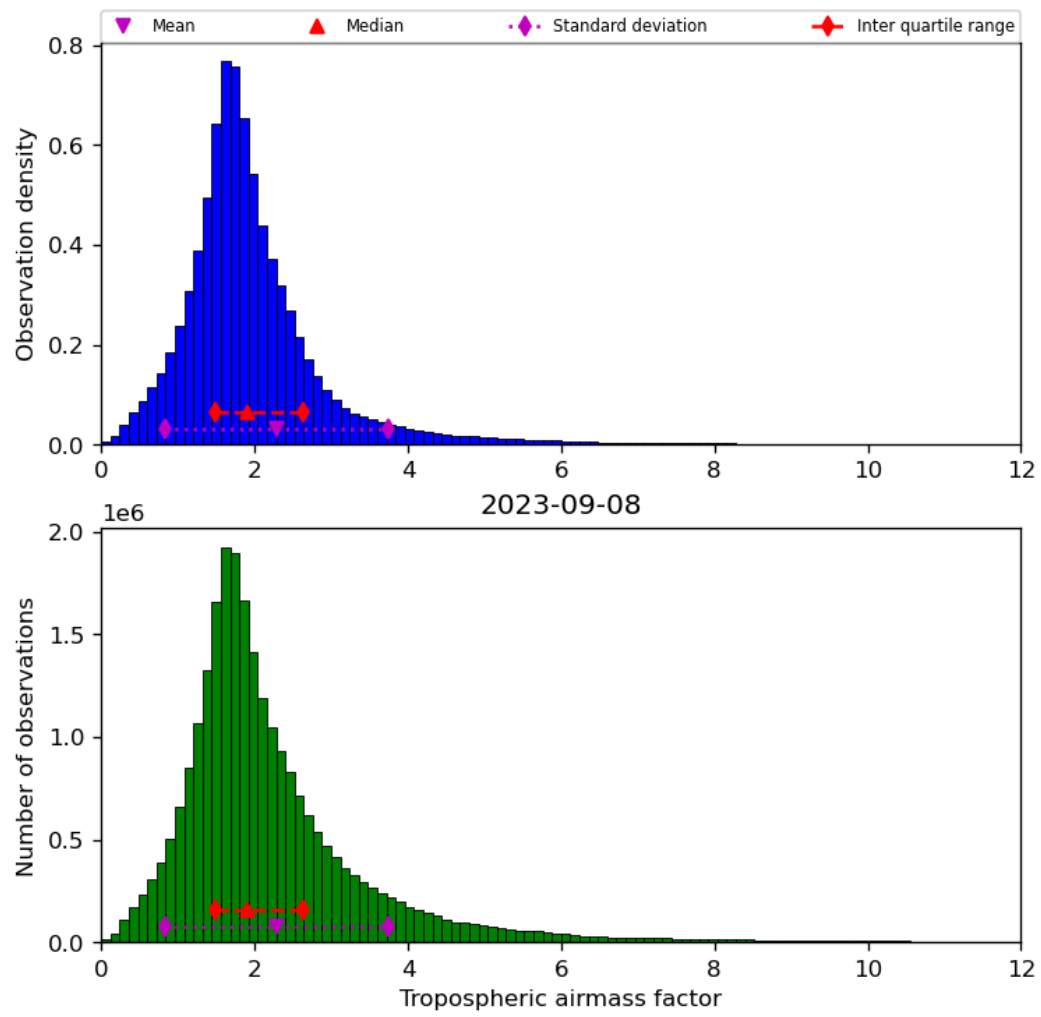
Figure 31: Histogram of “Tropospheric airmass factor” for 2023-09-07 to 2023-09-09
