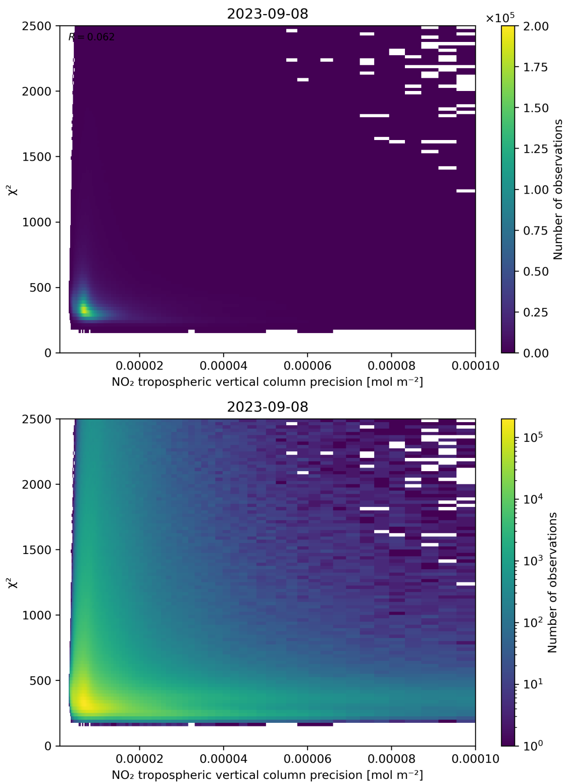
Figure 134: Scatter density plot of “NO 2 tropospheric vertical column precision” against “ \chi^2 ” for 2023-09-07 to 2023-09-09.
