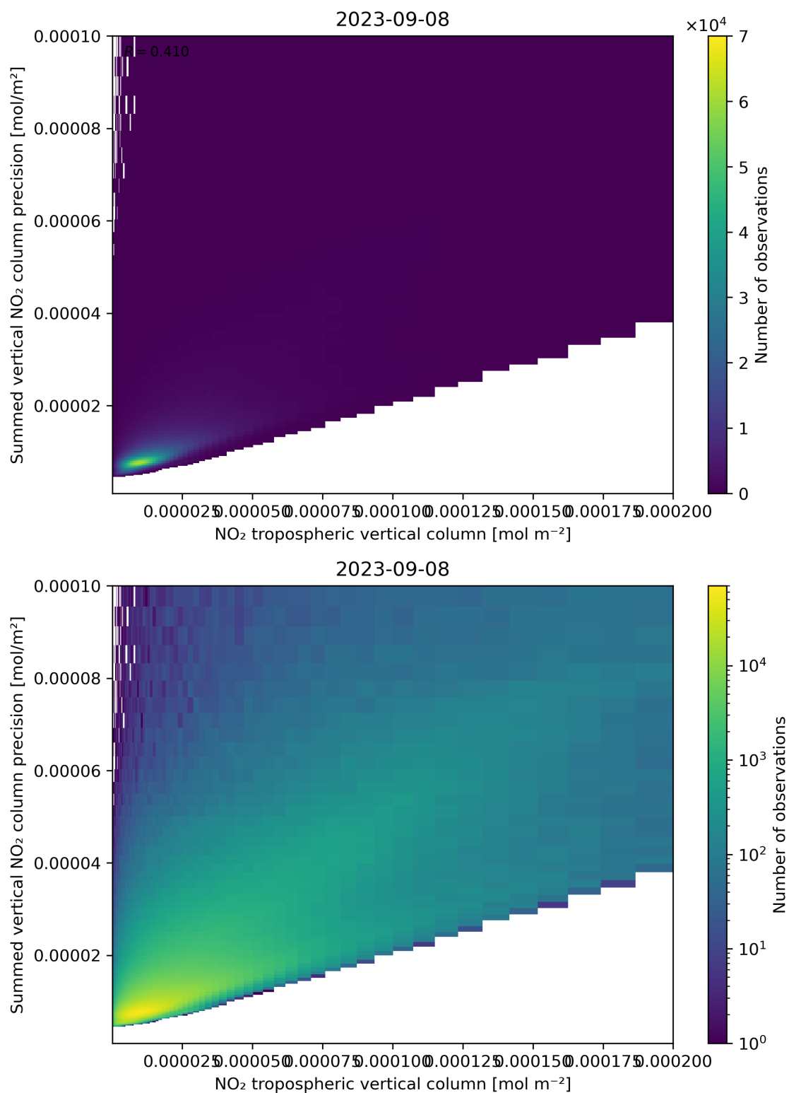
Figure 127: Scatter density plot of “NO 2 tropospheric vertical column” against “Summed vertical NO 2 column precision” for 2023-09-07 to 2023-09-09.
