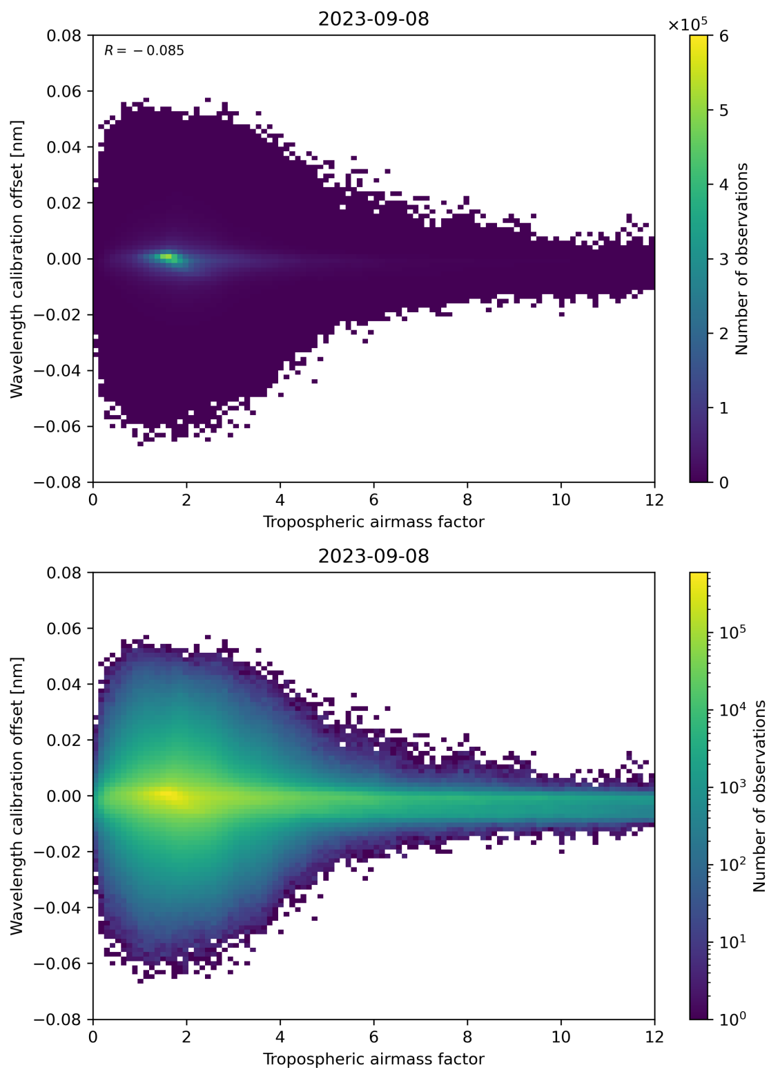
Figure 80: Scatter density plot of “Tropospheric airmass factor” against “Wavelength calibration offset” for 2023-09-07 to 2023-09-09.
