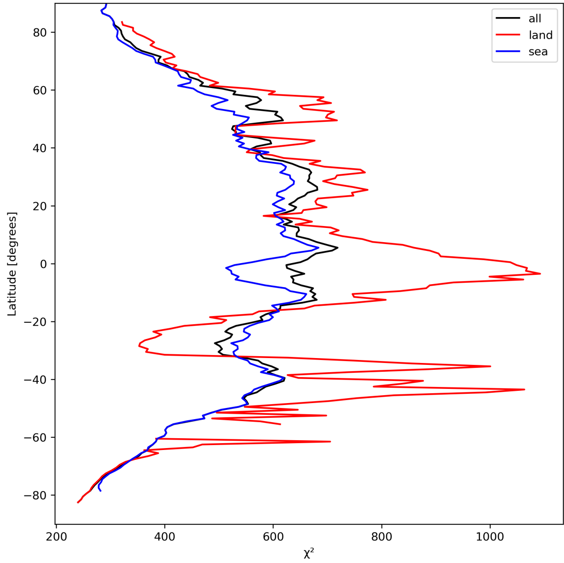
Figure 25: Zonal average of “ \chi^2 ” for 2023-09-07 to 2023-09-09.
