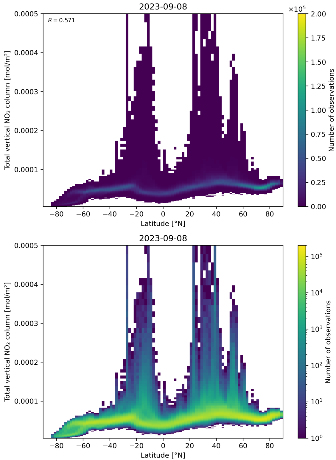
Figure 90: Scatter density plot of “Latitude” against “Total vertical NO 2 column” for 2023-09-07 to 2023-09-09.
