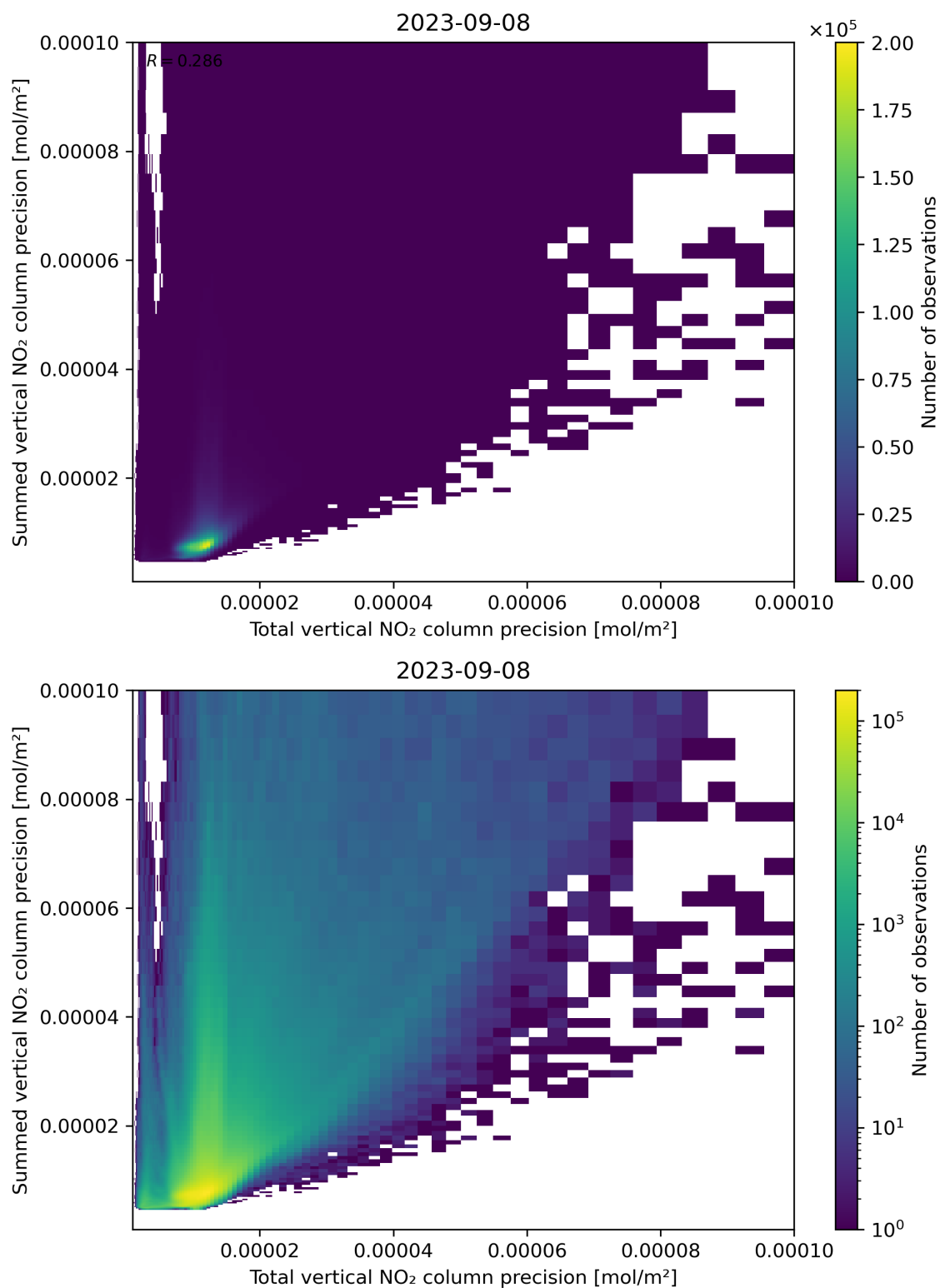
Figure 118: Scatter density plot of “Total vertical NO 2 column precision” against “Summed vertical NO 2 column precision” for 2023-09-07 to 2023-09-09.
