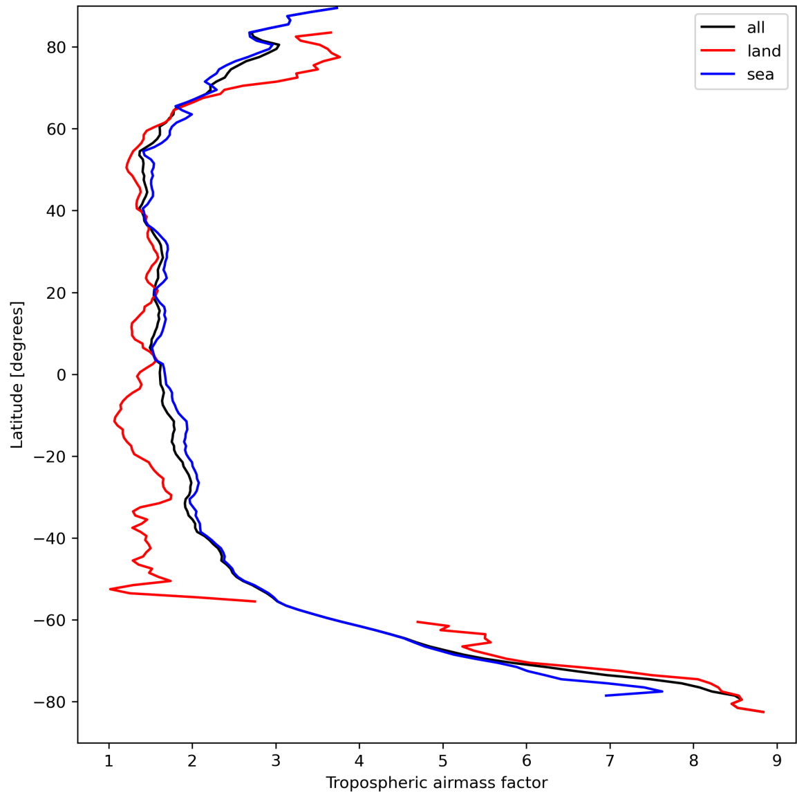
Figure 14: Zonal average of “Tropospheric air mass factor” for 2023-09-07 to 2023-09-09.
