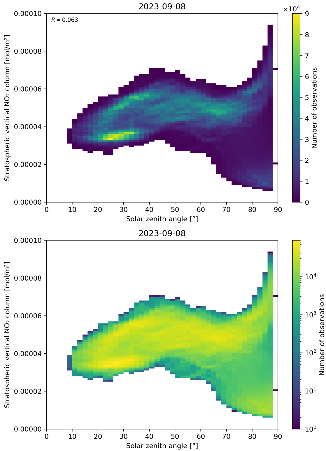
Figure 150: Scatter density plot of “Solar zenith angle” against “Stratospheric vertical NO 2 column” for 2023-09-07 to 2023-09-09.
