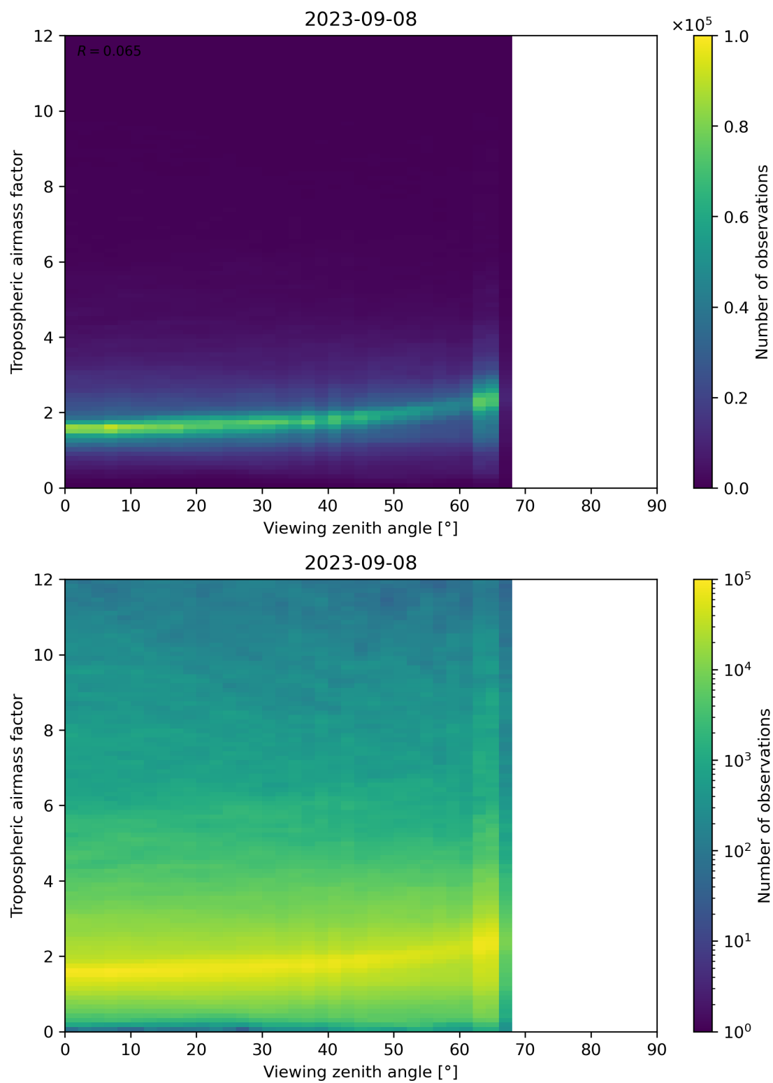
Figure 161: Scatter density plot of “Viewing zenith angle” against “Tropospheric airmass factor” for 2023-09-07 to 2023-09-09.
