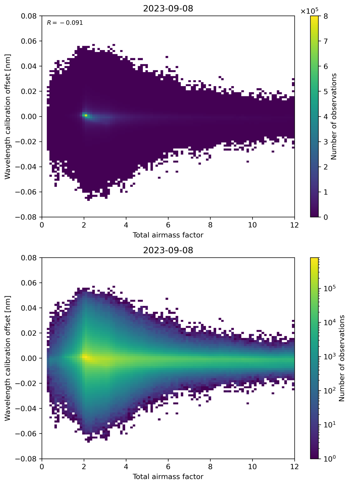
Figure 70: Scatter density plot of “Total airmass factor” against “Wavelength calibration offset” for 2023-09-07 to 2023-09-09.
