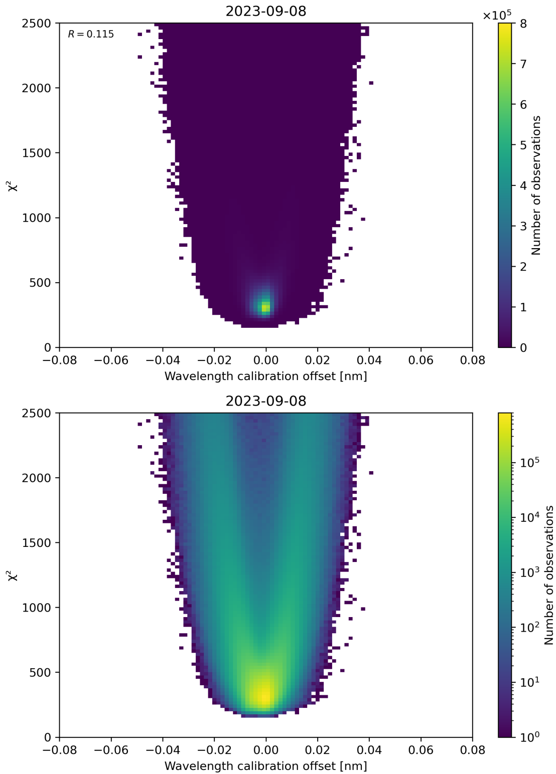
Figure 175: Scatter density plot of “Wavelength calibration offset” against “ \chi^2 ” for 2023-09-07 to 2023-09-09.
