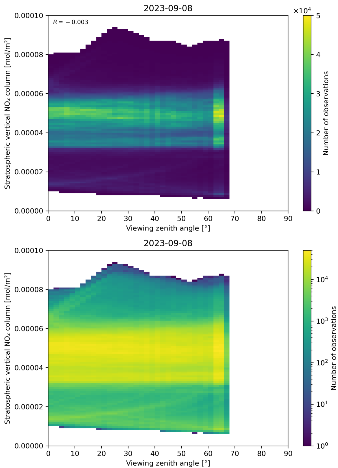
Figure 164: Scatter density plot of “Viewing zenith angle” against “Stratospheric vertical NO 2 column” for 2023-09-07 to 2023-09-09.
