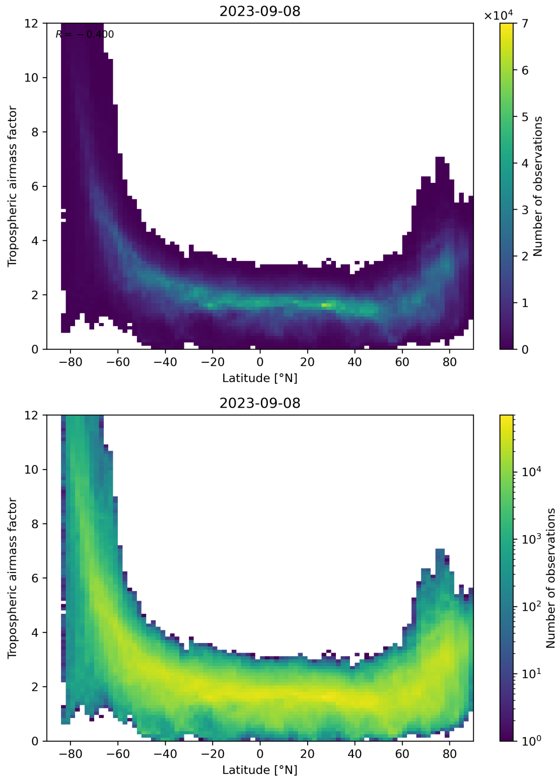
Figure 85: Scatter density plot of “Latitude” against “Tropospheric air mass factor” for 2023-09-07 to 2023-09-09.
