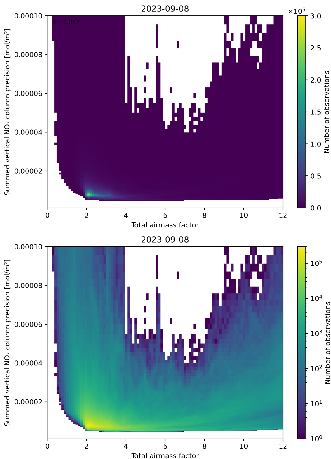
Figure 66: Scatter density plot of “Total airmass factor” against “Summed vertical NO 2 column precision” for 2023-09-07 to 2023-09-09.
