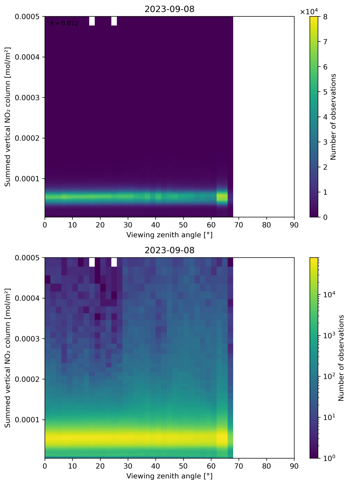
Figure 165: Scatter density plot of “Viewing zenith angle” against “Summed vertical NO 2 column” for 2023-09-07 to 2023-09-09.
