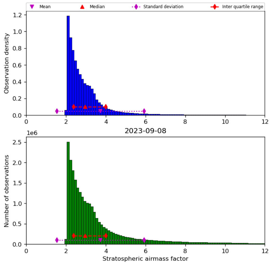
Figure 44: Histogram of “Stratospheric airmass factor” for 2023-09-07 to 2023-09-09
