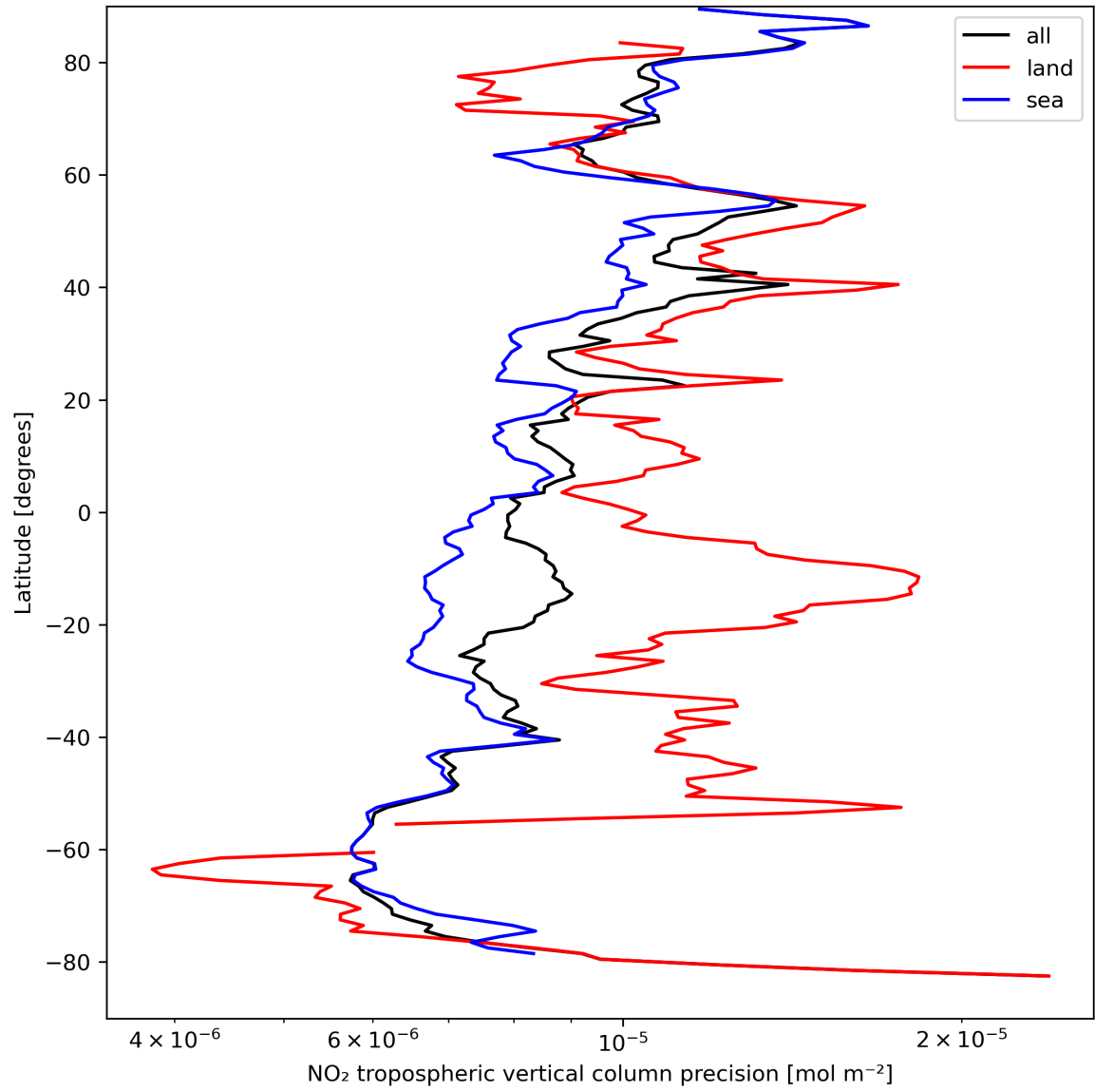
Figure 13: Zonal average of “NO 2 tropospheric vertical column precision” for 2023-09-07 to 2023-09-09.
