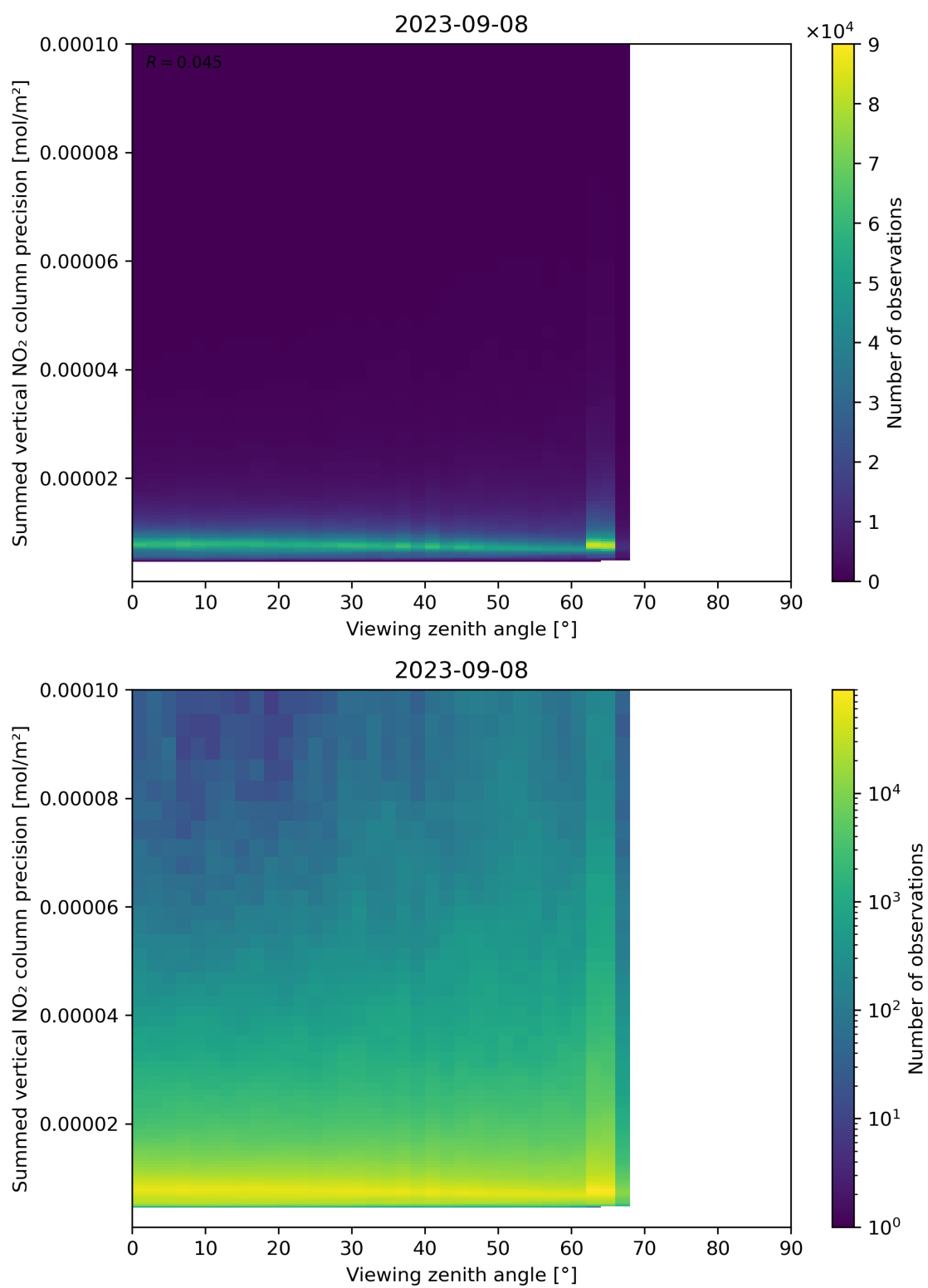
Figure 166: Scatter density plot of “Viewing zenith angle” against “Summed vertical NO 2 column precision” for 2023-09-07 to 2023-09-09.
