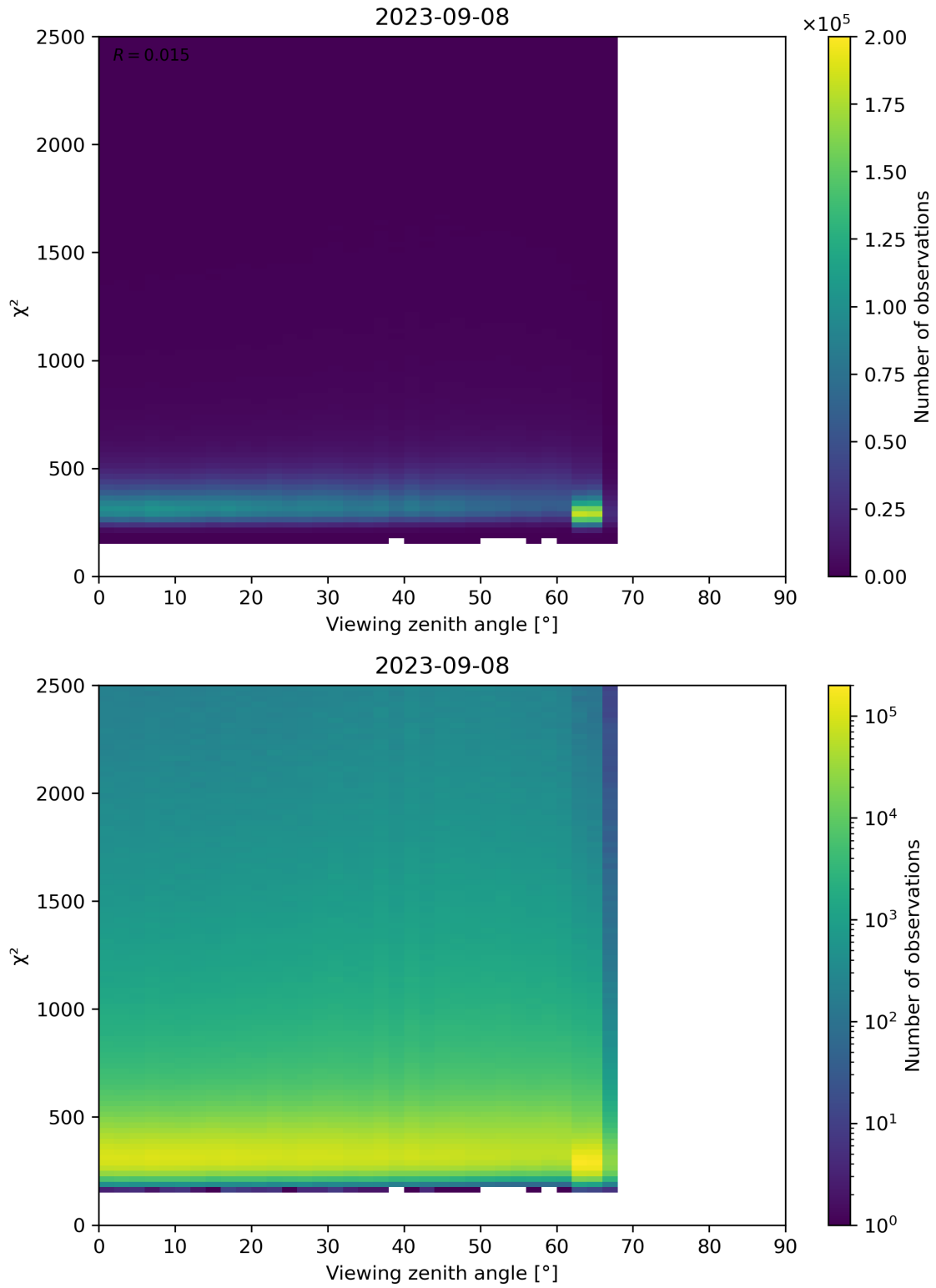
Figure 162: Scatter density plot of “Viewing zenith angle” against “ \chi^2 ” for 2023-09-07 to 2023-09-09.
