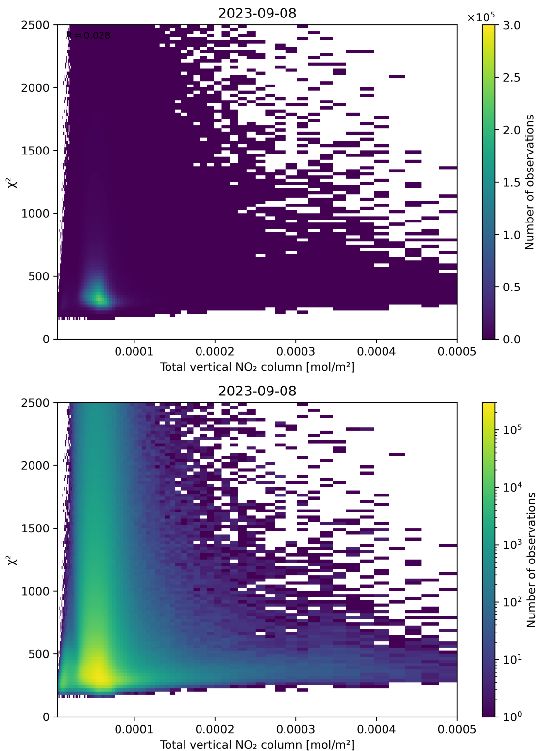
Figure 111: Scatter density plot of “Total vertical NO 2 column” against “ \chi^2 ” for 2023-09-07 to 2023-09-09.
