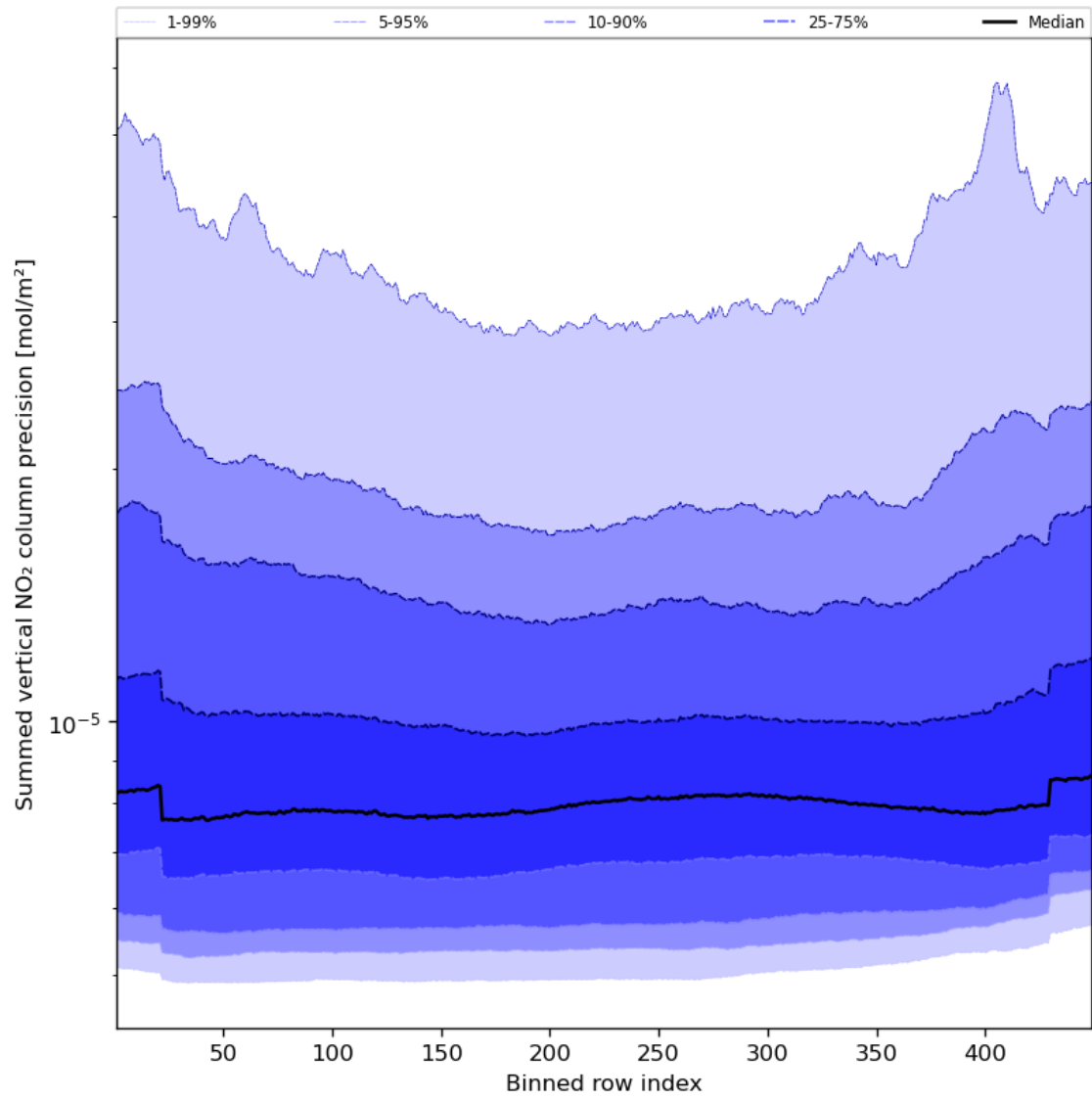
Figure 58: Along track statistics of “Summed vertical NO 2 column precision” for 2023-09-07 to 2023-09-09
