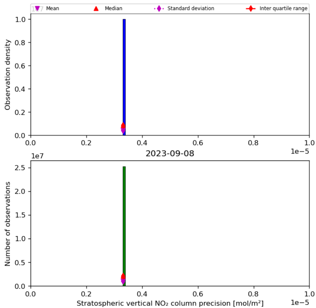
Figure 37: Histogram of “Stratospheric vertical NO 2 column precision” for 2023-09-07 to 2023-09-09
