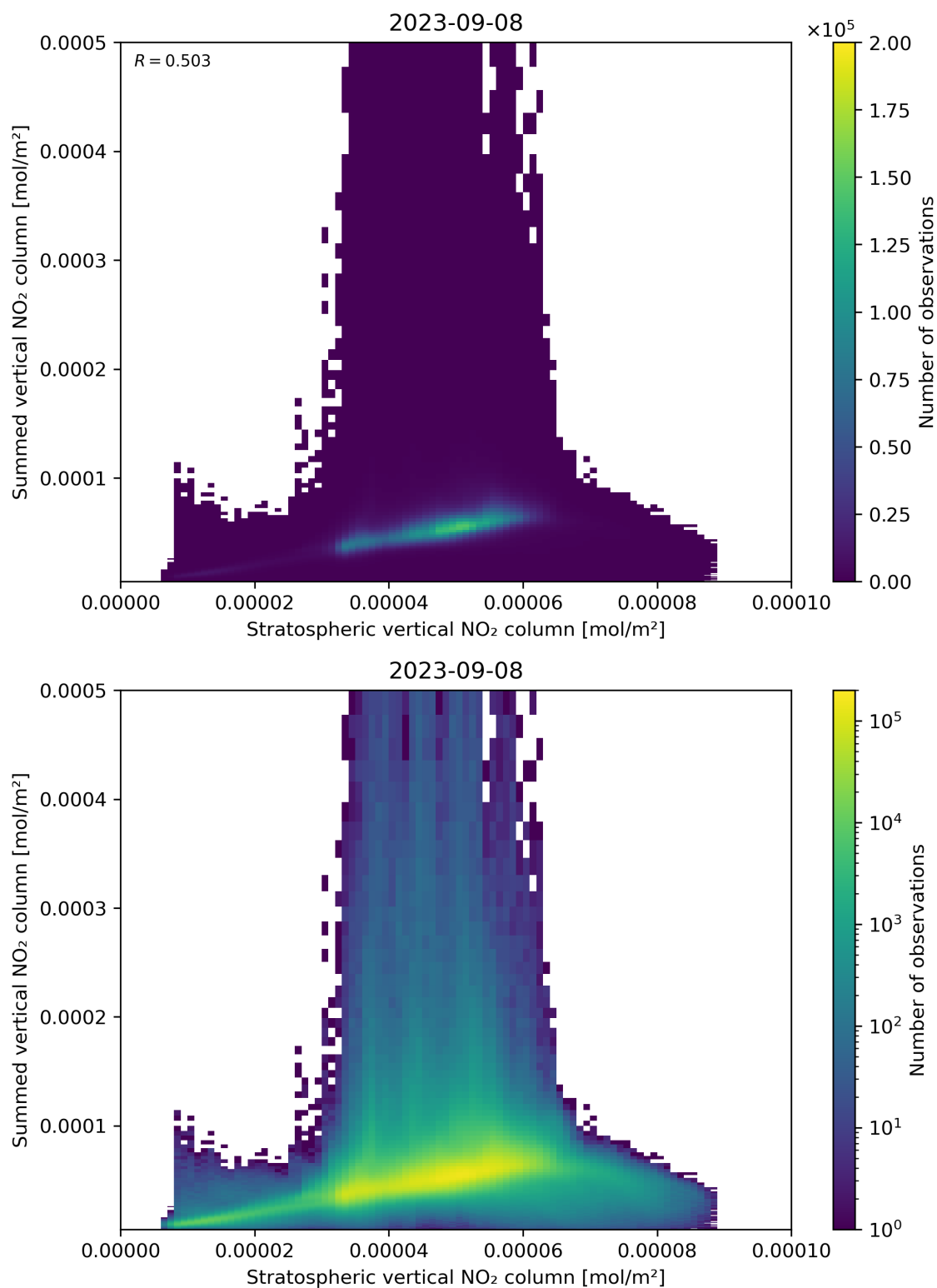
Figure 98: Scatter density plot of “Stratospheric vertical NO 2 column” against “Summed vertical NO 2 column” for 2023-09-07 to 2023-09-09.
