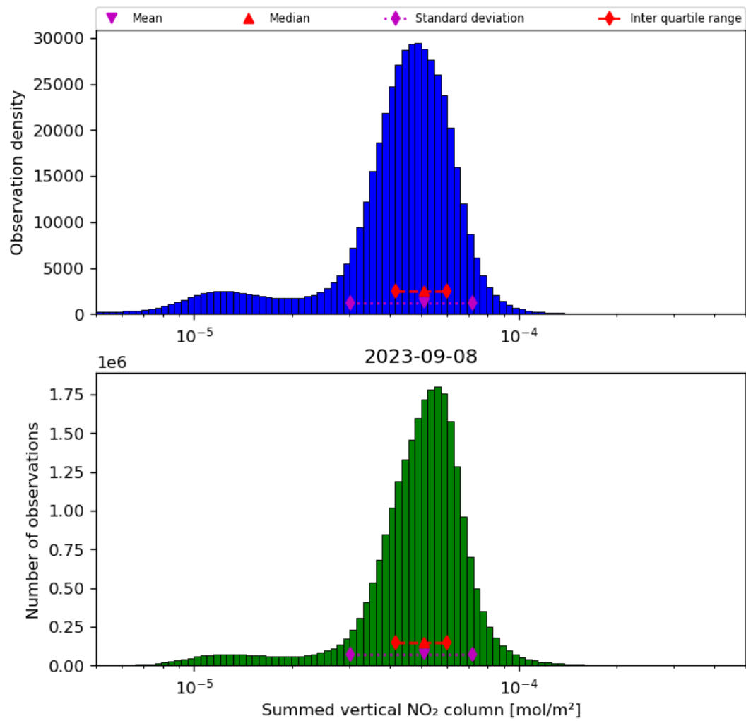
Figure 40: Histogram of “Summed vertical NO 2 column” for 2023-09-07 to 2023-09-09
