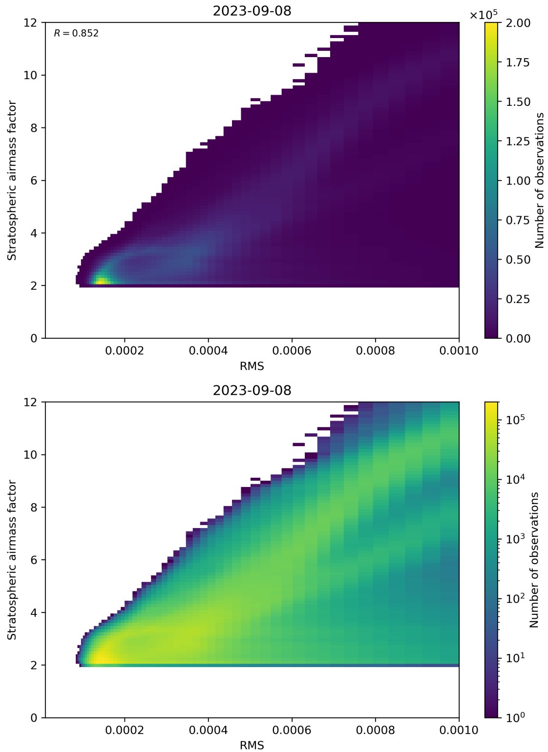
Figure 144: Scatter density plot of “RMS” against “Stratospheric airmass factor” for 2023-09-07 to 2023-09-09.
