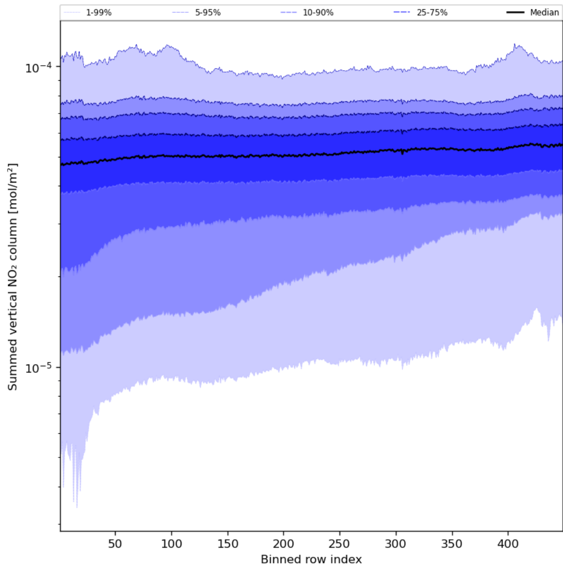
Figure 57: Along track statistics of “Summed vertical NO 2 column” for 2023-09-07 to 2023-09-09
