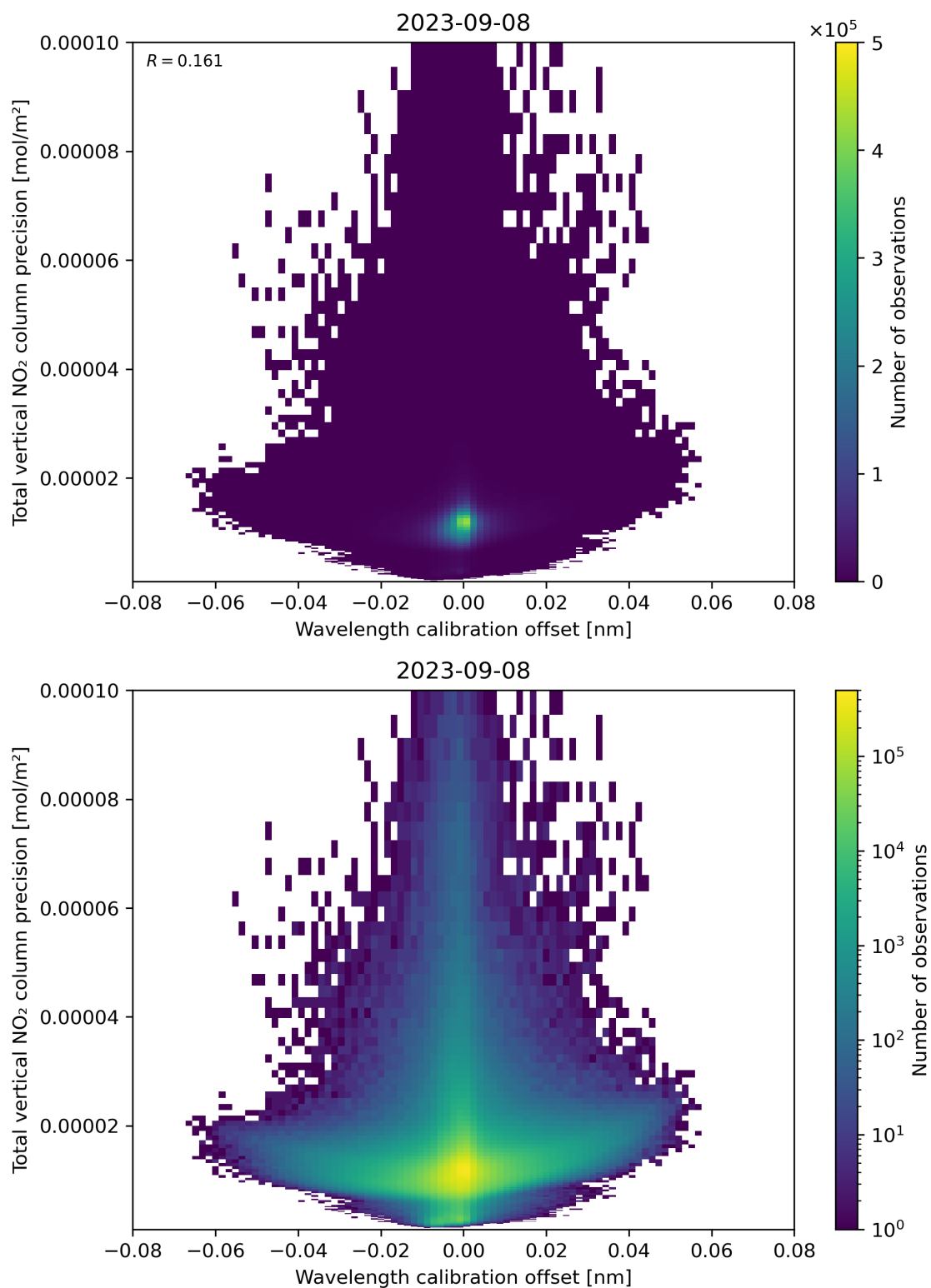
Figure 180: Scatter density plot of “Wavelength calibration offset” against “Total vertical NO 2 column precision” for 2023-09-07 to 2023-09-09.
