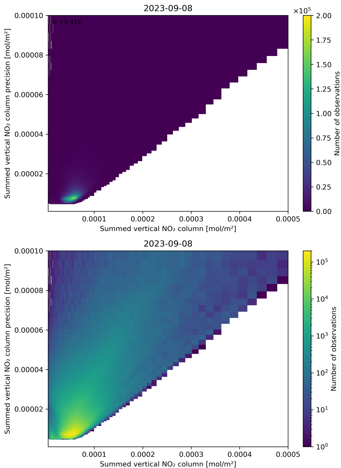
Figure 105: Scatter density plot of “Summed vertical NO 2 column” against “Summed vertical NO 2 column precision” for 2023-09-07 to 2023-09-09.
