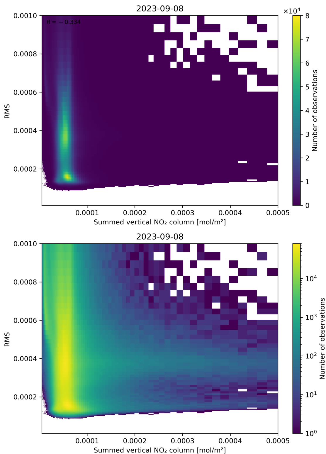
Figure 109: Scatter density plot of “Summed vertical NO 2 column” against “RMS” for 2023-09-07 to 2023-09-09.
