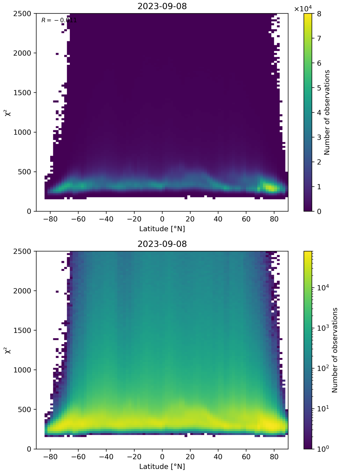
Figure 86: Scatter density plot of “Latitude” against “ \chi^2 ” for 2023-09-07 to 2023-09-09.
