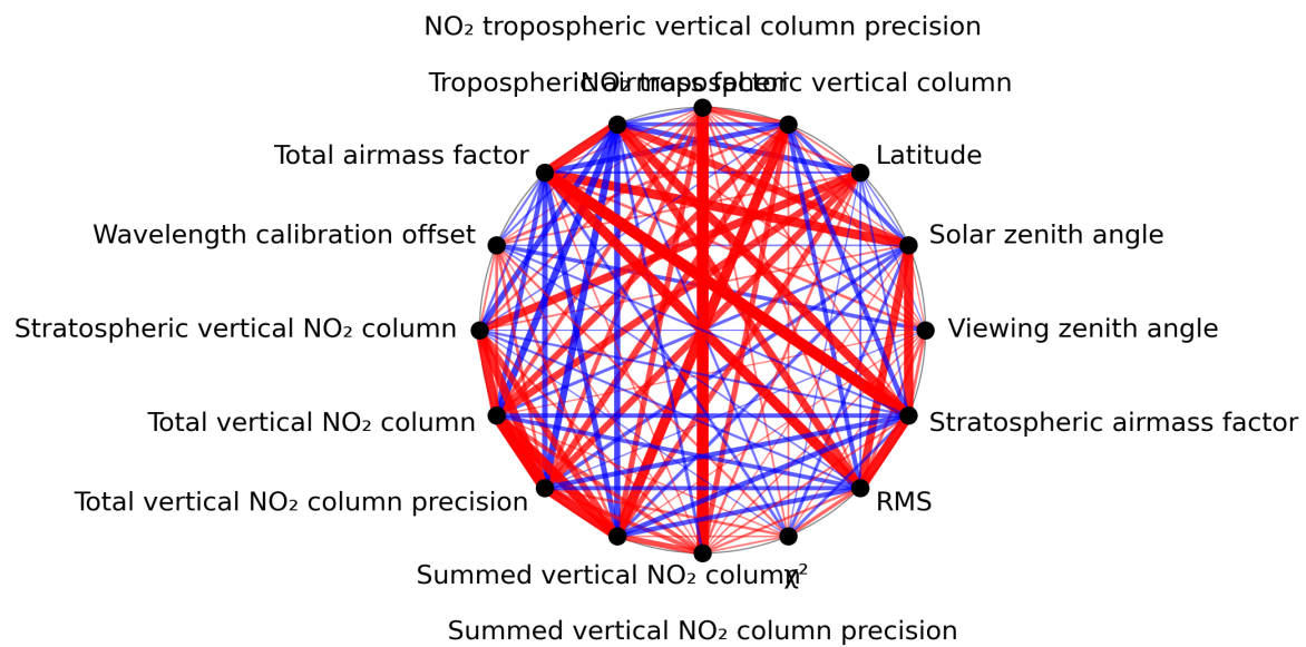
Figure 1: Map of correlation graph for 2023-09-07 to 2023-09-09.
