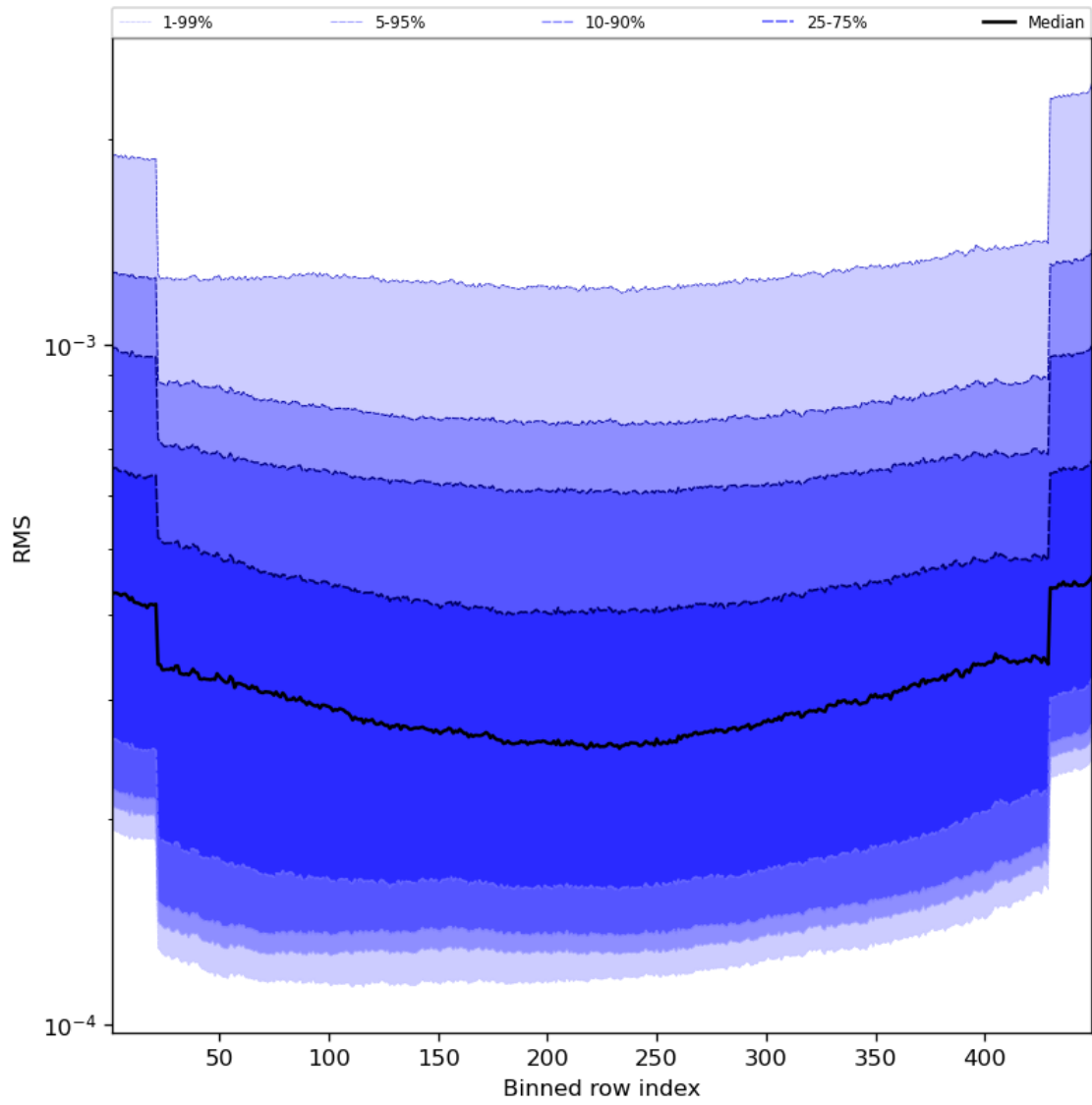
Figure 60: Along track statistics of “RMS” for 2023-09-07 to 2023-09-09
