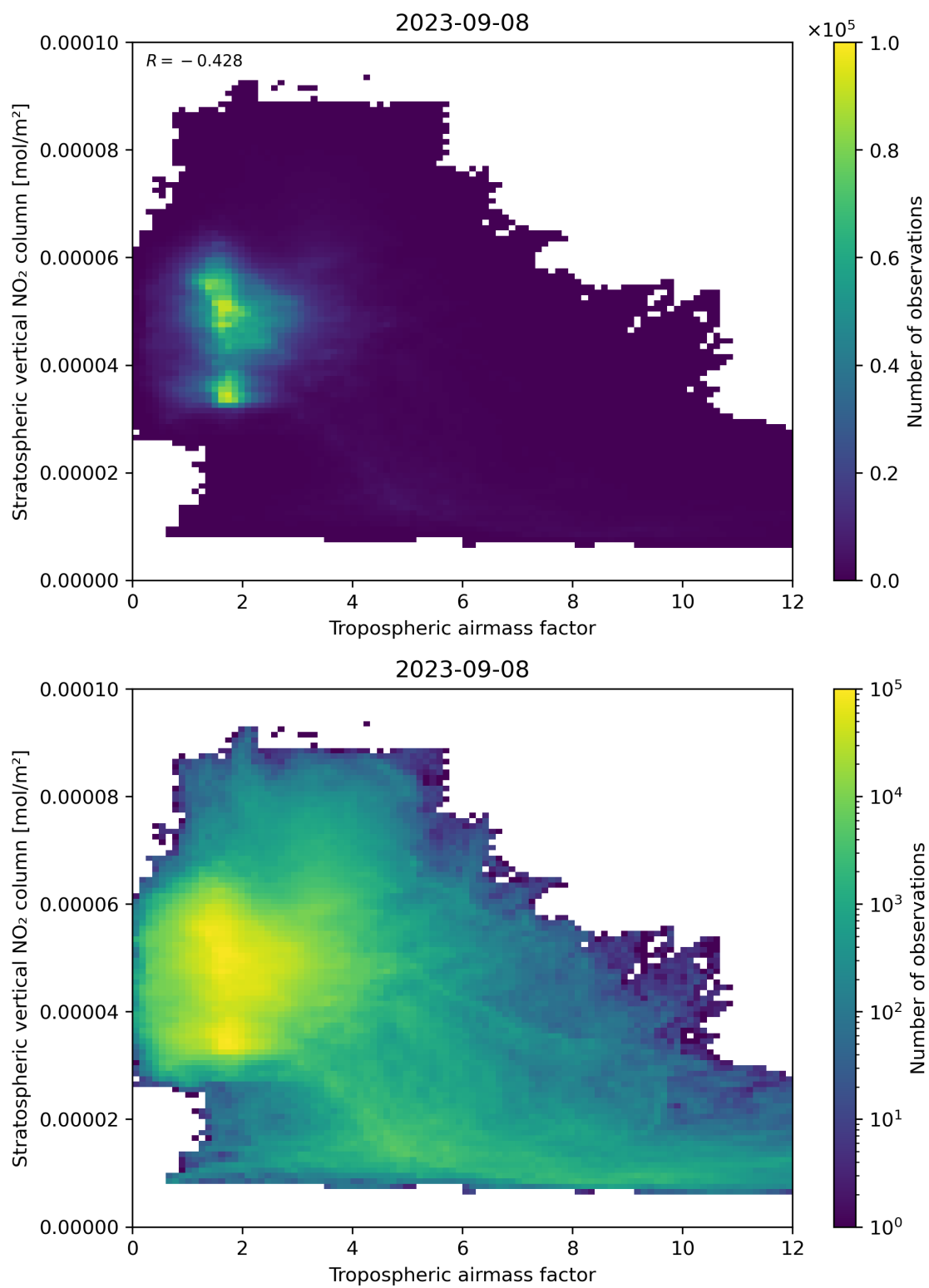
Figure 74: Scatter density plot of “Tropospheric air mass factor” against “Stratospheric vertical NO 2 column” for 2023-09-07 to 2023-09-09.
