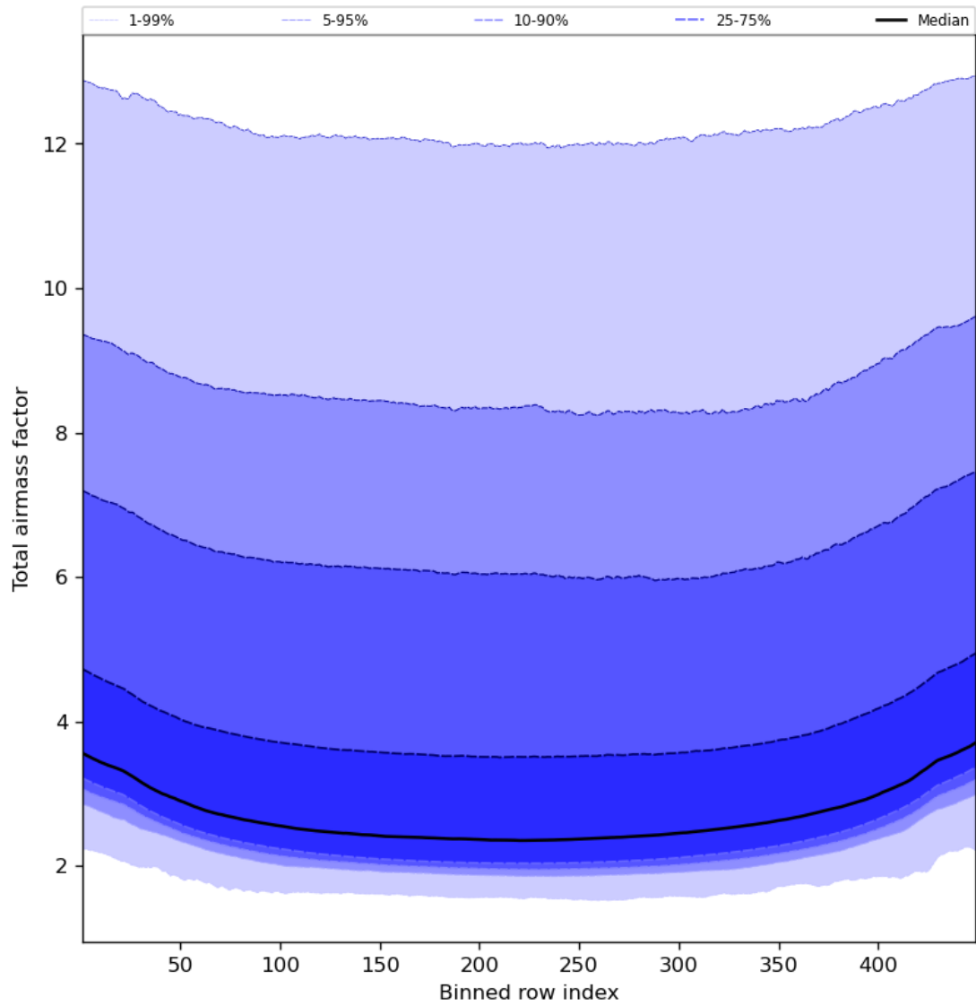
Figure 49: Along track statistics of “Total airmass factor” for 2023-09-07 to 2023-09-09
