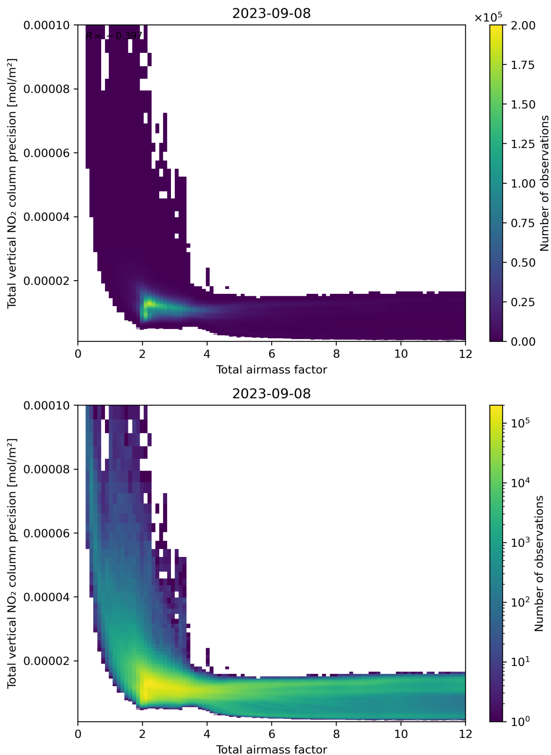
Figure 68: Scatter density plot of “Total airmass factor” against “Total vertical NO 2 column precision” for 2023-09-07 to 2023-09-09.
