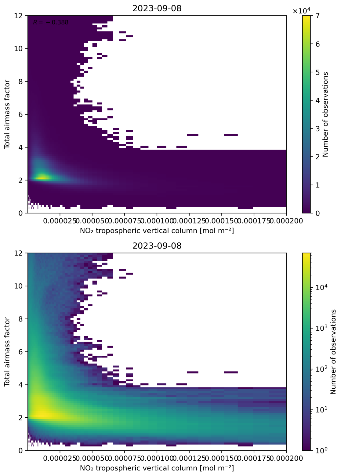
Figure 122: Scatter density plot of “NO 2 tropospheric vertical column” against “Total airmass factor” for 2023-09-07 to 2023-09-09.
