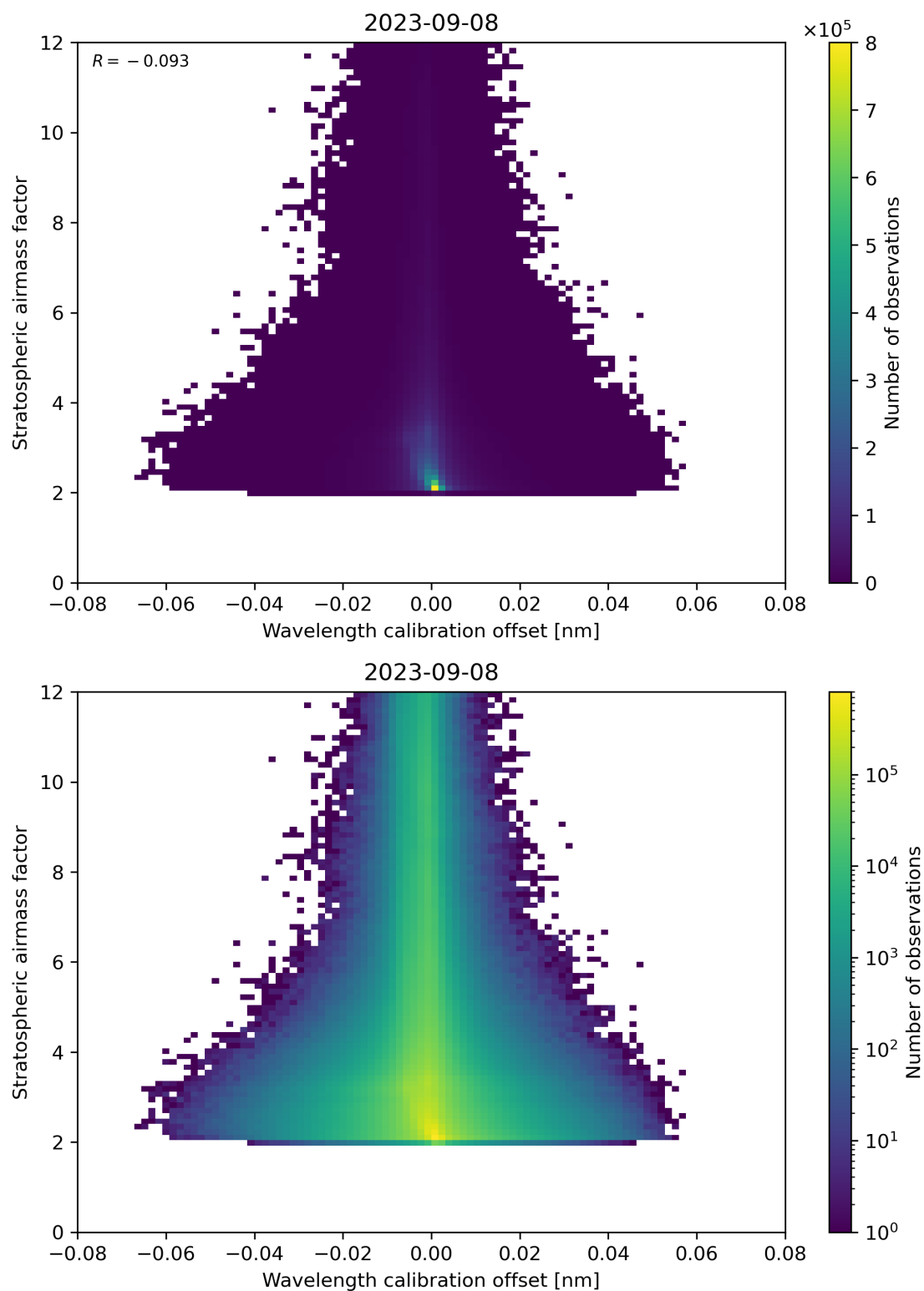
Figure 174: Scatter density plot of “Wavelength calibration offset” against “Stratospheric airmass factor” for 2023-09-07 to 2023-09-09.
