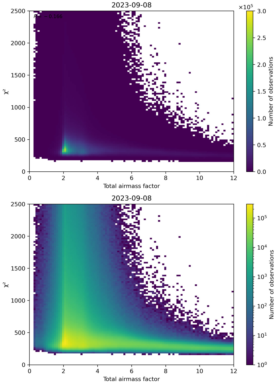
Figure 63: Scatter density plot of “Total airmass factor” against “ \chi^2 ” for 2023-09-07 to 2023-09-09.
