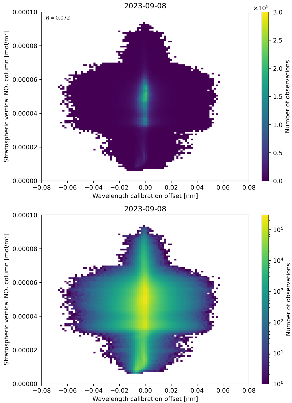
Figure 176: Scatter density plot of “Wavelength calibration offset” against “Stratospheric vertical NO 2 column” for 2023-09-07 to 2023-09-09.
