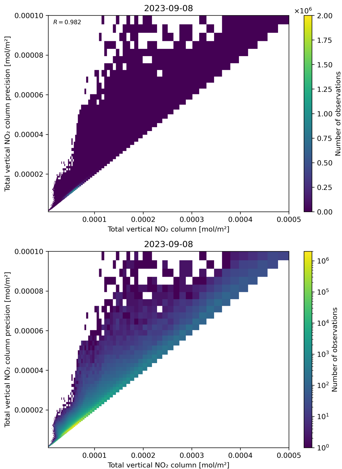
Figure 114: Scatter density plot of “Total vertical NO 2 column” against “Total vertical NO 2 column precision” for 2023-09-07 to 2023-09-09.
