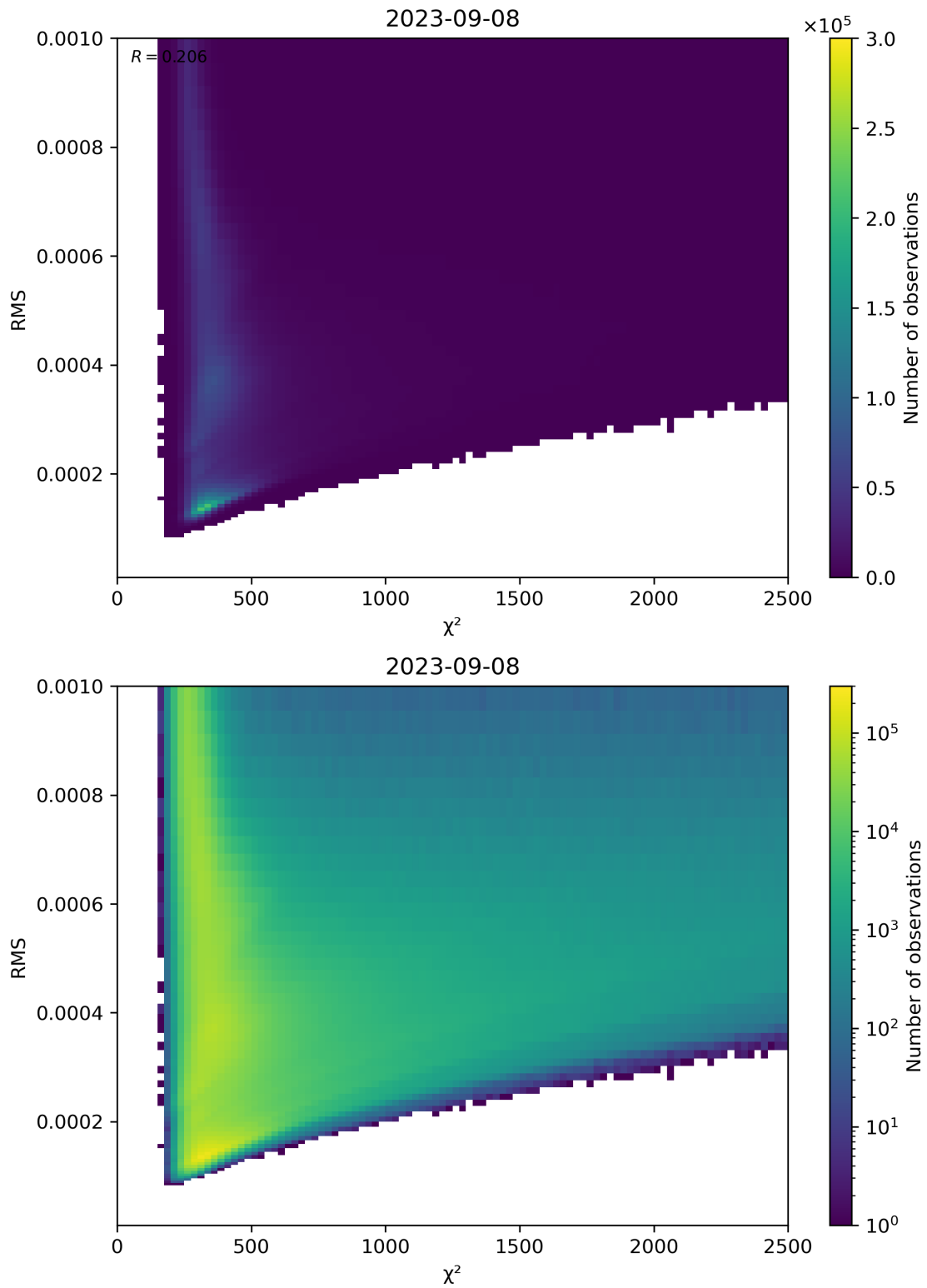
Figure 82: Scatter density plot of “ \chi^2 ” against “RMS” for 2023-09-07 to 2023-09-09.
