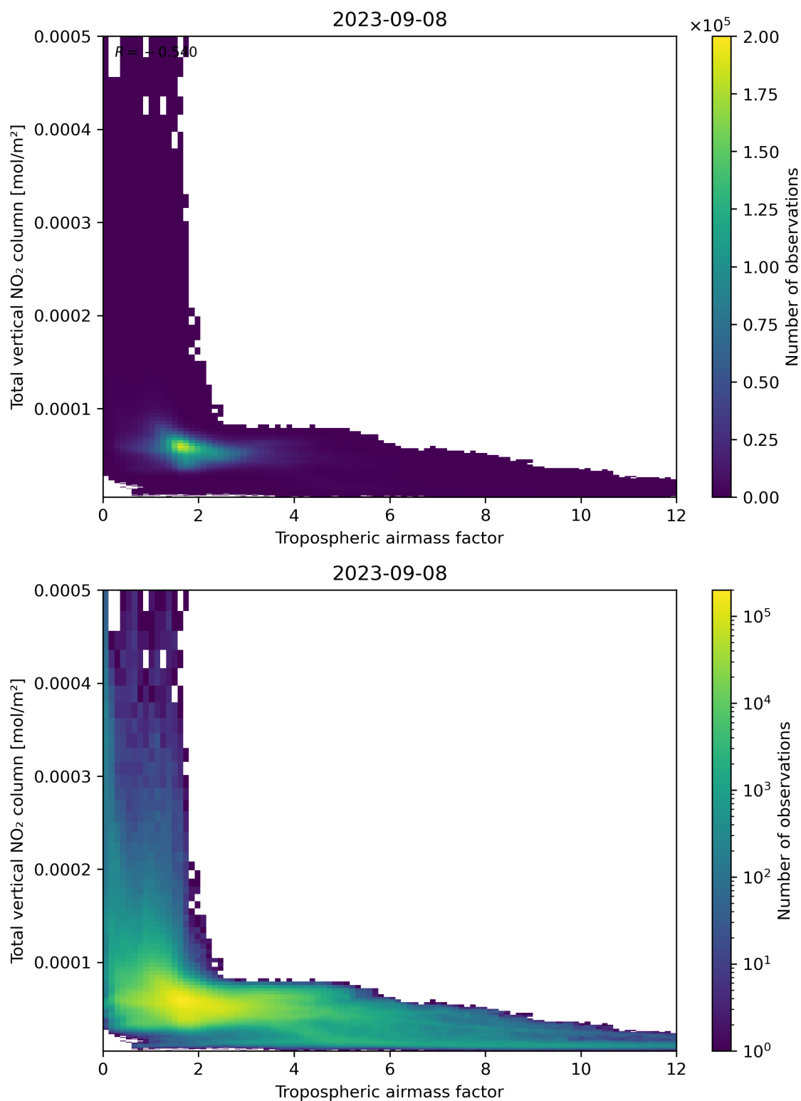
Figure 77: Scatter density plot of “Tropospheric airmass factor” against “Total vertical NO 2 column” for 2023-09-07 to 2023-09-09.
