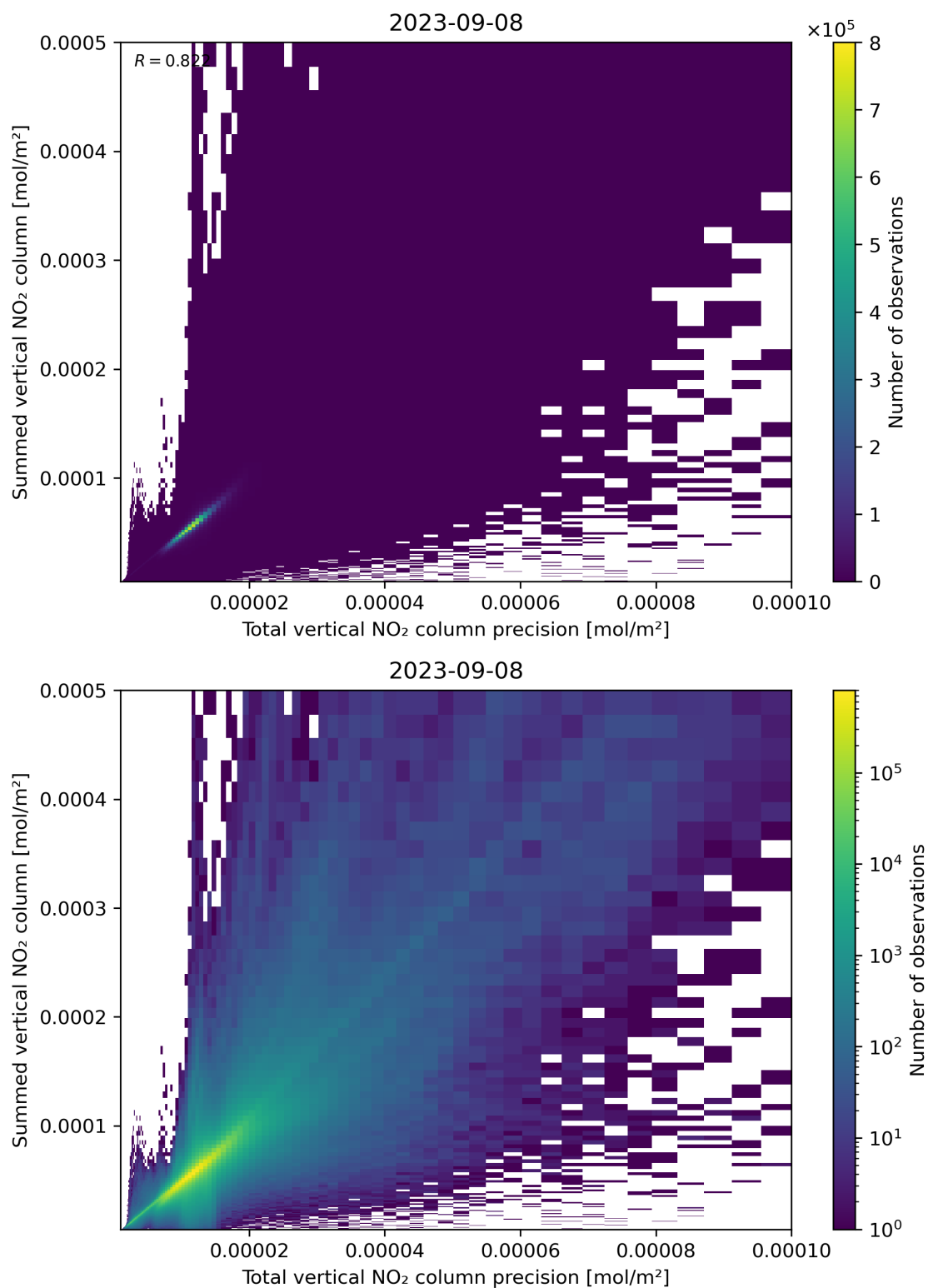
Figure 117: Scatter density plot of “Total vertical NO 2 column precision” against “Summed vertical NO 2 column” for 2023-09-07 to 2023-09-09.
