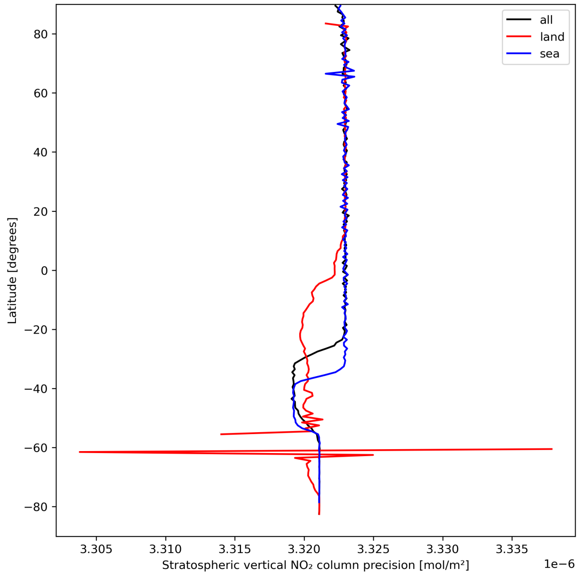
Figure 20: Zonal average of “Stratospheric vertical NO 2 column precision” for 2023-09-07 to 2023-09-09.
