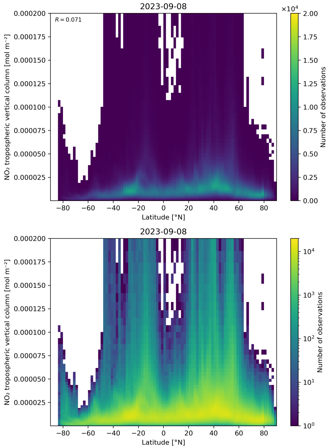
Figure 92: Scatter density plot of “Latitude” against “NO 2 tropospheric vertical column” for 2023-09-07 to 2023-09-09.
