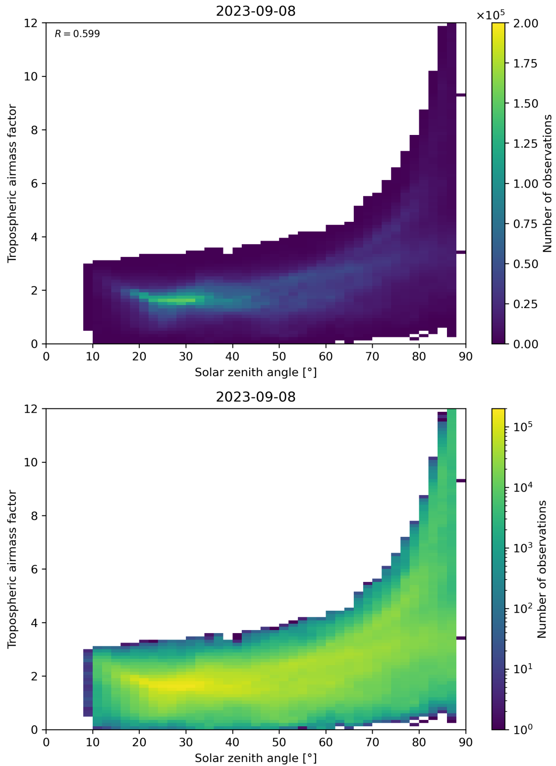
Figure 147: Scatter density plot of “Solar zenith angle” against “Tropospheric airmass factor” for 2023-09-07 to 2023-09-09.
