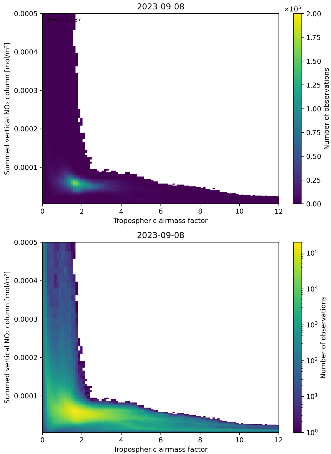
Figure 75: Scatter density plot of “Tropospheric air mass factor” against “Summed vertical NO 2 column” for 2023-09-07 to 2023-09-09.
