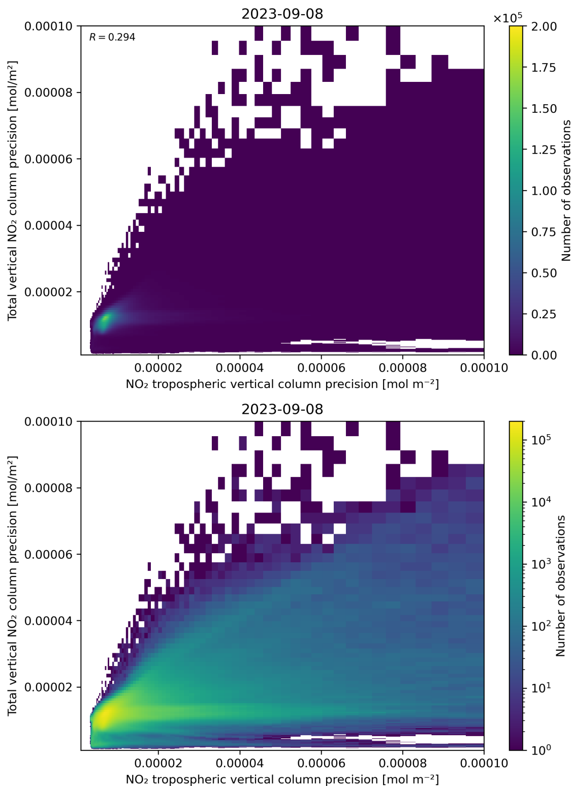
Figure 139: Scatter density plot of “NO 2 tropospheric vertical column precision” against “Total vertical NO 2 column precision” for 2023-09-07 to 2023-09-09.
