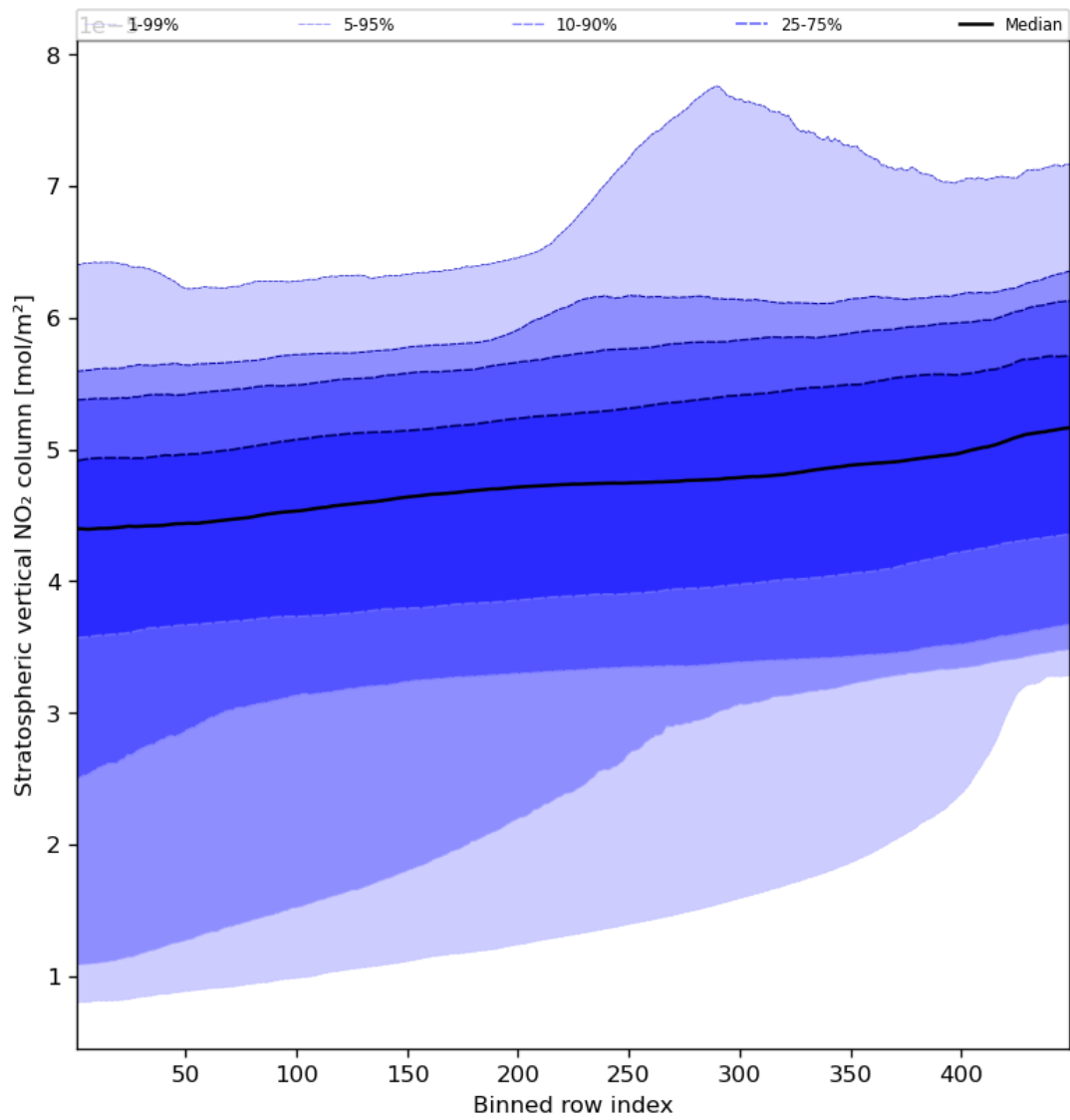
Figure 53: Along track statistics of “Stratospheric vertical NO 2 column” for 2023-09-07 to 2023-09-09
