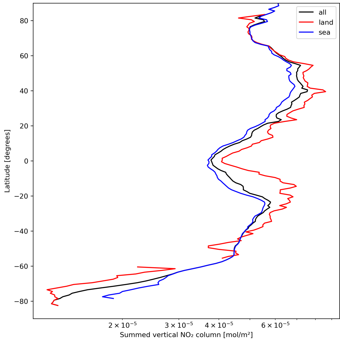
Figure 23: Zonal average of “Summed vertical NO 2 column” for 2023-09-07 to 2023-09-09.
