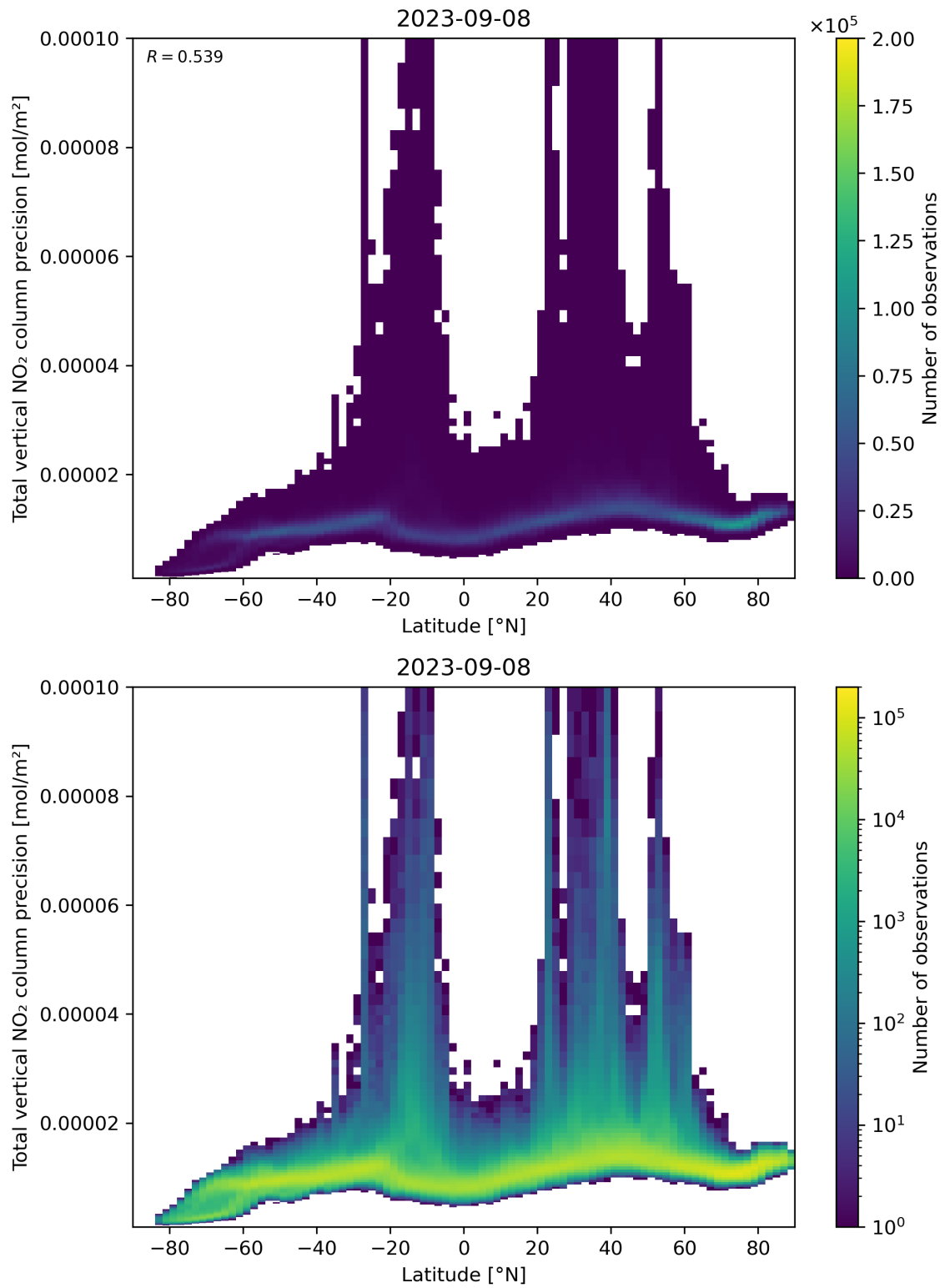
Figure 91: Scatter density plot of “Latitude” against “Total vertical NO 2 column precision” for 2023-09-07 to 2023-09-09.
