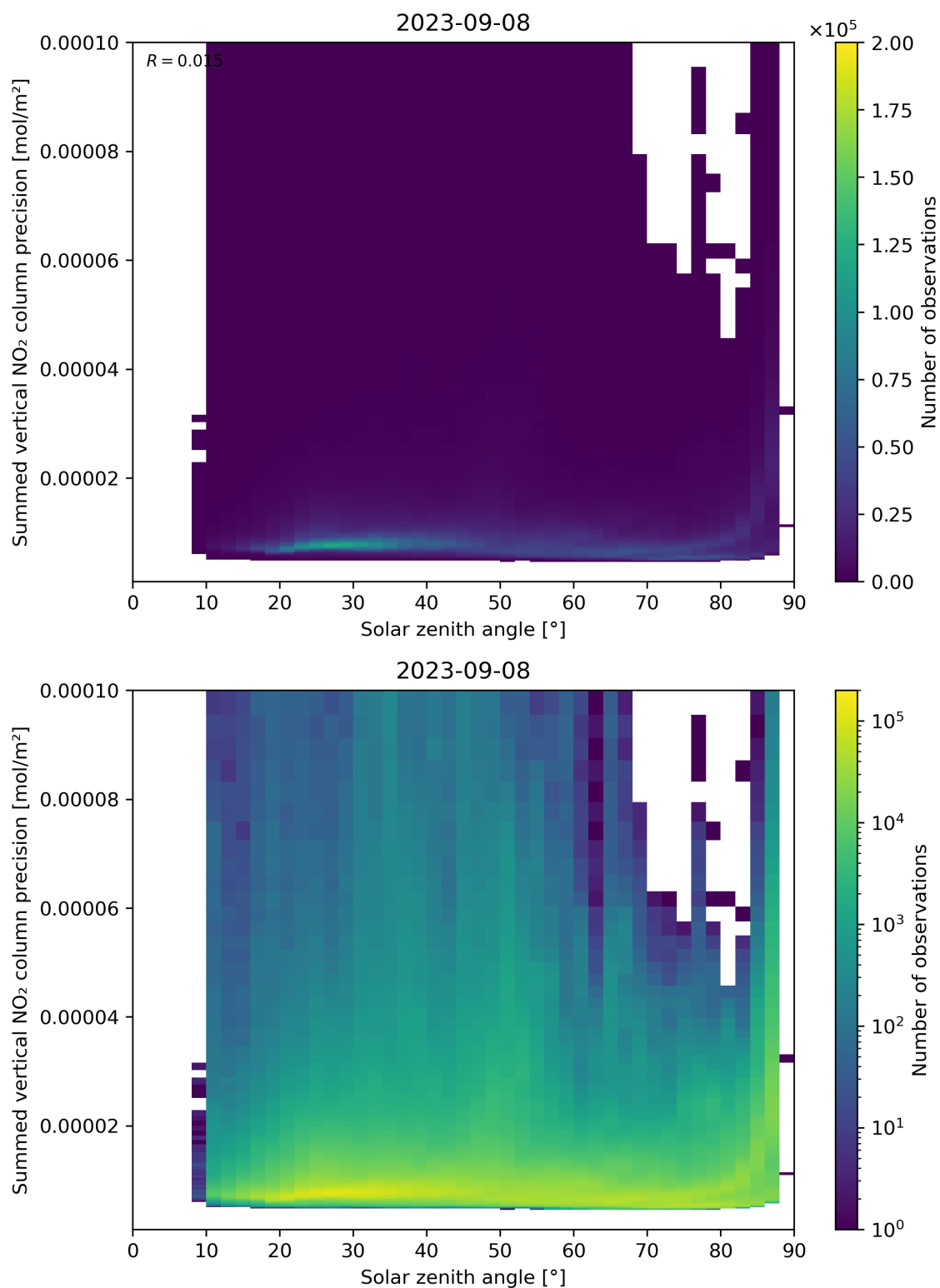
Figure 152: Scatter density plot of “Solar zenith angle” against “Summed vertical NO 2 column precision” for 2023-09-07 to 2023-09-09.
