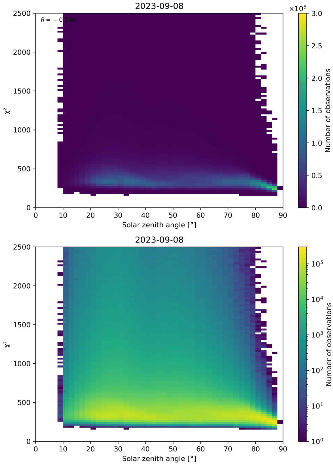
Figure 148: Scatter density plot of “Solar zenith angle” against “ \chi^2 ” for 2023-09-07 to 2023-09-09.
