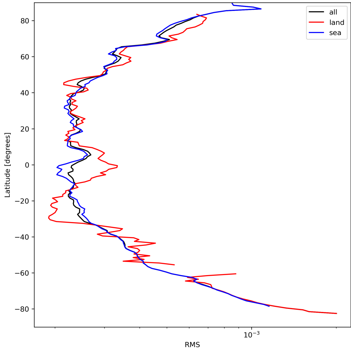
Figure 26: Zonal average of “RMS” for 2023-09-07 to 2023-09-09.
