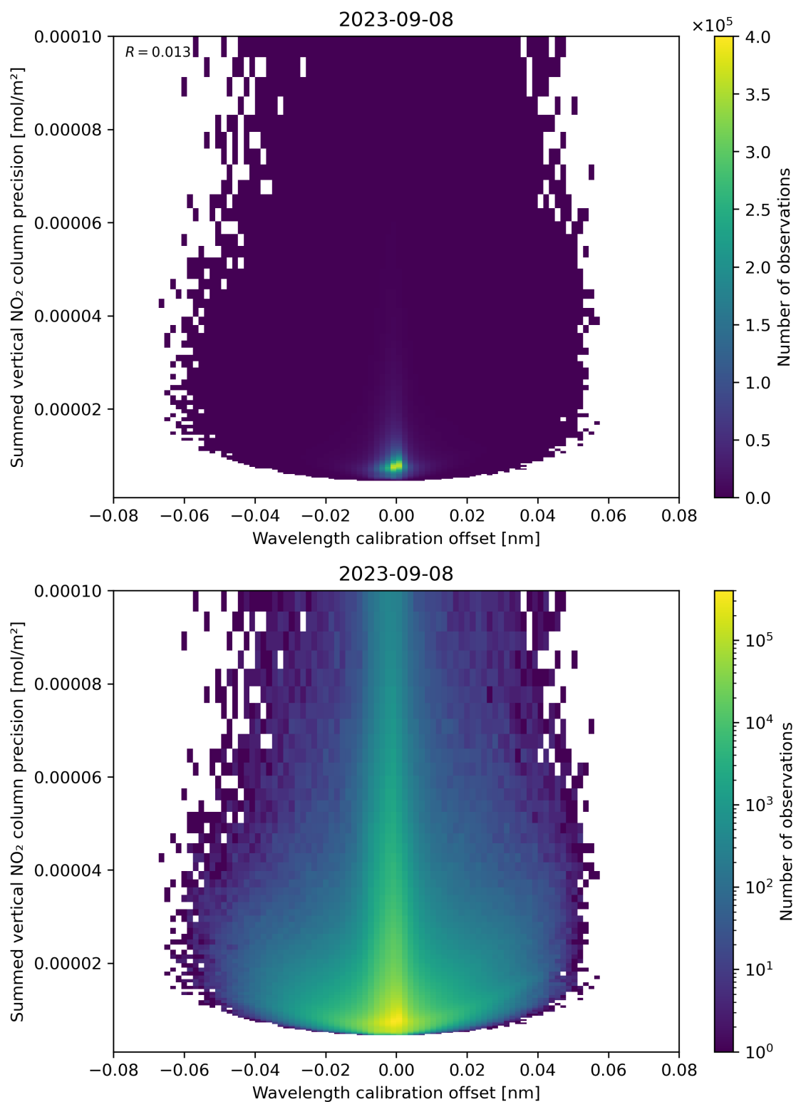
Figure 178: Scatter density plot of “Wavelength calibration offset” against “Summed vertical NO 2 column precision” for 2023-09-07 to 2023-09-09.
