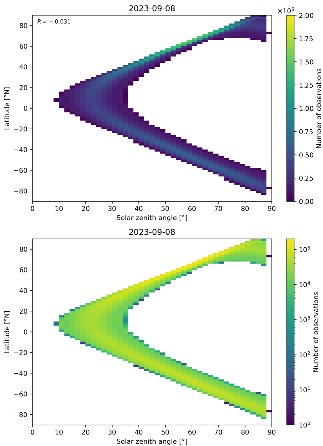
Figure 149: Scatter density plot of “Solar zenith angle” against “Latitude” for 2023-09-07 to 2023-09-09.
