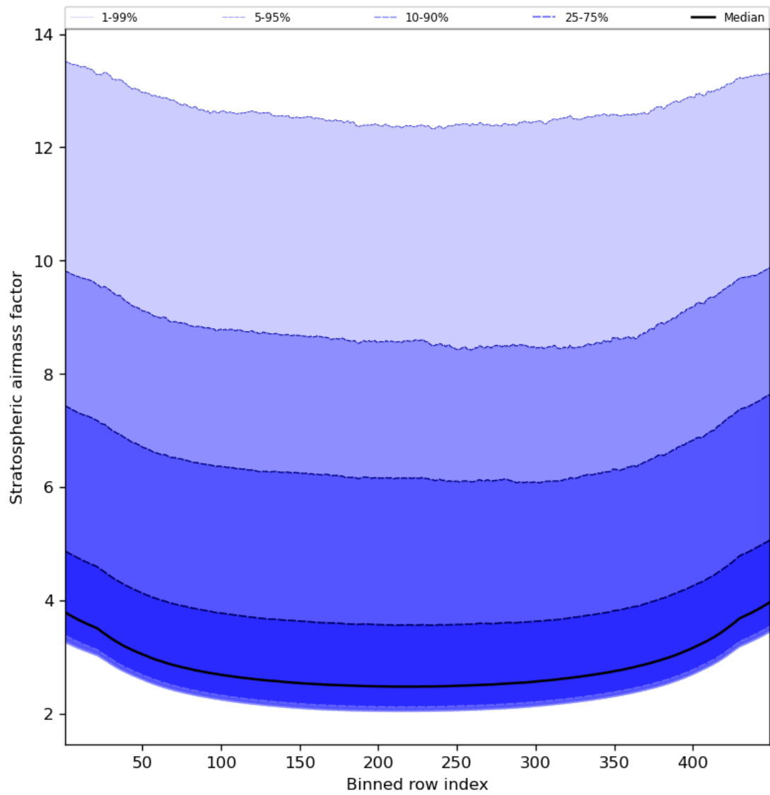
Figure 61: Along track statistics of “Stratospheric air mass factor” for 2023-09-07 to 2023-09-09
