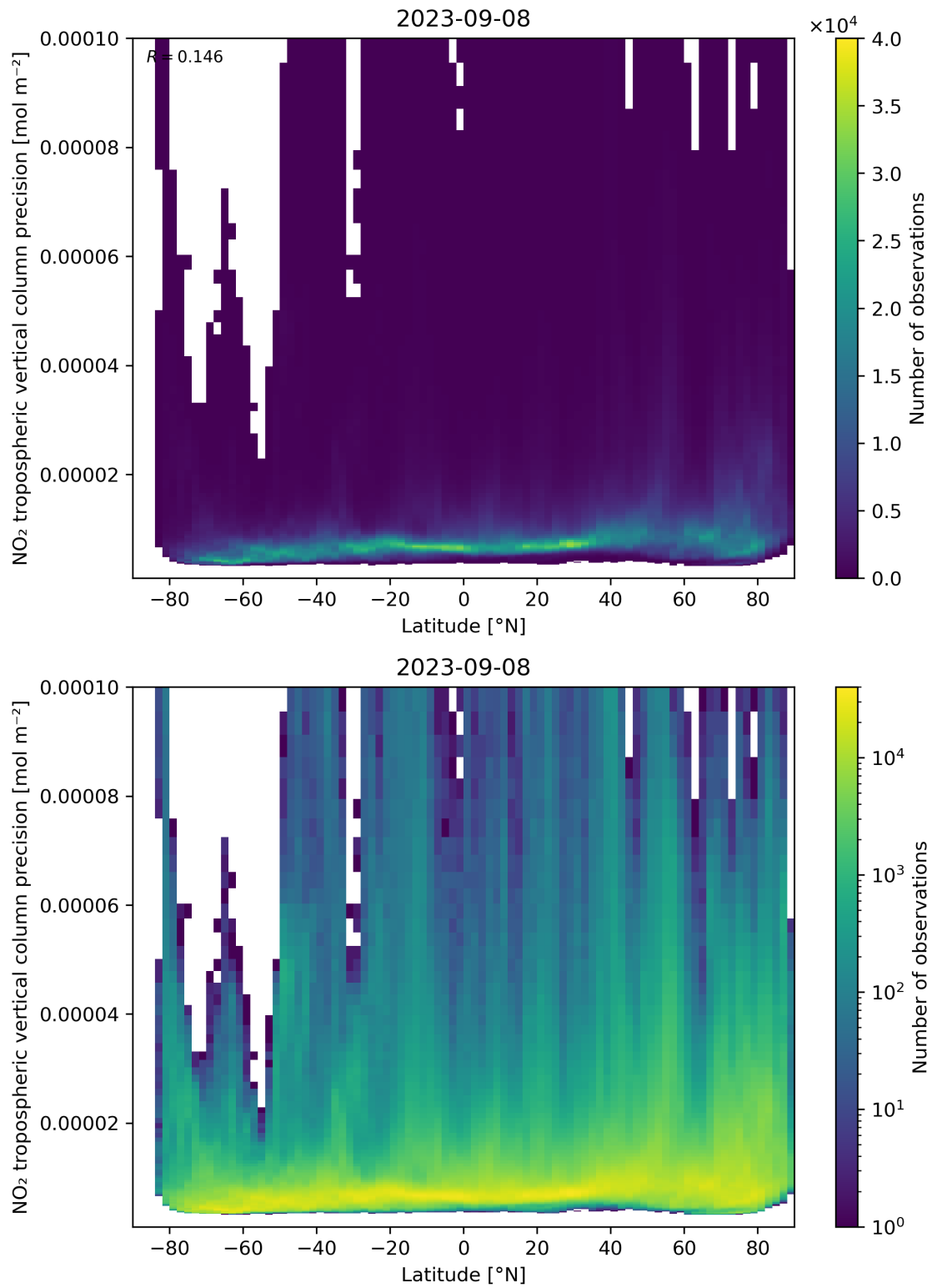
Figure 93: Scatter density plot of “Latitude” against “NO 2 tropospheric vertical column precision” for 2023-09-07 to 2023-09-09.
