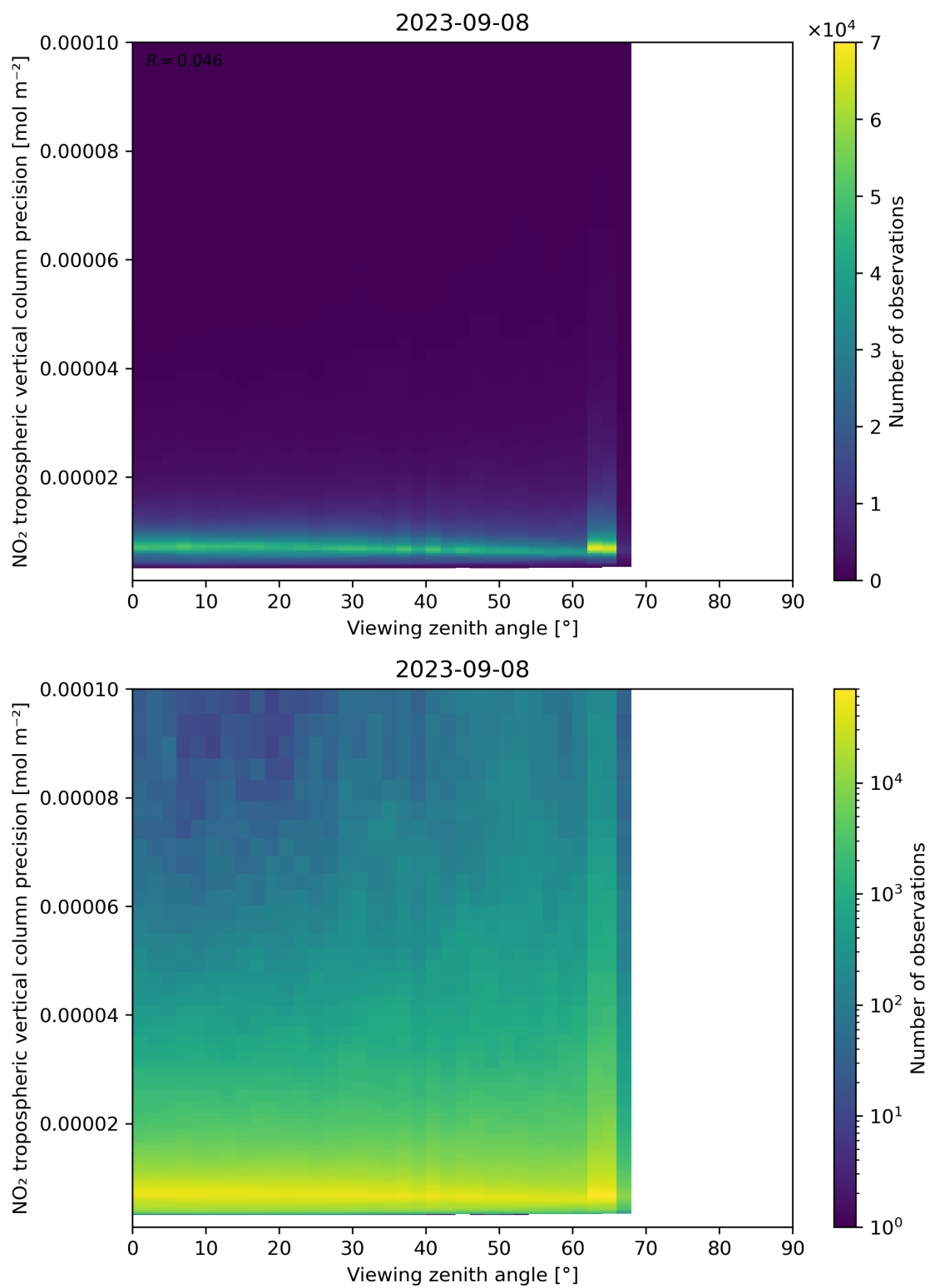
Figure 170: Scatter density plot of “Viewing zenith angle” against “NO 2 tropospheric vertical column precision” for 2023-09-07 to 2023-09-09.
