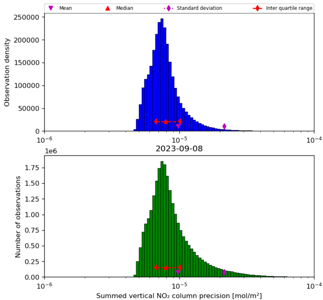
Figure 41: Histogram of “Summed vertical NO 2 column precision” for 2023-09-07 to 2023-09-09
