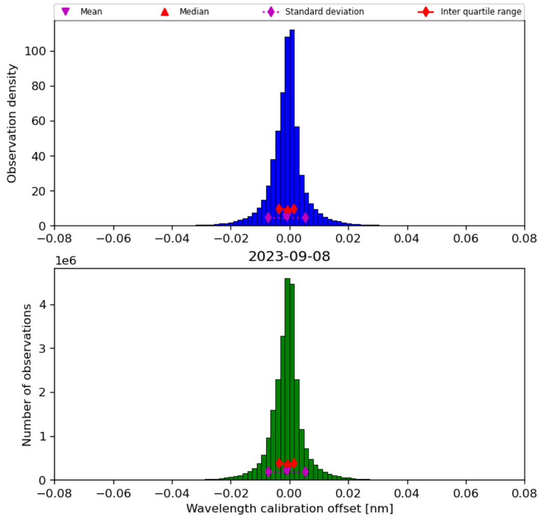
Figure 35: Histogram of “Wavelength calibration offset” for 2023-09-07 to 2023-09-09
