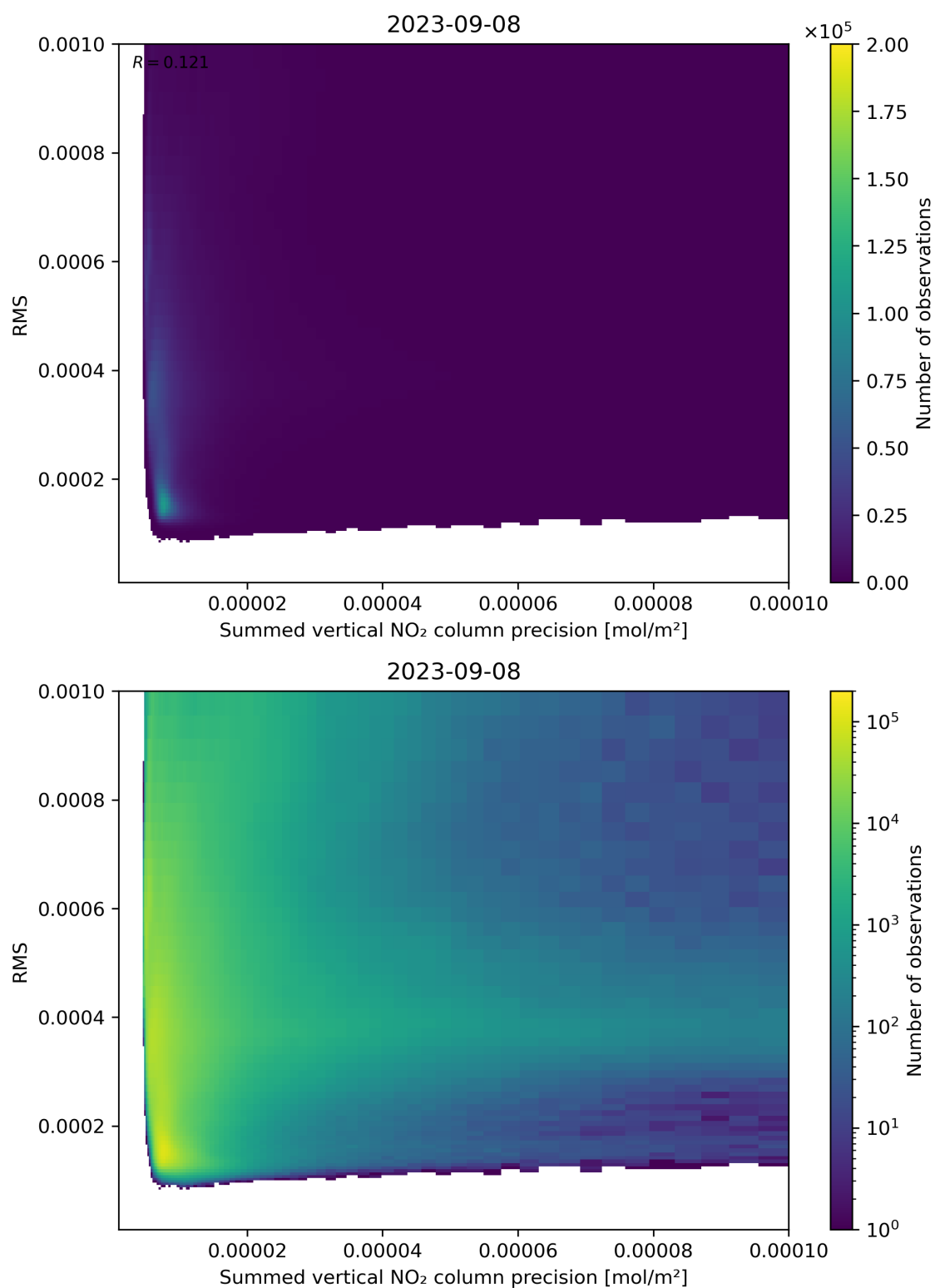
Figure 108: Scatter density plot of “Summed vertical NO 2 column precision” against “RMS” for 2023-09-07 to 2023-09-09.
