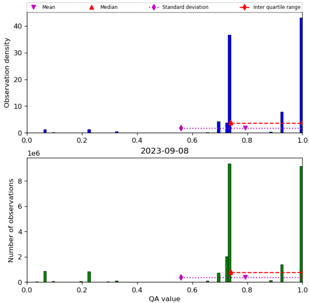
Figure 28: Histogram of “QA value” for 2023-09-07 to 2023-09-09
