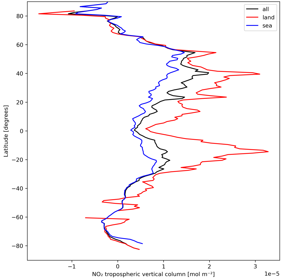
Figure 12: Zonal average of “NO 2 tropospheric vertical column” for 2023-09-07 to 2023-09-09.
