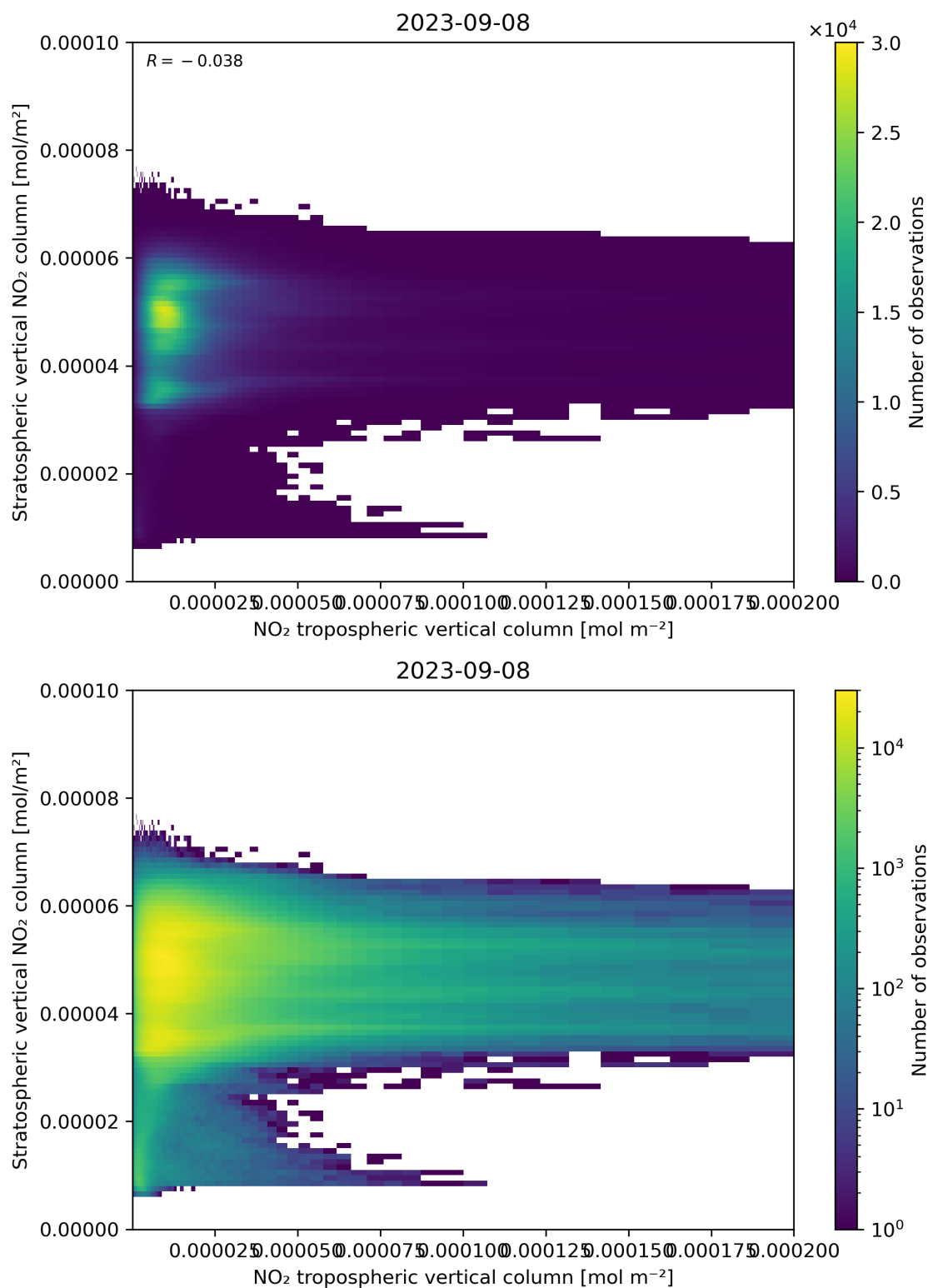
Figure 125: Scatter density plot of “NO 2 tropospheric vertical column” against “Stratospheric vertical NO 2 column” for 2023-09-07 to 2023-09-09.
