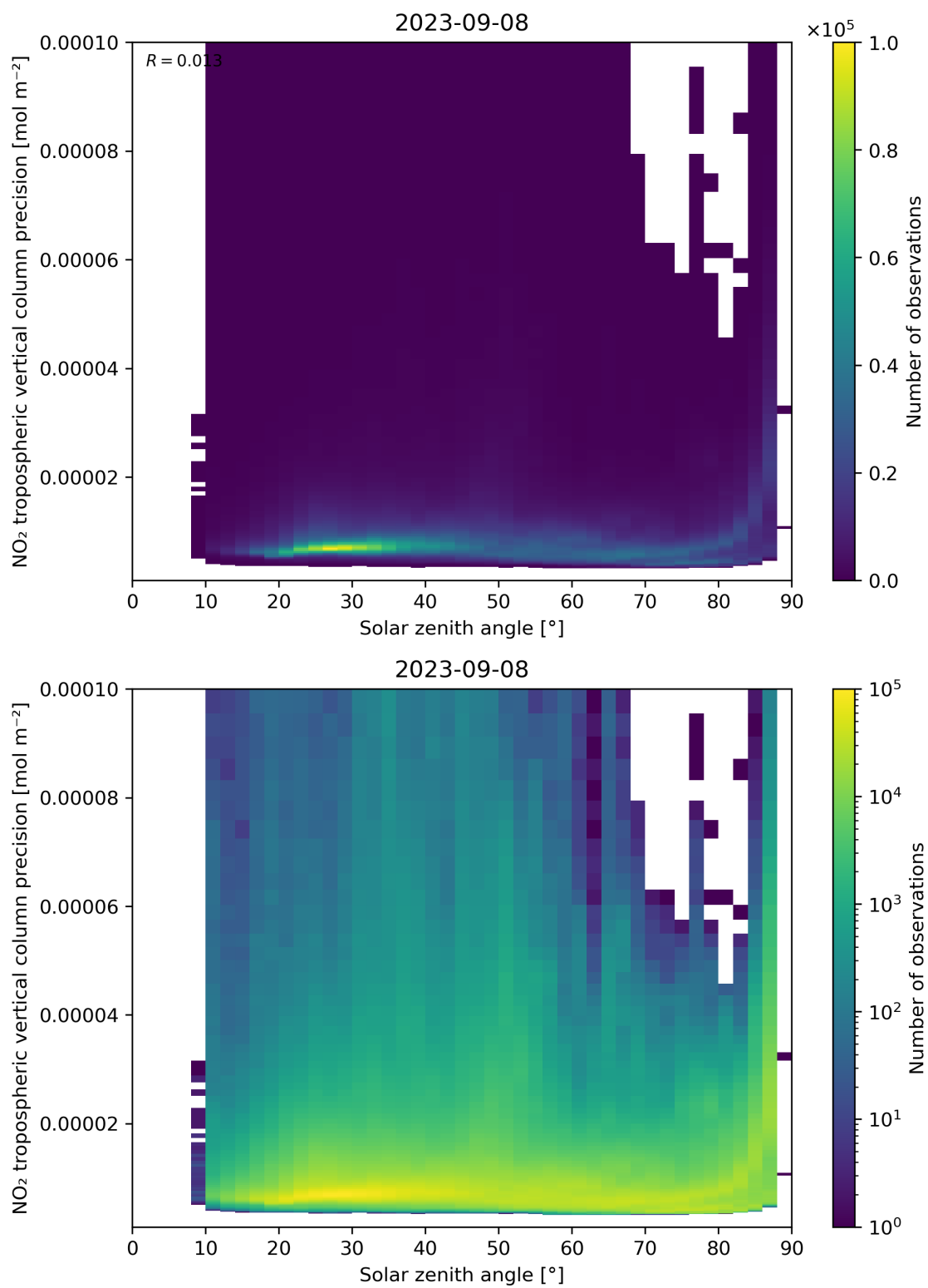
Figure 156: Scatter density plot of “Solar zenith angle” against “NO 2 tropospheric vertical column precision” for 2023-09-07 to 2023-09-09.
