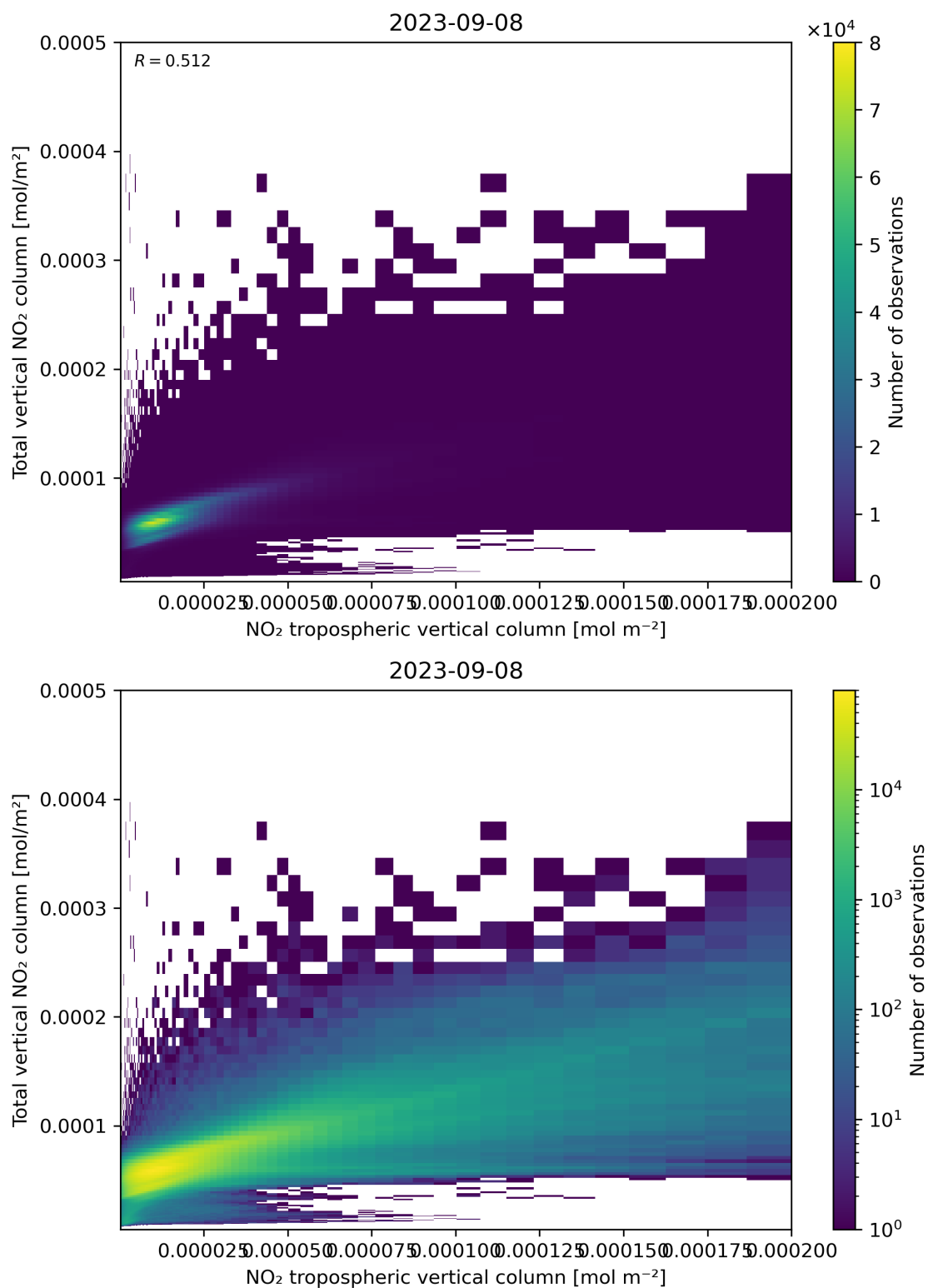
Figure 128: Scatter density plot of “NO 2 tropospheric vertical column” against “Total vertical NO 2 column” for 2023-09-07 to 2023-09-09.
