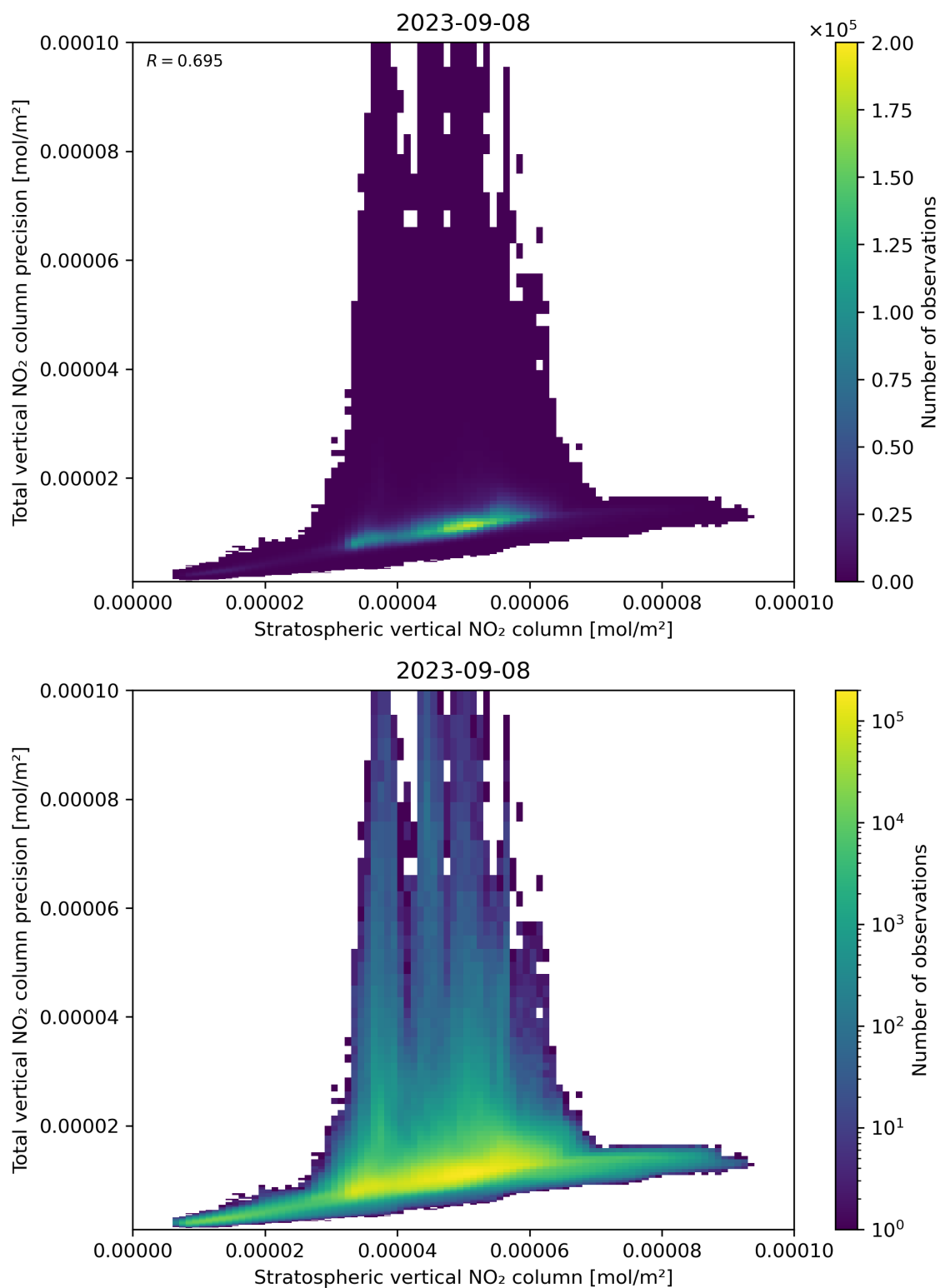
Figure 101: Scatter density plot of “Stratospheric vertical NO 2 column” against “Total vertical NO 2 column precision” for 2023-09-07 to 2023-09-09.
