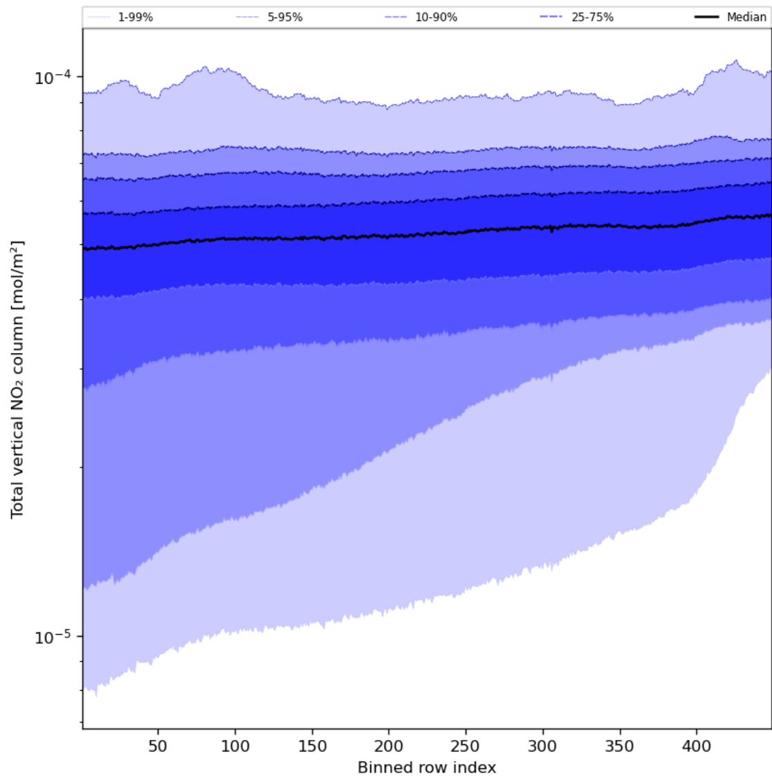
Figure 55: Along track statistics of “Total vertical NO 2 column” for 2023-09-07 to 2023-09-09
