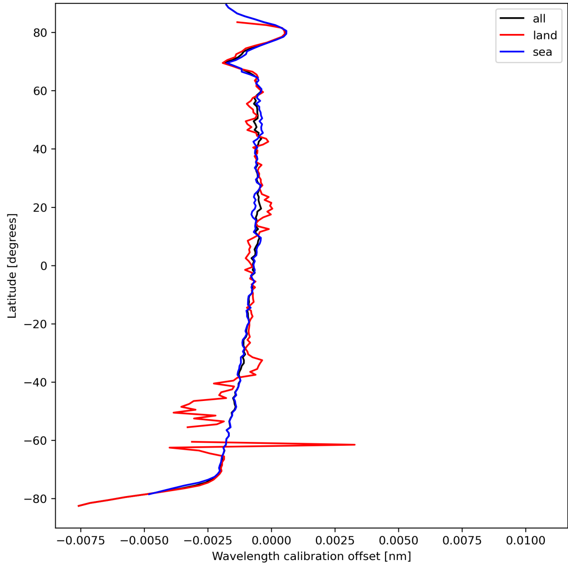
Figure 18: Zonal average of “Wavelength calibration offset” for 2023-09-07 to 2023-09-09.
