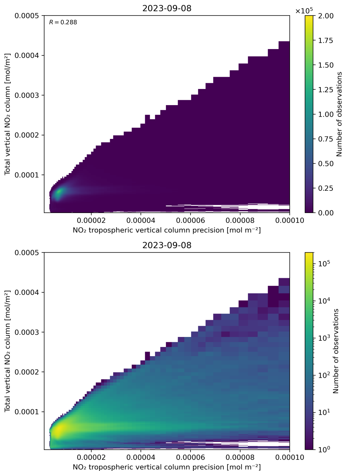
Figure 138: Scatter density plot of “NO 2 tropospheric vertical column precision” against “Total vertical NO 2 column” for 2023-09-07 to 2023-09-09.
