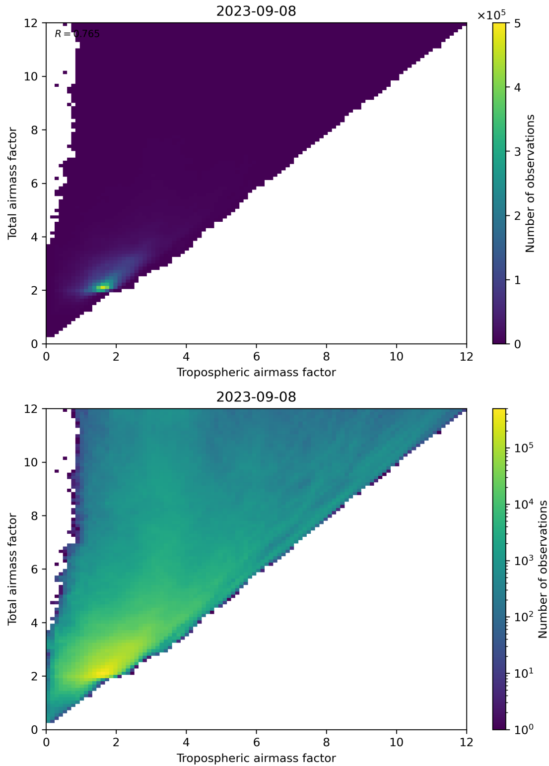
Figure 72: Scatter density plot of “Tropospheric airmass factor” against “Total airmass factor” for 2023-09-07 to 2023-09-09.
