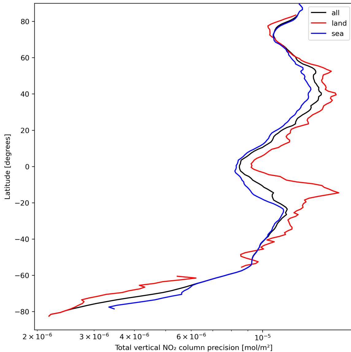
Figure 22: Zonal average of “Total vertical NO 2 column precision” for 2023-09-07 to 2023-09-09.
