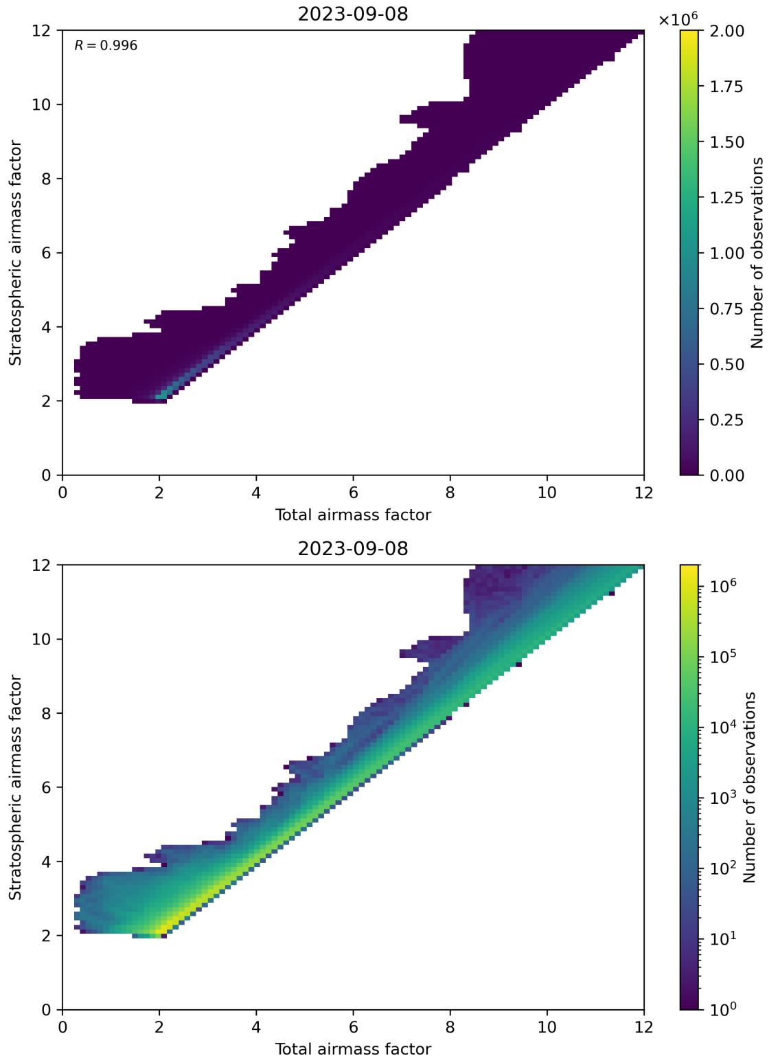
Figure 62: Scatter density plot of “Total airmass factor” against “Stratospheric airmass factor” for 2023-09-07 to 2023-09-09.
