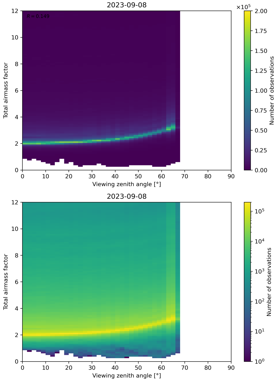
Figure 160: Scatter density plot of “Viewing zenith angle” against “Total airmass factor” for 2023-09-07 to 2023-09-09.
