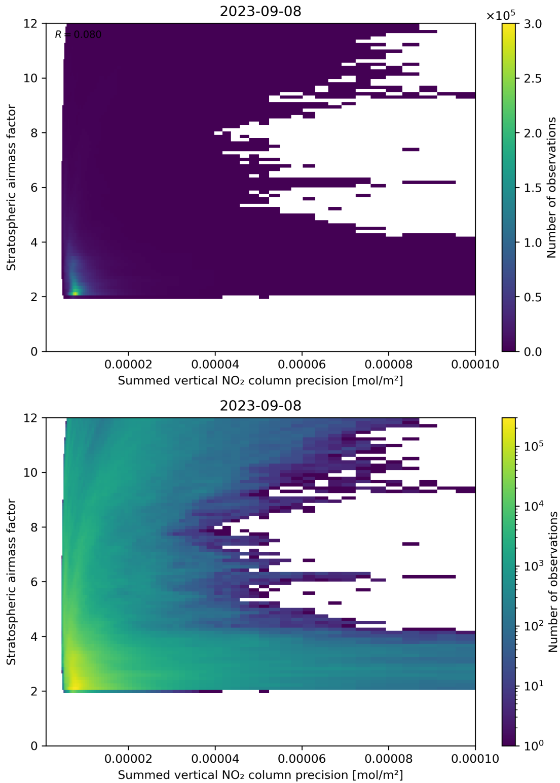
Figure 106: Scatter density plot of “Summed vertical NO 2 column precision” against “Stratospheric airmass factor” for 2023-09-07 to 2023-09-09.
