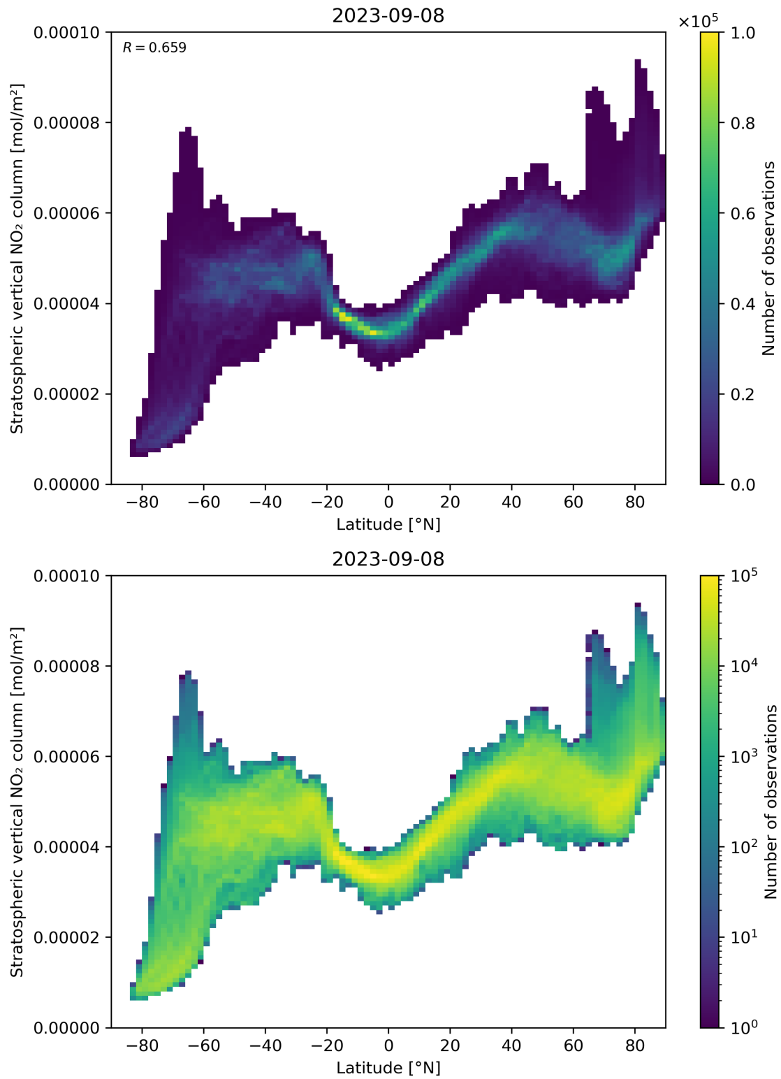
Figure 87: Scatter density plot of “Latitude” against “Stratospheric vertical NO 2 column” for 2023-09-07 to 2023-09-09.
