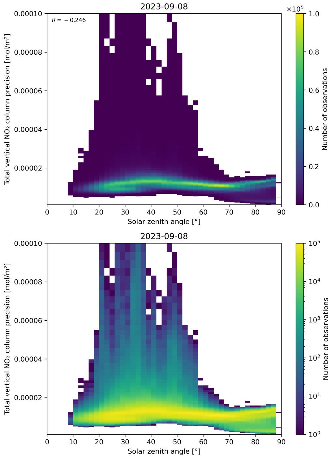
Figure 154: Scatter density plot of “Solar zenith angle” against “Total vertical NO 2 column precision” for 2023-09-07 to 2023-09-09.
