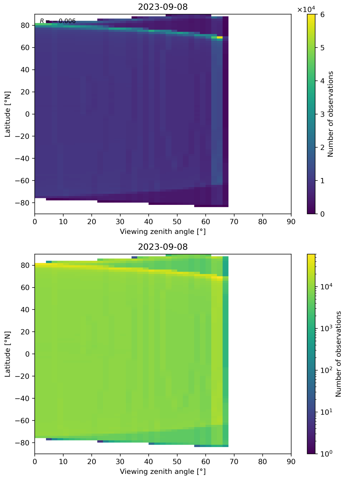
Figure 163: Scatter density plot of “Viewing zenith angle” against “Latitude” for 2023-09-07 to 2023-09-09.
