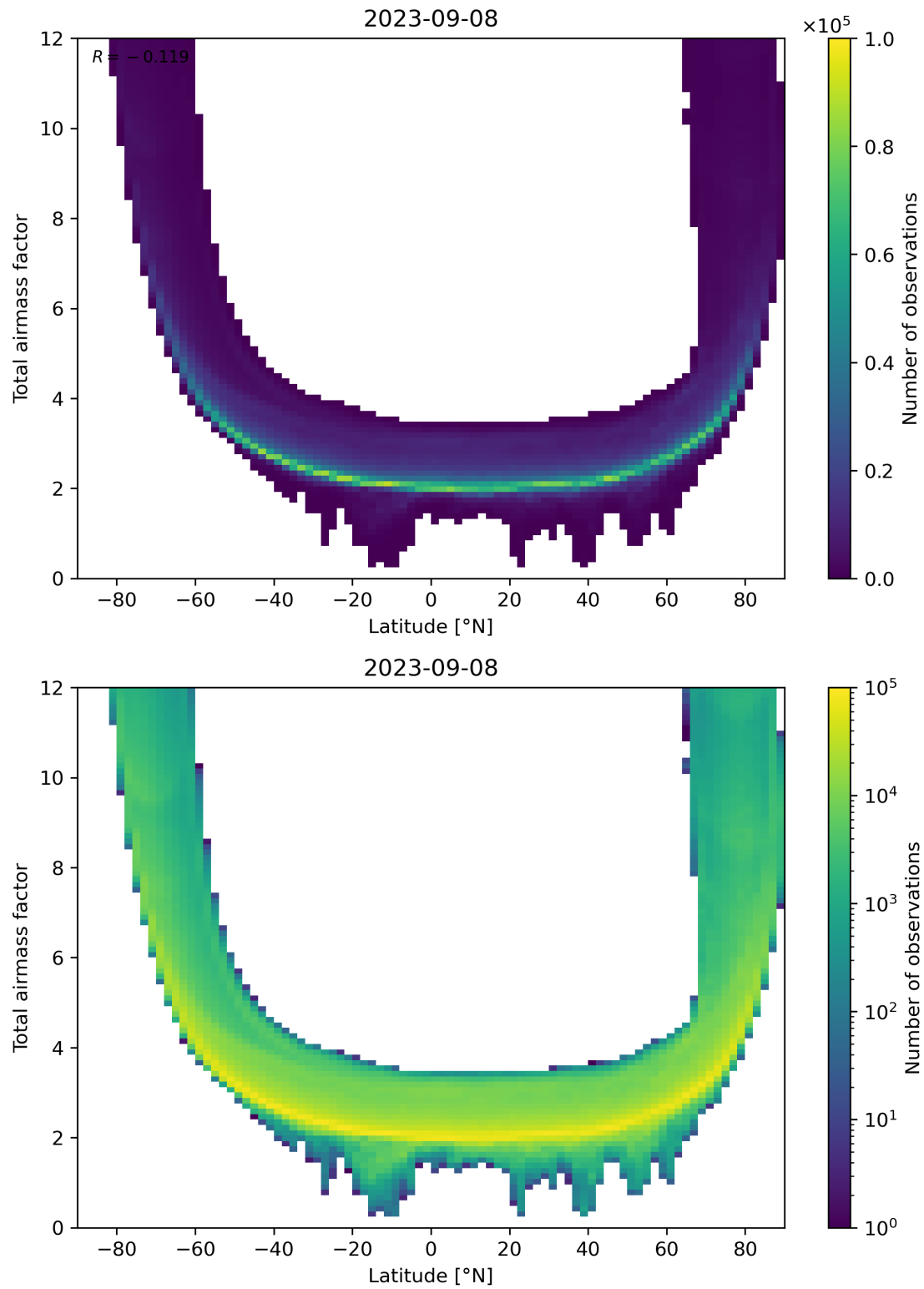
Figure 84: Scatter density plot of “Latitude” against “Total airmass factor” for 2023-09-07 to 2023-09-09.
