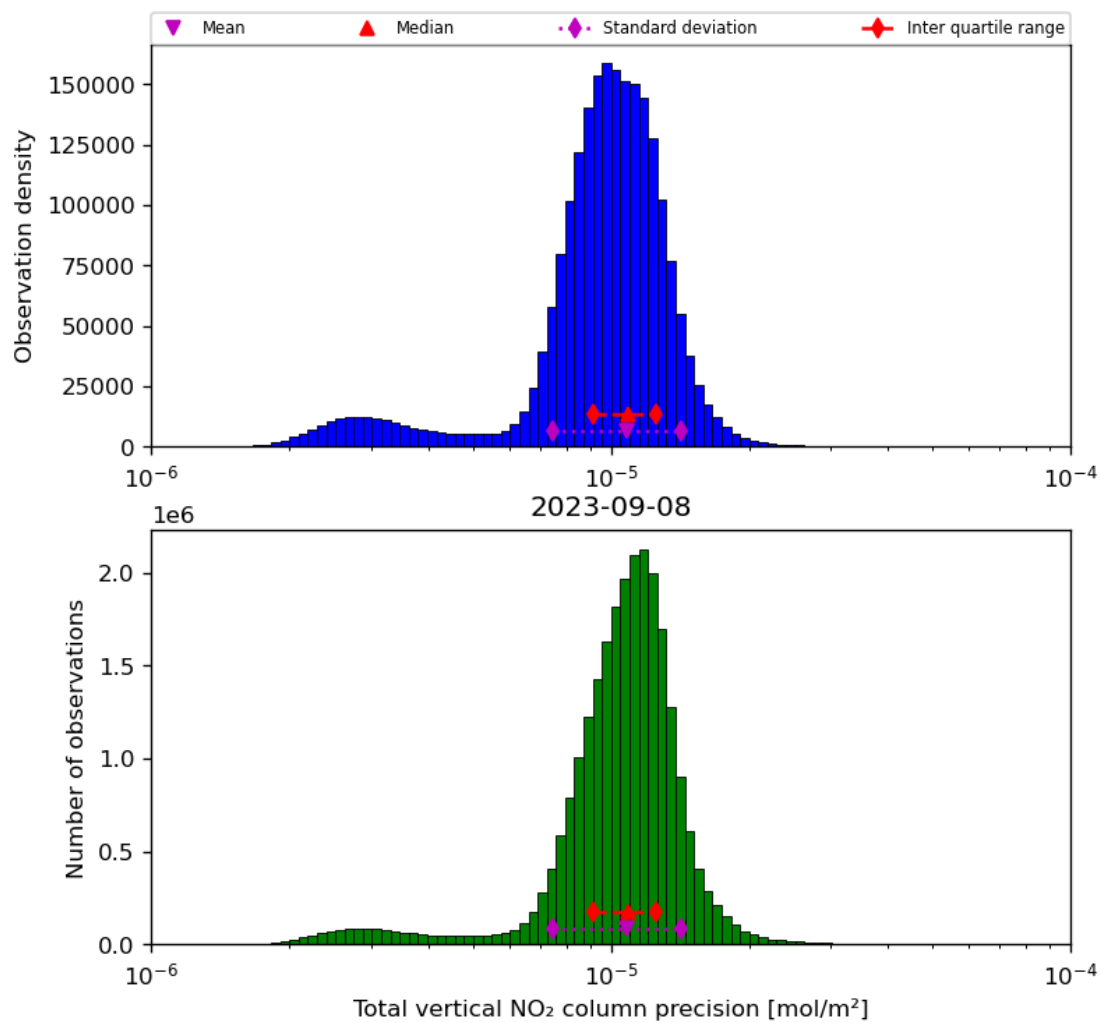
Figure 39: Histogram of "Total vertical NO 2 column precision" for 2023-09-07 to 2023-09-09
