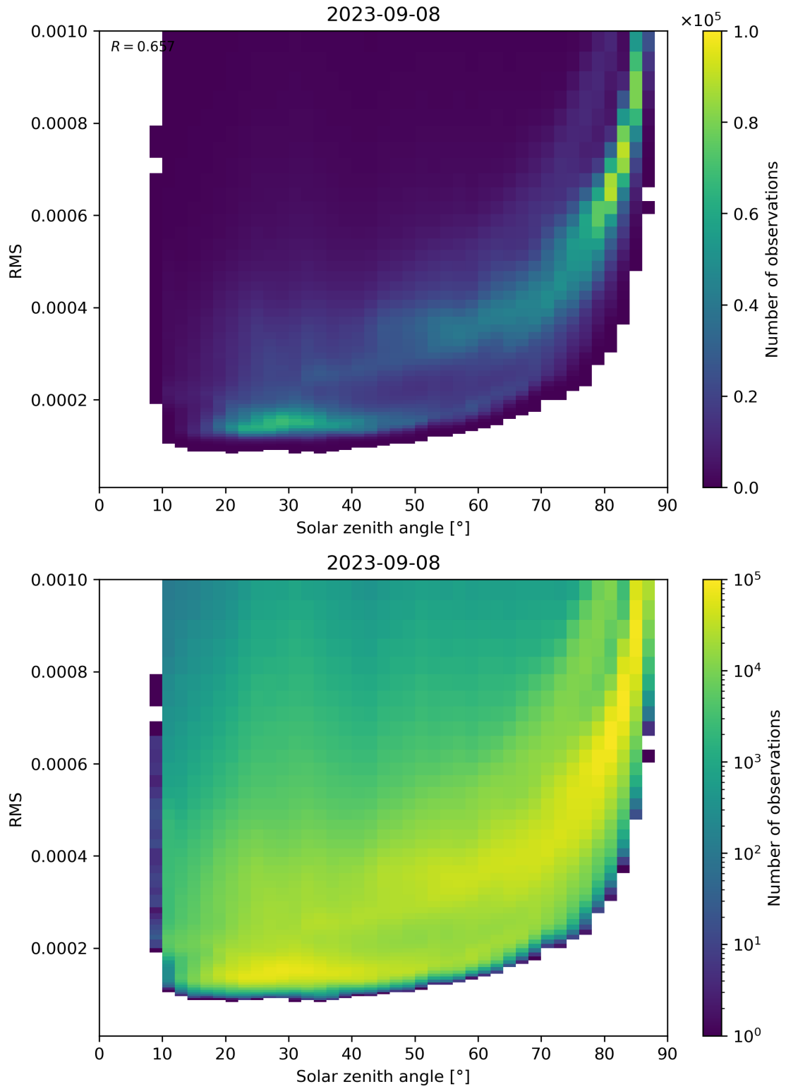
Figure 157: Scatter density plot of “Solar zenith angle” against “RMS” for 2023-09-07 to 2023-09-09.
