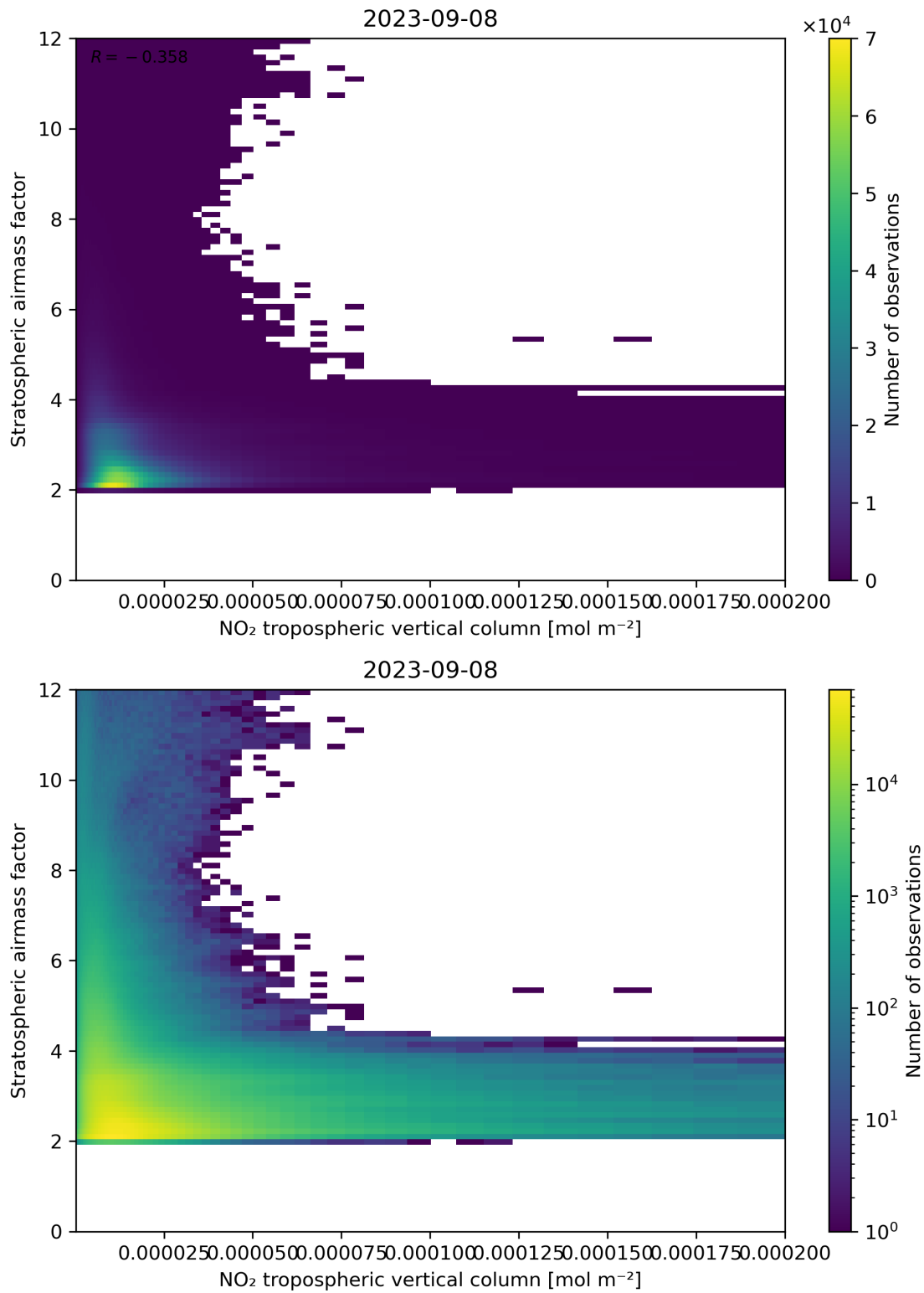
Figure 121: Scatter density plot of “NO 2 tropospheric vertical column” against “Stratospheric air mass factor” for 2023-09-07 to 2023-09-09.
