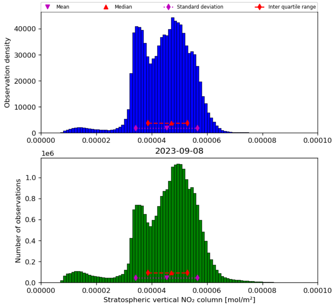
Figure 36: Histogram of “Stratospheric vertical NO 2 column” for 2023-09-07 to 2023-09-09
