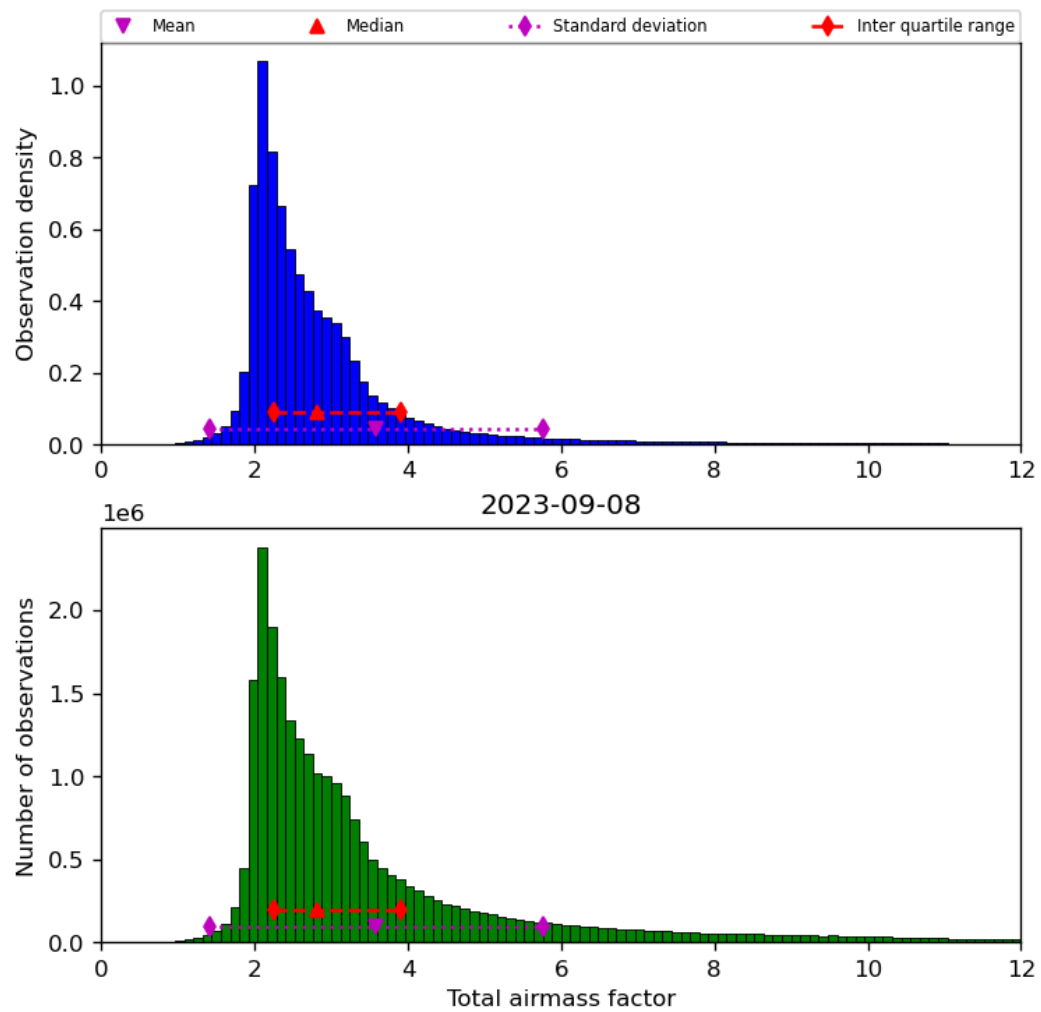
Figure 32: Histogram of “Total airmass factor” for 2023-09-07 to 2023-09-09
