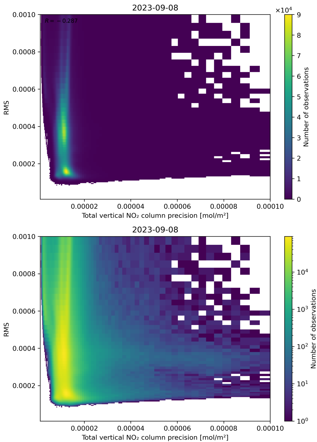
Figure 119: Scatter density plot of “Total vertical NO 2 column precision” against “RMS” for 2023-09-07 to 2023-09-09.
