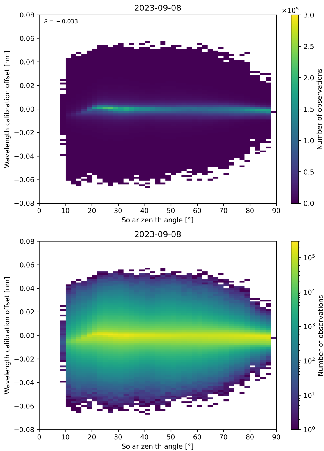
Figure 158: Scatter density plot of “Solar zenith angle” against “Wavelength calibration offset” for 2023-09-07 to 2023-09-09.
