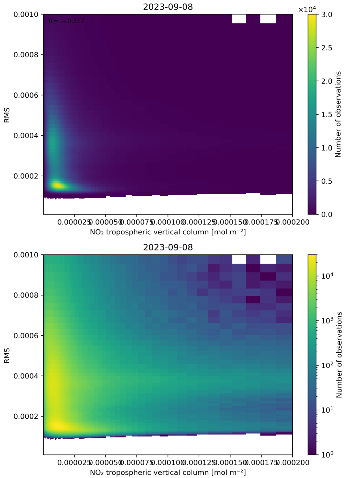
Figure 142: Scatter density plot of “NO 2 tropospheric vertical column” against “RMS” for 2023-09-07 to 2023-09-09.
