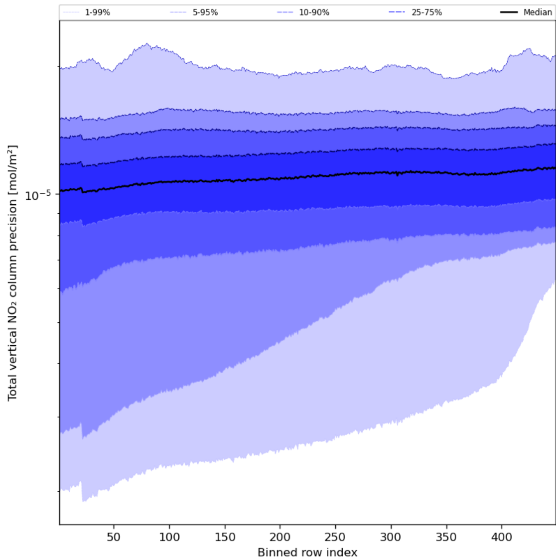
Figure 56: Along track statistics of “Total vertical NO 2 column precision” for 2023-09-07 to 2023-09-09
