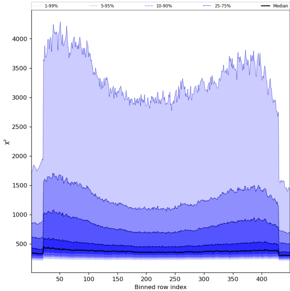
Figure 59: Along track statistics of “ \chi^2 ” for 2023-09-07 to 2023-09-09
