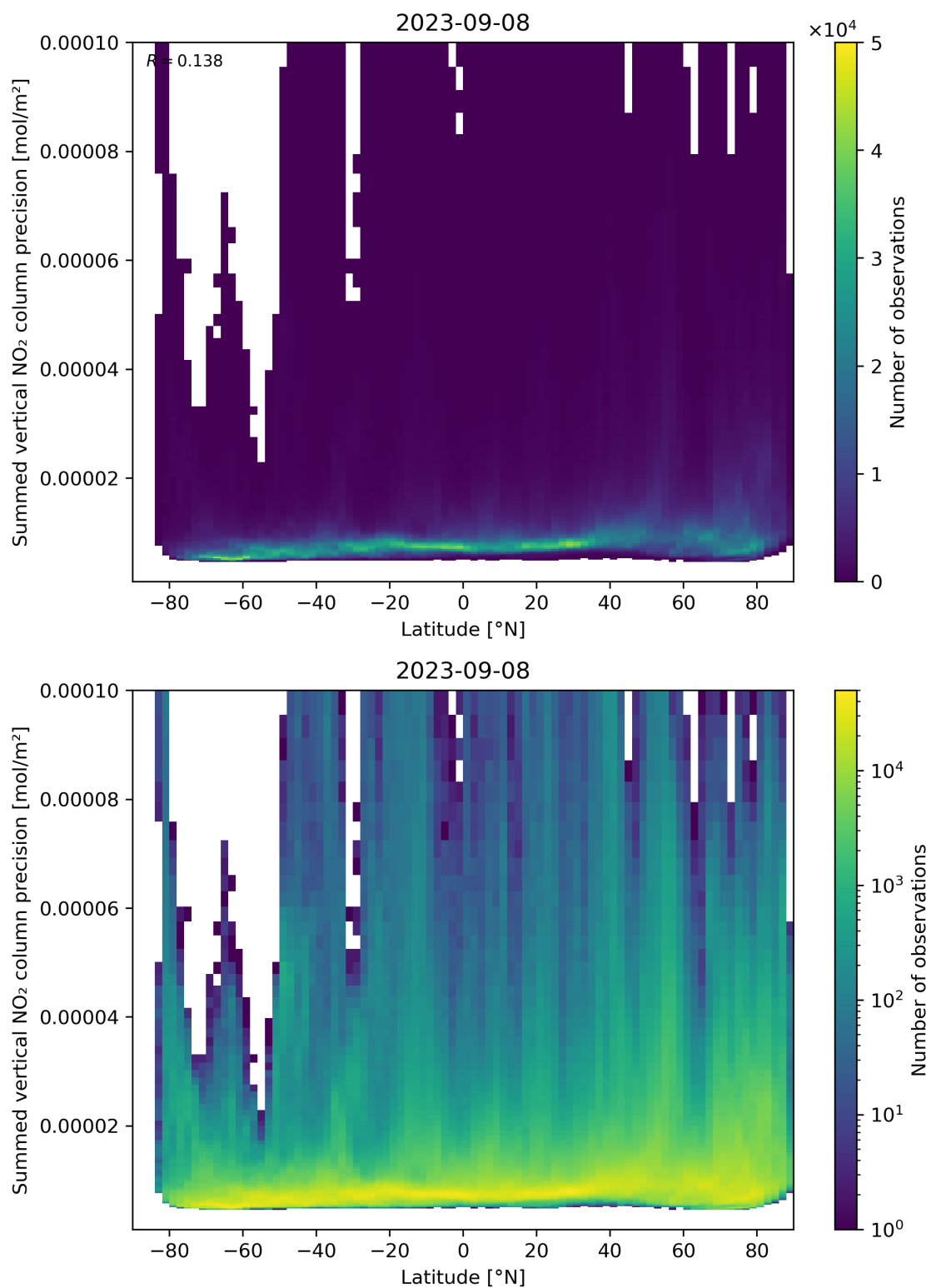
Figure 89: Scatter density plot of “Latitude” against “Summed vertical NO 2 column precision” for 2023-09-07 to 2023-09-09.
