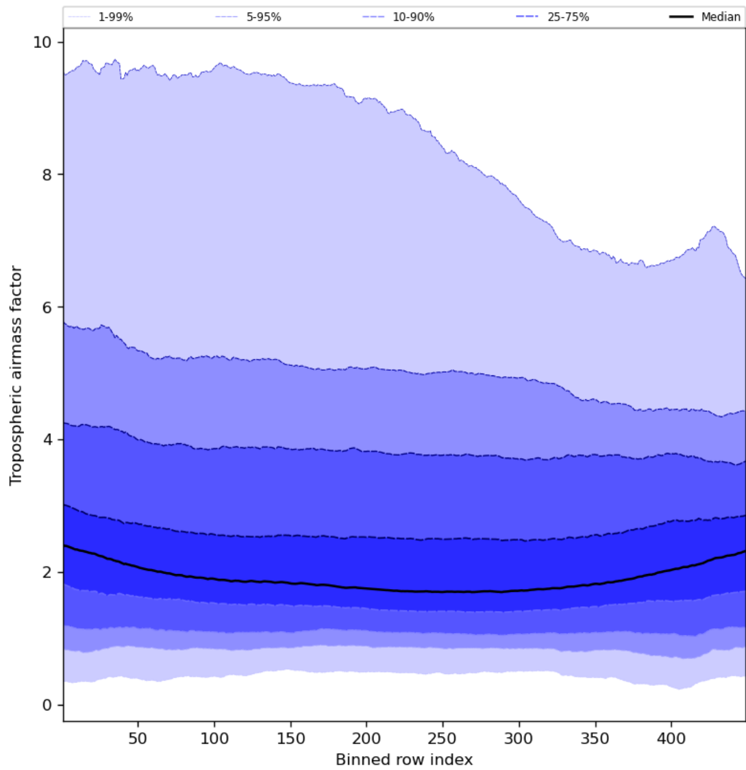
Figure 48: Along track statistics of “Tropospheric air mass factor” for 2023-09-07 to 2023-09-09
