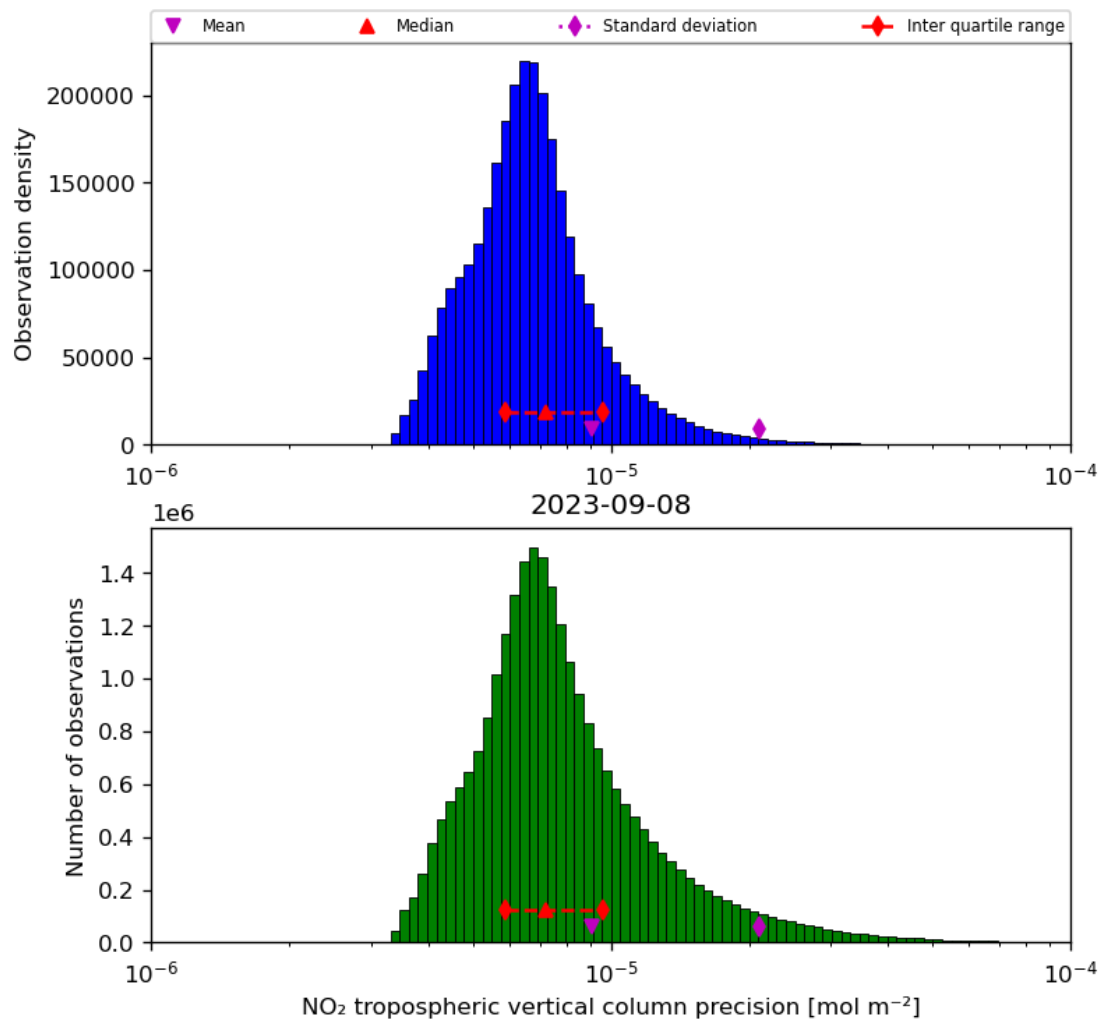
Figure 30: Histogram of “NO 2 tropospheric vertical column precision” for 2023-09-07 to 2023-09-09
