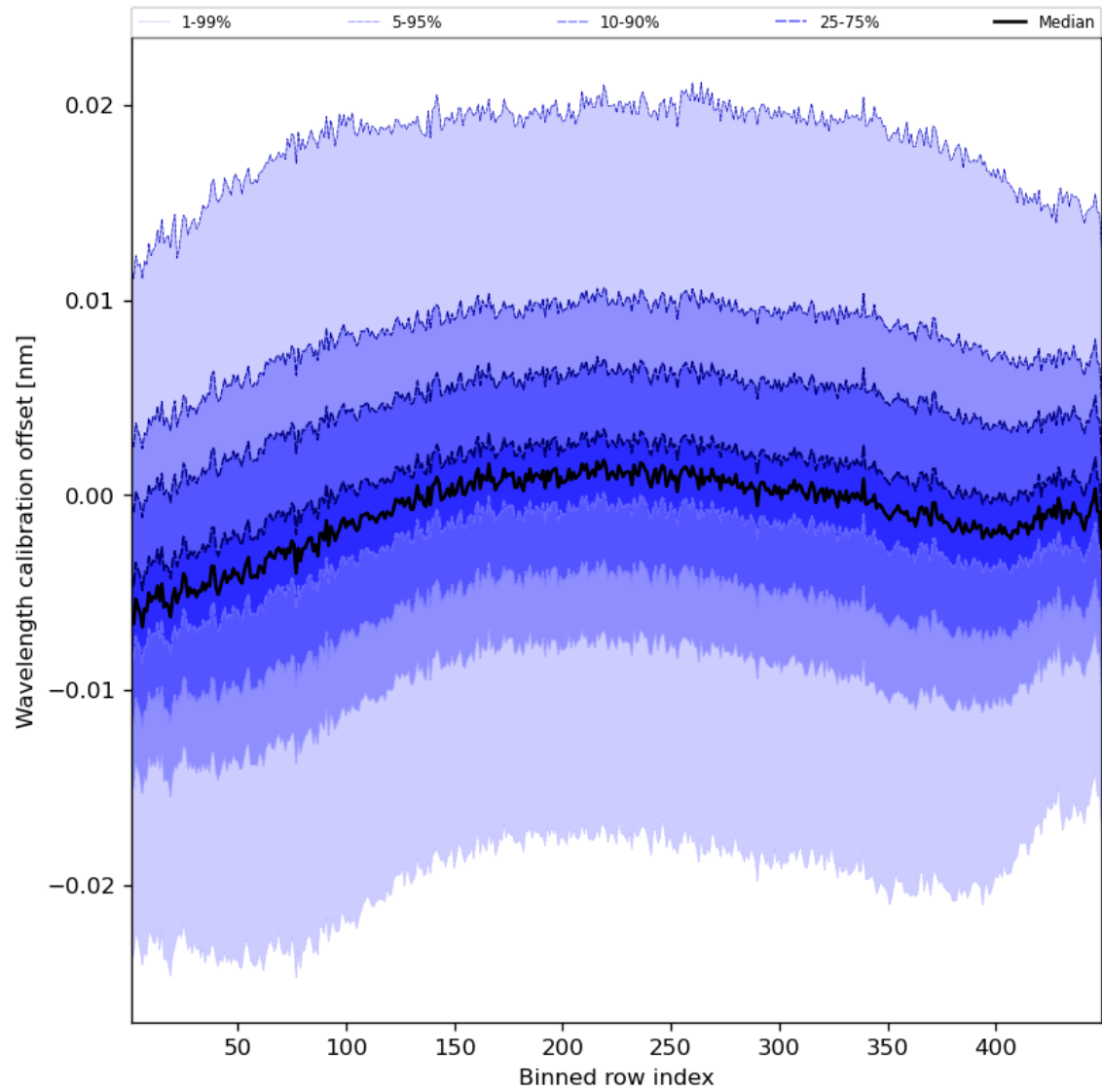
Figure 52: Along track statistics of “Wavelength calibration offset” for 2023-09-07 to 2023-09-09
