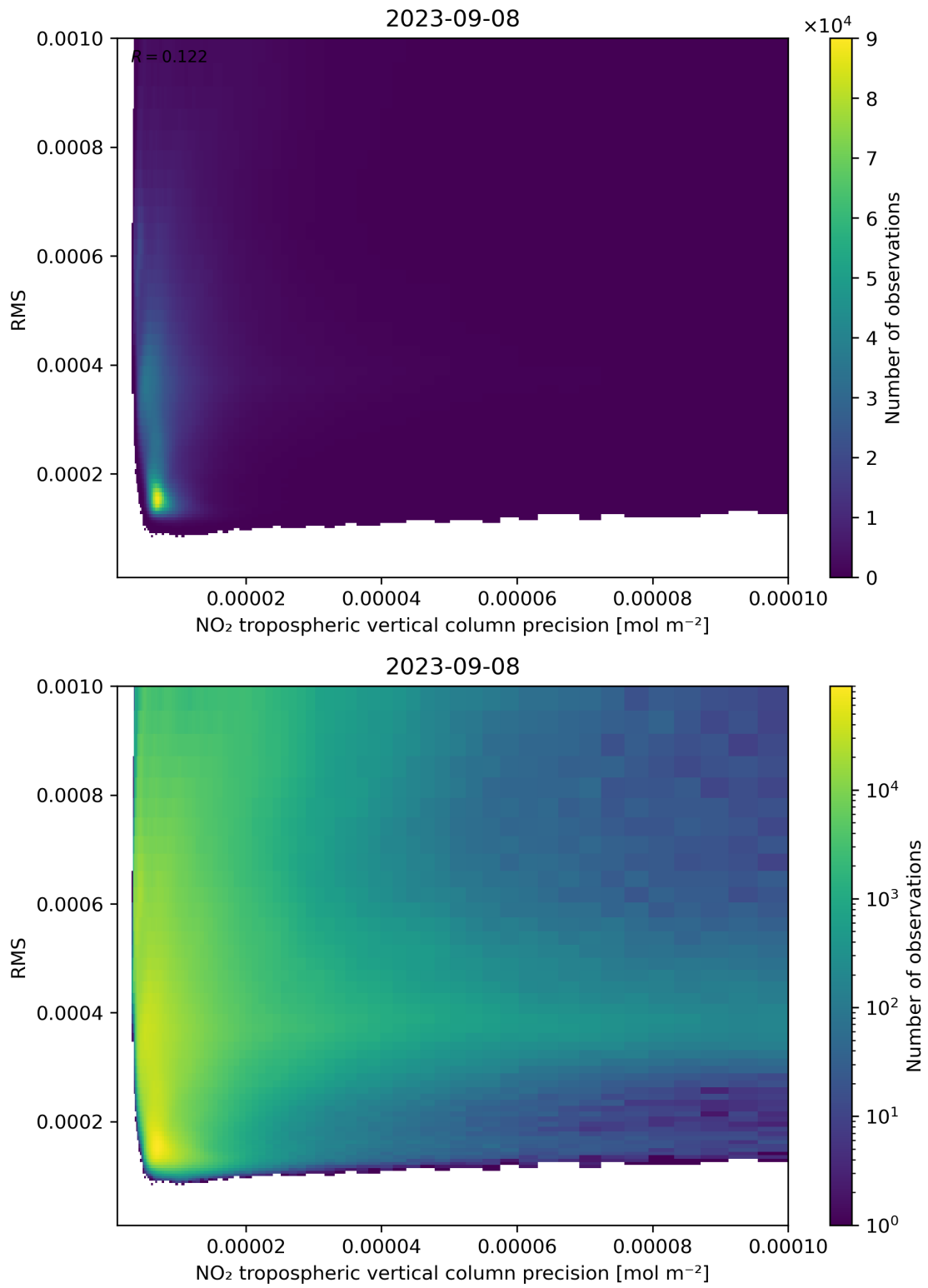
Figure 140: Scatter density plot of “NO 2 tropospheric vertical column precision” against “RMS” for 2023-09-07 to 2023-09-09.
