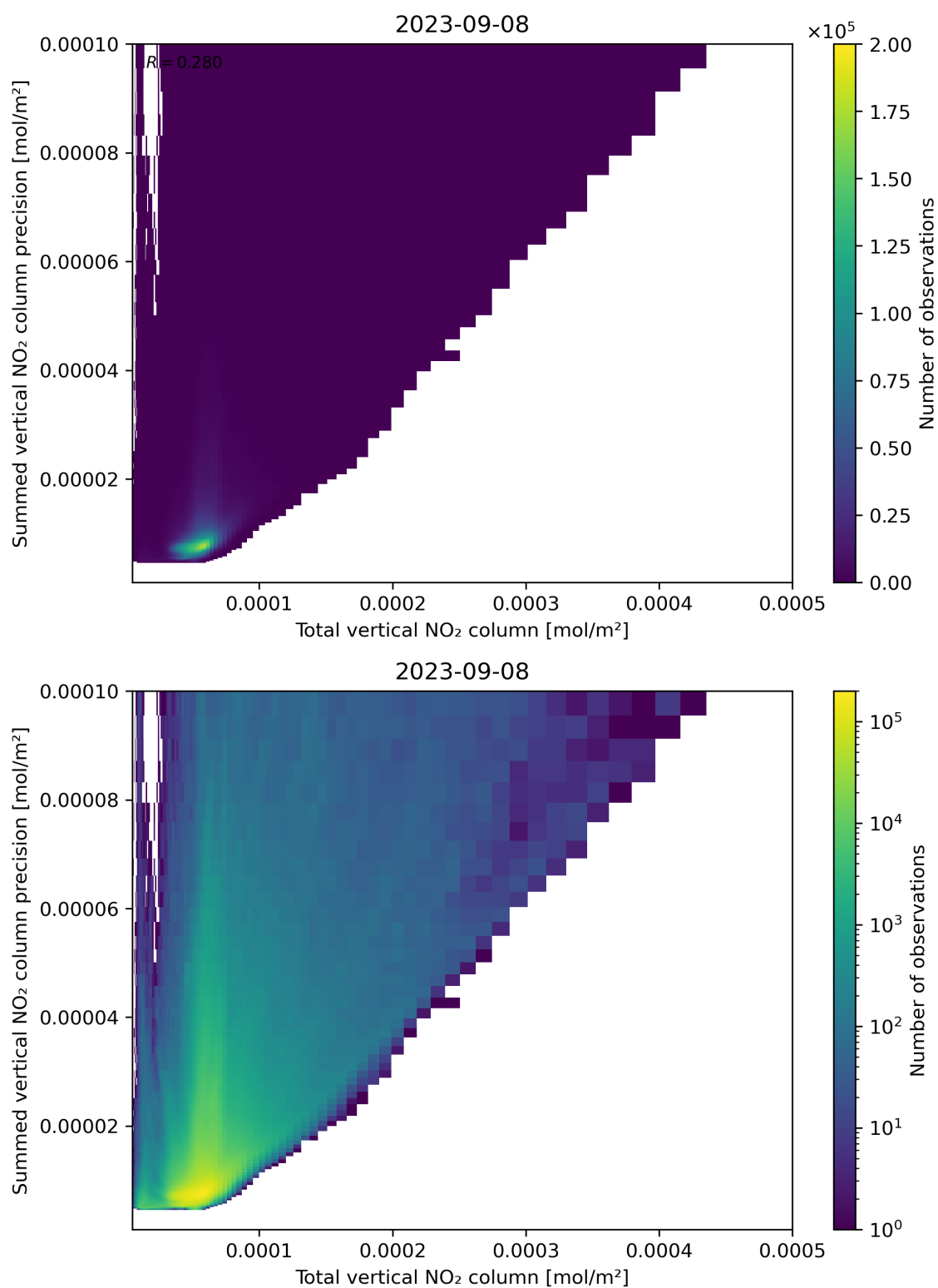
Figure 113: Scatter density plot of “Total vertical NO 2 column” against “Summed vertical NO 2 column precision” for 2023-09-07 to 2023-09-09.
