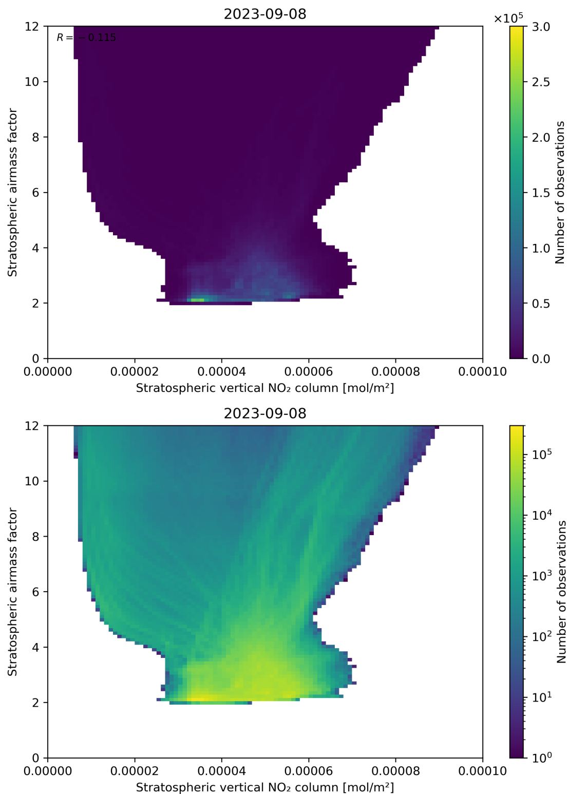
Figure 96: Scatter density plot of “Stratospheric vertical NO 2 column” against “Stratospheric airmass factor” for 2023-09-07 to 2023-09-09.
