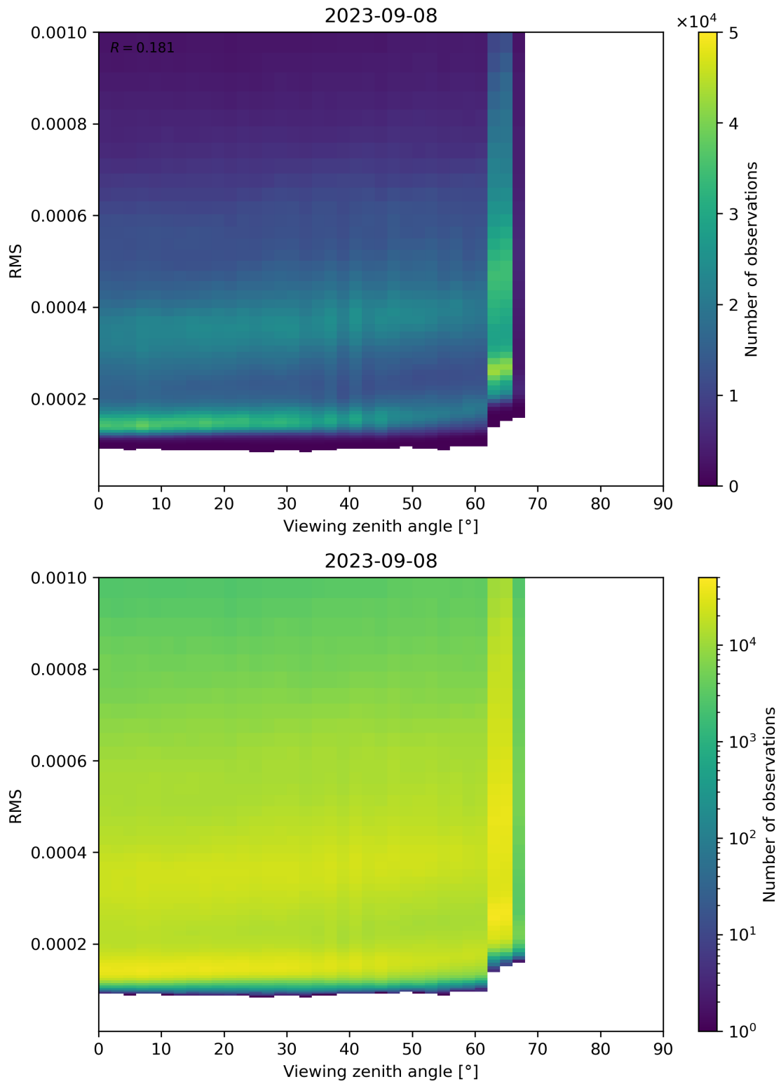
Figure 171: Scatter density plot of “Viewing zenith angle” against “RMS” for 2023-09-07 to 2023-09-09.
