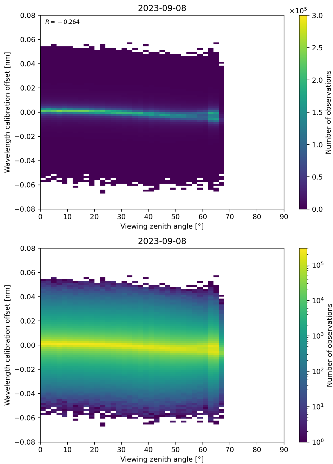
Figure 173: Scatter density plot of “Viewing zenith angle” against “Wavelength calibration offset” for 2023-09-07 to 2023-09-09.
