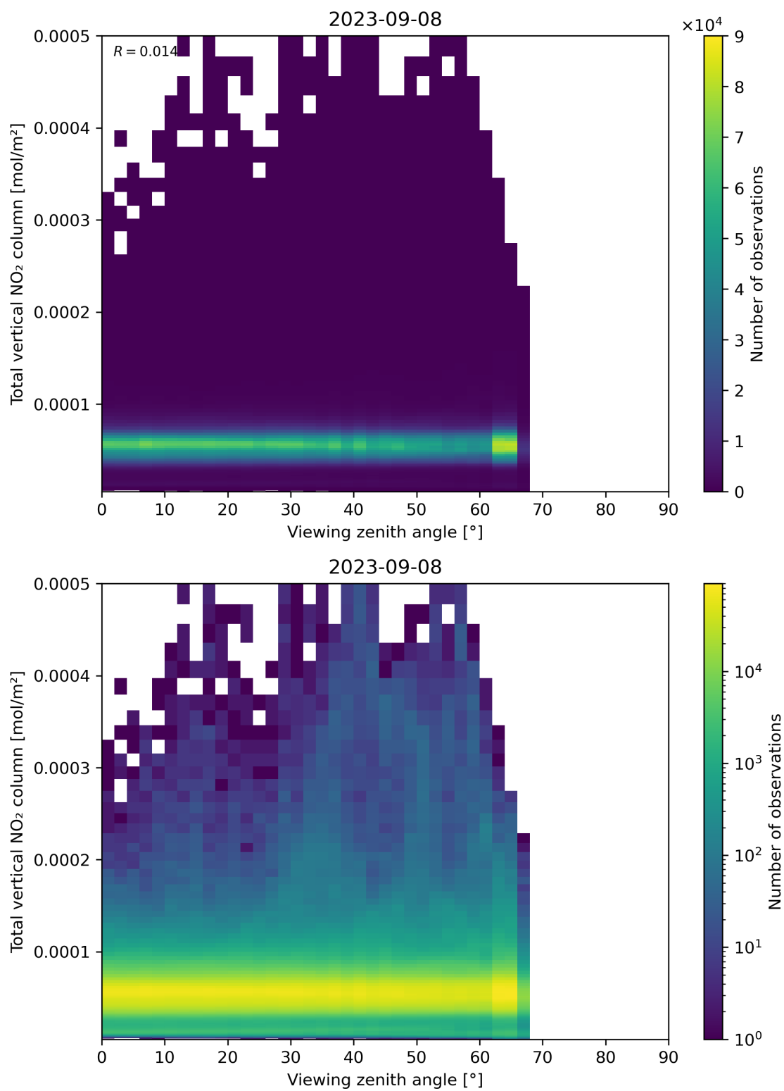
Figure 167: Scatter density plot of “Viewing zenith angle” against “Total vertical NO 2 column” for 2023-09-07 to 2023-09-09.
