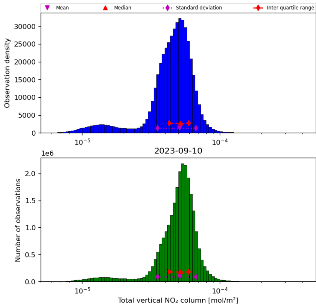
Figure 38: Histogram of "Total vertical NO 2 column" for 2023-09-10 to 2023-09-11
