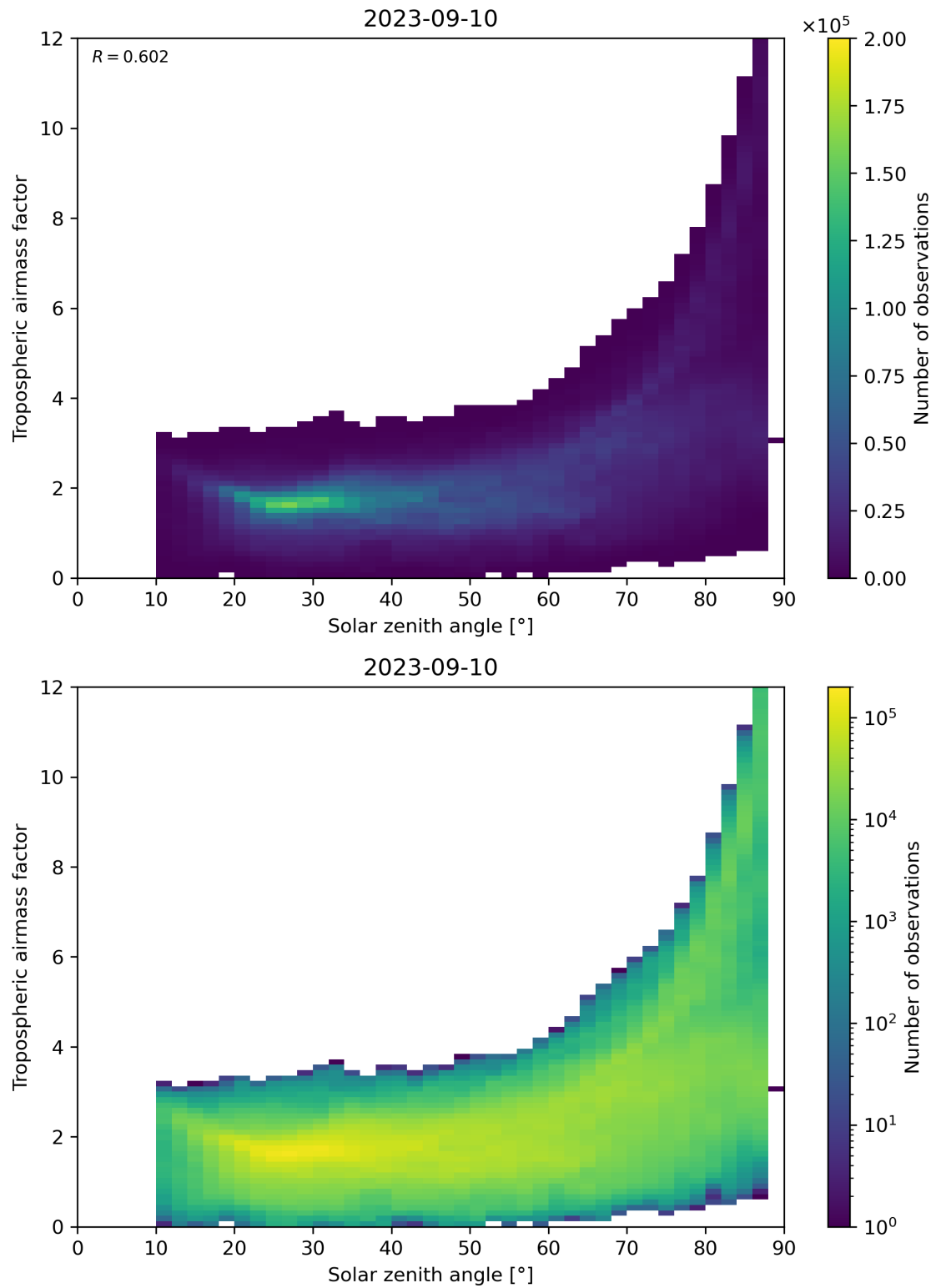
Figure 147: Scatter density plot of “Solar zenith angle” against “Tropospheric airmass factor” for 2023-09-10 to 2023-09-11.
