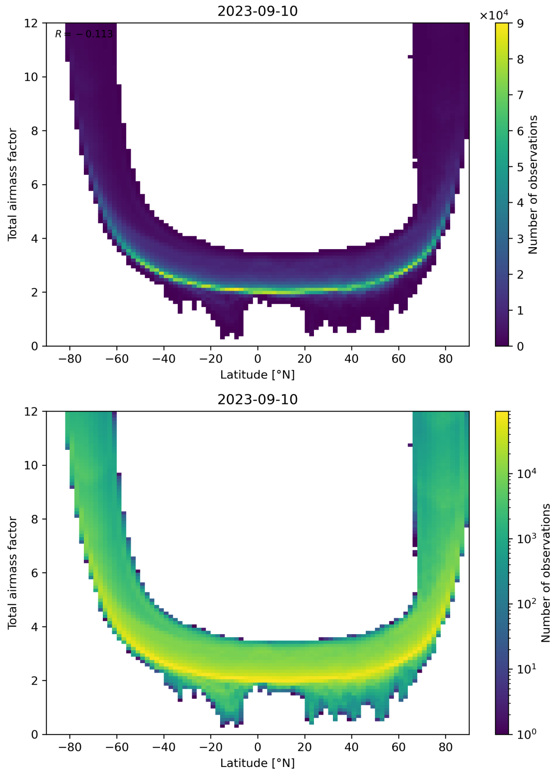
Figure 84: Scatter density plot of “Latitude” against “Total airmass factor” for 2023-09-10 to 2023-09-11.
