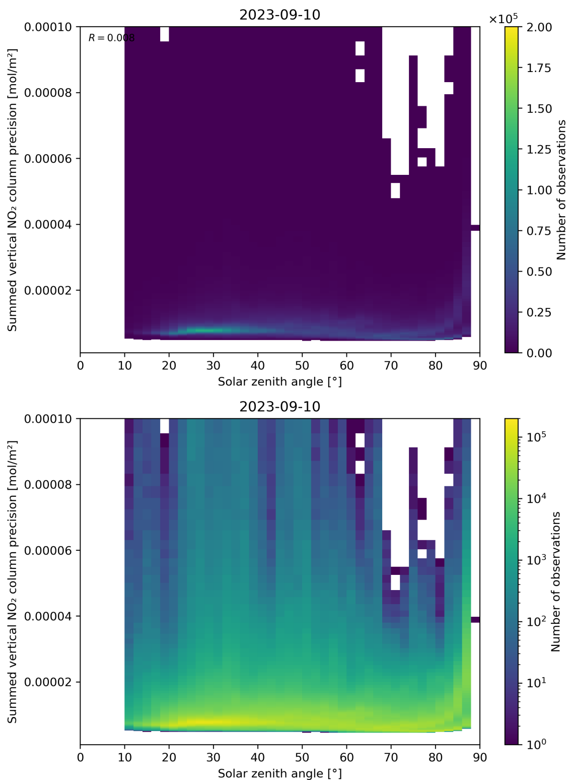
Figure 152: Scatter density plot of “Solar zenith angle” against “Summed vertical NO 2 column precision” for 2023-09-10 to 2023-09-11.
