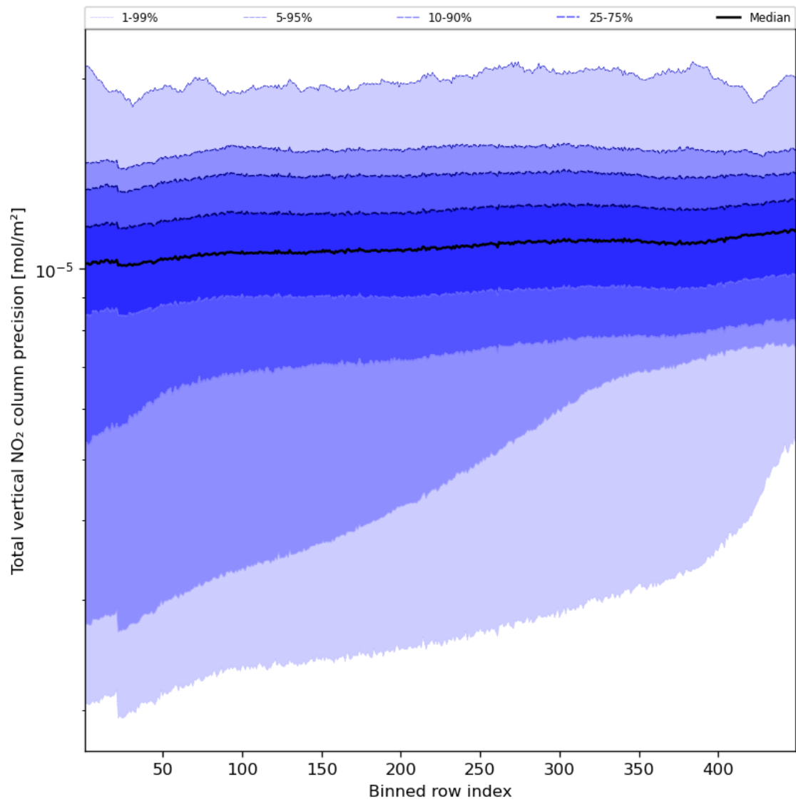
Figure 56: Along track statistics of “Total vertical NO 2 column precision” for 2023-09-10 to 2023-09-11
