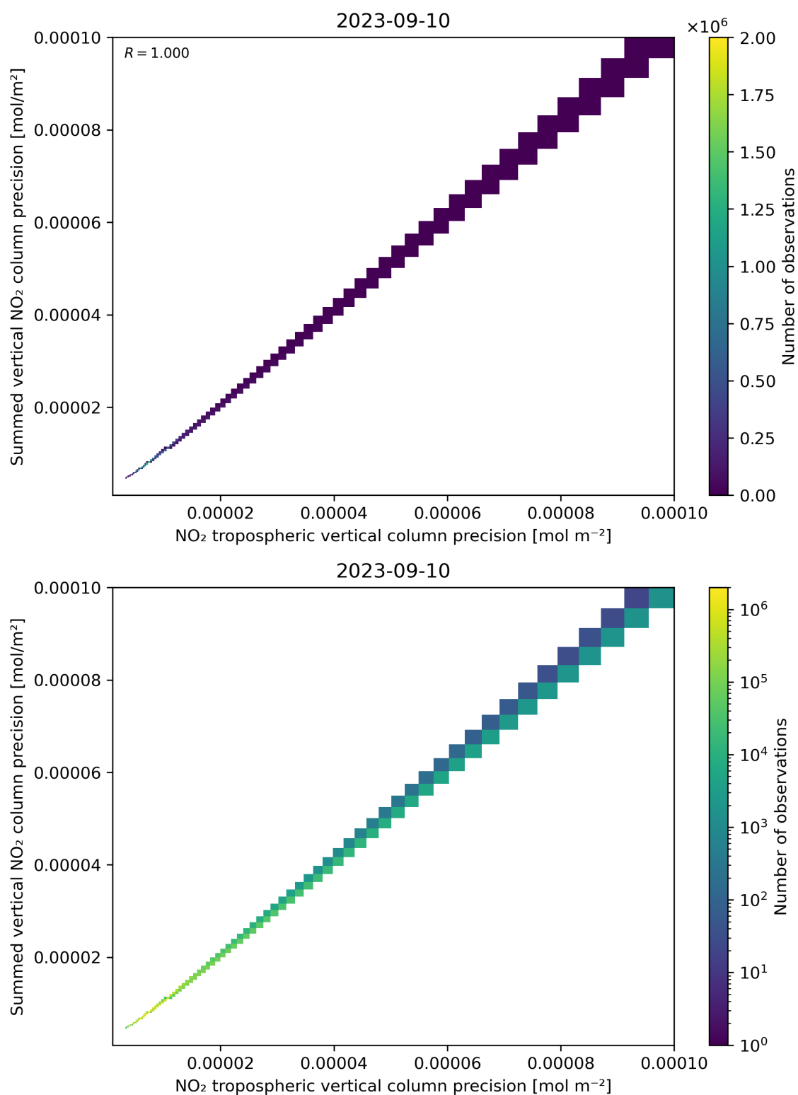
Figure 137: Scatter density plot of “NO 2 tropospheric vertical column precision” against “Summed vertical NO 2 column precision” for 2023-09-10 to 2023-09-11.
