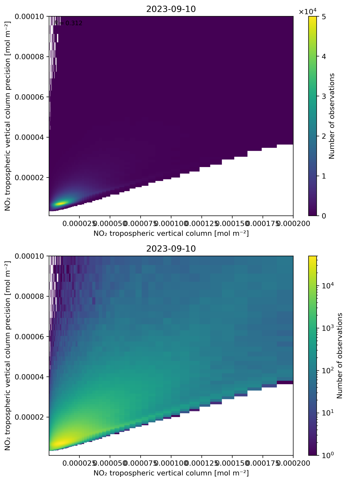
Figure 130: Scatter density plot of “NO 2 tropospheric vertical column” against “NO 2 tropospheric vertical column precision” for 2023-09-10 to 2023-09-11.
