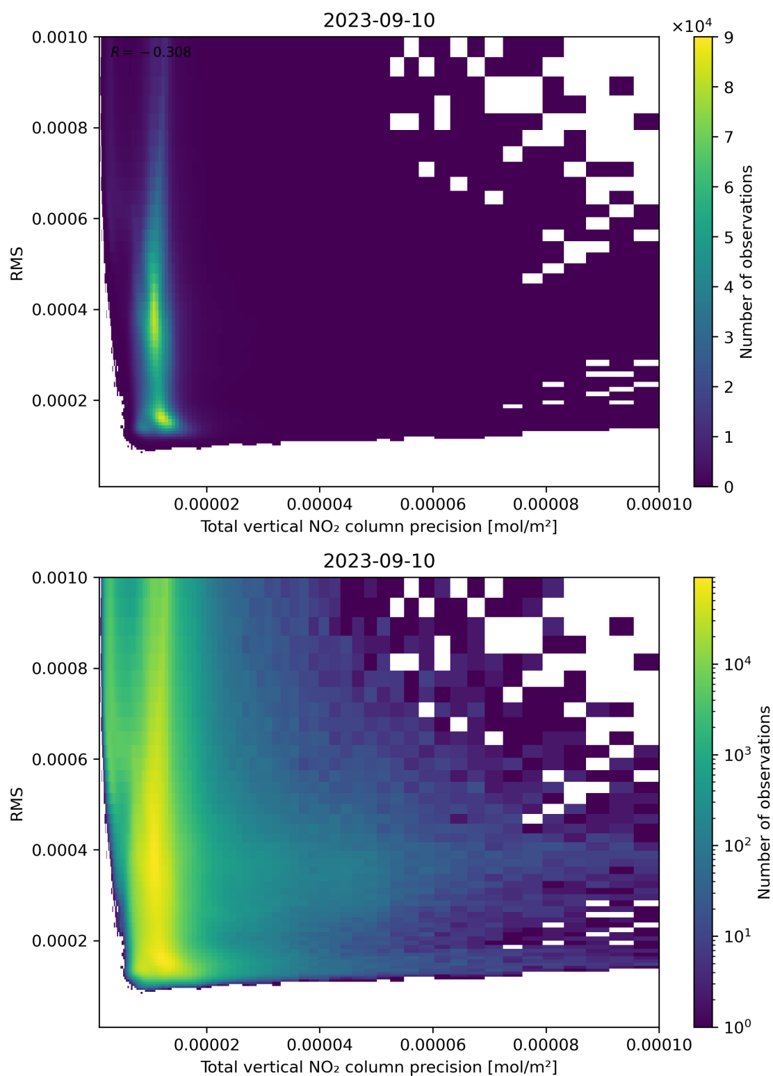
Figure 119: Scatter density plot of “Total vertical NO 2 column precision” against “RMS” for 2023-09-10 to 2023-09-11.
