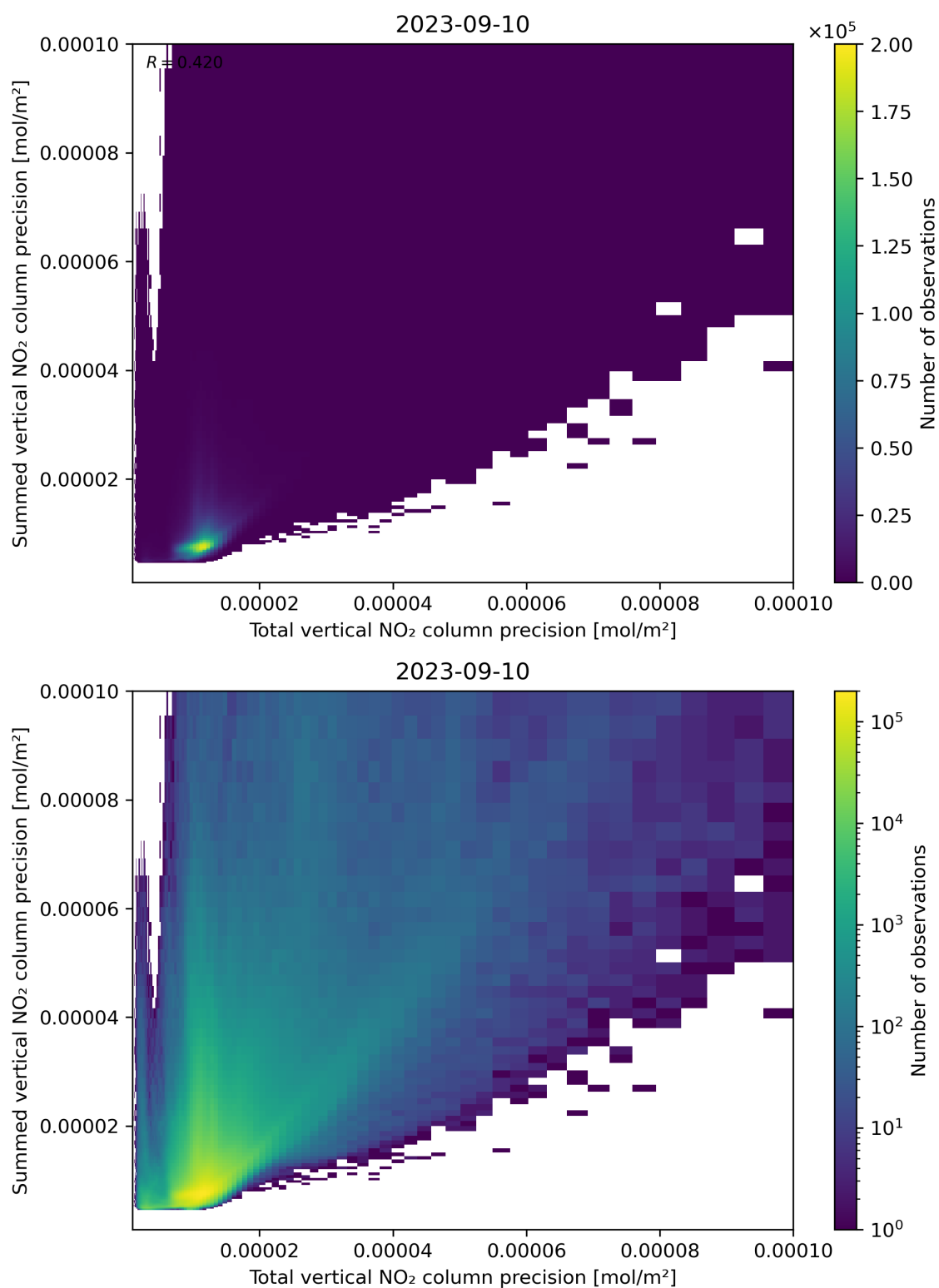
Figure 118: Scatter density plot of “Total vertical NO 2 column precision” against “Summed vertical NO 2 column precision” for 2023-09-10 to 2023-09-11.
