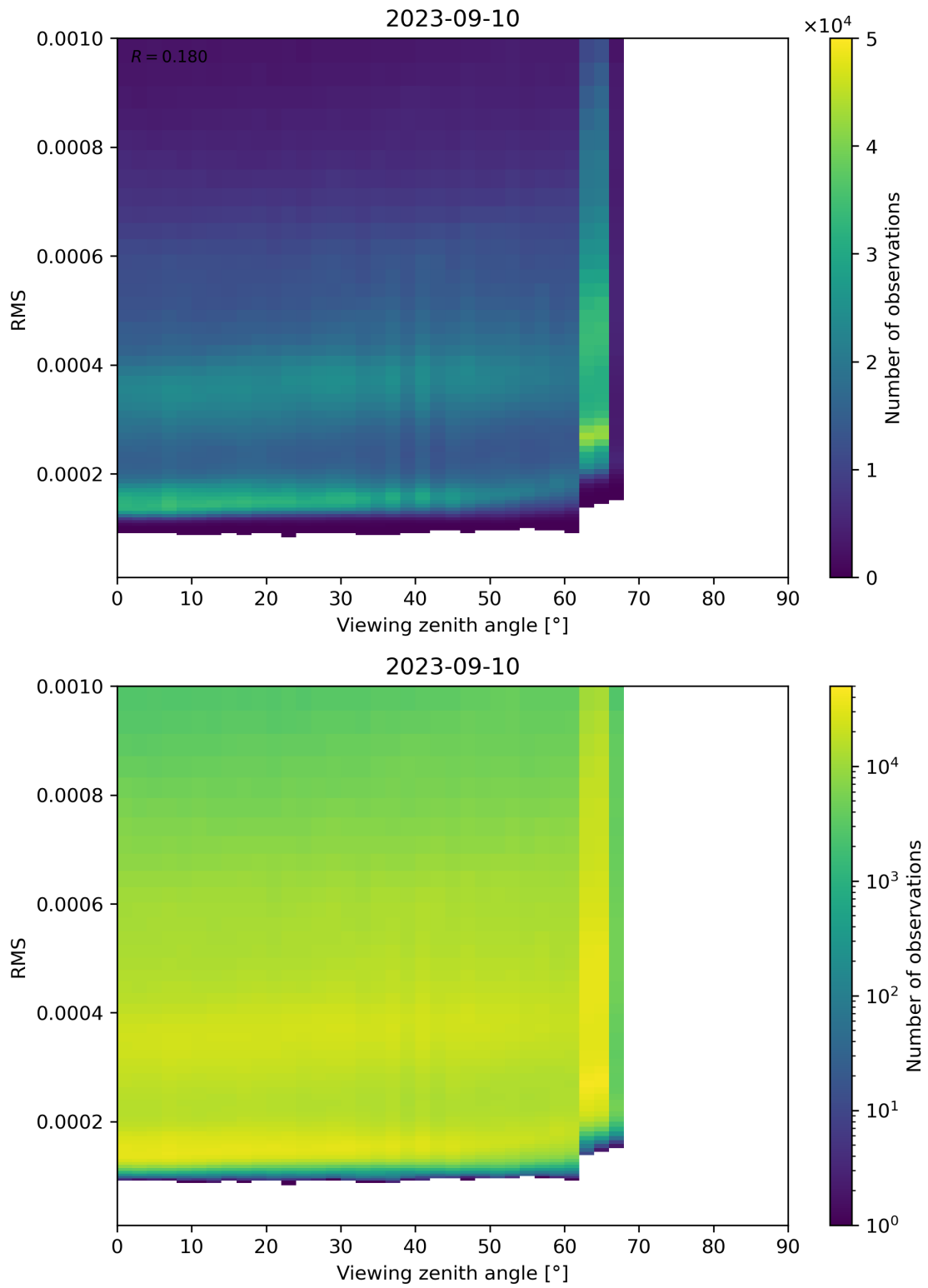
Figure 171: Scatter density plot of “Viewing zenith angle” against “RMS” for 2023-09-10 to 2023-09-11.
