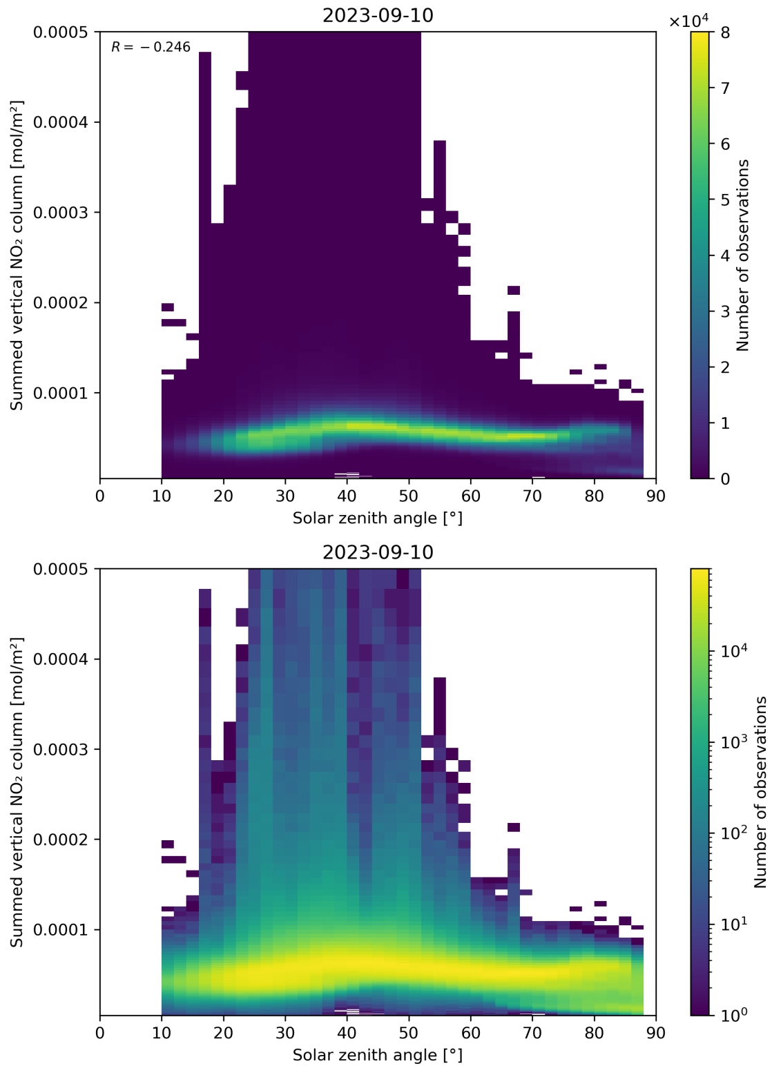
Figure 151: Scatter density plot of “Solar zenith angle” against “Summed vertical NO 2 column” for 2023-09-10 to 2023-09-11.
