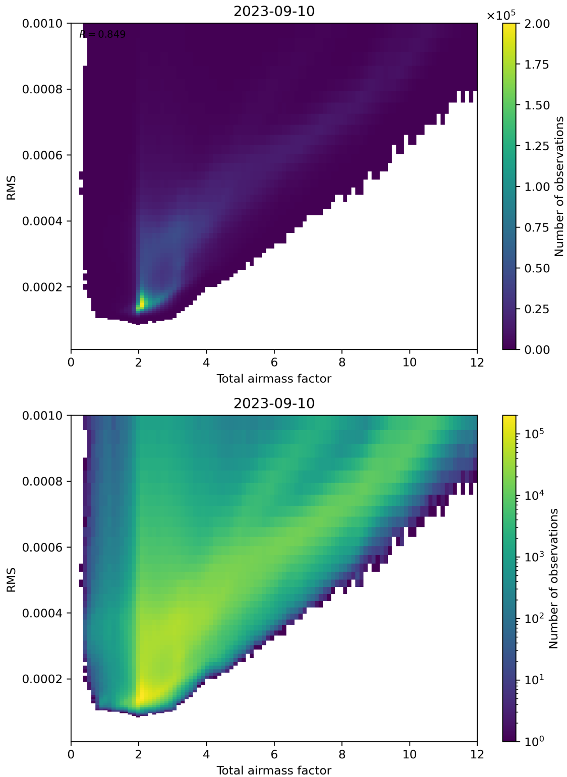
Figure 69: Scatter density plot of “Total airmass factor” against “RMS” for 2023-09-10 to 2023-09-11.
