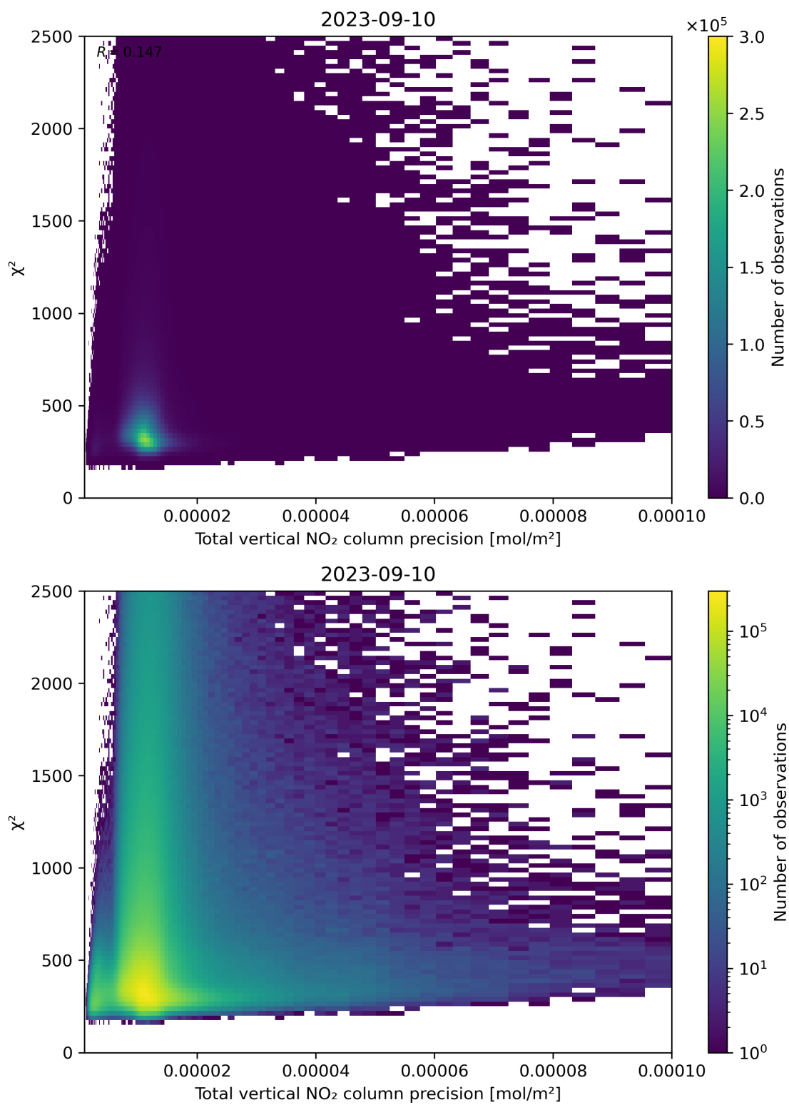
Figure 116: Scatter density plot of “Total vertical NO 2 column precision” against “ \chi^2 ” for 2023-09-10 to 2023-09-11.
