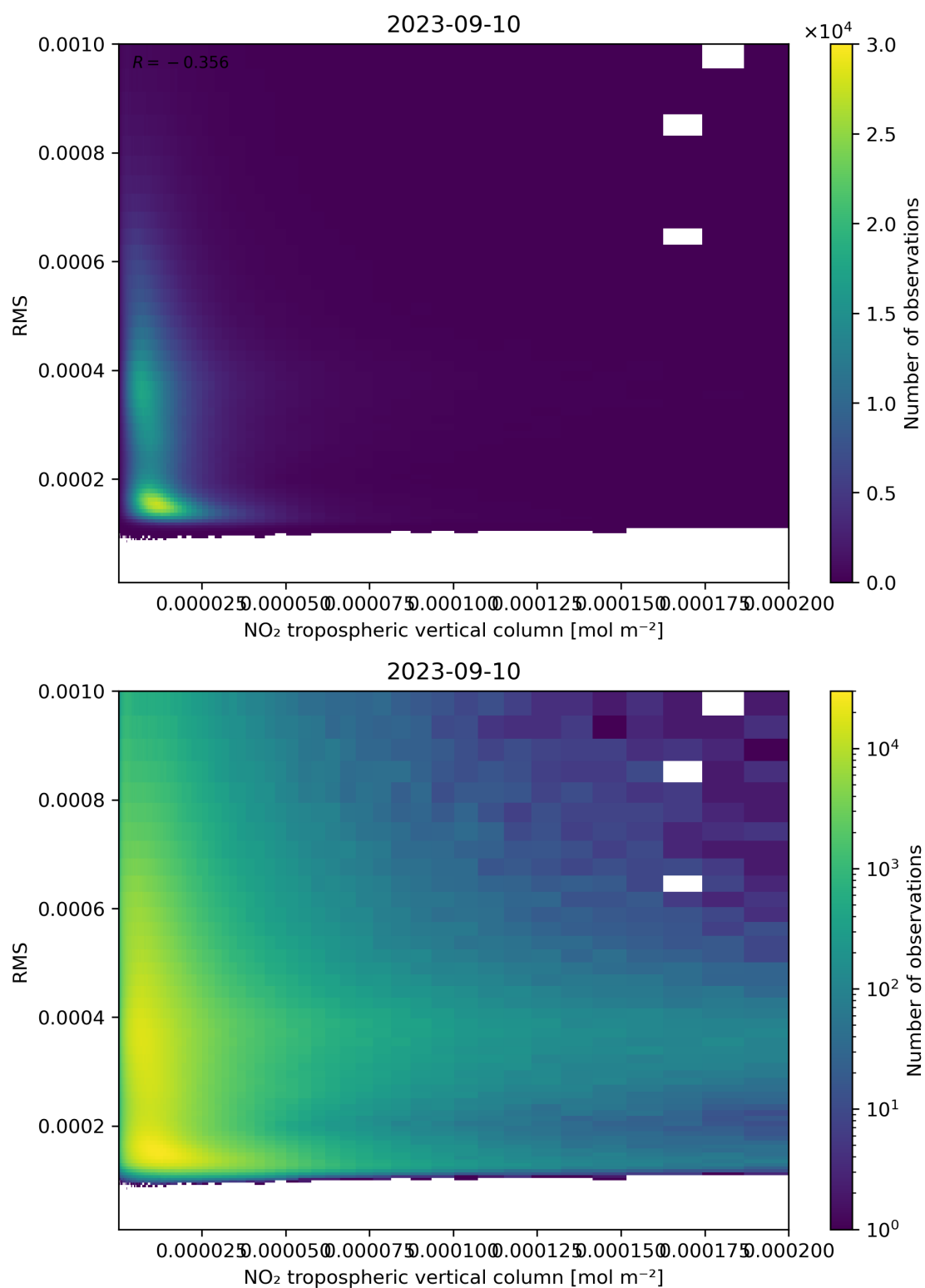
Figure 142: Scatter density plot of “NO 2 tropospheric vertical column” against “RMS” for 2023-09-10 to 2023-09-11.
