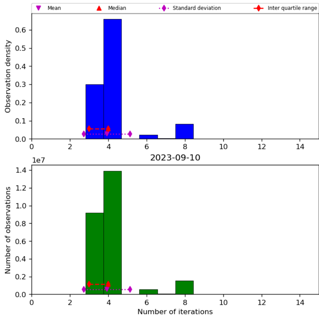
Figure 34: Histogram of “Number of iterations” for 2023-09-10 to 2023-09-11
