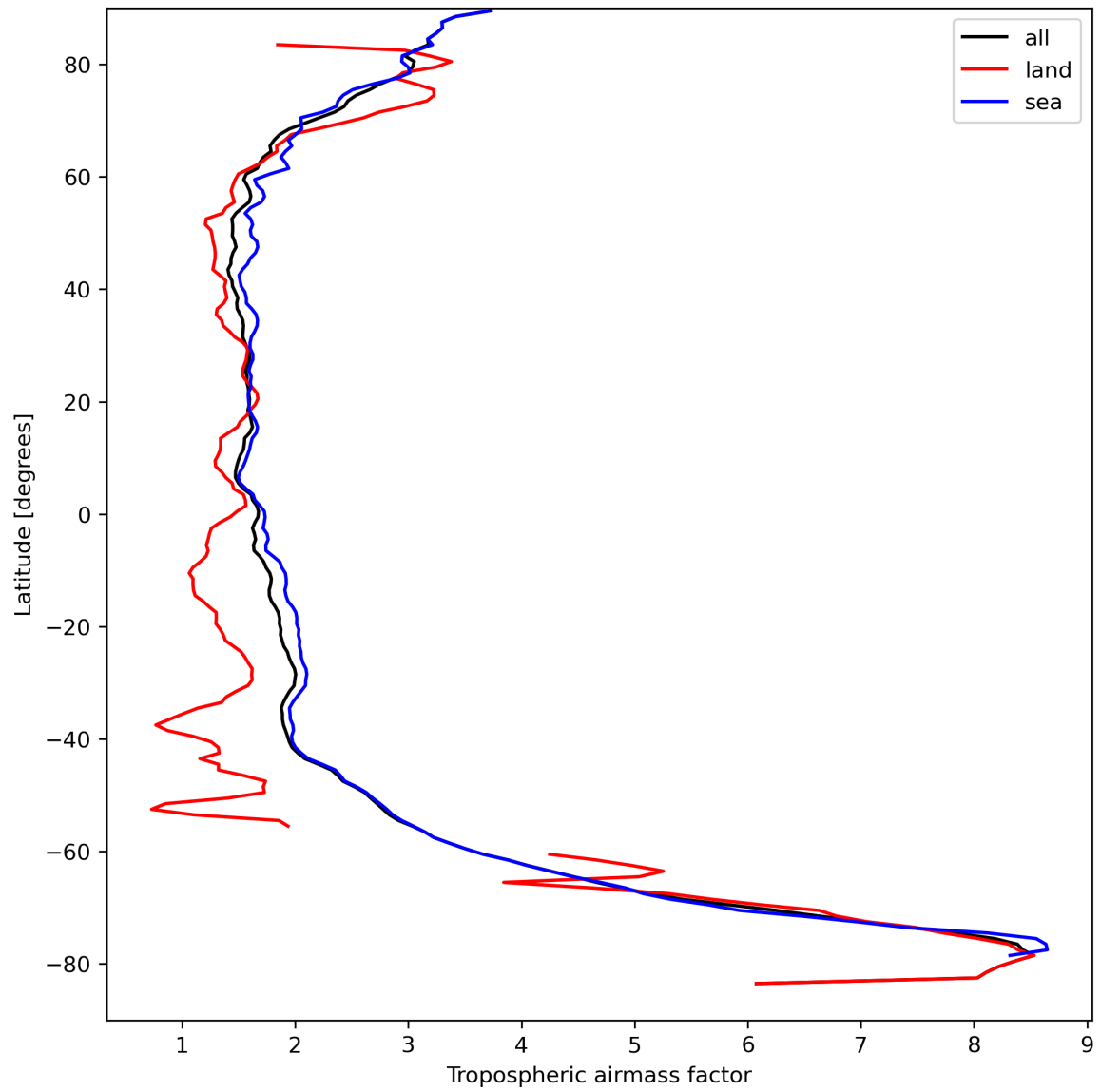
Figure 14: Zonal average of “Tropospheric air mass factor” for 2023-09-10 to 2023-09-11.
