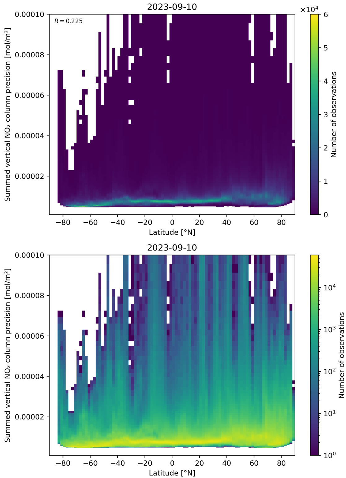
Figure 89: Scatter density plot of “Latitude” against “Summed vertical NO 2 column precision” for 2023-09-10 to 2023-09-11.
