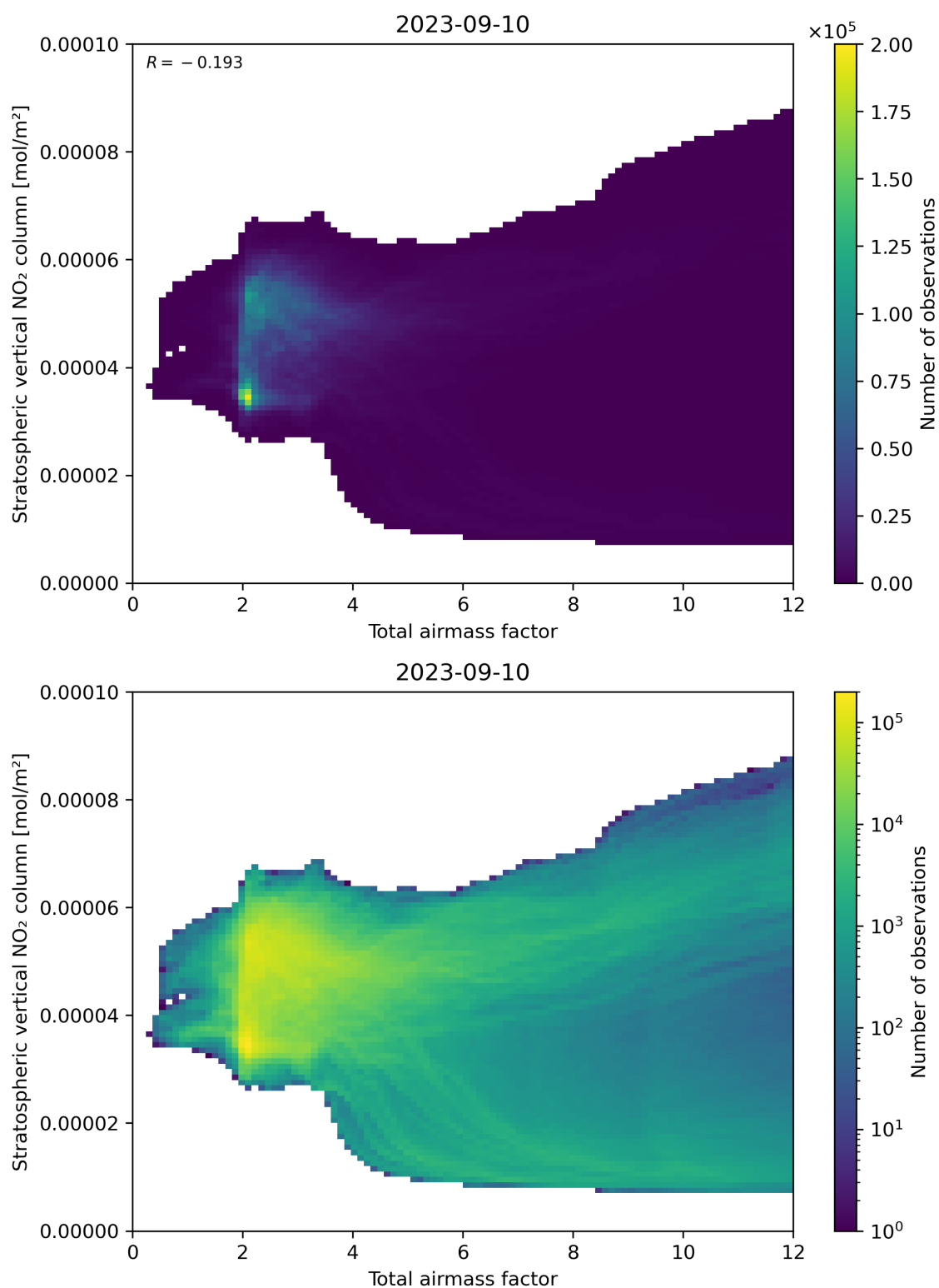
Figure 64: Scatter density plot of “Total airmass factor” against “Stratospheric vertical NO 2 column” for 2023-09-10 to 2023-09-11.
