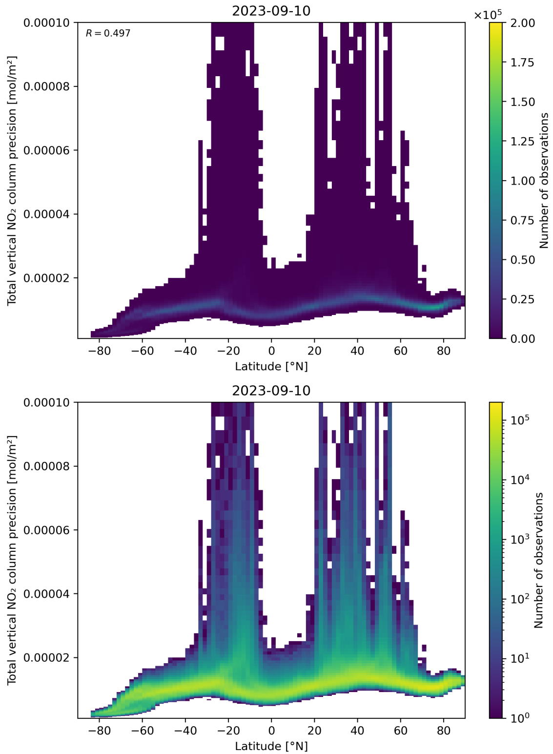
Figure 91: Scatter density plot of “Latitude” against “Total vertical NO 2 column precision” for 2023-09-10 to 2023-09-11.
