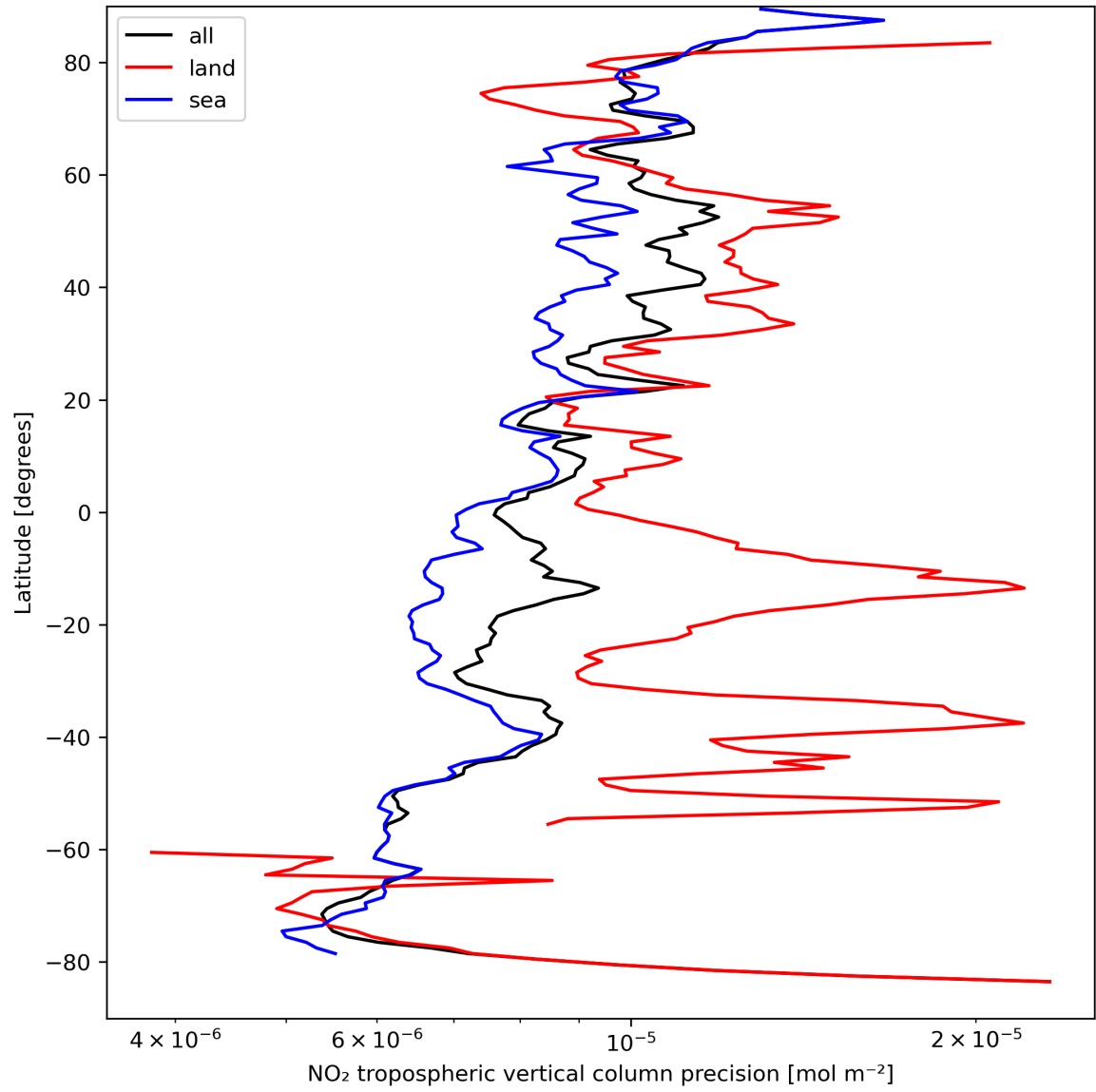
Figure 13: Zonal average of “NO 2 tropospheric vertical column precision” for 2023-09-10 to 2023-09-11.
