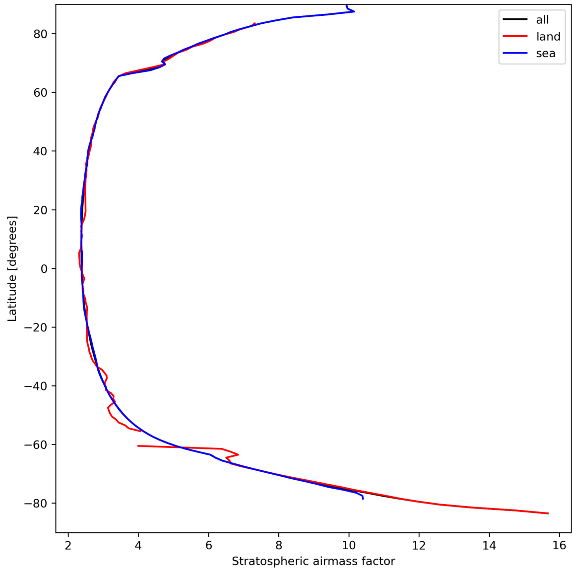
Figure 27: Zonal average of “Stratospheric airmass factor” for 2023-09-10 to 2023-09-11.
