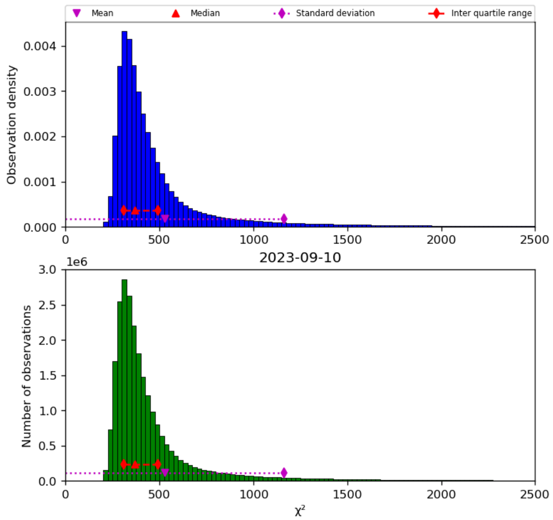
Figure 42: Histogram of “ \chi^2 ” for 2023-09-10 to 2023-09-11
