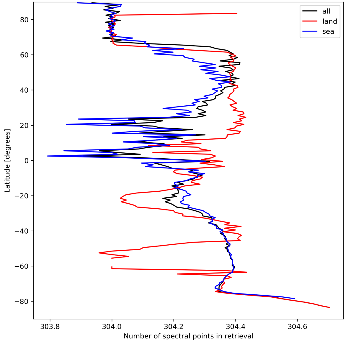
Figure 16: Zonal average of “Number of spectral points in retrieval” for 2023-09-10 to 2023-09-11.
