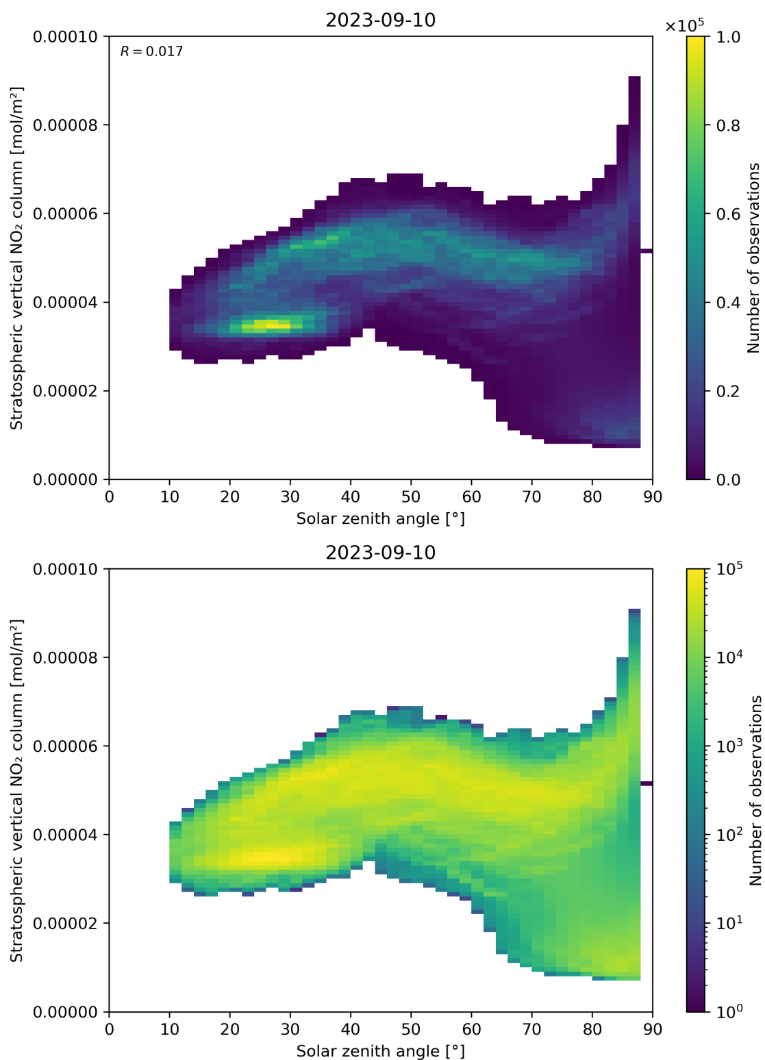
Figure 150: Scatter density plot of “Solar zenith angle” against “Stratospheric vertical NO 2 column” for 2023-09-10 to 2023-09-11.
