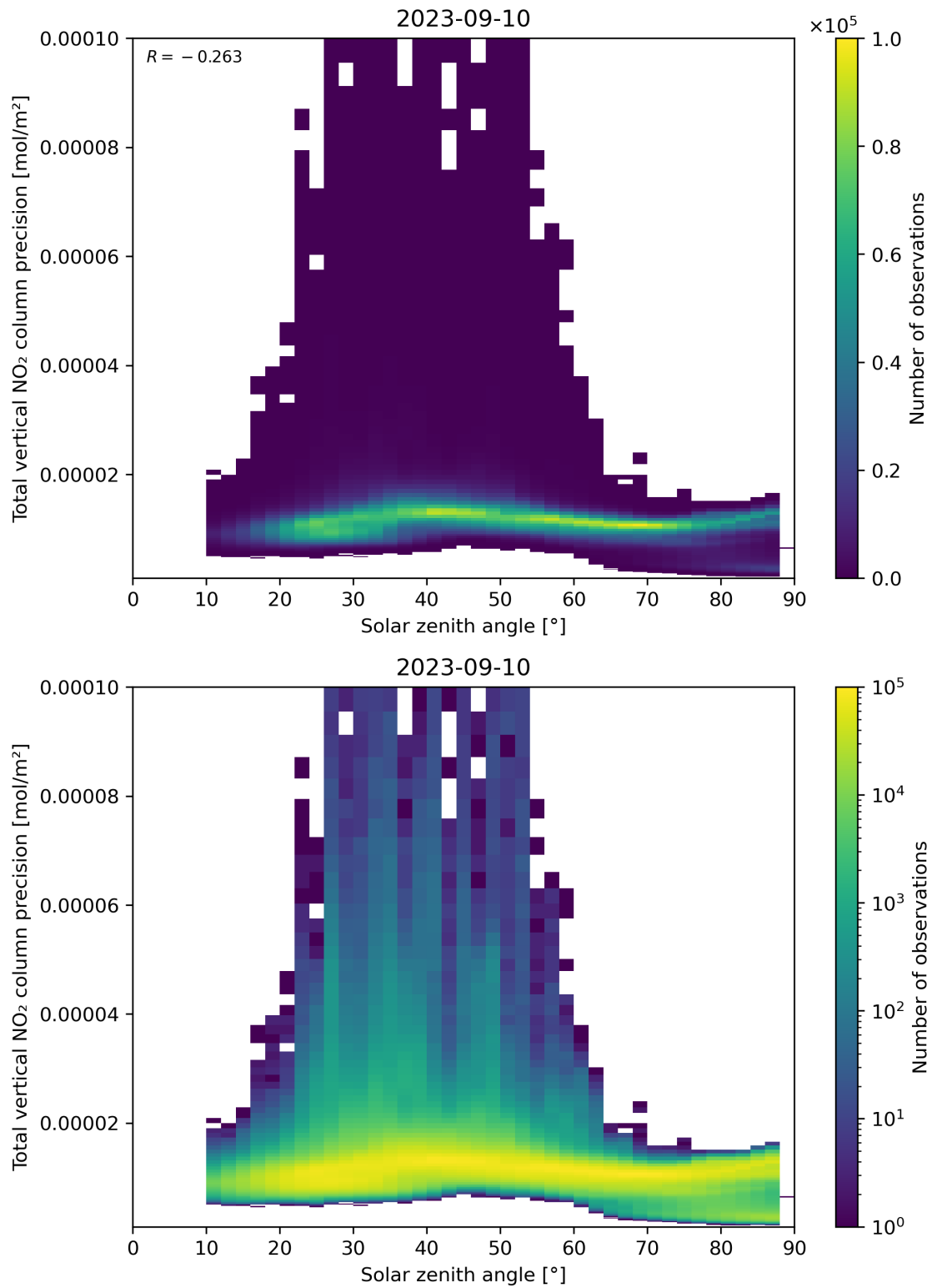
Figure 154: Scatter density plot of “Solar zenith angle” against “Total vertical NO 2 column precision” for 2023-09-10 to 2023-09-11.
