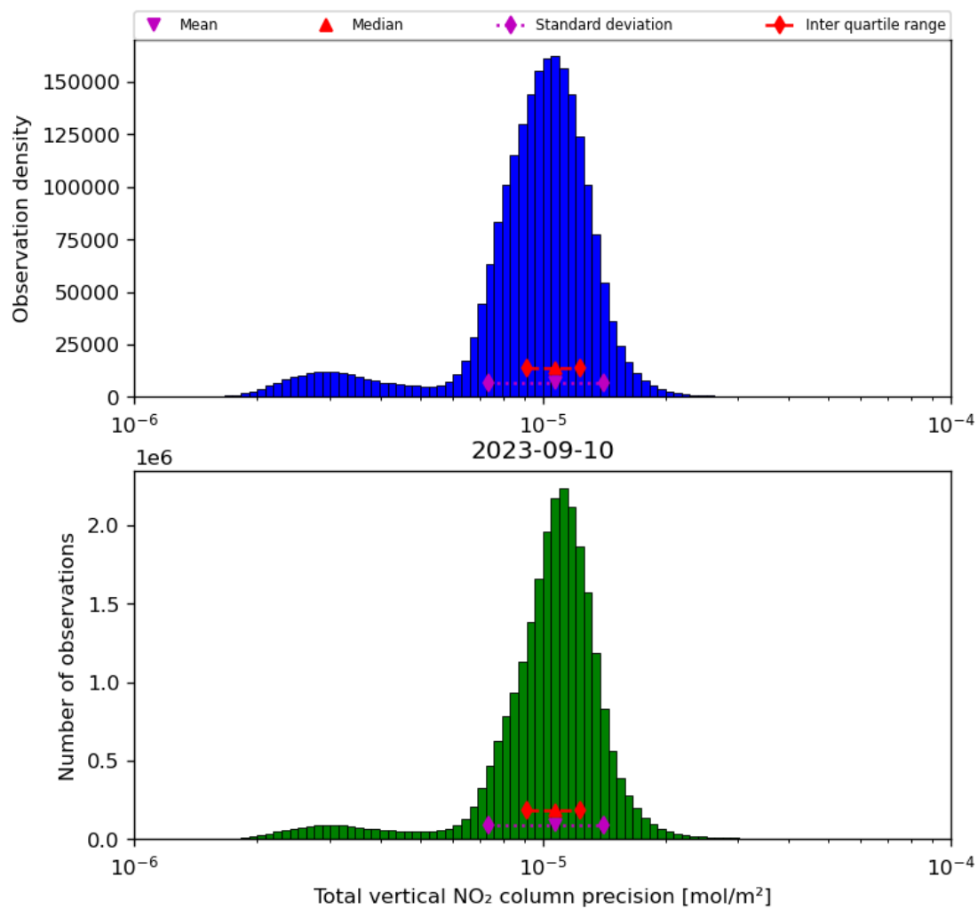
Figure 39: Histogram of “Total vertical NO 2 column precision” for 2023-09-10 to 2023-09-11
