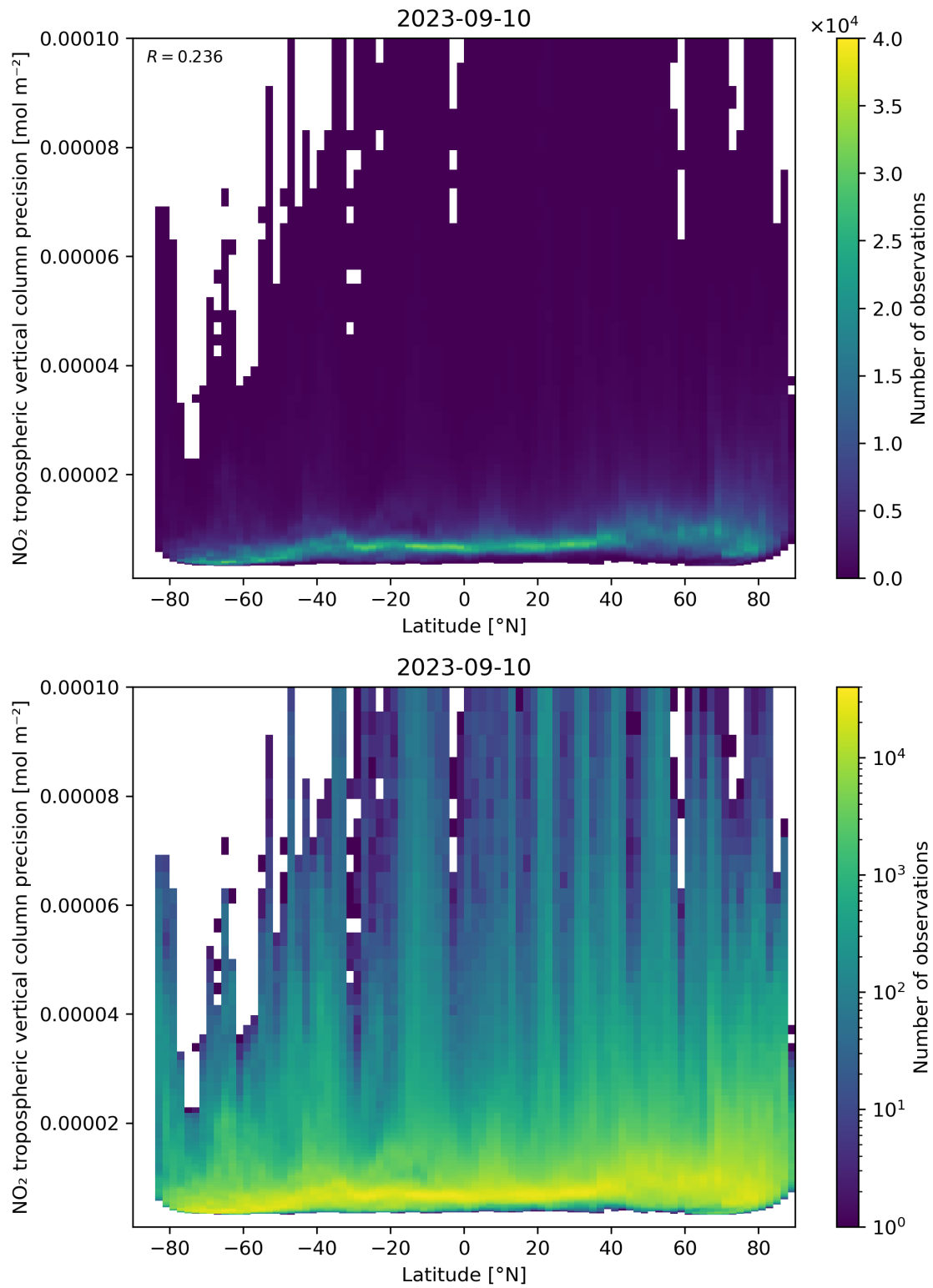
Figure 93: Scatter density plot of “Latitude” against “NO 2 tropospheric vertical column precision” for 2023-09-10 to 2023-09-11.
