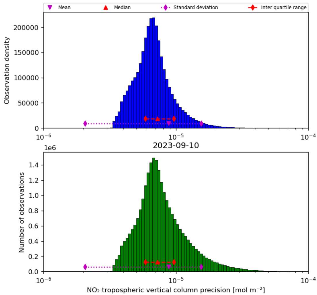
Figure 30: Histogram of “NO 2 tropospheric vertical column precision” for 2023-09-10 to 2023-09-11
