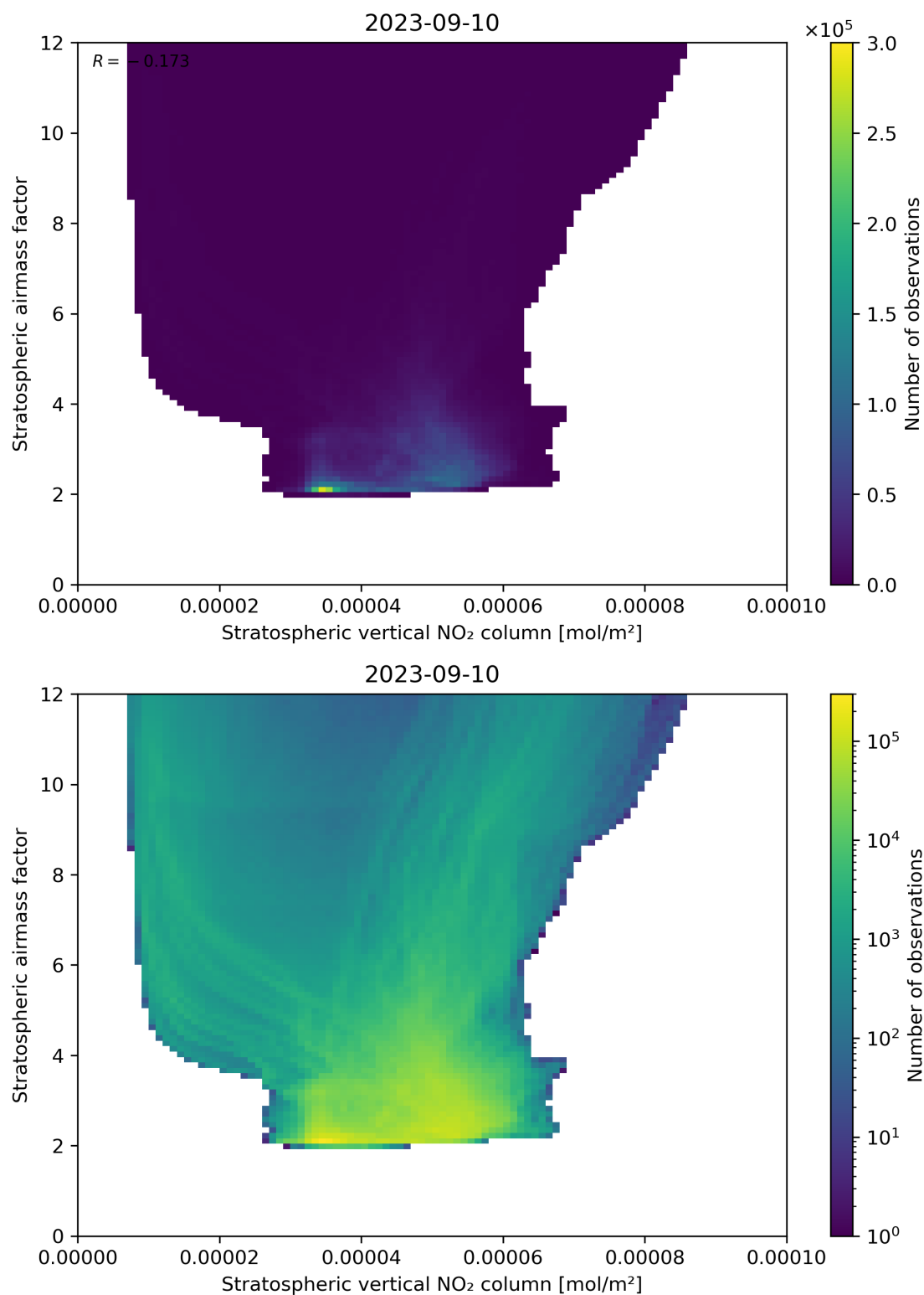
Figure 96: Scatter density plot of “Stratospheric vertical NO 2 column” against “Stratospheric airmass factor” for 2023-09-10 to 2023-09-11.
