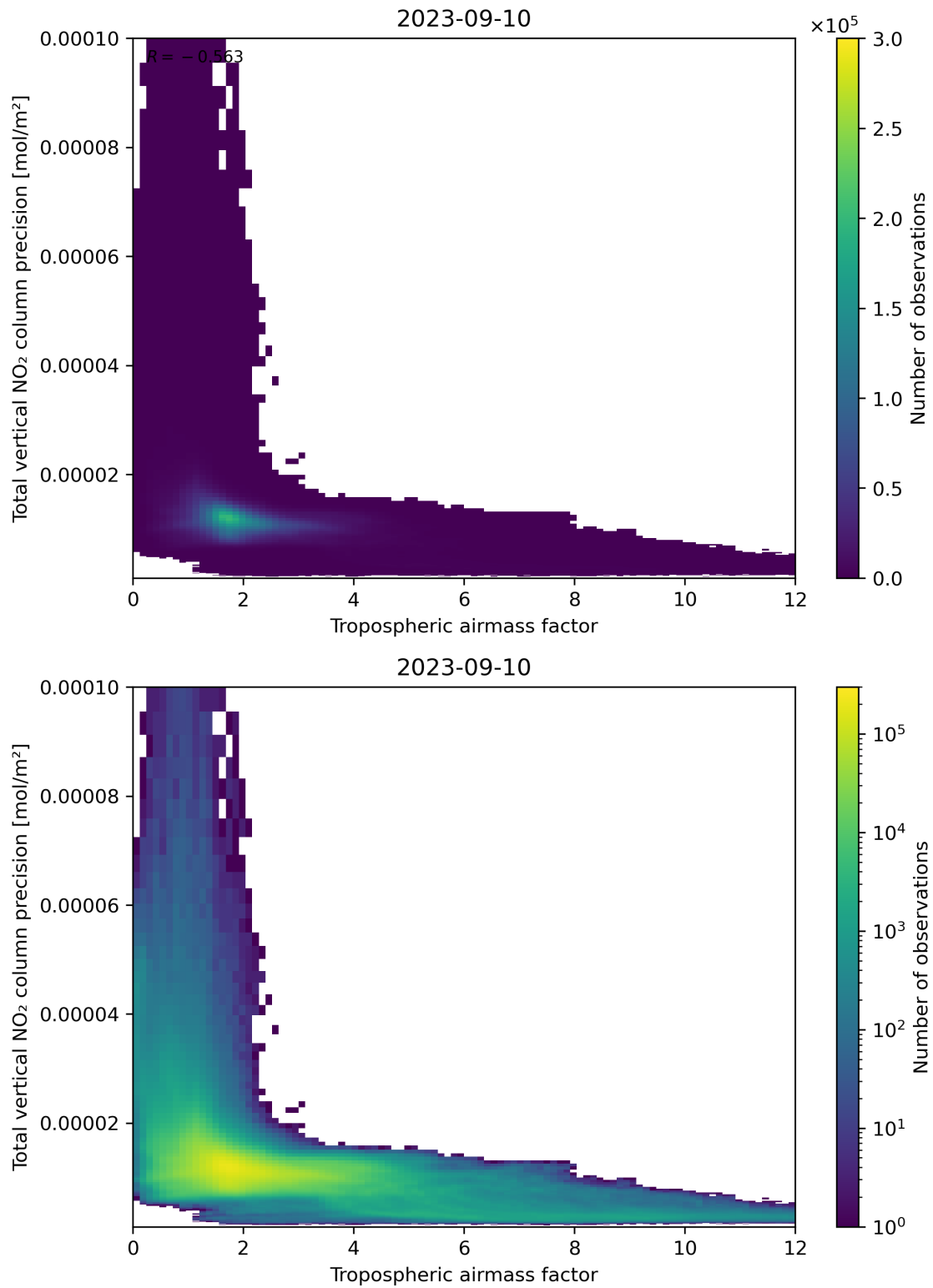
Figure 78: Scatter density plot of “Tropospheric air mass factor” against “Total vertical NO 2 column precision” for 2023-09-10 to 2023-09-11.
