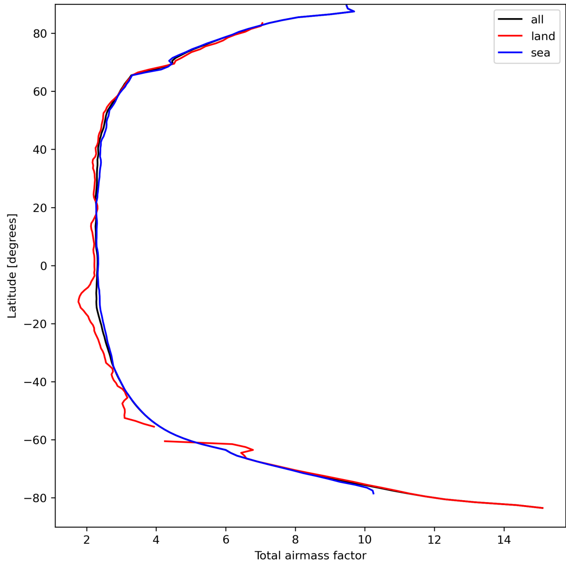
Figure 15: Zonal average of “Total airmass factor” for 2023-09-10 to 2023-09-11.
