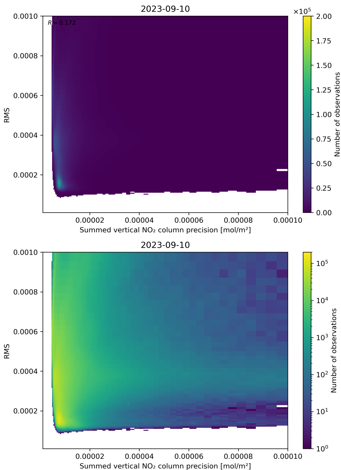
Figure 108: Scatter density plot of “Summed vertical NO 2 column precision” against “RMS” for 2023-09-10 to 2023-09-11.
