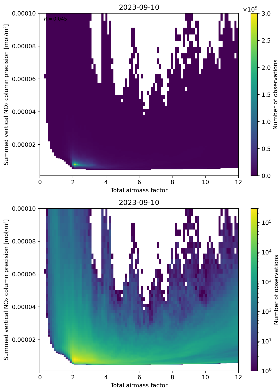
Figure 66: Scatter density plot of “Total airmass factor” against “Summed vertical NO 2 column precision” for 2023-09-10 to 2023-09-11.
