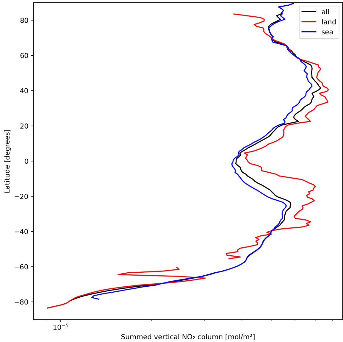
Figure 23: Zonal average of “Summed vertical NO 2 column” for 2023-09-10 to 2023-09-11.
