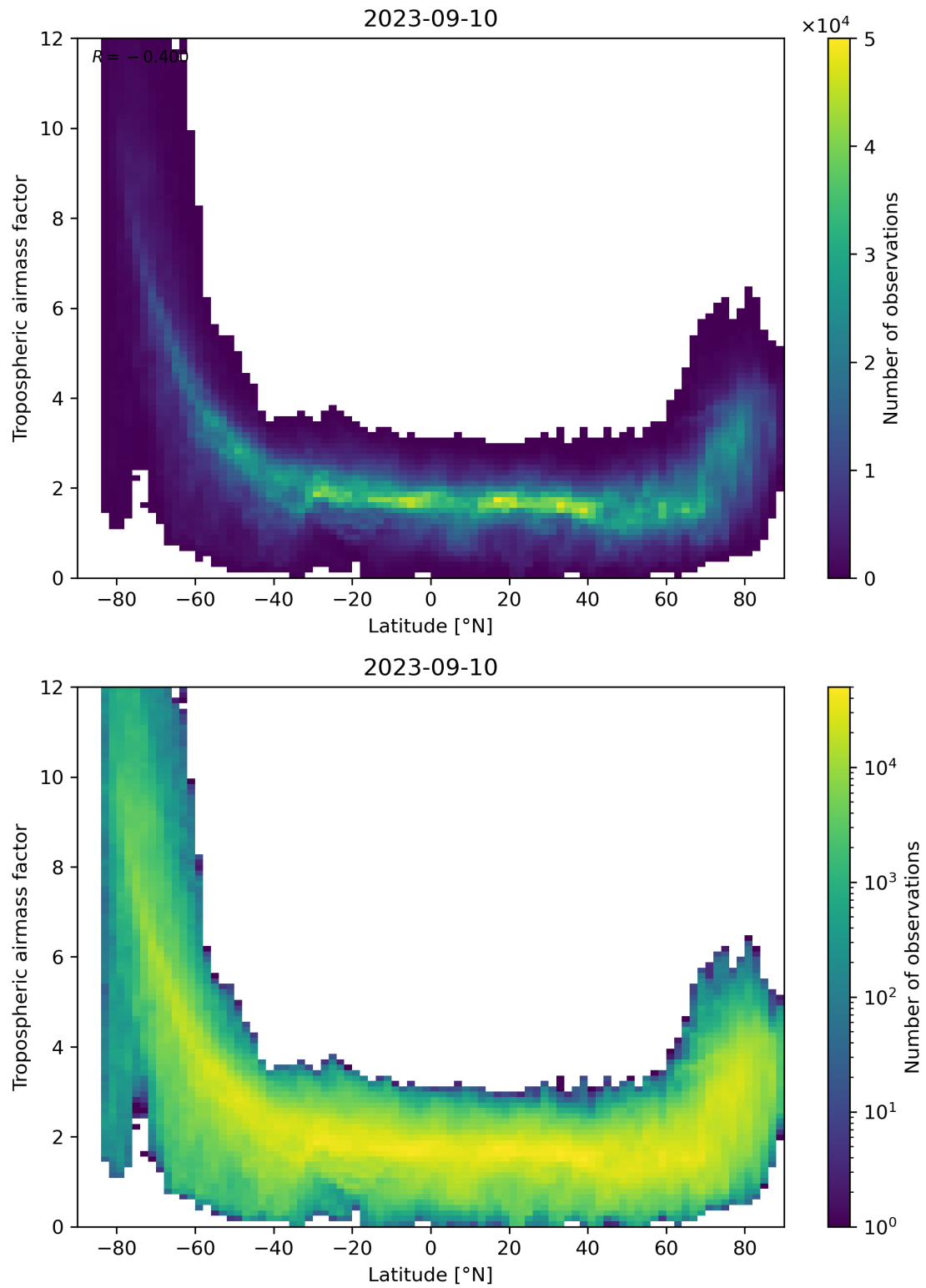
Figure 85: Scatter density plot of “Latitude” against “Tropospheric airmass factor” for 2023-09-10 to 2023-09-11.
