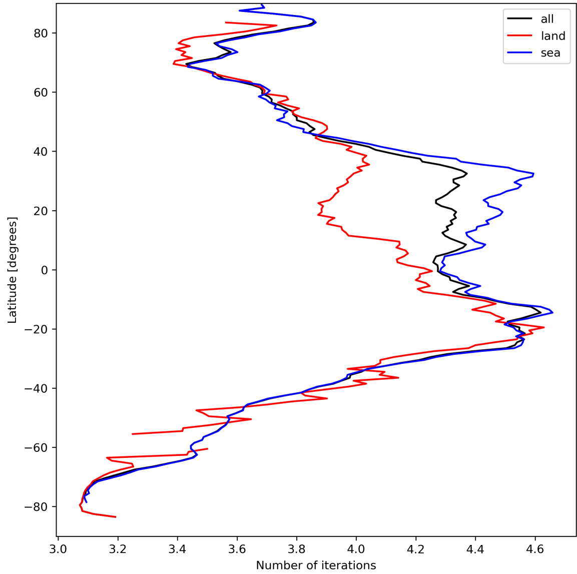
Figure 17: Zonal average of “Number of iterations” for 2023-09-10 to 2023-09-11.
