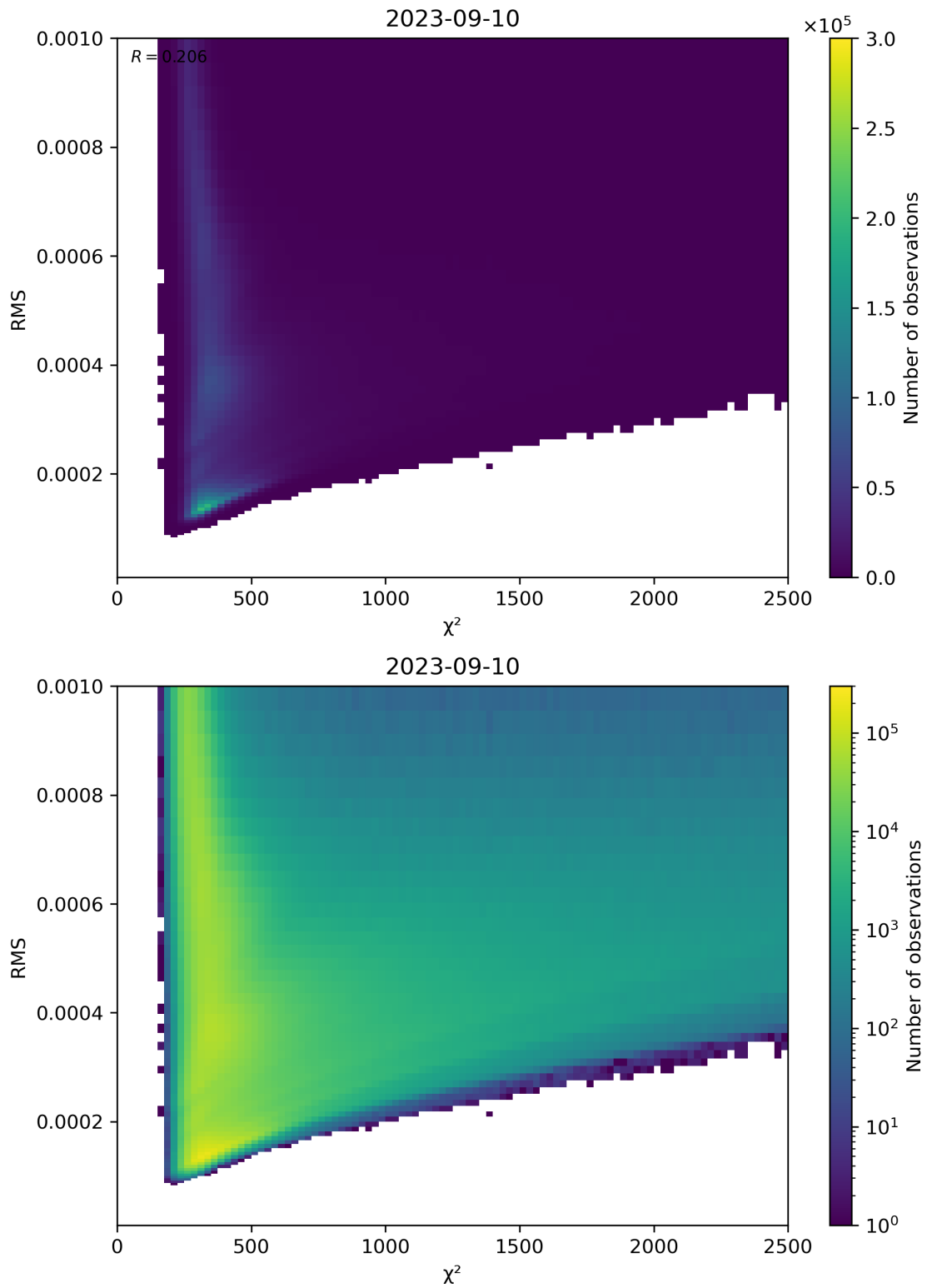
Figure 82: Scatter density plot of " \chi^2 " against "RMS" for 2023-09-10 to 2023-09-11.
