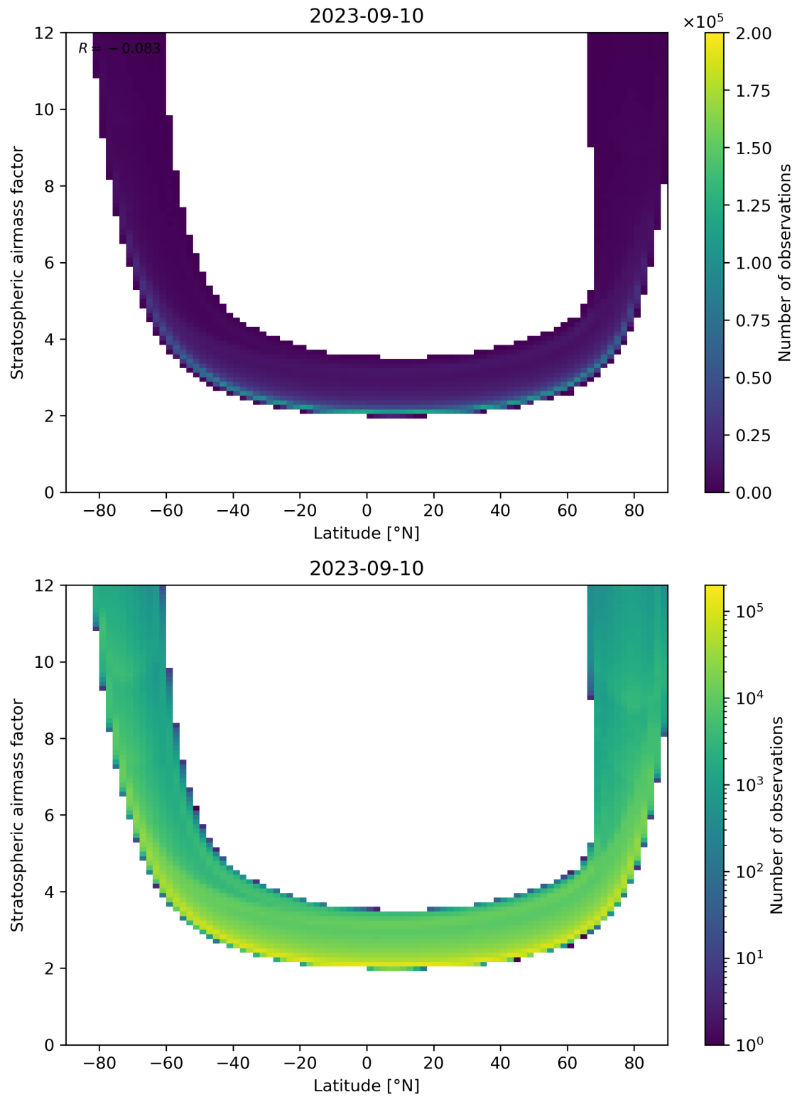
Figure 83: Scatter density plot of “Latitude” against “Stratospheric air mass factor” for 2023-09-10 to 2023-09-11.
