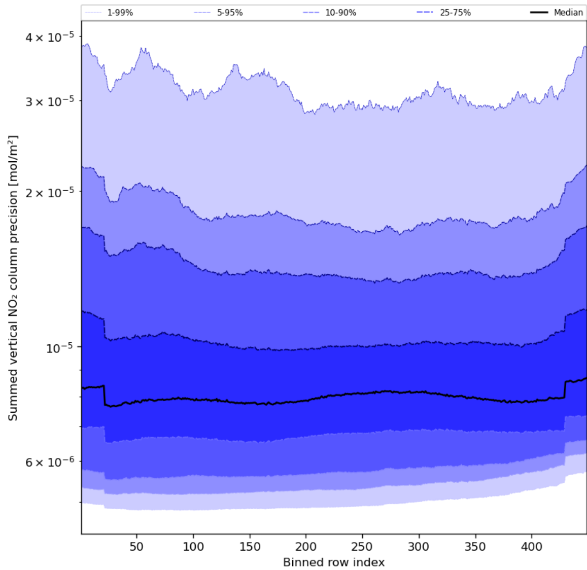
Figure 58: Along track statistics of “Summed vertical NO 2 column precision” for 2023-09-10 to 2023-09-11
