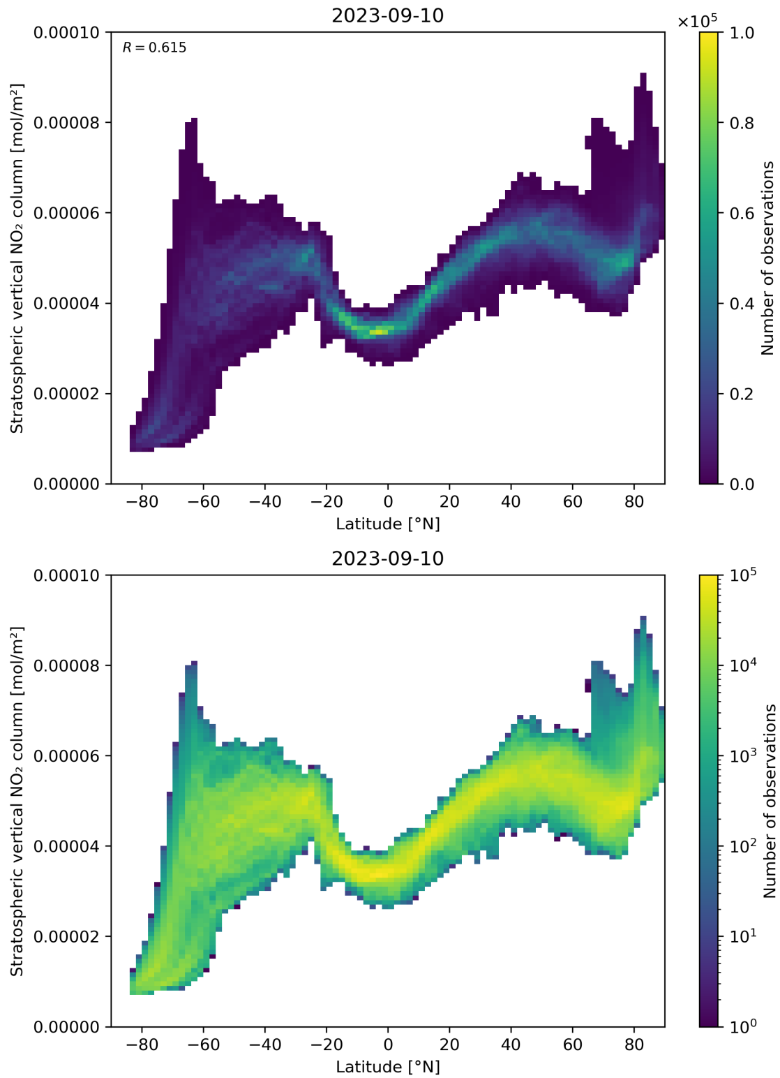
Figure 87: Scatter density plot of “Latitude” against “Stratospheric vertical \text{NO}_2 column” for 2023-09-10 to 2023-09-11.
