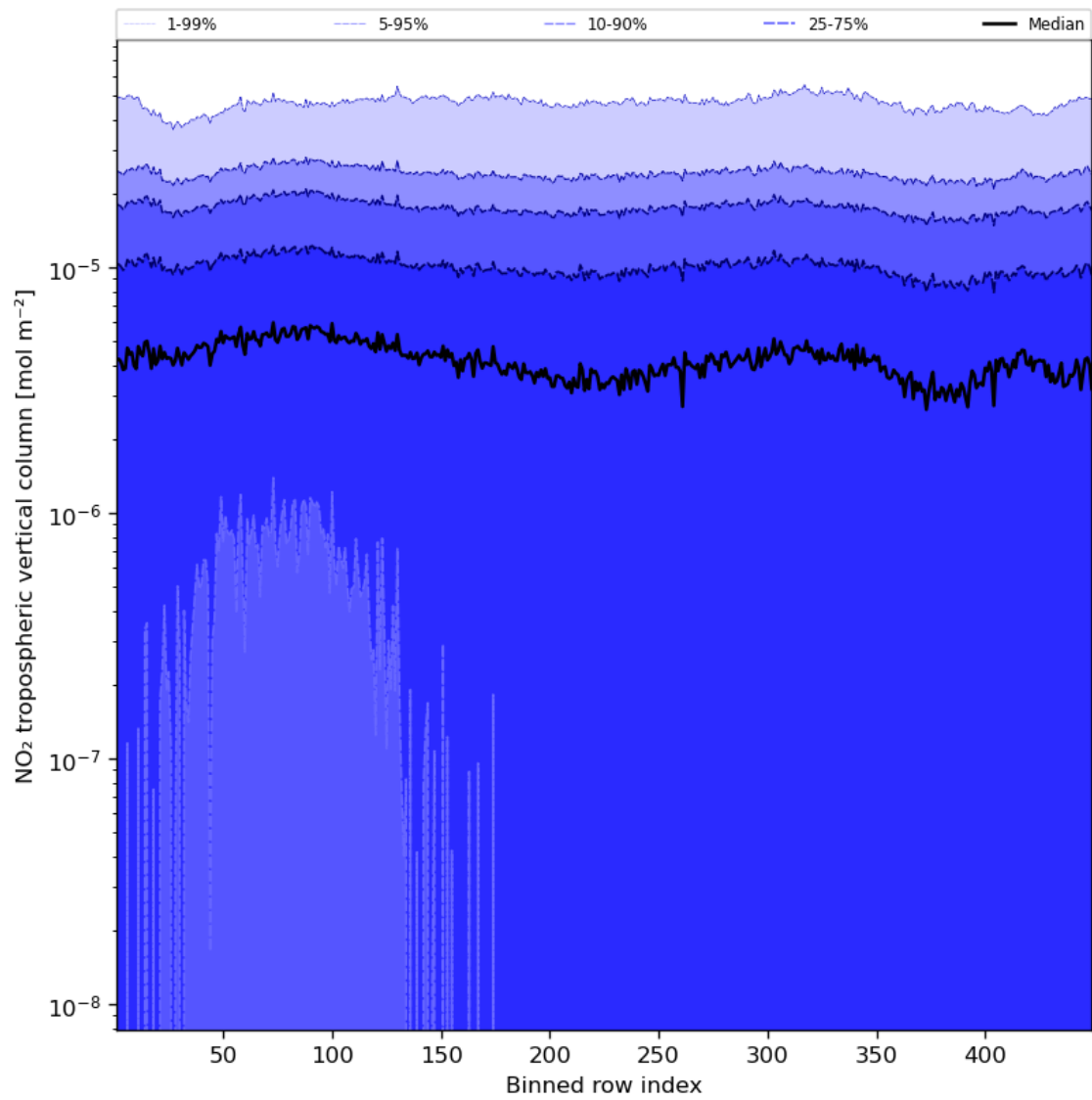
Figure 46: Along track statistics of “NO 2 tropospheric vertical column” for 2023-09-10 to 2023-09-11
