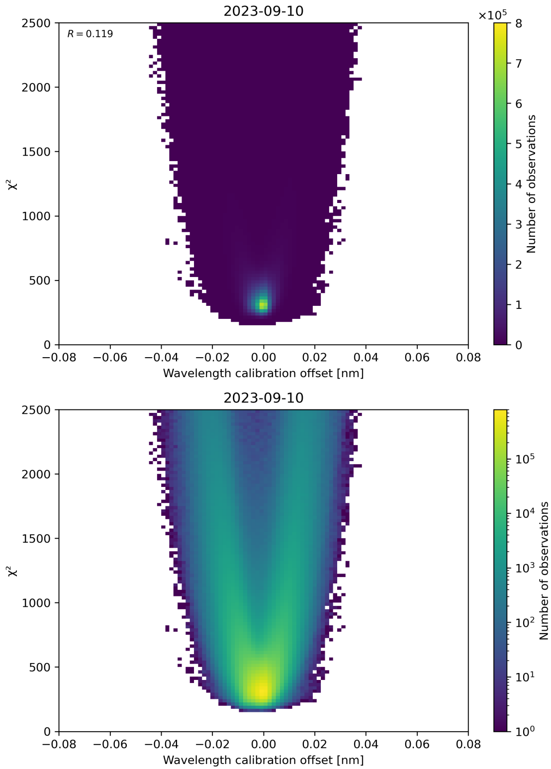
Figure 175: Scatter density plot of “Wavelength calibration offset” against “ \chi^2 ” for 2023-09-10 to 2023-09-11.
