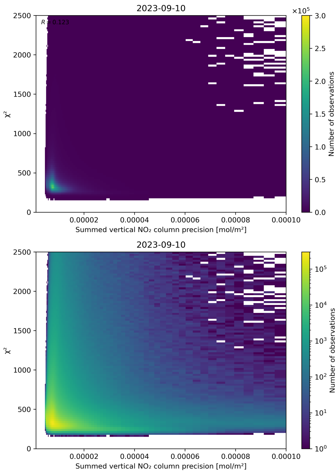
Figure 107: Scatter density plot of “Summed vertical NO 2 column precision” against “ \chi^2 ” for 2023-09-10 to 2023-09-11.
