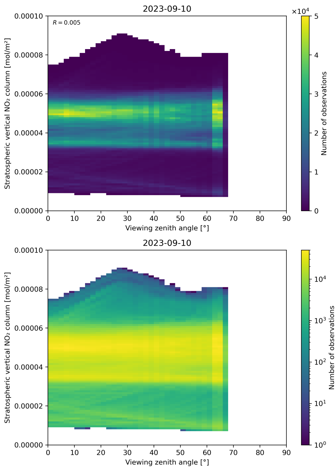
Figure 164: Scatter density plot of “Viewing zenith angle” against “Stratospheric vertical NO 2 column” for 2023-09-10 to 2023-09-11.
