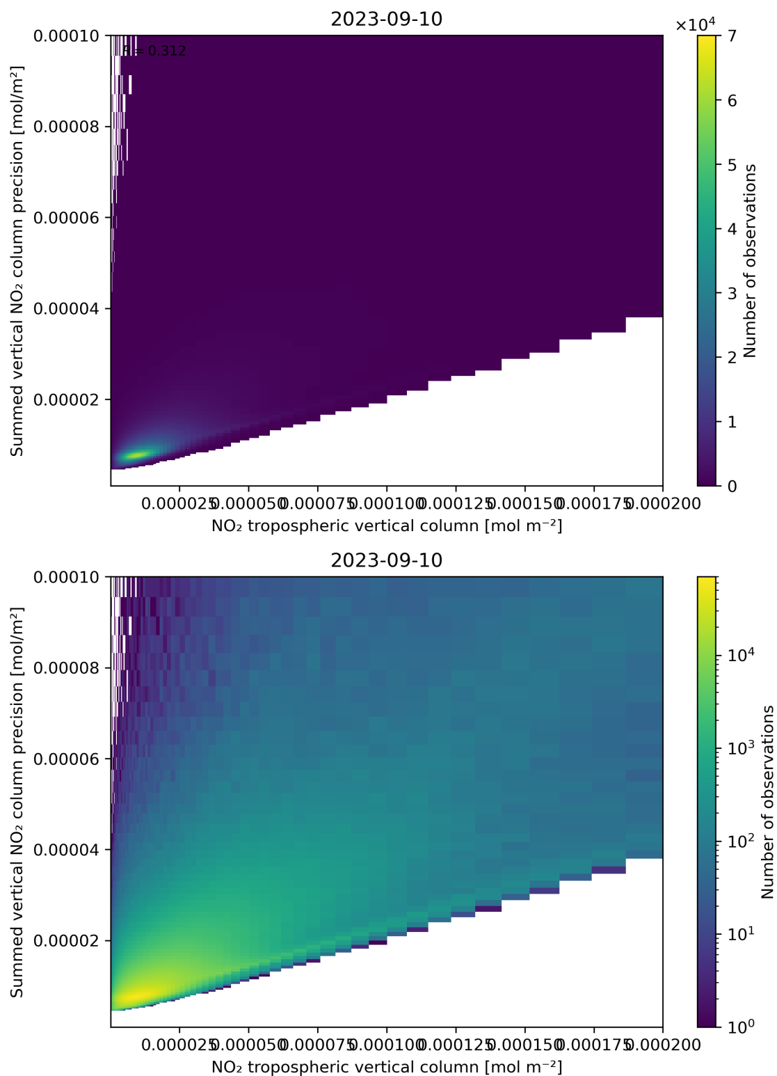
Figure 127: Scatter density plot of “NO 2 tropospheric vertical column” against “Summed vertical NO 2 column precision” for 2023-09-10 to 2023-09-11.
