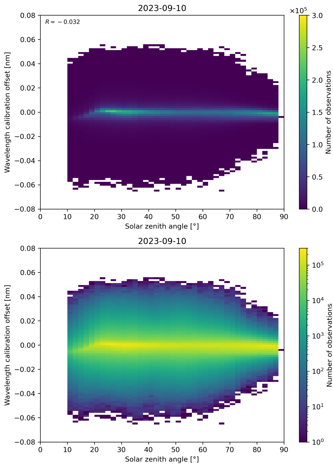
Figure 158: Scatter density plot of “Solar zenith angle” against “Wavelength calibration offset” for 2023-09-10 to 2023-09-11.
