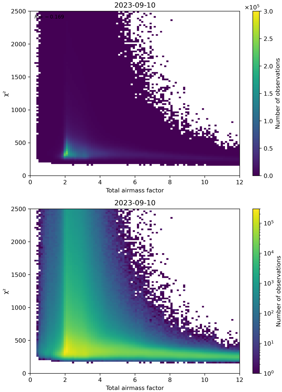
Figure 63: Scatter density plot of “Total airmass factor” against “ \chi^2 ” for 2023-09-10 to 2023-09-11.
