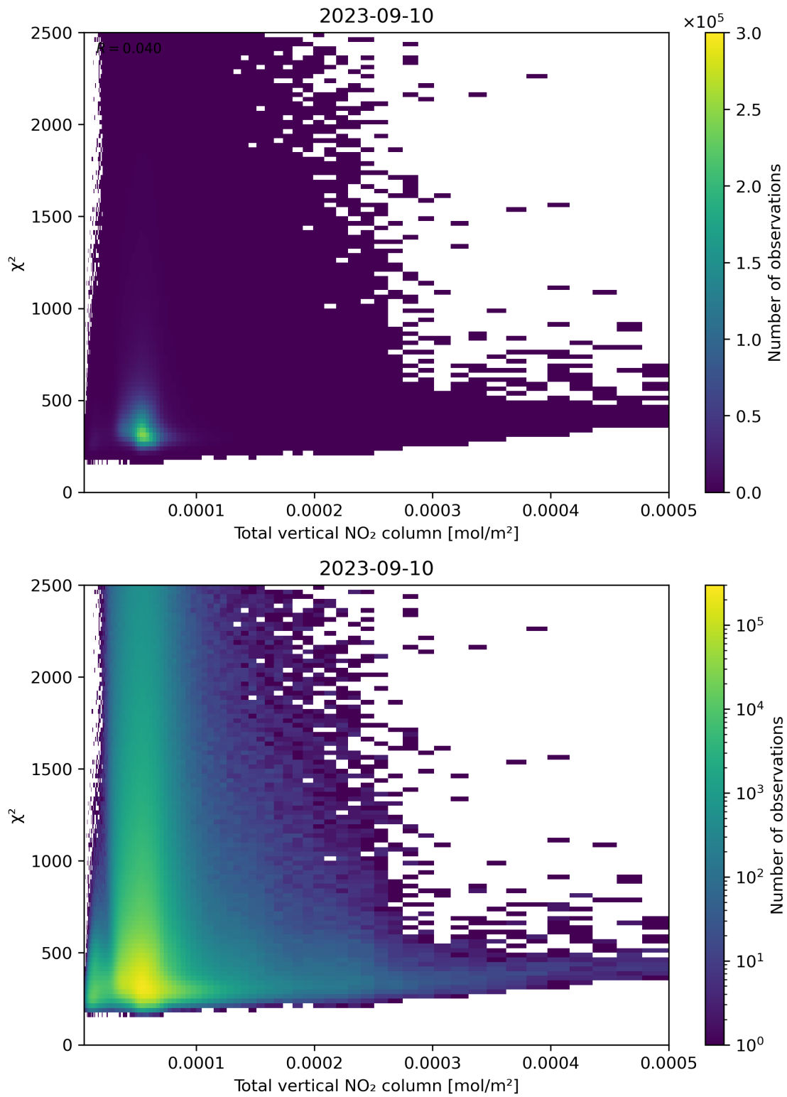
Figure 111: Scatter density plot of “Total vertical NO 2 column” against “ \chi^2 ” for 2023-09-10 to 2023-09-11.
