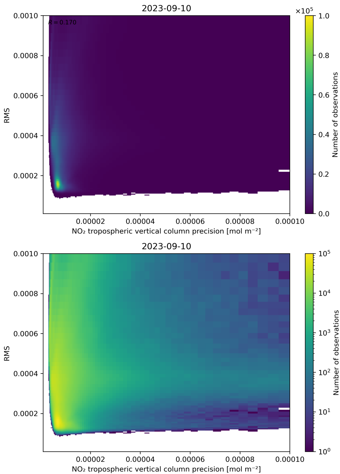
Figure 140: Scatter density plot of “NO 2 tropospheric vertical column precision” against “RMS” for 2023-09-10 to 2023-09-11.
