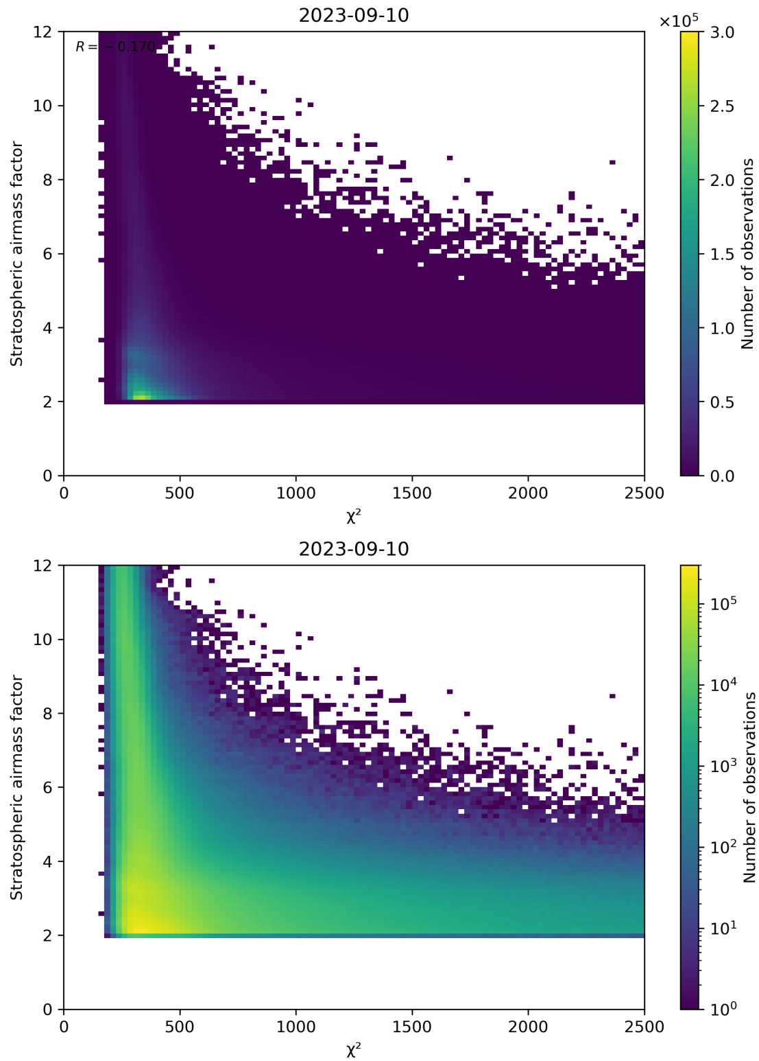
Figure 81: Scatter density plot of “ \chi^2 ” against “Stratospheric airmass factor” for 2023-09-10 to 2023-09-11.
