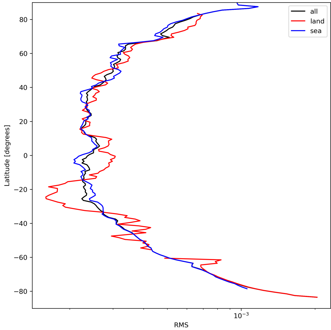
Figure 26: Zonal average of “RMS” for 2023-09-10 to 2023-09-11.
