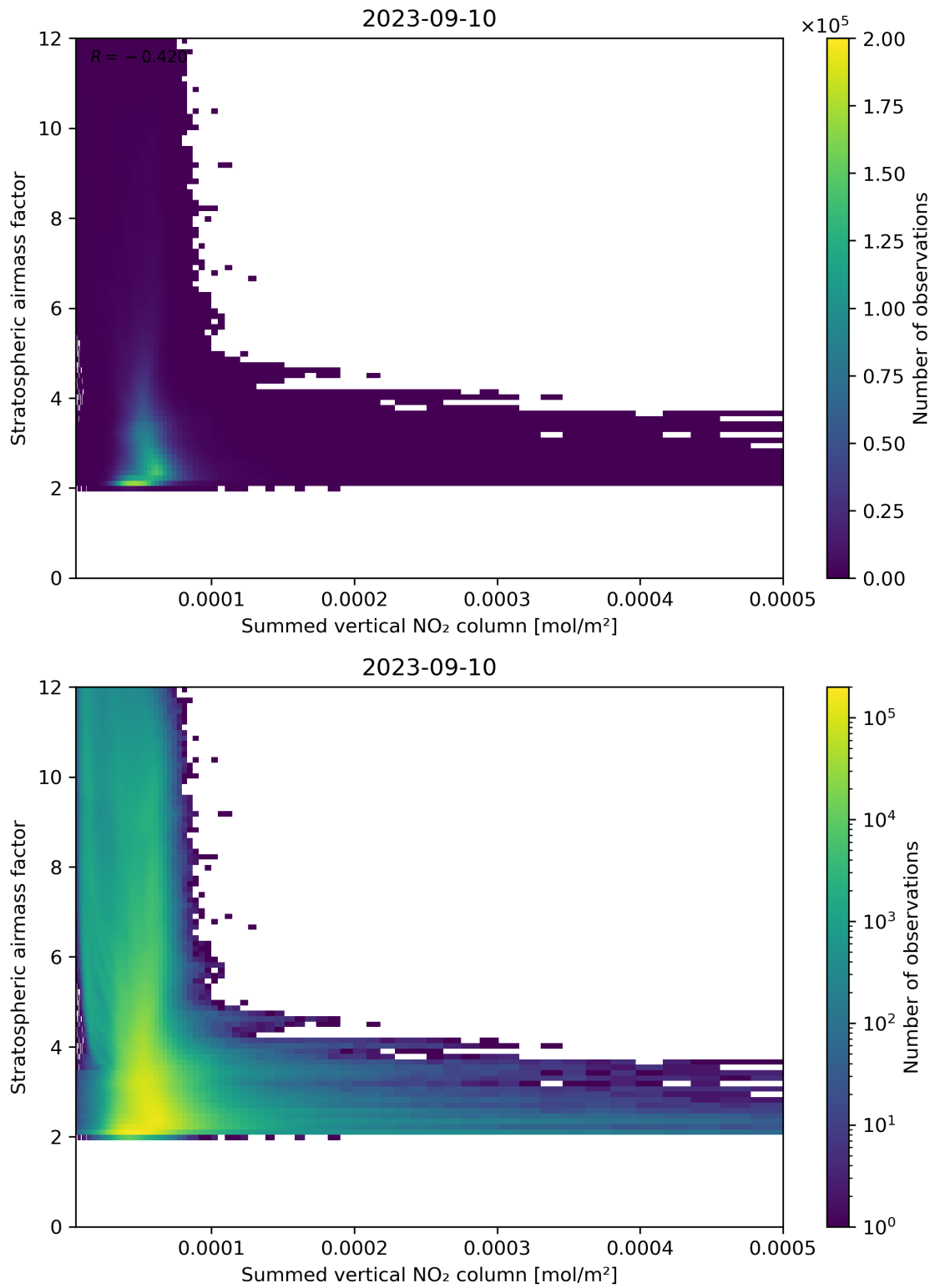
Figure 103: Scatter density plot of “Summed vertical NO 2 column” against “Stratospheric airmass factor” for 2023-09-10 to 2023-09-11.
