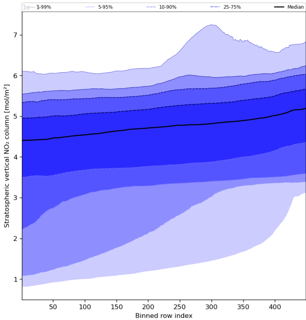
Figure 53: Along track statistics of “Stratospheric vertical NO 2 column” for 2023-09-10 to 2023-09-11
