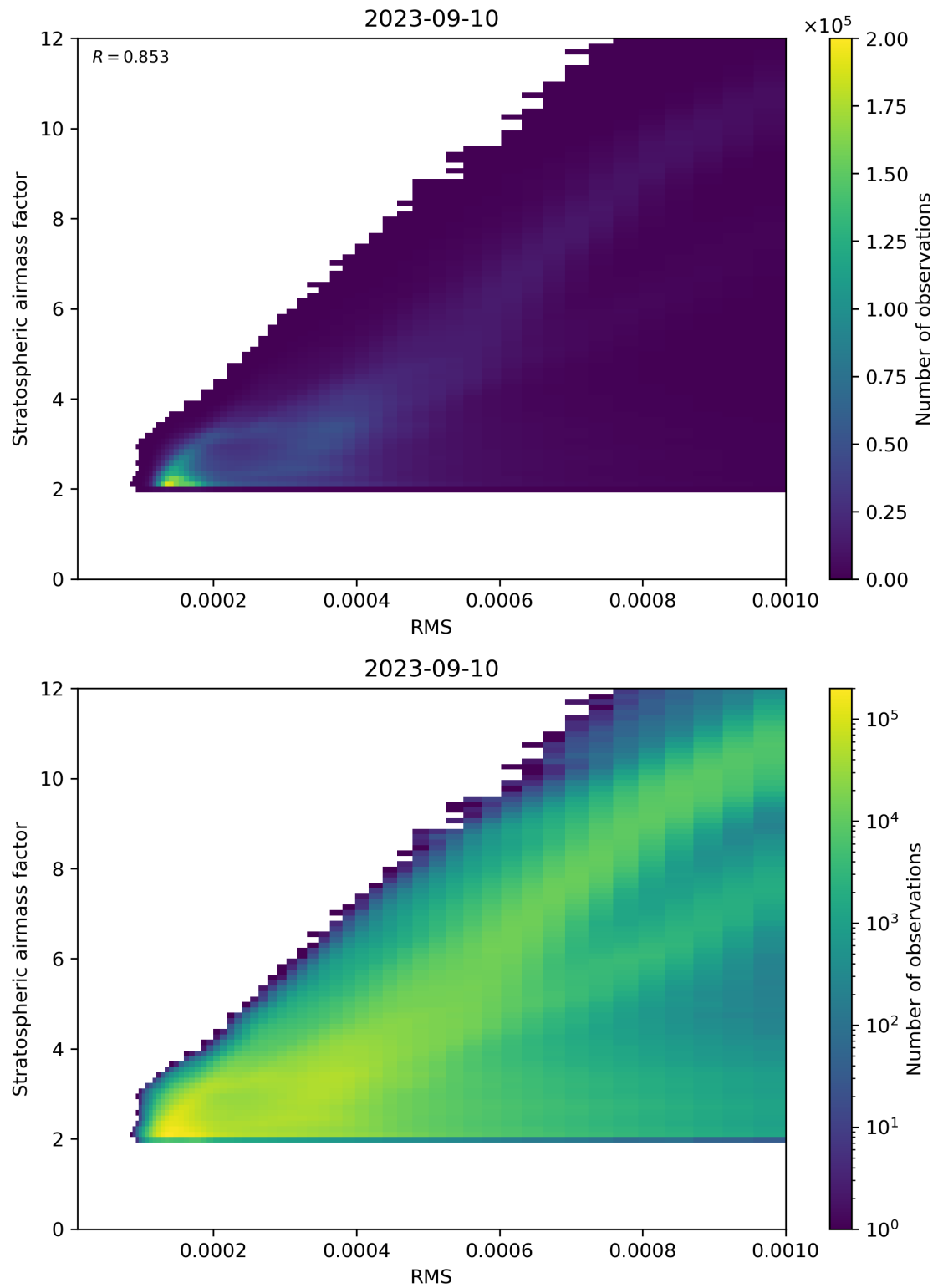
Figure 144: Scatter density plot of “RMS” against “Stratospheric airmass factor” for 2023-09-10 to 2023-09-11.
