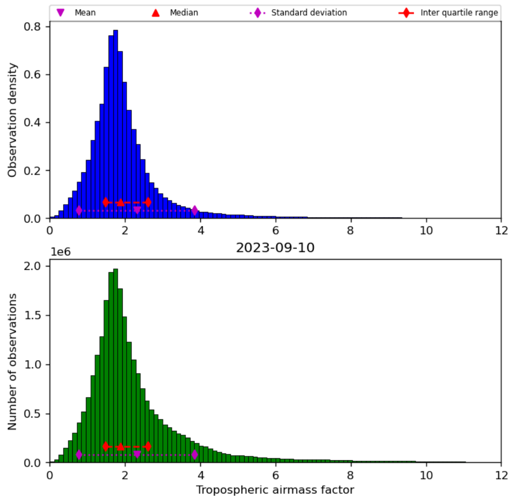
Figure 31: Histogram of “Tropospheric airmass factor” for 2023-09-10 to 2023-09-11
