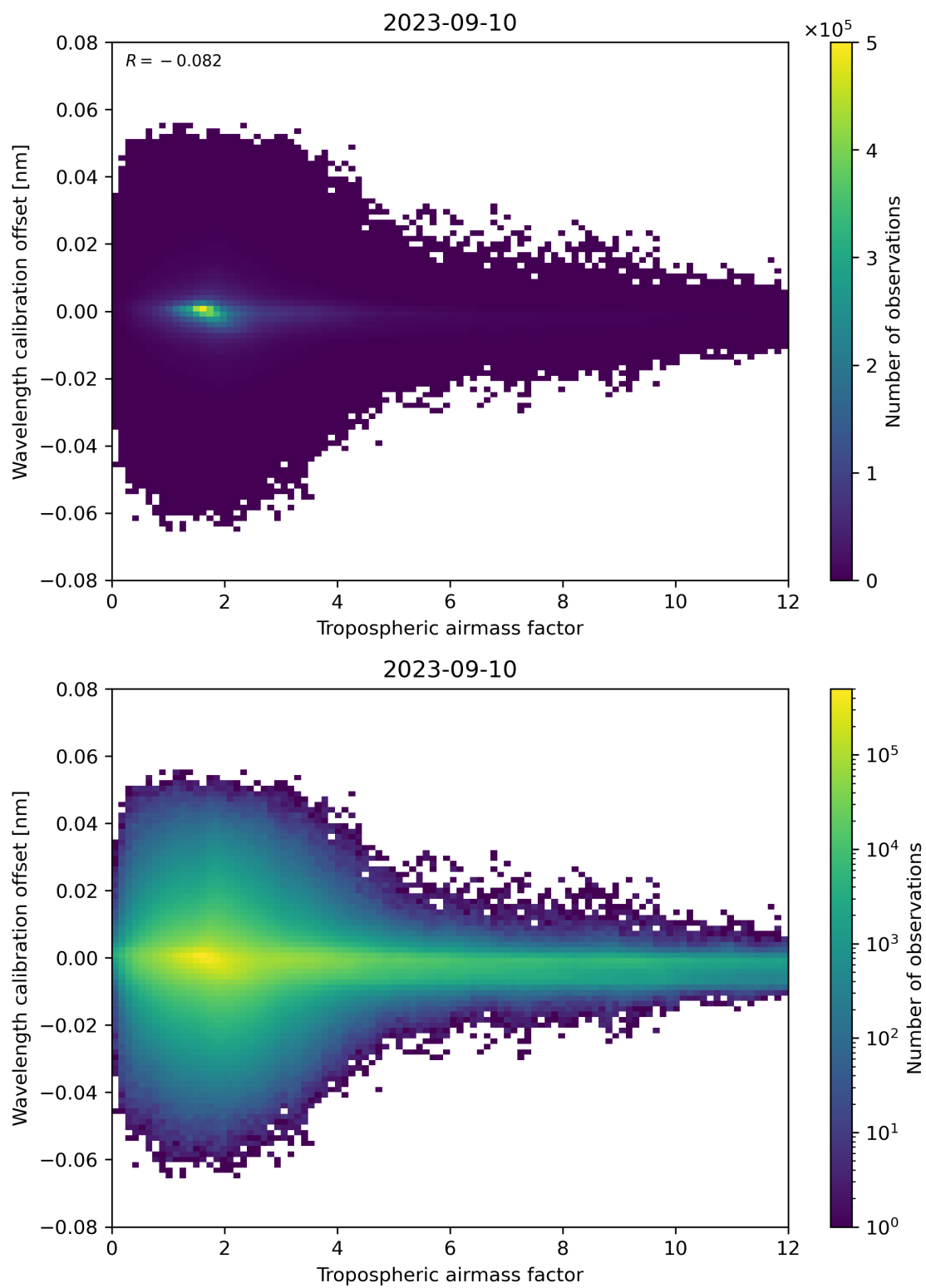
Figure 80: Scatter density plot of “Tropospheric airmass factor” against “Wavelength calibration offset” for 2023-09-10 to 2023-09-11.
