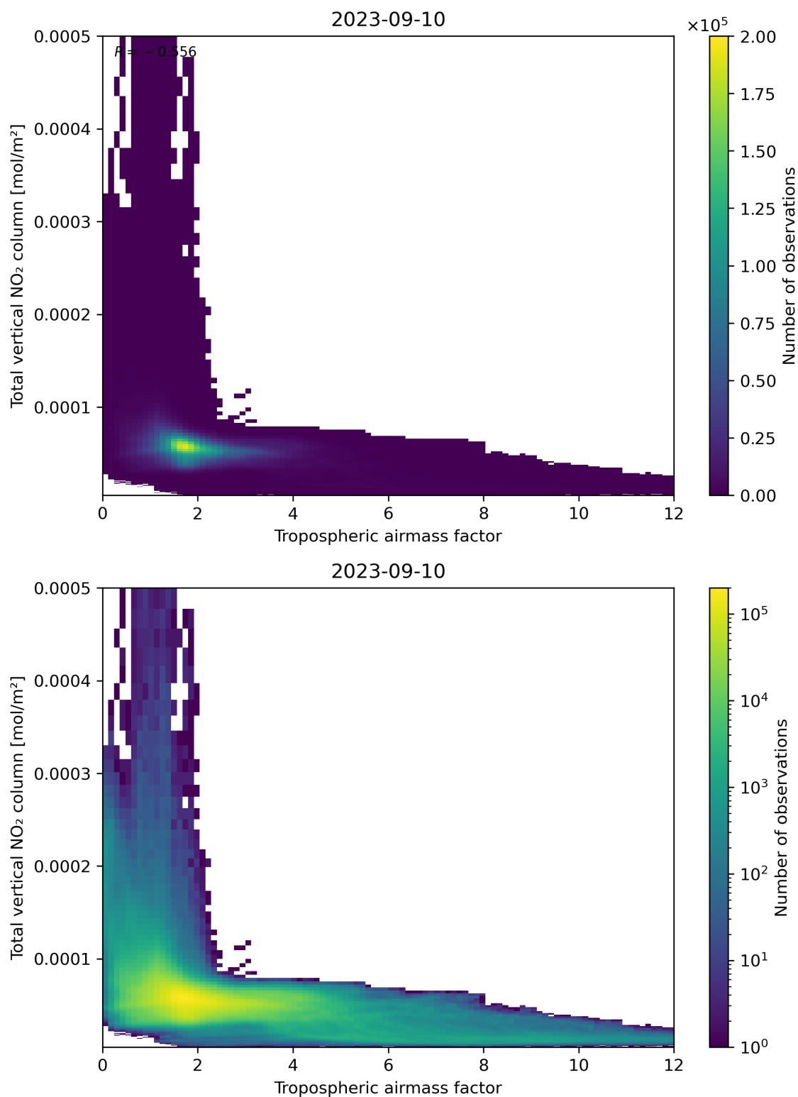
Figure 77: Scatter density plot of “Tropospheric airmass factor” against “Total vertical NO 2 column” for 2023-09-10 to 2023-09-11.
