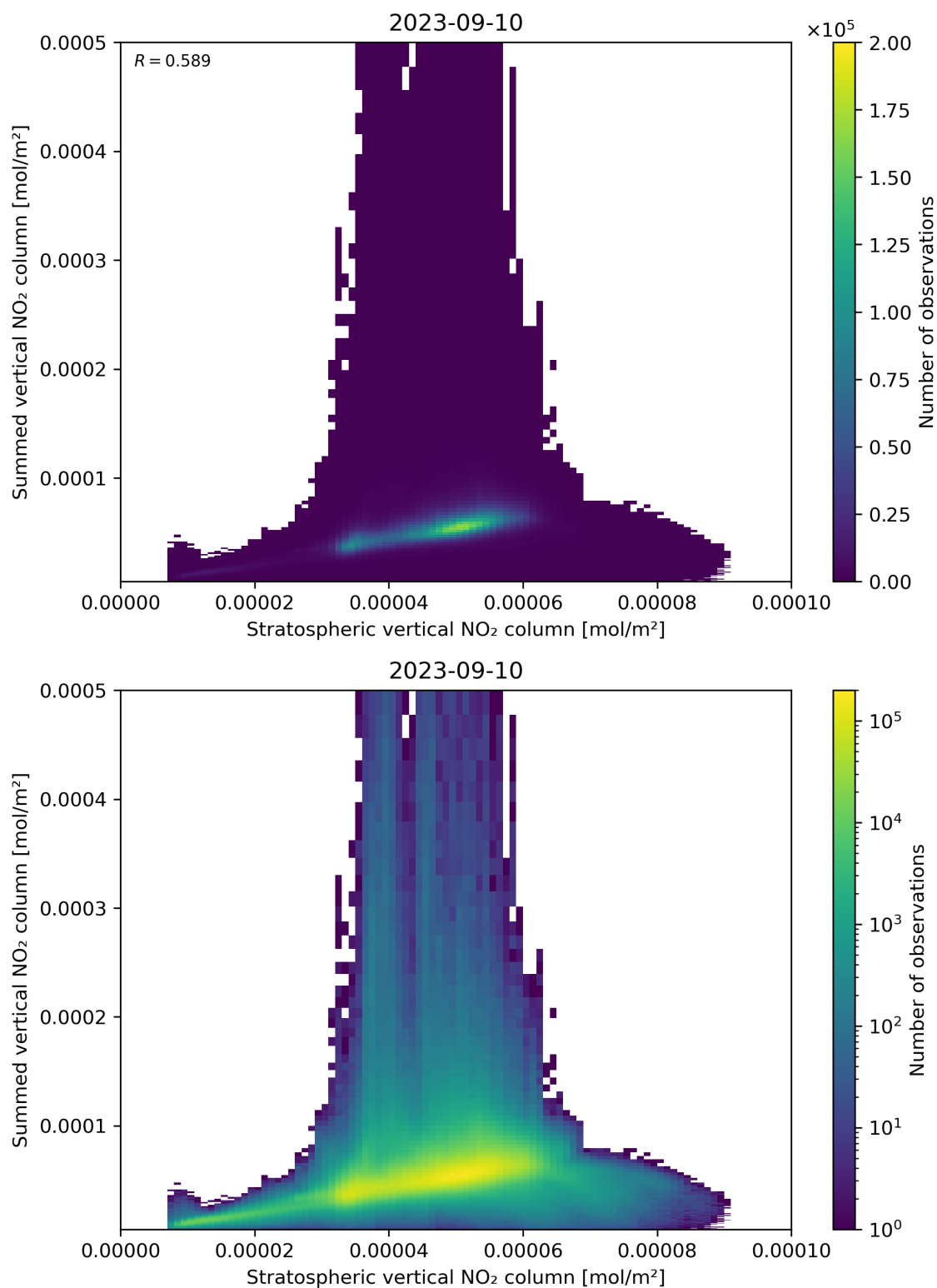
Figure 98: Scatter density plot of “Stratospheric vertical NO 2 column” against “Summed vertical NO 2 column” for 2023-09-10 to 2023-09-11.
