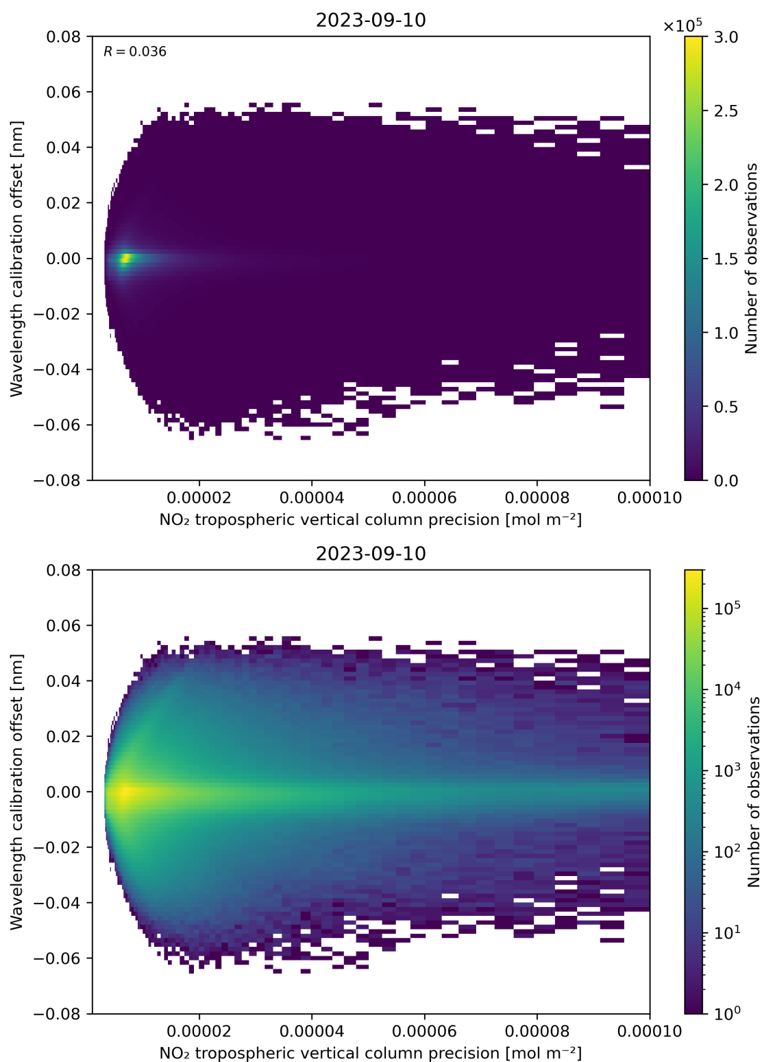
Figure 141: Scatter density plot of “NO 2 tropospheric vertical column precision” against “Wavelength calibration offset” for 2023-09-10 to 2023-09-11.
