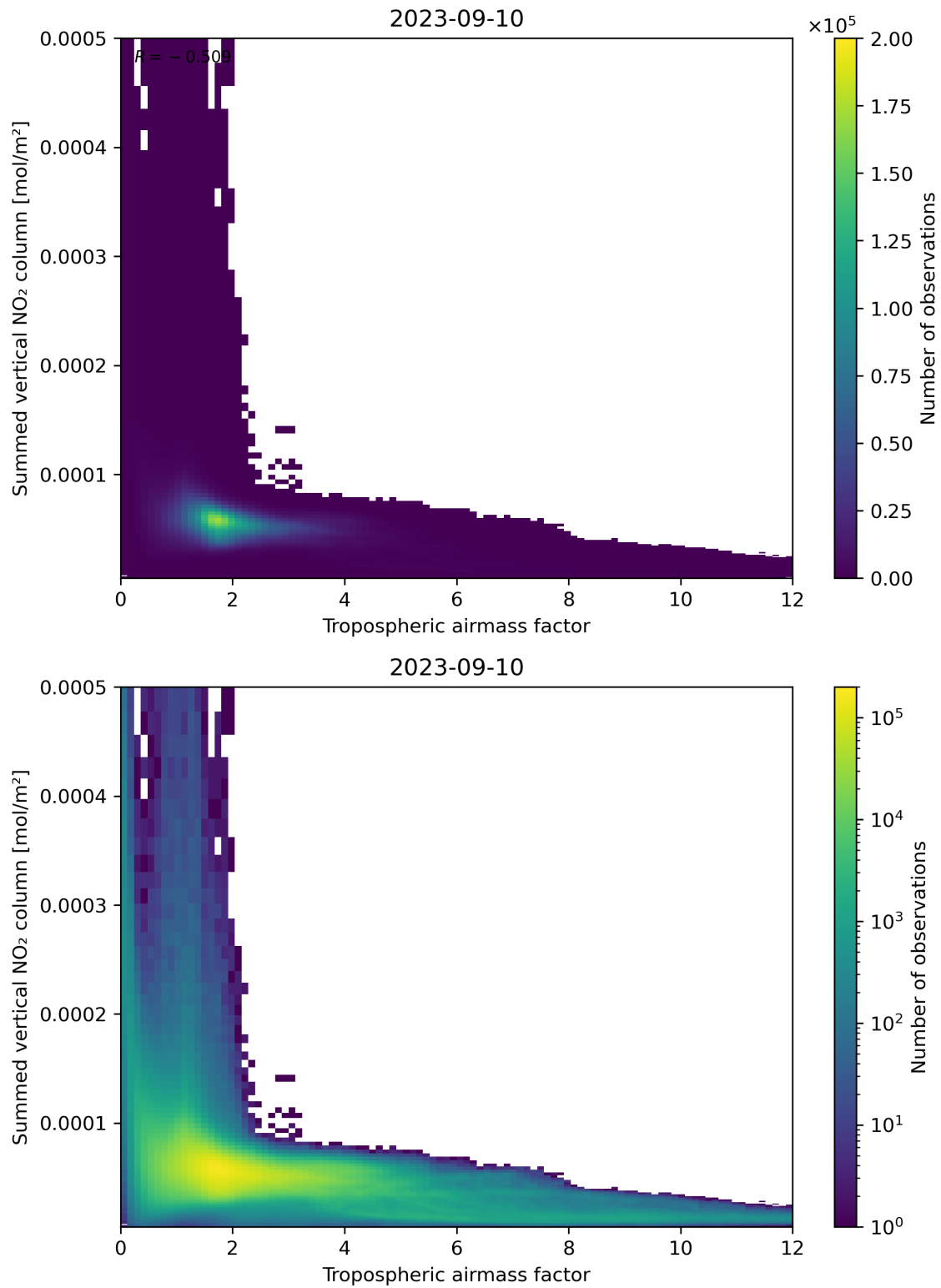
Figure 75: Scatter density plot of “Tropospheric air mass factor” against “Summed vertical NO 2 column” for 2023-09-10 to 2023-09-11.
