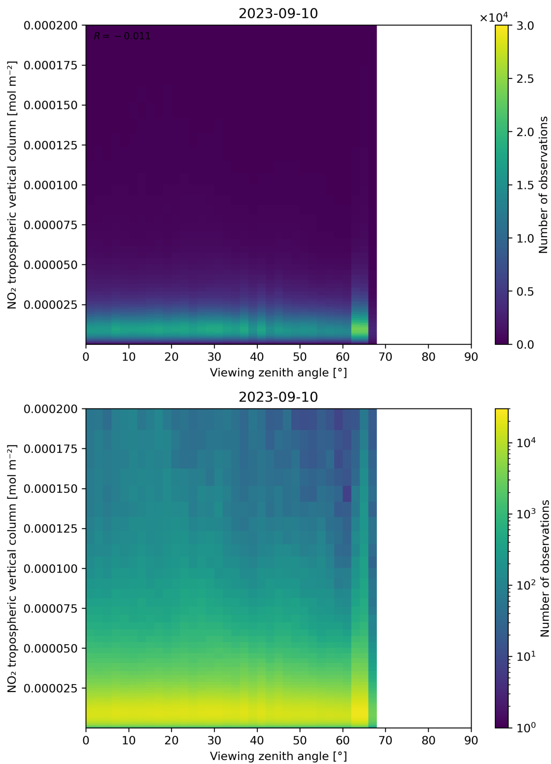
Figure 169: Scatter density plot of “Viewing zenith angle” against “NO 2 tropospheric vertical column” for 2023-09-10 to 2023-09-11.
