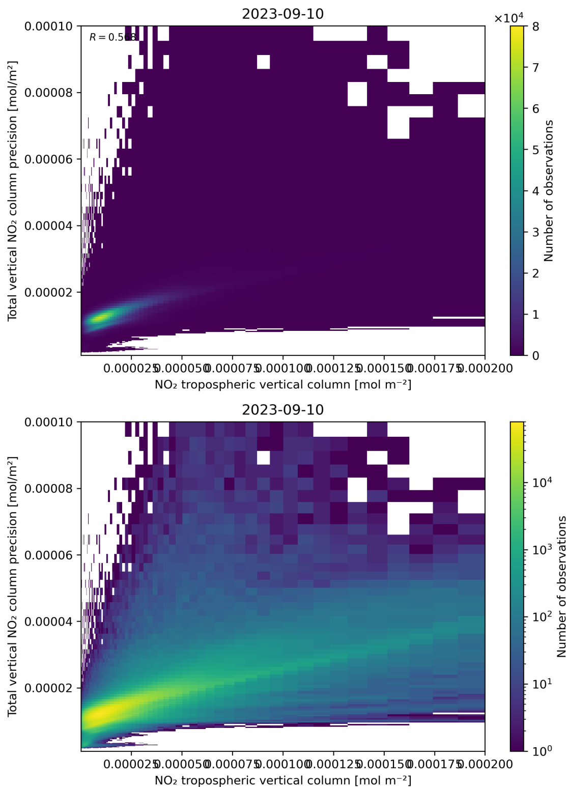
Figure 129: Scatter density plot of “NO 2 tropospheric vertical column” against “Total vertical NO 2 column precision” for 2023-09-10 to 2023-09-11.
