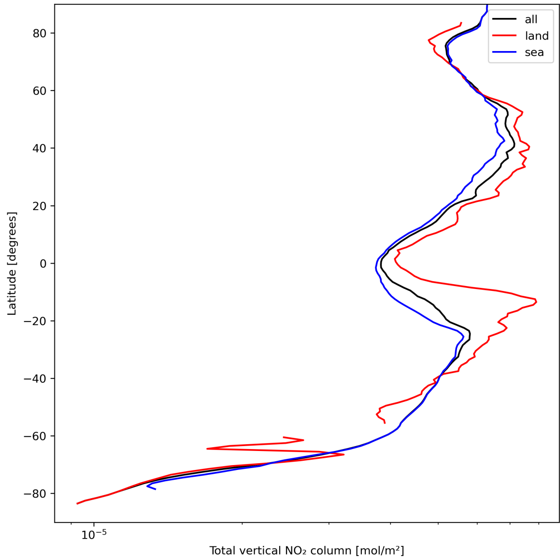
Figure 21: Zonal average of “Total vertical NO 2 column” for 2023-09-10 to 2023-09-11.
