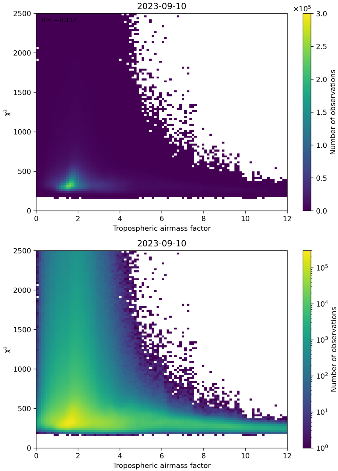
Figure 73: Scatter density plot of “Tropospheric airmass factor” against “ \chi^2 ” for 2023-09-10 to 2023-09-11.
