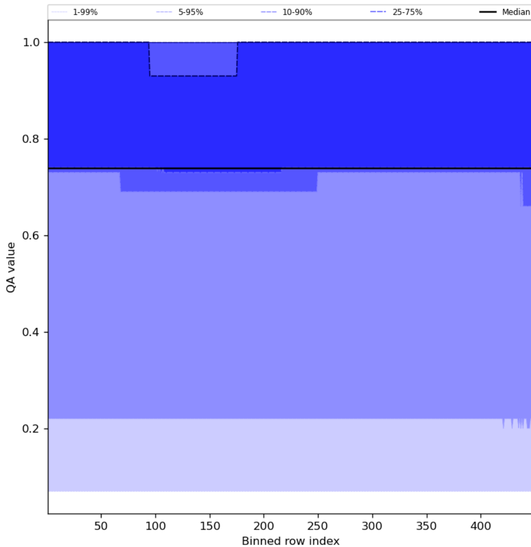
Figure 45: Along track statistics of “QA value” for 2023-09-10 to 2023-09-11
