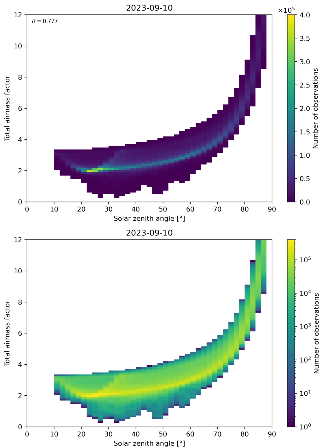
Figure 146: Scatter density plot of “Solar zenith angle” against “Total air mass factor” for 2023-09-10 to 2023-09-11.
