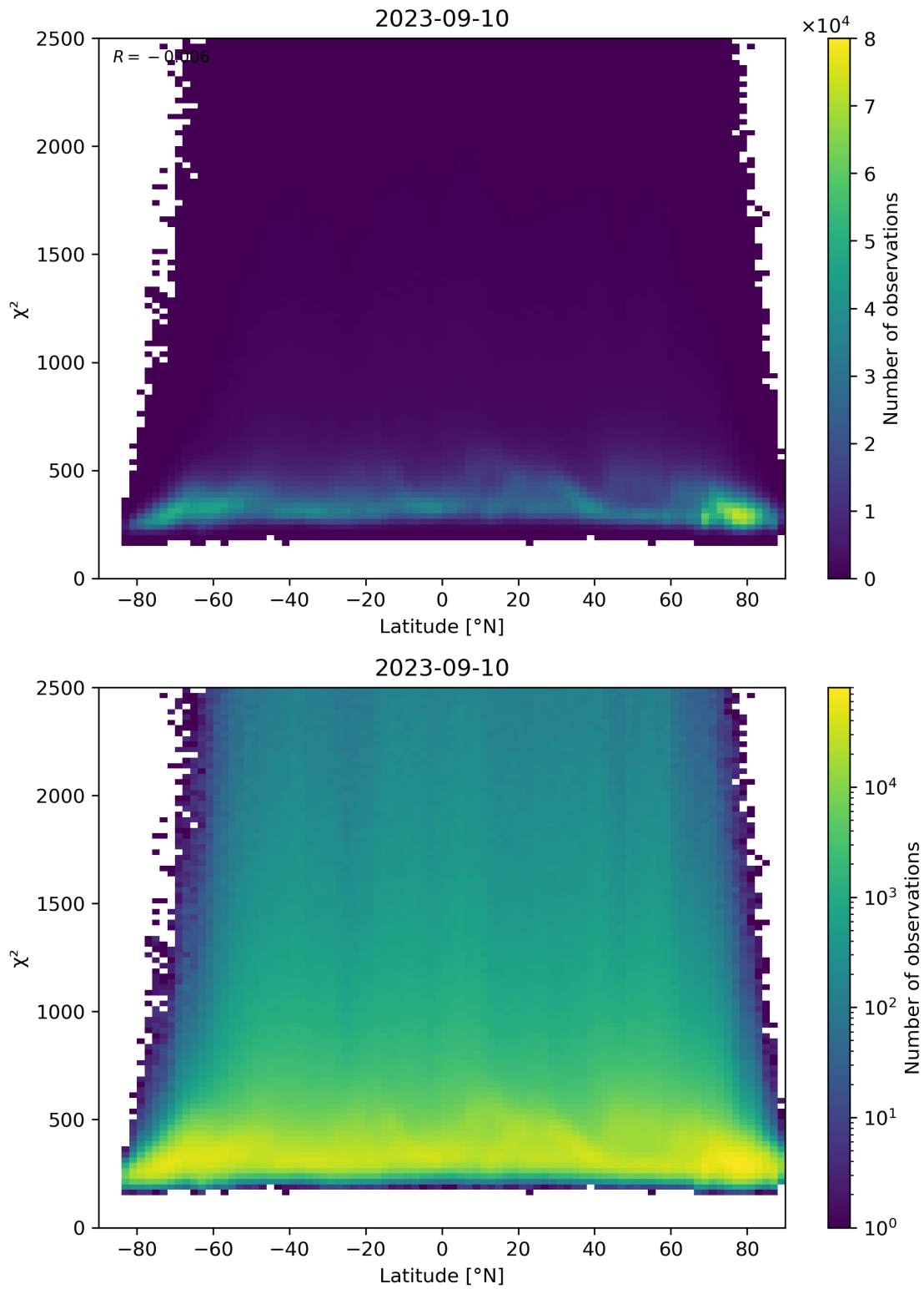
Figure 86: Scatter density plot of “Latitude” against “ \chi^2 ” for 2023-09-10 to 2023-09-11.
