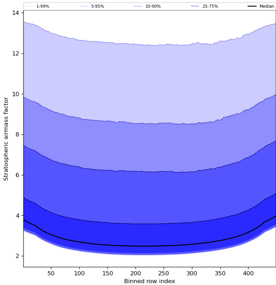
Figure 61: Along track statistics of “Stratospheric airmass factor” for 2023-09-10 to 2023-09-11
