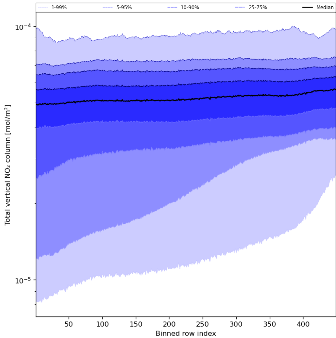
Figure 55: Along track statistics of “Total vertical NO 2 column” for 2023-09-10 to 2023-09-11
