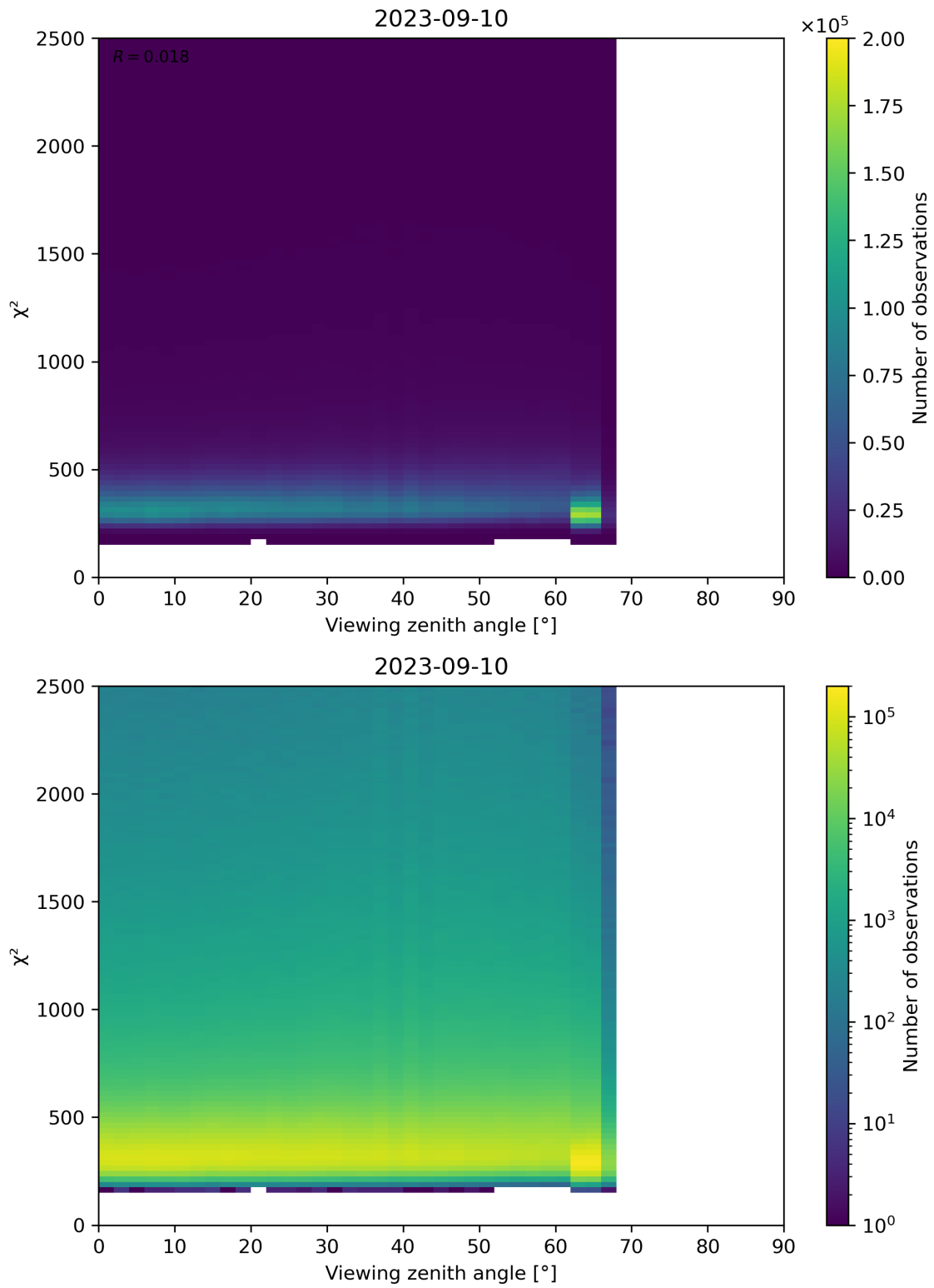
Figure 162: Scatter density plot of “Viewing zenith angle” against “ \chi^2 ” for 2023-09-10 to 2023-09-11.
