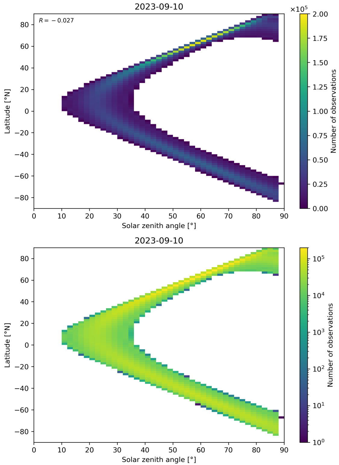
Figure 149: Scatter density plot of “Solar zenith angle” against “Latitude” for 2023-09-10 to 2023-09-11.
