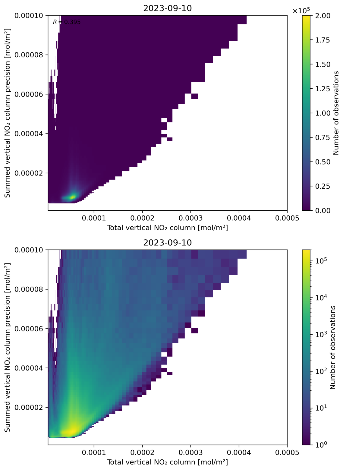
Figure 113: Scatter density plot of “Total vertical NO 2 column” against “Summed vertical NO 2 column precision” for 2023-09-10 to 2023-09-11.
