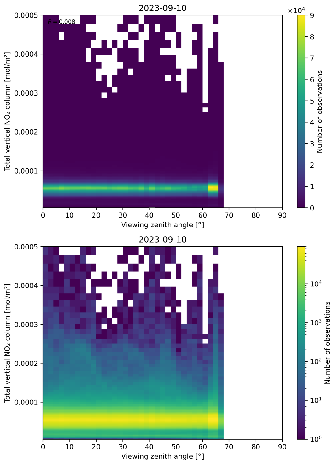
Figure 167: Scatter density plot of “Viewing zenith angle” against “Total vertical NO 2 column” for 2023-09-10 to 2023-09-11.
