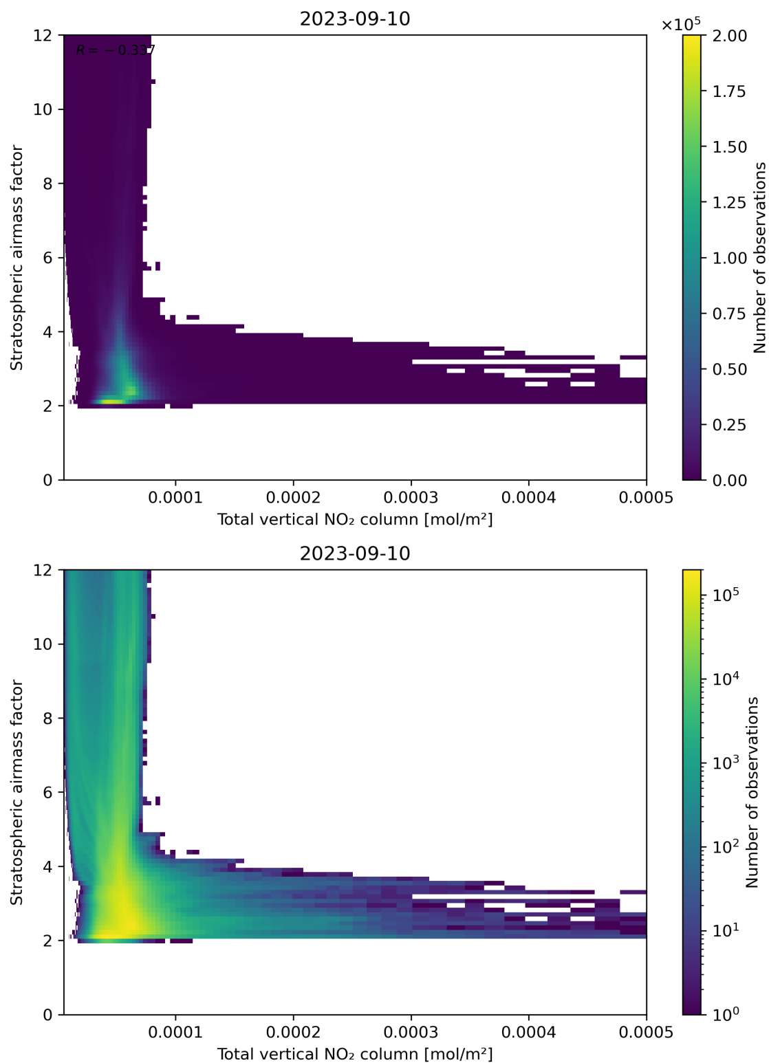
Figure 110: Scatter density plot of “Total vertical NO 2 column” against “Stratospheric airmass factor” for 2023-09-10 to 2023-09-11.
