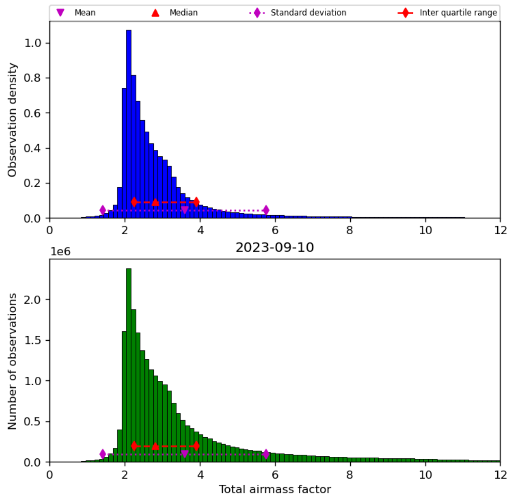
Figure 32: Histogram of “Total airmass factor” for 2023-09-10 to 2023-09-11
