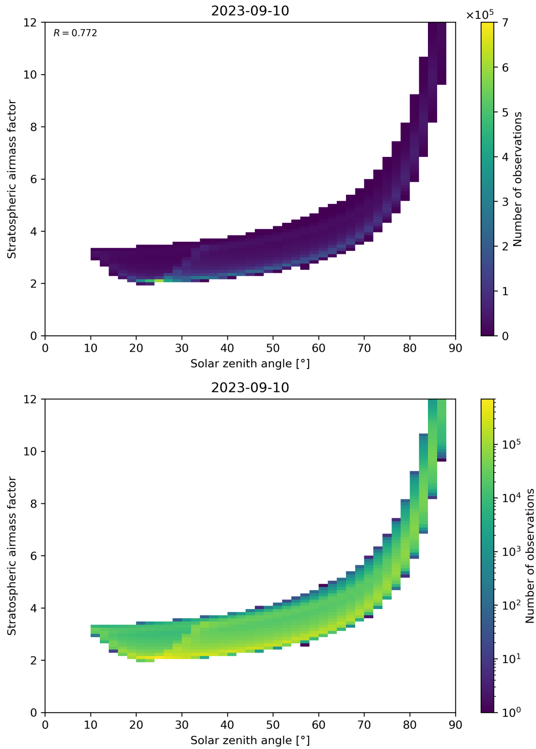
Figure 145: Scatter density plot of “Solar zenith angle” against “Stratospheric airmass factor” for 2023-09-10 to 2023-09-11.
