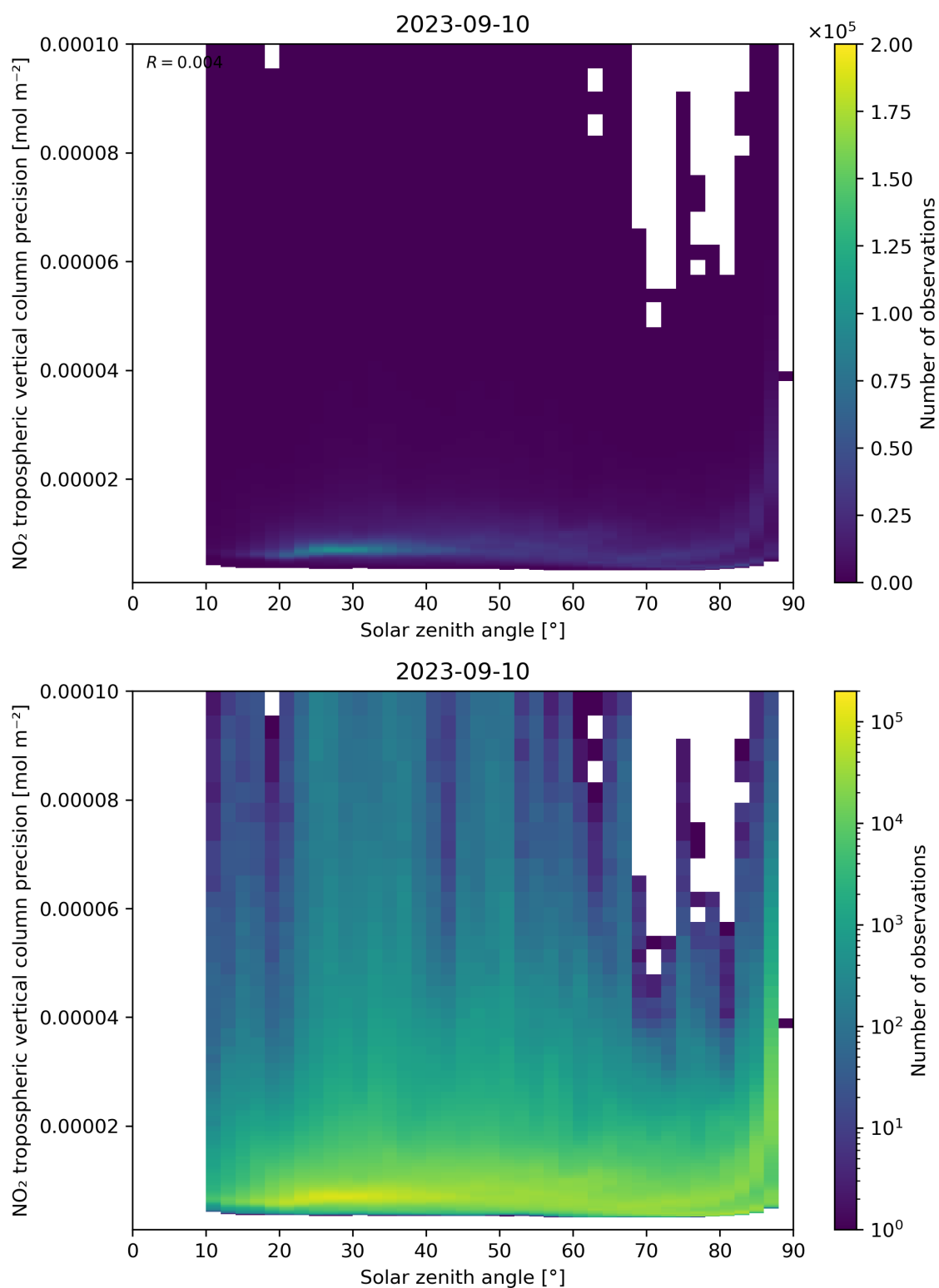
Figure 156: Scatter density plot of “Solar zenith angle” against “NO 2 tropospheric vertical column precision” for 2023-09-10 to 2023-09-11.
