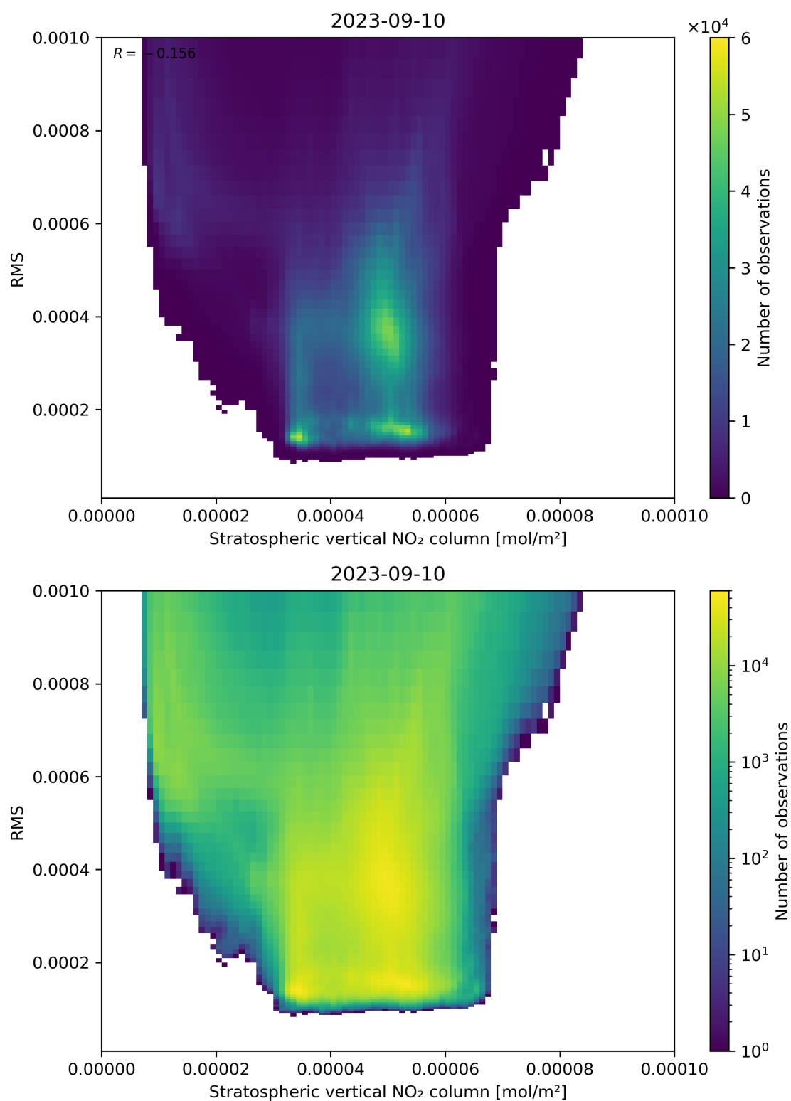
Figure 102: Scatter density plot of “Stratospheric vertical NO 2 column” against “RMS” for 2023-09-10 to 2023-09-11.
