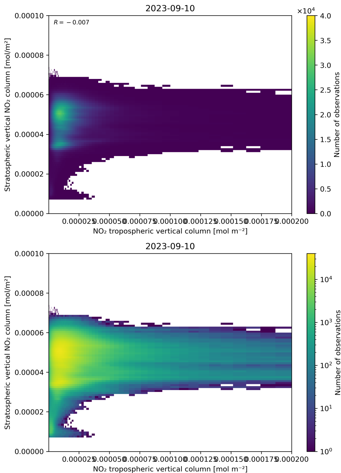
Figure 125: Scatter density plot of “NO 2 tropospheric vertical column” against “Stratospheric vertical NO 2 column” for 2023-09-10 to 2023-09-11.
