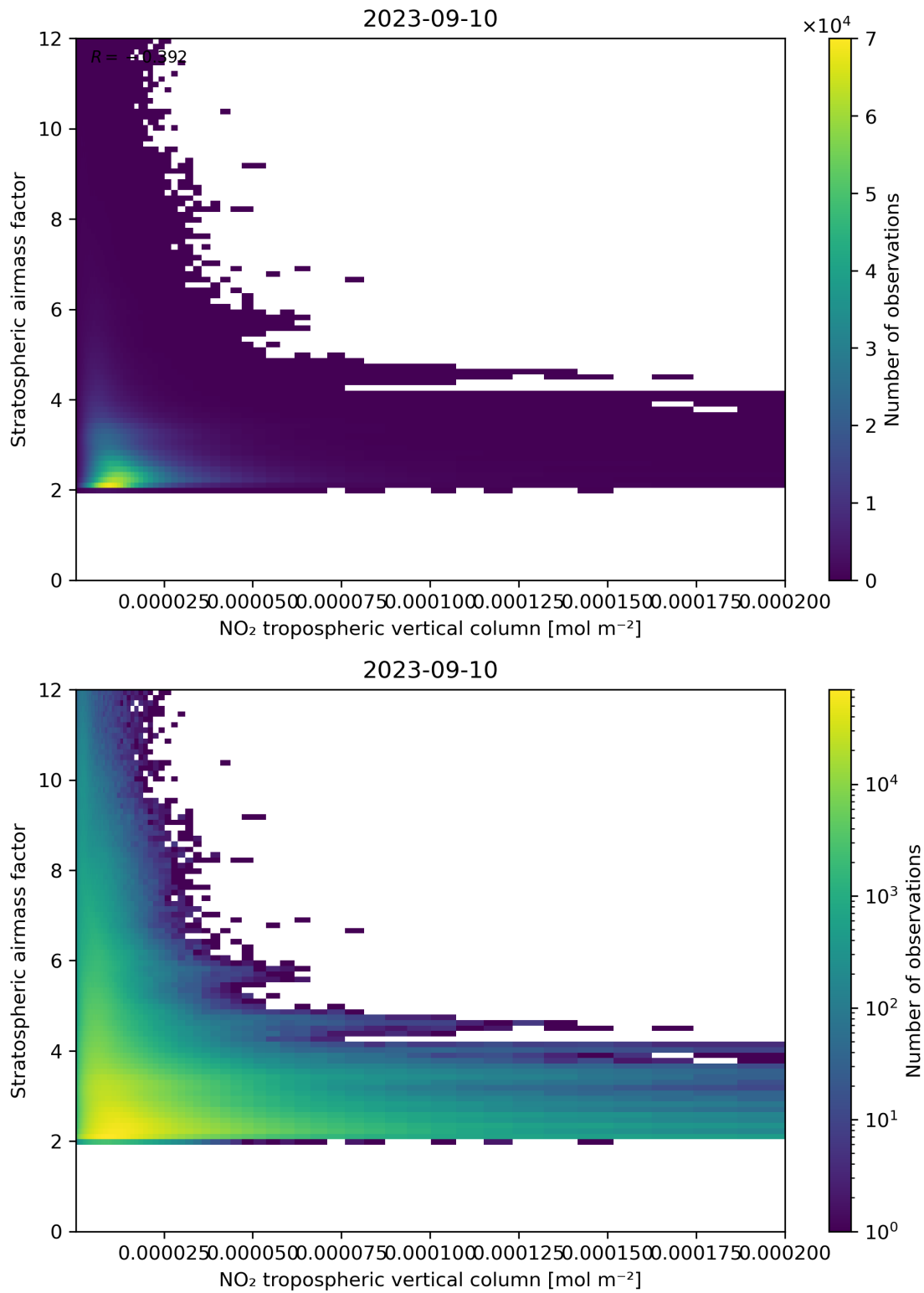
Figure 121: Scatter density plot of “NO 2 tropospheric vertical column” against “Stratospheric air mass factor” for 2023-09-10 to 2023-09-11.
