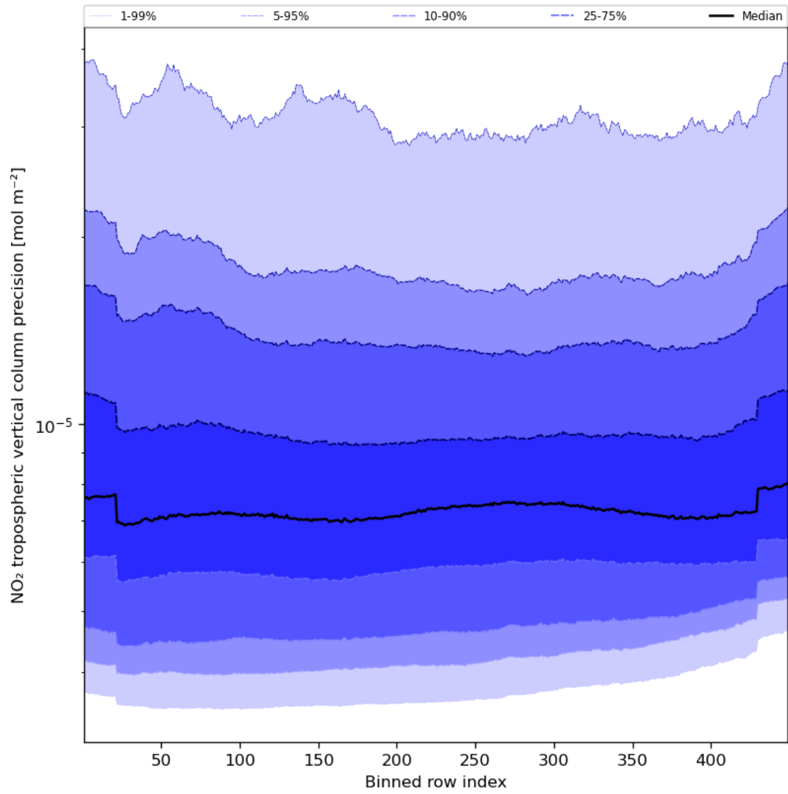
Figure 47: Along track statistics of “NO 2 tropospheric vertical column precision” for 2023-09-10 to 2023-09-11
