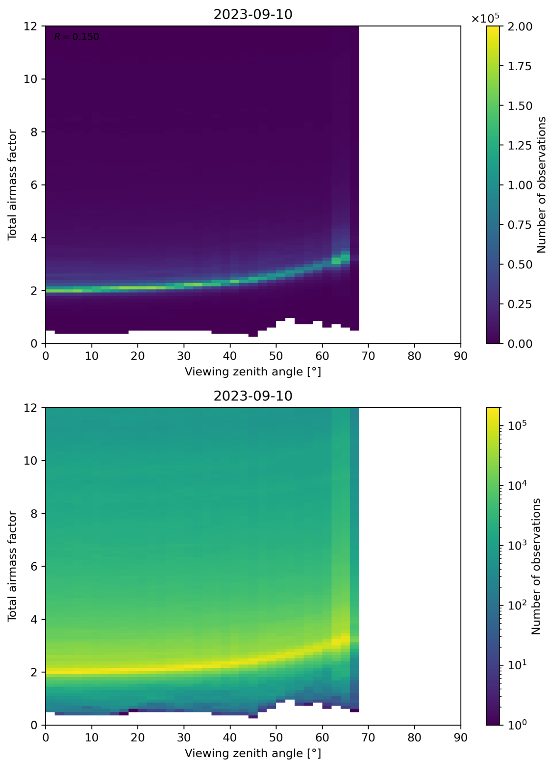
Figure 160: Scatter density plot of “Viewing zenith angle” against “Total airmass factor” for 2023-09-10 to 2023-09-11.
