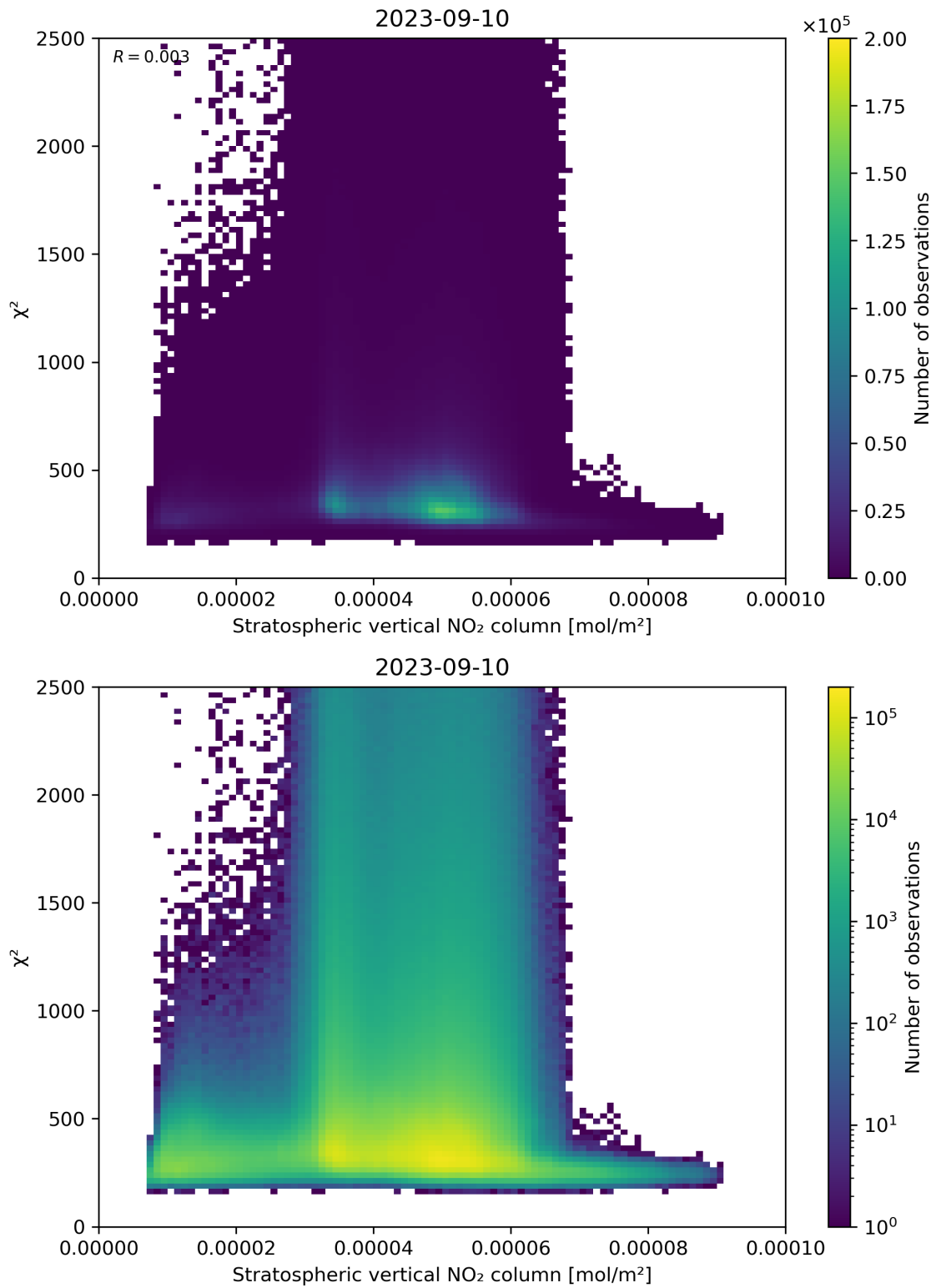
Figure 97: Scatter density plot of “Stratospheric vertical NO 2 column” against “ \chi^2 ” for 2023-09-10 to 2023-09-11.
