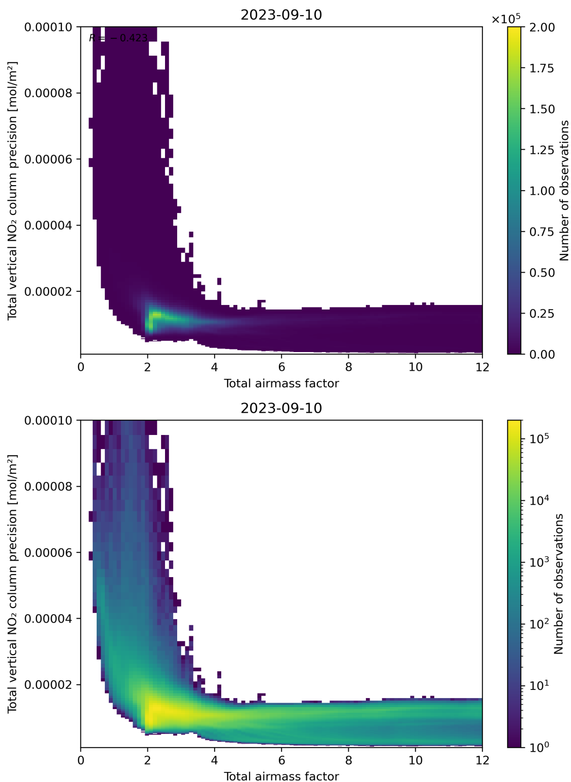
Figure 68: Scatter density plot of “Total airmass factor” against “Total vertical NO 2 column precision” for 2023-09-10 to 2023-09-11.
