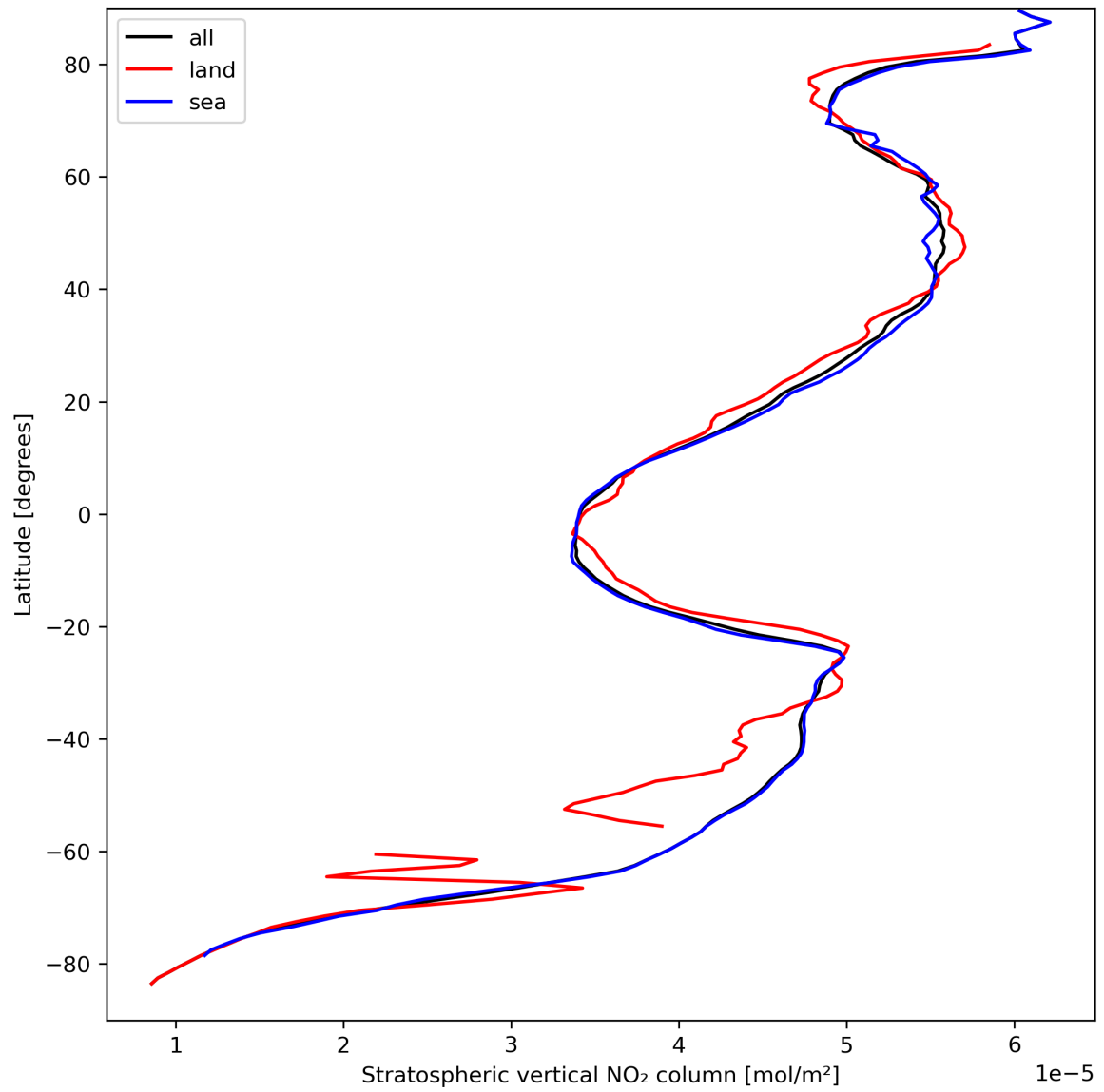
Figure 19: Zonal average of “Stratospheric vertical NO 2 column” for 2023-09-10 to 2023-09-11.
