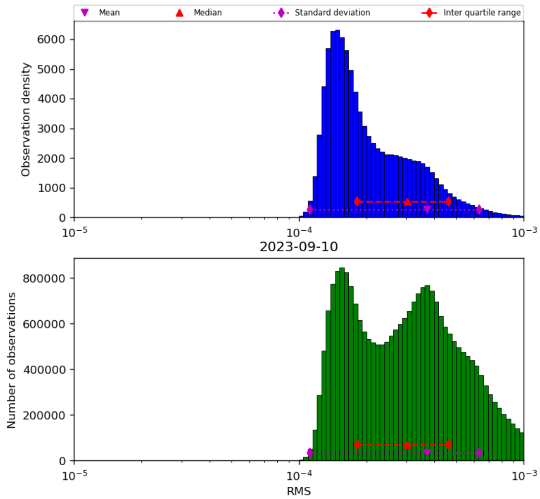
Figure 43: Histogram of “RMS” for 2023-09-10 to 2023-09-11
