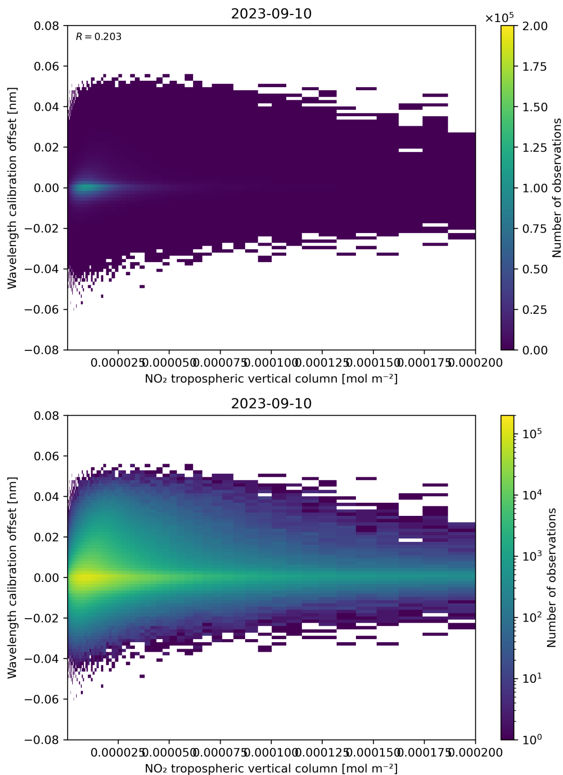
Figure 143: Scatter density plot of “NO 2 tropospheric vertical column” against “Wavelength calibration offset” for 2023-09-10 to 2023-09-11.
