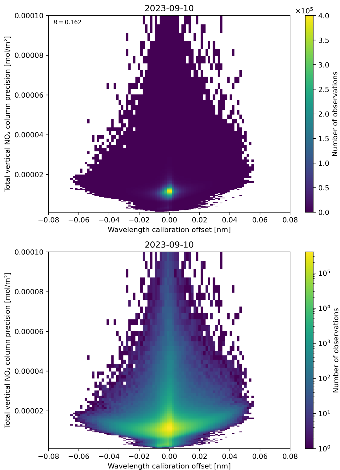
Figure 180: Scatter density plot of “Wavelength calibration offset” against “Total vertical NO 2 column precision” for 2023-09-10 to 2023-09-11.
