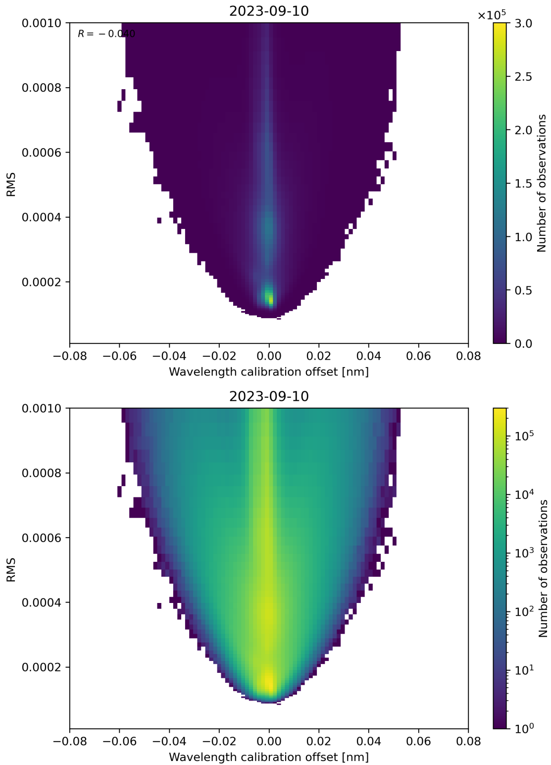
Figure 181: Scatter density plot of “Wavelength calibration offset” against “RMS” for 2023-09-10 to 2023-09-11.
