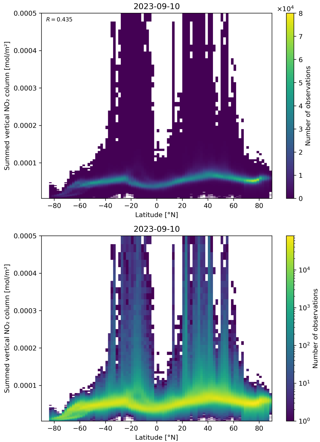
Figure 88: Scatter density plot of “Latitude” against “Summed vertical NO 2 column” for 2023-09-10 to 2023-09-11.
