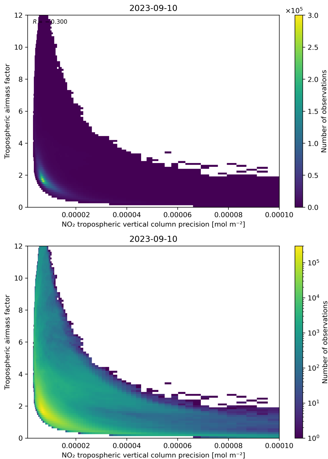
Figure 133: Scatter density plot of “NO 2 tropospheric vertical column precision” against “Tropospheric air mass factor” for 2023-09-10 to 2023-09-11.
