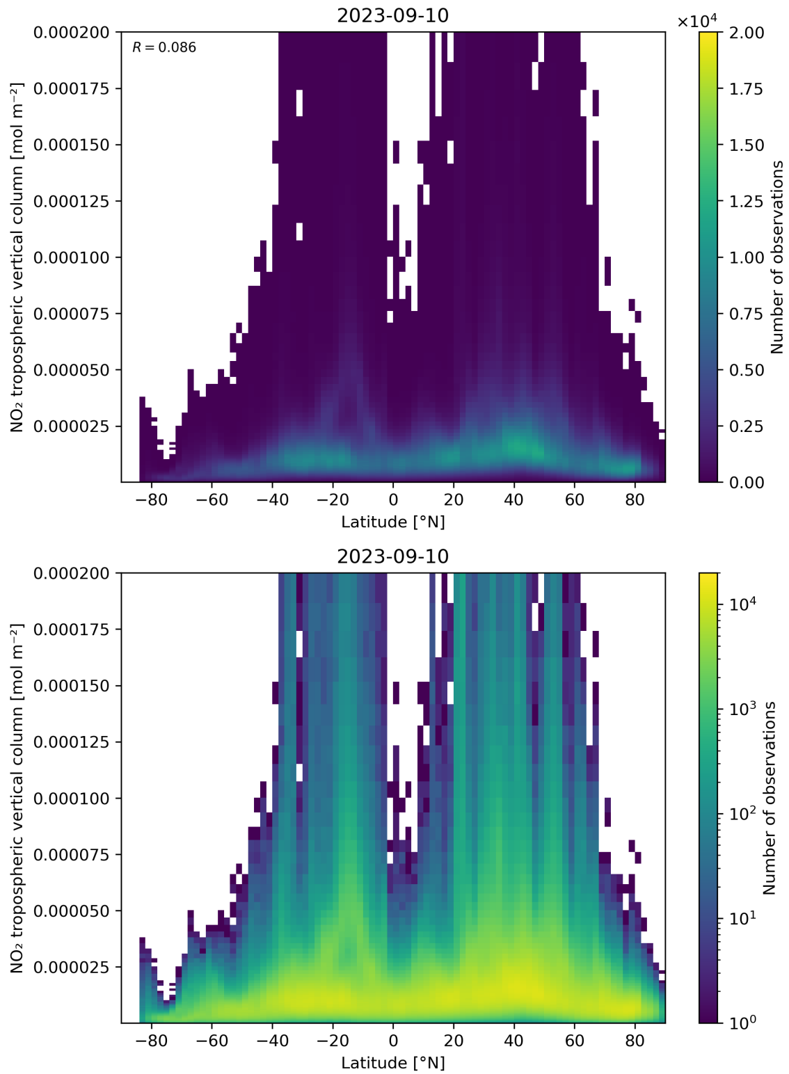
Figure 92: Scatter density plot of “Latitude” against “NO 2 tropospheric vertical column” for 2023-09-10 to 2023-09-11.
