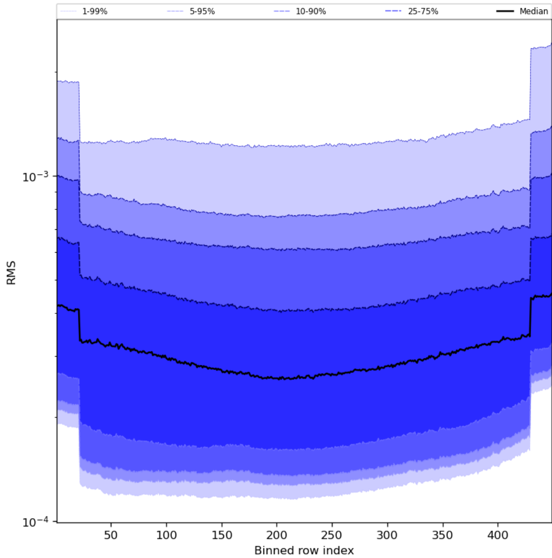
Figure 60: Along track statistics of “RMS” for 2023-09-10 to 2023-09-11
