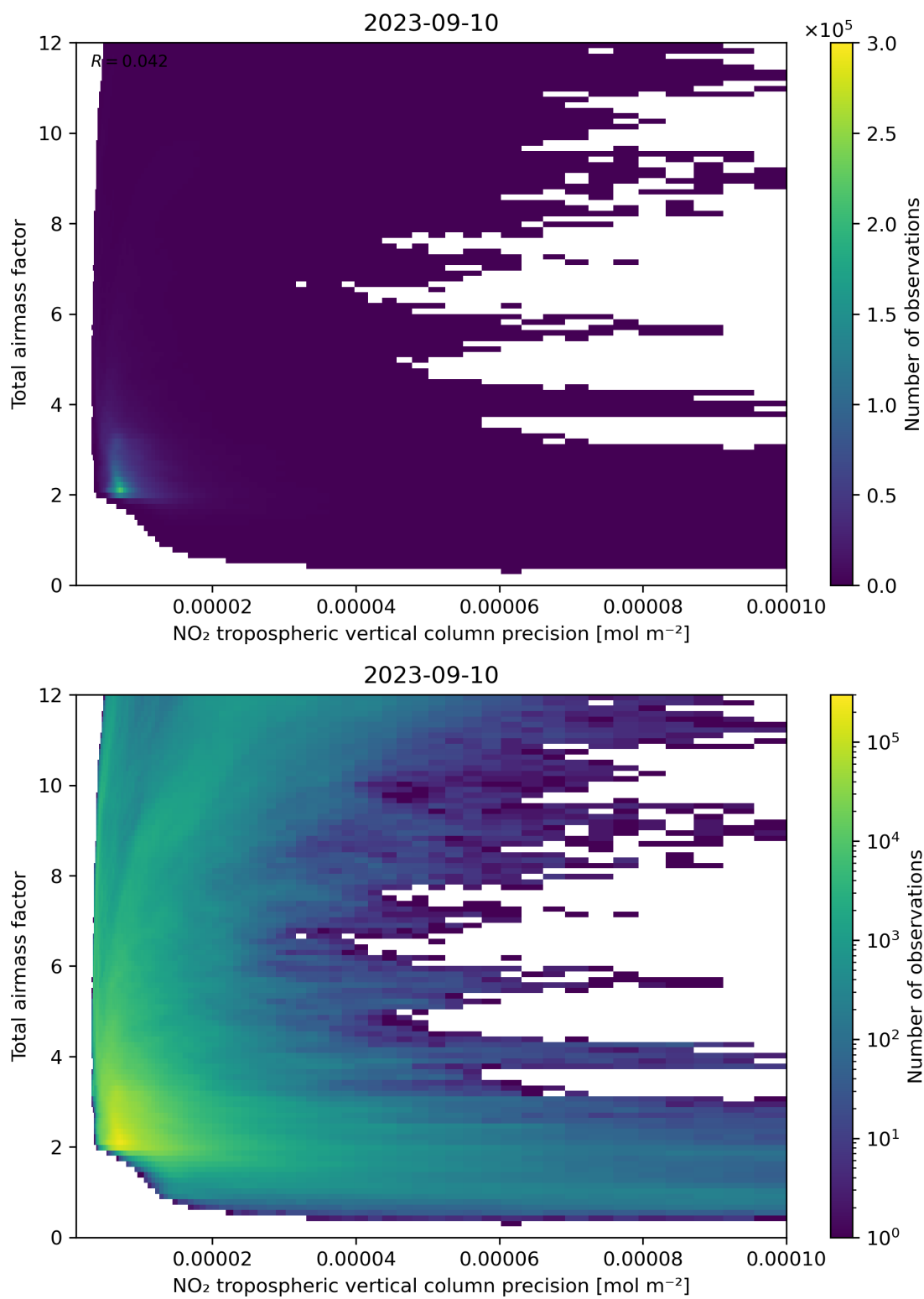
Figure 132: Scatter density plot of “NO 2 tropospheric vertical column precision” against “Total air mass factor” for 2023-09-10 to 2023-09-11.
