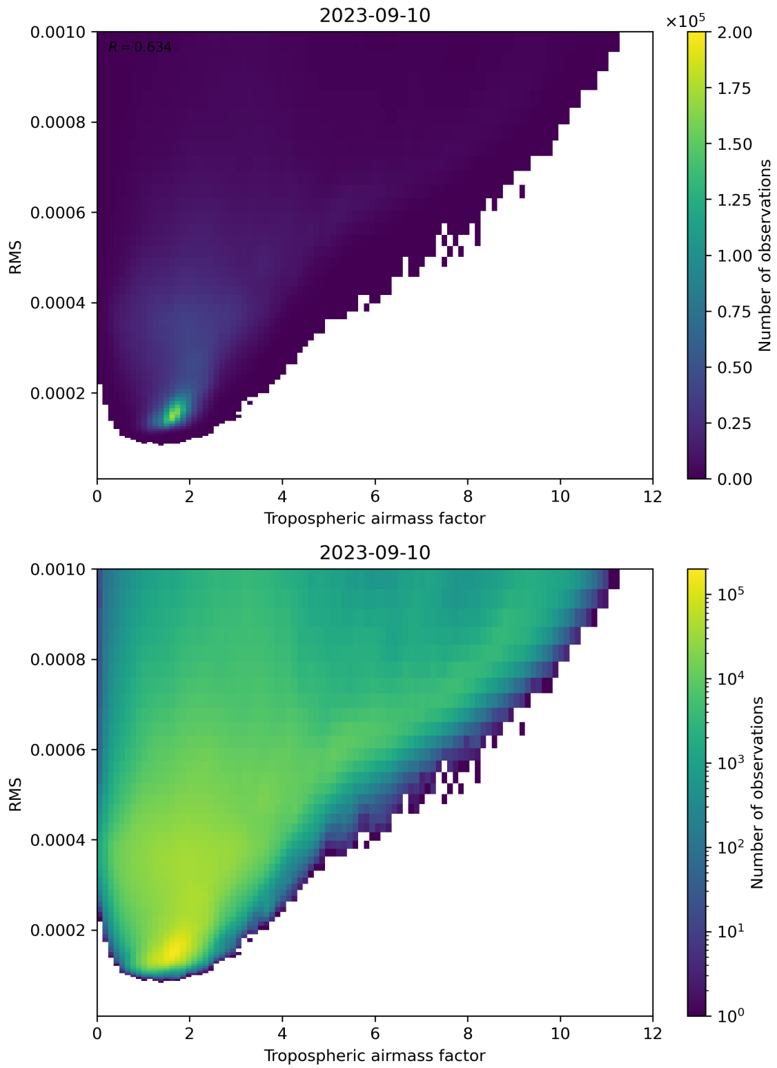
Figure 79: Scatter density plot of “Tropospheric airmass factor” against “RMS” for 2023-09-10 to 2023-09-11.
