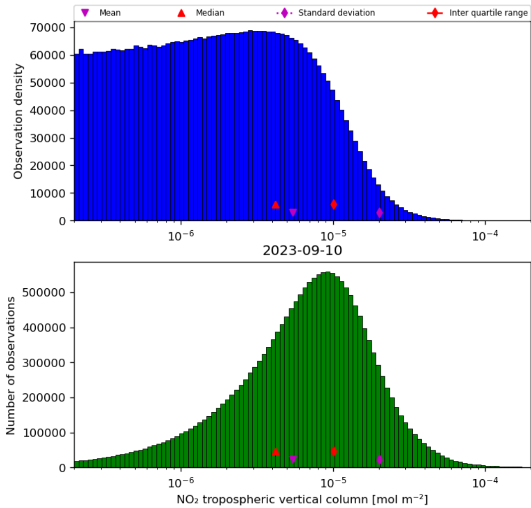
Figure 29: Histogram of “NO 2 tropospheric vertical column” for 2023-09-10 to 2023-09-11
