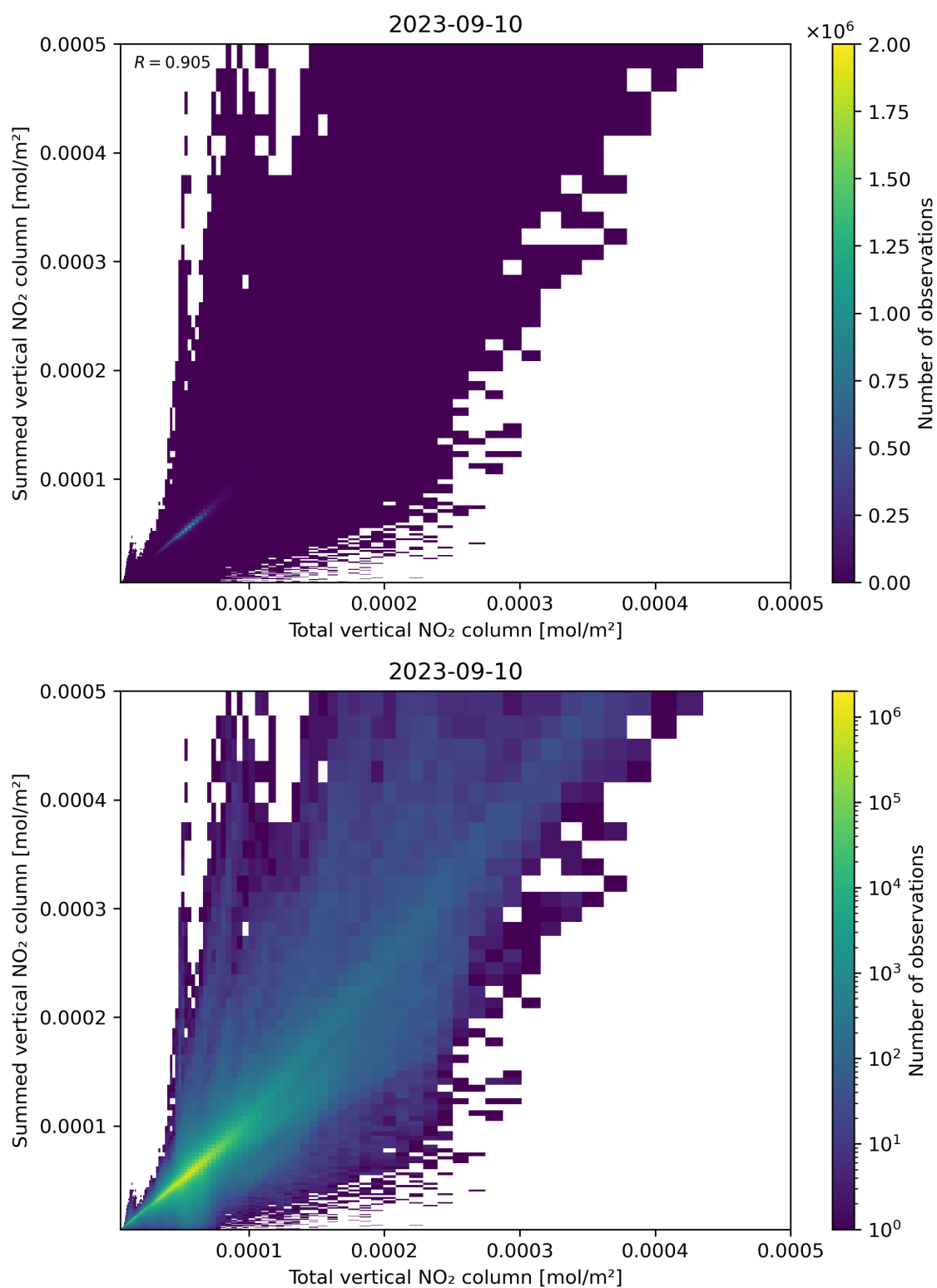
Figure 112: Scatter density plot of “Total vertical NO 2 column” against “Summed vertical NO 2 column” for 2023-09-10 to 2023-09-11.
