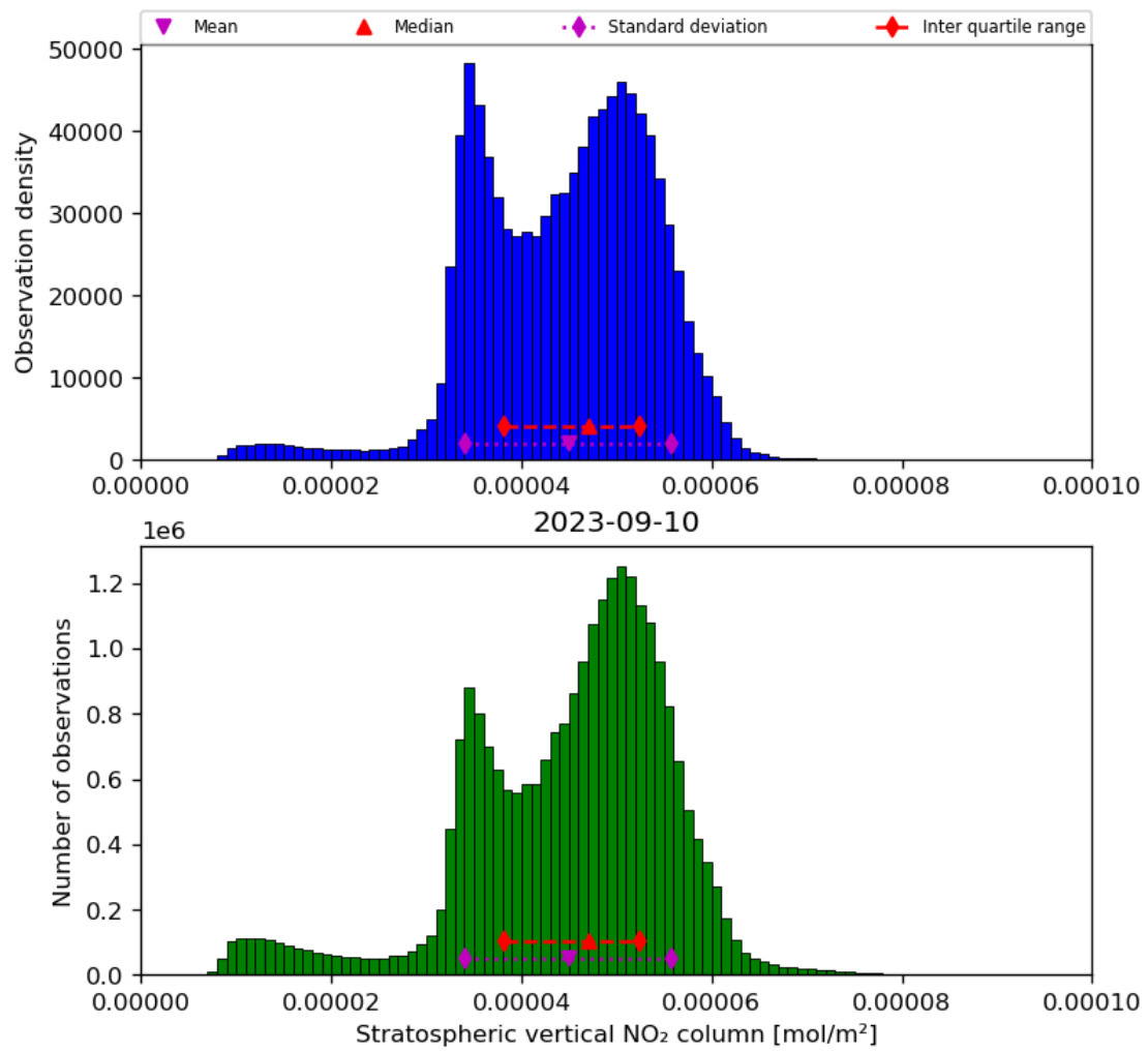
Figure 36: Histogram of “Stratospheric vertical NO 2 column” for 2023-09-10 to 2023-09-11
