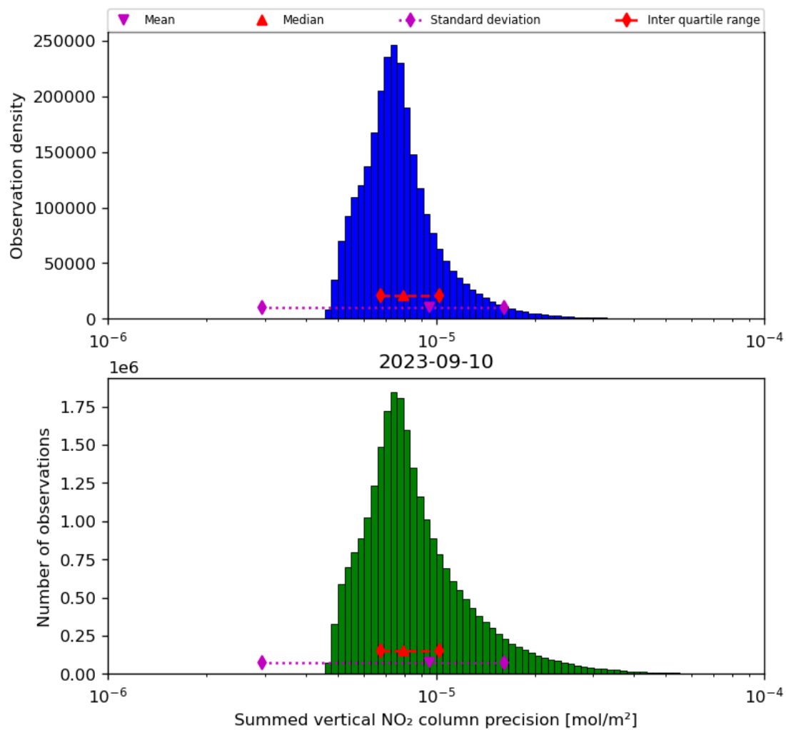
Figure 41: Histogram of “Summed vertical NO 2 column precision” for 2023-09-10 to 2023-09-11
