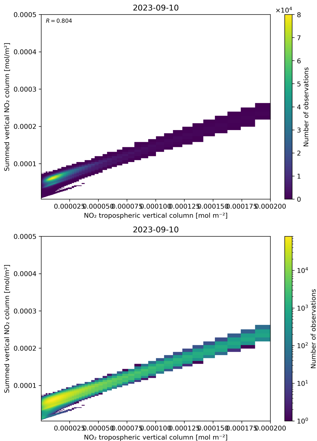
Figure 126: Scatter density plot of “NO 2 tropospheric vertical column” against “Summed vertical NO 2 column” for 2023-09-10 to 2023-09-11.
