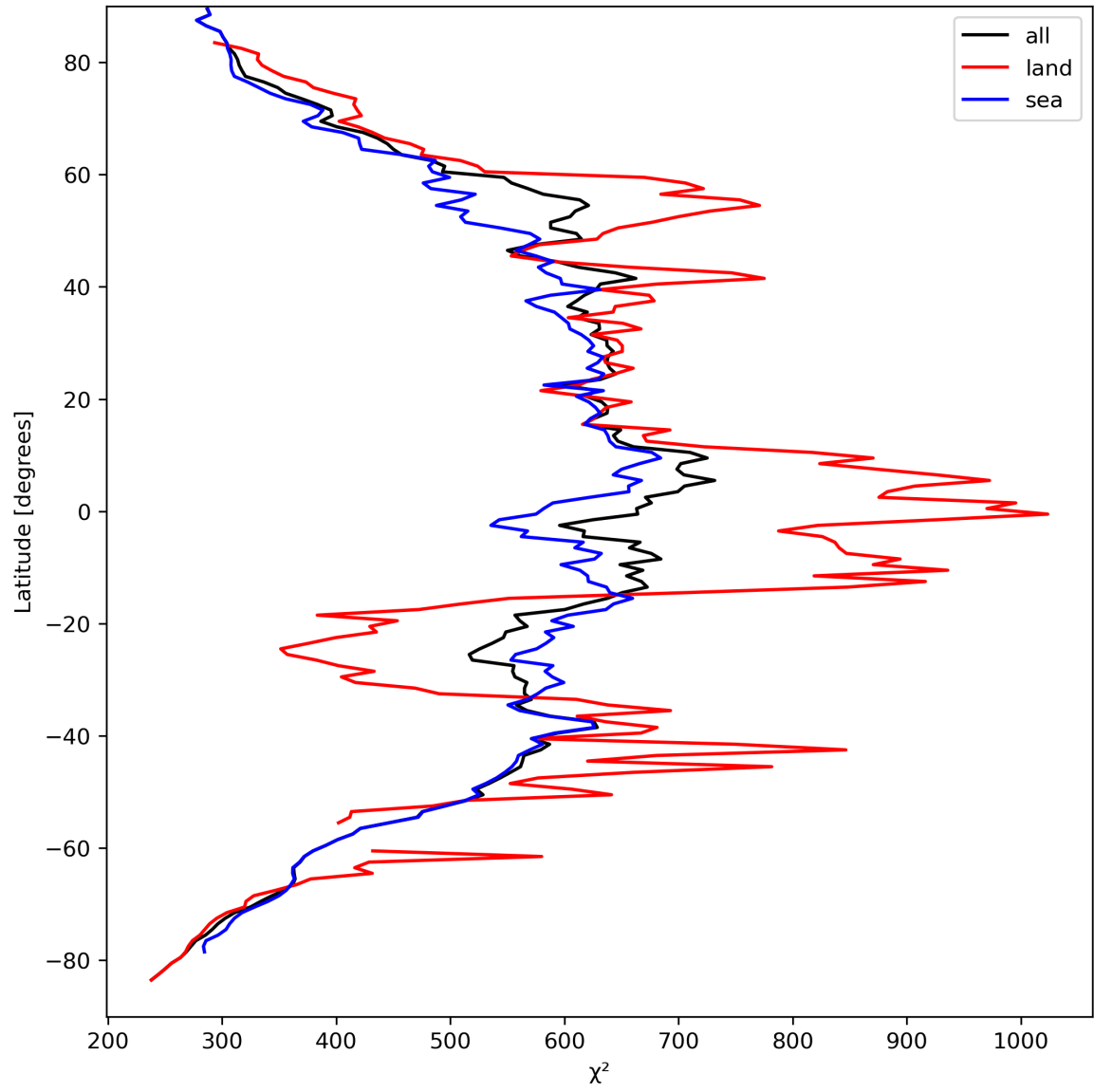
Figure 25: Zonal average of “ \chi^2 ” for 2023-09-10 to 2023-09-11.
