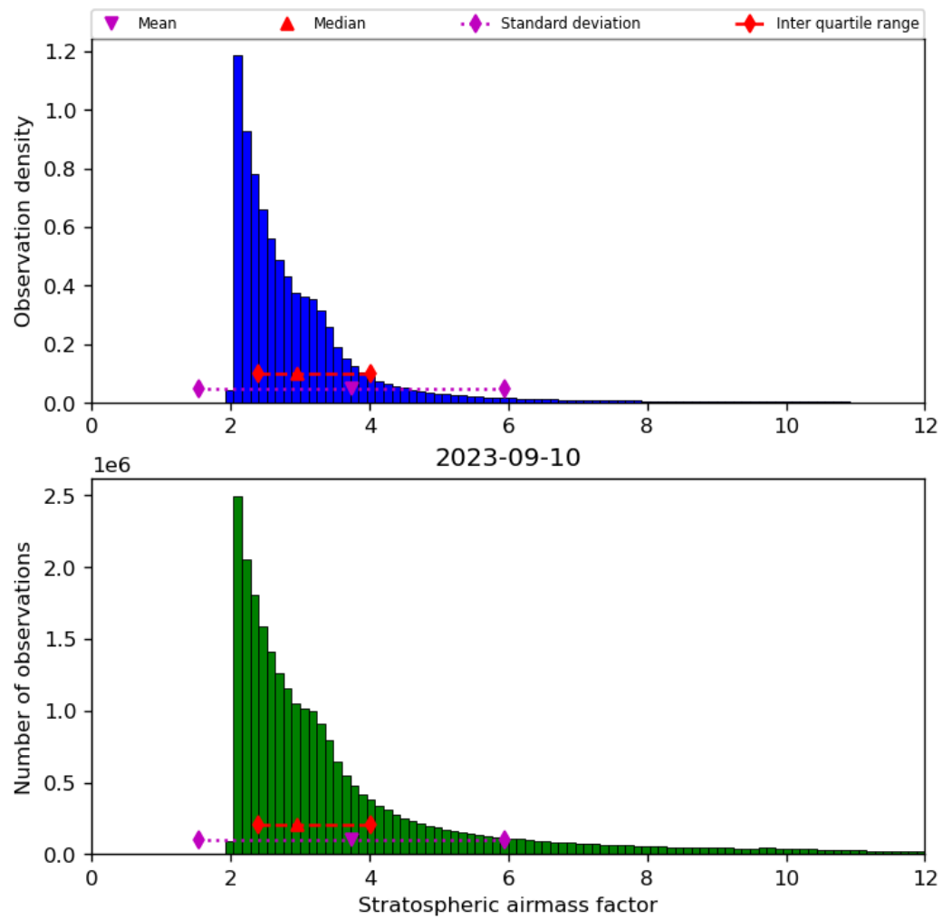
Figure 44: Histogram of “Stratospheric airmass factor” for 2023-09-10 to 2023-09-11
