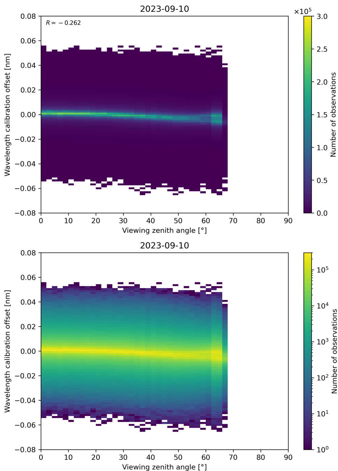
Figure 173: Scatter density plot of “Viewing zenith angle” against “Wavelength calibration offset” for 2023-09-10 to 2023-09-11.
