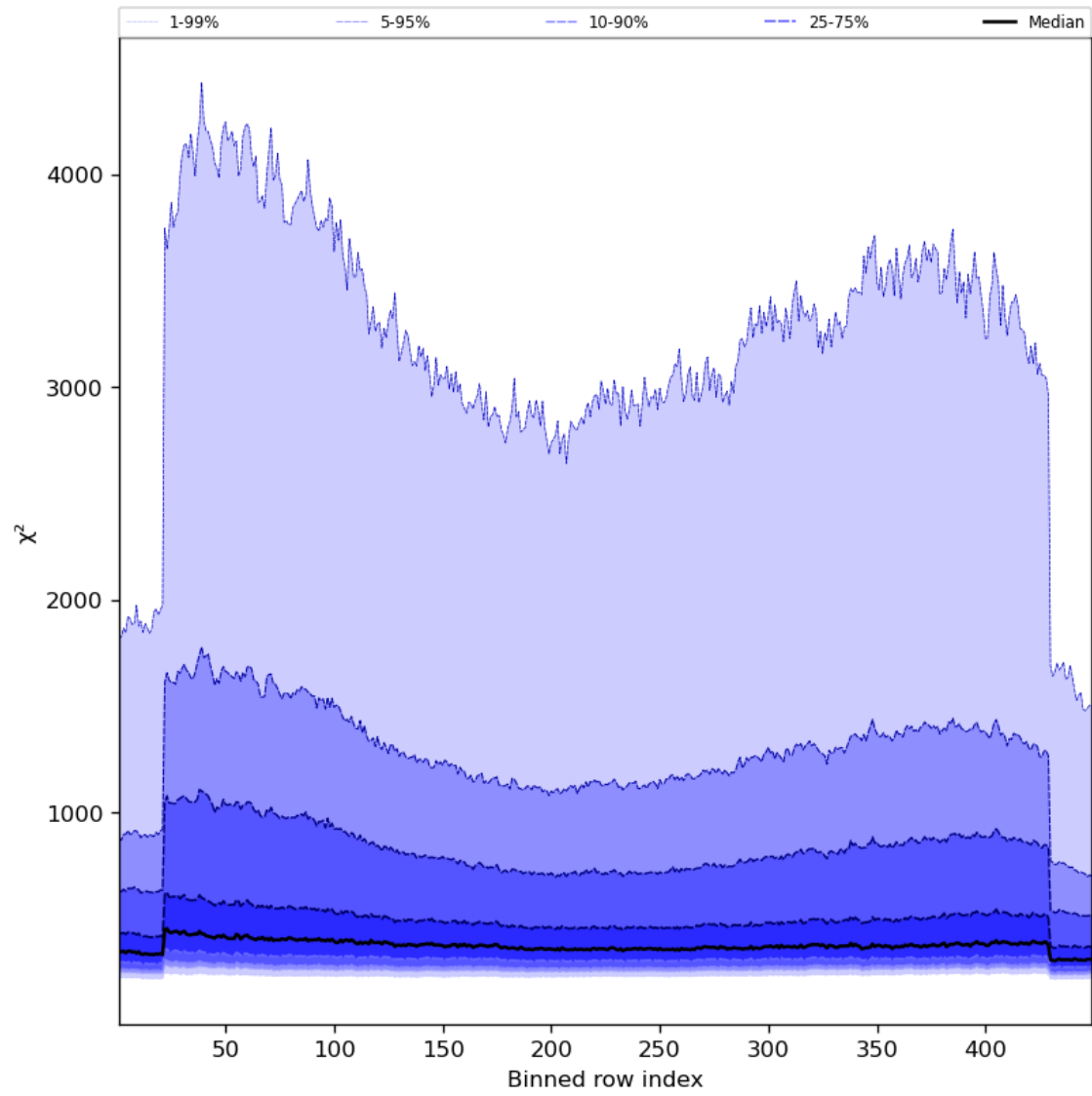
Figure 59: Along track statistics of “ \chi^2 ” for 2023-09-10 to 2023-09-11
