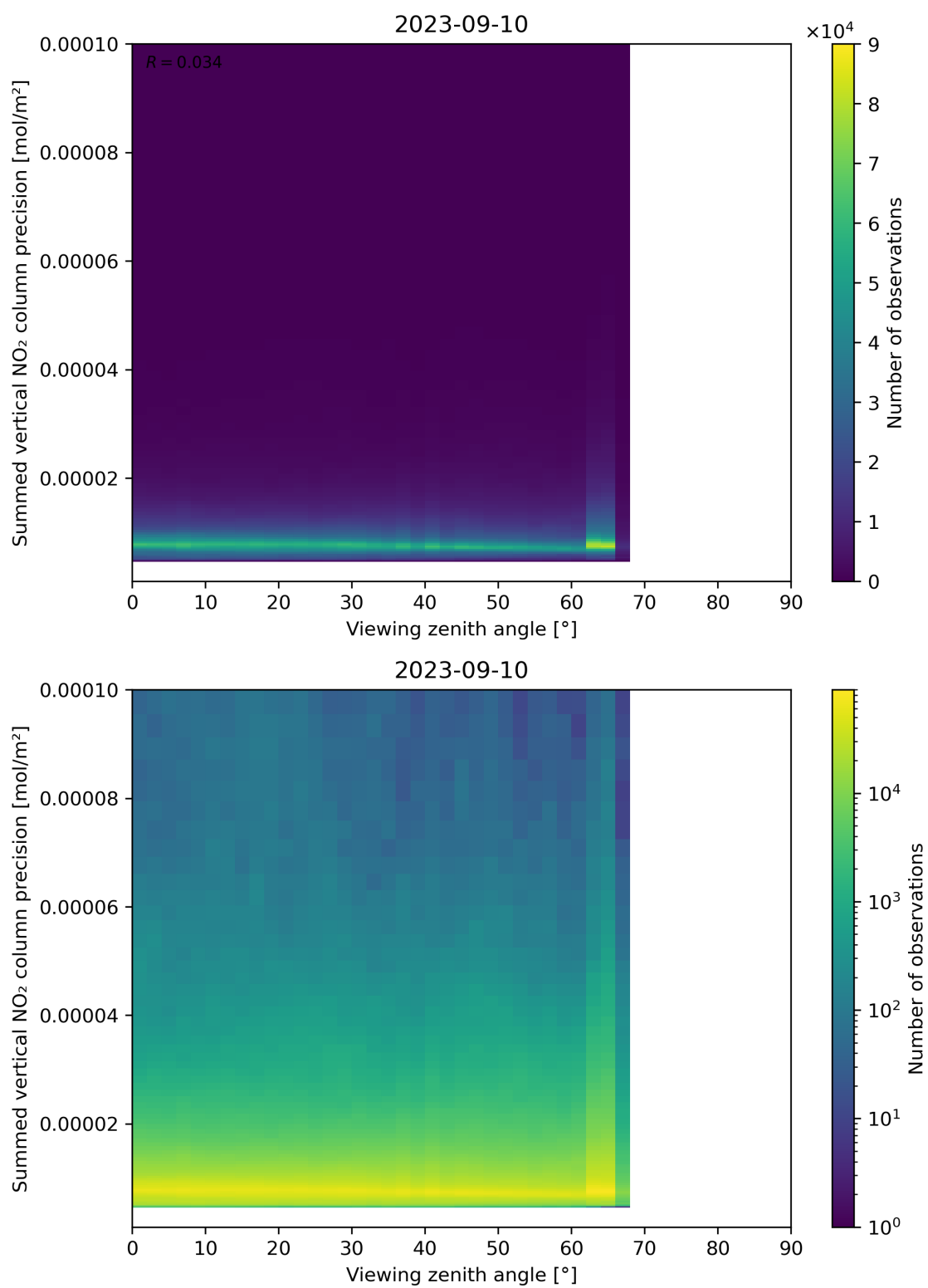
Figure 166: Scatter density plot of “Viewing zenith angle” against “Summed vertical NO 2 column precision” for 2023-09-10 to 2023-09-11.
