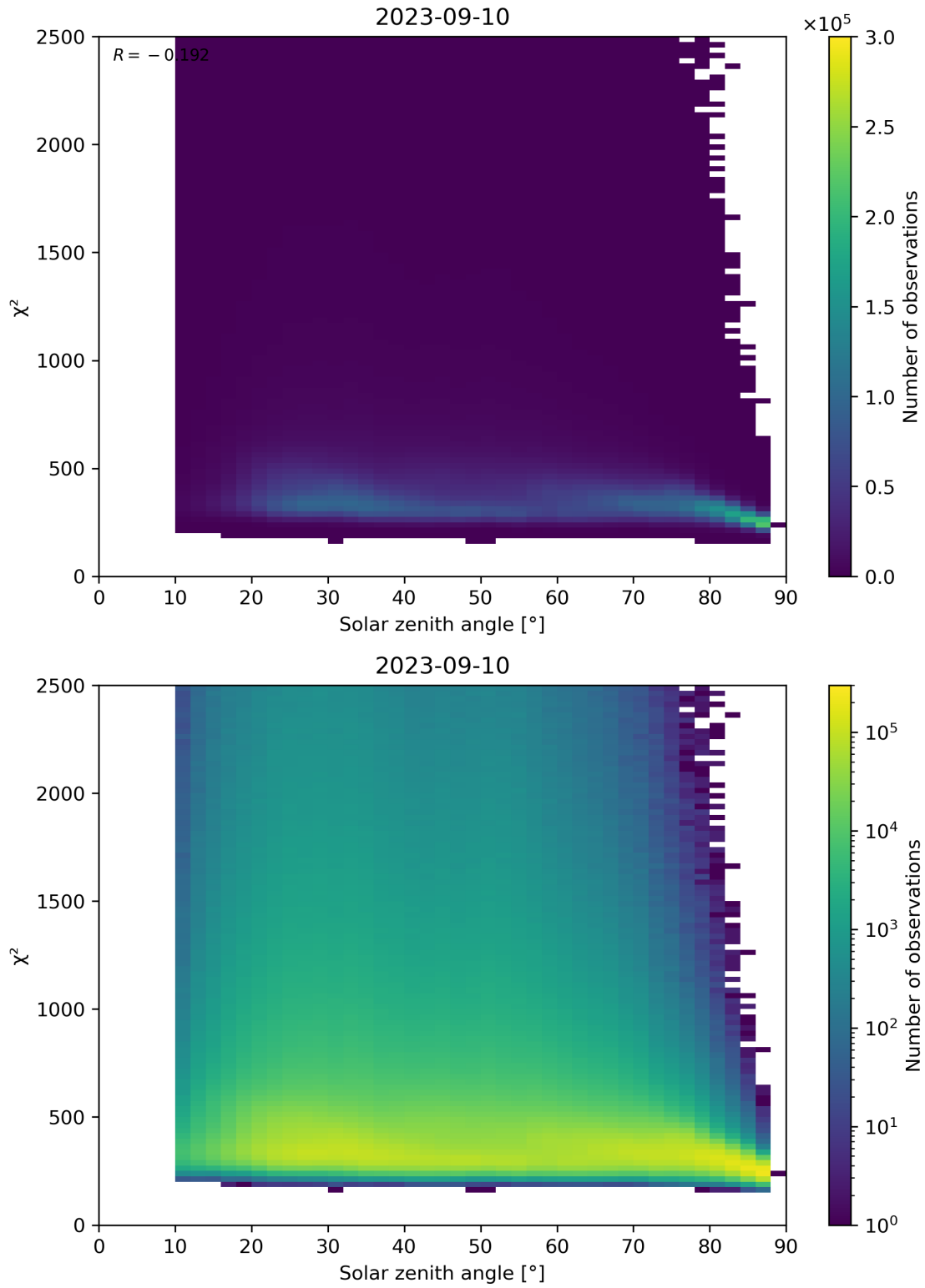
Figure 148: Scatter density plot of “Solar zenith angle” against “ \chi^2 ” for 2023-09-10 to 2023-09-11.
