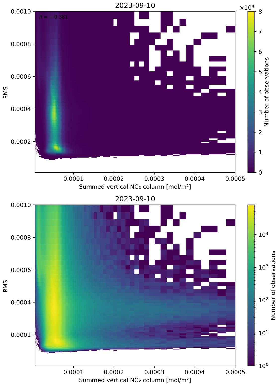
Figure 109: Scatter density plot of “Summed vertical NO 2 column” against “RMS” for 2023-09-10 to 2023-09-11.
