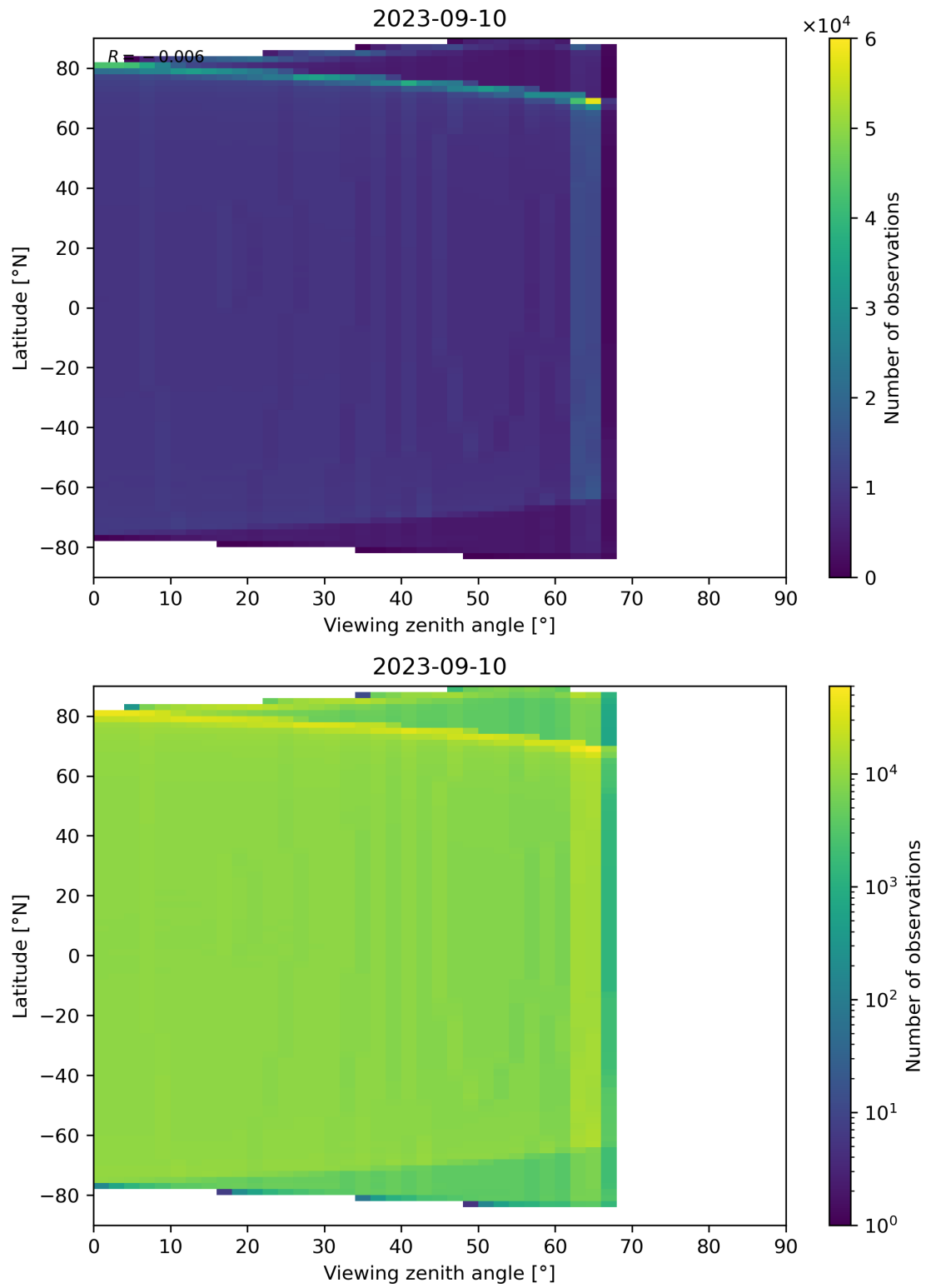
Figure 163: Scatter density plot of “Viewing zenith angle” against “Latitude” for 2023-09-10 to 2023-09-11.
