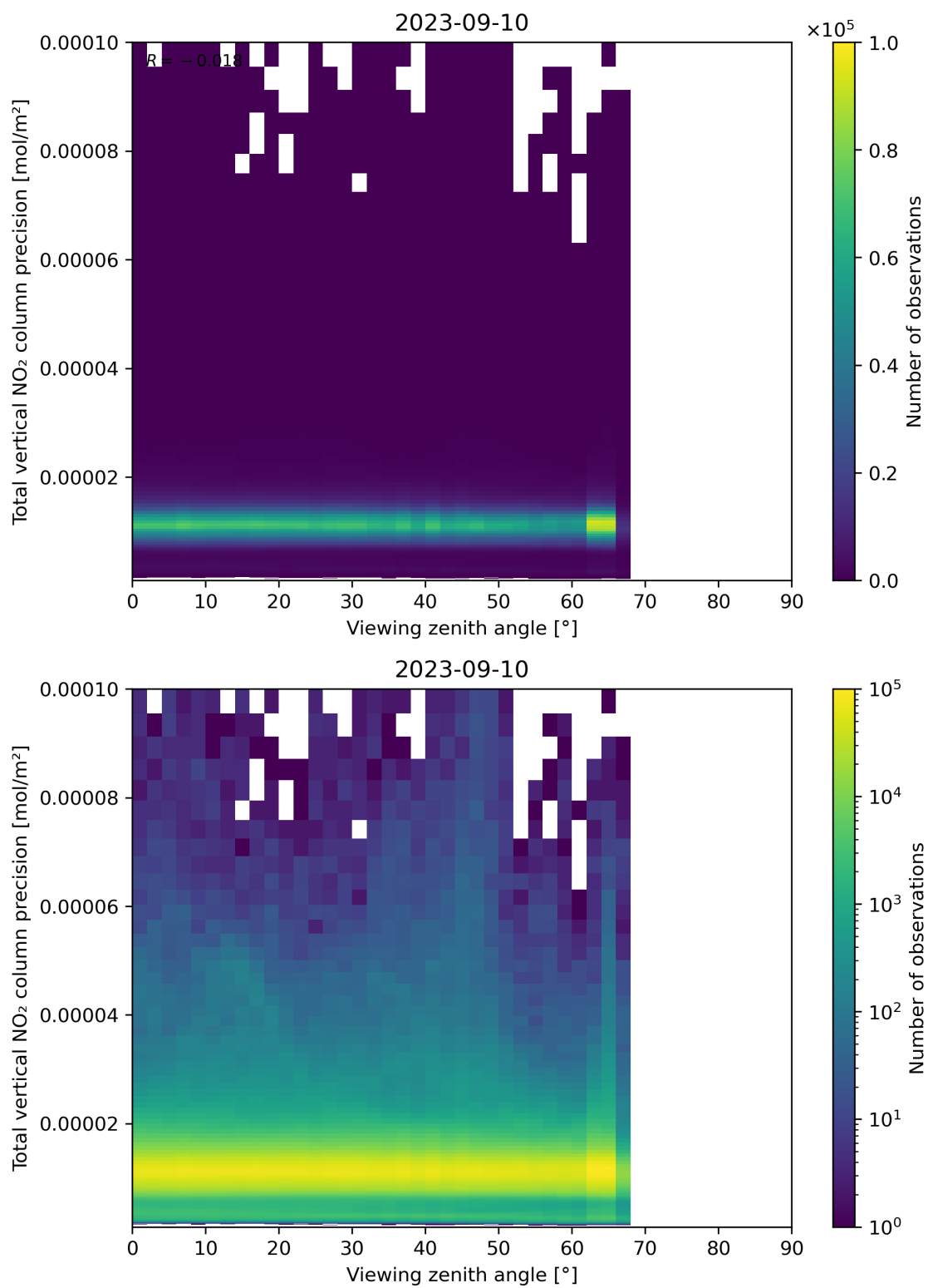
Figure 168: Scatter density plot of “Viewing zenith angle” against “Total vertical NO 2 column precision” for 2023-09-10 to 2023-09-11.
