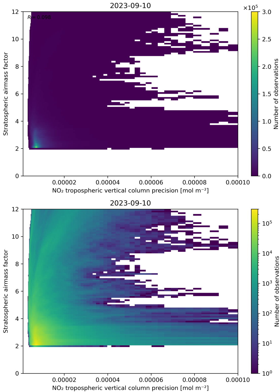
Figure 131: Scatter density plot of “NO 2 tropospheric vertical column precision” against “Stratospheric airmass factor” for 2023-09-10 to 2023-09-11.
