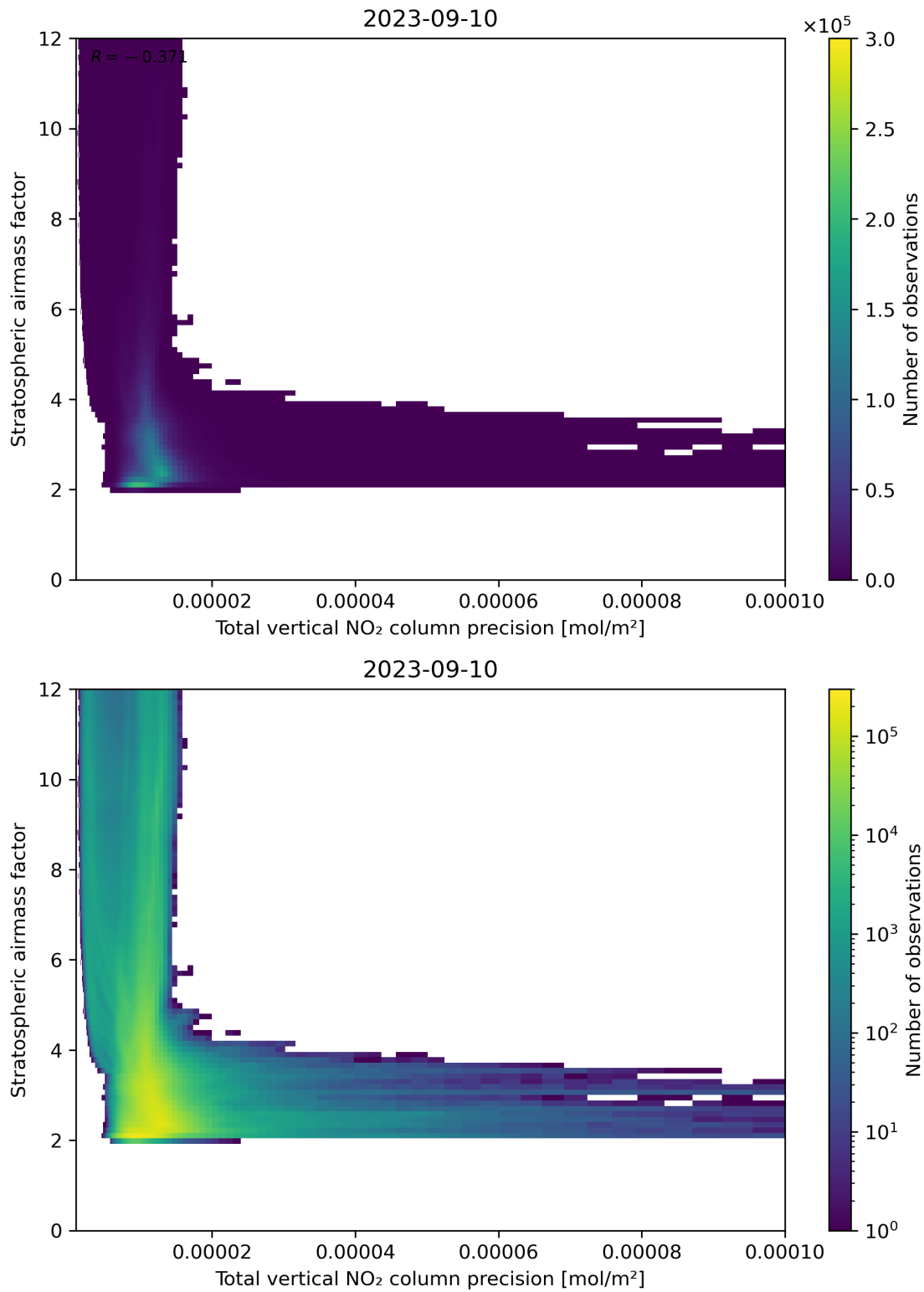
Figure 115: Scatter density plot of “Total vertical NO 2 column precision” against “Stratospheric air mass factor” for 2023-09-10 to 2023-09-11.
