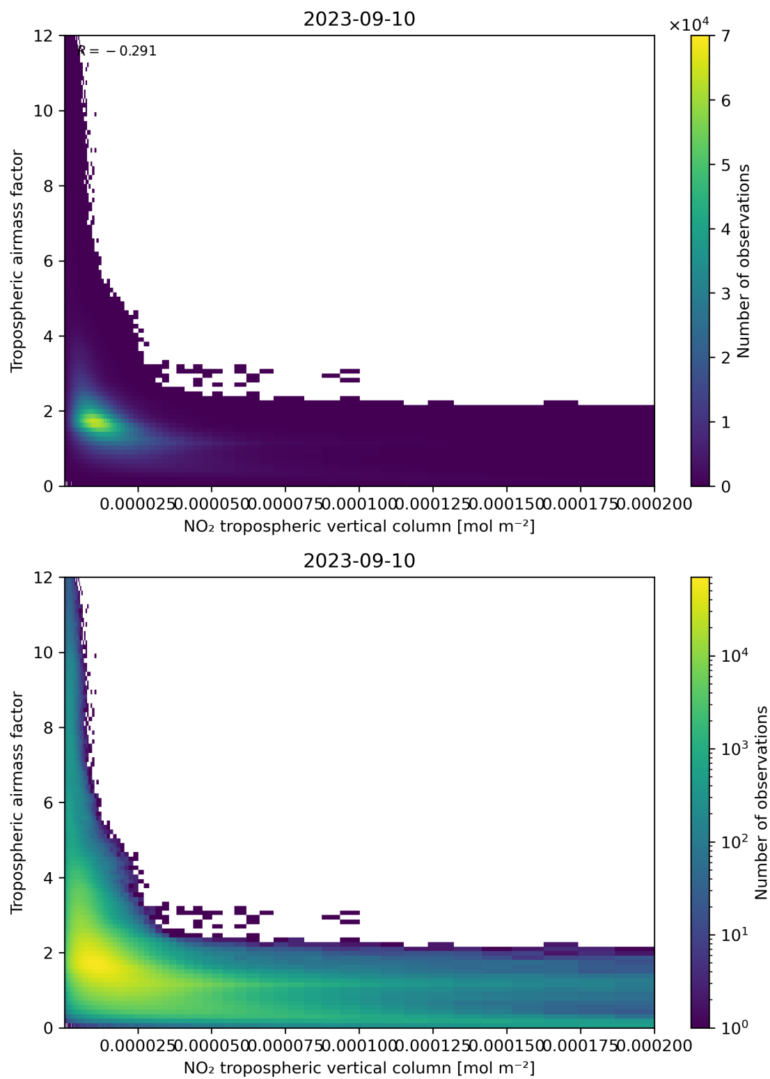
Figure 123: Scatter density plot of “NO 2 tropospheric vertical column” against “Tropospheric air mass factor” for 2023-09-10 to 2023-09-11.
