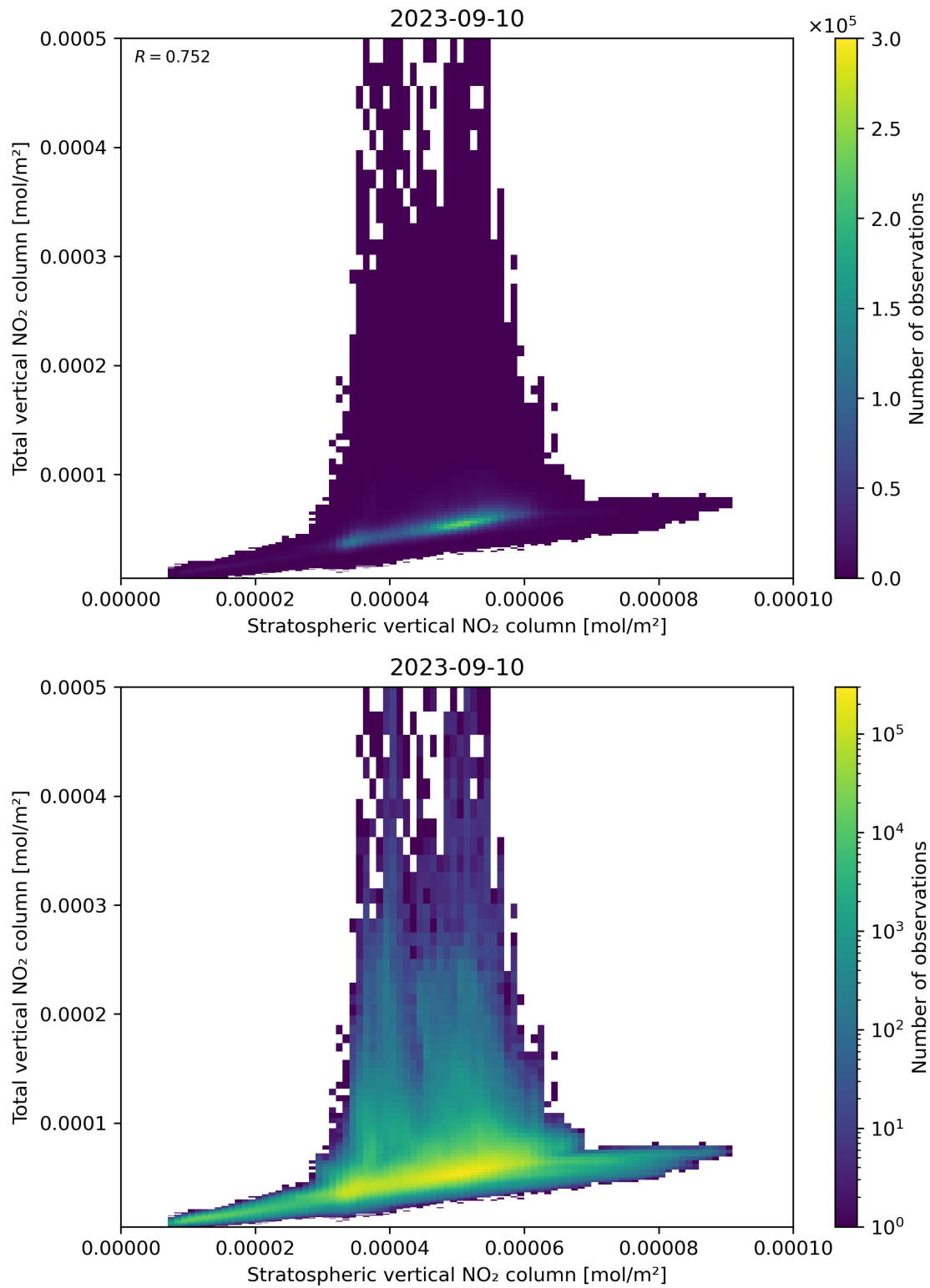
Figure 100: Scatter density plot of “Stratospheric vertical NO 2 column” against “Total vertical NO 2 column” for 2023-09-10 to 2023-09-11.
