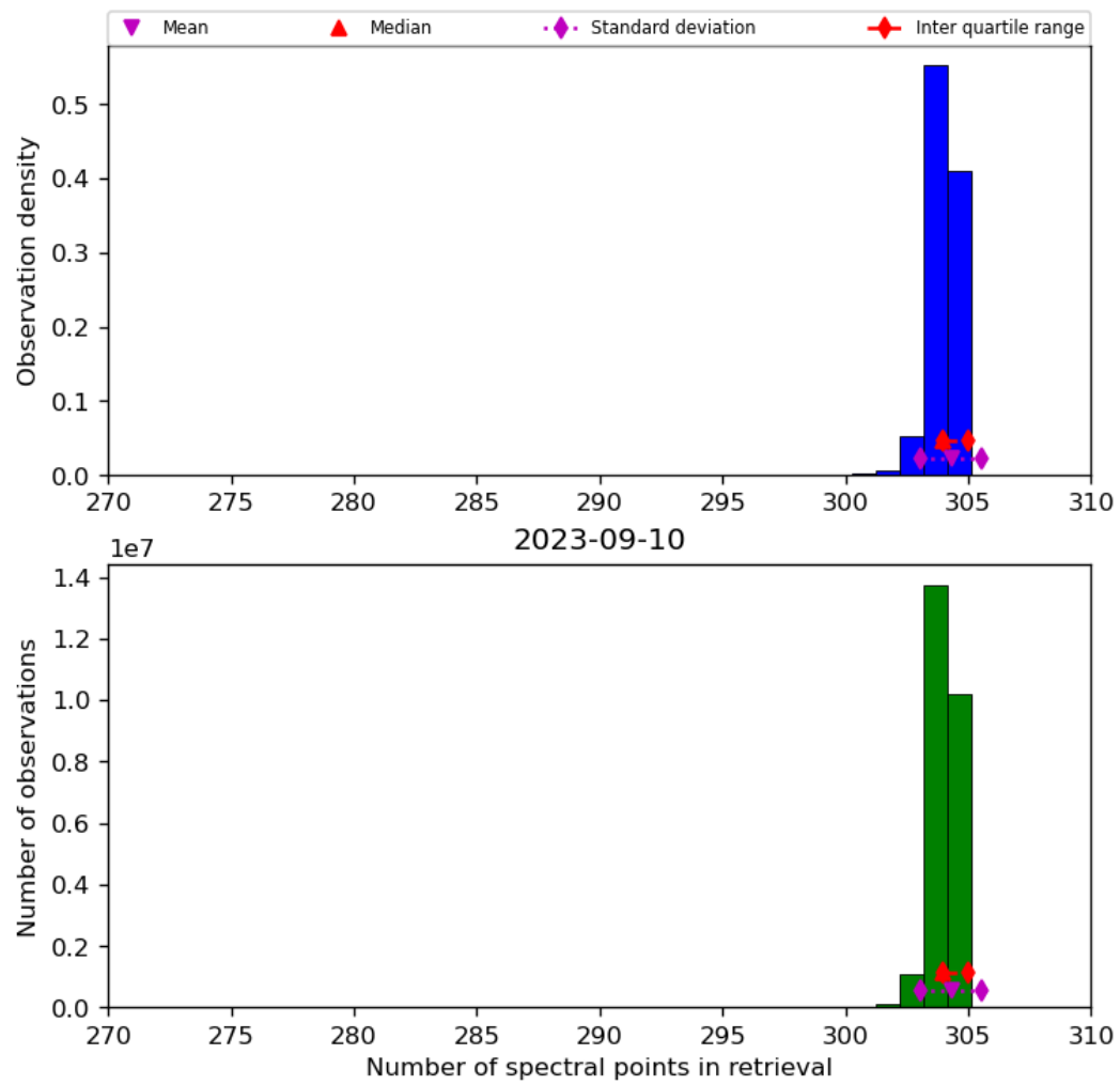
Figure 33: Histogram of “Number of spectral points in retrieval” for 2023-09-10 to 2023-09-11
