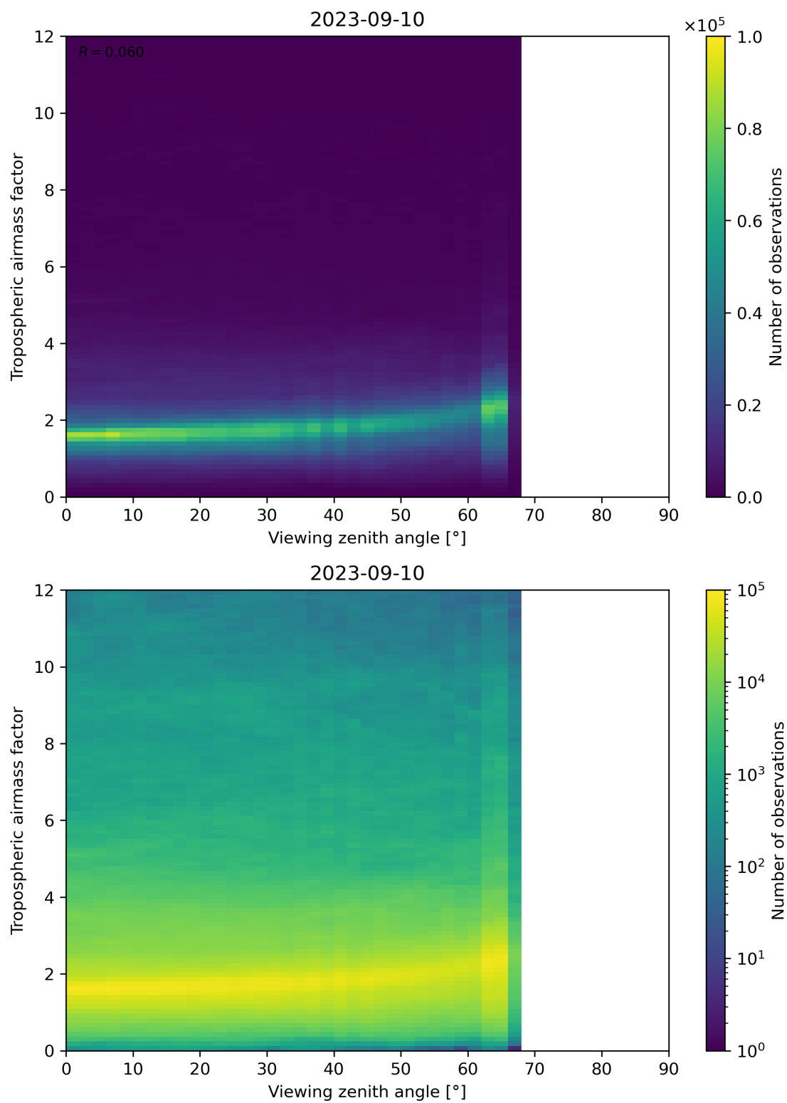
Figure 161: Scatter density plot of “Viewing zenith angle” against “Tropospheric airmass factor” for 2023-09-10 to 2023-09-11.
