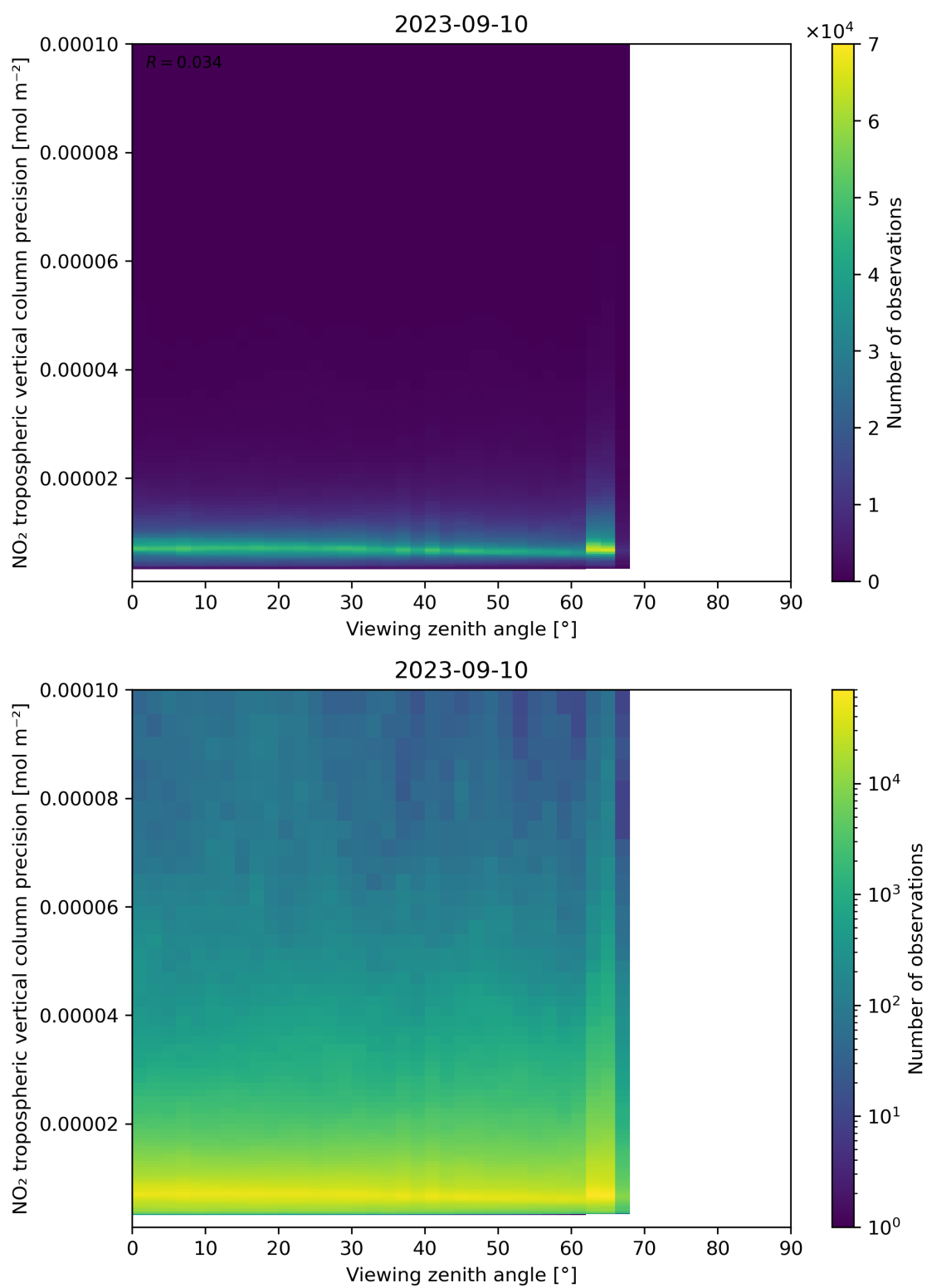
Figure 170: Scatter density plot of “Viewing zenith angle” against “NO 2 tropospheric vertical column precision” for 2023-09-10 to 2023-09-11.
