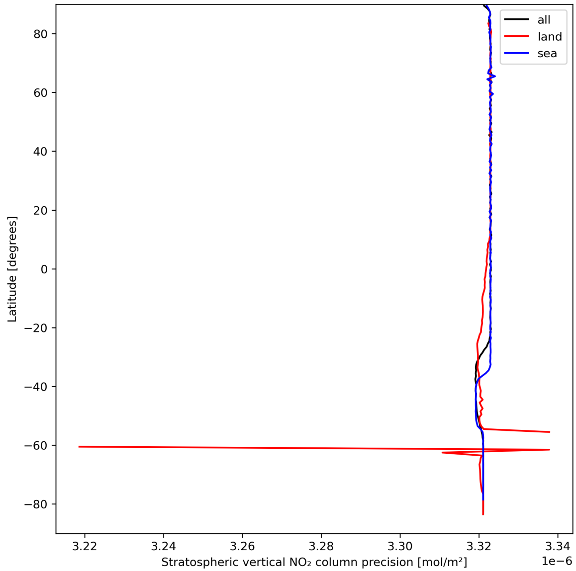
Figure 20: Zonal average of “Stratospheric vertical NO 2 column precision” for 2023-09-10 to 2023-09-11.
