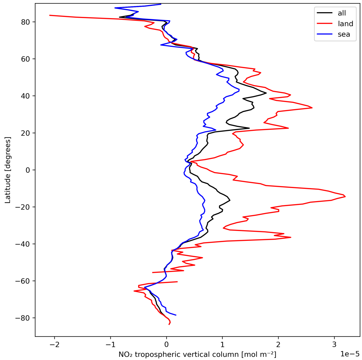
Figure 12: Zonal average of “NO 2 tropospheric vertical column” for 2023-09-10 to 2023-09-11.
