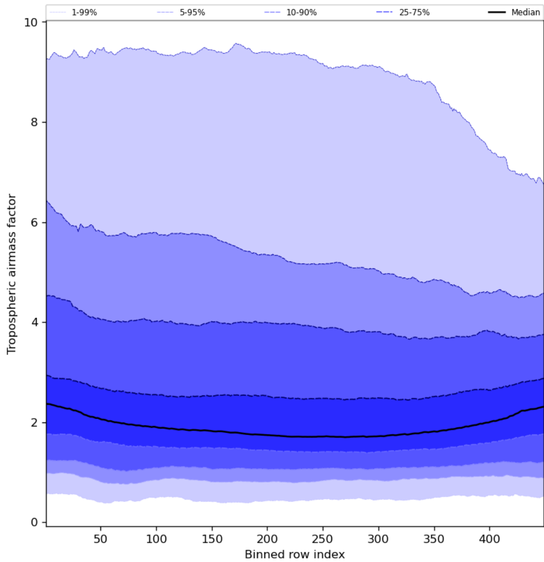
Figure 48: Along track statistics of “Tropospheric air mass factor” for 2023-09-10 to 2023-09-11
