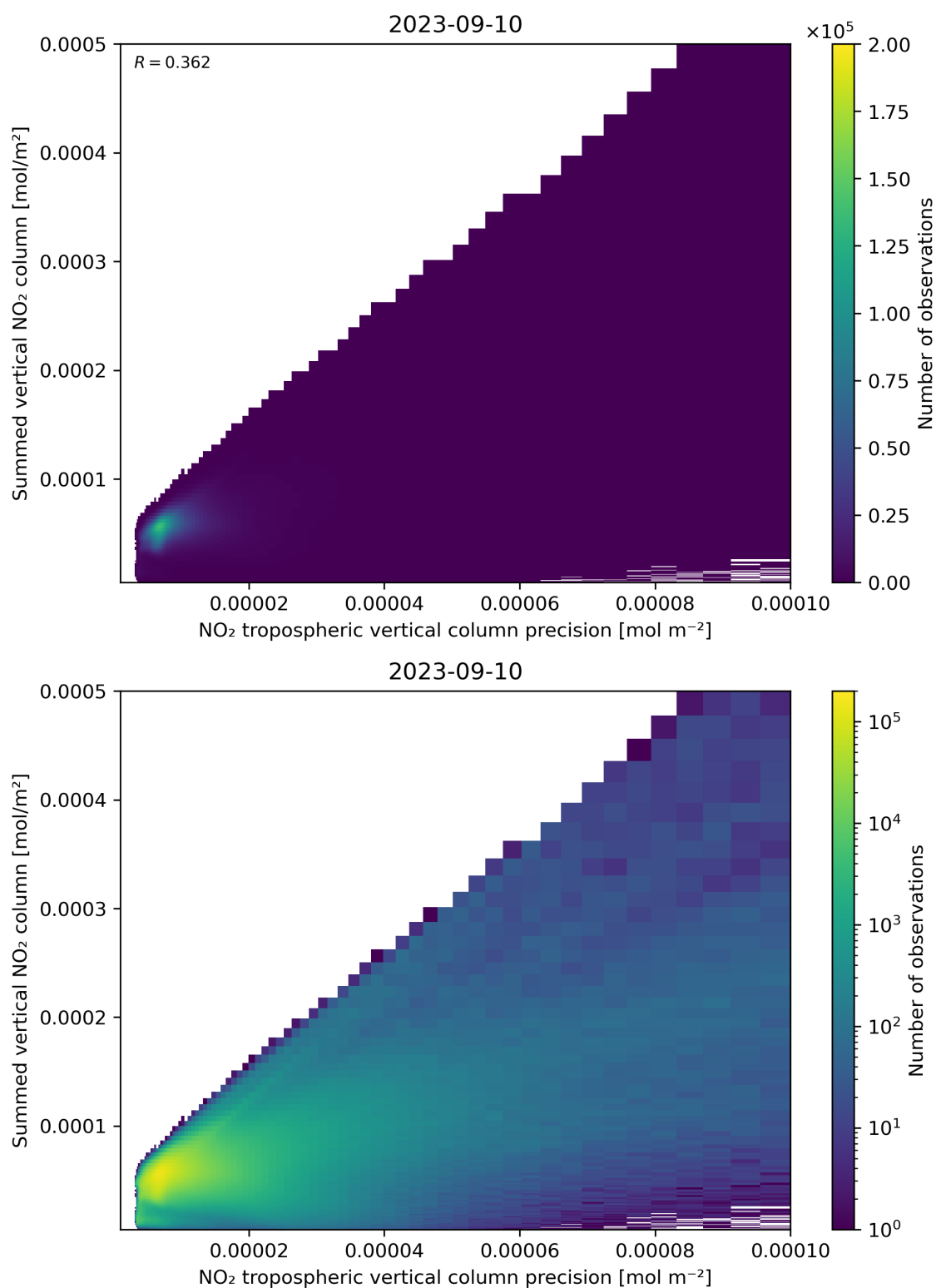
Figure 136: Scatter density plot of “NO 2 tropospheric vertical column precision” against “Summed vertical NO 2 column” for 2023-09-10 to 2023-09-11.
