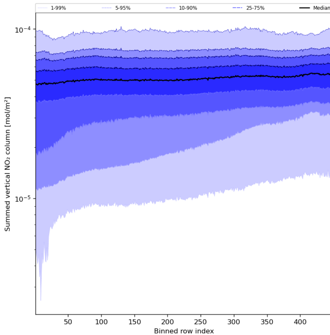
Figure 57: Along track statistics of “Summed vertical NO 2 column” for 2023-09-10 to 2023-09-11
