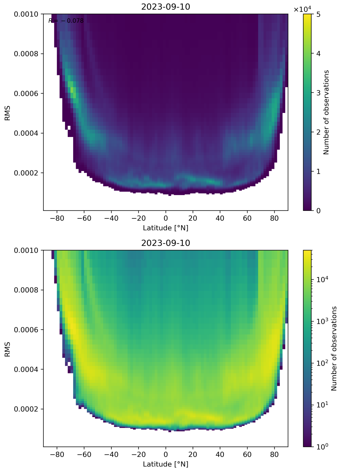
Figure 94: Scatter density plot of “Latitude” against “RMS” for 2023-09-10 to 2023-09-11.
