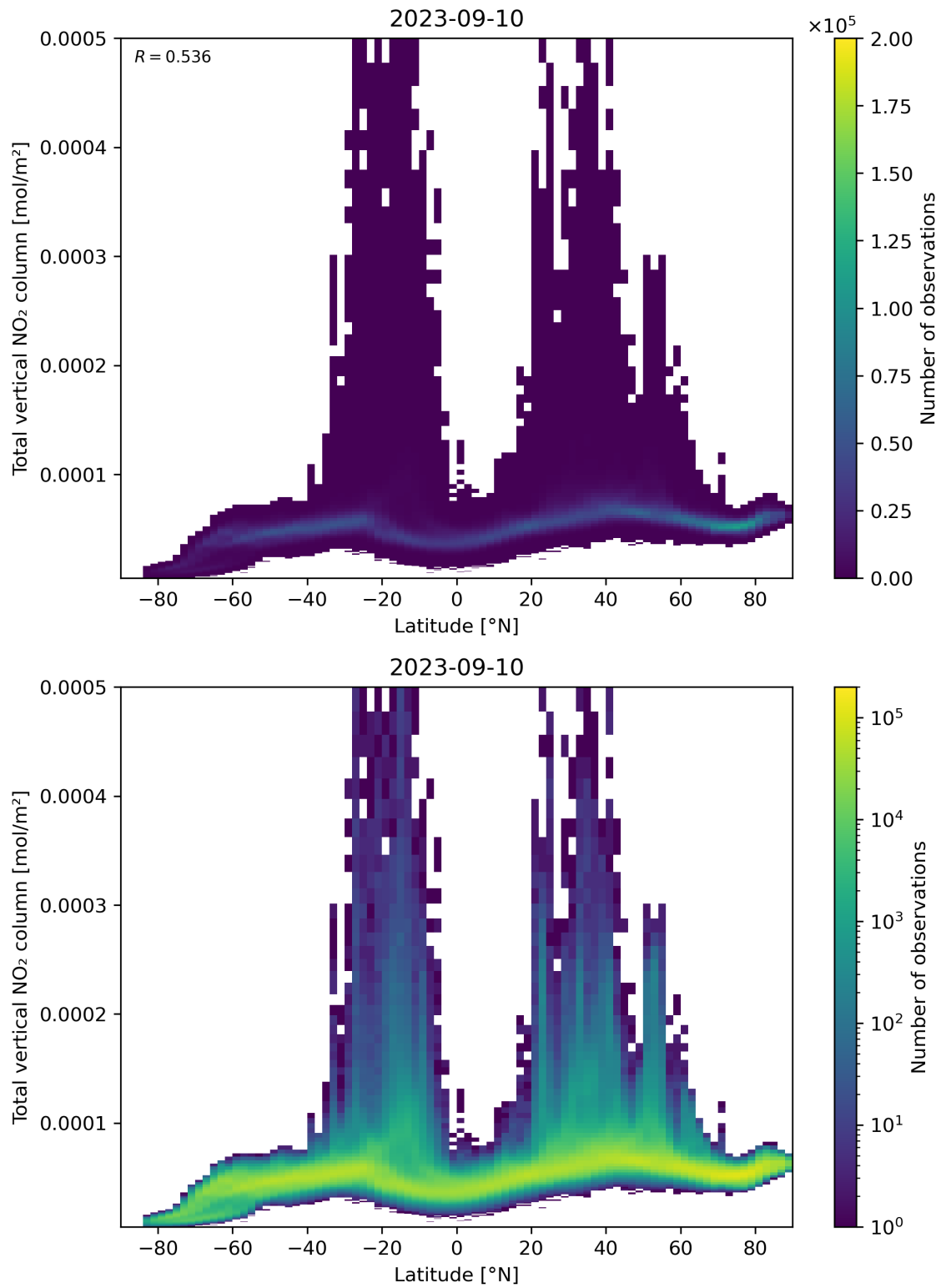
Figure 90: Scatter density plot of “Latitude” against “Total vertical NO 2 column” for 2023-09-10 to 2023-09-11.
