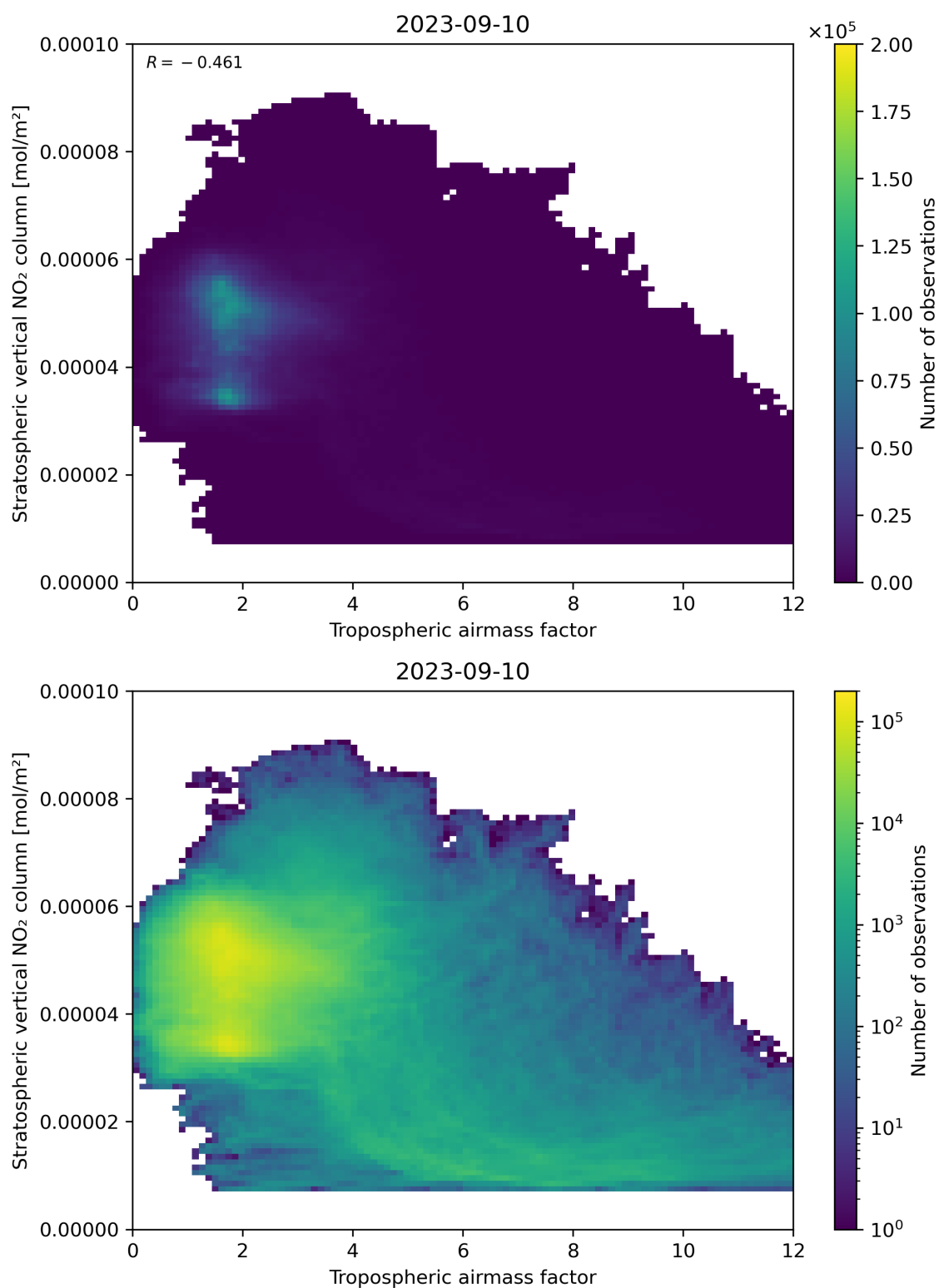
Figure 74: Scatter density plot of “Tropospheric air mass factor” against “Stratospheric vertical NO 2 column” for 2023-09-10 to 2023-09-11.
