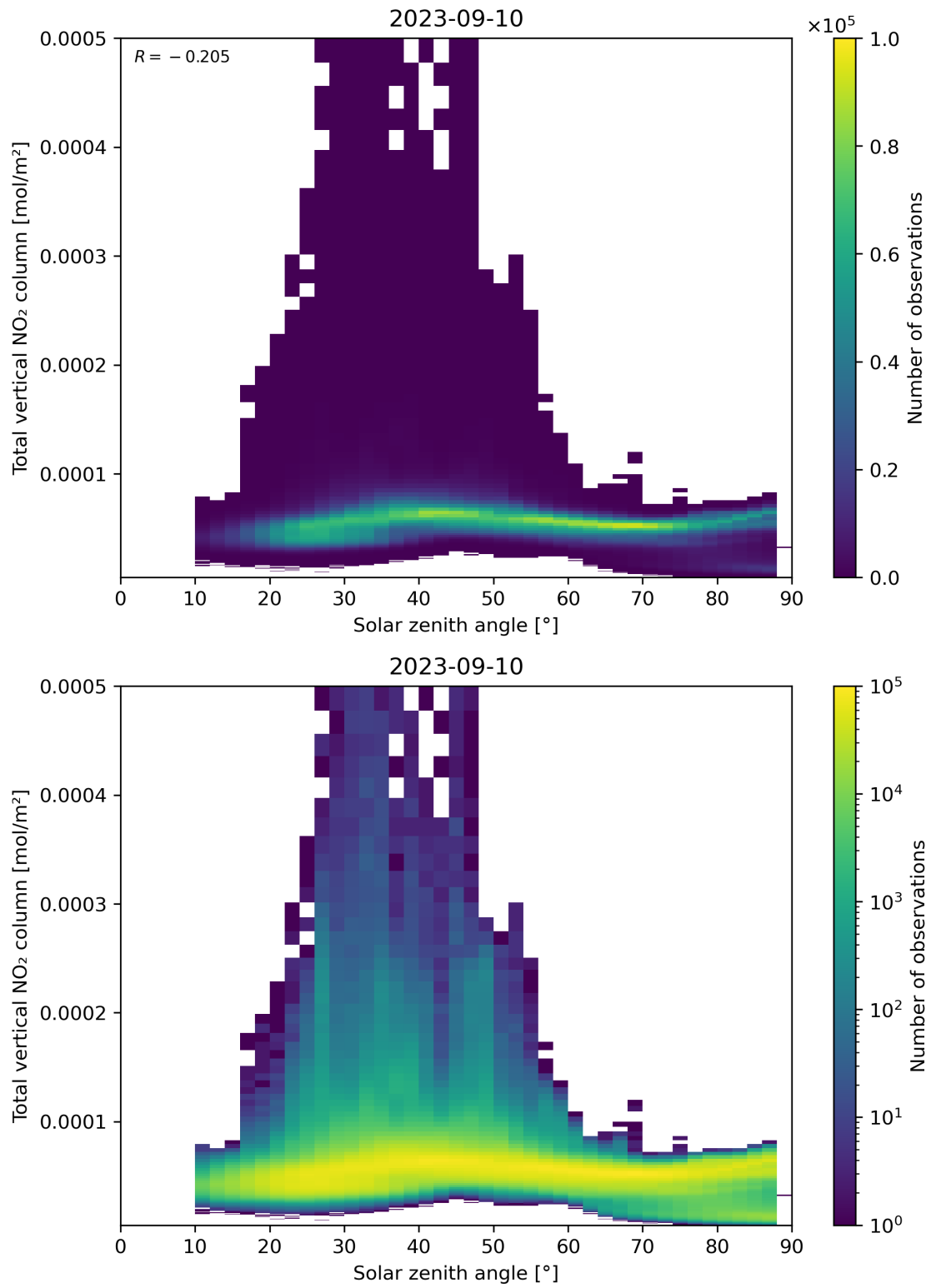
Figure 153: Scatter density plot of “Solar zenith angle” against “Total vertical NO 2 column” for 2023-09-10 to 2023-09-11.
