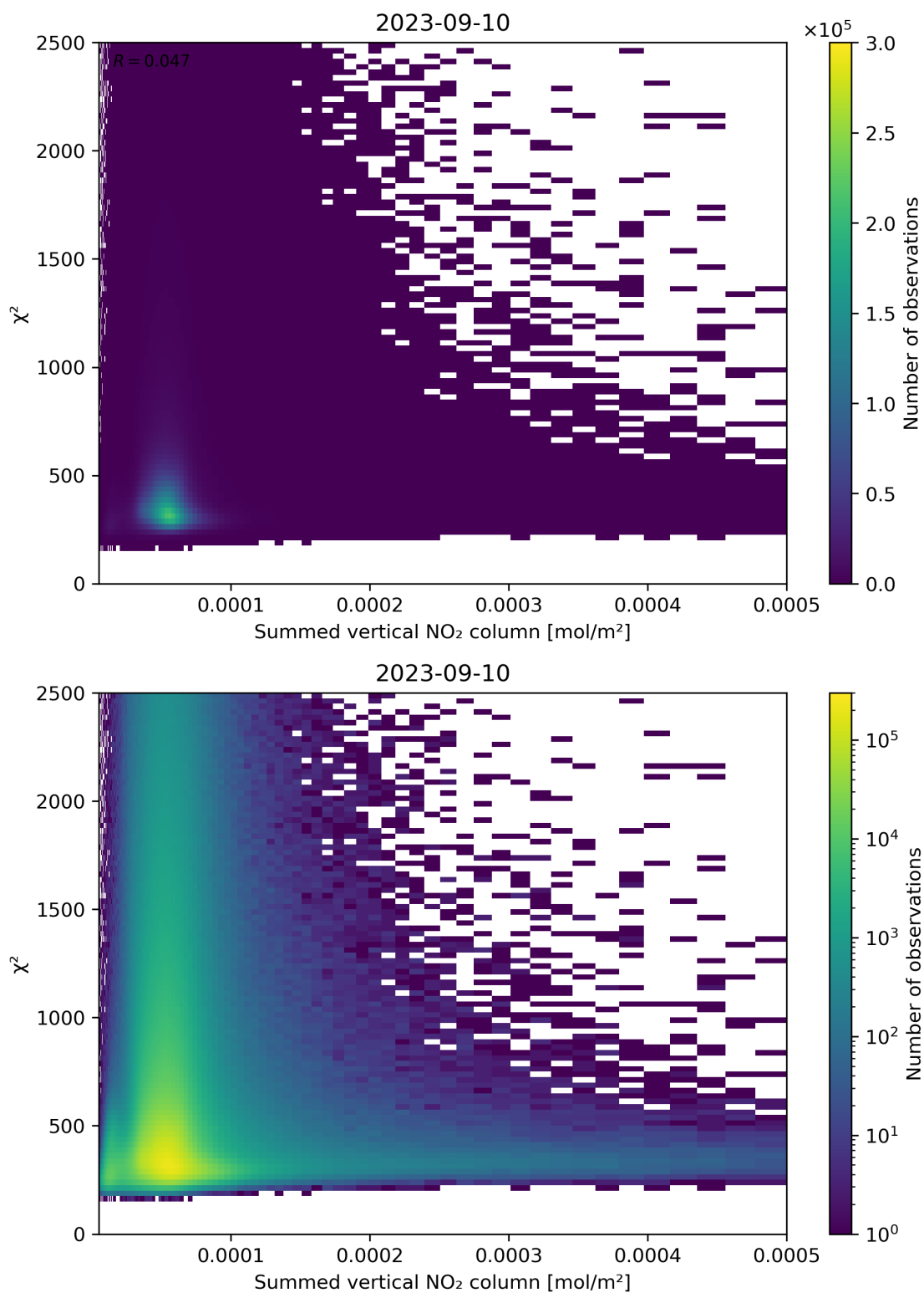
Figure 104: Scatter density plot of “Summed vertical NO 2 column” against “ \chi^2 ” for 2023-09-10 to 2023-09-11.
