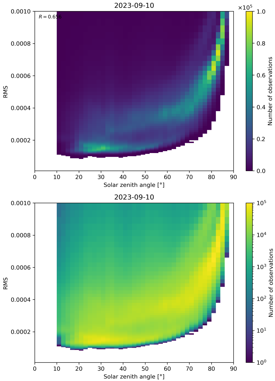
Figure 157: Scatter density plot of “Solar zenith angle” against “RMS” for 2023-09-10 to 2023-09-11.
