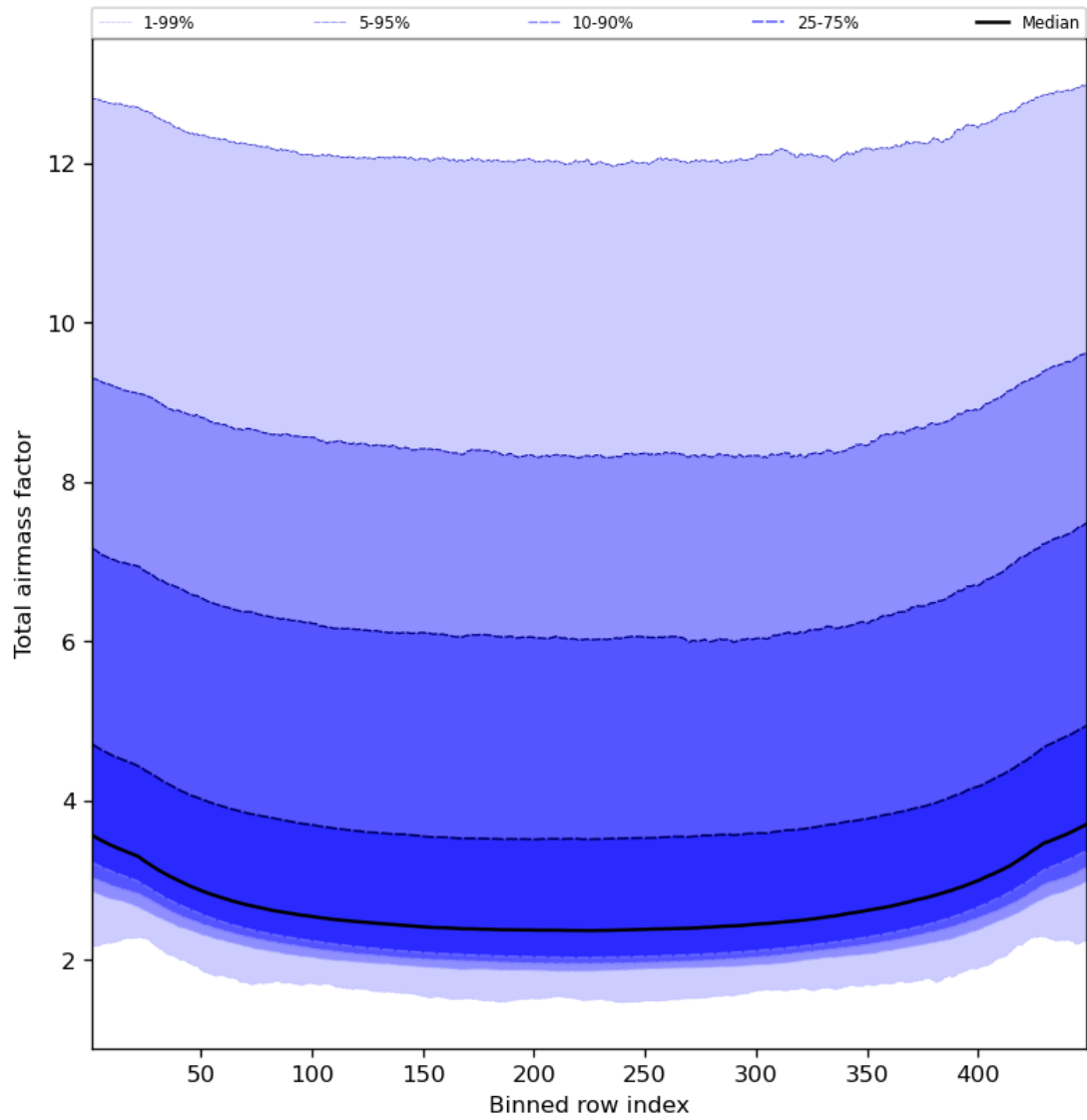
Figure 49: Along track statistics of “Total airmass factor” for 2023-09-10 to 2023-09-11
