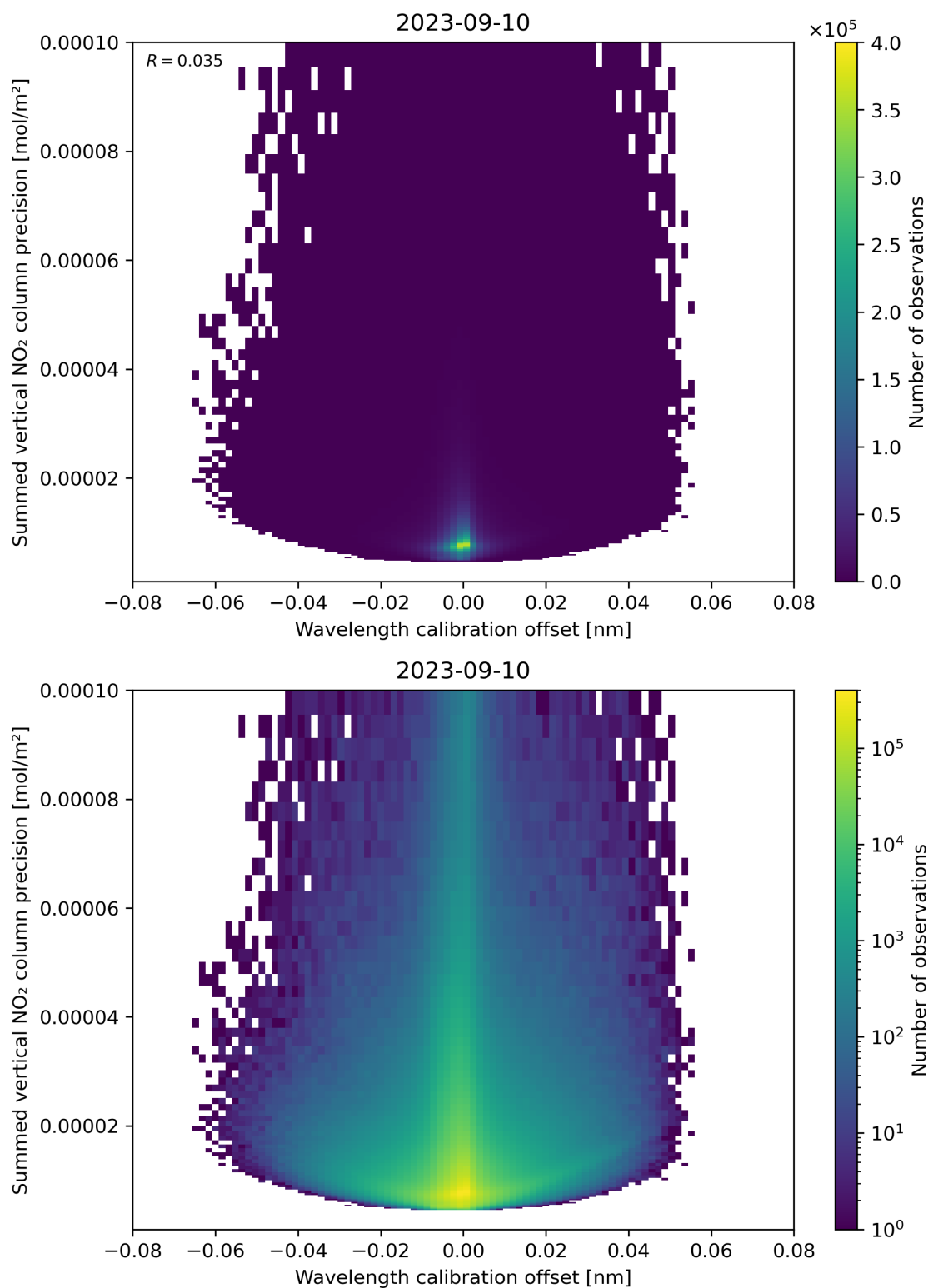
Figure 178: Scatter density plot of “Wavelength calibration offset” against “Summed vertical NO 2 column precision” for 2023-09-10 to 2023-09-11.
