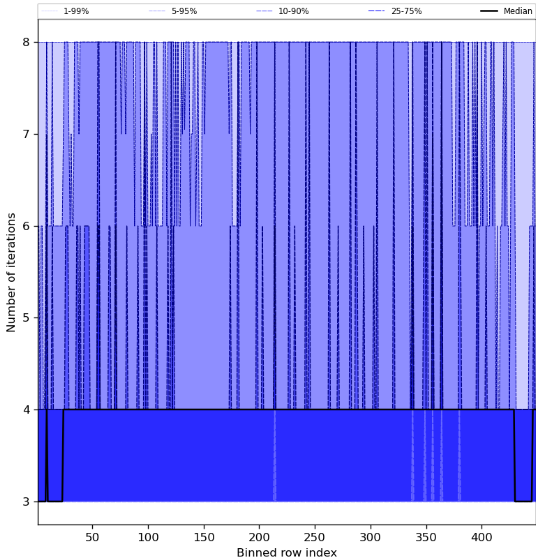
Figure 51: Along track statistics of “Number of iterations” for 2023-09-10 to 2023-09-11
