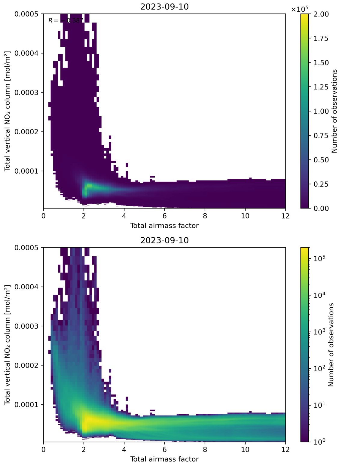
Figure 67: Scatter density plot of “Total airmass factor” against “Total vertical NO 2 column” for 2023-09-10 to 2023-09-11.
