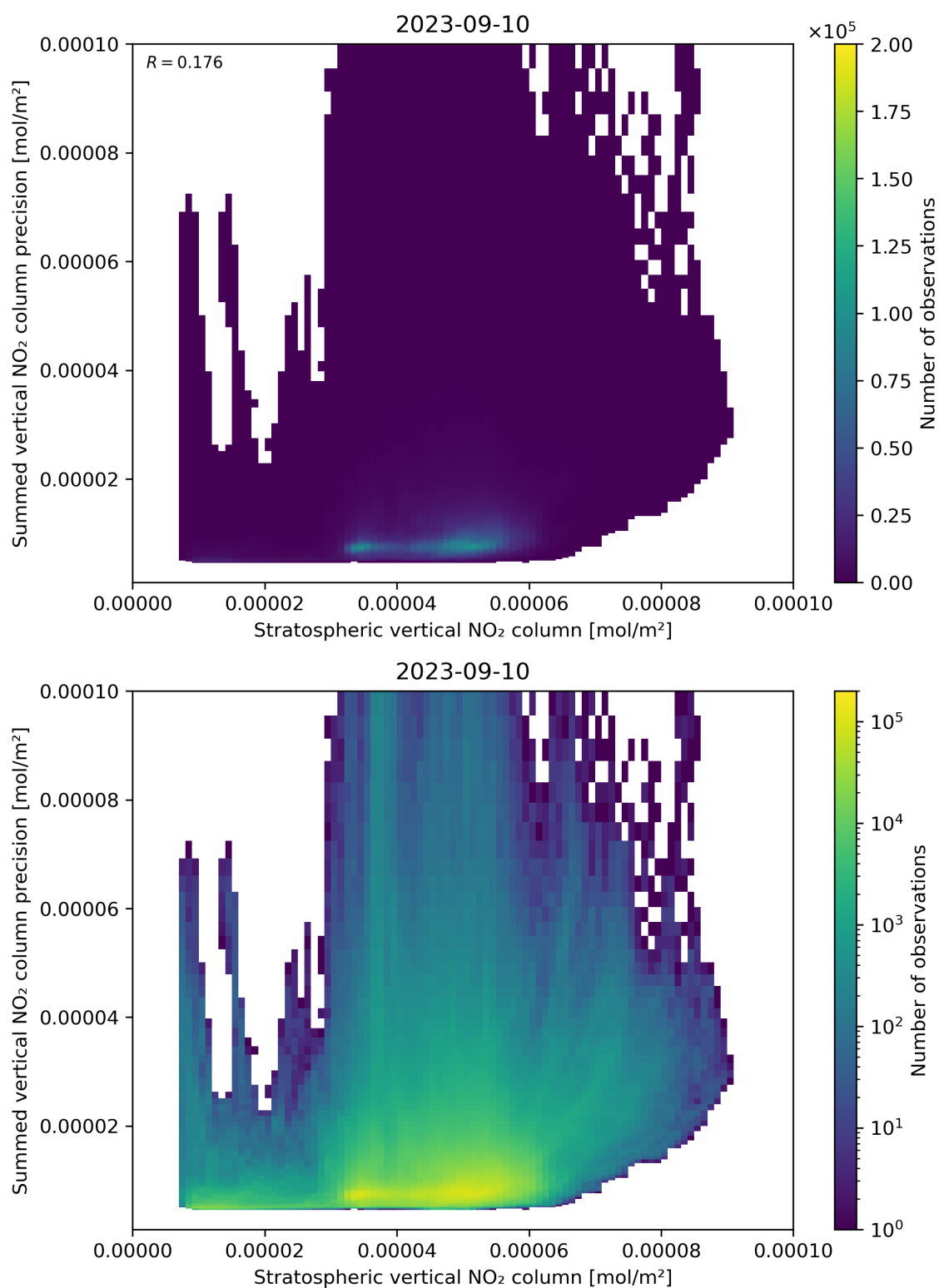
Figure 99: Scatter density plot of “Stratospheric vertical NO 2 column” against “Summed vertical NO 2 column precision” for 2023-09-10 to 2023-09-11.
