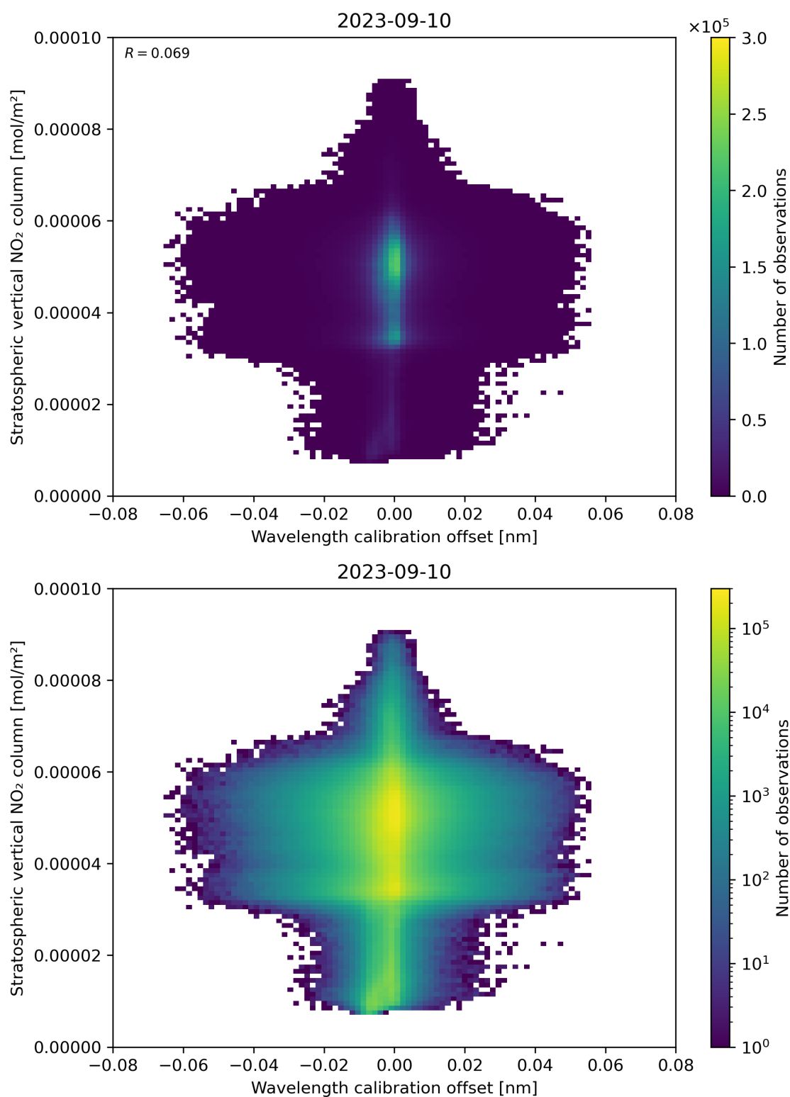
Figure 176: Scatter density plot of “Wavelength calibration offset” against “Stratospheric vertical NO 2 column” for 2023-09-10 to 2023-09-11.
