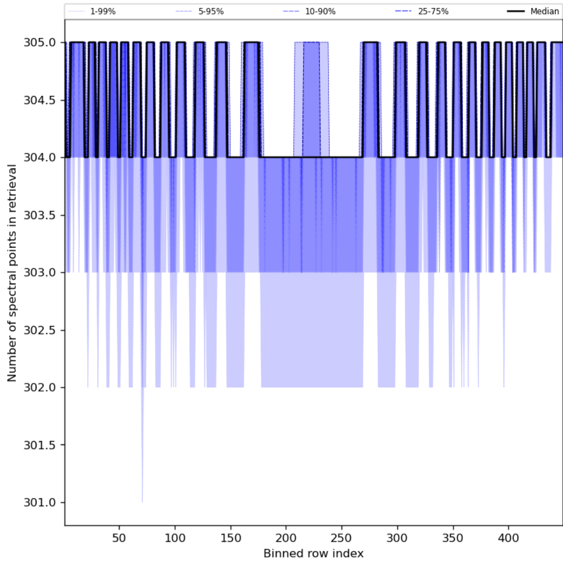
Figure 50: Along track statistics of “Number of spectral points in retrieval” for 2023-09-10 to 2023-09-11
