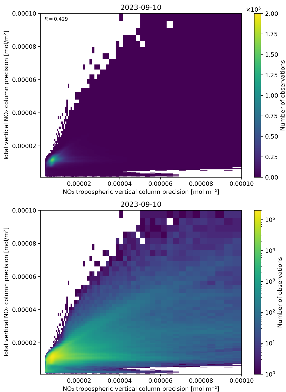
Figure 139: Scatter density plot of “NO 2 tropospheric vertical column precision” against “Total vertical NO 2 column precision” for 2023-09-10 to 2023-09-11.
