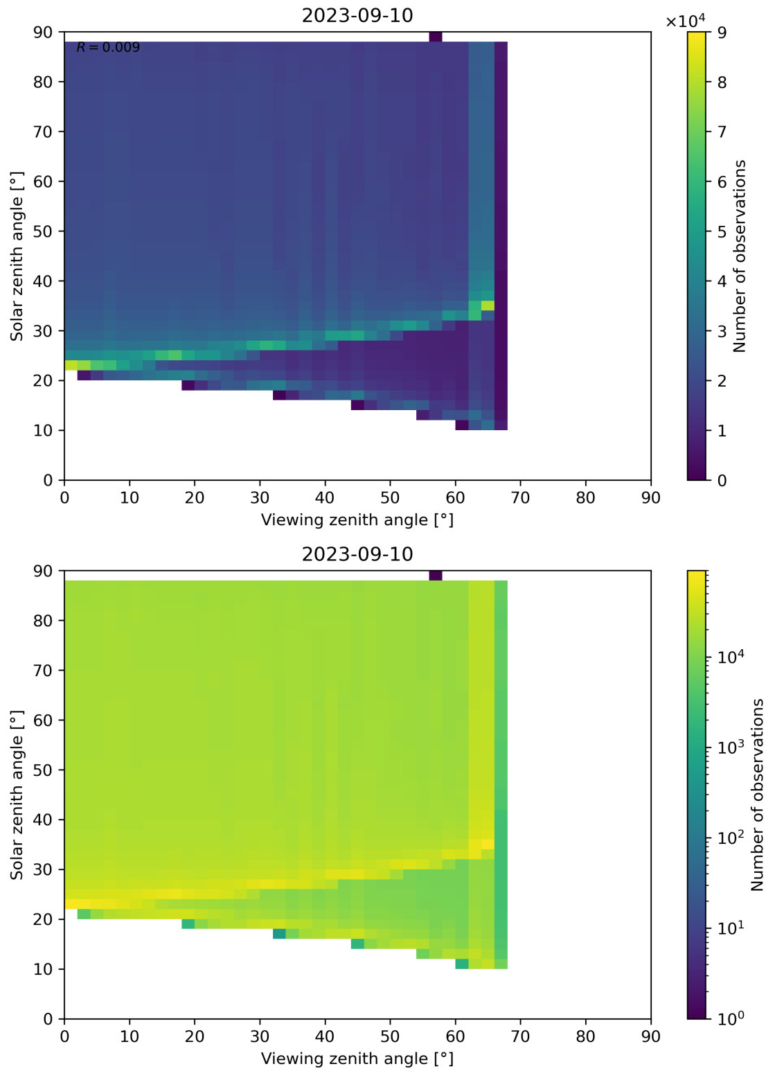
Figure 172: Scatter density plot of “Viewing zenith angle” against “Solar zenith angle” for 2023-09-10 to 2023-09-11.
