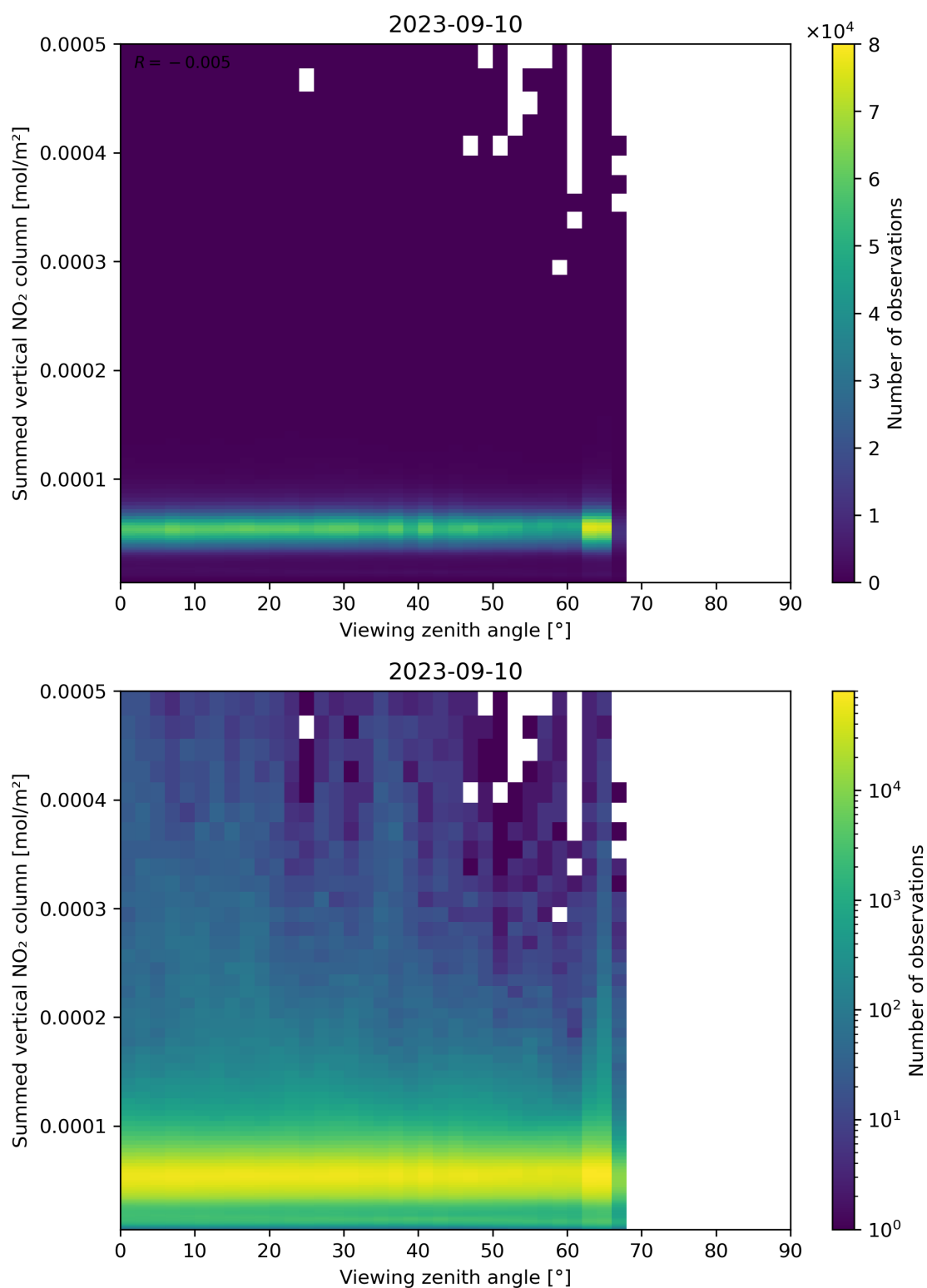
Figure 165: Scatter density plot of “Viewing zenith angle” against “Summed vertical NO 2 column” for 2023-09-10 to 2023-09-11.
