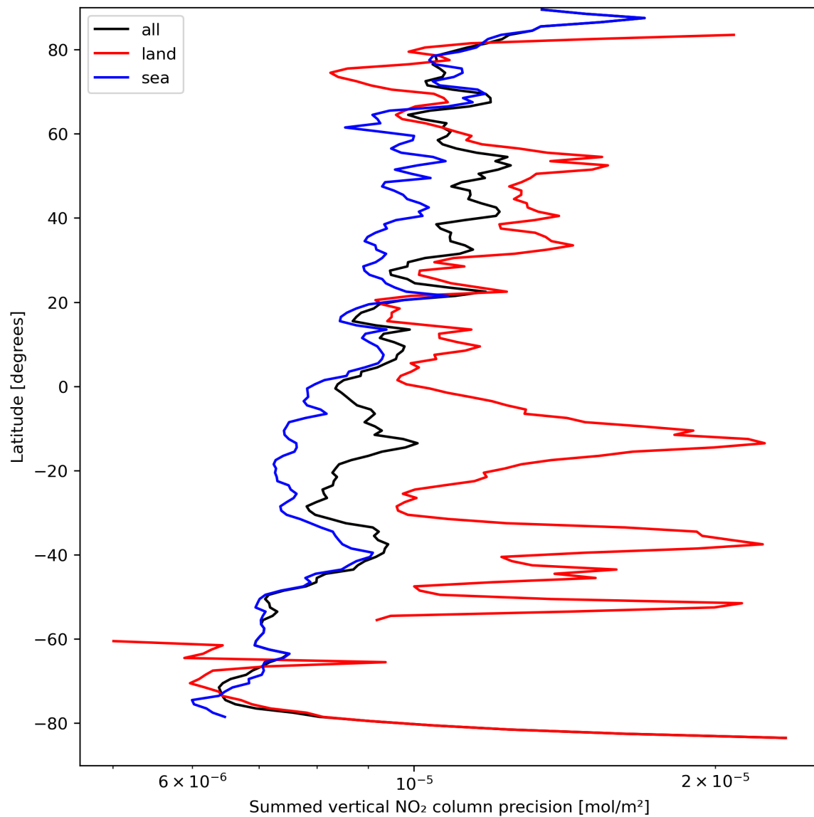
Figure 24: Zonal average of “Summed vertical NO 2 column precision” for 2023-09-10 to 2023-09-11.
