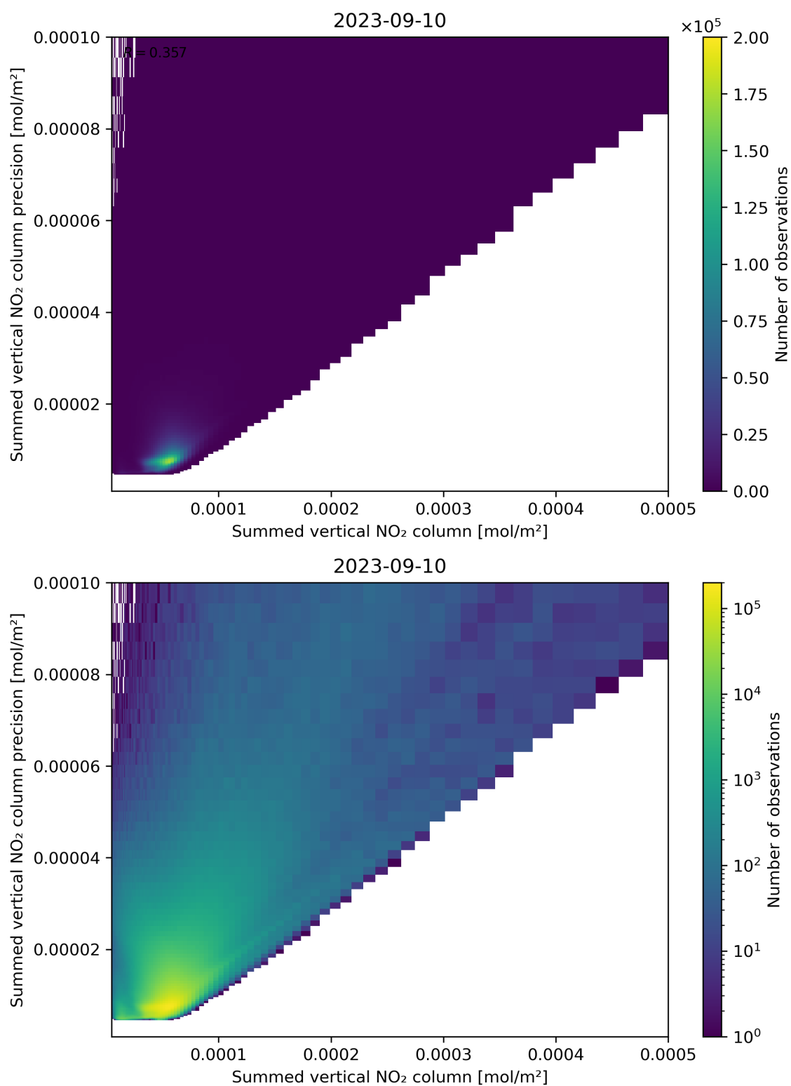
Figure 105: Scatter density plot of “Summed vertical NO 2 column” against “Summed vertical NO 2 column precision” for 2023-09-10 to 2023-09-11.
