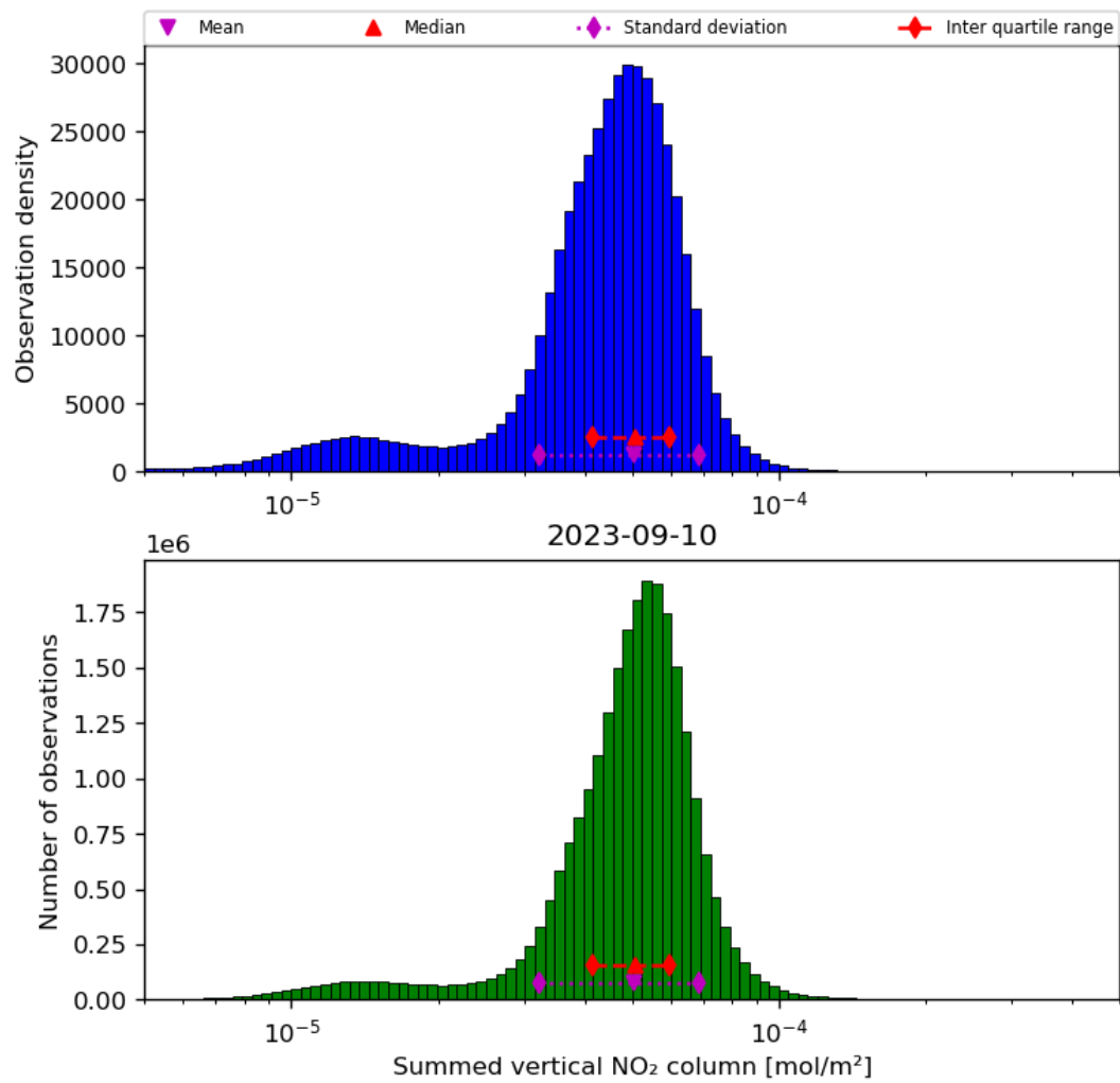
Figure 40: Histogram of “Summed vertical NO 2 column” for 2023-09-10 to 2023-09-11
