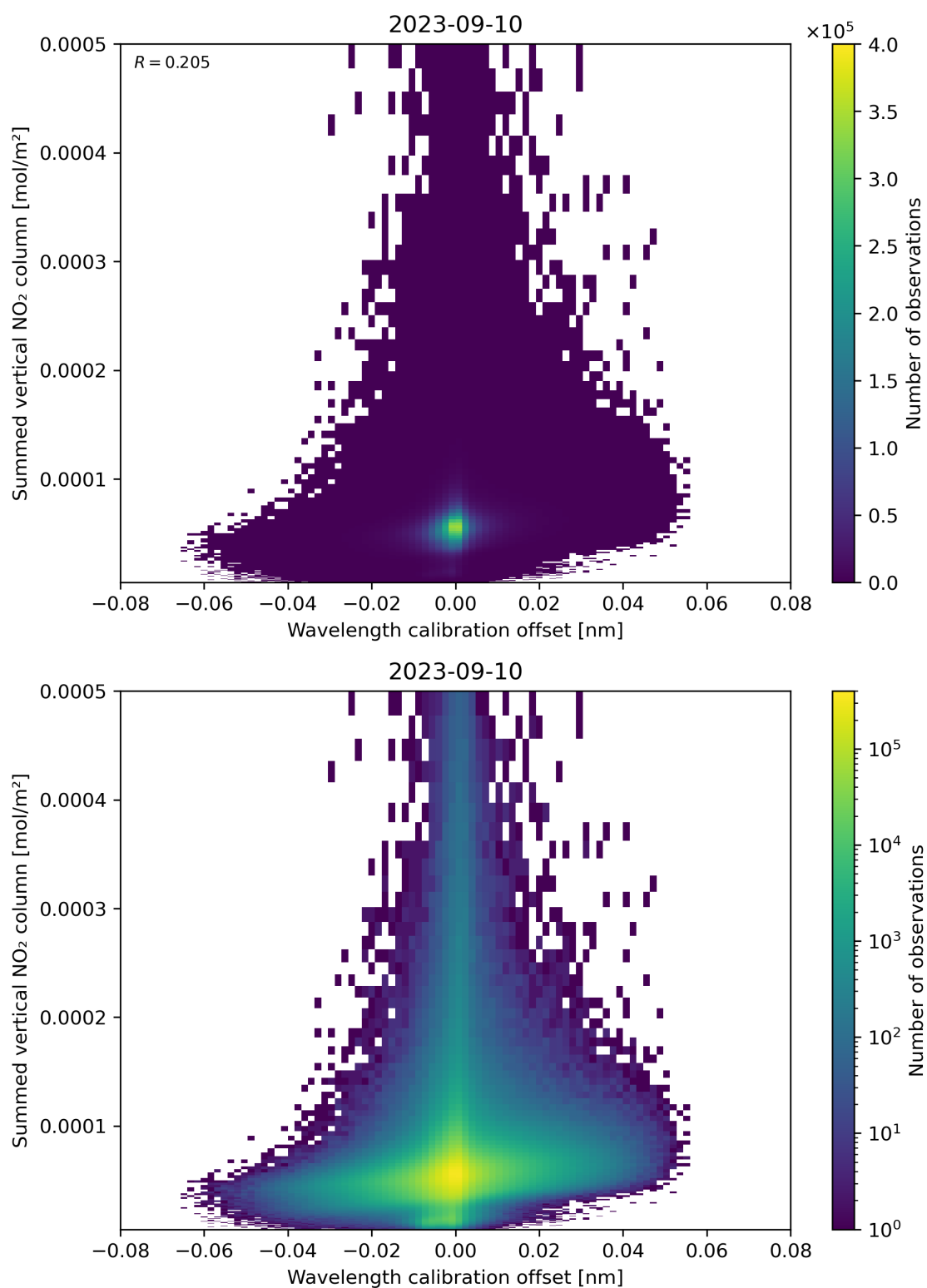
Figure 177: Scatter density plot of “Wavelength calibration offset” against “Summed vertical NO 2 column” for 2023-09-10 to 2023-09-11.
