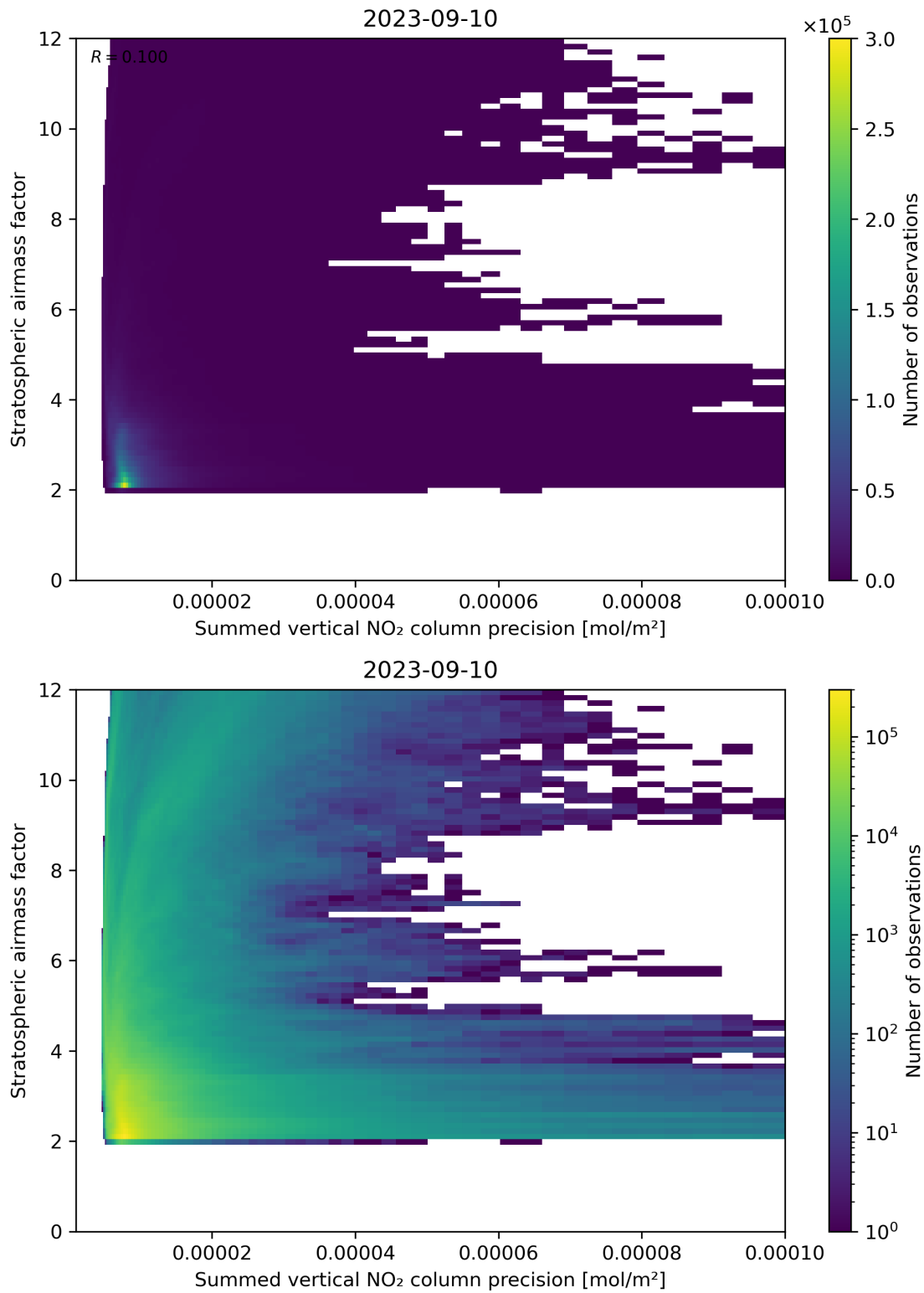
Figure 106: Scatter density plot of “Summed vertical NO 2 column precision” against “Stratospheric airmass factor” for 2023-09-10 to 2023-09-11.
