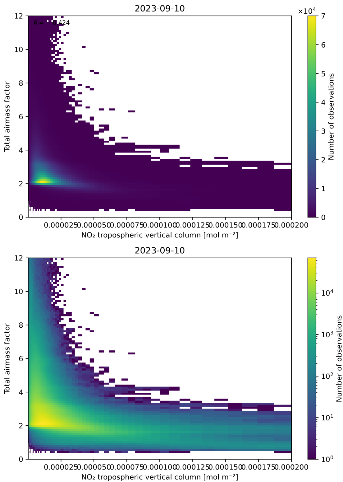
Figure 122: Scatter density plot of “NO 2 tropospheric vertical column” against “Total airmass factor” for 2023-09-10 to 2023-09-11.
