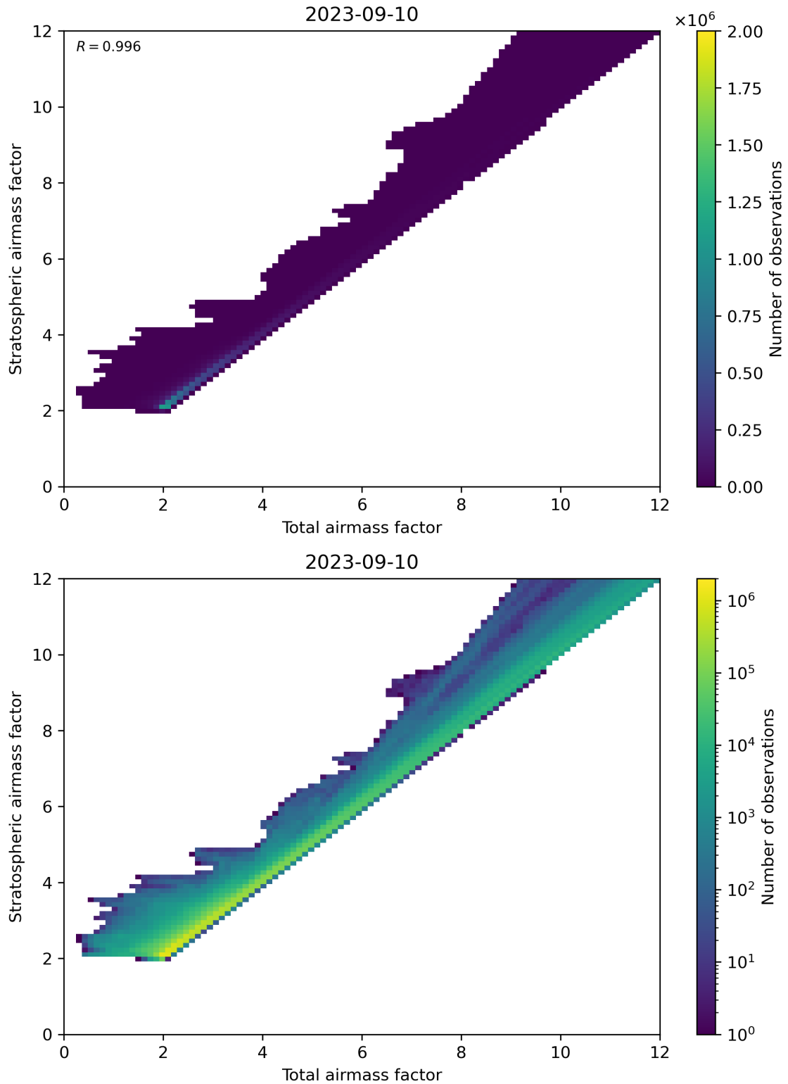
Figure 62: Scatter density plot of “Total airmass factor” against “Stratospheric airmass factor” for 2023-09-10 to 2023-09-11.
