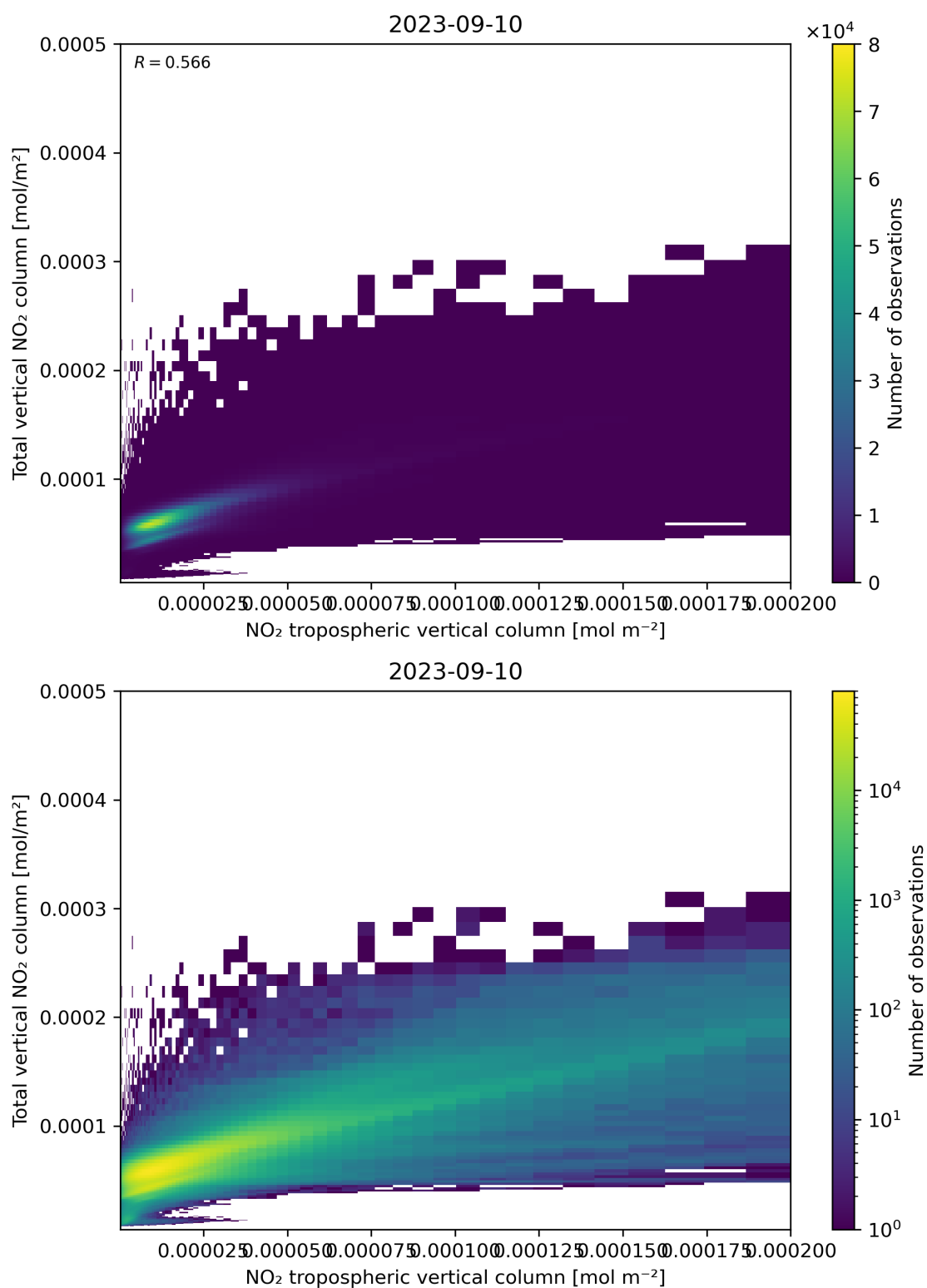
Figure 128: Scatter density plot of “NO 2 tropospheric vertical column” against “Total vertical NO 2 column” for 2023-09-10 to 2023-09-11.
