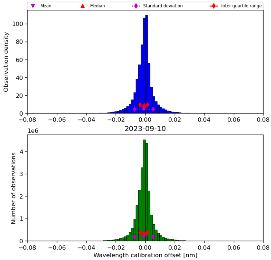
Figure 35: Histogram of “Wavelength calibration offset” for 2023-09-10 to 2023-09-11
