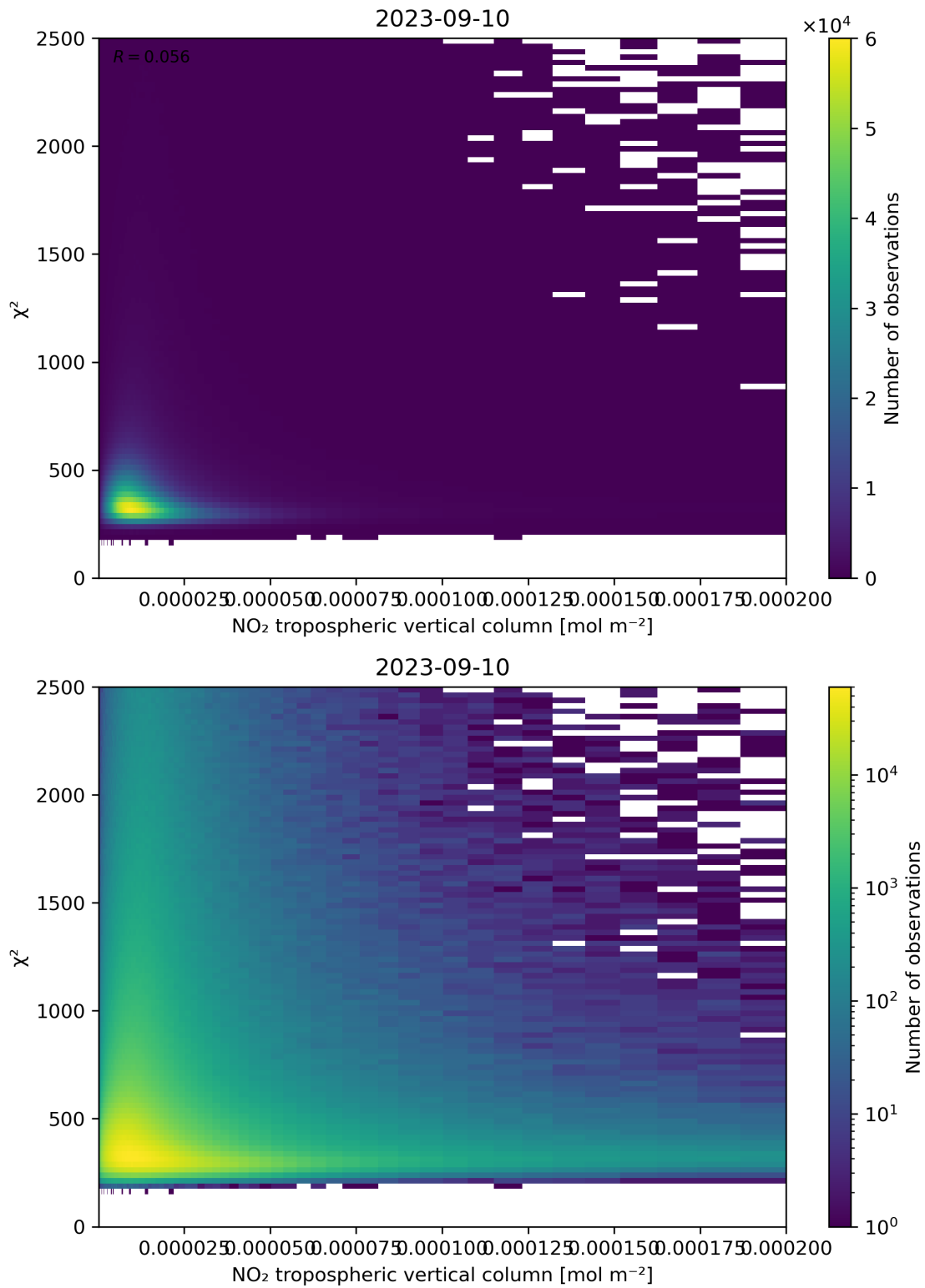
Figure 124: Scatter density plot of “NO 2 tropospheric vertical column” against “ \chi^2 ” for 2023-09-10 to 2023-09-11.
