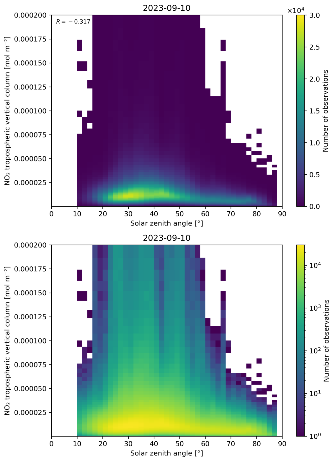
Figure 155: Scatter density plot of “Solar zenith angle” against “NO 2 tropospheric vertical column” for 2023-09-10 to 2023-09-11.
