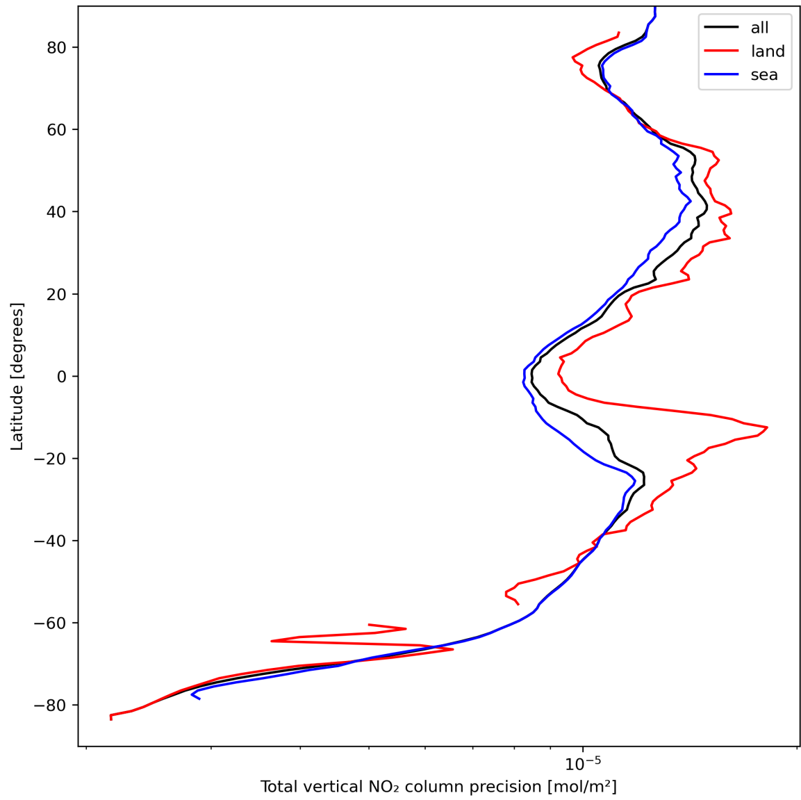
Figure 22: Zonal average of “Total vertical NO 2 column precision” for 2023-09-10 to 2023-09-11.
