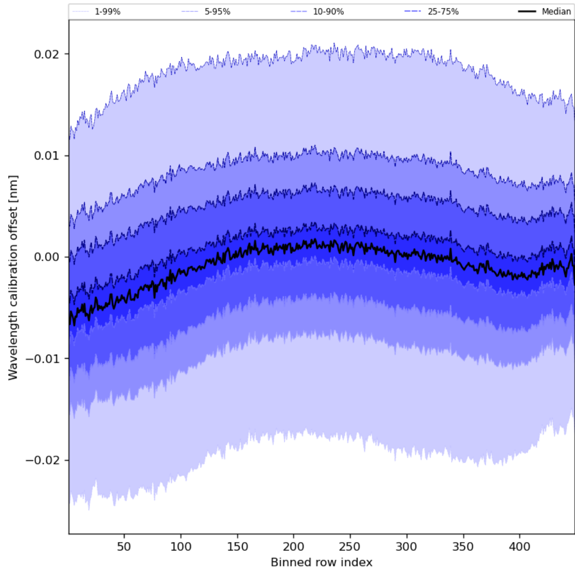
Figure 52: Along track statistics of “Wavelength calibration offset” for 2023-09-10 to 2023-09-11
