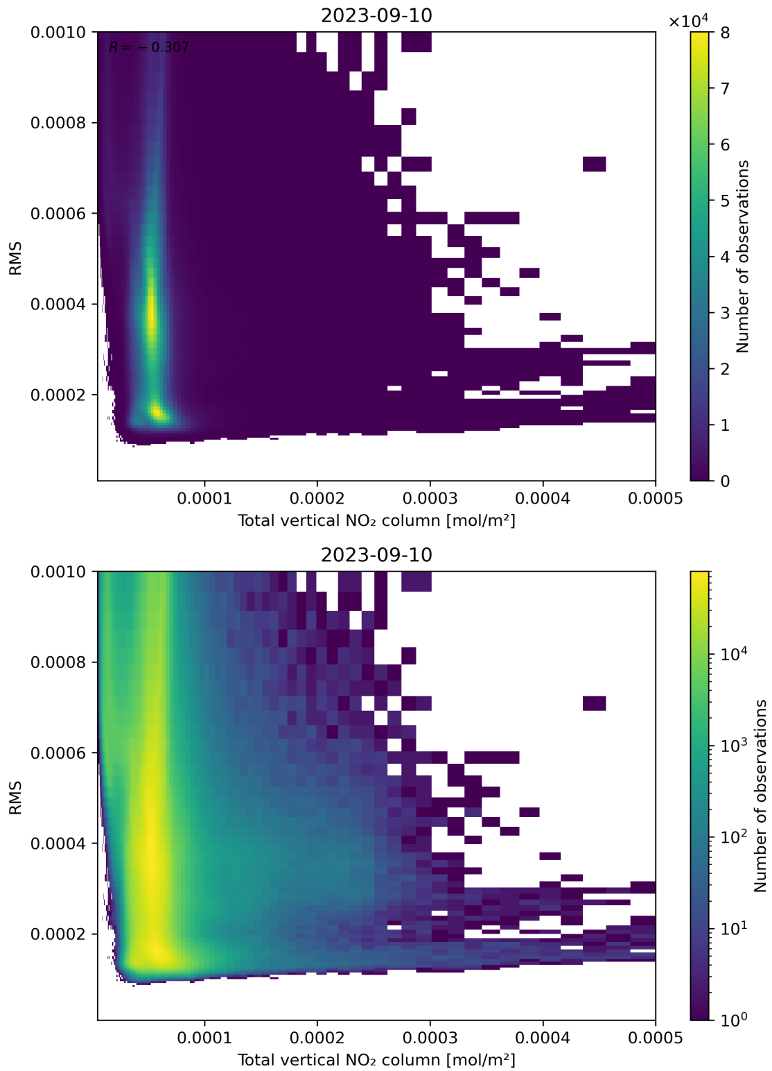
Figure 120: Scatter density plot of “Total vertical NO 2 column” against “RMS” for 2023-09-10 to 2023-09-11.
