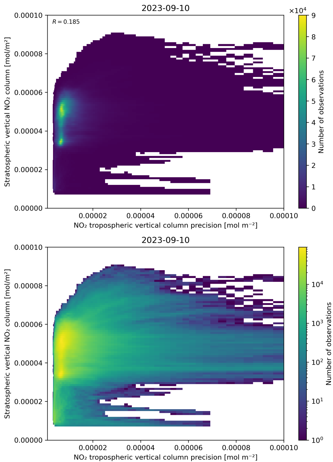
Figure 135: Scatter density plot of “NO 2 tropospheric vertical column precision” against “Stratospheric vertical NO 2 column” for 2023-09-10 to 2023-09-11.
