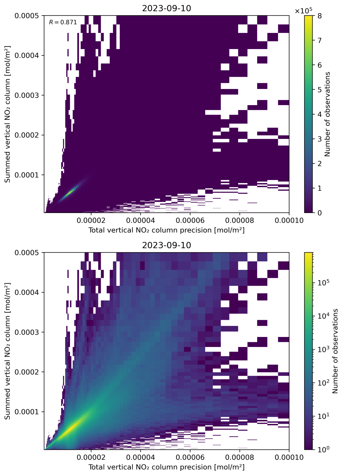
Figure 117: Scatter density plot of “Total vertical NO 2 column precision” against “Summed vertical NO 2 column” for 2023-09-10 to 2023-09-11.
