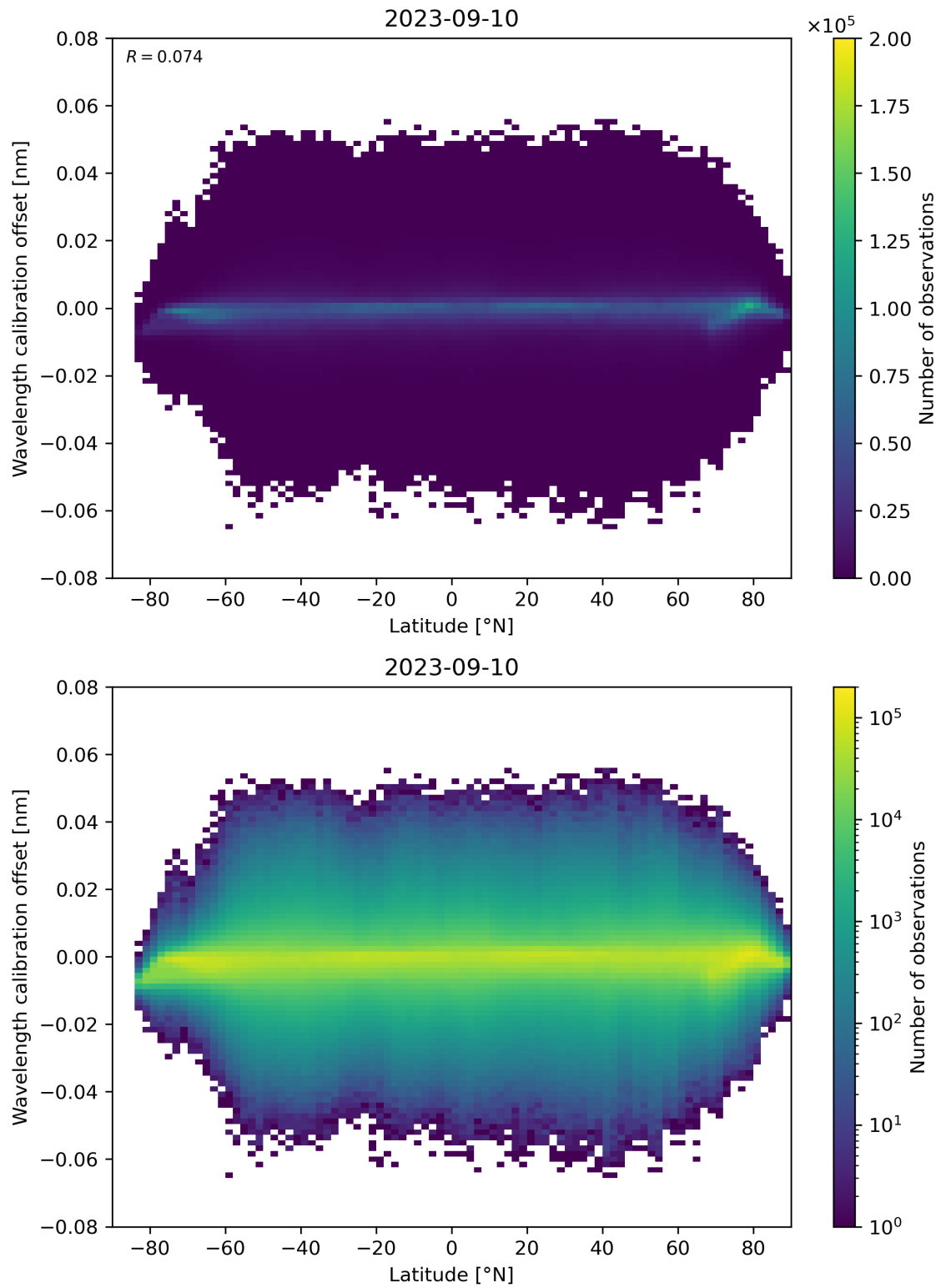
Figure 95: Scatter density plot of “Latitude” against “Wavelength calibration offset” for 2023-09-10 to 2023-09-11.
