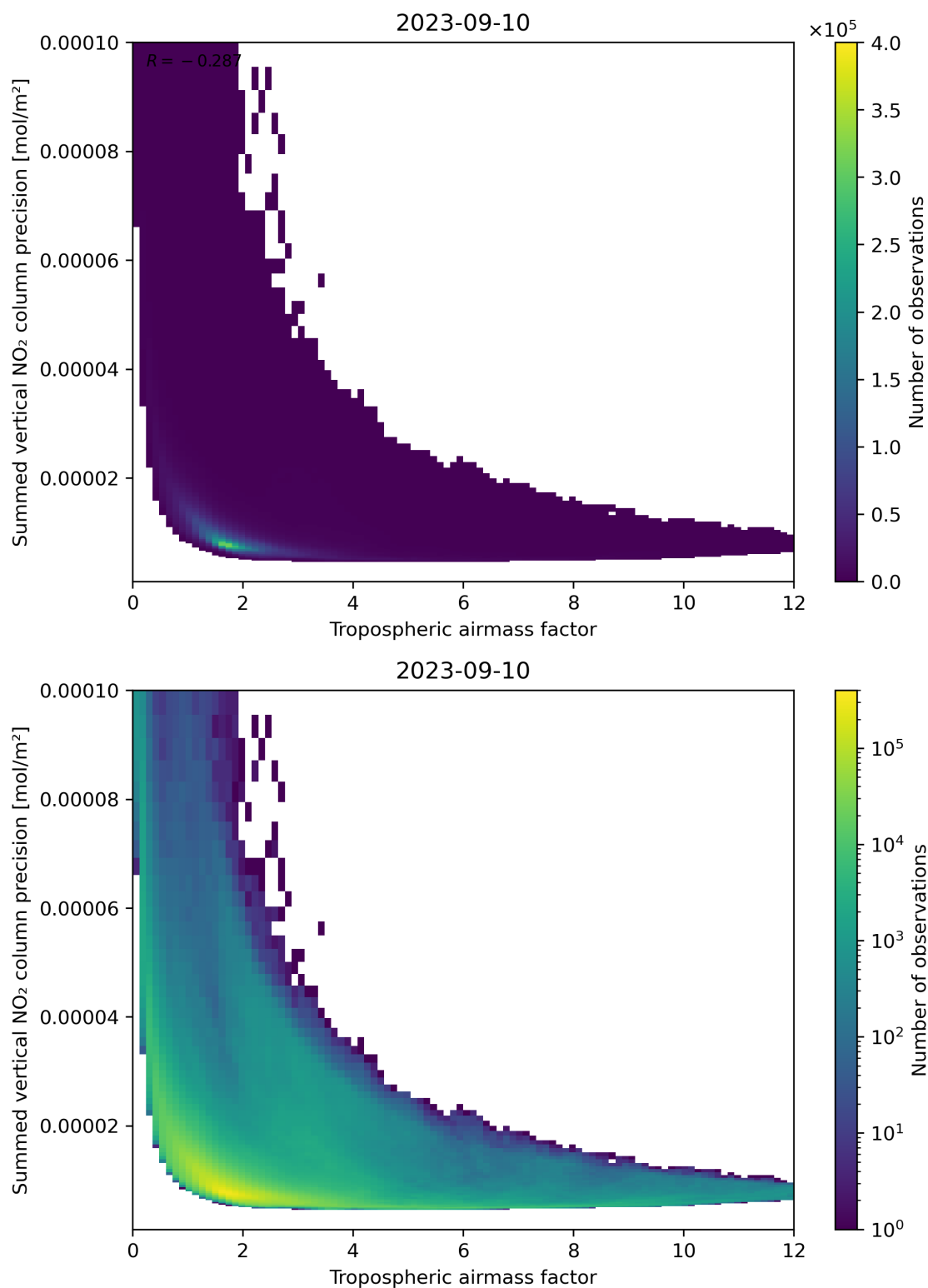
Figure 76: Scatter density plot of “Tropospheric air mass factor” against “Summed vertical NO 2 column precision” for 2023-09-10 to 2023-09-11.
