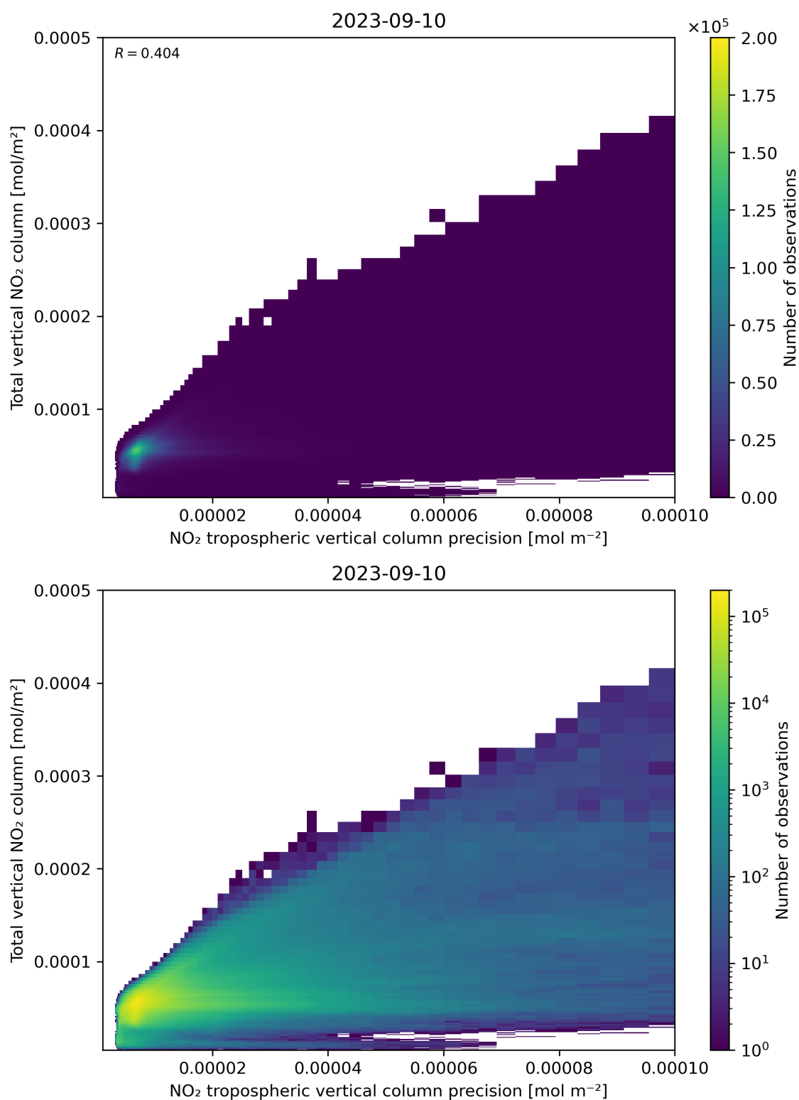
Figure 138: Scatter density plot of “NO 2 tropospheric vertical column precision” against “Total vertical NO 2 column” for 2023-09-10 to 2023-09-11.
