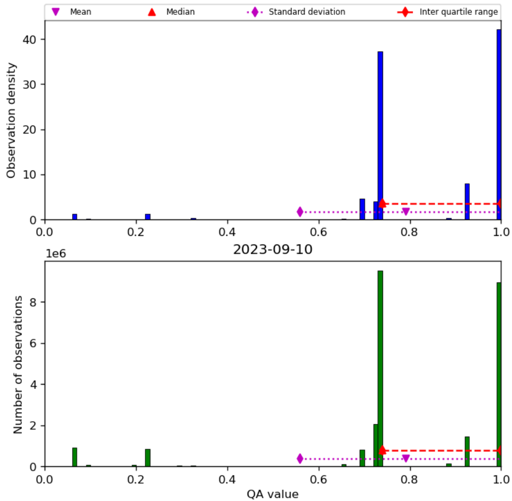
Figure 28: Histogram of “QA value” for 2023-09-10 to 2023-09-11
