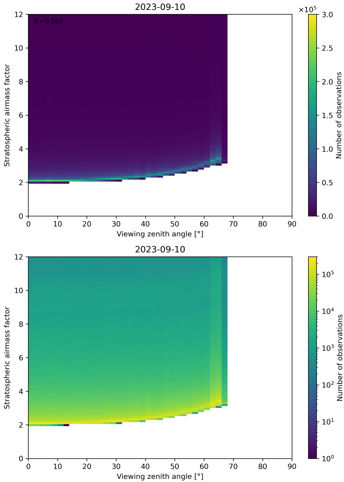
Figure 159: Scatter density plot of “Viewing zenith angle” against “Stratospheric airmass factor” for 2023-09-10 to 2023-09-11.
