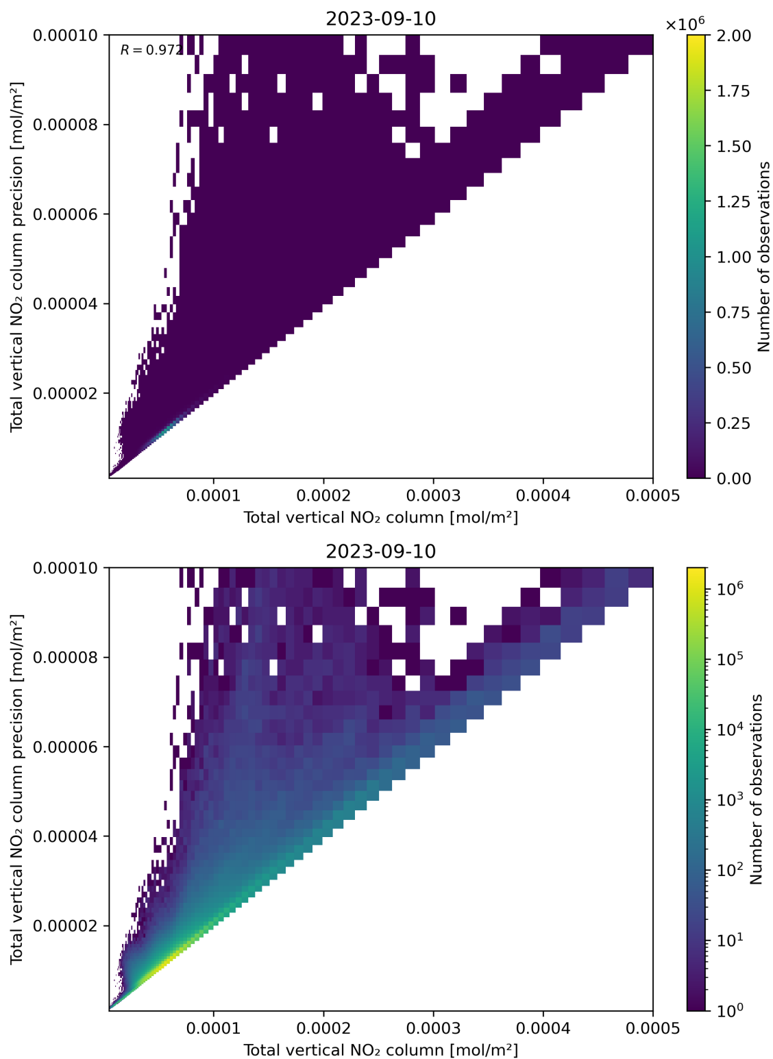
Figure 114: Scatter density plot of “Total vertical NO 2 column” against “Total vertical NO 2 column precision” for 2023-09-10 to 2023-09-11.
