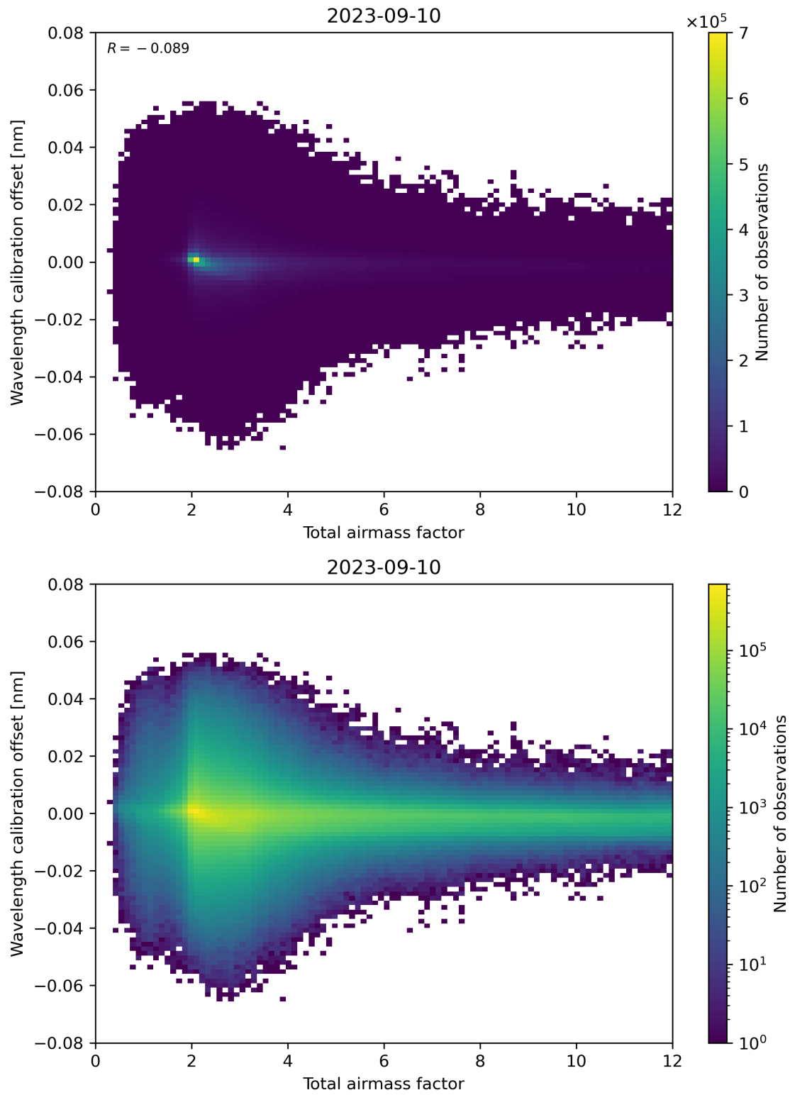
Figure 70: Scatter density plot of “Total airmass factor” against “Wavelength calibration offset” for 2023-09-10 to 2023-09-11.
