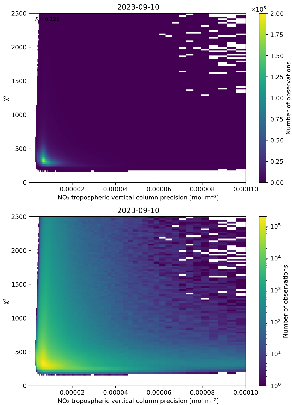
Figure 134: Scatter density plot of “NO 2 tropospheric vertical column precision” against “ \chi^2 ” for 2023-09-10 to 2023-09-11.
