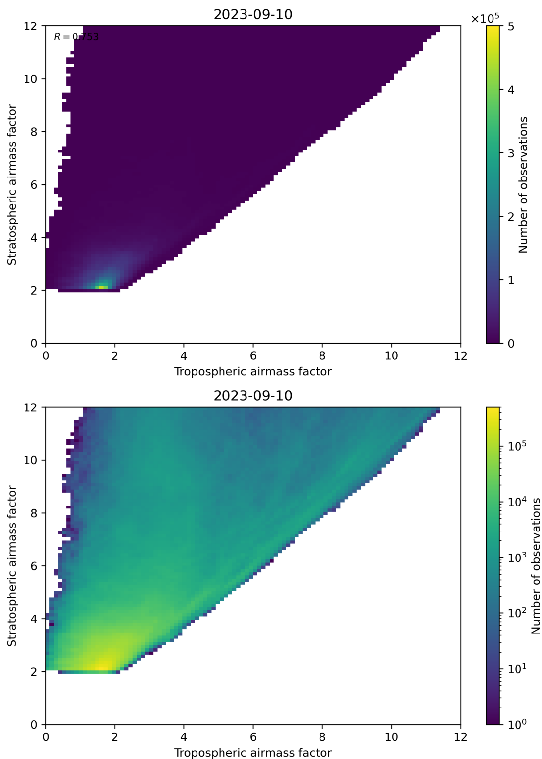
Figure 71: Scatter density plot of “Tropospheric airmass factor” against “Stratospheric airmass factor” for 2023-09-10 to 2023-09-11.
