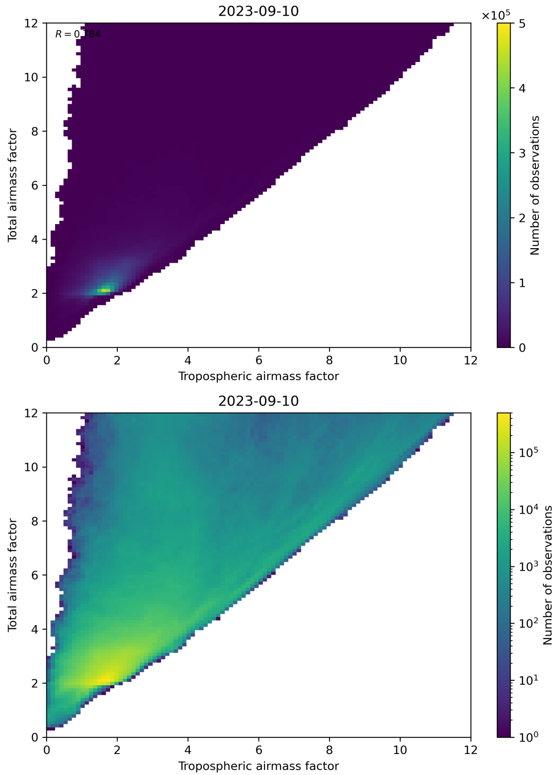
Figure 72: Scatter density plot of “Tropospheric airmass factor” against “Total airmass factor” for 2023-09-10 to 2023-09-11.
