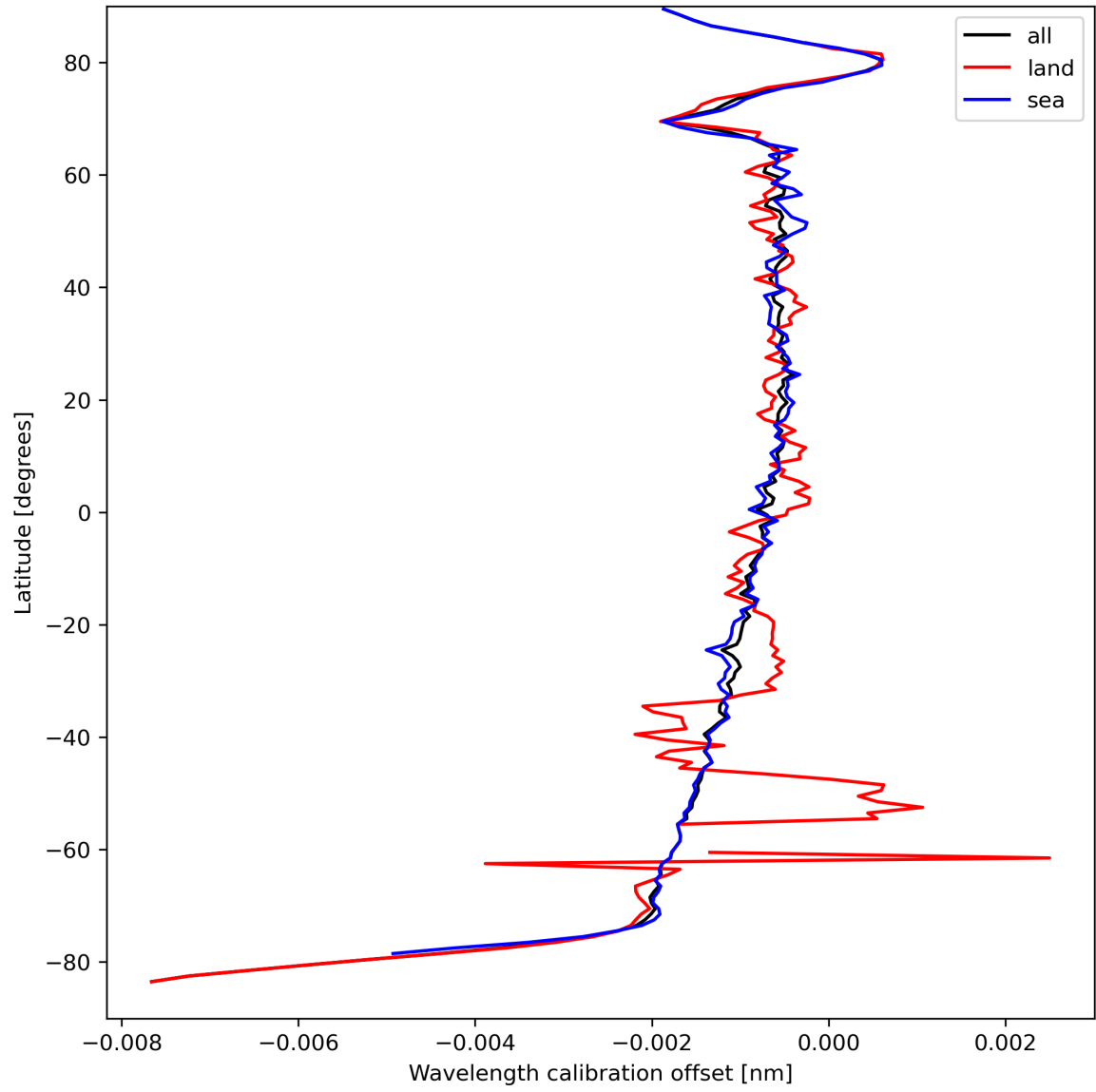
Figure 18: Zonal average of “Wavelength calibration offset” for 2023-09-10 to 2023-09-11.
