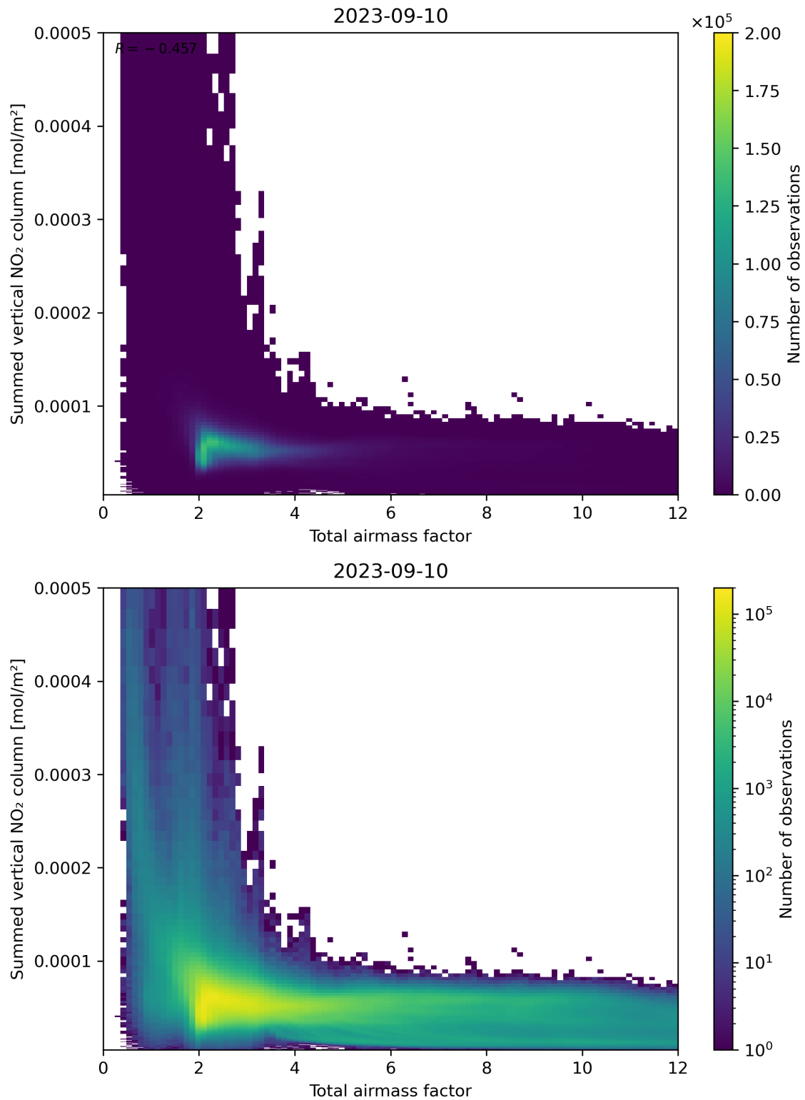
Figure 65: Scatter density plot of “Total airmass factor” against “Summed vertical NO 2 column” for 2023-09-10 to 2023-09-11.
