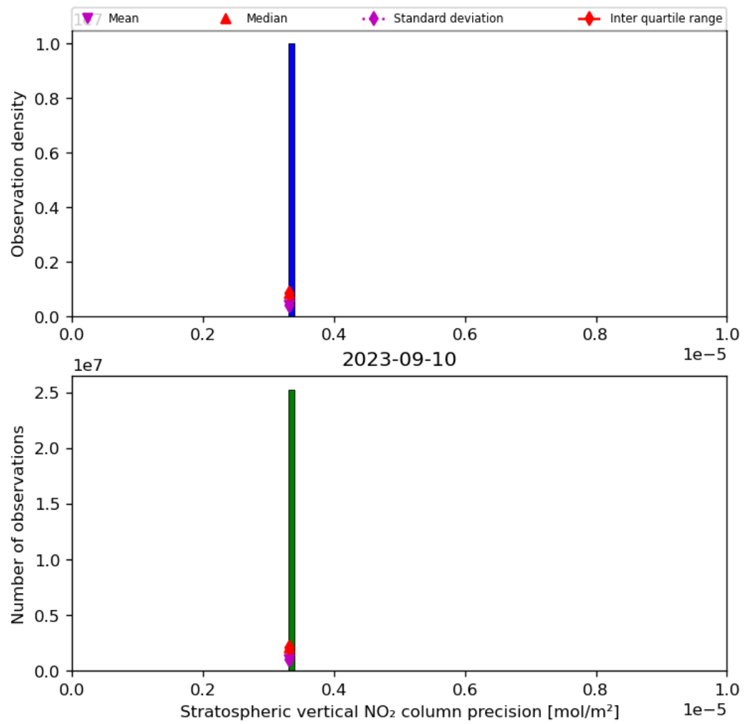
Figure 37: Histogram of “Stratospheric vertical NO 2 column precision” for 2023-09-10 to 2023-09-11
