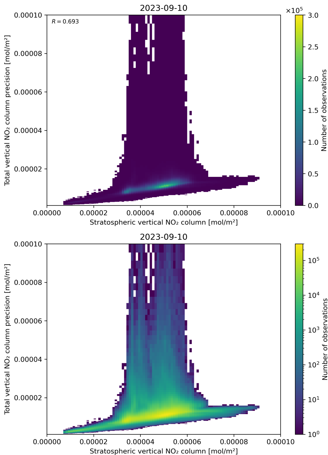
Figure 101: Scatter density plot of “Stratospheric vertical NO 2 column” against “Total vertical NO 2 column precision” for 2023-09-10 to 2023-09-11.
