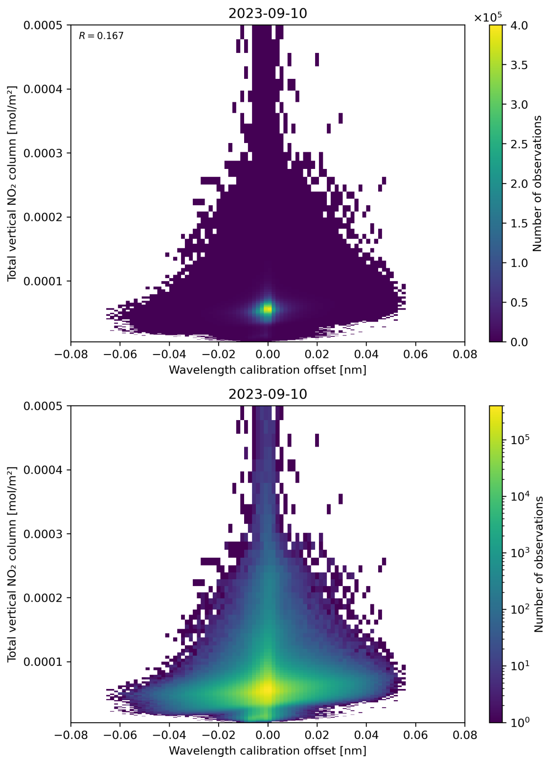
Figure 179: Scatter density plot of “Wavelength calibration offset” against “Total vertical NO 2 column” for 2023-09-10 to 2023-09-11.
