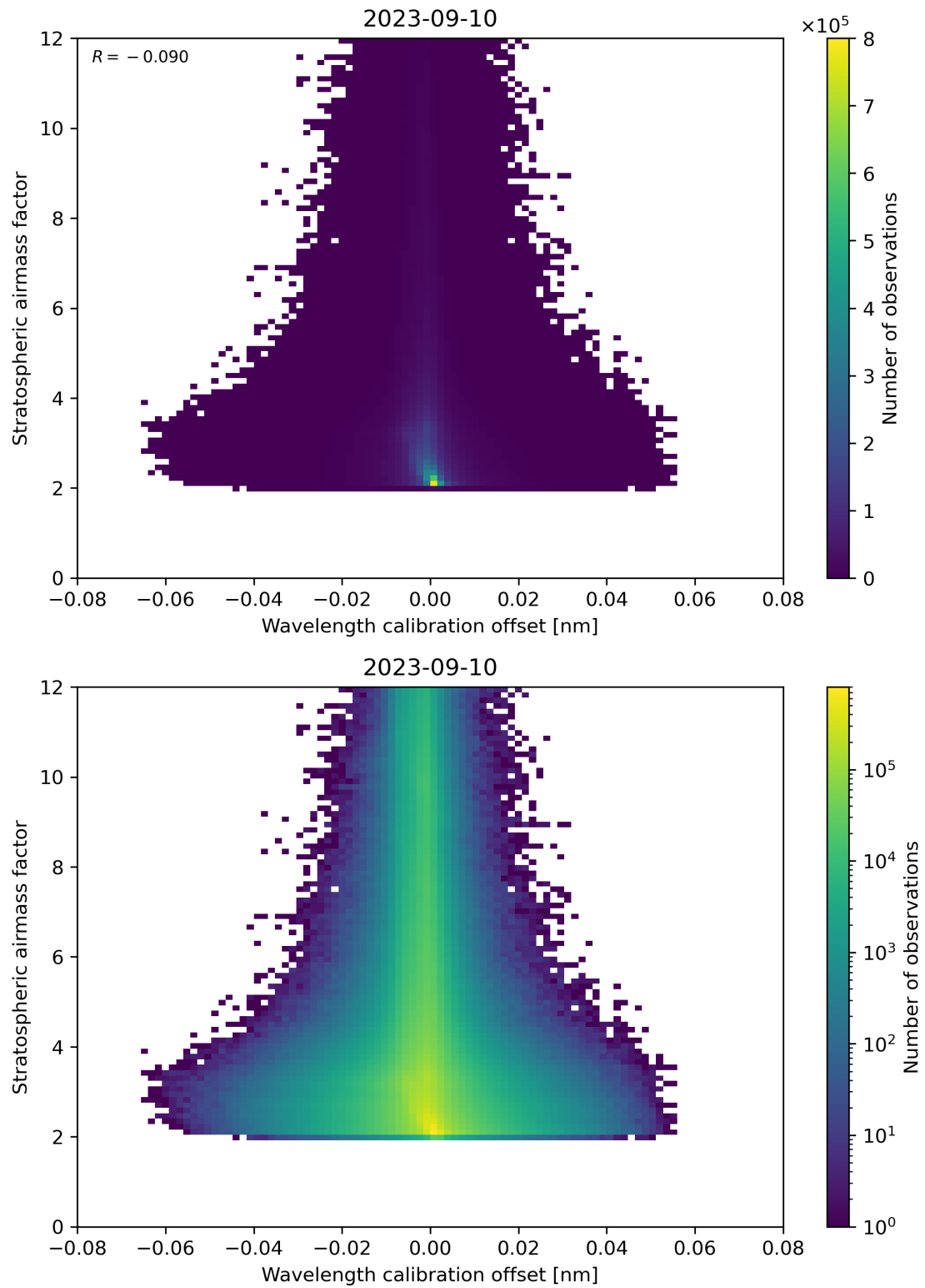
Figure 174: Scatter density plot of “Wavelength calibration offset” against “Stratospheric air mass factor” for 2023-09-10 to 2023-09-11.
