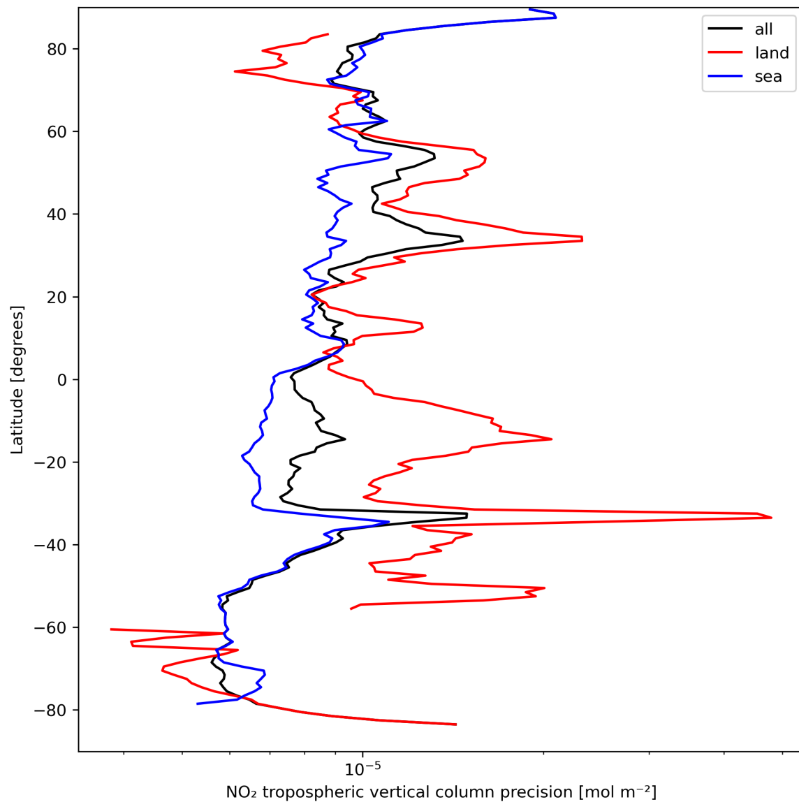
Figure 13: Zonal average of “NO 2 tropospheric vertical column precision” for 2023-09-10 to 2023-09-12.
