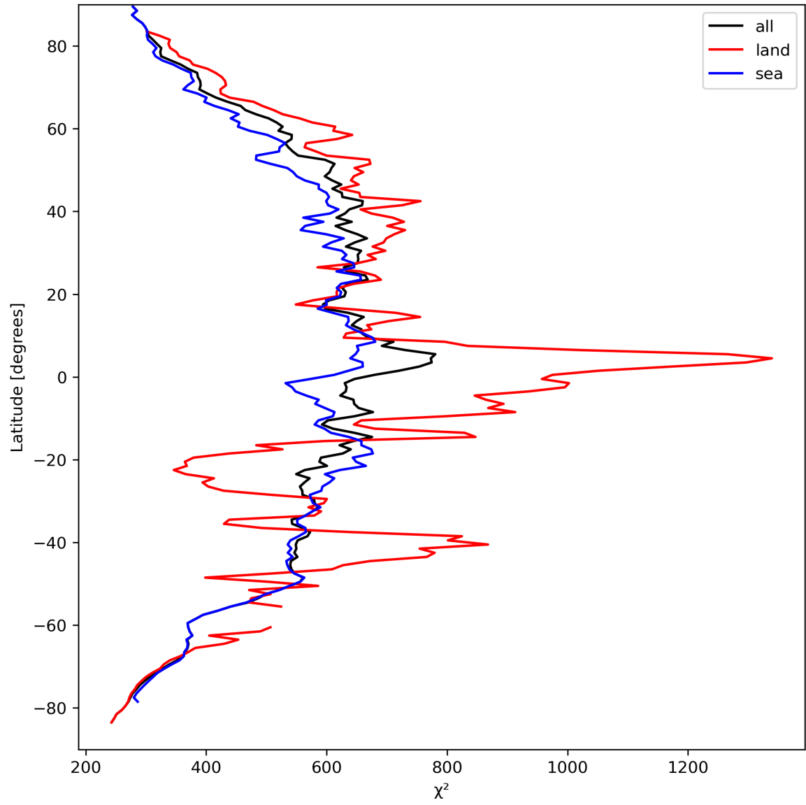
Figure 25: Zonal average of “ \chi^2 ” for 2023-09-10 to 2023-09-12.
