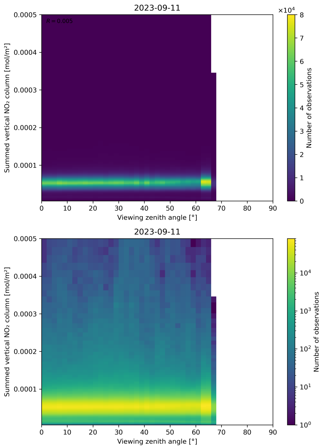
Figure 165: Scatter density plot of “Viewing zenith angle” against “Summed vertical NO 2 column” for 2023-09-10 to 2023-09-12.
