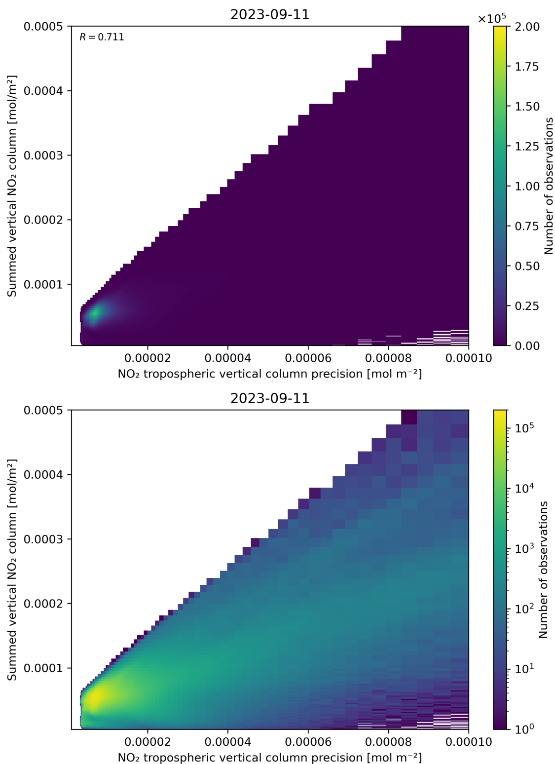
Figure 136: Scatter density plot of “NO 2 tropospheric vertical column precision” against “Summed vertical NO 2 column” for 2023-09-10 to 2023-09-12.
