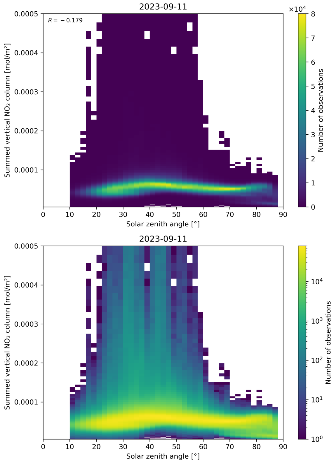
Figure 151: Scatter density plot of “Solar zenith angle” against “Summed vertical NO 2 column” for 2023-09-10 to 2023-09-12.
