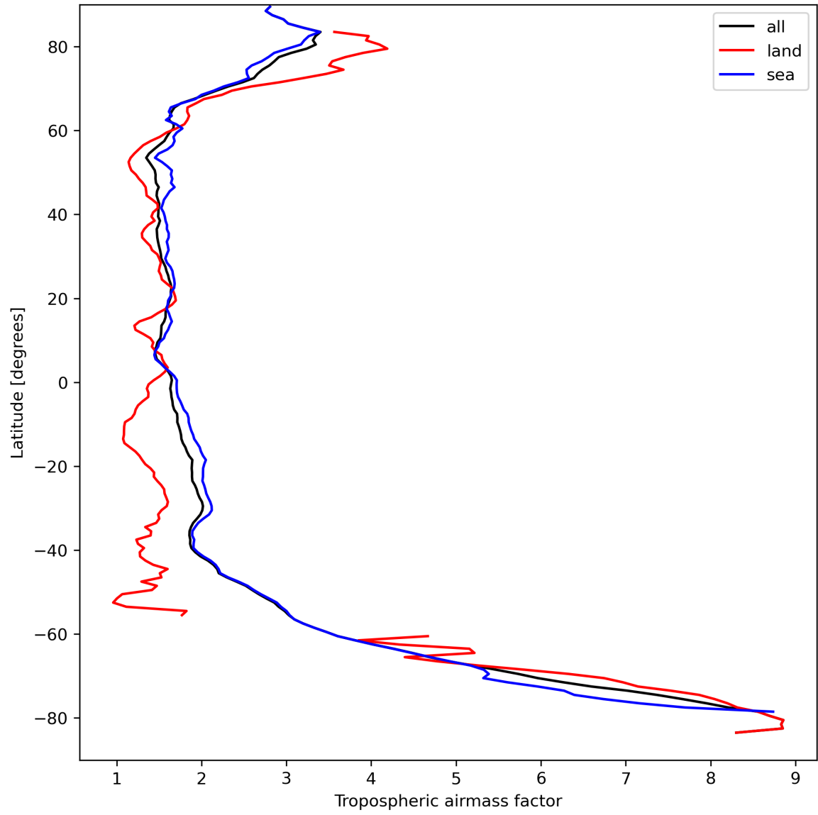
Figure 14: Zonal average of “Tropospheric airmass factor” for 2023-09-10 to 2023-09-12.
