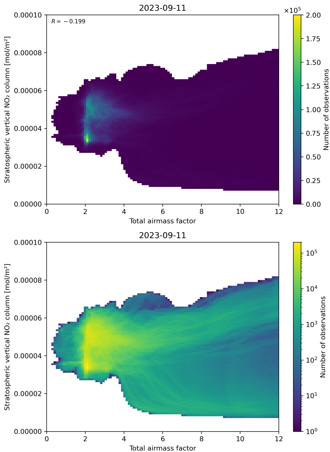
Figure 64: Scatter density plot of “Total airmass factor” against “Stratospheric vertical NO 2 column” for 2023-09-10 to 2023-09-12.
