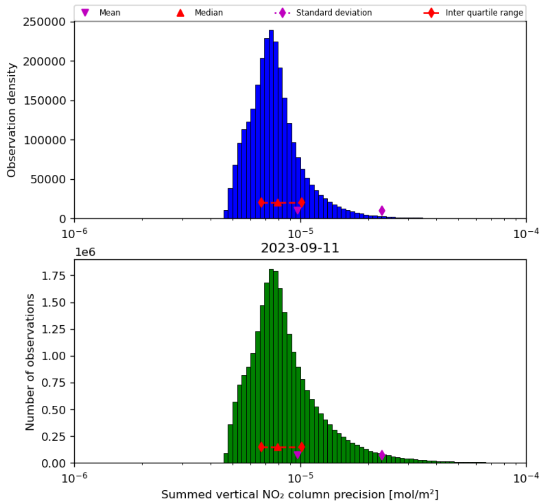
Figure 41: Histogram of "Summed vertical NO 2 column precision" for 2023-09-10 to 2023-09-12
