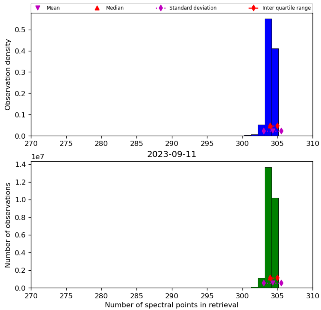
Figure 33: Histogram of “Number of spectral points in retrieval” for 2023-09-10 to 2023-09-12
