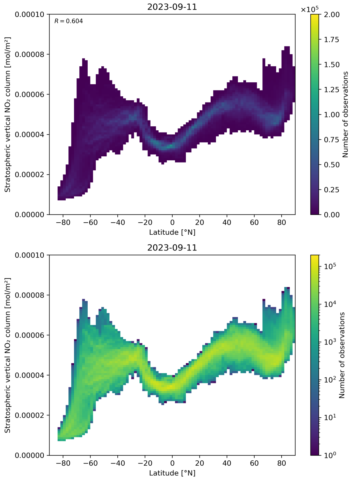
Figure 87: Scatter density plot of “Latitude” against “Stratospheric vertical NO 2 column” for 2023-09-10 to 2023-09-12.
