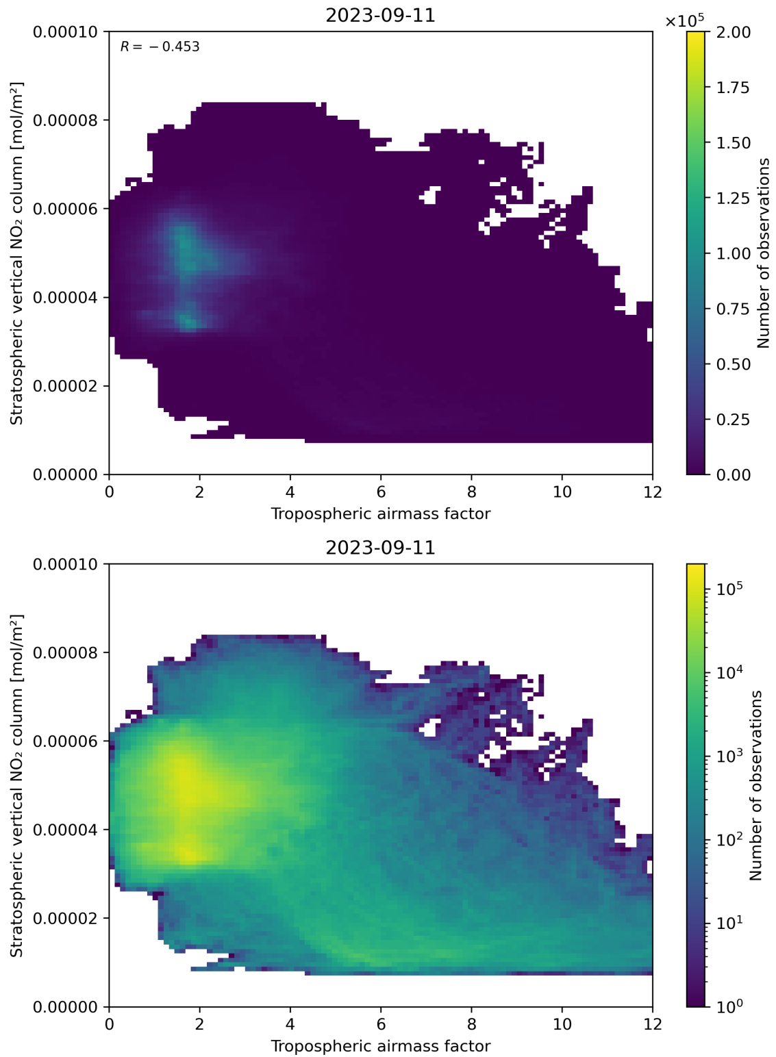
Figure 74: Scatter density plot of “Tropospheric air mass factor” against “Stratospheric vertical NO 2 column” for 2023-09-10 to 2023-09-12.
