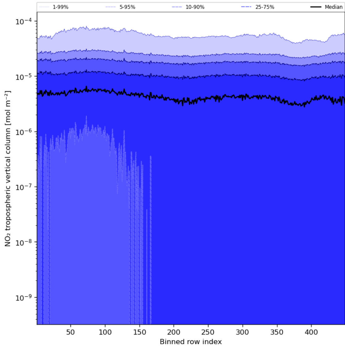
Figure 46: Along track statistics of “NO 2 tropospheric vertical column” for 2023-09-10 to 2023-09-12
