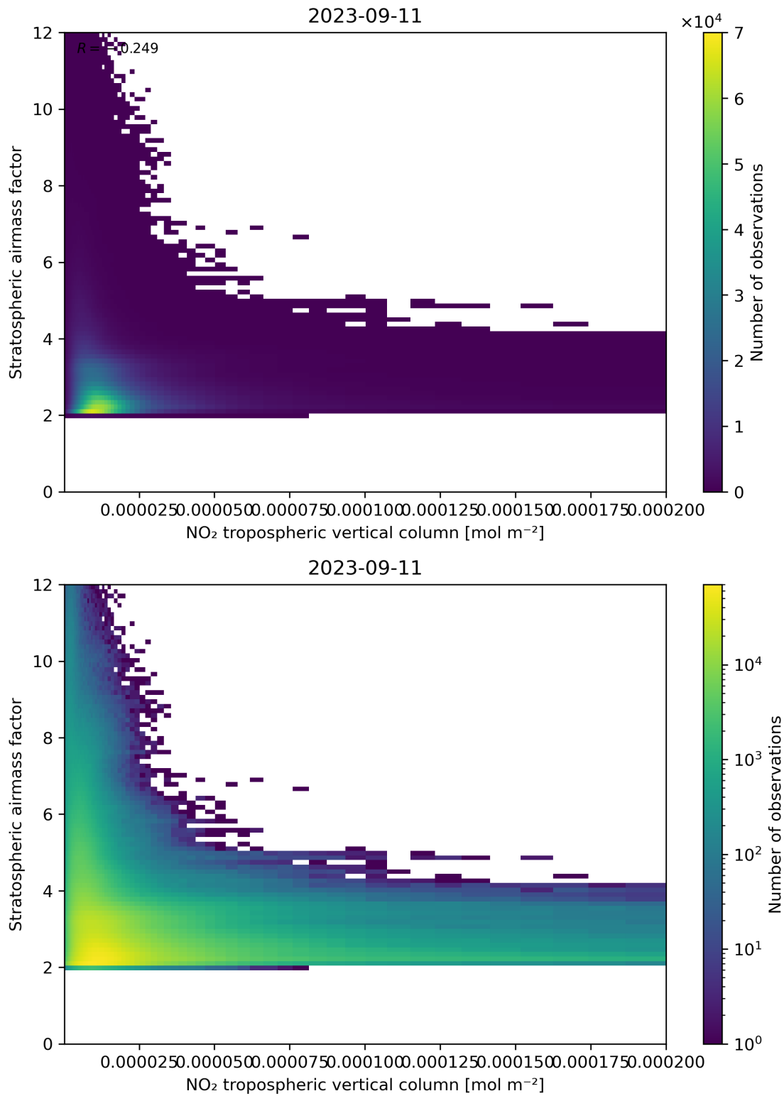
Figure 121: Scatter density plot of “NO 2 tropospheric vertical column” against “Stratospheric air mass factor” for 2023-09-10 to 2023-09-12.
