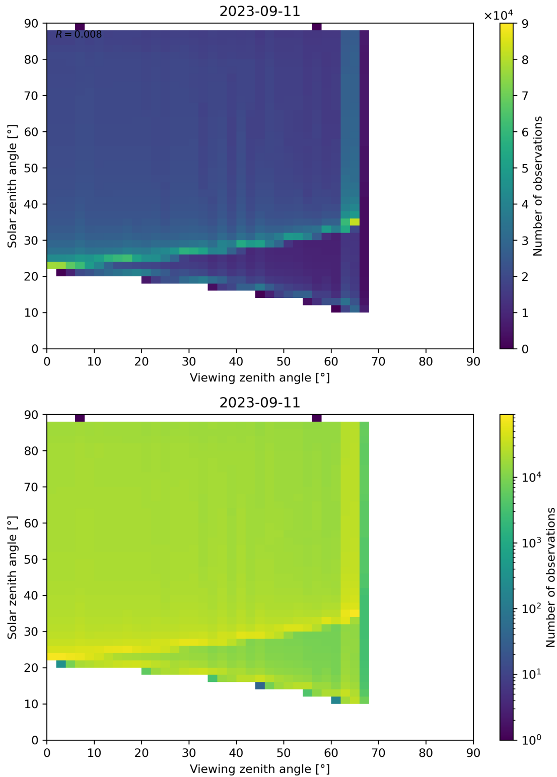
Figure 172: Scatter density plot of “Viewing zenith angle” against “Solar zenith angle” for 2023-09-10 to 2023-09-12.
