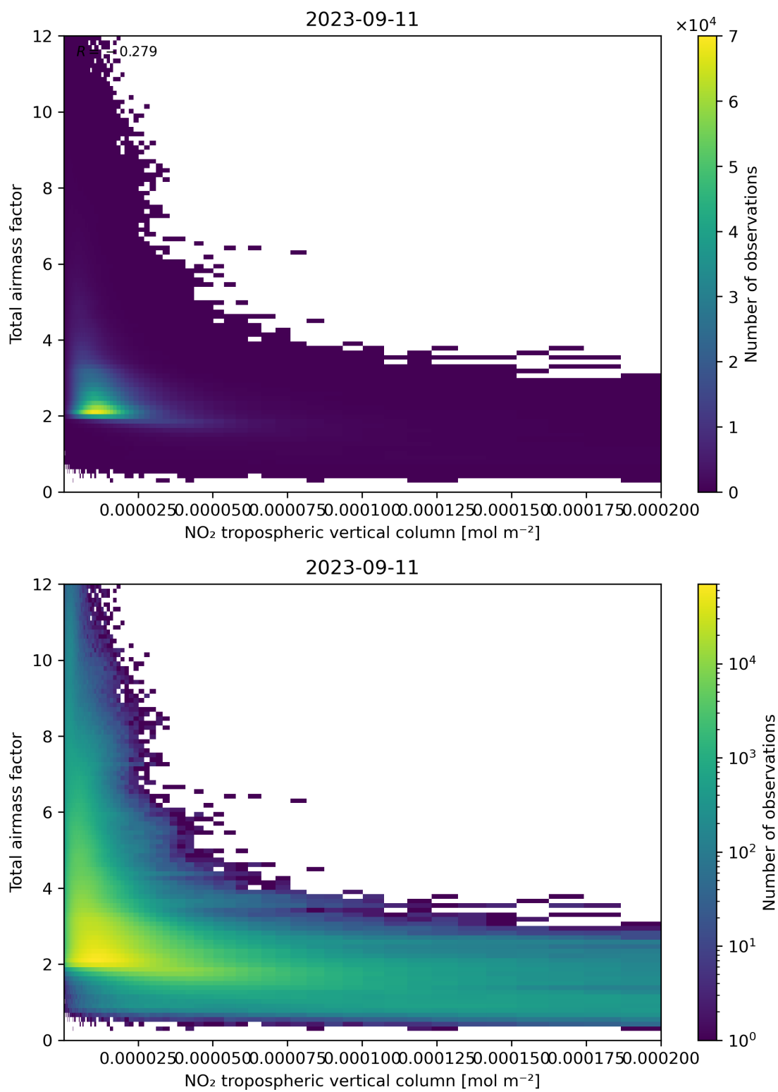
Figure 122: Scatter density plot of “NO 2 tropospheric vertical column” against “Total air mass factor” for 2023-09-10 to 2023-09-12.
