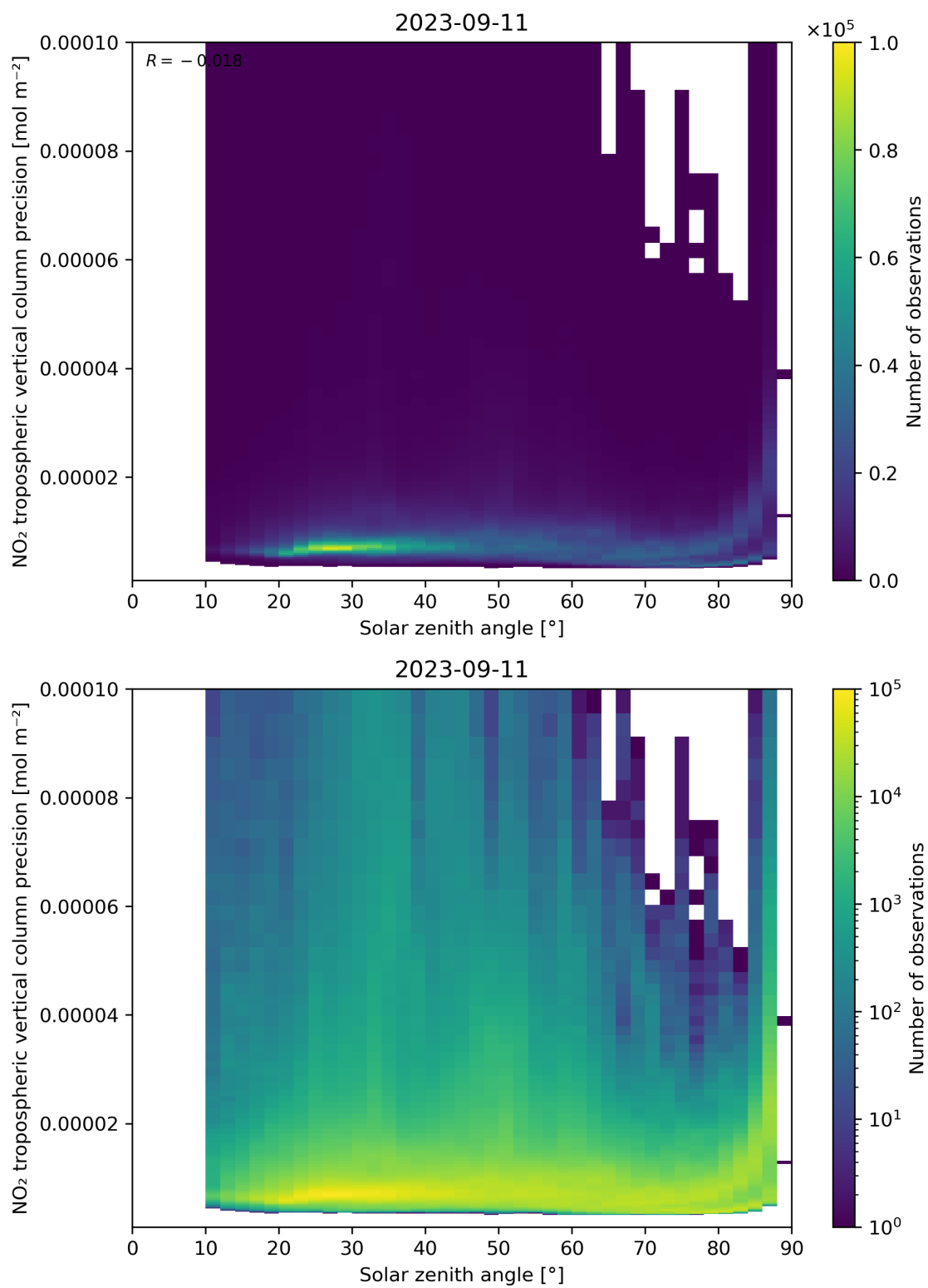
Figure 156: Scatter density plot of “Solar zenith angle” against “NO 2 tropospheric vertical column precision” for 2023-09-10 to 2023-09-12.
