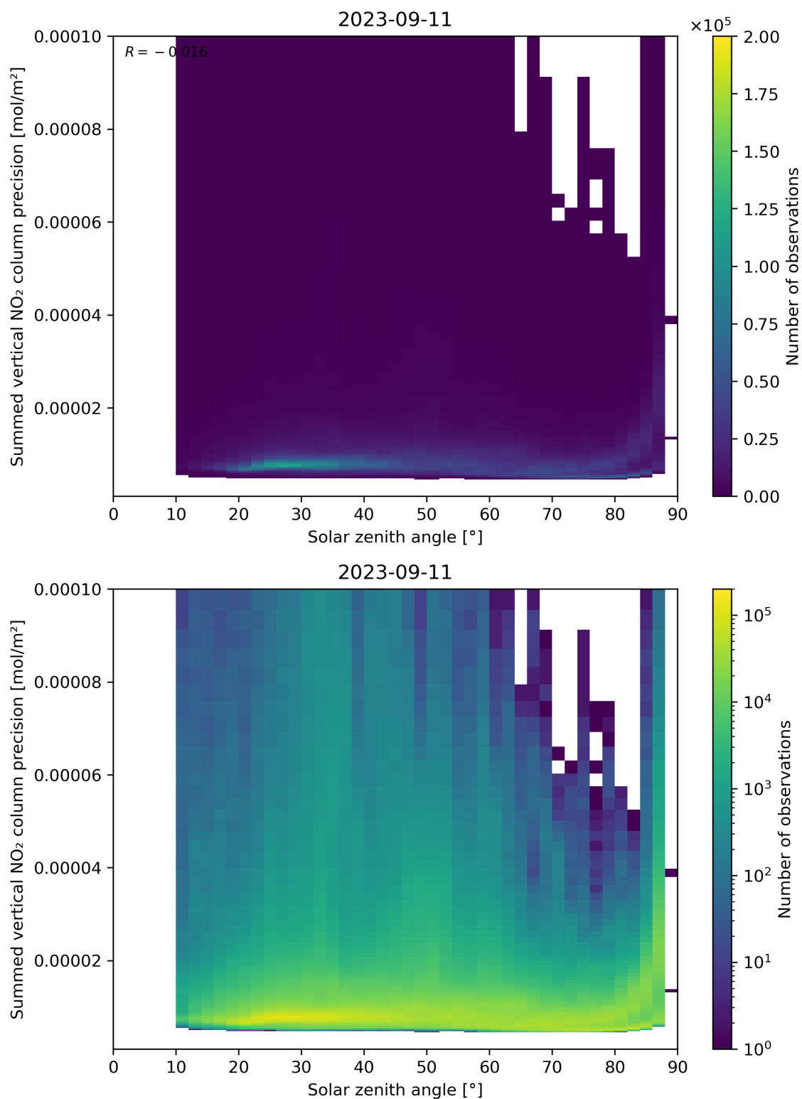
Figure 152: Scatter density plot of “Solar zenith angle” against “Summed vertical NO 2 column precision” for 2023-09-10 to 2023-09-12.
