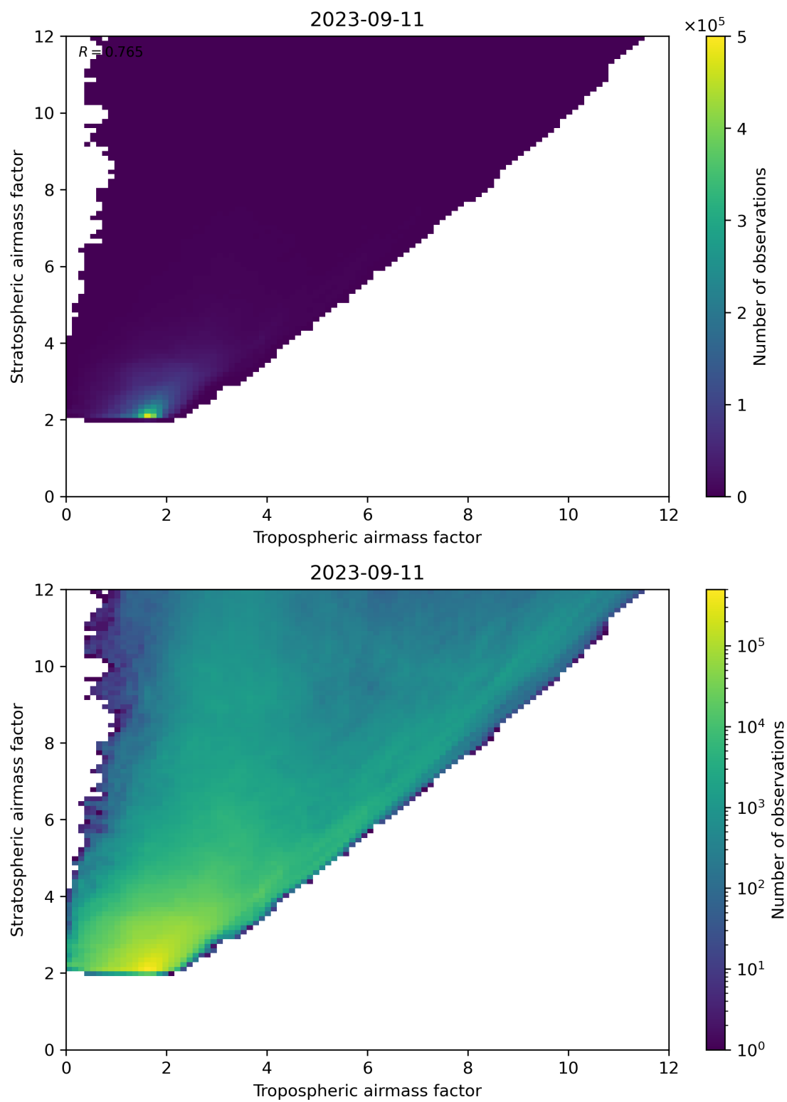
Figure 71: Scatter density plot of “Tropospheric airmass factor” against “Stratospheric airmass factor” for 2023-09-10 to 2023-09-12.
