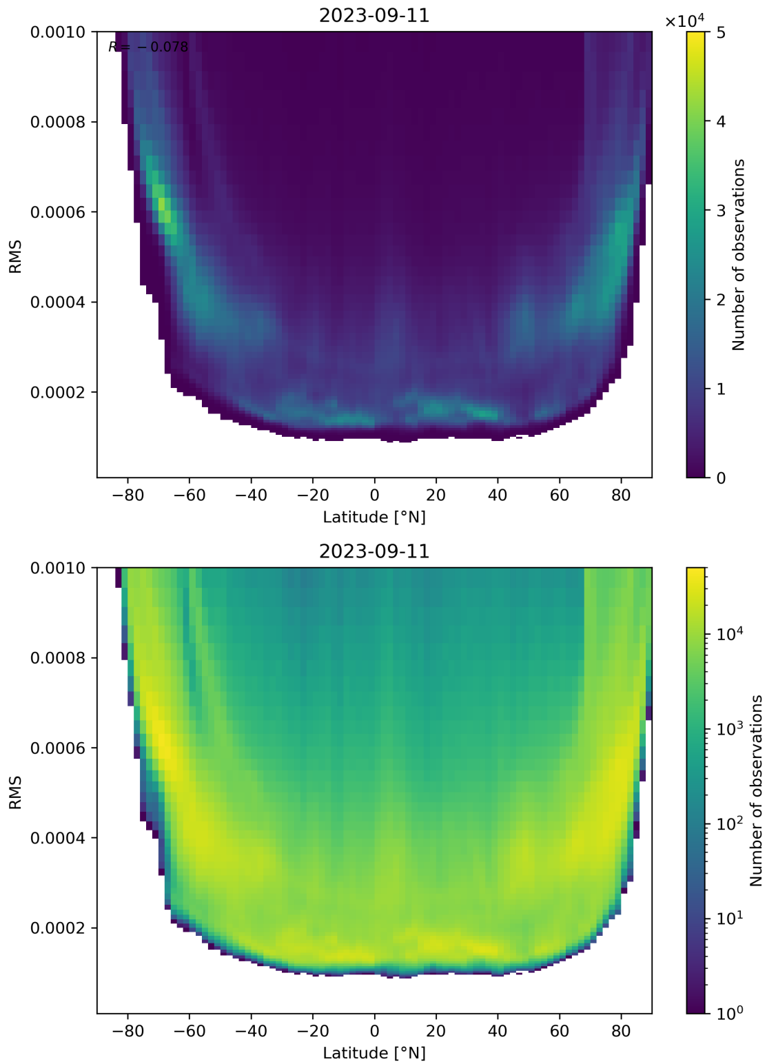
Figure 94: Scatter density plot of “Latitude” against “RMS” for 2023-09-10 to 2023-09-12.
