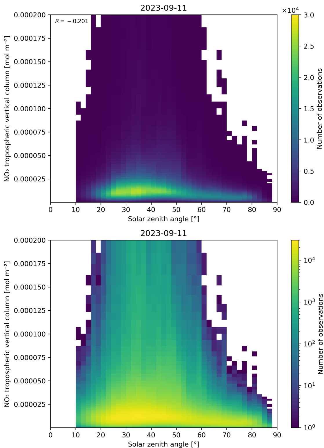
Figure 155: Scatter density plot of “Solar zenith angle” against “NO 2 tropospheric vertical column” for 2023-09-10 to 2023-09-12.
