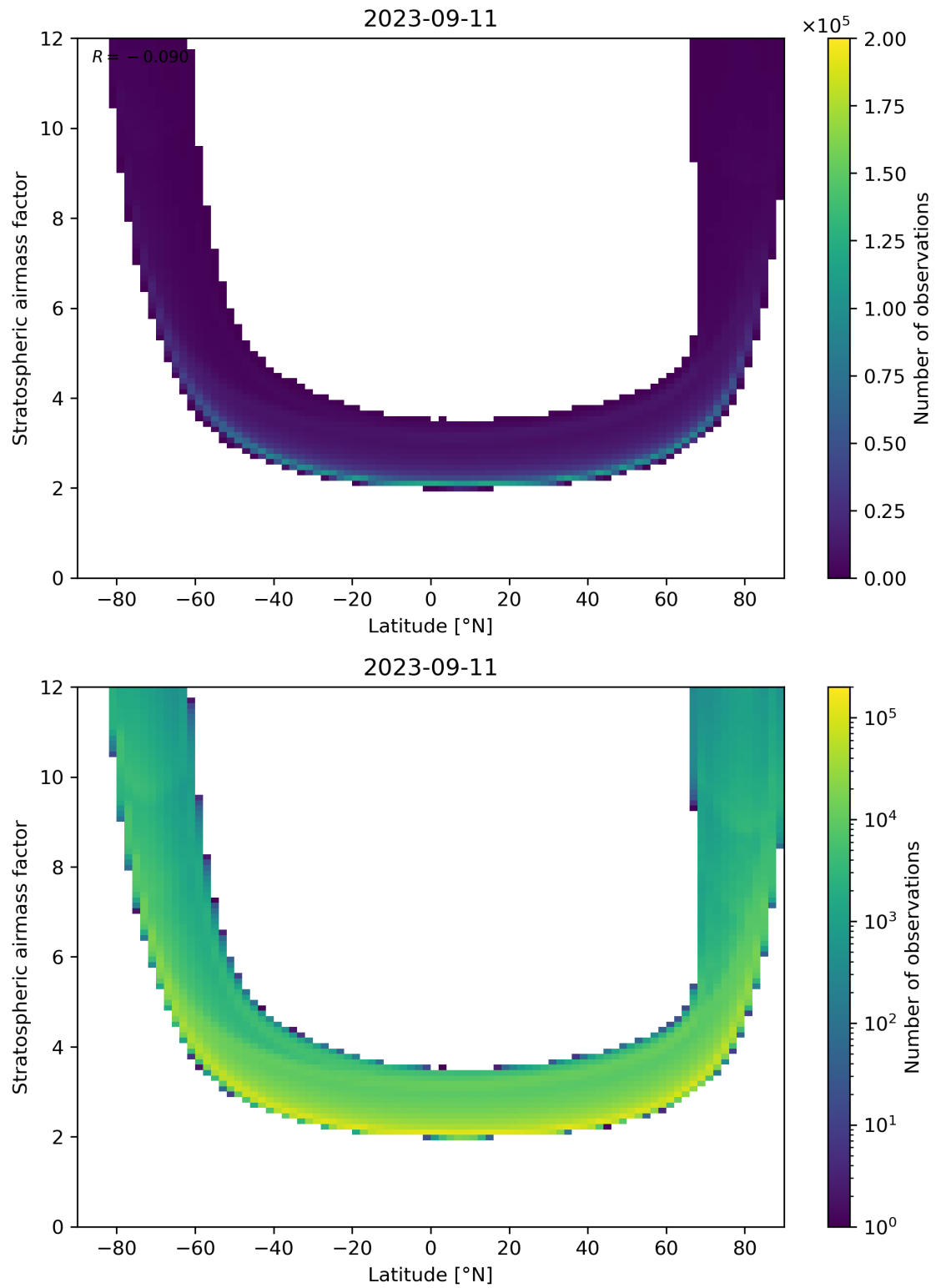
Figure 83: Scatter density plot of “Latitude” against “Stratospheric airmass factor” for 2023-09-10 to 2023-09-12.
