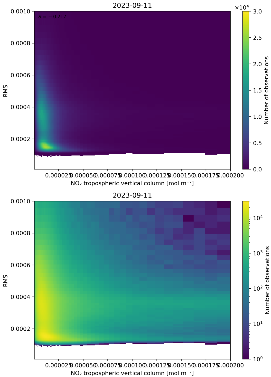
Figure 142: Scatter density plot of “NO 2 tropospheric vertical column” against “RMS” for 2023-09-10 to 2023-09-12.
