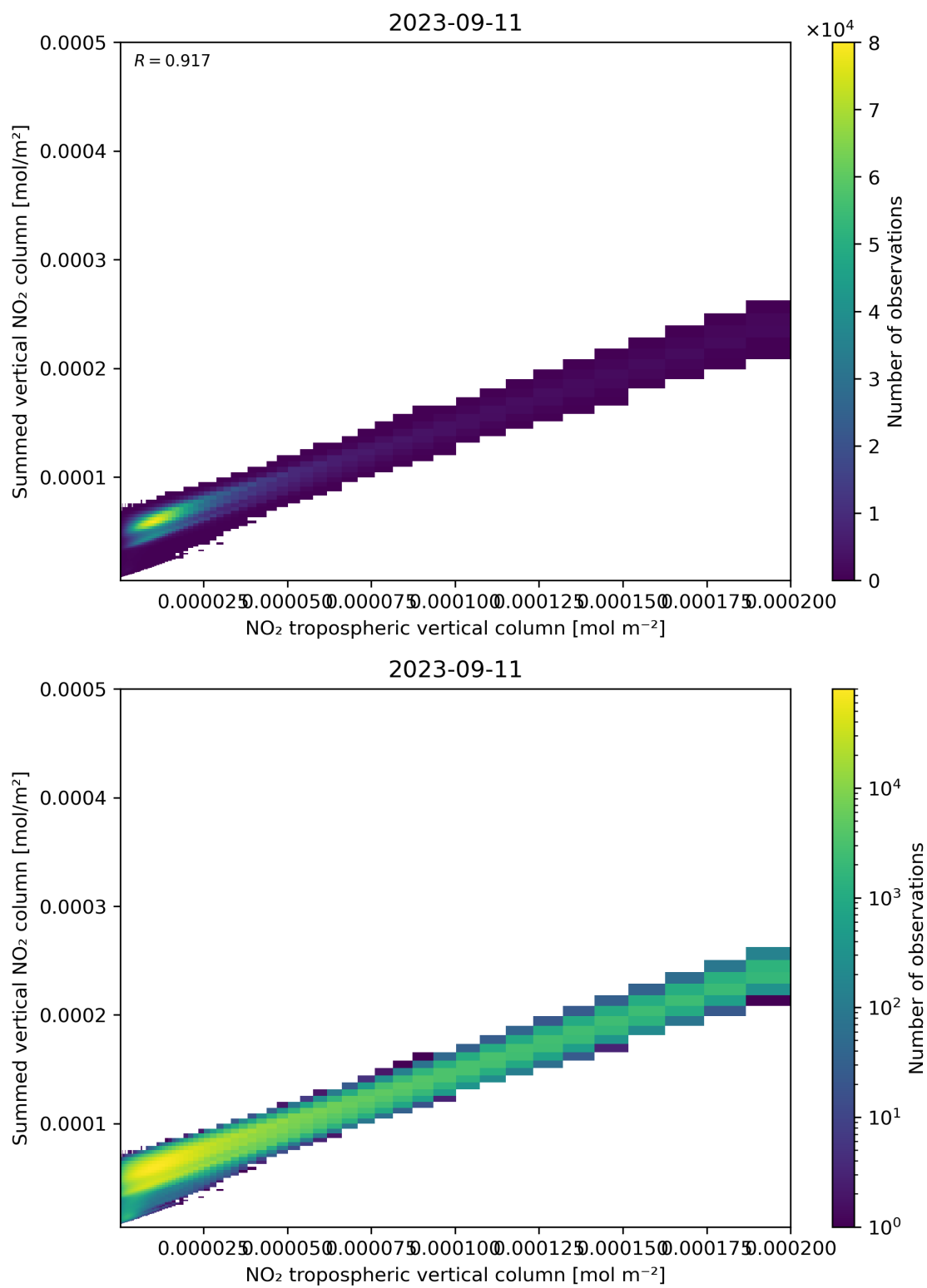
Figure 126: Scatter density plot of “NO 2 tropospheric vertical column” against “Summed vertical NO 2 column” for 2023-09-10 to 2023-09-12.
