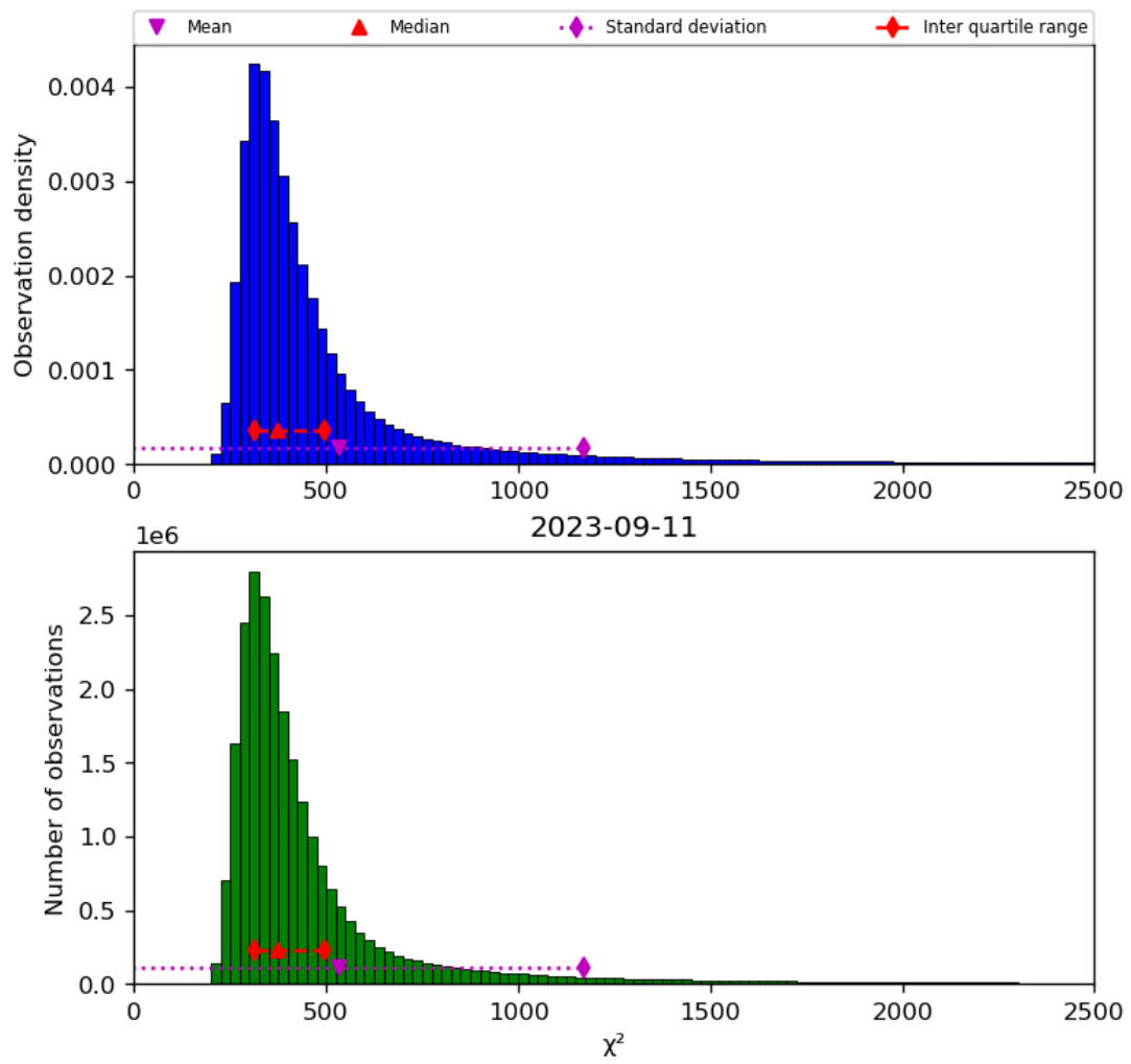
Figure 42: Histogram of “ \chi^2 ” for 2023-09-10 to 2023-09-12
