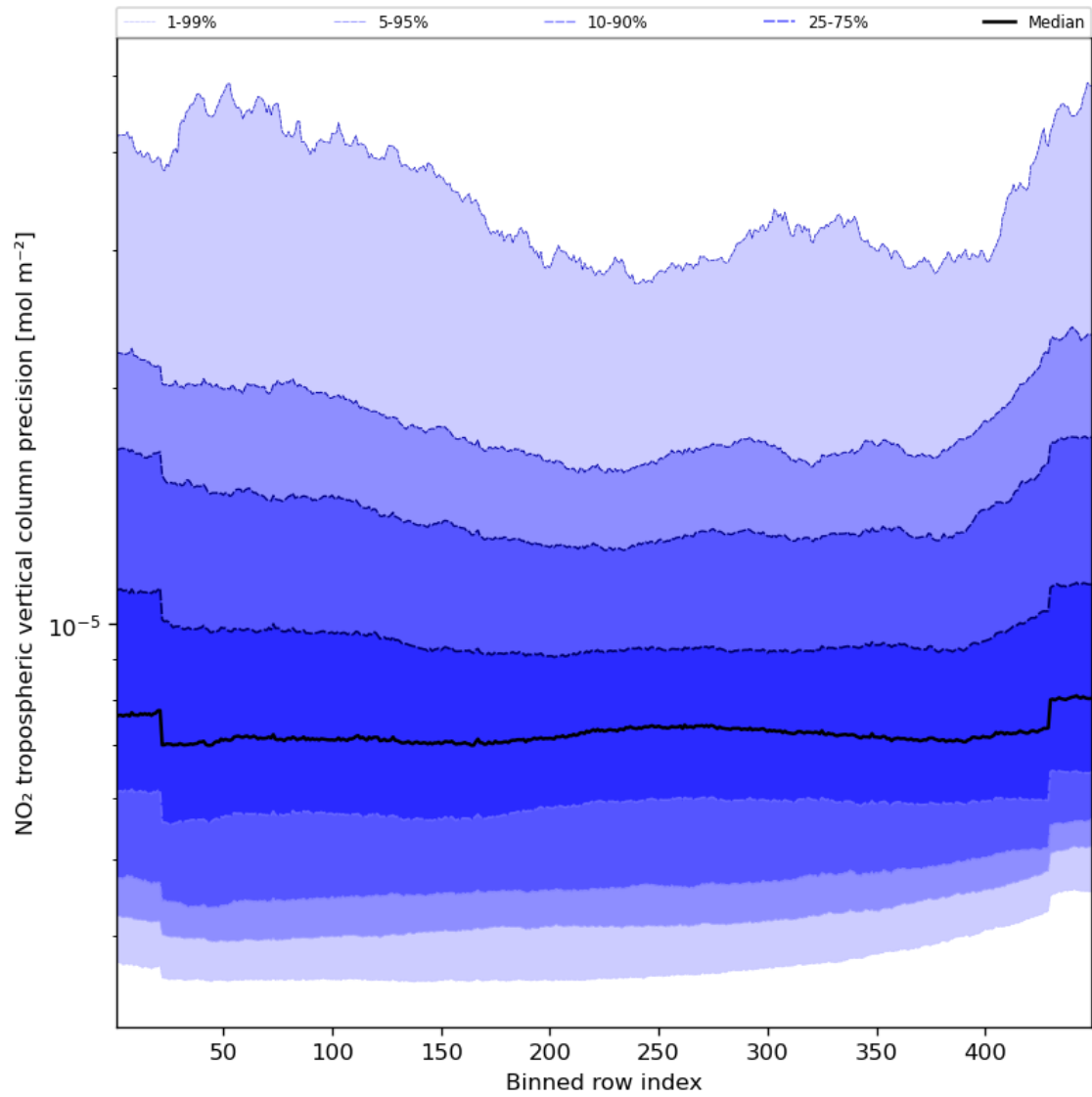
Figure 47: Along track statistics of “NO 2 tropospheric vertical column precision” for 2023-09-10 to 2023-09-12
