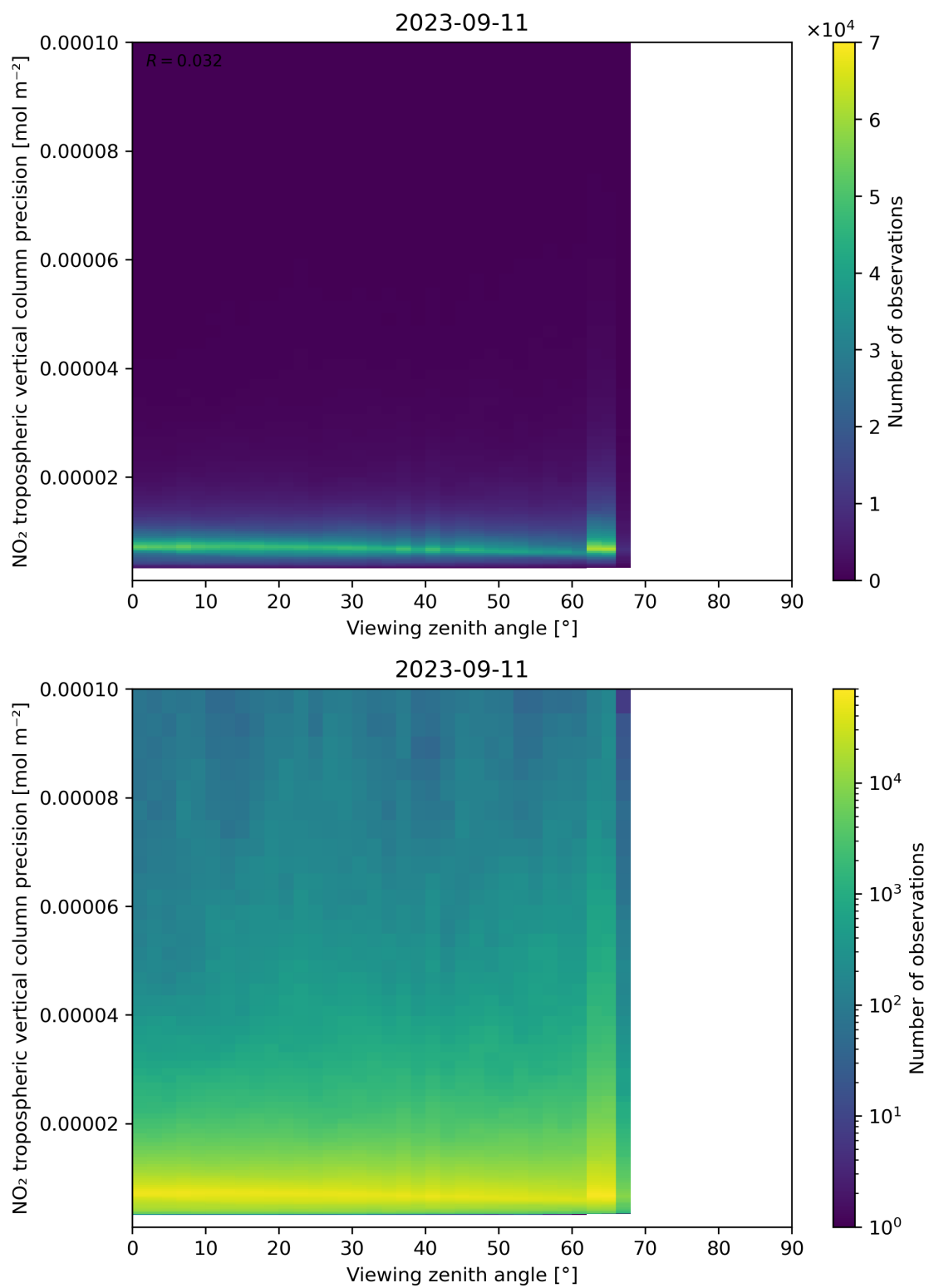
Figure 170: Scatter density plot of “Viewing zenith angle” against “NO 2 tropospheric vertical column precision” for 2023-09-10 to 2023-09-12.
