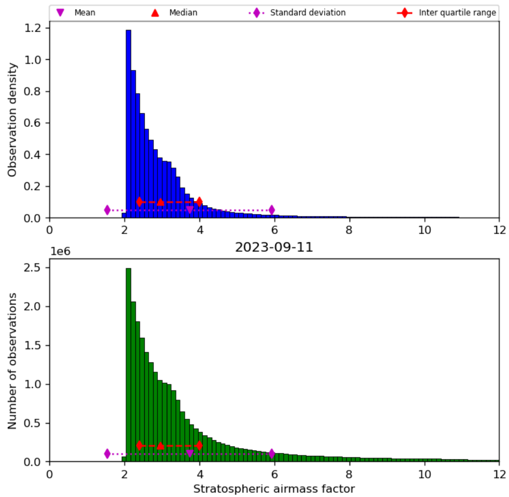
Figure 44: Histogram of “Stratospheric airmass factor” for 2023-09-10 to 2023-09-12
