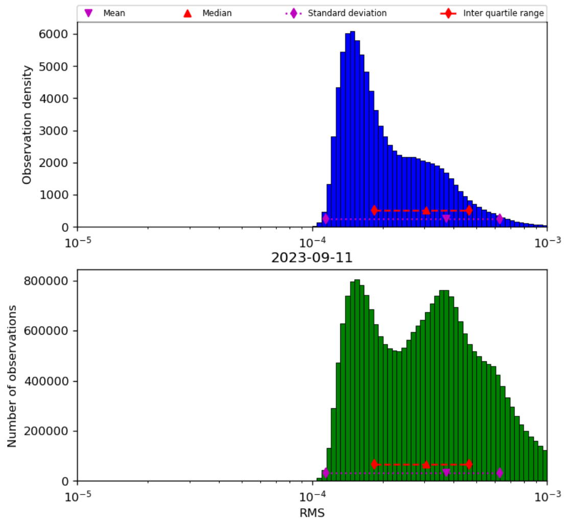
Figure 43: Histogram of “RMS” for 2023-09-10 to 2023-09-12
