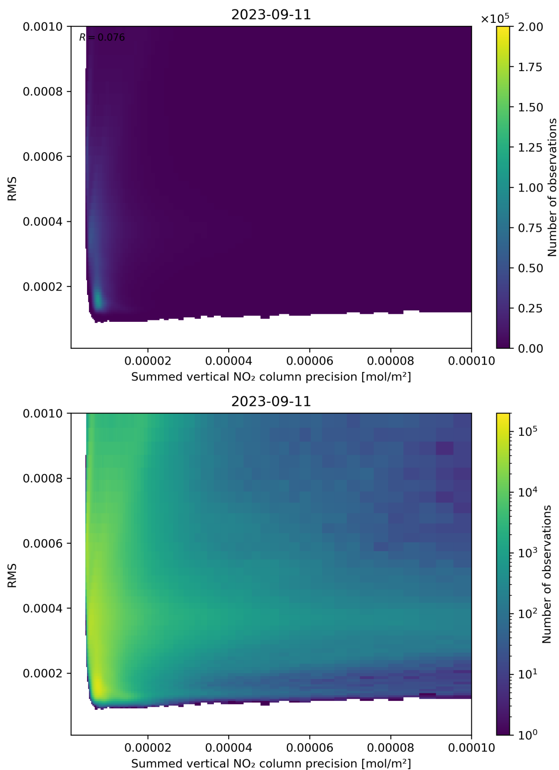
Figure 108: Scatter density plot of “Summed vertical NO 2 column precision” against “RMS” for 2023-09-10 to 2023-09-12.
