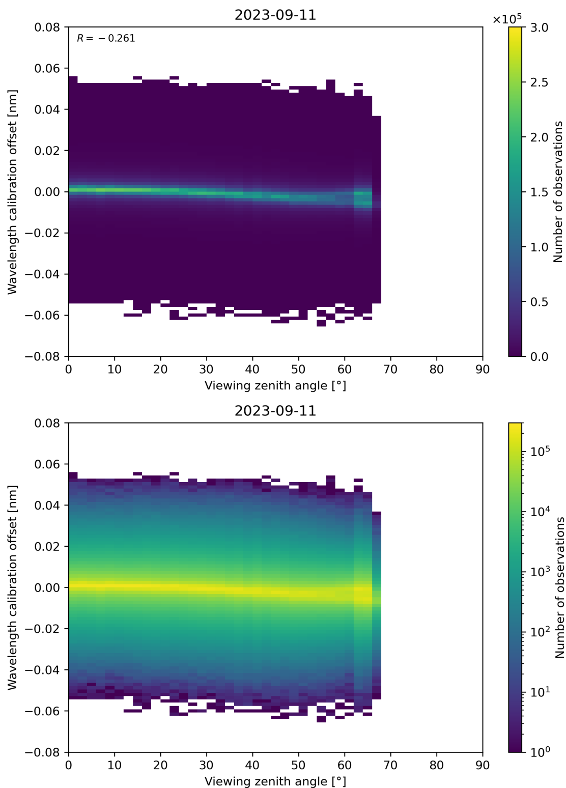
Figure 173: Scatter density plot of “Viewing zenith angle” against “Wavelength calibration offset” for 2023-09-10 to 2023-09-12.
