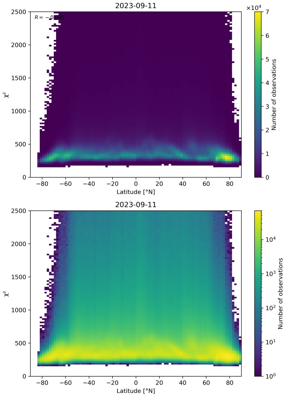
Figure 86: Scatter density plot of “Latitude” against “ \chi^2 ” for 2023-09-10 to 2023-09-12.
