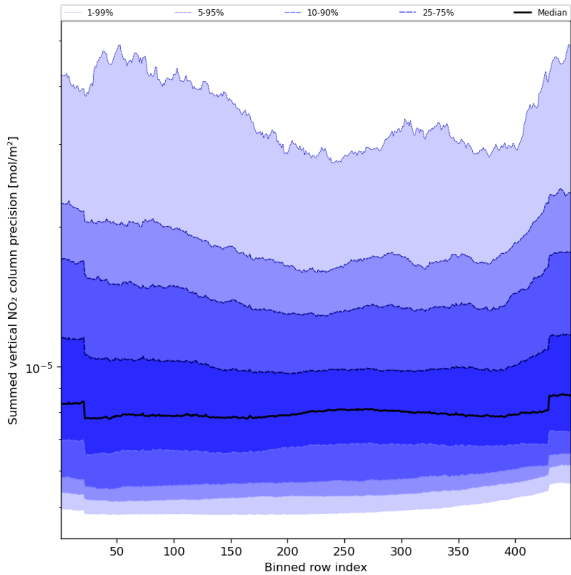
Figure 58: Along track statistics of “Summed vertical NO 2 column precision” for 2023-09-10 to 2023-09-12
