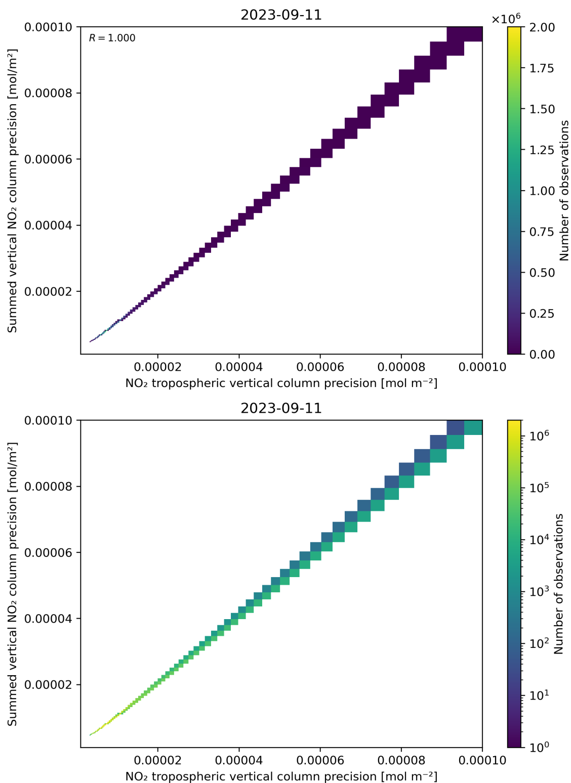
Figure 137: Scatter density plot of “NO 2 tropospheric vertical column precision” against “Summed vertical NO 2 column precision” for 2023-09-10 to 2023-09-12.
