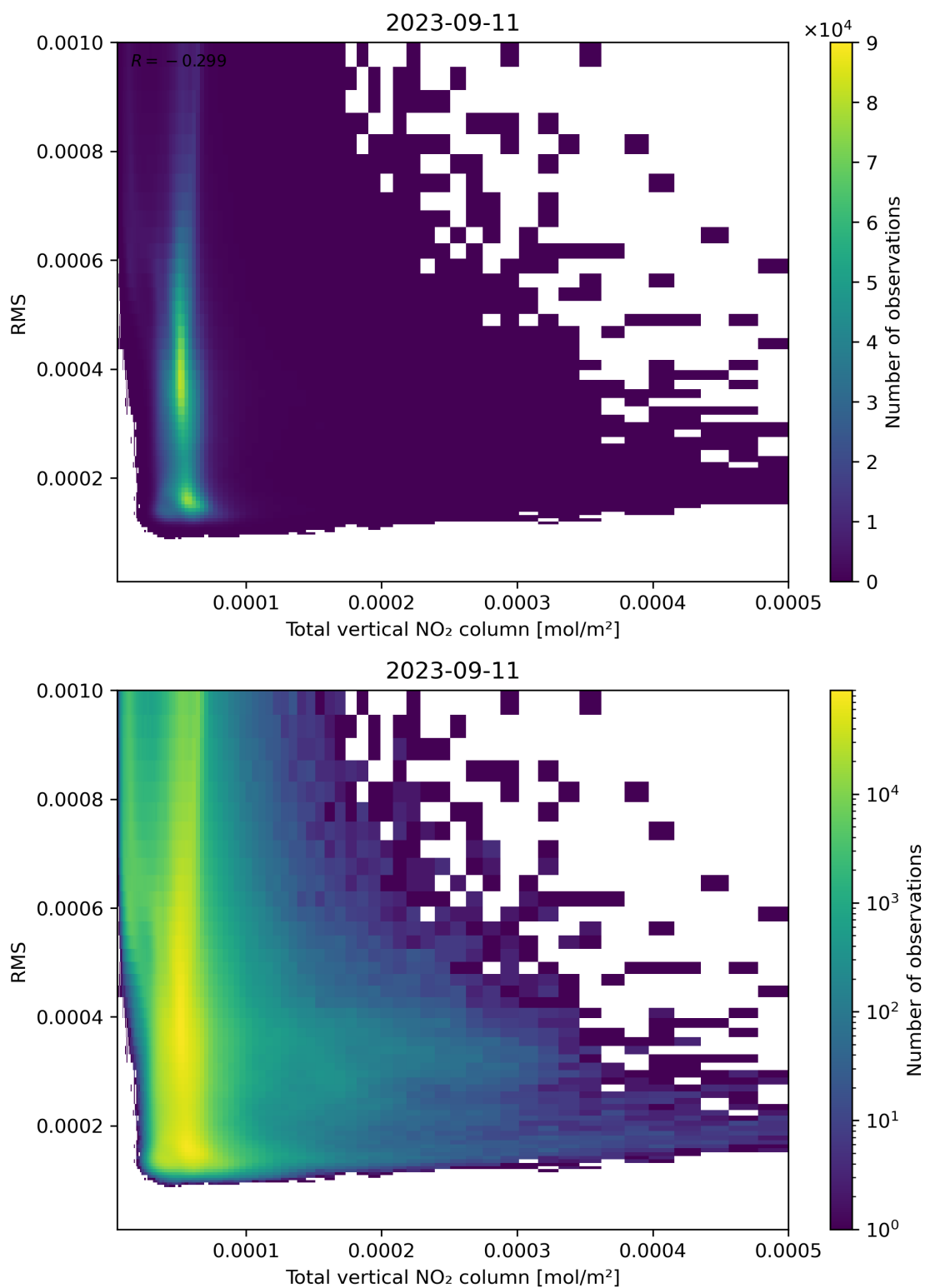
Figure 120: Scatter density plot of “Total vertical NO 2 column” against “RMS” for 2023-09-10 to 2023-09-12.
