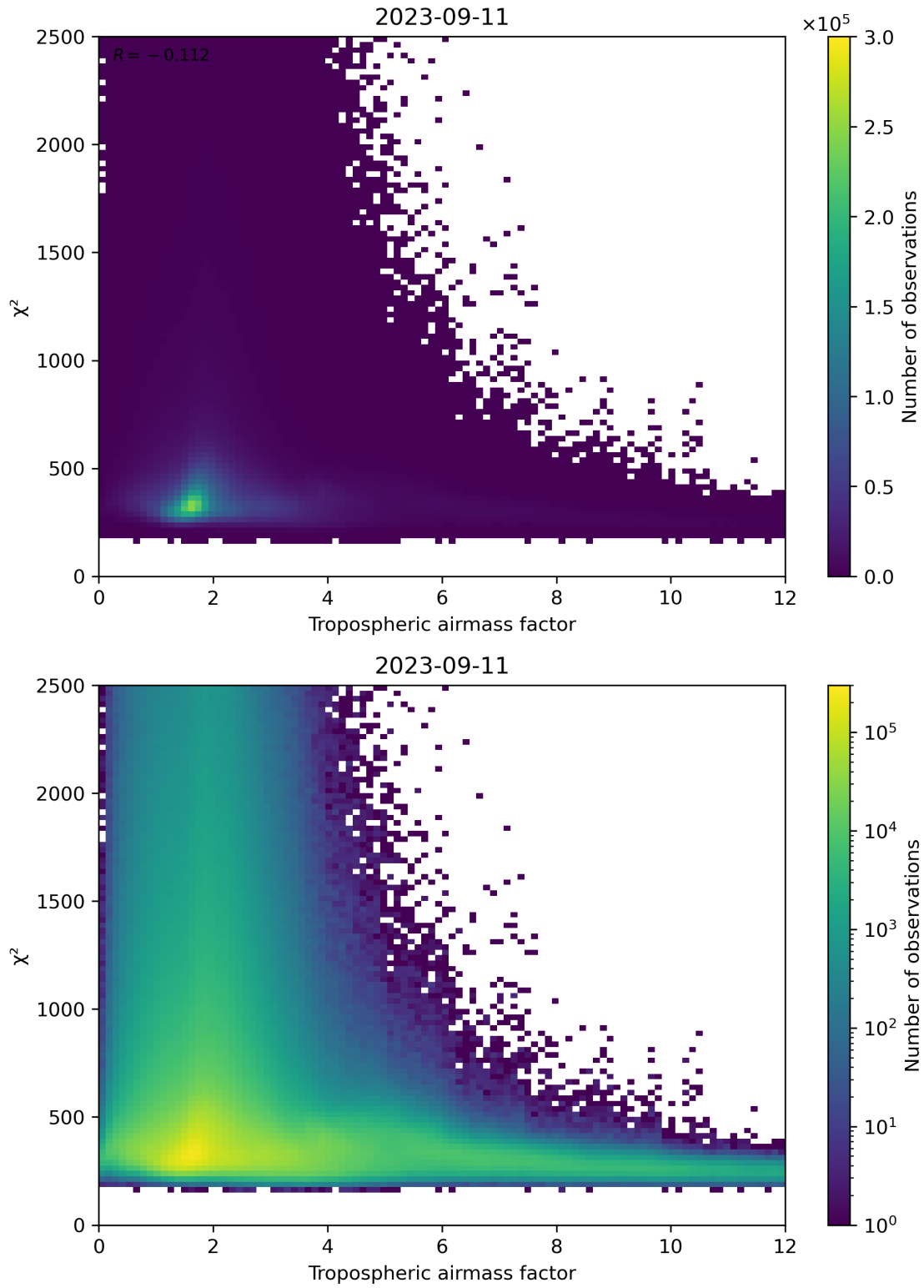
Figure 73: Scatter density plot of “Tropospheric airmass factor” against “ \chi^2 ” for 2023-09-10 to 2023-09-12.
