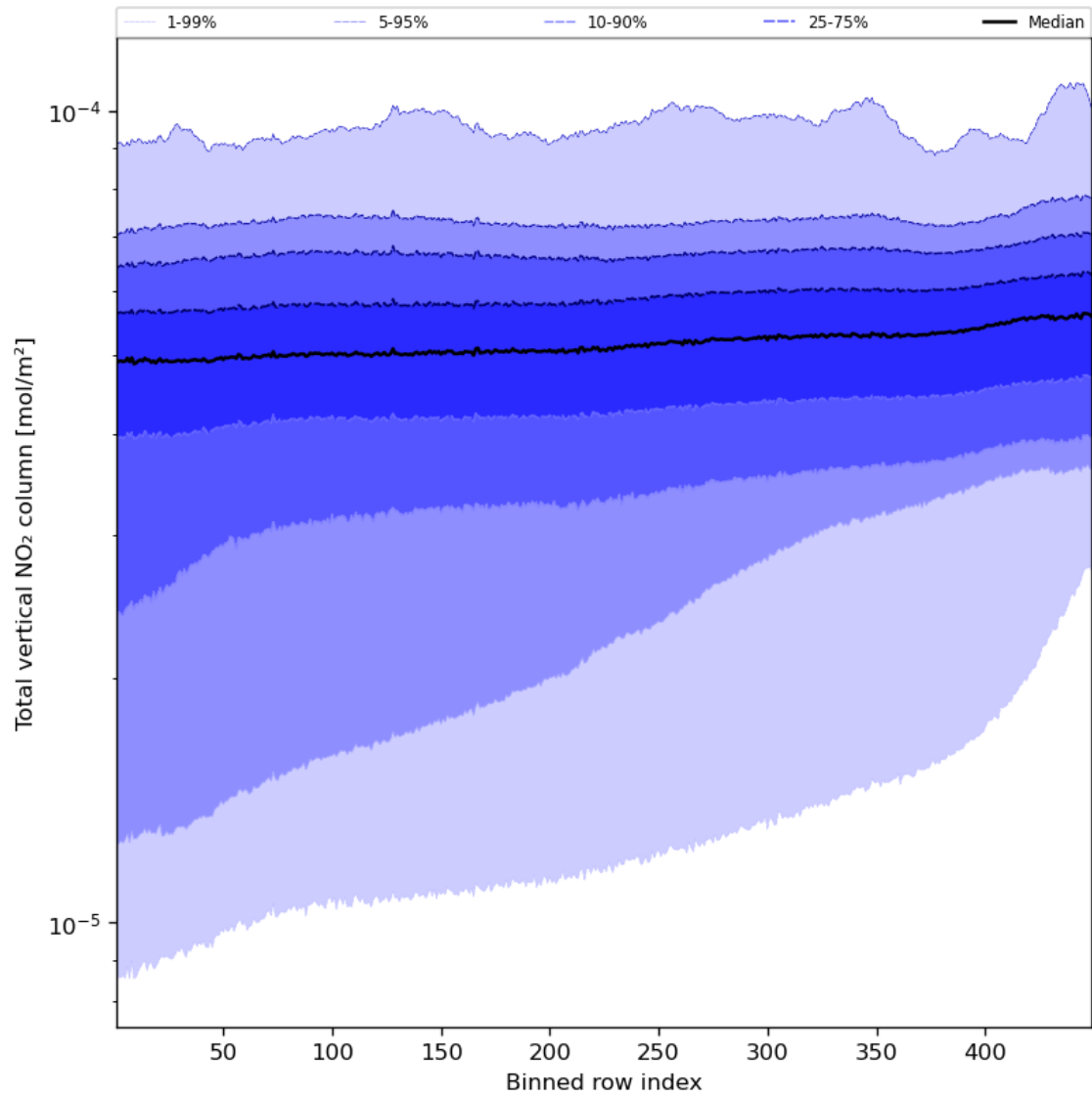
Figure 55: Along track statistics of “Total vertical NO 2 column” for 2023-09-10 to 2023-09-12
