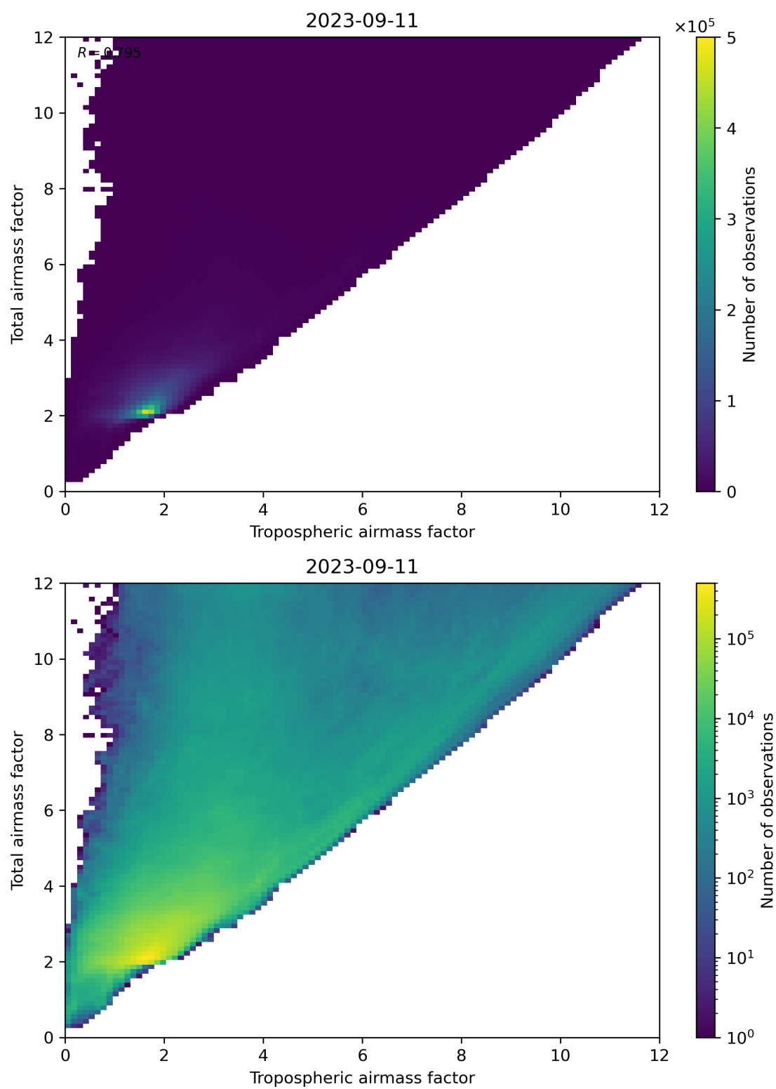
Figure 72: Scatter density plot of “Tropospheric airmass factor” against “Total airmass factor” for 2023-09-10 to 2023-09-12.
