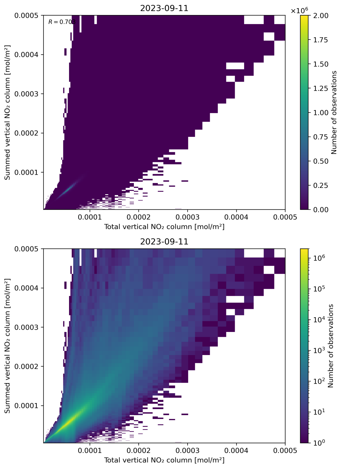
Figure 112: Scatter density plot of “Total vertical NO 2 column” against “Summed vertical NO 2 column” for 2023-09-10 to 2023-09-12.
