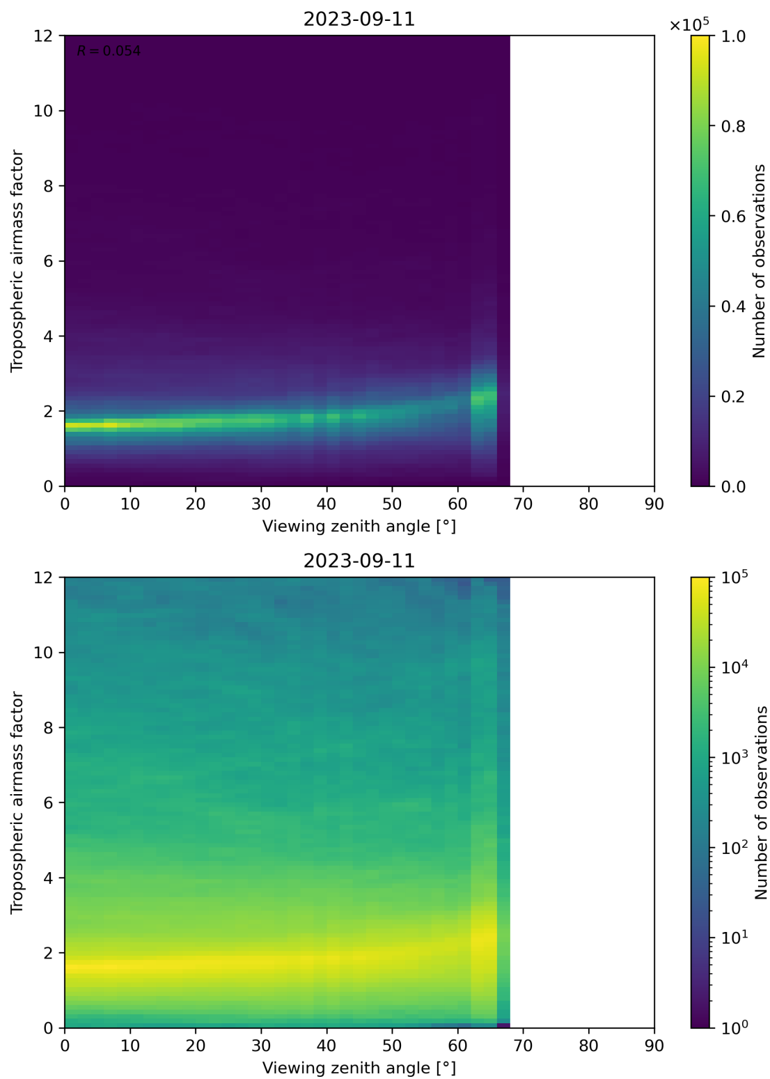
Figure 161: Scatter density plot of “Viewing zenith angle” against “Tropospheric airmass factor” for 2023-09-10 to 2023-09-12.
