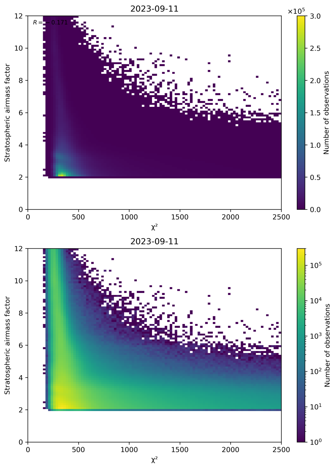
Figure 81: Scatter density plot of “ \chi^2 ” against “Stratospheric airmass factor” for 2023-09-10 to 2023-09-12.
