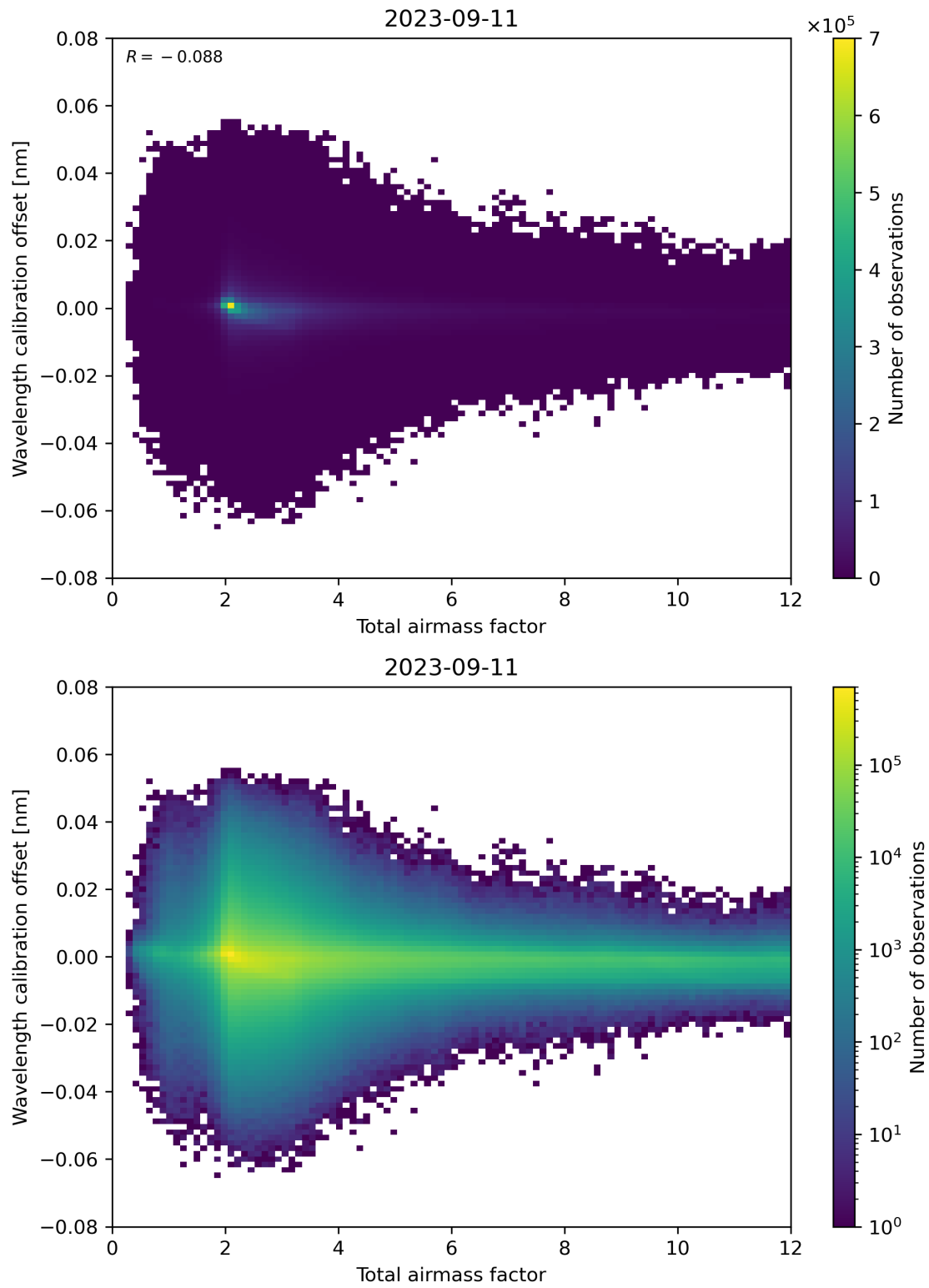
Figure 70: Scatter density plot of “Total airmass factor” against “Wavelength calibration offset” for 2023-09-10 to 2023-09-12.
