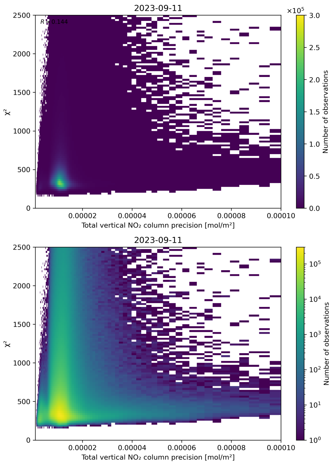
Figure 116: Scatter density plot of “Total vertical NO 2 column precision” against “ \chi^2 ” for 2023-09-10 to 2023-09-12.
