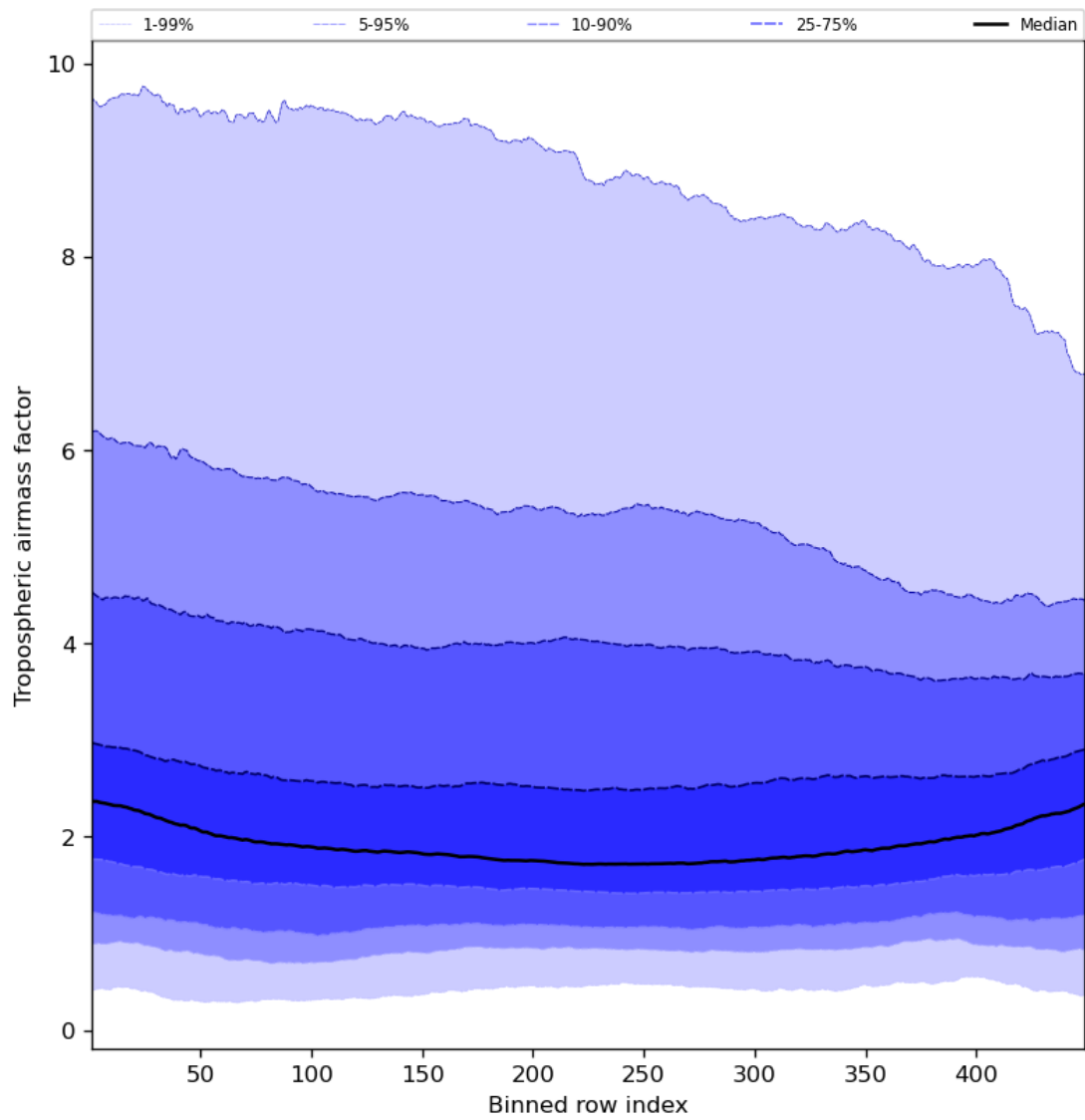
Figure 48: Along track statistics of “Tropospheric airmass factor” for 2023-09-10 to 2023-09-12
