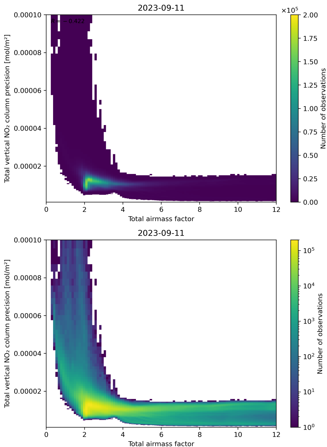
Figure 68: Scatter density plot of “Total airmass factor” against “Total vertical NO 2 column precision” for 2023-09-10 to 2023-09-12.
