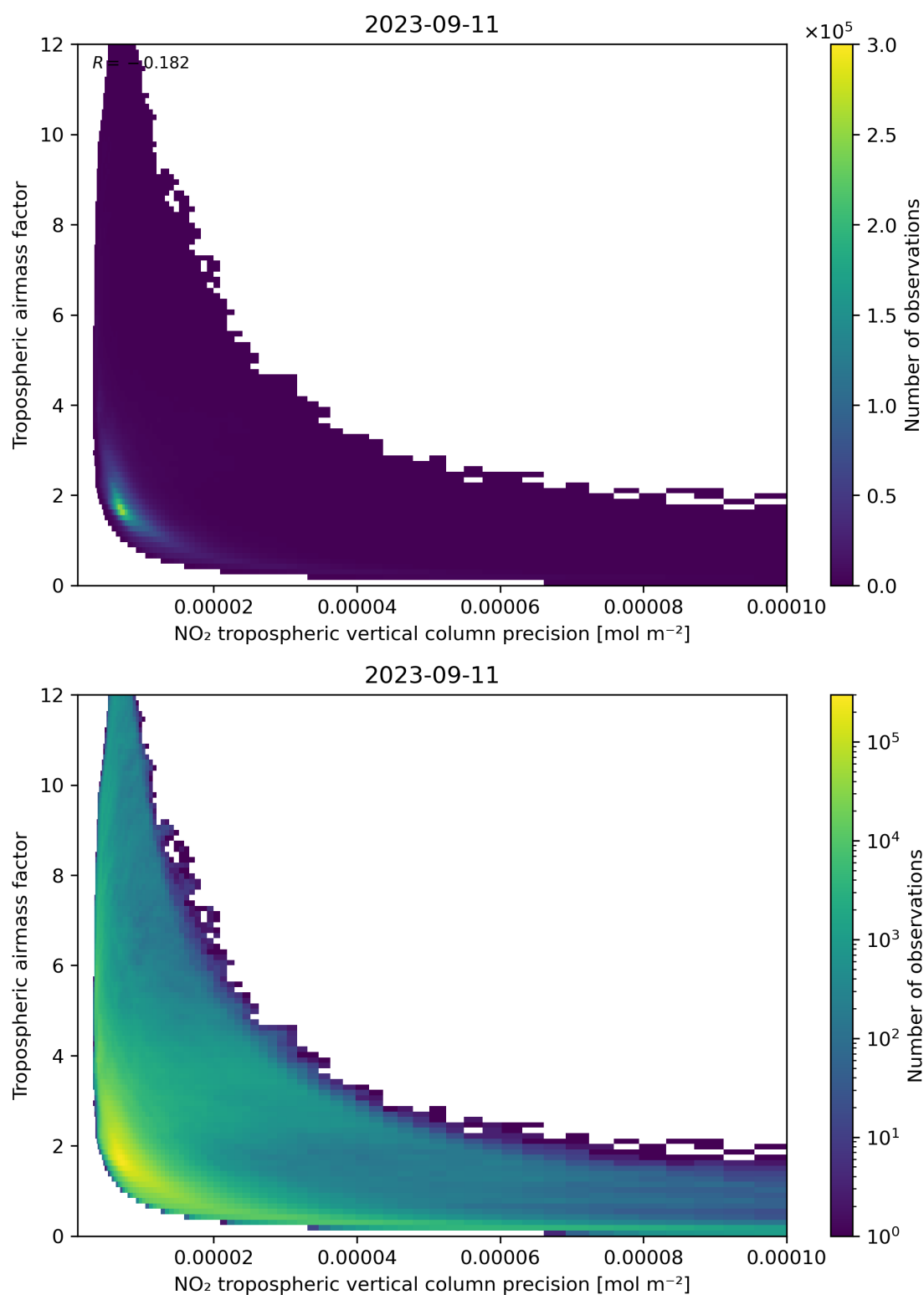
Figure 133: Scatter density plot of “NO 2 tropospheric vertical column precision” against “Tropospheric air mass factor” for 2023-09-10 to 2023-09-12.
