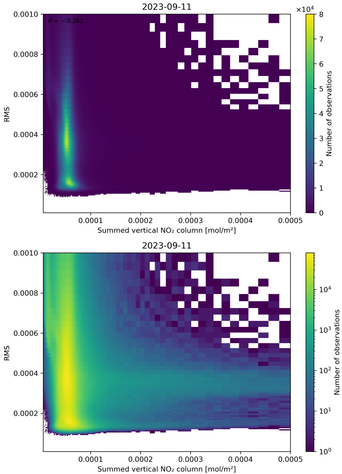
Figure 109: Scatter density plot of “Summed vertical NO 2 column” against “RMS” for 2023-09-10 to 2023-09-12.
