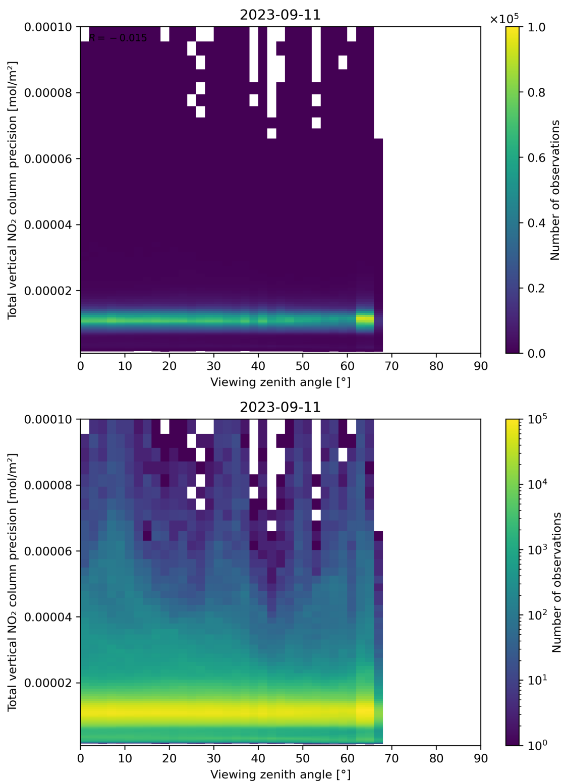
Figure 168: Scatter density plot of “Viewing zenith angle” against “Total vertical NO 2 column precision” for 2023-09-10 to 2023-09-12.
