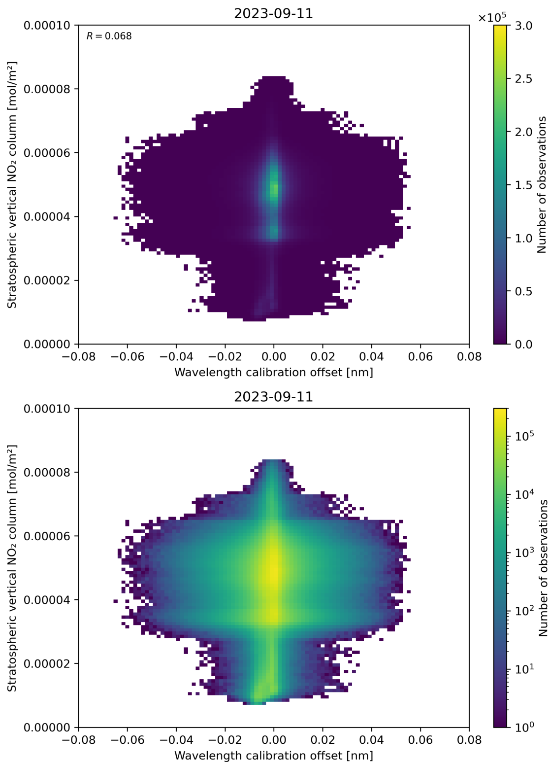
Figure 176: Scatter density plot of “Wavelength calibration offset” against “Stratospheric vertical NO 2 column” for 2023-09-10 to 2023-09-12.
