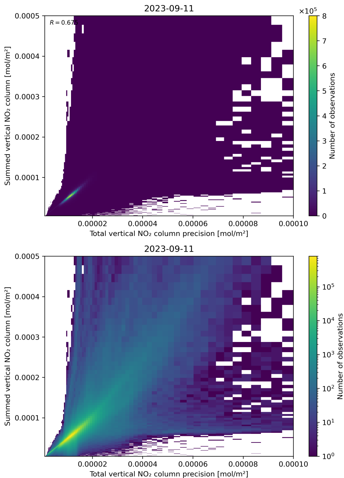
Figure 117: Scatter density plot of “Total vertical NO 2 column precision” against “Summed vertical NO 2 column” for 2023-09-10 to 2023-09-12.
