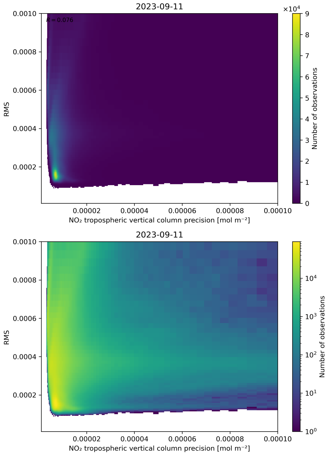
Figure 140: Scatter density plot of “NO 2 tropospheric vertical column precision” against “RMS” for 2023-09-10 to 2023-09-12.
