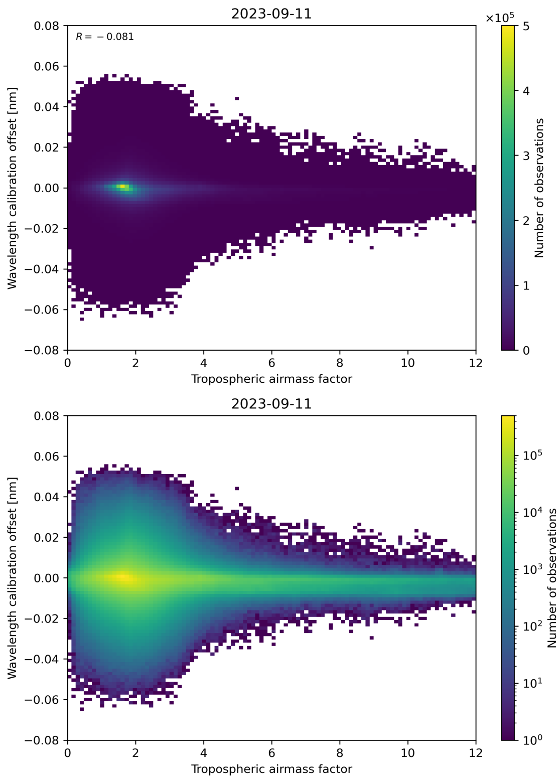
Figure 80: Scatter density plot of “Tropospheric airmass factor” against “Wavelength calibration offset” for 2023-09-10 to 2023-09-12.
