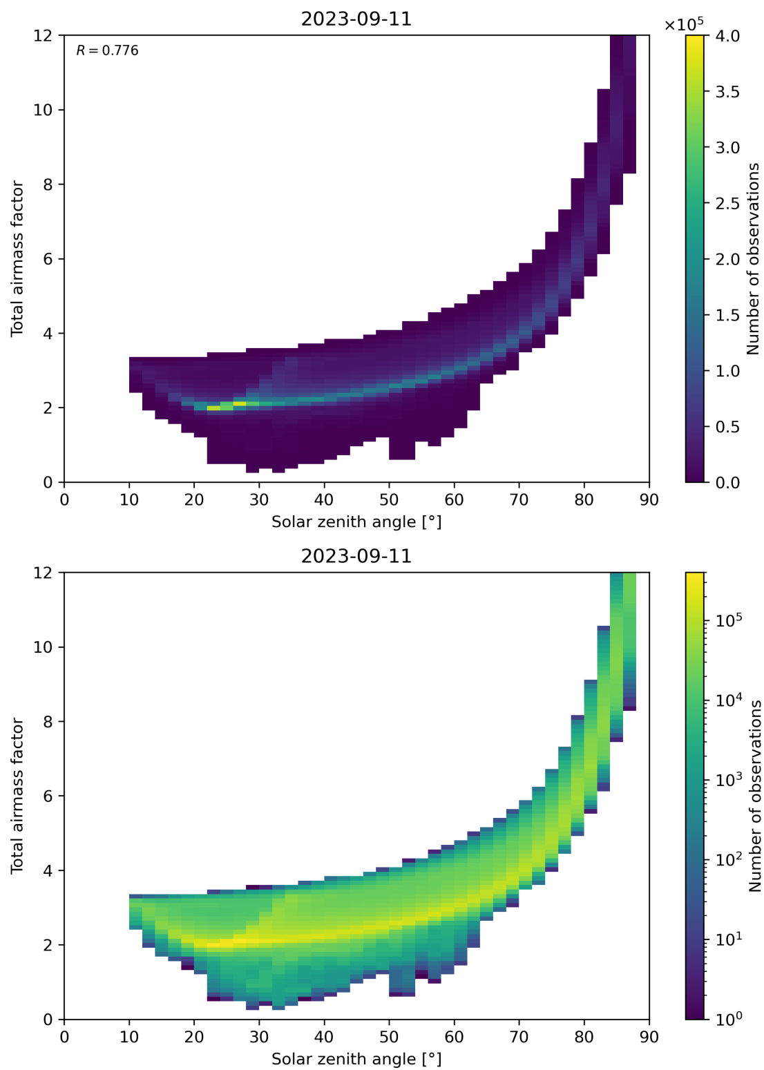
Figure 146: Scatter density plot of “Solar zenith angle” against “Total air mass factor” for 2023-09-10 to 2023-09-12.
