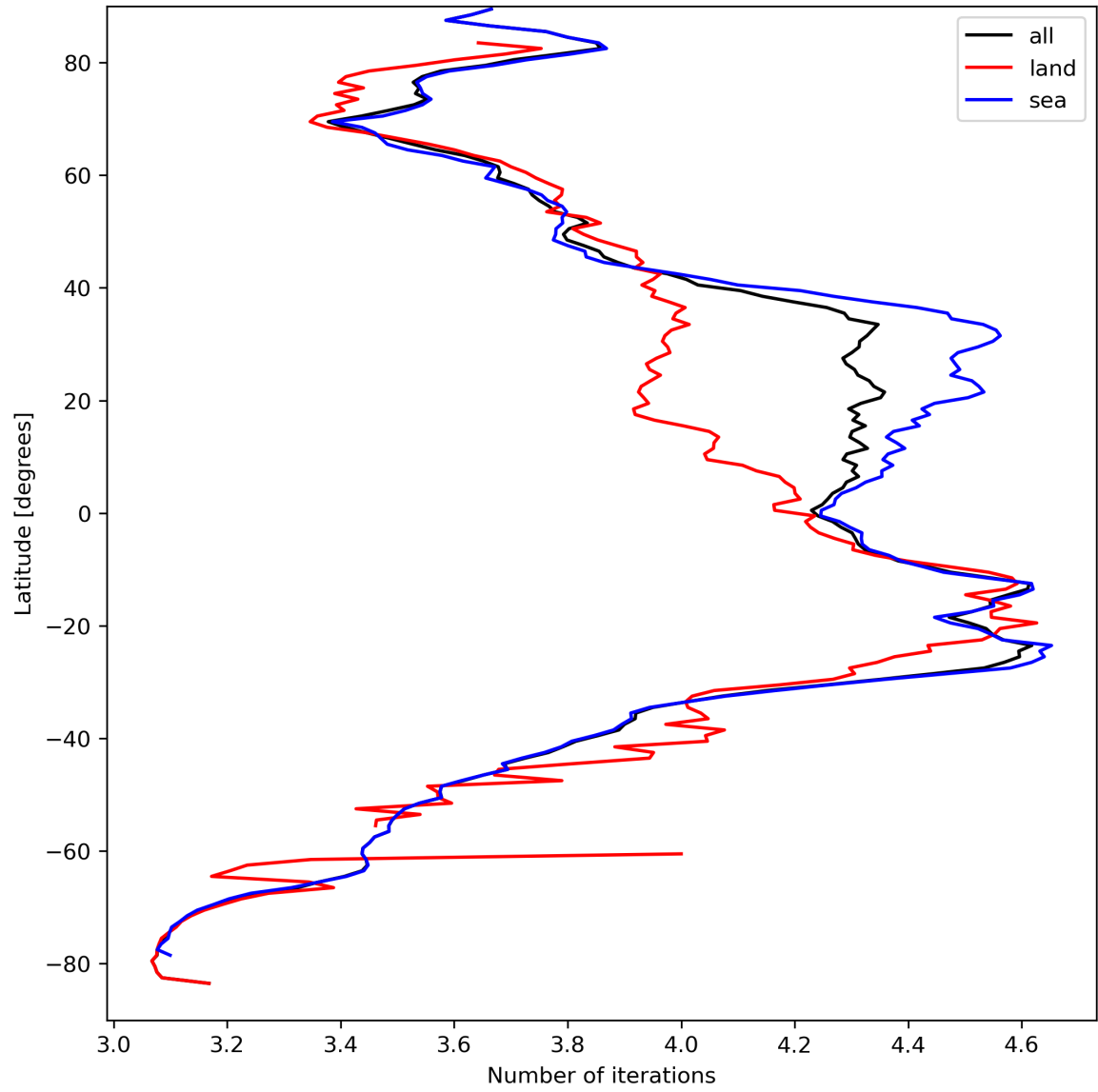
Figure 17: Zonal average of “Number of iterations” for 2023-09-10 to 2023-09-12.
