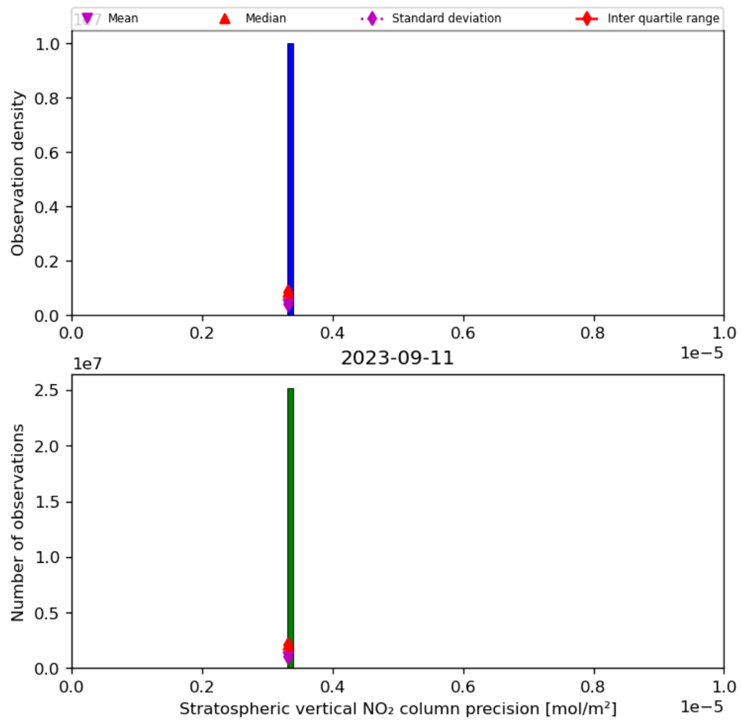
Figure 37: Histogram of “Stratospheric vertical NO 2 column precision” for 2023-09-10 to 2023-09-12
