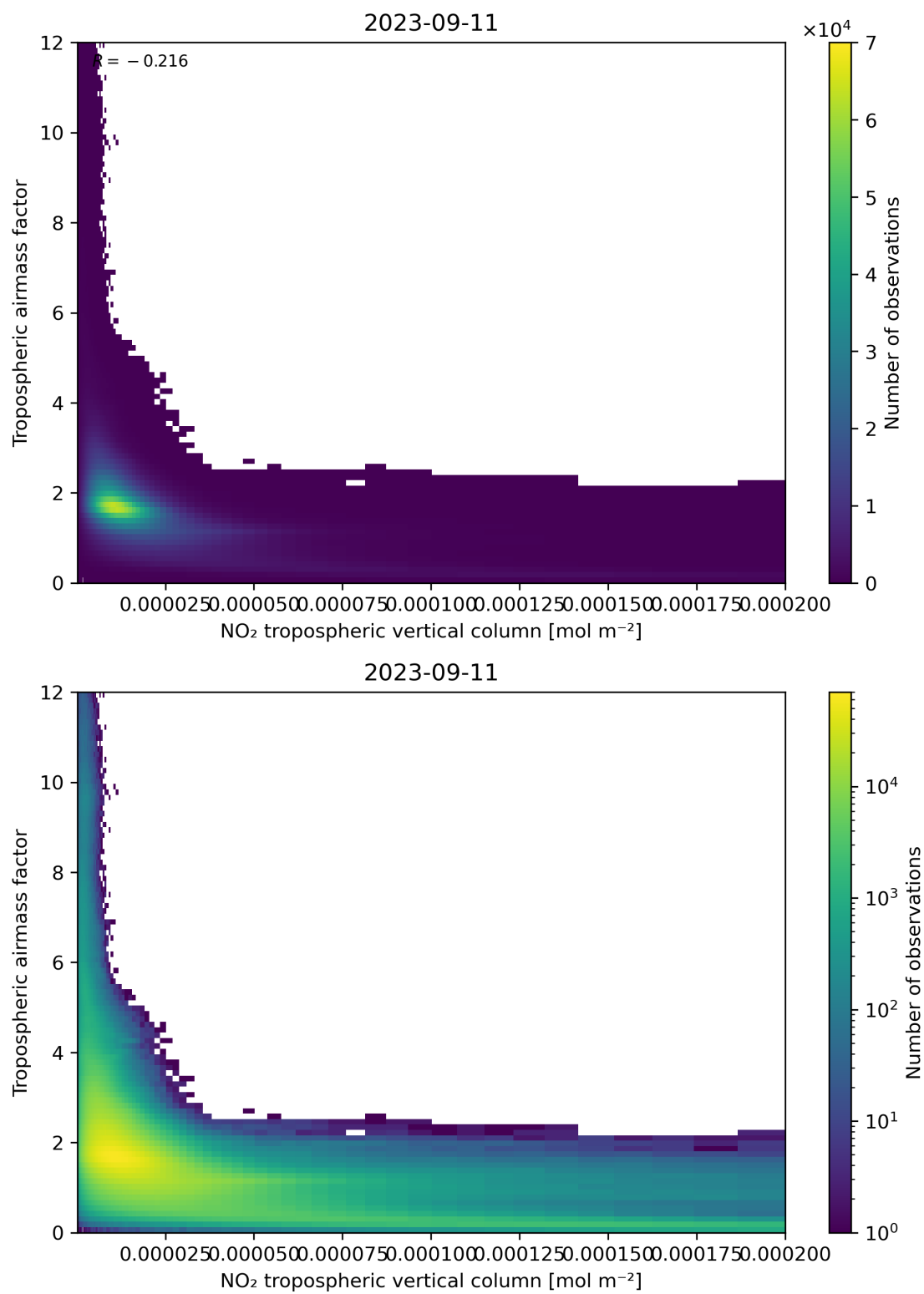
Figure 123: Scatter density plot of “NO 2 tropospheric vertical column” against “Tropospheric air mass factor” for 2023-09-10 to 2023-09-12.
