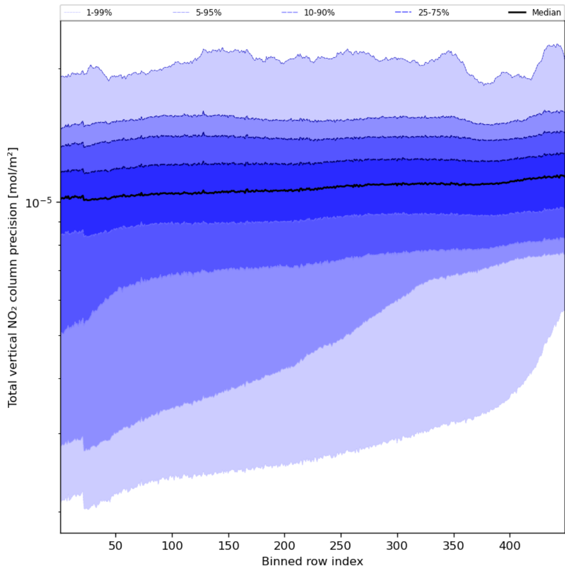
Figure 56: Along track statistics of “Total vertical NO 2 column precision” for 2023-09-10 to 2023-09-12
