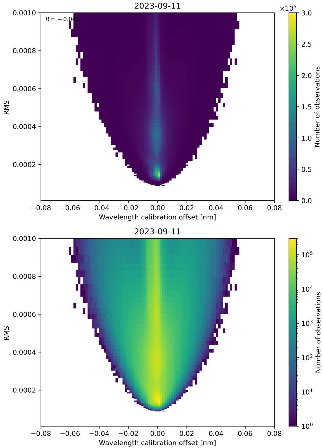
Figure 181: Scatter density plot of “Wavelength calibration offset” against “RMS” for 2023-09-10 to 2023-09-12.
