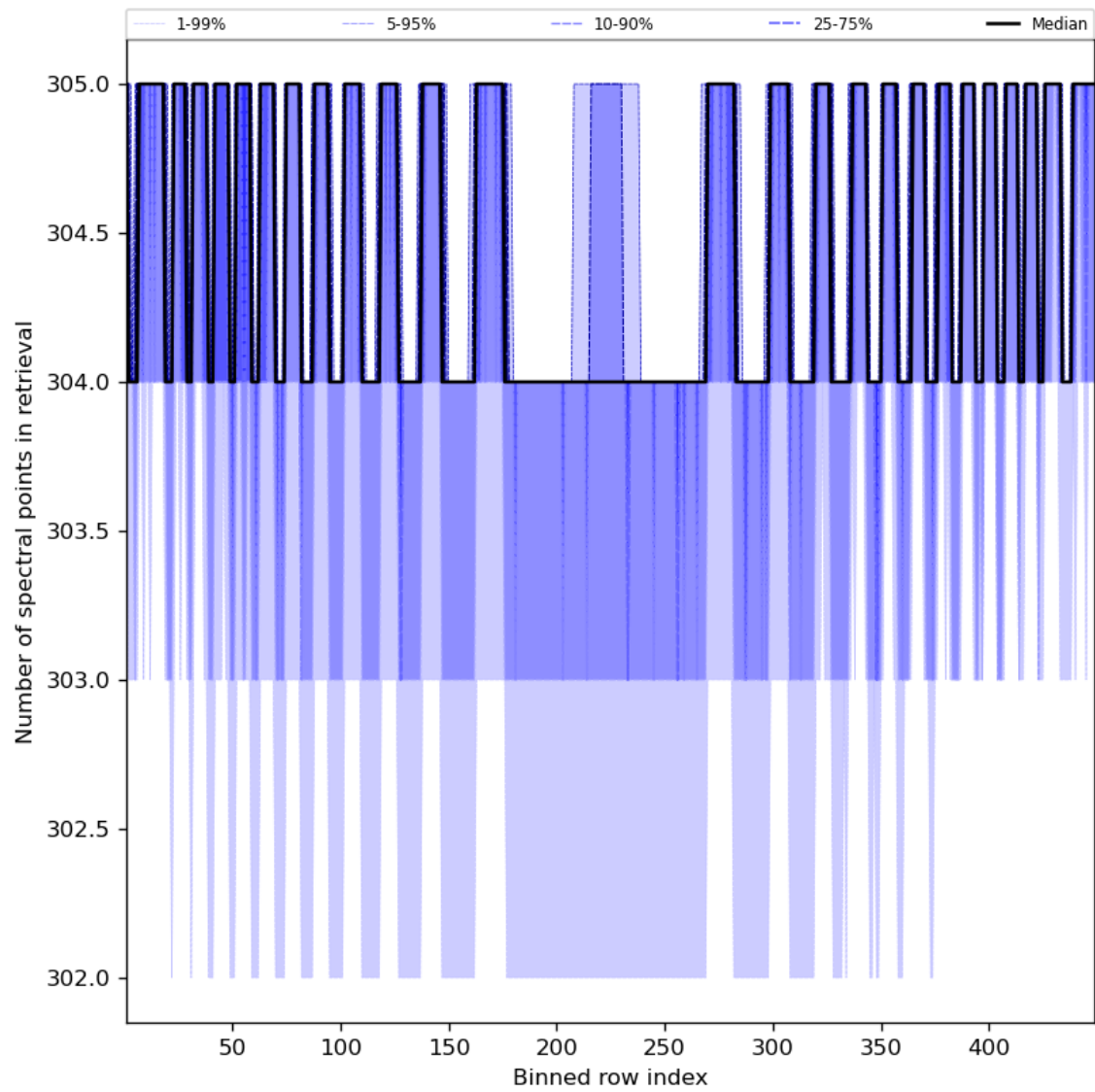
Figure 50: Along track statistics of “Number of spectral points in retrieval” for 2023-09-10 to 2023-09-12
