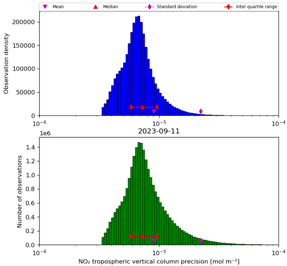
Figure 30: Histogram of “NO 2 tropospheric vertical column precision” for 2023-09-10 to 2023-09-12
