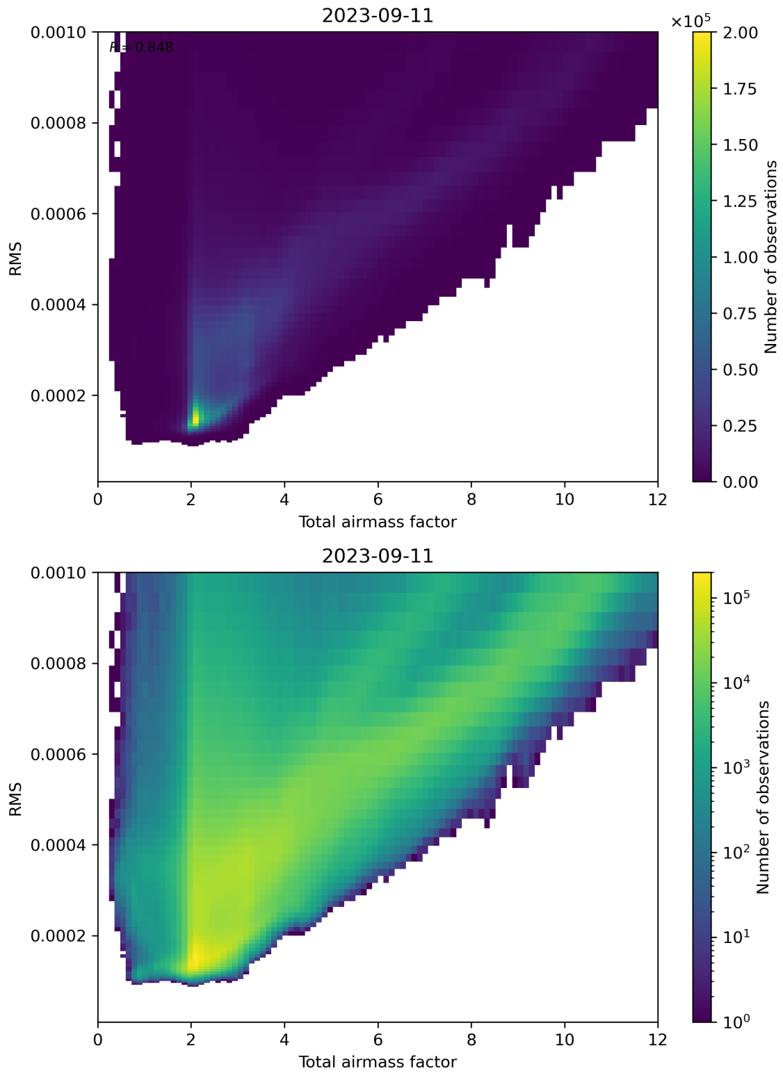
Figure 69: Scatter density plot of “Total airmass factor” against “RMS” for 2023-09-10 to 2023-09-12.
