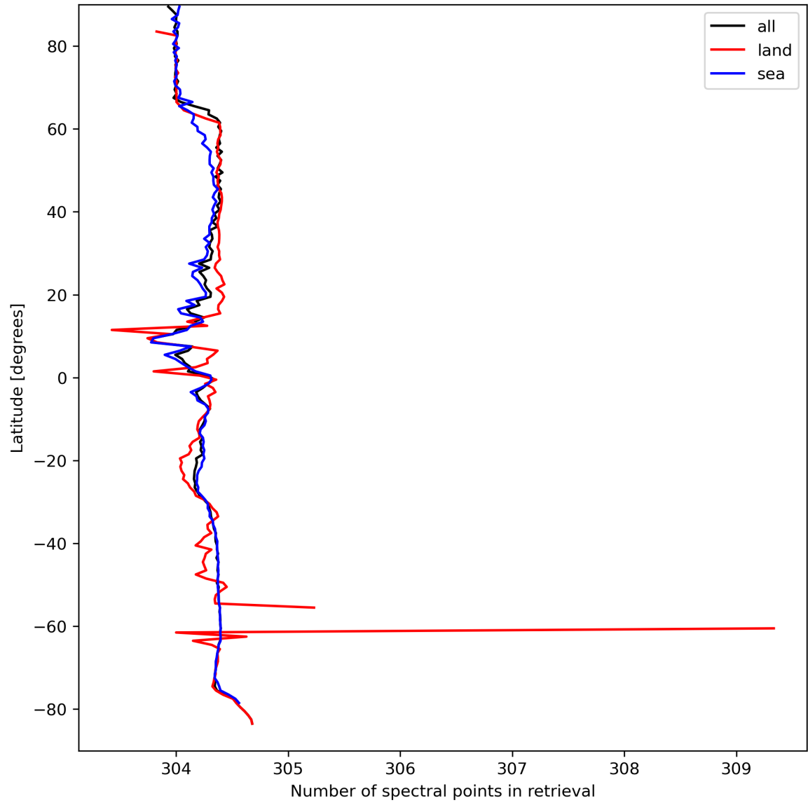
Figure 16: Zonal average of “Number of spectral points in retrieval” for 2023-09-10 to 2023-09-12.
