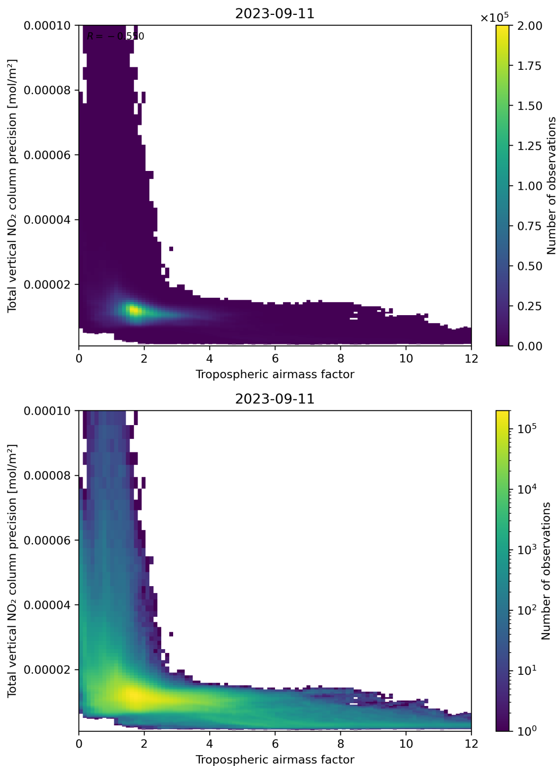
Figure 78: Scatter density plot of “Tropospheric air mass factor” against “Total vertical NO 2 column precision” for 2023-09-10 to 2023-09-12.
