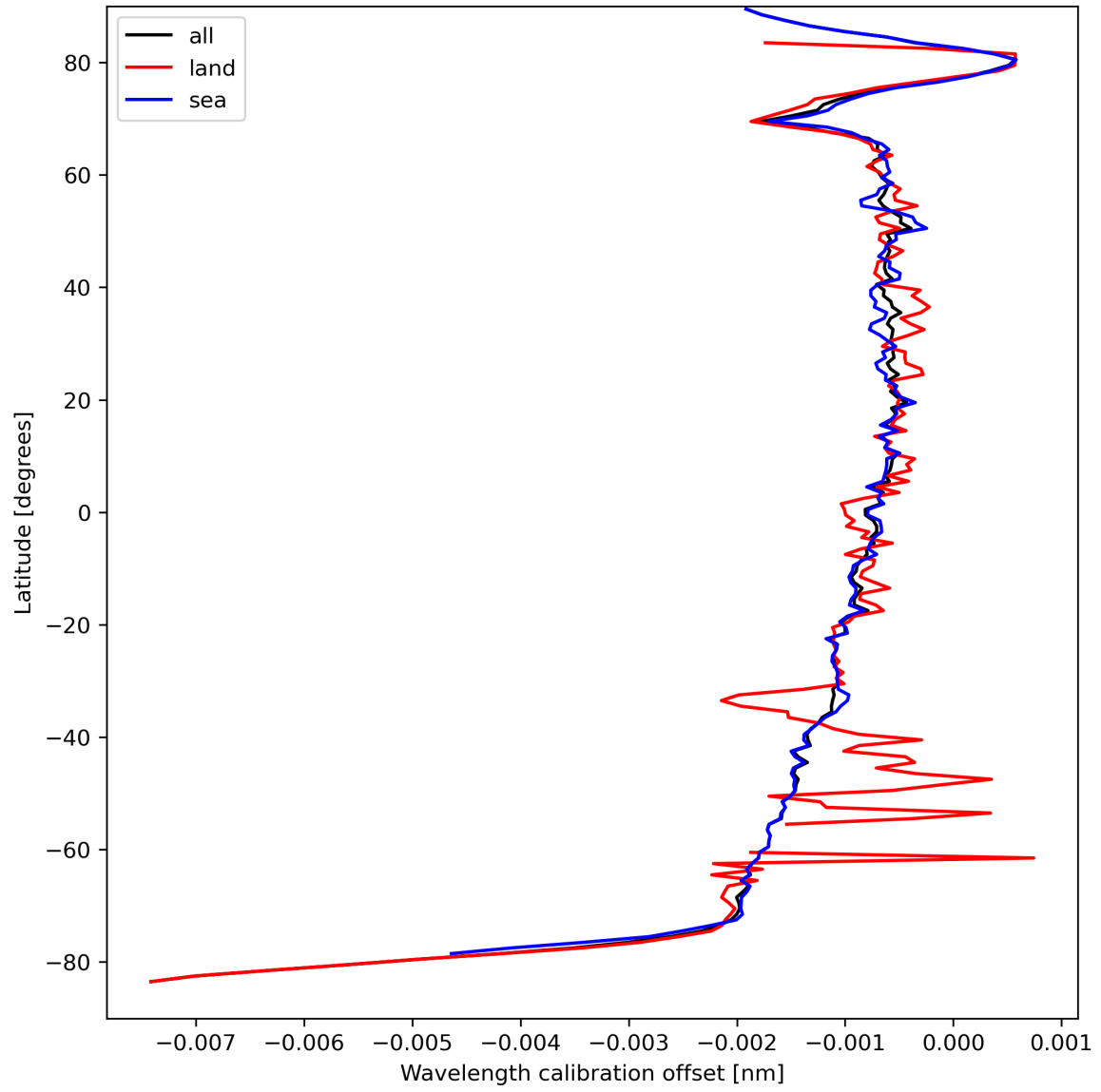
Figure 18: Zonal average of “Wavelength calibration offset” for 2023-09-10 to 2023-09-12.
