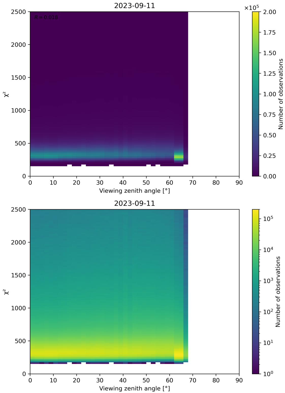
Figure 162: Scatter density plot of “Viewing zenith angle” against “ \chi^2 ” for 2023-09-10 to 2023-09-12.
