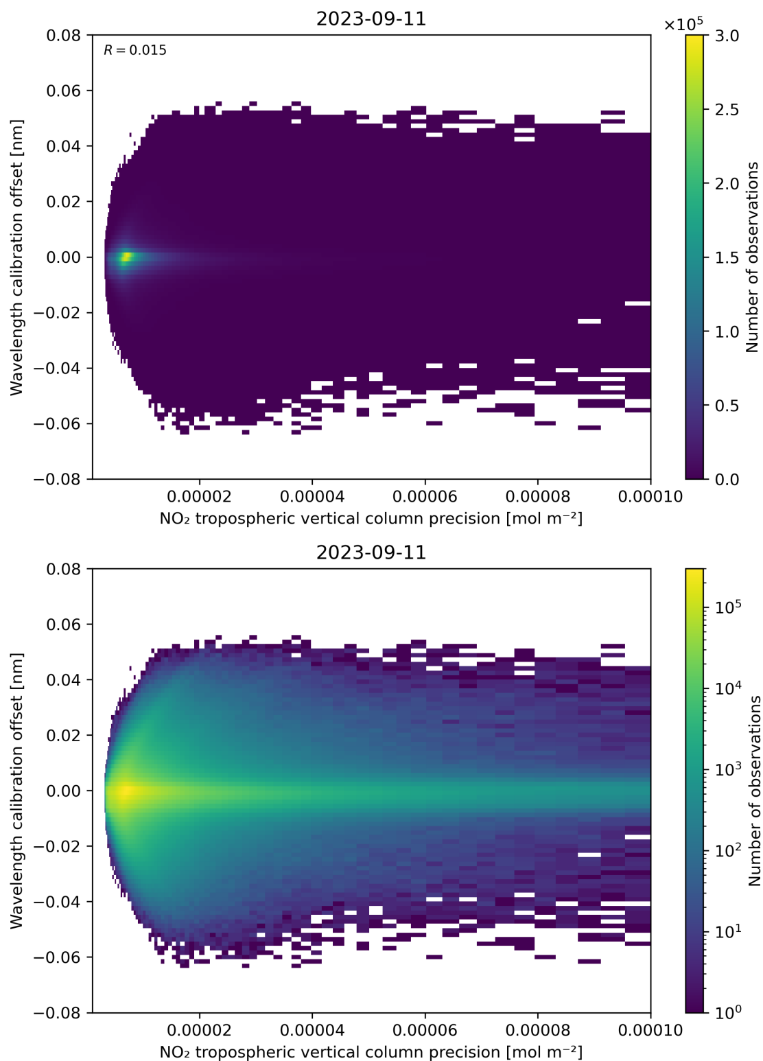
Figure 141: Scatter density plot of “NO 2 tropospheric vertical column precision” against “Wavelength calibration offset” for 2023-09-10 to 2023-09-12.
