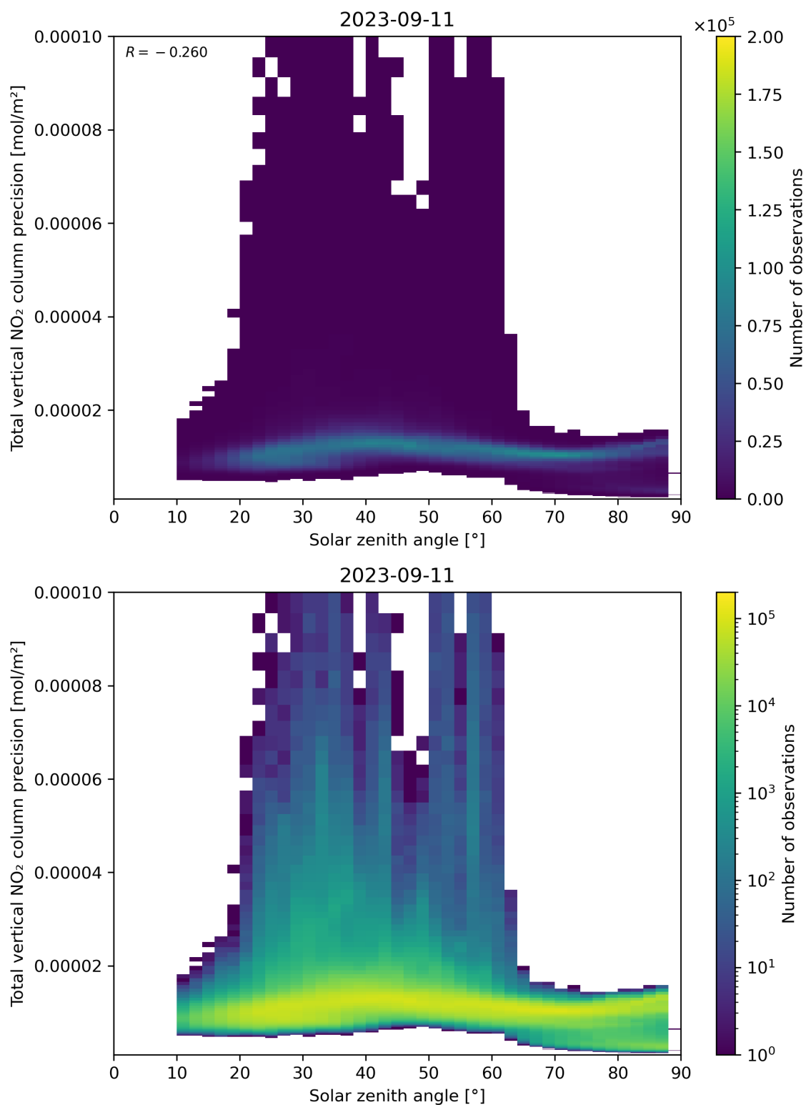
Figure 154: Scatter density plot of “Solar zenith angle” against “Total vertical NO 2 column precision” for 2023-09-10 to 2023-09-12.
