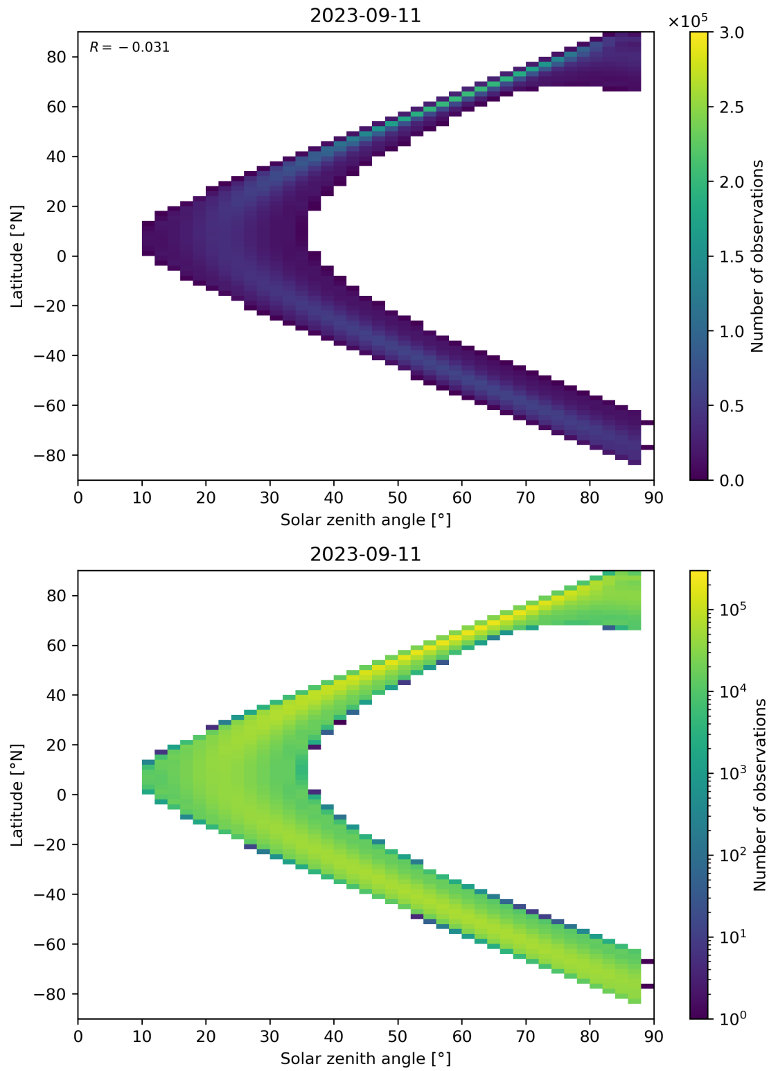
Figure 149: Scatter density plot of “Solar zenith angle” against “Latitude” for 2023-09-10 to 2023-09-12.
