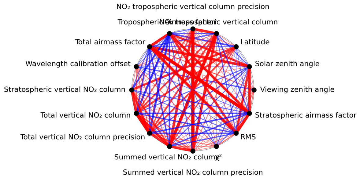
Figure 1: Map of correlation graph for 2023-09-10 to 2023-09-12.
