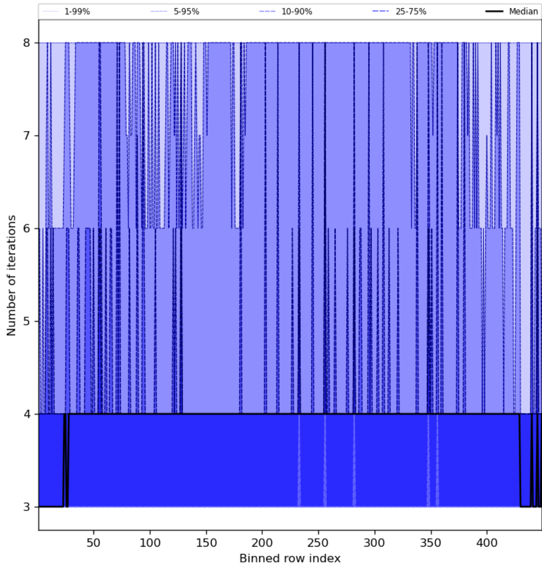
Figure 51: Along track statistics of “Number of iterations” for 2023-09-10 to 2023-09-12
