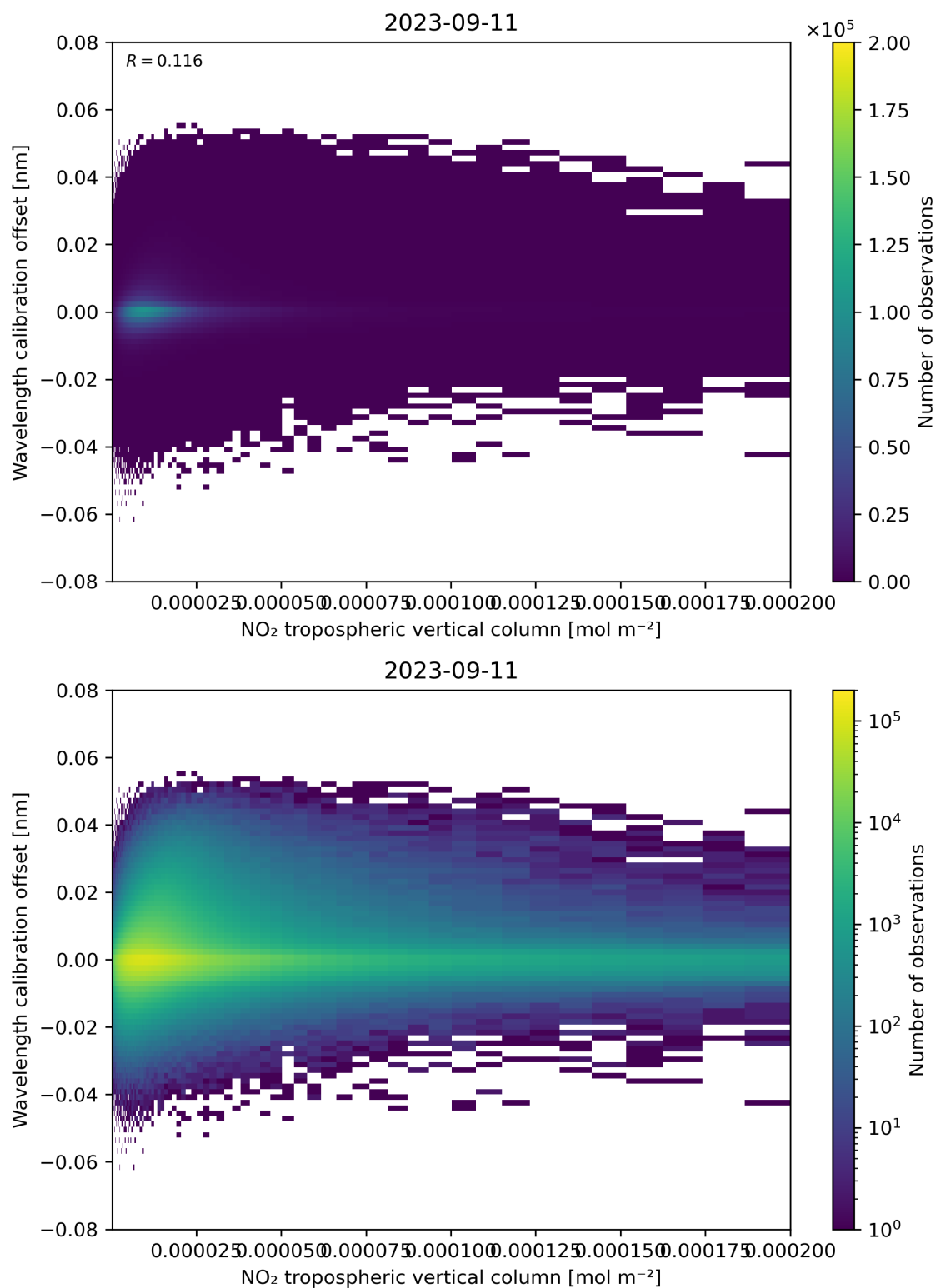
Figure 143: Scatter density plot of “NO 2 tropospheric vertical column” against “Wavelength calibration offset” for 2023-09-10 to 2023-09-12.
