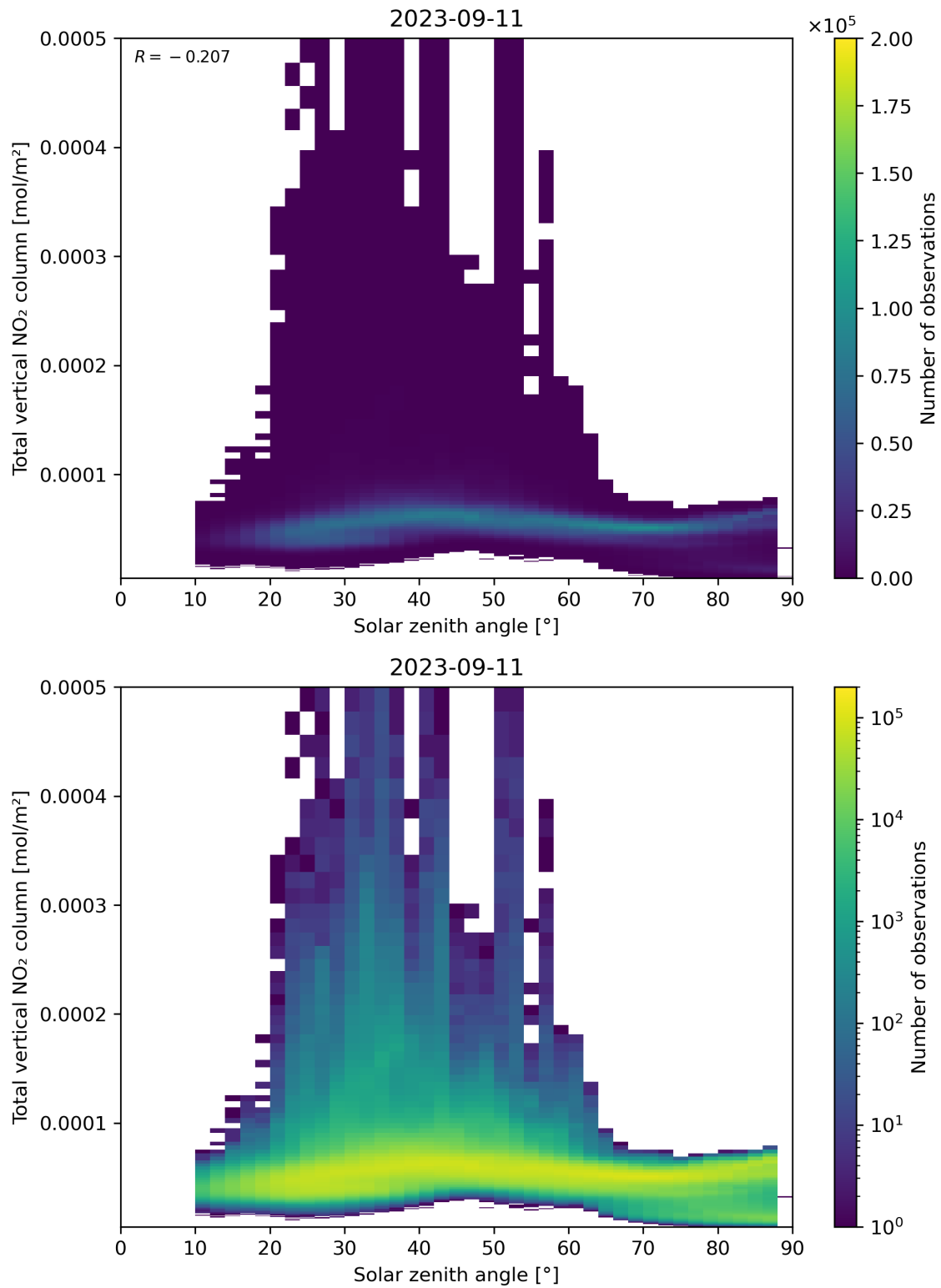
Figure 153: Scatter density plot of “Solar zenith angle” against “Total vertical NO 2 column” for 2023-09-10 to 2023-09-12.
