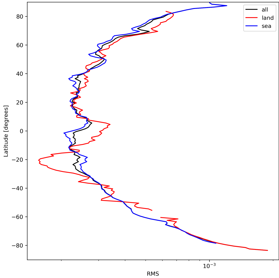
Figure 26: Zonal average of “RMS” for 2023-09-10 to 2023-09-12.
