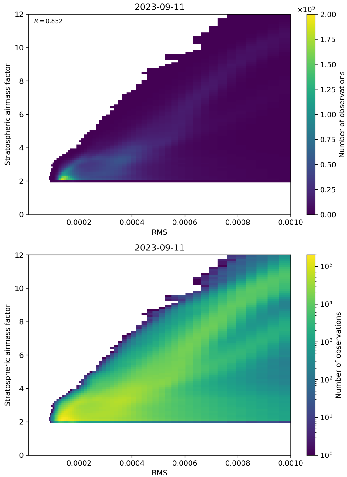
Figure 144: Scatter density plot of “RMS” against “Stratospheric airmass factor” for 2023-09-10 to 2023-09-12.
