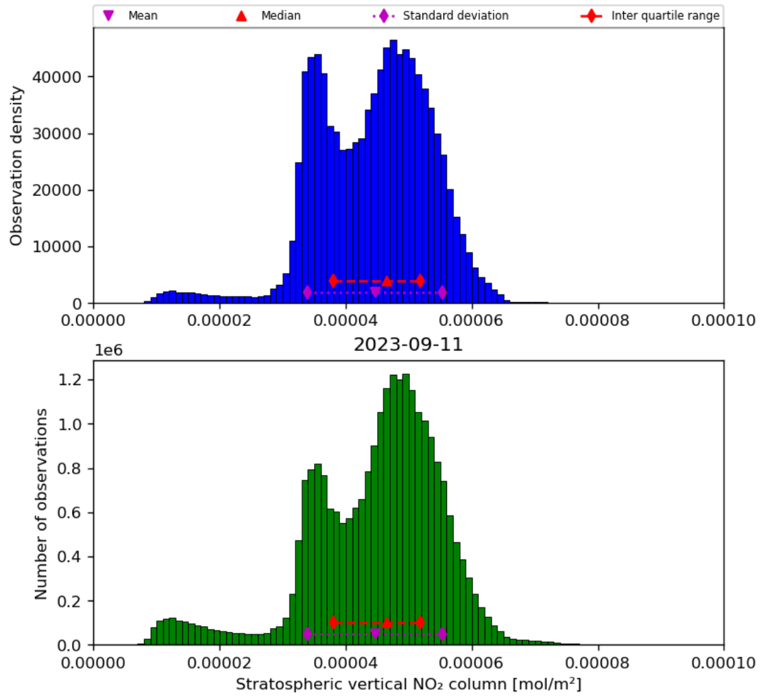
Figure 36: Histogram of “Stratospheric vertical NO 2 column” for 2023-09-10 to 2023-09-12
