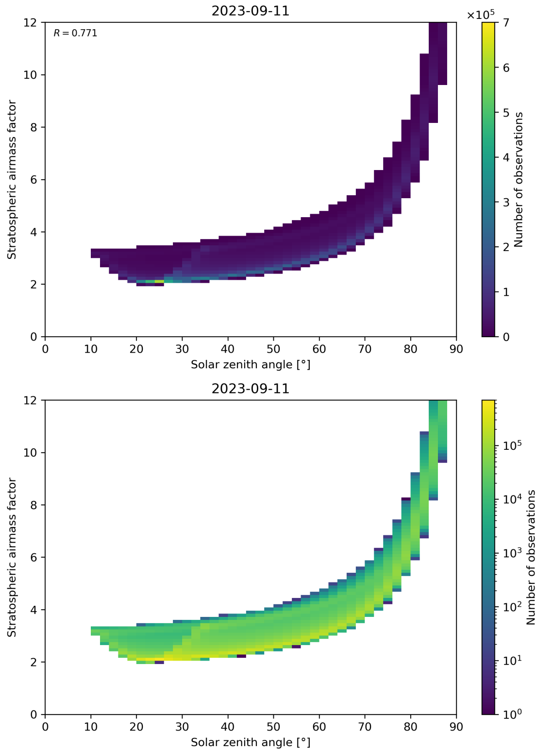
Figure 145: Scatter density plot of “Solar zenith angle” against “Stratospheric airmass factor” for 2023-09-10 to 2023-09-12.
