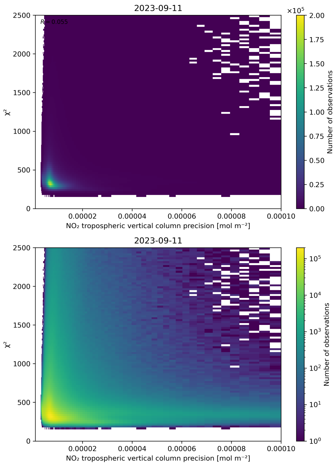
Figure 134: Scatter density plot of “NO 2 tropospheric vertical column precision” against “ \chi^2 ” for 2023-09-10 to 2023-09-12.
