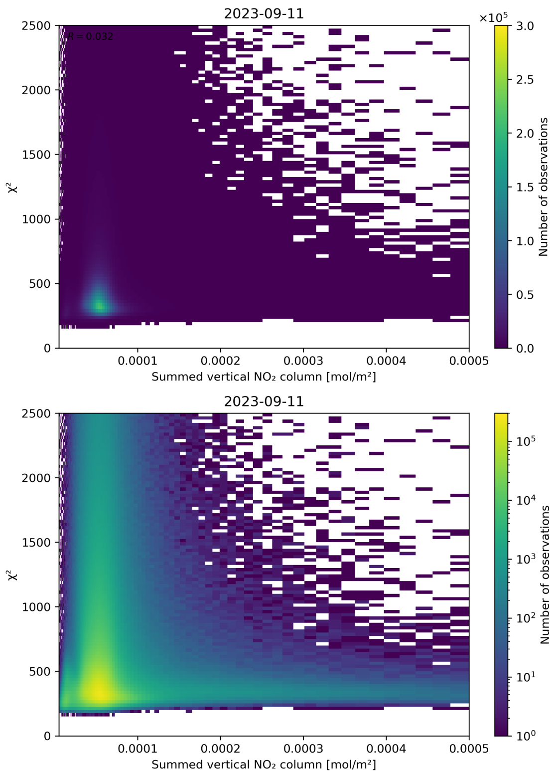
Figure 104: Scatter density plot of “Summed vertical NO 2 column” against “ \chi^2 ” for 2023-09-10 to 2023-09-12.
