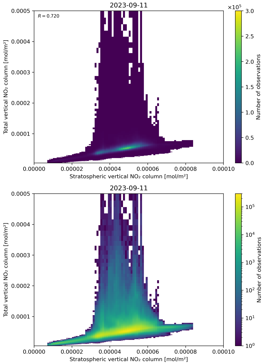
Figure 100: Scatter density plot of “Stratospheric vertical NO 2 column” against “Total vertical NO 2 column” for 2023-09-10 to 2023-09-12.
