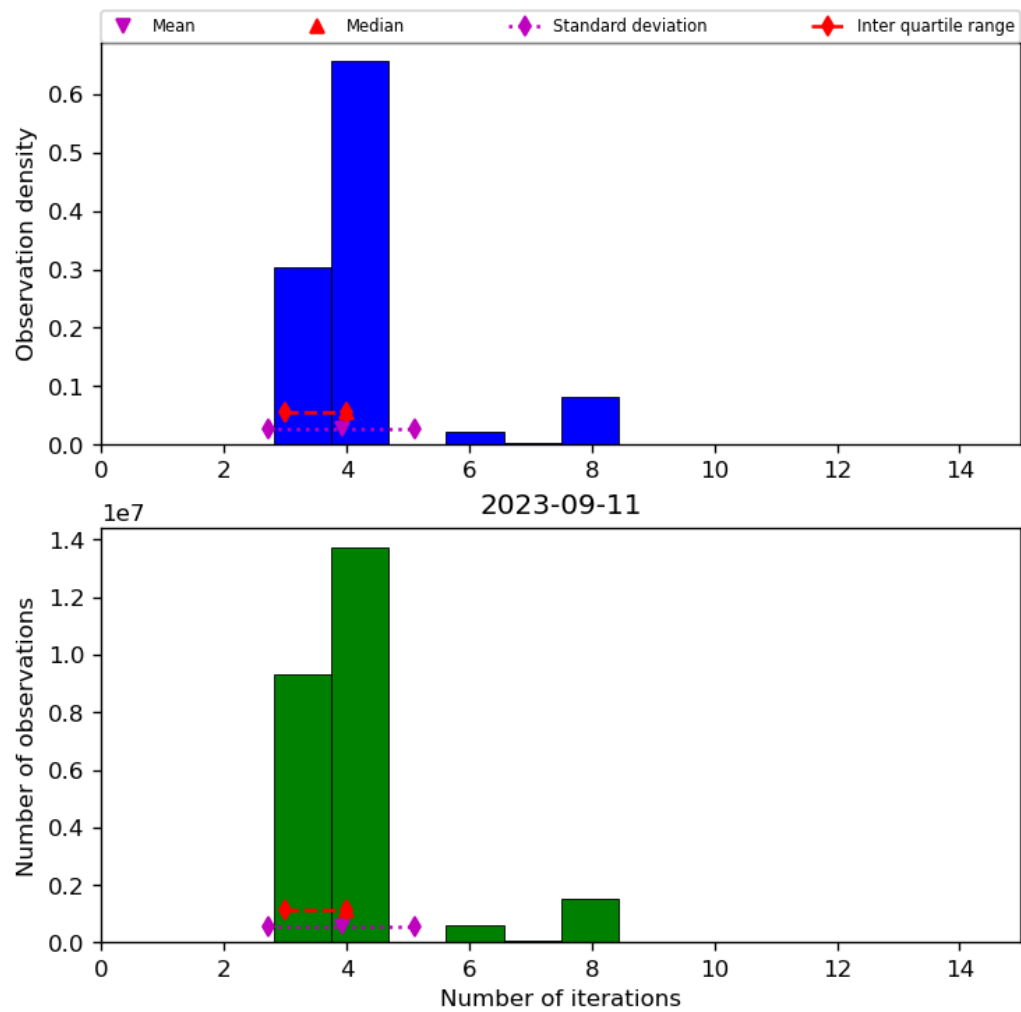
Figure 34: Histogram of “Number of iterations” for 2023-09-10 to 2023-09-12
