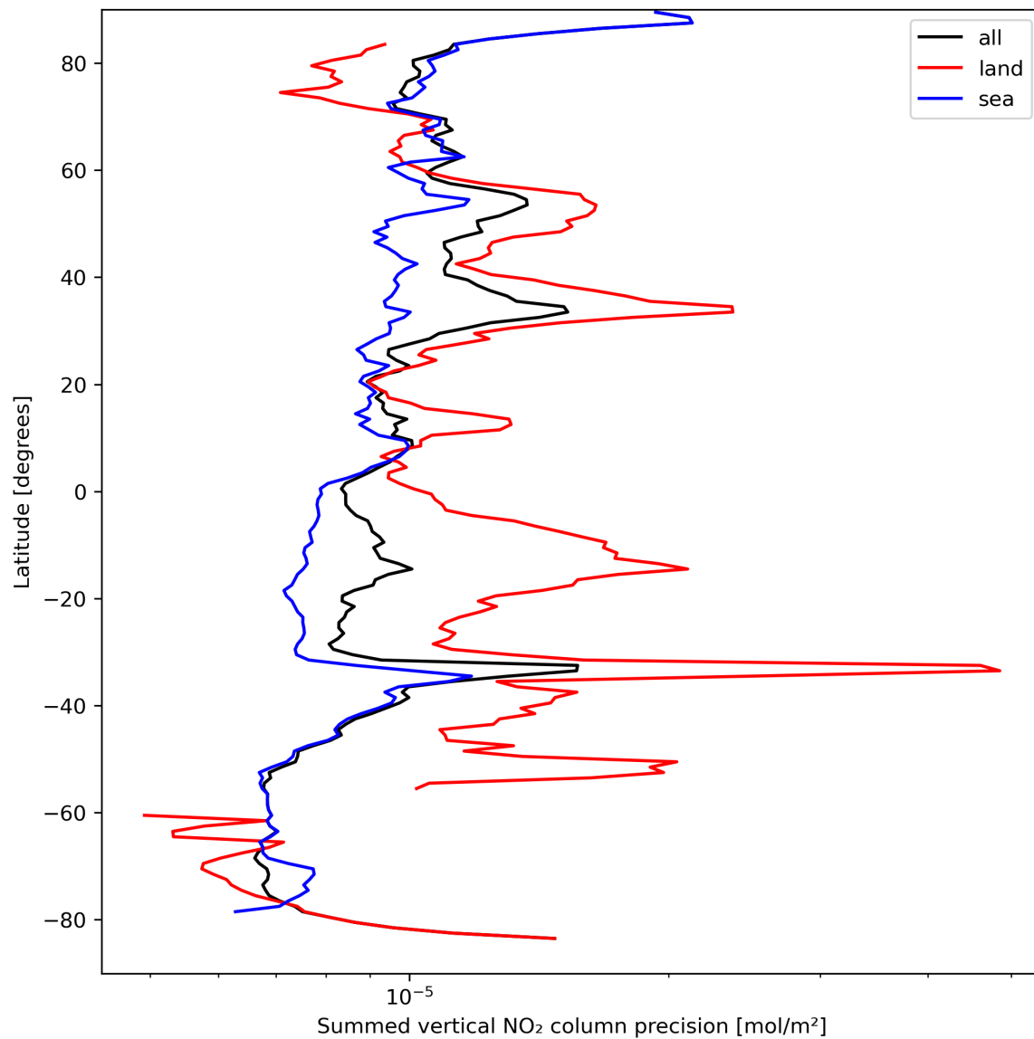
Figure 24: Zonal average of “Summed vertical NO 2 column precision” for 2023-09-10 to 2023-09-12.
