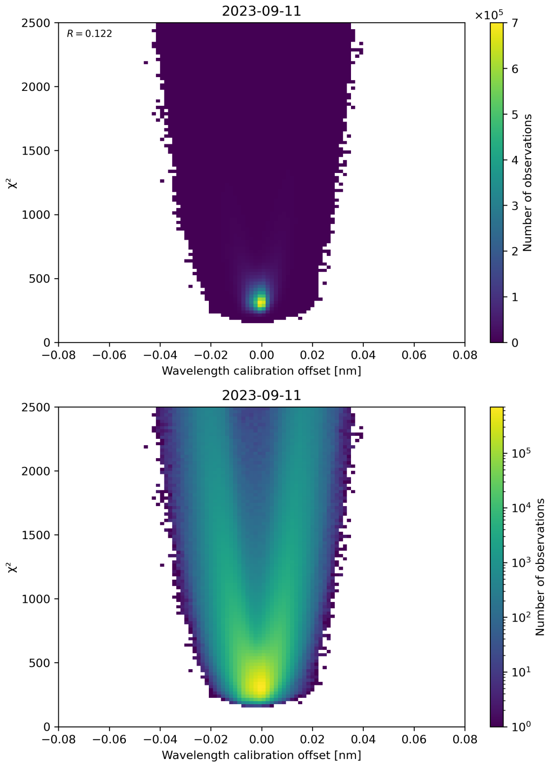
Figure 175: Scatter density plot of “Wavelength calibration offset” against “ \chi^2 ” for 2023-09-10 to 2023-09-12.
