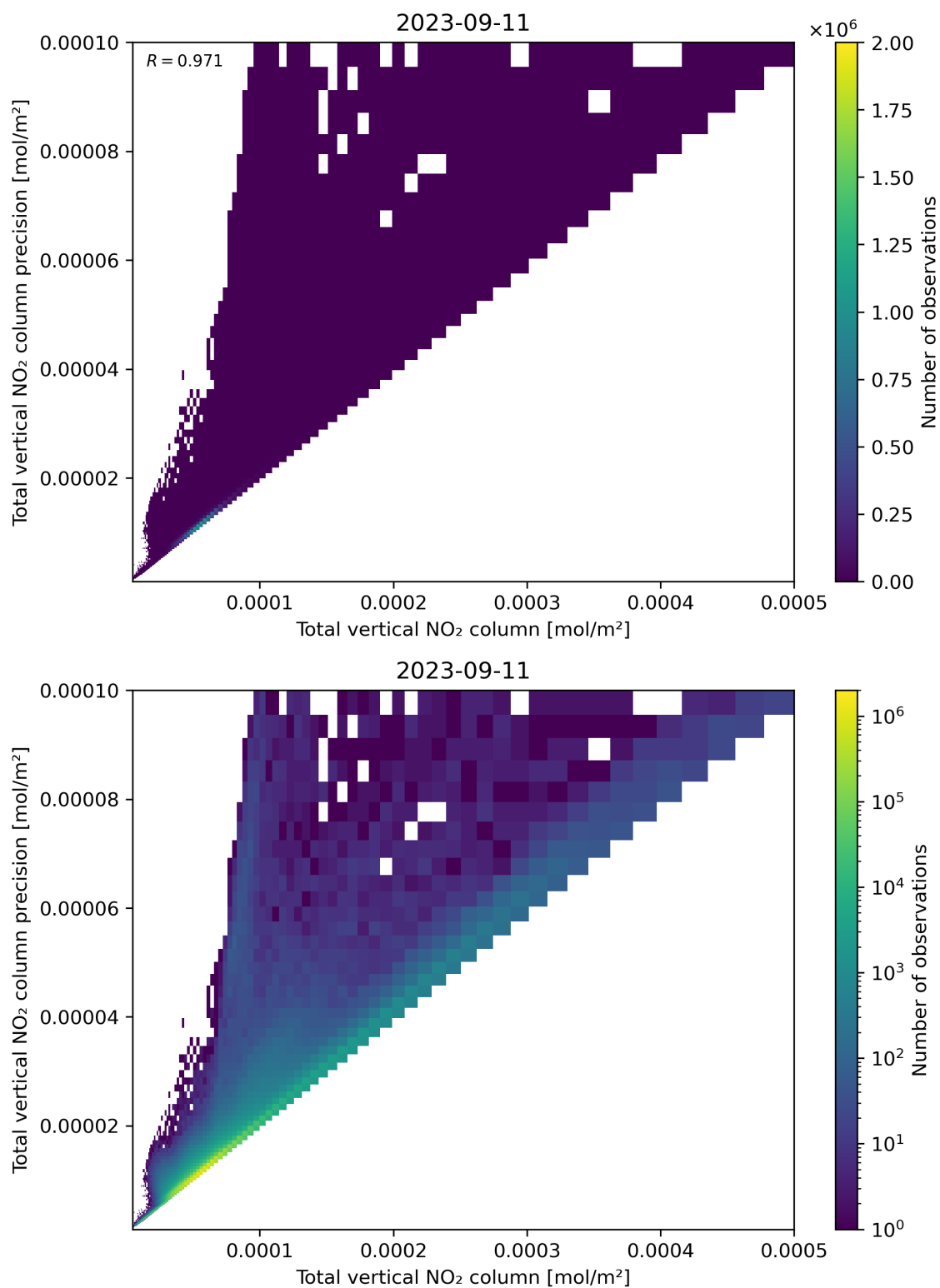
Figure 114: Scatter density plot of “Total vertical NO 2 column” against “Total vertical NO 2 column precision” for 2023-09-10 to 2023-09-12.
