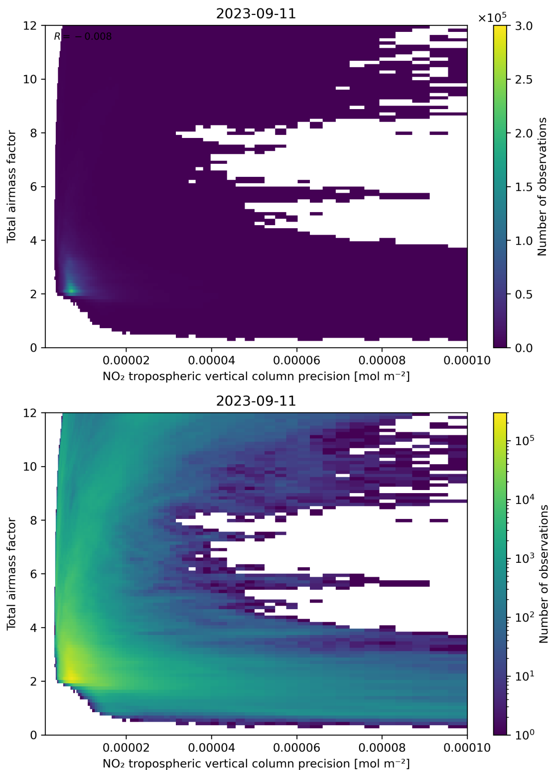
Figure 132: Scatter density plot of “NO 2 tropospheric vertical column precision” against “Total air mass factor” for 2023-09-10 to 2023-09-12.
