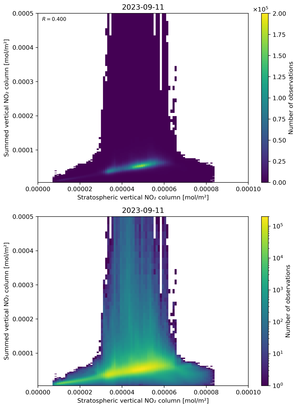
Figure 98: Scatter density plot of “Stratospheric vertical NO 2 column” against “Summed vertical NO 2 column” for 2023-09-10 to 2023-09-12.
