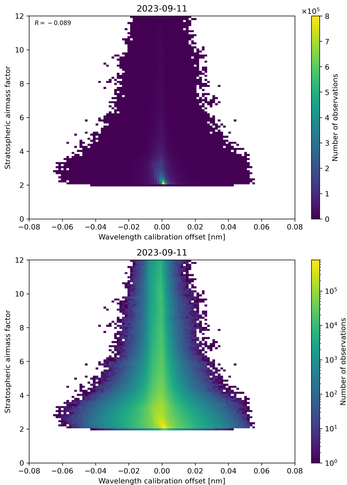
Figure 174: Scatter density plot of “Wavelength calibration offset” against “Stratospheric air mass factor” for 2023-09-10 to 2023-09-12.
