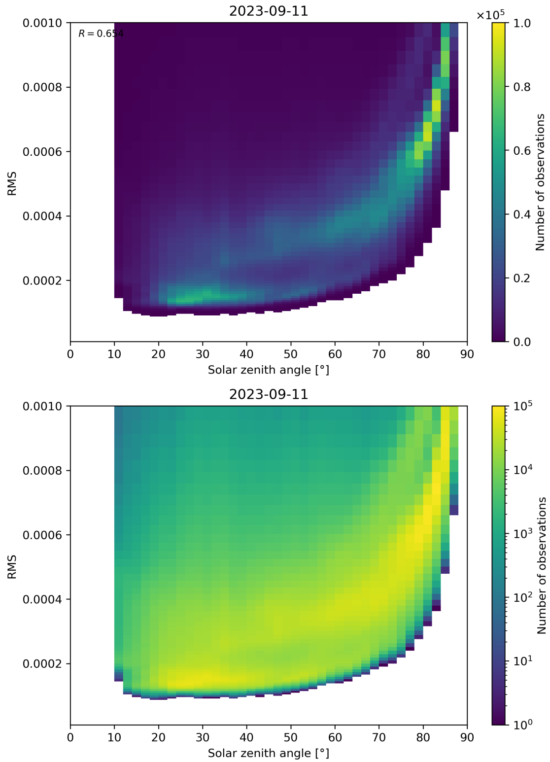
Figure 157: Scatter density plot of “Solar zenith angle” against “RMS” for 2023-09-10 to 2023-09-12.
