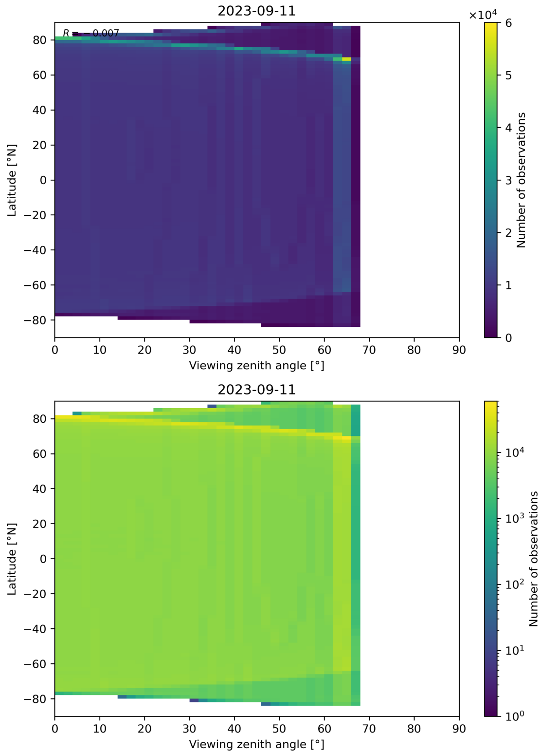
Figure 163: Scatter density plot of “Viewing zenith angle” against “Latitude” for 2023-09-10 to 2023-09-12.
