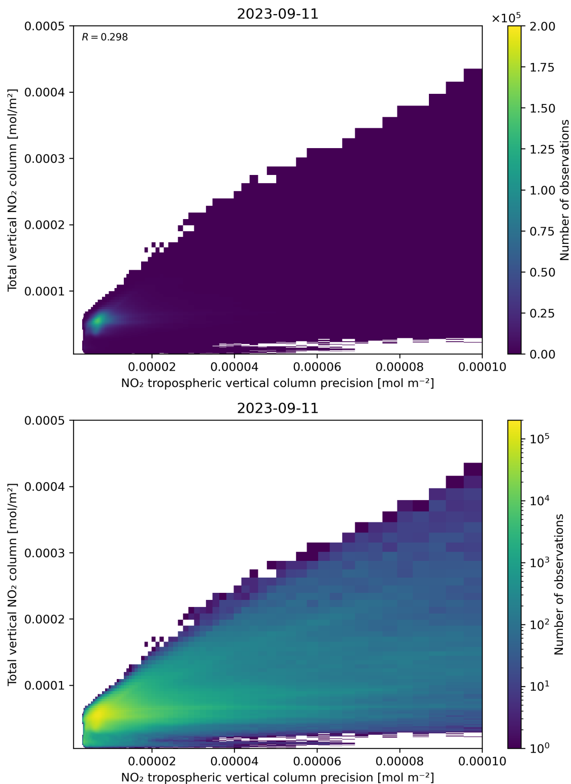
Figure 138: Scatter density plot of “NO 2 tropospheric vertical column precision” against “Total vertical NO 2 column” for 2023-09-10 to 2023-09-12.
