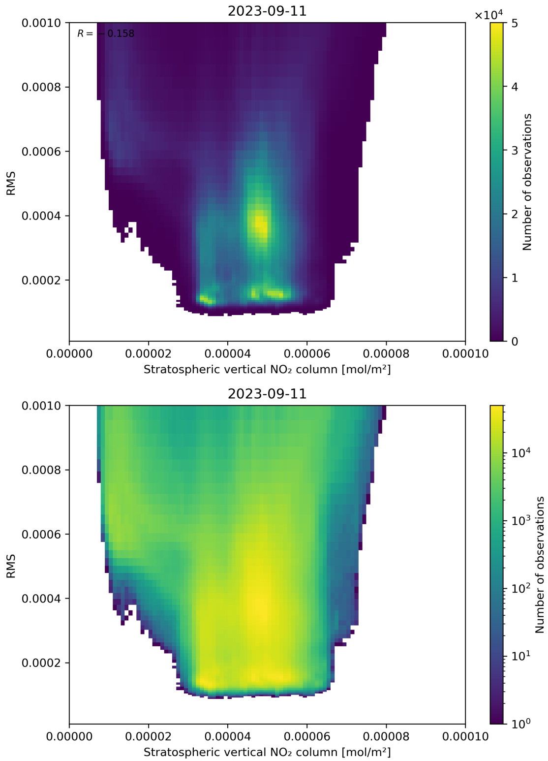
Figure 102: Scatter density plot of “Stratospheric vertical NO 2 column” against “RMS” for 2023-09-10 to 2023-09-12.
