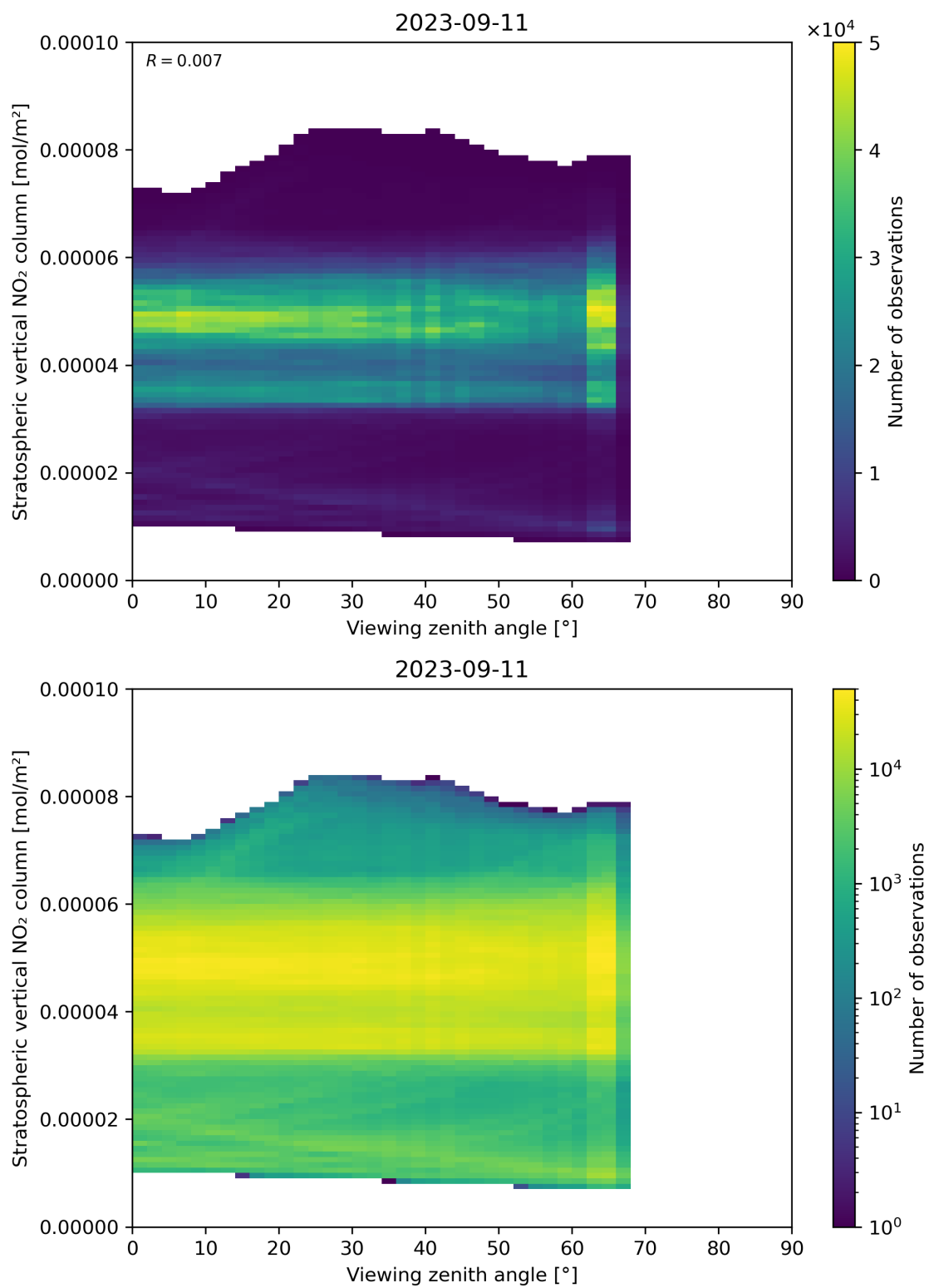
Figure 164: Scatter density plot of “Viewing zenith angle” against “Stratospheric vertical NO 2 column” for 2023-09-10 to 2023-09-12.
