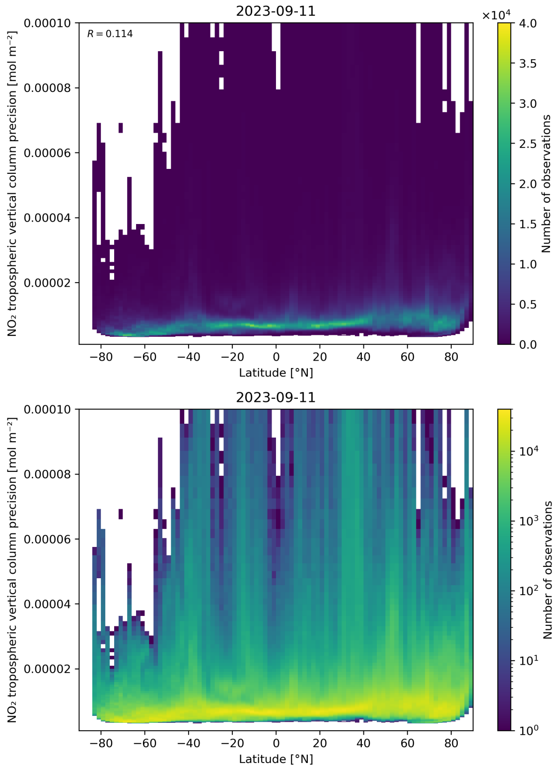
Figure 93: Scatter density plot of “Latitude” against “NO 2 tropospheric vertical column precision” for 2023-09-10 to 2023-09-12.
