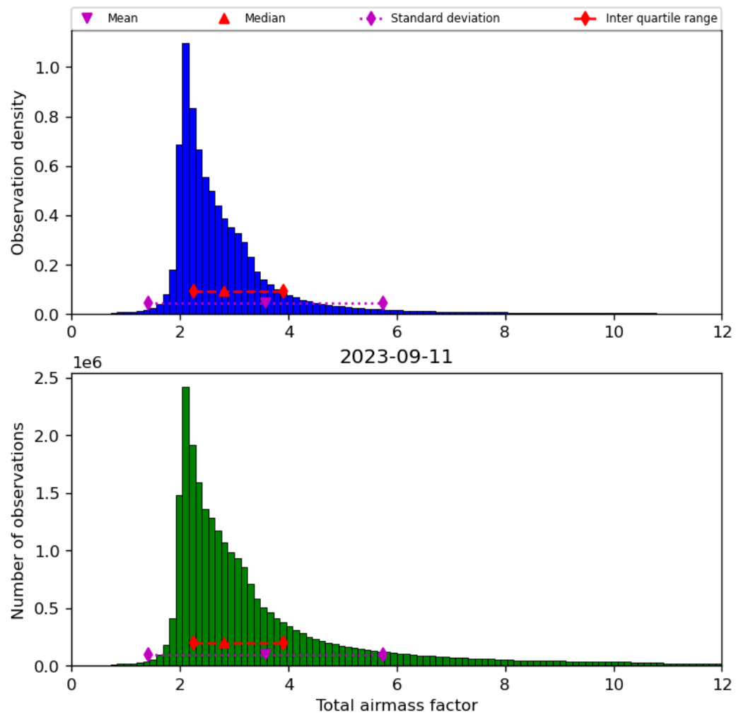
Figure 32: Histogram of “Total airmass factor” for 2023-09-10 to 2023-09-12
