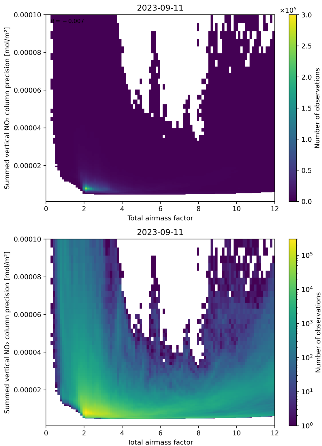
Figure 66: Scatter density plot of “Total airmass factor” against “Summed vertical NO 2 column precision” for 2023-09-10 to 2023-09-12.
