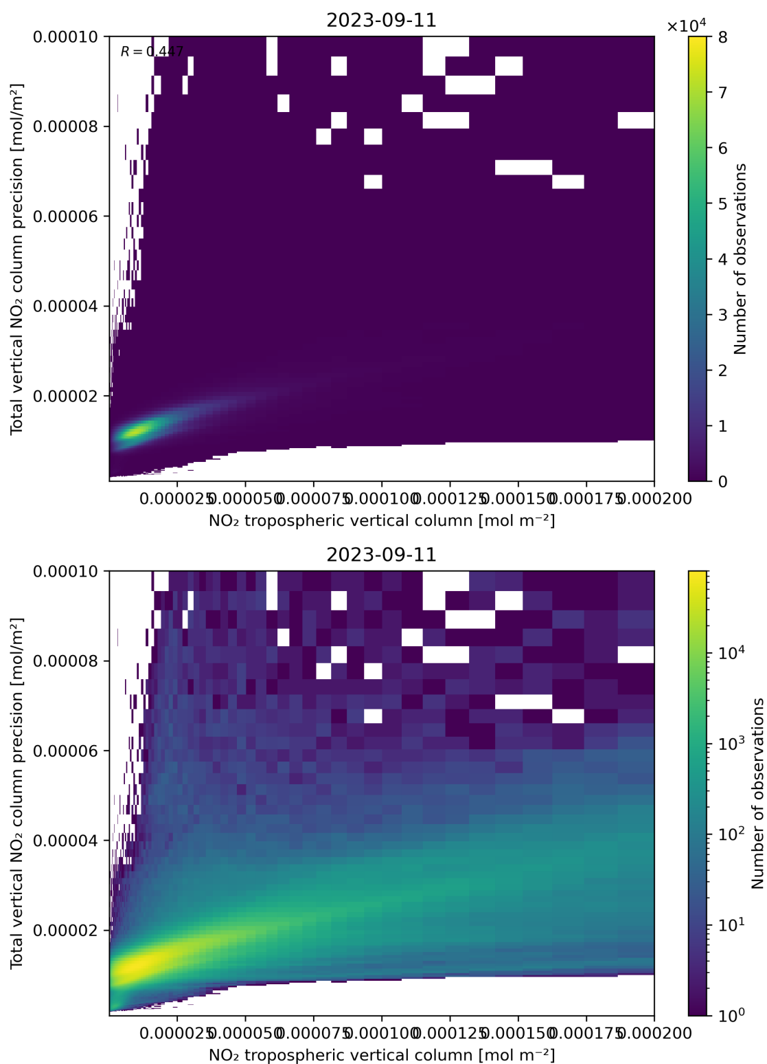
Figure 129: Scatter density plot of “NO 2 tropospheric vertical column” against “Total vertical NO 2 column precision” for 2023-09-10 to 2023-09-12.
