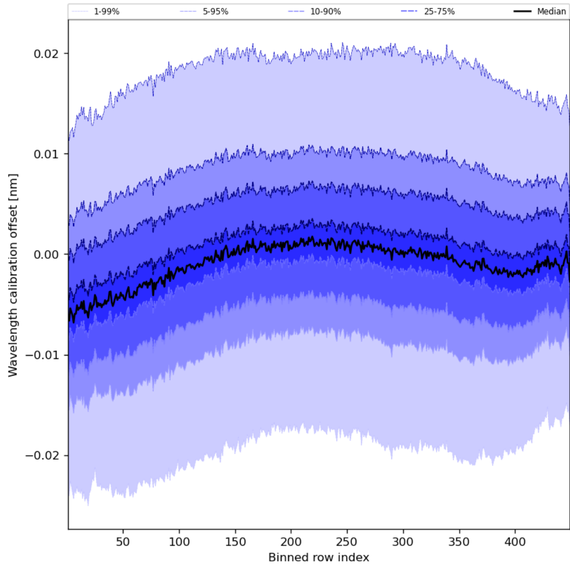
Figure 52: Along track statistics of “Wavelength calibration offset” for 2023-09-10 to 2023-09-12
