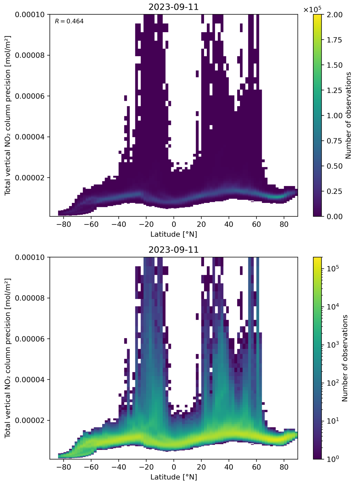
Figure 91: Scatter density plot of “Latitude” against “Total vertical NO 2 column precision” for 2023-09-10 to 2023-09-12.
