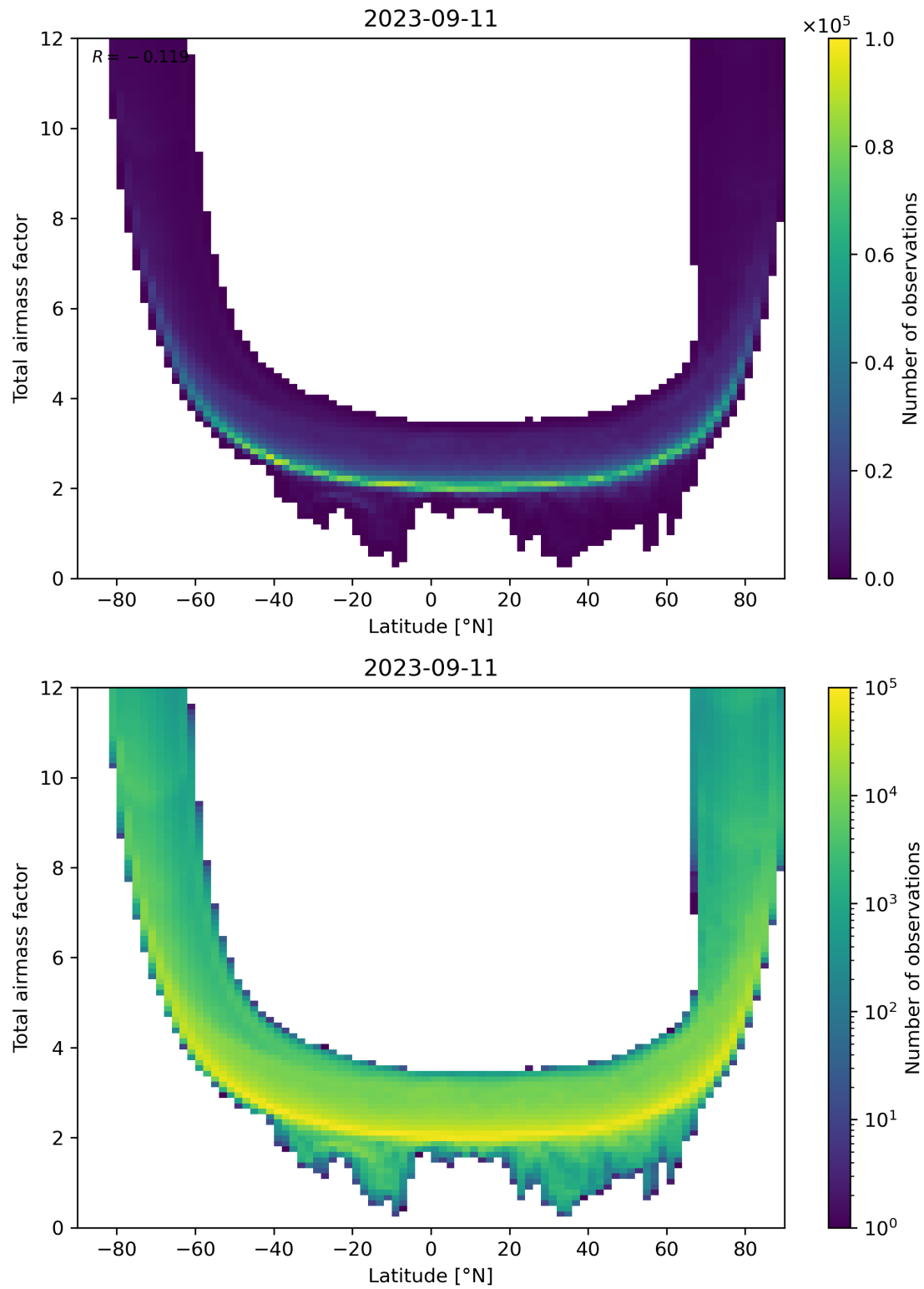
Figure 84: Scatter density plot of “Latitude” against “Total airmass factor” for 2023-09-10 to 2023-09-12.
