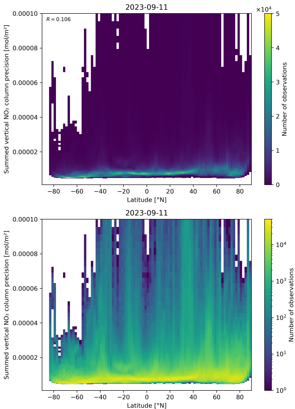
Figure 89: Scatter density plot of “Latitude” against “Summed vertical NO 2 column precision” for 2023-09-10 to 2023-09-12.
