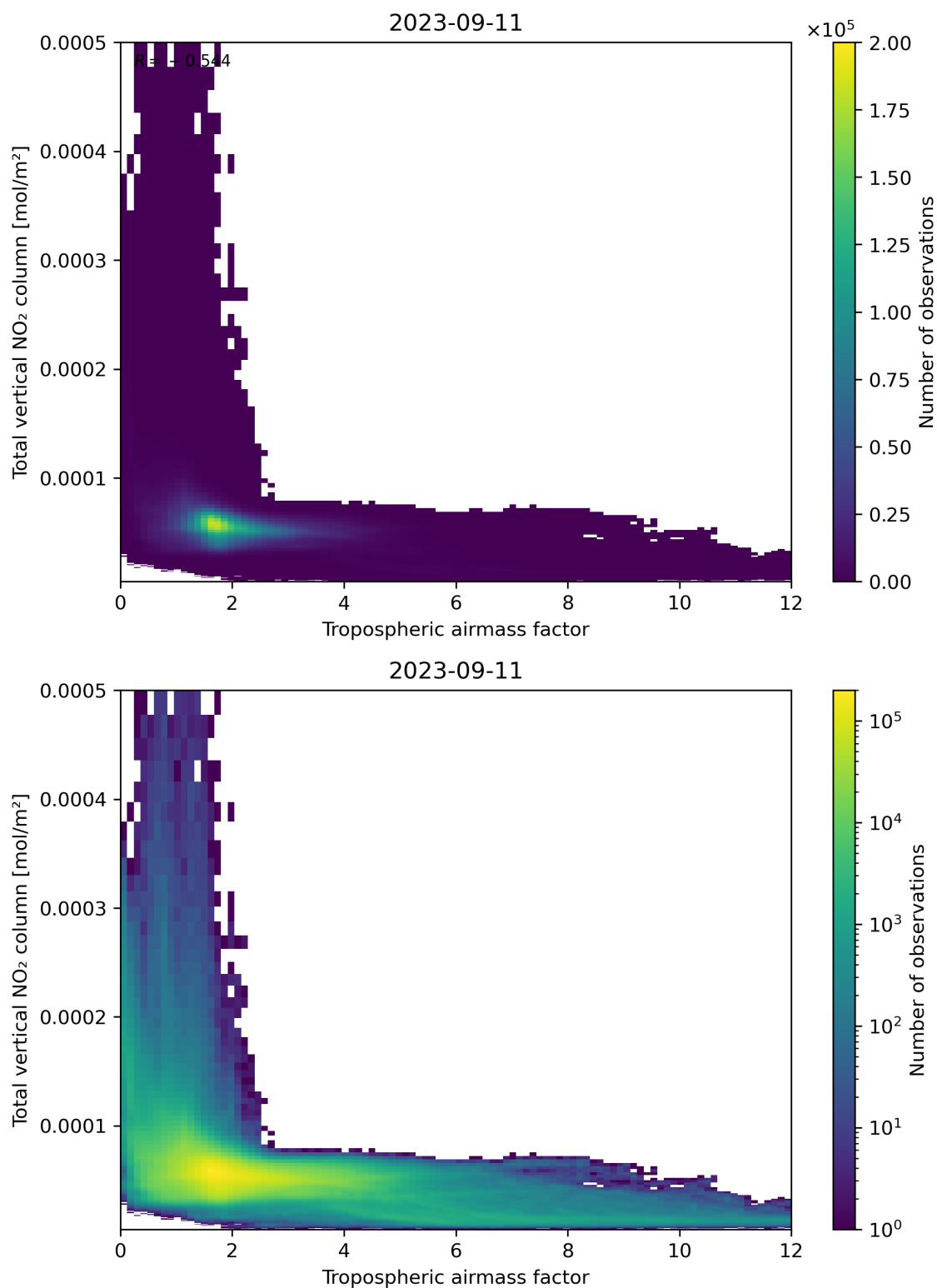
Figure 77: Scatter density plot of “Tropospheric airmass factor” against “Total vertical NO 2 column” for 2023-09-10 to 2023-09-12.
