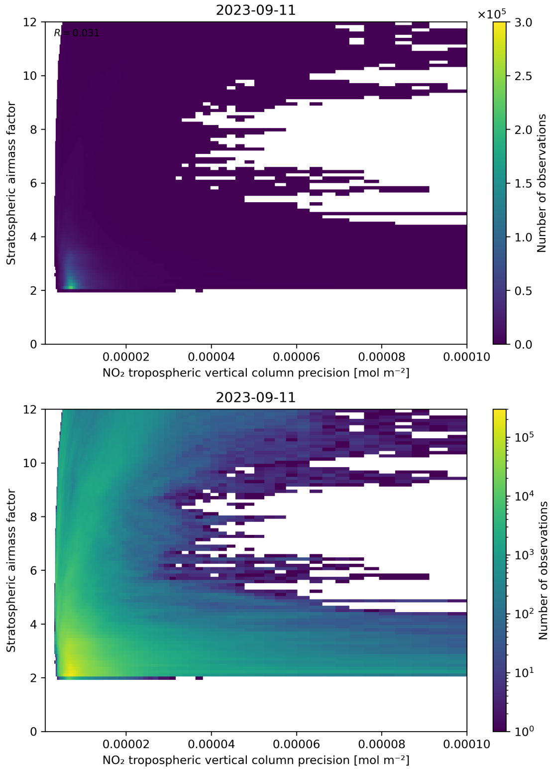
Figure 131: Scatter density plot of “NO 2 tropospheric vertical column precision” against “Stratospheric airmass factor” for 2023-09-10 to 2023-09-12.
