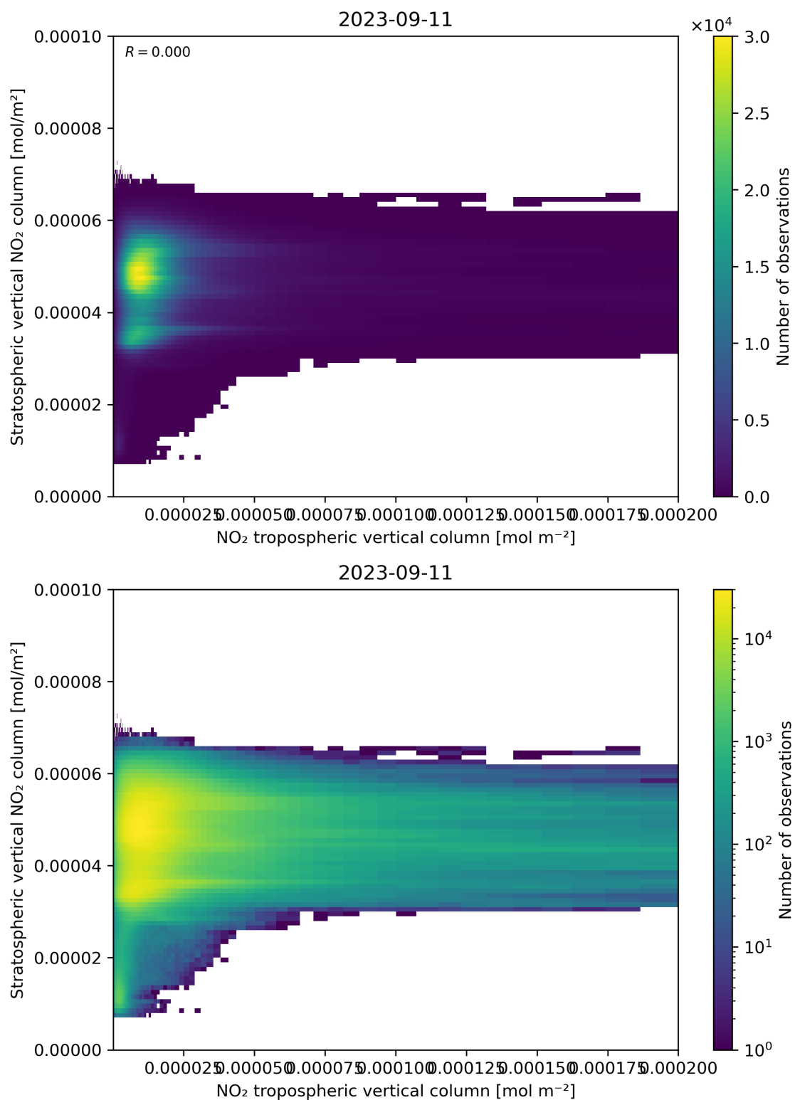
Figure 125: Scatter density plot of “NO 2 tropospheric vertical column” against “Stratospheric vertical NO 2 column” for 2023-09-10 to 2023-09-12.
