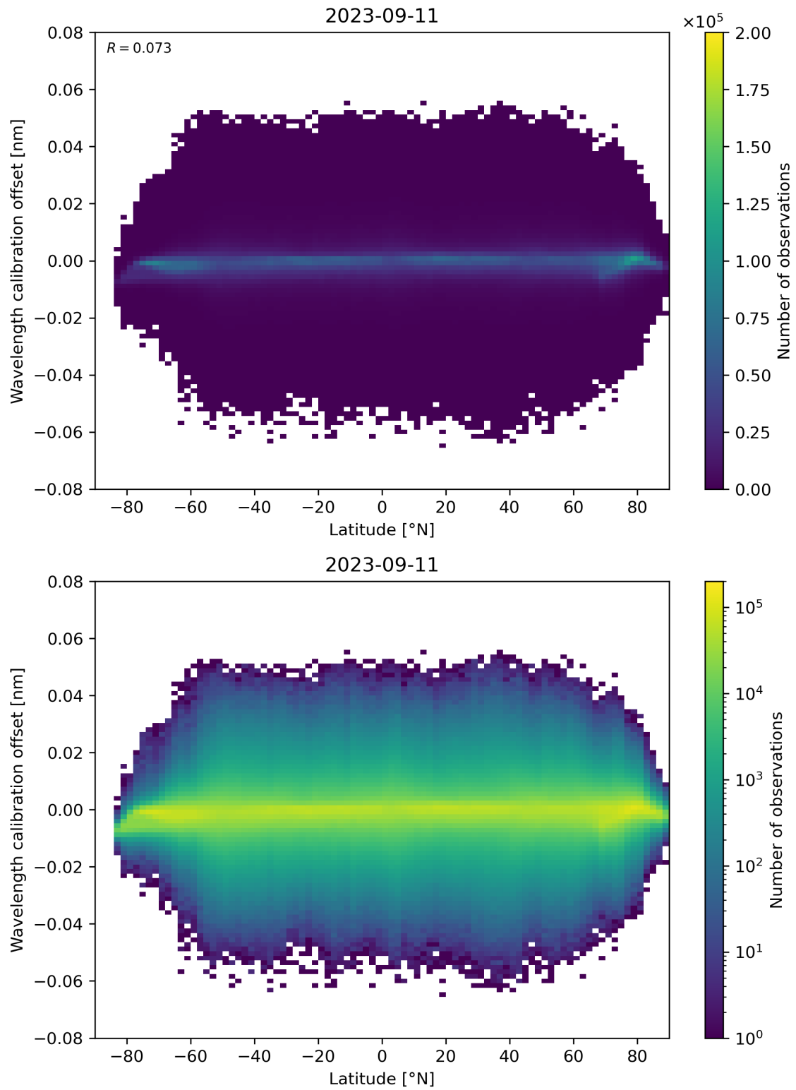
Figure 95: Scatter density plot of “Latitude” against “Wavelength calibration offset” for 2023-09-10 to 2023-09-12.
