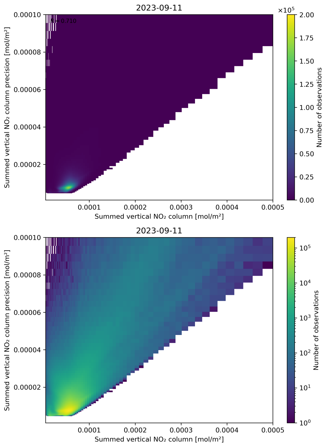
Figure 105: Scatter density plot of “Summed vertical NO 2 column” against “Summed vertical NO 2 column precision” for 2023-09-10 to 2023-09-12.
