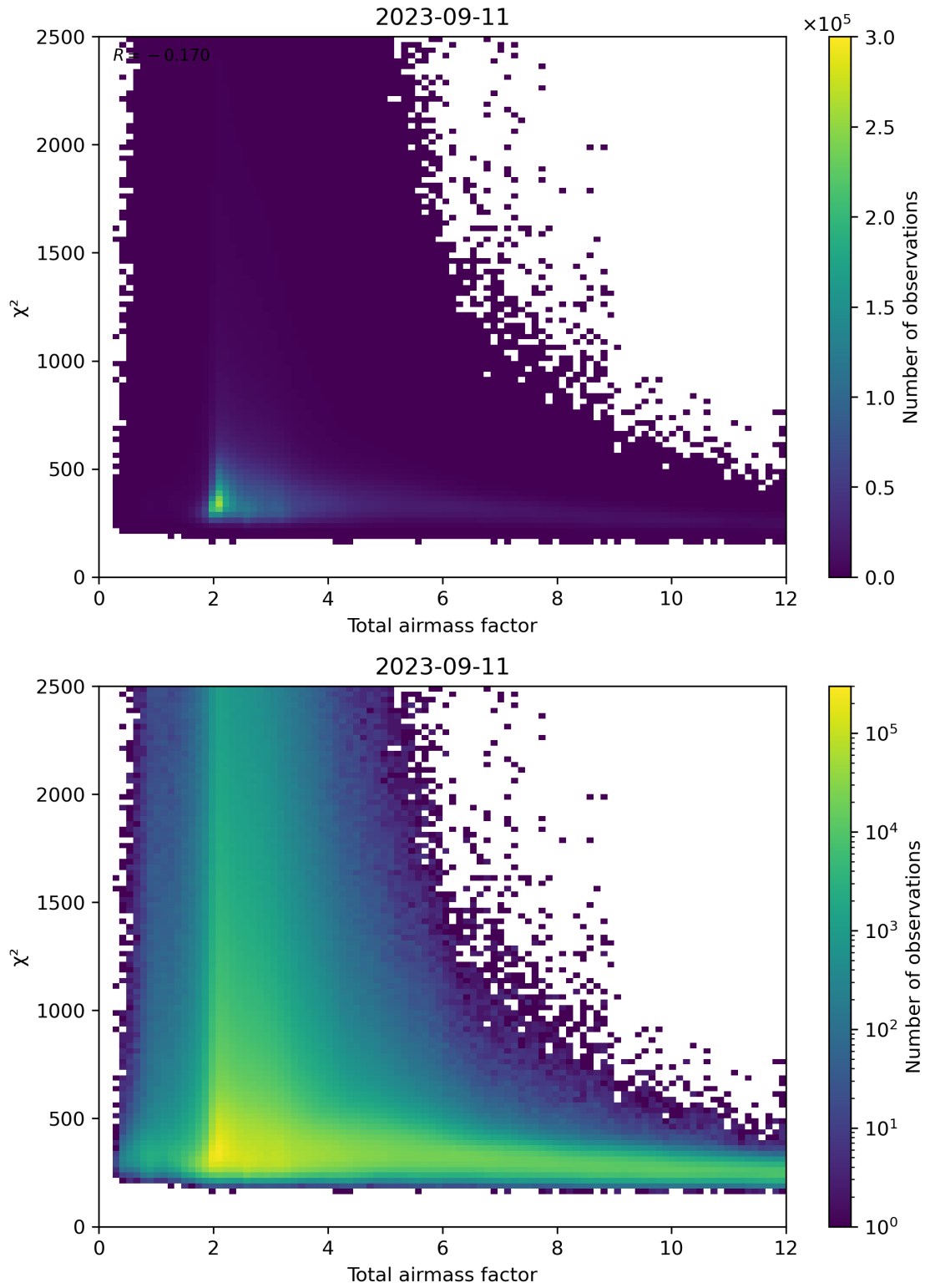
Figure 63: Scatter density plot of “Total airmass factor” against “ \chi^2 ” for 2023-09-10 to 2023-09-12.
