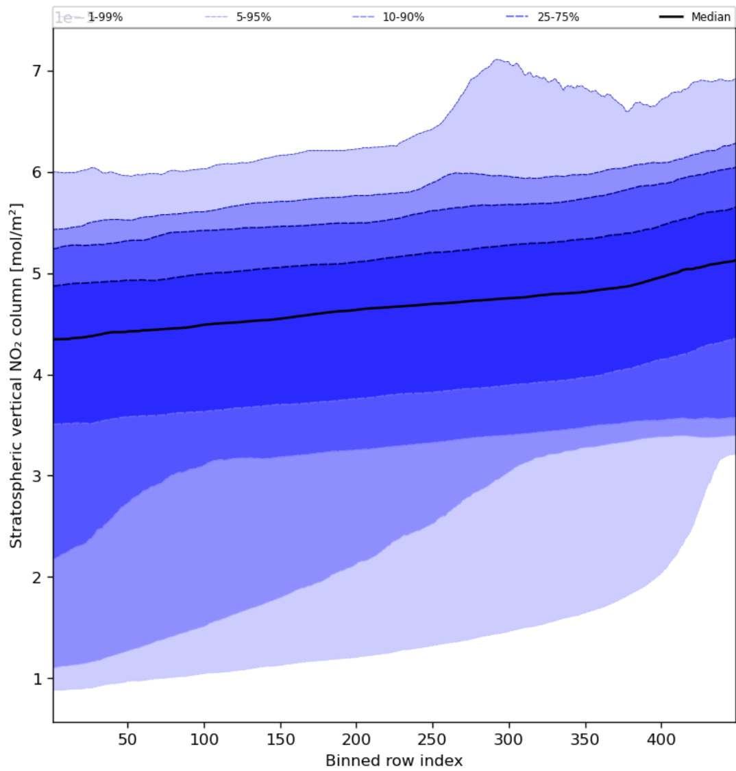
Figure 53: Along track statistics of “Stratospheric vertical NO 2 column” for 2023-09-10 to 2023-09-12
