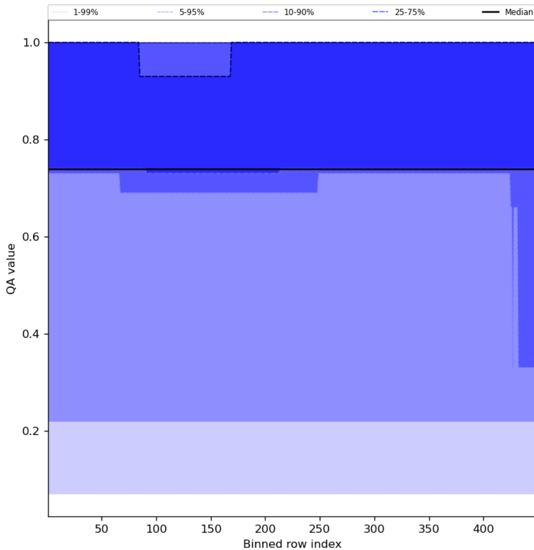
Figure 45: Along track statistics of “QA value” for 2023-09-10 to 2023-09-12
