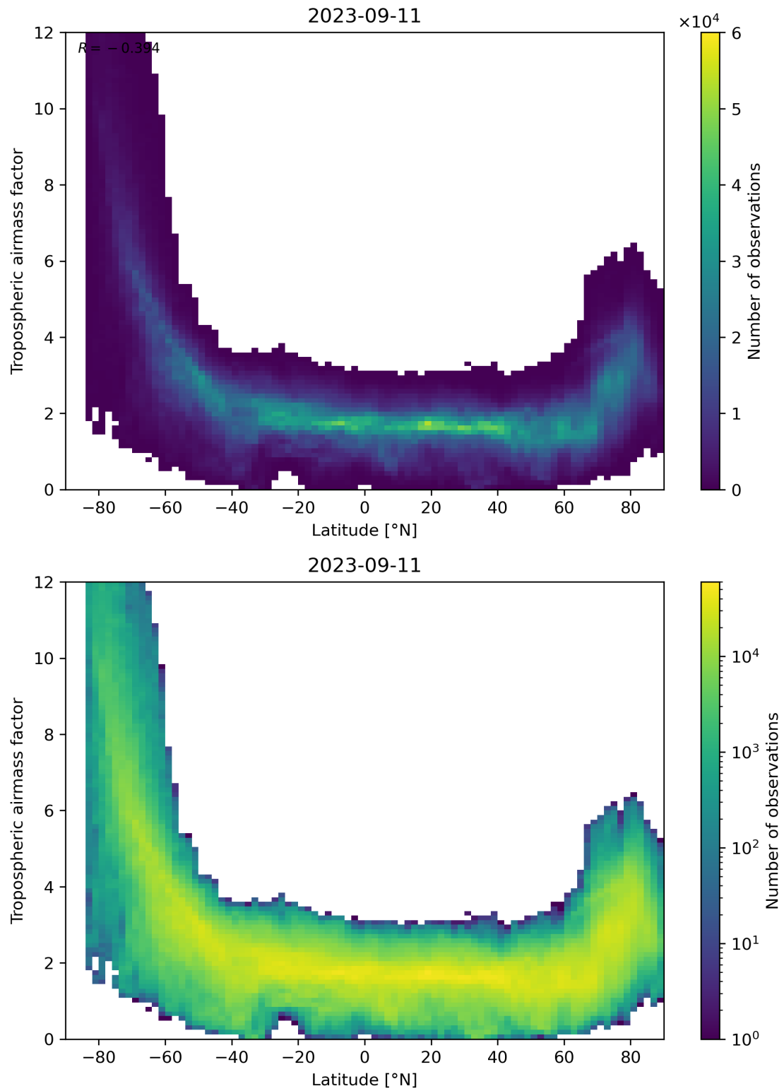
Figure 85: Scatter density plot of “Latitude” against “Tropospheric airmass factor” for 2023-09-10 to 2023-09-12.
