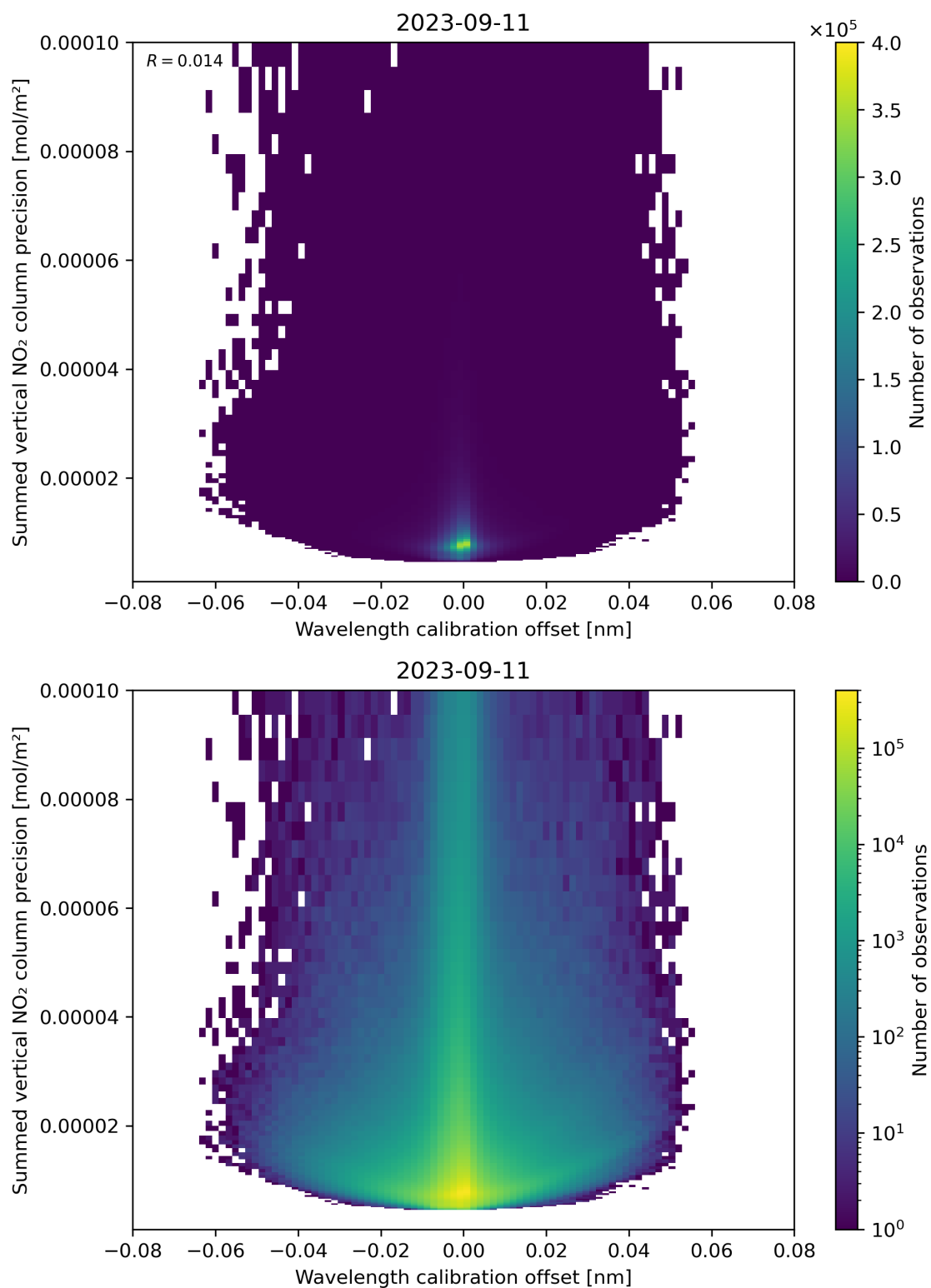
Figure 178: Scatter density plot of “Wavelength calibration offset” against “Summed vertical NO 2 column precision” for 2023-09-10 to 2023-09-12.
