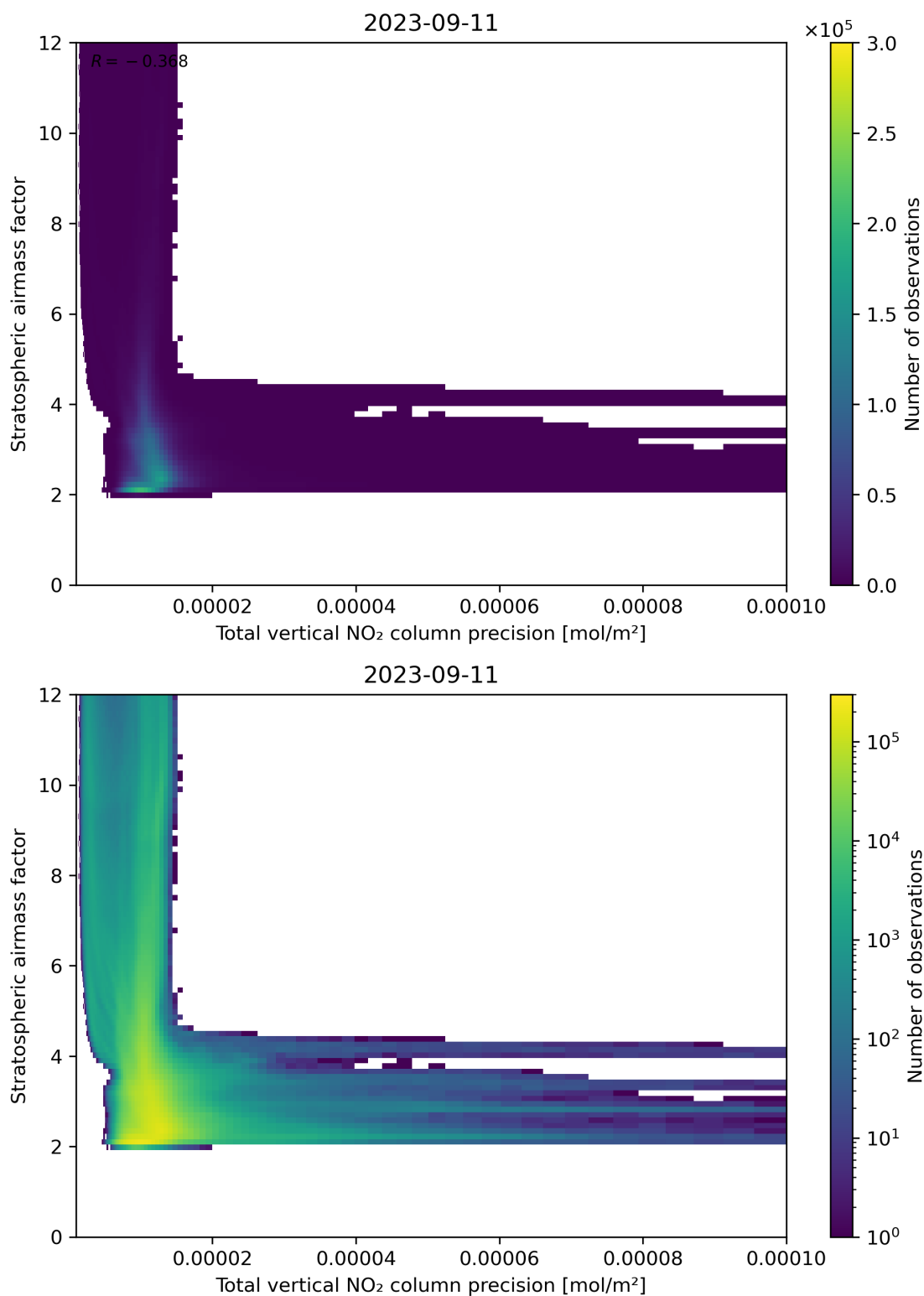
Figure 115: Scatter density plot of “Total vertical NO 2 column precision” against “Stratospheric air mass factor” for 2023-09-10 to 2023-09-12.
