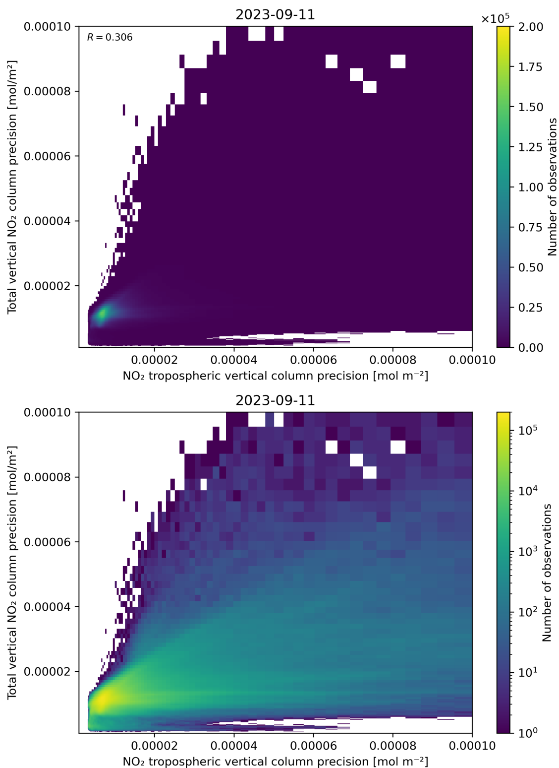
Figure 139: Scatter density plot of “NO 2 tropospheric vertical column precision” against “Total vertical NO 2 column precision” for 2023-09-10 to 2023-09-12.
