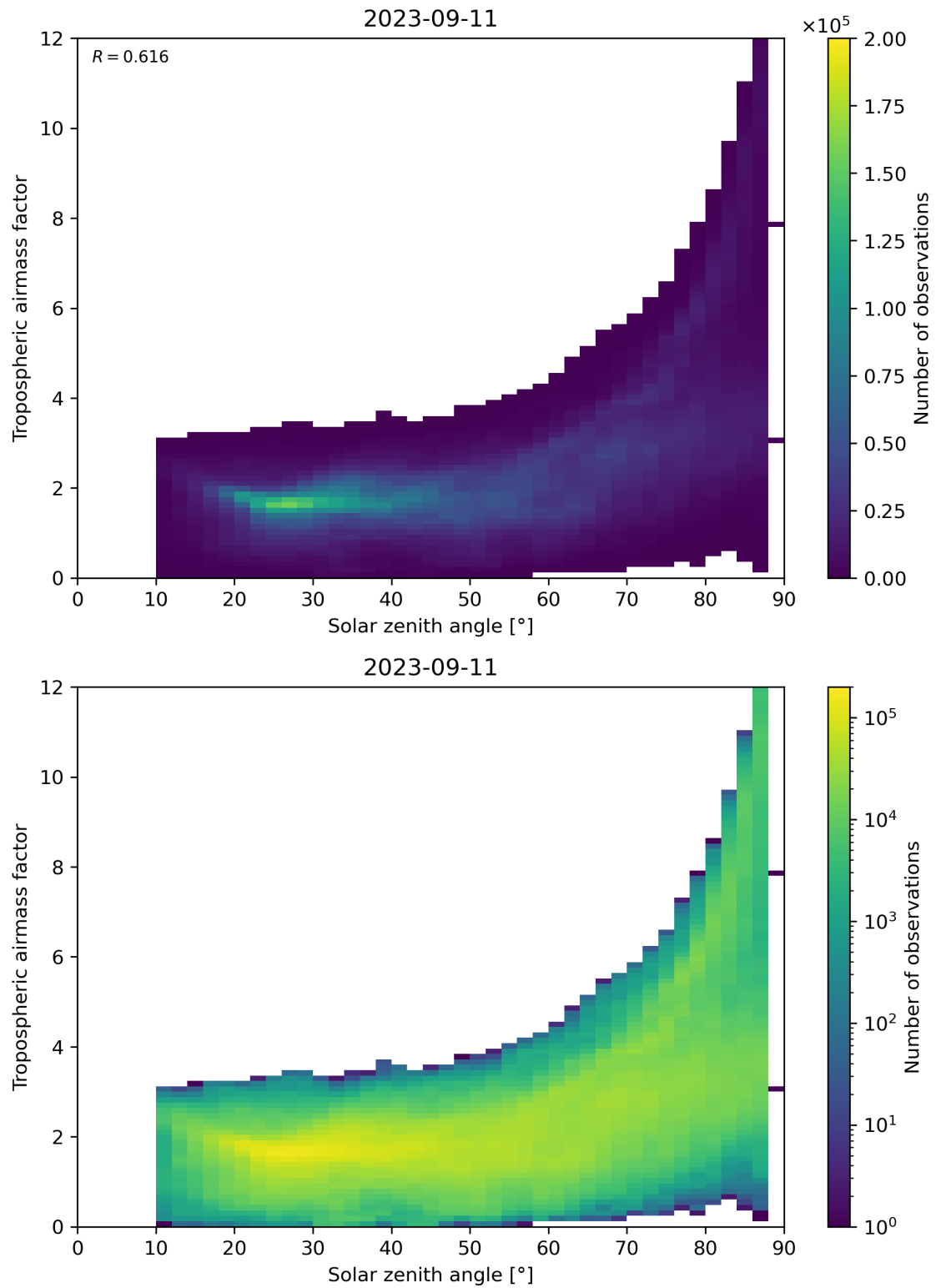
Figure 147: Scatter density plot of “Solar zenith angle” against “Tropospheric airmass factor” for 2023-09-10 to 2023-09-12.
