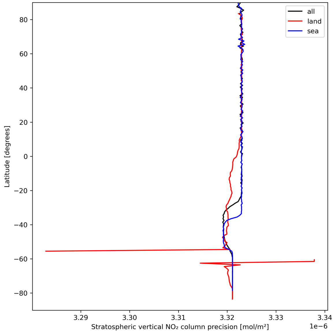
Figure 20: Zonal average of “Stratospheric vertical NO 2 column precision” for 2023-09-10 to 2023-09-12.
