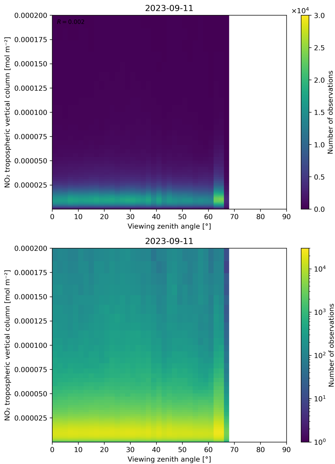
Figure 169: Scatter density plot of “Viewing zenith angle” against “NO 2 tropospheric vertical column” for 2023-09-10 to 2023-09-12.
