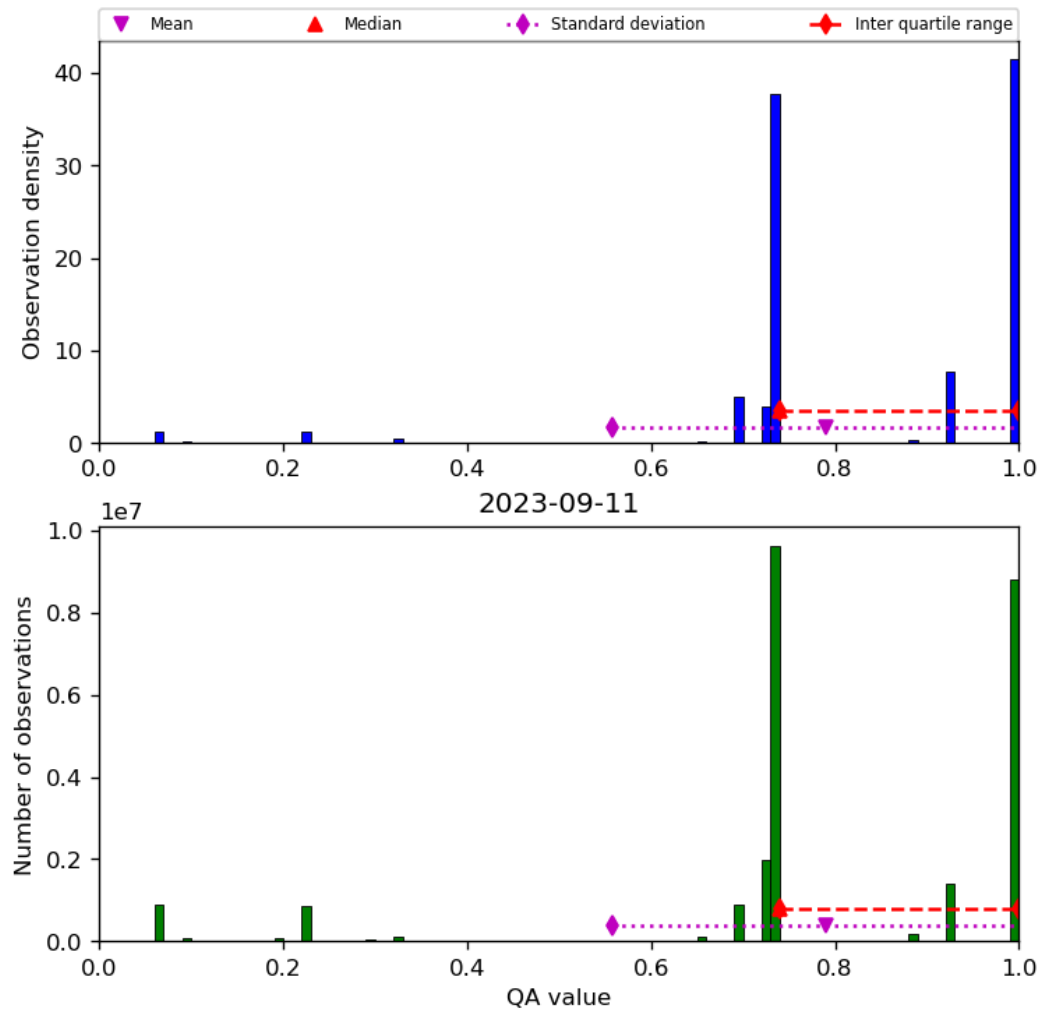
Figure 28: Histogram of “QA value” for 2023-09-10 to 2023-09-12
