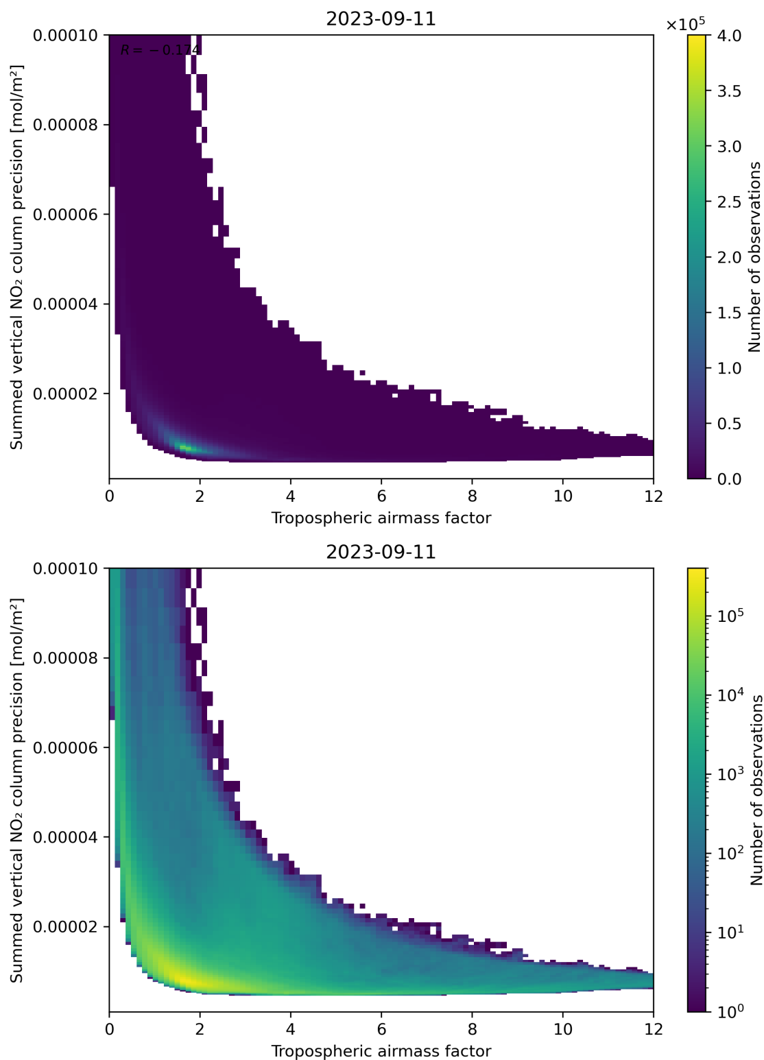
Figure 76: Scatter density plot of “Tropospheric air mass factor” against “Summed vertical NO 2 column precision” for 2023-09-10 to 2023-09-12.
