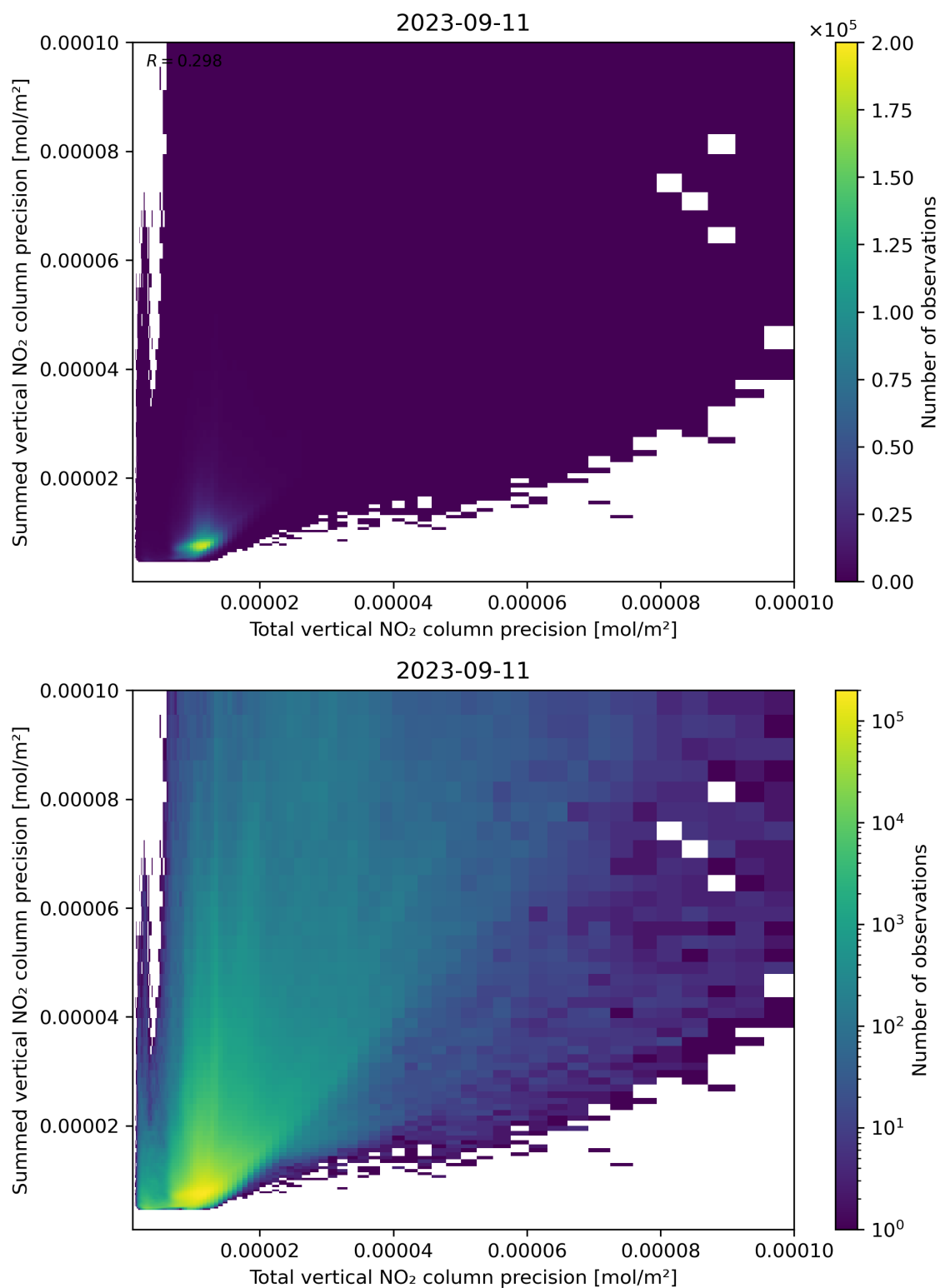
Figure 118: Scatter density plot of “Total vertical NO 2 column precision” against “Summed vertical NO 2 column precision” for 2023-09-10 to 2023-09-12.
