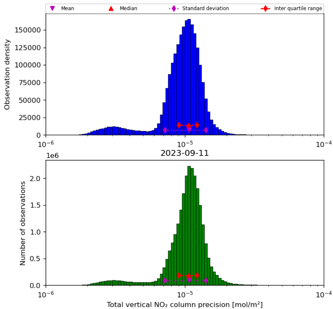
Figure 39: Histogram of “Total vertical NO 2 column precision” for 2023-09-10 to 2023-09-12
