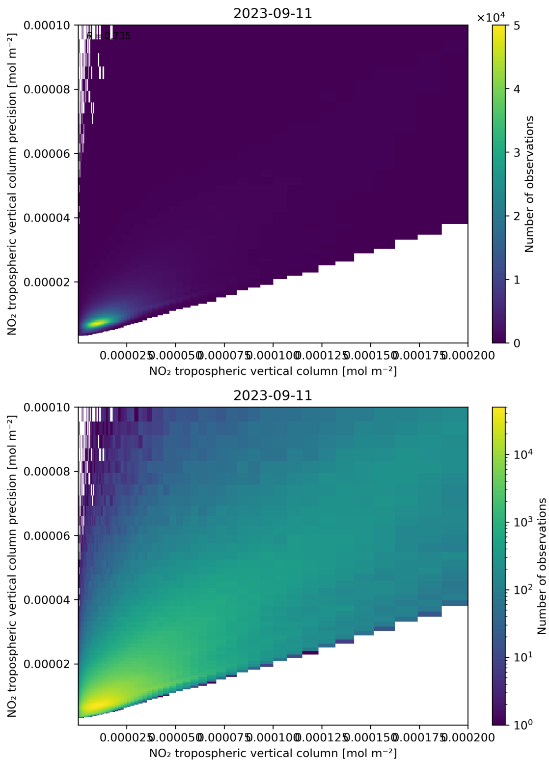
Figure 130: Scatter density plot of “NO 2 tropospheric vertical column” against “NO 2 tropospheric vertical column precision” for 2023-09-10 to 2023-09-12.
