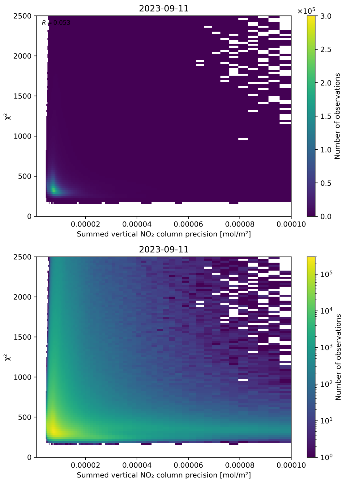
Figure 107: Scatter density plot of “Summed vertical NO 2 column precision” against “ \chi^2 ” for 2023-09-10 to 2023-09-12.
