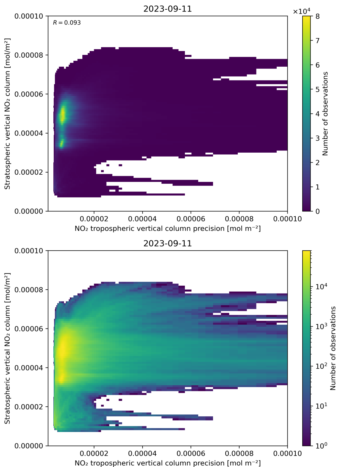
Figure 135: Scatter density plot of “NO 2 tropospheric vertical column precision” against “Stratospheric vertical NO 2 column” for 2023-09-10 to 2023-09-12.
