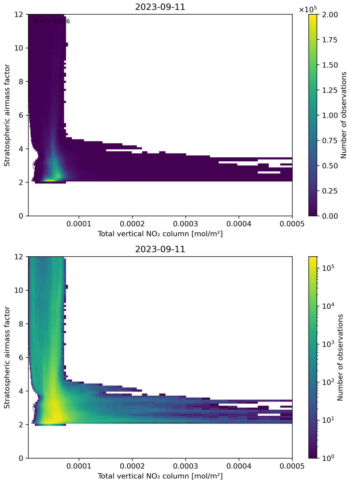
Figure 110: Scatter density plot of “Total vertical NO 2 column” against “Stratospheric airmass factor” for 2023-09-10 to 2023-09-12.
