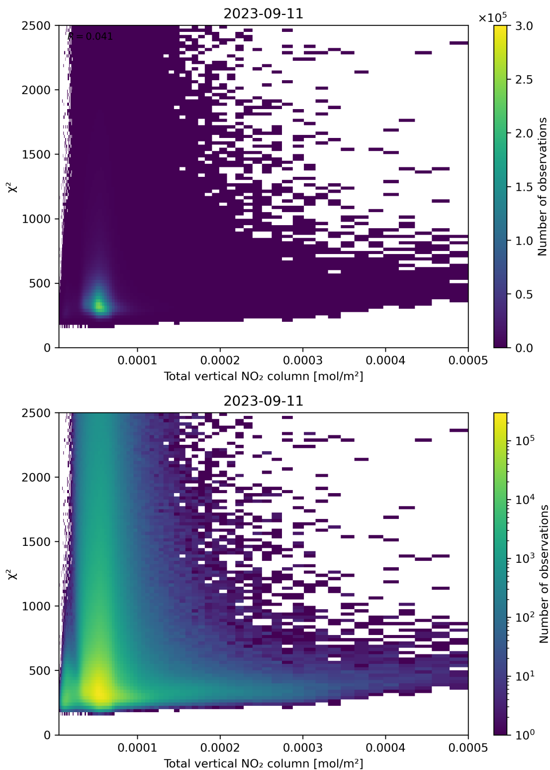
Figure 111: Scatter density plot of “Total vertical NO 2 column” against “ \chi^2 ” for 2023-09-10 to 2023-09-12.
