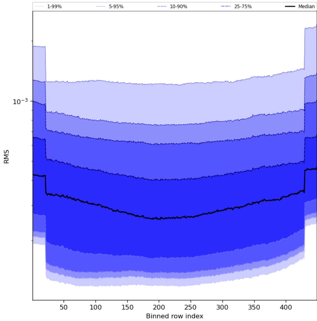
Figure 60: Along track statistics of “RMS” for 2023-09-10 to 2023-09-12
