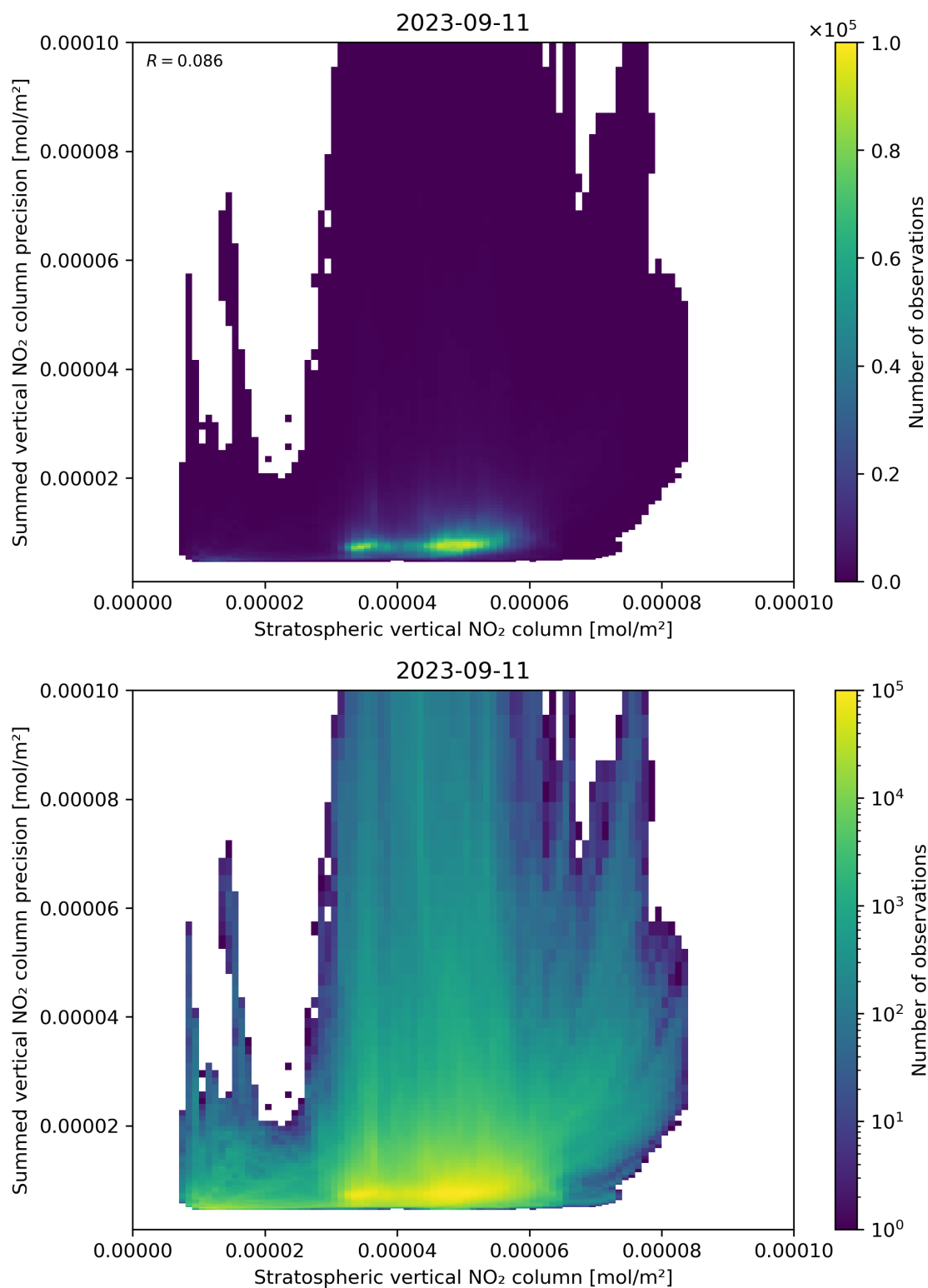
Figure 99: Scatter density plot of “Stratospheric vertical NO 2 column” against “Summed vertical NO 2 column precision” for 2023-09-10 to 2023-09-12.
