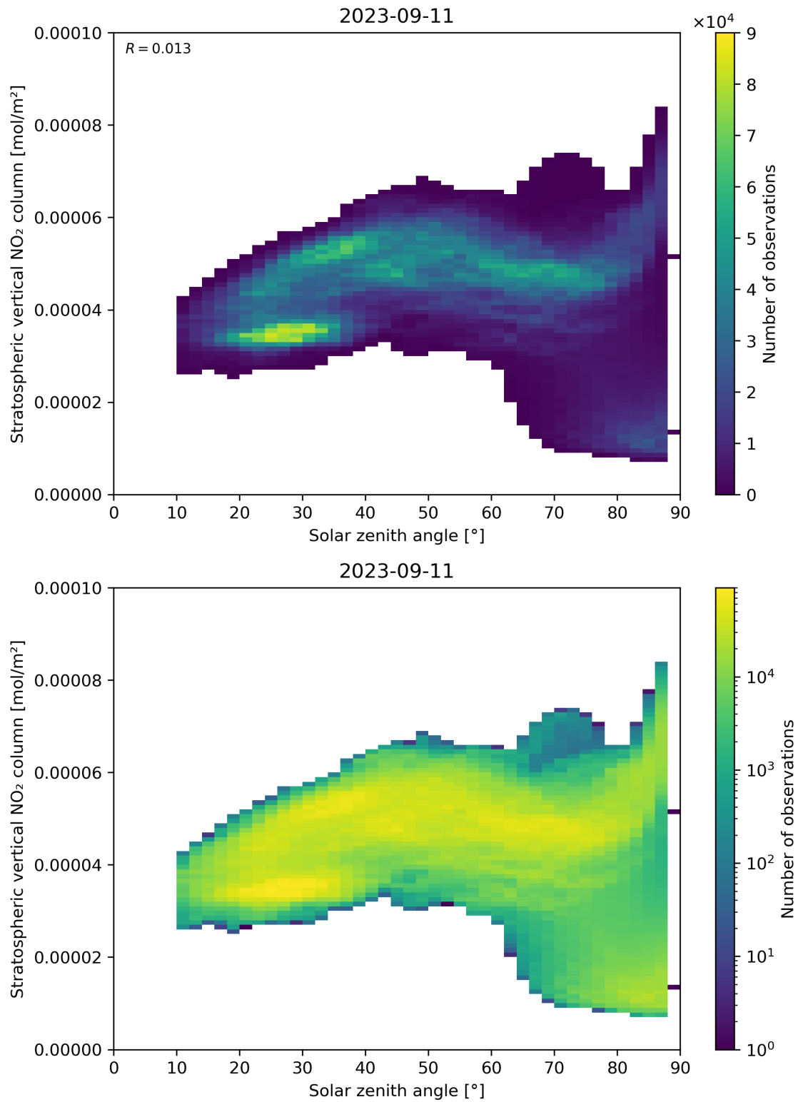
Figure 150: Scatter density plot of “Solar zenith angle” against “Stratospheric vertical NO 2 column” for 2023-09-10 to 2023-09-12.
