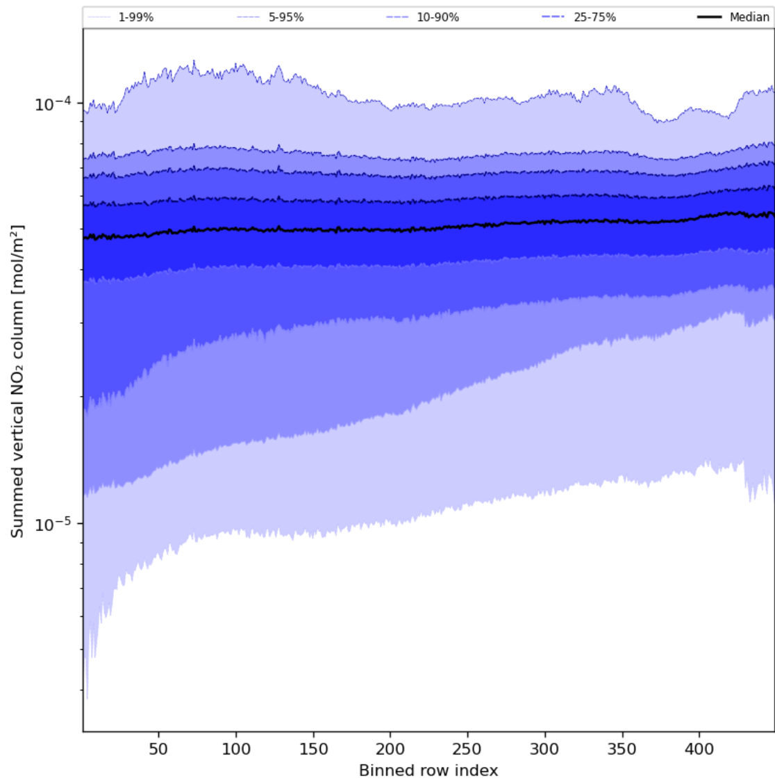
Figure 57: Along track statistics of “Summed vertical NO 2 column” for 2023-09-10 to 2023-09-12
