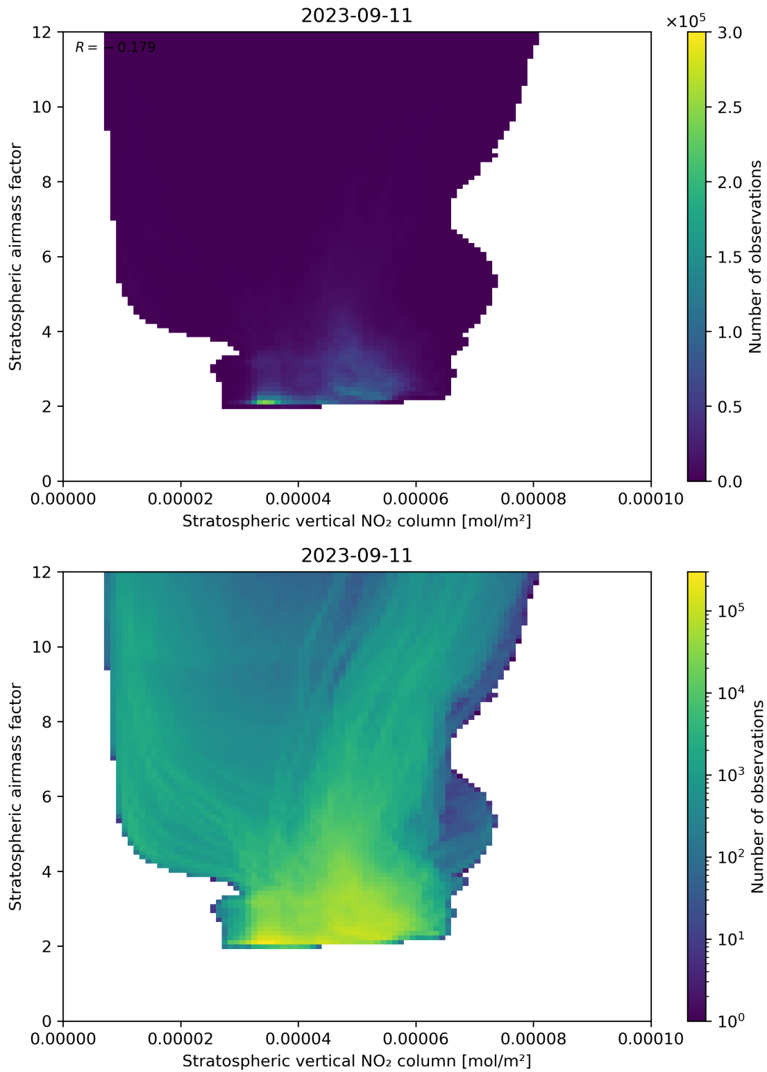
Figure 96: Scatter density plot of “Stratospheric vertical NO 2 column” against “Stratospheric airmass factor” for 2023-09-10 to 2023-09-12.
