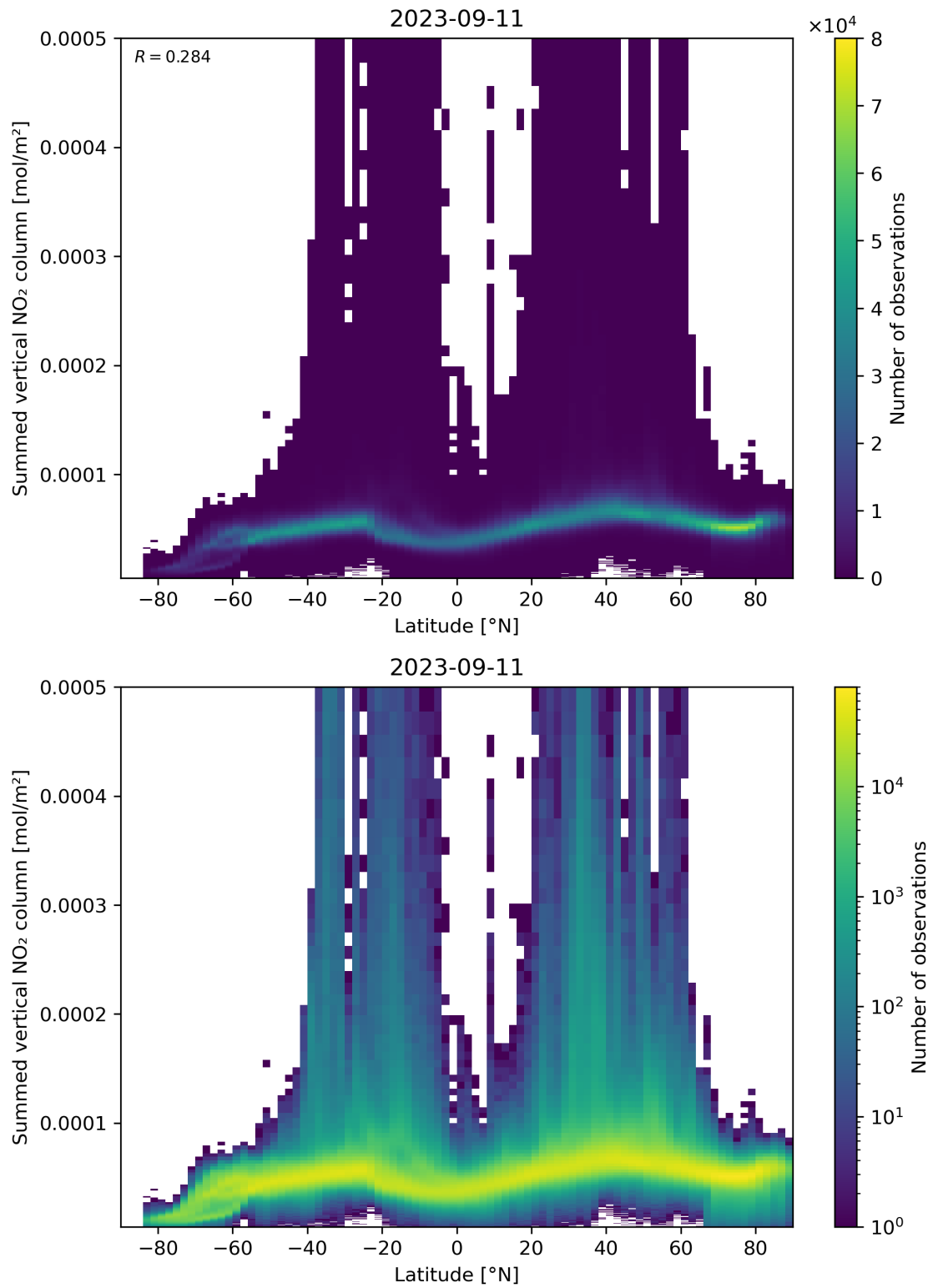
Figure 88: Scatter density plot of “Latitude” against “Summed vertical NO 2 column” for 2023-09-10 to 2023-09-12.
