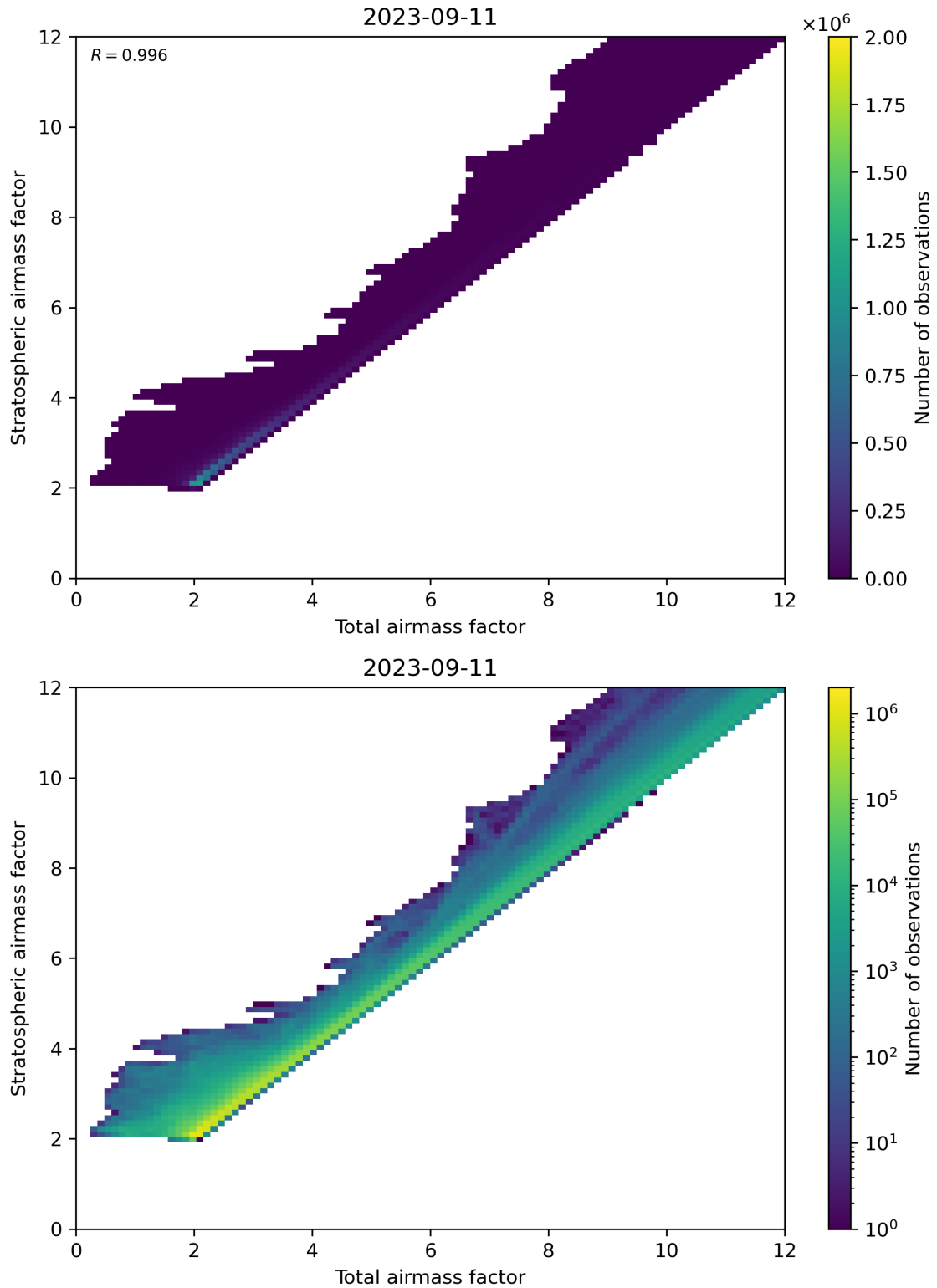
Figure 62: Scatter density plot of “Total airmass factor” against “Stratospheric airmass factor” for 2023-09-10 to 2023-09-12.
