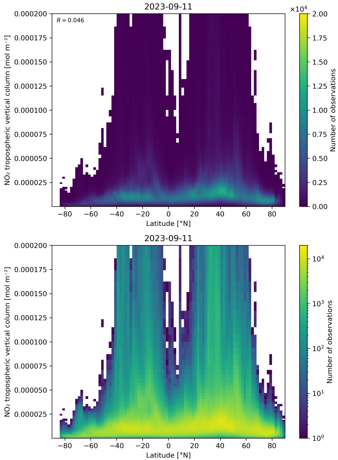
Figure 92: Scatter density plot of “Latitude” against “NO 2 tropospheric vertical column” for 2023-09-10 to 2023-09-12.
