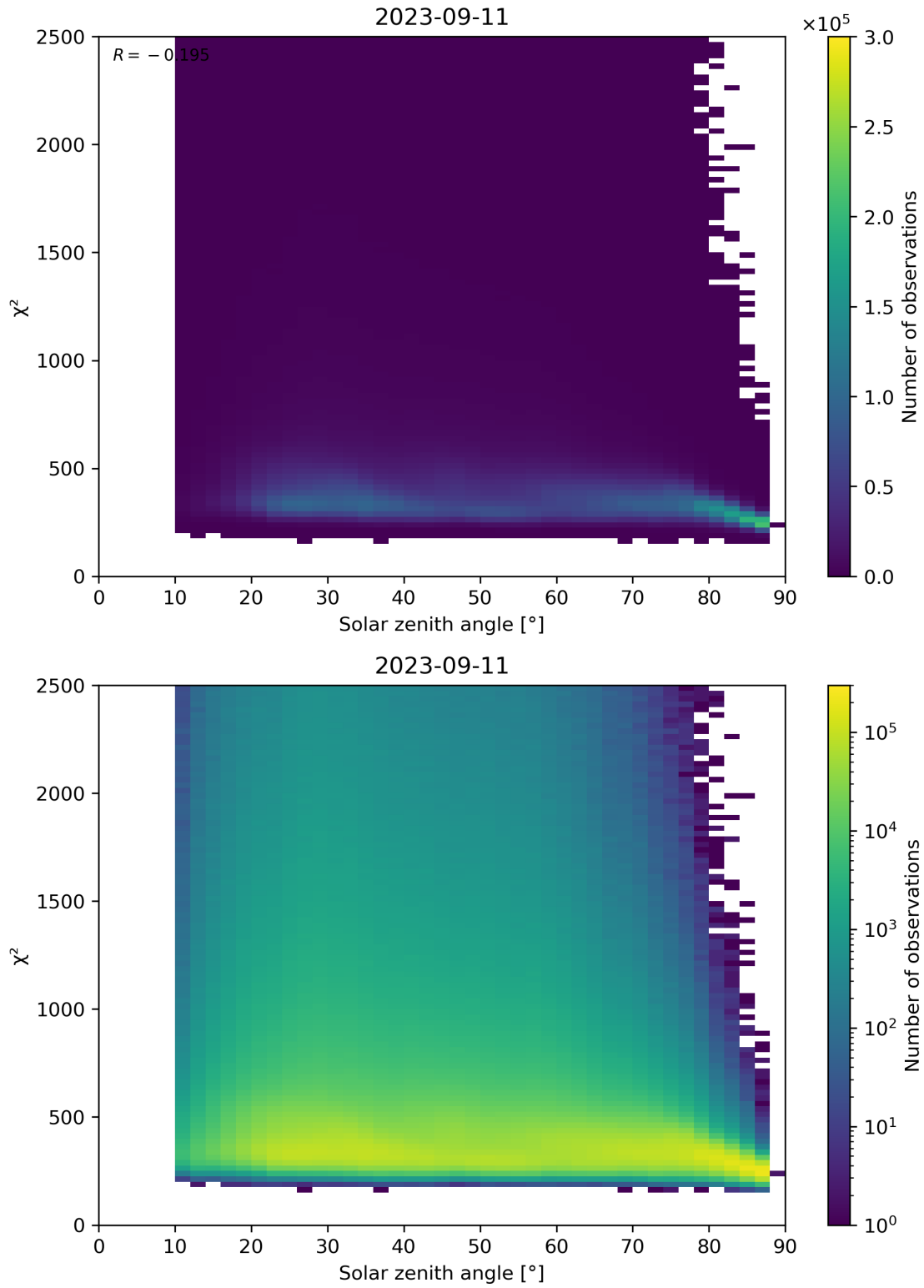
Figure 148: Scatter density plot of “Solar zenith angle” against “ \chi^2 ” for 2023-09-10 to 2023-09-12.
