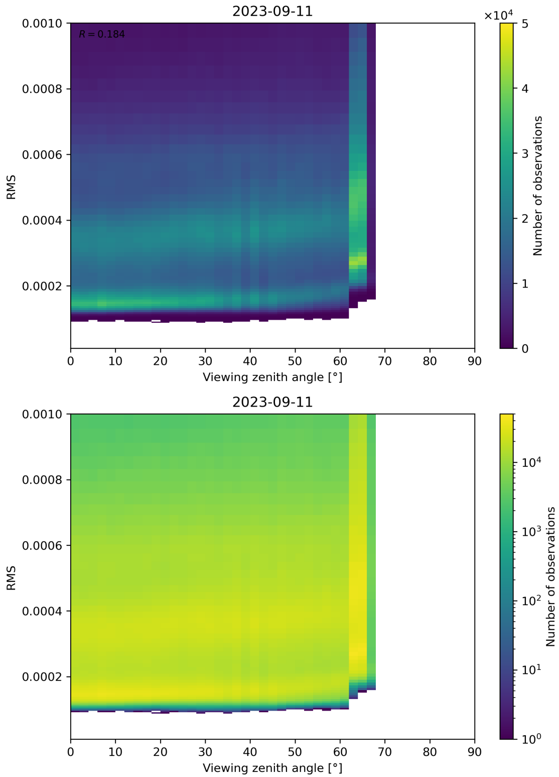
Figure 171: Scatter density plot of “Viewing zenith angle” against “RMS” for 2023-09-10 to 2023-09-12.
