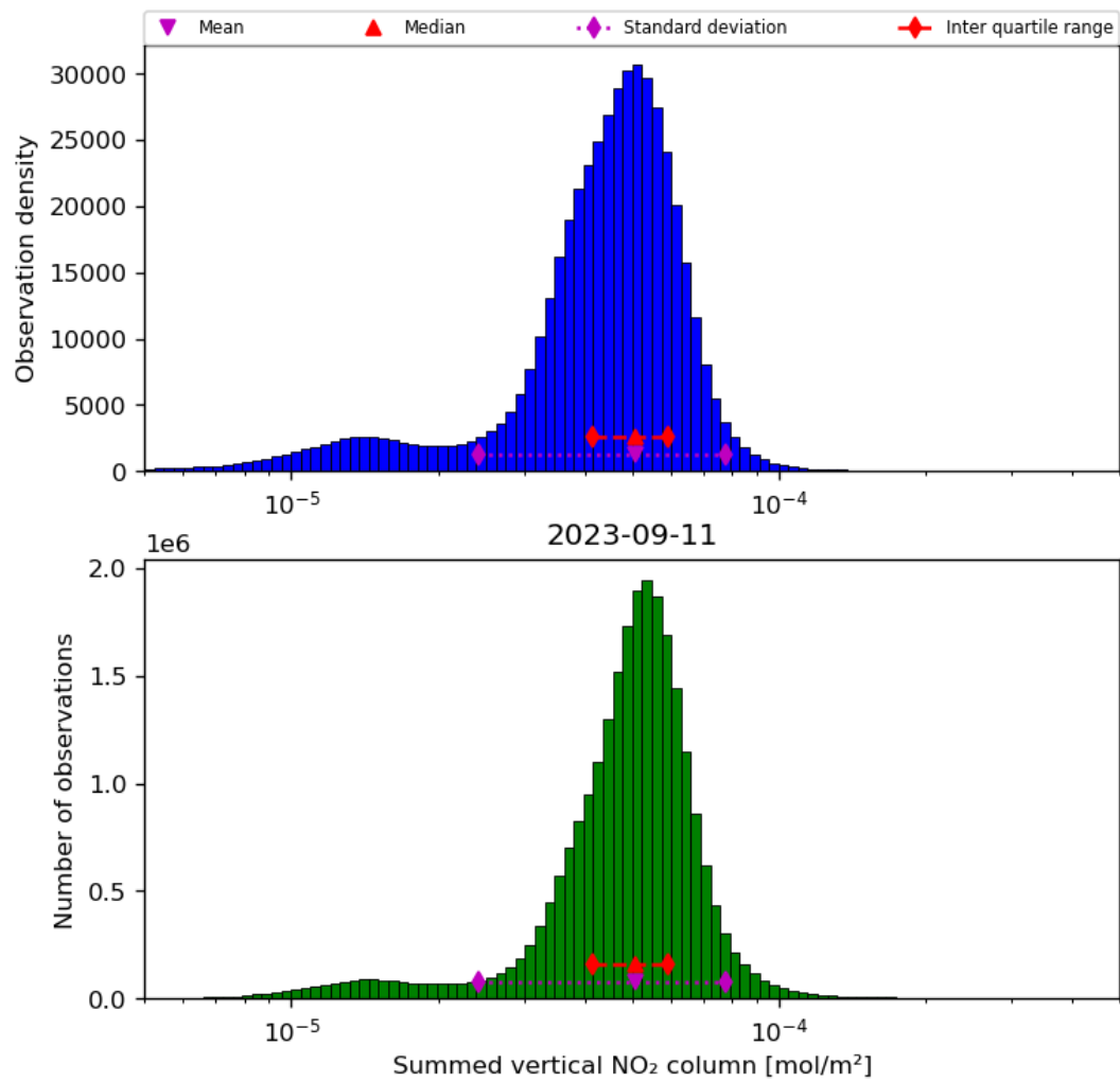
Figure 40: Histogram of “Summed vertical NO 2 column” for 2023-09-10 to 2023-09-12
