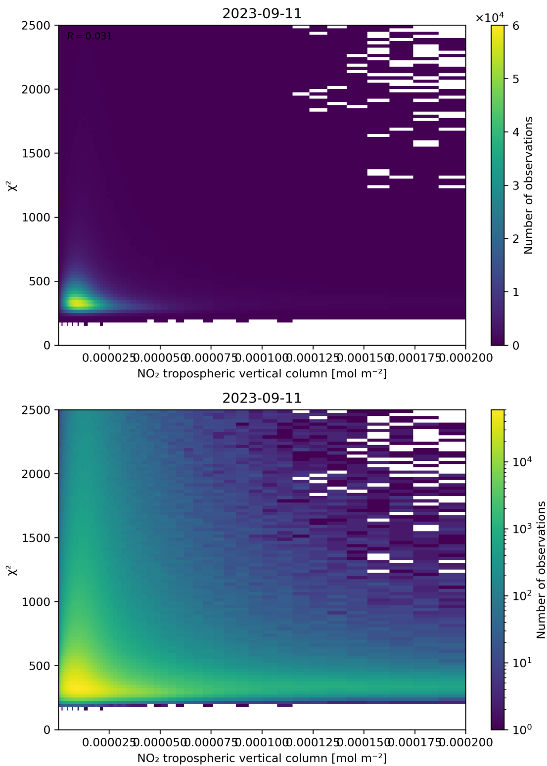
Figure 124: Scatter density plot of “NO 2 tropospheric vertical column” against “ \chi^2 ” for 2023-09-10 to 2023-09-12.
