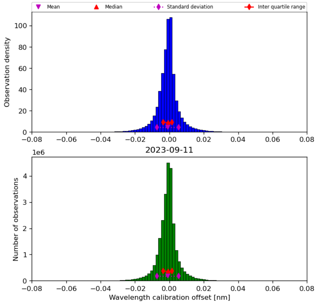
Figure 35: Histogram of “Wavelength calibration offset” for 2023-09-10 to 2023-09-12
