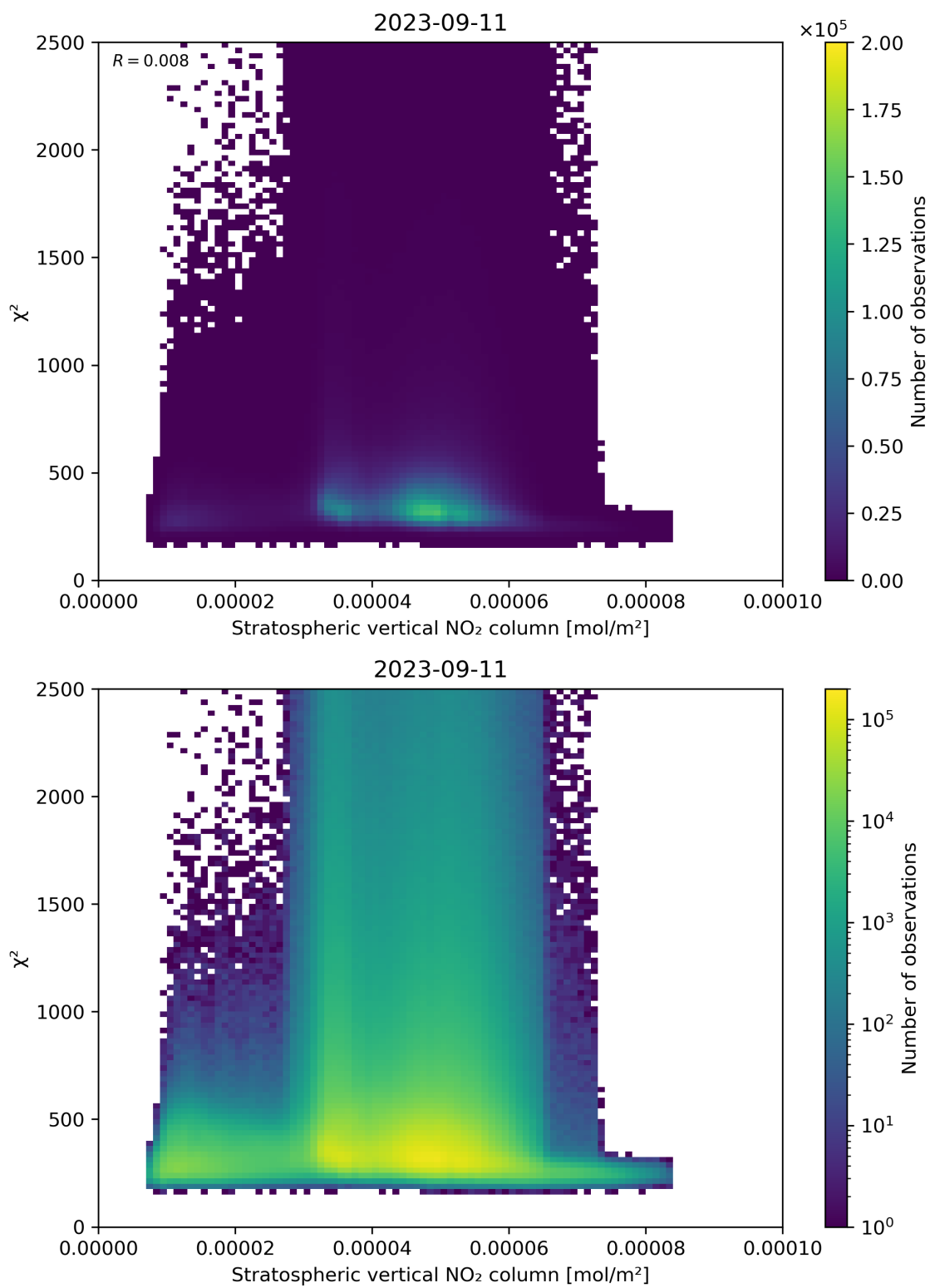
Figure 97: Scatter density plot of “Stratospheric vertical NO 2 column” against “ \chi^2 ” for 2023-09-10 to 2023-09-12.
