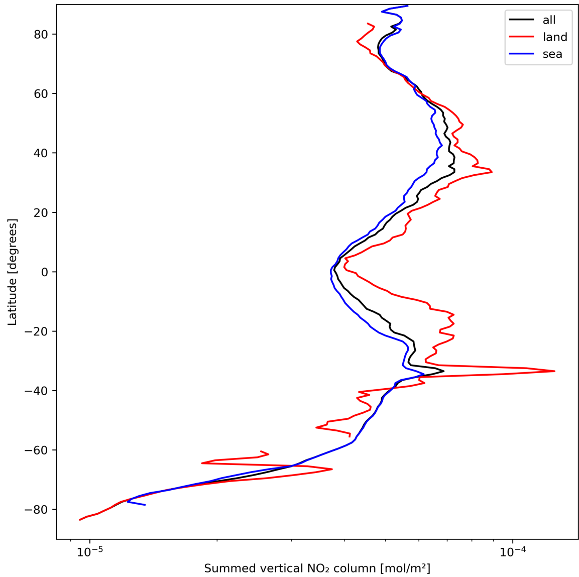
Figure 23: Zonal average of “Summed vertical NO 2 column” for 2023-09-10 to 2023-09-12.
