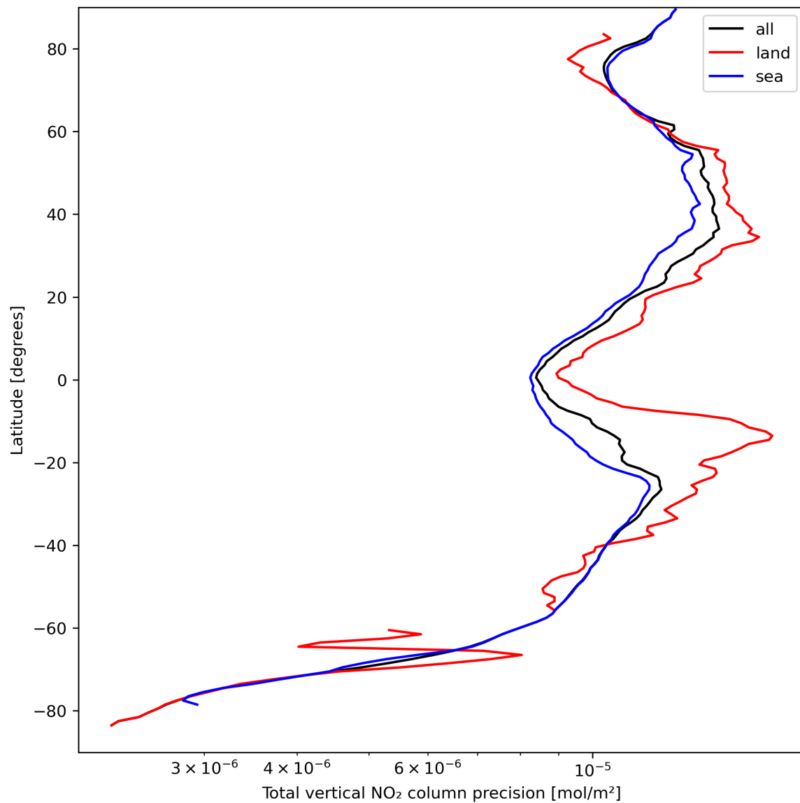
Figure 22: Zonal average of “Total vertical NO 2 column precision” for 2023-09-10 to 2023-09-12.
