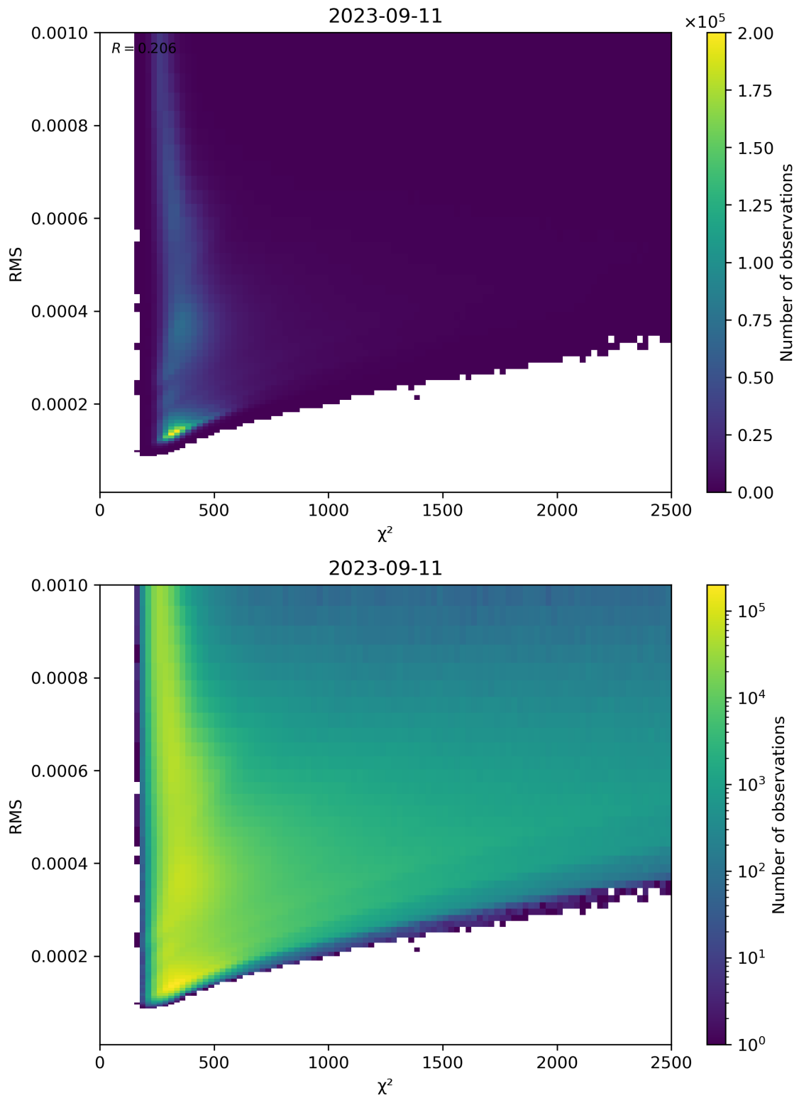
Figure 82: Scatter density plot of “ \chi^2 ” against “RMS” for 2023-09-10 to 2023-09-12.
