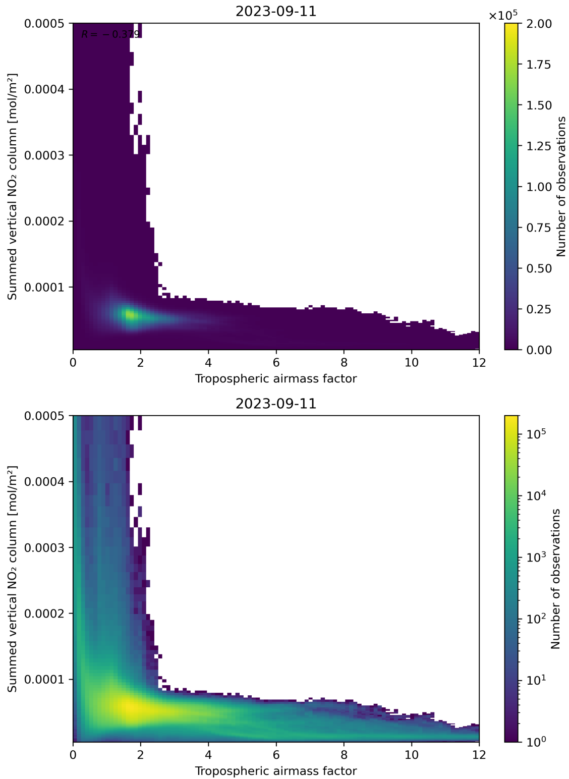
Figure 75: Scatter density plot of “Tropospheric air mass factor” against “Summed vertical NO 2 column” for 2023-09-10 to 2023-09-12.
