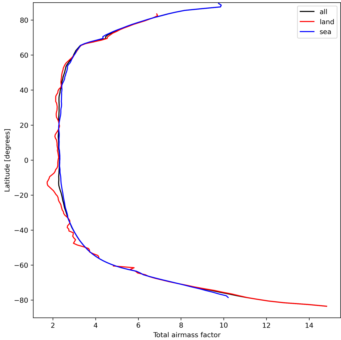
Figure 15: Zonal average of “Total airmass factor” for 2023-09-10 to 2023-09-12.
