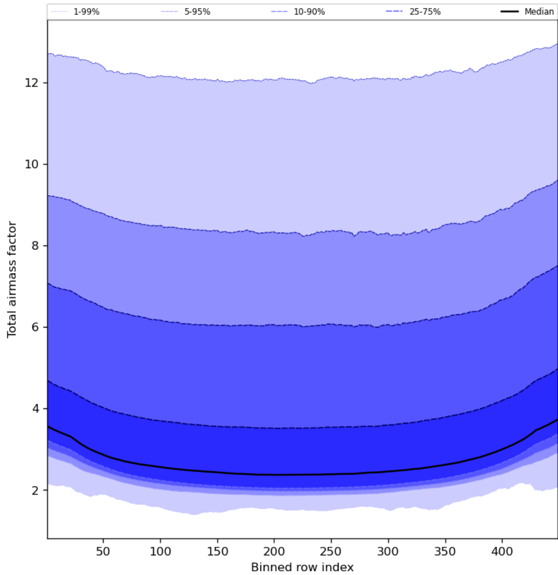
Figure 49: Along track statistics of “Total airmass factor” for 2023-09-10 to 2023-09-12
