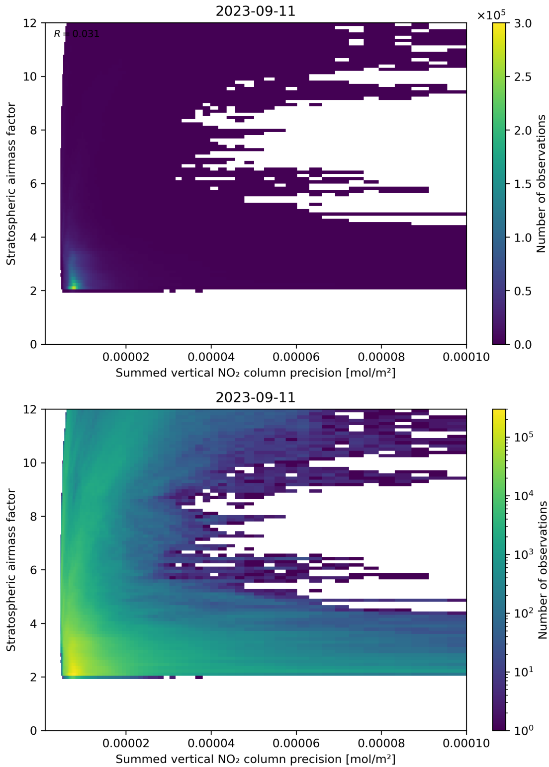
Figure 106: Scatter density plot of “Summed vertical NO 2 column precision” against “Stratospheric airmass factor” for 2023-09-10 to 2023-09-12.
