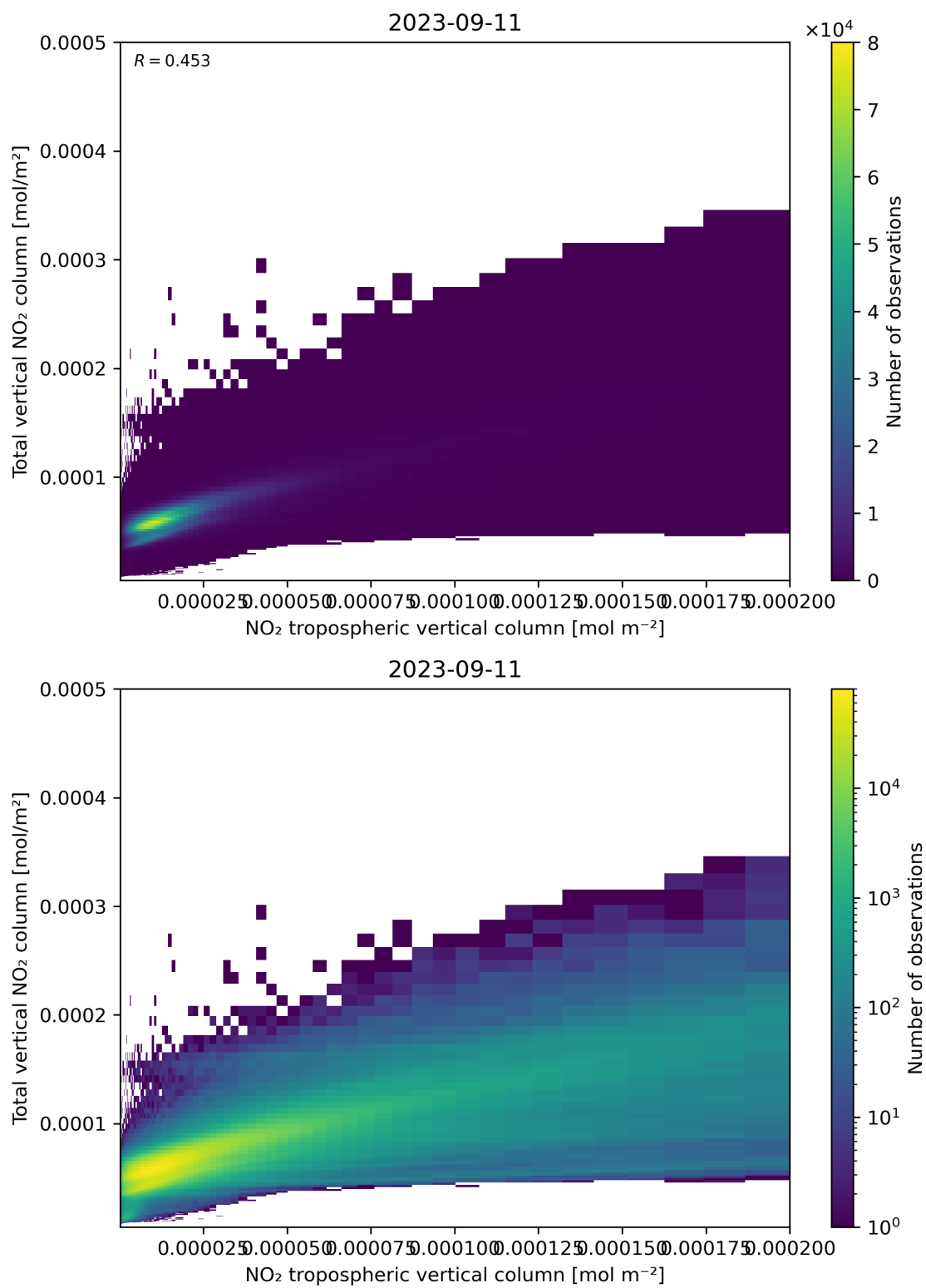
Figure 128: Scatter density plot of “NO 2 tropospheric vertical column” against “Total vertical NO 2 column” for 2023-09-10 to 2023-09-12.
