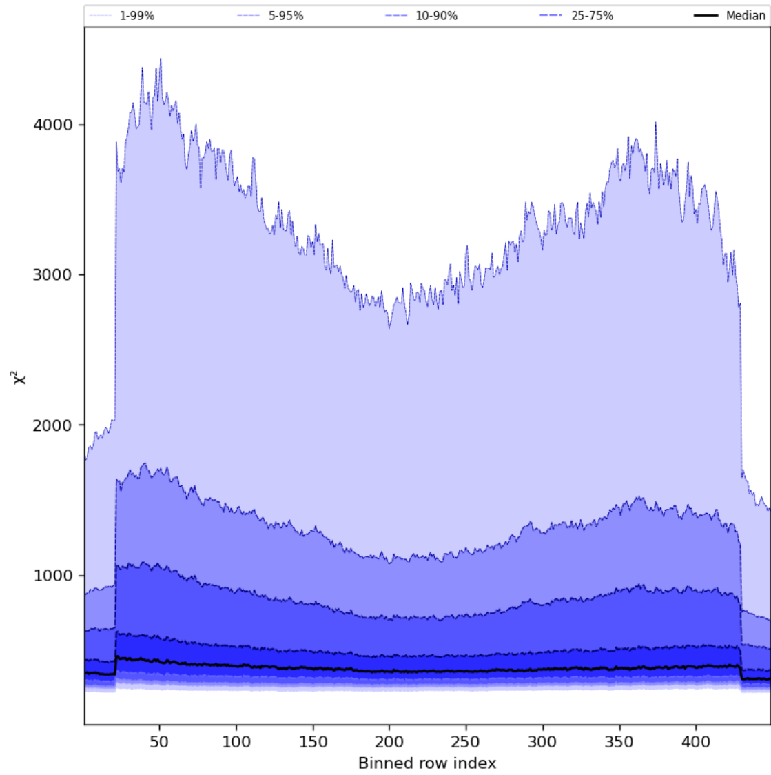
Figure 59: Along track statistics of “ \chi^2 ” for 2023-09-10 to 2023-09-12
