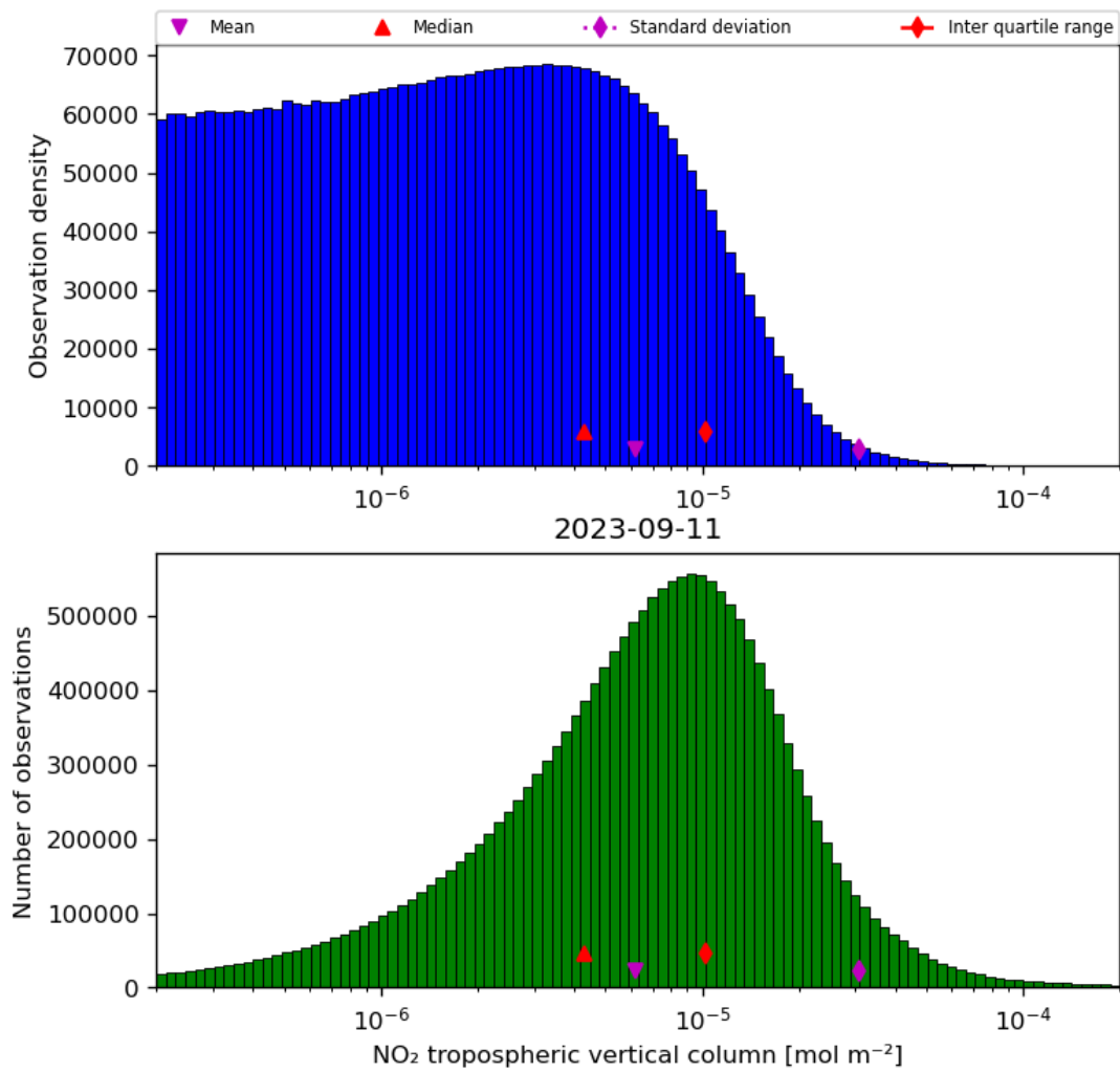
Figure 29: Histogram of “NO 2 tropospheric vertical column” for 2023-09-10 to 2023-09-12
