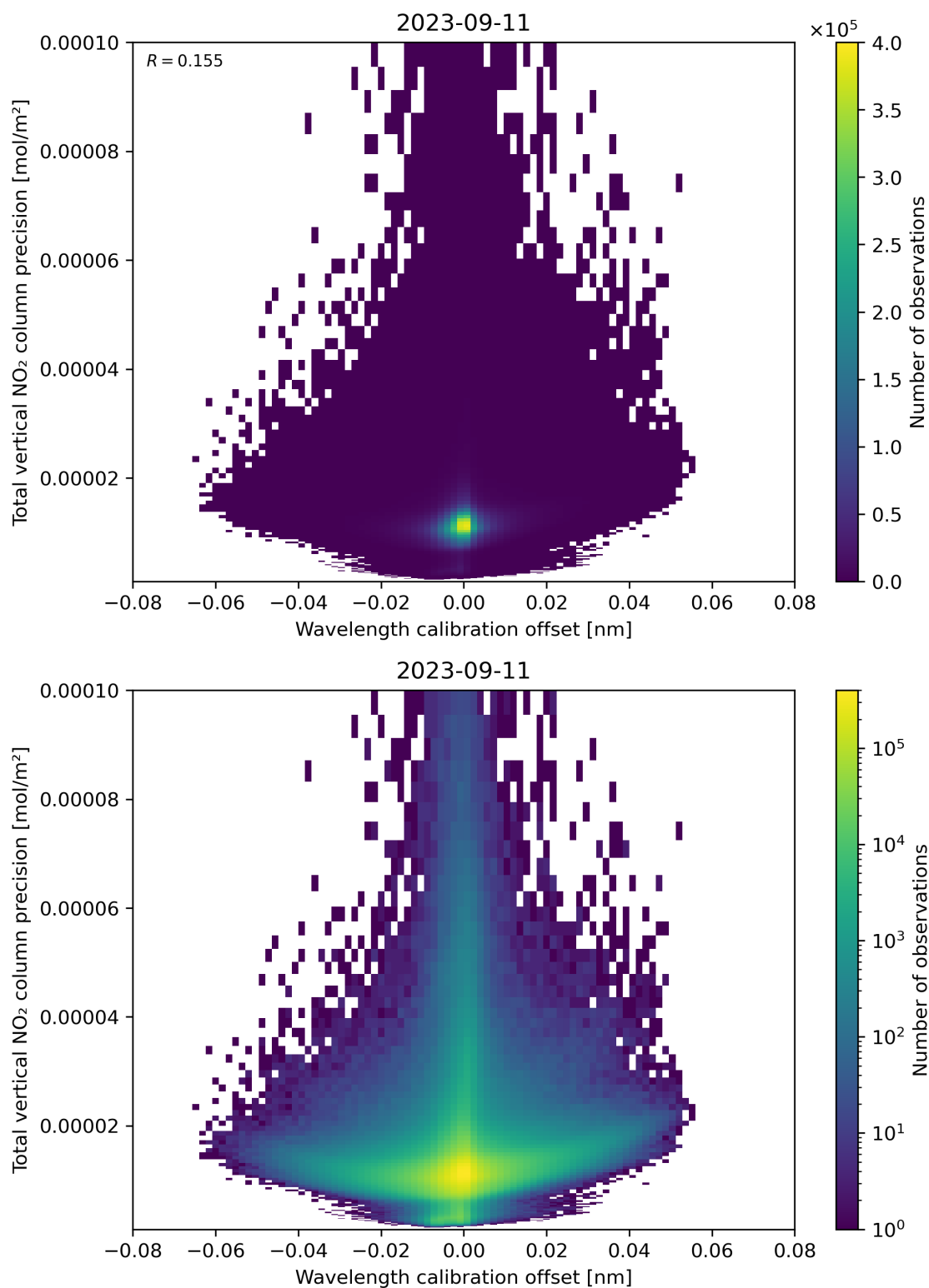
Figure 180: Scatter density plot of “Wavelength calibration offset” against “Total vertical NO 2 column precision” for 2023-09-10 to 2023-09-12.
