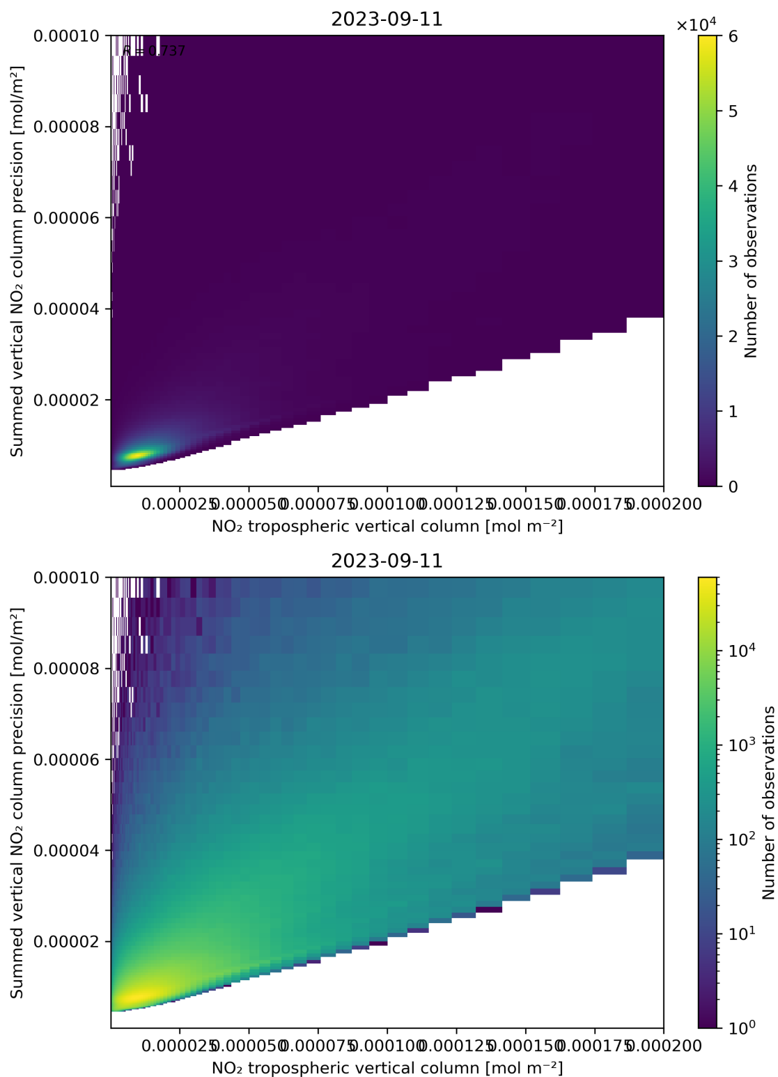
Figure 127: Scatter density plot of “NO 2 tropospheric vertical column” against “Summed vertical NO 2 column precision” for 2023-09-10 to 2023-09-12.
