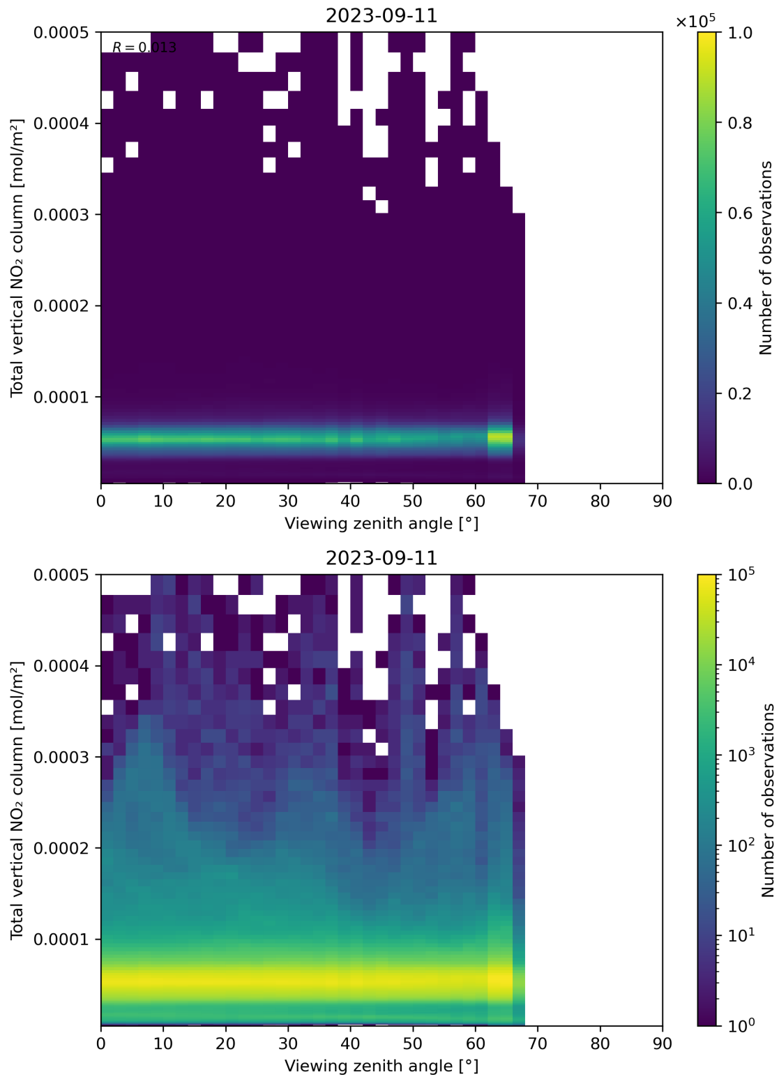
Figure 167: Scatter density plot of “Viewing zenith angle” against “Total vertical NO 2 column” for 2023-09-10 to 2023-09-12.
