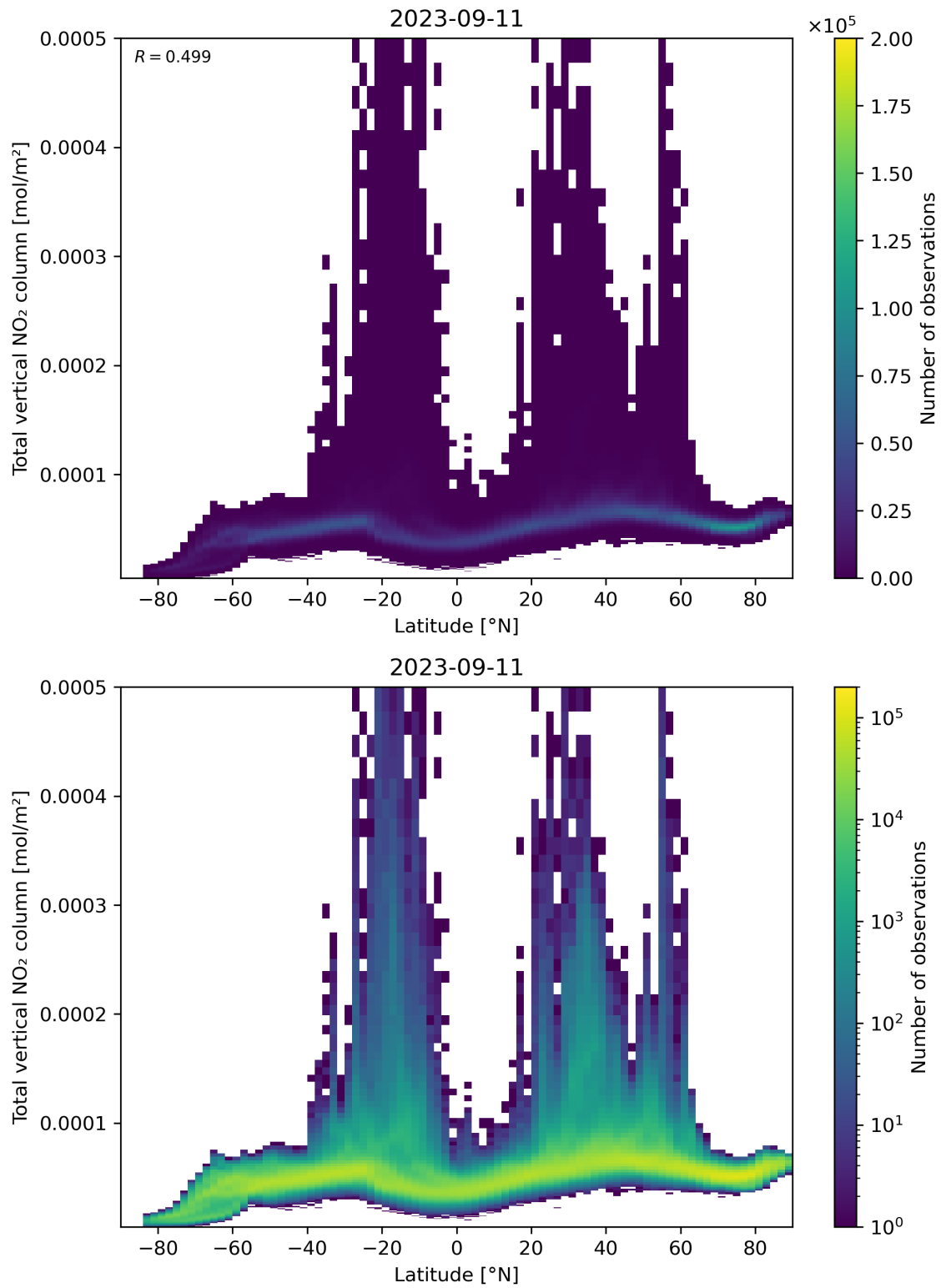
Figure 90: Scatter density plot of “Latitude” against “Total vertical NO 2 column” for 2023-09-10 to 2023-09-12.
