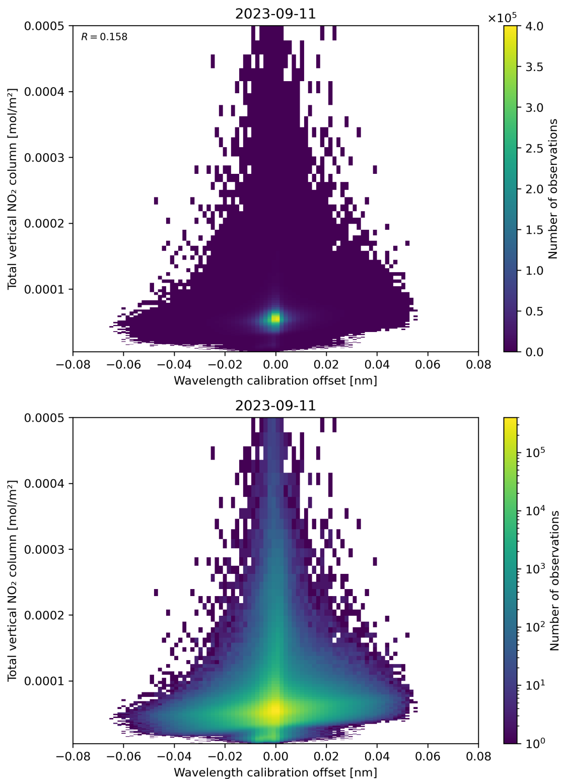
Figure 179: Scatter density plot of “Wavelength calibration offset” against “Total vertical NO 2 column” for 2023-09-10 to 2023-09-12.
