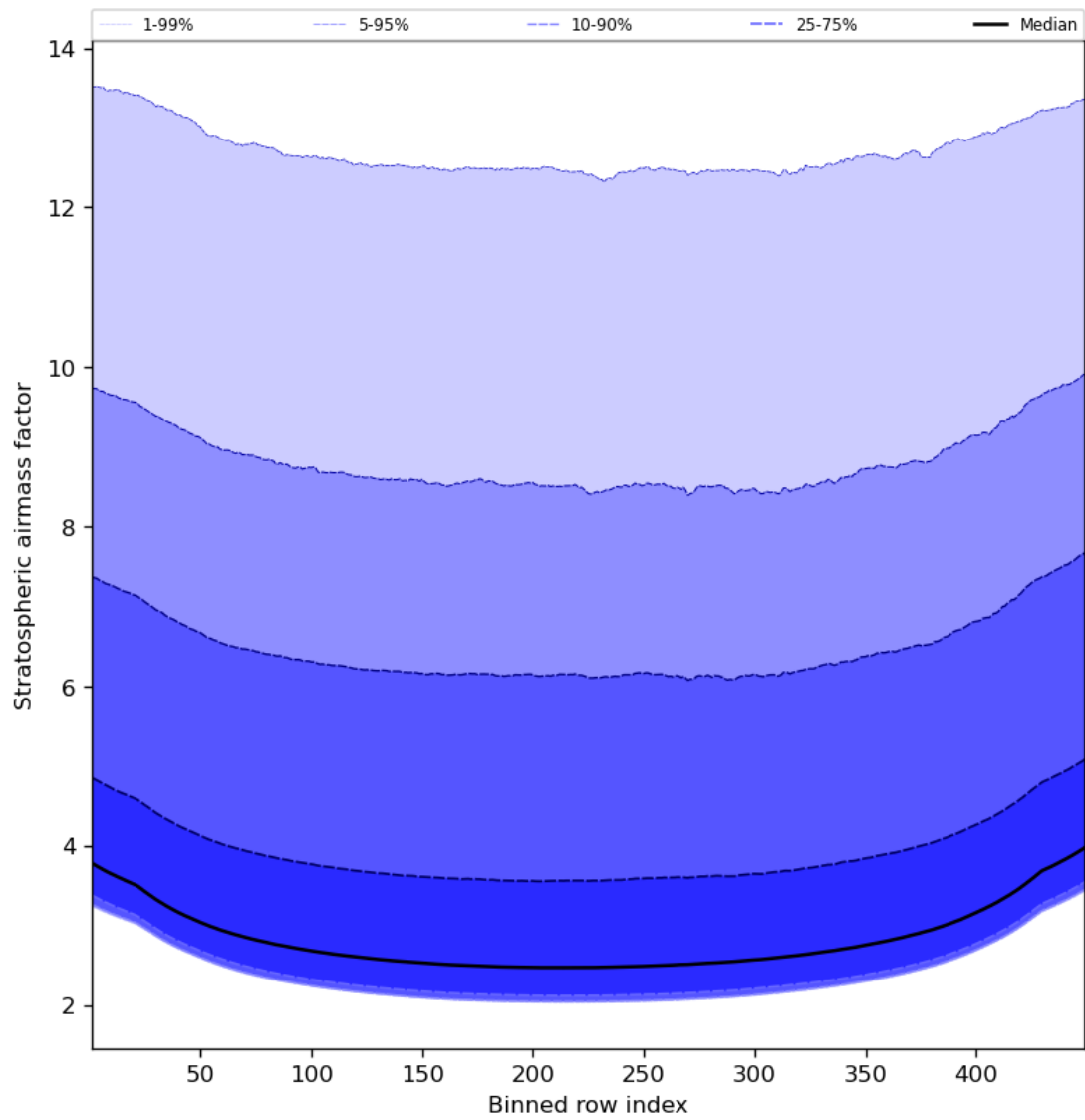
Figure 61: Along track statistics of “Stratospheric airmass factor” for 2023-09-10 to 2023-09-12
