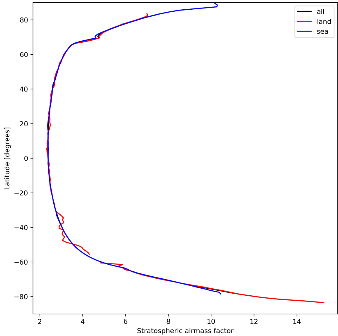
Figure 27: Zonal average of “Stratospheric airmass factor” for 2023-09-10 to 2023-09-12.
