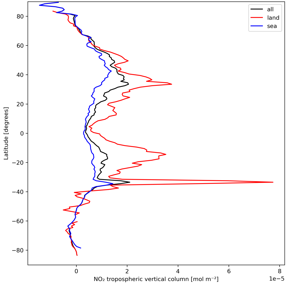
Figure 12: Zonal average of “NO 2 tropospheric vertical column” for 2023-09-10 to 2023-09-12.
