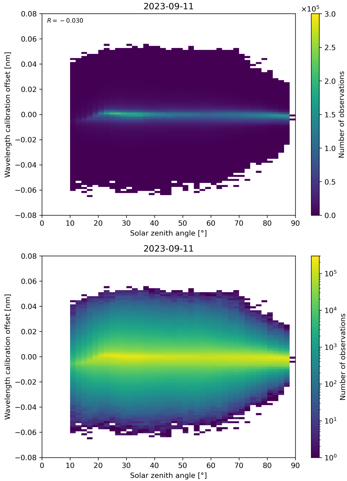
Figure 158: Scatter density plot of “Solar zenith angle” against “Wavelength calibration offset” for 2023-09-10 to 2023-09-12.
