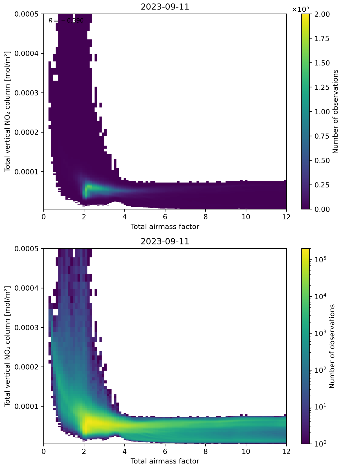
Figure 67: Scatter density plot of “Total airmass factor” against “Total vertical NO 2 column” for 2023-09-10 to 2023-09-12.
