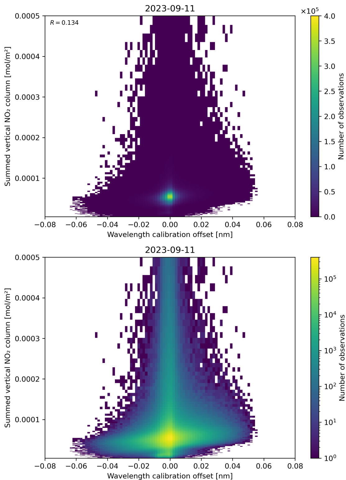
Figure 177: Scatter density plot of “Wavelength calibration offset” against “Summed vertical NO 2 column” for 2023-09-10 to 2023-09-12.
