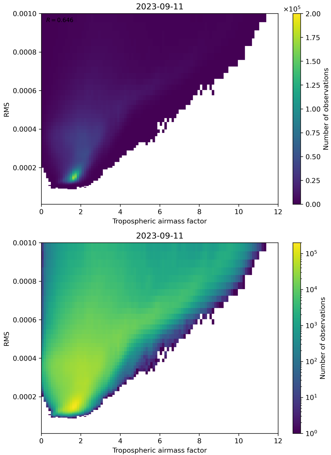
Figure 79: Scatter density plot of “Tropospheric airmass factor” against “RMS” for 2023-09-10 to 2023-09-12.
