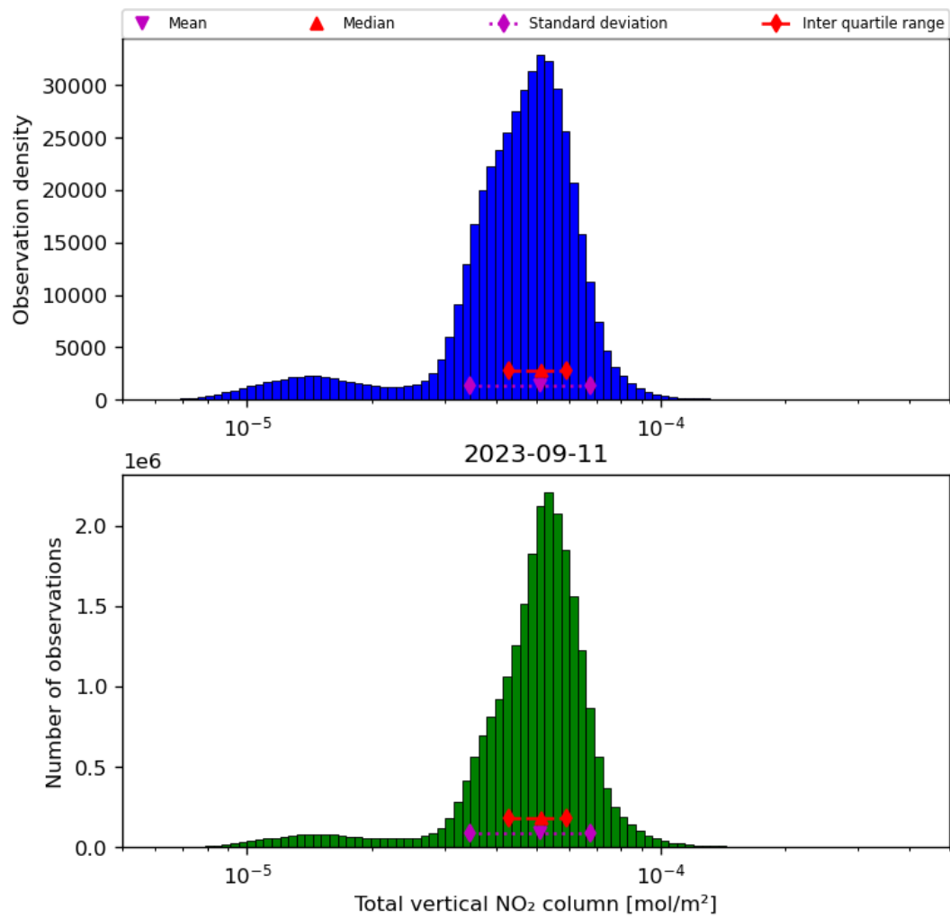
Figure 38: Histogram of "Total vertical NO 2 column" for 2023-09-10 to 2023-09-12
