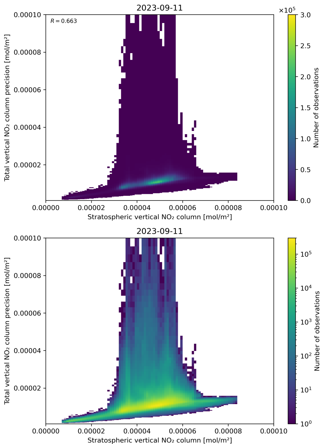
Figure 101: Scatter density plot of “Stratospheric vertical NO 2 column” against “Total vertical NO 2 column precision” for 2023-09-10 to 2023-09-12.
