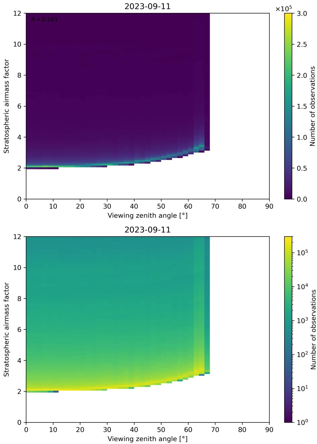
Figure 159: Scatter density plot of “Viewing zenith angle” against “Stratospheric airmass factor” for 2023-09-10 to 2023-09-12.
