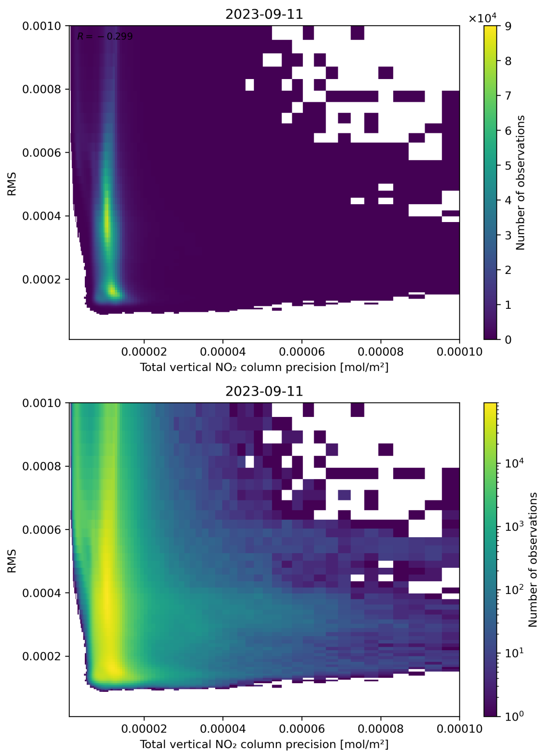
Figure 119: Scatter density plot of “Total vertical NO 2 column precision” against “RMS” for 2023-09-10 to 2023-09-12.
