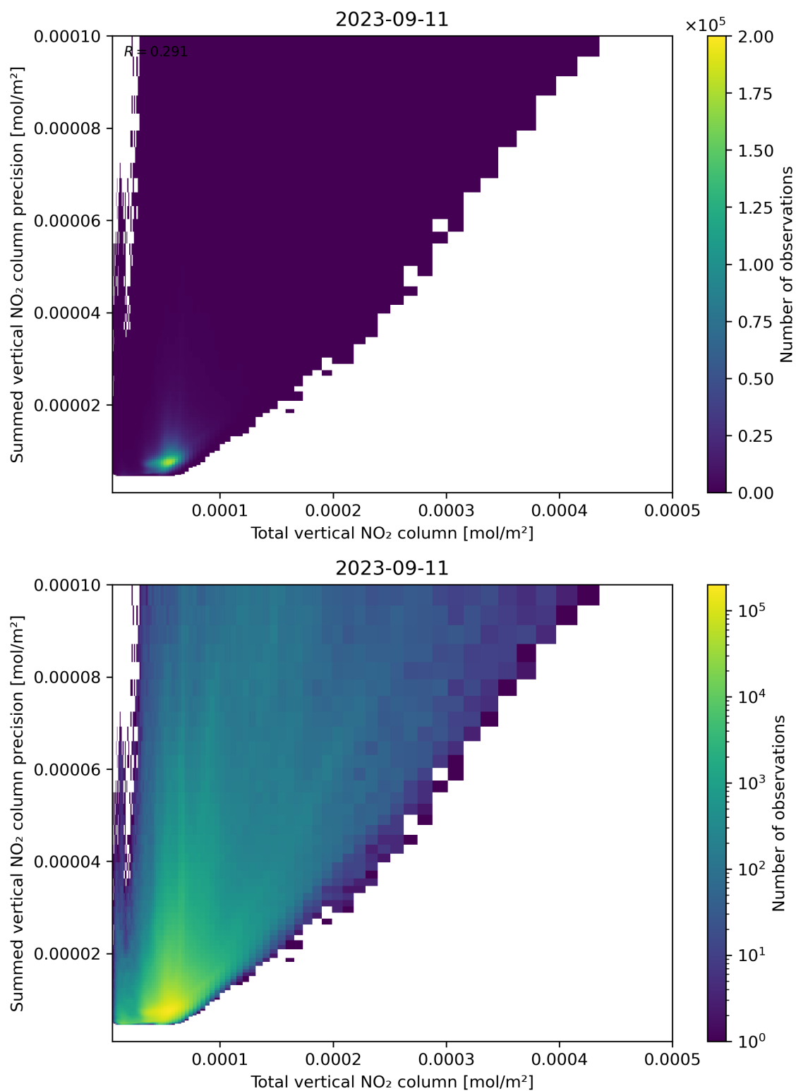
Figure 113: Scatter density plot of “Total vertical NO 2 column” against “Summed vertical NO 2 column precision” for 2023-09-10 to 2023-09-12.
