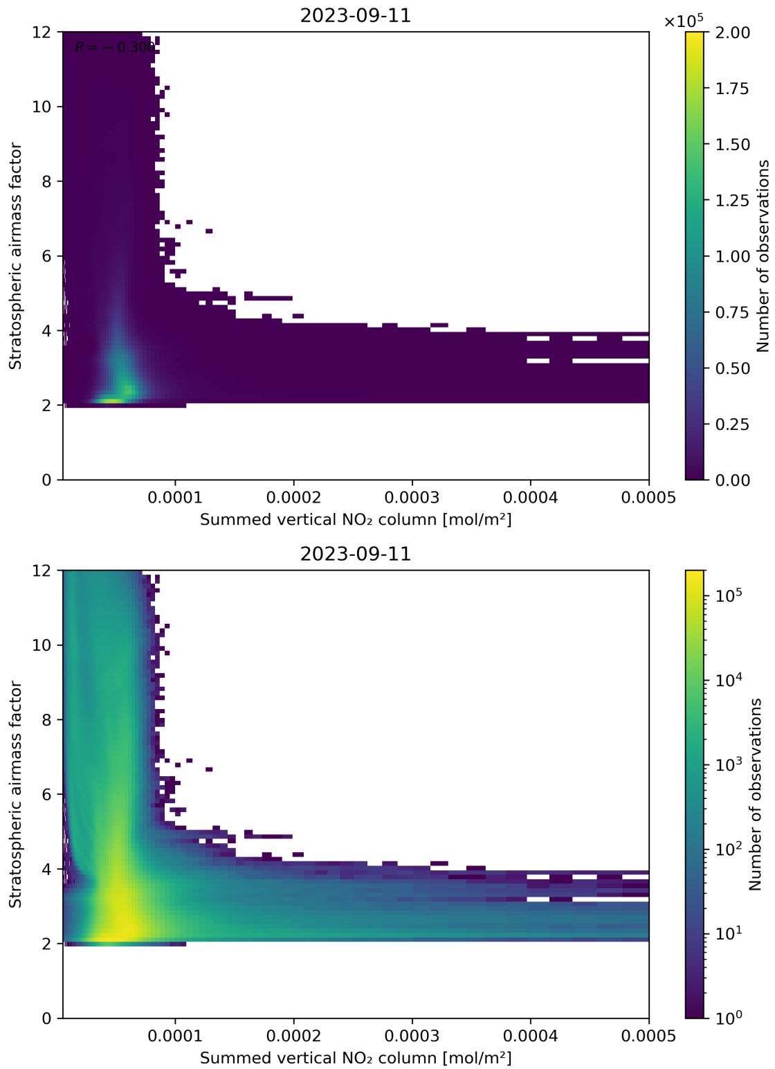
Figure 103: Scatter density plot of “Summed vertical NO 2 column” against “Stratospheric air mass factor” for 2023-09-10 to 2023-09-12.
