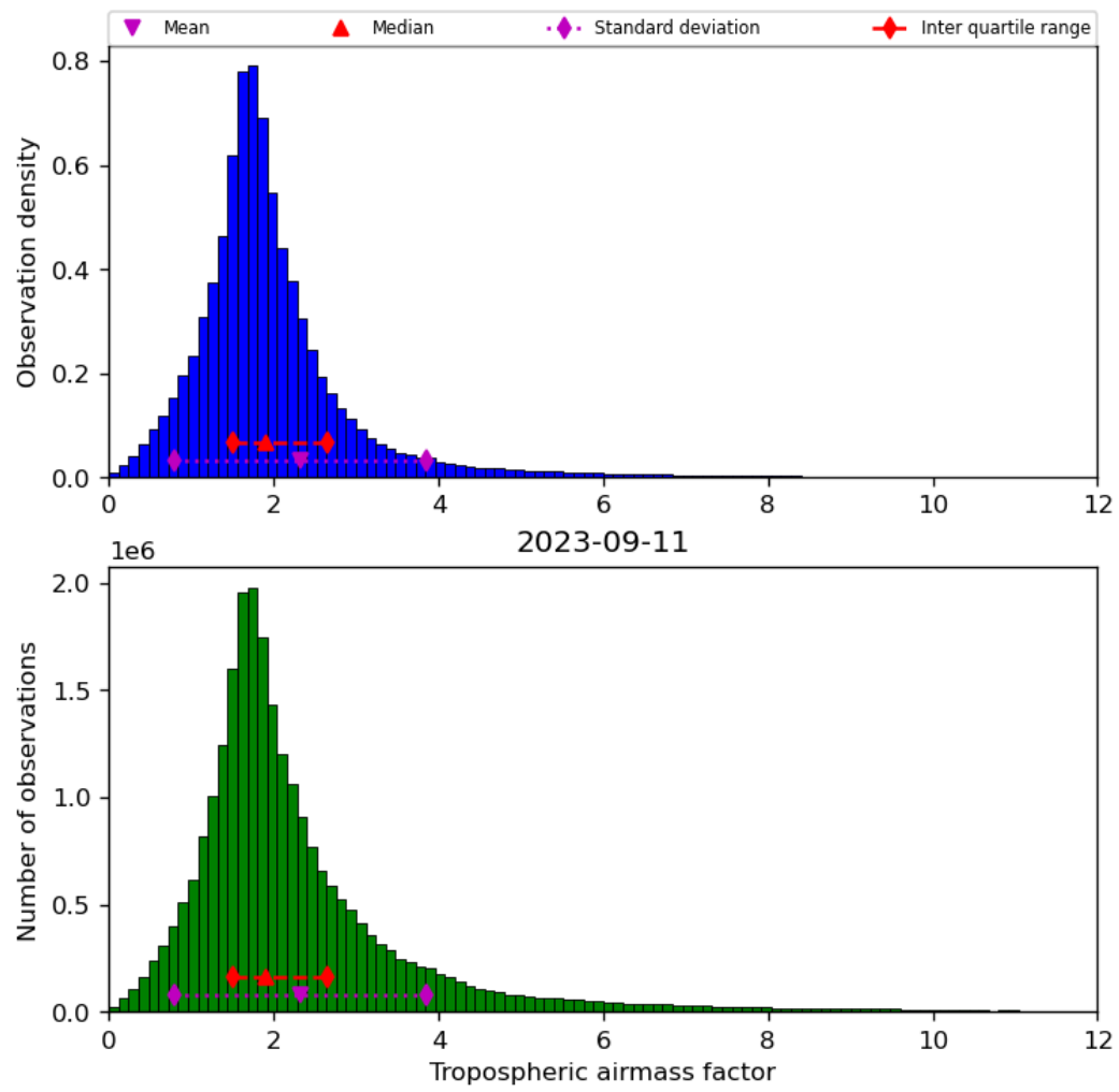
Figure 31: Histogram of “Tropospheric airmass factor” for 2023-09-10 to 2023-09-12
