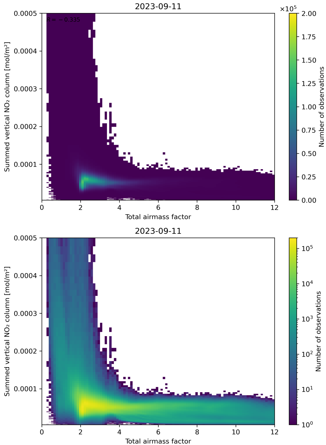
Figure 65: Scatter density plot of “Total airmass factor” against “Summed vertical NO 2 column” for 2023-09-10 to 2023-09-12.
