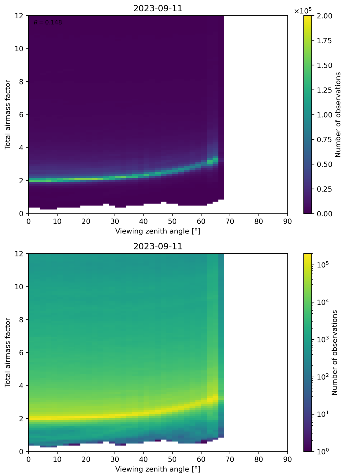
Figure 160: Scatter density plot of “Viewing zenith angle” against “Total airmass factor” for 2023-09-10 to 2023-09-12.
