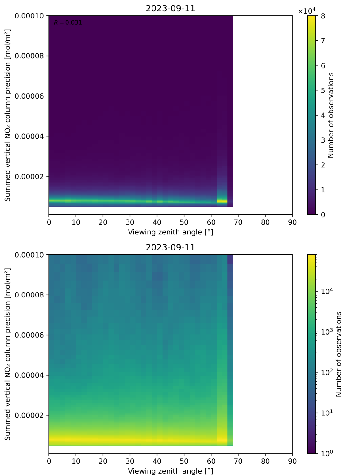
Figure 166: Scatter density plot of “Viewing zenith angle” against “Summed vertical NO 2 column precision” for 2023-09-10 to 2023-09-12.
