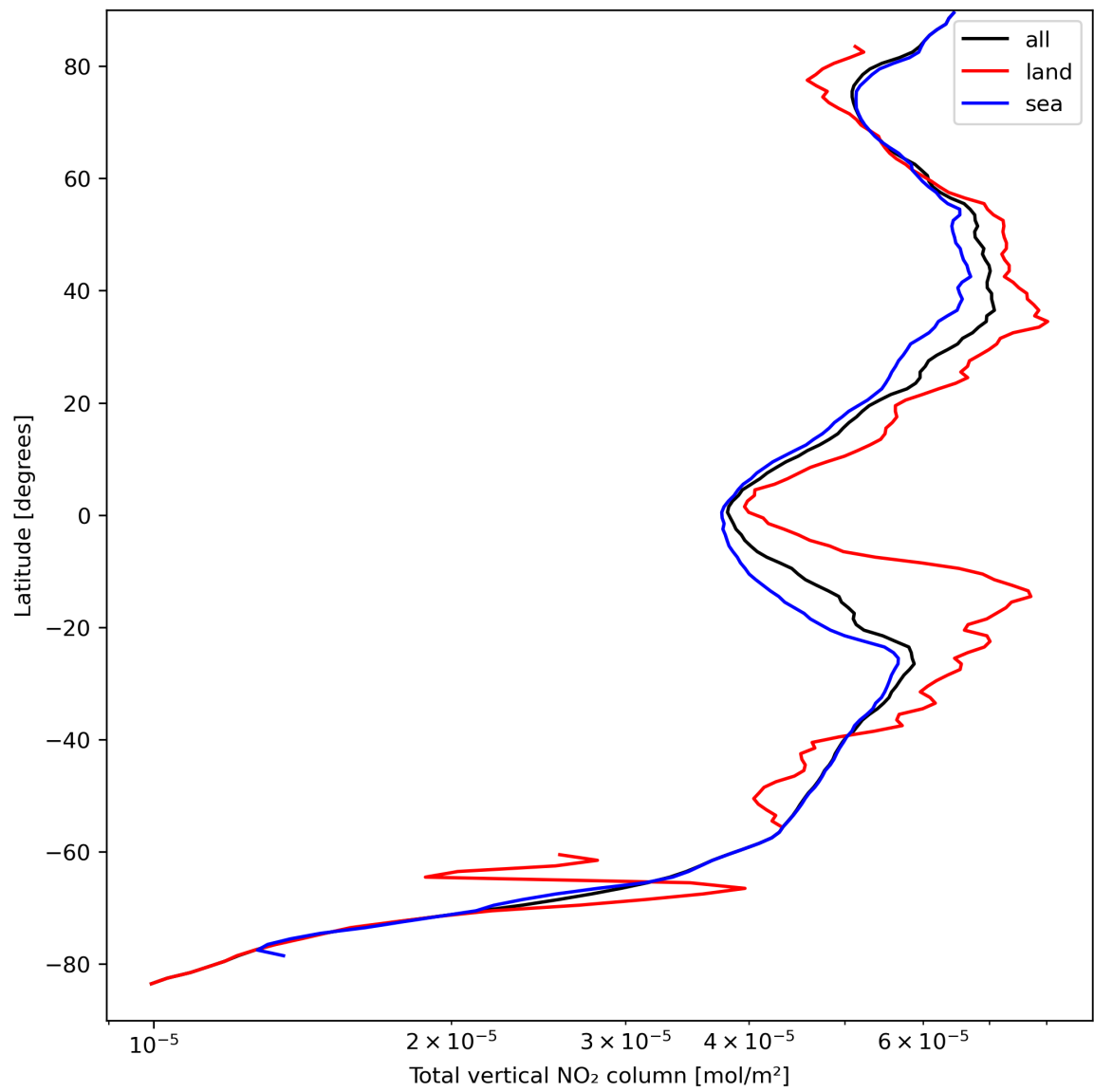
Figure 21: Zonal average of “Total vertical NO 2 column” for 2023-09-10 to 2023-09-12.
