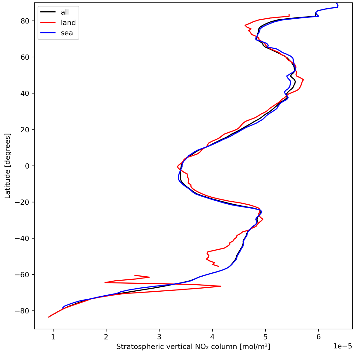
Figure 19: Zonal average of “Stratospheric vertical NO 2 column” for 2023-09-10 to 2023-09-12.
