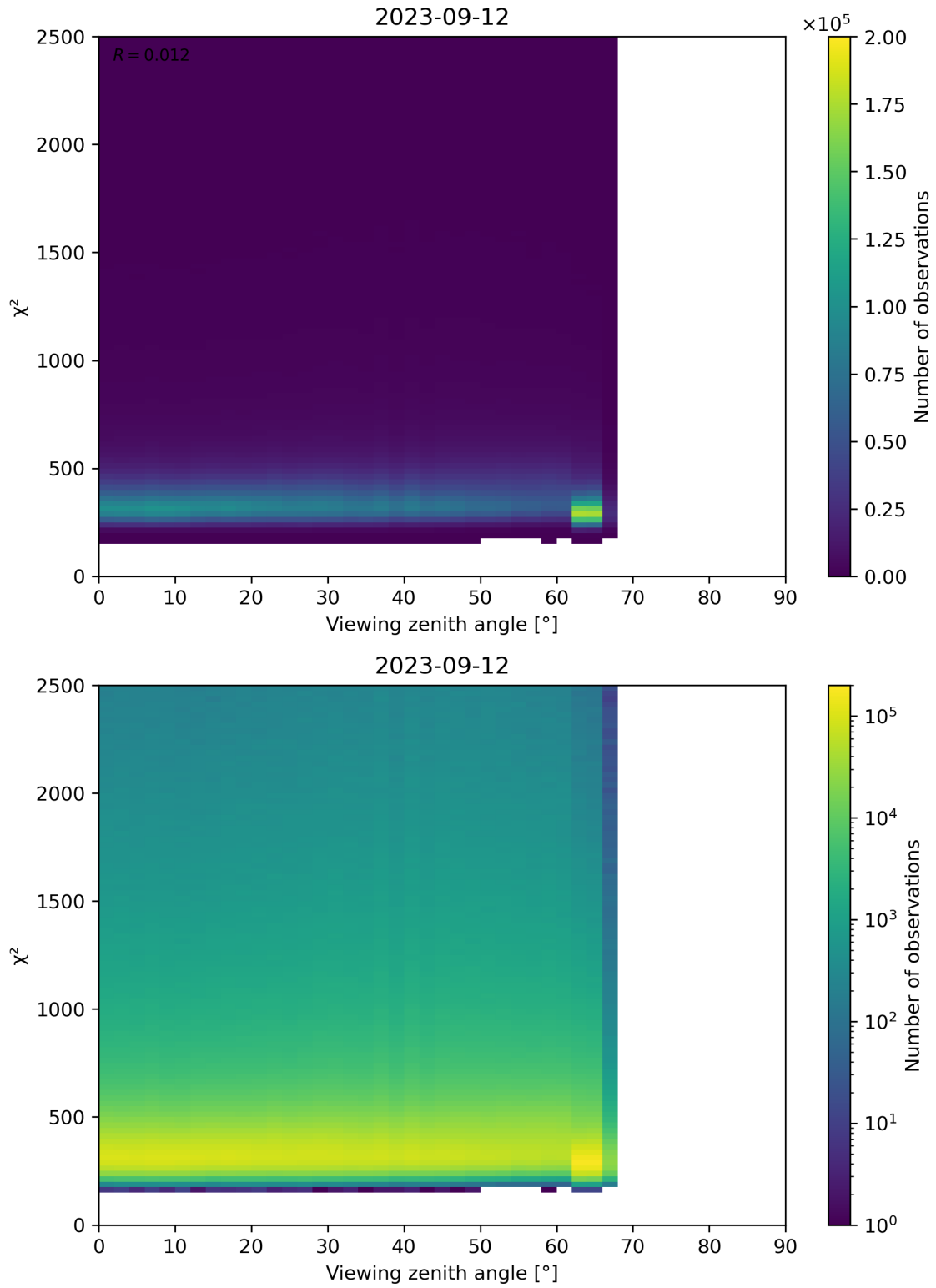
Figure 162: Scatter density plot of “Viewing zenith angle” against “ \chi^2 ” for 2023-09-11 to 2023-09-13.
