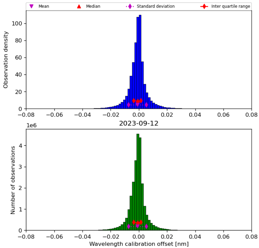
Figure 35: Histogram of “Wavelength calibration offset” for 2023-09-11 to 2023-09-13
