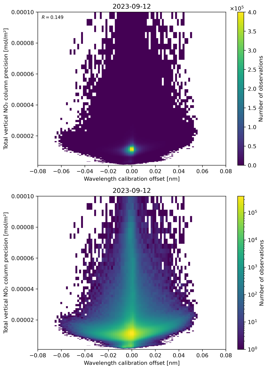
Figure 180: Scatter density plot of “Wavelength calibration offset” against “Total vertical NO 2 column precision” for 2023-09-11 to 2023-09-13.
