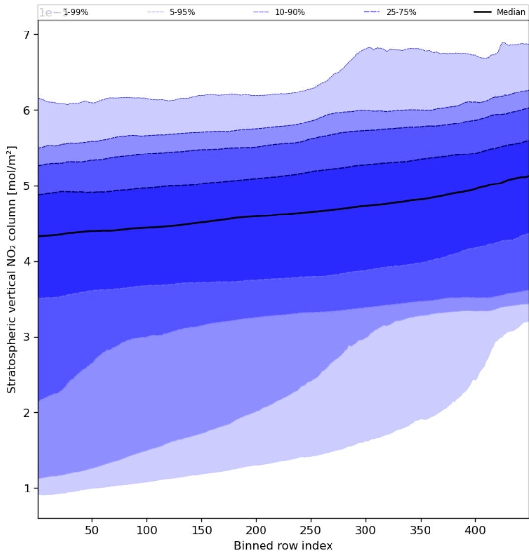
Figure 53: Along track statistics of “Stratospheric vertical NO 2 column” for 2023-09-11 to 2023-09-13
