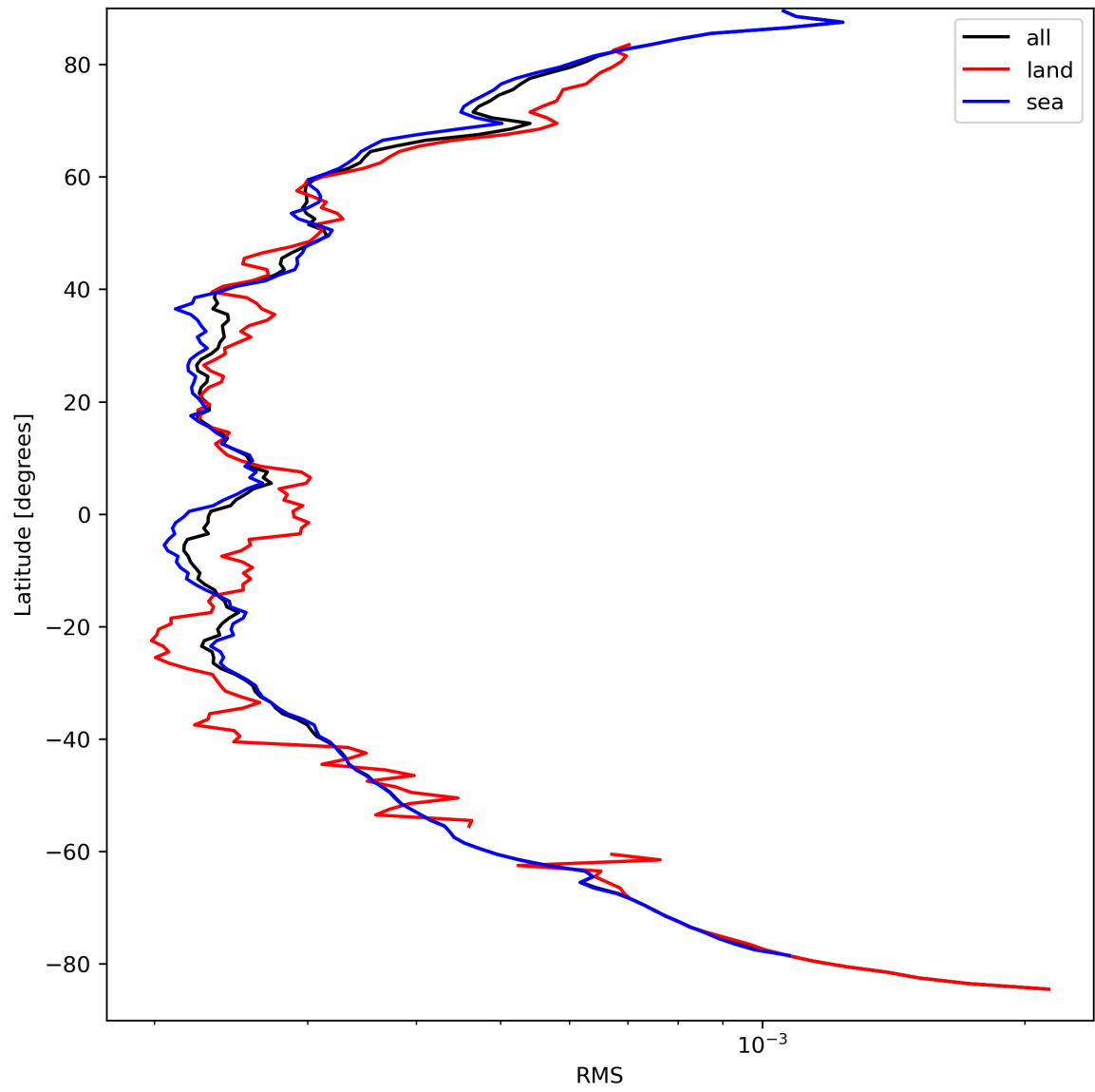
Figure 26: Zonal average of “RMS” for 2023-09-11 to 2023-09-13.
