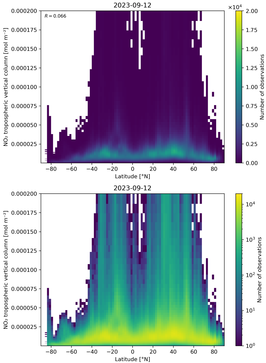
Figure 92: Scatter density plot of “Latitude” against “NO 2 tropospheric vertical column” for 2023-09-11 to 2023-09-13.
