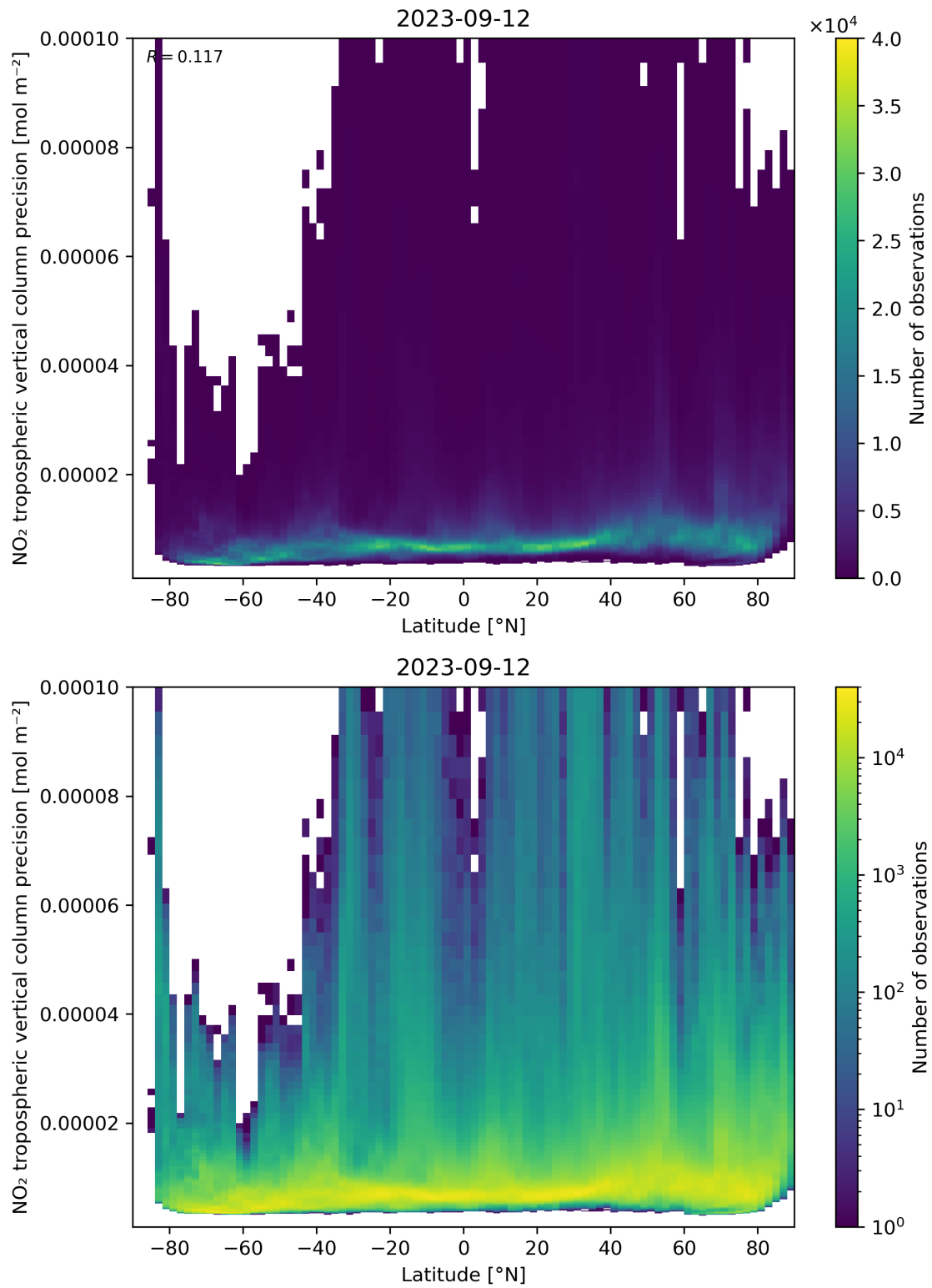
Figure 93: Scatter density plot of “Latitude” against “NO 2 tropospheric vertical column precision” for 2023-09-11 to 2023-09-13.
