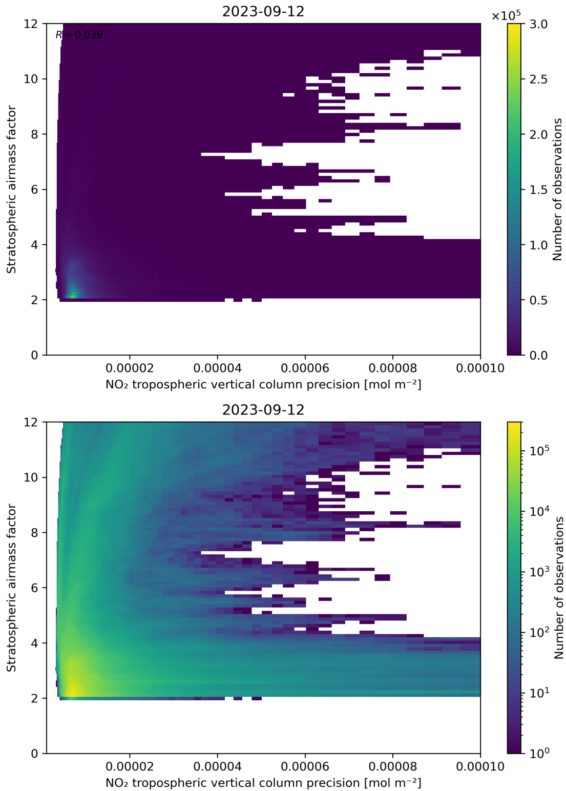
Figure 131: Scatter density plot of “NO 2 tropospheric vertical column precision” against “Stratospheric airmass factor” for 2023-09-11 to 2023-09-13.
