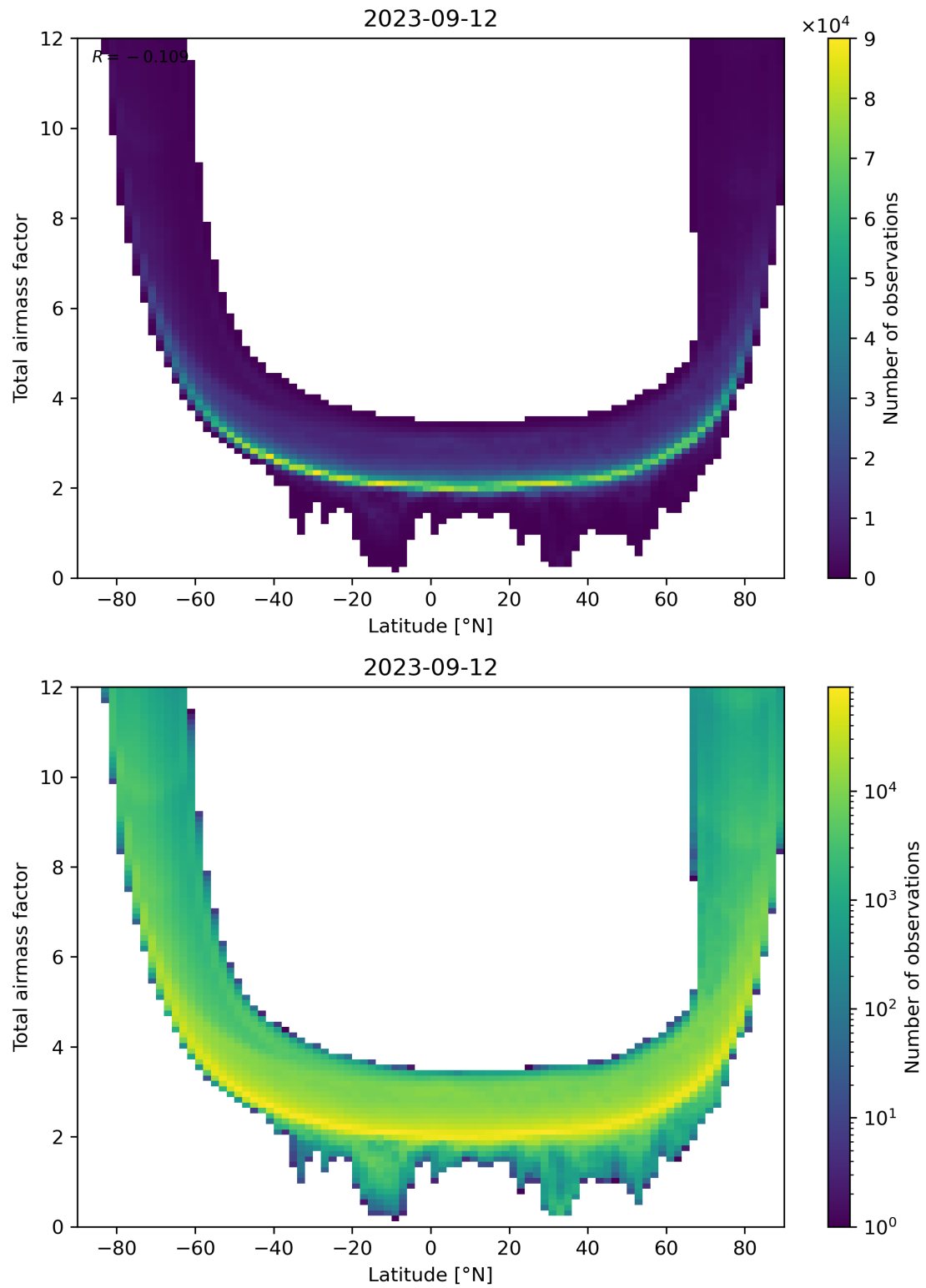
Figure 84: Scatter density plot of “Latitude” against “Total airmass factor” for 2023-09-11 to 2023-09-13.
