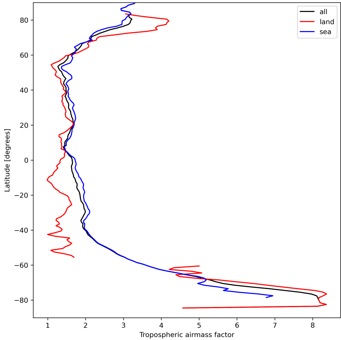
Figure 14: Zonal average of “Tropospheric airmass factor” for 2023-09-11 to 2023-09-13.
