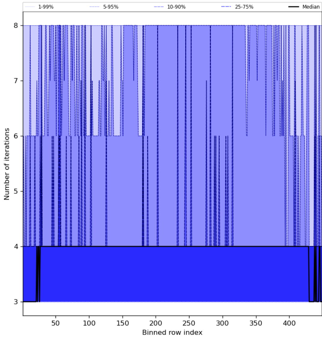
Figure 51: Along track statistics of “Number of iterations” for 2023-09-11 to 2023-09-13
