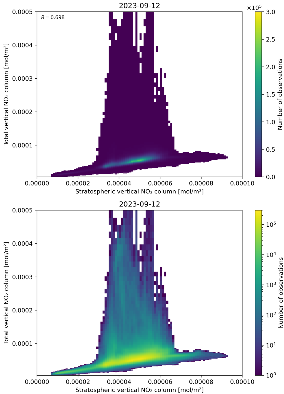
Figure 100: Scatter density plot of “Stratospheric vertical NO 2 column” against “Total vertical NO 2 column” for 2023-09-11 to 2023-09-13.
