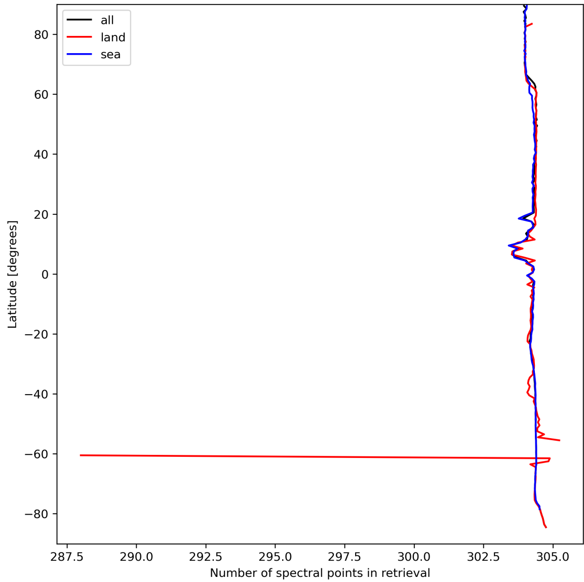
Figure 16: Zonal average of “Number of spectral points in retrieval” for 2023-09-11 to 2023-09-13.
