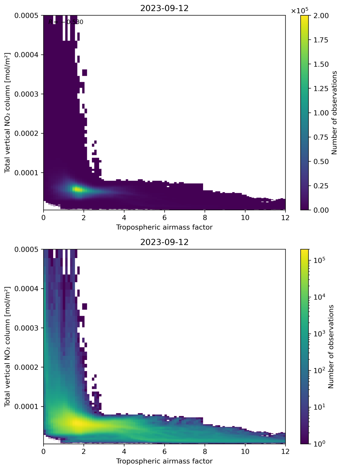
Figure 77: Scatter density plot of “Tropospheric airmass factor” against “Total vertical NO 2 column” for 2023-09-11 to 2023-09-13.
