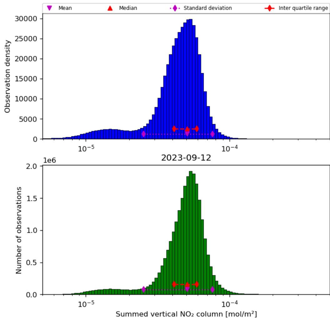
Figure 40: Histogram of “Summed vertical NO 2 column” for 2023-09-11 to 2023-09-13
