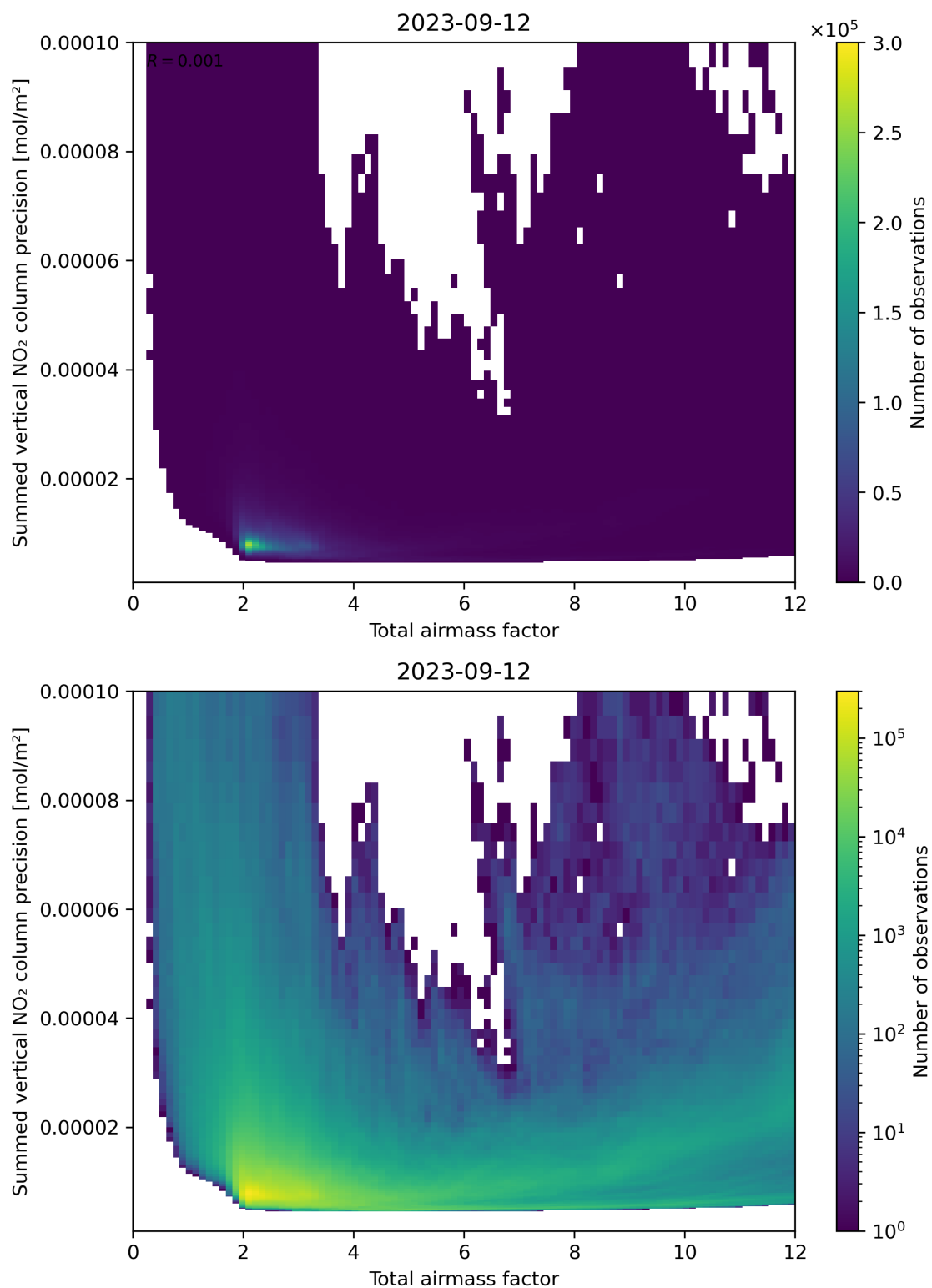
Figure 66: Scatter density plot of “Total airmass factor” against “Summed vertical NO 2 column precision” for 2023-09-11 to 2023-09-13.
