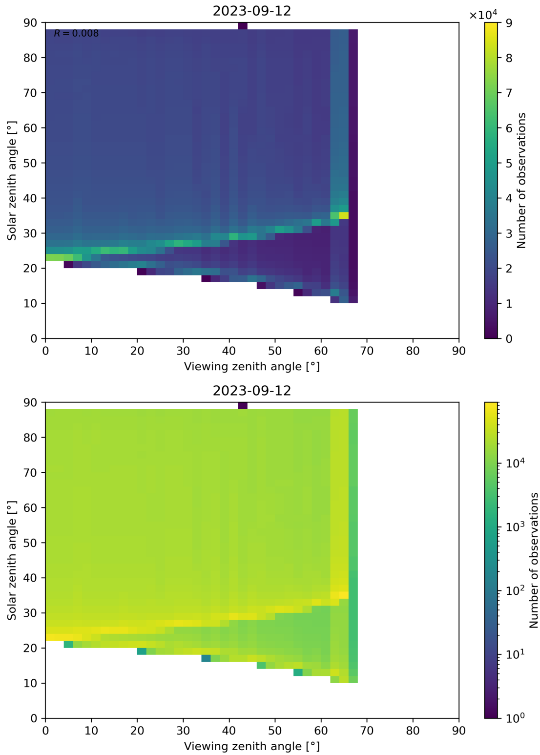
Figure 172: Scatter density plot of “Viewing zenith angle” against “Solar zenith angle” for 2023-09-11 to 2023-09-13.
