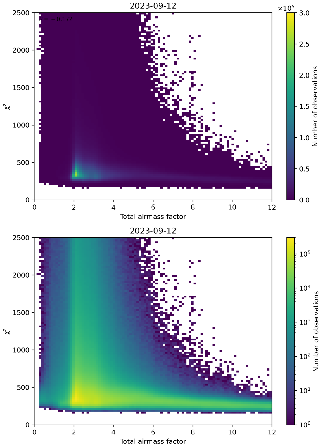
Figure 63: Scatter density plot of “Total airmass factor” against “ \chi^2 ” for 2023-09-11 to 2023-09-13.
