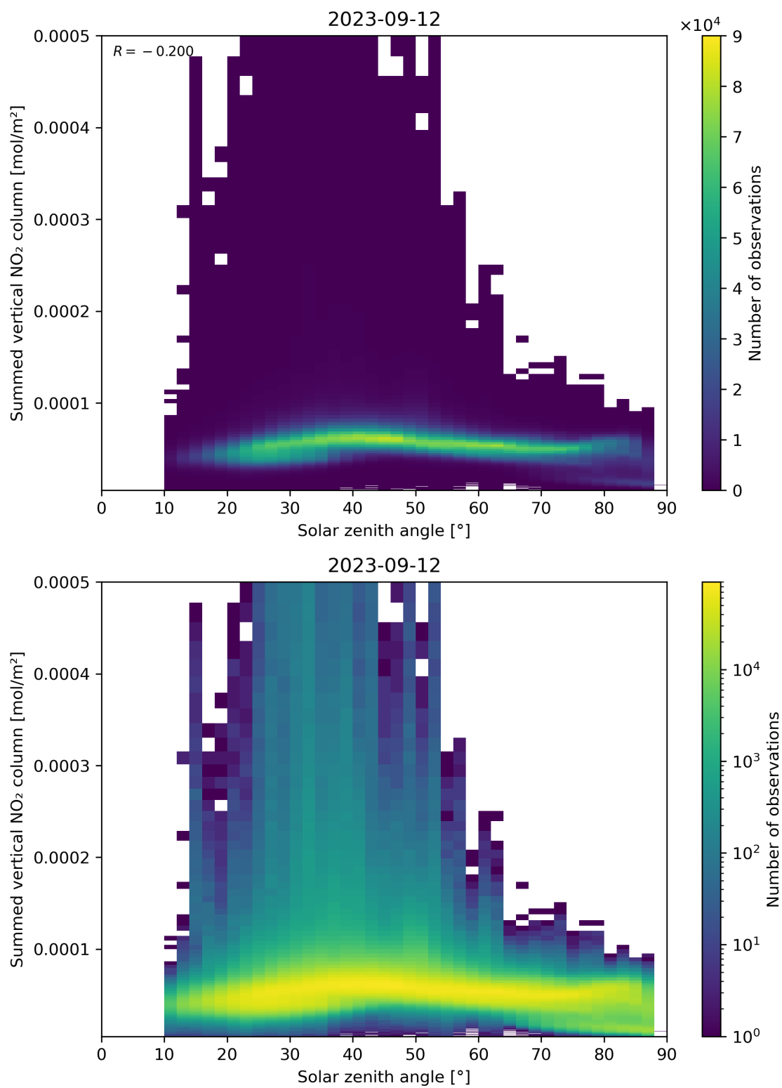
Figure 151: Scatter density plot of “Solar zenith angle” against “Summed vertical NO 2 column” for 2023-09-11 to 2023-09-13.
