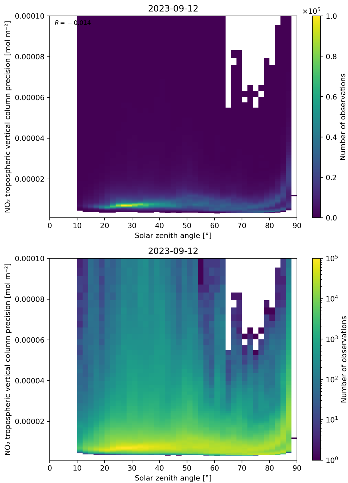
Figure 156: Scatter density plot of “Solar zenith angle” against “NO 2 tropospheric vertical column precision” for 2023-09-11 to 2023-09-13.
