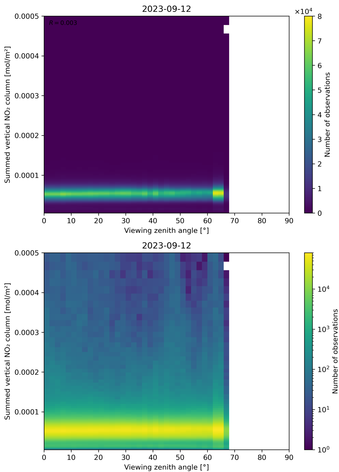
Figure 165: Scatter density plot of “Viewing zenith angle” against “Summed vertical NO 2 column” for 2023-09-11 to 2023-09-13.
