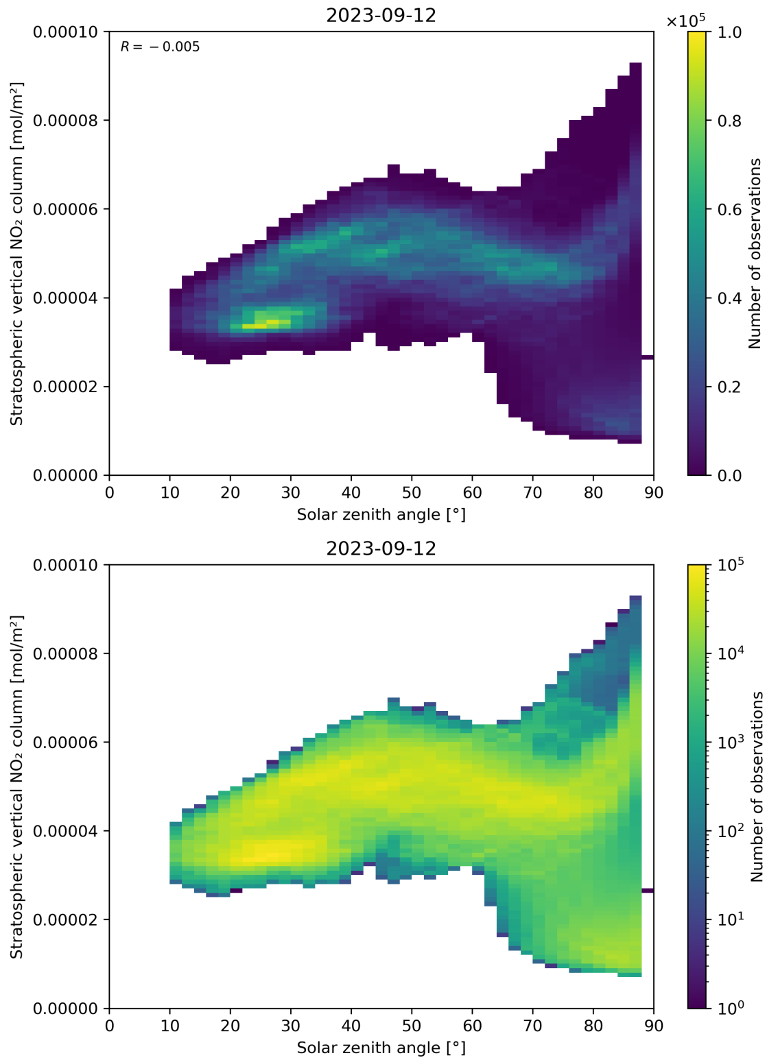
Figure 150: Scatter density plot of “Solar zenith angle” against “Stratospheric vertical NO 2 column” for 2023-09-11 to 2023-09-13.
