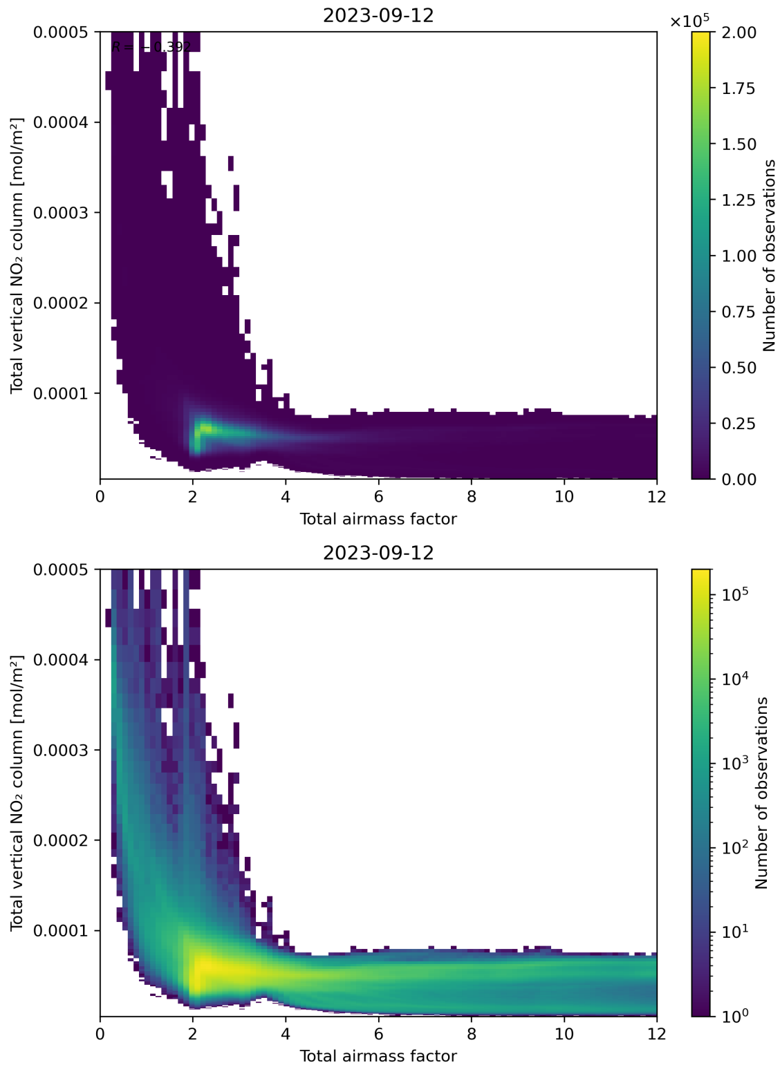
Figure 67: Scatter density plot of “Total airmass factor” against “Total vertical NO 2 column” for 2023-09-11 to 2023-09-13.
