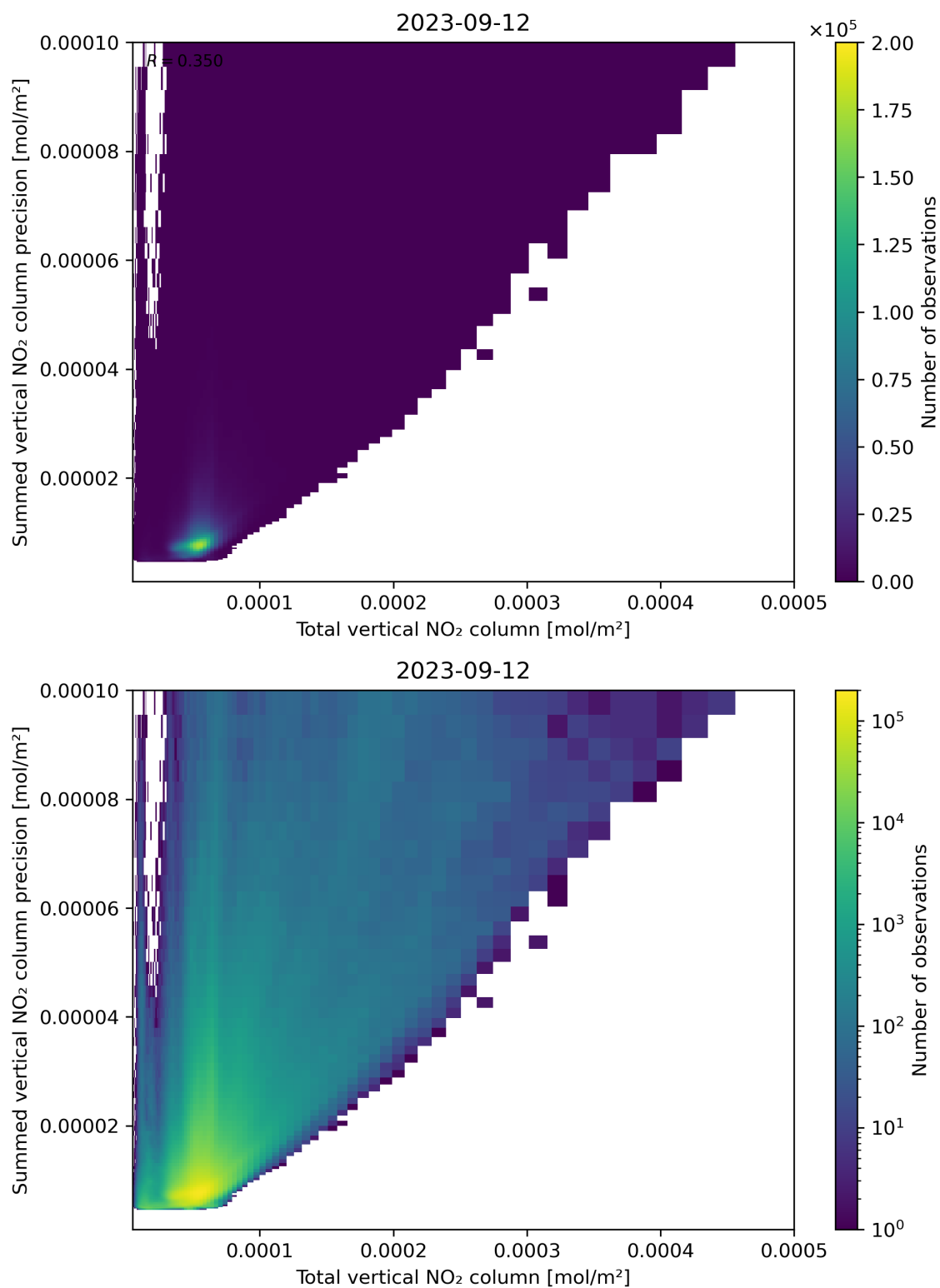
Figure 113: Scatter density plot of “Total vertical NO 2 column” against “Summed vertical NO 2 column precision” for 2023-09-11 to 2023-09-13.
