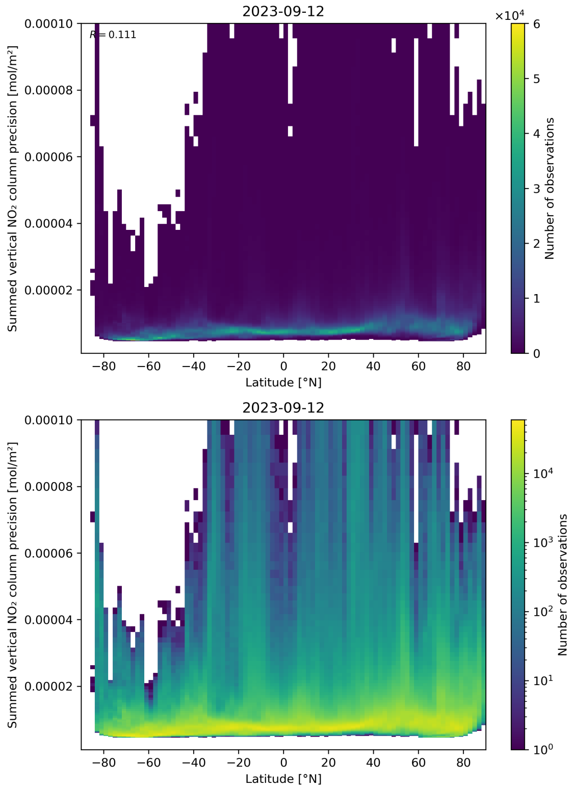
Figure 89: Scatter density plot of “Latitude” against “Summed vertical NO 2 column precision” for 2023-09-11 to 2023-09-13.
