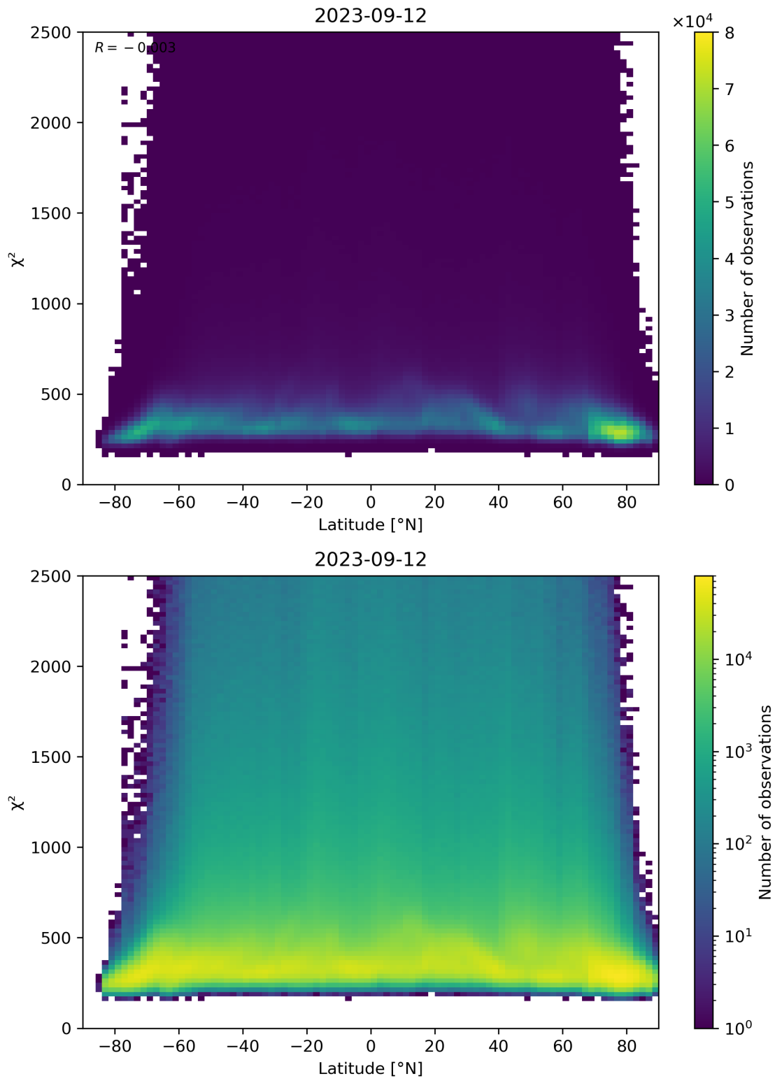
Figure 86: Scatter density plot of “Latitude” against “ \chi^2 ” for 2023-09-11 to 2023-09-13.
