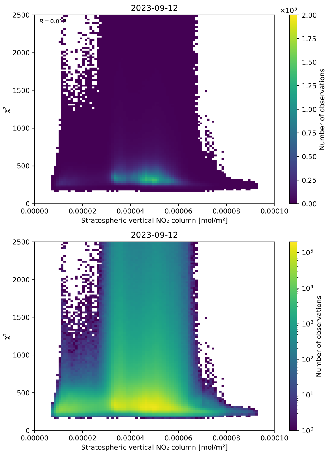
Figure 97: Scatter density plot of “Stratospheric vertical NO 2 column” against “ \chi^2 ” for 2023-09-11 to 2023-09-13.
