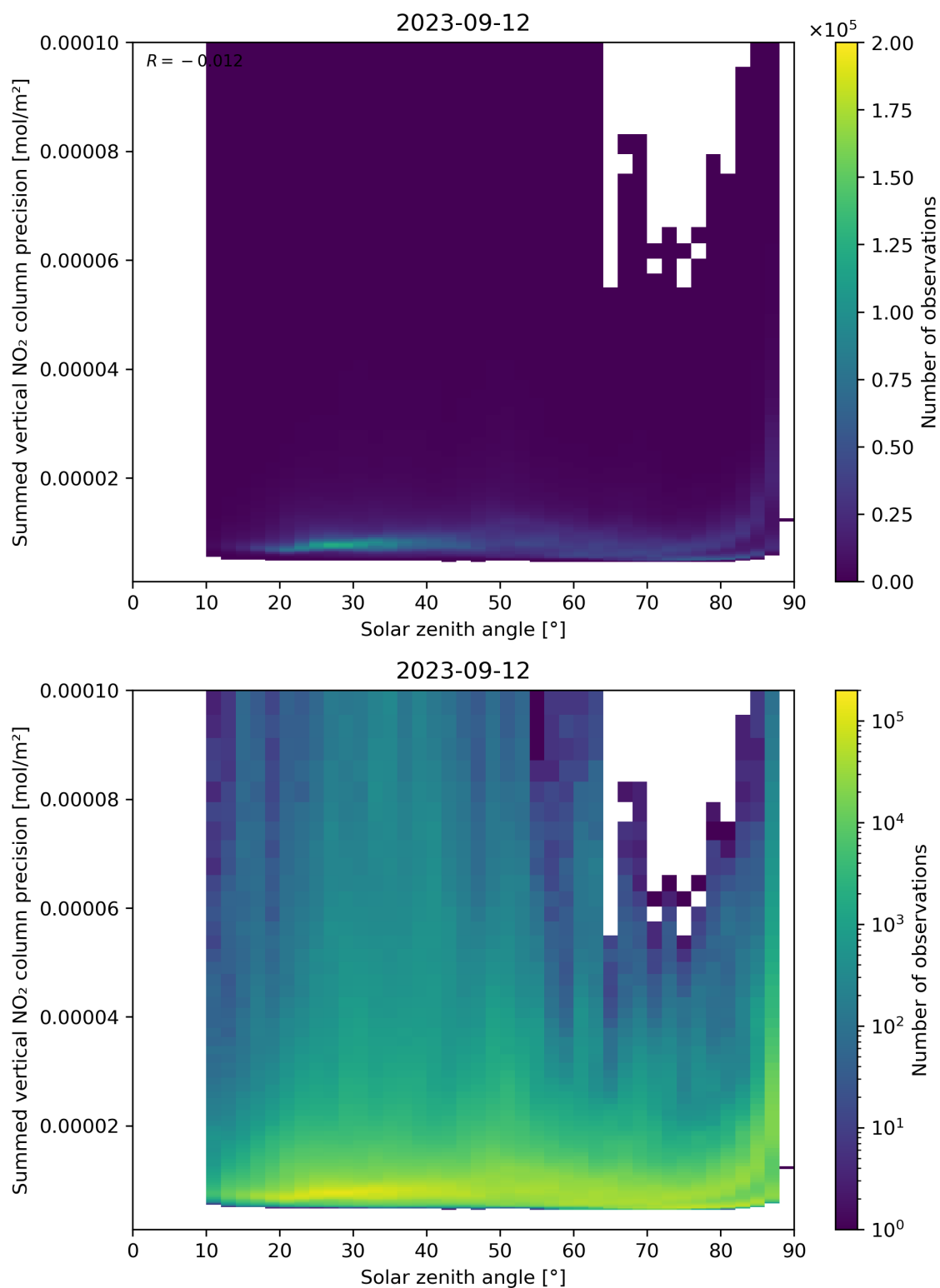
Figure 152: Scatter density plot of “Solar zenith angle” against “Summed vertical NO 2 column precision” for 2023-09-11 to 2023-09-13.
