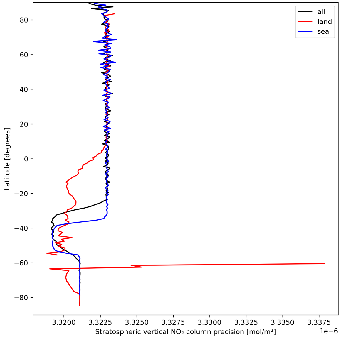
Figure 20: Zonal average of “Stratospheric vertical NO 2 column precision” for 2023-09-11 to 2023-09-13.
