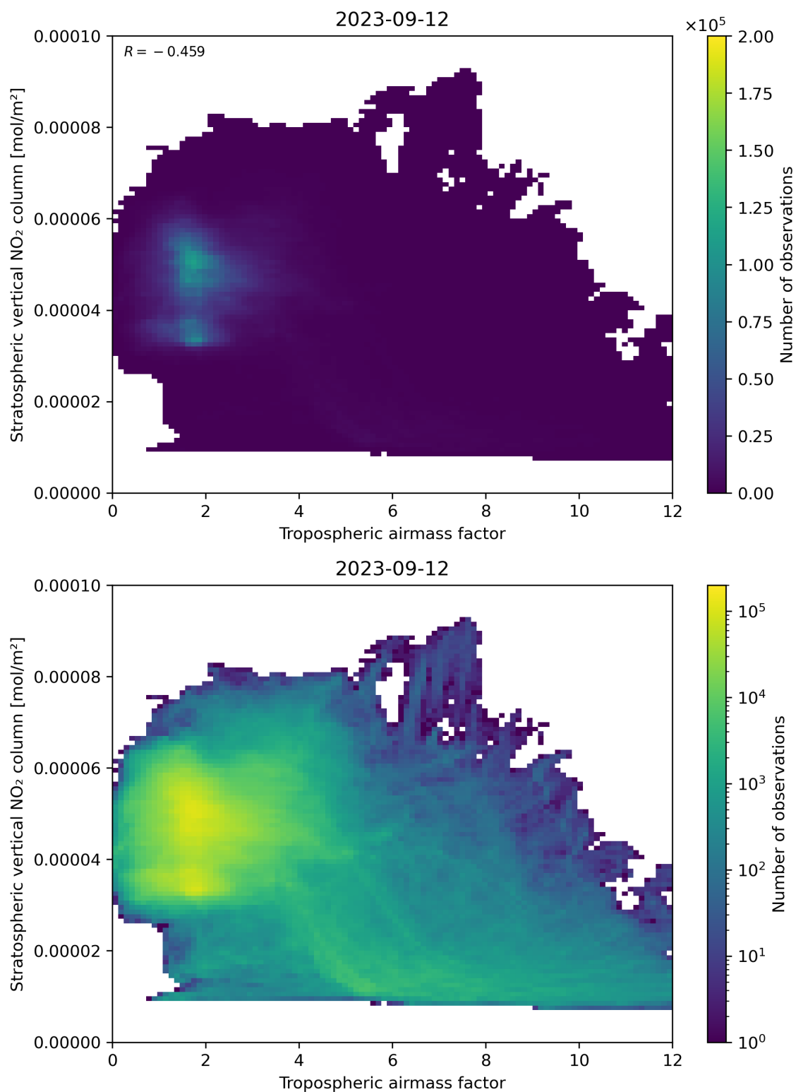
Figure 74: Scatter density plot of “Tropospheric air mass factor” against “Stratospheric vertical NO 2 column” for 2023-09-11 to 2023-09-13.
