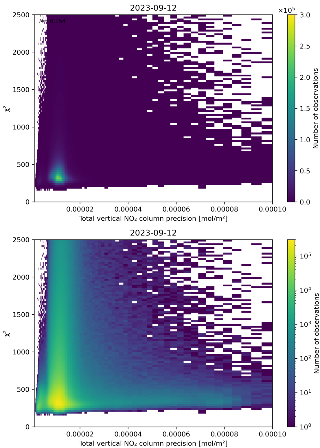
Figure 116: Scatter density plot of “Total vertical NO 2 column precision” against “ \chi^2 ” for 2023-09-11 to 2023-09-13.
