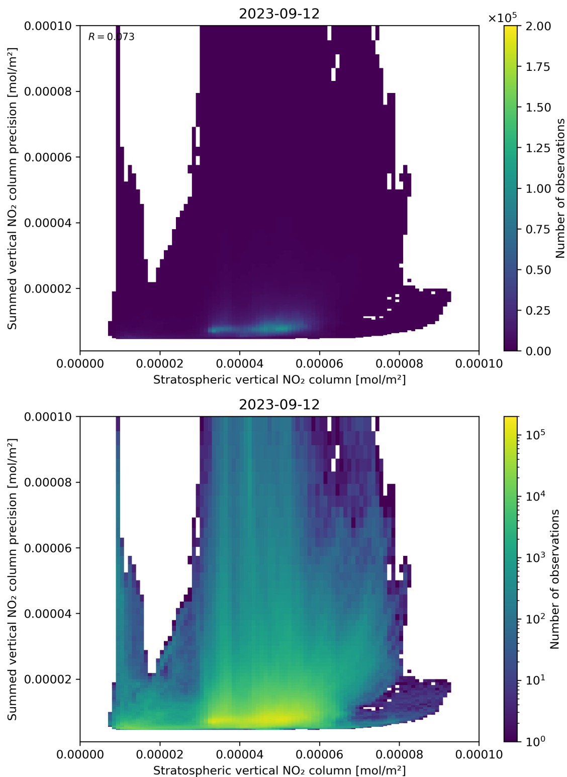
Figure 99: Scatter density plot of “Stratospheric vertical NO 2 column” against “Summed vertical NO 2 column precision” for 2023-09-11 to 2023-09-13.
