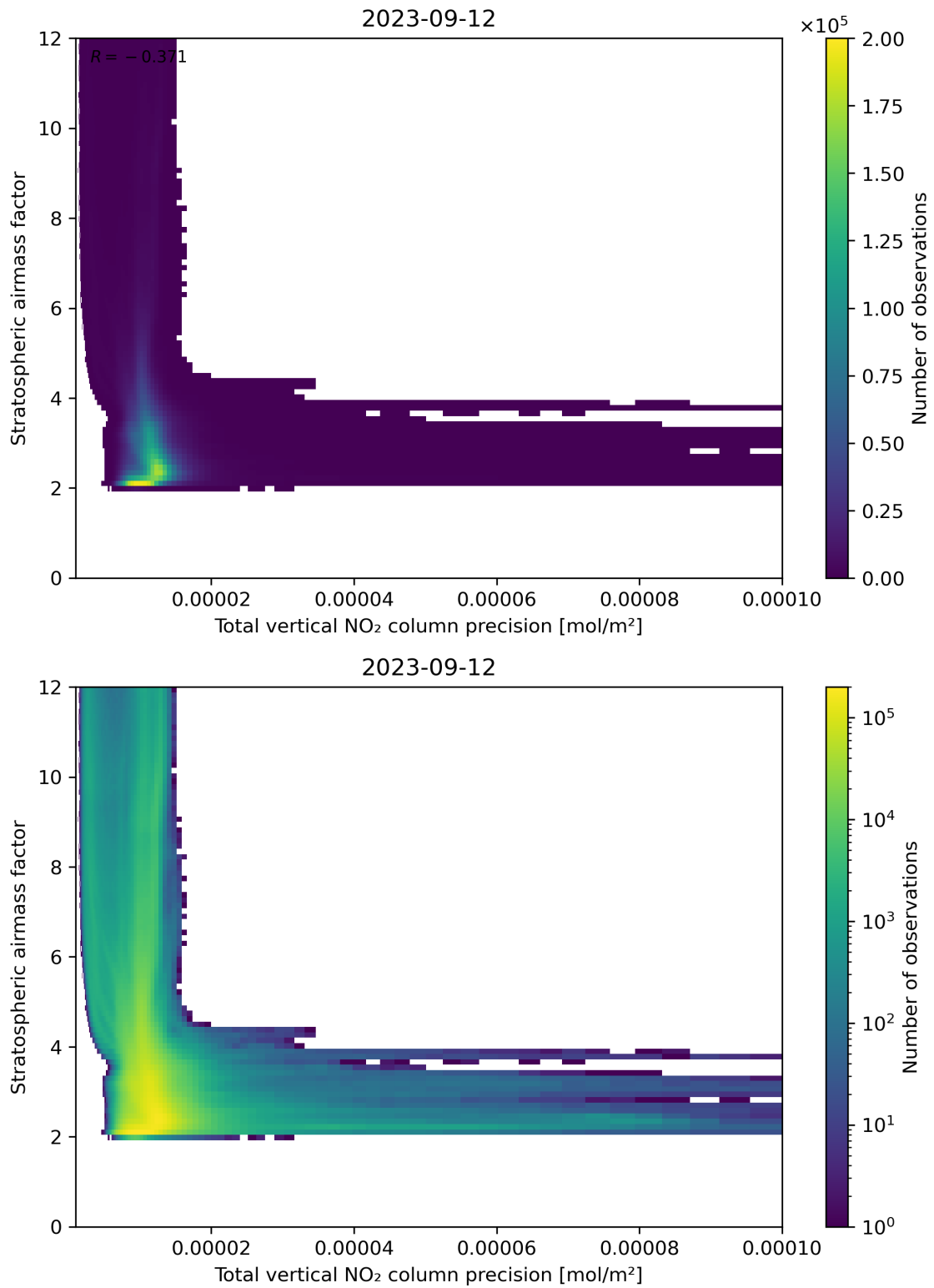
Figure 115: Scatter density plot of “Total vertical NO 2 column precision” against “Stratospheric airmass factor” for 2023-09-11 to 2023-09-13.
