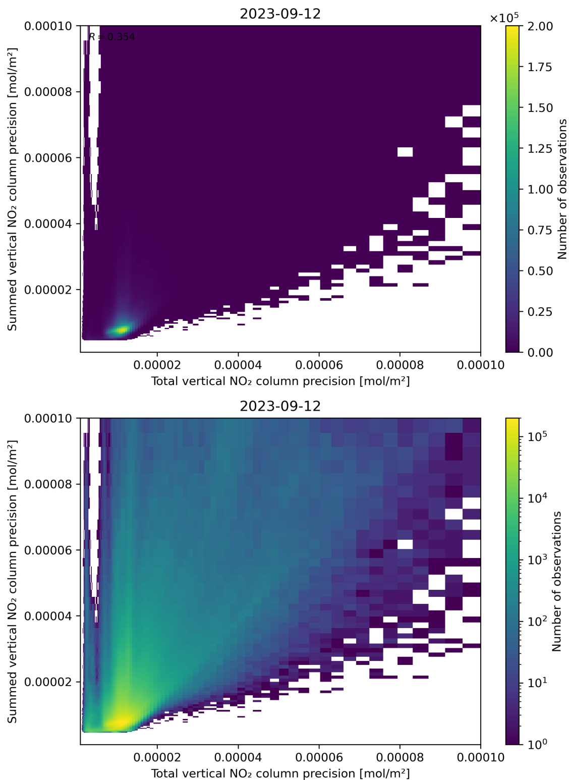
Figure 118: Scatter density plot of “Total vertical NO 2 column precision” against “Summed vertical NO 2 column precision” for 2023-09-11 to 2023-09-13.
