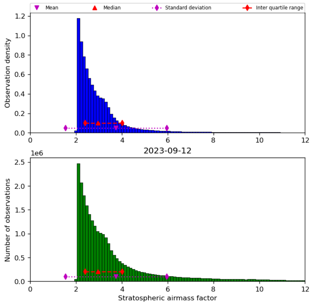
Figure 44: Histogram of “Stratospheric airmass factor” for 2023-09-11 to 2023-09-13
