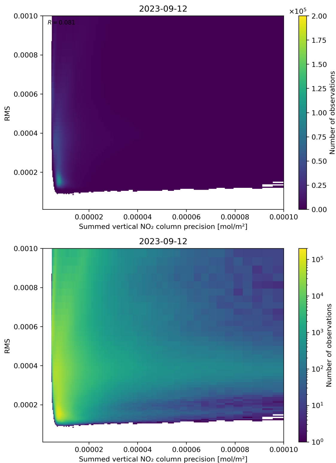
Figure 108: Scatter density plot of “Summed vertical NO 2 column precision” against “RMS” for 2023-09-11 to 2023-09-13.
