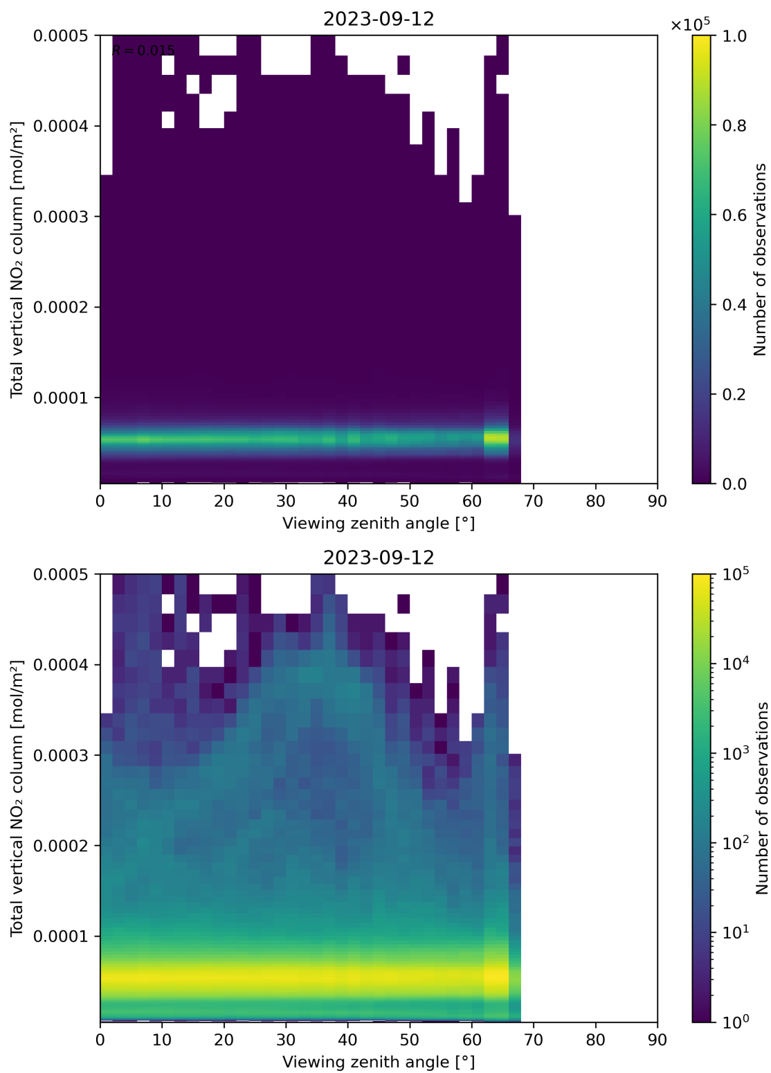
Figure 167: Scatter density plot of “Viewing zenith angle” against “Total vertical NO 2 column” for 2023-09-11 to 2023-09-13.
