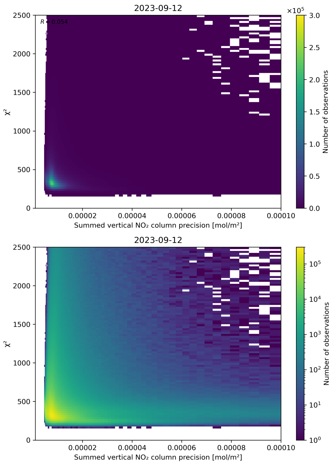
Figure 107: Scatter density plot of “Summed vertical NO 2 column precision” against “ \chi^2 ” for 2023-09-11 to 2023-09-13.
