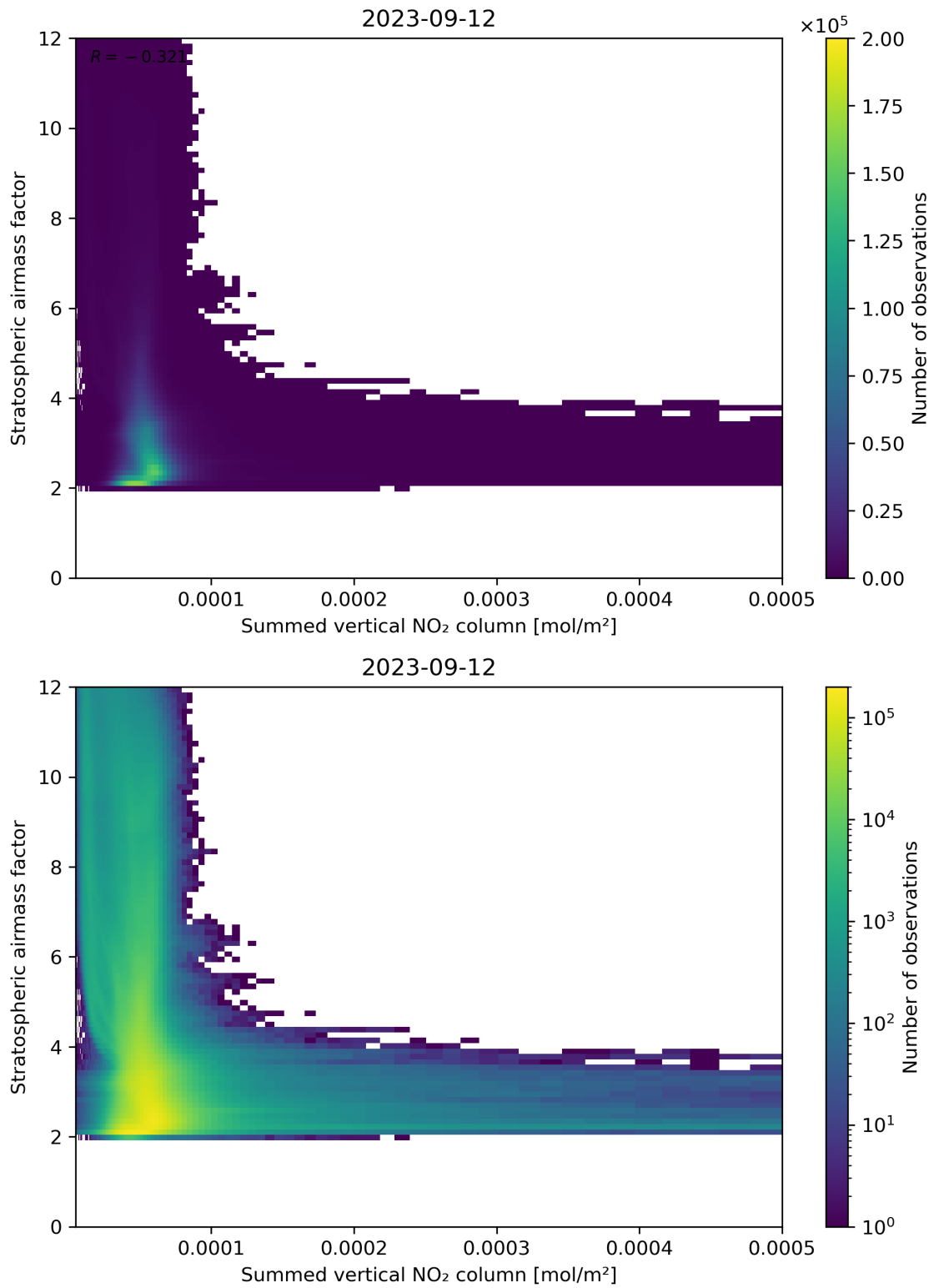
Figure 103: Scatter density plot of “Summed vertical NO 2 column” against “Stratospheric airmass factor” for 2023-09-11 to 2023-09-13.
