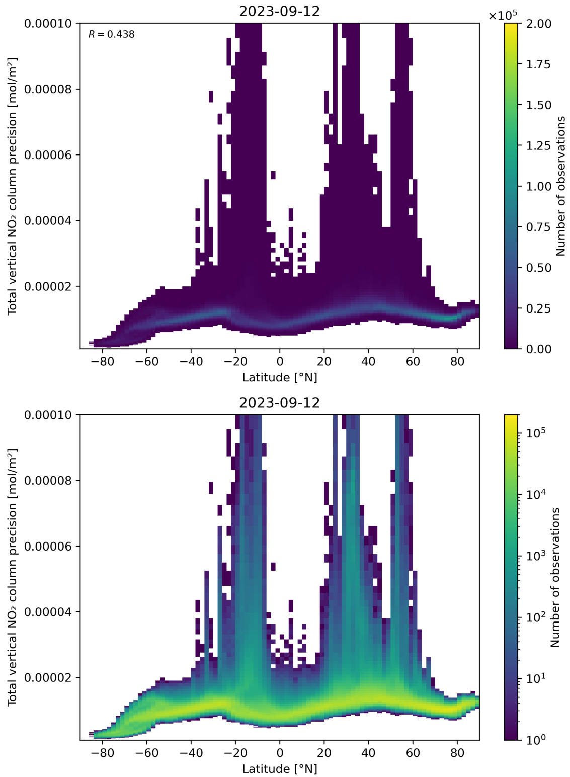
Figure 91: Scatter density plot of “Latitude” against “Total vertical NO 2 column precision” for 2023-09-11 to 2023-09-13.
