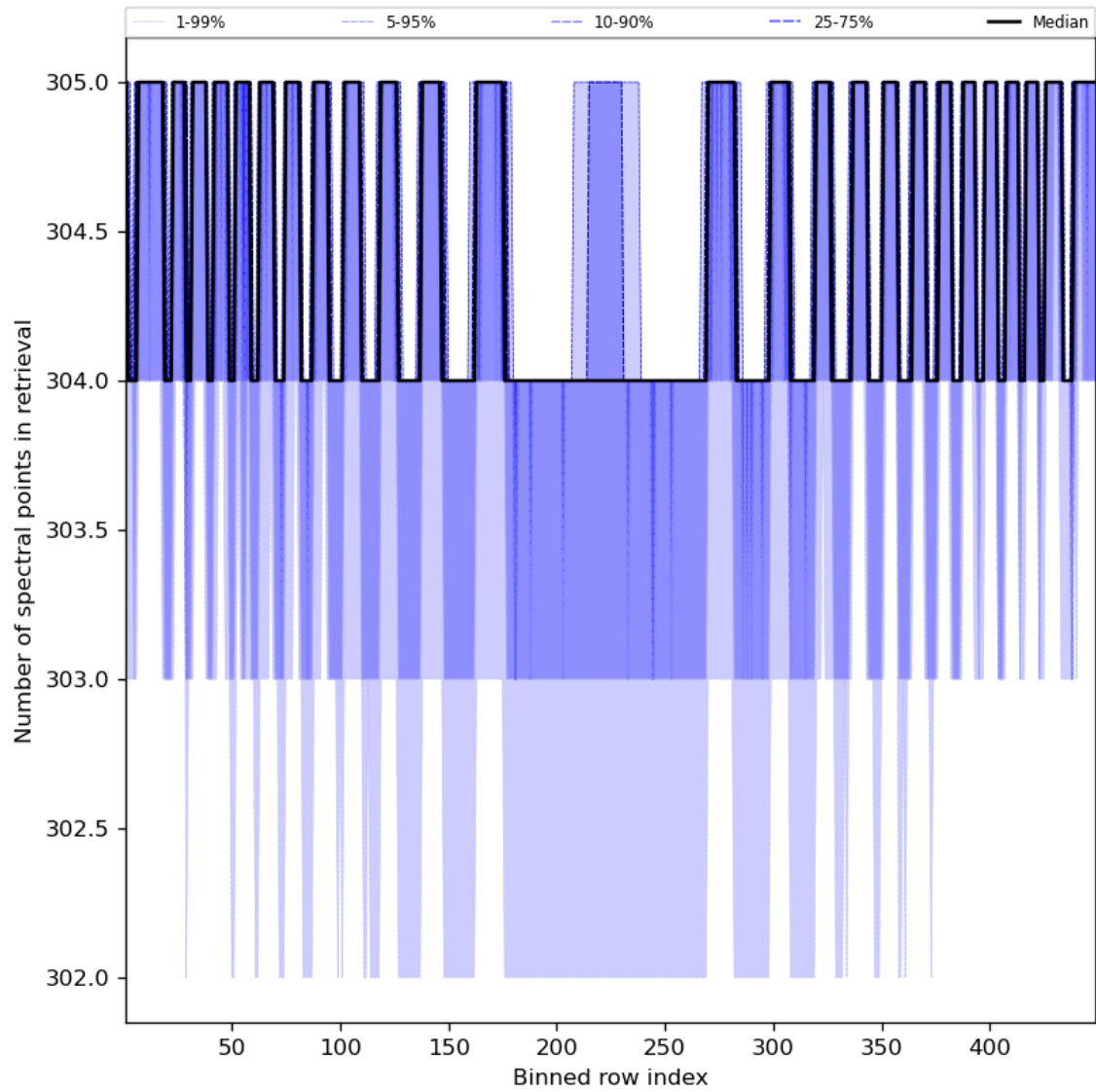
Figure 50: Along track statistics of “Number of spectral points in retrieval” for 2023-09-11 to 2023-09-13
