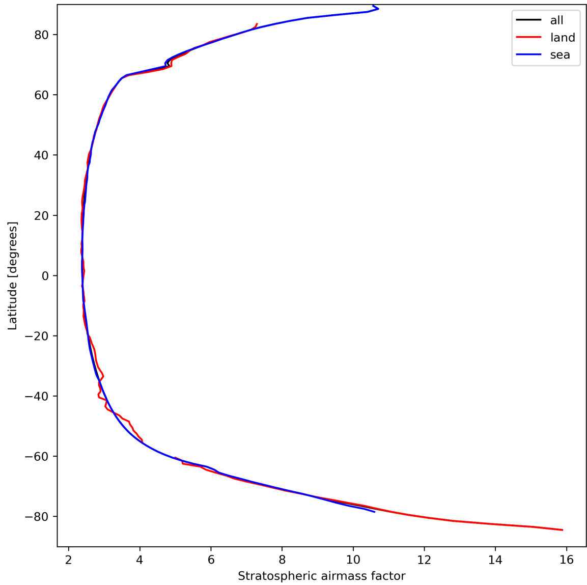
Figure 27: Zonal average of “Stratospheric airmass factor” for 2023-09-11 to 2023-09-13.
