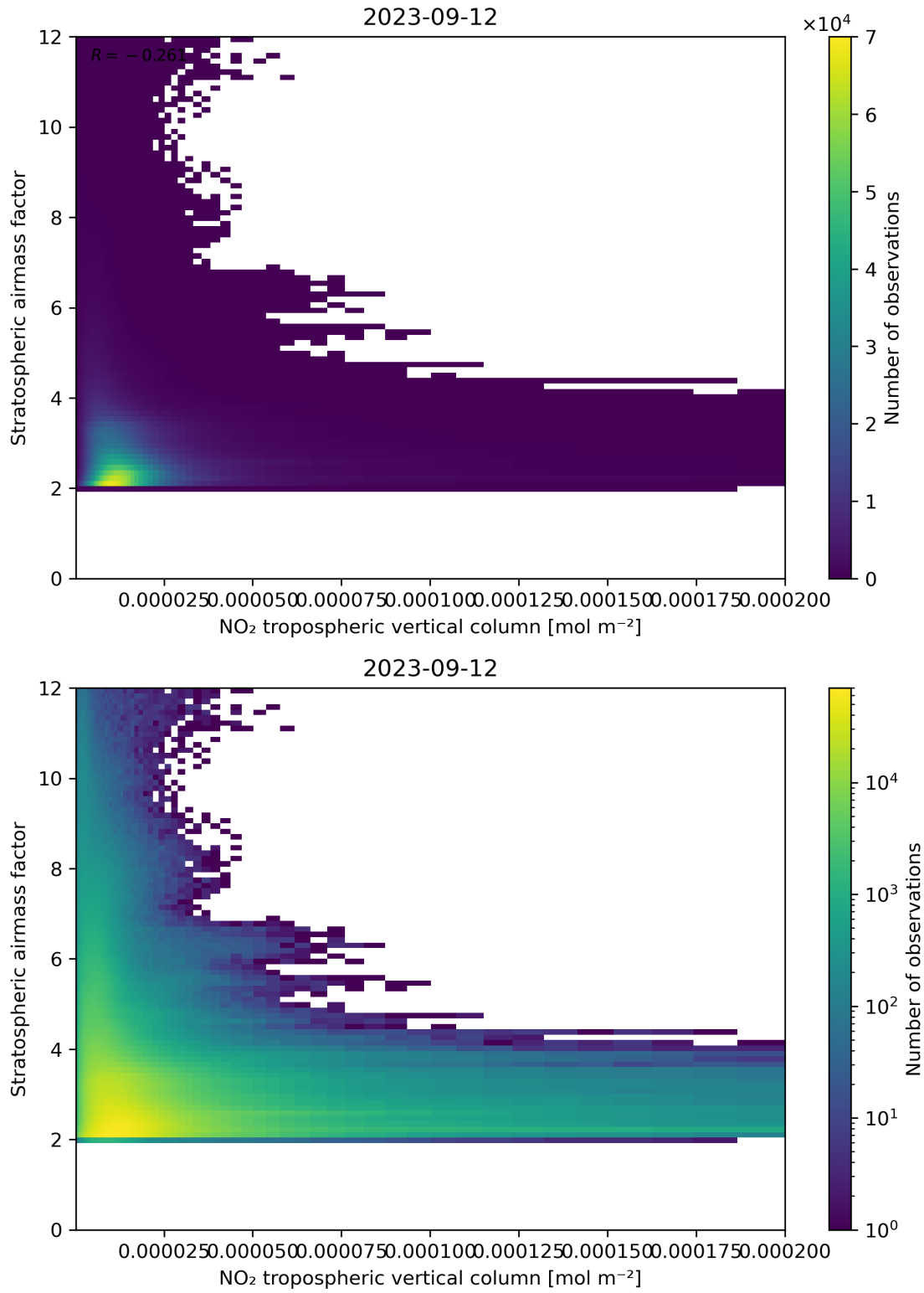
Figure 121: Scatter density plot of “NO 2 tropospheric vertical column” against “Stratospheric air mass factor” for 2023-09-11 to 2023-09-13.
