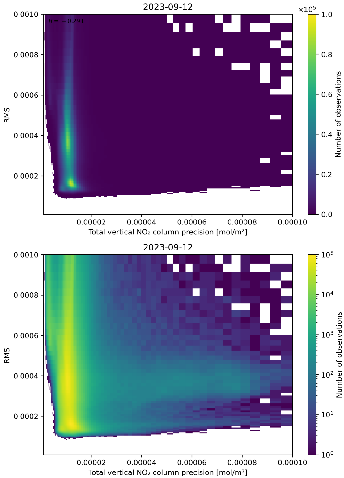
Figure 119: Scatter density plot of “Total vertical NO 2 column precision” against “RMS” for 2023-09-11 to 2023-09-13.
