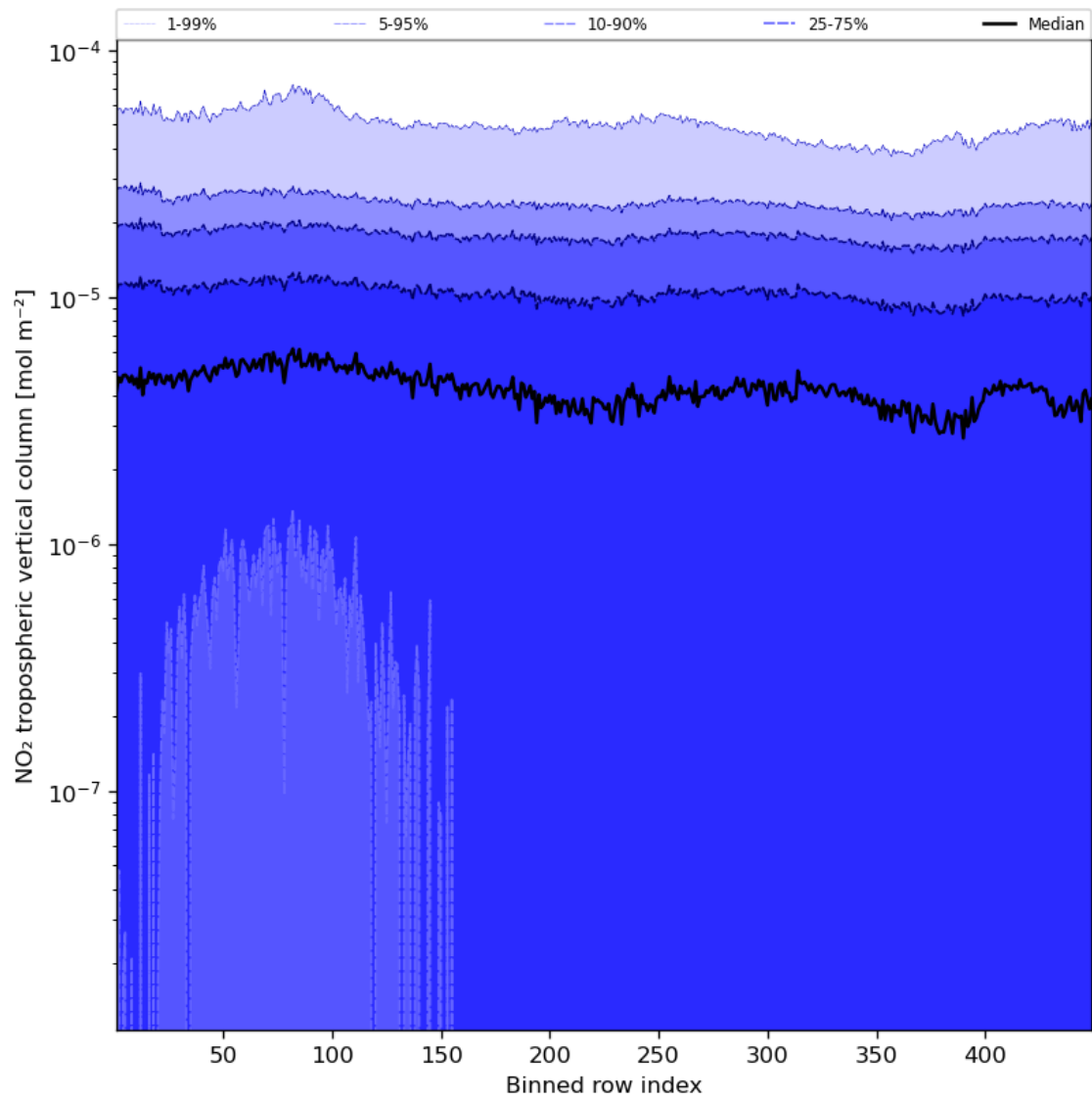
Figure 46: Along track statistics of “NO 2 tropospheric vertical column” for 2023-09-11 to 2023-09-13
