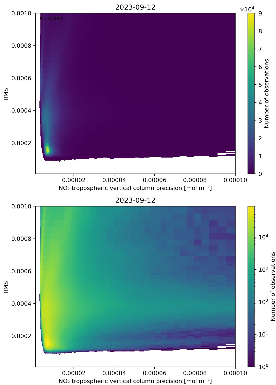
Figure 140: Scatter density plot of “NO 2 tropospheric vertical column precision” against “RMS” for 2023-09-11 to 2023-09-13.
