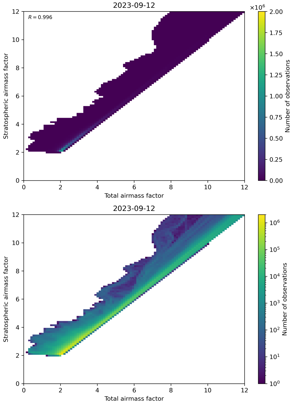
Figure 62: Scatter density plot of “Total airmass factor” against “Stratospheric airmass factor” for 2023-09-11 to 2023-09-13.
