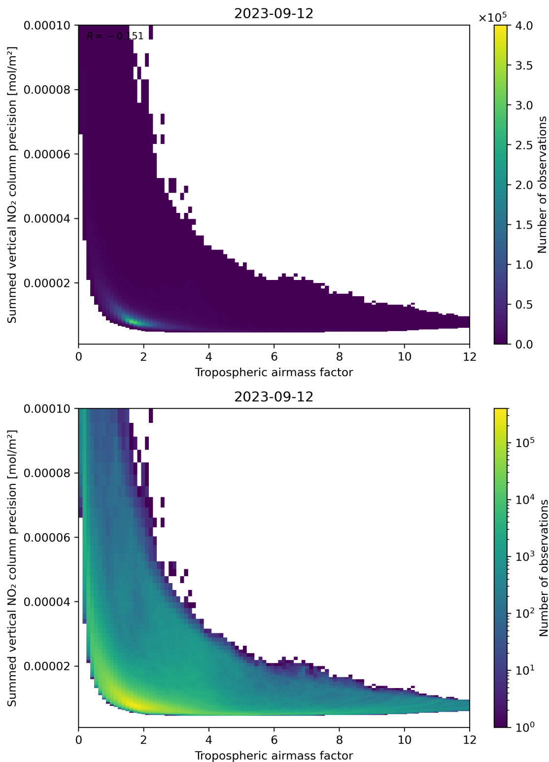
Figure 76: Scatter density plot of “Tropospheric air mass factor” against “Summed vertical NO 2 column precision” for 2023-09-11 to 2023-09-13.
