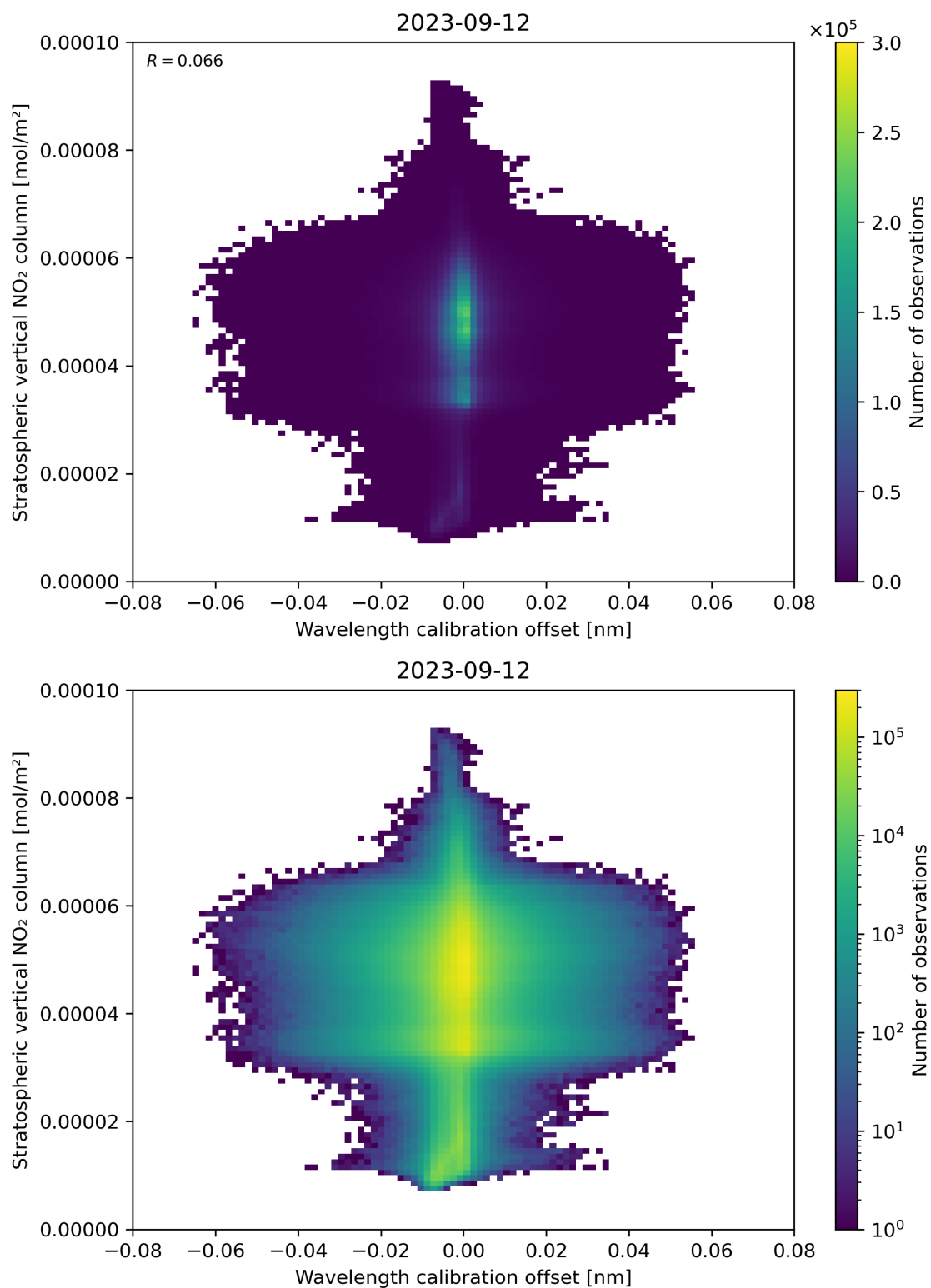
Figure 176: Scatter density plot of “Wavelength calibration offset” against “Stratospheric vertical NO 2 column” for 2023-09-11 to 2023-09-13.
