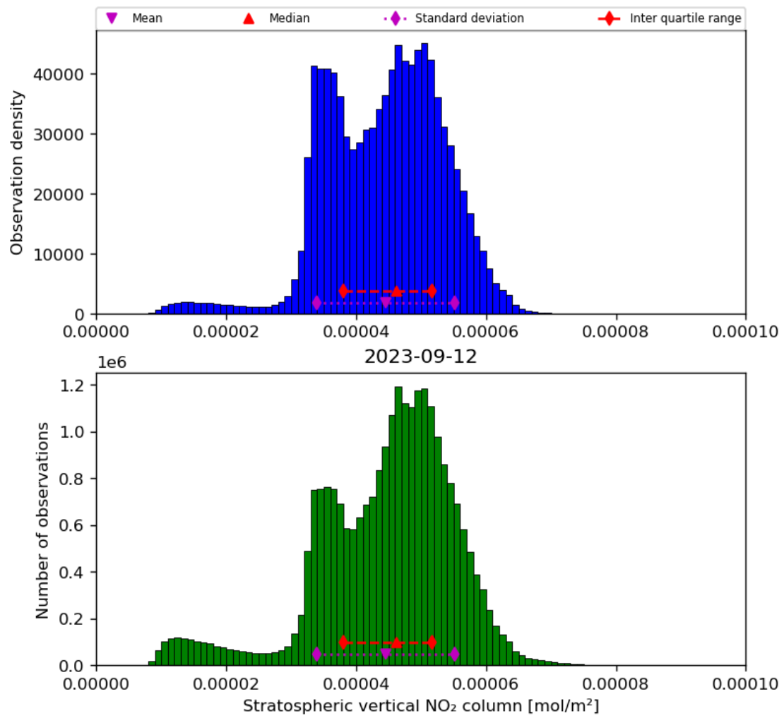
Figure 36: Histogram of “Stratospheric vertical NO 2 column” for 2023-09-11 to 2023-09-13
