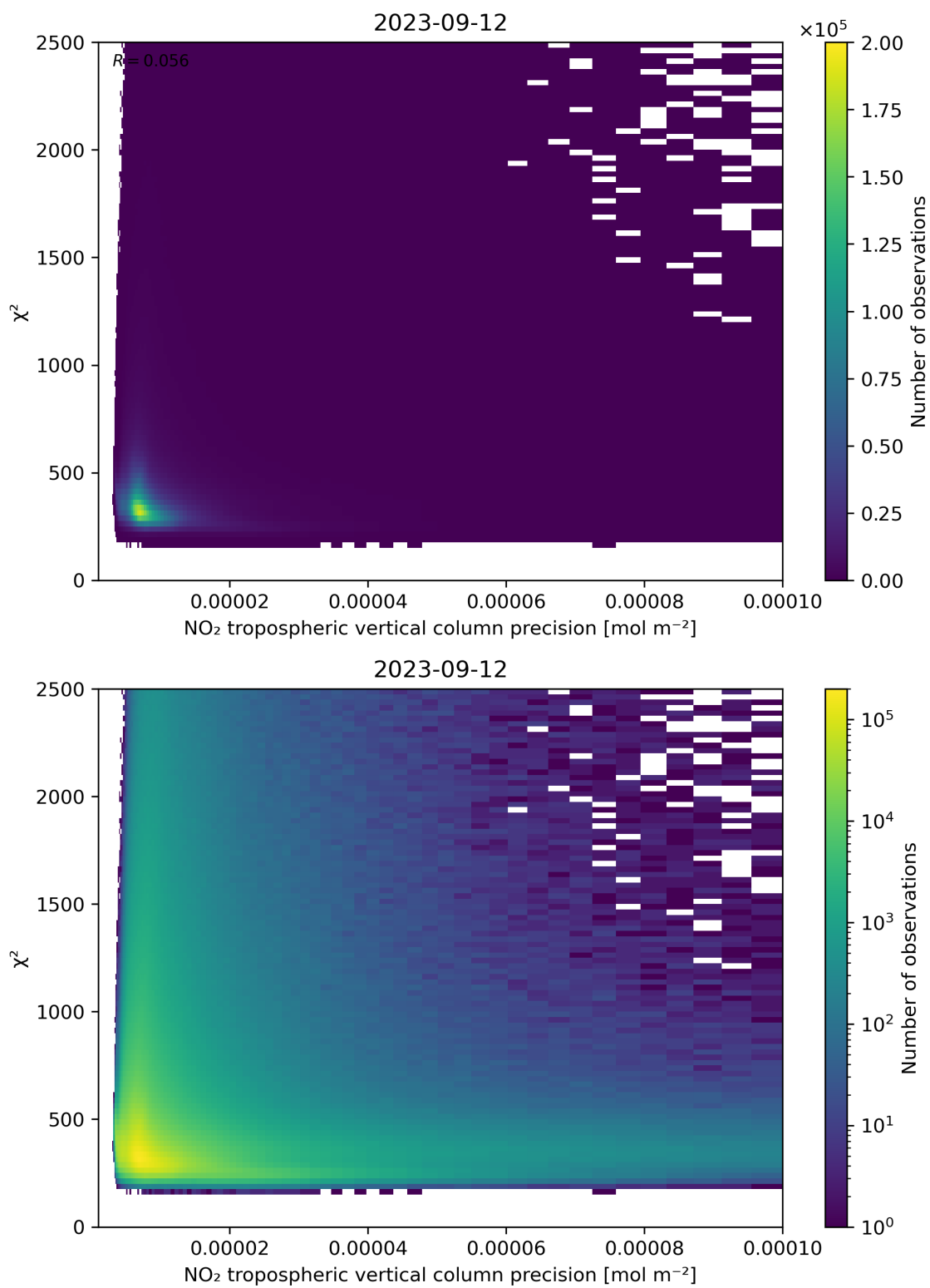
Figure 134: Scatter density plot of “NO 2 tropospheric vertical column precision” against “ \chi^2 ” for 2023-09-11 to 2023-09-13.
