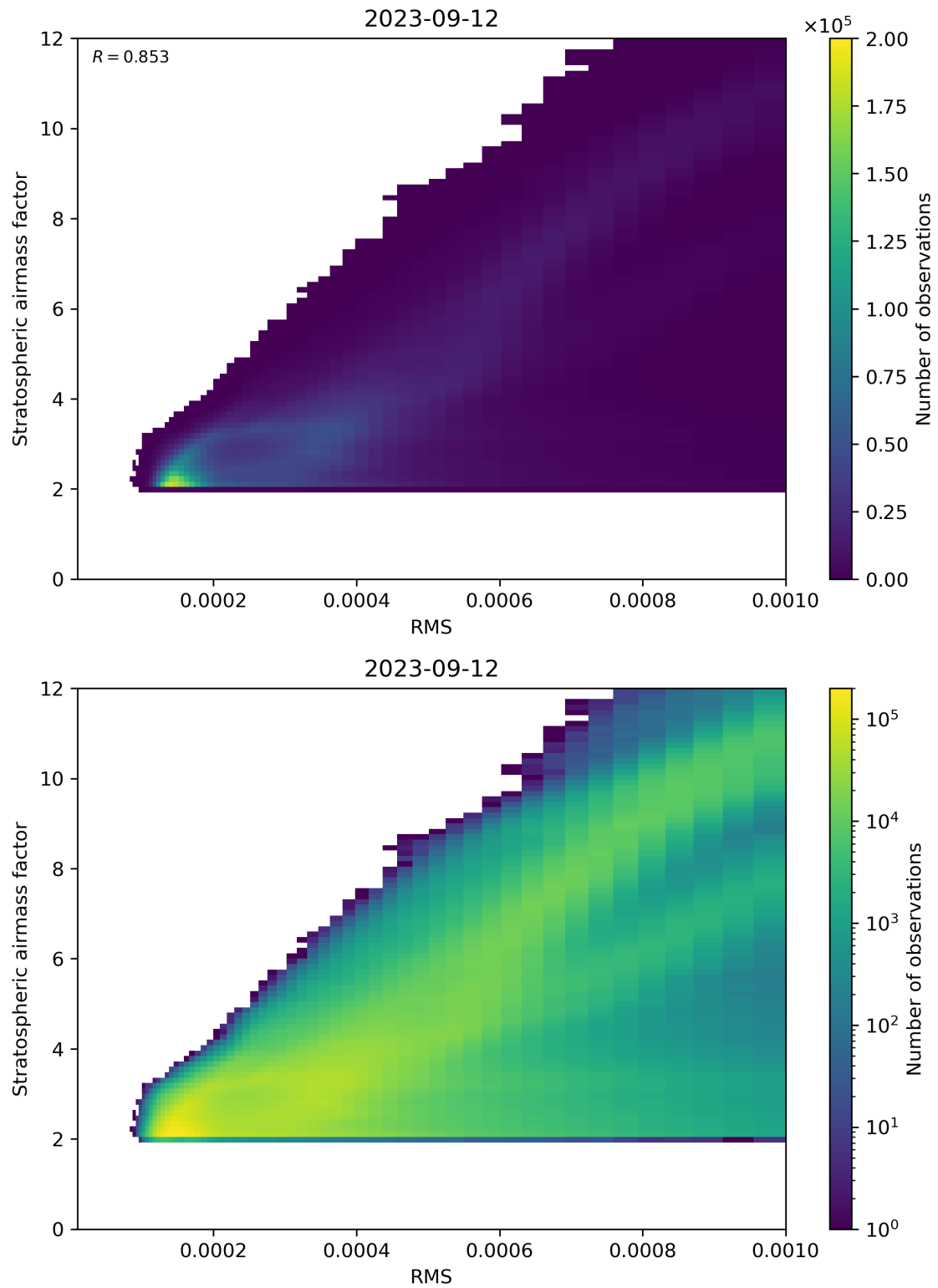
Figure 144: Scatter density plot of “RMS” against “Stratospheric airmass factor” for 2023-09-11 to 2023-09-13.
