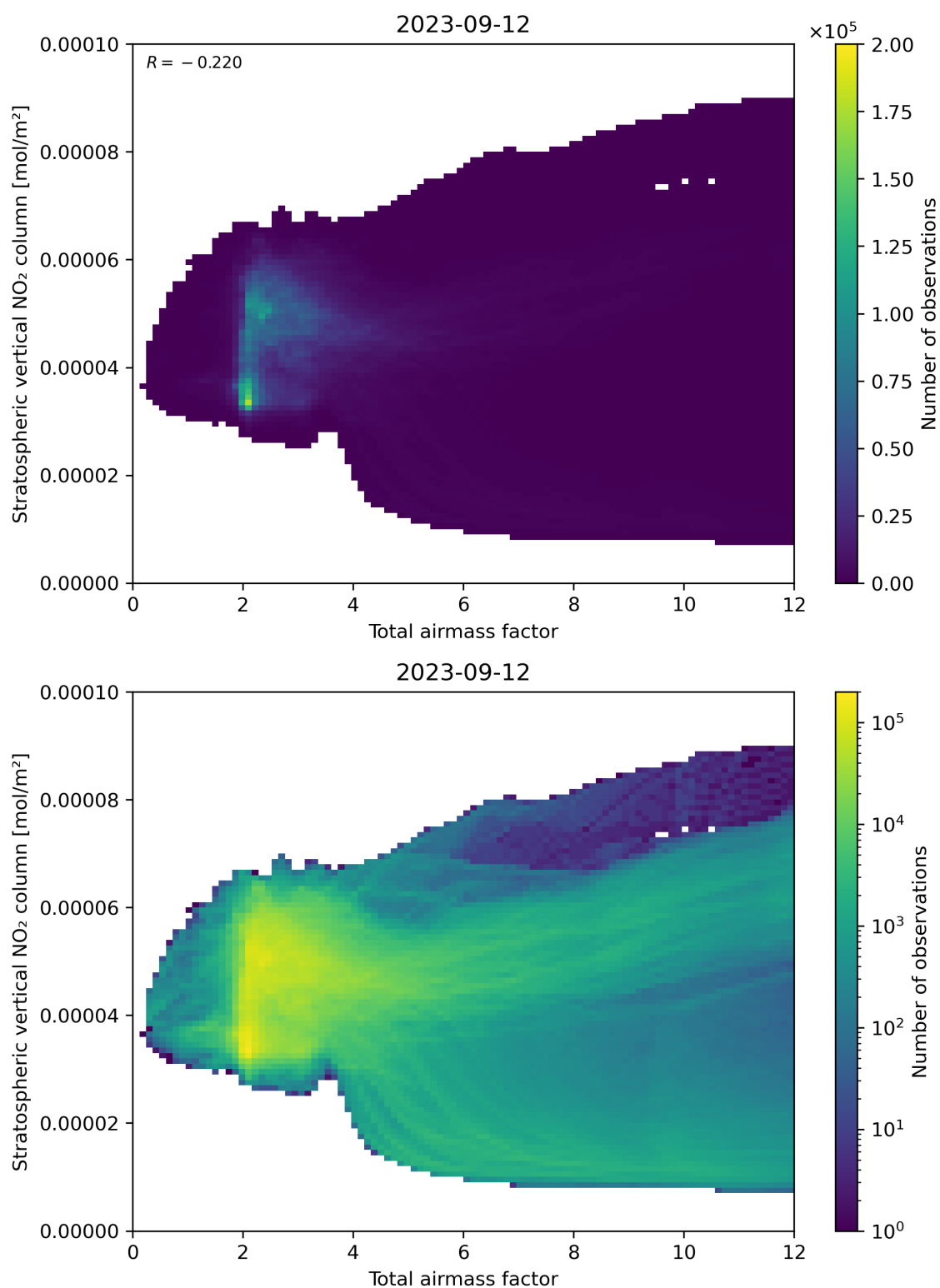
Figure 64: Scatter density plot of “Total airmass factor” against “Stratospheric vertical NO 2 column” for 2023-09-11 to 2023-09-13.
