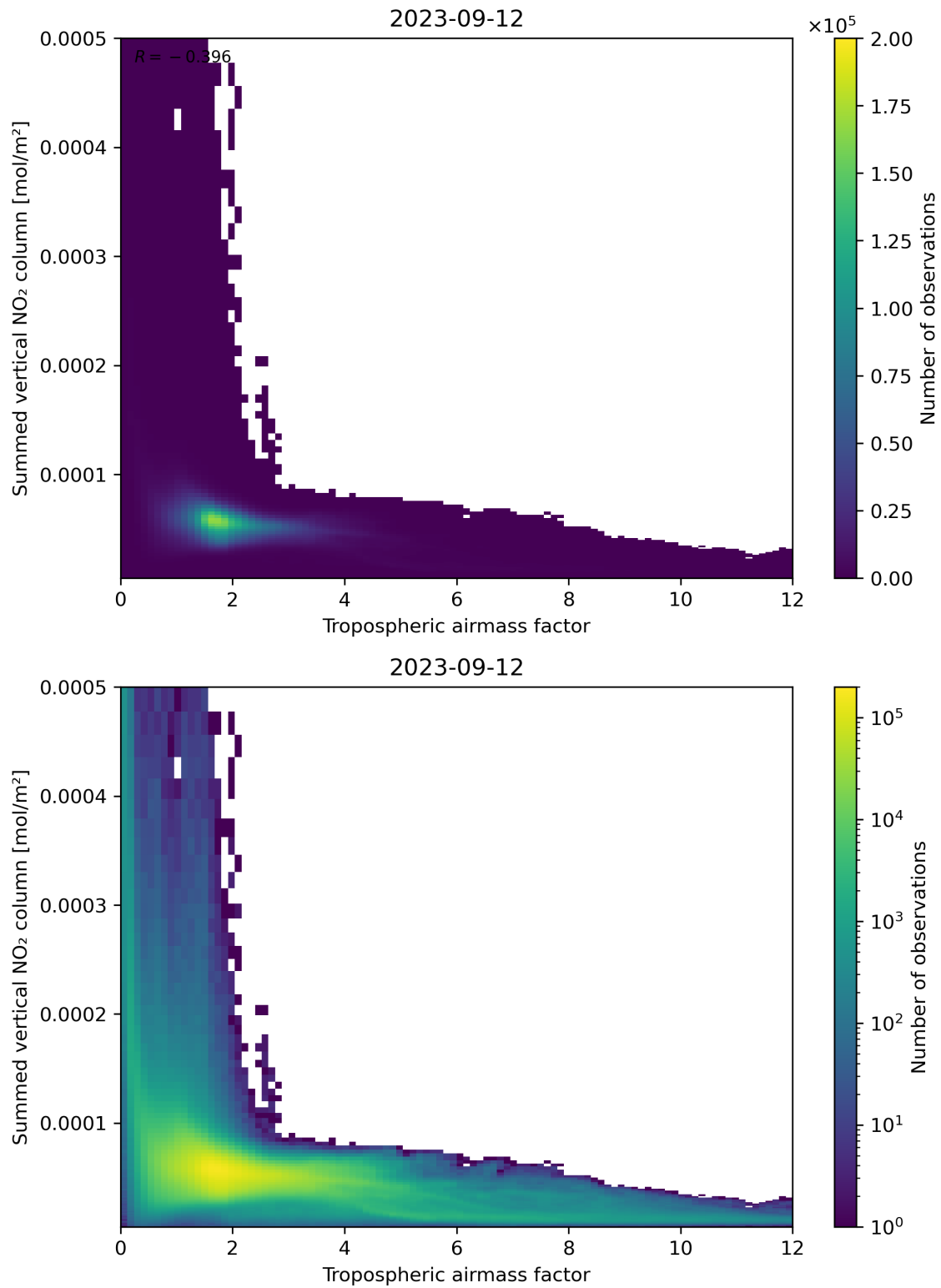
Figure 75: Scatter density plot of “Tropospheric airmass factor” against “Summed vertical NO 2 column” for 2023-09-11 to 2023-09-13.
