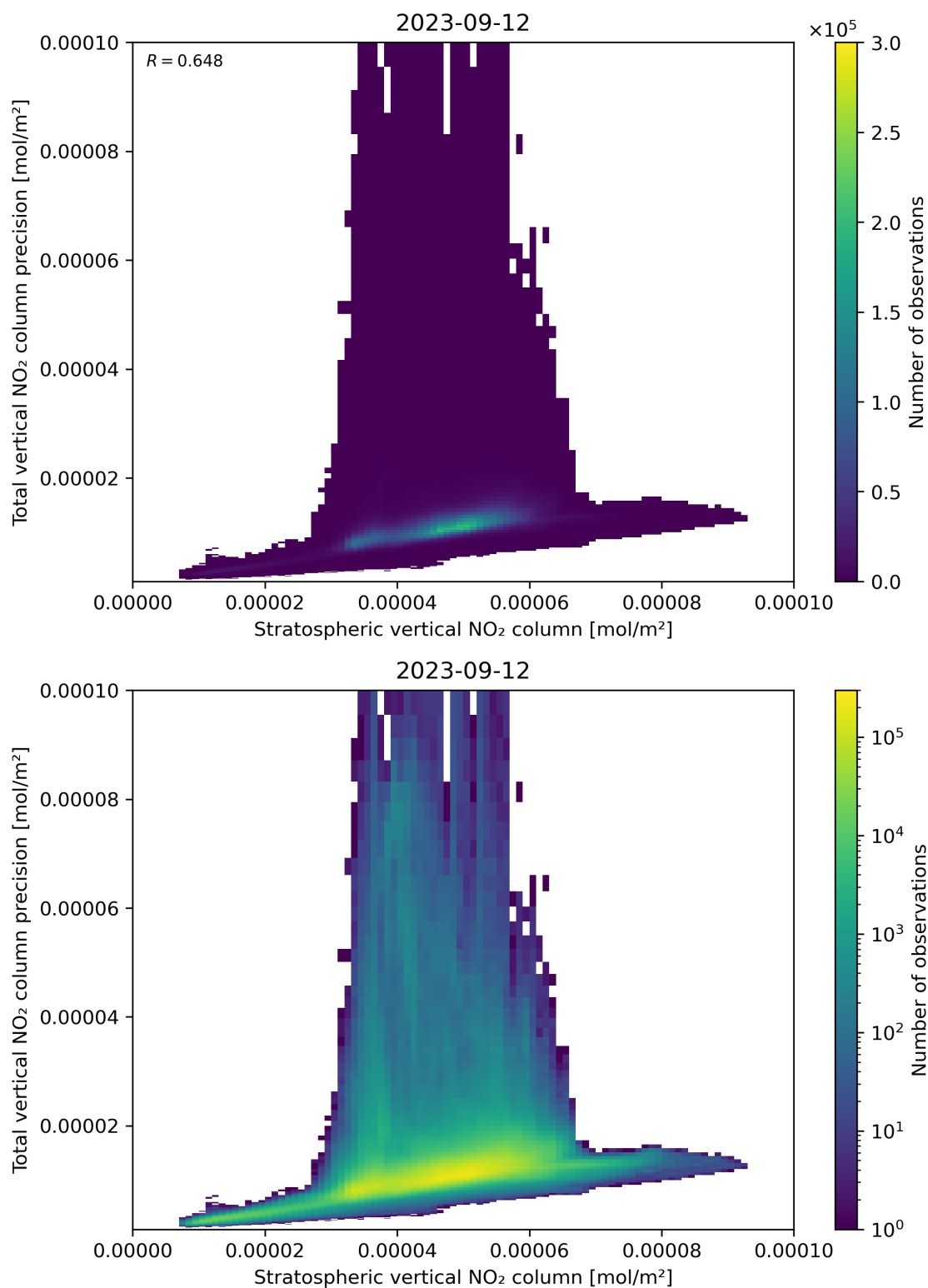
Figure 101: Scatter density plot of “Stratospheric vertical NO 2 column” against “Total vertical NO 2 column precision” for 2023-09-11 to 2023-09-13.
