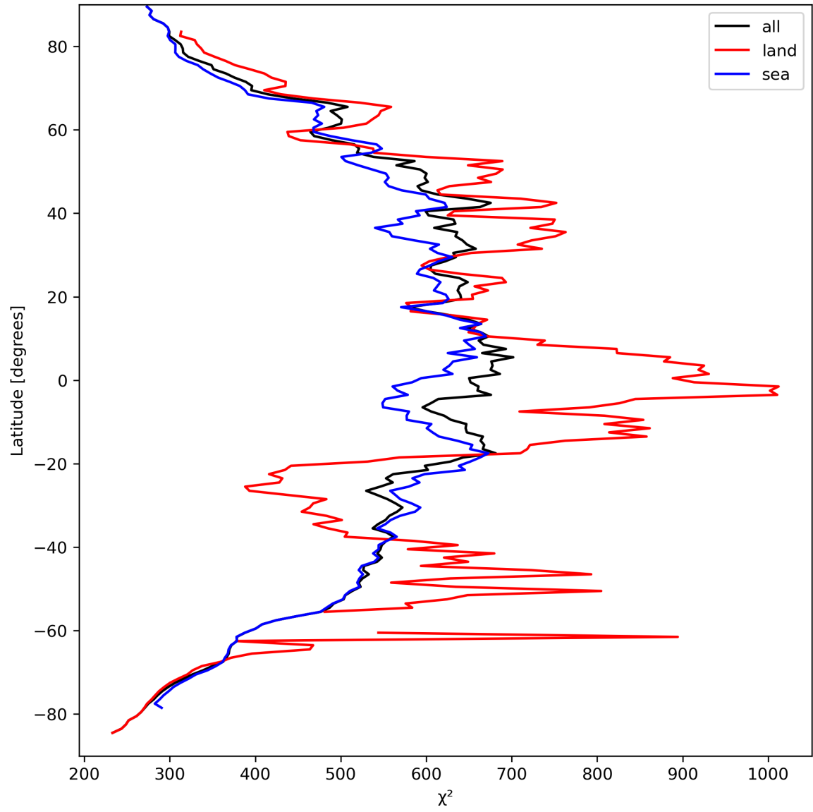
Figure 25: Zonal average of “ \chi^2 ” for 2023-09-11 to 2023-09-13.
