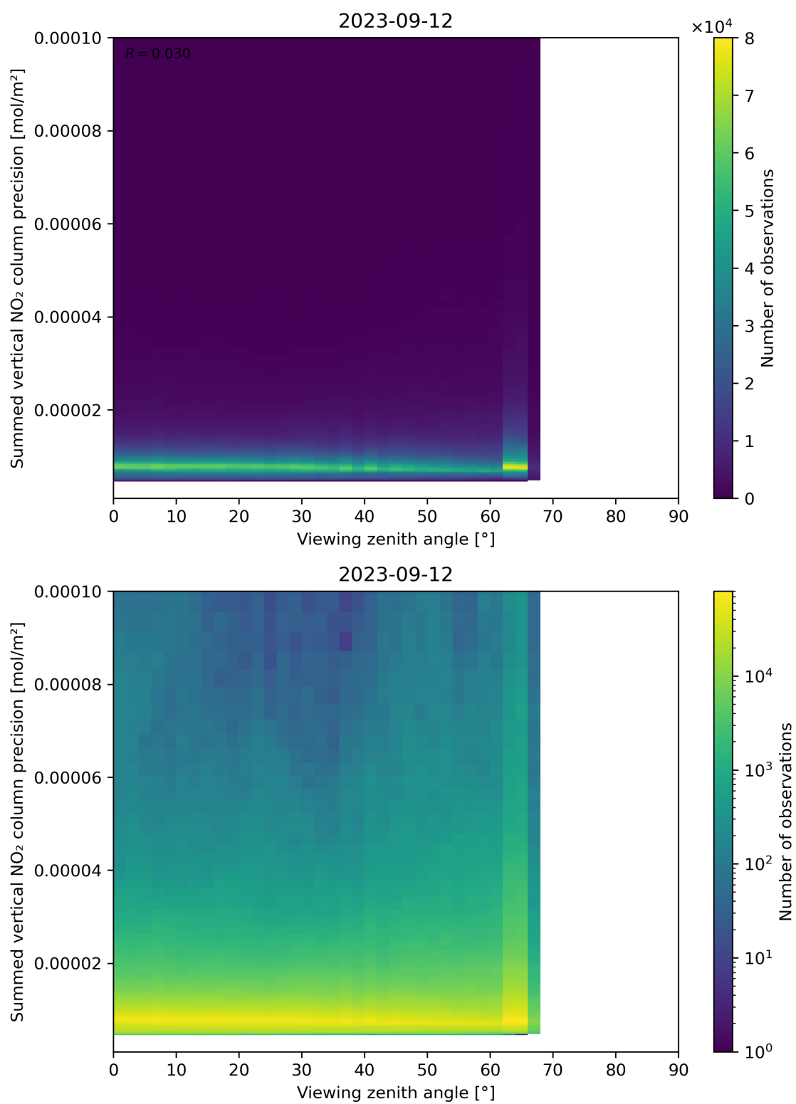
Figure 166: Scatter density plot of “Viewing zenith angle” against “Summed vertical NO 2 column precision” for 2023-09-11 to 2023-09-13.
