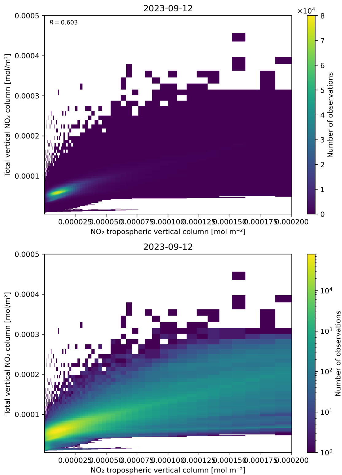
Figure 128: Scatter density plot of “NO 2 tropospheric vertical column” against “Total vertical NO 2 column” for 2023-09-11 to 2023-09-13.
