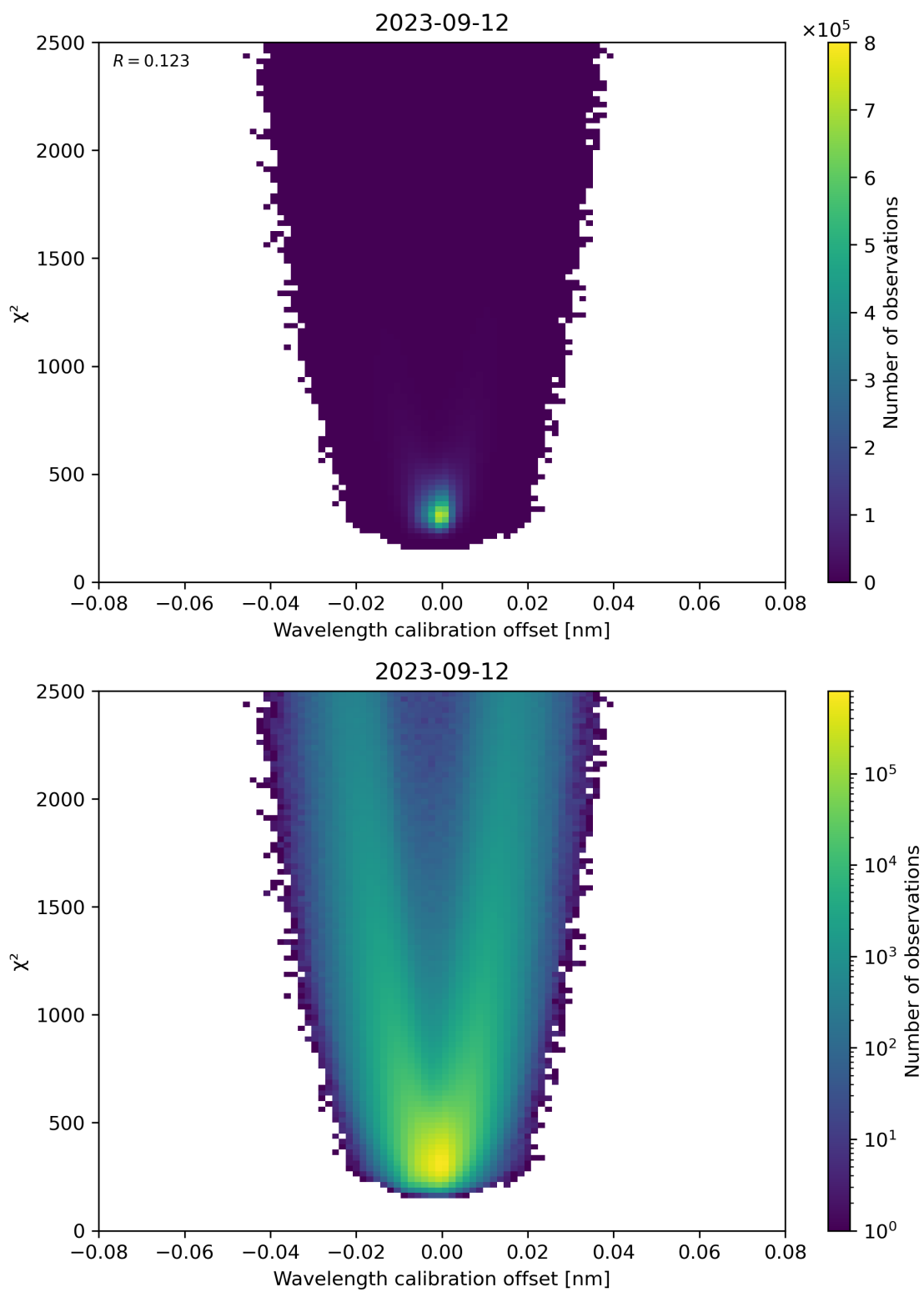
Figure 175: Scatter density plot of “Wavelength calibration offset” against “ \chi^2 ” for 2023-09-11 to 2023-09-13.
