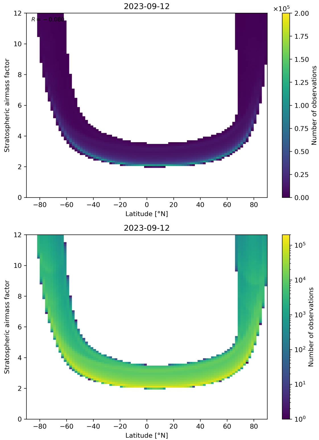
Figure 83: Scatter density plot of “Latitude” against “Stratospheric air mass factor” for 2023-09-11 to 2023-09-13.
