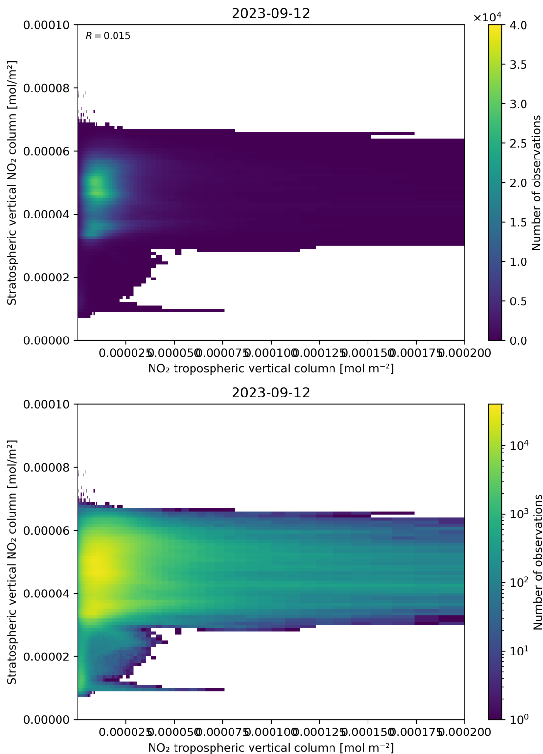
Figure 125: Scatter density plot of “NO 2 tropospheric vertical column” against “Stratospheric vertical NO 2 column” for 2023-09-11 to 2023-09-13.
