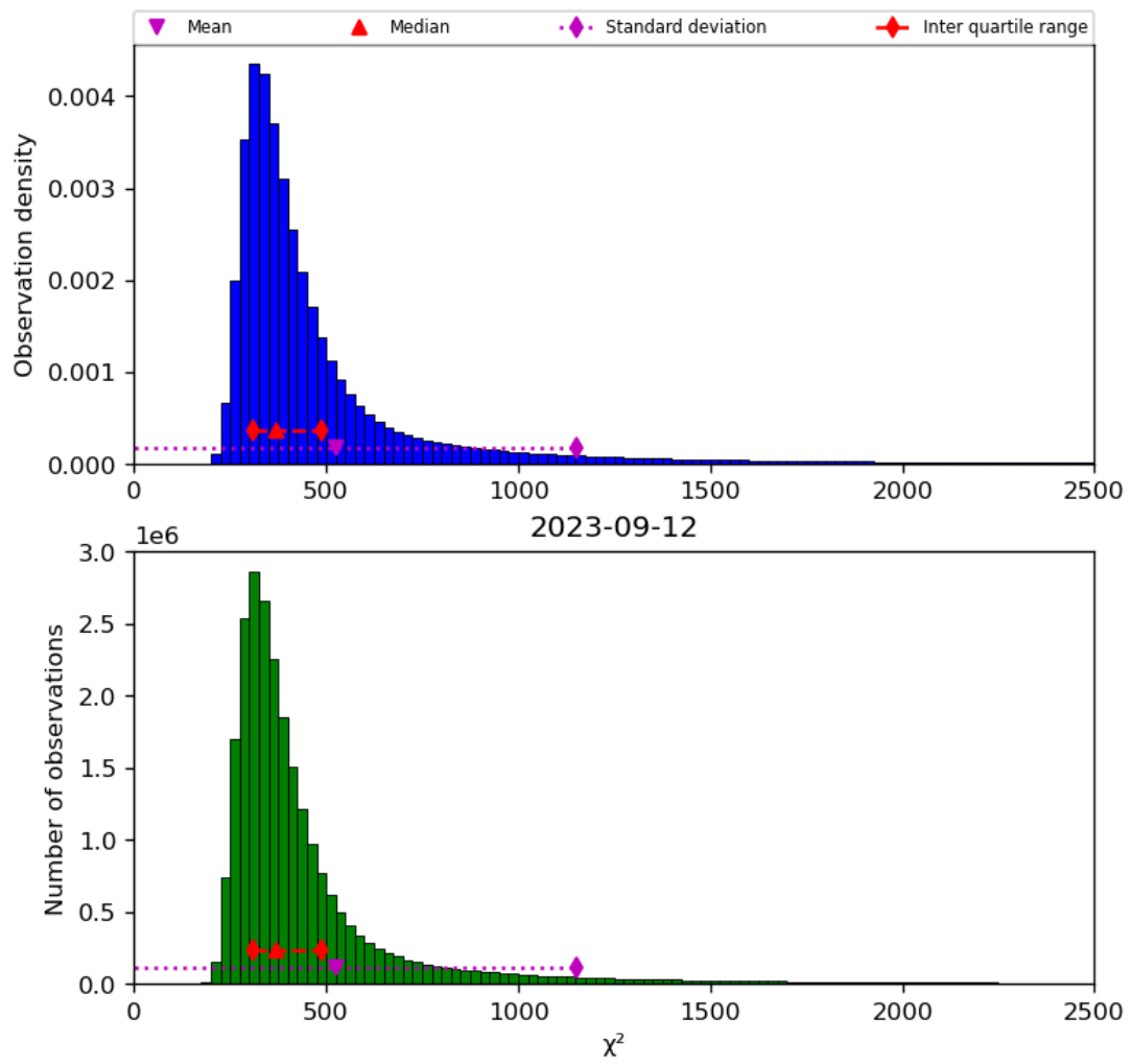
Figure 42: Histogram of “ \chi^2 ” for 2023-09-11 to 2023-09-13
