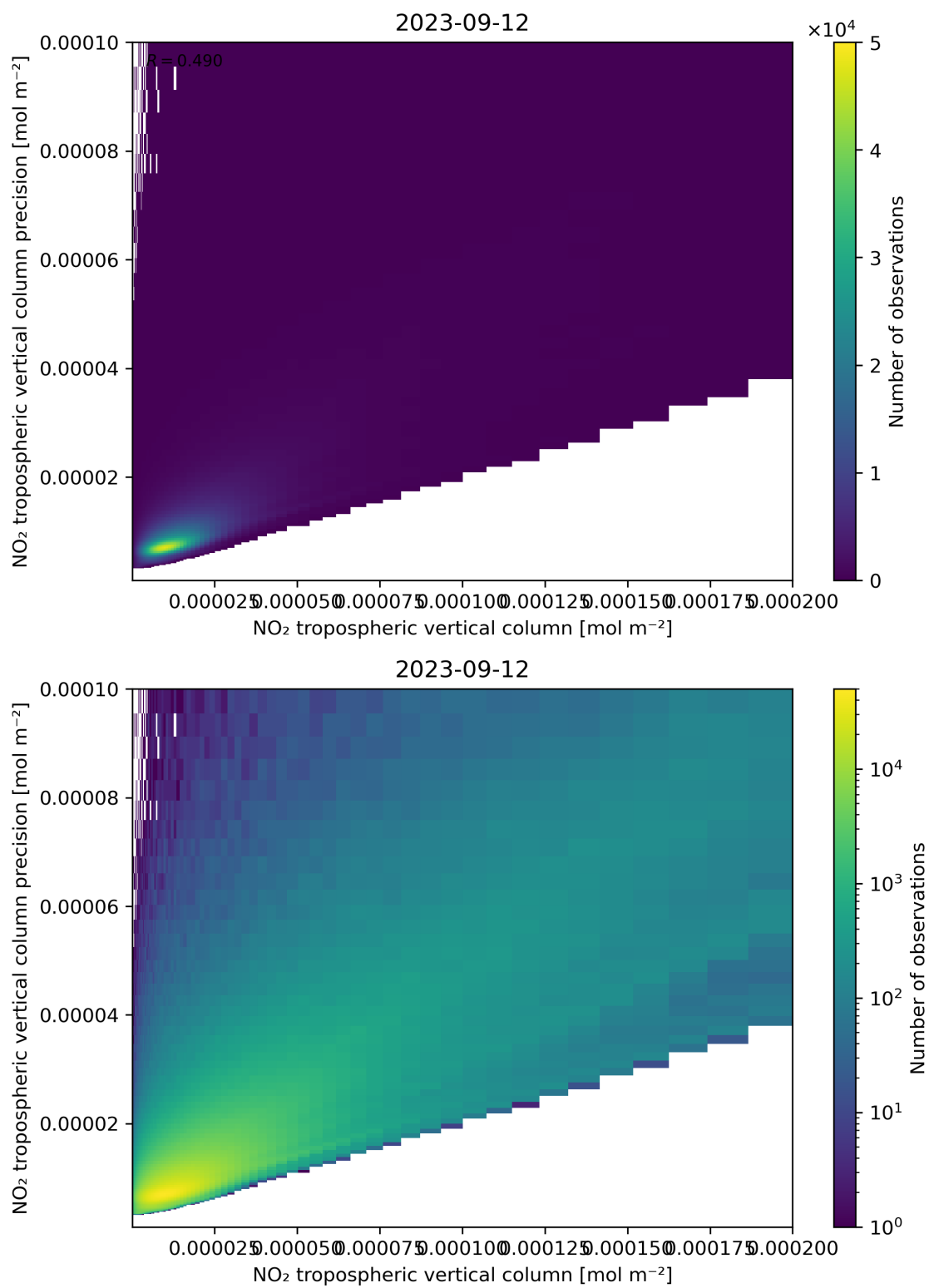
Figure 130: Scatter density plot of “NO 2 tropospheric vertical column” against “NO 2 tropospheric vertical column precision” for 2023-09-11 to 2023-09-13.
