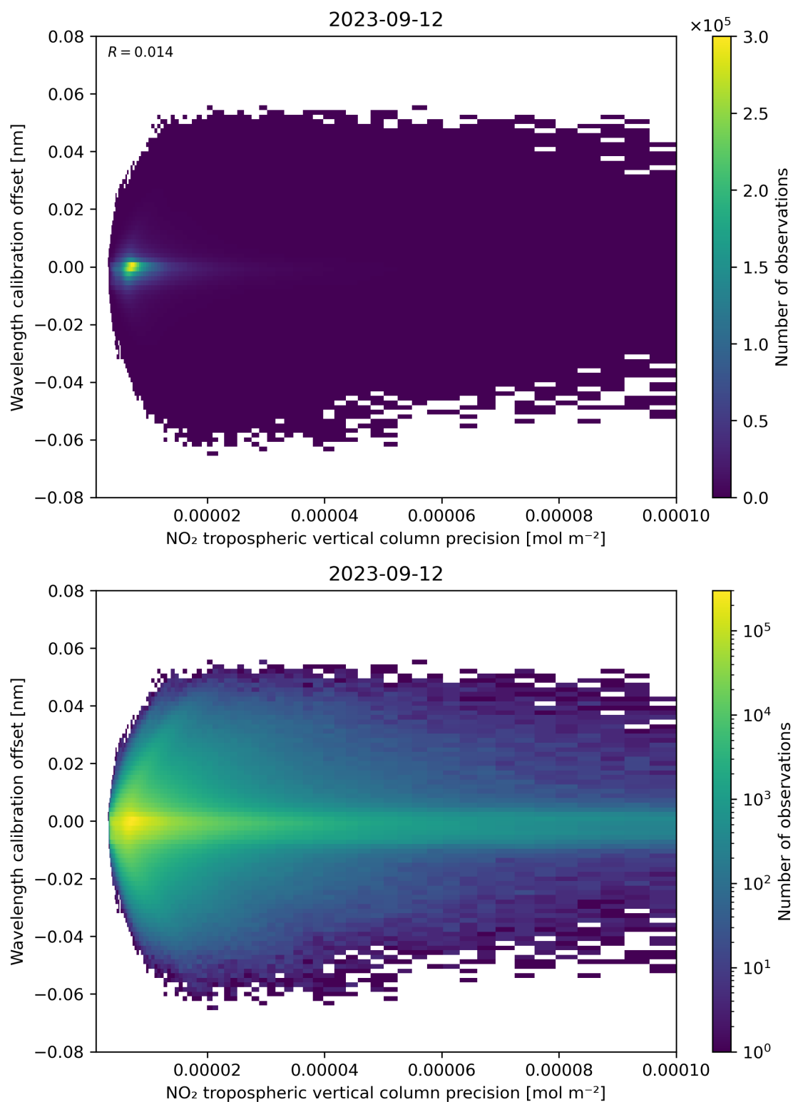
Figure 141: Scatter density plot of “NO 2 tropospheric vertical column precision” against “Wavelength calibration offset” for 2023-09-11 to 2023-09-13.
