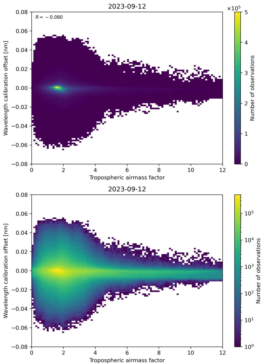
Figure 80: Scatter density plot of “Tropospheric airmass factor” against “Wavelength calibration offset” for 2023-09-11 to 2023-09-13.
