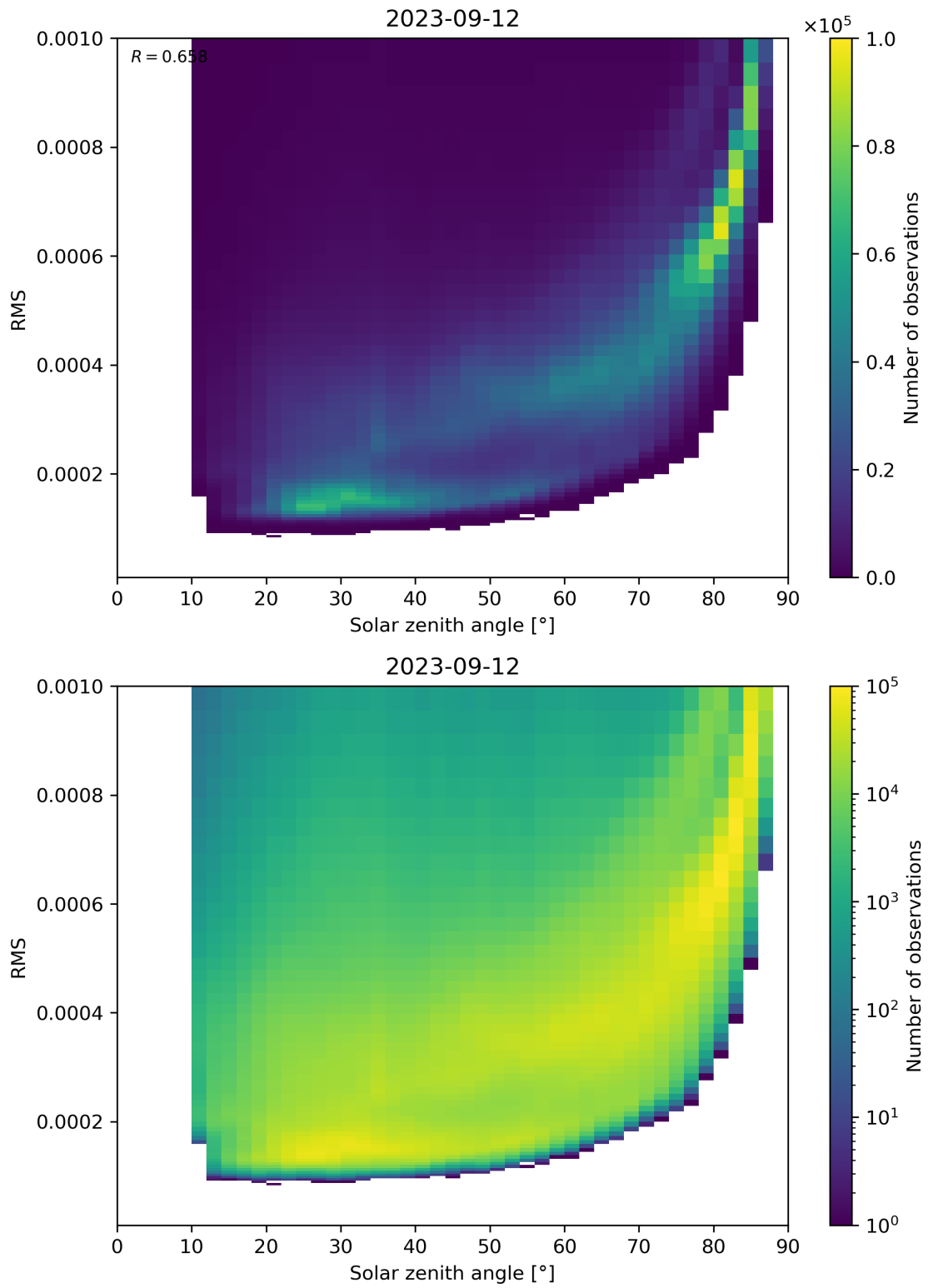
Figure 157: Scatter density plot of “Solar zenith angle” against “RMS” for 2023-09-11 to 2023-09-13.
