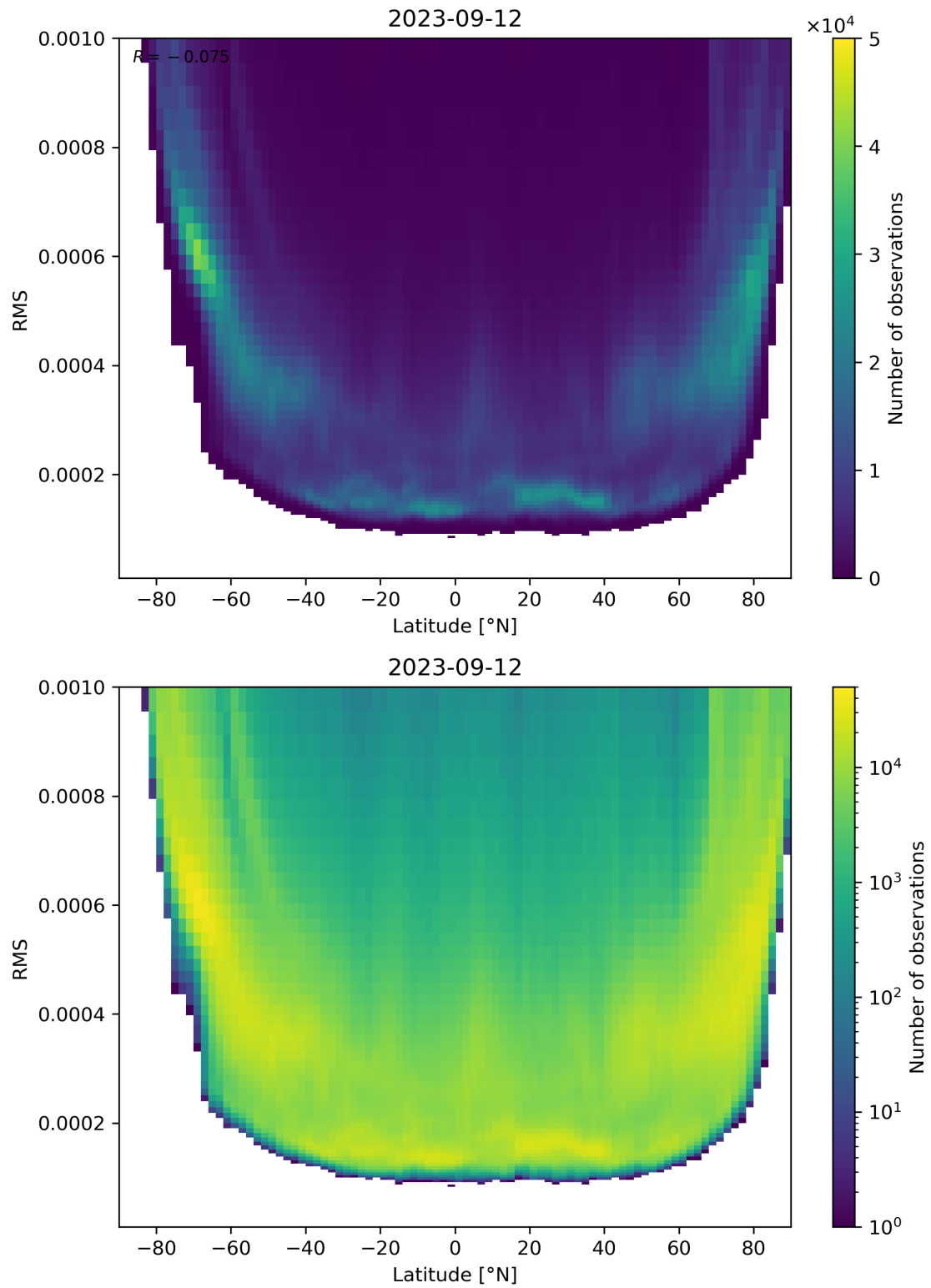
Figure 94: Scatter density plot of “Latitude” against “RMS” for 2023-09-11 to 2023-09-13.
