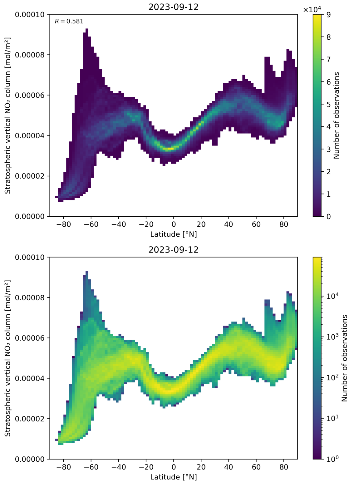
Figure 87: Scatter density plot of “Latitude” against “Stratospheric vertical NO 2 column” for 2023-09-11 to 2023-09-13.
