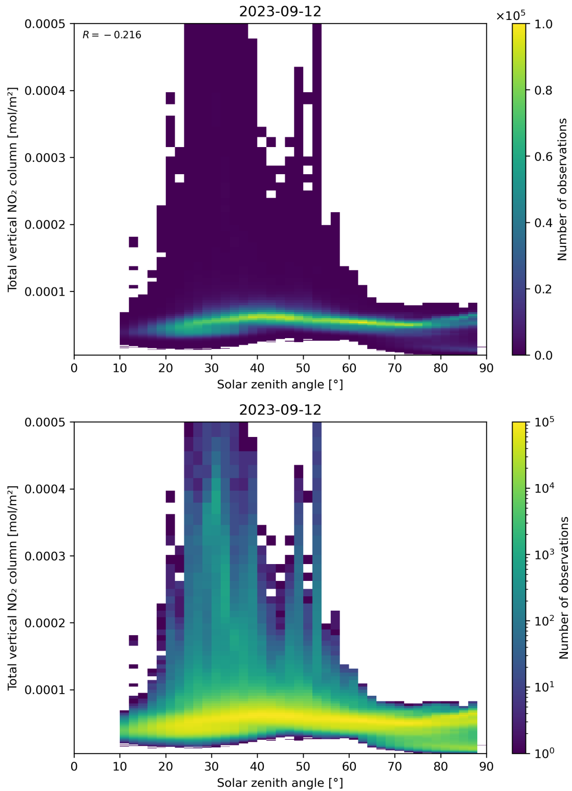
Figure 153: Scatter density plot of “Solar zenith angle” against “Total vertical NO 2 column” for 2023-09-11 to 2023-09-13.
