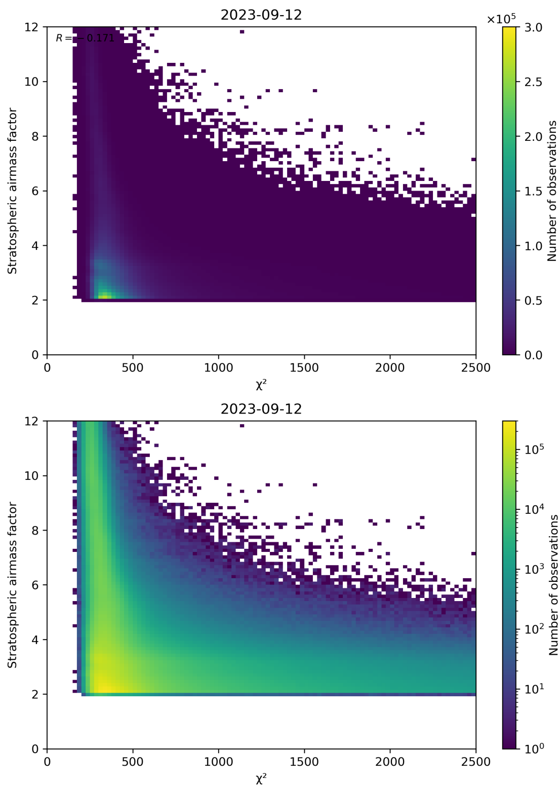
Figure 81: Scatter density plot of “ \chi^2 ” against “Stratospheric airmass factor” for 2023-09-11 to 2023-09-13.
