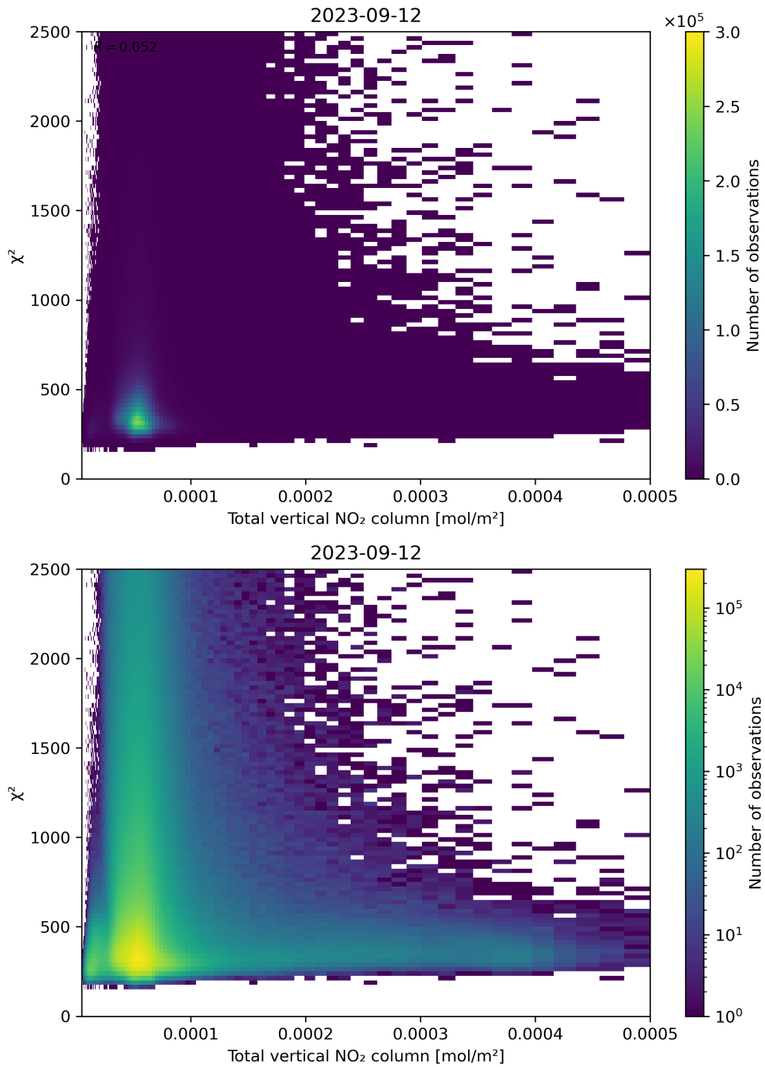
Figure 111: Scatter density plot of “Total vertical NO 2 column” against “ \chi^2 ” for 2023-09-11 to 2023-09-13.
