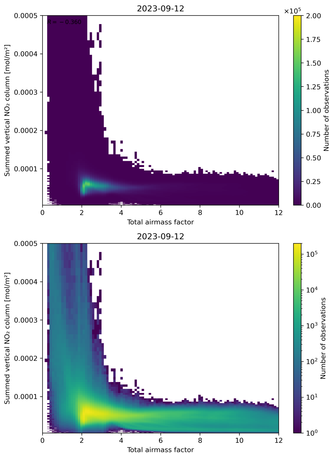
Figure 65: Scatter density plot of “Total airmass factor” against “Summed vertical NO 2 column” for 2023-09-11 to 2023-09-13.
