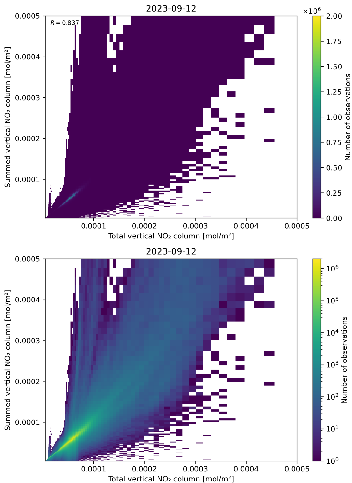
Figure 112: Scatter density plot of “Total vertical NO 2 column” against “Summed vertical NO 2 column” for 2023-09-11 to 2023-09-13.
