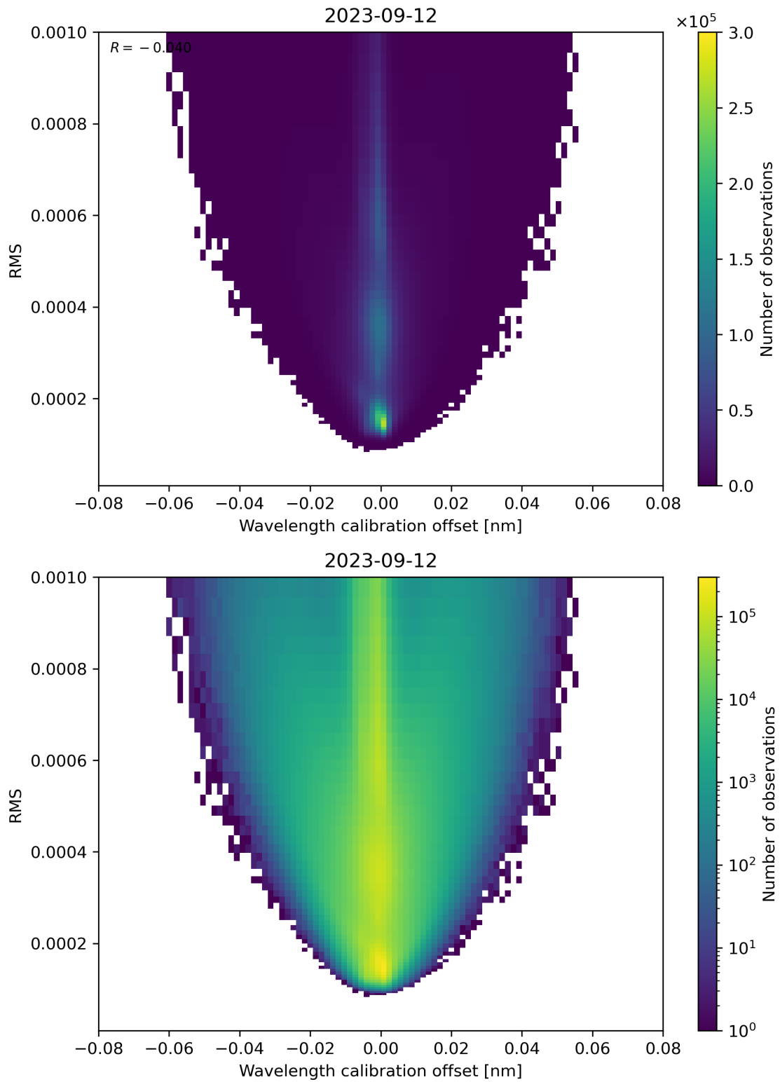
Figure 181: Scatter density plot of “Wavelength calibration offset” against “RMS” for 2023-09-11 to 2023-09-13.
