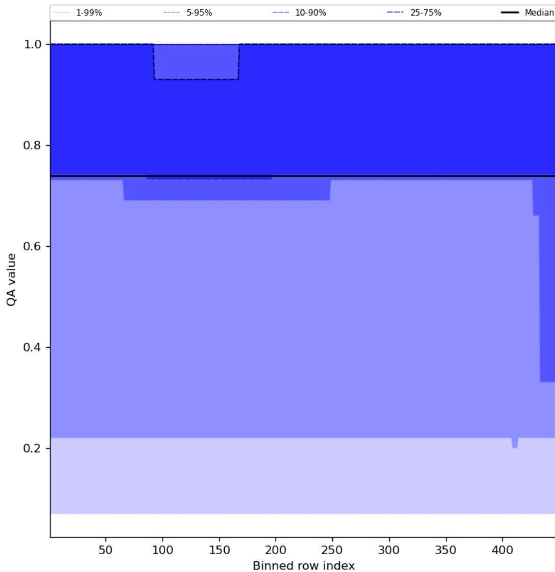
Figure 45: Along track statistics of “QA value” for 2023-09-11 to 2023-09-13
