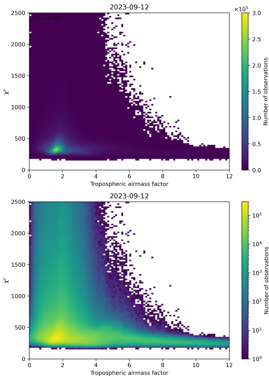
Figure 73: Scatter density plot of “Tropospheric airmass factor” against “ \chi^2 ” for 2023-09-11 to 2023-09-13.
