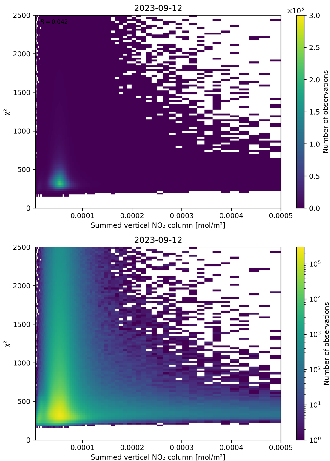
Figure 104: Scatter density plot of “Summed vertical NO 2 column” against “ \chi^2 ” for 2023-09-11 to 2023-09-13.
