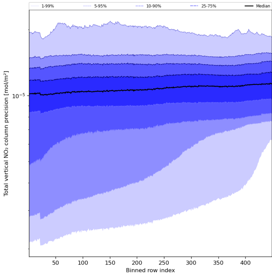
Figure 56: Along track statistics of “Total vertical NO 2 column precision” for 2023-09-11 to 2023-09-13
