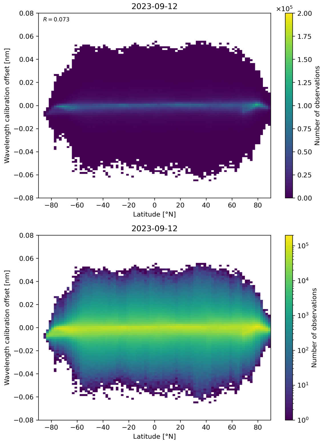
Figure 95: Scatter density plot of “Latitude” against “Wavelength calibration offset” for 2023-09-11 to 2023-09-13.
