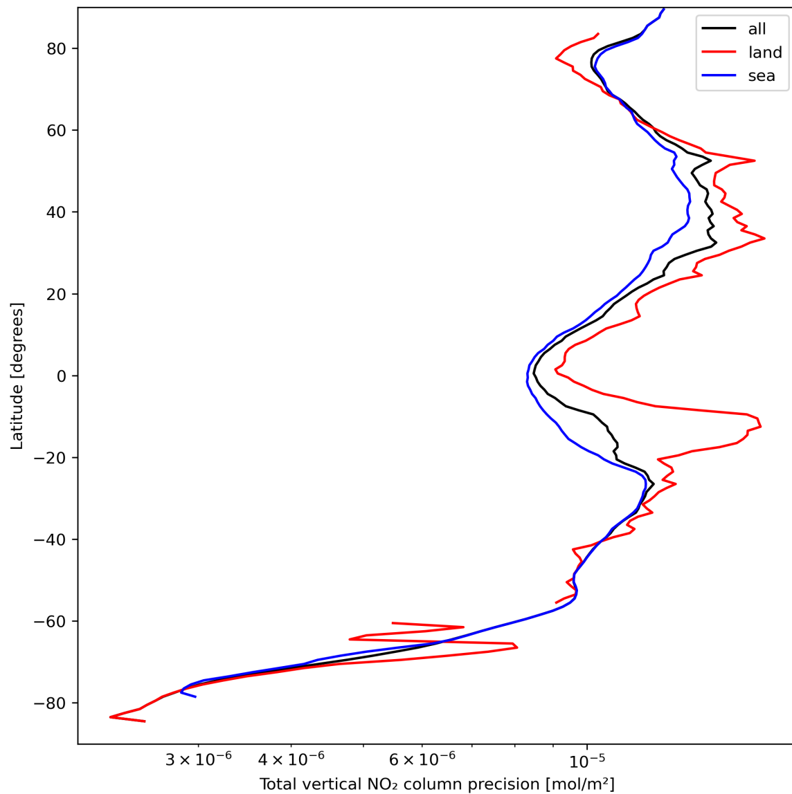
Figure 22: Zonal average of “Total vertical NO 2 column precision” for 2023-09-11 to 2023-09-13.
