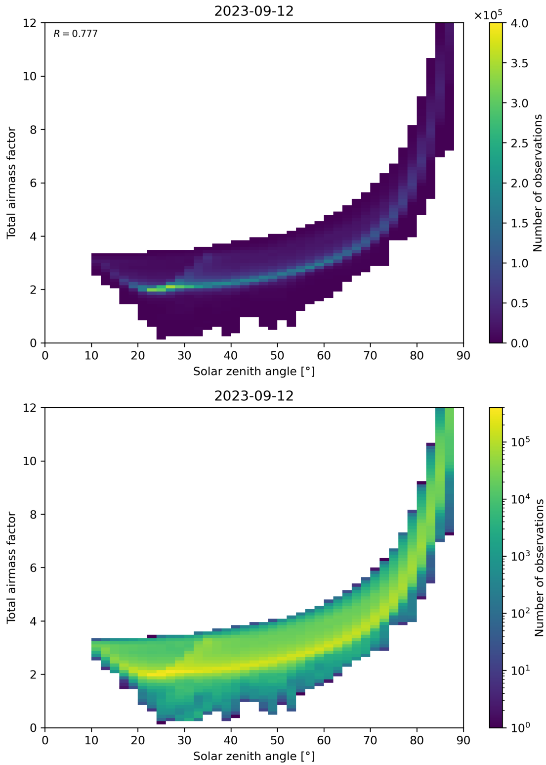
Figure 146: Scatter density plot of “Solar zenith angle” against “Total air mass factor” for 2023-09-11 to 2023-09-13.
