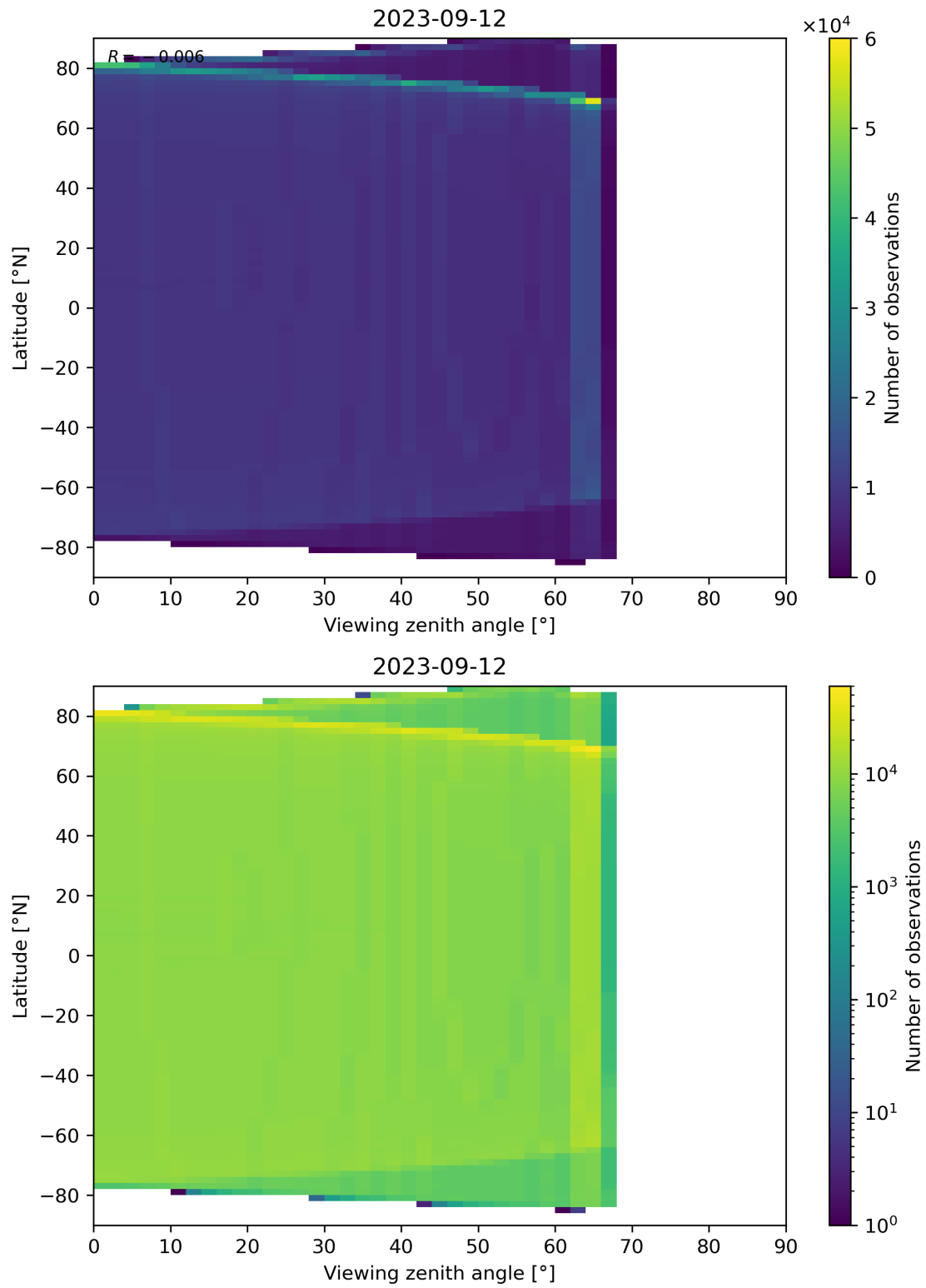
Figure 163: Scatter density plot of “Viewing zenith angle” against “Latitude” for 2023-09-11 to 2023-09-13.
