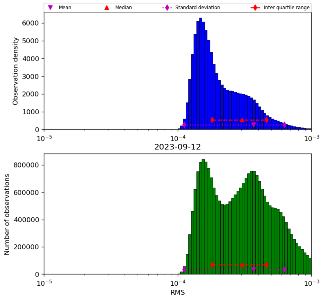
Figure 43: Histogram of “RMS” for 2023-09-11 to 2023-09-13
