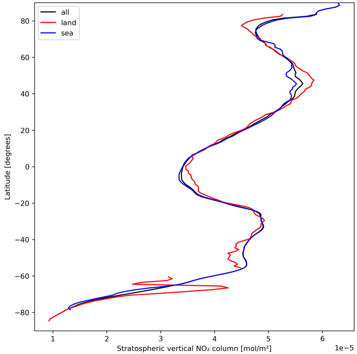
Figure 19: Zonal average of “Stratospheric vertical NO 2 column” for 2023-09-11 to 2023-09-13.
