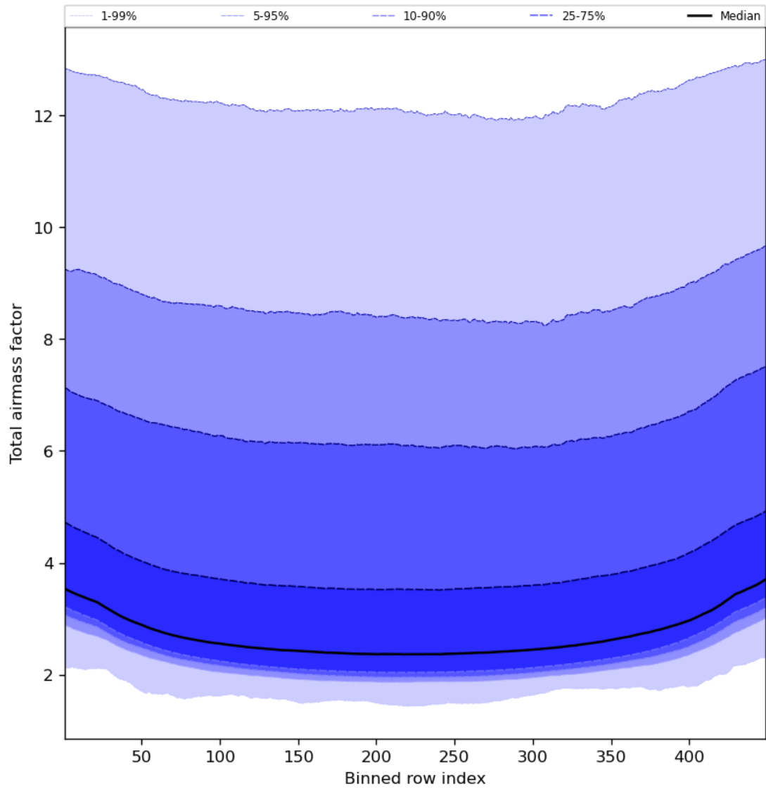
Figure 49: Along track statistics of “Total airmass factor” for 2023-09-11 to 2023-09-13
