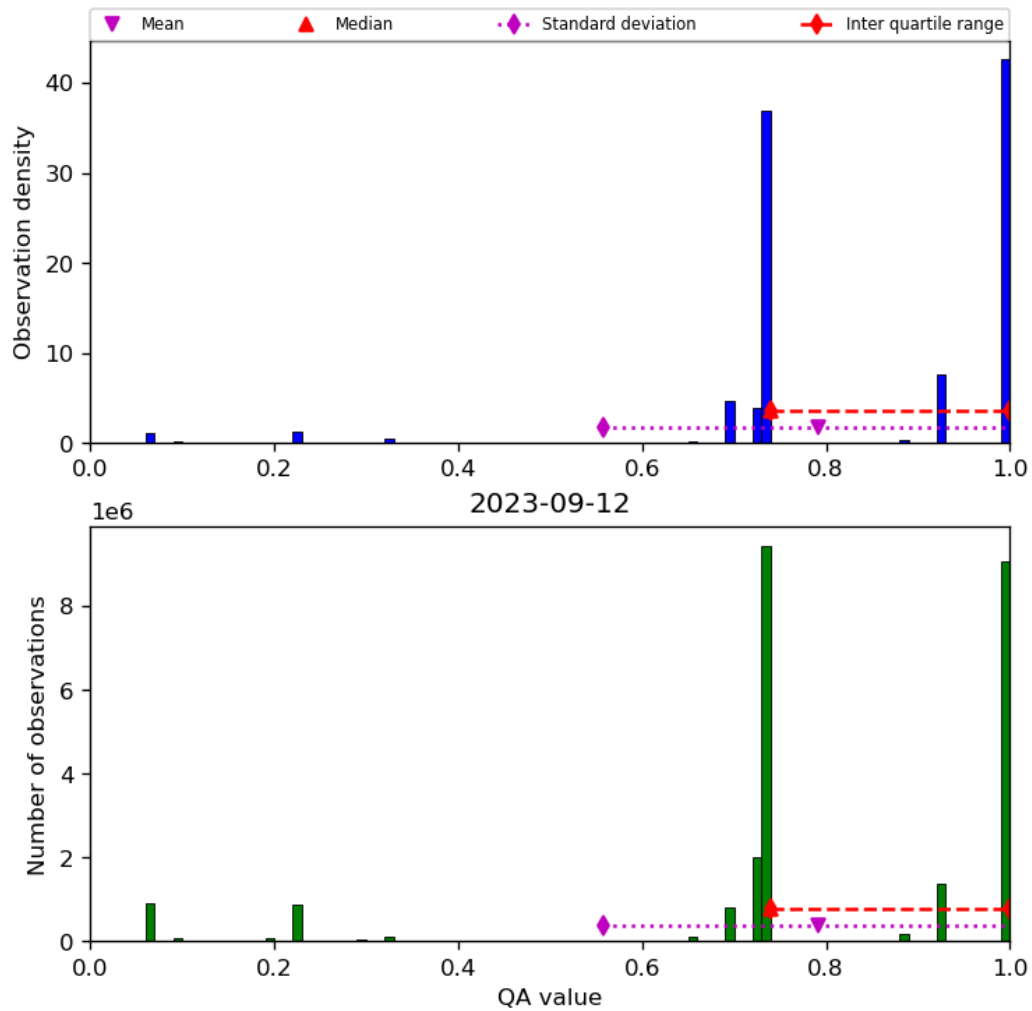
Figure 28: Histogram of “QA value” for 2023-09-11 to 2023-09-13
