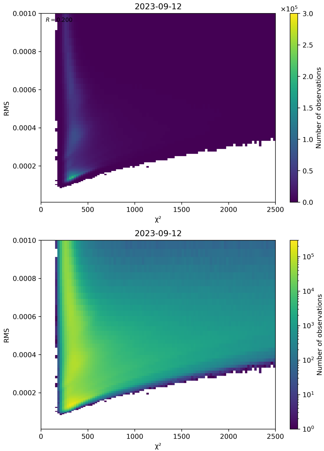
Figure 82: Scatter density plot of “ \chi^2 ” against “RMS” for 2023-09-11 to 2023-09-13.
