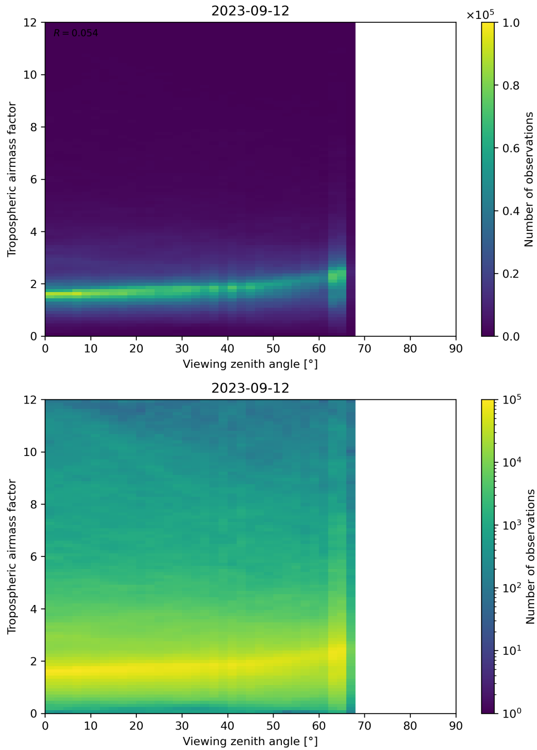
Figure 161: Scatter density plot of “Viewing zenith angle” against “Tropospheric airmass factor” for 2023-09-11 to 2023-09-13.
