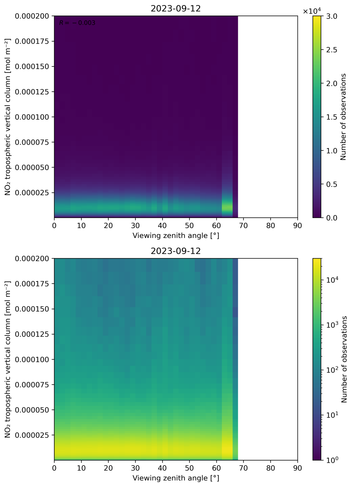
Figure 169: Scatter density plot of “Viewing zenith angle” against “NO 2 tropospheric vertical column” for 2023-09-11 to 2023-09-13.
