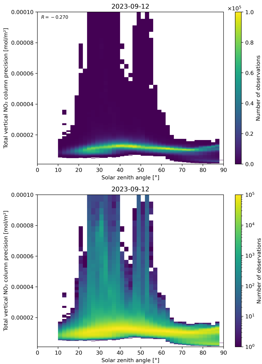
Figure 154: Scatter density plot of “Solar zenith angle” against “Total vertical NO 2 column precision” for 2023-09-11 to 2023-09-13.
