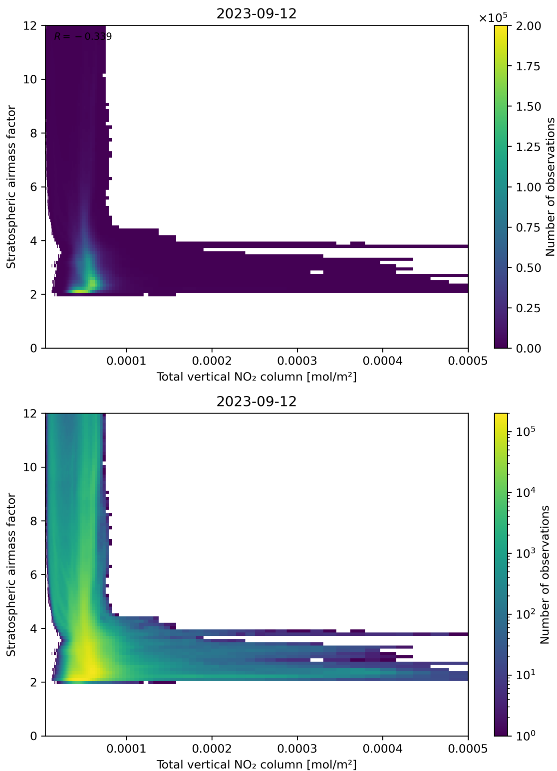
Figure 110: Scatter density plot of “Total vertical NO 2 column” against “Stratospheric airmass factor” for 2023-09-11 to 2023-09-13.
