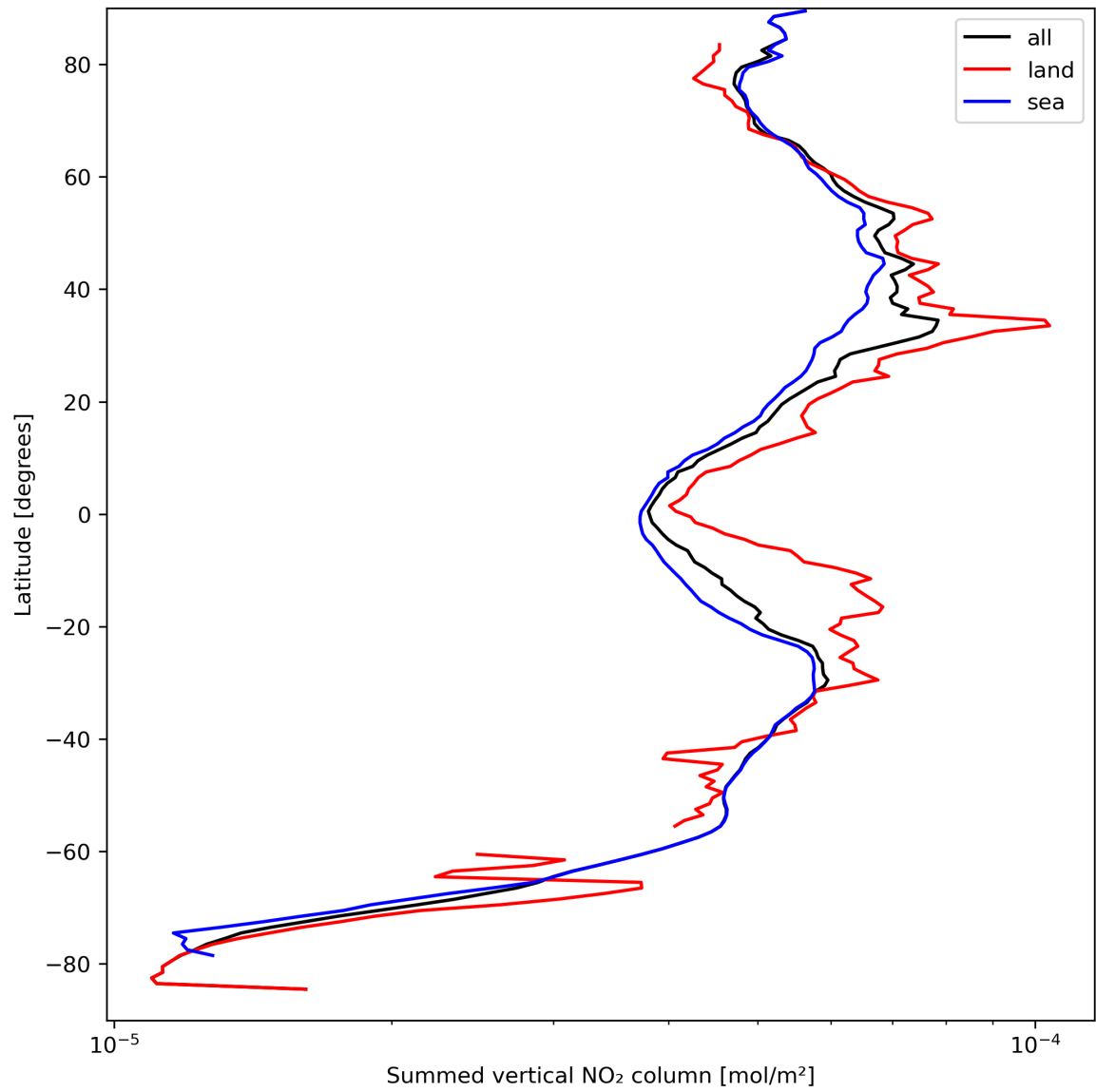
Figure 23: Zonal average of “Summed vertical NO 2 column” for 2023-09-11 to 2023-09-13.
