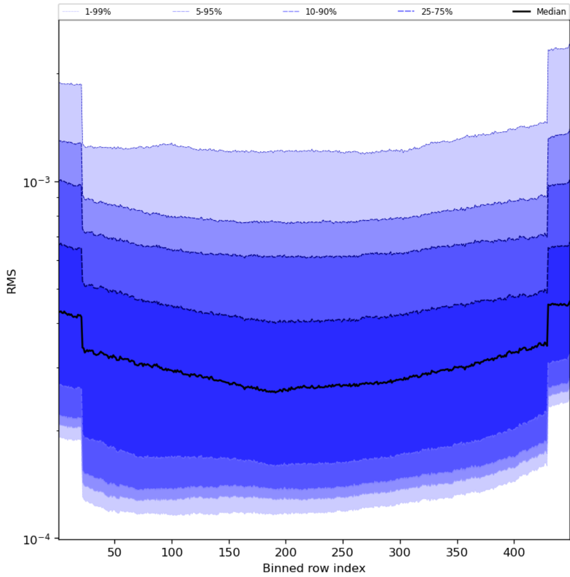
Figure 60: Along track statistics of “RMS” for 2023-09-11 to 2023-09-13
