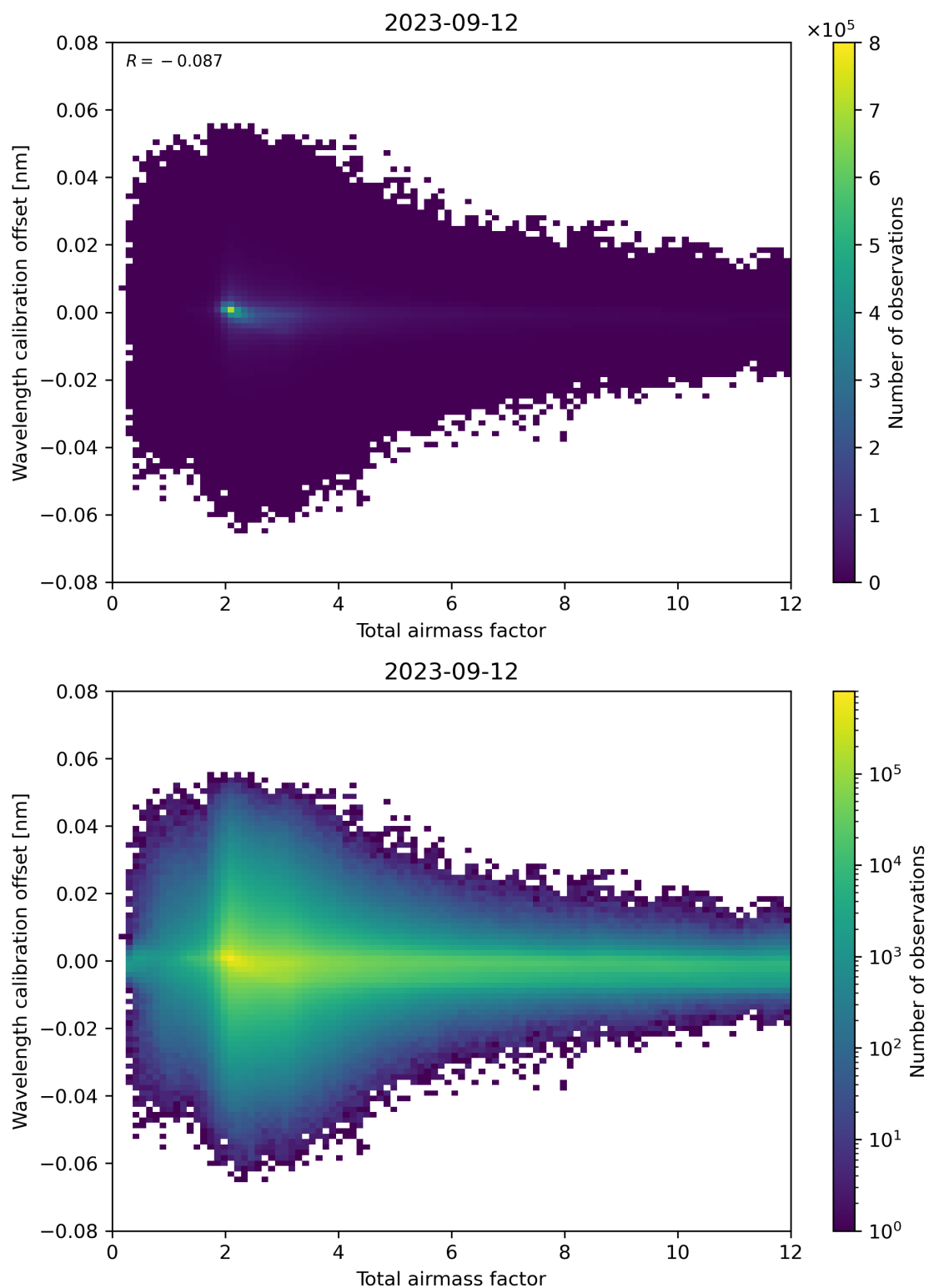
Figure 70: Scatter density plot of “Total airmass factor” against “Wavelength calibration offset” for 2023-09-11 to 2023-09-13.
