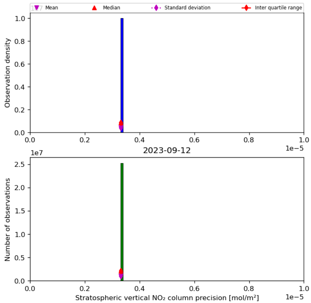
Figure 37: Histogram of “Stratospheric vertical NO 2 column precision” for 2023-09-11 to 2023-09-13
