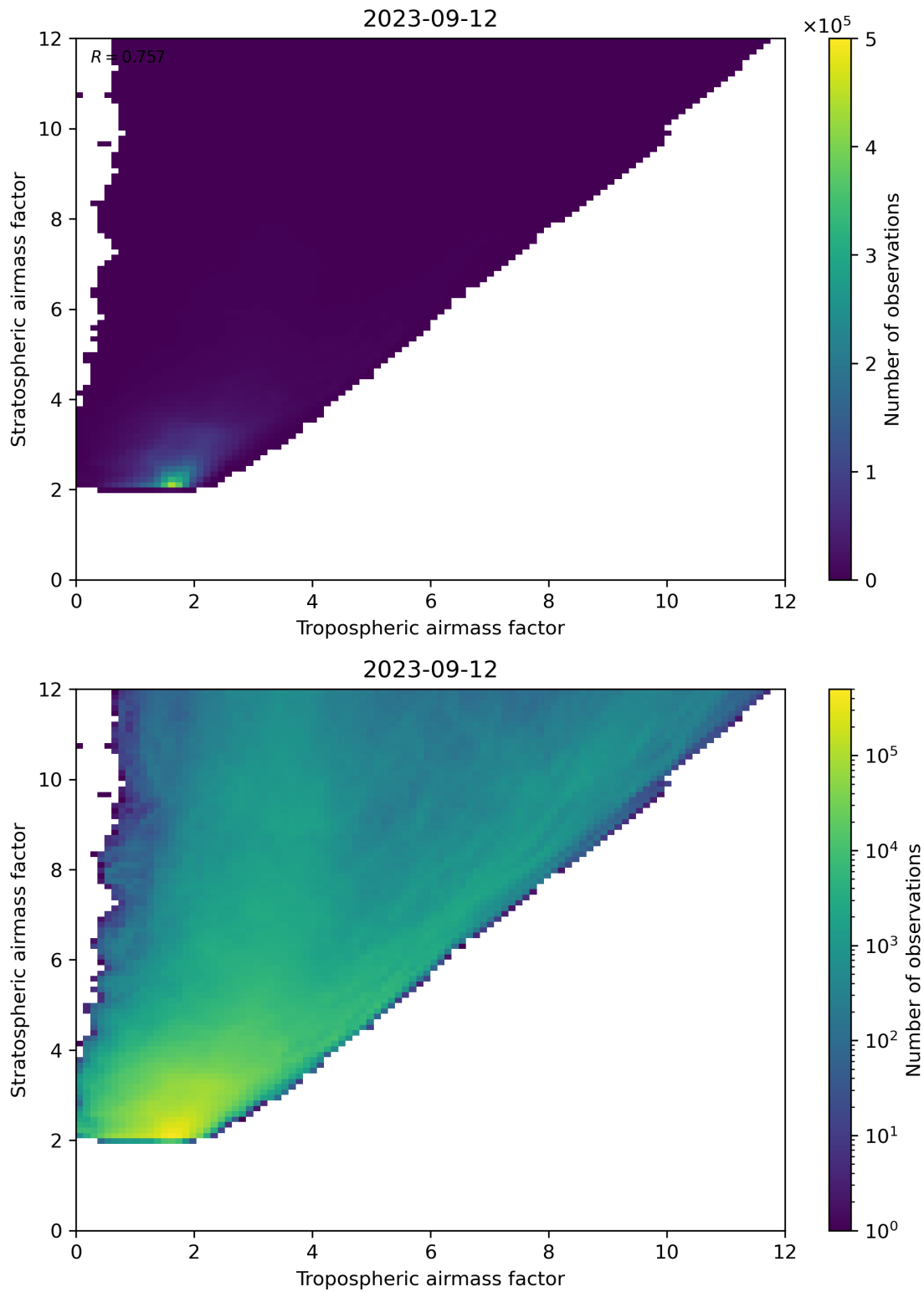
Figure 71: Scatter density plot of “Tropospheric airmass factor” against “Stratospheric airmass factor” for 2023-09-11 to 2023-09-13.
