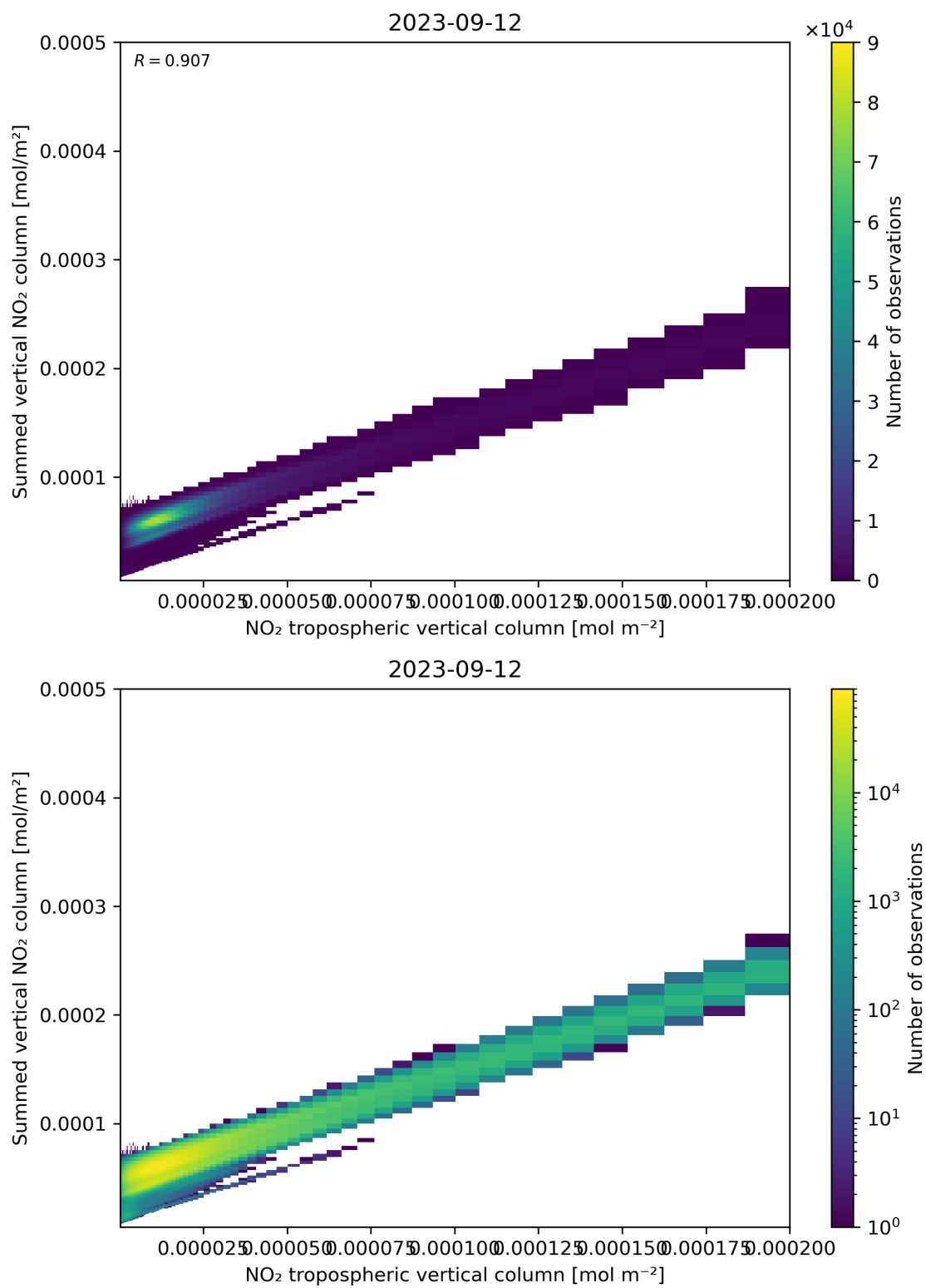
Figure 126: Scatter density plot of “NO 2 tropospheric vertical column” against “Summed vertical NO 2 column” for 2023-09-11 to 2023-09-13.
