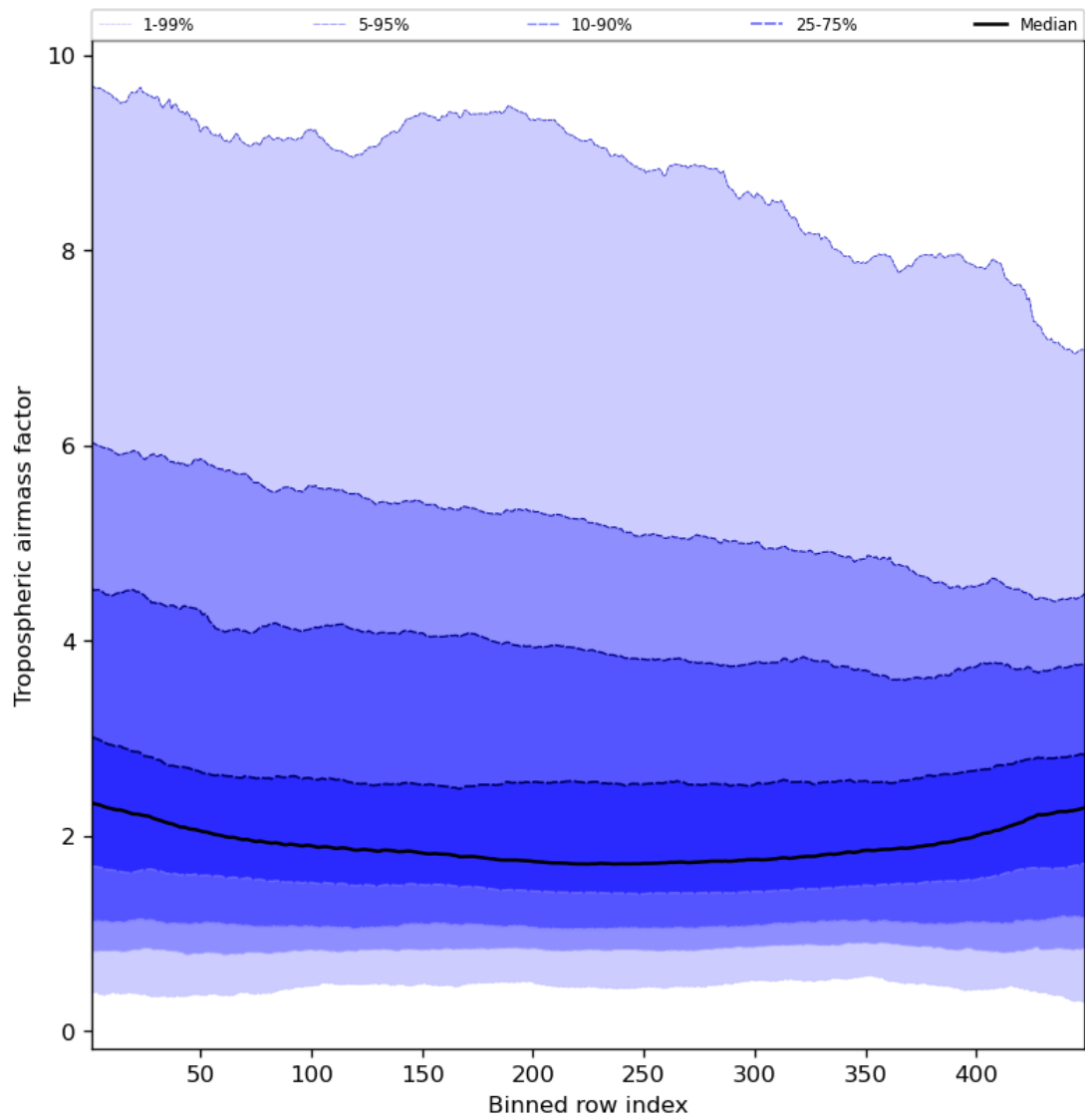
Figure 48: Along track statistics of “Tropospheric airmass factor” for 2023-09-11 to 2023-09-13
