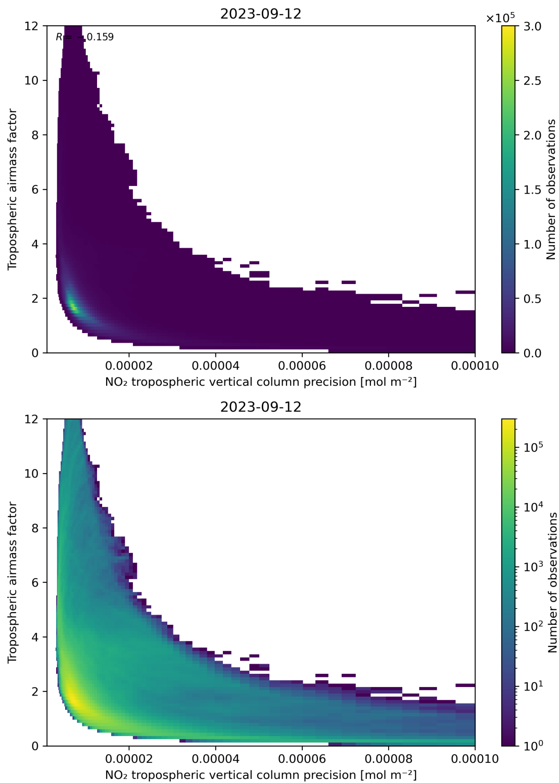
Figure 133: Scatter density plot of “NO 2 tropospheric vertical column precision” against “Tropospheric airmass factor” for 2023-09-11 to 2023-09-13.
