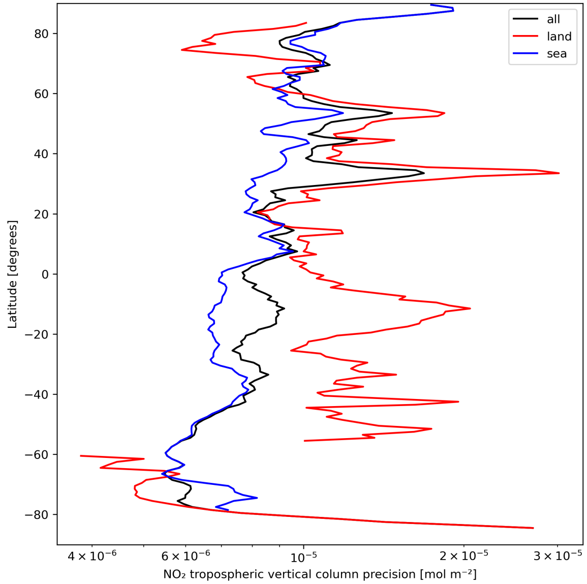
Figure 13: Zonal average of “NO 2 tropospheric vertical column precision” for 2023-09-11 to 2023-09-13.
