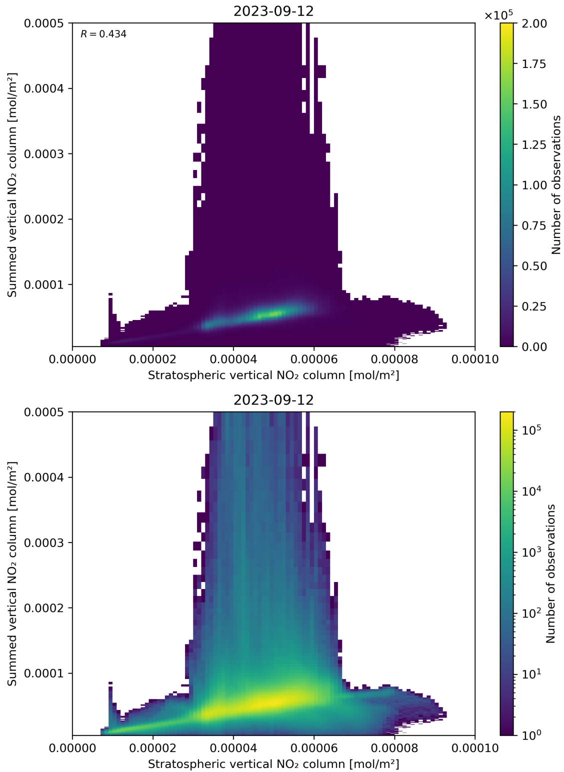
Figure 98: Scatter density plot of “Stratospheric vertical NO 2 column” against “Summed vertical NO 2 column” for 2023-09-11 to 2023-09-13.
