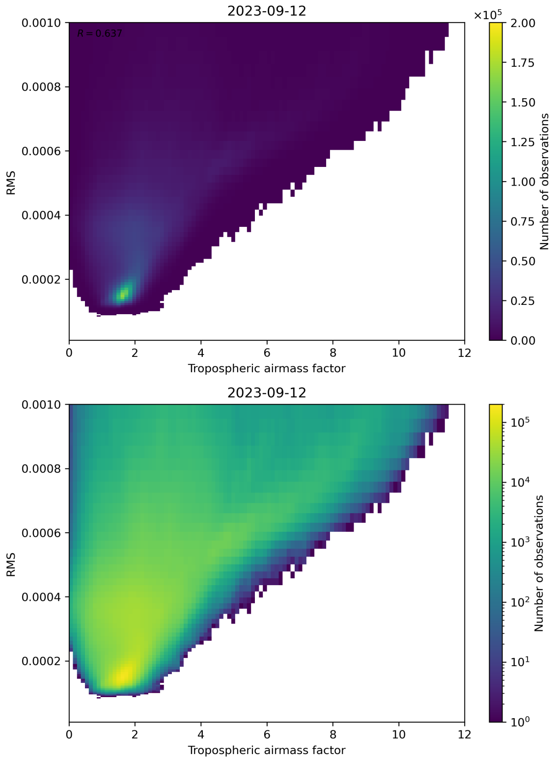
Figure 79: Scatter density plot of “Tropospheric airmass factor” against “RMS” for 2023-09-11 to 2023-09-13.
