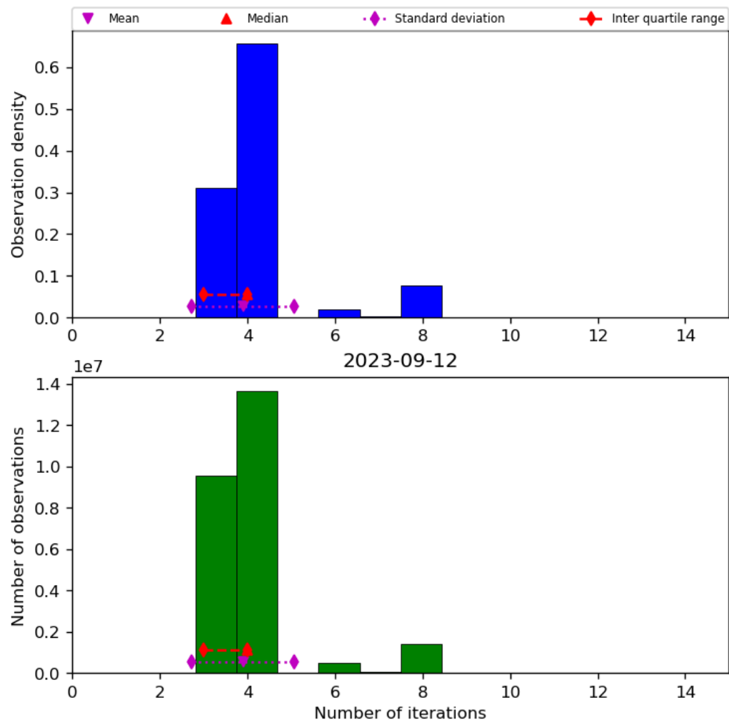
Figure 34: Histogram of “Number of iterations” for 2023-09-11 to 2023-09-13
