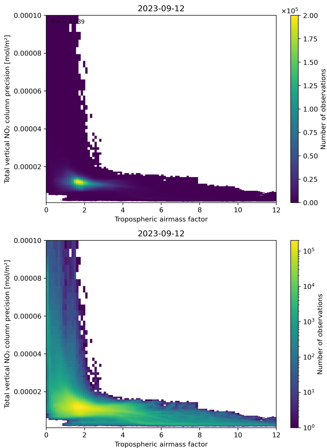
Figure 78: Scatter density plot of “Tropospheric air mass factor” against “Total vertical NO 2 column precision” for 2023-09-11 to 2023-09-13.
