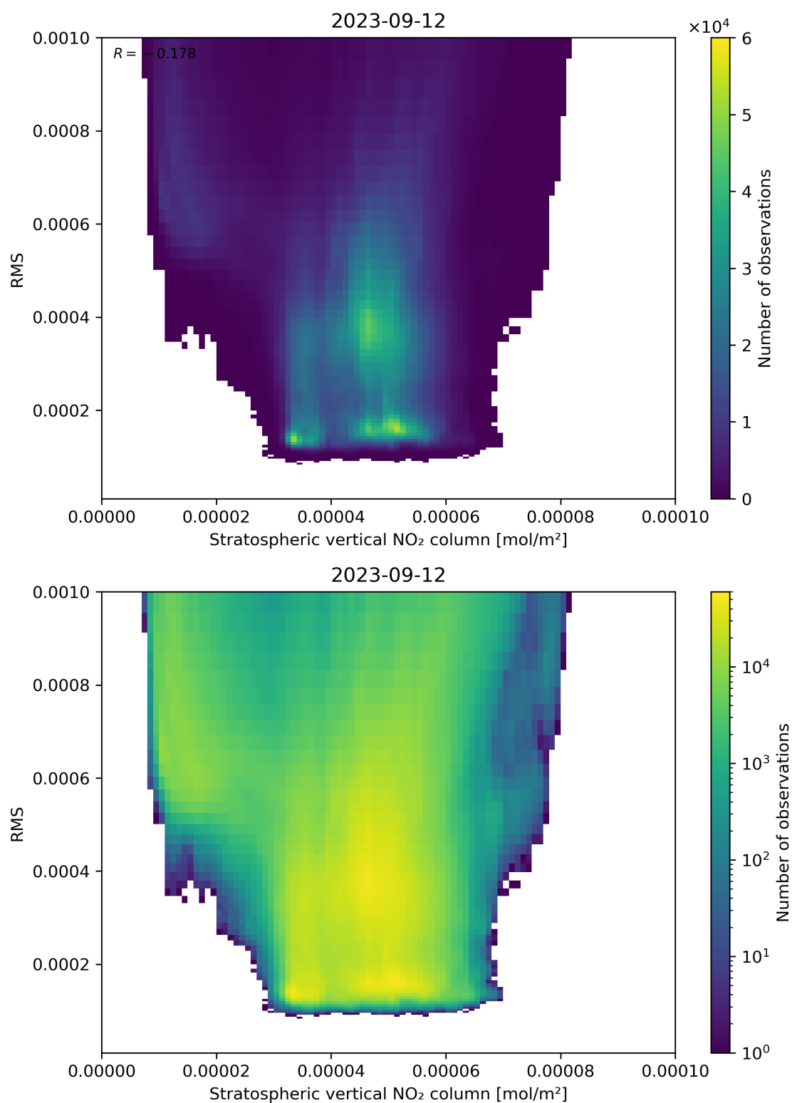
Figure 102: Scatter density plot of “Stratospheric vertical NO 2 column” against “RMS” for 2023-09-11 to 2023-09-13.
