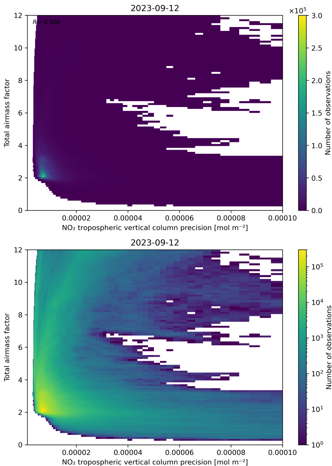
Figure 132: Scatter density plot of “NO 2 tropospheric vertical column precision” against “Total air mass factor” for 2023-09-11 to 2023-09-13.
