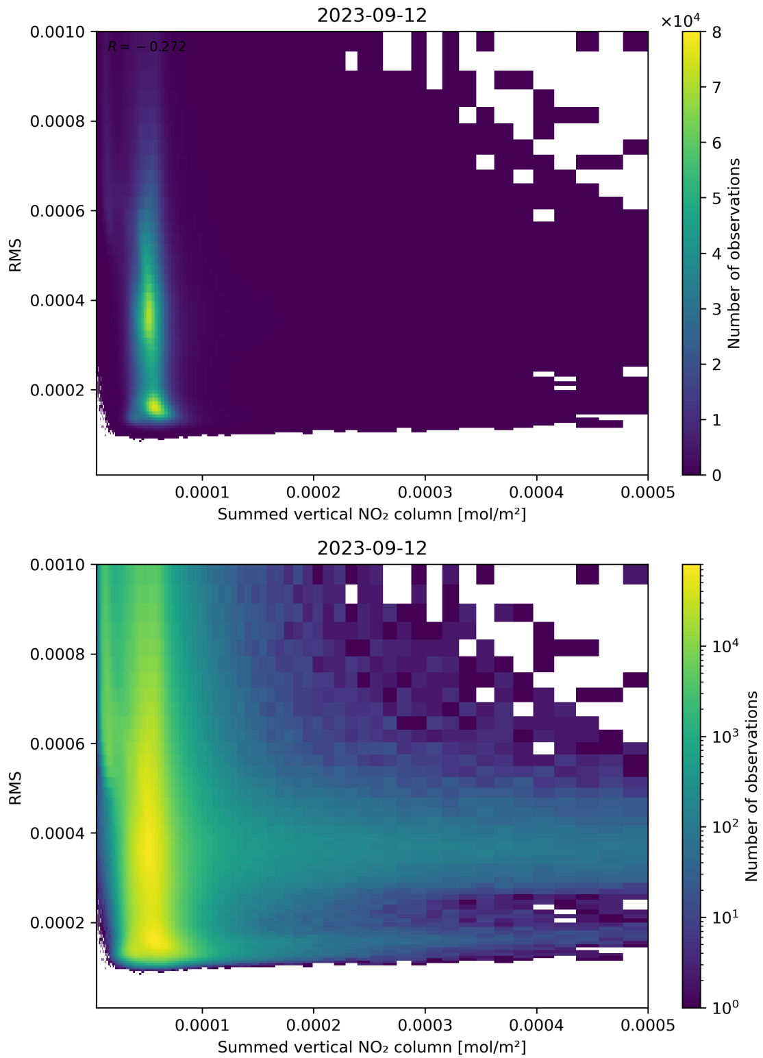
Figure 109: Scatter density plot of “Summed vertical NO 2 column” against “RMS” for 2023-09-11 to 2023-09-13.
