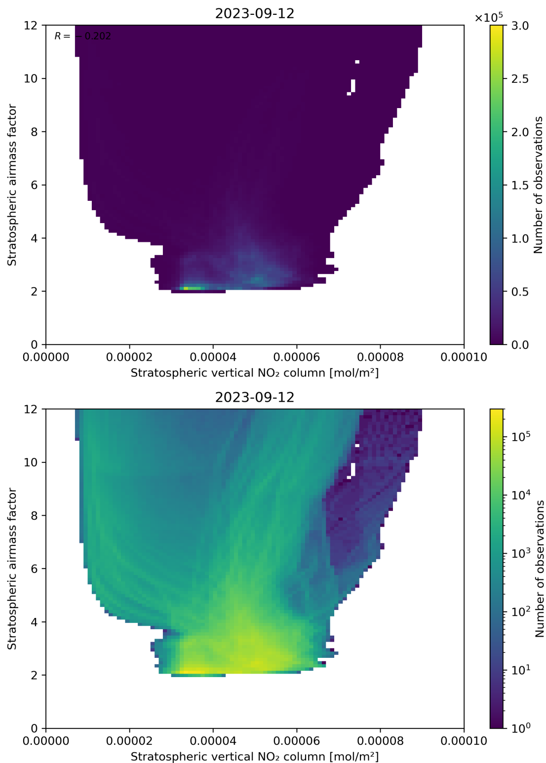
Figure 96: Scatter density plot of “Stratospheric vertical NO 2 column” against “Stratospheric airmass factor” for 2023-09-11 to 2023-09-13.
