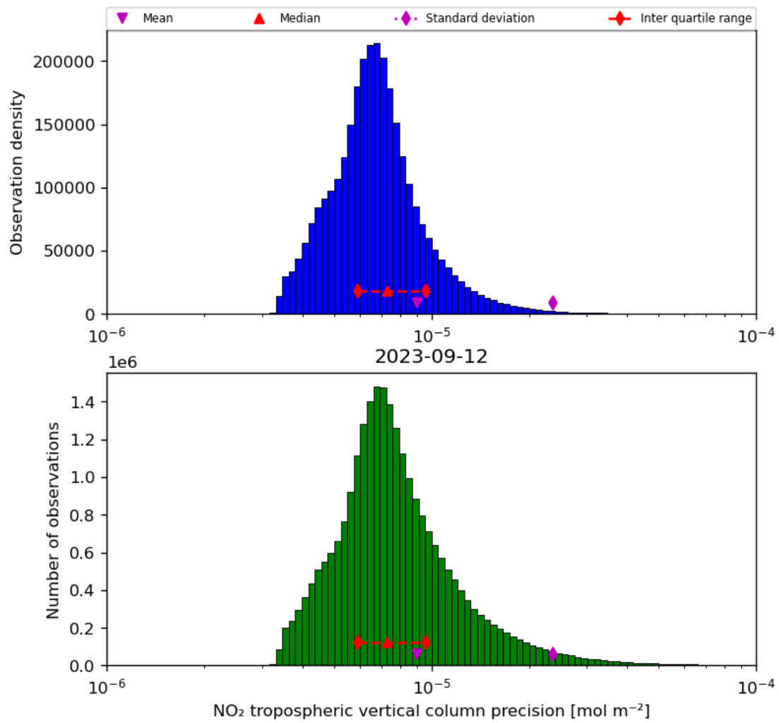
Figure 30: Histogram of “NO 2 tropospheric vertical column precision” for 2023-09-11 to 2023-09-13
