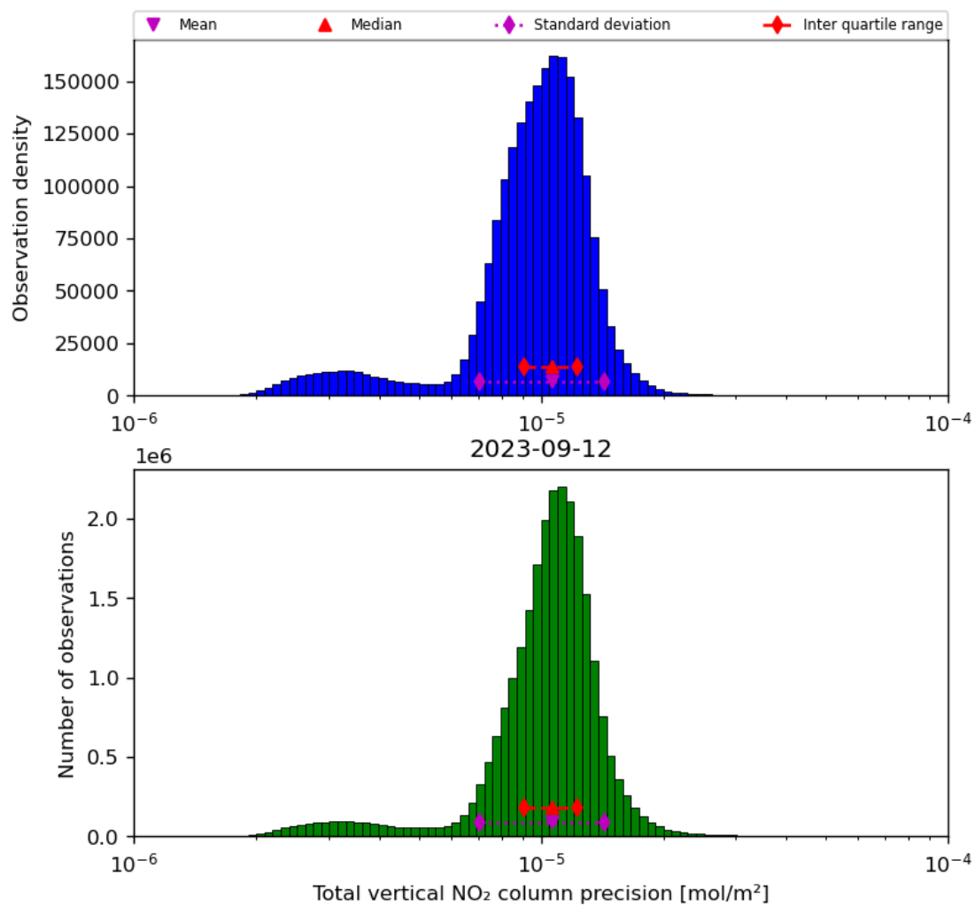
Figure 39: Histogram of "Total vertical NO 2 column precision" for 2023-09-11 to 2023-09-13
