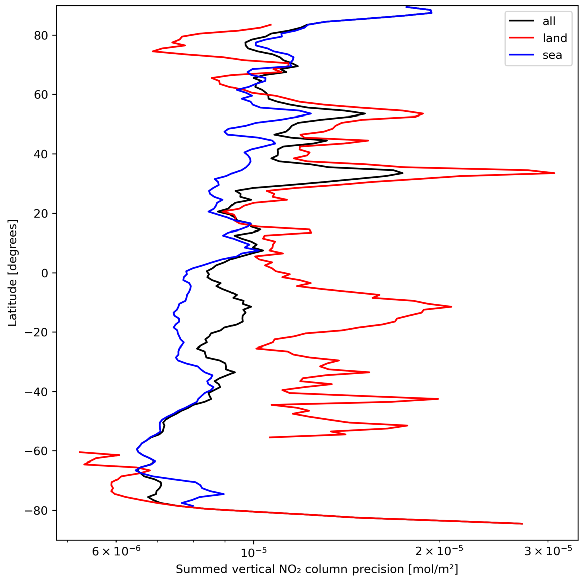
Figure 24: Zonal average of “Summed vertical NO 2 column precision” for 2023-09-11 to 2023-09-13.
