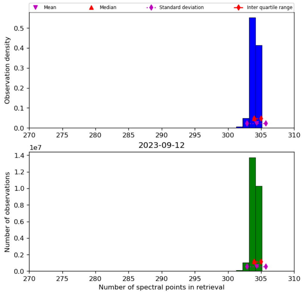
Figure 33: Histogram of “Number of spectral points in retrieval” for 2023-09-11 to 2023-09-13
