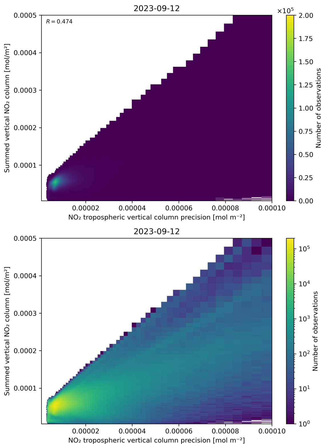
Figure 136: Scatter density plot of “NO 2 tropospheric vertical column precision” against “Summed vertical NO 2 column” for 2023-09-11 to 2023-09-13.
