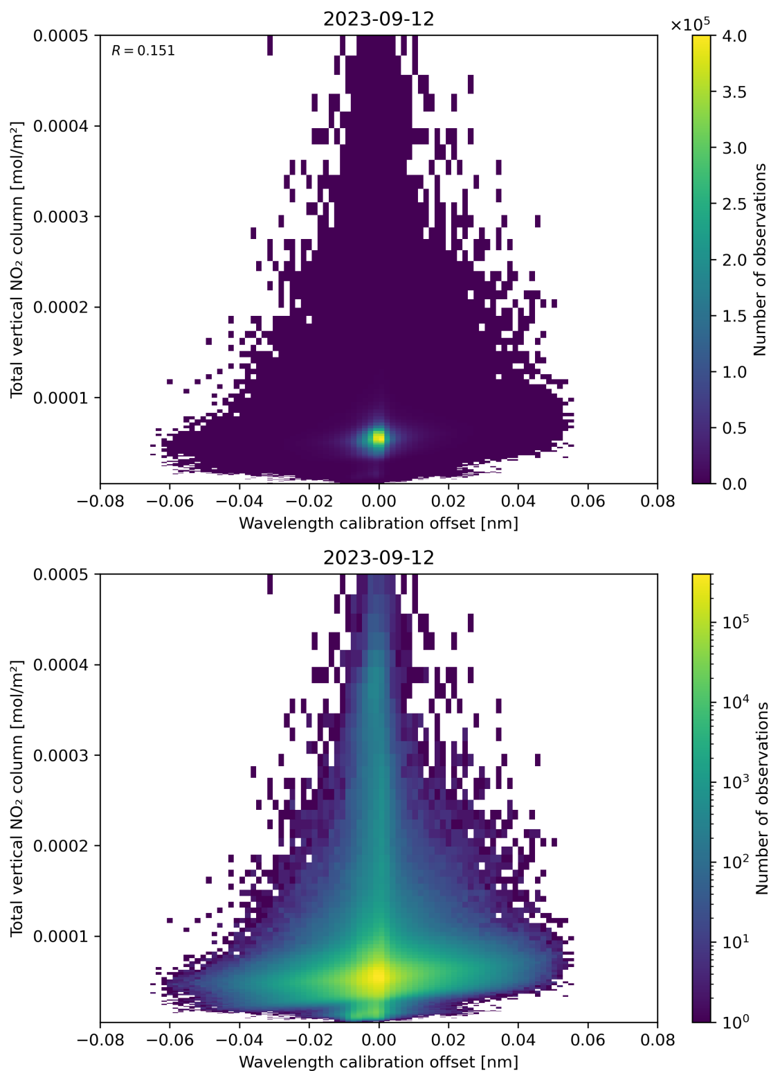
Figure 179: Scatter density plot of “Wavelength calibration offset” against “Total vertical NO 2 column” for 2023-09-11 to 2023-09-13.
