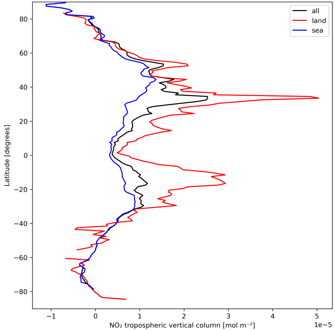
Figure 12: Zonal average of “NO 2 tropospheric vertical column” for 2023-09-11 to 2023-09-13.
