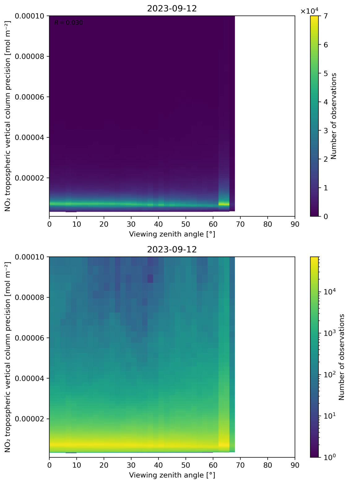
Figure 170: Scatter density plot of “Viewing zenith angle” against “NO 2 tropospheric vertical column precision” for 2023-09-11 to 2023-09-13.
