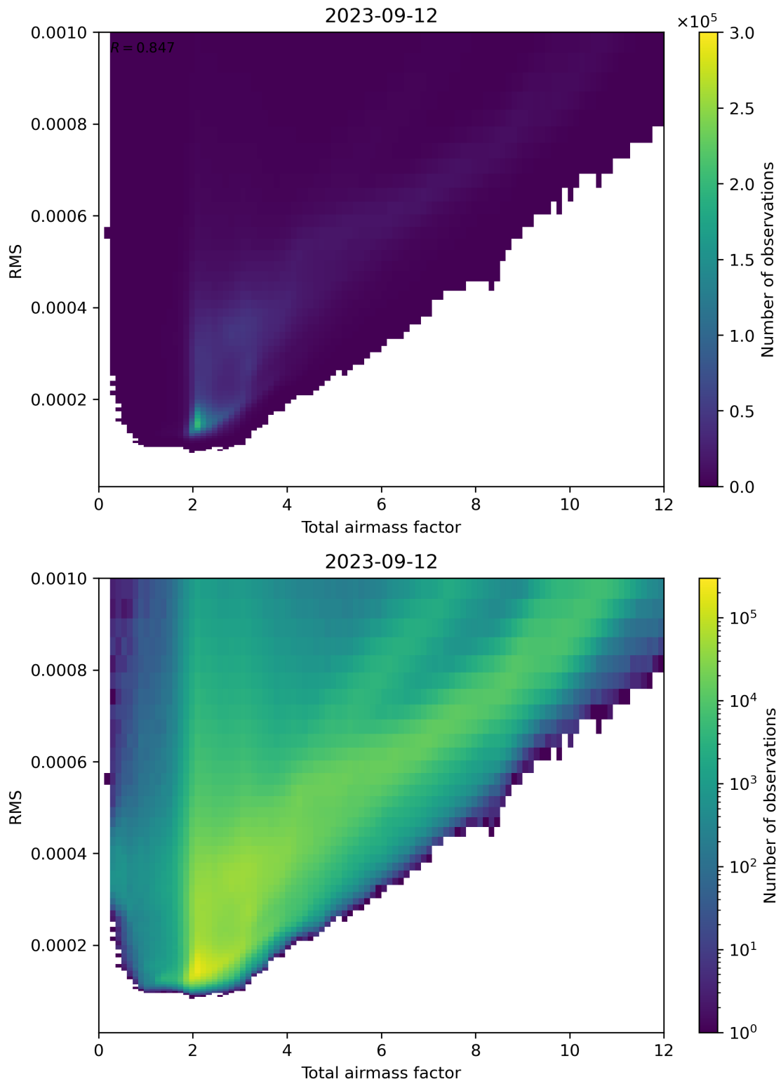
Figure 69: Scatter density plot of “Total airmass factor” against “RMS” for 2023-09-11 to 2023-09-13.
