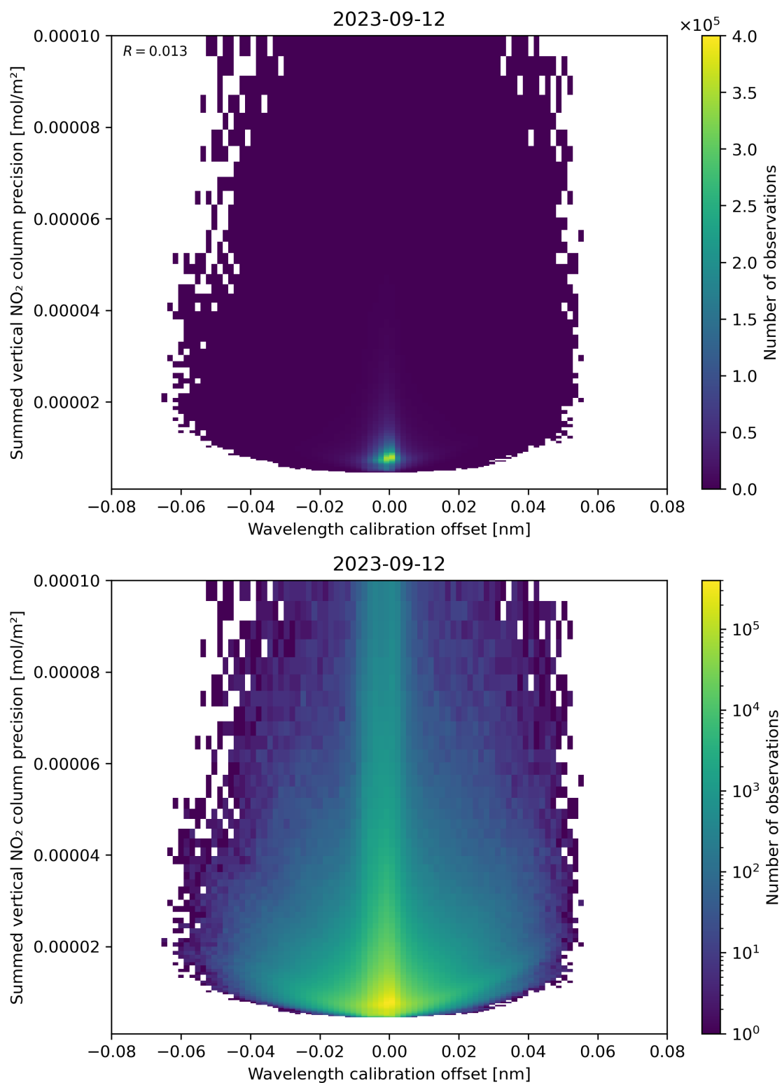
Figure 178: Scatter density plot of “Wavelength calibration offset” against “Summed vertical NO 2 column precision” for 2023-09-11 to 2023-09-13.
