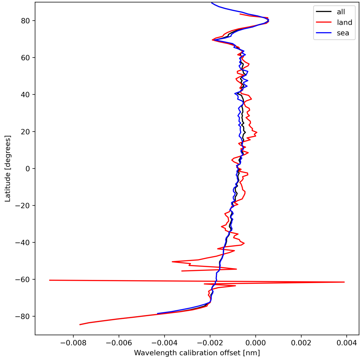
Figure 18: Zonal average of “Wavelength calibration offset” for 2023-09-11 to 2023-09-13.
