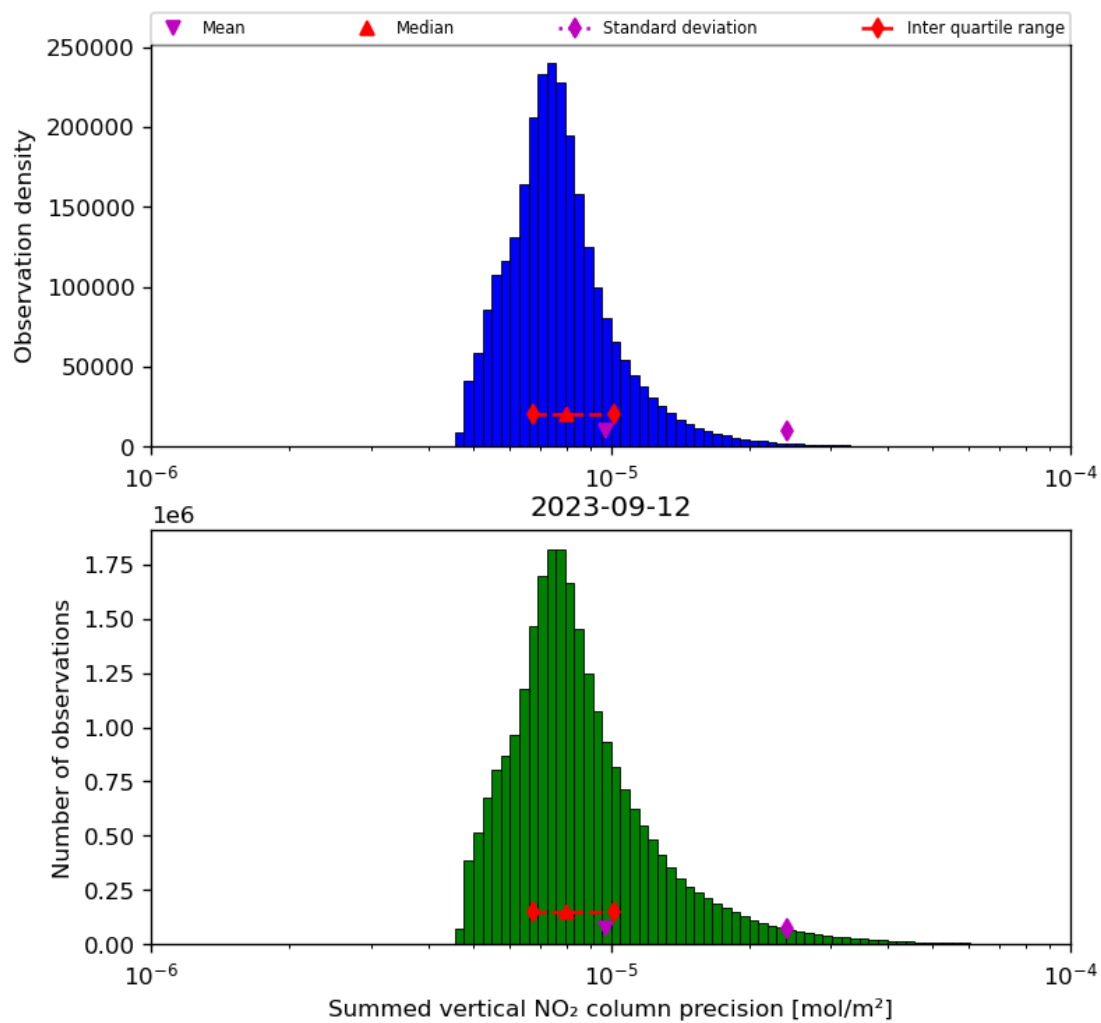
Figure 41: Histogram of “Summed vertical NO 2 column precision” for 2023-09-11 to 2023-09-13
