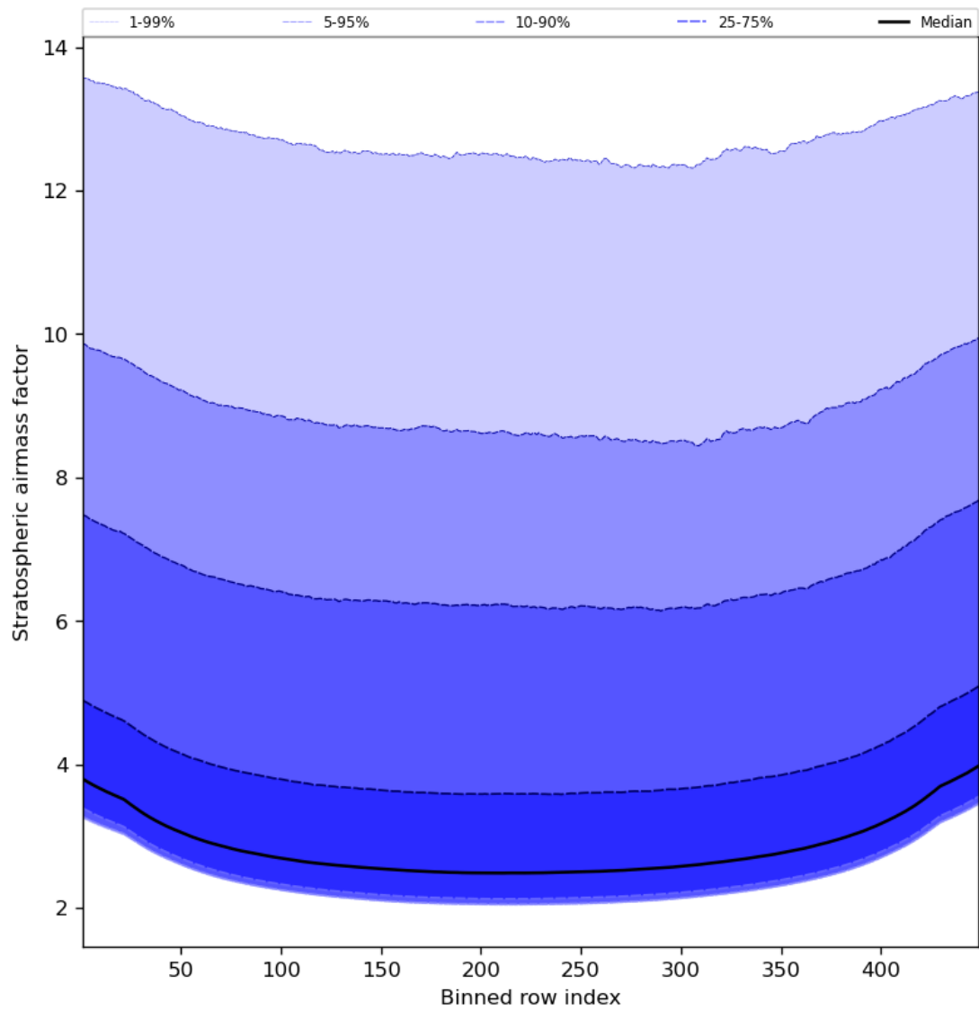
Figure 61: Along track statistics of “Stratospheric airmass factor” for 2023-09-11 to 2023-09-13
