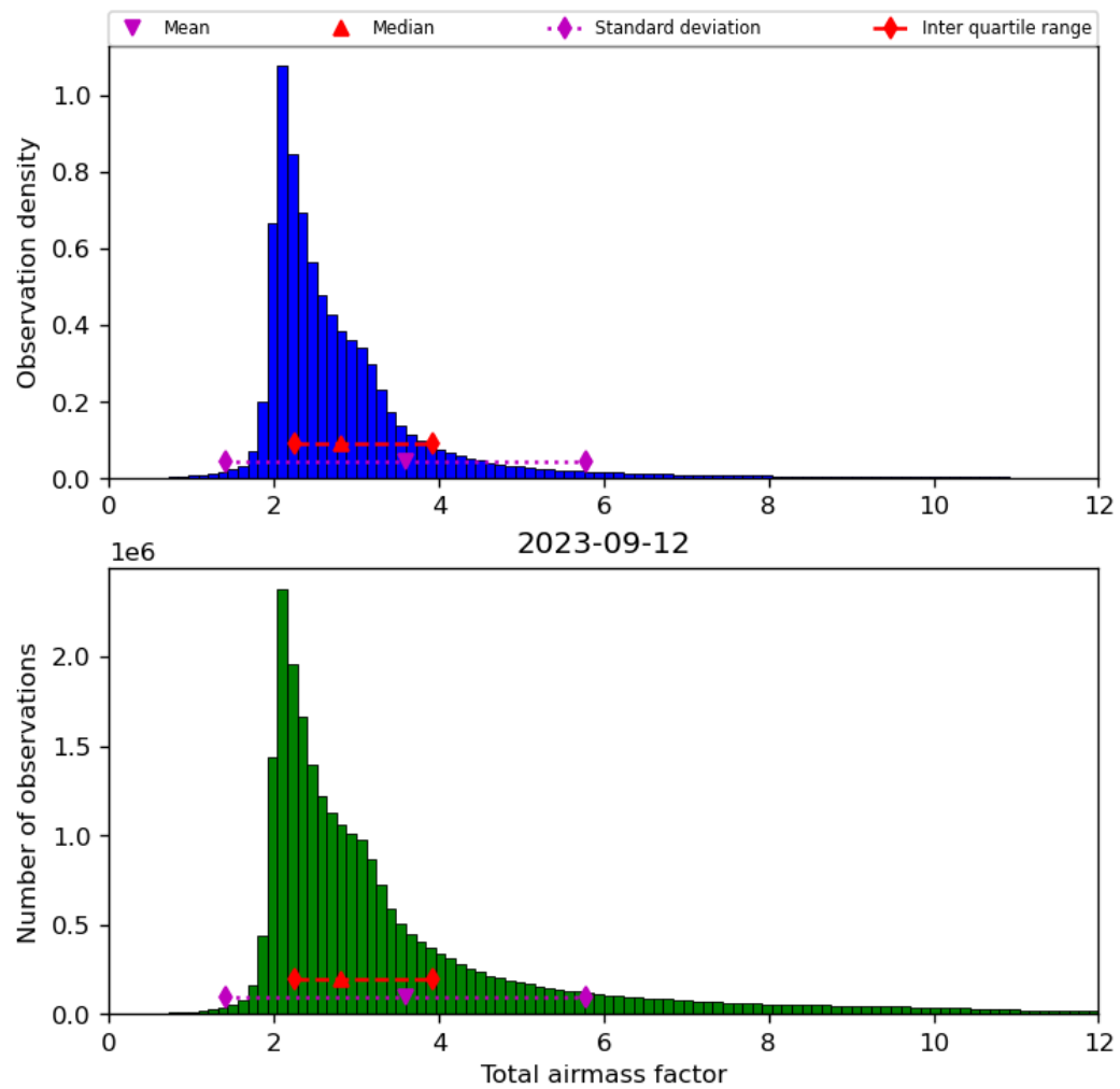
Figure 32: Histogram of “Total airmass factor” for 2023-09-11 to 2023-09-13
