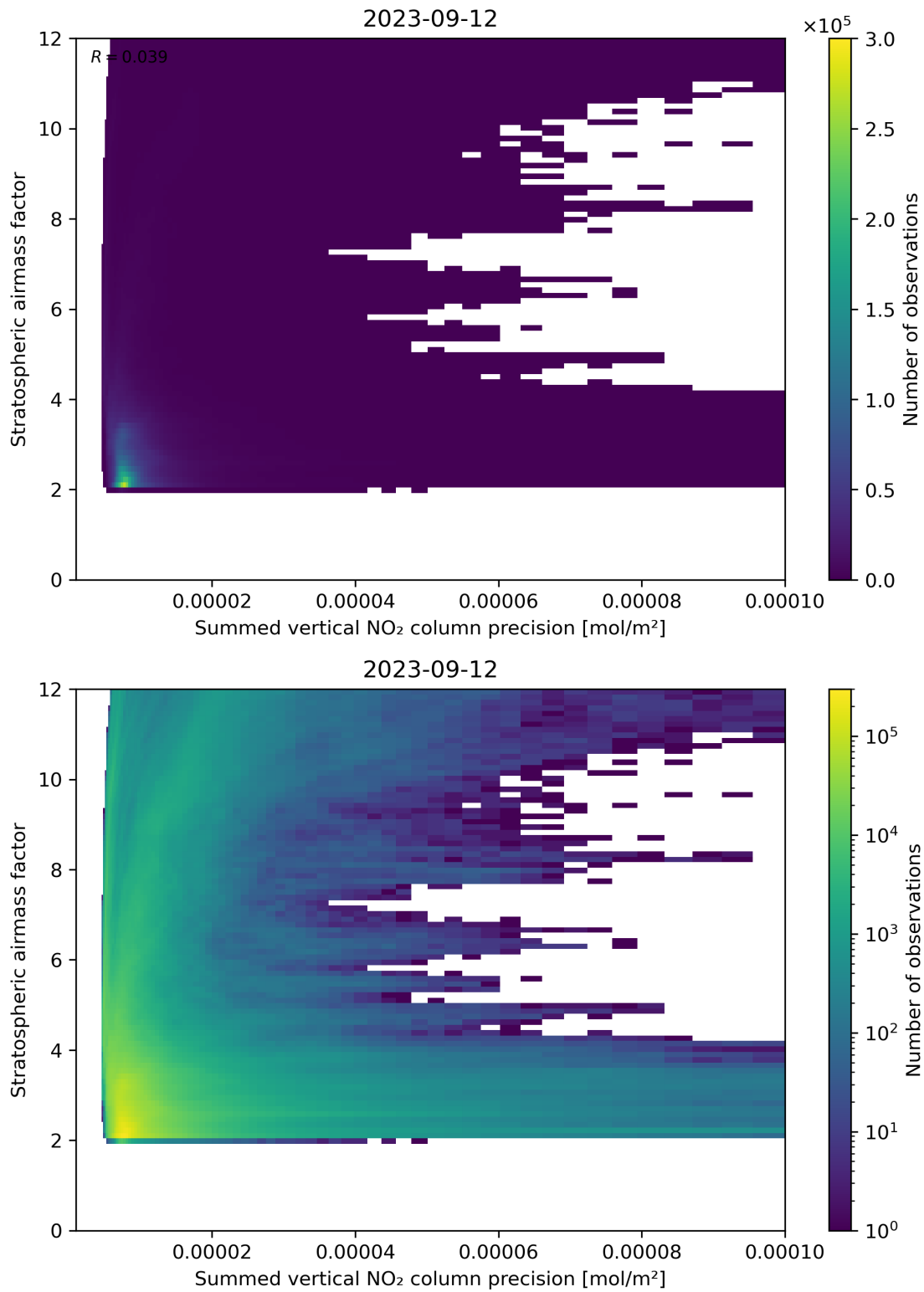
Figure 106: Scatter density plot of “Summed vertical NO 2 column precision” against “Stratospheric airmass factor” for 2023-09-11 to 2023-09-13.
