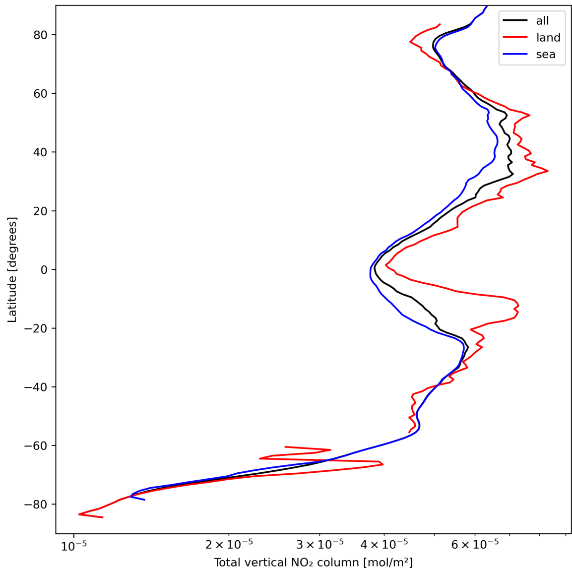
Figure 21: Zonal average of “Total vertical NO 2 column” for 2023-09-11 to 2023-09-13.
