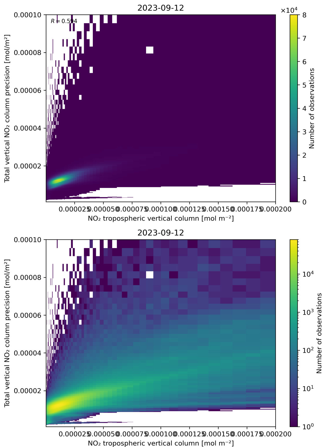
Figure 129: Scatter density plot of “NO 2 tropospheric vertical column” against “Total vertical NO 2 column precision” for 2023-09-11 to 2023-09-13.
