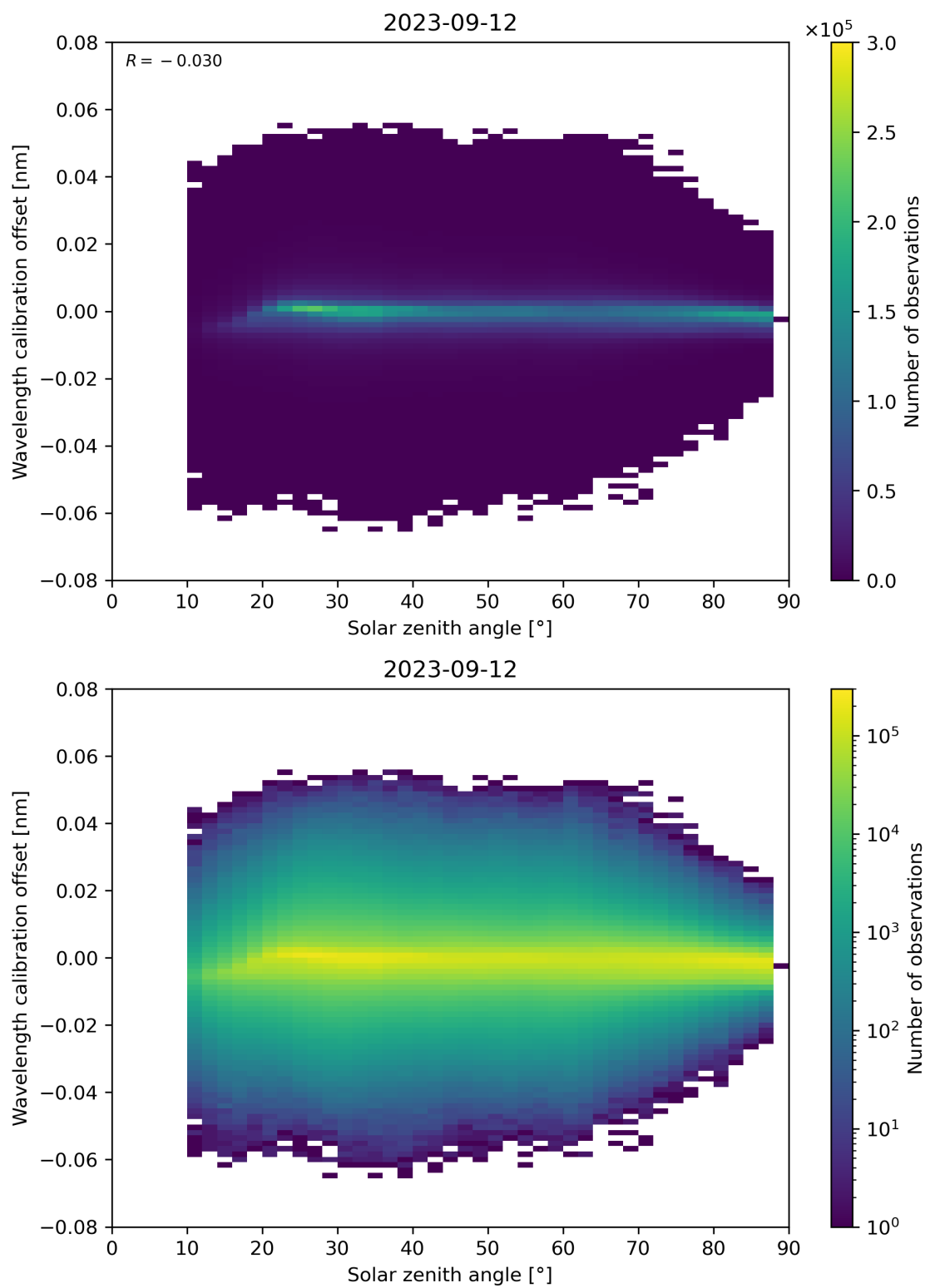
Figure 158: Scatter density plot of “Solar zenith angle” against “Wavelength calibration offset” for 2023-09-11 to 2023-09-13.
