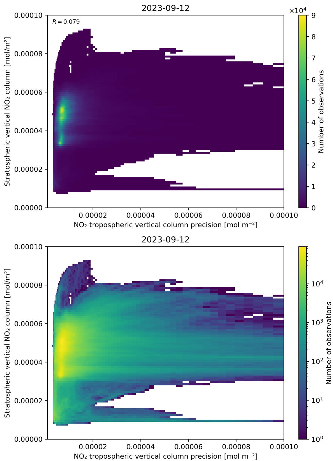
Figure 135: Scatter density plot of “NO 2 tropospheric vertical column precision” against “Stratospheric vertical NO 2 column” for 2023-09-11 to 2023-09-13.
