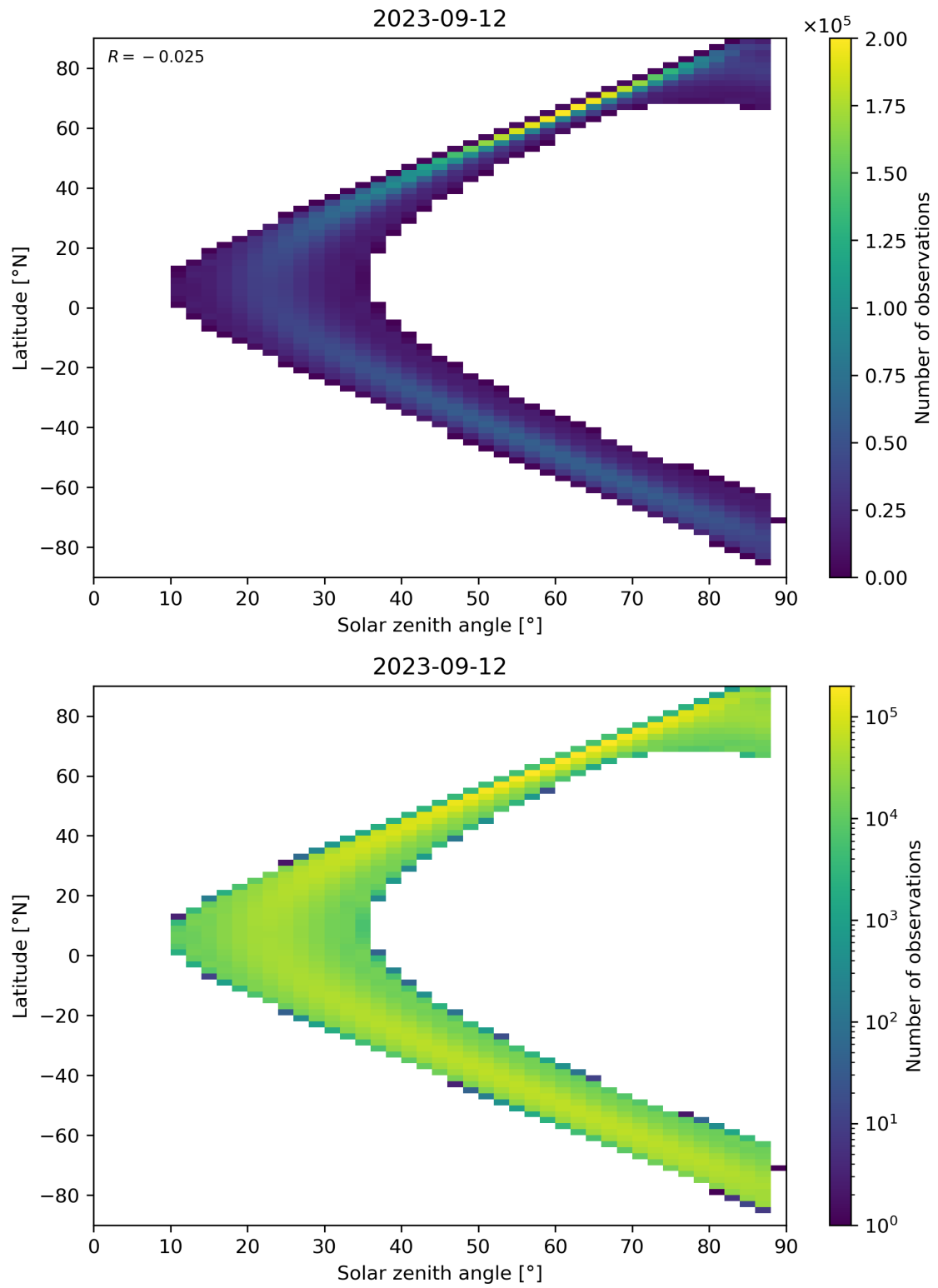
Figure 149: Scatter density plot of “Solar zenith angle” against “Latitude” for 2023-09-11 to 2023-09-13.
