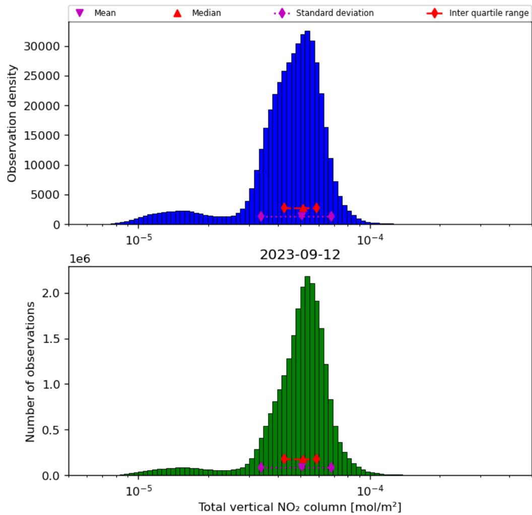
Figure 38: Histogram of “Total vertical NO 2 column” for 2023-09-11 to 2023-09-13
