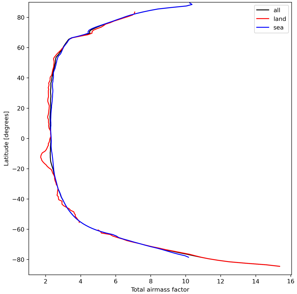
Figure 15: Zonal average of “Total airmass factor” for 2023-09-11 to 2023-09-13.
