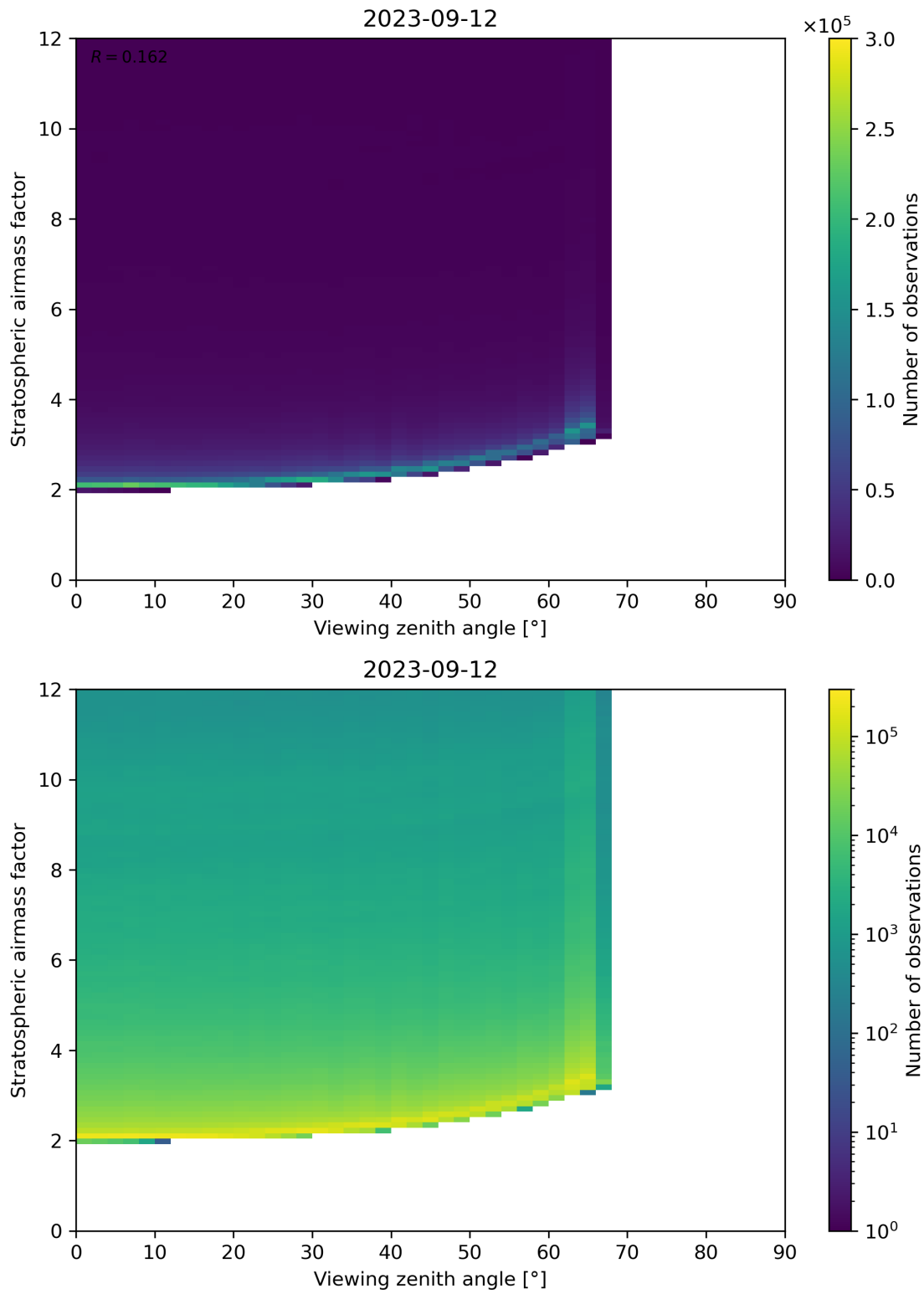
Figure 159: Scatter density plot of “Viewing zenith angle” against “Stratospheric airmass factor” for 2023-09-11 to 2023-09-13.
