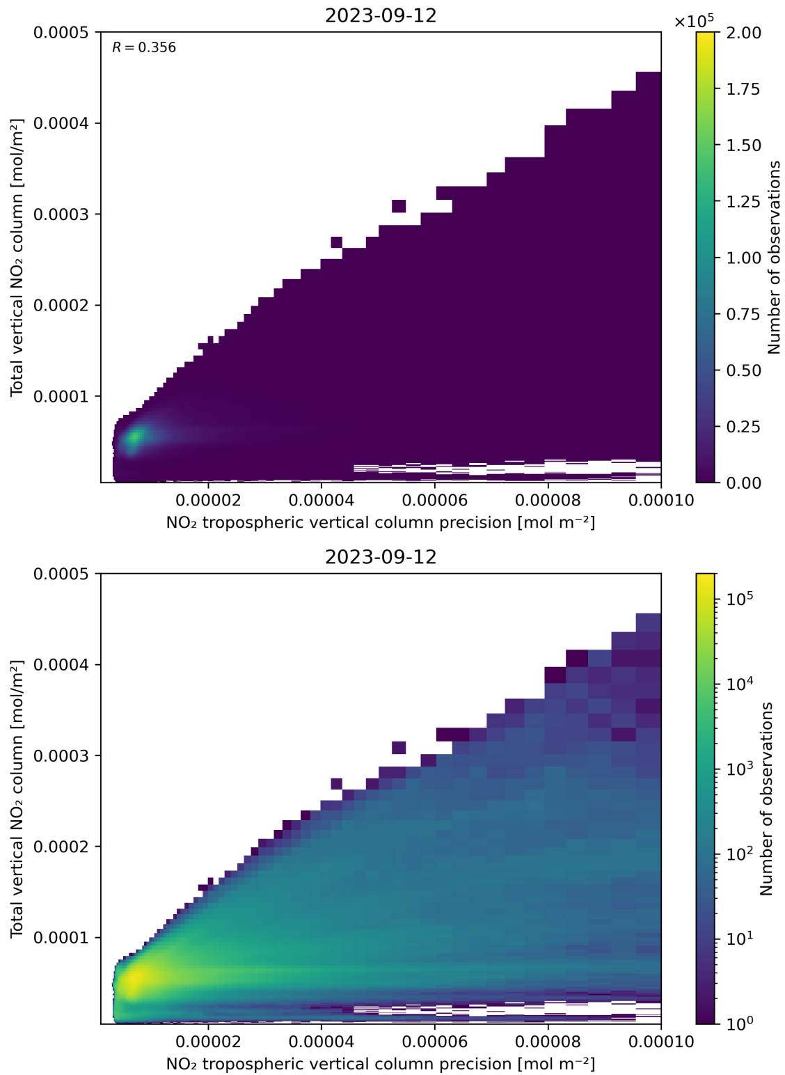
Figure 138: Scatter density plot of “NO 2 tropospheric vertical column precision” against “Total vertical NO 2 column” for 2023-09-11 to 2023-09-13.
