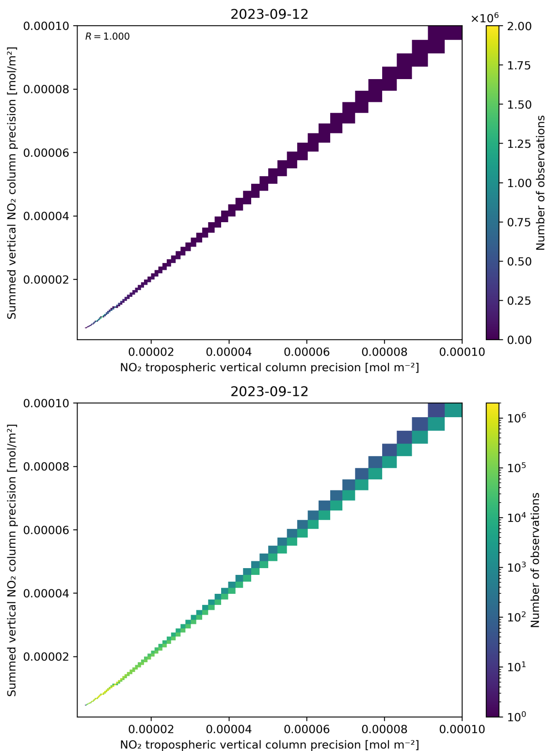
Figure 137: Scatter density plot of “NO 2 tropospheric vertical column precision” against “Summed vertical NO 2 column precision” for 2023-09-11 to 2023-09-13.
