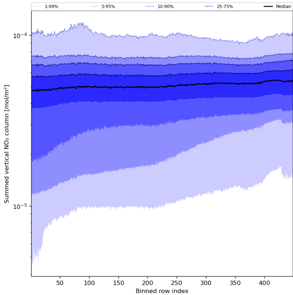
Figure 57: Along track statistics of “Summed vertical NO 2 column” for 2023-09-11 to 2023-09-13
