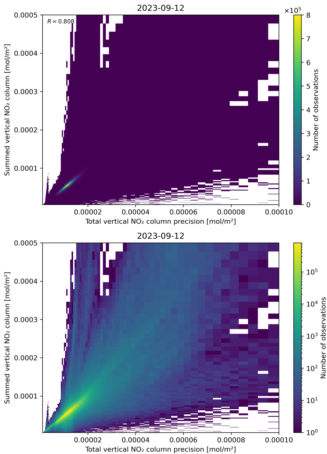
Figure 117: Scatter density plot of “Total vertical NO 2 column precision” against “Summed vertical NO 2 column” for 2023-09-11 to 2023-09-13.
