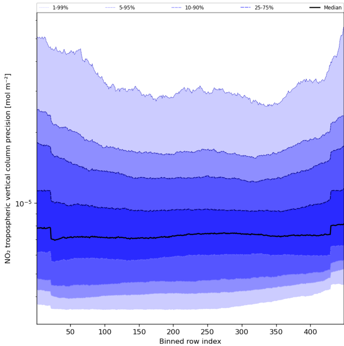
Figure 47: Along track statistics of “NO 2 tropospheric vertical column precision” for 2023-09-11 to 2023-09-13
