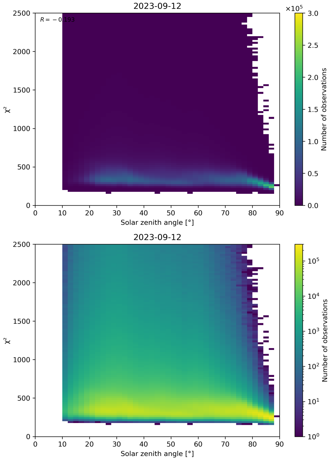
Figure 148: Scatter density plot of “Solar zenith angle” against “ \chi^2 ” for 2023-09-11 to 2023-09-13.
