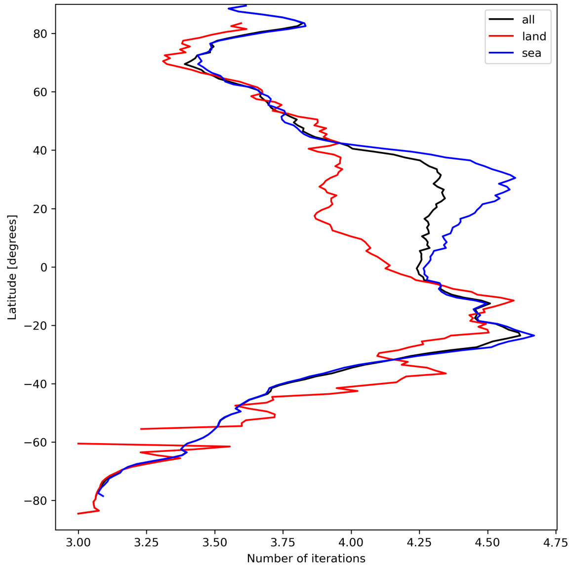
Figure 17: Zonal average of “Number of iterations” for 2023-09-11 to 2023-09-13.
