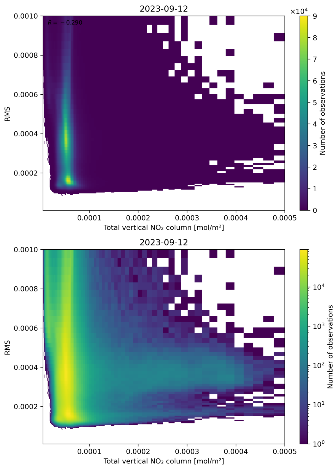
Figure 120: Scatter density plot of “Total vertical NO 2 column” against “RMS” for 2023-09-11 to 2023-09-13.
