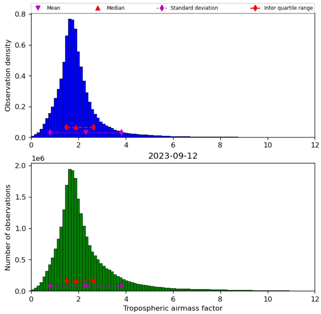
Figure 31: Histogram of “Tropospheric airmass factor” for 2023-09-11 to 2023-09-13
