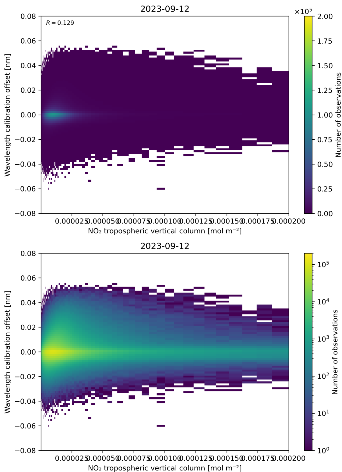
Figure 143: Scatter density plot of “NO 2 tropospheric vertical column” against “Wavelength calibration offset” for 2023-09-11 to 2023-09-13.
