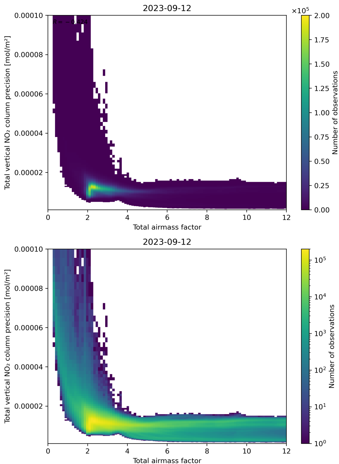
Figure 68: Scatter density plot of “Total airmass factor” against “Total vertical NO 2 column precision” for 2023-09-11 to 2023-09-13.
