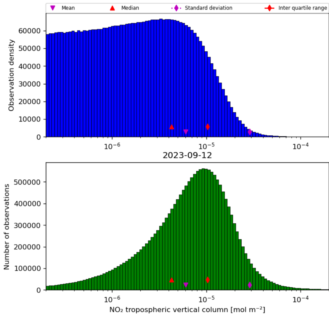
Figure 29: Histogram of “NO 2 tropospheric vertical column” for 2023-09-11 to 2023-09-13
