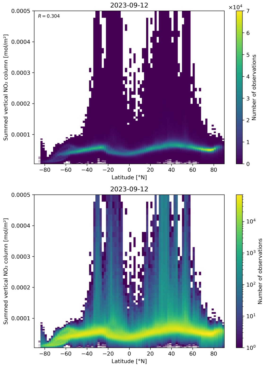
Figure 88: Scatter density plot of “Latitude” against “Summed vertical NO 2 column” for 2023-09-11 to 2023-09-13.
