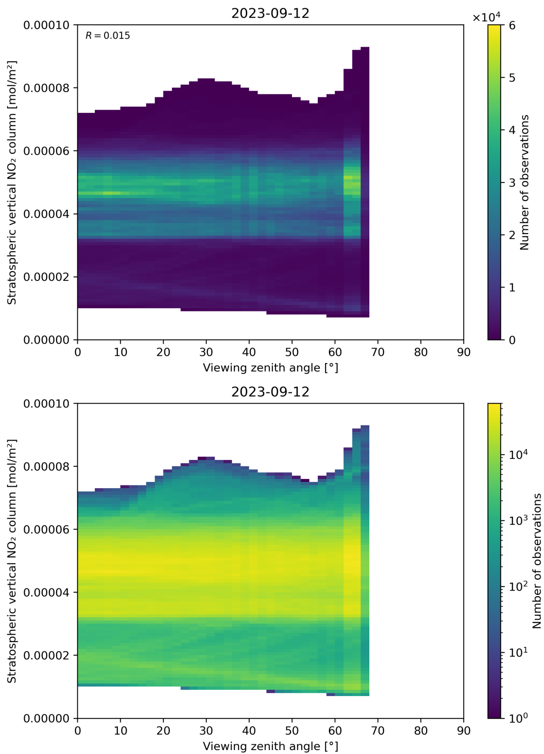
Figure 164: Scatter density plot of “Viewing zenith angle” against “Stratospheric vertical NO 2 column” for 2023-09-11 to 2023-09-13.
