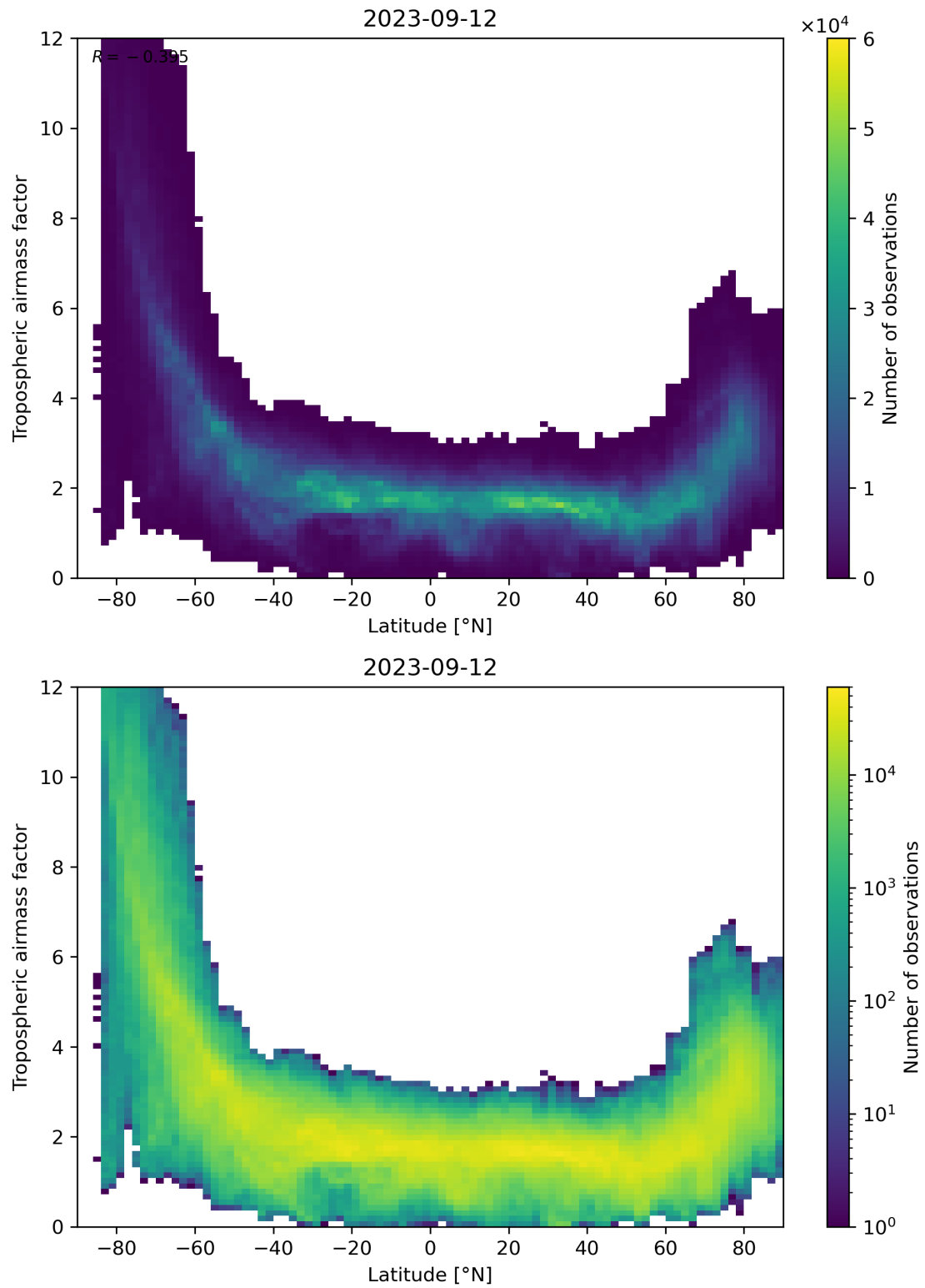
Figure 85: Scatter density plot of “Latitude” against “Tropospheric airmass factor” for 2023-09-11 to 2023-09-13.
