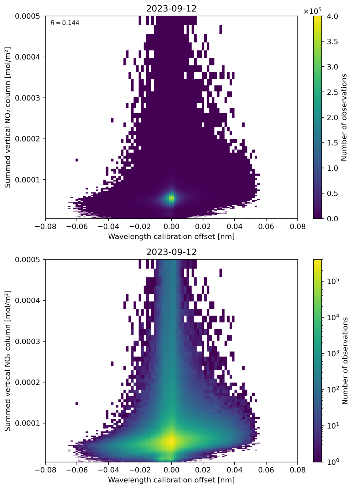
Figure 177: Scatter density plot of “Wavelength calibration offset” against “Summed vertical NO 2 column” for 2023-09-11 to 2023-09-13.
