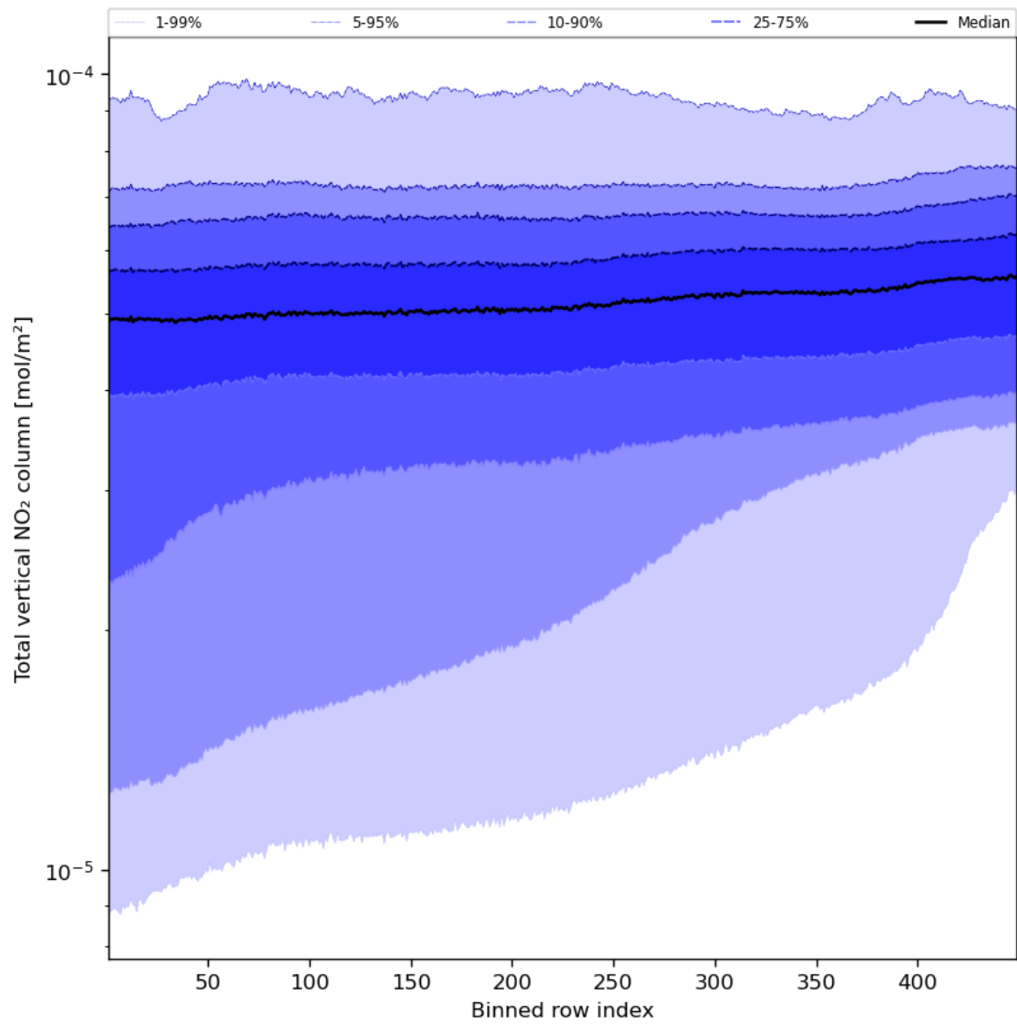
Figure 55: Along track statistics of “Total vertical NO 2 column” for 2023-09-11 to 2023-09-13
