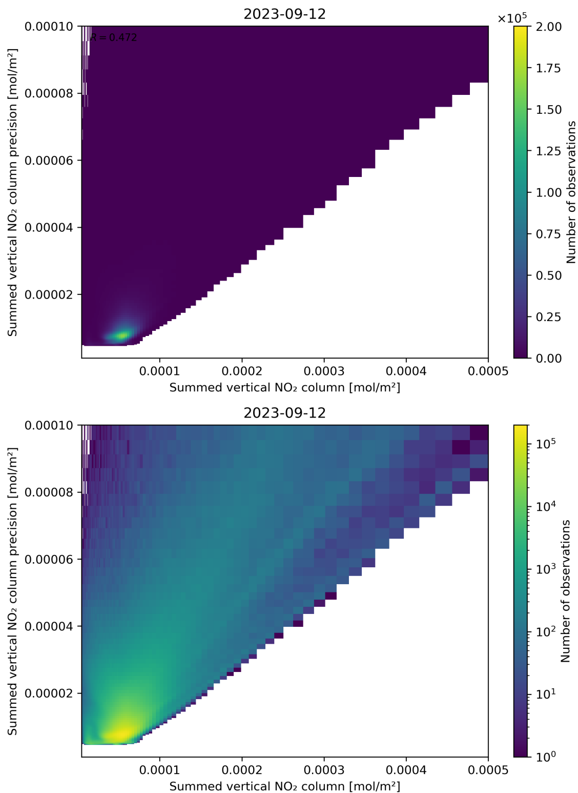
Figure 105: Scatter density plot of “Summed vertical NO 2 column” against “Summed vertical NO 2 column precision” for 2023-09-11 to 2023-09-13.
