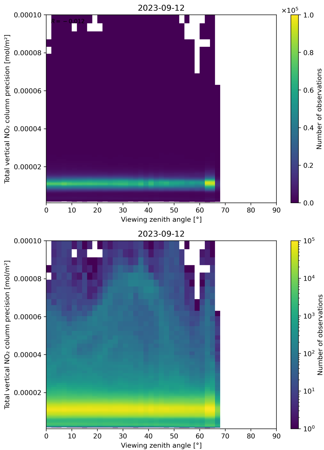
Figure 168: Scatter density plot of “Viewing zenith angle” against “Total vertical NO 2 column precision” for 2023-09-11 to 2023-09-13.
