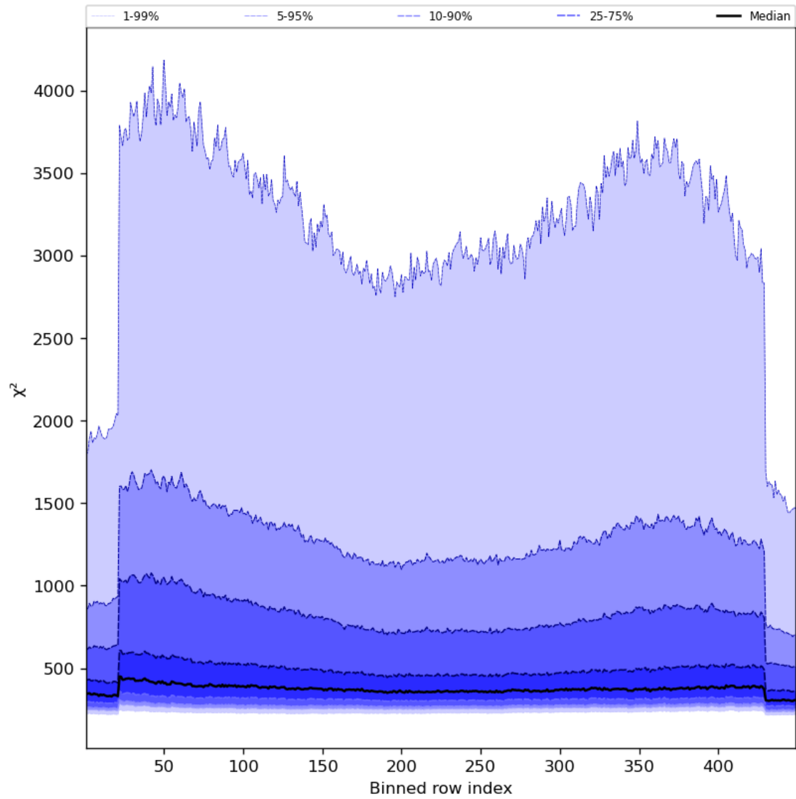
Figure 59: Along track statistics of “ \chi^2 ” for 2023-09-11 to 2023-09-13
