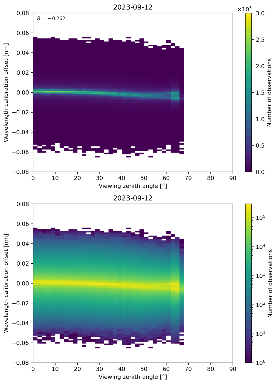
Figure 173: Scatter density plot of “Viewing zenith angle” against “Wavelength calibration offset” for 2023-09-11 to 2023-09-13.
