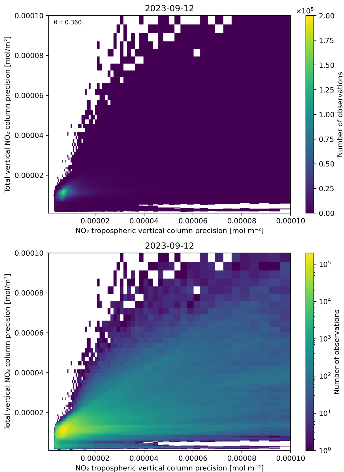
Figure 139: Scatter density plot of “NO 2 tropospheric vertical column precision” against “Total vertical NO 2 column precision” for 2023-09-11 to 2023-09-13.
