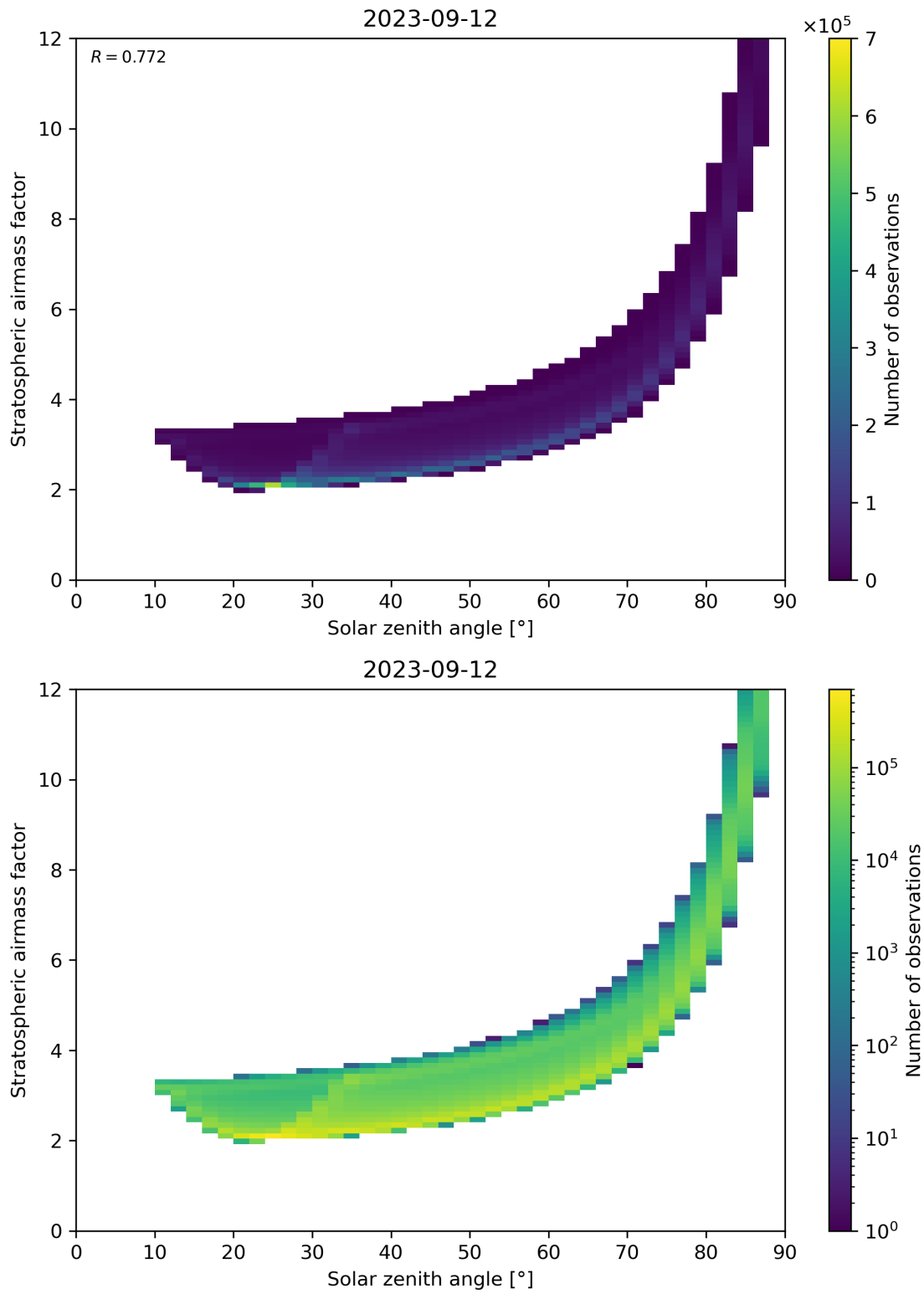
Figure 145: Scatter density plot of “Solar zenith angle” against “Stratospheric airmass factor” for 2023-09-11 to 2023-09-13.
