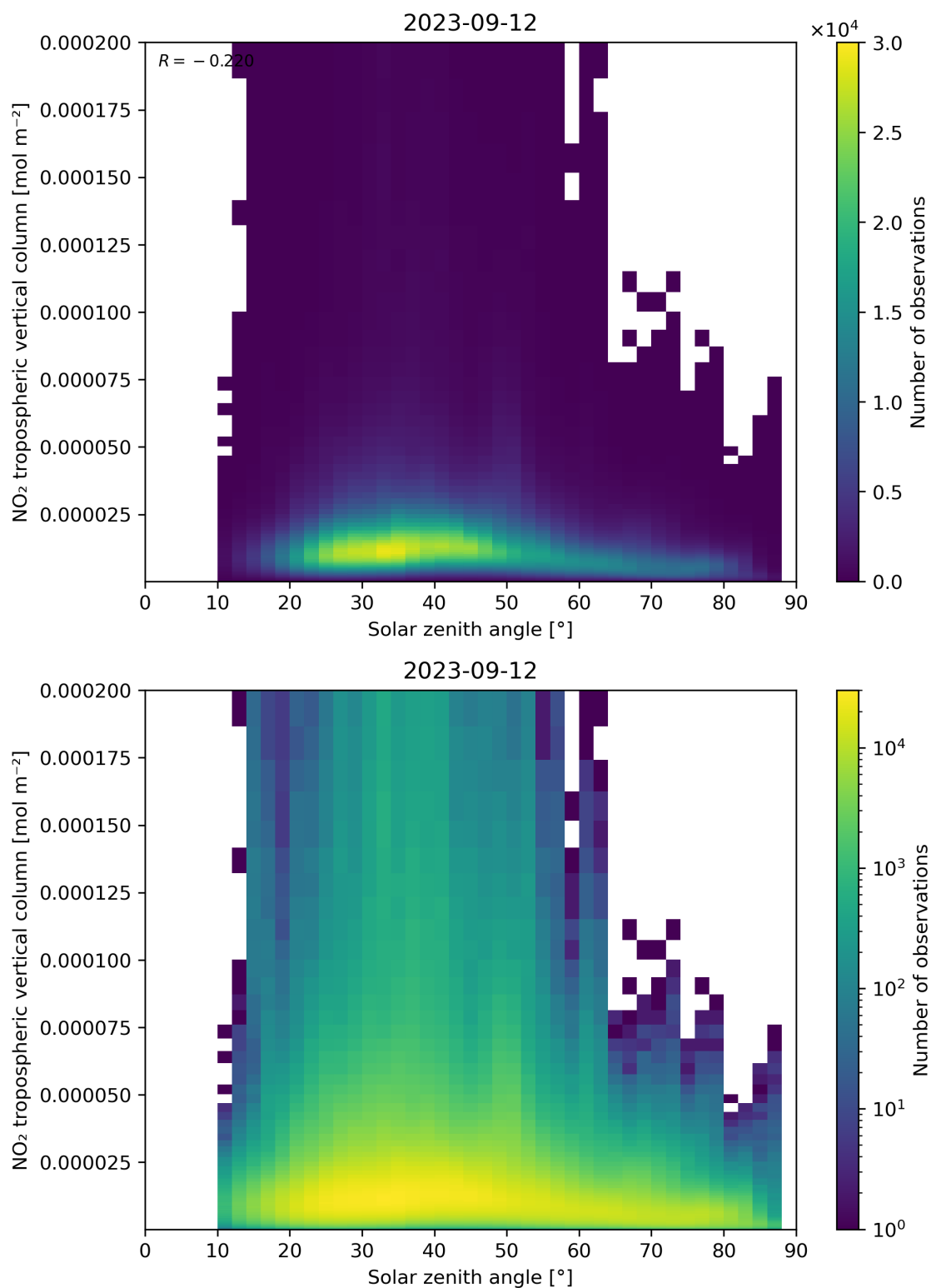
Figure 155: Scatter density plot of “Solar zenith angle” against “NO 2 tropospheric vertical column” for 2023-09-11 to 2023-09-13.
