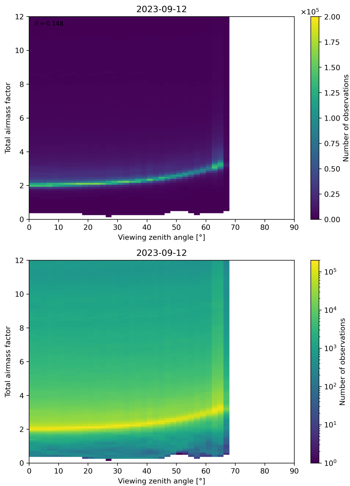
Figure 160: Scatter density plot of “Viewing zenith angle” against “Total airmass factor” for 2023-09-11 to 2023-09-13.
