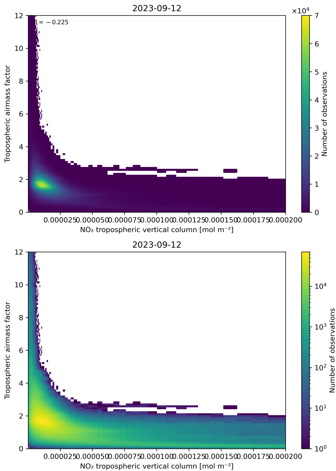
Figure 123: Scatter density plot of “NO 2 tropospheric vertical column” against “Tropospheric air mass factor” for 2023-09-11 to 2023-09-13.
