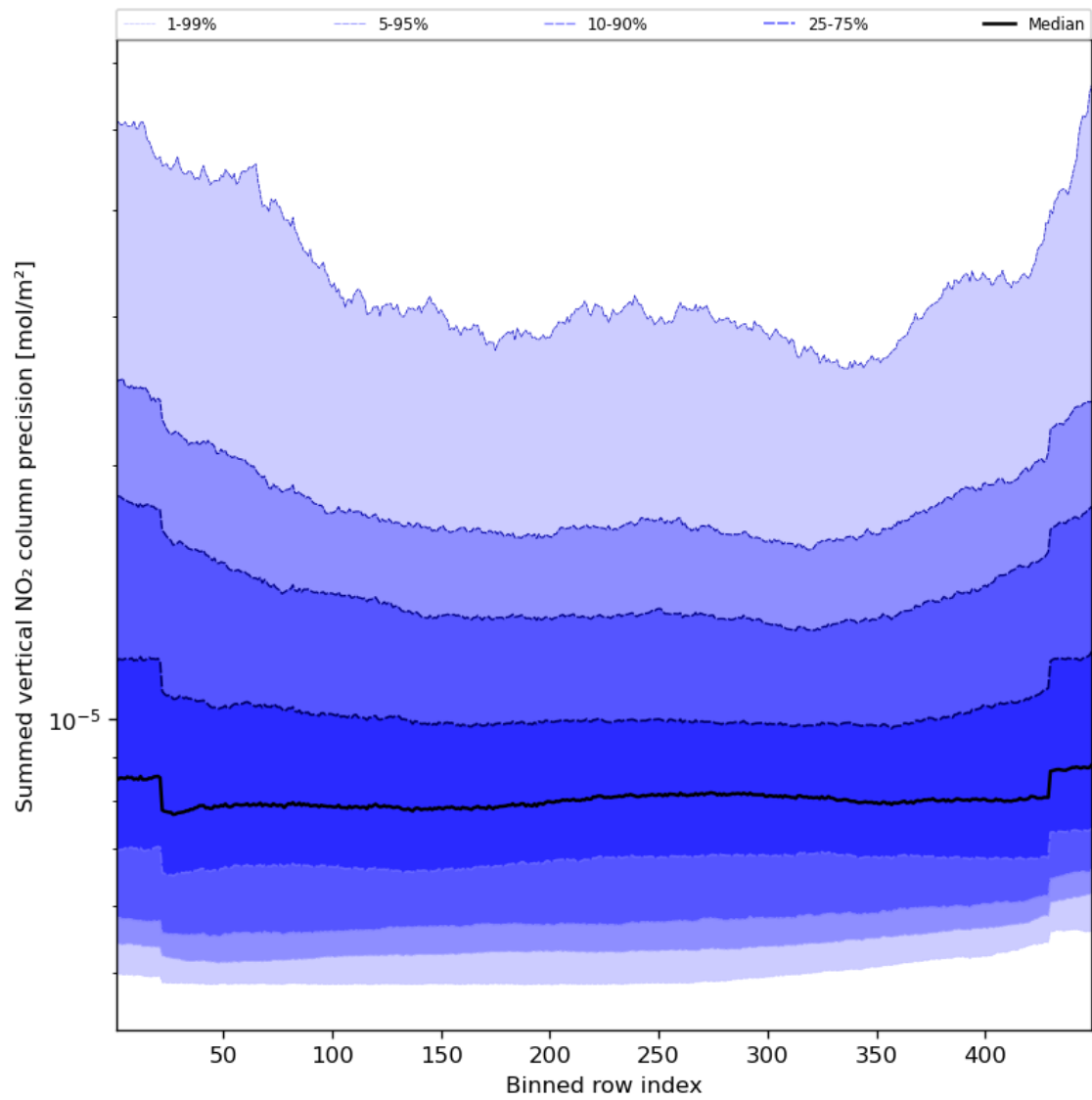
Figure 58: Along track statistics of “Summed vertical NO 2 column precision” for 2023-09-11 to 2023-09-13
