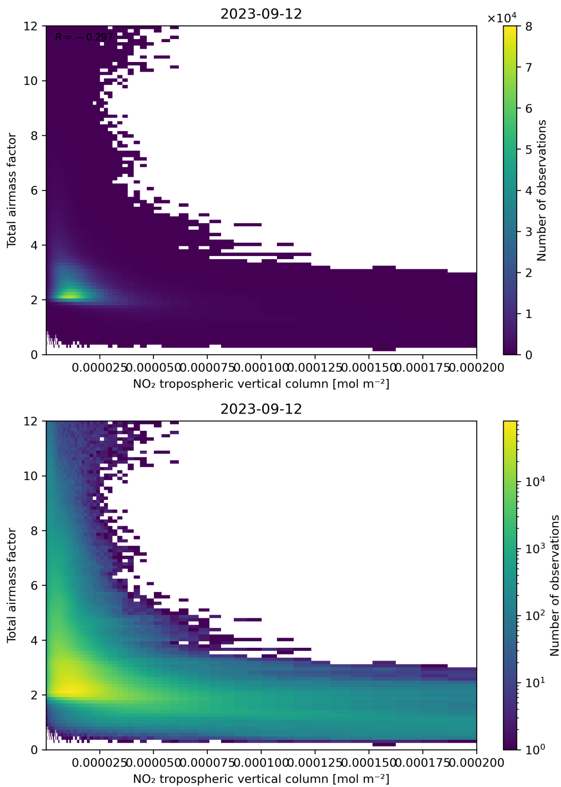
Figure 122: Scatter density plot of “NO 2 tropospheric vertical column” against “Total air mass factor” for 2023-09-11 to 2023-09-13.
