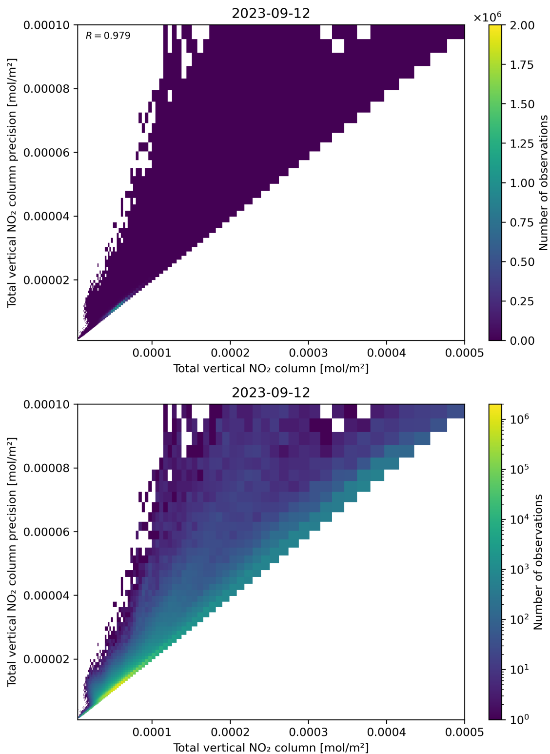
Figure 114: Scatter density plot of “Total vertical NO 2 column” against “Total vertical NO 2 column precision” for 2023-09-11 to 2023-09-13.
