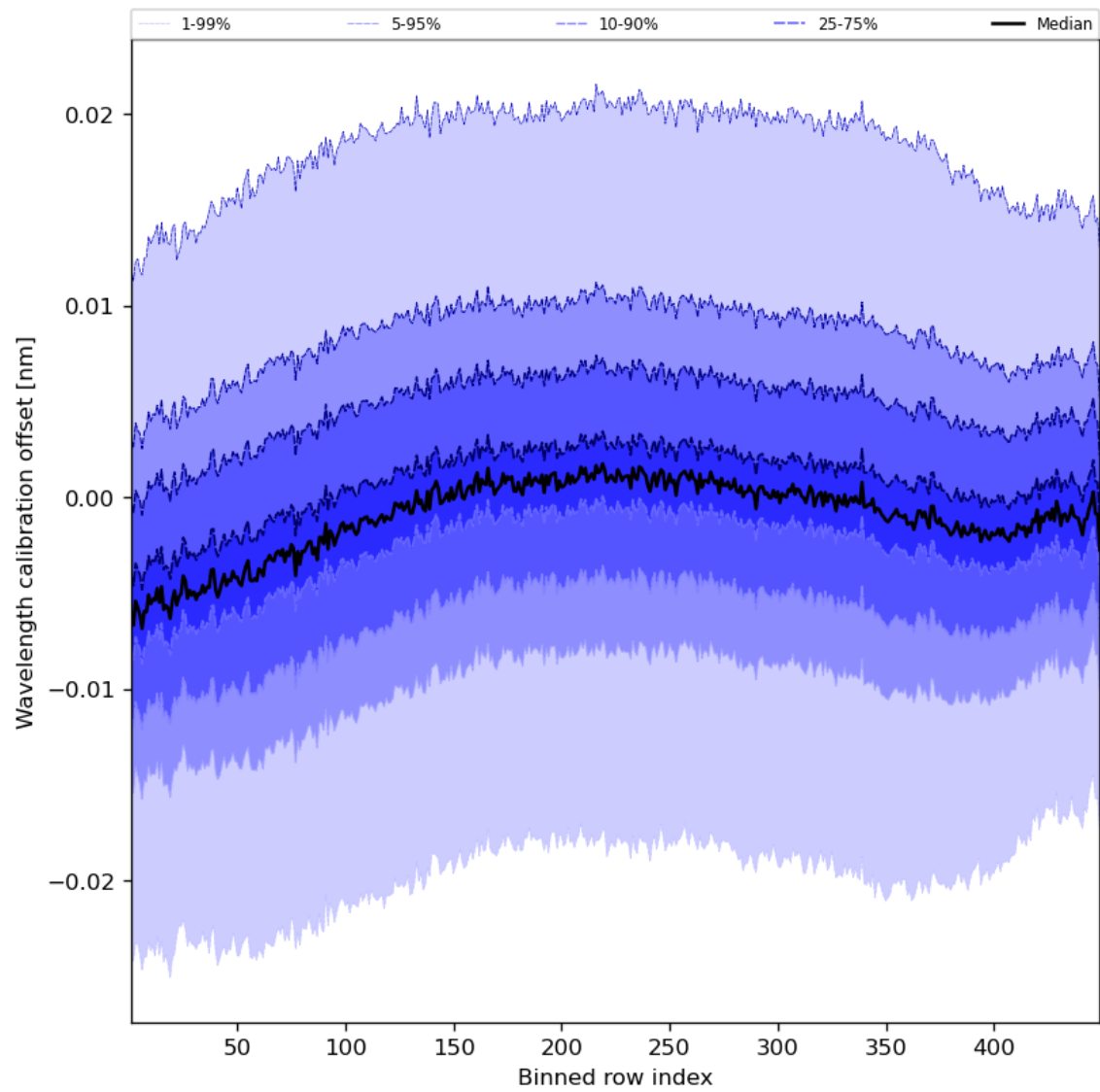
Figure 52: Along track statistics of “Wavelength calibration offset” for 2023-09-11 to 2023-09-13
