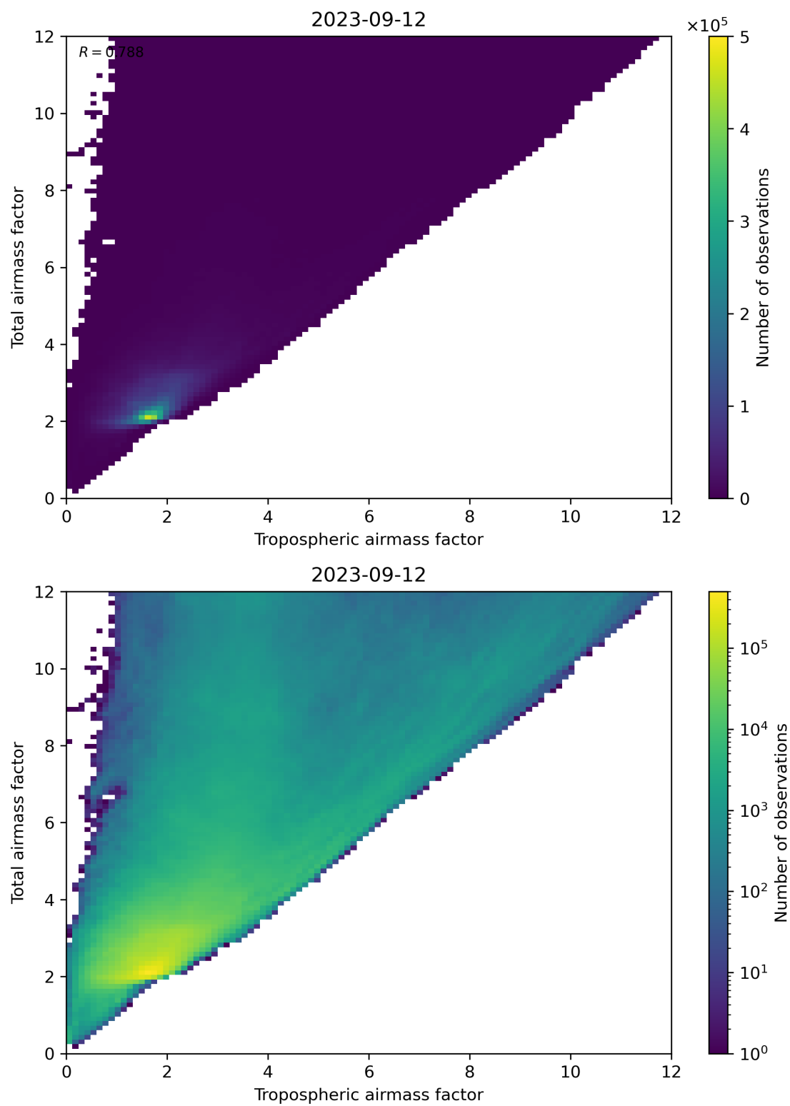
Figure 72: Scatter density plot of “Tropospheric airmass factor” against “Total airmass factor” for 2023-09-11 to 2023-09-13.
