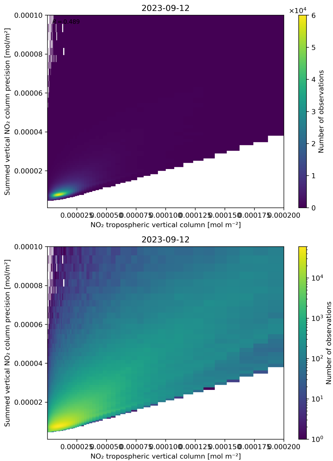
Figure 127: Scatter density plot of “NO 2 tropospheric vertical column” against “Summed vertical NO 2 column precision” for 2023-09-11 to 2023-09-13.
