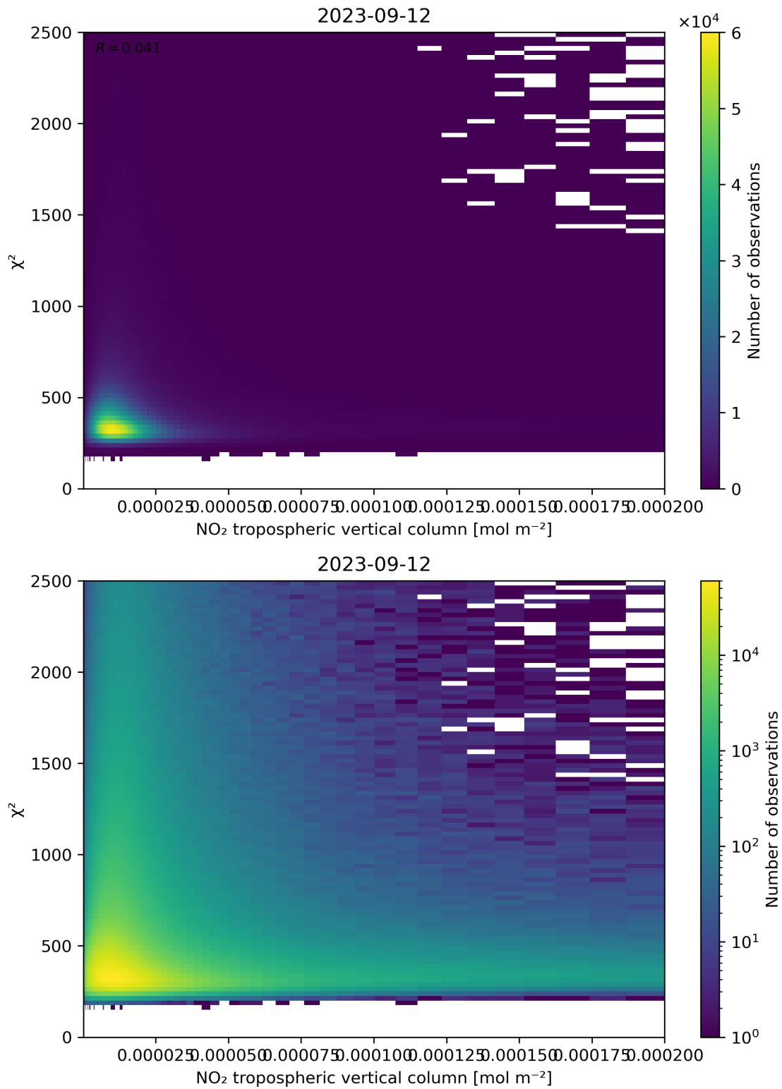
Figure 124: Scatter density plot of “NO 2 tropospheric vertical column” against “ \chi^2 ” for 2023-09-11 to 2023-09-13.
