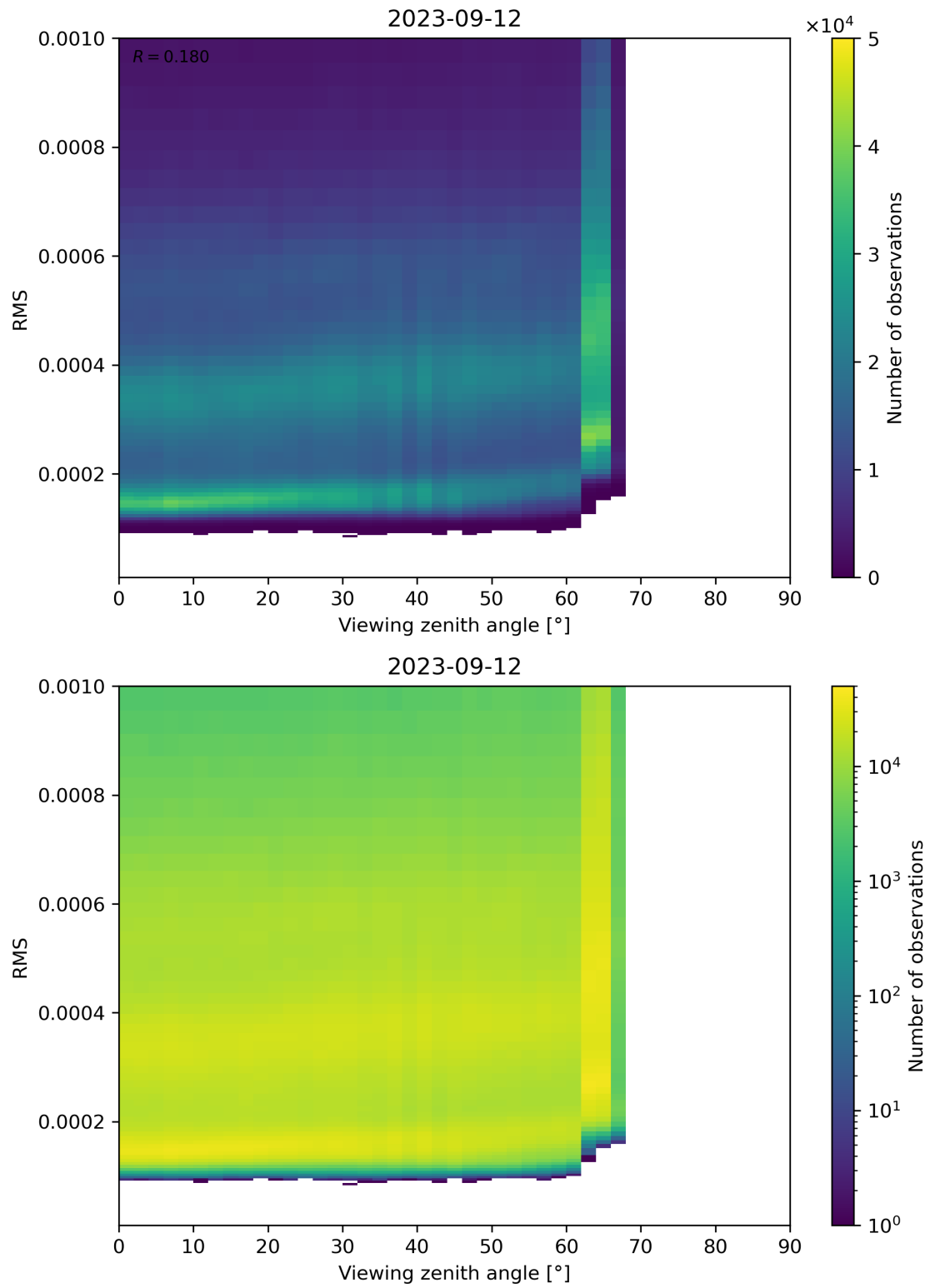
Figure 171: Scatter density plot of “Viewing zenith angle” against “RMS” for 2023-09-11 to 2023-09-13.
