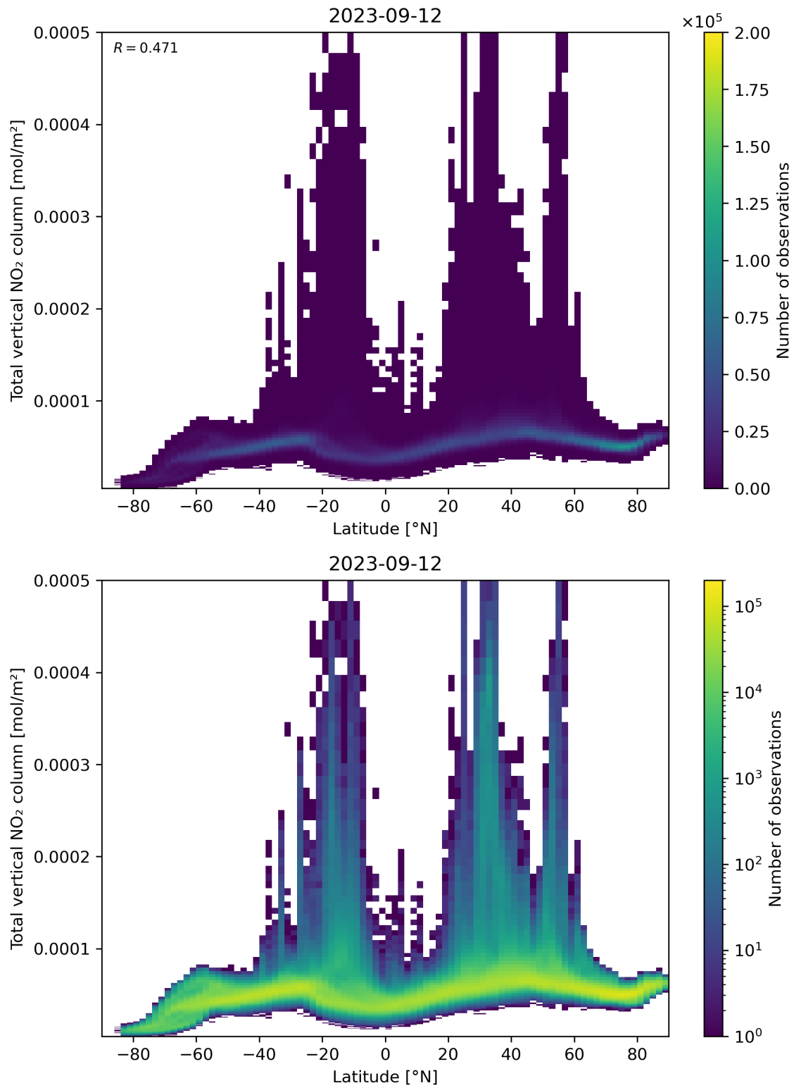
Figure 90: Scatter density plot of “Latitude” against “Total vertical NO 2 column” for 2023-09-11 to 2023-09-13.
