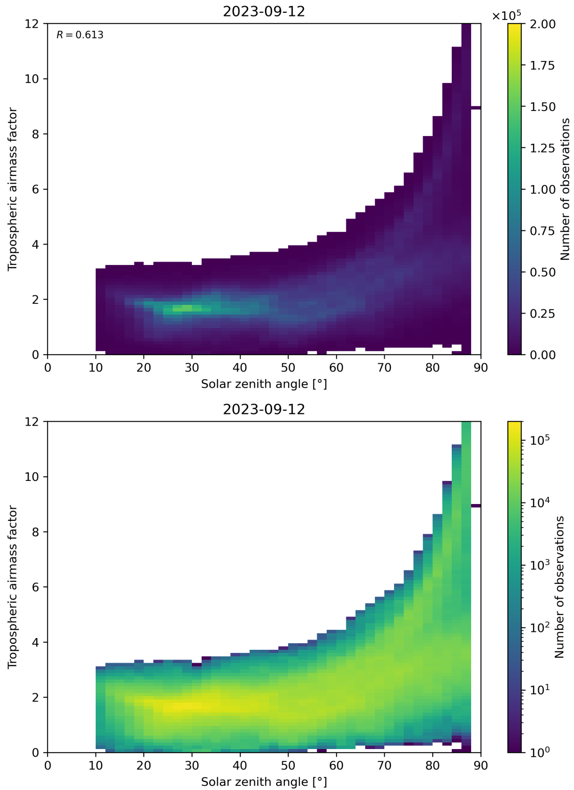
Figure 147: Scatter density plot of “Solar zenith angle” against “Tropospheric airmass factor” for 2023-09-11 to 2023-09-13.
