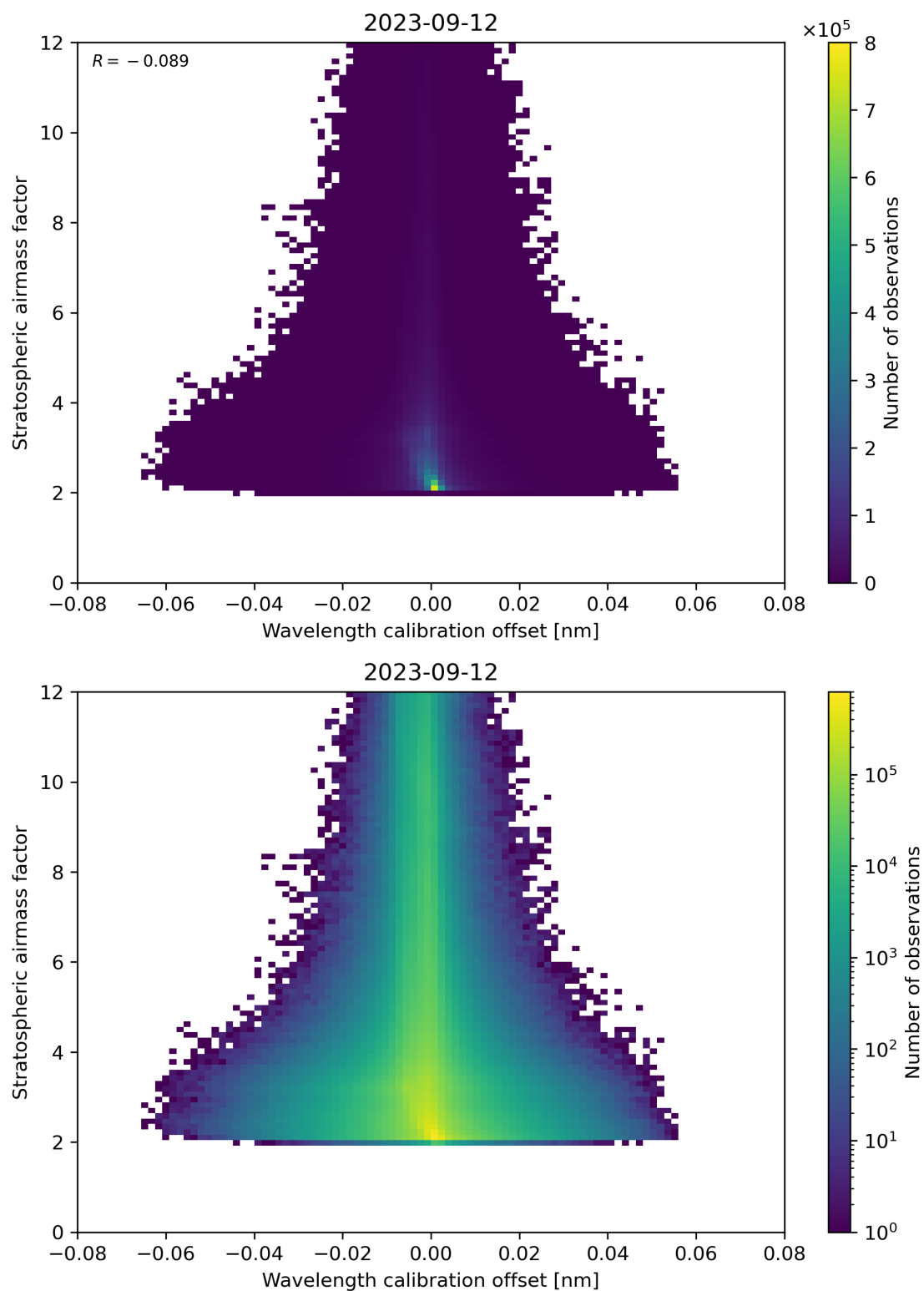
Figure 174: Scatter density plot of “Wavelength calibration offset” against “Stratospheric airmass factor” for 2023-09-11 to 2023-09-13.
