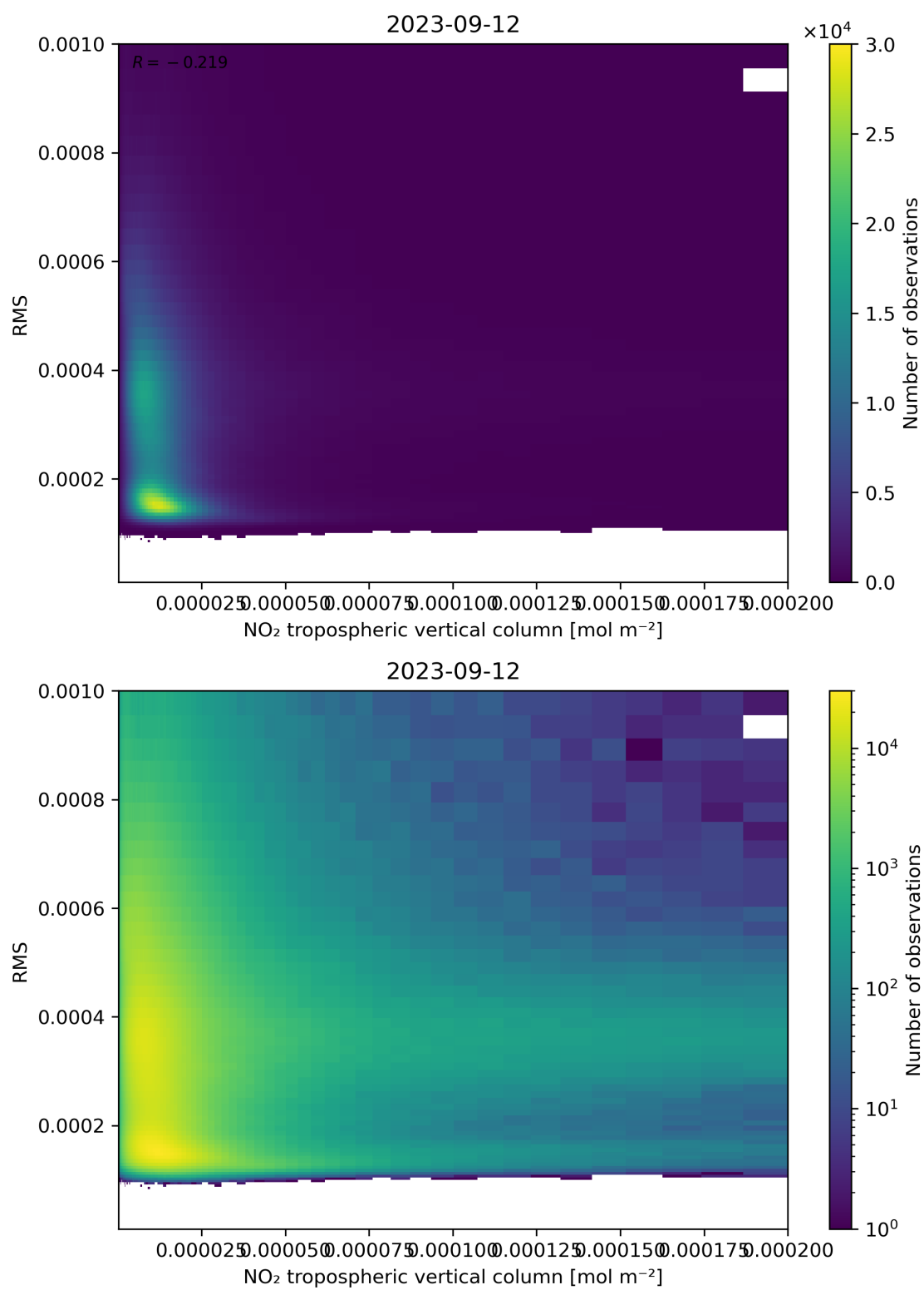
Figure 142: Scatter density plot of “NO 2 tropospheric vertical column” against “RMS” for 2023-09-11 to 2023-09-13.
