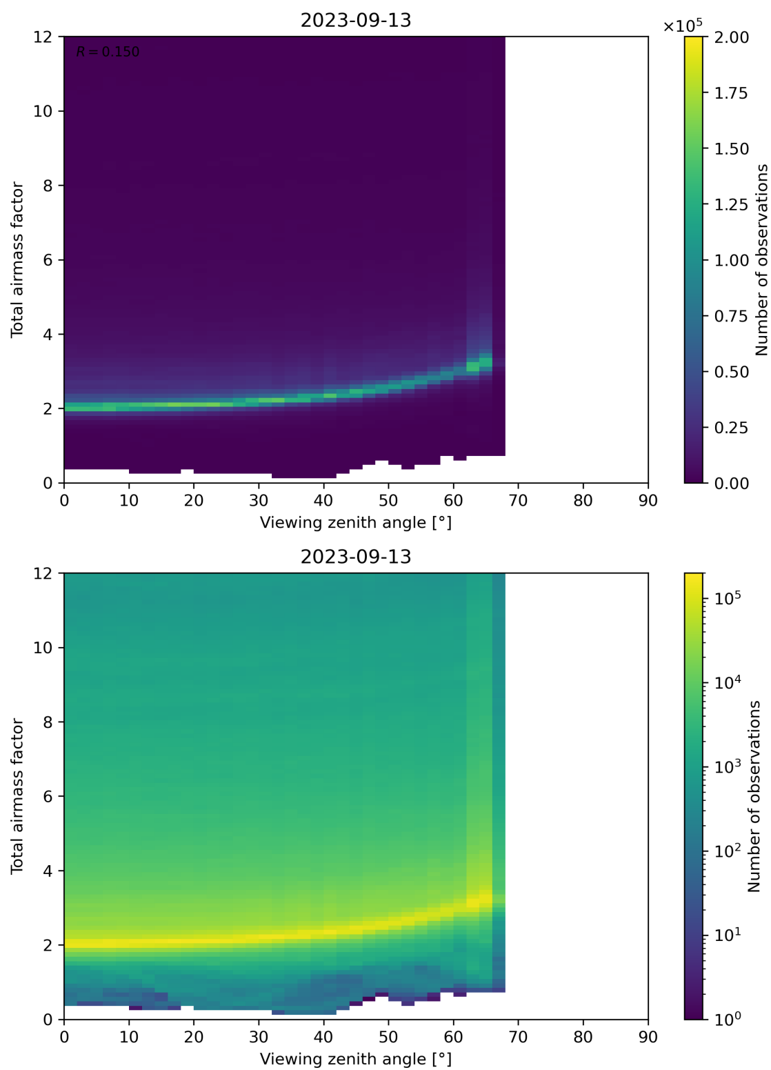
Figure 160: Scatter density plot of “Viewing zenith angle” against “Total airmass factor” for 2023-09-12 to 2023-09-14.
