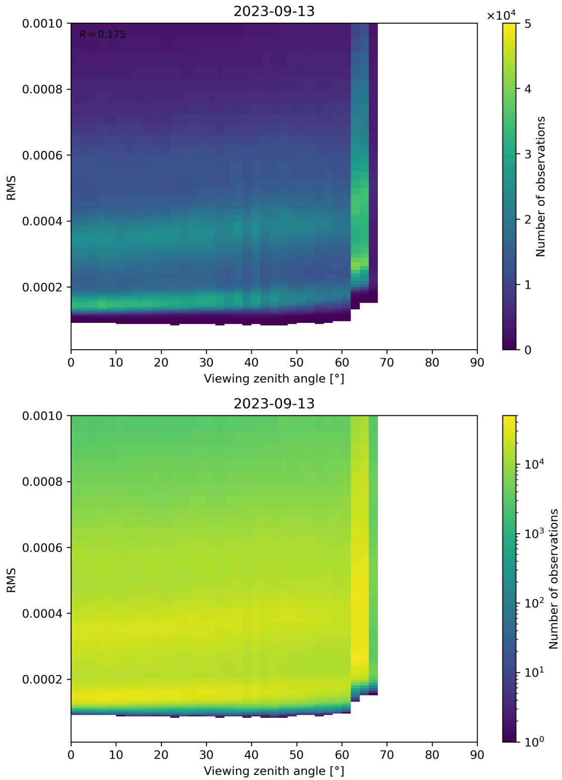
Figure 171: Scatter density plot of “Viewing zenith angle” against “RMS” for 2023-09-12 to 2023-09-14.
