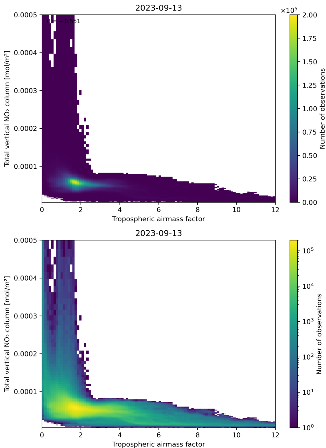
Figure 77: Scatter density plot of “Tropospheric airmass factor” against “Total vertical NO 2 column” for 2023-09-12 to 2023-09-14.
