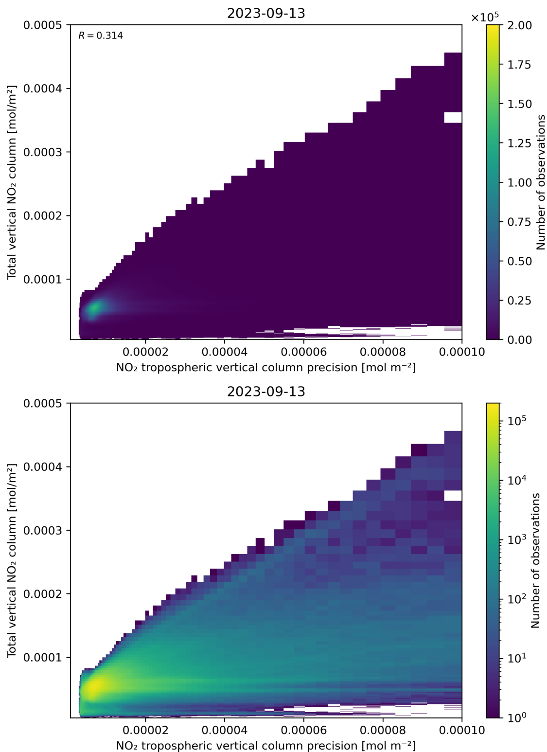
Figure 138: Scatter density plot of “NO 2 tropospheric vertical column precision” against “Total vertical NO 2 column” for 2023-09-12 to 2023-09-14.
