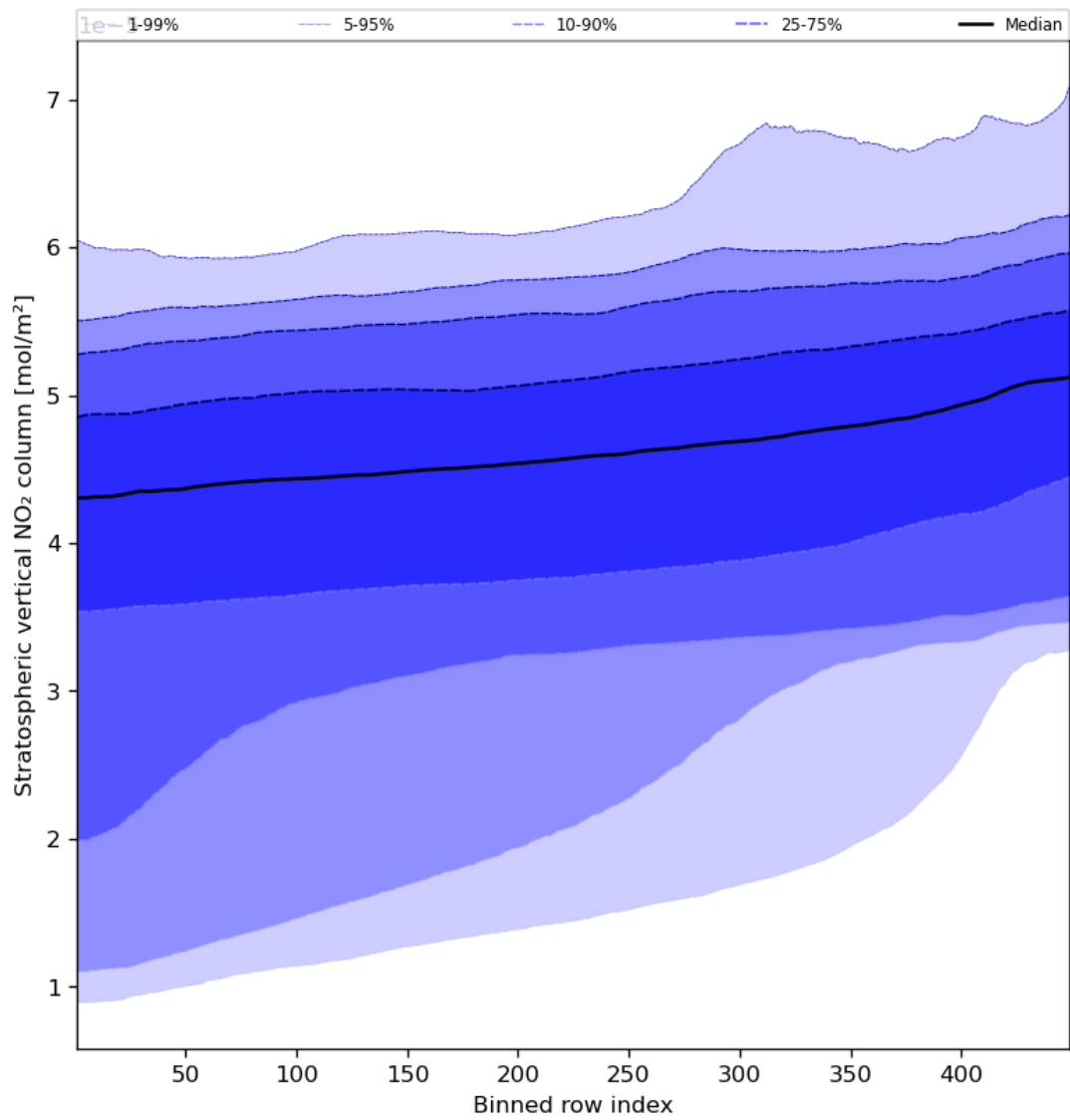
Figure 53: Along track statistics of “Stratospheric vertical NO 2 column” for 2023-09-12 to 2023-09-14
