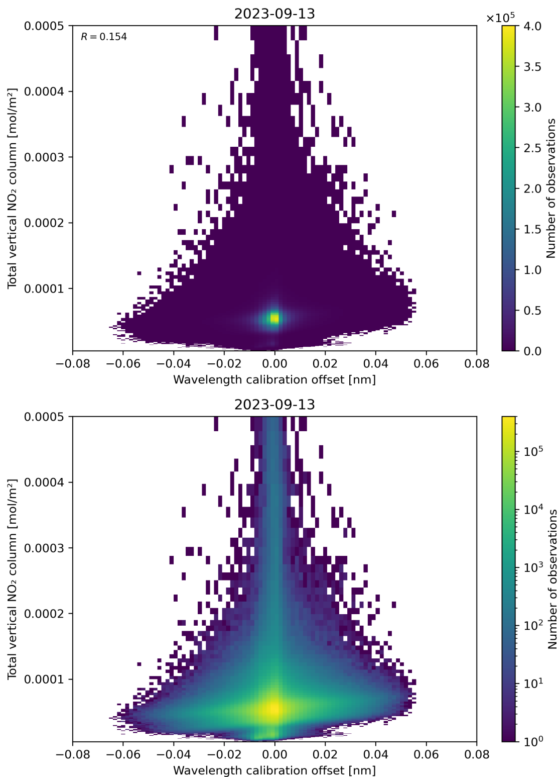
Figure 179: Scatter density plot of “Wavelength calibration offset” against “Total vertical NO 2 column” for 2023-09-12 to 2023-09-14.
