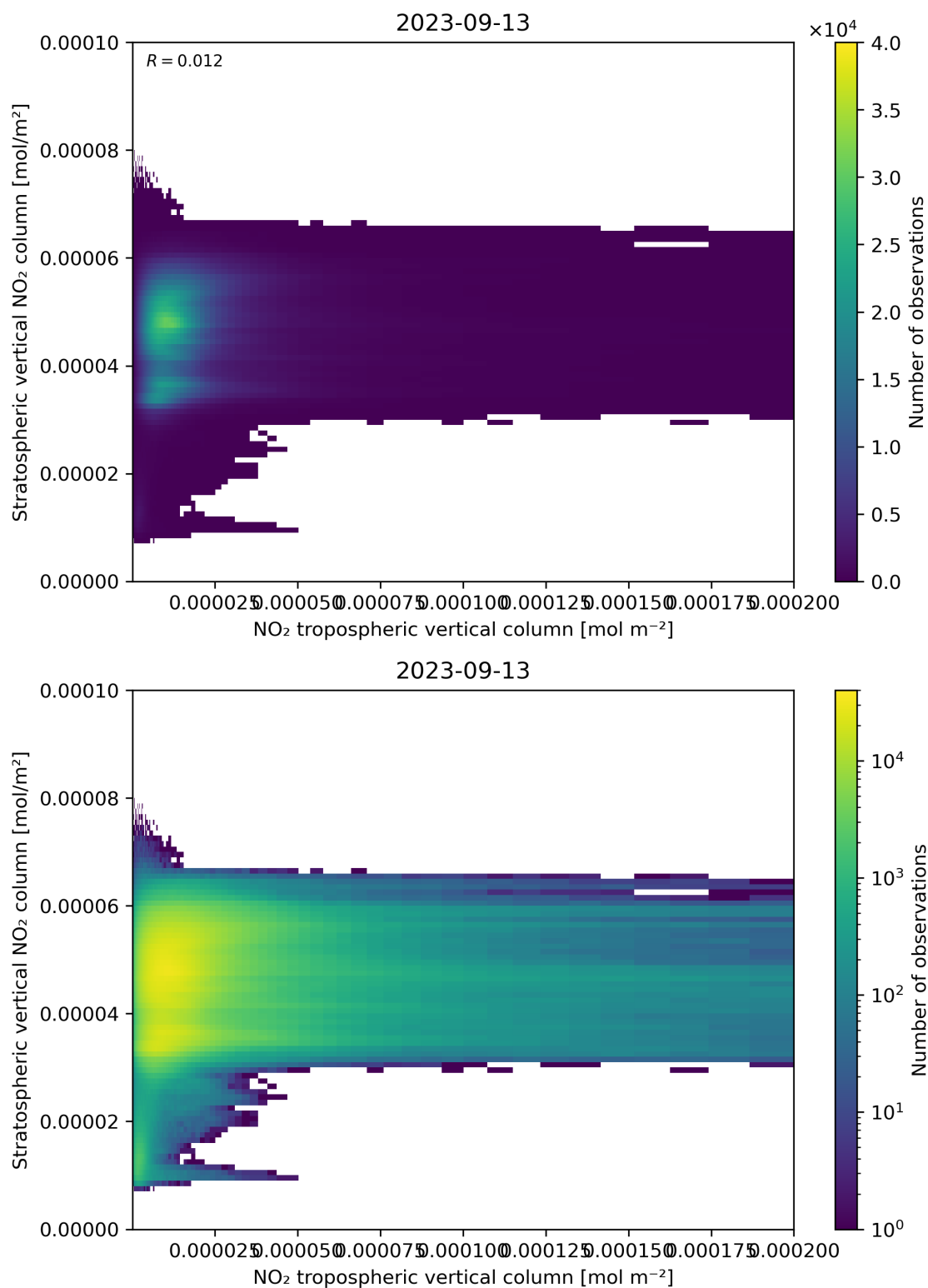
Figure 125: Scatter density plot of “NO 2 tropospheric vertical column” against “Stratospheric vertical NO 2 column” for 2023-09-12 to 2023-09-14.
