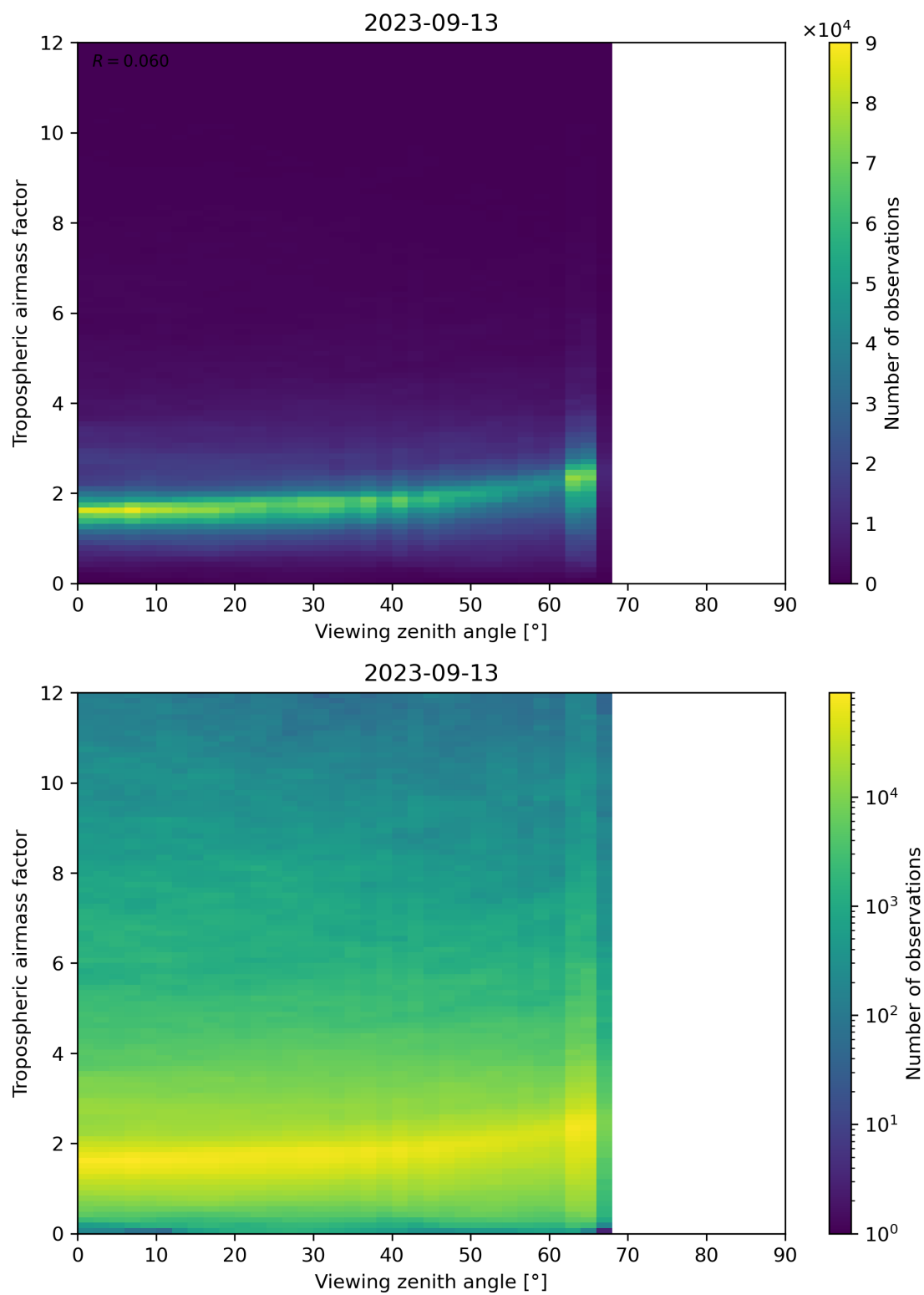
Figure 161: Scatter density plot of “Viewing zenith angle” against “Tropospheric airmass factor” for 2023-09-12 to 2023-09-14.
