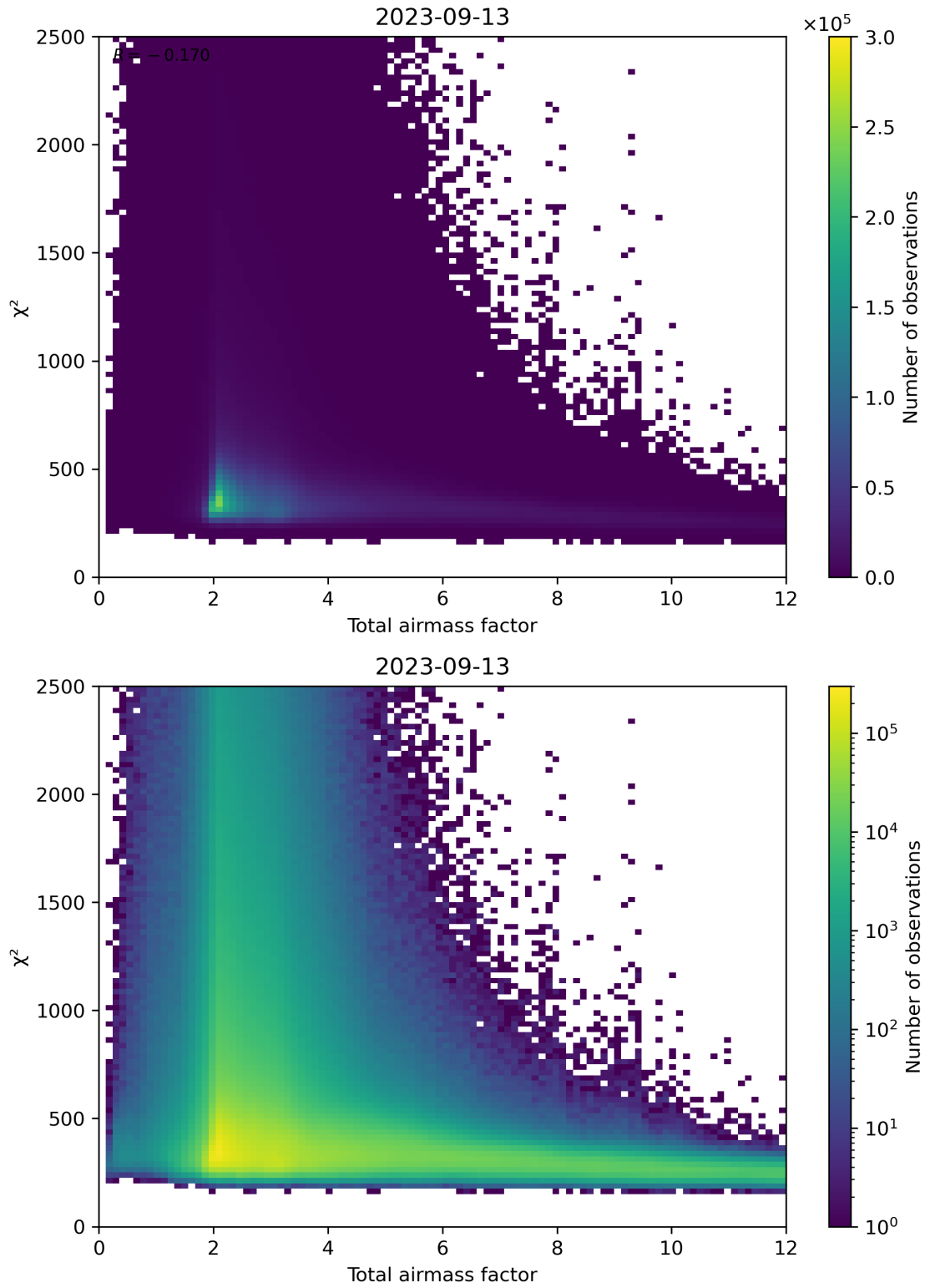
Figure 63: Scatter density plot of “Total airmass factor” against “ \chi^2 ” for 2023-09-12 to 2023-09-14.
