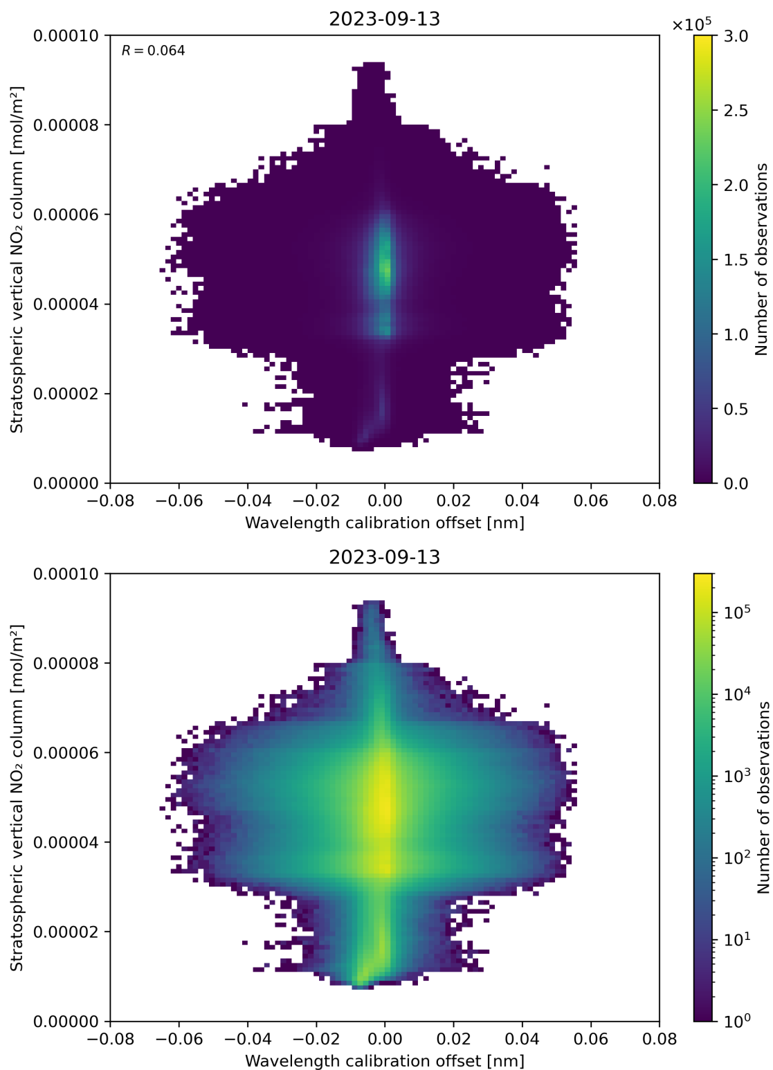
Figure 176: Scatter density plot of “Wavelength calibration offset” against “Stratospheric vertical NO 2 column” for 2023-09-12 to 2023-09-14.
