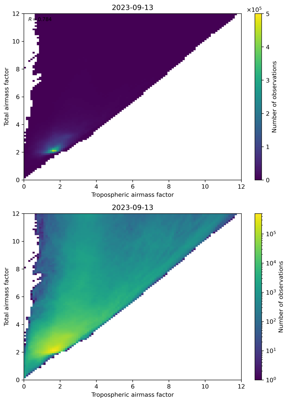
Figure 72: Scatter density plot of “Tropospheric airmass factor” against “Total airmass factor” for 2023-09-12 to 2023-09-14.
