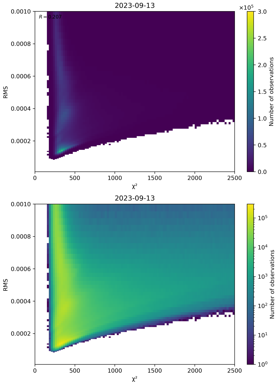
Figure 82: Scatter density plot of “ \chi^2 ” against “RMS” for 2023-09-12 to 2023-09-14.
