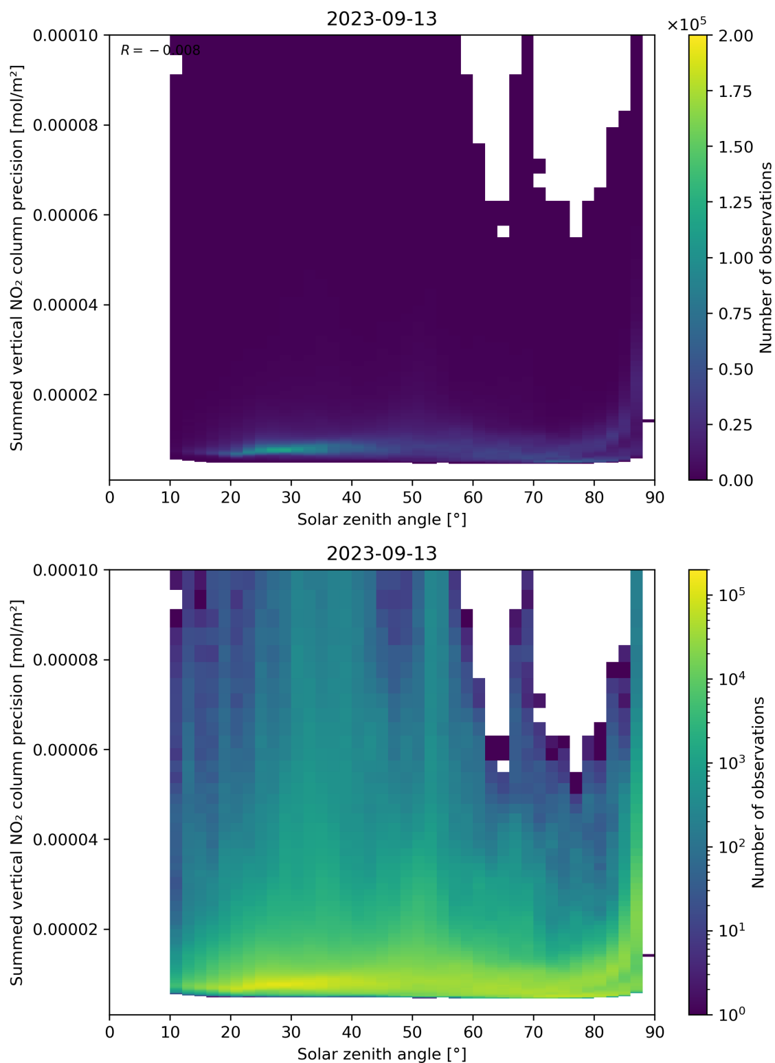
Figure 152: Scatter density plot of “Solar zenith angle” against “Summed vertical NO 2 column precision” for 2023-09-12 to 2023-09-14.
