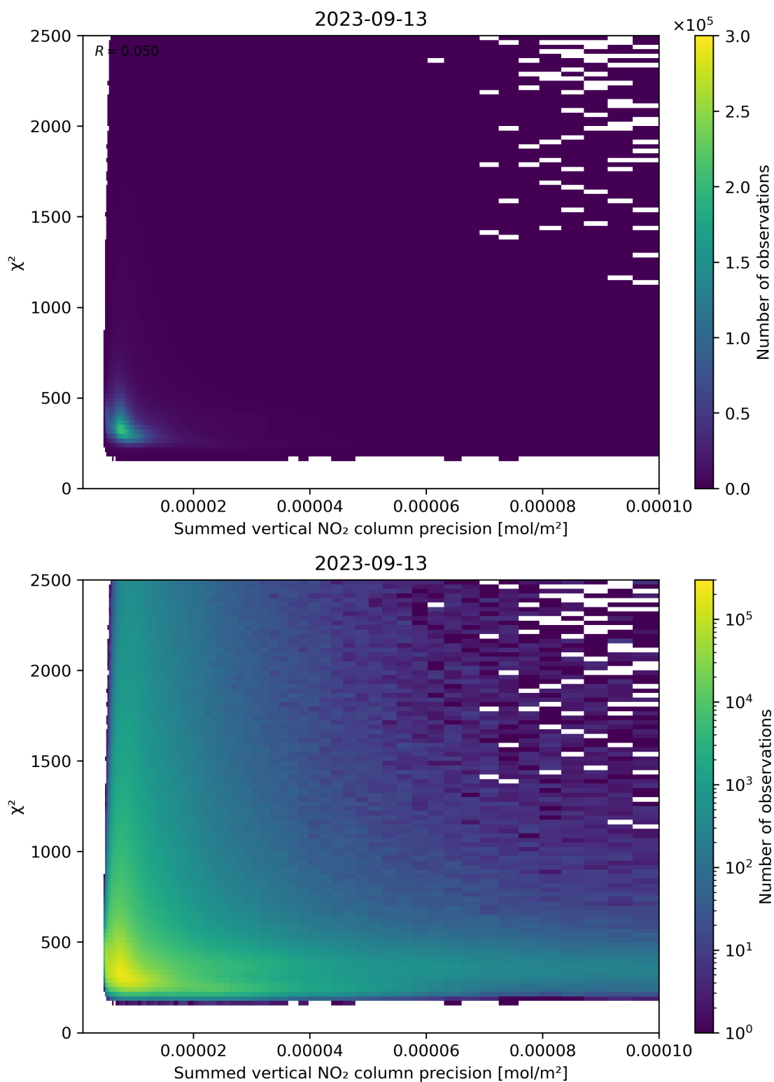
Figure 107: Scatter density plot of “Summed vertical NO 2 column precision” against “ \chi^2 ” for 2023-09-12 to 2023-09-14.
