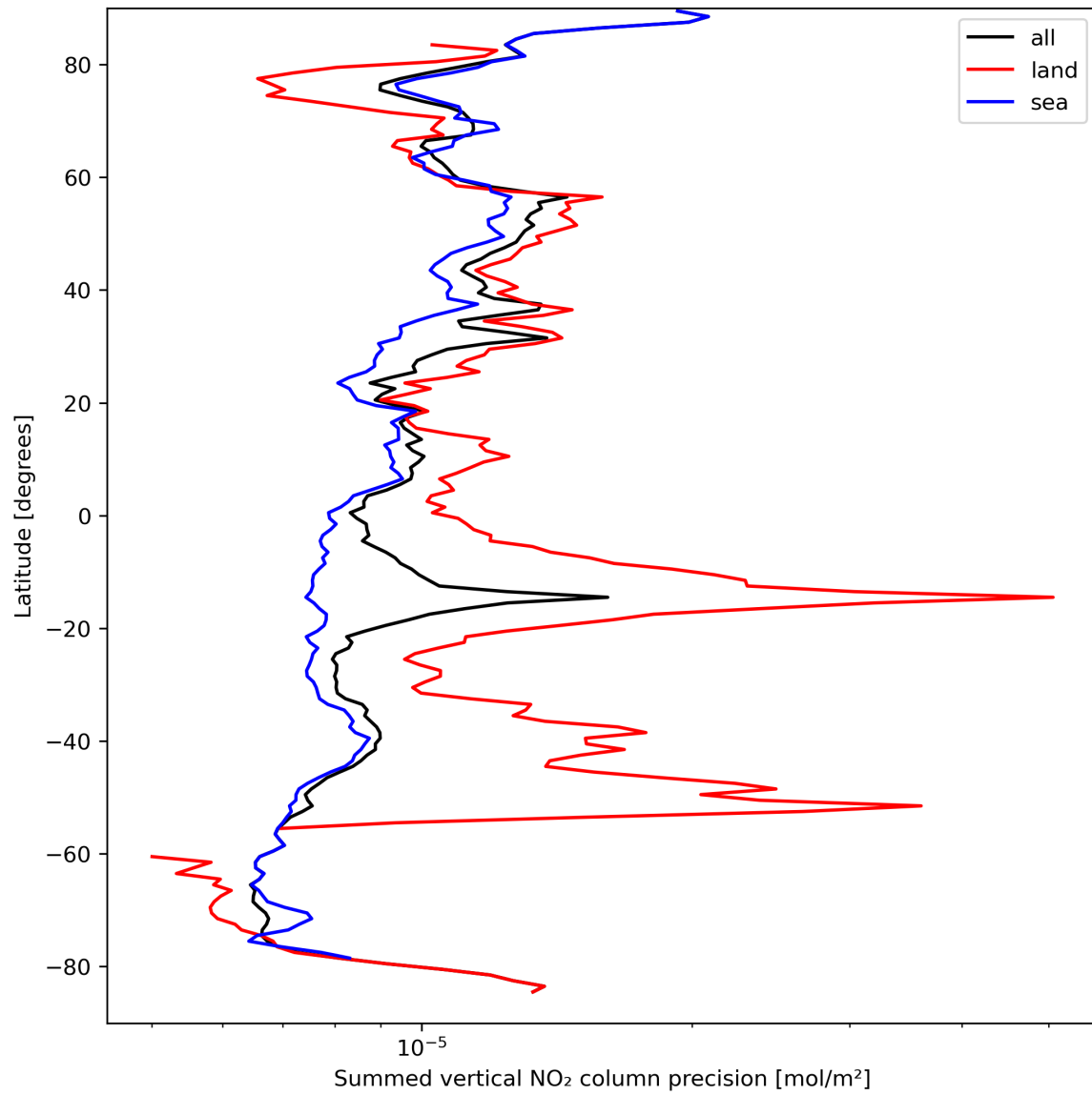
Figure 24: Zonal average of “Summed vertical NO 2 column precision” for 2023-09-12 to 2023-09-14.
