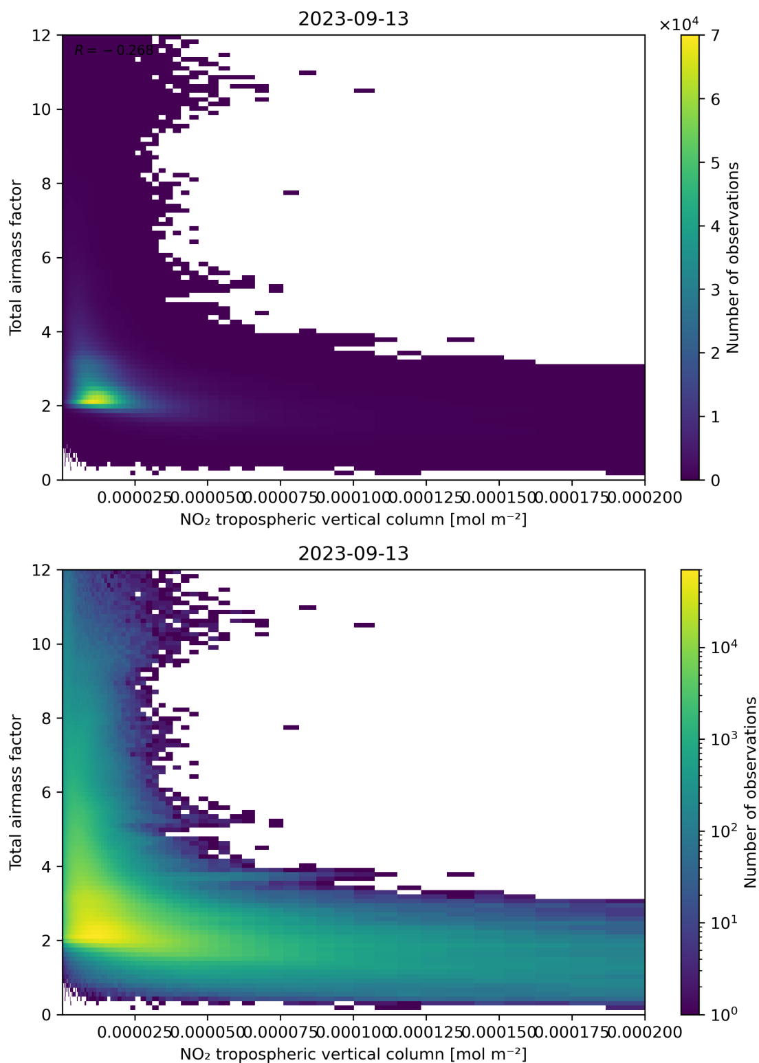
Figure 122: Scatter density plot of “NO 2 tropospheric vertical column” against “Total air mass factor” for 2023-09-12 to 2023-09-14.
