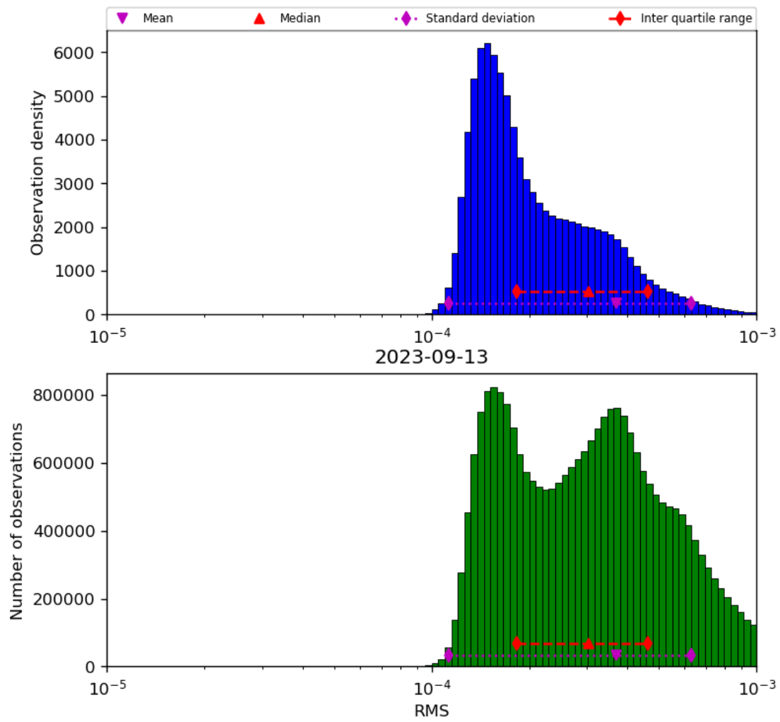
Figure 43: Histogram of “RMS” for 2023-09-12 to 2023-09-14
