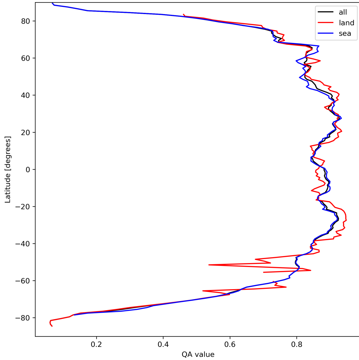
Figure 11: Zonal average of “QA value” for 2023-09-12 to 2023-09-14.
