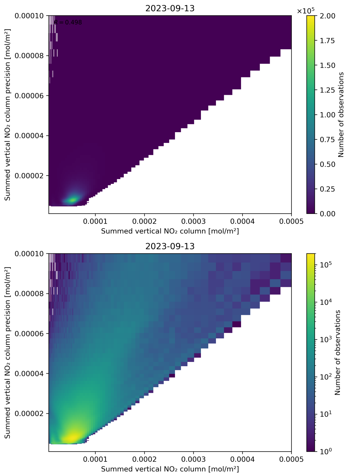
Figure 105: Scatter density plot of “Summed vertical NO 2 column” against “Summed vertical NO 2 column precision” for 2023-09-12 to 2023-09-14.
