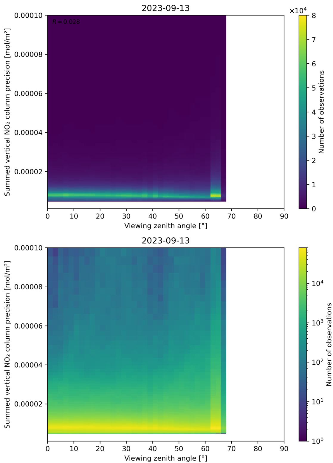
Figure 166: Scatter density plot of “Viewing zenith angle” against “Summed vertical NO 2 column precision” for 2023-09-12 to 2023-09-14.
