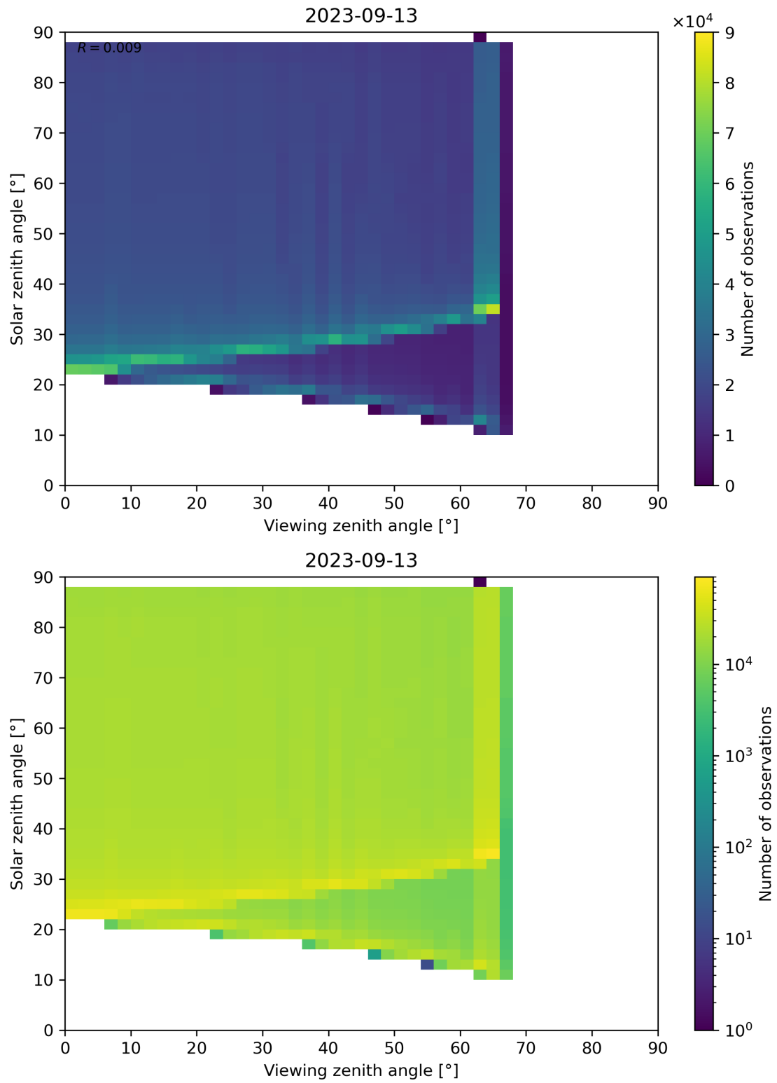
Figure 172: Scatter density plot of “Viewing zenith angle” against “Solar zenith angle” for 2023-09-12 to 2023-09-14.
