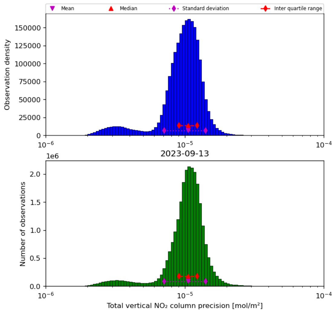
Figure 39: Histogram of “Total vertical NO 2 column precision” for 2023-09-12 to 2023-09-14
