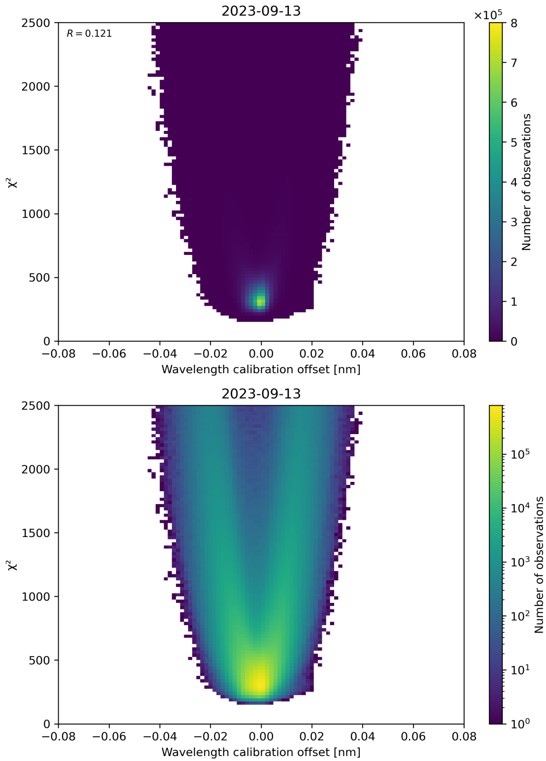
Figure 175: Scatter density plot of “Wavelength calibration offset” against “ \chi^2 ” for 2023-09-12 to 2023-09-14.
