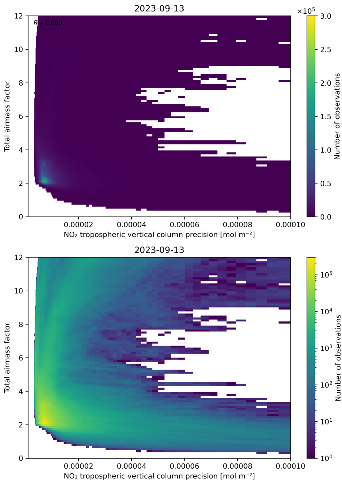
Figure 132: Scatter density plot of “NO 2 tropospheric vertical column precision” against “Total air mass factor” for 2023-09-12 to 2023-09-14.
