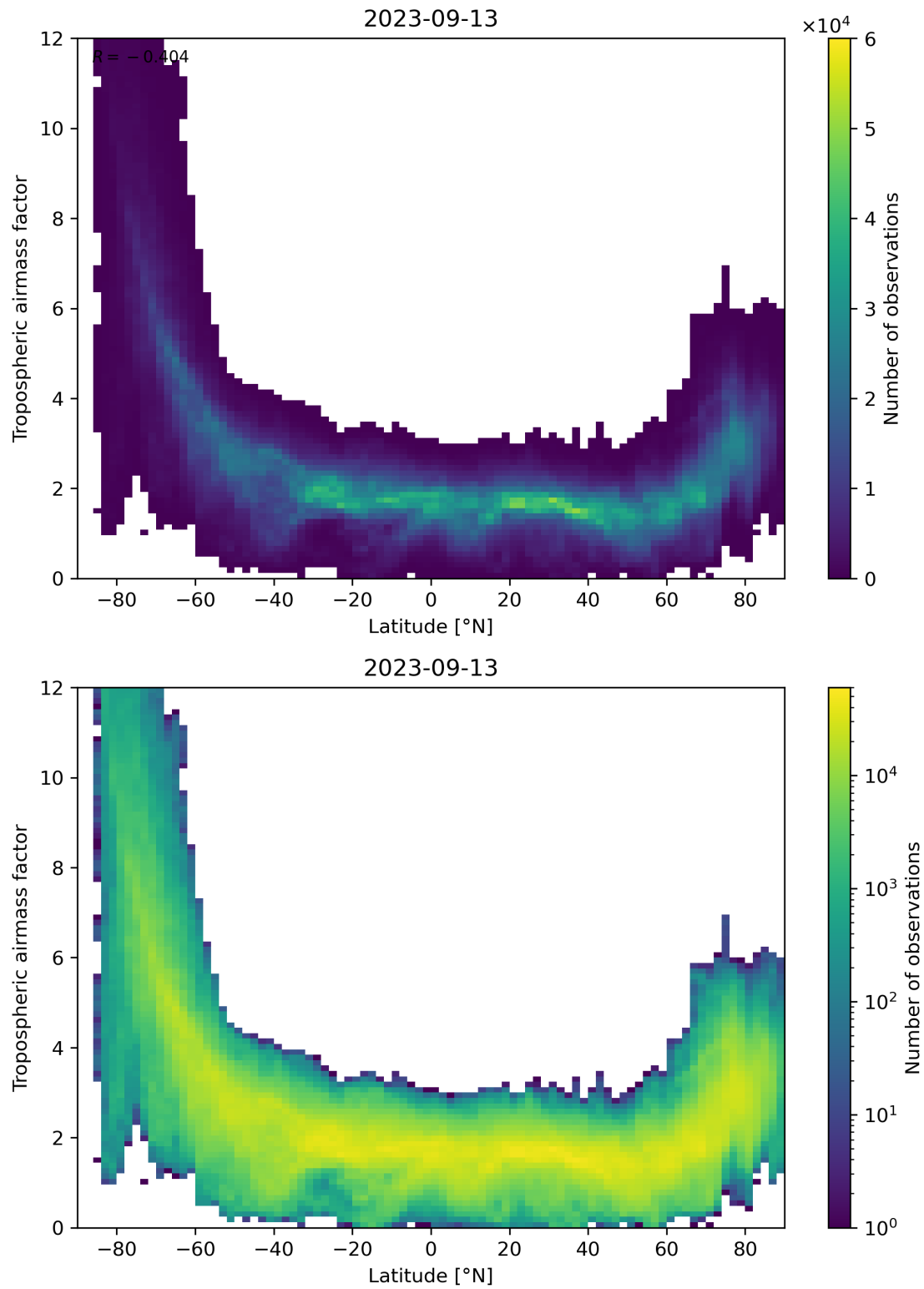
Figure 85: Scatter density plot of “Latitude” against “Tropospheric airmass factor” for 2023-09-12 to 2023-09-14.
