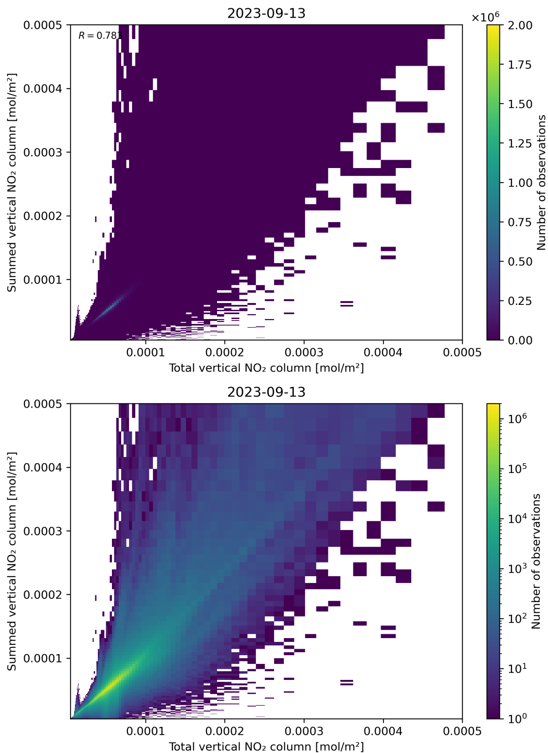
Figure 112: Scatter density plot of “Total vertical NO 2 column” against “Summed vertical NO 2 column” for 2023-09-12 to 2023-09-14.
