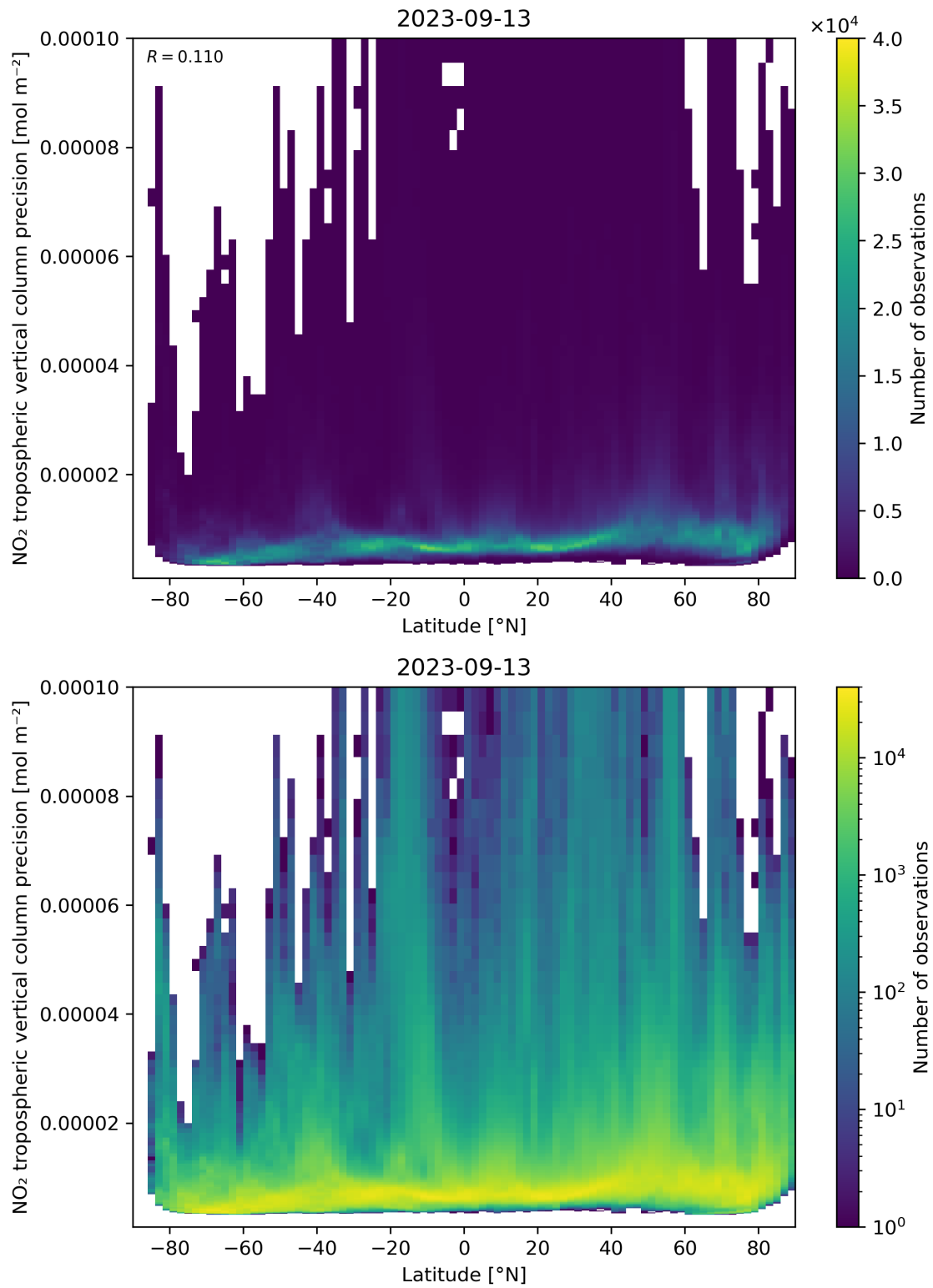
Figure 93: Scatter density plot of “Latitude” against “NO 2 tropospheric vertical column precision” for 2023-09-12 to 2023-09-14.
