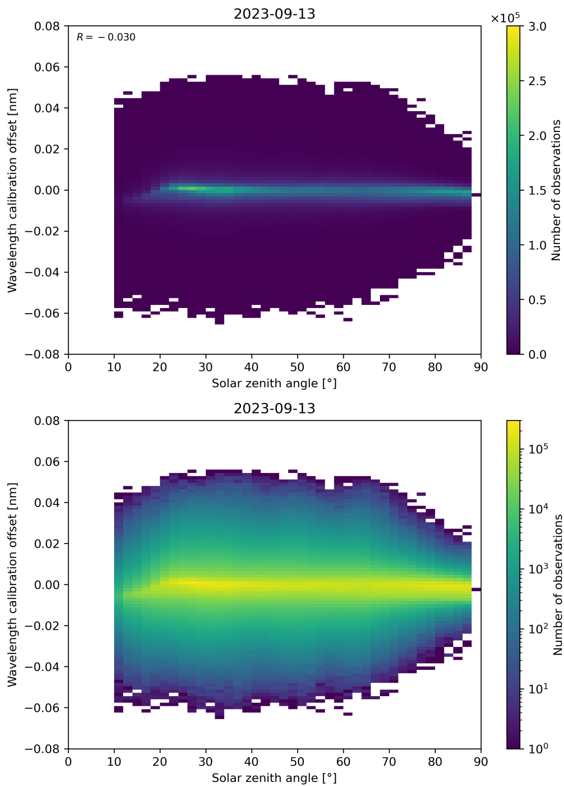
Figure 158: Scatter density plot of “Solar zenith angle” against “Wavelength calibration offset” for 2023-09-12 to 2023-09-14.
