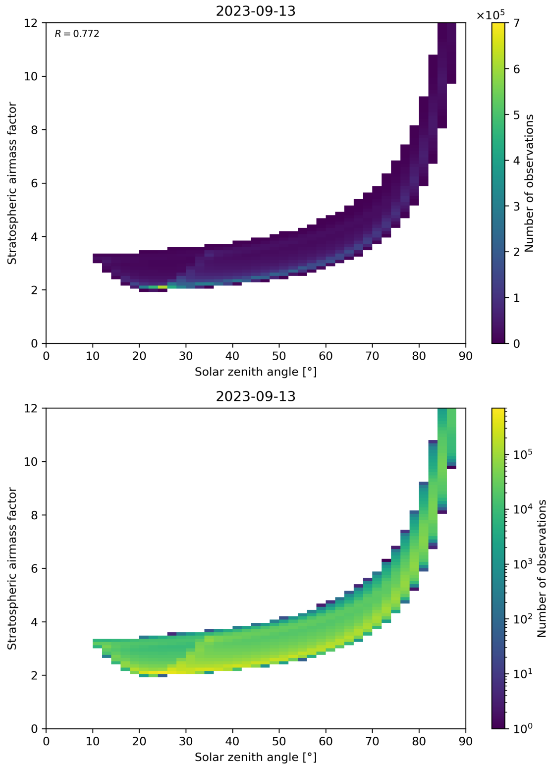
Figure 145: Scatter density plot of “Solar zenith angle” against “Stratospheric airmass factor” for 2023-09-12 to 2023-09-14.
