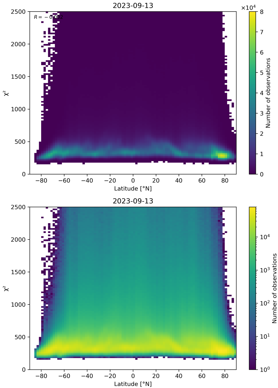
Figure 86: Scatter density plot of “Latitude” against “ \chi^2 ” for 2023-09-12 to 2023-09-14.
