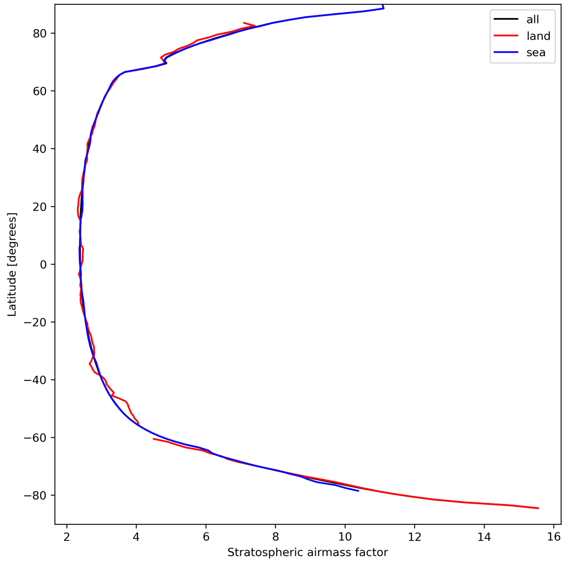
Figure 27: Zonal average of “Stratospheric airmass factor” for 2023-09-12 to 2023-09-14.
