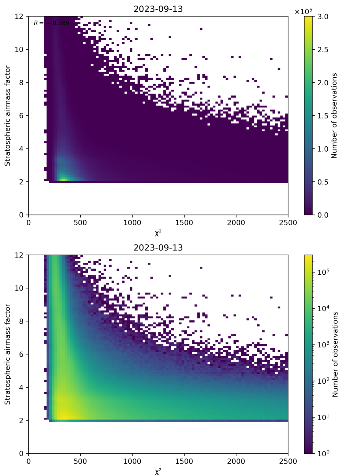
Figure 81: Scatter density plot of “ \chi^2 ” against “Stratospheric airmass factor” for 2023-09-12 to 2023-09-14.
