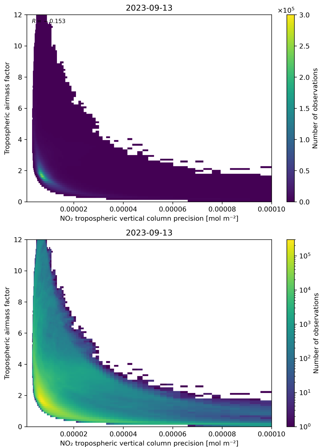
Figure 133: Scatter density plot of “NO 2 tropospheric vertical column precision” against “Tropospheric airmass factor” for 2023-09-12 to 2023-09-14.
