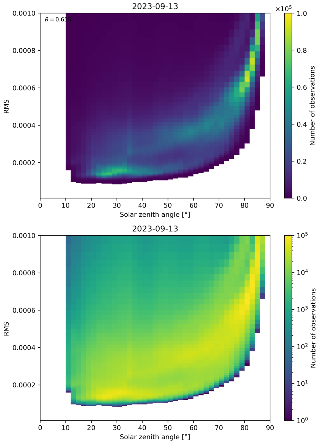
Figure 157: Scatter density plot of “Solar zenith angle” against “RMS” for 2023-09-12 to 2023-09-14.
