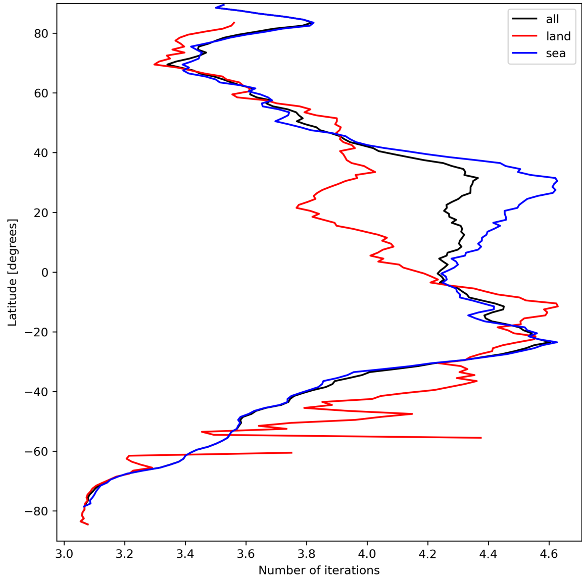
Figure 17: Zonal average of “Number of iterations” for 2023-09-12 to 2023-09-14.
