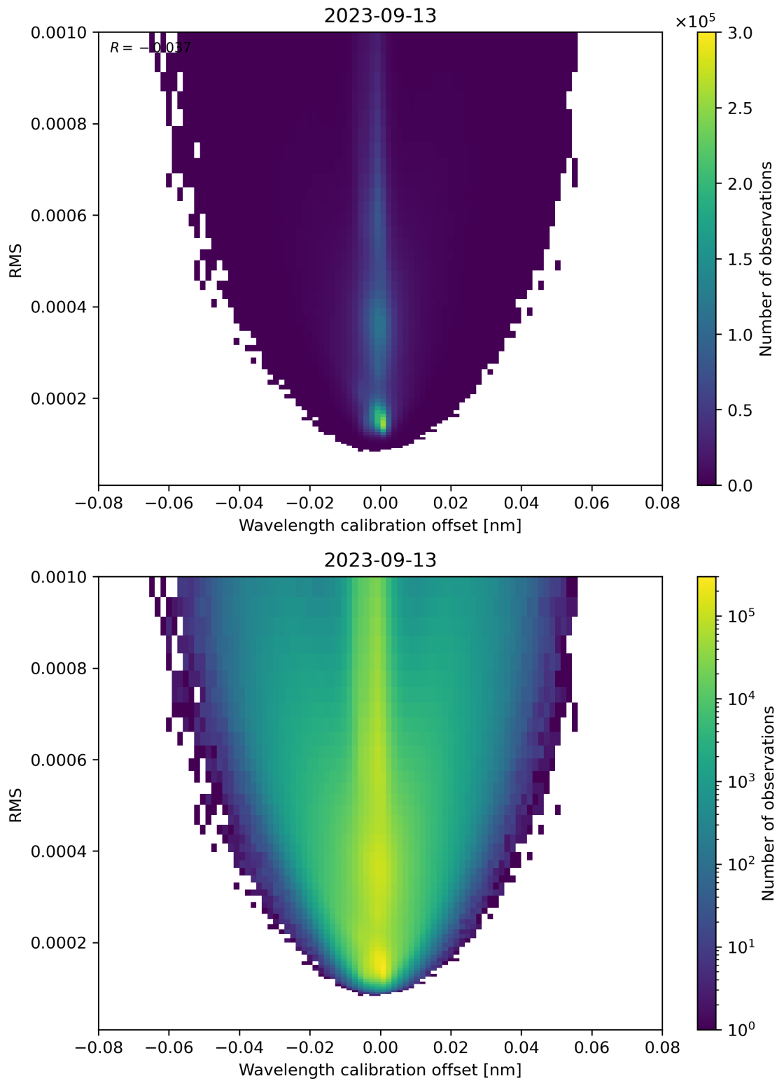
Figure 181: Scatter density plot of “Wavelength calibration offset” against “RMS” for 2023-09-12 to 2023-09-14.
