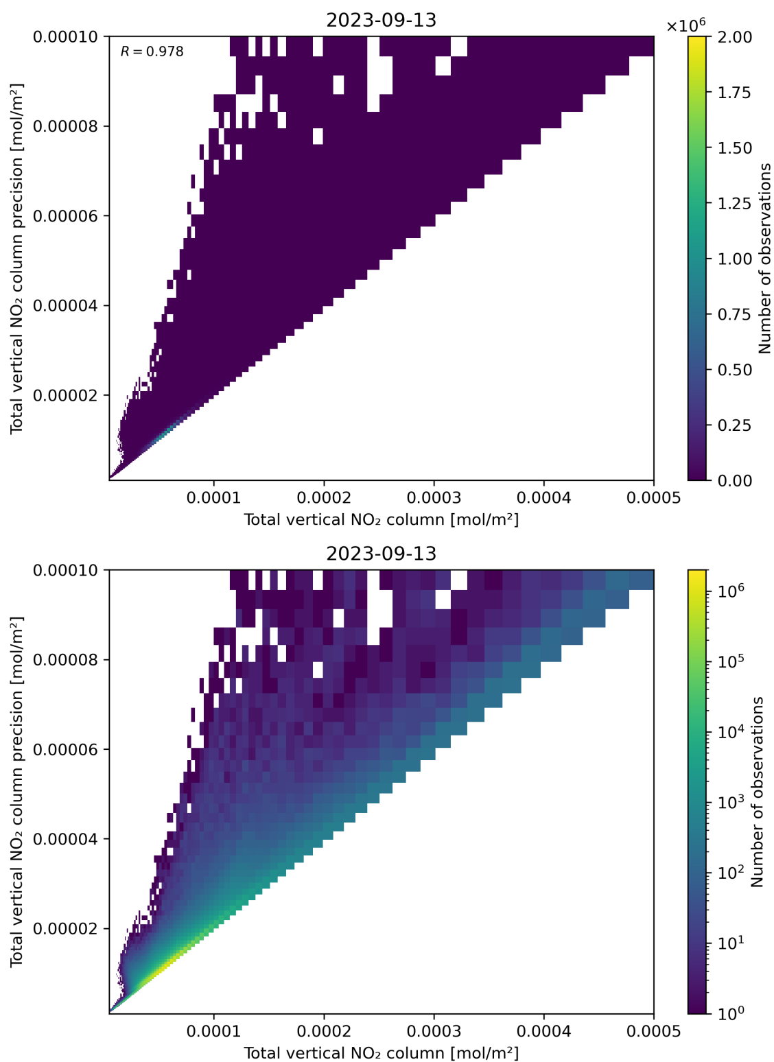
Figure 114: Scatter density plot of “Total vertical NO 2 column” against “Total vertical NO 2 column precision” for 2023-09-12 to 2023-09-14.
