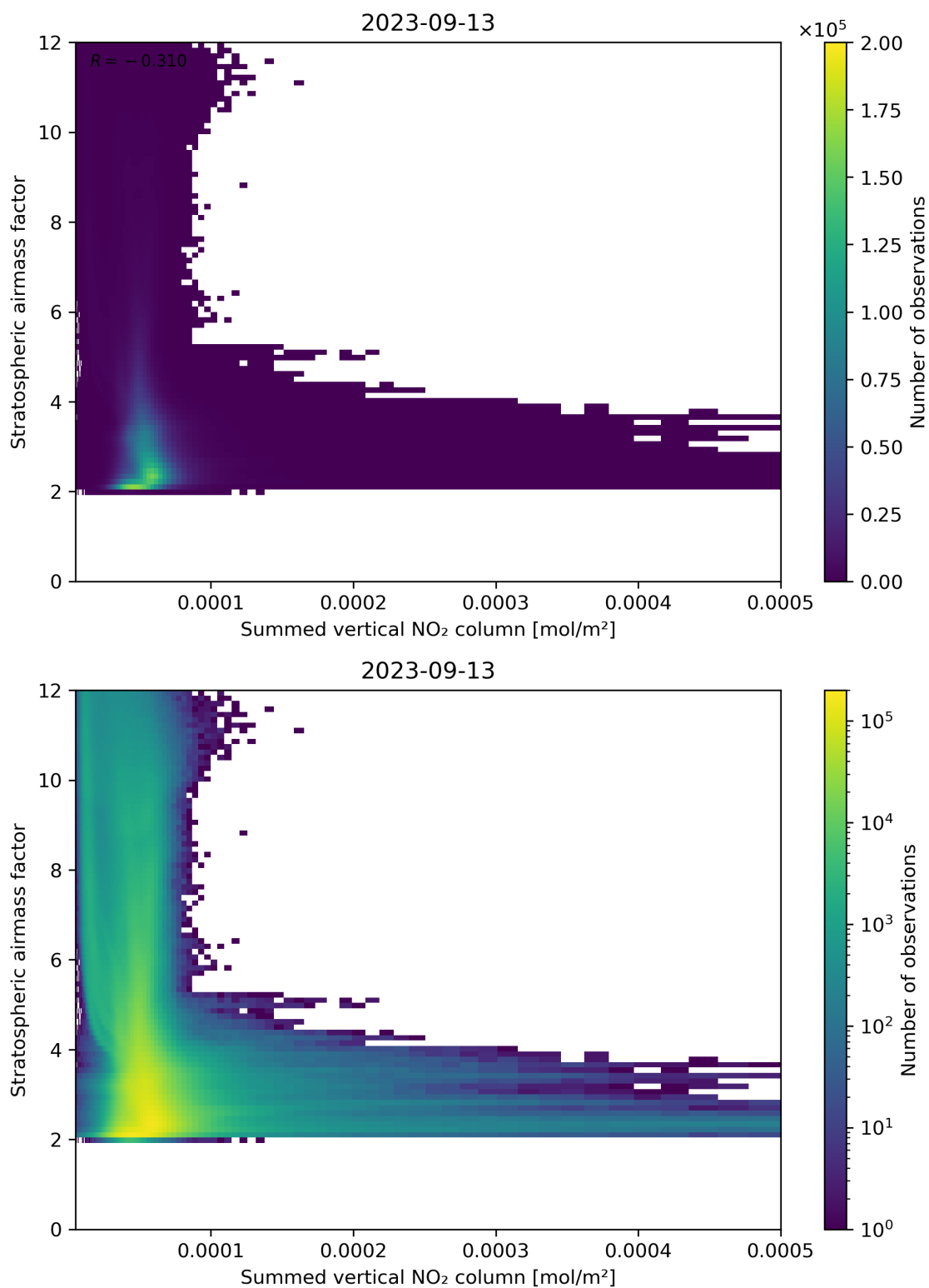
Figure 103: Scatter density plot of “Summed vertical NO 2 column” against “Stratospheric airmass factor” for 2023-09-12 to 2023-09-14.
