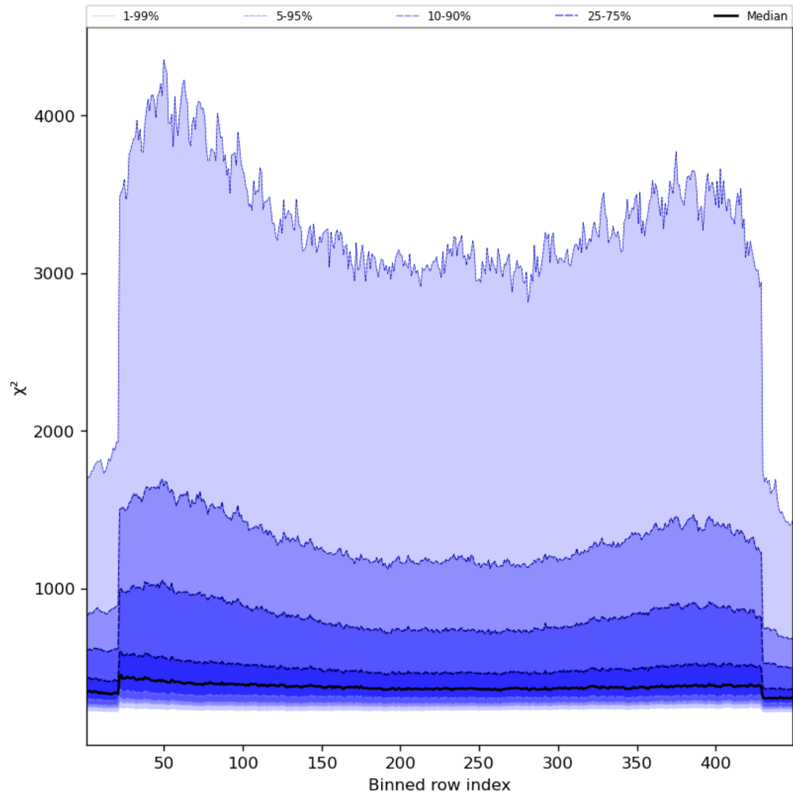
Figure 59: Along track statistics of “ \chi^2 ” for 2023-09-12 to 2023-09-14
