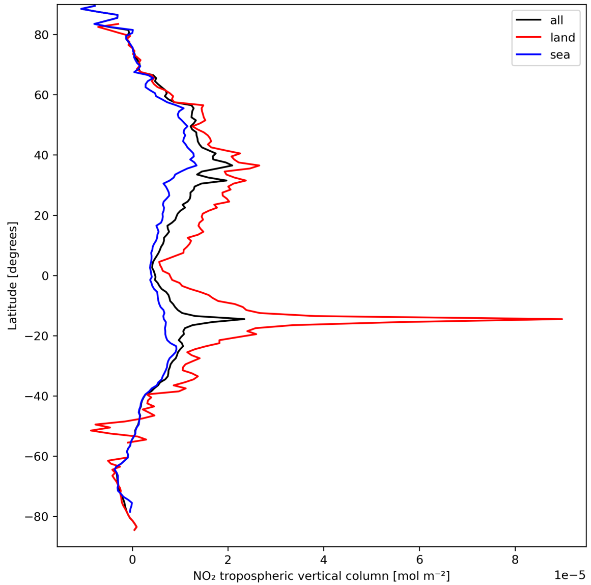
Figure 12: Zonal average of “NO 2 tropospheric vertical column” for 2023-09-12 to 2023-09-14.
