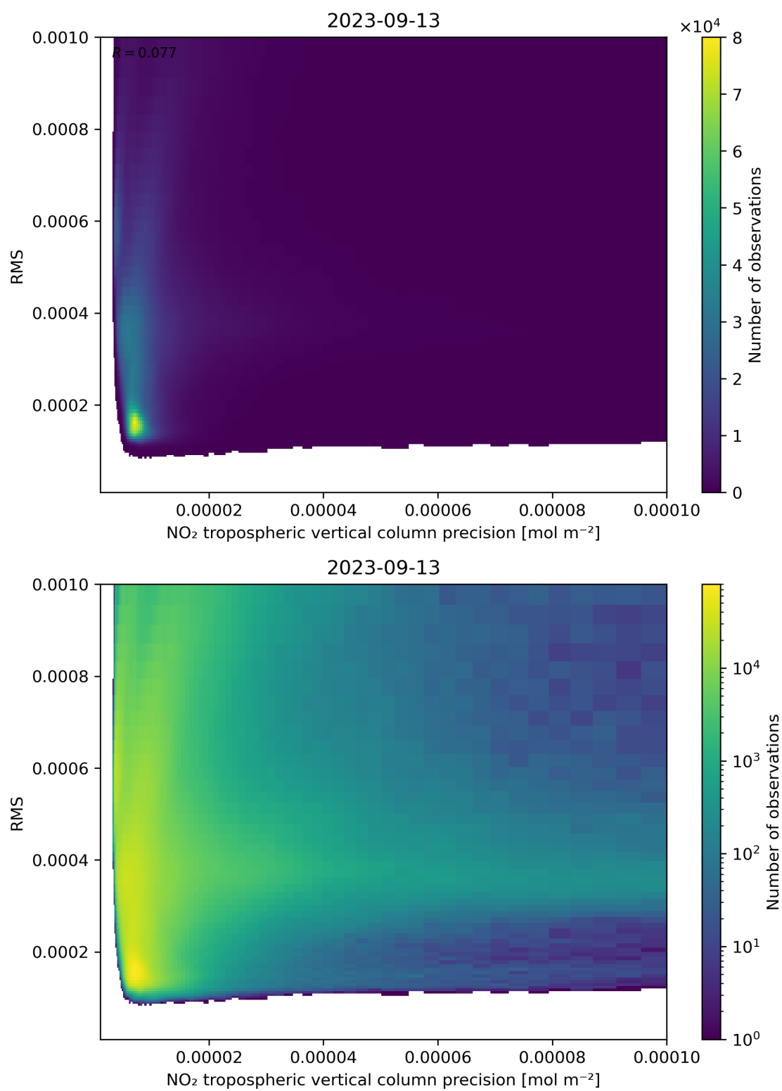
Figure 140: Scatter density plot of “NO 2 tropospheric vertical column precision” against “RMS” for 2023-09-12 to 2023-09-14.
