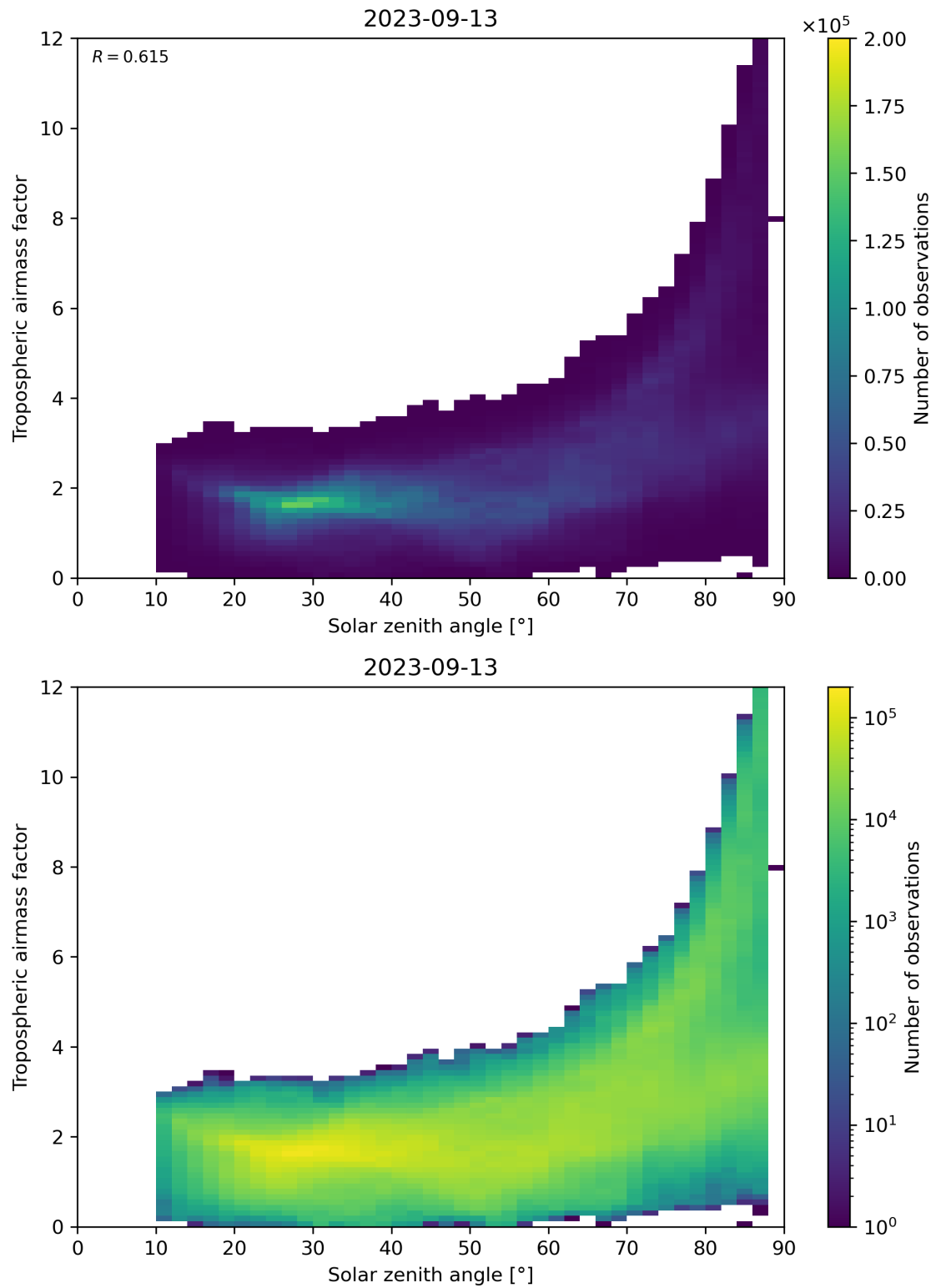
Figure 147: Scatter density plot of “Solar zenith angle” against “Tropospheric airmass factor” for 2023-09-12 to 2023-09-14.
