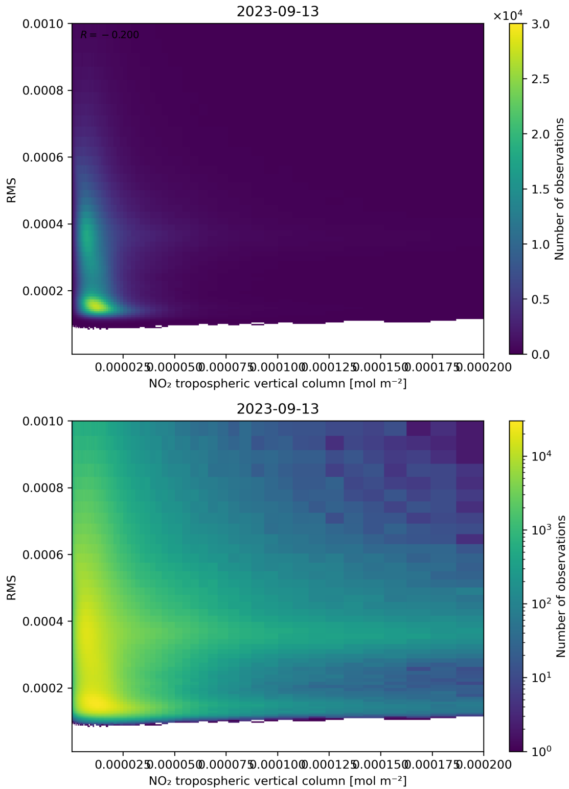
Figure 142: Scatter density plot of “NO 2 tropospheric vertical column” against “RMS” for 2023-09-12 to 2023-09-14.
