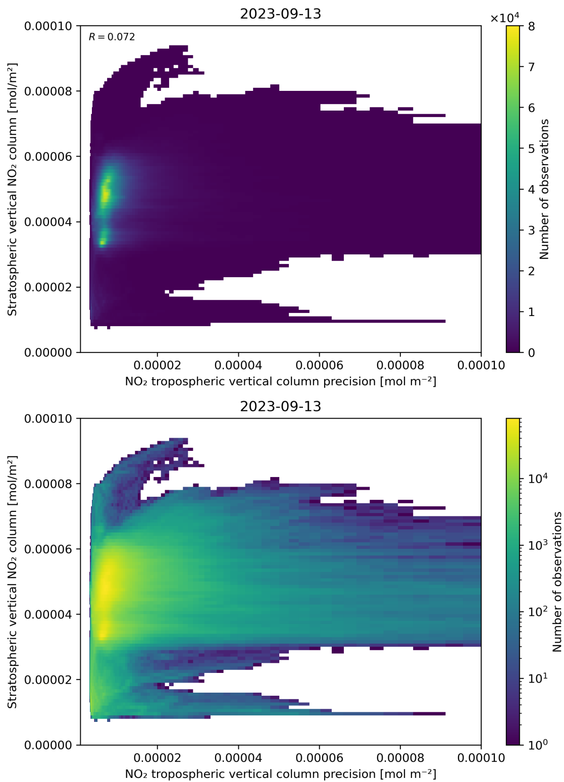
Figure 135: Scatter density plot of “NO 2 tropospheric vertical column precision” against “Stratospheric vertical NO 2 column” for 2023-09-12 to 2023-09-14.
