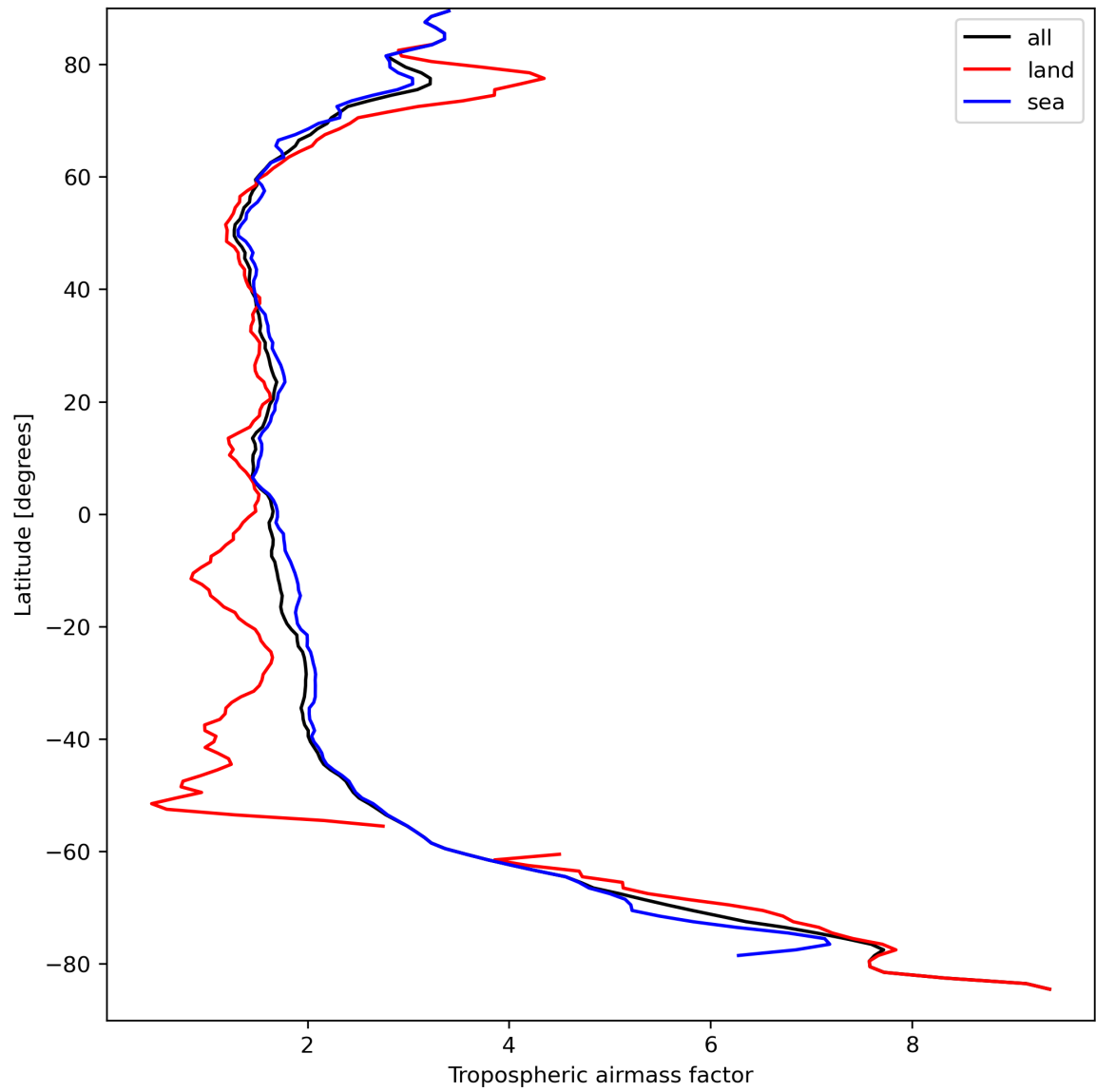
Figure 14: Zonal average of “Tropospheric airmass factor” for 2023-09-12 to 2023-09-14.
