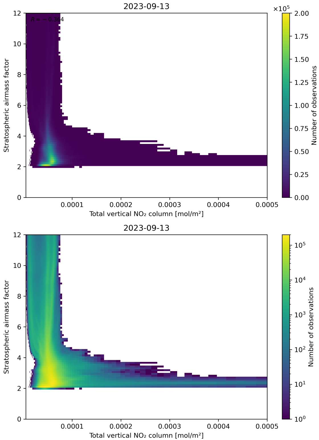
Figure 110: Scatter density plot of “Total vertical NO 2 column” against “Stratospheric airmass factor” for 2023-09-12 to 2023-09-14.
