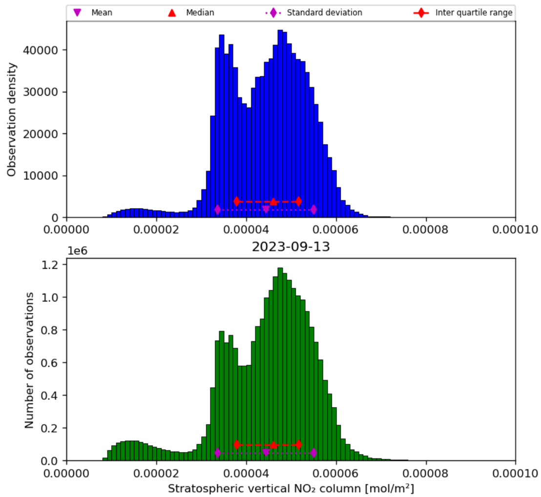
Figure 36: Histogram of “Stratospheric vertical NO 2 column” for 2023-09-12 to 2023-09-14
