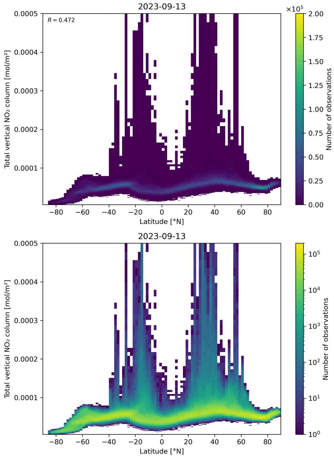
Figure 90: Scatter density plot of “Latitude” against “Total vertical NO 2 column” for 2023-09-12 to 2023-09-14.
