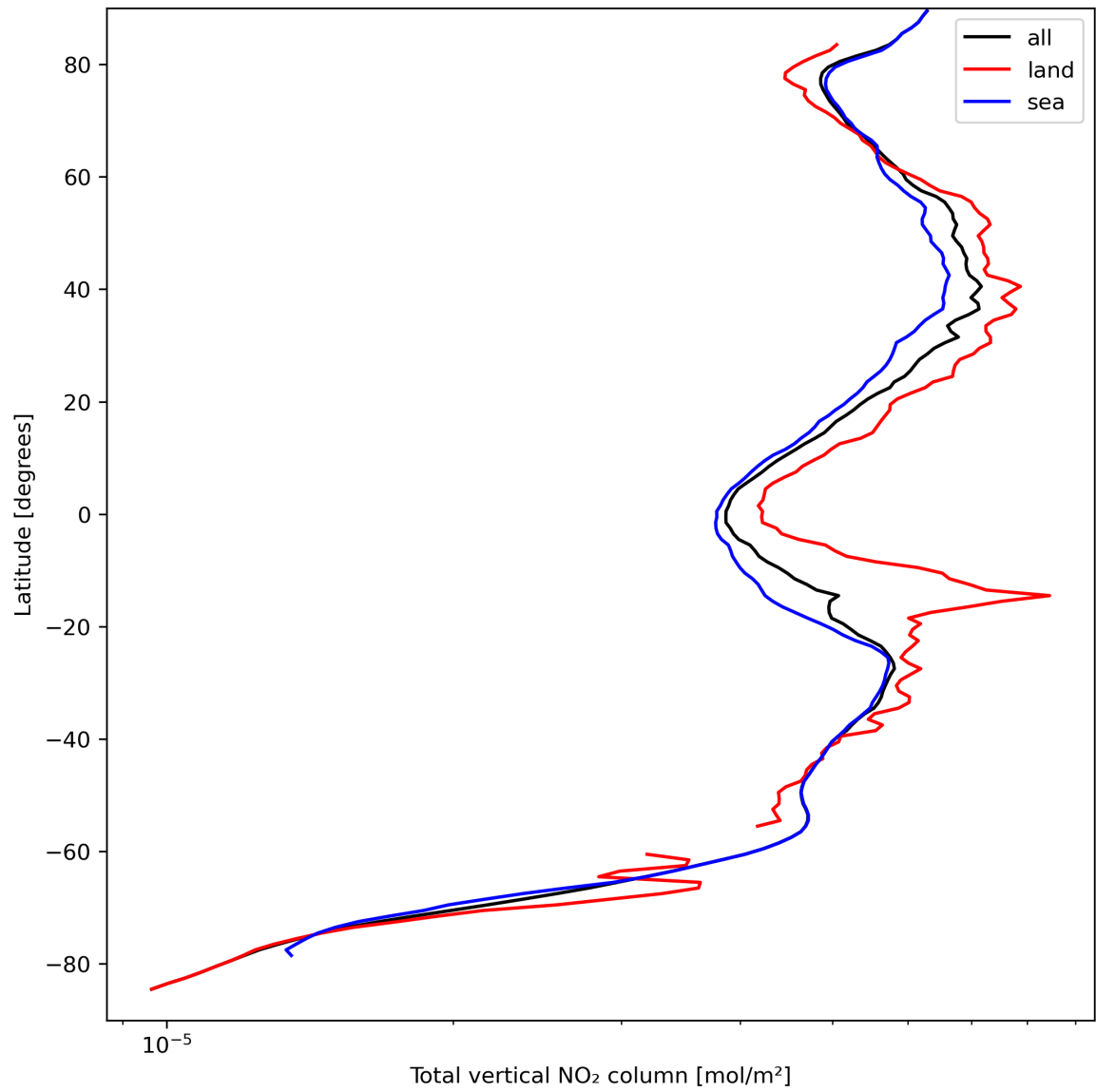
Figure 21: Zonal average of “Total vertical NO 2 column” for 2023-09-12 to 2023-09-14.
