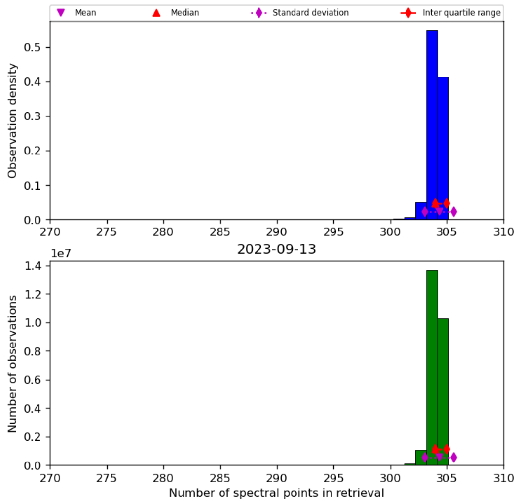
Figure 33: Histogram of “Number of spectral points in retrieval” for 2023-09-12 to 2023-09-14
