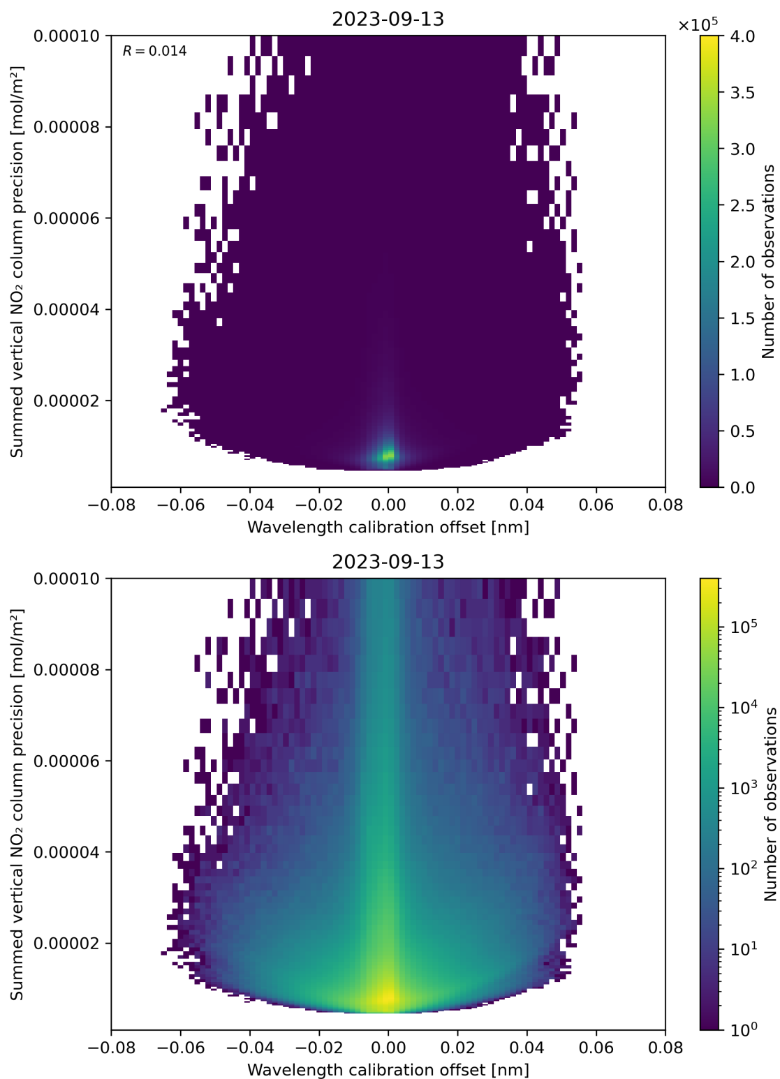
Figure 178: Scatter density plot of “Wavelength calibration offset” against “Summed vertical NO 2 column precision” for 2023-09-12 to 2023-09-14.
