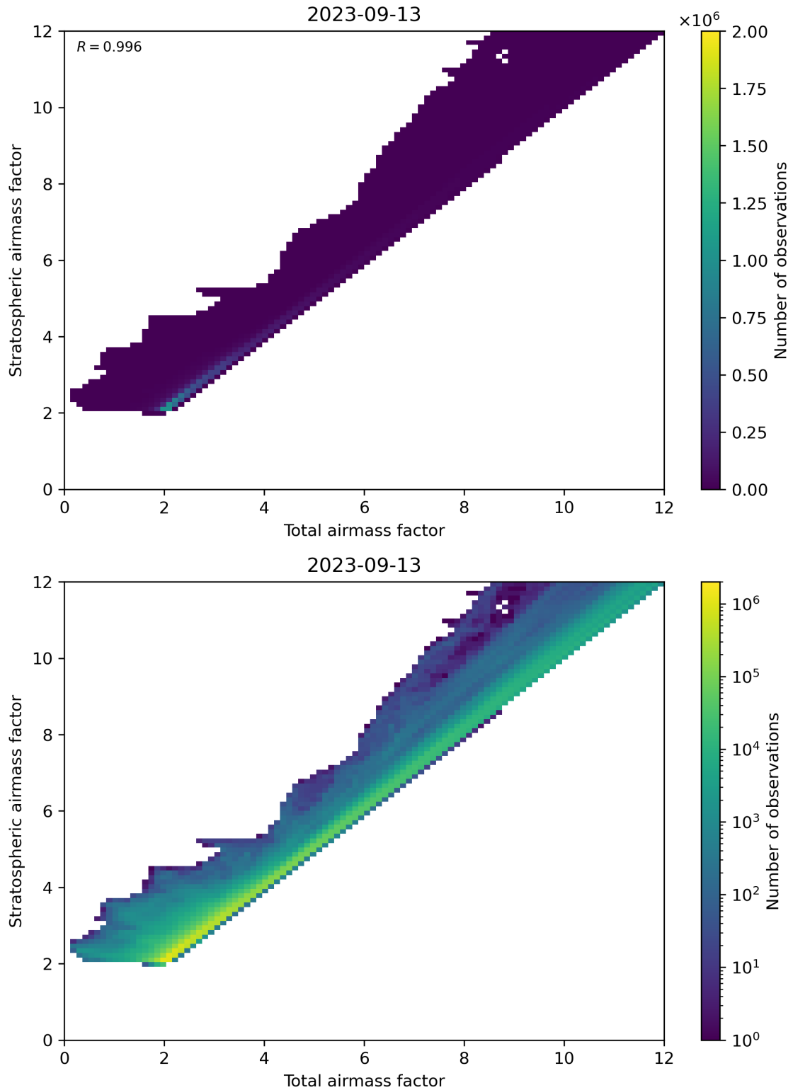
Figure 62: Scatter density plot of “Total airmass factor” against “Stratospheric airmass factor” for 2023-09-12 to 2023-09-14.
