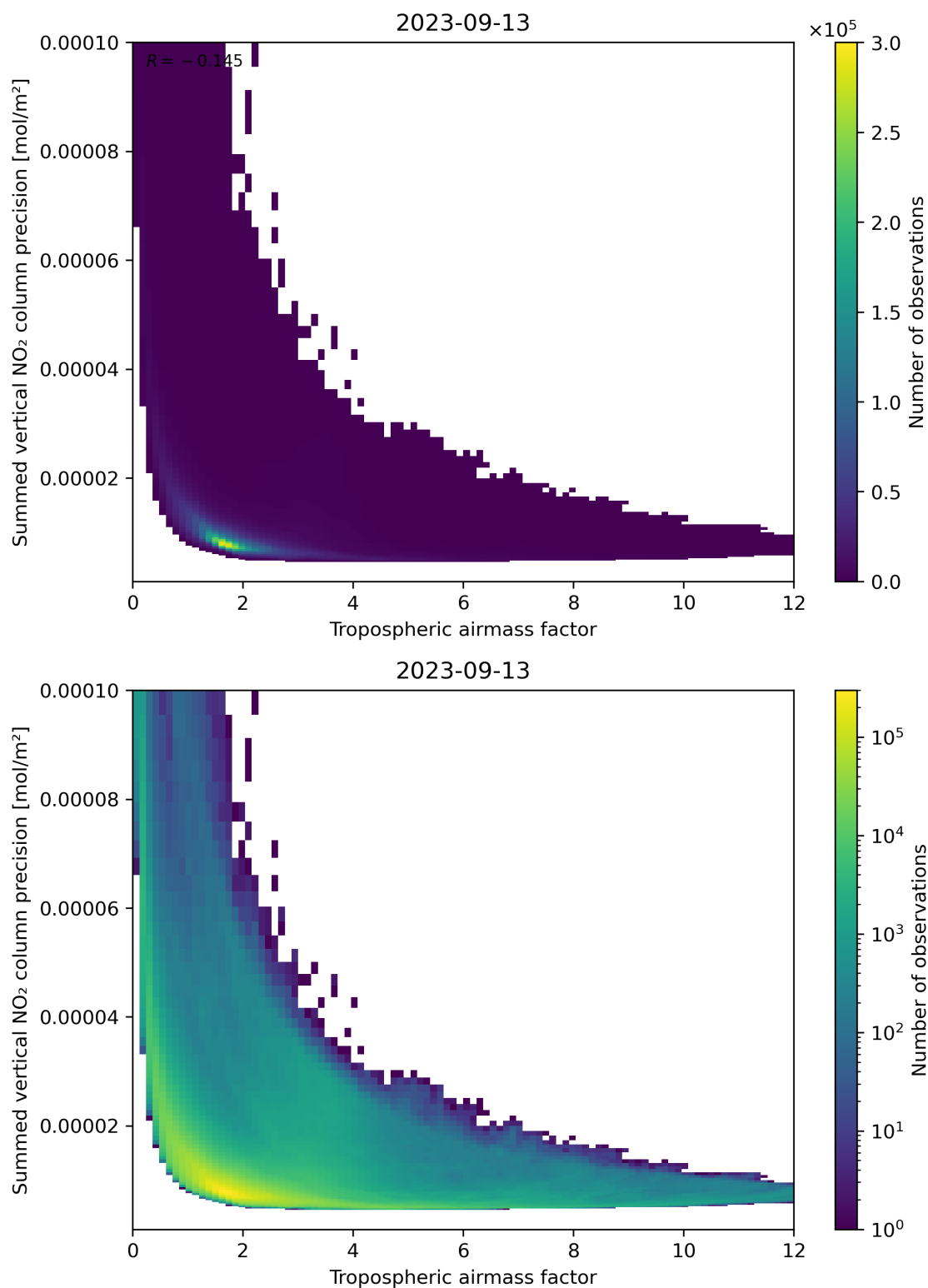
Figure 76: Scatter density plot of “Tropospheric air mass factor” against “Summed vertical NO 2 column precision” for 2023-09-12 to 2023-09-14.
