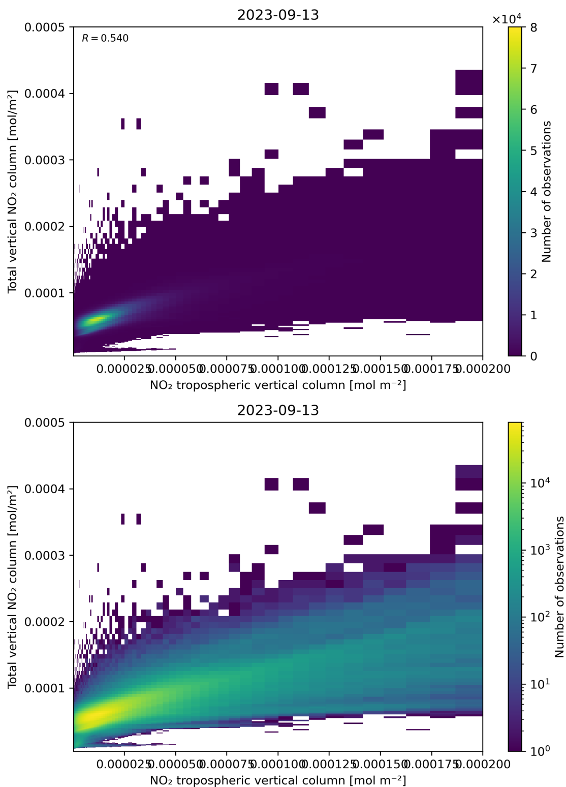
Figure 128: Scatter density plot of “NO 2 tropospheric vertical column” against “Total vertical NO 2 column” for 2023-09-12 to 2023-09-14.
