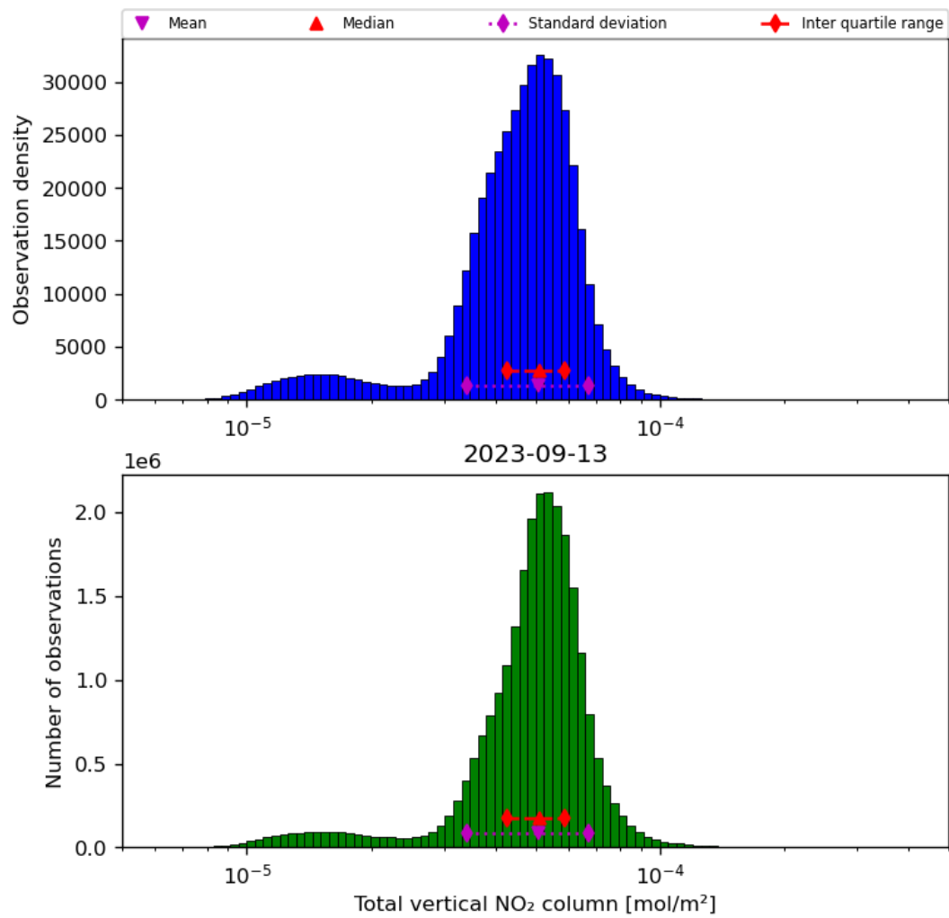
Figure 38: Histogram of "Total vertical NO 2 column" for 2023-09-12 to 2023-09-14
