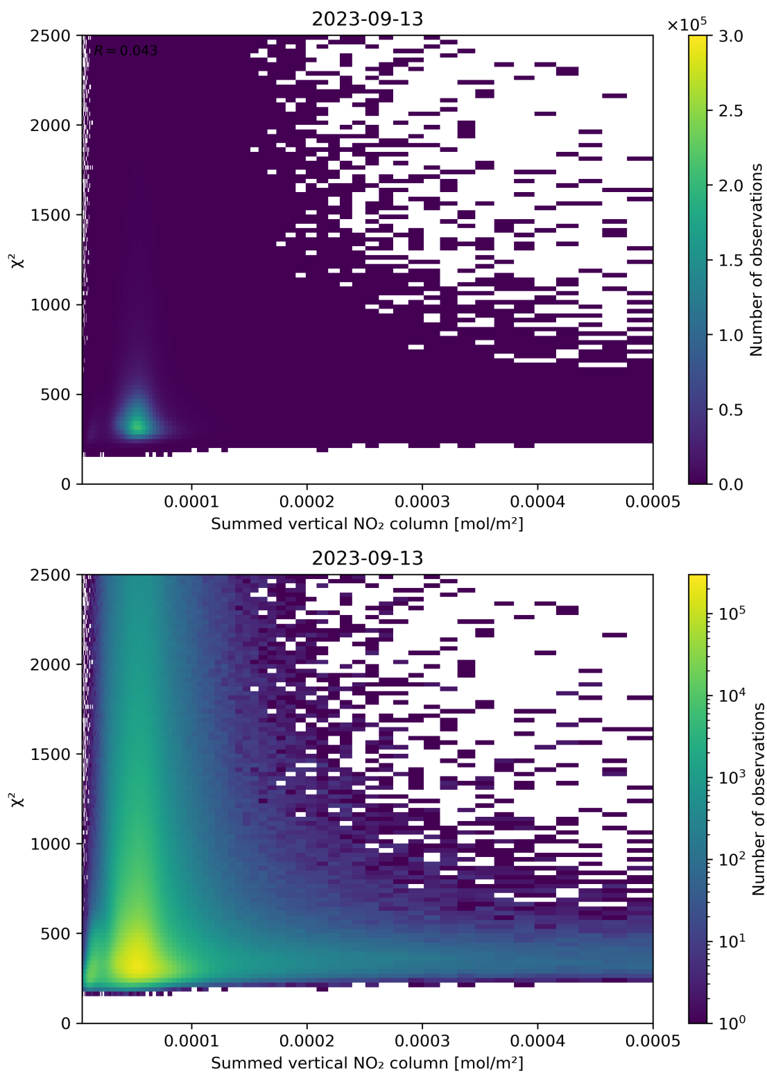
Figure 104: Scatter density plot of “Summed vertical NO 2 column” against “ \chi^2 ” for 2023-09-12 to 2023-09-14.
