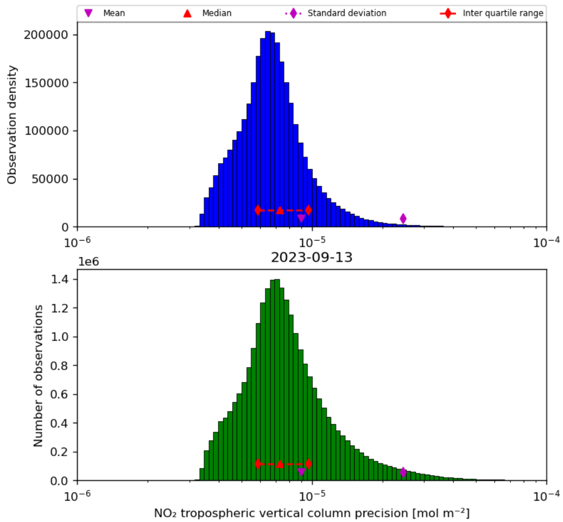
Figure 30: Histogram of “NO 2 tropospheric vertical column precision” for 2023-09-12 to 2023-09-14
