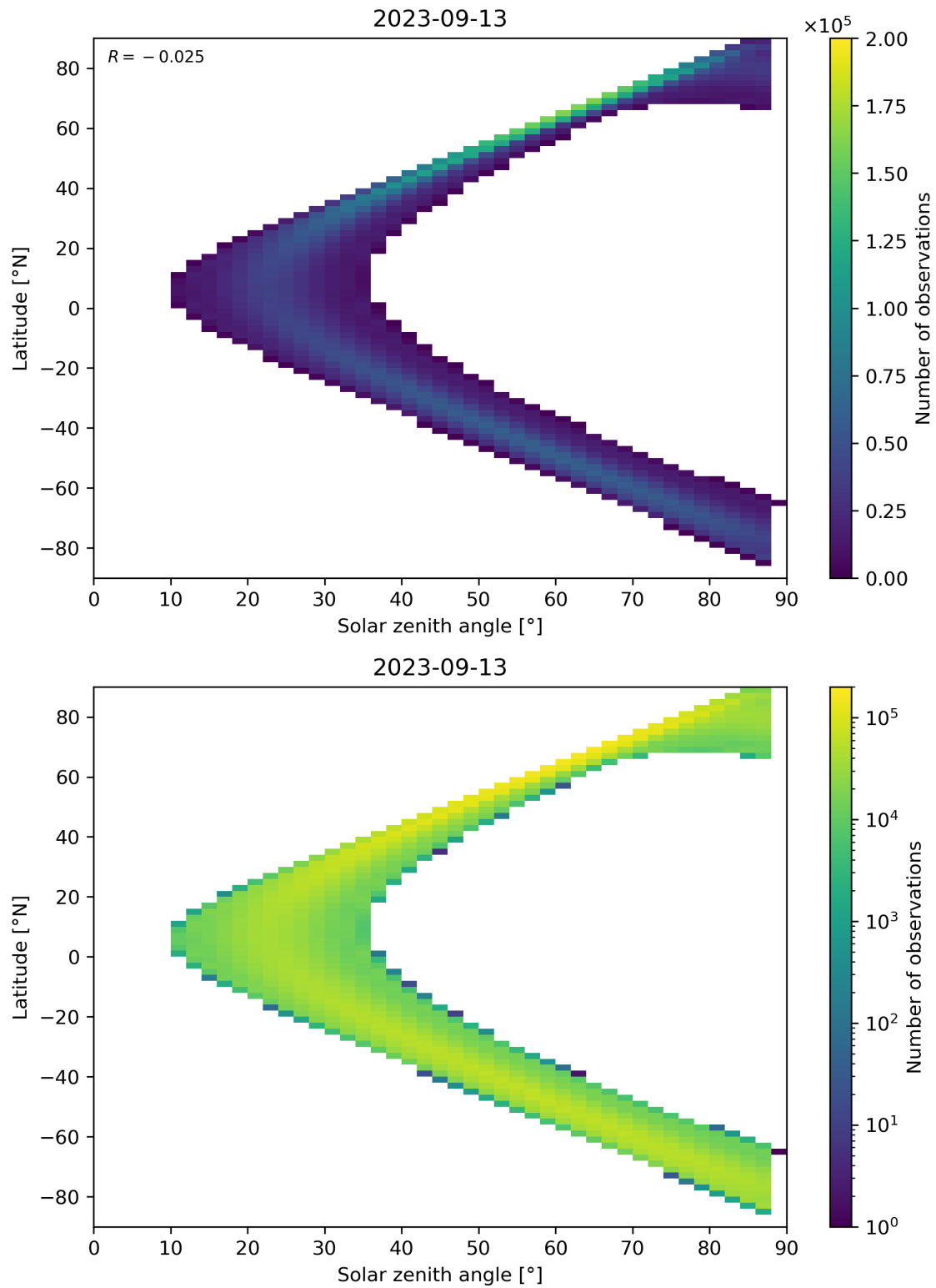
Figure 149: Scatter density plot of “Solar zenith angle” against “Latitude” for 2023-09-12 to 2023-09-14.
