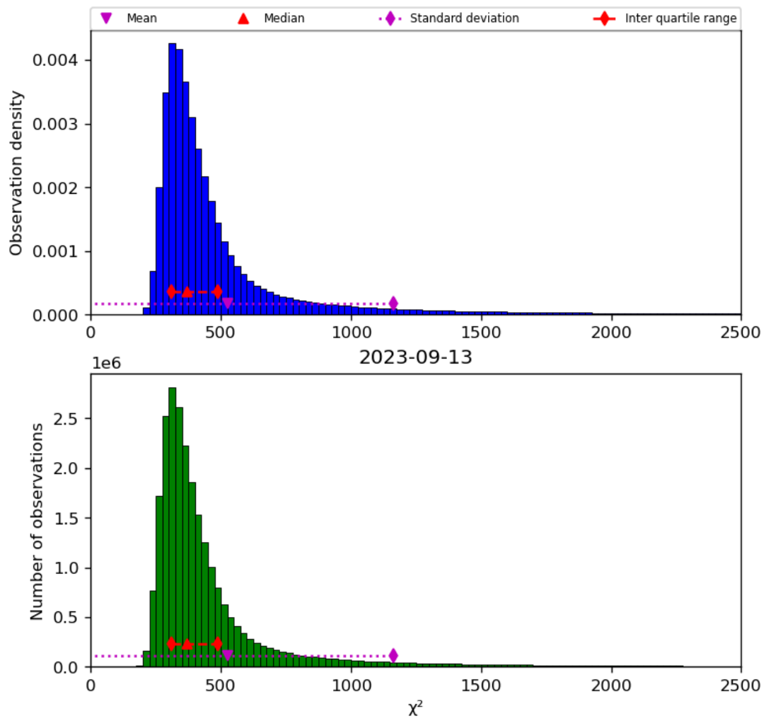
Figure 42: Histogram of “ \chi^2 ” for 2023-09-12 to 2023-09-14
