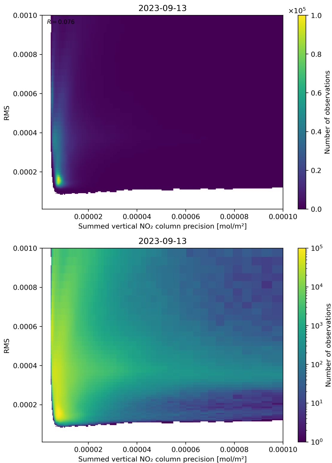
Figure 108: Scatter density plot of “Summed vertical NO 2 column precision” against “RMS” for 2023-09-12 to 2023-09-14.
