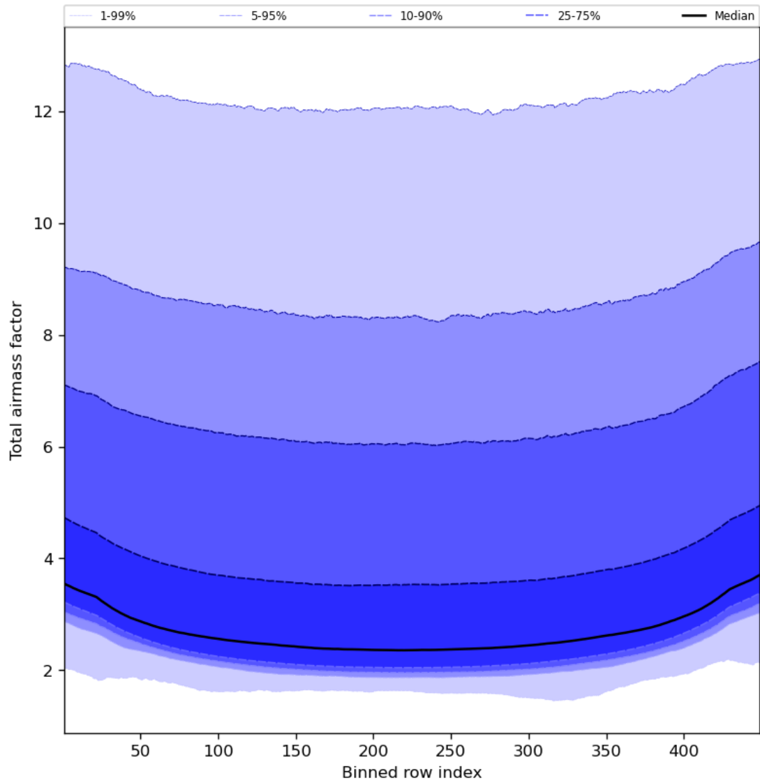
Figure 49: Along track statistics of “Total airmass factor” for 2023-09-12 to 2023-09-14
