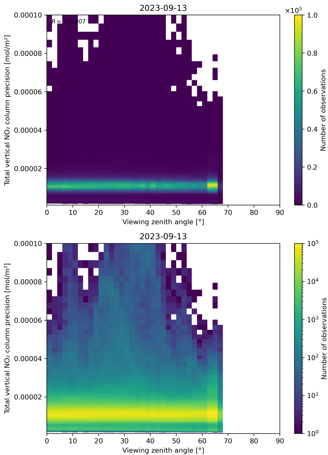
Figure 168: Scatter density plot of “Viewing zenith angle” against “Total vertical NO 2 column precision” for 2023-09-12 to 2023-09-14.
