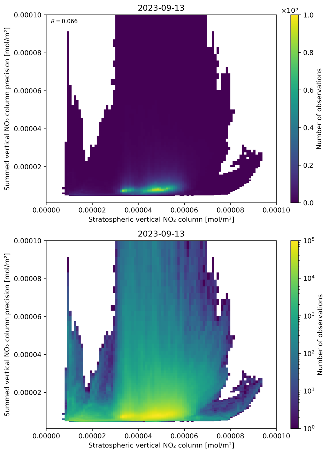
Figure 99: Scatter density plot of “Stratospheric vertical NO 2 column” against “Summed vertical NO 2 column precision” for 2023-09-12 to 2023-09-14.
