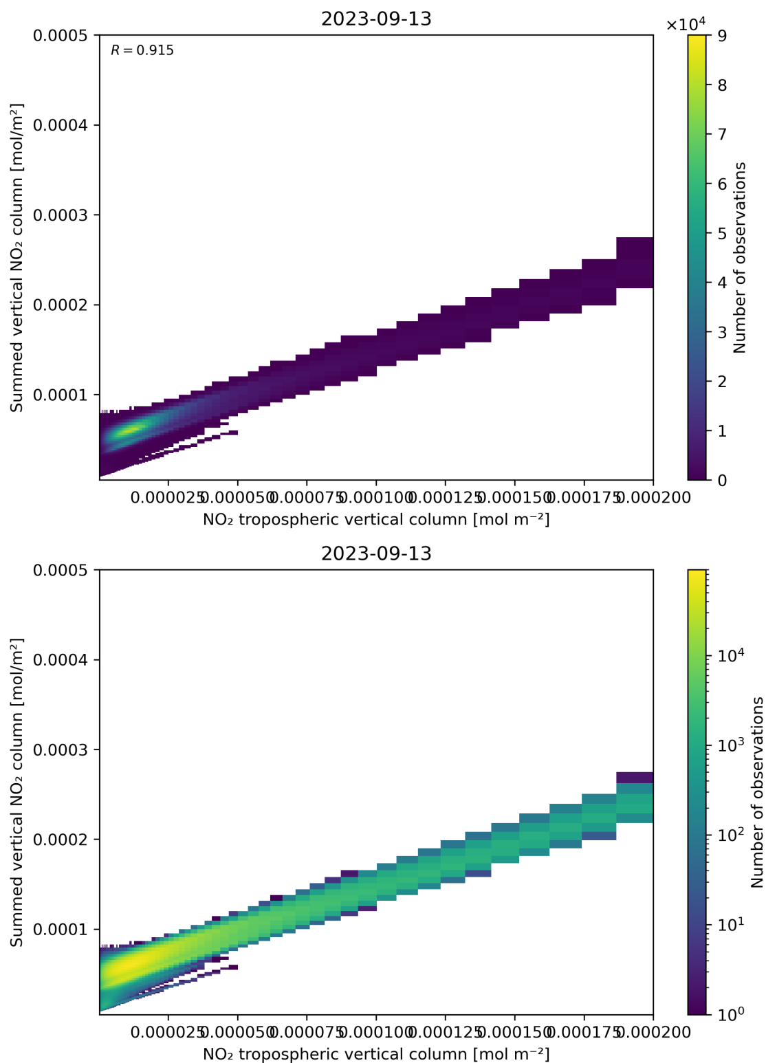
Figure 126: Scatter density plot of “NO 2 tropospheric vertical column” against “Summed vertical NO 2 column” for 2023-09-12 to 2023-09-14.
