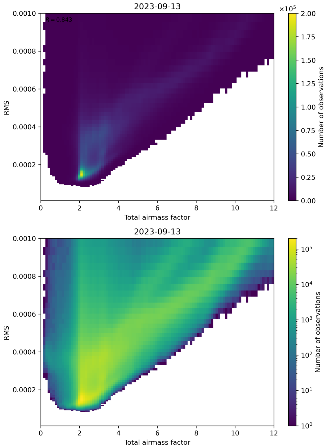
Figure 69: Scatter density plot of “Total airmass factor” against “RMS” for 2023-09-12 to 2023-09-14.
