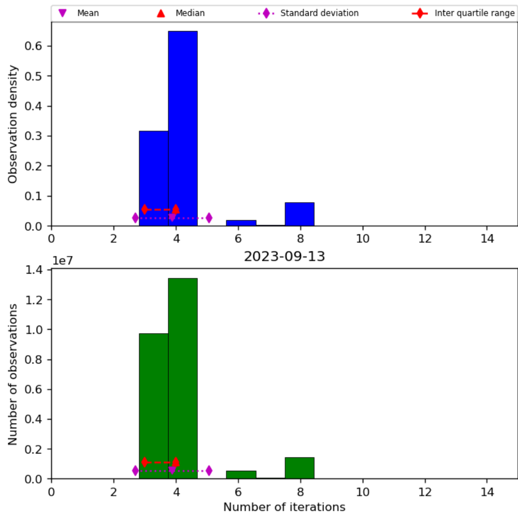
Figure 34: Histogram of “Number of iterations” for 2023-09-12 to 2023-09-14
