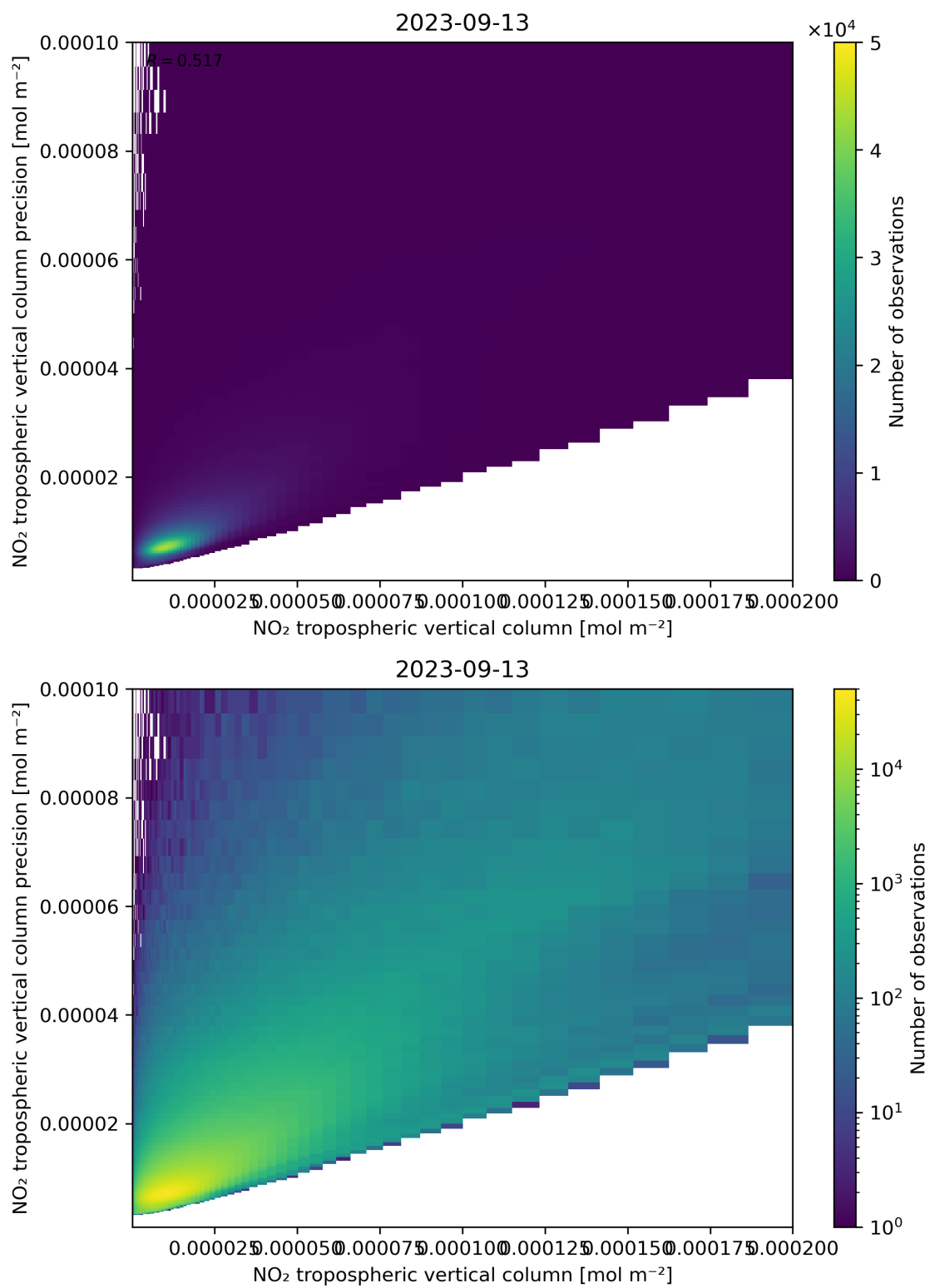
Figure 130: Scatter density plot of “NO 2 tropospheric vertical column” against “NO 2 tropospheric vertical column precision” for 2023-09-12 to 2023-09-14.
