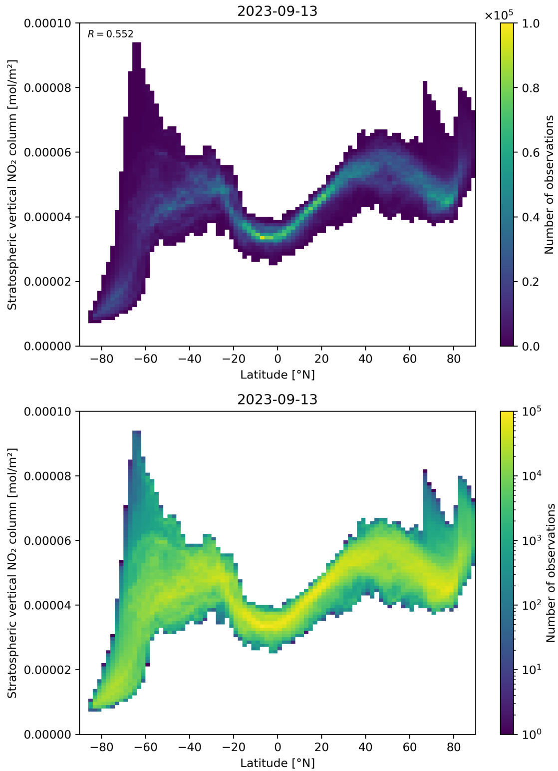
Figure 87: Scatter density plot of “Latitude” against “Stratospheric vertical NO 2 column” for 2023-09-12 to 2023-09-14.
