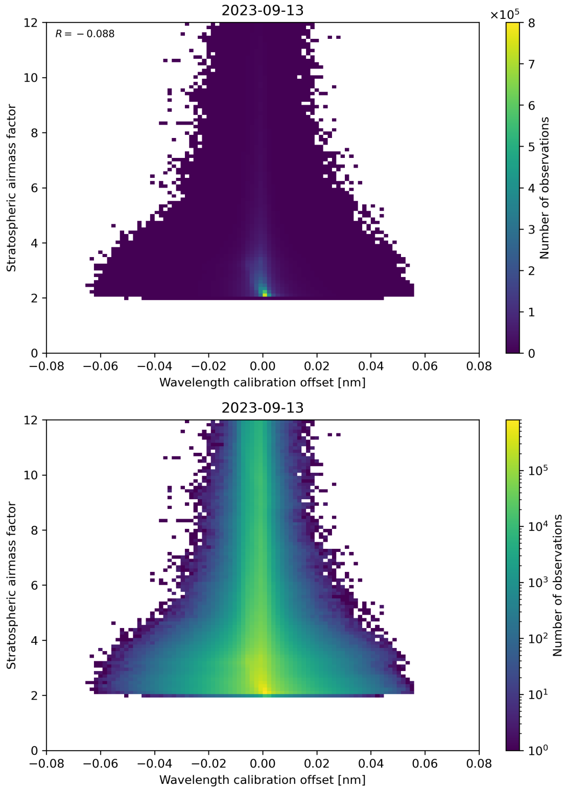
Figure 174: Scatter density plot of “Wavelength calibration offset” against “Stratospheric airmass factor” for 2023-09-12 to 2023-09-14.
