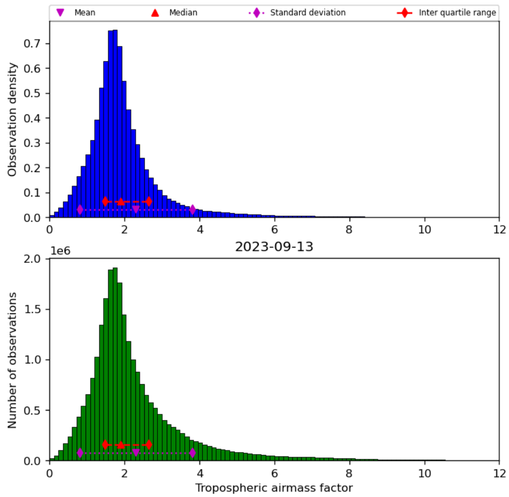
Figure 31: Histogram of “Tropospheric airmass factor” for 2023-09-12 to 2023-09-14
