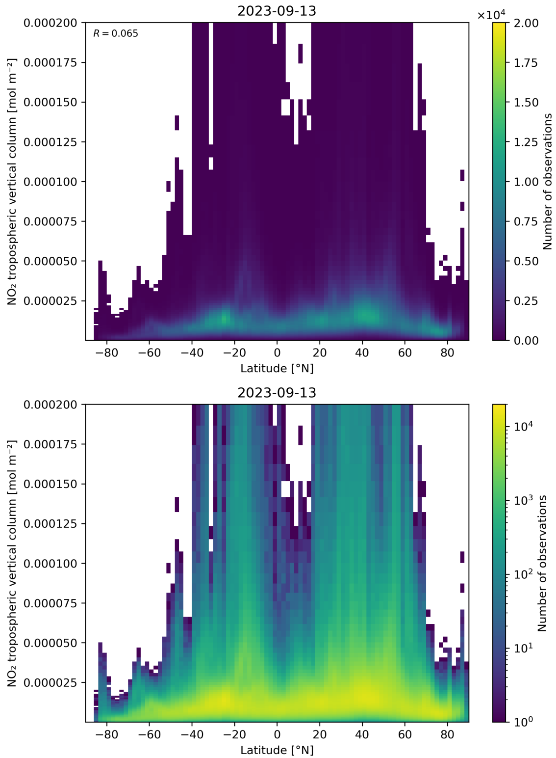
Figure 92: Scatter density plot of “Latitude” against “NO 2 tropospheric vertical column” for 2023-09-12 to 2023-09-14.
