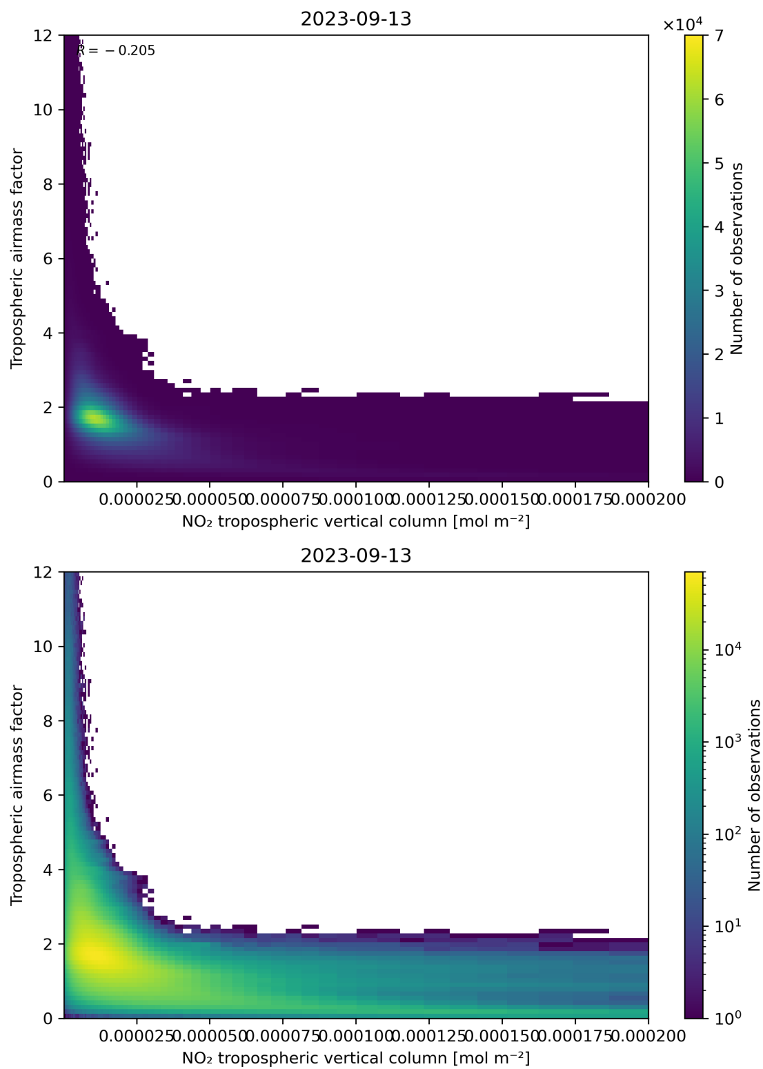
Figure 123: Scatter density plot of “NO 2 tropospheric vertical column” against “Tropospheric air mass factor” for 2023-09-12 to 2023-09-14.
