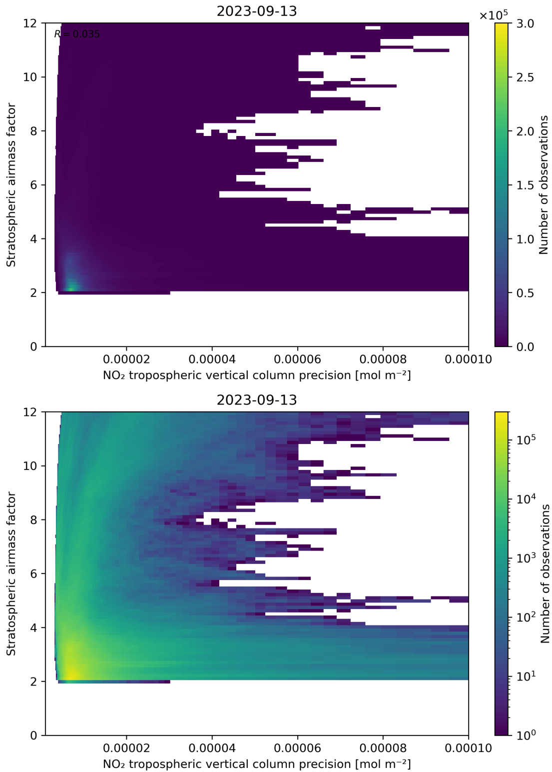
Figure 131: Scatter density plot of “NO 2 tropospheric vertical column precision” against “Stratospheric airmass factor” for 2023-09-12 to 2023-09-14.
