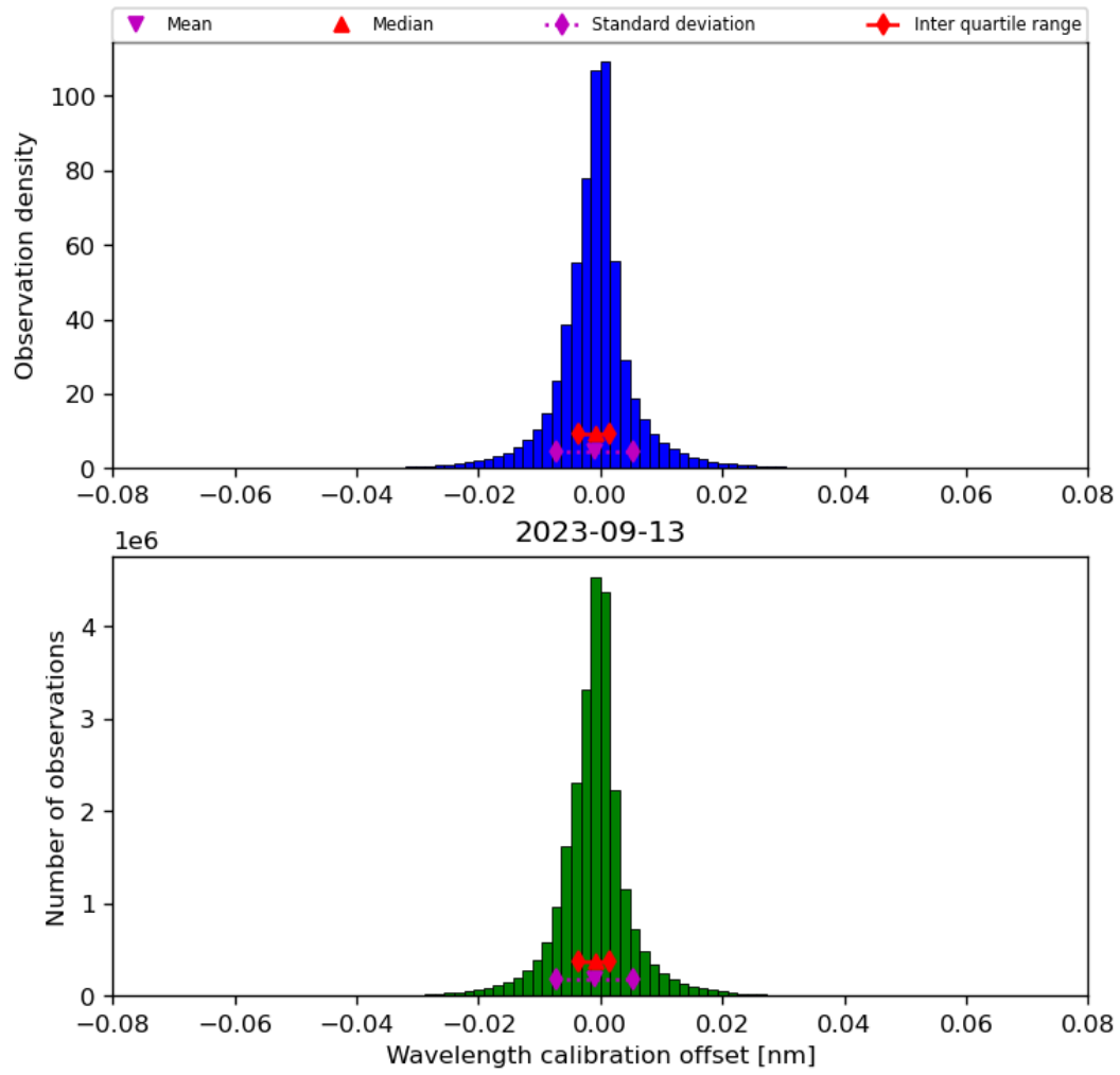
Figure 35: Histogram of “Wavelength calibration offset” for 2023-09-12 to 2023-09-14
