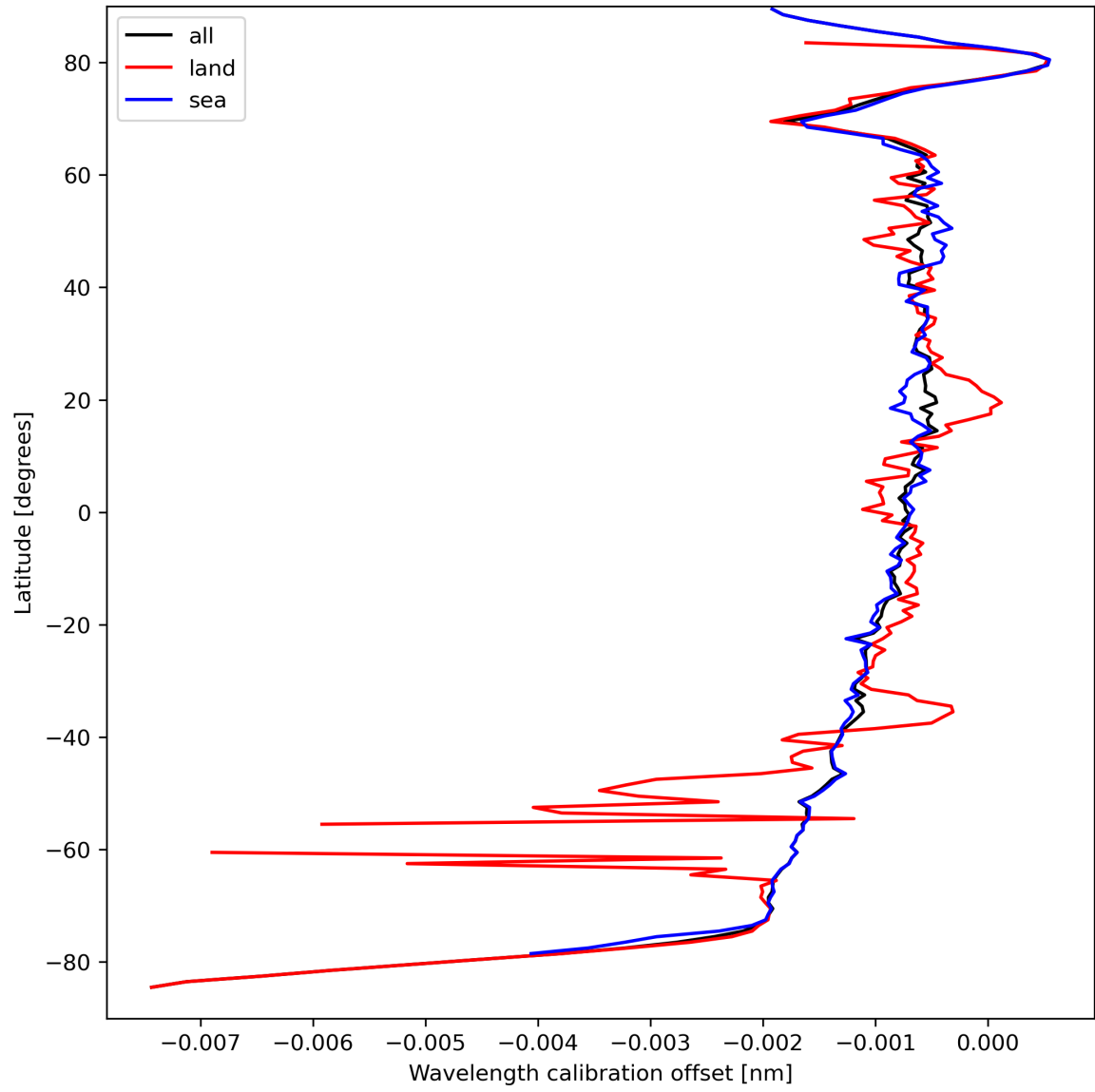
Figure 18: Zonal average of “Wavelength calibration offset” for 2023-09-12 to 2023-09-14.
