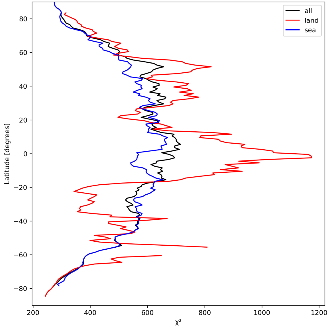
Figure 25: Zonal average of “ \chi^2 ” for 2023-09-12 to 2023-09-14.
