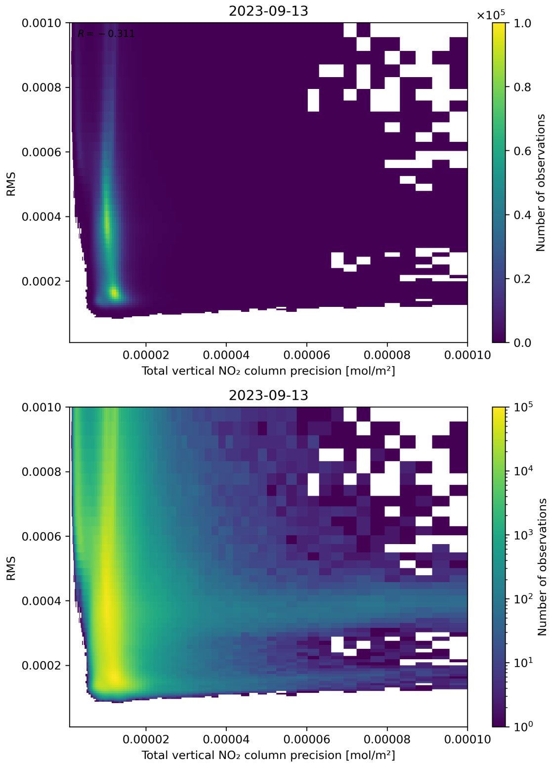
Figure 119: Scatter density plot of “Total vertical NO 2 column precision” against “RMS” for 2023-09-12 to 2023-09-14.
