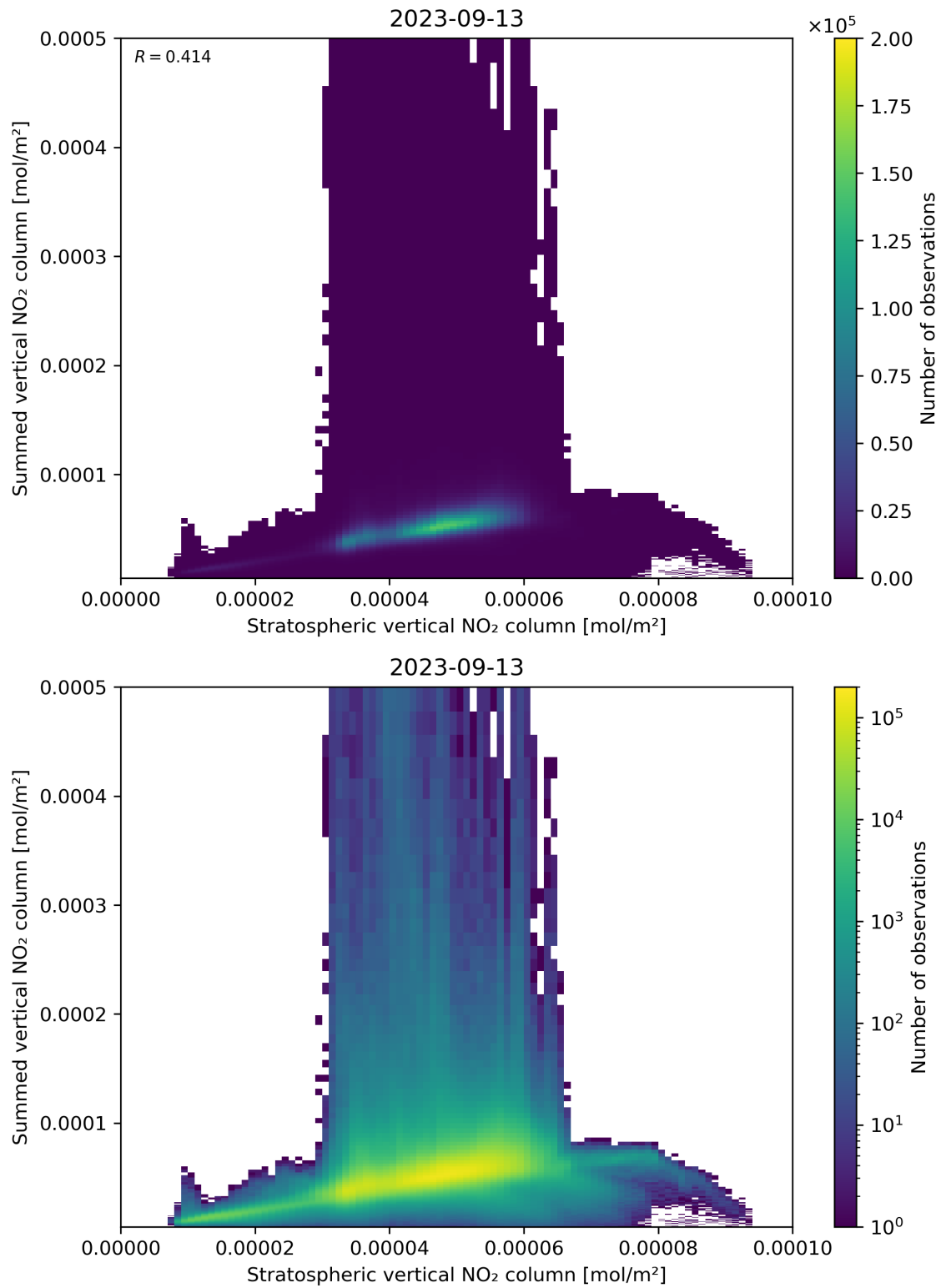
Figure 98: Scatter density plot of “Stratospheric vertical NO 2 column” against “Summed vertical NO 2 column” for 2023-09-12 to 2023-09-14.
