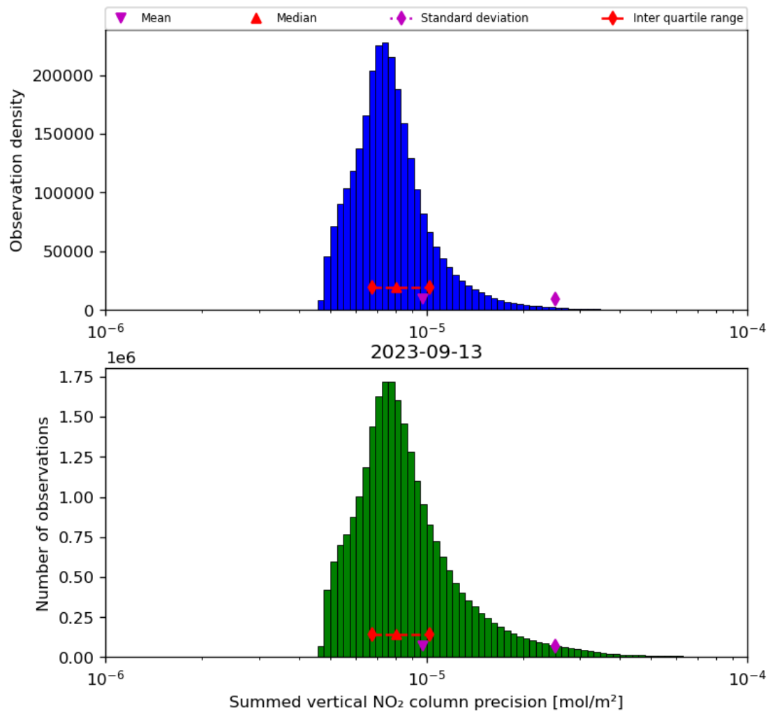
Figure 41: Histogram of "Summed vertical NO 2 column precision" for 2023-09-12 to 2023-09-14
