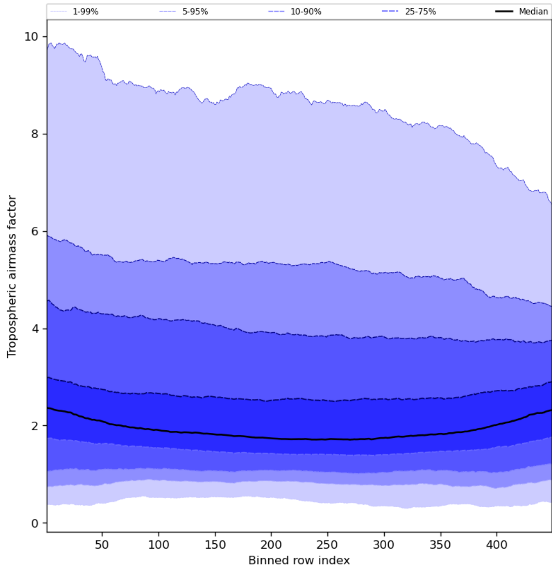
Figure 48: Along track statistics of “Tropospheric airmass factor” for 2023-09-12 to 2023-09-14
