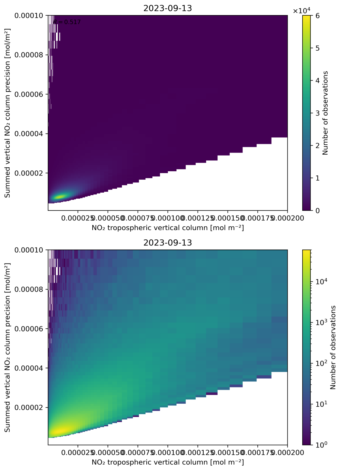
Figure 127: Scatter density plot of “NO 2 tropospheric vertical column” against “Summed vertical NO 2 column precision” for 2023-09-12 to 2023-09-14.
