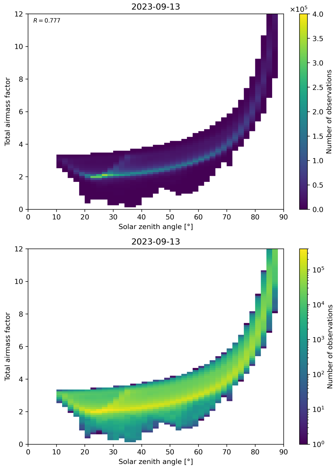
Figure 146: Scatter density plot of “Solar zenith angle” against “Total air mass factor” for 2023-09-12 to 2023-09-14.
