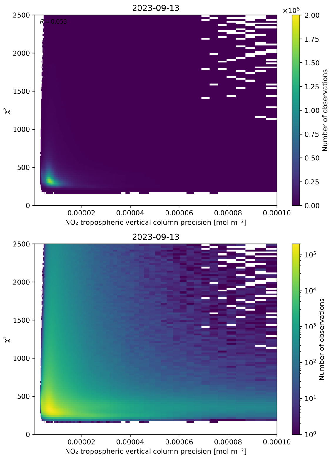
Figure 134: Scatter density plot of “NO 2 tropospheric vertical column precision” against “ \chi^2 ” for 2023-09-12 to 2023-09-14.
