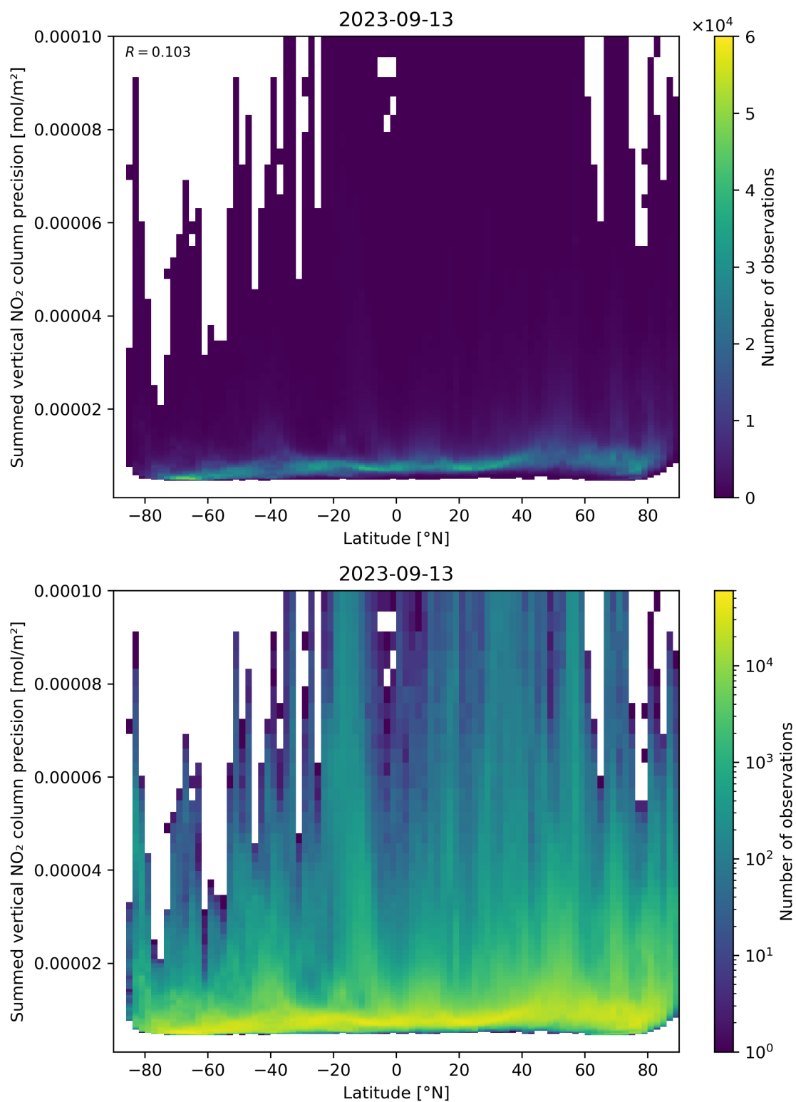
Figure 89: Scatter density plot of “Latitude” against “Summed vertical NO 2 column precision” for 2023-09-12 to 2023-09-14.
