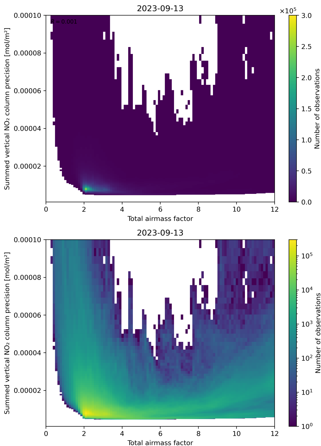
Figure 66: Scatter density plot of “Total airmass factor” against “Summed vertical NO 2 column precision” for 2023-09-12 to 2023-09-14.
