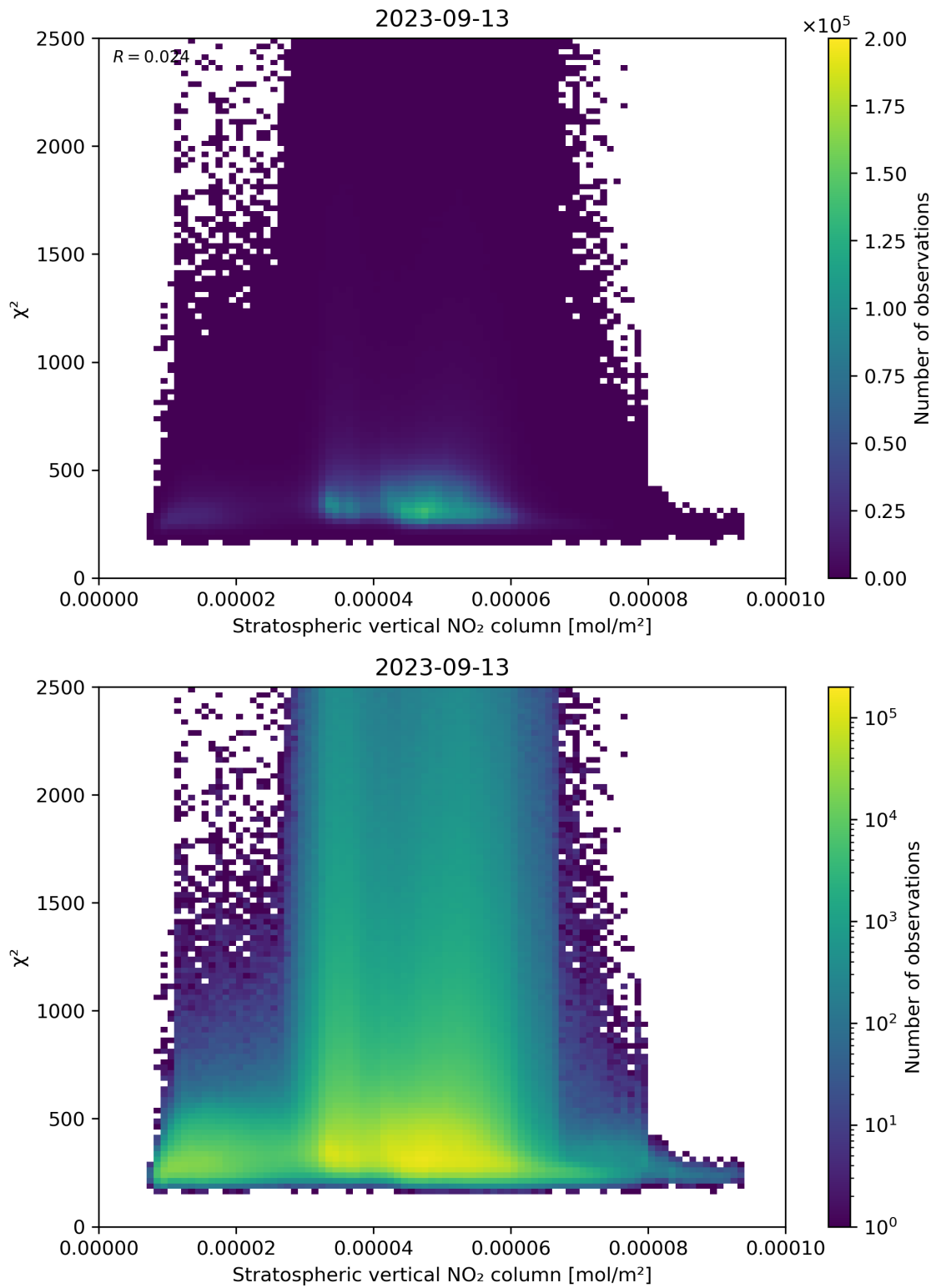
Figure 97: Scatter density plot of “Stratospheric vertical NO 2 column” against “ \chi^2 ” for 2023-09-12 to 2023-09-14.
