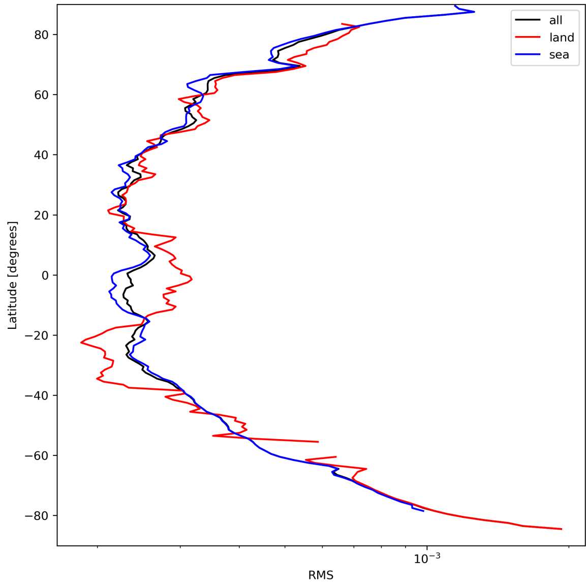
Figure 26: Zonal average of “RMS” for 2023-09-12 to 2023-09-14.
