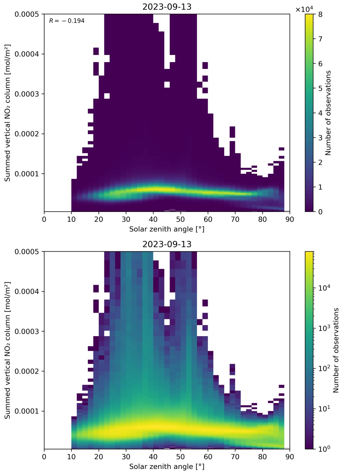
Figure 151: Scatter density plot of “Solar zenith angle” against “Summed vertical NO 2 column” for 2023-09-12 to 2023-09-14.
