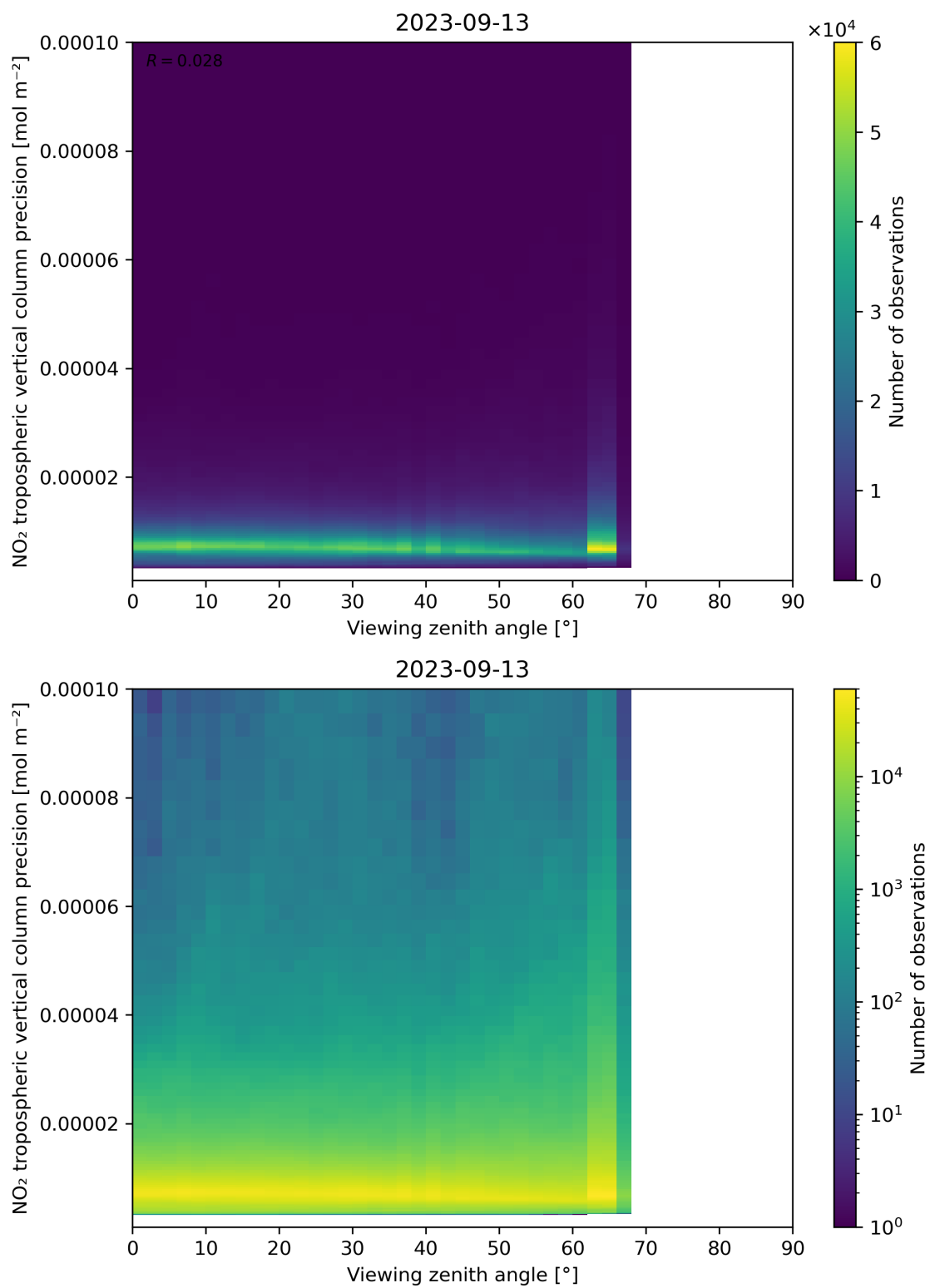
Figure 170: Scatter density plot of “Viewing zenith angle” against “NO 2 tropospheric vertical column precision” for 2023-09-12 to 2023-09-14.
