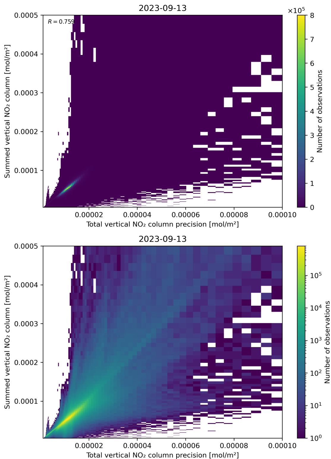
Figure 117: Scatter density plot of “Total vertical NO 2 column precision” against “Summed vertical NO 2 column” for 2023-09-12 to 2023-09-14.
