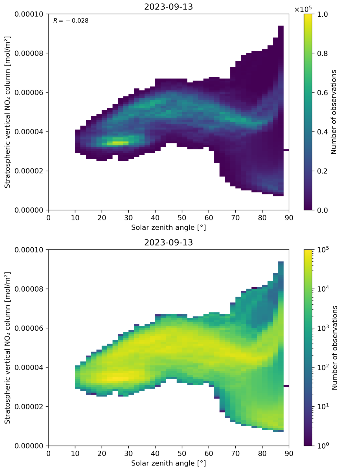
Figure 150: Scatter density plot of “Solar zenith angle” against “Stratospheric vertical NO 2 column” for 2023-09-12 to 2023-09-14.
