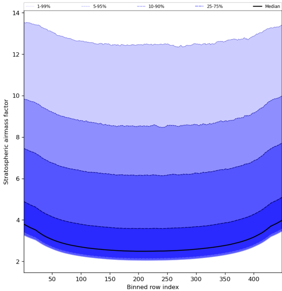
Figure 61: Along track statistics of “Stratospheric airmass factor” for 2023-09-12 to 2023-09-14
