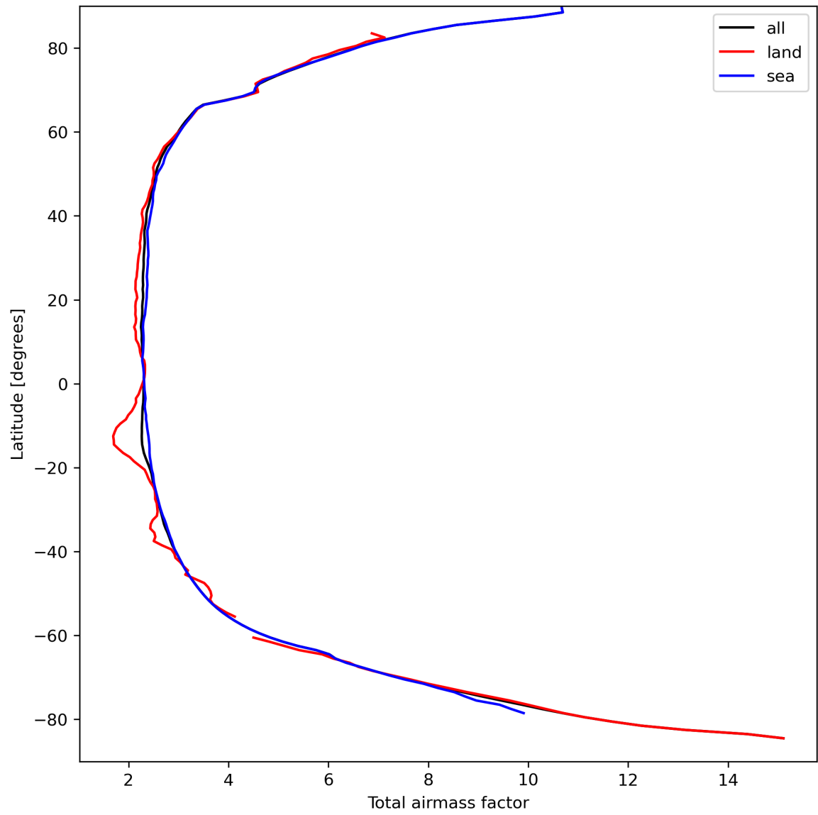
Figure 15: Zonal average of “Total airmass factor” for 2023-09-12 to 2023-09-14.
