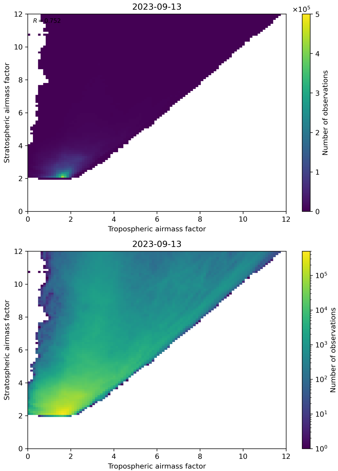
Figure 71: Scatter density plot of “Tropospheric airmass factor” against “Stratospheric airmass factor” for 2023-09-12 to 2023-09-14.
