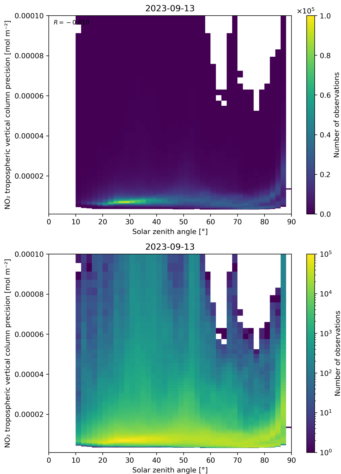
Figure 156: Scatter density plot of “Solar zenith angle” against “NO 2 tropospheric vertical column precision” for 2023-09-12 to 2023-09-14.
