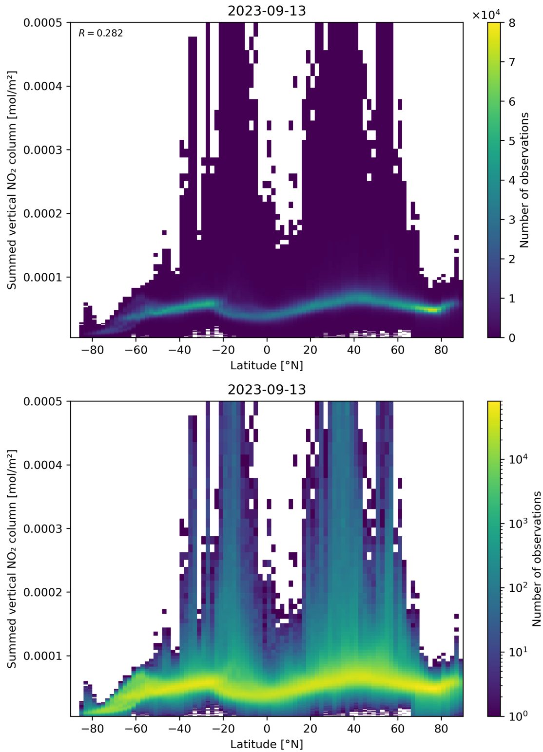
Figure 88: Scatter density plot of “Latitude” against “Summed vertical NO 2 column” for 2023-09-12 to 2023-09-14.
