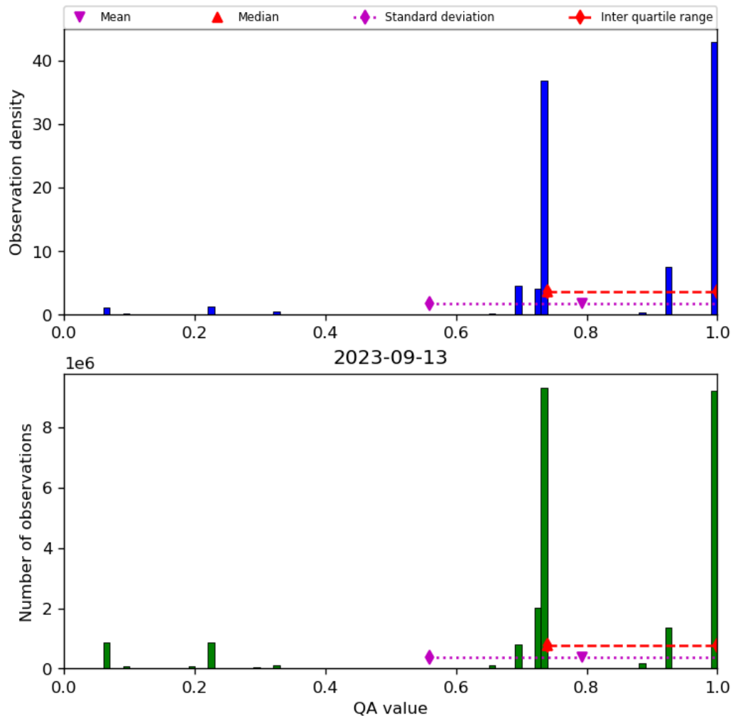
Figure 28: Histogram of “QA value” for 2023-09-12 to 2023-09-14
