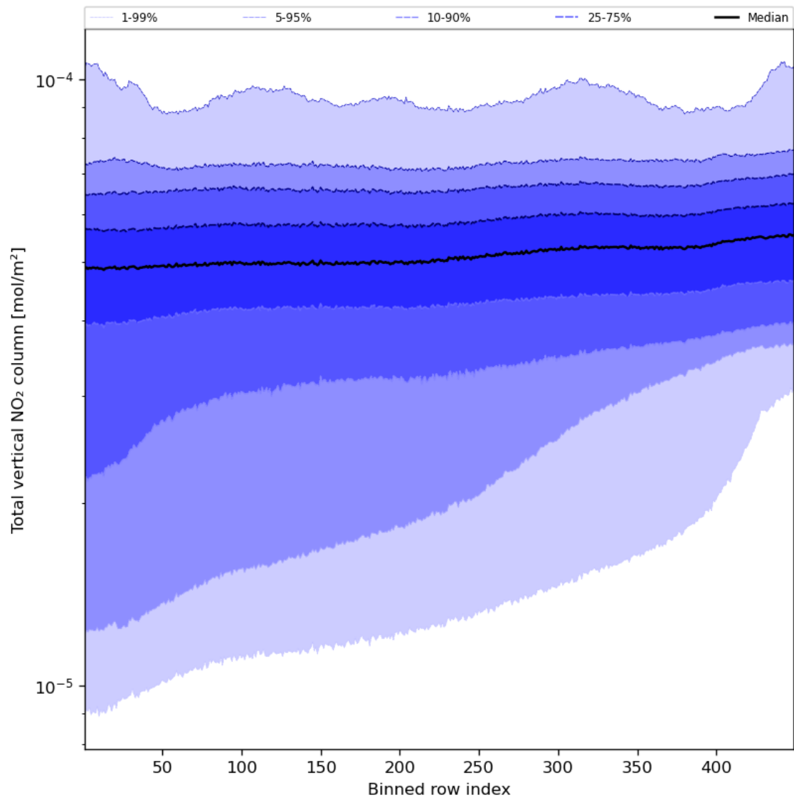
Figure 55: Along track statistics of “Total vertical NO 2 column” for 2023-09-12 to 2023-09-14
