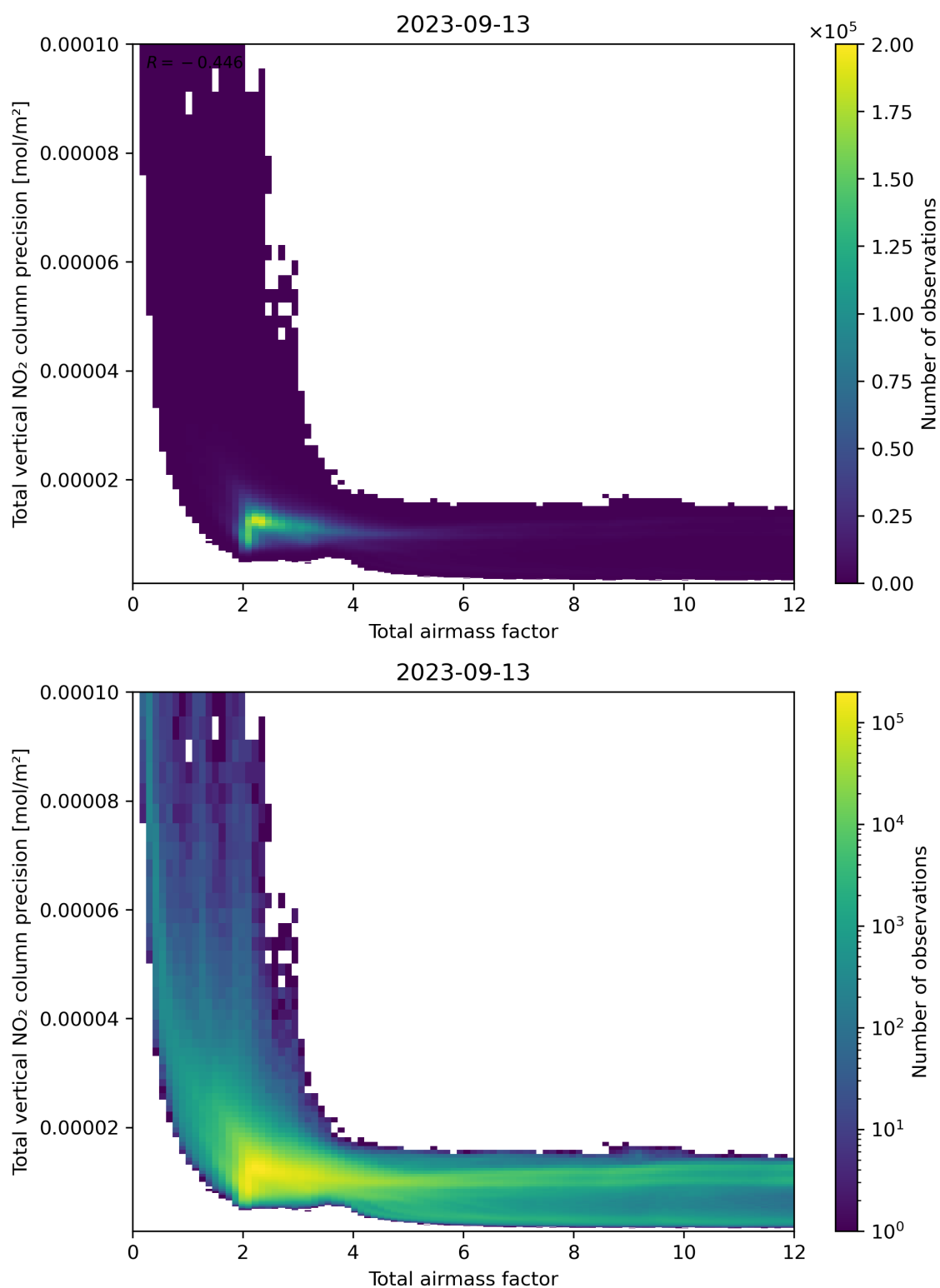
Figure 68: Scatter density plot of “Total airmass factor” against “Total vertical NO 2 column precision” for 2023-09-12 to 2023-09-14.
