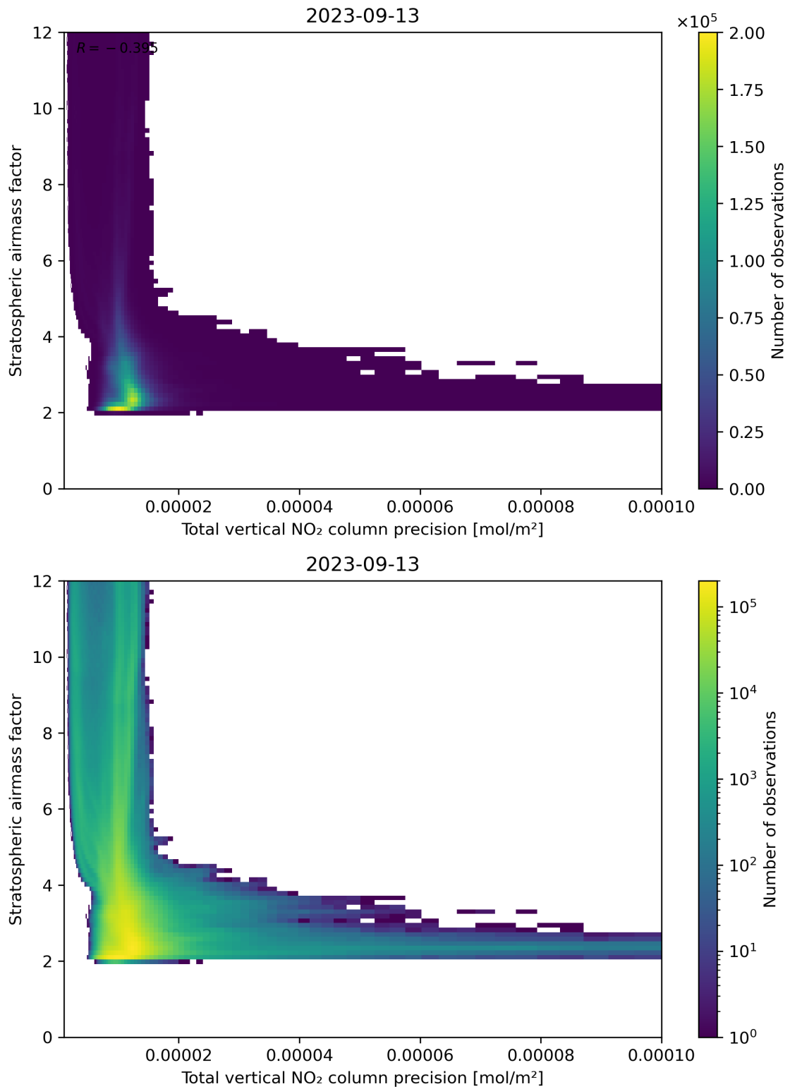
Figure 115: Scatter density plot of “Total vertical NO 2 column precision” against “Stratospheric air mass factor” for 2023-09-12 to 2023-09-14.
