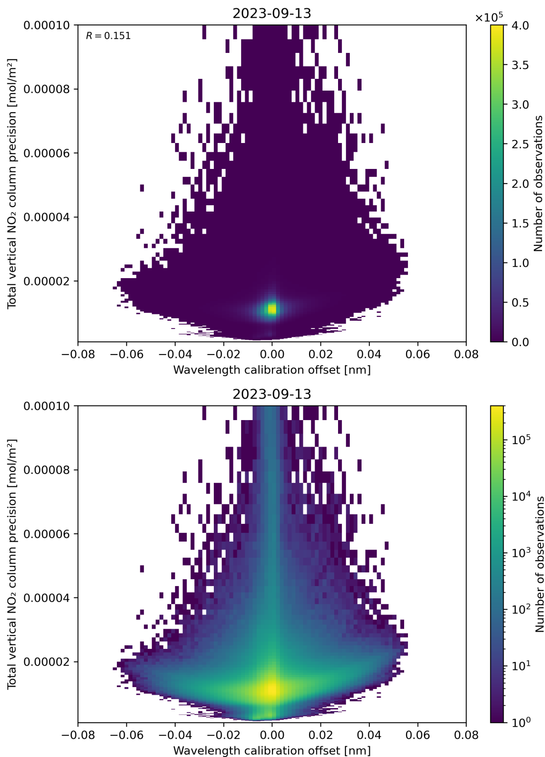
Figure 180: Scatter density plot of “Wavelength calibration offset” against “Total vertical NO 2 column precision” for 2023-09-12 to 2023-09-14.
