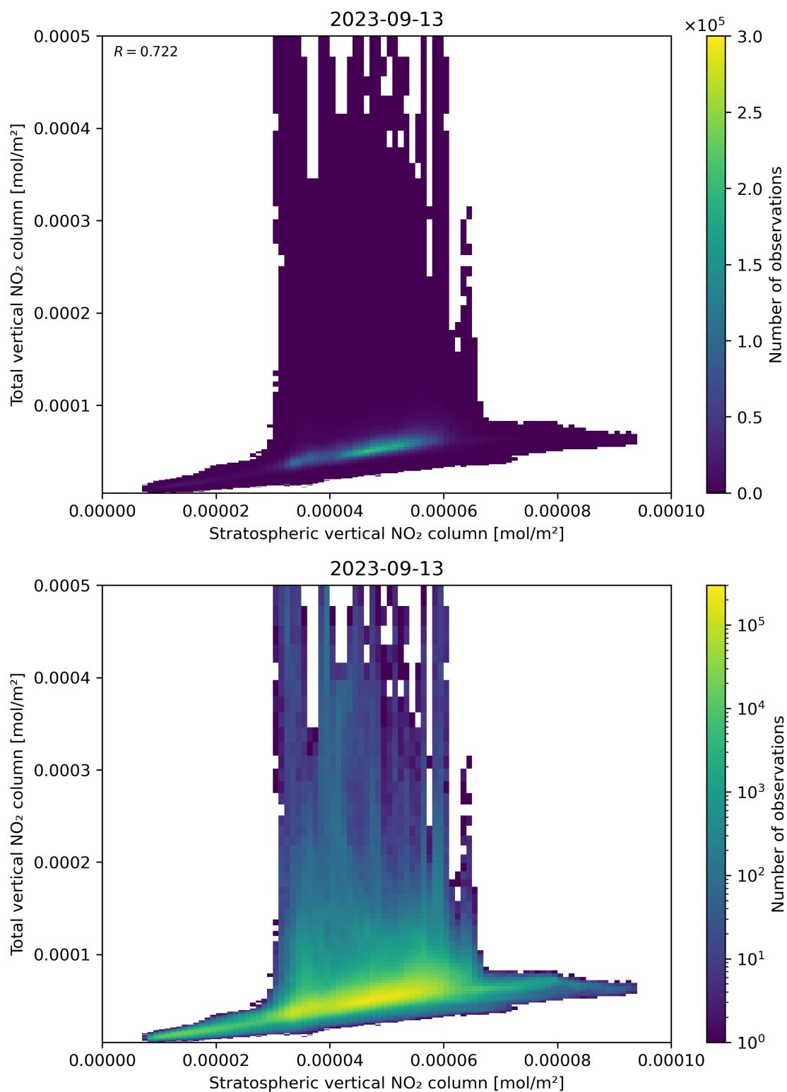
Figure 100: Scatter density plot of “Stratospheric vertical NO 2 column” against “Total vertical NO 2 column” for 2023-09-12 to 2023-09-14.
