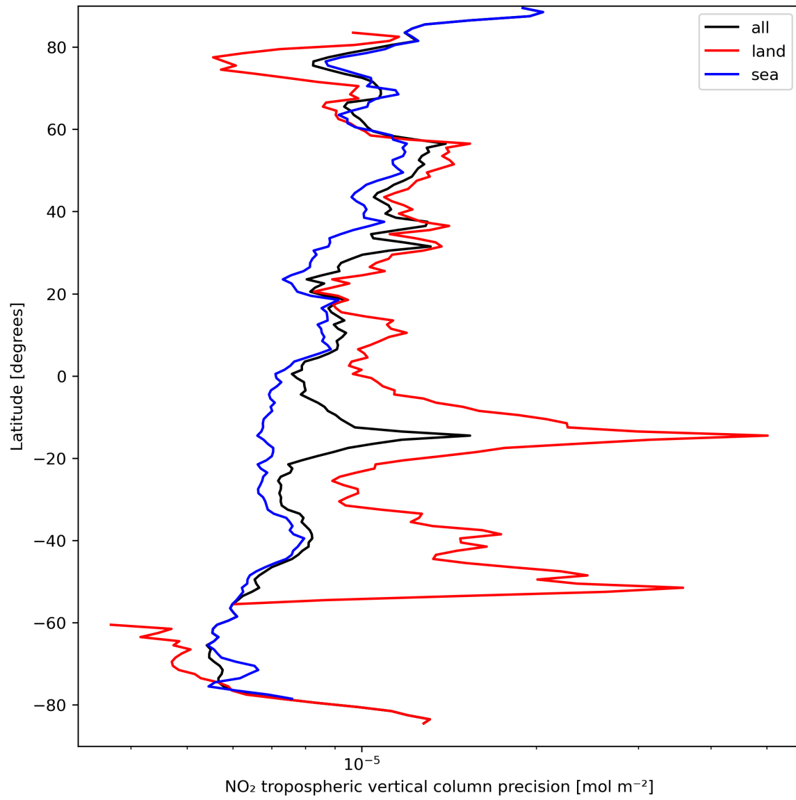
Figure 13: Zonal average of “NO 2 tropospheric vertical column precision” for 2023-09-12 to 2023-09-14.
