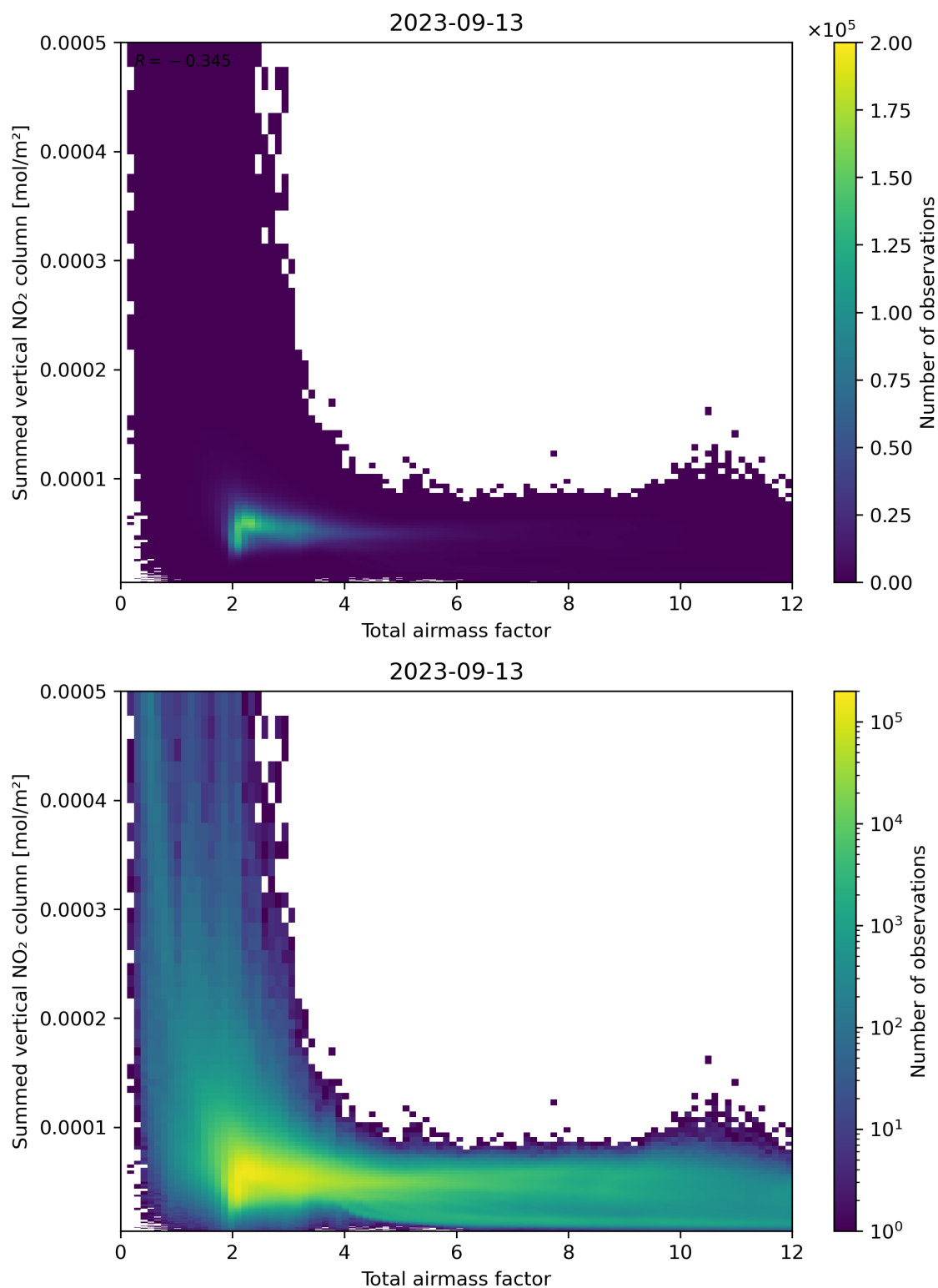
Figure 65: Scatter density plot of “Total airmass factor” against “Summed vertical NO 2 column” for 2023-09-12 to 2023-09-14.
