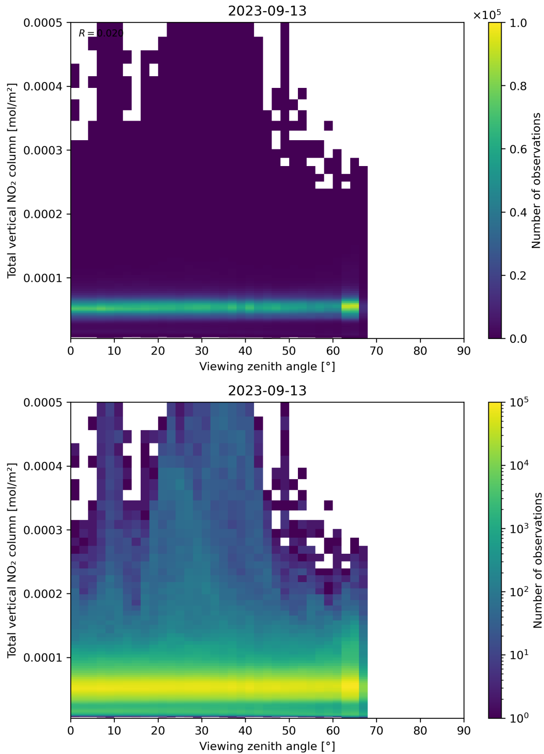
Figure 167: Scatter density plot of “Viewing zenith angle” against “Total vertical NO 2 column” for 2023-09-12 to 2023-09-14.
