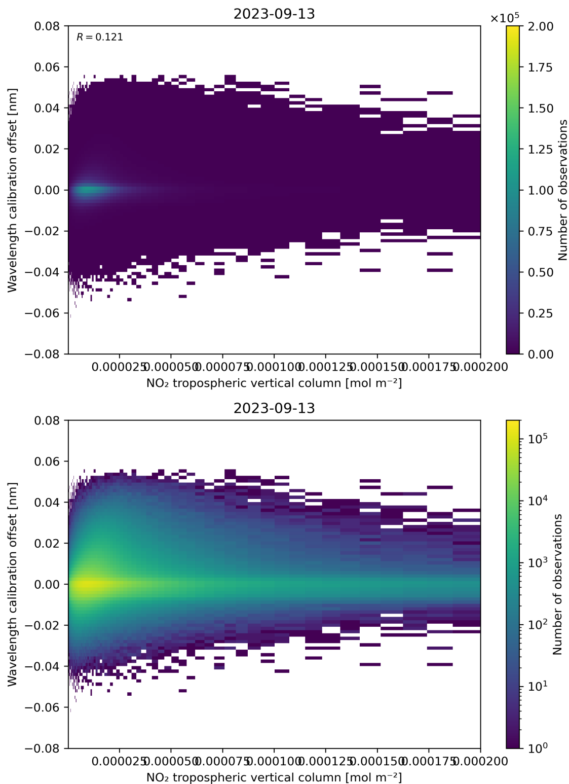
Figure 143: Scatter density plot of “NO 2 tropospheric vertical column” against “Wavelength calibration offset” for 2023-09-12 to 2023-09-14.
