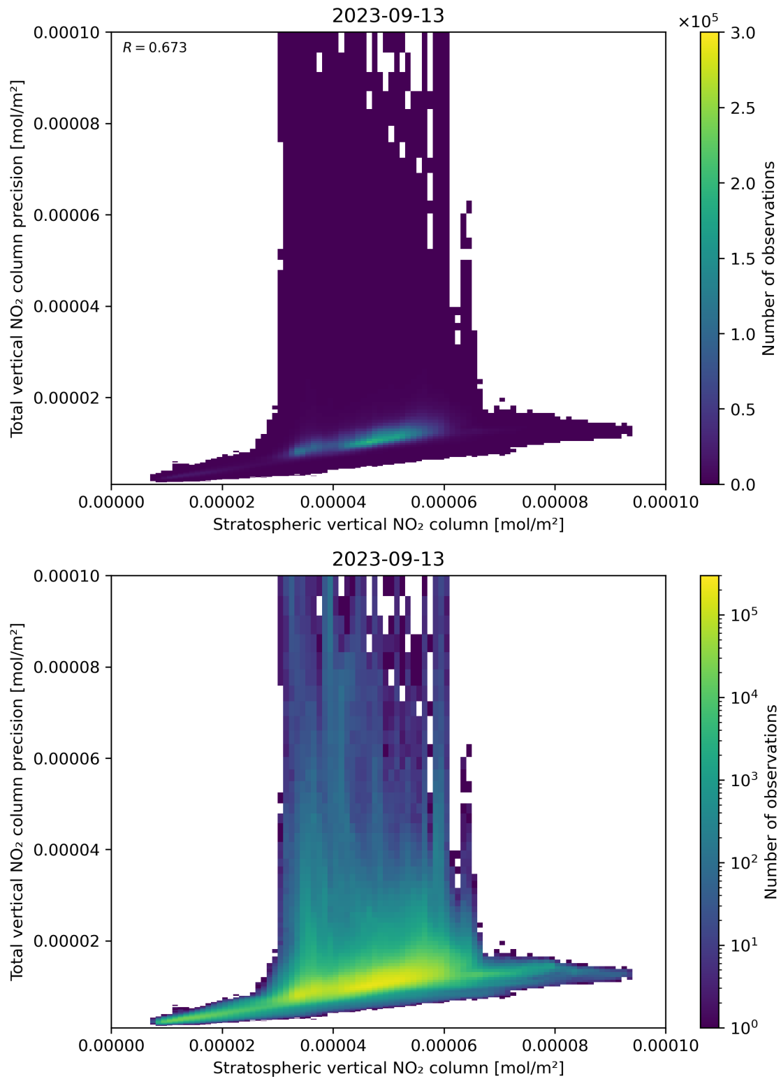
Figure 101: Scatter density plot of “Stratospheric vertical NO 2 column” against “Total vertical NO 2 column precision” for 2023-09-12 to 2023-09-14.
