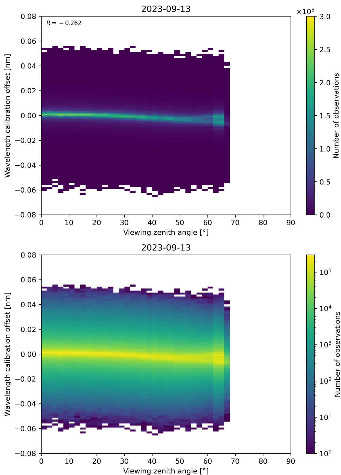
Figure 173: Scatter density plot of “Viewing zenith angle” against “Wavelength calibration offset” for 2023-09-12 to 2023-09-14.
