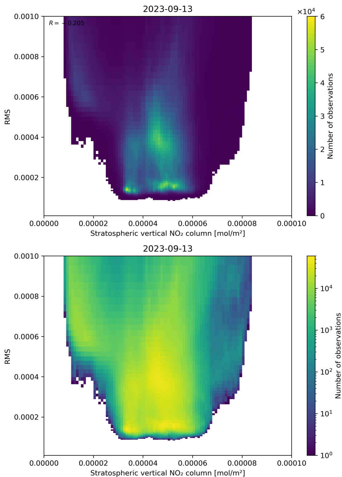
Figure 102: Scatter density plot of “Stratospheric vertical NO 2 column” against “RMS” for 2023-09-12 to 2023-09-14.
