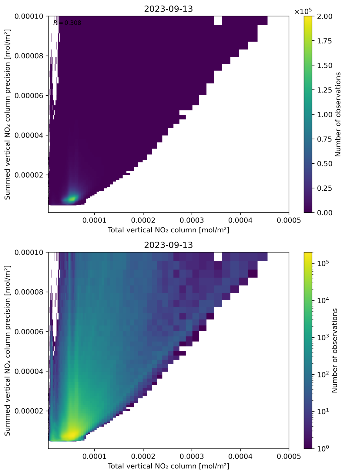
Figure 113: Scatter density plot of “Total vertical NO 2 column” against “Summed vertical NO 2 column precision” for 2023-09-12 to 2023-09-14.
