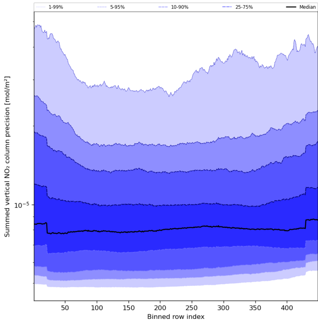
Figure 58: Along track statistics of “Summed vertical NO 2 column precision” for 2023-09-12 to 2023-09-14
