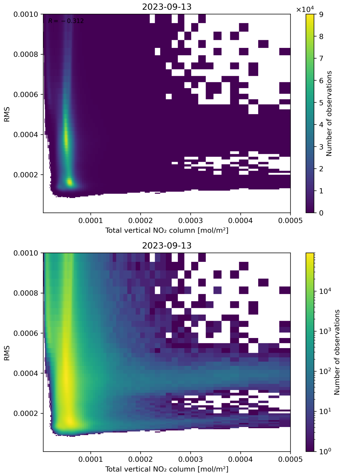
Figure 120: Scatter density plot of “Total vertical NO 2 column” against “RMS” for 2023-09-12 to 2023-09-14.
