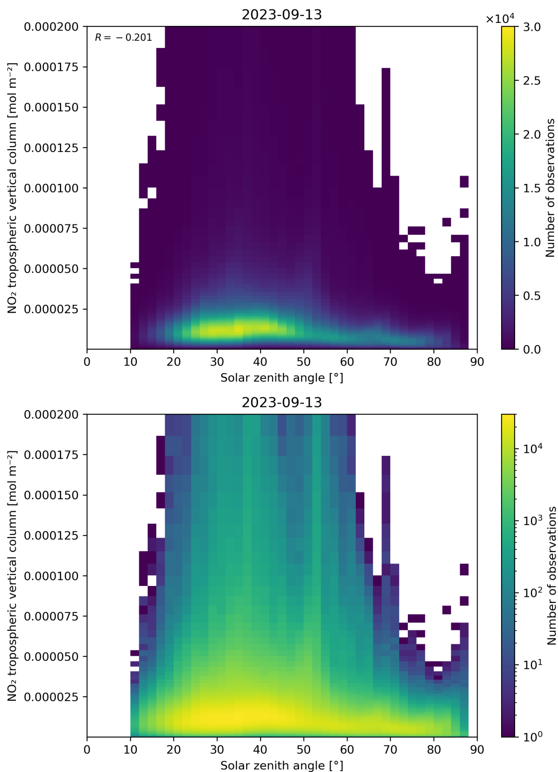
Figure 155: Scatter density plot of “Solar zenith angle” against “NO 2 tropospheric vertical column” for 2023-09-12 to 2023-09-14.
