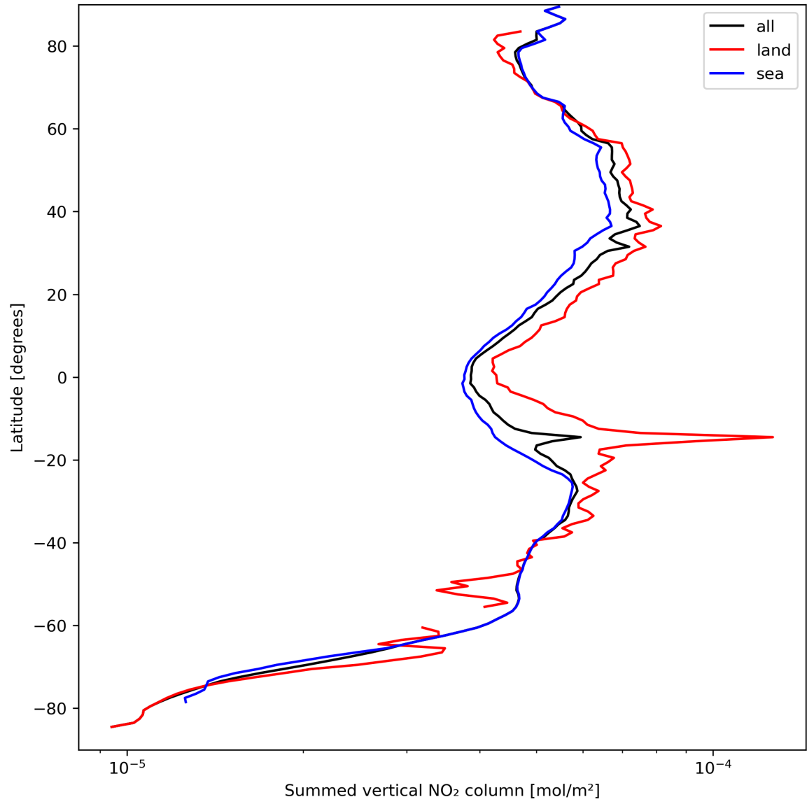
Figure 23: Zonal average of “Summed vertical NO 2 column” for 2023-09-12 to 2023-09-14.
