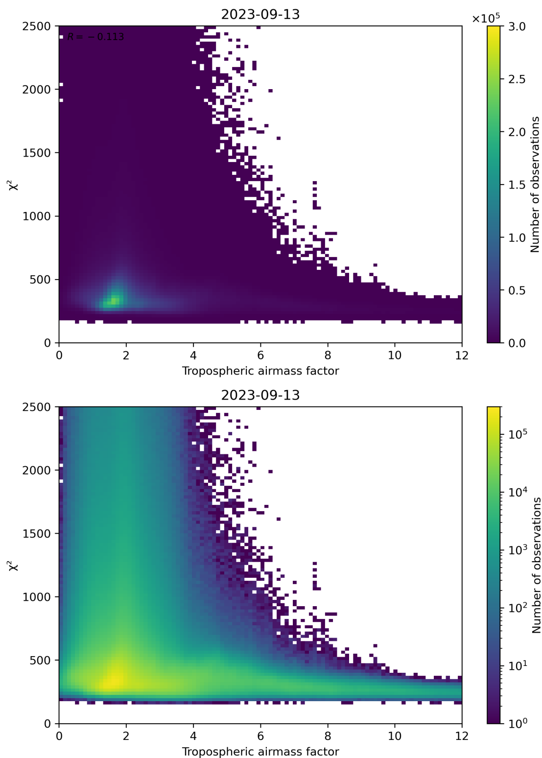
Figure 73: Scatter density plot of “Tropospheric airmass factor” against “ \chi^2 ” for 2023-09-12 to 2023-09-14.
