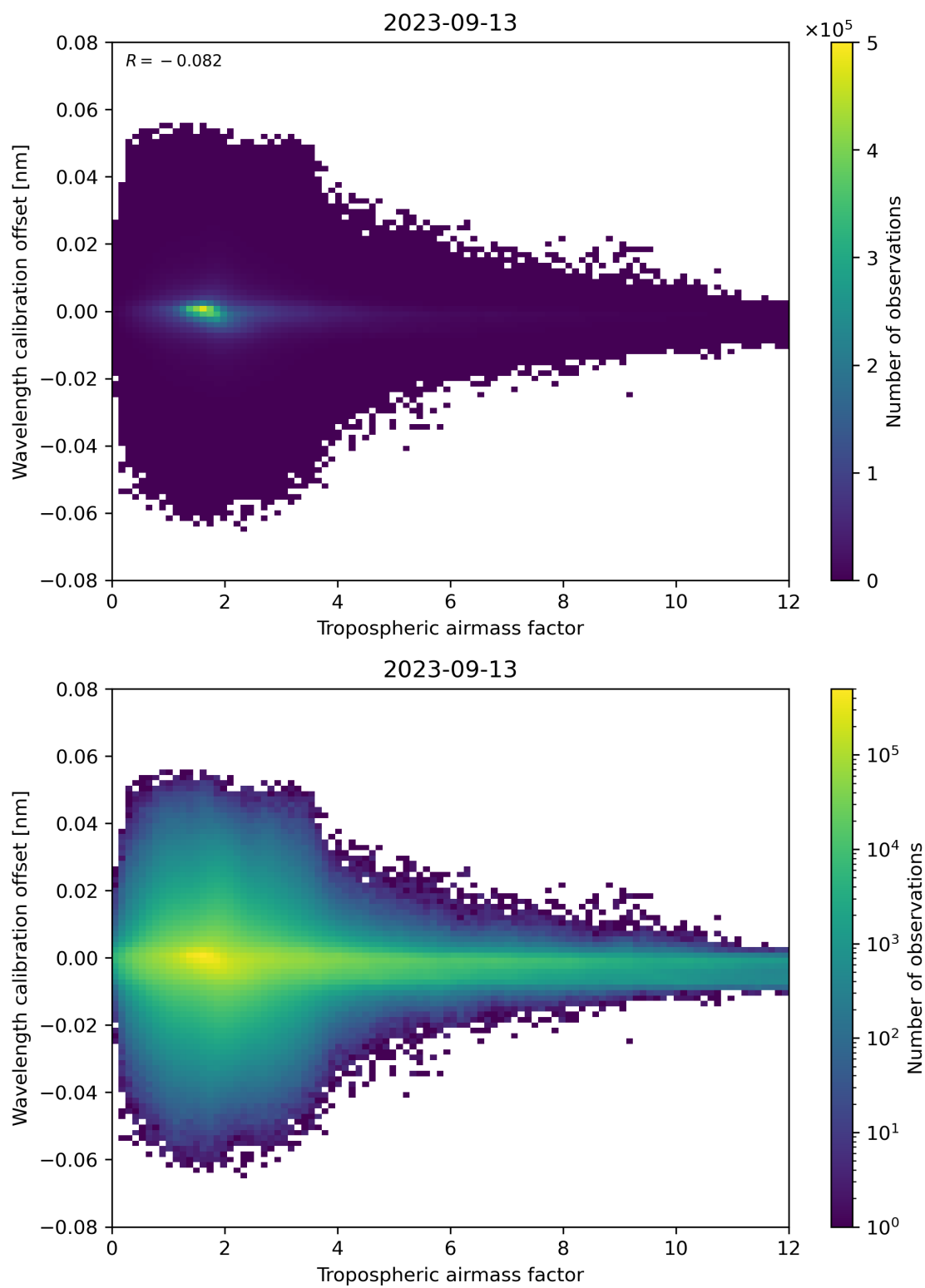
Figure 80: Scatter density plot of “Tropospheric airmass factor” against “Wavelength calibration offset” for 2023-09-12 to 2023-09-14.
