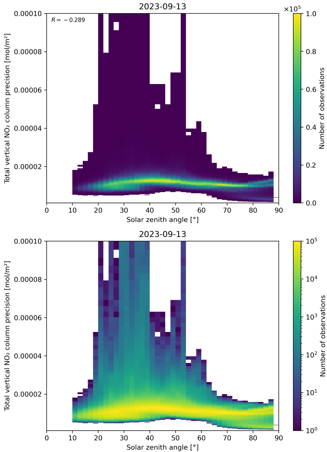
Figure 154: Scatter density plot of “Solar zenith angle” against “Total vertical NO 2 column precision” for 2023-09-12 to 2023-09-14.
