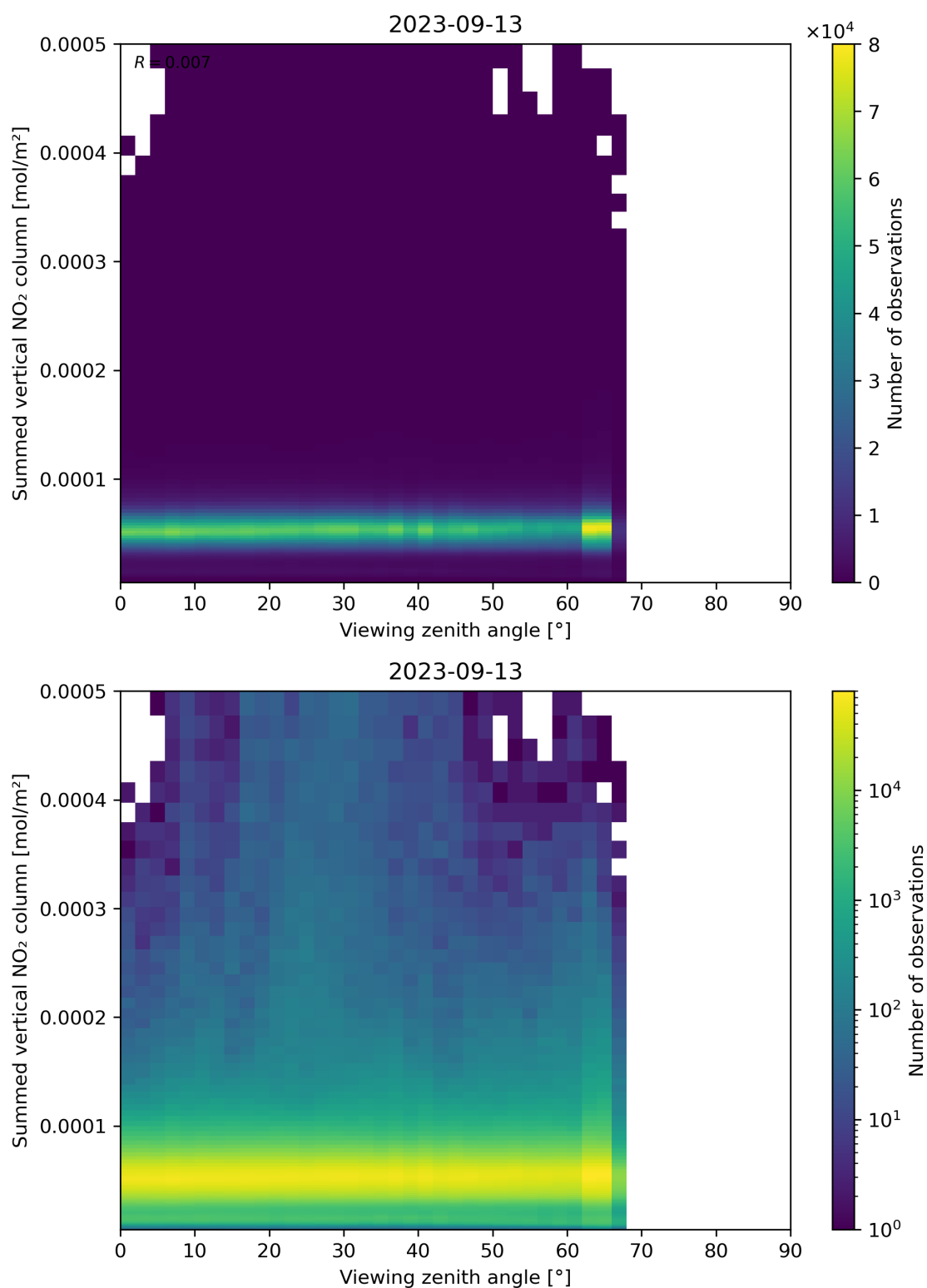
Figure 165: Scatter density plot of “Viewing zenith angle” against “Summed vertical NO 2 column” for 2023-09-12 to 2023-09-14.
