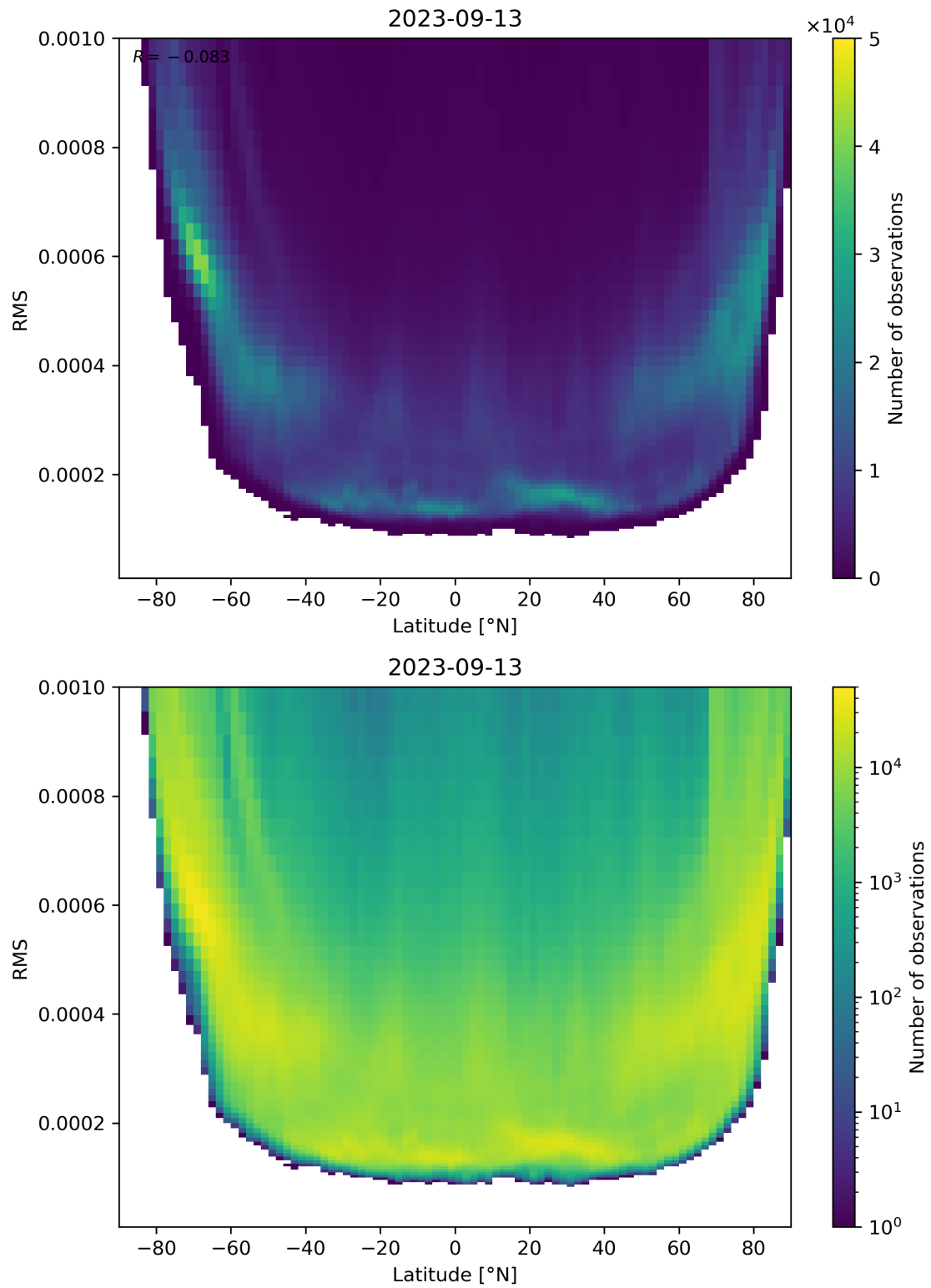
Figure 94: Scatter density plot of “Latitude” against “RMS” for 2023-09-12 to 2023-09-14.
