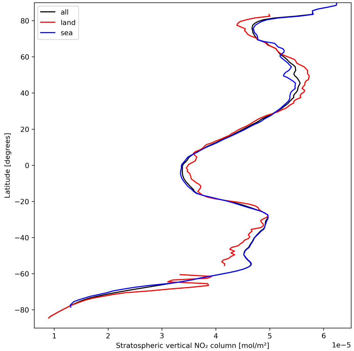
Figure 19: Zonal average of “Stratospheric vertical NO 2 column” for 2023-09-12 to 2023-09-14.
