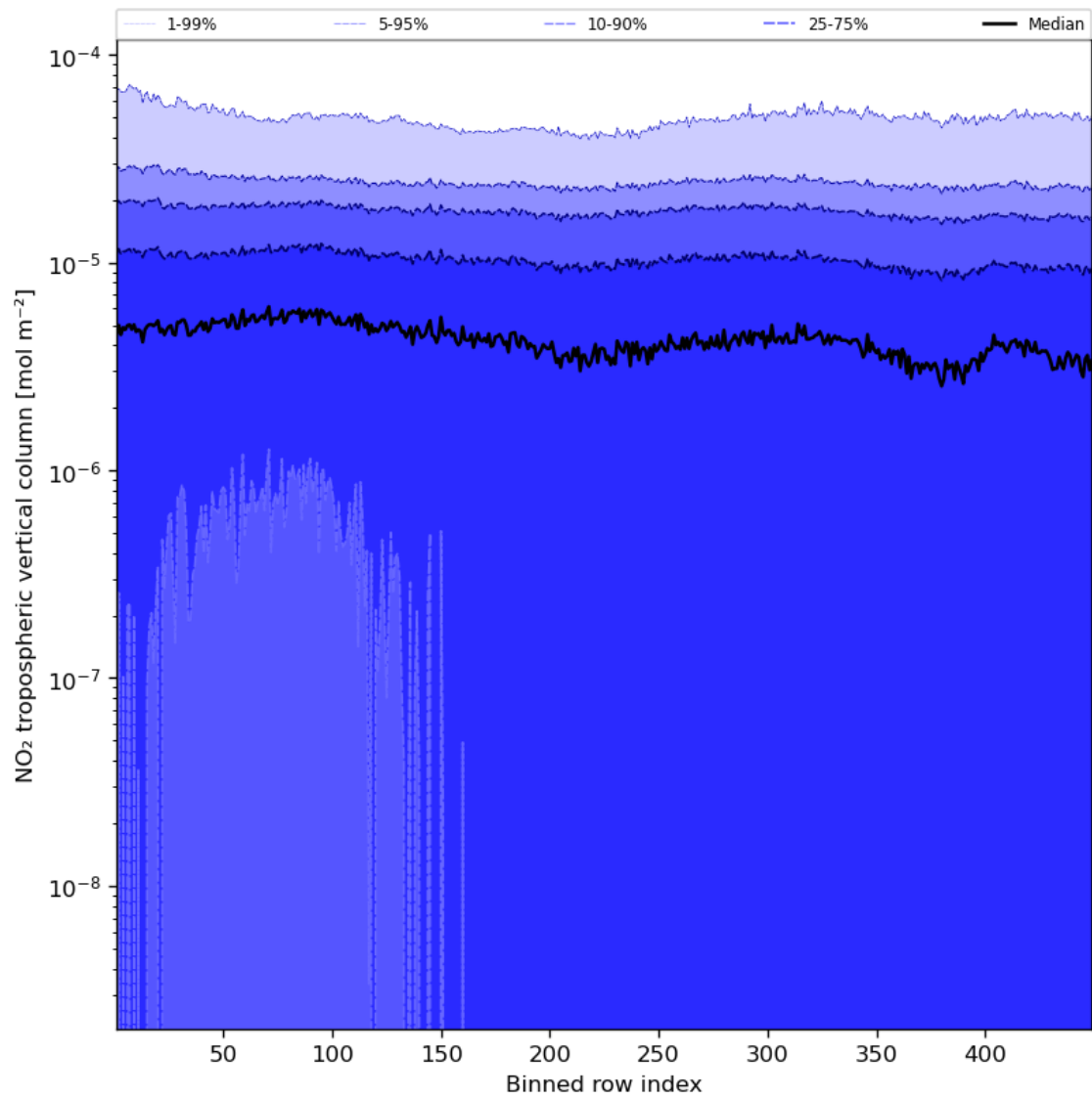
Figure 46: Along track statistics of “NO 2 tropospheric vertical column” for 2023-09-12 to 2023-09-14
