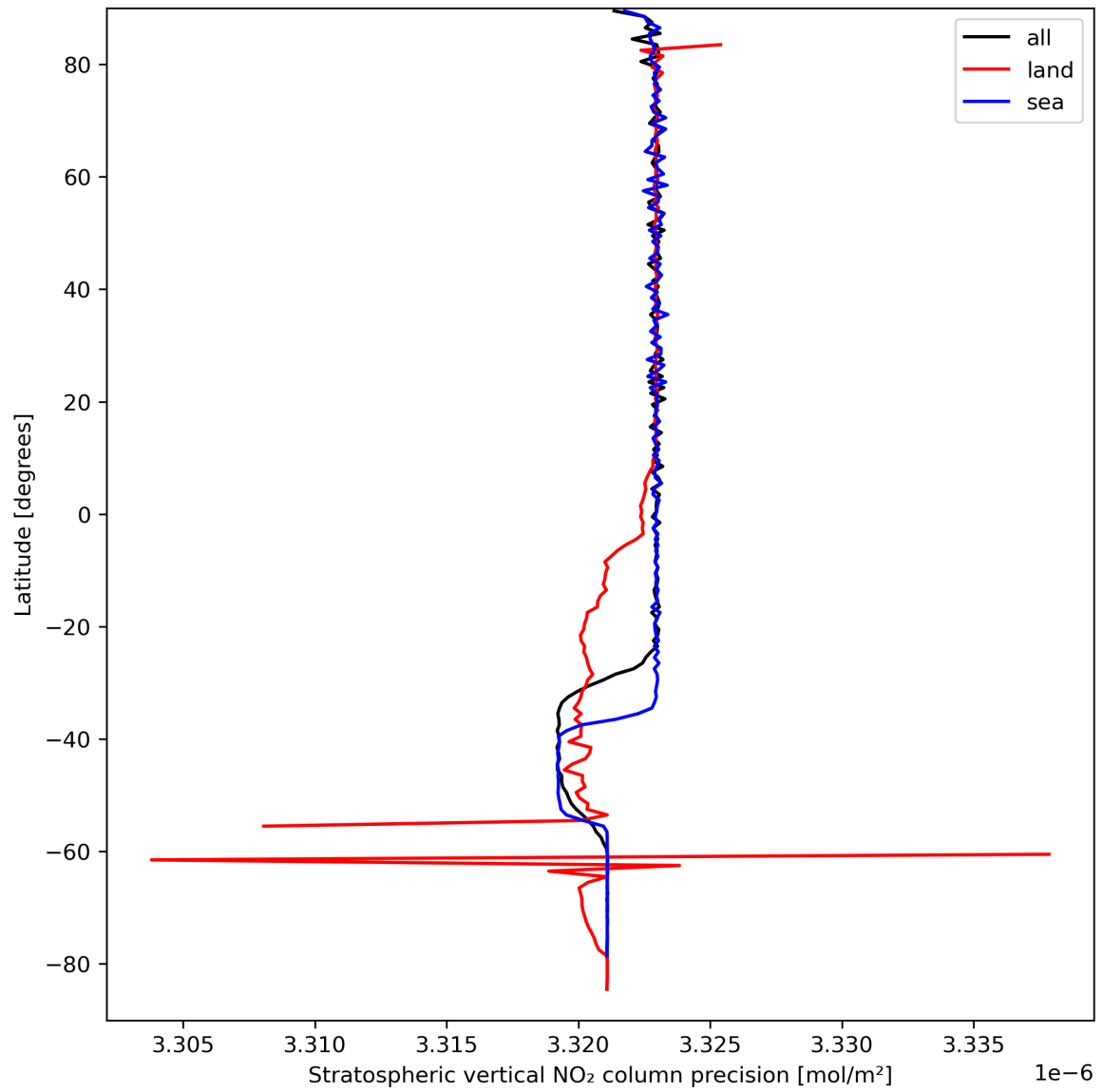
Figure 20: Zonal average of “Stratospheric vertical NO 2 column precision” for 2023-09-12 to 2023-09-14.
