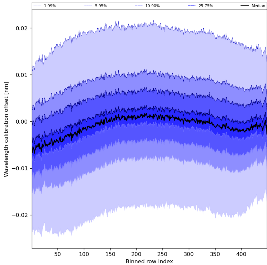
Figure 52: Along track statistics of “Wavelength calibration offset” for 2023-09-12 to 2023-09-14
