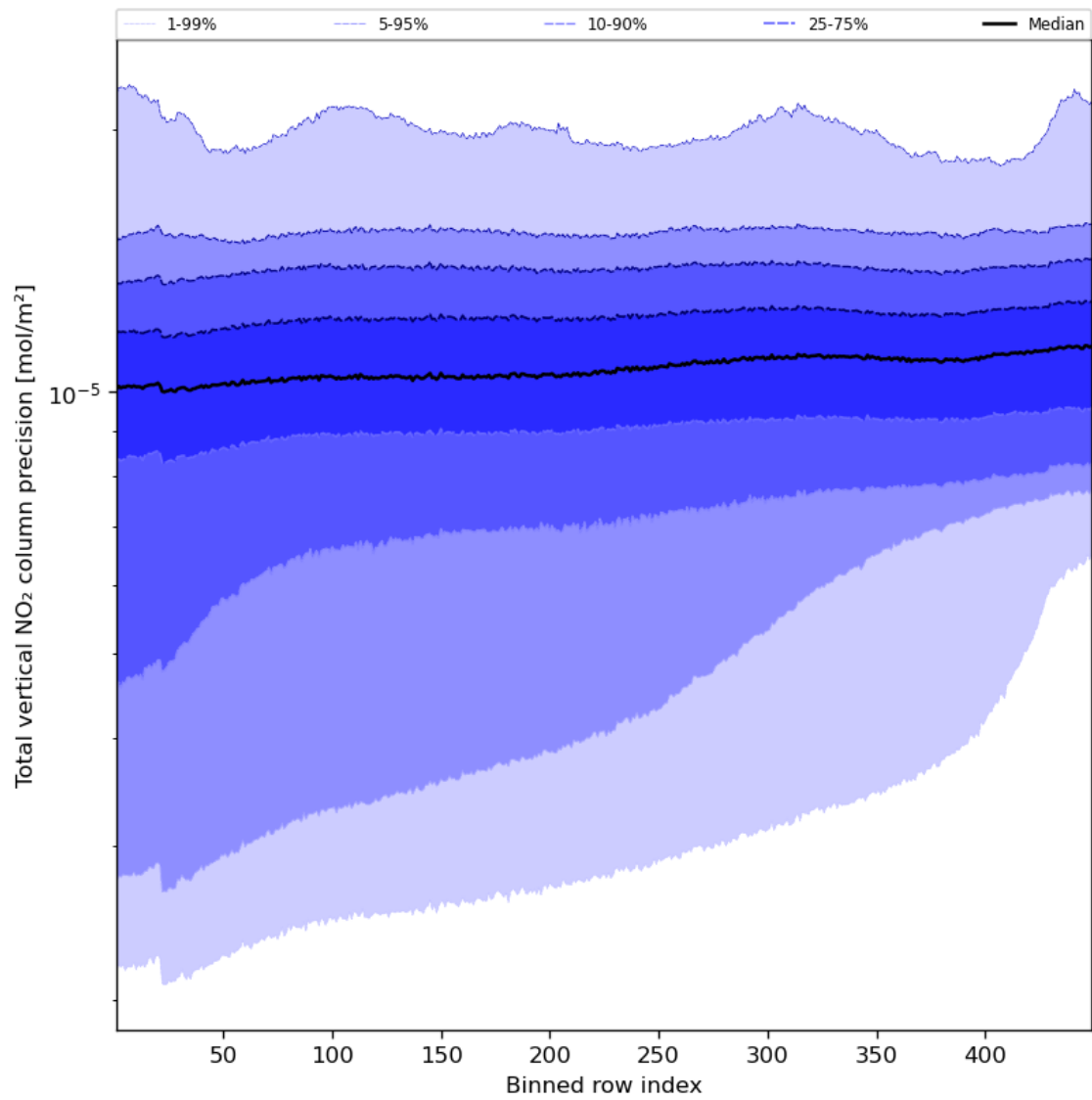
Figure 56: Along track statistics of “Total vertical NO 2 column precision” for 2023-09-12 to 2023-09-14
