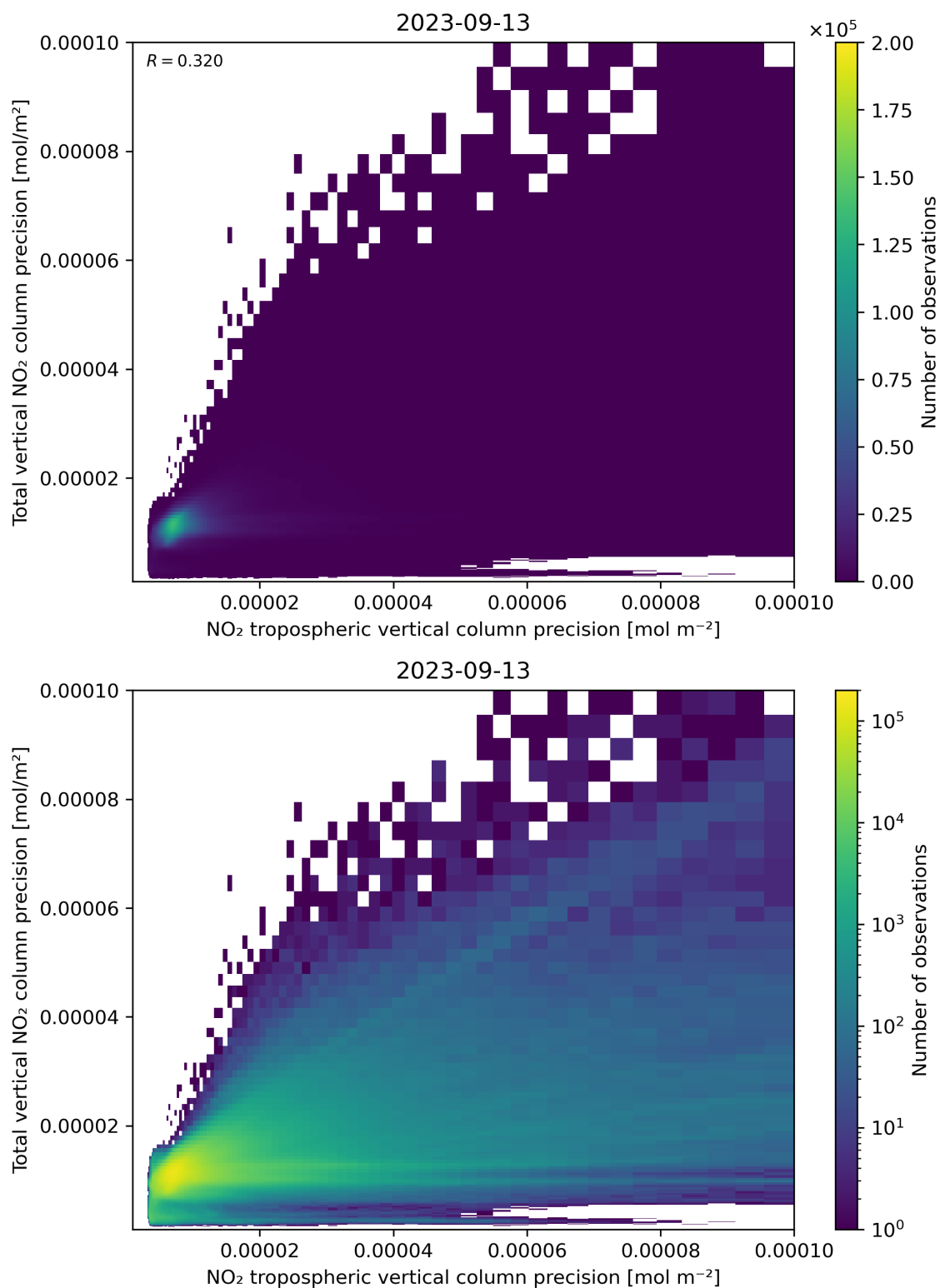
Figure 139: Scatter density plot of “NO 2 tropospheric vertical column precision” against “Total vertical NO 2 column precision” for 2023-09-12 to 2023-09-14.
