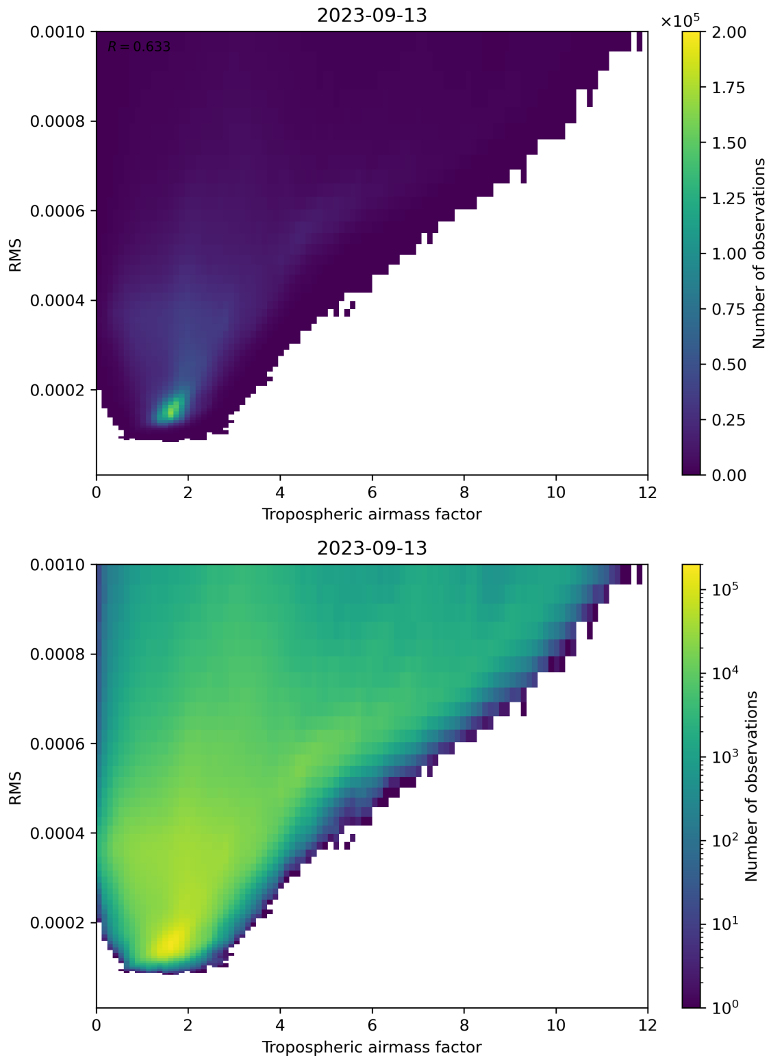
Figure 79: Scatter density plot of “Tropospheric airmass factor” against “RMS” for 2023-09-12 to 2023-09-14.
