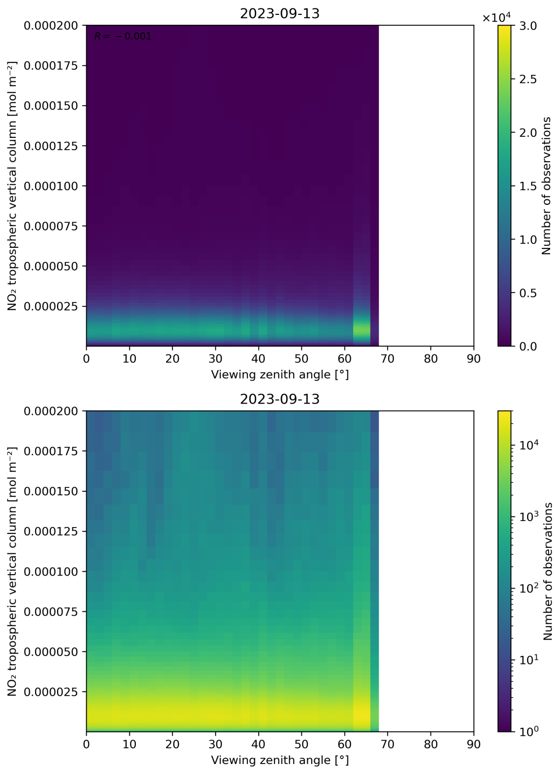
Figure 169: Scatter density plot of “Viewing zenith angle” against “NO 2 tropospheric vertical column” for 2023-09-12 to 2023-09-14.
