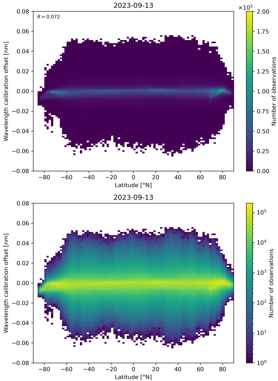
Figure 95: Scatter density plot of “Latitude” against “Wavelength calibration offset” for 2023-09-12 to 2023-09-14.
