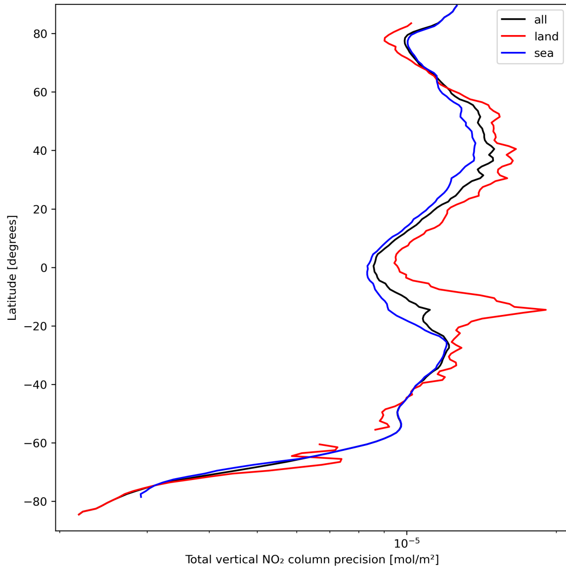
Figure 22: Zonal average of “Total vertical NO 2 column precision” for 2023-09-12 to 2023-09-14.
