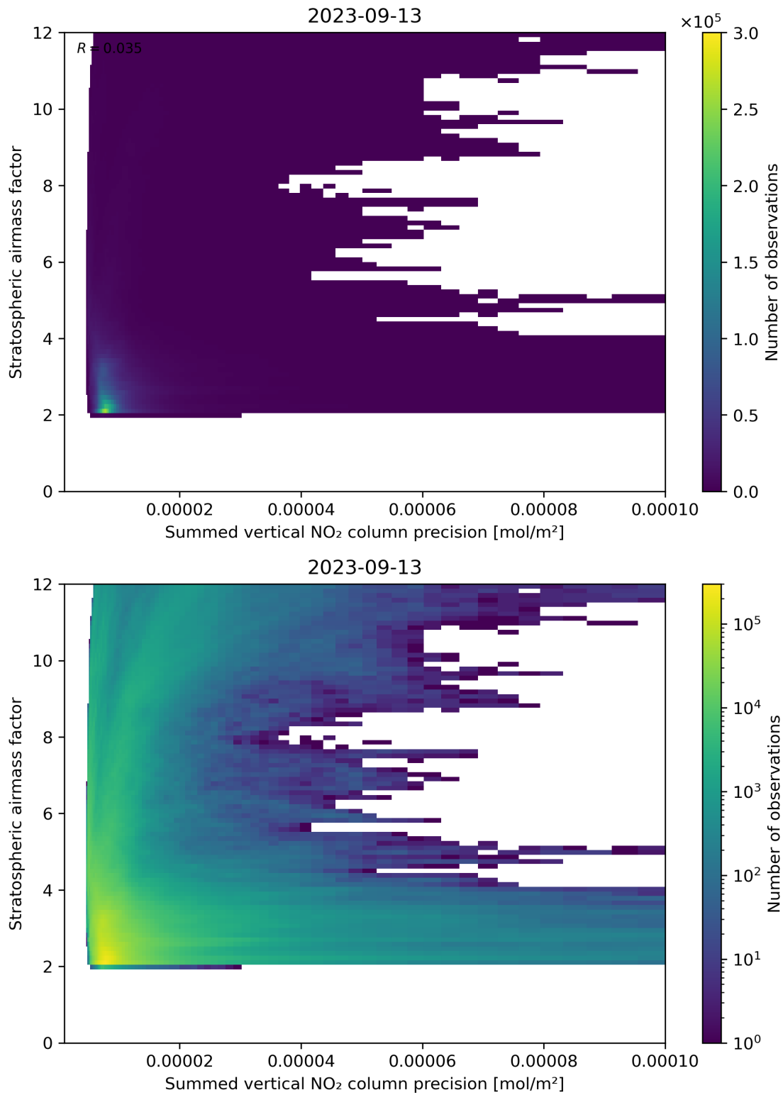
Figure 106: Scatter density plot of “Summed vertical NO 2 column precision” against “Stratospheric airmass factor” for 2023-09-12 to 2023-09-14.
