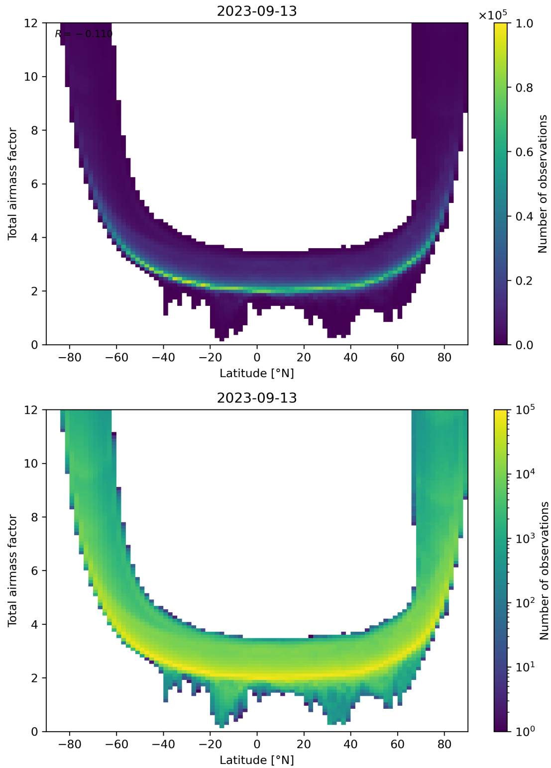
Figure 84: Scatter density plot of “Latitude” against “Total airmass factor” for 2023-09-12 to 2023-09-14.
