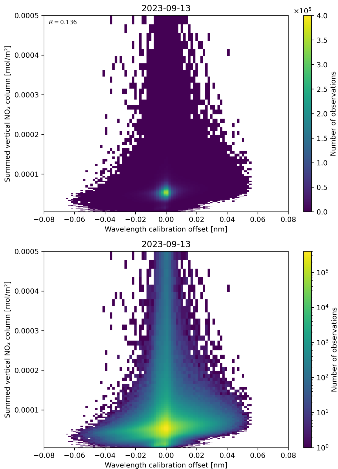
Figure 177: Scatter density plot of “Wavelength calibration offset” against “Summed vertical NO 2 column” for 2023-09-12 to 2023-09-14.
