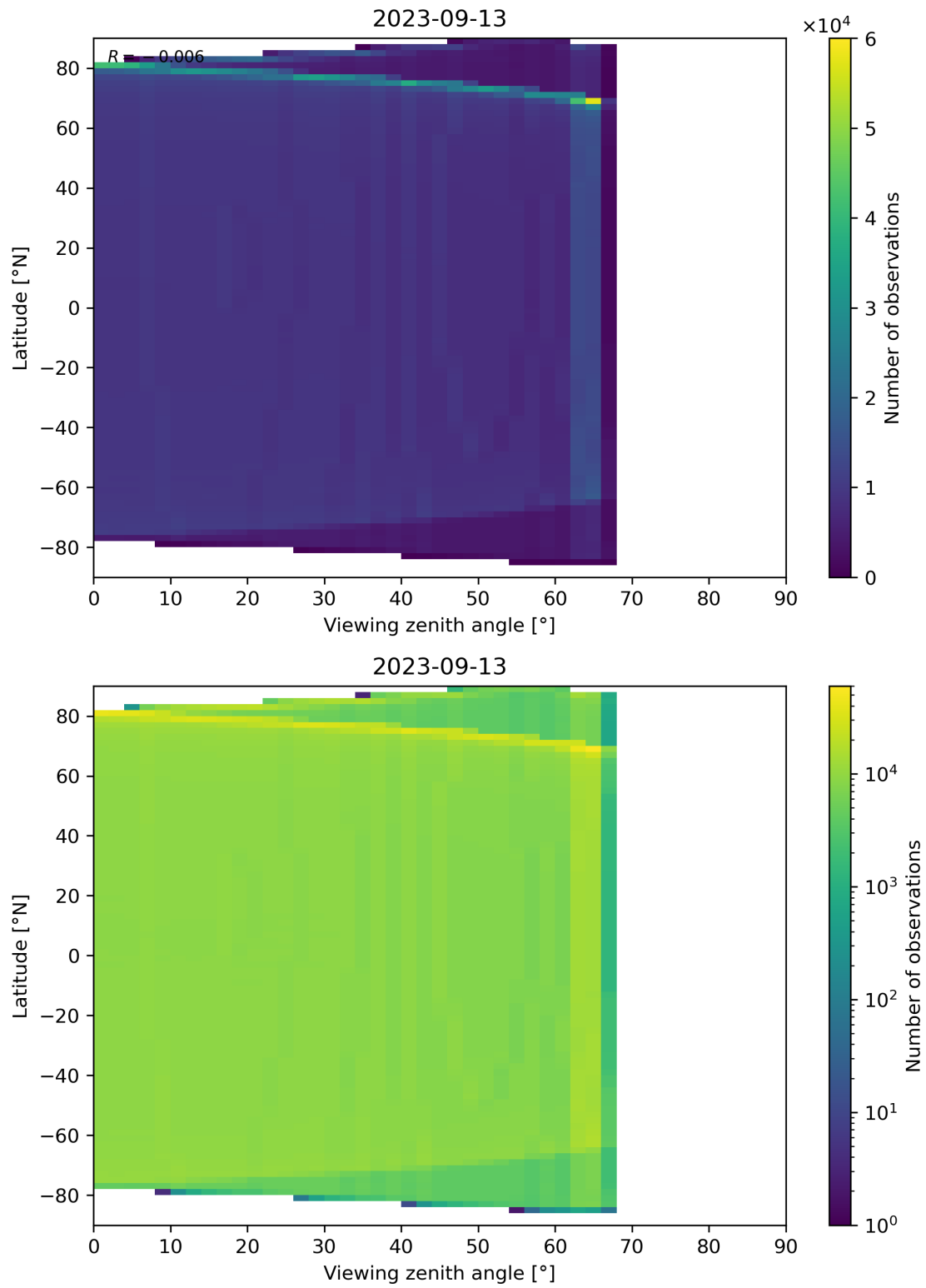
Figure 163: Scatter density plot of “Viewing zenith angle” against “Latitude” for 2023-09-12 to 2023-09-14.
