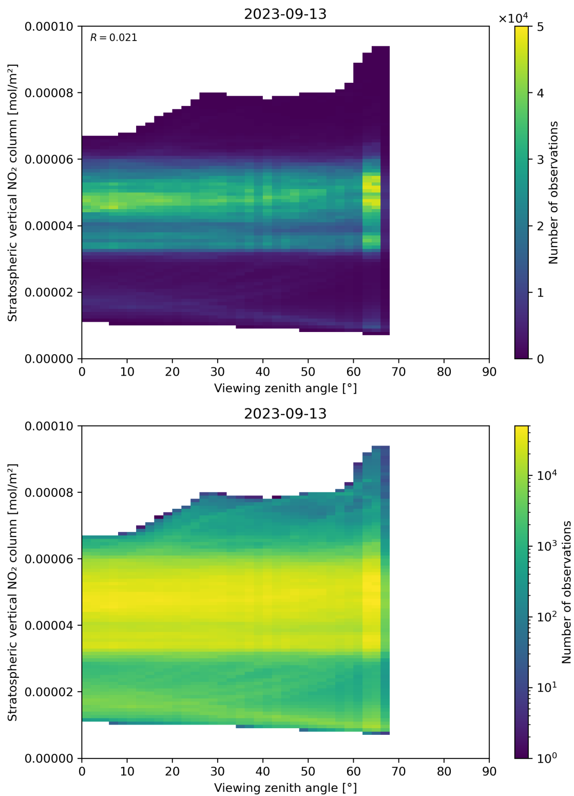
Figure 164: Scatter density plot of “Viewing zenith angle” against “Stratospheric vertical NO 2 column” for 2023-09-12 to 2023-09-14.
