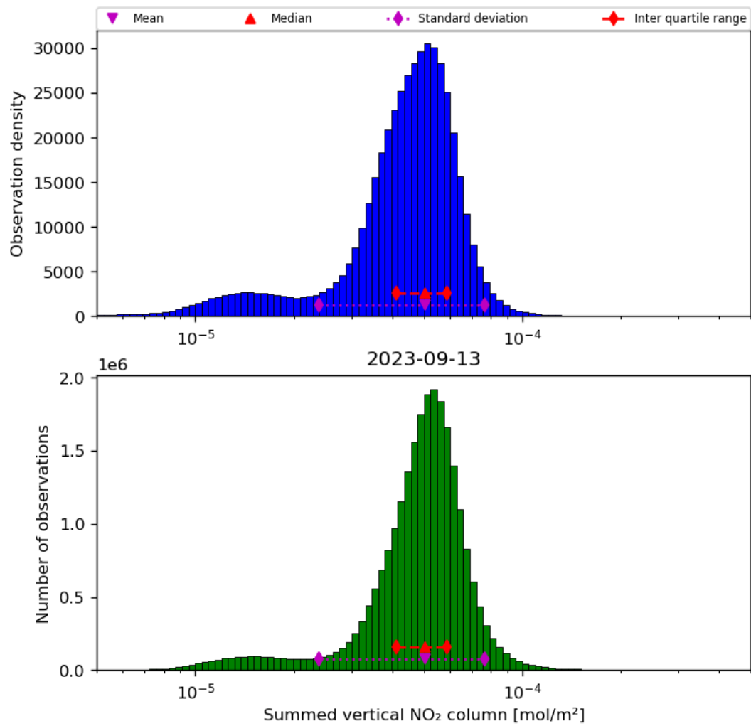
Figure 40: Histogram of “Summed vertical NO 2 column” for 2023-09-12 to 2023-09-14
