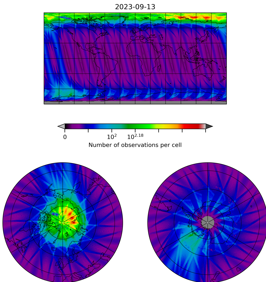
Figure 10: Map of the number of observations for 2023-09-12 to 2023-09-14
