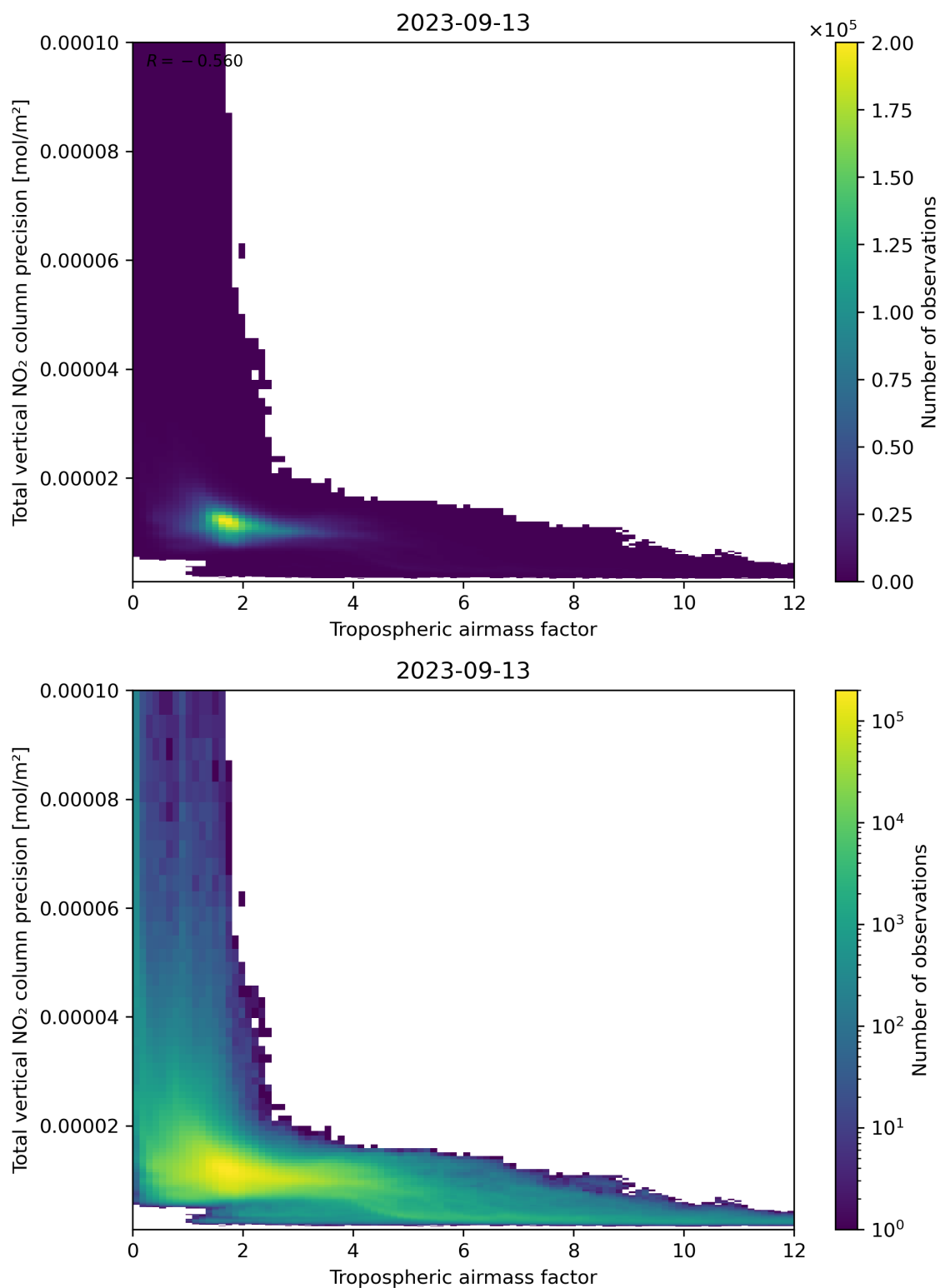
Figure 78: Scatter density plot of “Tropospheric air mass factor” against “Total vertical NO 2 column precision” for 2023-09-12 to 2023-09-14.
