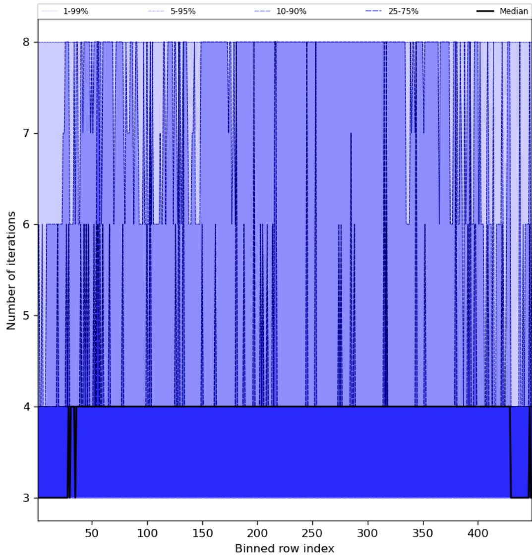
Figure 51: Along track statistics of “Number of iterations” for 2023-09-12 to 2023-09-14
