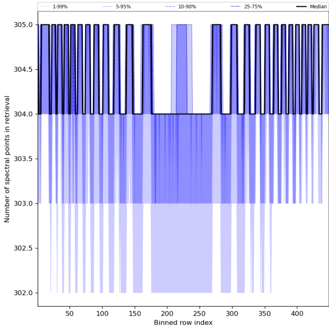
Figure 50: Along track statistics of “Number of spectral points in retrieval” for 2023-09-12 to 2023-09-14
