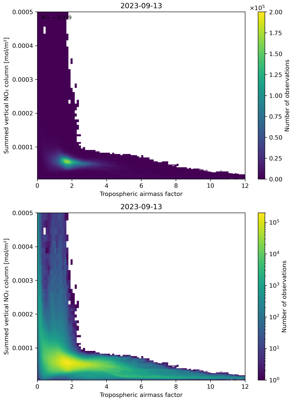
Figure 75: Scatter density plot of “Tropospheric airmass factor” against “Summed vertical NO 2 column” for 2023-09-12 to 2023-09-14.
