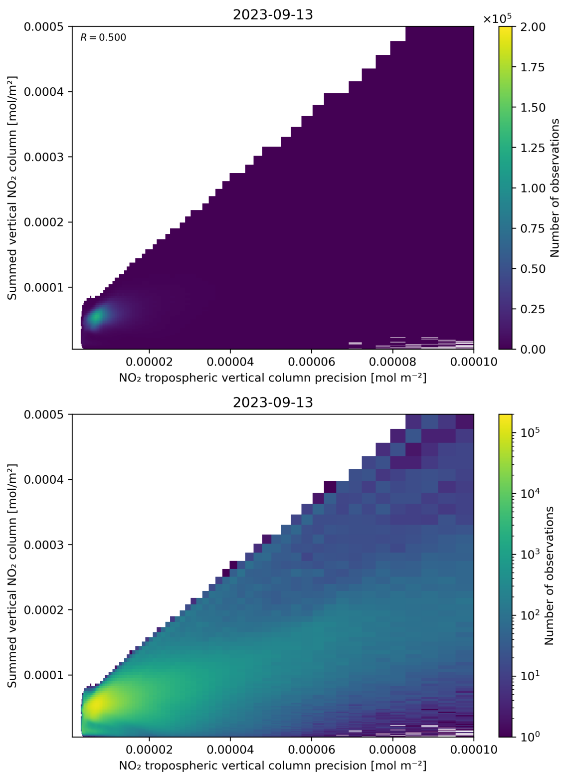
Figure 136: Scatter density plot of “NO 2 tropospheric vertical column precision” against “Summed vertical NO 2 column” for 2023-09-12 to 2023-09-14.
