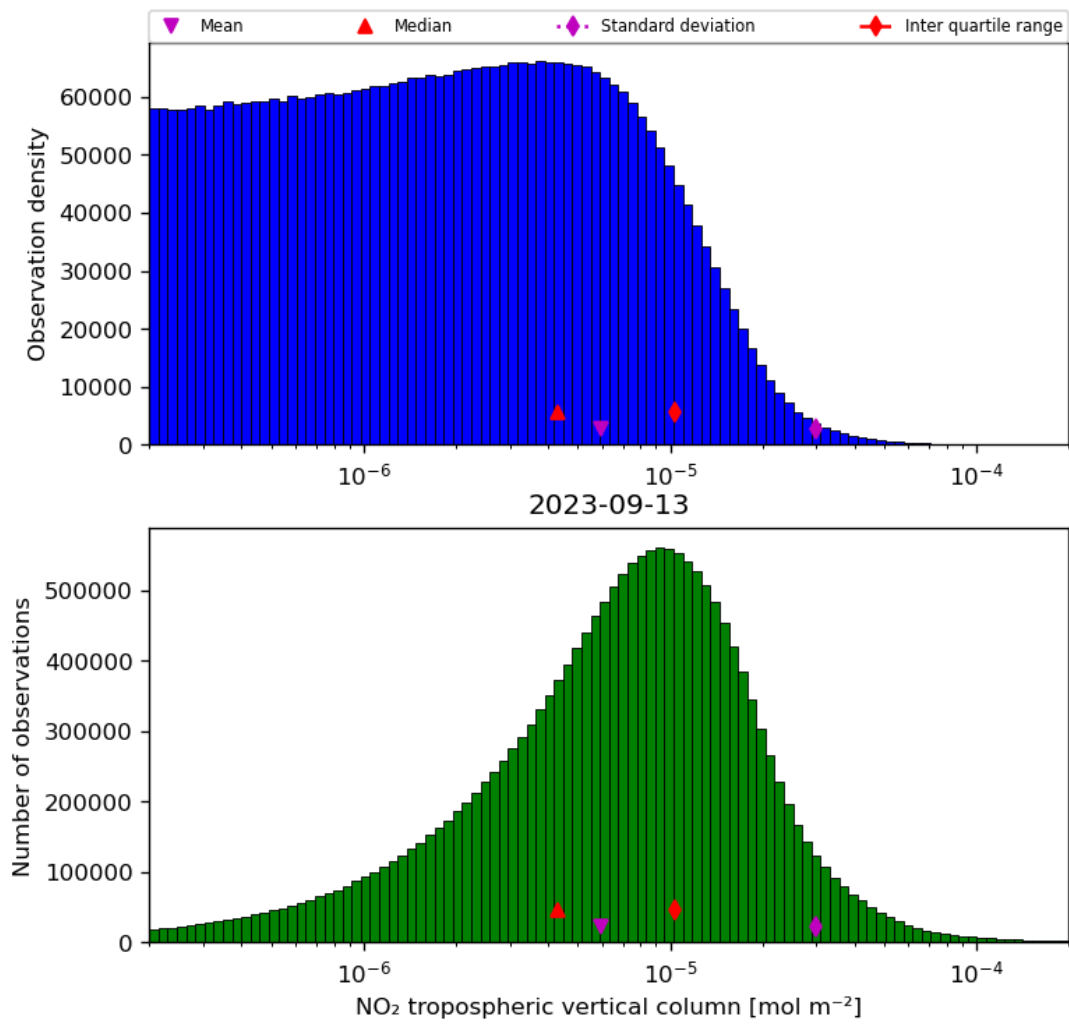
Figure 29: Histogram of “NO 2 tropospheric vertical column” for 2023-09-12 to 2023-09-14
