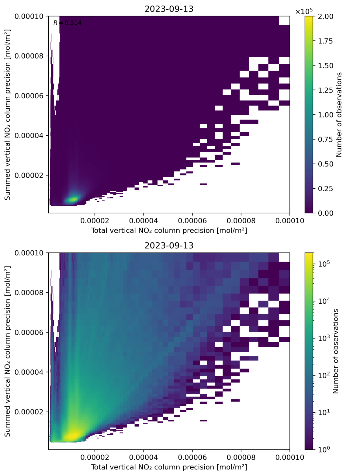
Figure 118: Scatter density plot of “Total vertical NO 2 column precision” against “Summed vertical NO 2 column precision” for 2023-09-12 to 2023-09-14.
