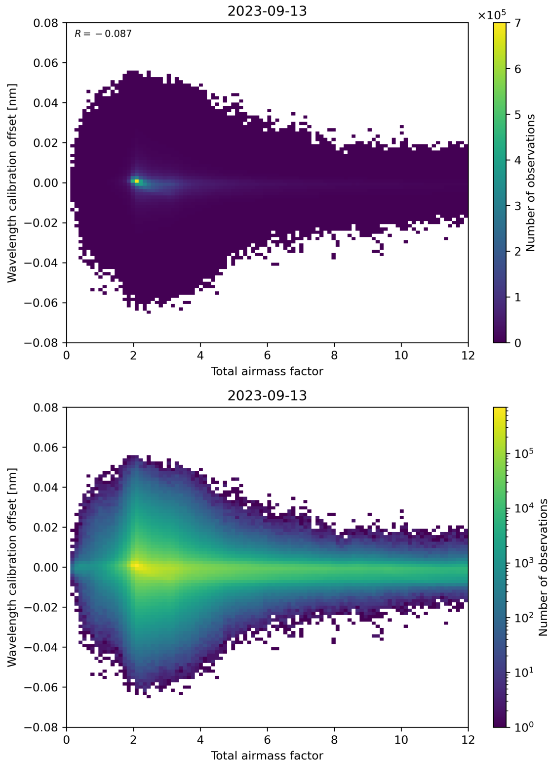
Figure 70: Scatter density plot of “Total airmass factor” against “Wavelength calibration offset” for 2023-09-12 to 2023-09-14.
