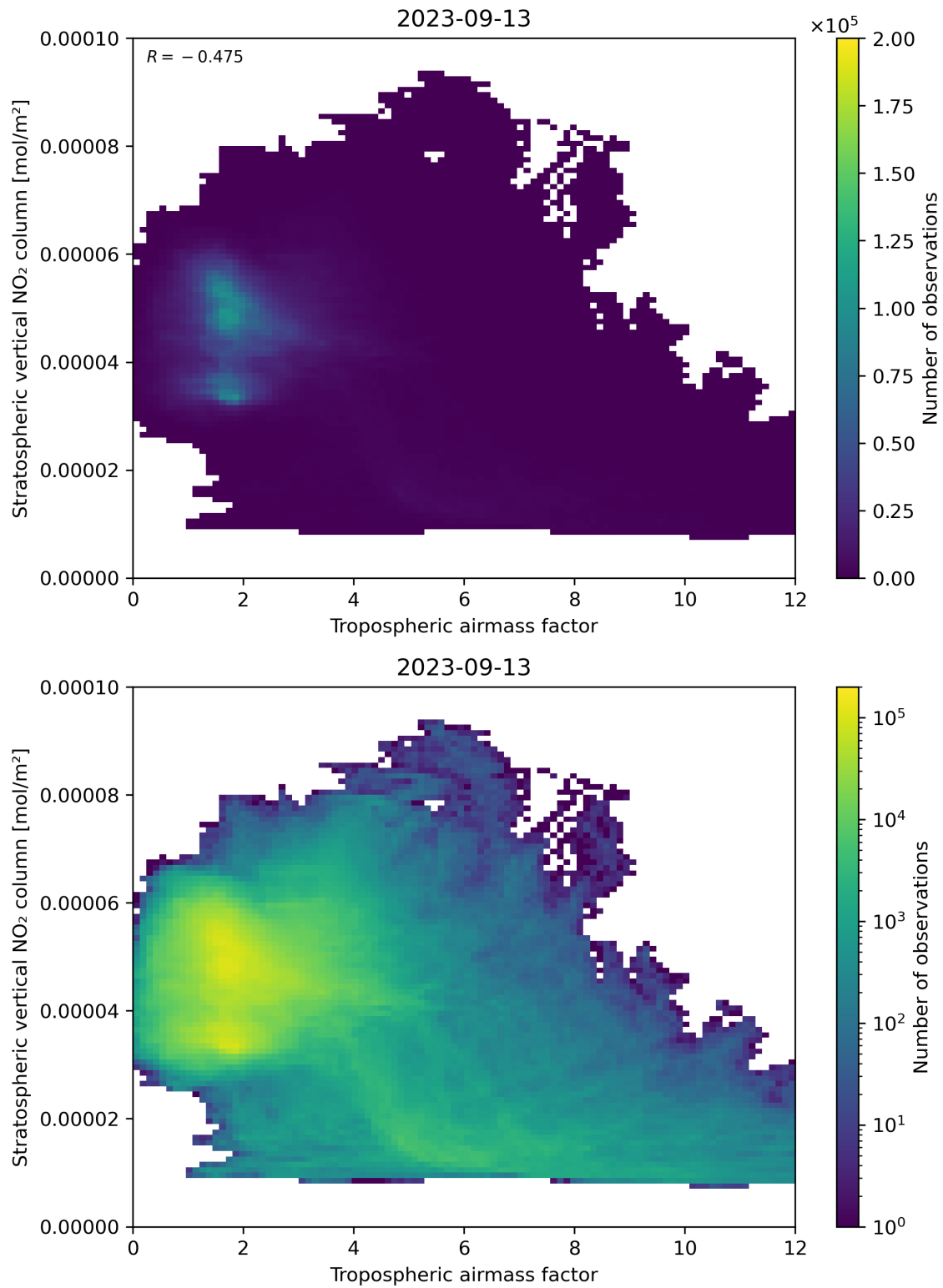
Figure 74: Scatter density plot of “Tropospheric air mass factor” against “Stratospheric vertical NO 2 column” for 2023-09-12 to 2023-09-14.
