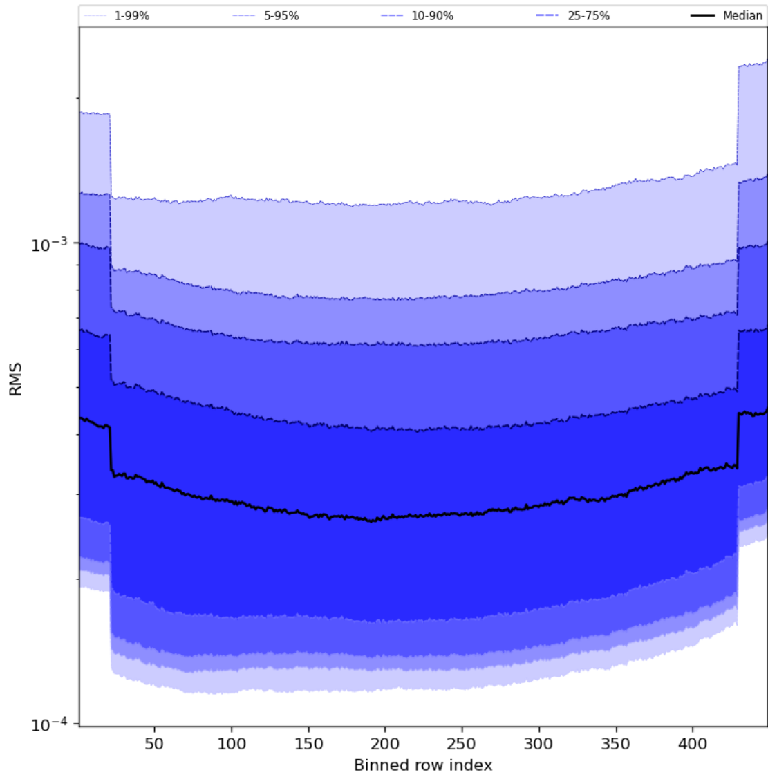
Figure 60: Along track statistics of “RMS” for 2023-09-12 to 2023-09-14
