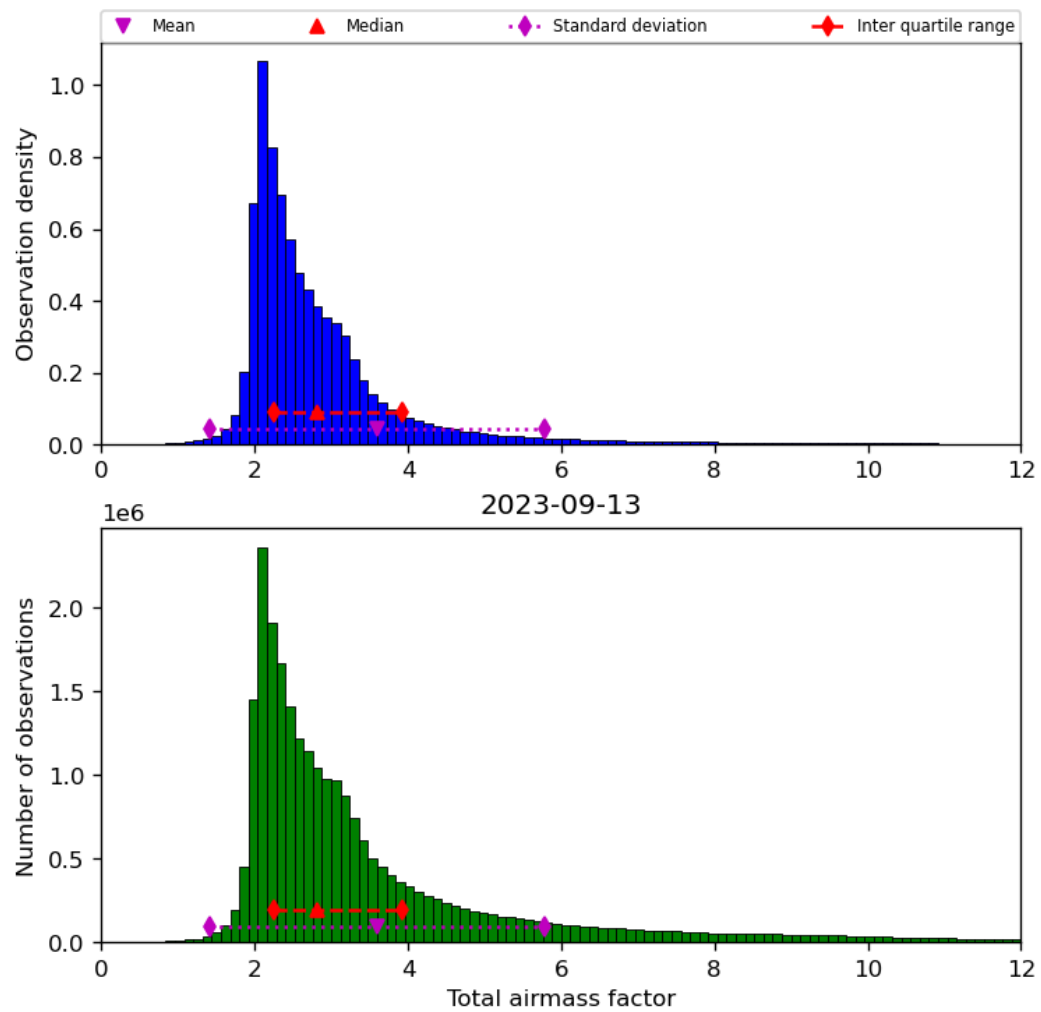
Figure 32: Histogram of “Total airmass factor” for 2023-09-12 to 2023-09-14
