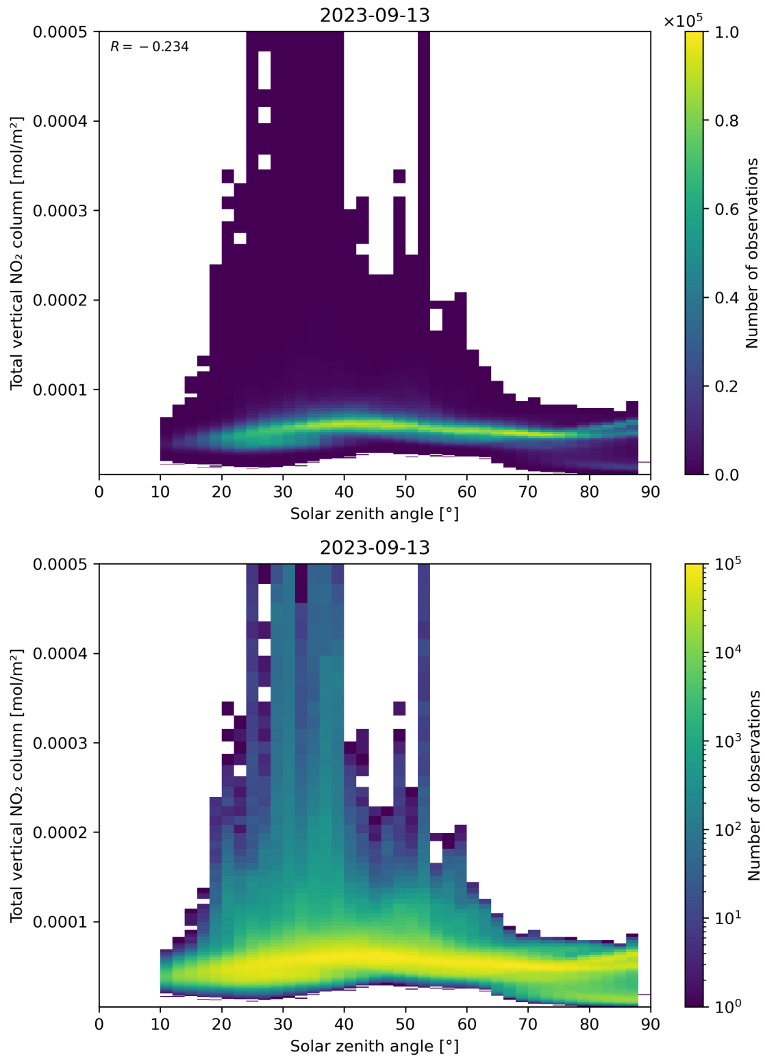
Figure 153: Scatter density plot of “Solar zenith angle” against “Total vertical NO 2 column” for 2023-09-12 to 2023-09-14.
