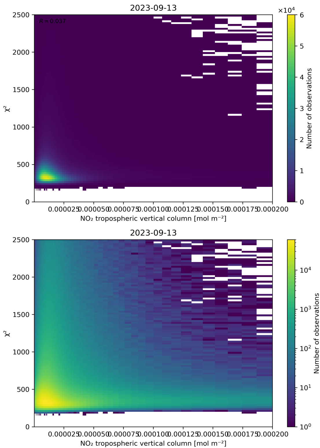
Figure 124: Scatter density plot of “NO 2 tropospheric vertical column” against “ \chi^2 ” for 2023-09-12 to 2023-09-14.
