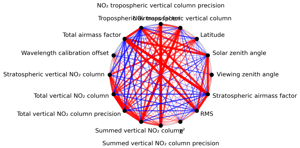
Figure 1: Map of correlation graph for 2023-09-12 to 2023-09-14.
