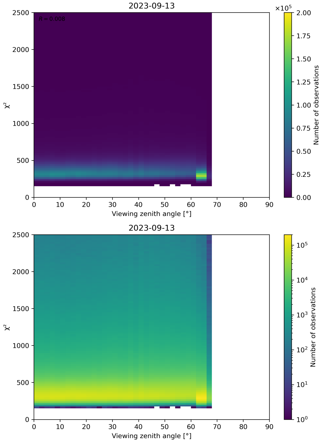
Figure 162: Scatter density plot of “Viewing zenith angle” against “ \chi^2 ” for 2023-09-12 to 2023-09-14.
