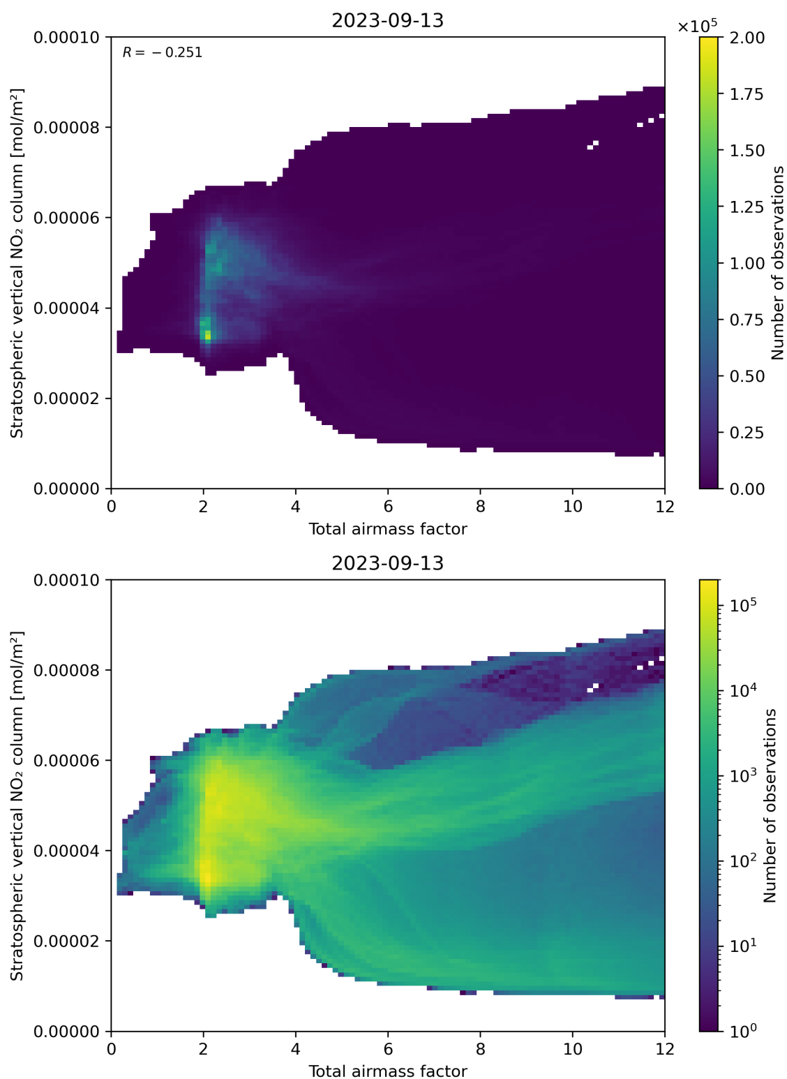
Figure 64: Scatter density plot of “Total airmass factor” against “Stratospheric vertical NO 2 column” for 2023-09-12 to 2023-09-14.
