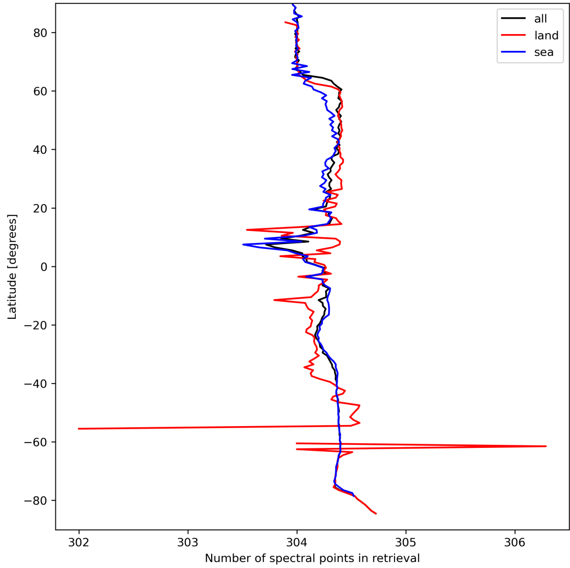
Figure 16: Zonal average of “Number of spectral points in retrieval” for 2023-09-12 to 2023-09-14.
