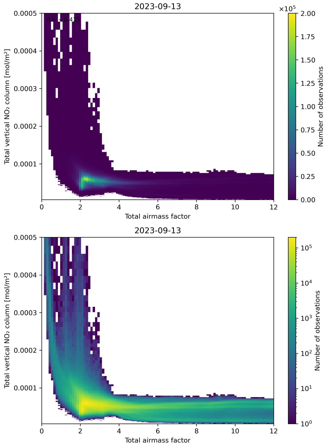
Figure 67: Scatter density plot of “Total airmass factor” against “Total vertical NO 2 column” for 2023-09-12 to 2023-09-14.
