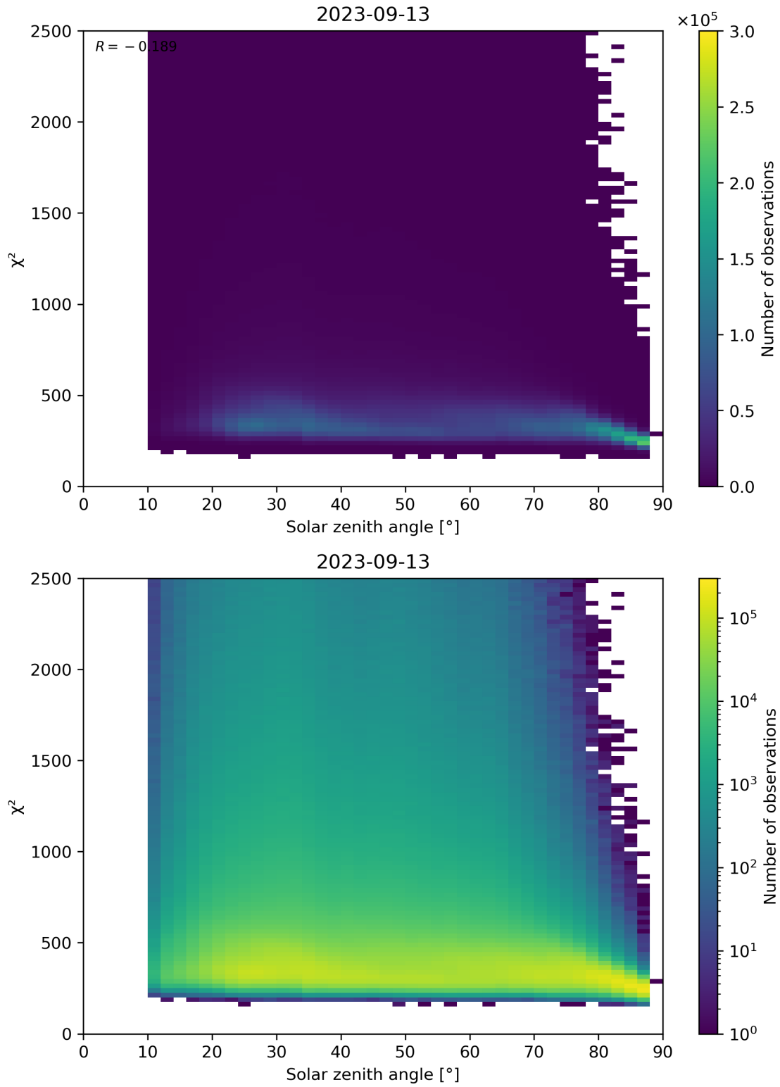
Figure 148: Scatter density plot of “Solar zenith angle” against “ \chi^2 ” for 2023-09-12 to 2023-09-14.
