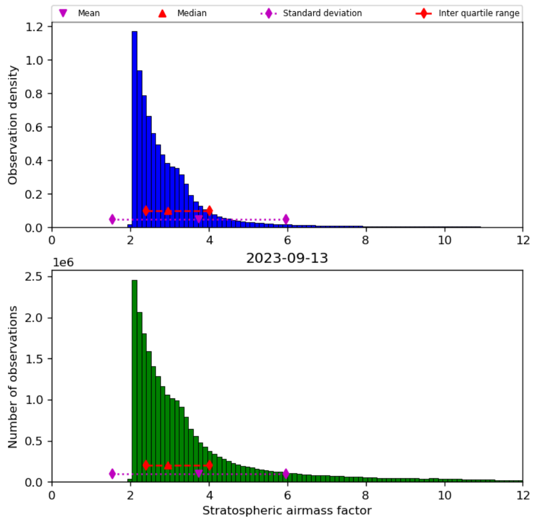
Figure 44: Histogram of “Stratospheric airmass factor” for 2023-09-12 to 2023-09-14
