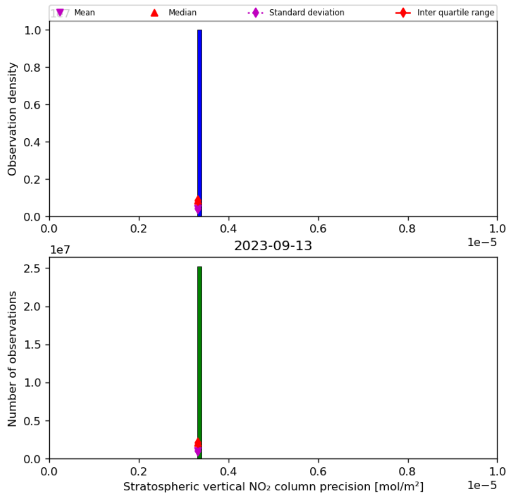
Figure 37: Histogram of “Stratospheric vertical NO 2 column precision” for 2023-09-12 to 2023-09-14
