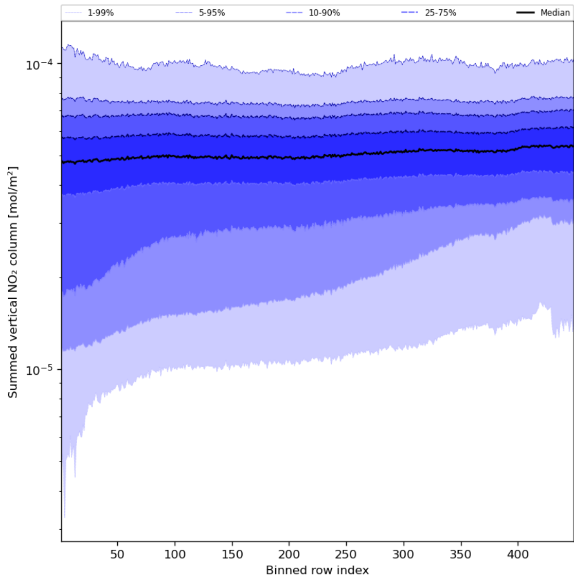
Figure 57: Along track statistics of “Summed vertical NO 2 column” for 2023-09-12 to 2023-09-14
