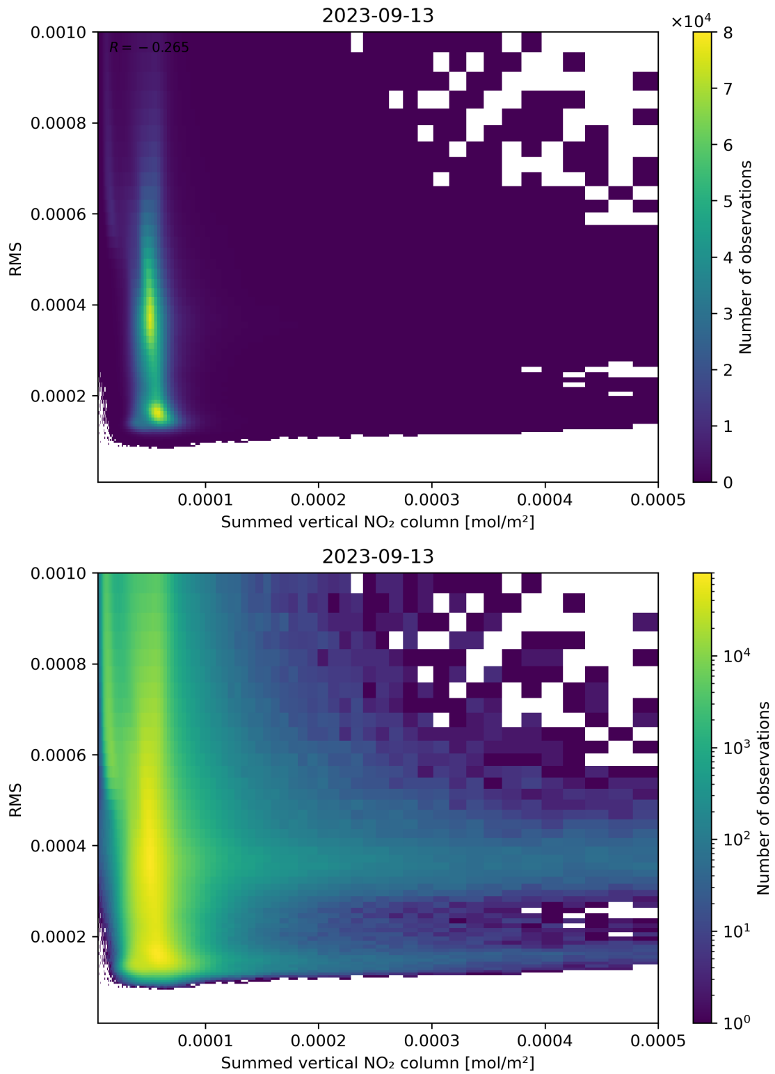
Figure 109: Scatter density plot of “Summed vertical NO 2 column” against “RMS” for 2023-09-12 to 2023-09-14.
