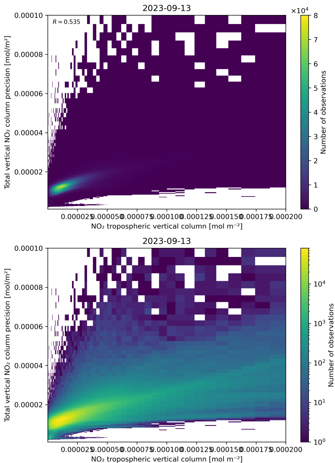
Figure 129: Scatter density plot of “NO 2 tropospheric vertical column” against “Total vertical NO 2 column precision” for 2023-09-12 to 2023-09-14.
