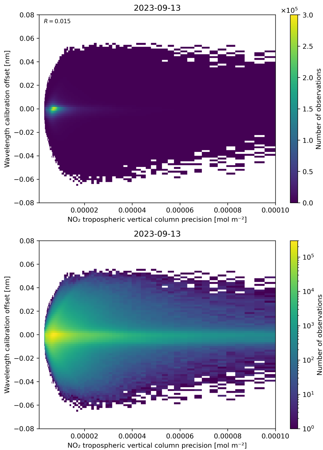
Figure 141: Scatter density plot of “NO 2 tropospheric vertical column precision” against “Wavelength calibration offset” for 2023-09-12 to 2023-09-14.
