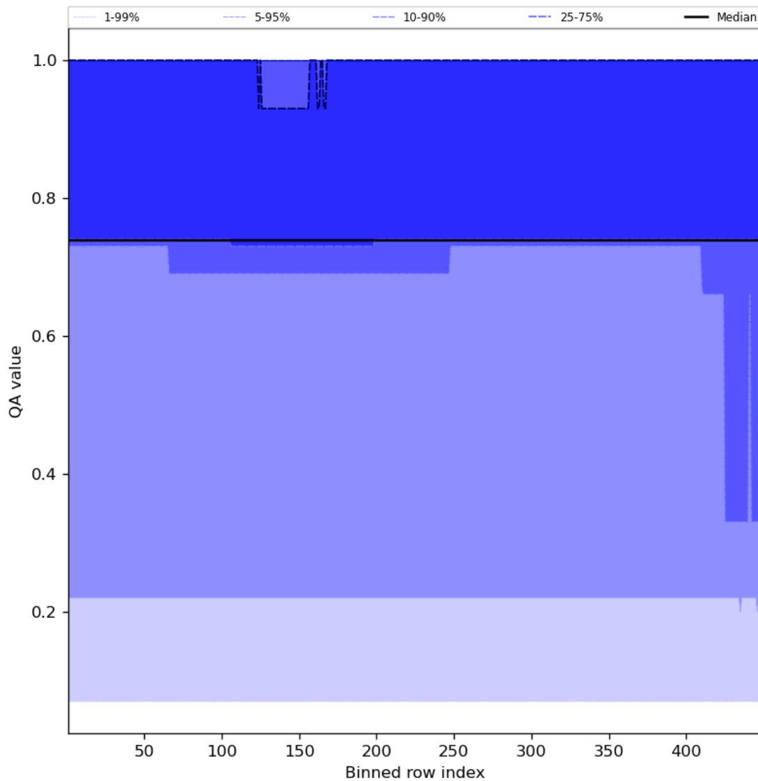
Figure 45: Along track statistics of "QA value" for 2023-09-12 to 2023-09-14
