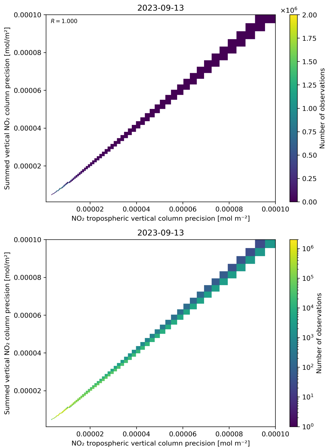
Figure 137: Scatter density plot of “NO 2 tropospheric vertical column precision” against “Summed vertical NO 2 column precision” for 2023-09-12 to 2023-09-14.
