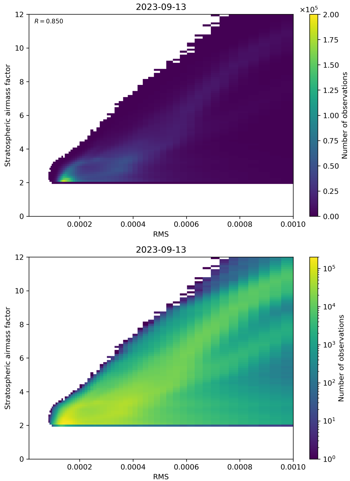
Figure 144: Scatter density plot of “RMS” against “Stratospheric airmass factor” for 2023-09-12 to 2023-09-14.
