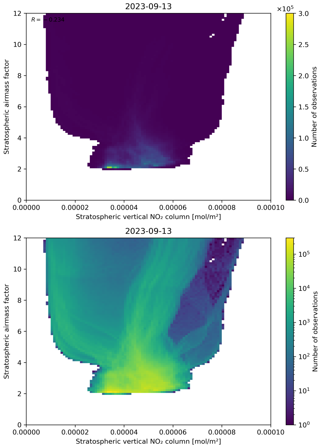
Figure 96: Scatter density plot of “Stratospheric vertical NO 2 column” against “Stratospheric airmass factor” for 2023-09-12 to 2023-09-14.
