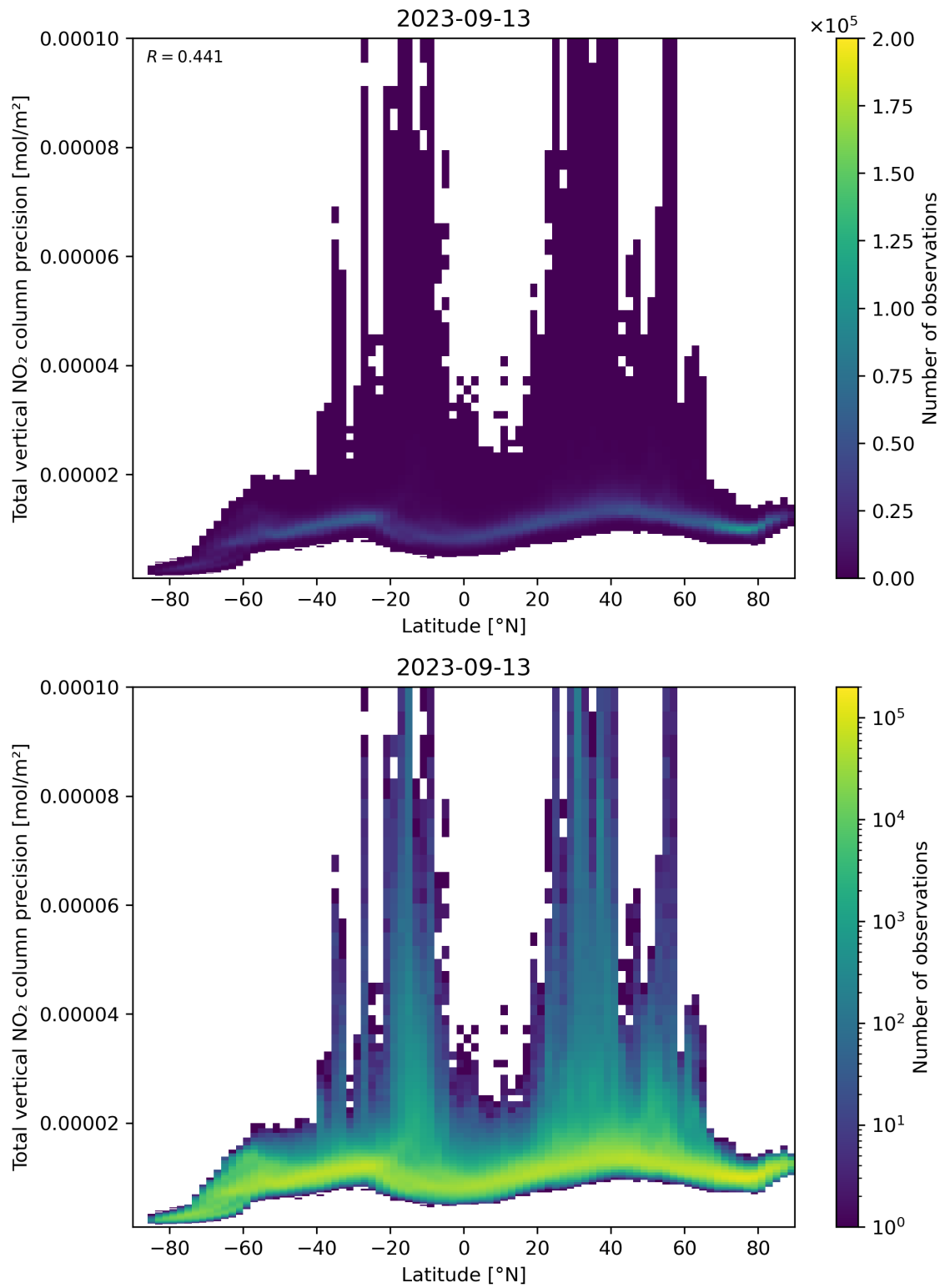
Figure 91: Scatter density plot of “Latitude” against “Total vertical NO 2 column precision” for 2023-09-12 to 2023-09-14.
