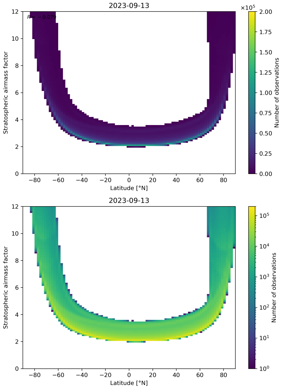
Figure 83: Scatter density plot of “Latitude” against “Stratospheric airmass factor” for 2023-09-12 to 2023-09-14.
