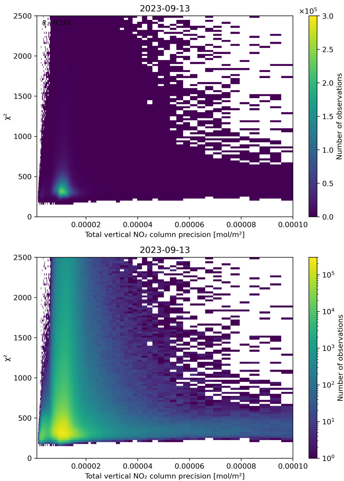
Figure 116: Scatter density plot of “Total vertical NO 2 column precision” against “ \chi^2 ” for 2023-09-12 to 2023-09-14.
