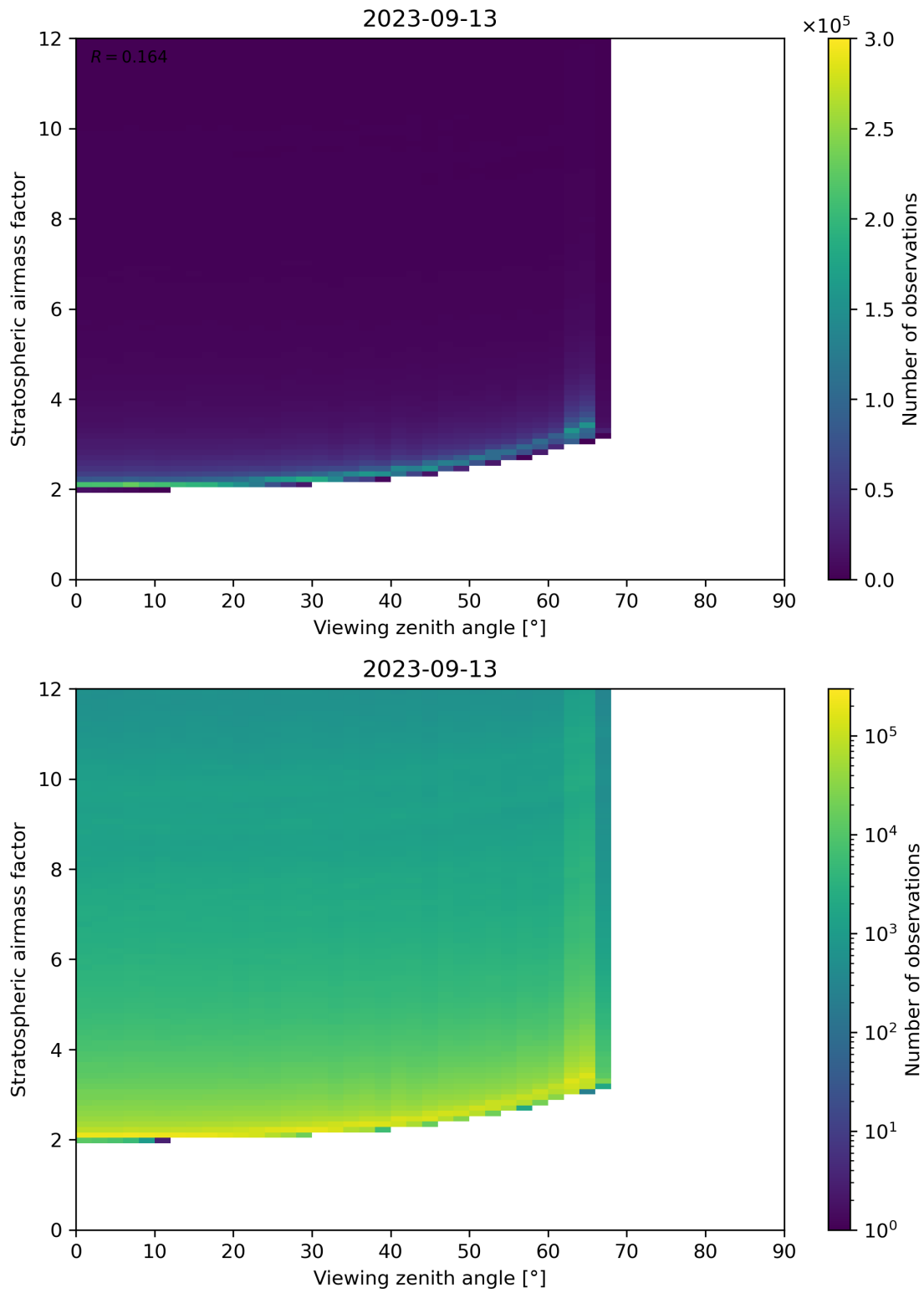
Figure 159: Scatter density plot of “Viewing zenith angle” against “Stratospheric airmass factor” for 2023-09-12 to 2023-09-14.
