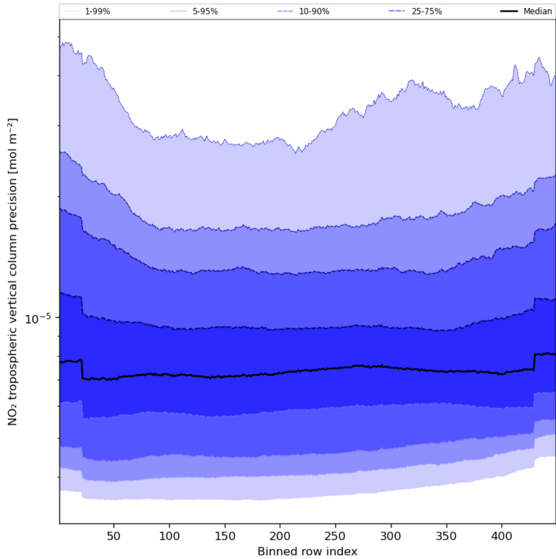
Figure 47: Along track statistics of “NO 2 tropospheric vertical column precision” for 2023-09-12 to 2023-09-14
