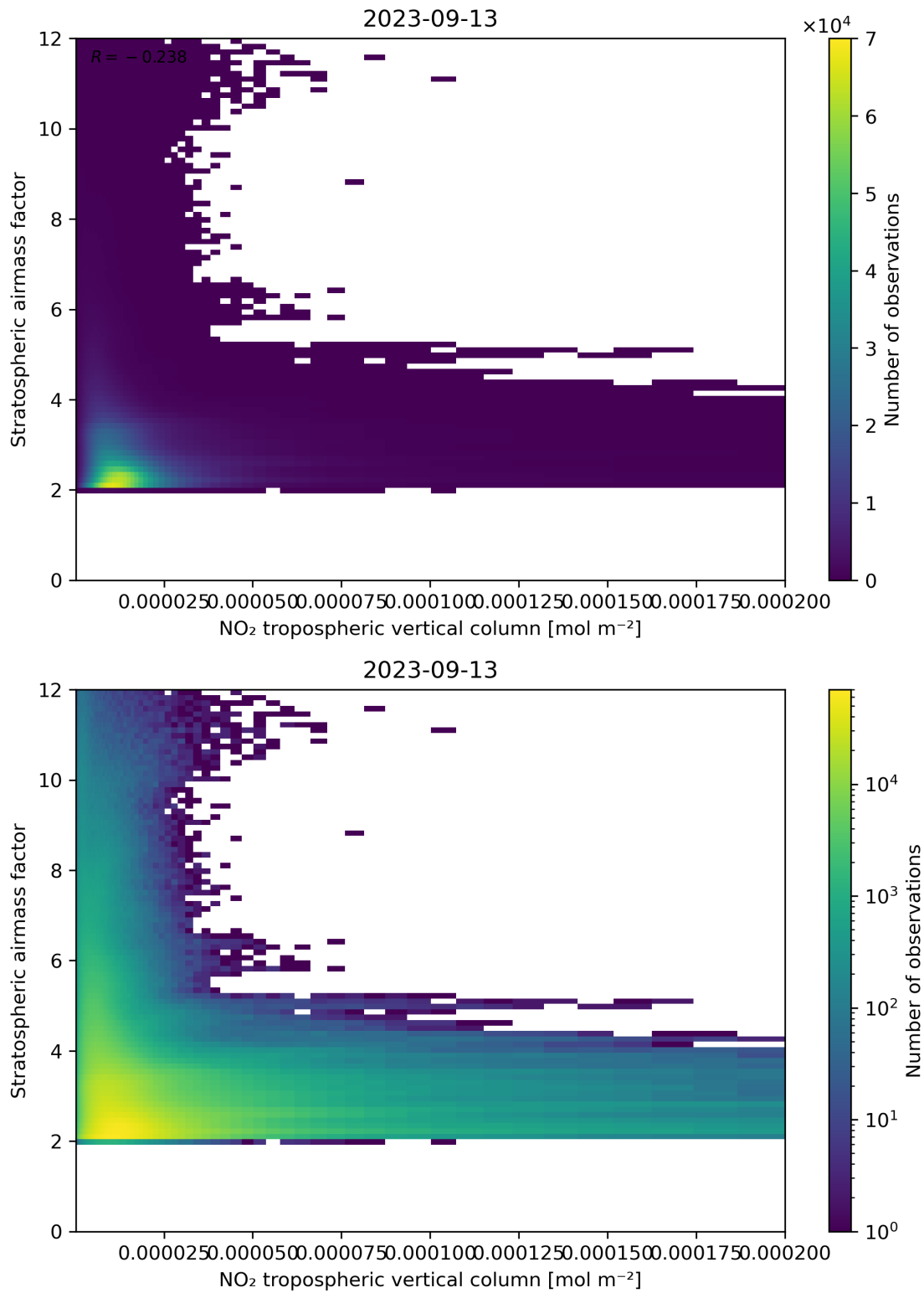
Figure 121: Scatter density plot of “NO 2 tropospheric vertical column” against “Stratospheric airmass factor” for 2023-09-12 to 2023-09-14.
