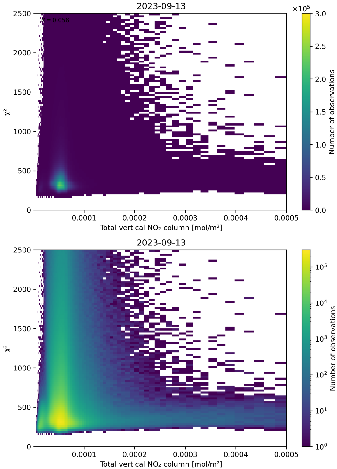
Figure 111: Scatter density plot of “Total vertical NO 2 column” against “ \chi^2 ” for 2023-09-12 to 2023-09-14.
