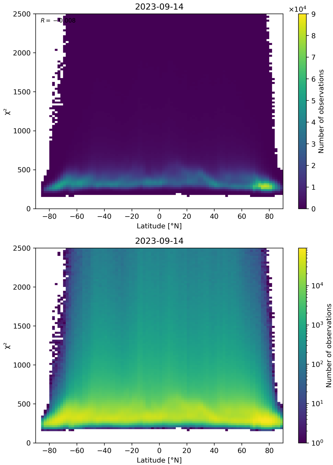
Figure 86: Scatter density plot of “Latitude” against “ \chi^2 ” for 2023-09-13 to 2023-09-15.
