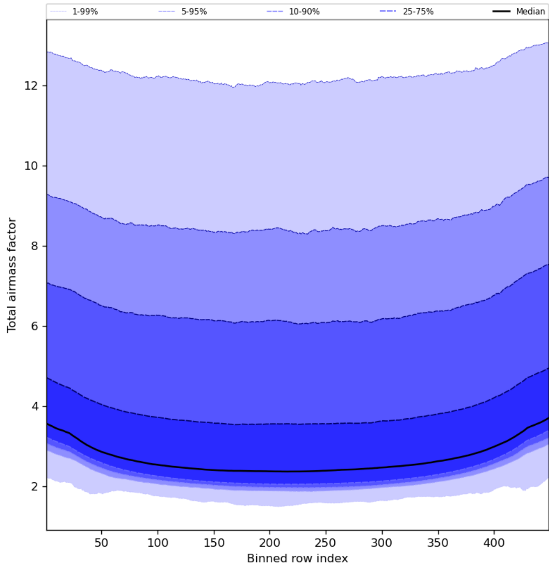
Figure 49: Along track statistics of “Total airmass factor” for 2023-09-13 to 2023-09-15
