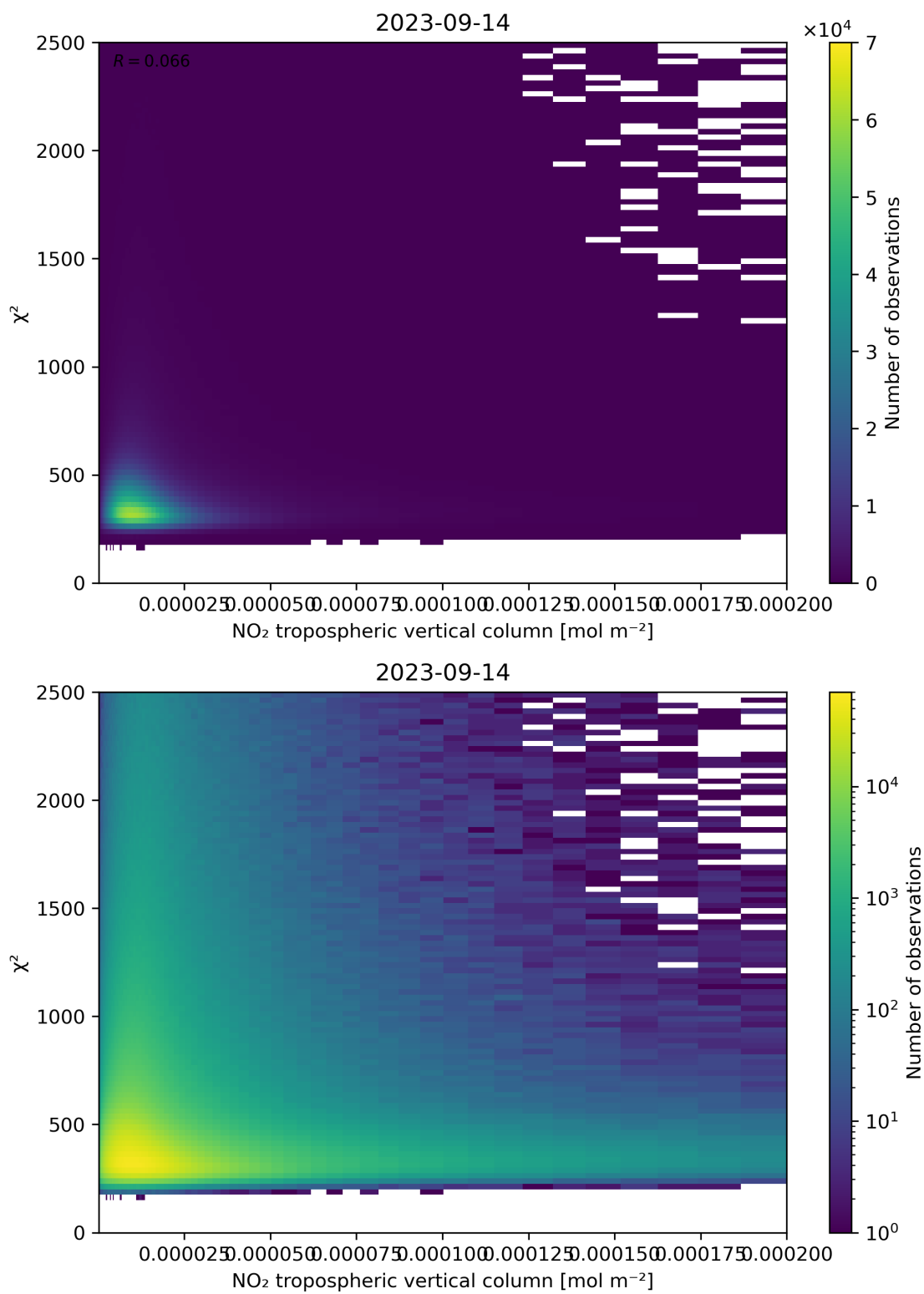
Figure 124: Scatter density plot of “NO 2 tropospheric vertical column” against “ \chi^2 ” for 2023-09-13 to 2023-09-15.
