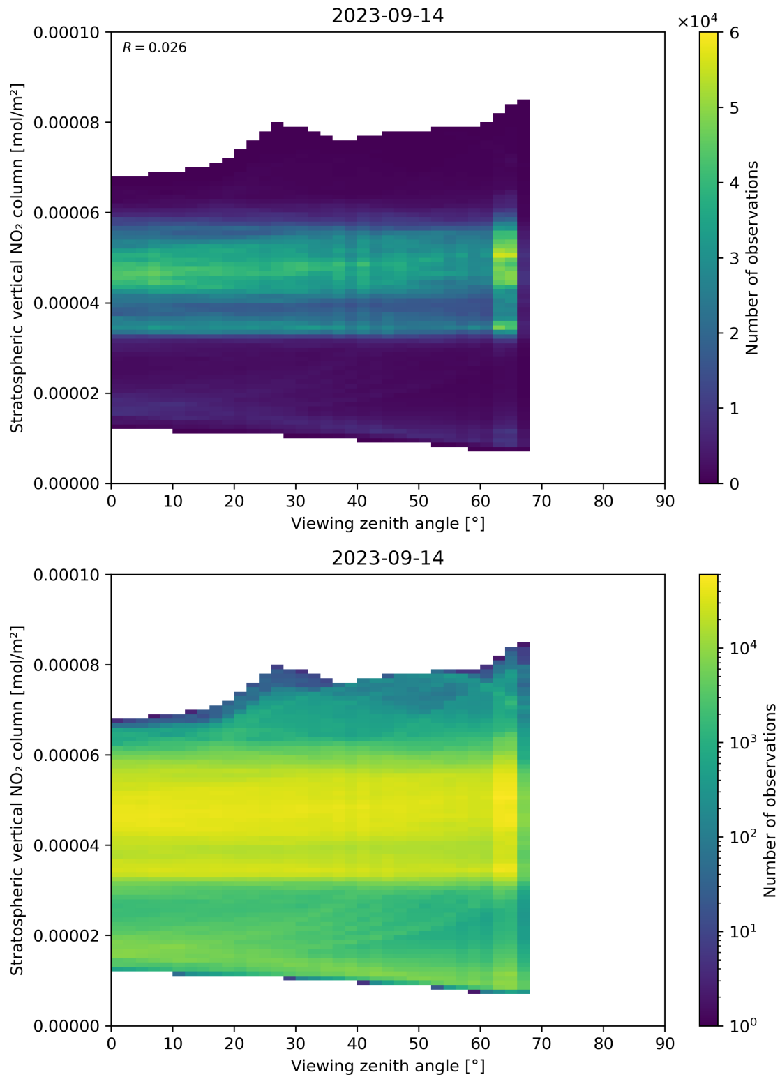
Figure 164: Scatter density plot of “Viewing zenith angle” against “Stratospheric vertical NO 2 column” for 2023-09-13 to 2023-09-15.
