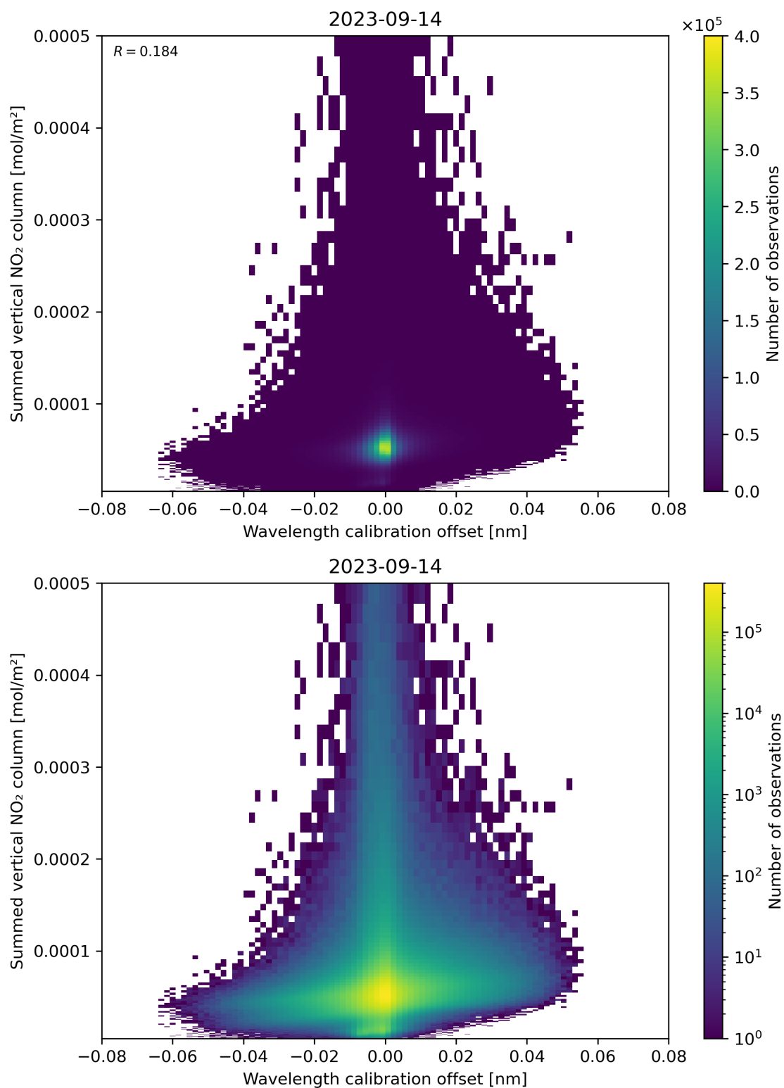
Figure 177: Scatter density plot of “Wavelength calibration offset” against “Summed vertical NO 2 column” for 2023-09-13 to 2023-09-15.
