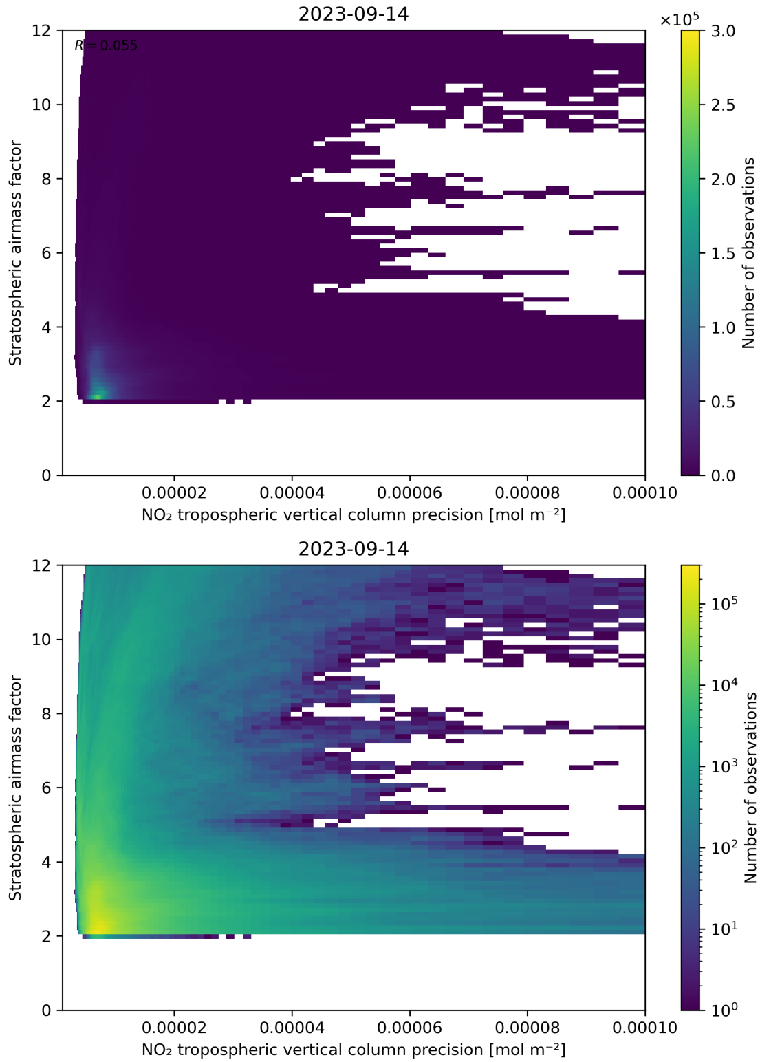
Figure 131: Scatter density plot of “NO 2 tropospheric vertical column precision” against “Stratospheric airmass factor” for 2023-09-13 to 2023-09-15.
