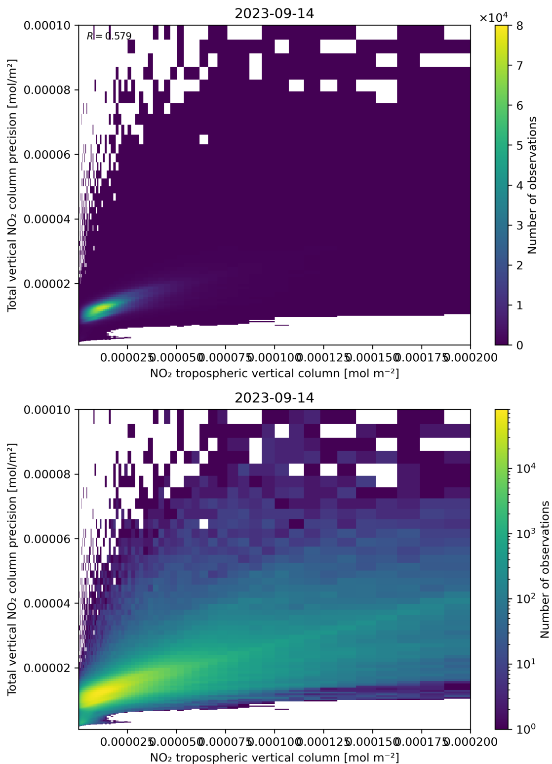
Figure 129: Scatter density plot of “NO 2 tropospheric vertical column” against “Total vertical NO 2 column precision” for 2023-09-13 to 2023-09-15.
