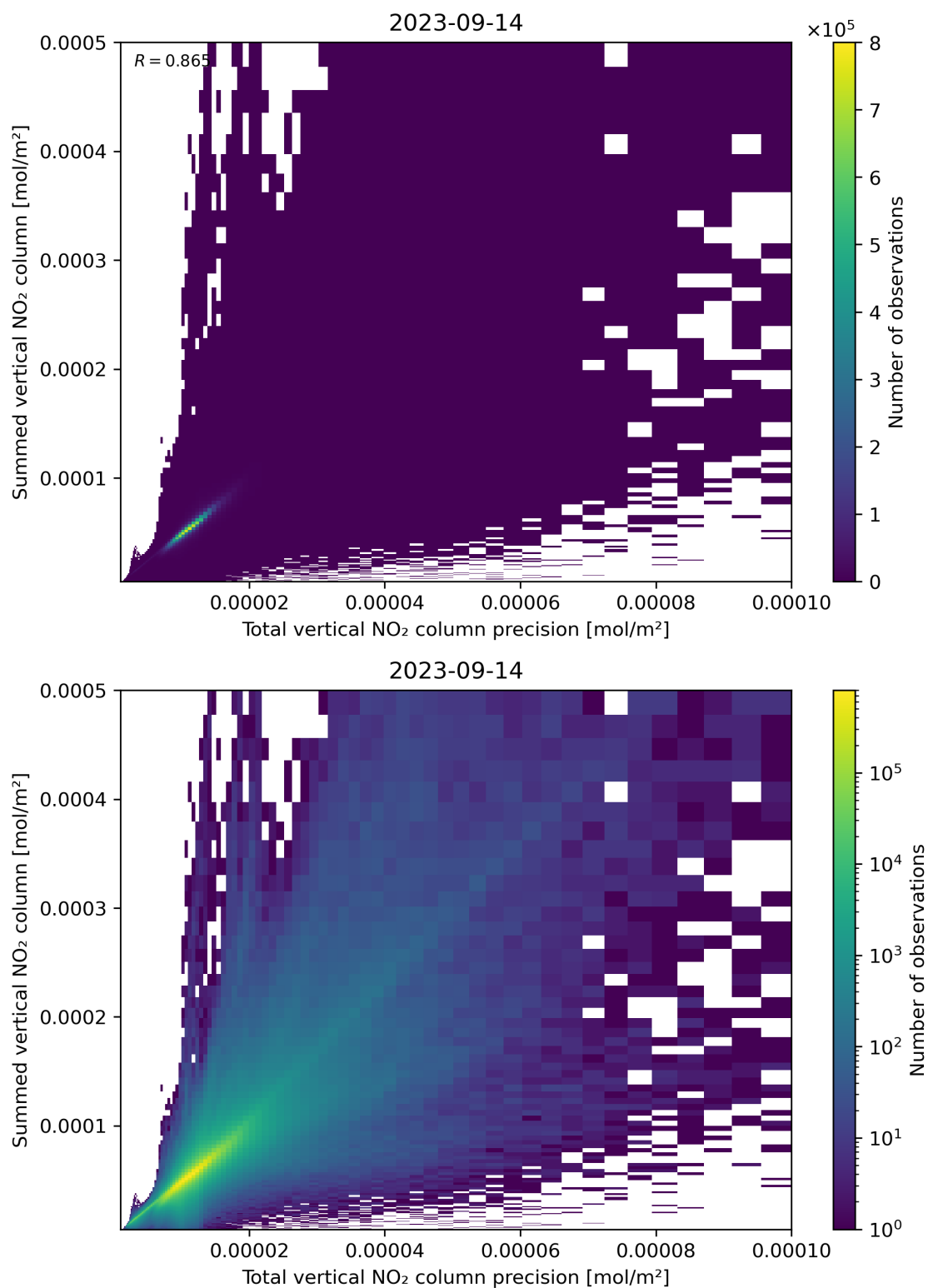
Figure 117: Scatter density plot of “Total vertical NO 2 column precision” against “Summed vertical NO 2 column” for 2023-09-13 to 2023-09-15.
