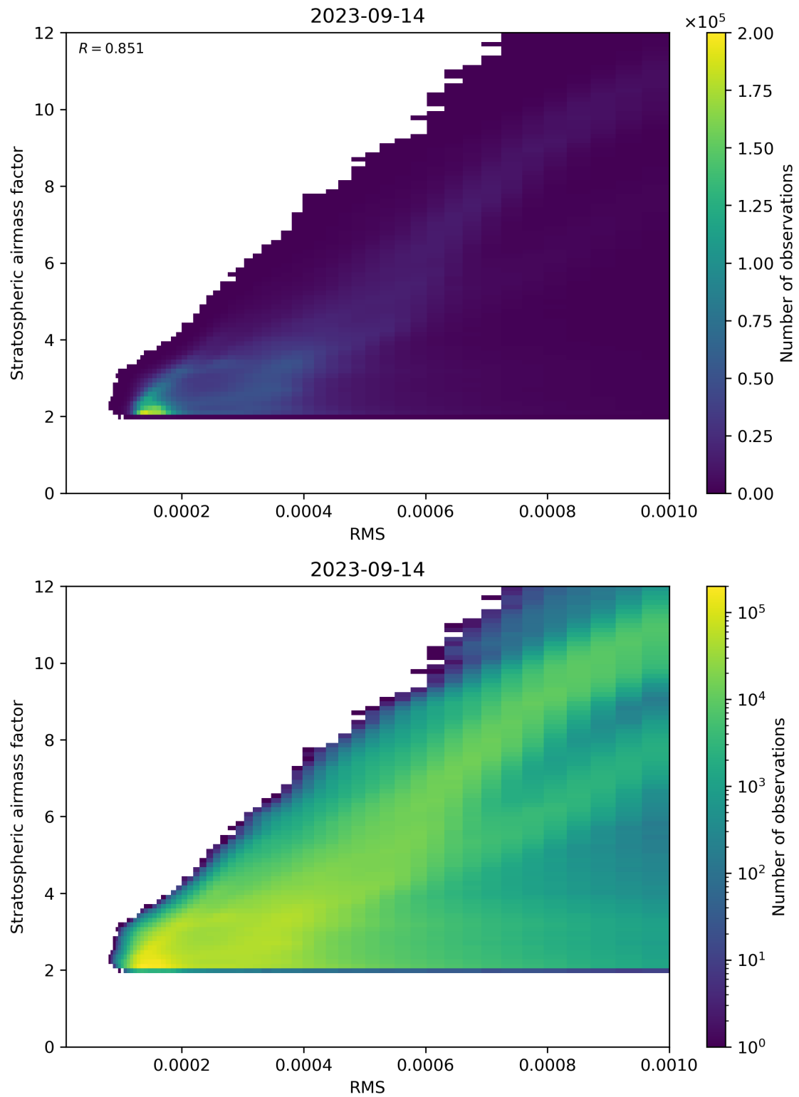
Figure 144: Scatter density plot of “RMS” against “Stratospheric airmass factor” for 2023-09-13 to 2023-09-15.
