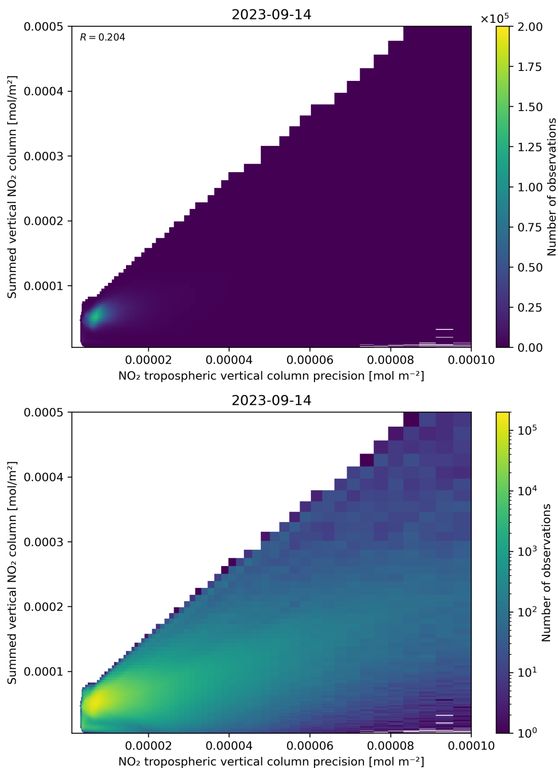
Figure 136: Scatter density plot of “NO 2 tropospheric vertical column precision” against “Summed vertical NO 2 column” for 2023-09-13 to 2023-09-15.
