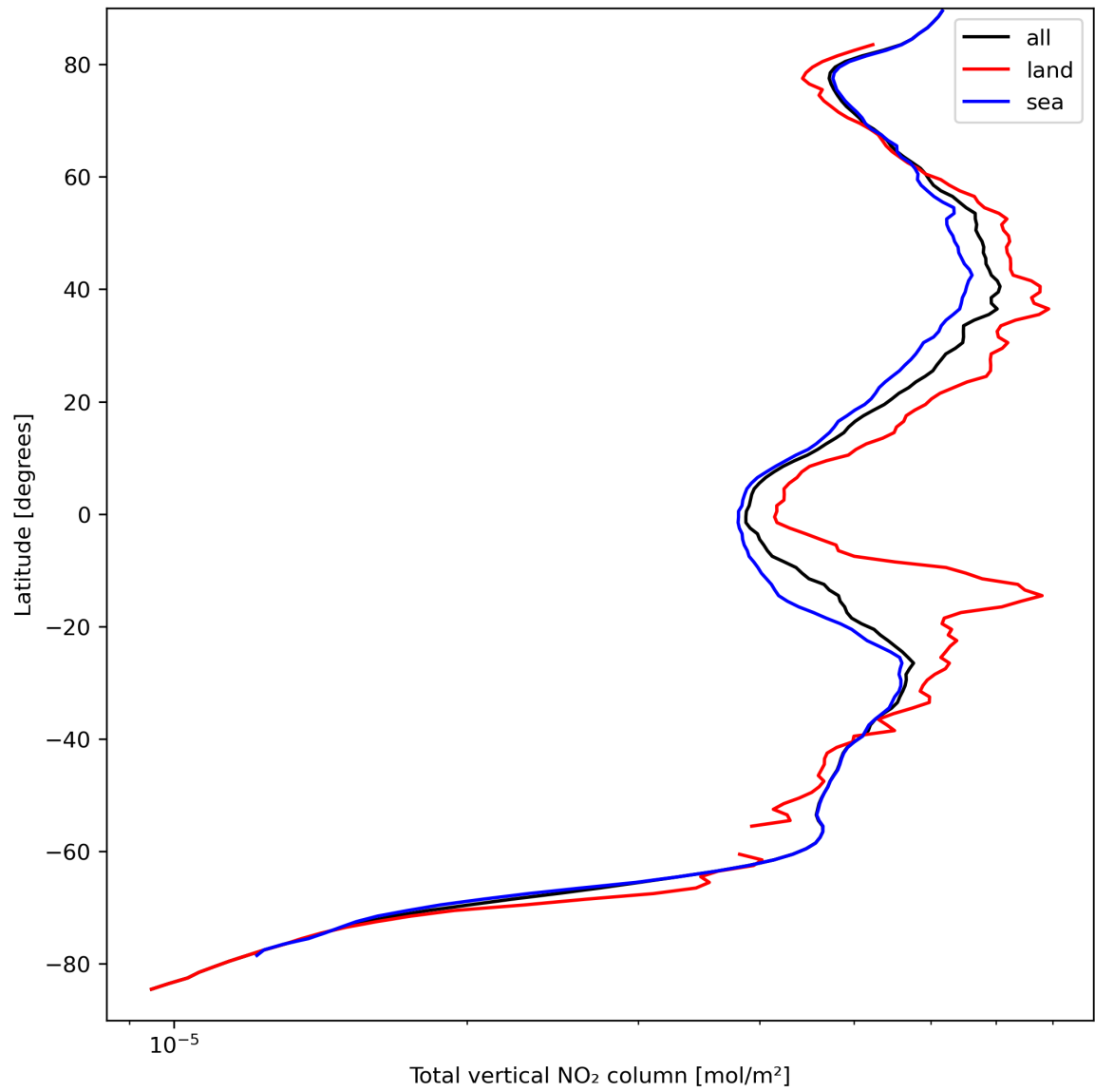
Figure 21: Zonal average of “Total vertical NO 2 column” for 2023-09-13 to 2023-09-15.
