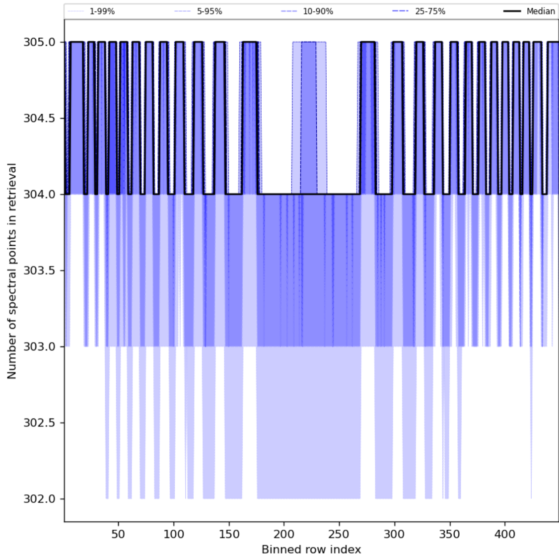
Figure 50: Along track statistics of “Number of spectral points in retrieval” for 2023-09-13 to 2023-09-15
