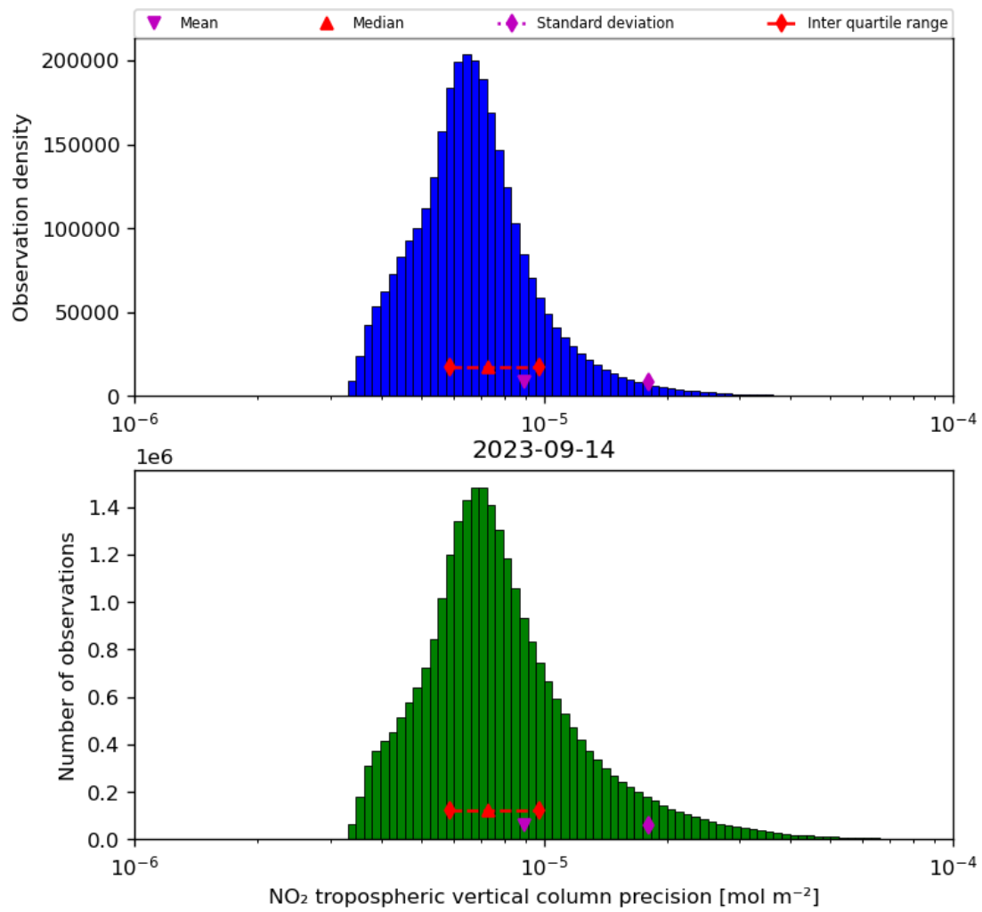
Figure 30: Histogram of “NO 2 tropospheric vertical column precision” for 2023-09-13 to 2023-09-15
