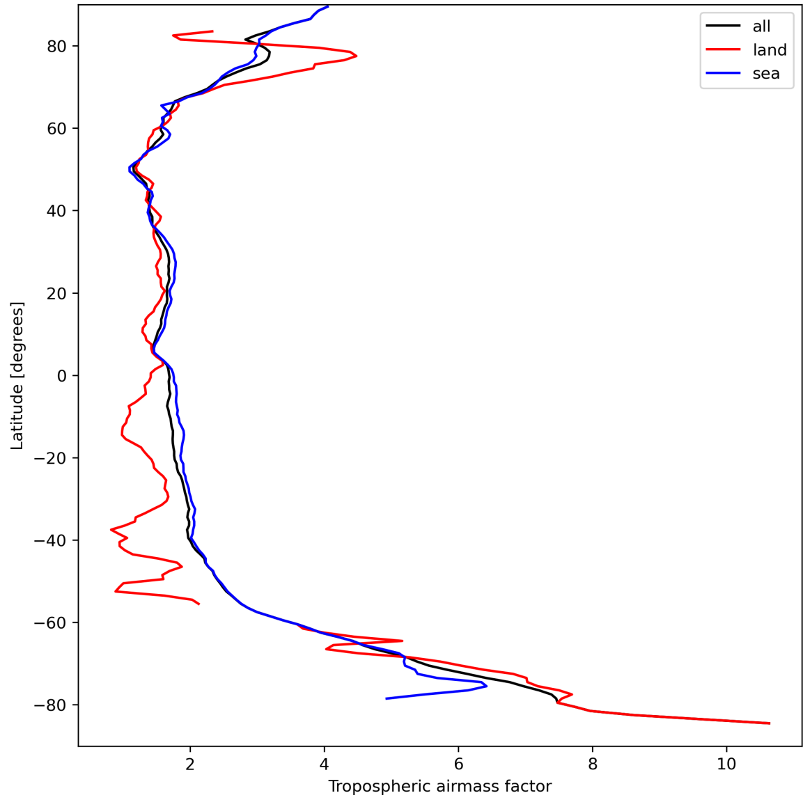
Figure 14: Zonal average of “Tropospheric airmass factor” for 2023-09-13 to 2023-09-15.
