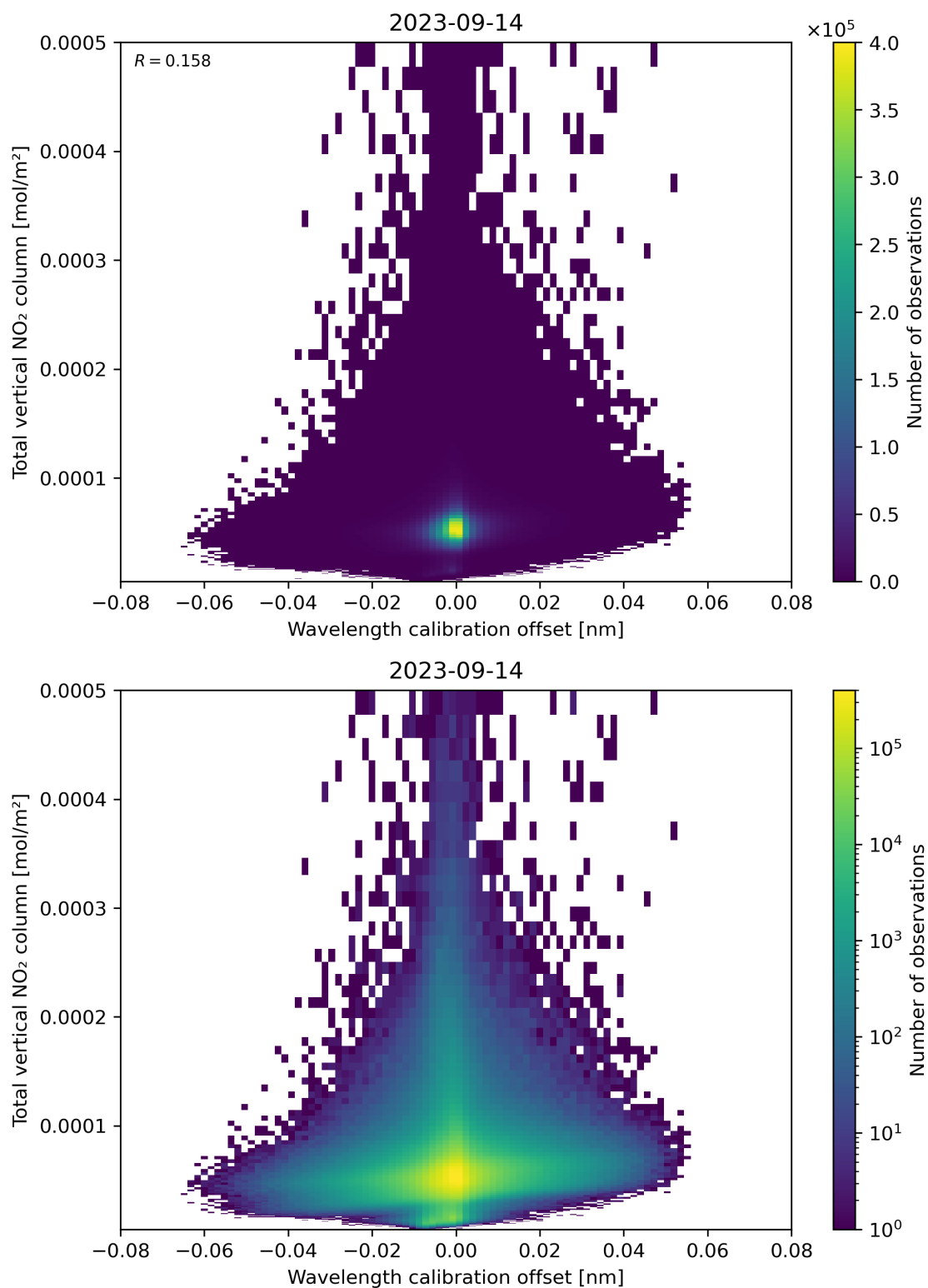
Figure 179: Scatter density plot of “Wavelength calibration offset” against “Total vertical NO 2 column” for 2023-09-13 to 2023-09-15.
