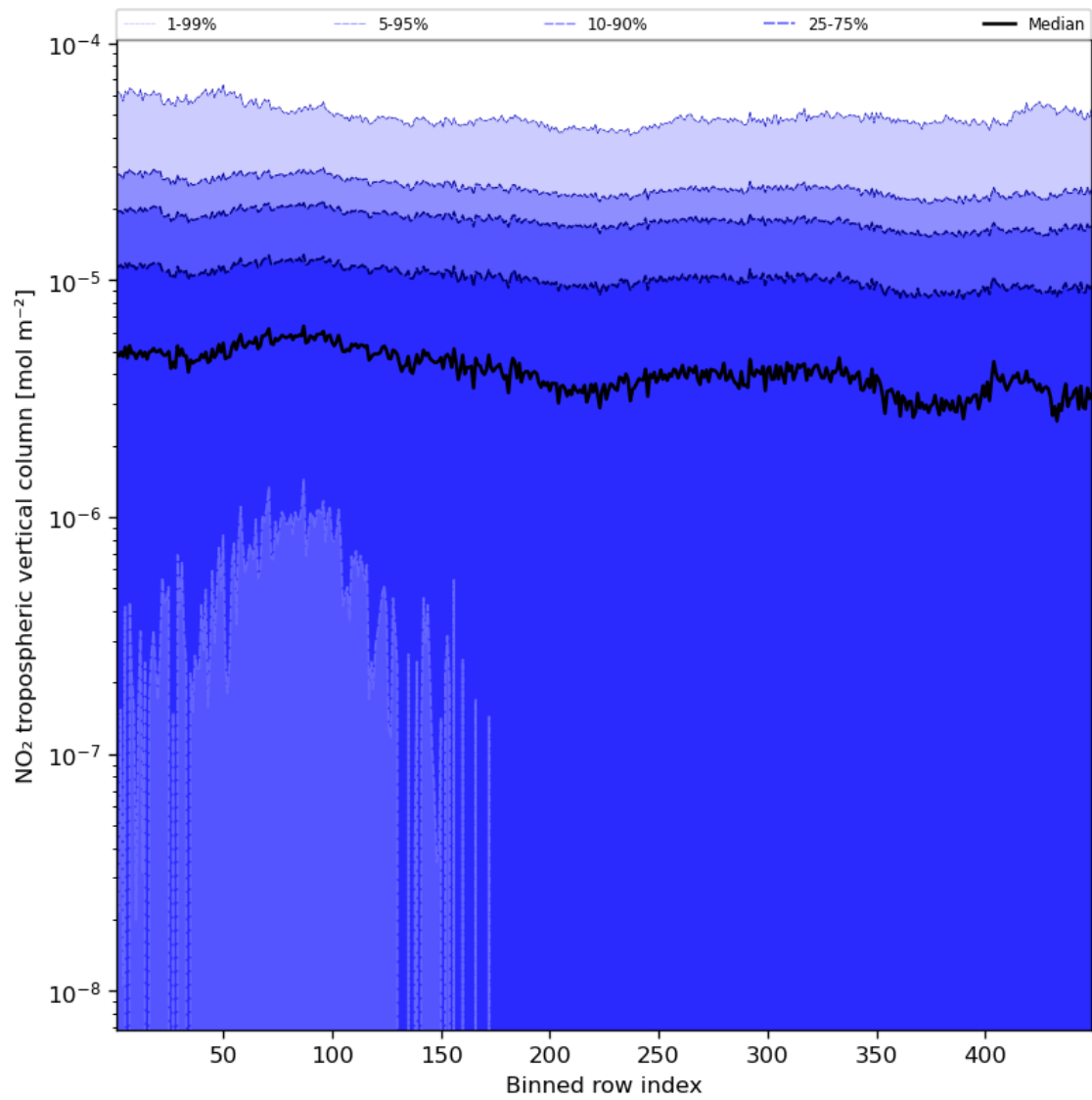
Figure 46: Along track statistics of “NO 2 tropospheric vertical column” for 2023-09-13 to 2023-09-15
