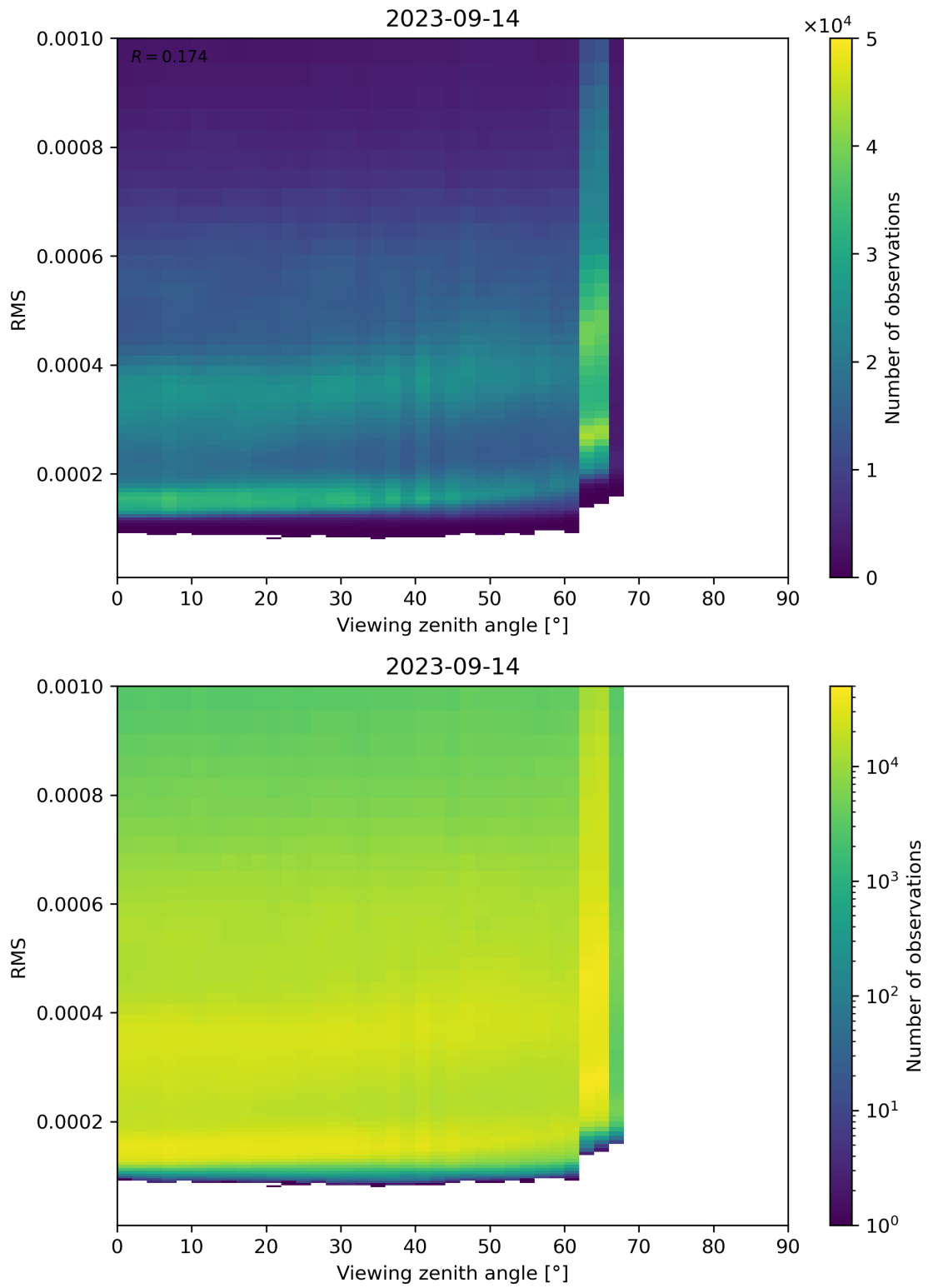
Figure 171: Scatter density plot of “Viewing zenith angle” against “RMS” for 2023-09-13 to 2023-09-15.
