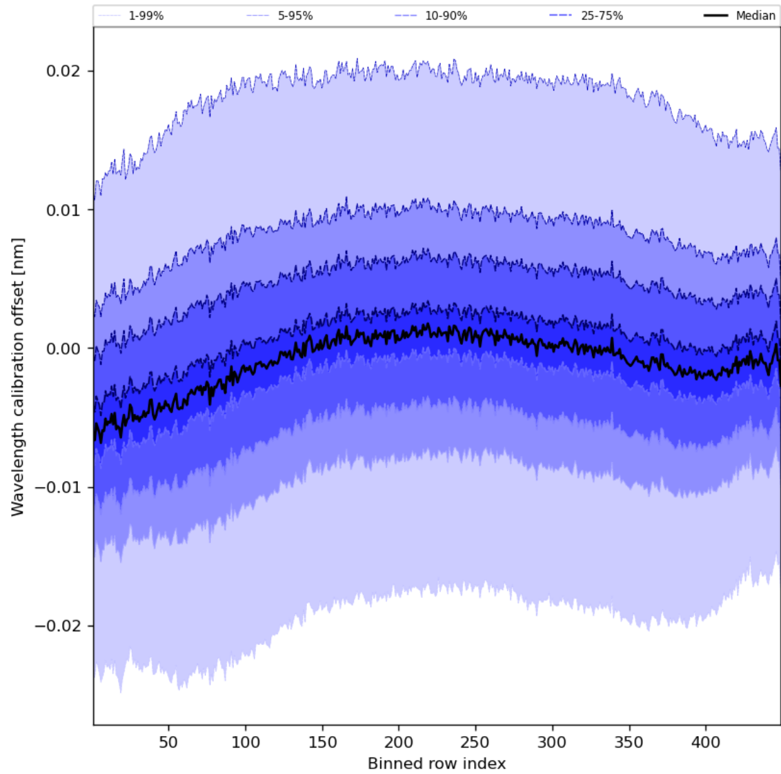
Figure 52: Along track statistics of “Wavelength calibration offset” for 2023-09-13 to 2023-09-15
