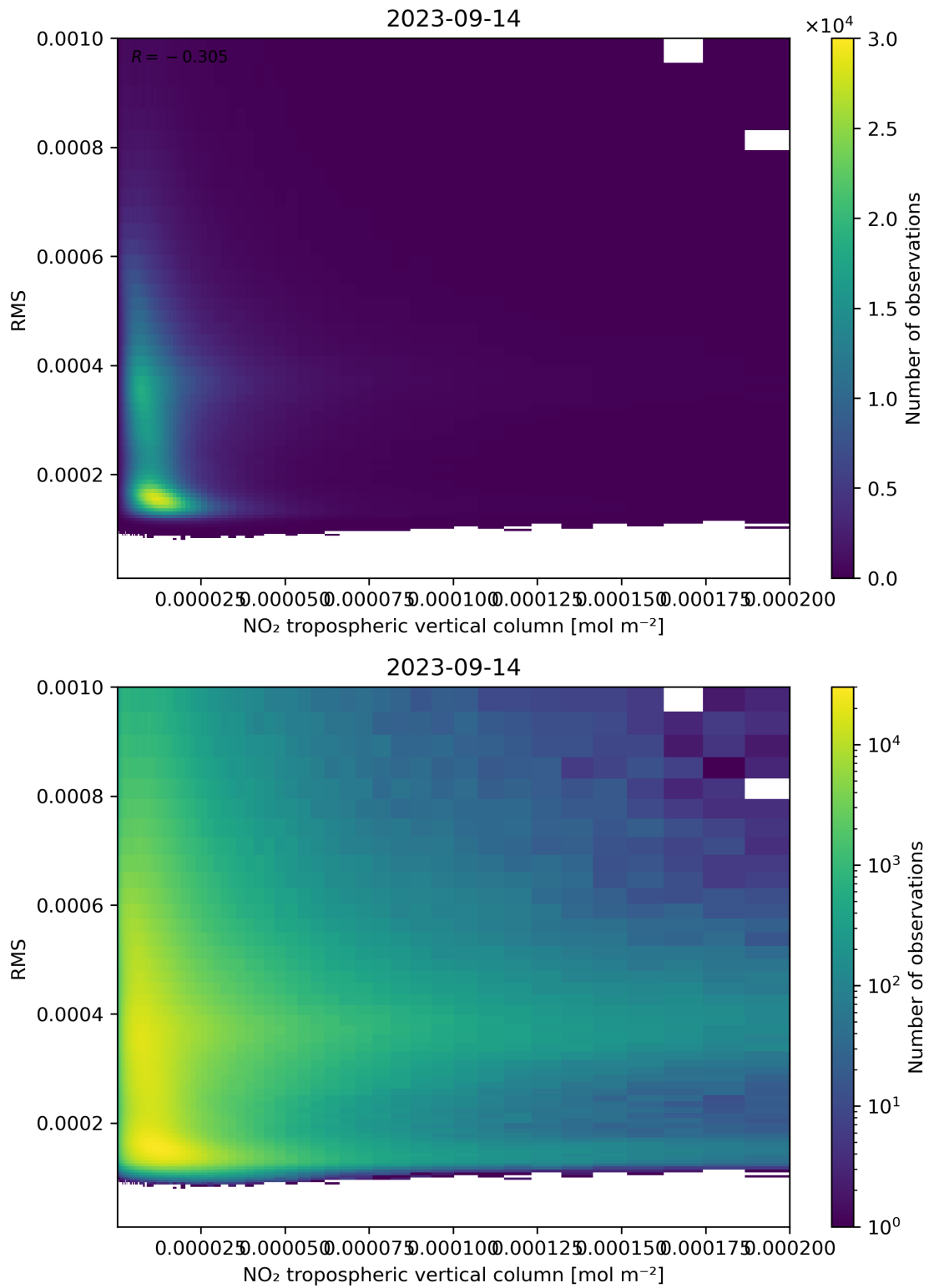
Figure 142: Scatter density plot of “NO 2 tropospheric vertical column” against “RMS” for 2023-09-13 to 2023-09-15.
