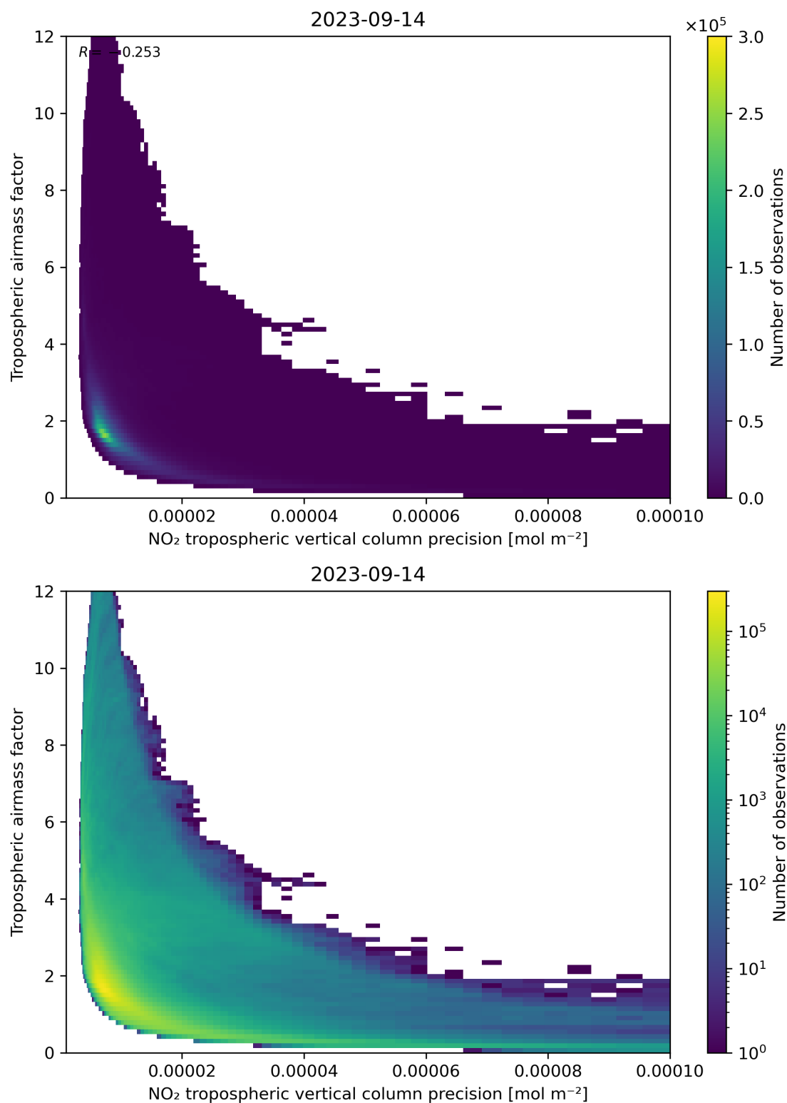
Figure 133: Scatter density plot of “NO 2 tropospheric vertical column precision” against “Tropospheric airmass factor” for 2023-09-13 to 2023-09-15.
