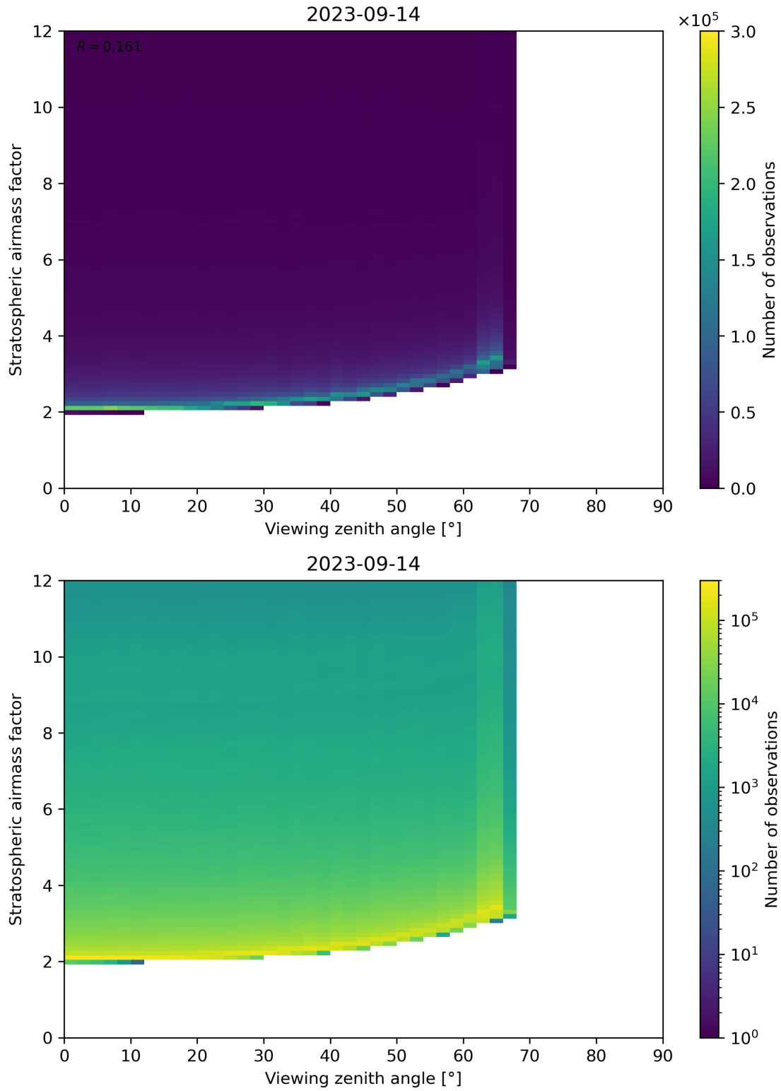
Figure 159: Scatter density plot of “Viewing zenith angle” against “Stratospheric airmass factor” for 2023-09-13 to 2023-09-15.
