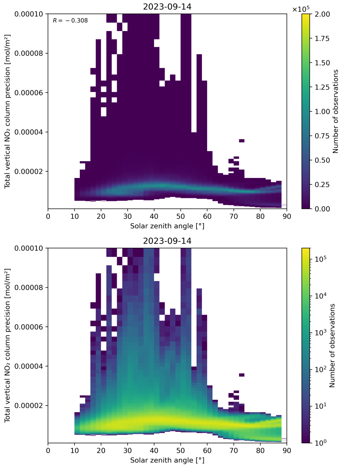
Figure 154: Scatter density plot of “Solar zenith angle” against “Total vertical NO 2 column precision” for 2023-09-13 to 2023-09-15.
