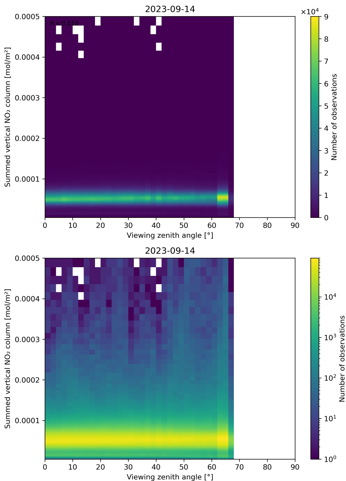
Figure 165: Scatter density plot of “Viewing zenith angle” against “Summed vertical NO 2 column” for 2023-09-13 to 2023-09-15.
