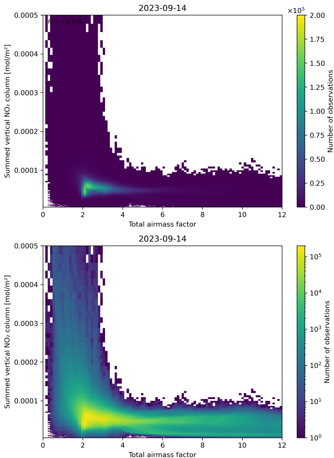
Figure 65: Scatter density plot of “Total airmass factor” against “Summed vertical NO 2 column” for 2023-09-13 to 2023-09-15.
