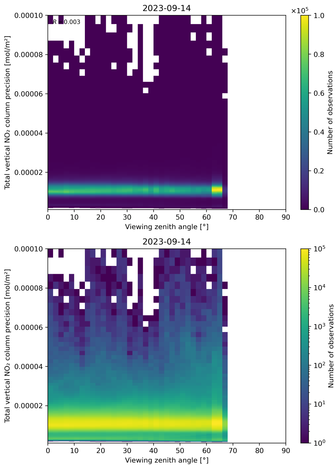
Figure 168: Scatter density plot of “Viewing zenith angle” against “Total vertical NO 2 column precision” for 2023-09-13 to 2023-09-15.
