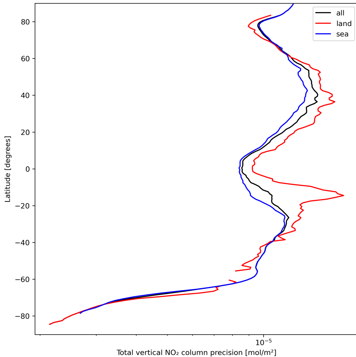
Figure 22: Zonal average of “Total vertical NO 2 column precision” for 2023-09-13 to 2023-09-15.
