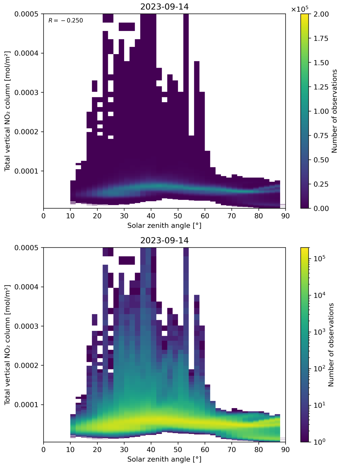
Figure 153: Scatter density plot of “Solar zenith angle” against “Total vertical NO 2 column” for 2023-09-13 to 2023-09-15.
