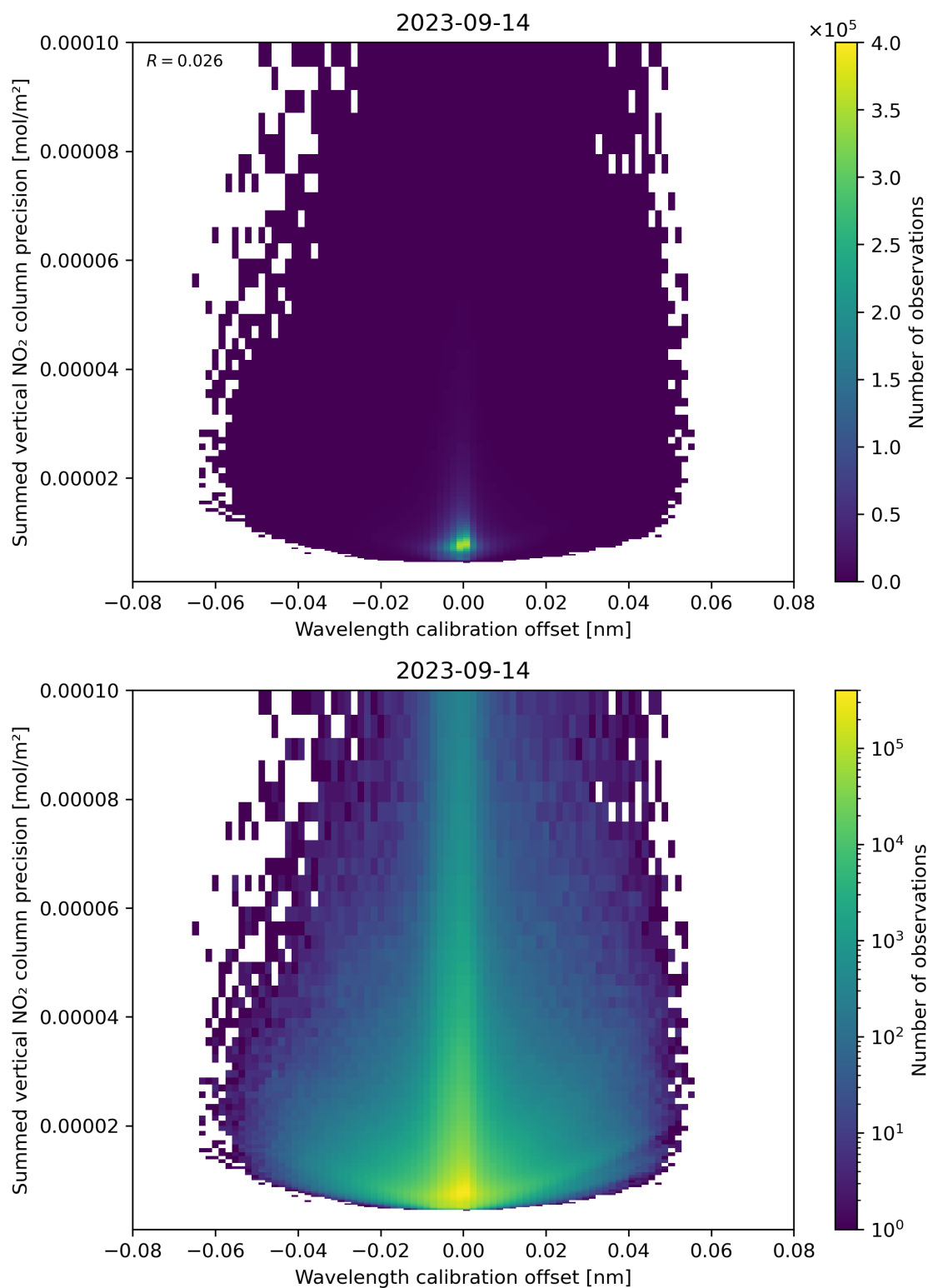
Figure 178: Scatter density plot of “Wavelength calibration offset” against “Summed vertical NO 2 column precision” for 2023-09-13 to 2023-09-15.
