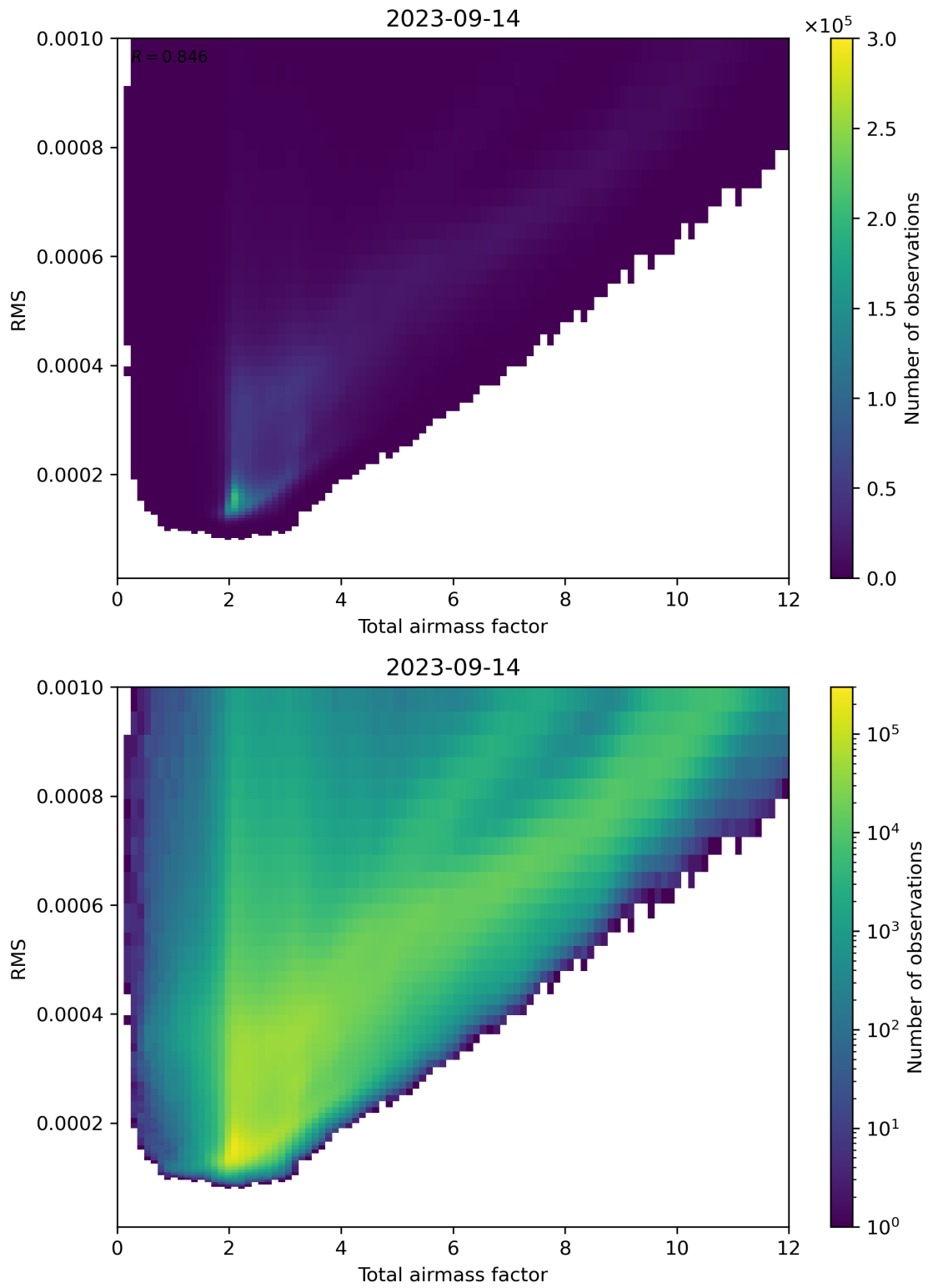
Figure 69: Scatter density plot of “Total airmass factor” against “RMS” for 2023-09-13 to 2023-09-15.
