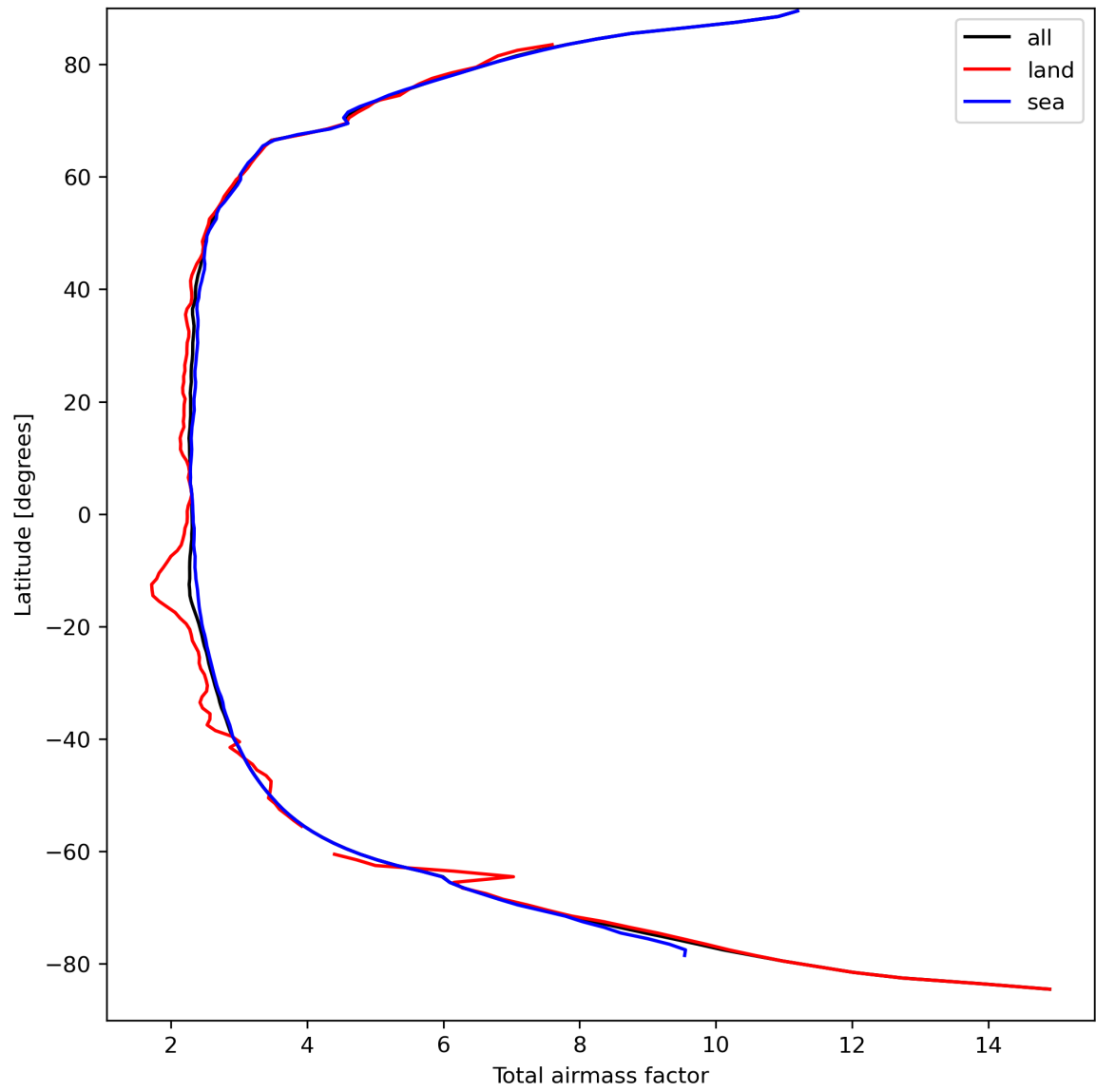
Figure 15: Zonal average of “Total airmass factor” for 2023-09-13 to 2023-09-15.
