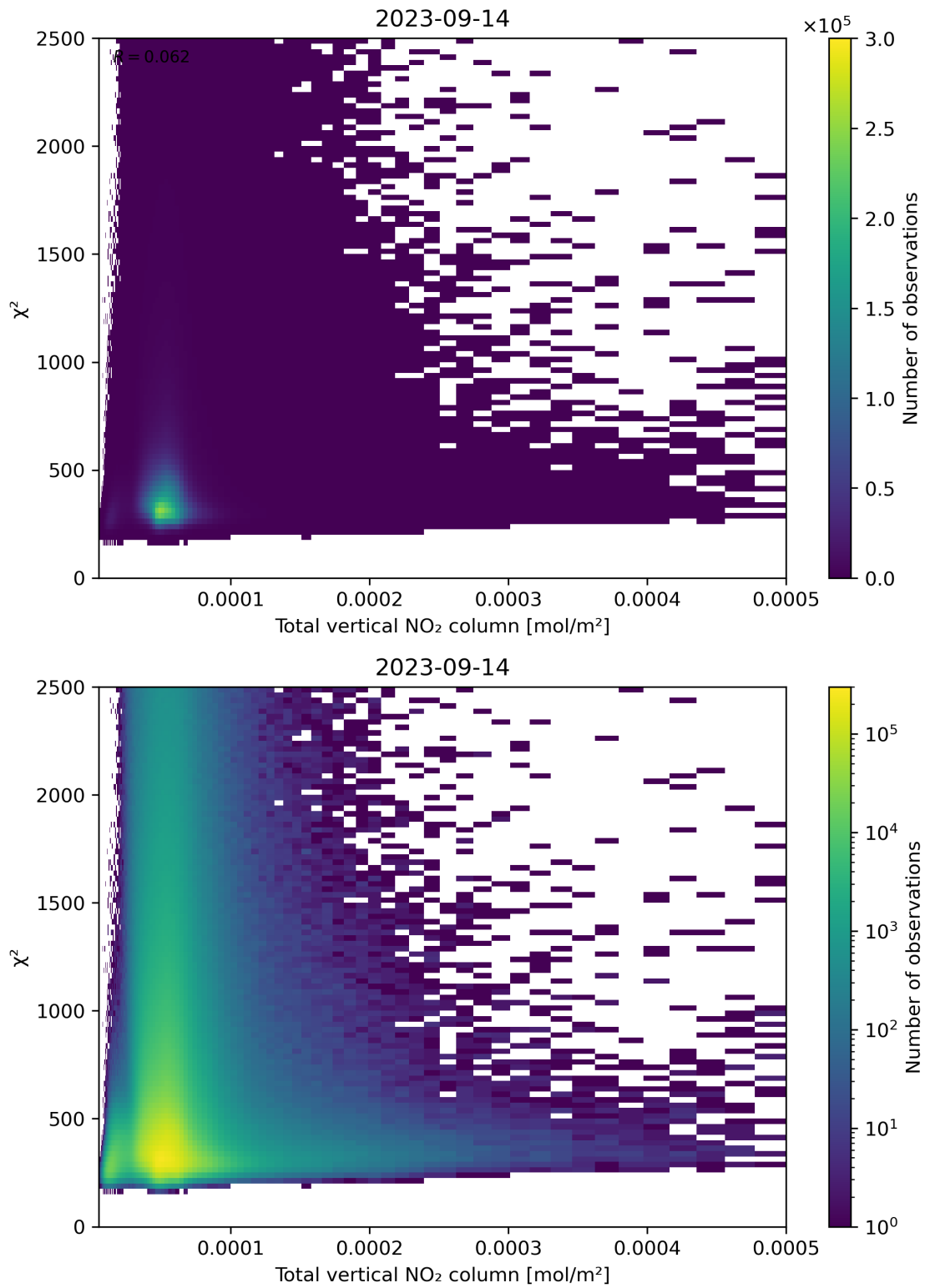
Figure 111: Scatter density plot of “Total vertical NO 2 column” against “ \chi^2 ” for 2023-09-13 to 2023-09-15.
