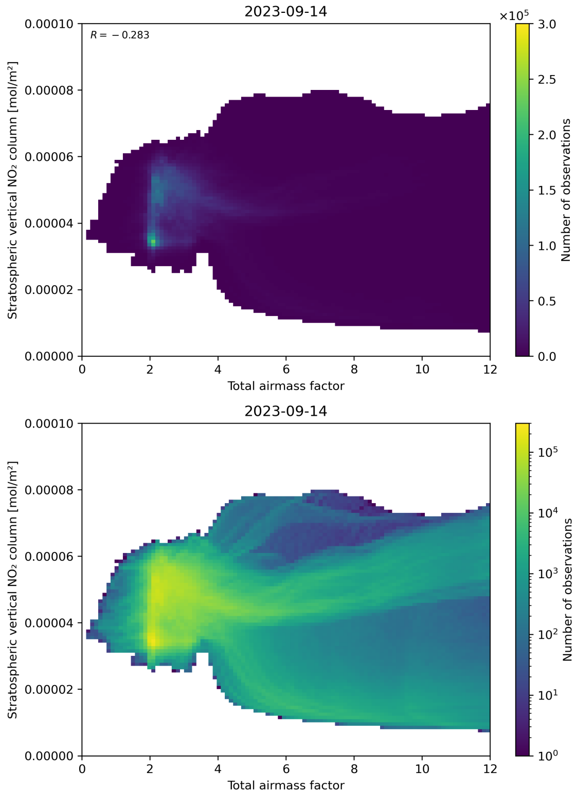
Figure 64: Scatter density plot of “Total airmass factor” against “Stratospheric vertical NO 2 column” for 2023-09-13 to 2023-09-15.
