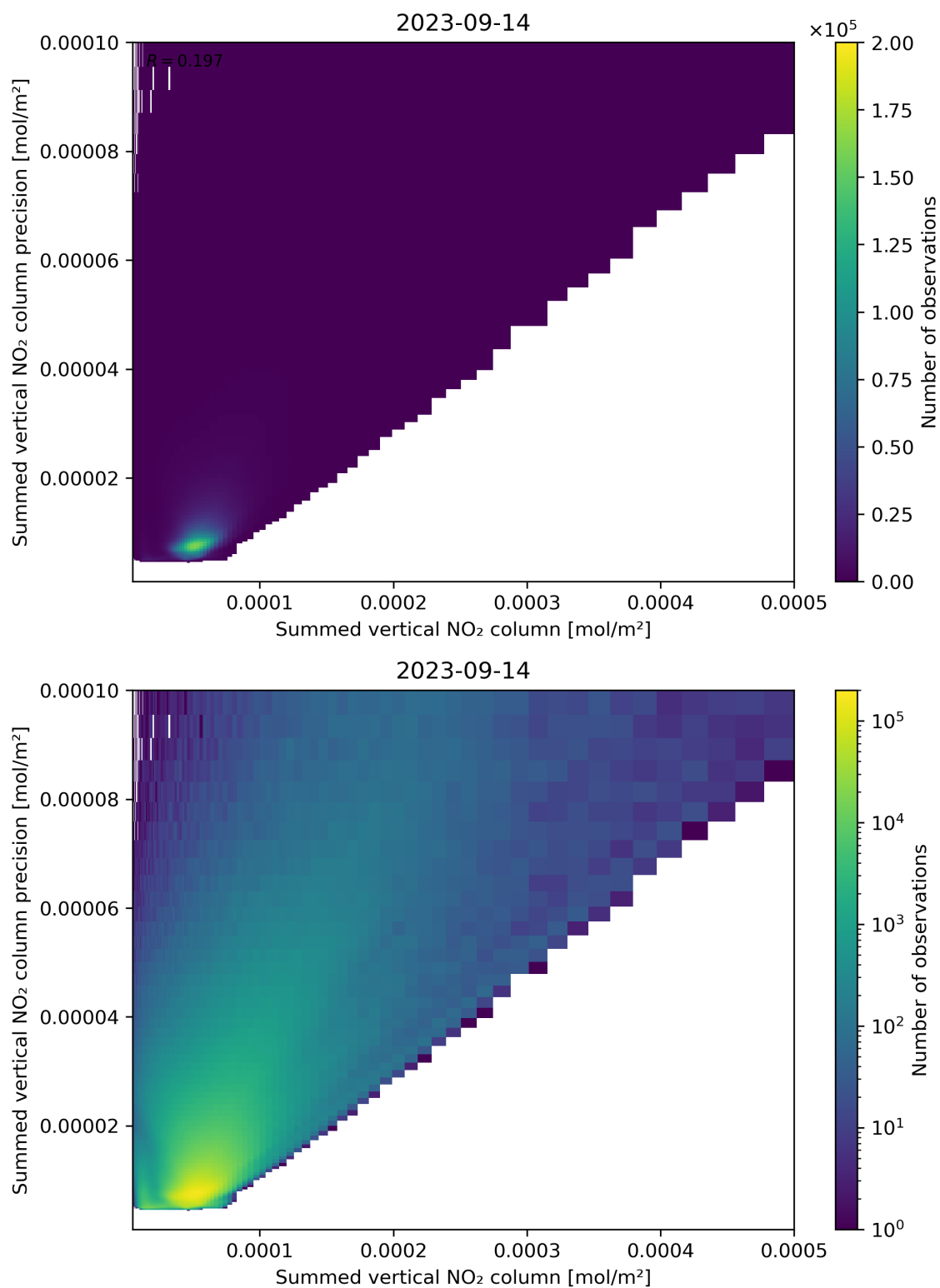
Figure 105: Scatter density plot of “Summed vertical NO 2 column” against “Summed vertical NO 2 column precision” for 2023-09-13 to 2023-09-15.
