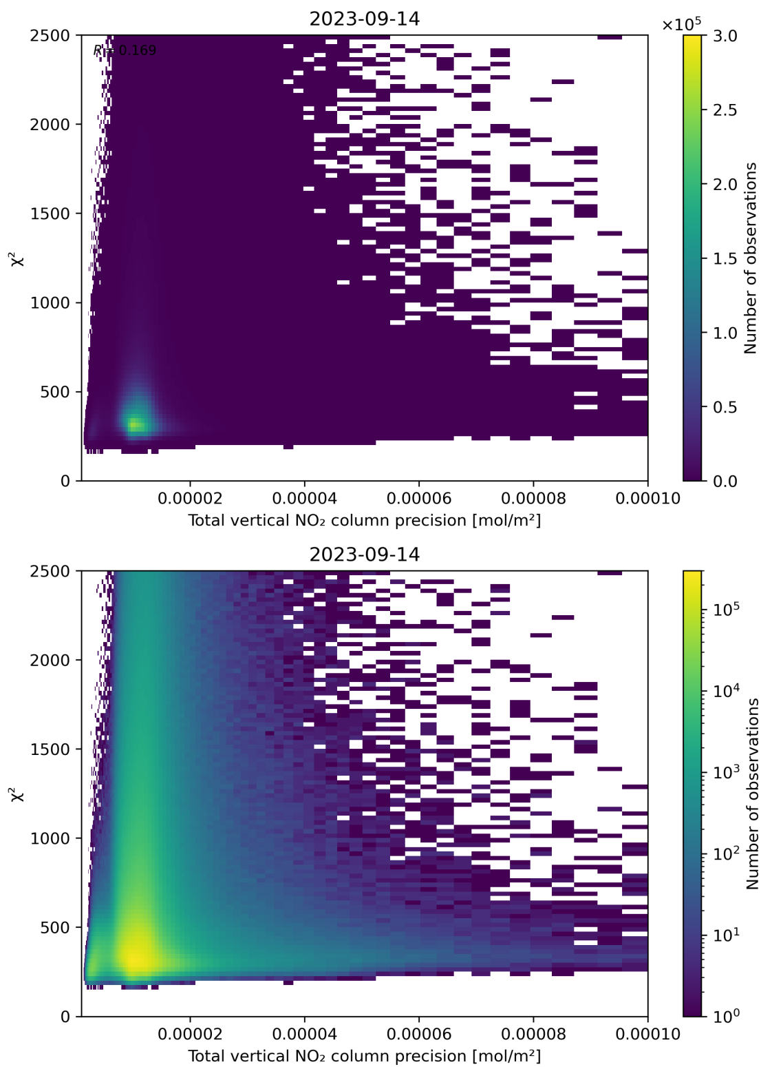
Figure 116: Scatter density plot of “Total vertical NO 2 column precision” against “ \chi^2 ” for 2023-09-13 to 2023-09-15.
