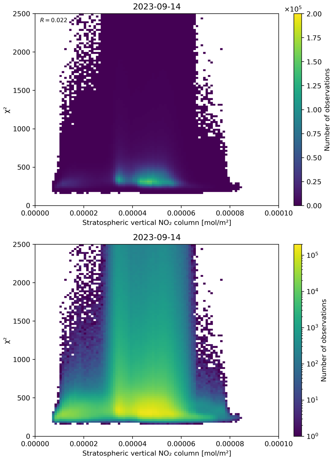
Figure 97: Scatter density plot of “Stratospheric vertical NO 2 column” against “ \chi^2 ” for 2023-09-13 to 2023-09-15.
