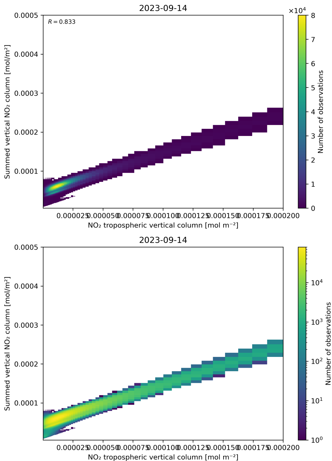
Figure 126: Scatter density plot of “NO 2 tropospheric vertical column” against “Summed vertical NO 2 column” for 2023-09-13 to 2023-09-15.
