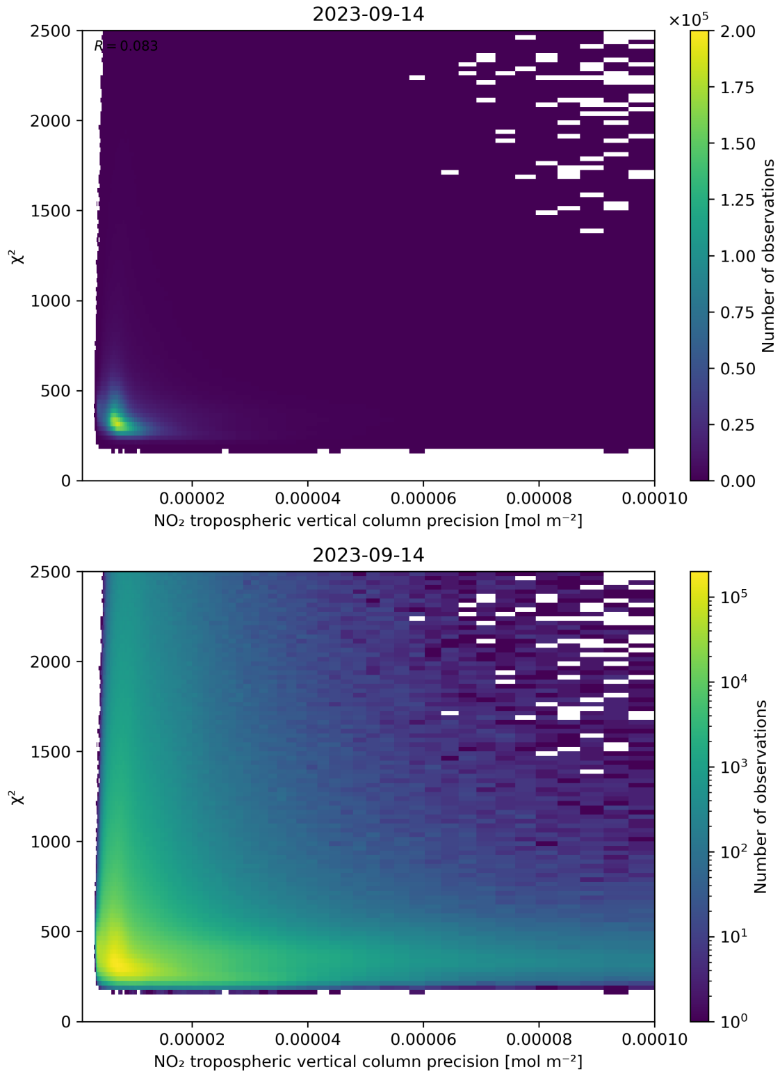
Figure 134: Scatter density plot of “NO 2 tropospheric vertical column precision” against “ \chi^2 ” for 2023-09-13 to 2023-09-15.
