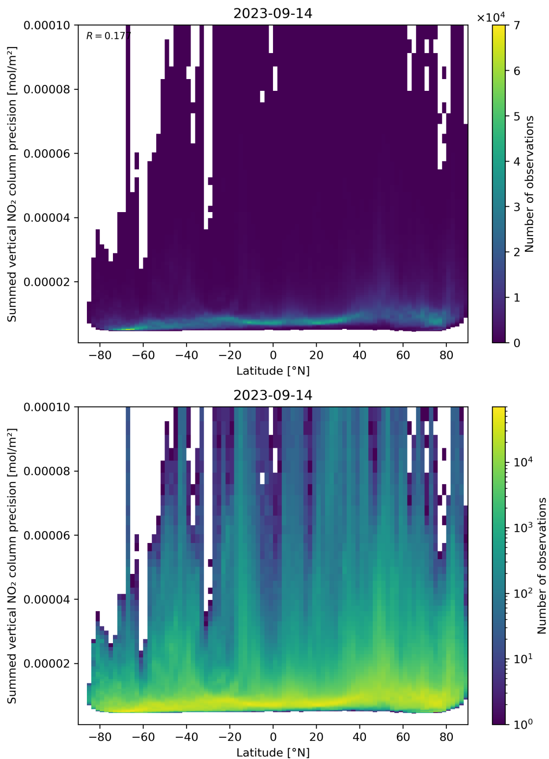
Figure 89: Scatter density plot of “Latitude” against “Summed vertical NO 2 column precision” for 2023-09-13 to 2023-09-15.
