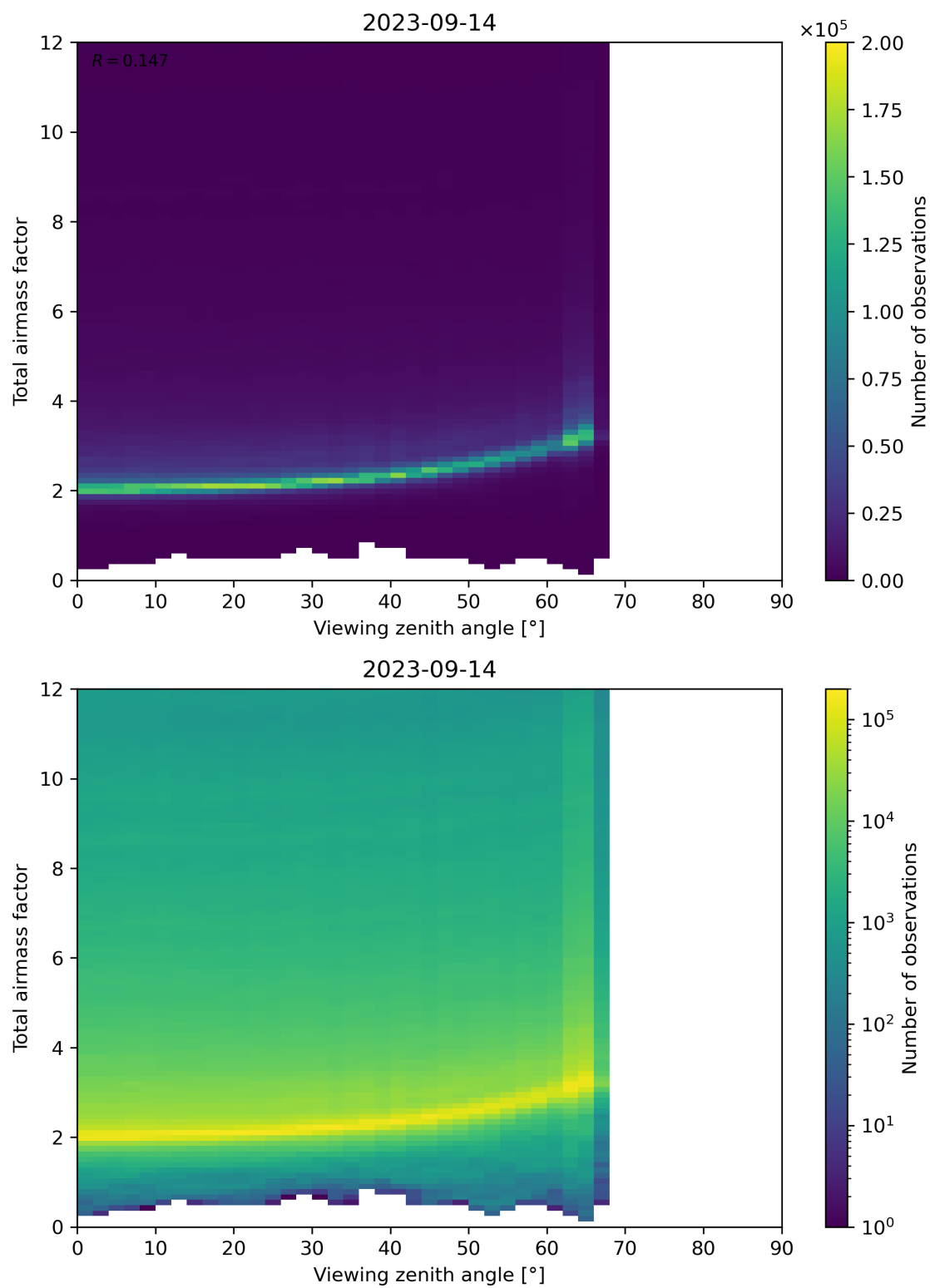
Figure 160: Scatter density plot of “Viewing zenith angle” against “Total airmass factor” for 2023-09-13 to 2023-09-15.
