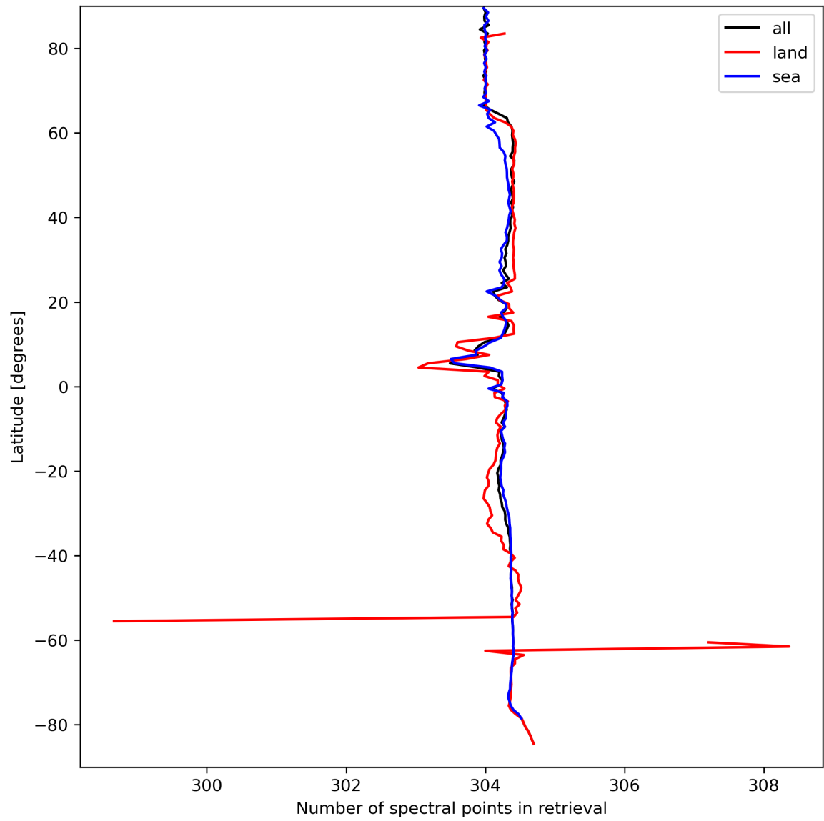
Figure 16: Zonal average of “Number of spectral points in retrieval” for 2023-09-13 to 2023-09-15.
