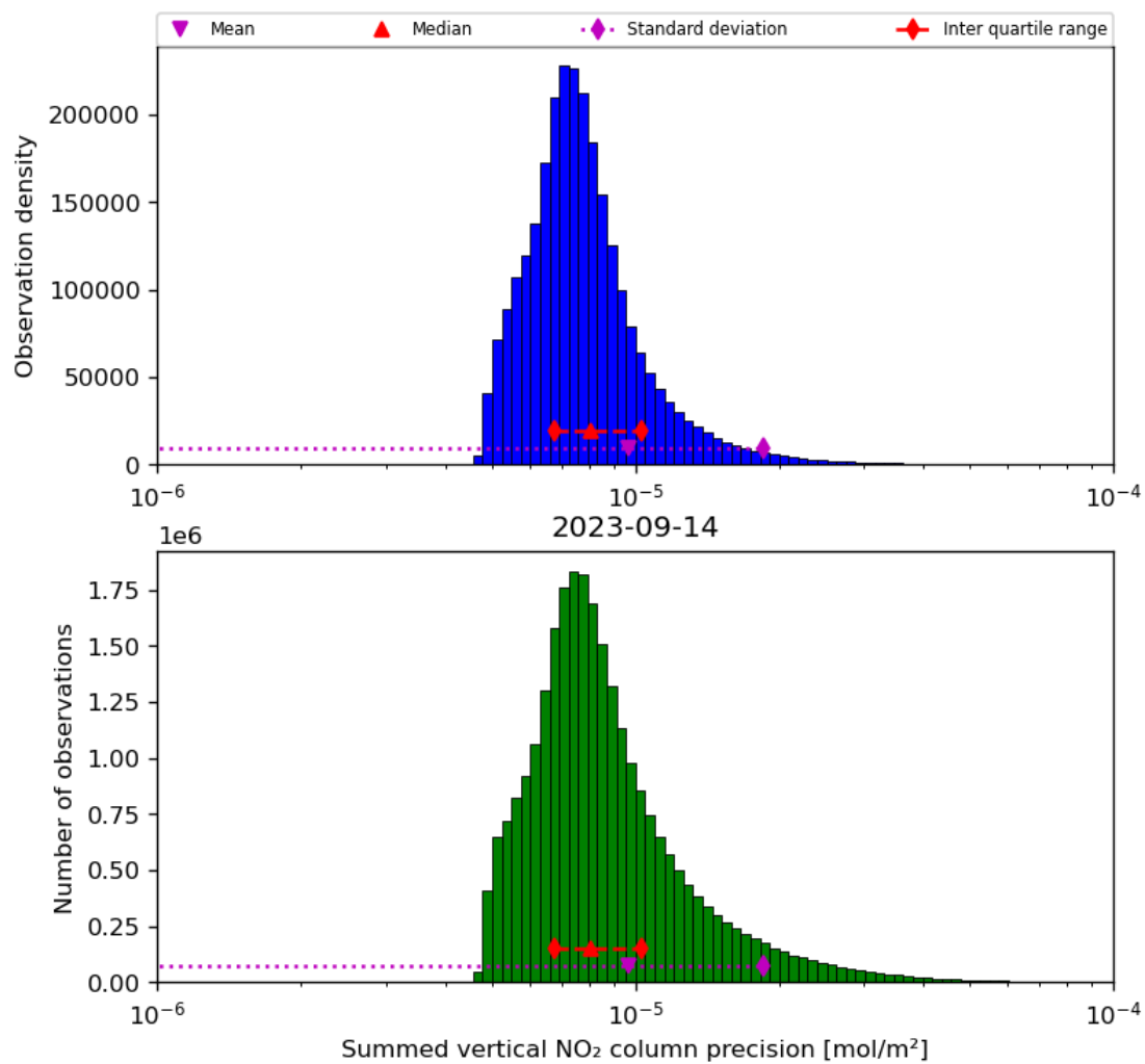
Figure 41: Histogram of "Summed vertical NO 2 column precision" for 2023-09-13 to 2023-09-15
