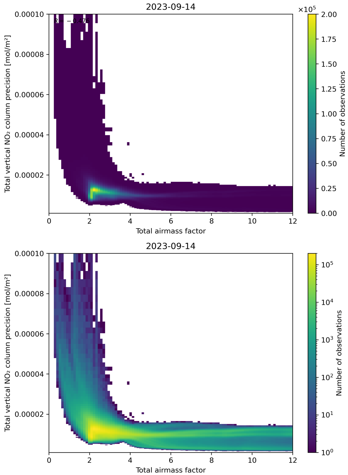
Figure 68: Scatter density plot of “Total airmass factor” against “Total vertical NO 2 column precision” for 2023-09-13 to 2023-09-15.
