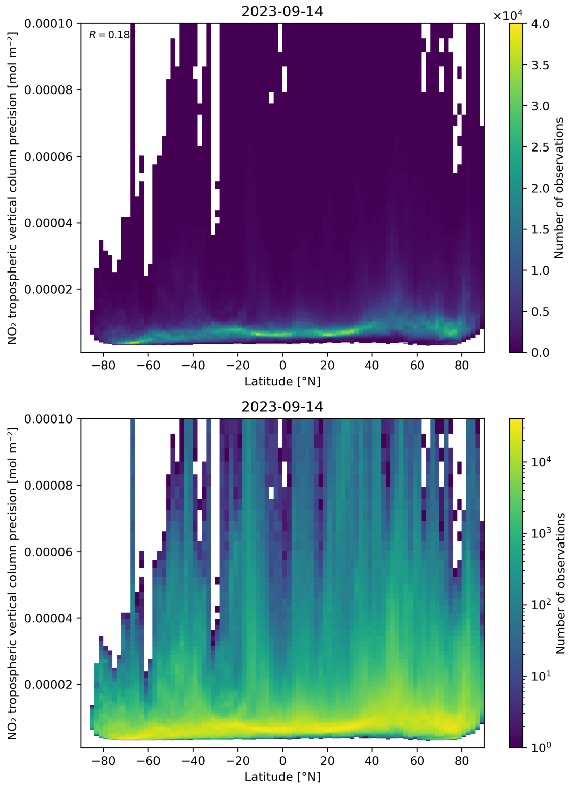
Figure 93: Scatter density plot of “Latitude” against “NO 2 tropospheric vertical column precision” for 2023-09-13 to 2023-09-15.
