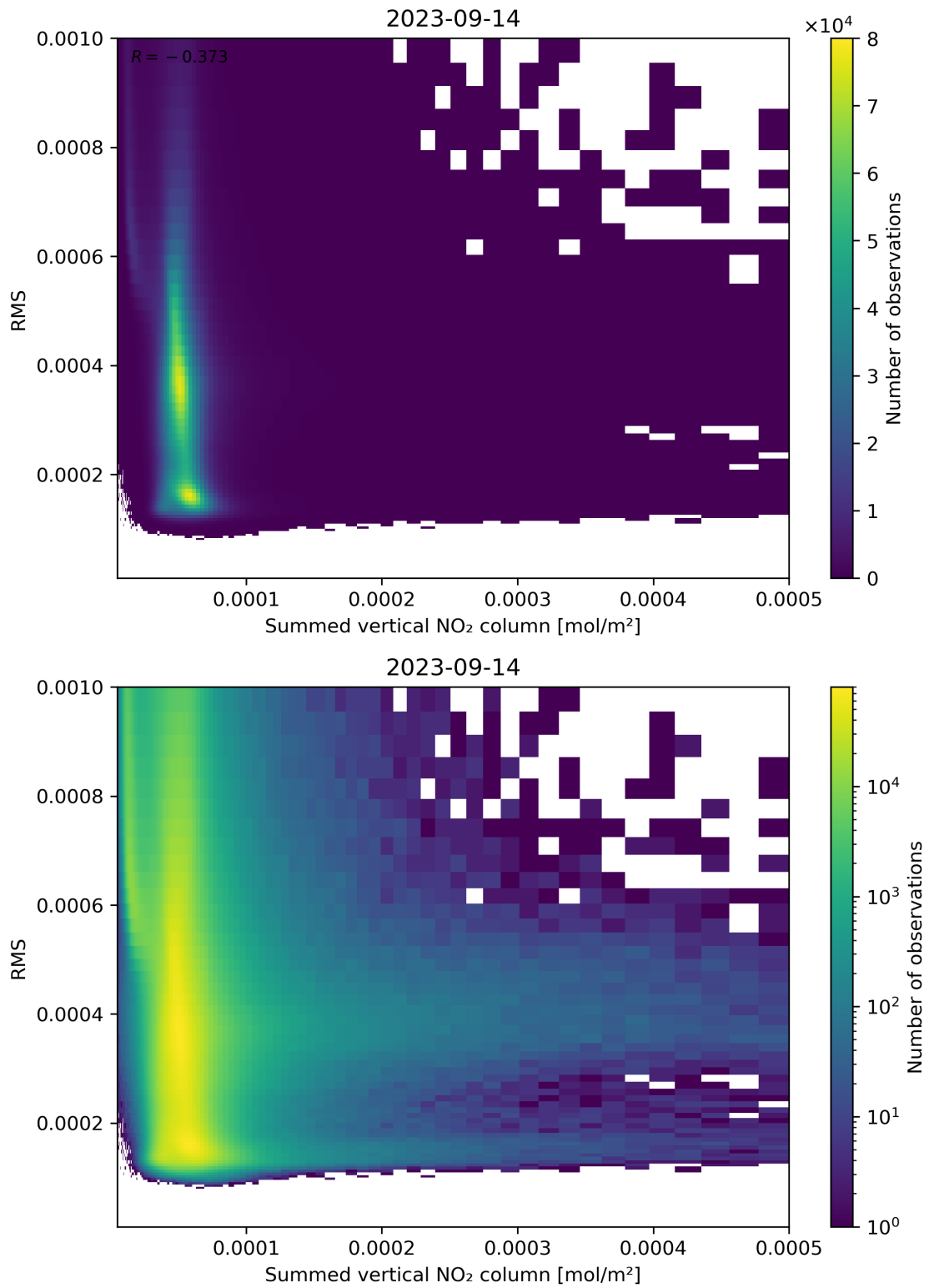
Figure 109: Scatter density plot of “Summed vertical NO 2 column” against “RMS” for 2023-09-13 to 2023-09-15.
