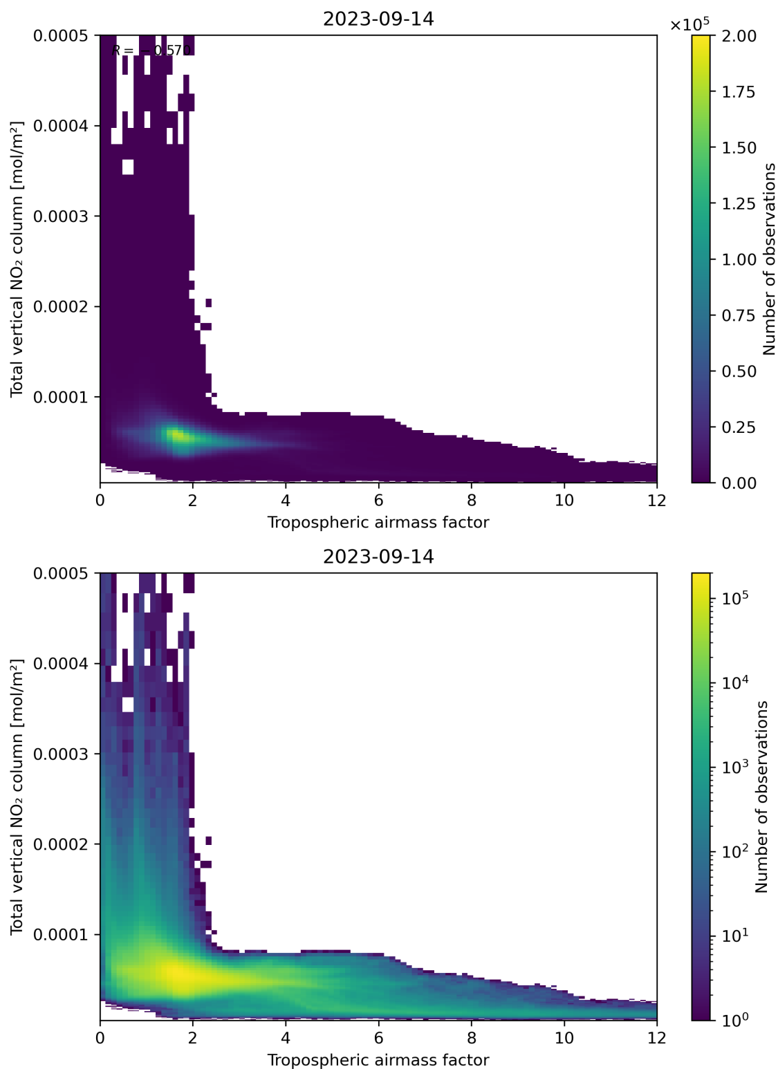
Figure 77: Scatter density plot of “Tropospheric airmass factor” against “Total vertical NO 2 column” for 2023-09-13 to 2023-09-15.
