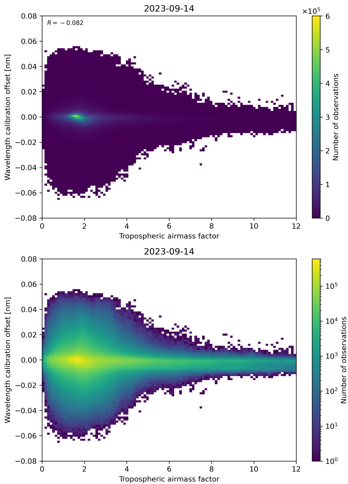
Figure 80: Scatter density plot of “Tropospheric airmass factor” against “Wavelength calibration offset” for 2023-09-13 to 2023-09-15.
