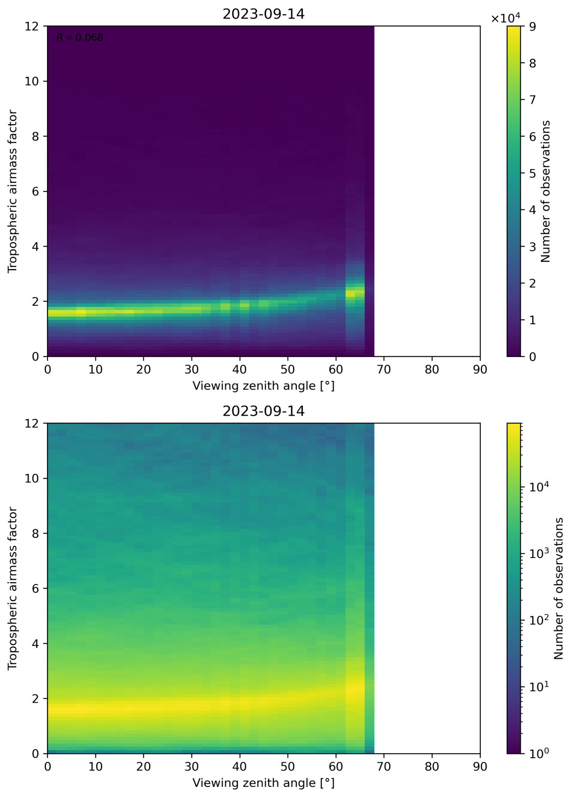
Figure 161: Scatter density plot of “Viewing zenith angle” against “Tropospheric airmass factor” for 2023-09-13 to 2023-09-15.
