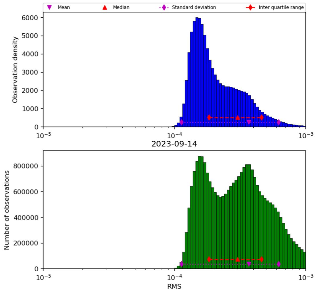
Figure 43: Histogram of “RMS” for 2023-09-13 to 2023-09-15
