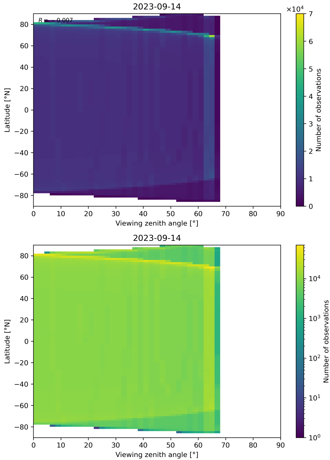
Figure 163: Scatter density plot of “Viewing zenith angle” against “Latitude” for 2023-09-13 to 2023-09-15.
