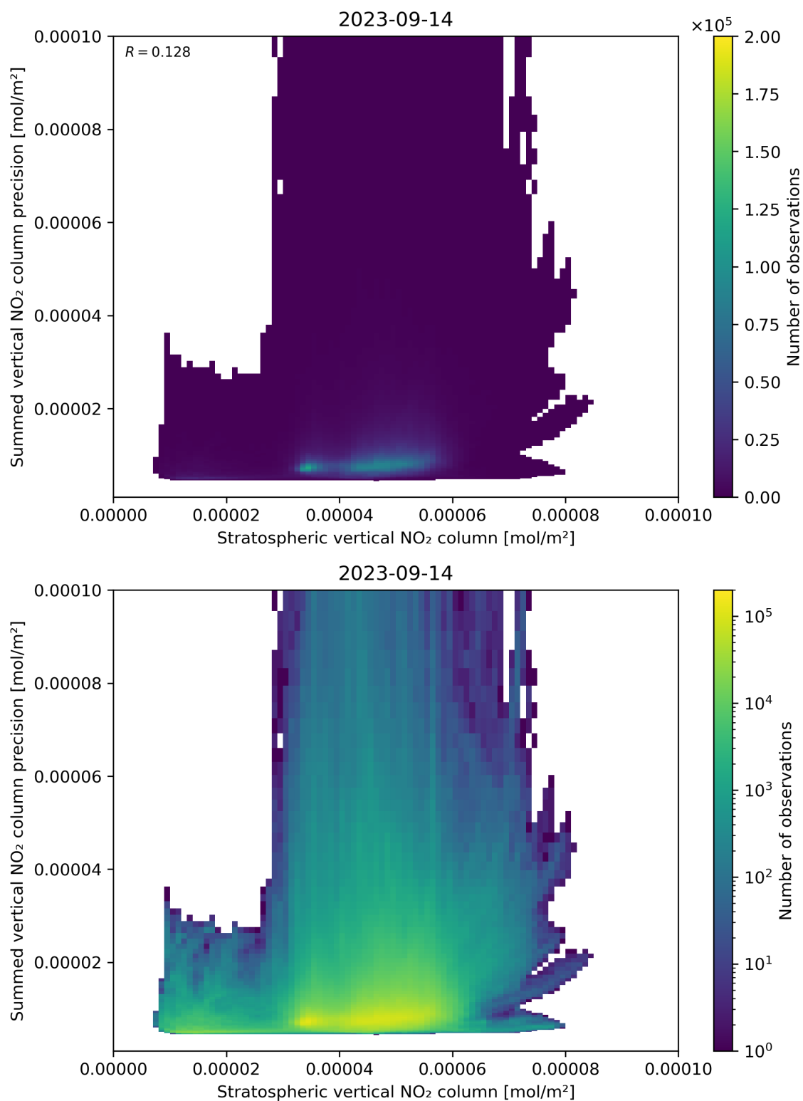
Figure 99: Scatter density plot of “Stratospheric vertical NO 2 column” against “Summed vertical NO 2 column precision” for 2023-09-13 to 2023-09-15.
