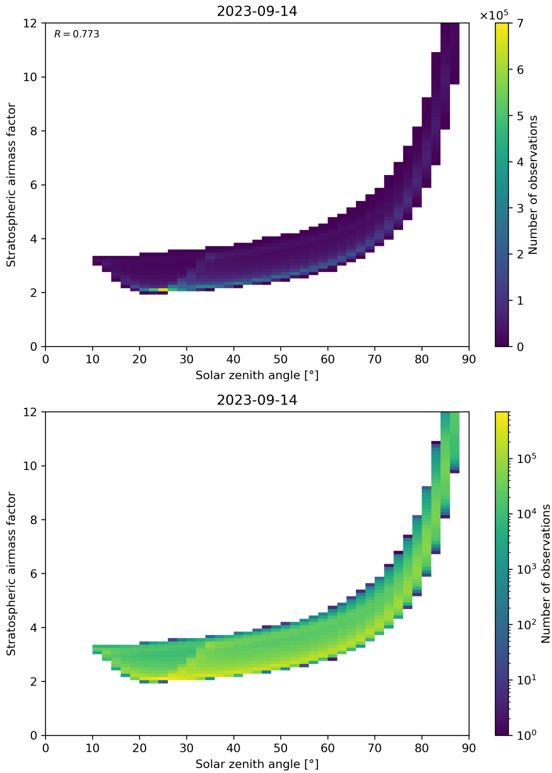
Figure 145: Scatter density plot of “Solar zenith angle” against “Stratospheric airmass factor” for 2023-09-13 to 2023-09-15.
