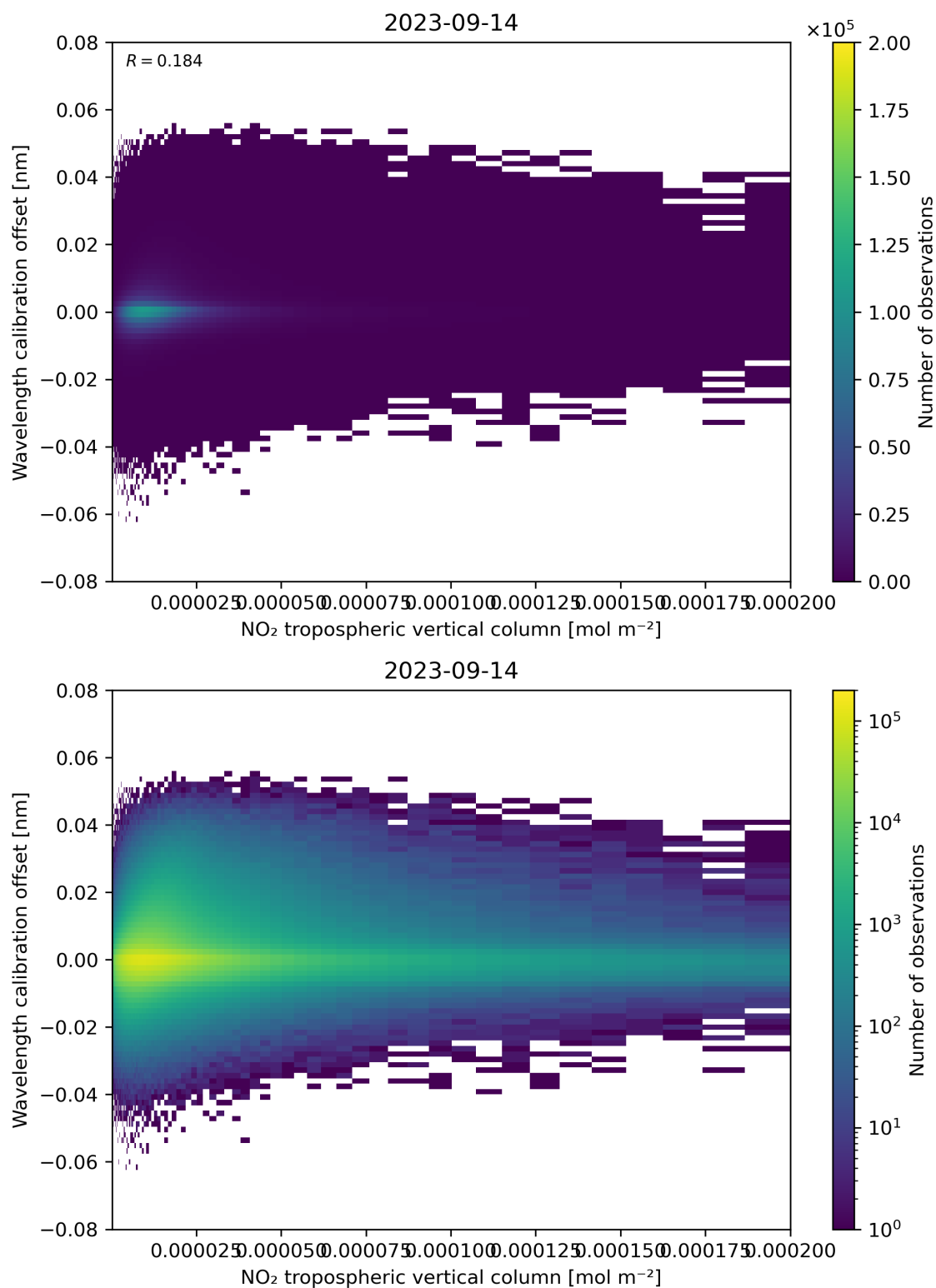
Figure 143: Scatter density plot of “NO 2 tropospheric vertical column” against “Wavelength calibration offset” for 2023-09-13 to 2023-09-15.
