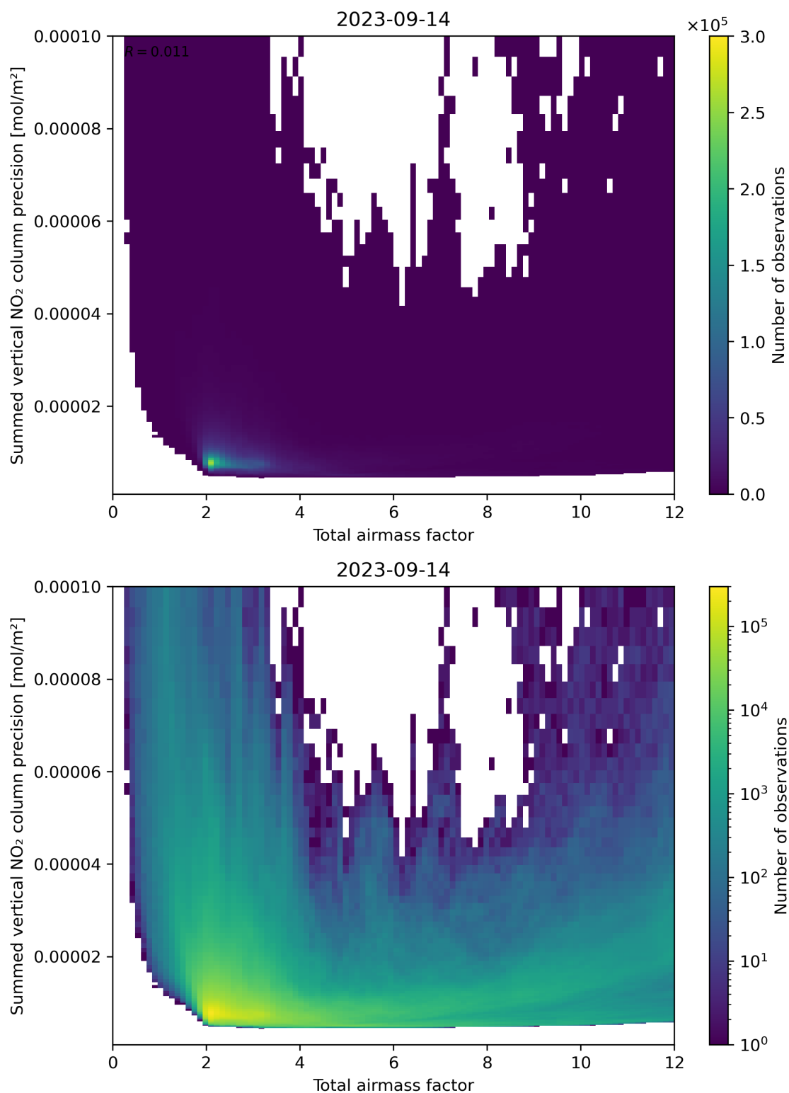
Figure 66: Scatter density plot of “Total airmass factor” against “Summed vertical NO 2 column precision” for 2023-09-13 to 2023-09-15.
