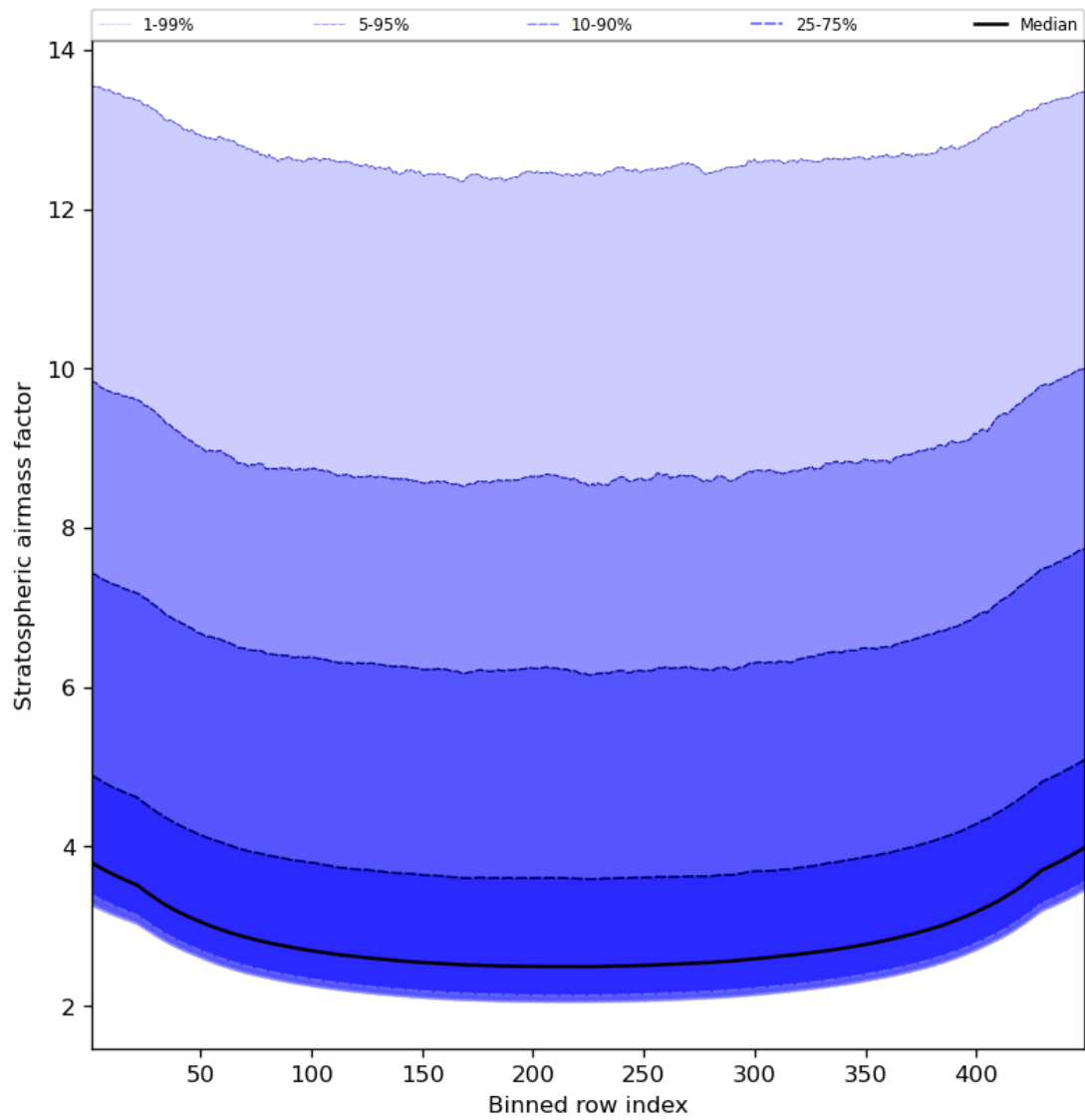
Figure 61: Along track statistics of “Stratospheric airmass factor” for 2023-09-13 to 2023-09-15
