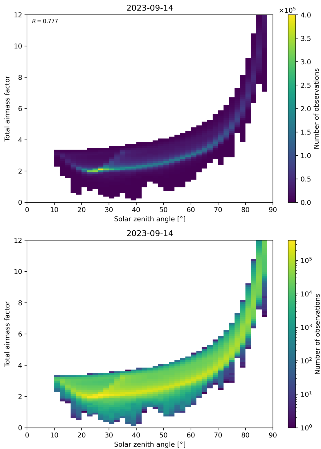
Figure 146: Scatter density plot of “Solar zenith angle” against “Total air mass factor” for 2023-09-13 to 2023-09-15.
