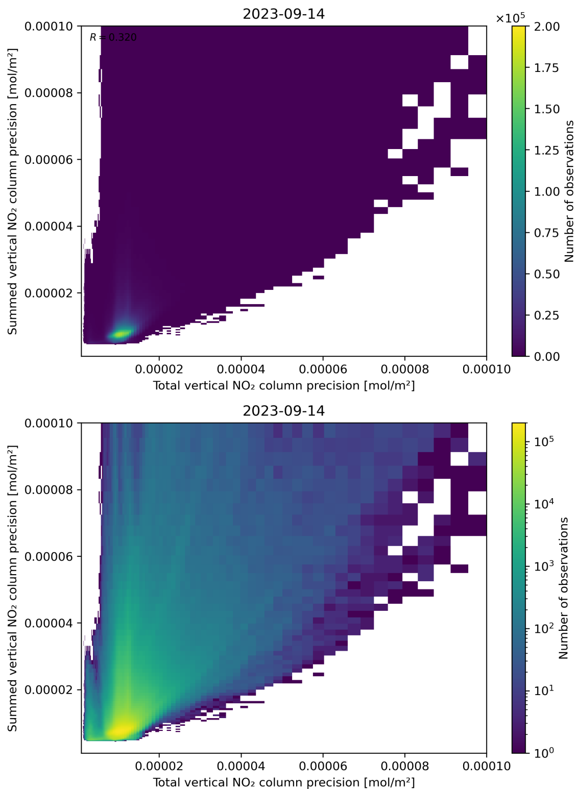
Figure 118: Scatter density plot of “Total vertical NO 2 column precision” against “Summed vertical NO 2 column precision” for 2023-09-13 to 2023-09-15.
