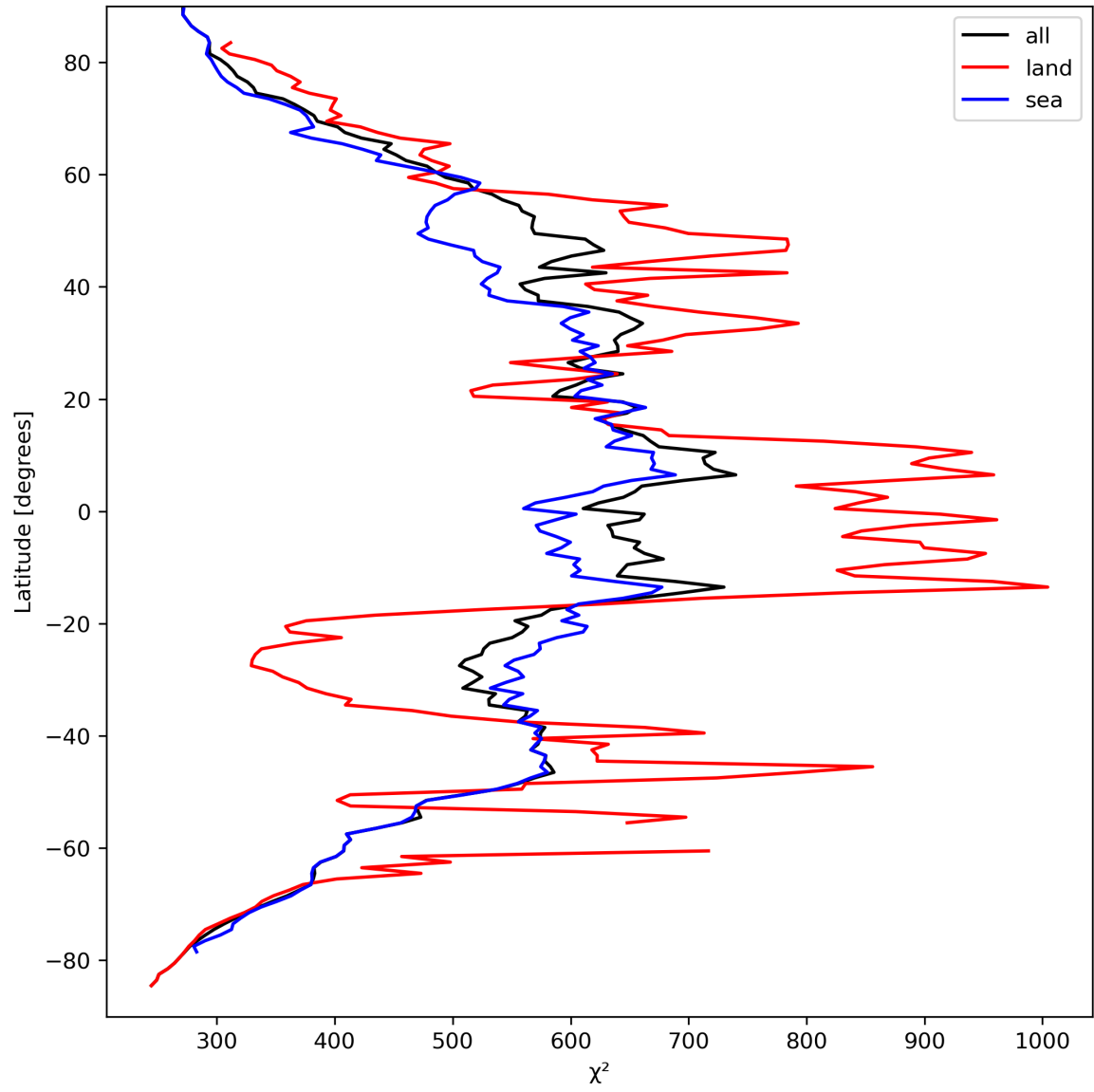
Figure 25: Zonal average of “ \chi^2 ” for 2023-09-13 to 2023-09-15.
