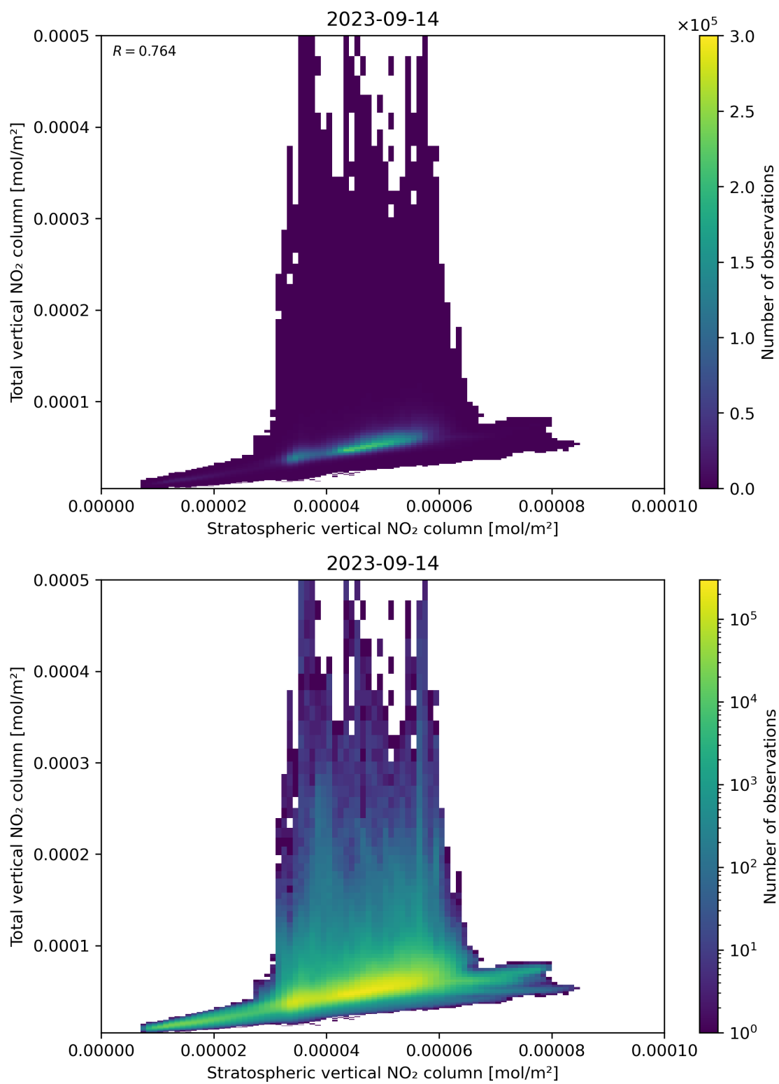
Figure 100: Scatter density plot of “Stratospheric vertical NO 2 column” against “Total vertical NO 2 column” for 2023-09-13 to 2023-09-15.
