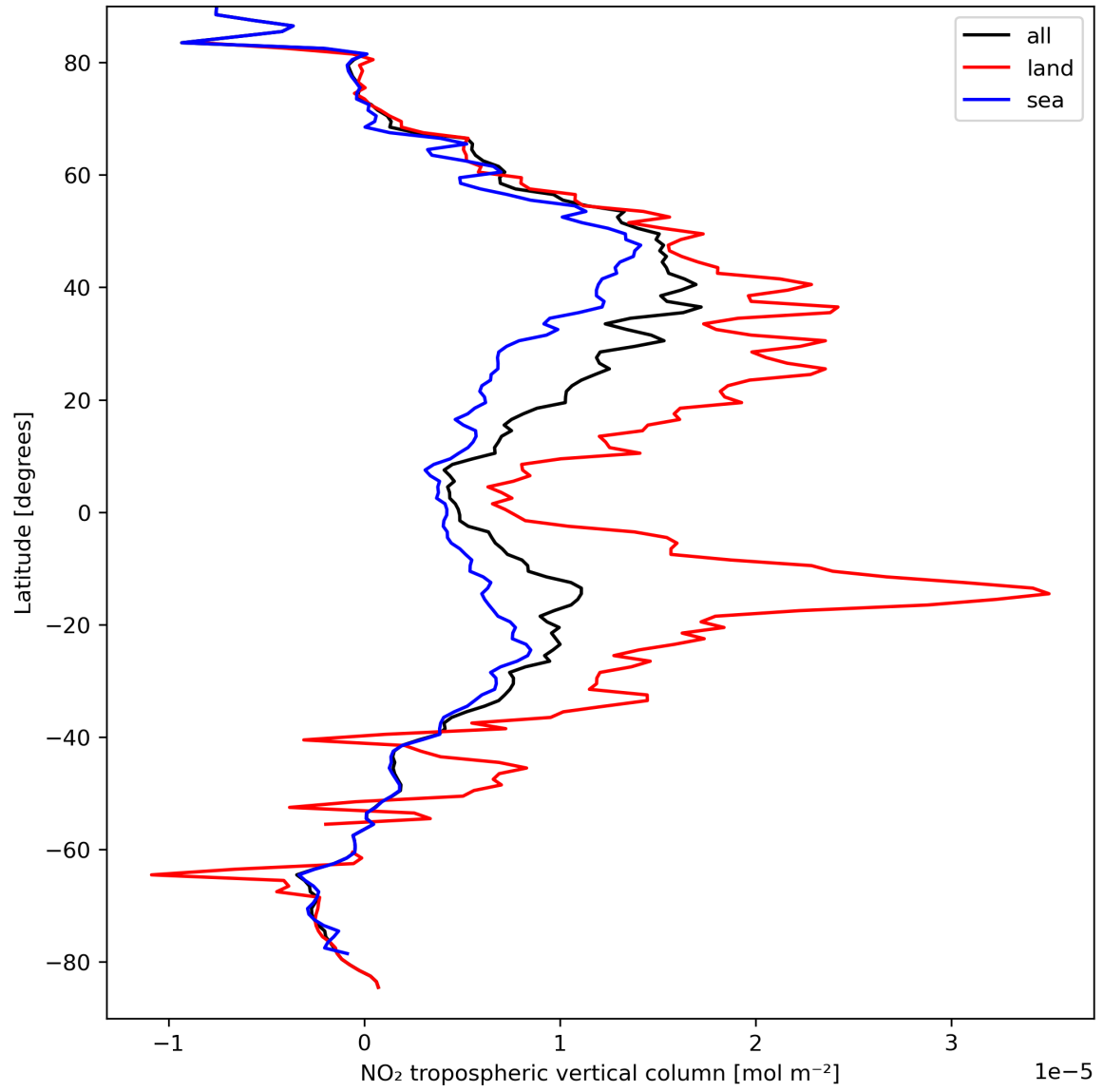
Figure 12: Zonal average of “NO 2 tropospheric vertical column” for 2023-09-13 to 2023-09-15.
