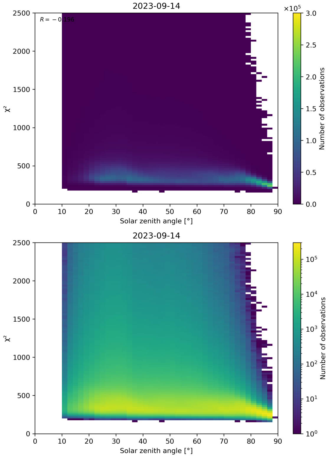
Figure 148: Scatter density plot of “Solar zenith angle” against “ \chi^2 ” for 2023-09-13 to 2023-09-15.
