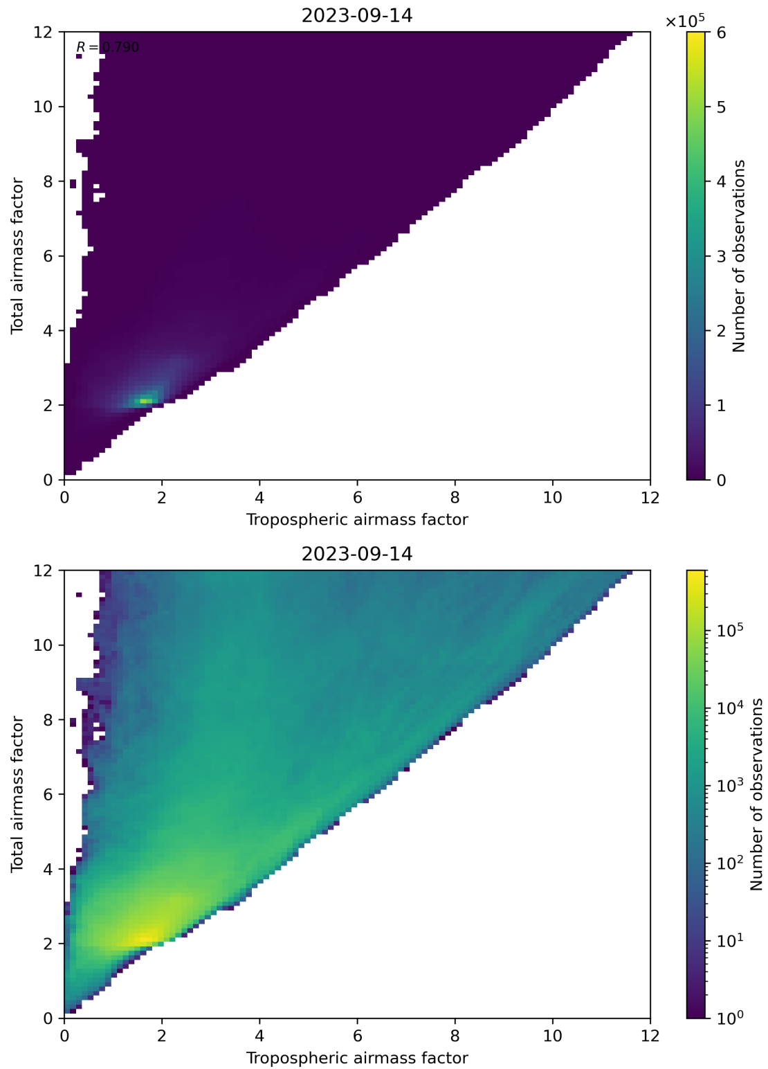
Figure 72: Scatter density plot of “Tropospheric airmass factor” against “Total airmass factor” for 2023-09-13 to 2023-09-15.
