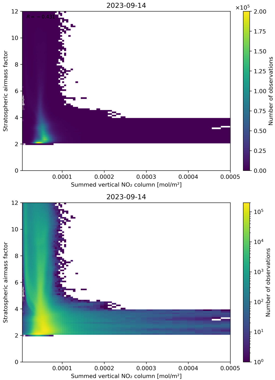
Figure 103: Scatter density plot of “Summed vertical NO 2 column” against “Stratospheric air mass factor” for 2023-09-13 to 2023-09-15.
