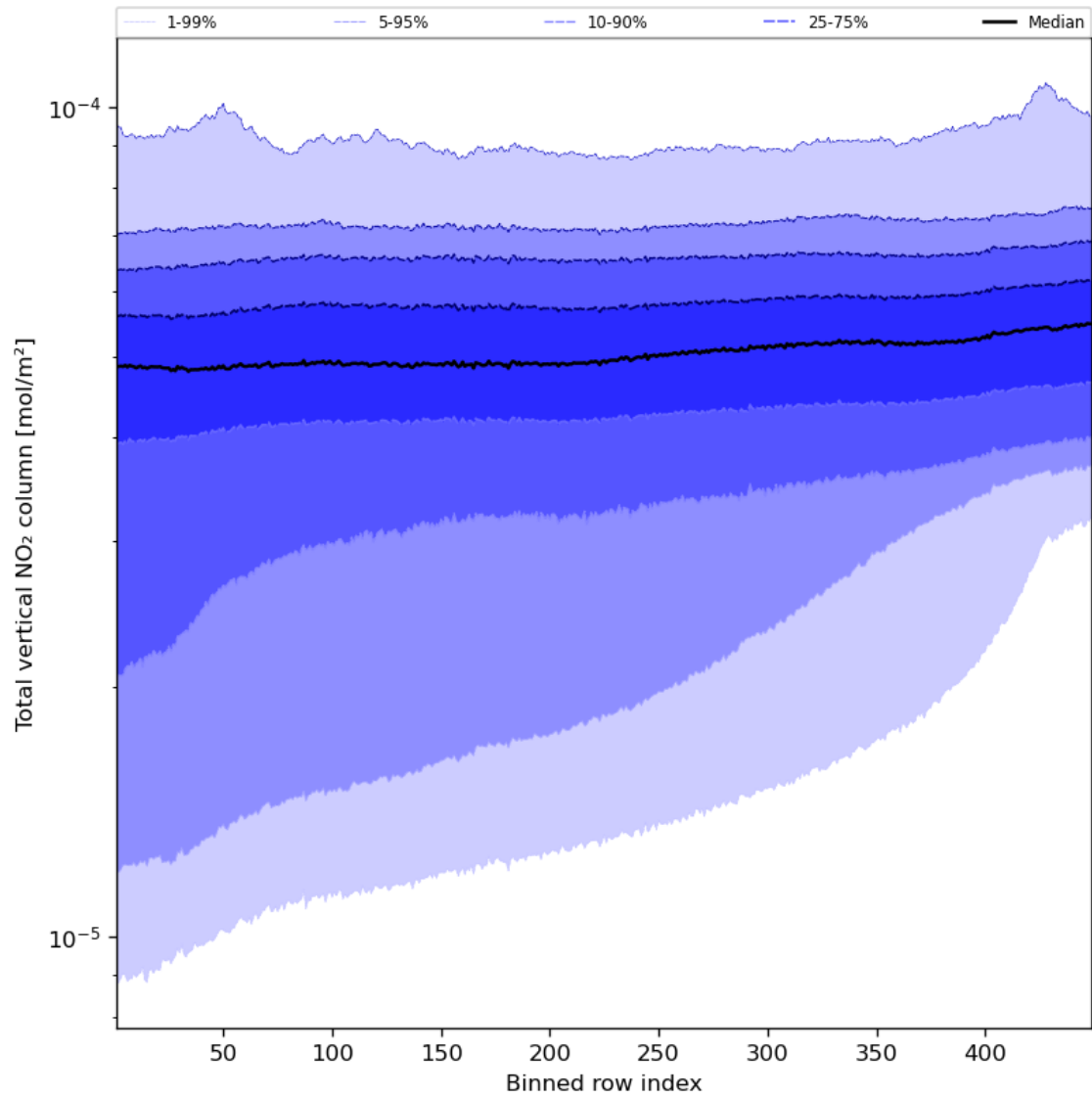
Figure 55: Along track statistics of "Total vertical NO 2 column" for 2023-09-13 to 2023-09-15
