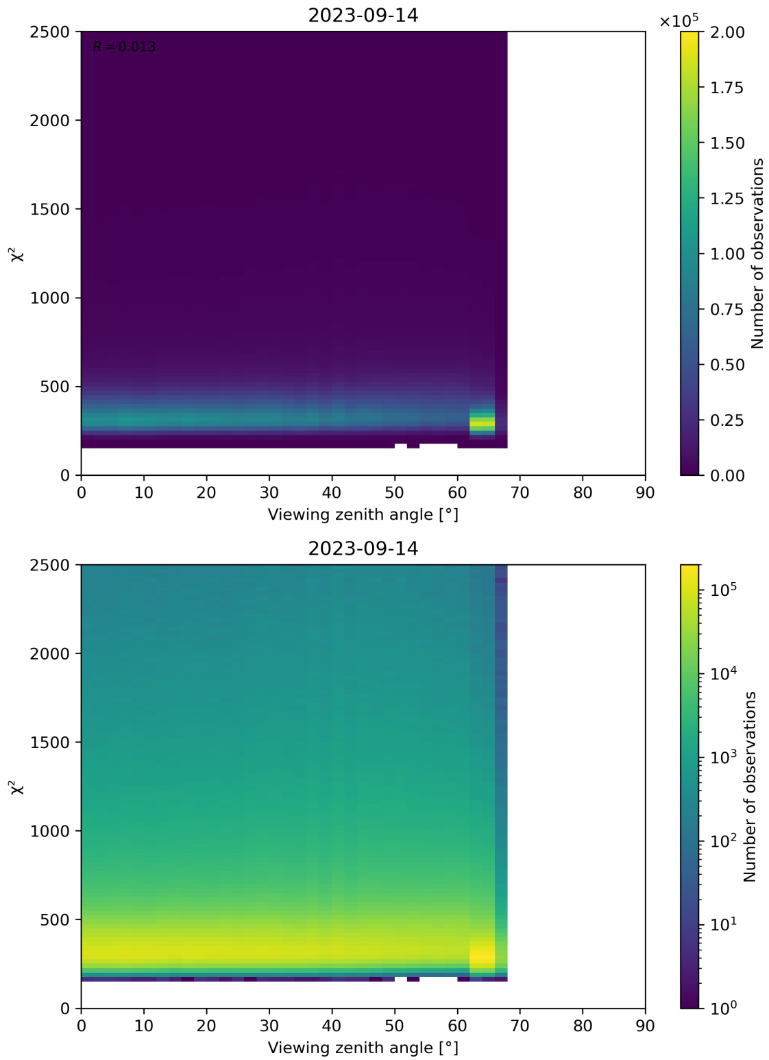
Figure 162: Scatter density plot of “Viewing zenith angle” against “ \chi^2 ” for 2023-09-13 to 2023-09-15.
