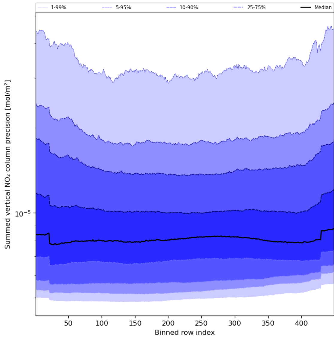
Figure 58: Along track statistics of “Summed vertical NO 2 column precision” for 2023-09-13 to 2023-09-15
