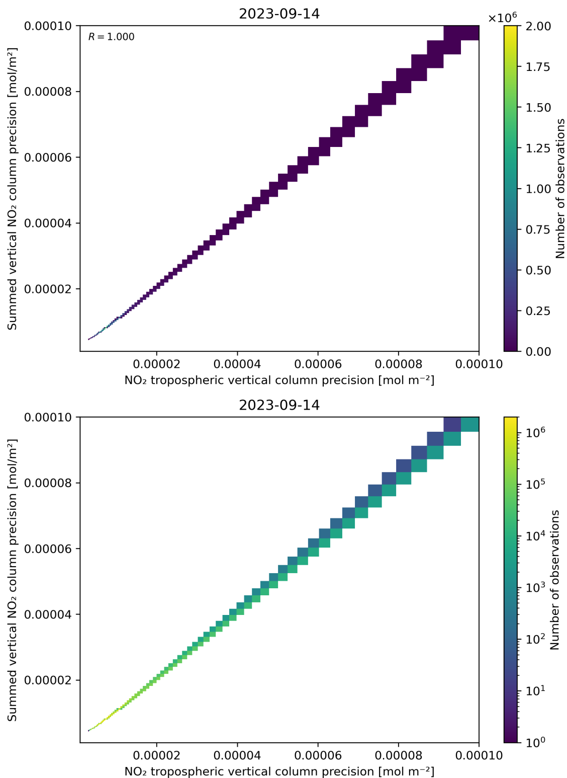
Figure 137: Scatter density plot of “NO 2 tropospheric vertical column precision” against “Summed vertical NO 2 column precision” for 2023-09-13 to 2023-09-15.
