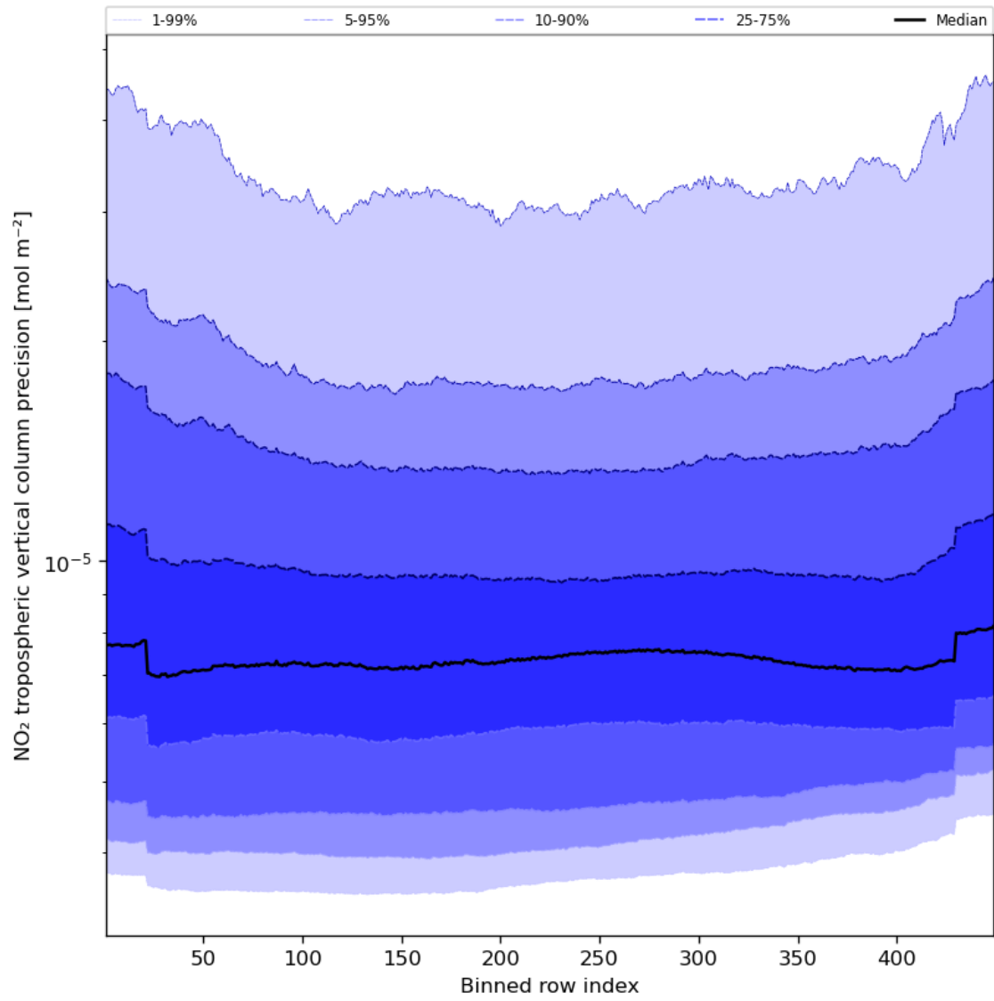
Figure 47: Along track statistics of “NO 2 tropospheric vertical column precision” for 2023-09-13 to 2023-09-15
