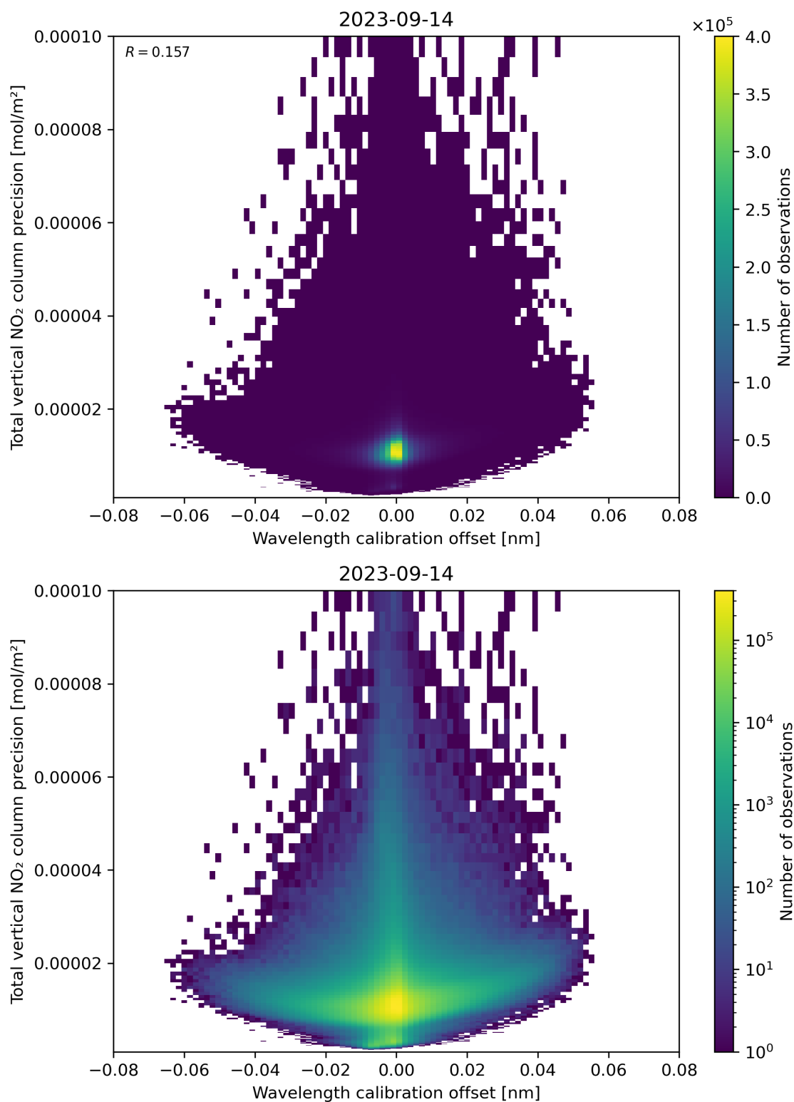
Figure 180: Scatter density plot of “Wavelength calibration offset” against “Total vertical NO 2 column precision” for 2023-09-13 to 2023-09-15.
