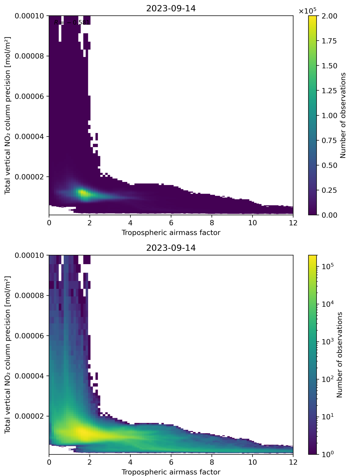
Figure 78: Scatter density plot of “Tropospheric air mass factor” against “Total vertical NO 2 column precision” for 2023-09-13 to 2023-09-15.
