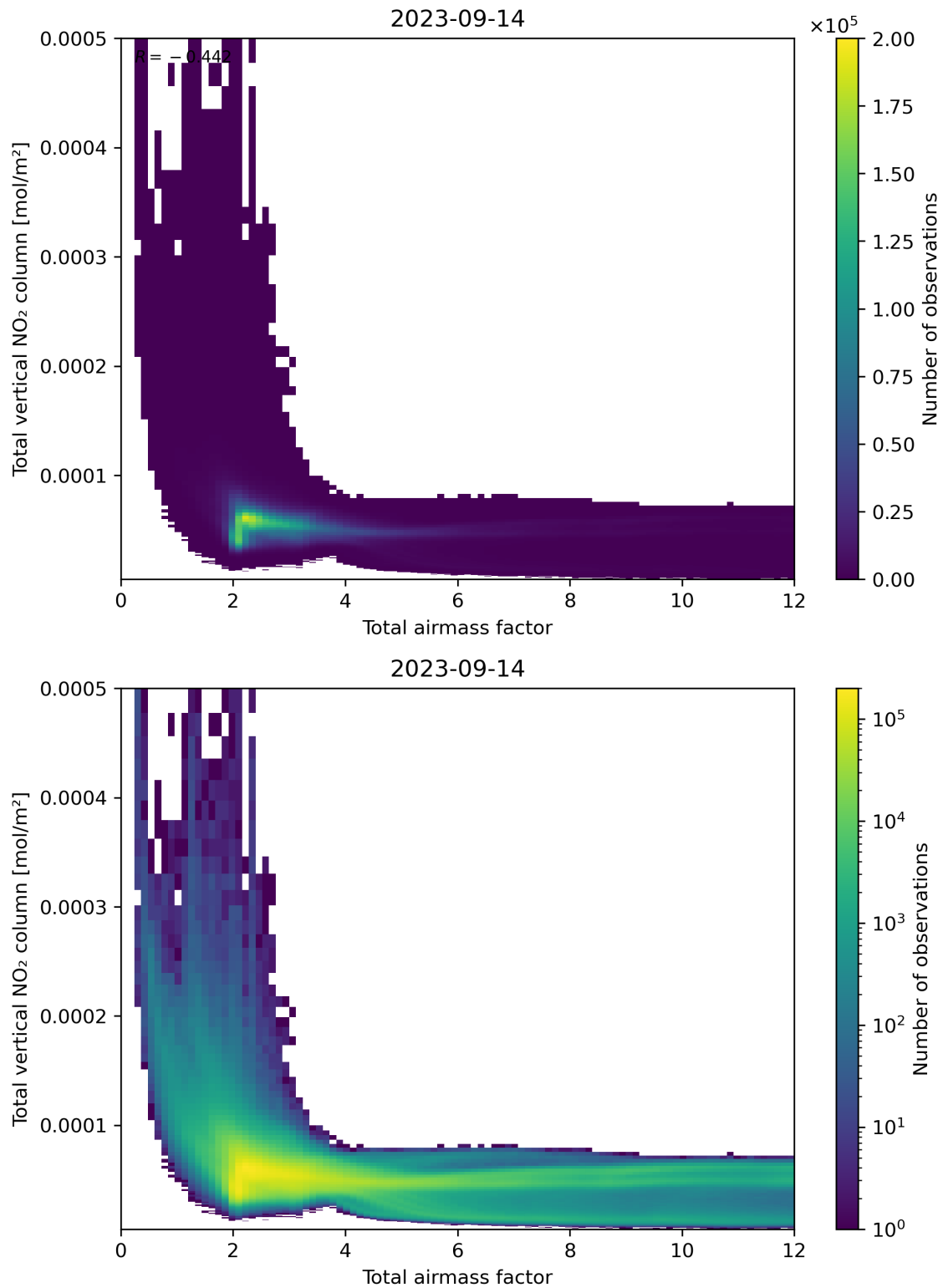
Figure 67: Scatter density plot of “Total airmass factor” against “Total vertical NO 2 column” for 2023-09-13 to 2023-09-15.
