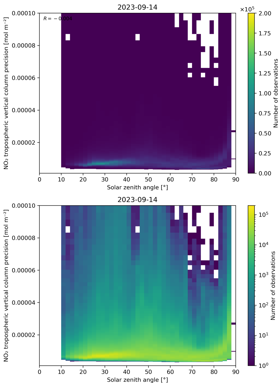
Figure 156: Scatter density plot of “Solar zenith angle” against “NO 2 tropospheric vertical column precision” for 2023-09-13 to 2023-09-15.
