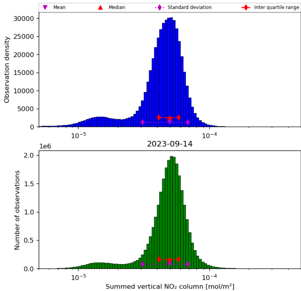
Figure 40: Histogram of “Summed vertical NO 2 column” for 2023-09-13 to 2023-09-15
