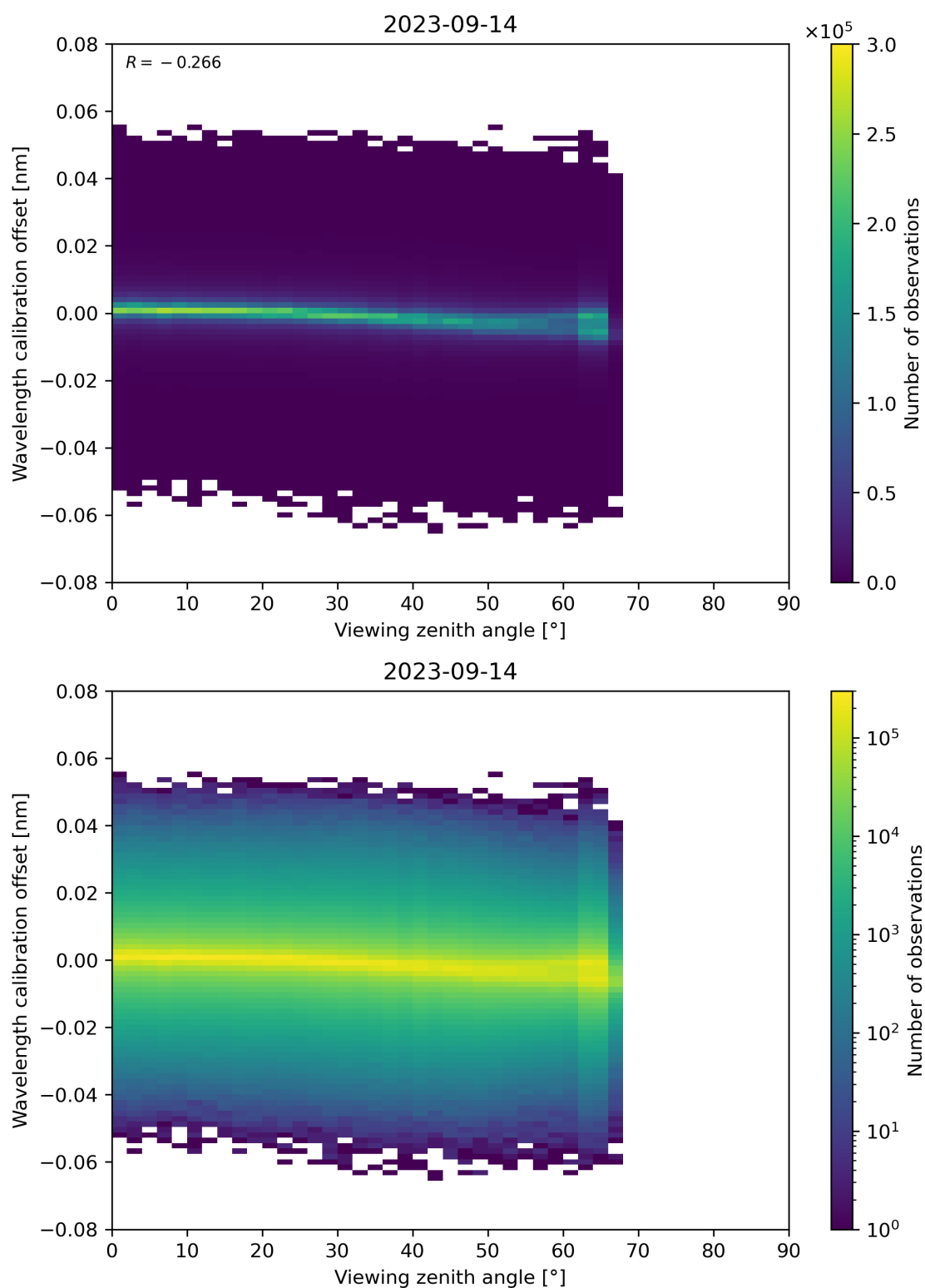
Figure 173: Scatter density plot of “Viewing zenith angle” against “Wavelength calibration offset” for 2023-09-13 to 2023-09-15.
