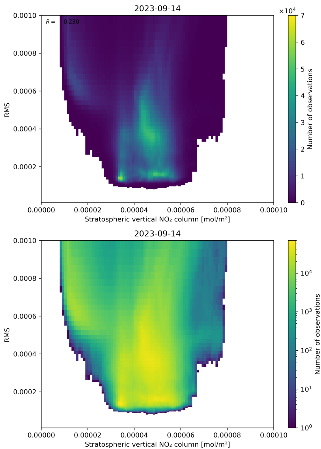
Figure 102: Scatter density plot of “Stratospheric vertical NO 2 column” against “RMS” for 2023-09-13 to 2023-09-15.
