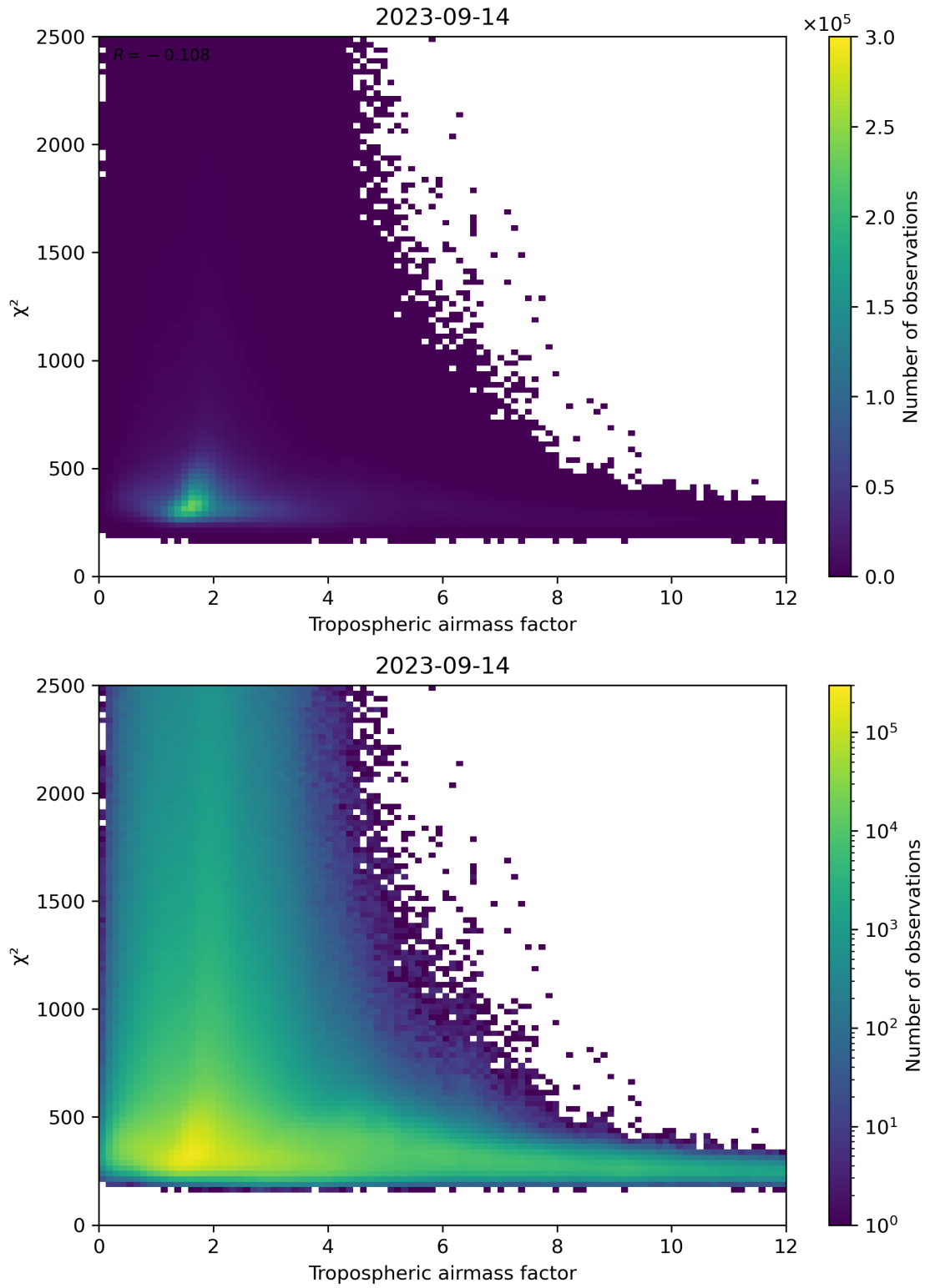
Figure 73: Scatter density plot of “Tropospheric airmass factor” against “ \chi^2 ” for 2023-09-13 to 2023-09-15.
