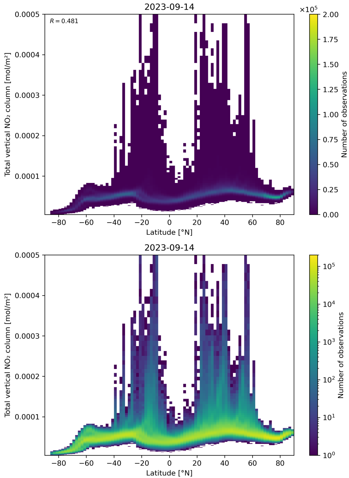
Figure 90: Scatter density plot of “Latitude” against “Total vertical NO 2 column” for 2023-09-13 to 2023-09-15.
