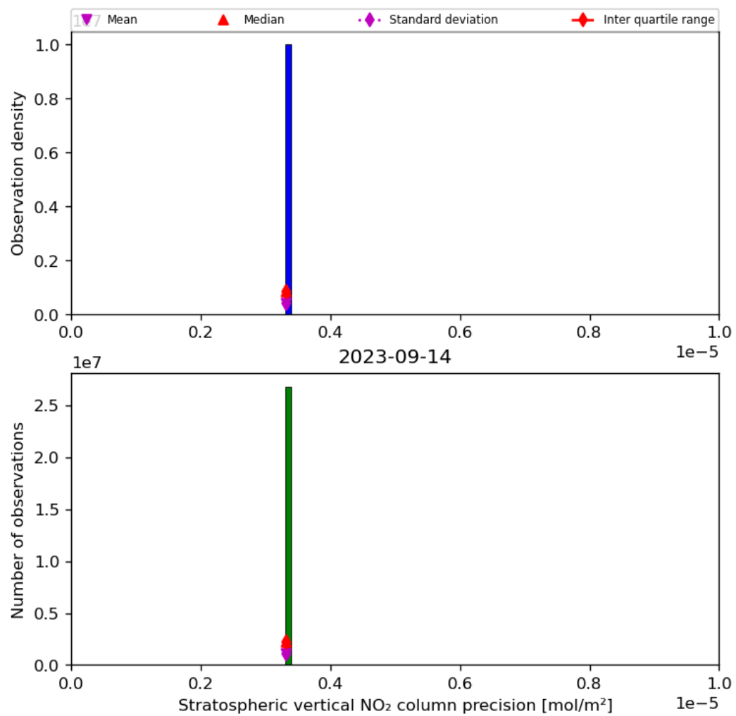
Figure 37: Histogram of “Stratospheric vertical NO 2 column precision” for 2023-09-13 to 2023-09-15
