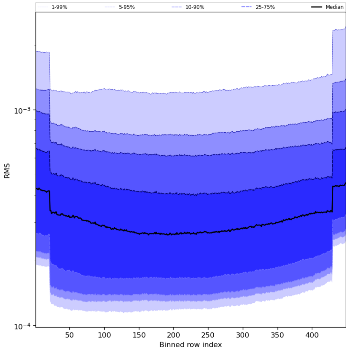
Figure 60: Along track statistics of “RMS” for 2023-09-13 to 2023-09-15
