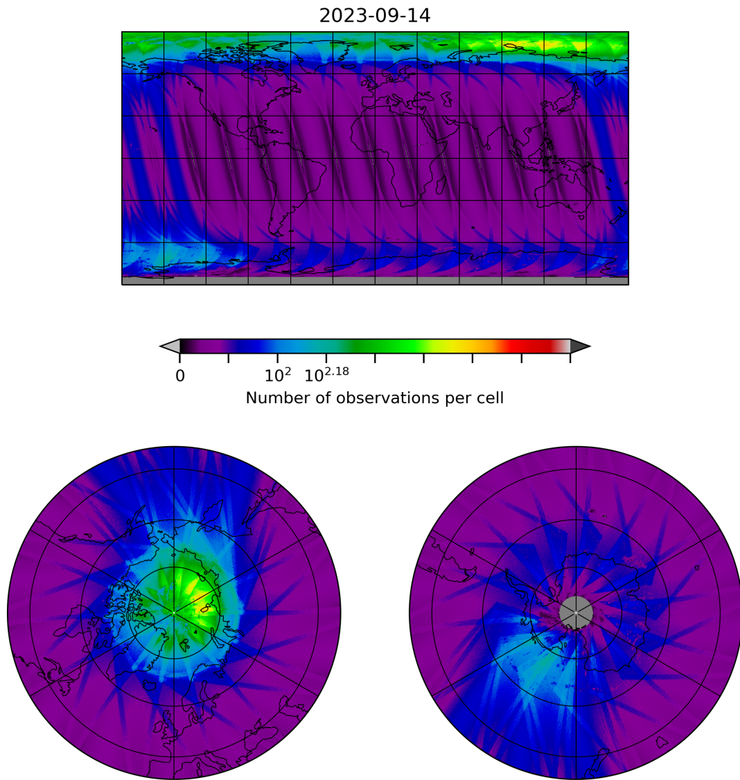
Figure 10: Map of the number of observations for 2023-09-13 to 2023-09-15
