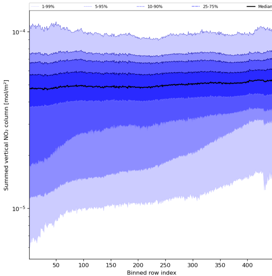
Figure 57: Along track statistics of “Summed vertical NO 2 column” for 2023-09-13 to 2023-09-15
