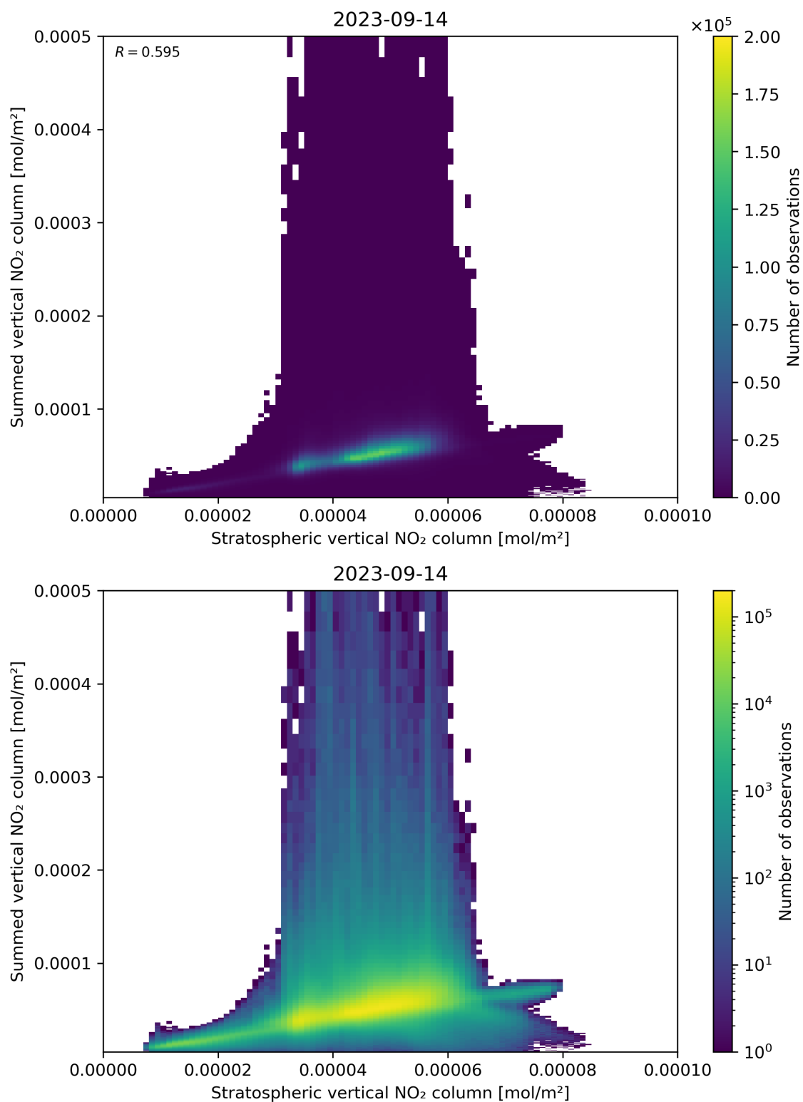
Figure 98: Scatter density plot of “Stratospheric vertical NO 2 column” against “Summed vertical NO 2 column” for 2023-09-13 to 2023-09-15.
