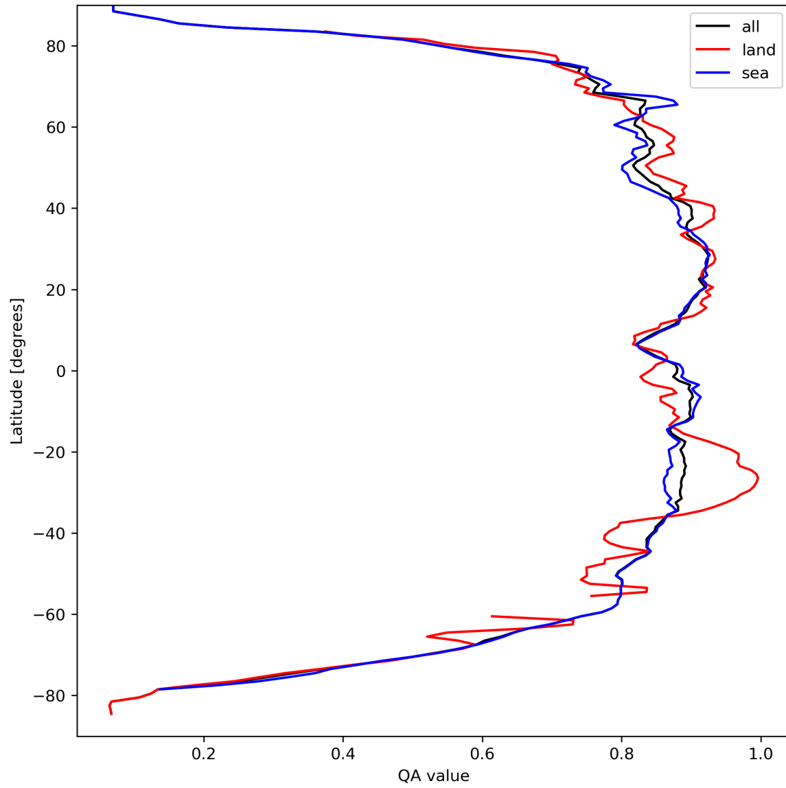
Figure 11: Zonal average of “QA value” for 2023-09-13 to 2023-09-15.
