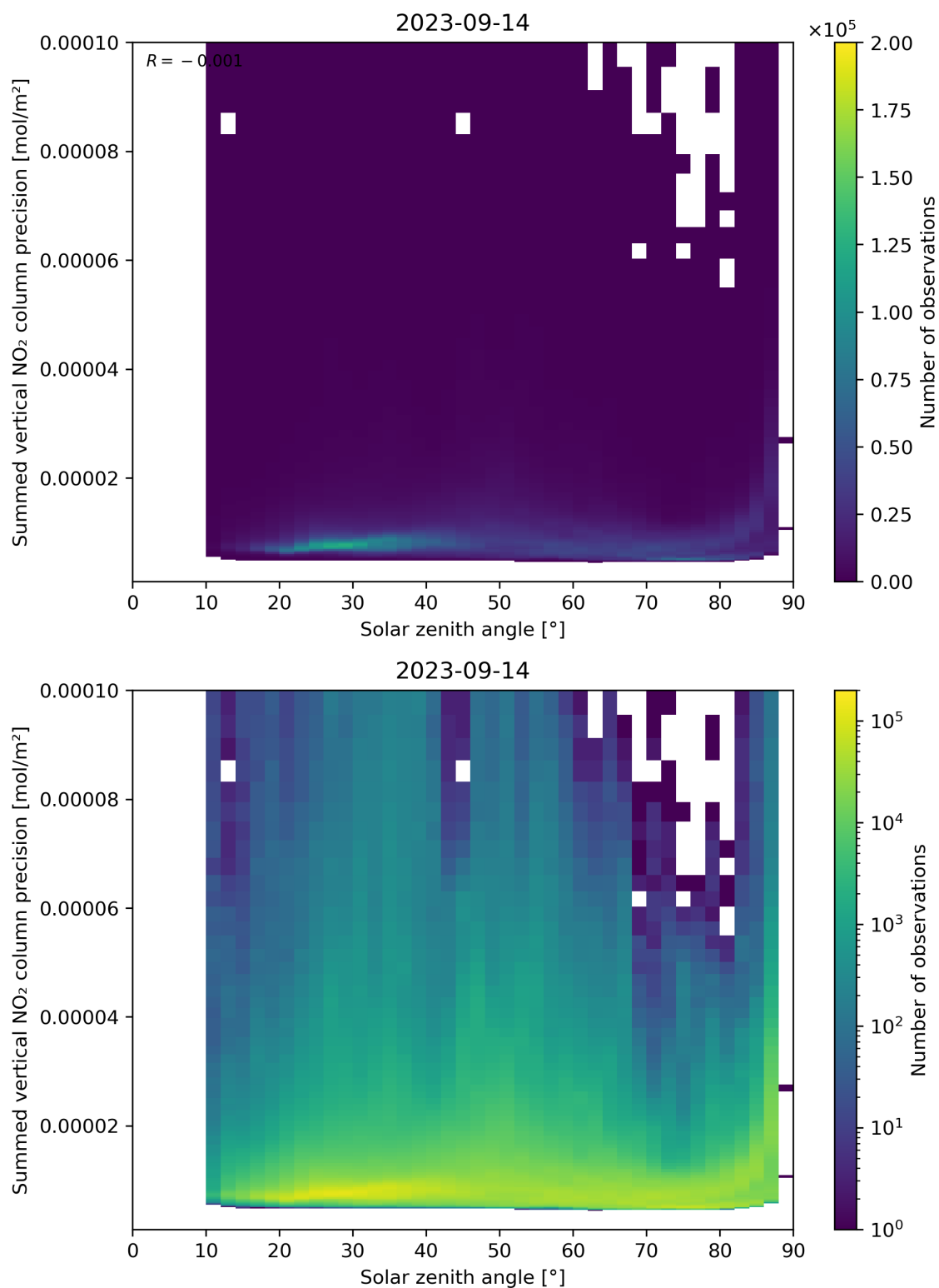
Figure 152: Scatter density plot of “Solar zenith angle” against “Summed vertical NO 2 column precision” for 2023-09-13 to 2023-09-15.
