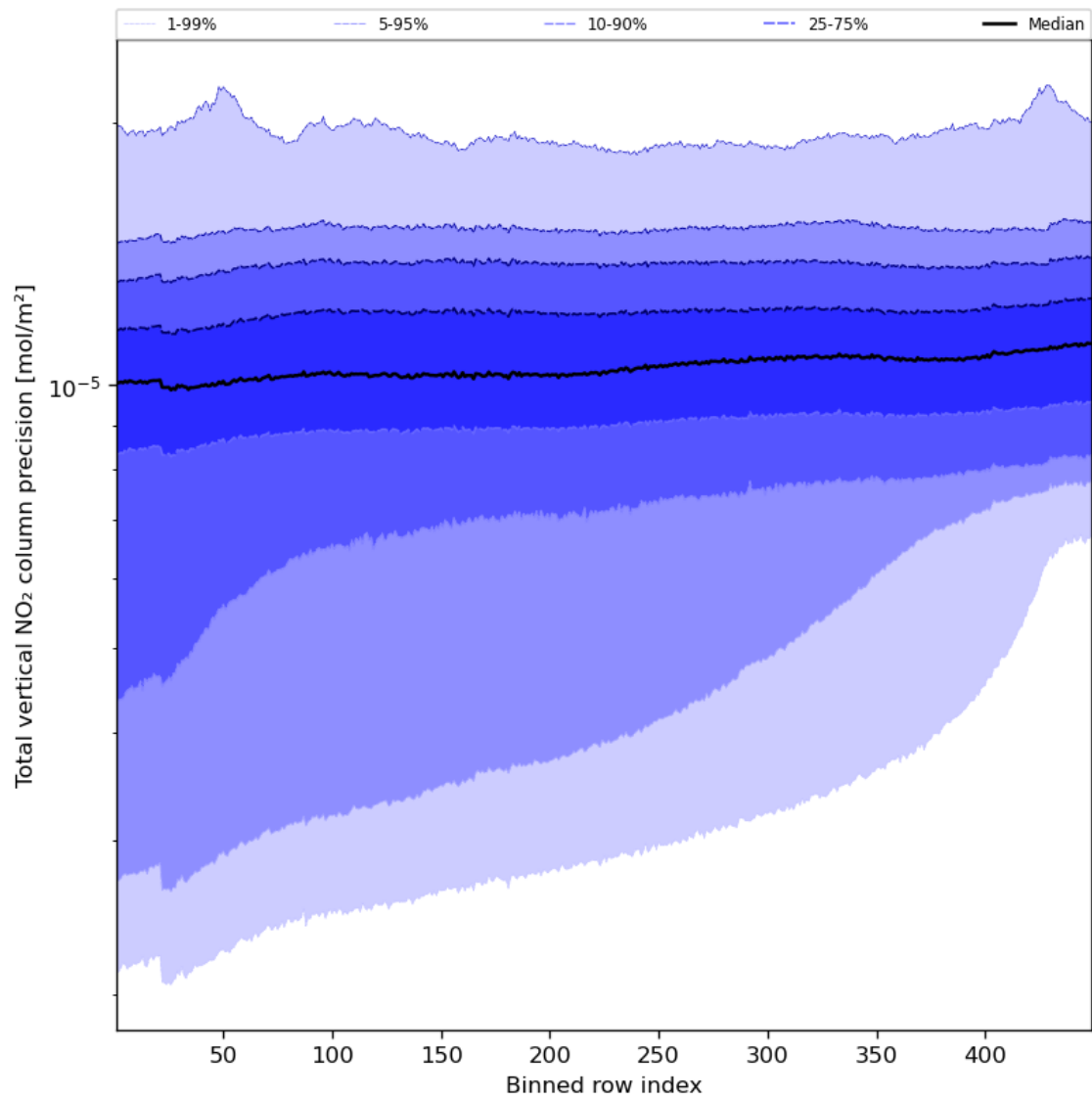
Figure 56: Along track statistics of “Total vertical NO 2 column precision” for 2023-09-13 to 2023-09-15
