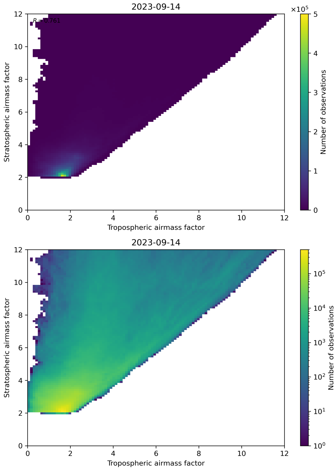
Figure 71: Scatter density plot of “Tropospheric airmass factor” against “Stratospheric airmass factor” for 2023-09-13 to 2023-09-15.
