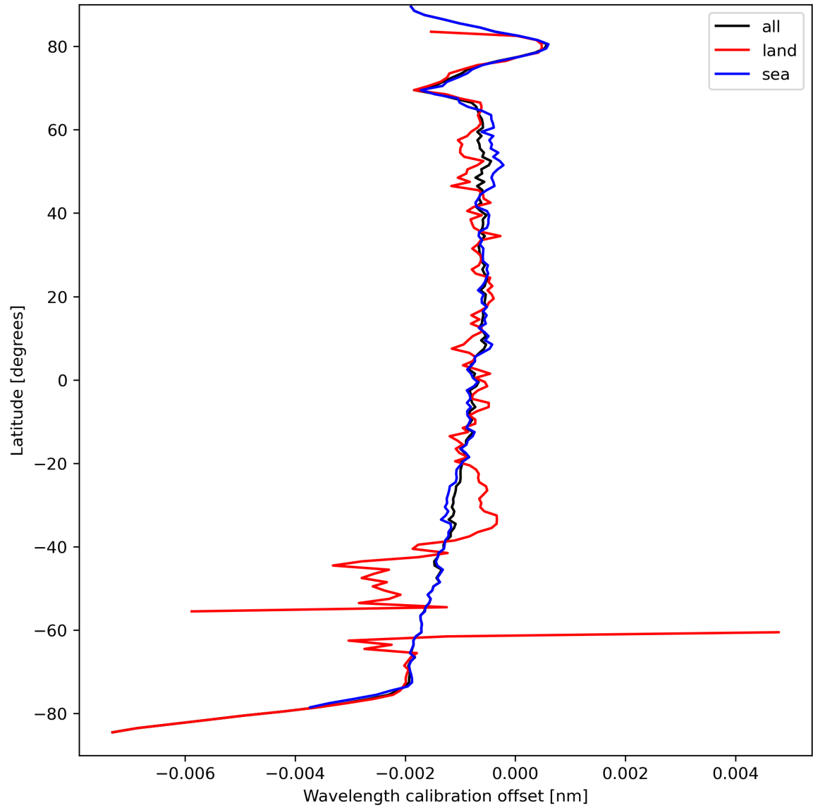
Figure 18: Zonal average of “Wavelength calibration offset” for 2023-09-13 to 2023-09-15.
