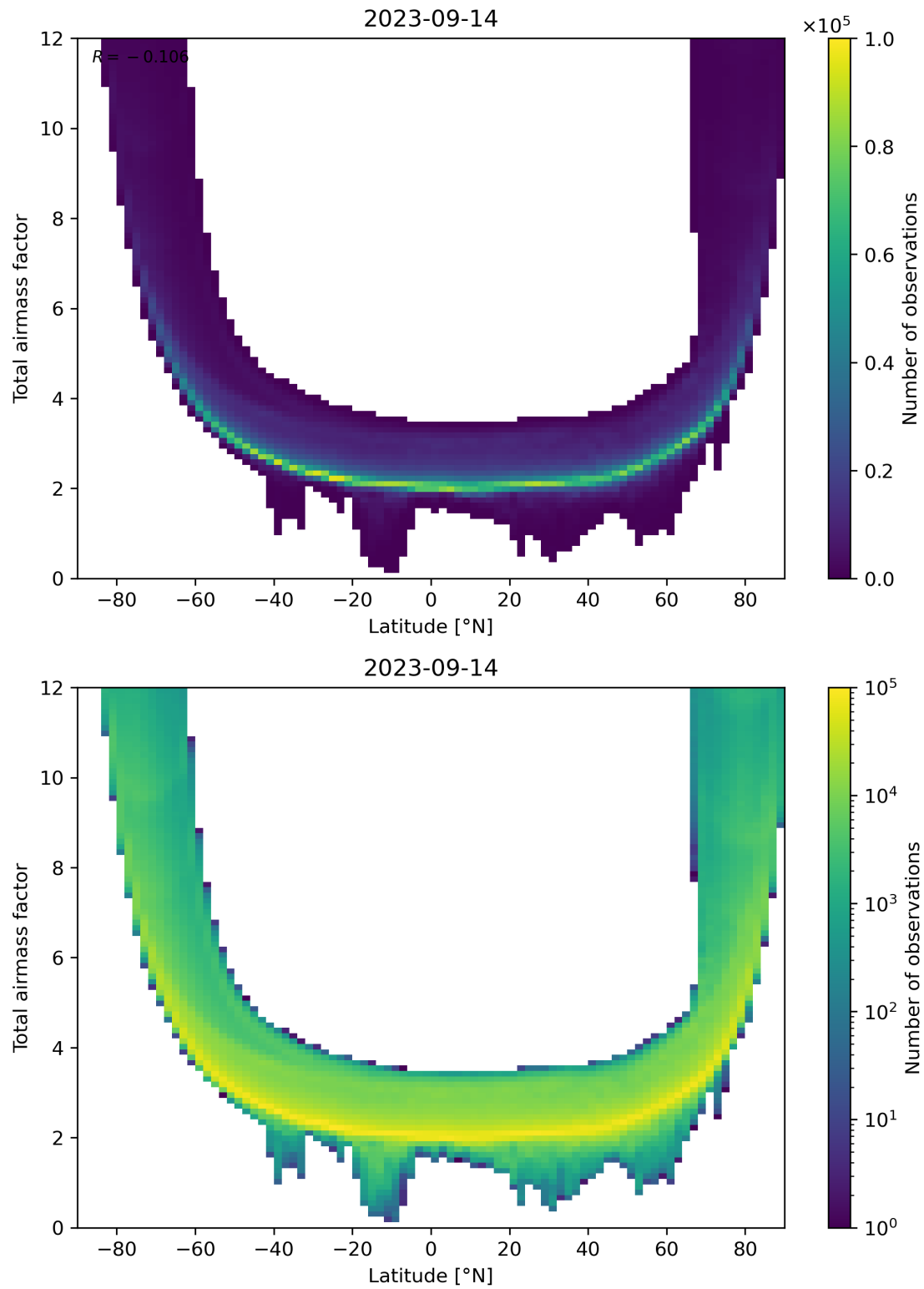
Figure 84: Scatter density plot of “Latitude” against “Total airmass factor” for 2023-09-13 to 2023-09-15.
