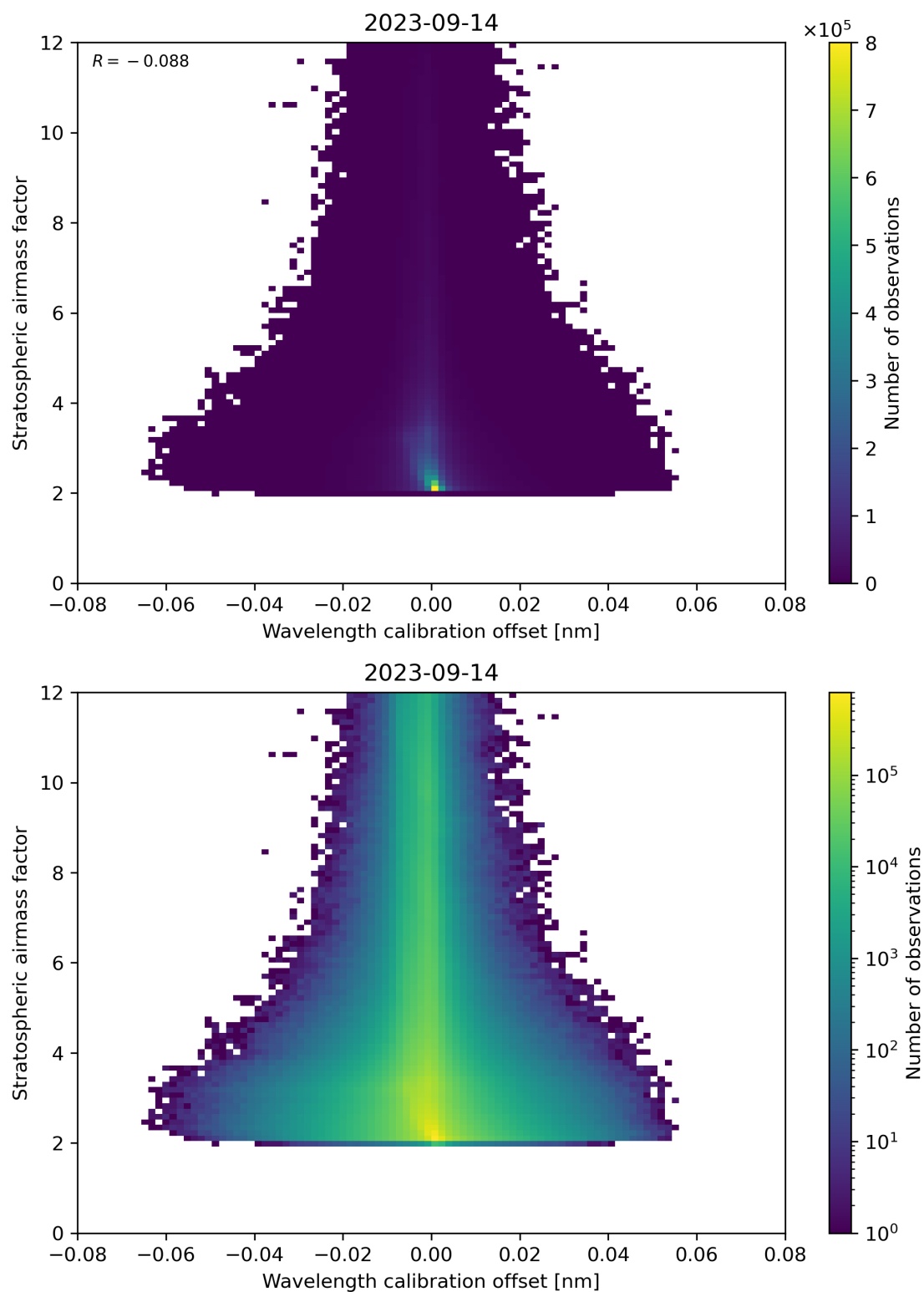
Figure 174: Scatter density plot of “Wavelength calibration offset” against “Stratospheric airmass factor” for 2023-09-13 to 2023-09-15.
