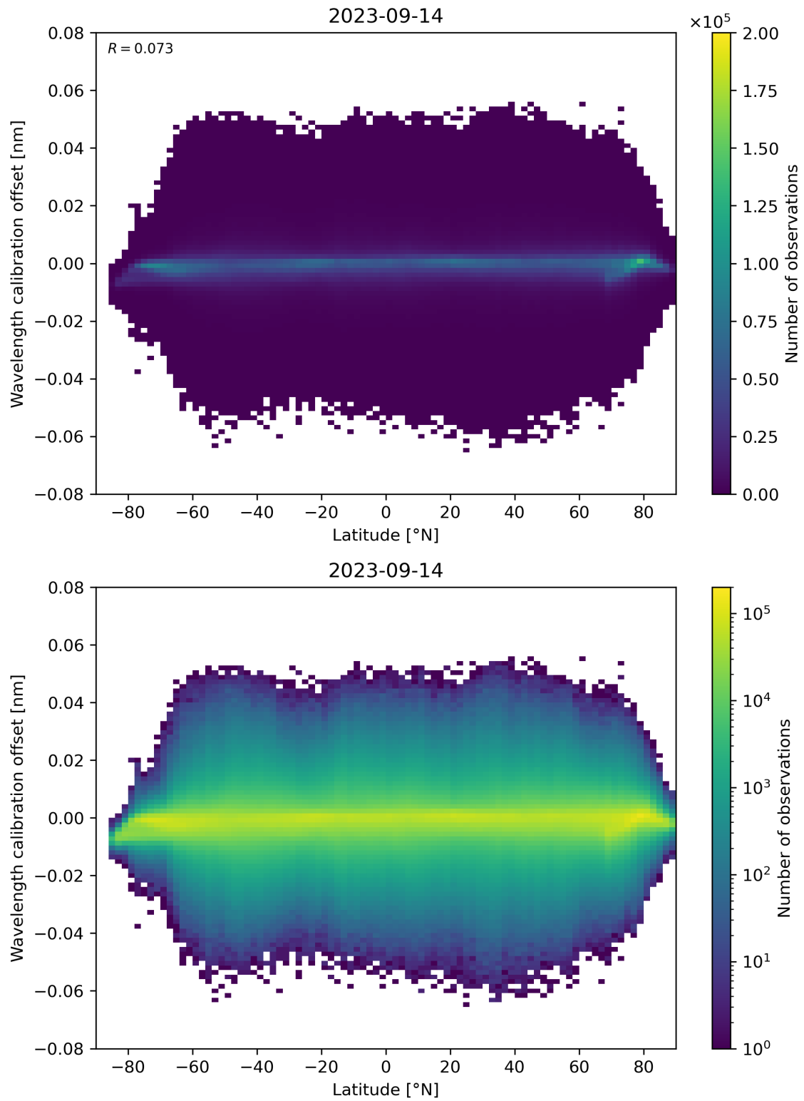
Figure 95: Scatter density plot of “Latitude” against “Wavelength calibration offset” for 2023-09-13 to 2023-09-15.
