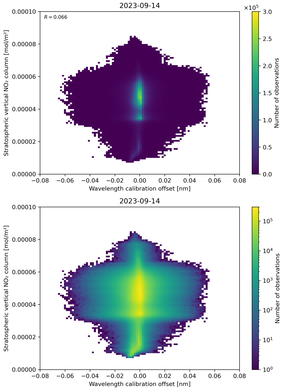
Figure 176: Scatter density plot of “Wavelength calibration offset” against “Stratospheric vertical NO 2 column” for 2023-09-13 to 2023-09-15.
