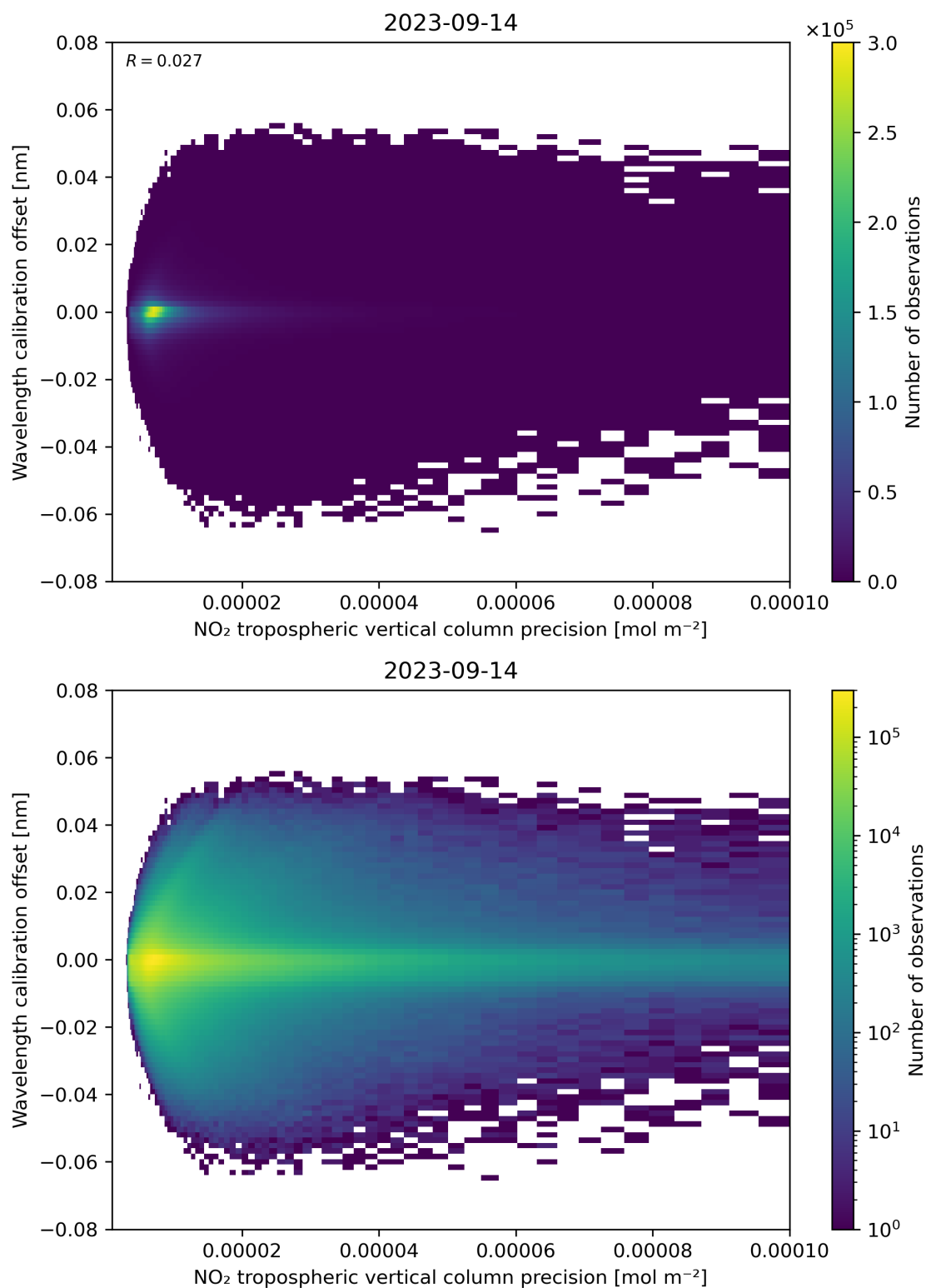
Figure 141: Scatter density plot of “NO 2 tropospheric vertical column precision” against “Wavelength calibration offset” for 2023-09-13 to 2023-09-15.
