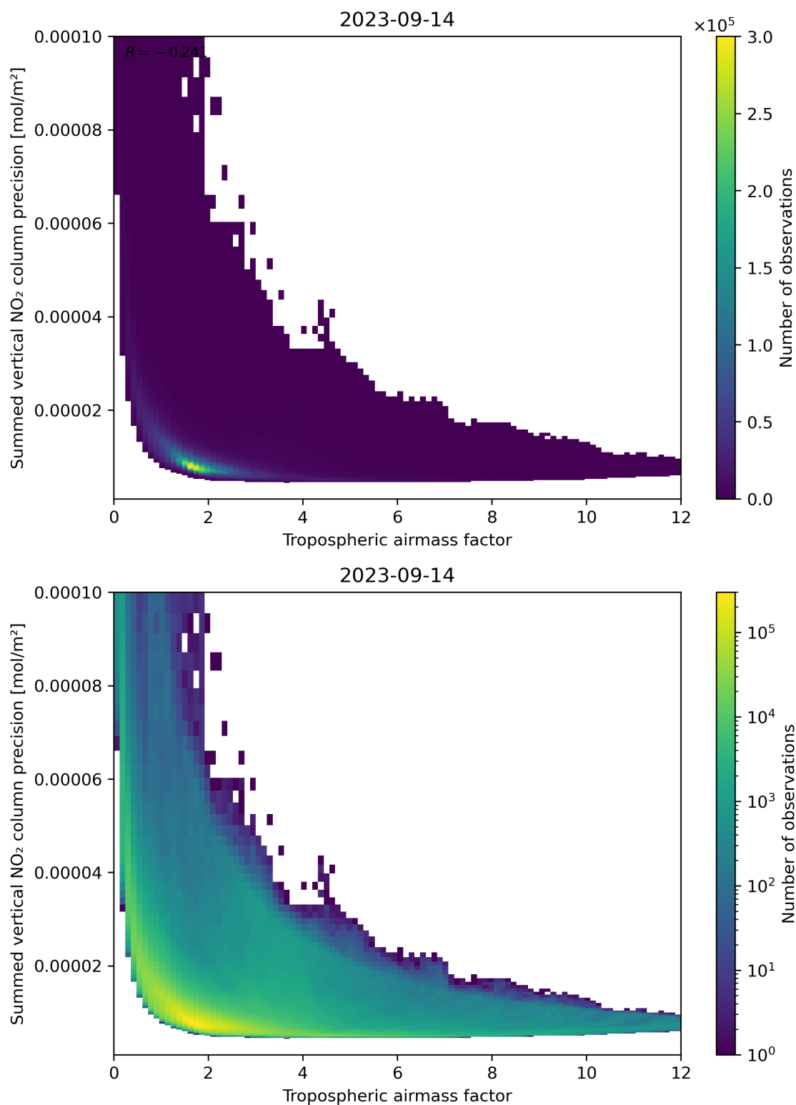
Figure 76: Scatter density plot of “Tropospheric air mass factor” against “Summed vertical NO 2 column precision” for 2023-09-13 to 2023-09-15.
