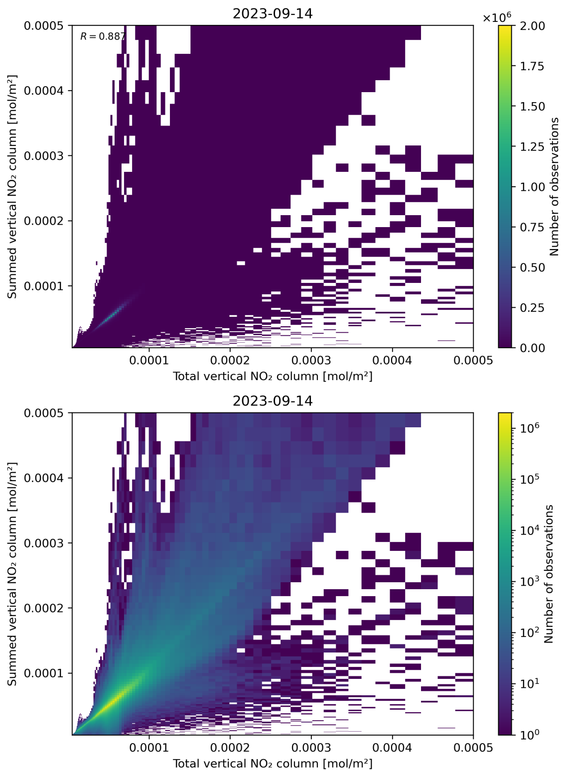
Figure 112: Scatter density plot of “Total vertical NO 2 column” against “Summed vertical NO 2 column” for 2023-09-13 to 2023-09-15.
