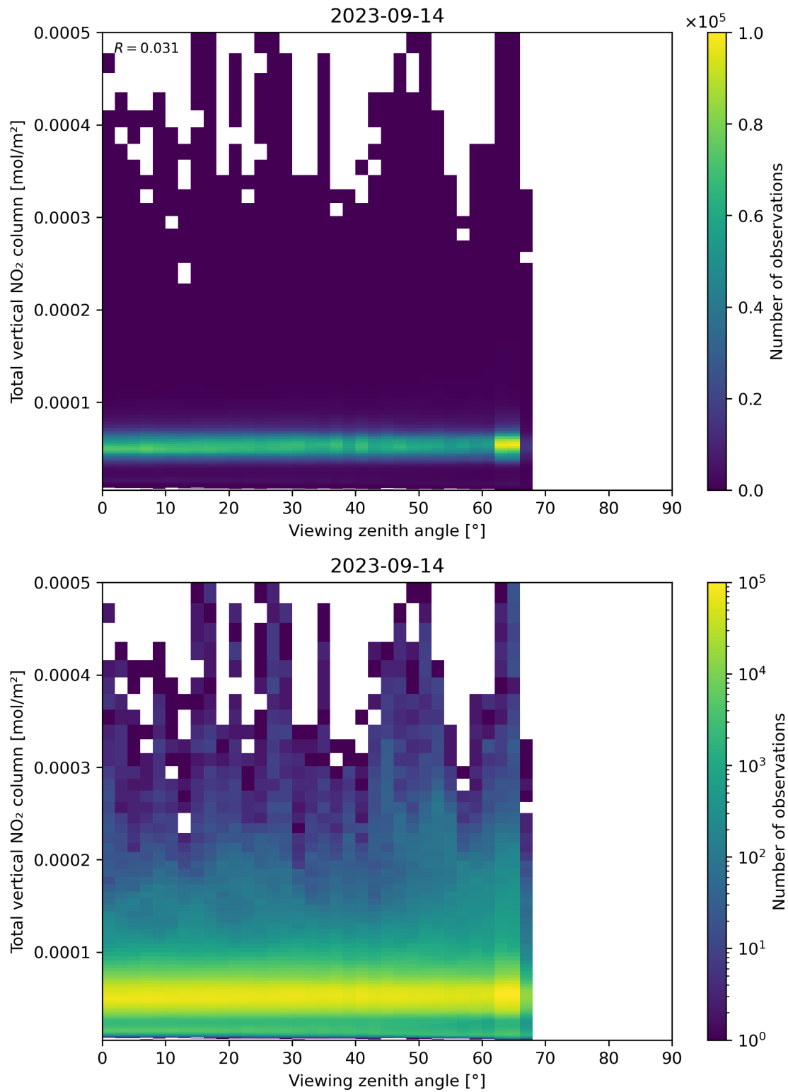
Figure 167: Scatter density plot of “Viewing zenith angle” against “Total vertical NO 2 column” for 2023-09-13 to 2023-09-15.
