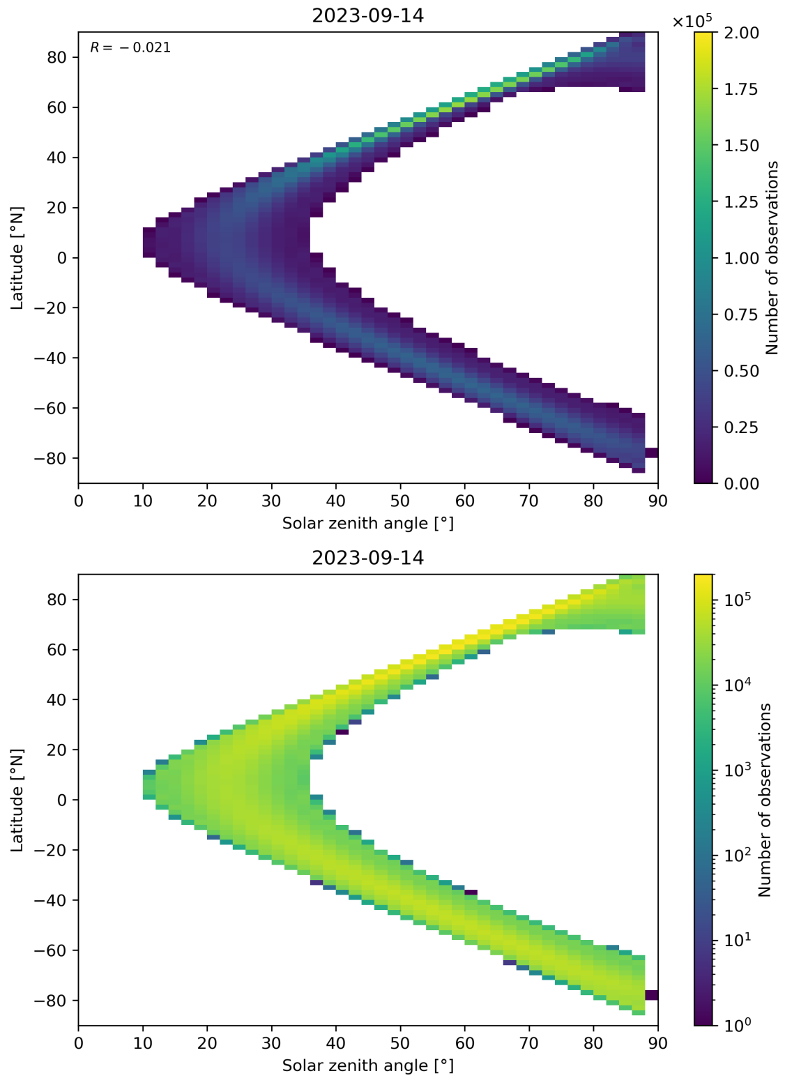
Figure 149: Scatter density plot of “Solar zenith angle” against “Latitude” for 2023-09-13 to 2023-09-15.
