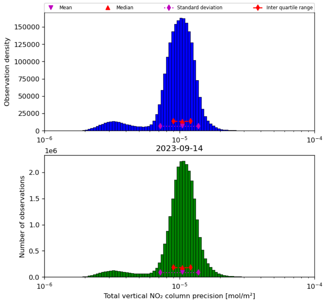
Figure 39: Histogram of “Total vertical NO 2 column precision” for 2023-09-13 to 2023-09-15
