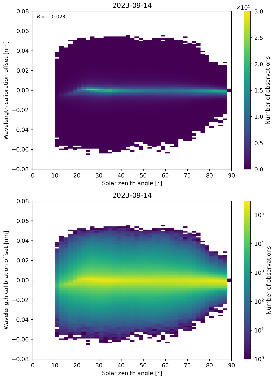
Figure 158: Scatter density plot of “Solar zenith angle” against “Wavelength calibration offset” for 2023-09-13 to 2023-09-15.
