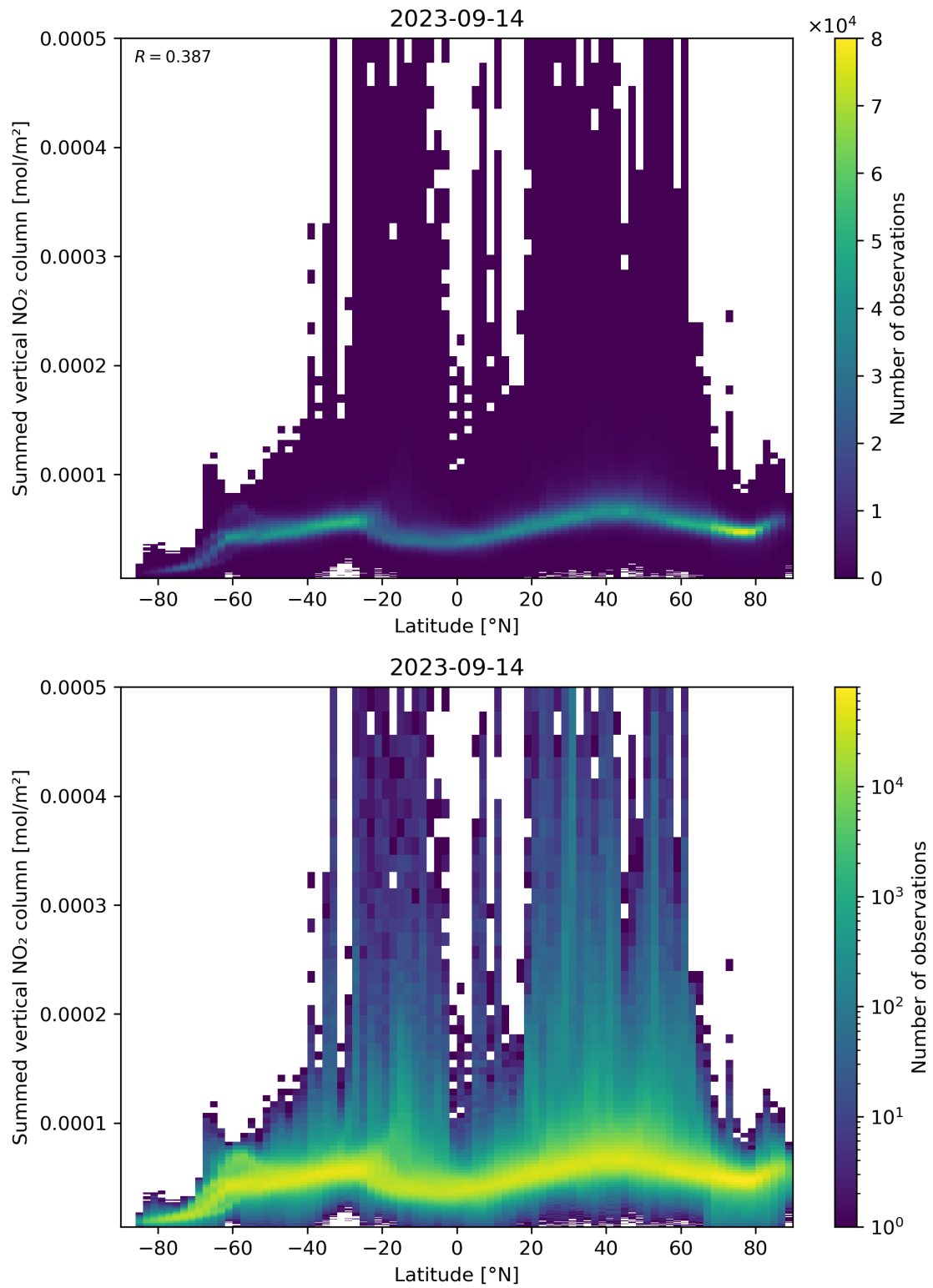
Figure 88: Scatter density plot of “Latitude” against “Summed vertical NO 2 column” for 2023-09-13 to 2023-09-15.
