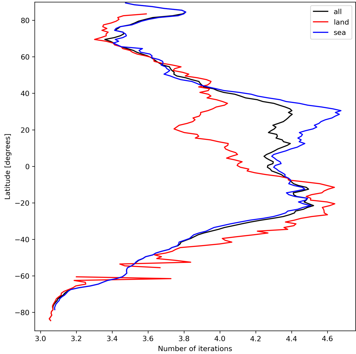
Figure 17: Zonal average of “Number of iterations” for 2023-09-13 to 2023-09-15.
