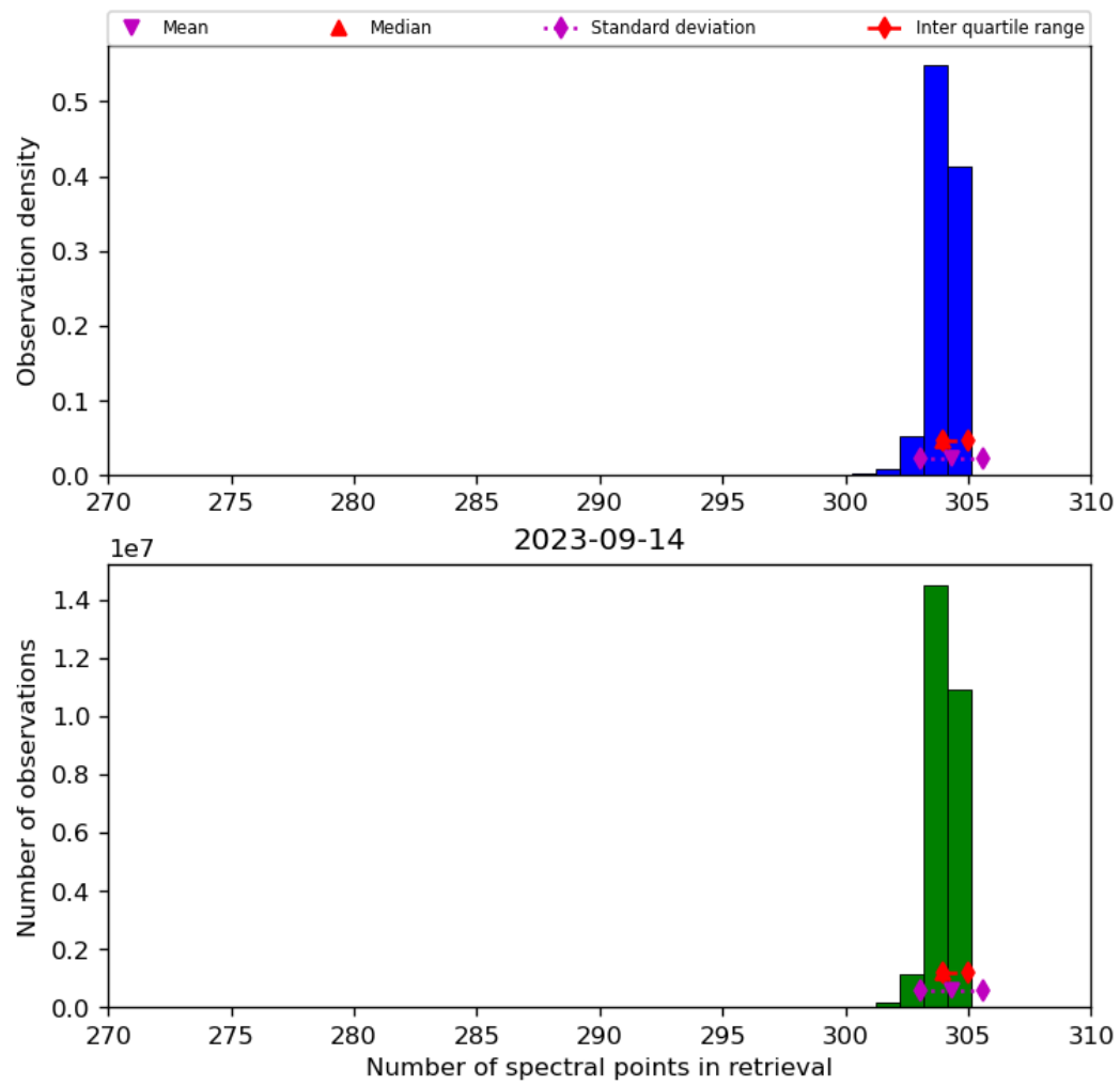
Figure 33: Histogram of “Number of spectral points in retrieval” for 2023-09-13 to 2023-09-15
