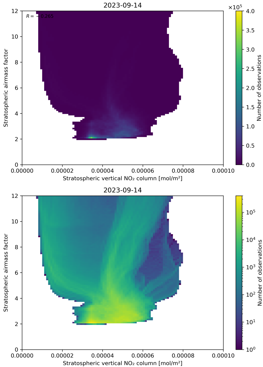
Figure 96: Scatter density plot of “Stratospheric vertical NO 2 column” against “Stratospheric airmass factor” for 2023-09-13 to 2023-09-15.
