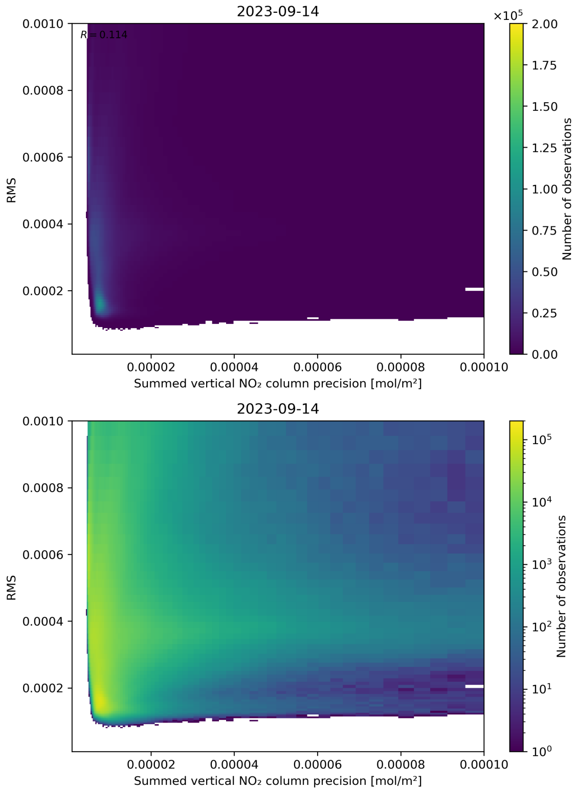
Figure 108: Scatter density plot of “Summed vertical NO 2 column precision” against “RMS” for 2023-09-13 to 2023-09-15.
