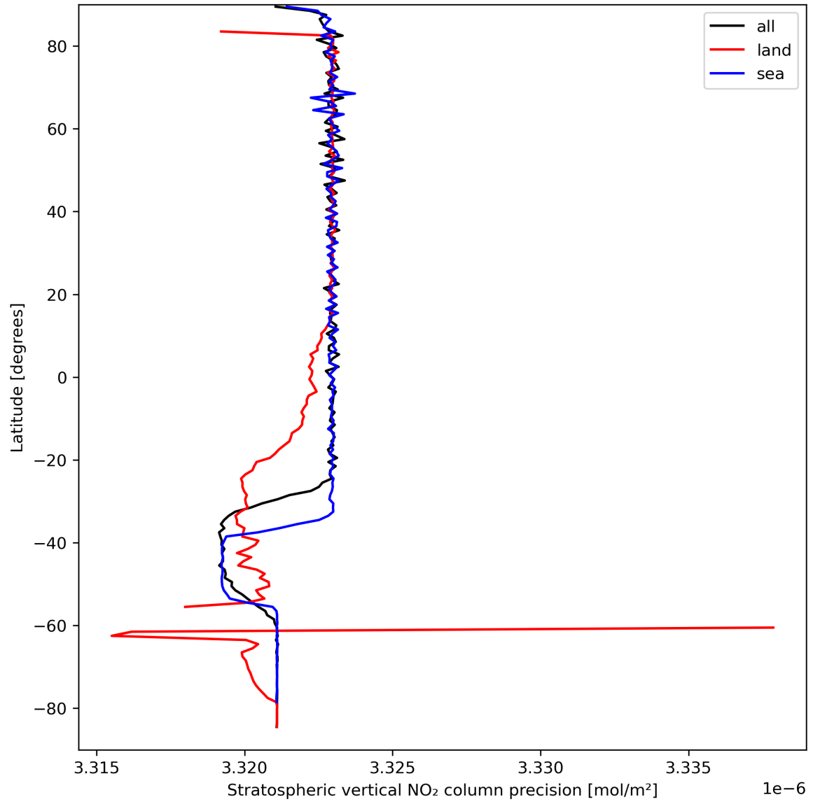
Figure 20: Zonal average of “Stratospheric vertical NO 2 column precision” for 2023-09-13 to 2023-09-15.
