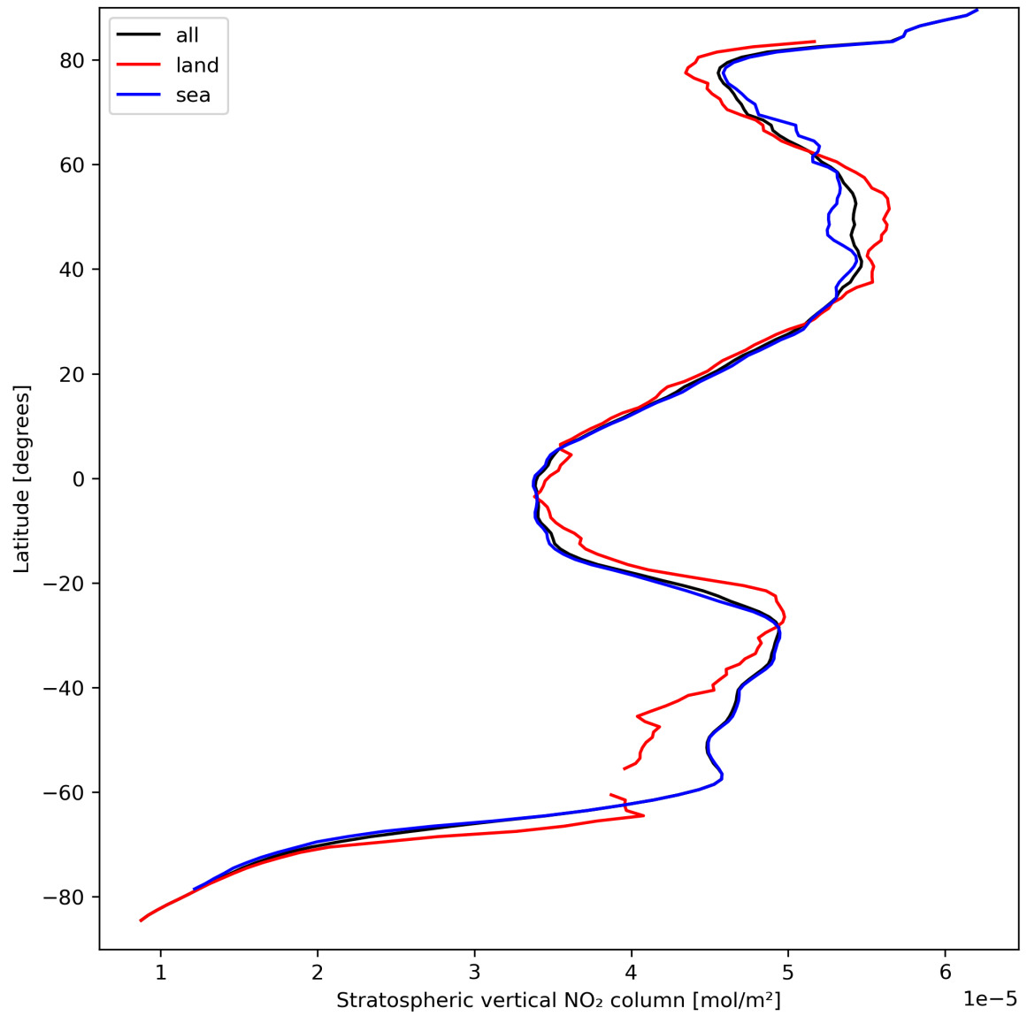
Figure 19: Zonal average of “Stratospheric vertical NO 2 column” for 2023-09-13 to 2023-09-15.
