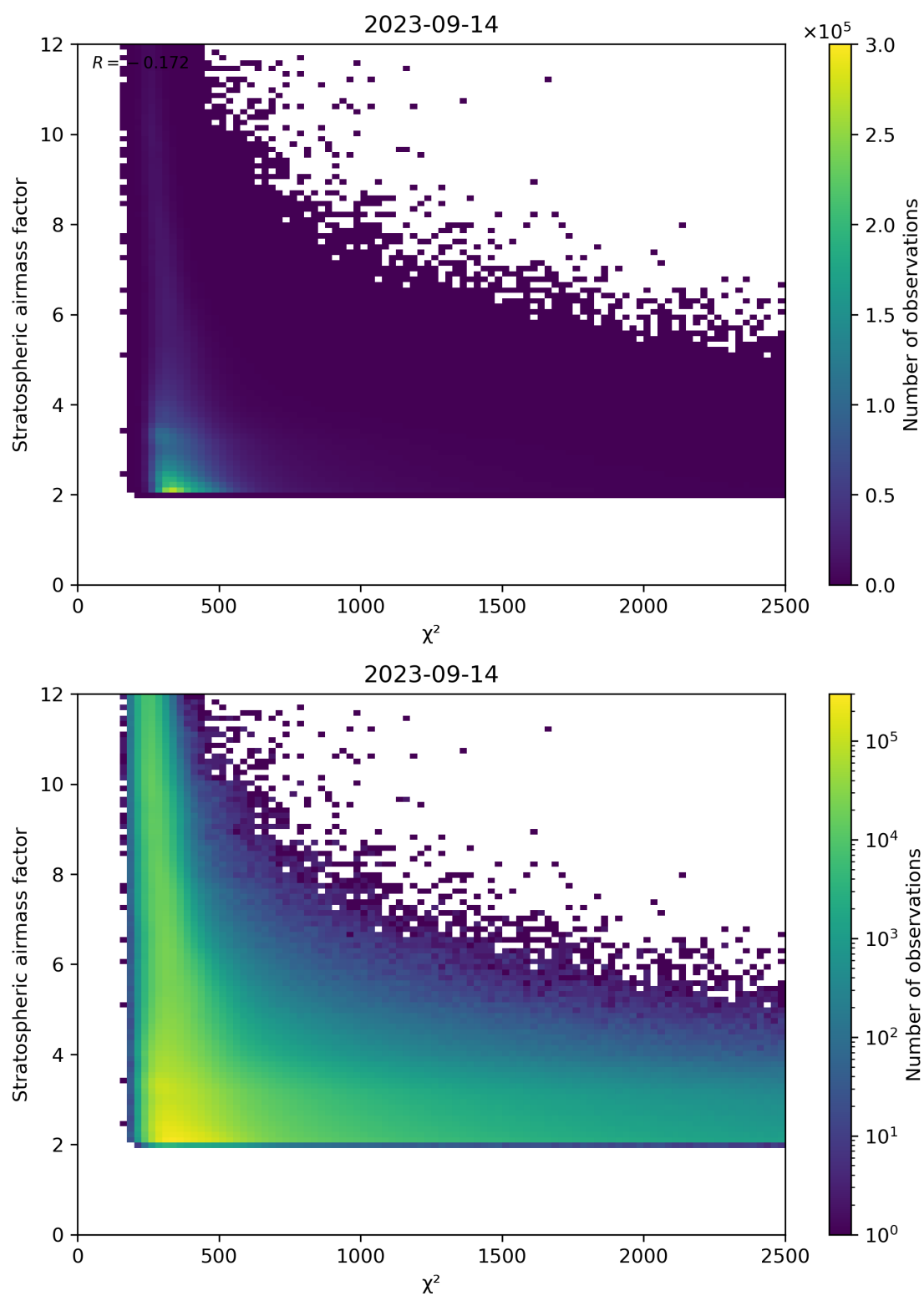
Figure 81: Scatter density plot of “ \chi^2 ” against “Stratospheric airmass factor” for 2023-09-13 to 2023-09-15.
