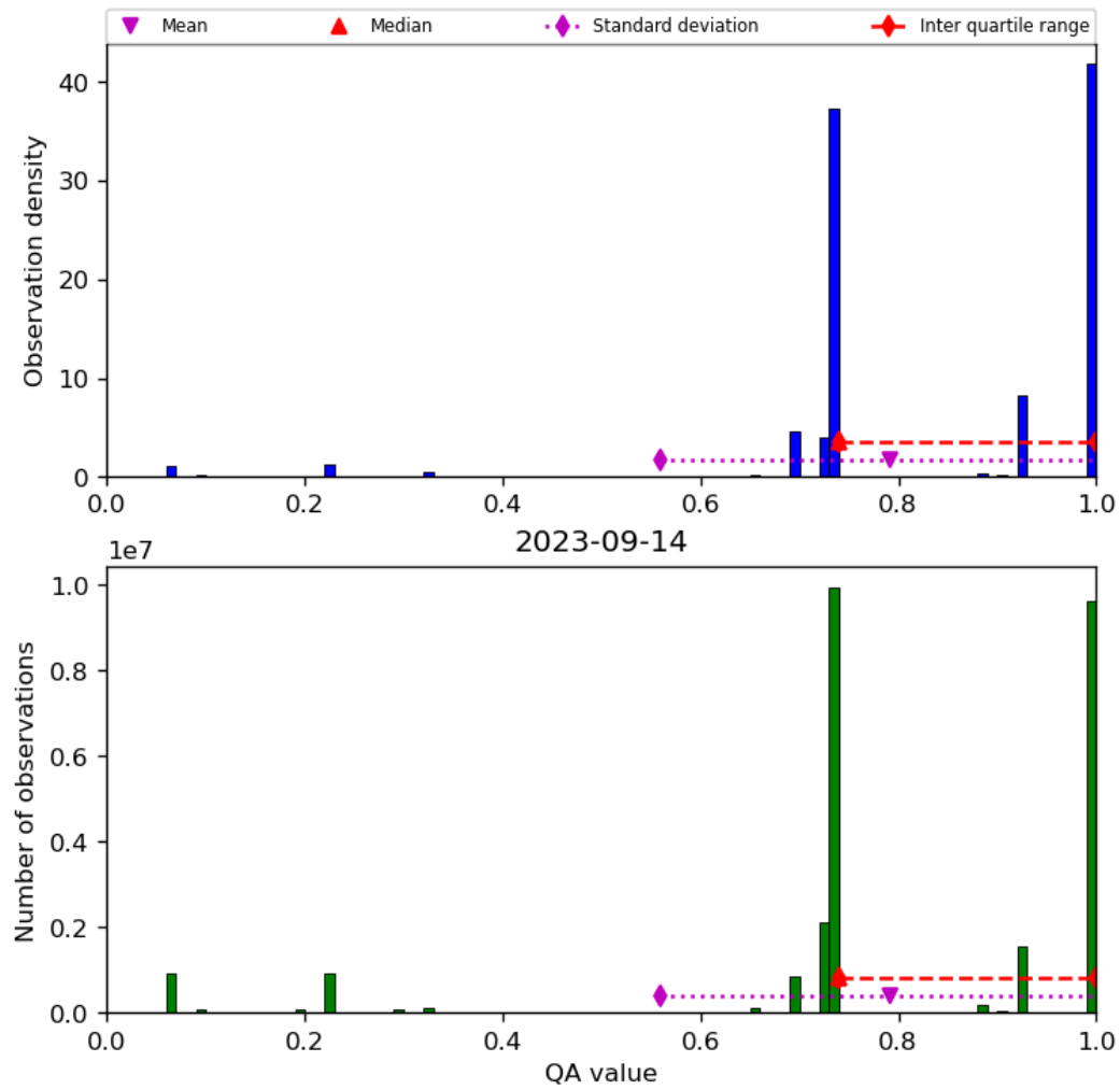
Figure 28: Histogram of “QA value” for 2023-09-13 to 2023-09-15
