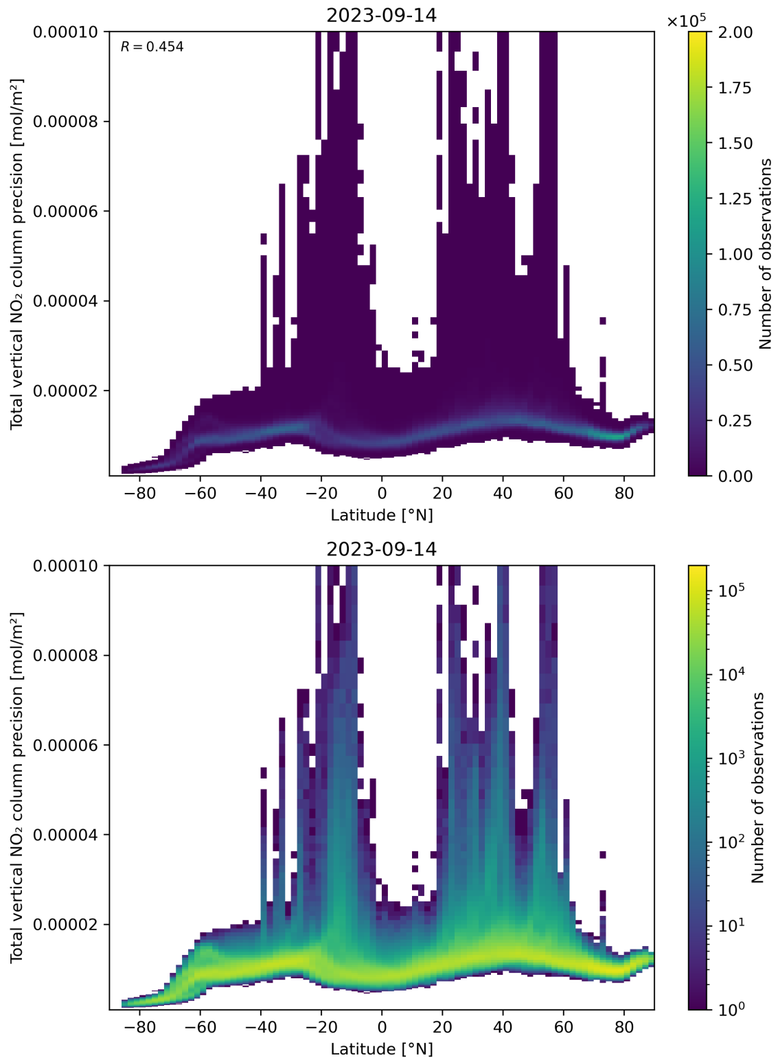
Figure 91: Scatter density plot of “Latitude” against “Total vertical NO 2 column precision” for 2023-09-13 to 2023-09-15.
