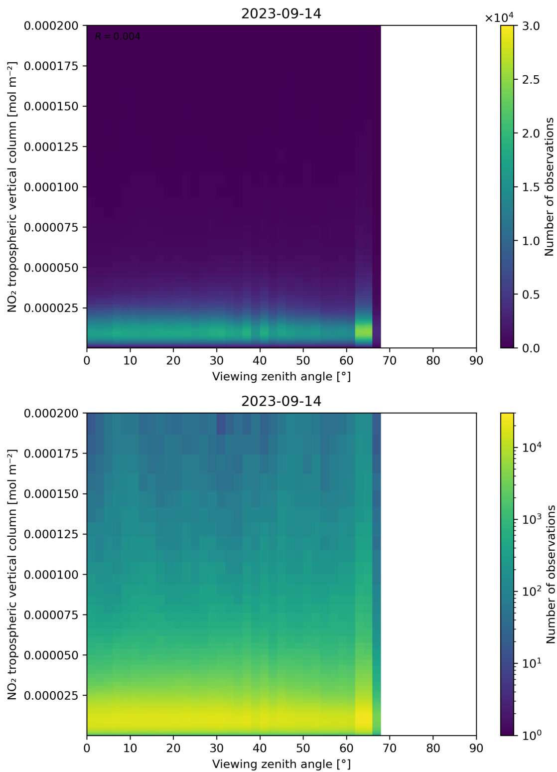
Figure 169: Scatter density plot of “Viewing zenith angle” against “NO 2 tropospheric vertical column” for 2023-09-13 to 2023-09-15.
