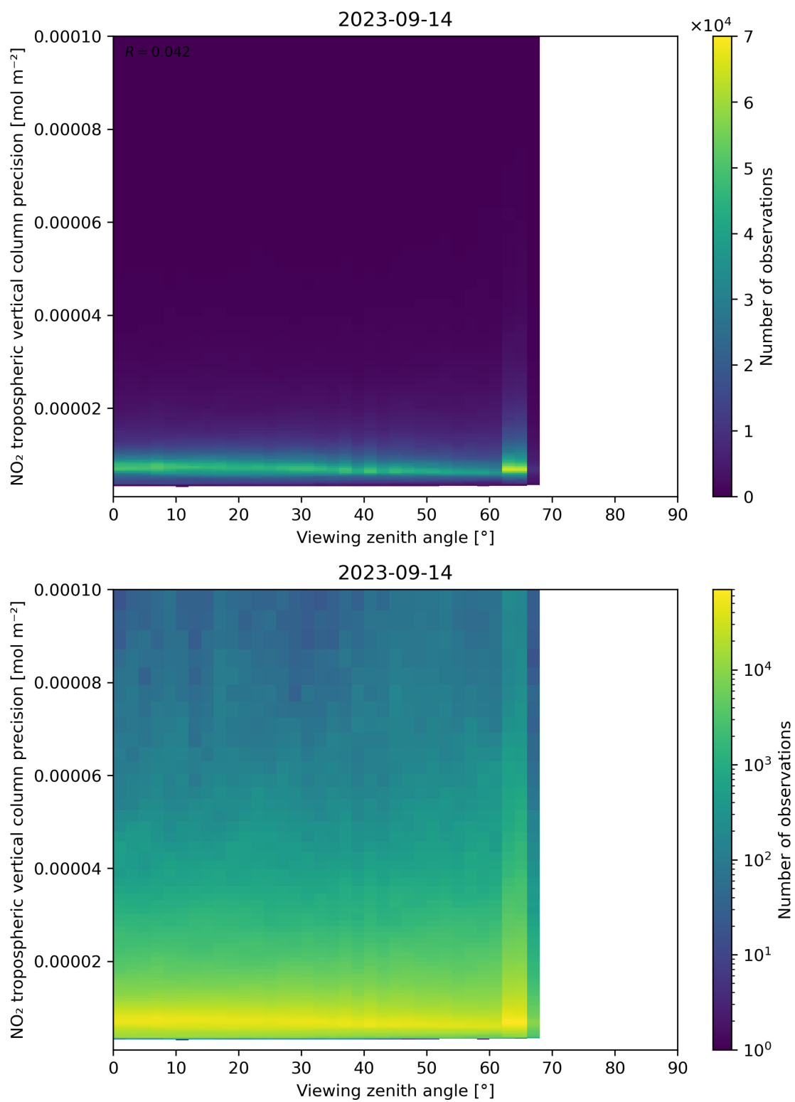
Figure 170: Scatter density plot of “Viewing zenith angle” against “NO 2 tropospheric vertical column precision” for 2023-09-13 to 2023-09-15.
