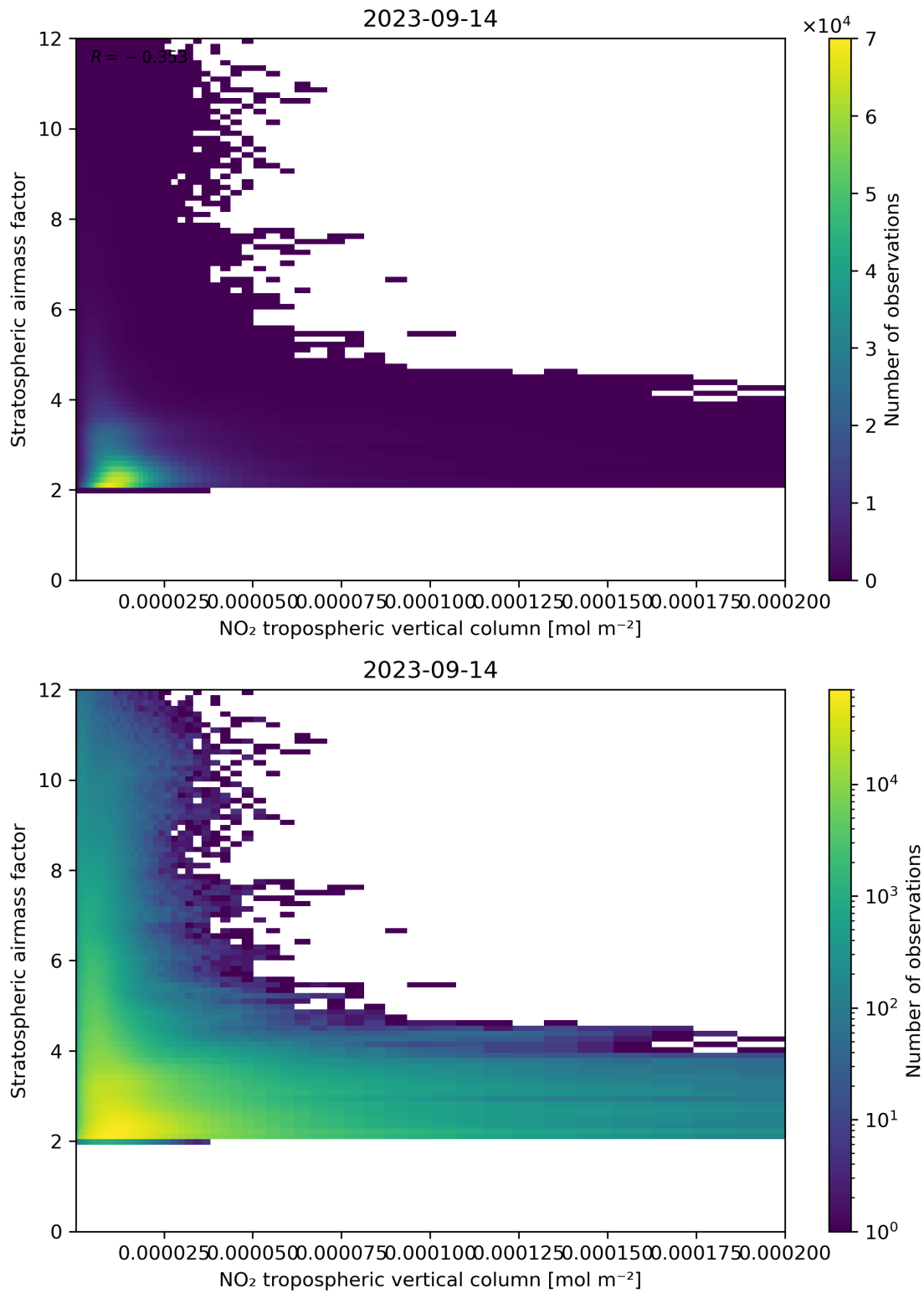
Figure 121: Scatter density plot of “NO 2 tropospheric vertical column” against “Stratospheric air mass factor” for 2023-09-13 to 2023-09-15.
