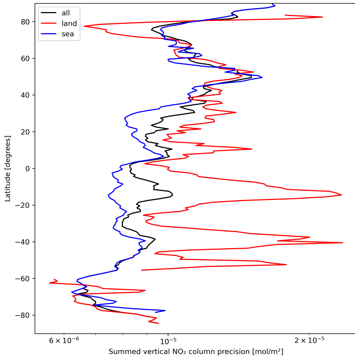
Figure 24: Zonal average of “Summed vertical NO 2 column precision” for 2023-09-13 to 2023-09-15.
