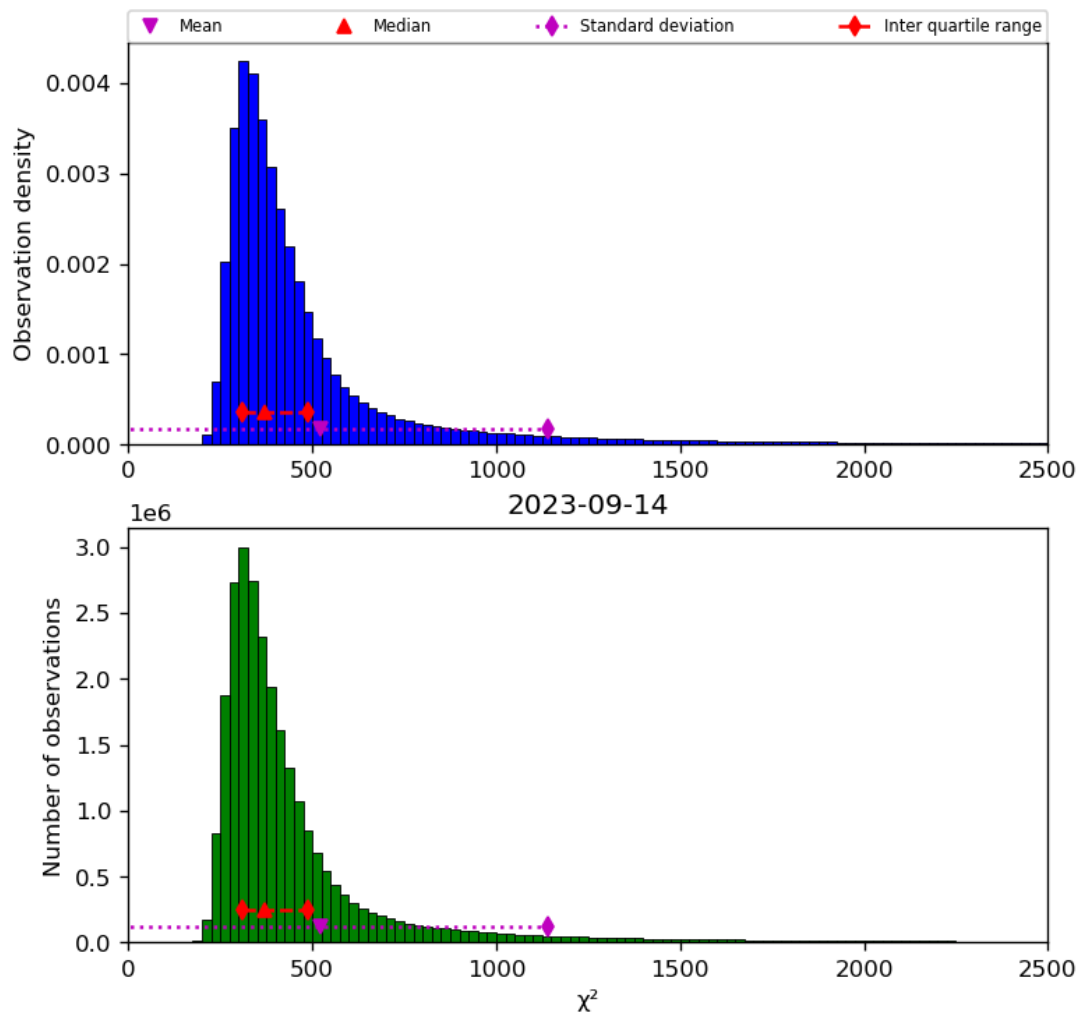
Figure 42: Histogram of “ \chi^2 ” for 2023-09-13 to 2023-09-15
