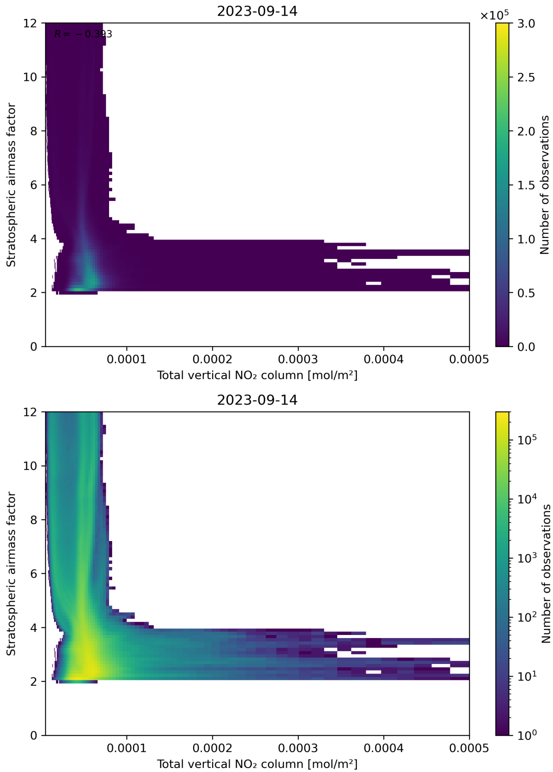
Figure 110: Scatter density plot of “Total vertical NO 2 column” against “Stratospheric airmass factor” for 2023-09-13 to 2023-09-15.
