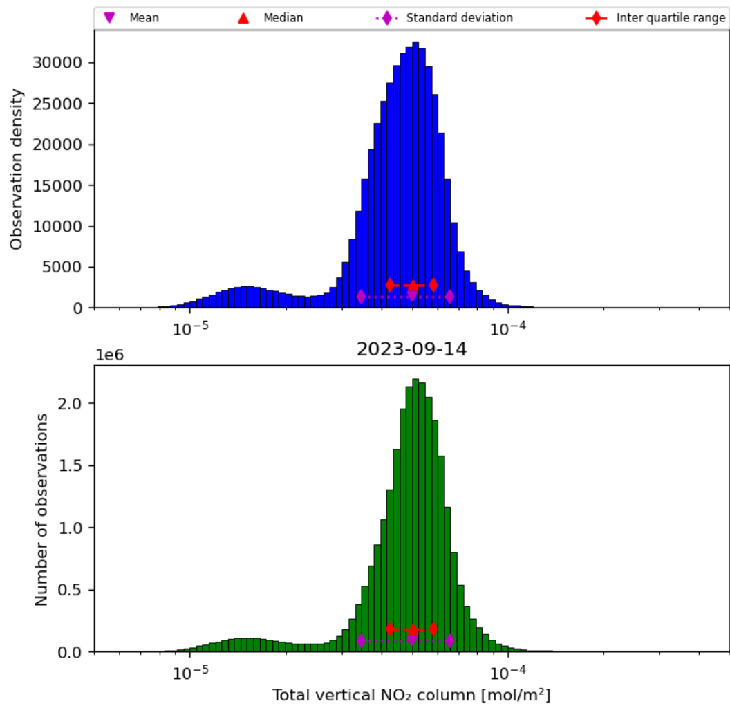
Figure 38: Histogram of “Total vertical NO 2 column” for 2023-09-13 to 2023-09-15
