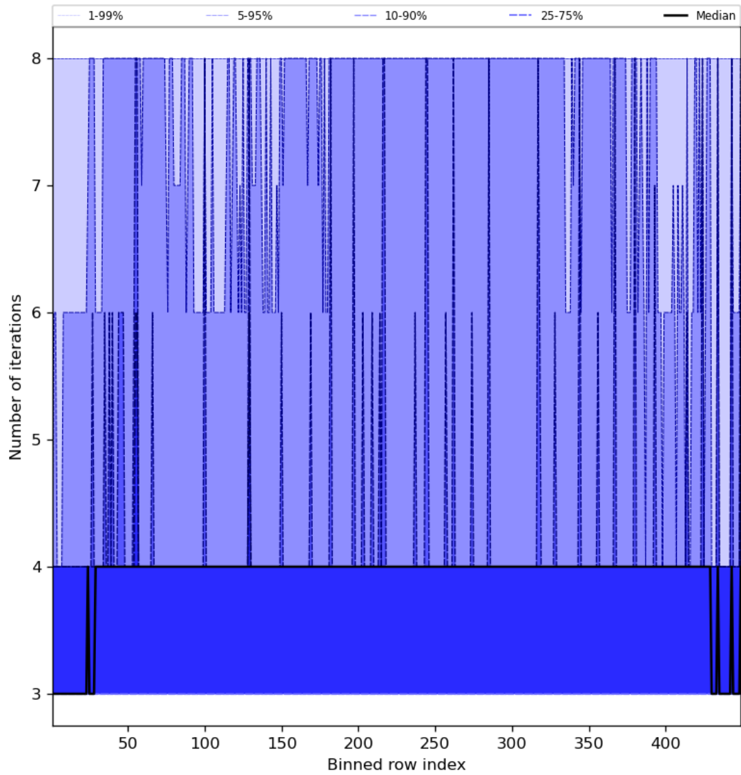
Figure 51: Along track statistics of “Number of iterations” for 2023-09-13 to 2023-09-15
