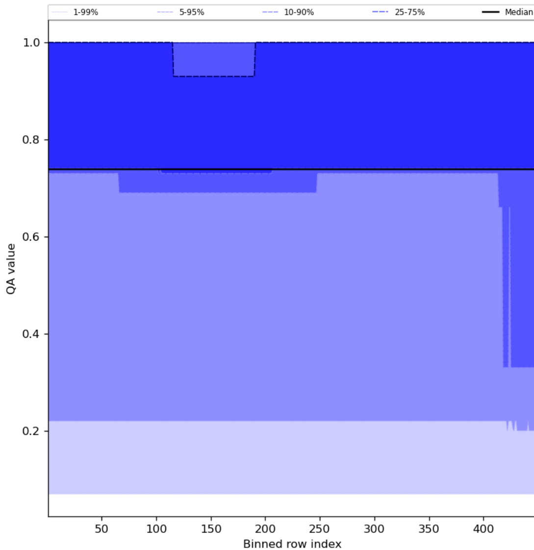
Figure 45: Along track statistics of “QA value” for 2023-09-13 to 2023-09-15
