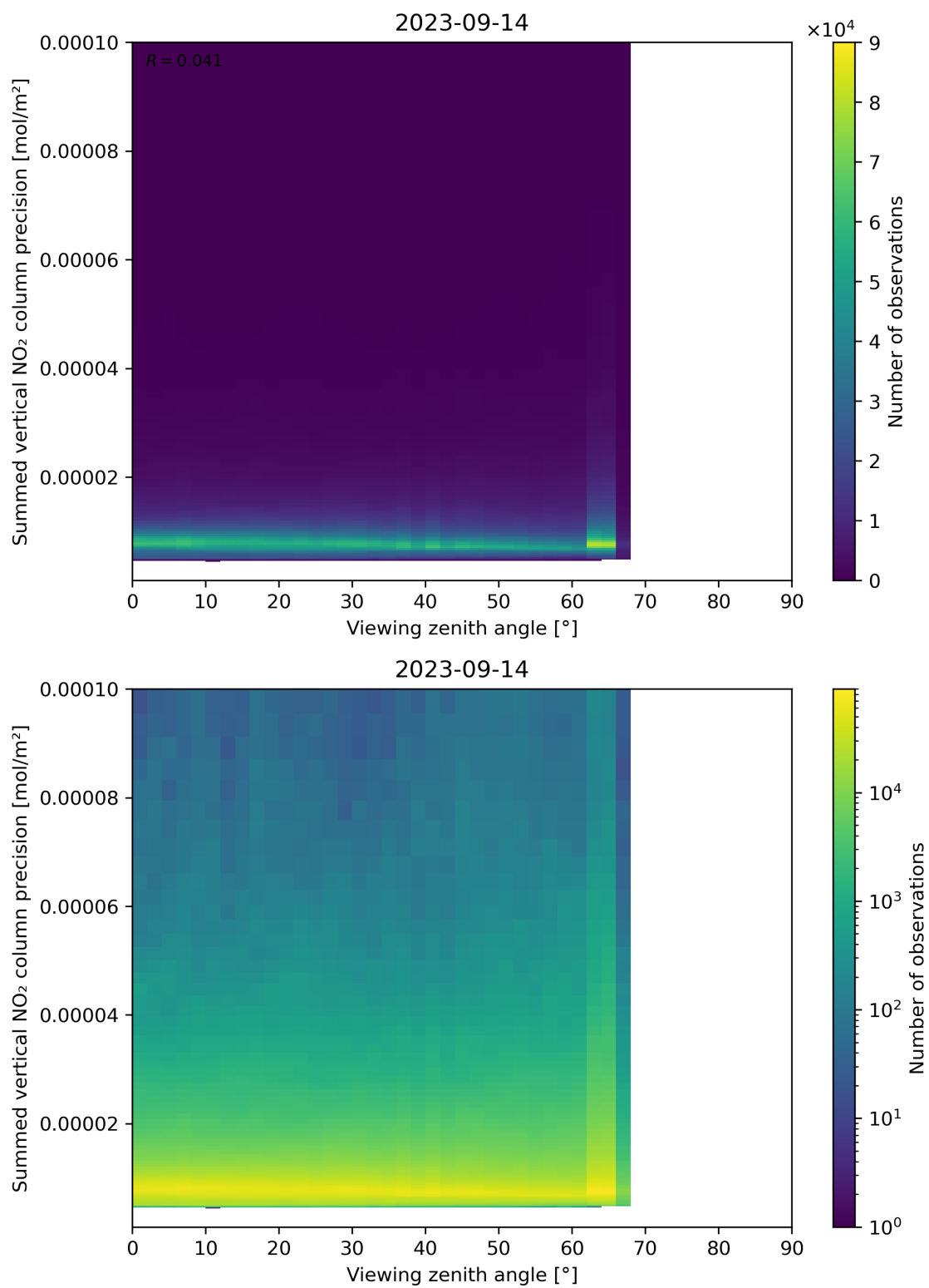
Figure 166: Scatter density plot of “Viewing zenith angle” against “Summed vertical NO 2 column precision” for 2023-09-13 to 2023-09-15.
