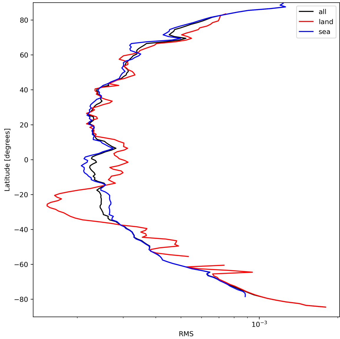
Figure 26: Zonal average of “RMS” for 2023-09-13 to 2023-09-15.
