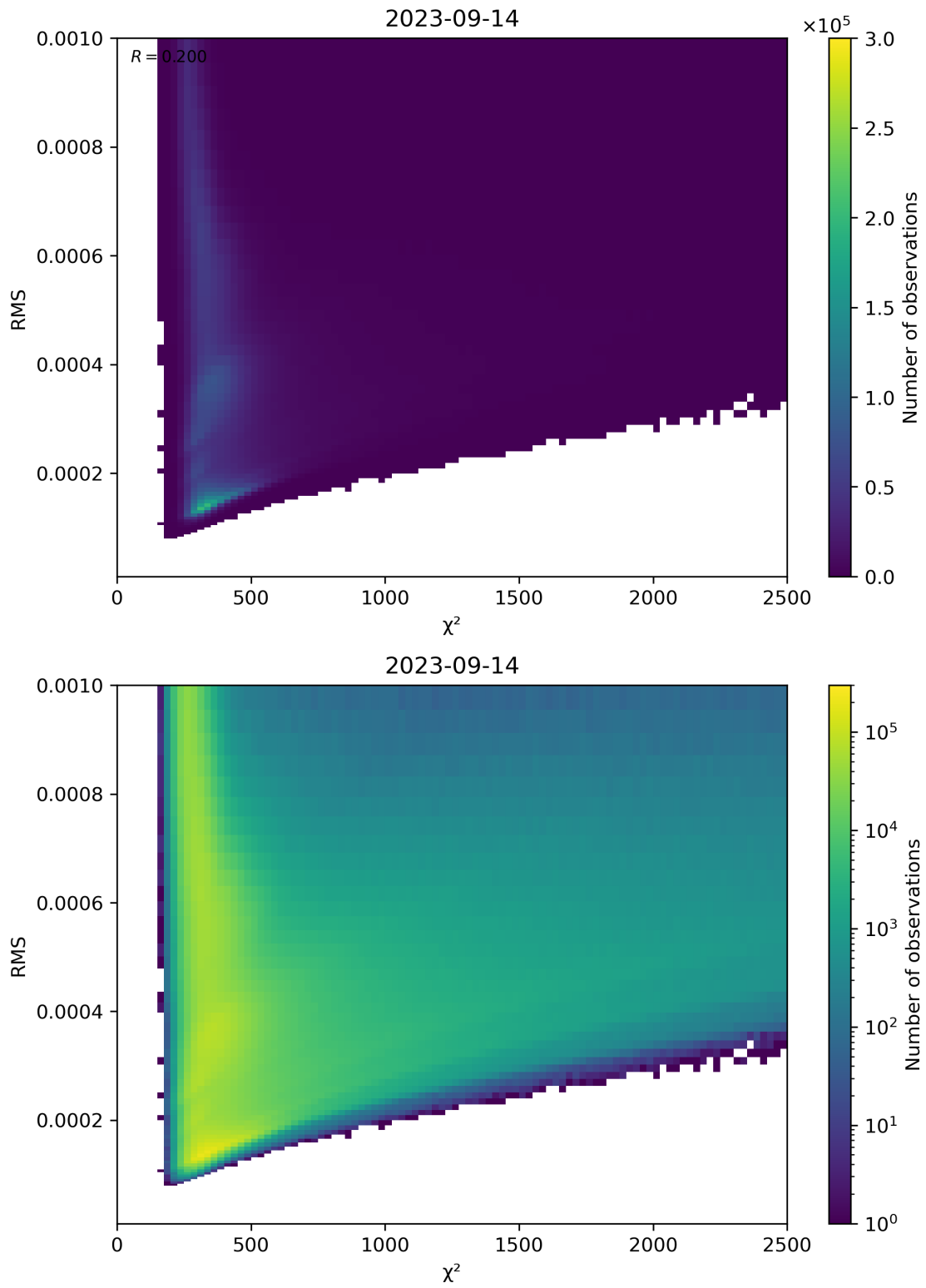
Figure 82: Scatter density plot of “ \chi^2 ” against “RMS” for 2023-09-13 to 2023-09-15.
