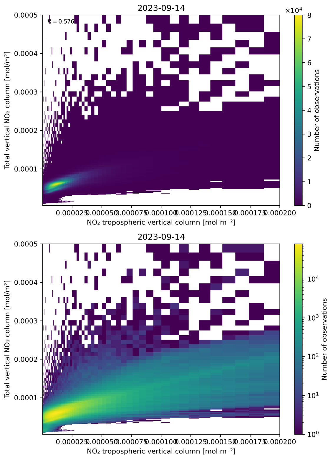
Figure 128: Scatter density plot of “NO 2 tropospheric vertical column” against “Total vertical NO 2 column” for 2023-09-13 to 2023-09-15.
