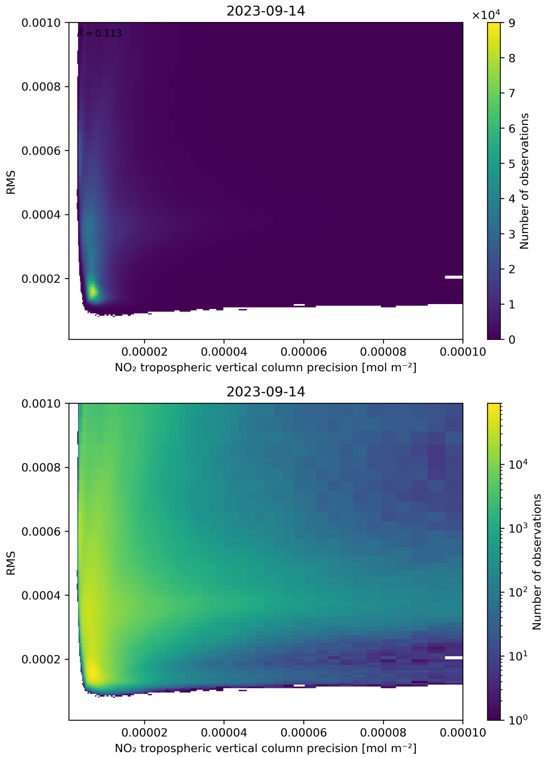
Figure 140: Scatter density plot of “NO 2 tropospheric vertical column precision” against “RMS” for 2023-09-13 to 2023-09-15.
