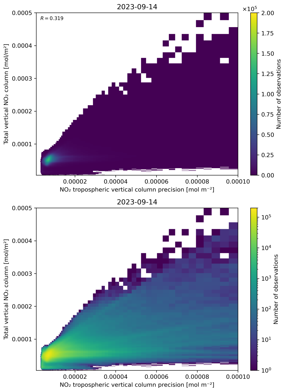
Figure 138: Scatter density plot of “NO 2 tropospheric vertical column precision” against “Total vertical NO 2 column” for 2023-09-13 to 2023-09-15.
