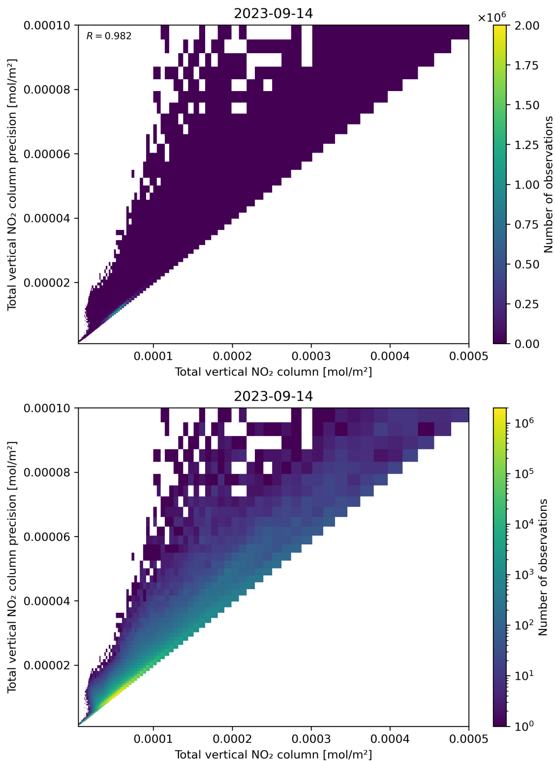
Figure 114: Scatter density plot of “Total vertical NO 2 column” against “Total vertical NO 2 column precision” for 2023-09-13 to 2023-09-15.
