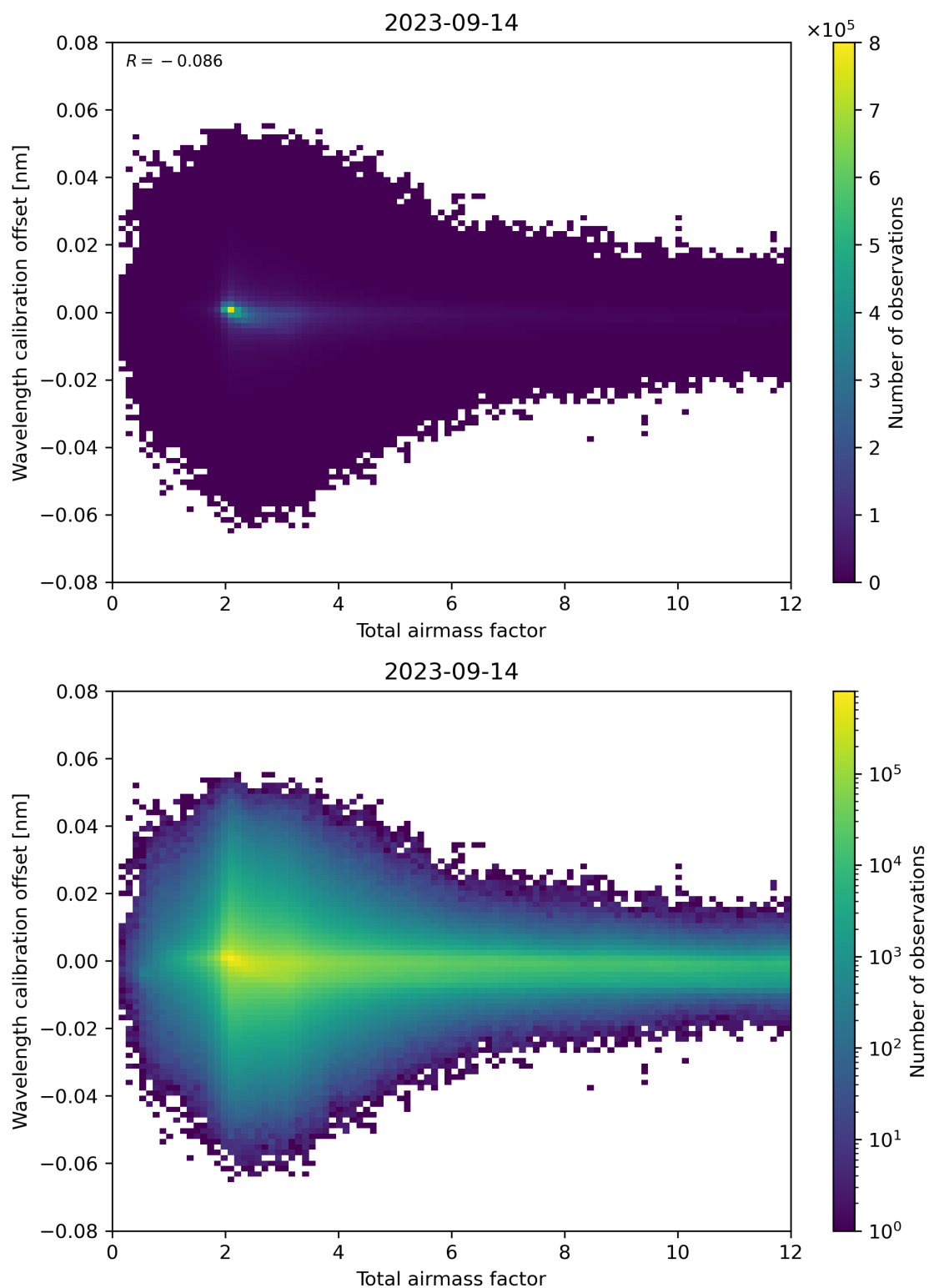
Figure 70: Scatter density plot of “Total airmass factor” against “Wavelength calibration offset” for 2023-09-13 to 2023-09-15.
