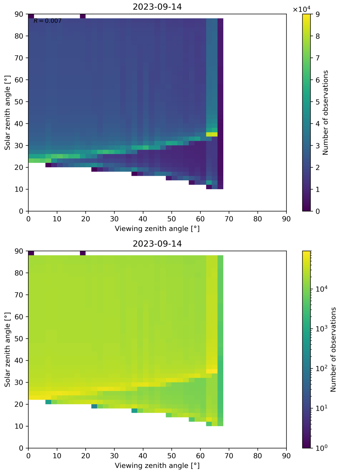
Figure 172: Scatter density plot of “Viewing zenith angle” against “Solar zenith angle” for 2023-09-13 to 2023-09-15.
