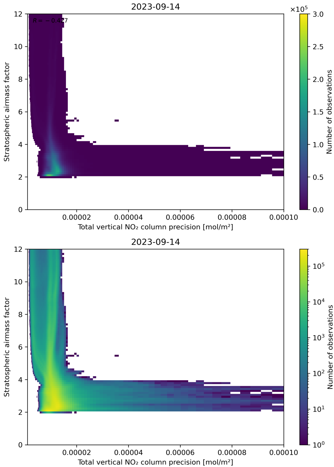
Figure 115: Scatter density plot of “Total vertical NO 2 column precision” against “Stratospheric air mass factor” for 2023-09-13 to 2023-09-15.
