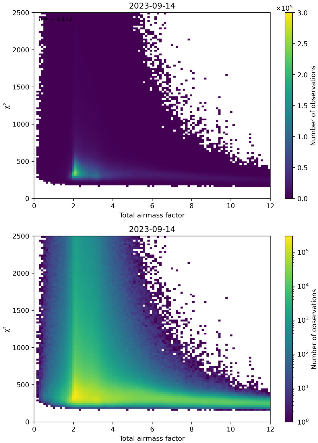
Figure 63: Scatter density plot of “Total airmass factor” against “ \chi^2 ” for 2023-09-13 to 2023-09-15.
