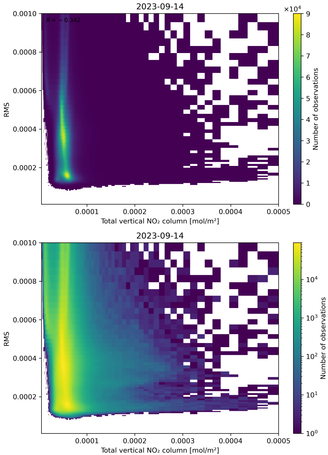
Figure 120: Scatter density plot of “Total vertical NO 2 column” against “RMS” for 2023-09-13 to 2023-09-15.
