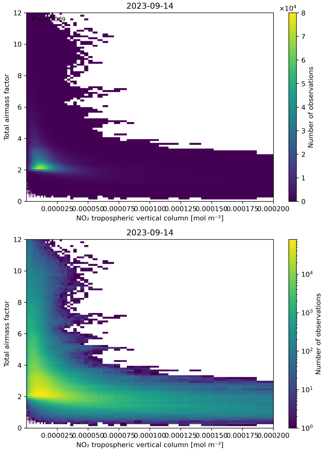
Figure 122: Scatter density plot of “NO 2 tropospheric vertical column” against “Total air mass factor” for 2023-09-13 to 2023-09-15.
