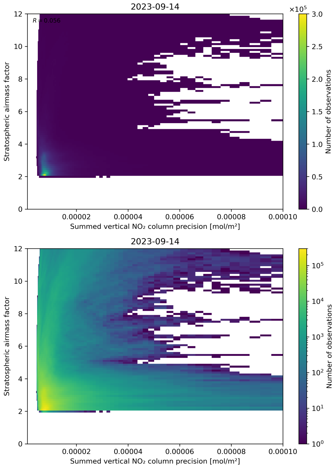
Figure 106: Scatter density plot of “Summed vertical NO 2 column precision” against “Stratospheric airmass factor” for 2023-09-13 to 2023-09-15.
