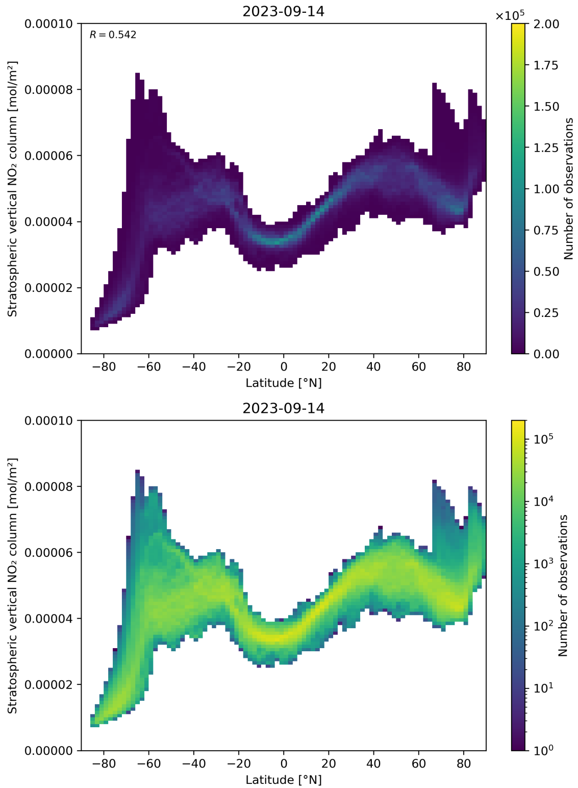
Figure 87: Scatter density plot of “Latitude” against “Stratospheric vertical \text{NO}_2 column” for 2023-09-13 to 2023-09-15.
