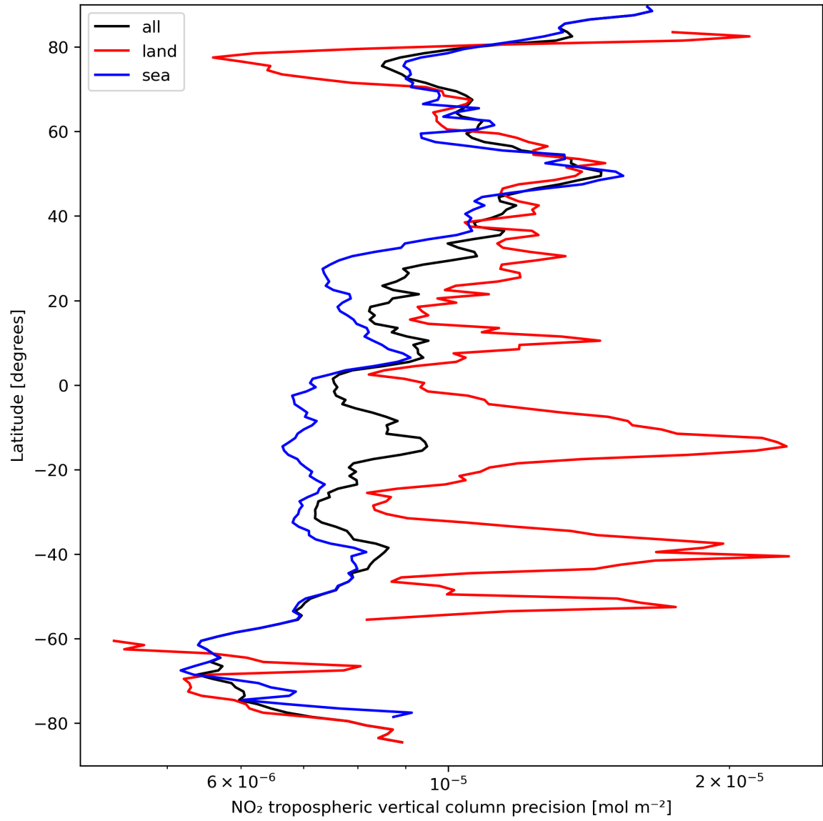
Figure 13: Zonal average of “NO 2 tropospheric vertical column precision” for 2023-09-13 to 2023-09-15.
