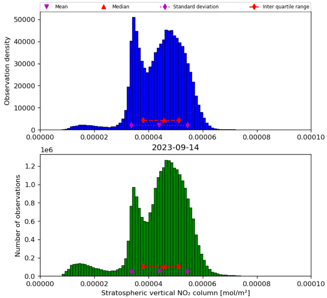
Figure 36: Histogram of “Stratospheric vertical NO 2 column” for 2023-09-13 to 2023-09-15
