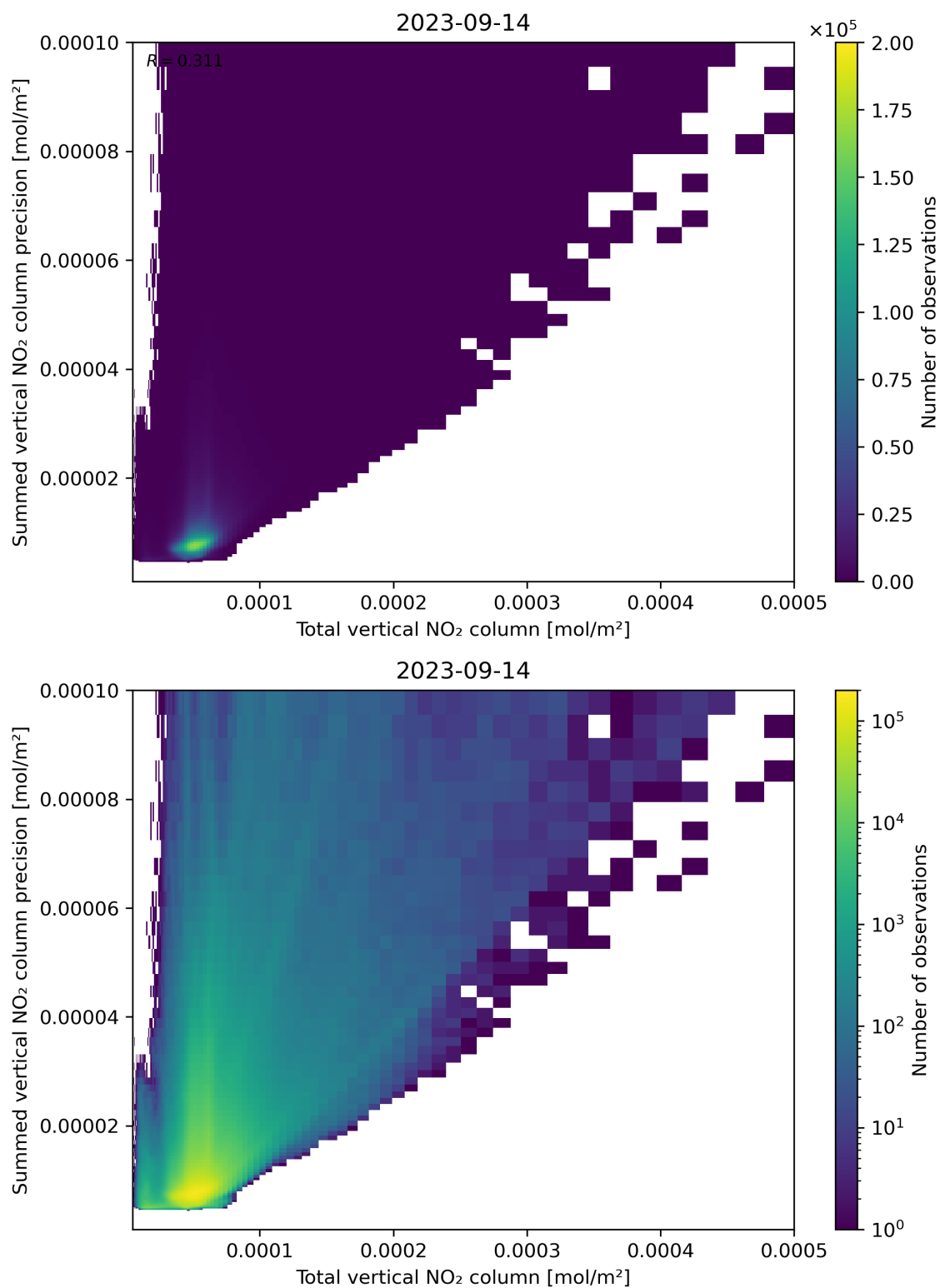
Figure 113: Scatter density plot of “Total vertical NO 2 column” against “Summed vertical NO 2 column precision” for 2023-09-13 to 2023-09-15.
