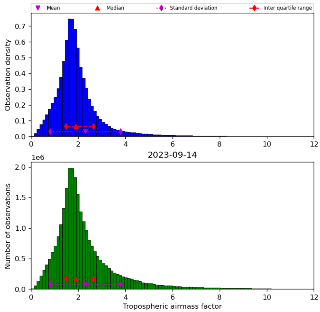
Figure 31: Histogram of “Tropospheric airmass factor” for 2023-09-13 to 2023-09-15
