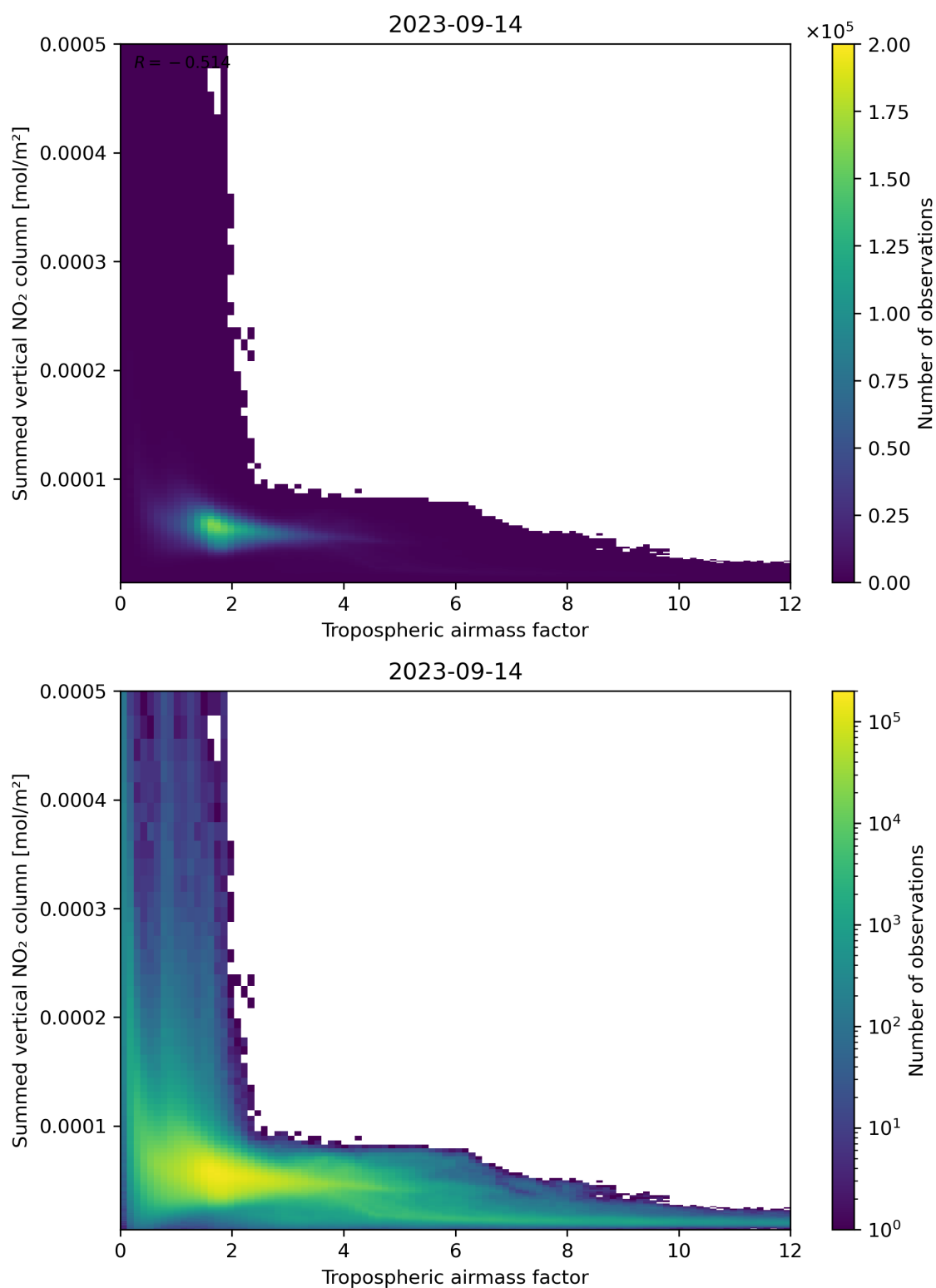
Figure 75: Scatter density plot of “Tropospheric air mass factor” against “Summed vertical NO 2 column” for 2023-09-13 to 2023-09-15.
