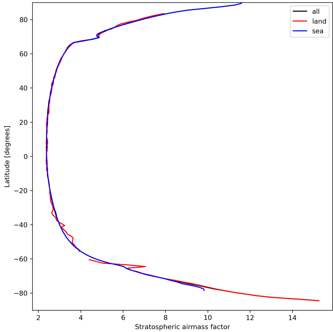
Figure 27: Zonal average of “Stratospheric airmass factor” for 2023-09-13 to 2023-09-15.
