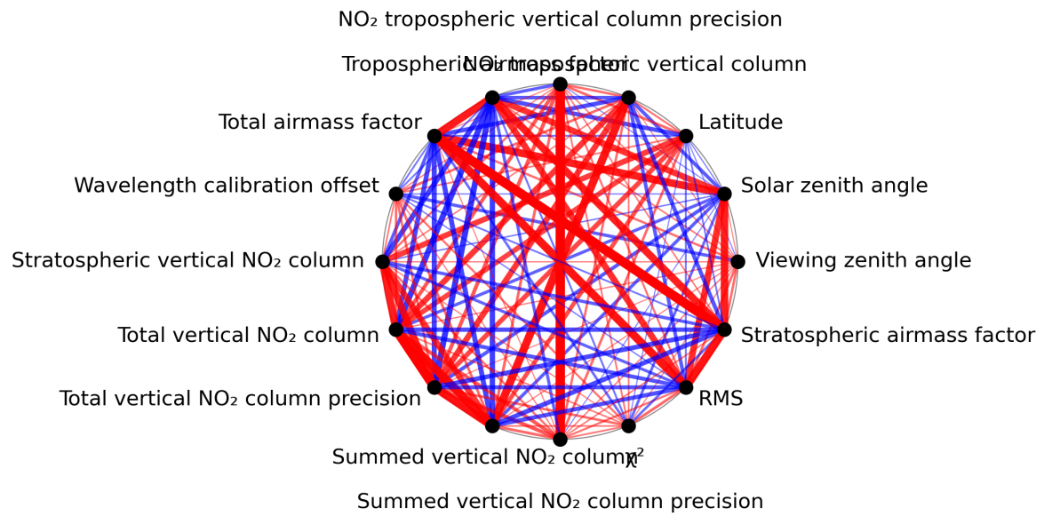
Figure 1: Map of correlation graph for 2023-09-13 to 2023-09-15.
