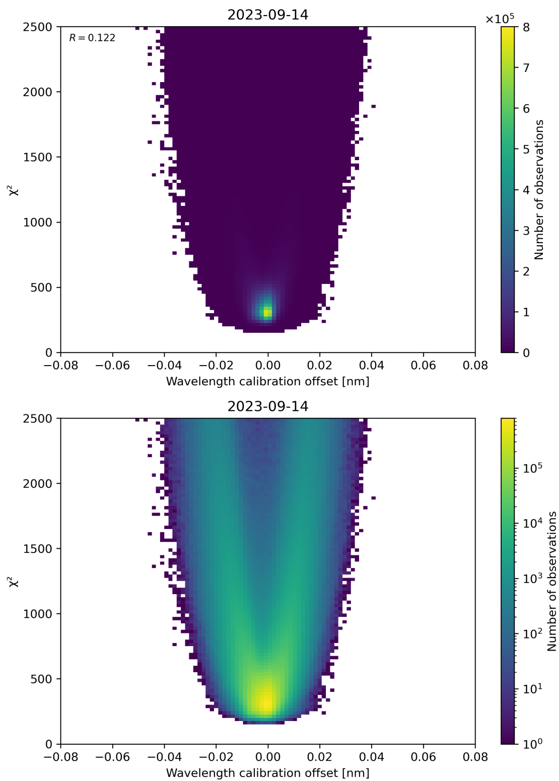
Figure 175: Scatter density plot of “Wavelength calibration offset” against “ \chi^2 ” for 2023-09-13 to 2023-09-15.
