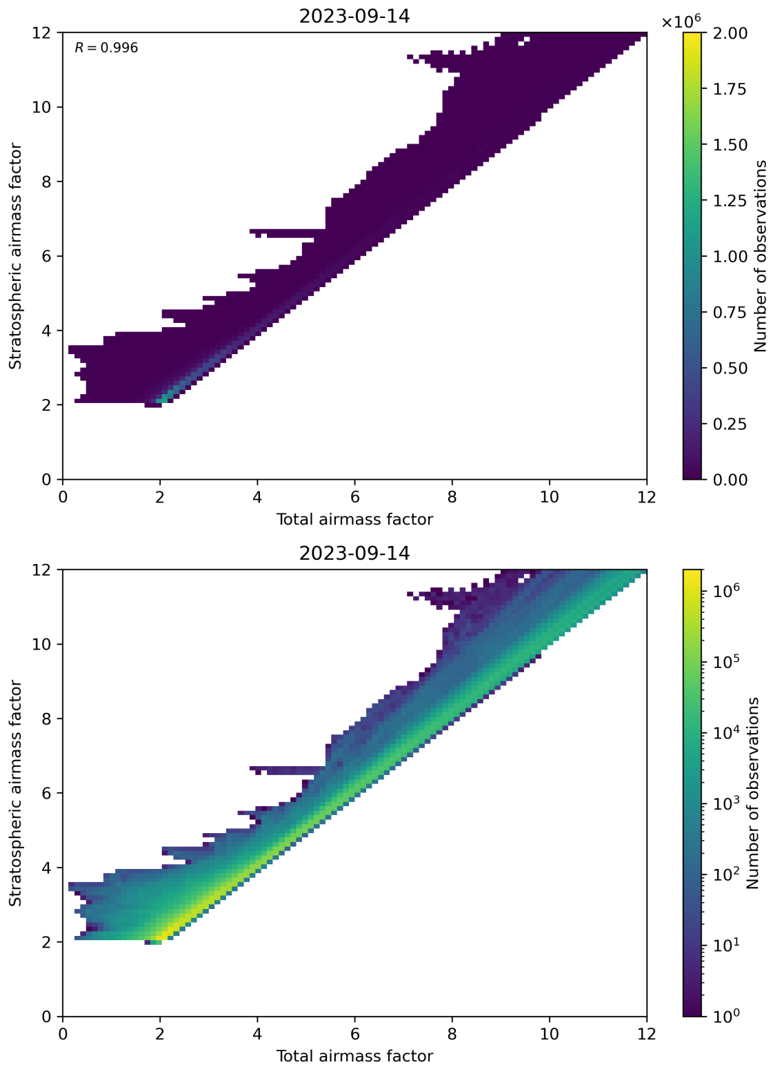
Figure 62: Scatter density plot of “Total airmass factor” against “Stratospheric airmass factor” for 2023-09-13 to 2023-09-15.
