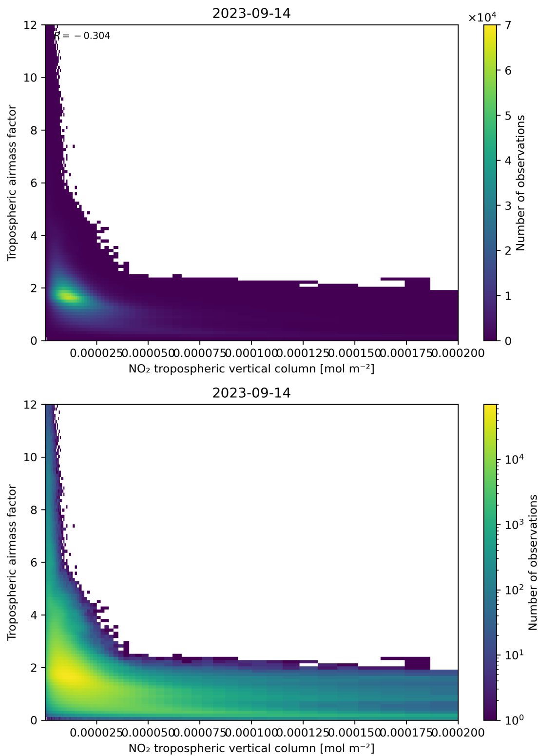
Figure 123: Scatter density plot of “NO 2 tropospheric vertical column” against “Tropospheric air mass factor” for 2023-09-13 to 2023-09-15.
