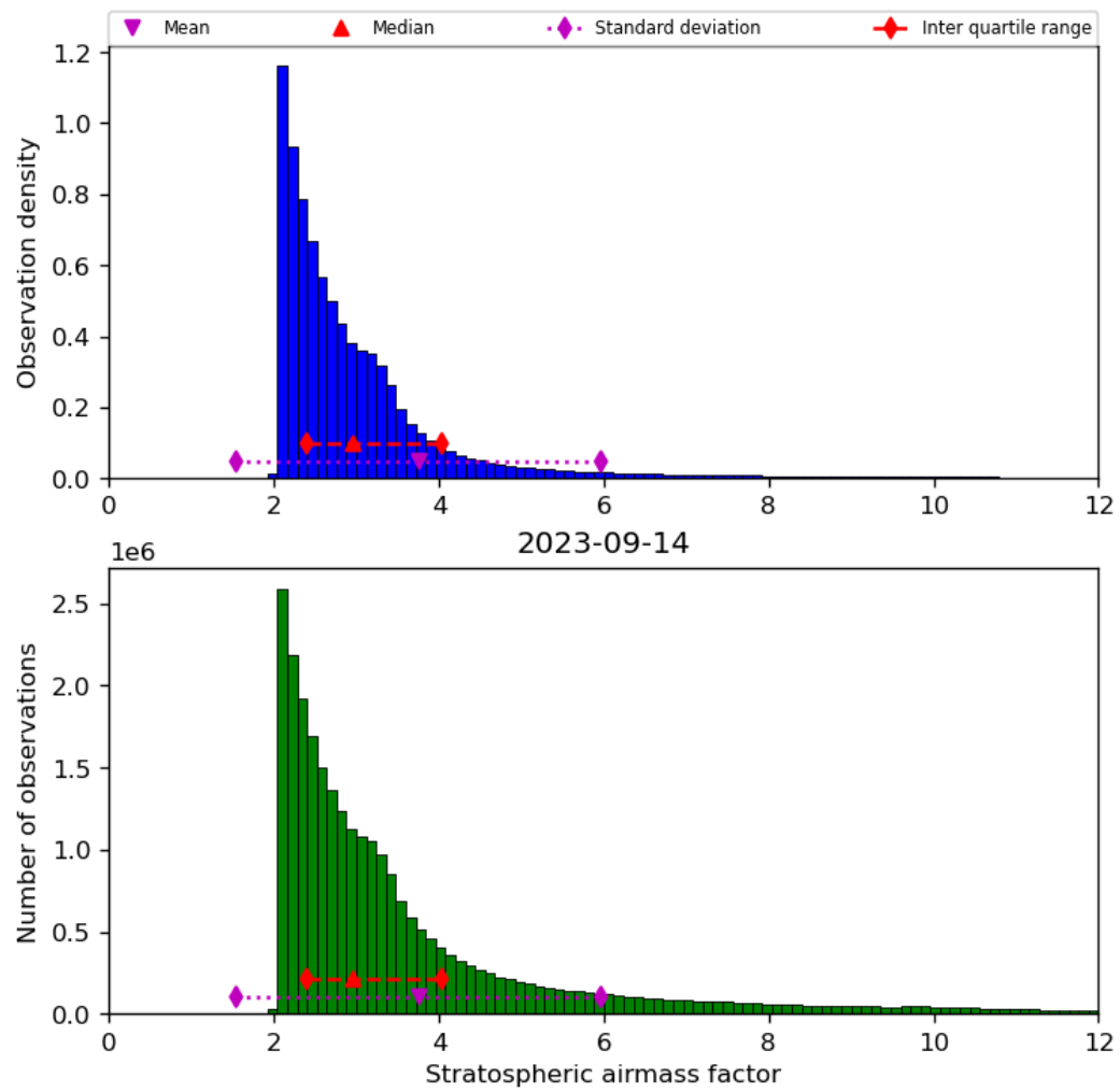
Figure 44: Histogram of “Stratospheric airmass factor” for 2023-09-13 to 2023-09-15
