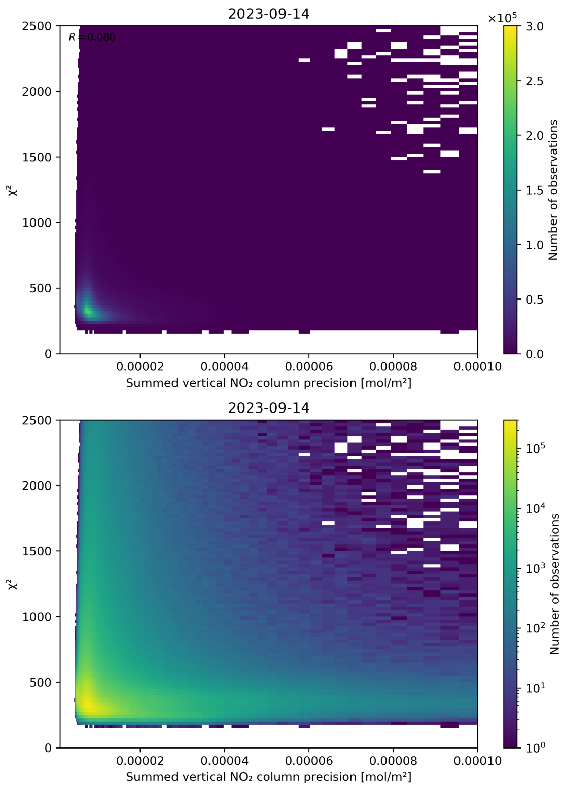
Figure 107: Scatter density plot of “Summed vertical NO 2 column precision” against “ \chi^2 ” for 2023-09-13 to 2023-09-15.
