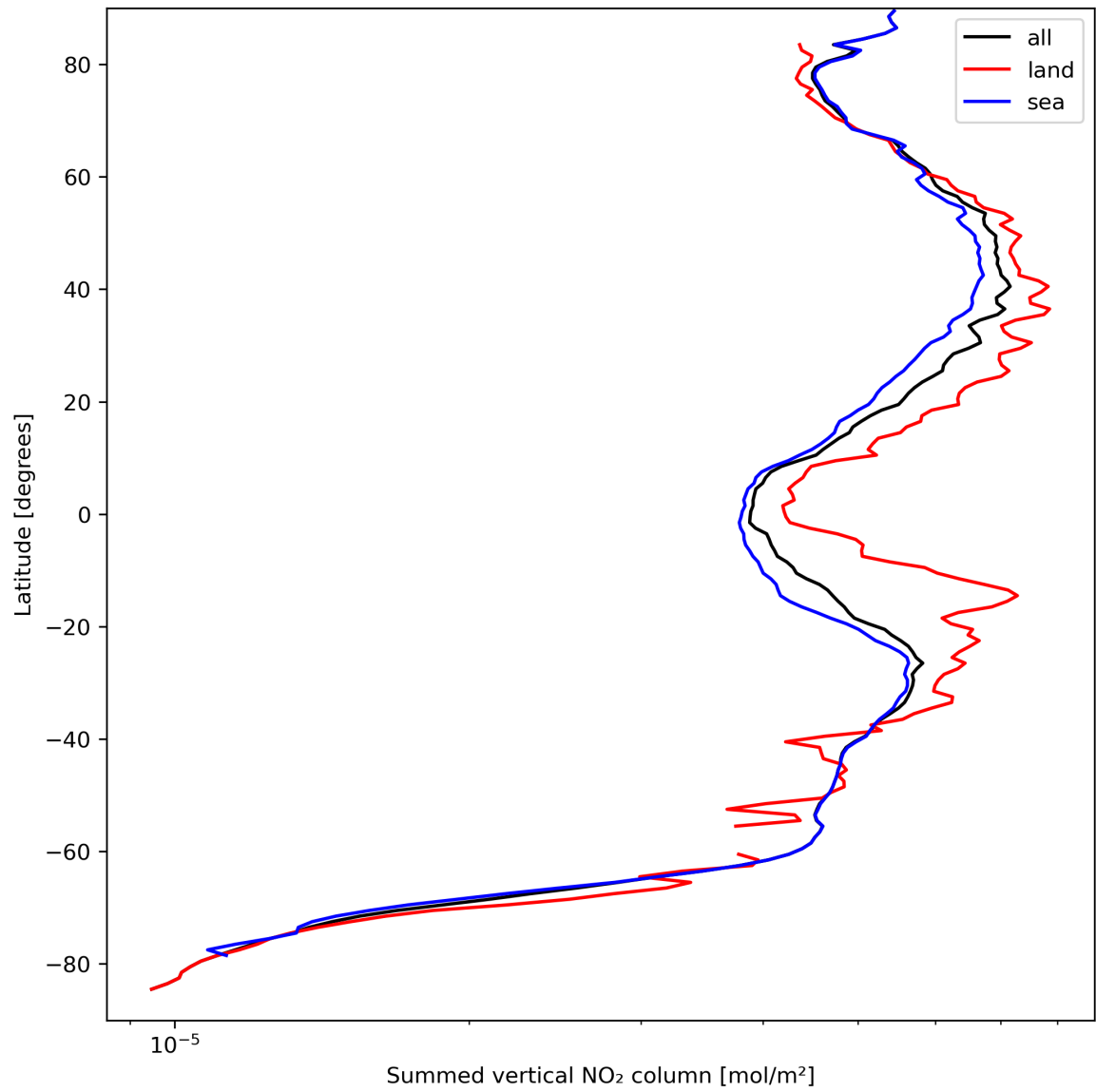
Figure 23: Zonal average of “Summed vertical NO 2 column” for 2023-09-13 to 2023-09-15.
