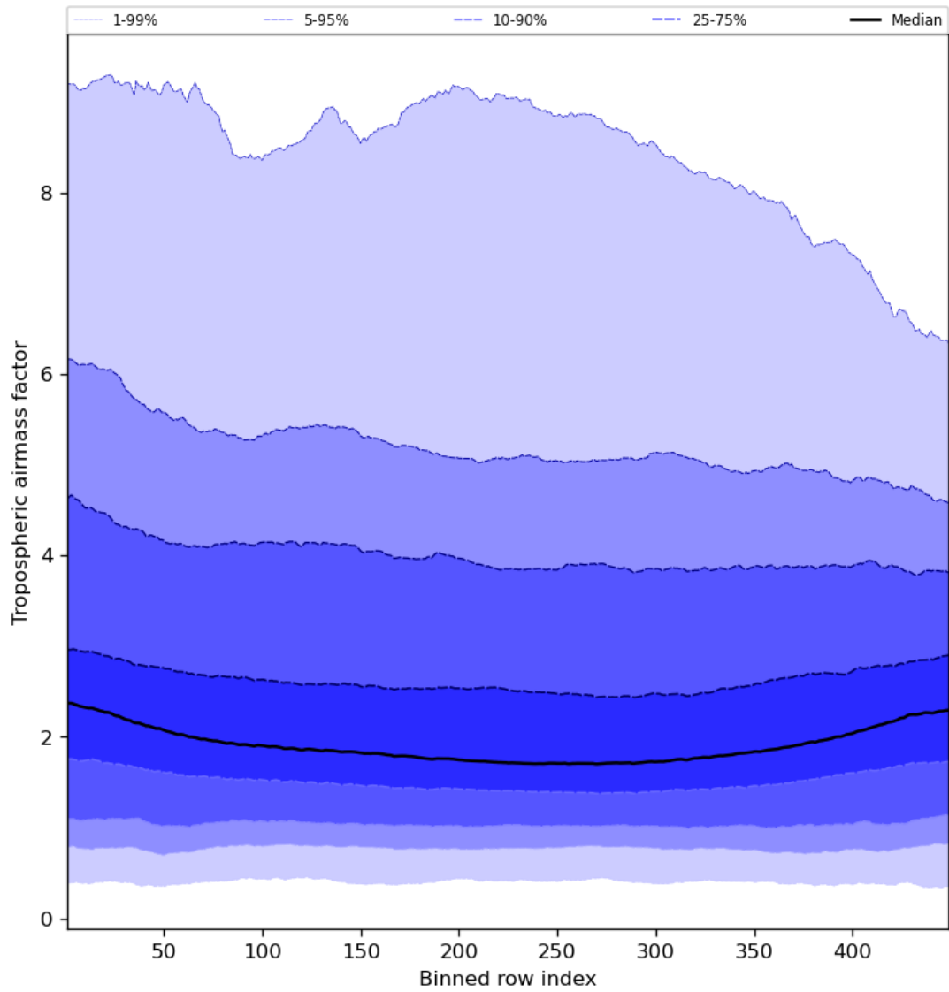
Figure 48: Along track statistics of “Tropospheric air mass factor” for 2023-09-13 to 2023-09-15
