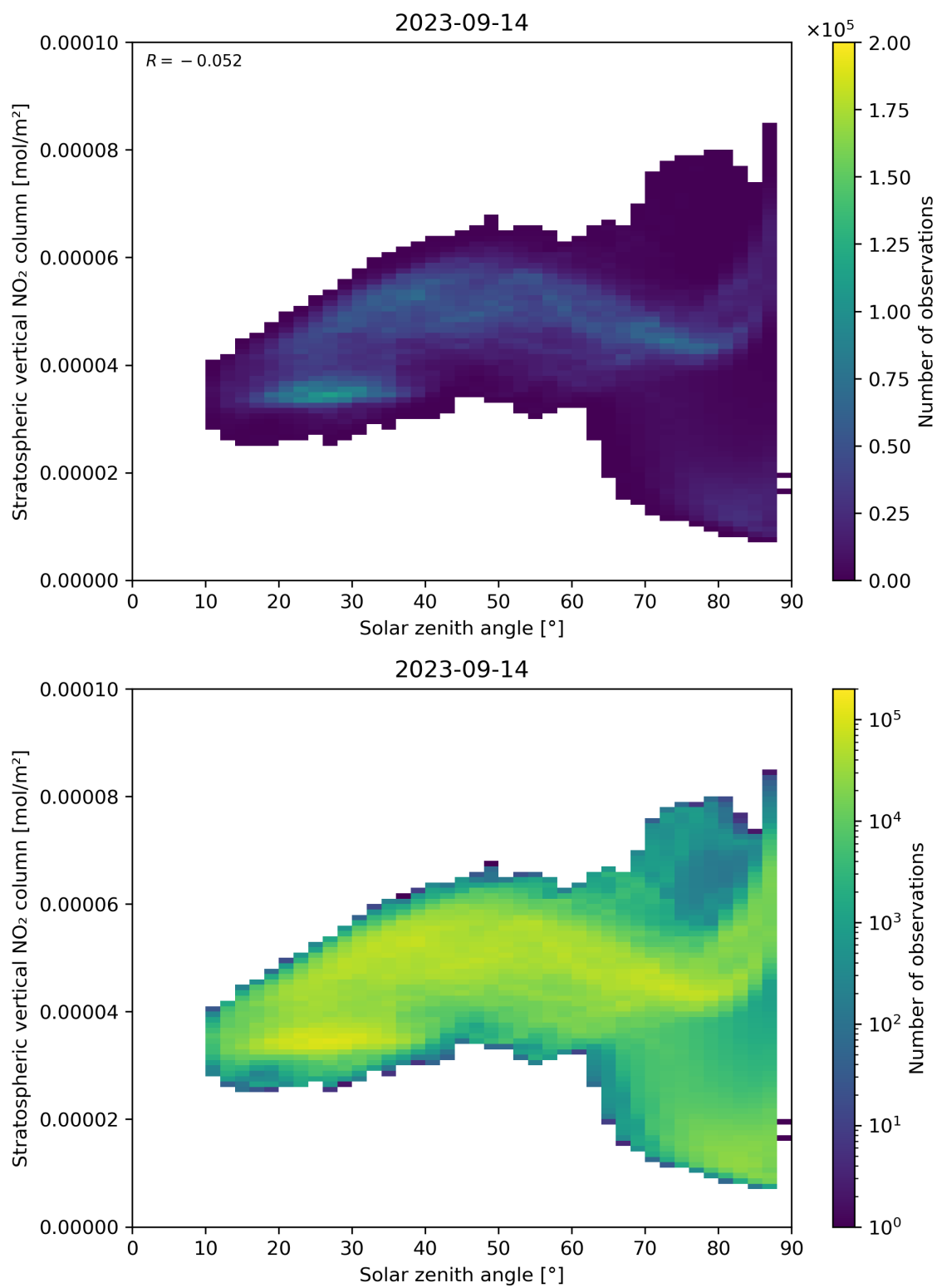
Figure 150: Scatter density plot of “Solar zenith angle” against “Stratospheric vertical NO 2 column” for 2023-09-13 to 2023-09-15.
