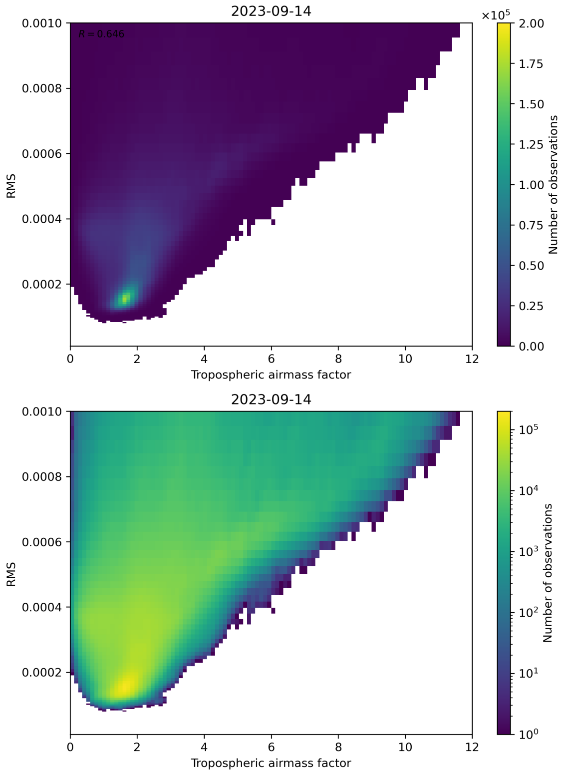
Figure 79: Scatter density plot of “Tropospheric airmass factor” against “RMS” for 2023-09-13 to 2023-09-15.
