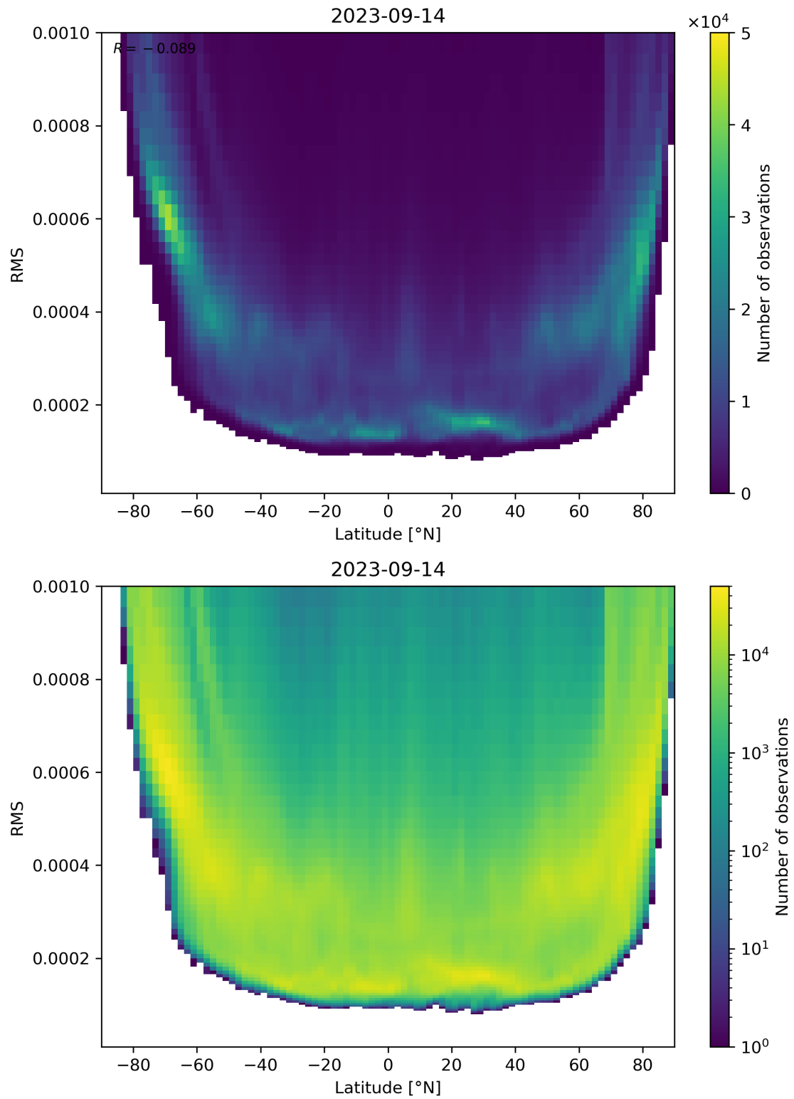
Figure 94: Scatter density plot of “Latitude” against “RMS” for 2023-09-13 to 2023-09-15.
