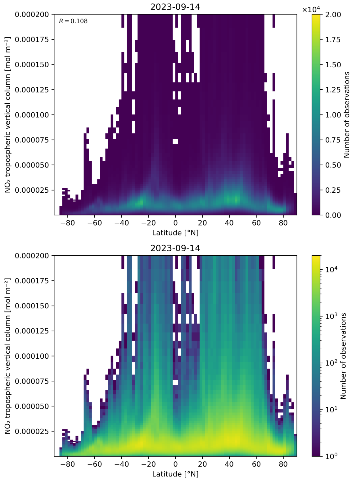
Figure 92: Scatter density plot of “Latitude” against “NO 2 tropospheric vertical column” for 2023-09-13 to 2023-09-15.
