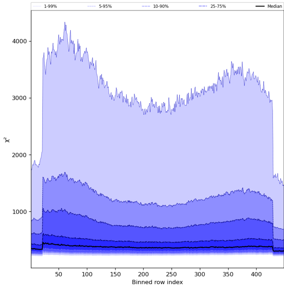
Figure 59: Along track statistics of “ \chi^2 ” for 2023-09-13 to 2023-09-15
