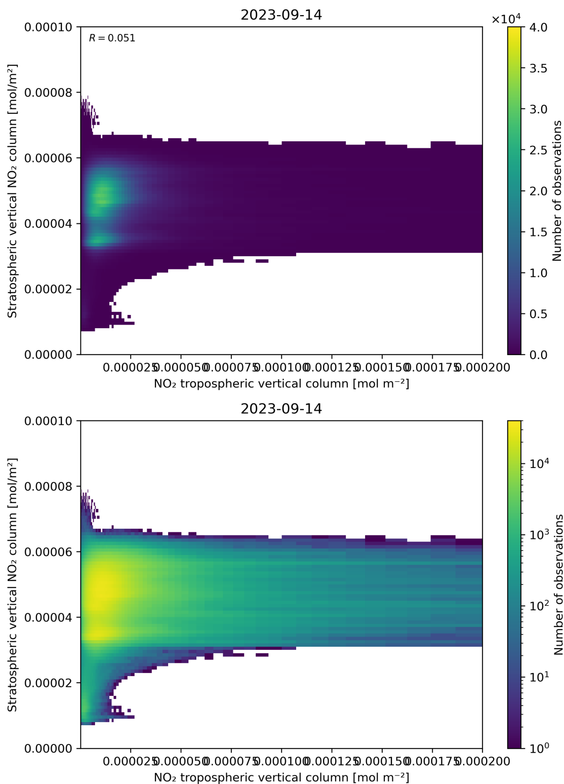
Figure 125: Scatter density plot of “NO 2 tropospheric vertical column” against “Stratospheric vertical NO 2 column” for 2023-09-13 to 2023-09-15.
