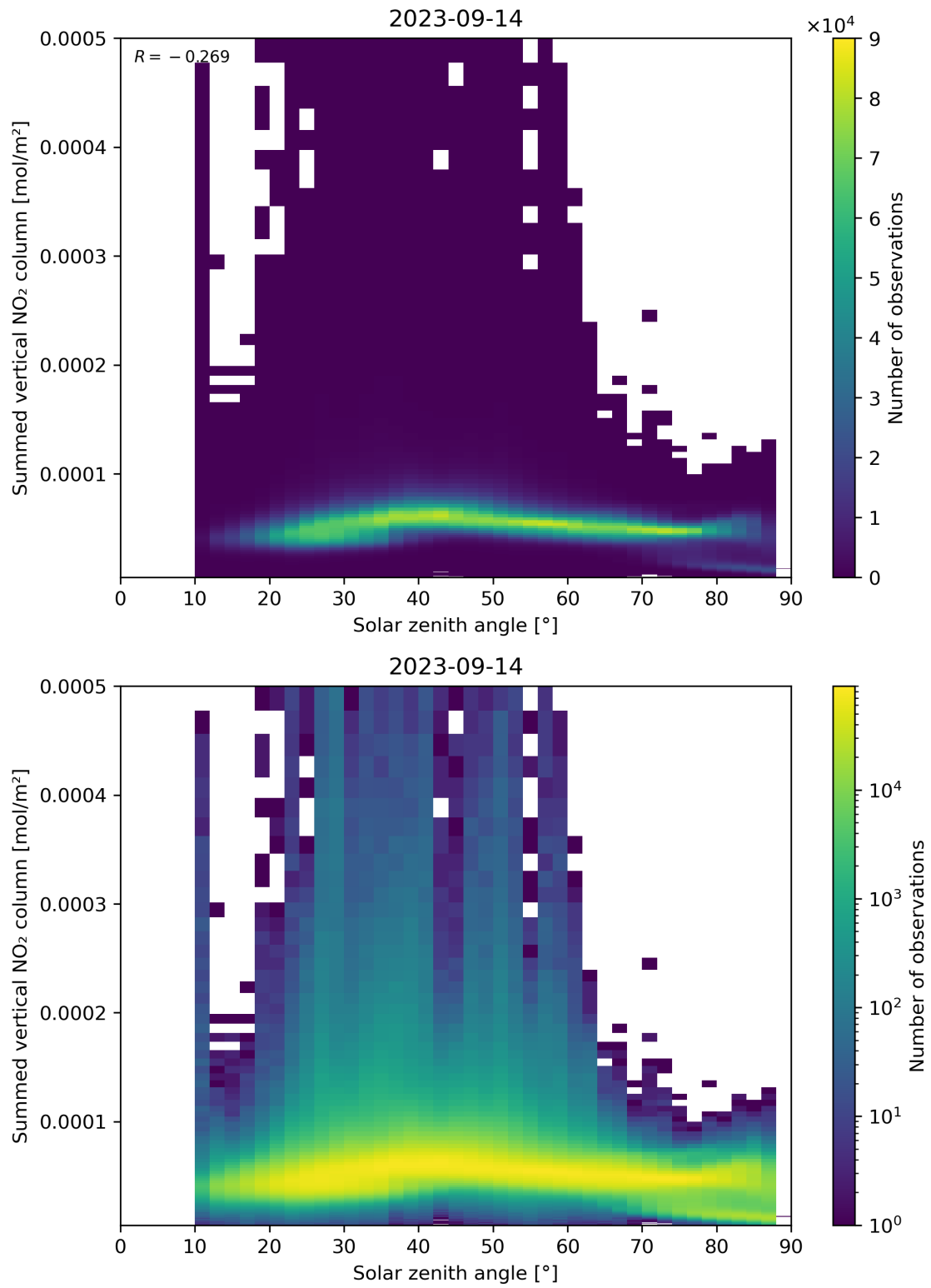
Figure 151: Scatter density plot of “Solar zenith angle” against “Summed vertical NO 2 column” for 2023-09-13 to 2023-09-15.
