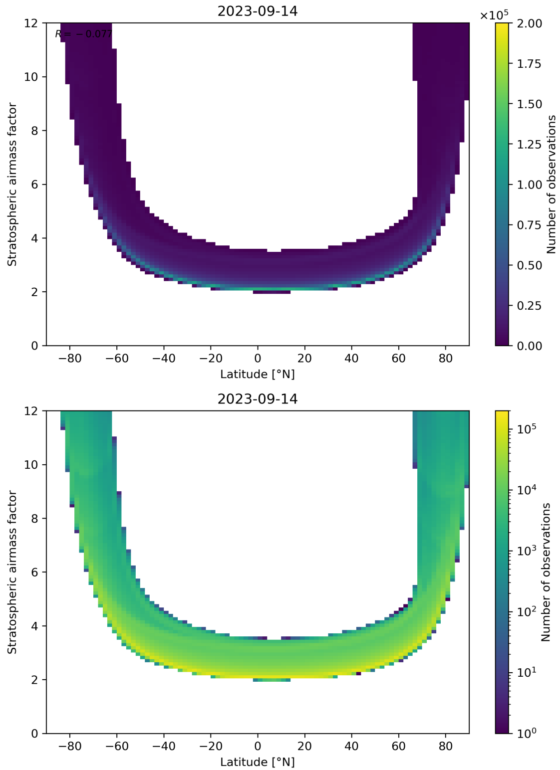
Figure 83: Scatter density plot of “Latitude” against “Stratospheric airmass factor” for 2023-09-13 to 2023-09-15.
