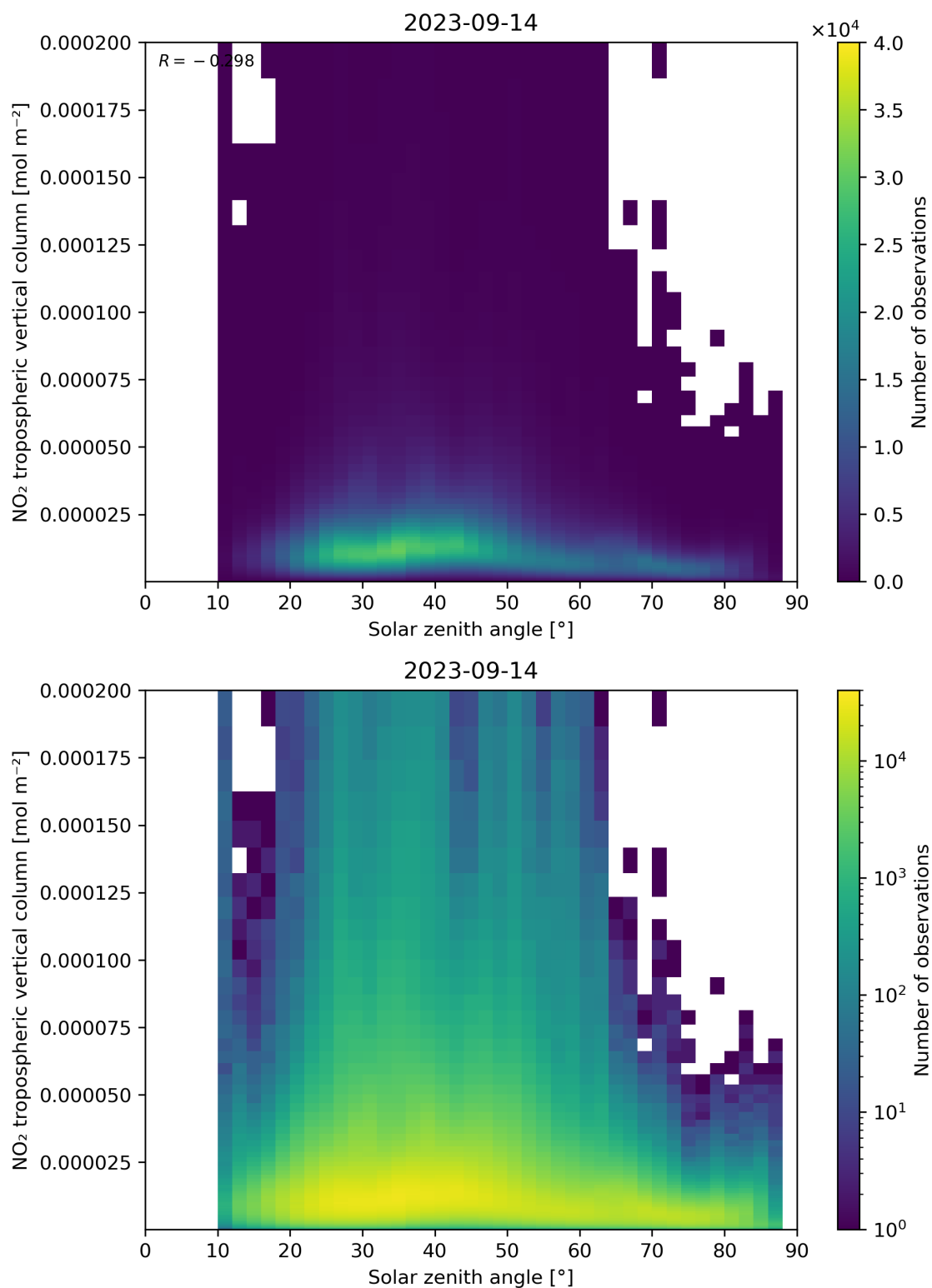
Figure 155: Scatter density plot of “Solar zenith angle” against “NO 2 tropospheric vertical column” for 2023-09-13 to 2023-09-15.
