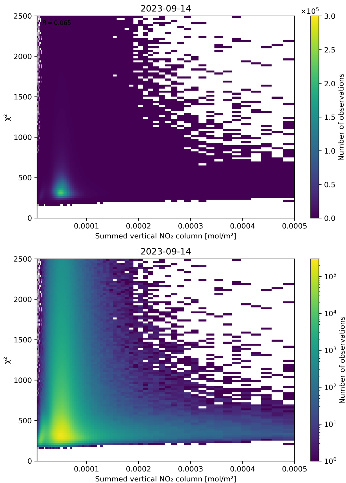
Figure 104: Scatter density plot of “Summed vertical NO 2 column” against “ \chi^2 ” for 2023-09-13 to 2023-09-15.
