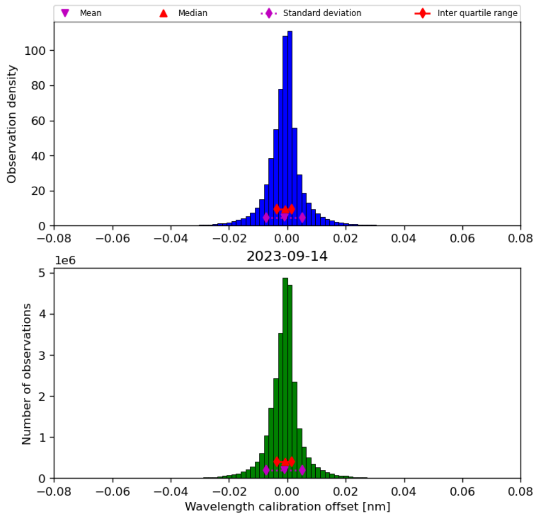
Figure 35: Histogram of “Wavelength calibration offset” for 2023-09-13 to 2023-09-15
