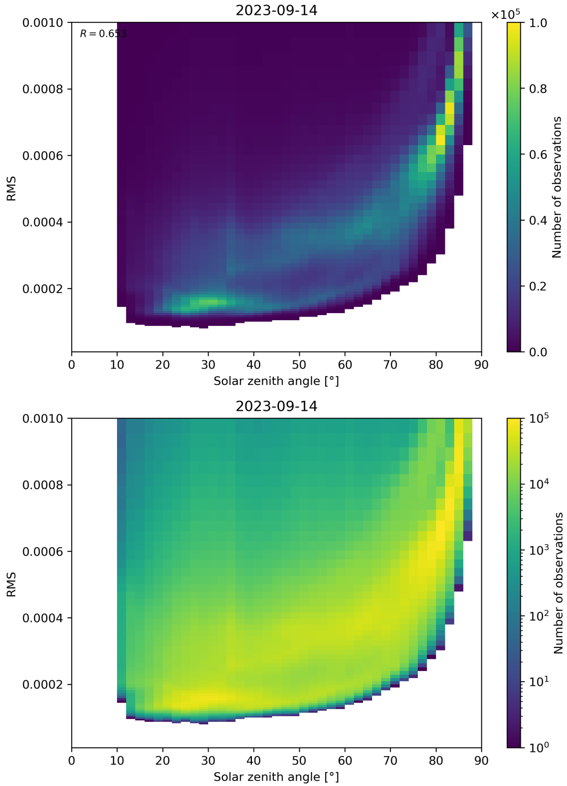
Figure 157: Scatter density plot of “Solar zenith angle” against “RMS” for 2023-09-13 to 2023-09-15.
