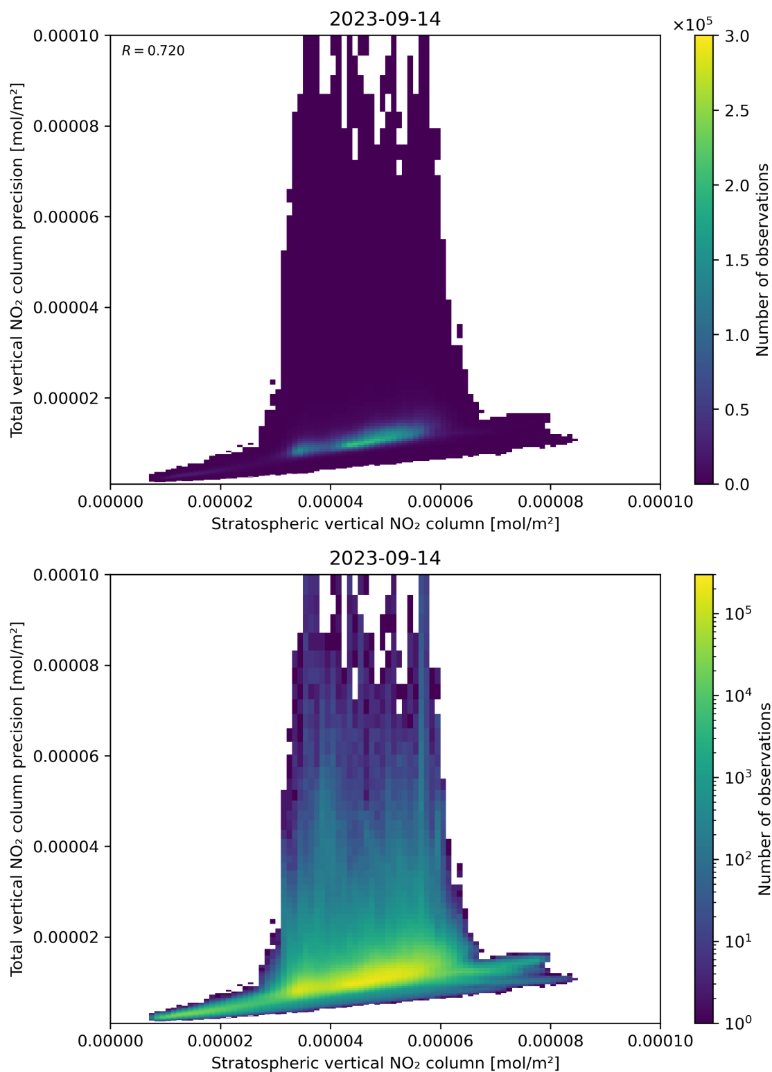
Figure 101: Scatter density plot of “Stratospheric vertical NO 2 column” against “Total vertical NO 2 column precision” for 2023-09-13 to 2023-09-15.
