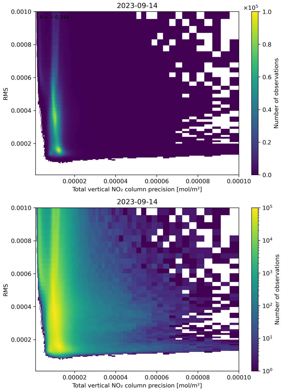
Figure 119: Scatter density plot of “Total vertical NO 2 column precision” against “RMS” for 2023-09-13 to 2023-09-15.
