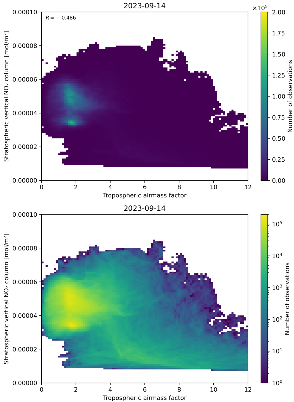
Figure 74: Scatter density plot of “Tropospheric air mass factor” against “Stratospheric vertical NO 2 column” for 2023-09-13 to 2023-09-15.
