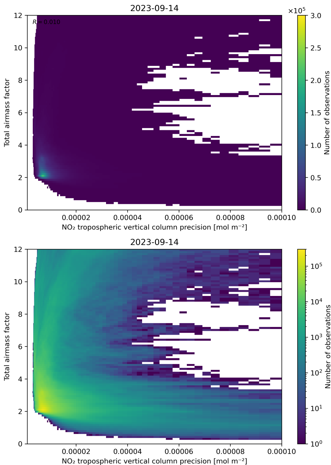
Figure 132: Scatter density plot of “NO 2 tropospheric vertical column precision” against “Total air mass factor” for 2023-09-13 to 2023-09-15.
