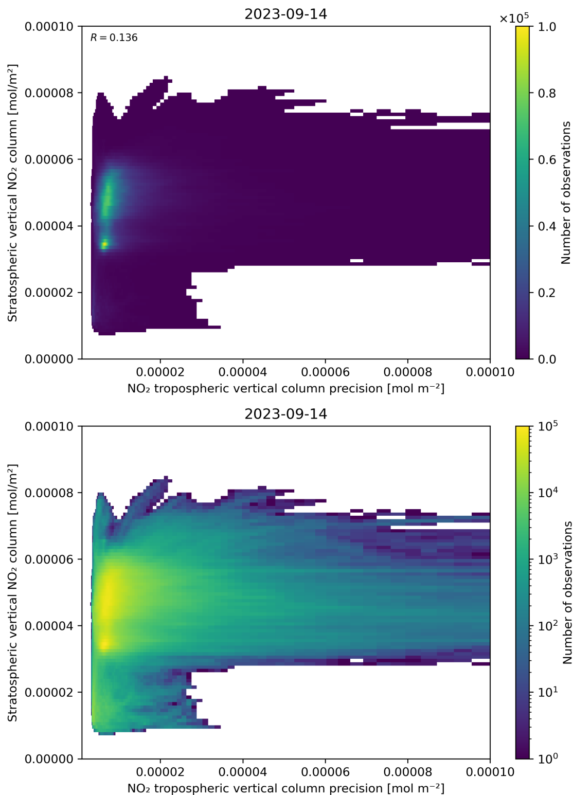
Figure 135: Scatter density plot of “NO 2 tropospheric vertical column precision” against “Stratospheric vertical NO 2 column” for 2023-09-13 to 2023-09-15.
