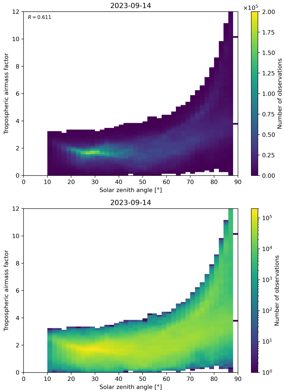
Figure 147: Scatter density plot of “Solar zenith angle” against “Tropospheric airmass factor” for 2023-09-13 to 2023-09-15.
