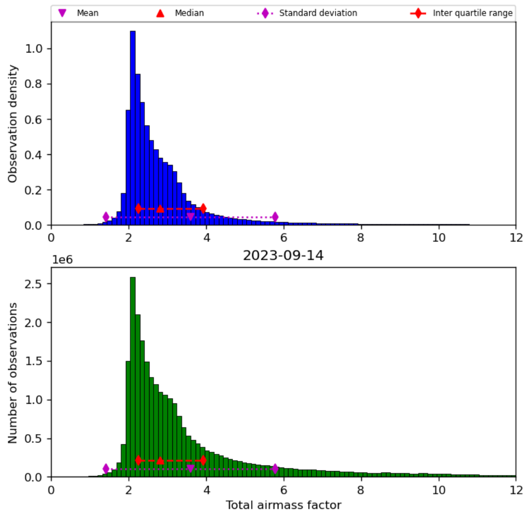
Figure 32: Histogram of “Total airmass factor” for 2023-09-13 to 2023-09-15
