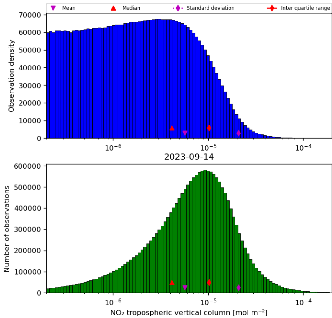
Figure 29: Histogram of “ \text{NO}_2 tropospheric vertical column” for 2023-09-13 to 2023-09-15
