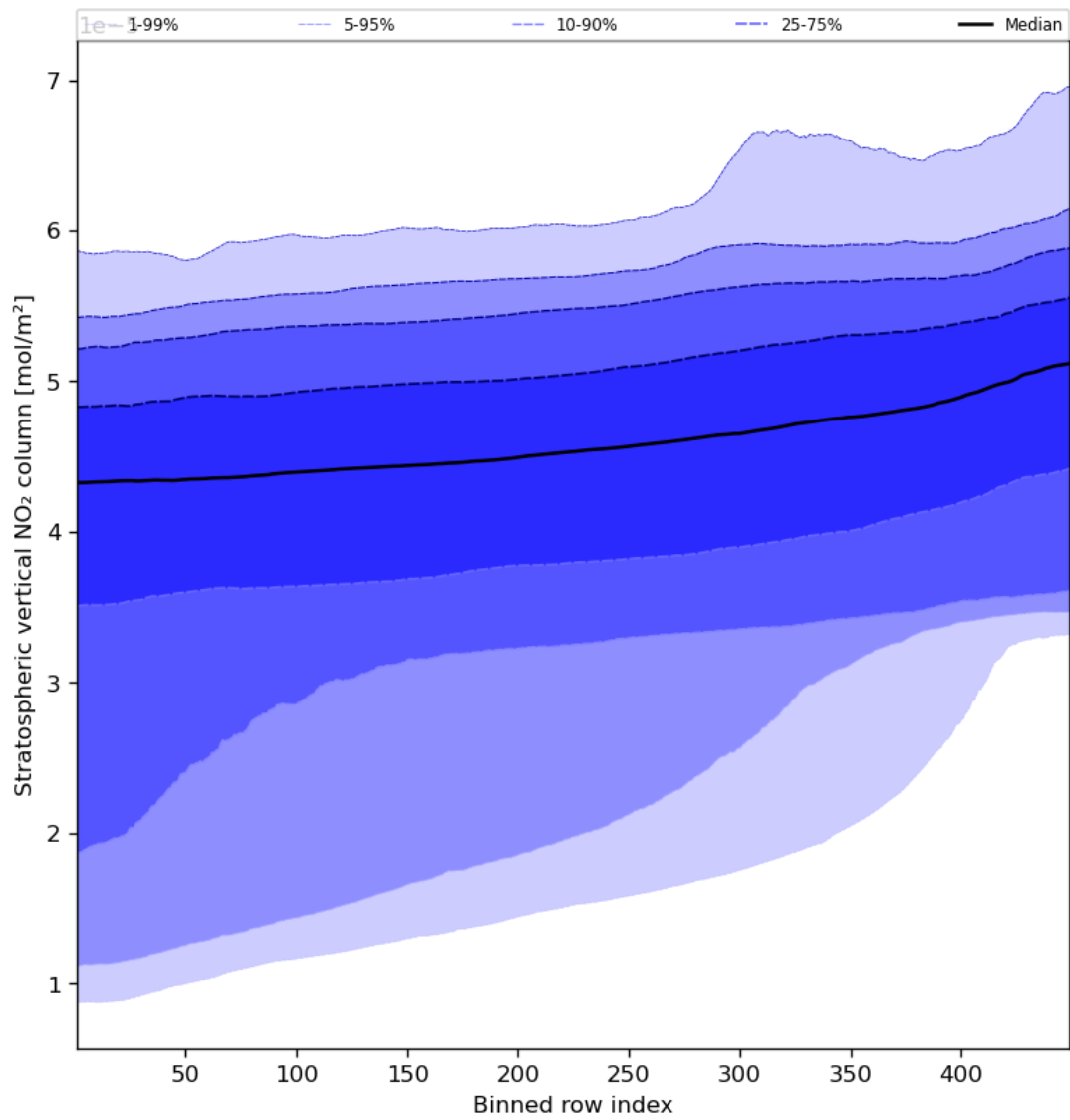
Figure 53: Along track statistics of “Stratospheric vertical NO 2 column” for 2023-09-13 to 2023-09-15
