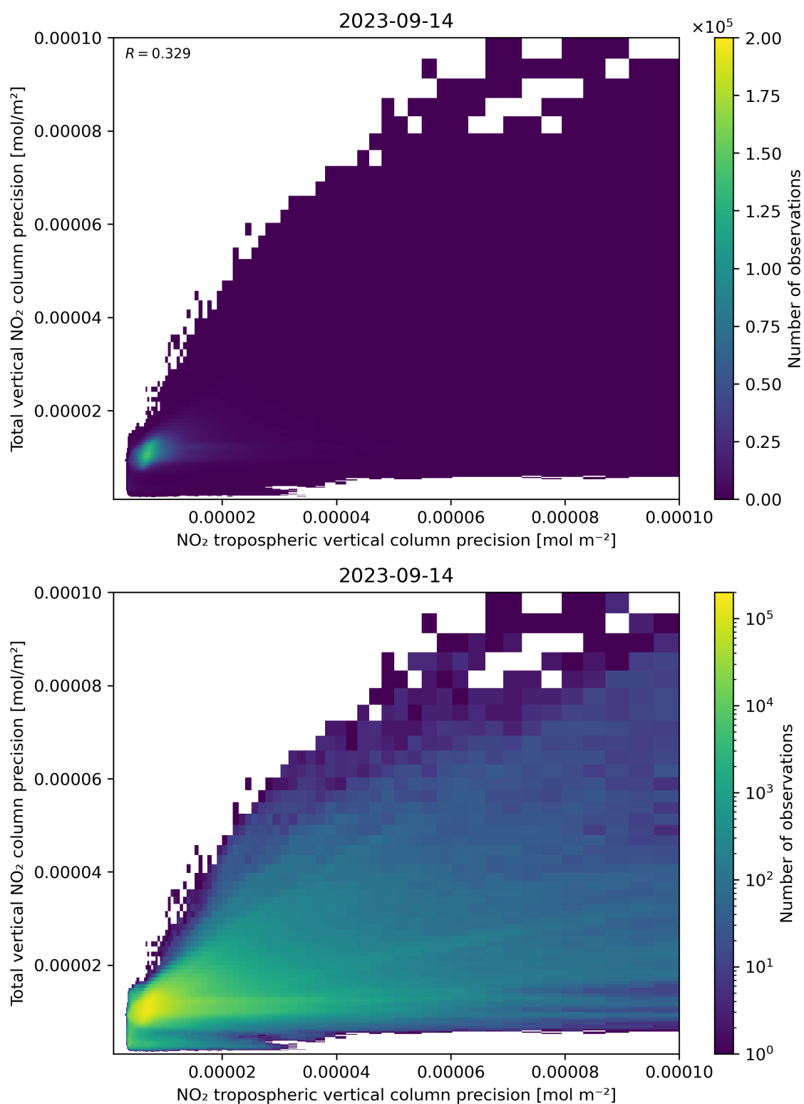
Figure 139: Scatter density plot of “NO 2 tropospheric vertical column precision” against “Total vertical NO 2 column precision” for 2023-09-13 to 2023-09-15.
