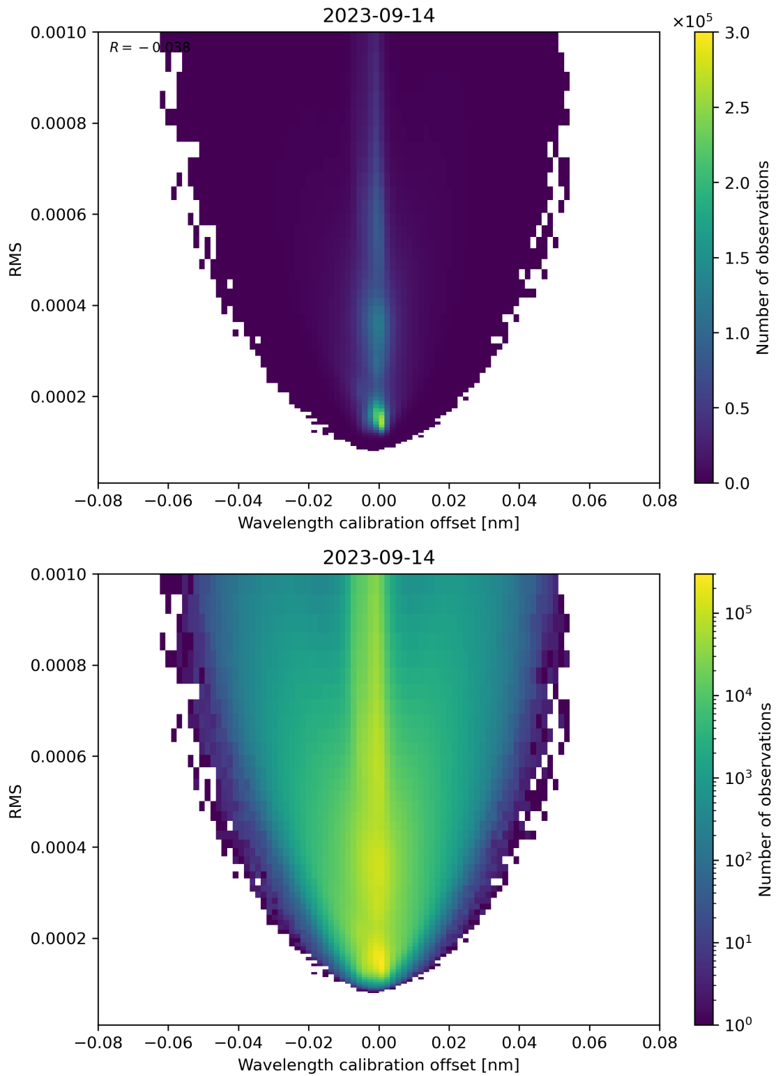
Figure 181: Scatter density plot of “Wavelength calibration offset” against “RMS” for 2023-09-13 to 2023-09-15.
