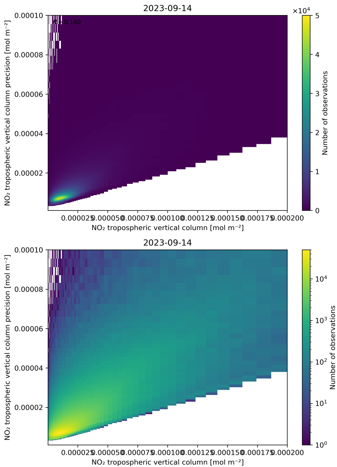
Figure 130: Scatter density plot of “NO 2 tropospheric vertical column” against “NO 2 tropospheric vertical column precision” for 2023-09-13 to 2023-09-15.
