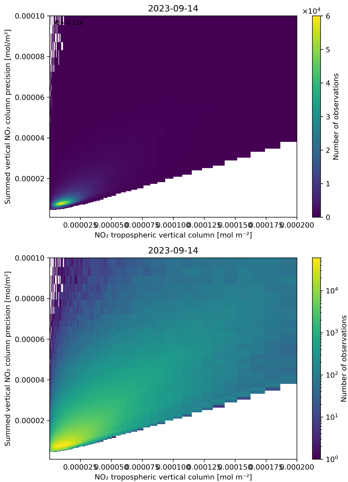
Figure 127: Scatter density plot of “NO 2 tropospheric vertical column” against “Summed vertical NO 2 column precision” for 2023-09-13 to 2023-09-15.
