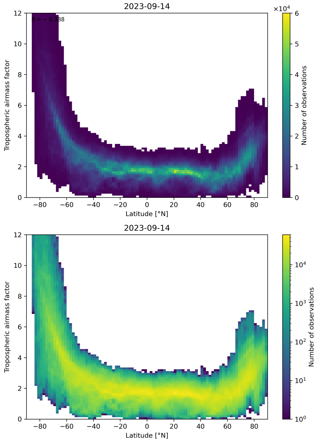
Figure 85: Scatter density plot of “Latitude” against “Tropospheric airmass factor” for 2023-09-13 to 2023-09-15.
