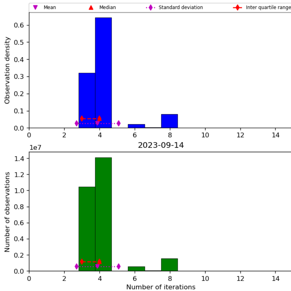
Figure 34: Histogram of “Number of iterations” for 2023-09-13 to 2023-09-15
