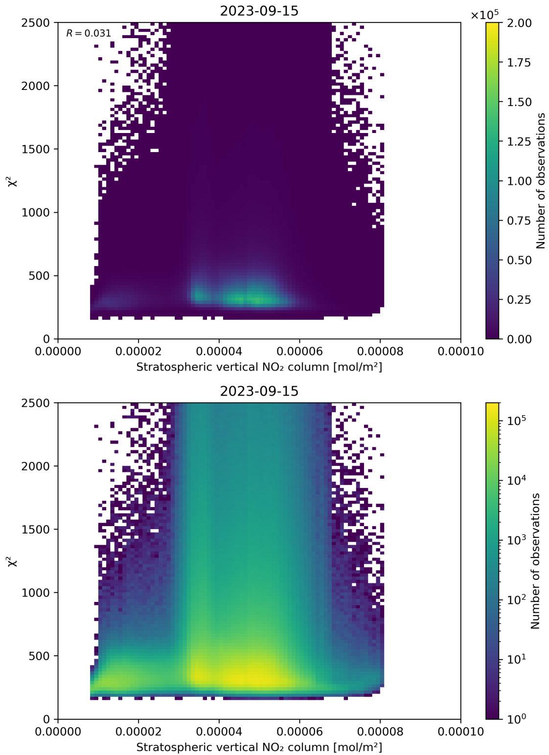
Figure 97: Scatter density plot of “Stratospheric vertical NO 2 column” against “ \chi^2 ” for 2023-09-15 to 2023-09-16.
