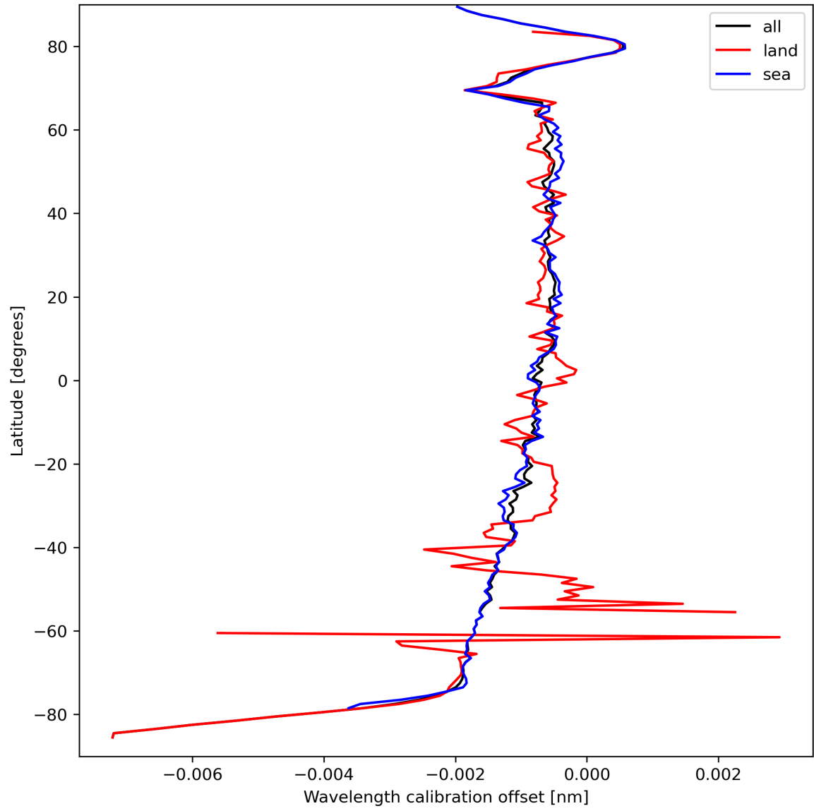
Figure 18: Zonal average of “Wavelength calibration offset” for 2023-09-15 to 2023-09-16.
