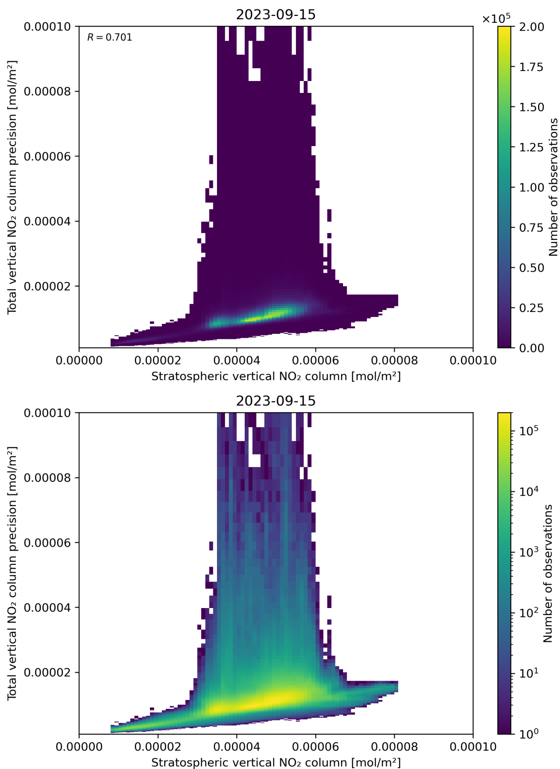
Figure 101: Scatter density plot of “Stratospheric vertical NO 2 column” against “Total vertical NO 2 column precision” for 2023-09-15 to 2023-09-16.
