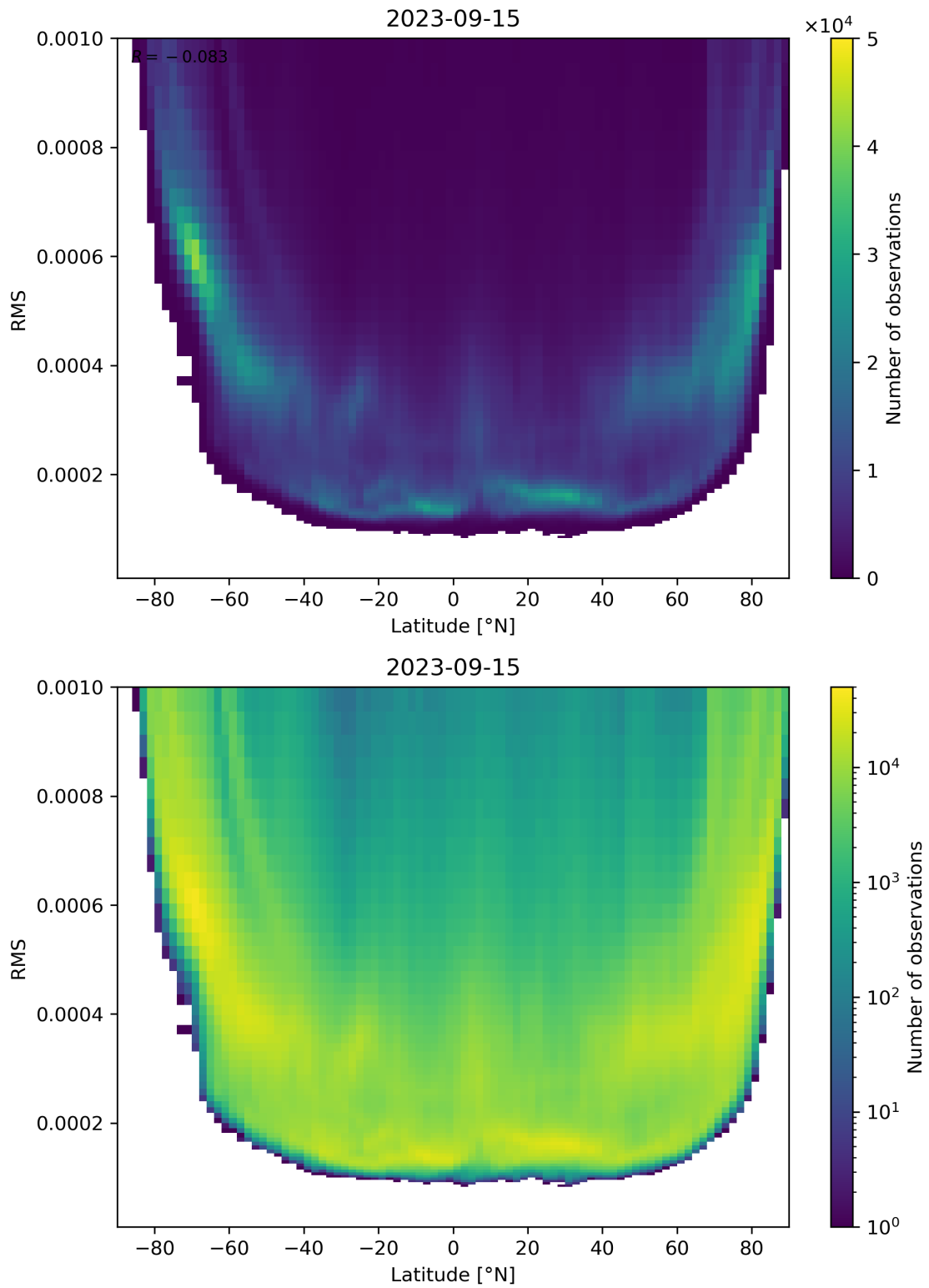
Figure 94: Scatter density plot of “Latitude” against “RMS” for 2023-09-15 to 2023-09-16.
