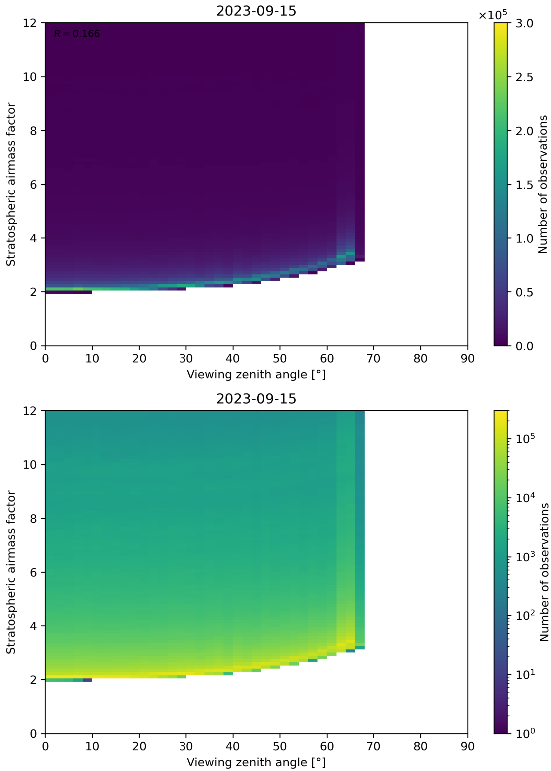
Figure 159: Scatter density plot of “Viewing zenith angle” against “Stratospheric airmass factor” for 2023-09-15 to 2023-09-16.
