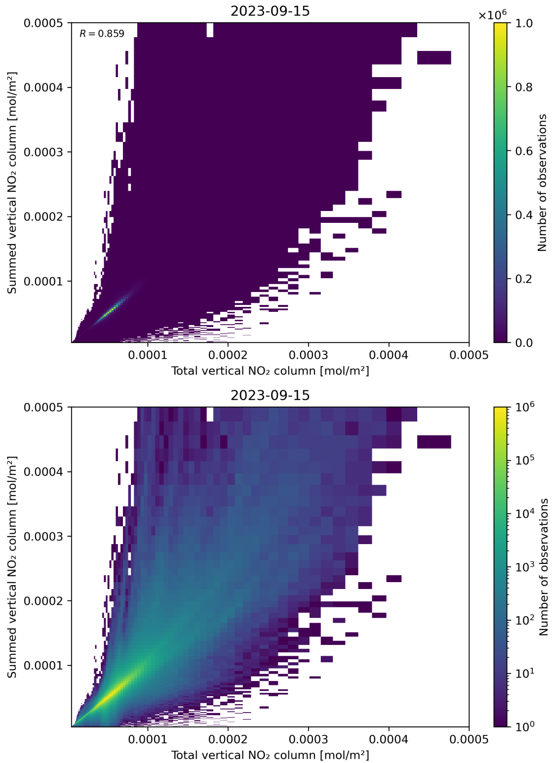
Figure 112: Scatter density plot of “Total vertical NO 2 column” against “Summed vertical NO 2 column” for 2023-09-15 to 2023-09-16.
