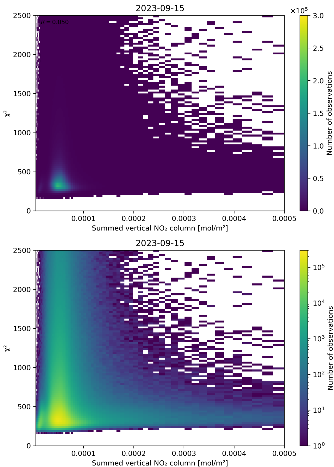
Figure 104: Scatter density plot of “Summed vertical NO 2 column” against “ \chi^2 ” for 2023-09-15 to 2023-09-16.
