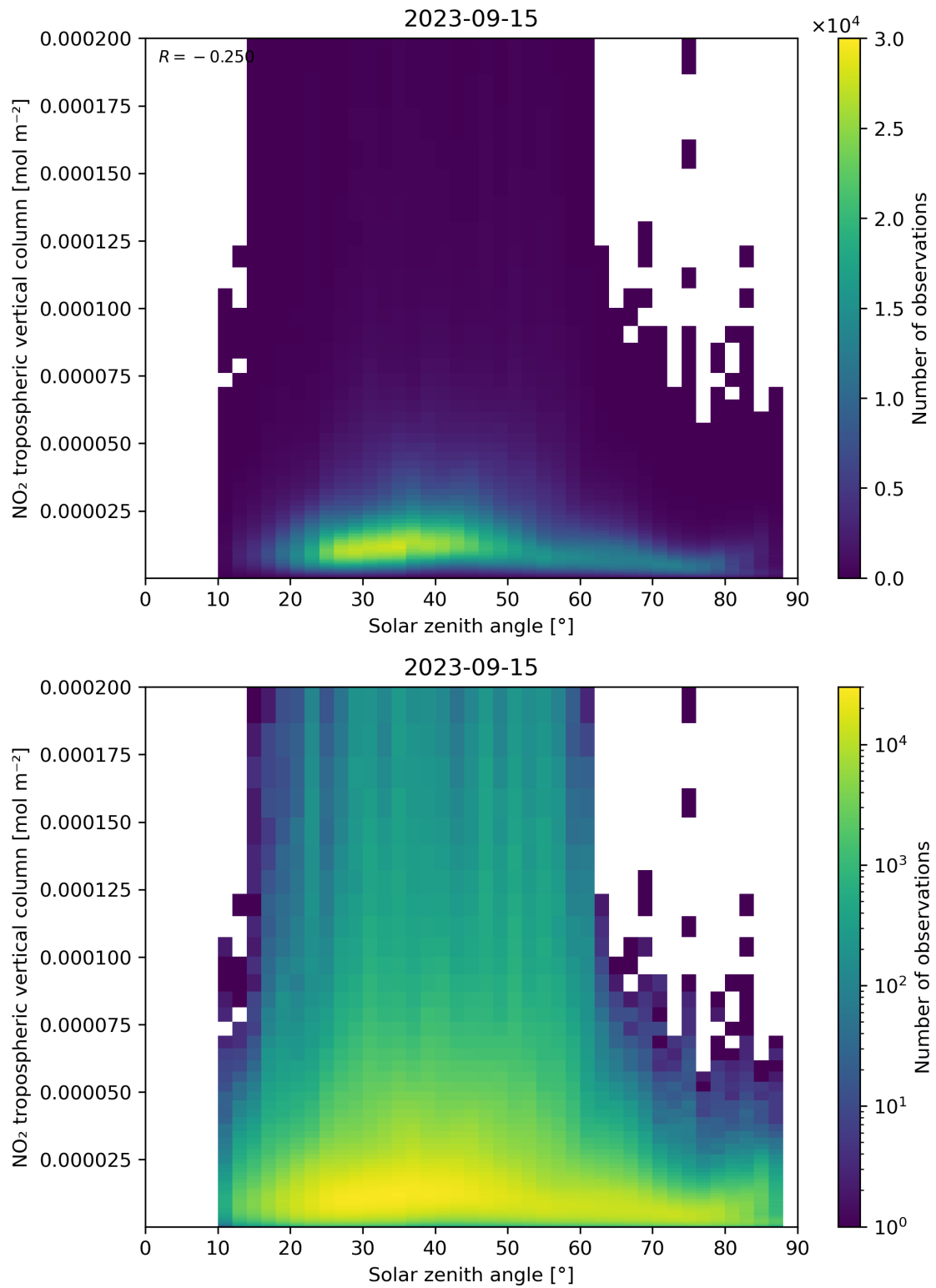
Figure 155: Scatter density plot of “Solar zenith angle” against “NO 2 tropospheric vertical column” for 2023-09-15 to 2023-09-16.
