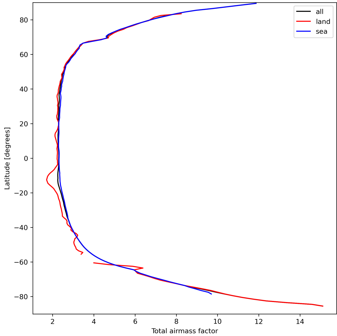
Figure 15: Zonal average of “Total airmass factor” for 2023-09-15 to 2023-09-16.
