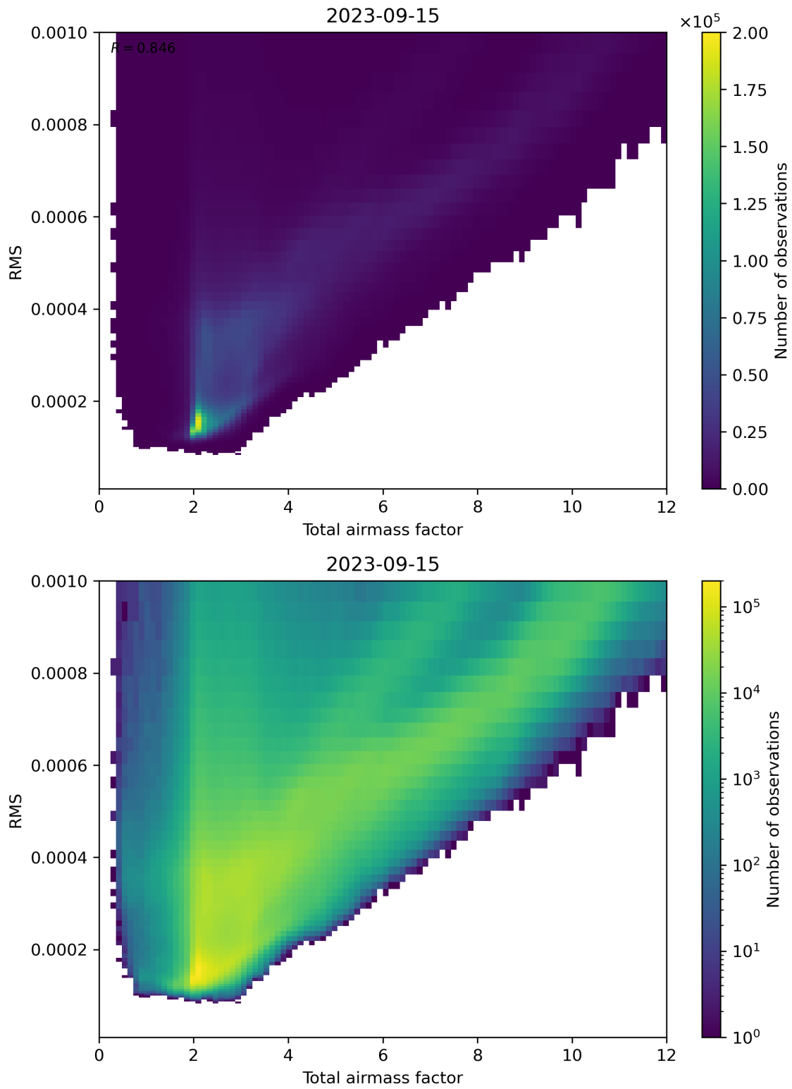
Figure 69: Scatter density plot of “Total airmass factor” against “RMS” for 2023-09-15 to 2023-09-16.
