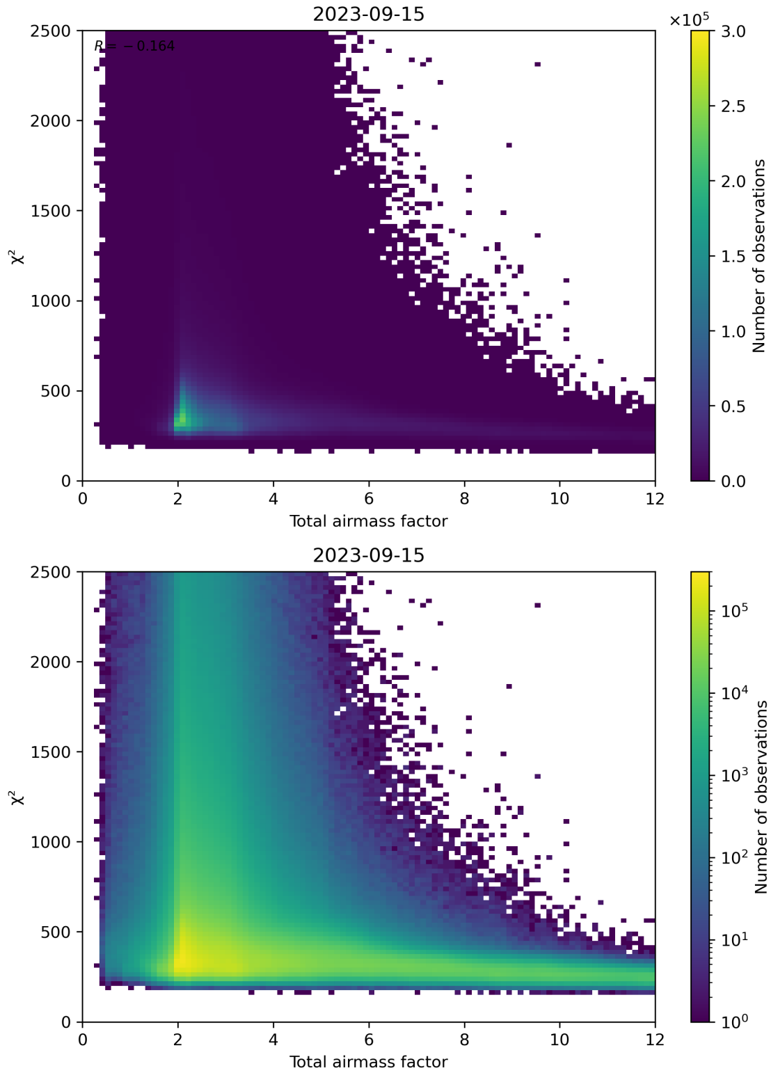
Figure 63: Scatter density plot of “Total airmass factor” against “ \chi^2 ” for 2023-09-15 to 2023-09-16.
