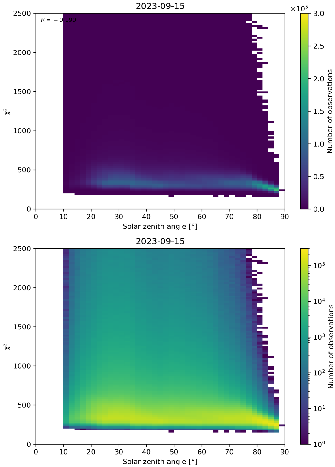
Figure 148: Scatter density plot of “Solar zenith angle” against “ \chi^2 ” for 2023-09-15 to 2023-09-16.
