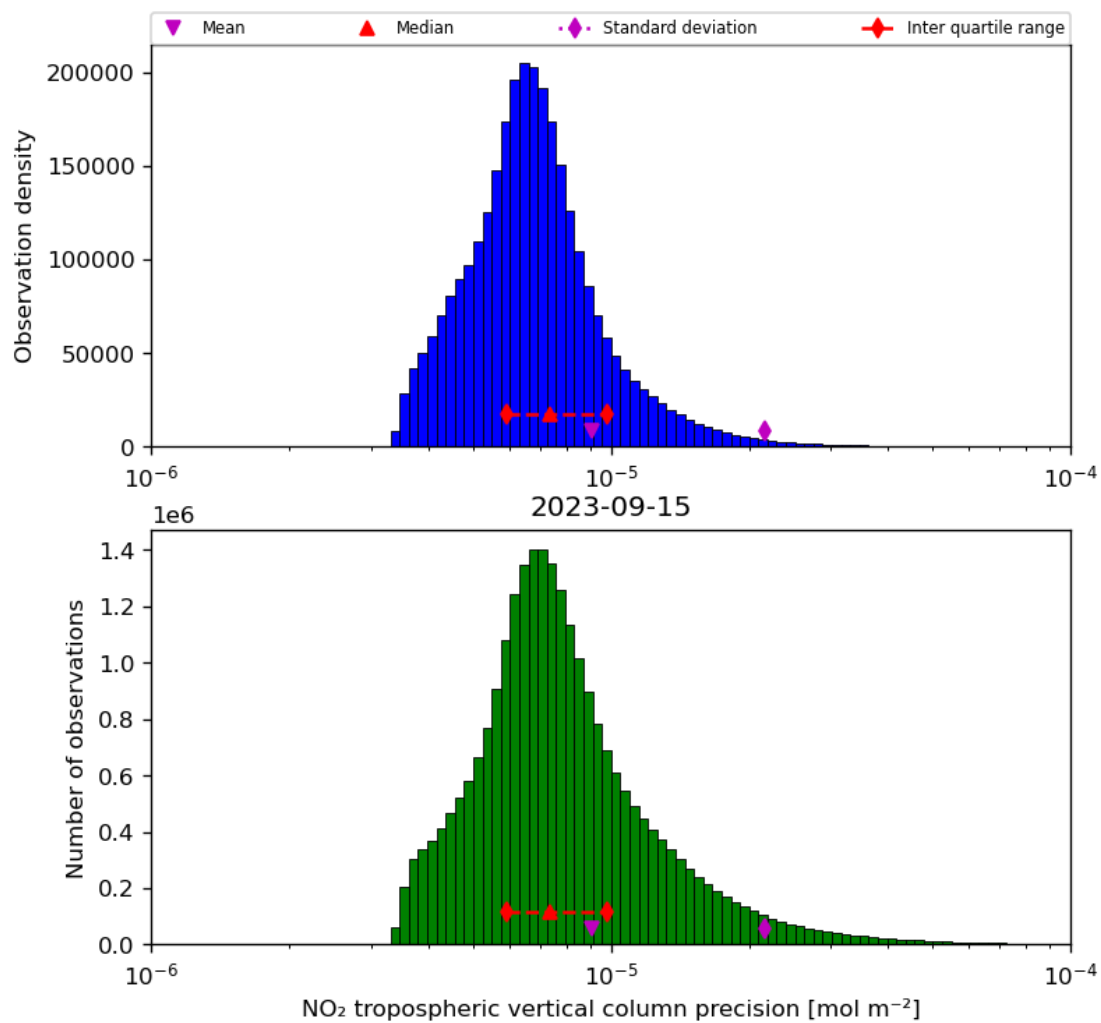
Figure 30: Histogram of “NO 2 tropospheric vertical column precision” for 2023-09-15 to 2023-09-16
