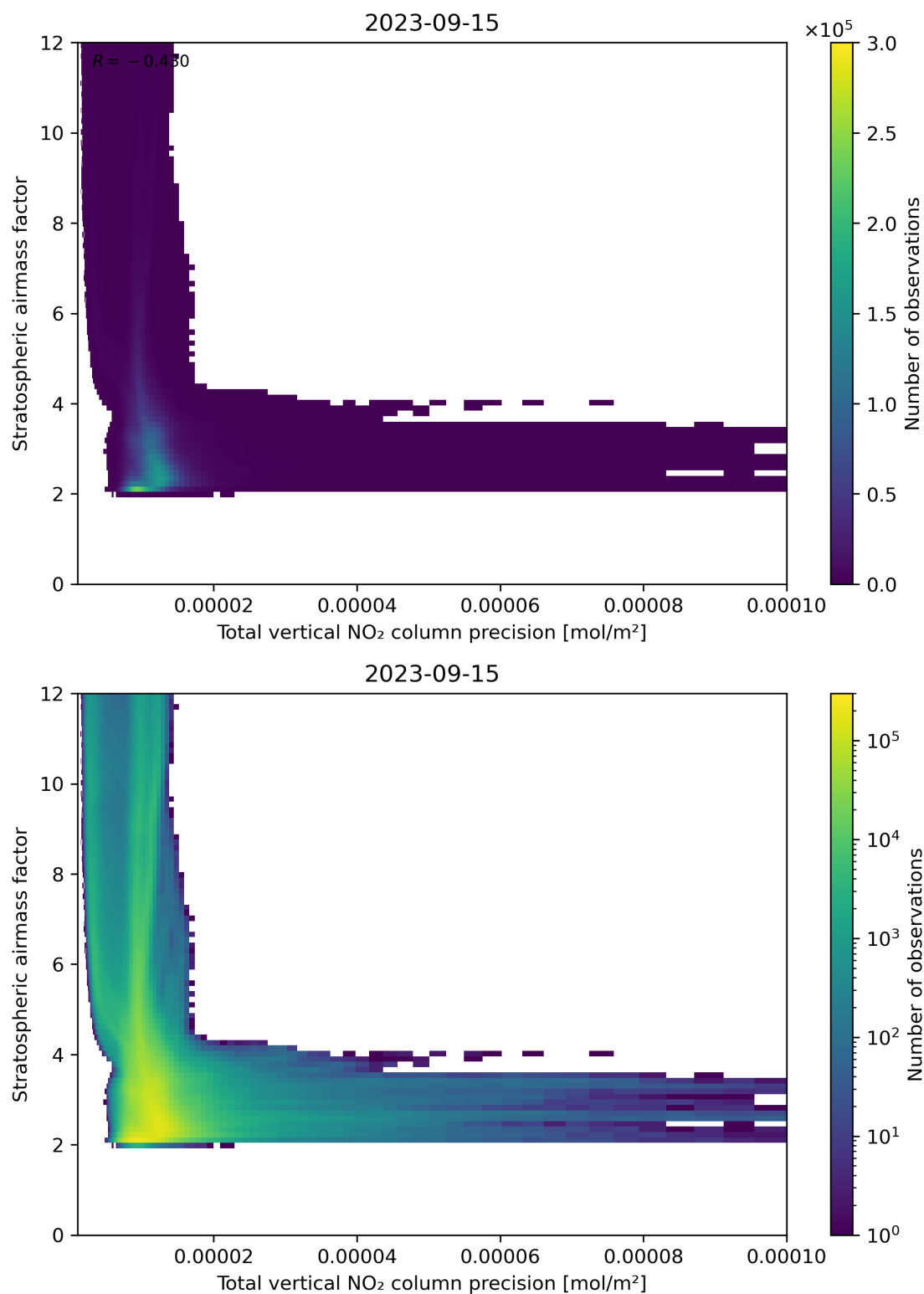
Figure 115: Scatter density plot of “Total vertical NO 2 column precision” against “Stratospheric air mass factor” for 2023-09-15 to 2023-09-16.
