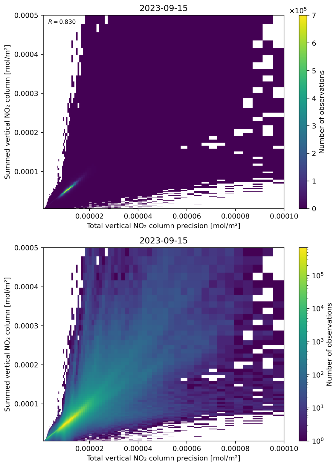
Figure 117: Scatter density plot of “Total vertical NO 2 column precision” against “Summed vertical NO 2 column” for 2023-09-15 to 2023-09-16.
