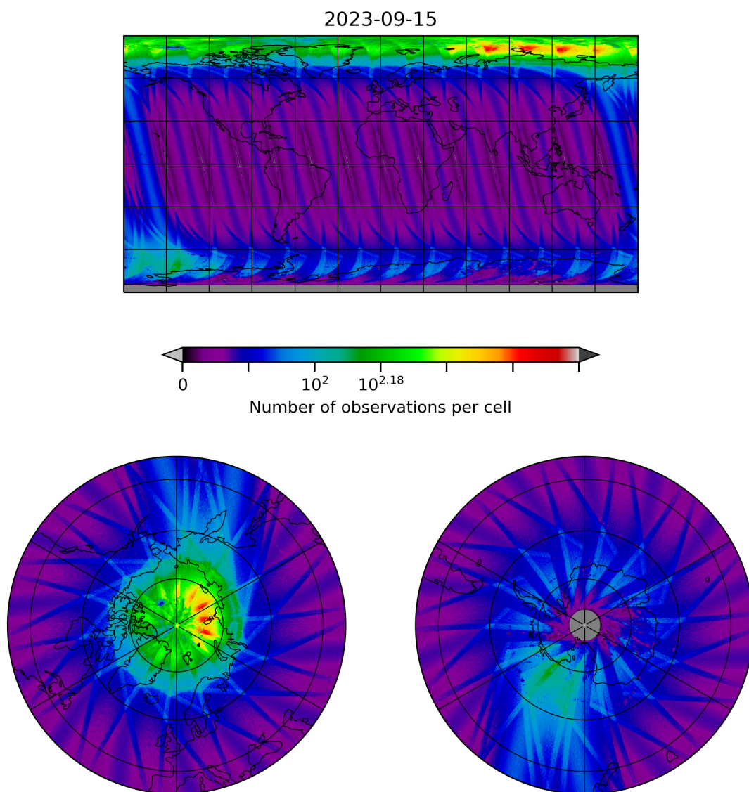
Figure 10: Map of the number of observations for 2023-09-15 to 2023-09-16
