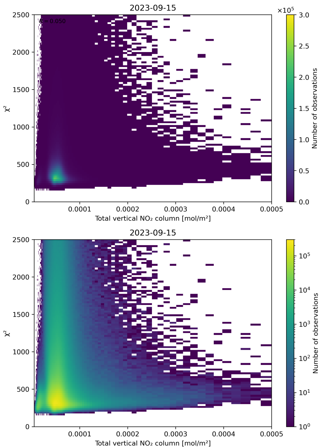
Figure 111: Scatter density plot of “Total vertical NO 2 column” against “ \chi^2 ” for 2023-09-15 to 2023-09-16.
