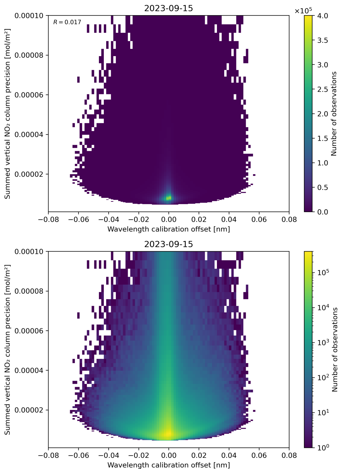
Figure 178: Scatter density plot of “Wavelength calibration offset” against “Summed vertical NO 2 column precision” for 2023-09-15 to 2023-09-16.
