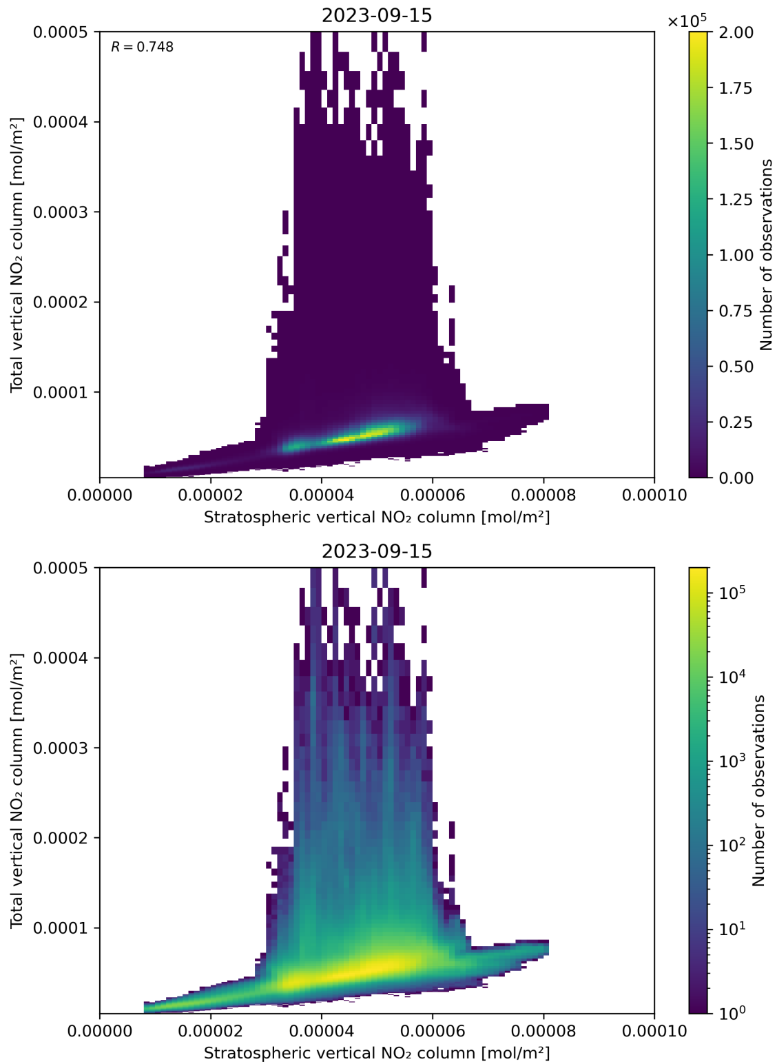
Figure 100: Scatter density plot of “Stratospheric vertical NO 2 column” against “Total vertical NO 2 column” for 2023-09-15 to 2023-09-16.
