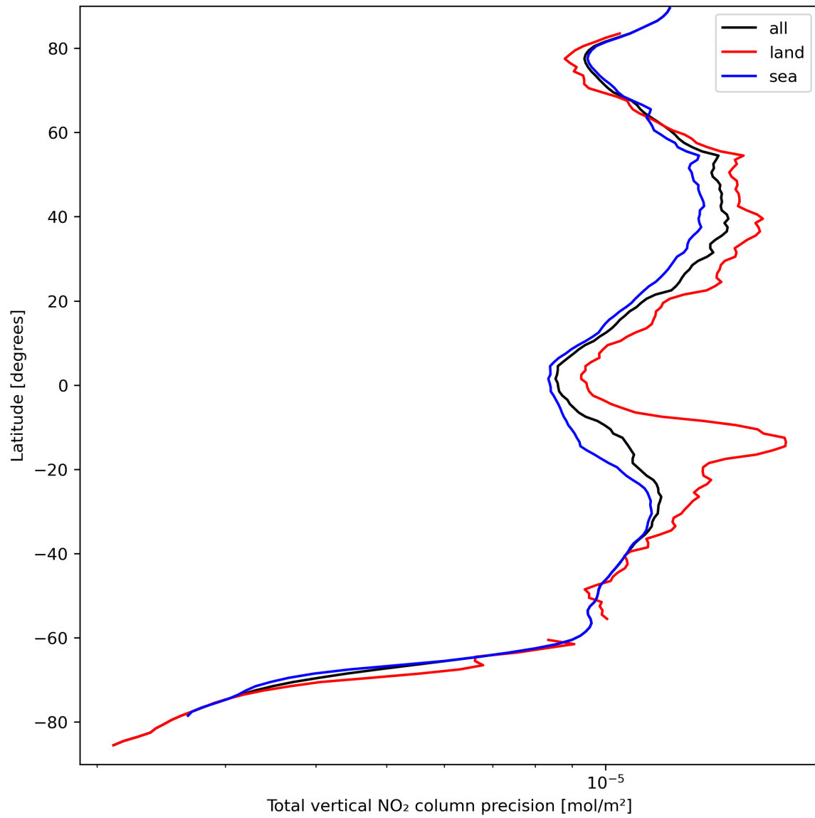
Figure 22: Zonal average of “Total vertical NO 2 column precision” for 2023-09-15 to 2023-09-16.
