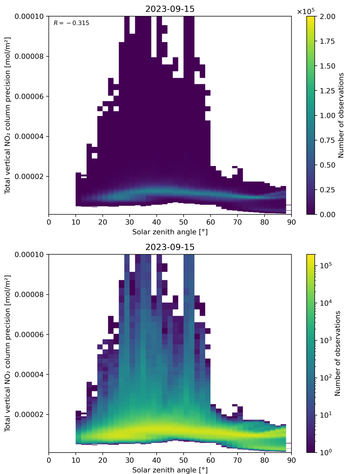
Figure 154: Scatter density plot of “Solar zenith angle” against “Total vertical NO 2 column precision” for 2023-09-15 to 2023-09-16.
