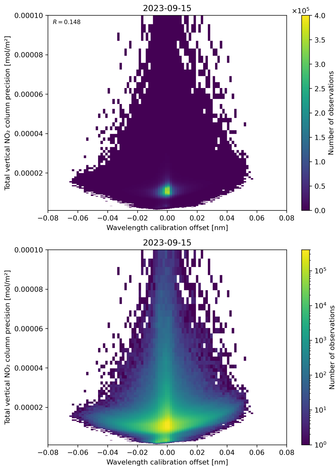
Figure 180: Scatter density plot of “Wavelength calibration offset” against “Total vertical NO 2 column precision” for 2023-09-15 to 2023-09-16.
