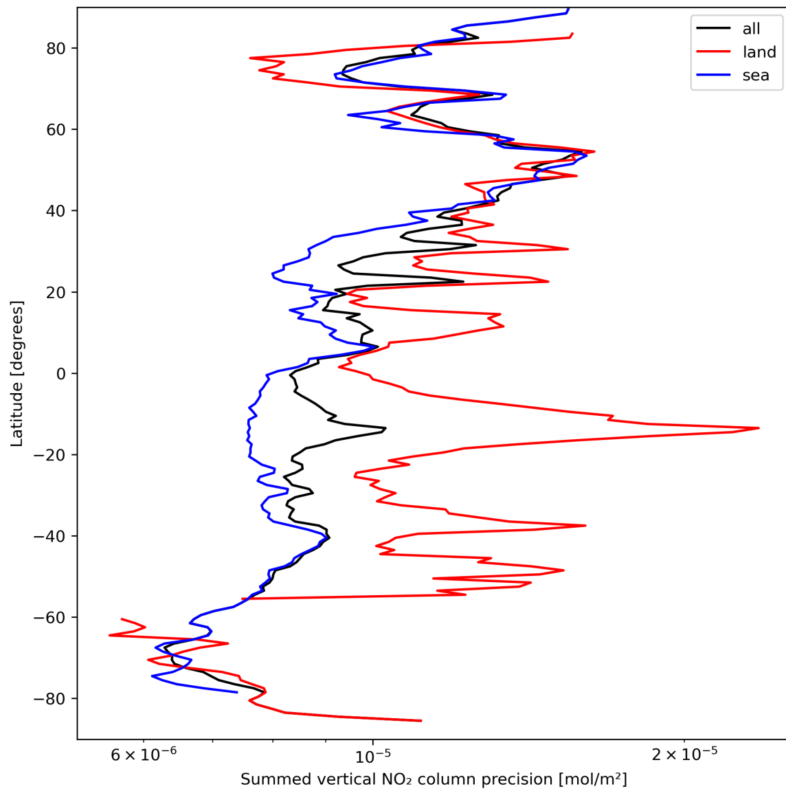
Figure 24: Zonal average of “Summed vertical NO 2 column precision” for 2023-09-15 to 2023-09-16.
