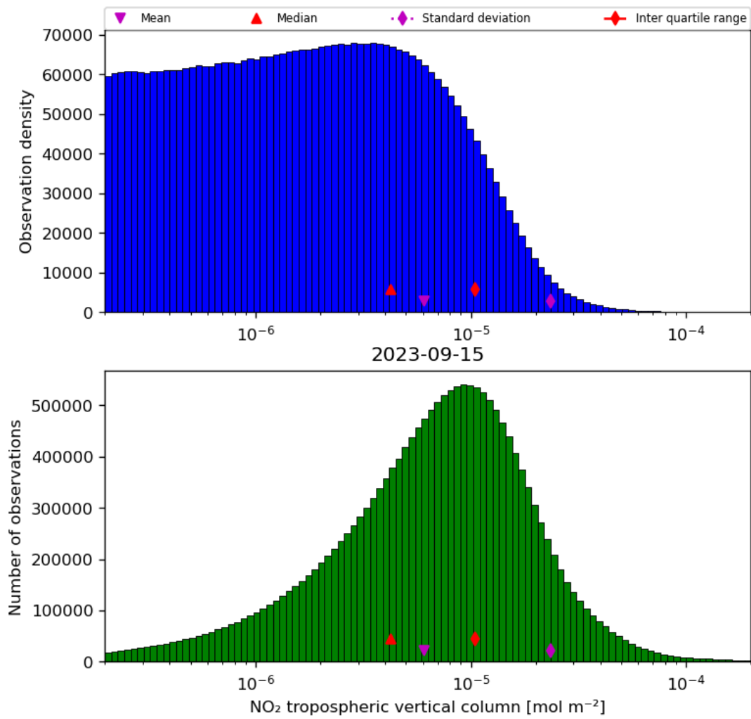
Figure 29: Histogram of “NO 2 tropospheric vertical column” for 2023-09-15 to 2023-09-16
