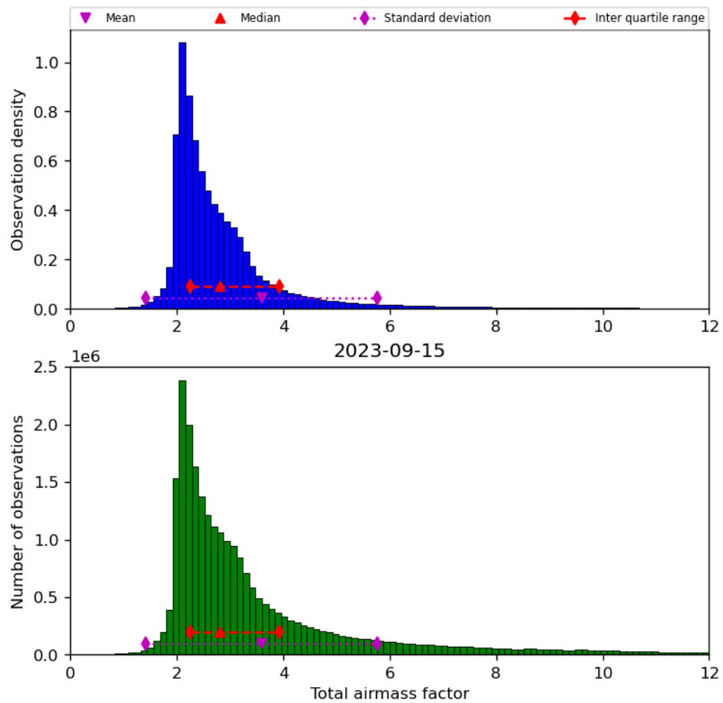
Figure 32: Histogram of “Total airmass factor” for 2023-09-15 to 2023-09-16
