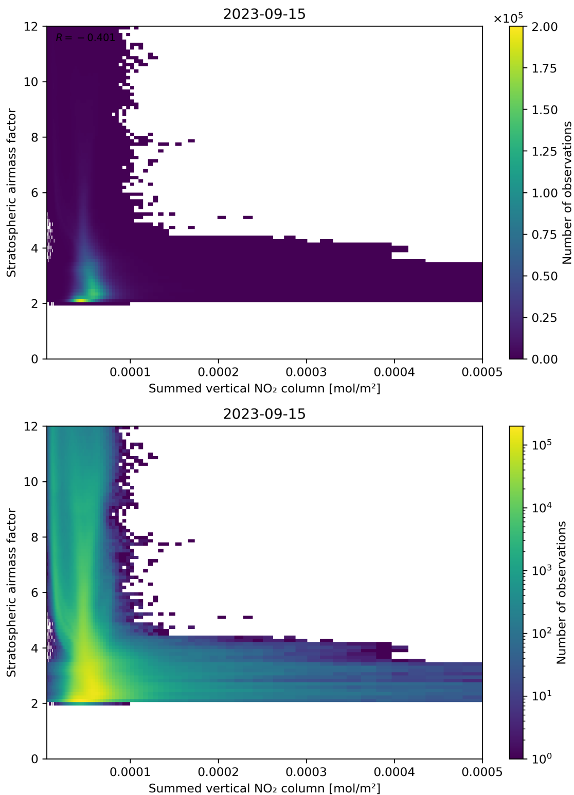
Figure 103: Scatter density plot of “Summed vertical NO 2 column” against “Stratospheric air mass factor” for 2023-09-15 to 2023-09-16.
