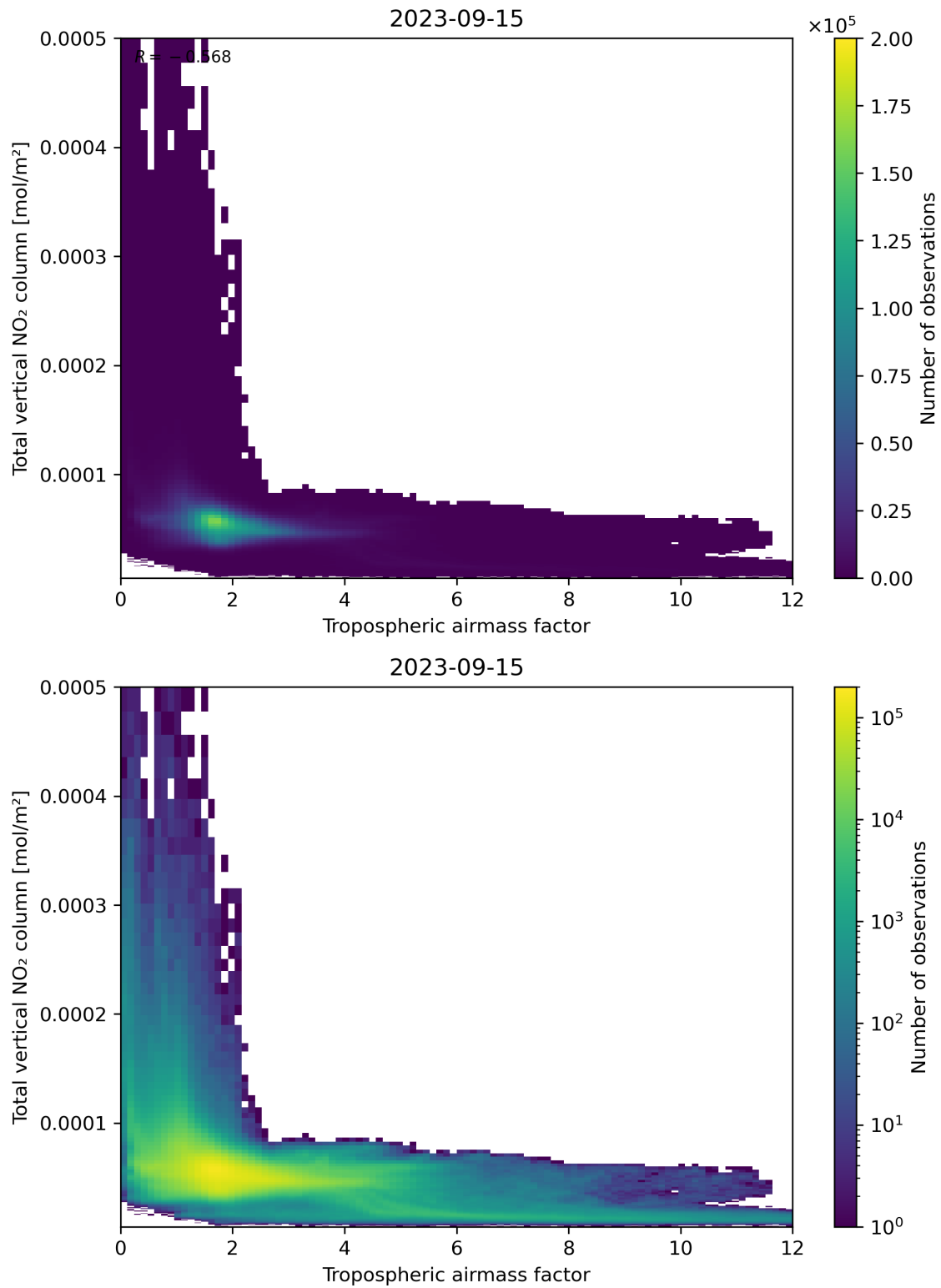
Figure 77: Scatter density plot of “Tropospheric airmass factor” against “Total vertical NO 2 column” for 2023-09-15 to 2023-09-16.
