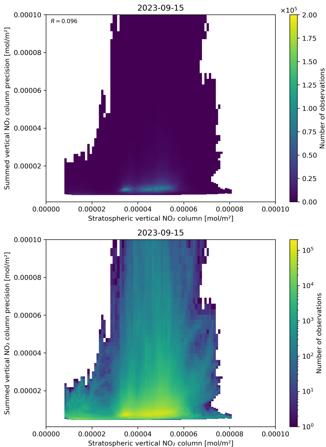
Figure 99: Scatter density plot of “Stratospheric vertical NO 2 column” against “Summed vertical NO 2 column precision” for 2023-09-15 to 2023-09-16.
