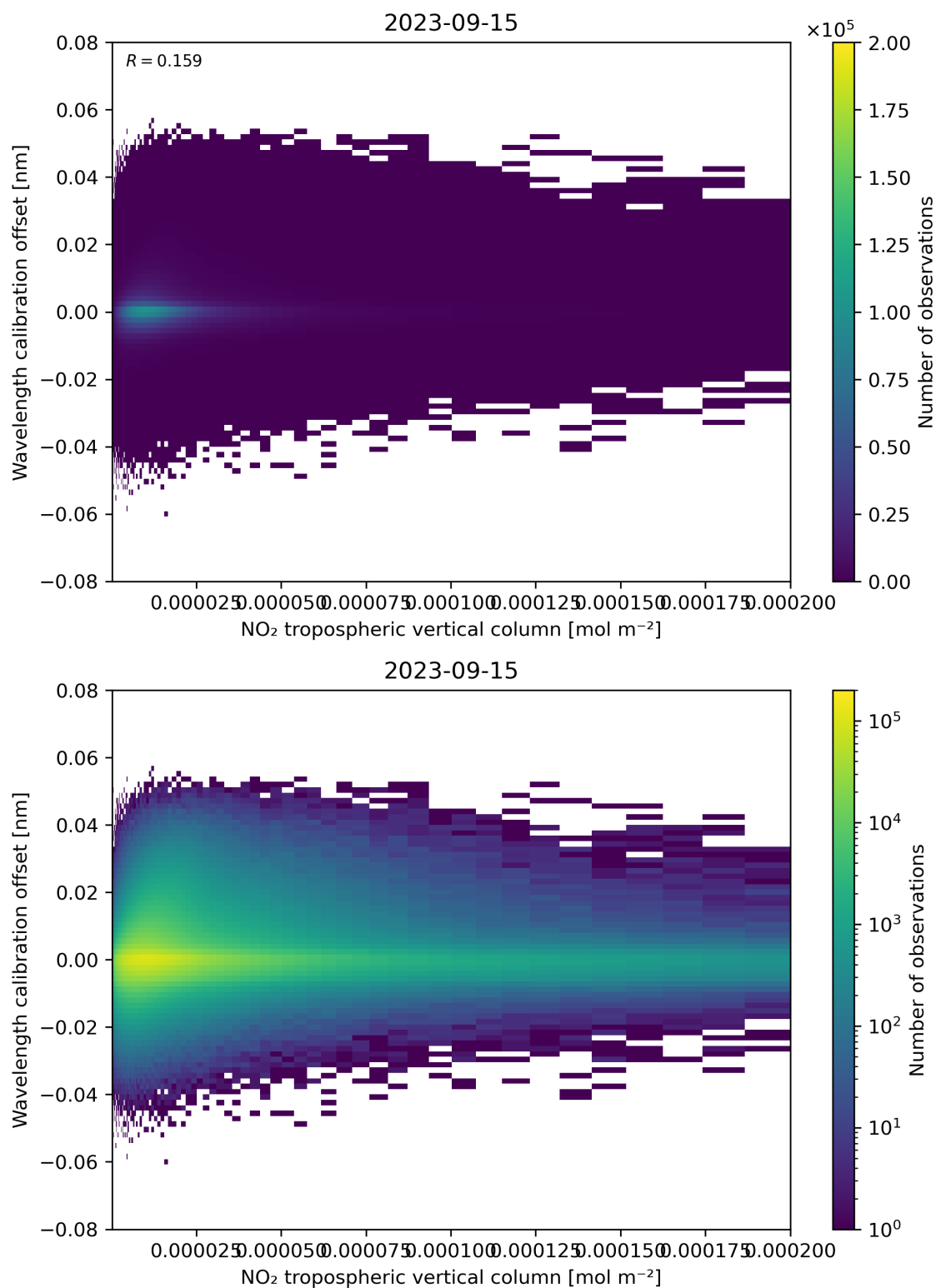
Figure 143: Scatter density plot of “NO 2 tropospheric vertical column” against “Wavelength calibration offset” for 2023-09-15 to 2023-09-16.
