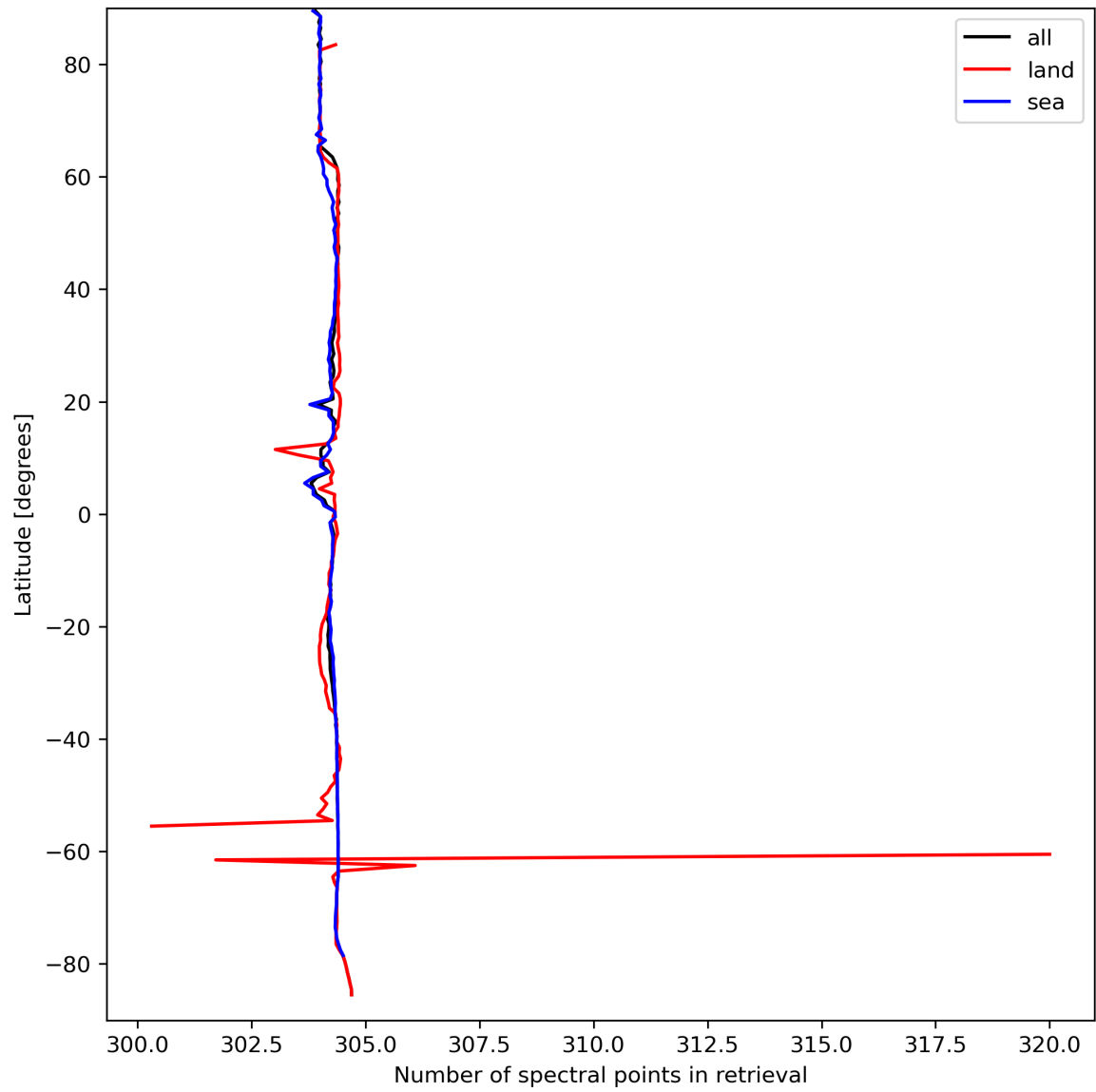
Figure 16: Zonal average of “Number of spectral points in retrieval” for 2023-09-15 to 2023-09-16.
