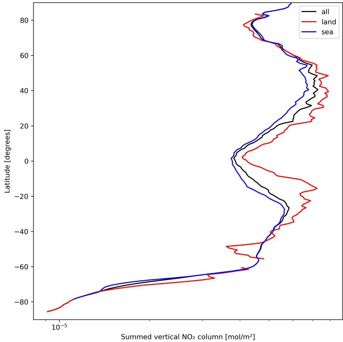
Figure 23: Zonal average of “Summed vertical NO 2 column” for 2023-09-15 to 2023-09-16.
