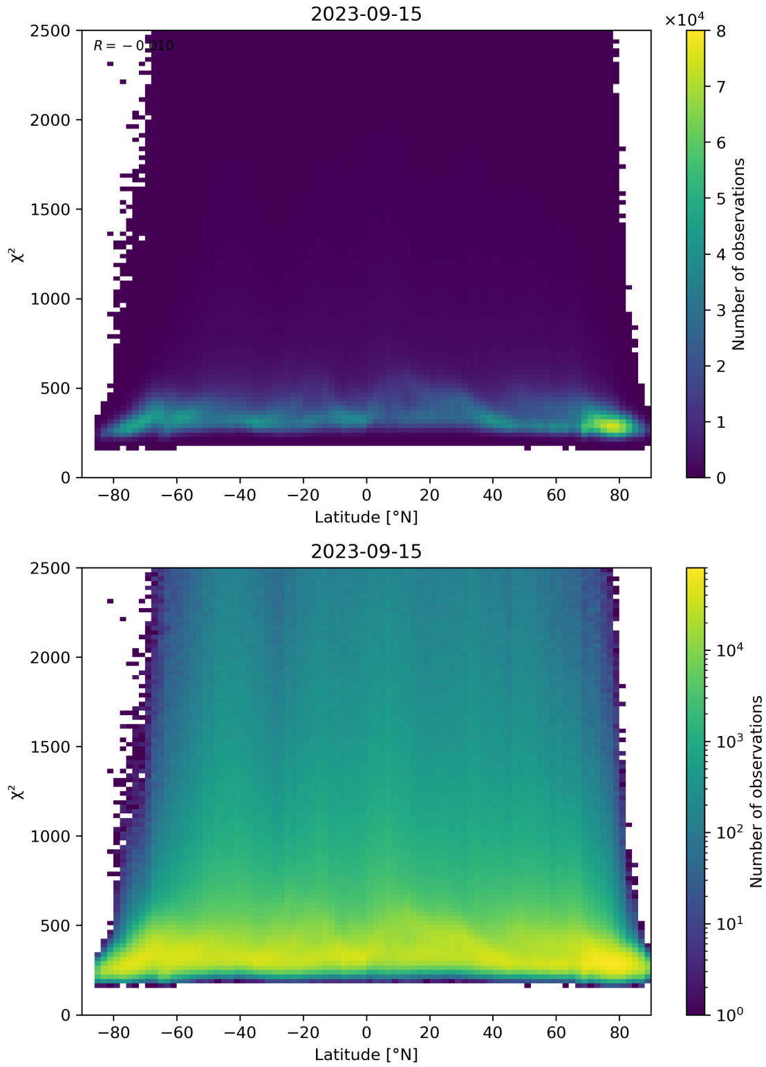
Figure 86: Scatter density plot of “Latitude” against “ \chi^2 ” for 2023-09-15 to 2023-09-16.
