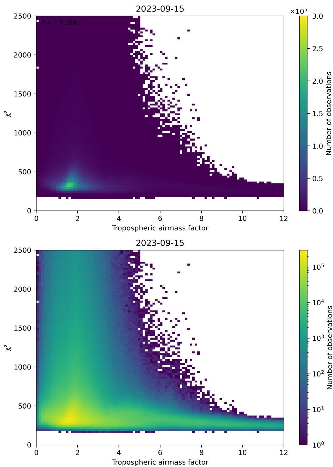
Figure 73: Scatter density plot of “Tropospheric airmass factor” against “ \chi^2 ” for 2023-09-15 to 2023-09-16.
