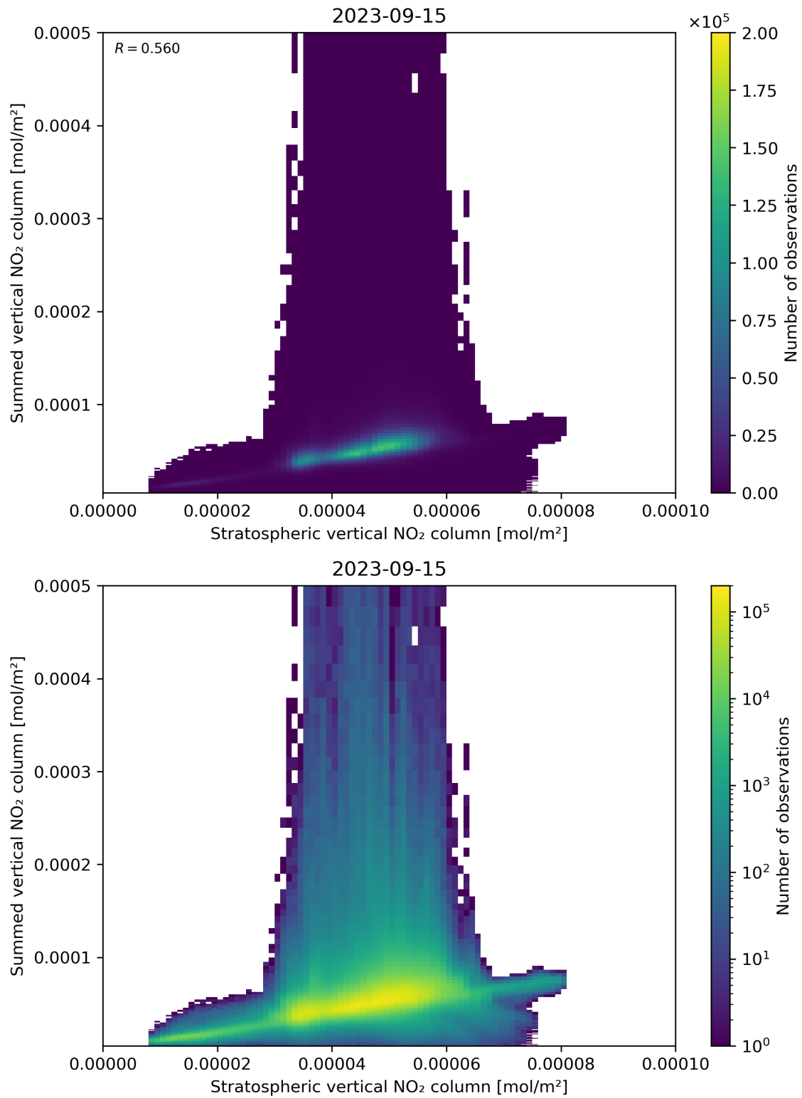
Figure 98: Scatter density plot of “Stratospheric vertical NO 2 column” against “Summed vertical NO 2 column” for 2023-09-15 to 2023-09-16.
