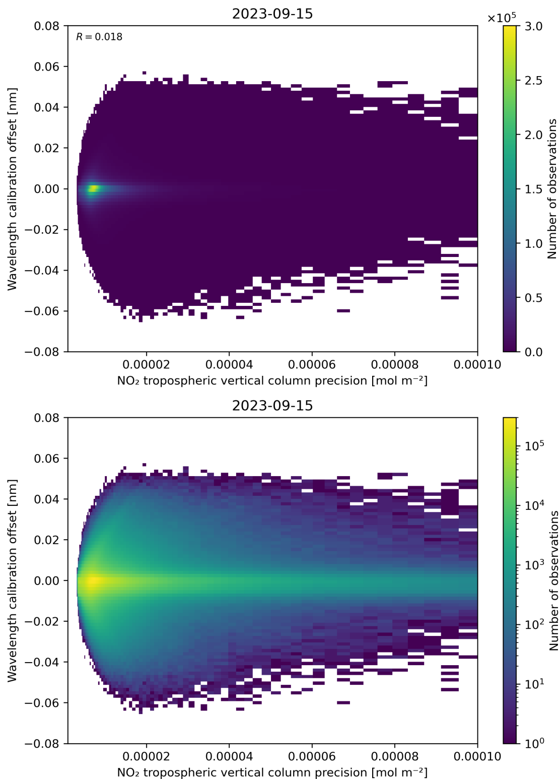
Figure 141: Scatter density plot of “NO 2 tropospheric vertical column precision” against “Wavelength calibration offset” for 2023-09-15 to 2023-09-16.
