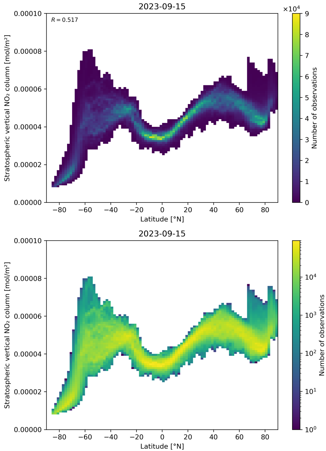
Figure 87: Scatter density plot of “Latitude” against “Stratospheric vertical \text{NO}_2 column” for 2023-09-15 to 2023-09-16.
