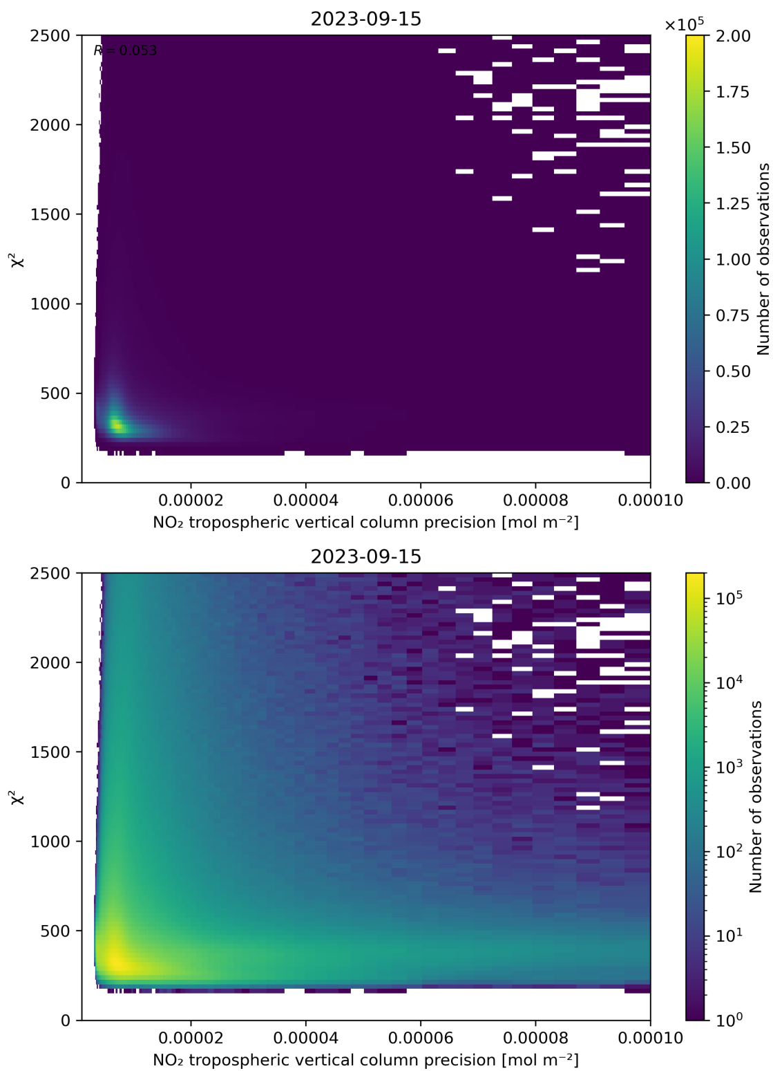
Figure 134: Scatter density plot of “NO 2 tropospheric vertical column precision” against “ \chi^2 ” for 2023-09-15 to 2023-09-16.
