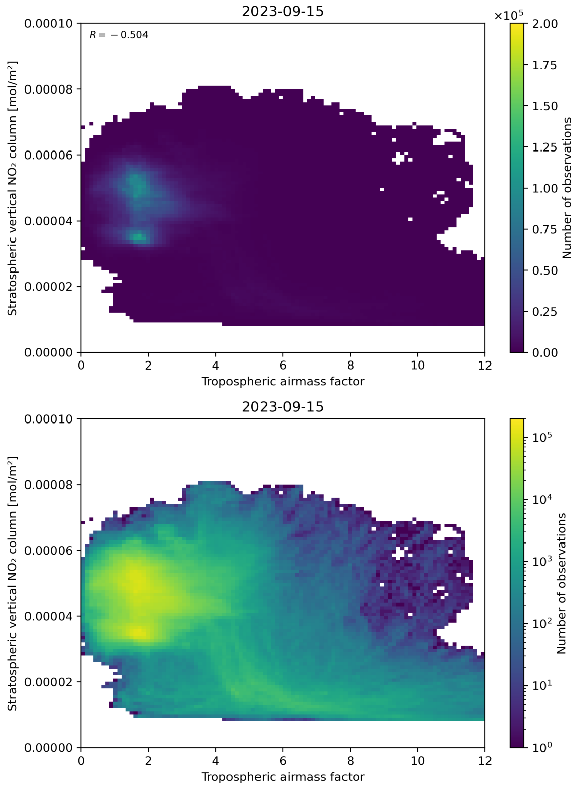
Figure 74: Scatter density plot of “Tropospheric air mass factor” against “Stratospheric vertical NO 2 column” for 2023-09-15 to 2023-09-16.
