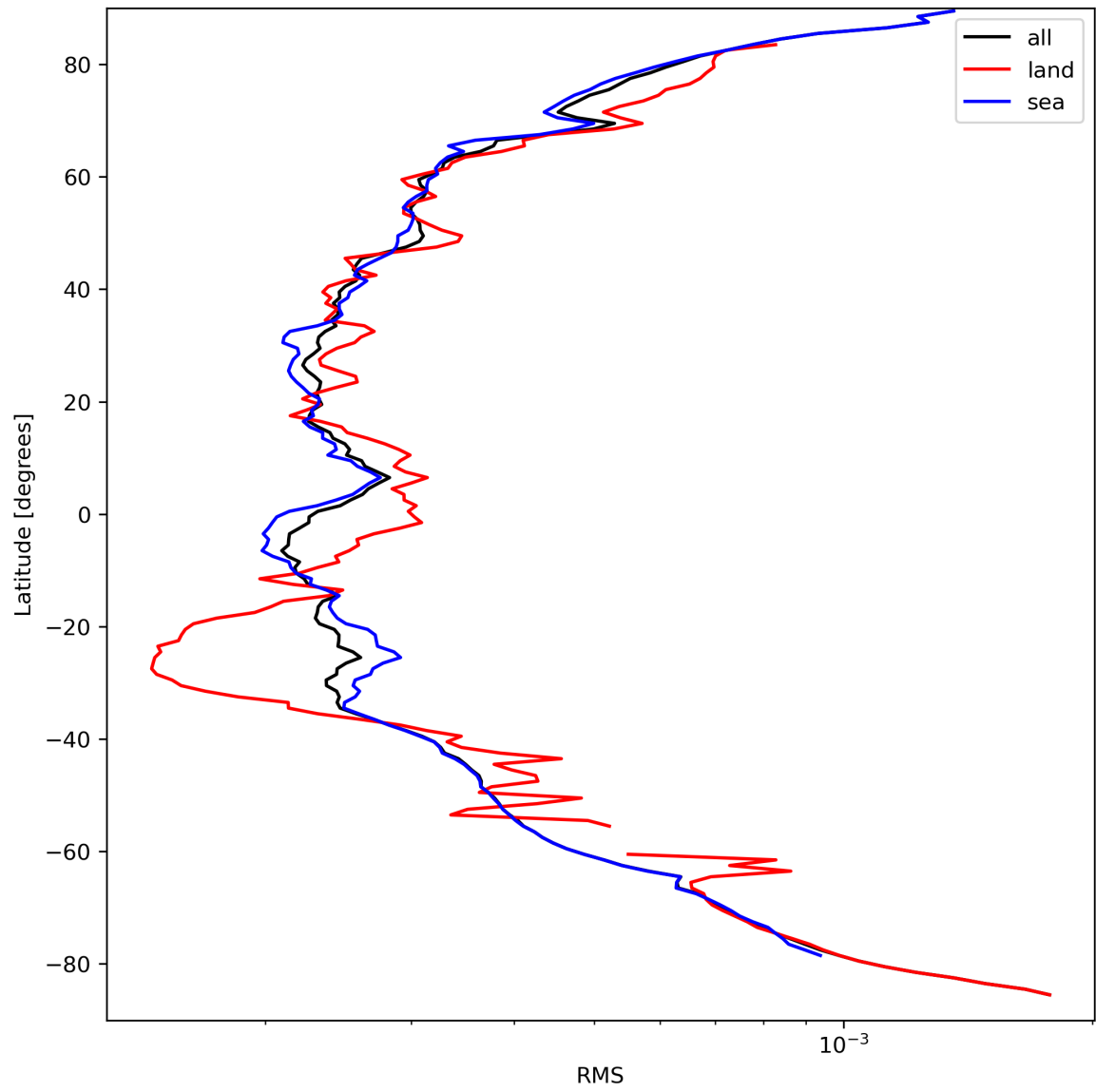
Figure 26: Zonal average of “RMS” for 2023-09-15 to 2023-09-16.
