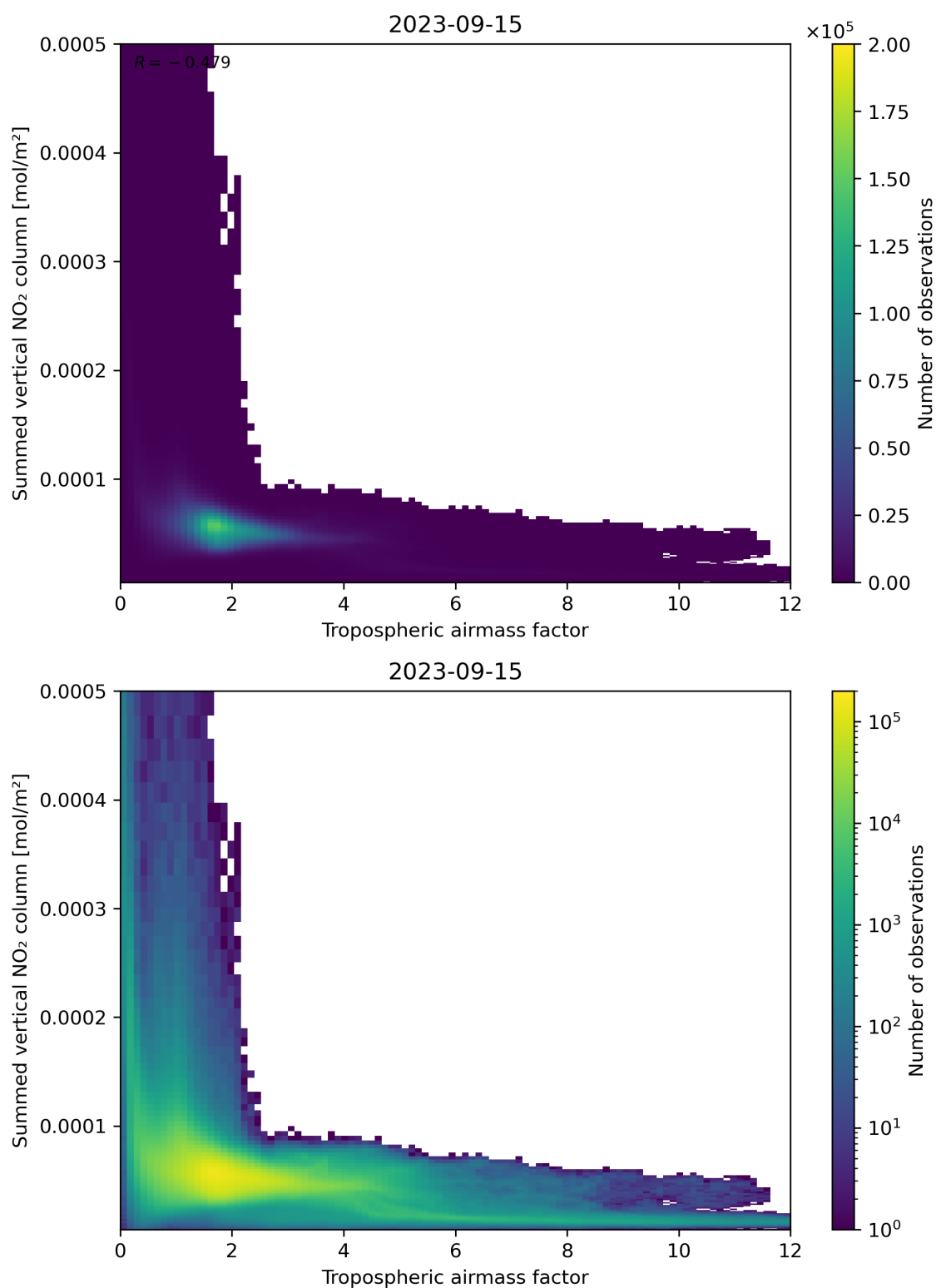
Figure 75: Scatter density plot of “Tropospheric air mass factor” against “Summed vertical NO 2 column” for 2023-09-15 to 2023-09-16.
