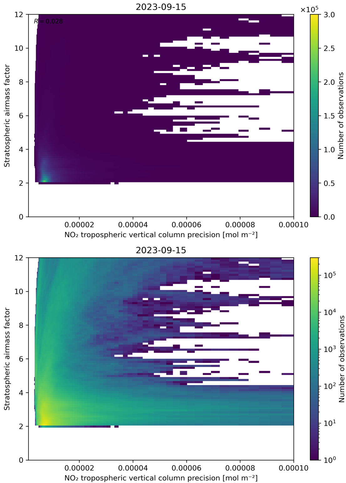
Figure 131: Scatter density plot of “NO 2 tropospheric vertical column precision” against “Stratospheric airmass factor” for 2023-09-15 to 2023-09-16.
