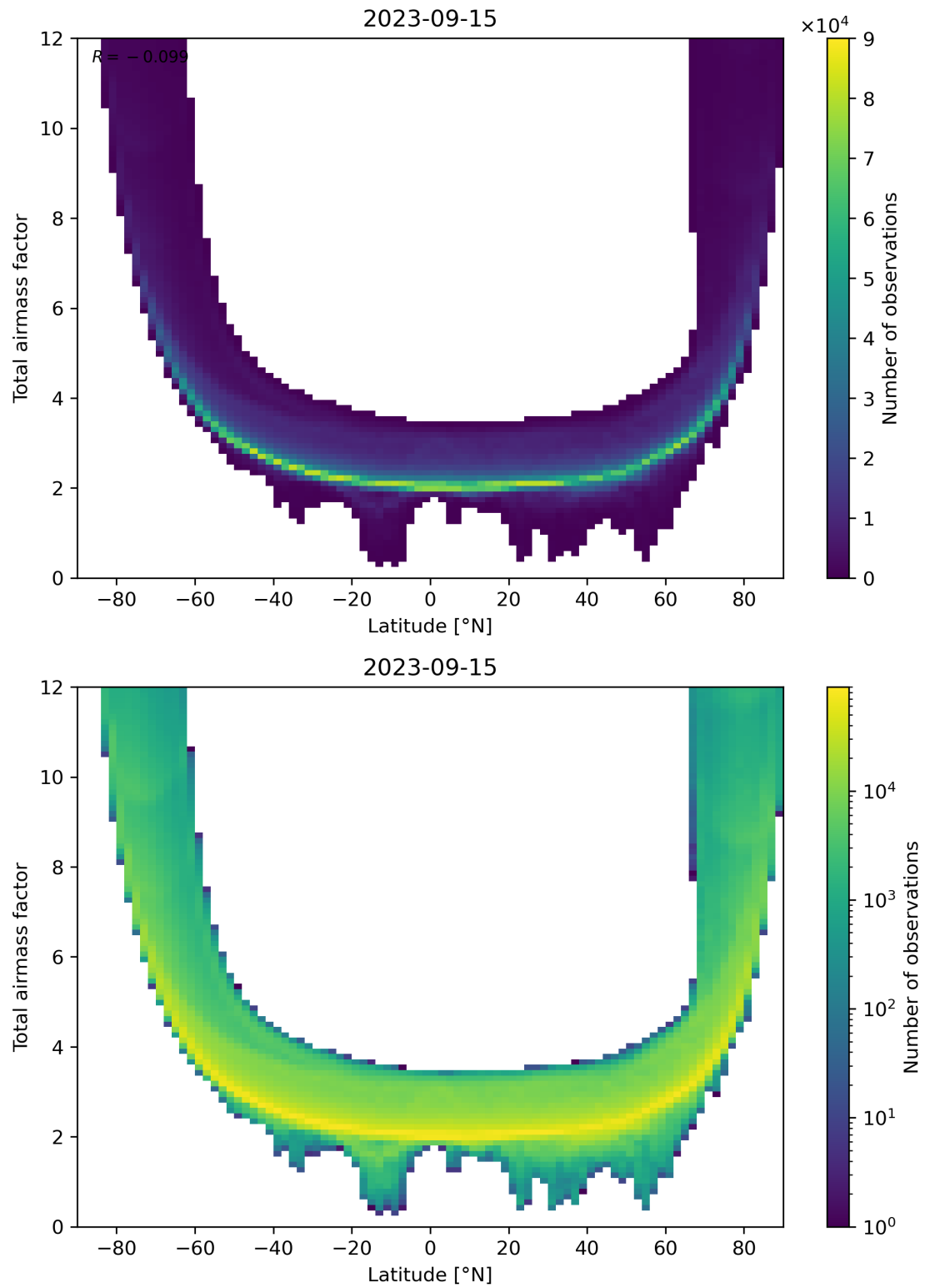
Figure 84: Scatter density plot of “Latitude” against “Total airmass factor” for 2023-09-15 to 2023-09-16.
