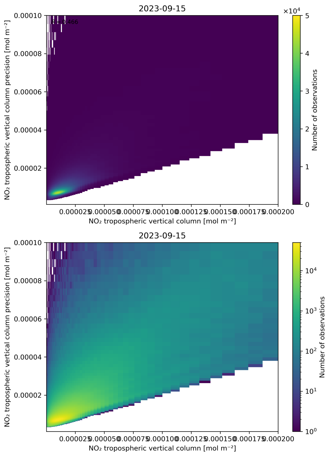
Figure 130: Scatter density plot of “NO 2 tropospheric vertical column” against “NO 2 tropospheric vertical column precision” for 2023-09-15 to 2023-09-16.
