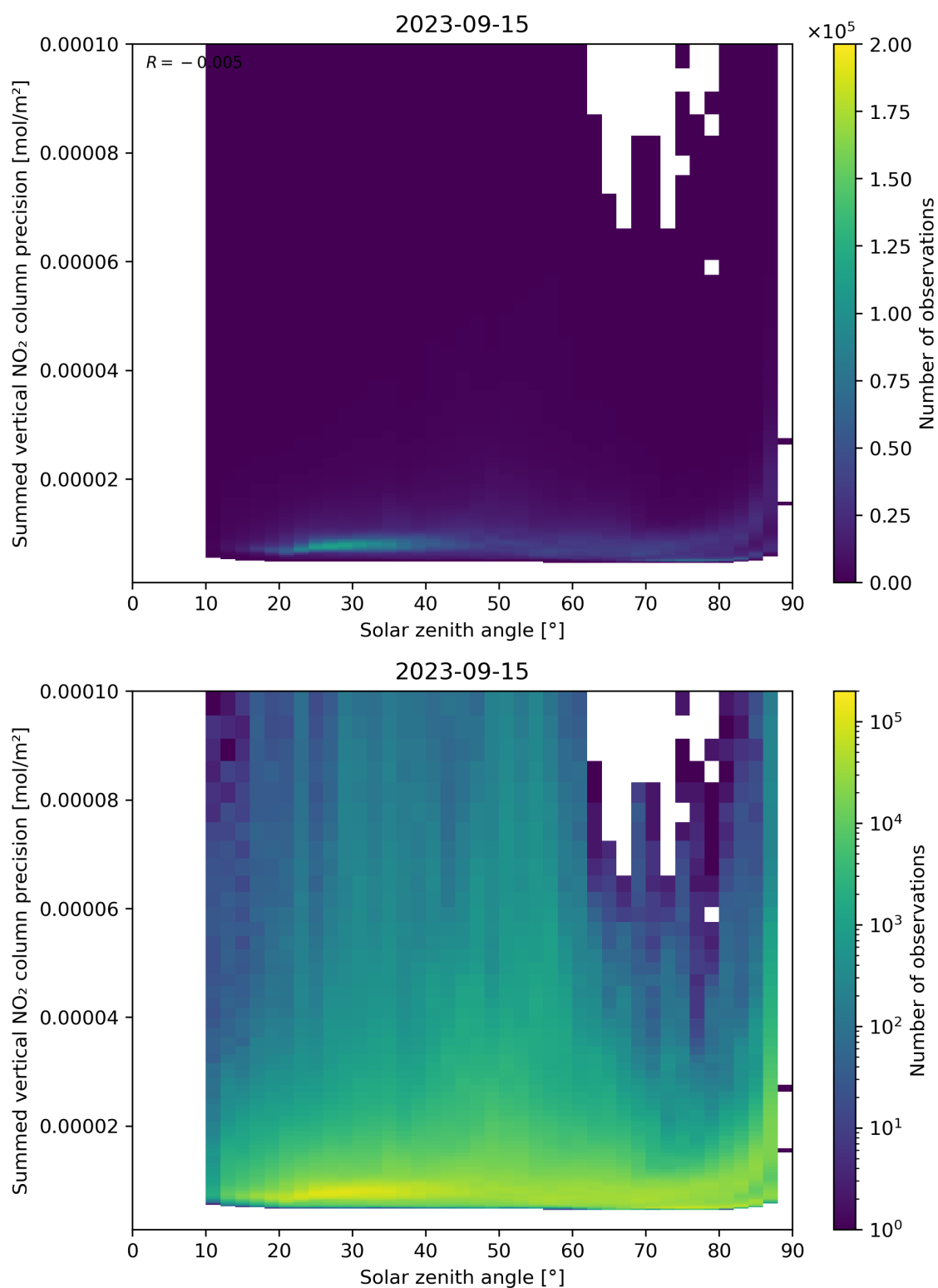
Figure 152: Scatter density plot of “Solar zenith angle” against “Summed vertical NO 2 column precision” for 2023-09-15 to 2023-09-16.
