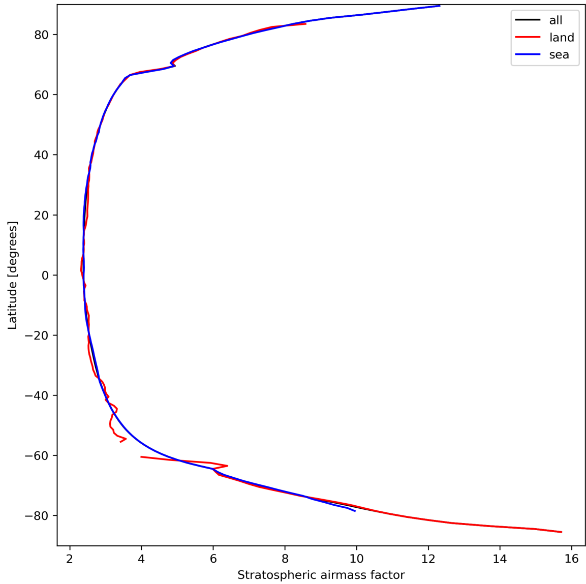
Figure 27: Zonal average of “Stratospheric air mass factor” for 2023-09-15 to 2023-09-16.
