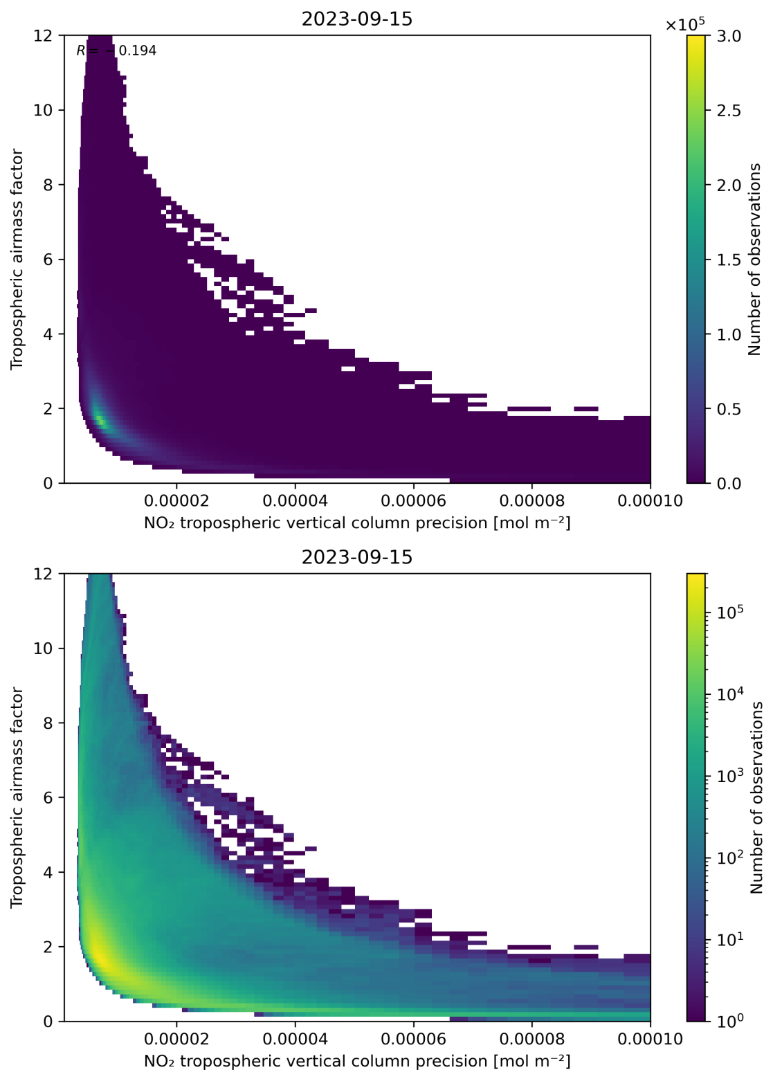
Figure 133: Scatter density plot of “NO 2 tropospheric vertical column precision” against “Tropospheric airmass factor” for 2023-09-15 to 2023-09-16.
