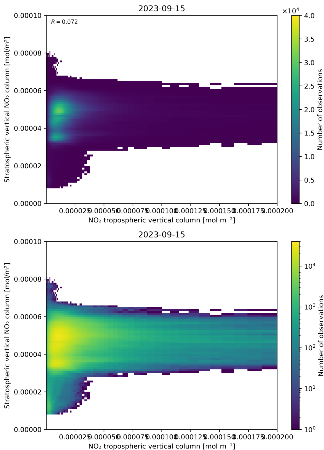
Figure 125: Scatter density plot of “NO 2 tropospheric vertical column” against “Stratospheric vertical NO 2 column” for 2023-09-15 to 2023-09-16.
