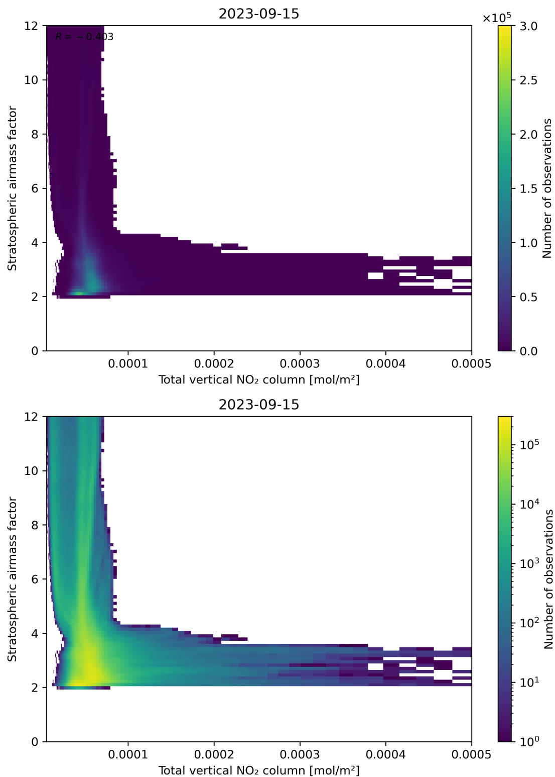
Figure 110: Scatter density plot of “Total vertical NO 2 column” against “Stratospheric air mass factor” for 2023-09-15 to 2023-09-16.
