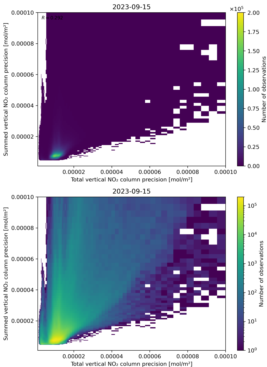
Figure 118: Scatter density plot of “Total vertical NO 2 column precision” against “Summed vertical NO 2 column precision” for 2023-09-15 to 2023-09-16.
