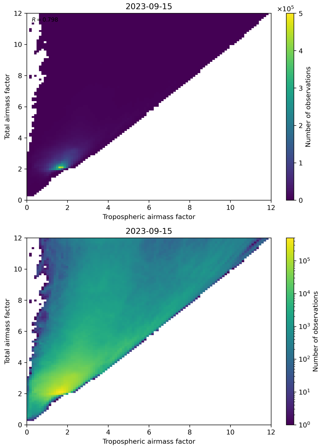
Figure 72: Scatter density plot of “Tropospheric airmass factor” against “Total airmass factor” for 2023-09-15 to 2023-09-16.
