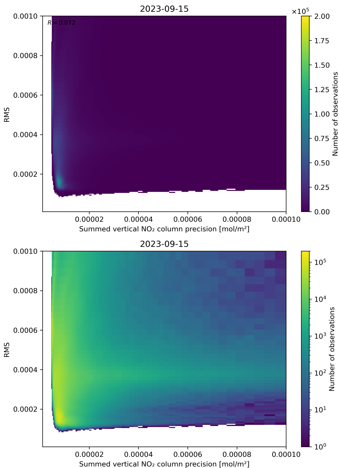
Figure 108: Scatter density plot of “Summed vertical NO 2 column precision” against “RMS” for 2023-09-15 to 2023-09-16.
