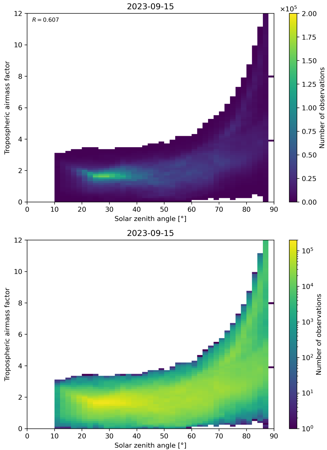
Figure 147: Scatter density plot of “Solar zenith angle” against “Tropospheric airmass factor” for 2023-09-15 to 2023-09-16.
