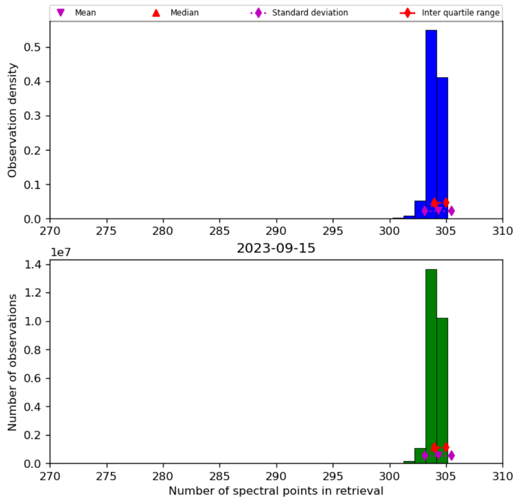
Figure 33: Histogram of “Number of spectral points in retrieval” for 2023-09-15 to 2023-09-16
