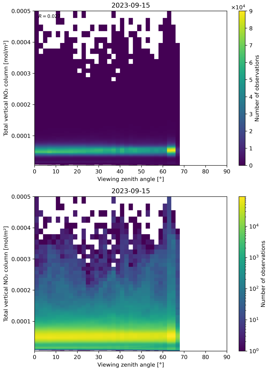
Figure 167: Scatter density plot of “Viewing zenith angle” against “Total vertical NO 2 column” for 2023-09-15 to 2023-09-16.
