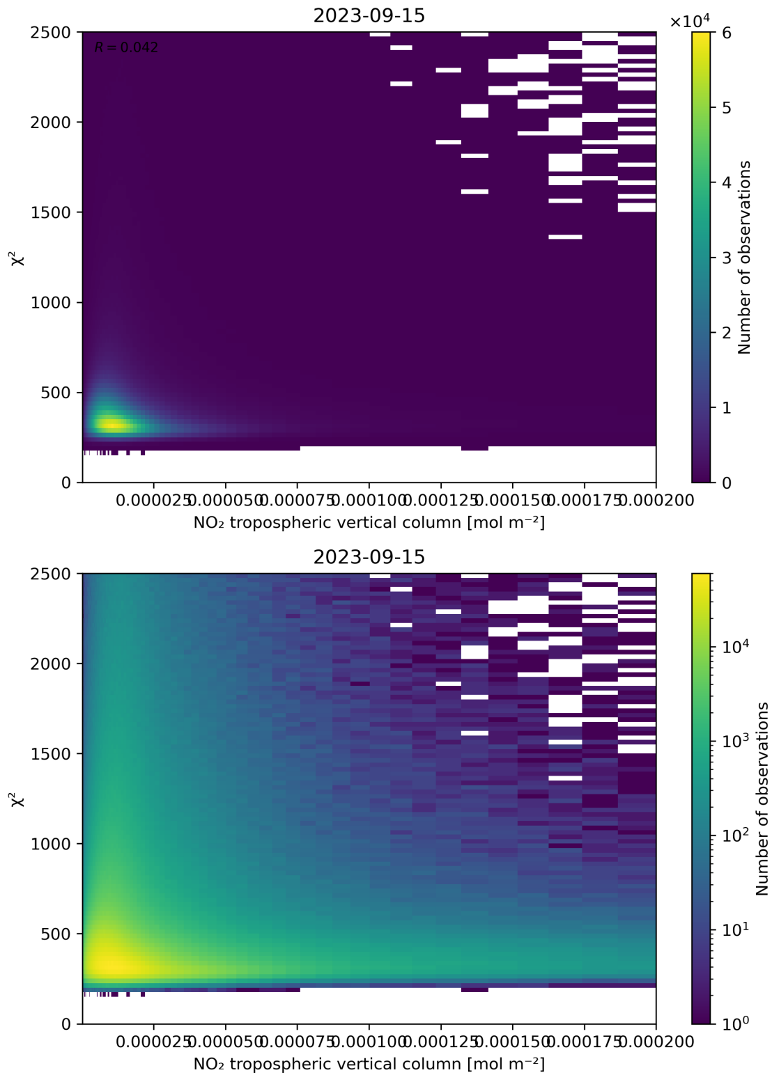
Figure 124: Scatter density plot of “NO 2 tropospheric vertical column” against “ \chi^2 ” for 2023-09-15 to 2023-09-16.
