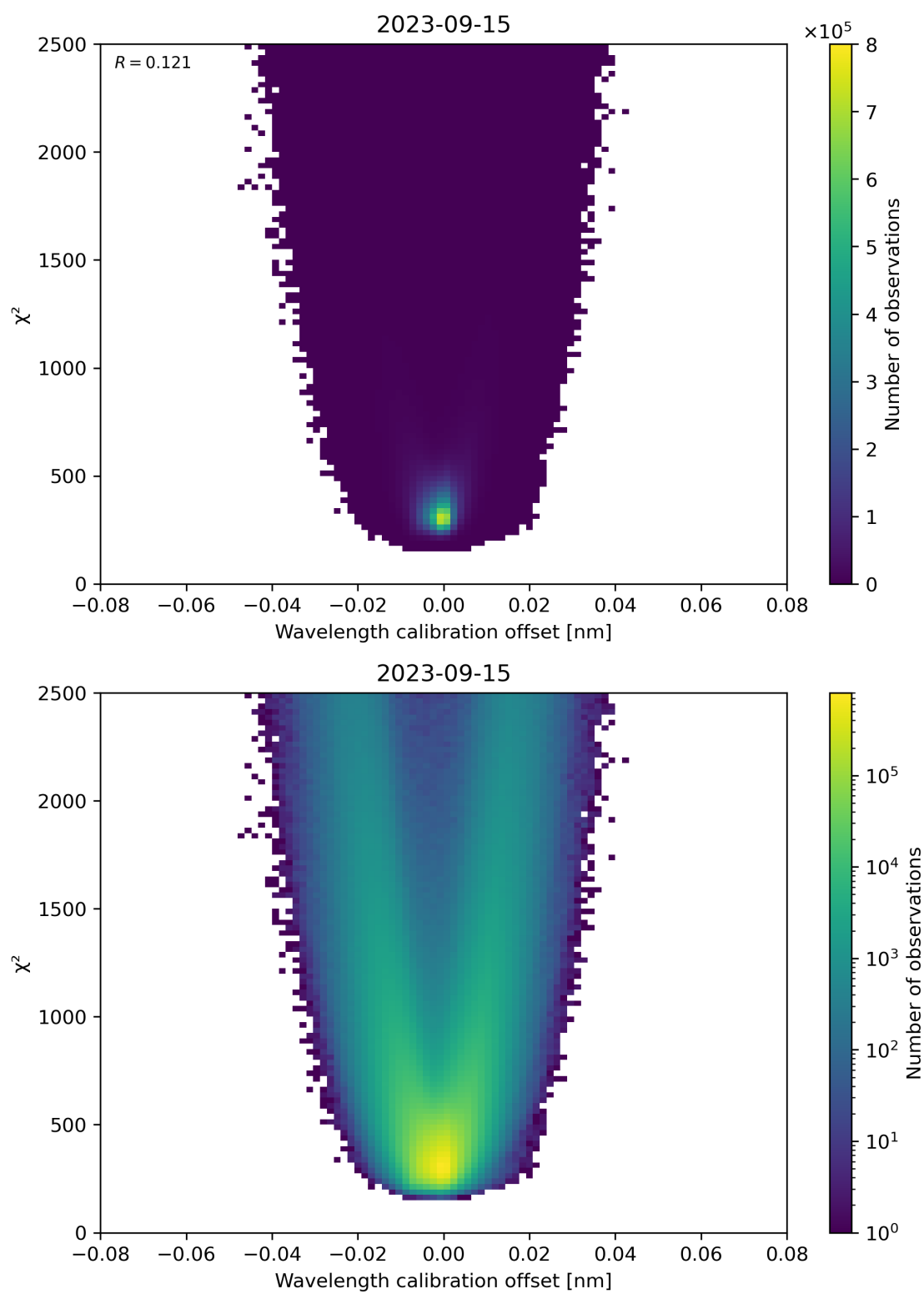
Figure 175: Scatter density plot of “Wavelength calibration offset” against “ \chi^2 ” for 2023-09-15 to 2023-09-16.
