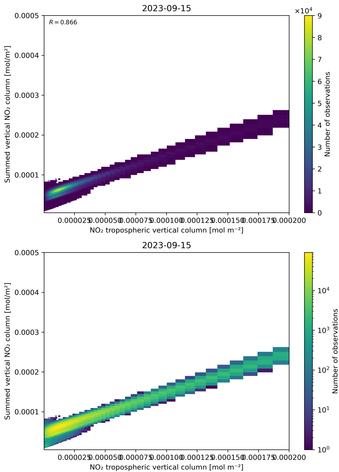
Figure 126: Scatter density plot of “NO 2 tropospheric vertical column” against “Summed vertical NO 2 column” for 2023-09-15 to 2023-09-16.
