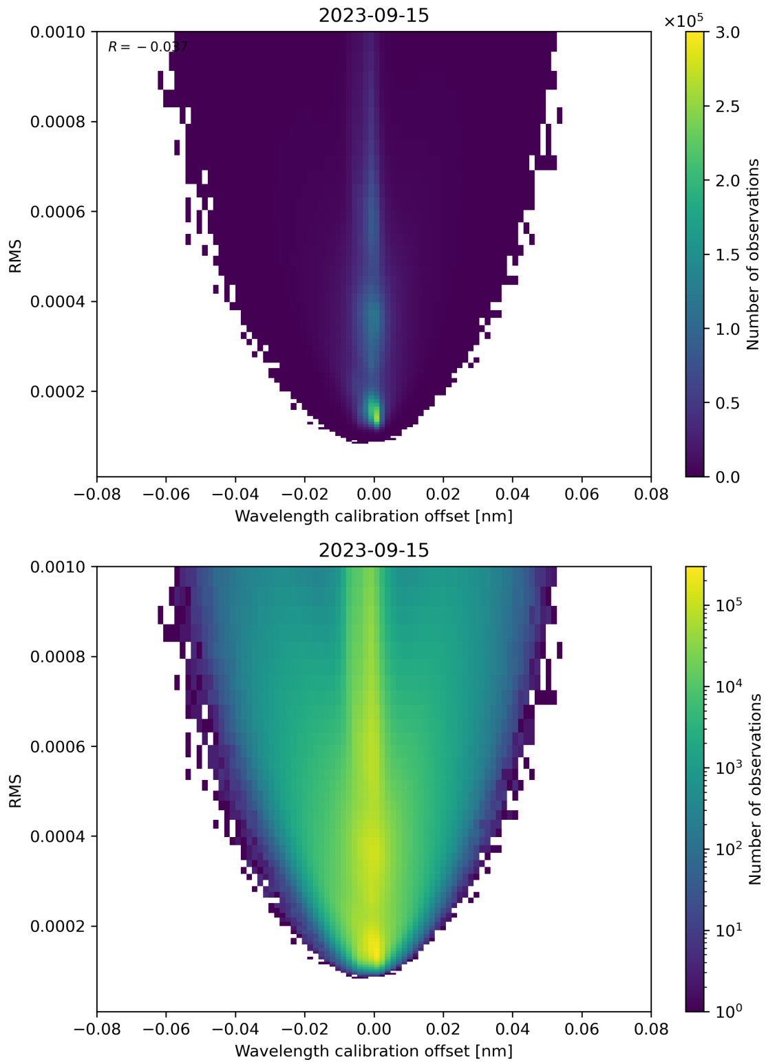
Figure 181: Scatter density plot of “Wavelength calibration offset” against “RMS” for 2023-09-15 to 2023-09-16.
