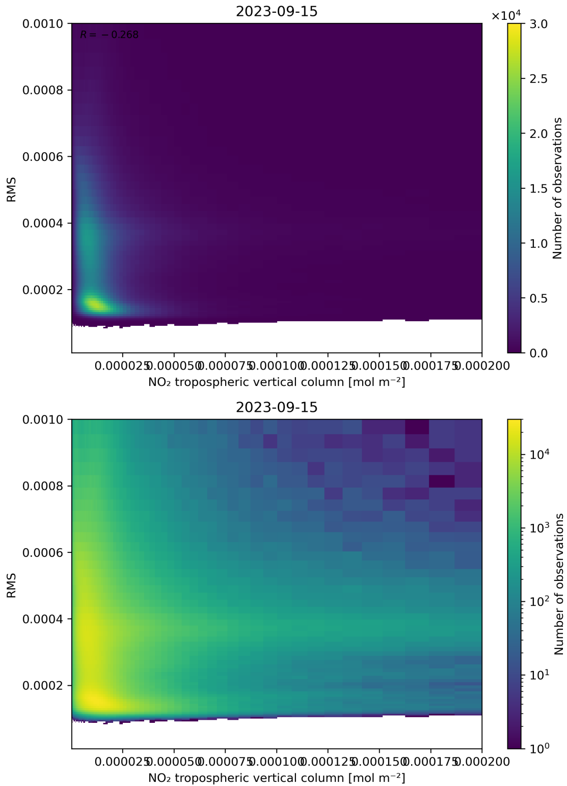
Figure 142: Scatter density plot of “NO 2 tropospheric vertical column” against “RMS” for 2023-09-15 to 2023-09-16.
