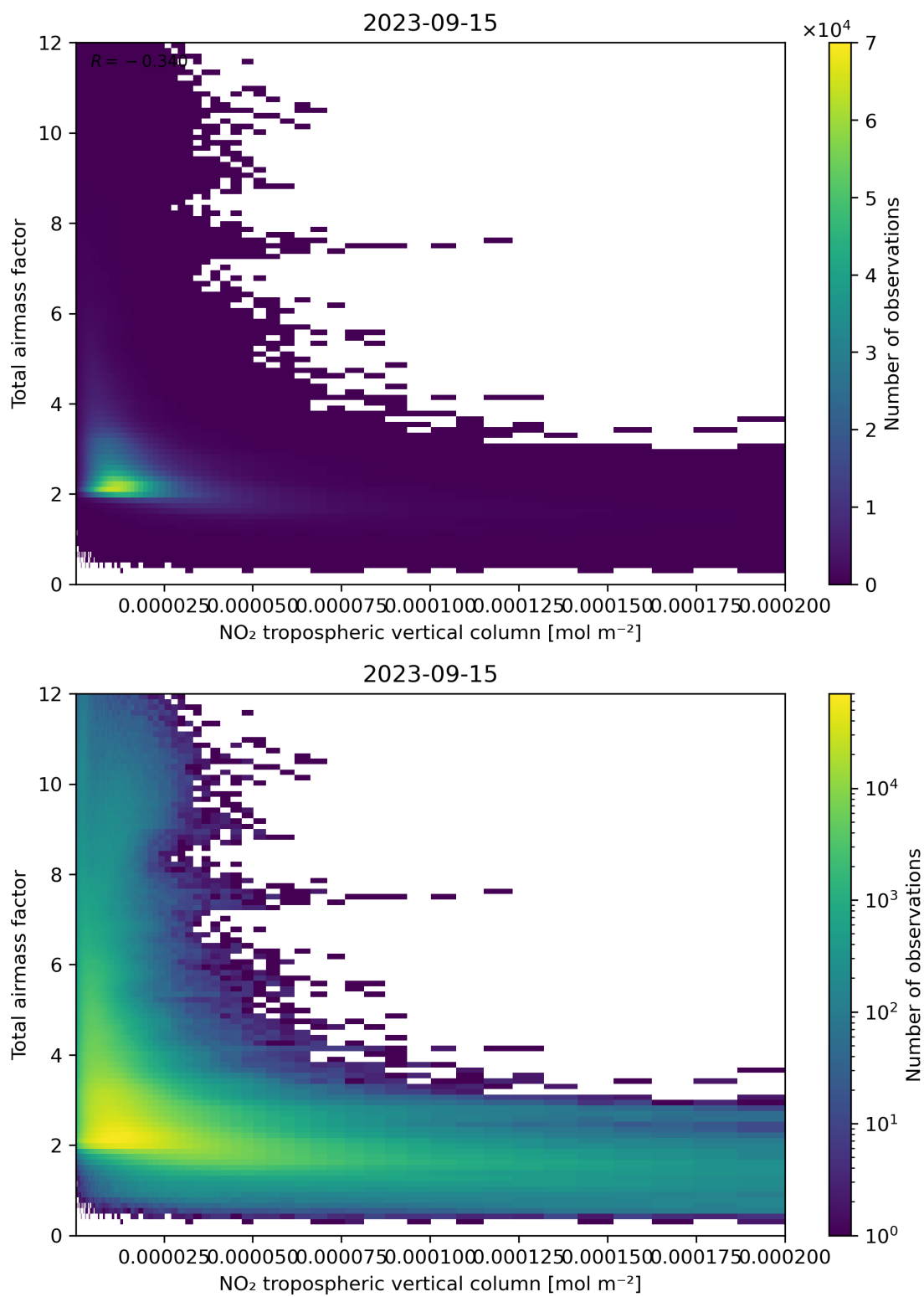
Figure 122: Scatter density plot of “NO 2 tropospheric vertical column” against “Total air mass factor” for 2023-09-15 to 2023-09-16.
