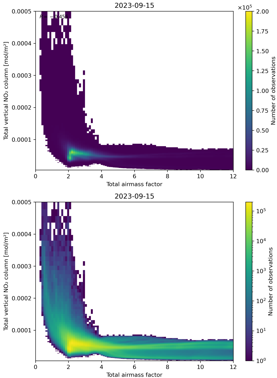
Figure 67: Scatter density plot of “Total airmass factor” against “Total vertical NO 2 column” for 2023-09-15 to 2023-09-16.
