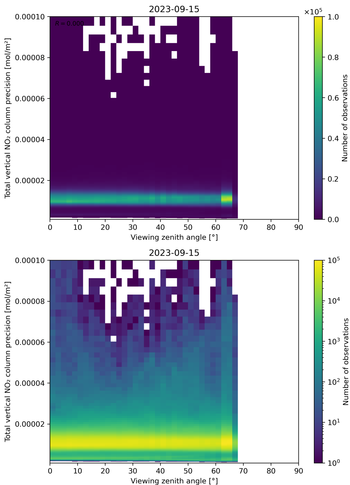
Figure 168: Scatter density plot of “Viewing zenith angle” against “Total vertical NO 2 column precision” for 2023-09-15 to 2023-09-16.
