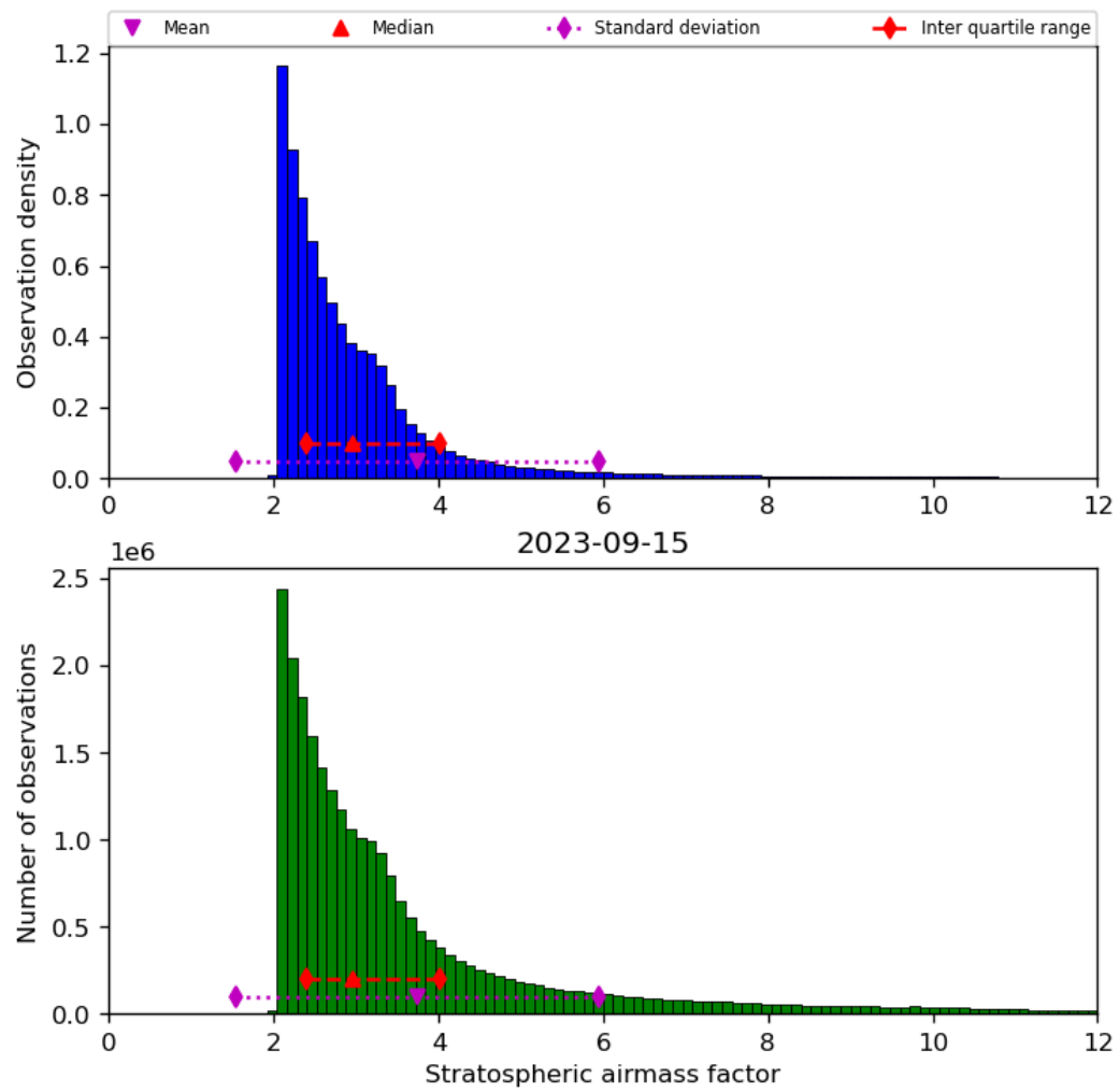
Figure 44: Histogram of “Stratospheric airmass factor” for 2023-09-15 to 2023-09-16
