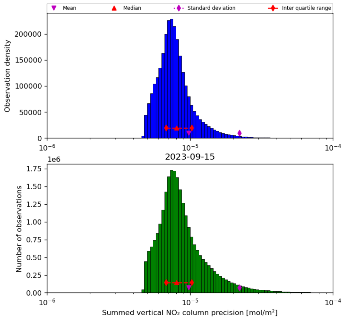
Figure 41: Histogram of “Summed vertical NO 2 column precision” for 2023-09-15 to 2023-09-16
