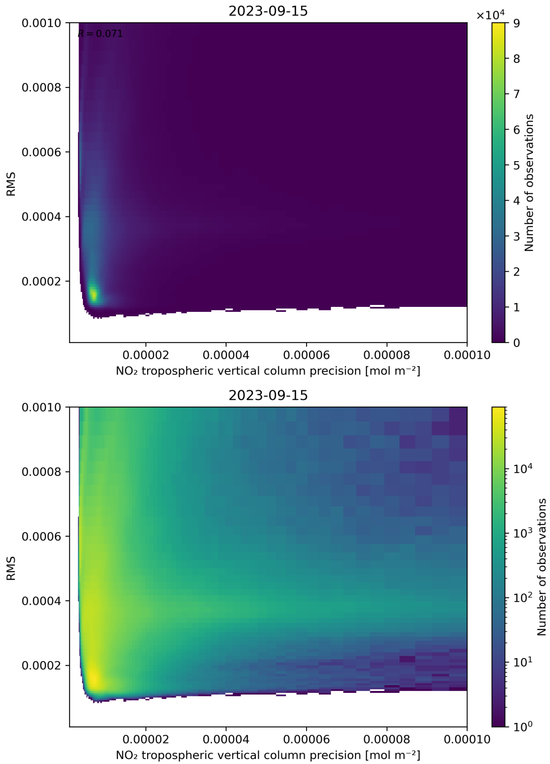
Figure 140: Scatter density plot of “NO 2 tropospheric vertical column precision” against “RMS” for 2023-09-15 to 2023-09-16.
