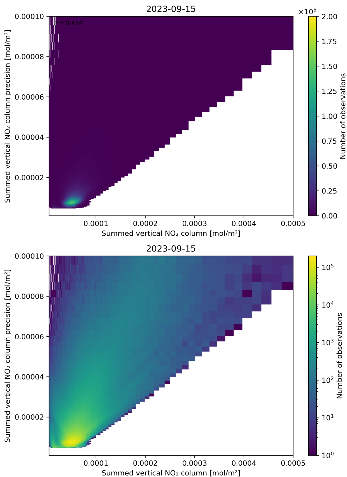
Figure 105: Scatter density plot of “Summed vertical NO 2 column” against “Summed vertical NO 2 column precision” for 2023-09-15 to 2023-09-16.
