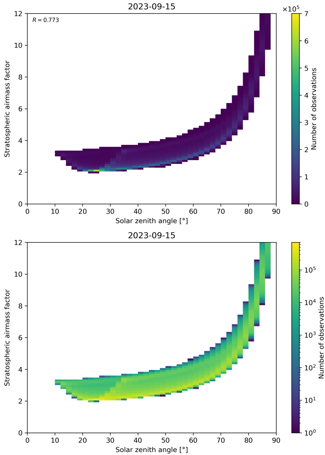
Figure 145: Scatter density plot of “Solar zenith angle” against “Stratospheric airmass factor” for 2023-09-15 to 2023-09-16.
