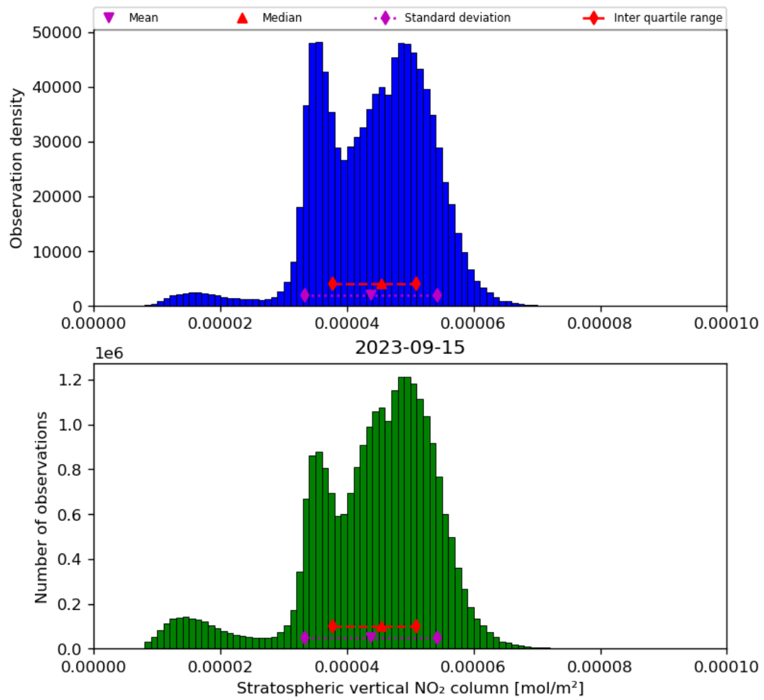
Figure 36: Histogram of “Stratospheric vertical NO 2 column” for 2023-09-15 to 2023-09-16
