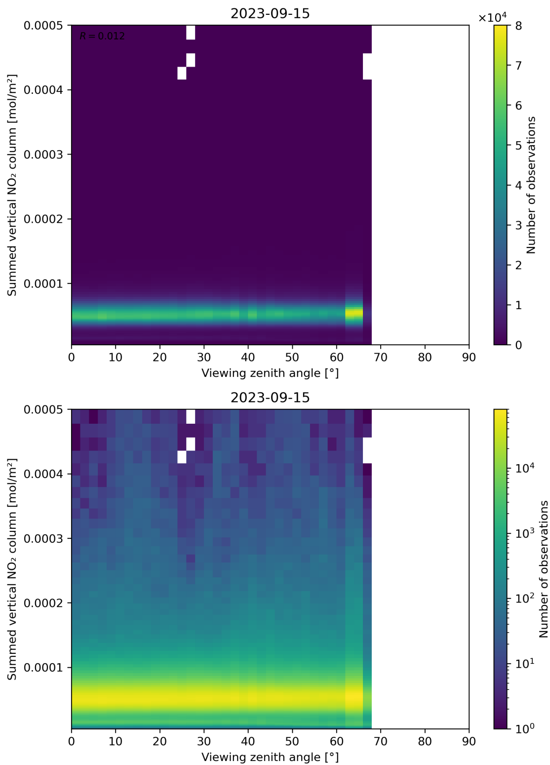
Figure 165: Scatter density plot of “Viewing zenith angle” against “Summed vertical NO 2 column” for 2023-09-15 to 2023-09-16.
