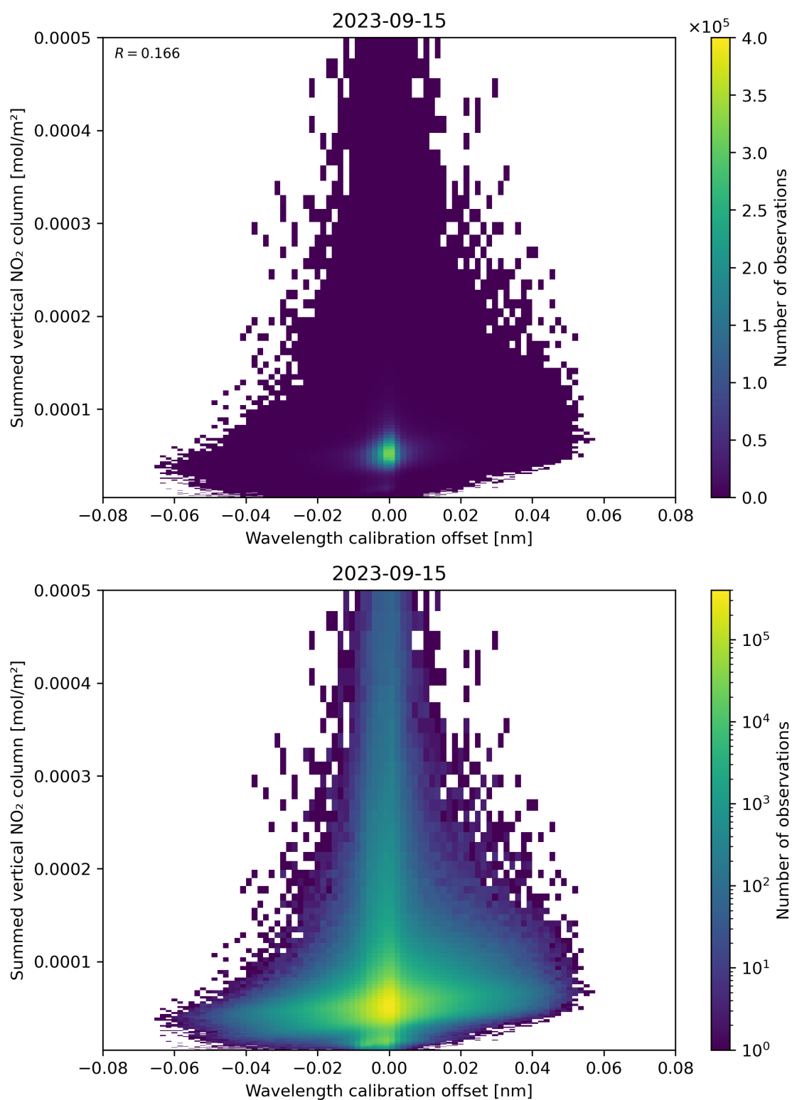
Figure 177: Scatter density plot of “Wavelength calibration offset” against “Summed vertical NO 2 column” for 2023-09-15 to 2023-09-16.
