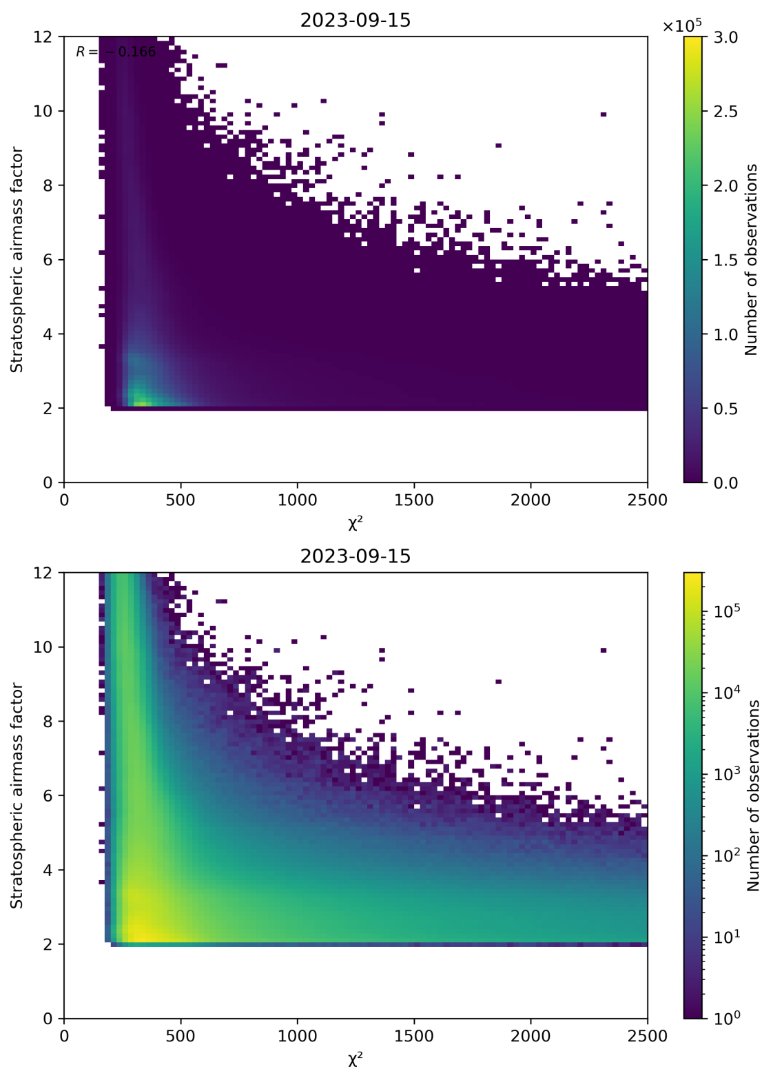
Figure 81: Scatter density plot of “ \chi^2 ” against “Stratospheric airmass factor” for 2023-09-15 to 2023-09-16.
