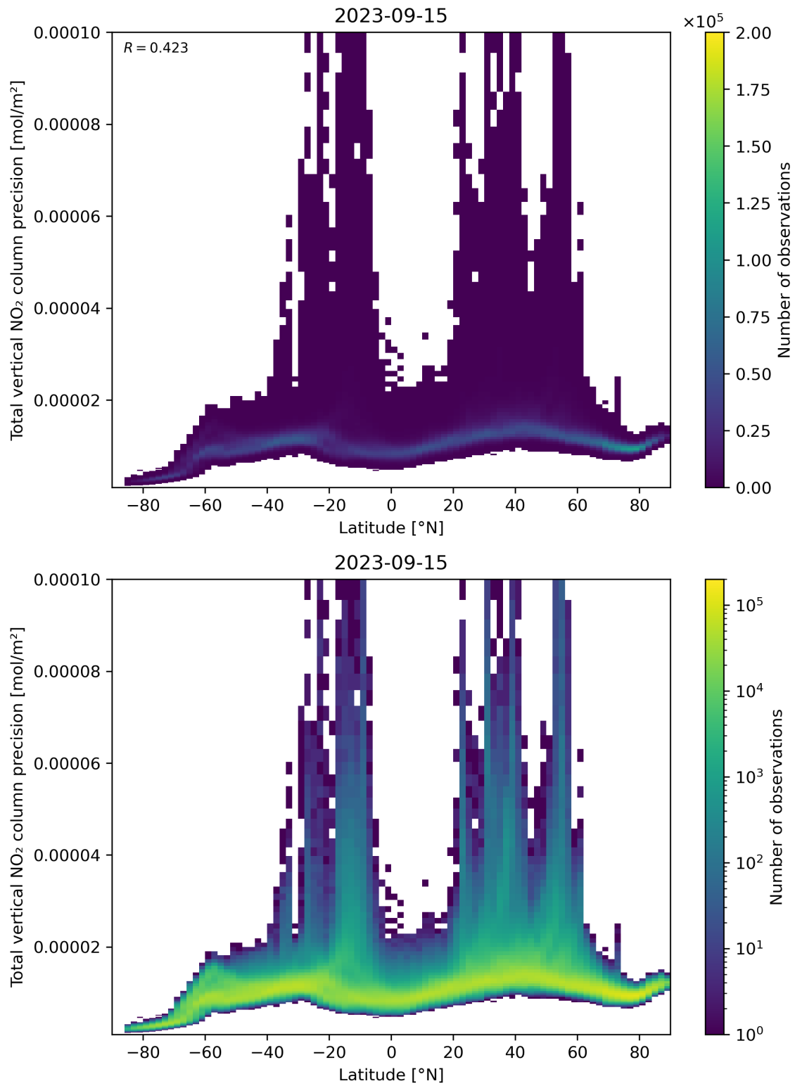
Figure 91: Scatter density plot of “Latitude” against “Total vertical NO 2 column precision” for 2023-09-15 to 2023-09-16.
