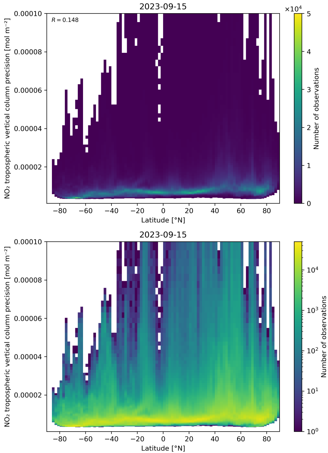
Figure 93: Scatter density plot of “Latitude” against “NO 2 tropospheric vertical column precision” for 2023-09-15 to 2023-09-16.
