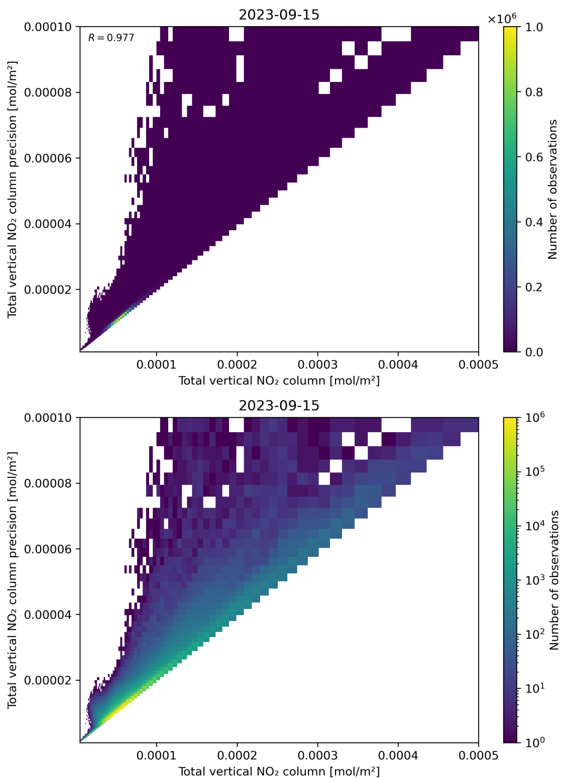
Figure 114: Scatter density plot of “Total vertical NO 2 column” against “Total vertical NO 2 column precision” for 2023-09-15 to 2023-09-16.
