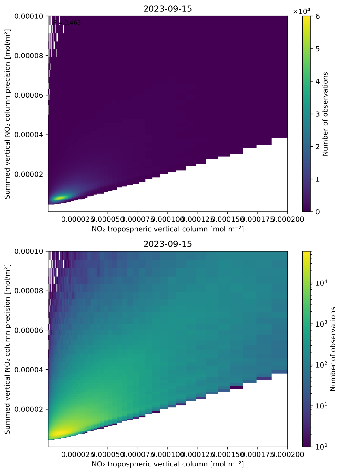
Figure 127: Scatter density plot of “NO 2 tropospheric vertical column” against “Summed vertical NO 2 column precision” for 2023-09-15 to 2023-09-16.
