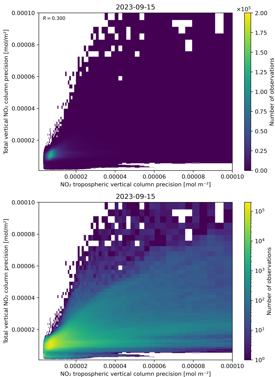
Figure 139: Scatter density plot of “NO 2 tropospheric vertical column precision” against “Total vertical NO 2 column precision” for 2023-09-15 to 2023-09-16.
