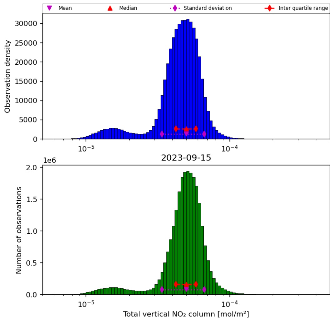
Figure 38: Histogram of “Total vertical NO 2 column” for 2023-09-15 to 2023-09-16
