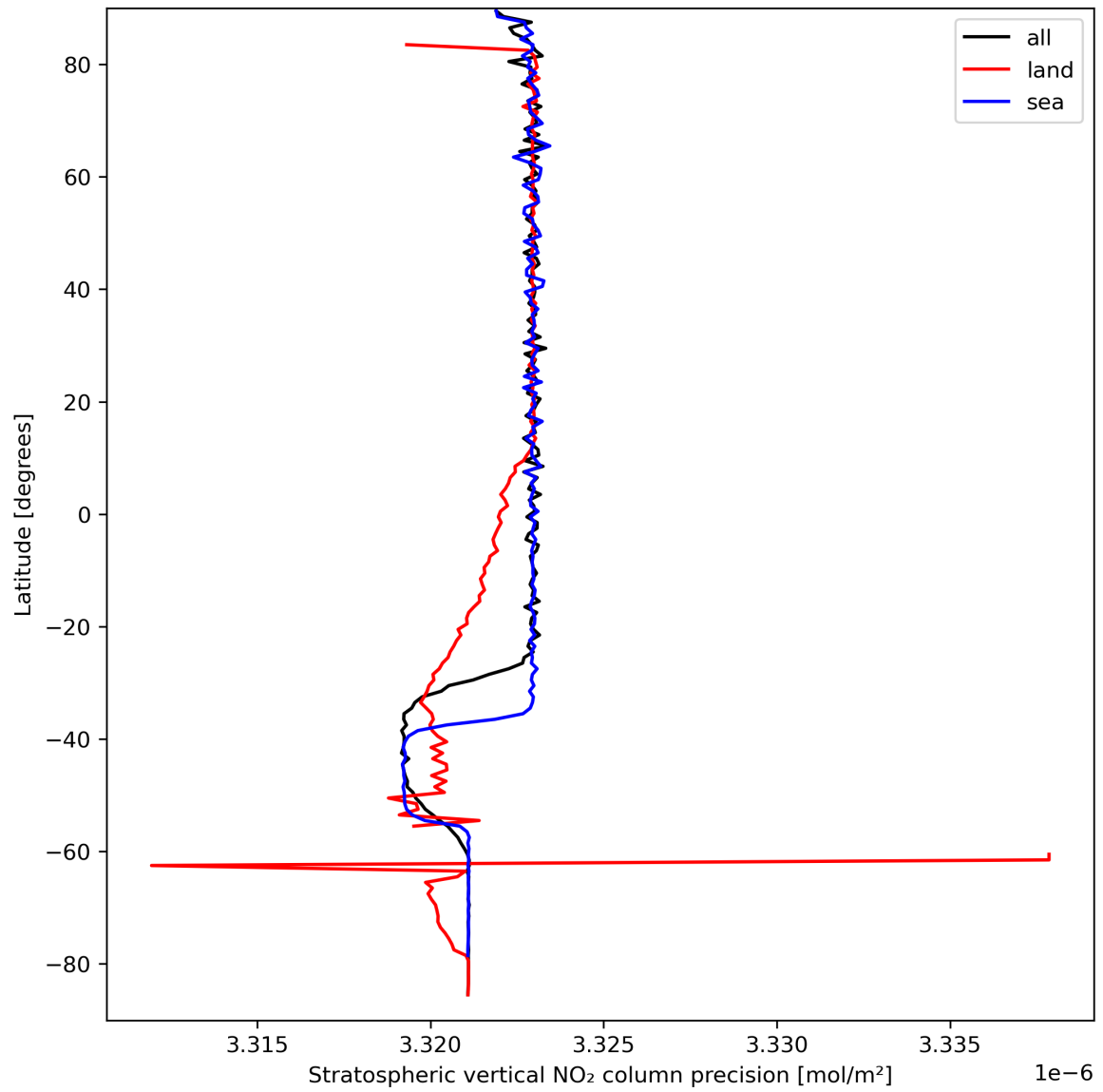
Figure 20: Zonal average of “Stratospheric vertical NO 2 column precision” for 2023-09-15 to 2023-09-16.
