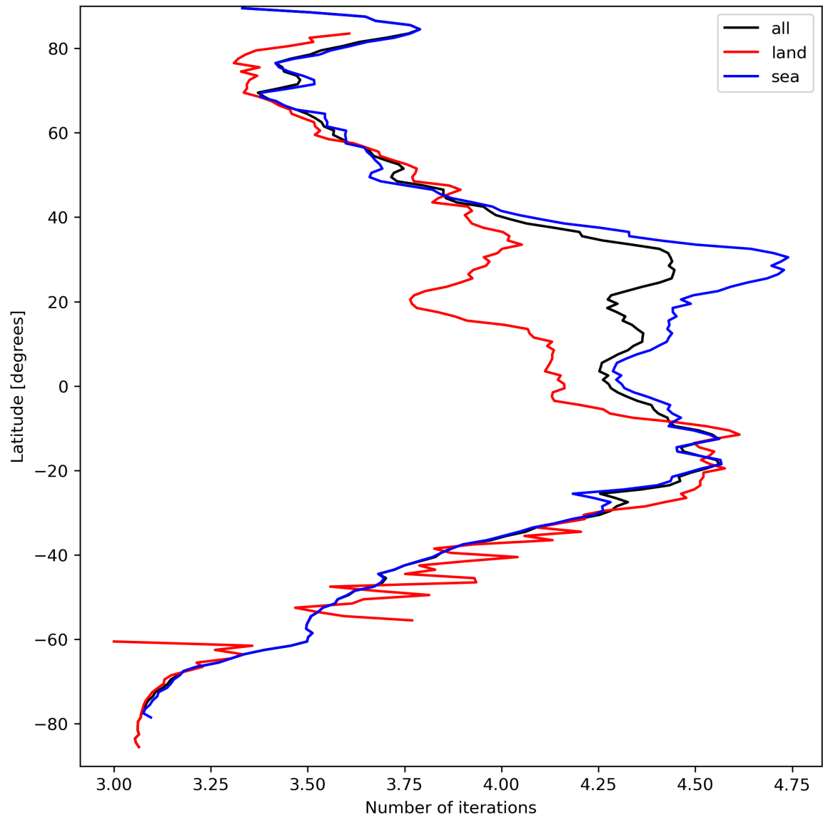
Figure 17: Zonal average of “Number of iterations” for 2023-09-15 to 2023-09-16.
