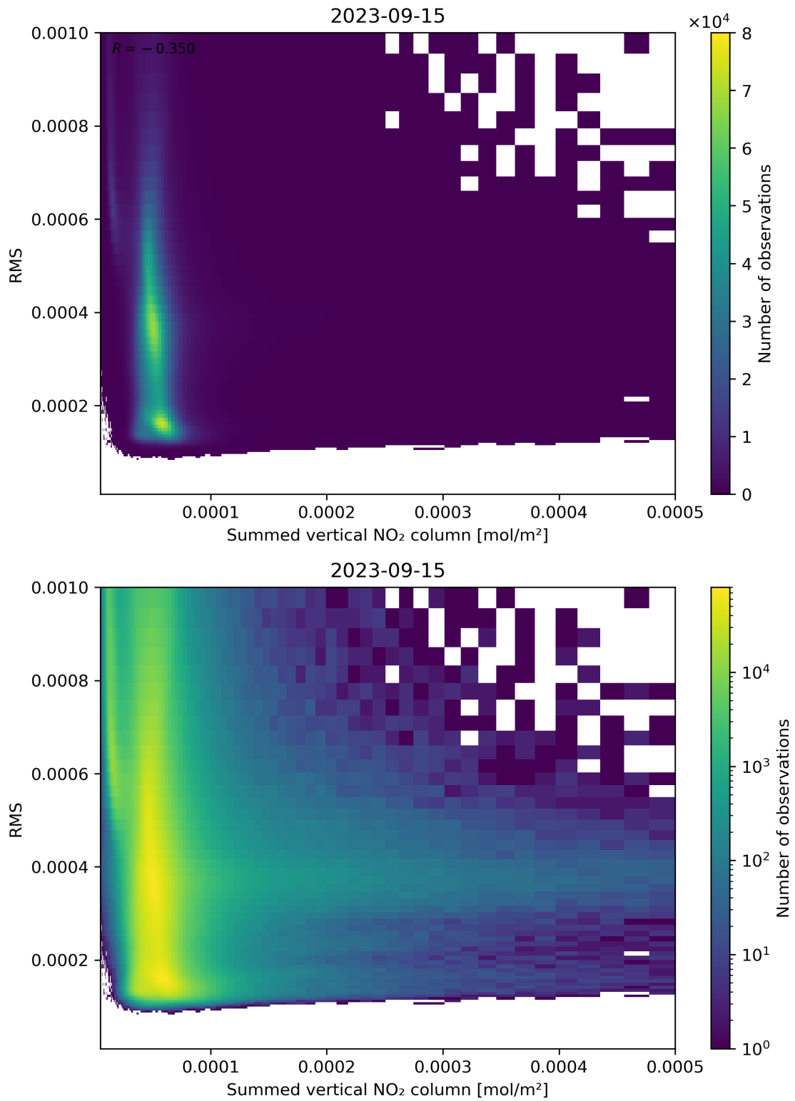
Figure 109: Scatter density plot of “Summed vertical NO 2 column” against “RMS” for 2023-09-15 to 2023-09-16.
