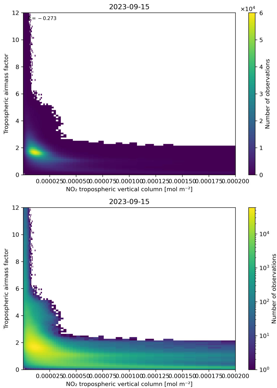
Figure 123: Scatter density plot of “NO 2 tropospheric vertical column” against “Tropospheric air mass factor” for 2023-09-15 to 2023-09-16.
