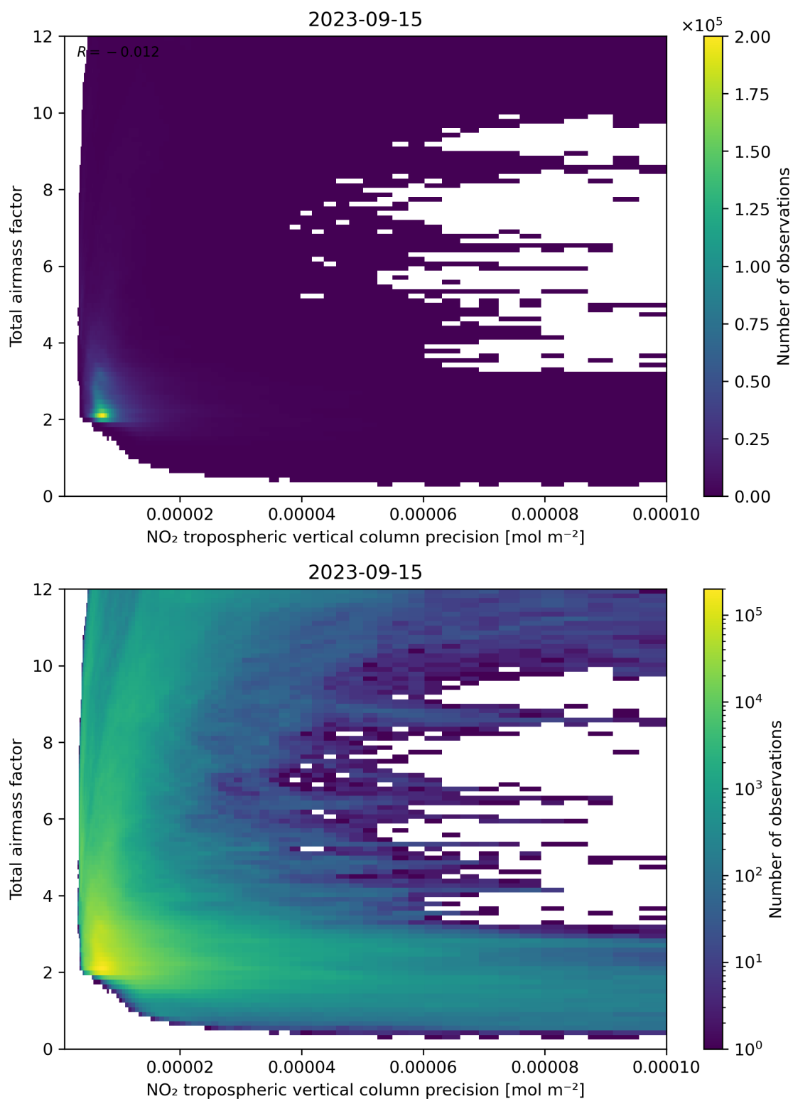
Figure 132: Scatter density plot of “NO 2 tropospheric vertical column precision” against “Total air mass factor” for 2023-09-15 to 2023-09-16.
