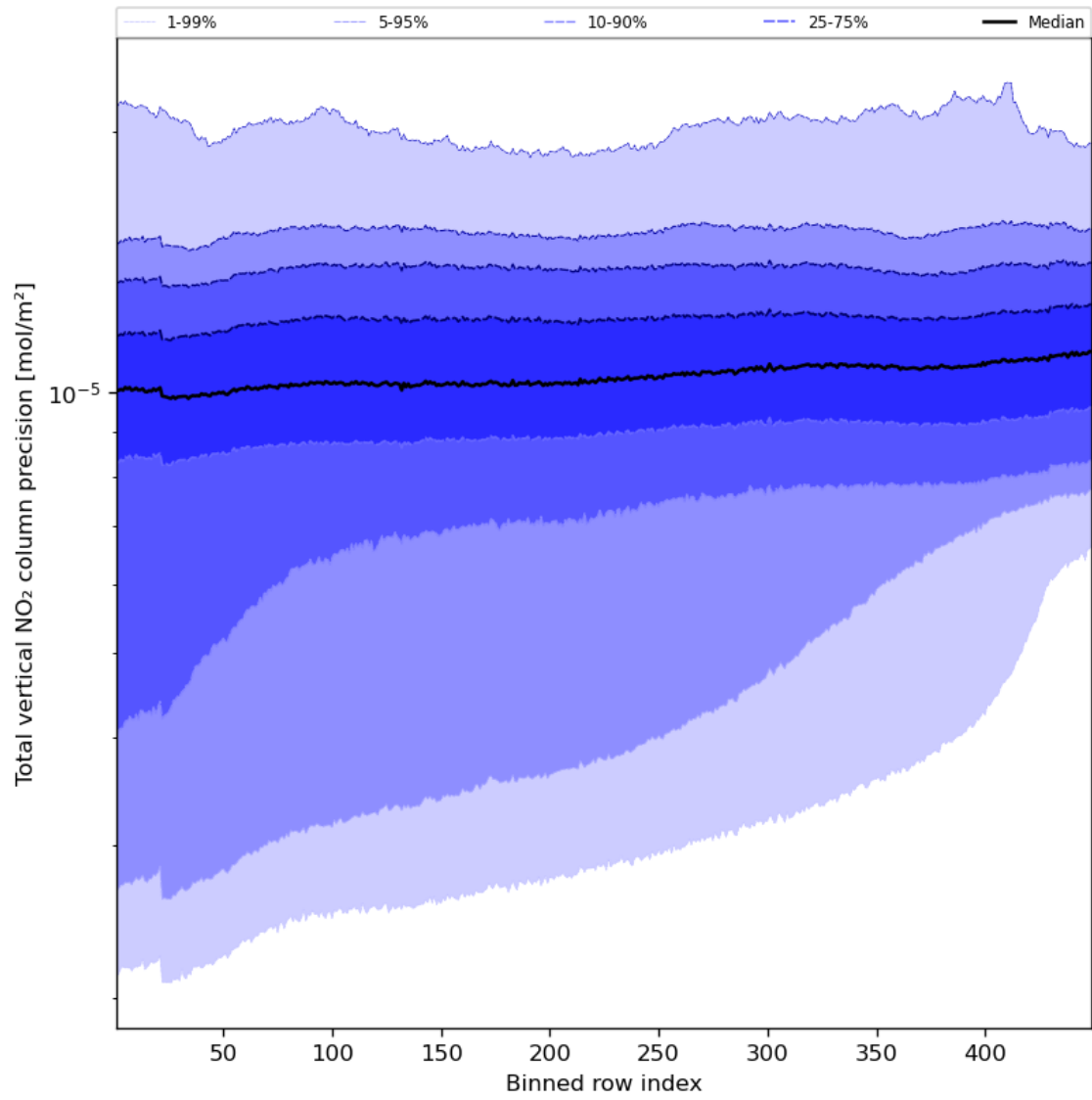
Figure 56: Along track statistics of “Total vertical NO 2 column precision” for 2023-09-15 to 2023-09-16
