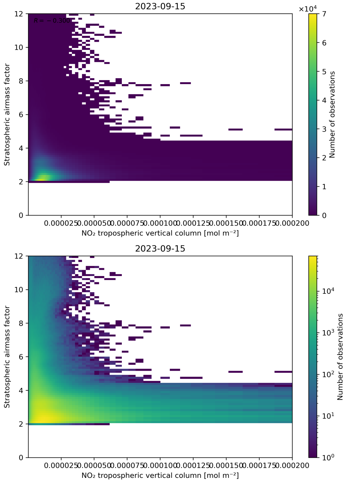
Figure 121: Scatter density plot of “NO 2 tropospheric vertical column” against “Stratospheric air mass factor” for 2023-09-15 to 2023-09-16.
