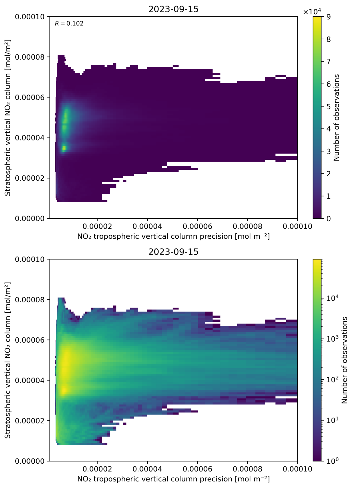
Figure 135: Scatter density plot of “ \text{NO}_2 tropospheric vertical column precision” against “Stratospheric vertical \text{NO}_2 column” for 2023-09-15 to 2023-09-16.
