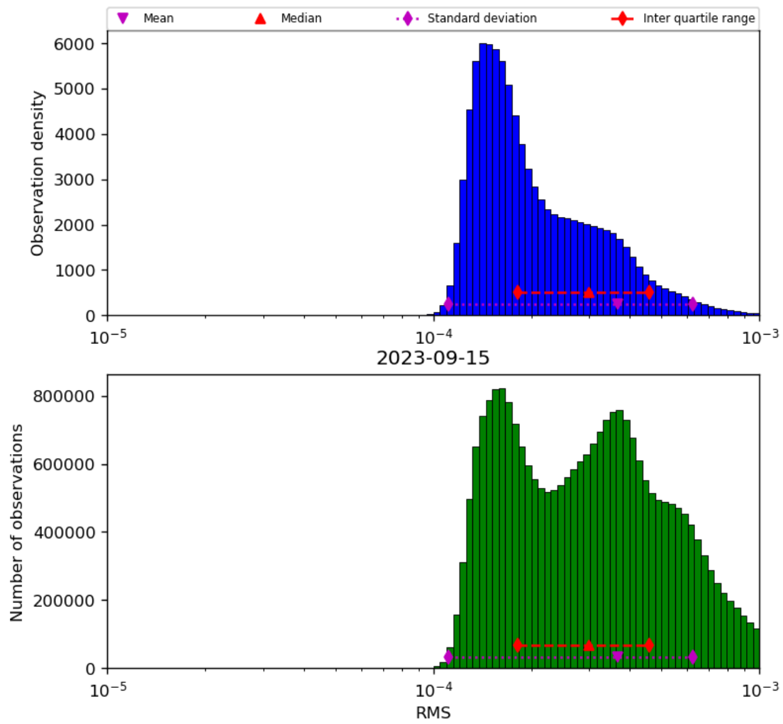
Figure 43: Histogram of “RMS” for 2023-09-15 to 2023-09-16
