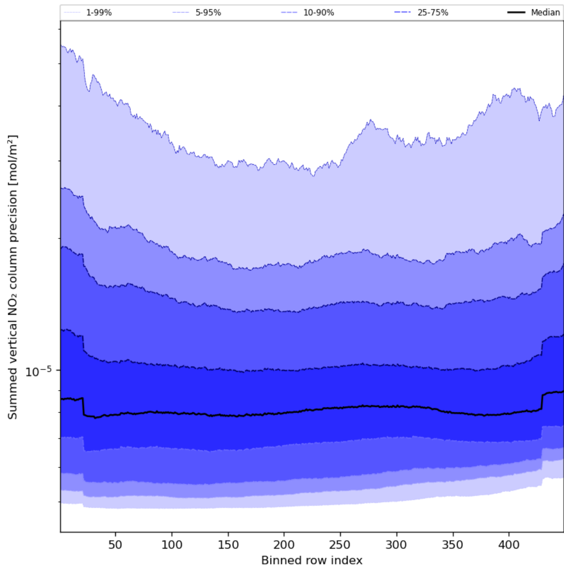
Figure 58: Along track statistics of “Summed vertical NO 2 column precision” for 2023-09-15 to 2023-09-16
