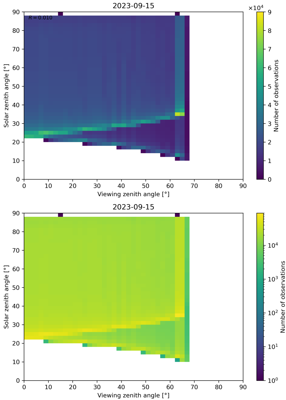
Figure 172: Scatter density plot of “Viewing zenith angle” against “Solar zenith angle” for 2023-09-15 to 2023-09-16.
