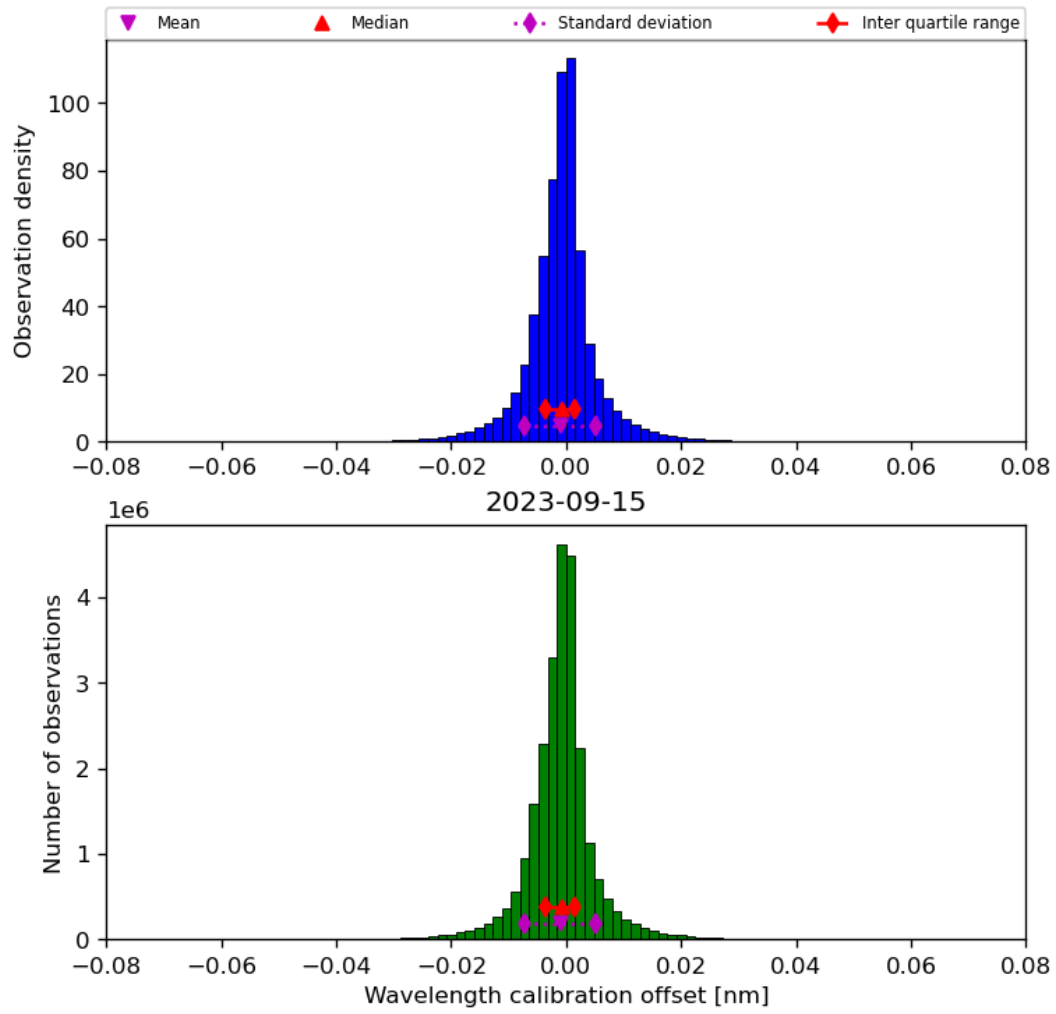
Figure 35: Histogram of “Wavelength calibration offset” for 2023-09-15 to 2023-09-16
