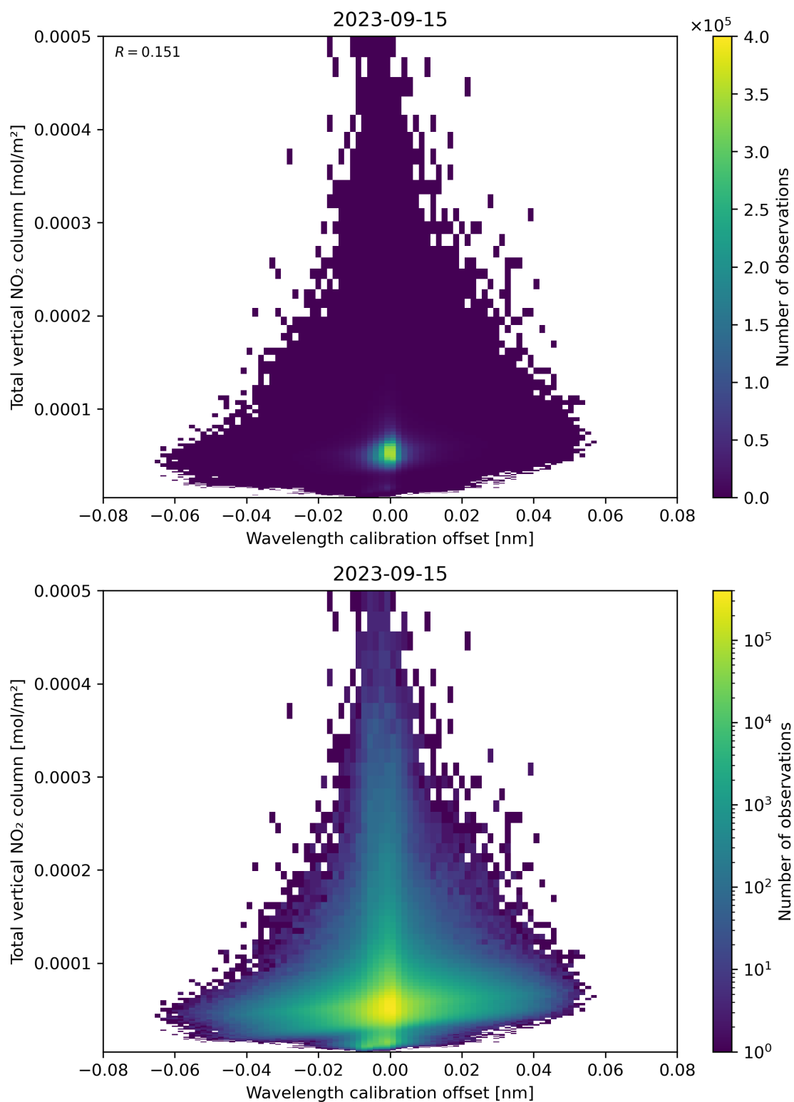
Figure 179: Scatter density plot of “Wavelength calibration offset” against “Total vertical NO 2 column” for 2023-09-15 to 2023-09-16.
