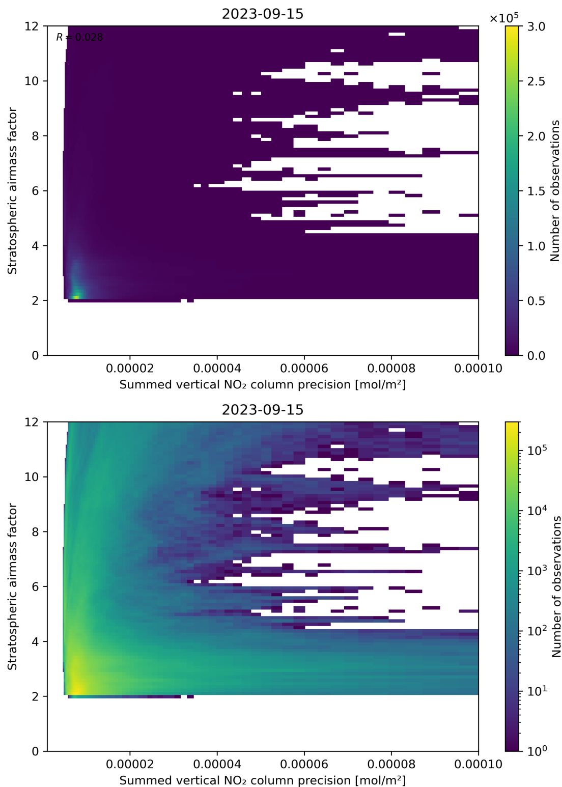
Figure 106: Scatter density plot of “Summed vertical NO 2 column precision” against “Stratospheric airmass factor” for 2023-09-15 to 2023-09-16.
