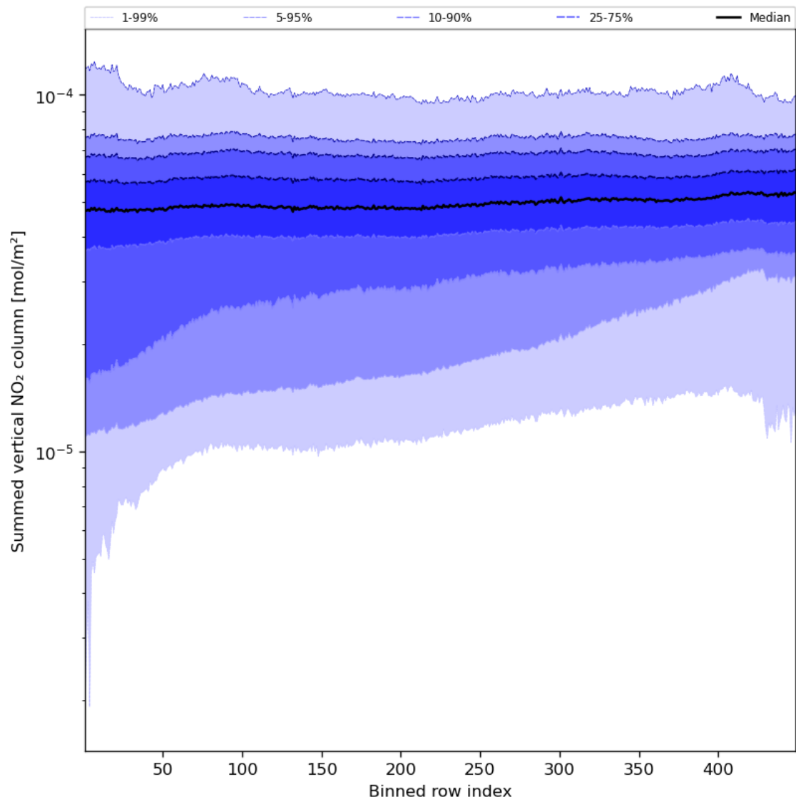
Figure 57: Along track statistics of “Summed vertical NO 2 column” for 2023-09-15 to 2023-09-16
