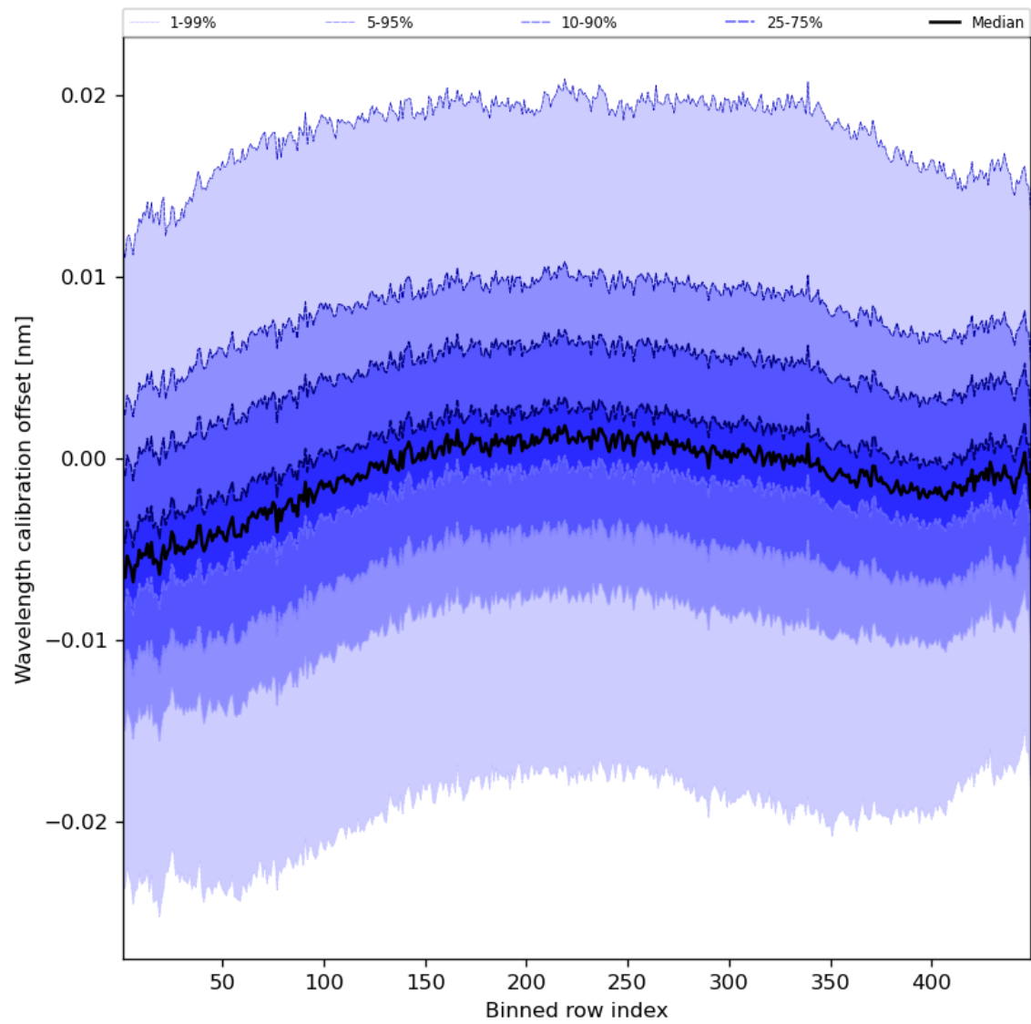
Figure 52: Along track statistics of “Wavelength calibration offset” for 2023-09-15 to 2023-09-16
