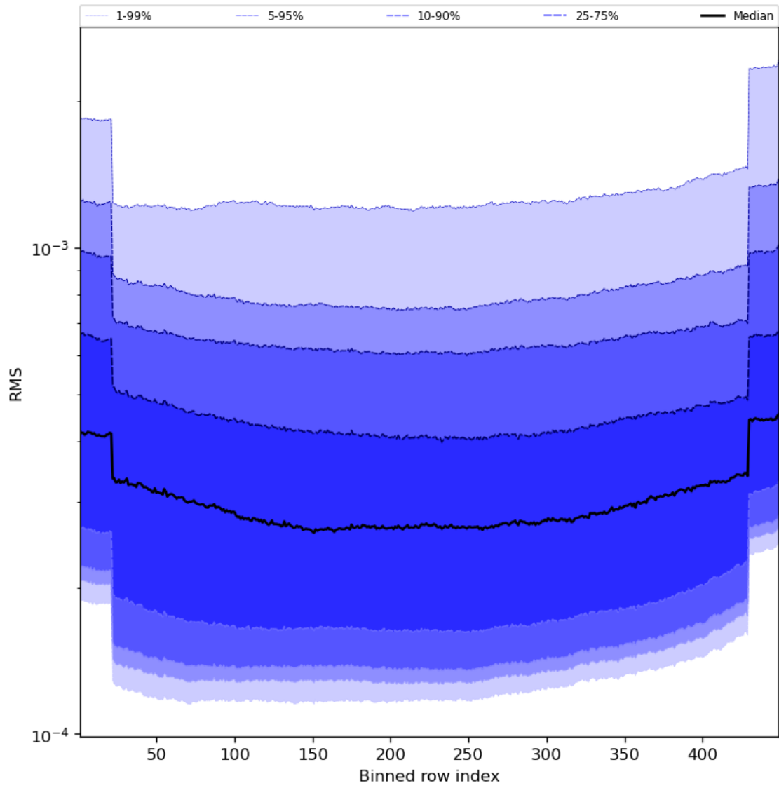
Figure 60: Along track statistics of “RMS” for 2023-09-15 to 2023-09-16
