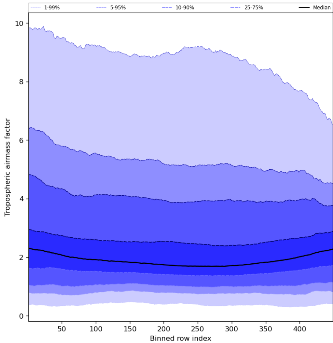
Figure 48: Along track statistics of “Tropospheric airmass factor” for 2023-09-15 to 2023-09-16
