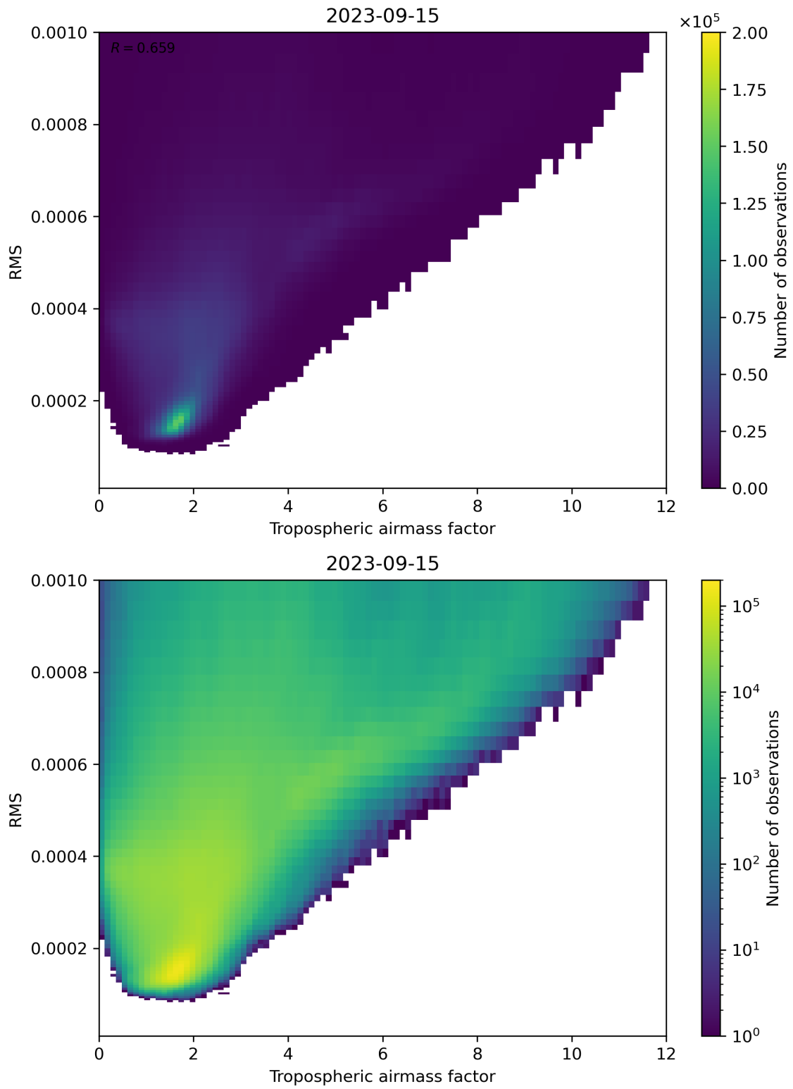
Figure 79: Scatter density plot of “Tropospheric airmass factor” against “RMS” for 2023-09-15 to 2023-09-16.
