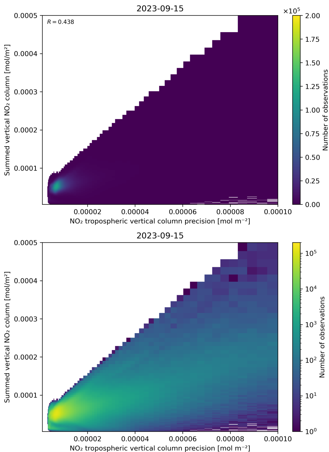
Figure 136: Scatter density plot of “NO 2 tropospheric vertical column precision” against “Summed vertical NO 2 column” for 2023-09-15 to 2023-09-16.
