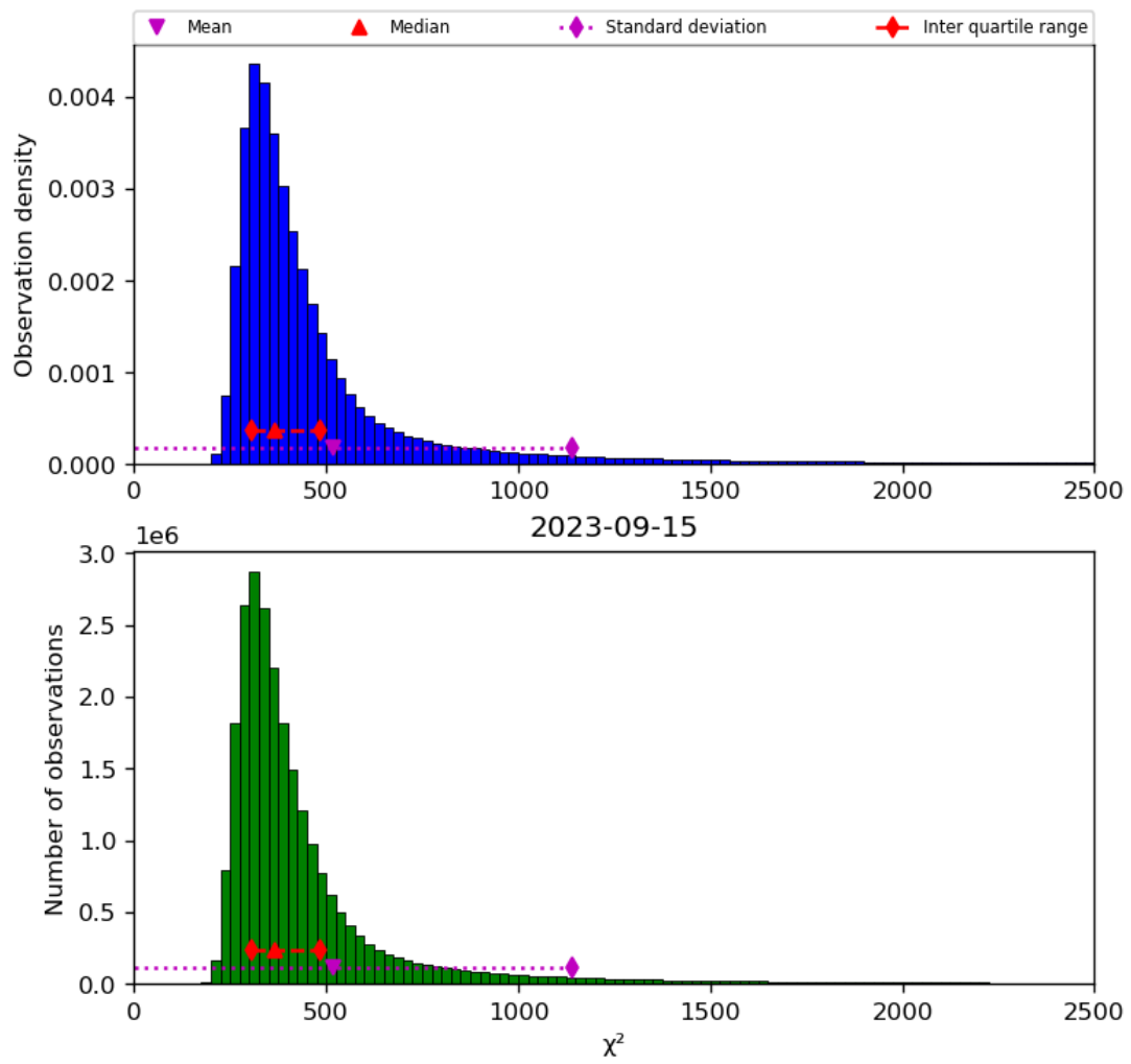
Figure 42: Histogram of “ \chi^2 ” for 2023-09-15 to 2023-09-16
