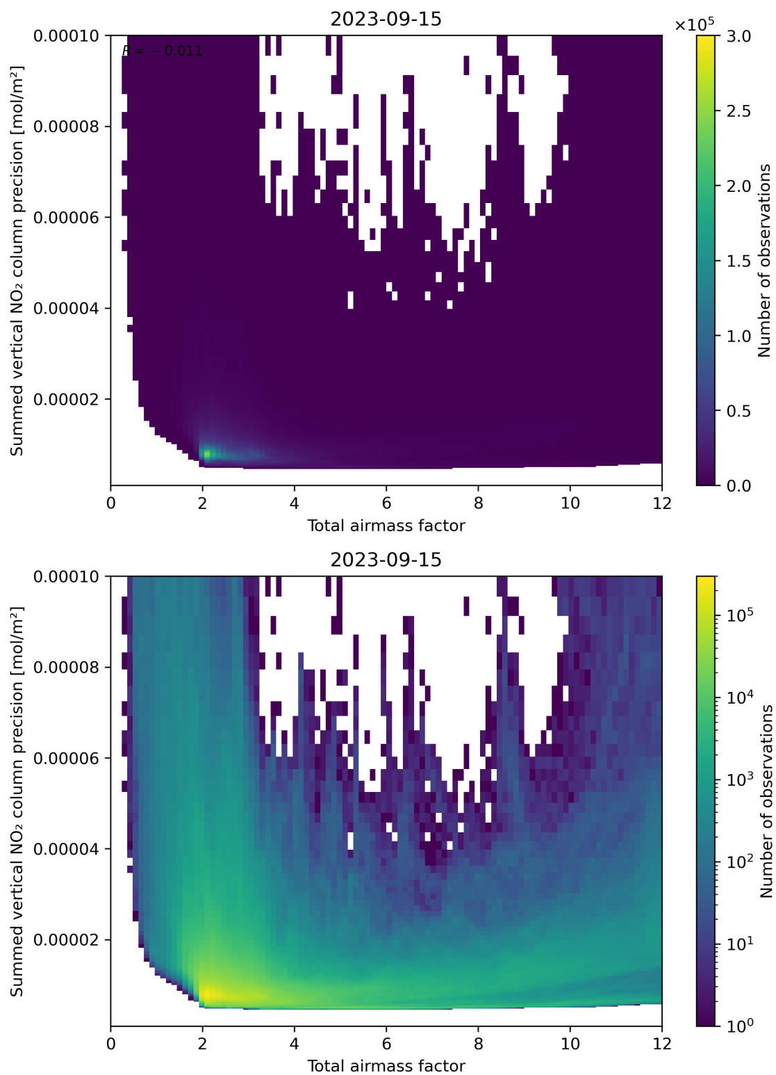
Figure 66: Scatter density plot of “Total airmass factor” against “Summed vertical NO 2 column precision” for 2023-09-15 to 2023-09-16.
