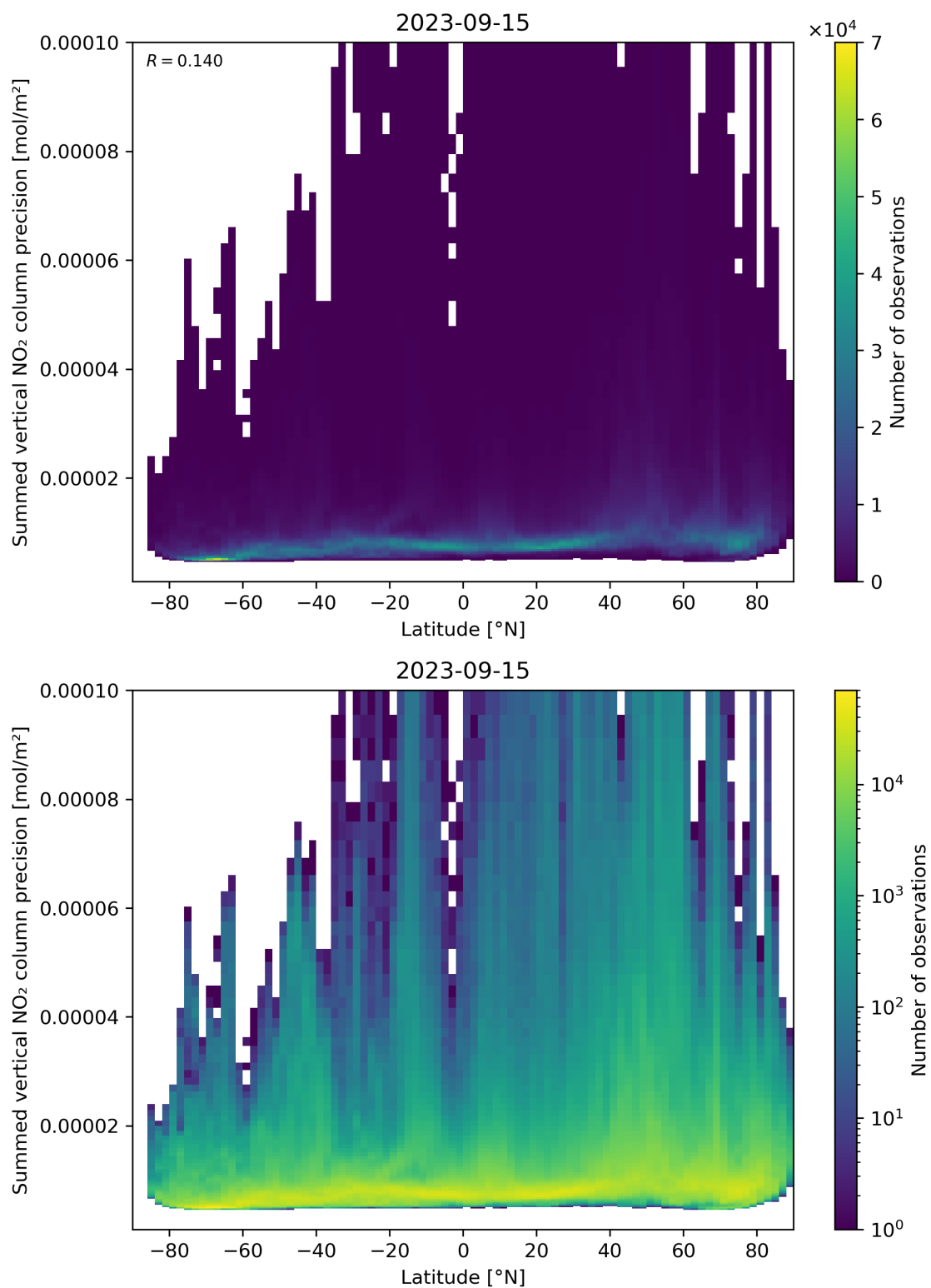
Figure 89: Scatter density plot of “Latitude” against “Summed vertical NO 2 column precision” for 2023-09-15 to 2023-09-16.
