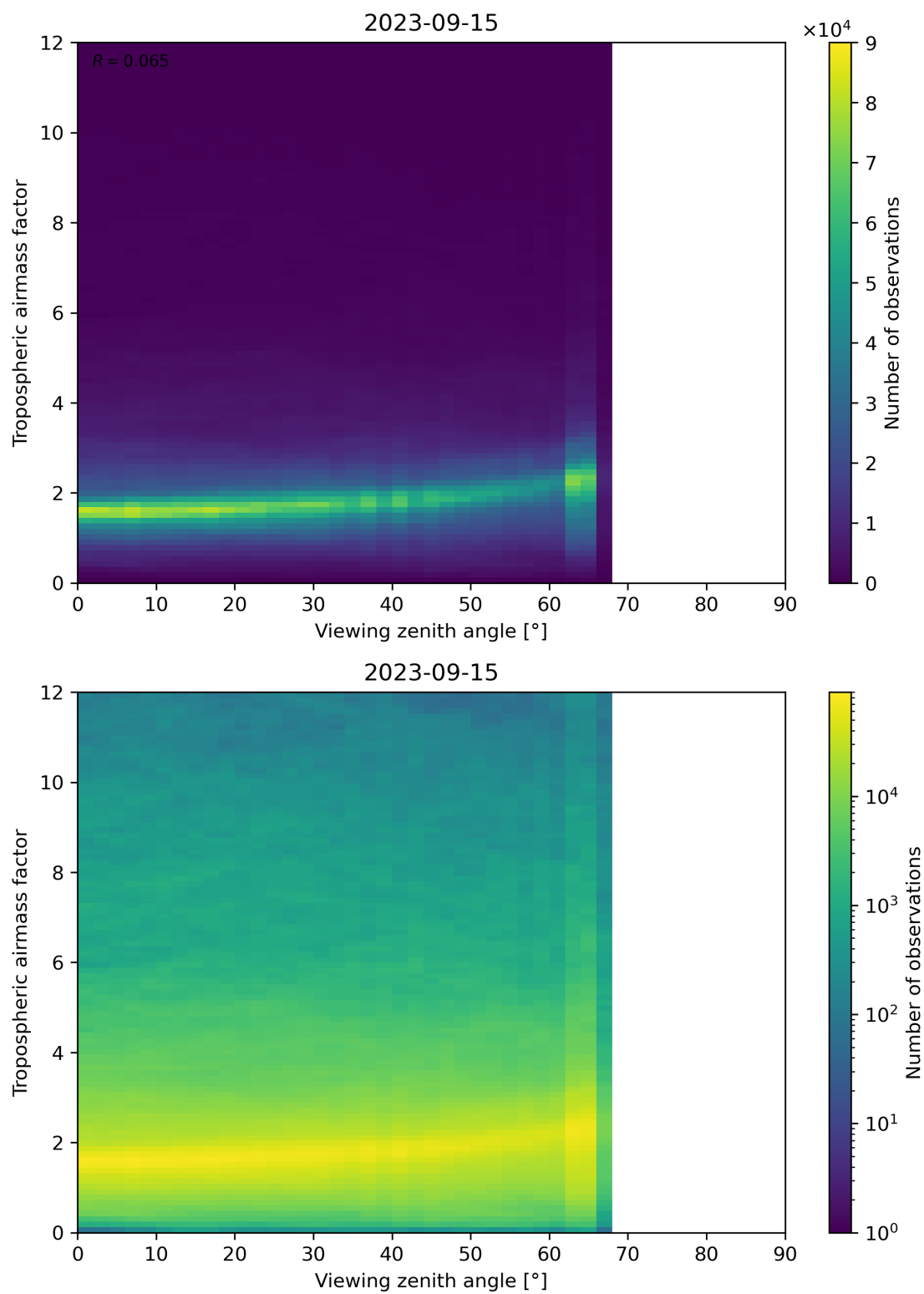
Figure 161: Scatter density plot of “Viewing zenith angle” against “Tropospheric airmass factor” for 2023-09-15 to 2023-09-16.
