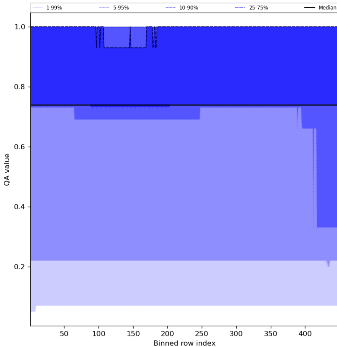
Figure 45: Along track statistics of “QA value” for 2023-09-15 to 2023-09-16
