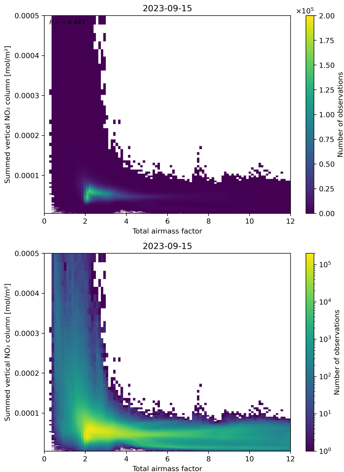
Figure 65: Scatter density plot of “Total airmass factor” against “Summed vertical NO 2 column” for 2023-09-15 to 2023-09-16.
