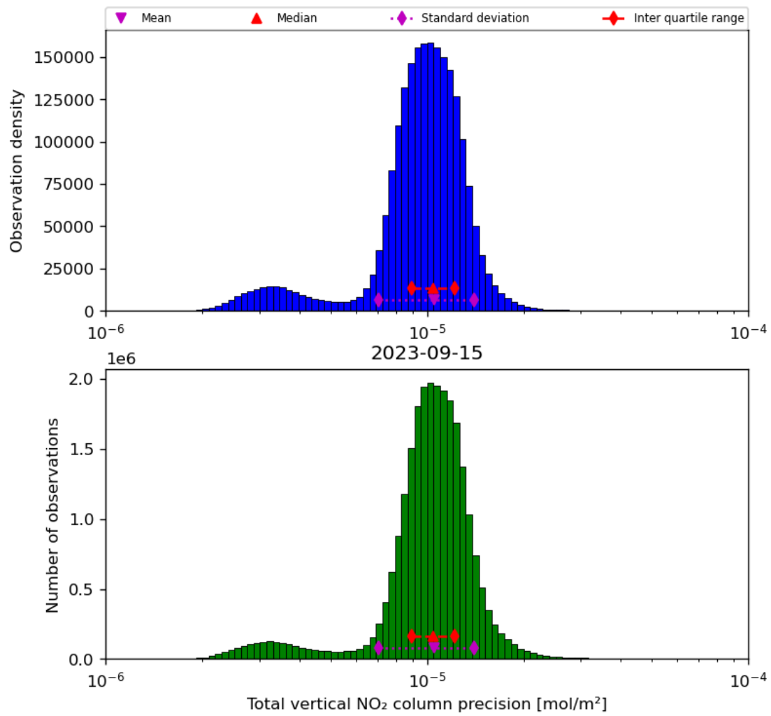
Figure 39: Histogram of "Total vertical NO 2 column precision" for 2023-09-15 to 2023-09-16
