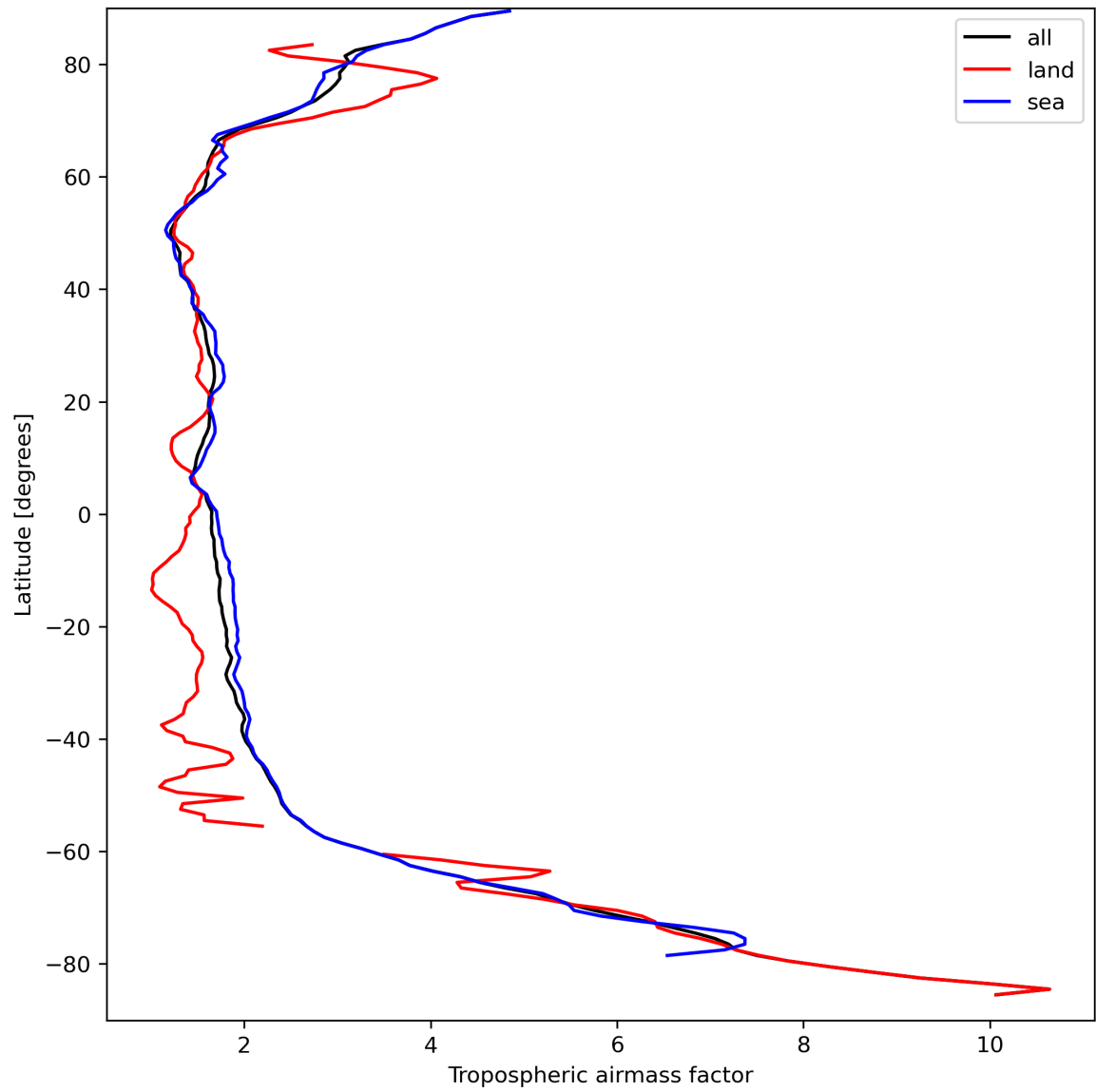
Figure 14: Zonal average of “Tropospheric airmass factor” for 2023-09-15 to 2023-09-16.
