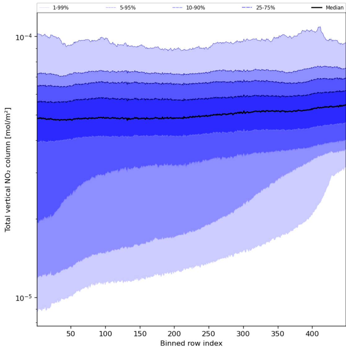
Figure 55: Along track statistics of "Total vertical NO 2 column" for 2023-09-15 to 2023-09-16
