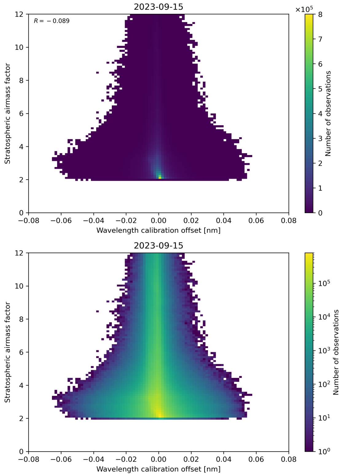
Figure 174: Scatter density plot of “Wavelength calibration offset” against “Stratospheric airmass factor” for 2023-09-15 to 2023-09-16.
