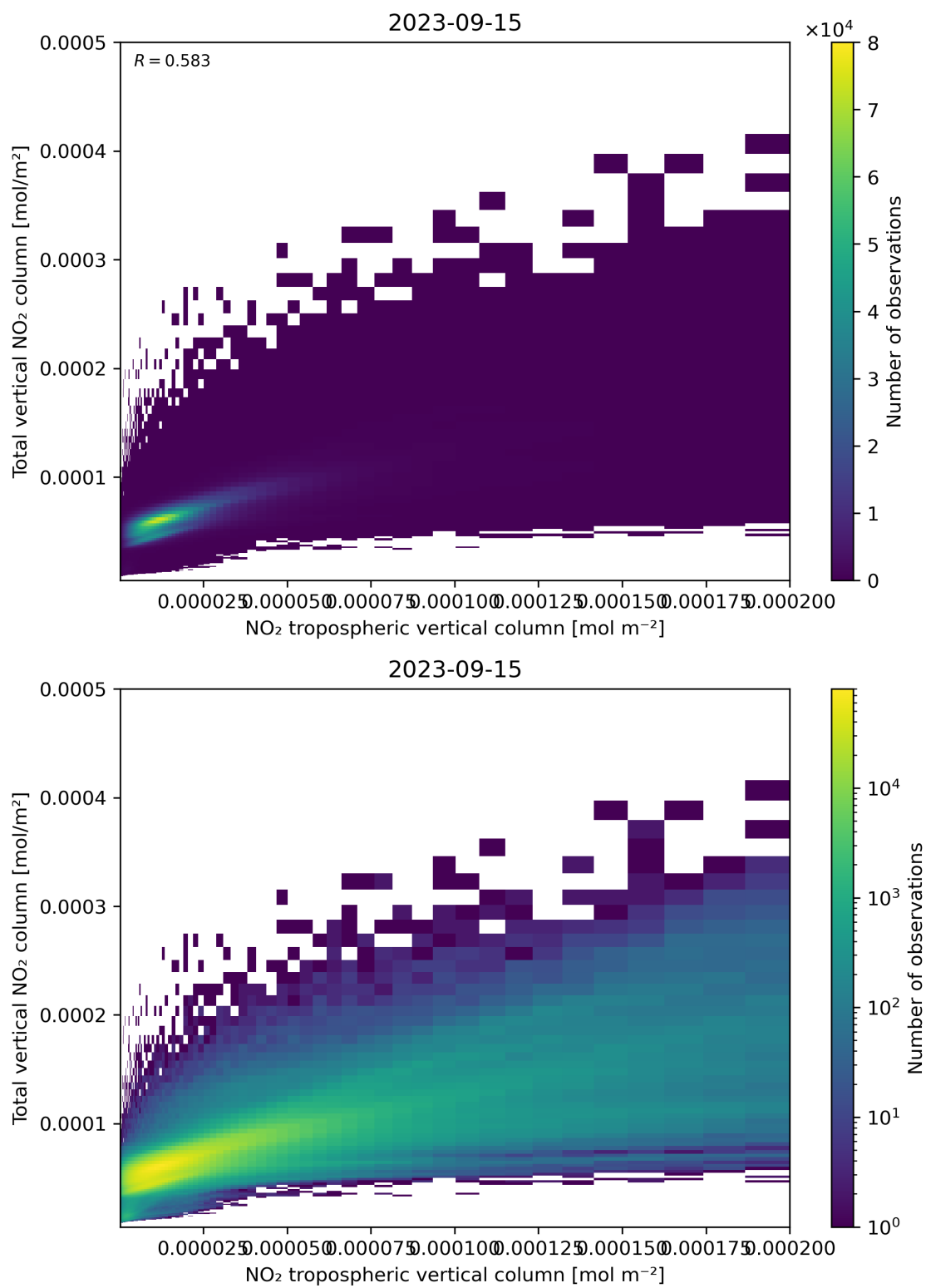
Figure 128: Scatter density plot of “NO 2 tropospheric vertical column” against “Total vertical NO 2 column” for 2023-09-15 to 2023-09-16.
