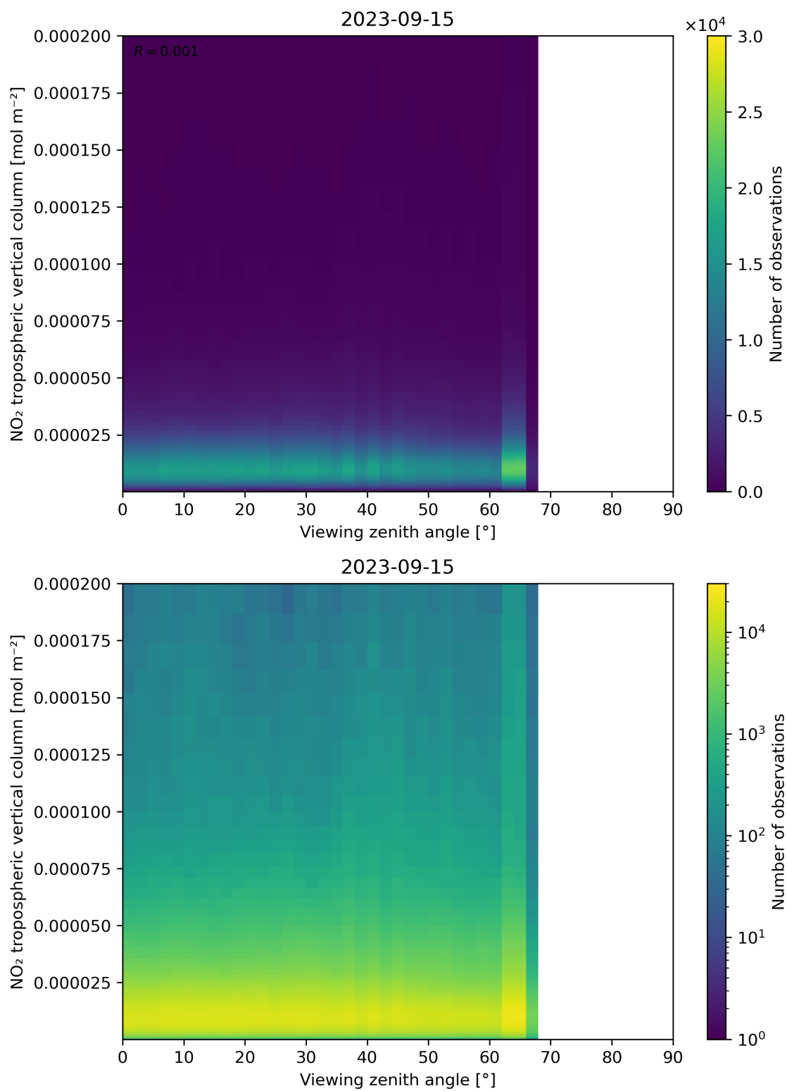
Figure 169: Scatter density plot of “Viewing zenith angle” against “NO 2 tropospheric vertical column” for 2023-09-15 to 2023-09-16.
