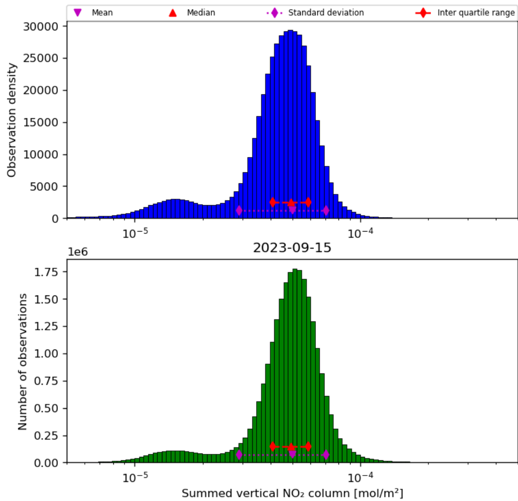
Figure 40: Histogram of "Summed vertical NO 2 column" for 2023-09-15 to 2023-09-16
