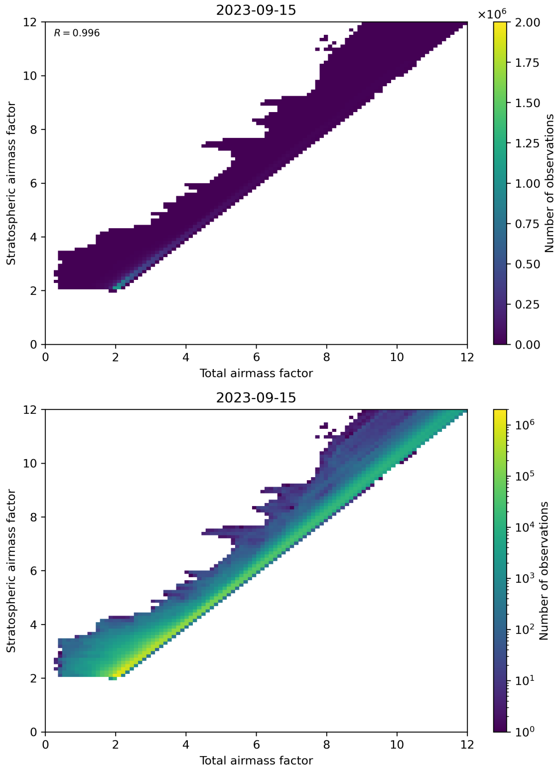
Figure 62: Scatter density plot of “Total airmass factor” against “Stratospheric airmass factor” for 2023-09-15 to 2023-09-16.
