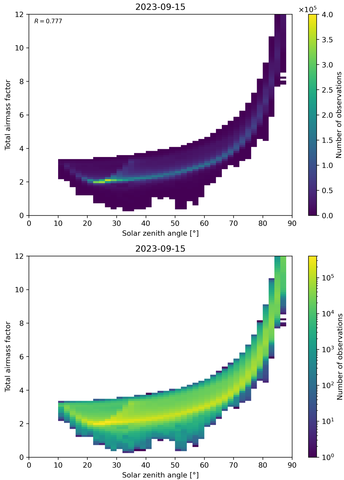
Figure 146: Scatter density plot of “Solar zenith angle” against “Total air mass factor” for 2023-09-15 to 2023-09-16.
