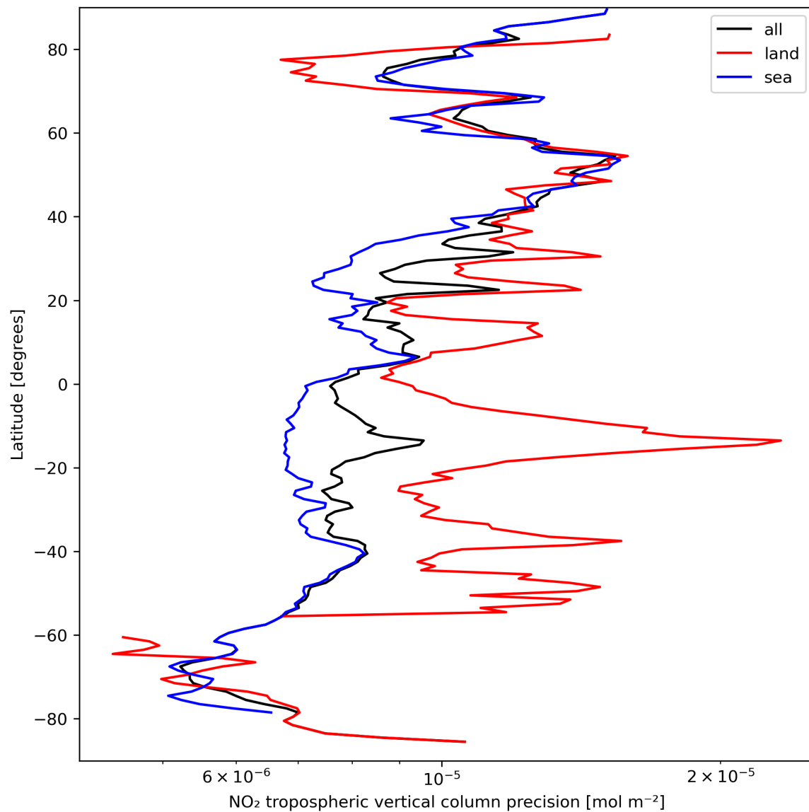
Figure 13: Zonal average of “NO 2 tropospheric vertical column precision” for 2023-09-15 to 2023-09-16.
