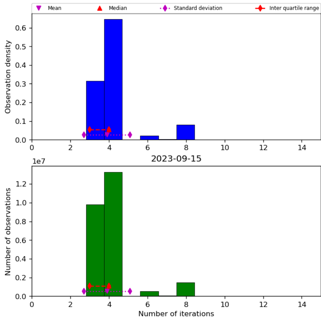
Figure 34: Histogram of “Number of iterations” for 2023-09-15 to 2023-09-16
