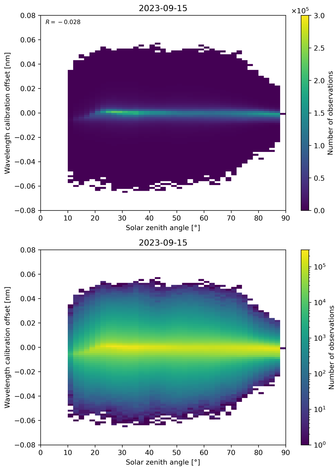
Figure 158: Scatter density plot of “Solar zenith angle” against “Wavelength calibration offset” for 2023-09-15 to 2023-09-16.
