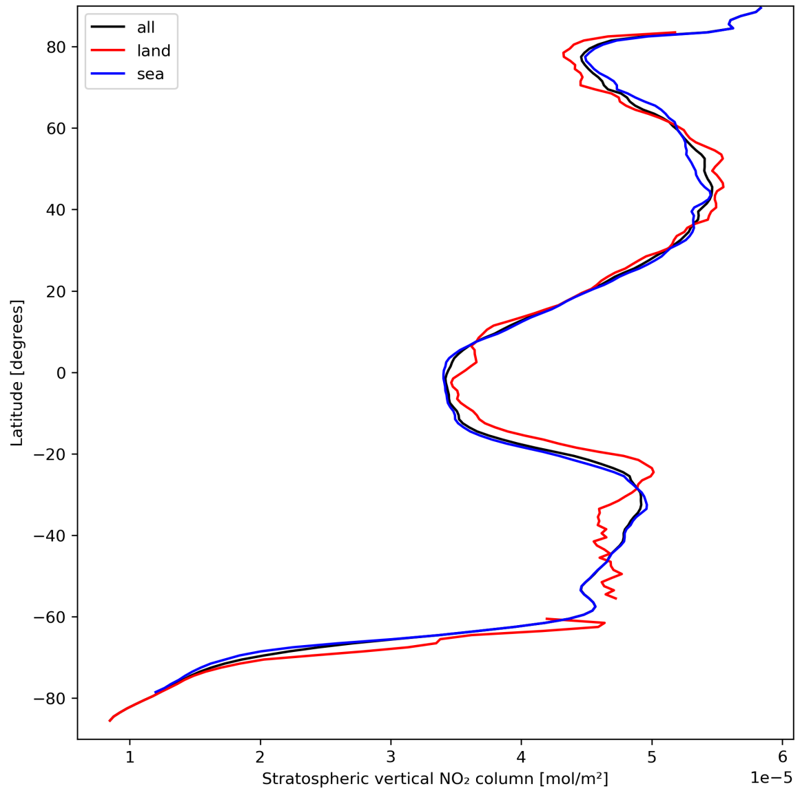
Figure 19: Zonal average of “Stratospheric vertical NO 2 column” for 2023-09-15 to 2023-09-16.
