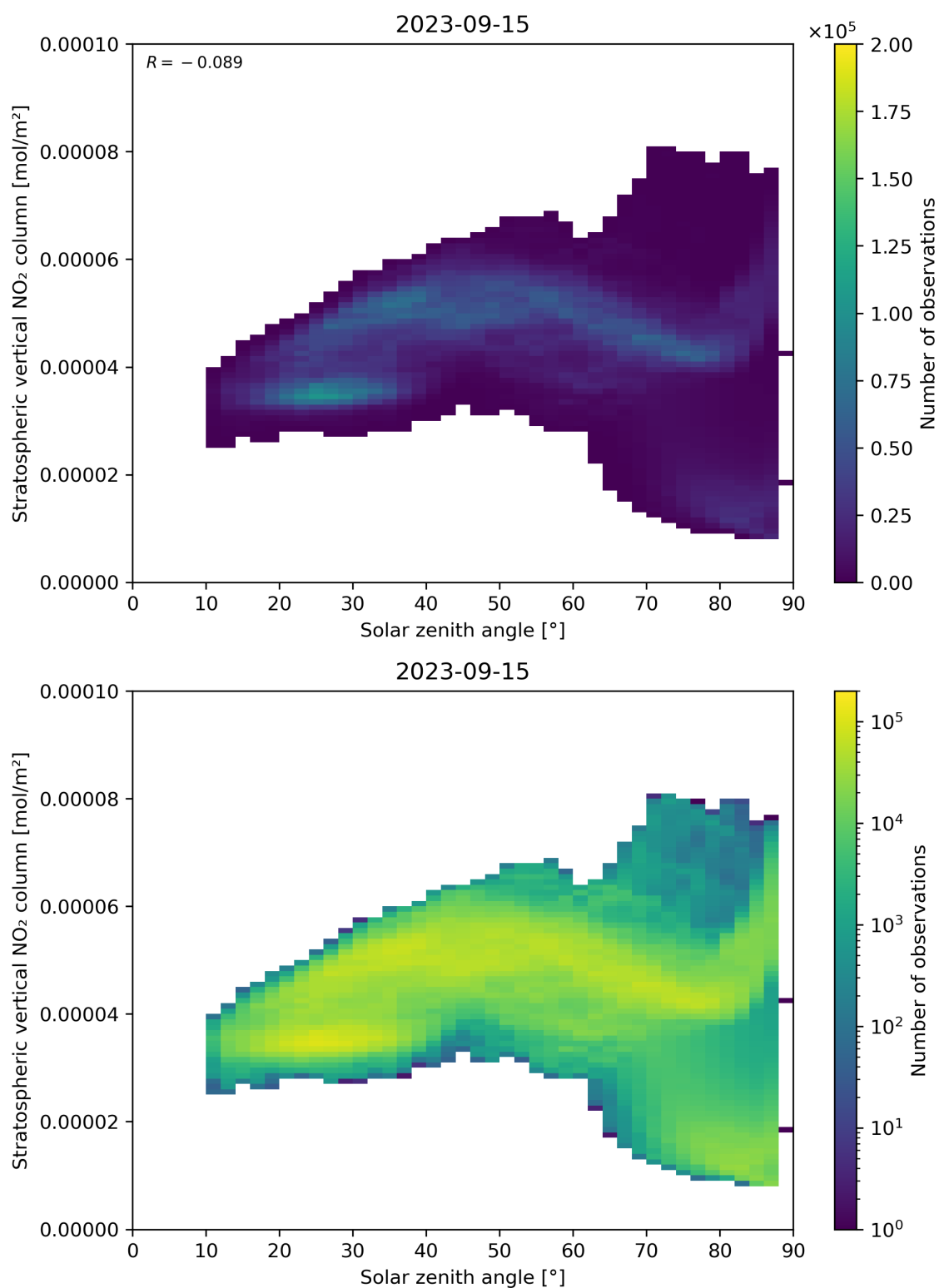
Figure 150: Scatter density plot of “Solar zenith angle” against “Stratospheric vertical NO 2 column” for 2023-09-15 to 2023-09-16.
