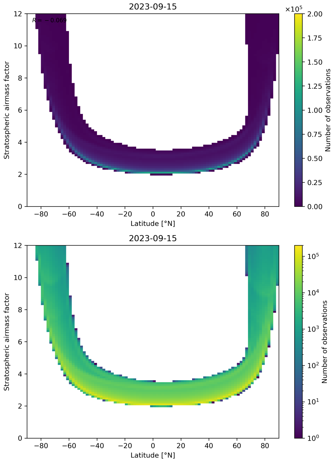
Figure 83: Scatter density plot of “Latitude” against “Stratospheric air mass factor” for 2023-09-15 to 2023-09-16.
