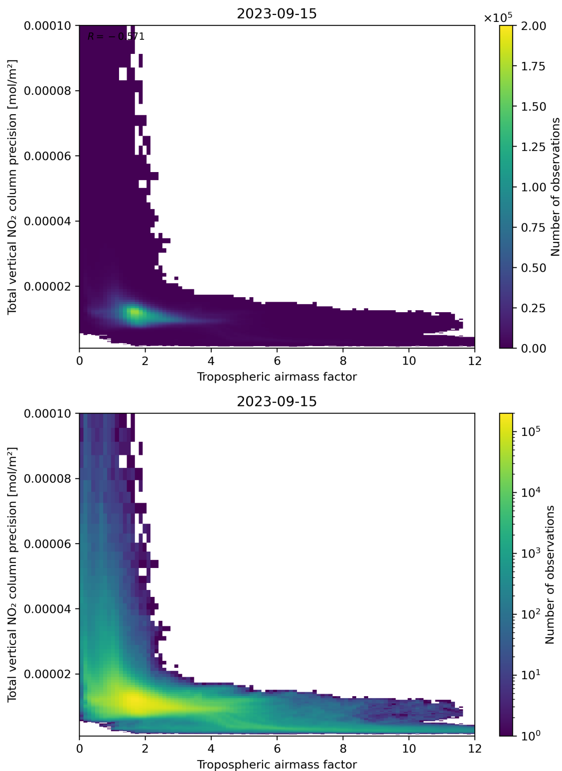
Figure 78: Scatter density plot of “Tropospheric air mass factor” against “Total vertical NO 2 column precision” for 2023-09-15 to 2023-09-16.
