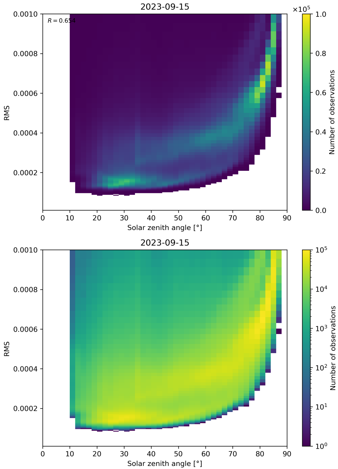
Figure 157: Scatter density plot of “Solar zenith angle” against “RMS” for 2023-09-15 to 2023-09-16.
