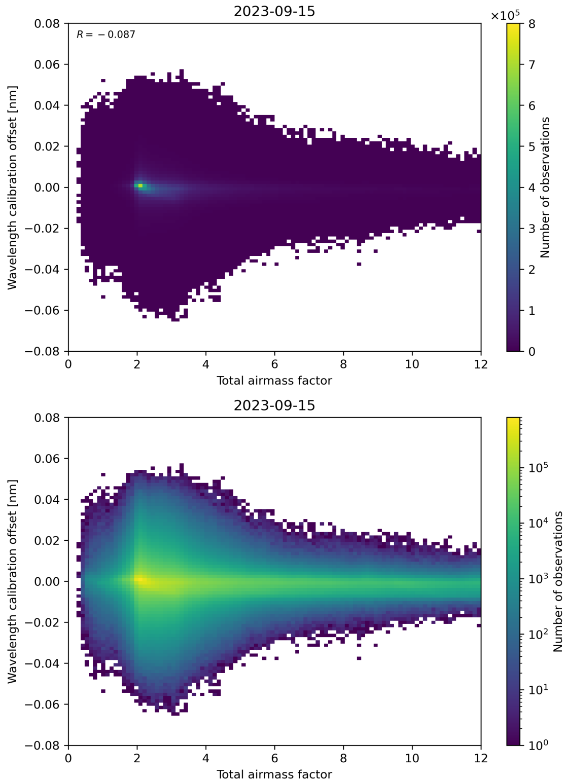
Figure 70: Scatter density plot of “Total airmass factor” against “Wavelength calibration offset” for 2023-09-15 to 2023-09-16.
