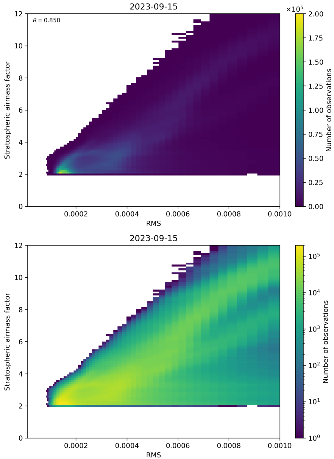
Figure 144: Scatter density plot of “RMS” against “Stratospheric airmass factor” for 2023-09-15 to 2023-09-16.
