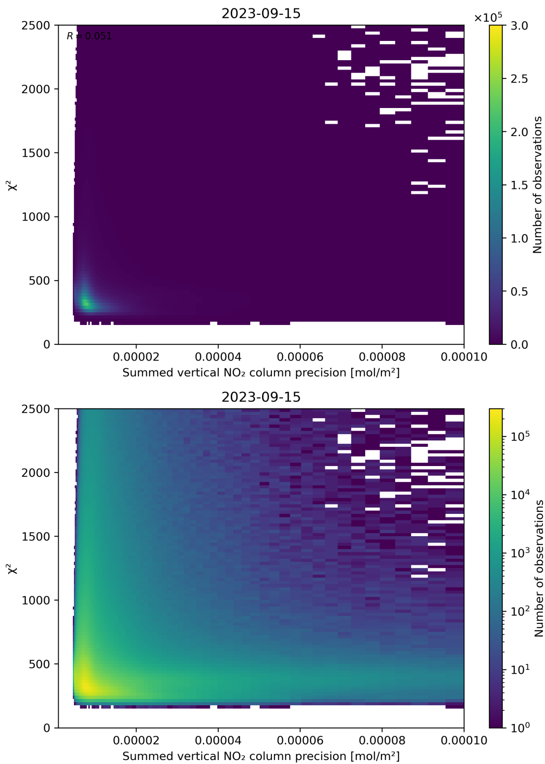
Figure 107: Scatter density plot of “Summed vertical NO 2 column precision” against “ \chi^2 ” for 2023-09-15 to 2023-09-16.
