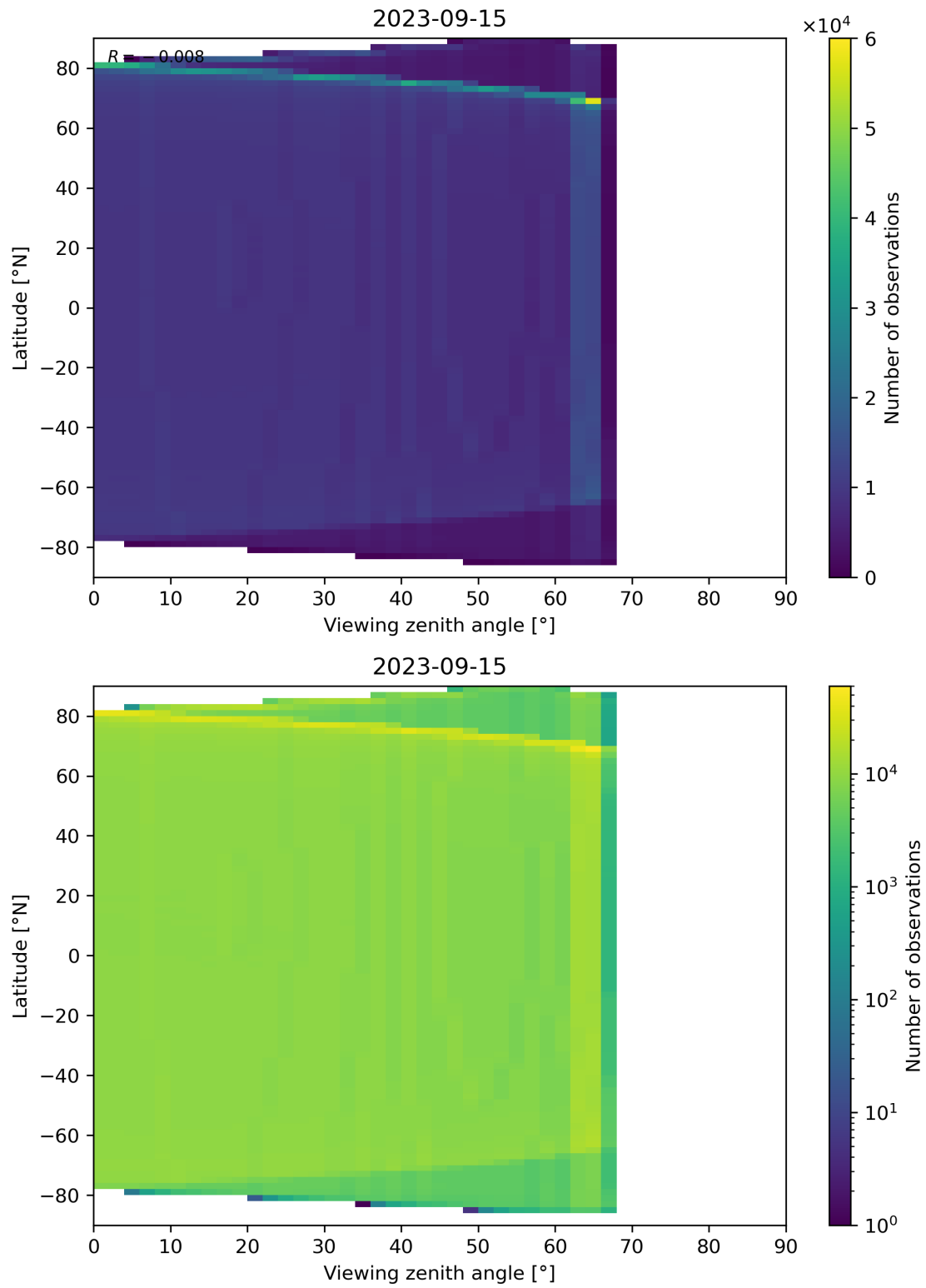
Figure 163: Scatter density plot of “Viewing zenith angle” against “Latitude” for 2023-09-15 to 2023-09-16.
