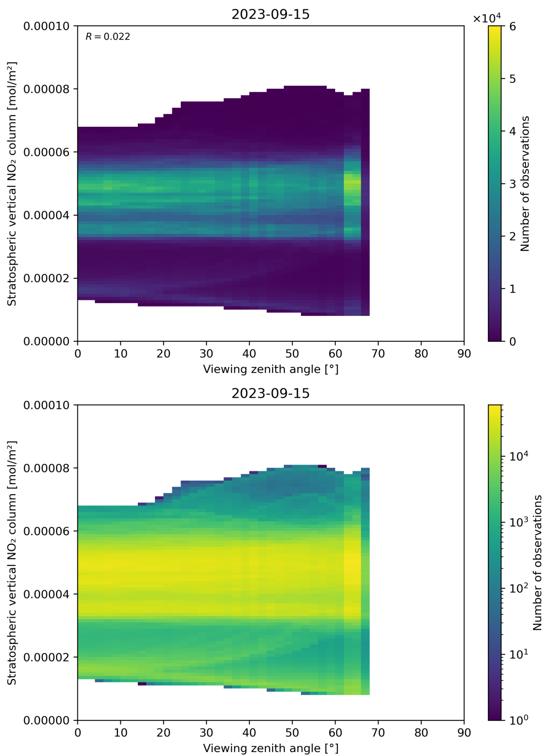
Figure 164: Scatter density plot of “Viewing zenith angle” against “Stratospheric vertical NO 2 column” for 2023-09-15 to 2023-09-16.
