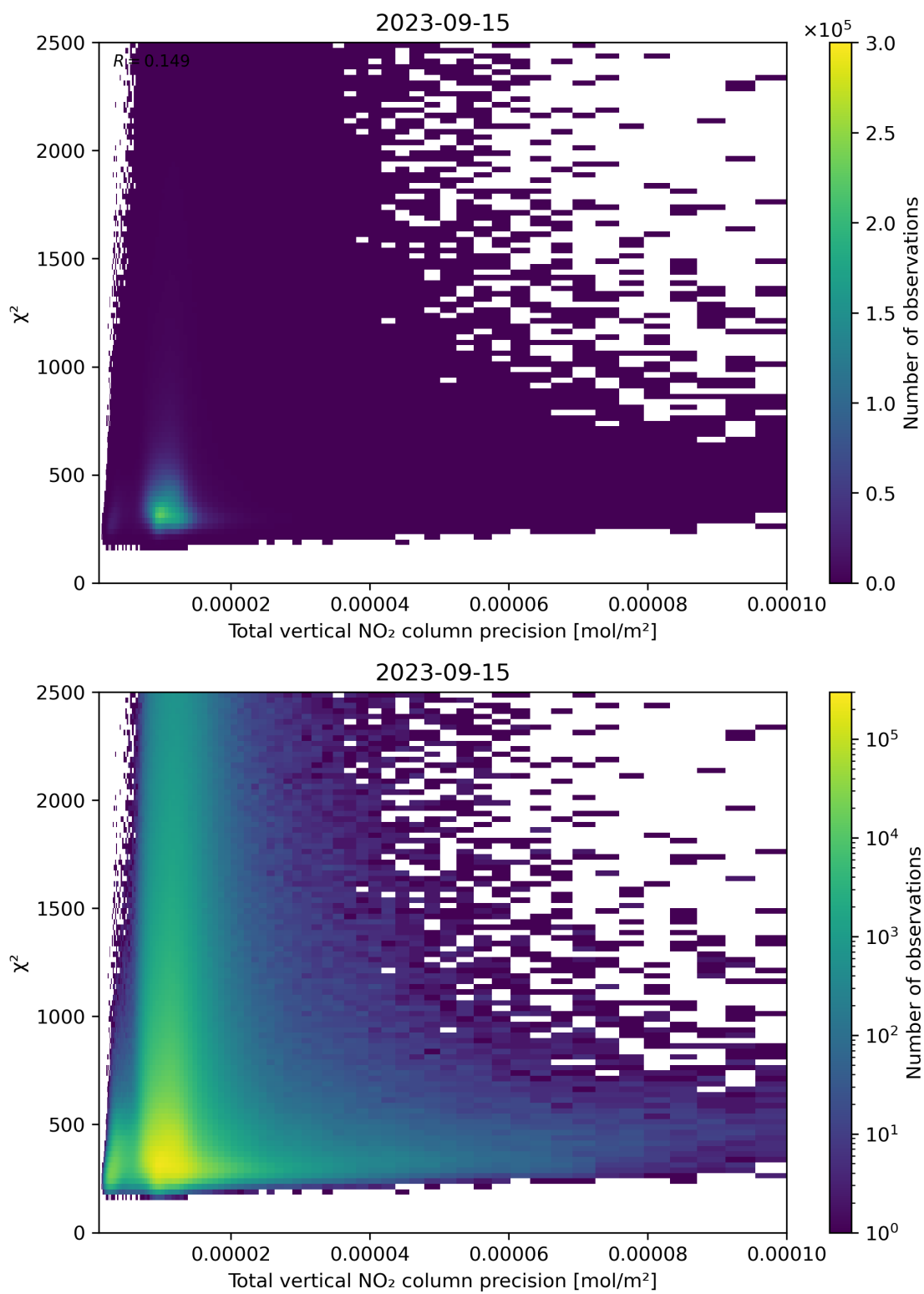
Figure 116: Scatter density plot of “Total vertical NO 2 column precision” against “ \chi^2 ” for 2023-09-15 to 2023-09-16.
