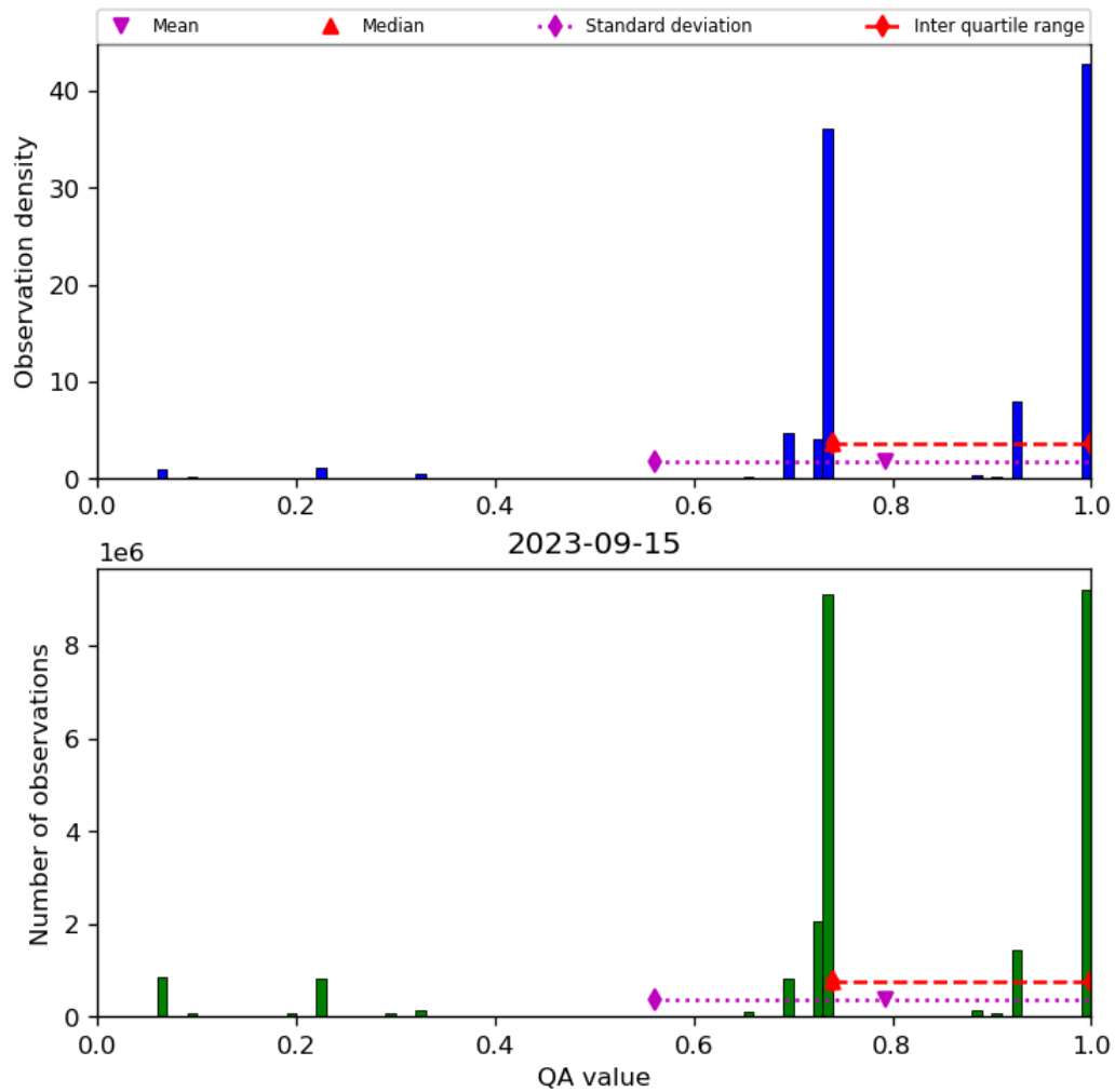
Figure 28: Histogram of “QA value” for 2023-09-15 to 2023-09-16
