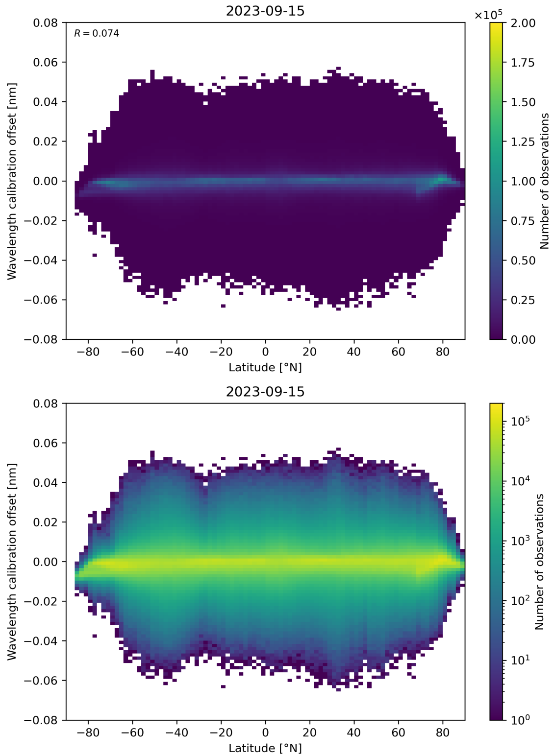
Figure 95: Scatter density plot of “Latitude” against “Wavelength calibration offset” for 2023-09-15 to 2023-09-16.
