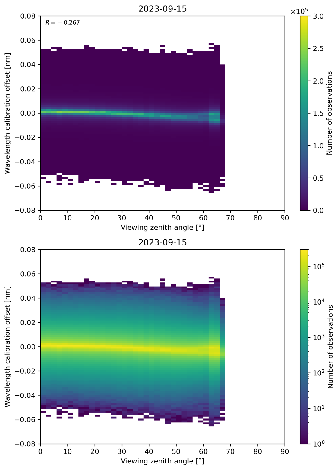
Figure 173: Scatter density plot of “Viewing zenith angle” against “Wavelength calibration offset” for 2023-09-15 to 2023-09-16.
