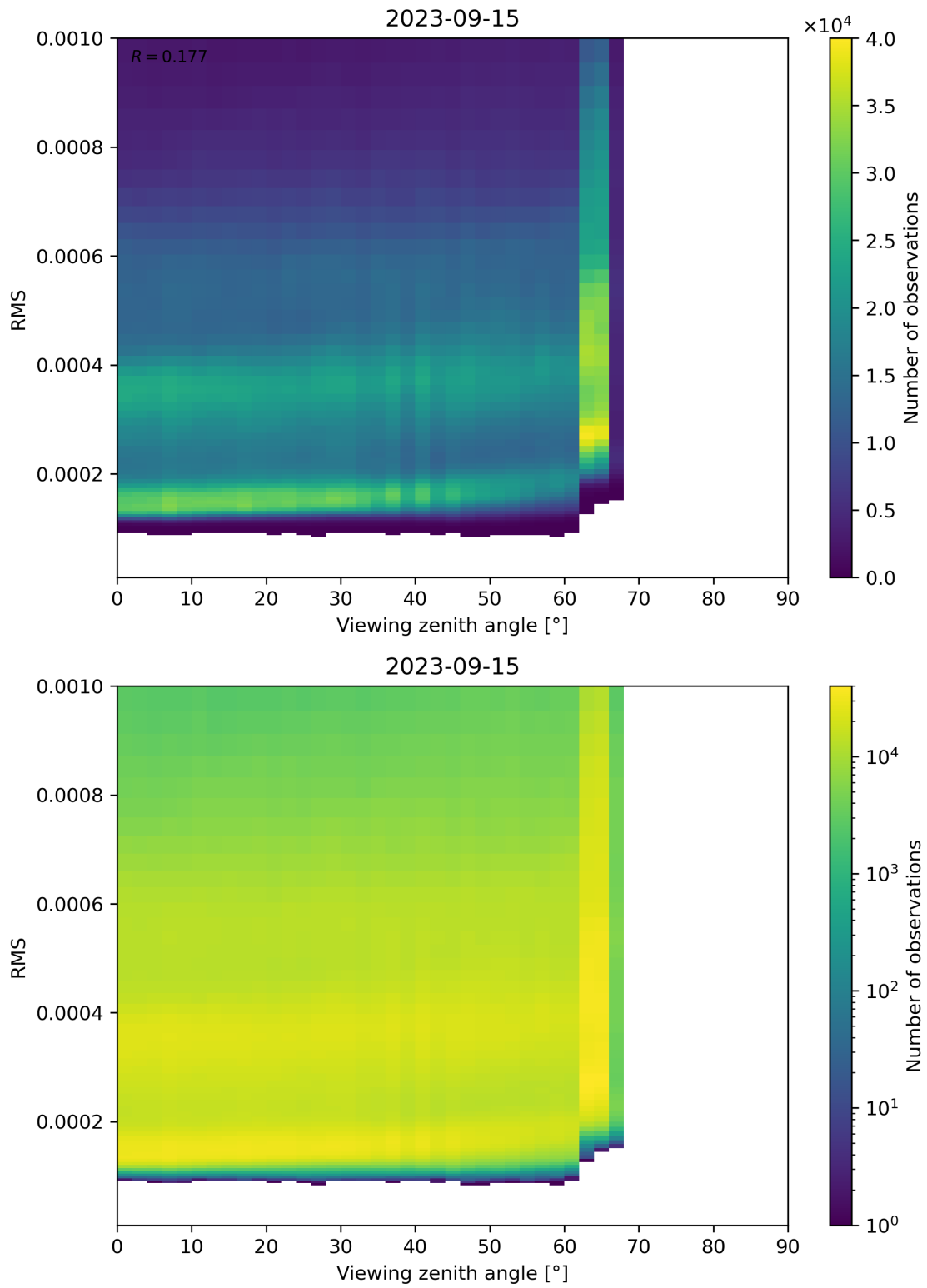
Figure 171: Scatter density plot of “Viewing zenith angle” against “RMS” for 2023-09-15 to 2023-09-16.
