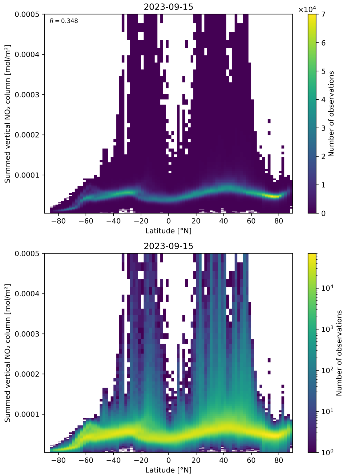
Figure 88: Scatter density plot of “Latitude” against “Summed vertical NO 2 column” for 2023-09-15 to 2023-09-16.
