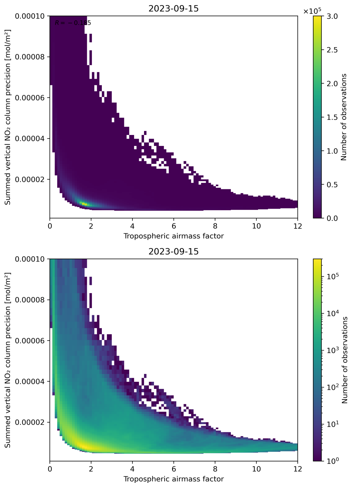
Figure 76: Scatter density plot of “Tropospheric air mass factor” against “Summed vertical NO 2 column precision” for 2023-09-15 to 2023-09-16.
