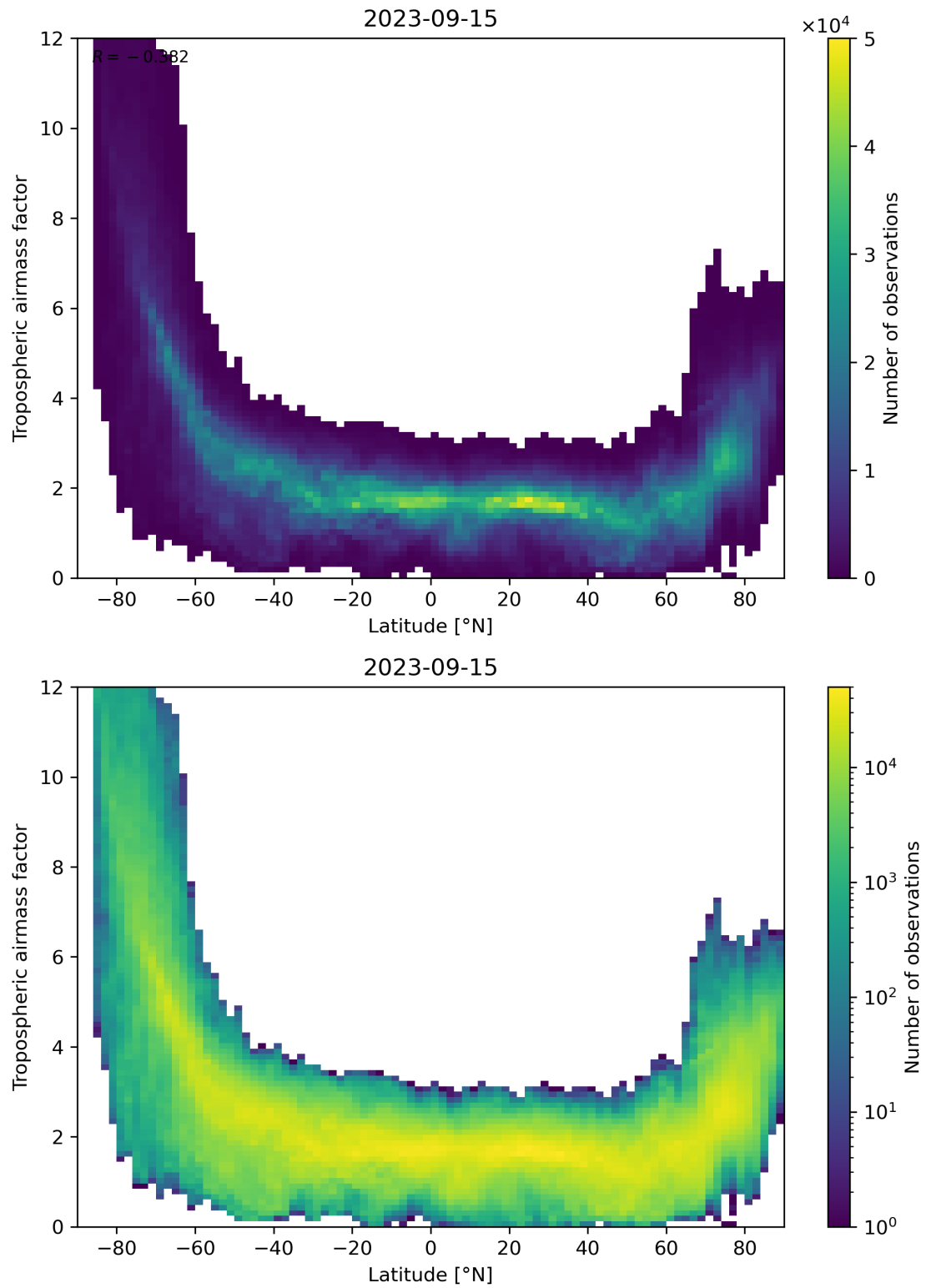
Figure 85: Scatter density plot of “Latitude” against “Tropospheric airmass factor” for 2023-09-15 to 2023-09-16.
