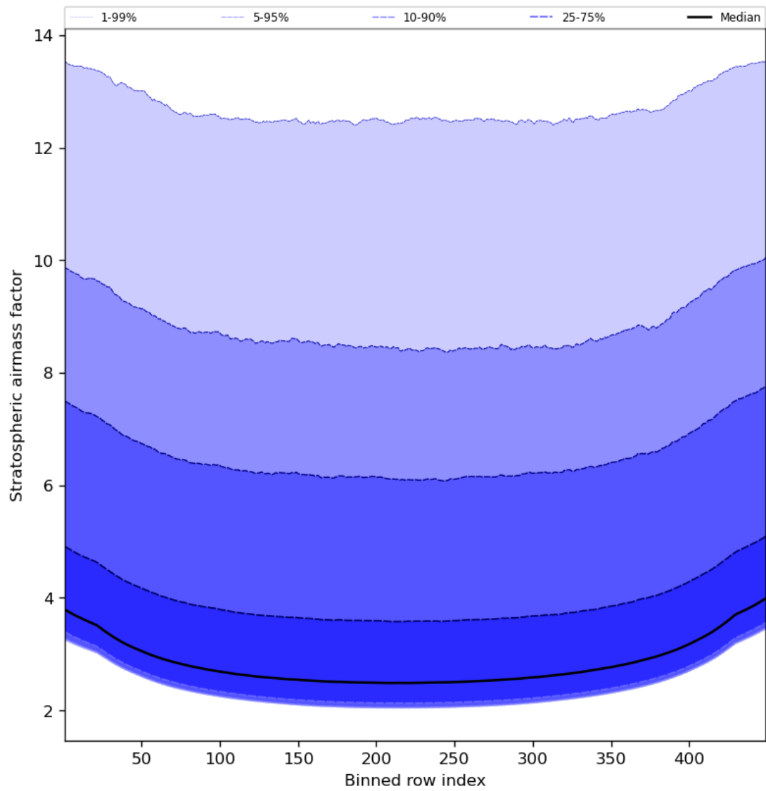
Figure 61: Along track statistics of “Stratospheric airmass factor” for 2023-09-15 to 2023-09-16
