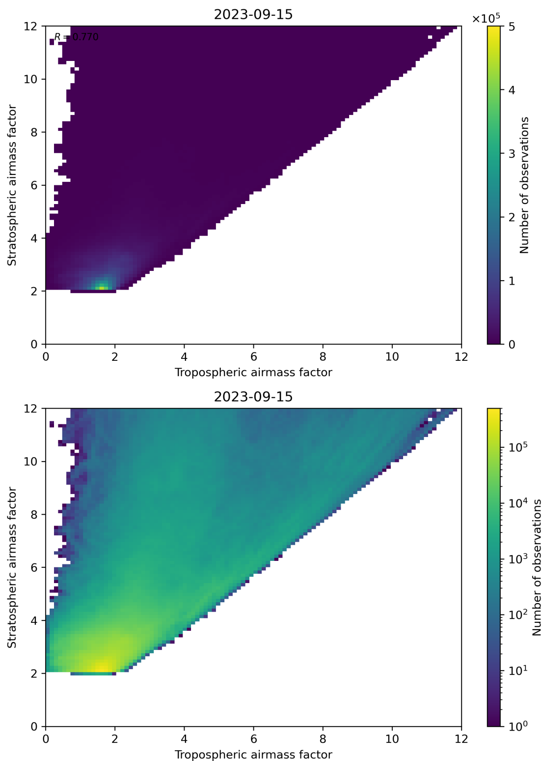
Figure 71: Scatter density plot of “Tropospheric airmass factor” against “Stratospheric airmass factor” for 2023-09-15 to 2023-09-16.
