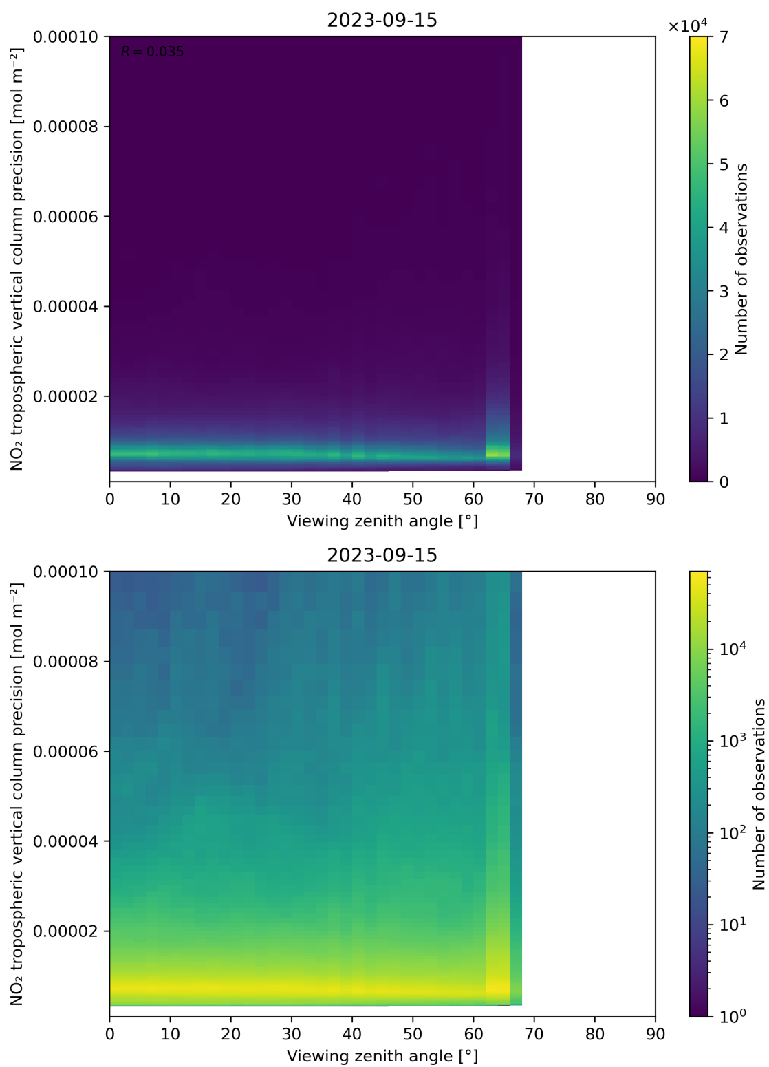
Figure 170: Scatter density plot of “Viewing zenith angle” against “NO 2 tropospheric vertical column precision” for 2023-09-15 to 2023-09-16.
