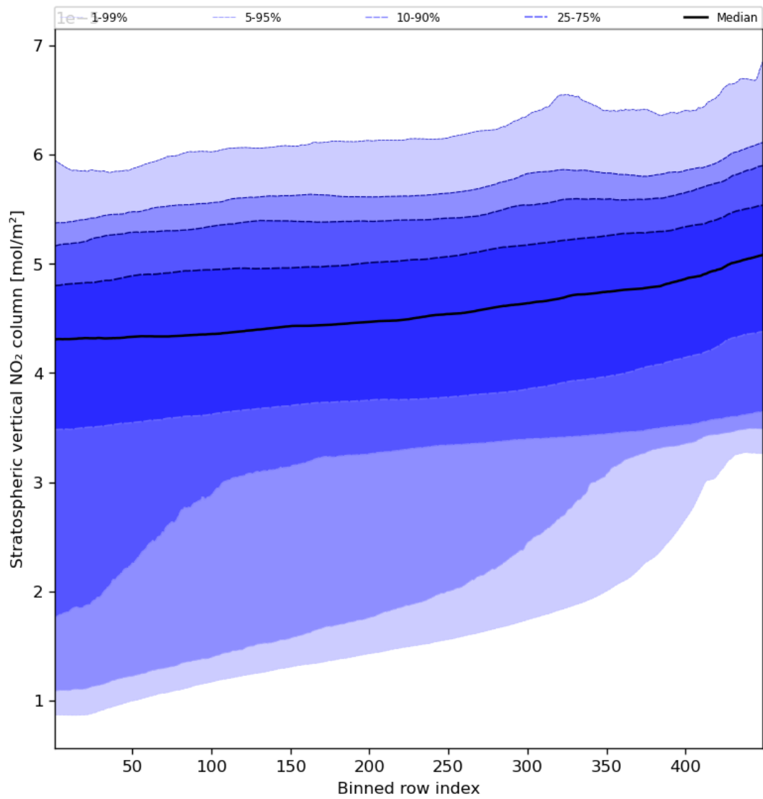
Figure 53: Along track statistics of “Stratospheric vertical NO 2 column” for 2023-09-15 to 2023-09-16
