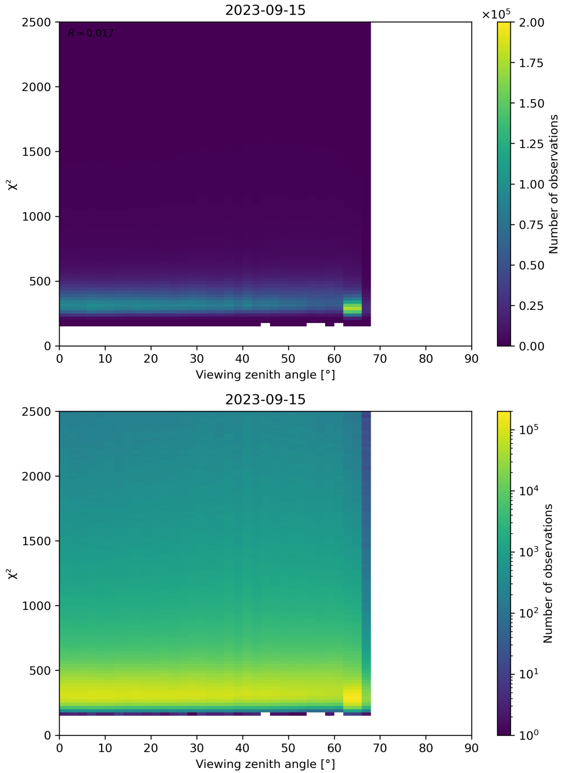
Figure 162: Scatter density plot of “Viewing zenith angle” against “ \chi^2 ” for 2023-09-15 to 2023-09-16.
