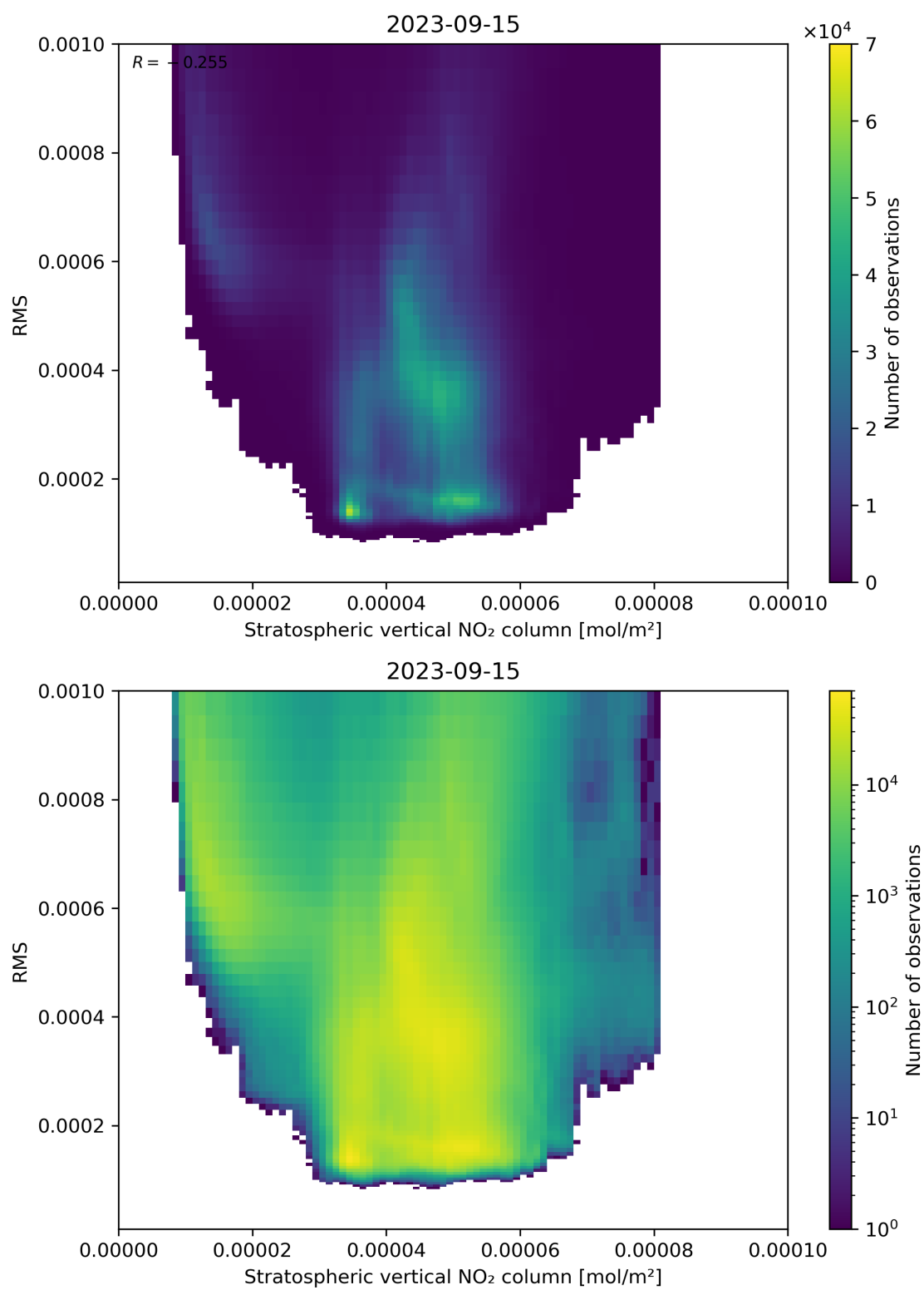
Figure 102: Scatter density plot of “Stratospheric vertical NO 2 column” against “RMS” for 2023-09-15 to 2023-09-16.
