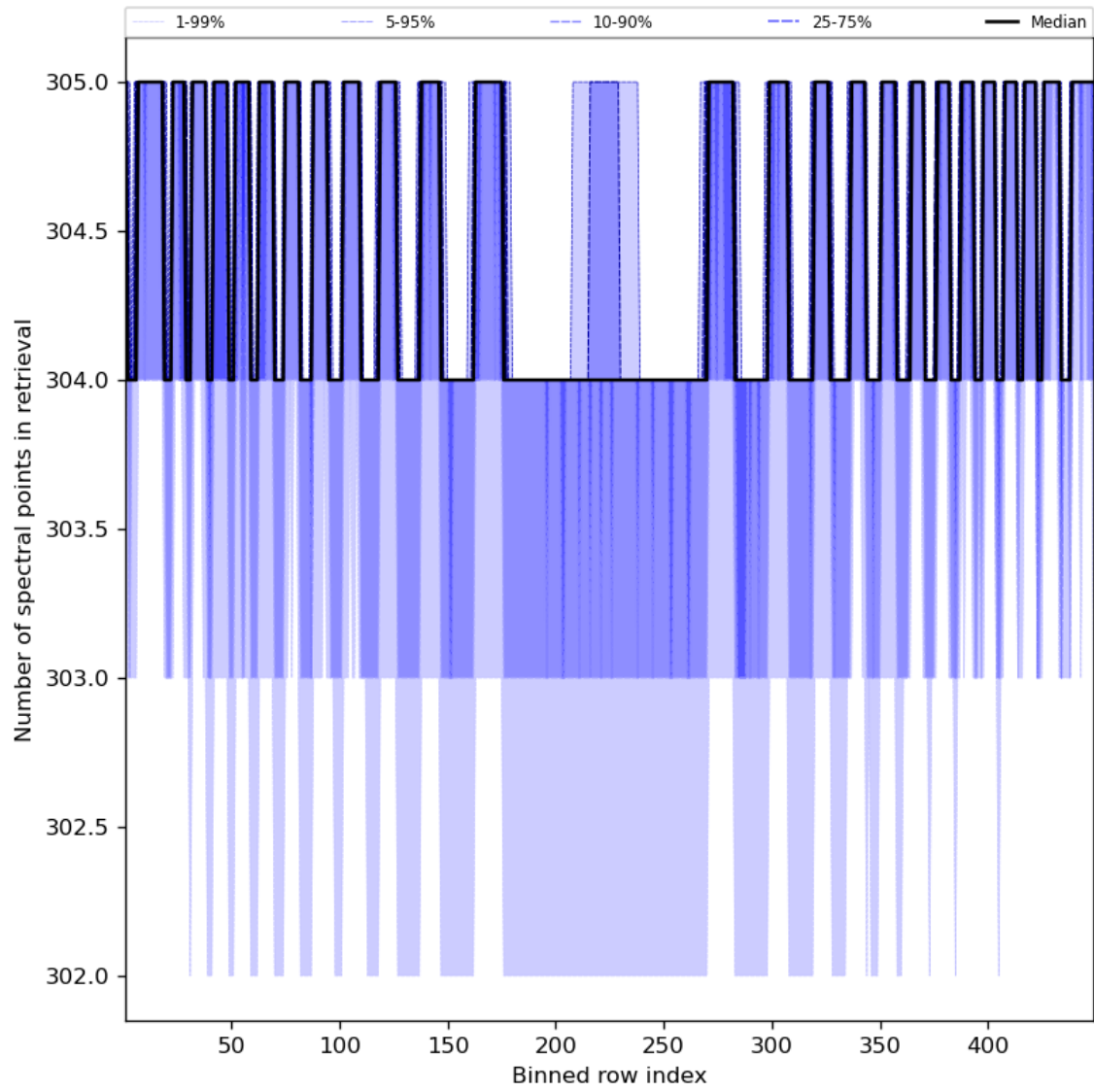
Figure 50: Along track statistics of “Number of spectral points in retrieval” for 2023-09-15 to 2023-09-16
