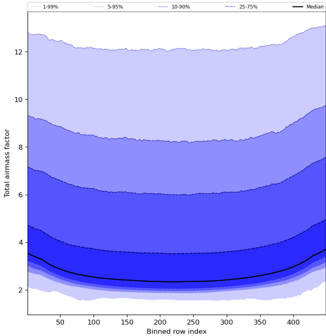
Figure 49: Along track statistics of “Total airmass factor” for 2023-09-15 to 2023-09-16
