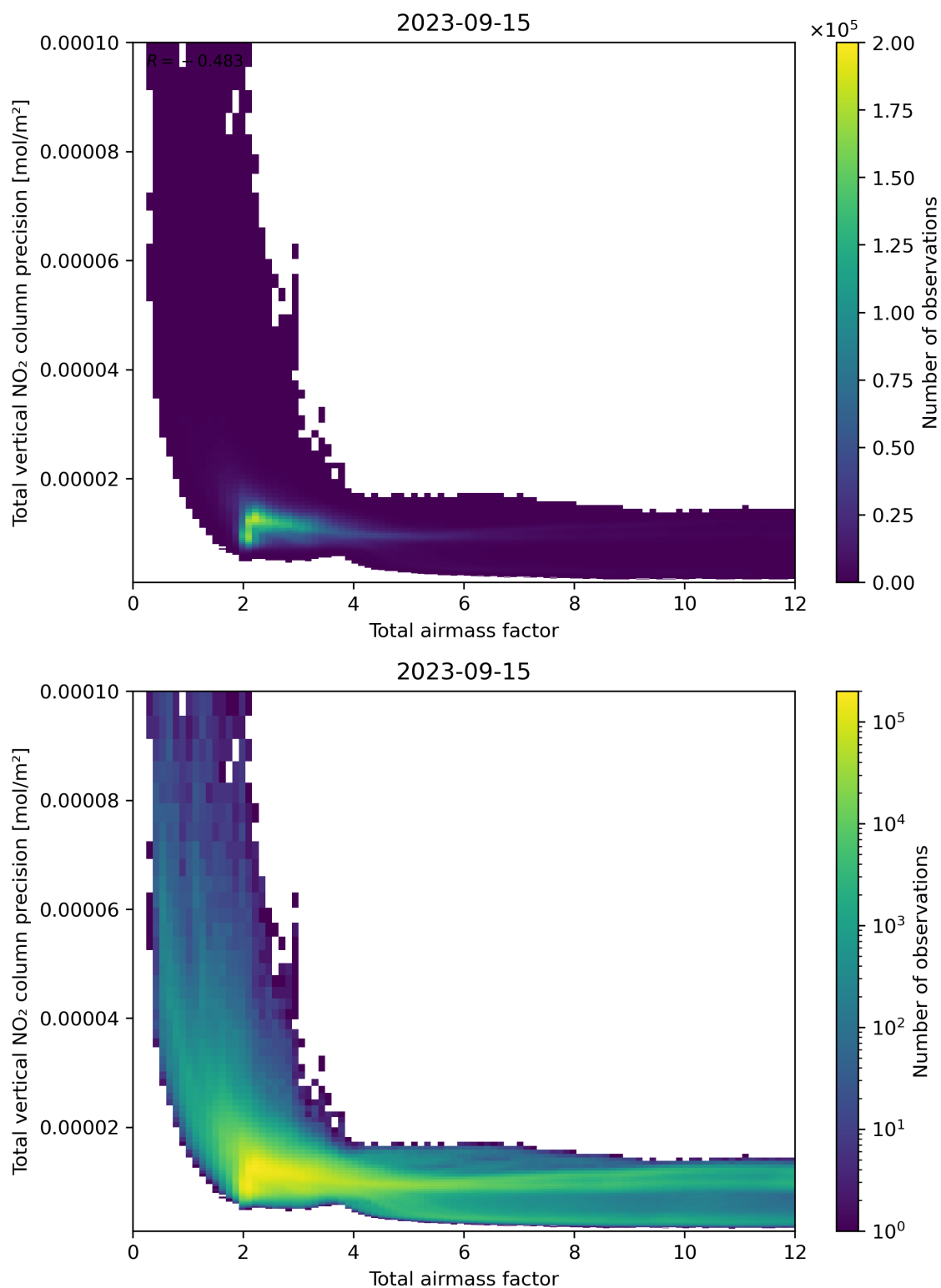
Figure 68: Scatter density plot of “Total airmass factor” against “Total vertical NO 2 column precision” for 2023-09-15 to 2023-09-16.
