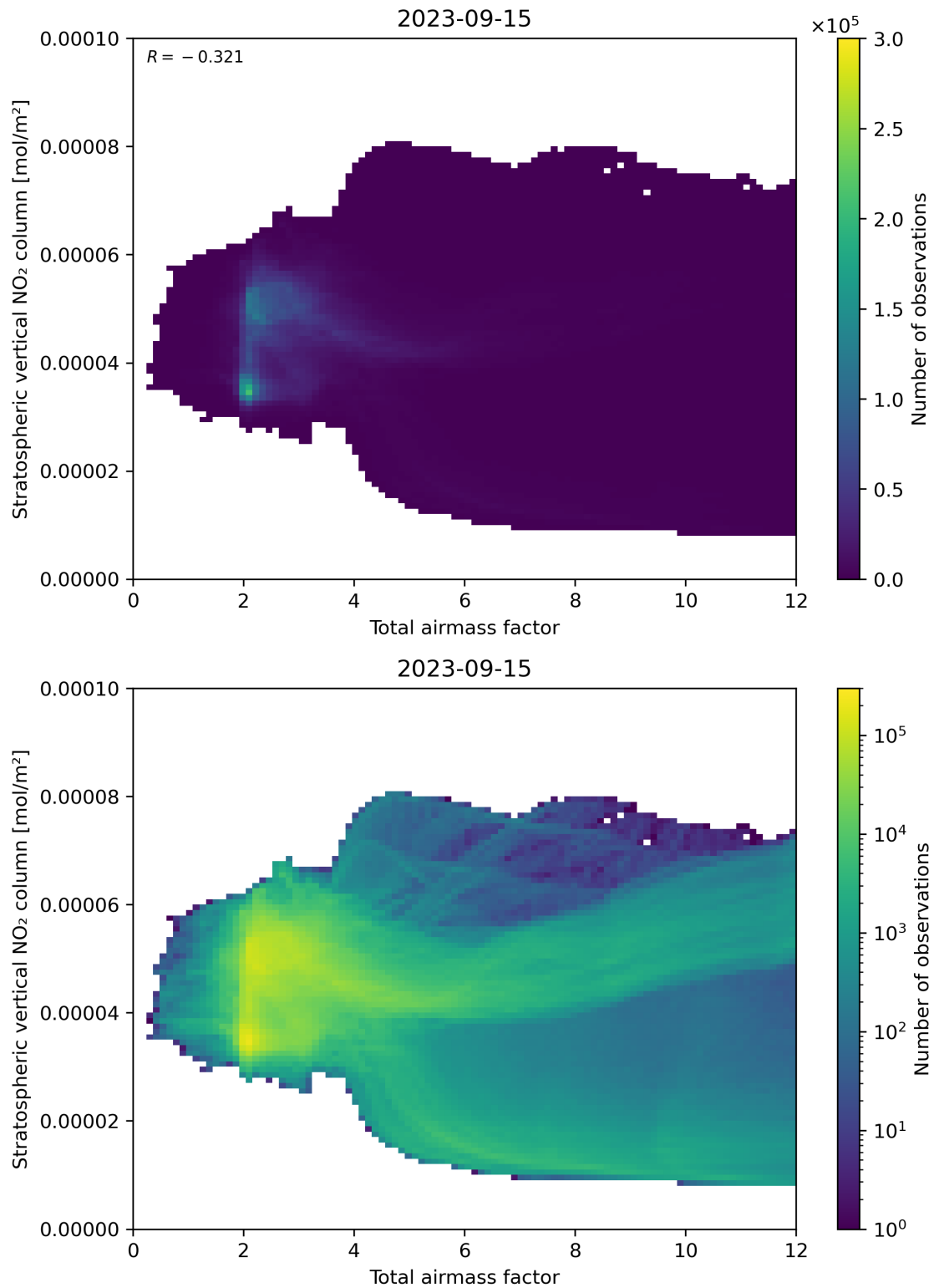
Figure 64: Scatter density plot of “Total airmass factor” against “Stratospheric vertical NO 2 column” for 2023-09-15 to 2023-09-16.
