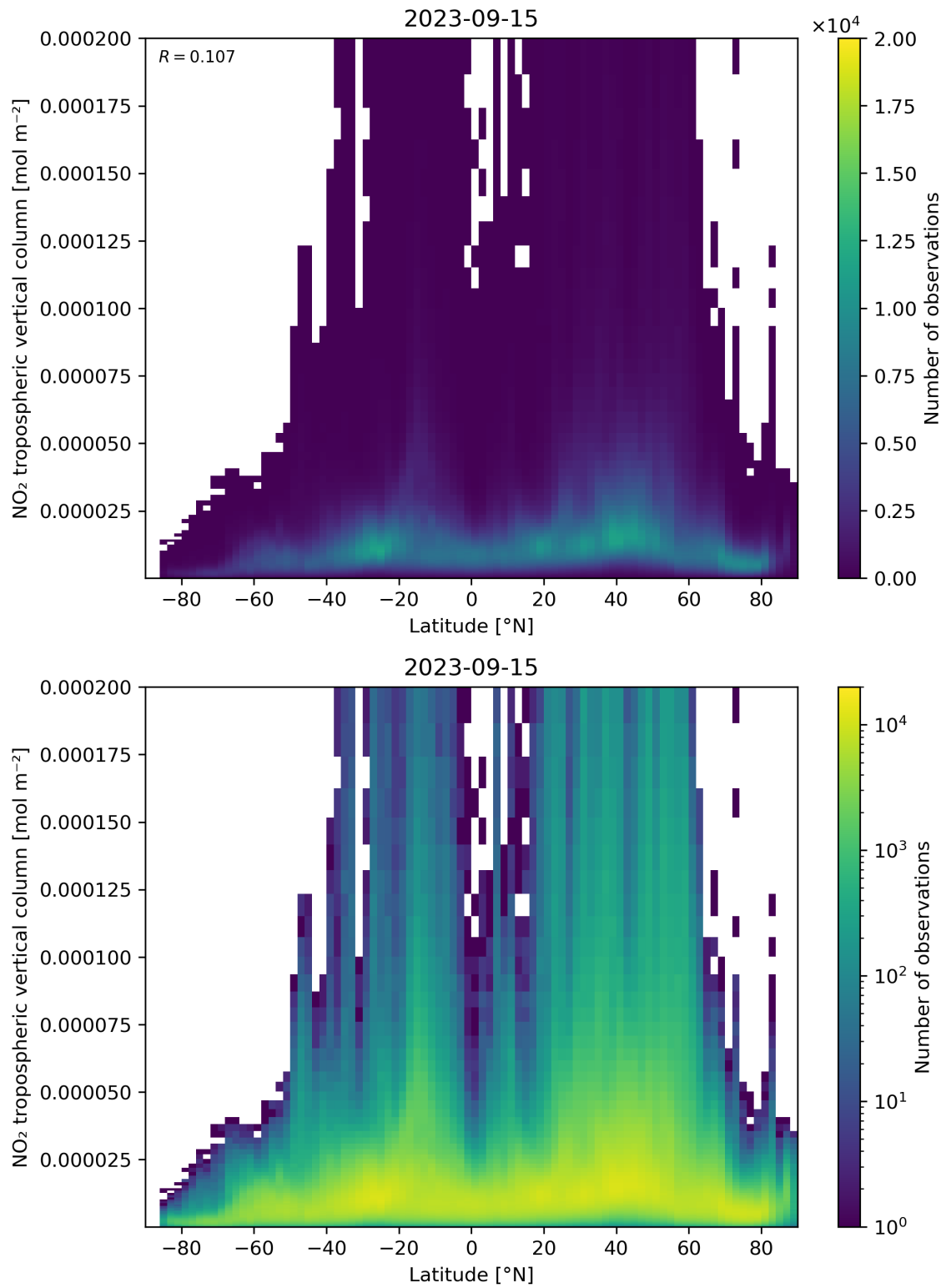
Figure 92: Scatter density plot of “Latitude” against “NO 2 tropospheric vertical column” for 2023-09-15 to 2023-09-16.
