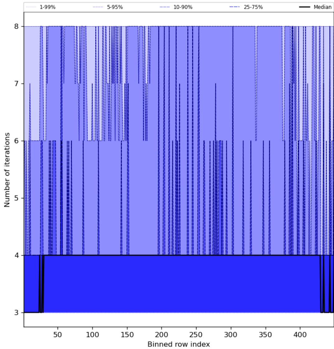
Figure 51: Along track statistics of “Number of iterations” for 2023-09-15 to 2023-09-16
