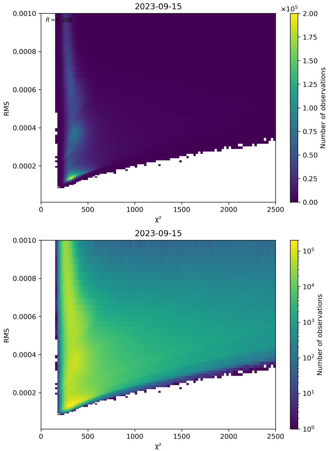
Figure 82: Scatter density plot of “ \chi^2 ” against “RMS” for 2023-09-15 to 2023-09-16.
