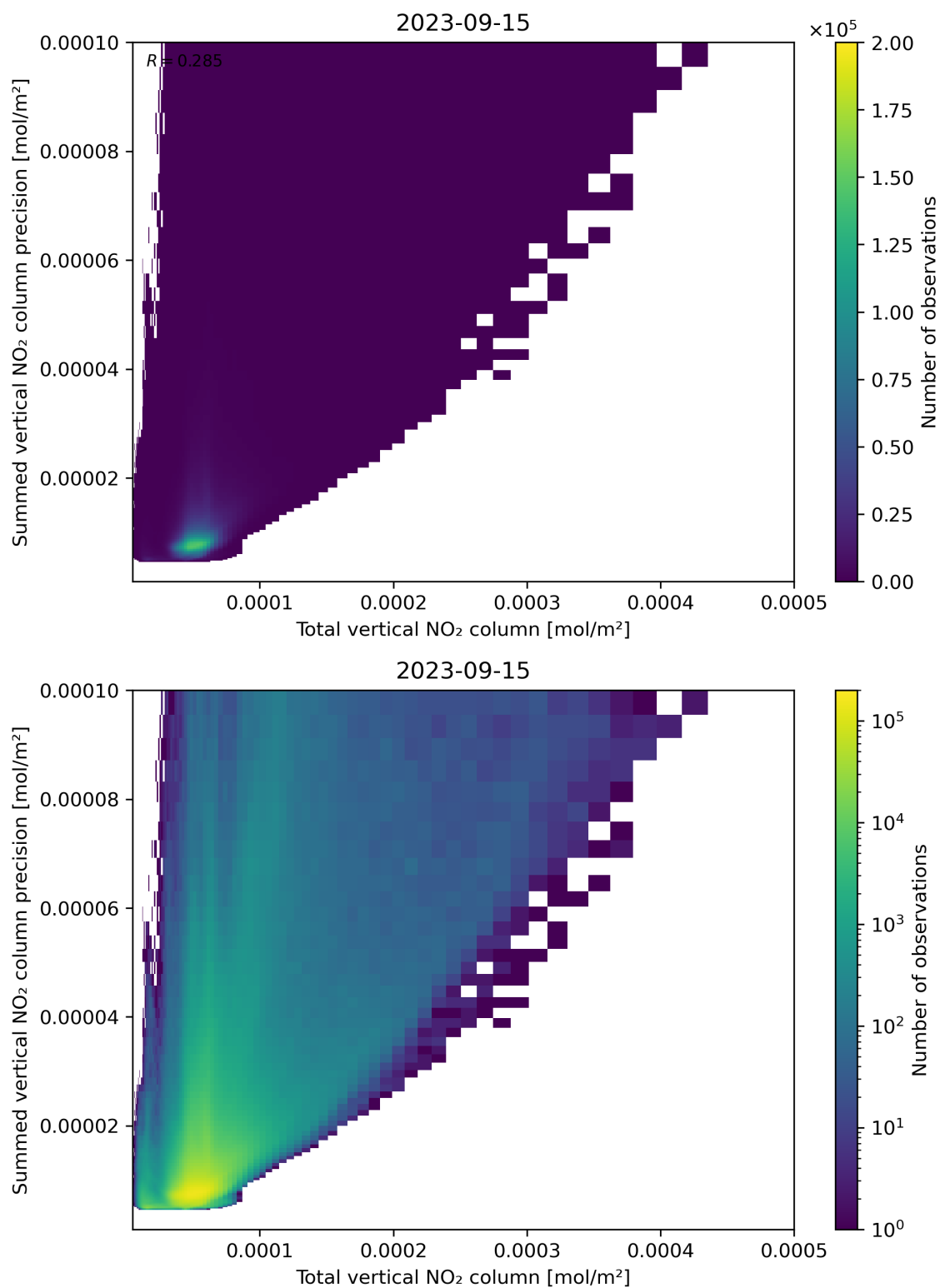
Figure 113: Scatter density plot of “Total vertical NO 2 column” against “Summed vertical NO 2 column precision” for 2023-09-15 to 2023-09-16.
