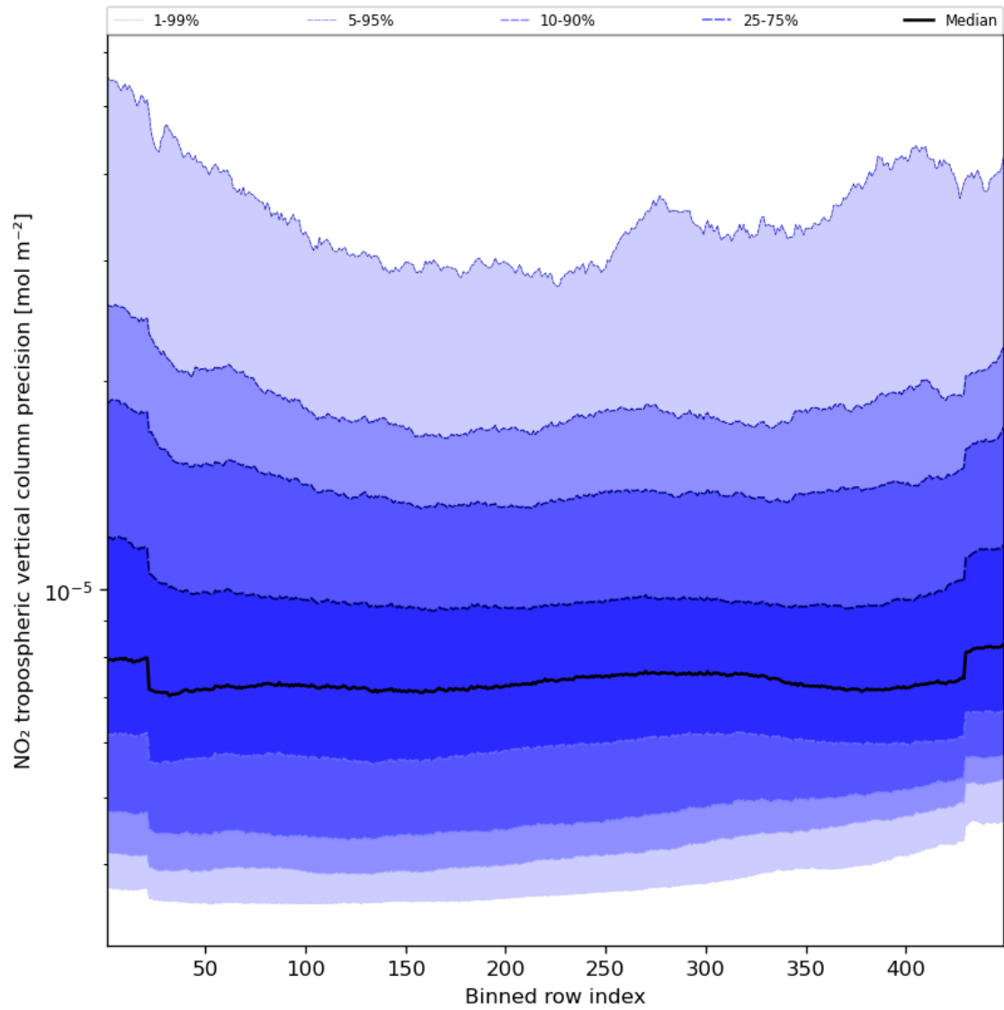
Figure 47: Along track statistics of “NO 2 tropospheric vertical column precision” for 2023-09-15 to 2023-09-16
