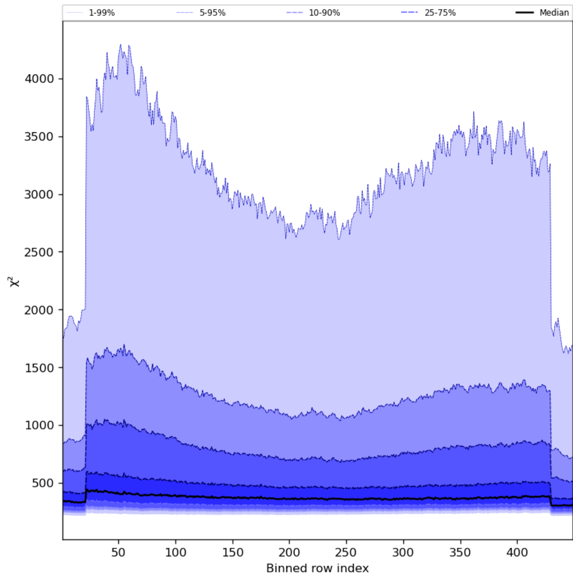
Figure 59: Along track statistics of “ \chi^2 ” for 2023-09-15 to 2023-09-16
