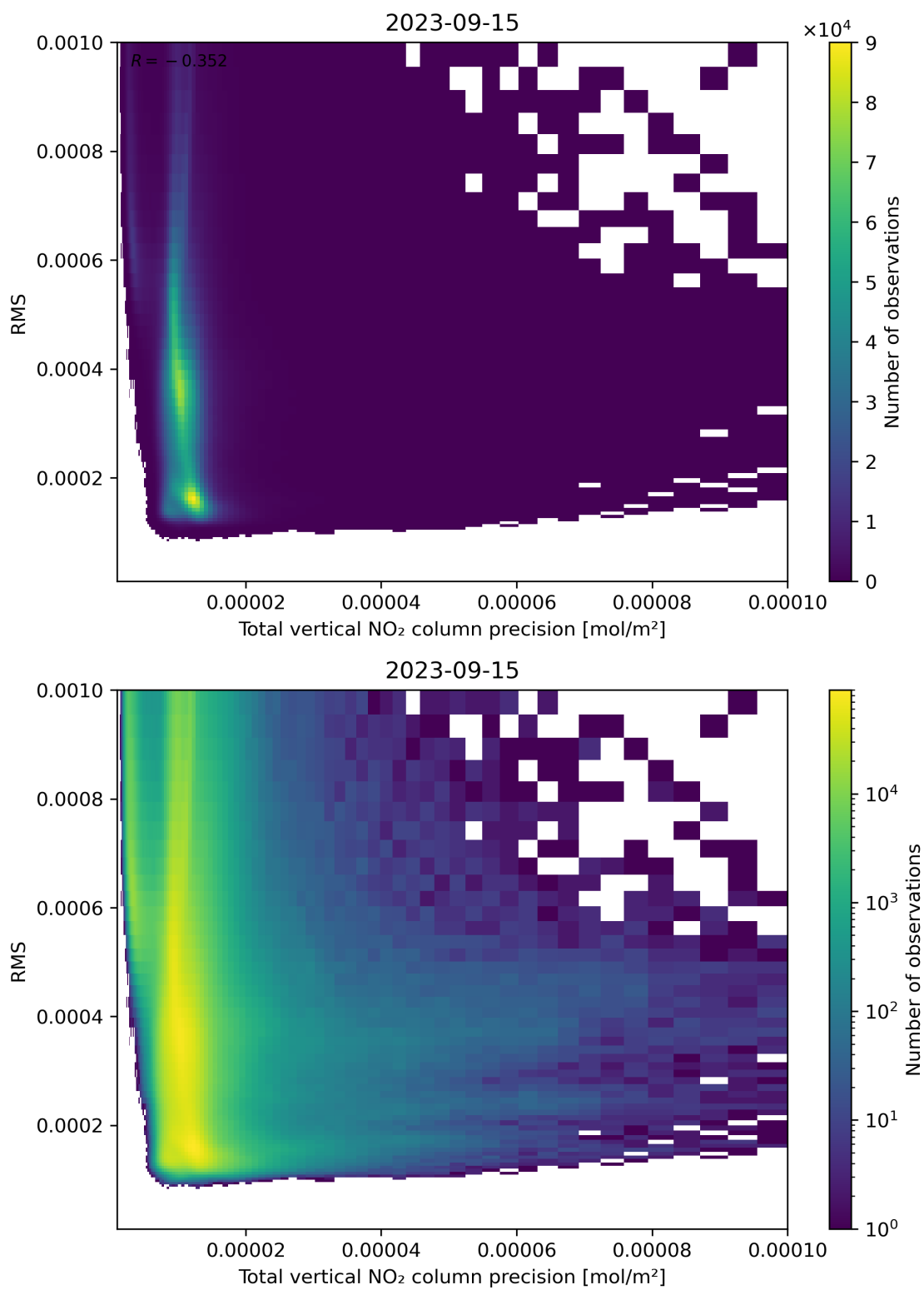
Figure 119: Scatter density plot of “Total vertical NO 2 column precision” against “RMS” for 2023-09-15 to 2023-09-16.
