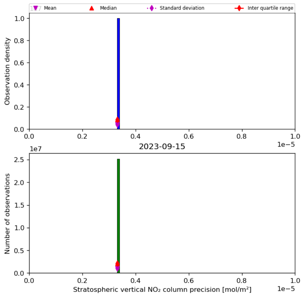
Figure 37: Histogram of “Stratospheric vertical NO 2 column precision” for 2023-09-15 to 2023-09-16
