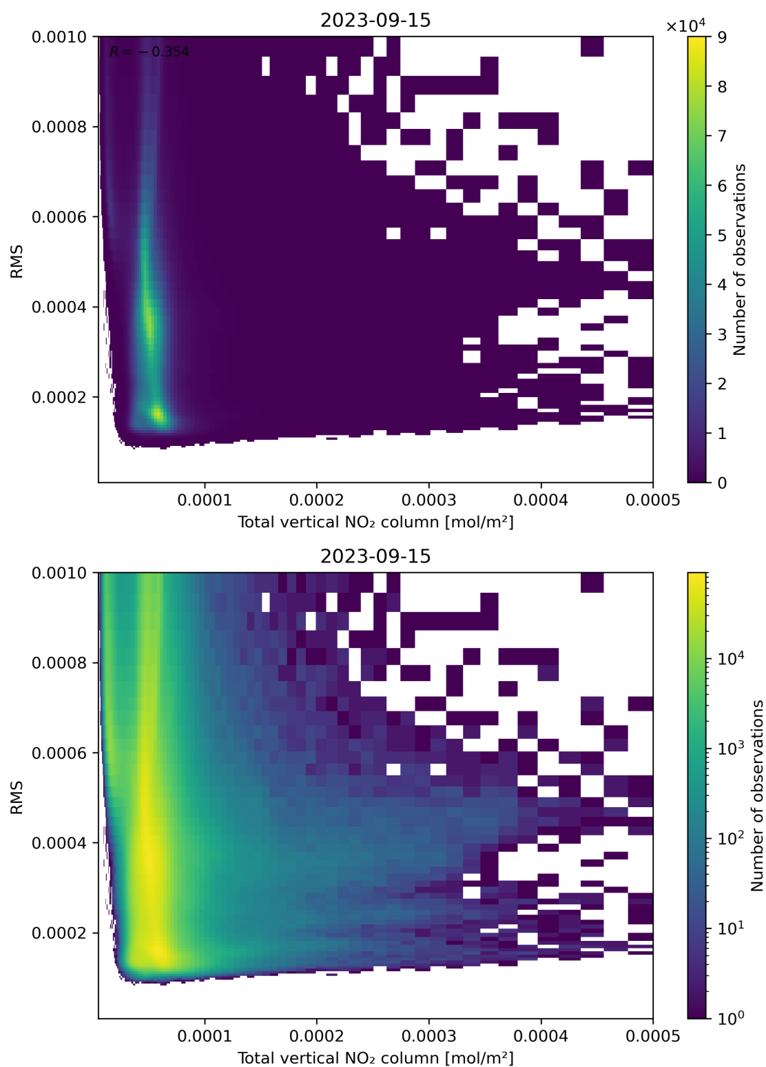
Figure 120: Scatter density plot of “Total vertical NO 2 column” against “RMS” for 2023-09-15 to 2023-09-16.
