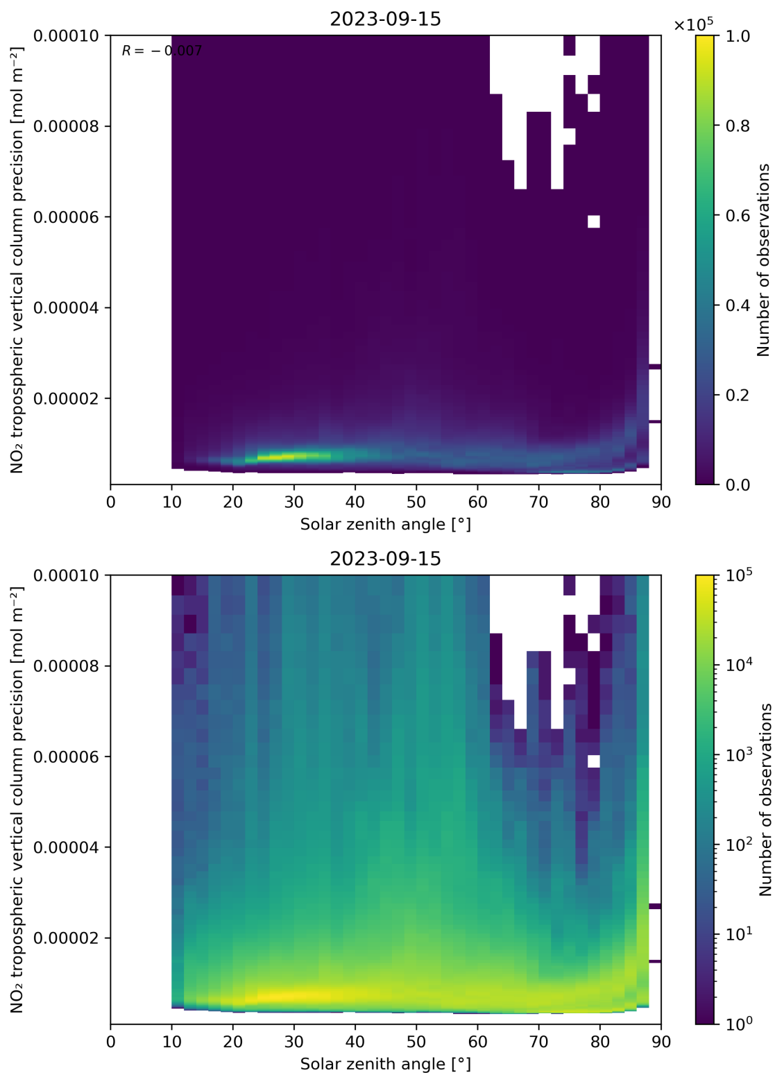
Figure 156: Scatter density plot of “Solar zenith angle” against “NO 2 tropospheric vertical column precision” for 2023-09-15 to 2023-09-16.
