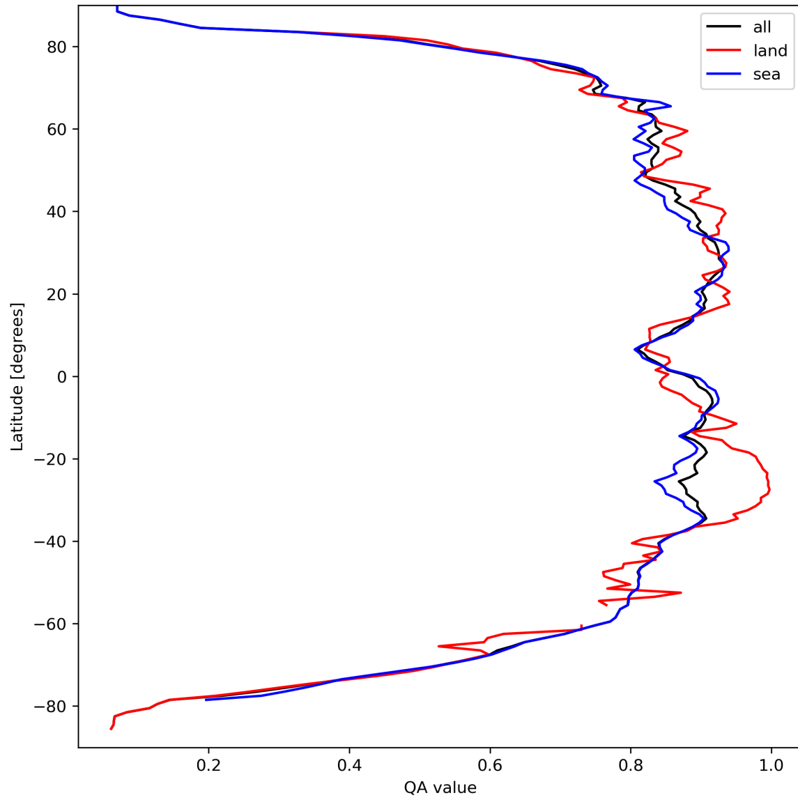
Figure 11: Zonal average of “QA value” for 2023-09-15 to 2023-09-16.
