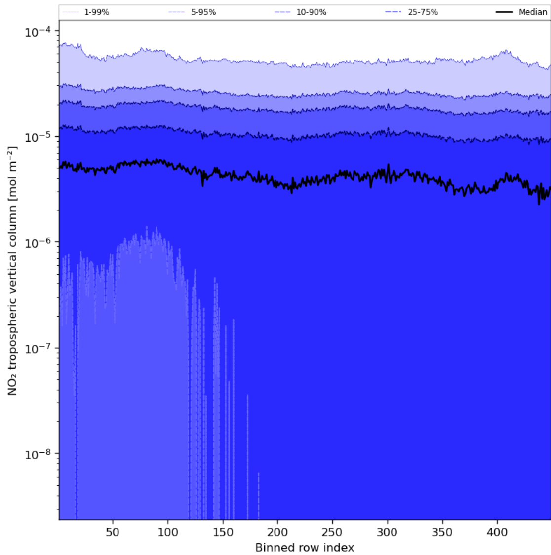
Figure 46: Along track statistics of “NO 2 tropospheric vertical column” for 2023-09-15 to 2023-09-16
