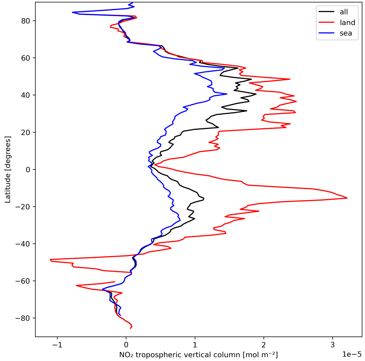
Figure 12: Zonal average of “NO 2 tropospheric vertical column” for 2023-09-15 to 2023-09-16.
