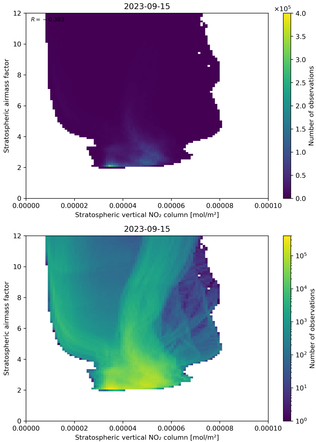
Figure 96: Scatter density plot of “Stratospheric vertical NO 2 column” against “Stratospheric airmass factor” for 2023-09-15 to 2023-09-16.
