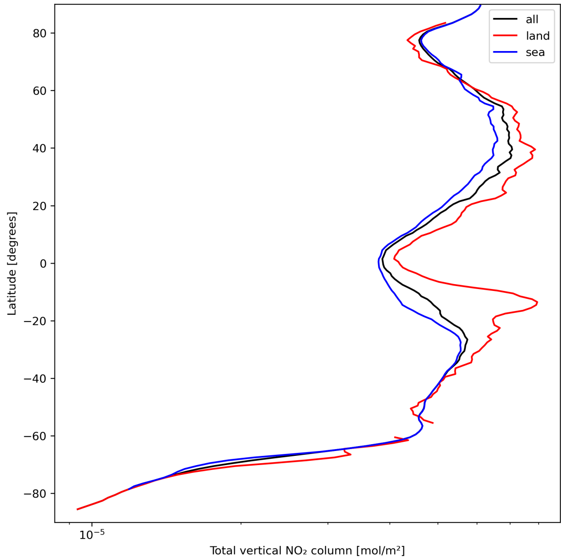
Figure 21: Zonal average of “Total vertical NO 2 column” for 2023-09-15 to 2023-09-16.
