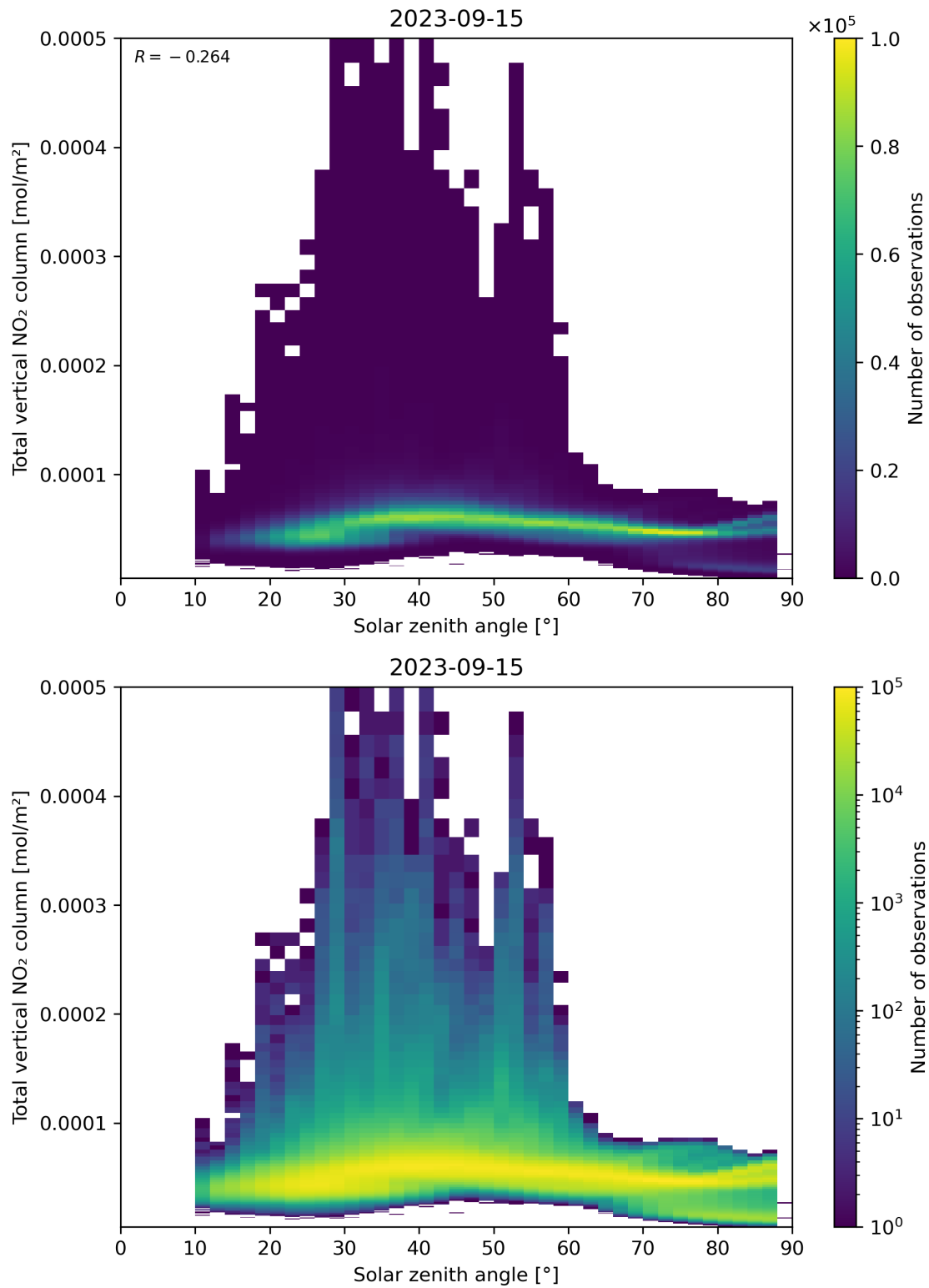
Figure 153: Scatter density plot of “Solar zenith angle” against “Total vertical NO 2 column” for 2023-09-15 to 2023-09-16.
