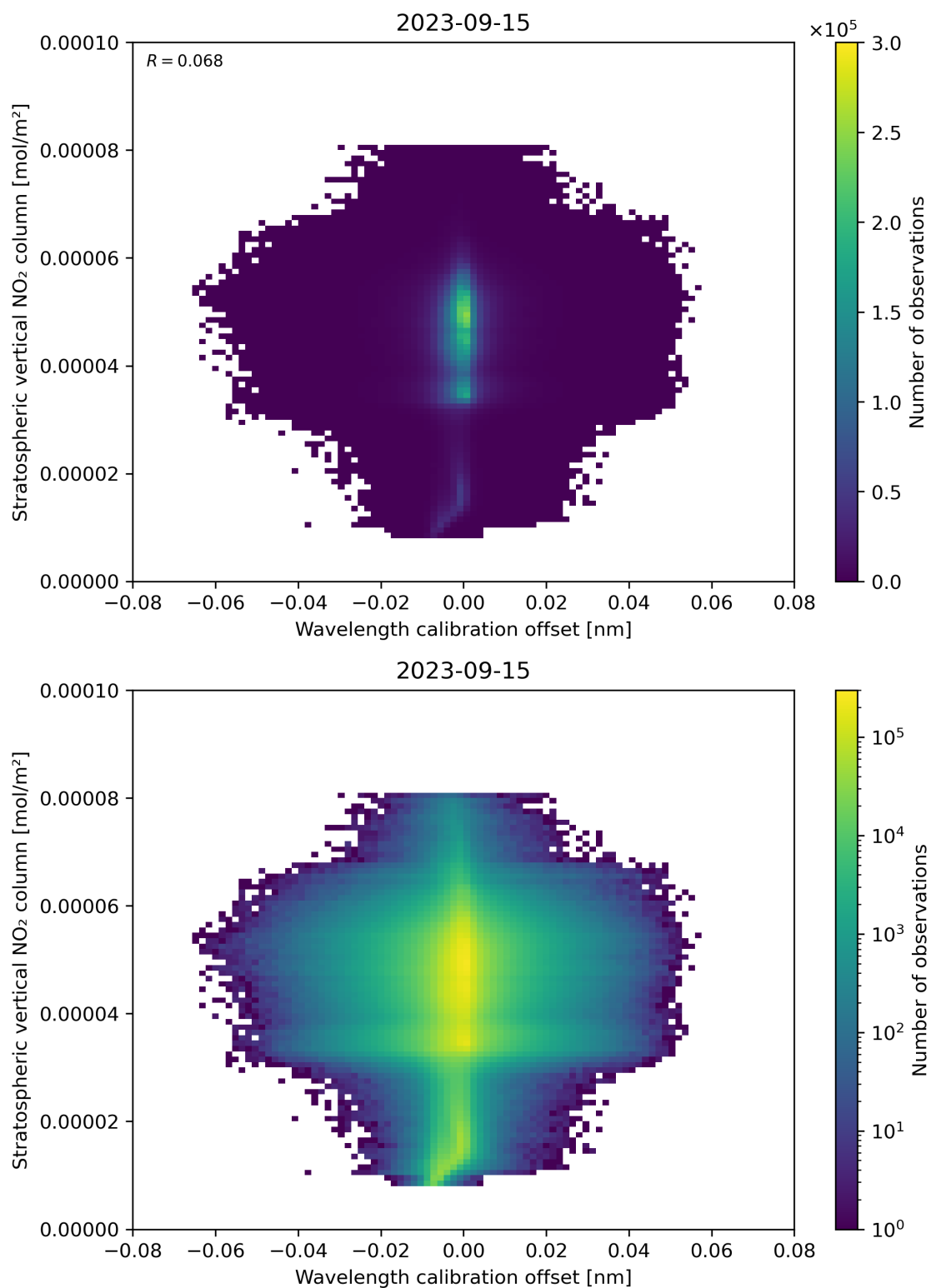
Figure 176: Scatter density plot of “Wavelength calibration offset” against “Stratospheric vertical NO 2 column” for 2023-09-15 to 2023-09-16.
