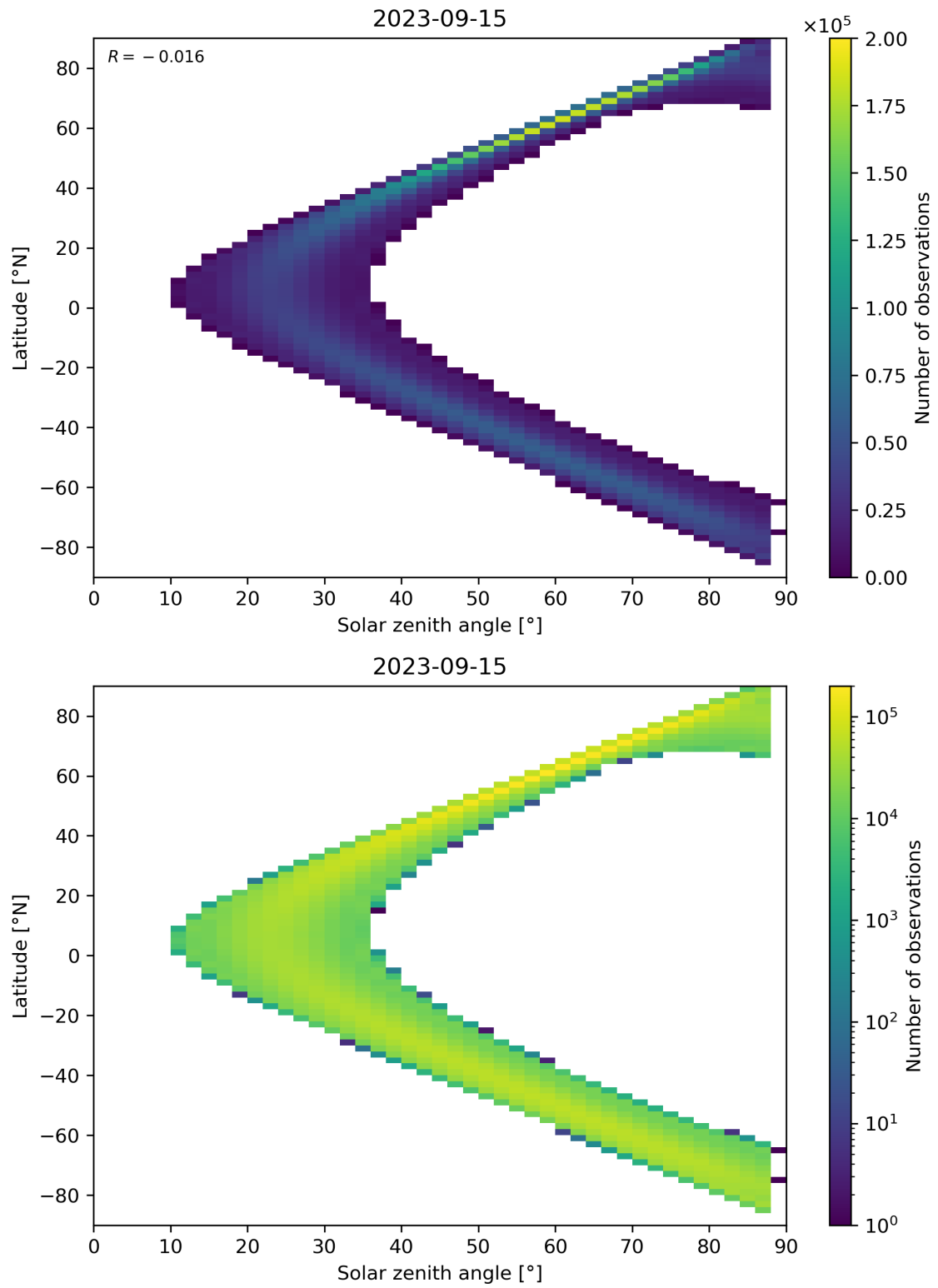
Figure 149: Scatter density plot of “Solar zenith angle” against “Latitude” for 2023-09-15 to 2023-09-16.
