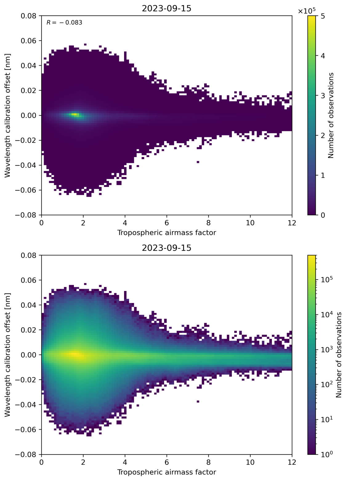
Figure 80: Scatter density plot of “Tropospheric airmass factor” against “Wavelength calibration offset” for 2023-09-15 to 2023-09-16.
