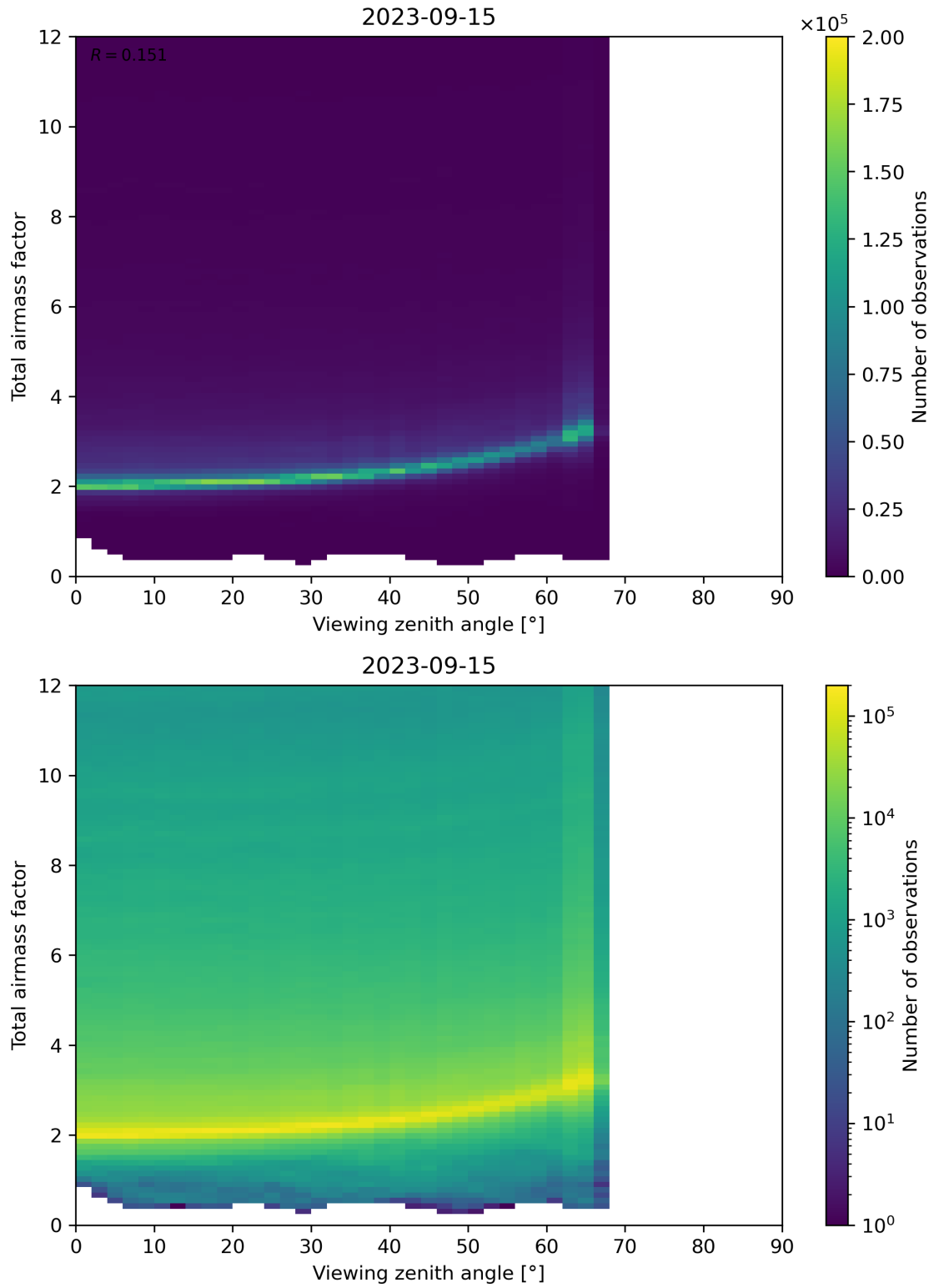
Figure 160: Scatter density plot of “Viewing zenith angle” against “Total airmass factor” for 2023-09-15 to 2023-09-16.
