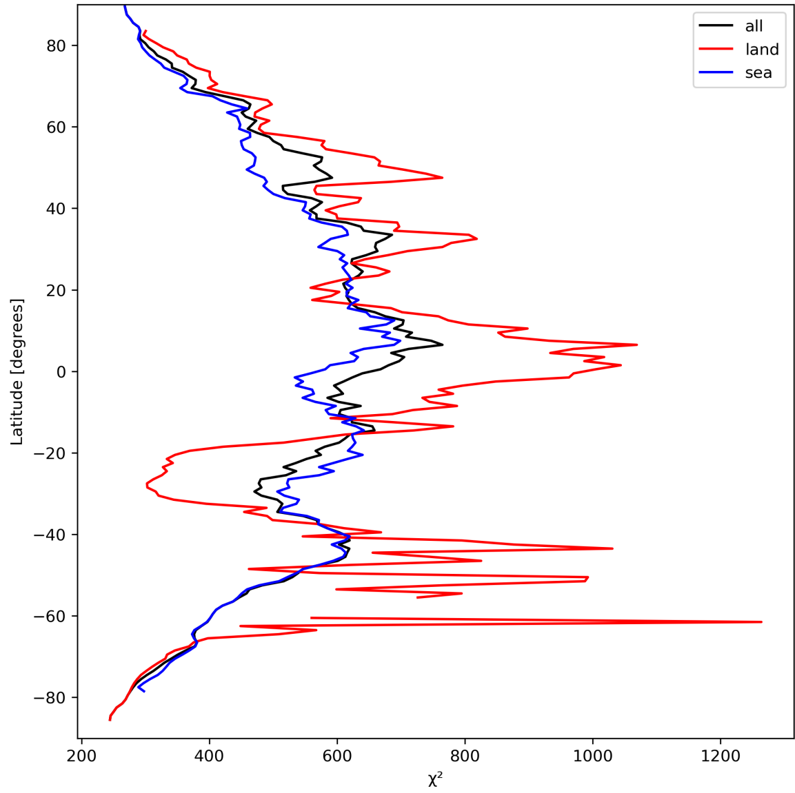
Figure 25: Zonal average of “ \chi^2 ” for 2023-09-15 to 2023-09-16.
