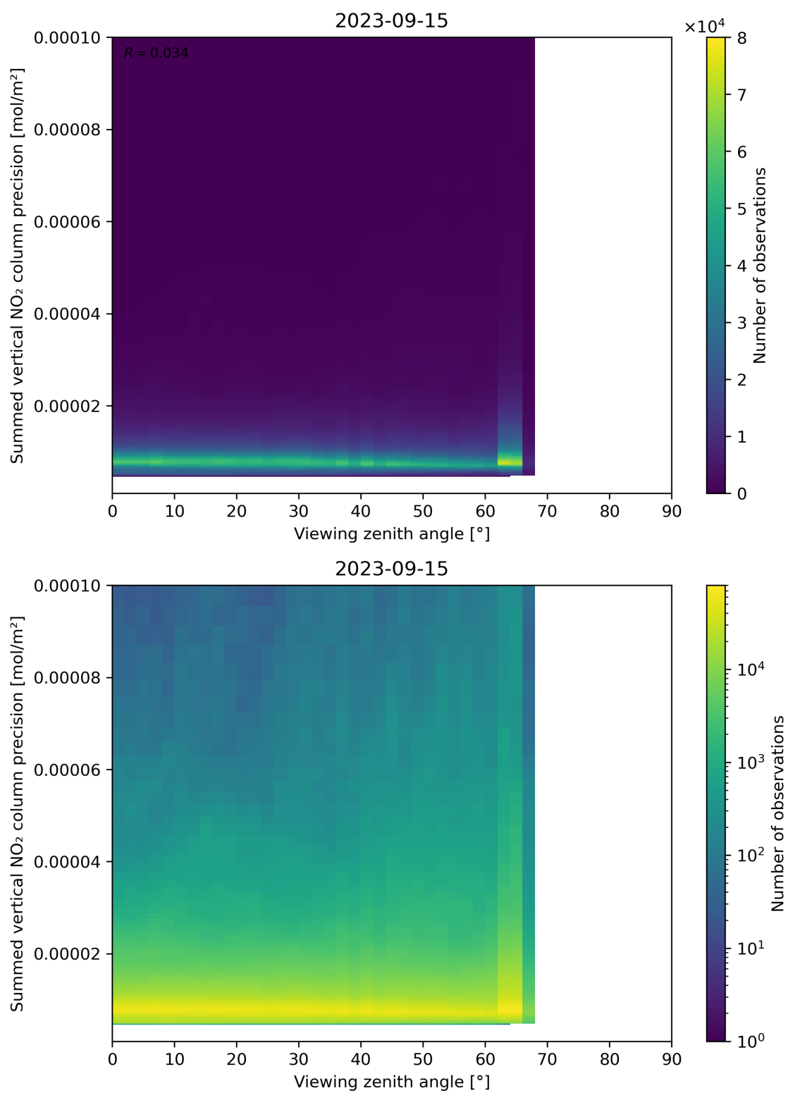
Figure 166: Scatter density plot of “Viewing zenith angle” against “Summed vertical NO 2 column precision” for 2023-09-15 to 2023-09-16.
