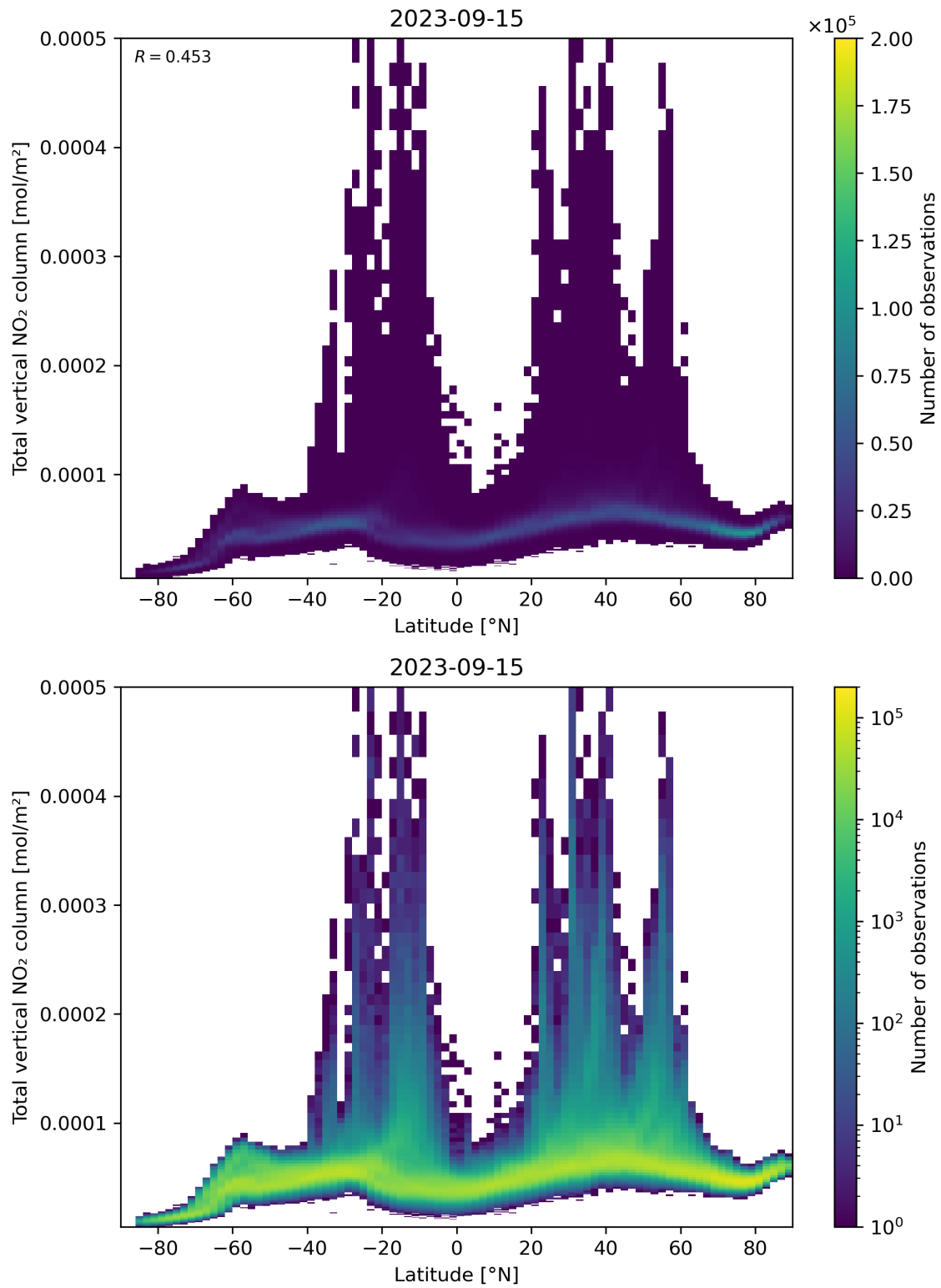
Figure 90: Scatter density plot of “Latitude” against “Total vertical NO 2 column” for 2023-09-15 to 2023-09-16.
