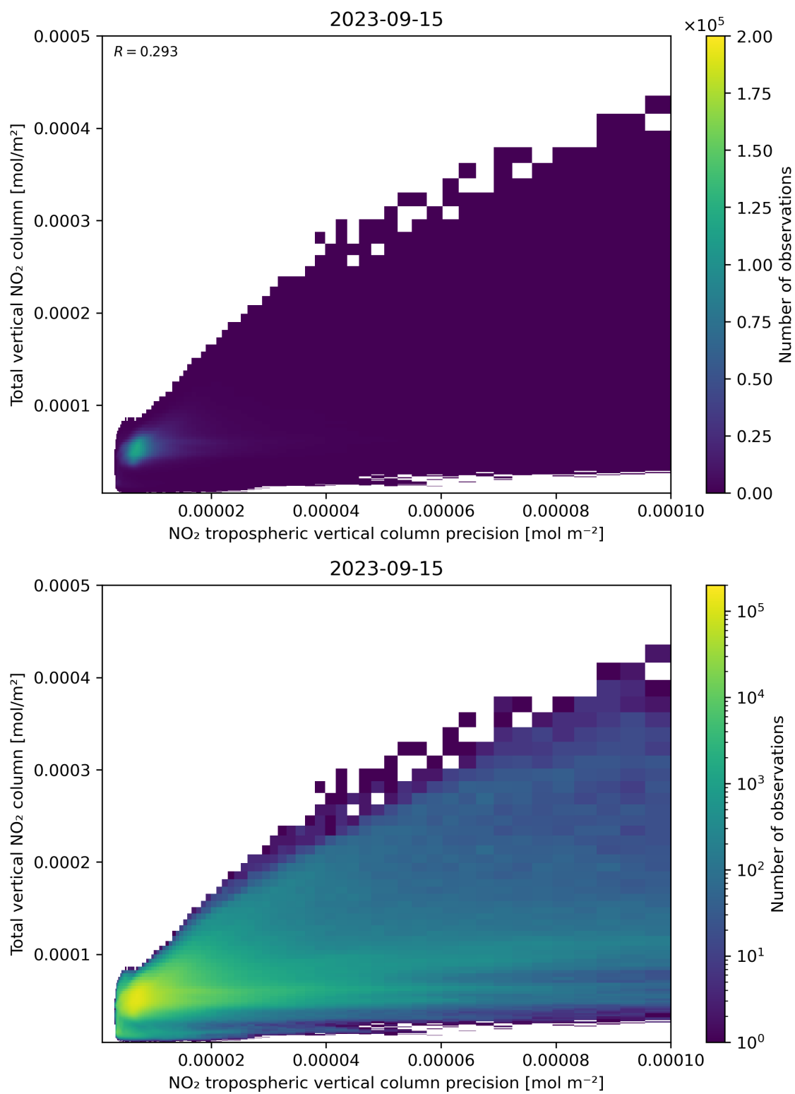
Figure 138: Scatter density plot of “NO 2 tropospheric vertical column precision” against “Total vertical NO 2 column” for 2023-09-15 to 2023-09-16.
