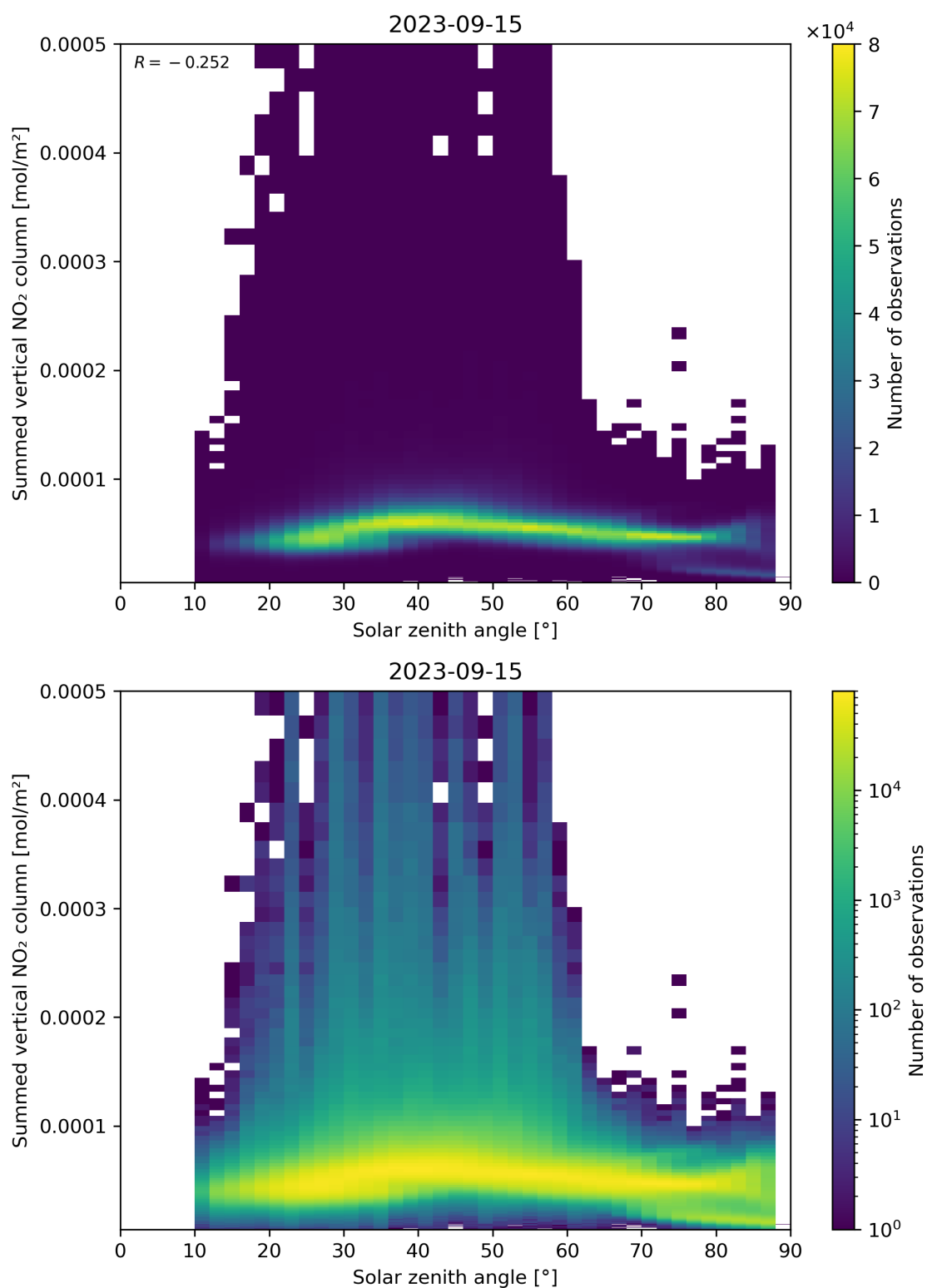
Figure 151: Scatter density plot of “Solar zenith angle” against “Summed vertical NO 2 column” for 2023-09-15 to 2023-09-16.
