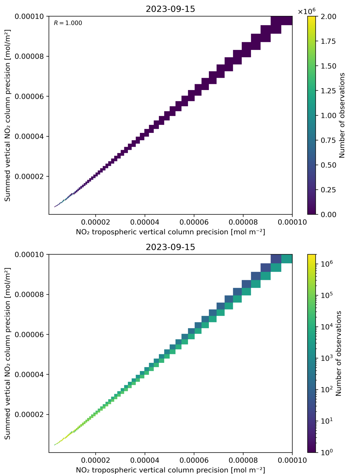
Figure 137: Scatter density plot of “NO 2 tropospheric vertical column precision” against “Summed vertical NO 2 column precision” for 2023-09-15 to 2023-09-16.
