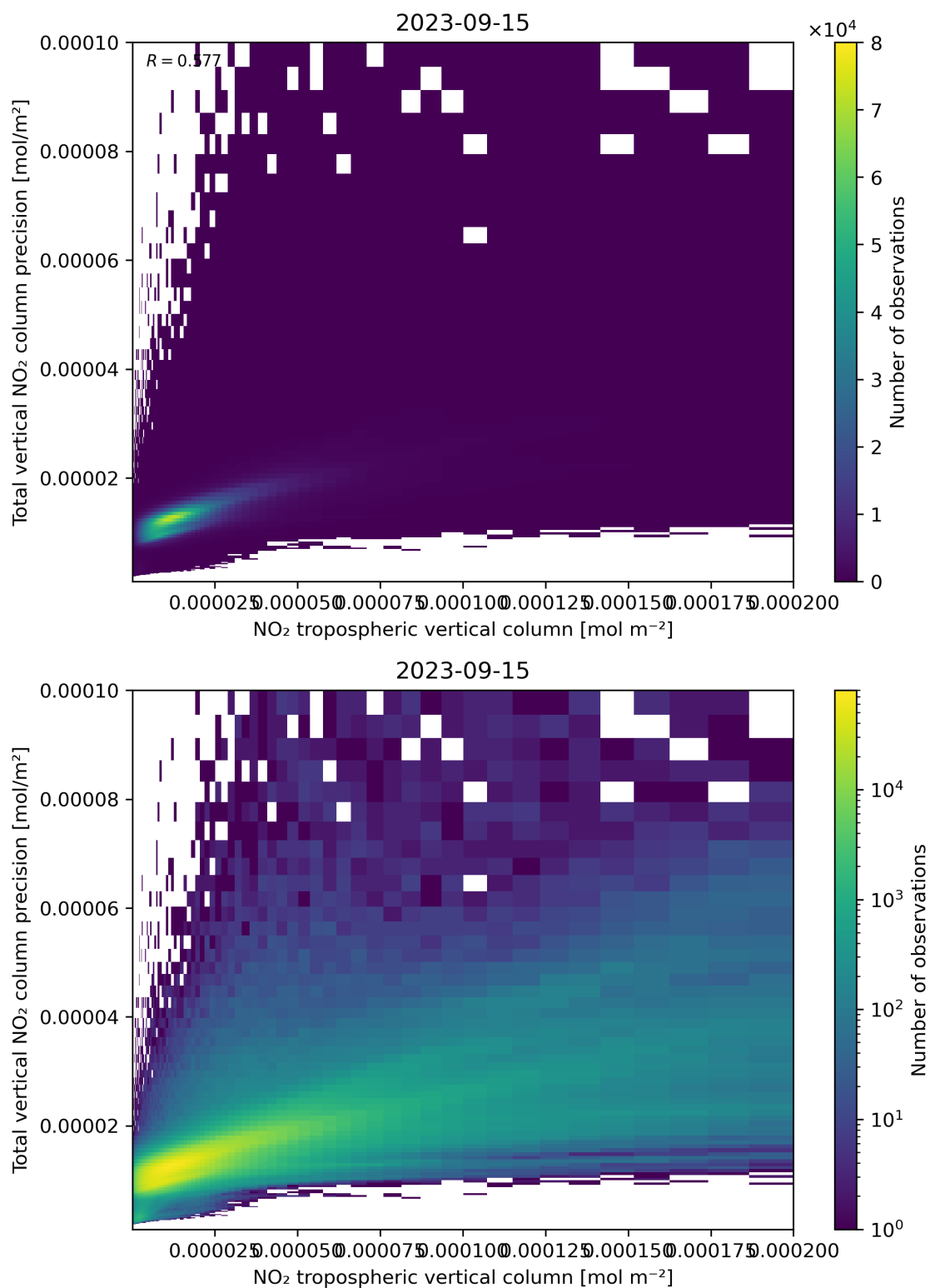
Figure 129: Scatter density plot of “NO 2 tropospheric vertical column” against “Total vertical NO 2 column precision” for 2023-09-15 to 2023-09-16.
