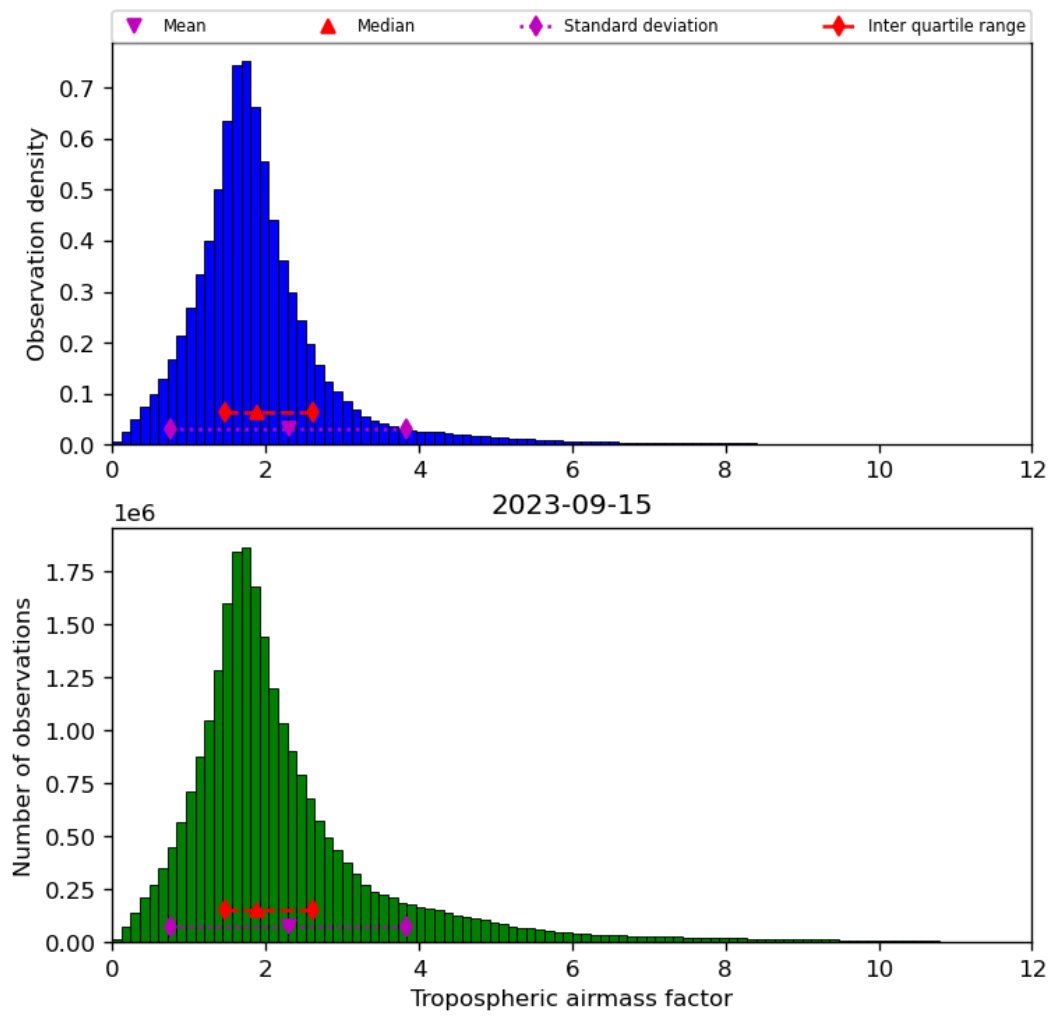
Figure 31: Histogram of “Tropospheric airmass factor” for 2023-09-15 to 2023-09-16
