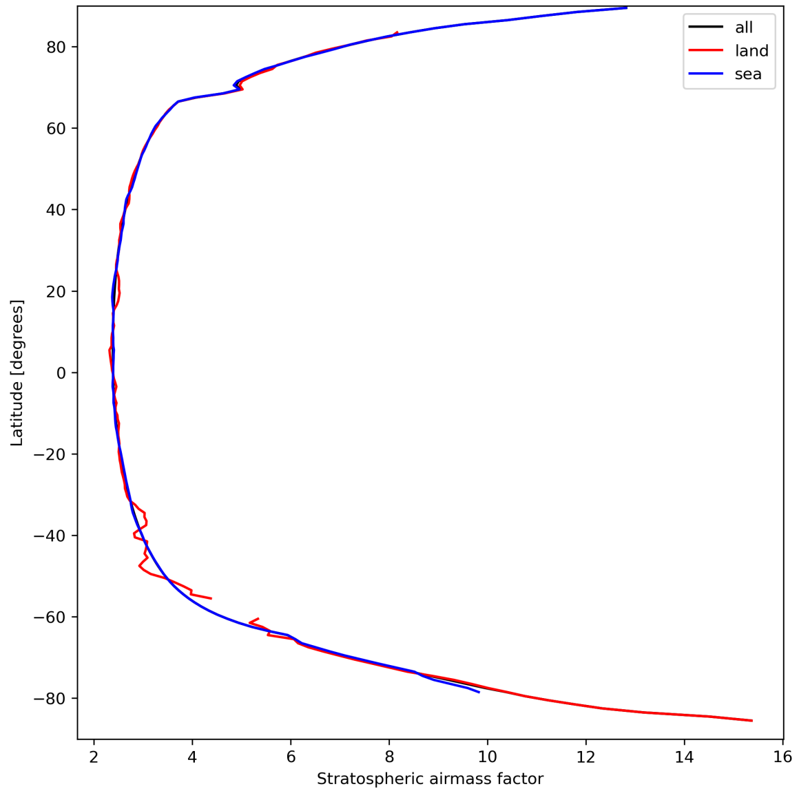
Figure 27: Zonal average of “Stratospheric airmass factor” for 2023-09-15 to 2023-09-17.
