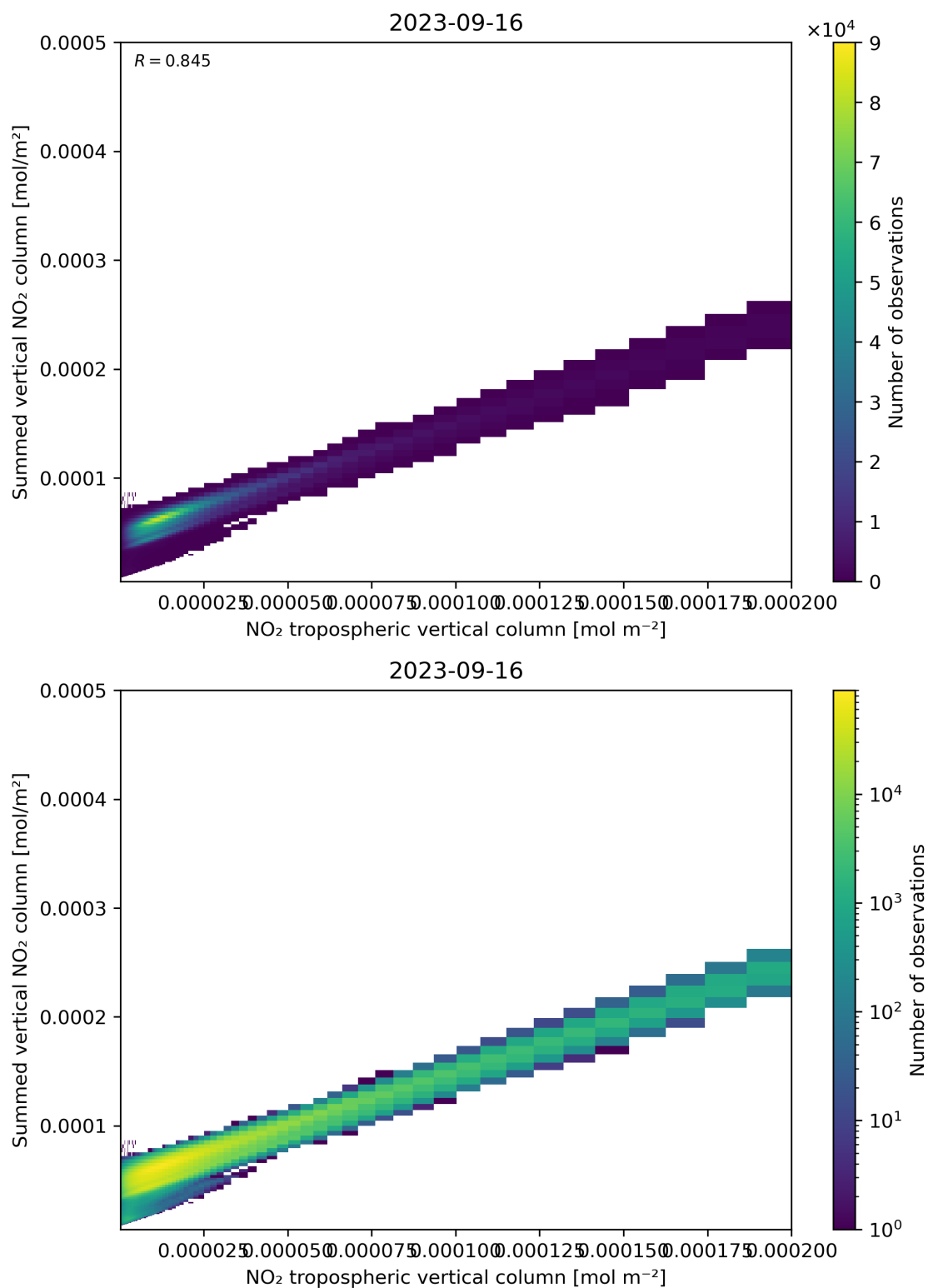
Figure 126: Scatter density plot of “NO 2 tropospheric vertical column” against “Summed vertical NO 2 column” for 2023-09-15 to 2023-09-17.
