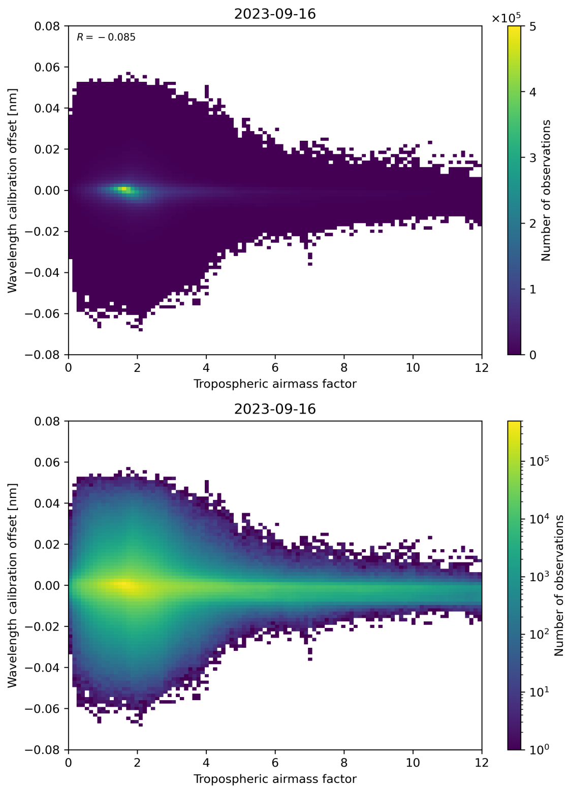
Figure 80: Scatter density plot of “Tropospheric airmass factor” against “Wavelength calibration offset” for 2023-09-15 to 2023-09-17.
