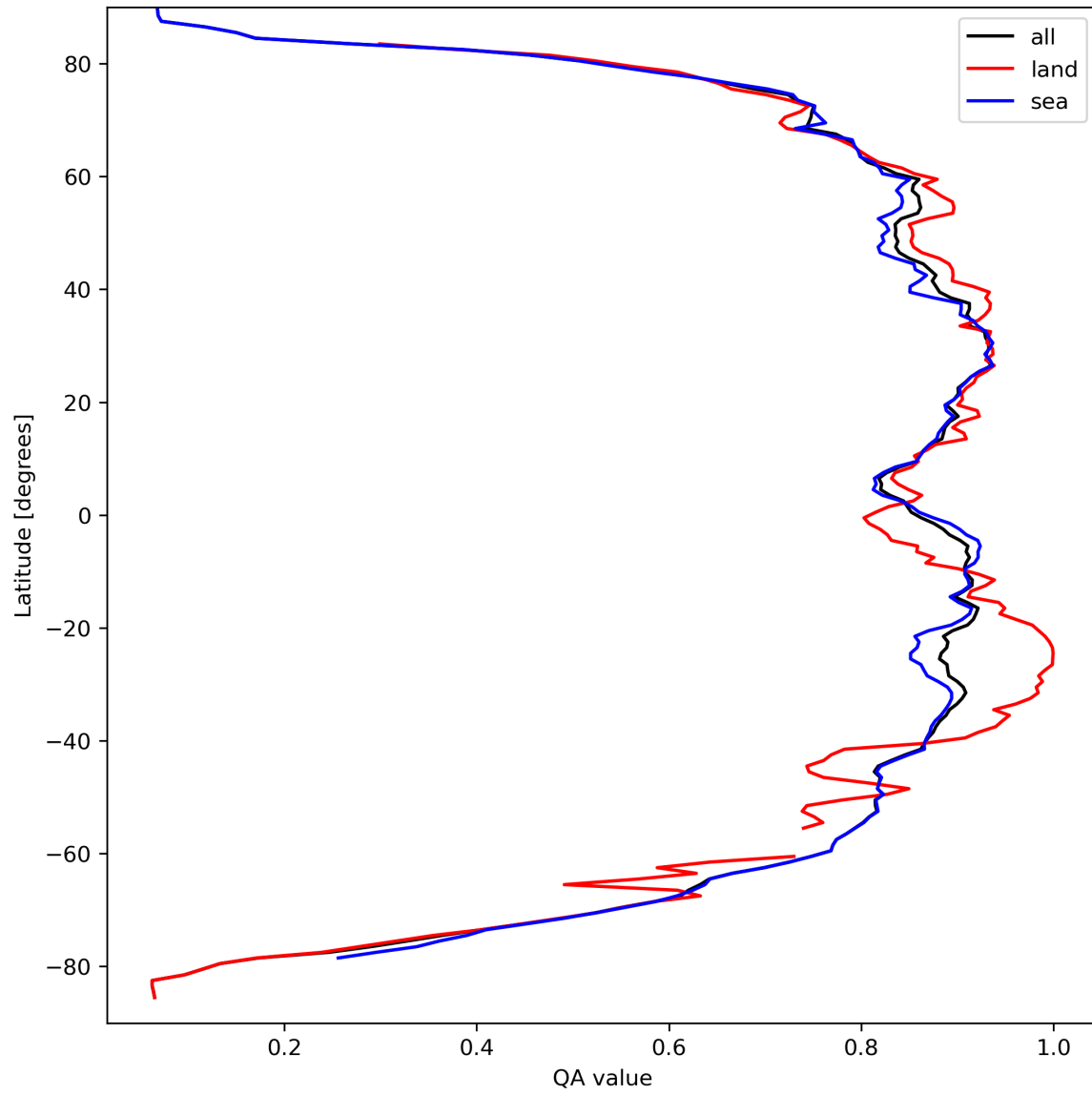
Figure 11: Zonal average of “QA value” for 2023-09-15 to 2023-09-17.
