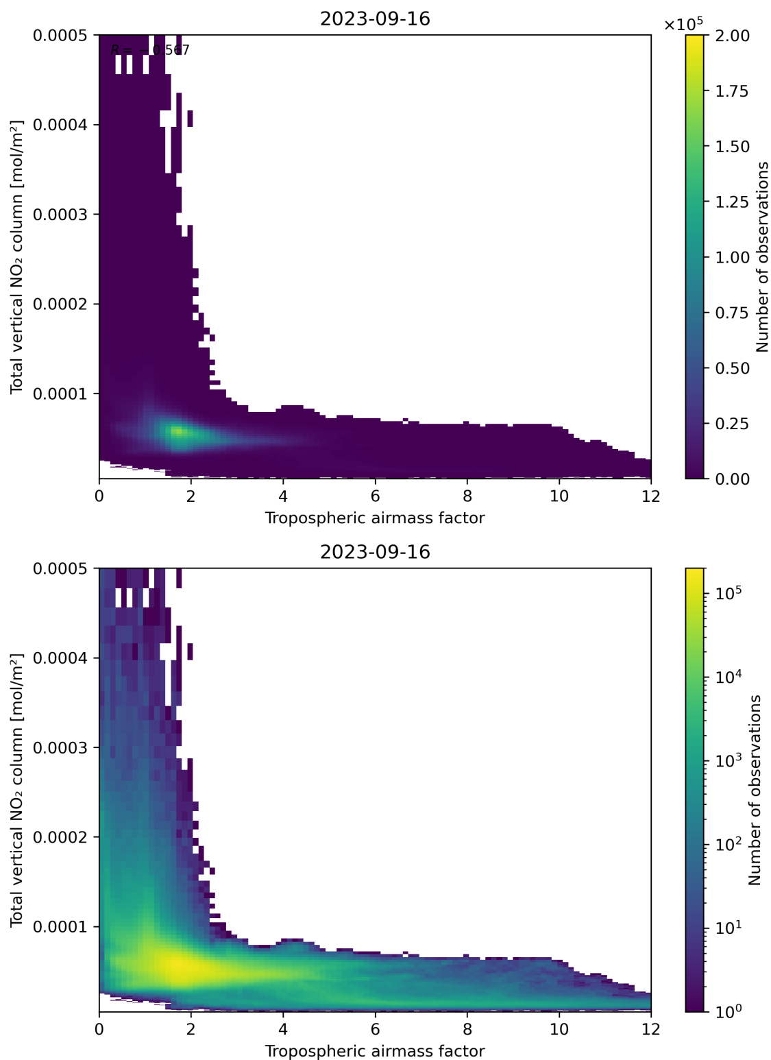
Figure 77: Scatter density plot of “Tropospheric airmass factor” against “Total vertical NO 2 column” for 2023-09-15 to 2023-09-17.
