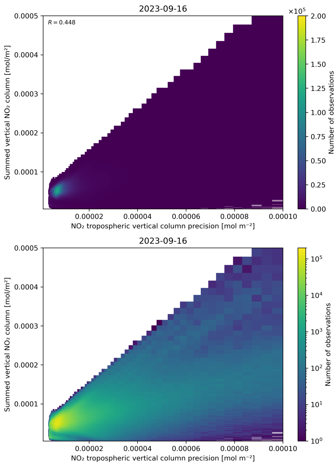
Figure 136: Scatter density plot of “NO 2 tropospheric vertical column precision” against “Summed vertical NO 2 column” for 2023-09-15 to 2023-09-17.
