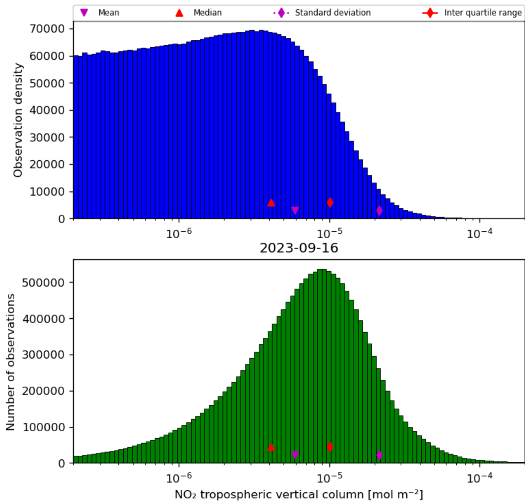
Figure 29: Histogram of “NO 2 tropospheric vertical column” for 2023-09-15 to 2023-09-17
