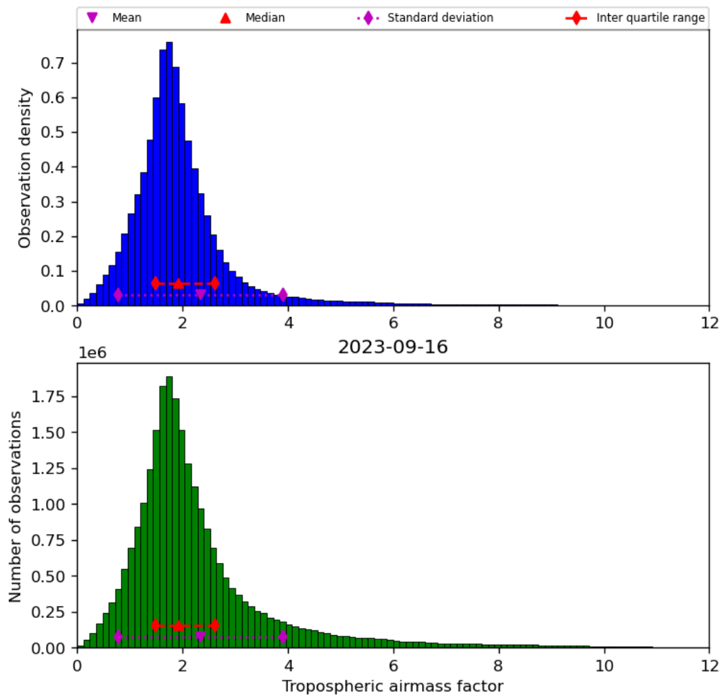
Figure 31: Histogram of “Tropospheric airmass factor” for 2023-09-15 to 2023-09-17
