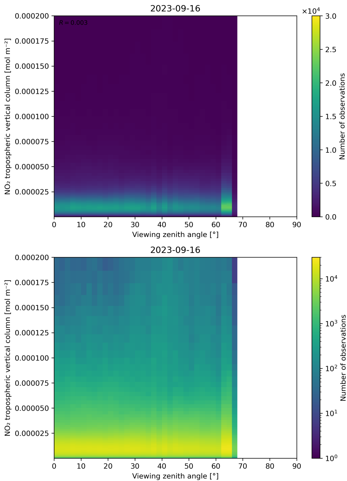
Figure 169: Scatter density plot of “Viewing zenith angle” against “NO 2 tropospheric vertical column” for 2023-09-15 to 2023-09-17.
