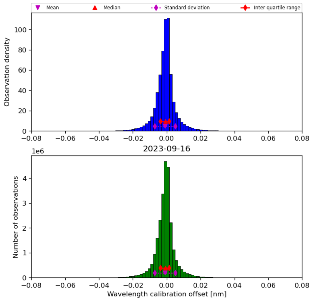
Figure 35: Histogram of “Wavelength calibration offset” for 2023-09-15 to 2023-09-17
