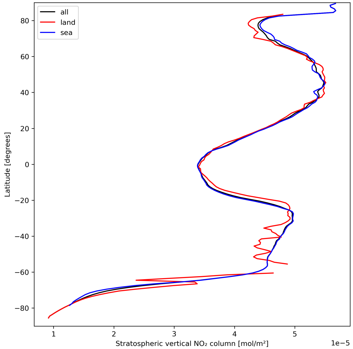
Figure 19: Zonal average of “Stratospheric vertical NO 2 column” for 2023-09-15 to 2023-09-17.
