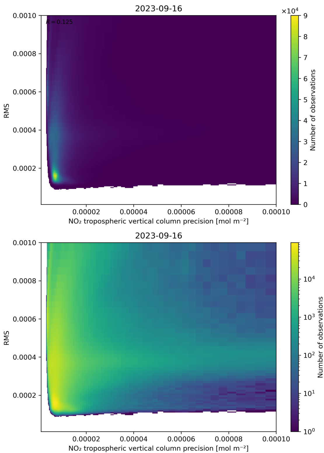
Figure 140: Scatter density plot of “NO 2 tropospheric vertical column precision” against “RMS” for 2023-09-15 to 2023-09-17.
