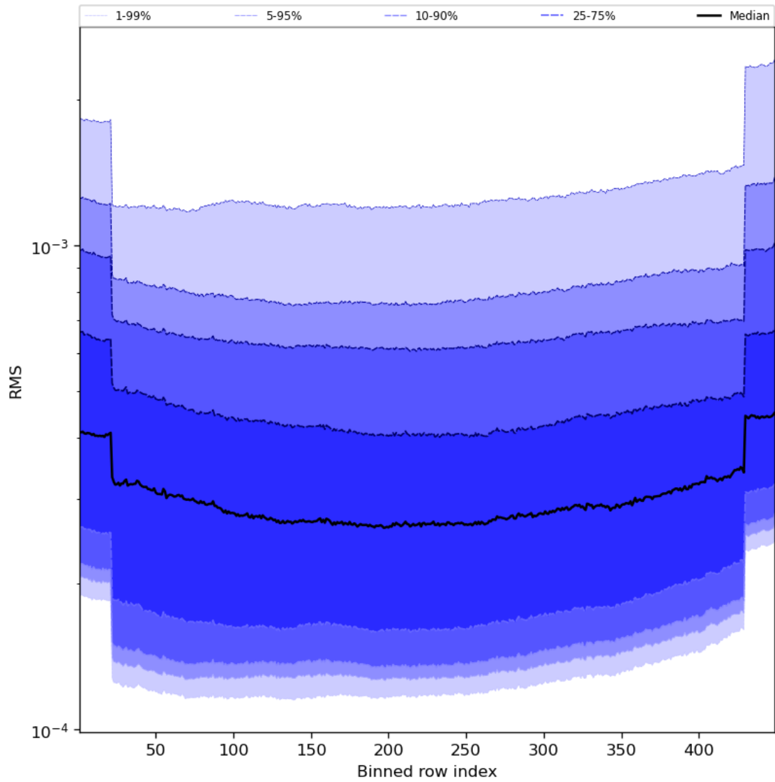
Figure 60: Along track statistics of “RMS” for 2023-09-15 to 2023-09-17
