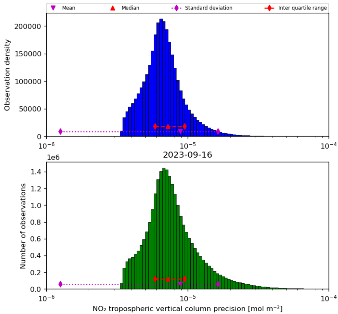
Figure 30: Histogram of “NO 2 tropospheric vertical column precision” for 2023-09-15 to 2023-09-17
