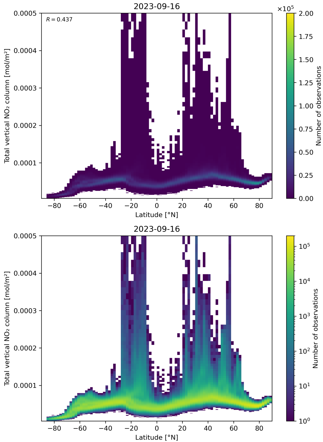
Figure 90: Scatter density plot of “Latitude” against “Total vertical NO 2 column” for 2023-09-15 to 2023-09-17.
