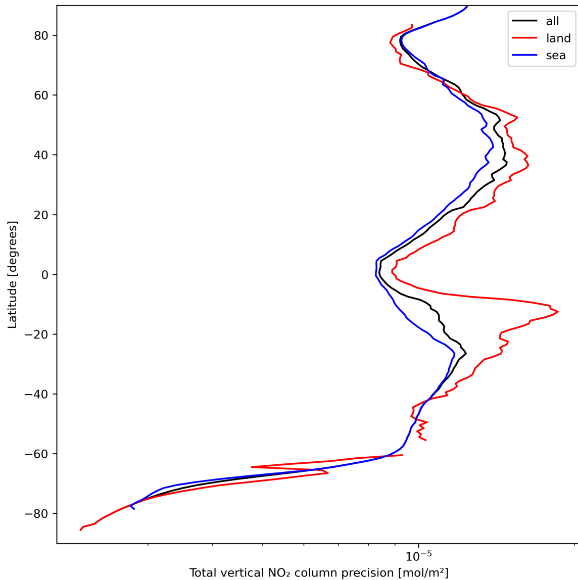
Figure 22: Zonal average of “Total vertical NO 2 column precision” for 2023-09-15 to 2023-09-17.
