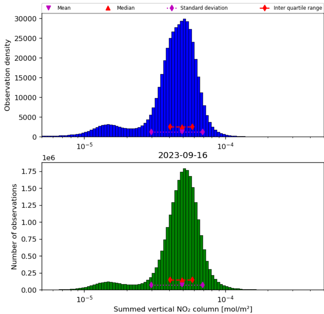
Figure 40: Histogram of "Summed vertical NO 2 column" for 2023-09-15 to 2023-09-17
