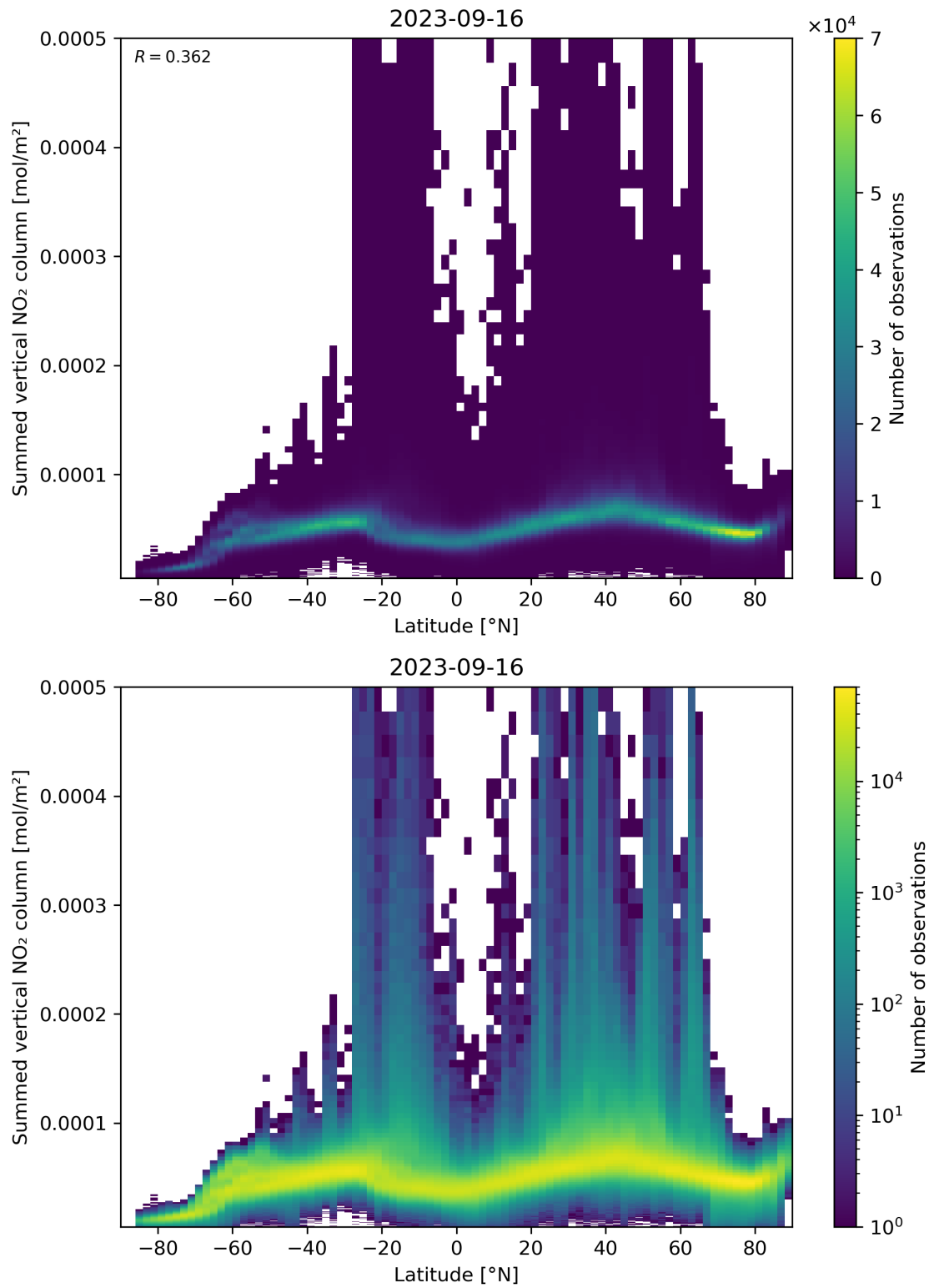
Figure 88: Scatter density plot of “Latitude” against “Summed vertical NO 2 column” for 2023-09-15 to 2023-09-17.
