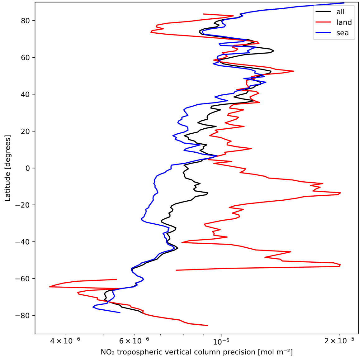
Figure 13: Zonal average of “NO 2 tropospheric vertical column precision” for 2023-09-15 to 2023-09-17.
