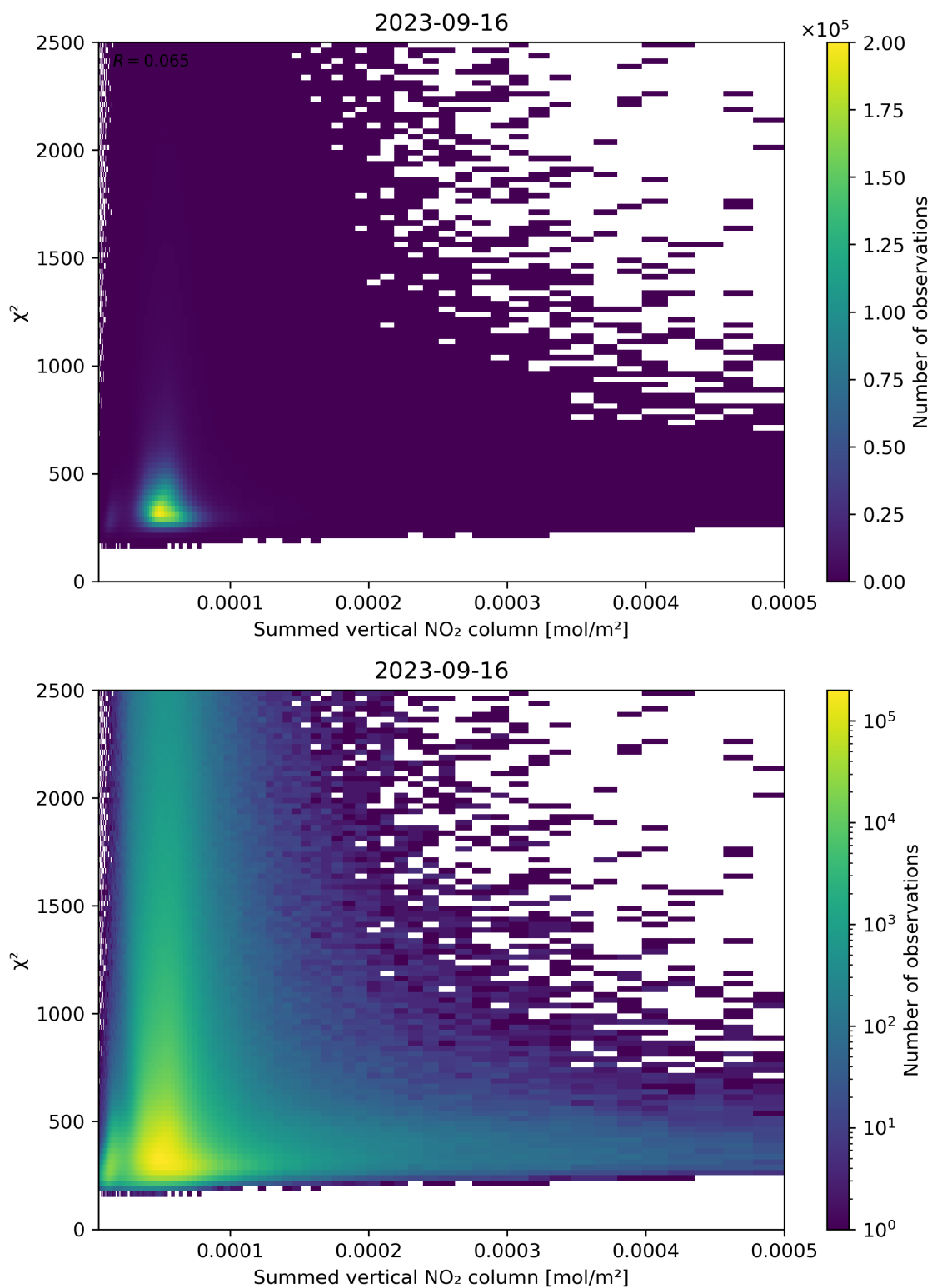
Figure 104: Scatter density plot of “Summed vertical NO 2 column” against “ \chi^2 ” for 2023-09-15 to 2023-09-17.
