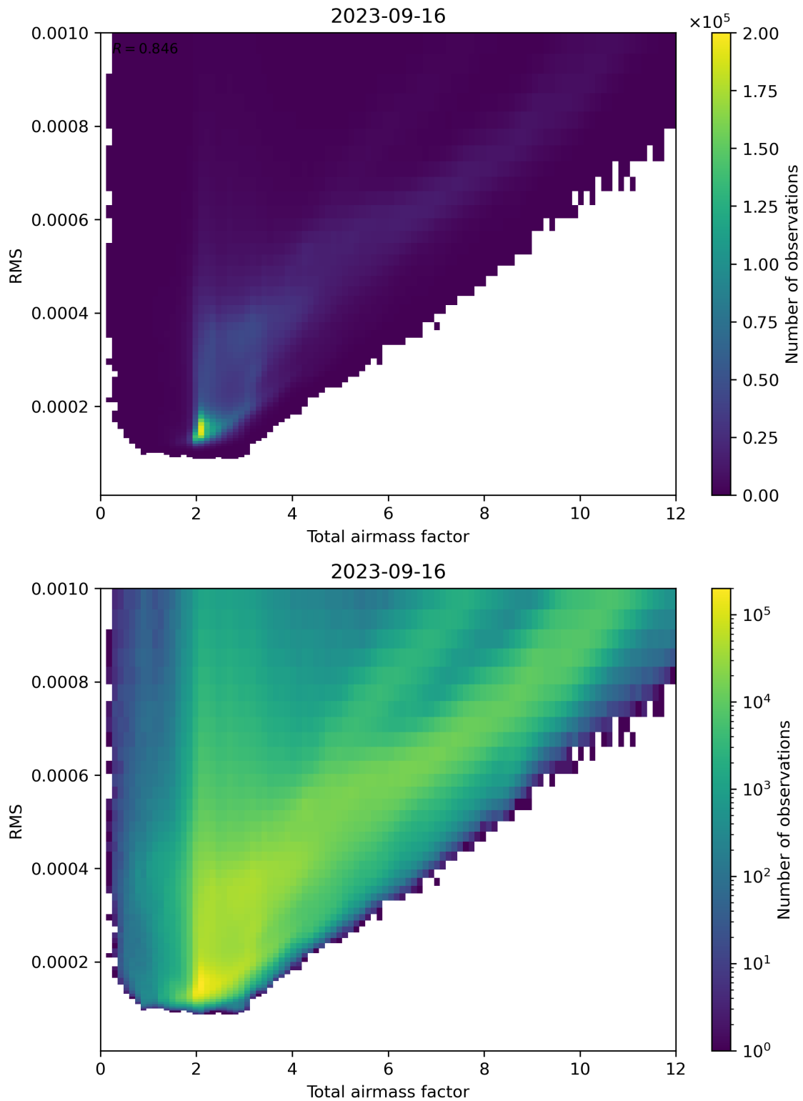
Figure 69: Scatter density plot of “Total airmass factor” against “RMS” for 2023-09-15 to 2023-09-17.
