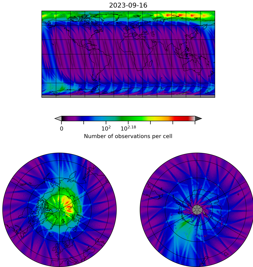
Figure 10: Map of the number of observations for 2023-09-15 to 2023-09-17
