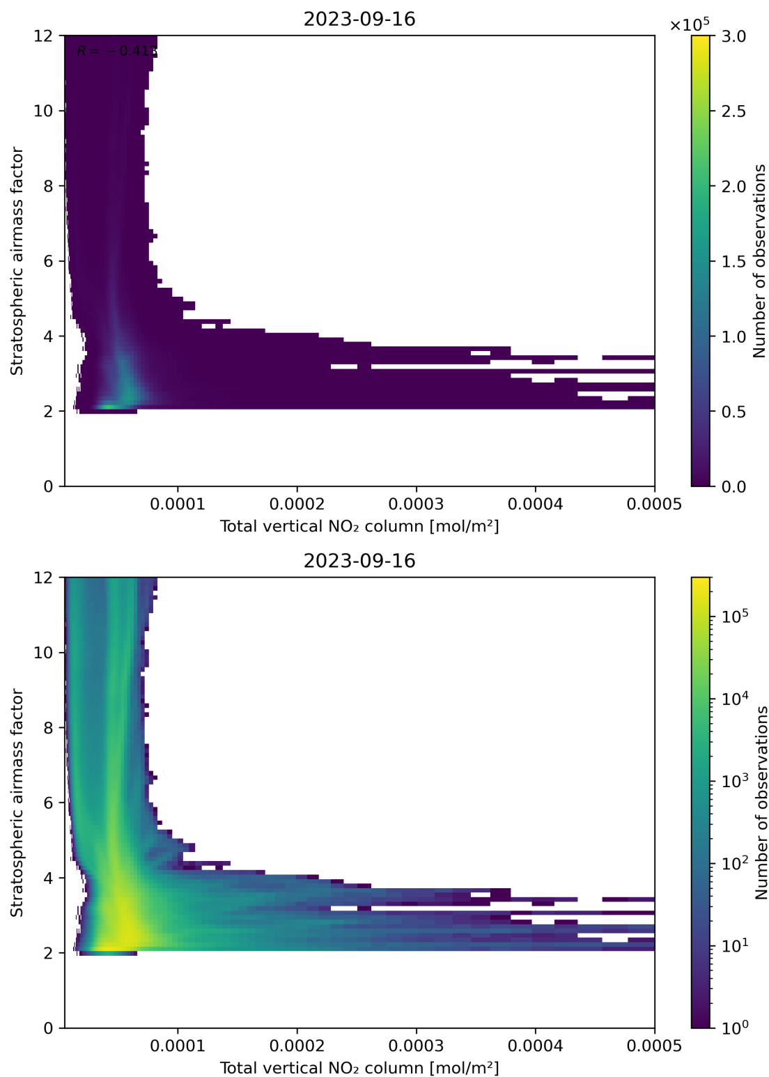
Figure 110: Scatter density plot of “Total vertical NO 2 column” against “Stratospheric air mass factor” for 2023-09-15 to 2023-09-17.
