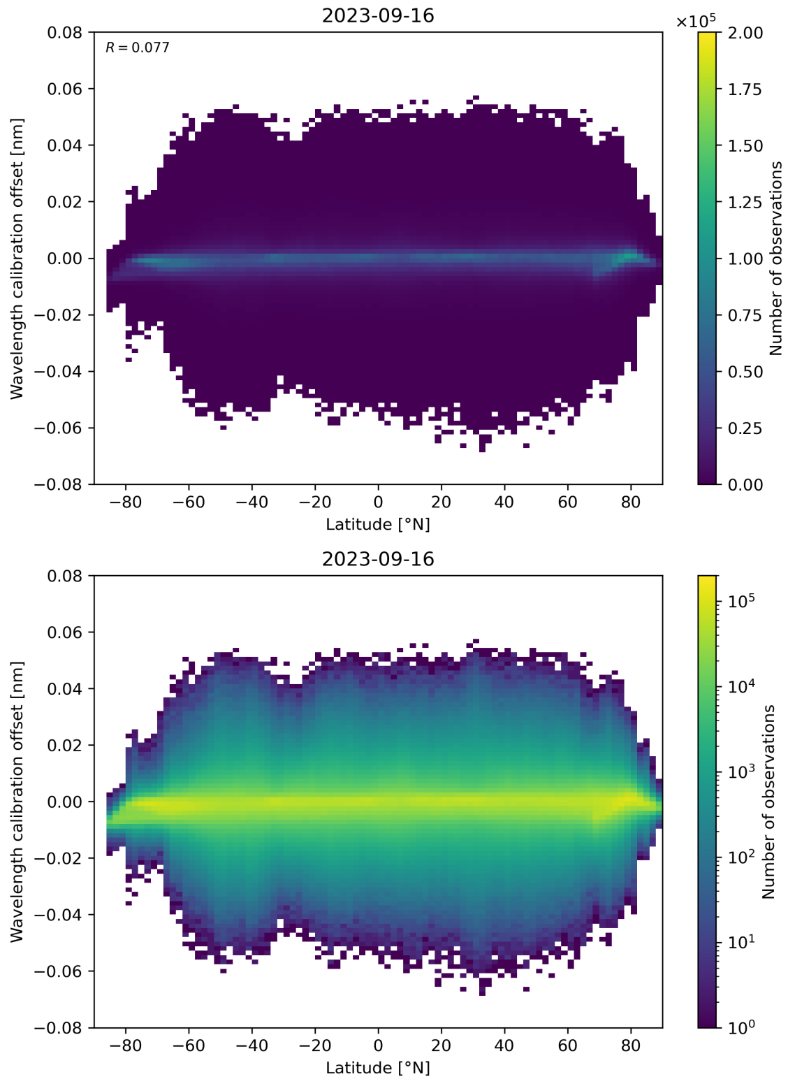
Figure 95: Scatter density plot of “Latitude” against “Wavelength calibration offset” for 2023-09-15 to 2023-09-17.
