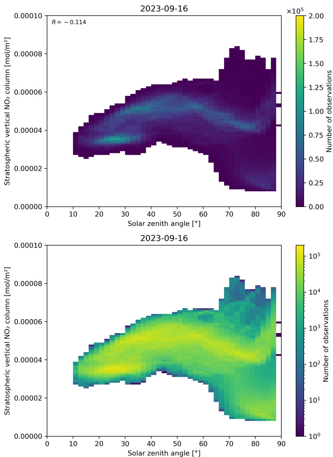
Figure 150: Scatter density plot of “Solar zenith angle” against “Stratospheric vertical NO 2 column” for 2023-09-15 to 2023-09-17.
