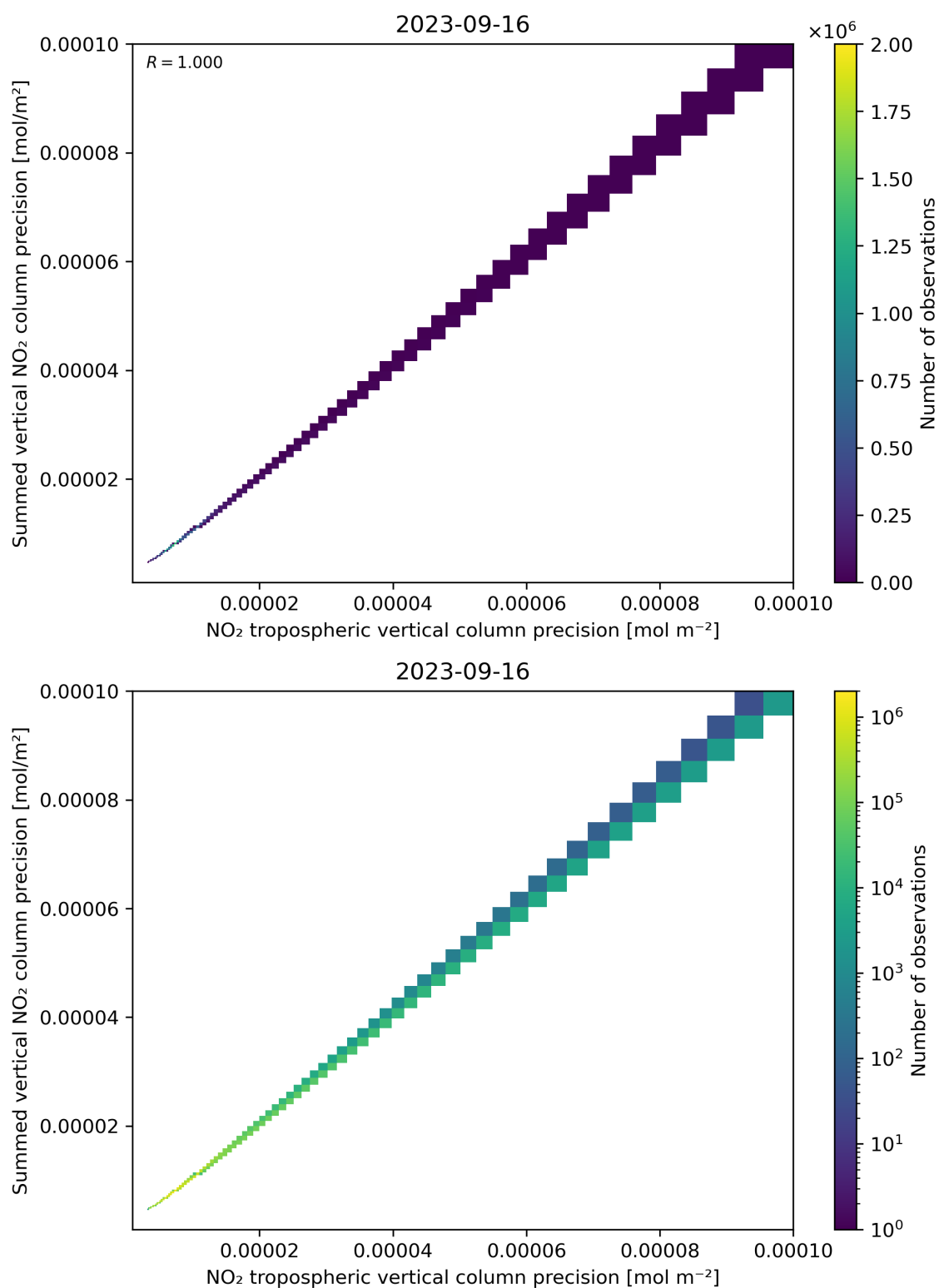
Figure 137: Scatter density plot of “NO 2 tropospheric vertical column precision” against “Summed vertical NO 2 column precision” for 2023-09-15 to 2023-09-17.
