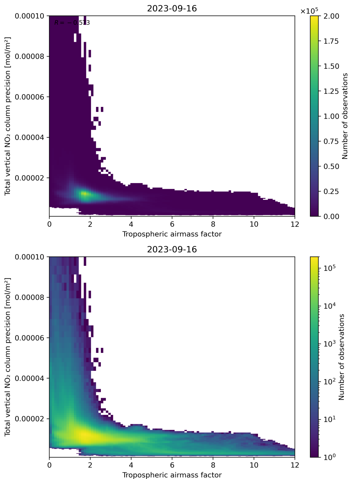
Figure 78: Scatter density plot of “Tropospheric air mass factor” against “Total vertical NO 2 column precision” for 2023-09-15 to 2023-09-17.
