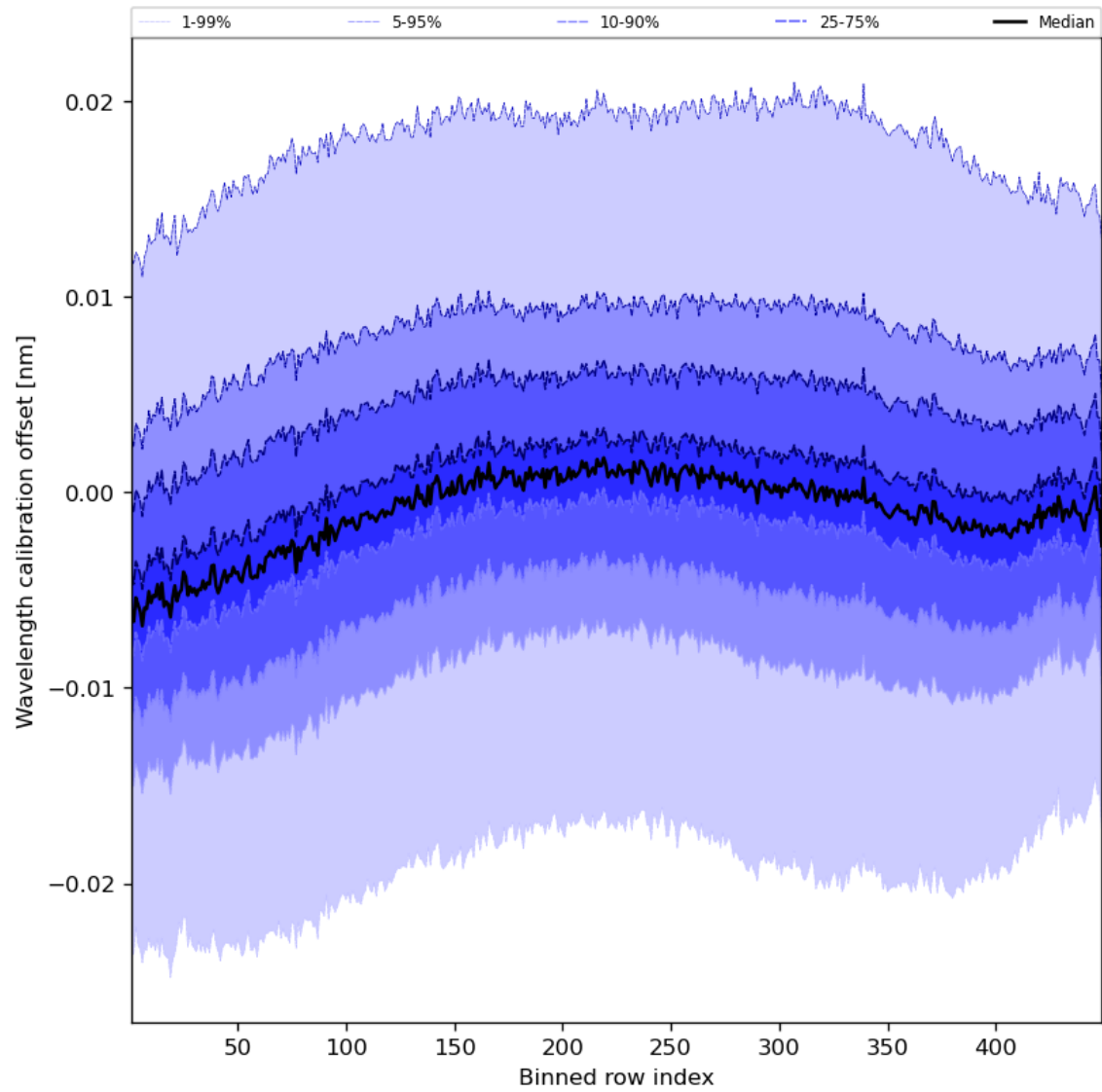
Figure 52: Along track statistics of “Wavelength calibration offset” for 2023-09-15 to 2023-09-17
