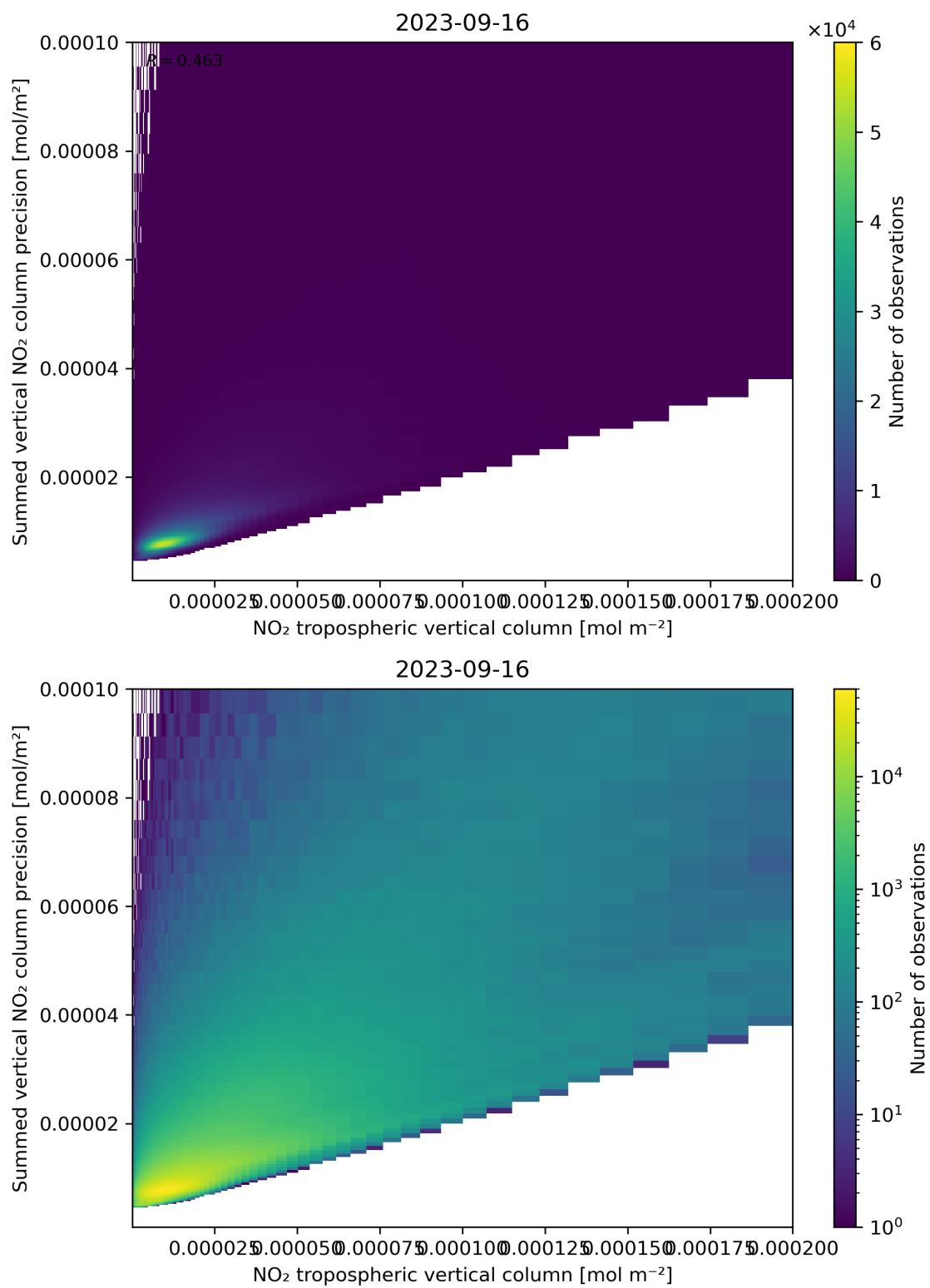
Figure 127: Scatter density plot of “NO 2 tropospheric vertical column” against “Summed vertical NO 2 column precision” for 2023-09-15 to 2023-09-17.
