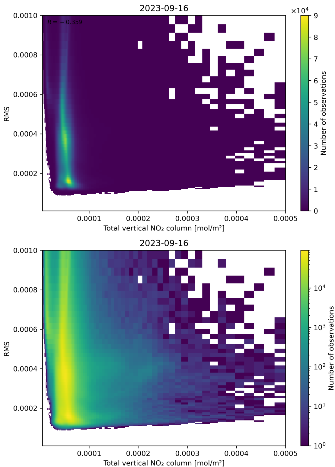
Figure 120: Scatter density plot of “Total vertical NO 2 column” against “RMS” for 2023-09-15 to 2023-09-17.
