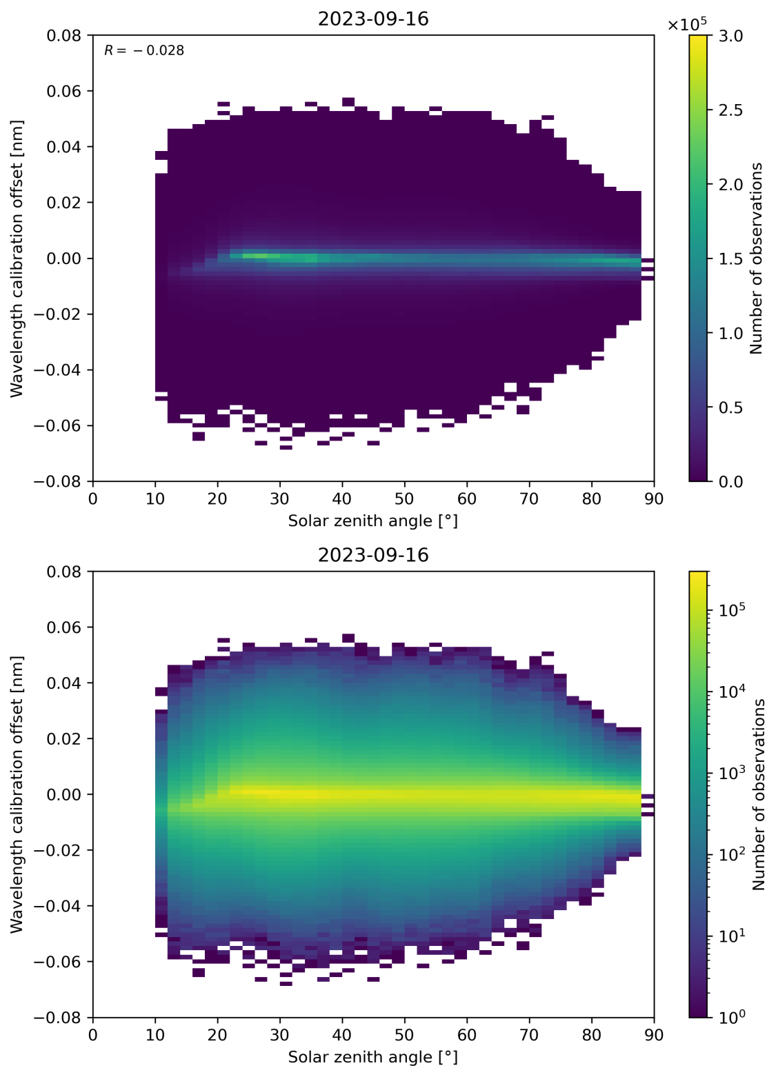
Figure 158: Scatter density plot of “Solar zenith angle” against “Wavelength calibration offset” for 2023-09-15 to 2023-09-17.
