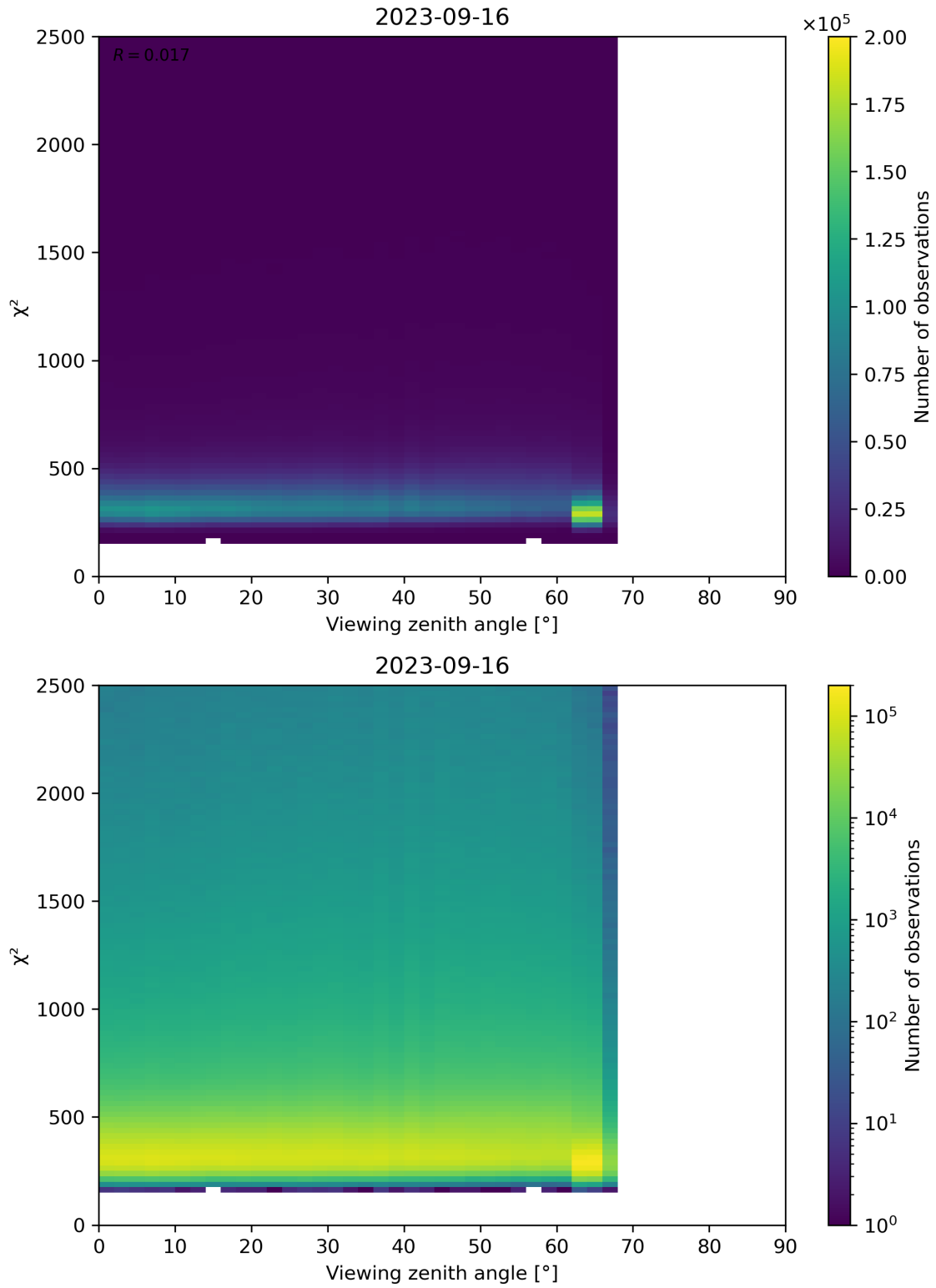
Figure 162: Scatter density plot of “Viewing zenith angle” against “ \chi^2 ” for 2023-09-15 to 2023-09-17.
