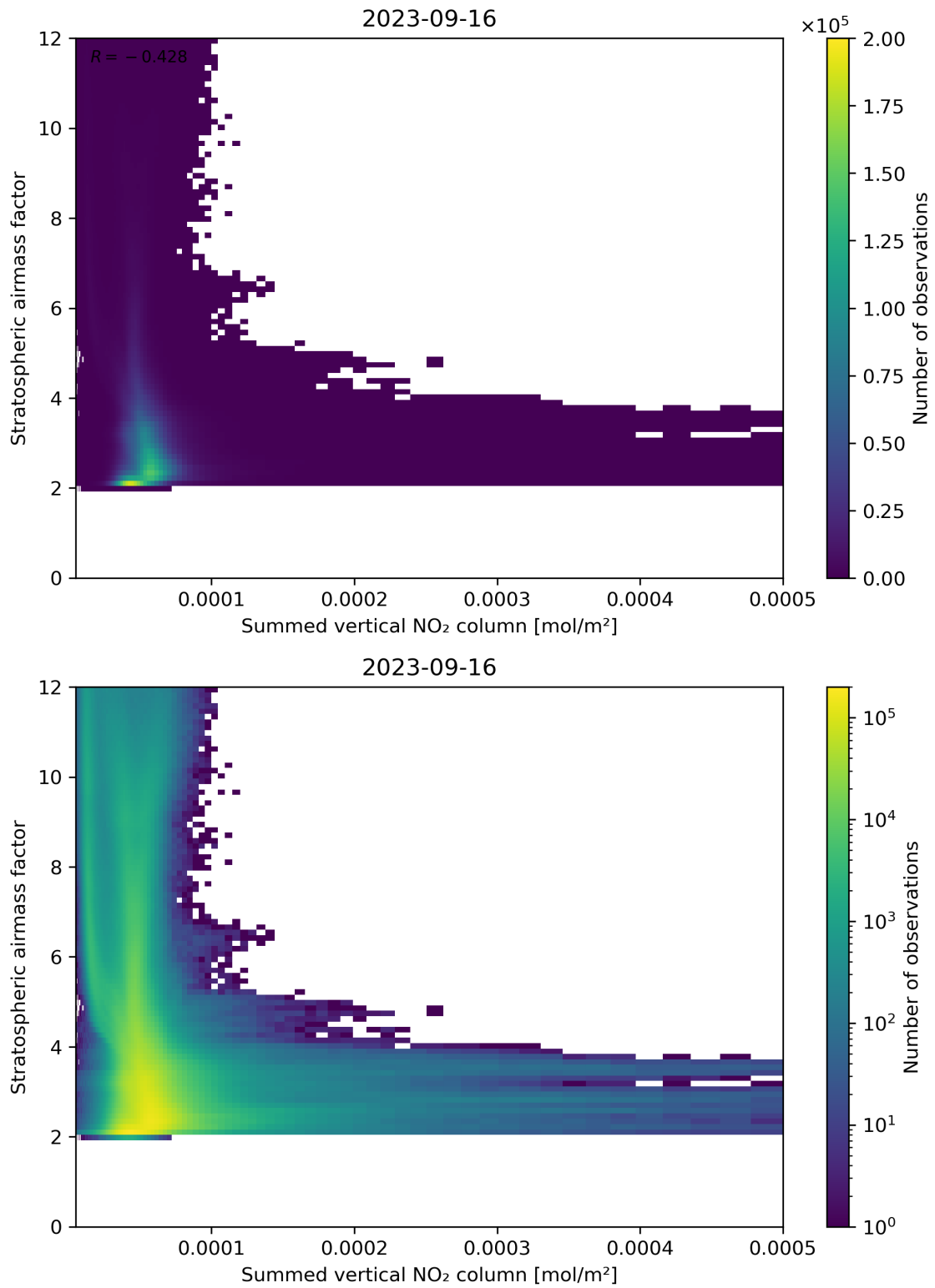
Figure 103: Scatter density plot of “Summed vertical NO 2 column” against “Stratospheric airmass factor” for 2023-09-15 to 2023-09-17.
