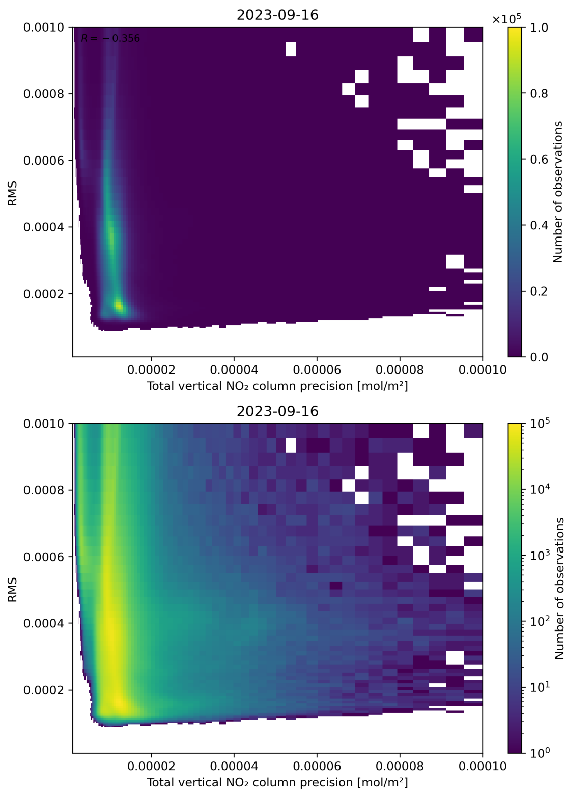
Figure 119: Scatter density plot of “Total vertical NO 2 column precision” against “RMS” for 2023-09-15 to 2023-09-17.
