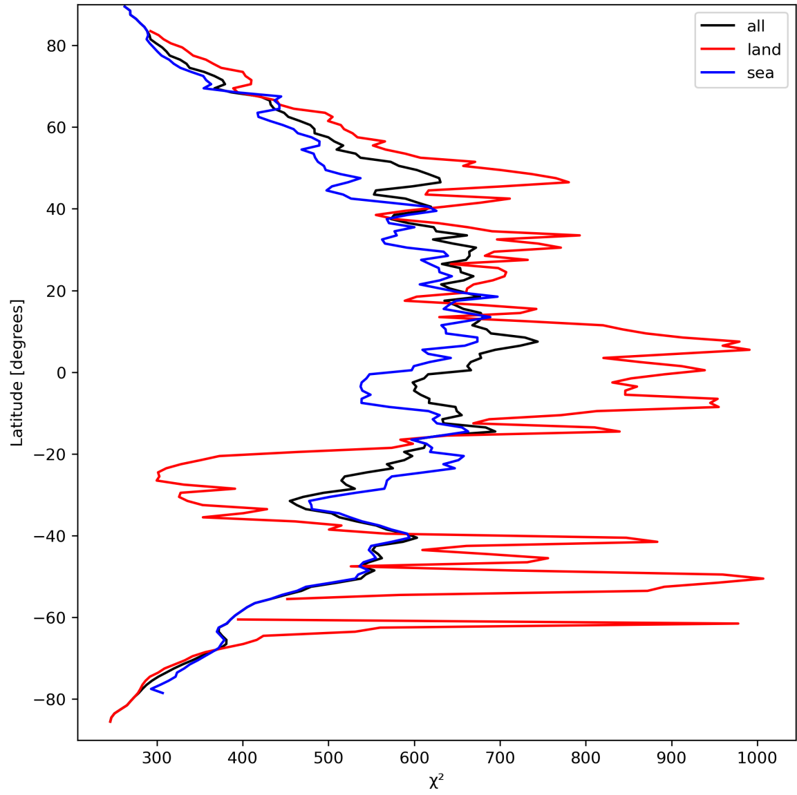
Figure 25: Zonal average of “ \chi^2 ” for 2023-09-15 to 2023-09-17.
