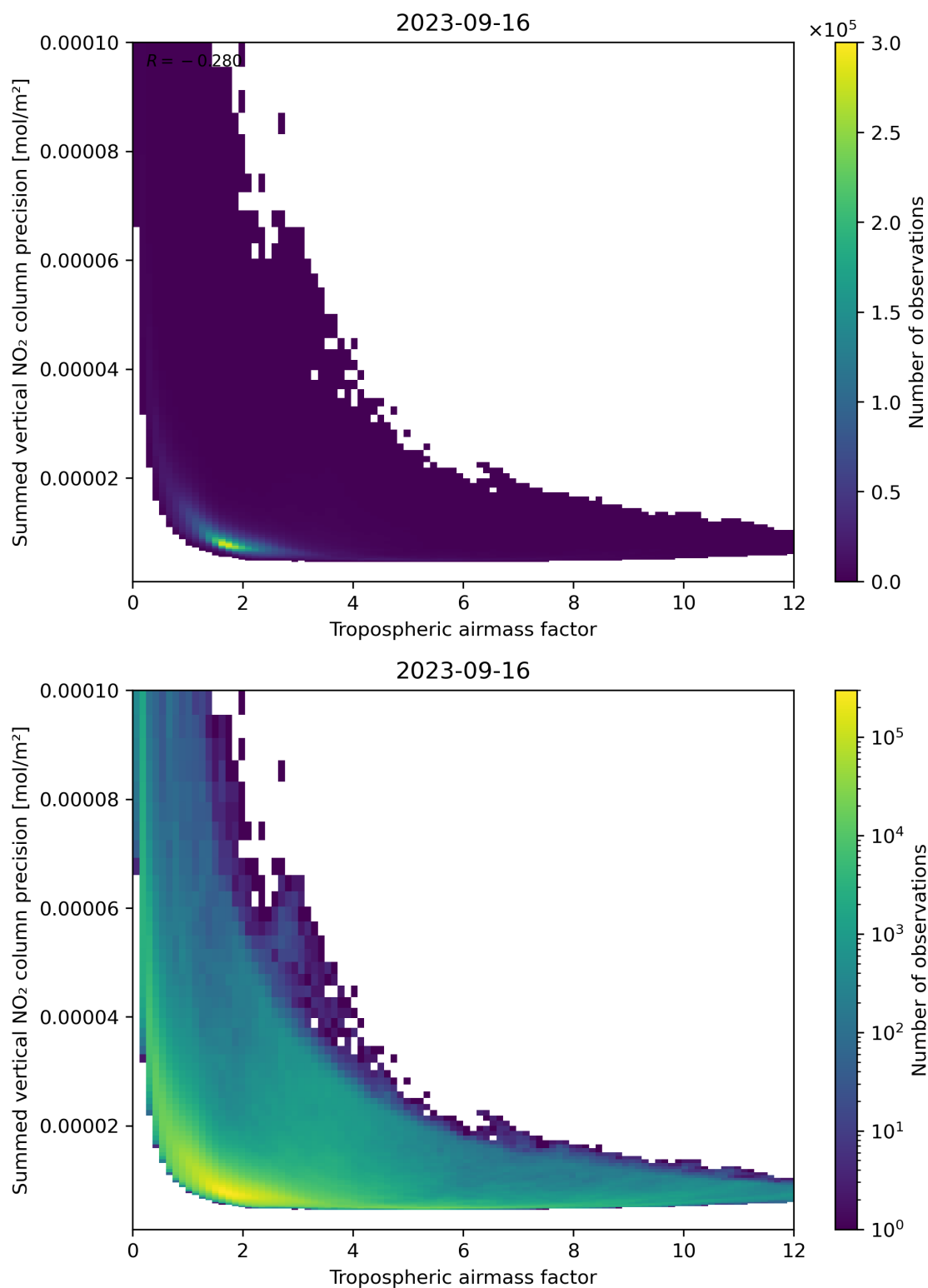
Figure 76: Scatter density plot of “Tropospheric air mass factor” against “Summed vertical NO 2 column precision” for 2023-09-15 to 2023-09-17.
