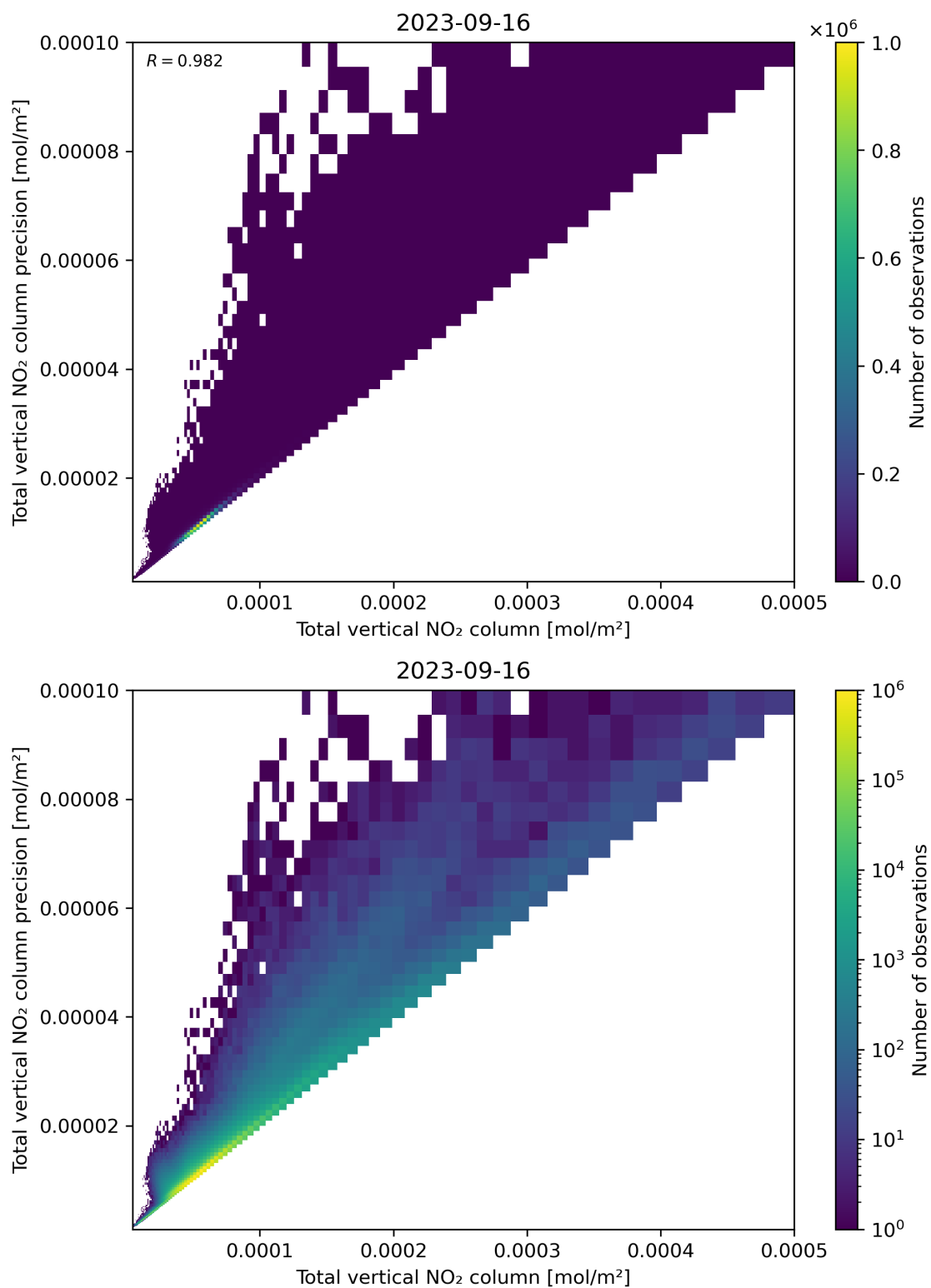
Figure 114: Scatter density plot of “Total vertical NO 2 column” against “Total vertical NO 2 column precision” for 2023-09-15 to 2023-09-17.
