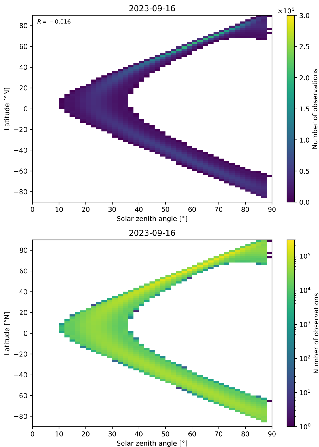
Figure 149: Scatter density plot of “Solar zenith angle” against “Latitude” for 2023-09-15 to 2023-09-17.
