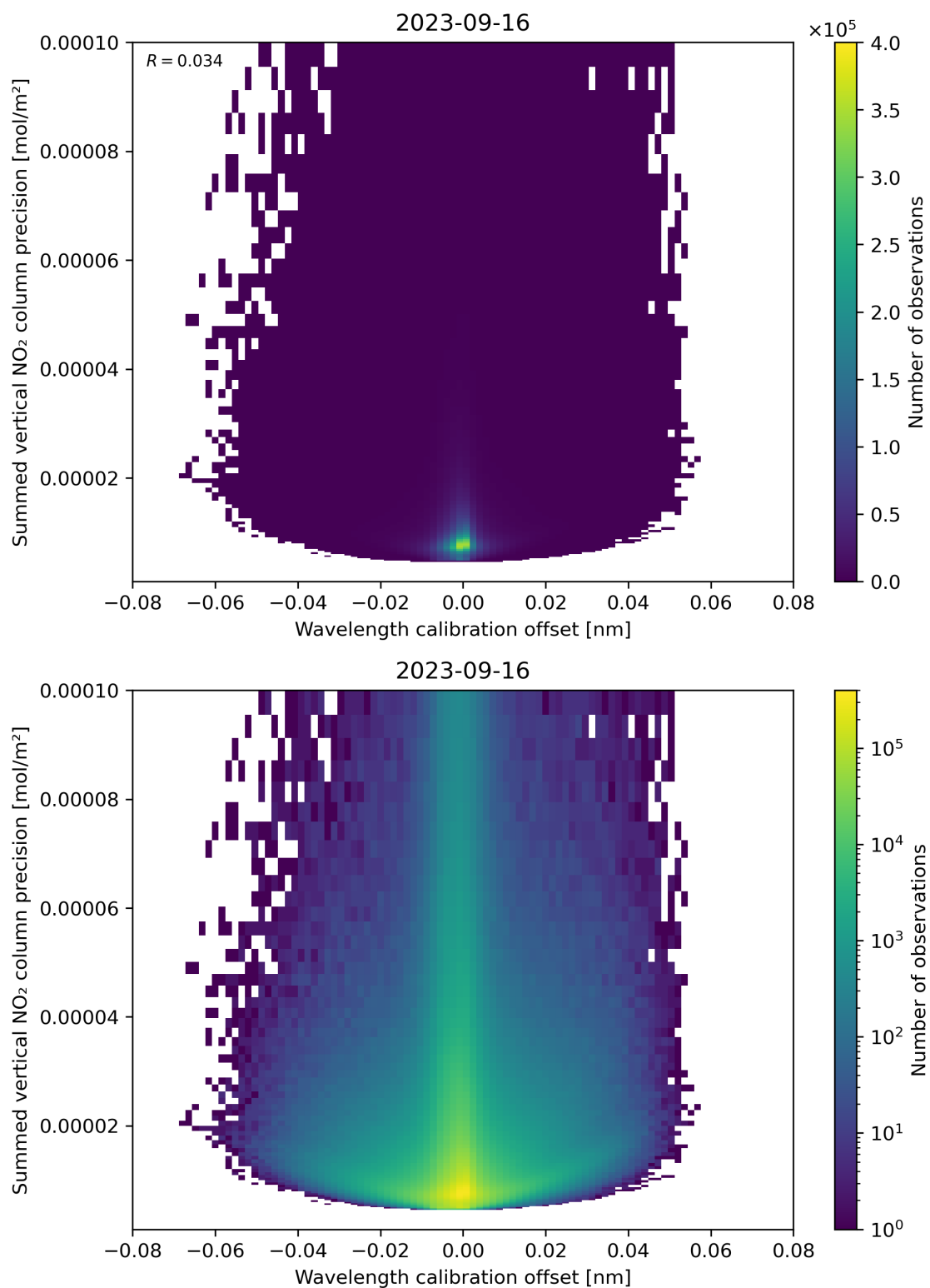
Figure 178: Scatter density plot of “Wavelength calibration offset” against “Summed vertical NO 2 column precision” for 2023-09-15 to 2023-09-17.
