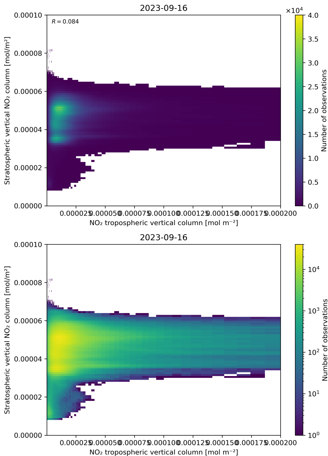
Figure 125: Scatter density plot of “NO 2 tropospheric vertical column” against “Stratospheric vertical NO 2 column” for 2023-09-15 to 2023-09-17.
