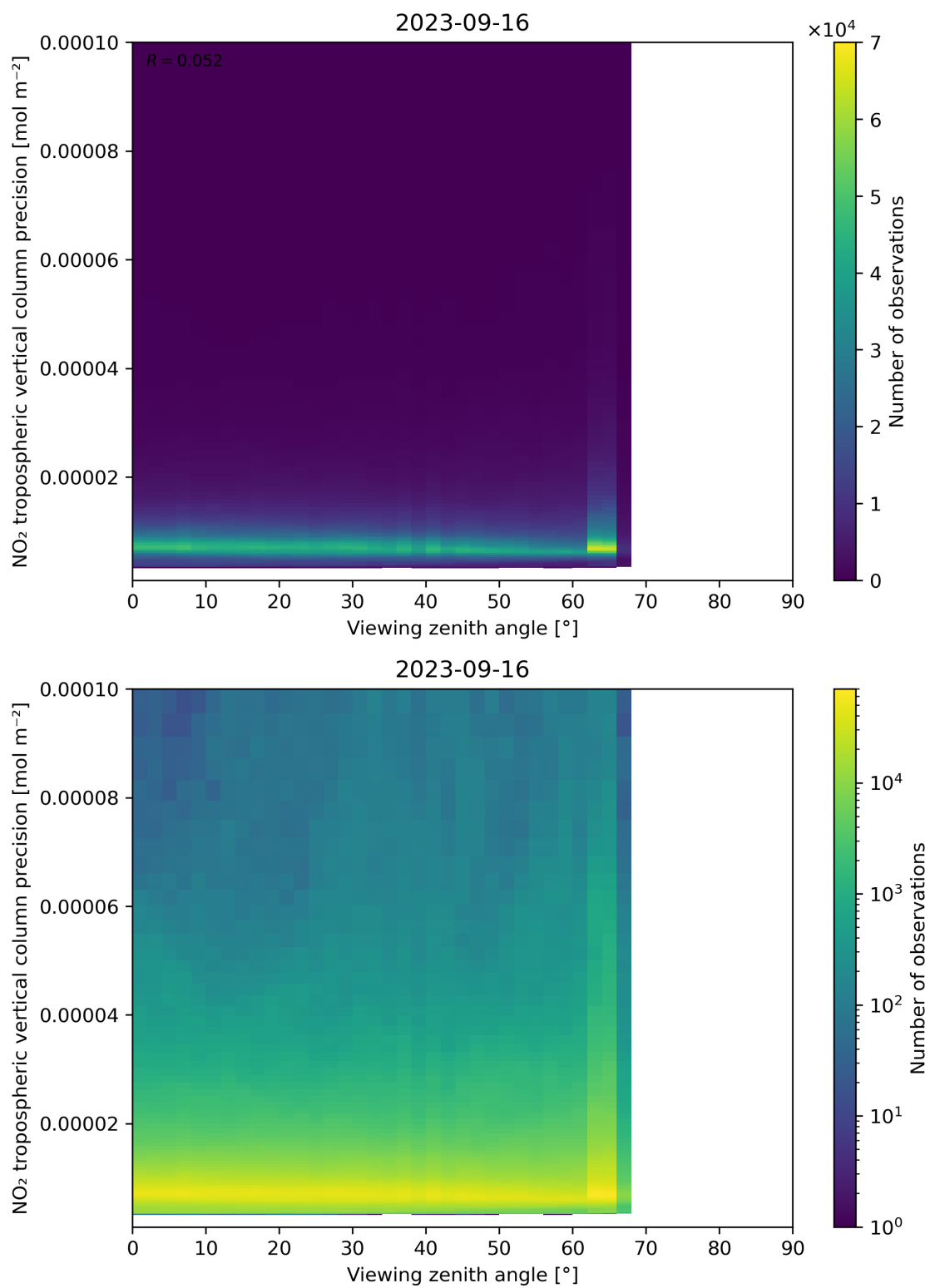
Figure 170: Scatter density plot of “Viewing zenith angle” against “NO 2 tropospheric vertical column precision” for 2023-09-15 to 2023-09-17.
