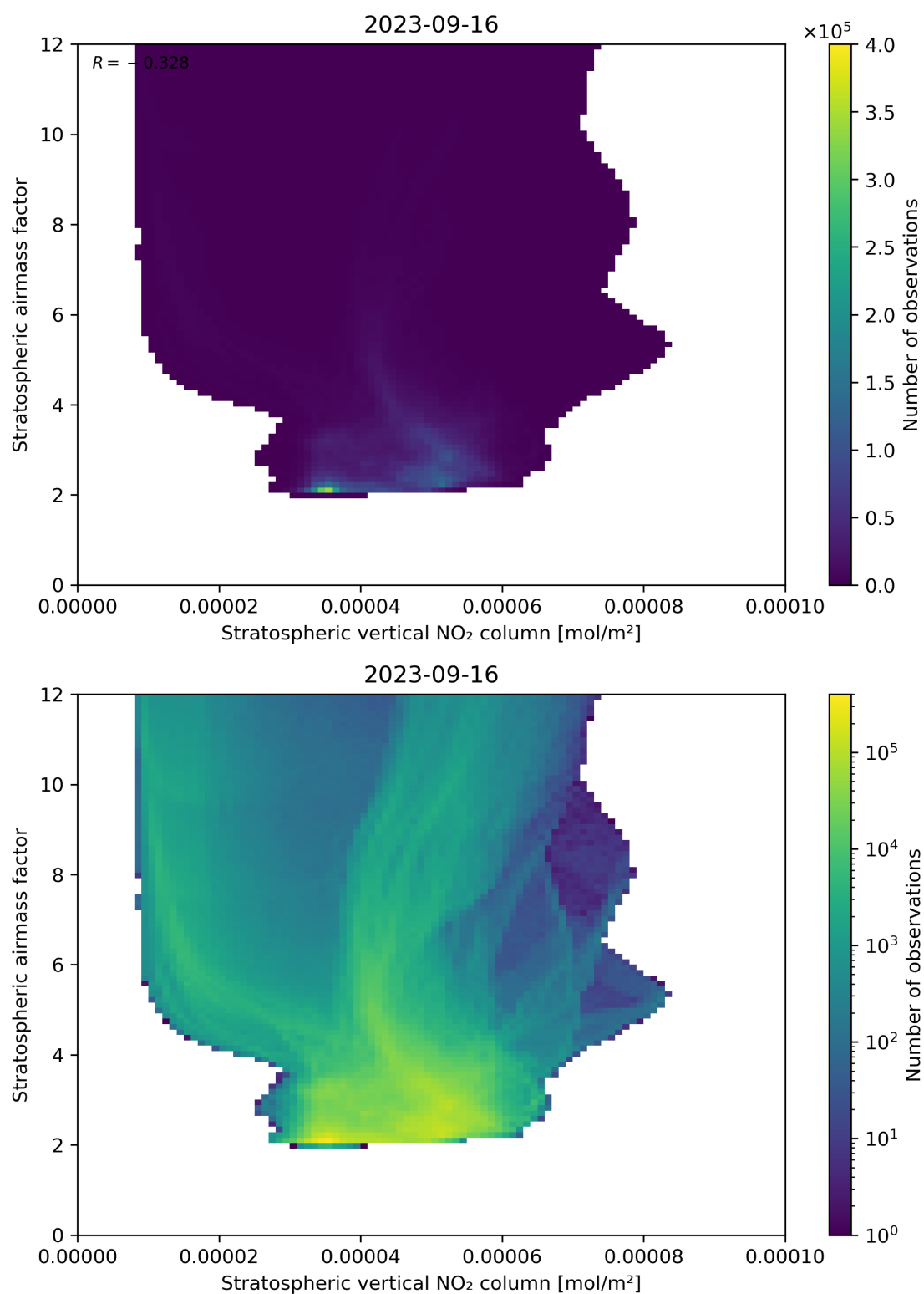
Figure 96: Scatter density plot of “Stratospheric vertical NO 2 column” against “Stratospheric airmass factor” for 2023-09-15 to 2023-09-17.
