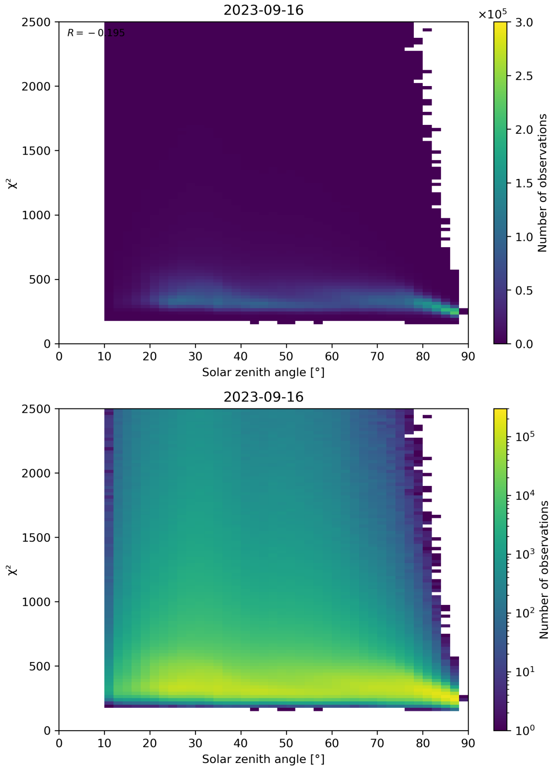
Figure 148: Scatter density plot of “Solar zenith angle” against “ \chi^2 ” for 2023-09-15 to 2023-09-17.
