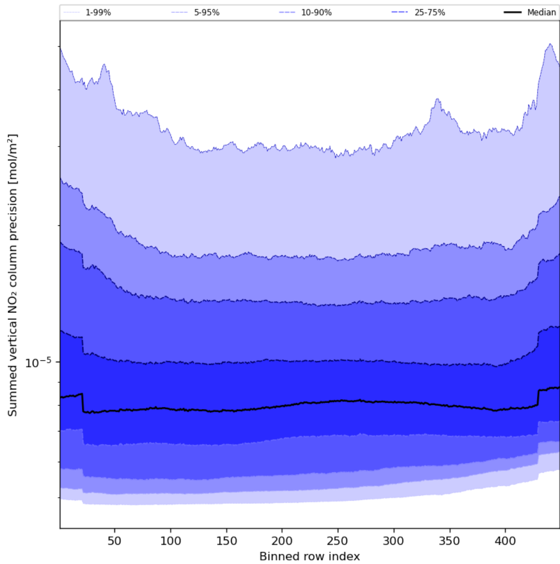
Figure 58: Along track statistics of “Summed vertical NO 2 column precision” for 2023-09-15 to 2023-09-17
