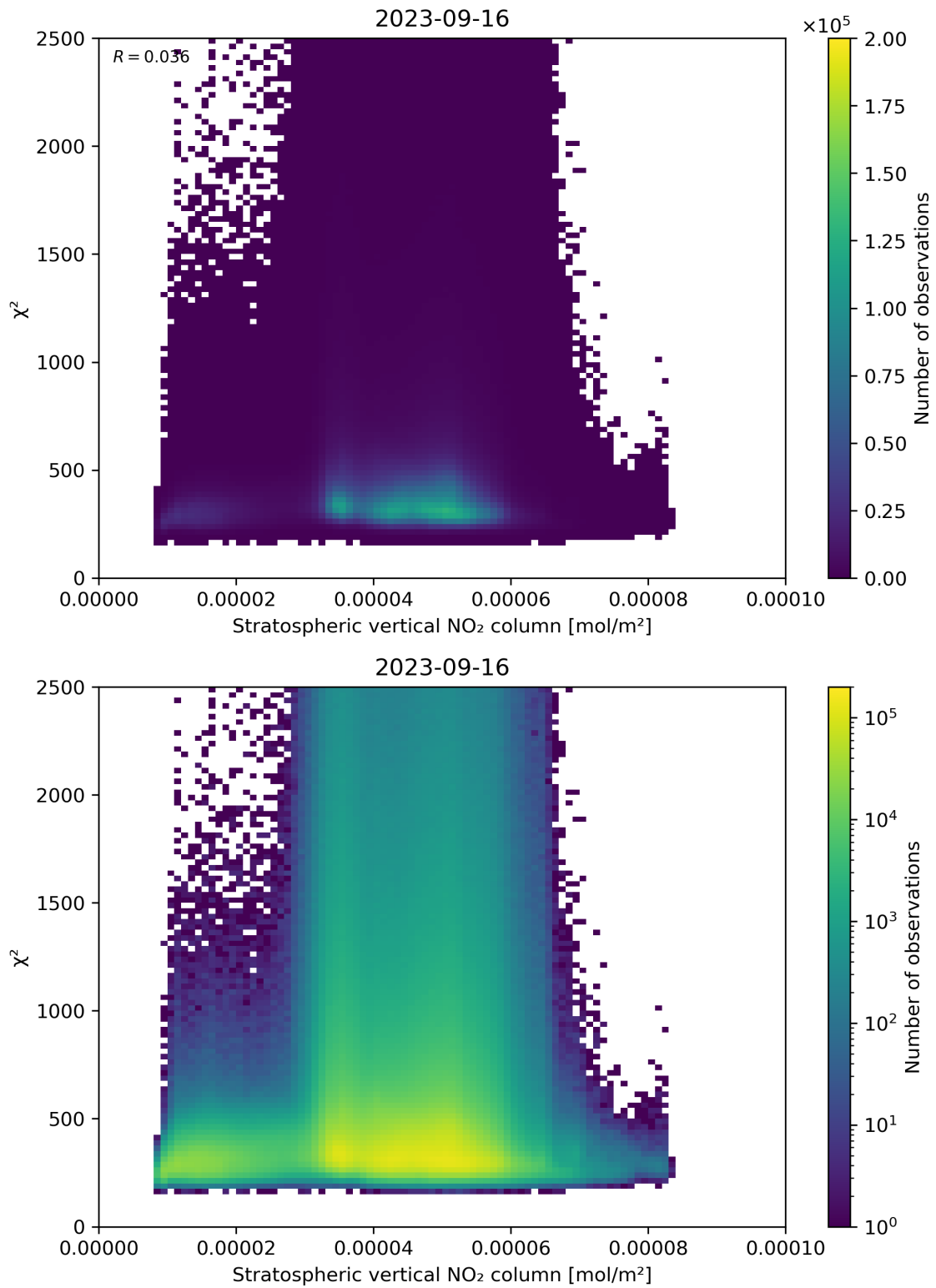
Figure 97: Scatter density plot of “Stratospheric vertical NO 2 column” against “ \chi^2 ” for 2023-09-15 to 2023-09-17.
