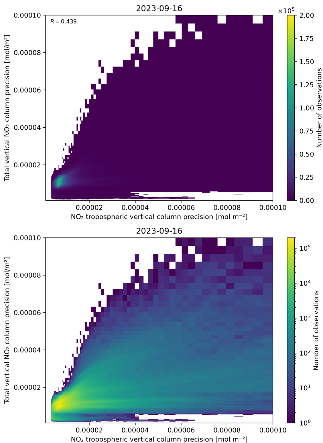
Figure 139: Scatter density plot of “NO 2 tropospheric vertical column precision” against “Total vertical NO 2 column precision” for 2023-09-15 to 2023-09-17.
