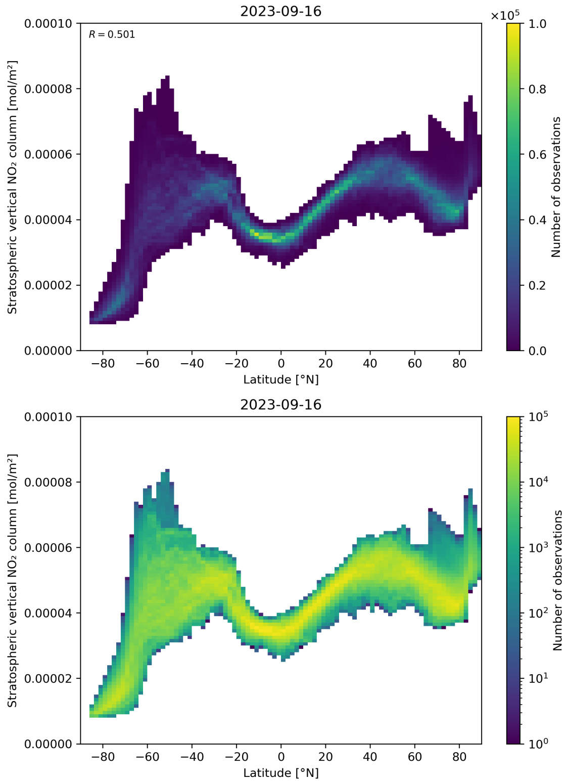
Figure 87: Scatter density plot of “Latitude” against “Stratospheric vertical NO 2 column” for 2023-09-15 to 2023-09-17.
