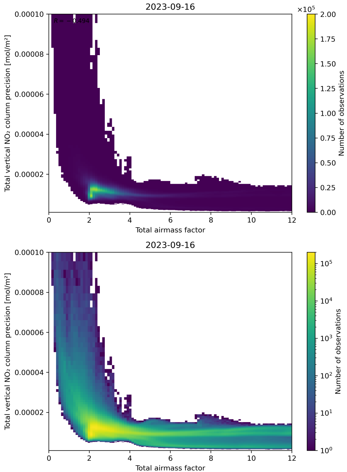
Figure 68: Scatter density plot of “Total airmass factor” against “Total vertical NO 2 column precision” for 2023-09-15 to 2023-09-17.
