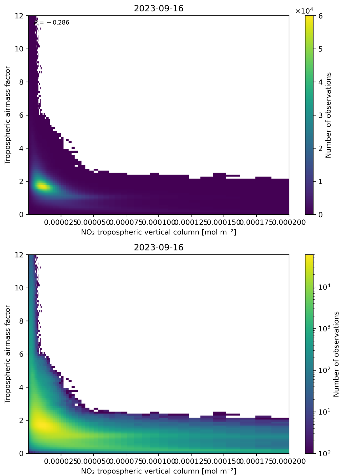
Figure 123: Scatter density plot of “NO 2 tropospheric vertical column” against “Tropospheric air mass factor” for 2023-09-15 to 2023-09-17.
