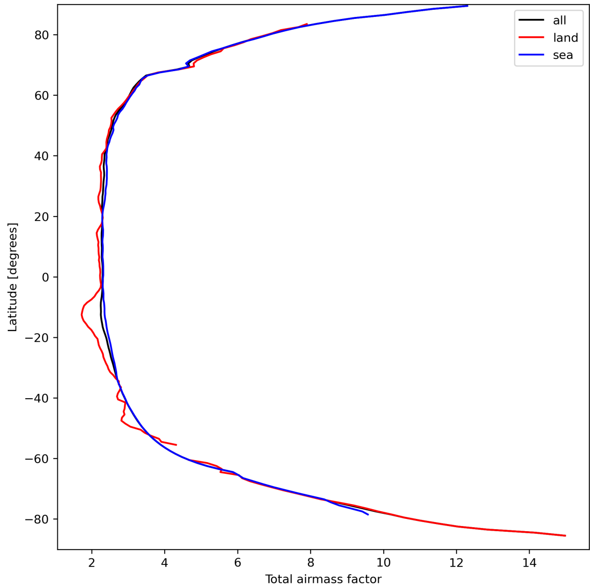
Figure 15: Zonal average of “Total airmass factor” for 2023-09-15 to 2023-09-17.
