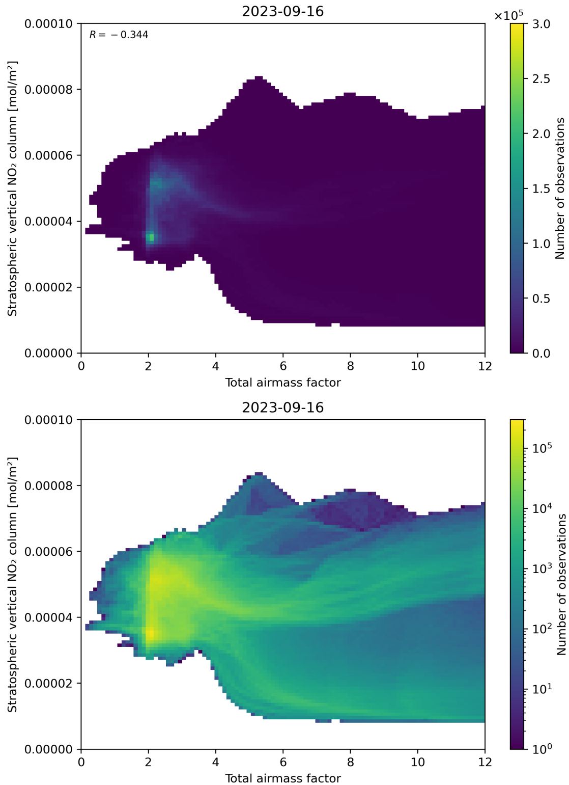
Figure 64: Scatter density plot of “Total airmass factor” against “Stratospheric vertical NO 2 column” for 2023-09-15 to 2023-09-17.
