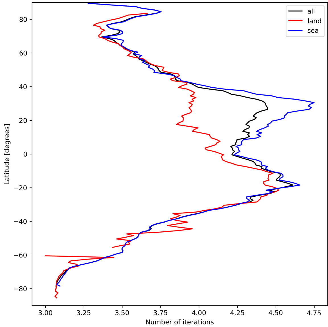
Figure 17: Zonal average of “Number of iterations” for 2023-09-15 to 2023-09-17.
