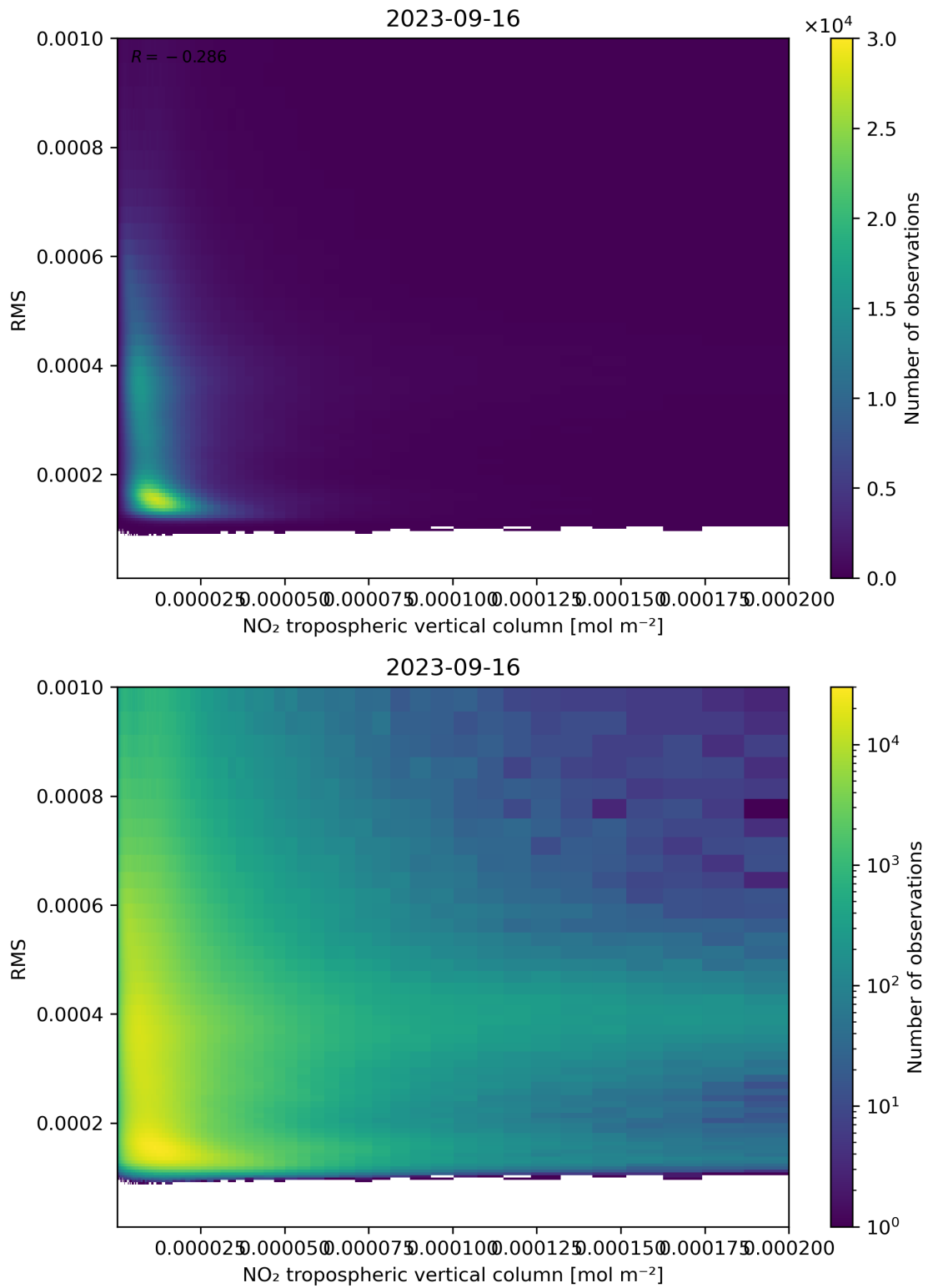
Figure 142: Scatter density plot of “NO 2 tropospheric vertical column” against “RMS” for 2023-09-15 to 2023-09-17.
