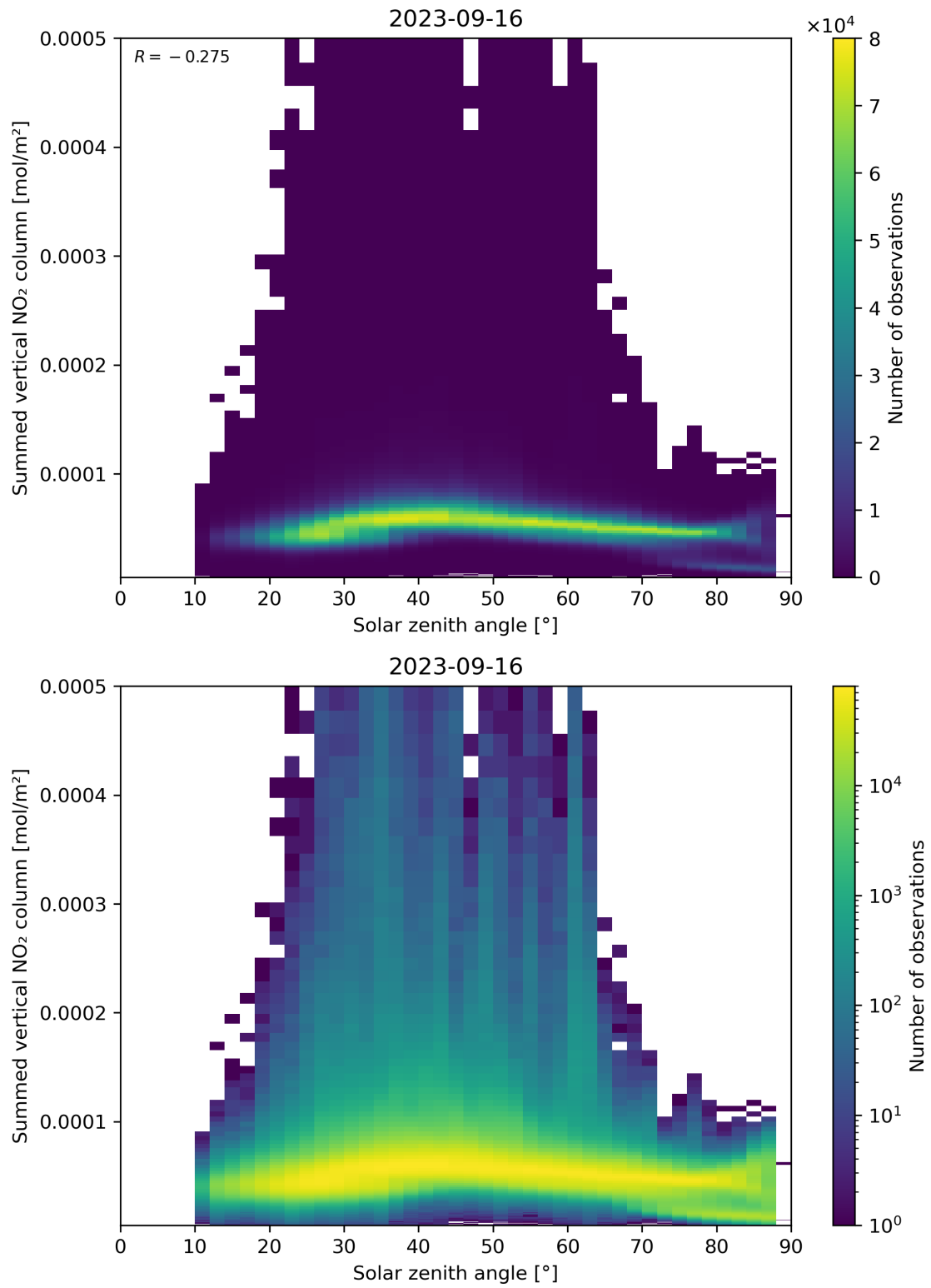
Figure 151: Scatter density plot of “Solar zenith angle” against “Summed vertical NO 2 column” for 2023-09-15 to 2023-09-17.
