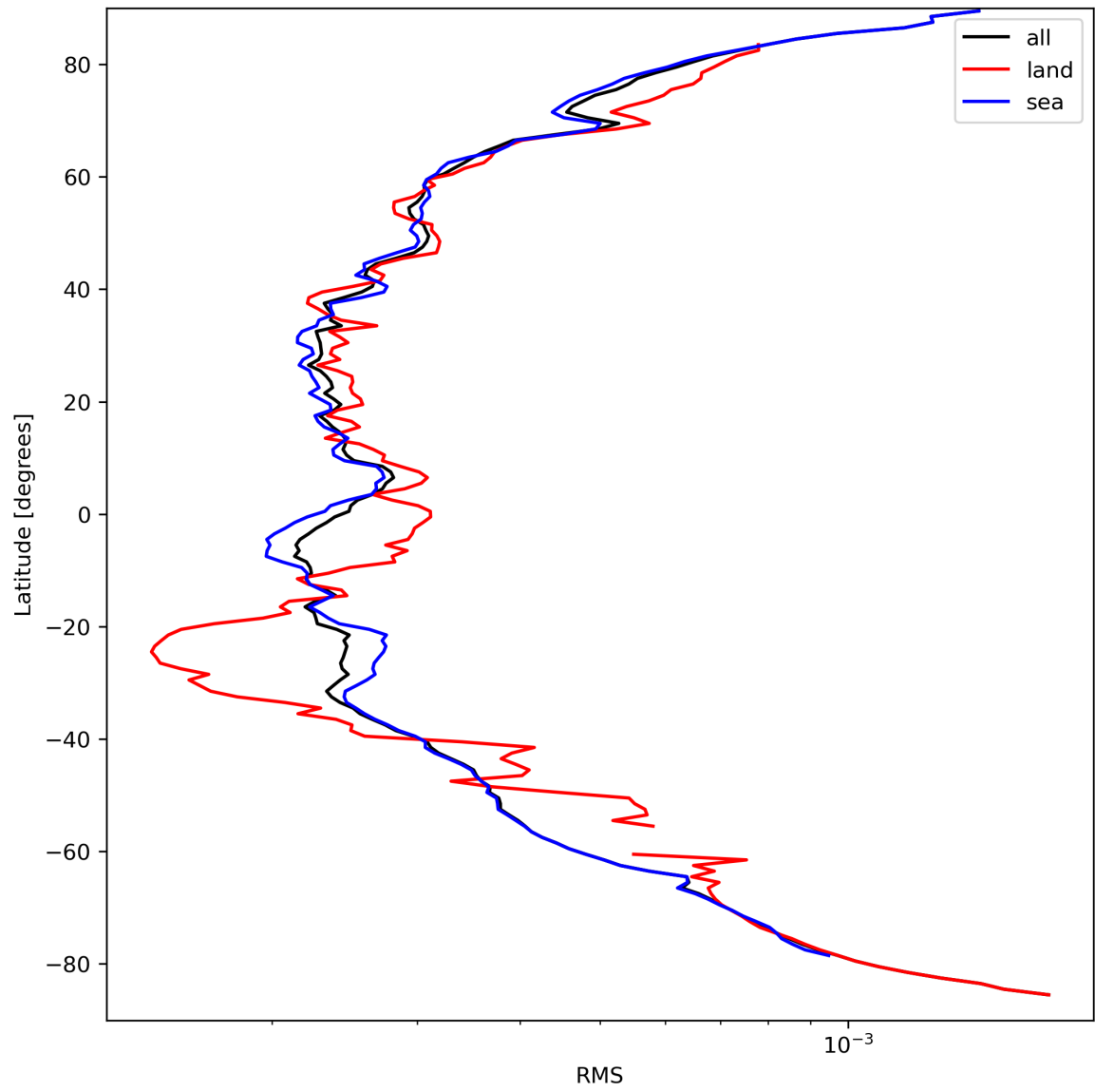
Figure 26: Zonal average of “RMS” for 2023-09-15 to 2023-09-17.
