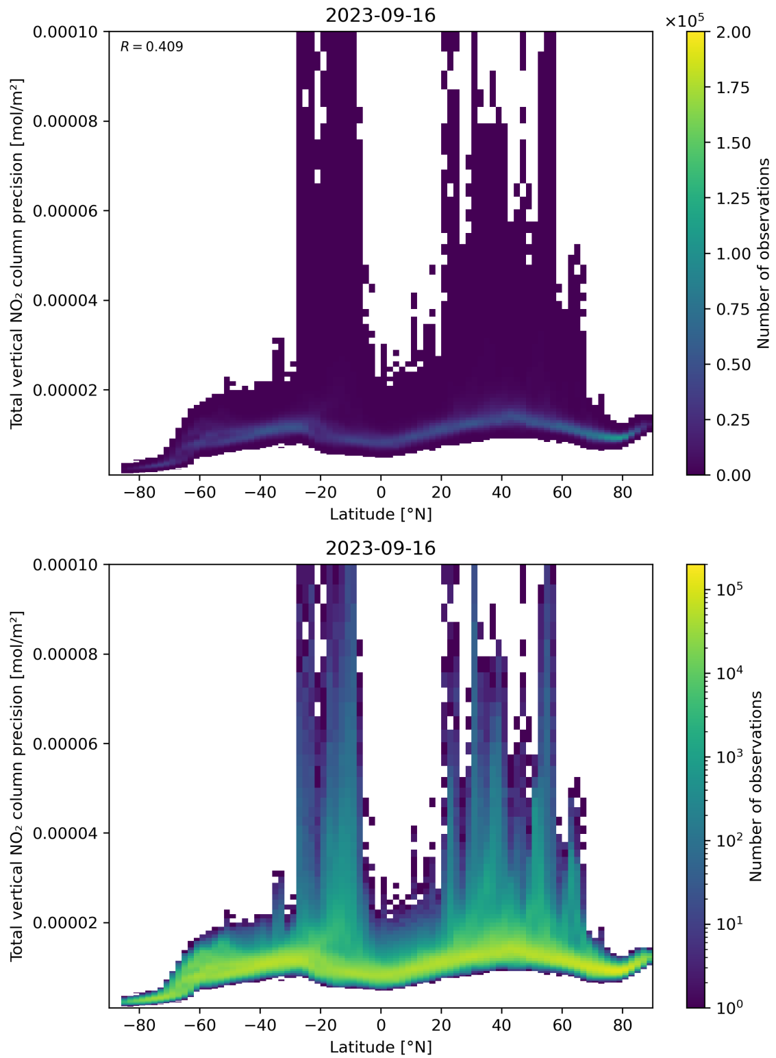
Figure 91: Scatter density plot of “Latitude” against “Total vertical NO 2 column precision” for 2023-09-15 to 2023-09-17.
