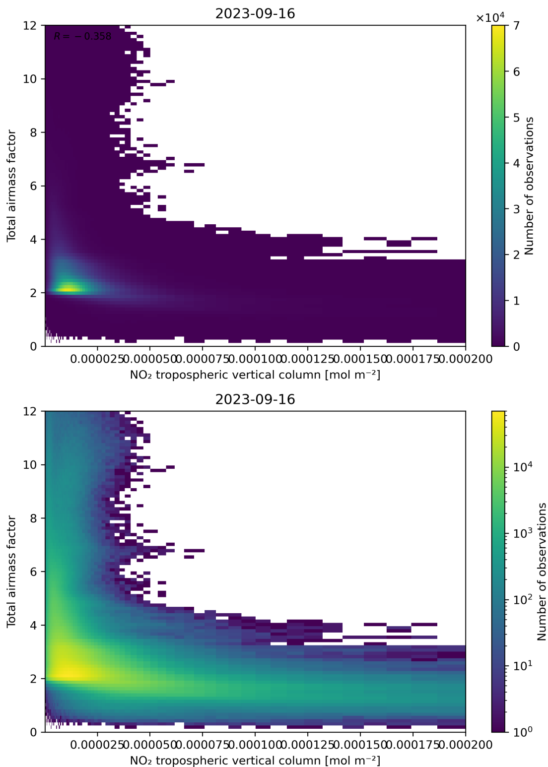
Figure 122: Scatter density plot of “NO 2 tropospheric vertical column” against “Total air mass factor” for 2023-09-15 to 2023-09-17.
