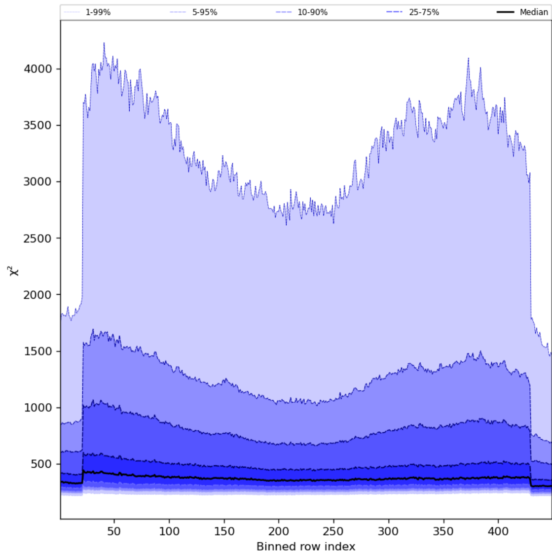
Figure 59: Along track statistics of “ \chi^2 ” for 2023-09-15 to 2023-09-17
