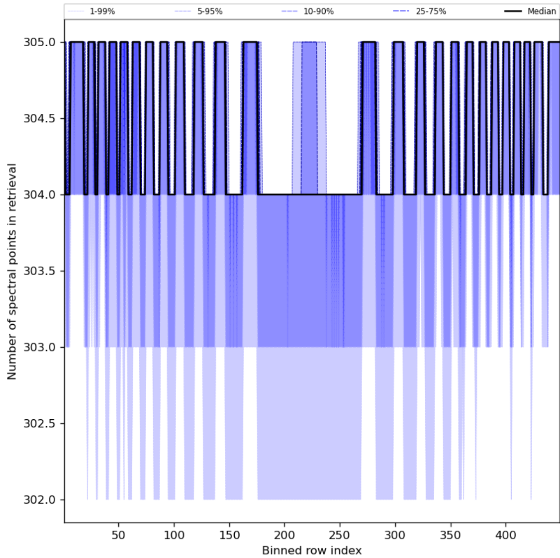
Figure 50: Along track statistics of “Number of spectral points in retrieval” for 2023-09-15 to 2023-09-17
