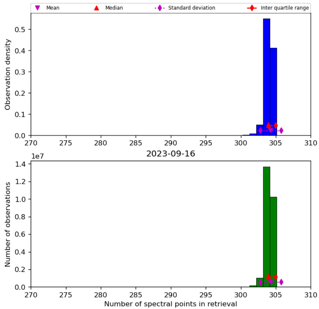
Figure 33: Histogram of “Number of spectral points in retrieval” for 2023-09-15 to 2023-09-17
