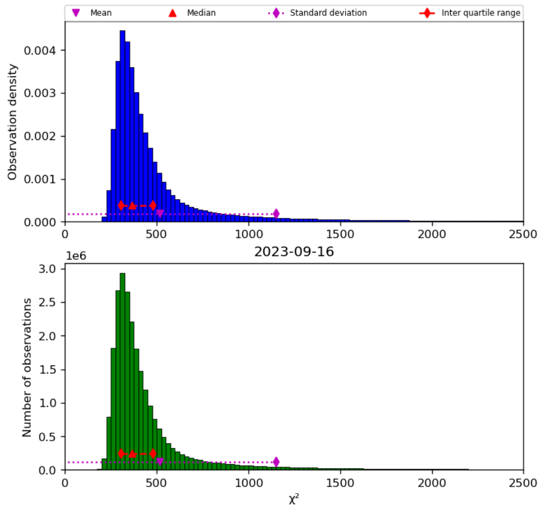
Figure 42: Histogram of “ \chi^2 ” for 2023-09-15 to 2023-09-17
