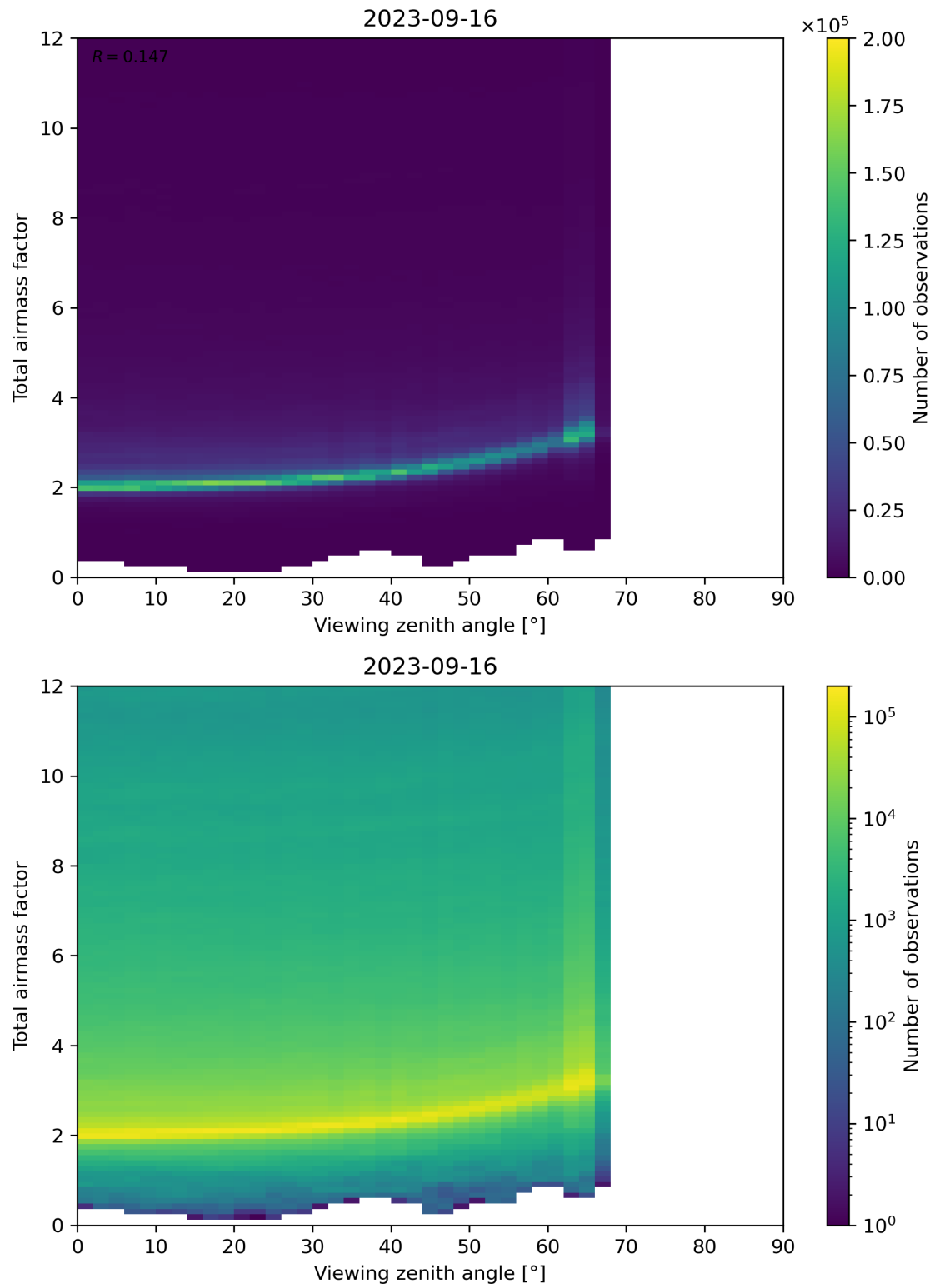
Figure 160: Scatter density plot of “Viewing zenith angle” against “Total airmass factor” for 2023-09-15 to 2023-09-17.
