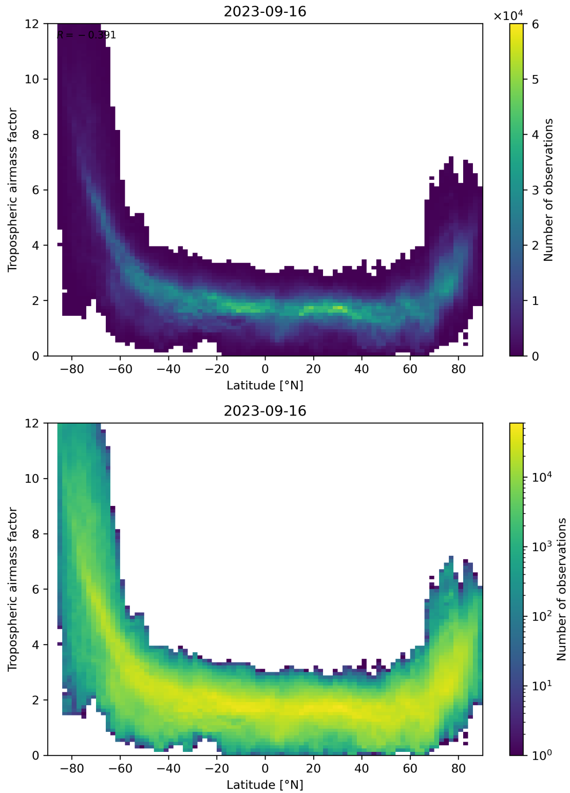
Figure 85: Scatter density plot of “Latitude” against “Tropospheric air mass factor” for 2023-09-15 to 2023-09-17.
