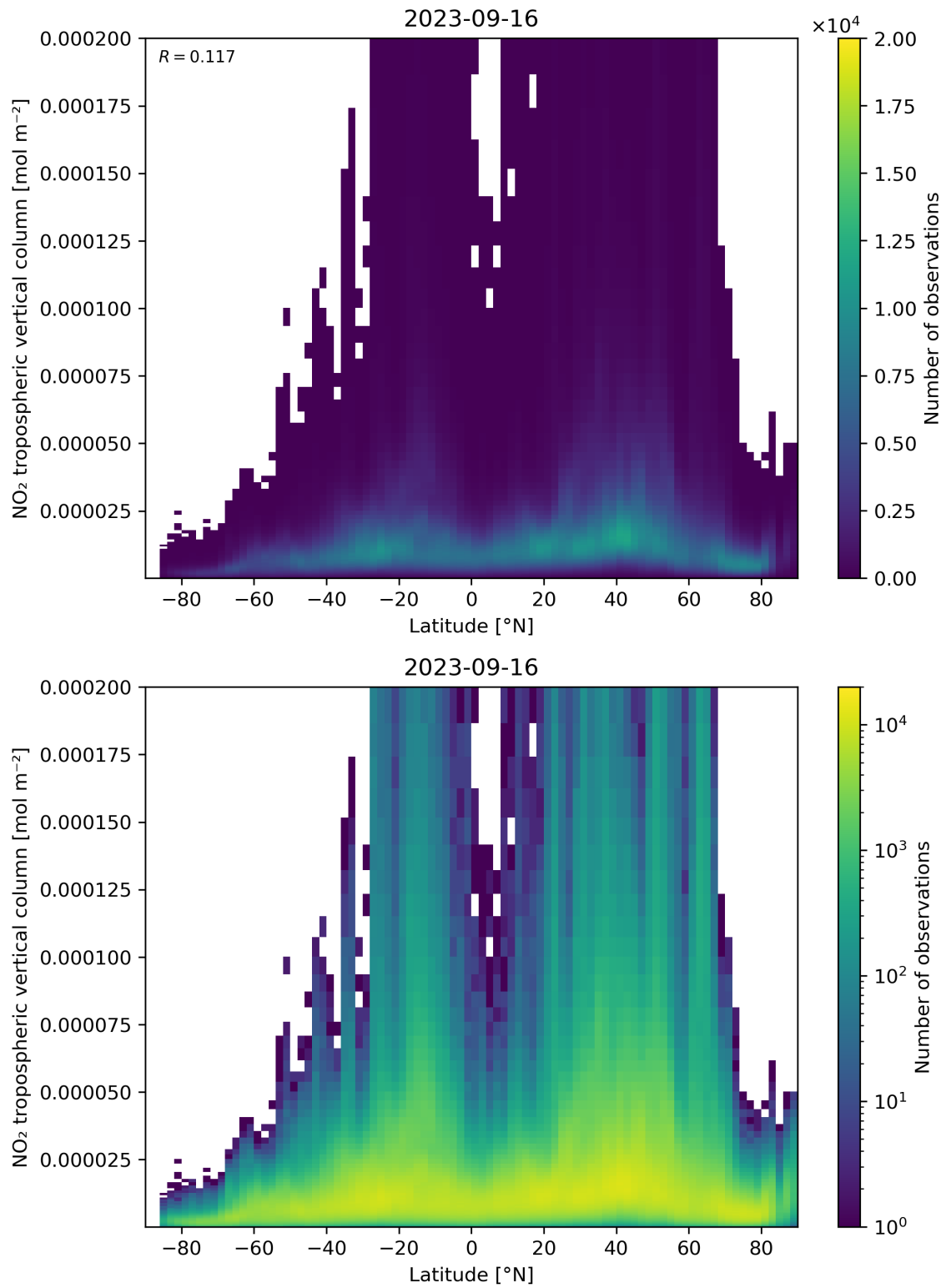
Figure 92: Scatter density plot of “Latitude” against “NO 2 tropospheric vertical column” for 2023-09-15 to 2023-09-17.
