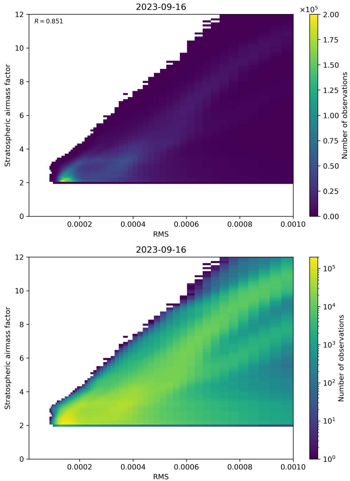
Figure 144: Scatter density plot of “RMS” against “Stratospheric airmass factor” for 2023-09-15 to 2023-09-17.
