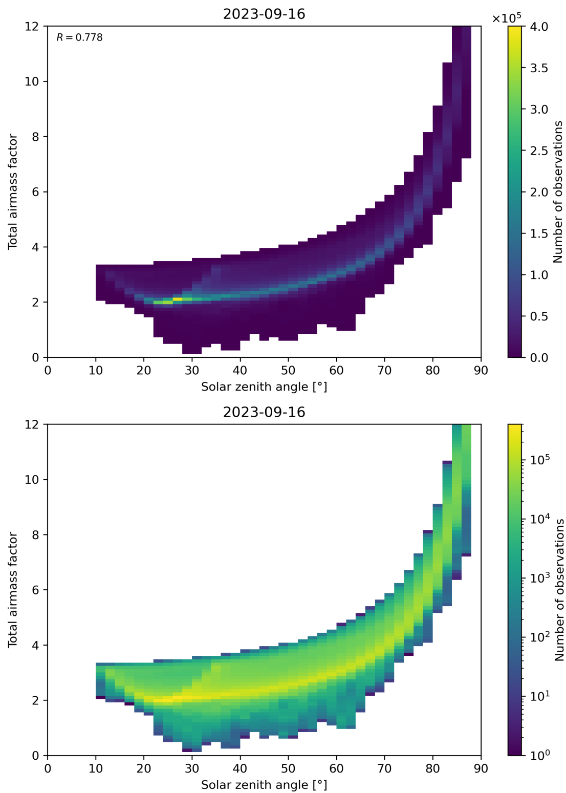
Figure 146: Scatter density plot of “Solar zenith angle” against “Total air mass factor” for 2023-09-15 to 2023-09-17.
