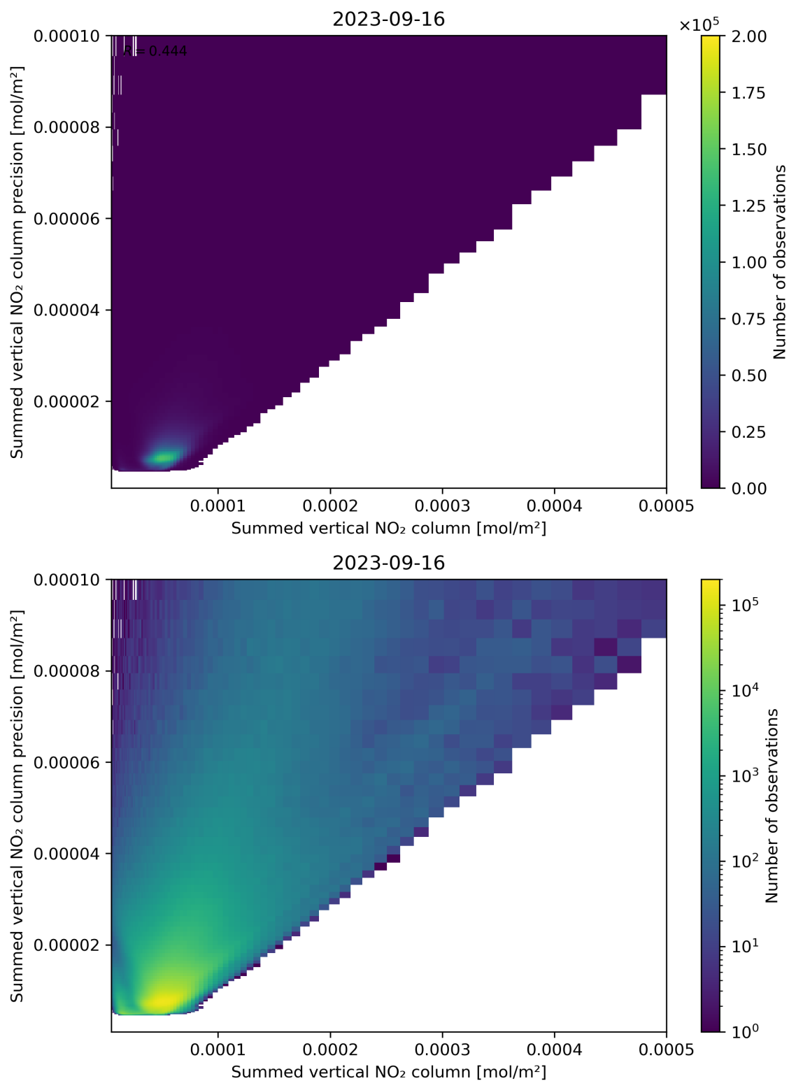
Figure 105: Scatter density plot of “Summed vertical NO 2 column” against “Summed vertical NO 2 column precision” for 2023-09-15 to 2023-09-17.
