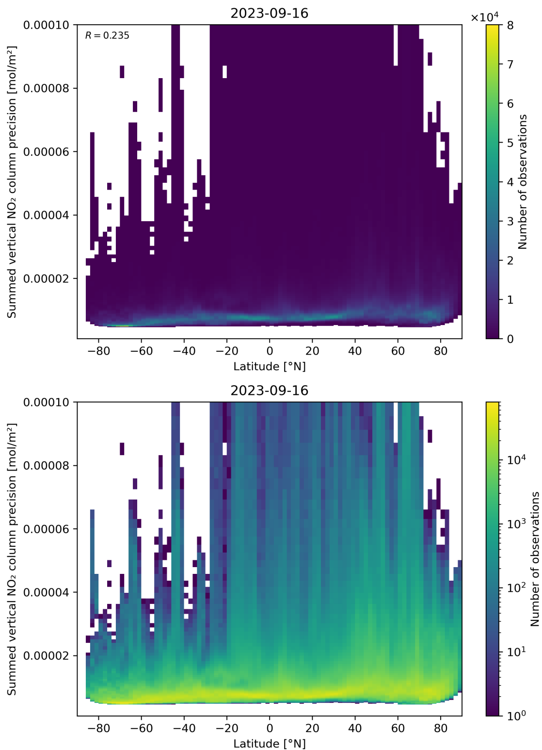
Figure 89: Scatter density plot of “Latitude” against “Summed vertical NO 2 column precision” for 2023-09-15 to 2023-09-17.
