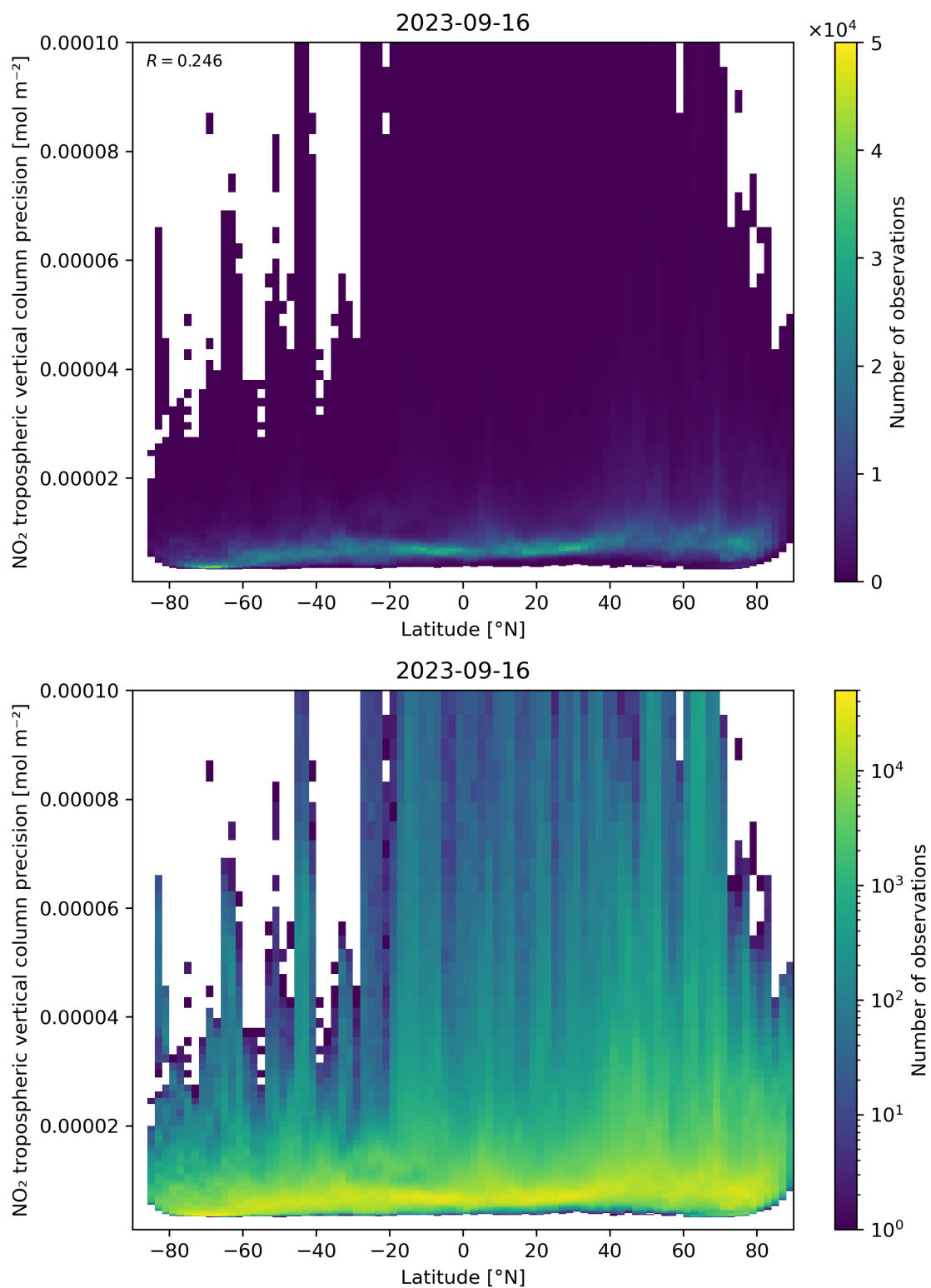
Figure 93: Scatter density plot of “Latitude” against “NO 2 tropospheric vertical column precision” for 2023-09-15 to 2023-09-17.
