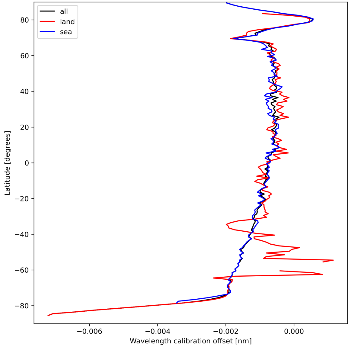
Figure 18: Zonal average of “Wavelength calibration offset” for 2023-09-15 to 2023-09-17.
