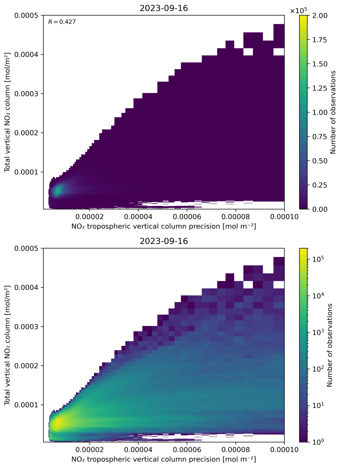
Figure 138: Scatter density plot of “NO 2 tropospheric vertical column precision” against “Total vertical NO 2 column” for 2023-09-15 to 2023-09-17.
