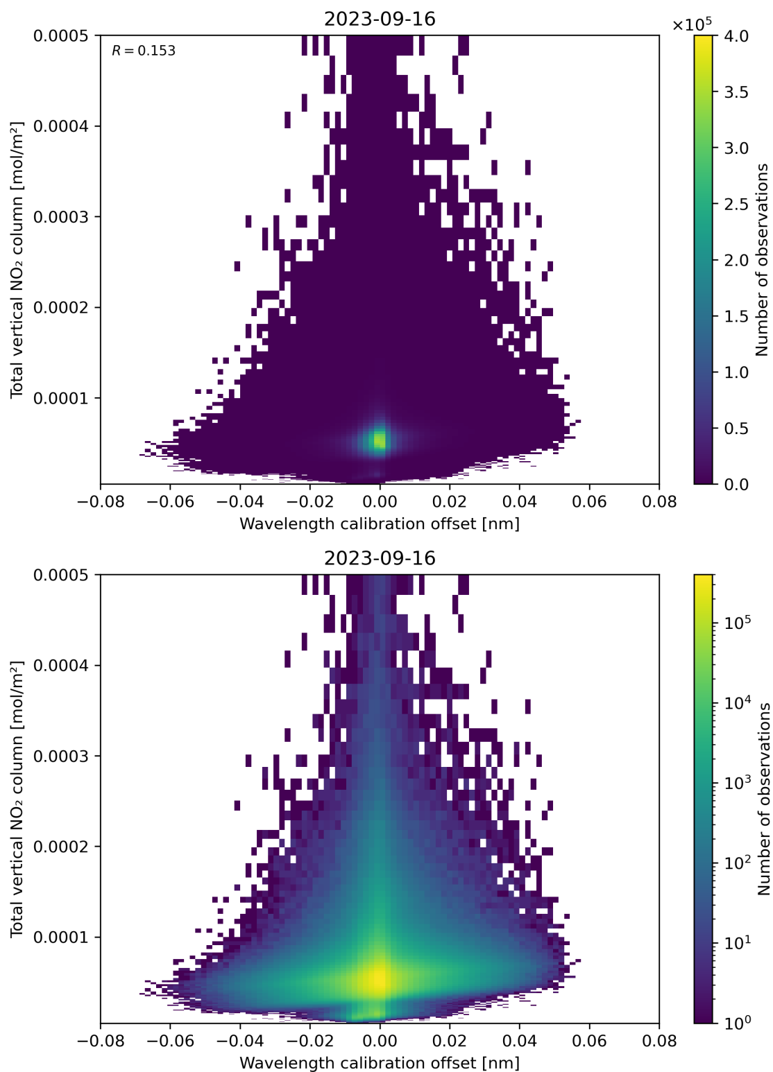
Figure 179: Scatter density plot of “Wavelength calibration offset” against “Total vertical NO 2 column” for 2023-09-15 to 2023-09-17.
