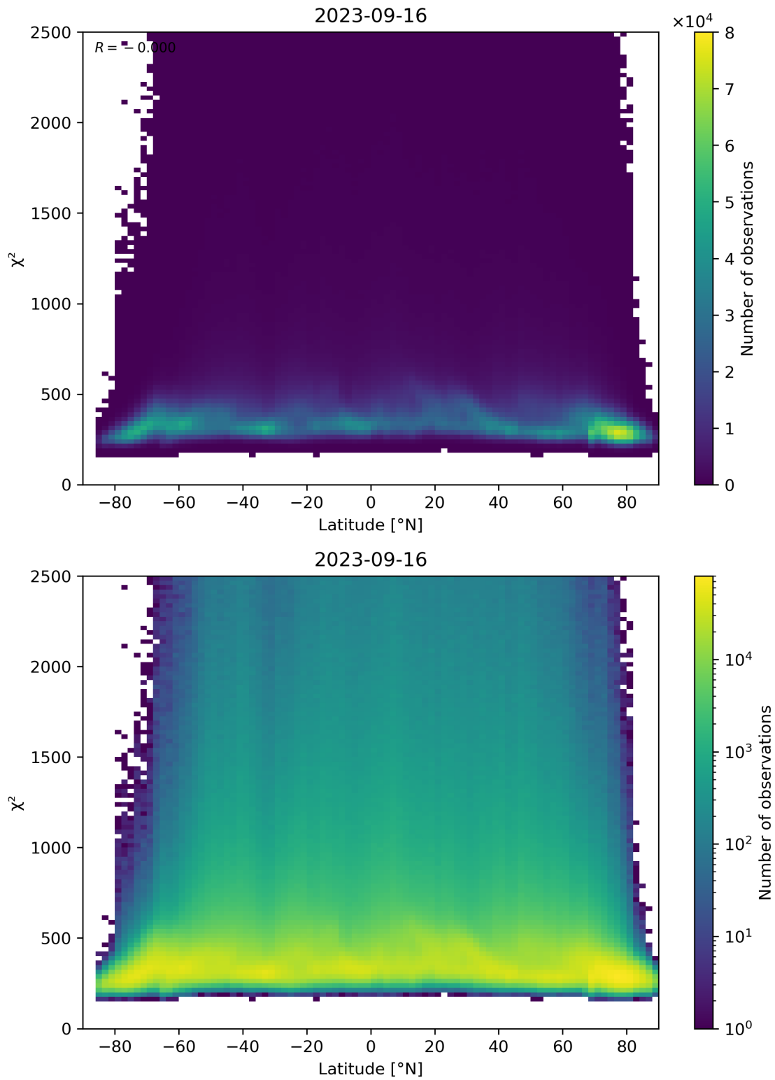
Figure 86: Scatter density plot of “Latitude” against “ \chi^2 ” for 2023-09-15 to 2023-09-17.
