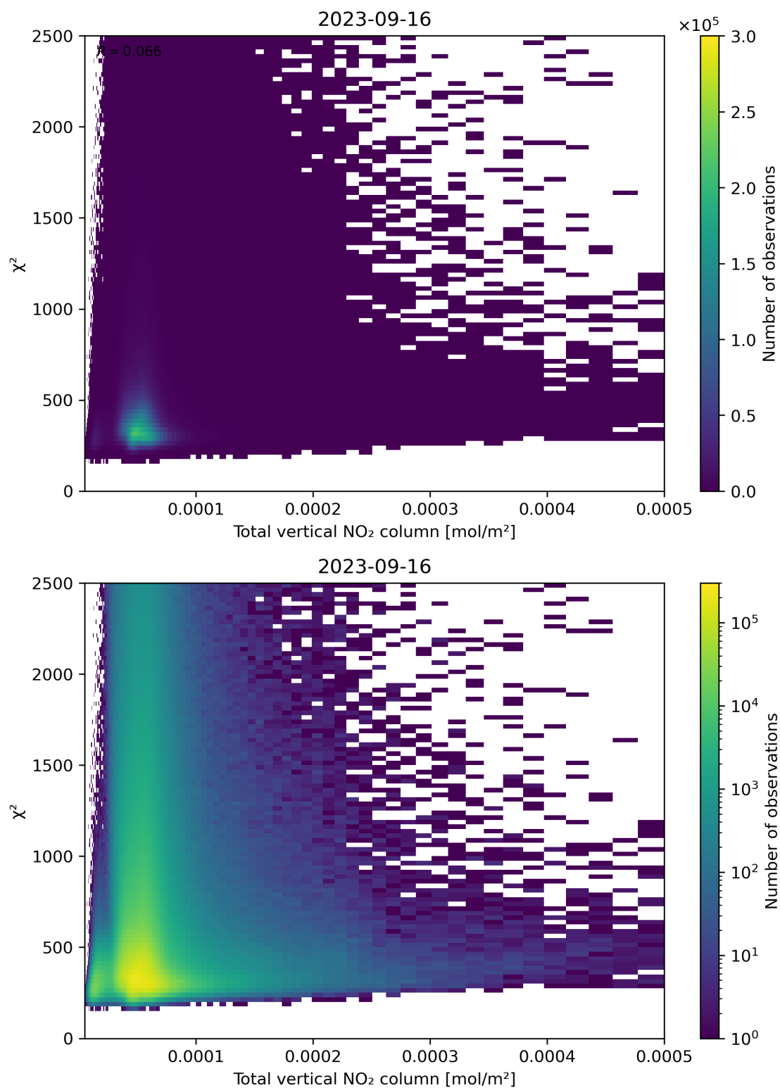
Figure 111: Scatter density plot of “Total vertical NO 2 column” against “ \chi^2 ” for 2023-09-15 to 2023-09-17.
