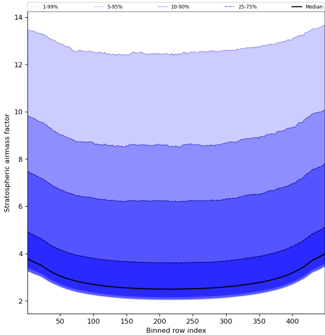
Figure 61: Along track statistics of “Stratospheric airmass factor” for 2023-09-15 to 2023-09-17
