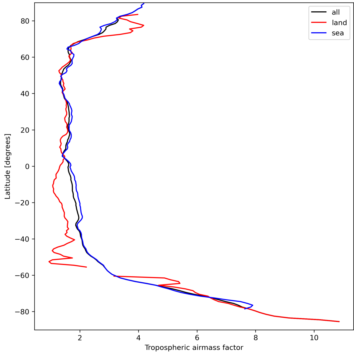
Figure 14: Zonal average of “Tropospheric airmass factor” for 2023-09-15 to 2023-09-17.
