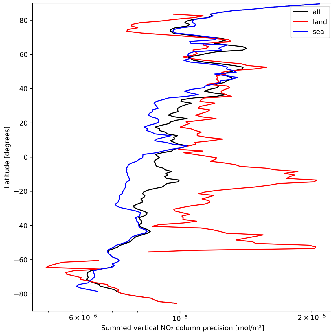
Figure 24: Zonal average of “Summed vertical NO 2 column precision” for 2023-09-15 to 2023-09-17.
