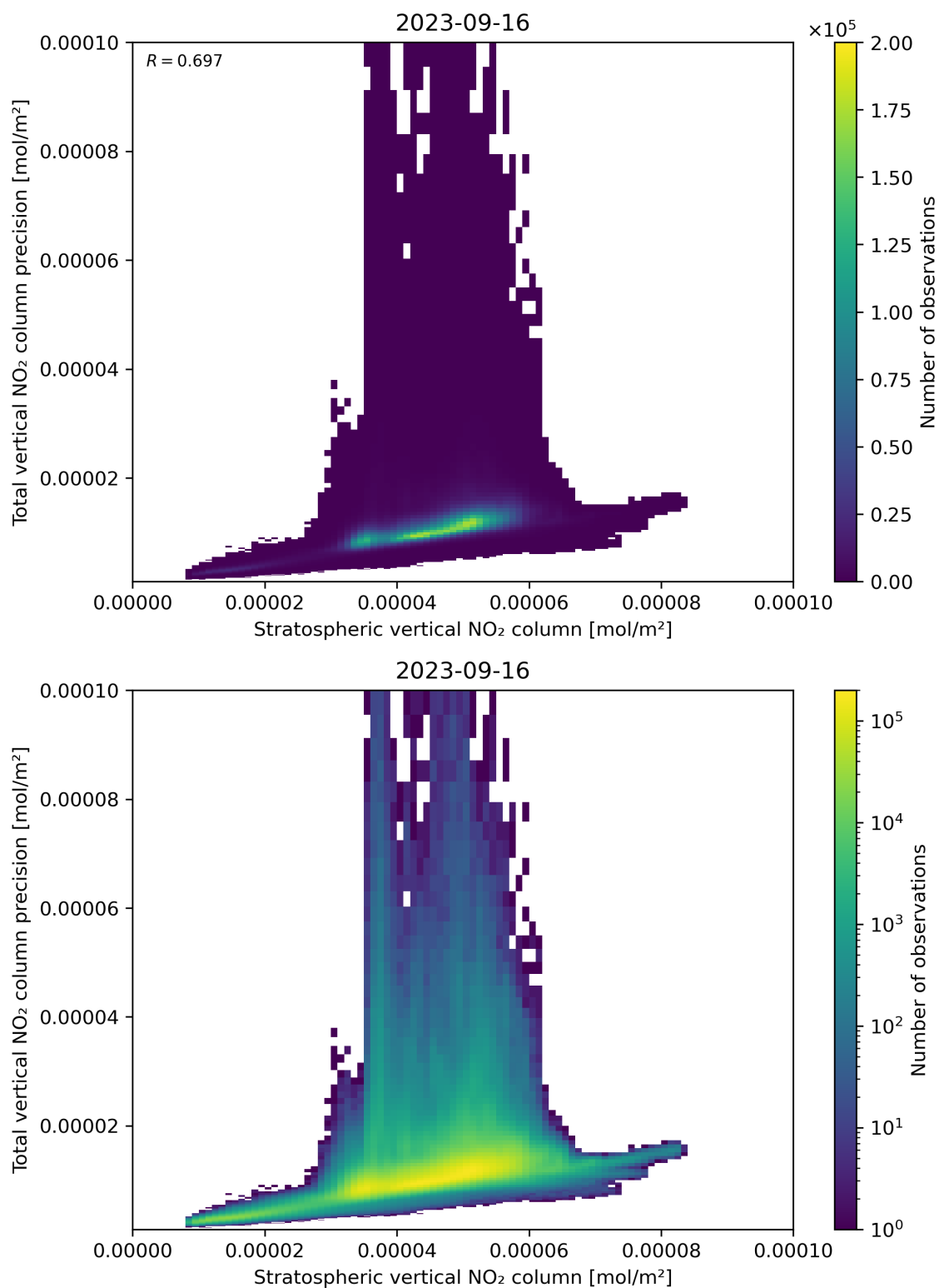
Figure 101: Scatter density plot of “Stratospheric vertical NO 2 column” against “Total vertical NO 2 column precision” for 2023-09-15 to 2023-09-17.
