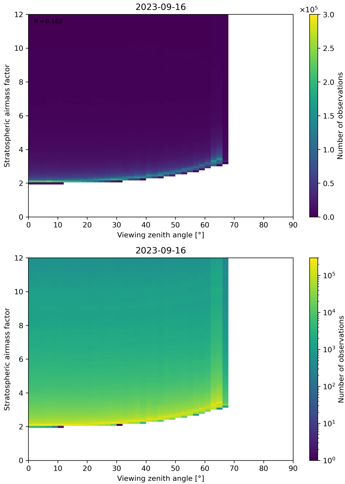
Figure 159: Scatter density plot of “Viewing zenith angle” against “Stratospheric airmass factor” for 2023-09-15 to 2023-09-17.
