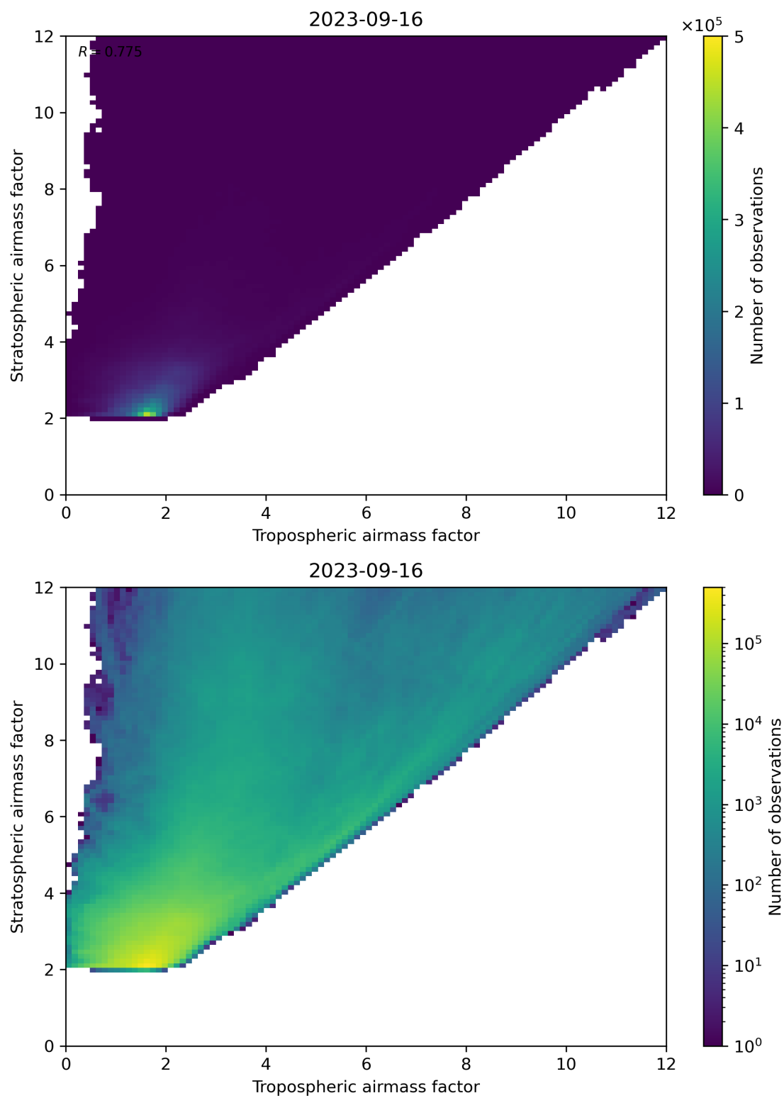
Figure 71: Scatter density plot of “Tropospheric airmass factor” against “Stratospheric airmass factor” for 2023-09-15 to 2023-09-17.
