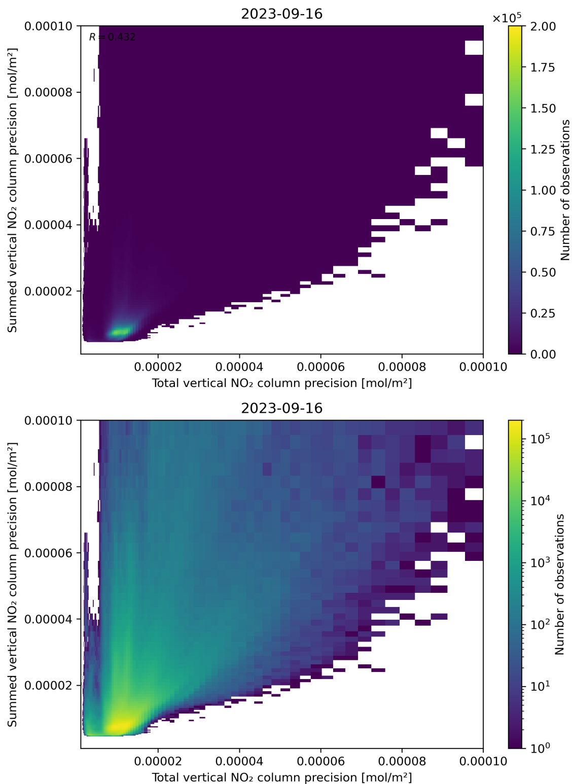
Figure 118: Scatter density plot of “Total vertical NO 2 column precision” against “Summed vertical NO 2 column precision” for 2023-09-15 to 2023-09-17.
