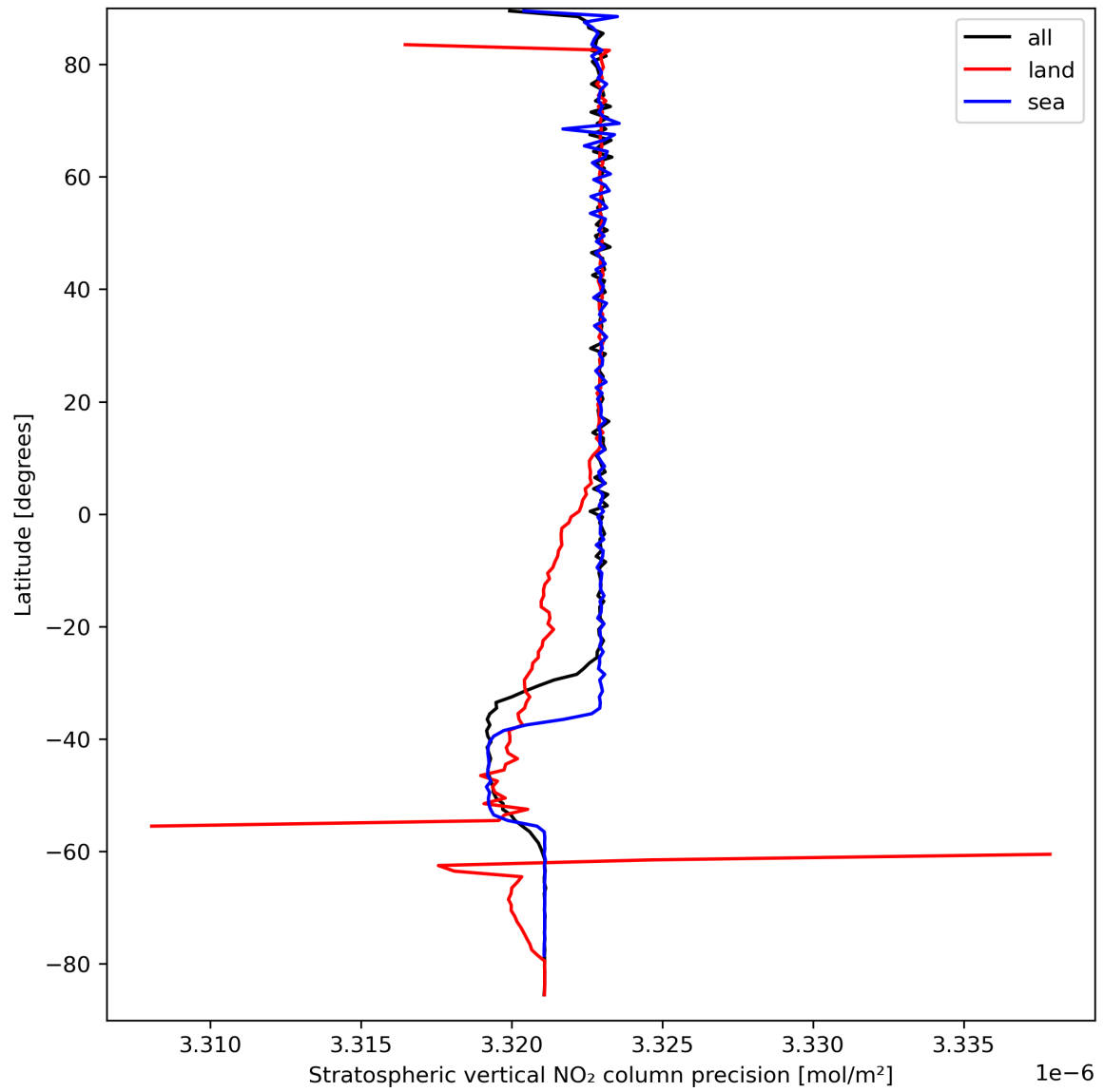
Figure 20: Zonal average of “Stratospheric vertical NO 2 column precision” for 2023-09-15 to 2023-09-17.
