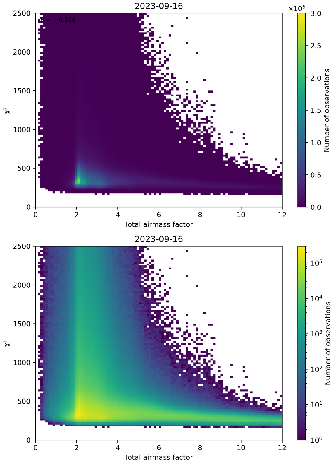
Figure 63: Scatter density plot of “Total airmass factor” against “ \chi^2 ” for 2023-09-15 to 2023-09-17.
