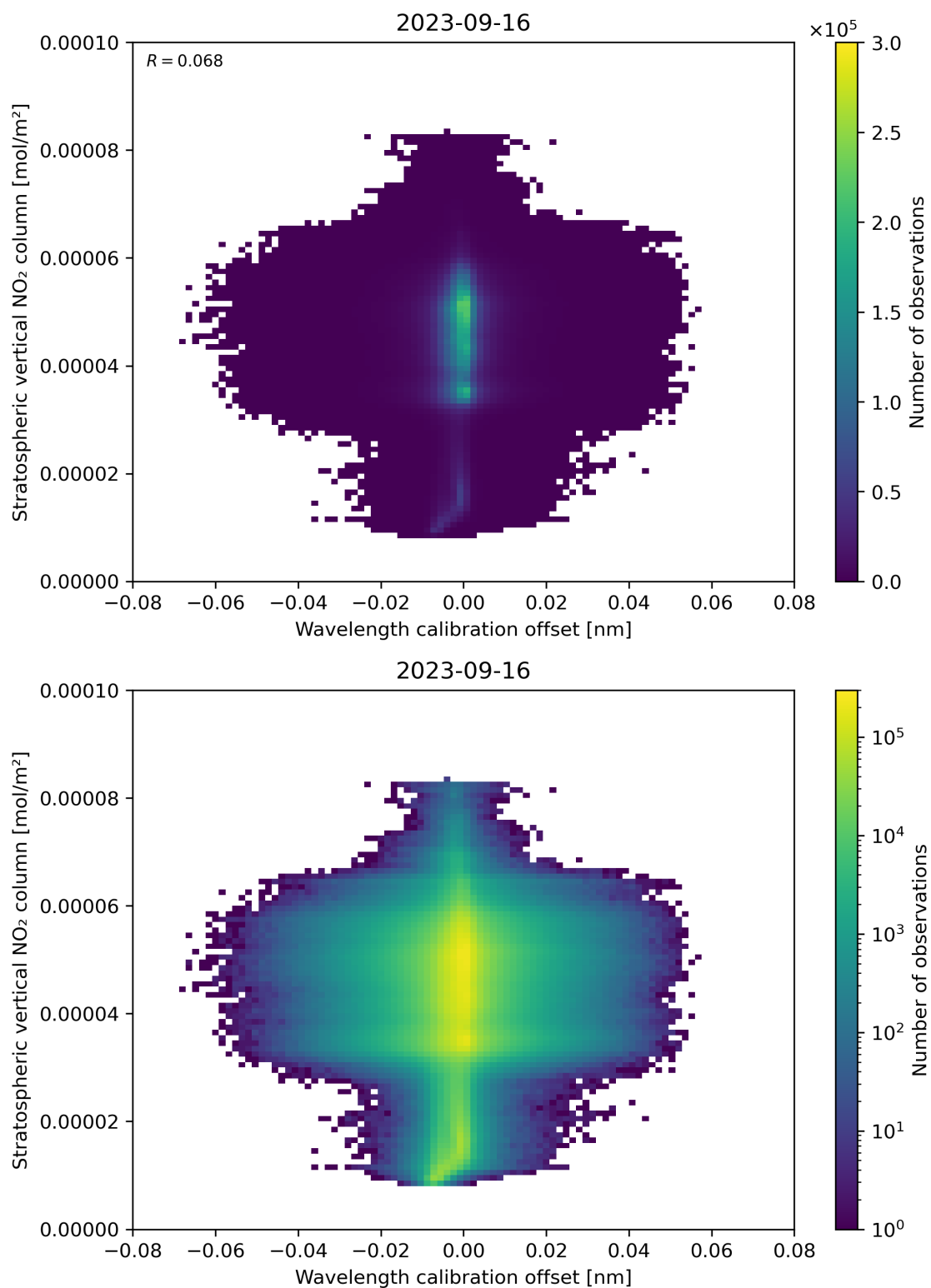
Figure 176: Scatter density plot of “Wavelength calibration offset” against “Stratospheric vertical NO 2 column” for 2023-09-15 to 2023-09-17.
