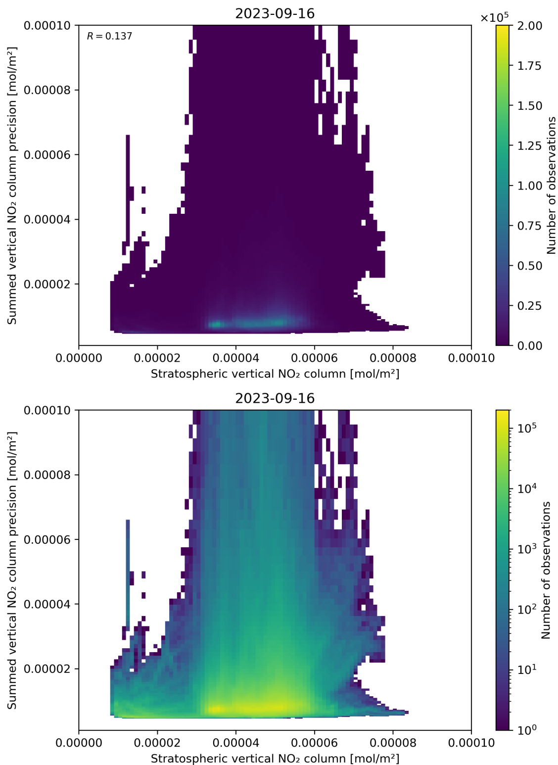
Figure 99: Scatter density plot of “Stratospheric vertical NO 2 column” against “Summed vertical NO 2 column precision” for 2023-09-15 to 2023-09-17.
