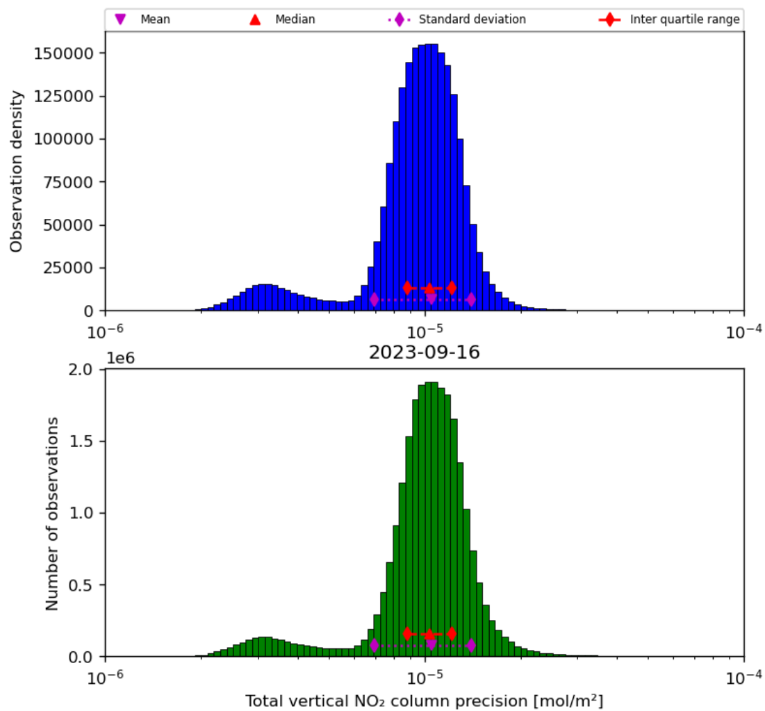
Figure 39: Histogram of “Total vertical NO 2 column precision” for 2023-09-15 to 2023-09-17
