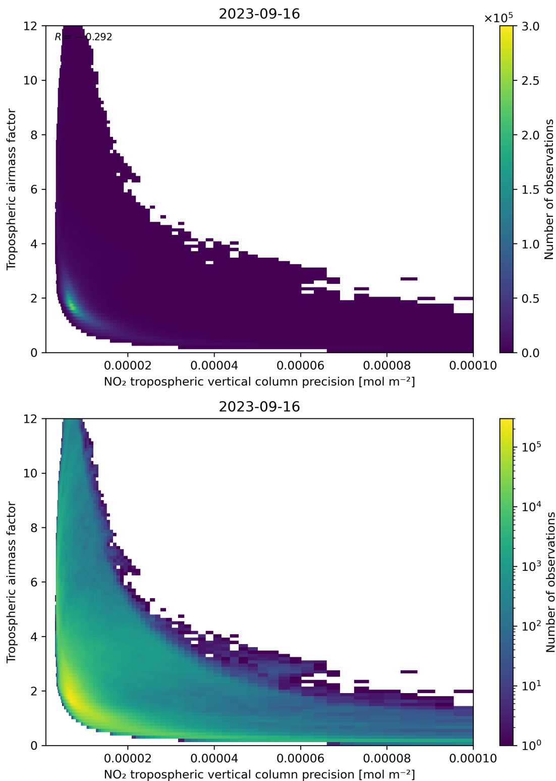
Figure 133: Scatter density plot of “NO 2 tropospheric vertical column precision” against “Tropospheric airmass factor” for 2023-09-15 to 2023-09-17.
