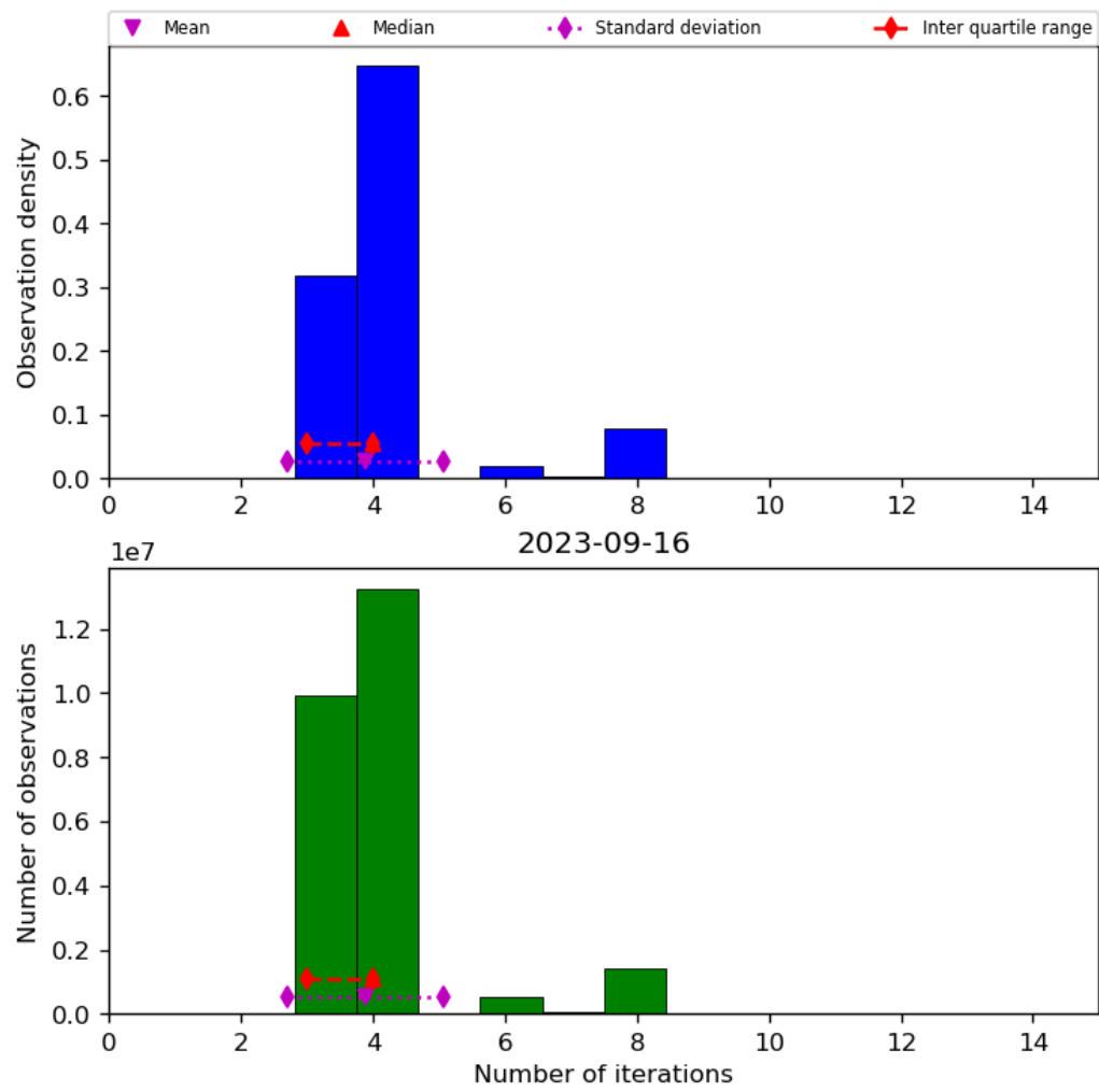
Figure 34: Histogram of “Number of iterations” for 2023-09-15 to 2023-09-17
