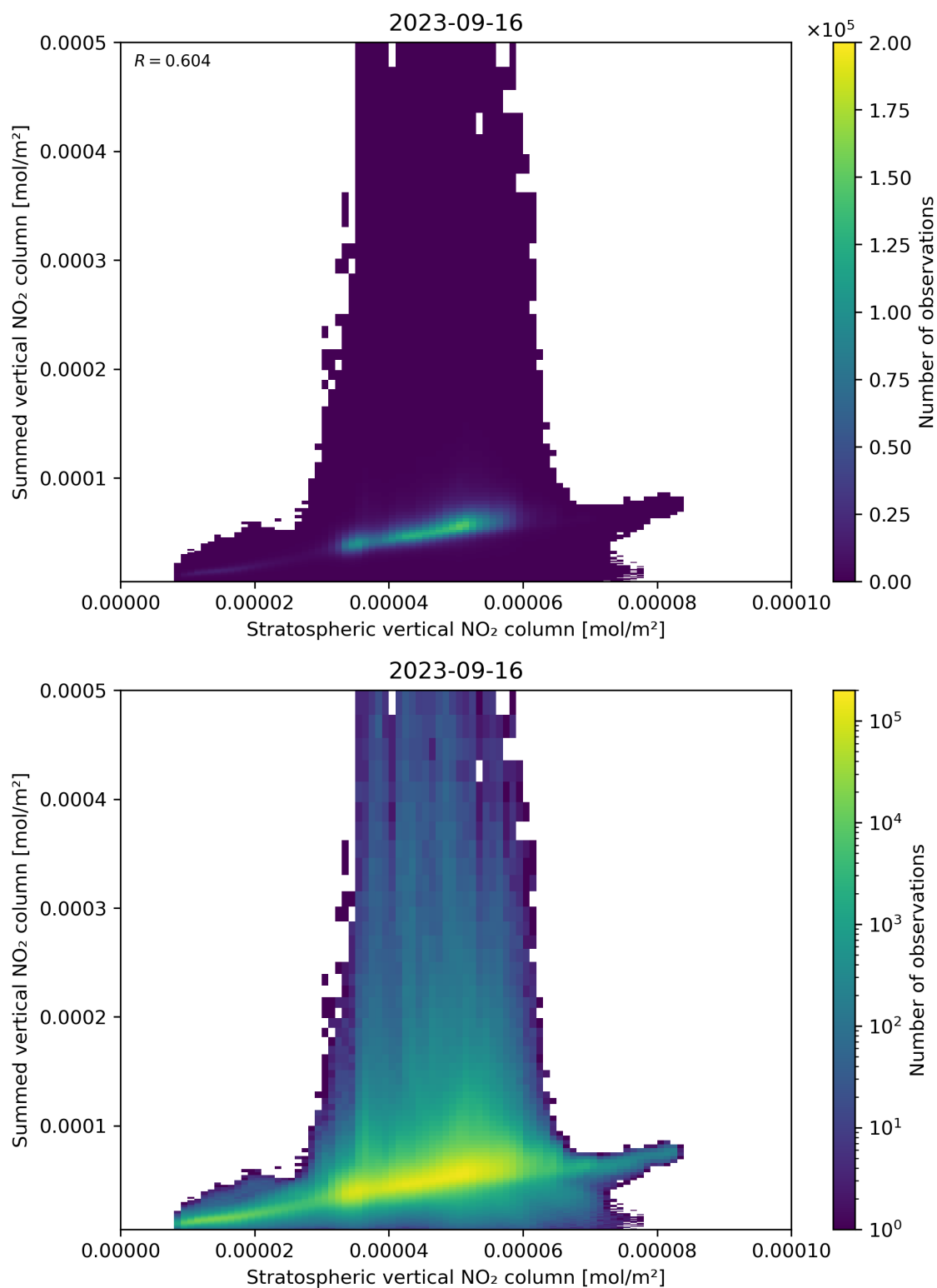
Figure 98: Scatter density plot of “Stratospheric vertical NO 2 column” against “Summed vertical NO 2 column” for 2023-09-15 to 2023-09-17.
