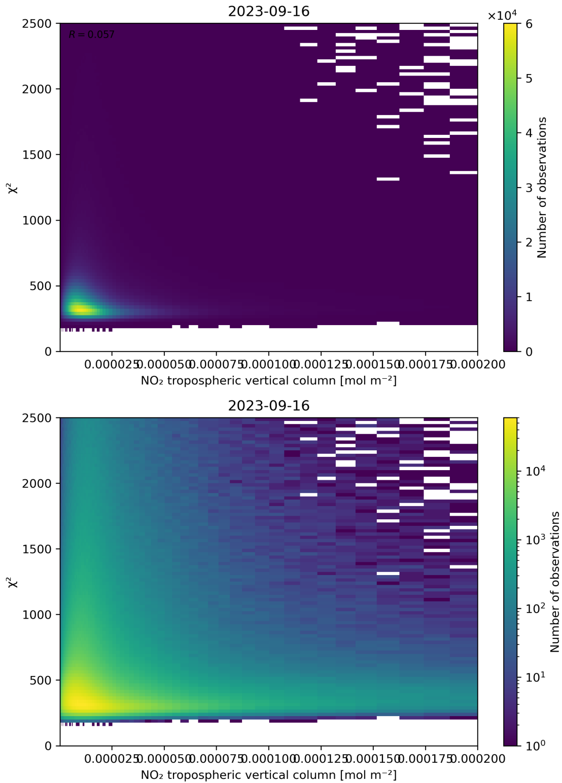
Figure 124: Scatter density plot of “NO 2 tropospheric vertical column” against “ \chi^2 ” for 2023-09-15 to 2023-09-17.
