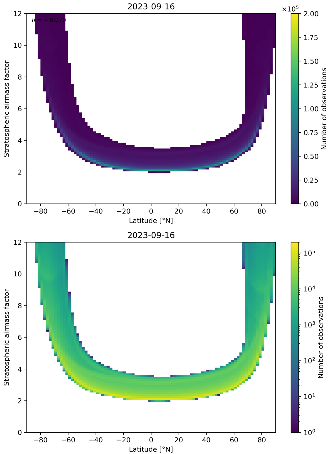
Figure 83: Scatter density plot of “Latitude” against “Stratospheric air mass factor” for 2023-09-15 to 2023-09-17.
