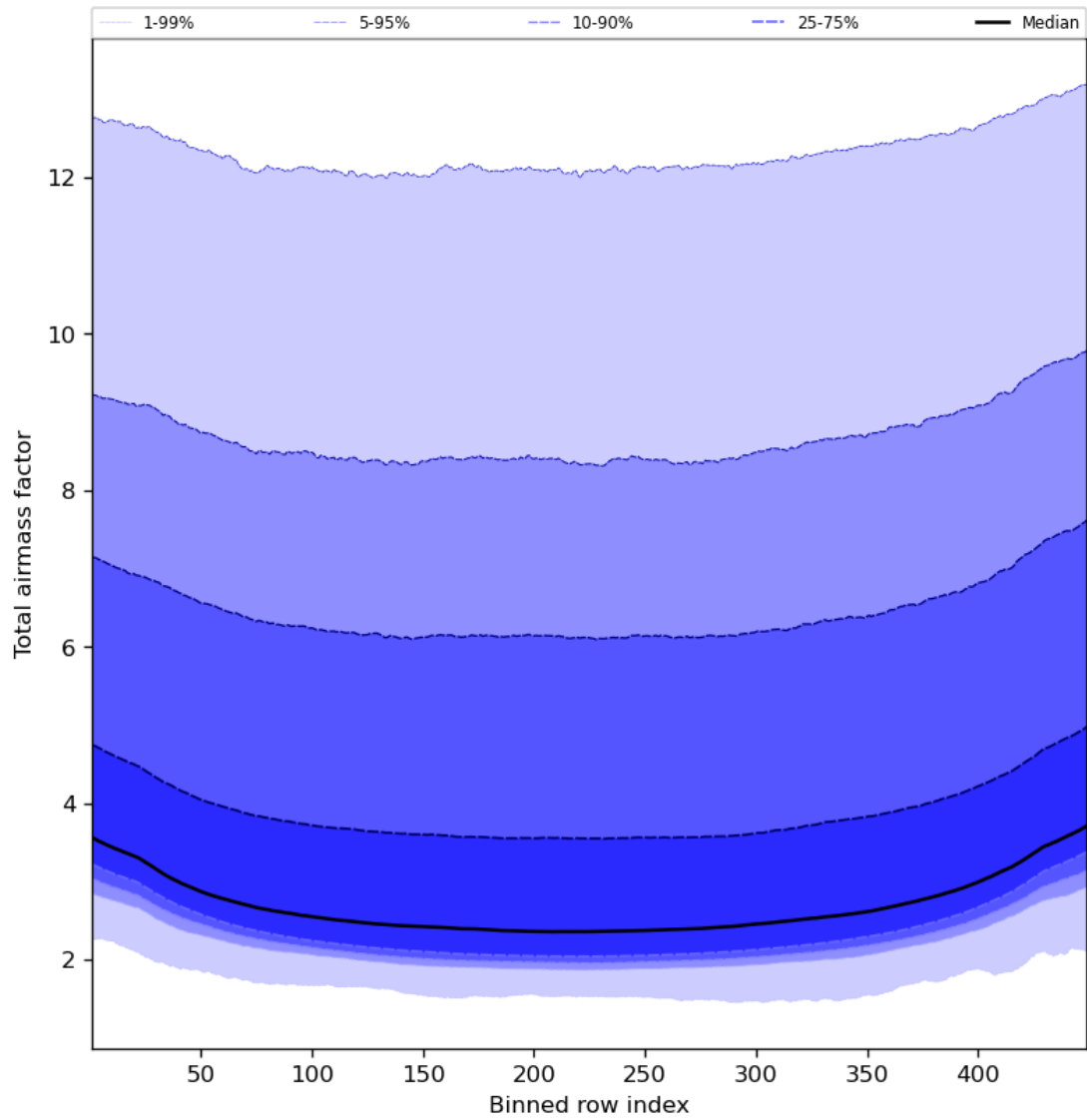
Figure 49: Along track statistics of “Total airmass factor” for 2023-09-15 to 2023-09-17
