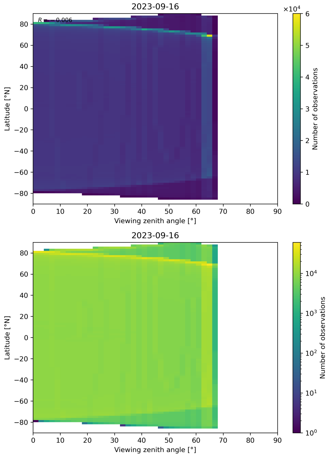
Figure 163: Scatter density plot of “Viewing zenith angle” against “Latitude” for 2023-09-15 to 2023-09-17.
