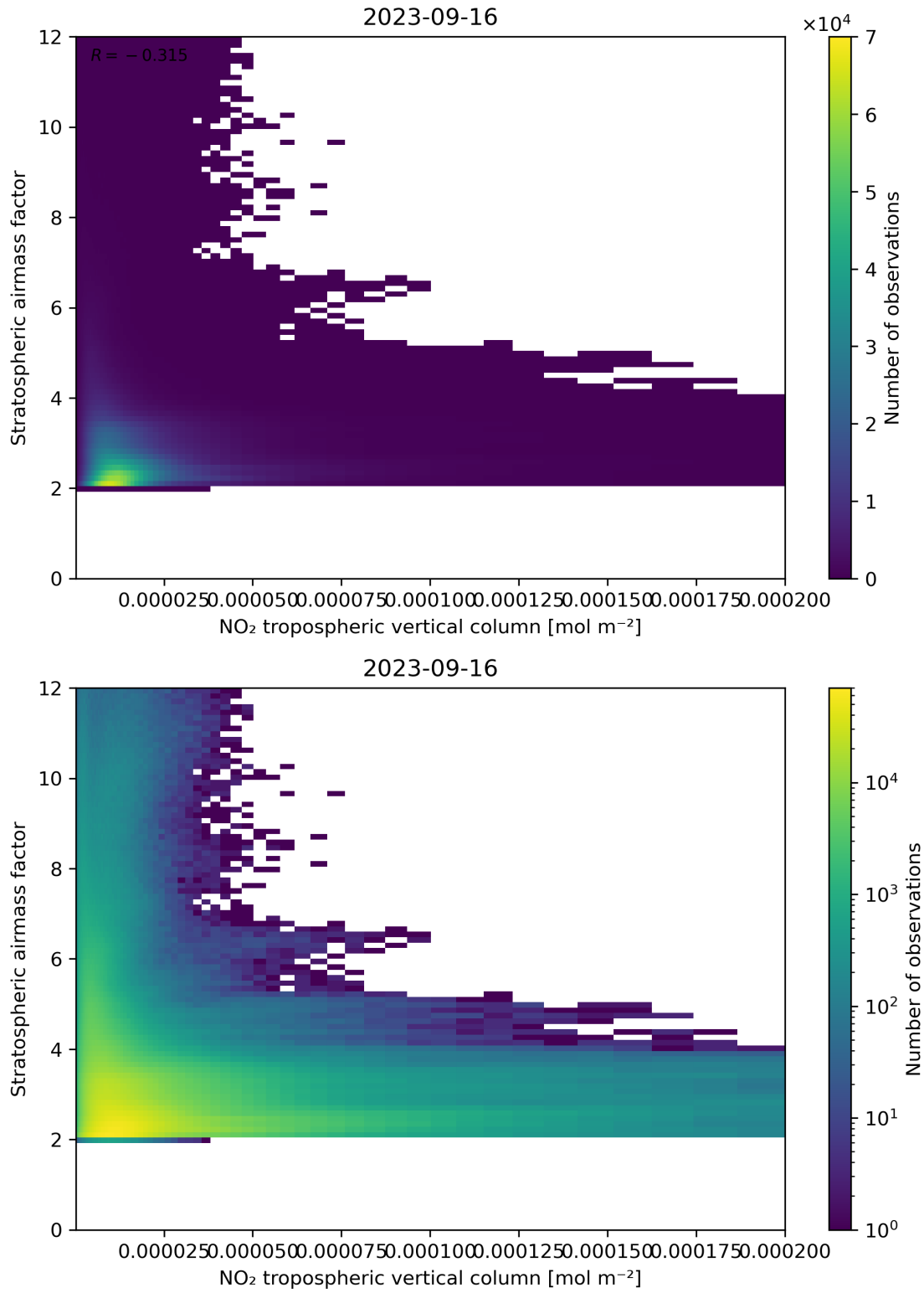
Figure 121: Scatter density plot of “NO 2 tropospheric vertical column” against “Stratospheric air mass factor” for 2023-09-15 to 2023-09-17.
