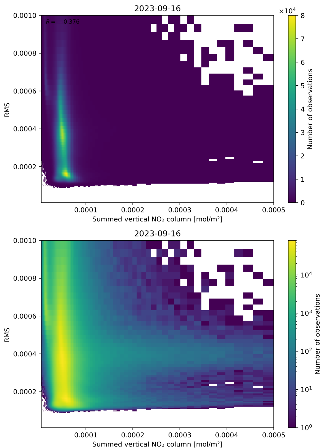
Figure 109: Scatter density plot of “Summed vertical NO 2 column” against “RMS” for 2023-09-15 to 2023-09-17.
