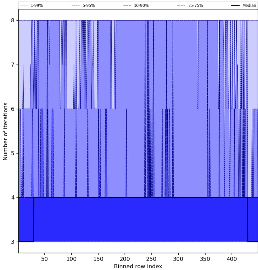
Figure 51: Along track statistics of “Number of iterations” for 2023-09-15 to 2023-09-17
