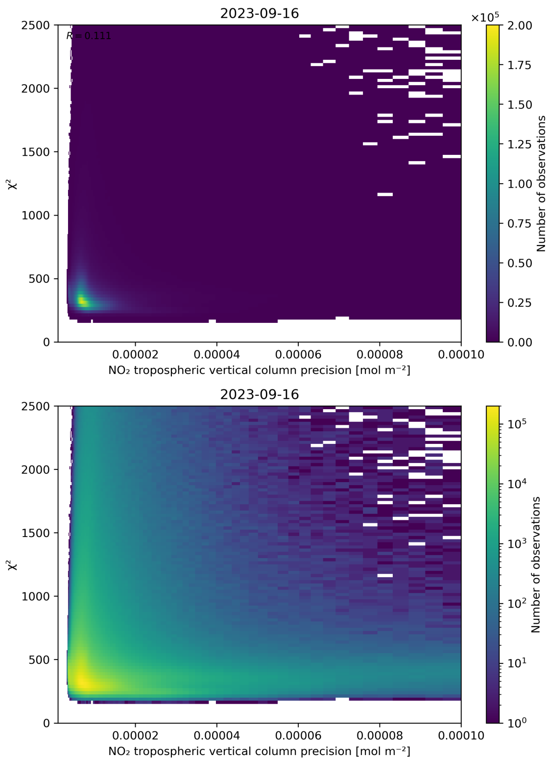
Figure 134: Scatter density plot of “NO 2 tropospheric vertical column precision” against “ \chi^2 ” for 2023-09-15 to 2023-09-17.
