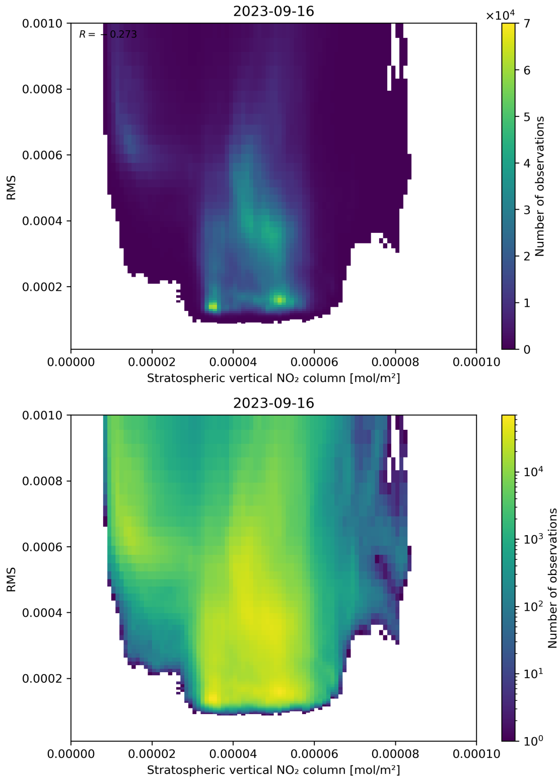
Figure 102: Scatter density plot of “Stratospheric vertical NO 2 column” against “RMS” for 2023-09-15 to 2023-09-17.
