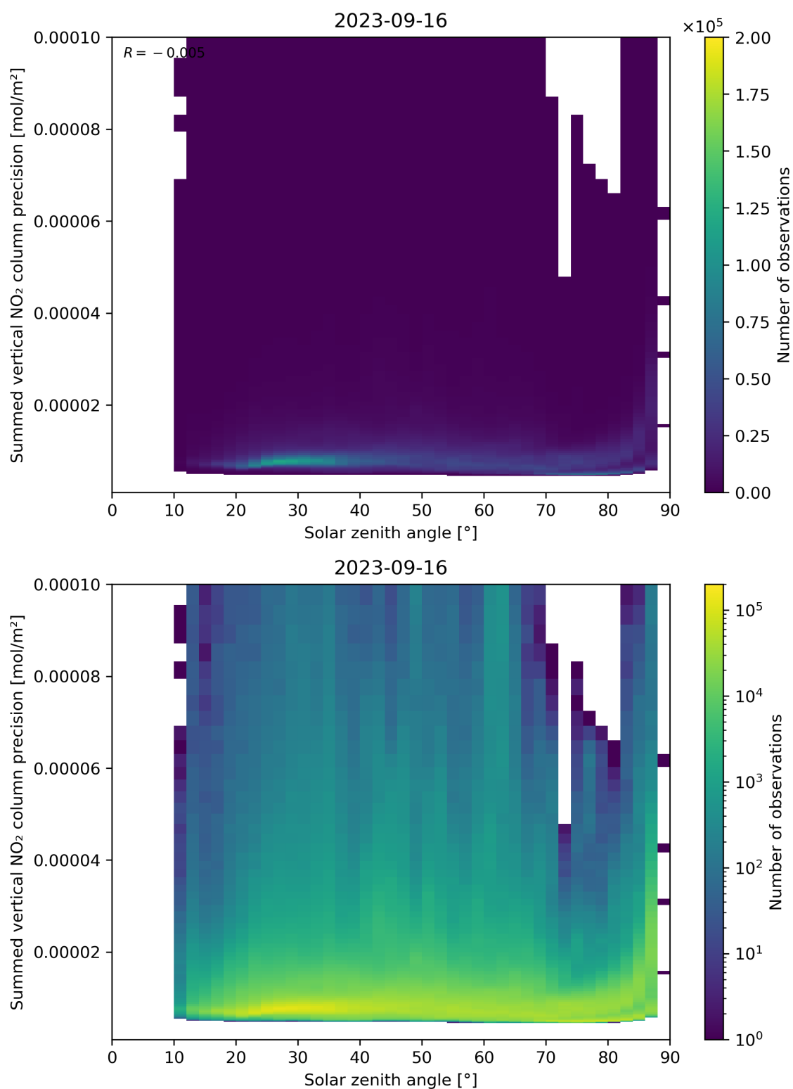
Figure 152: Scatter density plot of “Solar zenith angle” against “Summed vertical NO 2 column precision” for 2023-09-15 to 2023-09-17.
