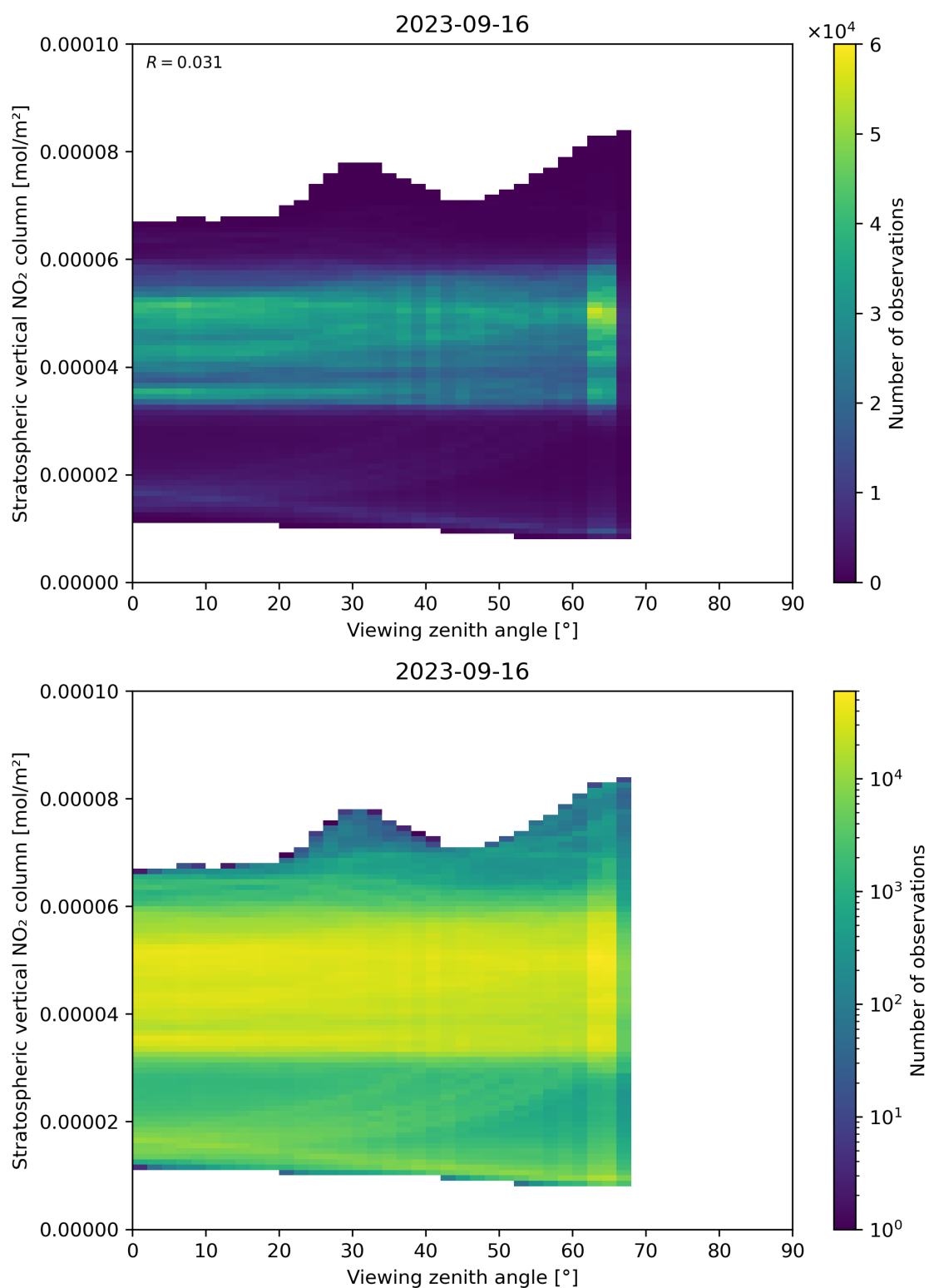
Figure 164: Scatter density plot of “Viewing zenith angle” against “Stratospheric vertical NO 2 column” for 2023-09-15 to 2023-09-17.
