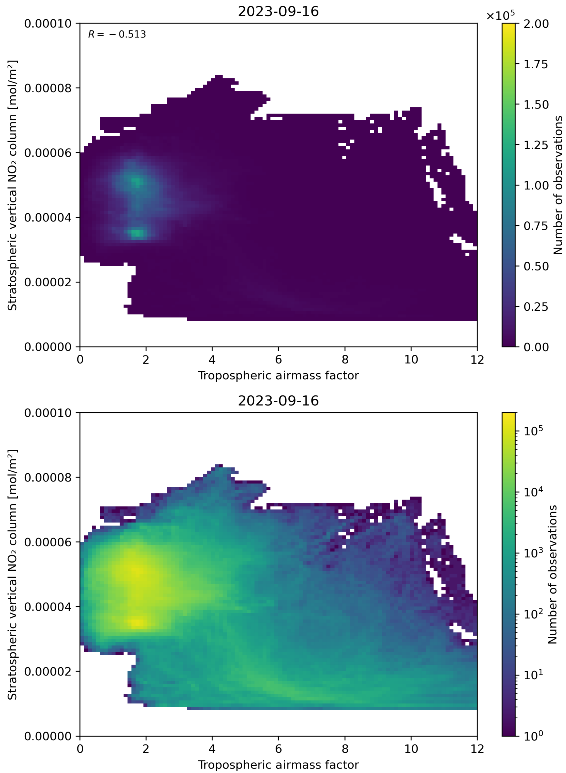
Figure 74: Scatter density plot of “Tropospheric air mass factor” against “Stratospheric vertical NO 2 column” for 2023-09-15 to 2023-09-17.
