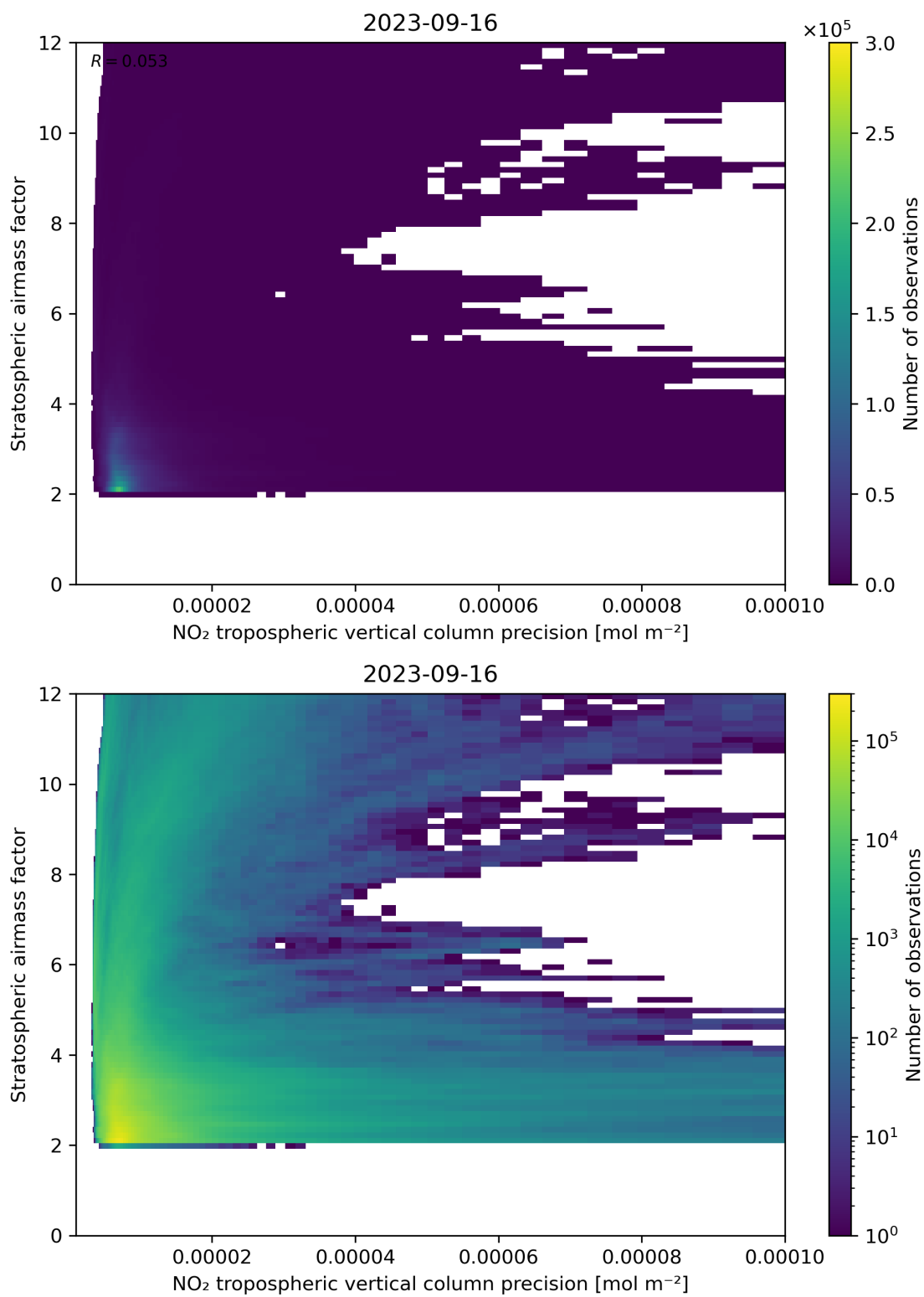
Figure 131: Scatter density plot of “NO 2 tropospheric vertical column precision” against “Stratospheric airmass factor” for 2023-09-15 to 2023-09-17.
