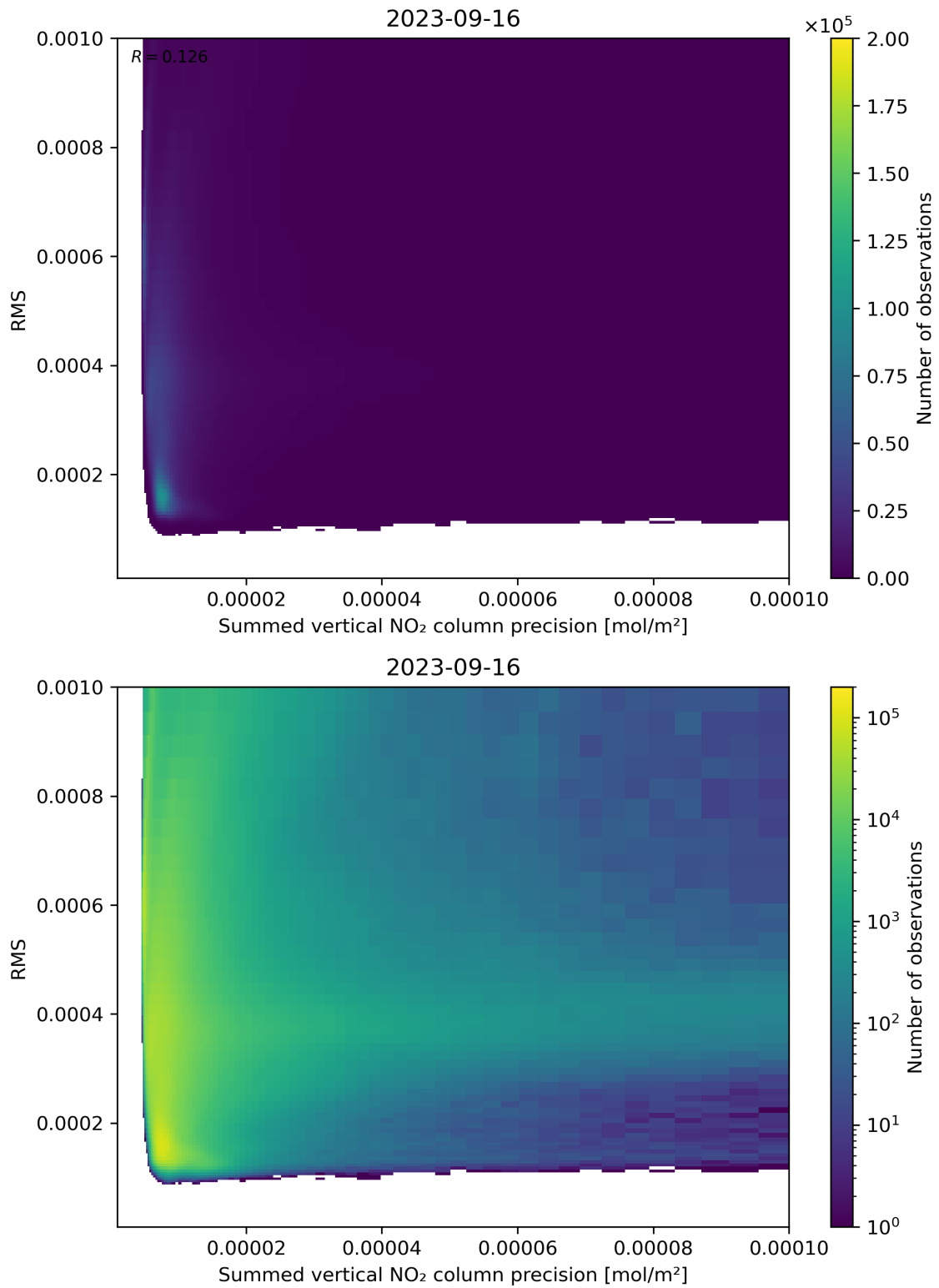
Figure 108: Scatter density plot of “Summed vertical NO 2 column precision” against “RMS” for 2023-09-15 to 2023-09-17.
