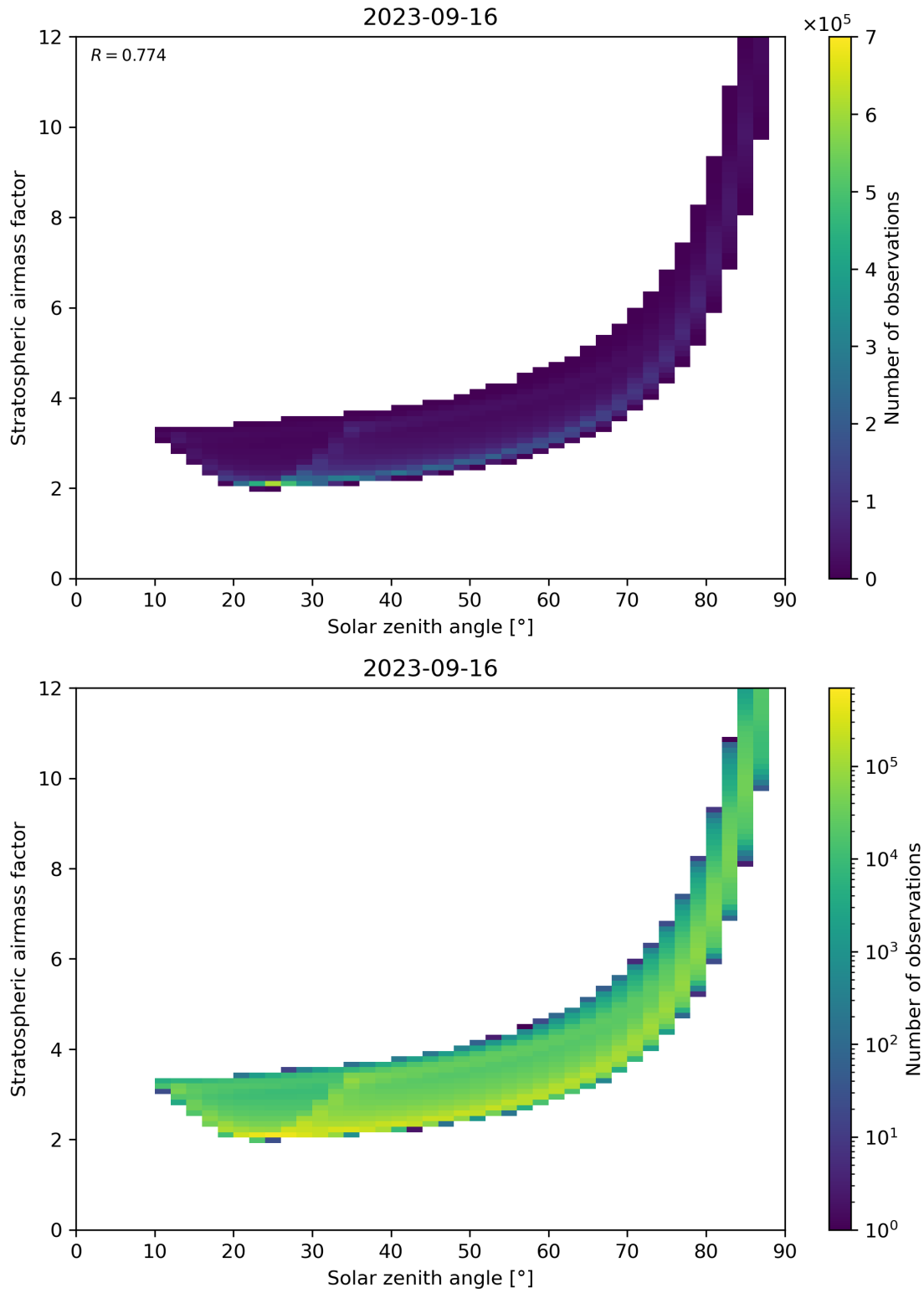
Figure 145: Scatter density plot of “Solar zenith angle” against “Stratospheric airmass factor” for 2023-09-15 to 2023-09-17.
