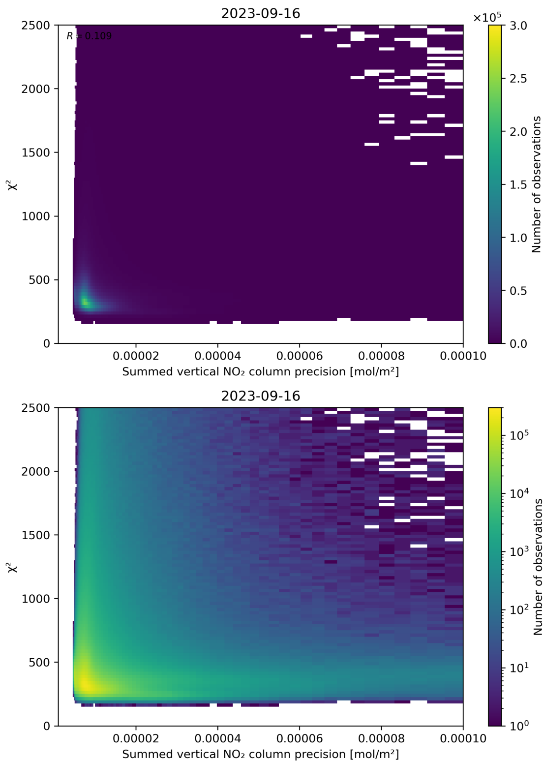
Figure 107: Scatter density plot of “Summed vertical NO 2 column precision” against “ \chi^2 ” for 2023-09-15 to 2023-09-17.
