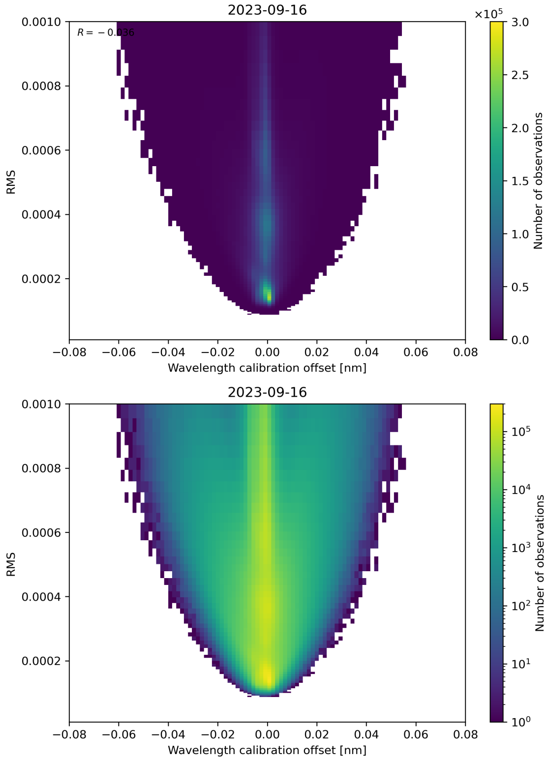
Figure 181: Scatter density plot of “Wavelength calibration offset” against “RMS” for 2023-09-15 to 2023-09-17.
