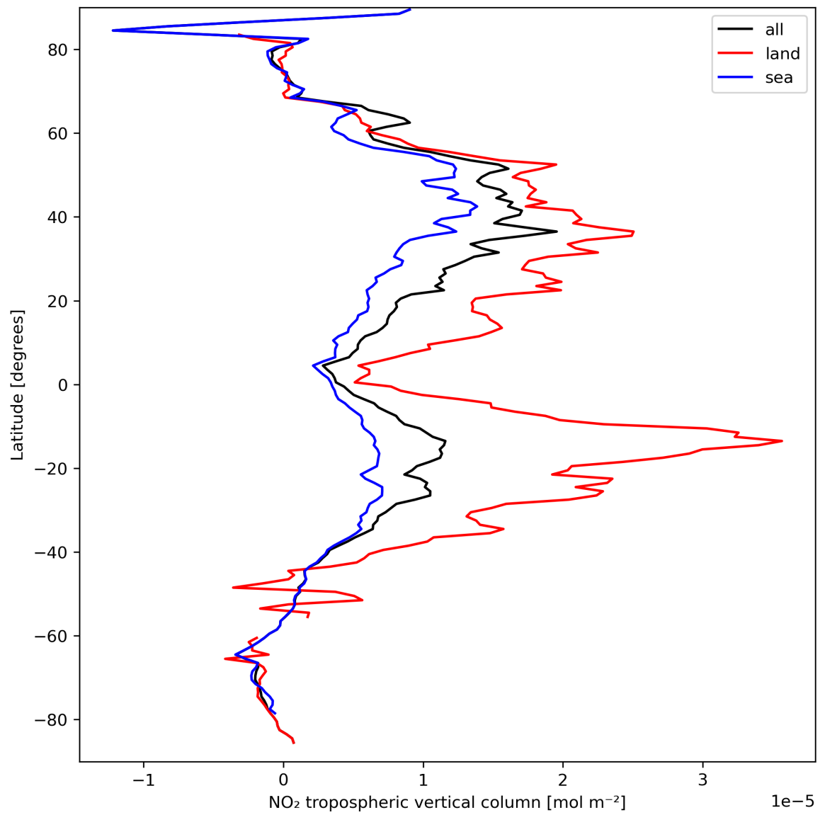
Figure 12: Zonal average of “NO 2 tropospheric vertical column” for 2023-09-15 to 2023-09-17.
