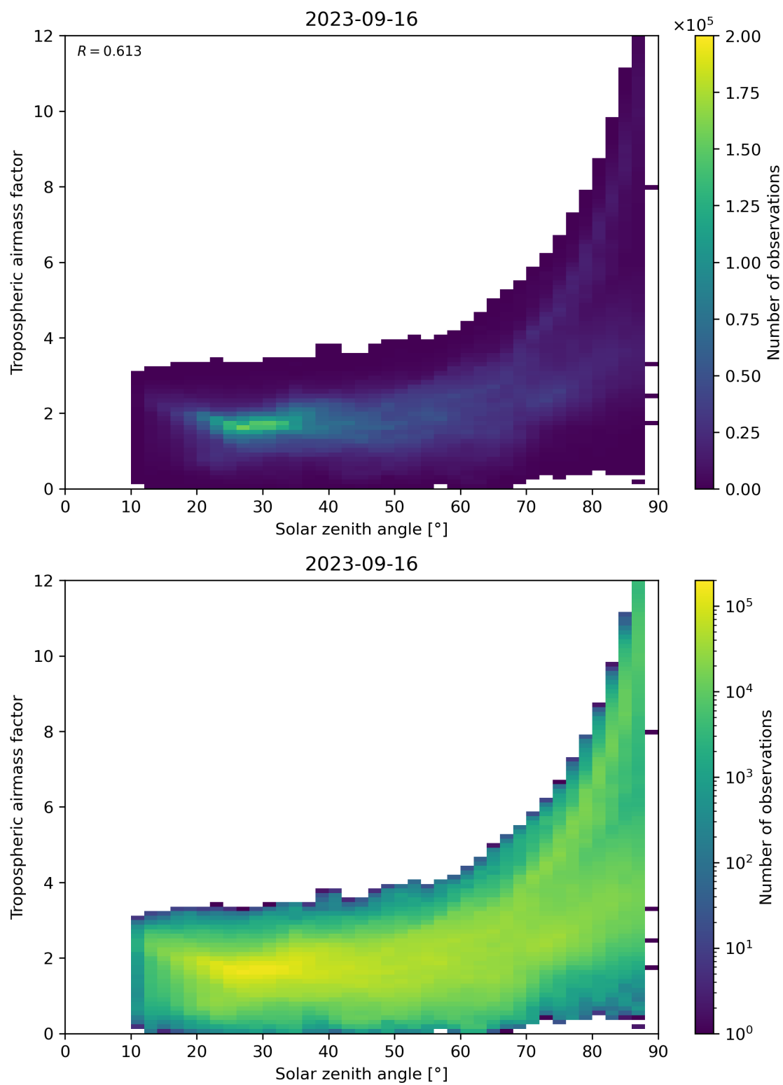
Figure 147: Scatter density plot of “Solar zenith angle” against “Tropospheric airmass factor” for 2023-09-15 to 2023-09-17.
