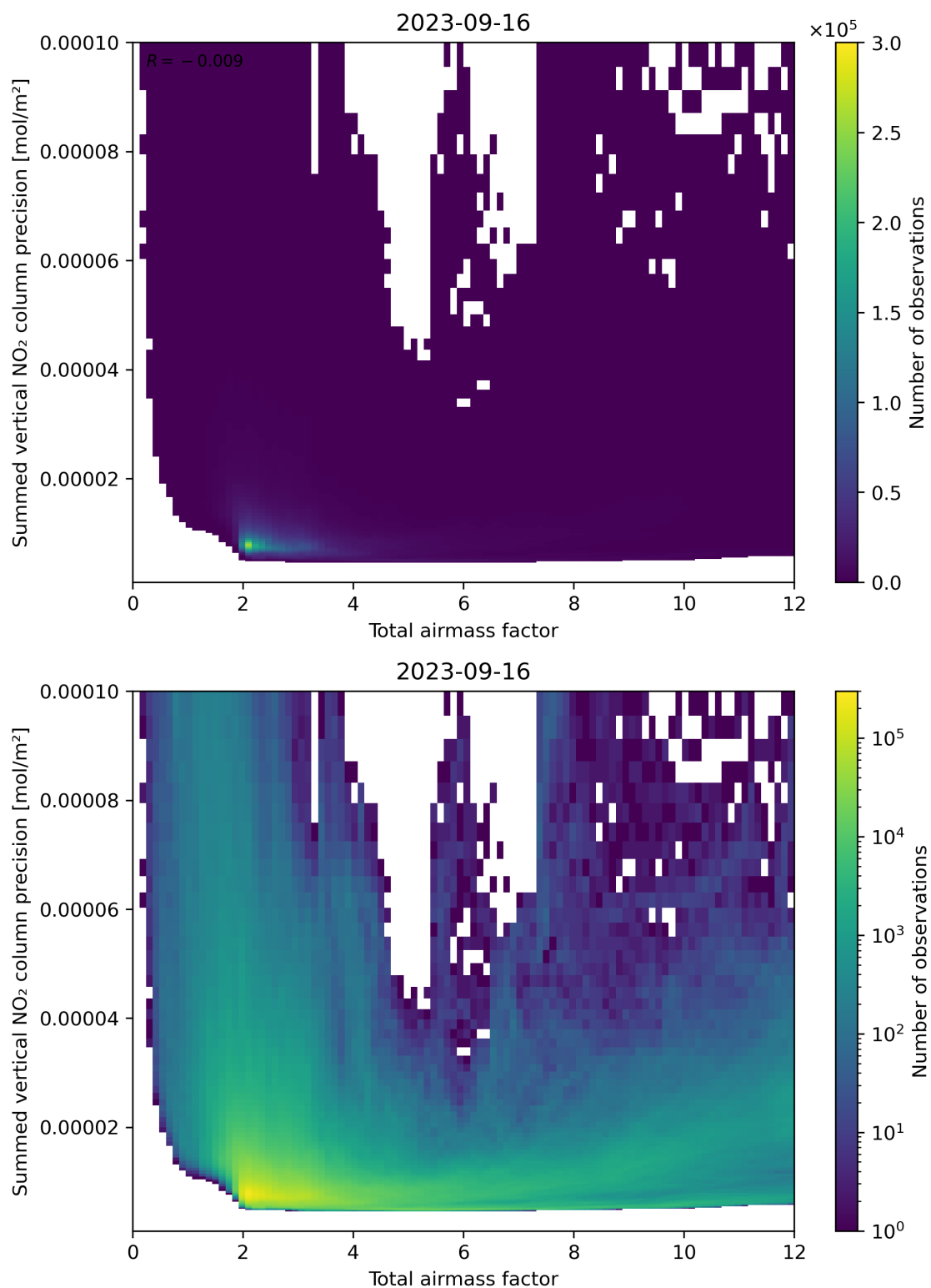
Figure 66: Scatter density plot of “Total airmass factor” against “Summed vertical NO 2 column precision” for 2023-09-15 to 2023-09-17.
