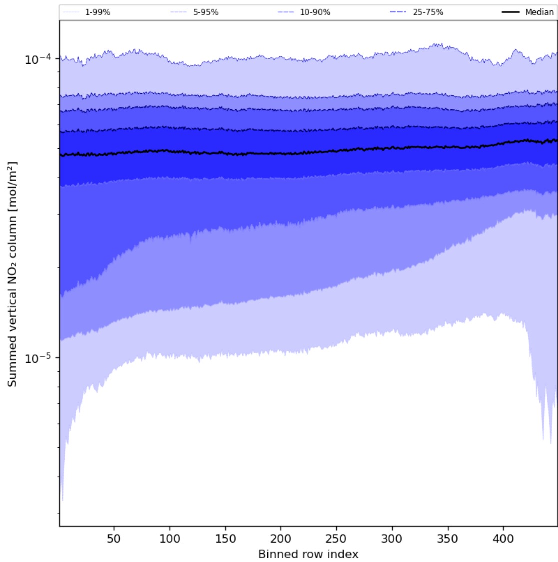
Figure 57: Along track statistics of “Summed vertical NO 2 column” for 2023-09-15 to 2023-09-17
