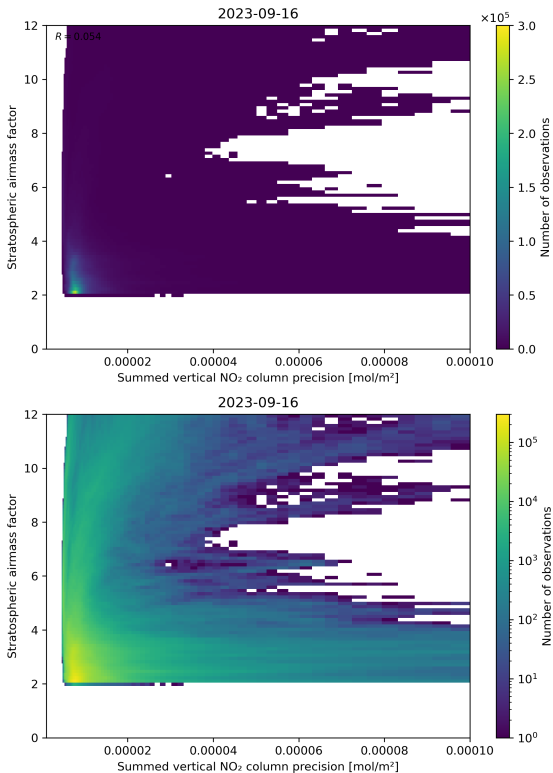
Figure 106: Scatter density plot of “Summed vertical NO 2 column precision” against “Stratospheric airmass factor” for 2023-09-15 to 2023-09-17.
