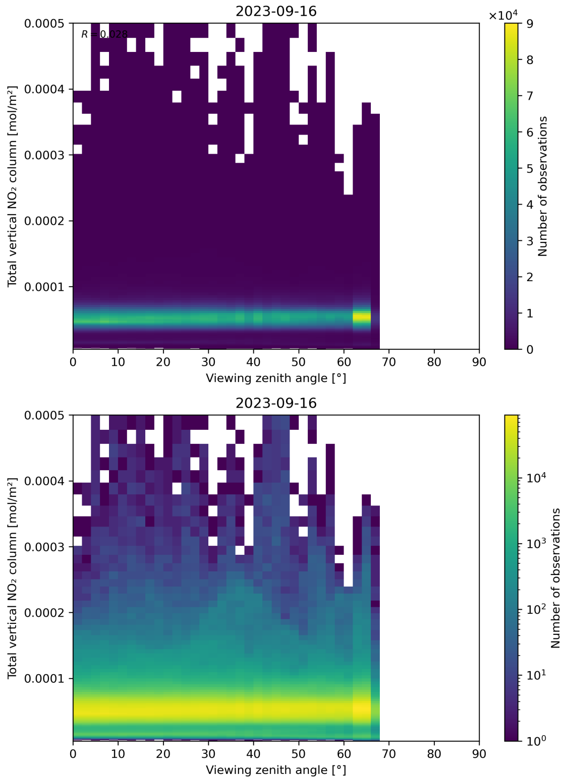
Figure 167: Scatter density plot of “Viewing zenith angle” against “Total vertical NO 2 column” for 2023-09-15 to 2023-09-17.
