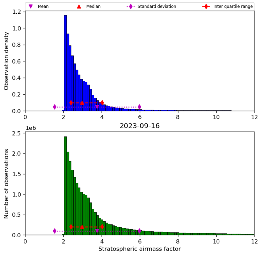
Figure 44: Histogram of “Stratospheric airmass factor” for 2023-09-15 to 2023-09-17
