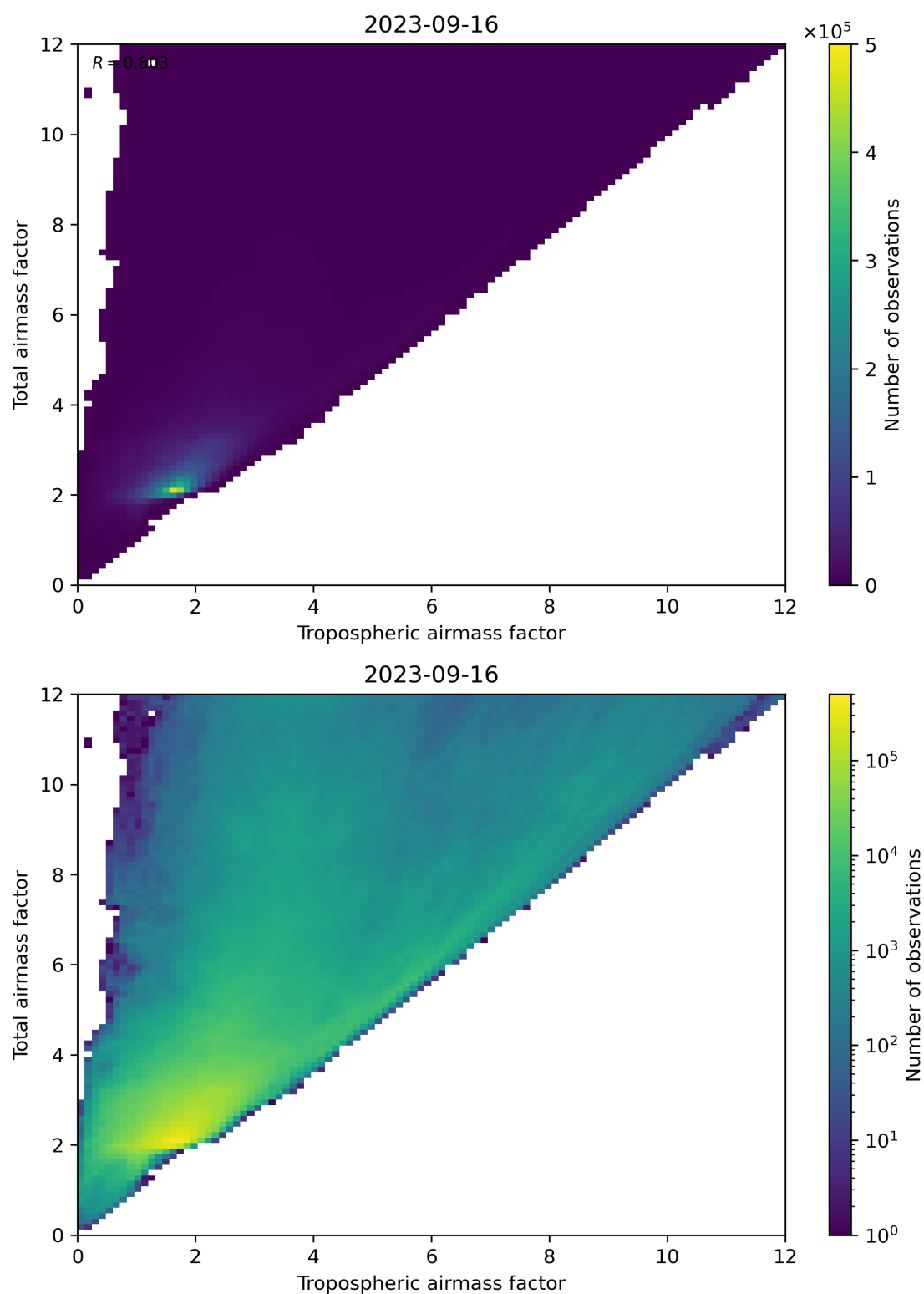
Figure 72: Scatter density plot of “Tropospheric airmass factor” against “Total airmass factor” for 2023-09-15 to 2023-09-17.
