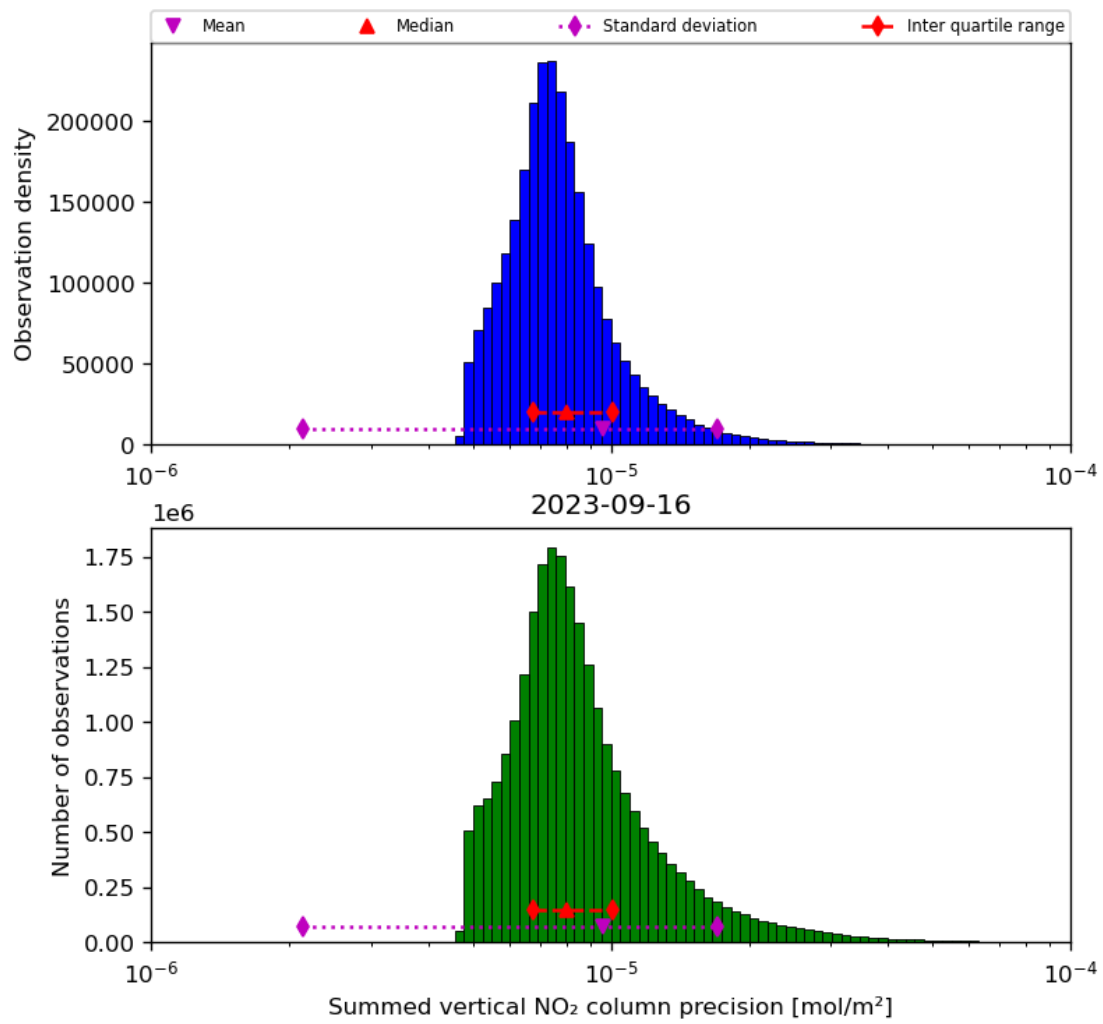
Figure 41: Histogram of "Summed vertical NO 2 column precision" for 2023-09-15 to 2023-09-17
