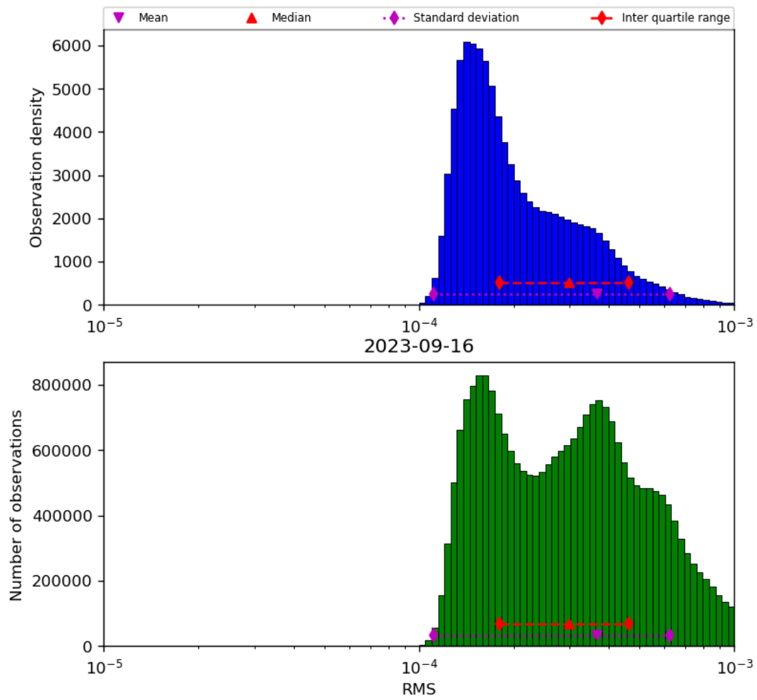
Figure 43: Histogram of “RMS” for 2023-09-15 to 2023-09-17
