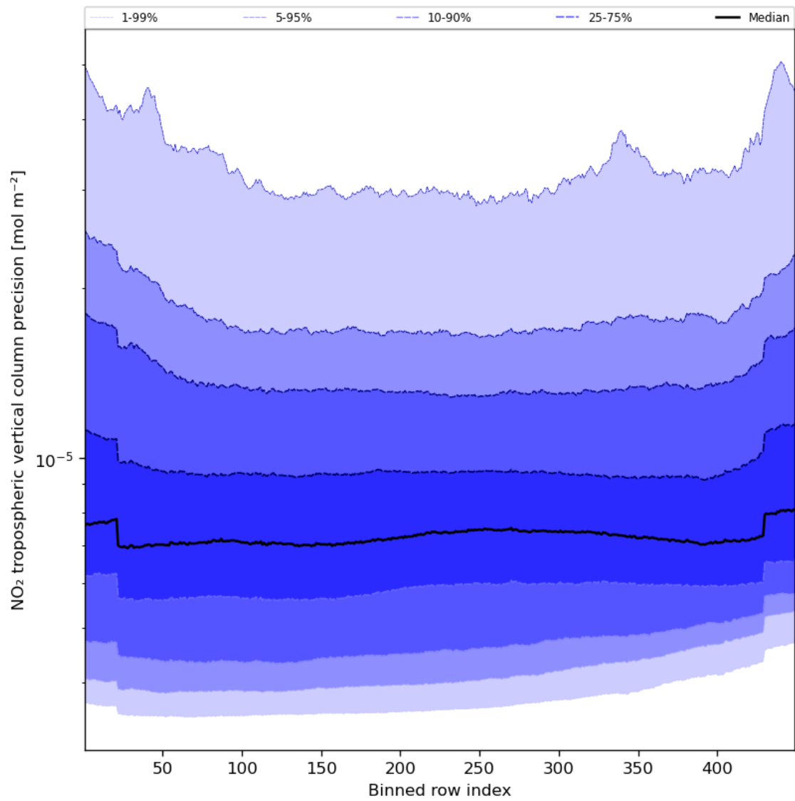
Figure 47: Along track statistics of “NO 2 tropospheric vertical column precision” for 2023-09-15 to 2023-09-17
