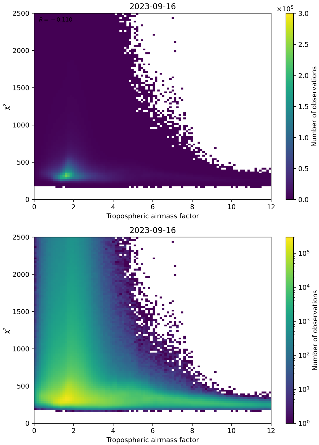
Figure 73: Scatter density plot of “Tropospheric airmass factor” against “ \chi^2 ” for 2023-09-15 to 2023-09-17.
