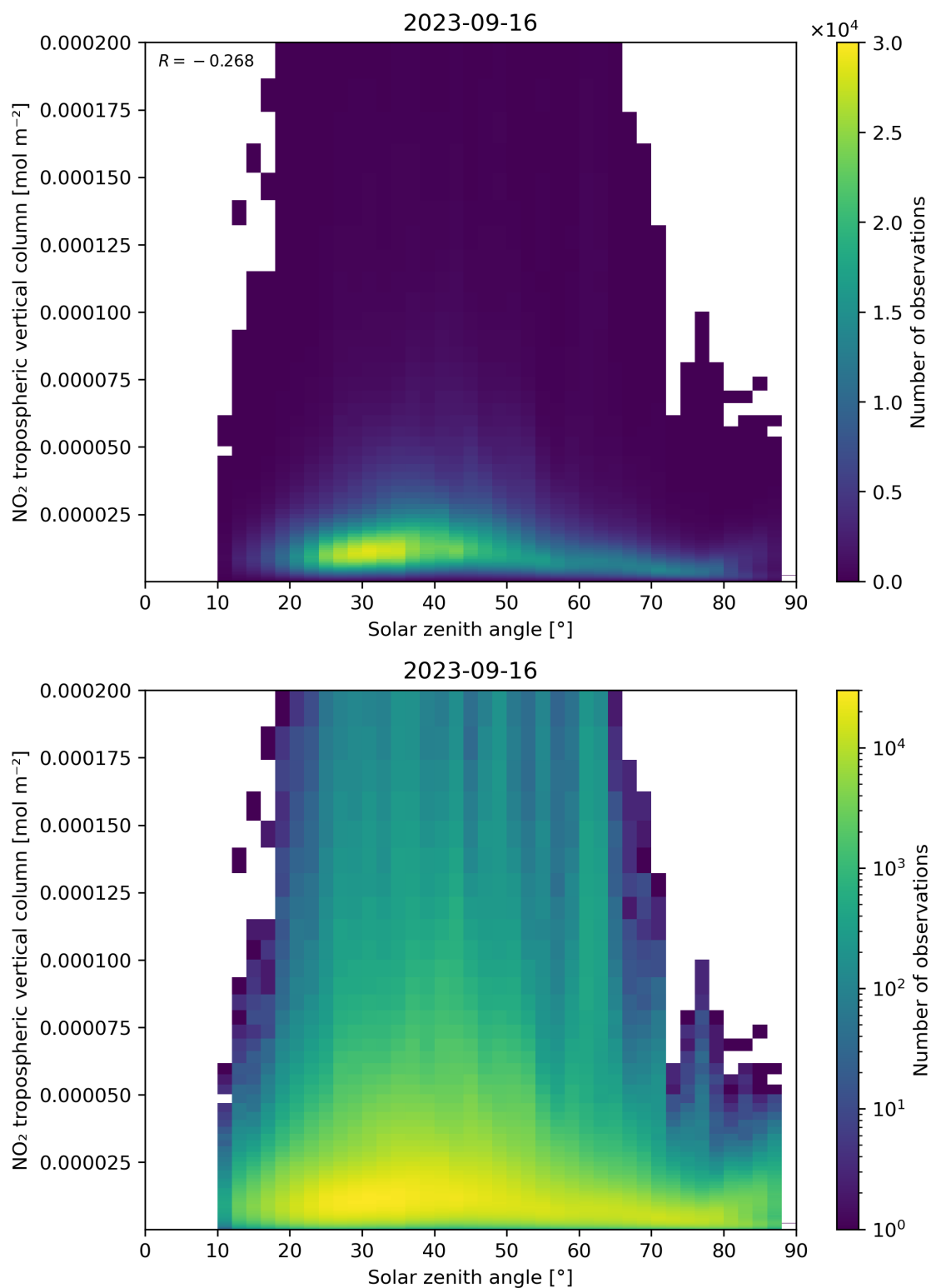
Figure 155: Scatter density plot of “Solar zenith angle” against “NO 2 tropospheric vertical column” for 2023-09-15 to 2023-09-17.
