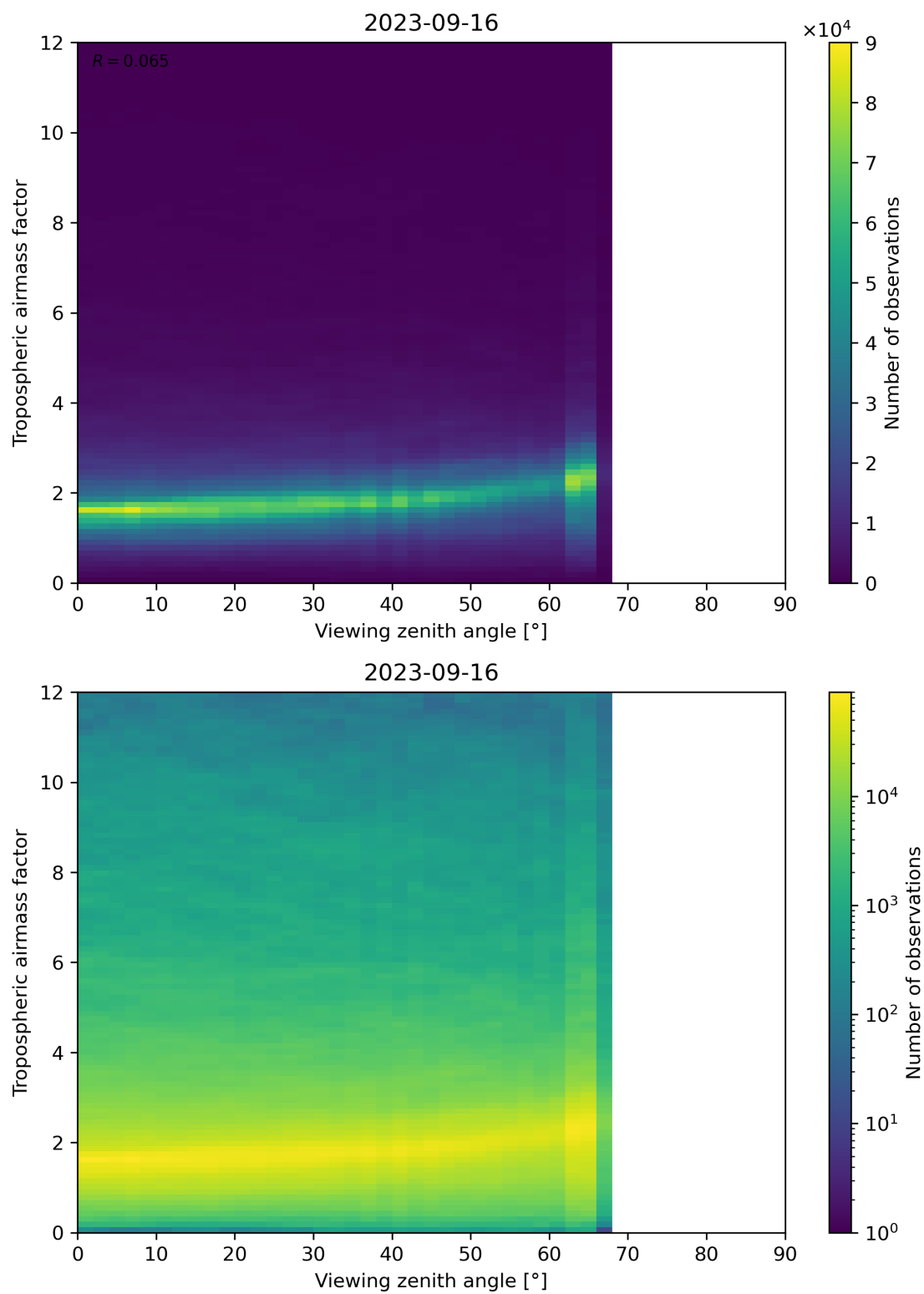
Figure 161: Scatter density plot of “Viewing zenith angle” against “Tropospheric airmass factor” for 2023-09-15 to 2023-09-17.
