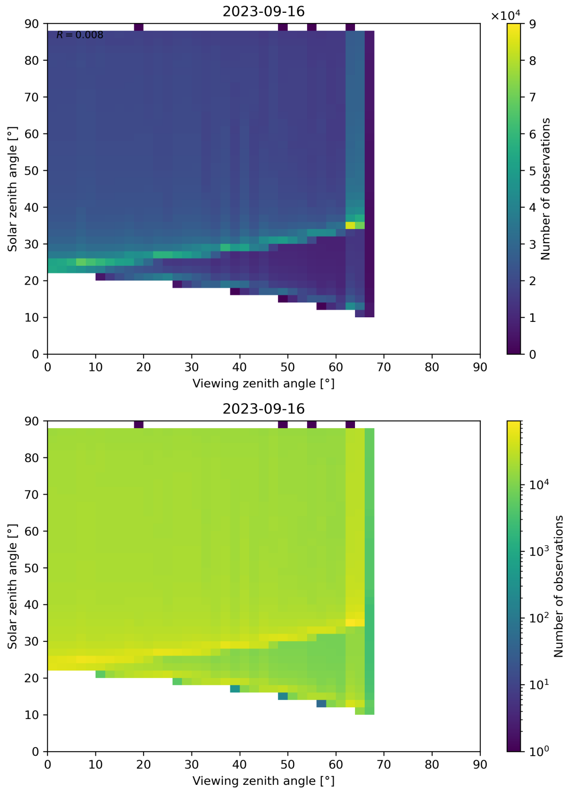
Figure 172: Scatter density plot of “Viewing zenith angle” against “Solar zenith angle” for 2023-09-15 to 2023-09-17.
