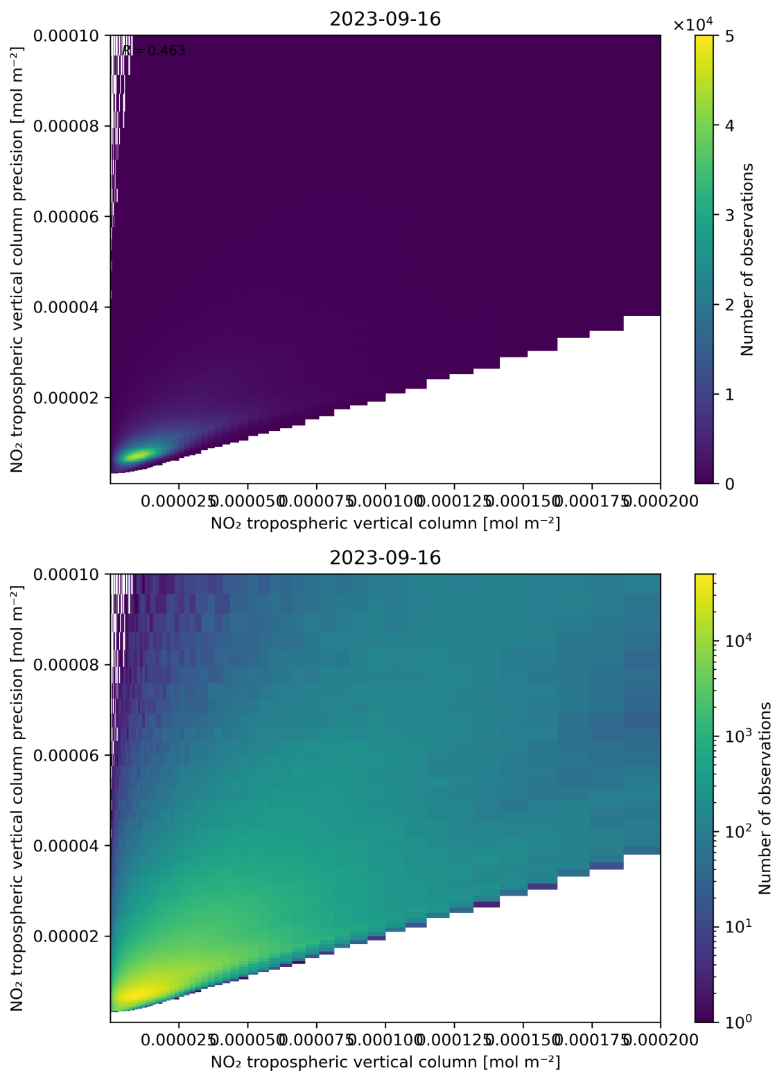
Figure 130: Scatter density plot of “NO 2 tropospheric vertical column” against “NO 2 tropospheric vertical column precision” for 2023-09-15 to 2023-09-17.
