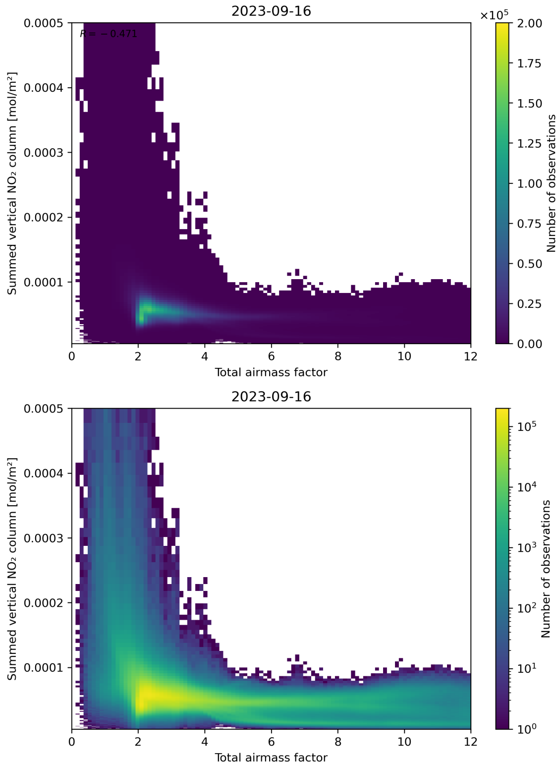
Figure 65: Scatter density plot of “Total airmass factor” against “Summed vertical NO 2 column” for 2023-09-15 to 2023-09-17.
