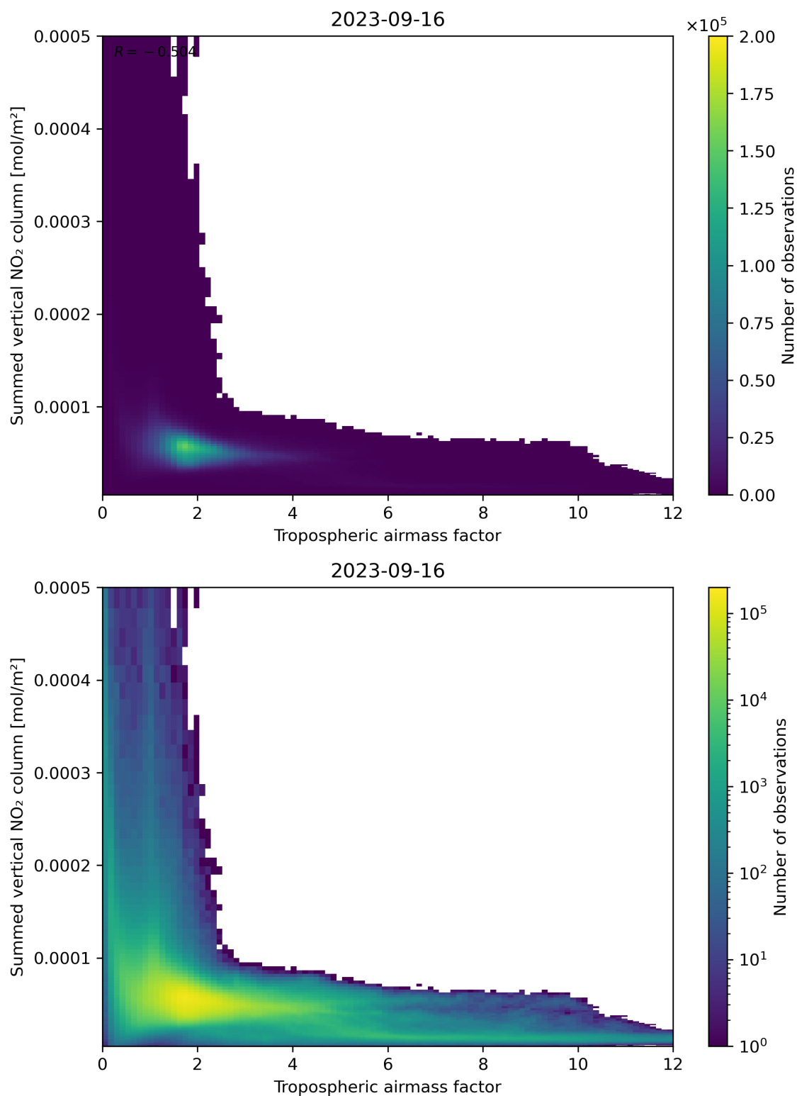
Figure 75: Scatter density plot of “Tropospheric air mass factor” against “Summed vertical NO 2 column” for 2023-09-15 to 2023-09-17.
