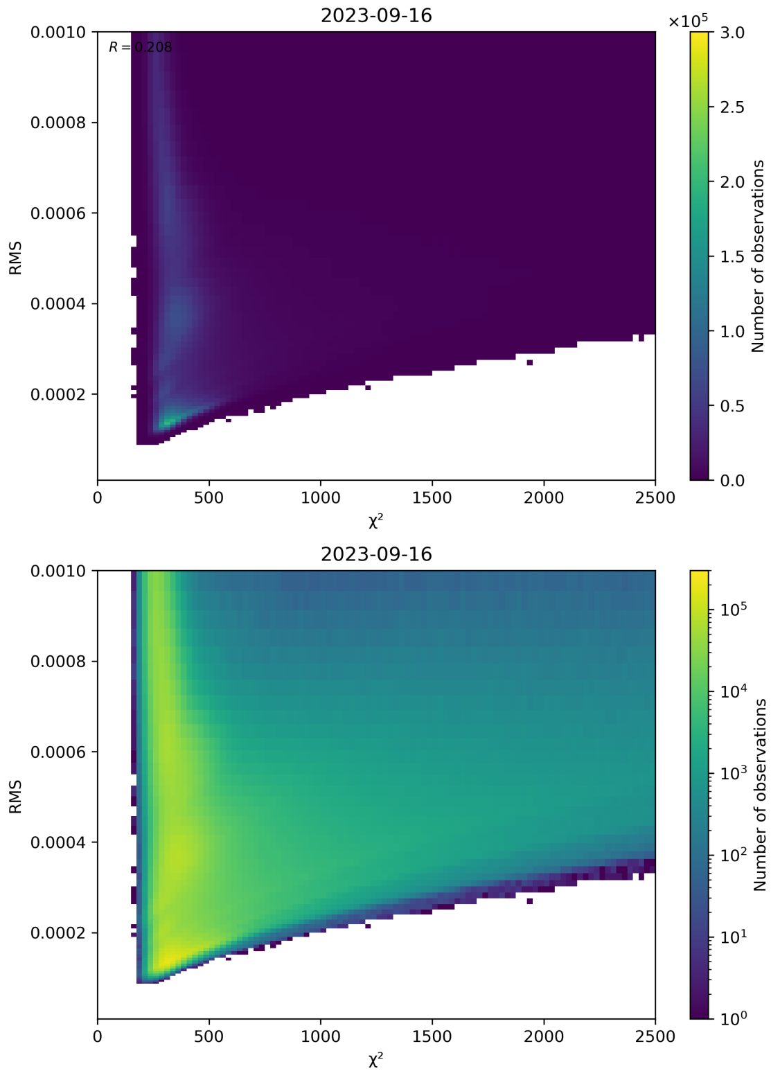
Figure 82: Scatter density plot of “ \chi^2 ” against “RMS” for 2023-09-15 to 2023-09-17.
