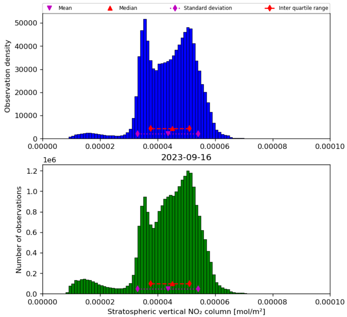
Figure 36: Histogram of “Stratospheric vertical NO 2 column” for 2023-09-15 to 2023-09-17
