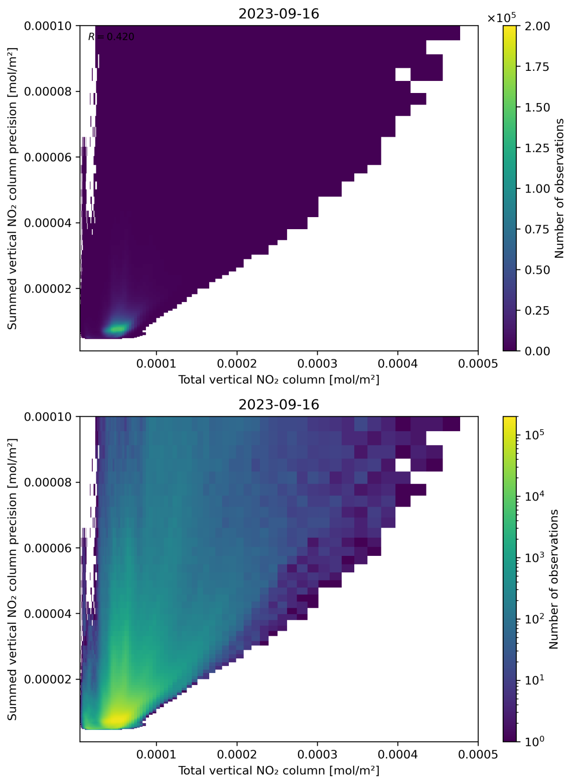
Figure 113: Scatter density plot of “Total vertical NO 2 column” against “Summed vertical NO 2 column precision” for 2023-09-15 to 2023-09-17.
