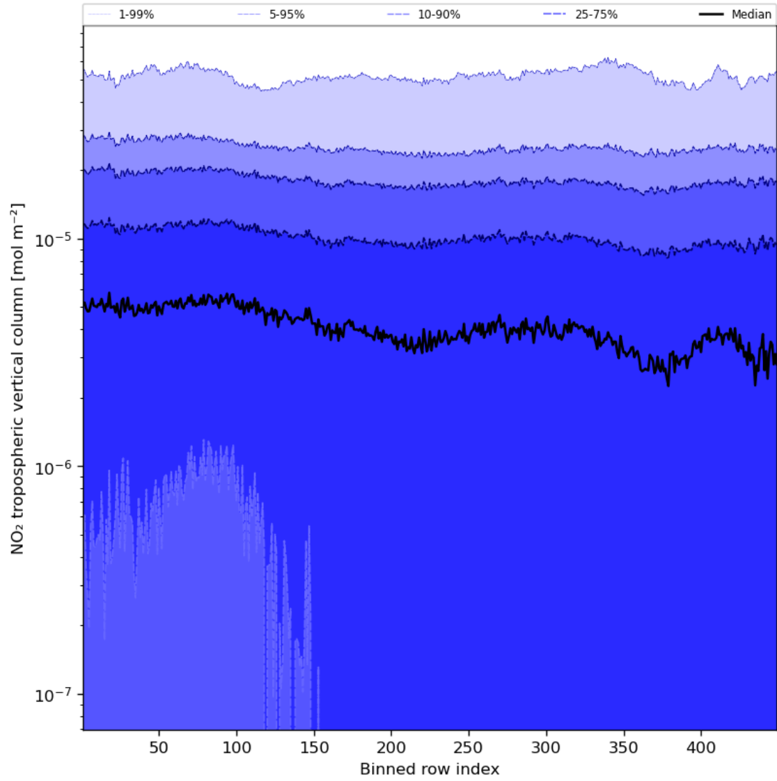
Figure 46: Along track statistics of “NO 2 tropospheric vertical column” for 2023-09-15 to 2023-09-17
