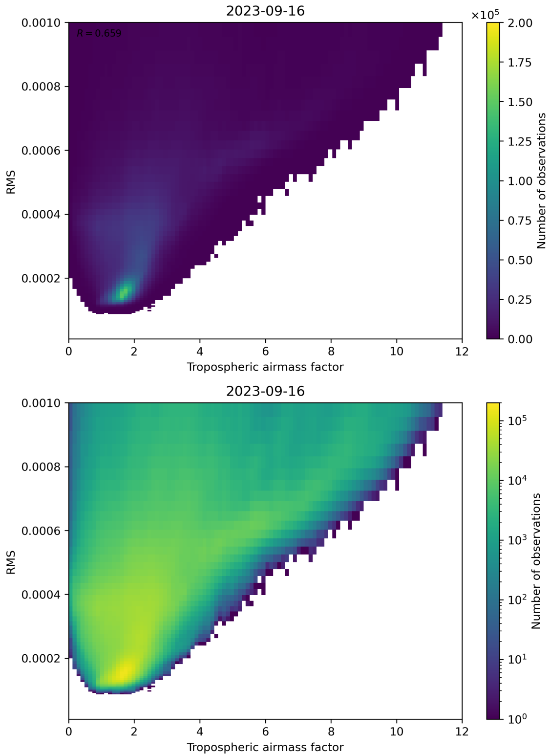
Figure 79: Scatter density plot of “Tropospheric airmass factor” against “RMS” for 2023-09-15 to 2023-09-17.
