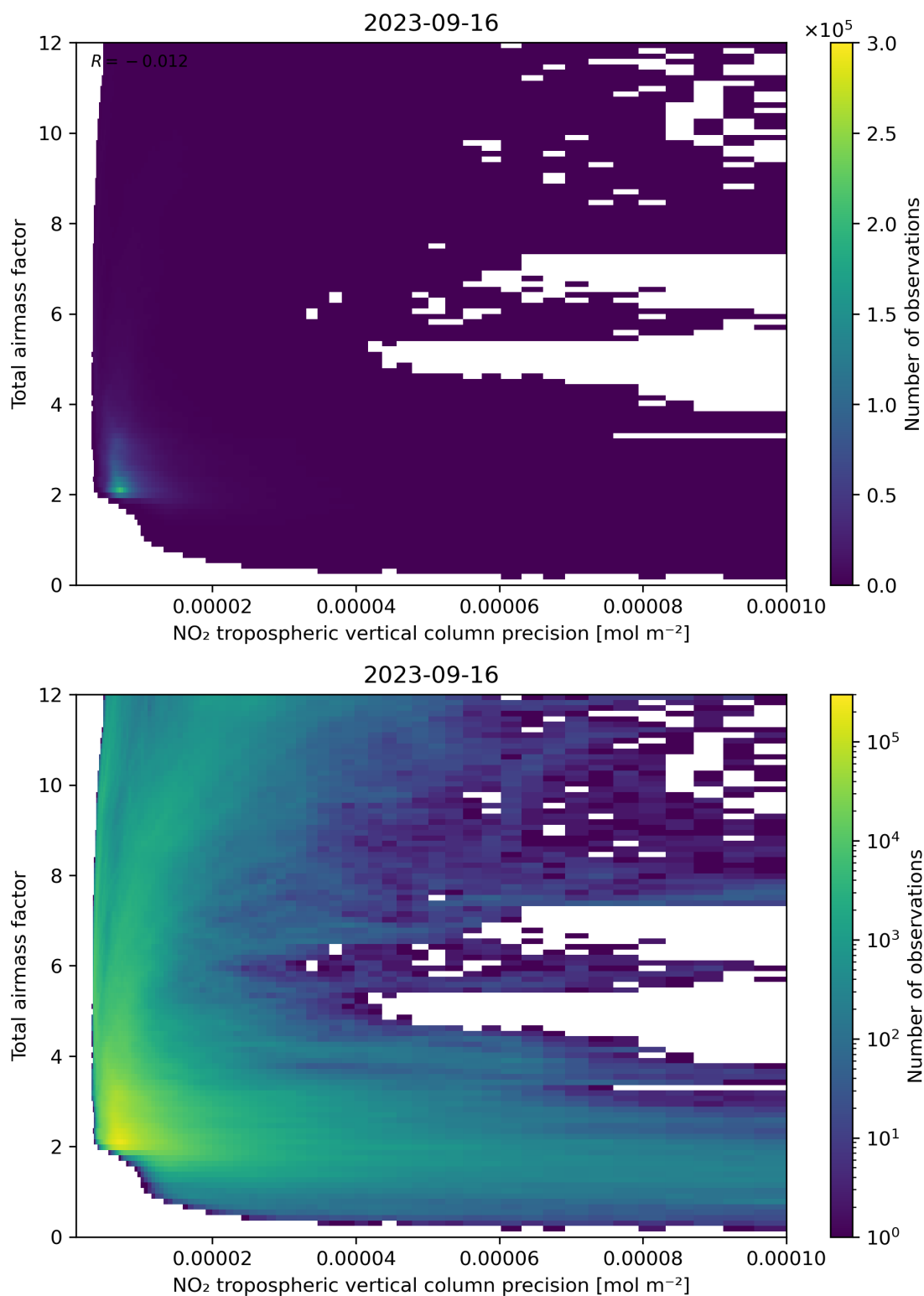
Figure 132: Scatter density plot of “NO 2 tropospheric vertical column precision” against “Total air mass factor” for 2023-09-15 to 2023-09-17.
