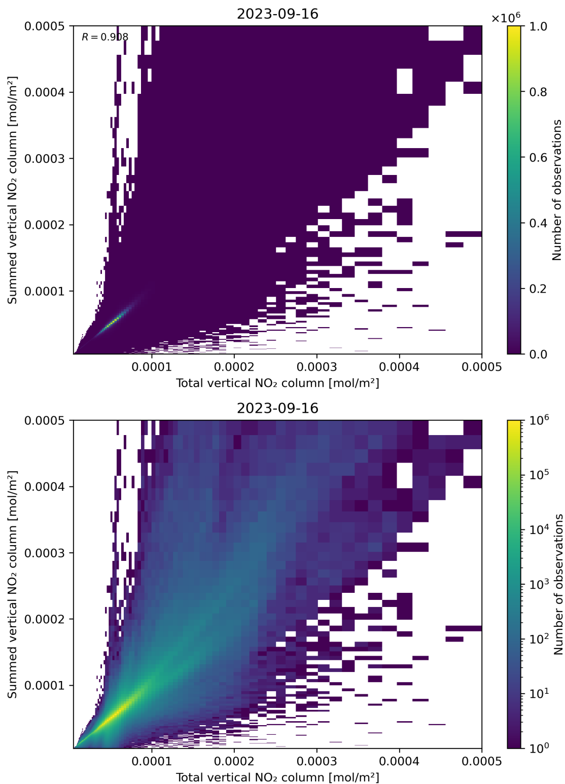
Figure 112: Scatter density plot of “Total vertical NO 2 column” against “Summed vertical NO 2 column” for 2023-09-15 to 2023-09-17.
