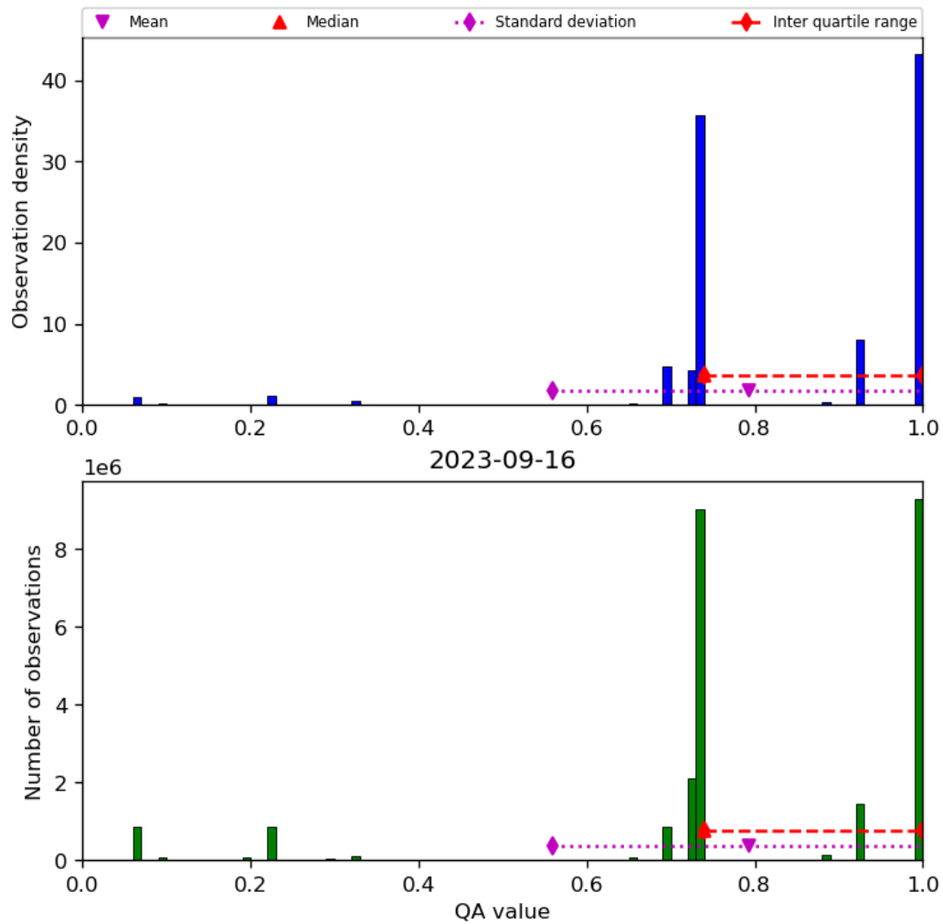
Figure 28: Histogram of “QA value” for 2023-09-15 to 2023-09-17
