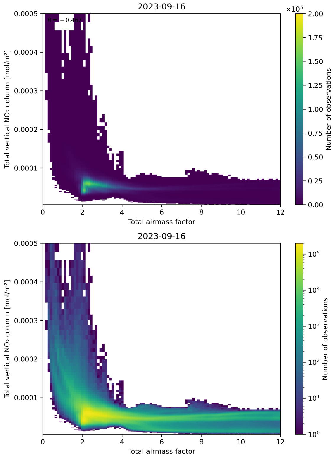
Figure 67: Scatter density plot of “Total airmass factor” against “Total vertical NO 2 column” for 2023-09-15 to 2023-09-17.
