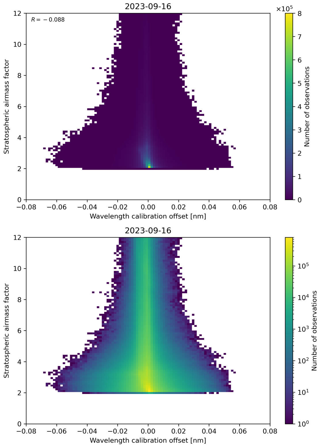
Figure 174: Scatter density plot of “Wavelength calibration offset” against “Stratospheric airmass factor” for 2023-09-15 to 2023-09-17.
