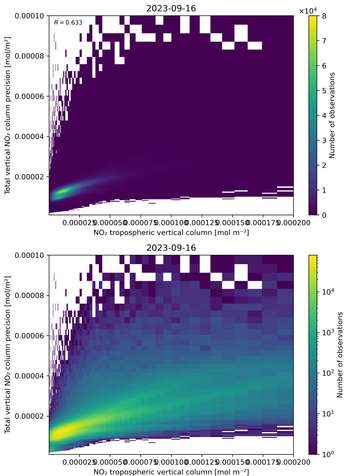
Figure 129: Scatter density plot of “NO 2 tropospheric vertical column” against “Total vertical NO 2 column precision” for 2023-09-15 to 2023-09-17.
