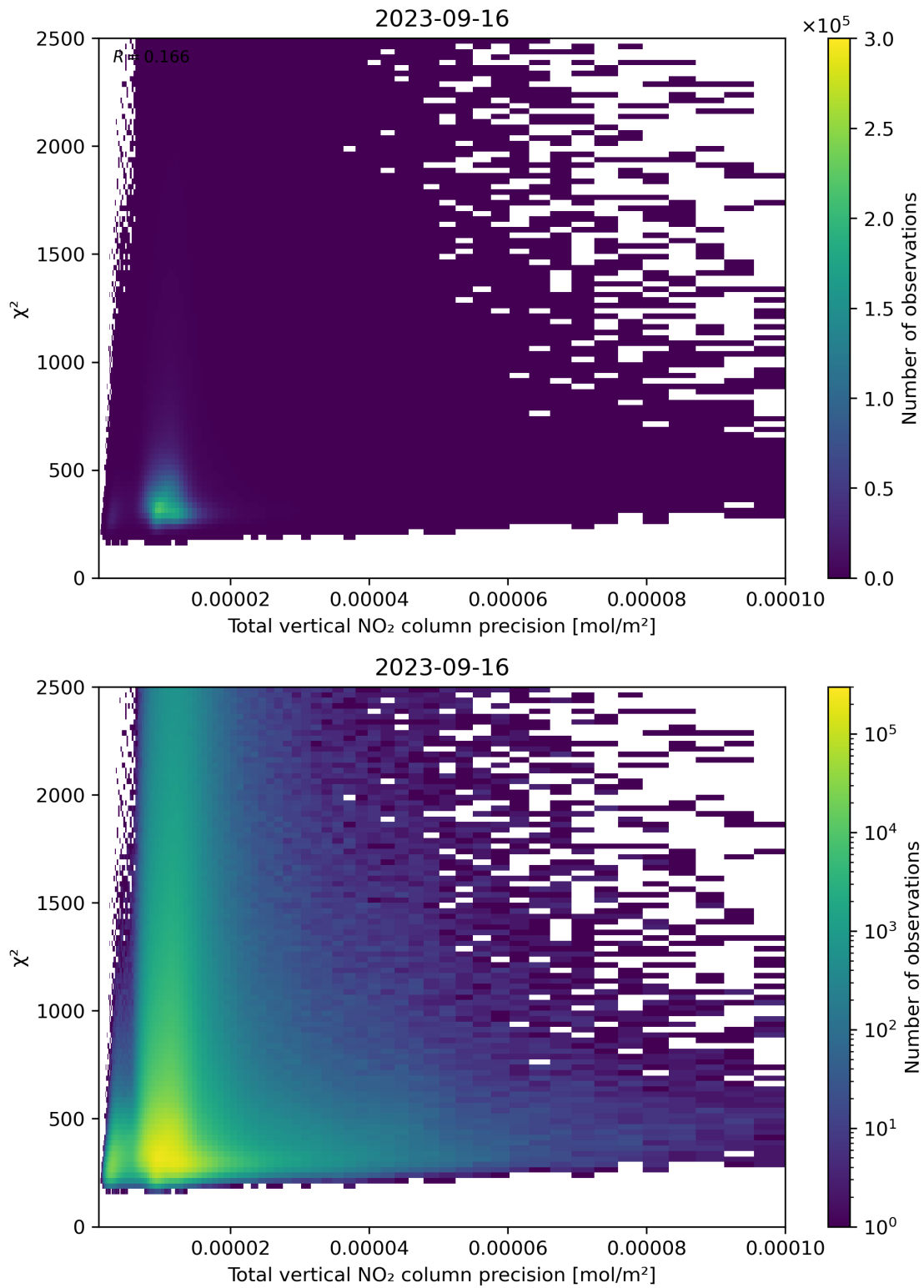
Figure 116: Scatter density plot of “Total vertical NO 2 column precision” against “ \chi^2 ” for 2023-09-15 to 2023-09-17.
