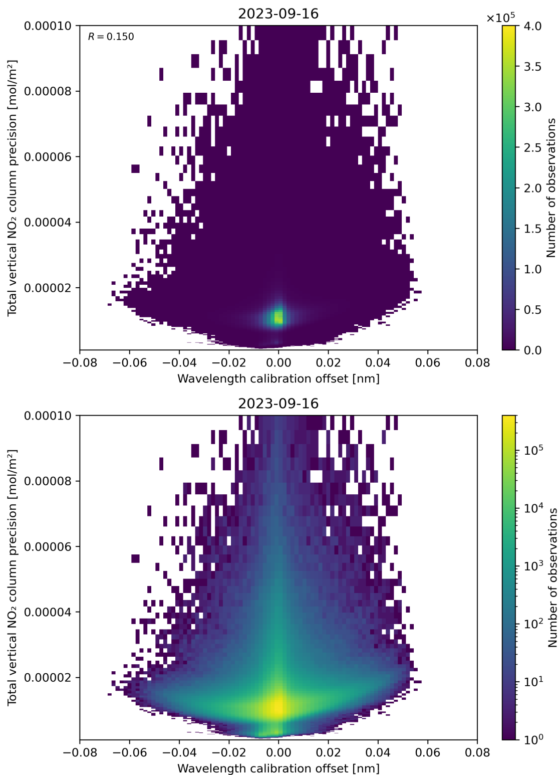
Figure 180: Scatter density plot of “Wavelength calibration offset” against “Total vertical NO 2 column precision” for 2023-09-15 to 2023-09-17.
