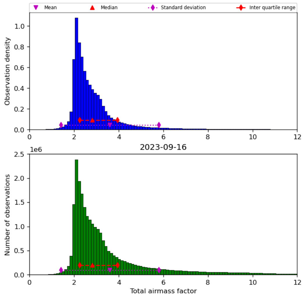
Figure 32: Histogram of “Total airmass factor” for 2023-09-15 to 2023-09-17
