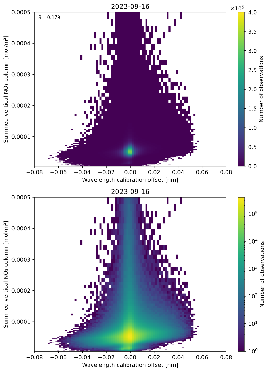
Figure 177: Scatter density plot of “Wavelength calibration offset” against “Summed vertical NO 2 column” for 2023-09-15 to 2023-09-17.
