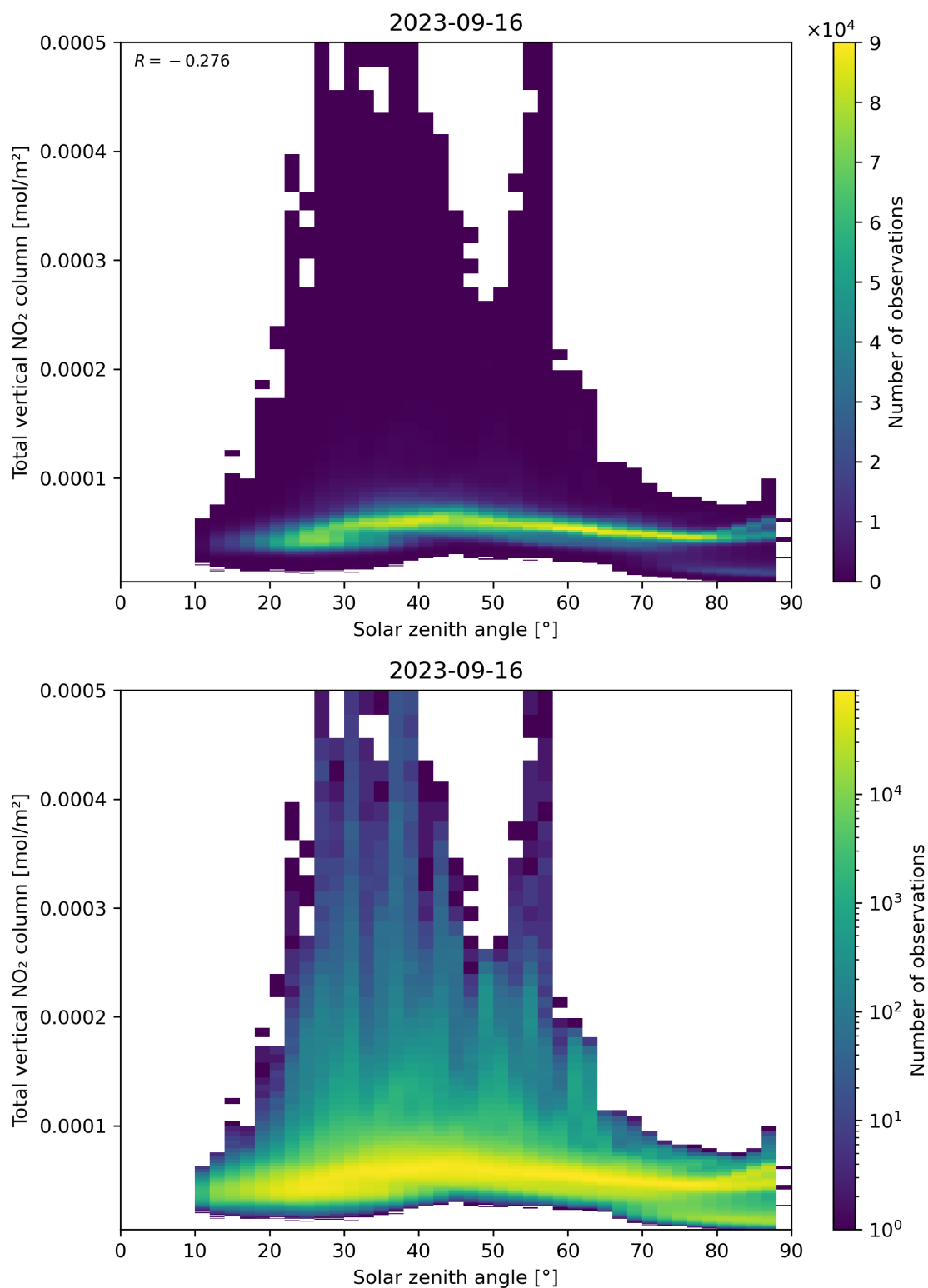
Figure 153: Scatter density plot of “Solar zenith angle” against “Total vertical NO 2 column” for 2023-09-15 to 2023-09-17.
