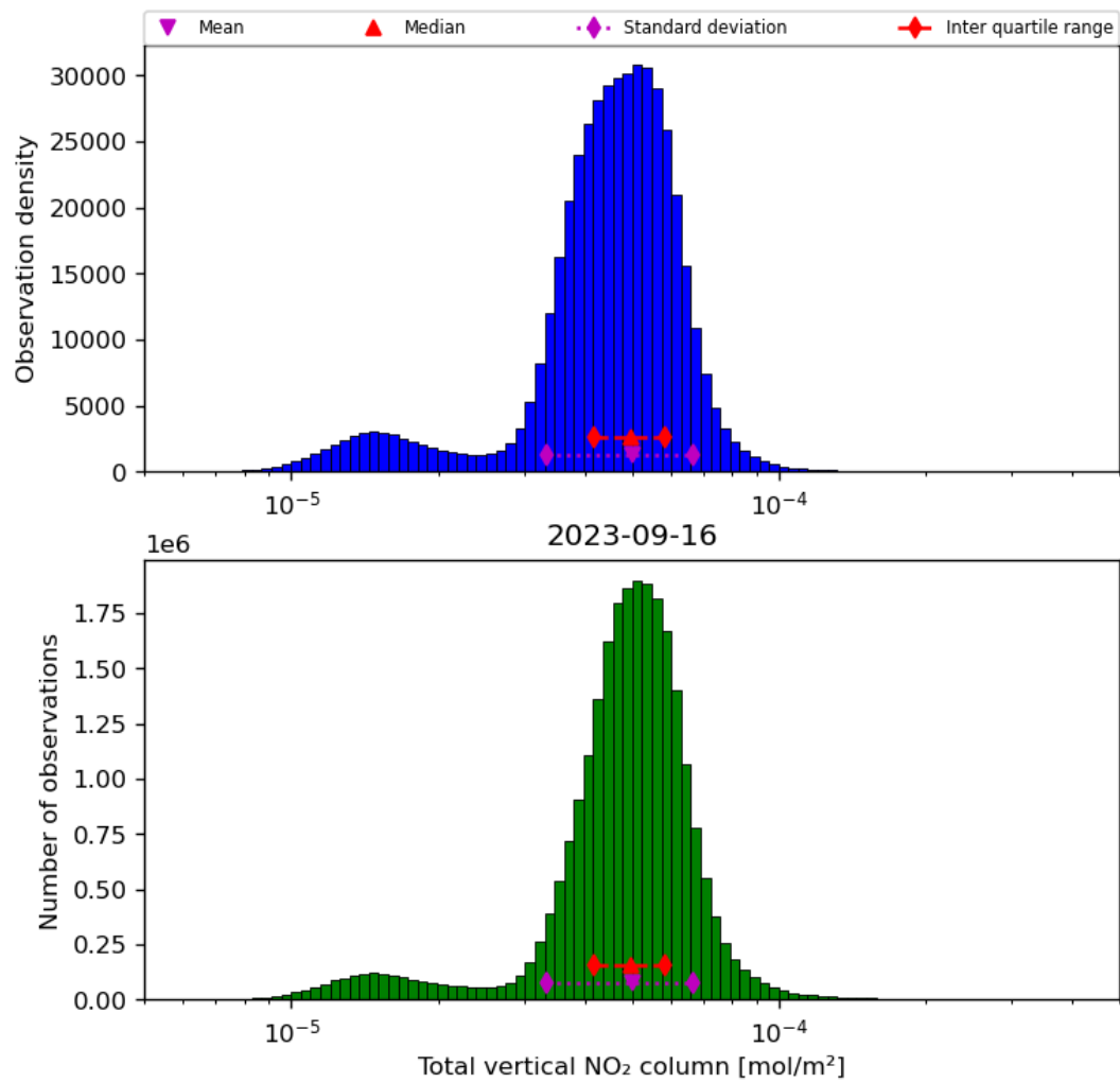
Figure 38: Histogram of "Total vertical NO 2 column" for 2023-09-15 to 2023-09-17
