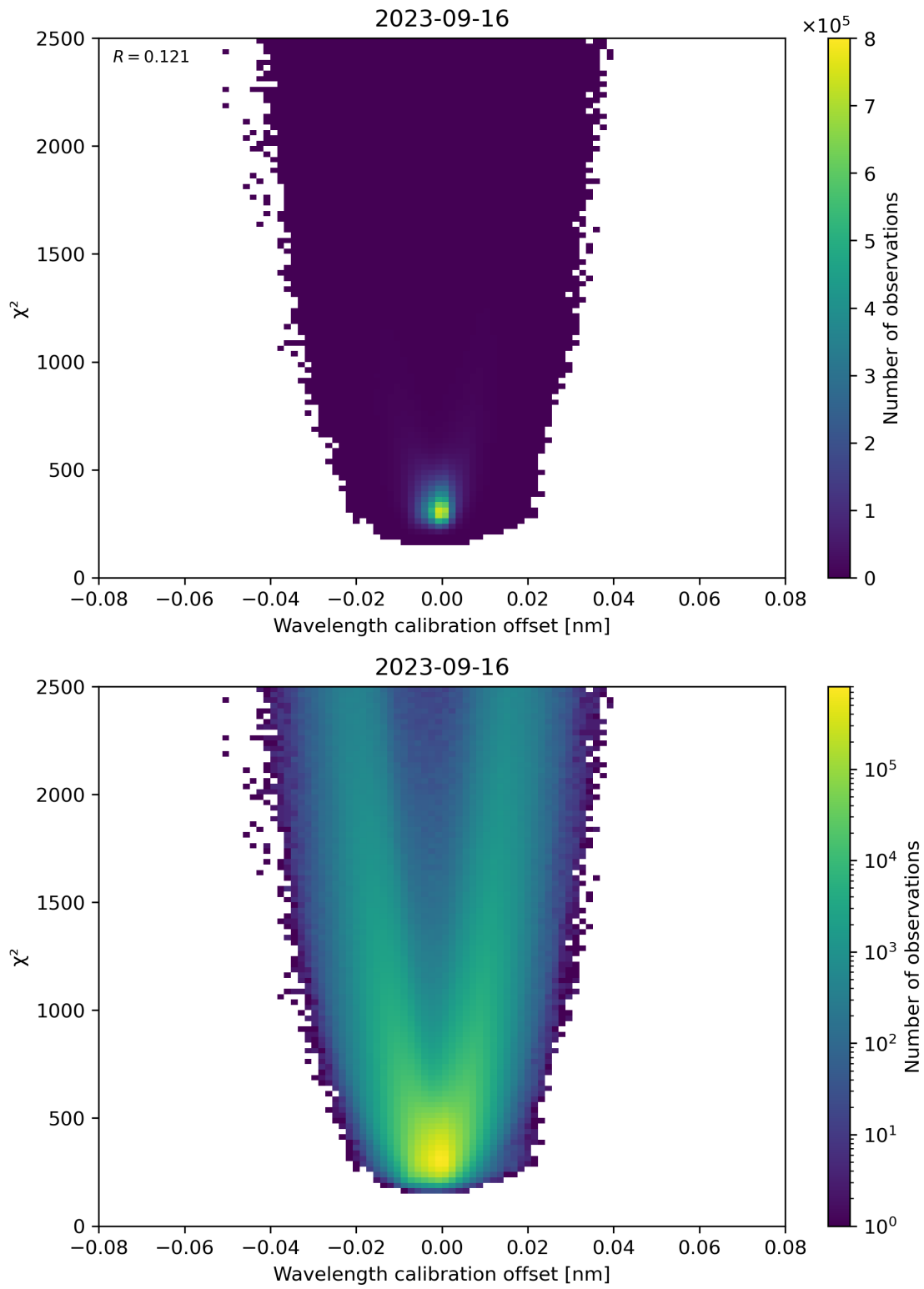
Figure 175: Scatter density plot of “Wavelength calibration offset” against “ \chi^2 ” for 2023-09-15 to 2023-09-17.
