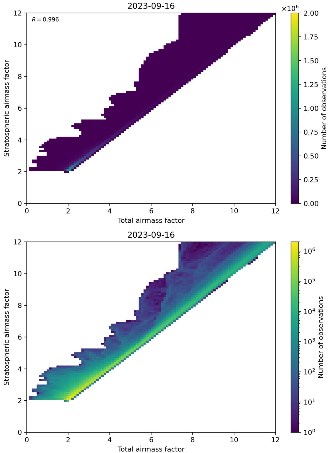
Figure 62: Scatter density plot of “Total airmass factor” against “Stratospheric airmass factor” for 2023-09-15 to 2023-09-17.
