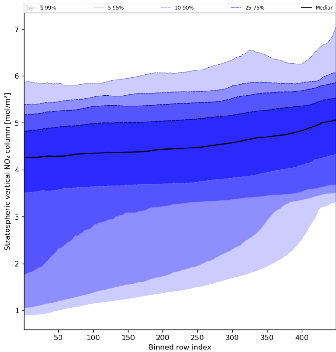
Figure 53: Along track statistics of “Stratospheric vertical NO 2 column” for 2023-09-15 to 2023-09-17
