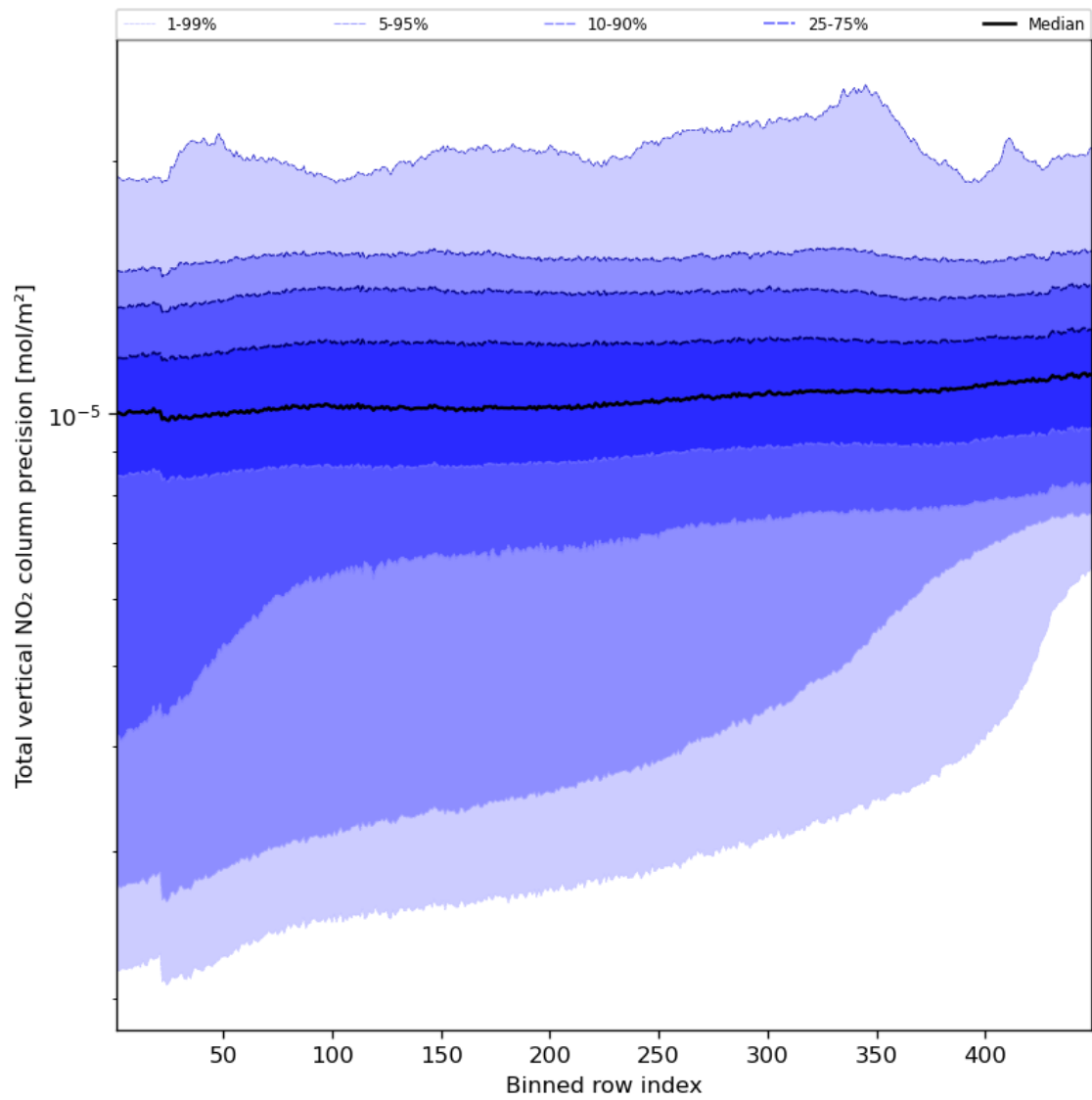
Figure 56: Along track statistics of “Total vertical NO 2 column precision” for 2023-09-15 to 2023-09-17
