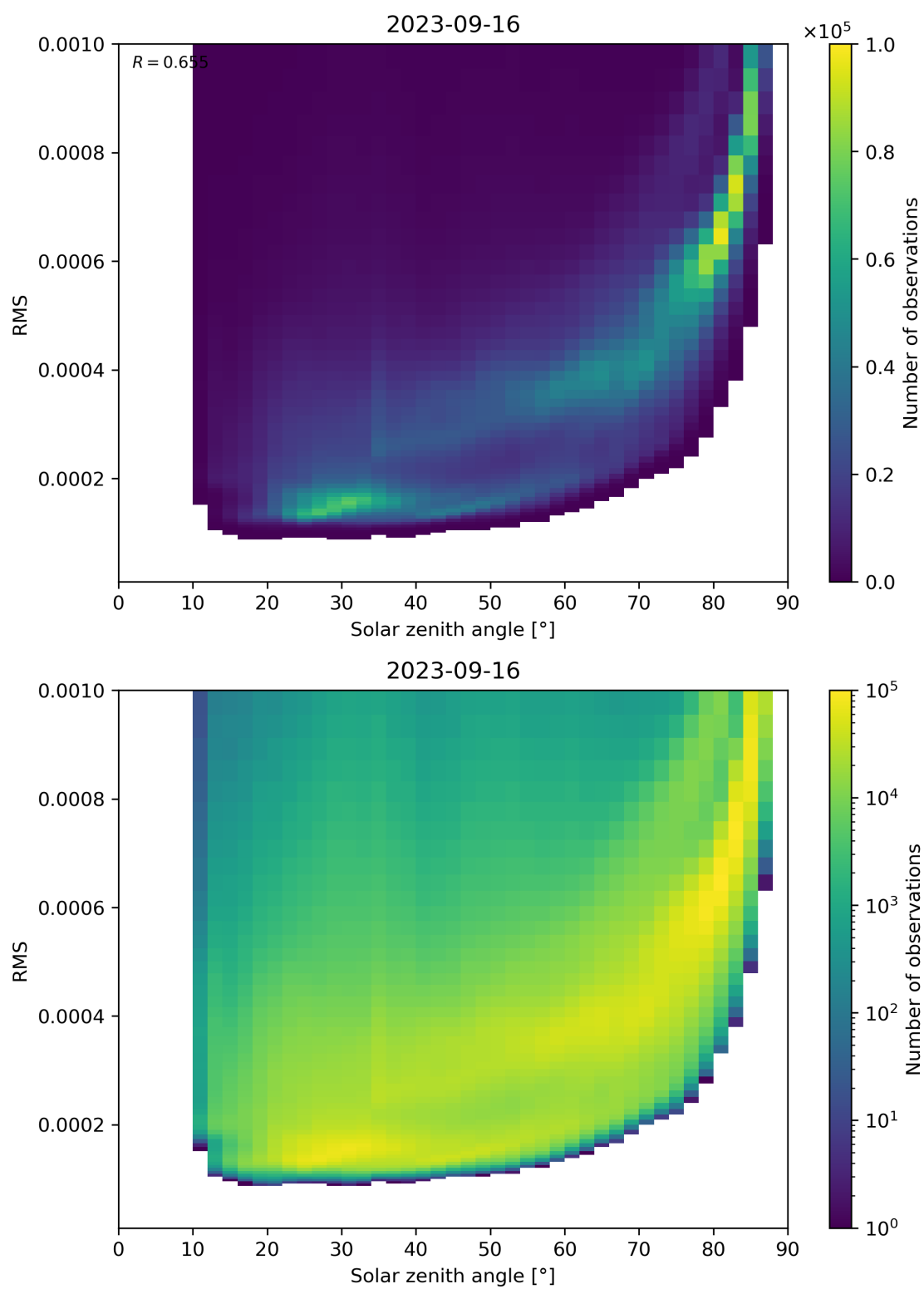
Figure 157: Scatter density plot of “Solar zenith angle” against “RMS” for 2023-09-15 to 2023-09-17.
