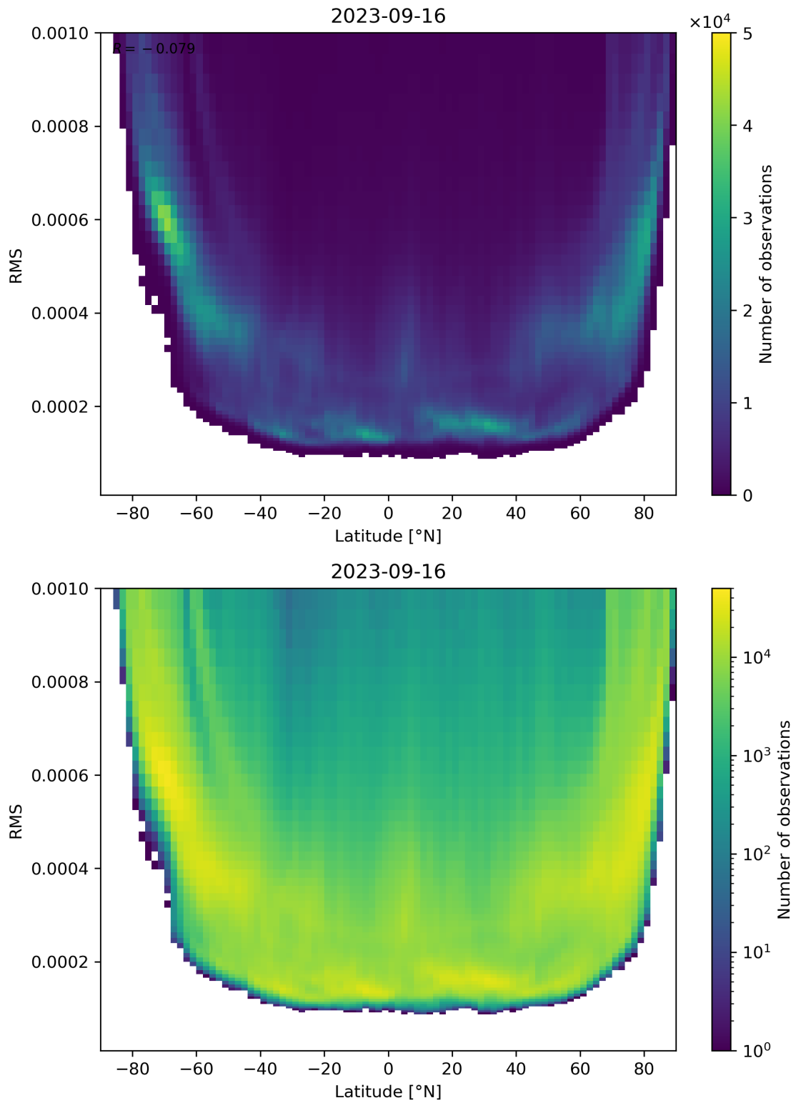
Figure 94: Scatter density plot of “Latitude” against “RMS” for 2023-09-15 to 2023-09-17.
