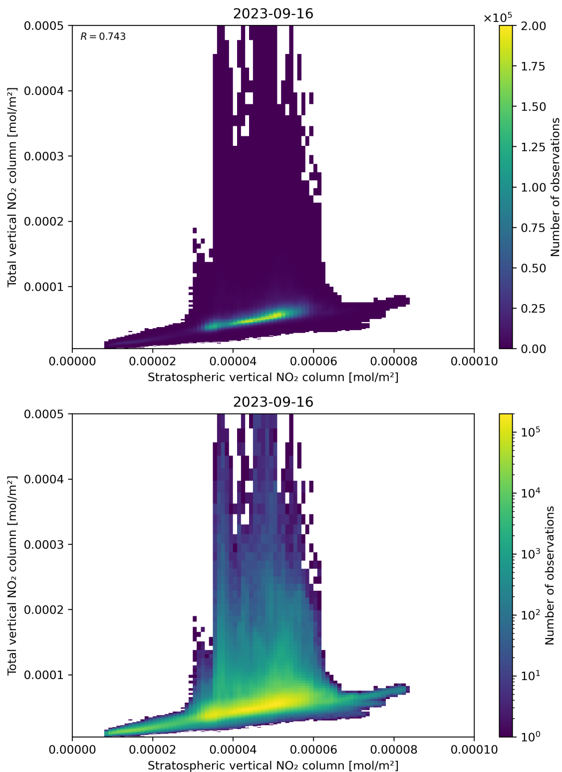
Figure 100: Scatter density plot of “Stratospheric vertical NO 2 column” against “Total vertical NO 2 column” for 2023-09-15 to 2023-09-17.
