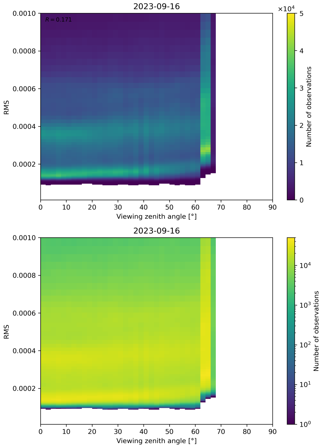
Figure 171: Scatter density plot of “Viewing zenith angle” against “RMS” for 2023-09-15 to 2023-09-17.
