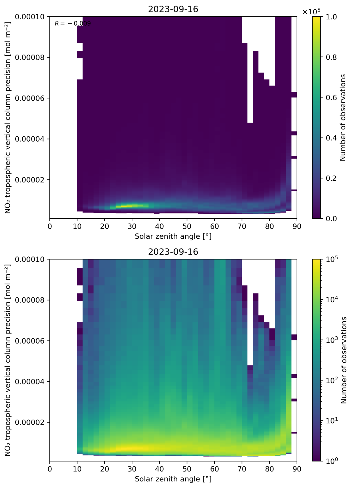
Figure 156: Scatter density plot of “Solar zenith angle” against “NO 2 tropospheric vertical column precision” for 2023-09-15 to 2023-09-17.
