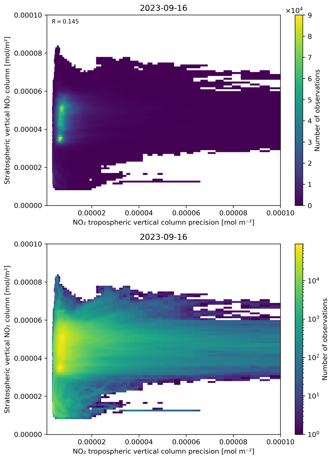
Figure 135: Scatter density plot of “NO 2 tropospheric vertical column precision” against “Stratospheric vertical NO 2 column” for 2023-09-15 to 2023-09-17.
