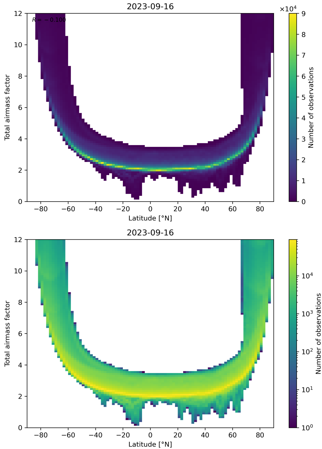
Figure 84: Scatter density plot of “Latitude” against “Total airmass factor” for 2023-09-15 to 2023-09-17.
