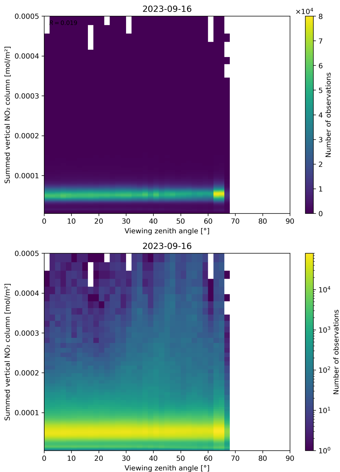
Figure 165: Scatter density plot of “Viewing zenith angle” against “Summed vertical NO 2 column” for 2023-09-15 to 2023-09-17.
