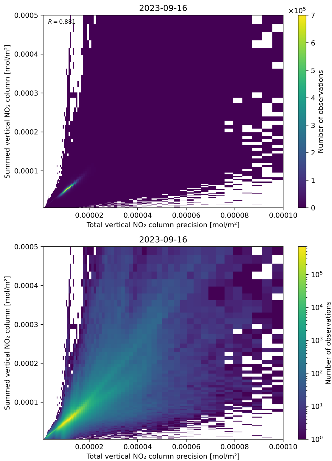
Figure 117: Scatter density plot of “Total vertical NO 2 column precision” against “Summed vertical NO 2 column” for 2023-09-15 to 2023-09-17.
