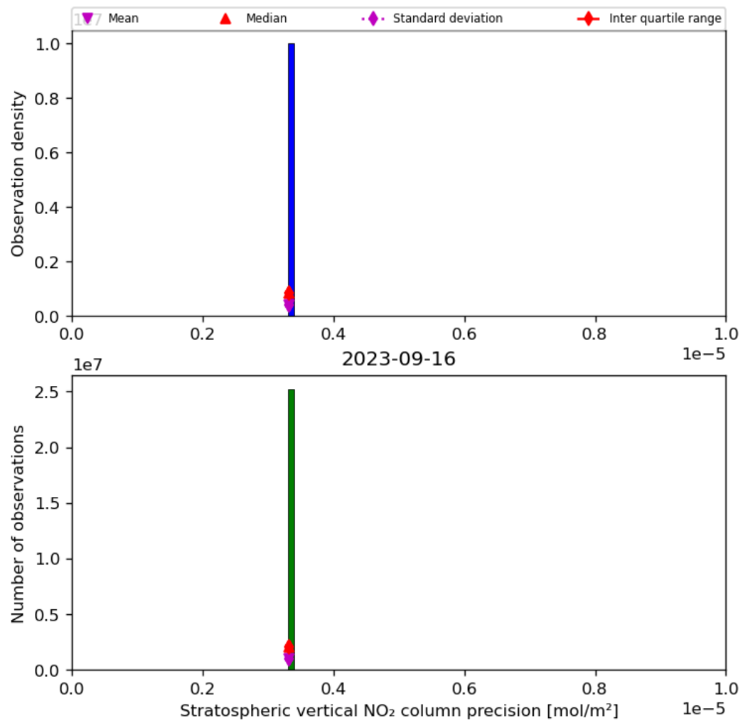
Figure 37: Histogram of “Stratospheric vertical NO 2 column precision” for 2023-09-15 to 2023-09-17
