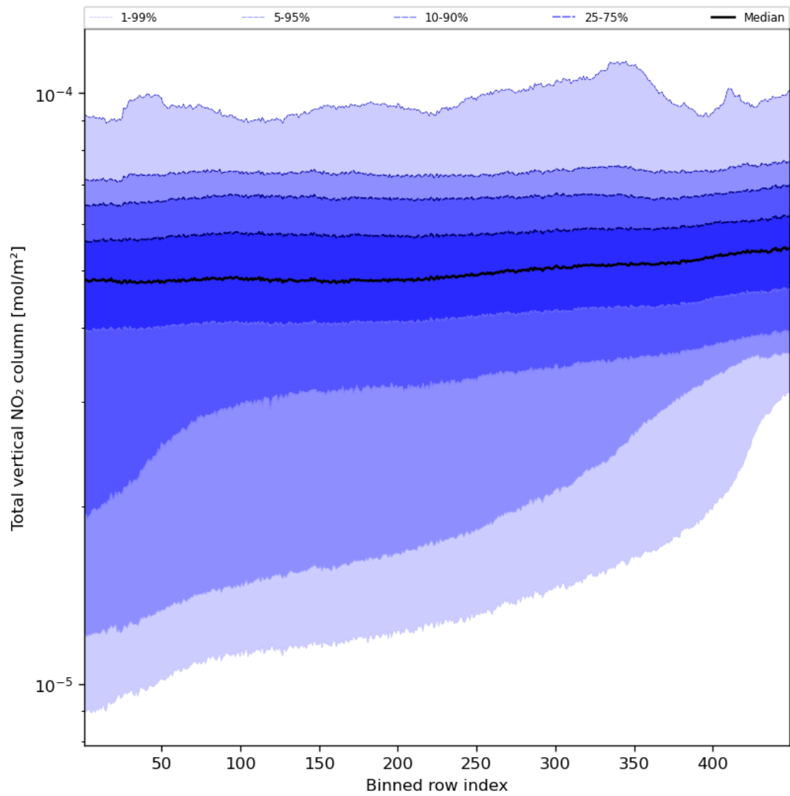
Figure 55: Along track statistics of “Total vertical NO 2 column” for 2023-09-15 to 2023-09-17
