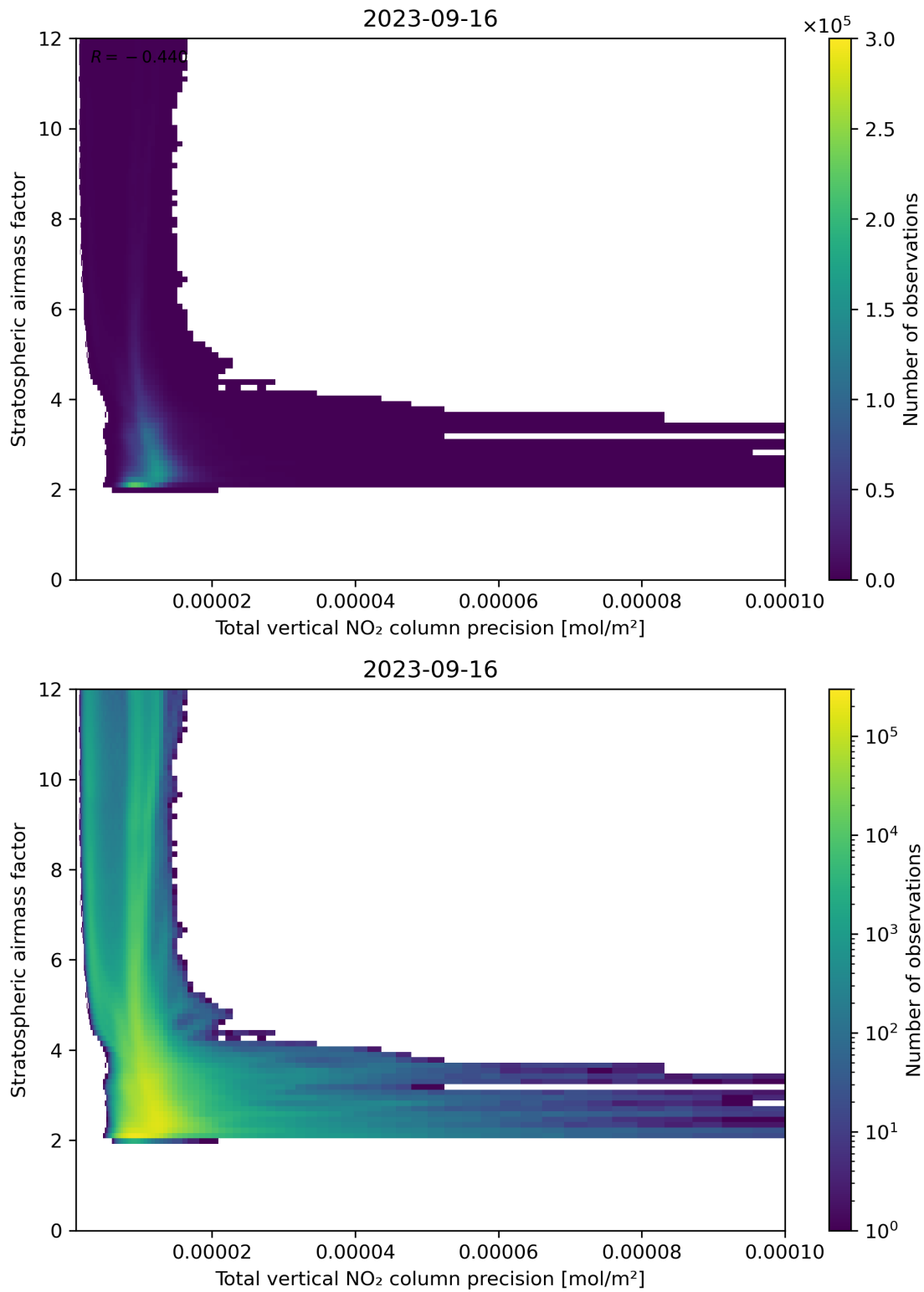
Figure 115: Scatter density plot of “Total vertical NO 2 column precision” against “Stratospheric air mass factor” for 2023-09-15 to 2023-09-17.
