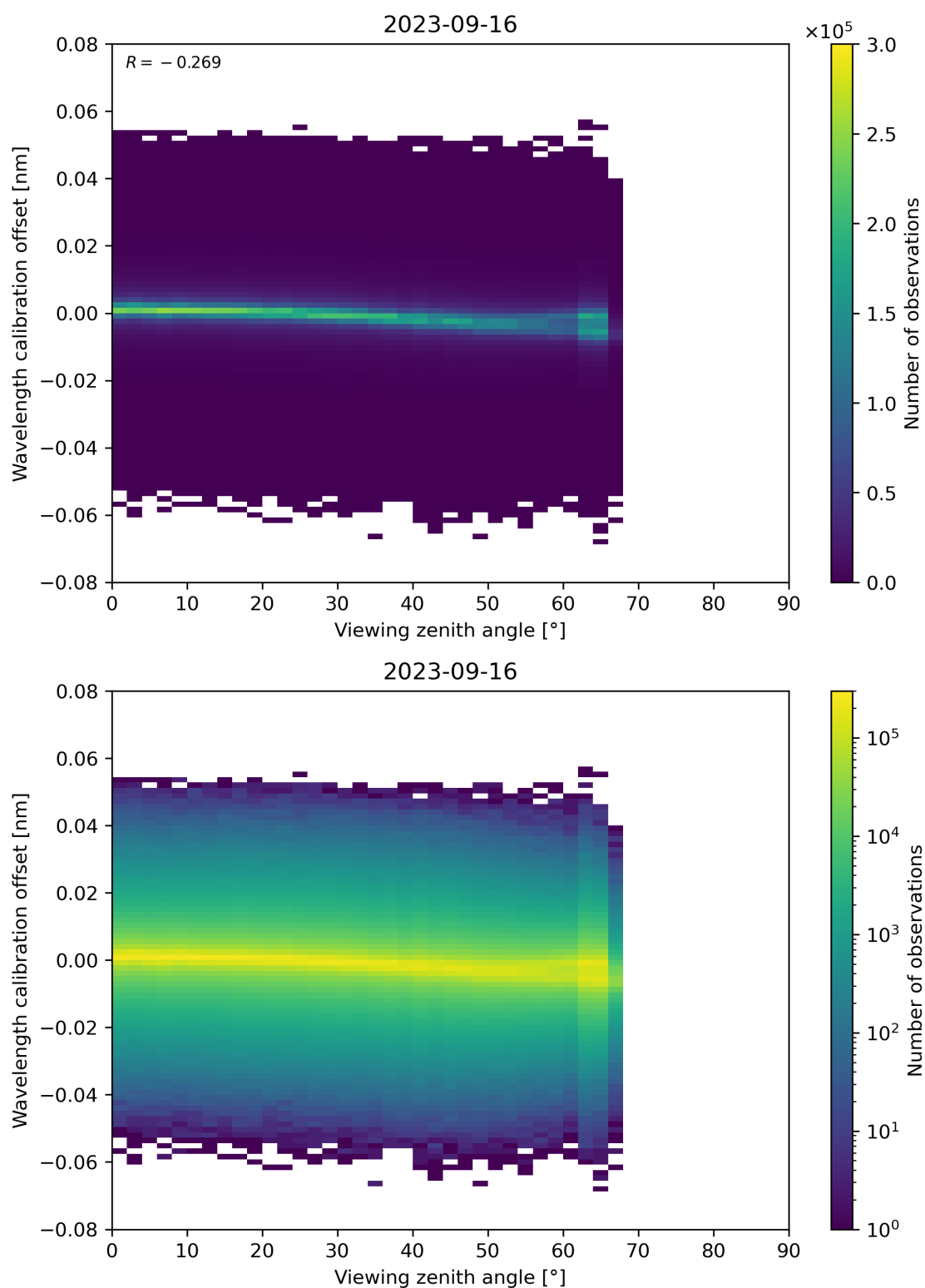
Figure 173: Scatter density plot of “Viewing zenith angle” against “Wavelength calibration offset” for 2023-09-15 to 2023-09-17.
