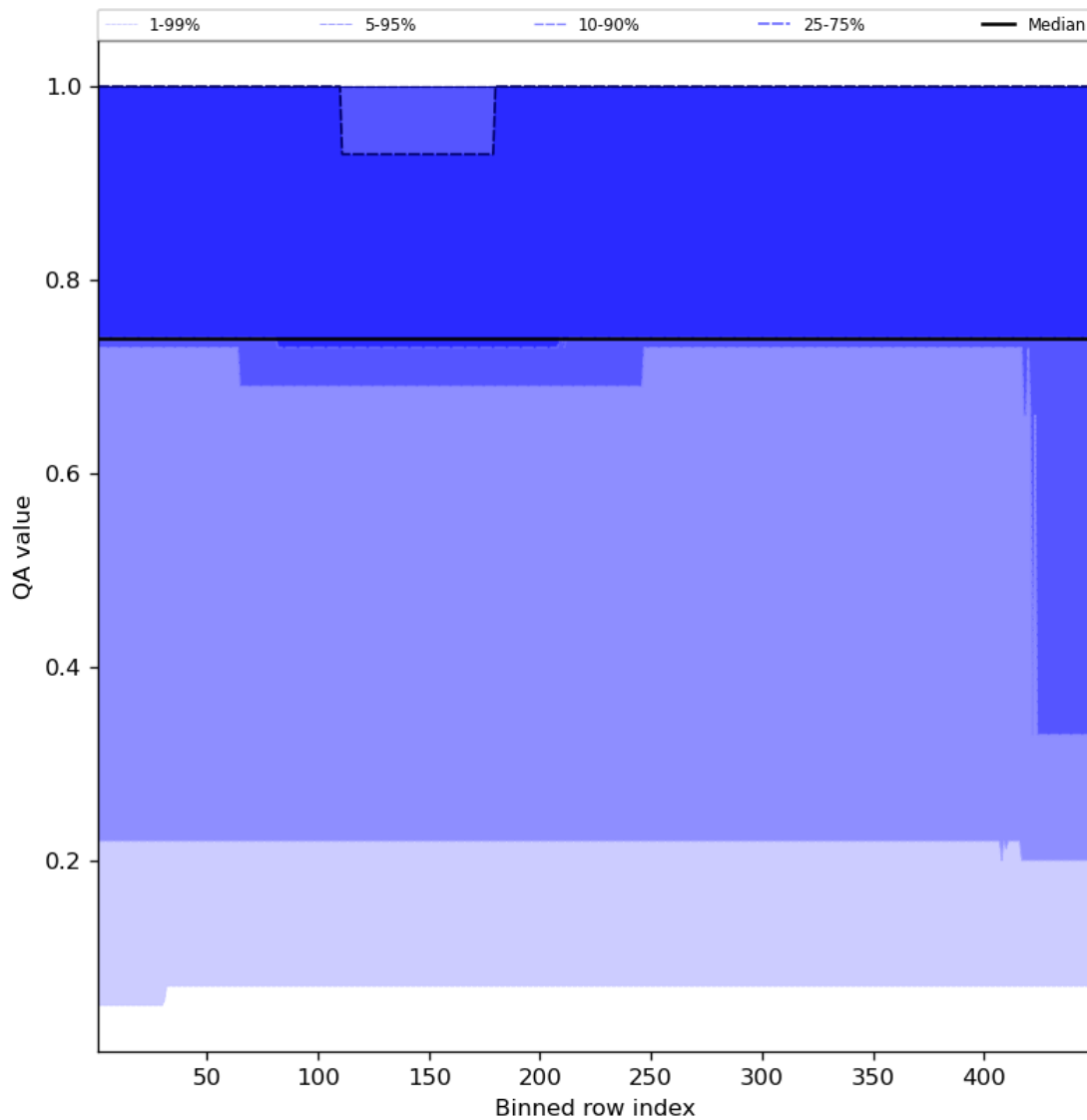
Figure 45: Along track statistics of “QA value” for 2023-09-15 to 2023-09-17
