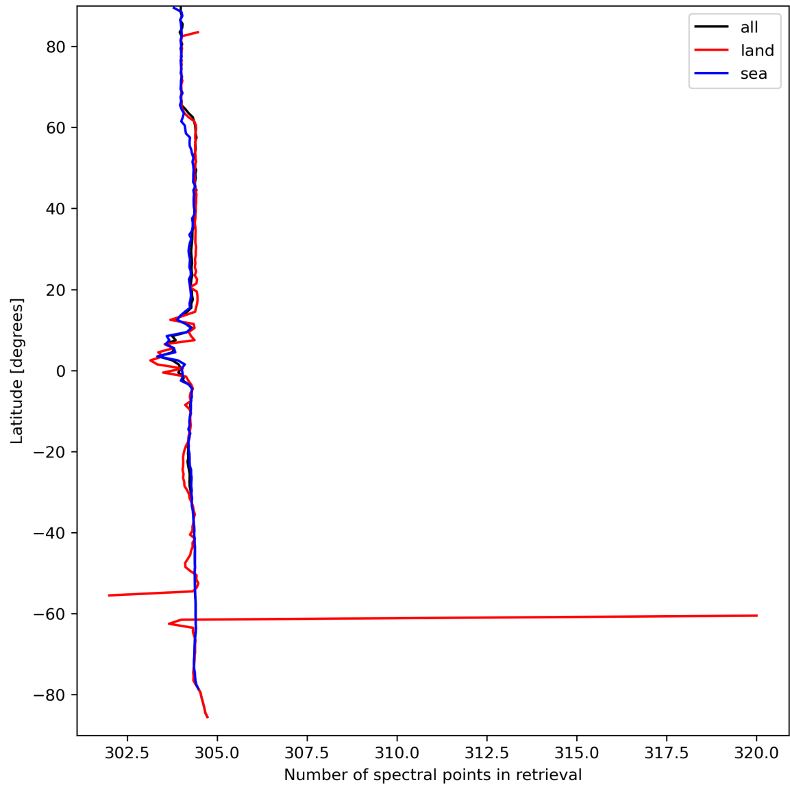
Figure 16: Zonal average of “Number of spectral points in retrieval” for 2023-09-15 to 2023-09-17.
