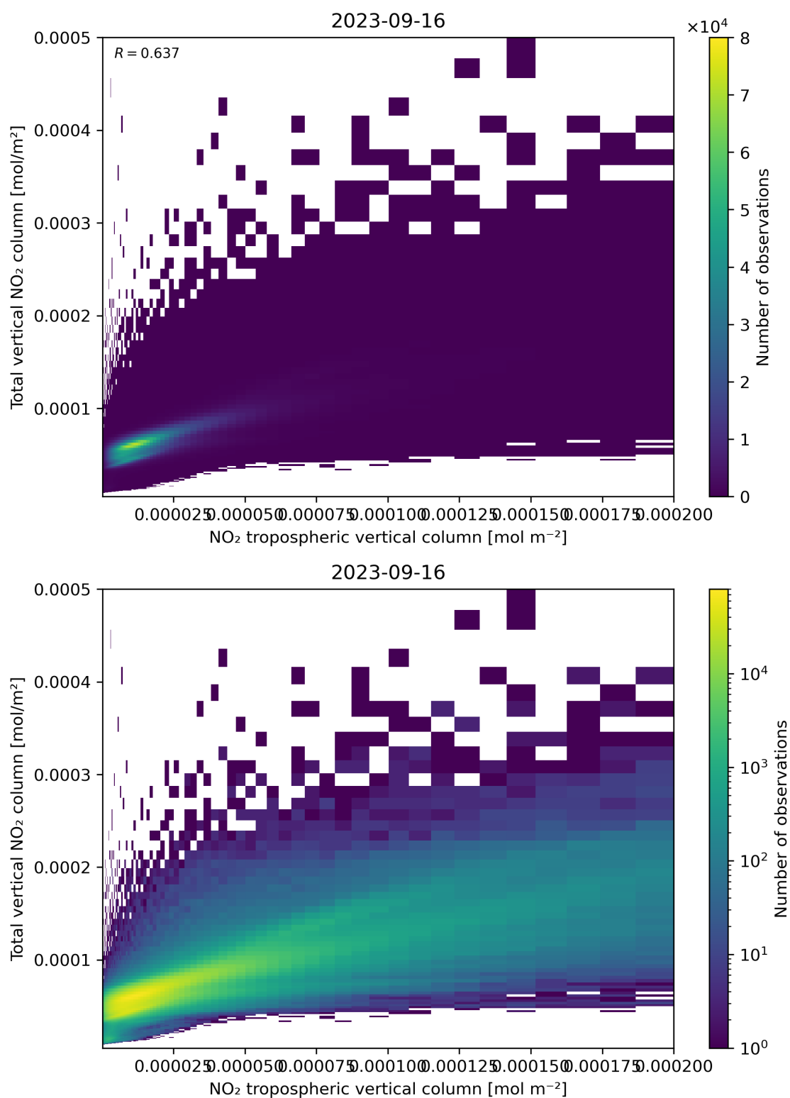
Figure 128: Scatter density plot of “NO 2 tropospheric vertical column” against “Total vertical NO 2 column” for 2023-09-15 to 2023-09-17.
