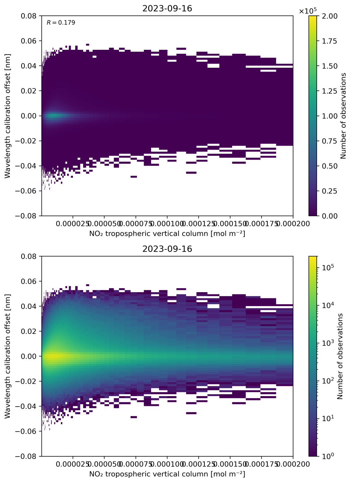
Figure 143: Scatter density plot of “NO 2 tropospheric vertical column” against “Wavelength calibration offset” for 2023-09-15 to 2023-09-17.
