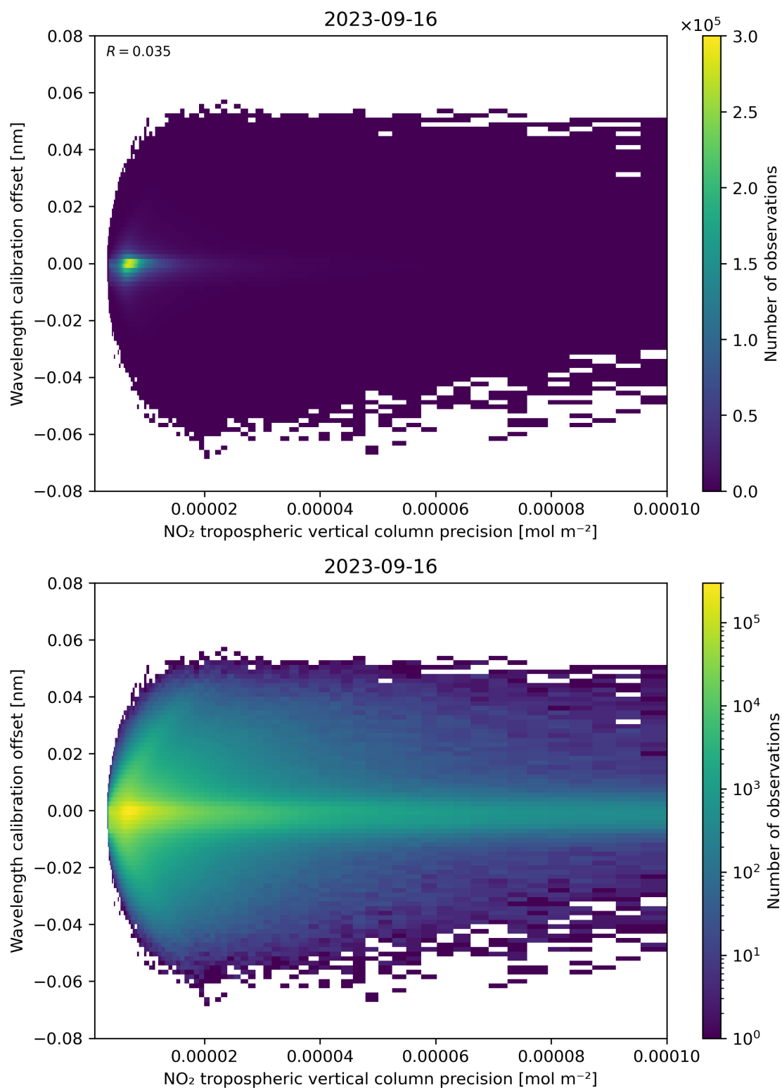
Figure 141: Scatter density plot of “NO 2 tropospheric vertical column precision” against “Wavelength calibration offset” for 2023-09-15 to 2023-09-17.
