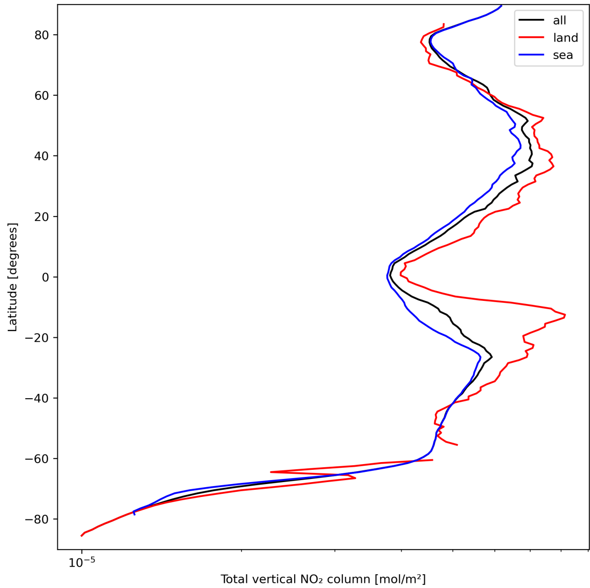
Figure 21: Zonal average of “Total vertical NO 2 column” for 2023-09-15 to 2023-09-17.
