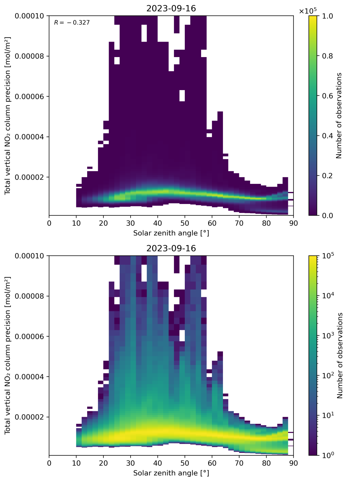
Figure 154: Scatter density plot of “Solar zenith angle” against “Total vertical NO 2 column precision” for 2023-09-15 to 2023-09-17.
