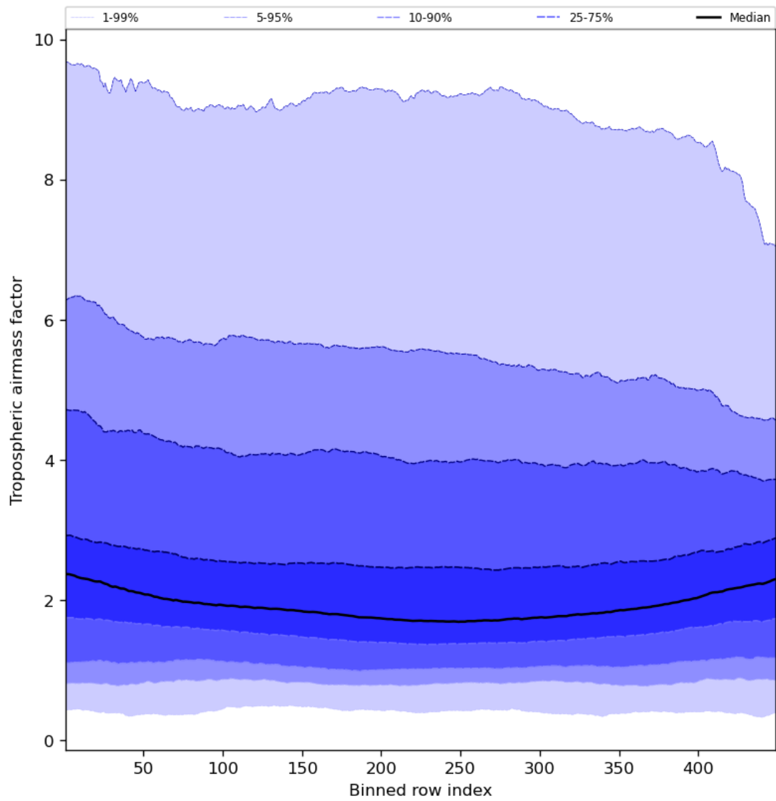
Figure 48: Along track statistics of “Tropospheric air mass factor” for 2023-09-15 to 2023-09-17
