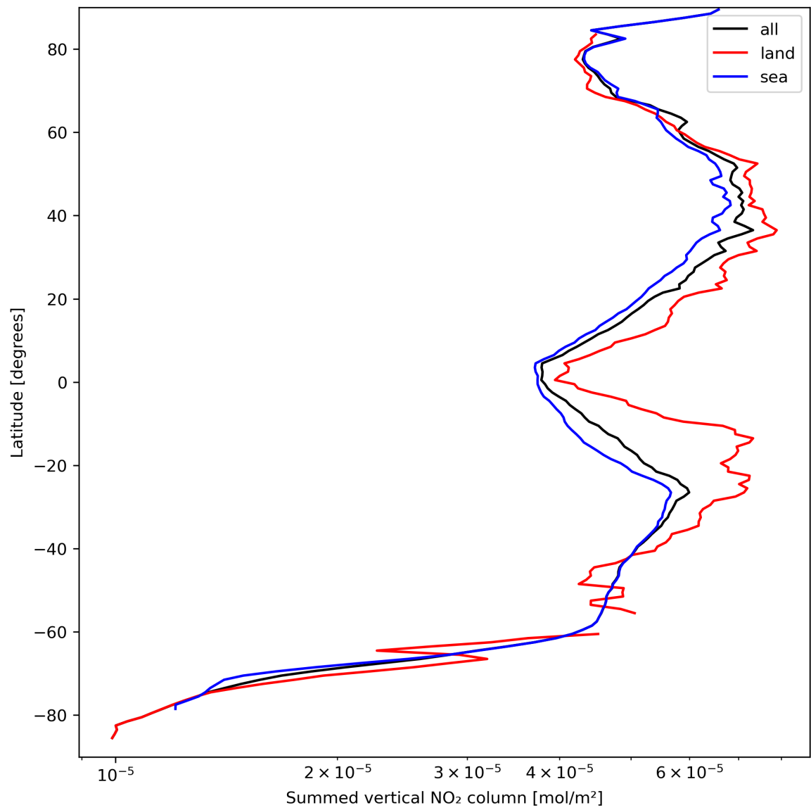
Figure 23: Zonal average of “Summed vertical NO 2 column” for 2023-09-15 to 2023-09-17.
