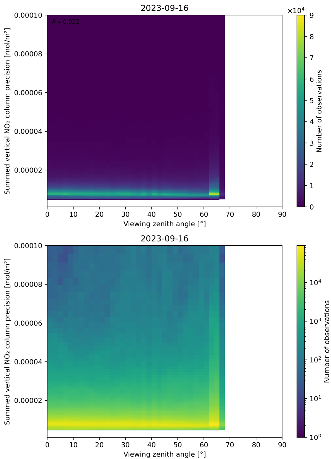
Figure 166: Scatter density plot of “Viewing zenith angle” against “Summed vertical NO 2 column precision” for 2023-09-15 to 2023-09-17.
