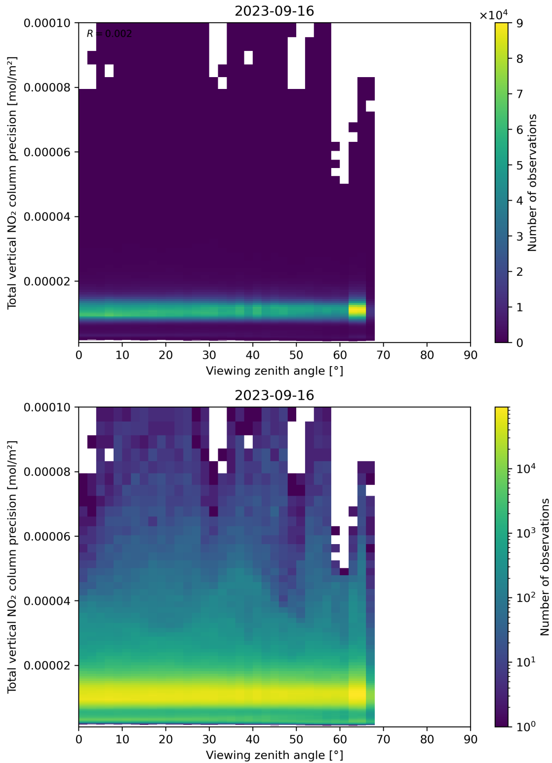
Figure 168: Scatter density plot of “Viewing zenith angle” against “Total vertical NO 2 column precision” for 2023-09-15 to 2023-09-17.
