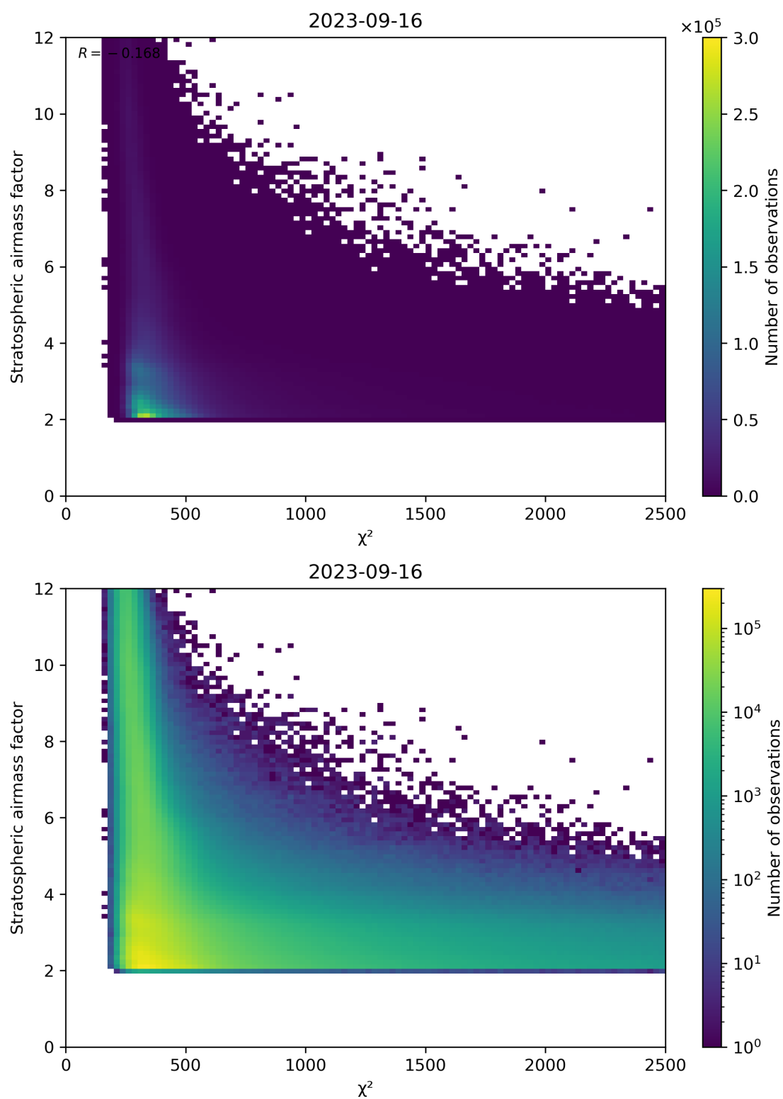
Figure 81: Scatter density plot of “ \chi^2 ” against “Stratospheric airmass factor” for 2023-09-15 to 2023-09-17.
