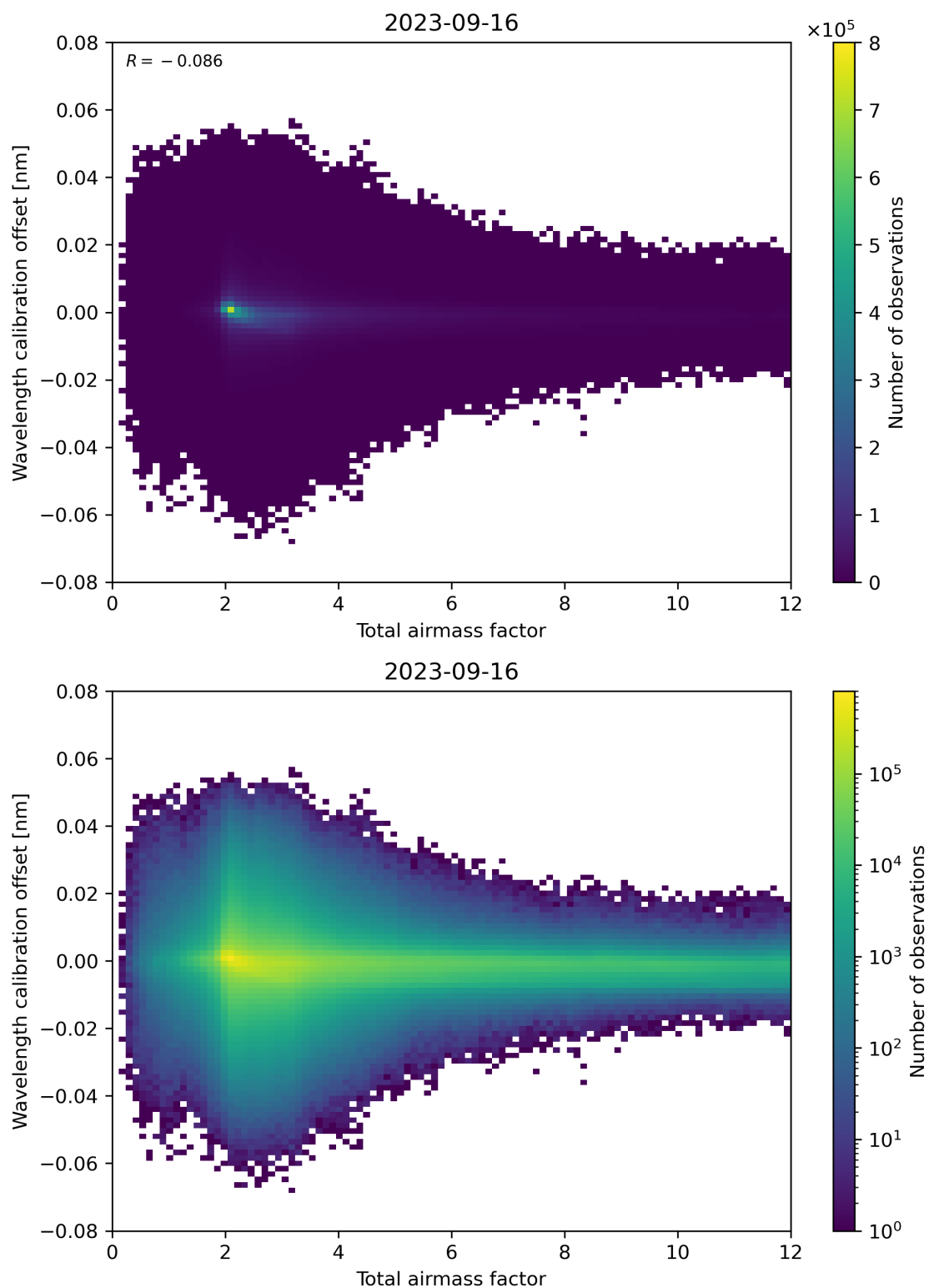
Figure 70: Scatter density plot of “Total airmass factor” against “Wavelength calibration offset” for 2023-09-15 to 2023-09-17.
